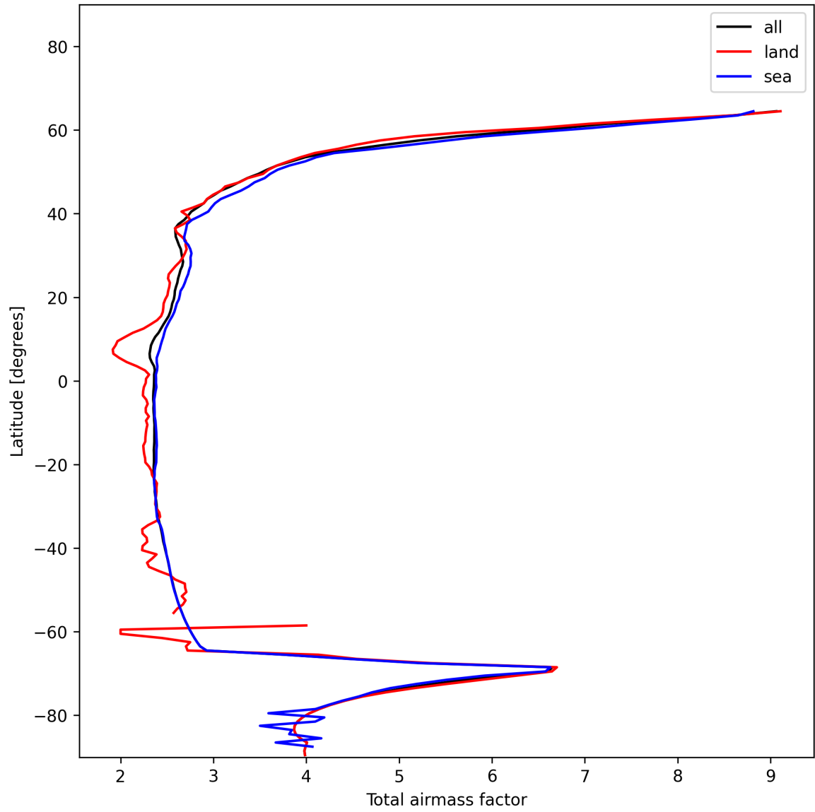
Figure 15: Zonal average of “Total airmass factor” for 2024-12-18 to 2024-12-20.
