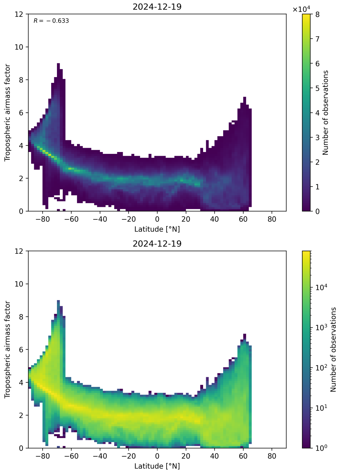
Figure 85: Scatter density plot of “Latitude” against “Tropospheric airmass factor” for 2024-12-18 to 2024-12-20.
