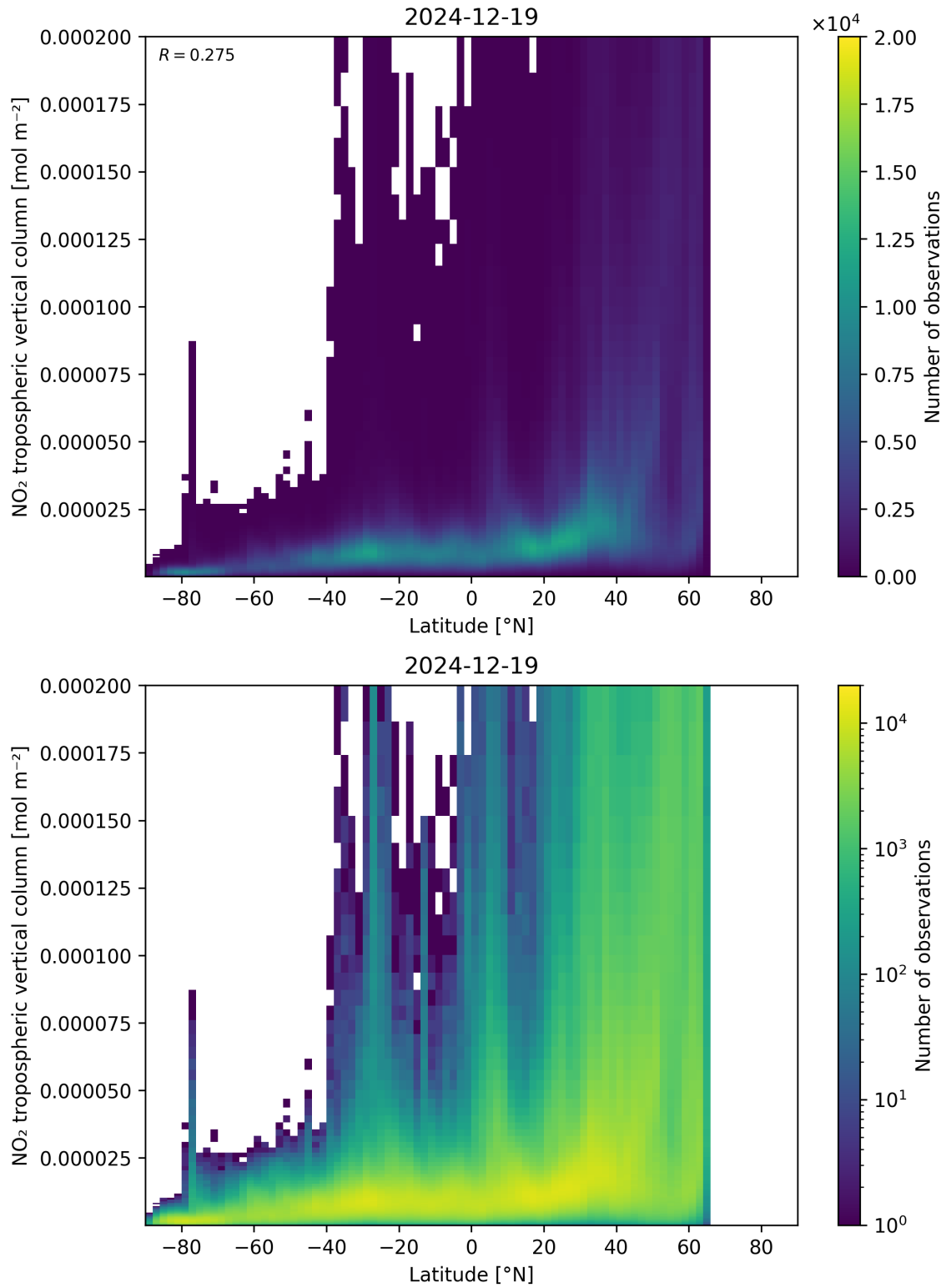
Figure 92: Scatter density plot of “Latitude” against “NO 2 tropospheric vertical column” for 2024-12-18 to 2024-12-20.
