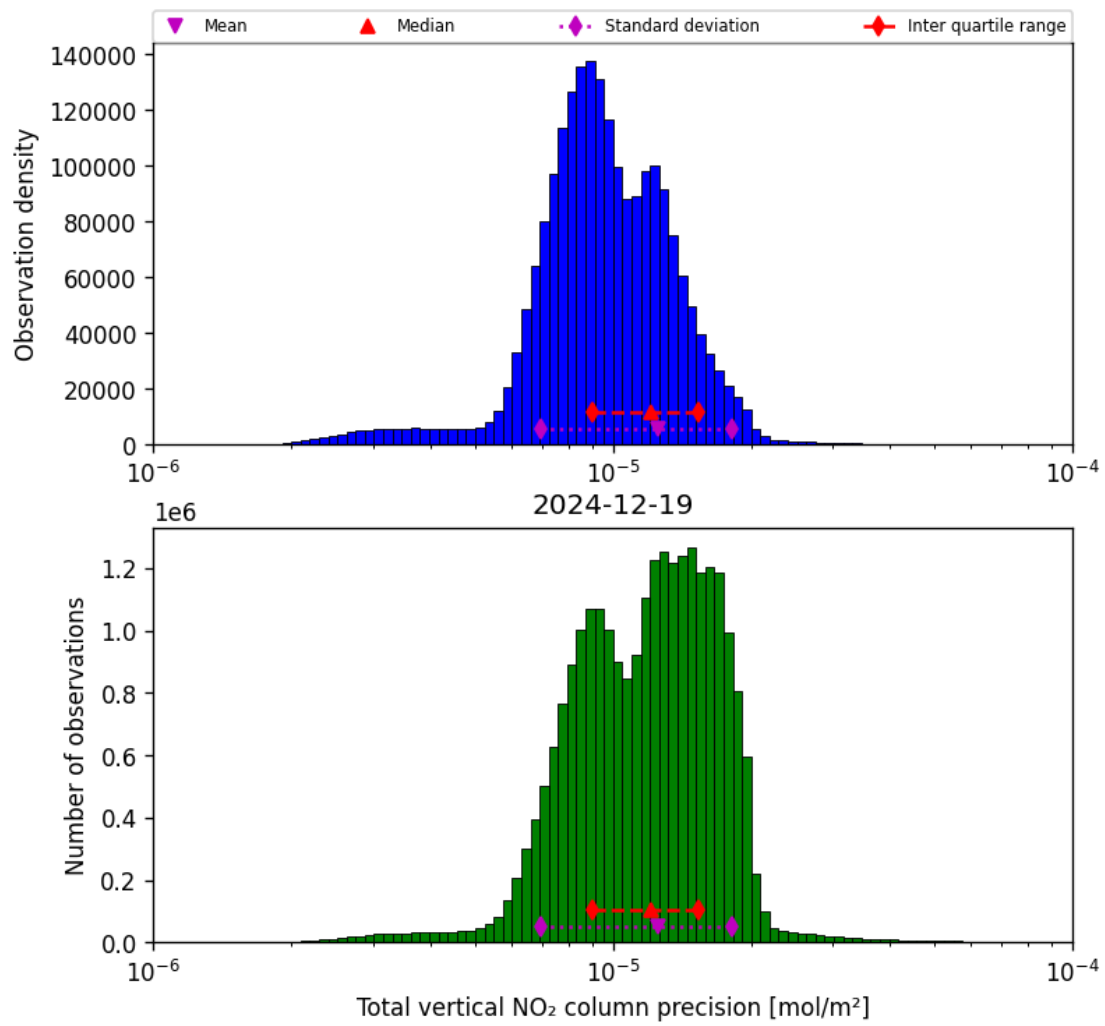
Figure 39: Histogram of “Total vertical NO 2 column precision” for 2024-12-18 to 2024-12-20
