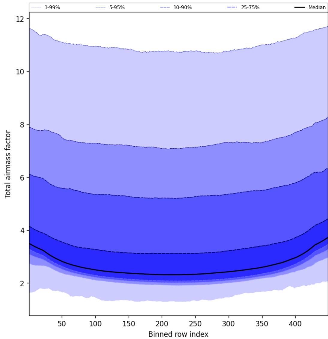
Figure 49: Along track statistics of “Total airmass factor” for 2024-12-18 to 2024-12-20
