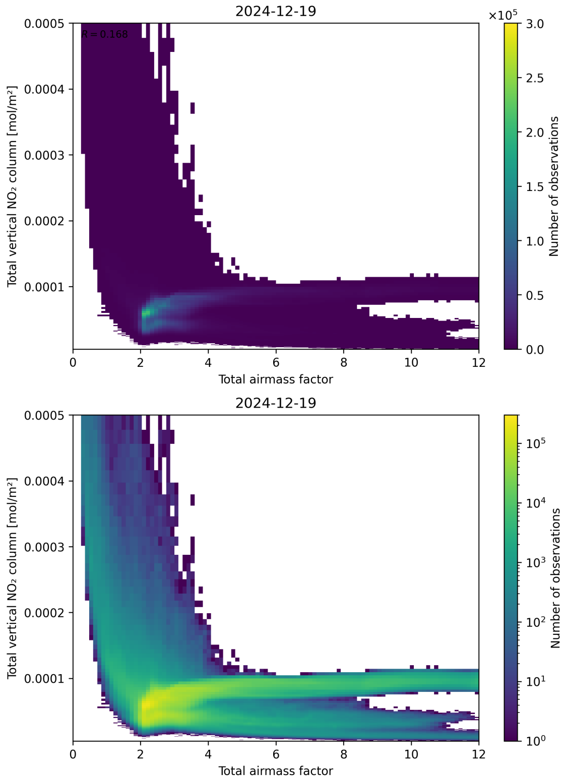
Figure 67: Scatter density plot of “Total air mass factor” against “Total vertical NO 2 column” for 2024-12-18 to 2024-12-20.
