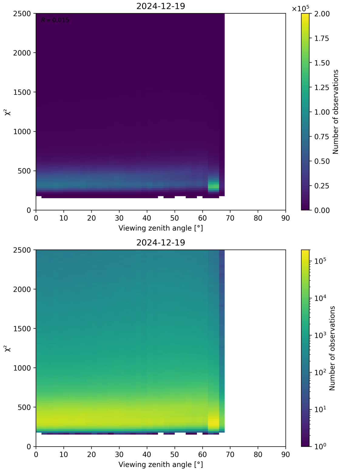
Figure 162: Scatter density plot of “Viewing zenith angle” against “ \chi^2 ” for 2024-12-18 to 2024-12-20.
