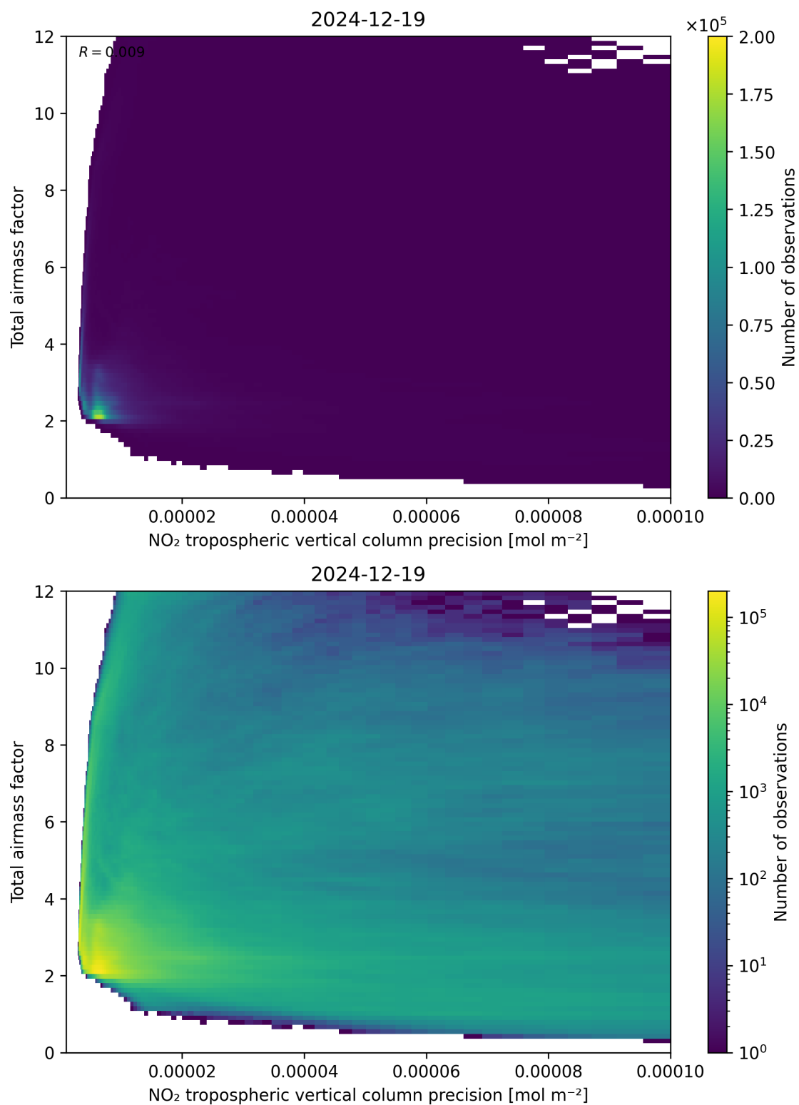
Figure 132: Scatter density plot of “NO 2 tropospheric vertical column precision” against “Total air mass factor” for 2024-12-18 to 2024-12-20.
