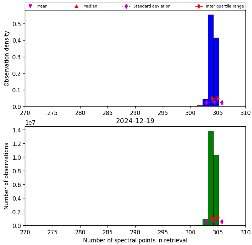
Figure 33: Histogram of “Number of spectral points in retrieval” for 2024-12-18 to 2024-12-20
