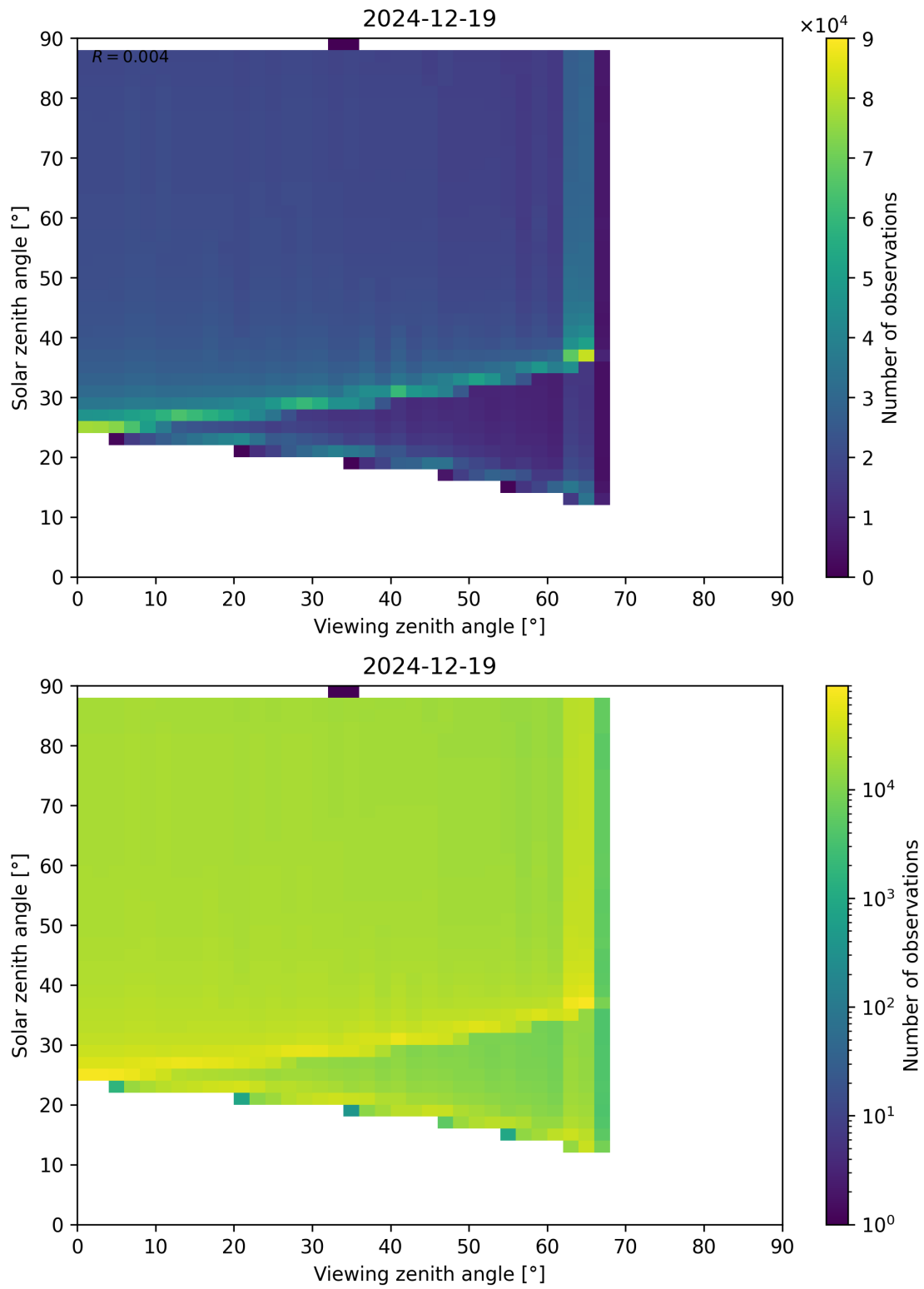
Figure 172: Scatter density plot of “Viewing zenith angle” against “Solar zenith angle” for 2024-12-18 to 2024-12-20.
