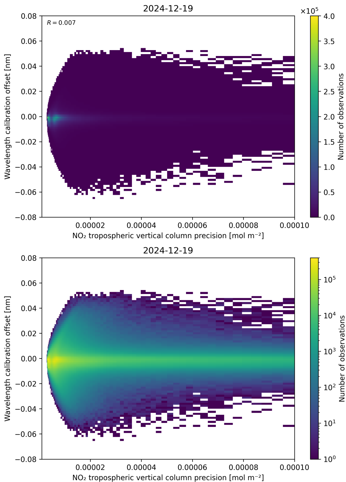
Figure 141: Scatter density plot of “NO 2 tropospheric vertical column precision” against “Wavelength calibration offset” for 2024-12-18 to 2024-12-20.
