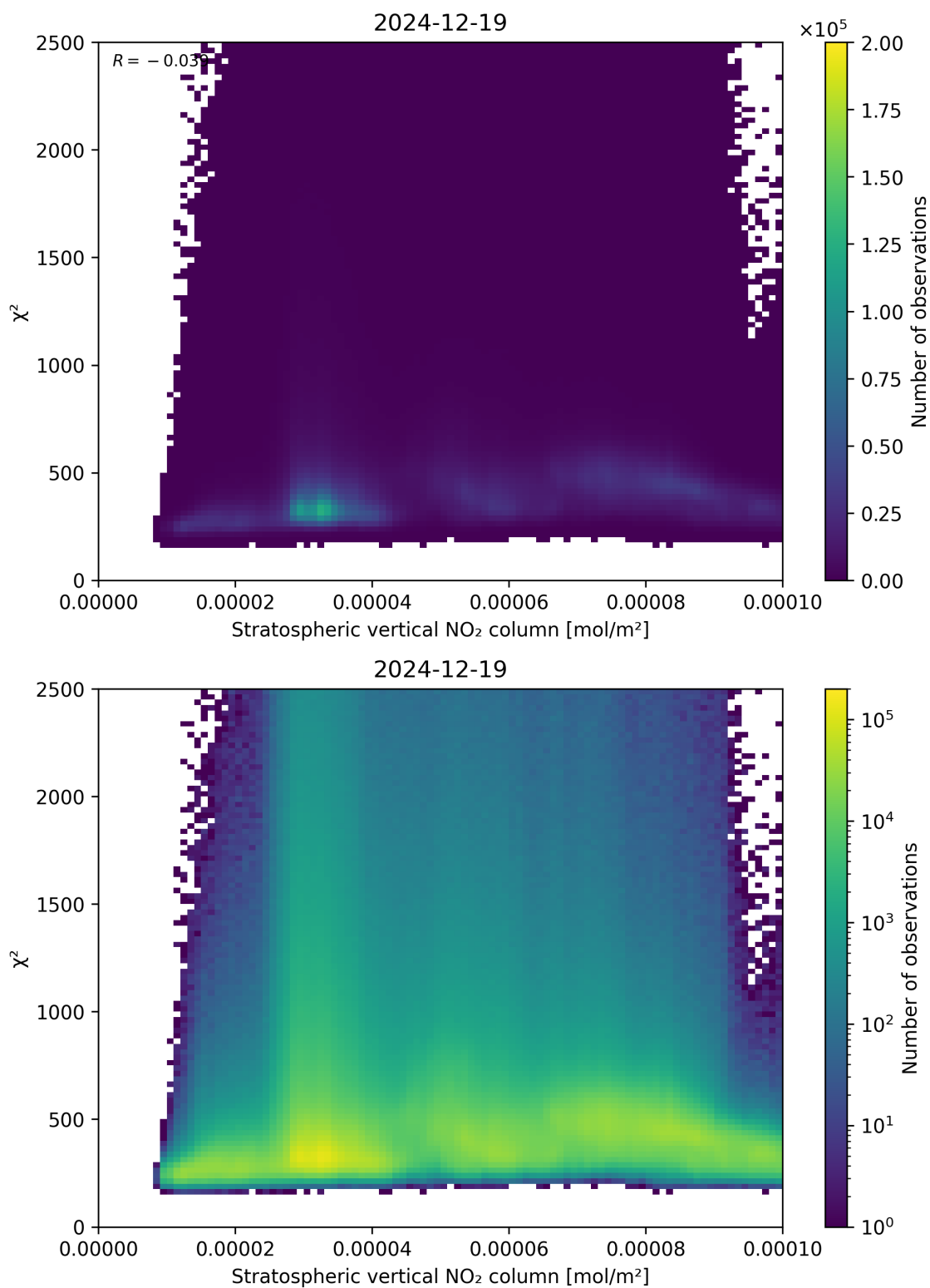
Figure 97: Scatter density plot of “Stratospheric vertical NO 2 column” against “ \chi^2 ” for 2024-12-18 to 2024-12-20.
