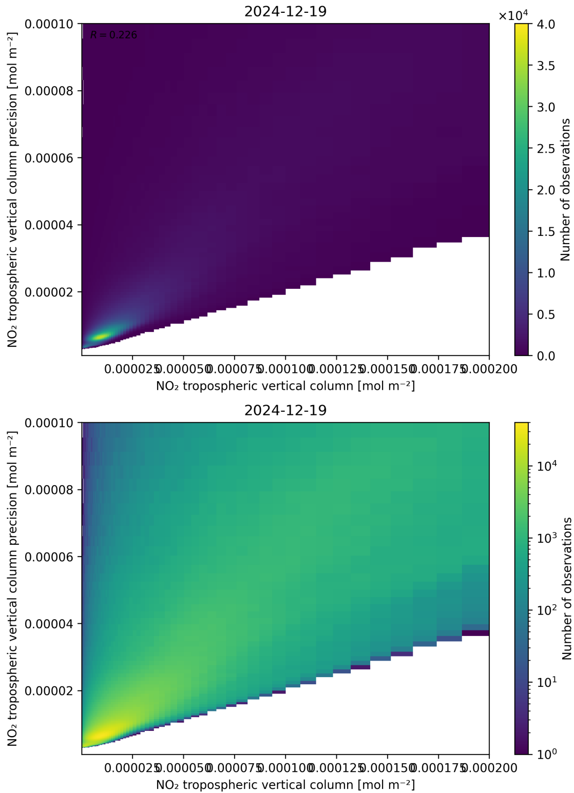
Figure 130: Scatter density plot of “NO 2 tropospheric vertical column” against “NO 2 tropospheric vertical column precision” for 2024-12-18 to 2024-12-20.
