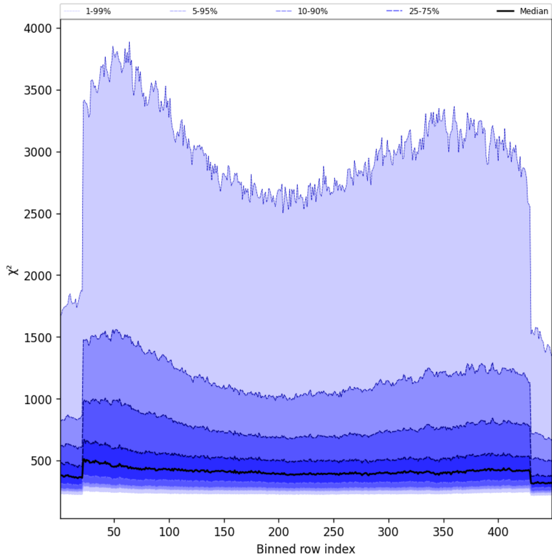
Figure 59: Along track statistics of “ \chi^2 ” for 2024-12-18 to 2024-12-20
