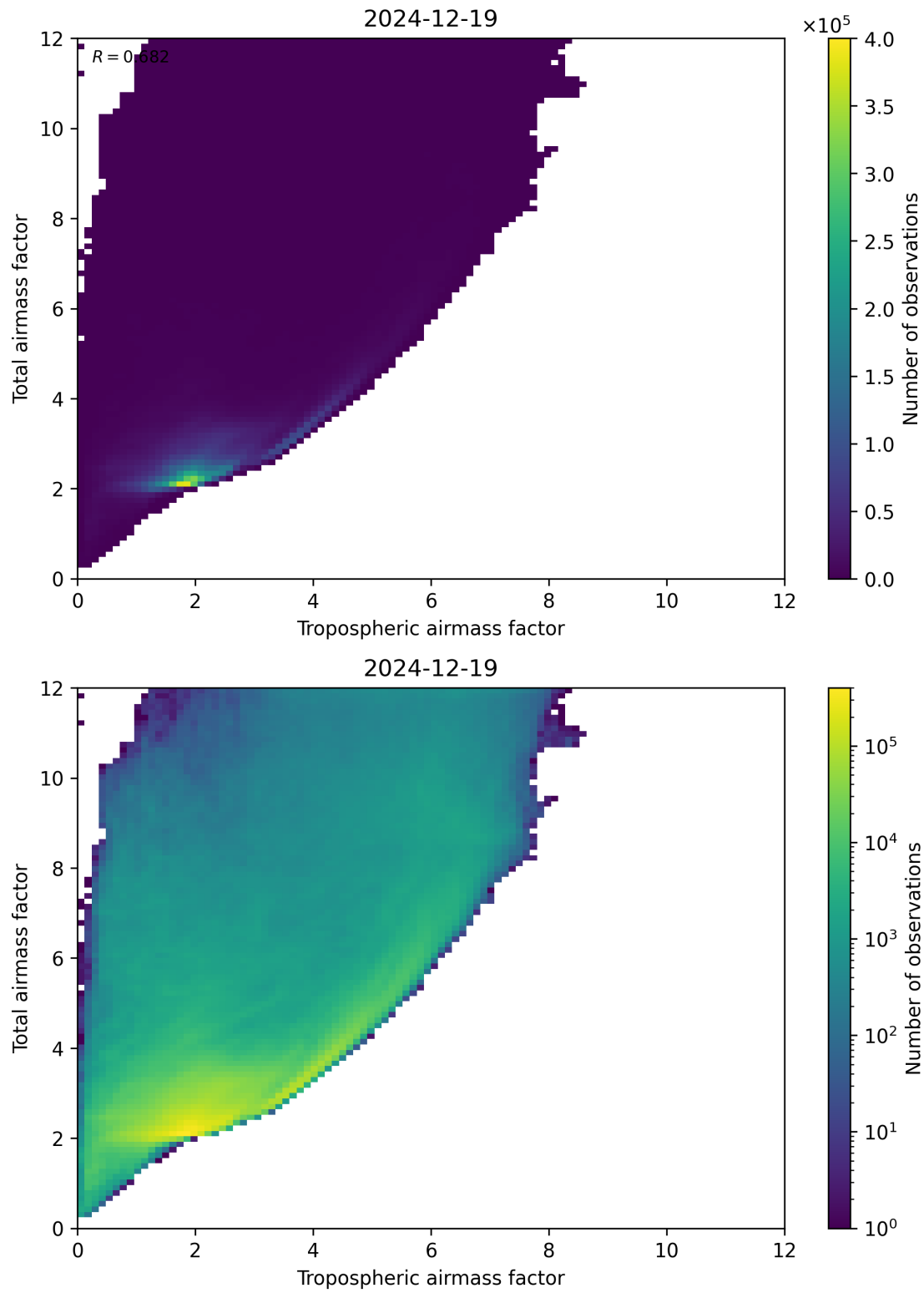
Figure 72: Scatter density plot of “Tropospheric airmass factor” against “Total airmass factor” for 2024-12-18 to 2024-12-20.
