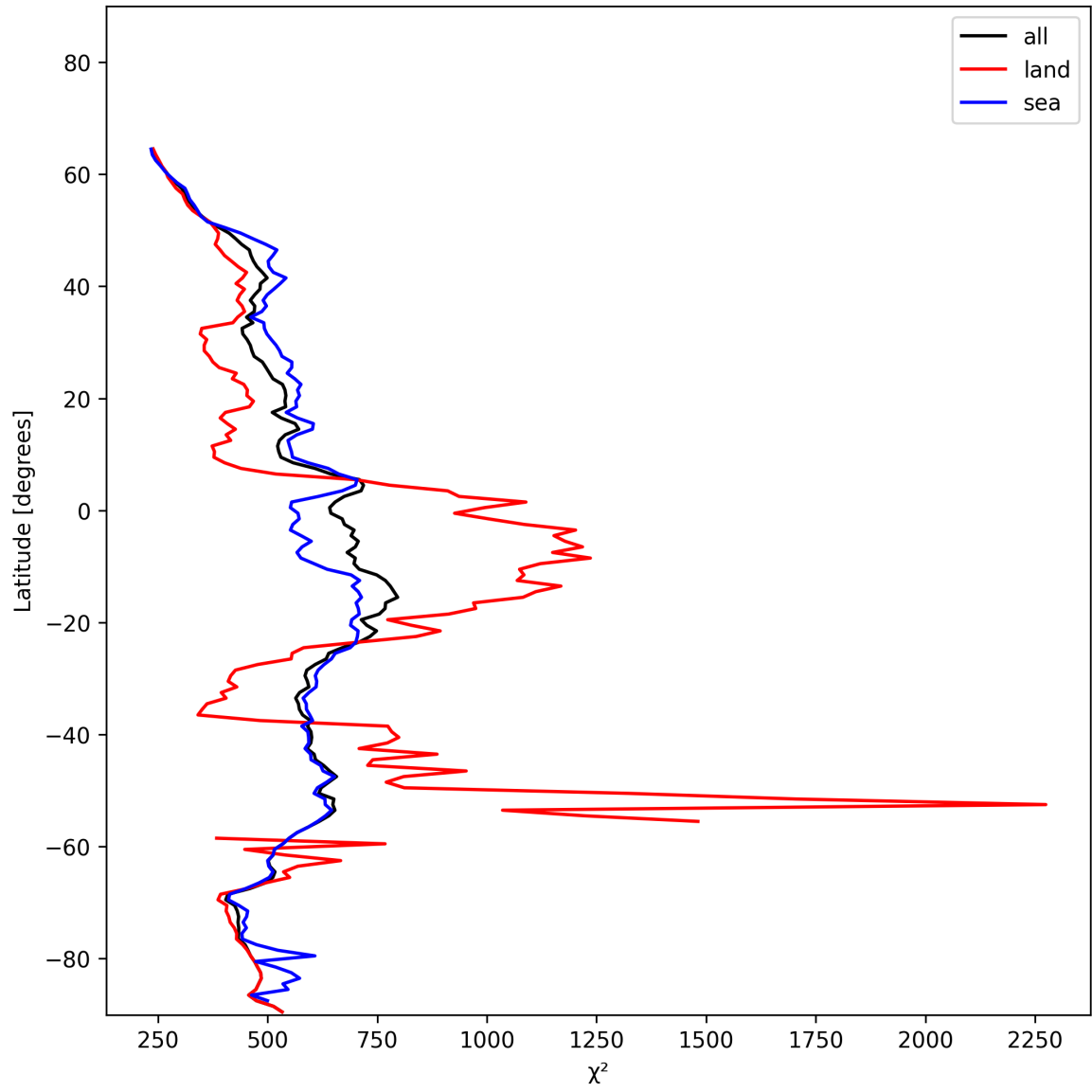
Figure 25: Zonal average of “ \chi^2 ” for 2024-12-18 to 2024-12-20.
