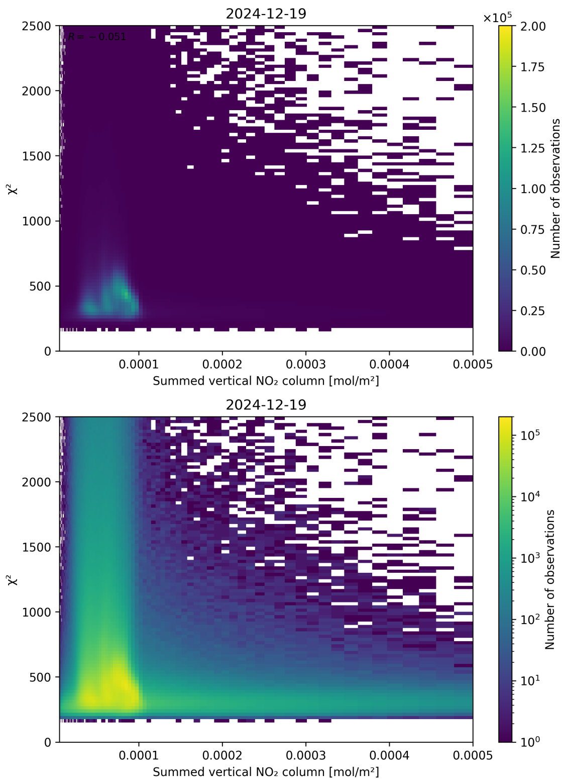
Figure 104: Scatter density plot of “Summed vertical NO 2 column” against “ \chi^2 ” for 2024-12-18 to 2024-12-20.
