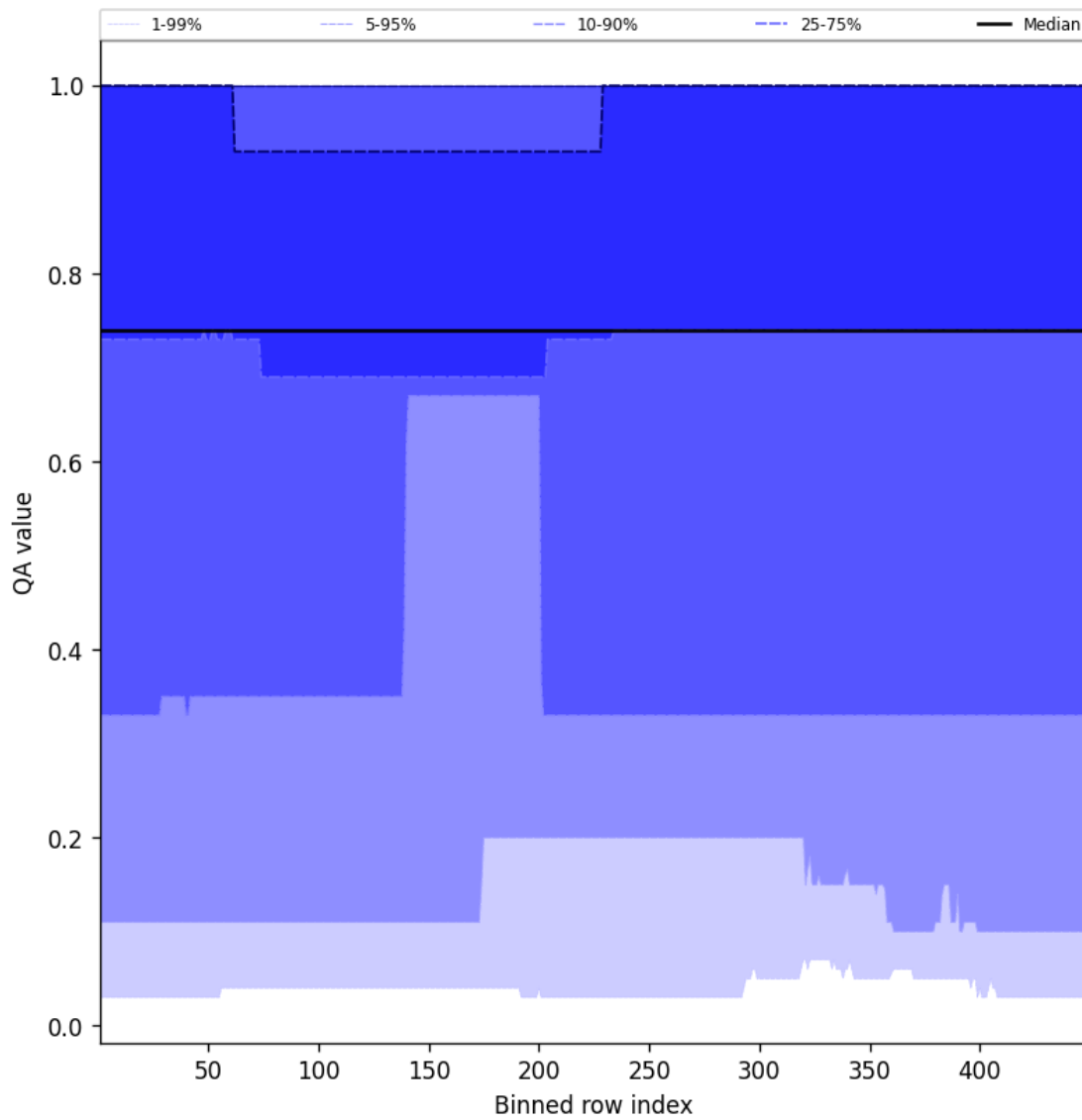
Figure 45: Along track statistics of “QA value” for 2024-12-18 to 2024-12-20
