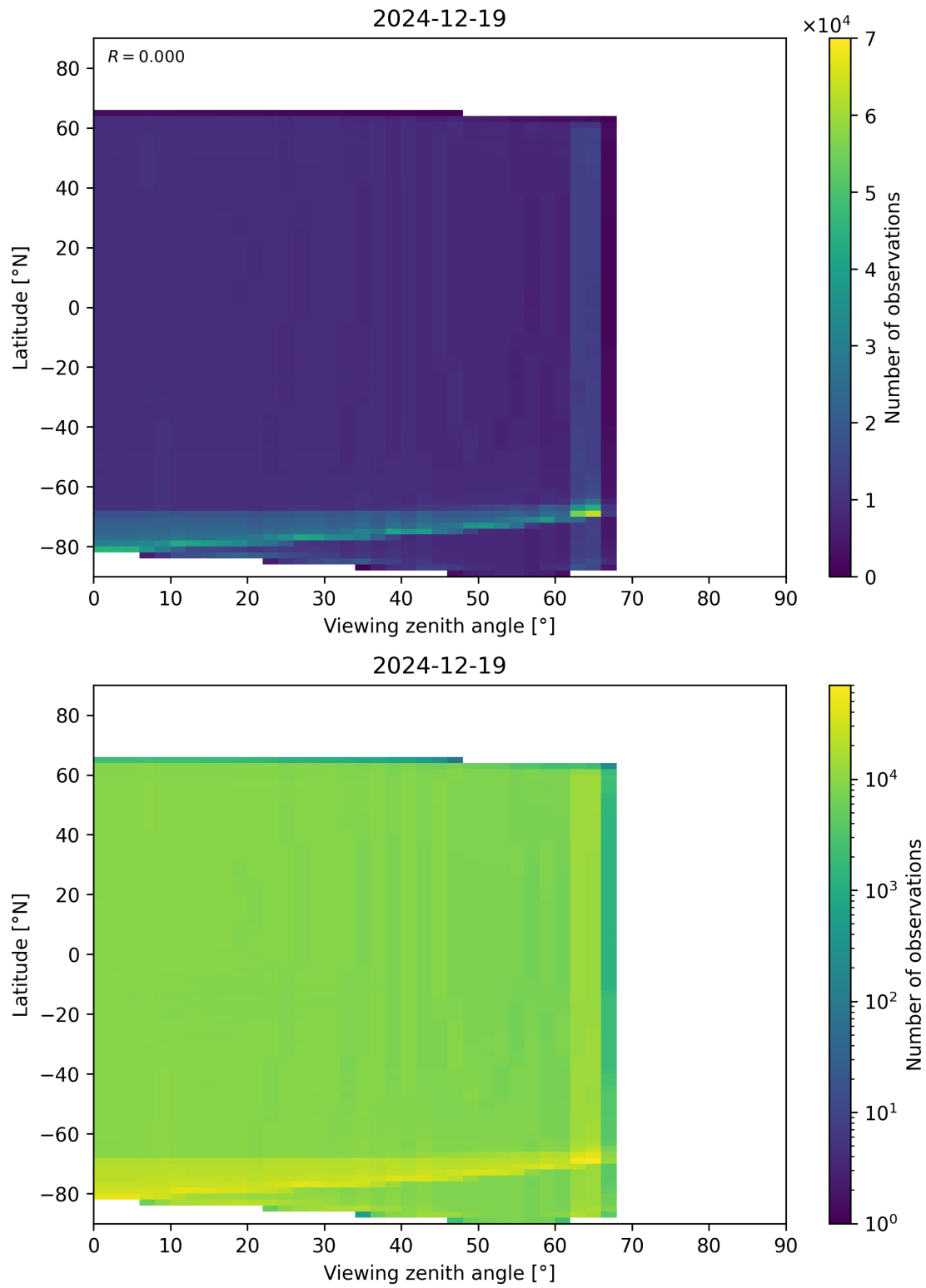
Figure 163: Scatter density plot of “Viewing zenith angle” against “Latitude” for 2024-12-18 to 2024-12-20.
