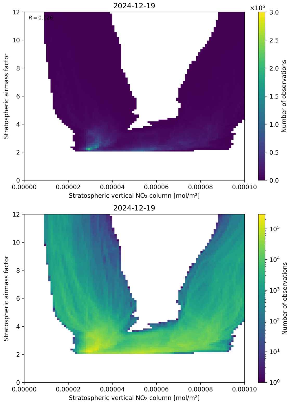
Figure 96: Scatter density plot of “Stratospheric vertical NO 2 column” against “Stratospheric airmass factor” for 2024-12-18 to 2024-12-20.
