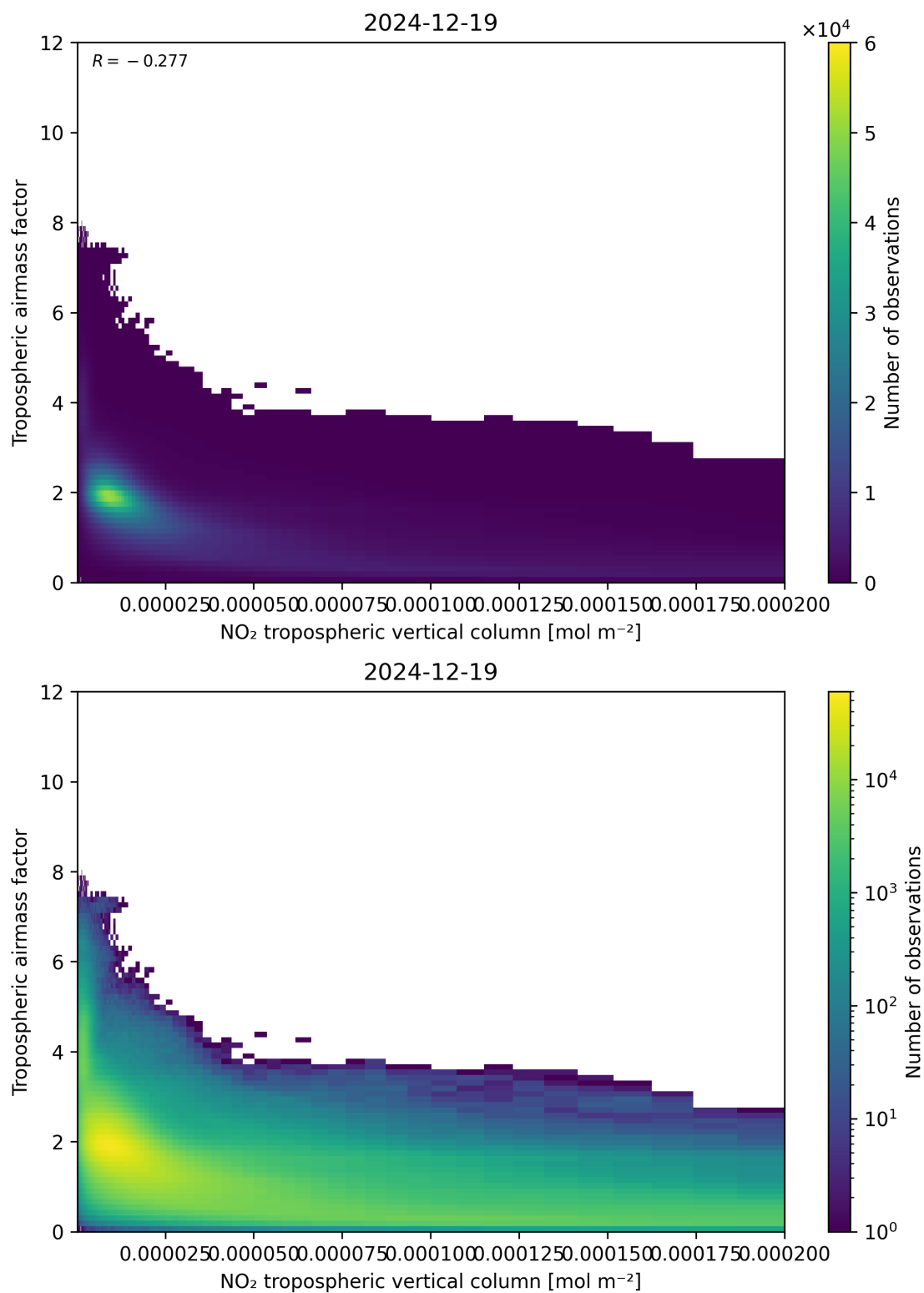
Figure 123: Scatter density plot of “NO 2 tropospheric vertical column” against “Tropospheric air mass factor” for 2024-12-18 to 2024-12-20.
