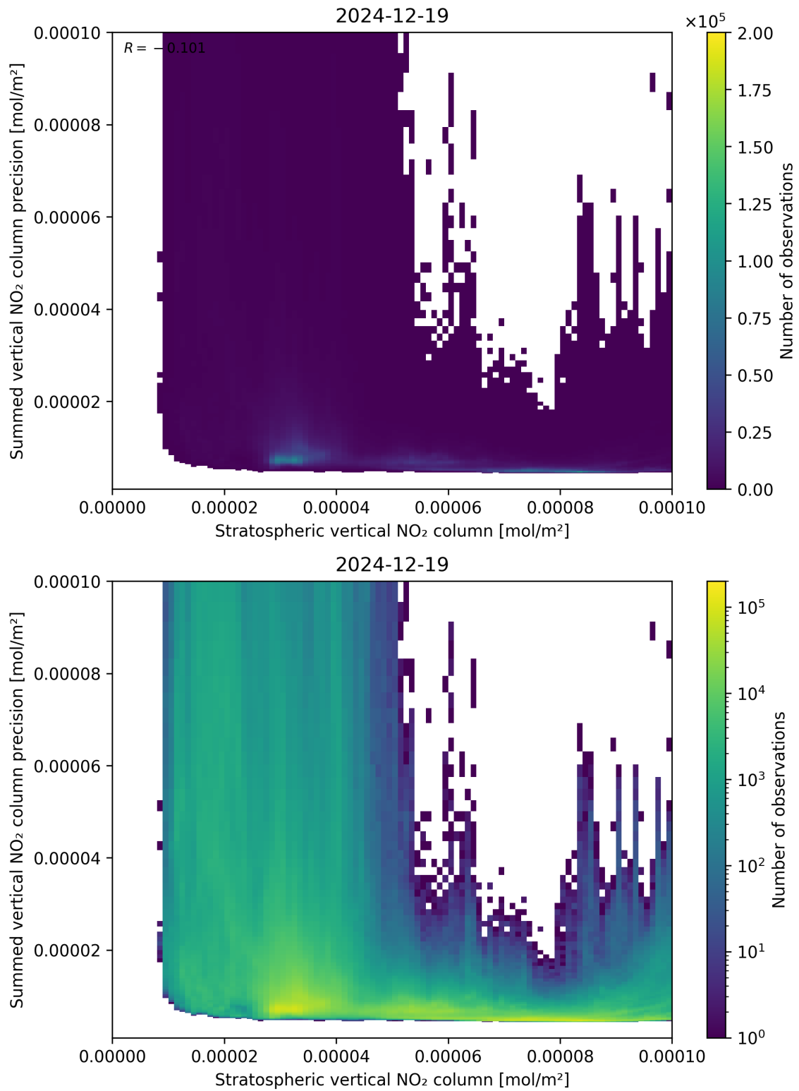
Figure 99: Scatter density plot of “Stratospheric vertical NO 2 column” against “Summed vertical NO 2 column precision” for 2024-12-18 to 2024-12-20.
