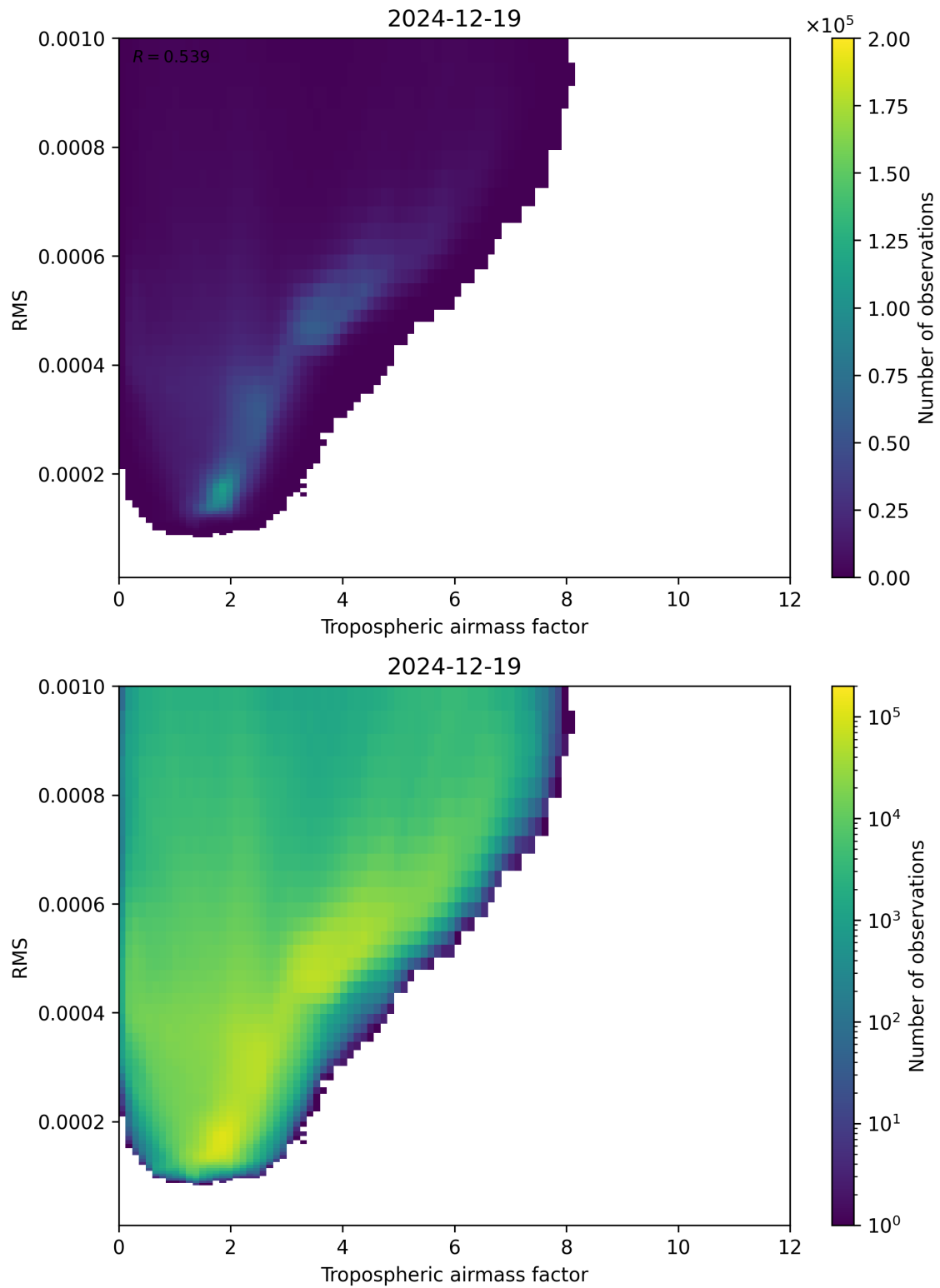
Figure 79: Scatter density plot of “Tropospheric airmass factor” against “RMS” for 2024-12-18 to 2024-12-20.
