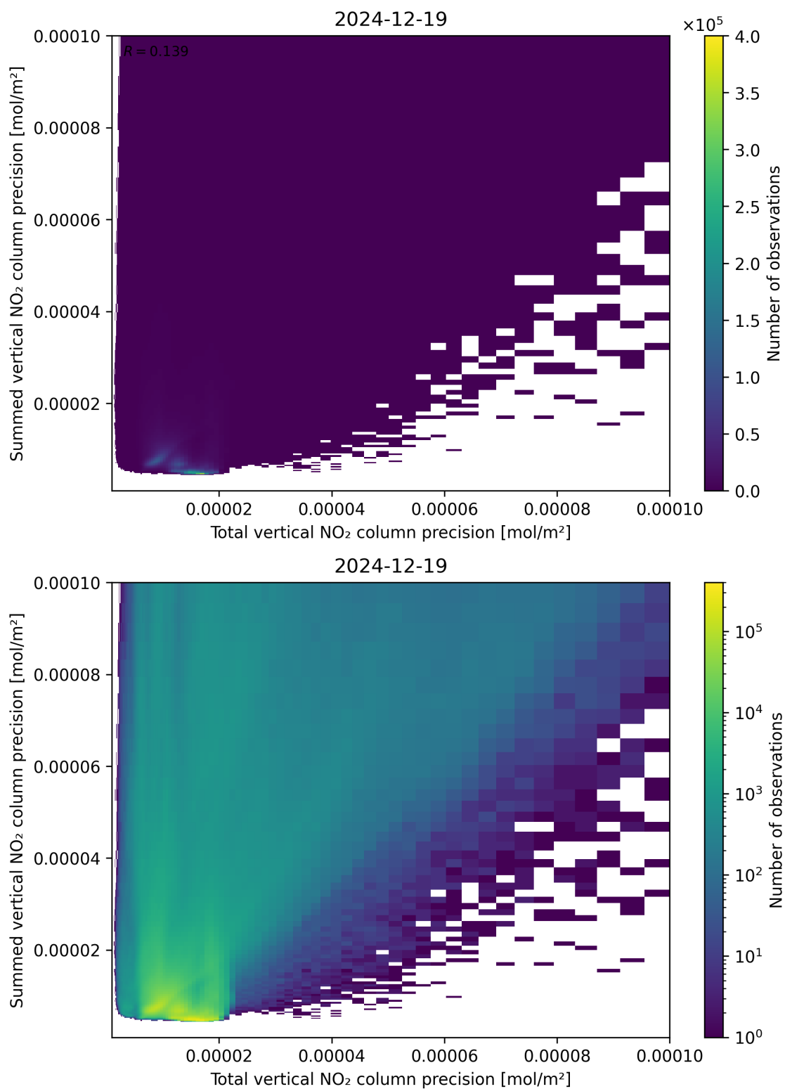
Figure 118: Scatter density plot of “Total vertical NO 2 column precision” against “Summed vertical NO 2 column precision” for 2024-12-18 to 2024-12-20.
