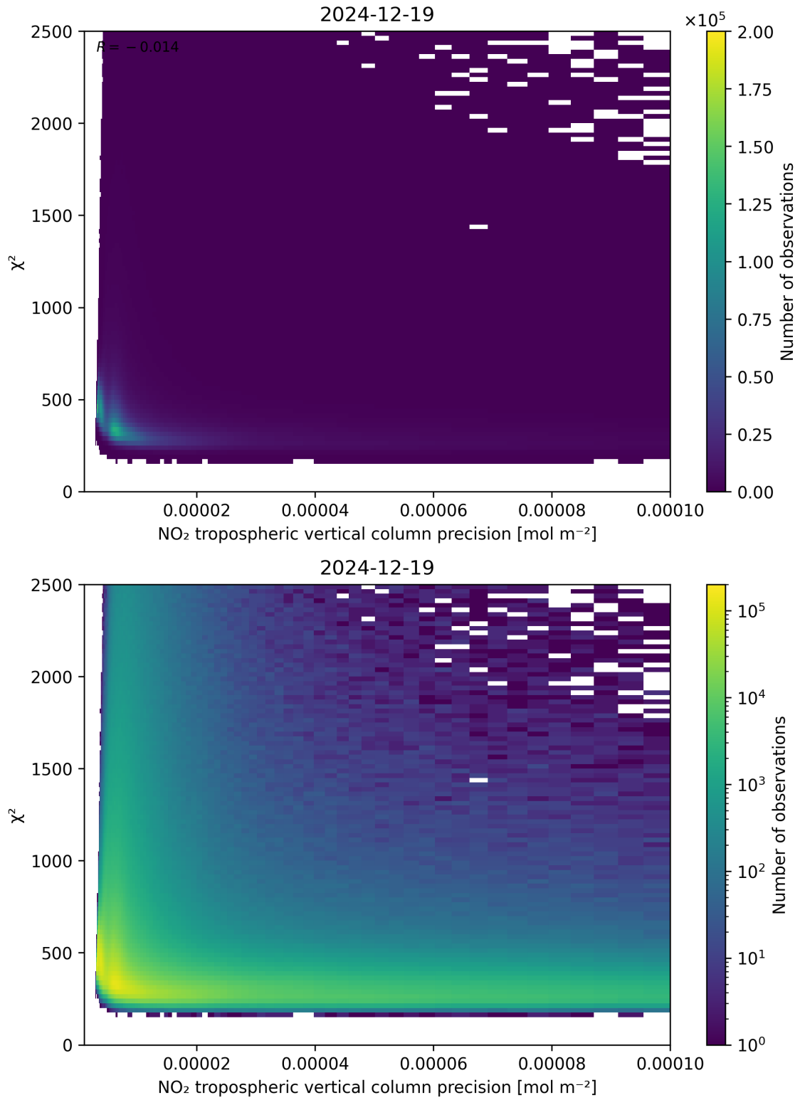
Figure 134: Scatter density plot of “NO 2 tropospheric vertical column precision” against “ \chi^2 ” for 2024-12-18 to 2024-12-20.
