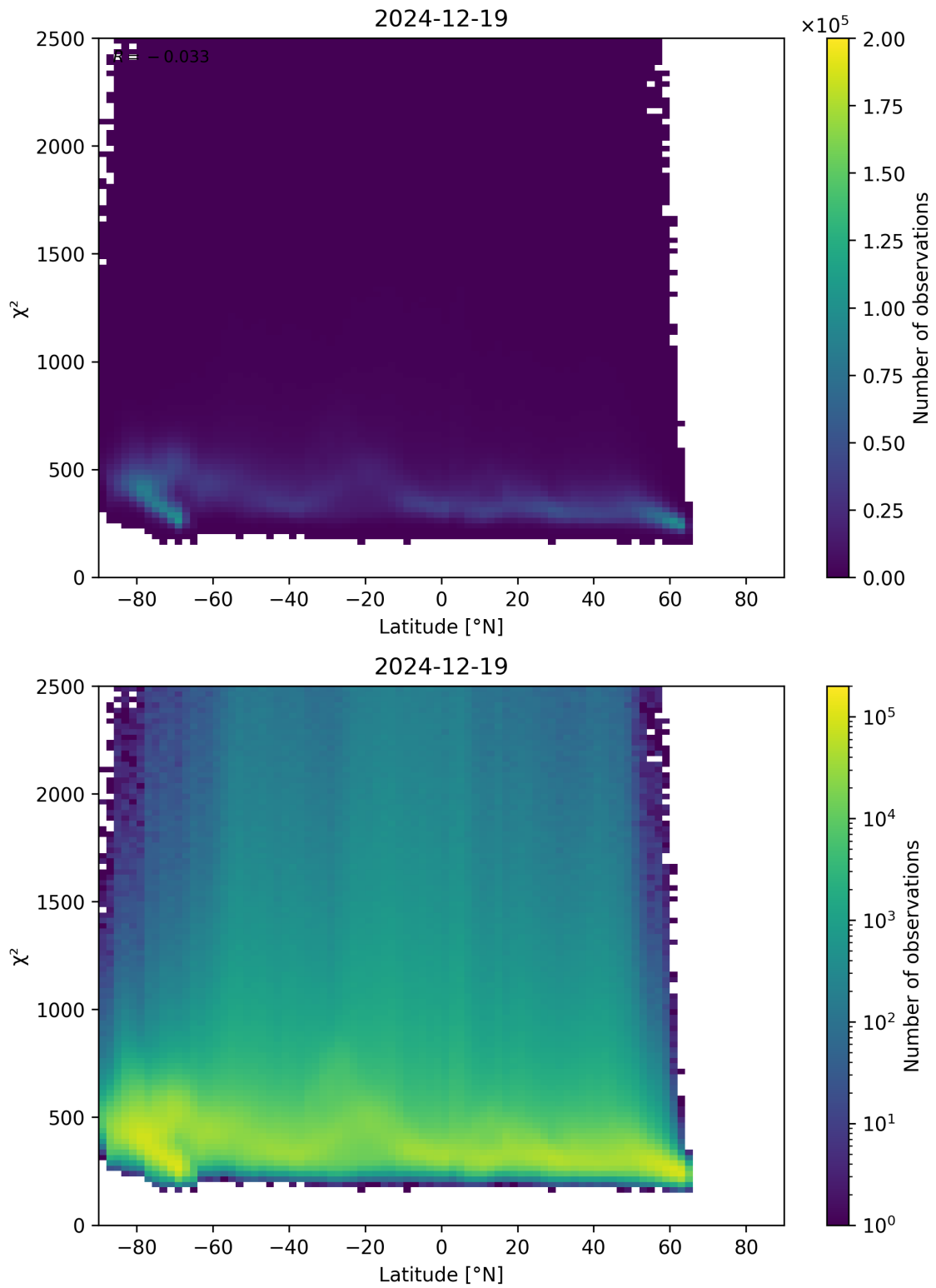
Figure 86: Scatter density plot of “Latitude” against “ \chi^2 ” for 2024-12-18 to 2024-12-20.
