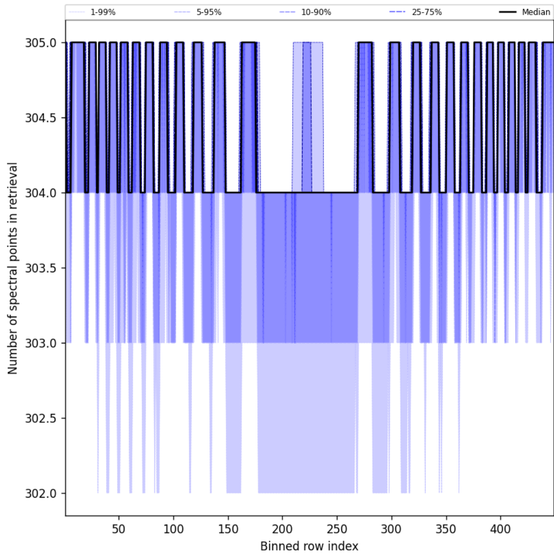
Figure 50: Along track statistics of “Number of spectral points in retrieval” for 2024-12-18 to 2024-12-20
