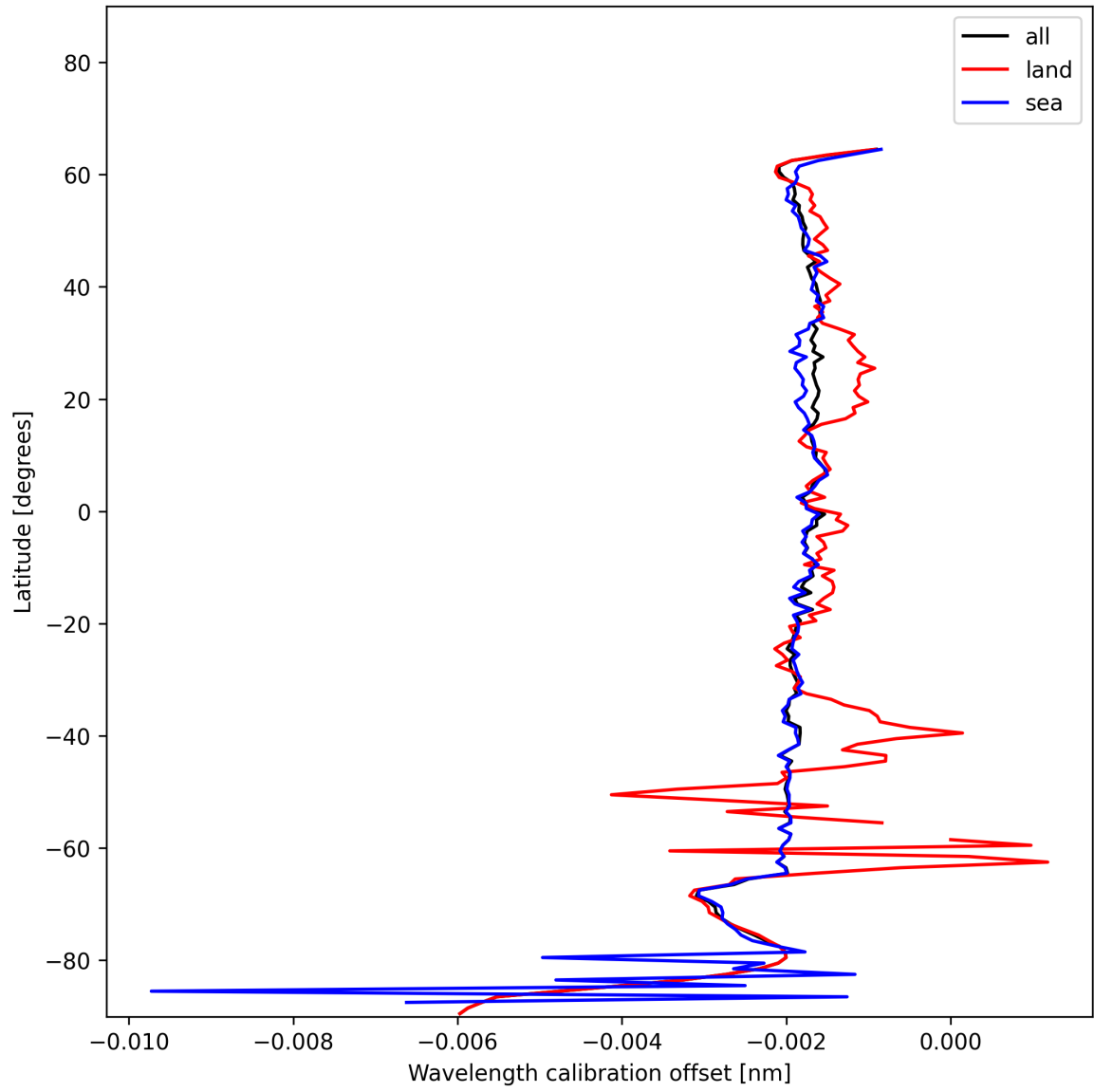
Figure 18: Zonal average of “Wavelength calibration offset” for 2024-12-18 to 2024-12-20.
