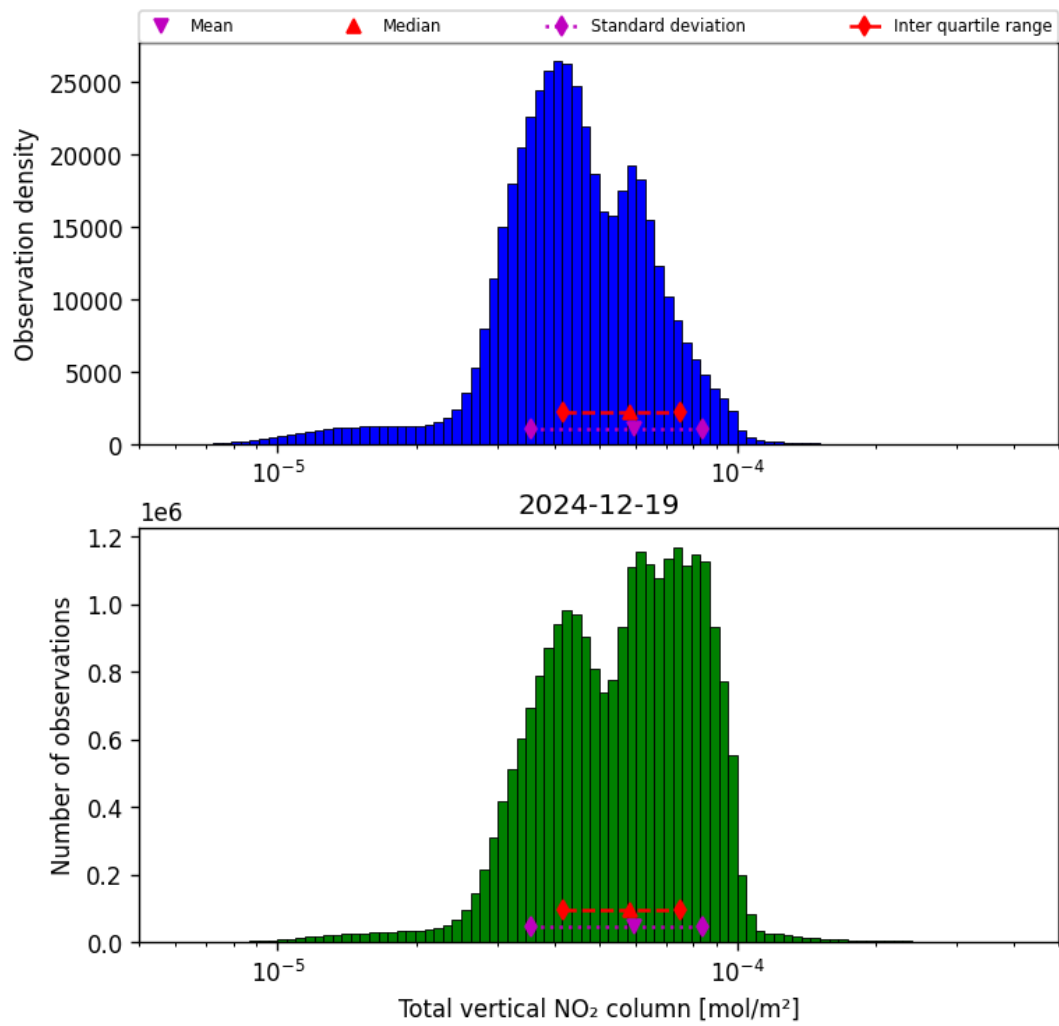
Figure 38: Histogram of “Total vertical NO 2 column” for 2024-12-18 to 2024-12-20
