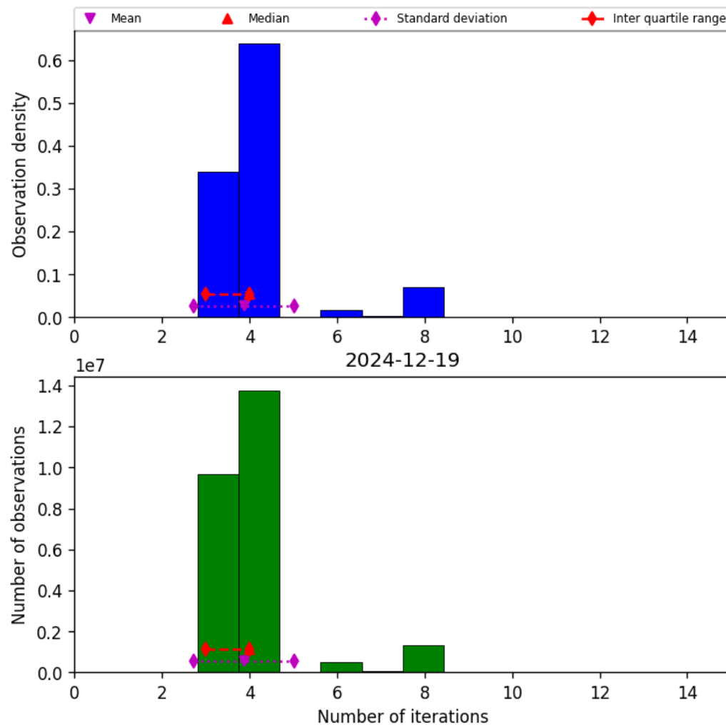
Figure 34: Histogram of “Number of iterations” for 2024-12-18 to 2024-12-20
