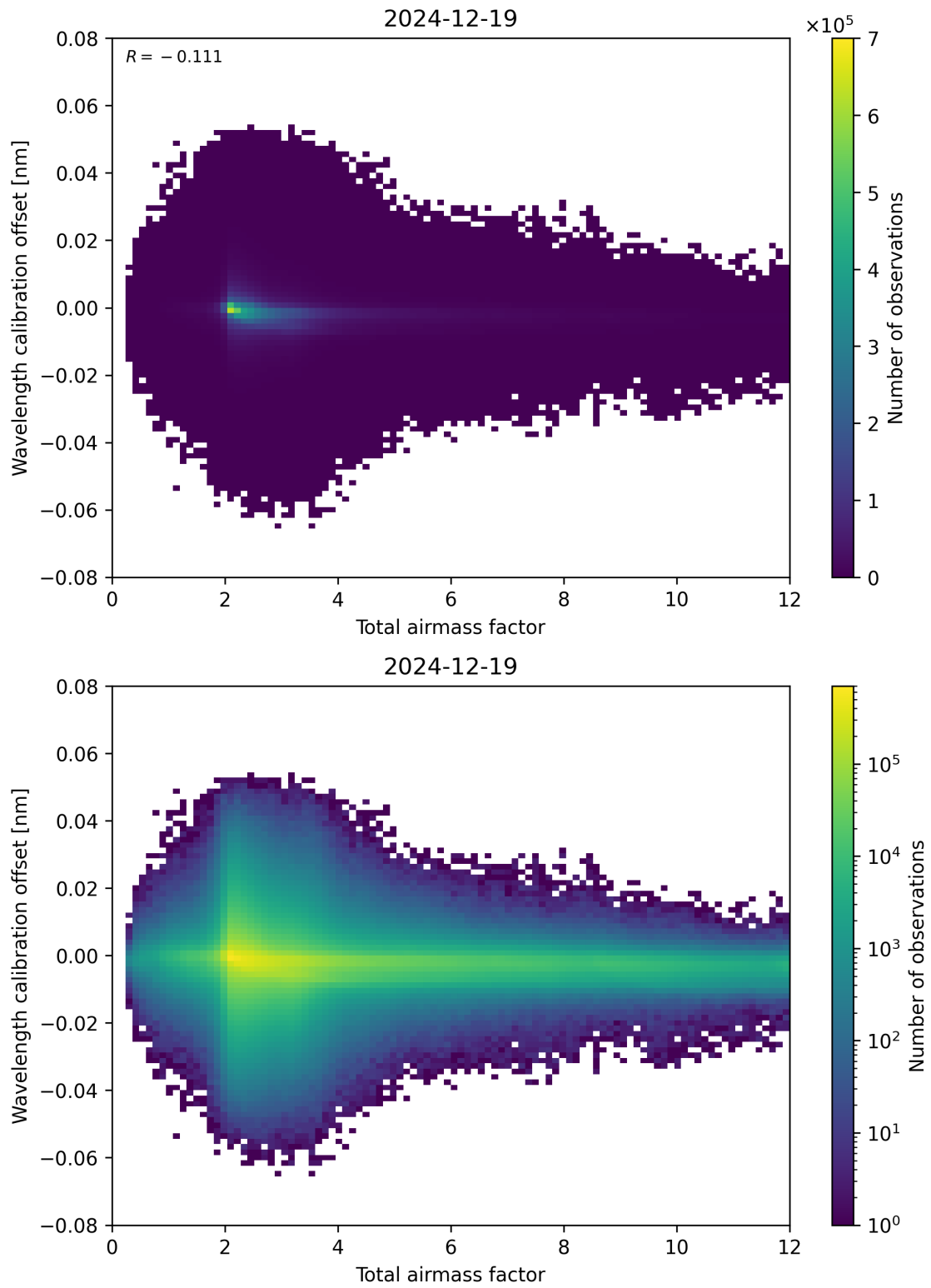
Figure 70: Scatter density plot of “Total airmass factor” against “Wavelength calibration offset” for 2024-12-18 to 2024-12-20.
