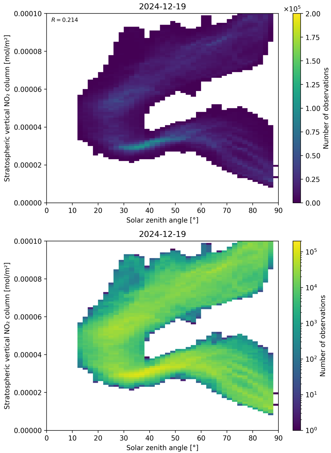
Figure 150: Scatter density plot of “Solar zenith angle” against “Stratospheric vertical NO 2 column” for 2024-12-18 to 2024-12-20.
