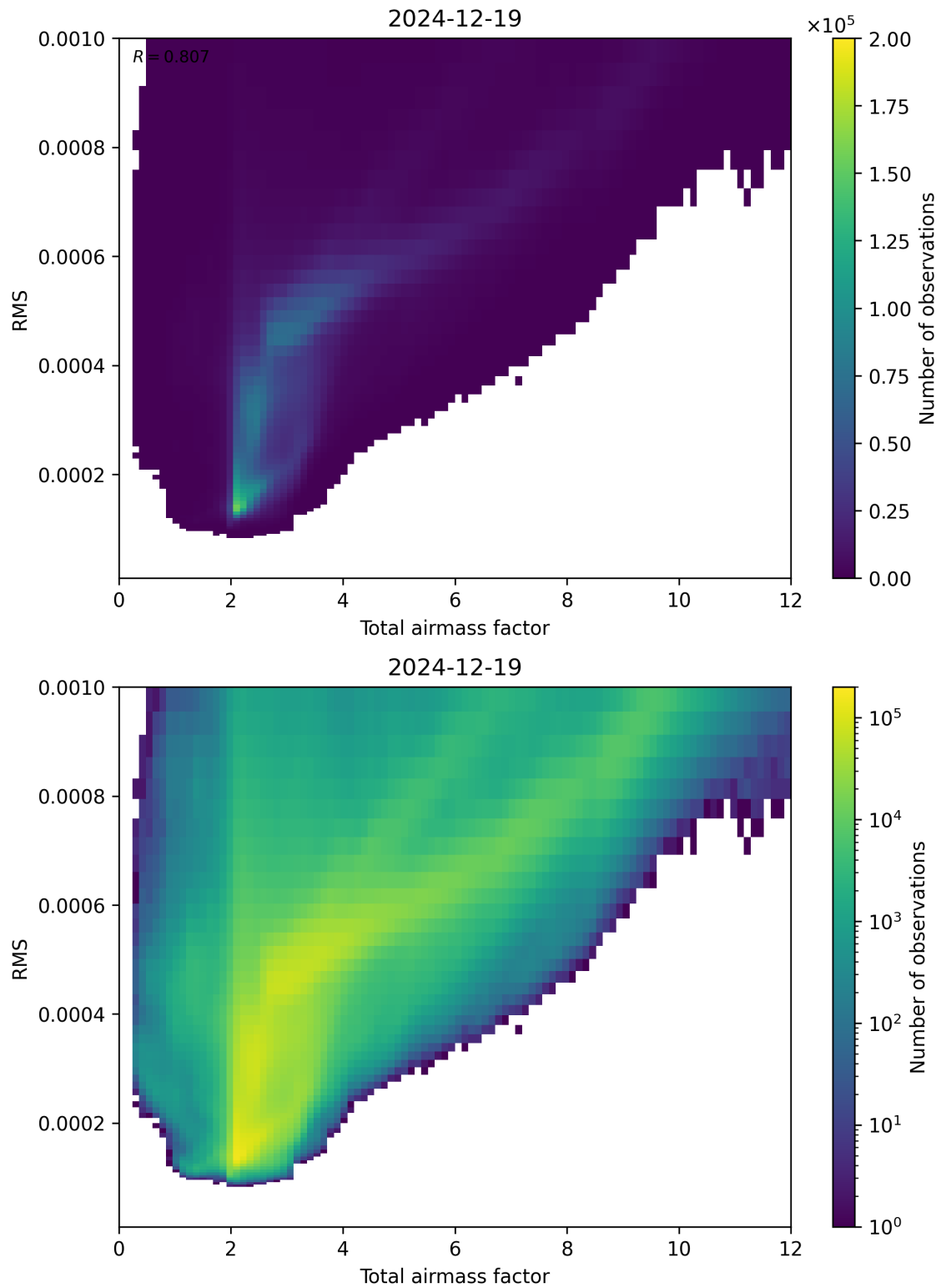
Figure 69: Scatter density plot of “Total airmass factor” against “RMS” for 2024-12-18 to 2024-12-20.
