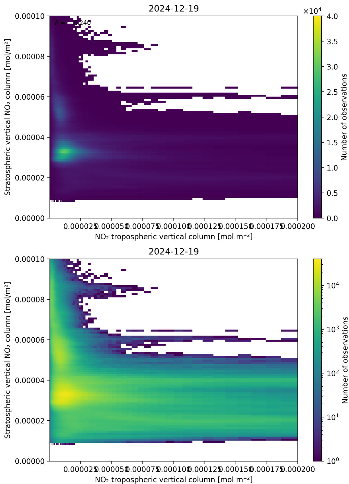
Figure 125: Scatter density plot of “NO 2 tropospheric vertical column” against “Stratospheric vertical NO 2 column” for 2024-12-18 to 2024-12-20.
