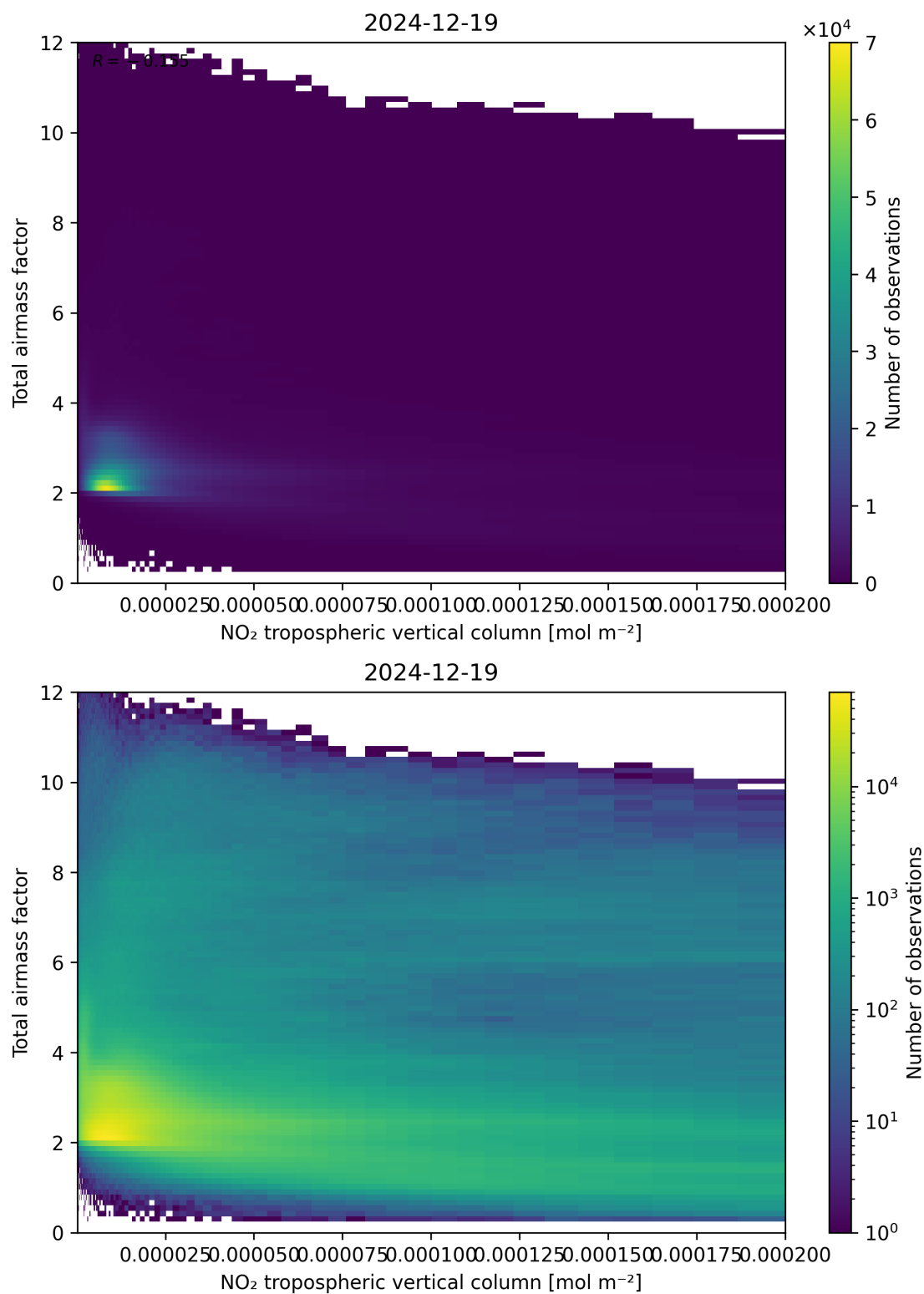
Figure 122: Scatter density plot of “NO 2 tropospheric vertical column” against “Total air mass factor” for 2024-12-18 to 2024-12-20.
