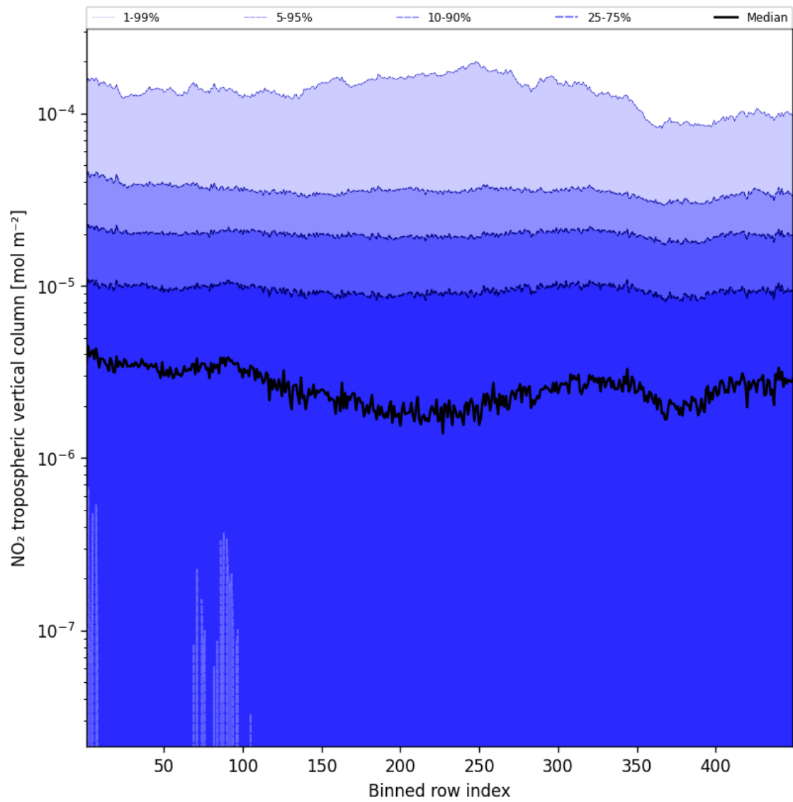
Figure 46: Along track statistics of “NO 2 tropospheric vertical column” for 2024-12-18 to 2024-12-20
