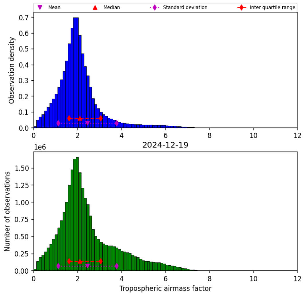
Figure 31: Histogram of “Tropospheric airmass factor” for 2024-12-18 to 2024-12-20
