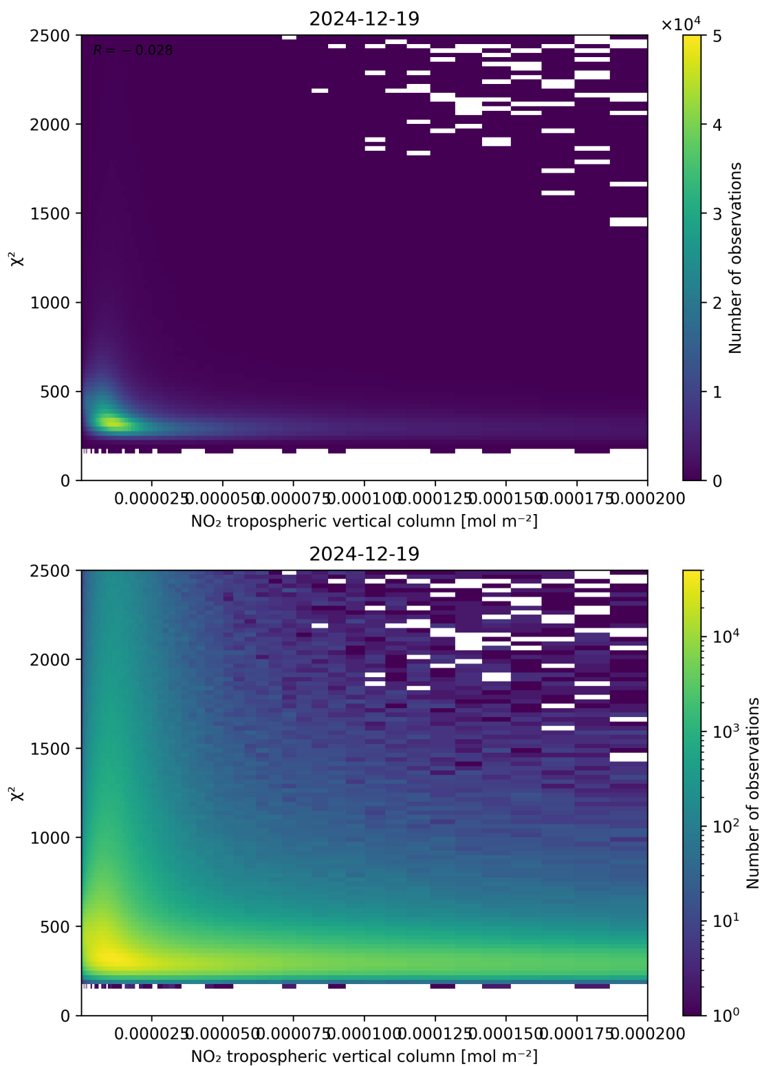
Figure 124: Scatter density plot of “NO 2 tropospheric vertical column” against “ \chi^2 ” for 2024-12-18 to 2024-12-20.
