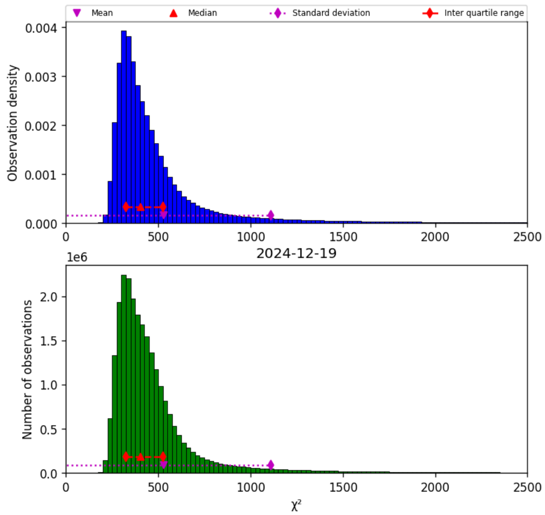
Figure 42: Histogram of “ \chi^2 ” for 2024-12-18 to 2024-12-20
