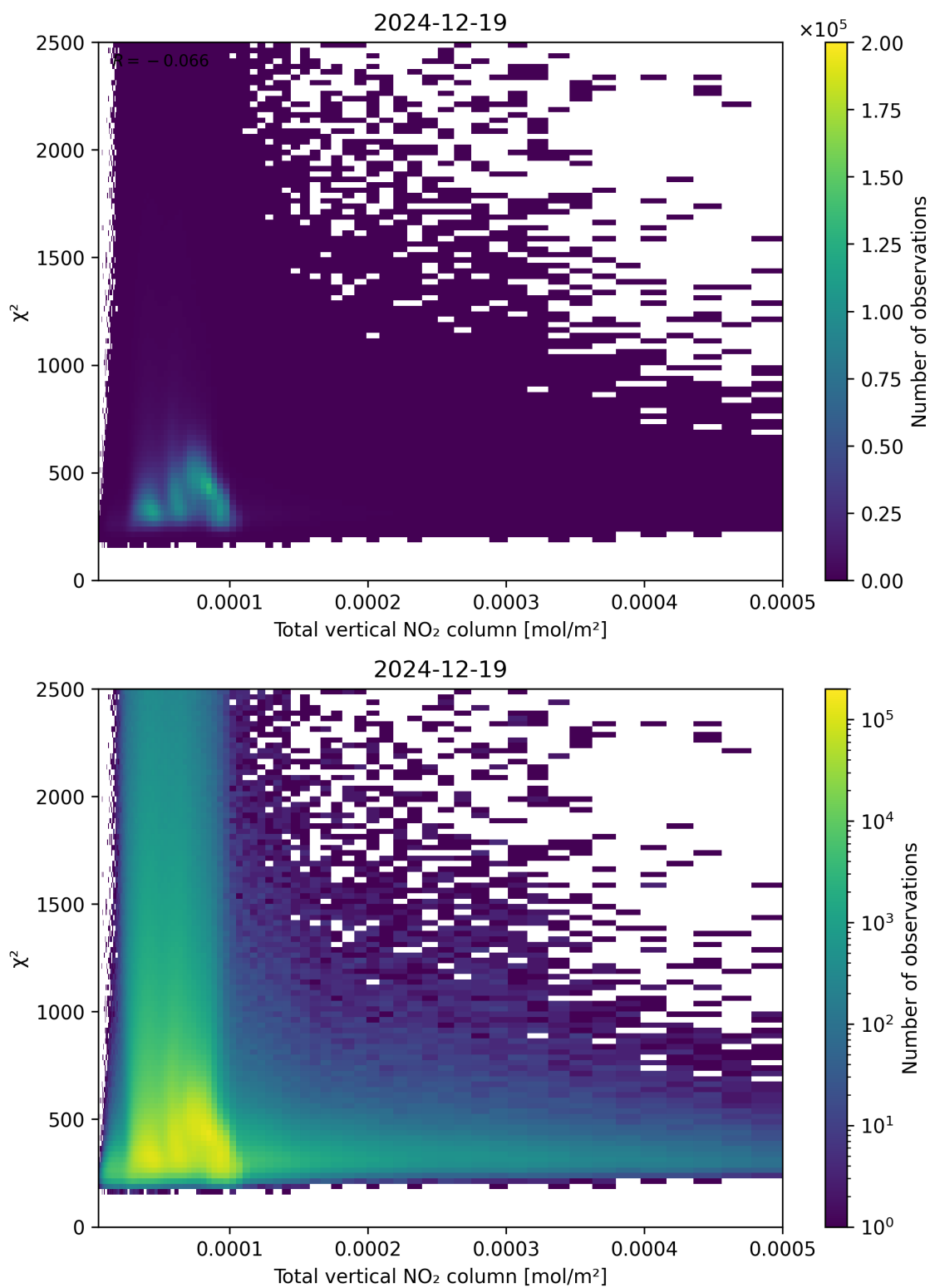
Figure 111: Scatter density plot of “Total vertical NO 2 column” against “ \chi^2 ” for 2024-12-18 to 2024-12-20.
