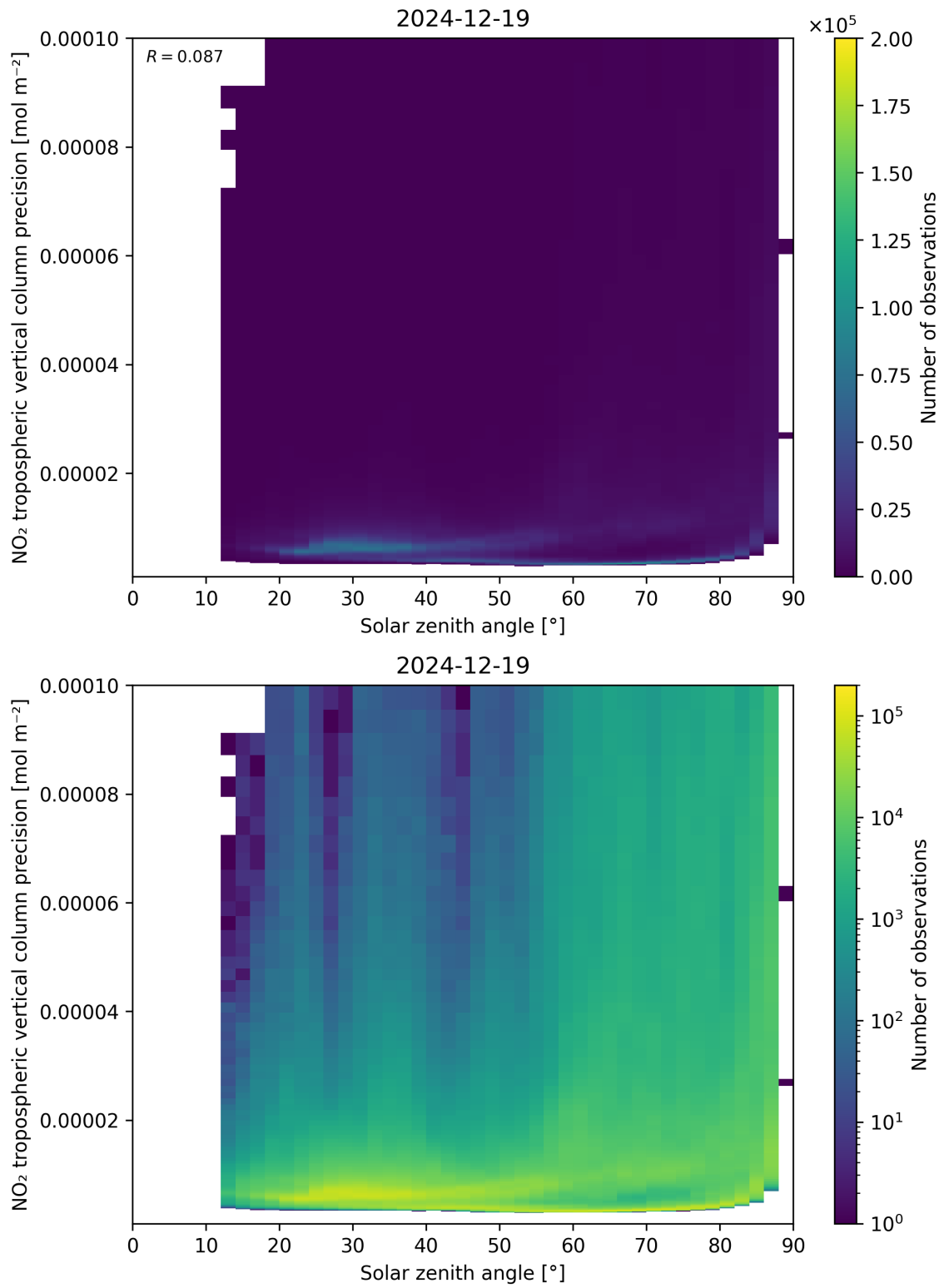
Figure 156: Scatter density plot of “Solar zenith angle” against “NO 2 tropospheric vertical column precision” for 2024-12-18 to 2024-12-20.
