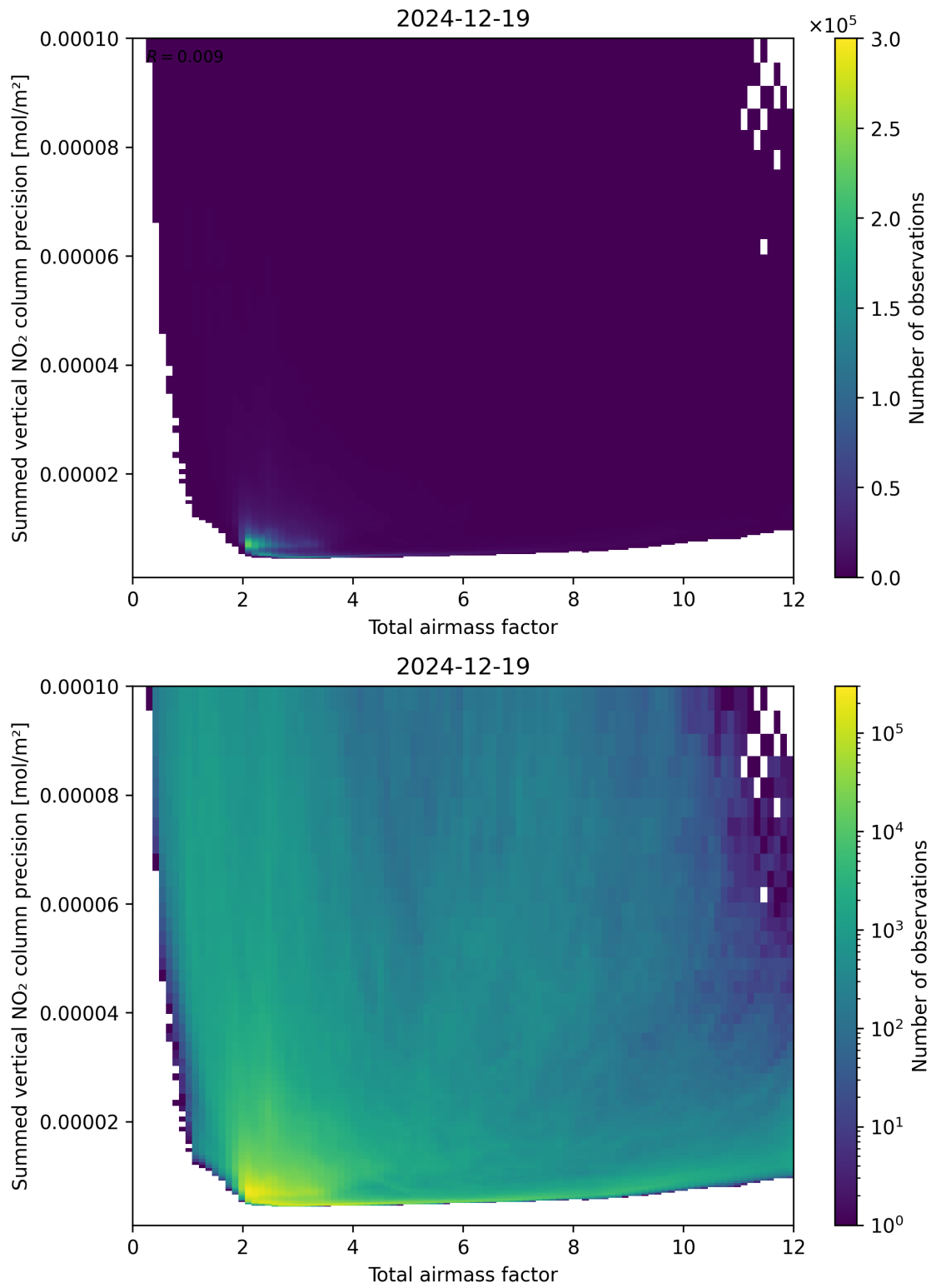
Figure 66: Scatter density plot of “Total airmass factor” against “Summed vertical NO 2 column precision” for 2024-12-18 to 2024-12-20.
