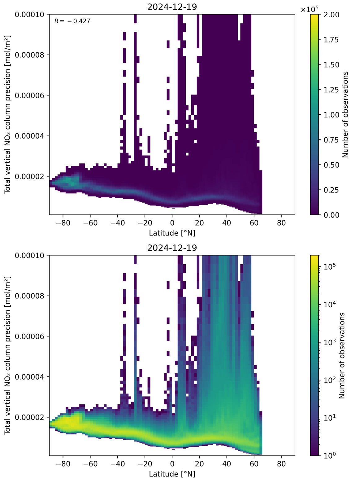
Figure 91: Scatter density plot of “Latitude” against “Total vertical NO 2 column precision” for 2024-12-18 to 2024-12-20.
