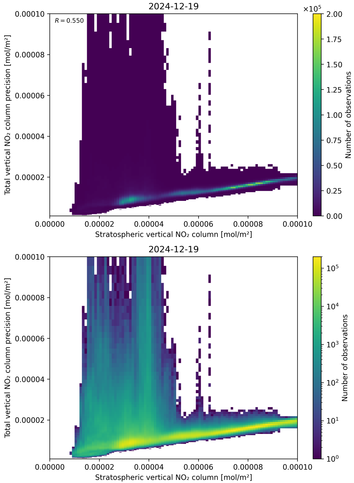
Figure 101: Scatter density plot of “Stratospheric vertical NO 2 column” against “Total vertical NO 2 column precision” for 2024-12-18 to 2024-12-20.
