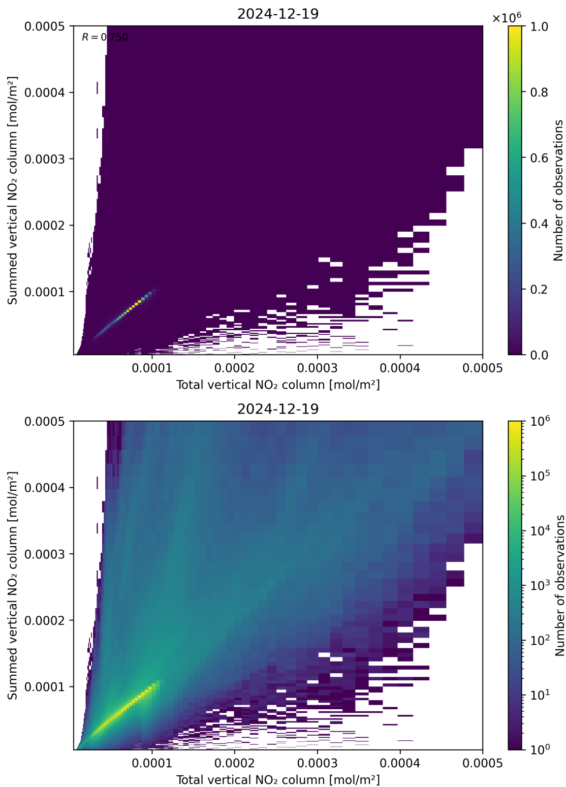
Figure 112: Scatter density plot of “Total vertical NO 2 column” against “Summed vertical NO 2 column” for 2024-12-18 to 2024-12-20.
