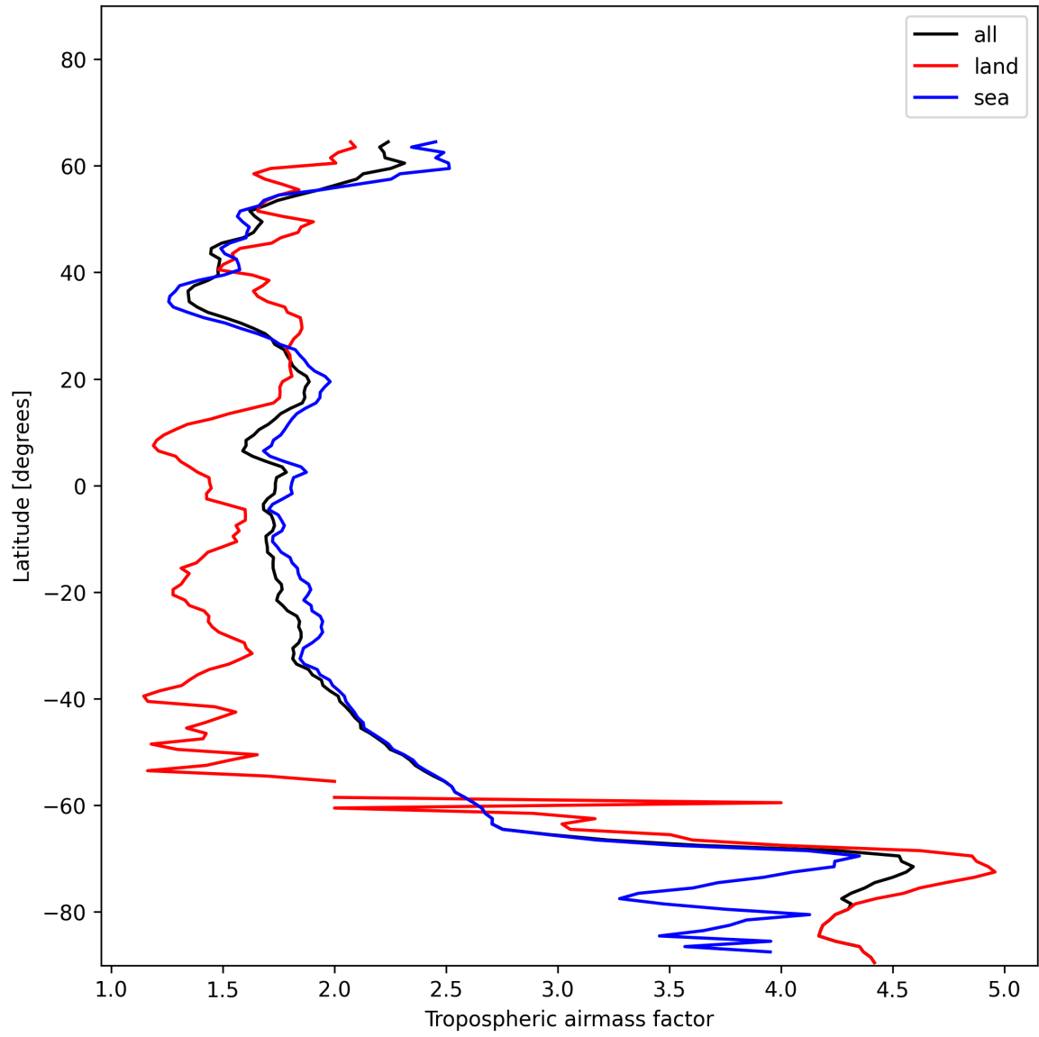
Figure 14: Zonal average of “Tropospheric airmass factor” for 2024-12-18 to 2024-12-20.
