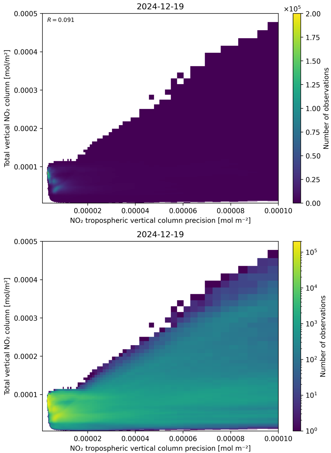
Figure 138: Scatter density plot of “NO 2 tropospheric vertical column precision” against “Total vertical NO 2 column” for 2024-12-18 to 2024-12-20.
