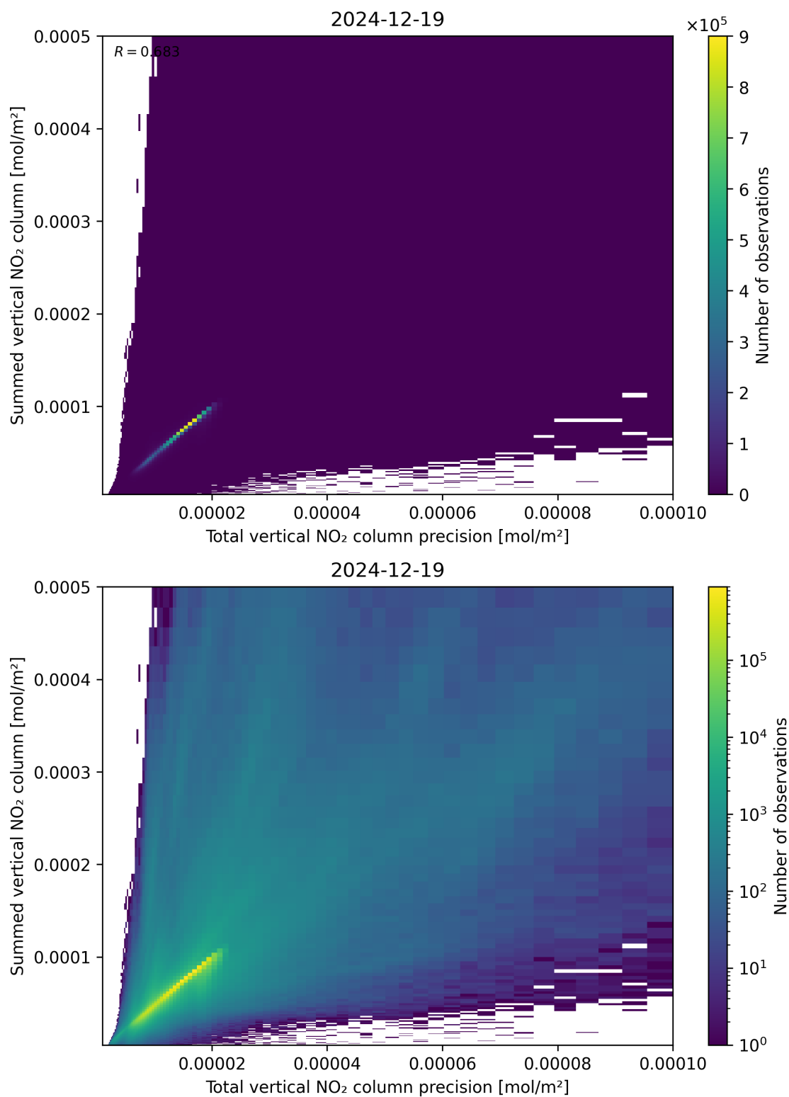
Figure 117: Scatter density plot of “Total vertical NO 2 column precision” against “Summed vertical NO 2 column” for 2024-12-18 to 2024-12-20.
