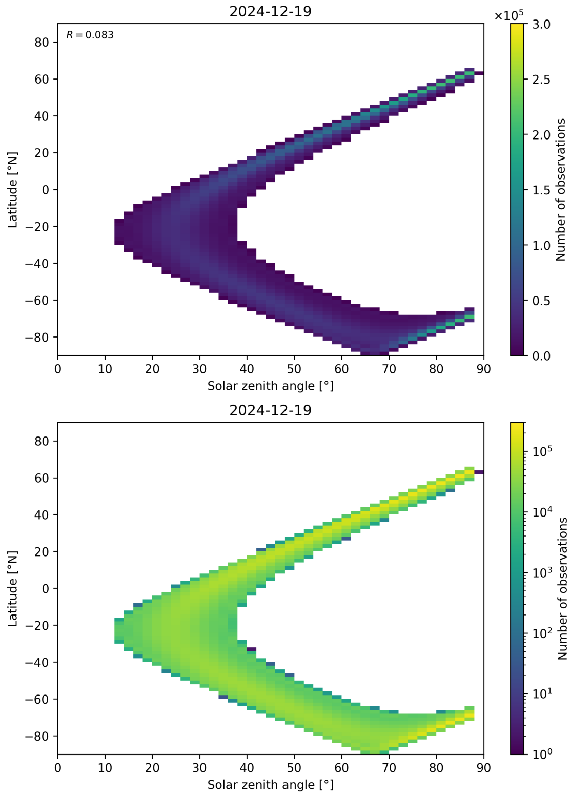
Figure 149: Scatter density plot of “Solar zenith angle” against “Latitude” for 2024-12-18 to 2024-12-20.
