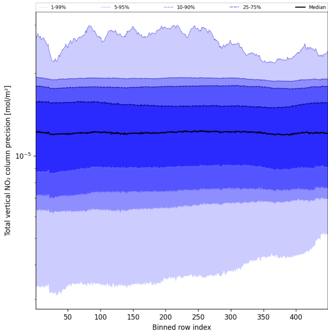
Figure 56: Along track statistics of “Total vertical NO 2 column precision” for 2024-12-18 to 2024-12-20
