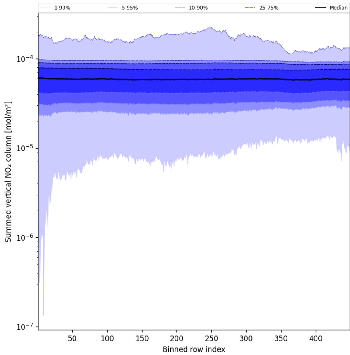
Figure 57: Along track statistics of “Summed vertical NO 2 column” for 2024-12-18 to 2024-12-20
