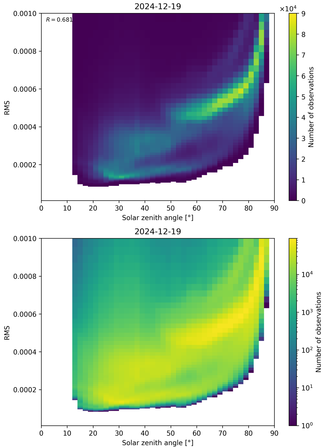
Figure 157: Scatter density plot of “Solar zenith angle” against “RMS” for 2024-12-18 to 2024-12-20.
