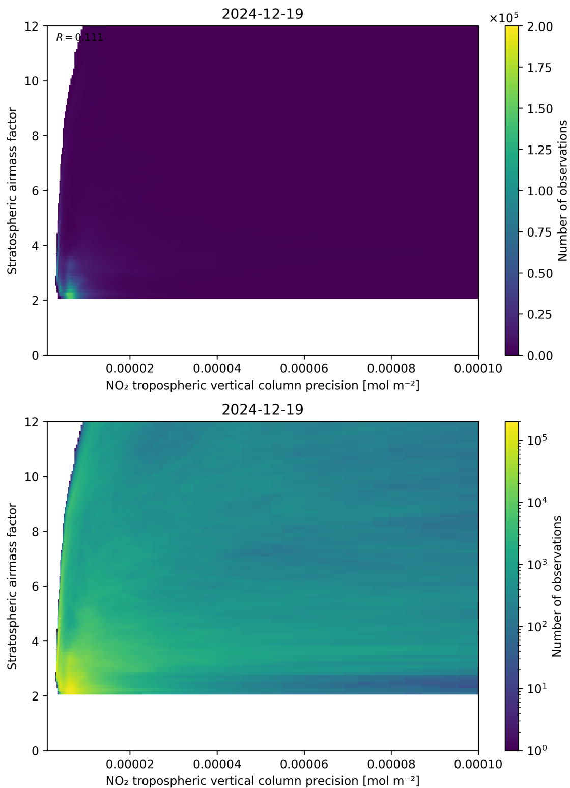
Figure 131: Scatter density plot of “NO 2 tropospheric vertical column precision” against “Stratospheric airmass factor” for 2024-12-18 to 2024-12-20.
