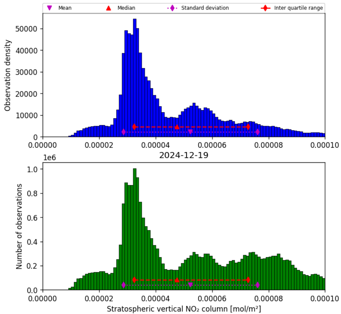
Figure 36: Histogram of “Stratospheric vertical NO 2 column” for 2024-12-18 to 2024-12-20
