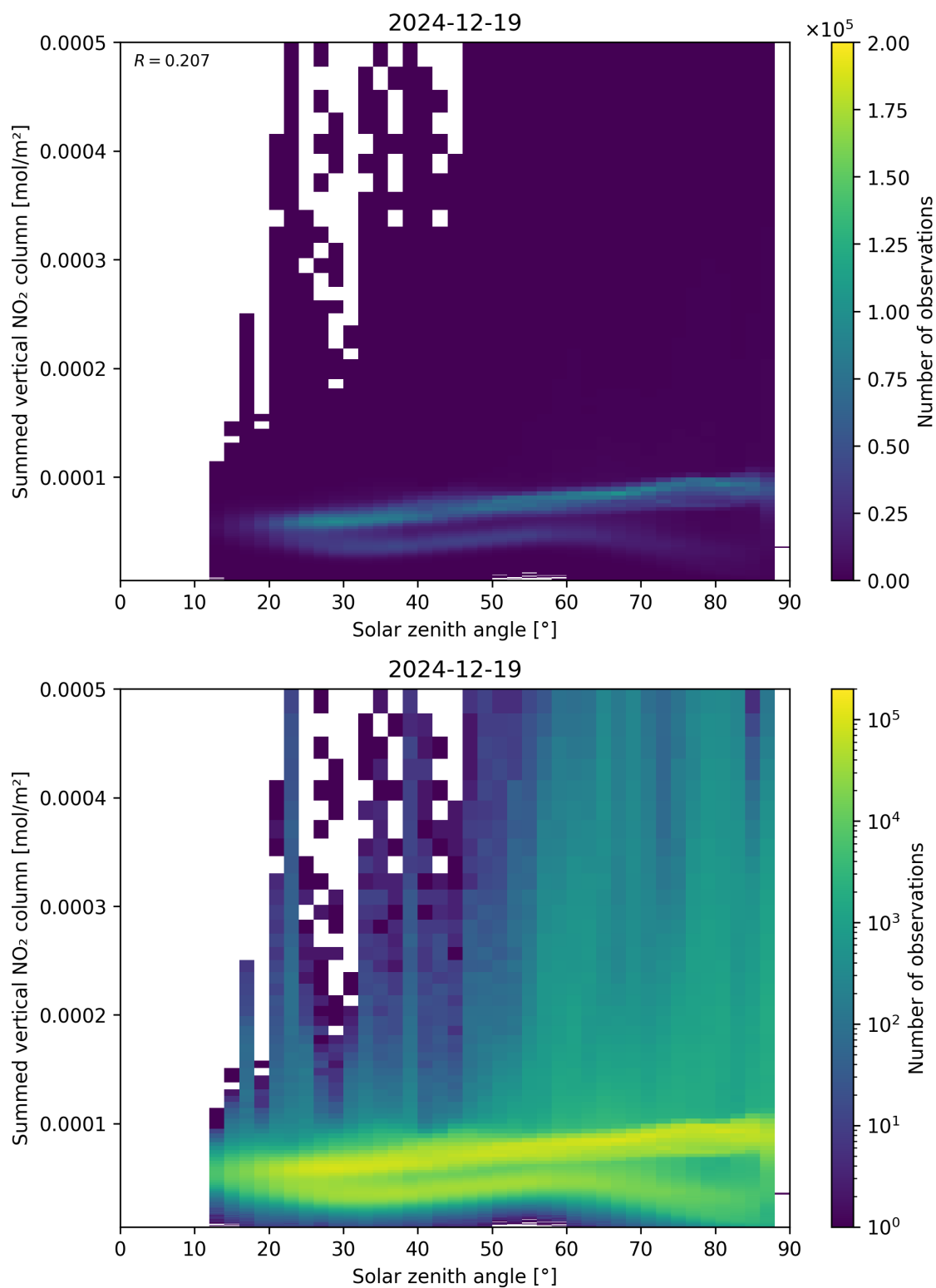
Figure 151: Scatter density plot of “Solar zenith angle” against “Summed vertical NO 2 column” for 2024-12-18 to 2024-12-20.
