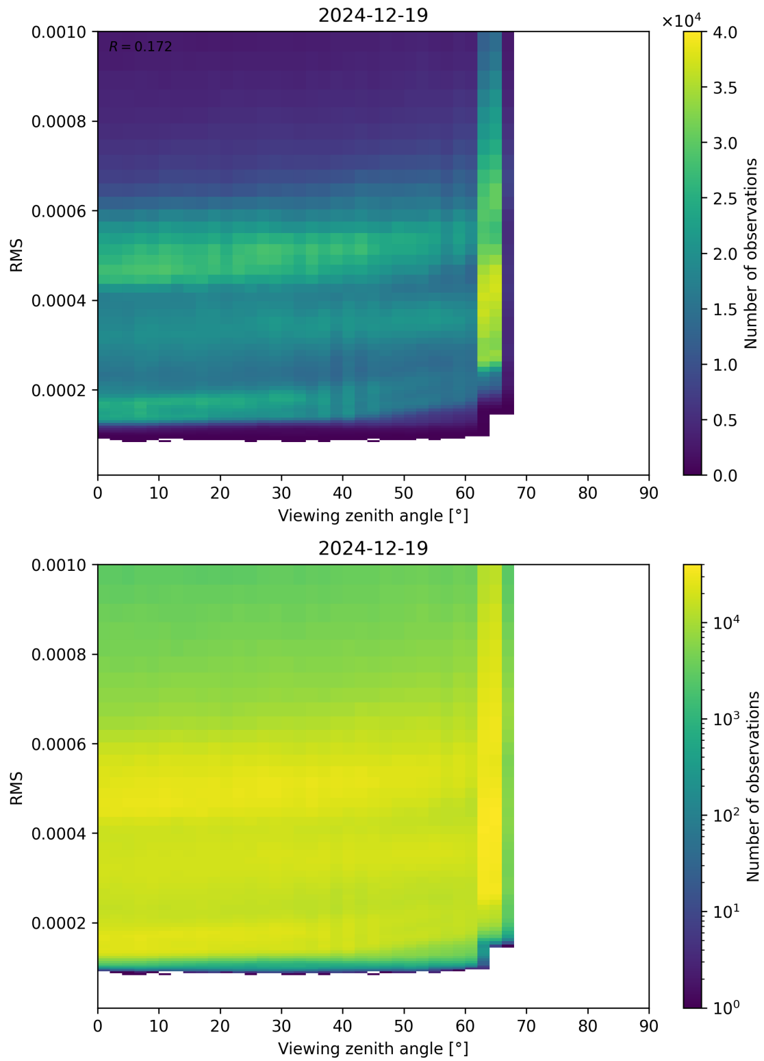
Figure 171: Scatter density plot of “Viewing zenith angle” against “RMS” for 2024-12-18 to 2024-12-20.
