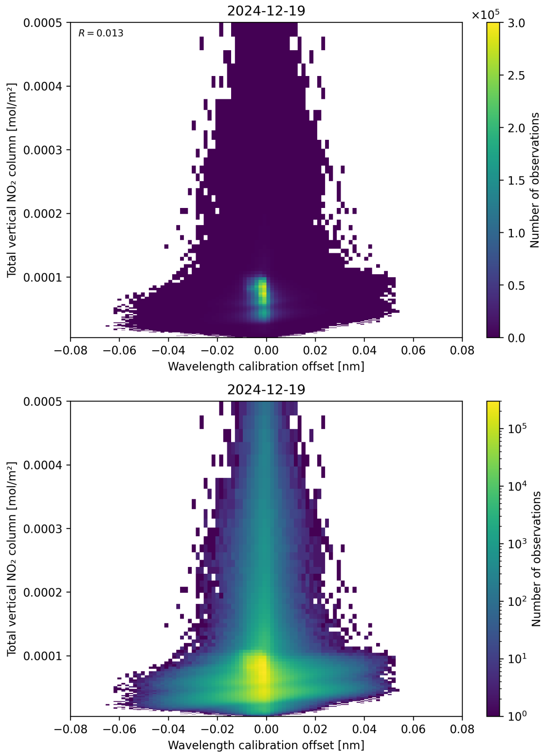
Figure 179: Scatter density plot of “Wavelength calibration offset” against “Total vertical NO 2 column” for 2024-12-18 to 2024-12-20.
