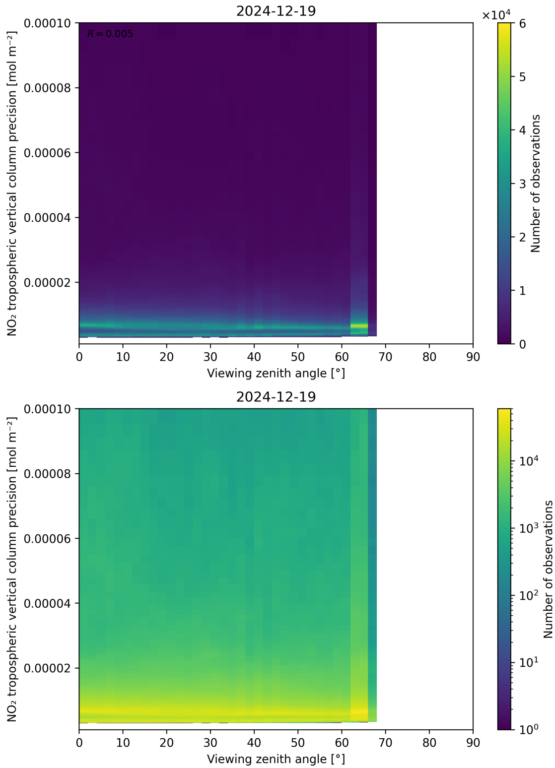
Figure 170: Scatter density plot of “Viewing zenith angle” against “NO 2 tropospheric vertical column precision” for 2024-12-18 to 2024-12-20.
