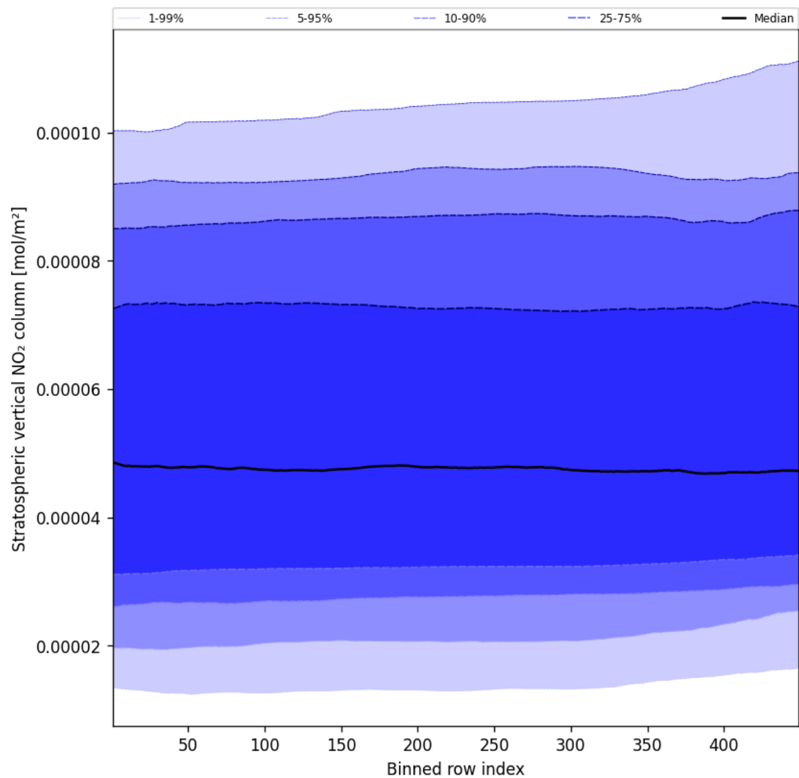
Figure 53: Along track statistics of “Stratospheric vertical NO 2 column” for 2024-12-18 to 2024-12-20
