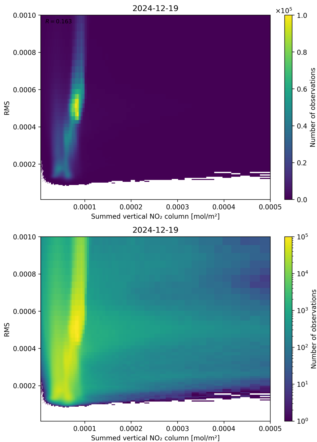
Figure 109: Scatter density plot of “Summed vertical NO 2 column” against “RMS” for 2024-12-18 to 2024-12-20.
