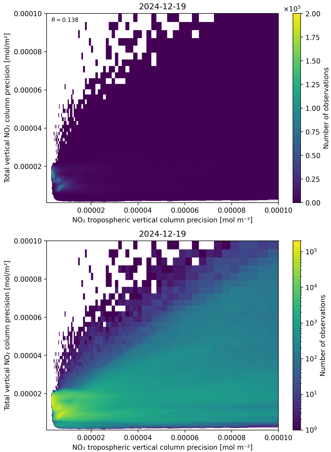
Figure 139: Scatter density plot of “NO 2 tropospheric vertical column precision” against “Total vertical NO 2 column precision” for 2024-12-18 to 2024-12-20.
