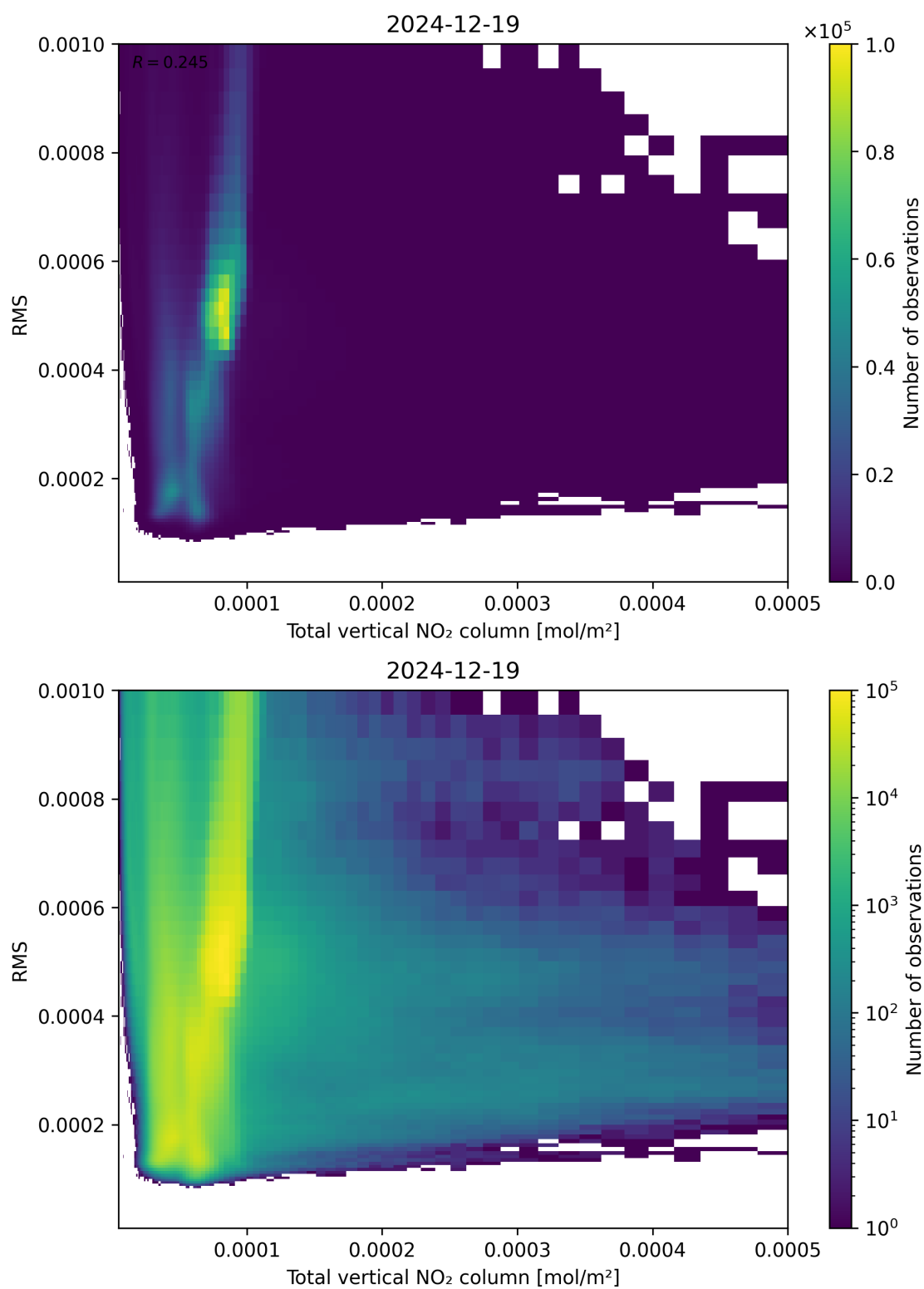
Figure 120: Scatter density plot of “Total vertical NO 2 column” against “RMS” for 2024-12-18 to 2024-12-20.
