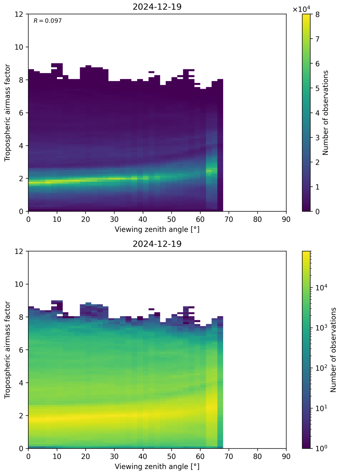
Figure 161: Scatter density plot of “Viewing zenith angle” against “Tropospheric airmass factor” for 2024-12-18 to 2024-12-20.
