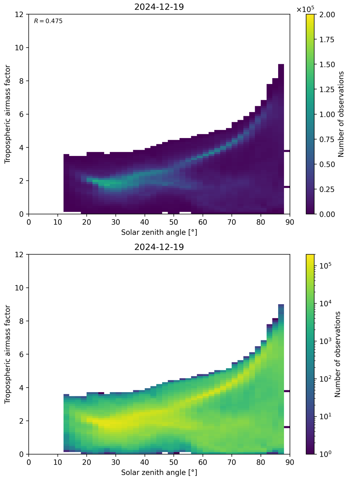
Figure 147: Scatter density plot of “Solar zenith angle” against “Tropospheric airmass factor” for 2024-12-18 to 2024-12-20.
