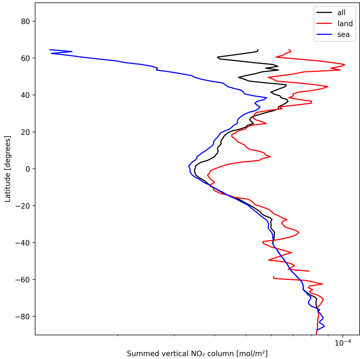
Figure 23: Zonal average of “Summed vertical NO 2 column” for 2024-12-18 to 2024-12-20.
