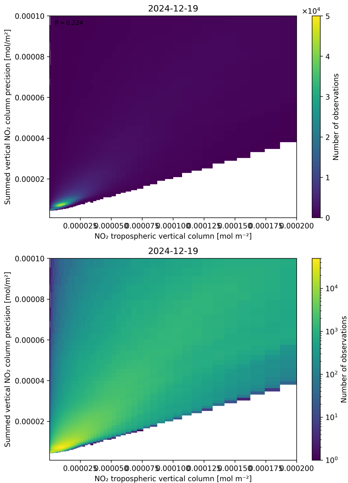
Figure 127: Scatter density plot of “NO 2 tropospheric vertical column” against “Summed vertical NO 2 column precision” for 2024-12-18 to 2024-12-20.
