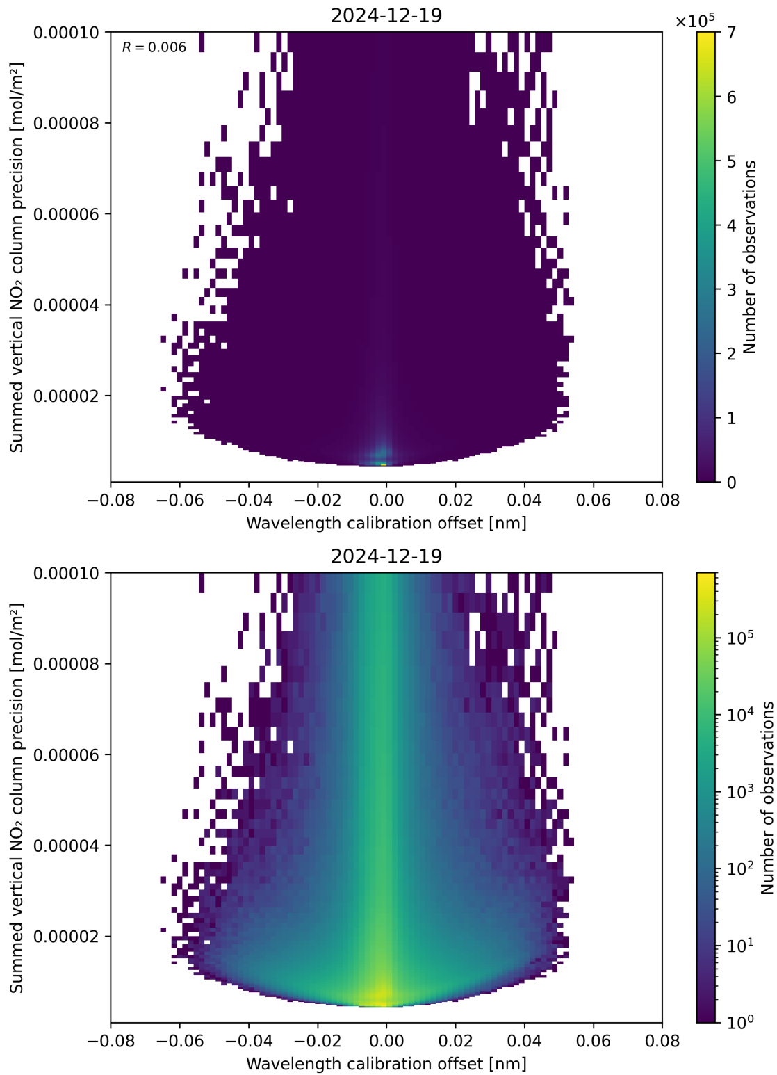
Figure 178: Scatter density plot of “Wavelength calibration offset” against “Summed vertical NO 2 column precision” for 2024-12-18 to 2024-12-20.
