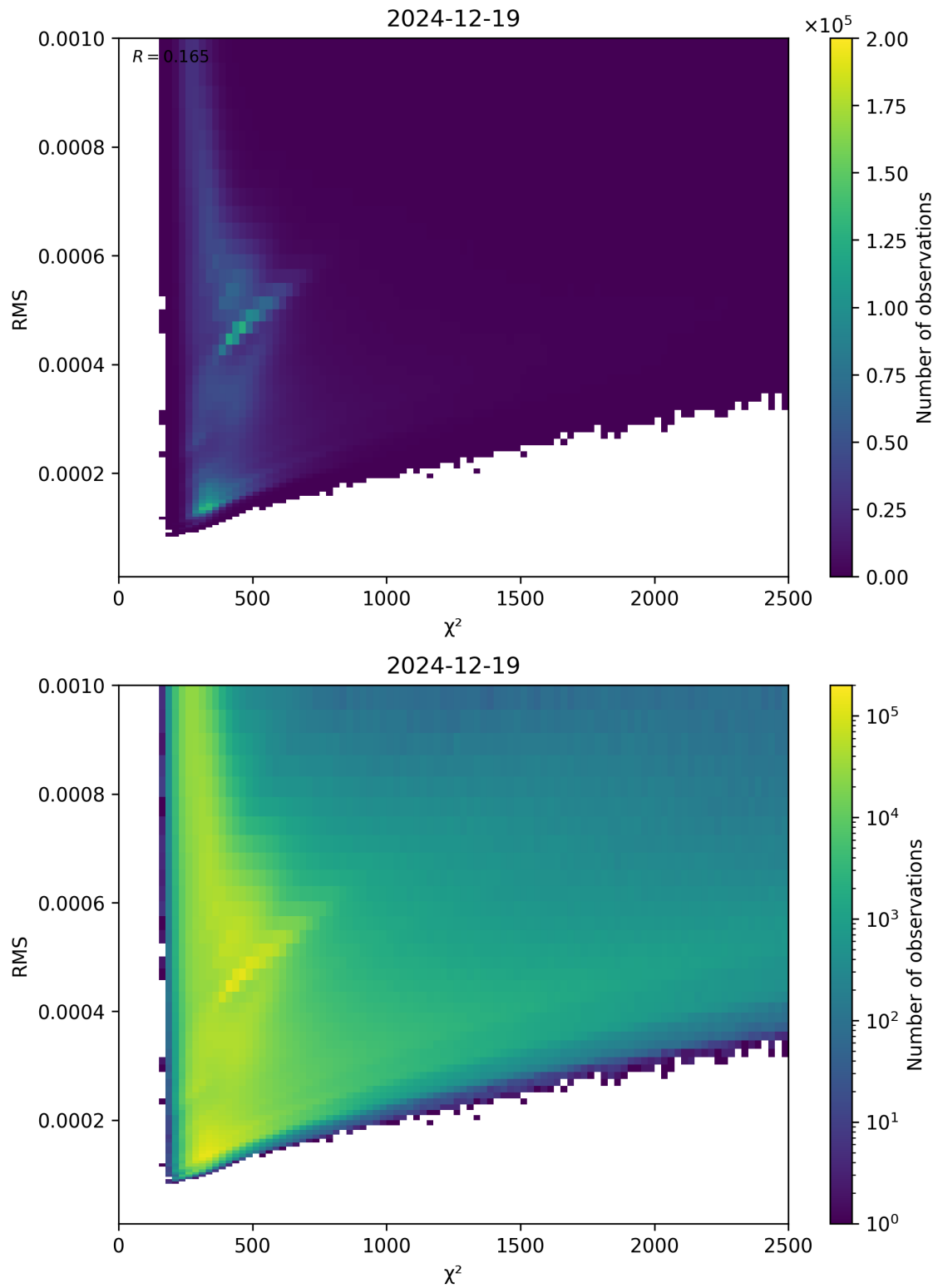
Figure 82: Scatter density plot of “ \chi^2 ” against “RMS” for 2024-12-18 to 2024-12-20.
