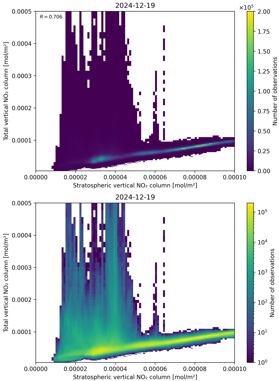
Figure 100: Scatter density plot of “Stratospheric vertical NO 2 column” against “Total vertical NO 2 column” for 2024-12-18 to 2024-12-20.
