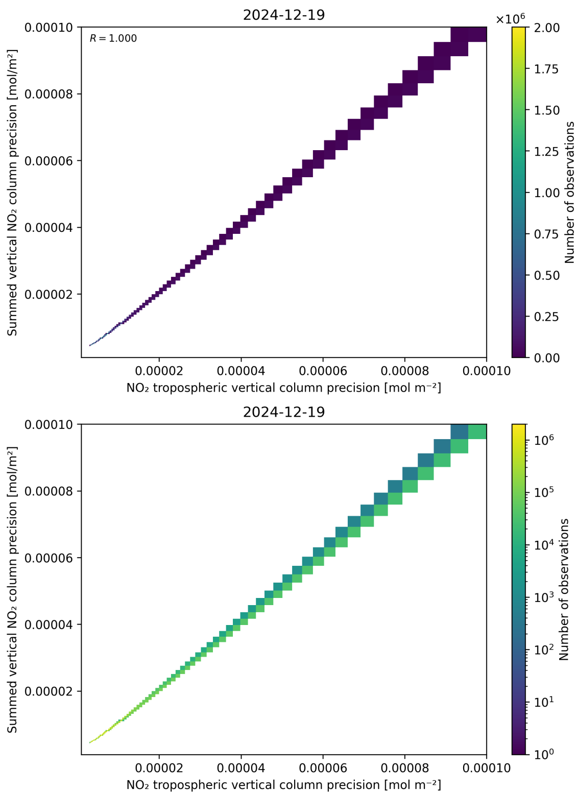
Figure 137: Scatter density plot of “NO 2 tropospheric vertical column precision” against “Summed vertical NO 2 column precision” for 2024-12-18 to 2024-12-20.
