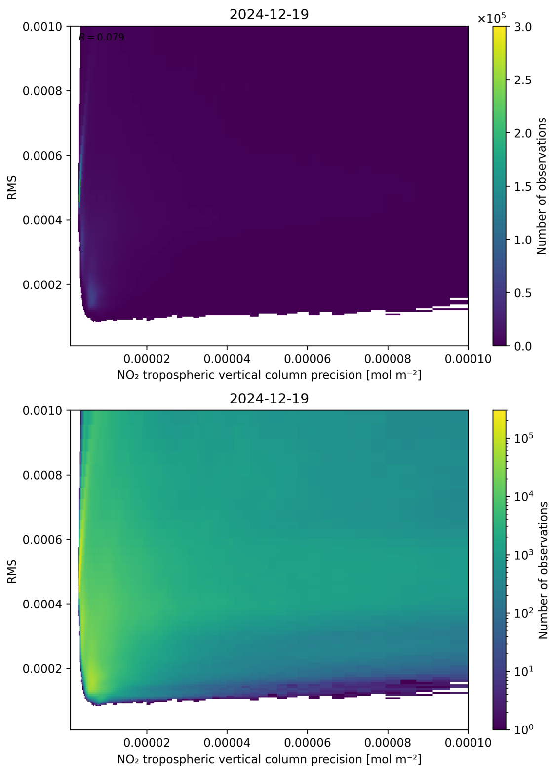
Figure 140: Scatter density plot of “NO 2 tropospheric vertical column precision” against “RMS” for 2024-12-18 to 2024-12-20.
