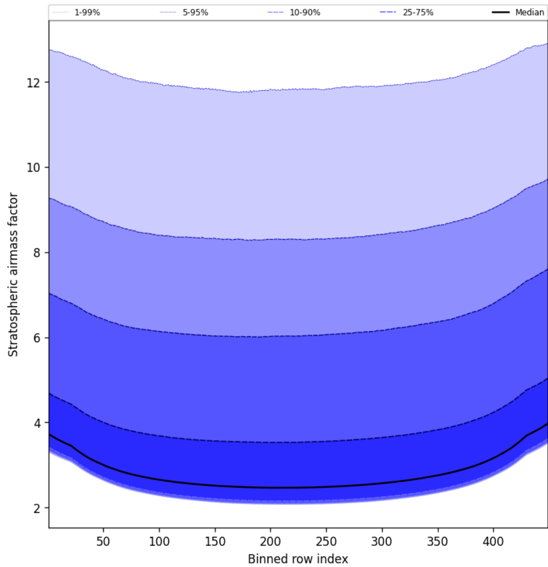
Figure 61: Along track statistics of “Stratospheric airmass factor” for 2024-12-18 to 2024-12-20
