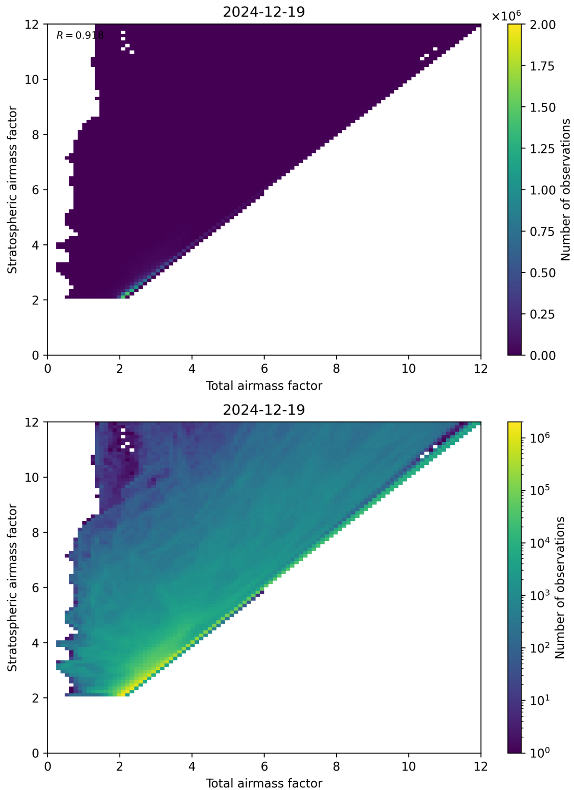
Figure 62: Scatter density plot of “Total airmass factor” against “Stratospheric airmass factor” for 2024-12-18 to 2024-12-20.
