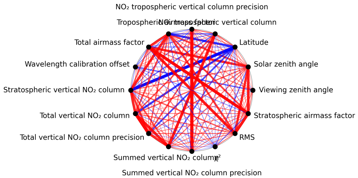
Figure 1: Map of correlation graph for 2024-12-18 to 2024-12-20.
