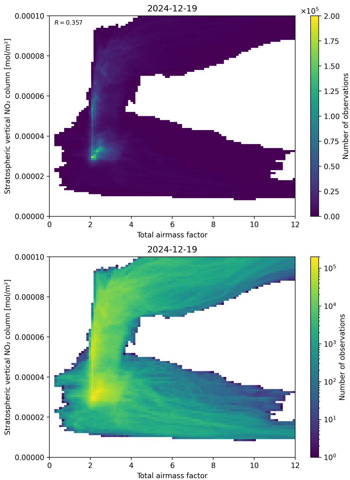
Figure 64: Scatter density plot of “Total airmass factor” against “Stratospheric vertical \text{NO}_2 column” for 2024-12-18 to 2024-12-20.
