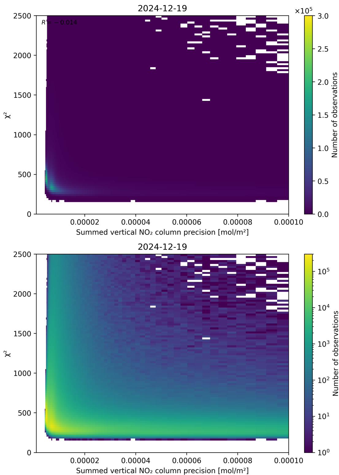
Figure 107: Scatter density plot of “Summed vertical NO 2 column precision” against “ \chi^2 ” for 2024-12-18 to 2024-12-20.
