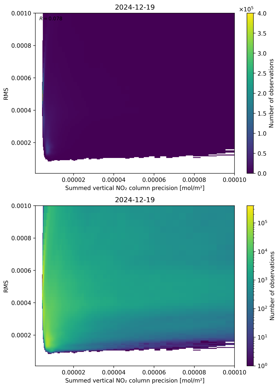
Figure 108: Scatter density plot of “Summed vertical NO 2 column precision” against “RMS” for 2024-12-18 to 2024-12-20.
