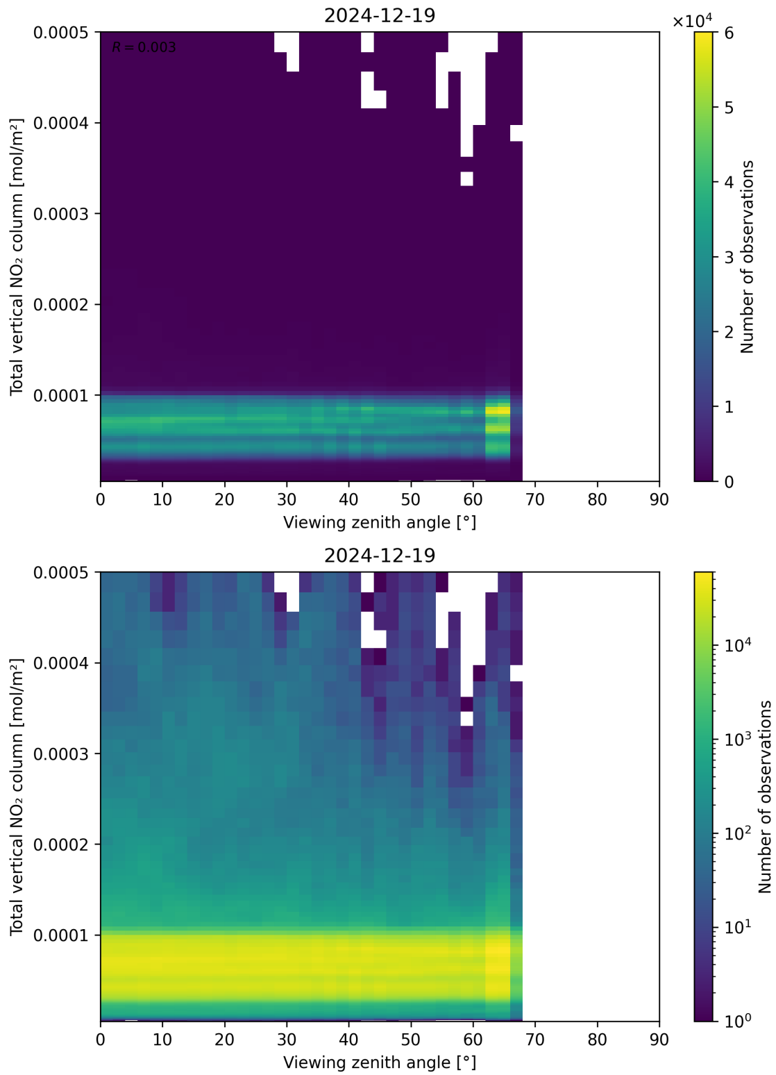
Figure 167: Scatter density plot of “Viewing zenith angle” against “Total vertical NO 2 column” for 2024-12-18 to 2024-12-20.
