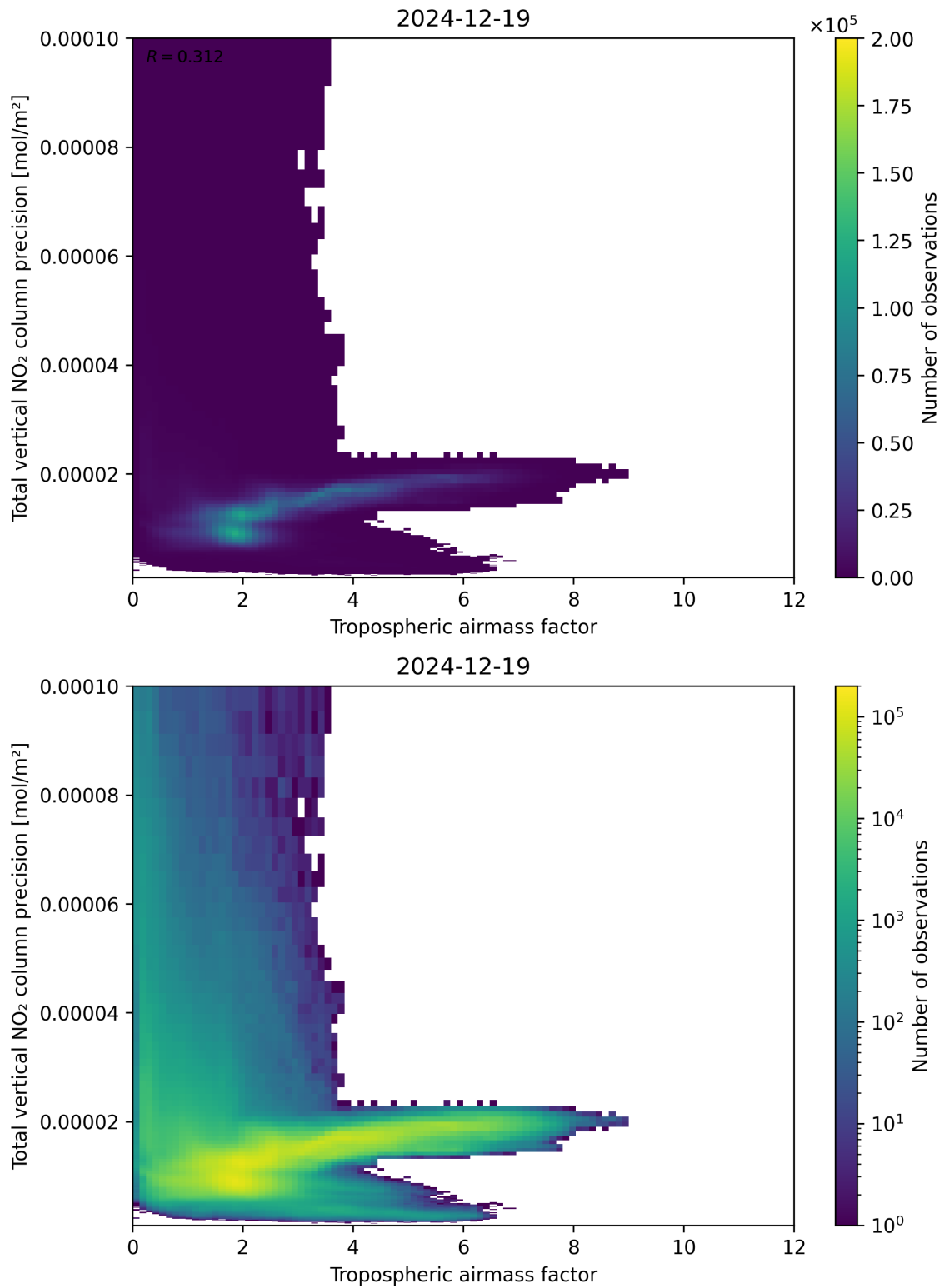
Figure 78: Scatter density plot of “Tropospheric air mass factor” against “Total vertical NO 2 column precision” for 2024-12-18 to 2024-12-20.
