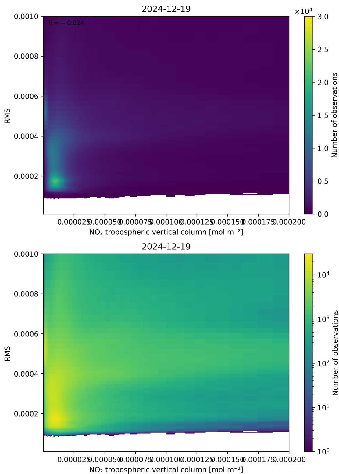
Figure 142: Scatter density plot of “NO 2 tropospheric vertical column” against “RMS” for 2024-12-18 to 2024-12-20.
