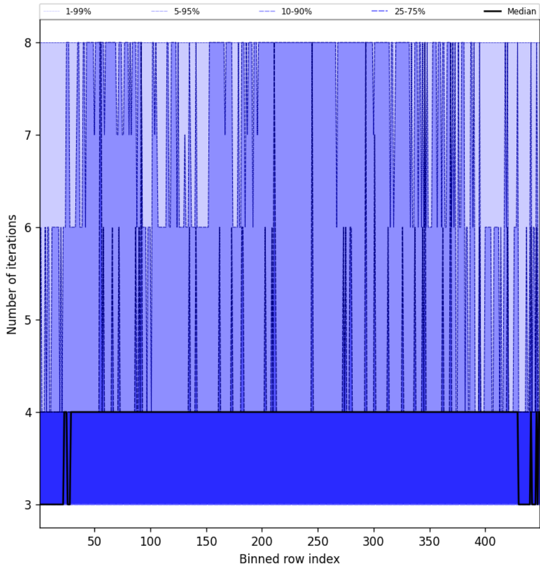
Figure 51: Along track statistics of “Number of iterations” for 2024-12-18 to 2024-12-20
