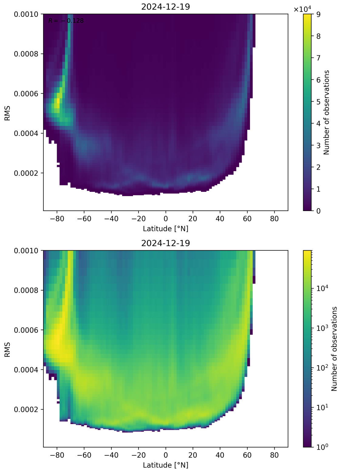
Figure 94: Scatter density plot of “Latitude” against “RMS” for 2024-12-18 to 2024-12-20.
