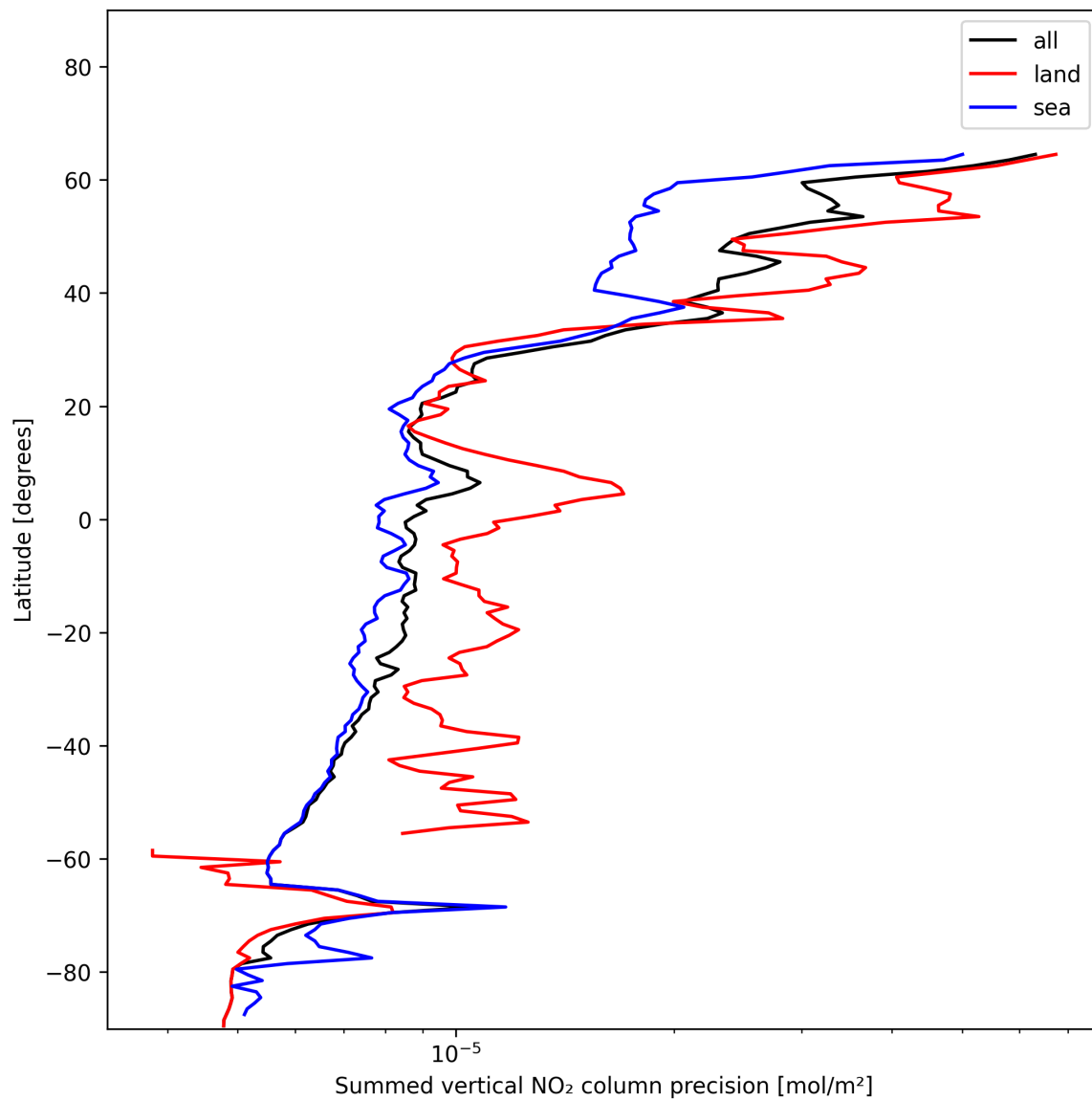
Figure 24: Zonal average of “Summed vertical NO 2 column precision” for 2024-12-18 to 2024-12-20.
