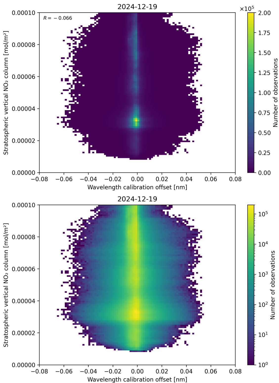
Figure 176: Scatter density plot of “Wavelength calibration offset” against “Stratospheric vertical NO 2 column” for 2024-12-18 to 2024-12-20.
