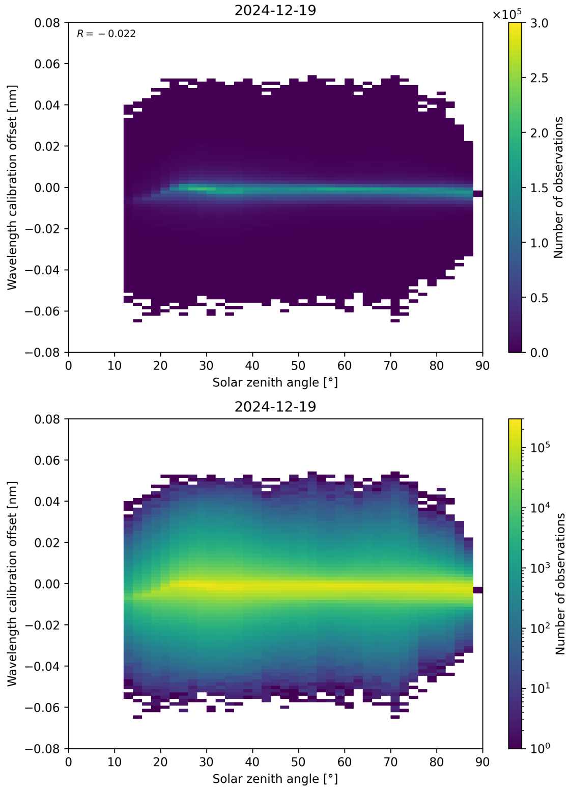
Figure 158: Scatter density plot of “Solar zenith angle” against “Wavelength calibration offset” for 2024-12-18 to 2024-12-20.
