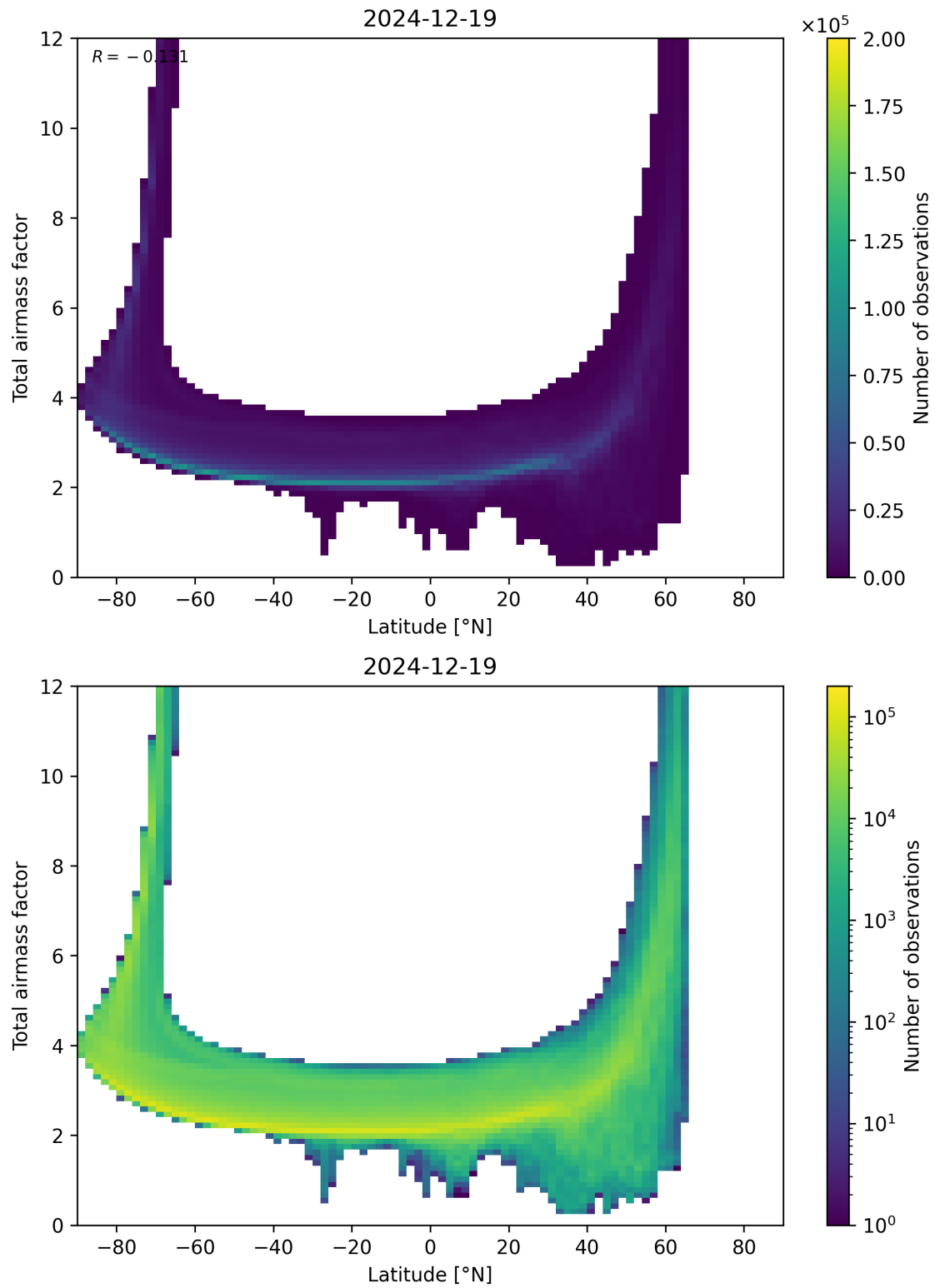
Figure 84: Scatter density plot of “Latitude” against “Total airmass factor” for 2024-12-18 to 2024-12-20.
