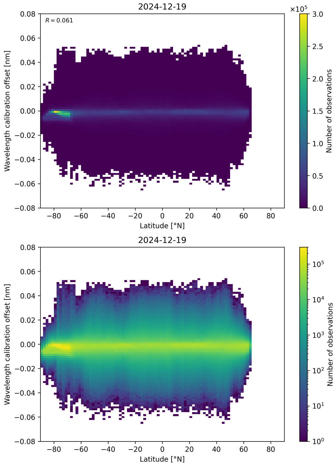
Figure 95: Scatter density plot of “Latitude” against “Wavelength calibration offset” for 2024-12-18 to 2024-12-20.
