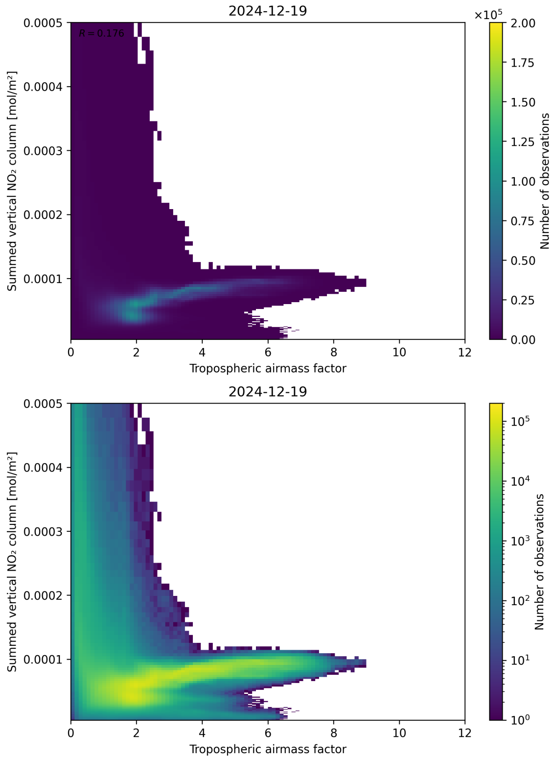
Figure 75: Scatter density plot of “Tropospheric air mass factor” against “Summed vertical NO 2 column” for 2024-12-18 to 2024-12-20.
