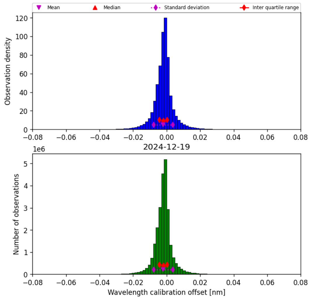
Figure 35: Histogram of "Wavelength calibration offset" for 2024-12-18 to 2024-12-20
