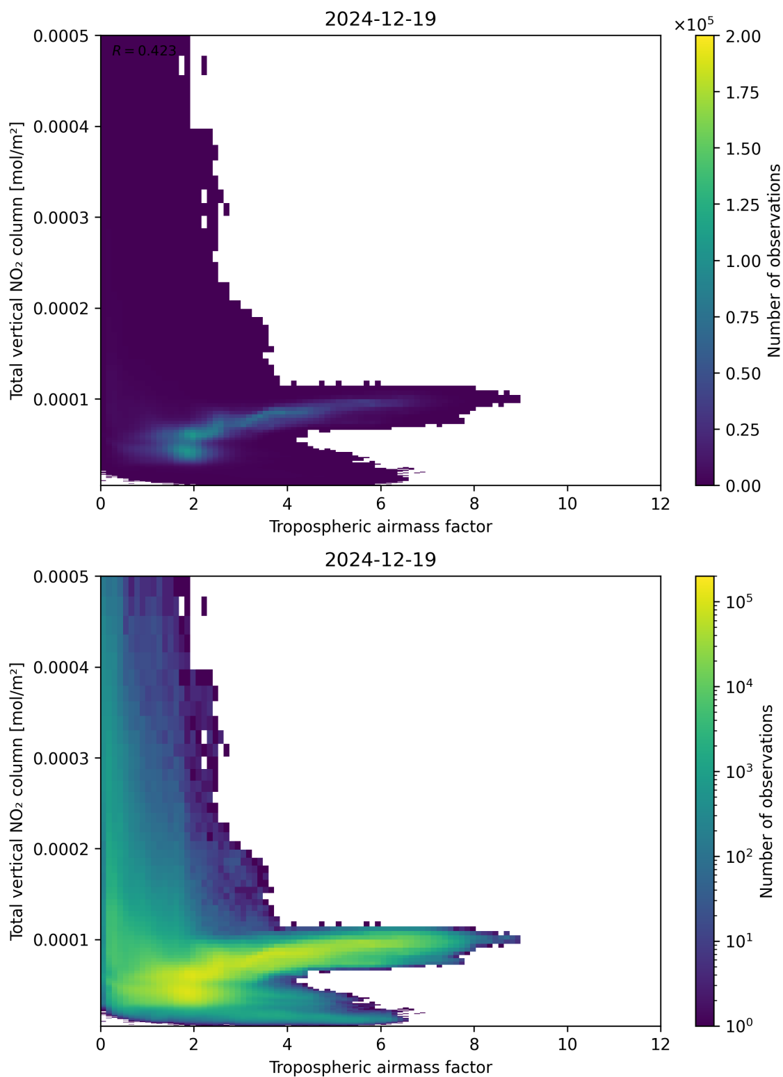
Figure 77: Scatter density plot of “Tropospheric airmass factor” against “Total vertical NO 2 column” for 2024-12-18 to 2024-12-20.
