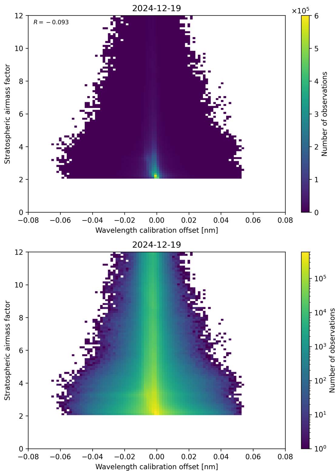
Figure 174: Scatter density plot of “Wavelength calibration offset” against “Stratospheric airmass factor” for 2024-12-18 to 2024-12-20.
