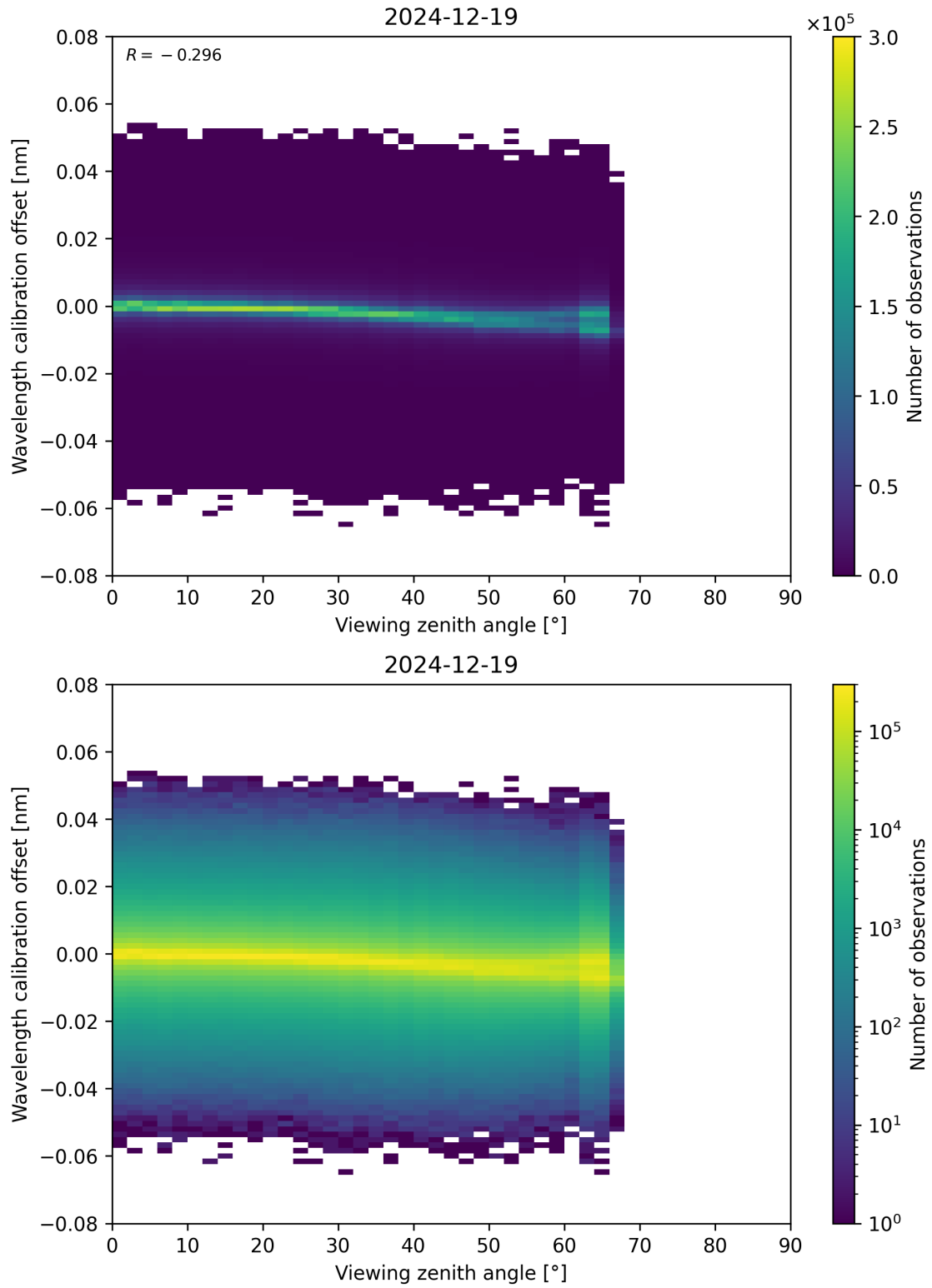
Figure 173: Scatter density plot of “Viewing zenith angle” against “Wavelength calibration offset” for 2024-12-18 to 2024-12-20.
