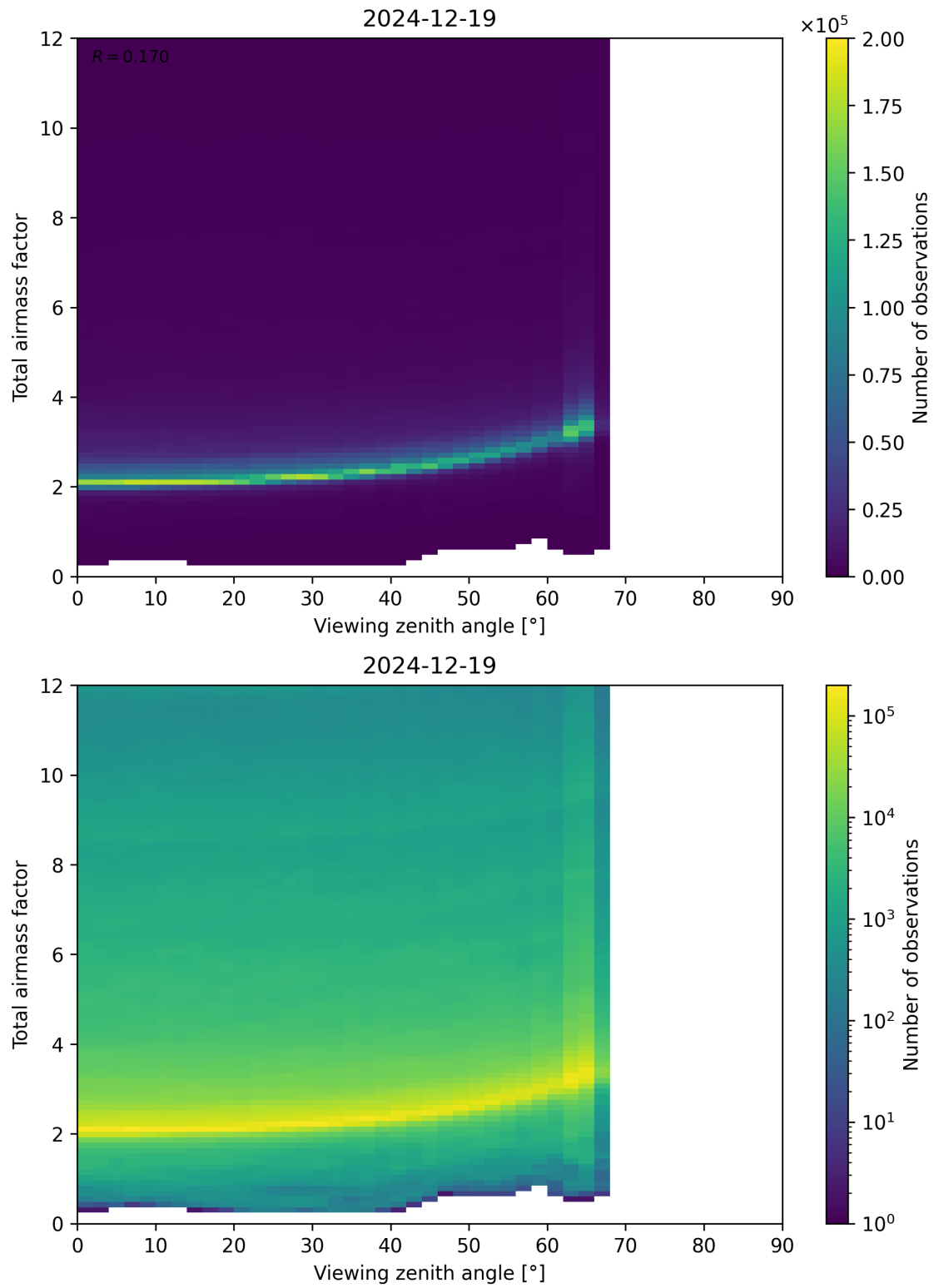
Figure 160: Scatter density plot of “Viewing zenith angle” against “Total airmass factor” for 2024-12-18 to 2024-12-20.
