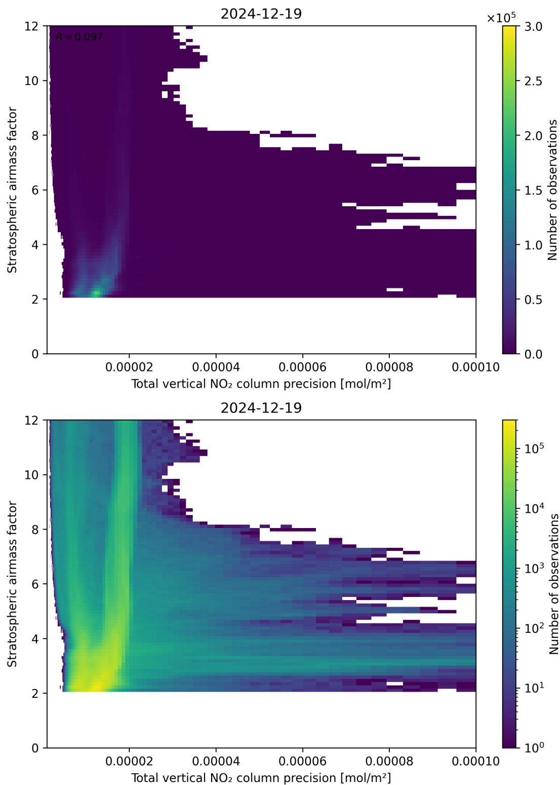
Figure 115: Scatter density plot of “Total vertical NO 2 column precision” against “Stratospheric air mass factor” for 2024-12-18 to 2024-12-20.
