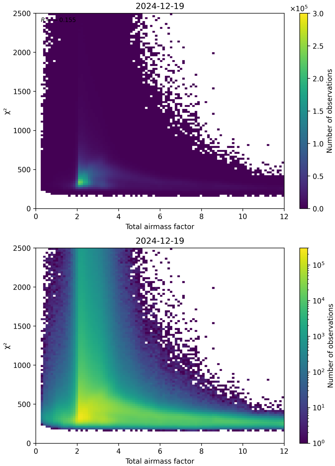
Figure 63: Scatter density plot of “Total airmass factor” against “ \chi^2 ” for 2024-12-18 to 2024-12-20.
