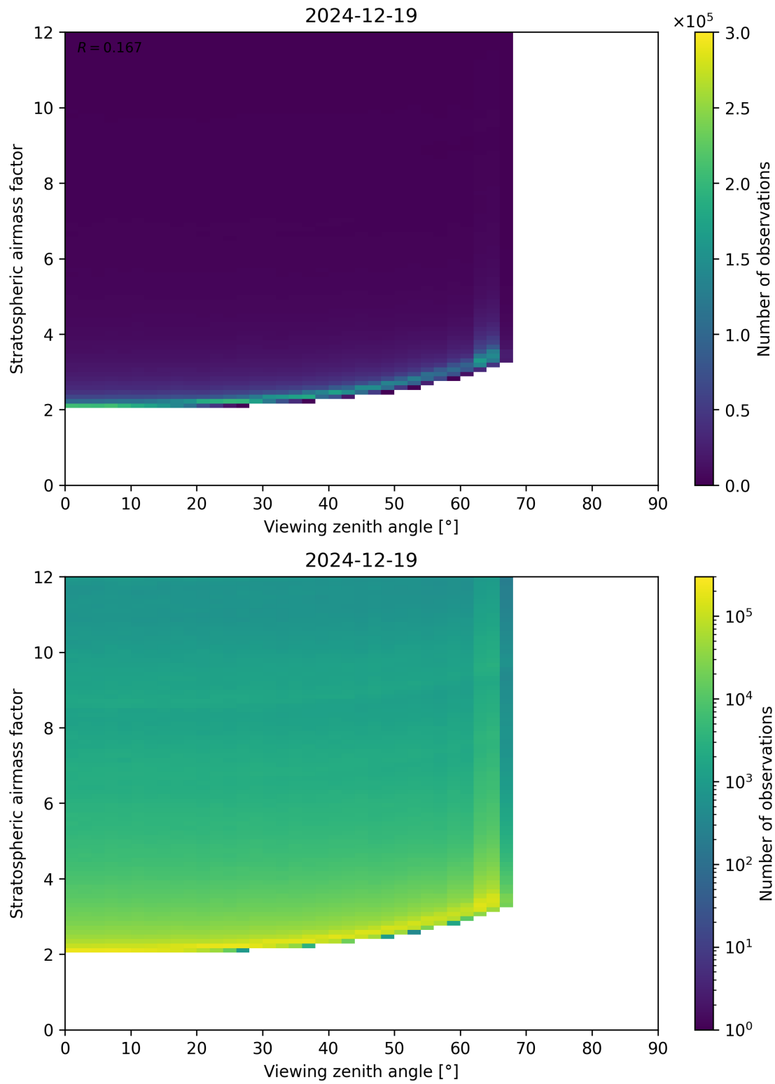
Figure 159: Scatter density plot of “Viewing zenith angle” against “Stratospheric airmass factor” for 2024-12-18 to 2024-12-20.
