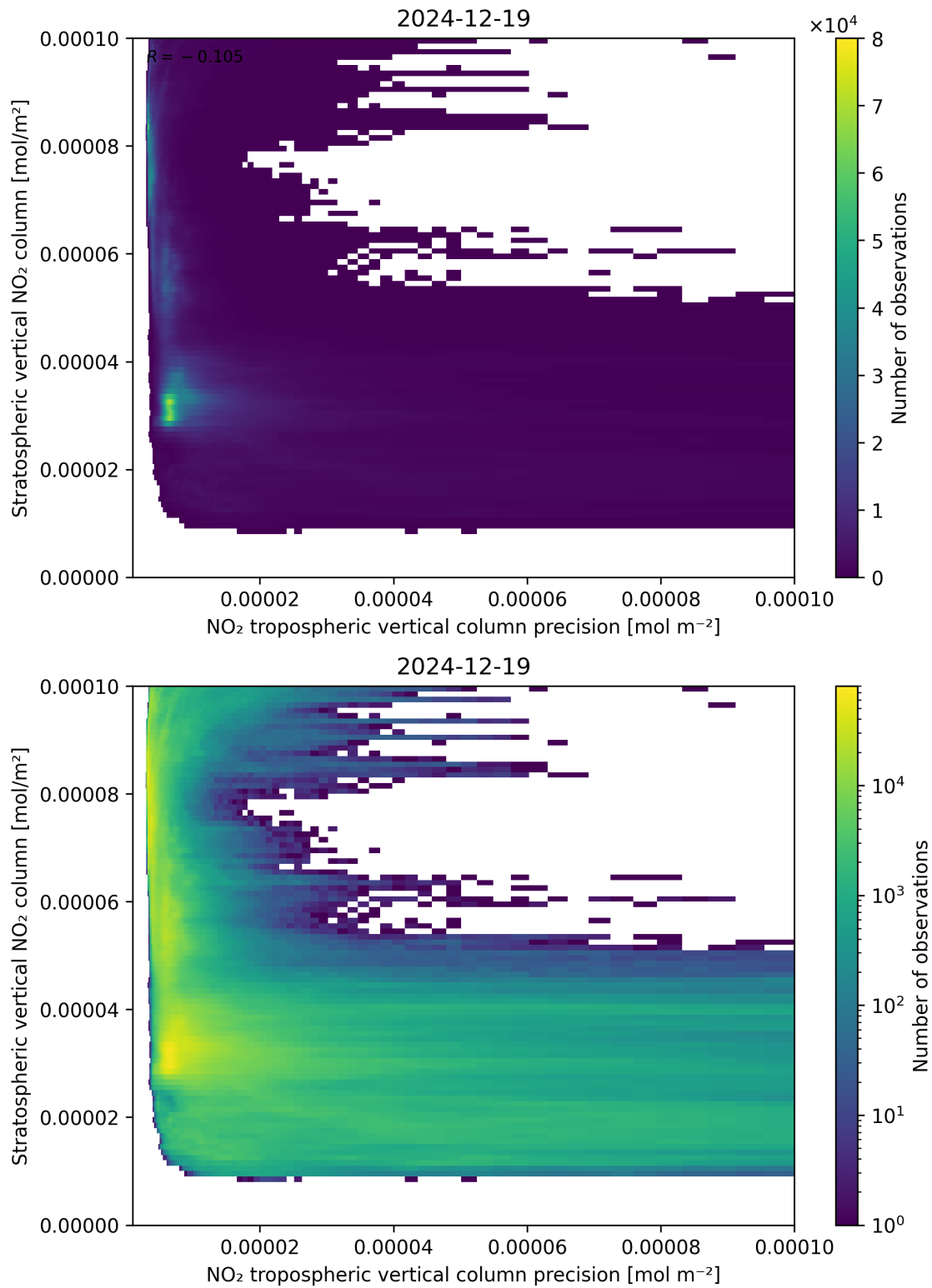
Figure 135: Scatter density plot of “NO 2 tropospheric vertical column precision” against “Stratospheric vertical NO 2 column” for 2024-12-18 to 2024-12-20.
