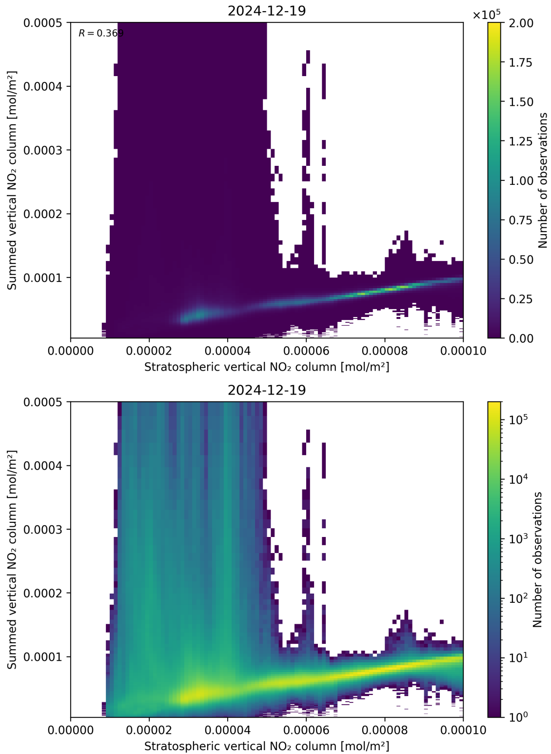
Figure 98: Scatter density plot of “Stratospheric vertical NO 2 column” against “Summed vertical NO 2 column” for 2024-12-18 to 2024-12-20.
