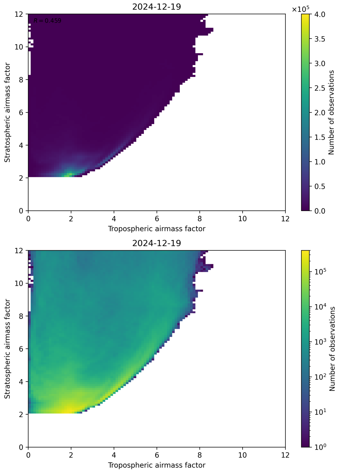
Figure 71: Scatter density plot of “Tropospheric airmass factor” against “Stratospheric airmass factor” for 2024-12-18 to 2024-12-20.
