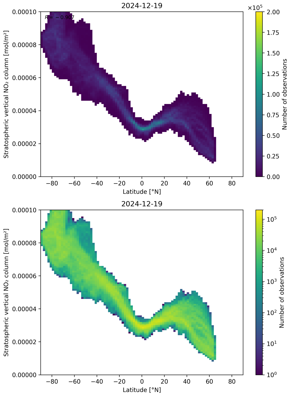
Figure 87: Scatter density plot of “Latitude” against “Stratospheric vertical NO 2 column” for 2024-12-18 to 2024-12-20.
