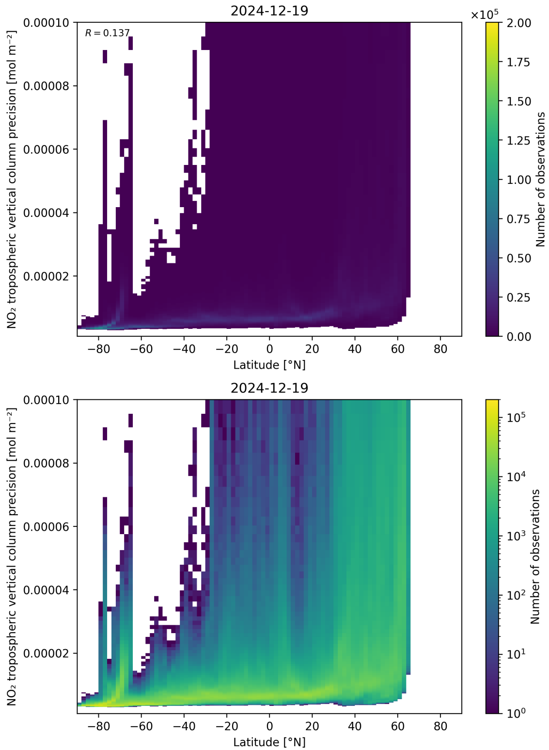
Figure 93: Scatter density plot of “Latitude” against “NO 2 tropospheric vertical column precision” for 2024-12-18 to 2024-12-20.
