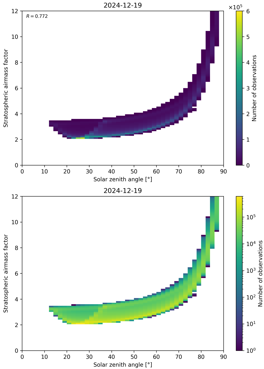
Figure 145: Scatter density plot of “Solar zenith angle” against “Stratospheric airmass factor” for 2024-12-18 to 2024-12-20.
