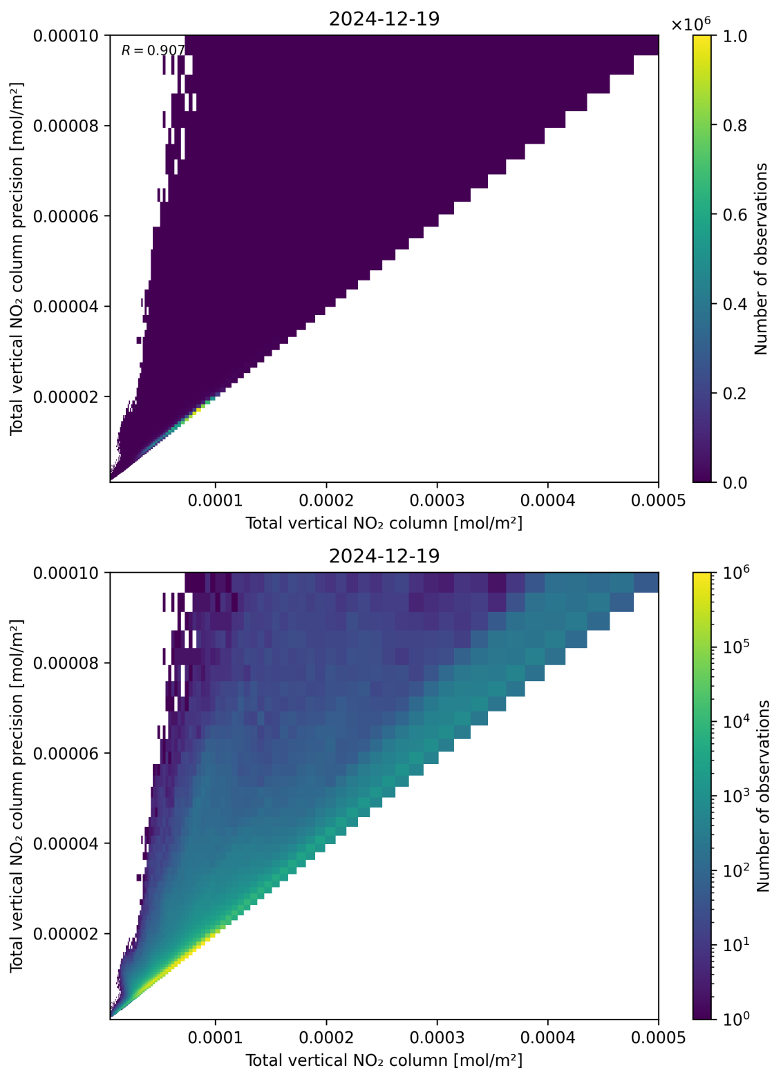
Figure 114: Scatter density plot of “Total vertical NO 2 column” against “Total vertical NO 2 column precision” for 2024-12-18 to 2024-12-20.
