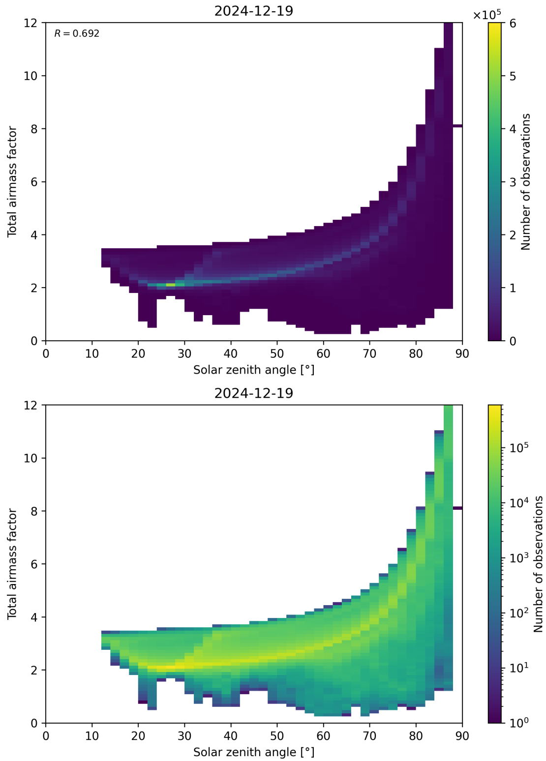
Figure 146: Scatter density plot of “Solar zenith angle” against “Total airmass factor” for 2024-12-18 to 2024-12-20.
