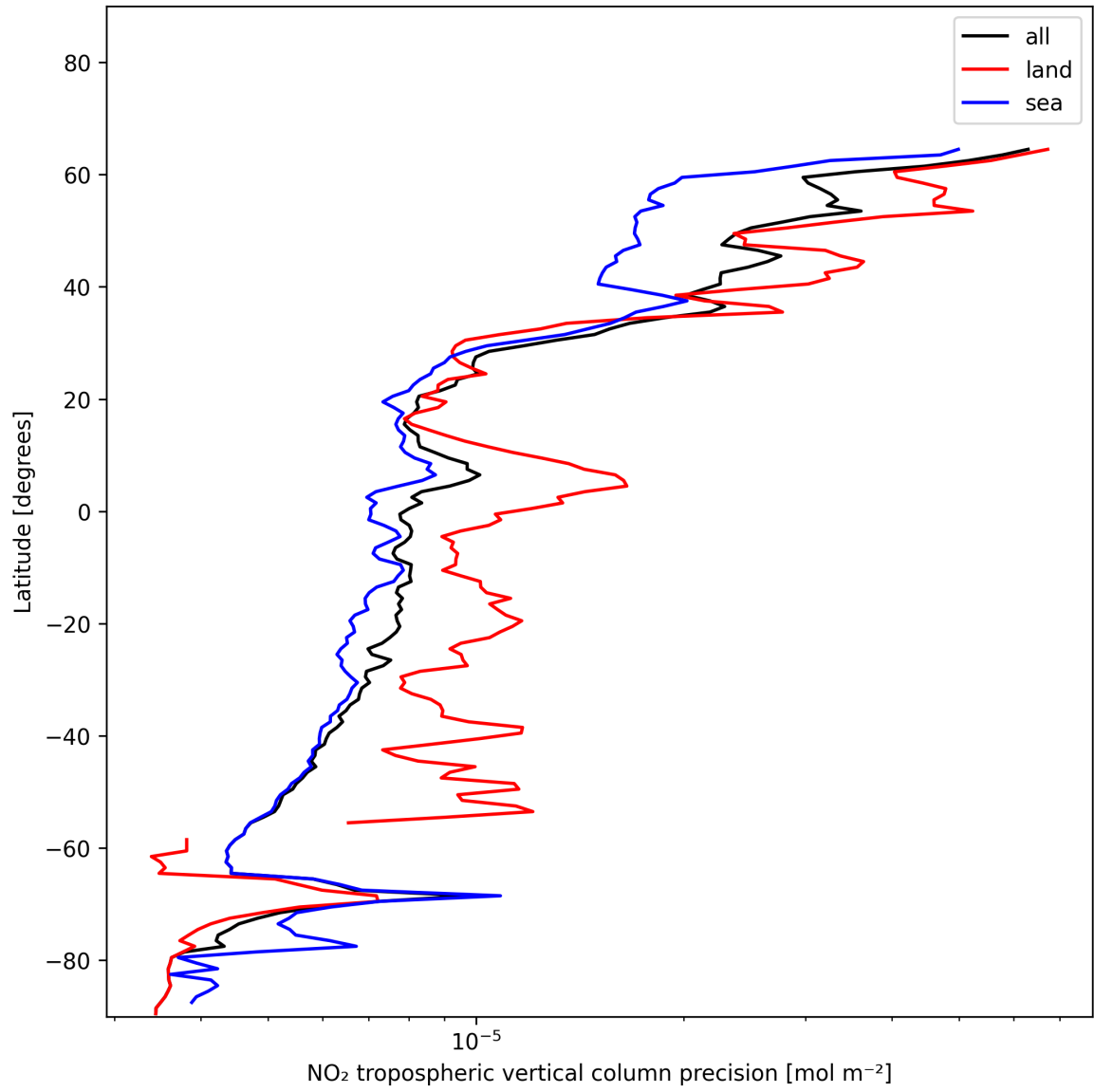
Figure 13: Zonal average of “NO 2 tropospheric vertical column precision” for 2024-12-18 to 2024-12-20.
