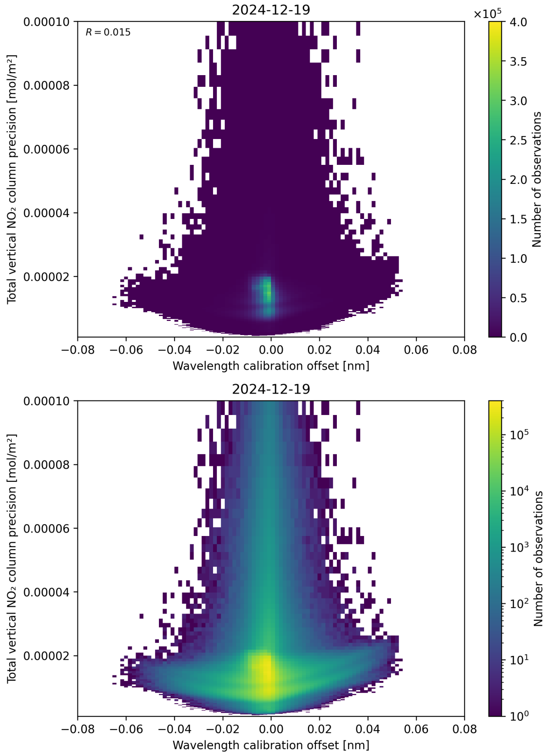
Figure 180: Scatter density plot of “Wavelength calibration offset” against “Total vertical NO 2 column precision” for 2024-12-18 to 2024-12-20.
