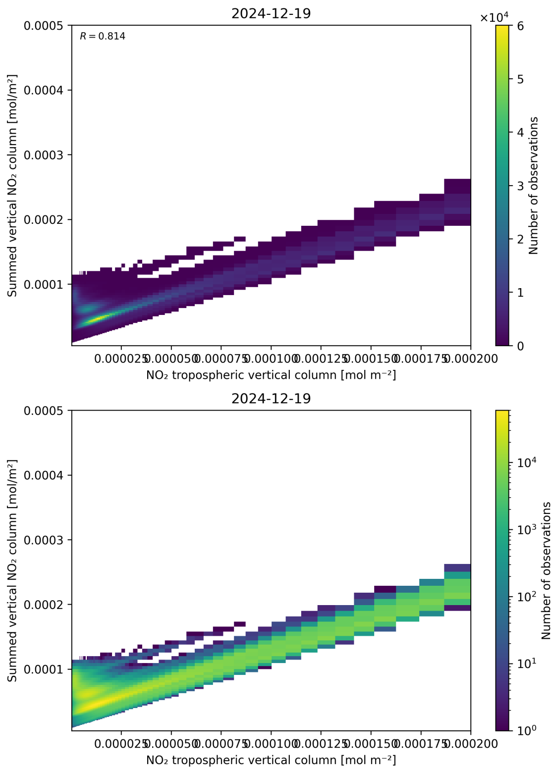
Figure 126: Scatter density plot of “NO 2 tropospheric vertical column” against “Summed vertical NO 2 column” for 2024-12-18 to 2024-12-20.
