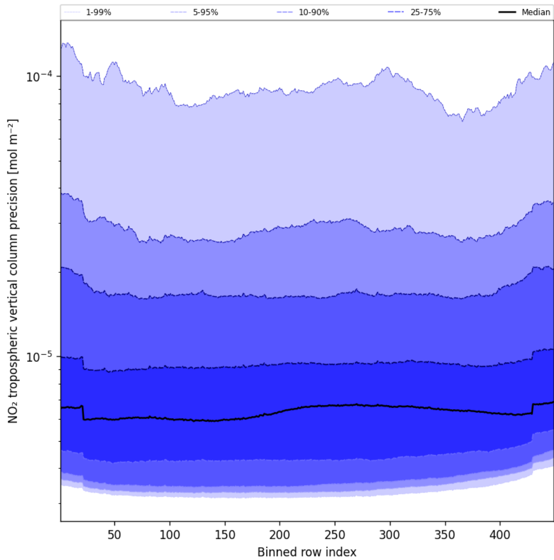
Figure 47: Along track statistics of “NO 2 tropospheric vertical column precision” for 2024-12-18 to 2024-12-20
