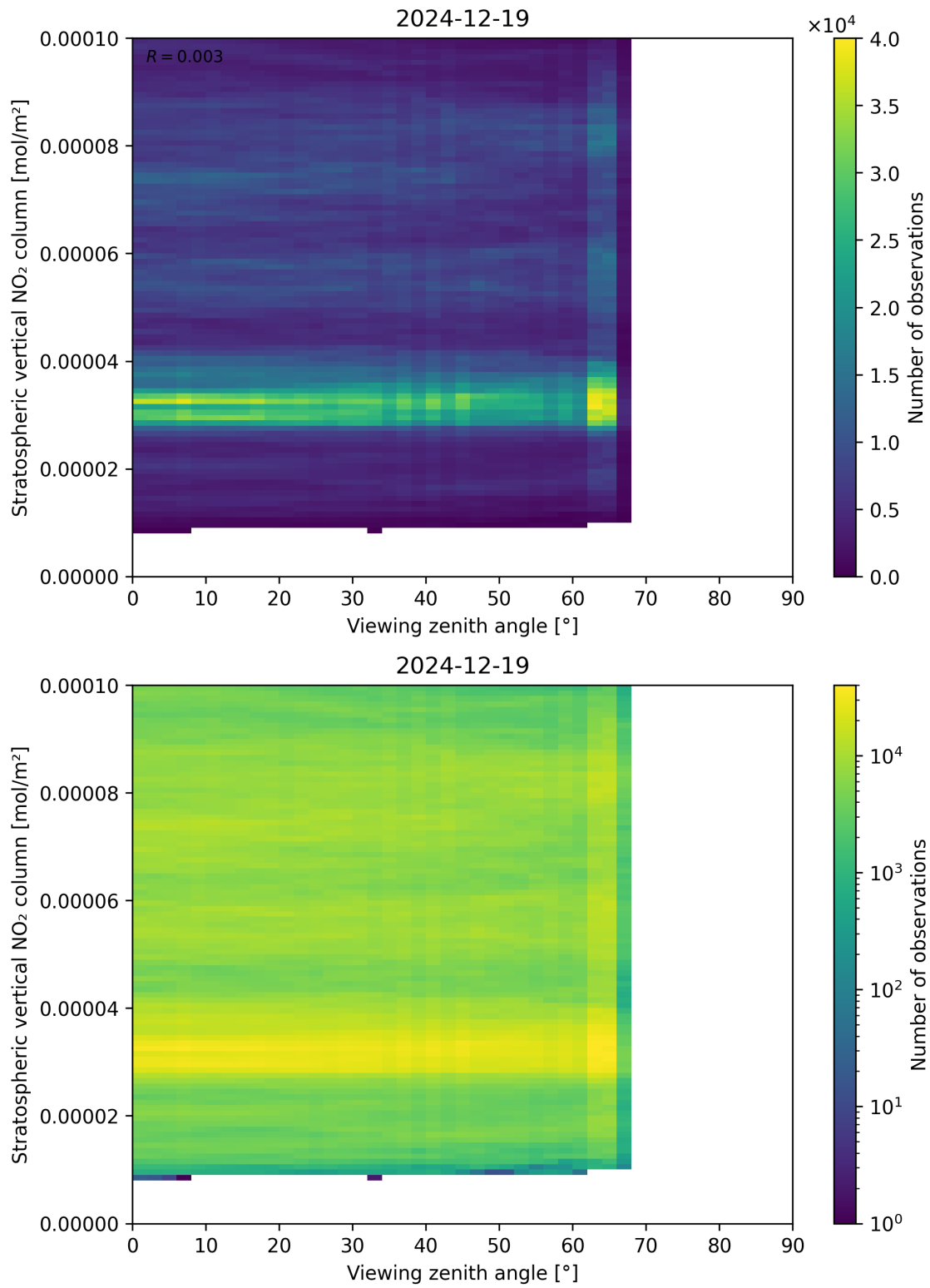
Figure 164: Scatter density plot of “Viewing zenith angle” against “Stratospheric vertical NO 2 column” for 2024-12-18 to 2024-12-20.
