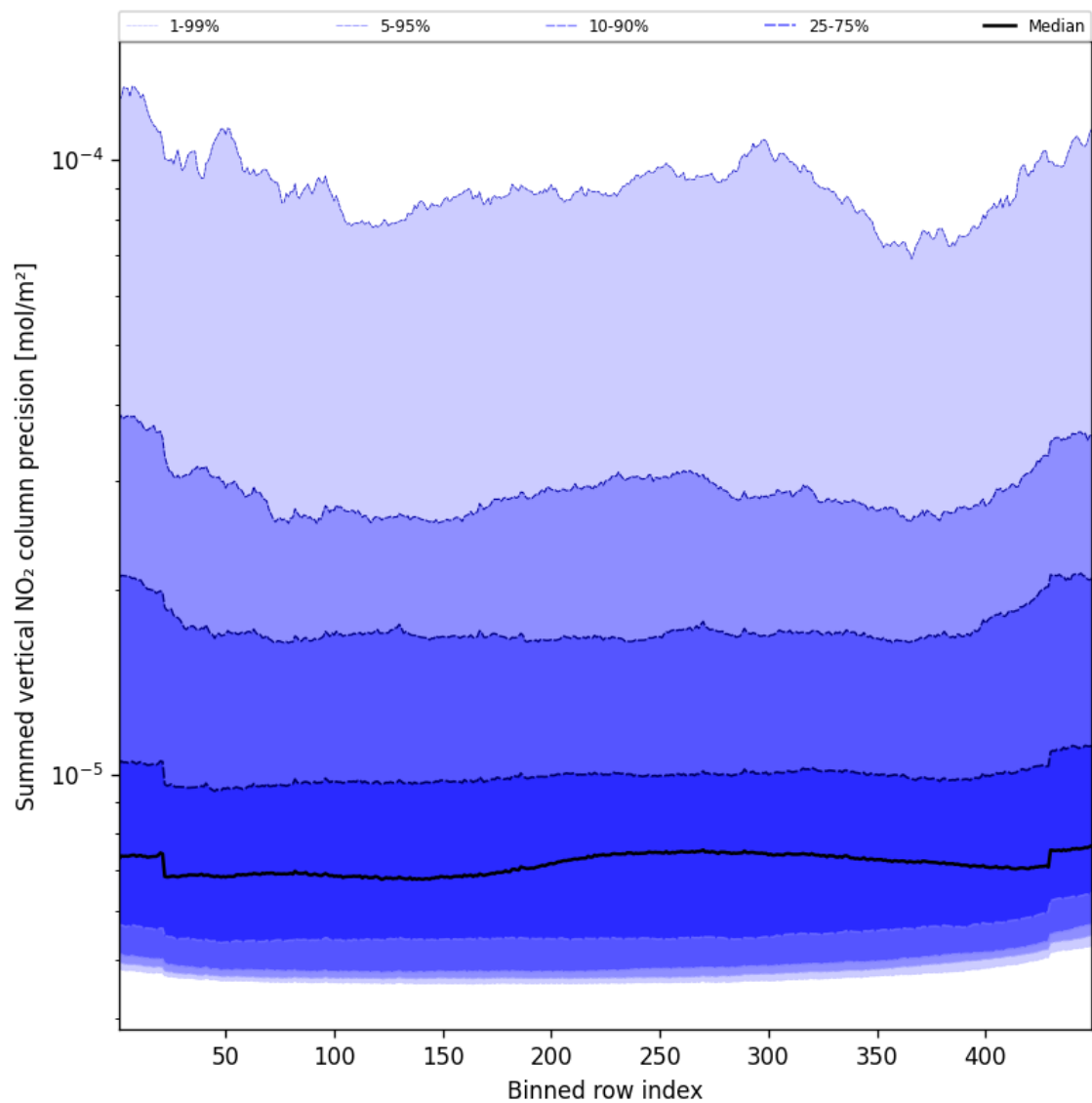
Figure 58: Along track statistics of “Summed vertical NO 2 column precision” for 2024-12-18 to 2024-12-20
