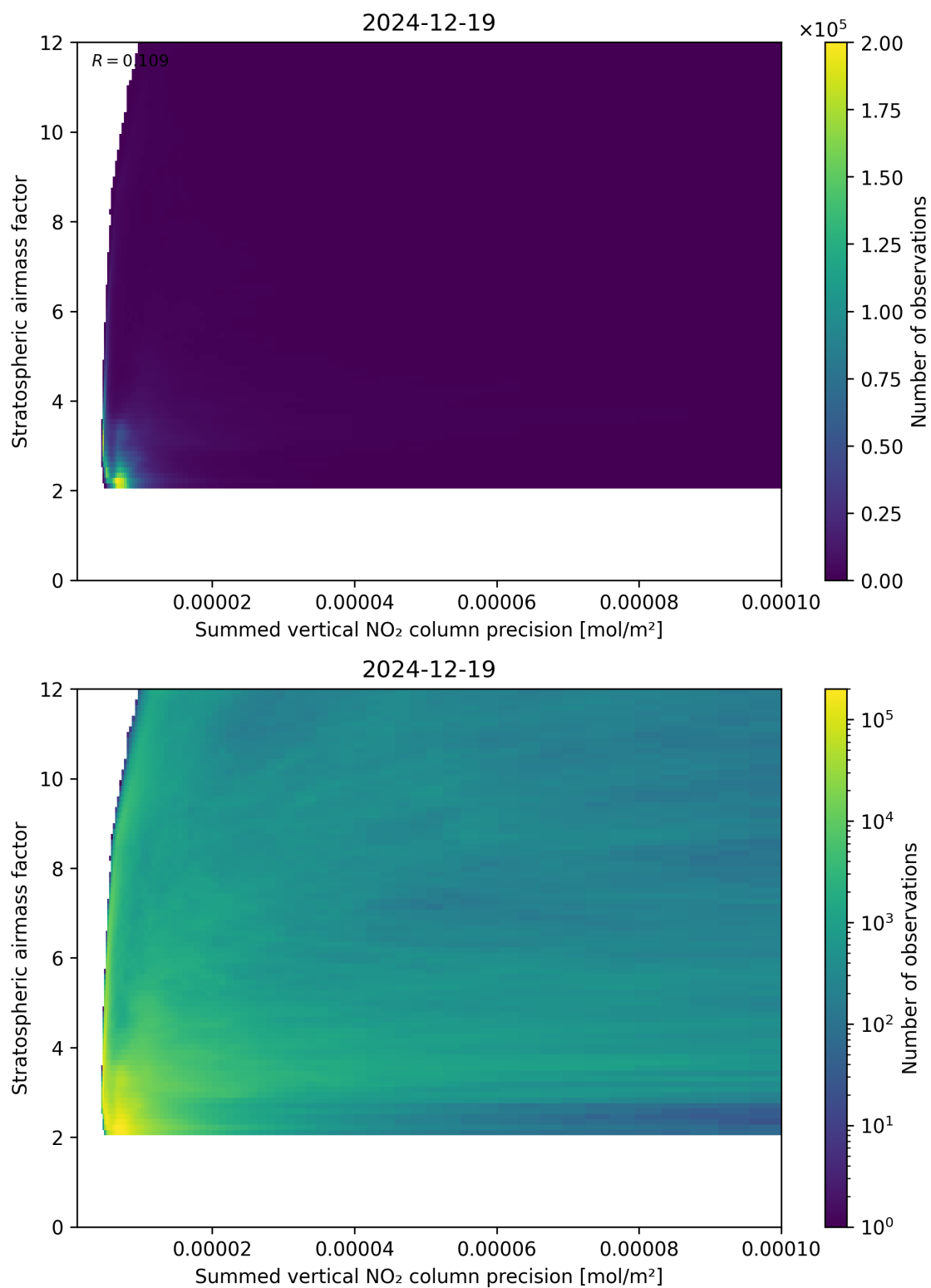
Figure 106: Scatter density plot of “Summed vertical NO 2 column precision” against “Stratospheric airmass factor” for 2024-12-18 to 2024-12-20.
