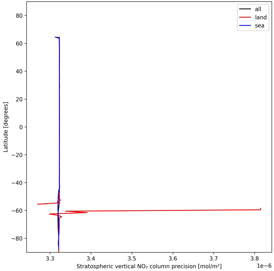
Figure 20: Zonal average of “Stratospheric vertical NO 2 column precision” for 2024-12-18 to 2024-12-20.
