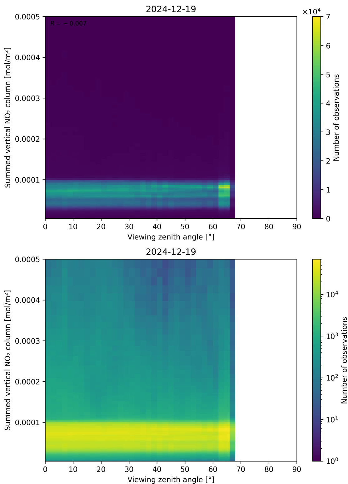
Figure 165: Scatter density plot of “Viewing zenith angle” against “Summed vertical NO 2 column” for 2024-12-18 to 2024-12-20.
