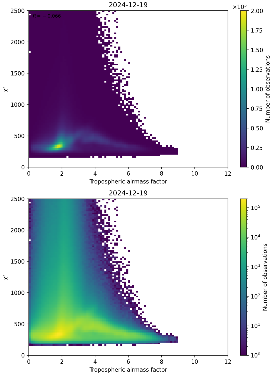
Figure 73: Scatter density plot of “Tropospheric airmass factor” against “ \chi^2 ” for 2024-12-18 to 2024-12-20.
