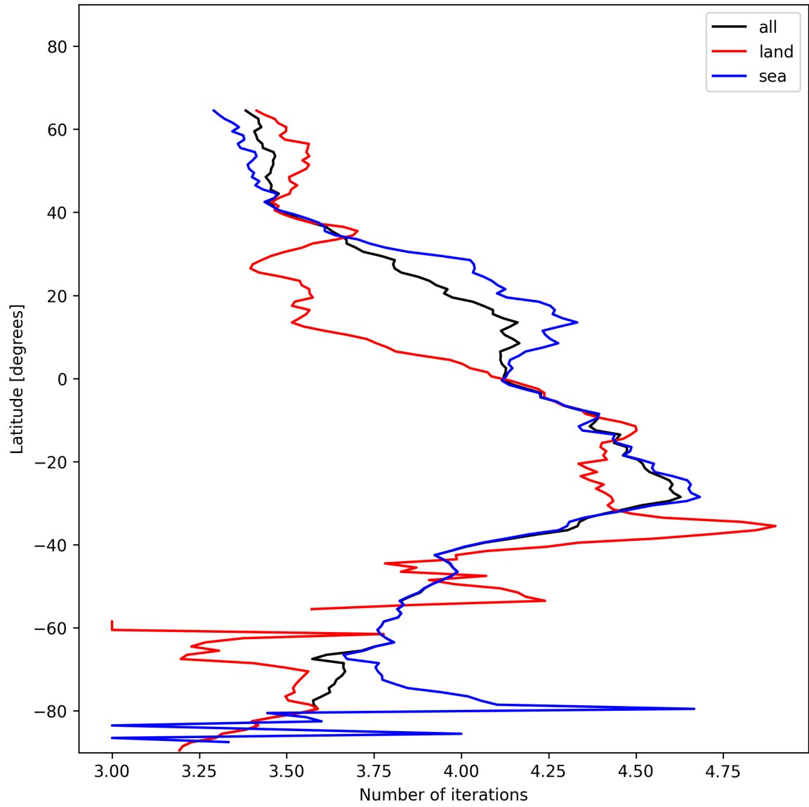
Figure 17: Zonal average of “Number of iterations” for 2024-12-18 to 2024-12-20.
