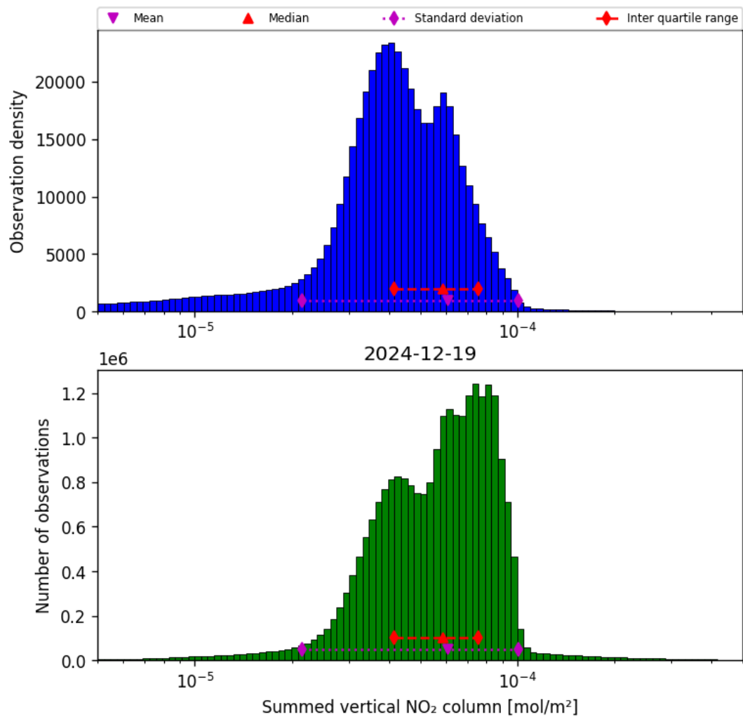
Figure 40: Histogram of “Summed vertical NO 2 column” for 2024-12-18 to 2024-12-20
