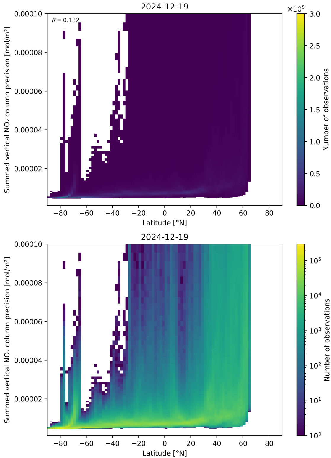
Figure 89: Scatter density plot of “Latitude” against “Summed vertical NO 2 column precision” for 2024-12-18 to 2024-12-20.
