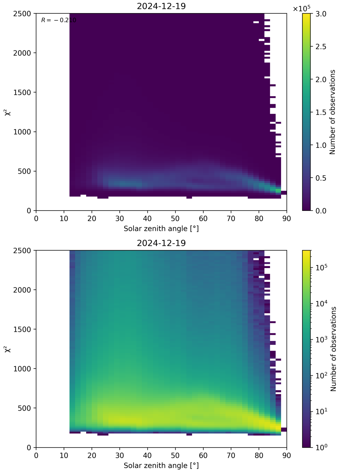
Figure 148: Scatter density plot of “Solar zenith angle” against “ \chi^2 ” for 2024-12-18 to 2024-12-20.
