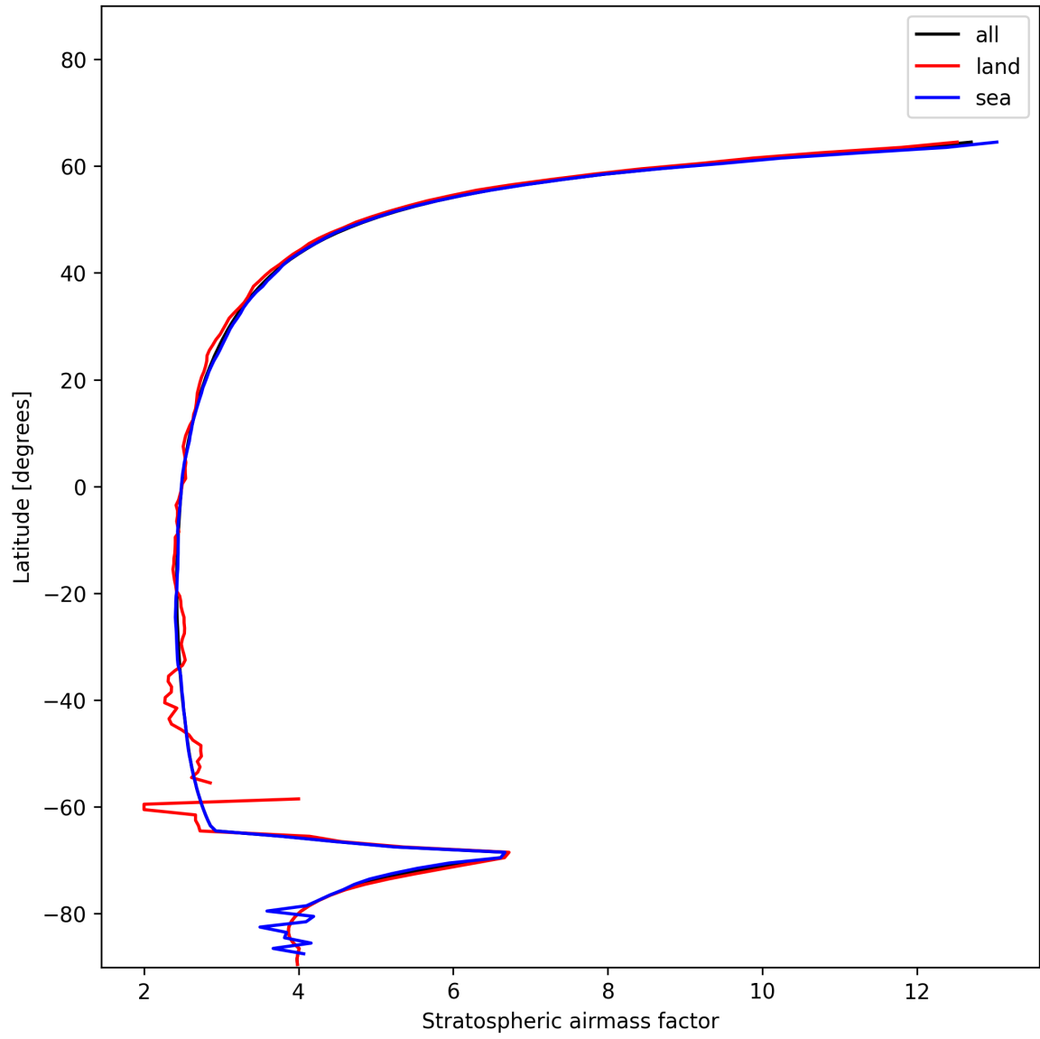
Figure 27: Zonal average of “Stratospheric airmass factor” for 2024-12-18 to 2024-12-20.
