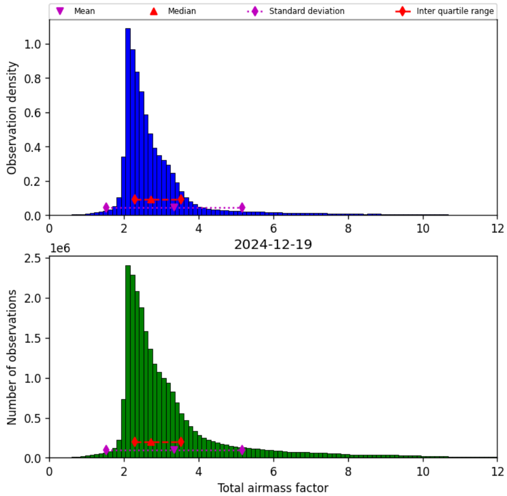
Figure 32: Histogram of “Total airmass factor” for 2024-12-18 to 2024-12-20
