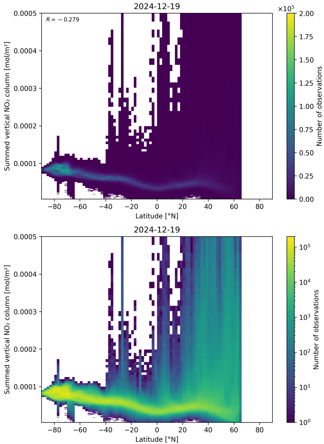
Figure 88: Scatter density plot of “Latitude” against “Summed vertical NO 2 column” for 2024-12-18 to 2024-12-20.
