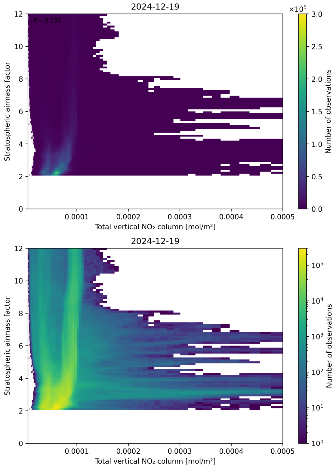
Figure 110: Scatter density plot of “Total vertical NO 2 column” against “Stratospheric air mass factor” for 2024-12-18 to 2024-12-20.
