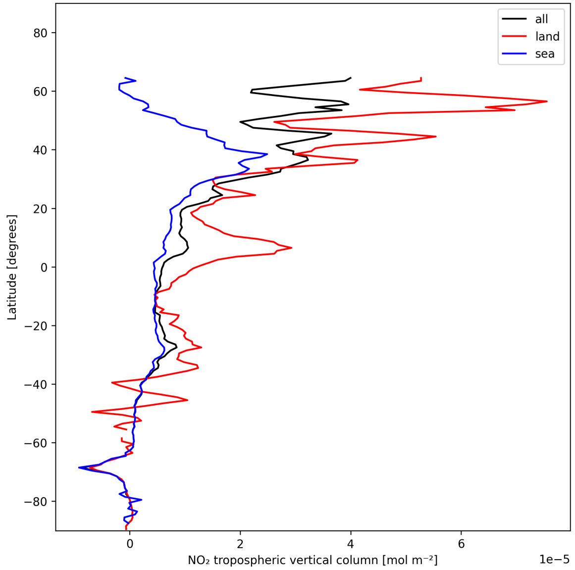
Figure 12: Zonal average of “NO 2 tropospheric vertical column” for 2024-12-18 to 2024-12-20.
