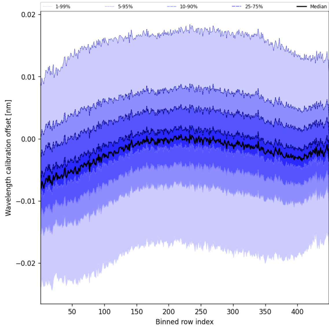
Figure 52: Along track statistics of “Wavelength calibration offset” for 2024-12-18 to 2024-12-20
