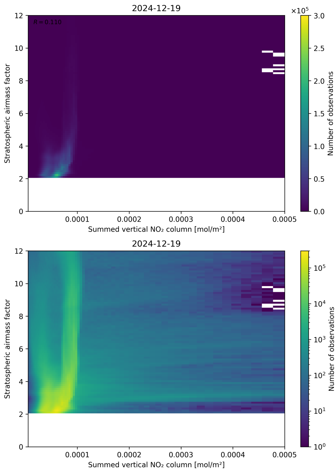
Figure 103: Scatter density plot of “Summed vertical NO 2 column” against “Stratospheric airmass factor” for 2024-12-18 to 2024-12-20.
