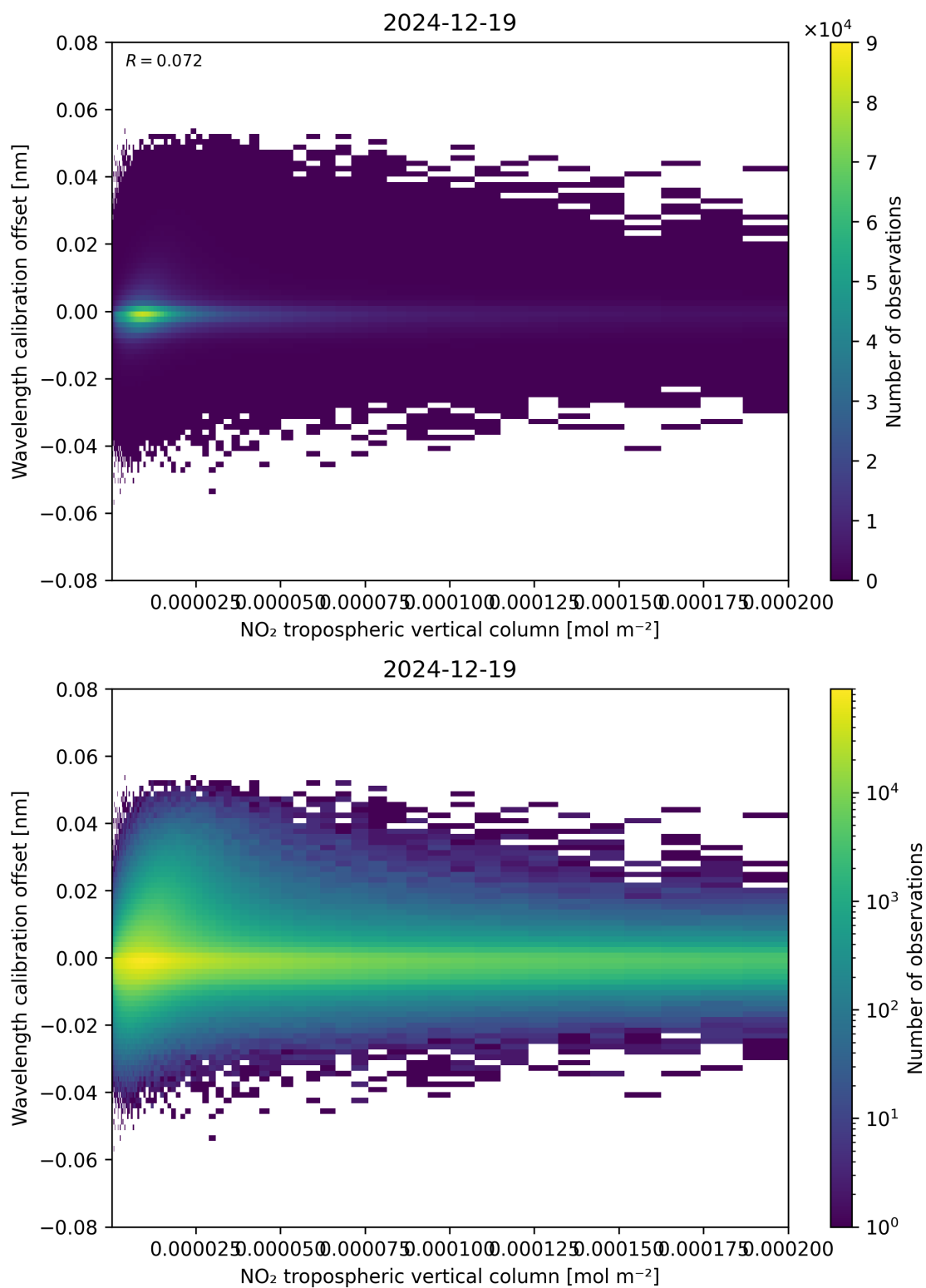
Figure 143: Scatter density plot of “NO 2 tropospheric vertical column” against “Wavelength calibration offset” for 2024-12-18 to 2024-12-20.
