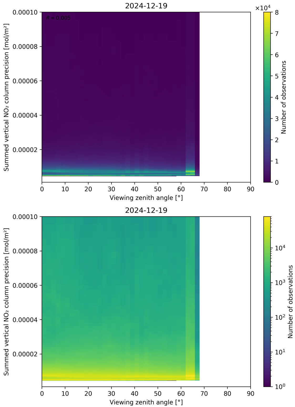
Figure 166: Scatter density plot of “Viewing zenith angle” against “Summed vertical NO 2 column precision” for 2024-12-18 to 2024-12-20.
