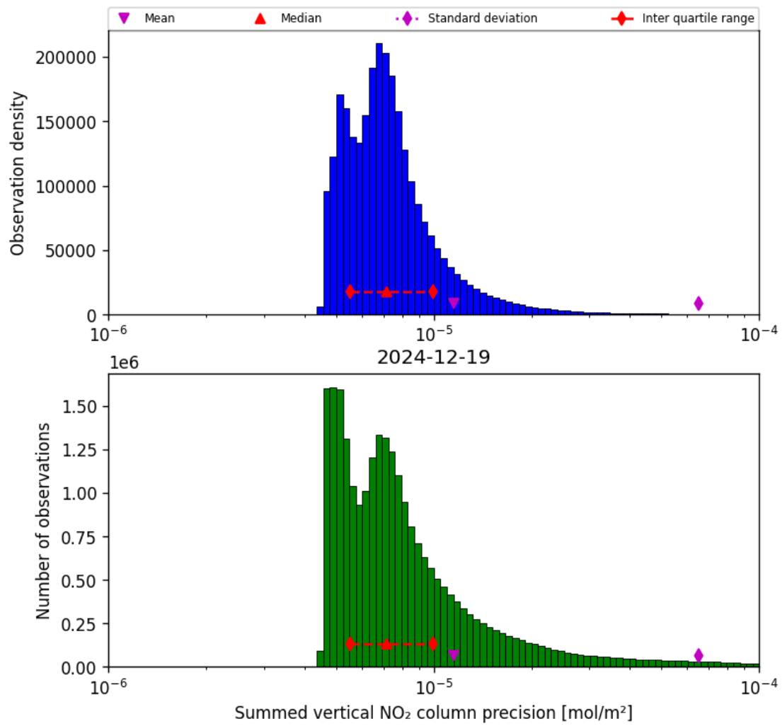
Figure 41: Histogram of “Summed vertical NO 2 column precision” for 2024-12-18 to 2024-12-20
