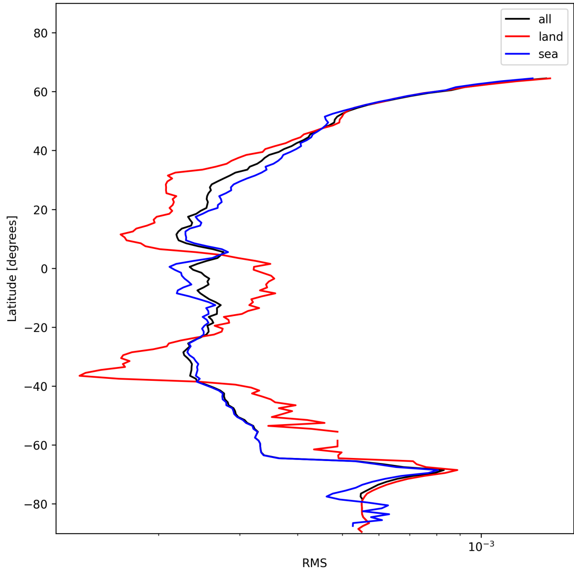
Figure 26: Zonal average of “RMS” for 2024-12-18 to 2024-12-20.
