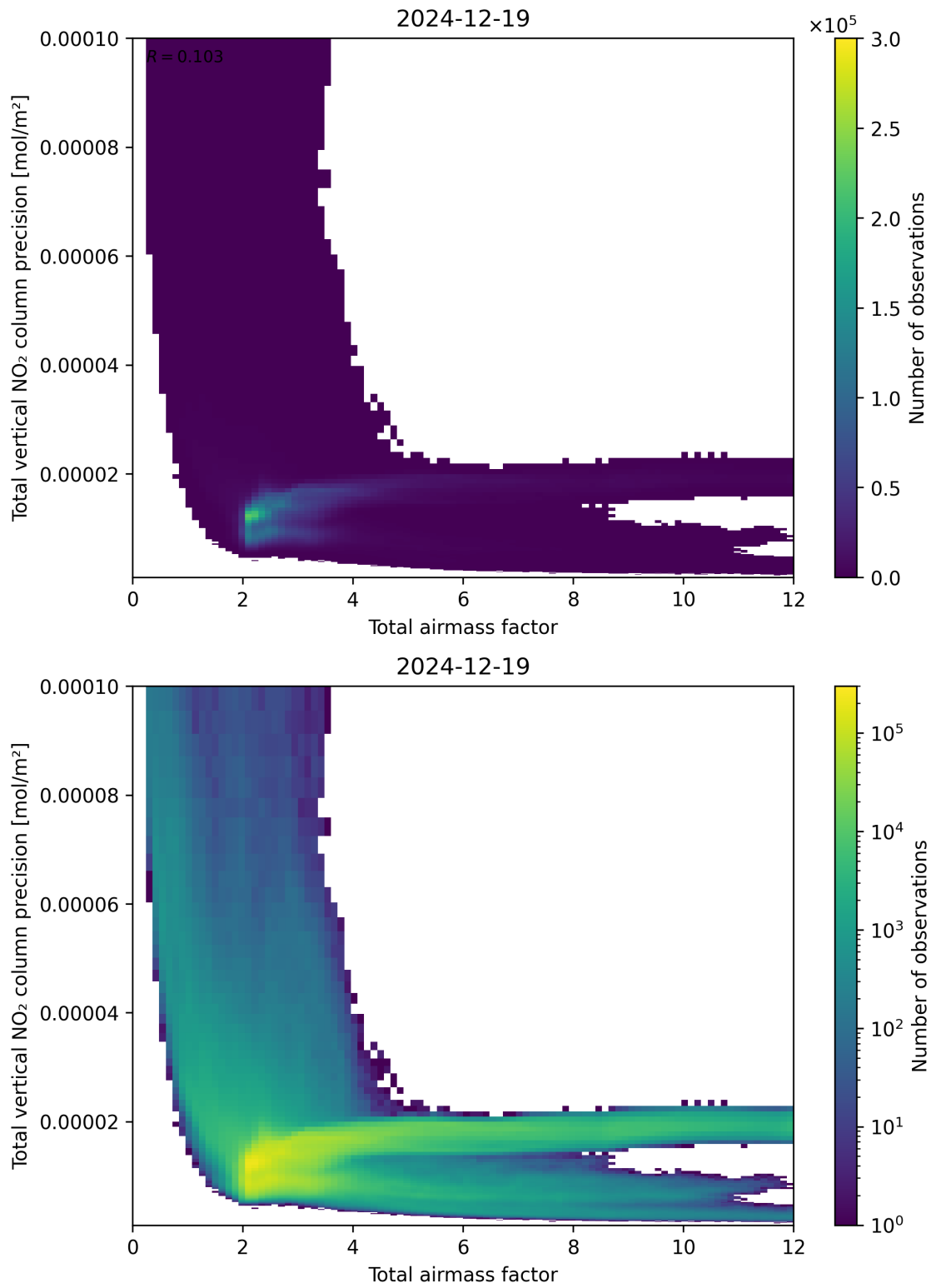
Figure 68: Scatter density plot of “Total airmass factor” against “Total vertical NO 2 column precision” for 2024-12-18 to 2024-12-20.
