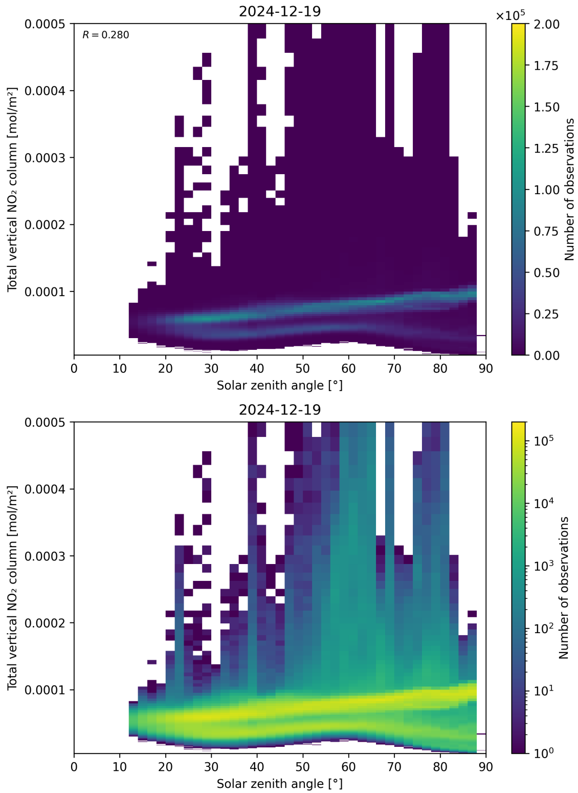
Figure 153: Scatter density plot of “Solar zenith angle” against “Total vertical NO 2 column” for 2024-12-18 to 2024-12-20.
