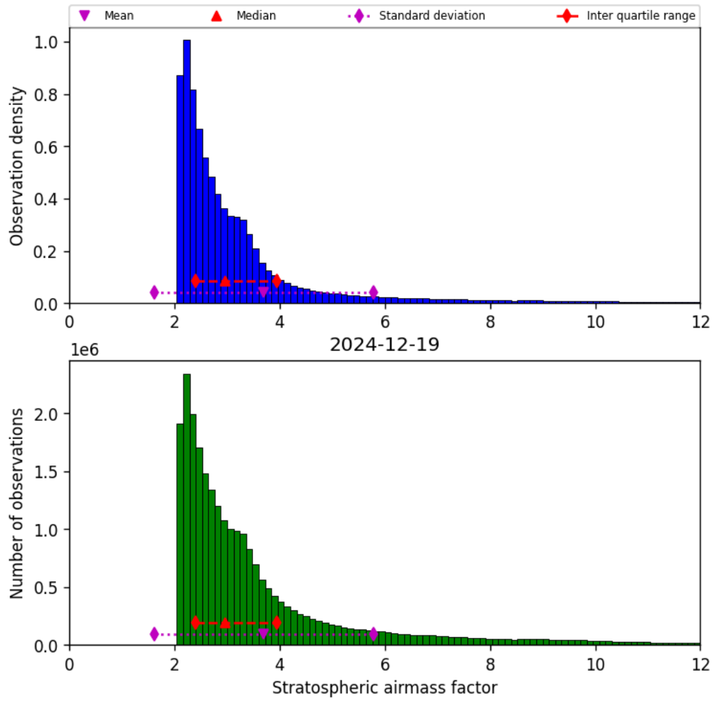
Figure 44: Histogram of “Stratospheric airmass factor” for 2024-12-18 to 2024-12-20
