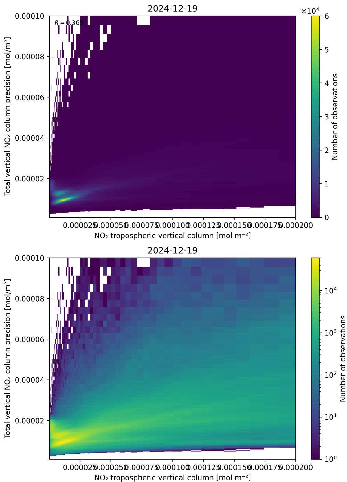
Figure 129: Scatter density plot of “NO 2 tropospheric vertical column” against “Total vertical NO 2 column precision” for 2024-12-18 to 2024-12-20.
