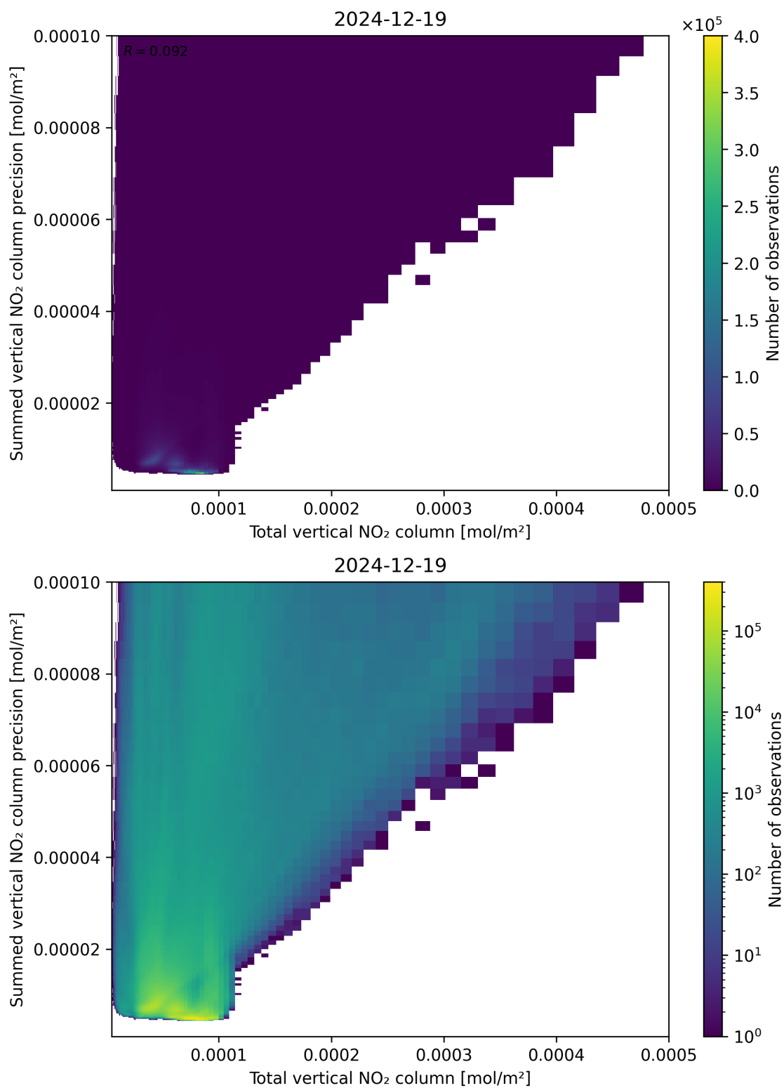
Figure 113: Scatter density plot of “Total vertical NO 2 column” against “Summed vertical NO 2 column precision” for 2024-12-18 to 2024-12-20.
