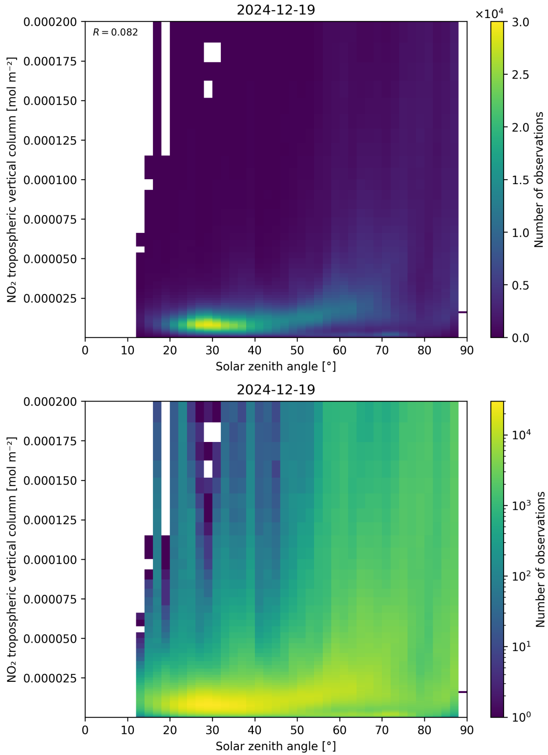
Figure 155: Scatter density plot of “Solar zenith angle” against “NO 2 tropospheric vertical column” for 2024-12-18 to 2024-12-20.
