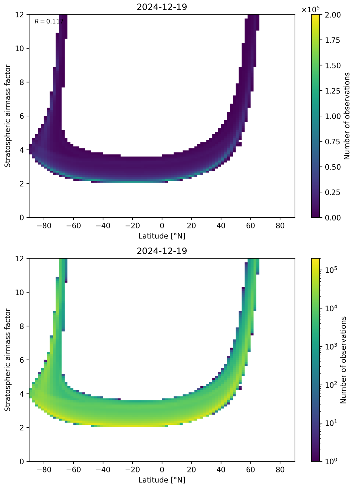
Figure 83: Scatter density plot of “Latitude” against “Stratospheric airmass factor” for 2024-12-18 to 2024-12-20.
