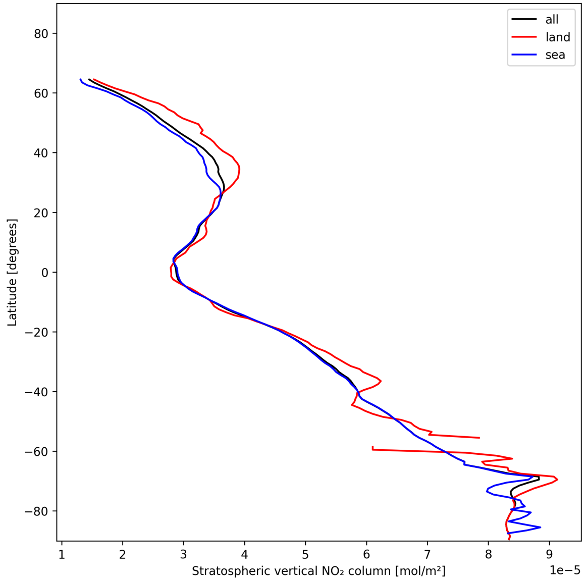
Figure 19: Zonal average of “Stratospheric vertical NO 2 column” for 2024-12-18 to 2024-12-20.
