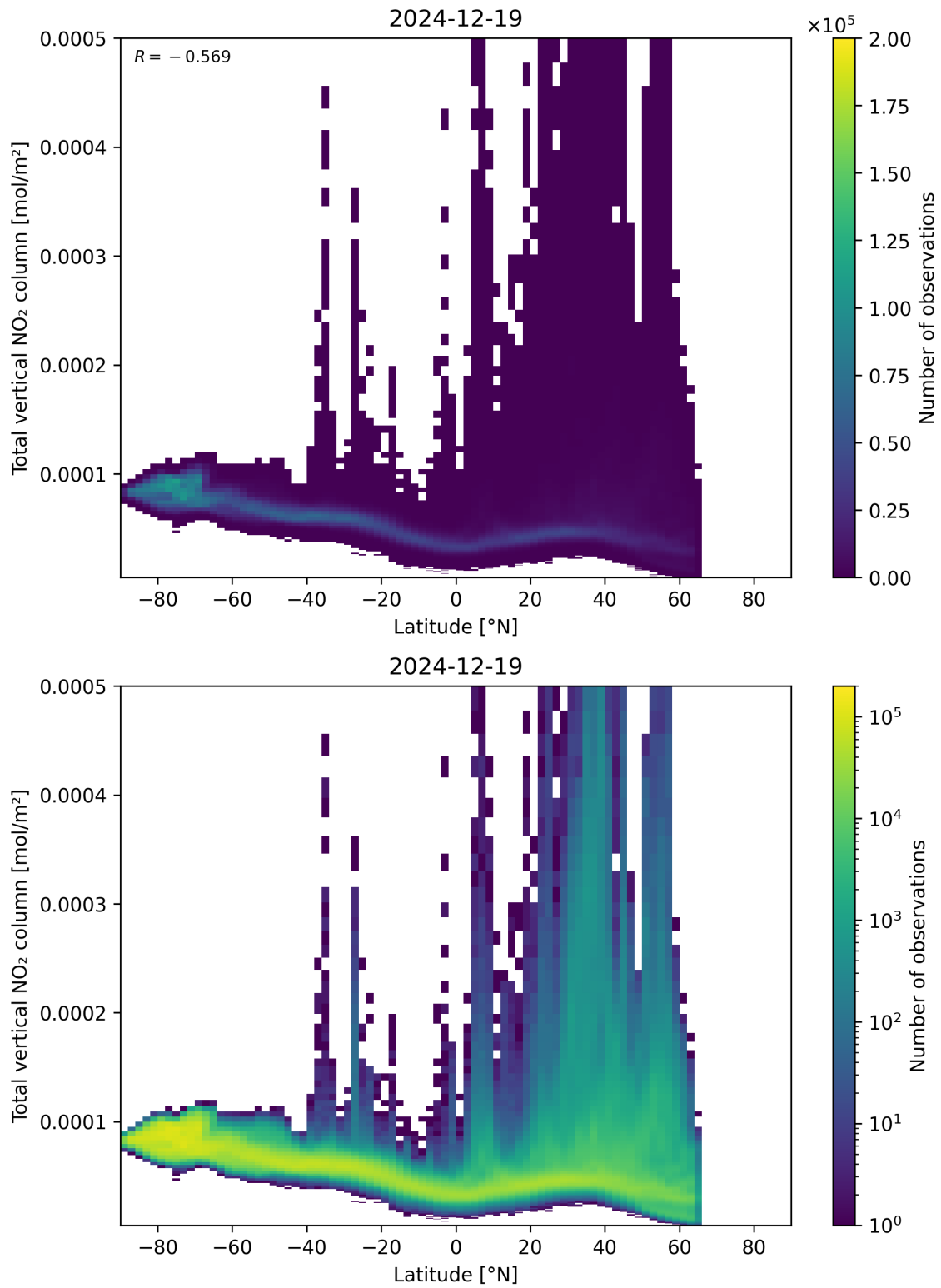
Figure 90: Scatter density plot of “Latitude” against “Total vertical NO 2 column” for 2024-12-18 to 2024-12-20.
