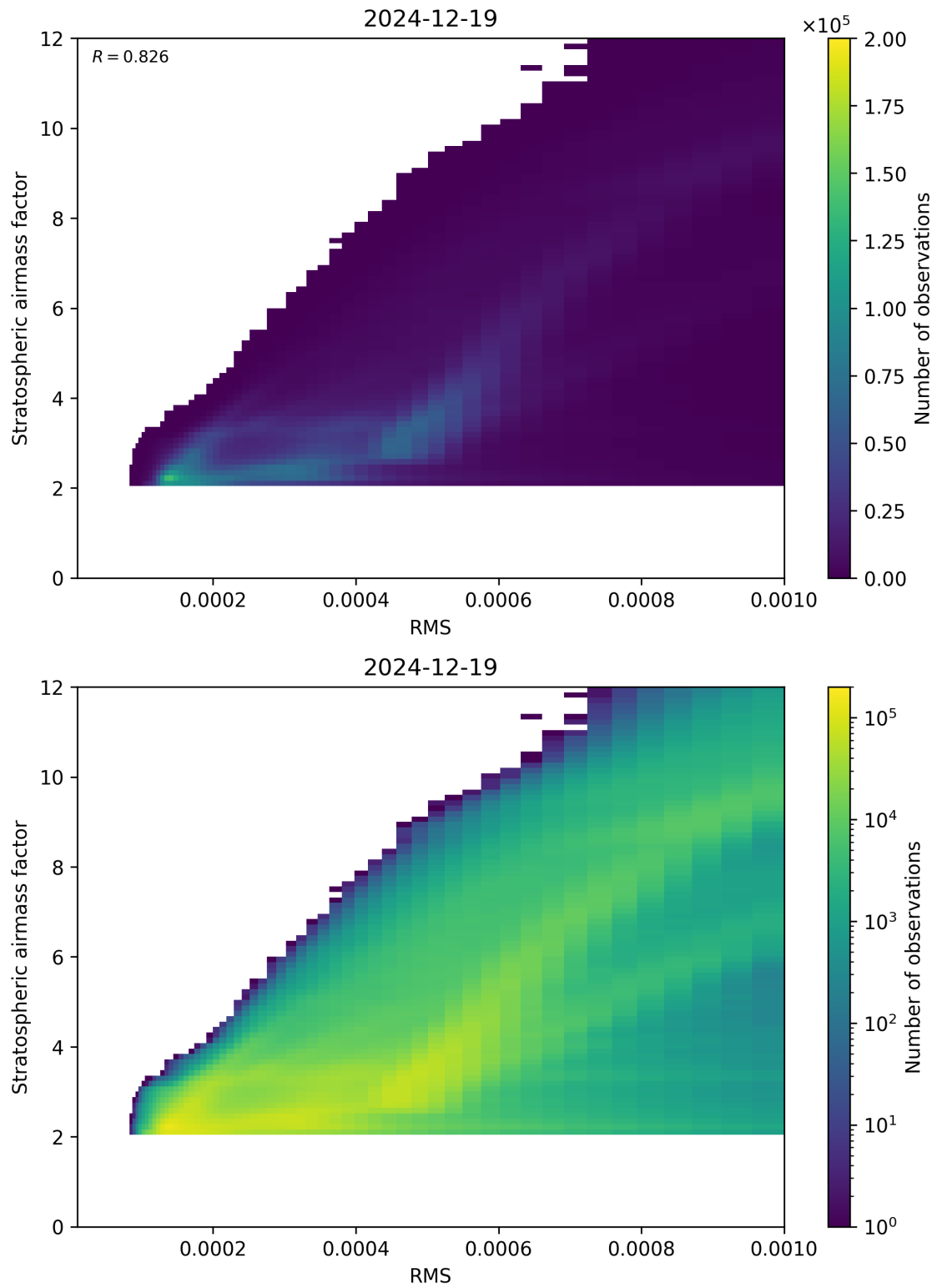
Figure 144: Scatter density plot of “RMS” against “Stratospheric airmass factor” for 2024-12-18 to 2024-12-20.
