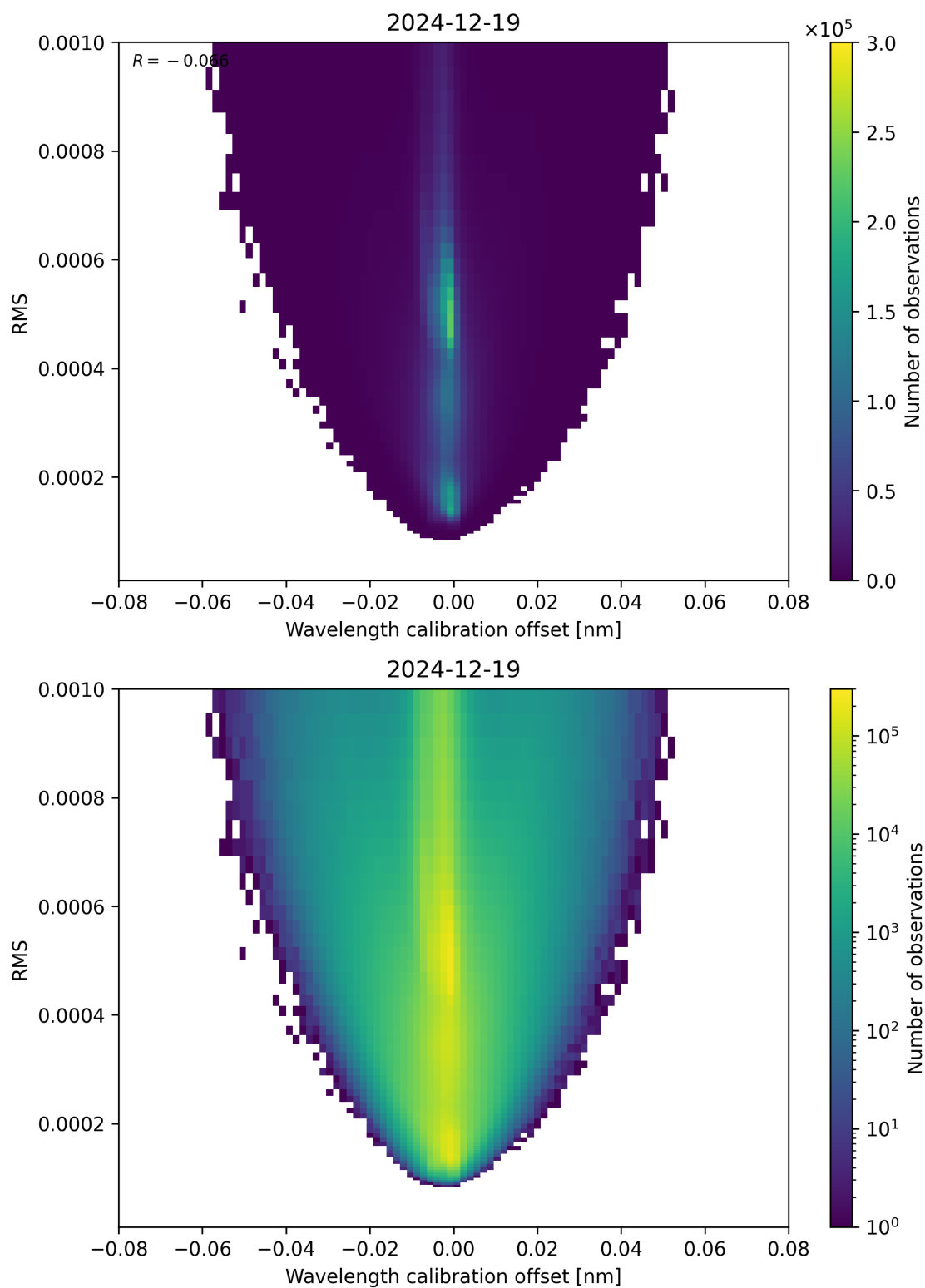
Figure 181: Scatter density plot of “Wavelength calibration offset” against “RMS” for 2024-12-18 to 2024-12-20.
