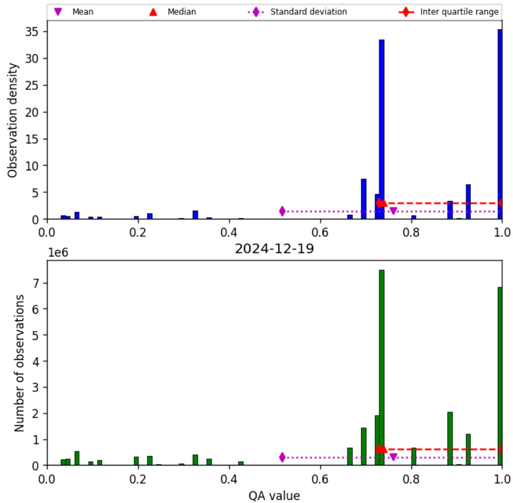
Figure 28: Histogram of “QA value” for 2024-12-18 to 2024-12-20
