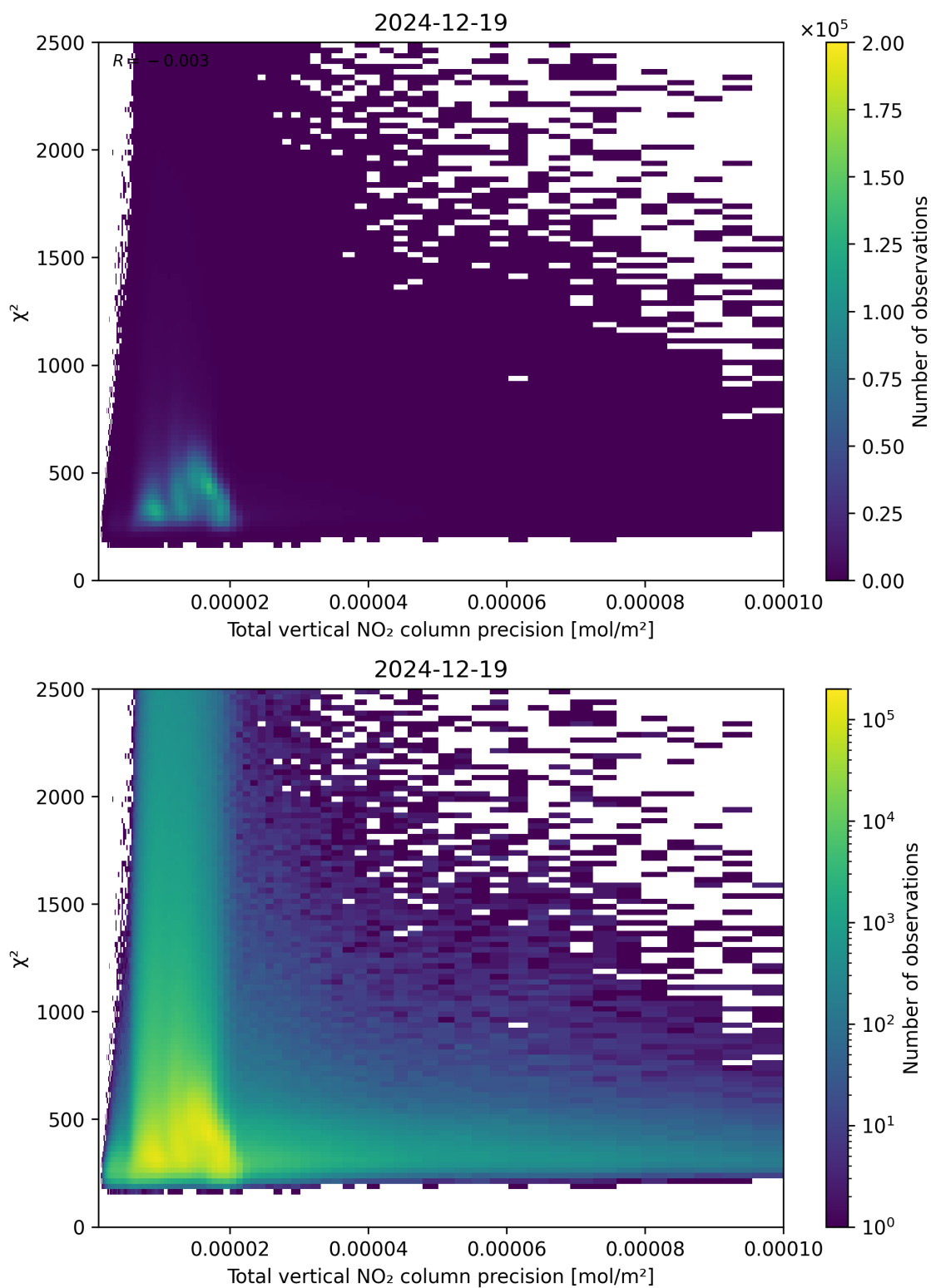
Figure 116: Scatter density plot of “Total vertical NO 2 column precision” against “ \chi^2 ” for 2024-12-18 to 2024-12-20.
