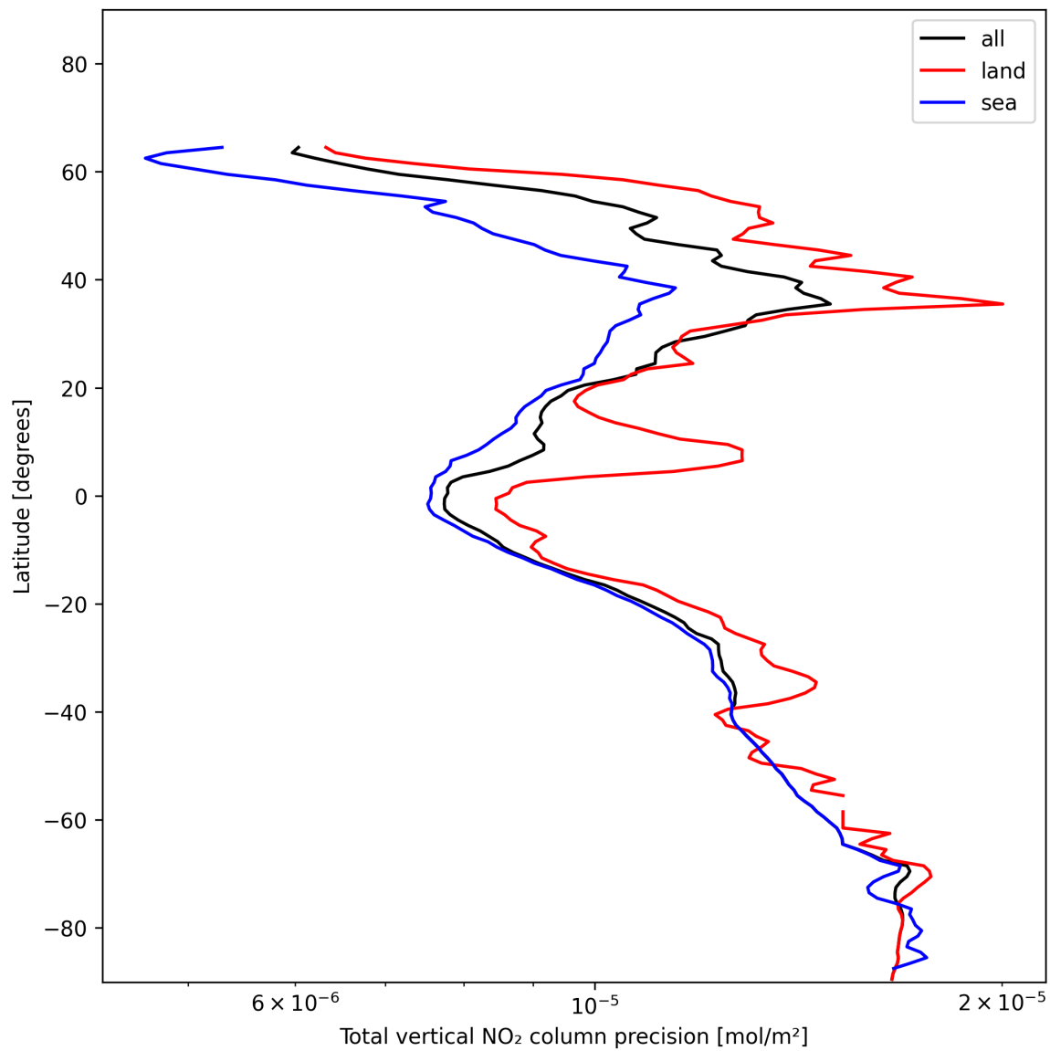
Figure 22: Zonal average of “Total vertical NO 2 column precision” for 2024-12-18 to 2024-12-20.
