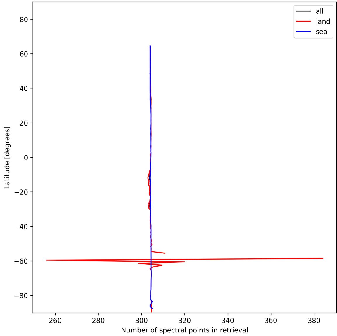
Figure 16: Zonal average of “Number of spectral points in retrieval” for 2024-12-18 to 2024-12-20.
