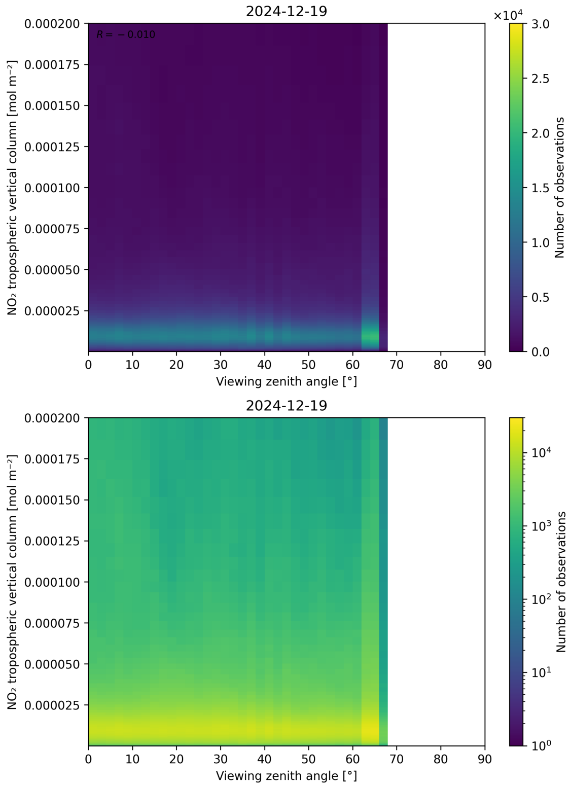
Figure 169: Scatter density plot of “Viewing zenith angle” against “NO 2 tropospheric vertical column” for 2024-12-18 to 2024-12-20.
