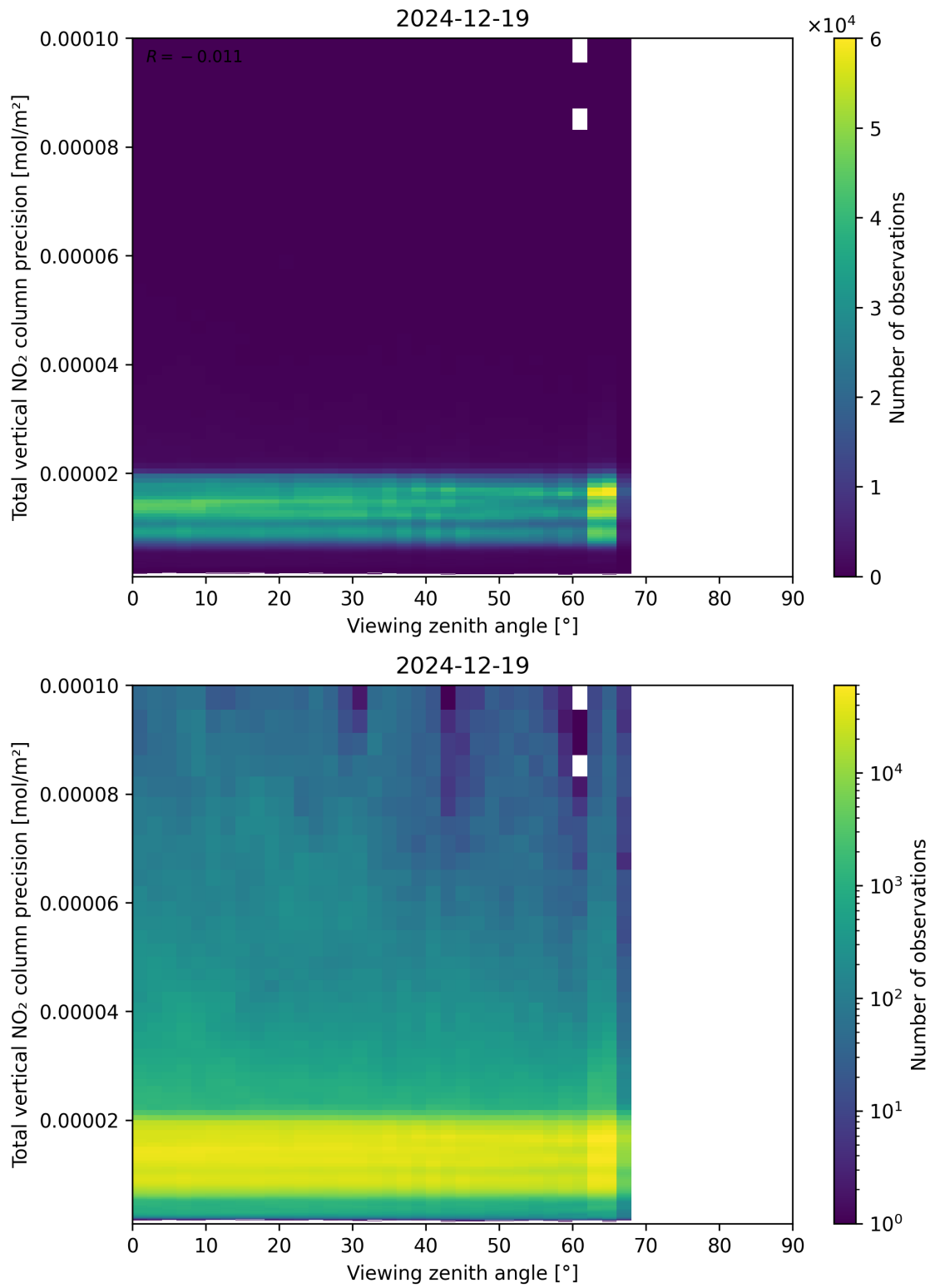
Figure 168: Scatter density plot of “Viewing zenith angle” against “Total vertical NO 2 column precision” for 2024-12-18 to 2024-12-20.
