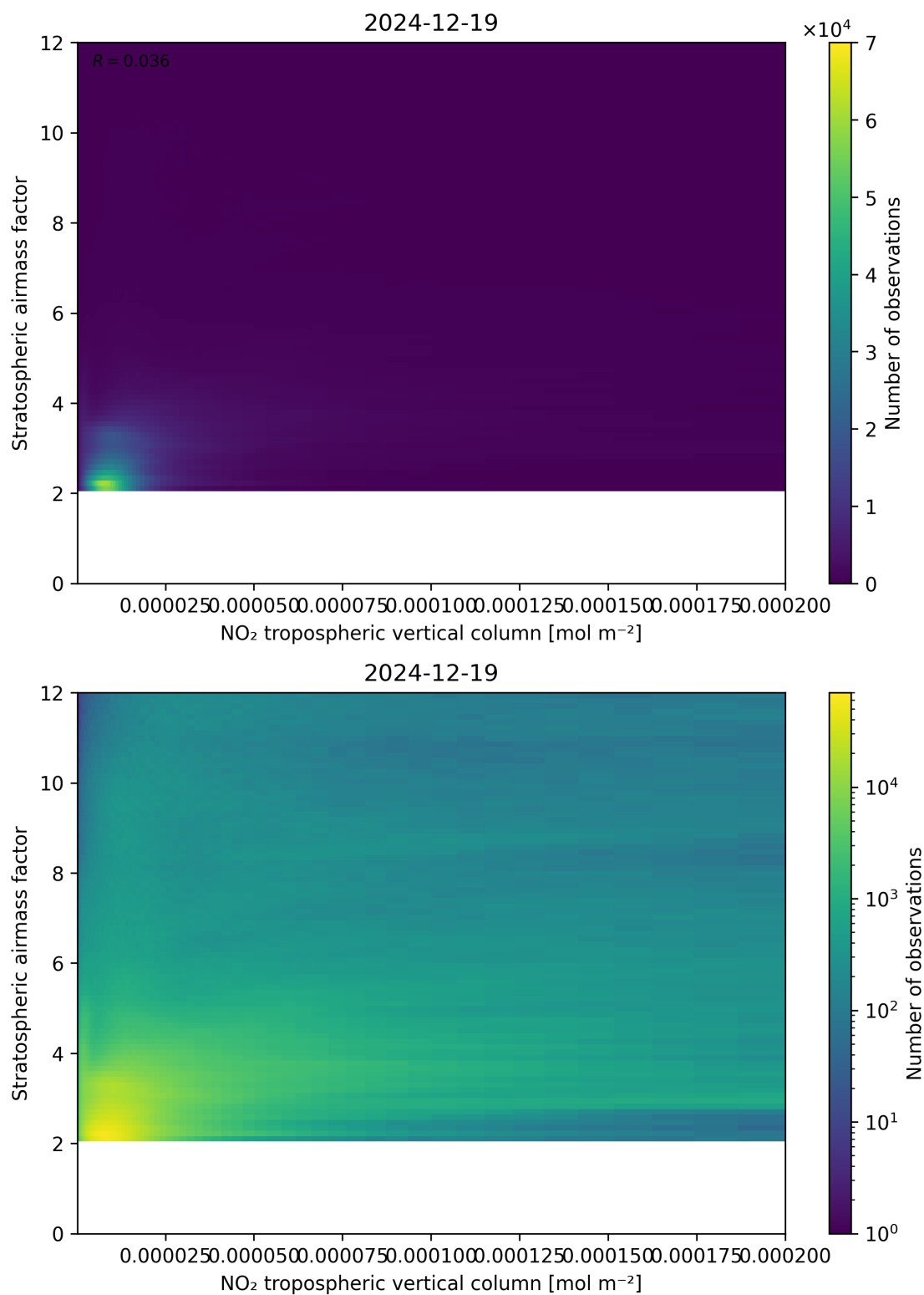
Figure 121: Scatter density plot of “NO 2 tropospheric vertical column” against “Stratospheric airmass factor” for 2024-12-18 to 2024-12-20.
