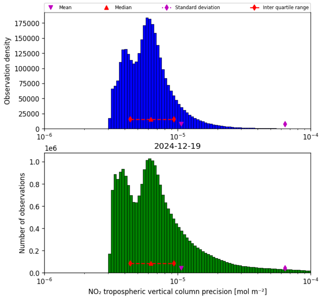
Figure 30: Histogram of “NO 2 tropospheric vertical column precision” for 2024-12-18 to 2024-12-20
