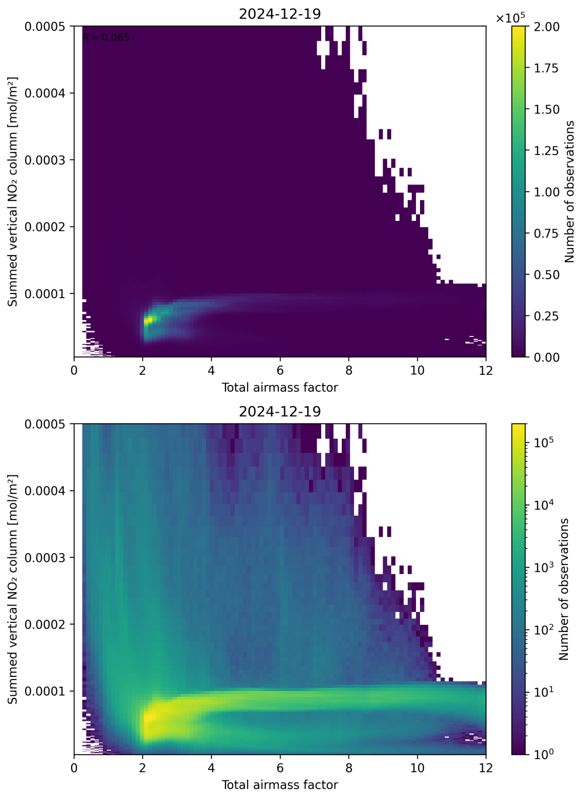
Figure 65: Scatter density plot of “Total airmass factor” against “Summed vertical NO 2 column” for 2024-12-18 to 2024-12-20.
