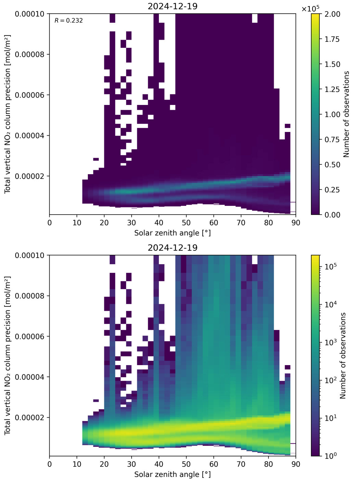
Figure 154: Scatter density plot of “Solar zenith angle” against “Total vertical NO 2 column precision” for 2024-12-18 to 2024-12-20.
