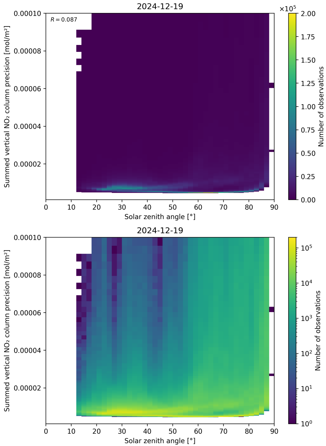
Figure 152: Scatter density plot of “Solar zenith angle” against “Summed vertical NO 2 column precision” for 2024-12-18 to 2024-12-20.
