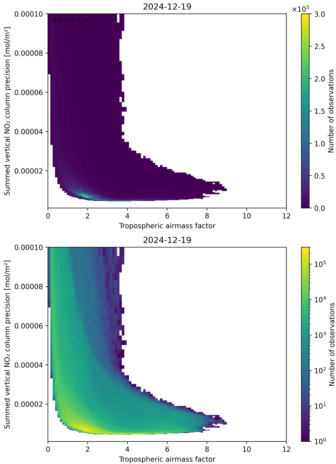
Figure 76: Scatter density plot of “Tropospheric air mass factor” against “Summed vertical NO 2 column precision” for 2024-12-18 to 2024-12-20.
