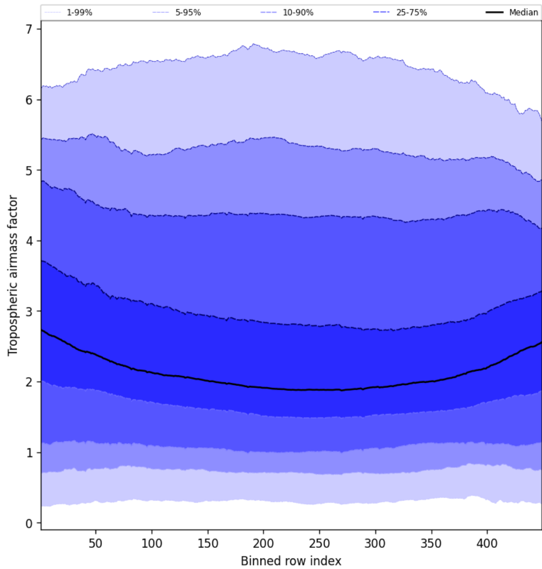
Figure 48: Along track statistics of “Tropospheric air mass factor” for 2024-12-18 to 2024-12-20
