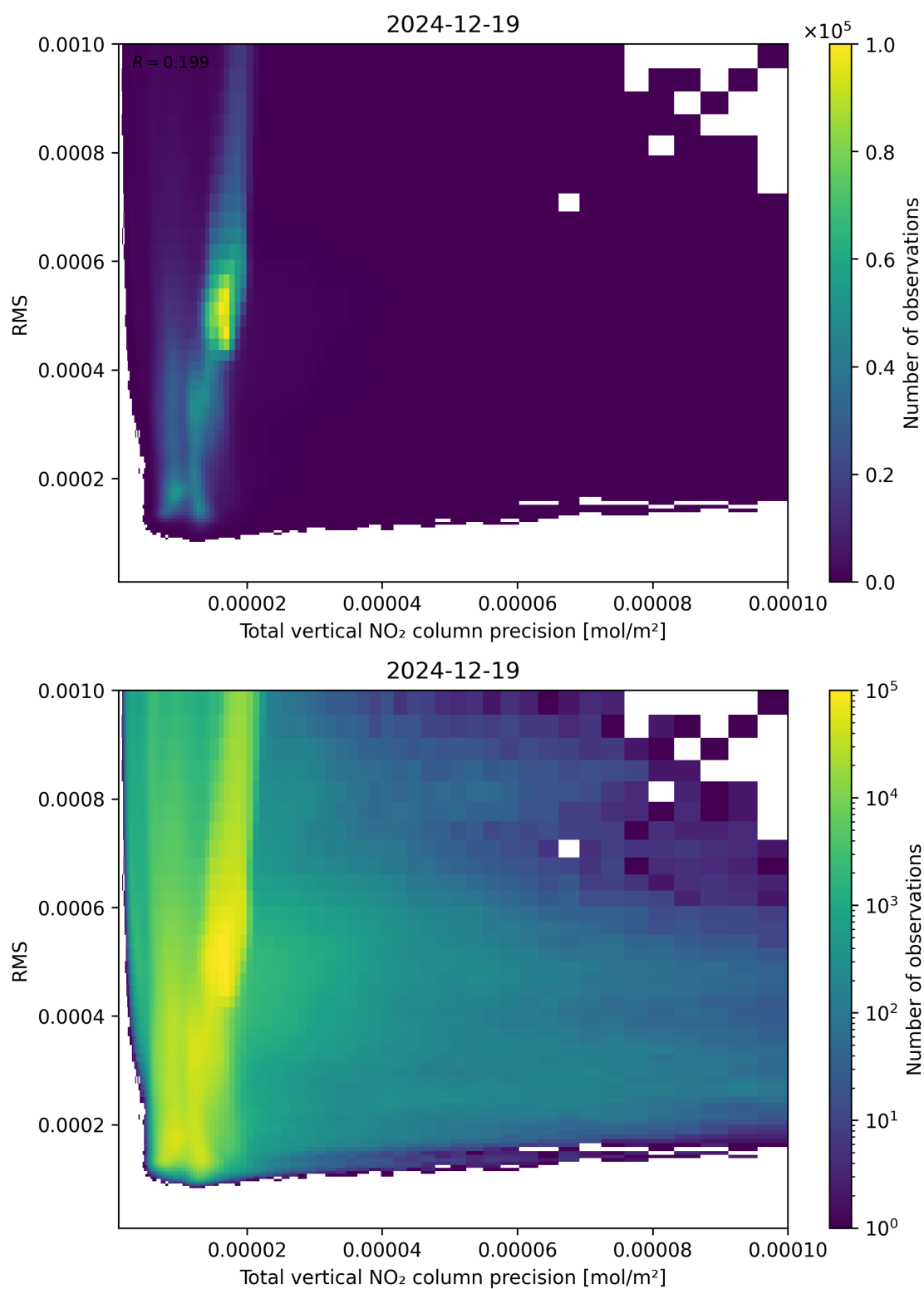
Figure 119: Scatter density plot of “Total vertical NO 2 column precision” against “RMS” for 2024-12-18 to 2024-12-20.
