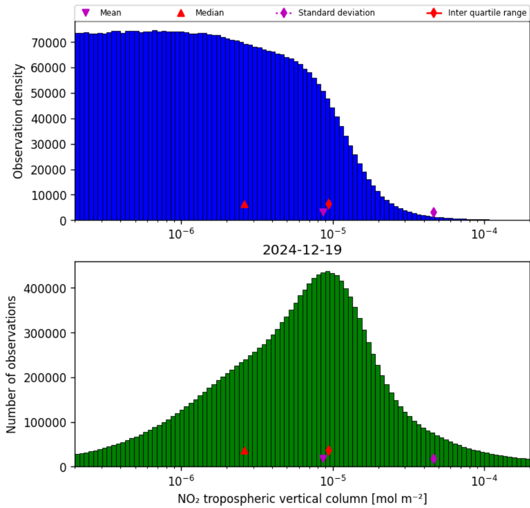
Figure 29: Histogram of “NO 2 tropospheric vertical column” for 2024-12-18 to 2024-12-20
