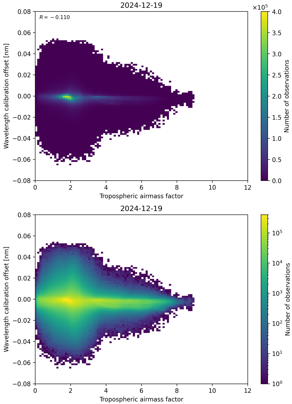
Figure 80: Scatter density plot of “Tropospheric airmass factor” against “Wavelength calibration offset” for 2024-12-18 to 2024-12-20.
