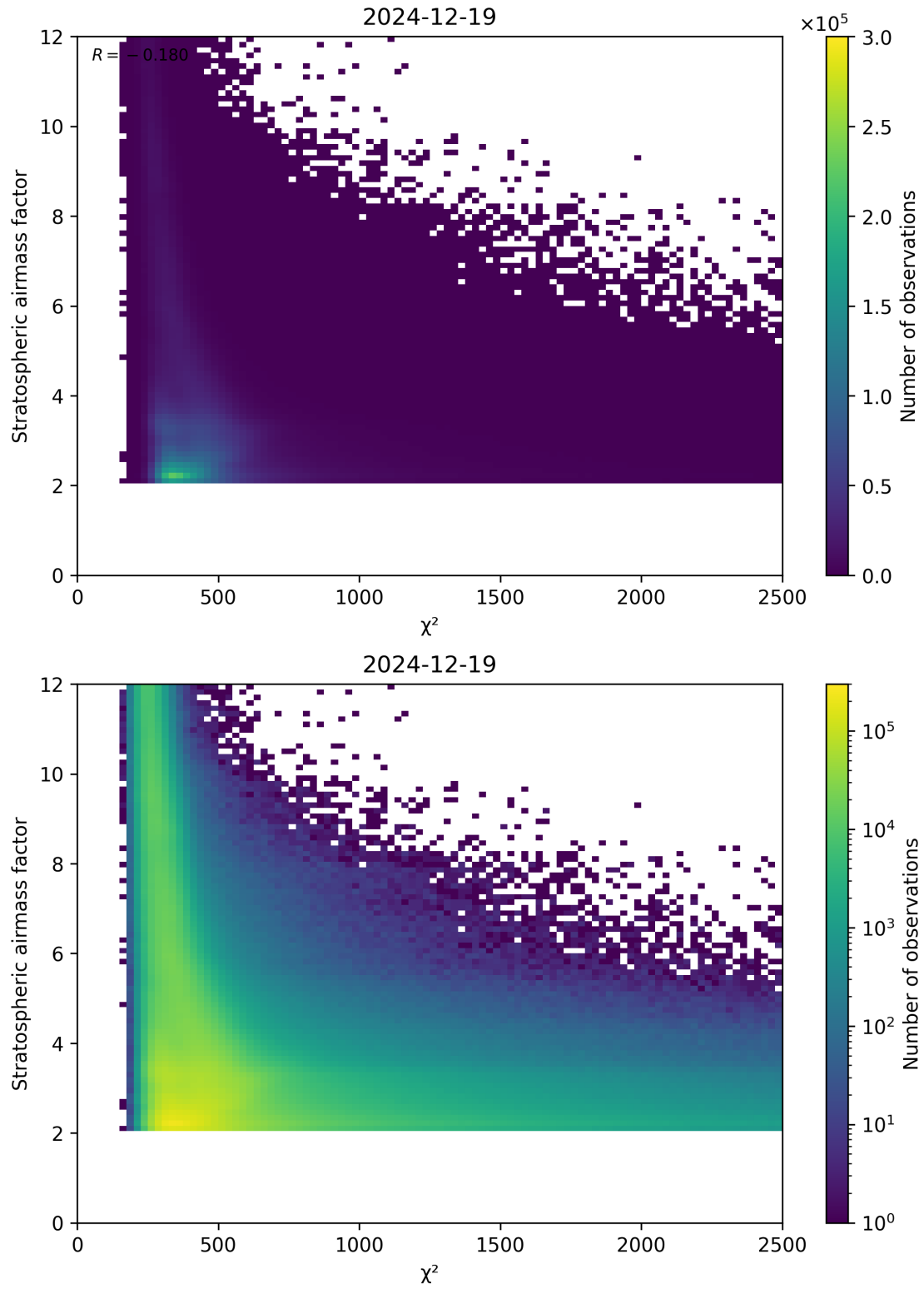
Figure 81: Scatter density plot of “ \chi^2 ” against “Stratospheric airmass factor” for 2024-12-18 to 2024-12-20.
