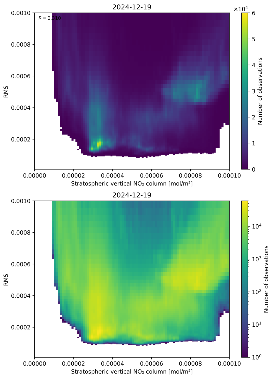
Figure 102: Scatter density plot of “Stratospheric vertical NO 2 column” against “RMS” for 2024-12-18 to 2024-12-20.
