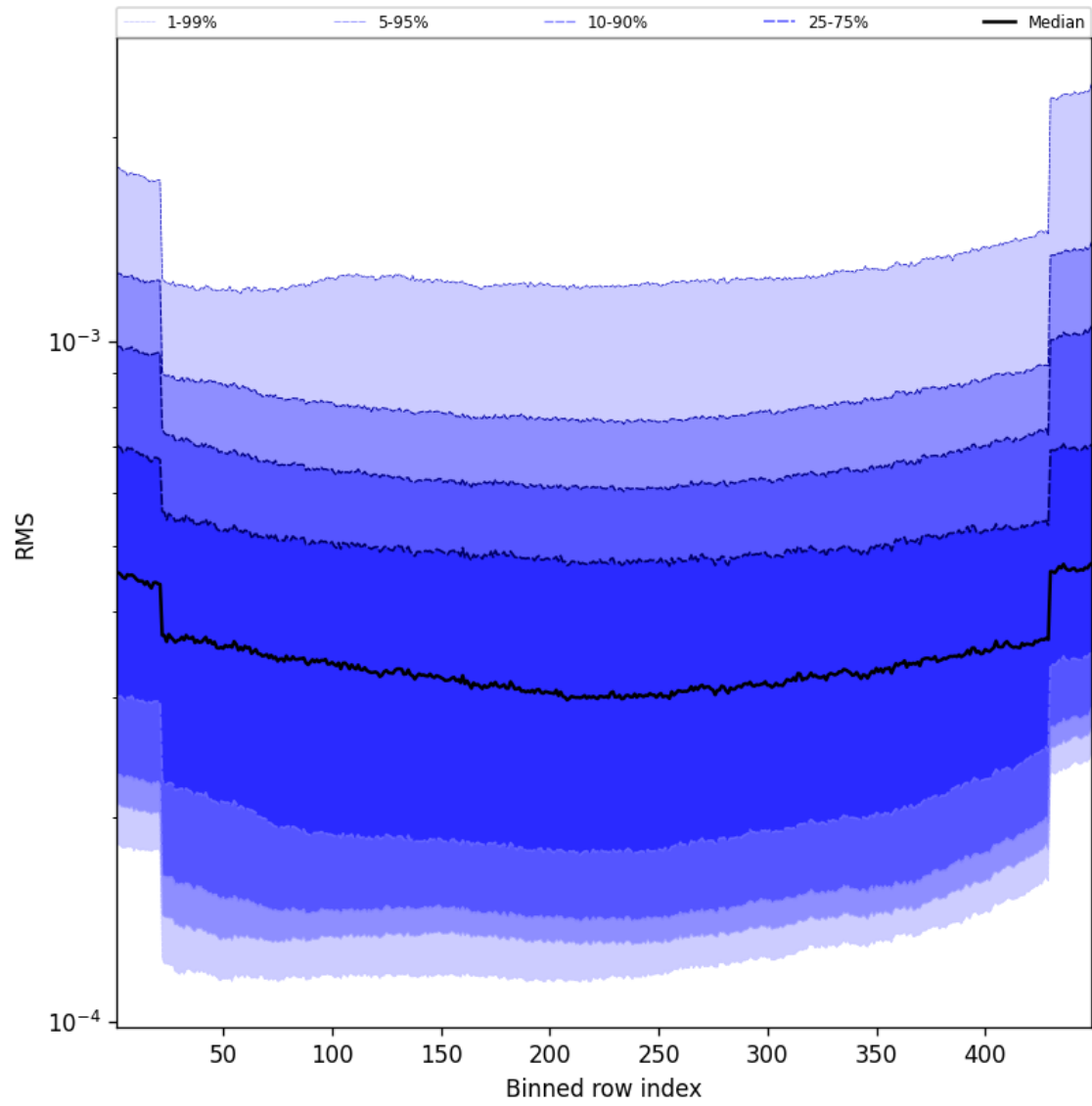
Figure 60: Along track statistics of “RMS” for 2024-12-18 to 2024-12-20
