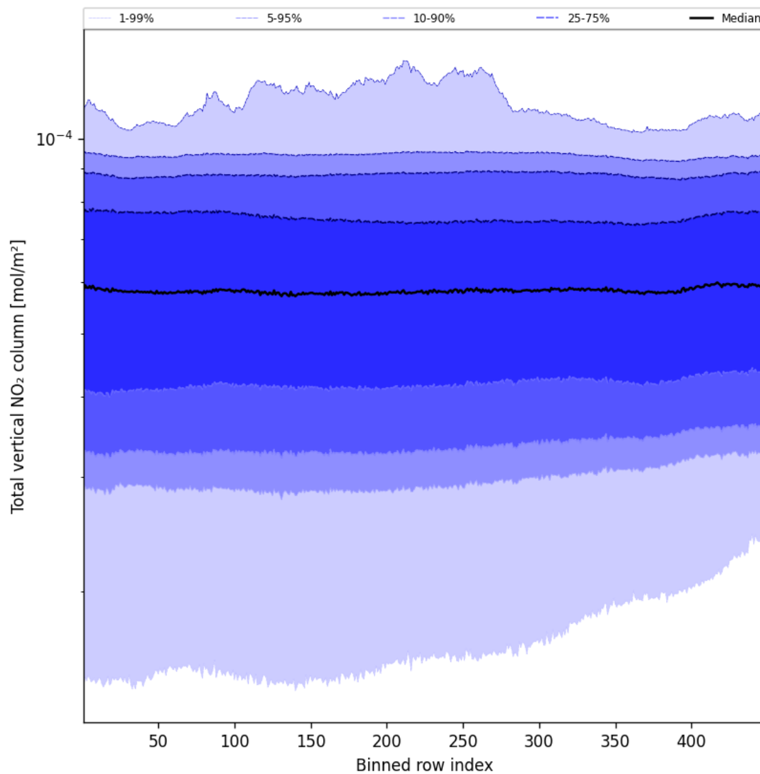
Figure 55: Along track statistics of “Total vertical NO 2 column” for 2024-12-18 to 2024-12-20
