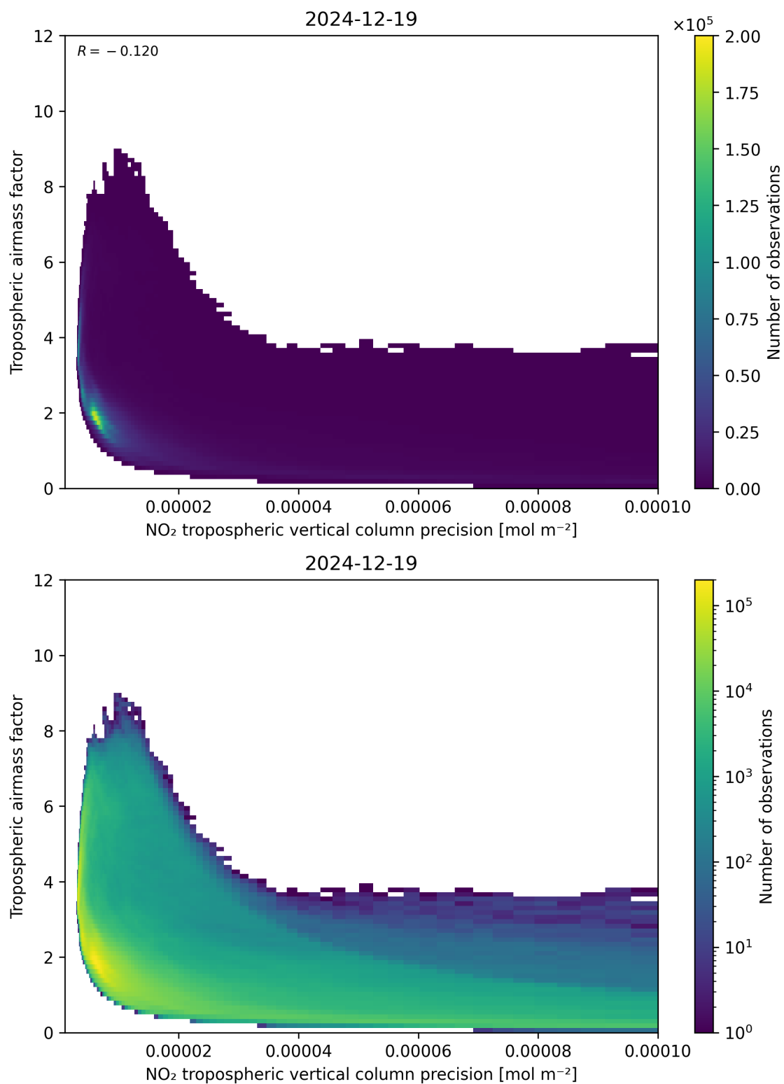
Figure 133: Scatter density plot of “NO 2 tropospheric vertical column precision” against “Tropospheric airmass factor” for 2024-12-18 to 2024-12-20.
