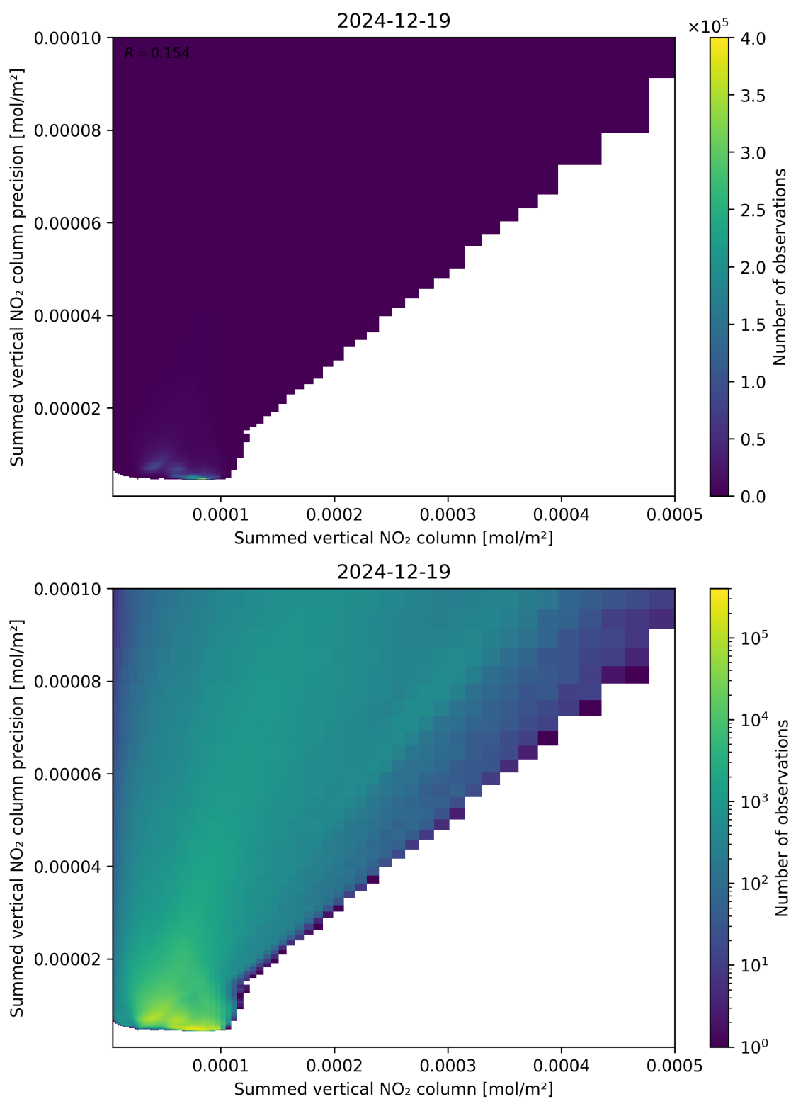
Figure 105: Scatter density plot of “Summed vertical NO 2 column” against “Summed vertical NO 2 column precision” for 2024-12-18 to 2024-12-20.
