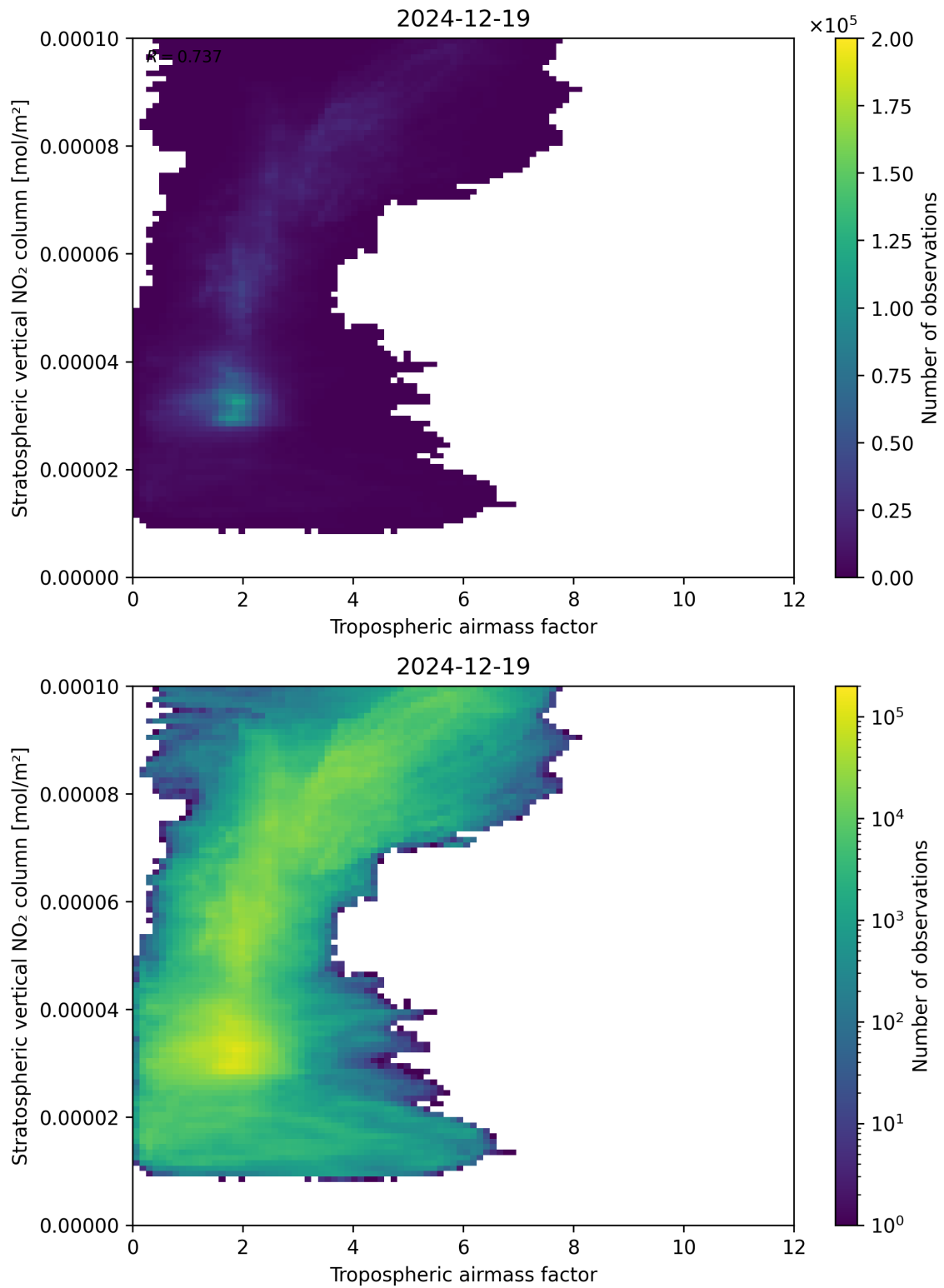
Figure 74: Scatter density plot of “Tropospheric air mass factor” against “Stratospheric vertical NO 2 column” for 2024-12-18 to 2024-12-20.
