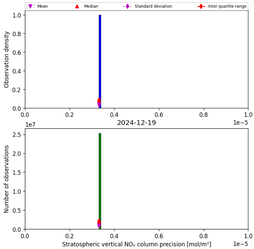
Figure 37: Histogram of “Stratospheric vertical NO 2 column precision” for 2024-12-18 to 2024-12-20
