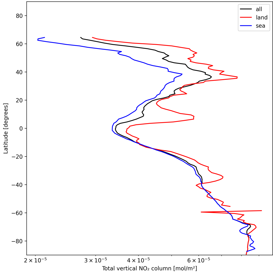
Figure 21: Zonal average of “Total vertical NO 2 column” for 2024-12-18 to 2024-12-20.
