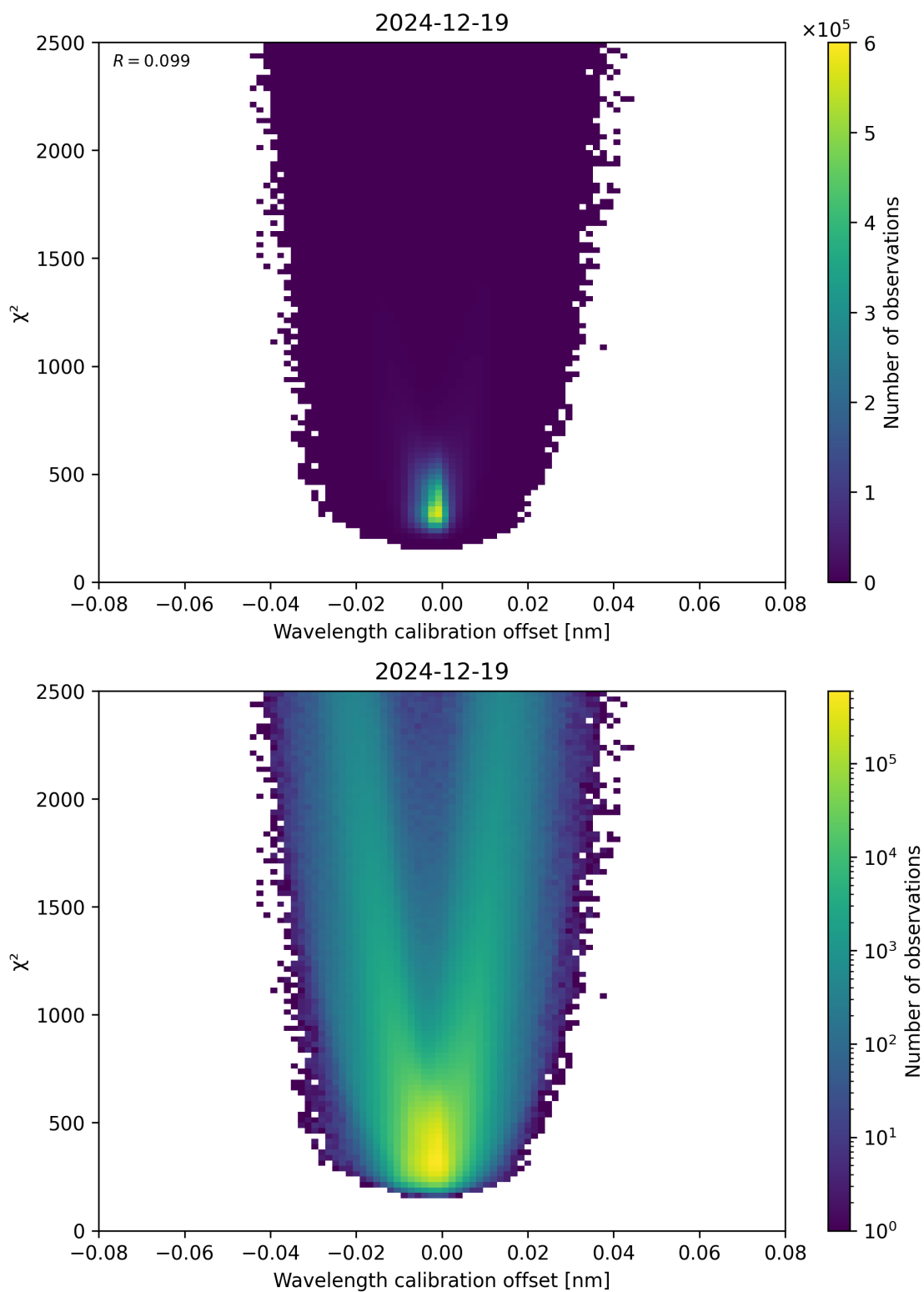
Figure 175: Scatter density plot of “Wavelength calibration offset” against “ \chi^2 ” for 2024-12-18 to 2024-12-20.
