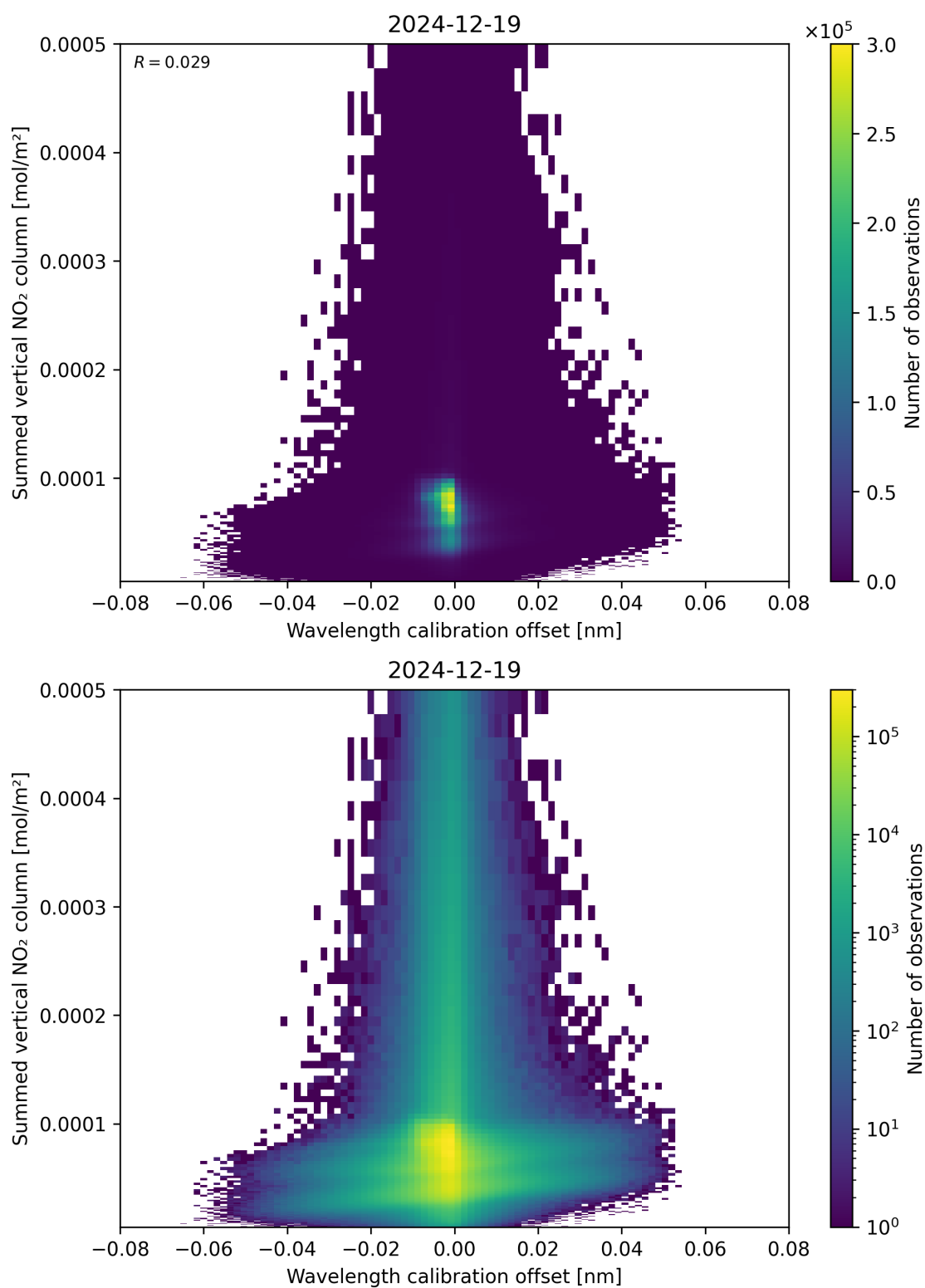
Figure 177: Scatter density plot of “Wavelength calibration offset” against “Summed vertical NO 2 column” for 2024-12-18 to 2024-12-20.
