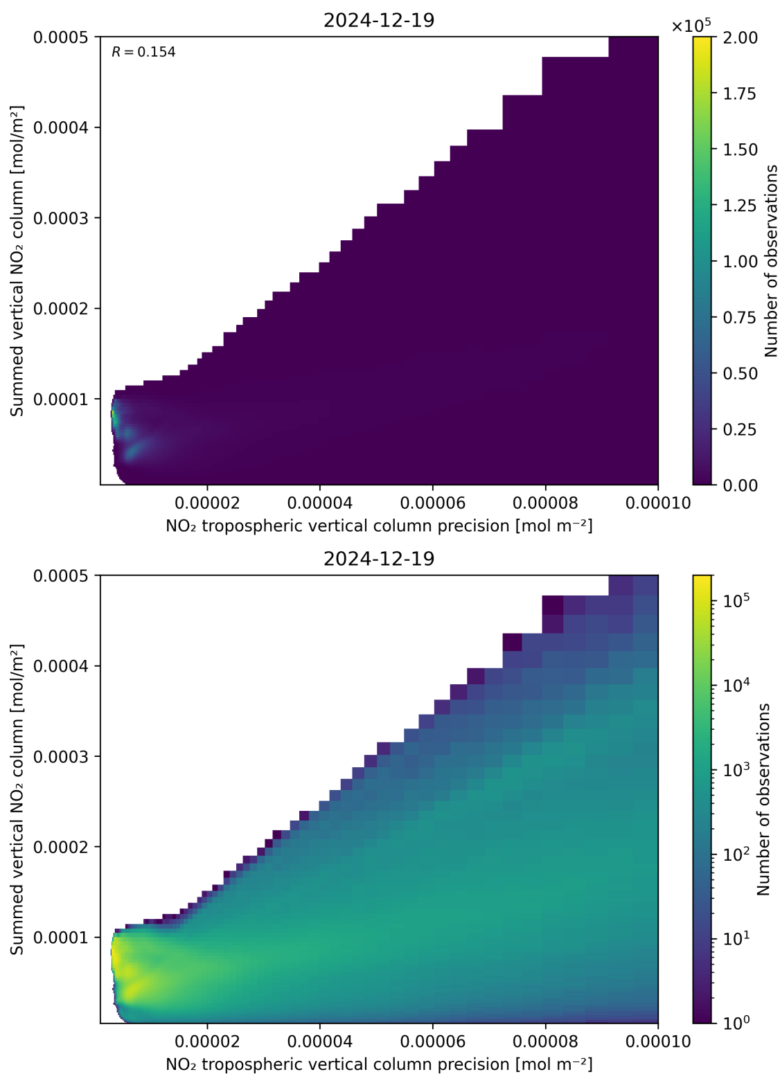
Figure 136: Scatter density plot of “NO 2 tropospheric vertical column precision” against “Summed vertical NO 2 column” for 2024-12-18 to 2024-12-20.
