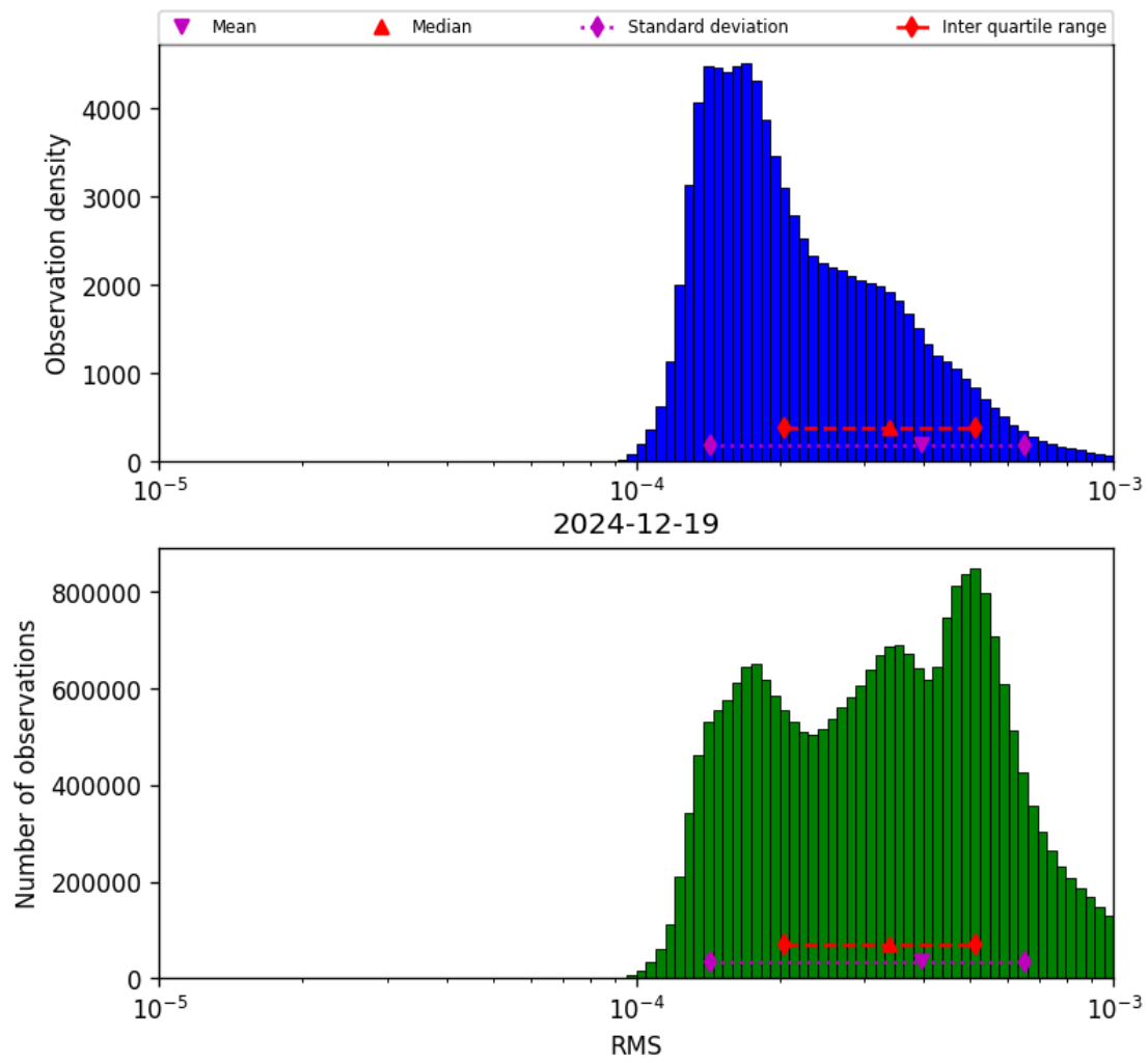
Figure 43: Histogram of “RMS” for 2024-12-18 to 2024-12-20
