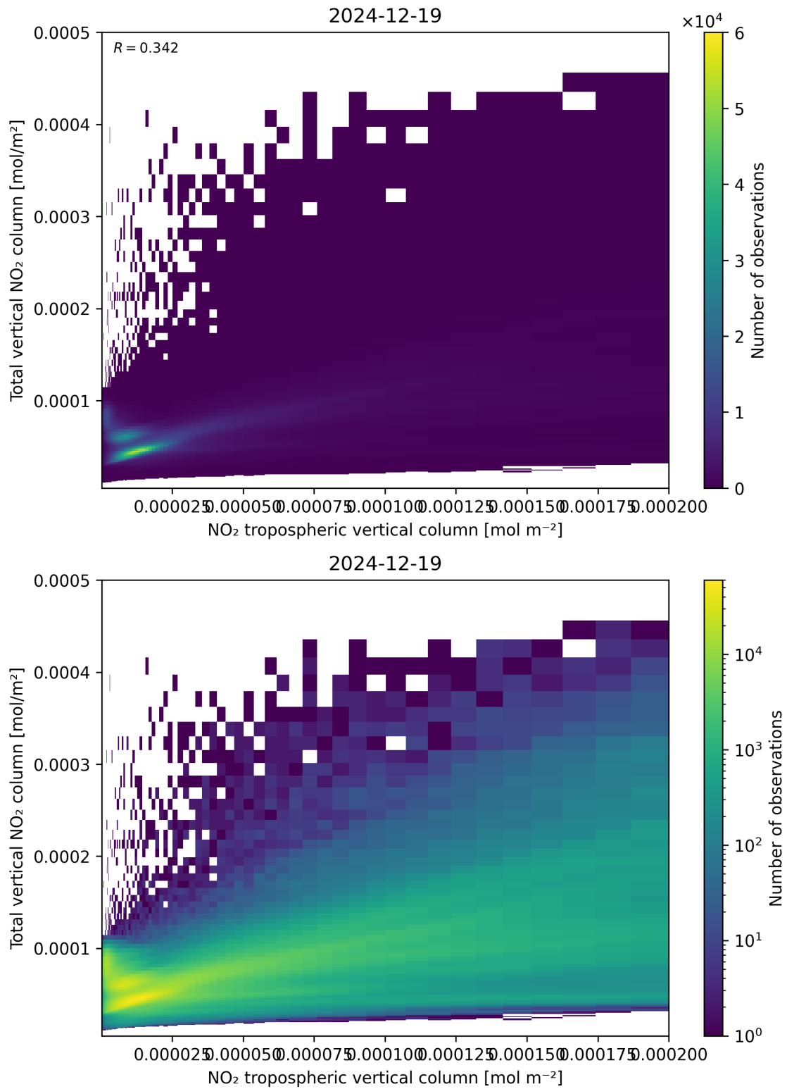
Figure 128: Scatter density plot of “NO 2 tropospheric vertical column” against “Total vertical NO 2 column” for 2024-12-18 to 2024-12-20.
