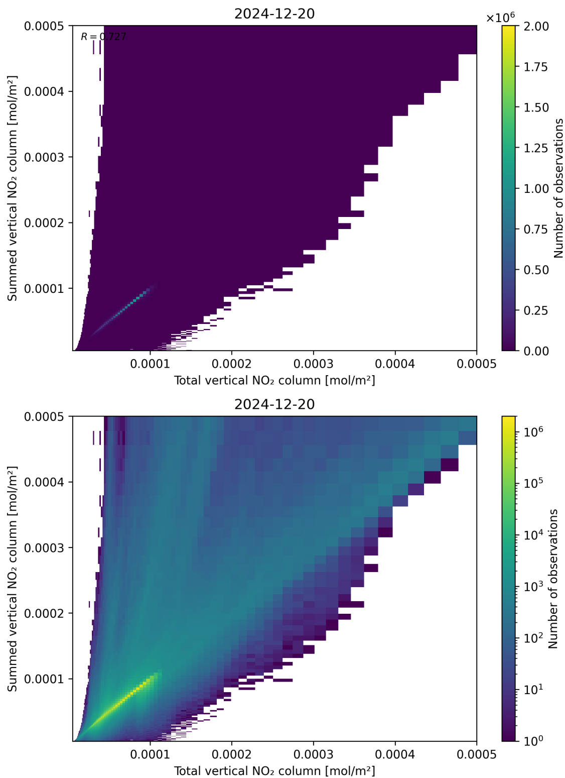
Figure 112: Scatter density plot of “Total vertical NO 2 column” against “Summed vertical NO 2 column” for 2024-12-19 to 2024-12-21.
