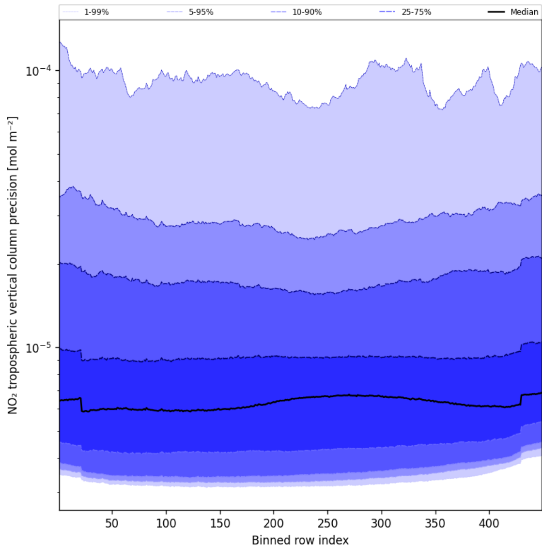
Figure 47: Along track statistics of “NO 2 tropospheric vertical column precision” for 2024-12-19 to 2024-12-21
