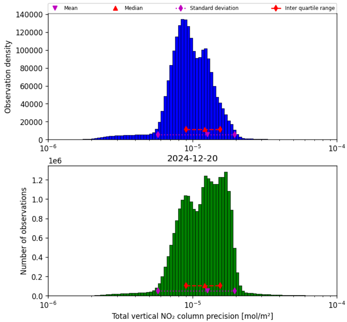
Figure 39: Histogram of “Total vertical NO 2 column precision” for 2024-12-19 to 2024-12-21
