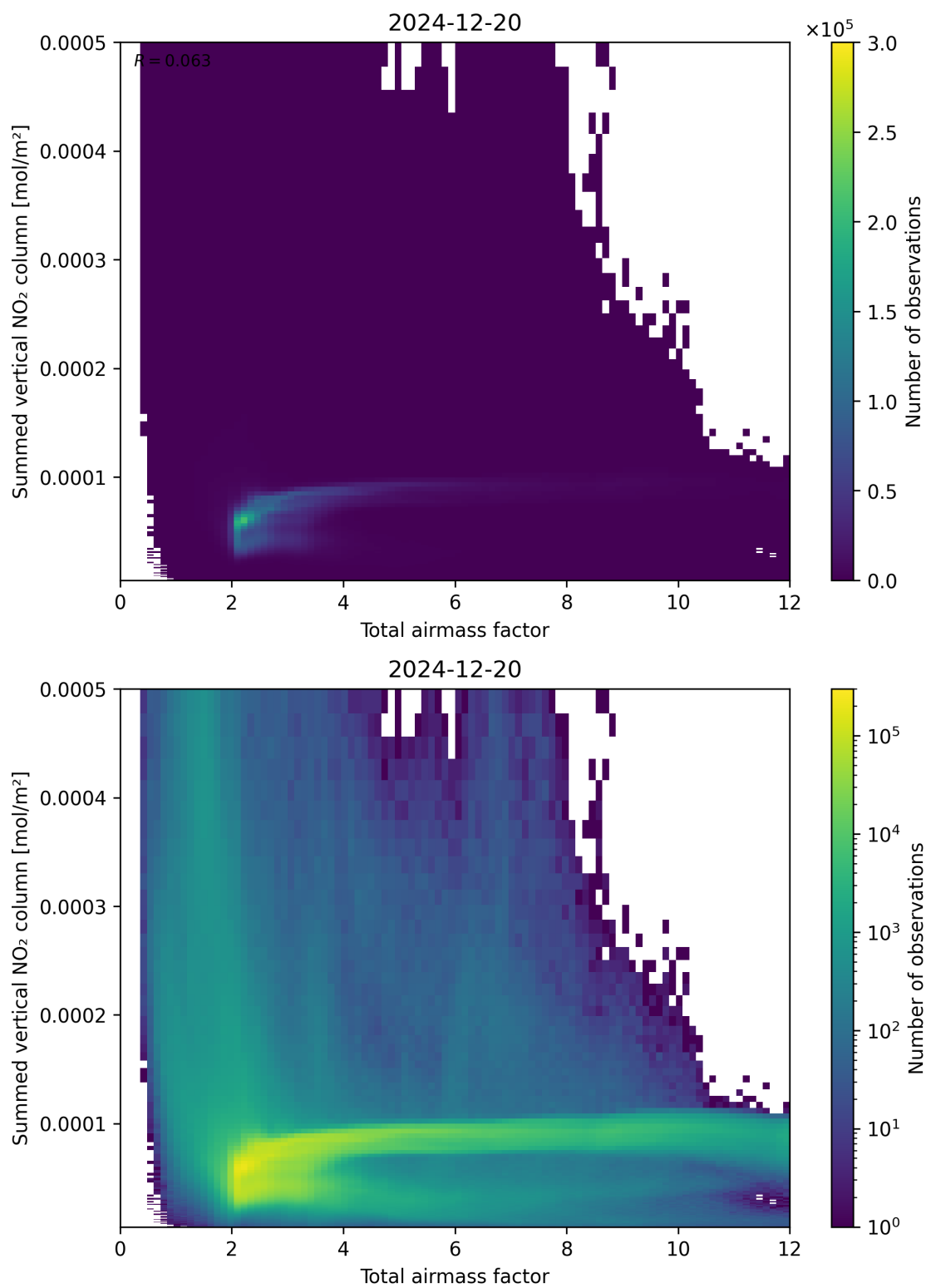
Figure 65: Scatter density plot of “Total airmass factor” against “Summed vertical NO 2 column” for 2024-12-19 to 2024-12-21.
