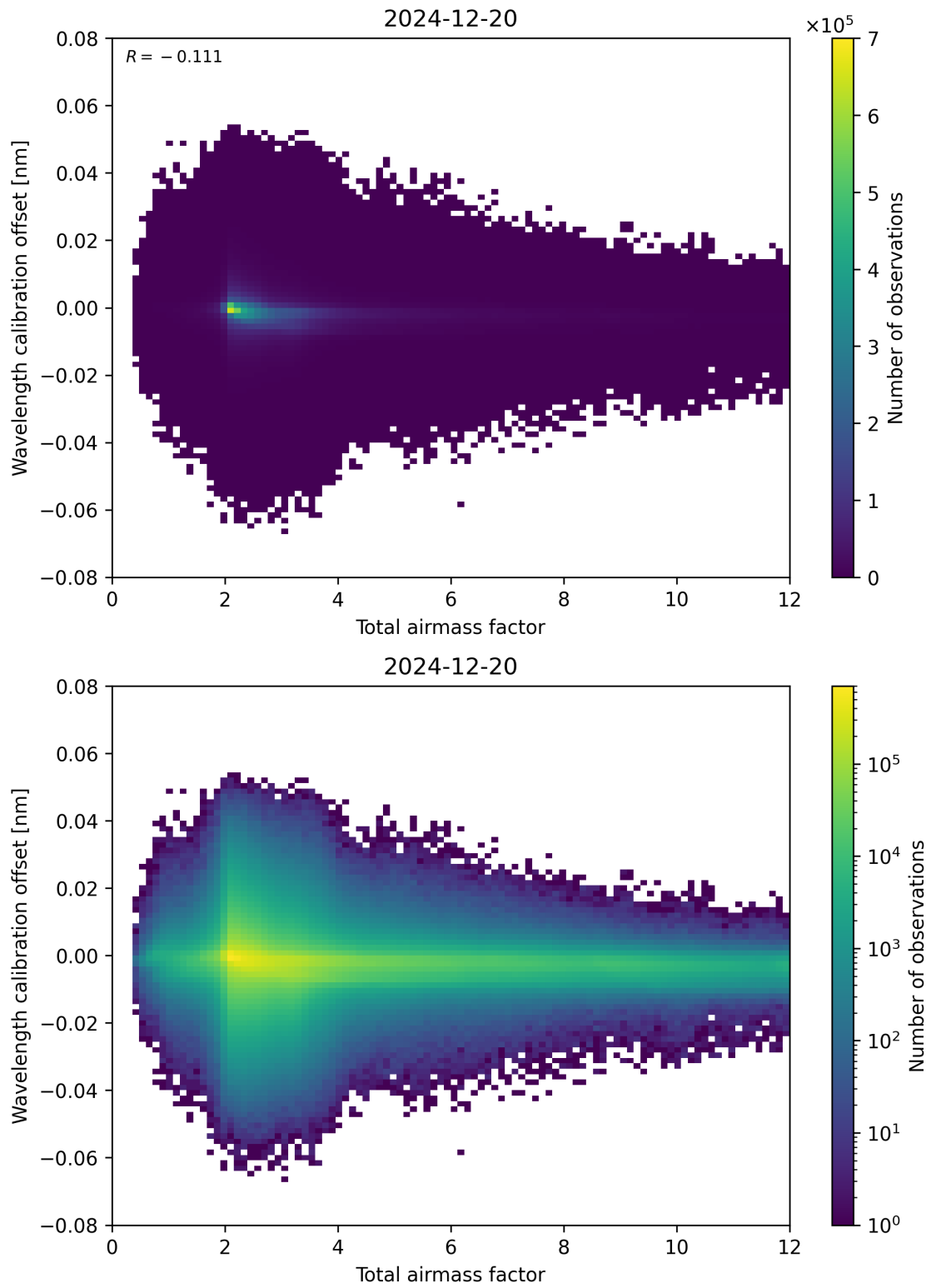
Figure 70: Scatter density plot of “Total airmass factor” against “Wavelength calibration offset” for 2024-12-19 to 2024-12-21.
