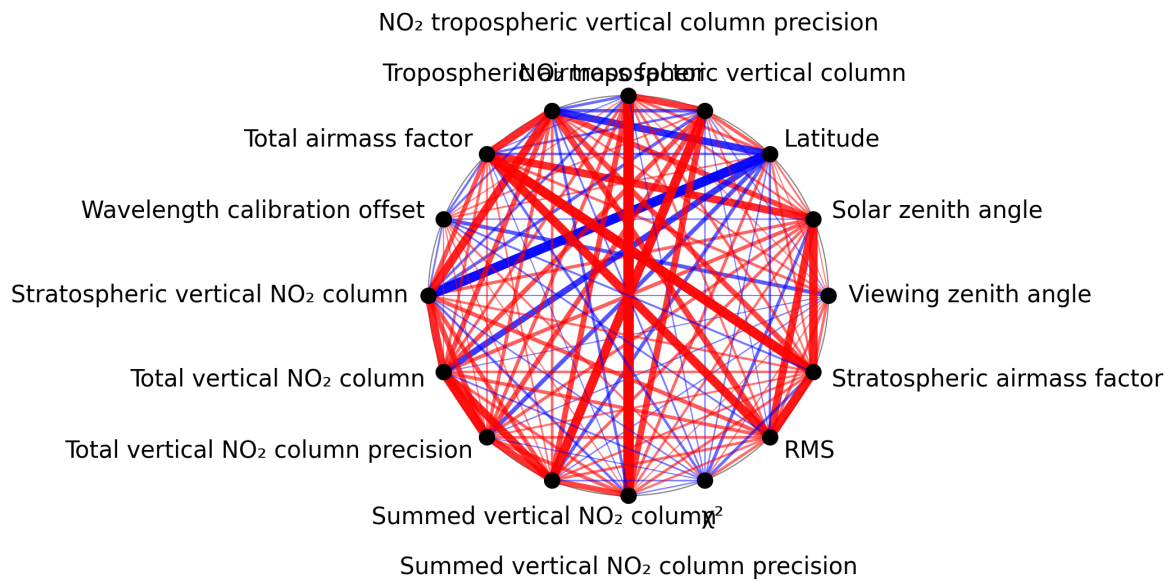
Figure 1: Map of correlation graph for 2024-12-19 to 2024-12-21.
