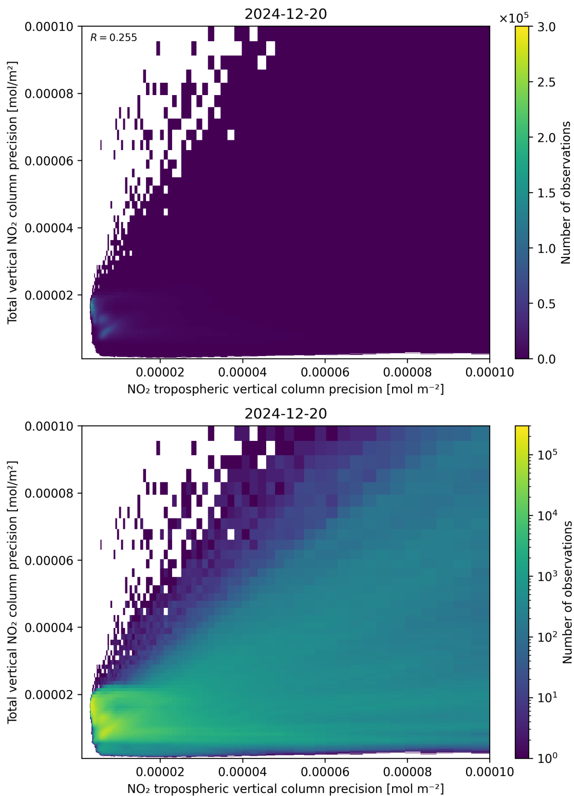
Figure 139: Scatter density plot of “NO 2 tropospheric vertical column precision” against “Total vertical NO 2 column precision” for 2024-12-19 to 2024-12-21.
