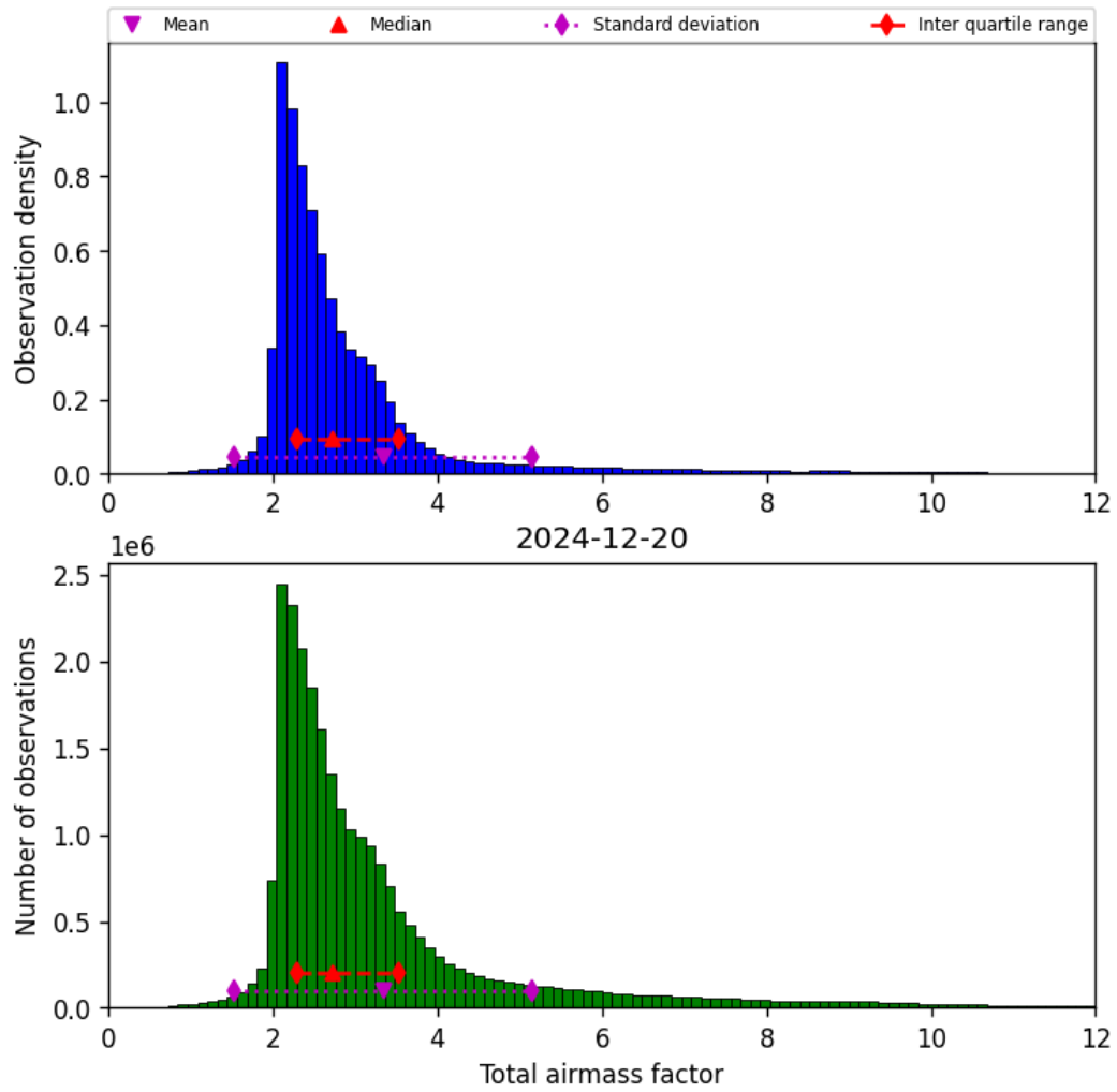
Figure 32: Histogram of “Total airmass factor” for 2024-12-19 to 2024-12-21
