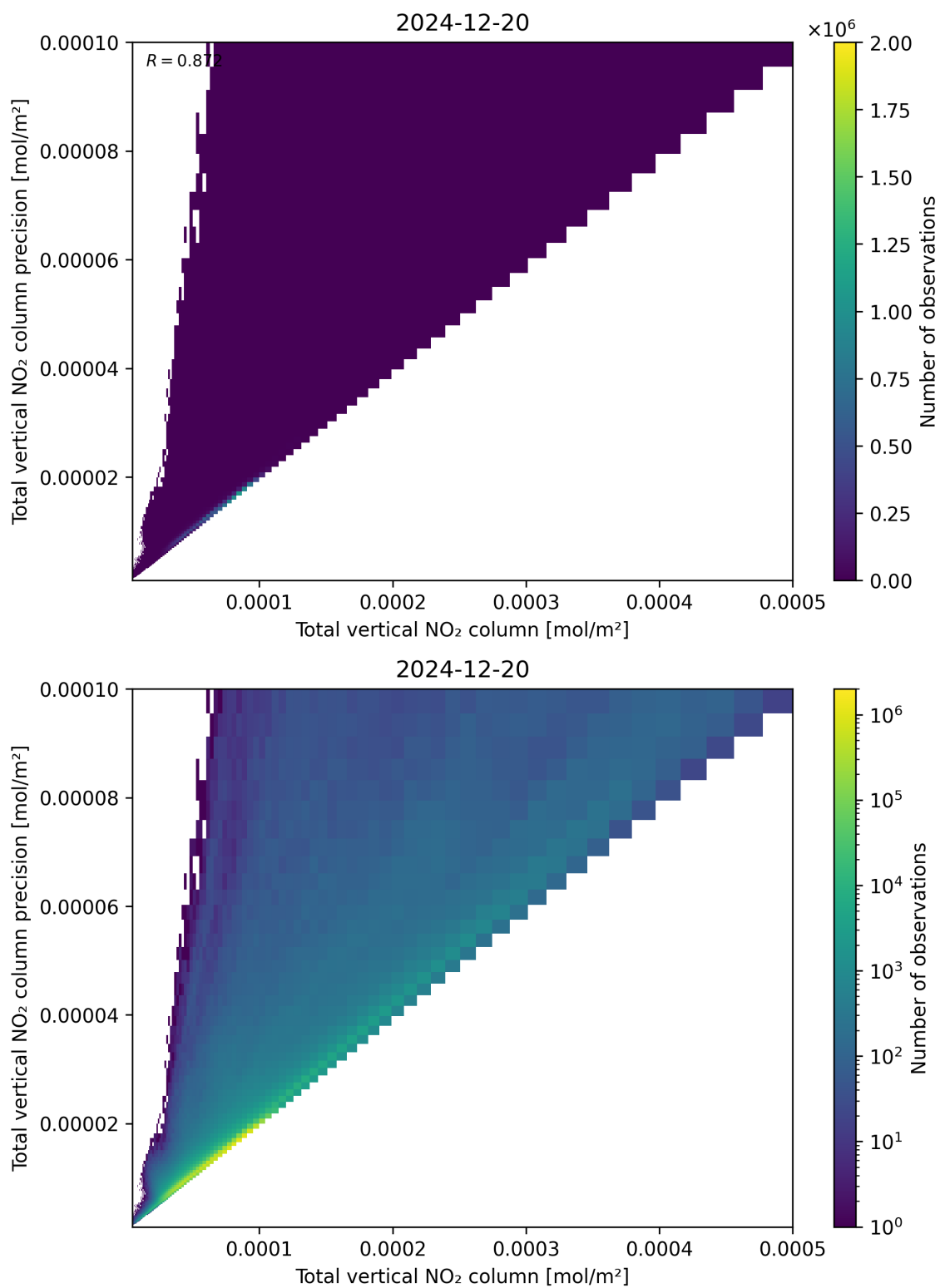
Figure 114: Scatter density plot of “Total vertical NO 2 column” against “Total vertical NO 2 column precision” for 2024-12-19 to 2024-12-21.
