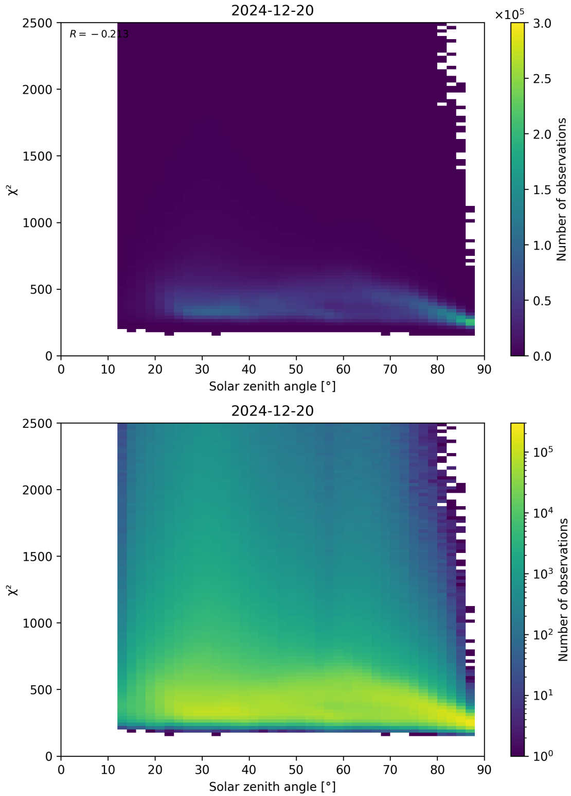
Figure 148: Scatter density plot of “Solar zenith angle” against “ \chi^2 ” for 2024-12-19 to 2024-12-21.
