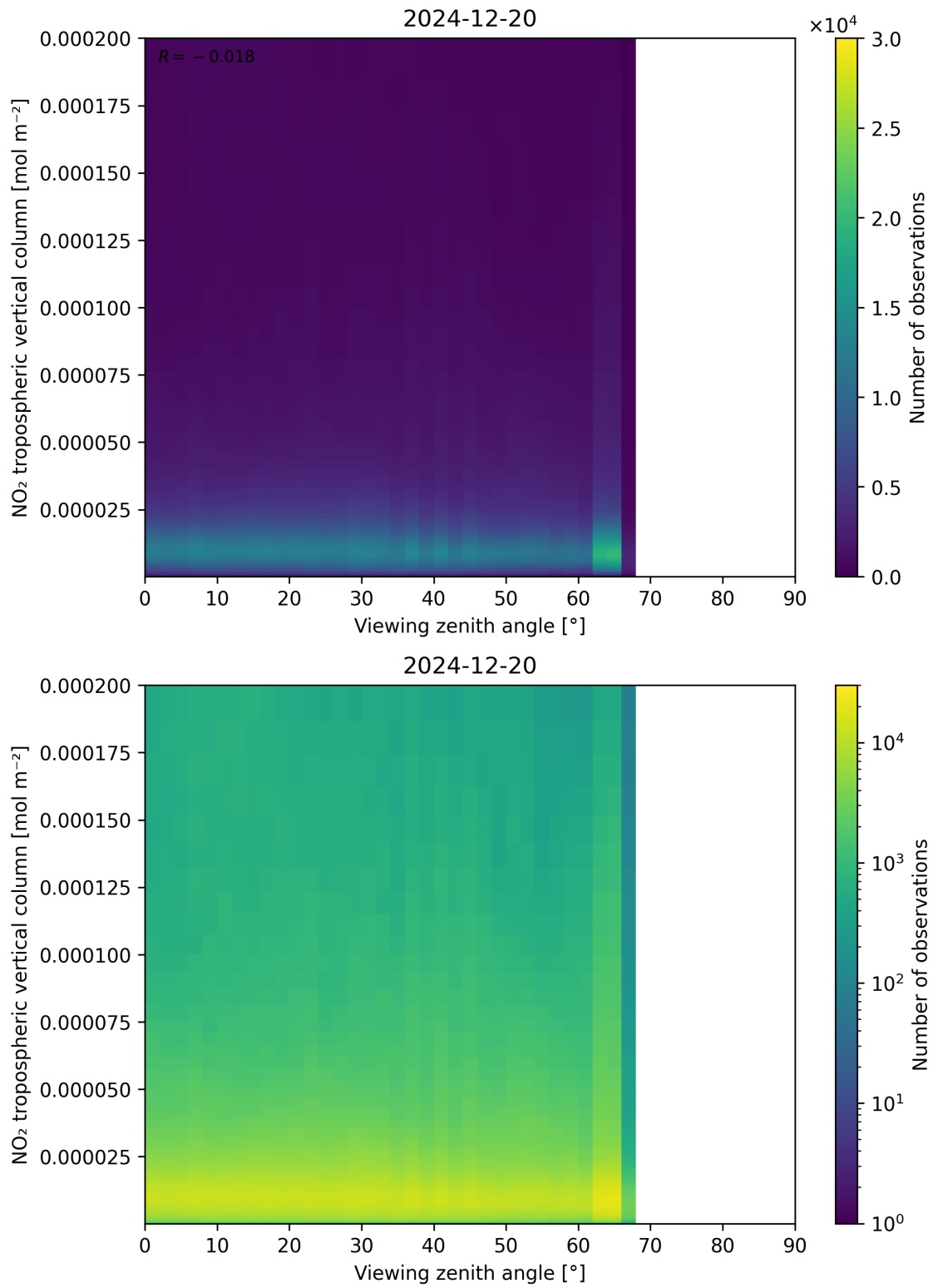
Figure 169: Scatter density plot of “Viewing zenith angle” against “NO 2 tropospheric vertical column” for 2024-12-19 to 2024-12-21.
