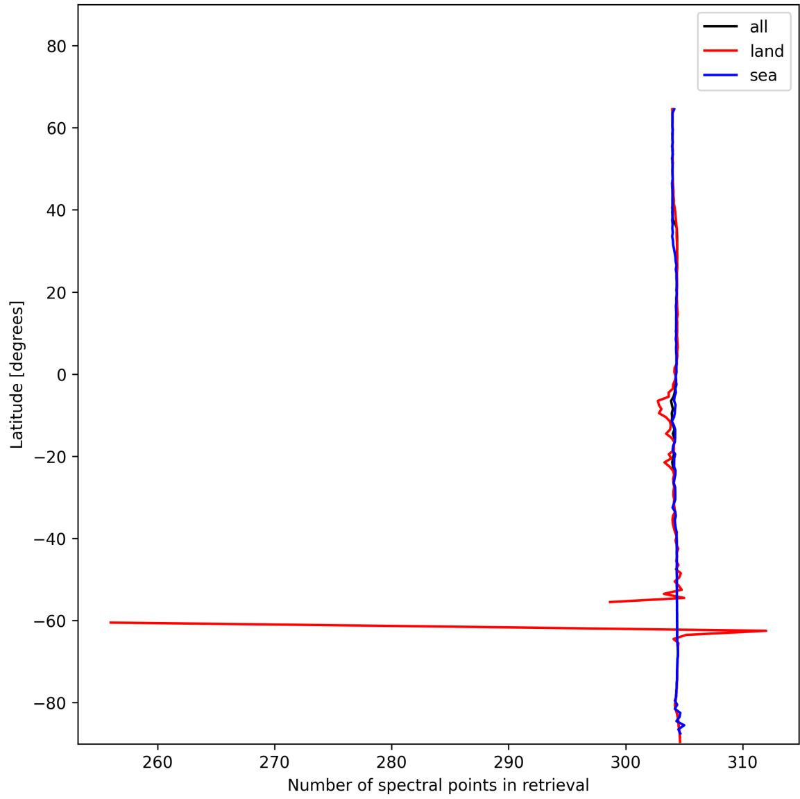
Figure 16: Zonal average of “Number of spectral points in retrieval” for 2024-12-19 to 2024-12-21.
