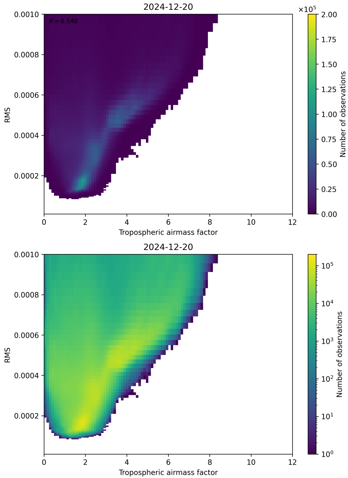
Figure 79: Scatter density plot of “Tropospheric airmass factor” against “RMS” for 2024-12-19 to 2024-12-21.
