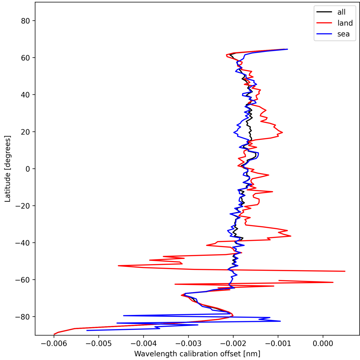
Figure 18: Zonal average of “Wavelength calibration offset” for 2024-12-19 to 2024-12-21.
