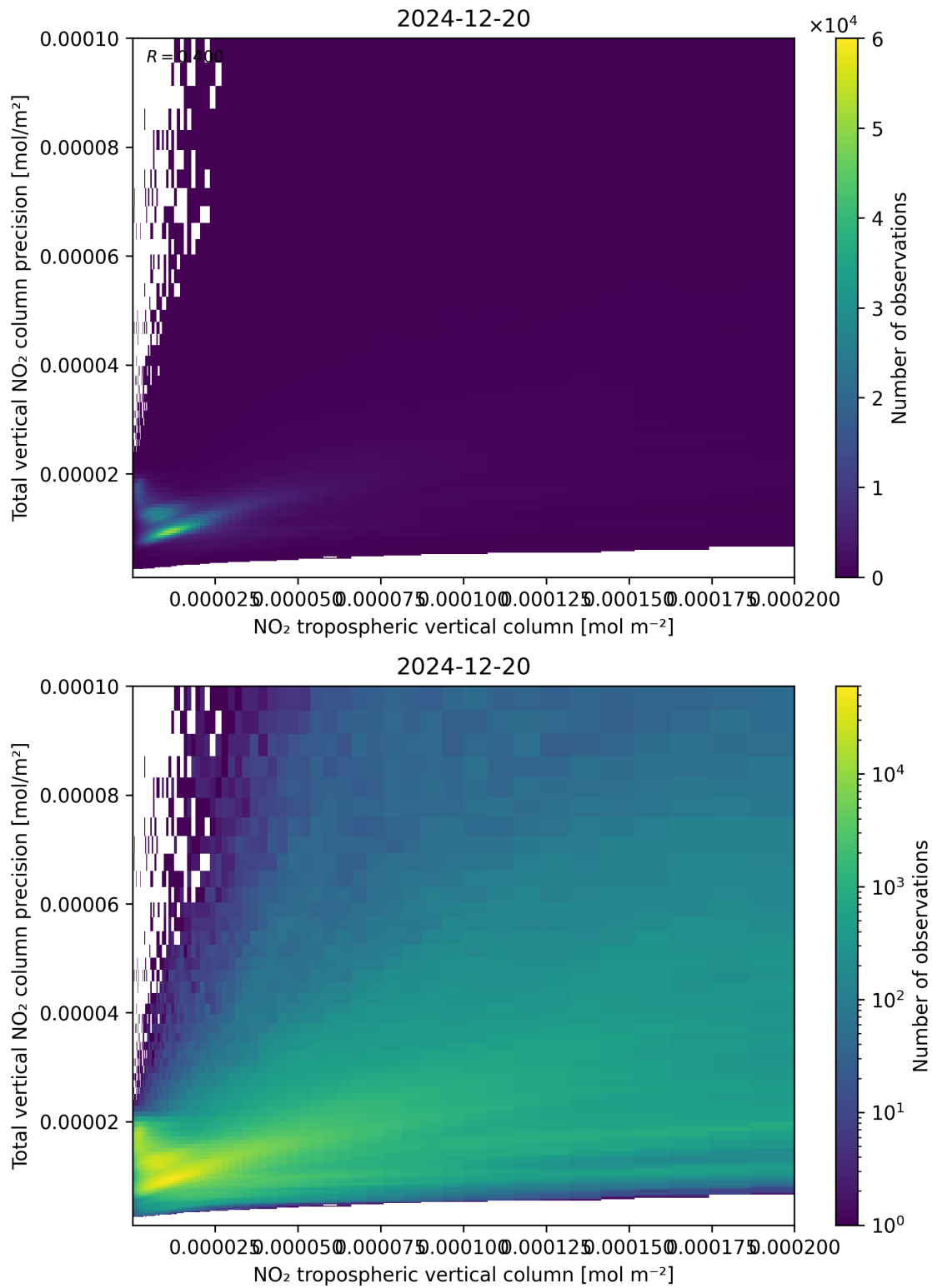
Figure 129: Scatter density plot of “NO 2 tropospheric vertical column” against “Total vertical NO 2 column precision” for 2024-12-19 to 2024-12-21.
