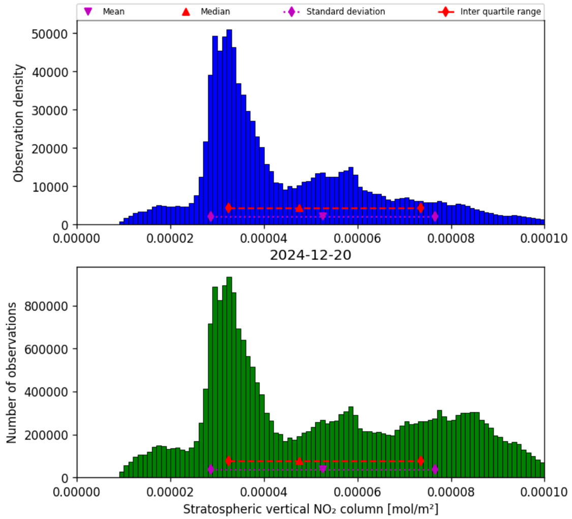
Figure 36: Histogram of “Stratospheric vertical NO 2 column” for 2024-12-19 to 2024-12-21
