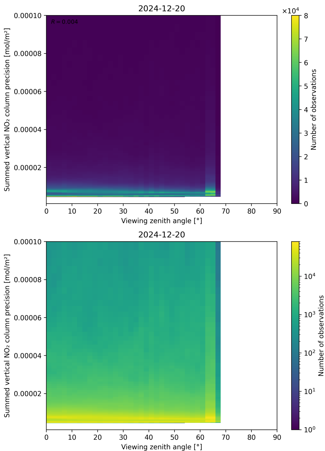
Figure 166: Scatter density plot of “Viewing zenith angle” against “Summed vertical NO 2 column precision” for 2024-12-19 to 2024-12-21.
