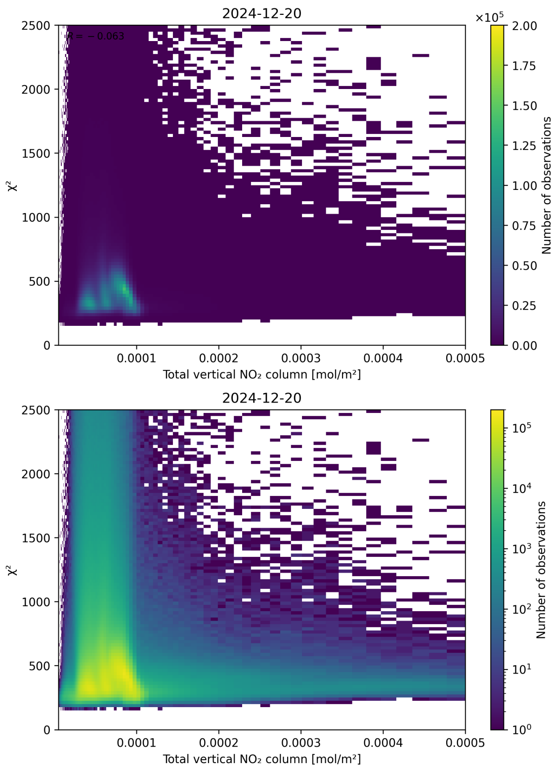
Figure 111: Scatter density plot of “Total vertical NO 2 column” against “ \chi^2 ” for 2024-12-19 to 2024-12-21.
