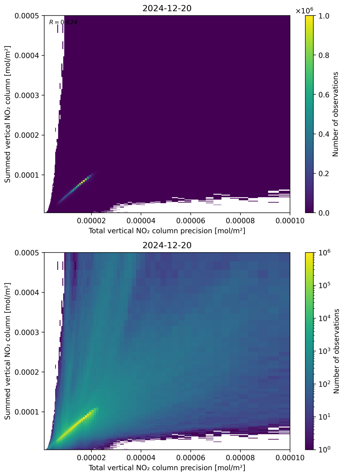
Figure 117: Scatter density plot of “Total vertical NO 2 column precision” against “Summed vertical NO 2 column” for 2024-12-19 to 2024-12-21.
