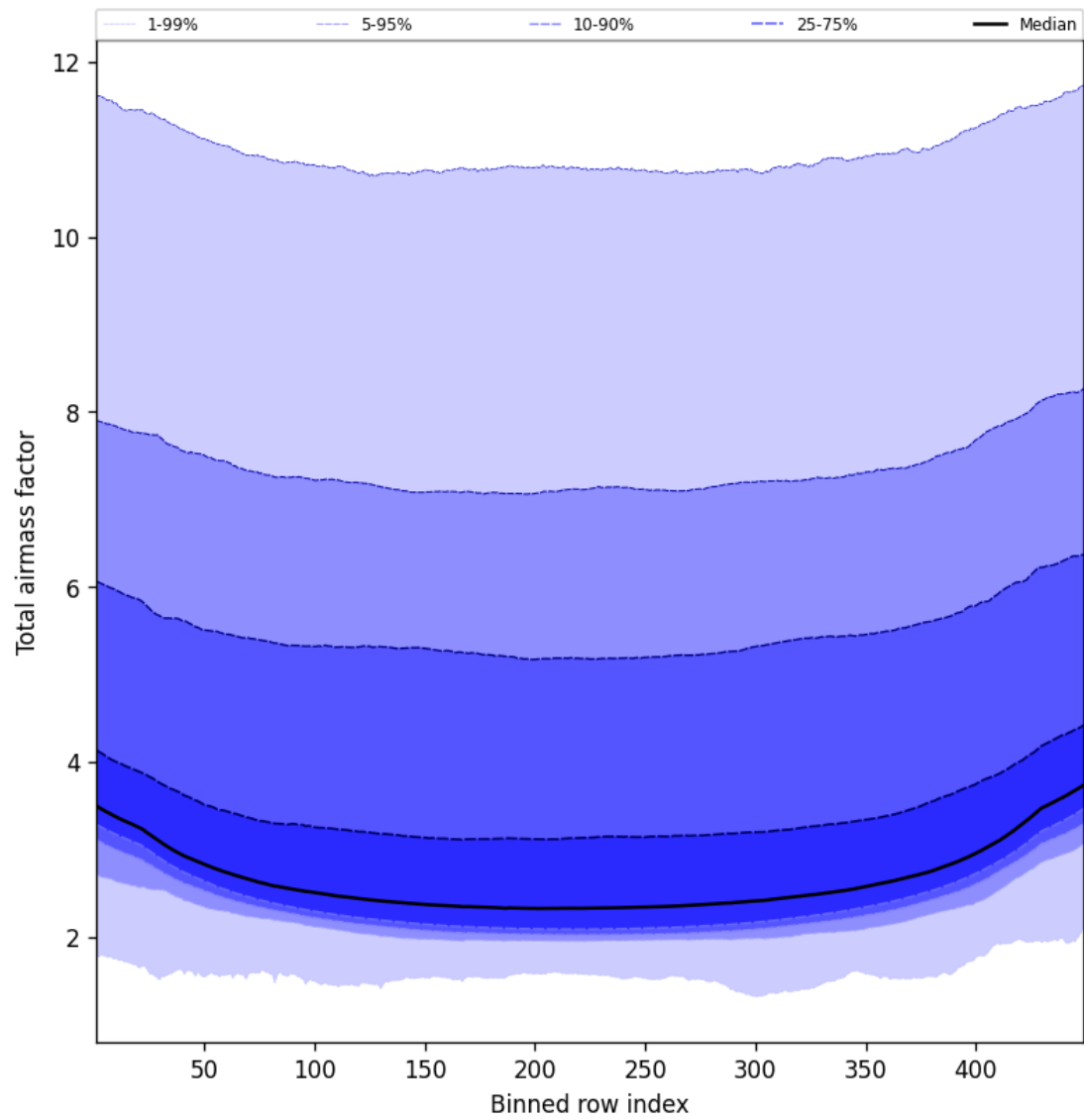
Figure 49: Along track statistics of “Total airmass factor” for 2024-12-19 to 2024-12-21
