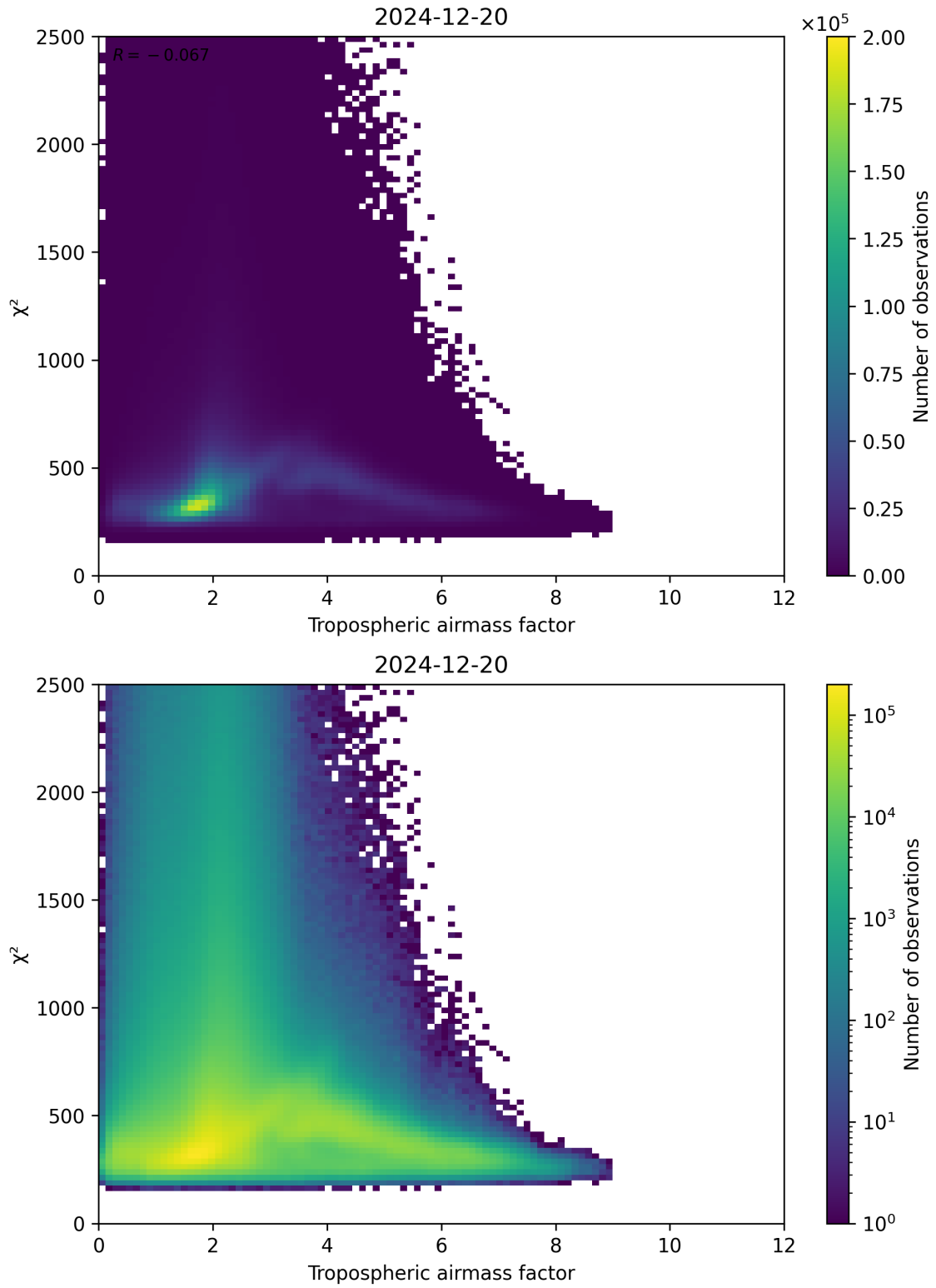
Figure 73: Scatter density plot of “Tropospheric airmass factor” against “ \chi^2 ” for 2024-12-19 to 2024-12-21.
