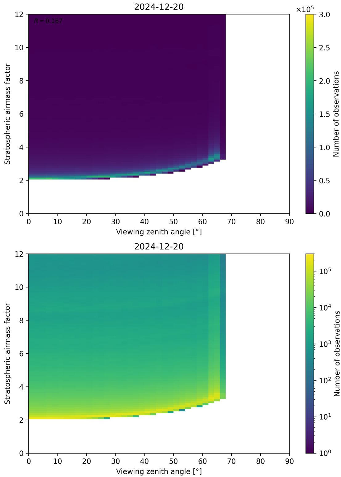
Figure 159: Scatter density plot of “Viewing zenith angle” against “Stratospheric airmass factor” for 2024-12-19 to 2024-12-21.
