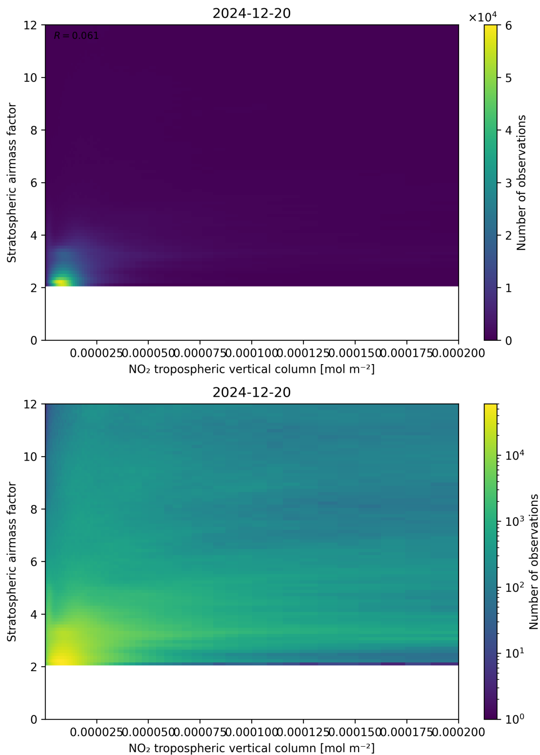
Figure 121: Scatter density plot of “NO 2 tropospheric vertical column” against “Stratospheric airmass factor” for 2024-12-19 to 2024-12-21.
