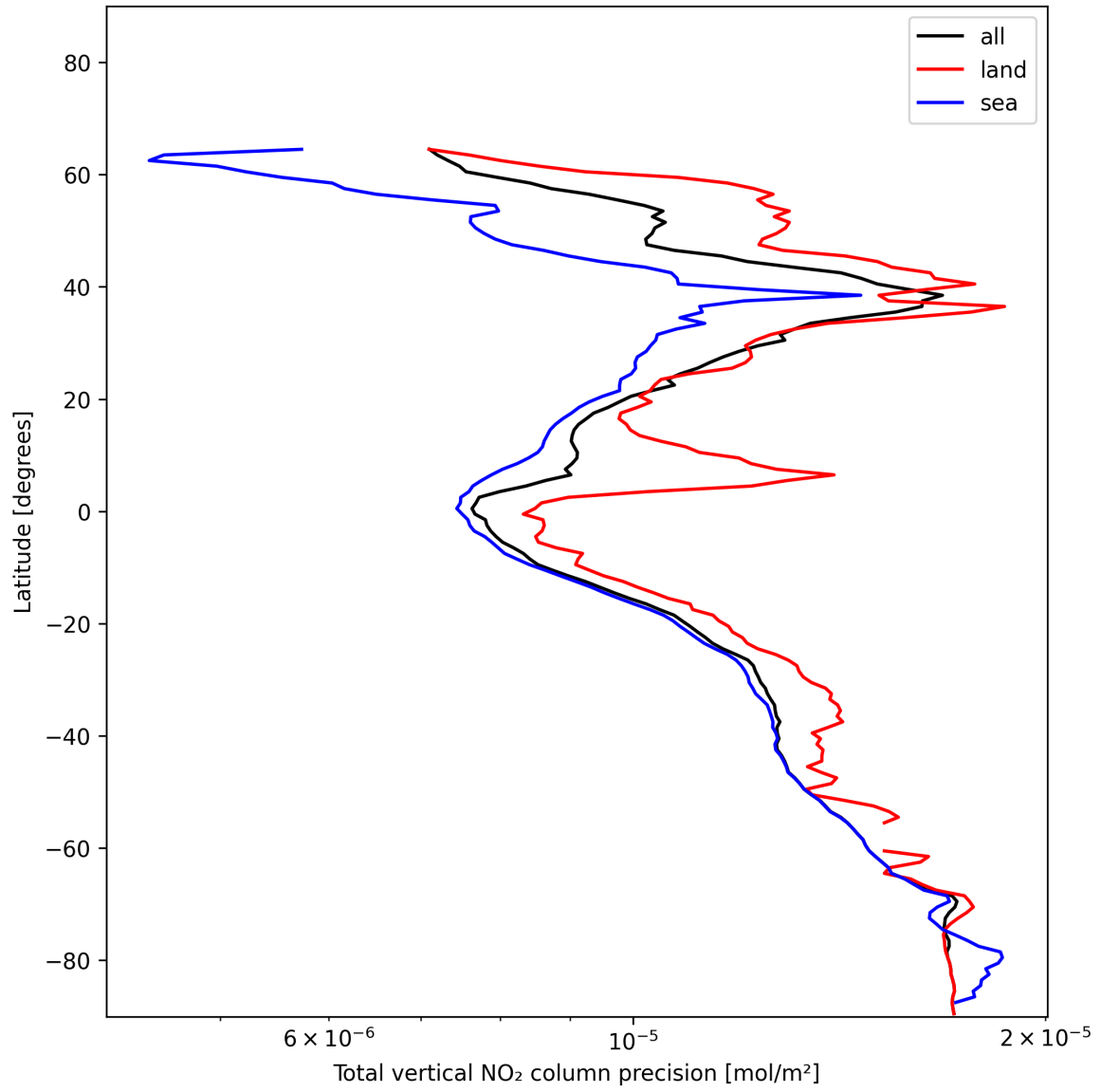
Figure 22: Zonal average of “Total vertical NO 2 column precision” for 2024-12-19 to 2024-12-21.
