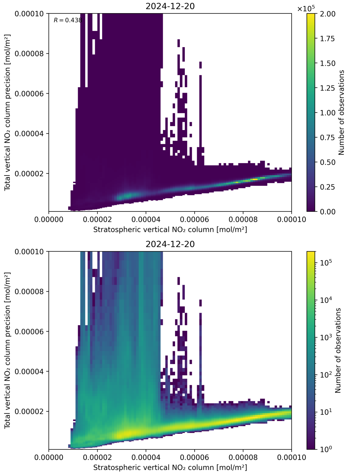
Figure 101: Scatter density plot of “Stratospheric vertical NO 2 column” against “Total vertical NO 2 column precision” for 2024-12-19 to 2024-12-21.
