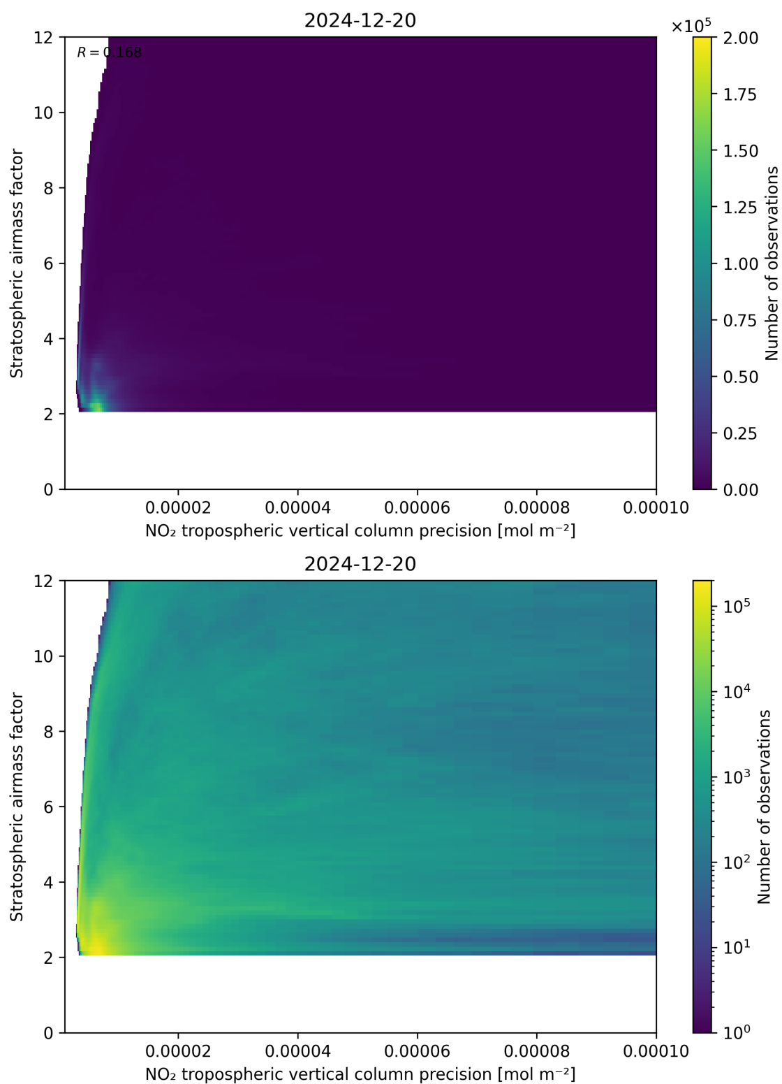
Figure 131: Scatter density plot of “NO 2 tropospheric vertical column precision” against “Stratospheric airmass factor” for 2024-12-19 to 2024-12-21.
