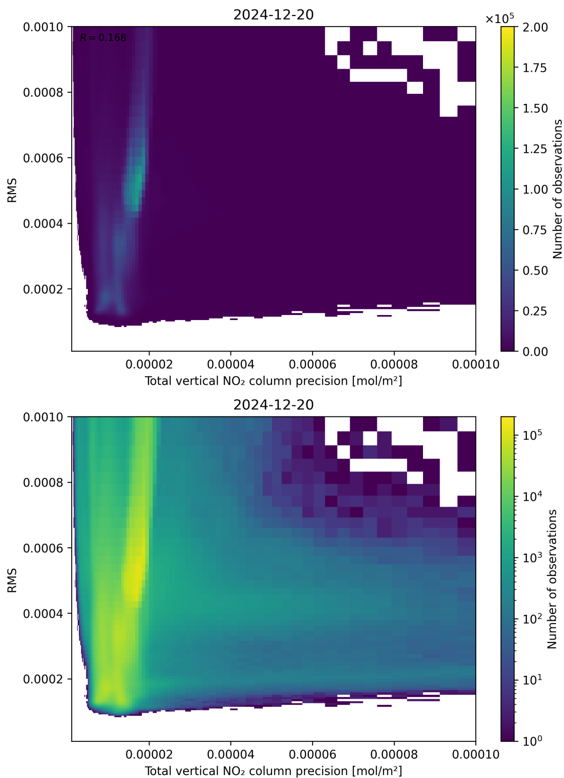
Figure 119: Scatter density plot of “Total vertical NO 2 column precision” against “RMS” for 2024-12-19 to 2024-12-21.
