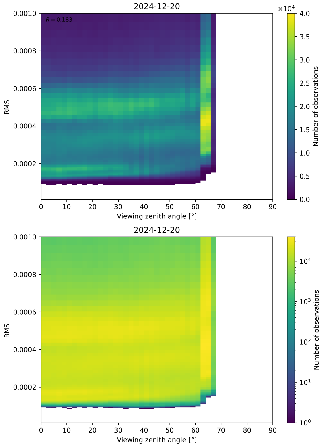
Figure 171: Scatter density plot of “Viewing zenith angle” against “RMS” for 2024-12-19 to 2024-12-21.
