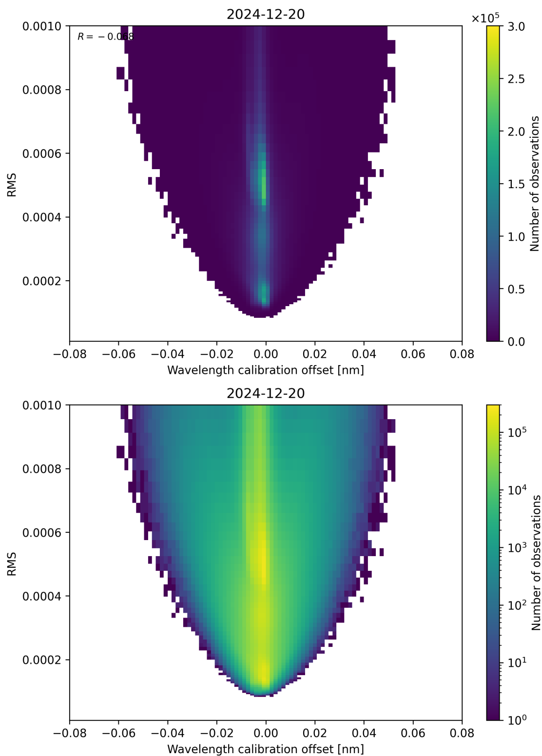
Figure 181: Scatter density plot of “Wavelength calibration offset” against “RMS” for 2024-12-19 to 2024-12-21.
