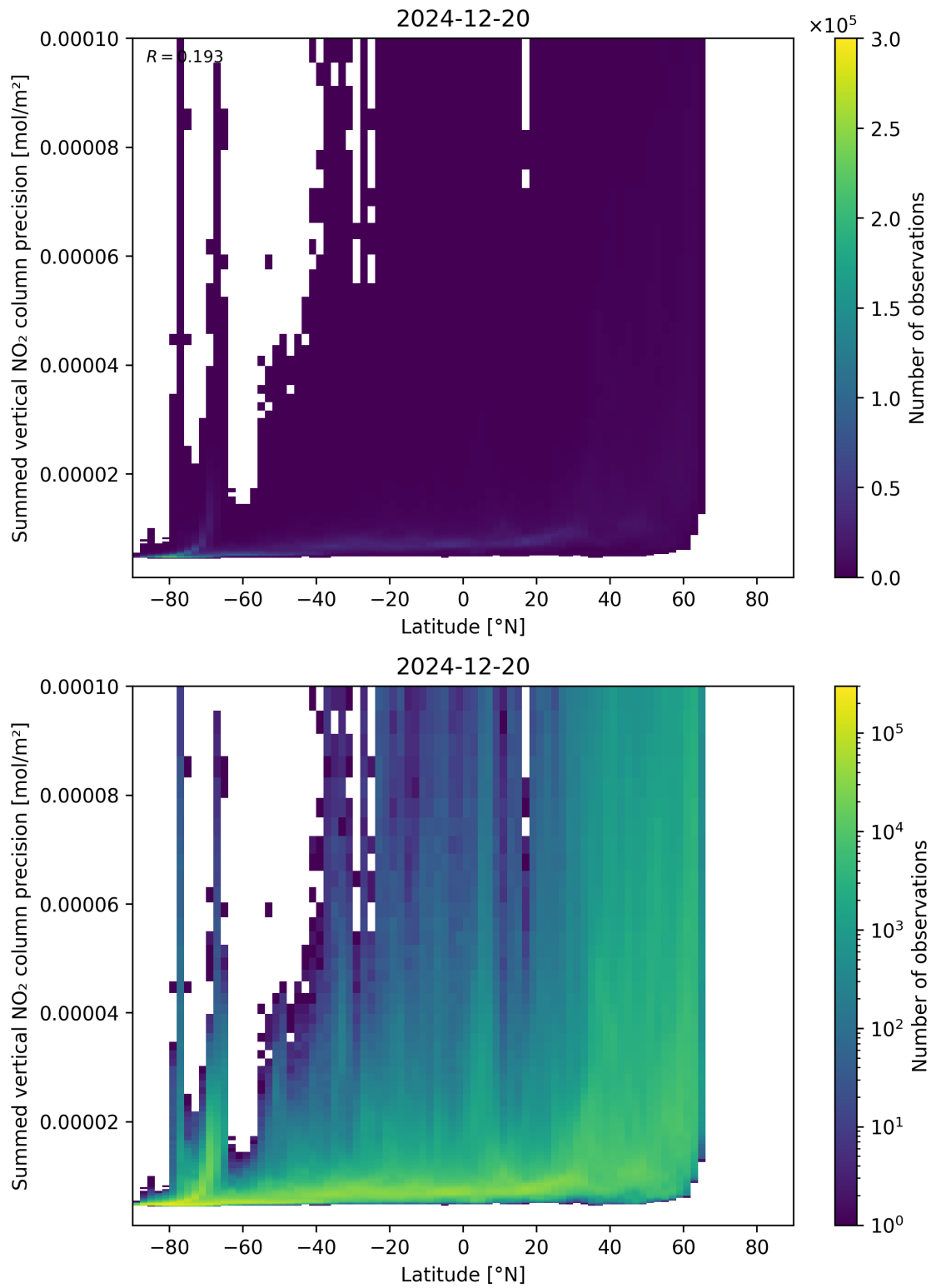
Figure 89: Scatter density plot of “Latitude” against “Summed vertical NO 2 column precision” for 2024-12-19 to 2024-12-21.
