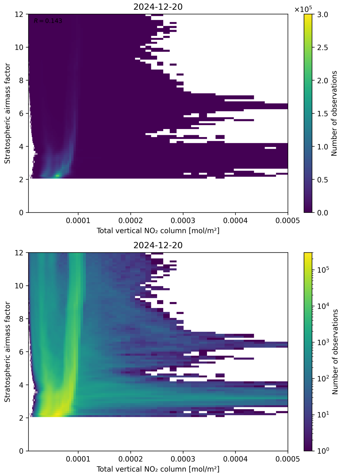
Figure 110: Scatter density plot of “Total vertical NO 2 column” against “Stratospheric airmass factor” for 2024-12-19 to 2024-12-21.
