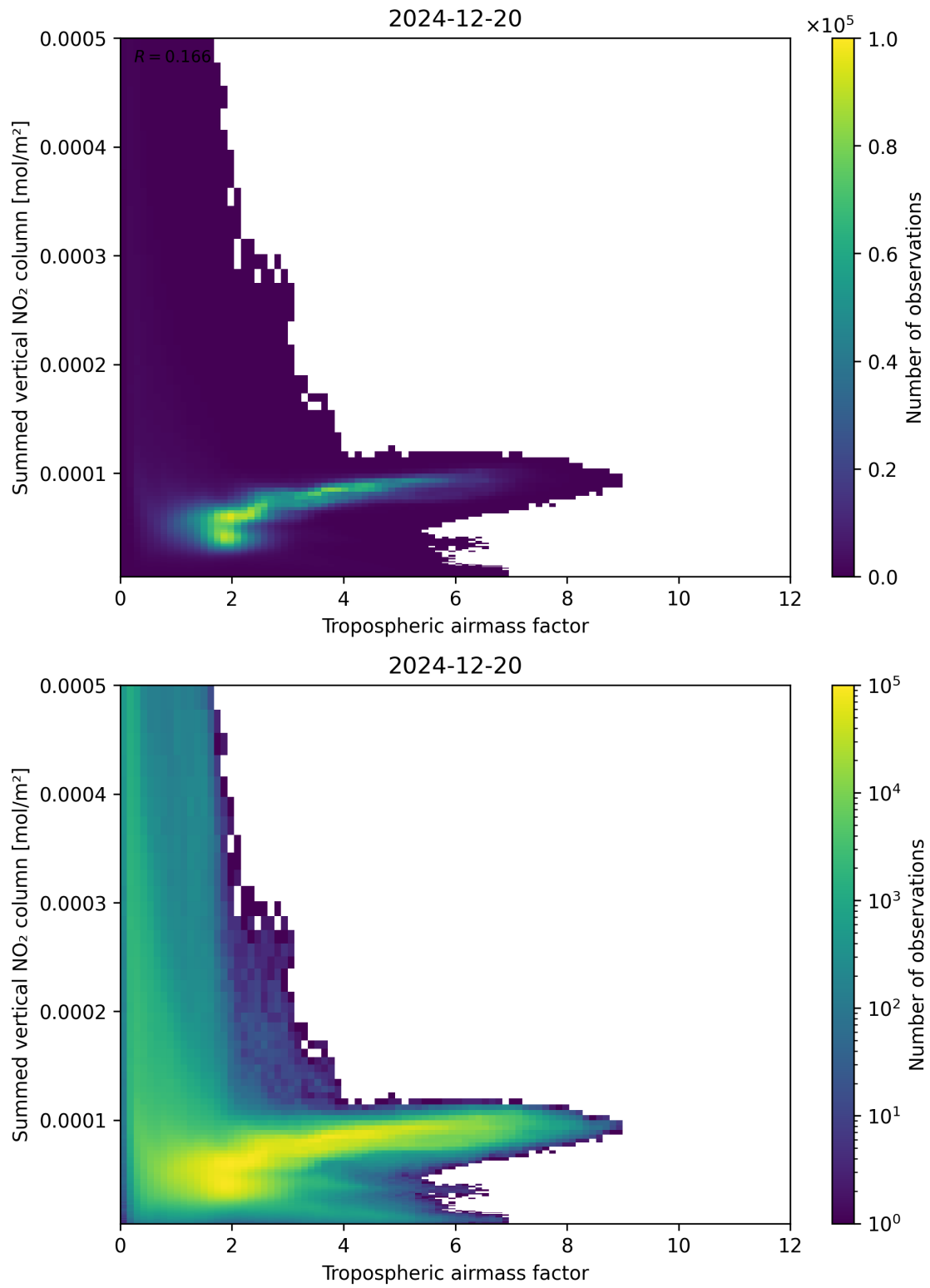
Figure 75: Scatter density plot of “Tropospheric airmass factor” against “Summed vertical NO 2 column” for 2024-12-19 to 2024-12-21.
