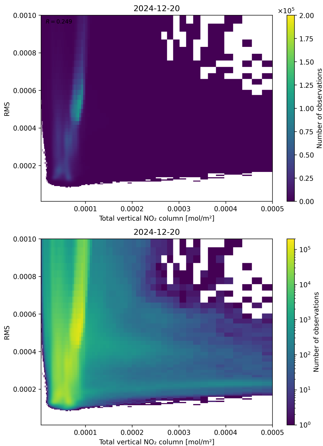
Figure 120: Scatter density plot of “Total vertical NO 2 column” against “RMS” for 2024-12-19 to 2024-12-21.
