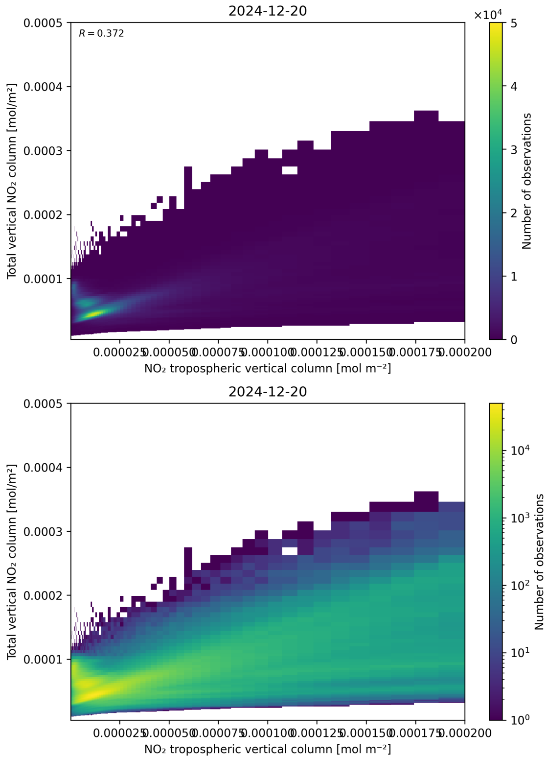
Figure 128: Scatter density plot of “NO 2 tropospheric vertical column” against “Total vertical NO 2 column” for 2024-12-19 to 2024-12-21.
