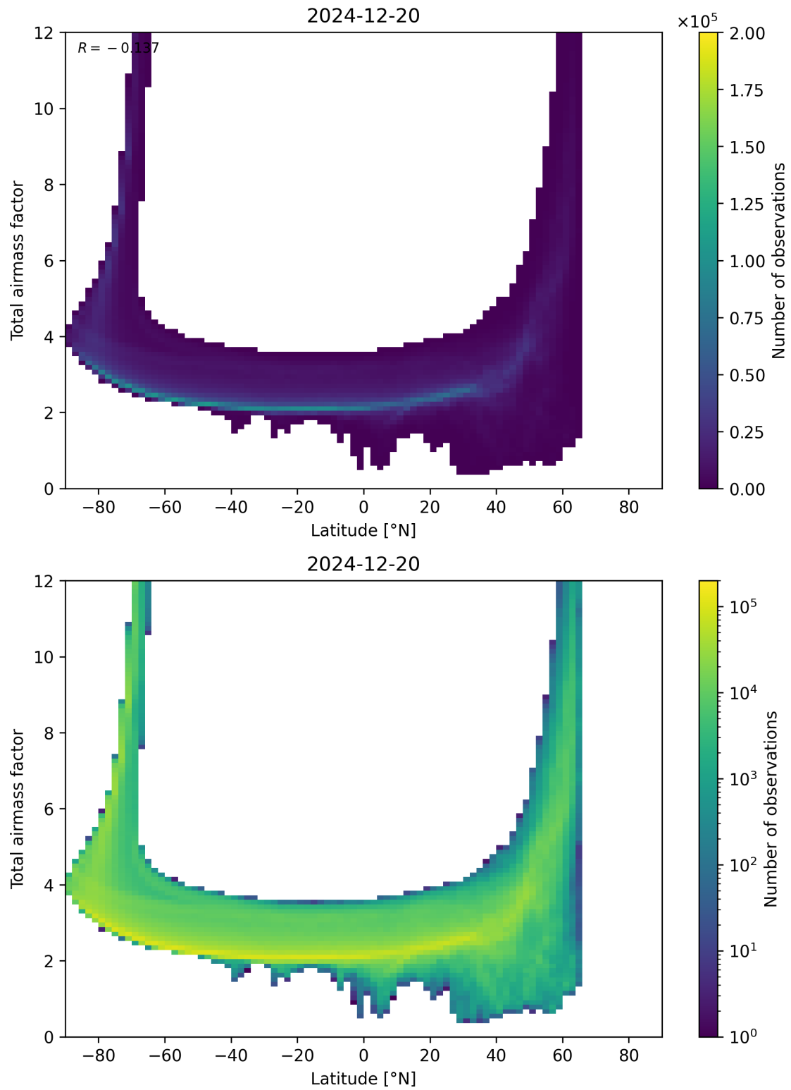
Figure 84: Scatter density plot of “Latitude” against “Total airmass factor” for 2024-12-19 to 2024-12-21.
