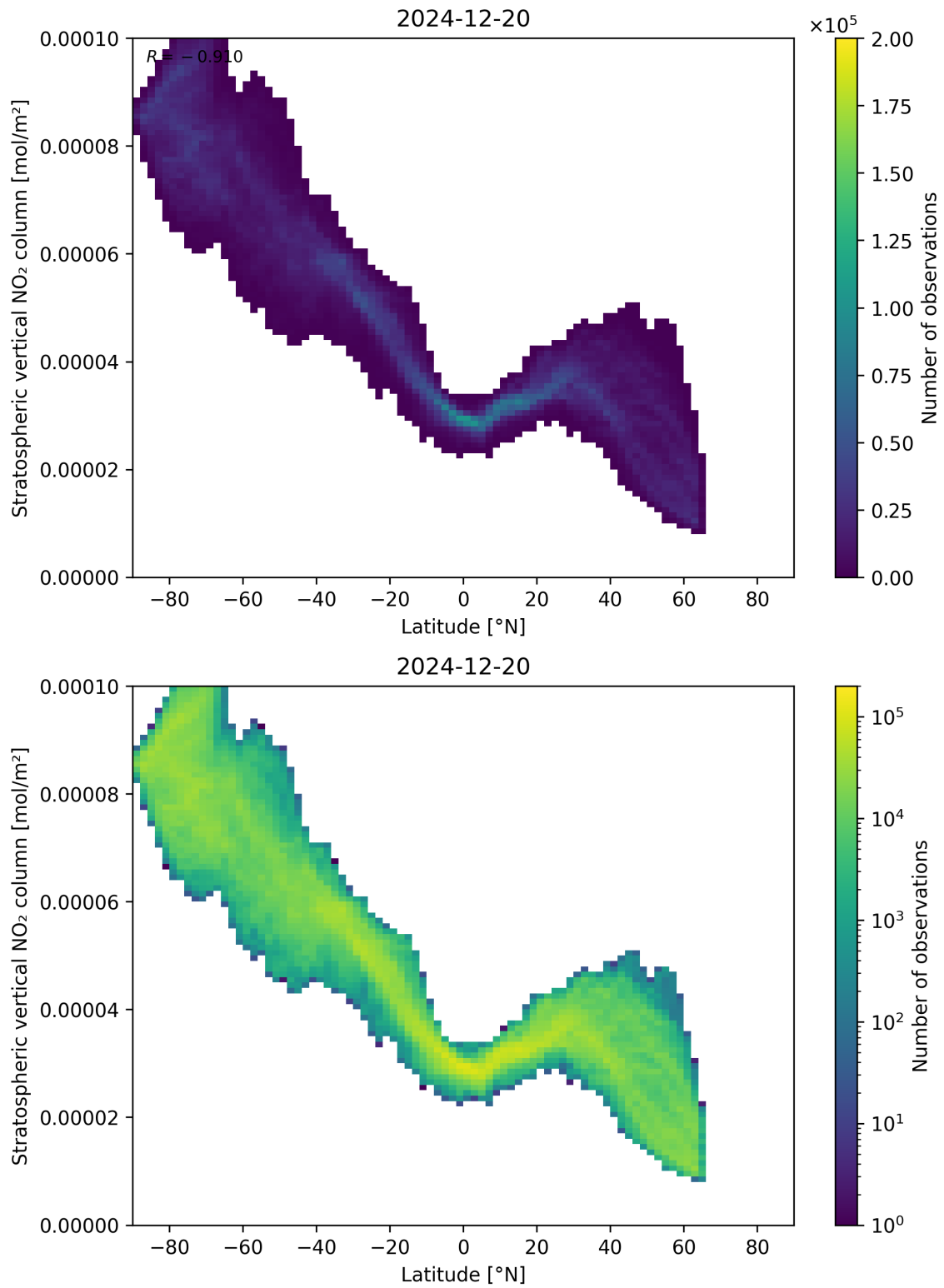
Figure 87: Scatter density plot of “Latitude” against “Stratospheric vertical NO 2 column” for 2024-12-19 to 2024-12-21.
