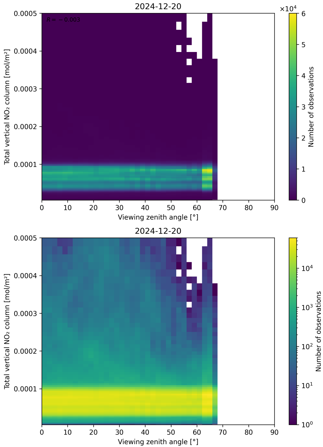
Figure 167: Scatter density plot of “Viewing zenith angle” against “Total vertical NO 2 column” for 2024-12-19 to 2024-12-21.
