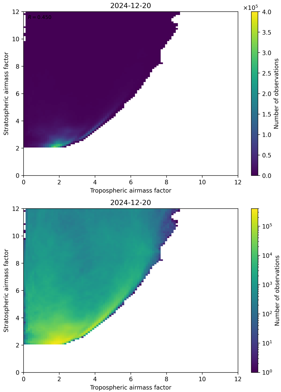
Figure 71: Scatter density plot of “Tropospheric airmass factor” against “Stratospheric airmass factor” for 2024-12-19 to 2024-12-21.
