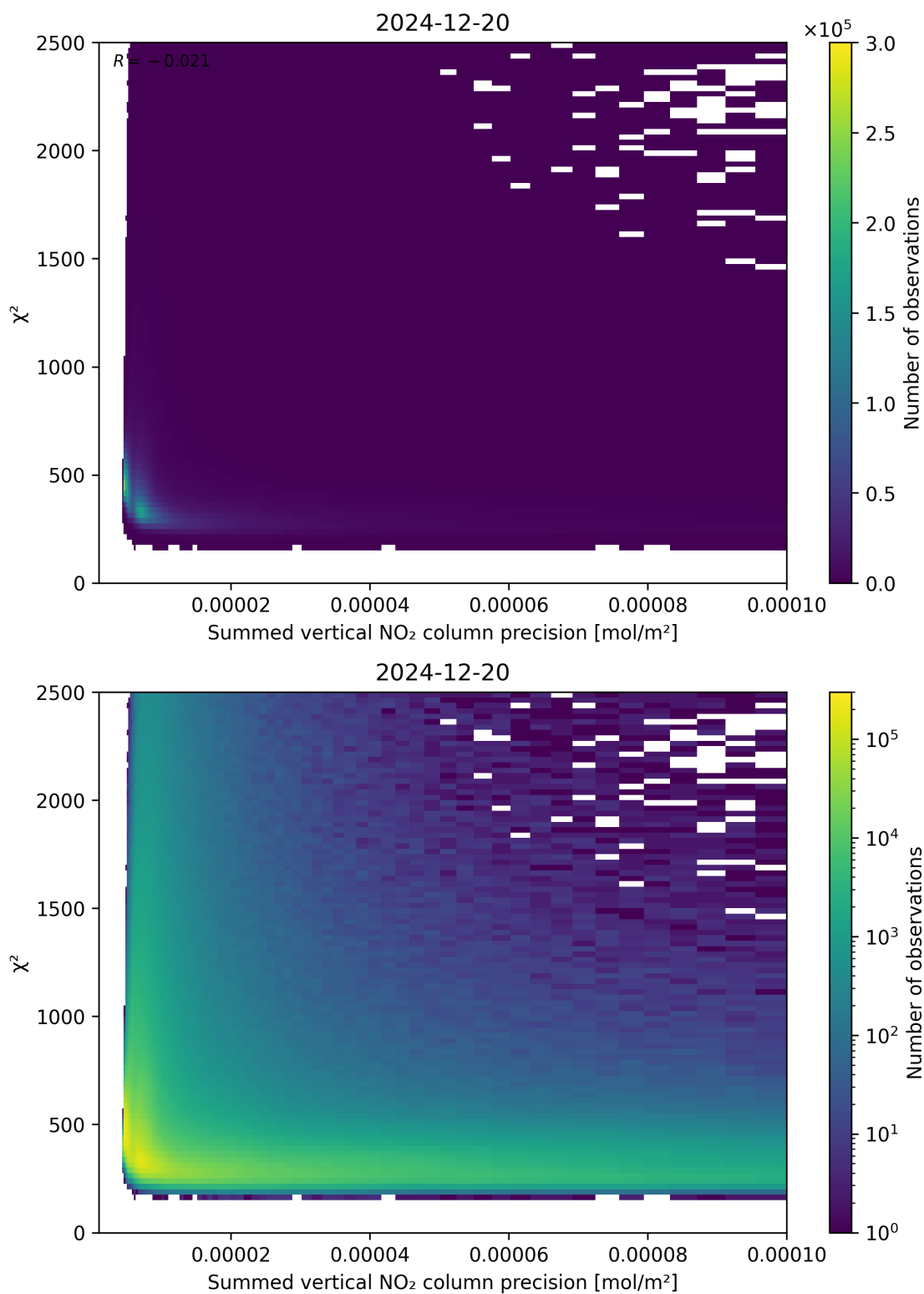
Figure 107: Scatter density plot of “Summed vertical NO 2 column precision” against “ \chi^2 ” for 2024-12-19 to 2024-12-21.
