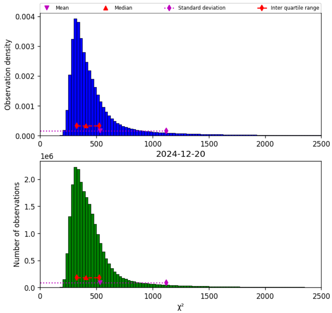
Figure 42: Histogram of “ \chi^2 ” for 2024-12-19 to 2024-12-21
