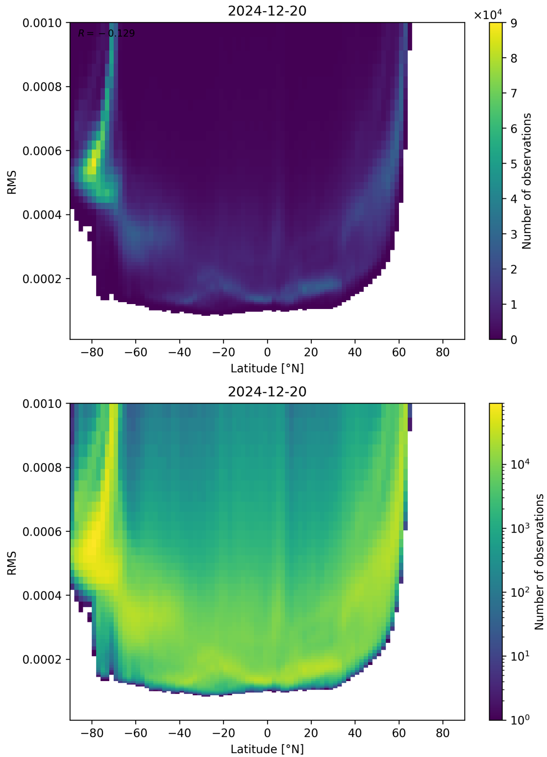
Figure 94: Scatter density plot of “Latitude” against “RMS” for 2024-12-19 to 2024-12-21.
