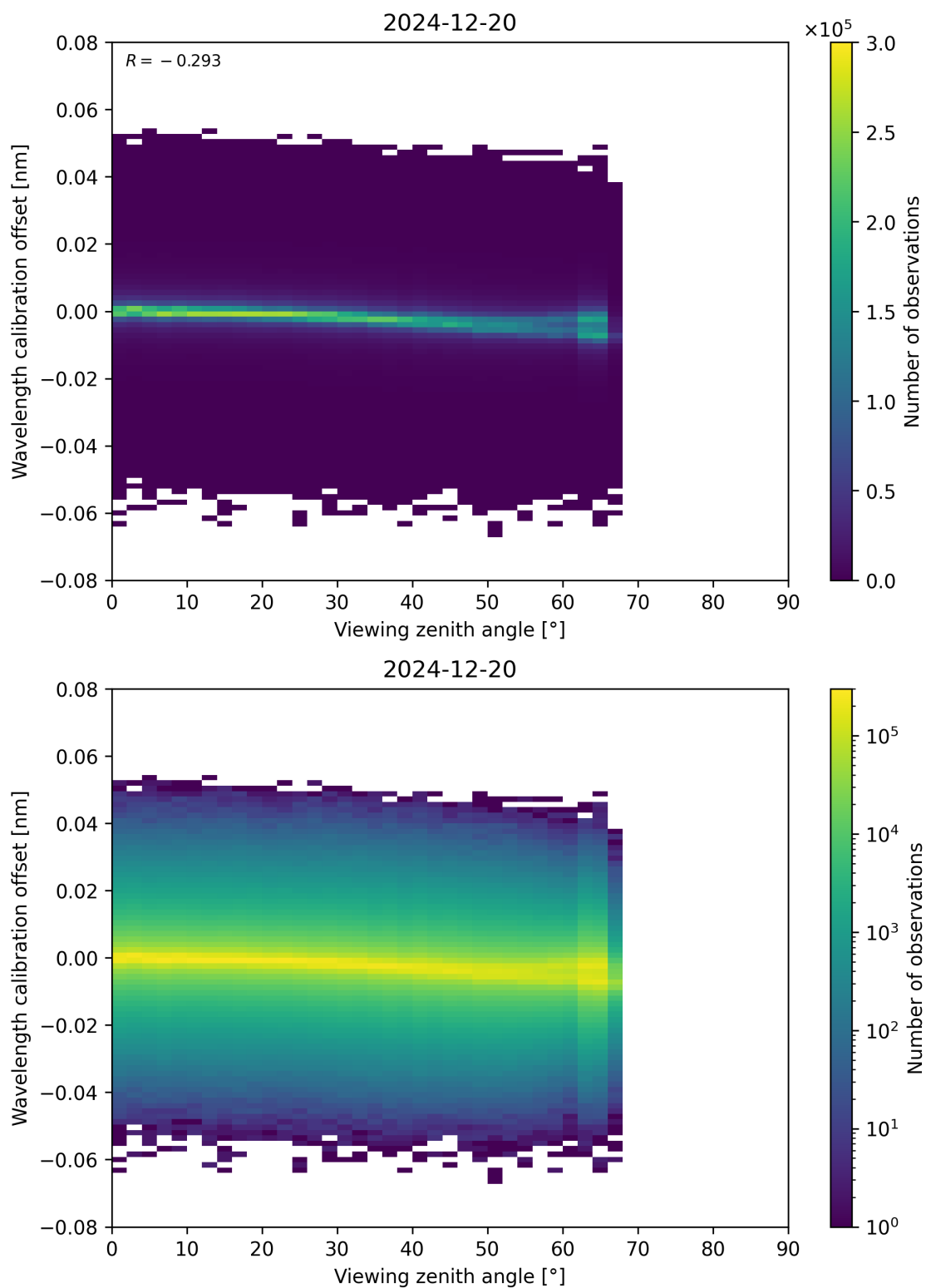
Figure 173: Scatter density plot of “Viewing zenith angle” against “Wavelength calibration offset” for 2024-12-19 to 2024-12-21.
