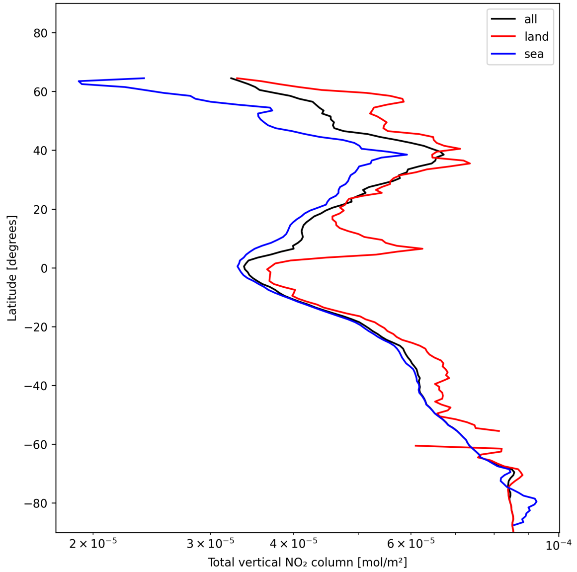
Figure 21: Zonal average of “Total vertical NO 2 column” for 2024-12-19 to 2024-12-21.
