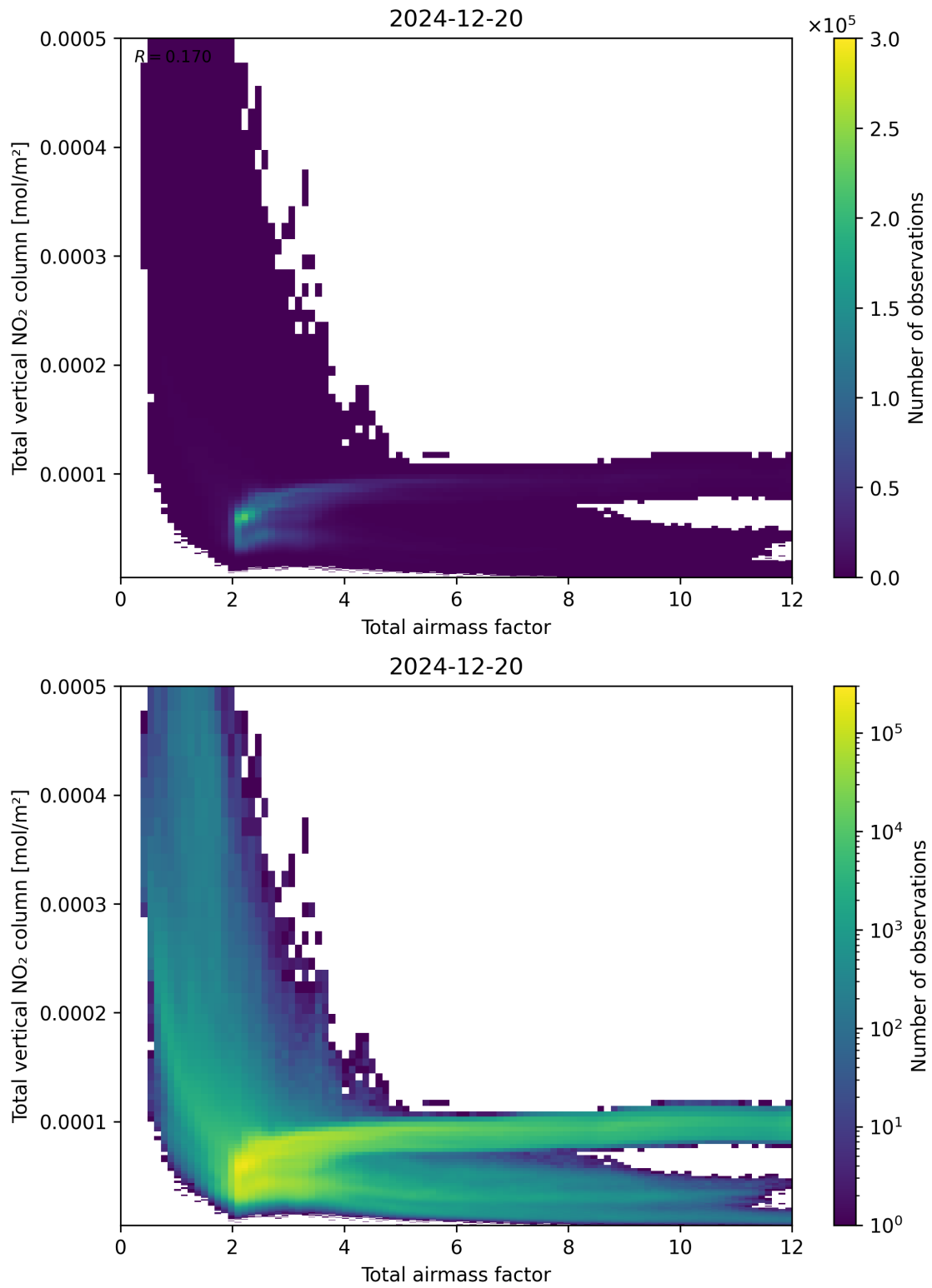
Figure 67: Scatter density plot of “Total airmass factor” against “Total vertical NO 2 column” for 2024-12-19 to 2024-12-21.
