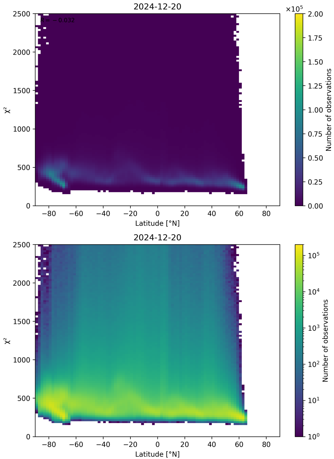
Figure 86: Scatter density plot of “Latitude” against “ \chi^2 ” for 2024-12-19 to 2024-12-21.
