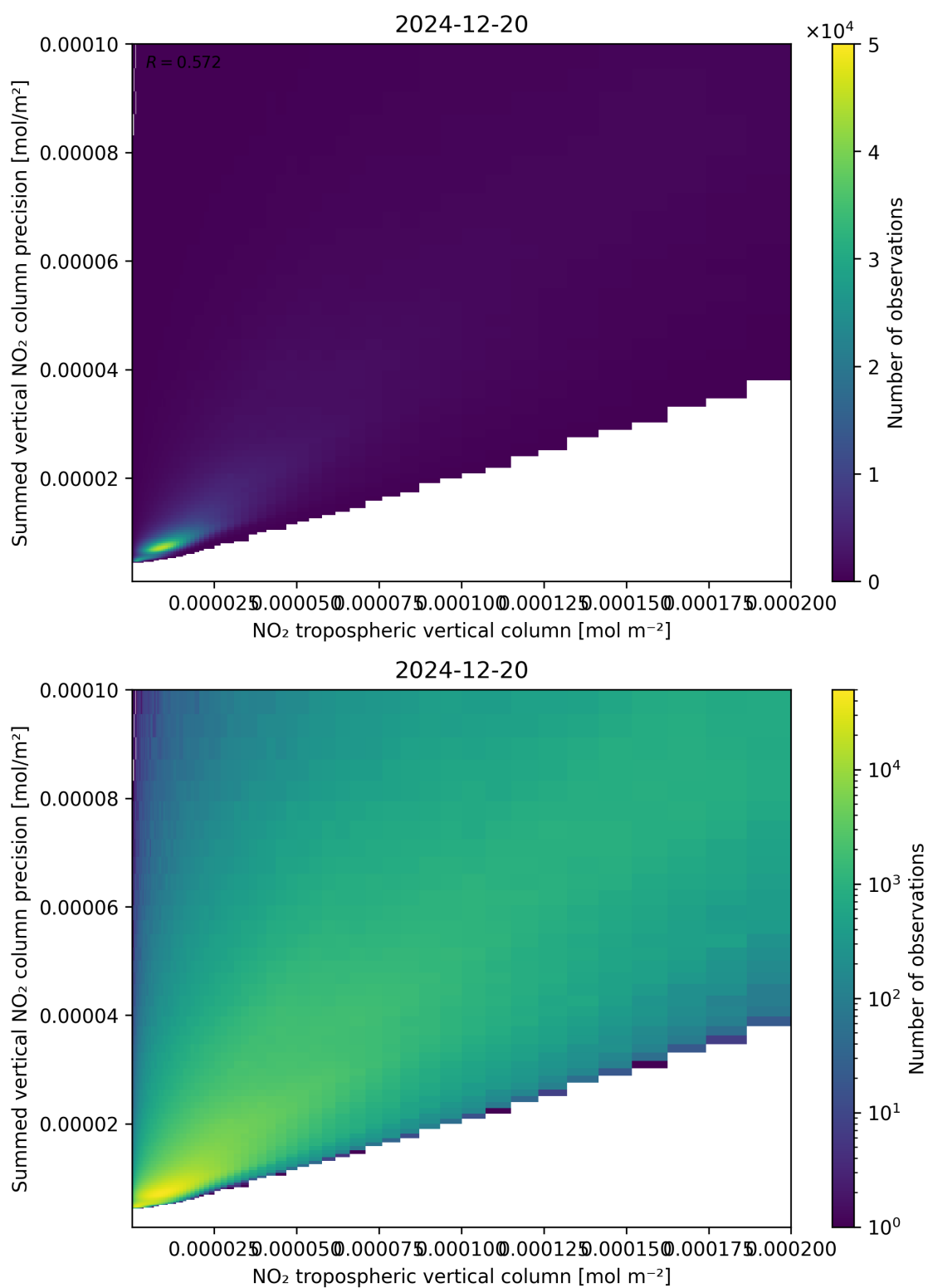
Figure 127: Scatter density plot of “NO 2 tropospheric vertical column” against “Summed vertical NO 2 column precision” for 2024-12-19 to 2024-12-21.
