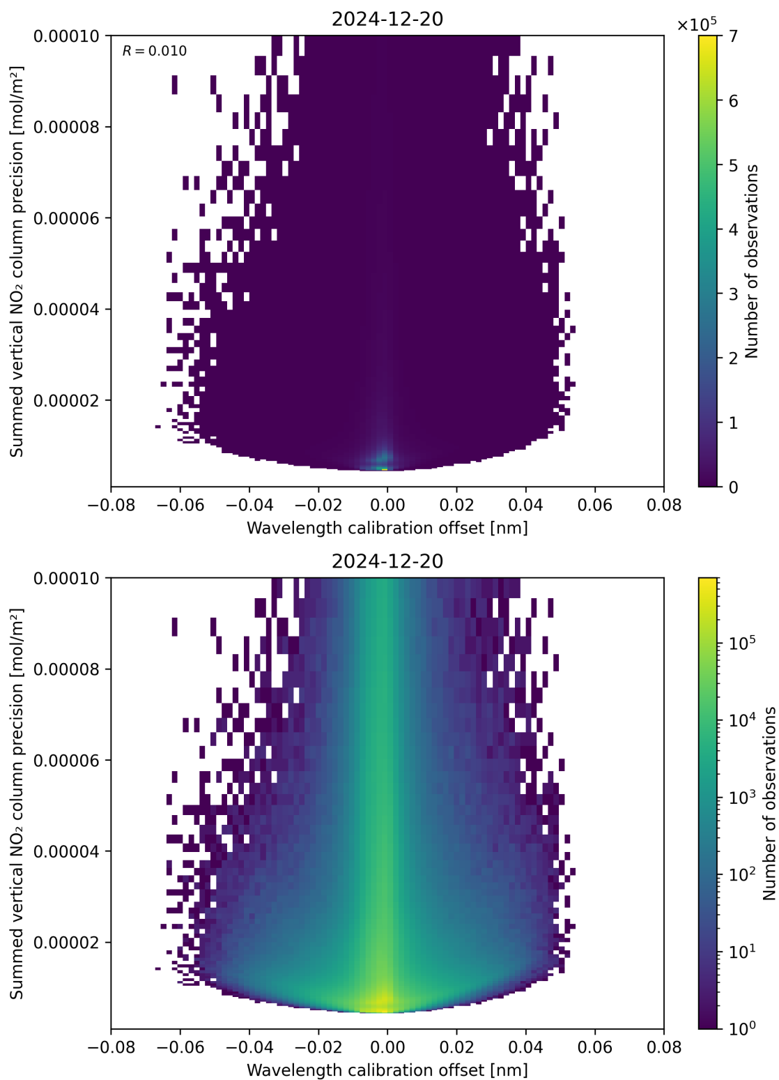
Figure 178: Scatter density plot of “Wavelength calibration offset” against “Summed vertical NO 2 column precision” for 2024-12-19 to 2024-12-21.
