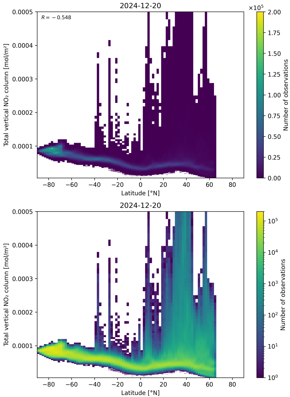
Figure 90: Scatter density plot of “Latitude” against “Total vertical NO 2 column” for 2024-12-19 to 2024-12-21.
