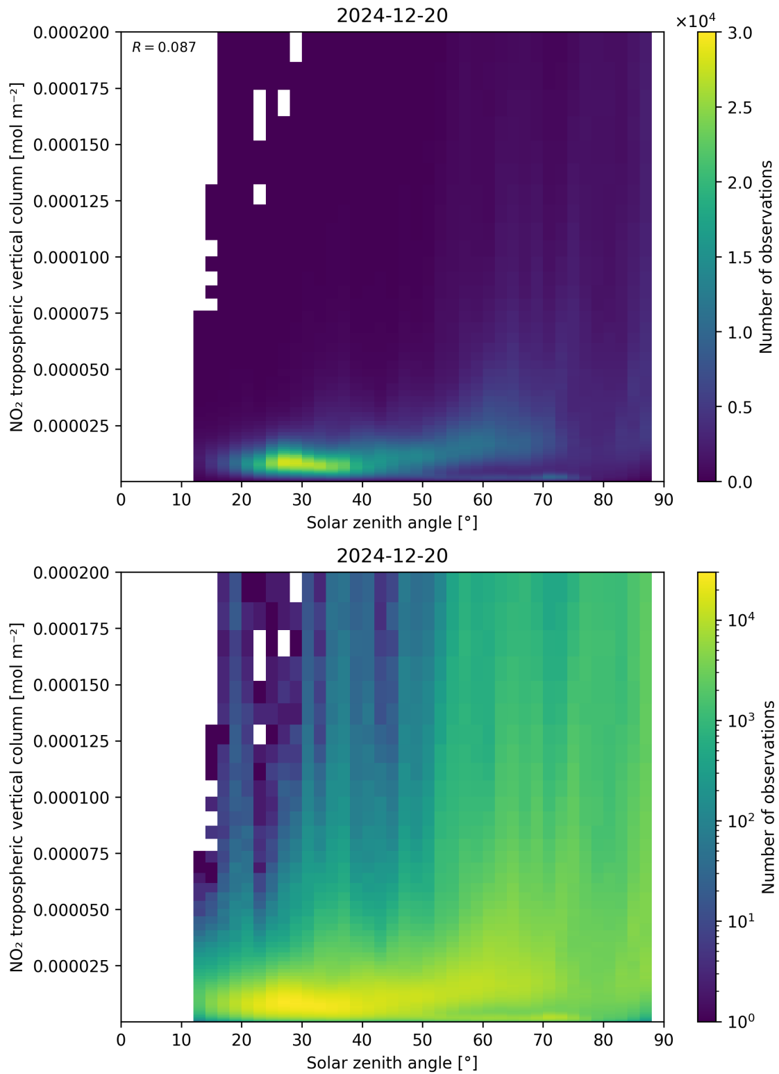
Figure 155: Scatter density plot of “Solar zenith angle” against “NO 2 tropospheric vertical column” for 2024-12-19 to 2024-12-21.
