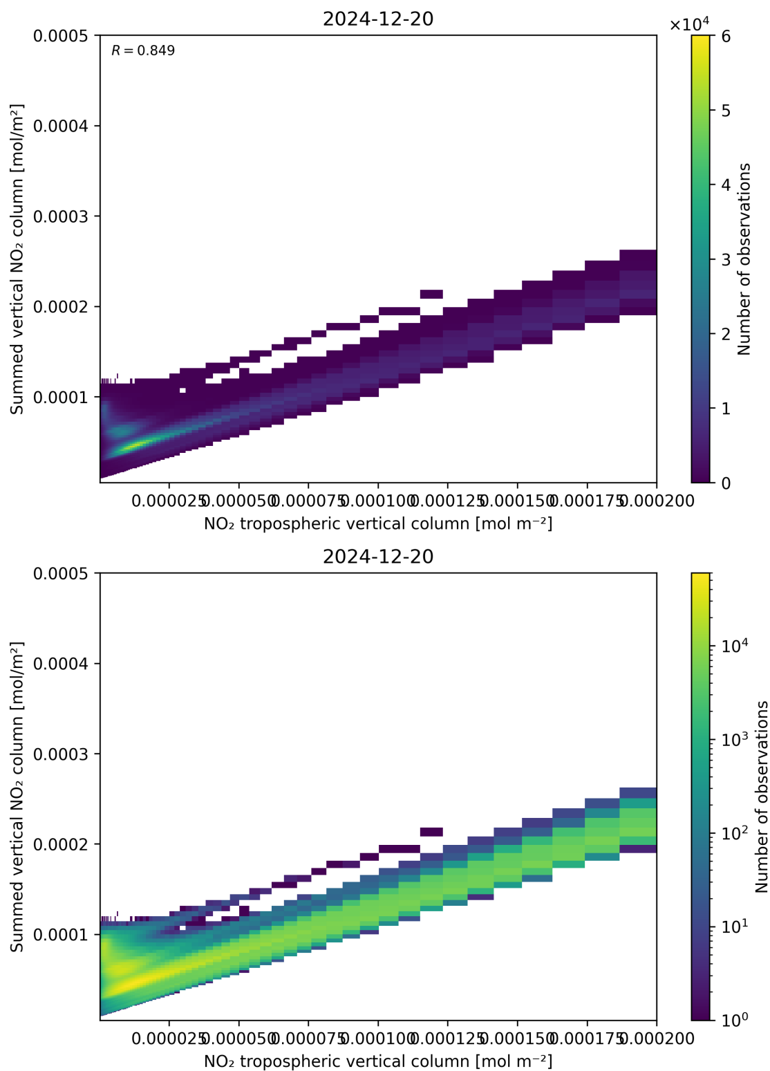
Figure 126: Scatter density plot of “NO 2 tropospheric vertical column” against “Summed vertical NO 2 column” for 2024-12-19 to 2024-12-21.
