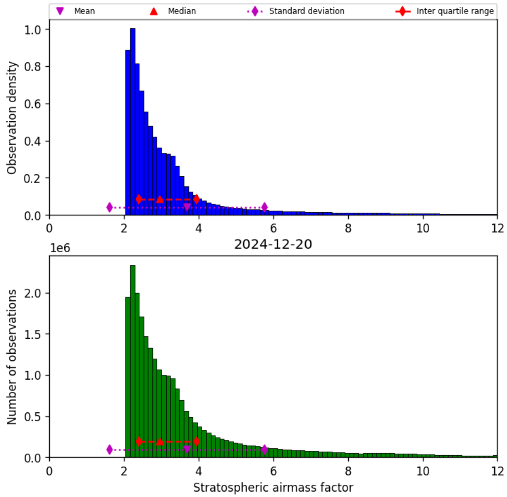
Figure 44: Histogram of “Stratospheric airmass factor” for 2024-12-19 to 2024-12-21
