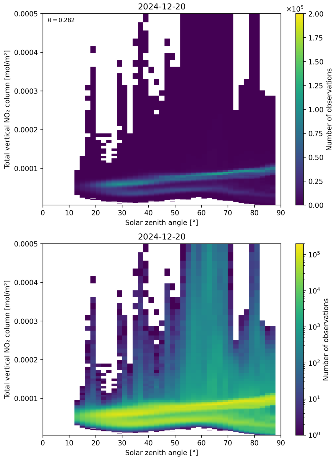
Figure 153: Scatter density plot of “Solar zenith angle” against “Total vertical NO 2 column” for 2024-12-19 to 2024-12-21.
