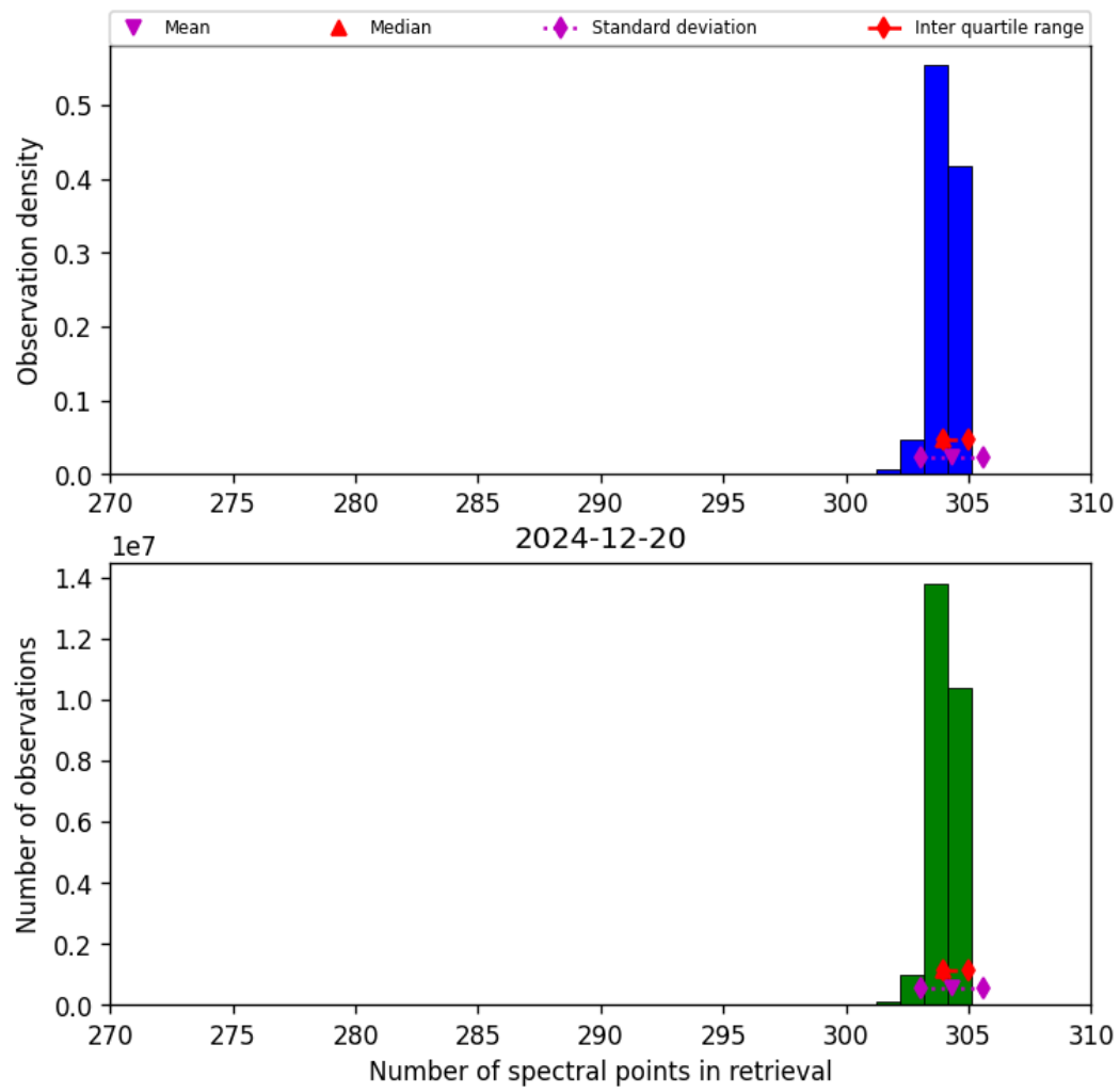
Figure 33: Histogram of “Number of spectral points in retrieval” for 2024-12-19 to 2024-12-21
