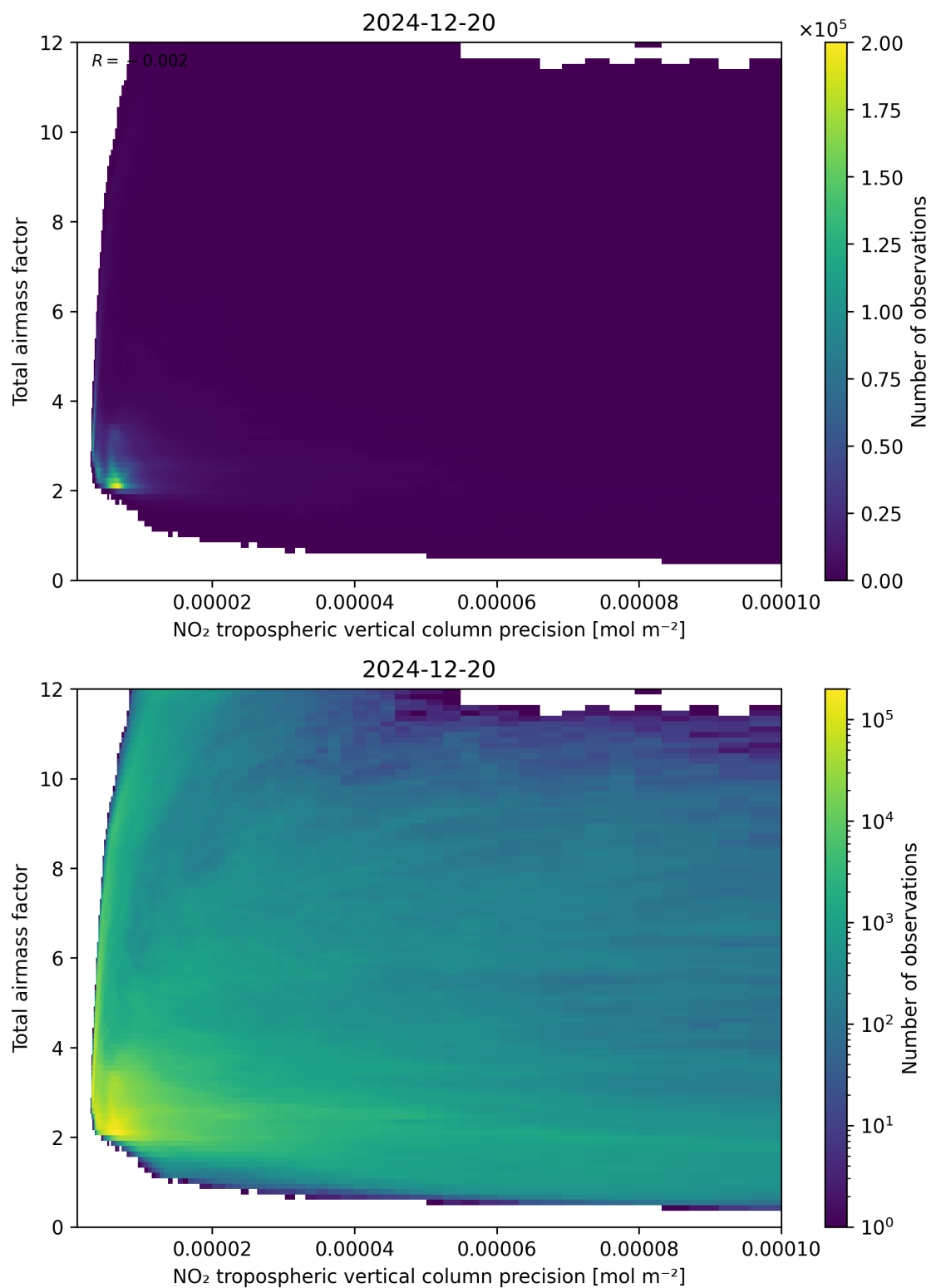
Figure 132: Scatter density plot of “NO 2 tropospheric vertical column precision” against “Total air mass factor” for 2024-12-19 to 2024-12-21.
