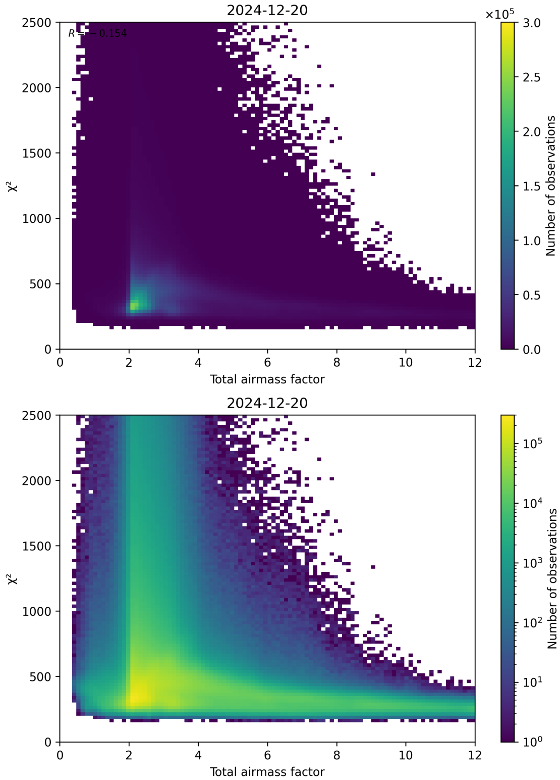
Figure 63: Scatter density plot of “Total airmass factor” against “ \chi^2 ” for 2024-12-19 to 2024-12-21.
