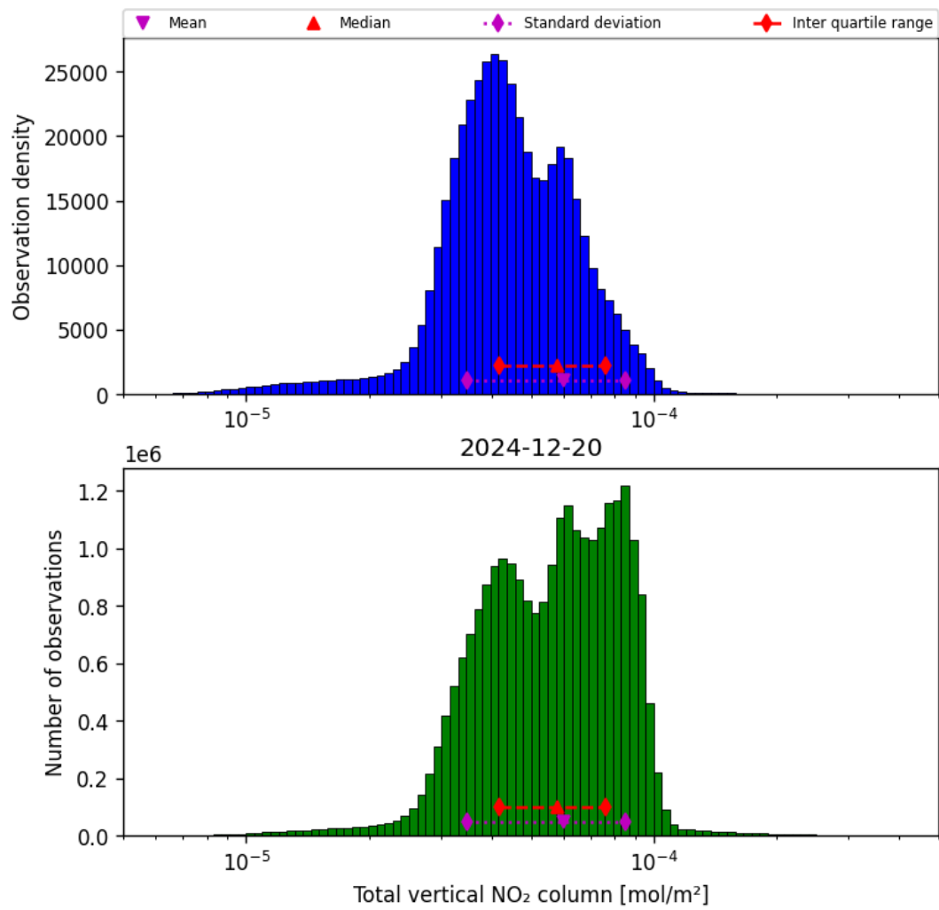
Figure 38: Histogram of “Total vertical NO 2 column” for 2024-12-19 to 2024-12-21
