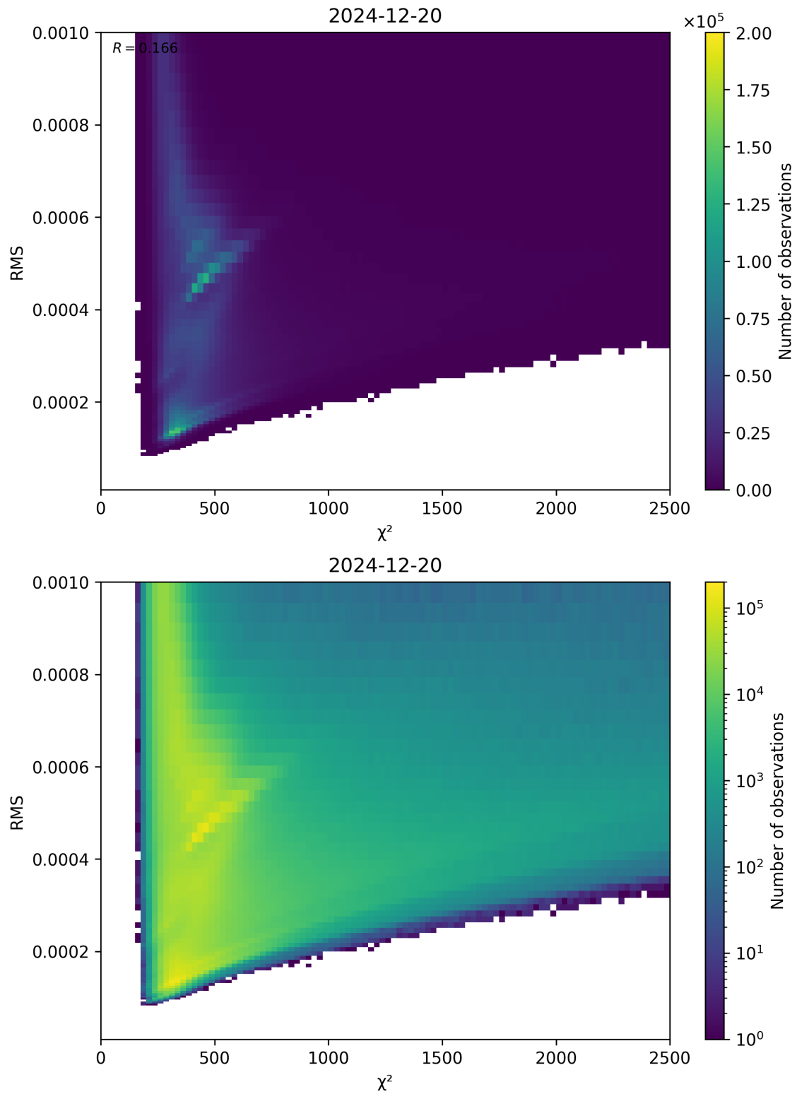
Figure 82: Scatter density plot of “ \chi^2 ” against “RMS” for 2024-12-19 to 2024-12-21.
