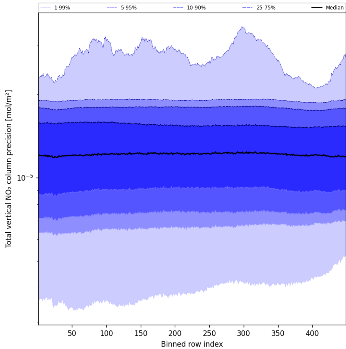
Figure 56: Along track statistics of “Total vertical NO 2 column precision” for 2024-12-19 to 2024-12-21
