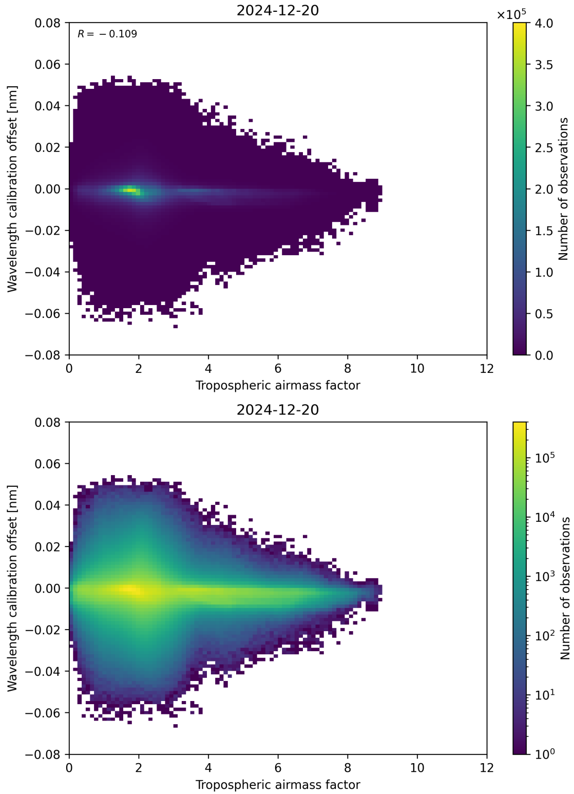
Figure 80: Scatter density plot of “Tropospheric airmass factor” against “Wavelength calibration offset” for 2024-12-19 to 2024-12-21.
