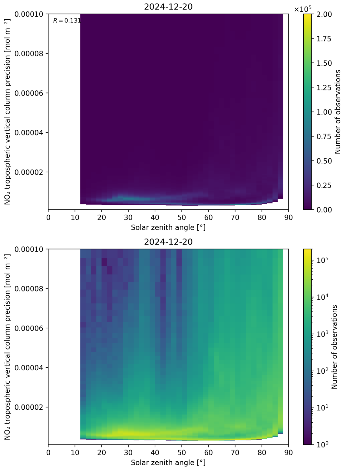
Figure 156: Scatter density plot of “Solar zenith angle” against “NO 2 tropospheric vertical column precision” for 2024-12-19 to 2024-12-21.
