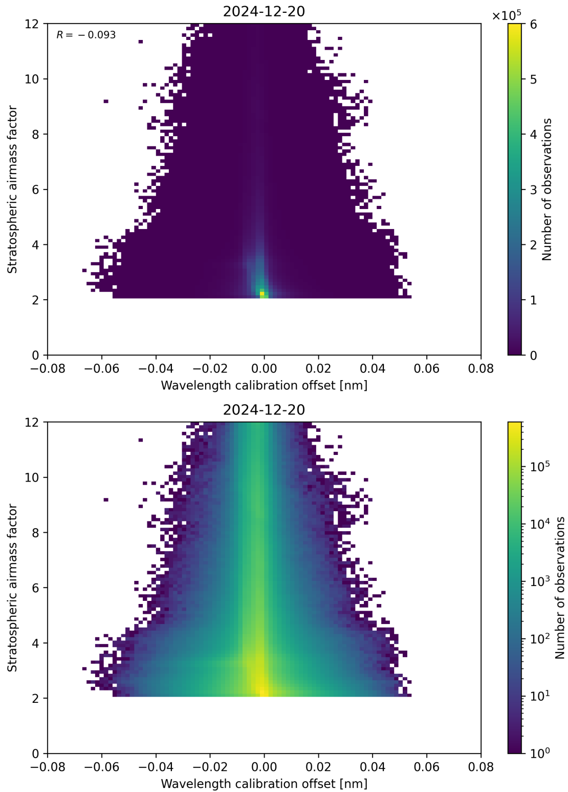
Figure 174: Scatter density plot of “Wavelength calibration offset” against “Stratospheric airmass factor” for 2024-12-19 to 2024-12-21.
