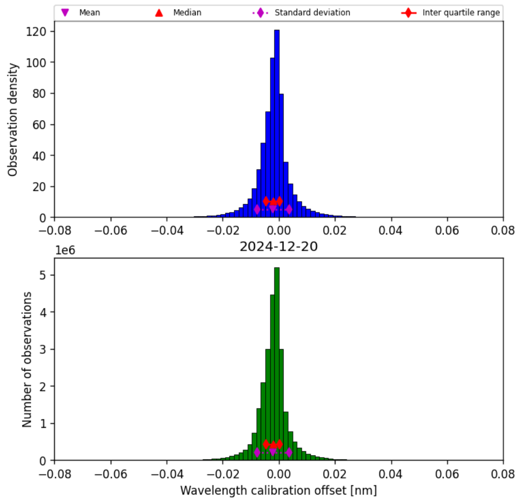
Figure 35: Histogram of “Wavelength calibration offset” for 2024-12-19 to 2024-12-21
