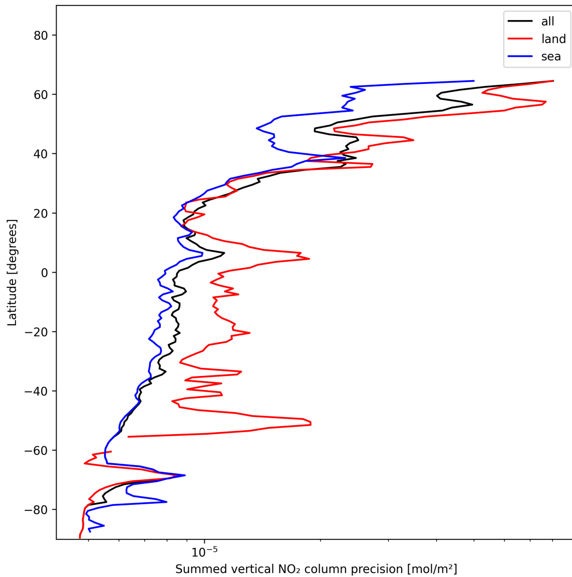
Figure 24: Zonal average of “Summed vertical NO 2 column precision” for 2024-12-19 to 2024-12-21.
