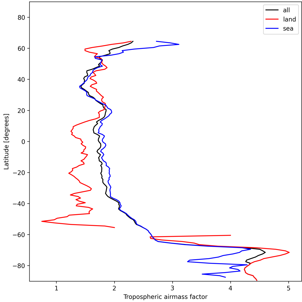
Figure 14: Zonal average of “Tropospheric airmass factor” for 2024-12-19 to 2024-12-21.
