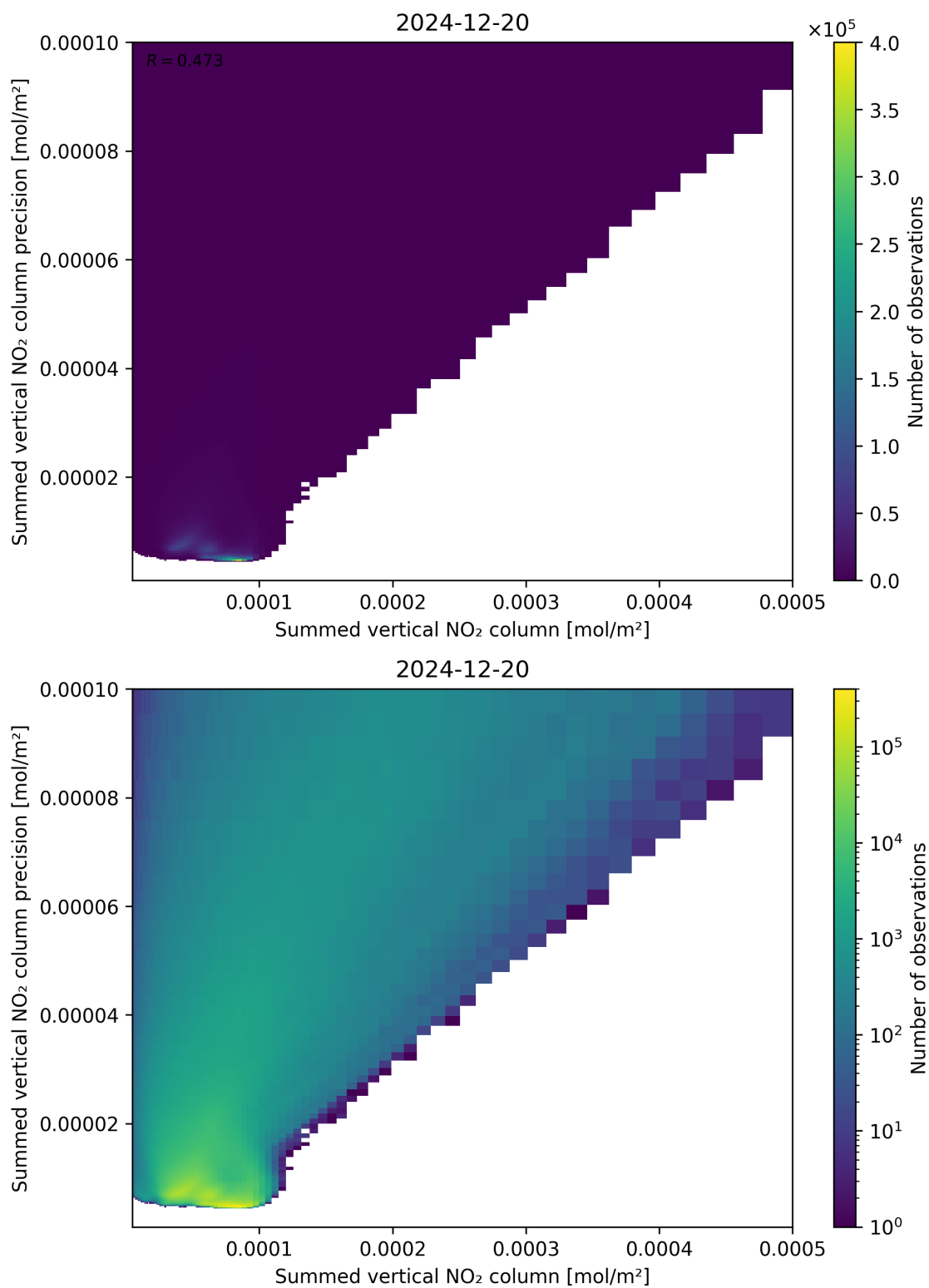
Figure 105: Scatter density plot of “Summed vertical NO 2 column” against “Summed vertical NO 2 column precision” for 2024-12-19 to 2024-12-21.
