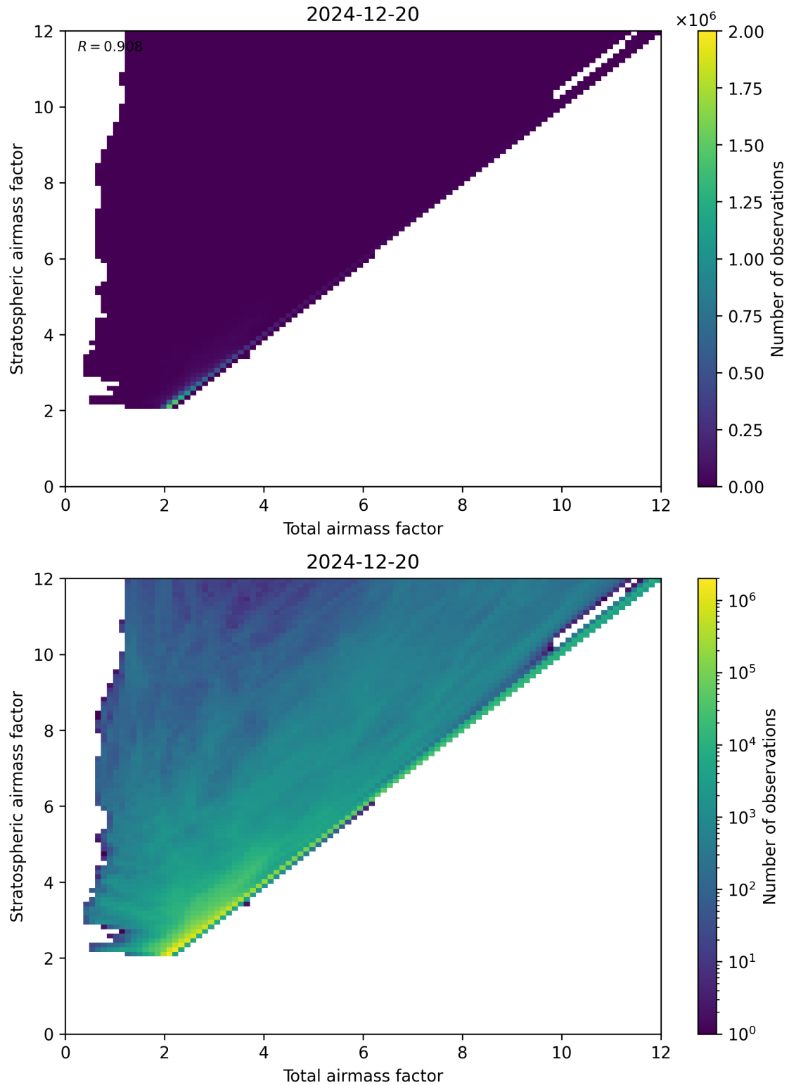
Figure 62: Scatter density plot of “Total airmass factor” against “Stratospheric airmass factor” for 2024-12-19 to 2024-12-21.
