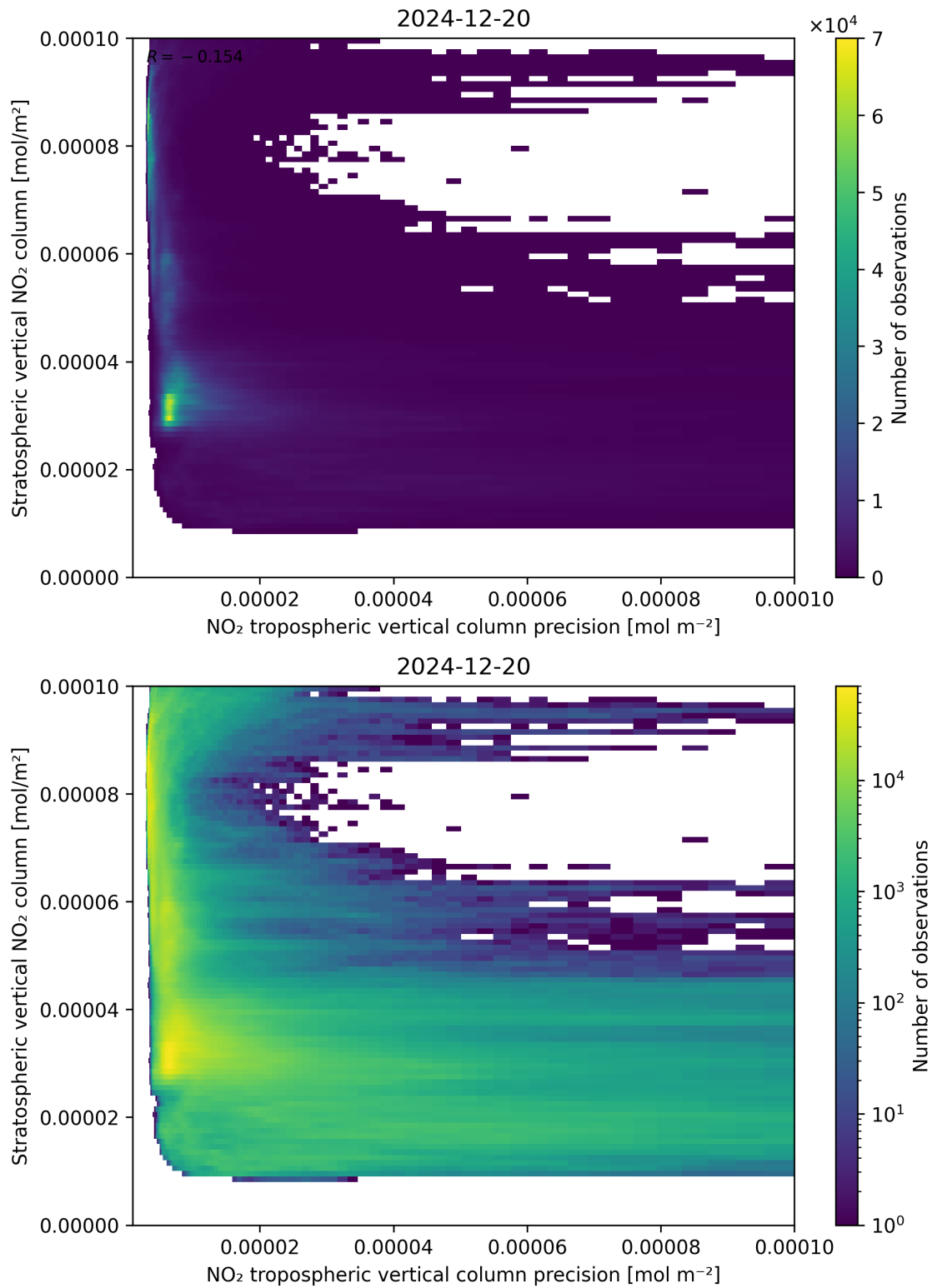
Figure 135: Scatter density plot of “NO 2 tropospheric vertical column precision” against “Stratospheric vertical NO 2 column” for 2024-12-19 to 2024-12-21.
