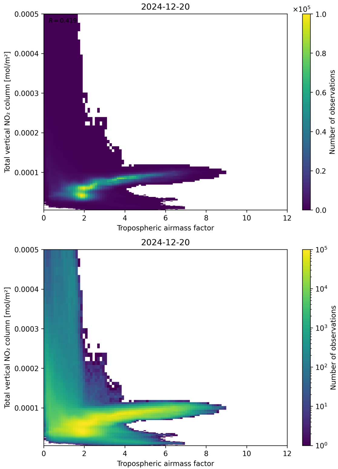
Figure 77: Scatter density plot of “Tropospheric airmass factor” against “Total vertical \text{NO}_2 column” for 2024-12-19 to 2024-12-21.
