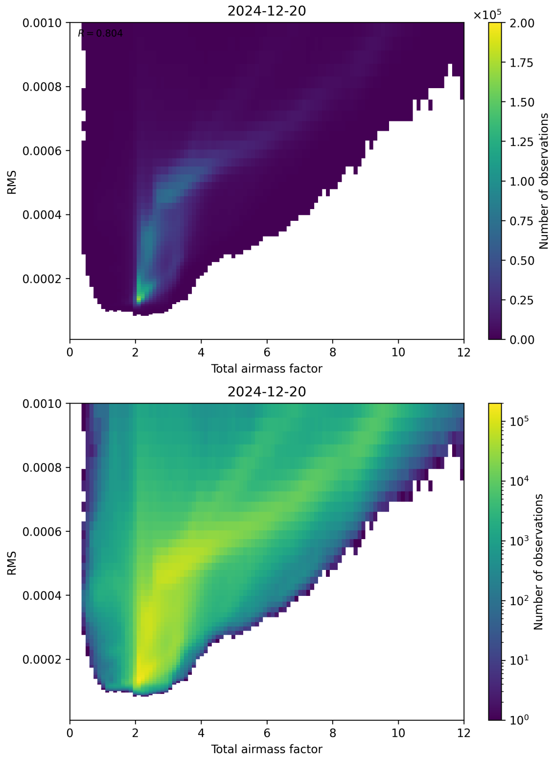
Figure 69: Scatter density plot of “Total airmass factor” against “RMS” for 2024-12-19 to 2024-12-21.
