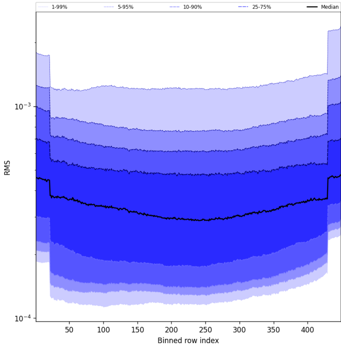
Figure 60: Along track statistics of “RMS” for 2024-12-19 to 2024-12-21
