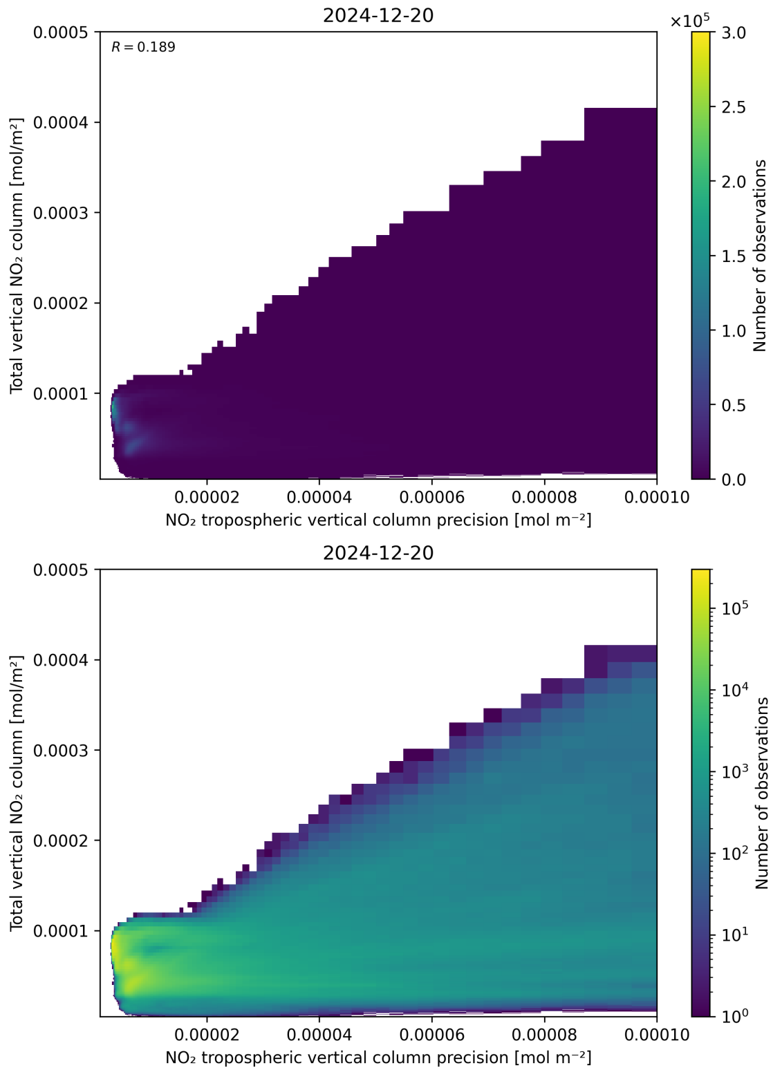
Figure 138: Scatter density plot of “NO 2 tropospheric vertical column precision” against “Total vertical NO 2 column” for 2024-12-19 to 2024-12-21.
