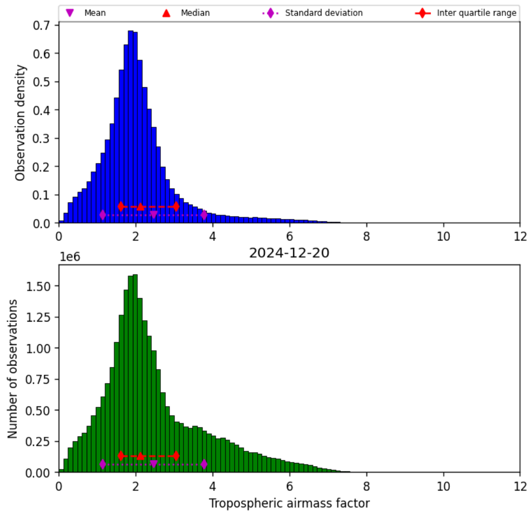
Figure 31: Histogram of “Tropospheric airmass factor” for 2024-12-19 to 2024-12-21
