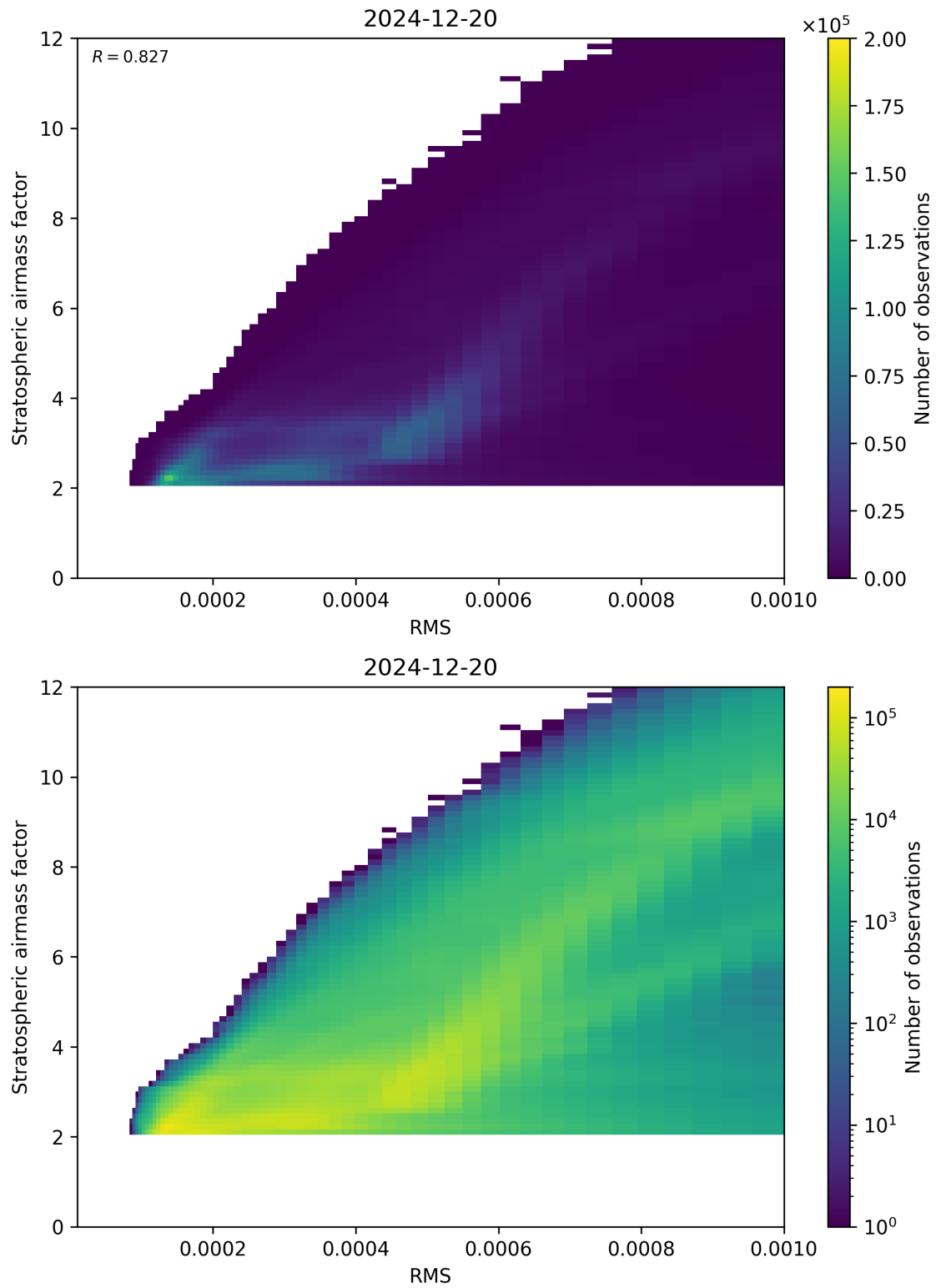
Figure 144: Scatter density plot of “RMS” against “Stratospheric airmass factor” for 2024-12-19 to 2024-12-21.
