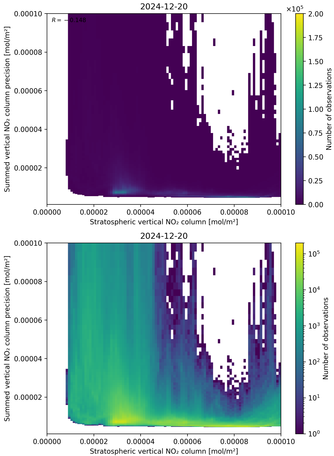
Figure 99: Scatter density plot of “Stratospheric vertical NO 2 column” against “Summed vertical NO 2 column precision” for 2024-12-19 to 2024-12-21.
