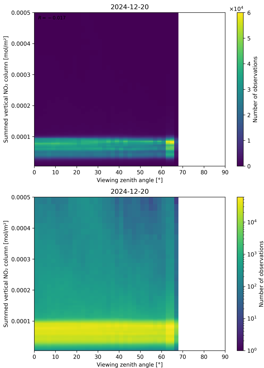
Figure 165: Scatter density plot of “Viewing zenith angle” against “Summed vertical NO 2 column” for 2024-12-19 to 2024-12-21.
