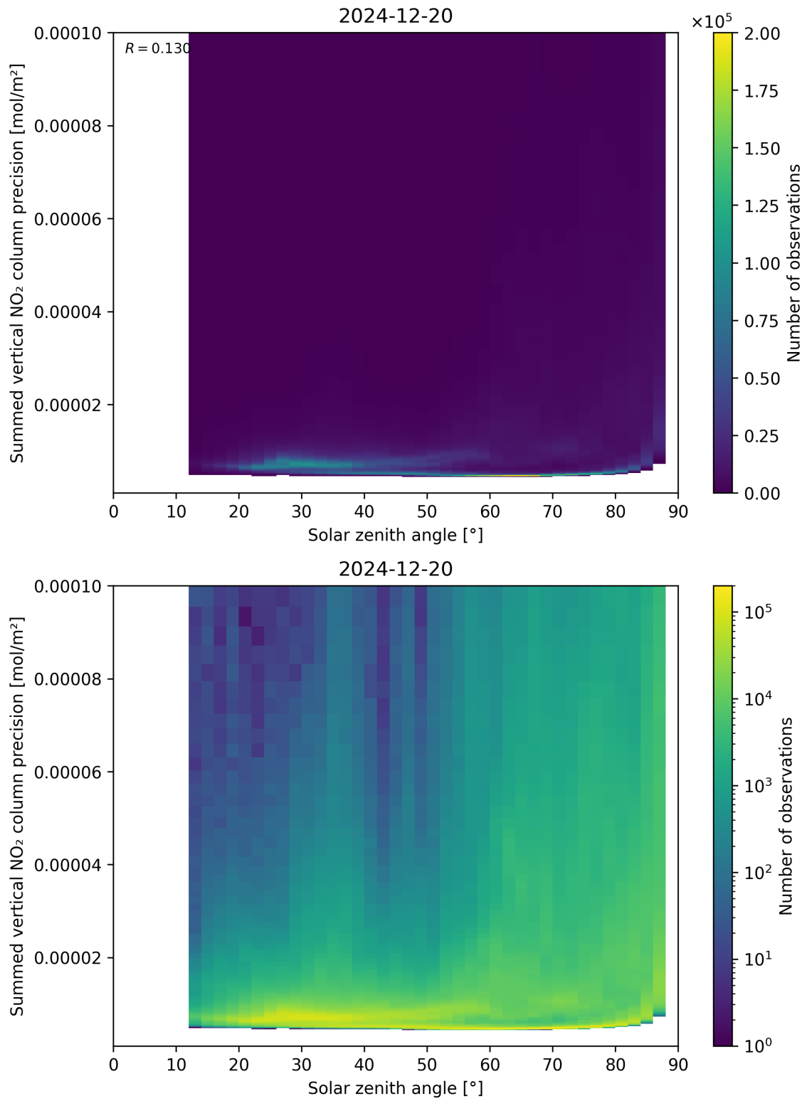
Figure 152: Scatter density plot of “Solar zenith angle” against “Summed vertical NO 2 column precision” for 2024-12-19 to 2024-12-21.
