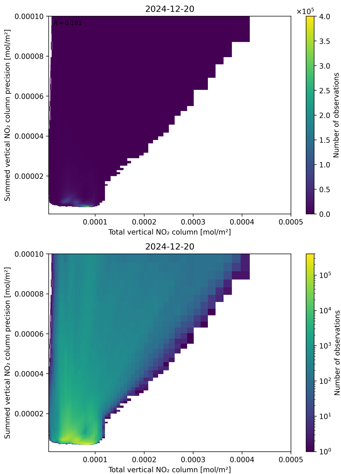
Figure 113: Scatter density plot of “Total vertical NO 2 column” against “Summed vertical NO 2 column precision” for 2024-12-19 to 2024-12-21.
