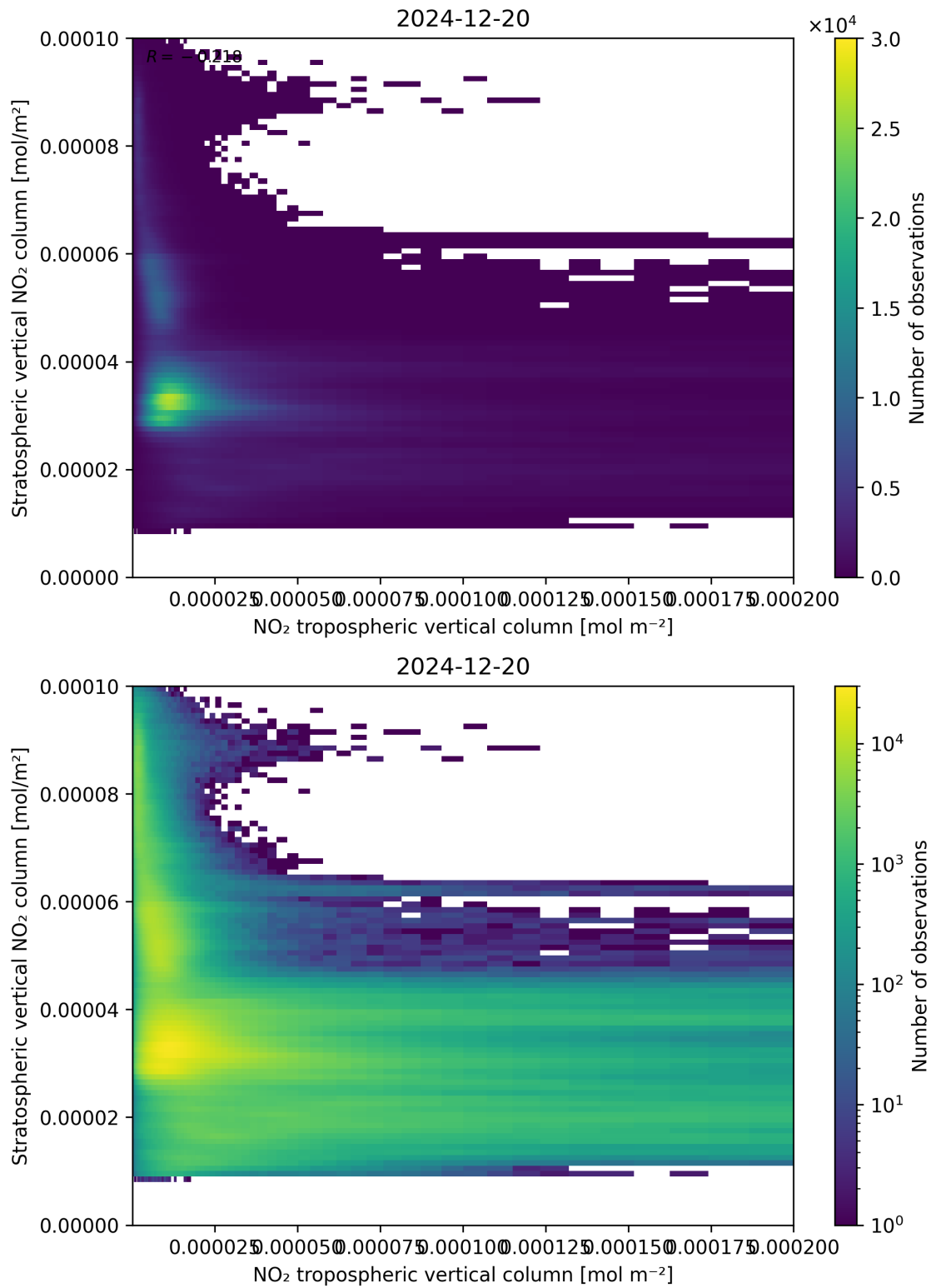
Figure 125: Scatter density plot of “NO 2 tropospheric vertical column” against “Stratospheric vertical NO 2 column” for 2024-12-19 to 2024-12-21.
