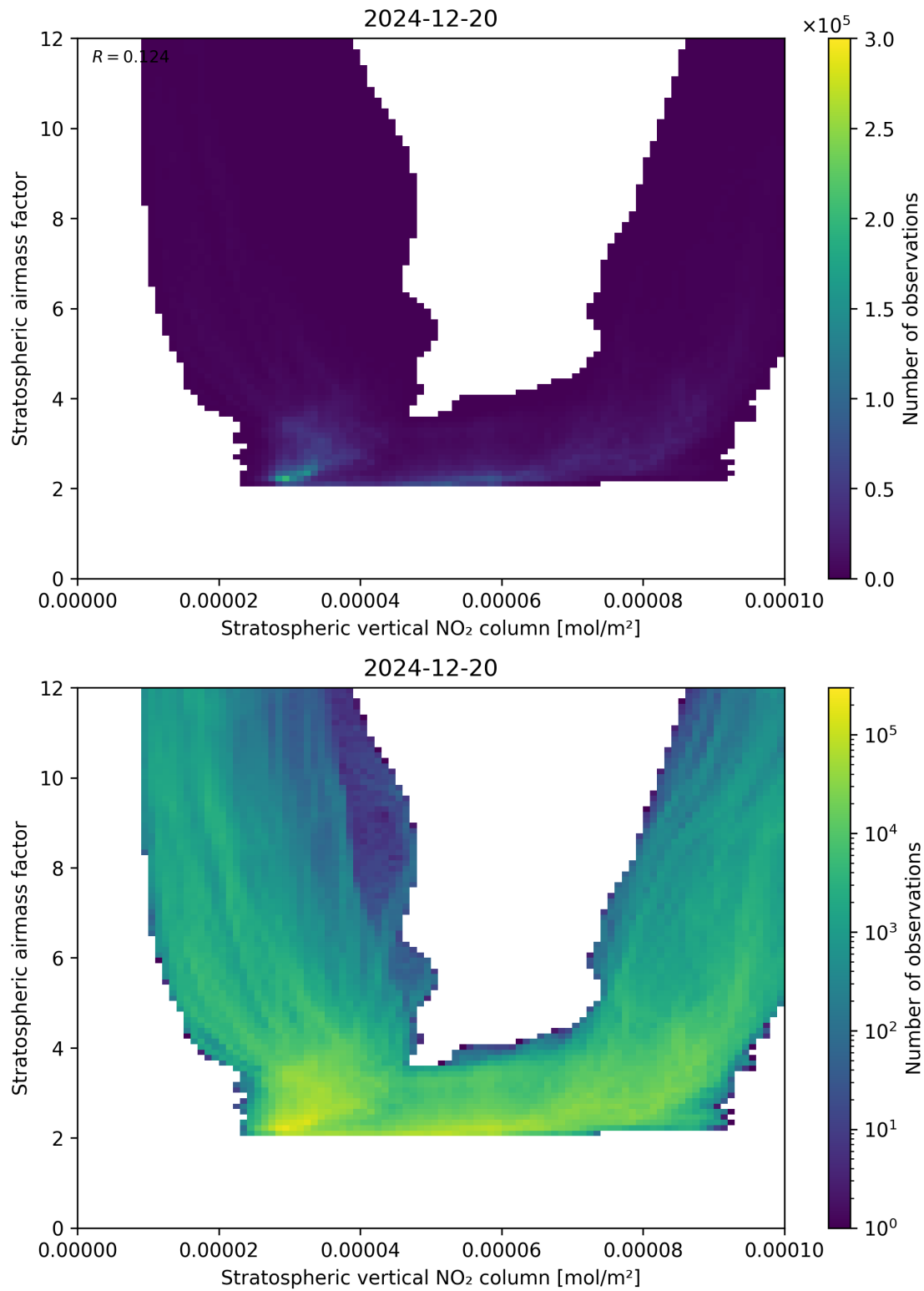
Figure 96: Scatter density plot of “Stratospheric vertical NO 2 column” against “Stratospheric airmass factor” for 2024-12-19 to 2024-12-21.
