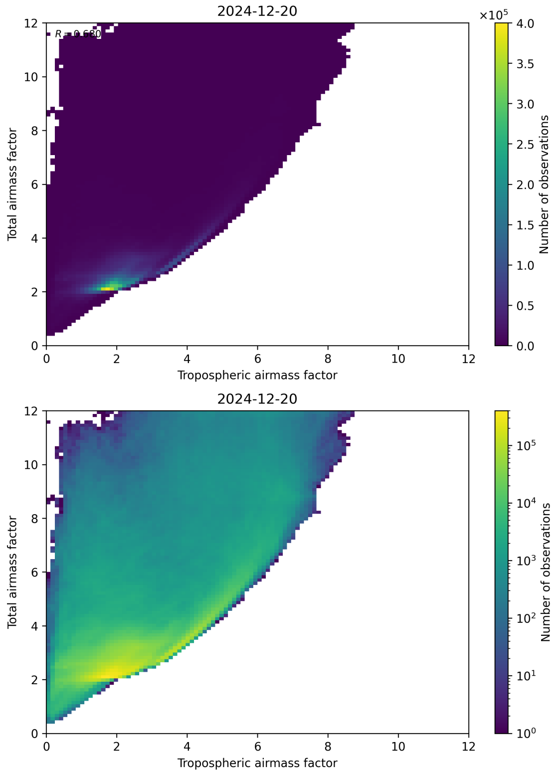
Figure 72: Scatter density plot of “Tropospheric airmass factor” against “Total airmass factor” for 2024-12-19 to 2024-12-21.
