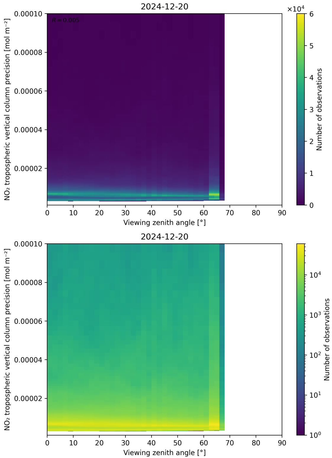
Figure 170: Scatter density plot of “Viewing zenith angle” against “NO 2 tropospheric vertical column precision” for 2024-12-19 to 2024-12-21.
