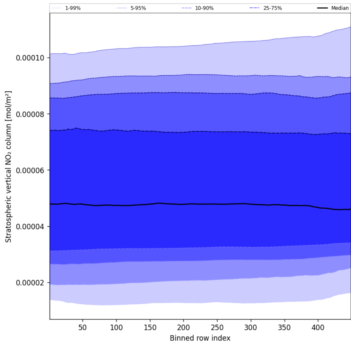
Figure 53: Along track statistics of “Stratospheric vertical NO 2 column” for 2024-12-19 to 2024-12-21
