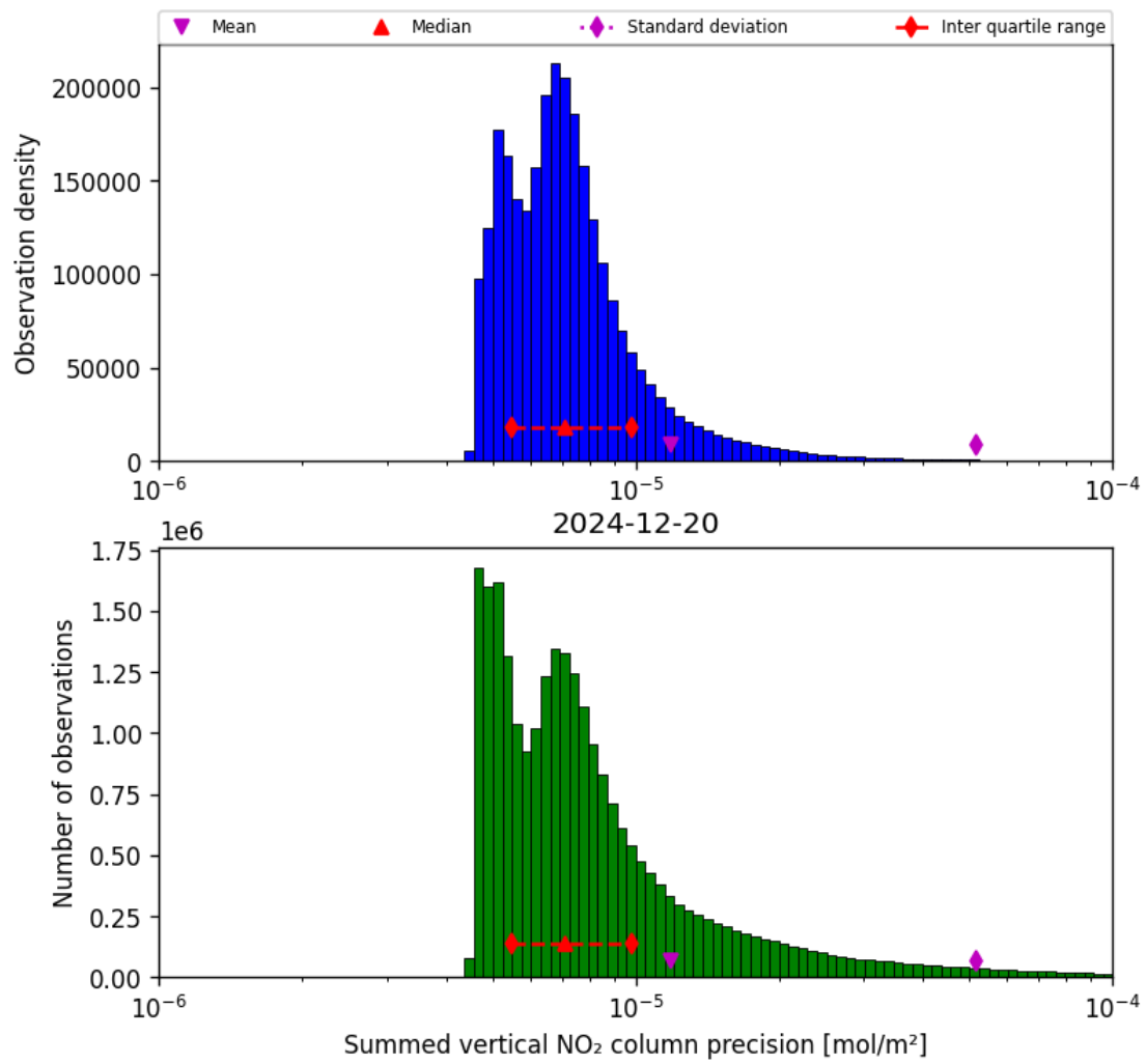
Figure 41: Histogram of “Summed vertical NO 2 column precision” for 2024-12-19 to 2024-12-21
