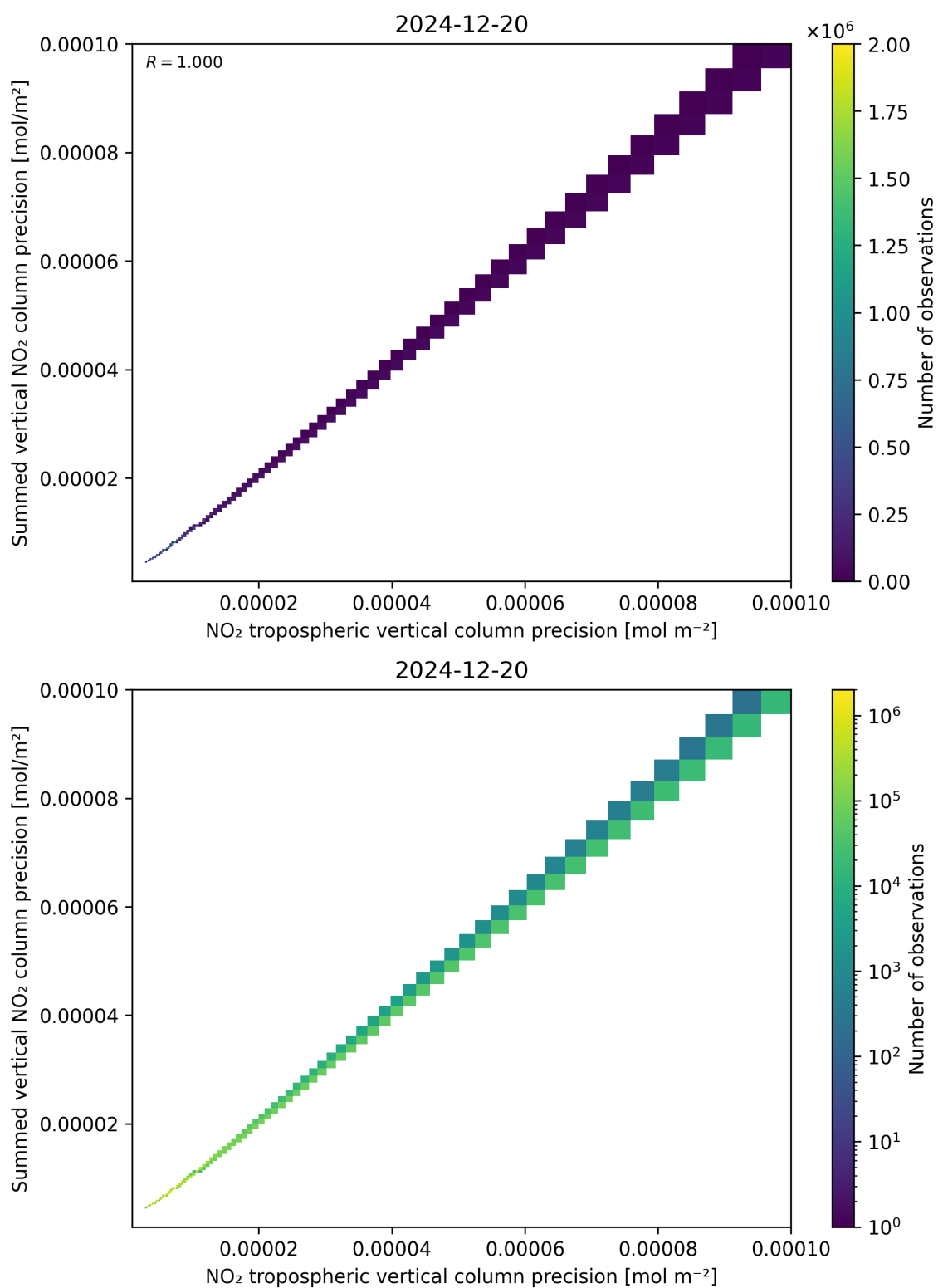
Figure 137: Scatter density plot of “NO 2 tropospheric vertical column precision” against “Summed vertical NO 2 column precision” for 2024-12-19 to 2024-12-21.
