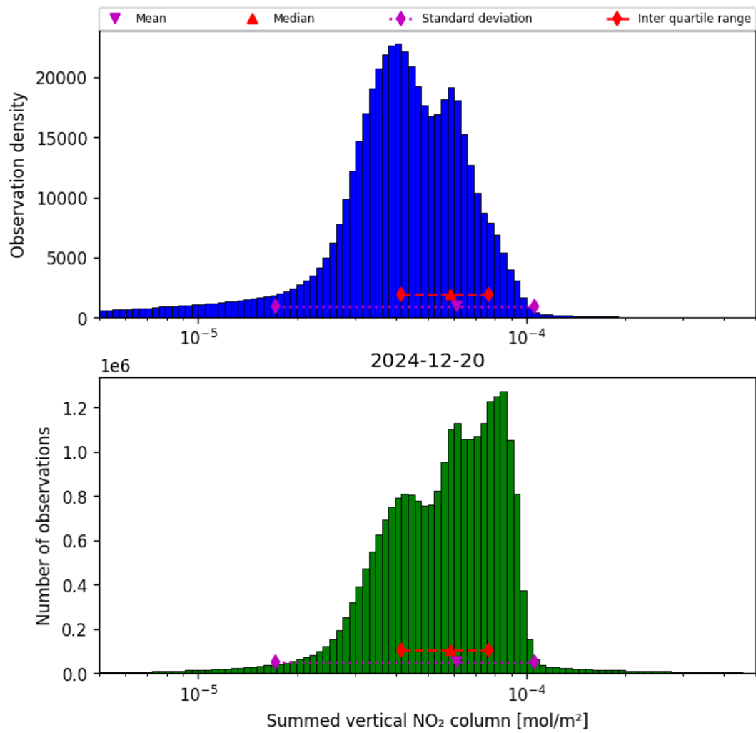
Figure 40: Histogram of “Summed vertical NO 2 column” for 2024-12-19 to 2024-12-21
