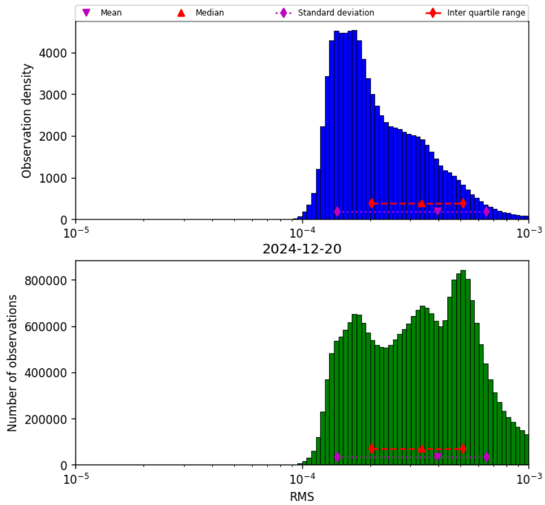
Figure 43: Histogram of “RMS” for 2024-12-19 to 2024-12-21
