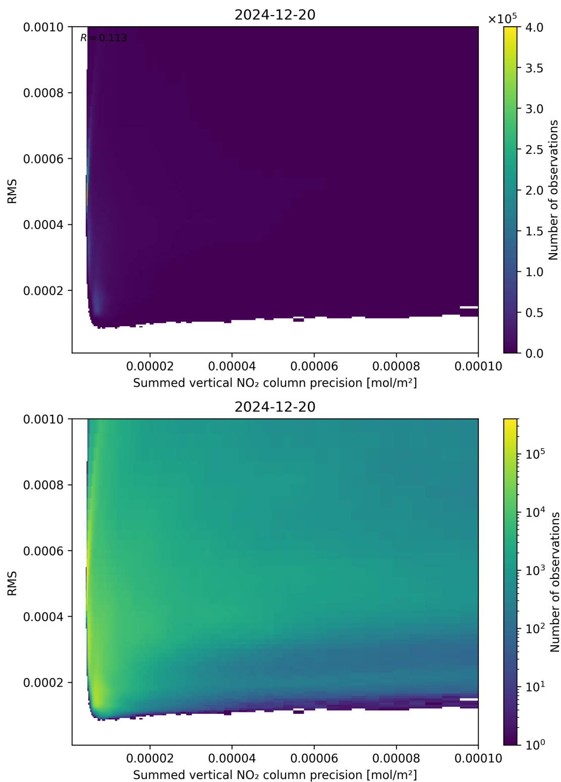
Figure 108: Scatter density plot of “Summed vertical NO 2 column precision” against “RMS” for 2024-12-19 to 2024-12-21.
