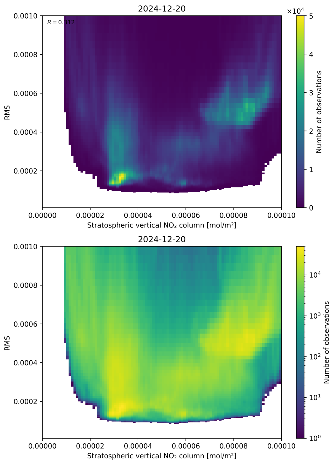
Figure 102: Scatter density plot of “Stratospheric vertical NO 2 column” against “RMS” for 2024-12-19 to 2024-12-21.
