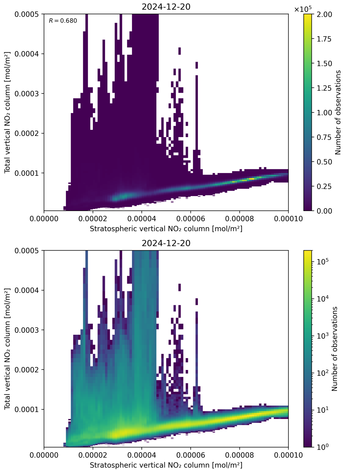
Figure 100: Scatter density plot of “Stratospheric vertical NO 2 column” against “Total vertical NO 2 column” for 2024-12-19 to 2024-12-21.
