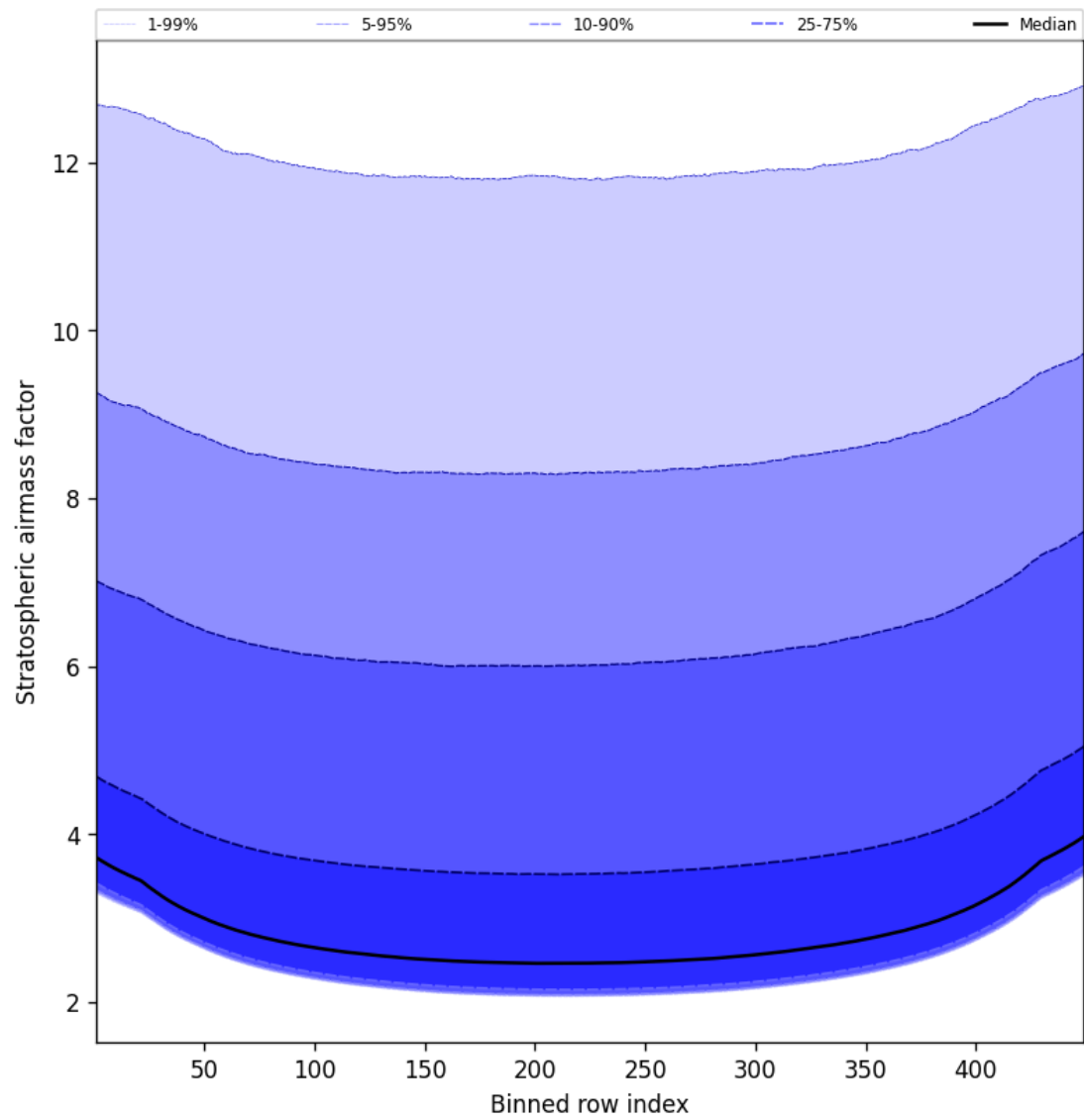
Figure 61: Along track statistics of “Stratospheric airmass factor” for 2024-12-19 to 2024-12-21
