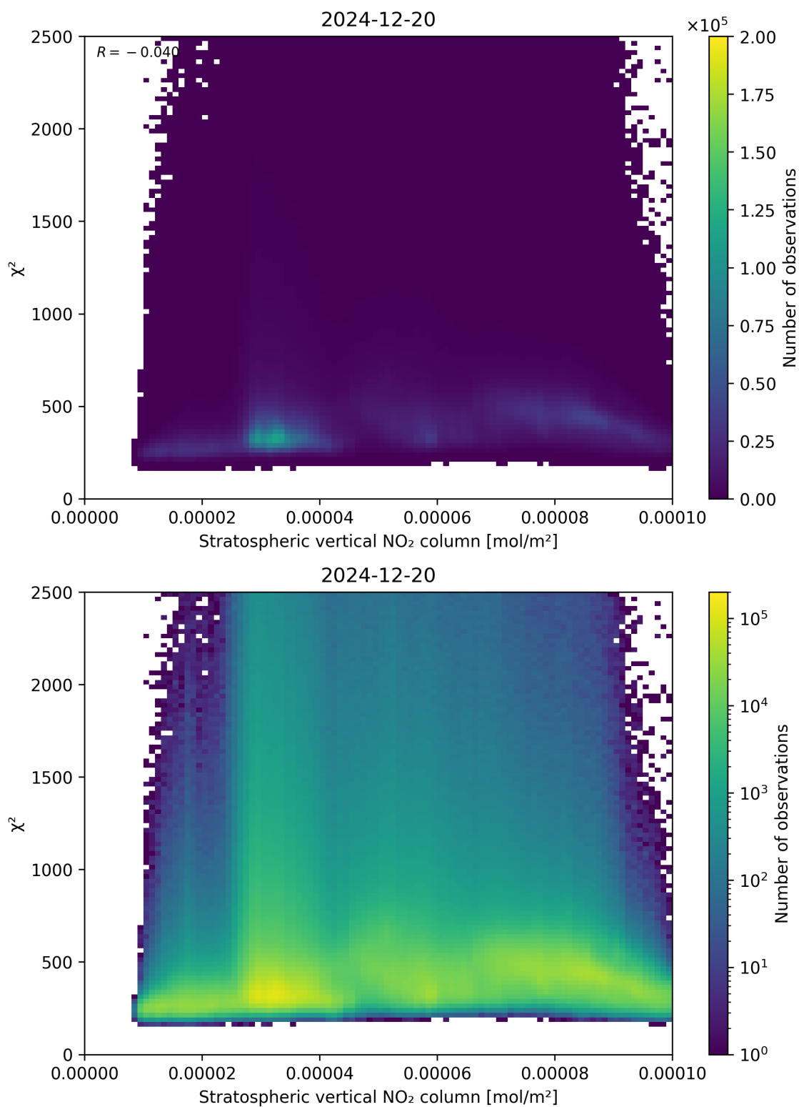
Figure 97: Scatter density plot of “Stratospheric vertical NO 2 column” against “ \chi^2 ” for 2024-12-19 to 2024-12-21.
