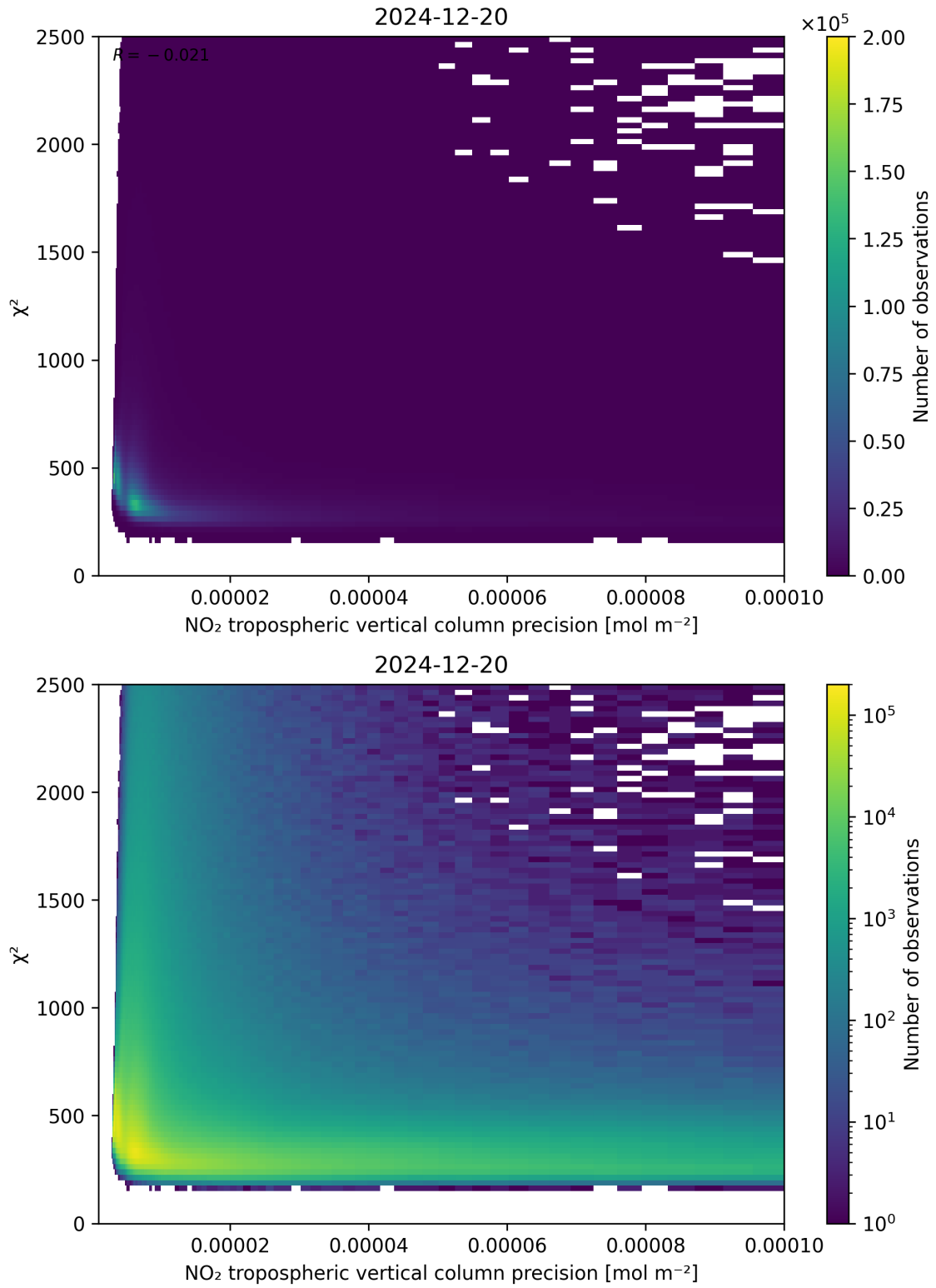
Figure 134: Scatter density plot of “NO 2 tropospheric vertical column precision” against “ \chi^2 ” for 2024-12-19 to 2024-12-21.
