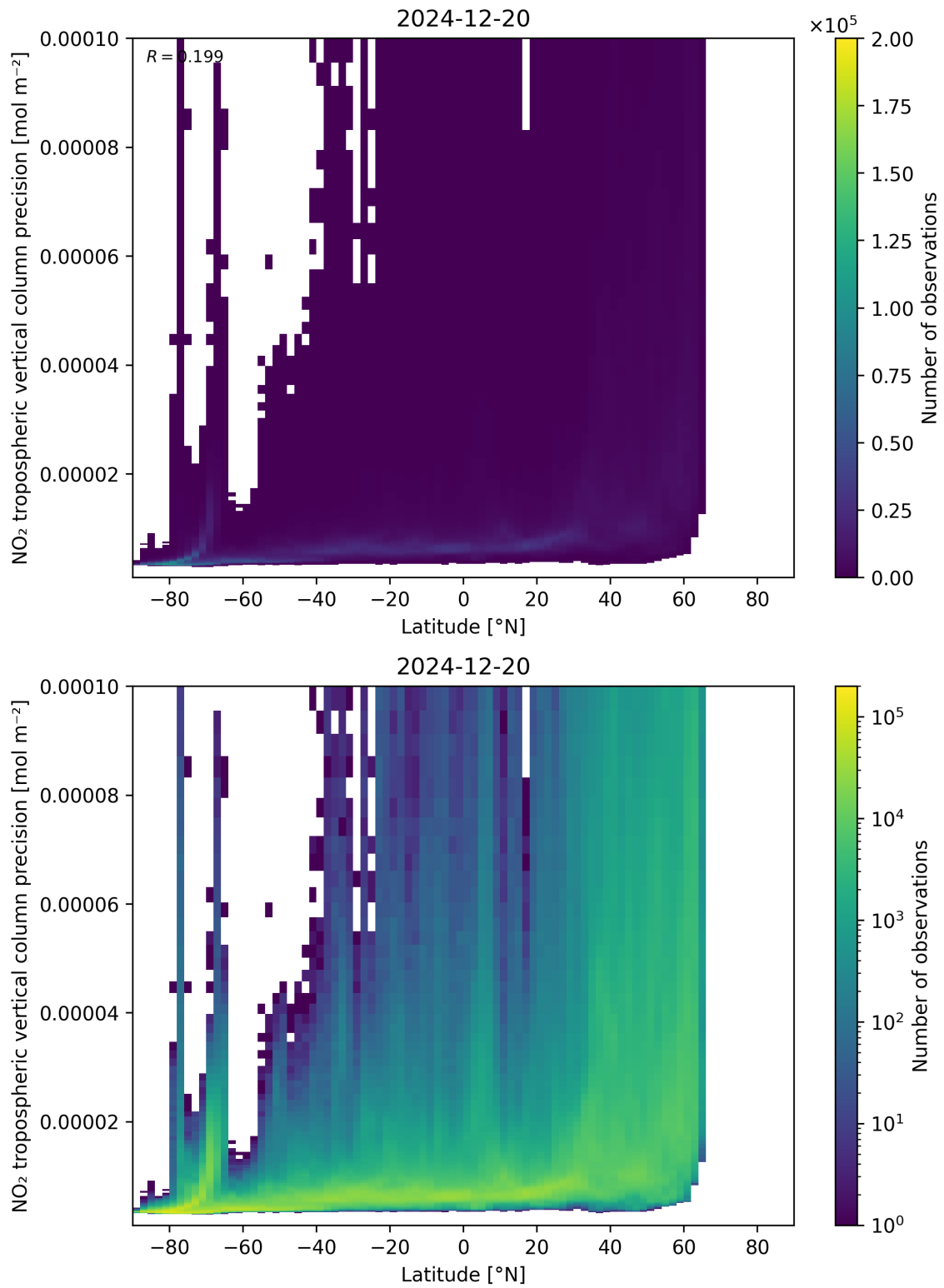
Figure 93: Scatter density plot of “Latitude” against “NO 2 tropospheric vertical column precision” for 2024-12-19 to 2024-12-21.
