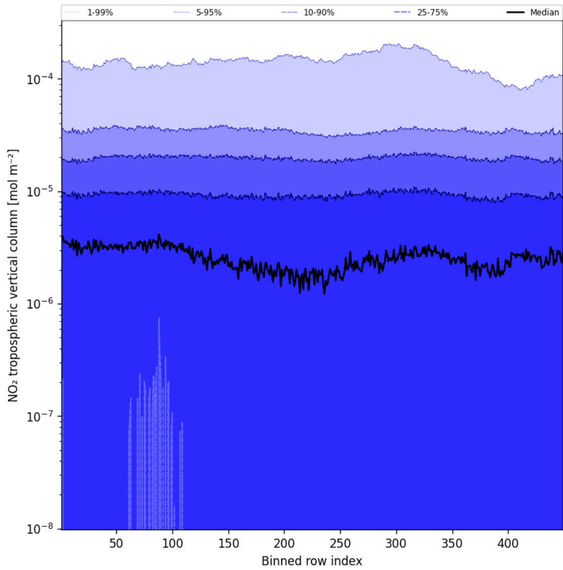
Figure 46: Along track statistics of “NO 2 tropospheric vertical column” for 2024-12-19 to 2024-12-21
