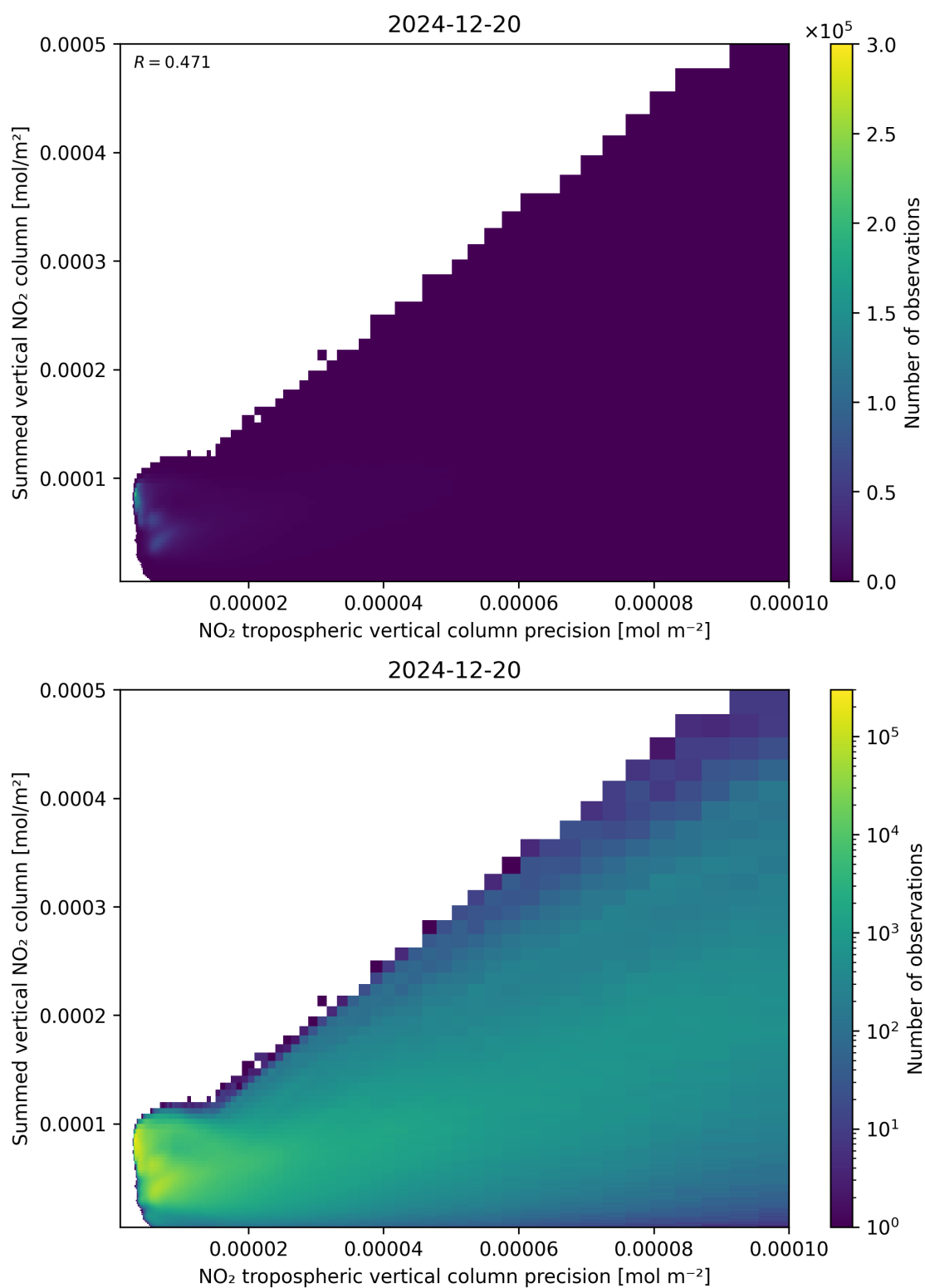
Figure 136: Scatter density plot of “NO 2 tropospheric vertical column precision” against “Summed vertical NO 2 column” for 2024-12-19 to 2024-12-21.
