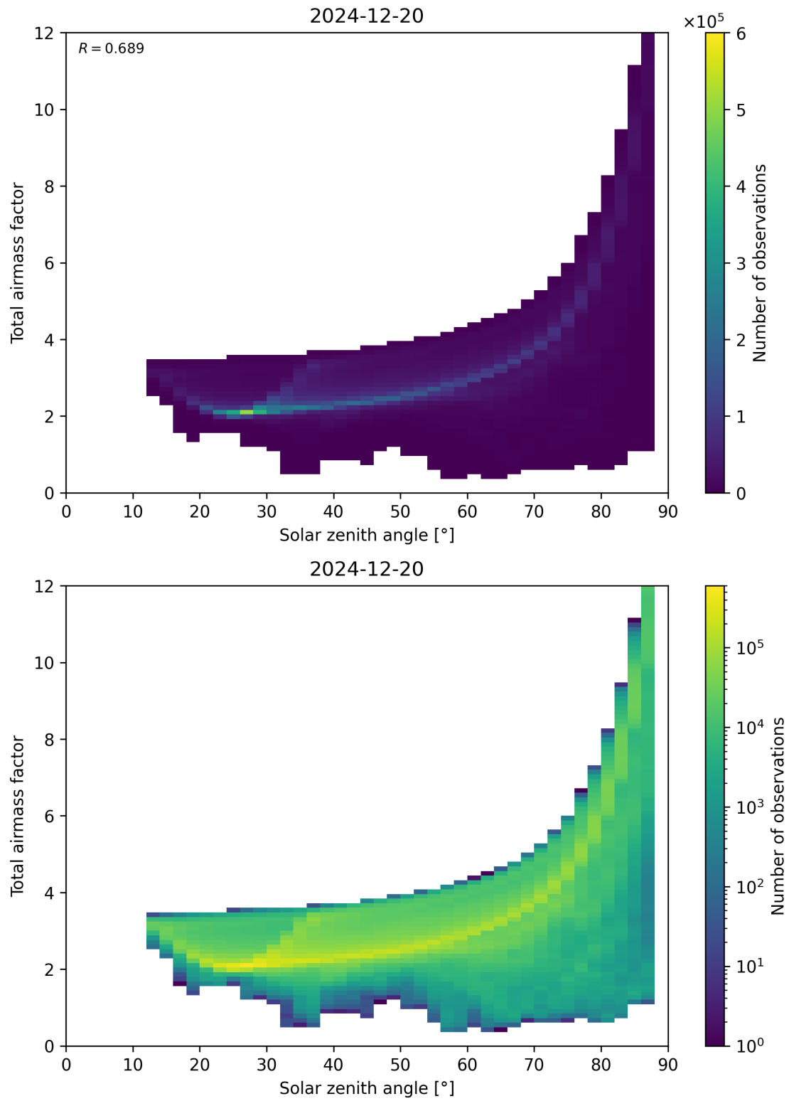
Figure 146: Scatter density plot of “Solar zenith angle” against “Total airmass factor” for 2024-12-19 to 2024-12-21.
