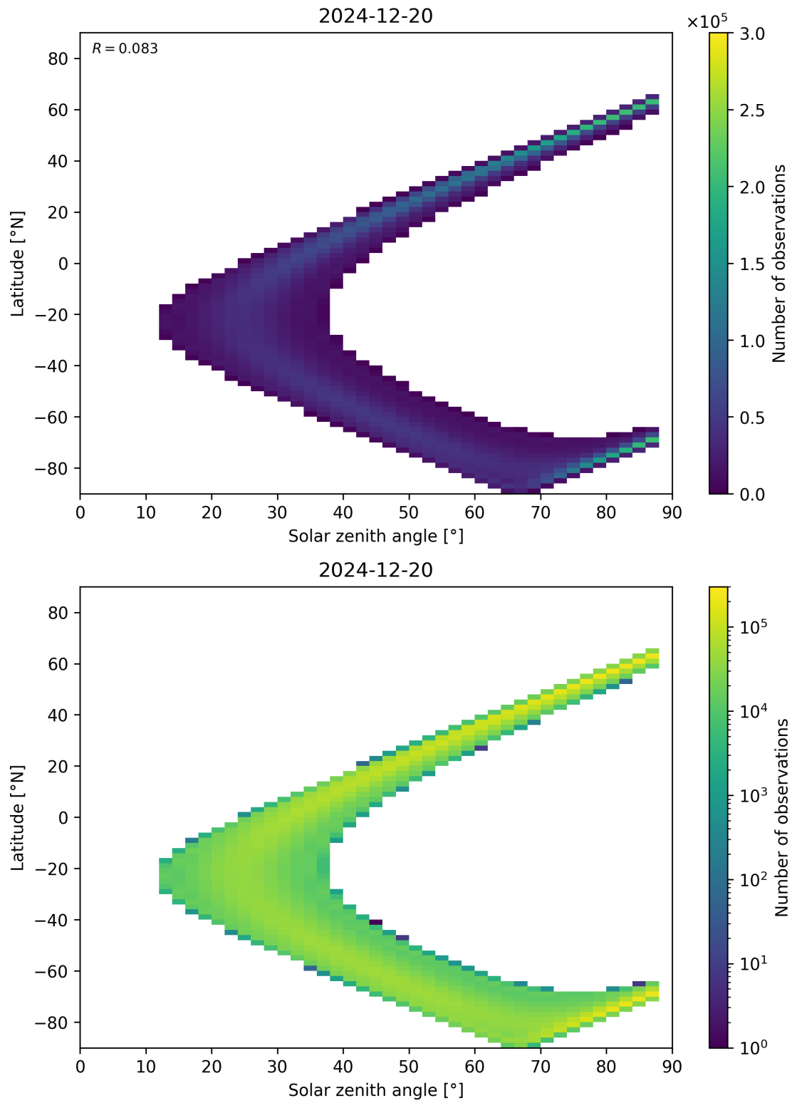
Figure 149: Scatter density plot of “Solar zenith angle” against “Latitude” for 2024-12-19 to 2024-12-21.
