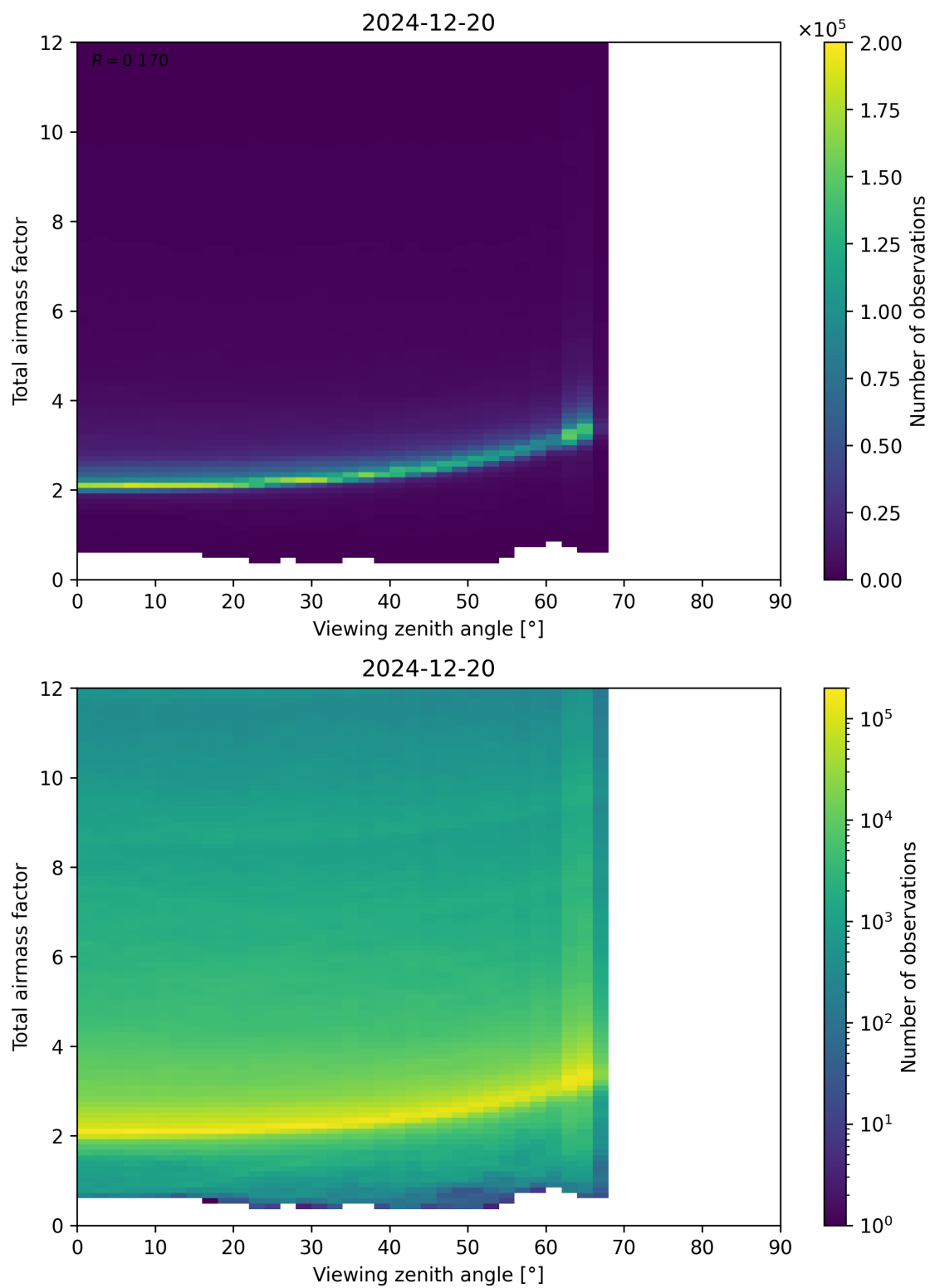
Figure 160: Scatter density plot of “Viewing zenith angle” against “Total airmass factor” for 2024-12-19 to 2024-12-21.
