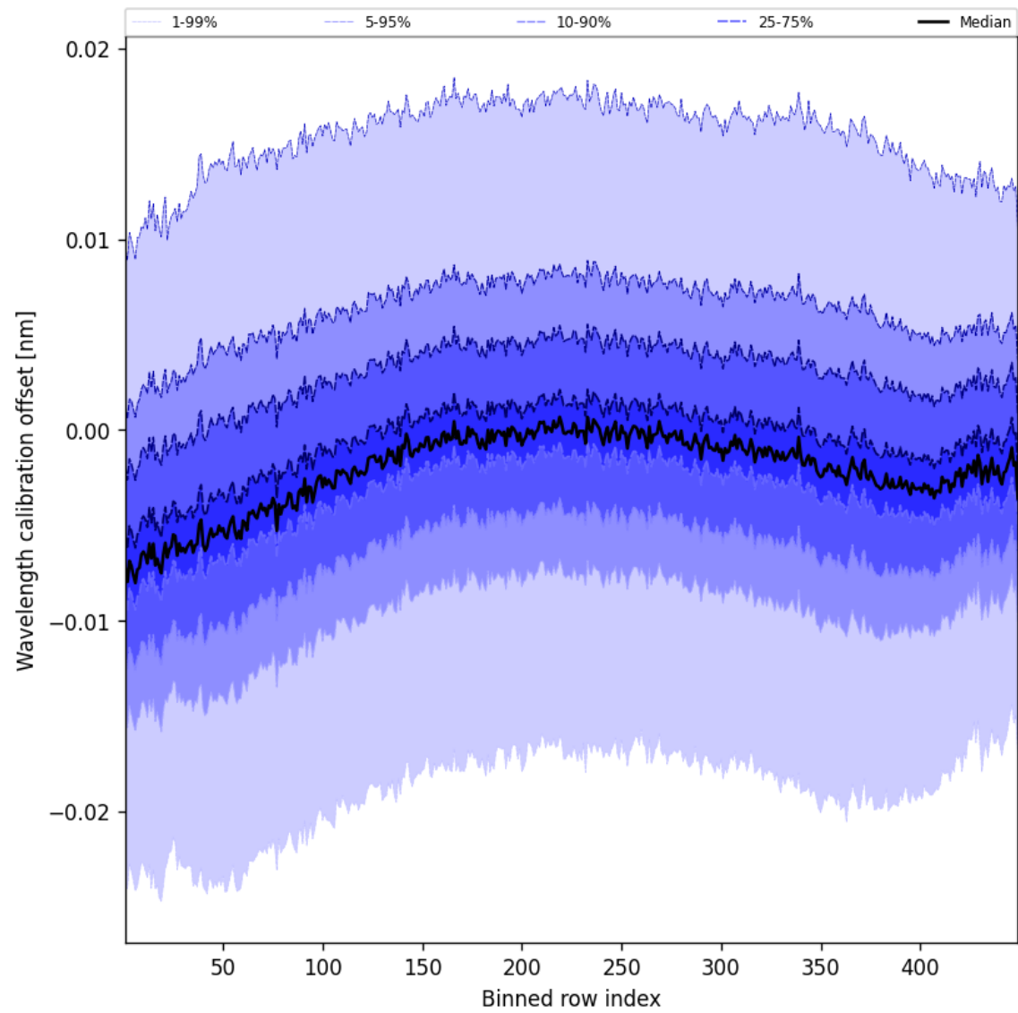
Figure 52: Along track statistics of “Wavelength calibration offset” for 2024-12-19 to 2024-12-21
