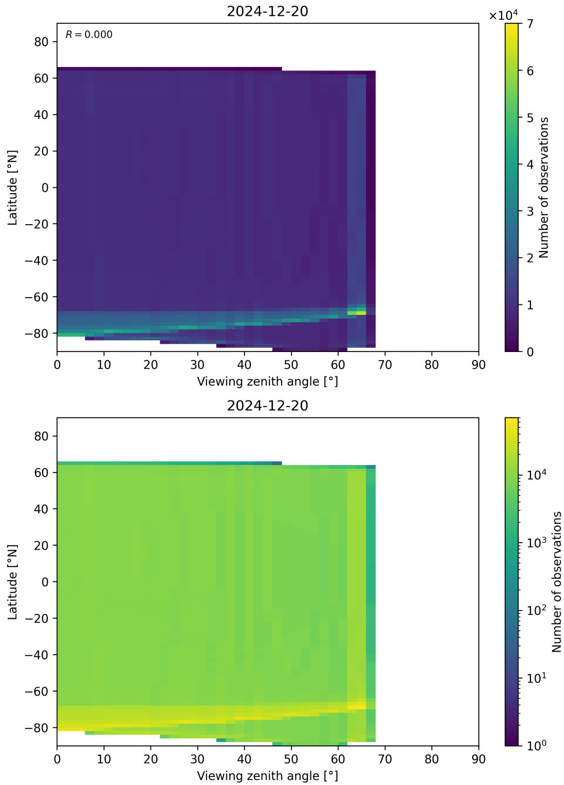
Figure 163: Scatter density plot of “Viewing zenith angle” against “Latitude” for 2024-12-19 to 2024-12-21.
