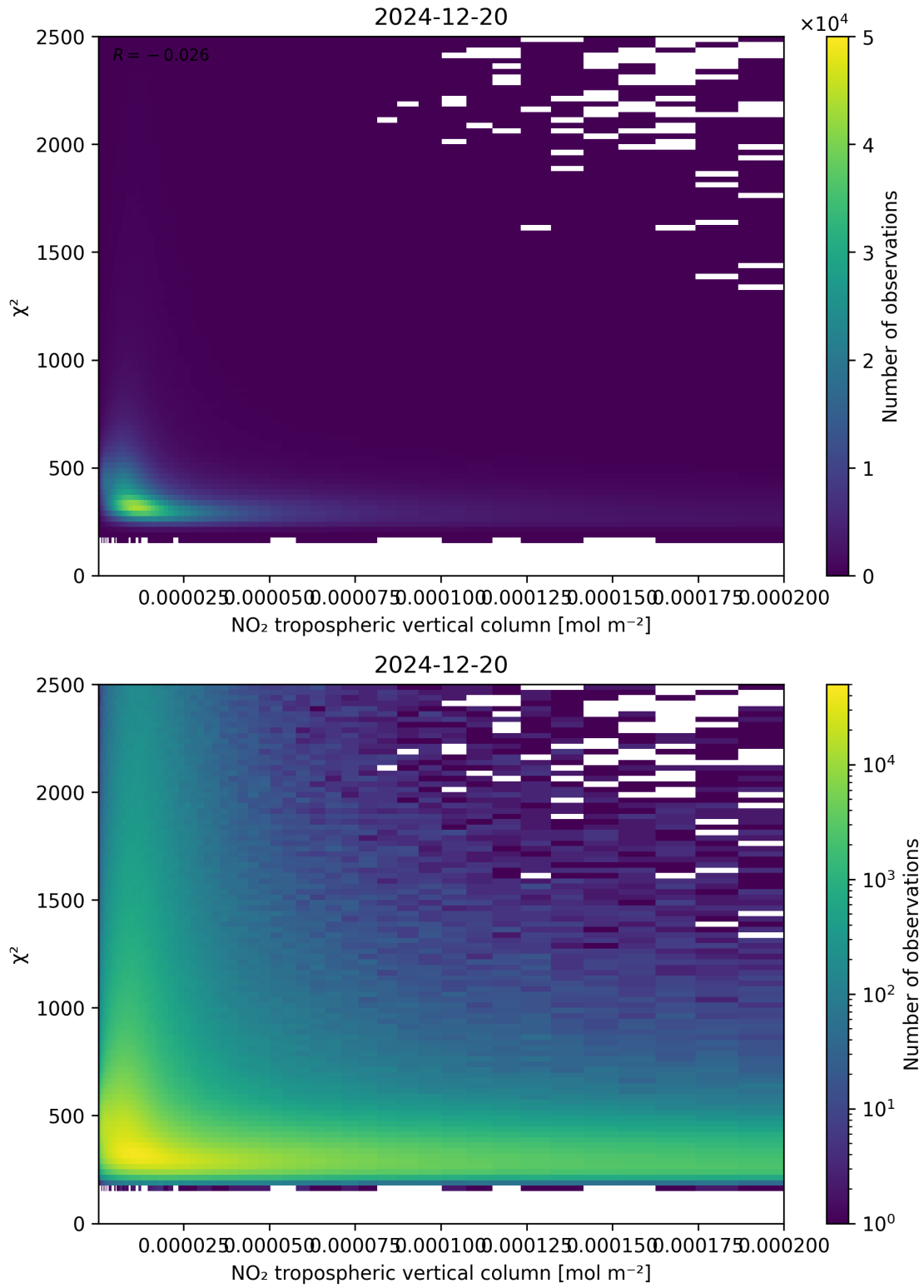
Figure 124: Scatter density plot of “NO 2 tropospheric vertical column” against “ \chi^2 ” for 2024-12-19 to 2024-12-21.
