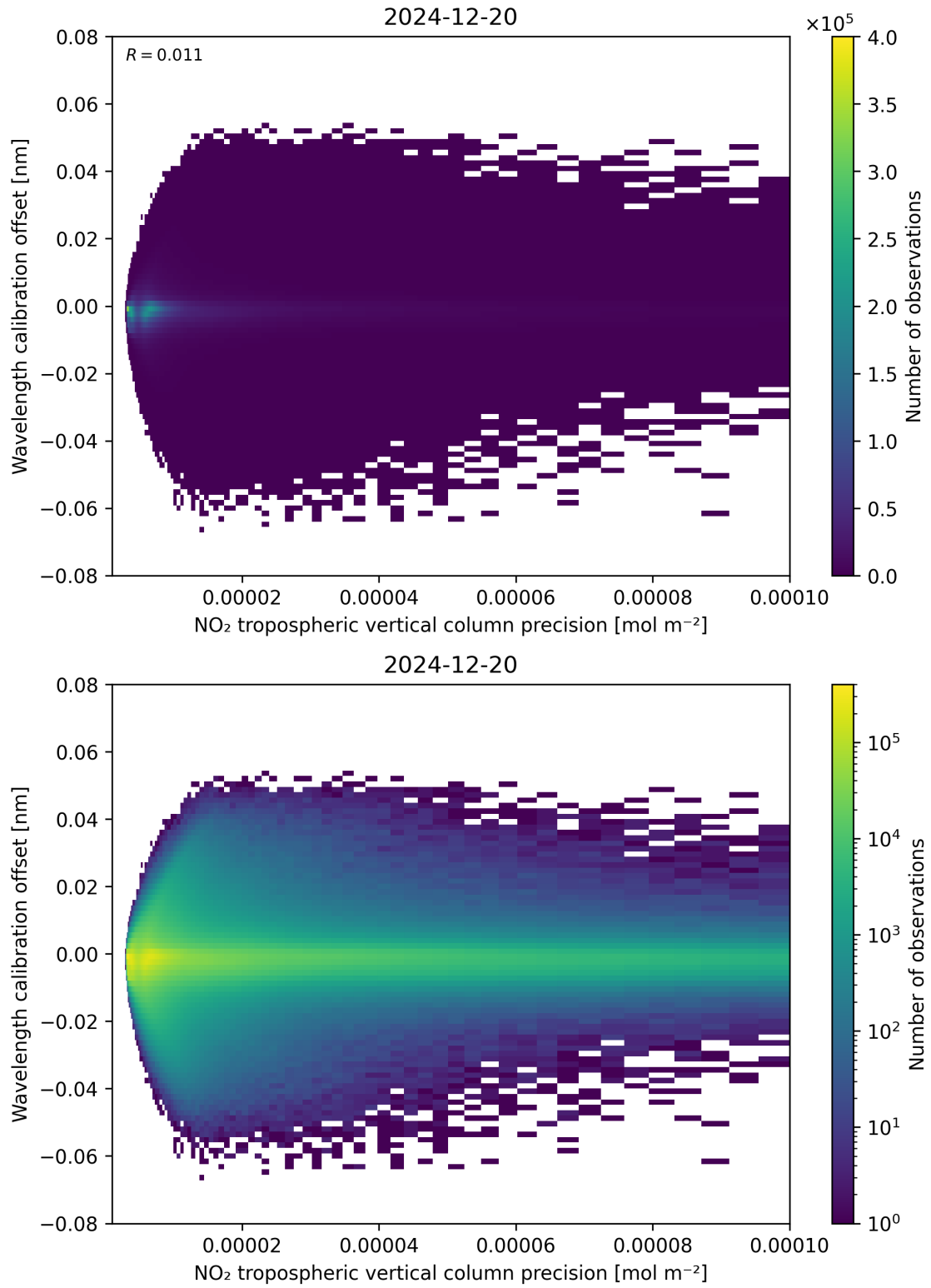
Figure 141: Scatter density plot of “NO 2 tropospheric vertical column precision” against “Wavelength calibration offset” for 2024-12-19 to 2024-12-21.
