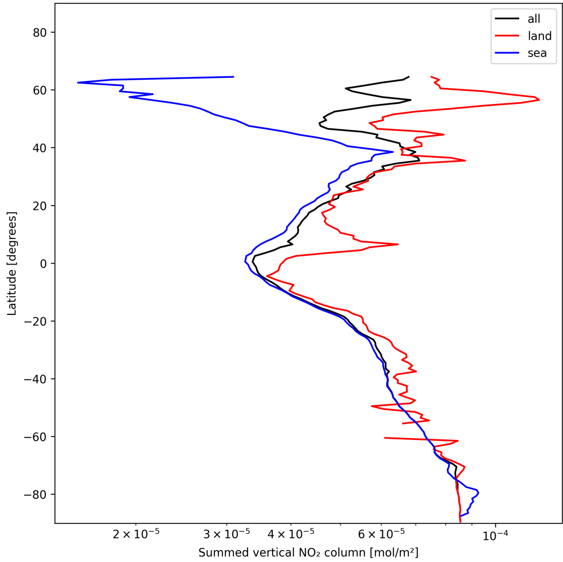
Figure 23: Zonal average of “Summed vertical NO 2 column” for 2024-12-19 to 2024-12-21.
