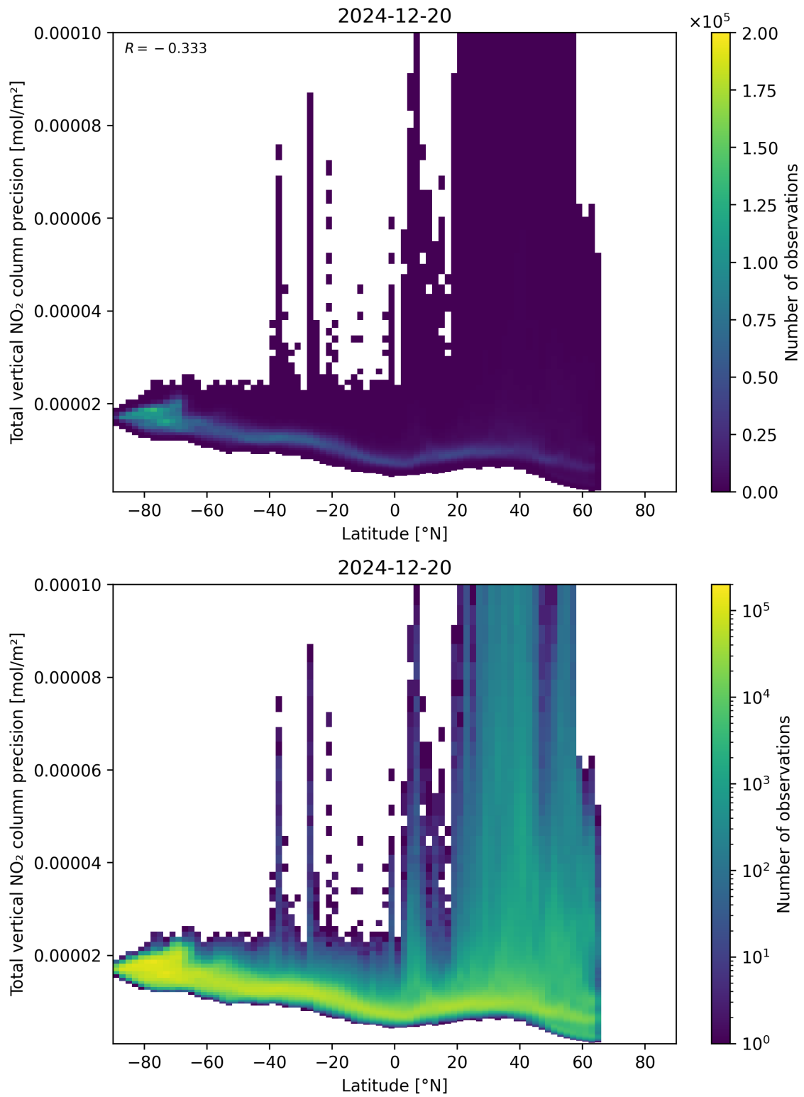
Figure 91: Scatter density plot of “Latitude” against “Total vertical NO 2 column precision” for 2024-12-19 to 2024-12-21.
