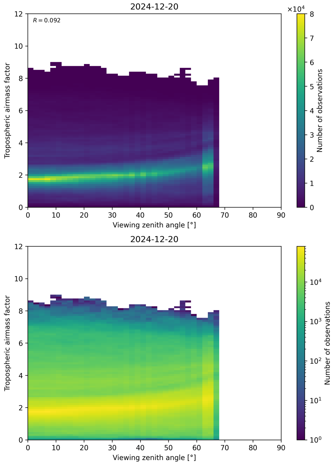
Figure 161: Scatter density plot of “Viewing zenith angle” against “Tropospheric airmass factor” for 2024-12-19 to 2024-12-21.
