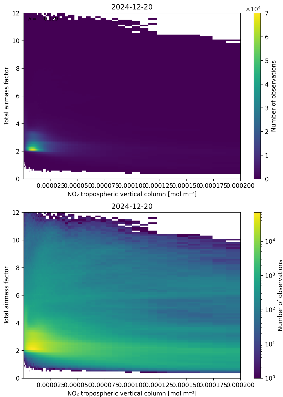
Figure 122: Scatter density plot of “NO 2 tropospheric vertical column” against “Total air mass factor” for 2024-12-19 to 2024-12-21.
