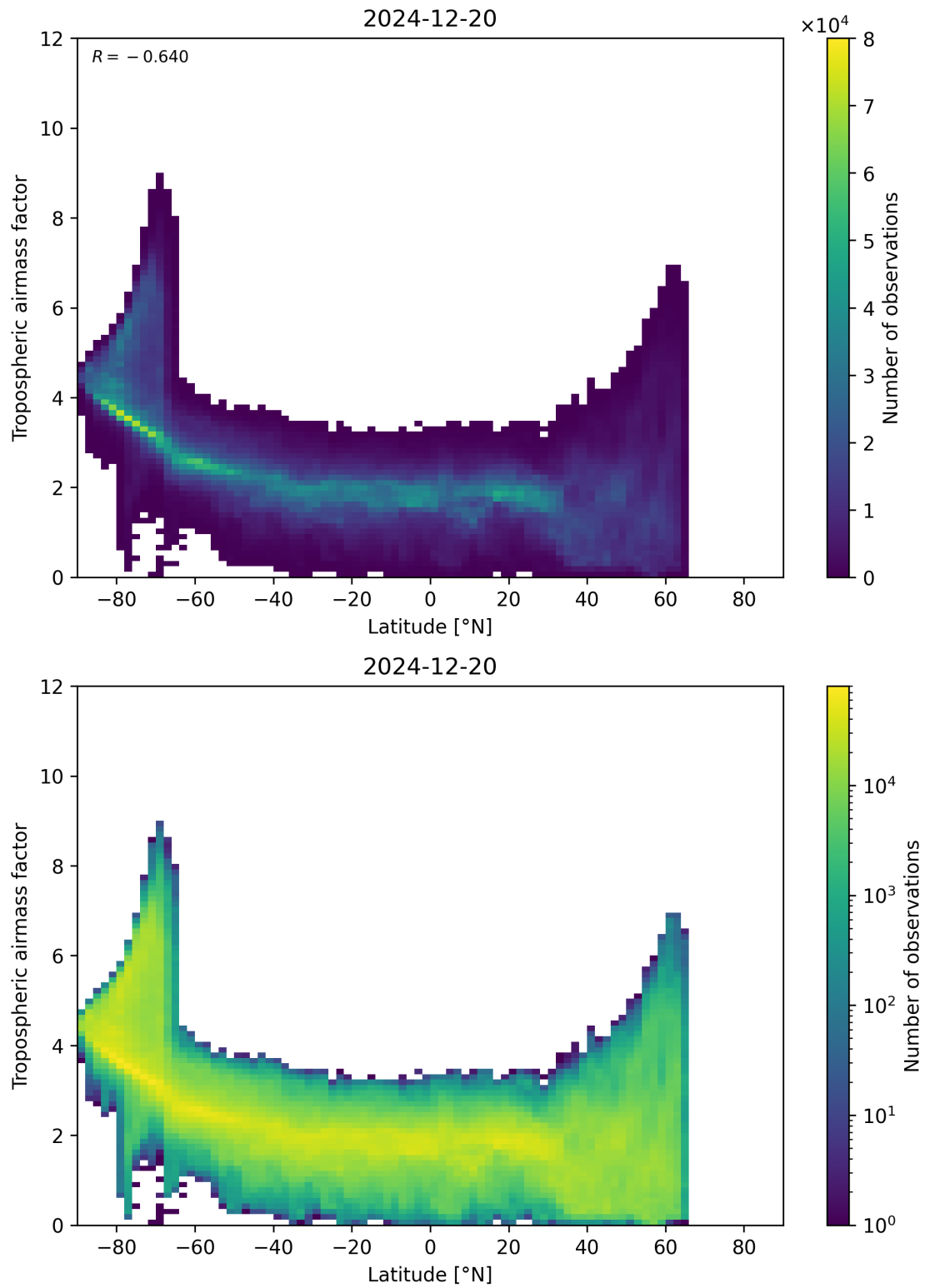
Figure 85: Scatter density plot of “Latitude” against “Tropospheric airmass factor” for 2024-12-19 to 2024-12-21.
