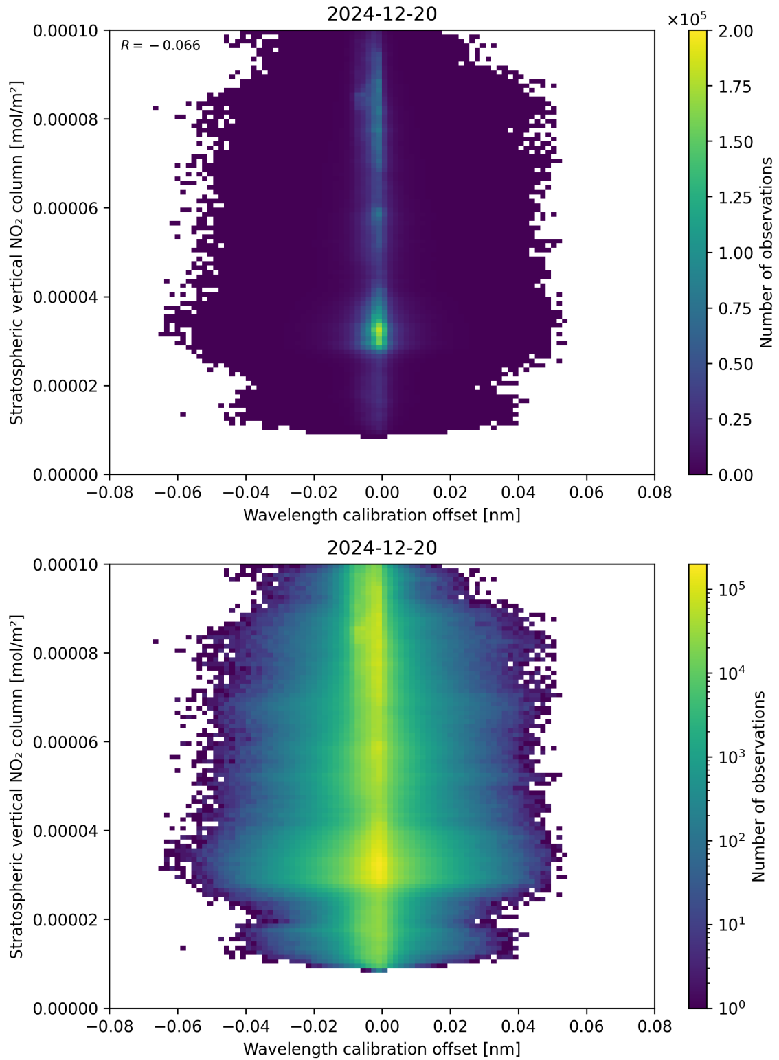
Figure 176: Scatter density plot of “Wavelength calibration offset” against “Stratospheric vertical NO 2 column” for 2024-12-19 to 2024-12-21.
