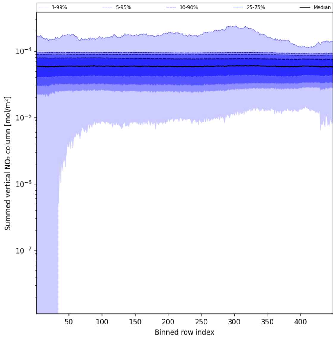
Figure 57: Along track statistics of “Summed vertical NO 2 column” for 2024-12-19 to 2024-12-21
