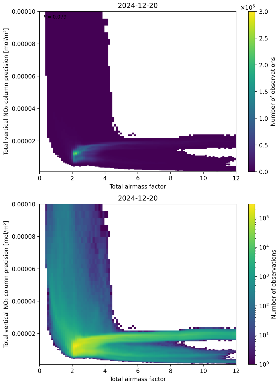
Figure 68: Scatter density plot of “Total airmass factor” against “Total vertical NO 2 column precision” for 2024-12-19 to 2024-12-21.
