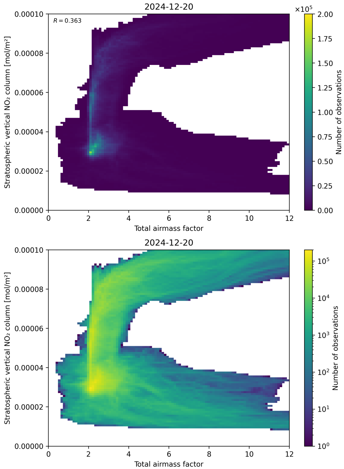
Figure 64: Scatter density plot of “Total airmass factor” against “Stratospheric vertical NO 2 column” for 2024-12-19 to 2024-12-21.
