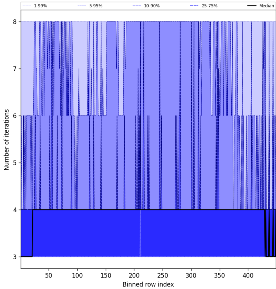
Figure 51: Along track statistics of “Number of iterations” for 2024-12-19 to 2024-12-21
