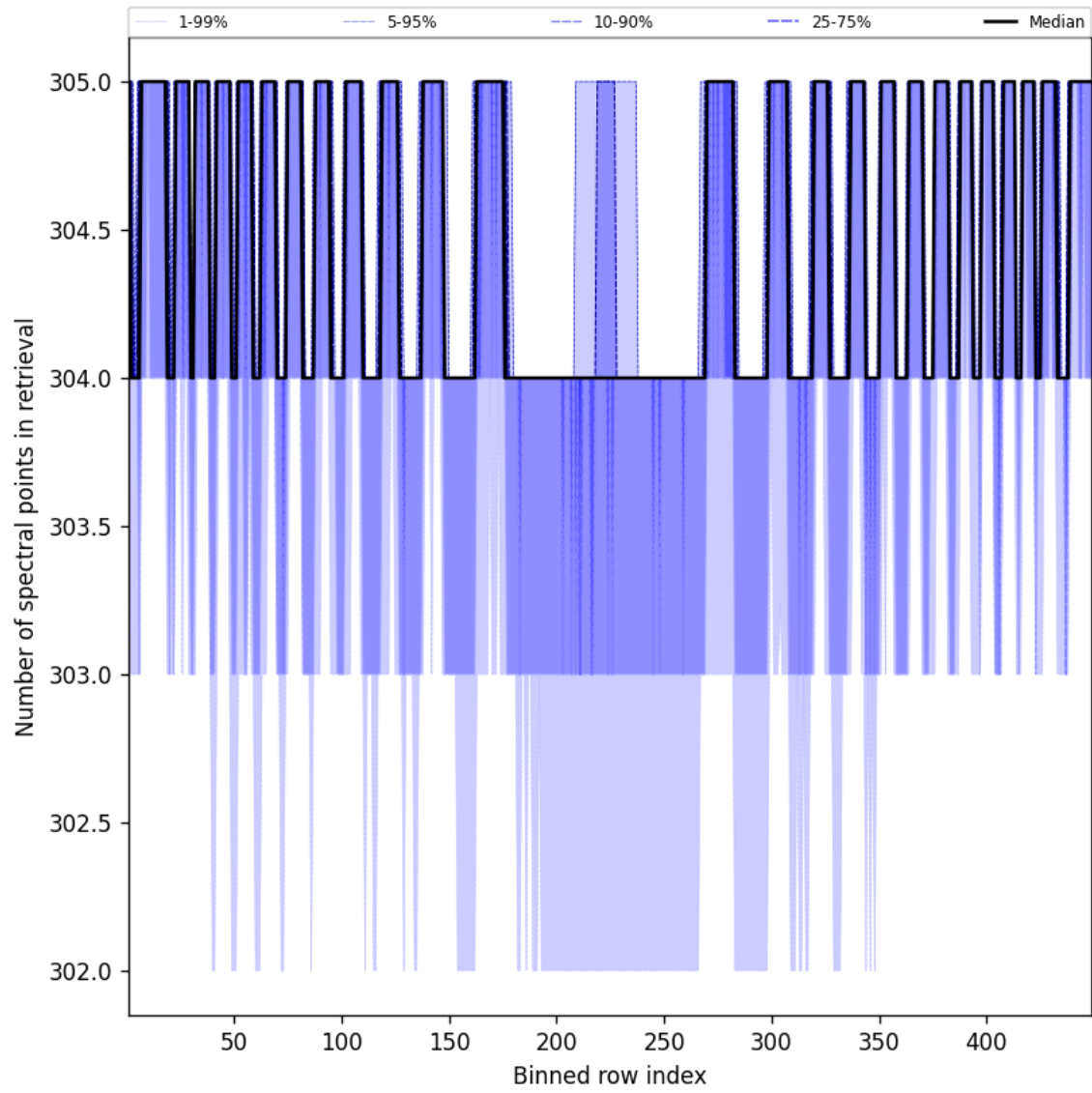
Figure 50: Along track statistics of “Number of spectral points in retrieval” for 2024-12-19 to 2024-12-21
