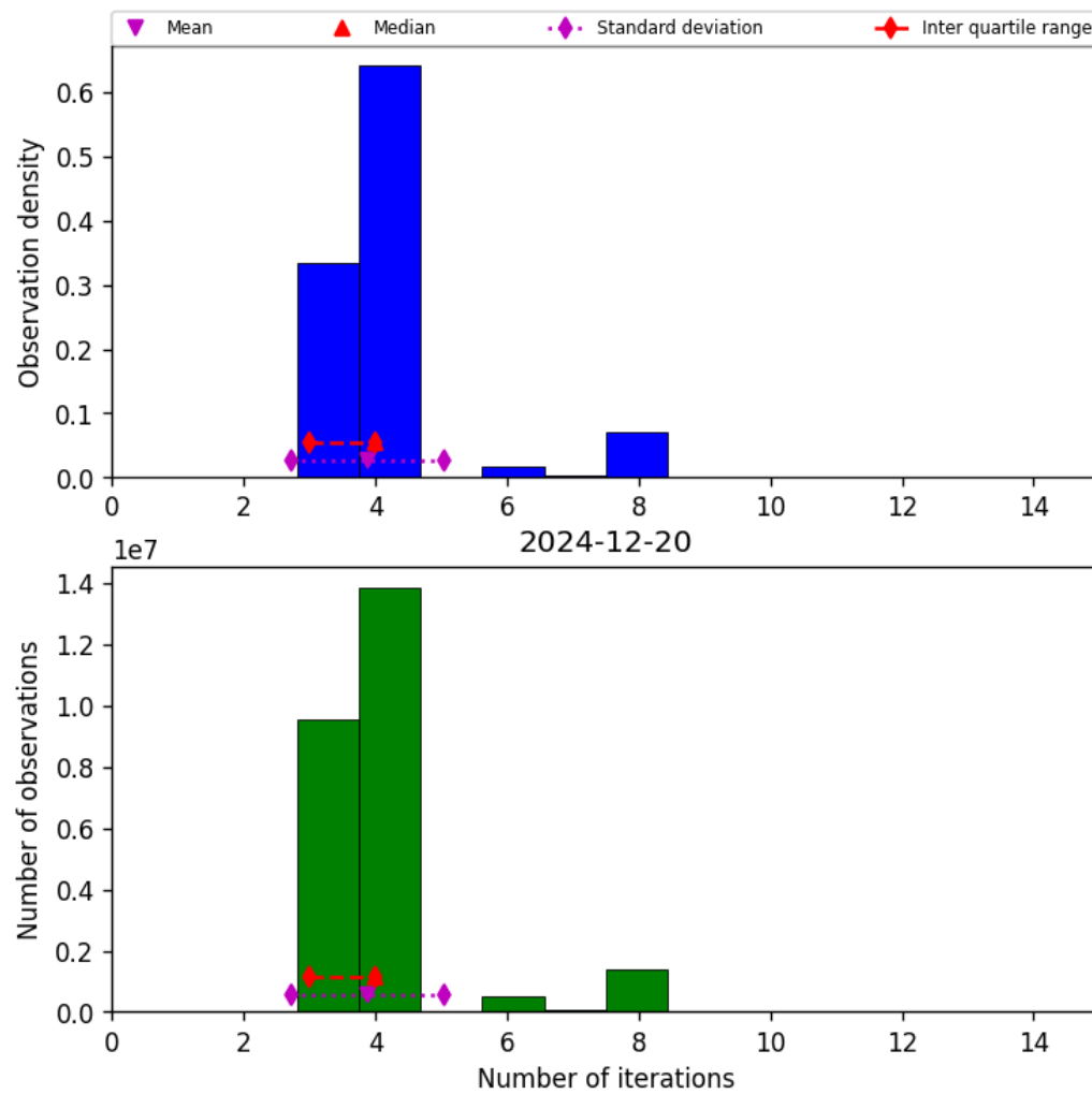
Figure 34: Histogram of “Number of iterations” for 2024-12-19 to 2024-12-21
