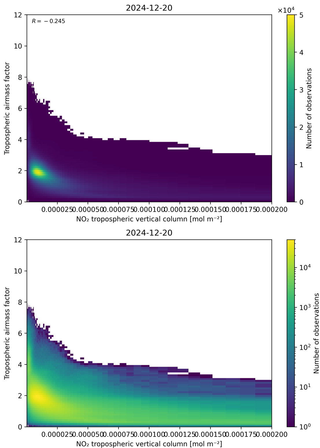
Figure 123: Scatter density plot of “NO 2 tropospheric vertical column” against “Tropospheric air mass factor” for 2024-12-19 to 2024-12-21.
