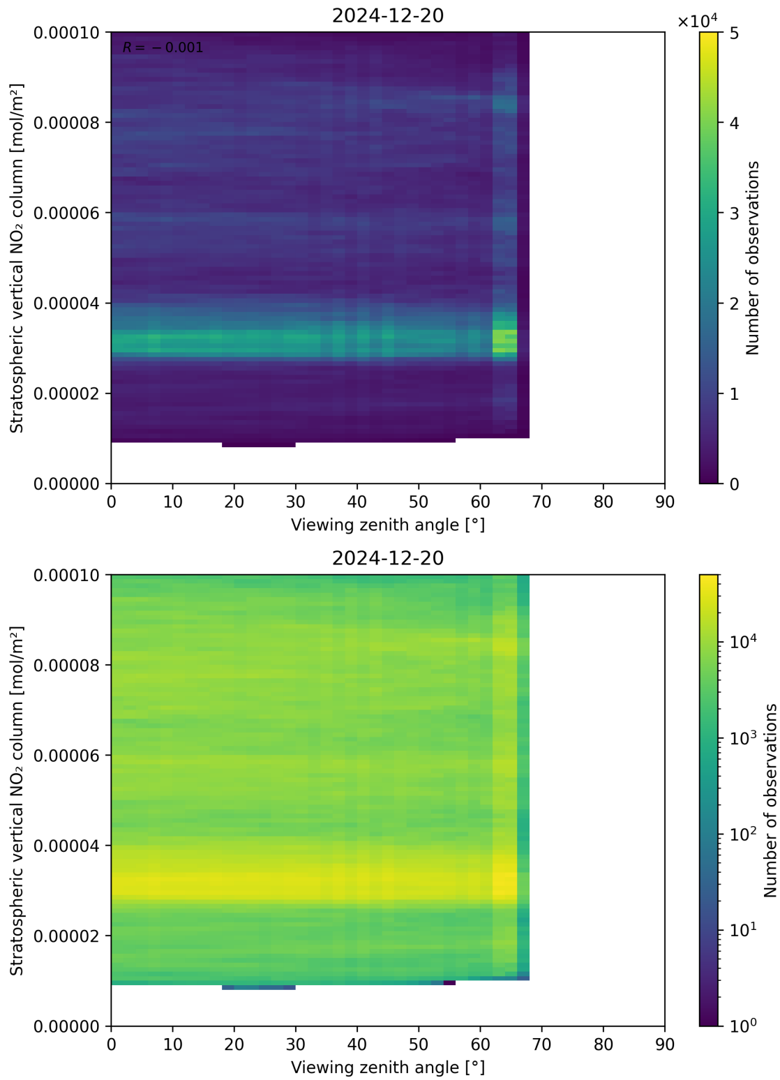
Figure 164: Scatter density plot of “Viewing zenith angle” against “Stratospheric vertical NO 2 column” for 2024-12-19 to 2024-12-21.
