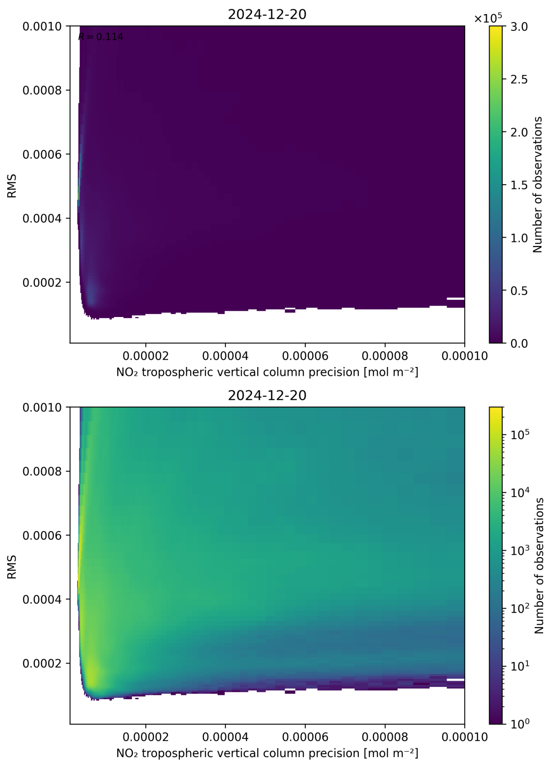
Figure 140: Scatter density plot of “NO 2 tropospheric vertical column precision” against “RMS” for 2024-12-19 to 2024-12-21.
