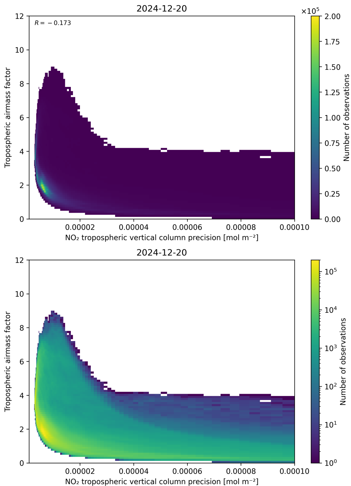
Figure 133: Scatter density plot of “NO 2 tropospheric vertical column precision” against “Tropospheric air mass factor” for 2024-12-19 to 2024-12-21.
