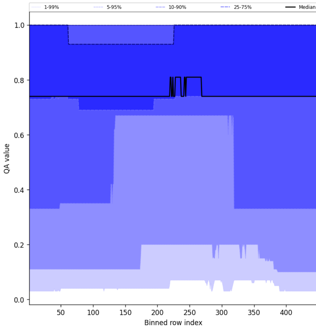
Figure 45: Along track statistics of “QA value” for 2024-12-19 to 2024-12-21
