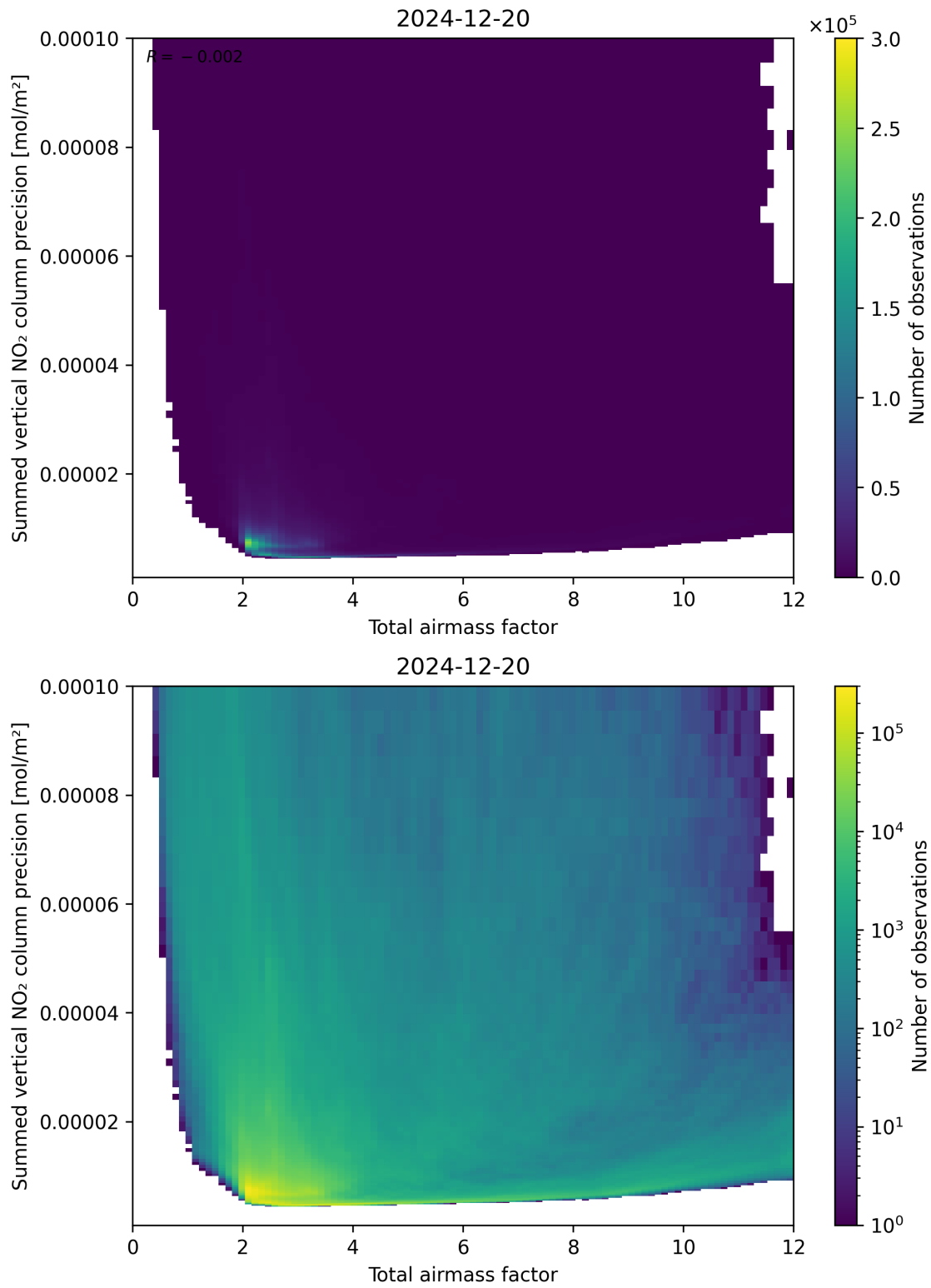
Figure 66: Scatter density plot of “Total airmass factor” against “Summed vertical NO 2 column precision” for 2024-12-19 to 2024-12-21.
