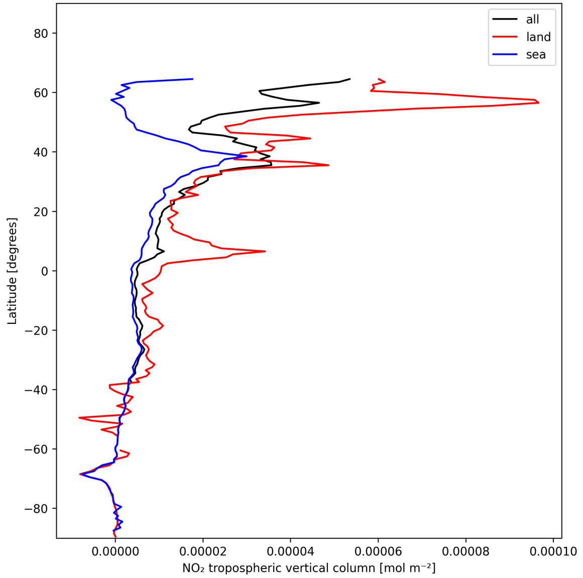
Figure 12: Zonal average of “NO 2 tropospheric vertical column” for 2024-12-19 to 2024-12-21.
