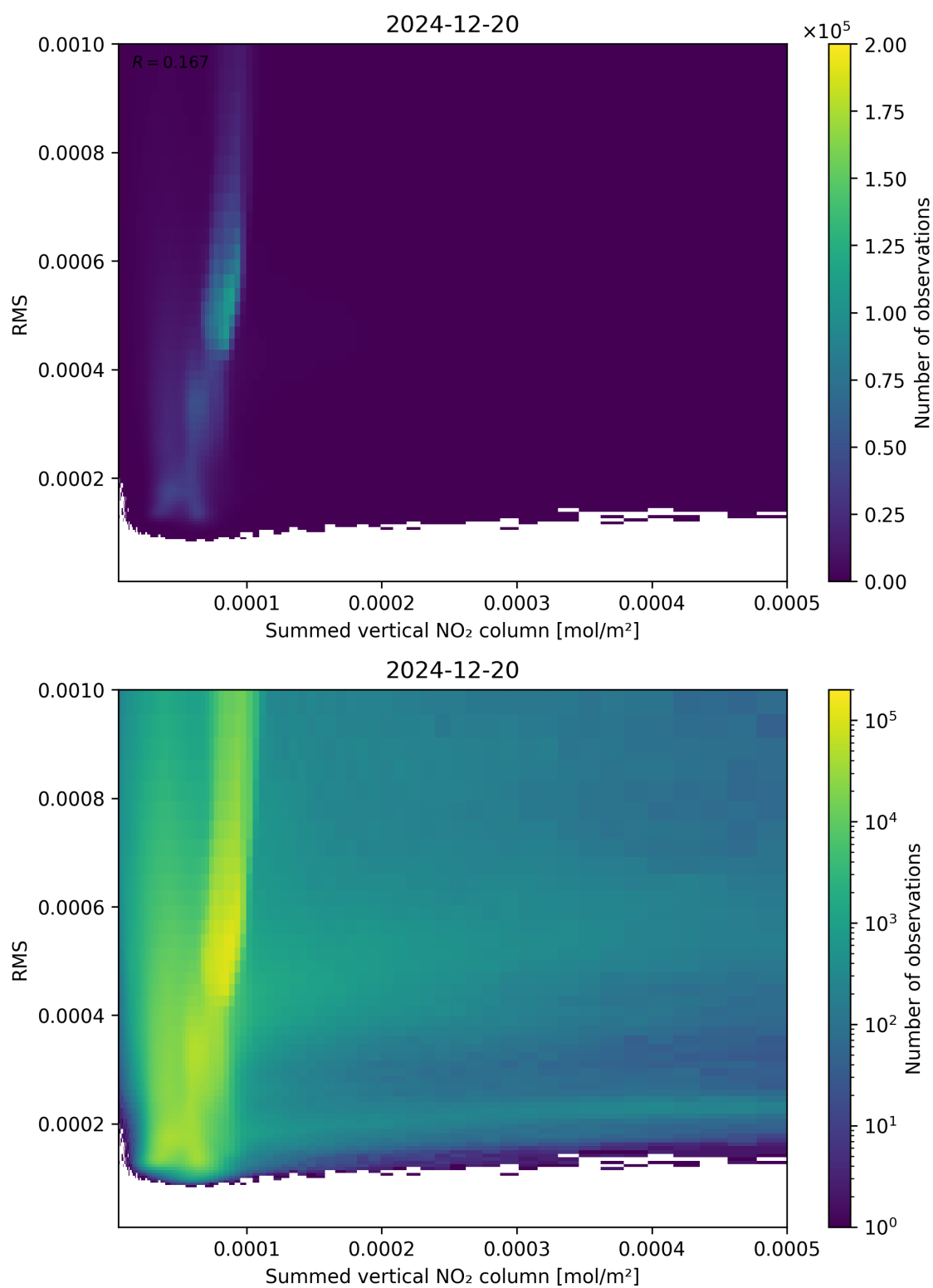
Figure 109: Scatter density plot of “Summed vertical NO 2 column” against “RMS” for 2024-12-19 to 2024-12-21.
