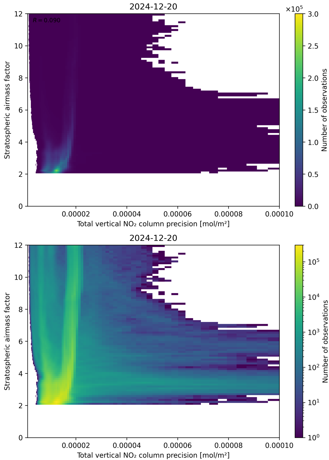
Figure 115: Scatter density plot of “Total vertical NO 2 column precision” against “Stratospheric air mass factor” for 2024-12-19 to 2024-12-21.
