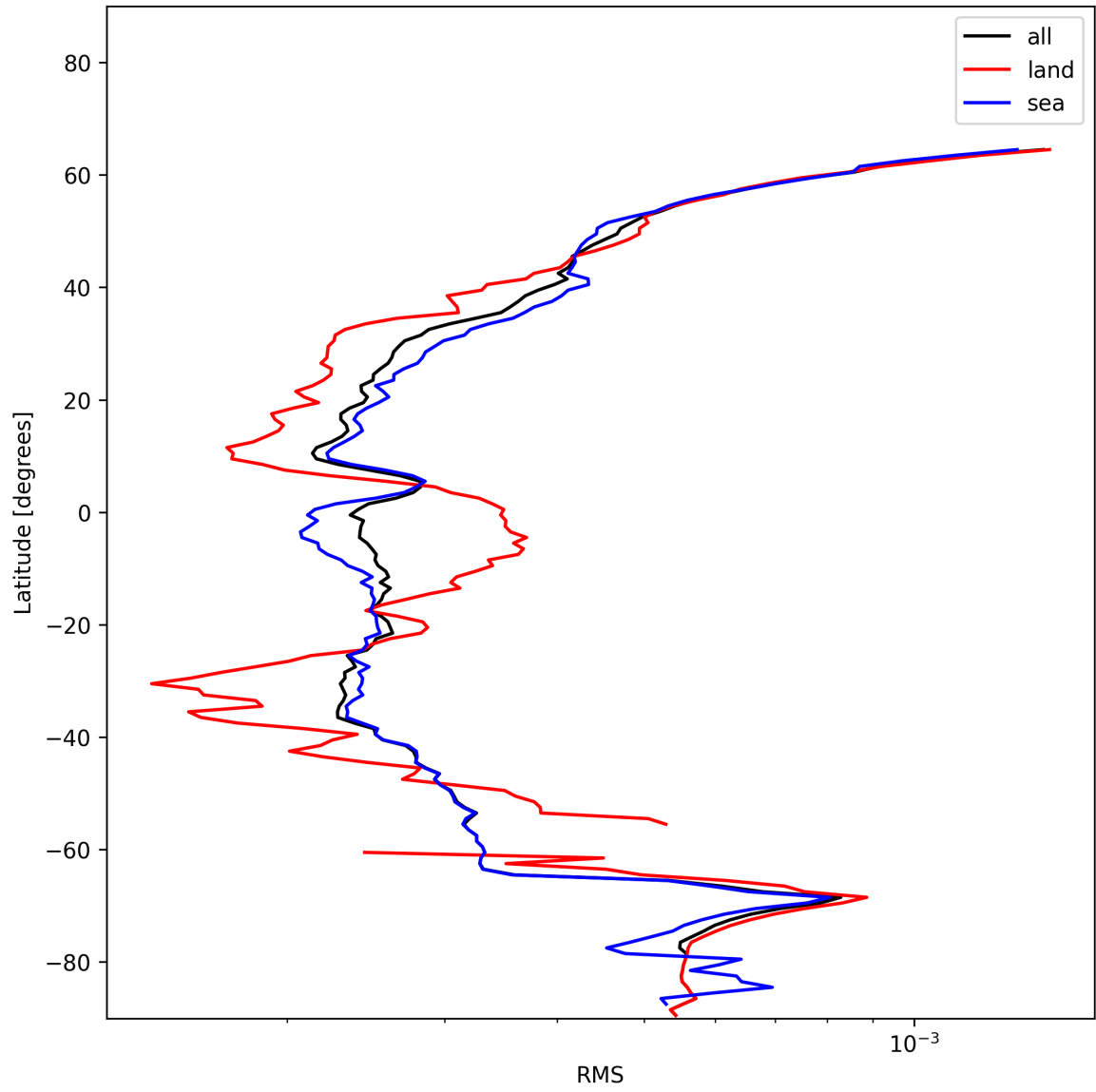
Figure 26: Zonal average of “RMS” for 2024-12-19 to 2024-12-21.
