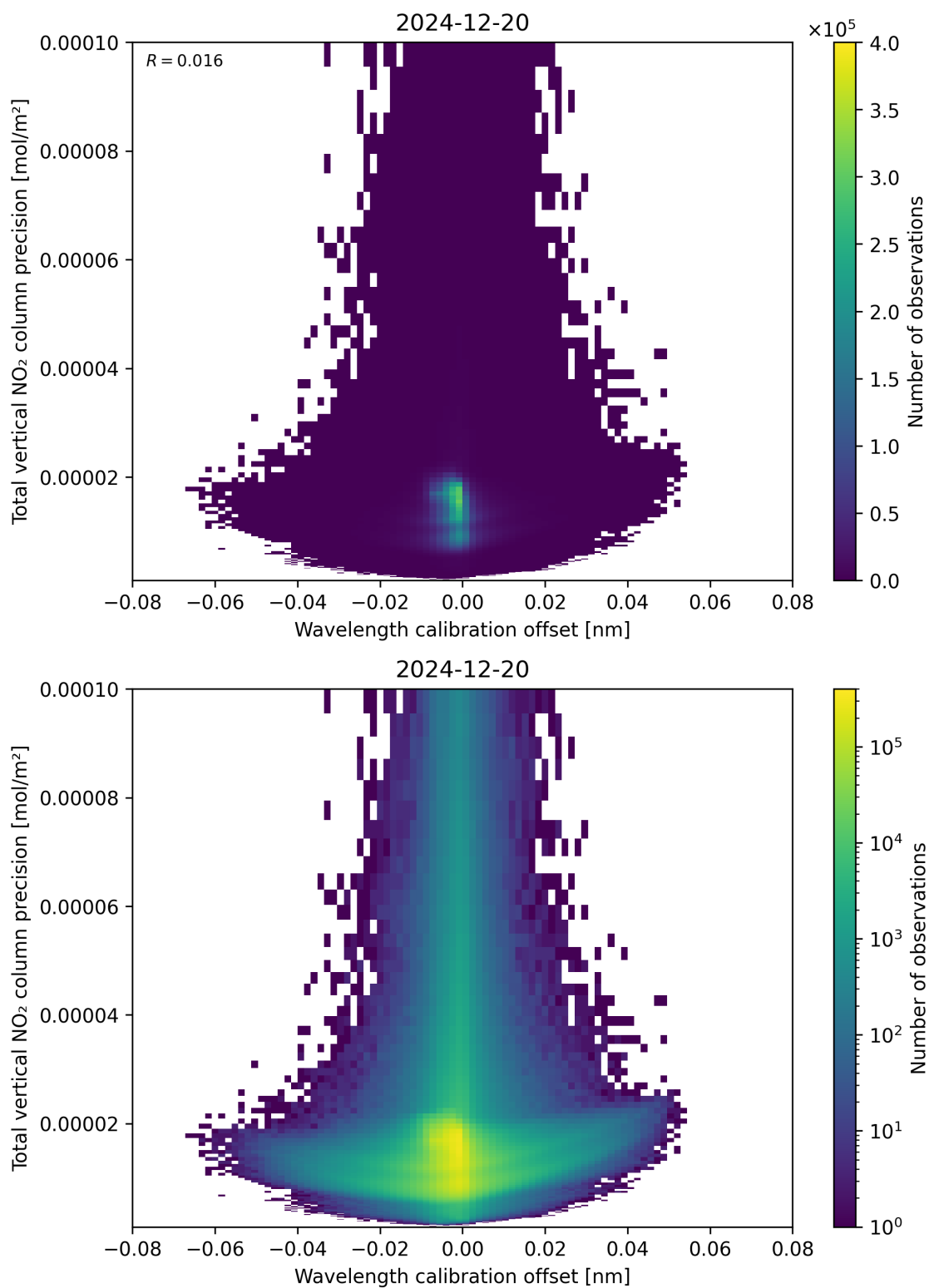
Figure 180: Scatter density plot of “Wavelength calibration offset” against “Total vertical NO 2 column precision” for 2024-12-19 to 2024-12-21.
