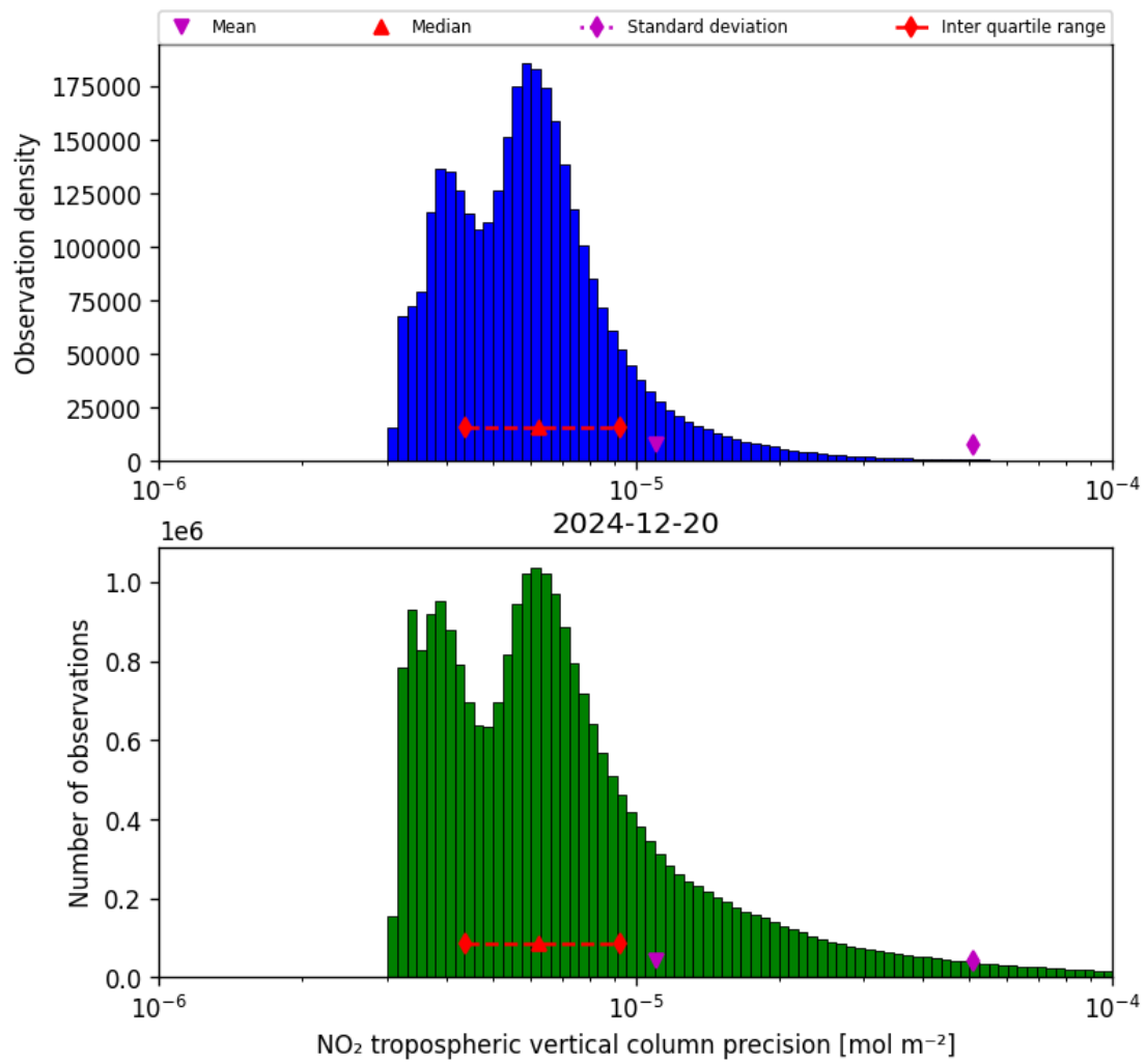
Figure 30: Histogram of “NO 2 tropospheric vertical column precision” for 2024-12-19 to 2024-12-21
