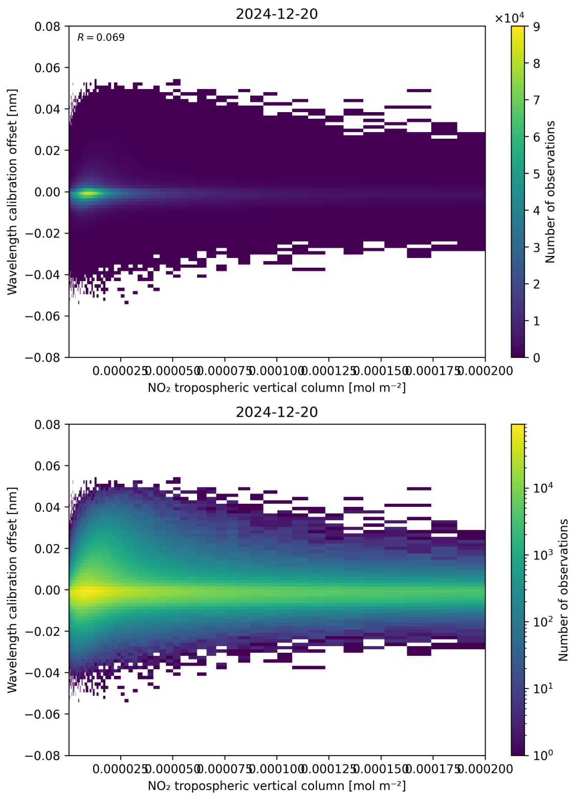
Figure 143: Scatter density plot of “NO 2 tropospheric vertical column” against “Wavelength calibration offset” for 2024-12-19 to 2024-12-21.
