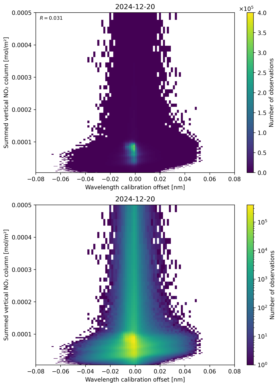
Figure 177: Scatter density plot of “Wavelength calibration offset” against “Summed vertical NO 2 column” for 2024-12-19 to 2024-12-21.
