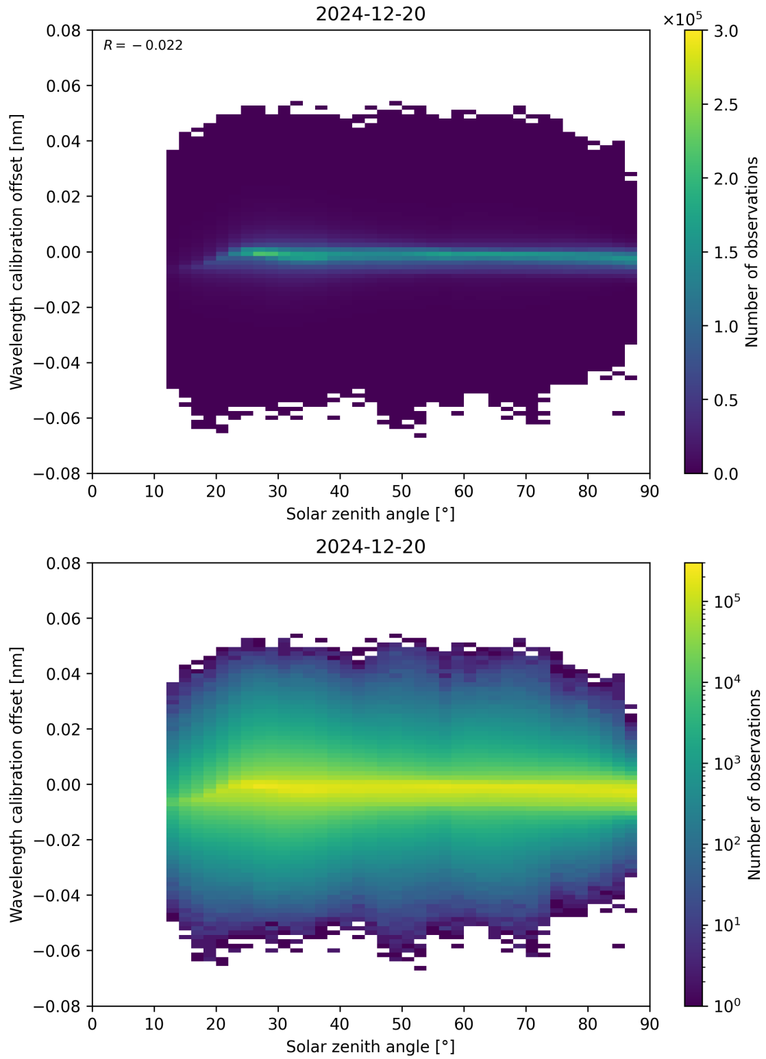
Figure 158: Scatter density plot of “Solar zenith angle” against “Wavelength calibration offset” for 2024-12-19 to 2024-12-21.
