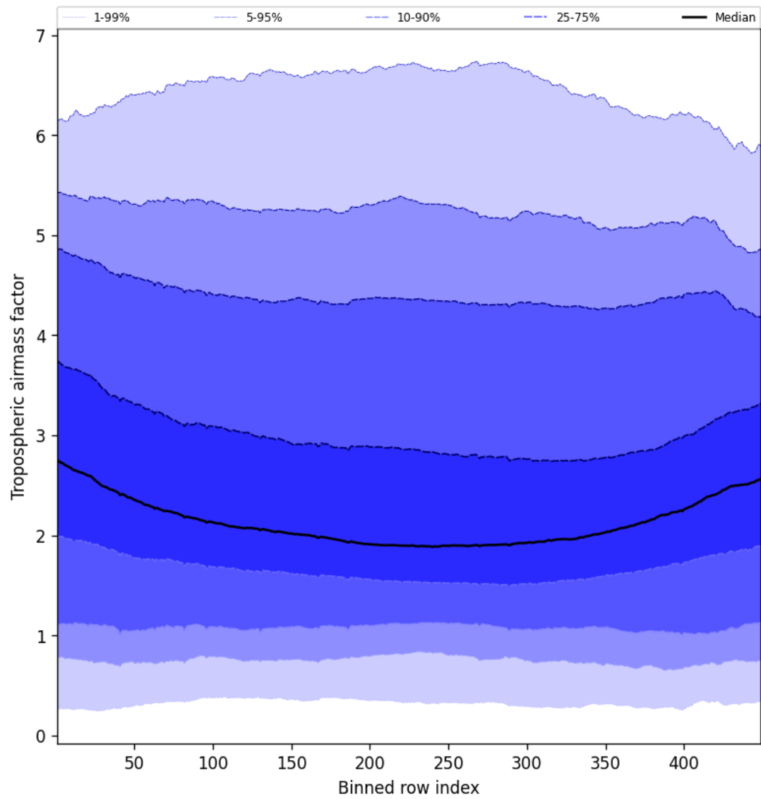
Figure 48: Along track statistics of “Tropospheric airmass factor” for 2024-12-19 to 2024-12-21
