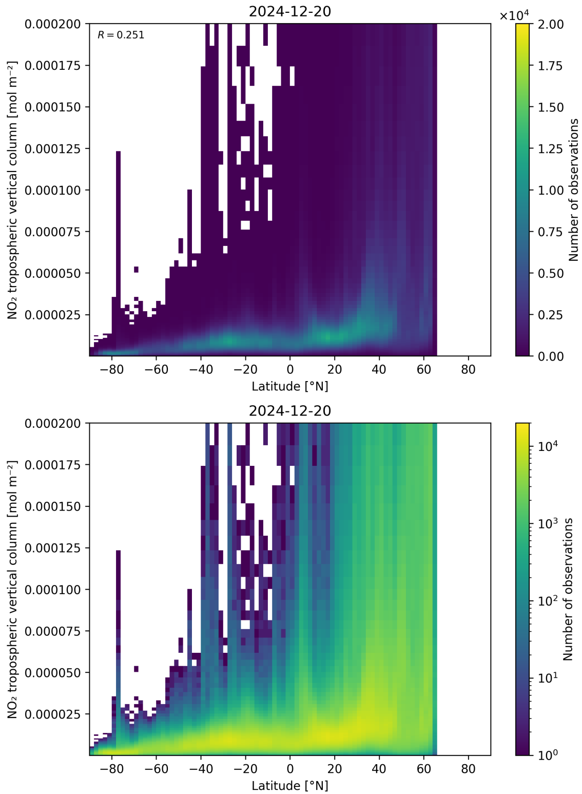
Figure 92: Scatter density plot of “Latitude” against “NO 2 tropospheric vertical column” for 2024-12-19 to 2024-12-21.
