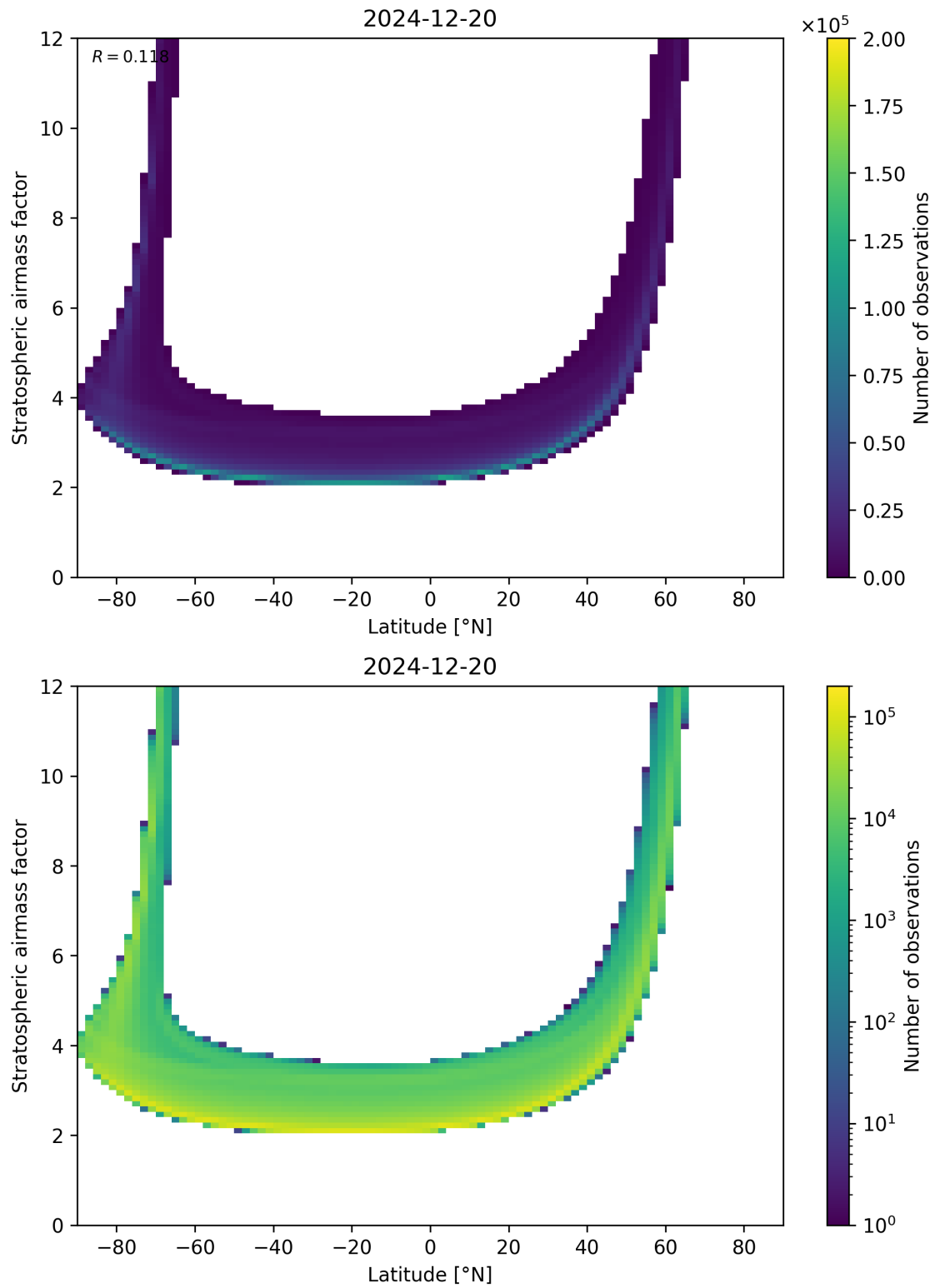
Figure 83: Scatter density plot of “Latitude” against “Stratospheric airmass factor” for 2024-12-19 to 2024-12-21.
