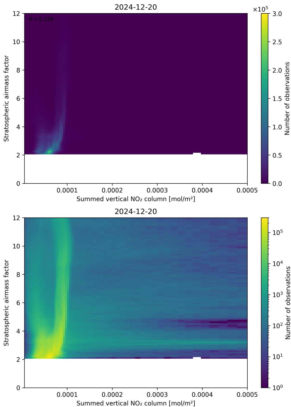
Figure 103: Scatter density plot of “Summed vertical NO 2 column” against “Stratospheric airmass factor” for 2024-12-19 to 2024-12-21.
