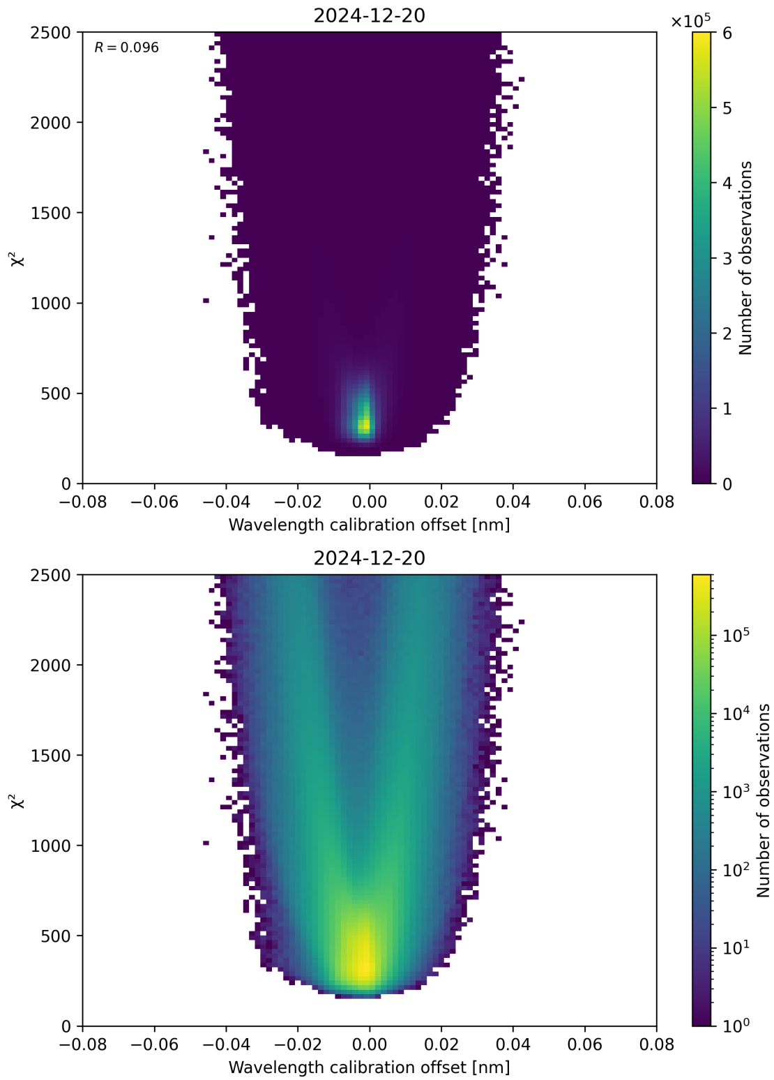
Figure 175: Scatter density plot of “Wavelength calibration offset” against “ \chi^2 ” for 2024-12-19 to 2024-12-21.
