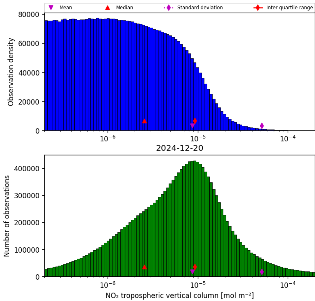
Figure 29: Histogram of “NO 2 tropospheric vertical column” for 2024-12-19 to 2024-12-21
