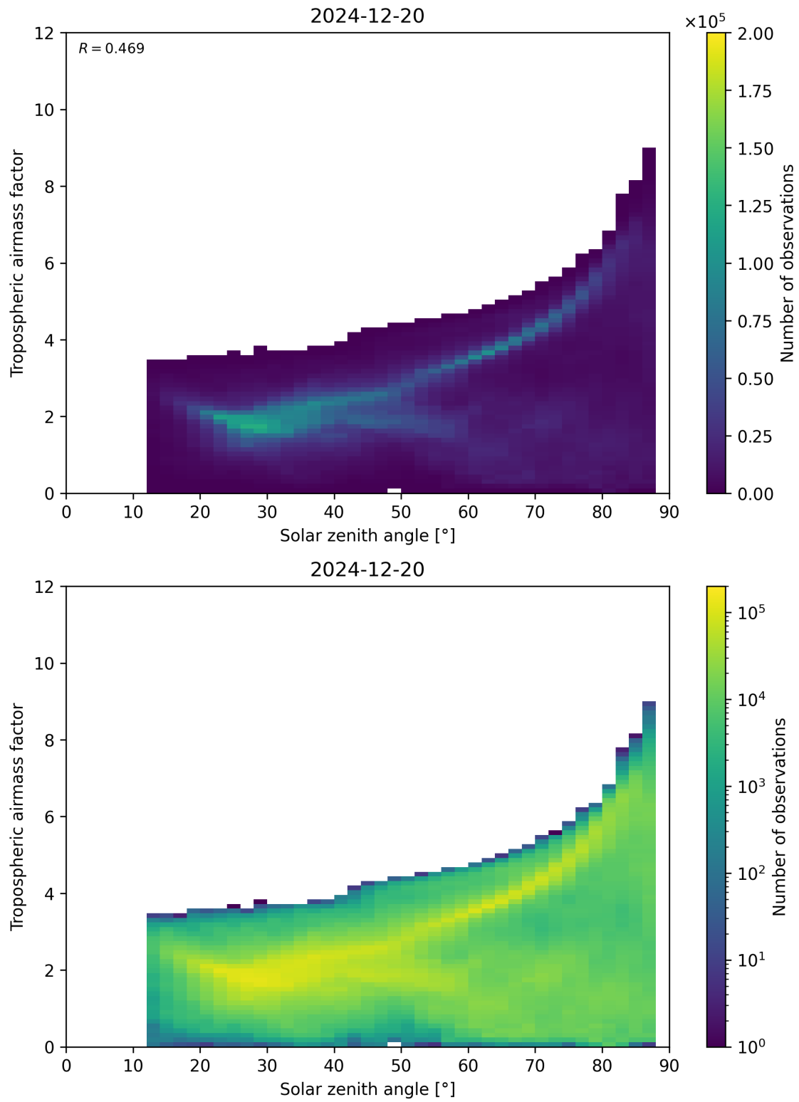
Figure 147: Scatter density plot of “Solar zenith angle” against “Tropospheric airmass factor” for 2024-12-19 to 2024-12-21.
