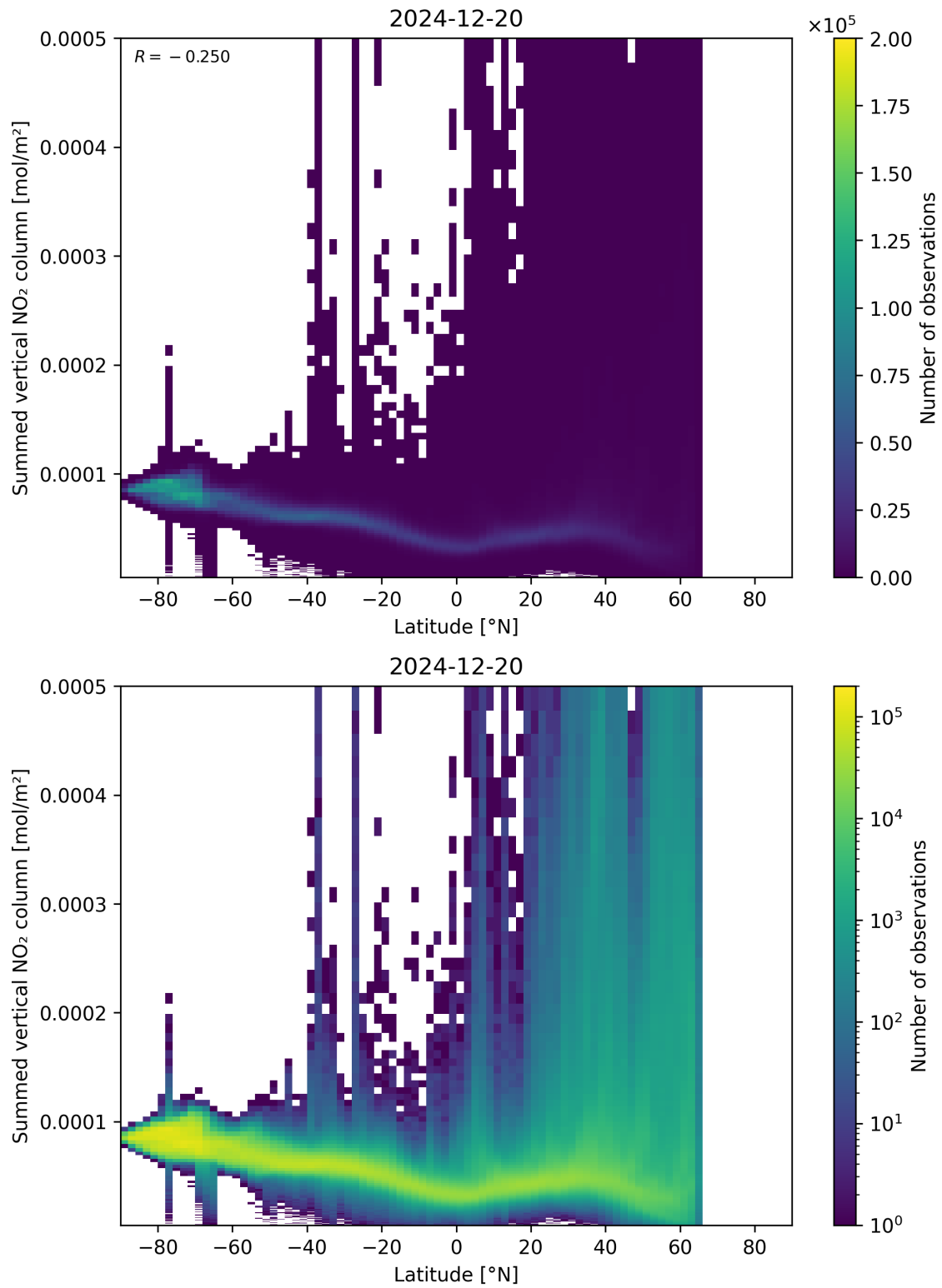
Figure 88: Scatter density plot of “Latitude” against “Summed vertical NO 2 column” for 2024-12-19 to 2024-12-21.
