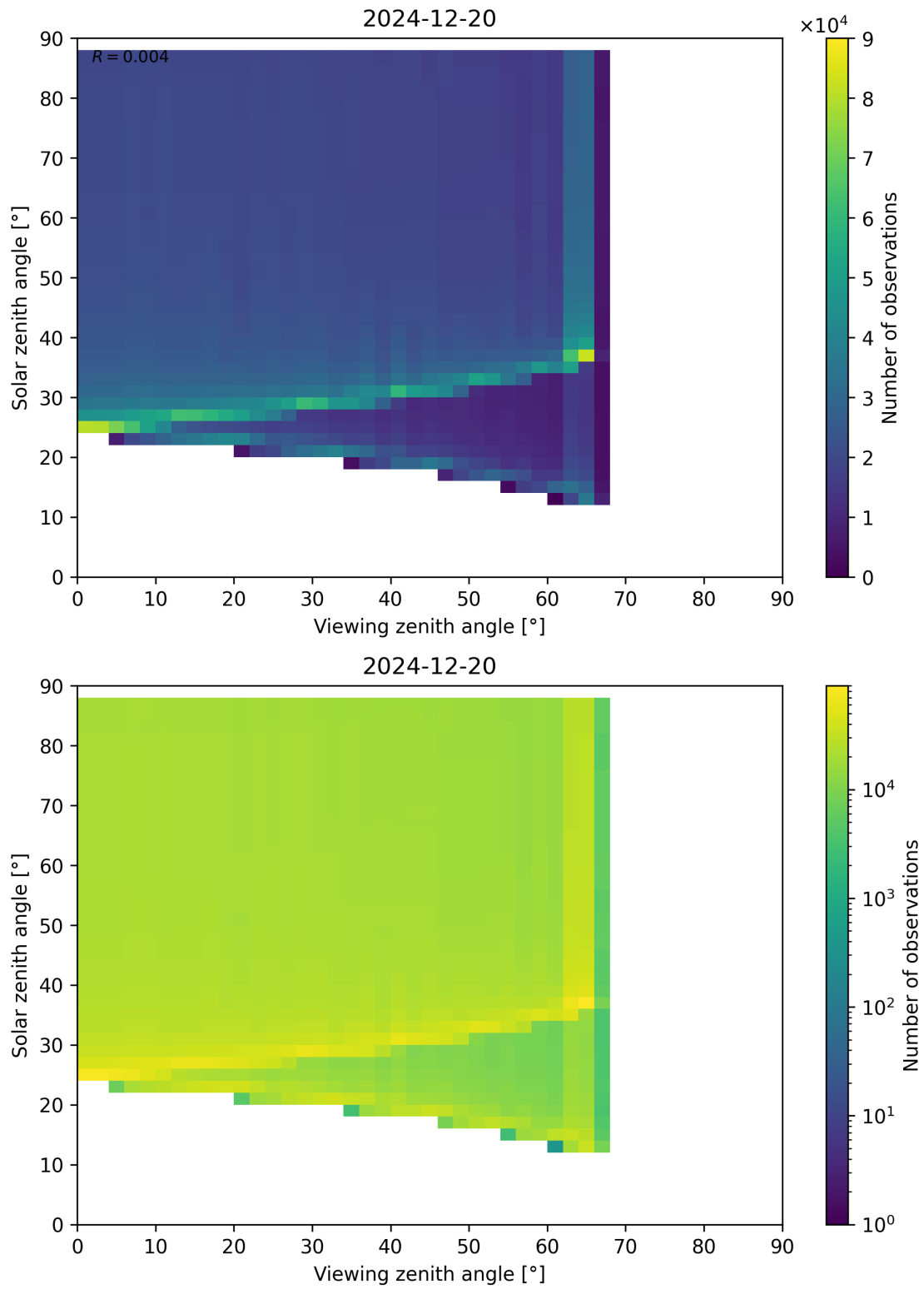
Figure 172: Scatter density plot of “Viewing zenith angle” against “Solar zenith angle” for 2024-12-19 to 2024-12-21.
