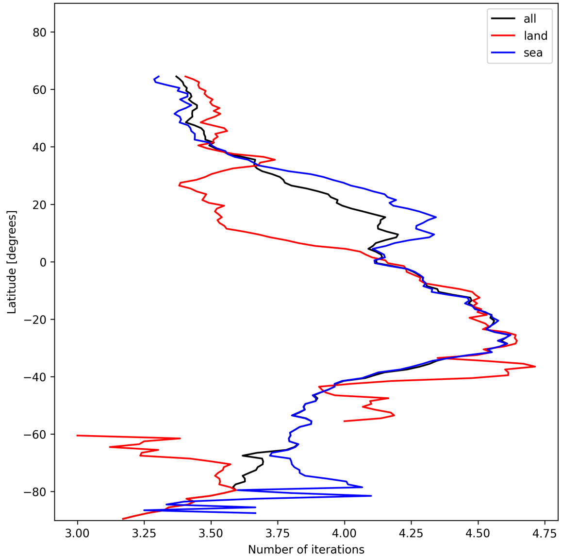
Figure 17: Zonal average of “Number of iterations” for 2024-12-19 to 2024-12-21.
