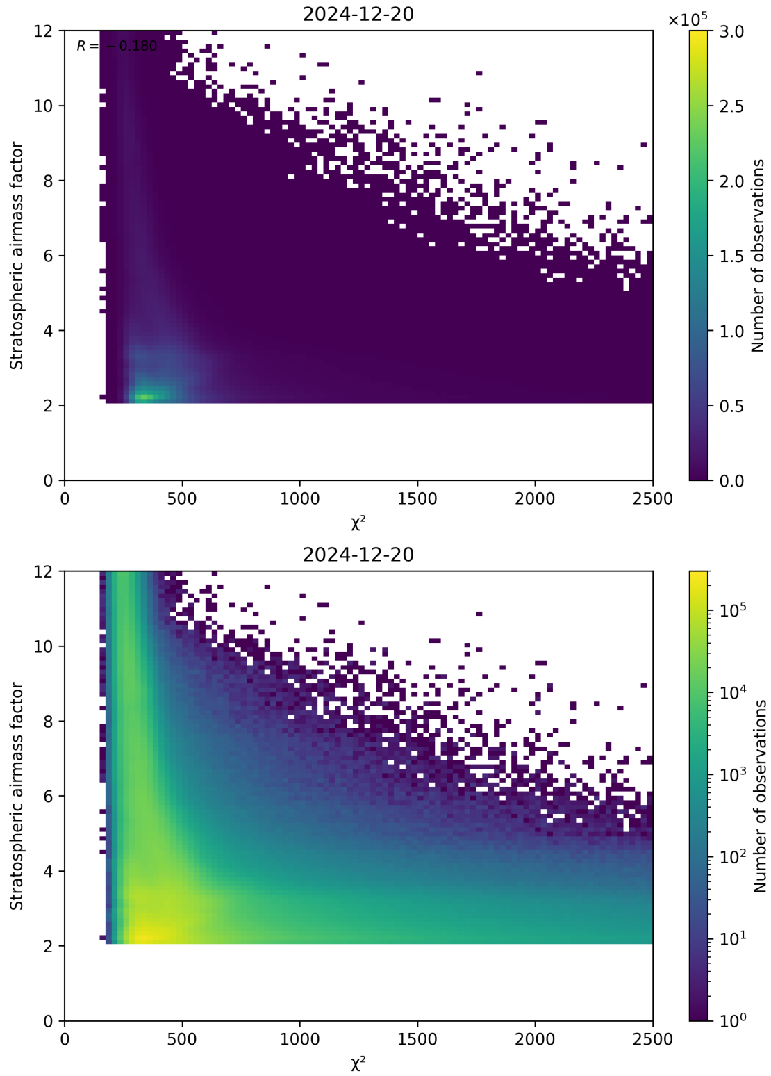
Figure 81: Scatter density plot of “ \chi^2 ” against “Stratospheric airmass factor” for 2024-12-19 to 2024-12-21.
