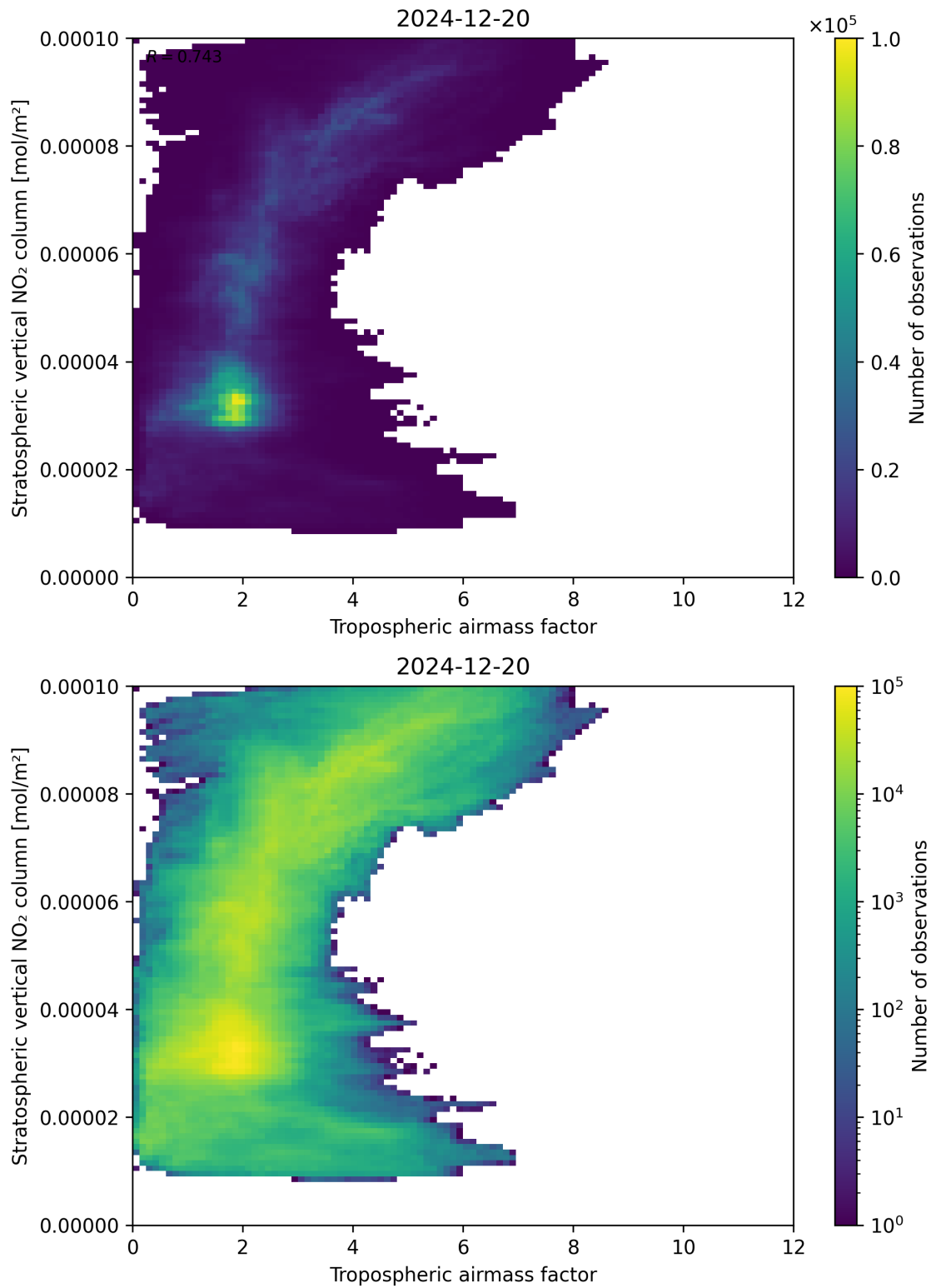
Figure 74: Scatter density plot of “Tropospheric air mass factor” against “Stratospheric vertical NO 2 column” for 2024-12-19 to 2024-12-21.
