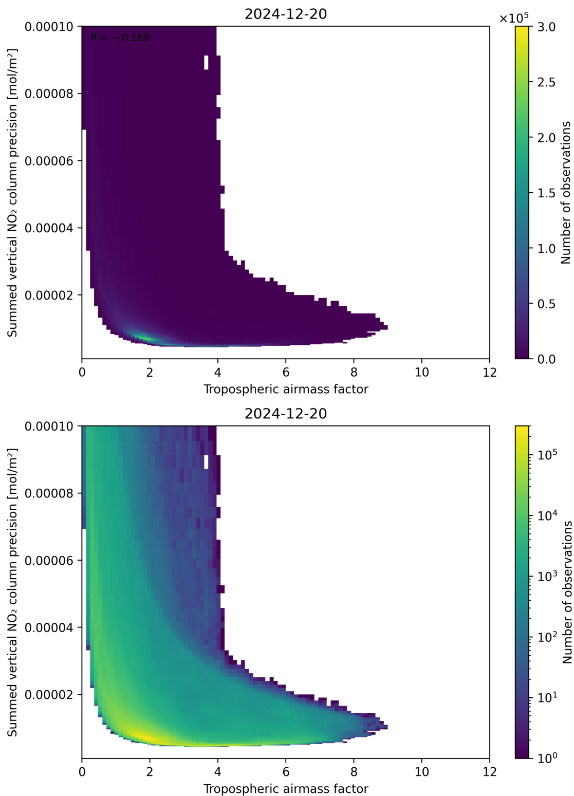
Figure 76: Scatter density plot of “Tropospheric air mass factor” against “Summed vertical NO 2 column precision” for 2024-12-19 to 2024-12-21.
