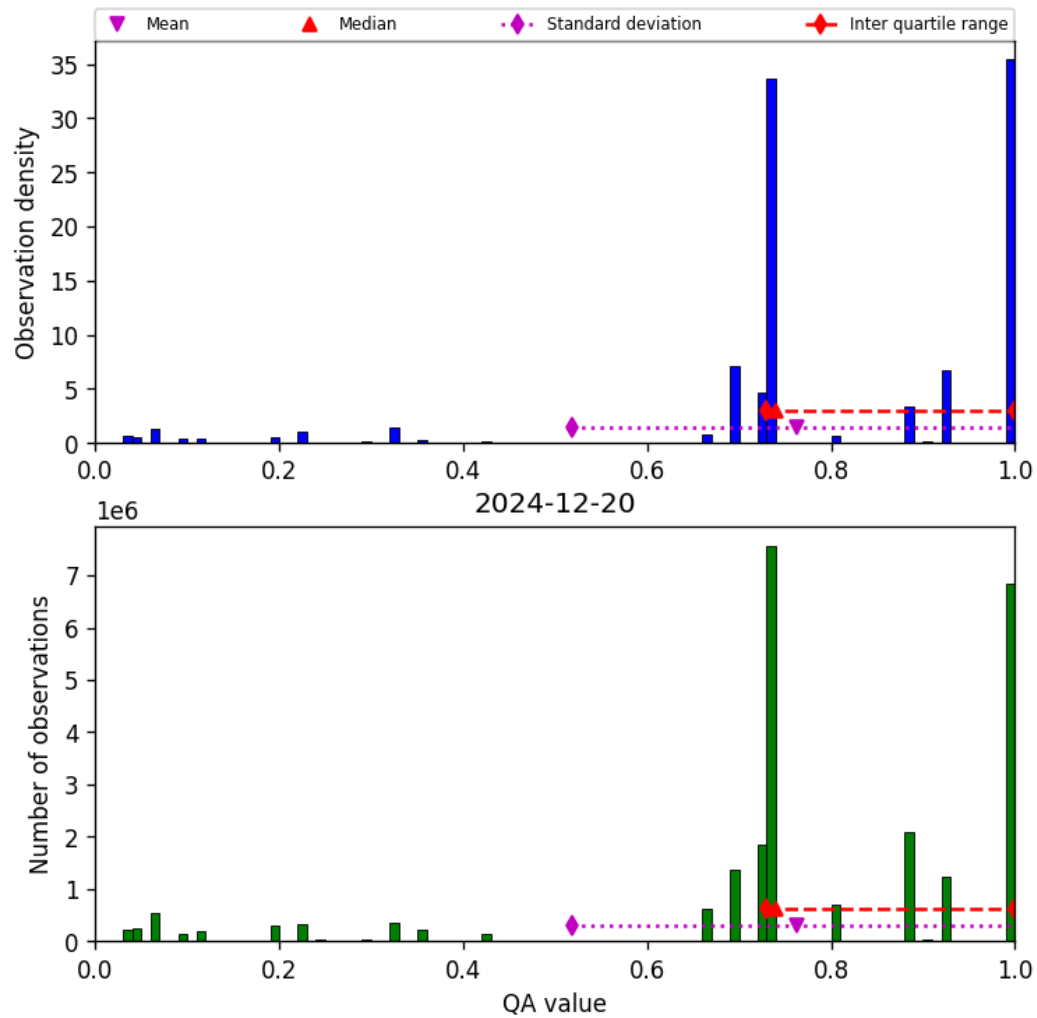
Figure 28: Histogram of “QA value” for 2024-12-19 to 2024-12-21
