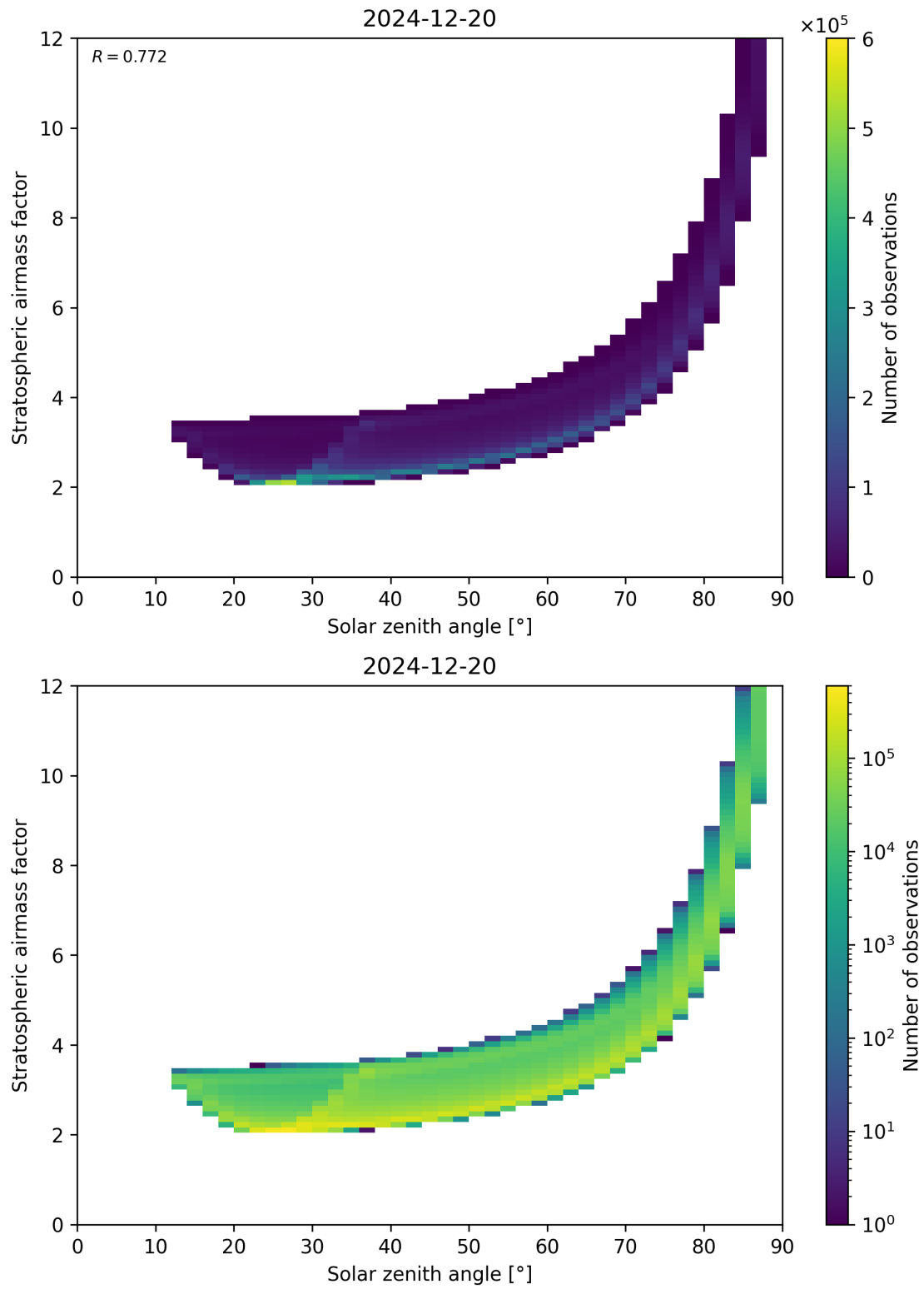
Figure 145: Scatter density plot of “Solar zenith angle” against “Stratospheric airmass factor” for 2024-12-19 to 2024-12-21.
