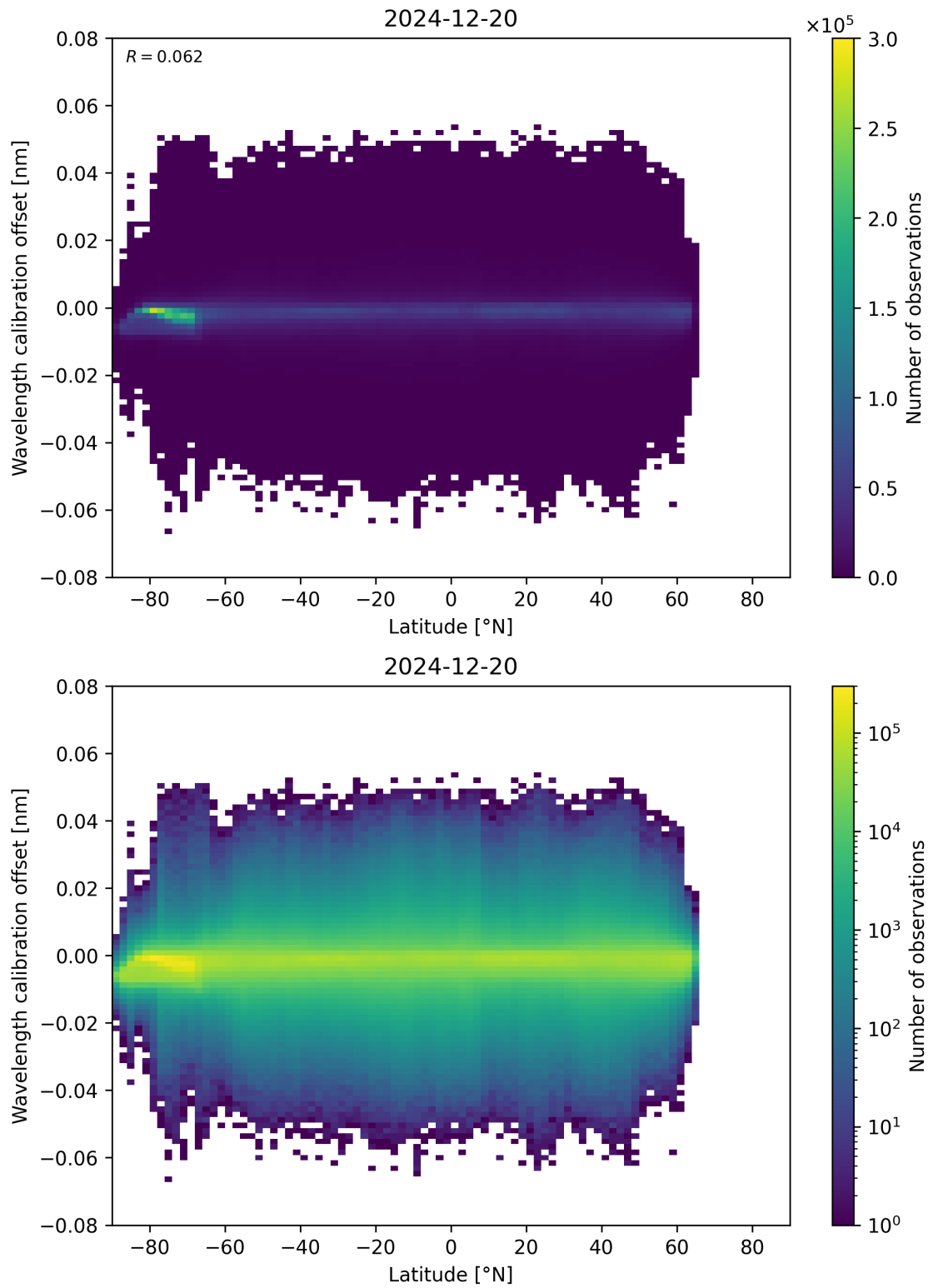
Figure 95: Scatter density plot of “Latitude” against “Wavelength calibration offset” for 2024-12-19 to 2024-12-21.
