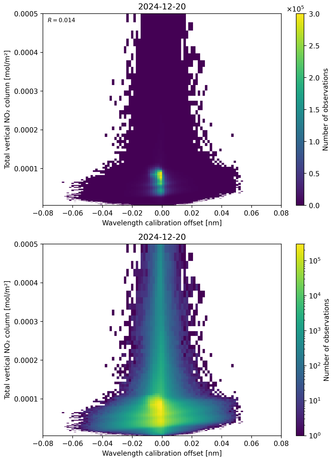
Figure 179: Scatter density plot of “Wavelength calibration offset” against “Total vertical NO 2 column” for 2024-12-19 to 2024-12-21.
