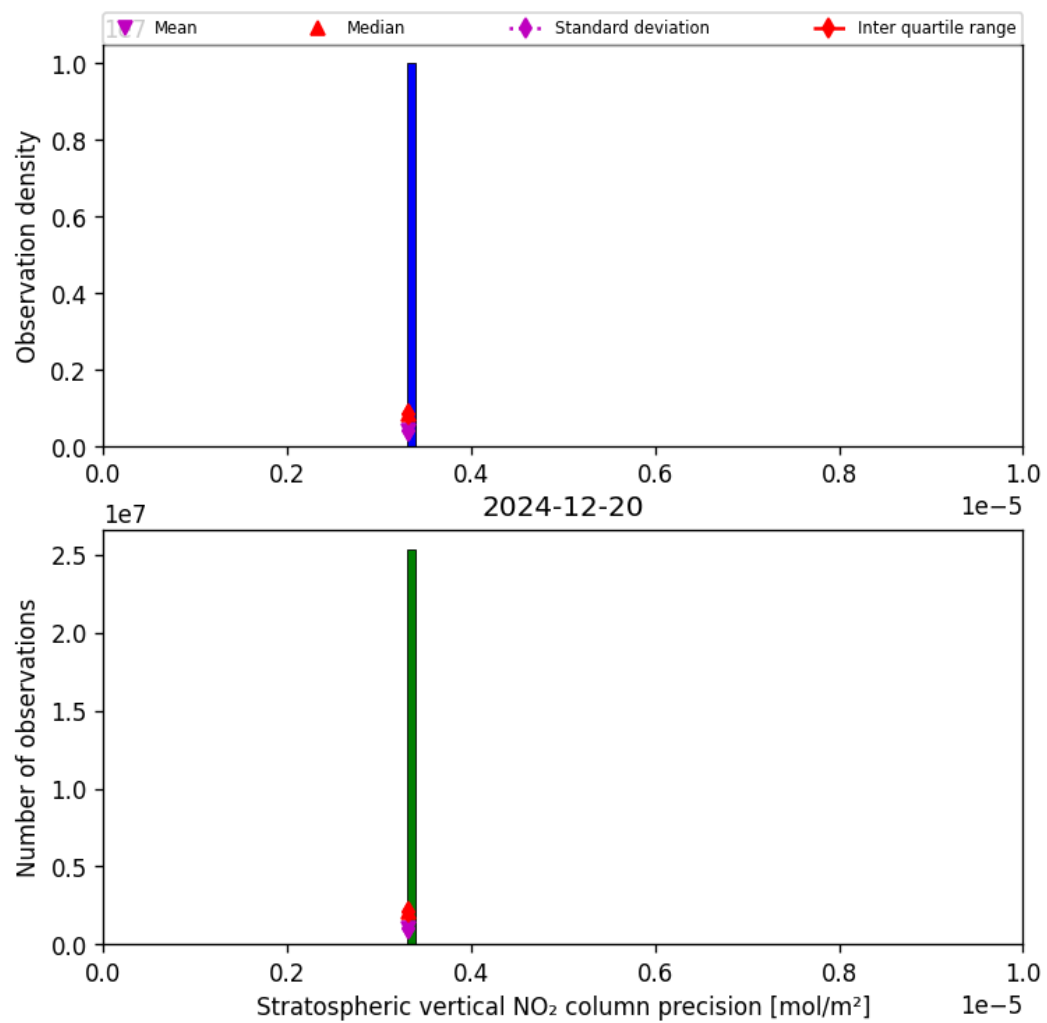
Figure 37: Histogram of “Stratospheric vertical NO 2 column precision” for 2024-12-19 to 2024-12-21
