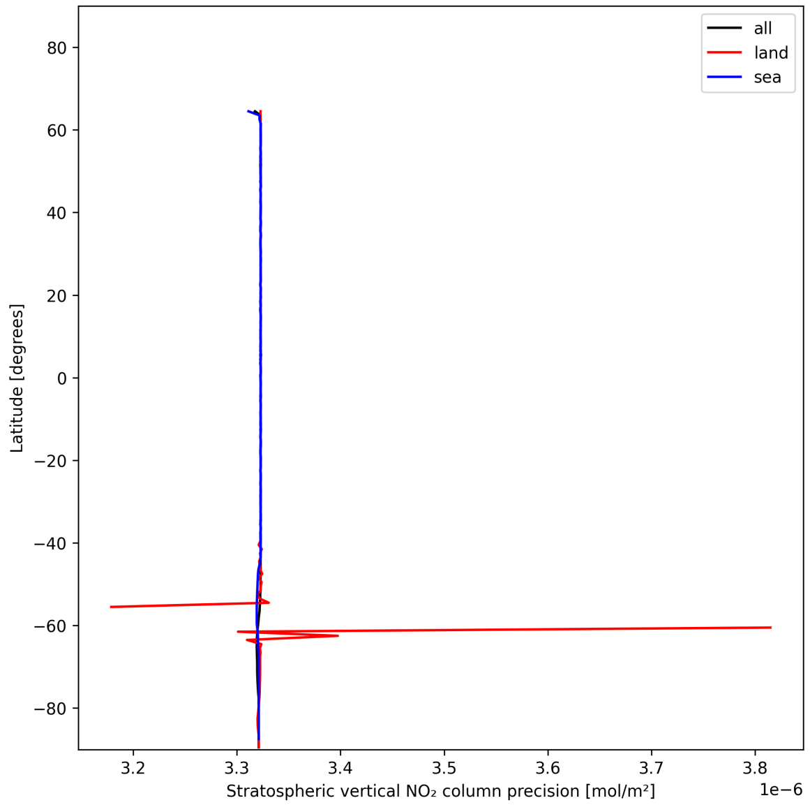
Figure 20: Zonal average of “Stratospheric vertical NO 2 column precision” for 2024-12-19 to 2024-12-21.
