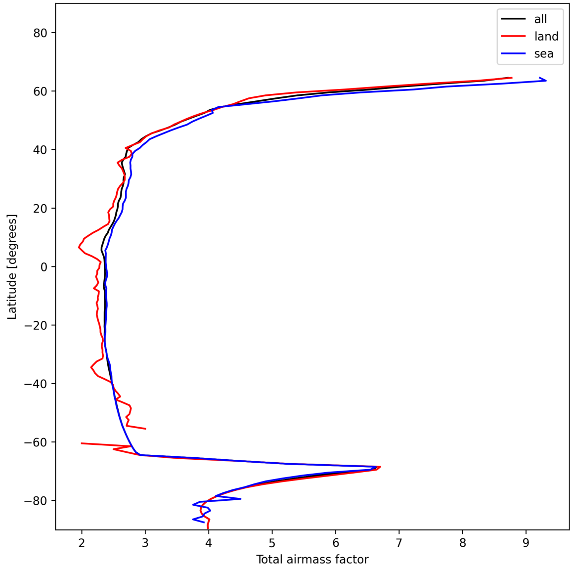
Figure 15: Zonal average of “Total airmass factor” for 2024-12-19 to 2024-12-21.
