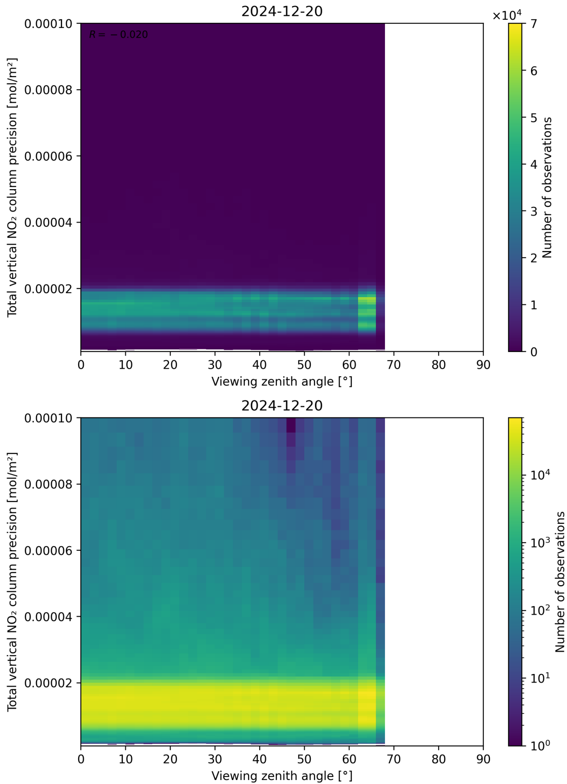
Figure 168: Scatter density plot of “Viewing zenith angle” against “Total vertical NO 2 column precision” for 2024-12-19 to 2024-12-21.
