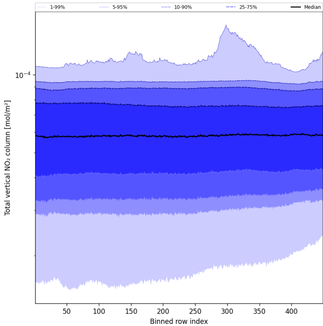
Figure 55: Along track statistics of “Total vertical NO 2 column” for 2024-12-19 to 2024-12-21
