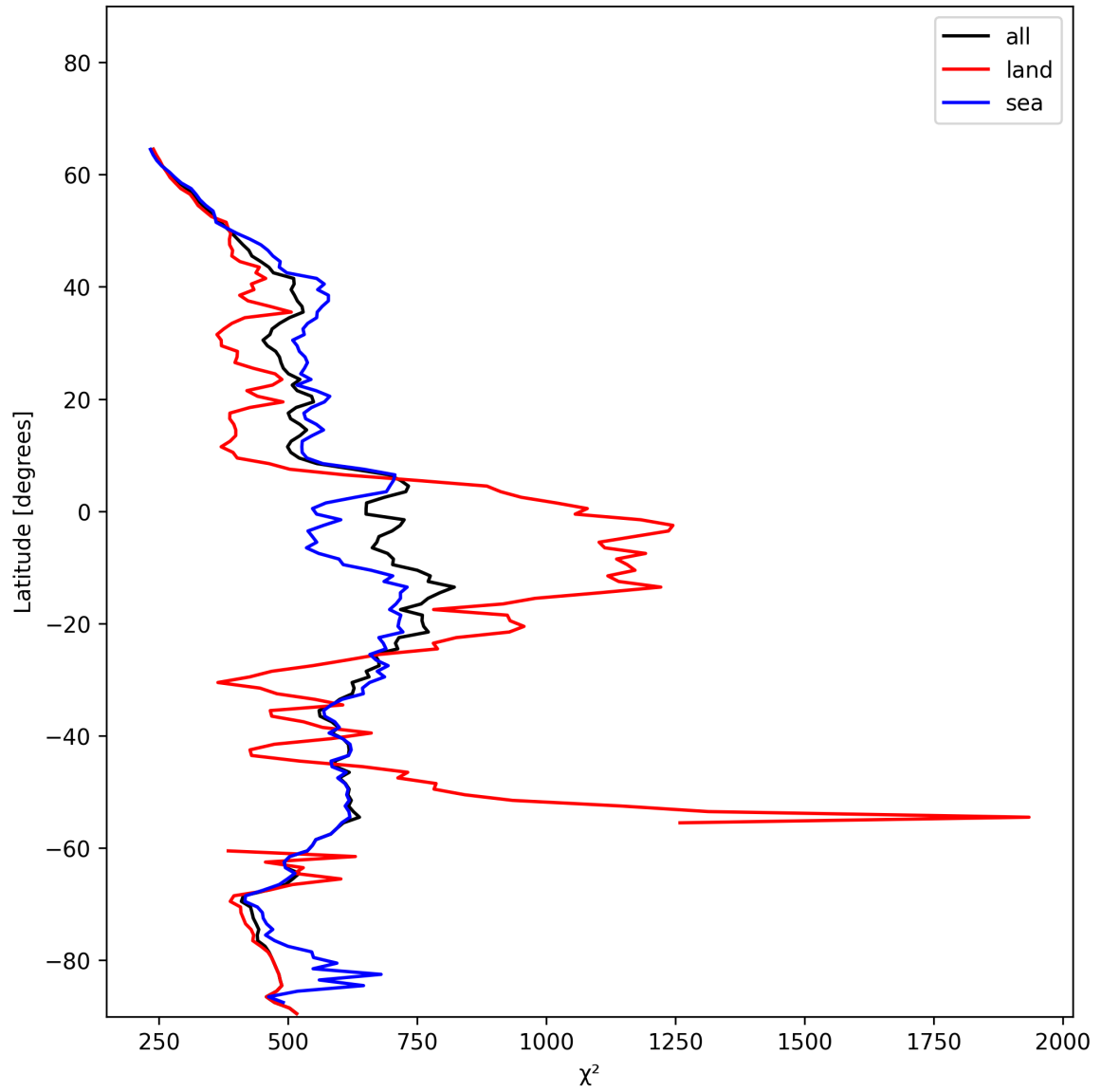
Figure 25: Zonal average of “ \chi^2 ” for 2024-12-19 to 2024-12-21.
