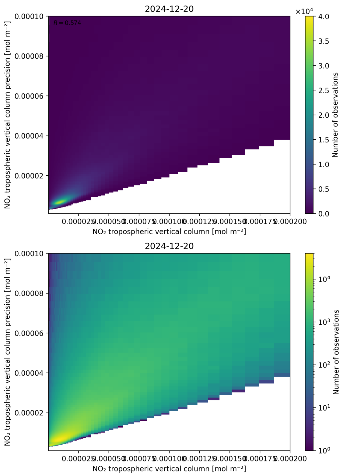
Figure 130: Scatter density plot of “NO 2 tropospheric vertical column” against “NO 2 tropospheric vertical column precision” for 2024-12-19 to 2024-12-21.
