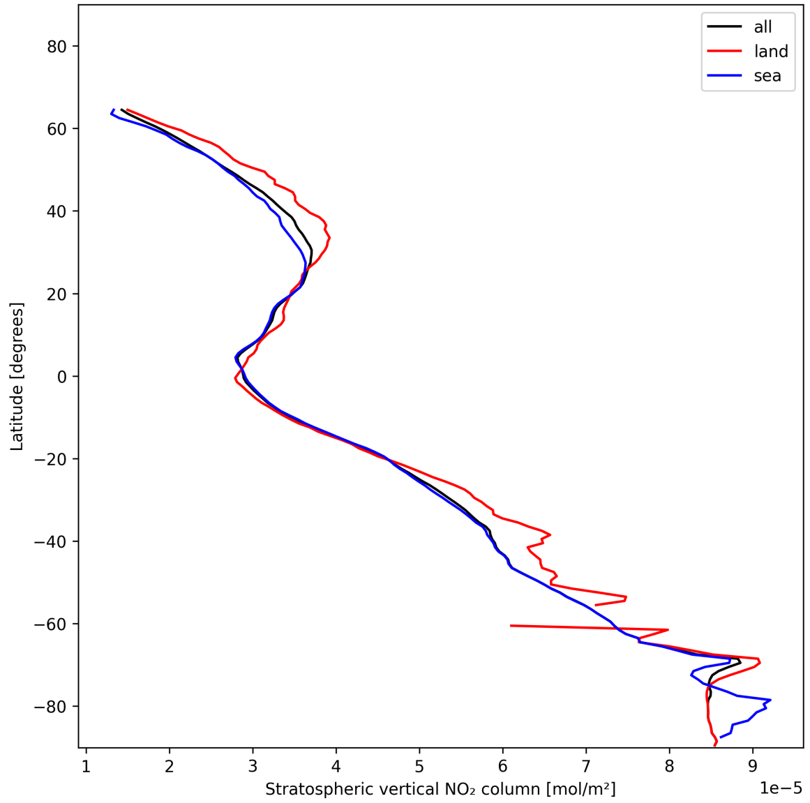
Figure 19: Zonal average of “Stratospheric vertical NO 2 column” for 2024-12-19 to 2024-12-21.
