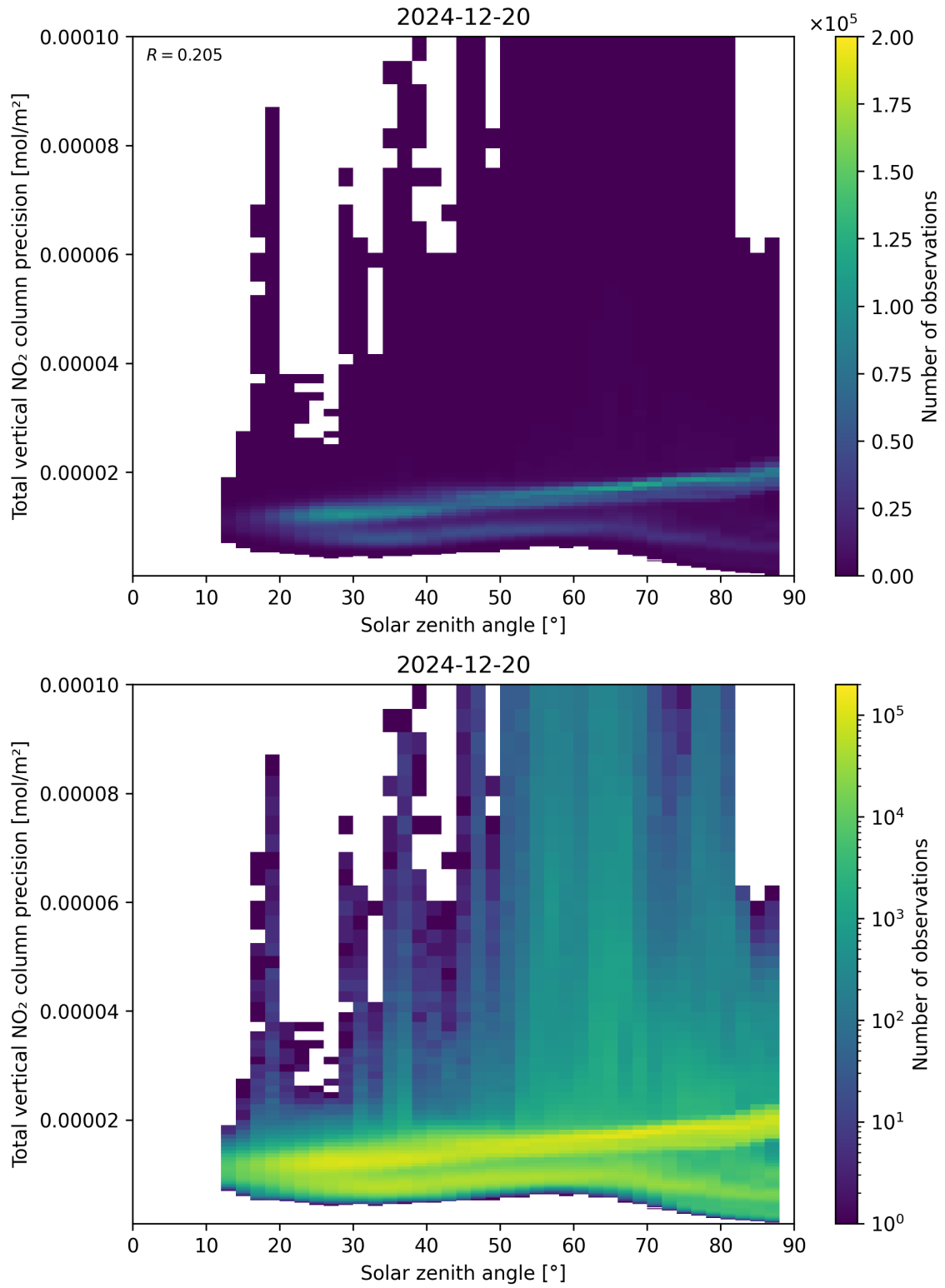
Figure 154: Scatter density plot of “Solar zenith angle” against “Total vertical NO 2 column precision” for 2024-12-19 to 2024-12-21.
