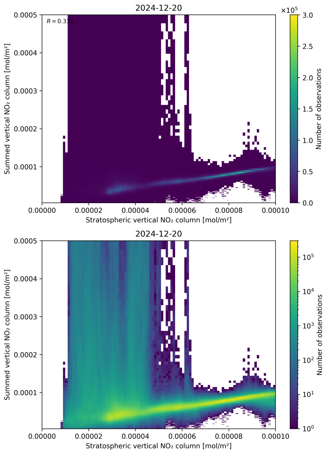
Figure 98: Scatter density plot of “Stratospheric vertical NO 2 column” against “Summed vertical NO 2 column” for 2024-12-19 to 2024-12-21.
