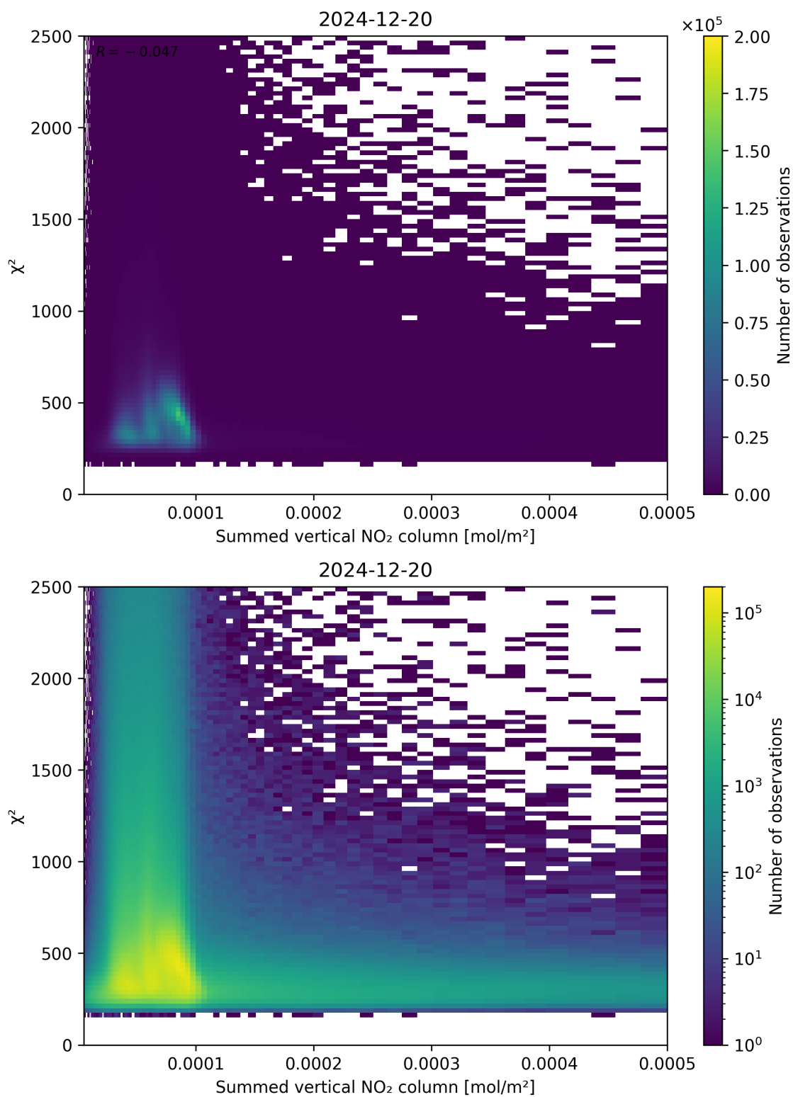
Figure 104: Scatter density plot of “Summed vertical NO 2 column” against “ \chi^2 ” for 2024-12-19 to 2024-12-21.
