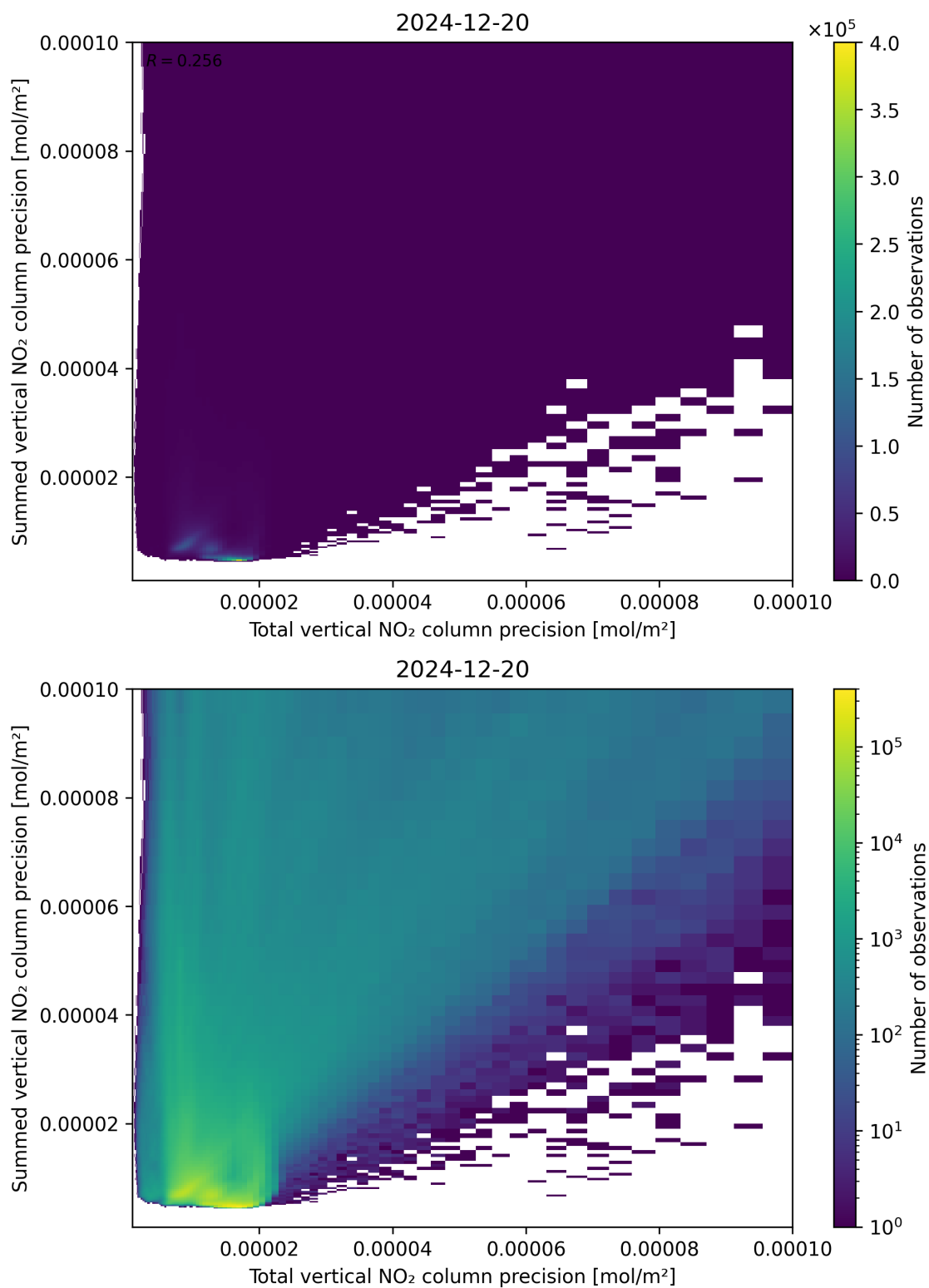
Figure 118: Scatter density plot of “Total vertical NO 2 column precision” against “Summed vertical NO 2 column precision” for 2024-12-19 to 2024-12-21.
