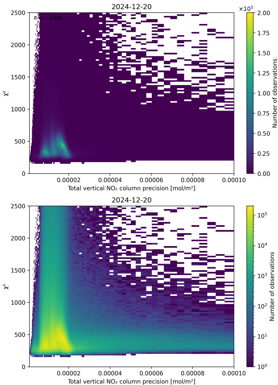
Figure 116: Scatter density plot of “Total vertical NO 2 column precision” against “ \chi^2 ” for 2024-12-19 to 2024-12-21.
