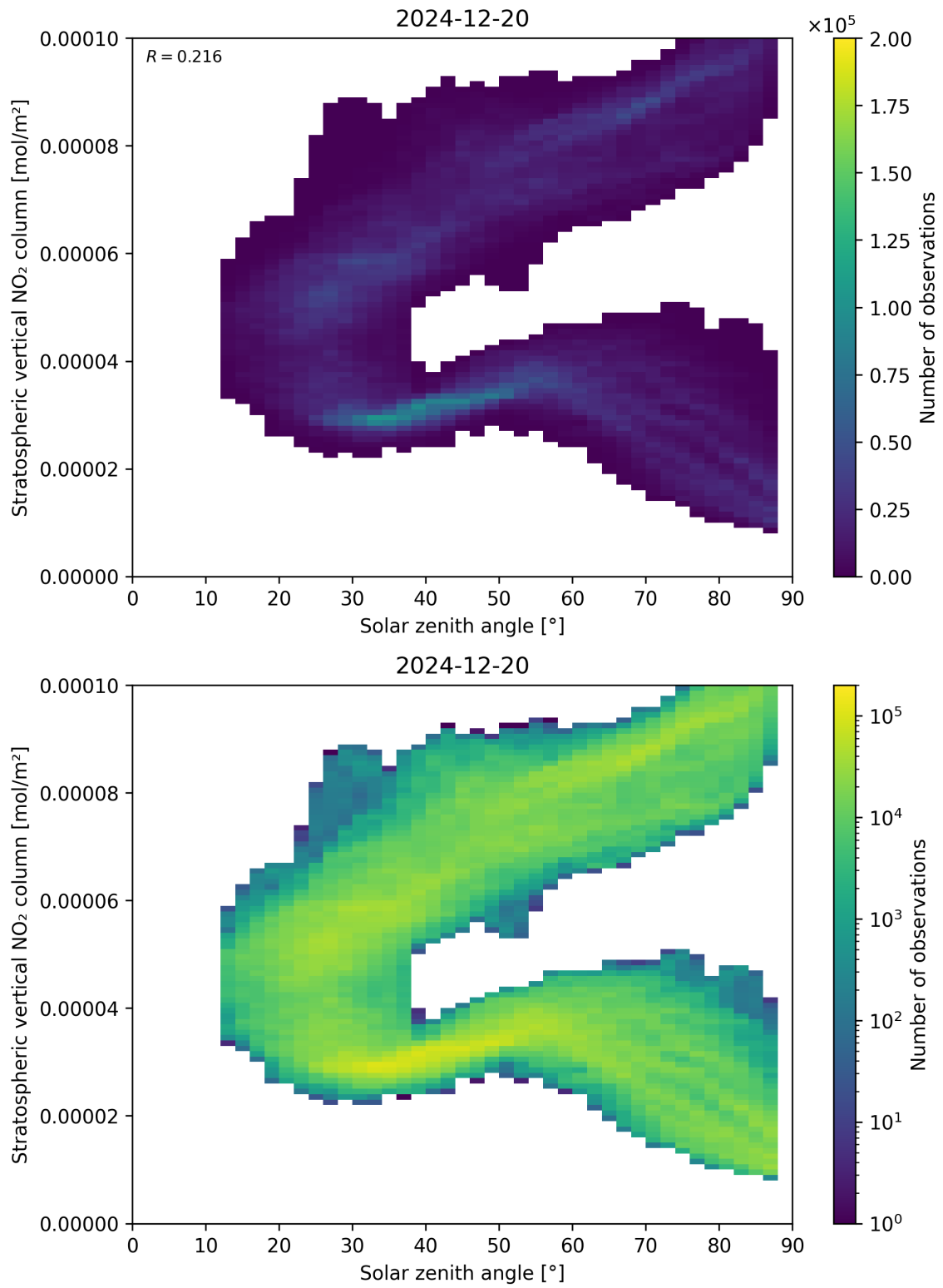
Figure 150: Scatter density plot of “Solar zenith angle” against “Stratospheric vertical NO 2 column” for 2024-12-19 to 2024-12-21.
