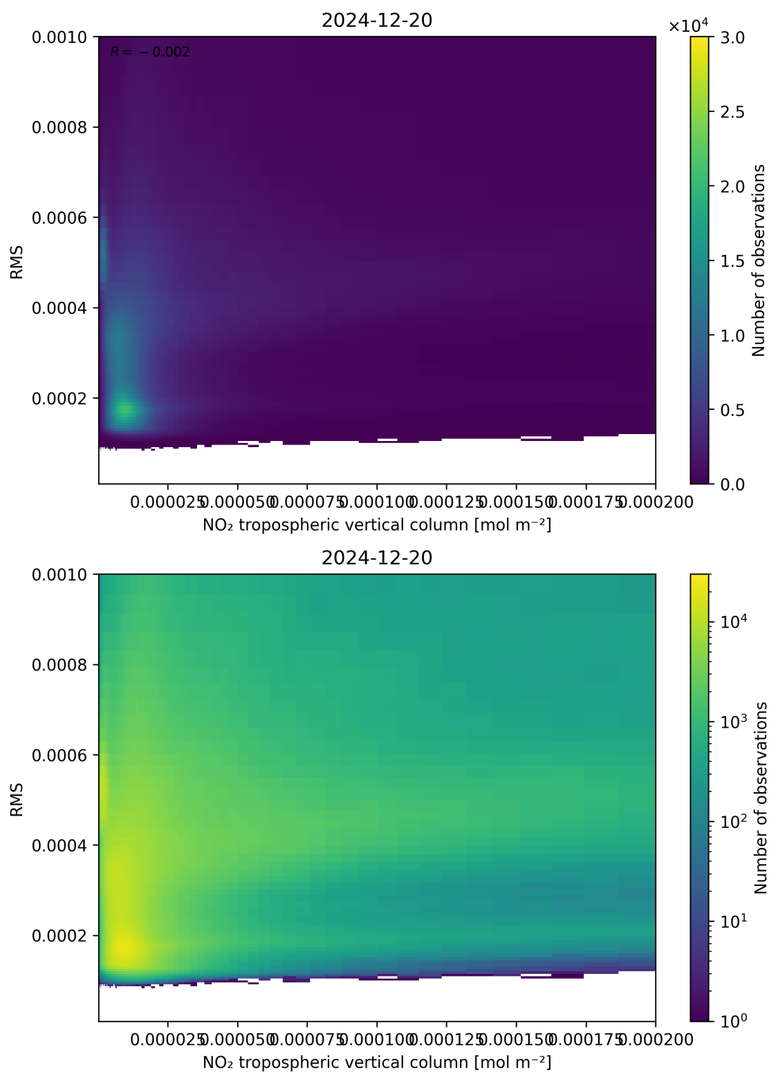
Figure 142: Scatter density plot of “NO 2 tropospheric vertical column” against “RMS” for 2024-12-19 to 2024-12-21.
