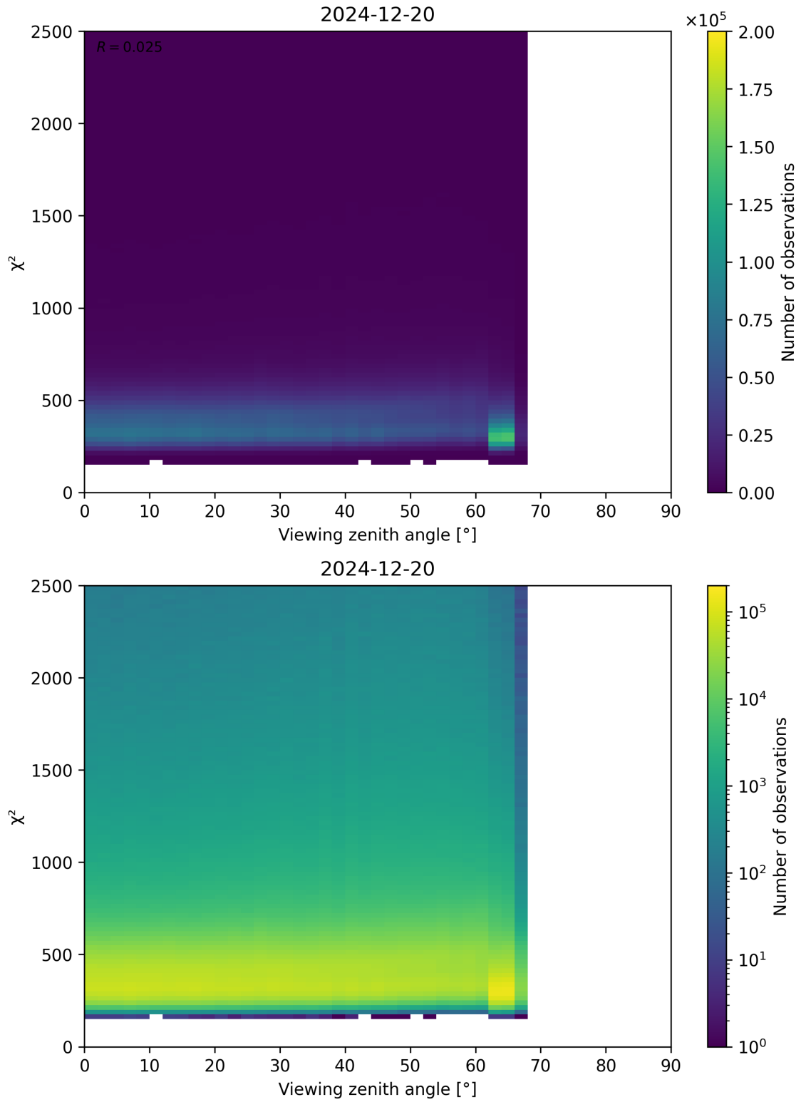
Figure 162: Scatter density plot of “Viewing zenith angle” against “ \chi^2 ” for 2024-12-19 to 2024-12-21.
