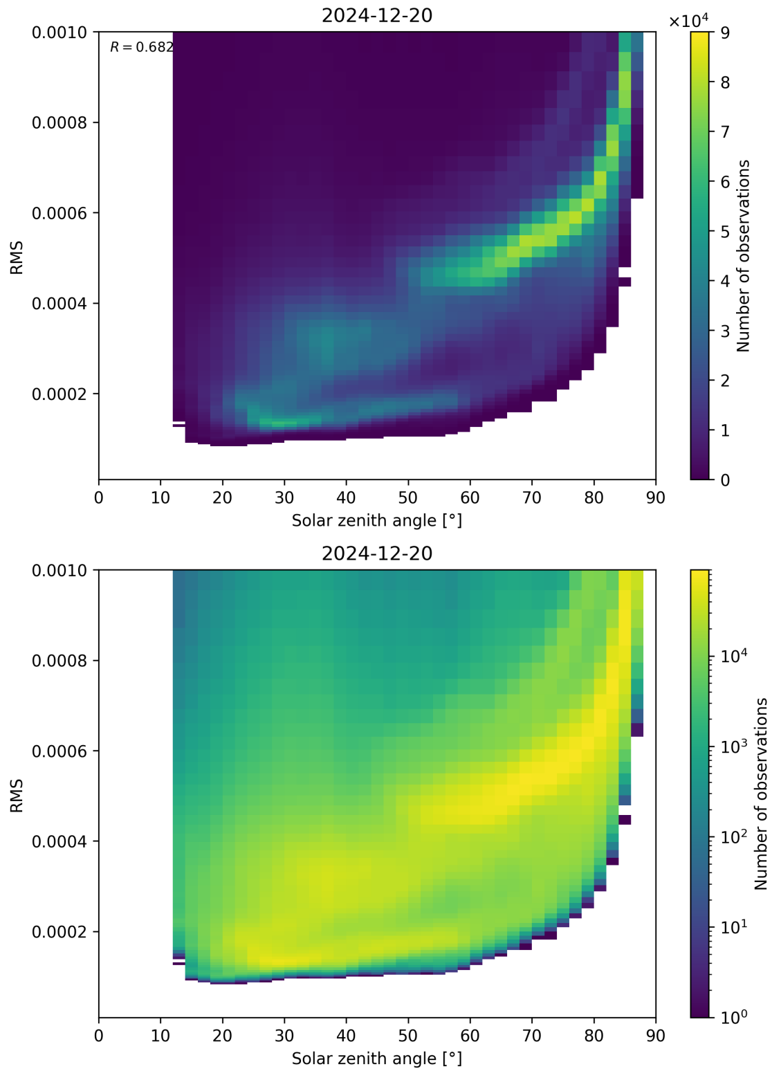
Figure 157: Scatter density plot of “Solar zenith angle” against “RMS” for 2024-12-19 to 2024-12-21.
