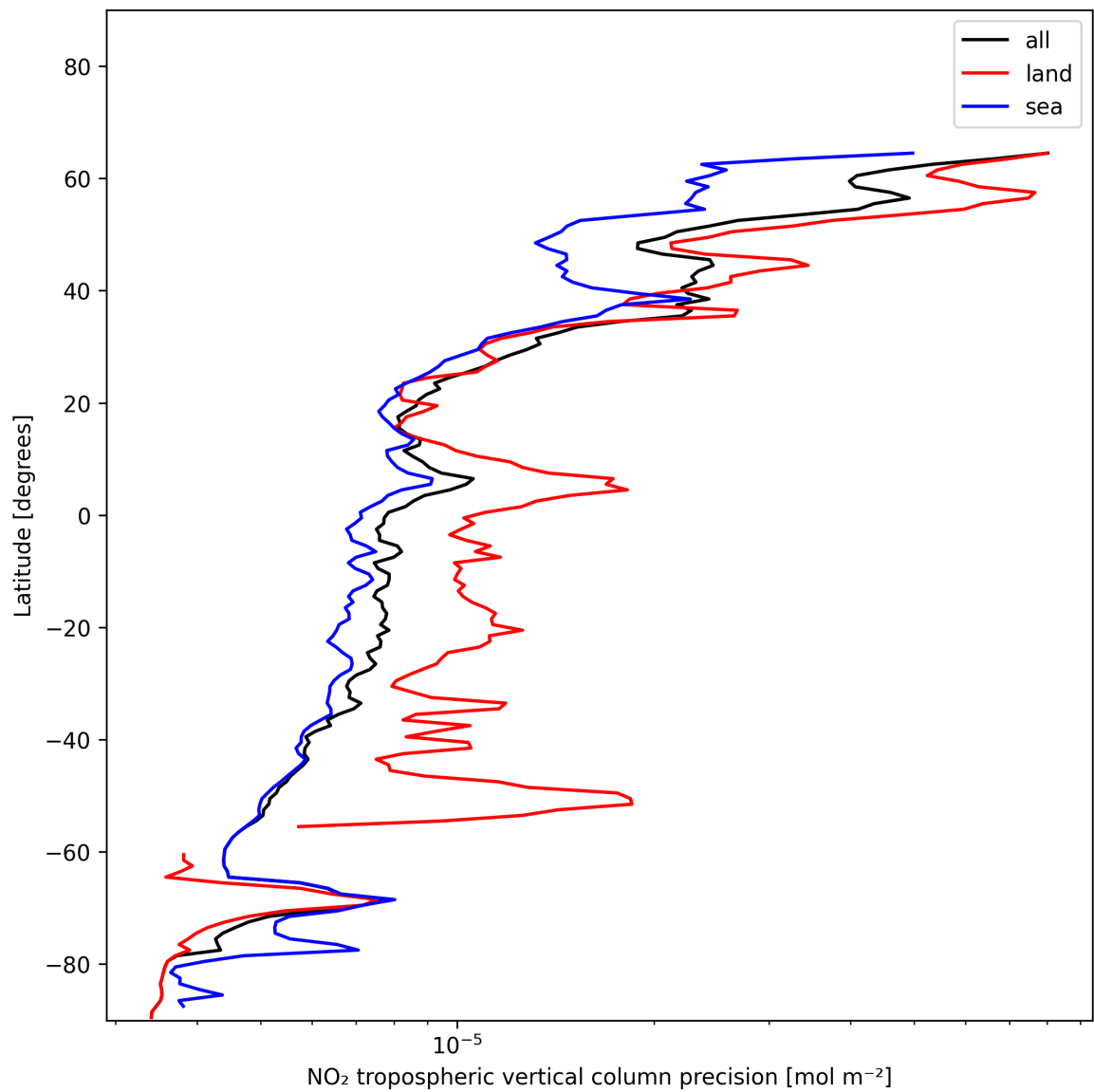
Figure 13: Zonal average of “NO 2 tropospheric vertical column precision” for 2024-12-19 to 2024-12-21.
