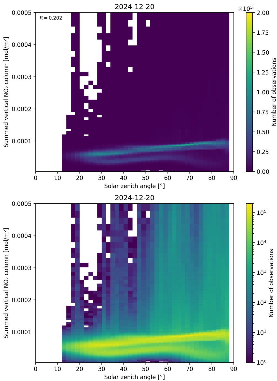
Figure 151: Scatter density plot of “Solar zenith angle” against “Summed vertical NO 2 column” for 2024-12-19 to 2024-12-21.
