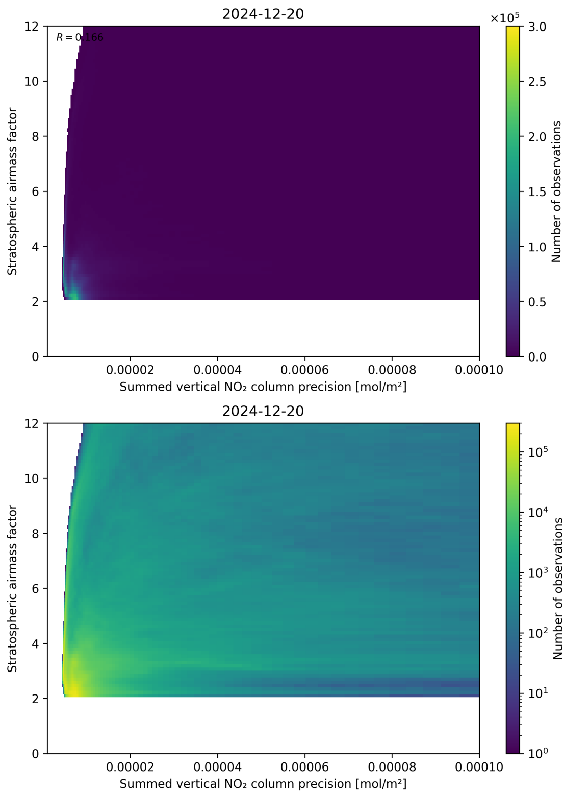
Figure 106: Scatter density plot of “Summed vertical NO 2 column precision” against “Stratospheric airmass factor” for 2024-12-19 to 2024-12-21.
