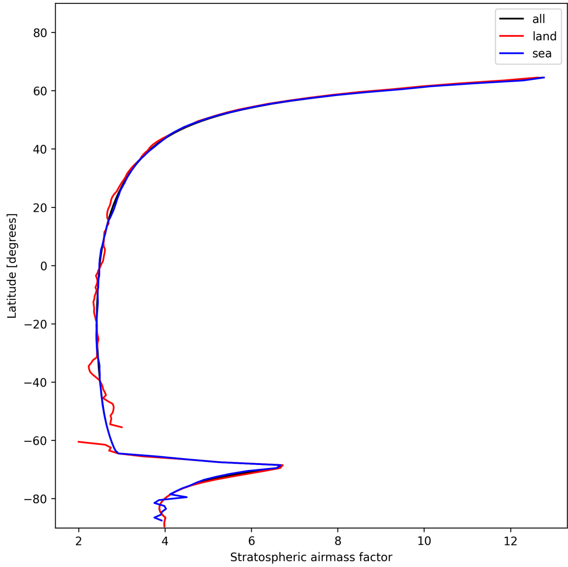
Figure 27: Zonal average of “Stratospheric airmass factor” for 2024-12-19 to 2024-12-21.
