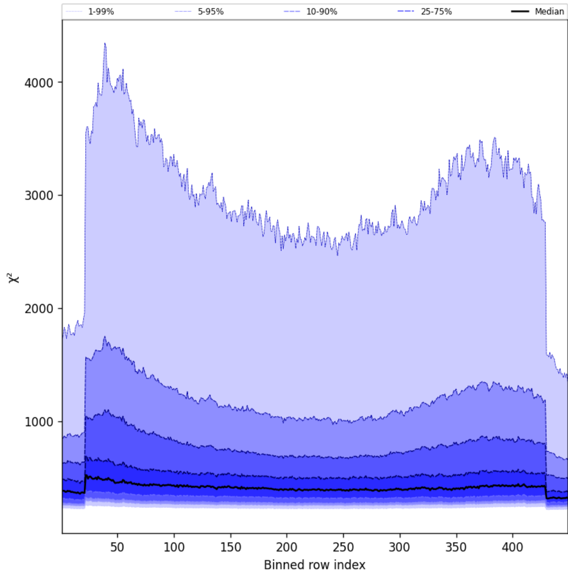
Figure 59: Along track statistics of “ \chi^2 ” for 2024-12-19 to 2024-12-21
