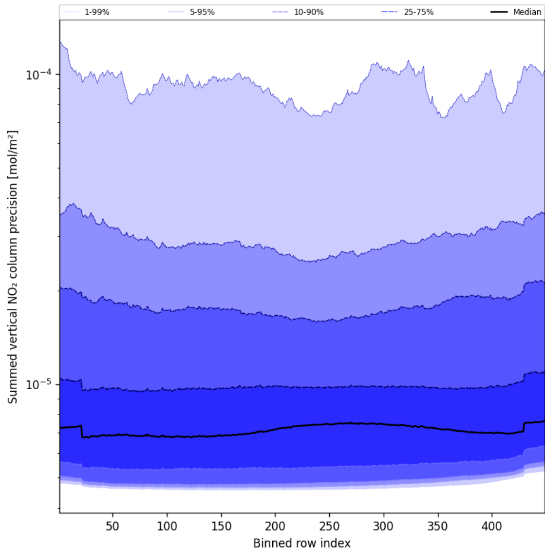
Figure 58: Along track statistics of “Summed vertical NO 2 column precision” for 2024-12-19 to 2024-12-21
