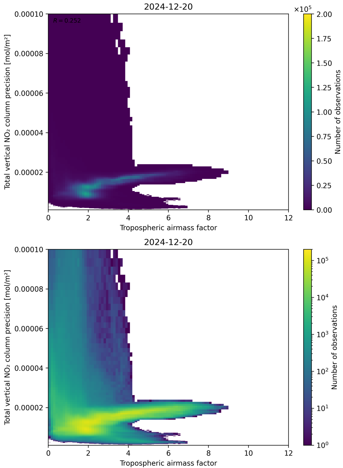
Figure 78: Scatter density plot of “Tropospheric air mass factor” against “Total vertical NO 2 column precision” for 2024-12-19 to 2024-12-21.
