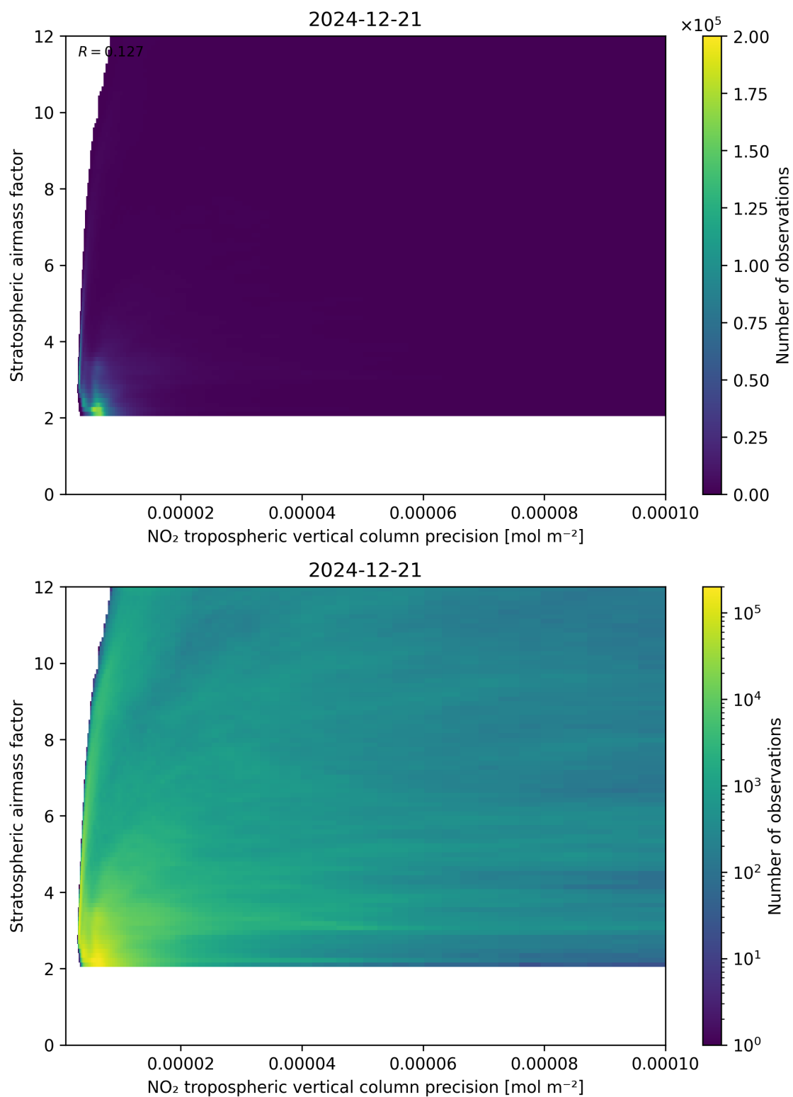
Figure 131: Scatter density plot of “NO 2 tropospheric vertical column precision” against “Stratospheric airmass factor” for 2024-12-20 to 2024-12-22.
