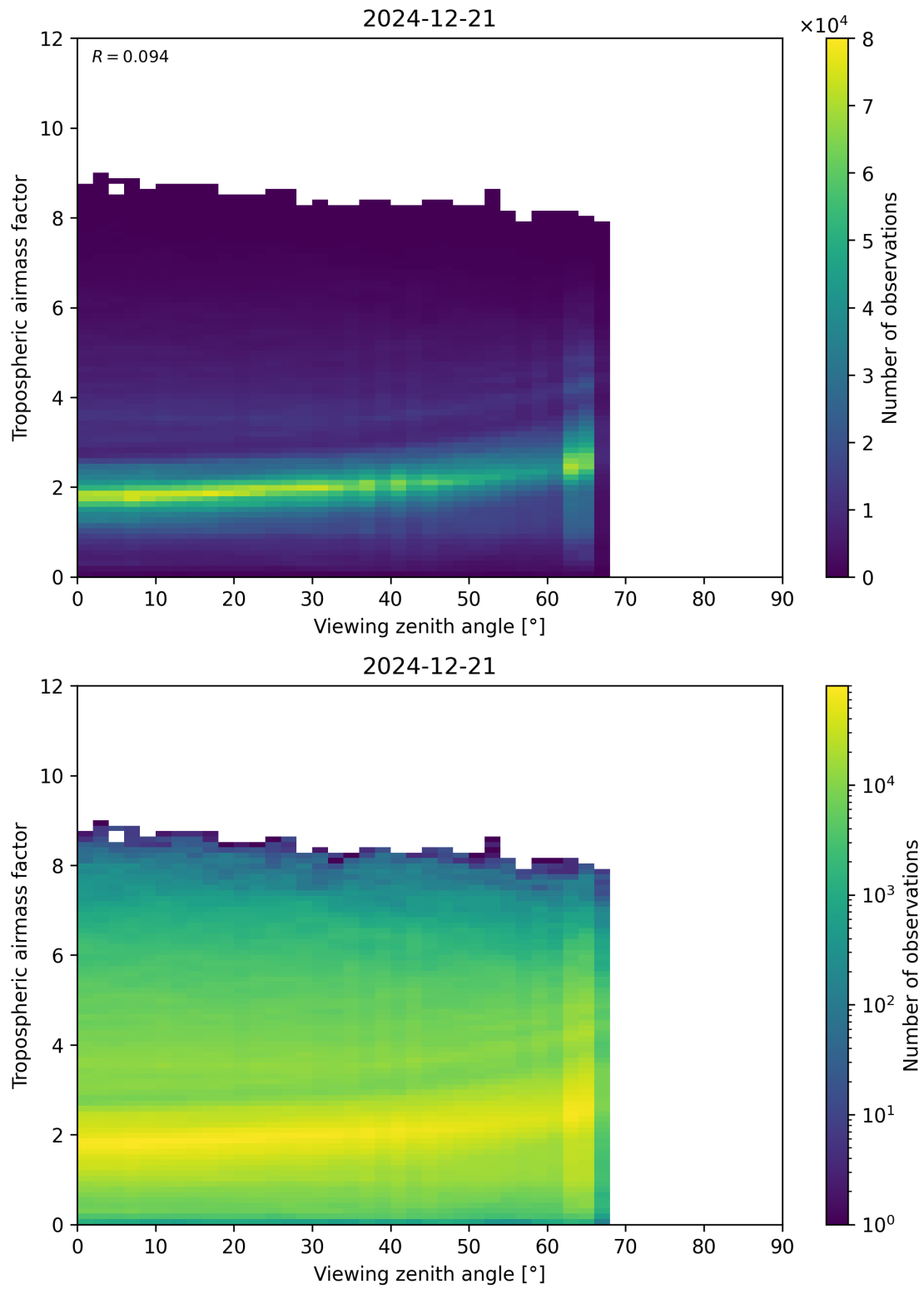
Figure 161: Scatter density plot of “Viewing zenith angle” against “Tropospheric airmass factor” for 2024-12-20 to 2024-12-22.
