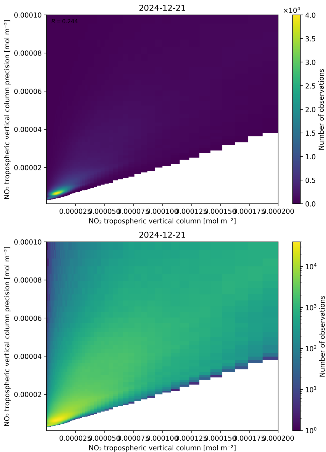
Figure 130: Scatter density plot of “NO 2 tropospheric vertical column” against “NO 2 tropospheric vertical column precision” for 2024-12-20 to 2024-12-22.
