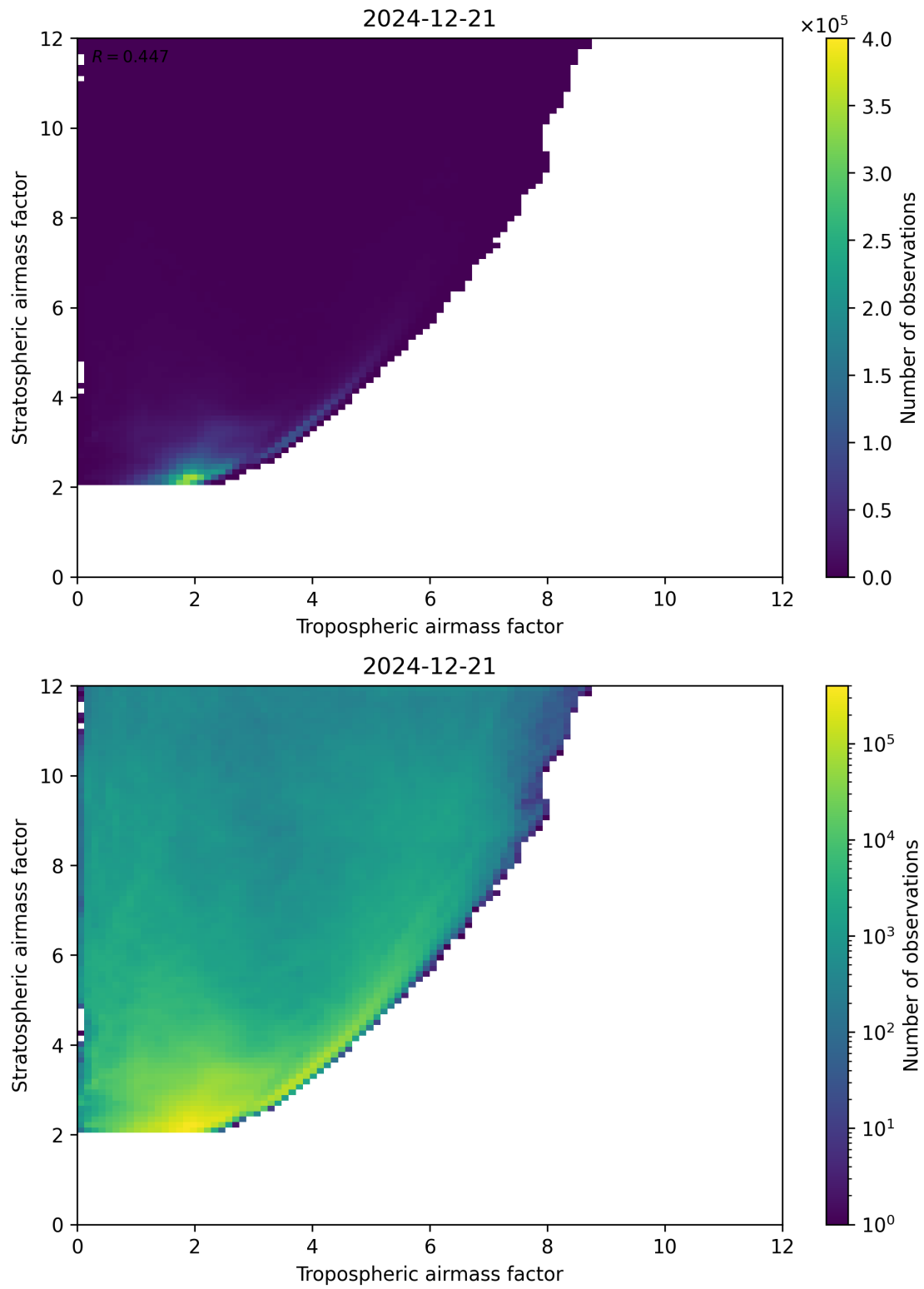
Figure 71: Scatter density plot of “Tropospheric airmass factor” against “Stratospheric airmass factor” for 2024-12-20 to 2024-12-22.
