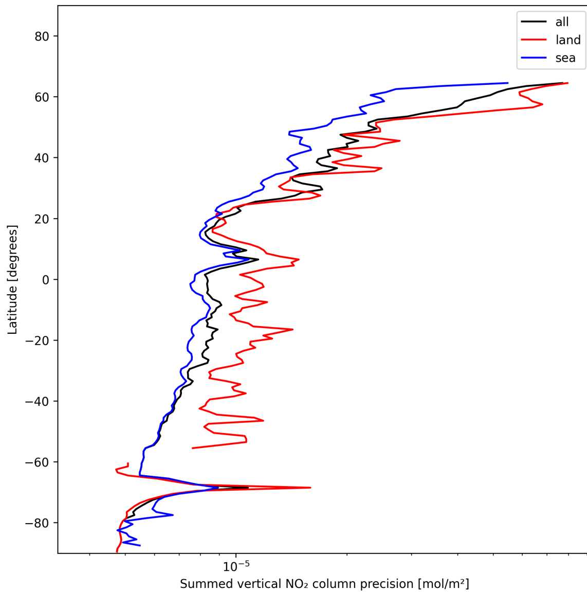
Figure 24: Zonal average of “Summed vertical NO 2 column precision” for 2024-12-20 to 2024-12-22.
