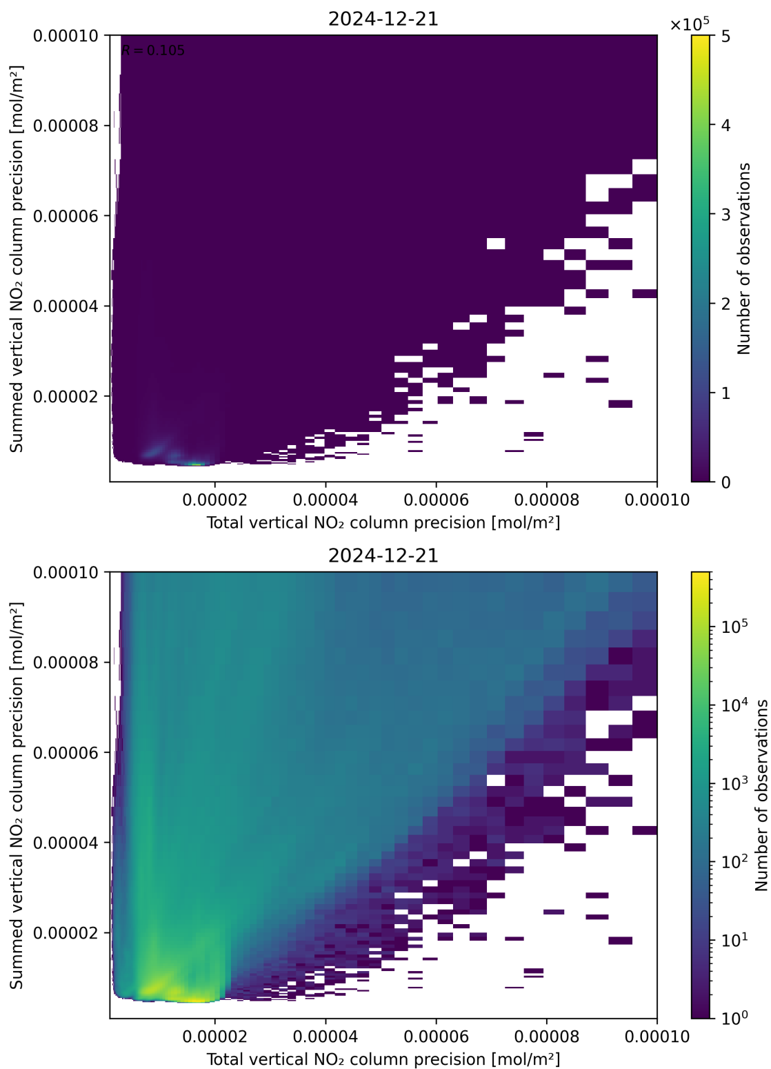
Figure 118: Scatter density plot of “Total vertical NO 2 column precision” against “Summed vertical NO 2 column precision” for 2024-12-20 to 2024-12-22.
