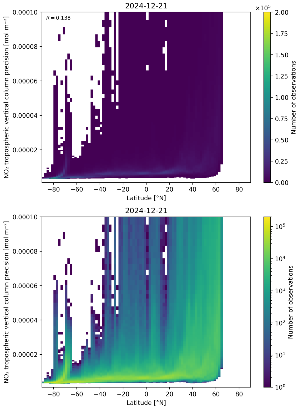
Figure 93: Scatter density plot of “Latitude” against “NO 2 tropospheric vertical column precision” for 2024-12-20 to 2024-12-22.
