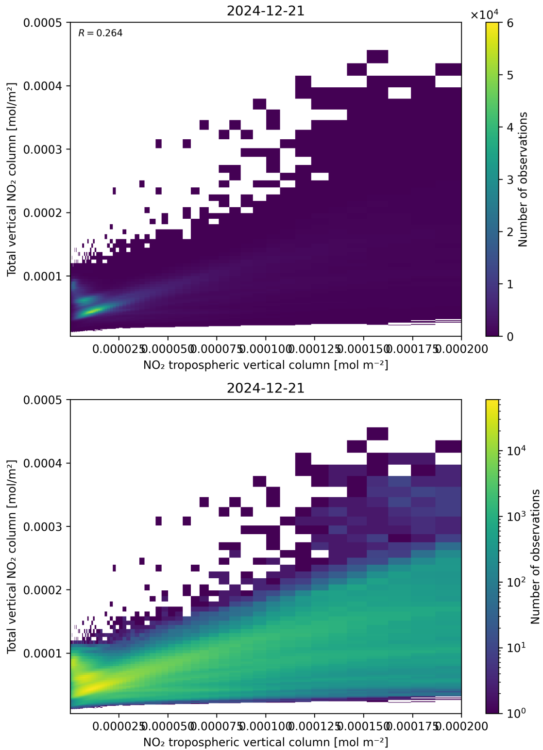
Figure 128: Scatter density plot of “NO 2 tropospheric vertical column” against “Total vertical NO 2 column” for 2024-12-20 to 2024-12-22.
