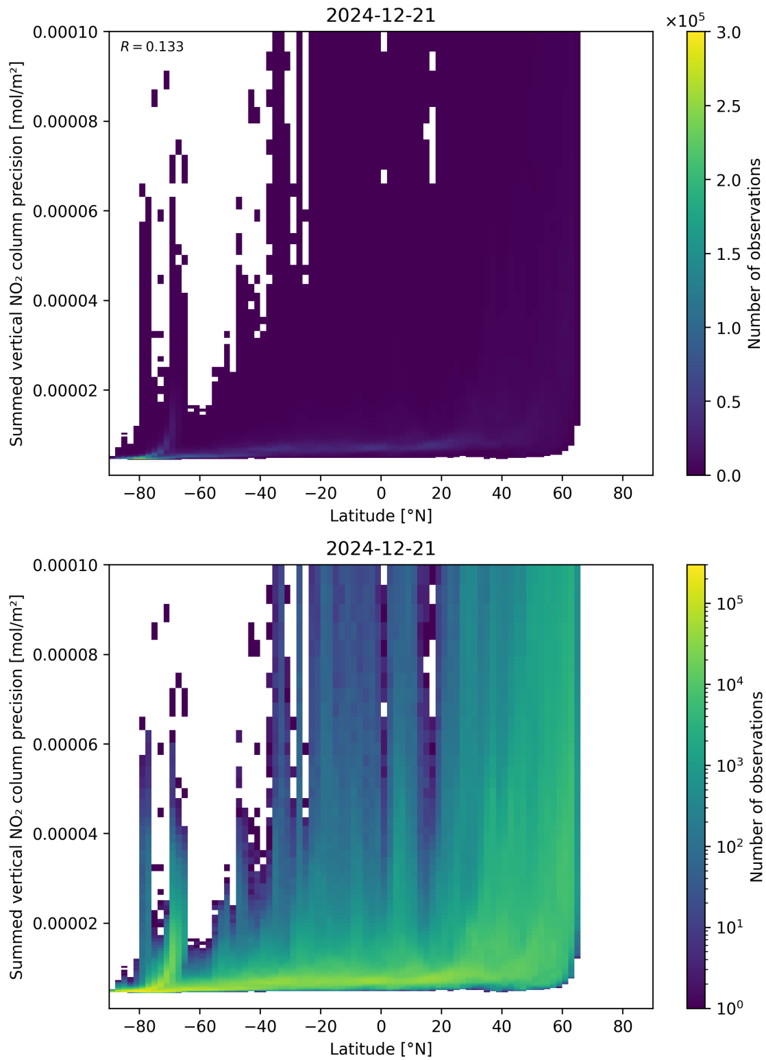
Figure 89: Scatter density plot of “Latitude” against “Summed vertical NO 2 column precision” for 2024-12-20 to 2024-12-22.
