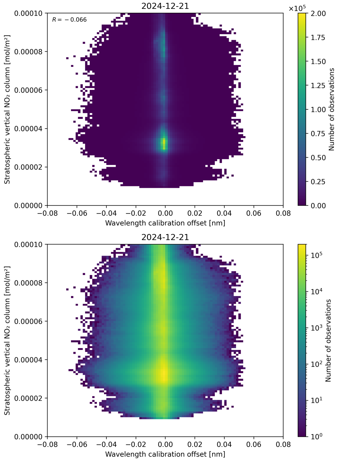
Figure 176: Scatter density plot of “Wavelength calibration offset” against “Stratospheric vertical NO 2 column” for 2024-12-20 to 2024-12-22.
