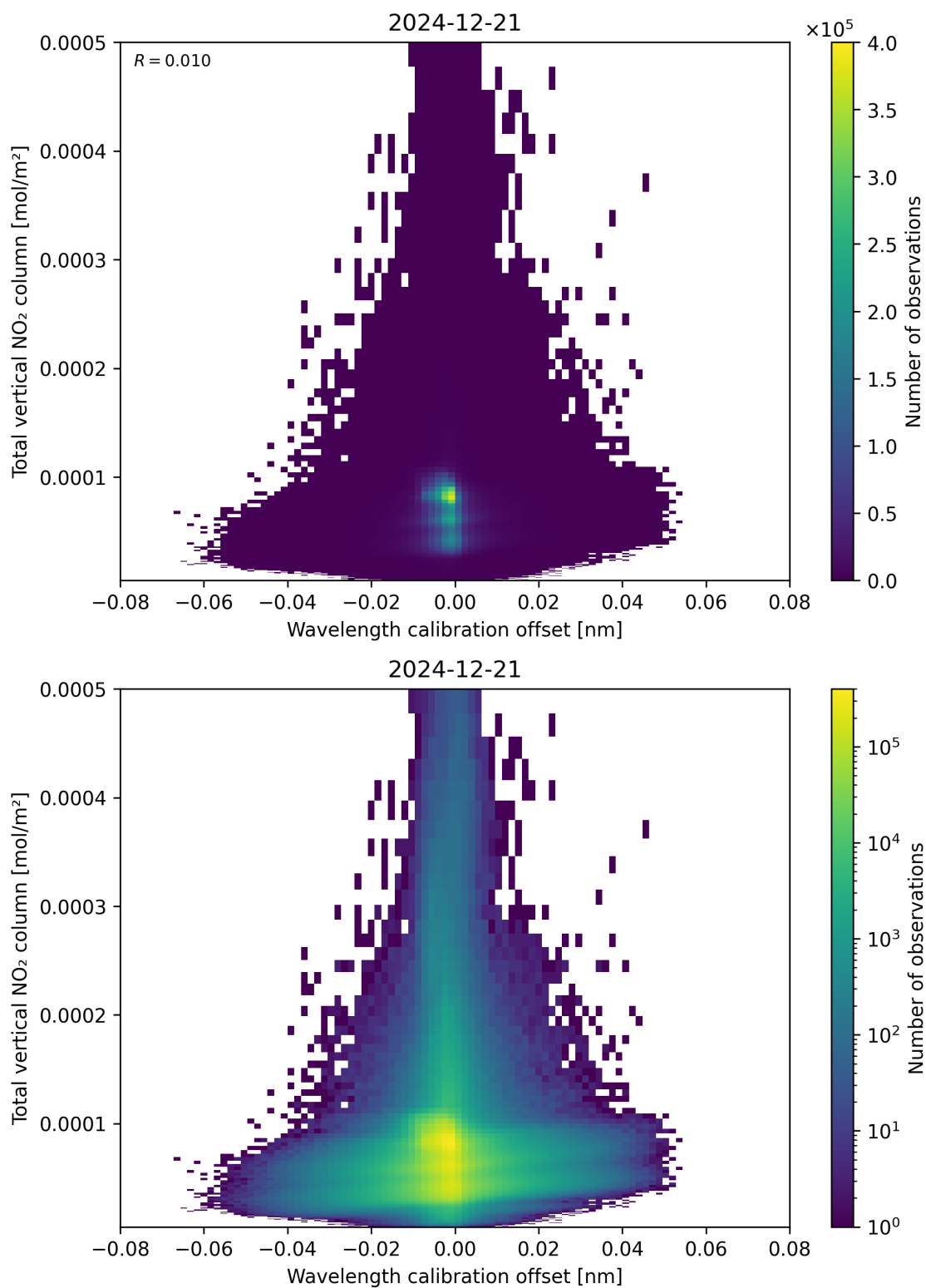
Figure 179: Scatter density plot of “Wavelength calibration offset” against “Total vertical NO 2 column” for 2024-12-20 to 2024-12-22.
