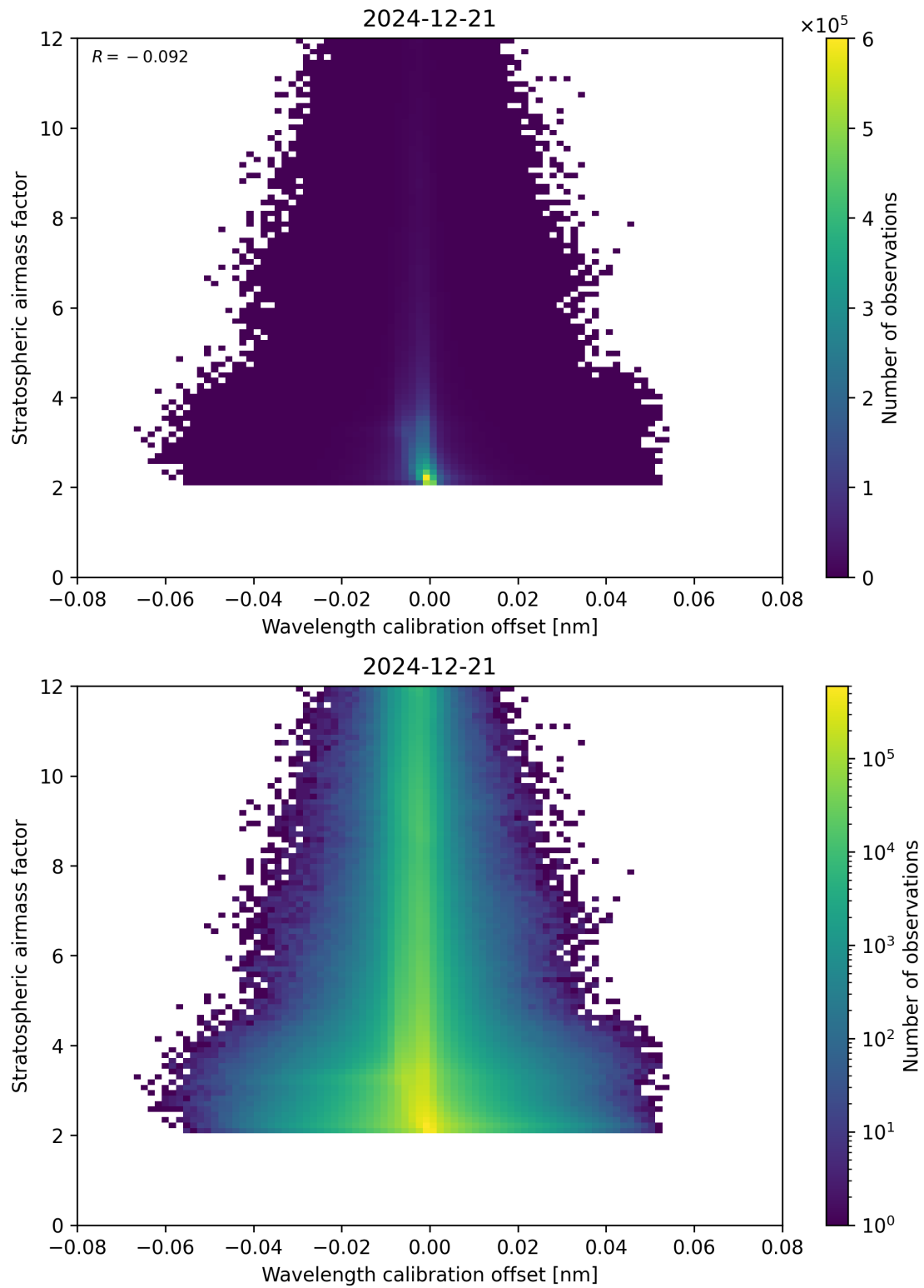
Figure 174: Scatter density plot of “Wavelength calibration offset” against “Stratospheric airmass factor” for 2024-12-20 to 2024-12-22.
