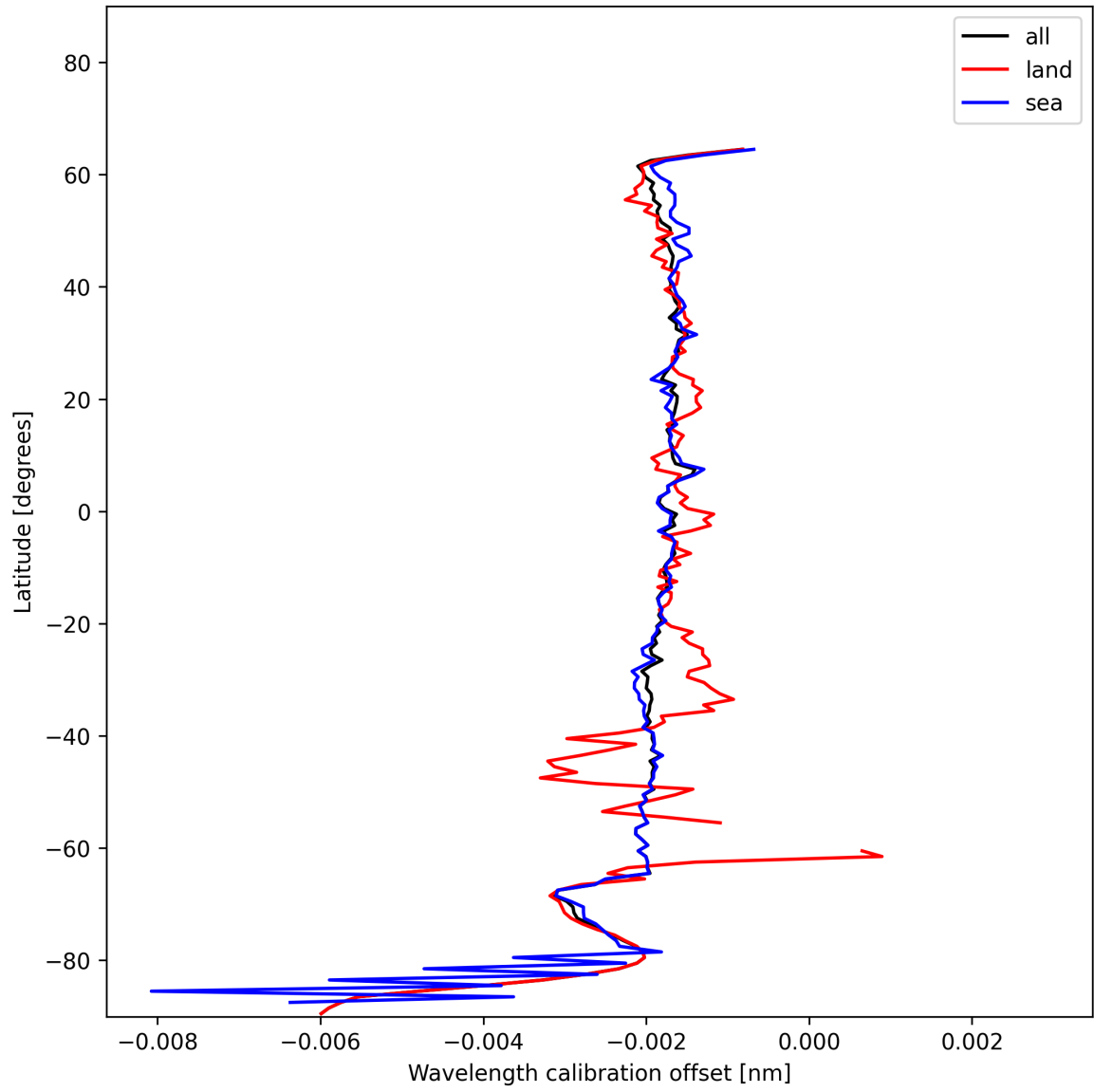
Figure 18: Zonal average of “Wavelength calibration offset” for 2024-12-20 to 2024-12-22.
