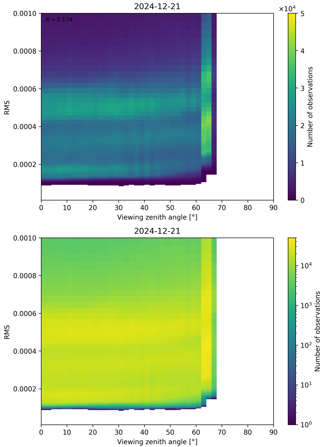
Figure 171: Scatter density plot of “Viewing zenith angle” against “RMS” for 2024-12-20 to 2024-12-22.
