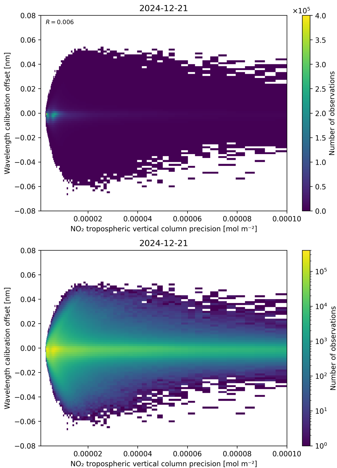
Figure 141: Scatter density plot of “NO 2 tropospheric vertical column precision” against “Wavelength calibration offset” for 2024-12-20 to 2024-12-22.
