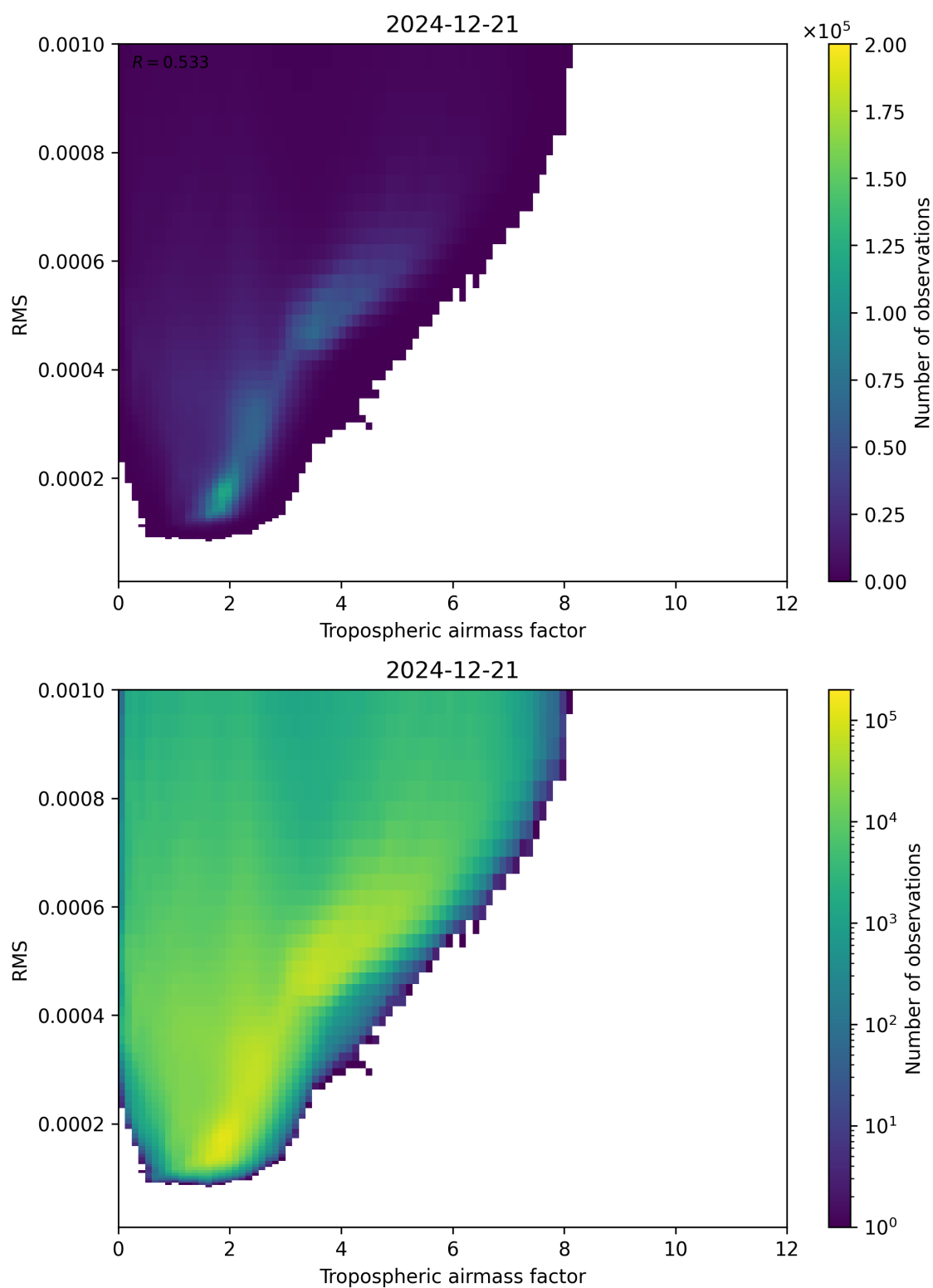
Figure 79: Scatter density plot of “Tropospheric airmass factor” against “RMS” for 2024-12-20 to 2024-12-22.
