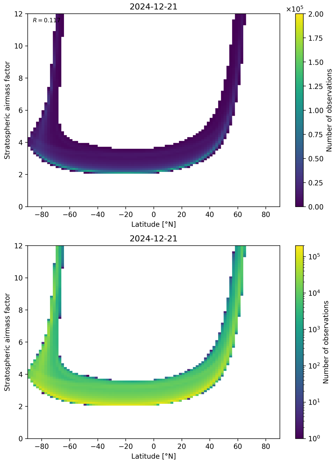
Figure 83: Scatter density plot of “Latitude” against “Stratospheric air mass factor” for 2024-12-20 to 2024-12-22.
