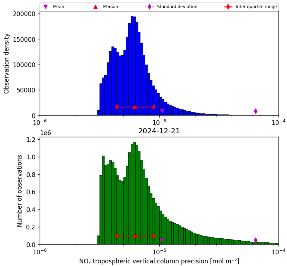
Figure 30: Histogram of “NO 2 tropospheric vertical column precision” for 2024-12-20 to 2024-12-22
