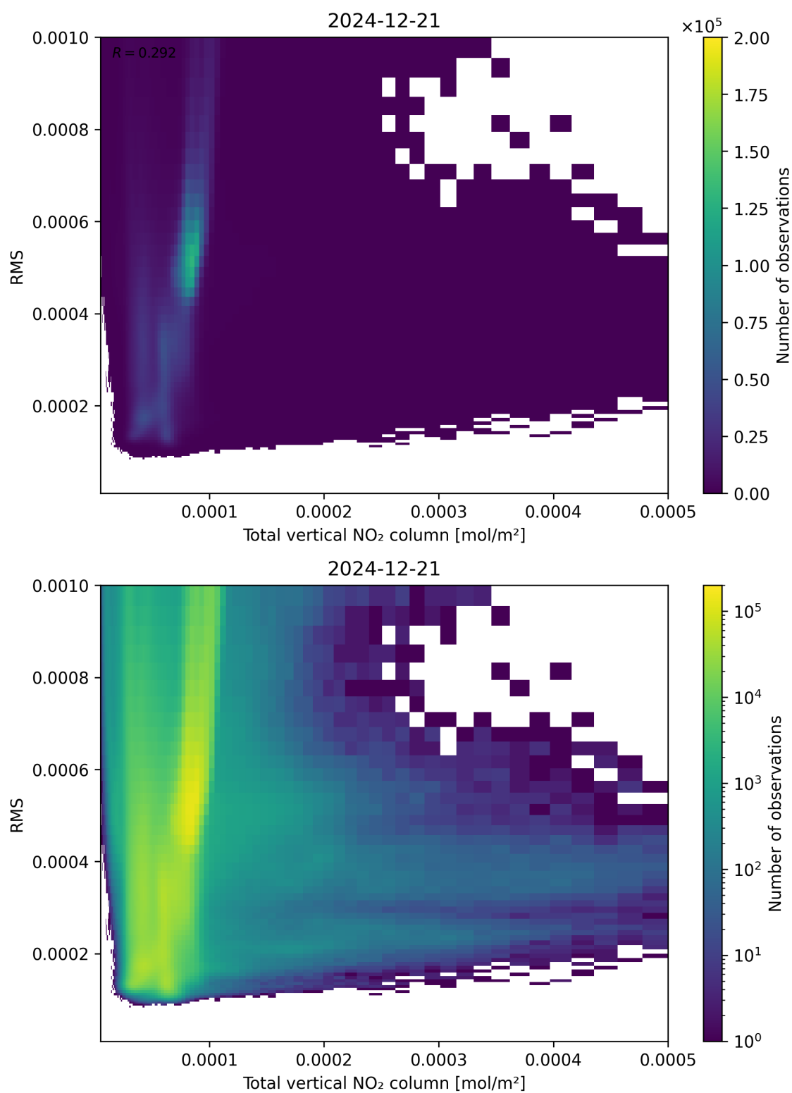
Figure 120: Scatter density plot of “Total vertical NO 2 column” against “RMS” for 2024-12-20 to 2024-12-22.
