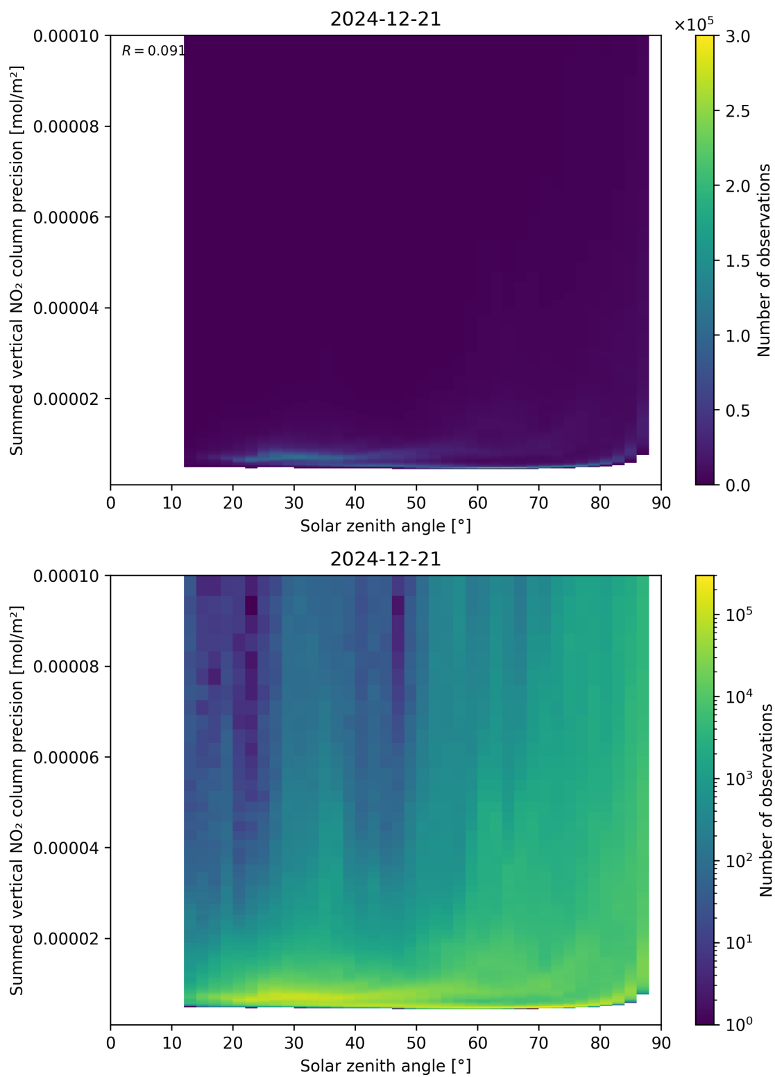
Figure 152: Scatter density plot of “Solar zenith angle” against “Summed vertical NO 2 column precision” for 2024-12-20 to 2024-12-22.
