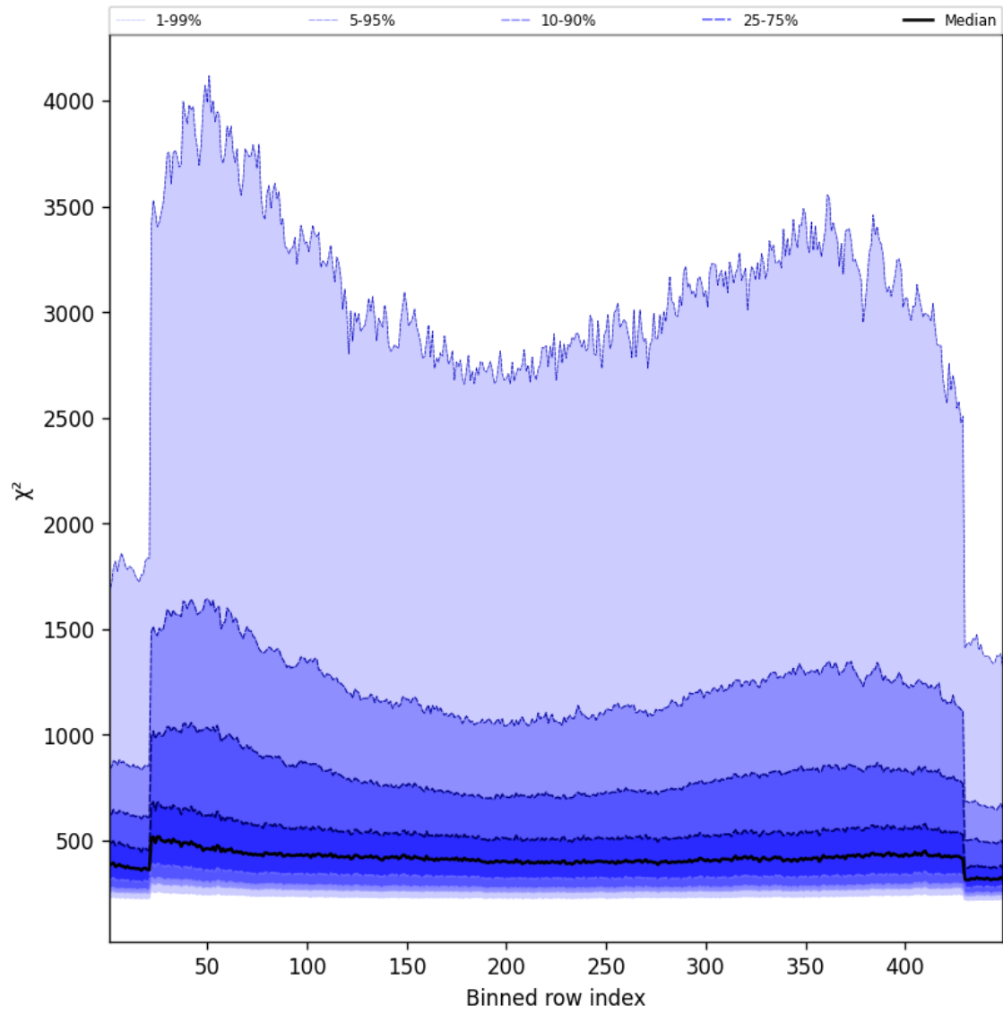
Figure 59: Along track statistics of “ \chi^2 ” for 2024-12-20 to 2024-12-22
