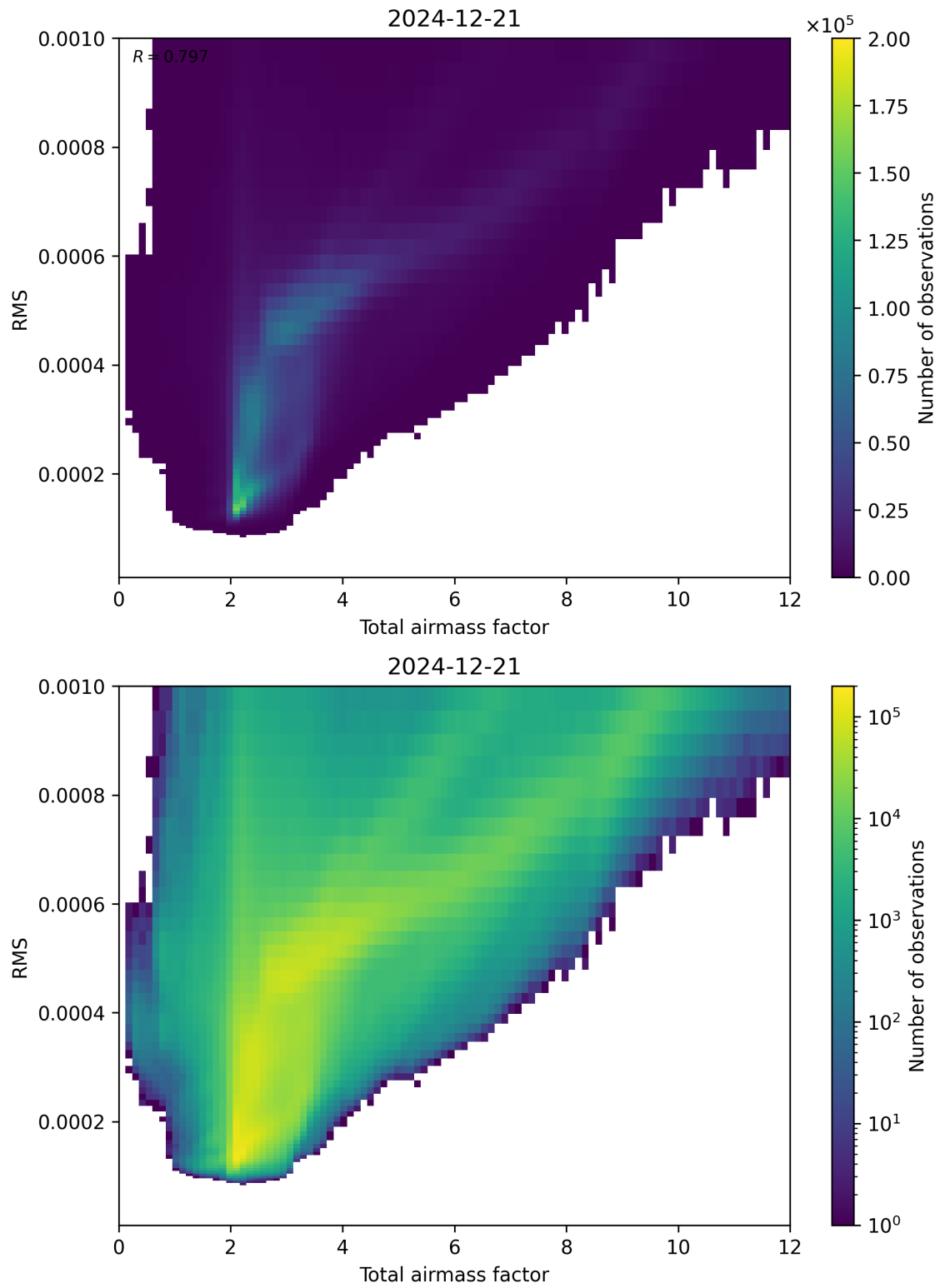
Figure 69: Scatter density plot of “Total airmass factor” against “RMS” for 2024-12-20 to 2024-12-22.
