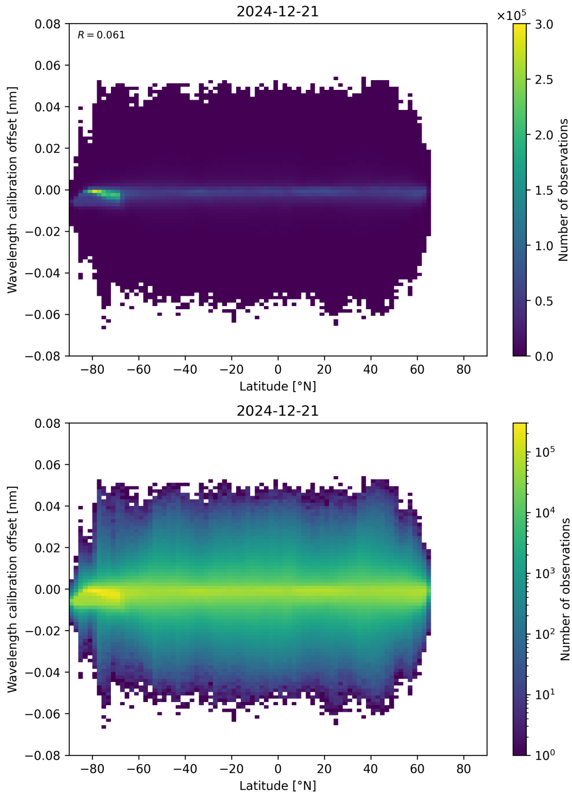
Figure 95: Scatter density plot of “Latitude” against “Wavelength calibration offset” for 2024-12-20 to 2024-12-22.
