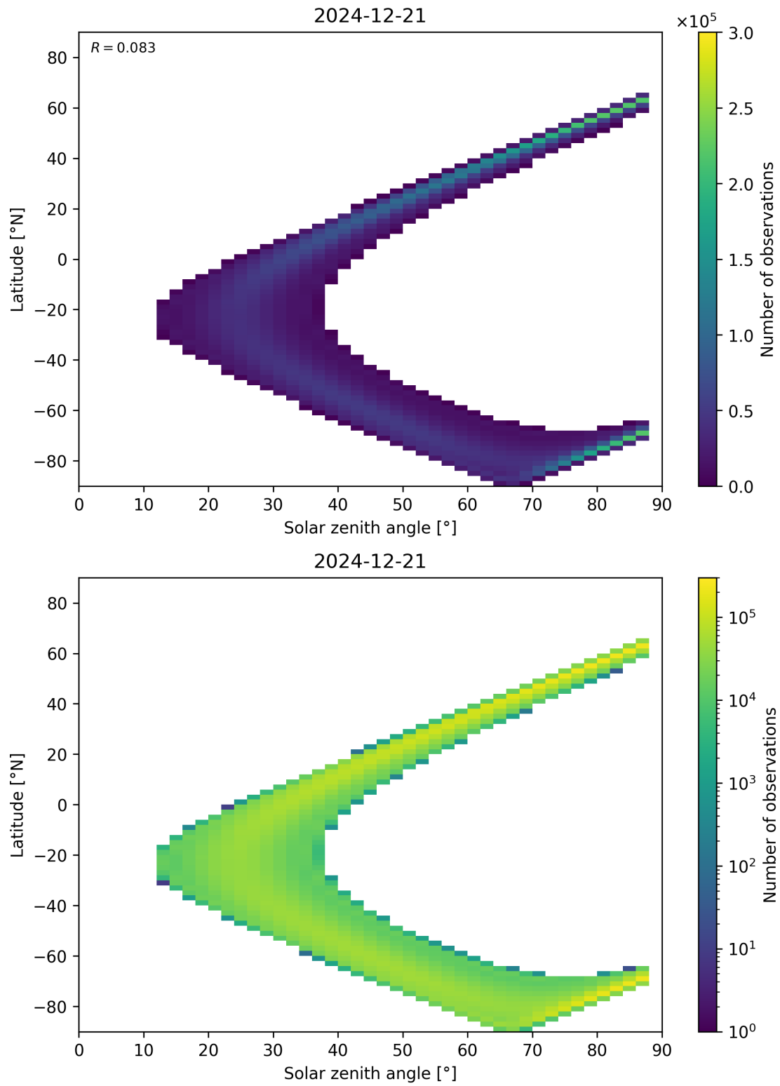
Figure 149: Scatter density plot of “Solar zenith angle” against “Latitude” for 2024-12-20 to 2024-12-22.
