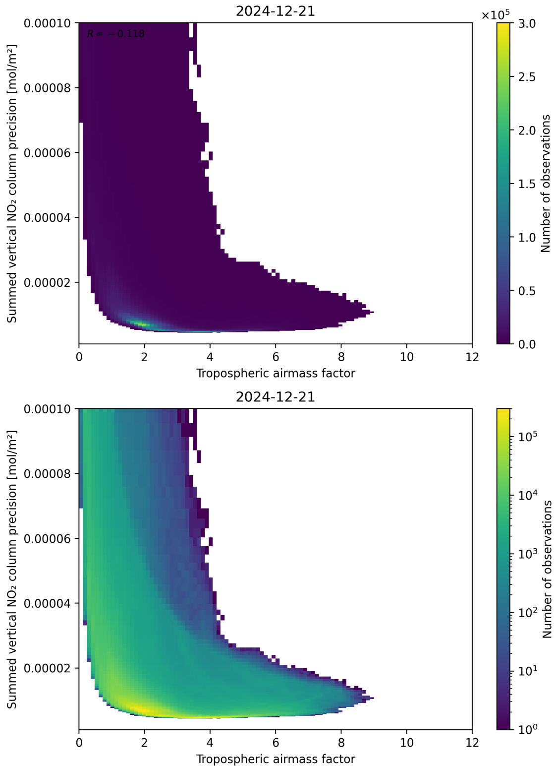
Figure 76: Scatter density plot of “Tropospheric air mass factor” against “Summed vertical NO 2 column precision” for 2024-12-20 to 2024-12-22.
