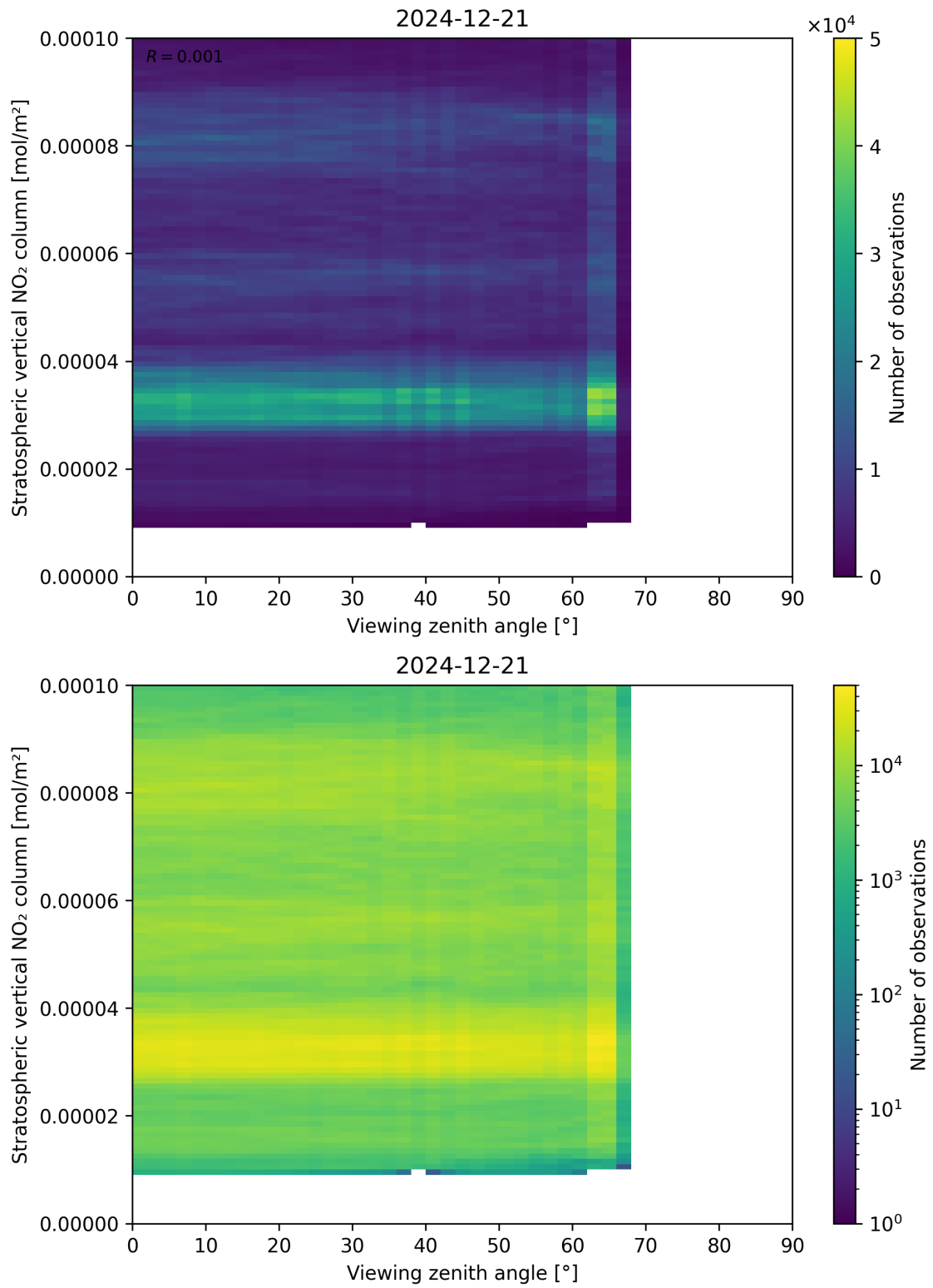
Figure 164: Scatter density plot of “Viewing zenith angle” against “Stratospheric vertical NO 2 column” for 2024-12-20 to 2024-12-22.
