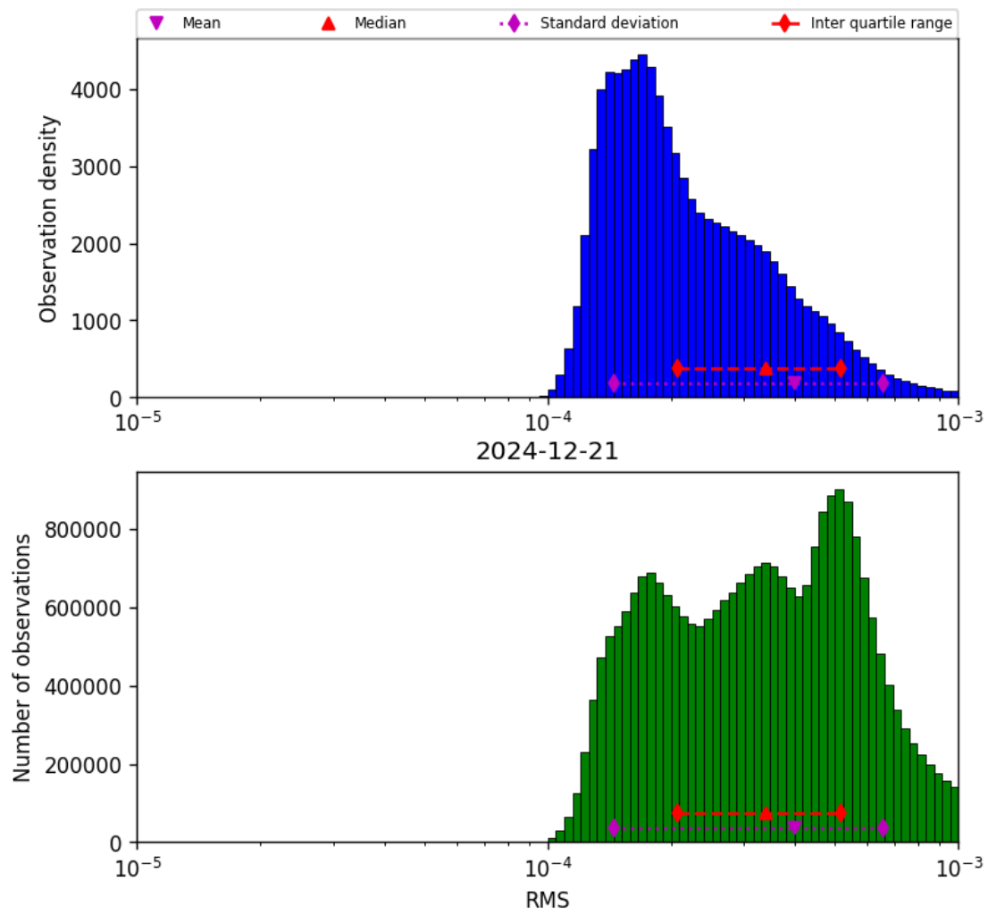
Figure 43: Histogram of “RMS” for 2024-12-20 to 2024-12-22
