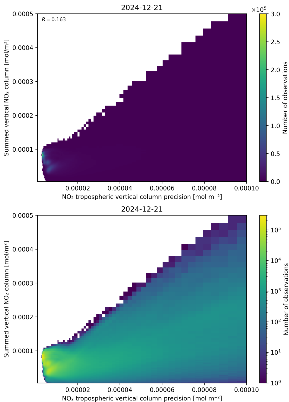
Figure 136: Scatter density plot of “NO 2 tropospheric vertical column precision” against “Summed vertical NO 2 column” for 2024-12-20 to 2024-12-22.
