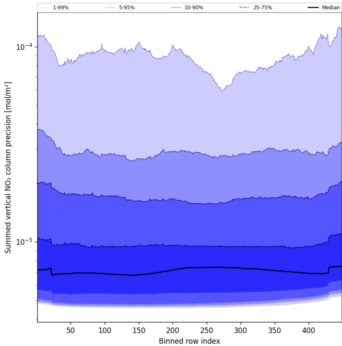
Figure 58: Along track statistics of “Summed vertical NO 2 column precision” for 2024-12-20 to 2024-12-22
