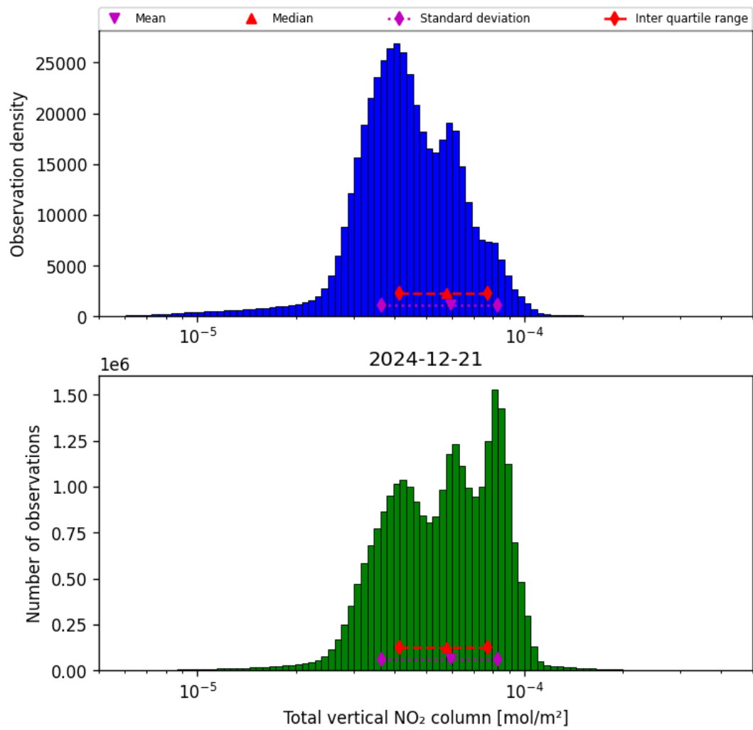
Figure 38: Histogram of “Total vertical NO 2 column” for 2024-12-20 to 2024-12-22
