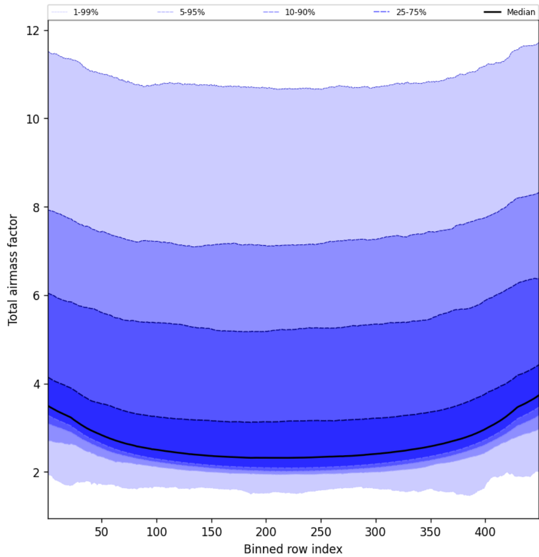
Figure 49: Along track statistics of “Total airmass factor” for 2024-12-20 to 2024-12-22
