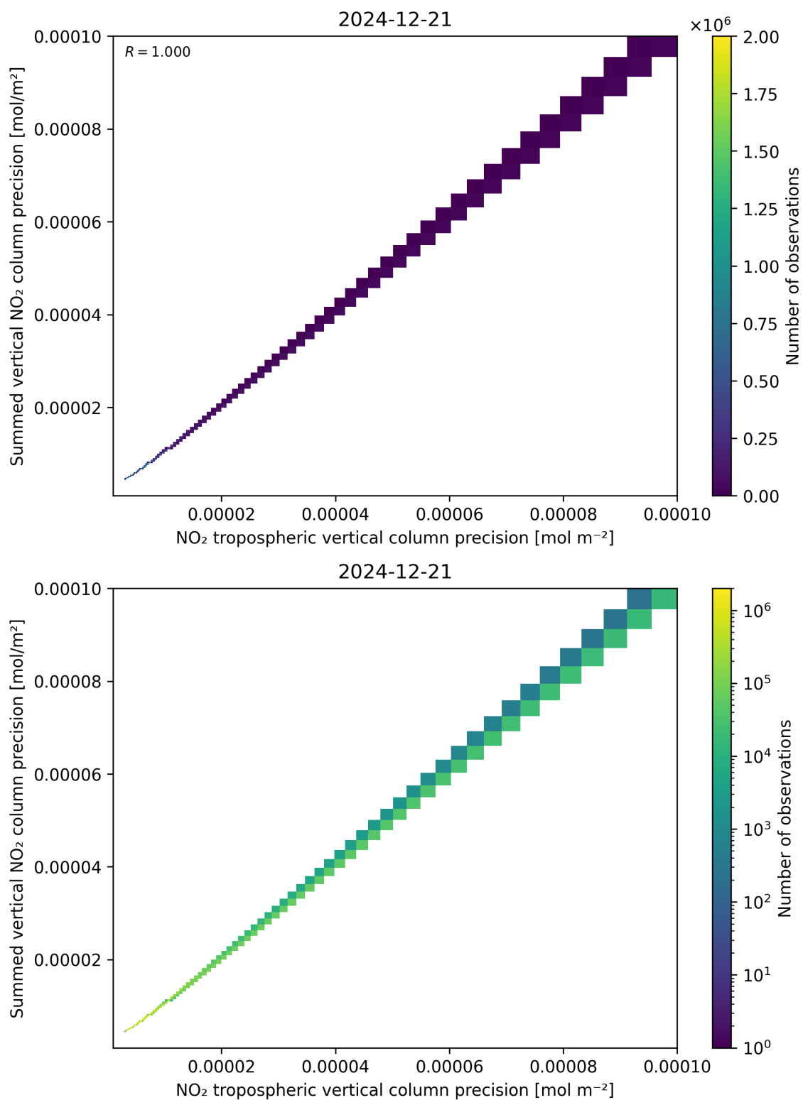
Figure 137: Scatter density plot of “NO 2 tropospheric vertical column precision” against “Summed vertical NO 2 column precision” for 2024-12-20 to 2024-12-22.
