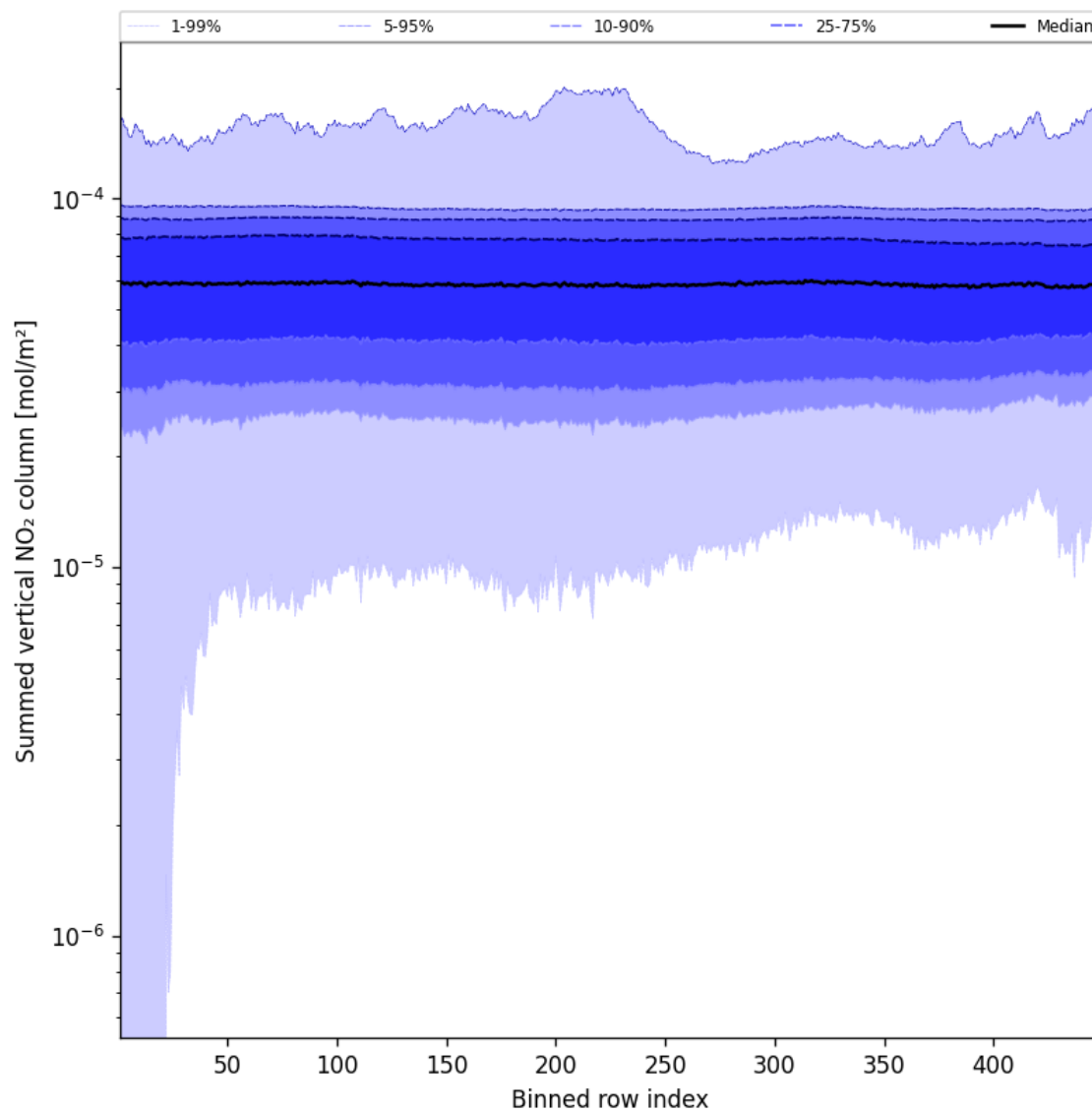
Figure 57: Along track statistics of “Summed vertical NO 2 column” for 2024-12-20 to 2024-12-22
