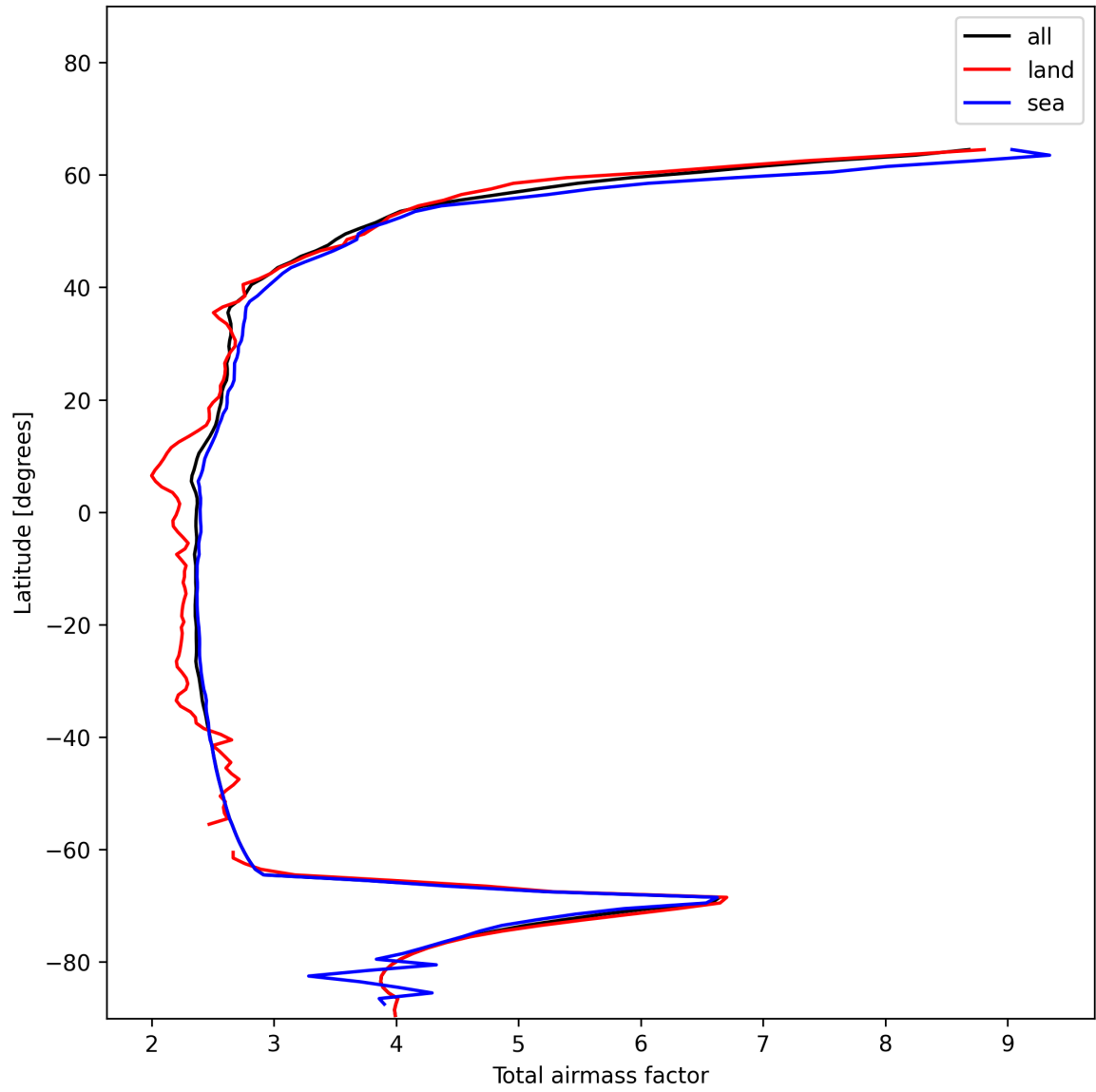
Figure 15: Zonal average of “Total airmass factor” for 2024-12-20 to 2024-12-22.
