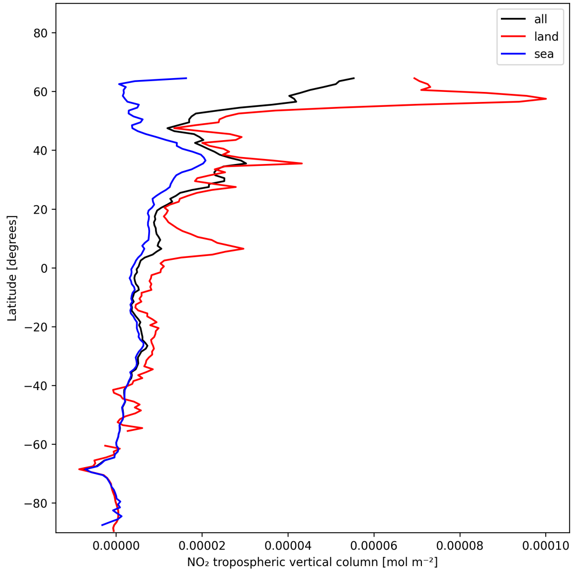
Figure 12: Zonal average of “NO 2 tropospheric vertical column” for 2024-12-20 to 2024-12-22.
