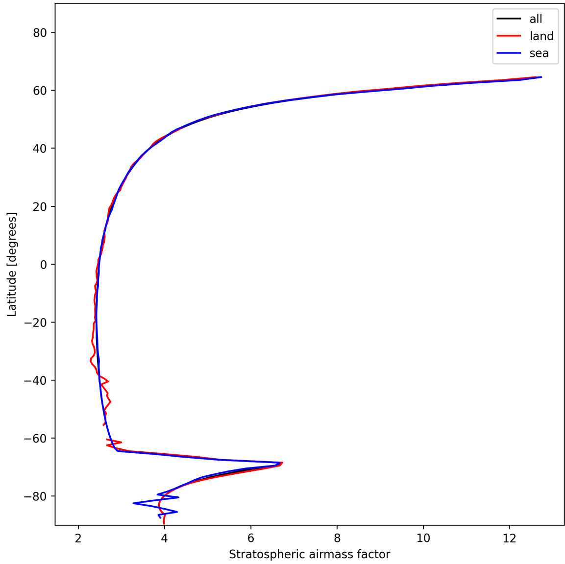
Figure 27: Zonal average of “Stratospheric airmass factor” for 2024-12-20 to 2024-12-22.
