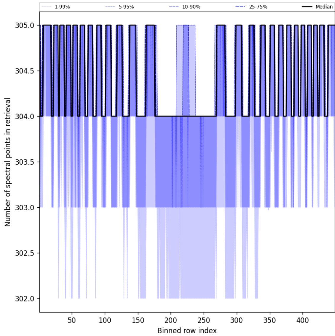
Figure 50: Along track statistics of “Number of spectral points in retrieval” for 2024-12-20 to 2024-12-22
