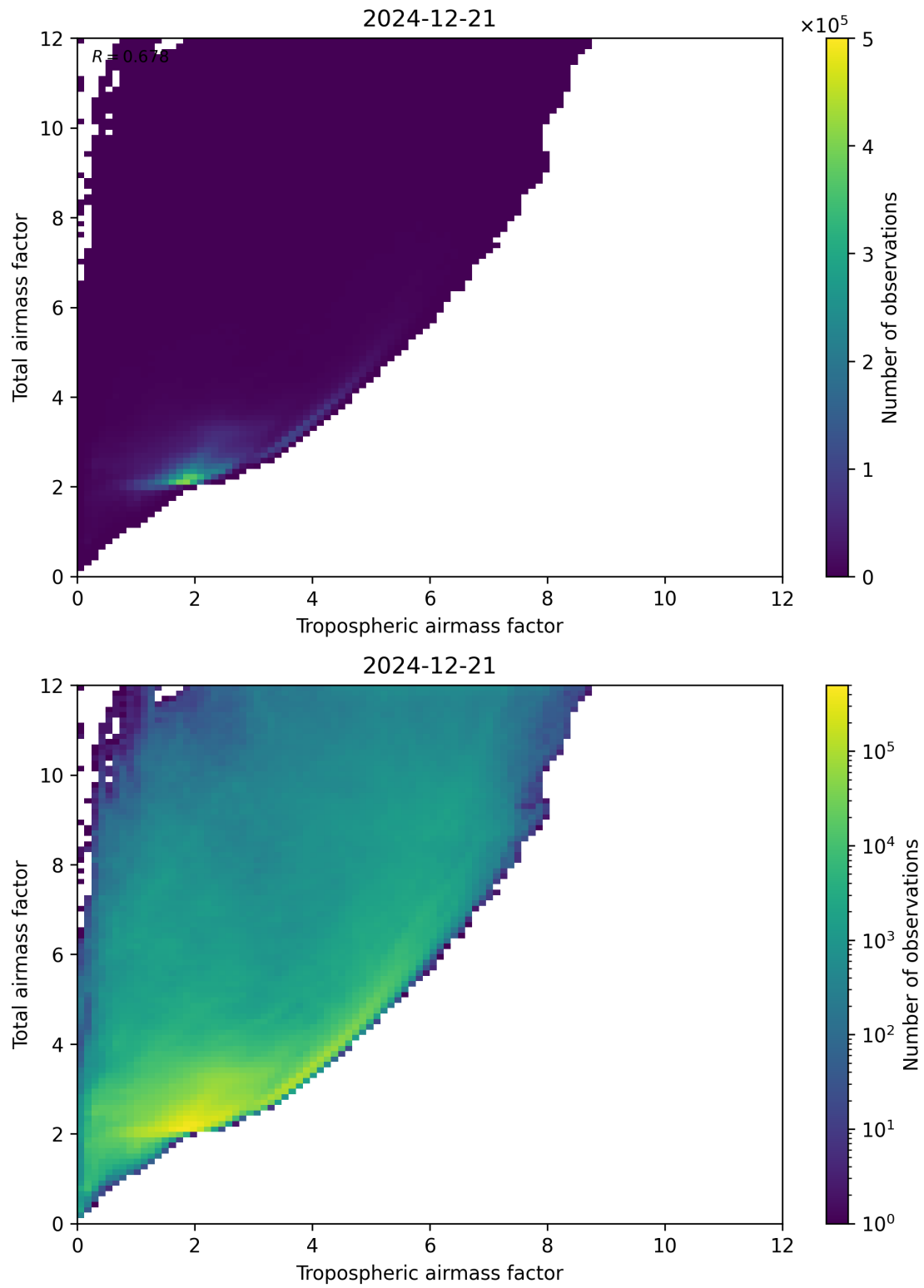
Figure 72: Scatter density plot of “Tropospheric airmass factor” against “Total airmass factor” for 2024-12-20 to 2024-12-22.
