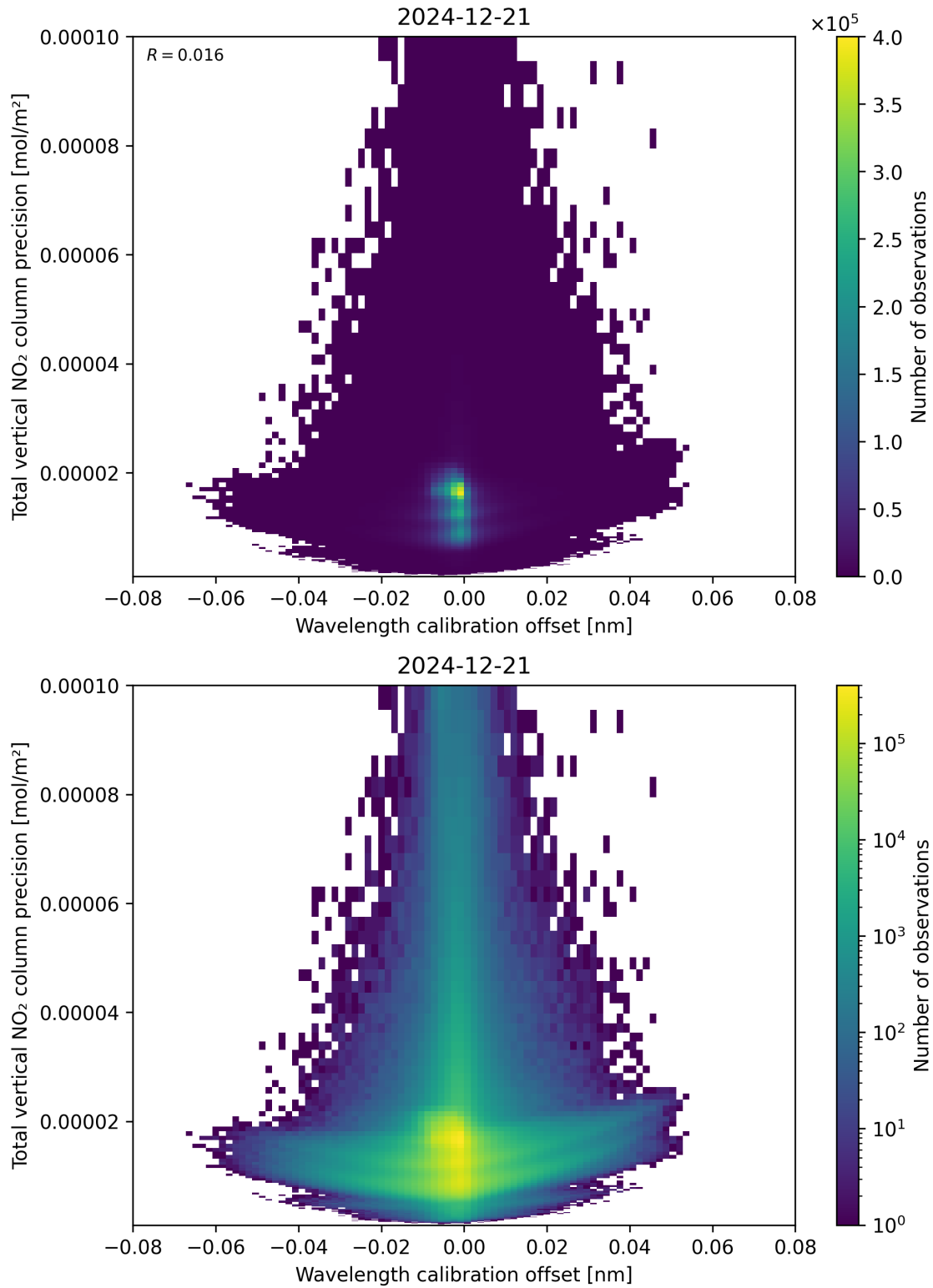
Figure 180: Scatter density plot of “Wavelength calibration offset” against “Total vertical NO 2 column precision” for 2024-12-20 to 2024-12-22.
