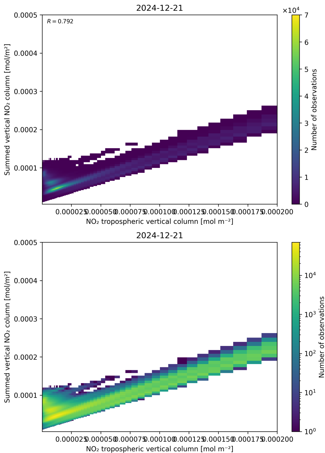
Figure 126: Scatter density plot of “NO 2 tropospheric vertical column” against “Summed vertical NO 2 column” for 2024-12-20 to 2024-12-22.
