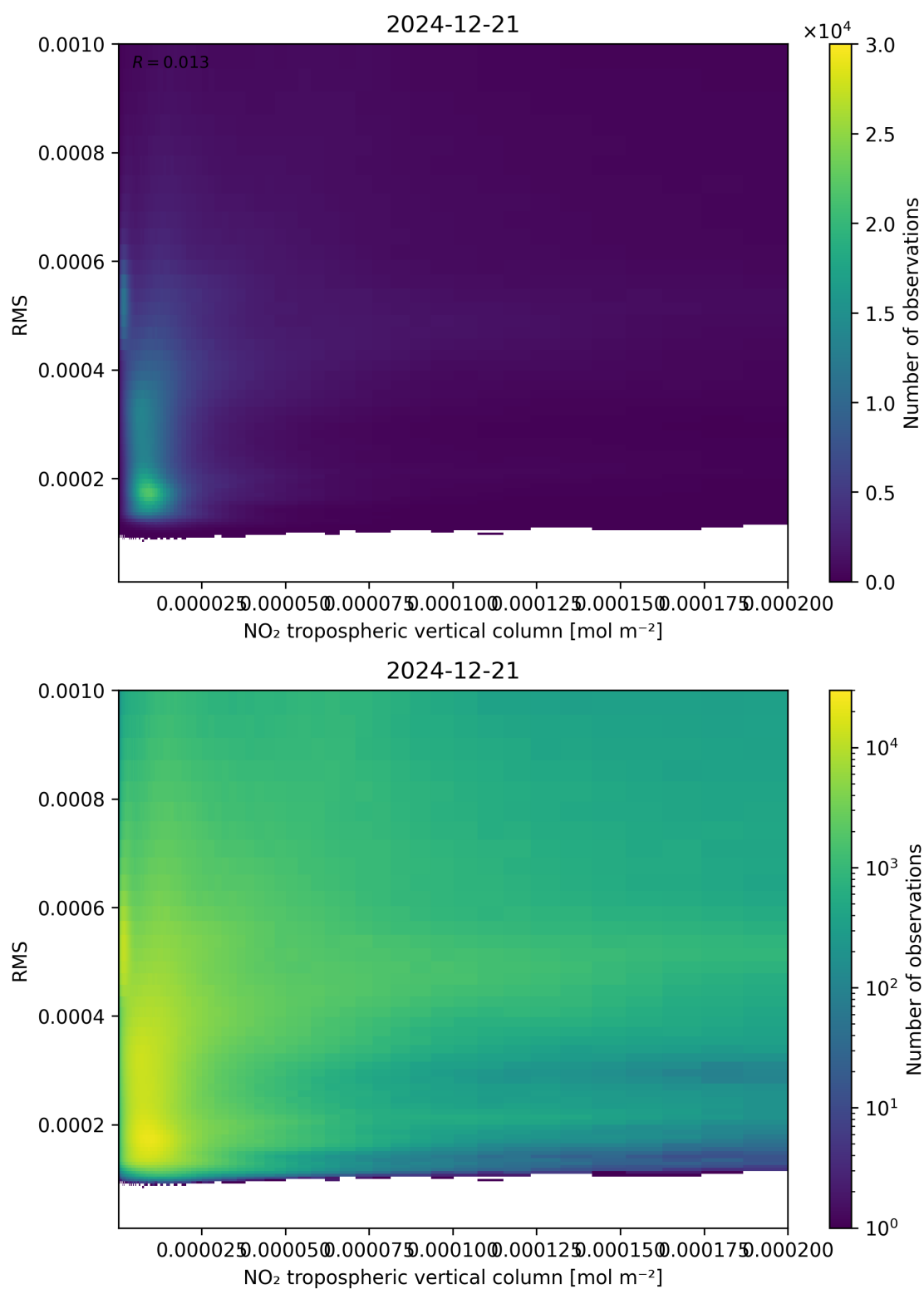
Figure 142: Scatter density plot of “NO 2 tropospheric vertical column” against “RMS” for 2024-12-20 to 2024-12-22.
