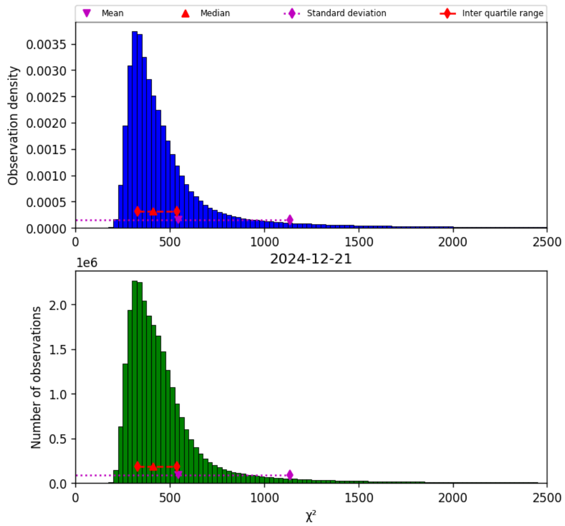
Figure 42: Histogram of “ \chi^2 ” for 2024-12-20 to 2024-12-22
