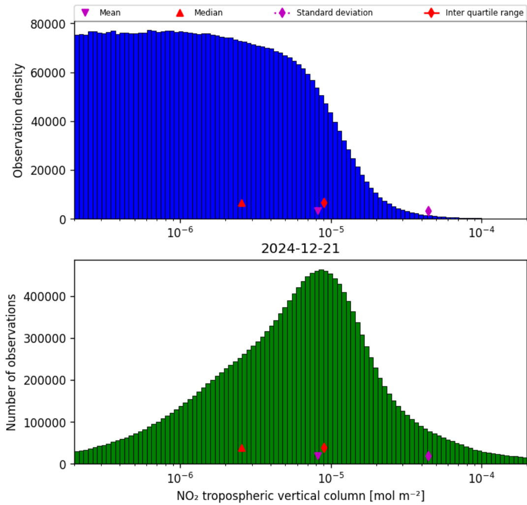
Figure 29: Histogram of “NO 2 tropospheric vertical column” for 2024-12-20 to 2024-12-22
