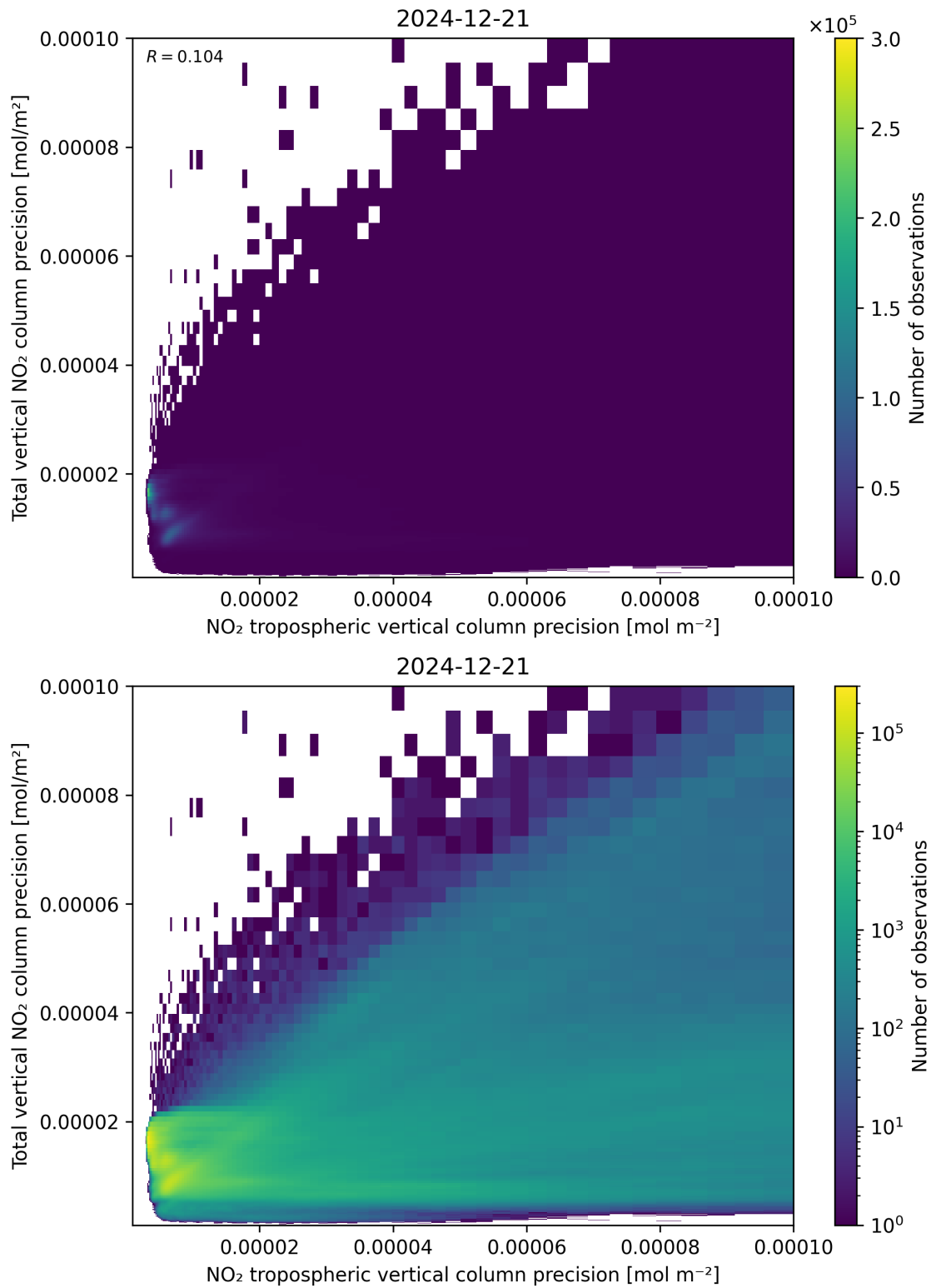
Figure 139: Scatter density plot of “NO 2 tropospheric vertical column precision” against “Total vertical NO 2 column precision” for 2024-12-20 to 2024-12-22.
