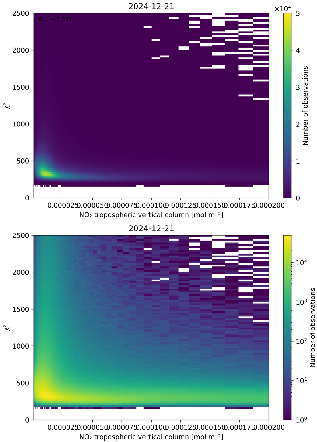
Figure 124: Scatter density plot of “NO 2 tropospheric vertical column” against “ \chi^2 ” for 2024-12-20 to 2024-12-22.
