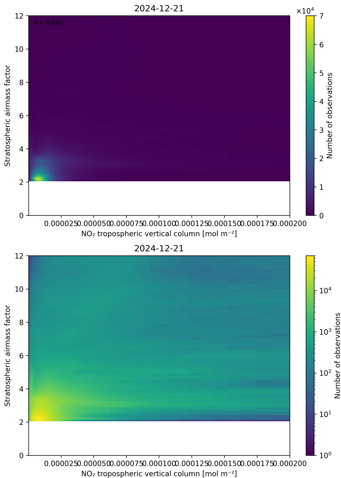
Figure 121: Scatter density plot of “NO 2 tropospheric vertical column” against “Stratospheric airmass factor” for 2024-12-20 to 2024-12-22.
