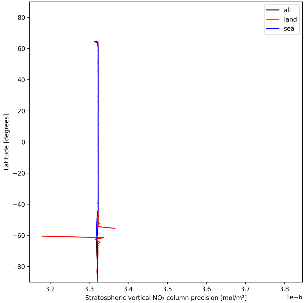
Figure 20: Zonal average of “Stratospheric vertical NO 2 column precision” for 2024-12-20 to 2024-12-22.
