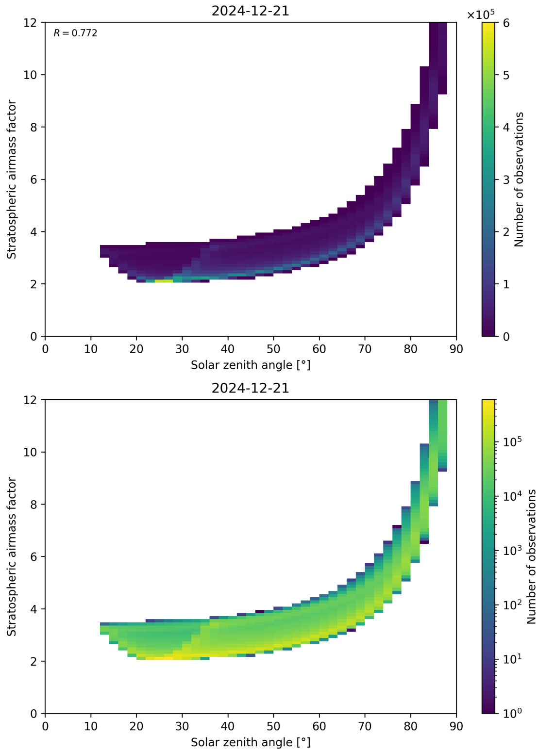
Figure 145: Scatter density plot of “Solar zenith angle” against “Stratospheric airmass factor” for 2024-12-20 to 2024-12-22.
