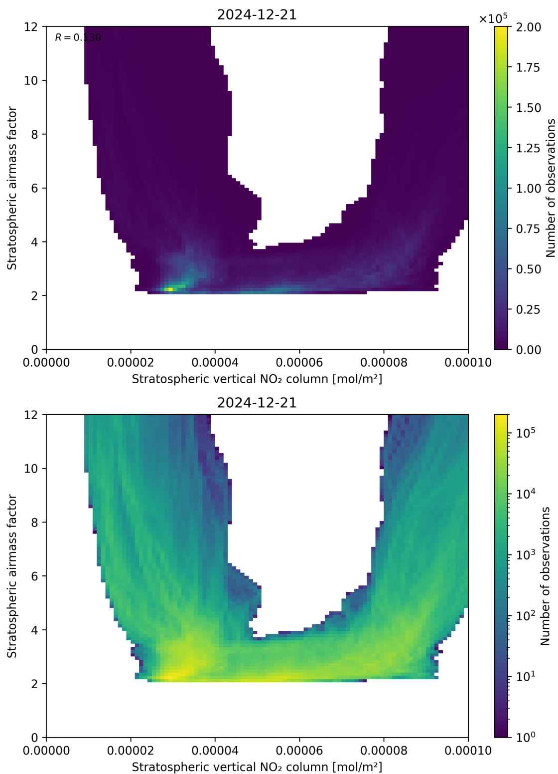
Figure 96: Scatter density plot of “Stratospheric vertical NO 2 column” against “Stratospheric airmass factor” for 2024-12-20 to 2024-12-22.
