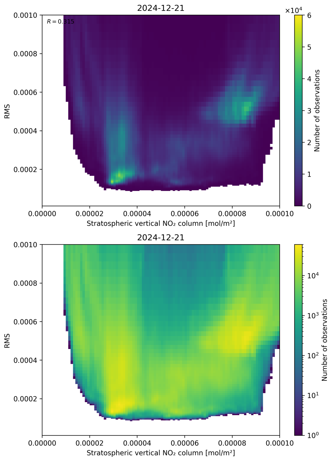
Figure 102: Scatter density plot of “Stratospheric vertical NO 2 column” against “RMS” for 2024-12-20 to 2024-12-22.
