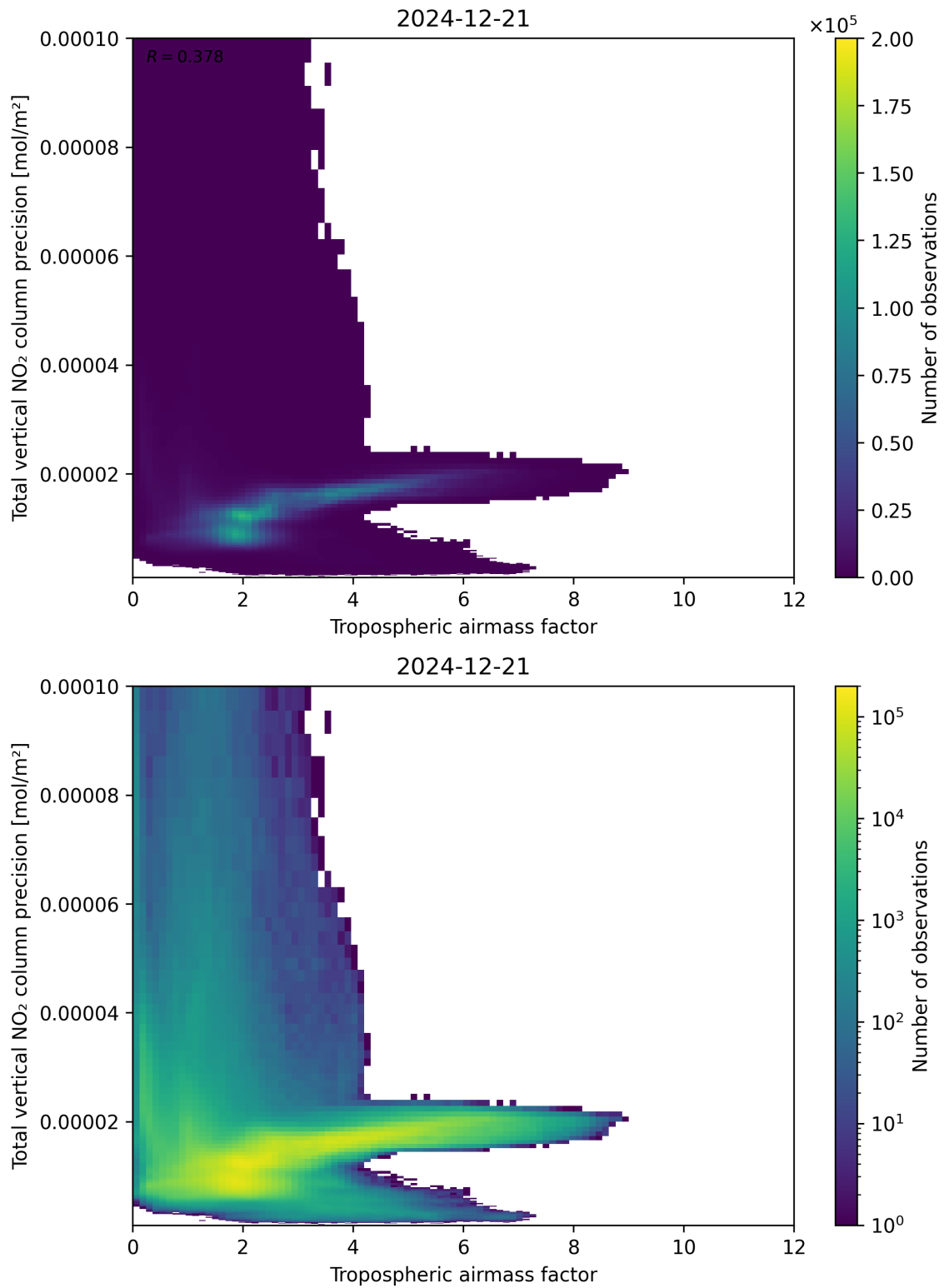
Figure 78: Scatter density plot of “Tropospheric air mass factor” against “Total vertical NO 2 column precision” for 2024-12-20 to 2024-12-22.
