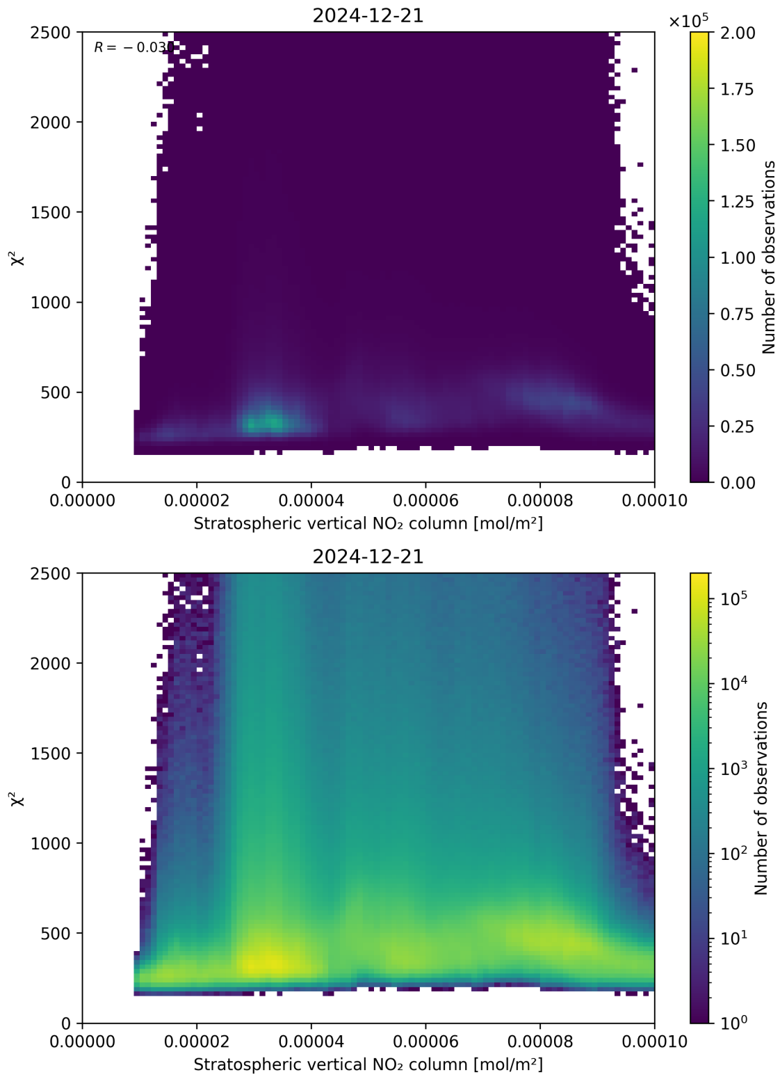
Figure 97: Scatter density plot of “Stratospheric vertical NO 2 column” against “ \chi^2 ” for 2024-12-20 to 2024-12-22.
