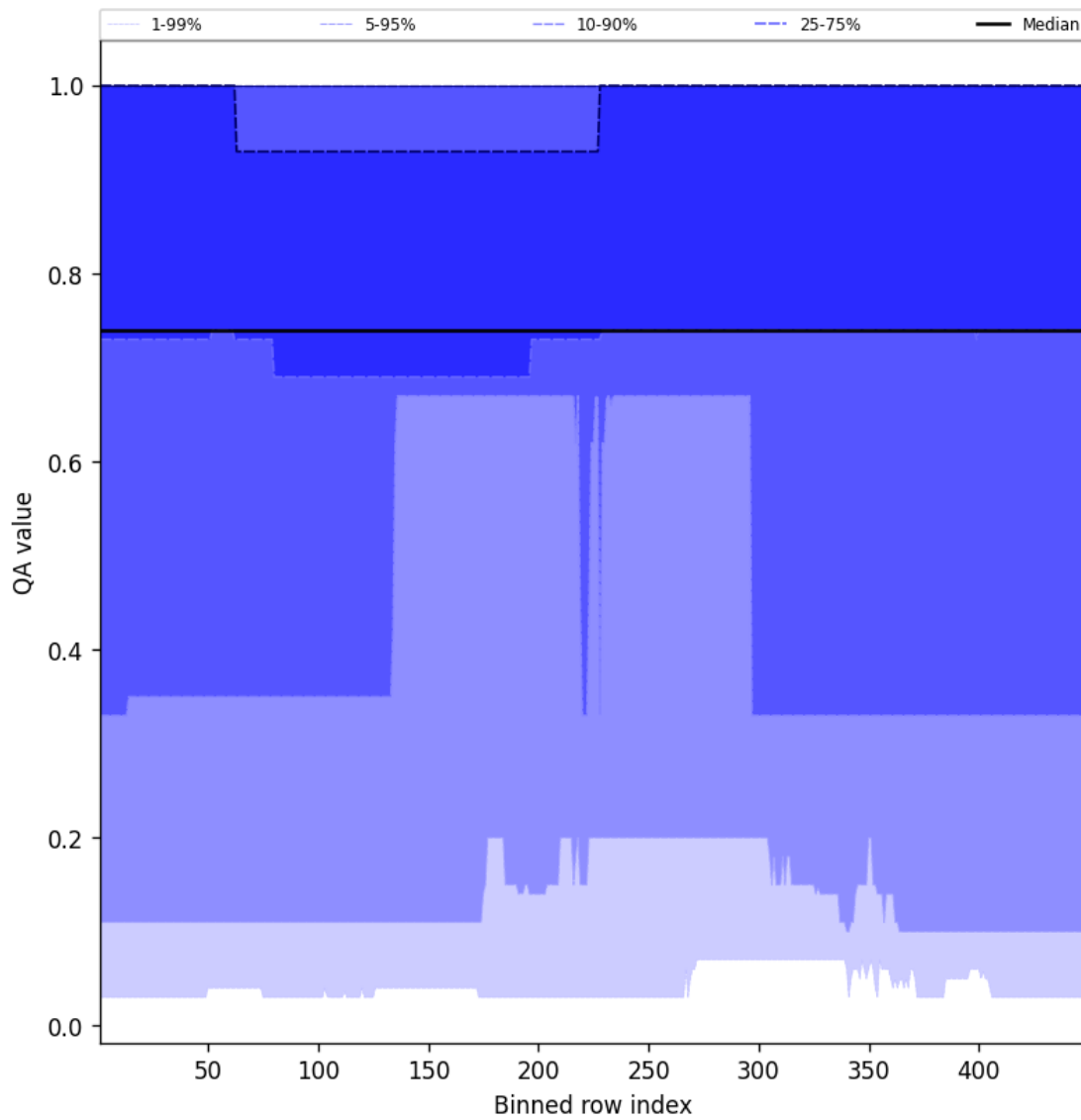
Figure 45: Along track statistics of “QA value” for 2024-12-20 to 2024-12-22
