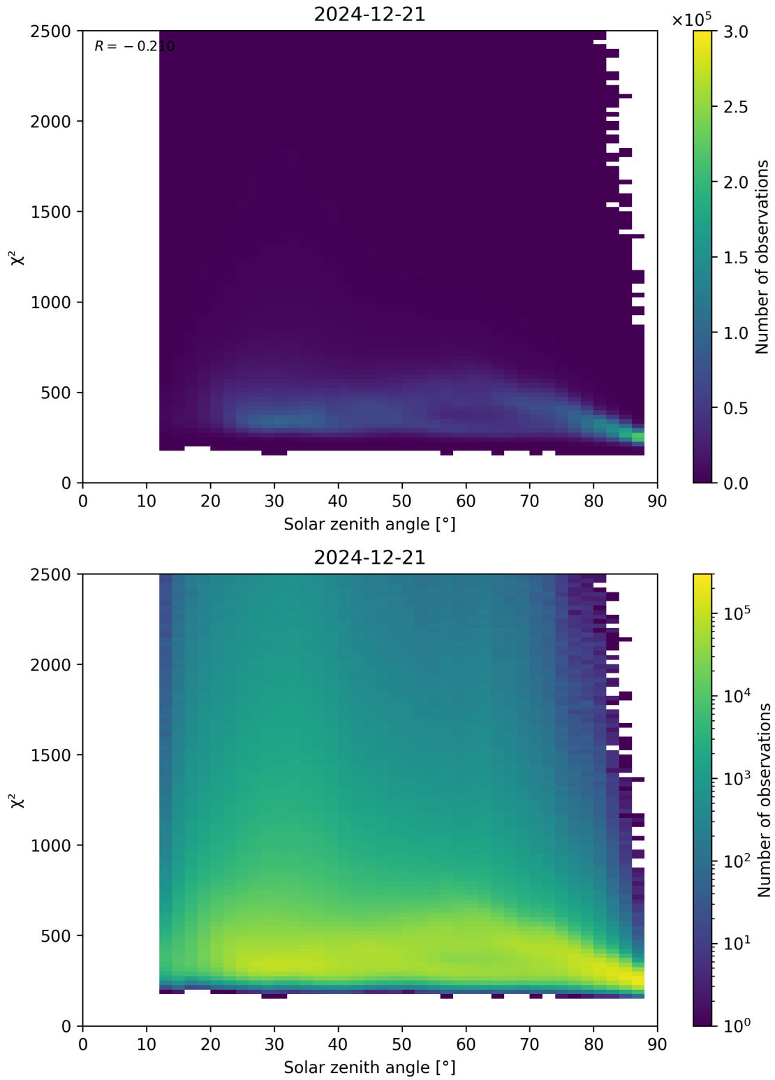
Figure 148: Scatter density plot of “Solar zenith angle” against “ \chi^2 ” for 2024-12-20 to 2024-12-22.
