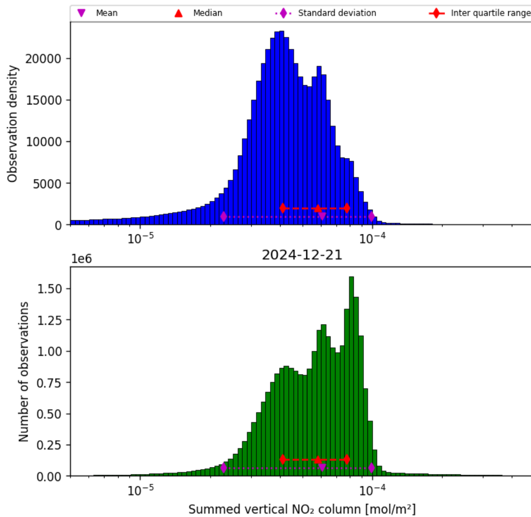
Figure 40: Histogram of “Summed vertical NO 2 column” for 2024-12-20 to 2024-12-22
