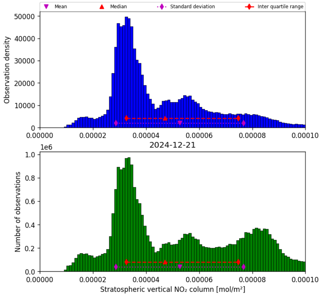
Figure 36: Histogram of “Stratospheric vertical NO 2 column” for 2024-12-20 to 2024-12-22
