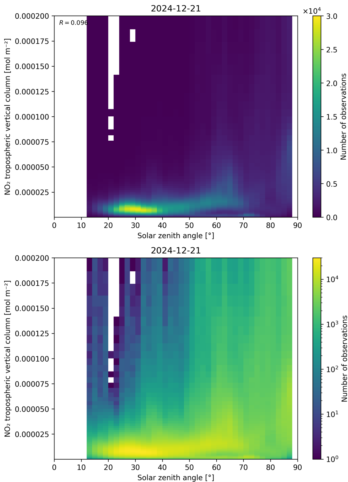
Figure 155: Scatter density plot of “Solar zenith angle” against “NO 2 tropospheric vertical column” for 2024-12-20 to 2024-12-22.
