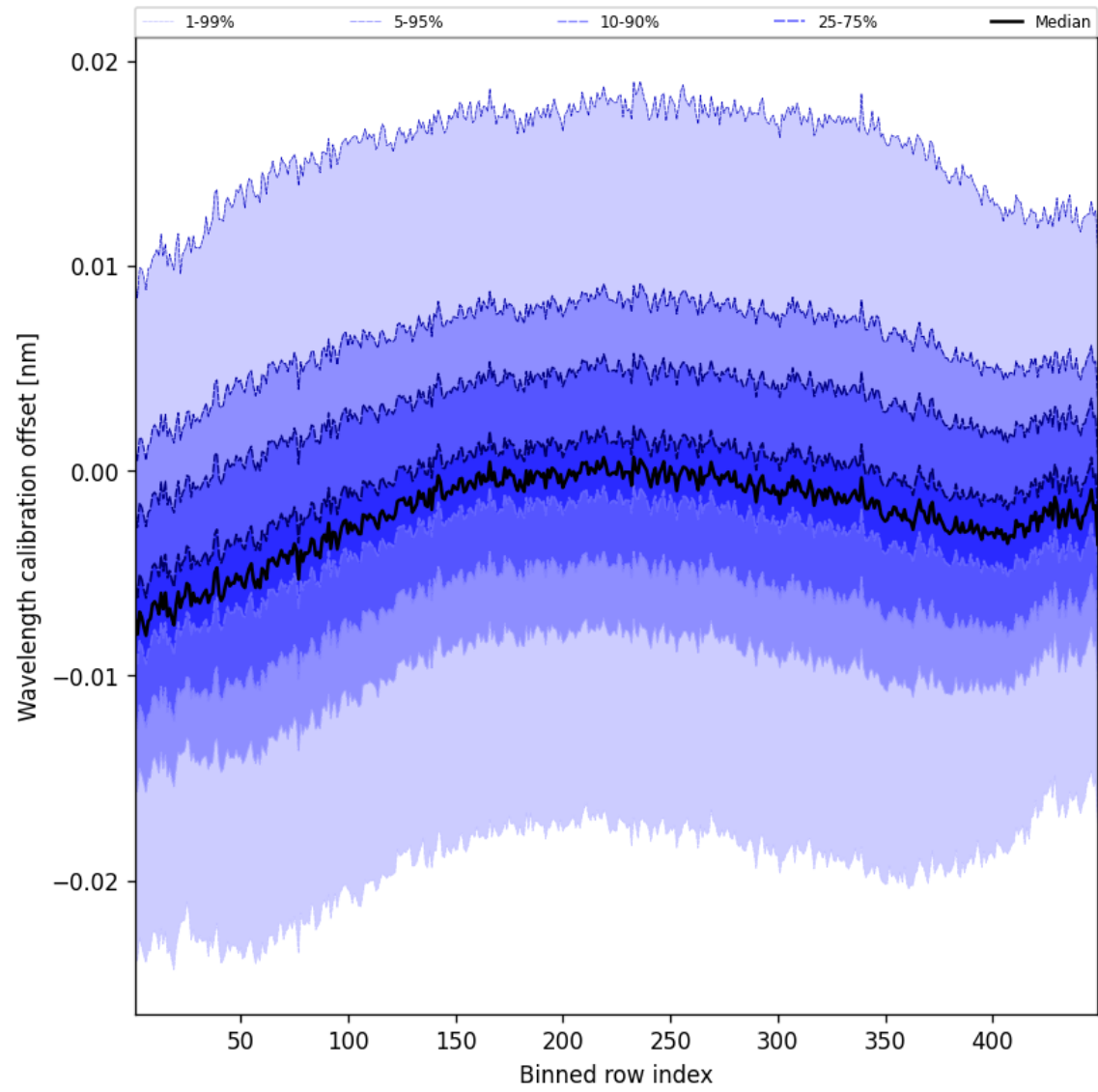
Figure 52: Along track statistics of “Wavelength calibration offset” for 2024-12-20 to 2024-12-22
