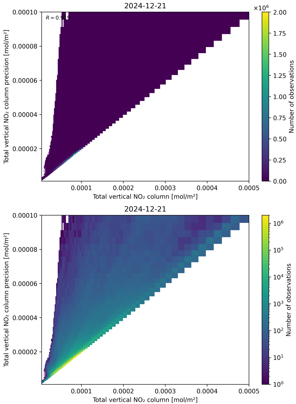
Figure 114: Scatter density plot of “Total vertical NO 2 column” against “Total vertical NO 2 column precision” for 2024-12-20 to 2024-12-22.
