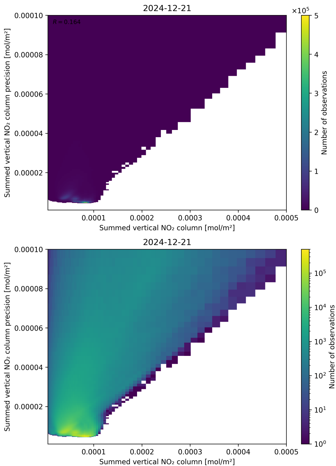
Figure 105: Scatter density plot of “Summed vertical NO 2 column” against “Summed vertical NO 2 column precision” for 2024-12-20 to 2024-12-22.
