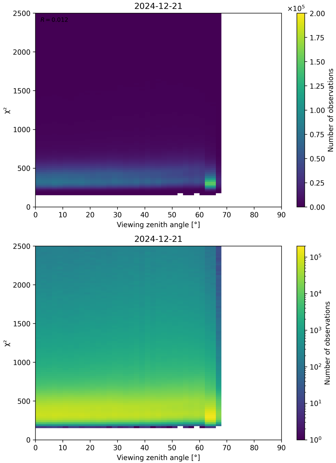
Figure 162: Scatter density plot of “Viewing zenith angle” against “ \chi^2 ” for 2024-12-20 to 2024-12-22.
