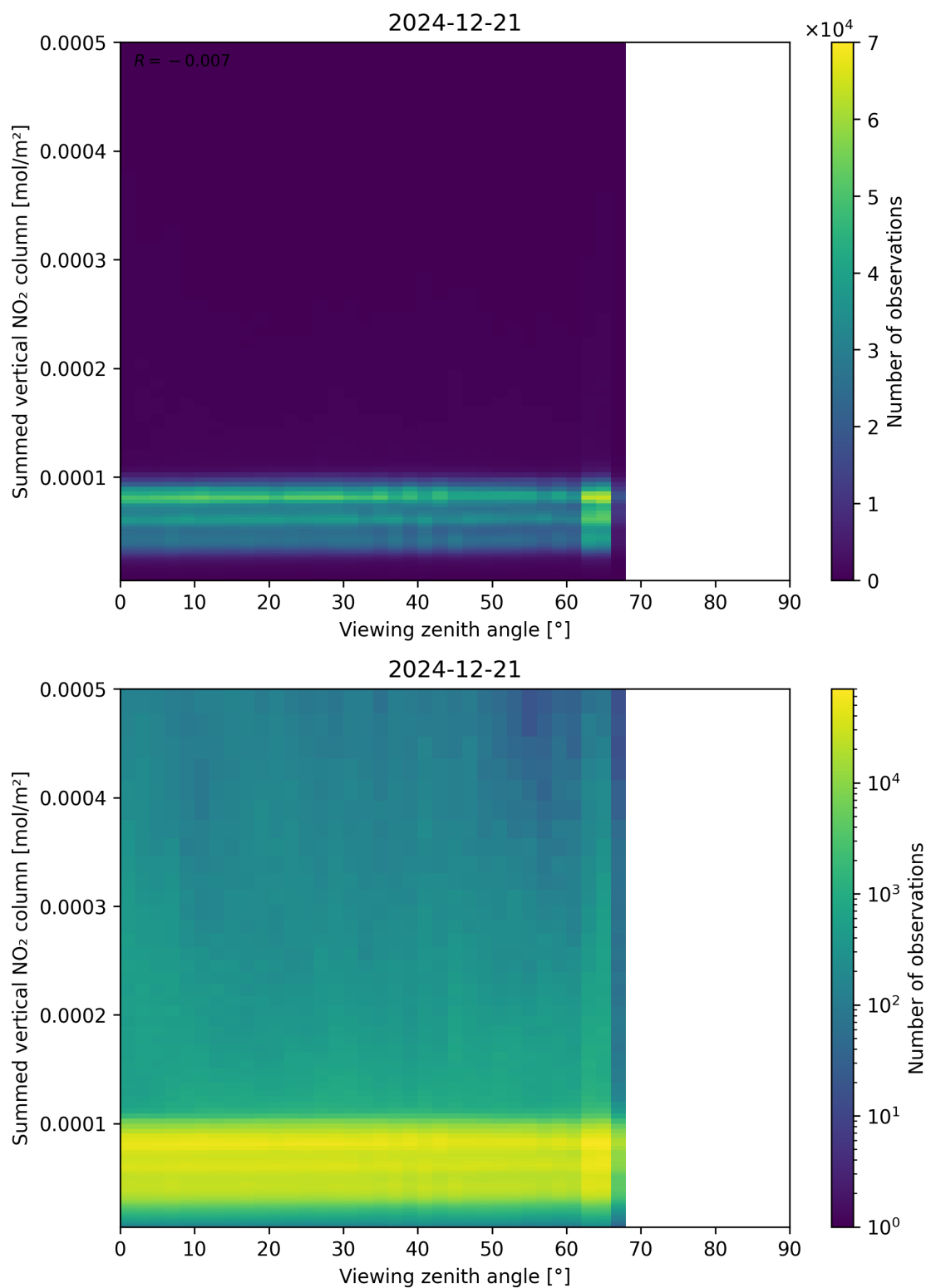
Figure 165: Scatter density plot of “Viewing zenith angle” against “Summed vertical NO 2 column” for 2024-12-20 to 2024-12-22.
