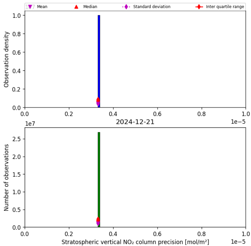
Figure 37: Histogram of “Stratospheric vertical NO 2 column precision” for 2024-12-20 to 2024-12-22
