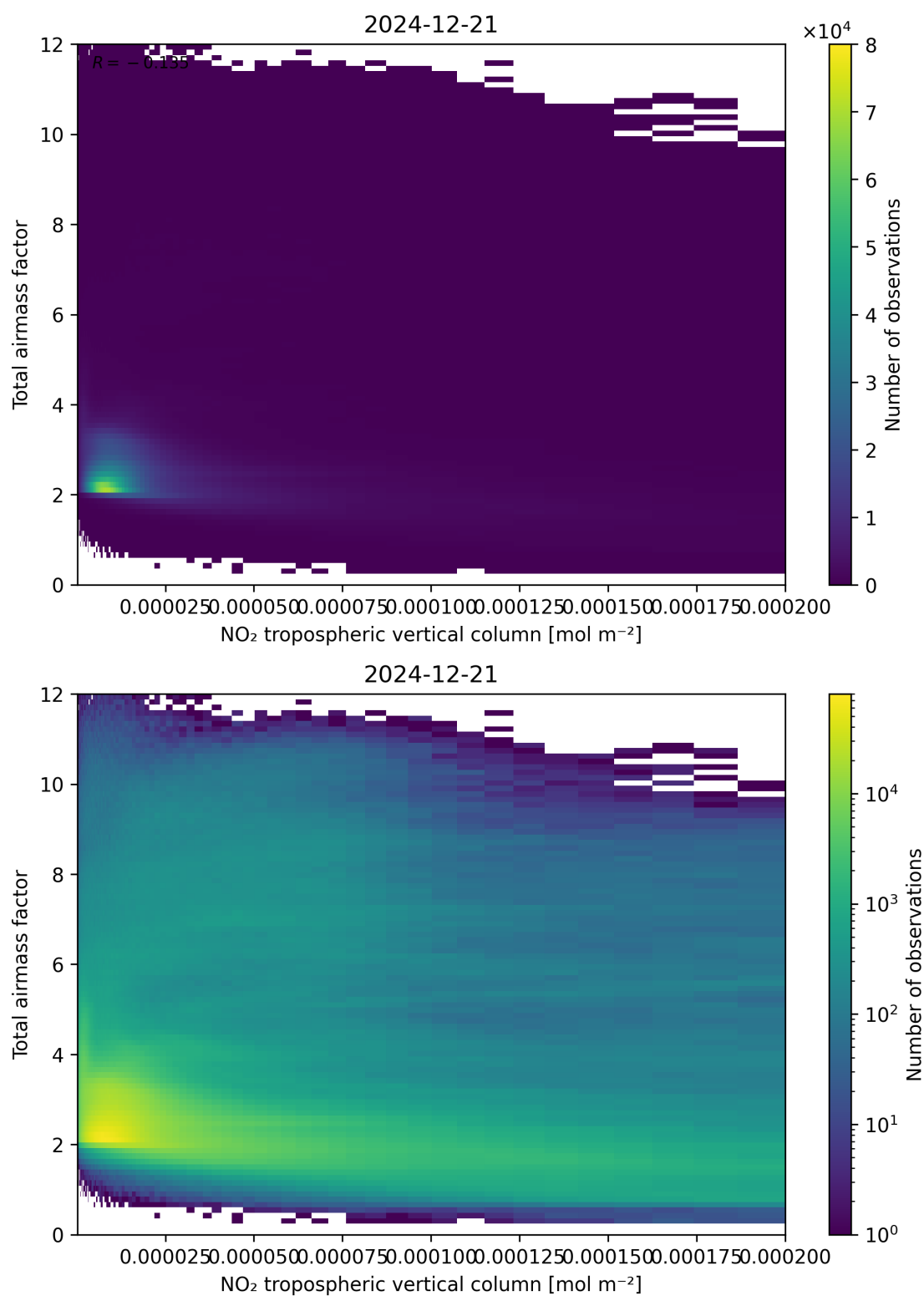
Figure 122: Scatter density plot of “NO 2 tropospheric vertical column” against “Total air mass factor” for 2024-12-20 to 2024-12-22.
