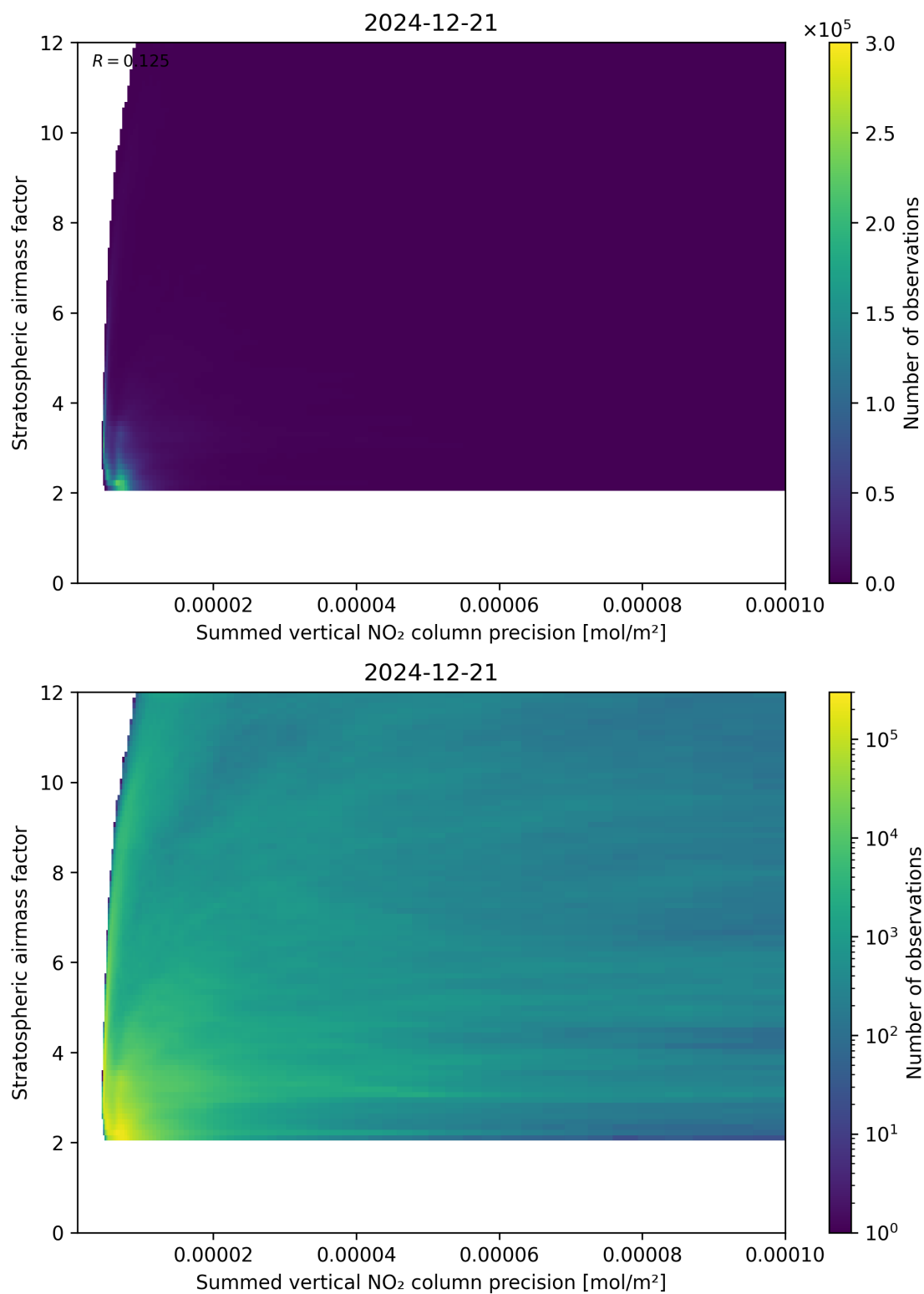
Figure 106: Scatter density plot of “Summed vertical NO 2 column precision” against “Stratospheric airmass factor” for 2024-12-20 to 2024-12-22.
