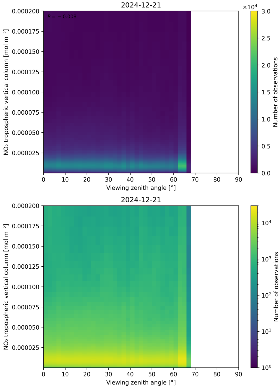
Figure 169: Scatter density plot of “Viewing zenith angle” against “NO 2 tropospheric vertical column” for 2024-12-20 to 2024-12-22.
