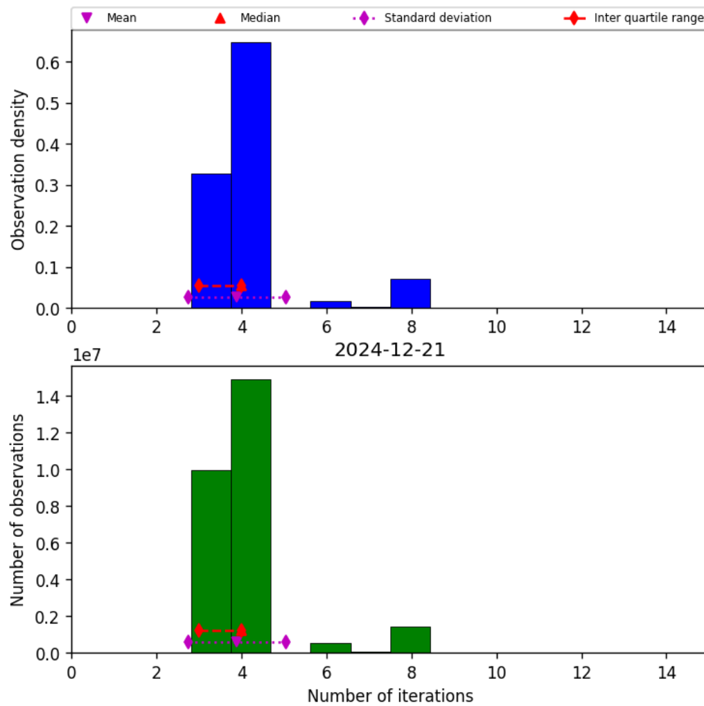
Figure 34: Histogram of “Number of iterations” for 2024-12-20 to 2024-12-22
