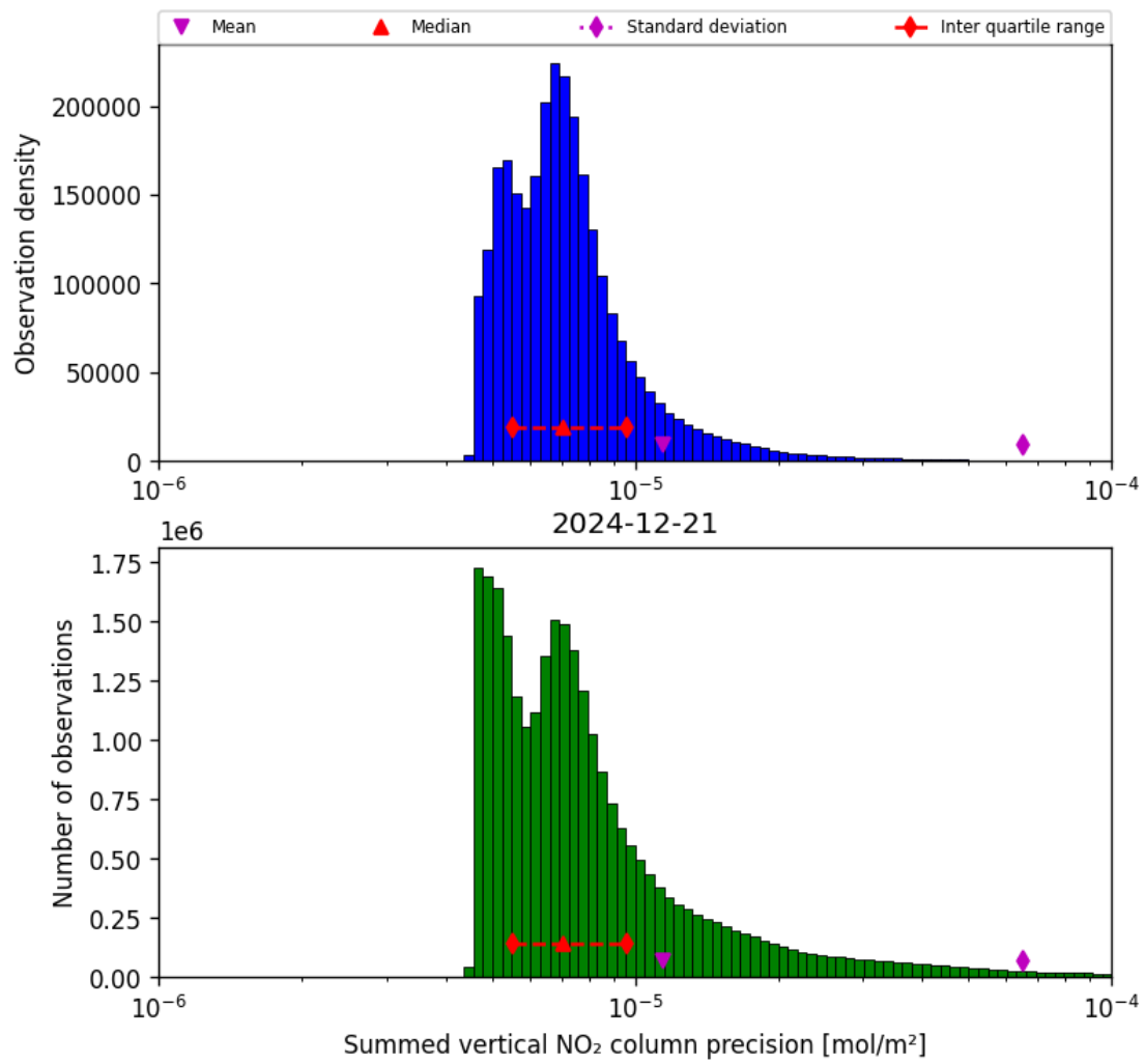
Figure 41: Histogram of "Summed vertical NO 2 column precision" for 2024-12-20 to 2024-12-22
