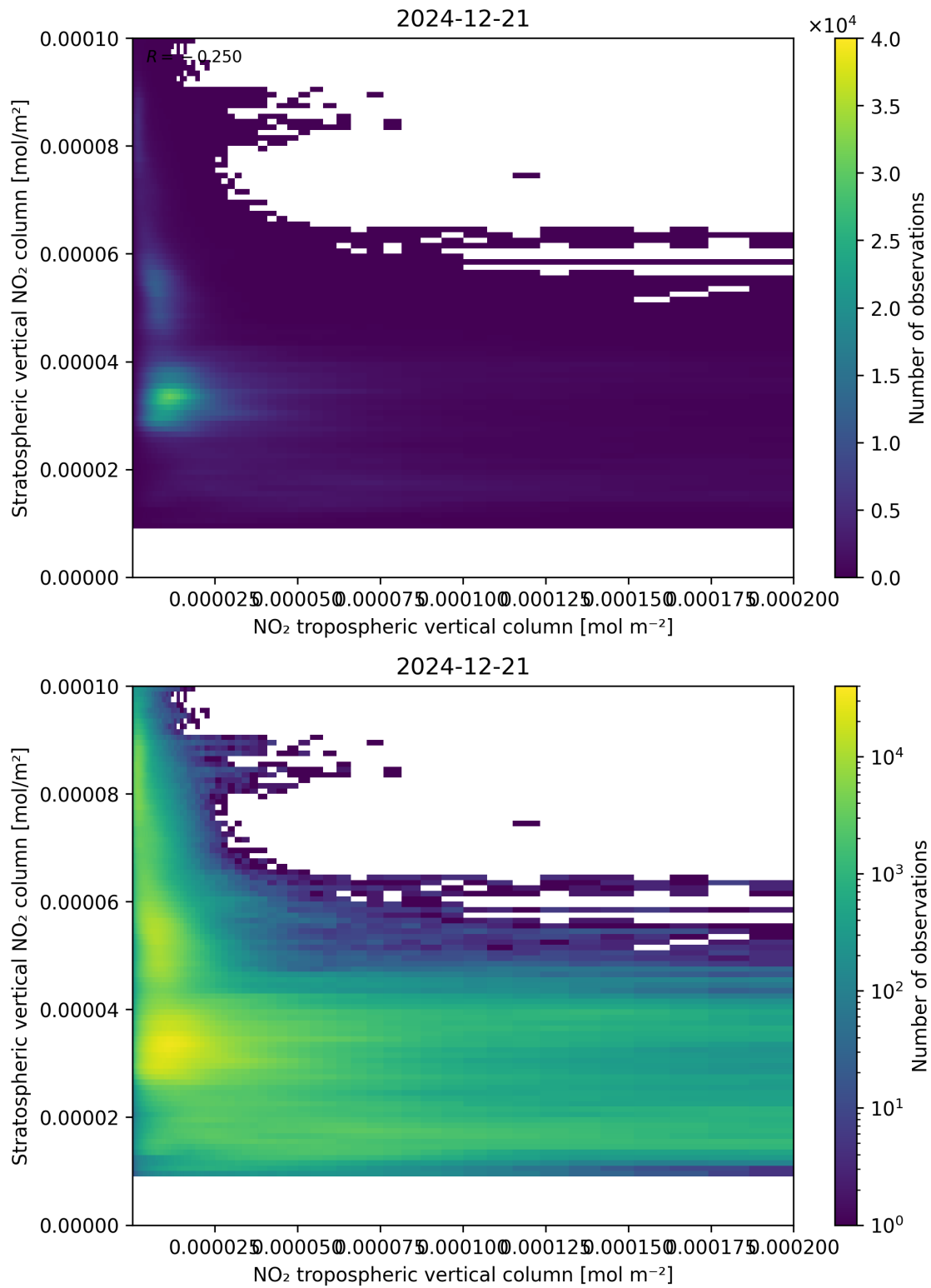
Figure 125: Scatter density plot of “NO 2 tropospheric vertical column” against “Stratospheric vertical NO 2 column” for 2024-12-20 to 2024-12-22.
