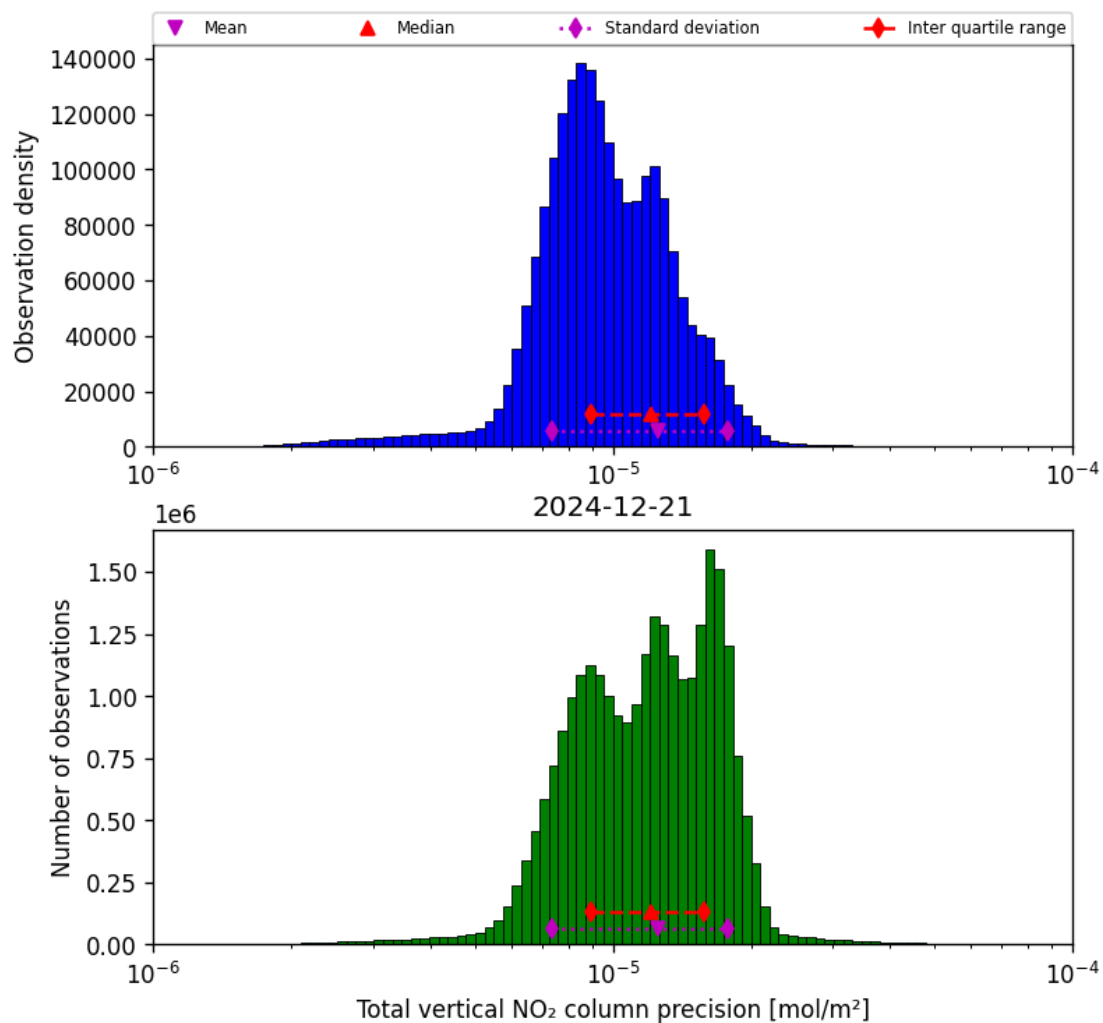
Figure 39: Histogram of “Total vertical NO 2 column precision” for 2024-12-20 to 2024-12-22
