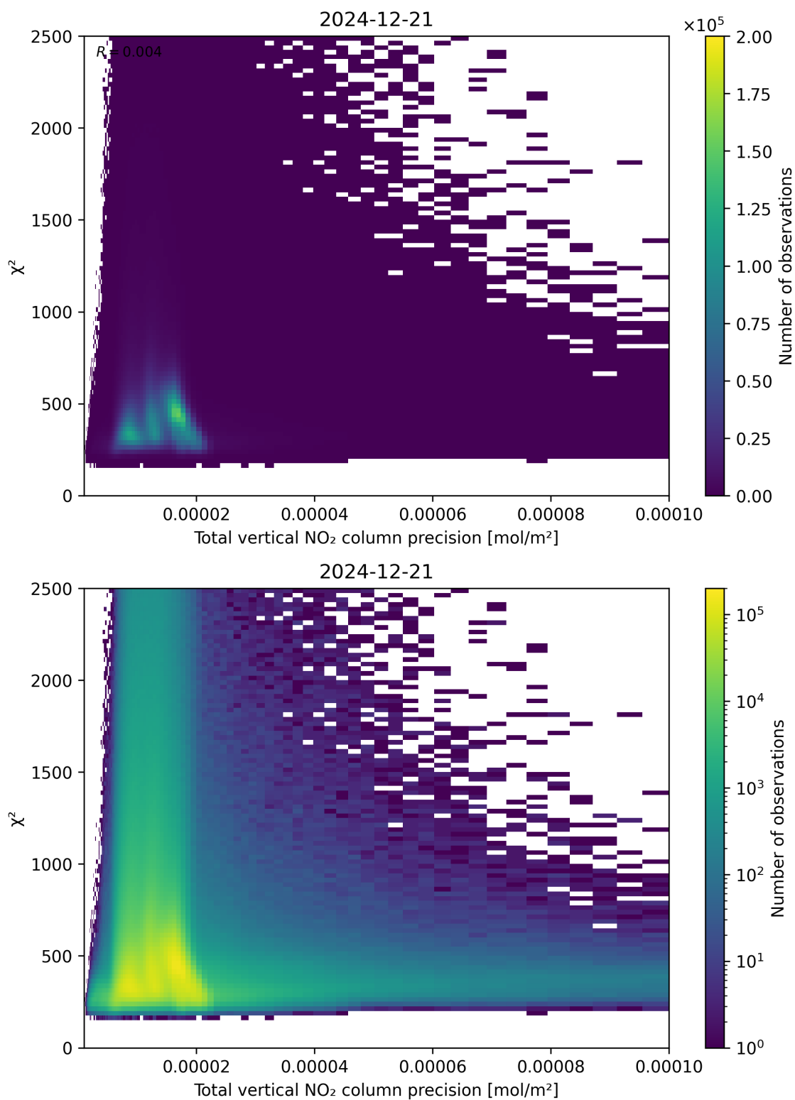
Figure 116: Scatter density plot of “Total vertical NO 2 column precision” against “ \chi^2 ” for 2024-12-20 to 2024-12-22.
