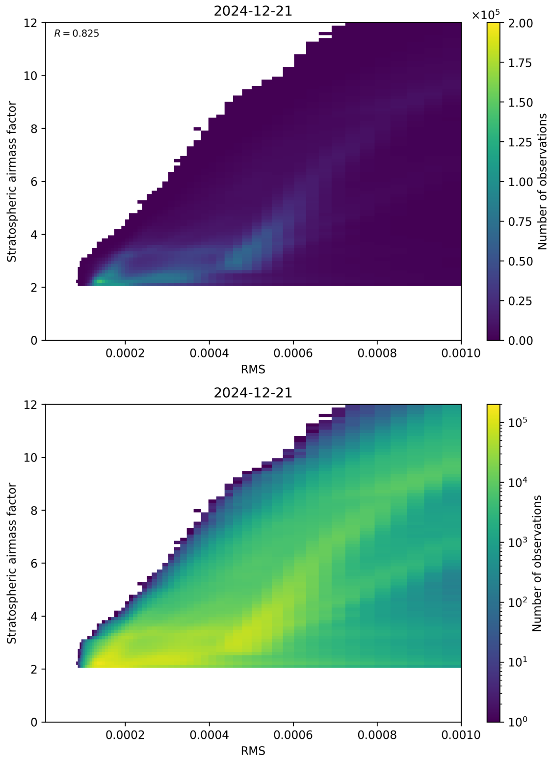
Figure 144: Scatter density plot of “RMS” against “Stratospheric airmass factor” for 2024-12-20 to 2024-12-22.
