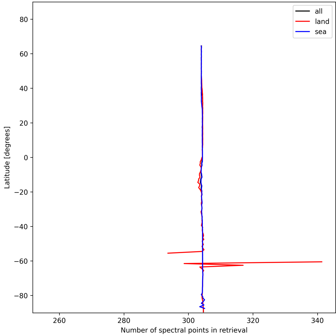
Figure 16: Zonal average of “Number of spectral points in retrieval” for 2024-12-20 to 2024-12-22.
