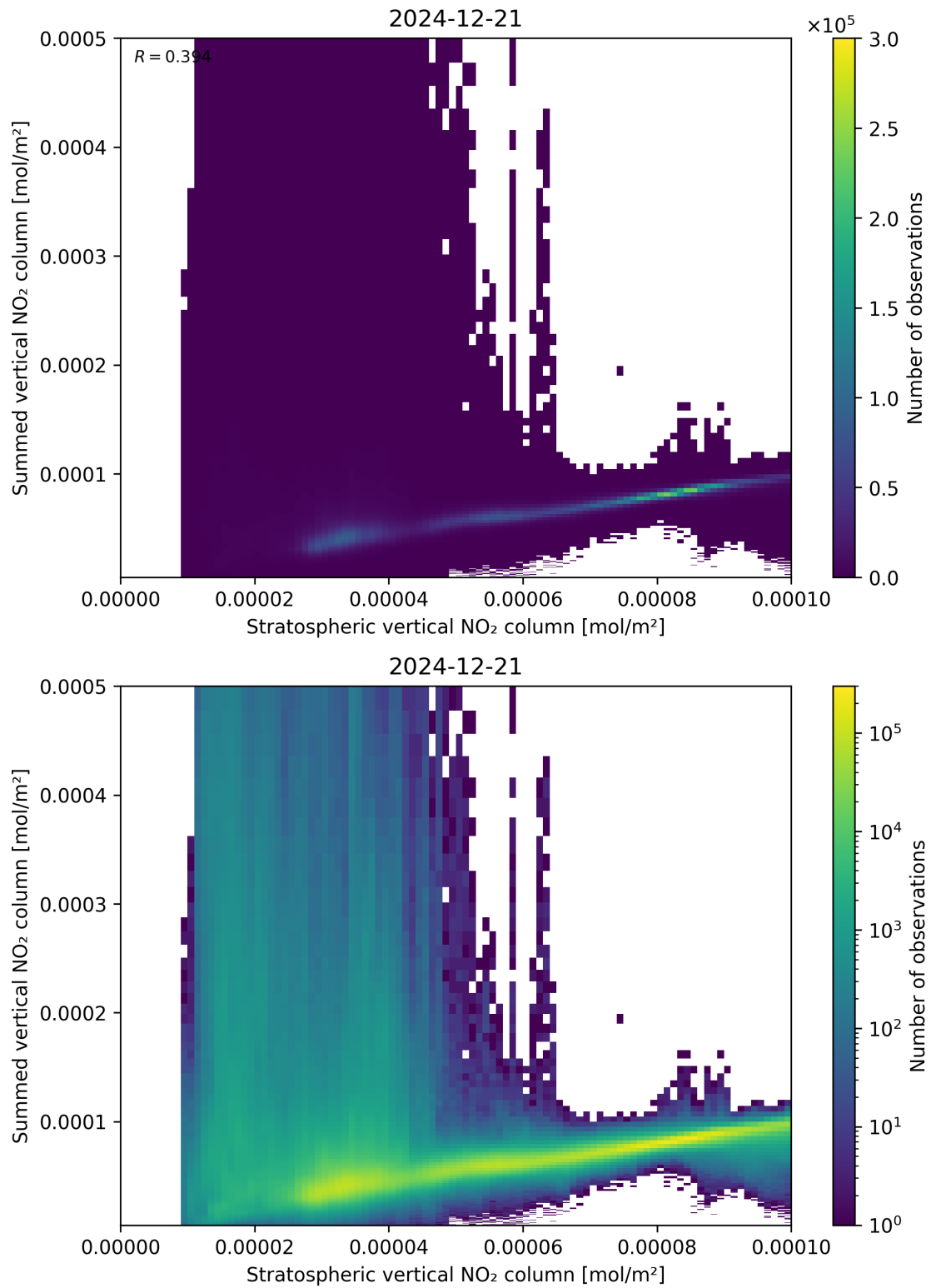
Figure 98: Scatter density plot of “Stratospheric vertical NO 2 column” against “Summed vertical NO 2 column” for 2024-12-20 to 2024-12-22.
