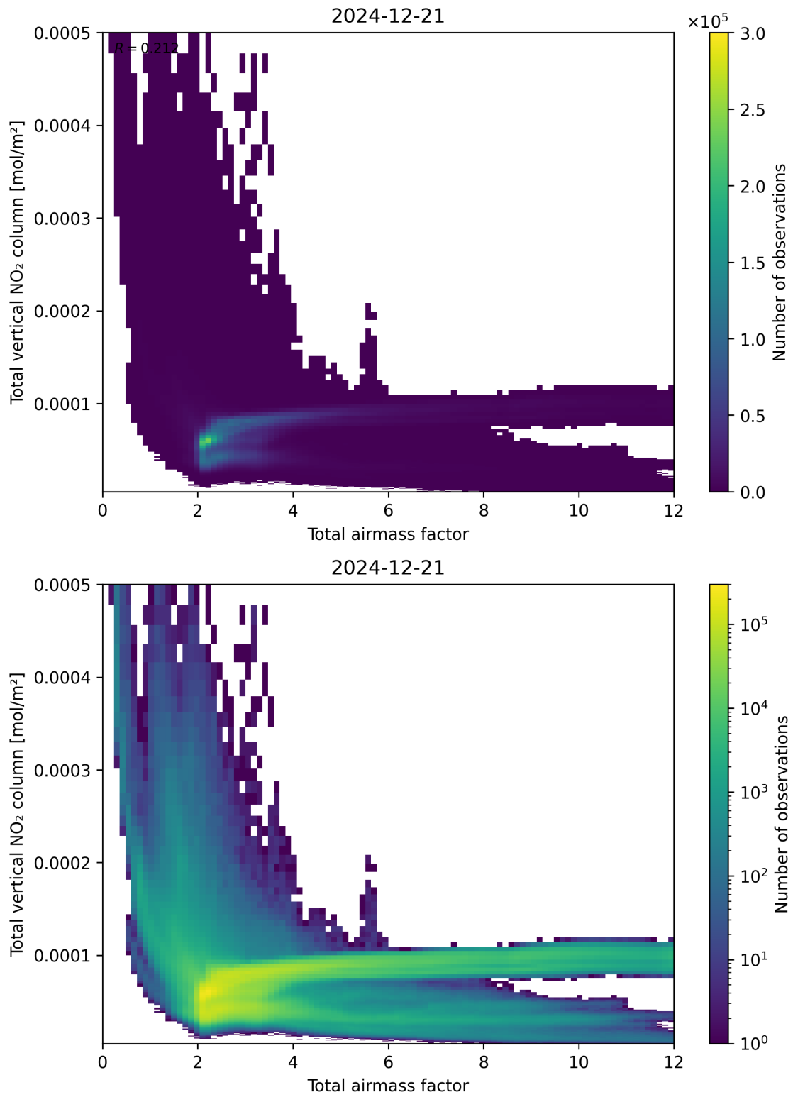
Figure 67: Scatter density plot of “Total airmass factor” against “Total vertical NO 2 column” for 2024-12-20 to 2024-12-22.
