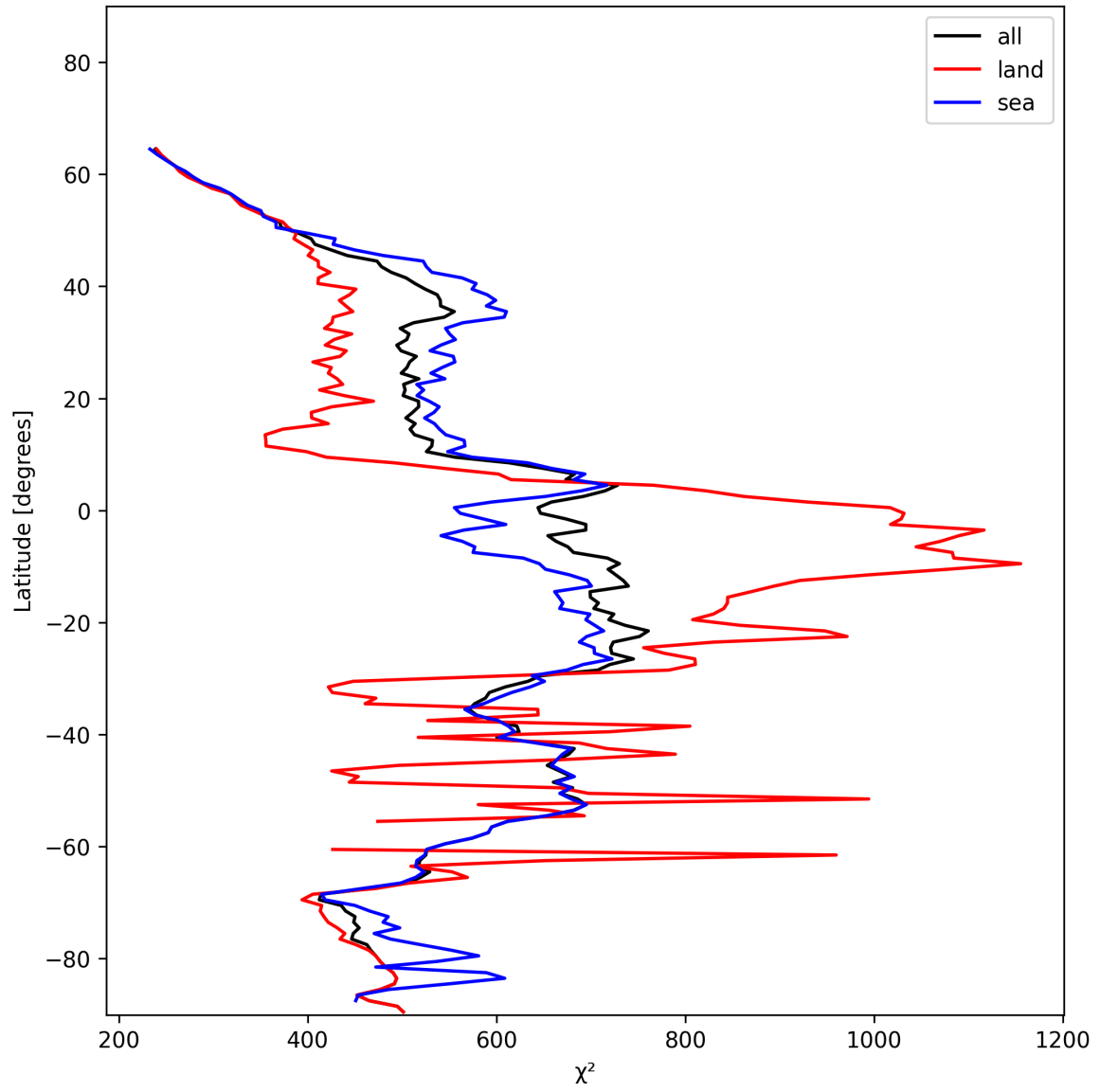
Figure 25: Zonal average of “ \chi^2 ” for 2024-12-20 to 2024-12-22.
