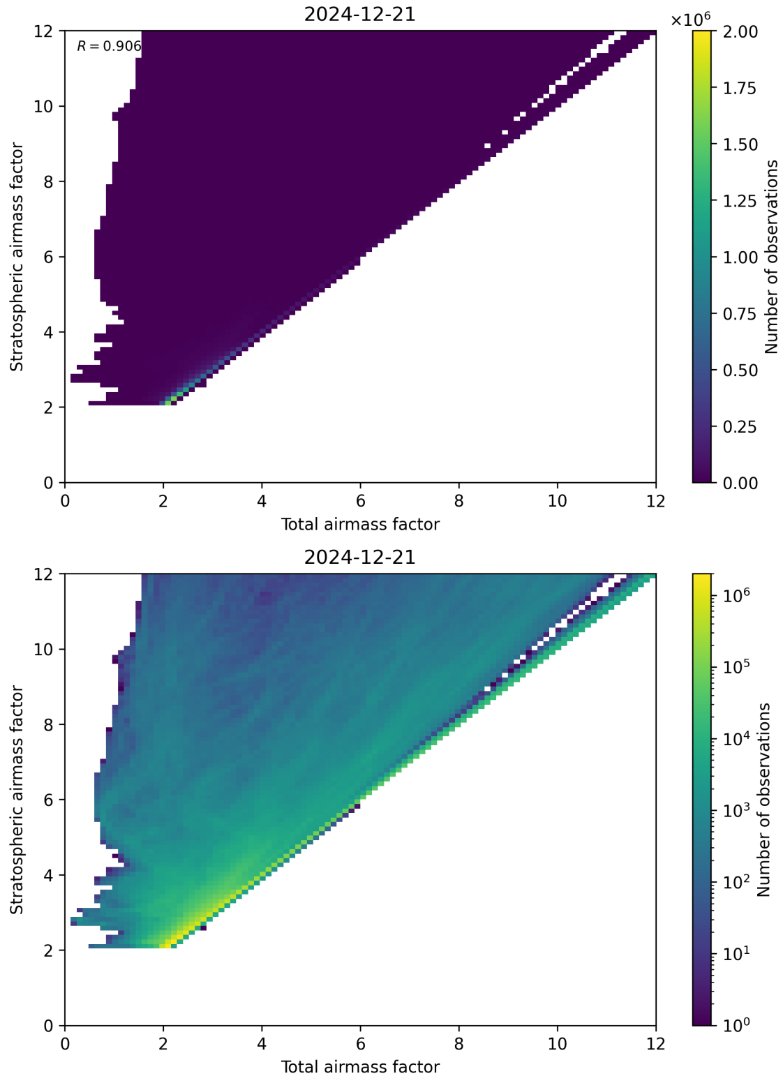
Figure 62: Scatter density plot of “Total airmass factor” against “Stratospheric airmass factor” for 2024-12-20 to 2024-12-22.
