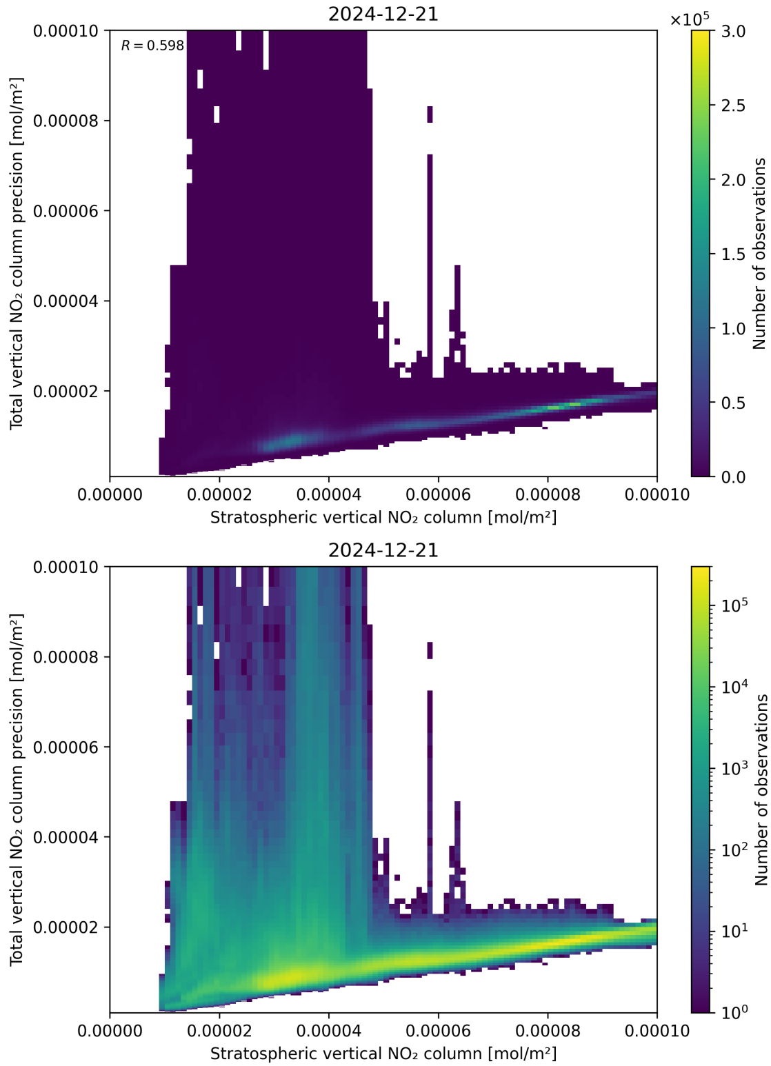
Figure 101: Scatter density plot of “Stratospheric vertical NO 2 column” against “Total vertical NO 2 column precision” for 2024-12-20 to 2024-12-22.
