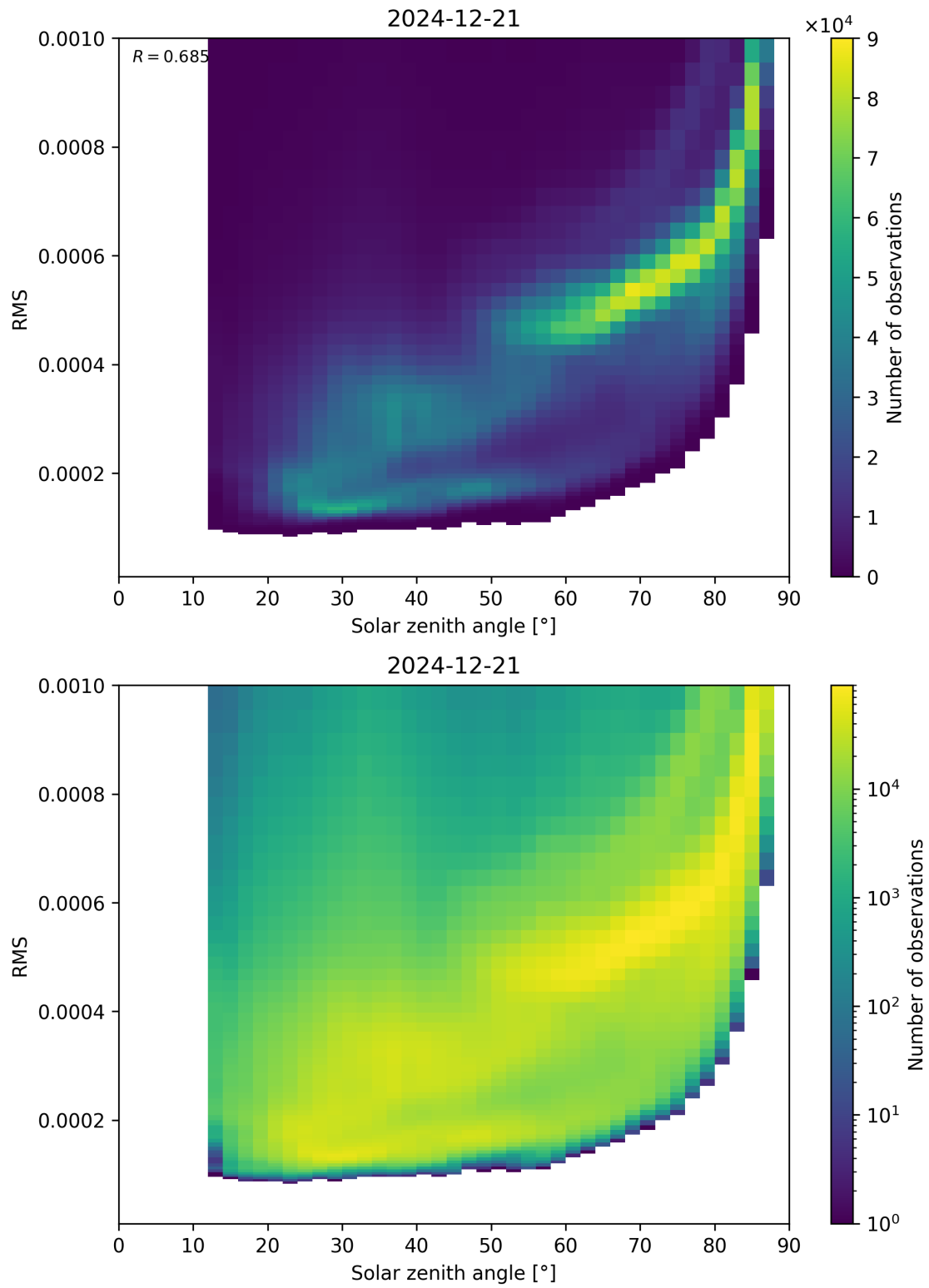
Figure 157: Scatter density plot of “Solar zenith angle” against “RMS” for 2024-12-20 to 2024-12-22.
