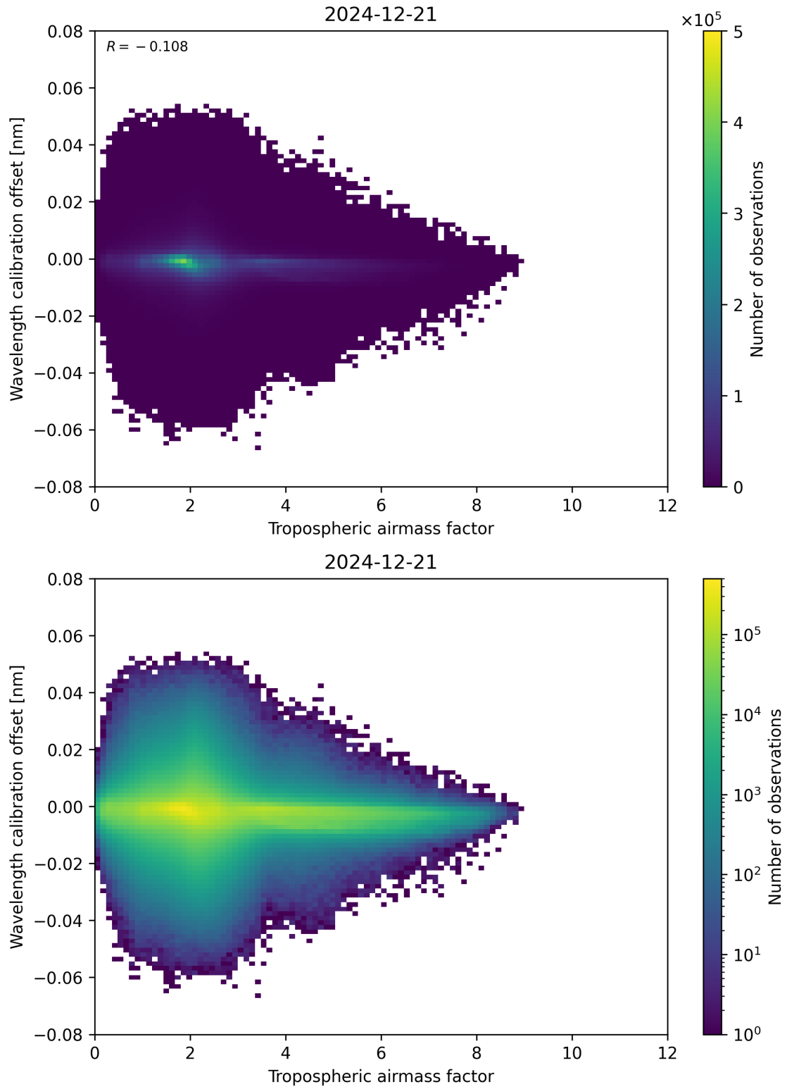
Figure 80: Scatter density plot of “Tropospheric air mass factor” against “Wavelength calibration offset” for 2024-12-20 to 2024-12-22.
