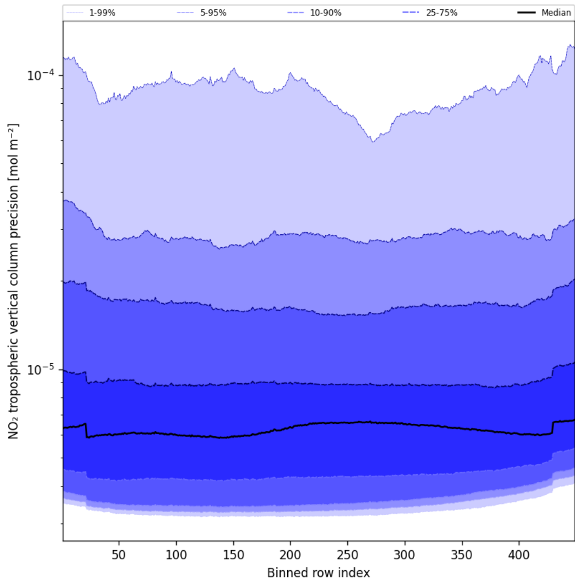
Figure 47: Along track statistics of “NO 2 tropospheric vertical column precision” for 2024-12-20 to 2024-12-22
