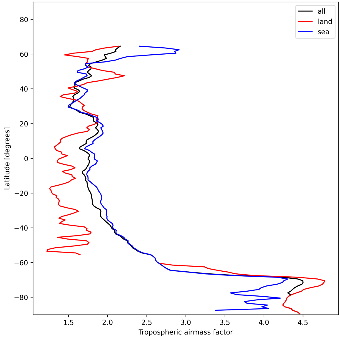
Figure 14: Zonal average of “Tropospheric airmass factor” for 2024-12-20 to 2024-12-22.
