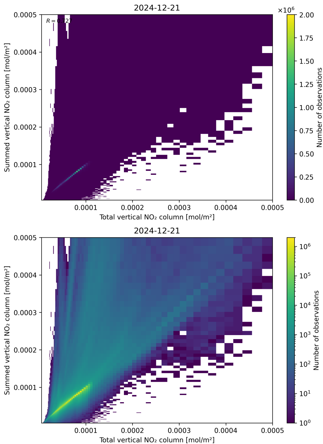
Figure 112: Scatter density plot of “Total vertical NO 2 column” against “Summed vertical NO 2 column” for 2024-12-20 to 2024-12-22.
