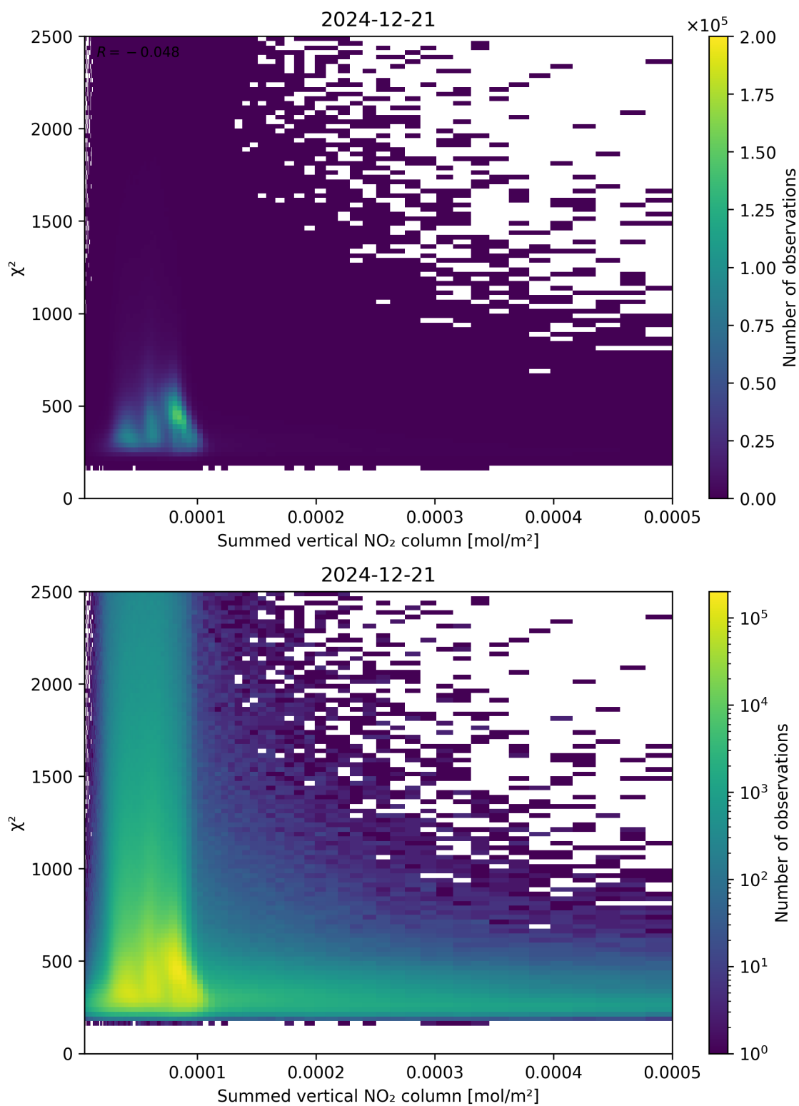
Figure 104: Scatter density plot of “Summed vertical NO 2 column” against “ \chi^2 ” for 2024-12-20 to 2024-12-22.
