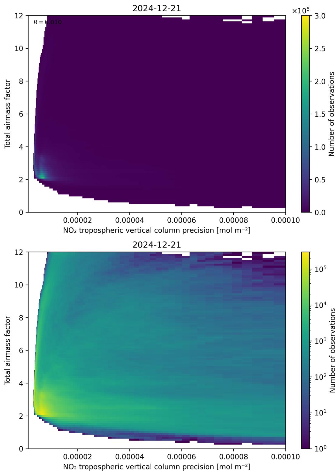
Figure 132: Scatter density plot of “NO 2 tropospheric vertical column precision” against “Total air mass factor” for 2024-12-20 to 2024-12-22.
