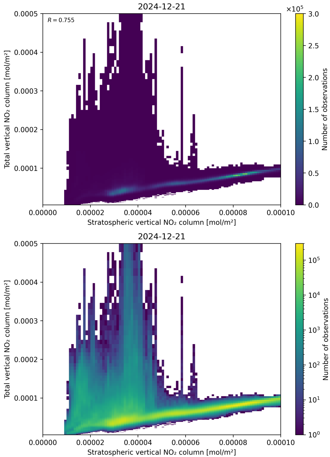
Figure 100: Scatter density plot of “Stratospheric vertical NO 2 column” against “Total vertical NO 2 column” for 2024-12-20 to 2024-12-22.
