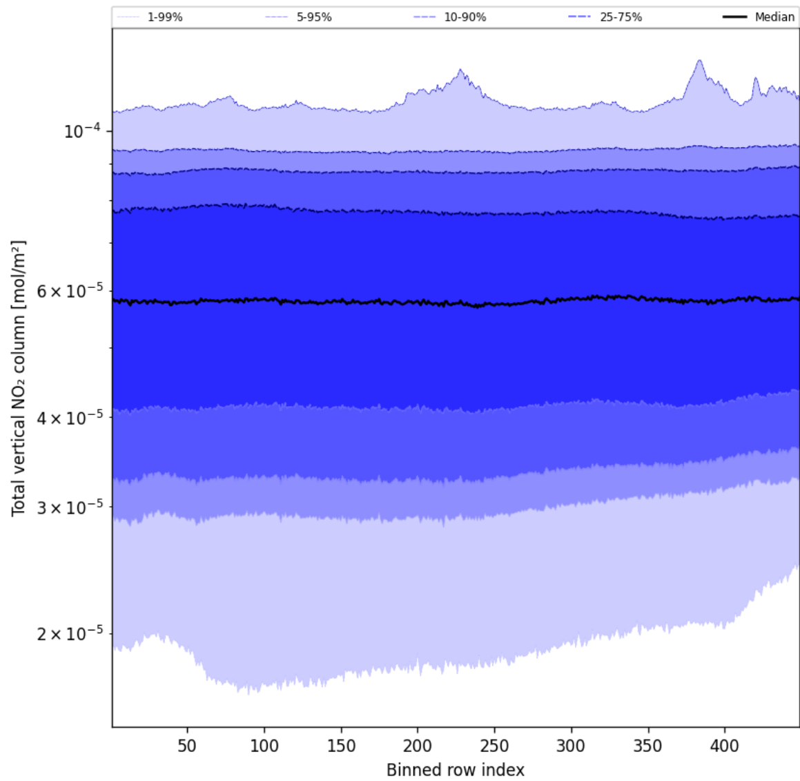
Figure 55: Along track statistics of “Total vertical NO 2 column” for 2024-12-20 to 2024-12-22
