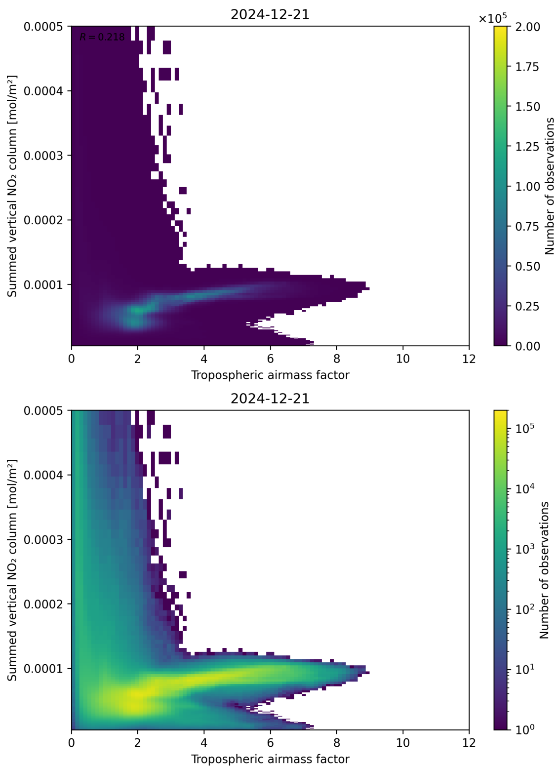
Figure 75: Scatter density plot of “Tropospheric air mass factor” against “Summed vertical NO 2 column” for 2024-12-20 to 2024-12-22.
