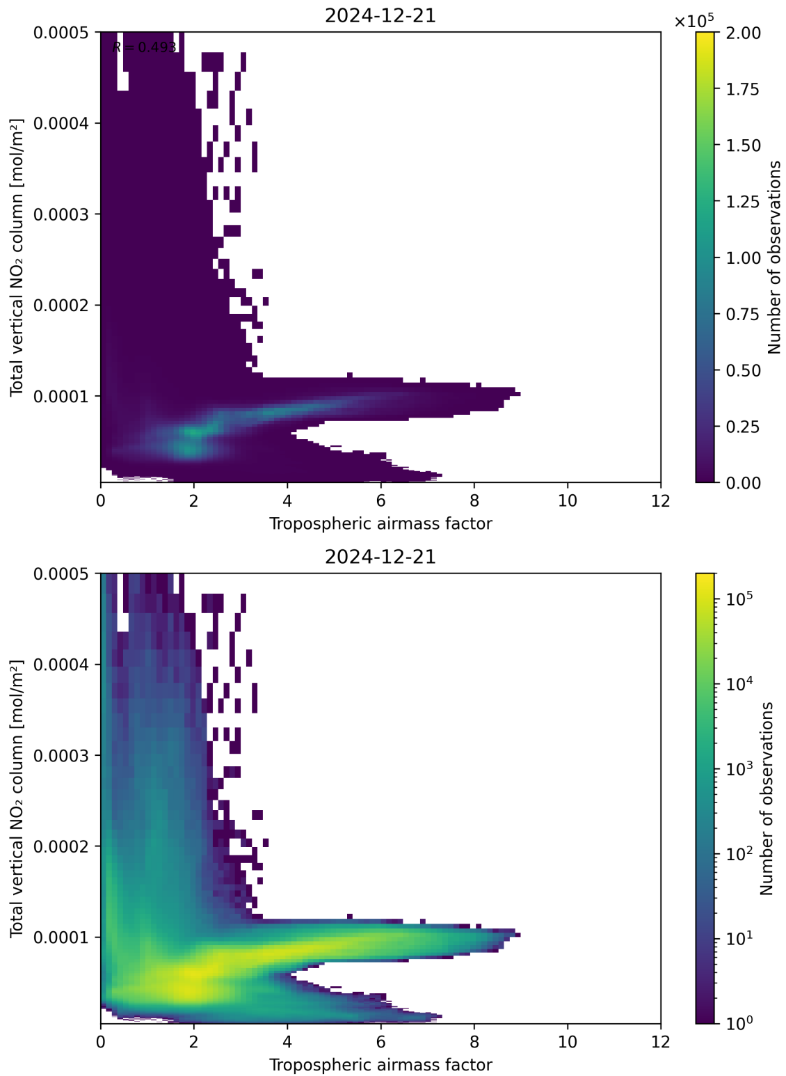
Figure 77: Scatter density plot of “Tropospheric airmass factor” against “Total vertical NO 2 column” for 2024-12-20 to 2024-12-22.
