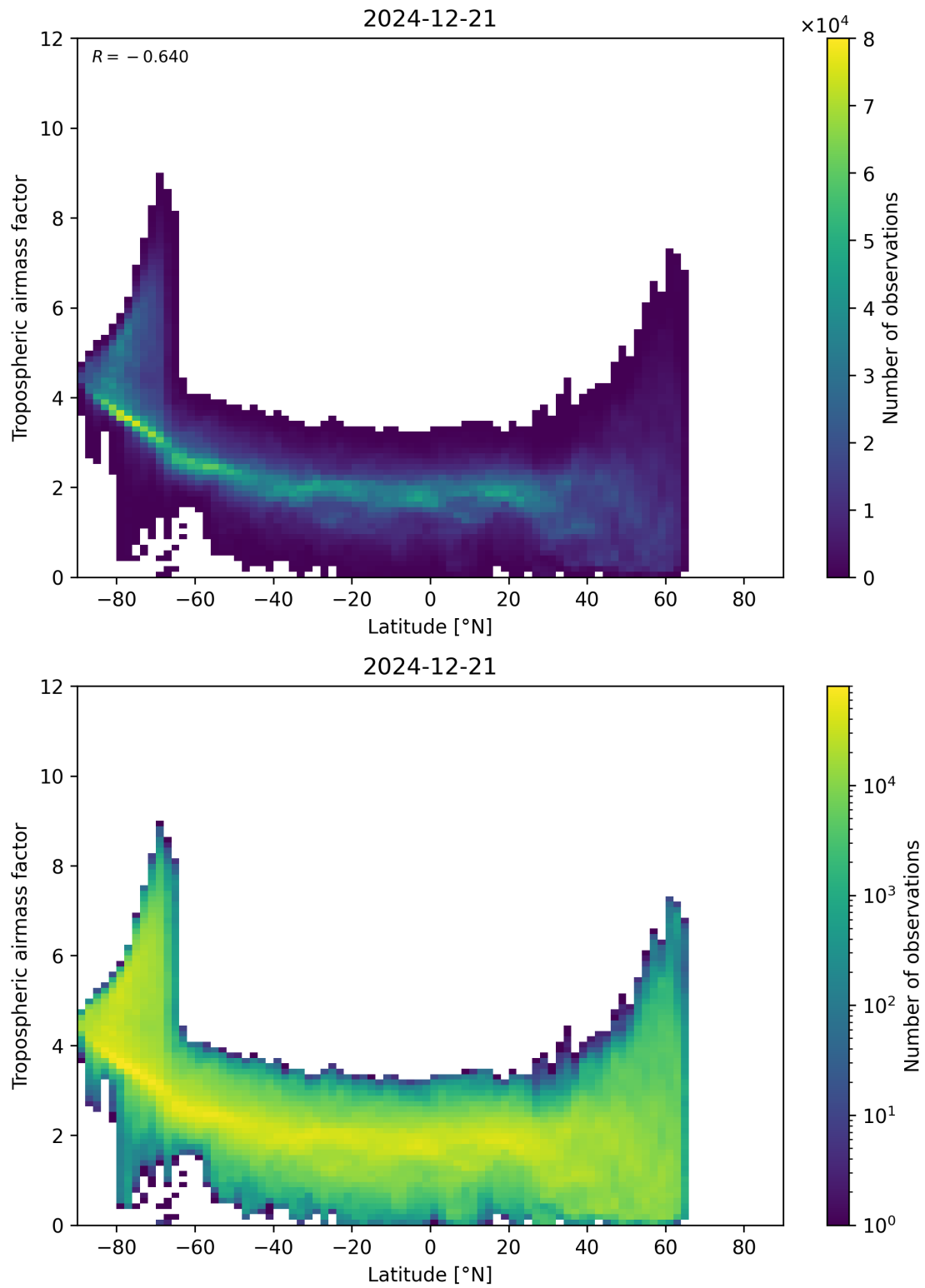
Figure 85: Scatter density plot of “Latitude” against “Tropospheric airmass factor” for 2024-12-20 to 2024-12-22.
