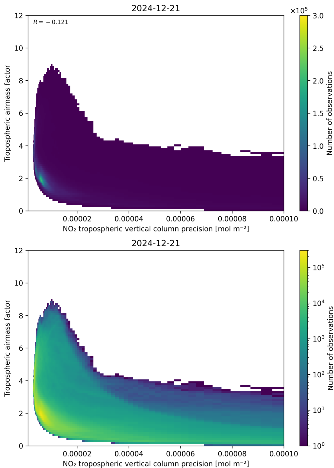
Figure 133: Scatter density plot of “NO 2 tropospheric vertical column precision” against “Tropospheric air mass factor” for 2024-12-20 to 2024-12-22.
