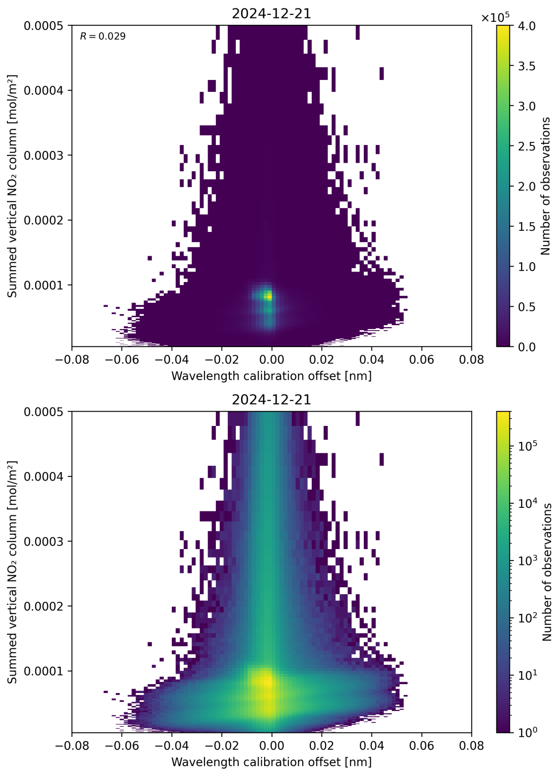
Figure 177: Scatter density plot of “Wavelength calibration offset” against “Summed vertical NO 2 column” for 2024-12-20 to 2024-12-22.
