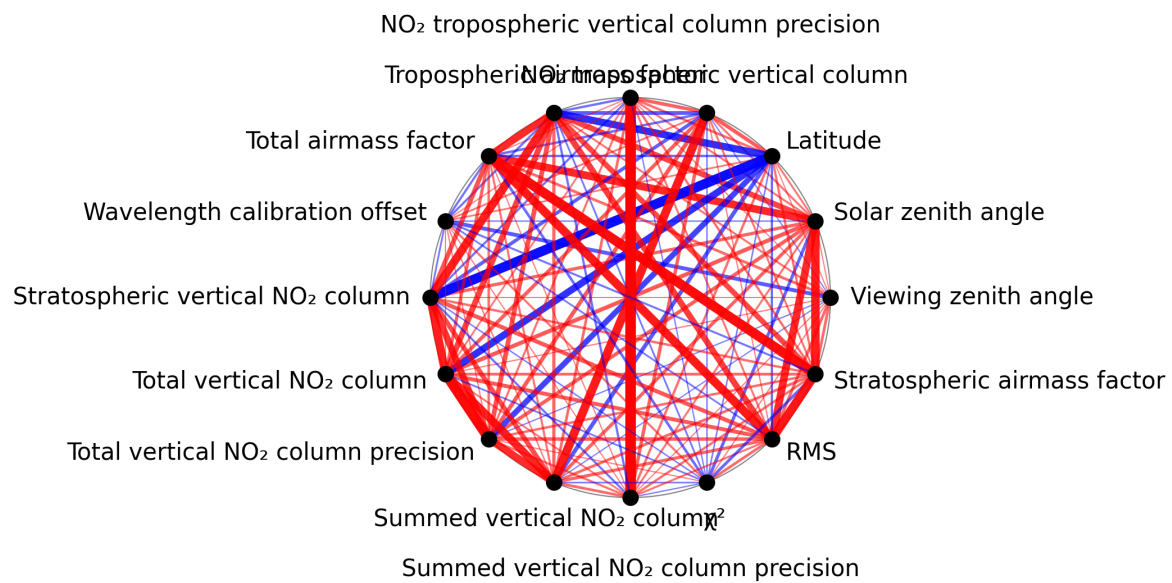
Figure 1: Map of correlation graph for 2024-12-20 to 2024-12-22.
