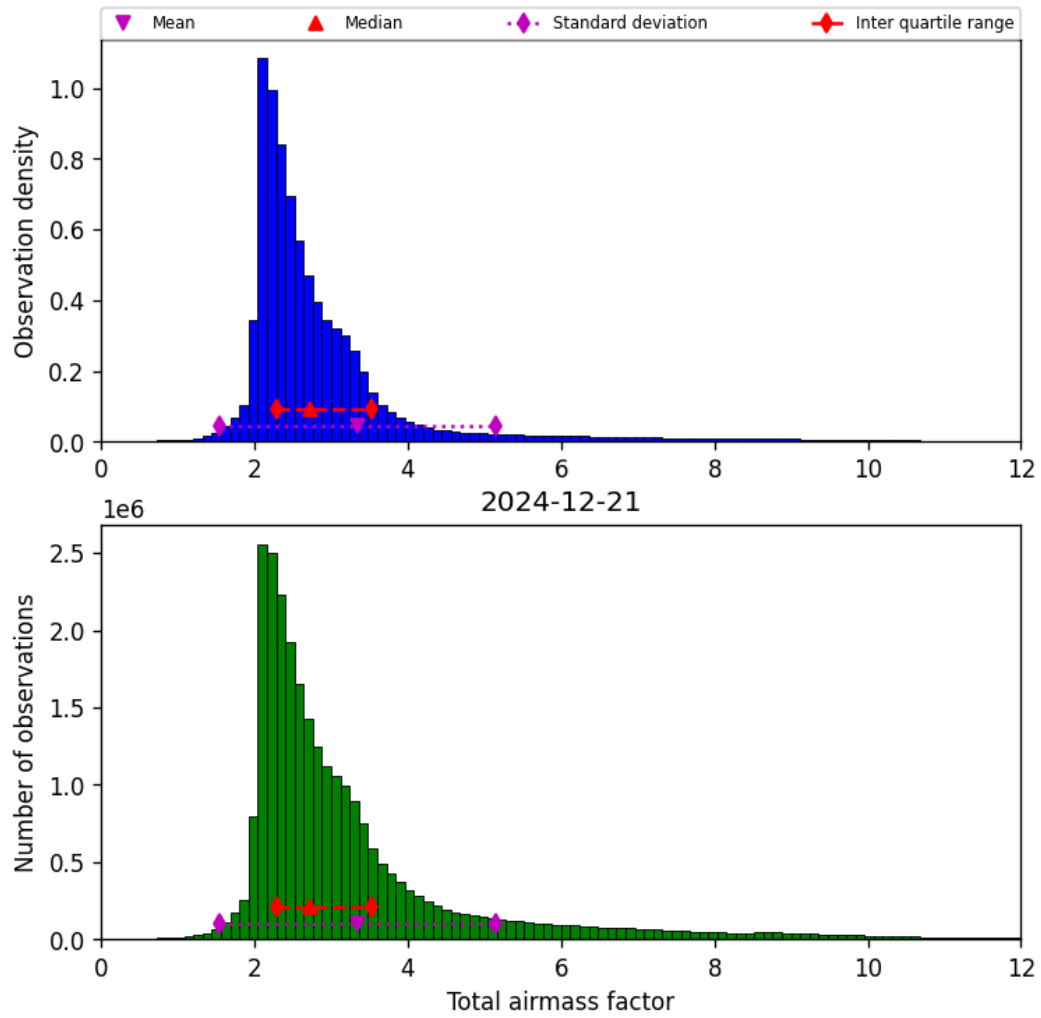
Figure 32: Histogram of “Total airmass factor” for 2024-12-20 to 2024-12-22
