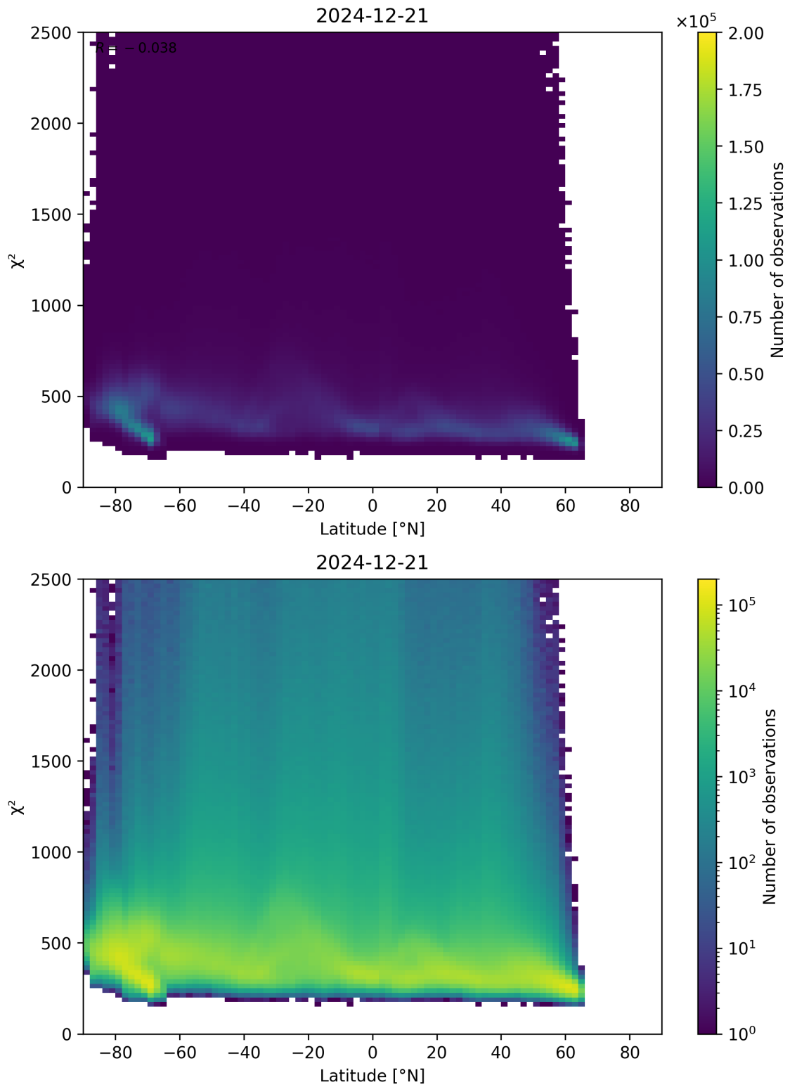
Figure 86: Scatter density plot of “Latitude” against “ \chi^2 ” for 2024-12-20 to 2024-12-22.
