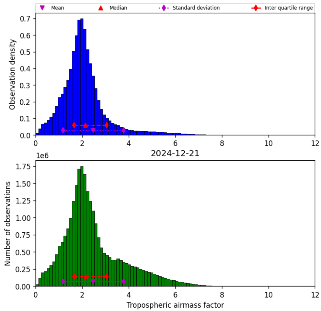
Figure 31: Histogram of “Tropospheric airmass factor” for 2024-12-20 to 2024-12-22
