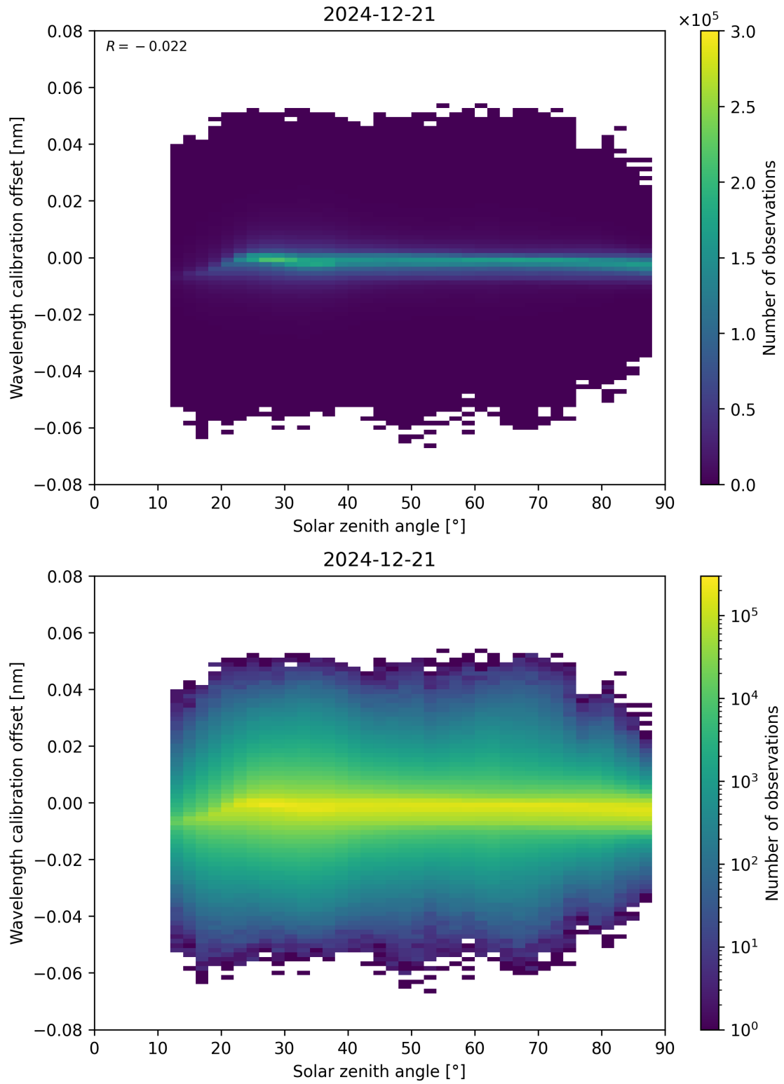
Figure 158: Scatter density plot of “Solar zenith angle” against “Wavelength calibration offset” for 2024-12-20 to 2024-12-22.
