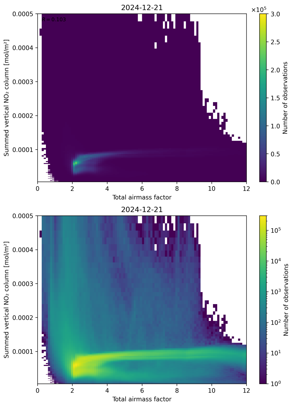
Figure 65: Scatter density plot of “Total airmass factor” against “Summed vertical NO 2 column” for 2024-12-20 to 2024-12-22.
