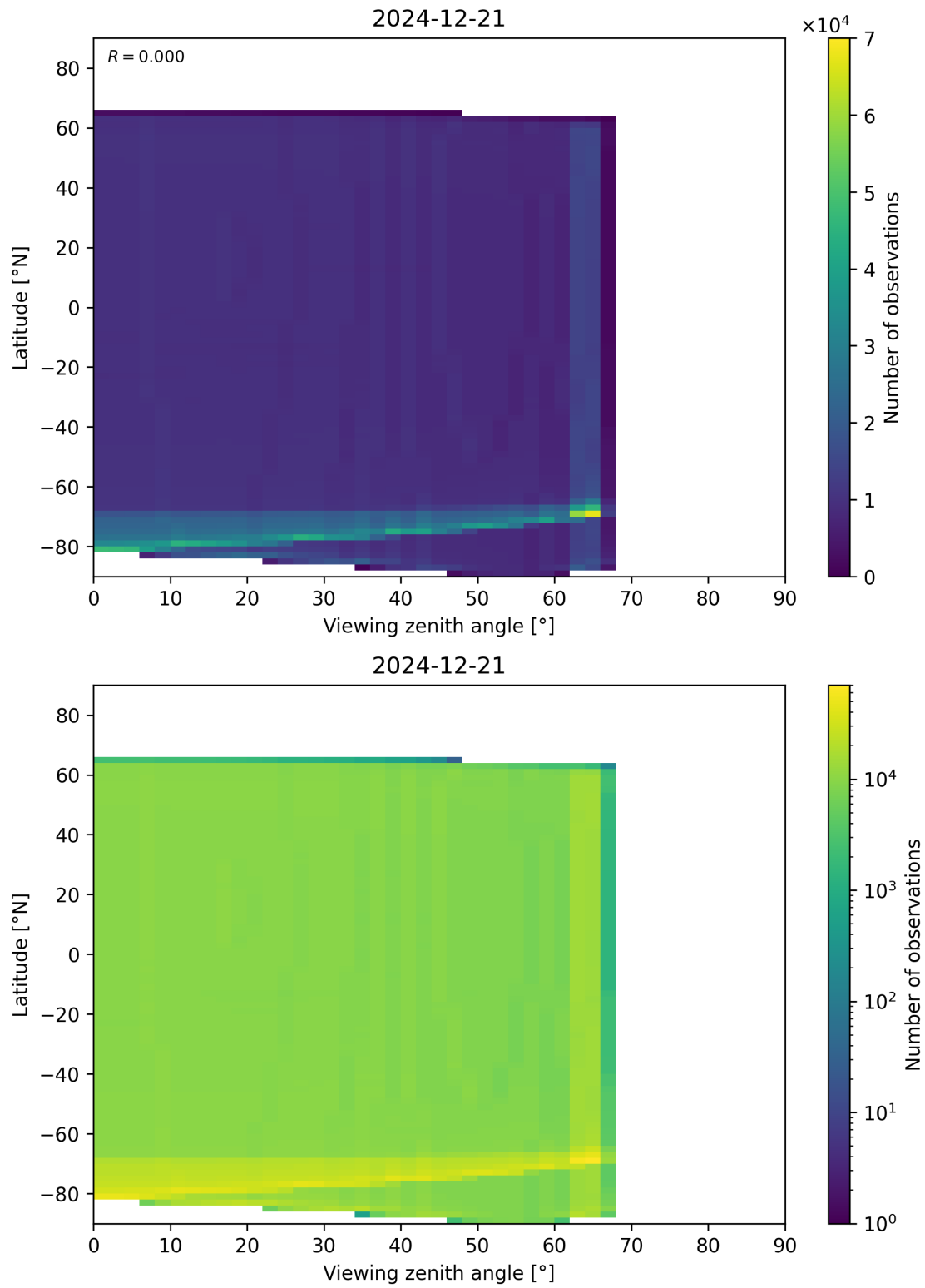
Figure 163: Scatter density plot of “Viewing zenith angle” against “Latitude” for 2024-12-20 to 2024-12-22.
