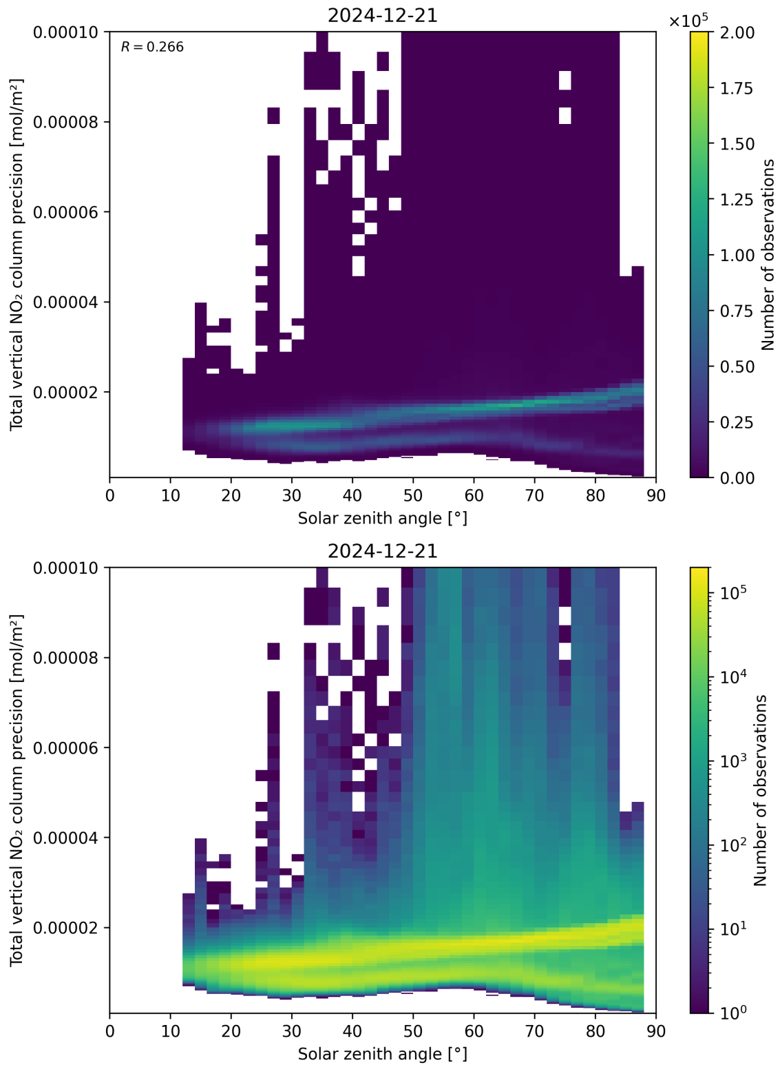
Figure 154: Scatter density plot of “Solar zenith angle” against “Total vertical NO 2 column precision” for 2024-12-20 to 2024-12-22.
