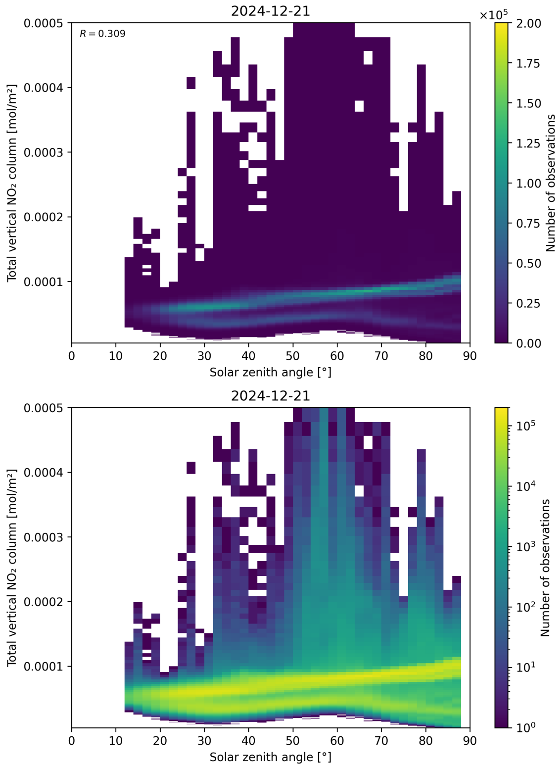
Figure 153: Scatter density plot of “Solar zenith angle” against “Total vertical NO 2 column” for 2024-12-20 to 2024-12-22.
