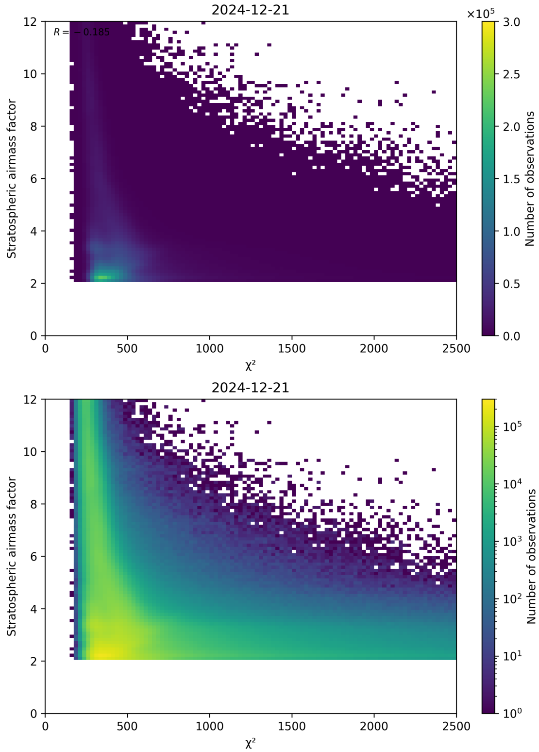
Figure 81: Scatter density plot of “ \chi^2 ” against “Stratospheric airmass factor” for 2024-12-20 to 2024-12-22.
