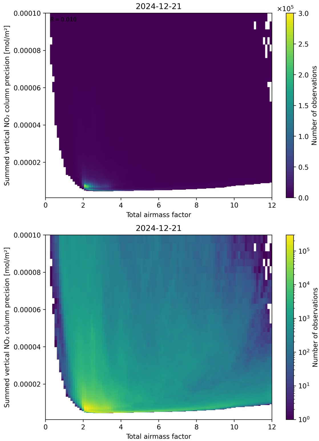
Figure 66: Scatter density plot of “Total airmass factor” against “Summed vertical NO 2 column precision” for 2024-12-20 to 2024-12-22.
