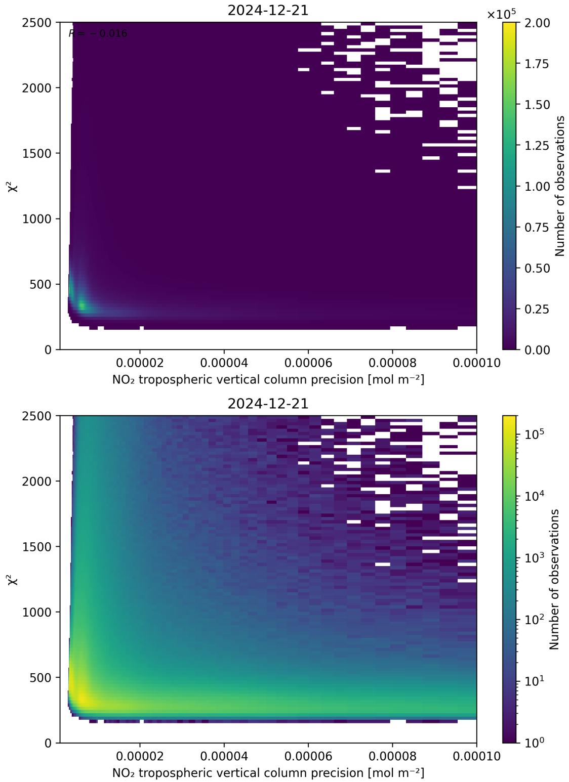
Figure 134: Scatter density plot of “NO 2 tropospheric vertical column precision” against “ \chi^2 ” for 2024-12-20 to 2024-12-22.
