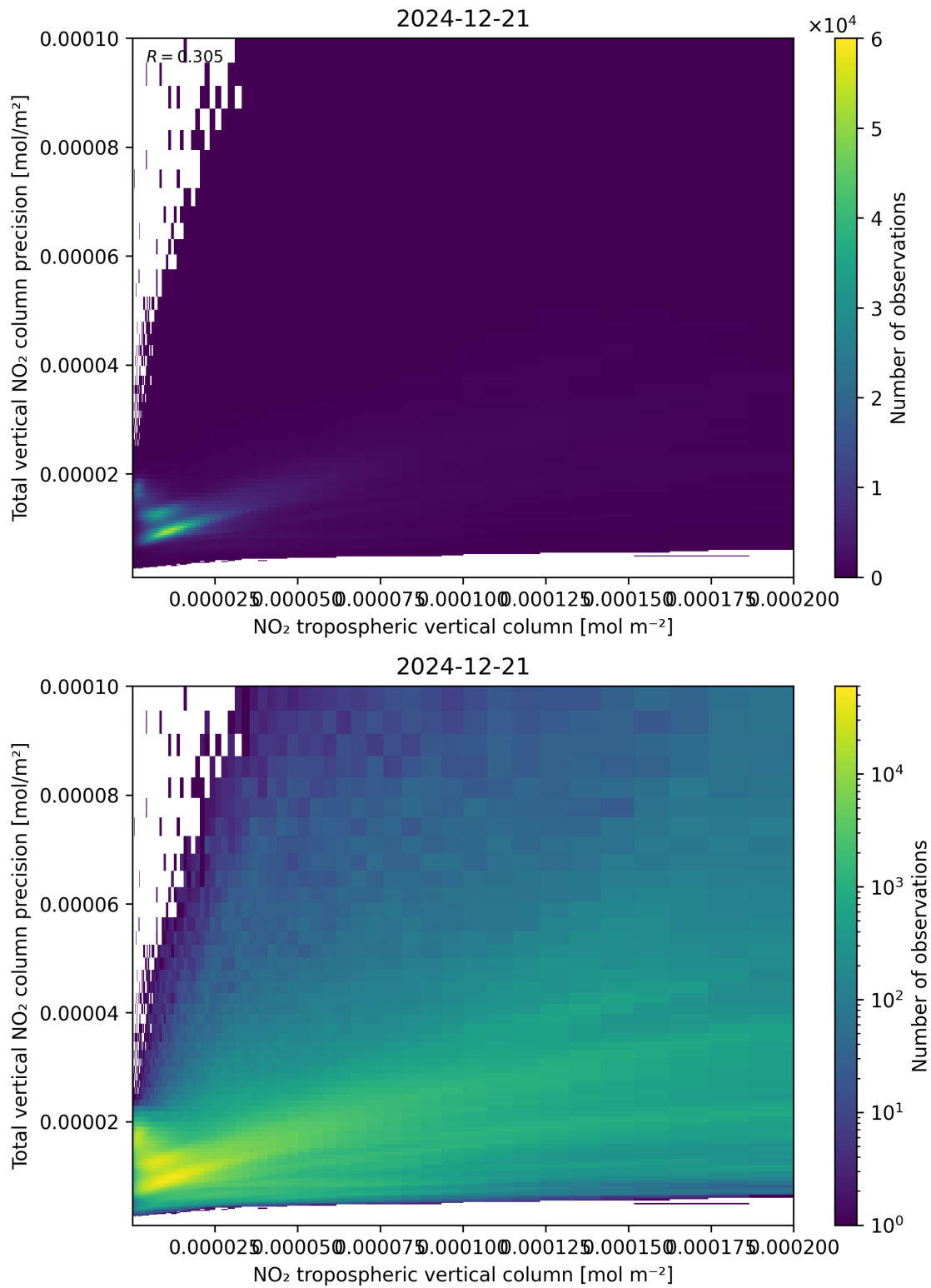
Figure 129: Scatter density plot of “NO 2 tropospheric vertical column” against “Total vertical NO 2 column precision” for 2024-12-20 to 2024-12-22.
