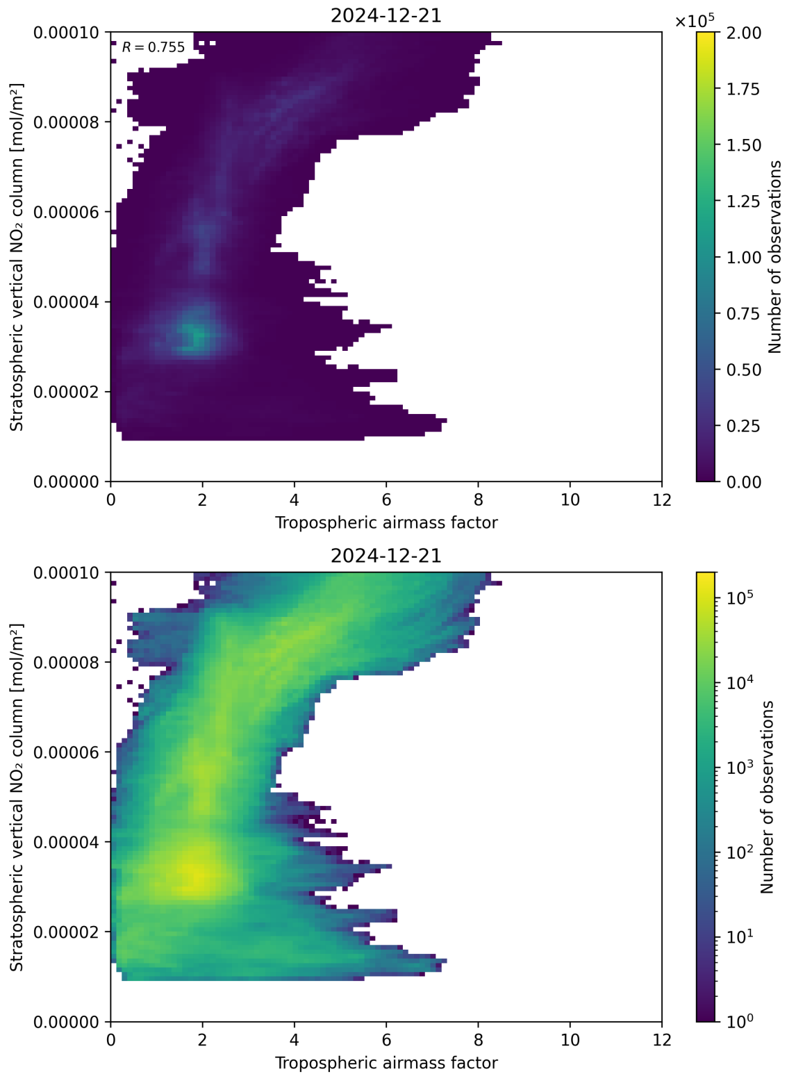
Figure 74: Scatter density plot of “Tropospheric air mass factor” against “Stratospheric vertical NO 2 column” for 2024-12-20 to 2024-12-22.
