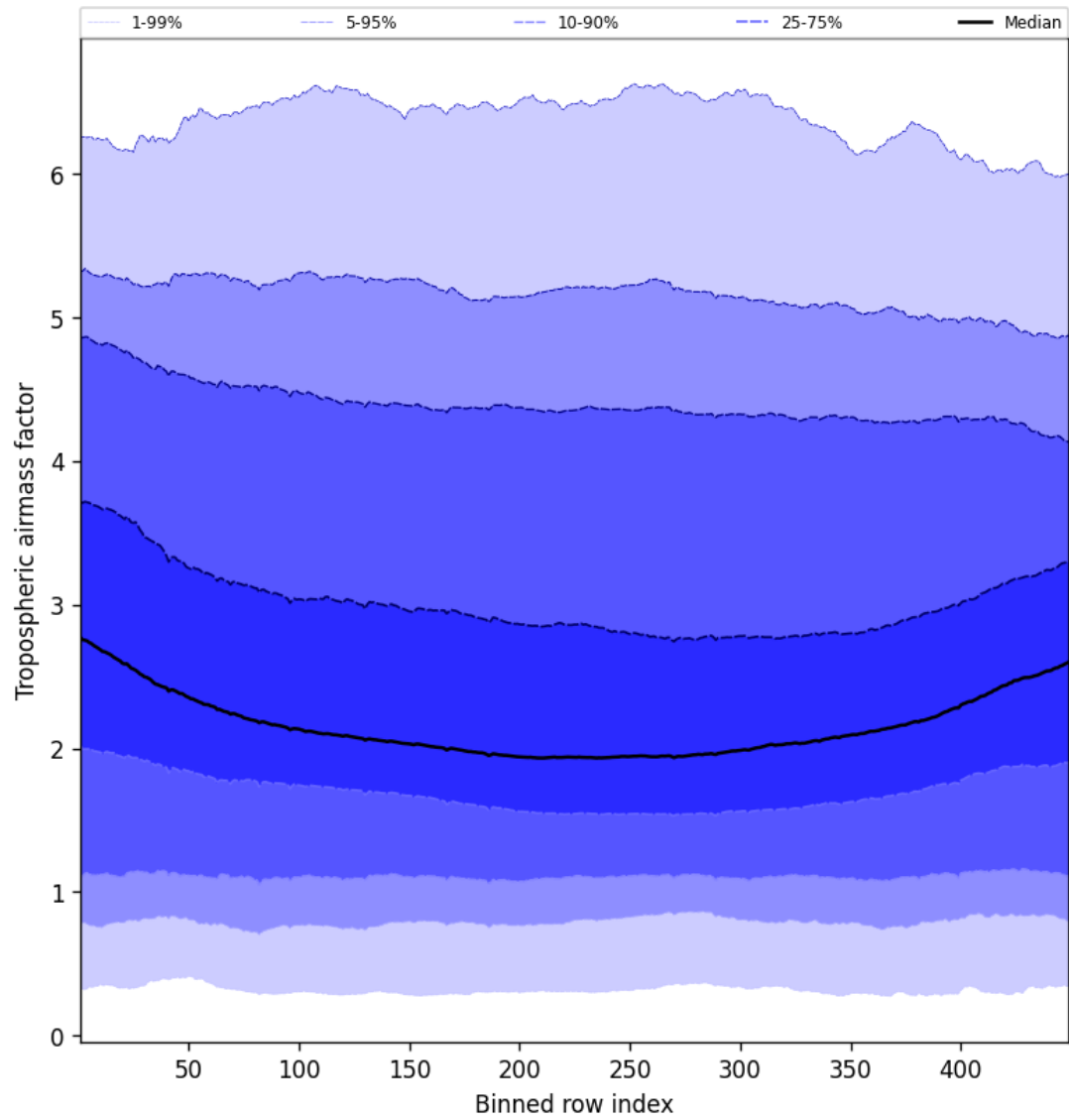
Figure 48: Along track statistics of “Tropospheric airmass factor” for 2024-12-20 to 2024-12-22
