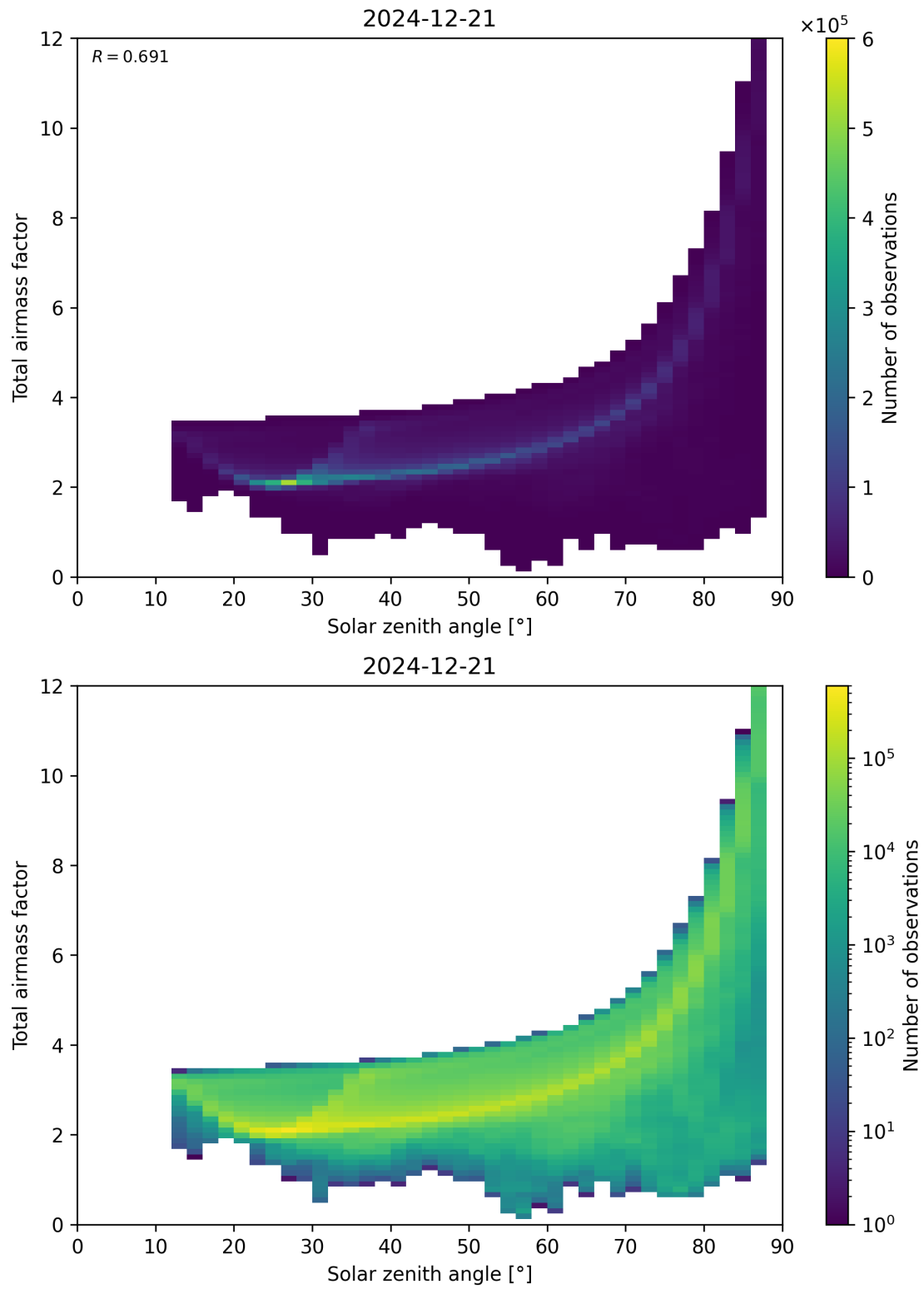
Figure 146: Scatter density plot of “Solar zenith angle” against “Total air mass factor” for 2024-12-20 to 2024-12-22.
