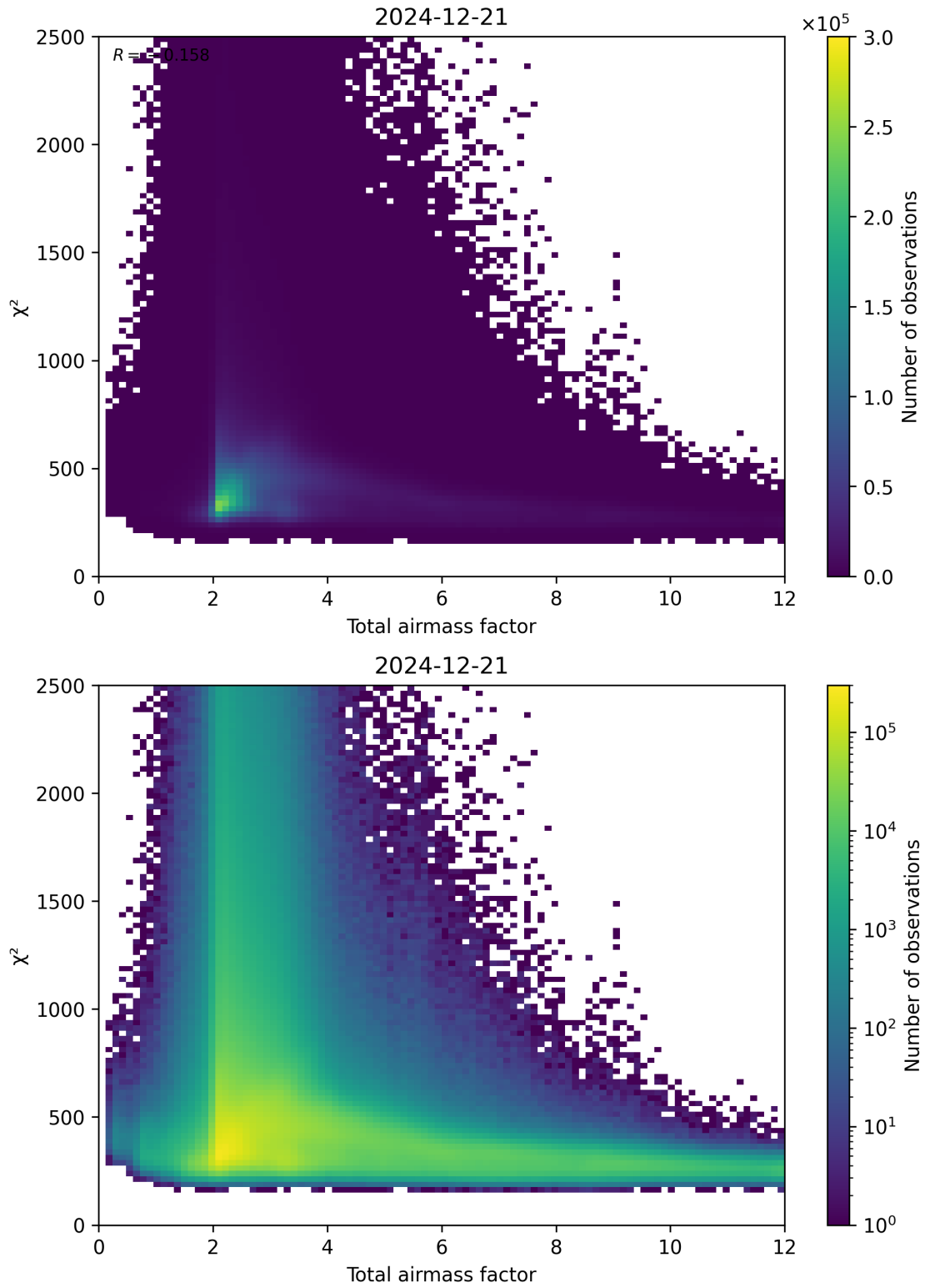
Figure 63: Scatter density plot of “Total airmass factor” against “ \chi^2 ” for 2024-12-20 to 2024-12-22.
