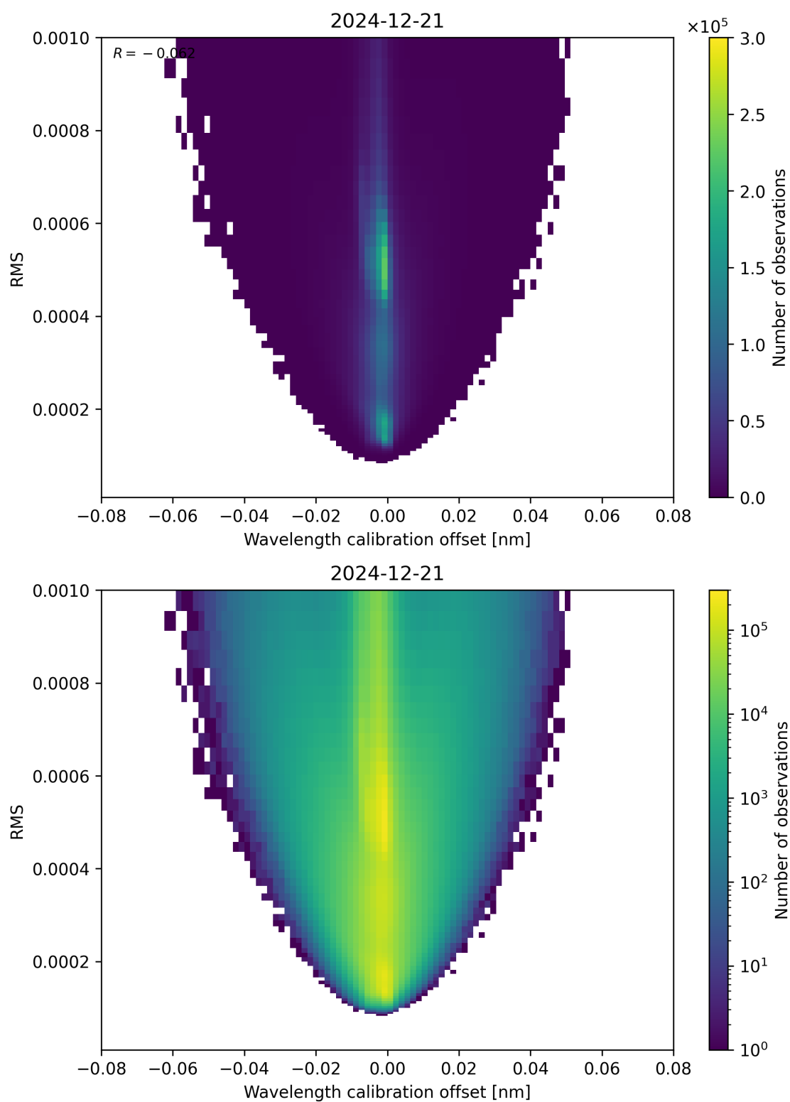
Figure 181: Scatter density plot of “Wavelength calibration offset” against “RMS” for 2024-12-20 to 2024-12-22.
