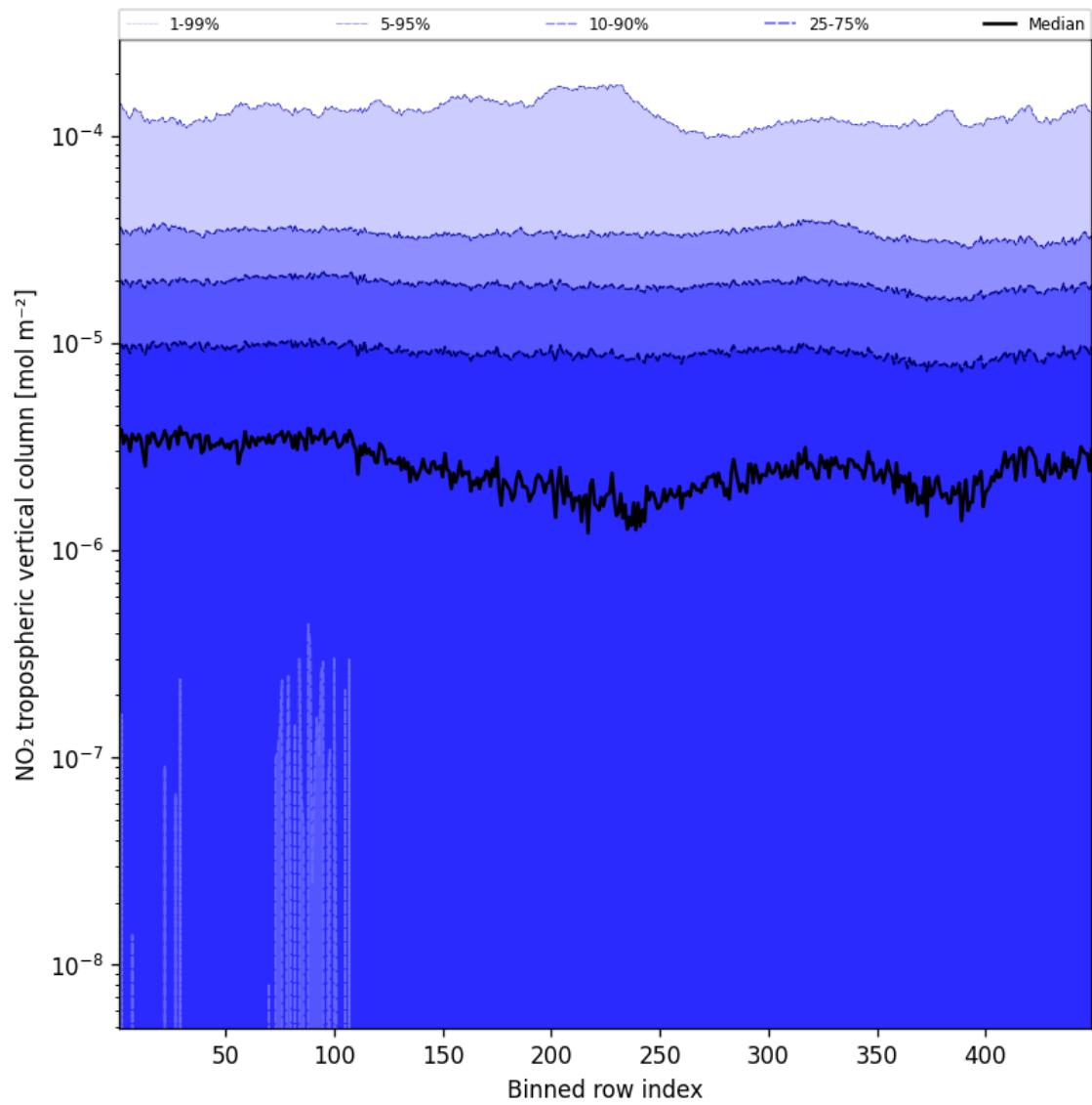
Figure 46: Along track statistics of “NO 2 tropospheric vertical column” for 2024-12-20 to 2024-12-22
