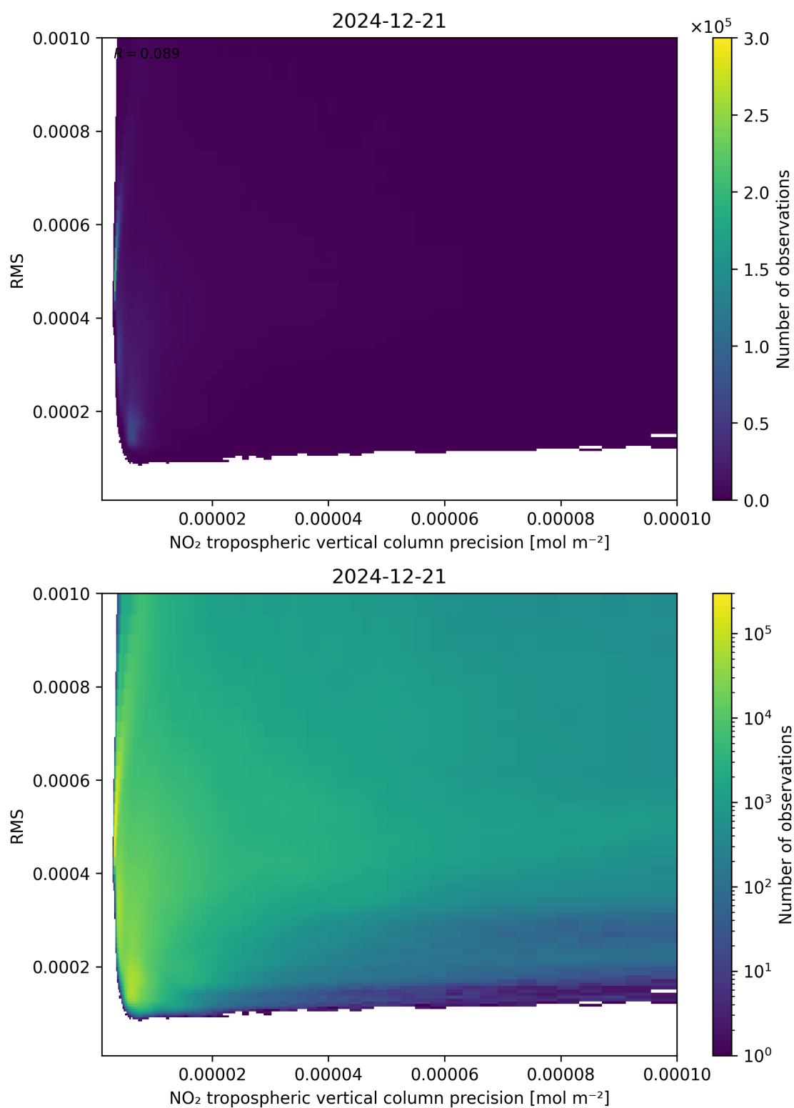
Figure 140: Scatter density plot of “NO 2 tropospheric vertical column precision” against “RMS” for 2024-12-20 to 2024-12-22.
