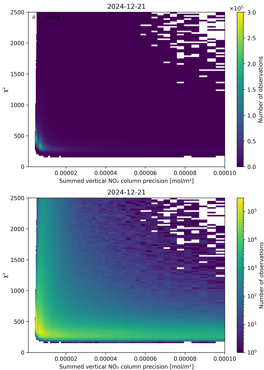
Figure 107: Scatter density plot of “Summed vertical NO 2 column precision” against “ \chi^2 ” for 2024-12-20 to 2024-12-22.
