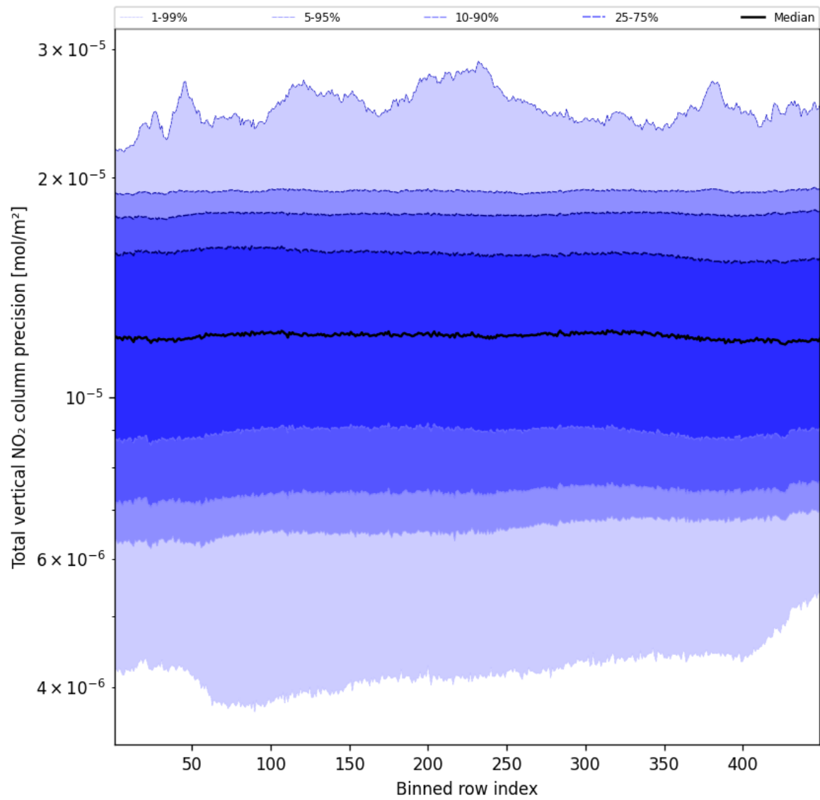
Figure 56: Along track statistics of "Total vertical NO 2 column precision" for 2024-12-20 to 2024-12-22
