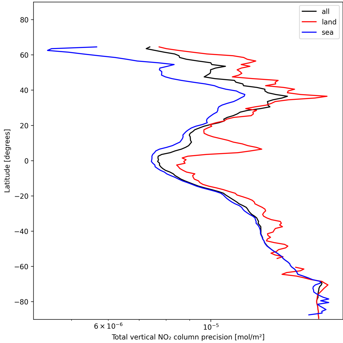
Figure 22: Zonal average of “Total vertical NO 2 column precision” for 2024-12-20 to 2024-12-22.
