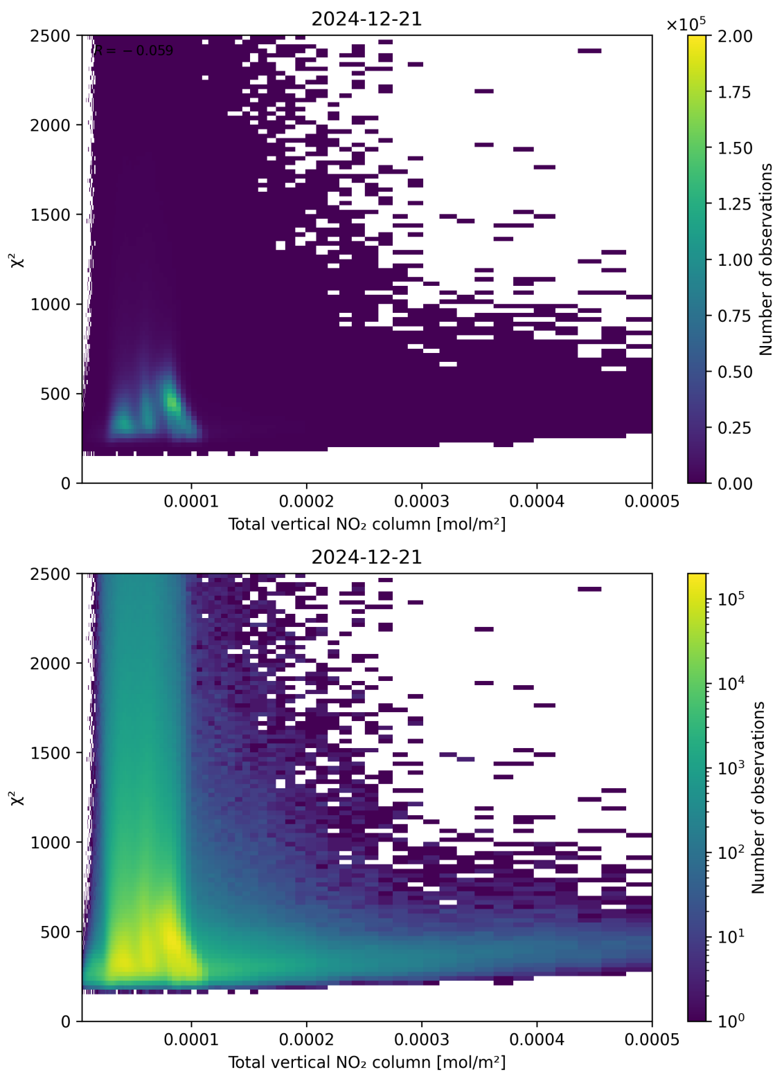
Figure 111: Scatter density plot of “Total vertical NO 2 column” against “ \chi^2 ” for 2024-12-20 to 2024-12-22.
