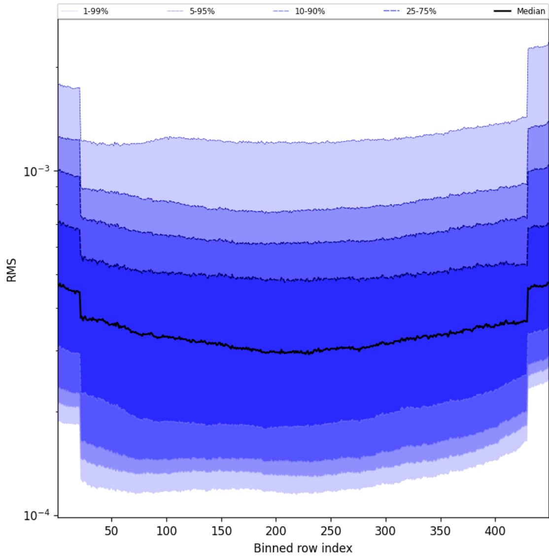
Figure 60: Along track statistics of “RMS” for 2024-12-20 to 2024-12-22
