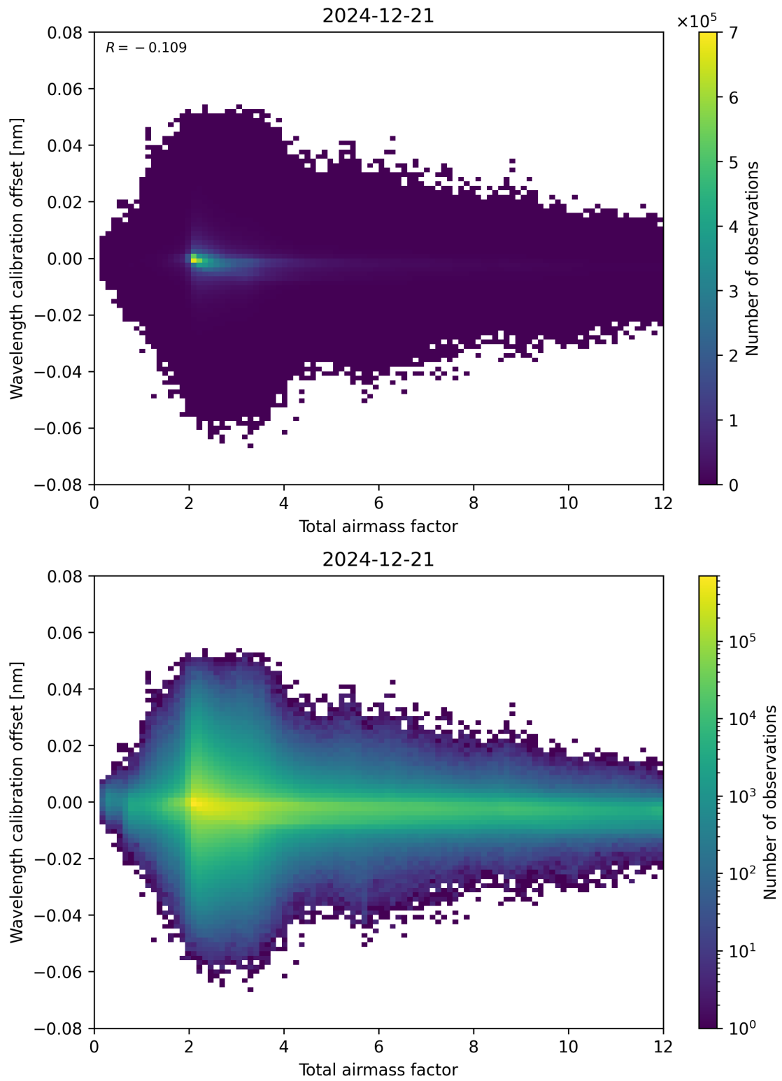
Figure 70: Scatter density plot of “Total airmass factor” against “Wavelength calibration offset” for 2024-12-20 to 2024-12-22.
