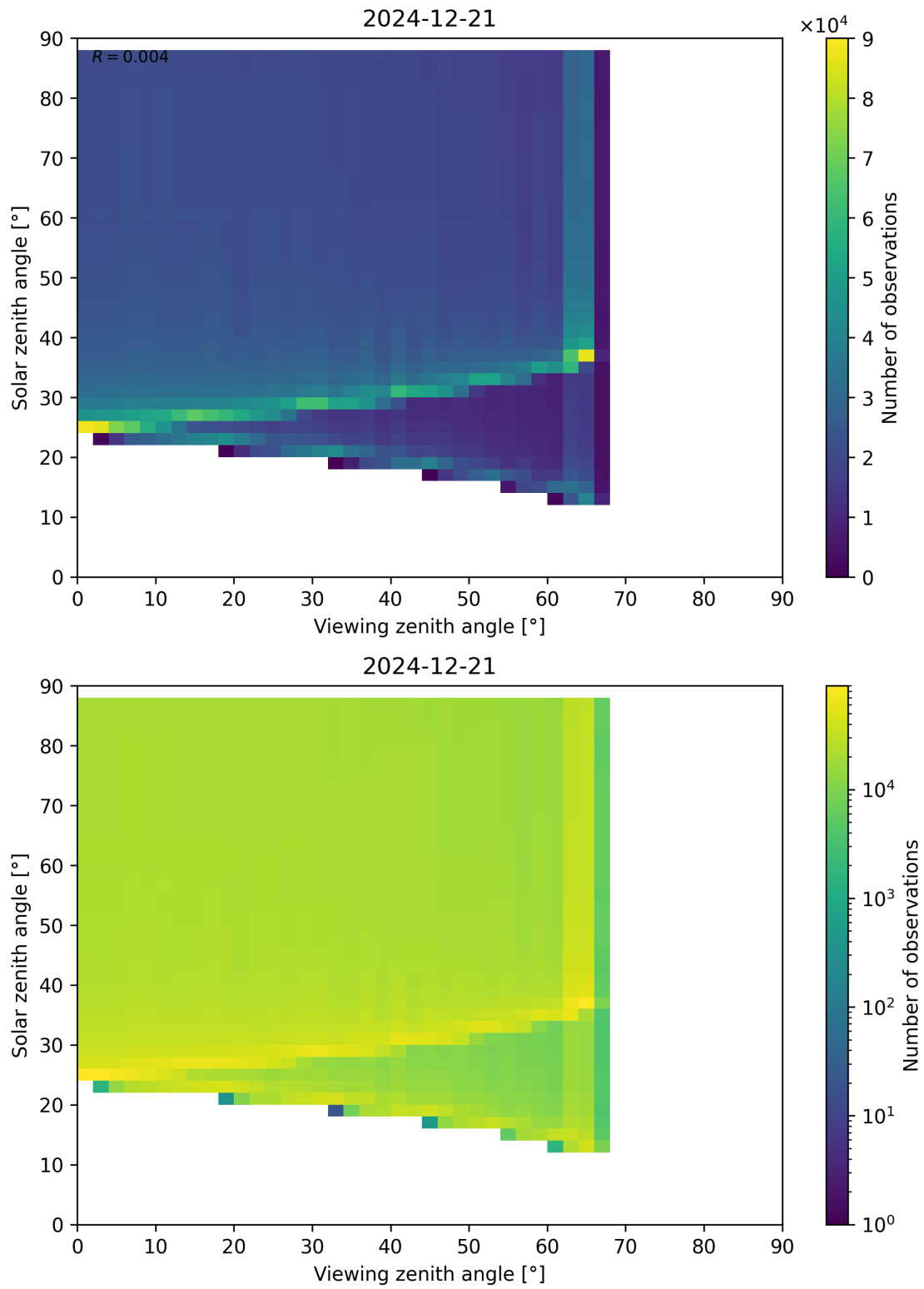
Figure 172: Scatter density plot of “Viewing zenith angle” against “Solar zenith angle” for 2024-12-20 to 2024-12-22.
