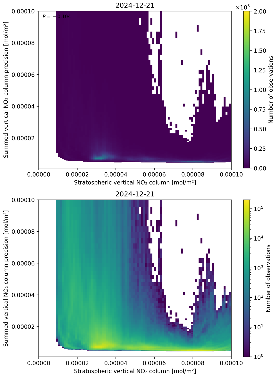
Figure 99: Scatter density plot of “Stratospheric vertical NO 2 column” against “Summed vertical NO 2 column precision” for 2024-12-20 to 2024-12-22.
