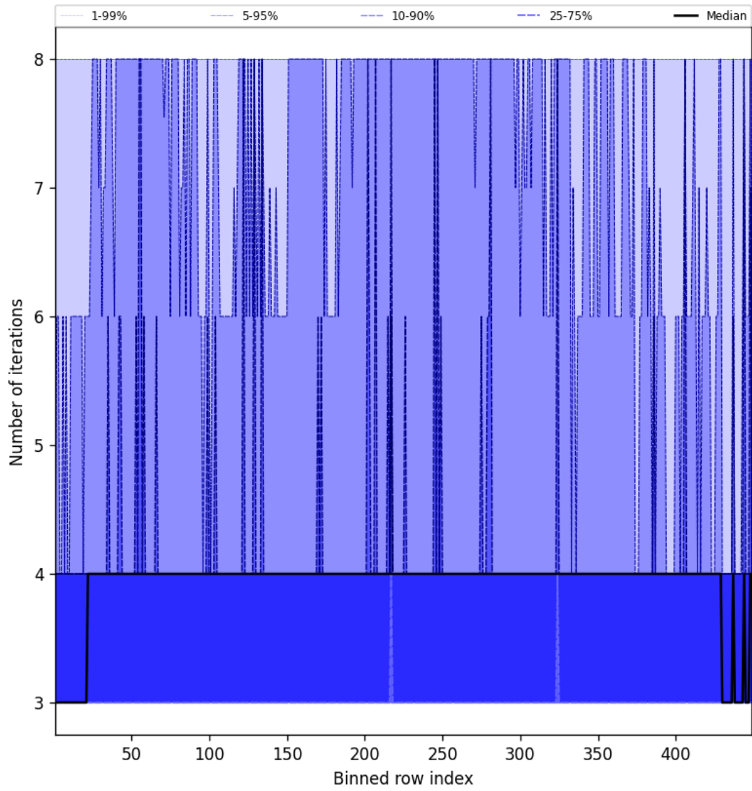
Figure 51: Along track statistics of “Number of iterations” for 2024-12-20 to 2024-12-22
