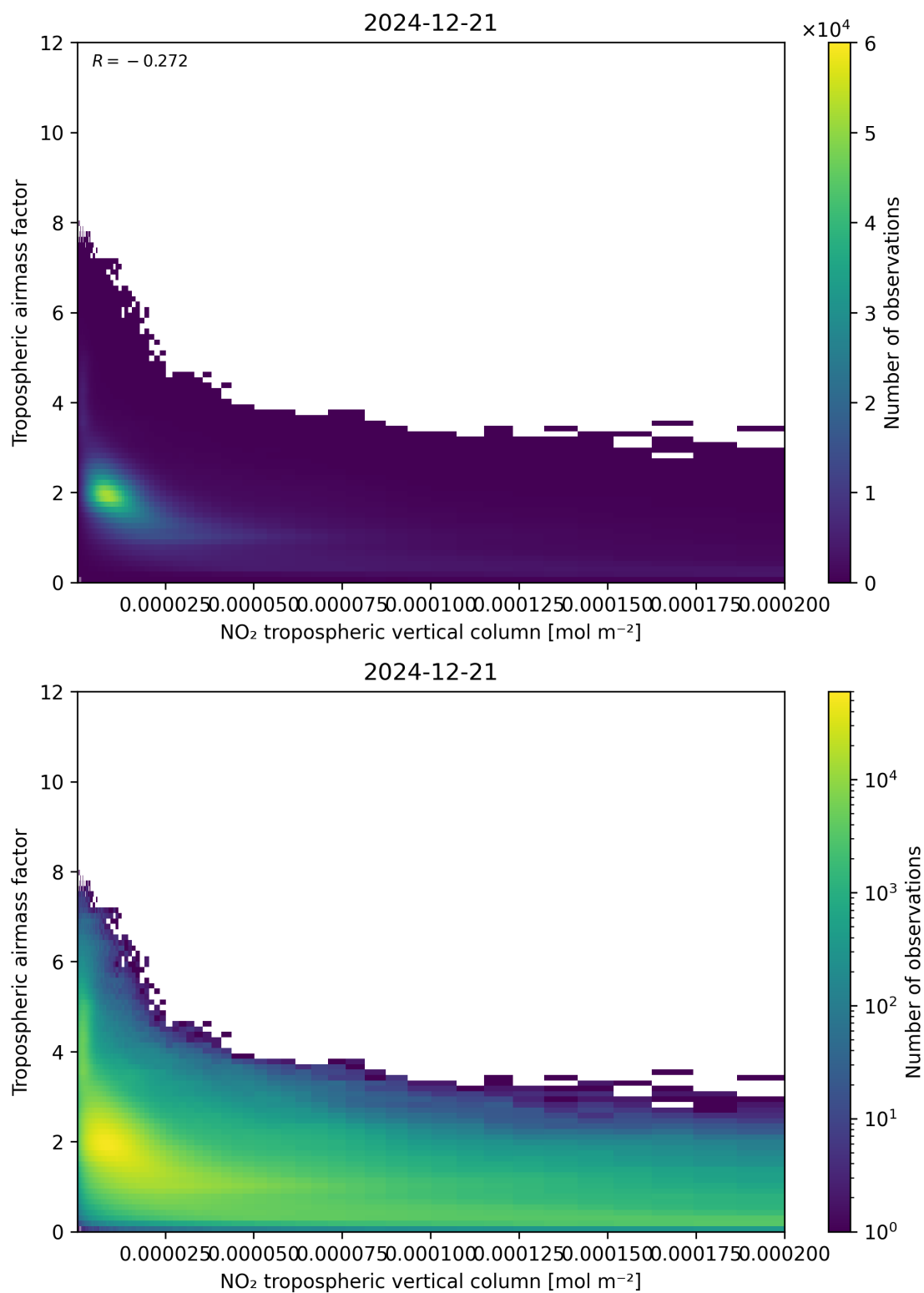
Figure 123: Scatter density plot of “NO 2 tropospheric vertical column” against “Tropospheric air mass factor” for 2024-12-20 to 2024-12-22.
