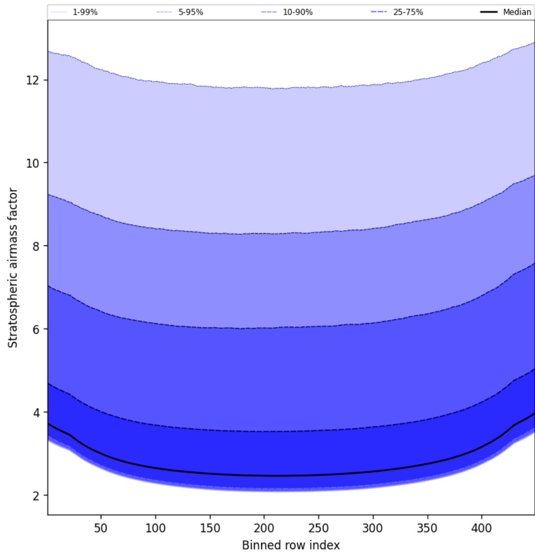
Figure 61: Along track statistics of “Stratospheric air mass factor” for 2024-12-20 to 2024-12-22
