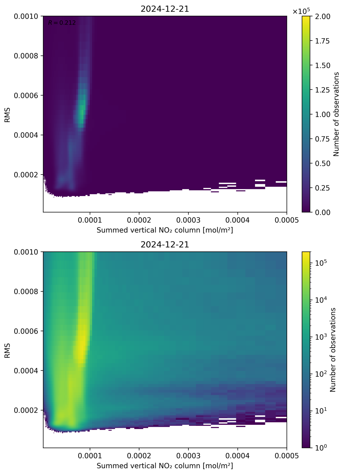
Figure 109: Scatter density plot of “Summed vertical NO 2 column” against “RMS” for 2024-12-20 to 2024-12-22.
