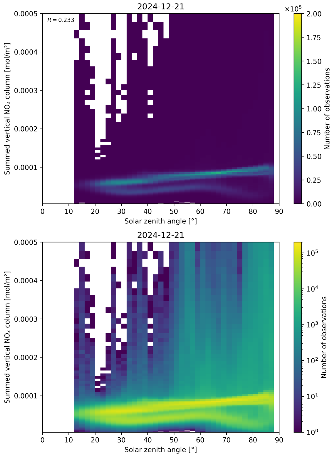
Figure 151: Scatter density plot of “Solar zenith angle” against “Summed vertical NO 2 column” for 2024-12-20 to 2024-12-22.
