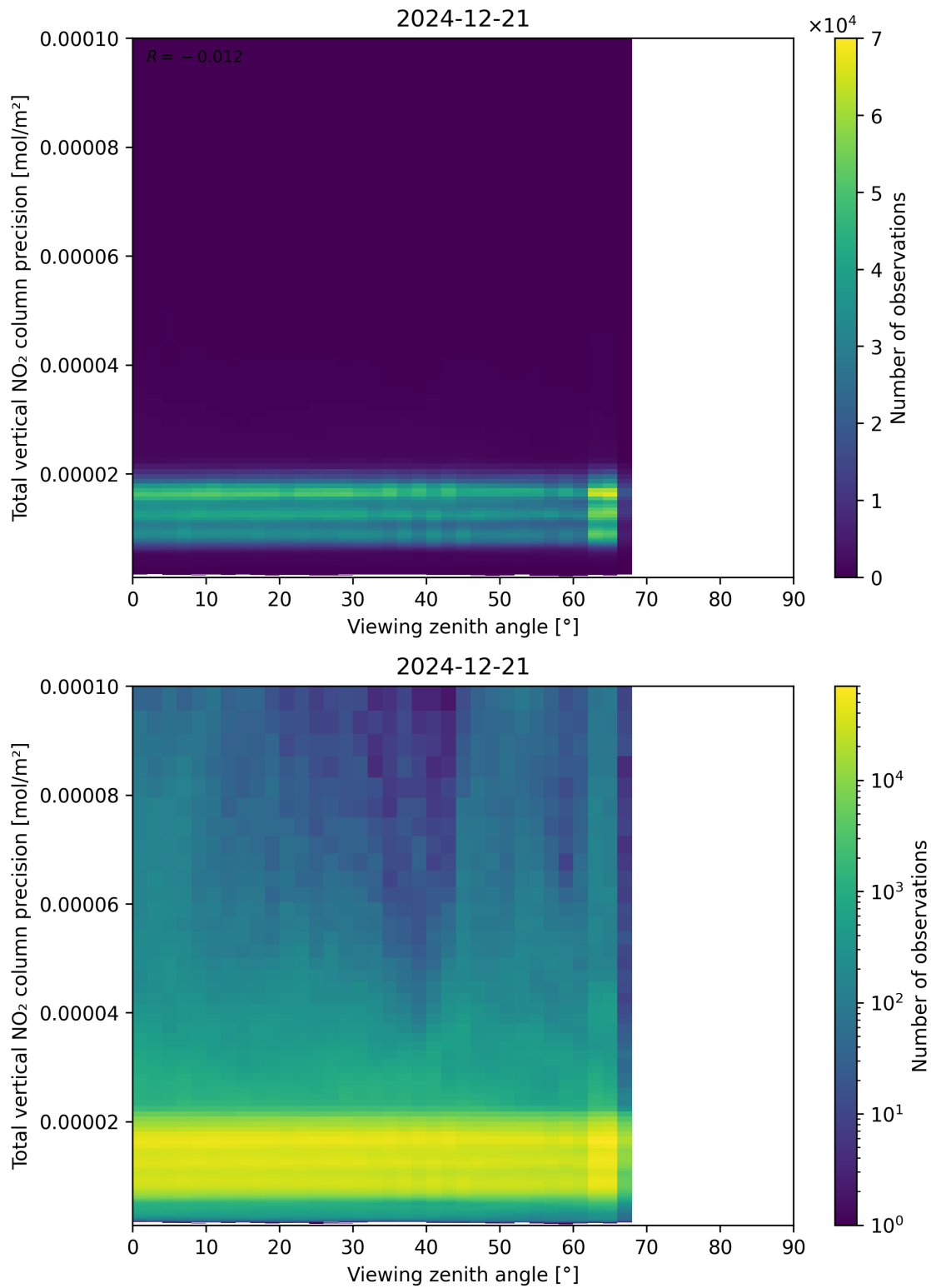
Figure 168: Scatter density plot of “Viewing zenith angle” against “Total vertical NO 2 column precision” for 2024-12-20 to 2024-12-22.
