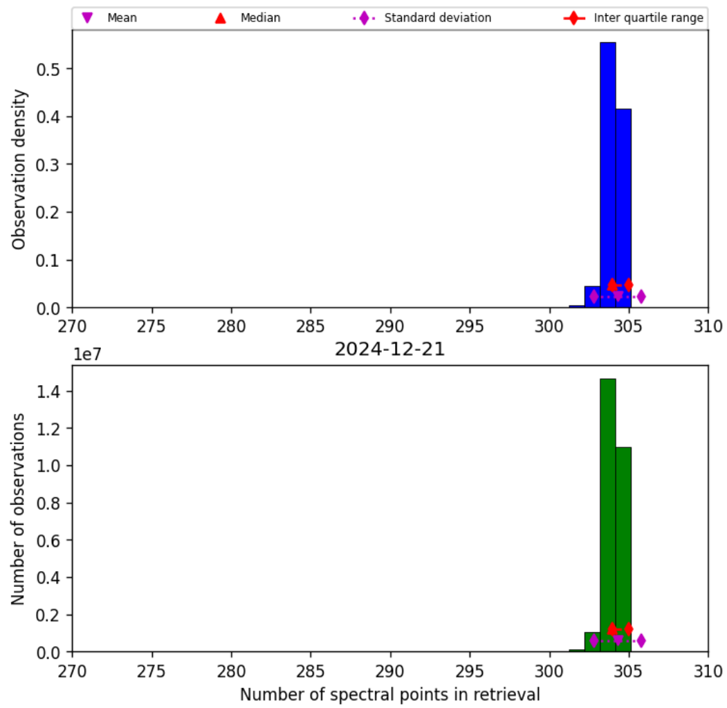
Figure 33: Histogram of “Number of spectral points in retrieval” for 2024-12-20 to 2024-12-22
