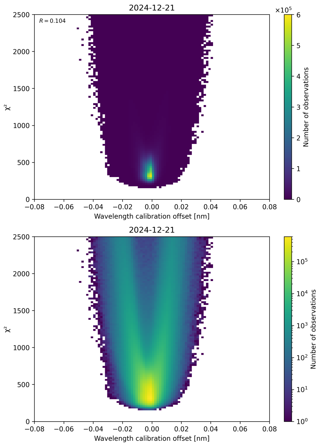
Figure 175: Scatter density plot of “Wavelength calibration offset” against “ \chi^2 ” for 2024-12-20 to 2024-12-22.
