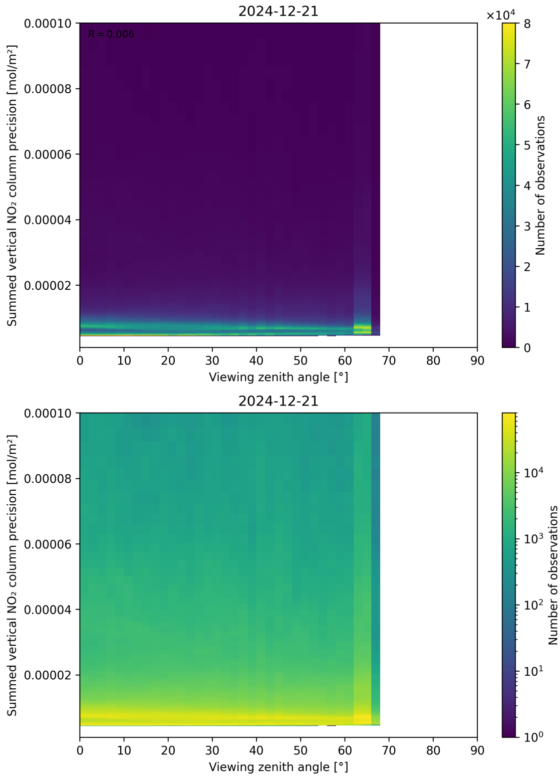
Figure 166: Scatter density plot of “Viewing zenith angle” against “Summed vertical NO 2 column precision” for 2024-12-20 to 2024-12-22.
