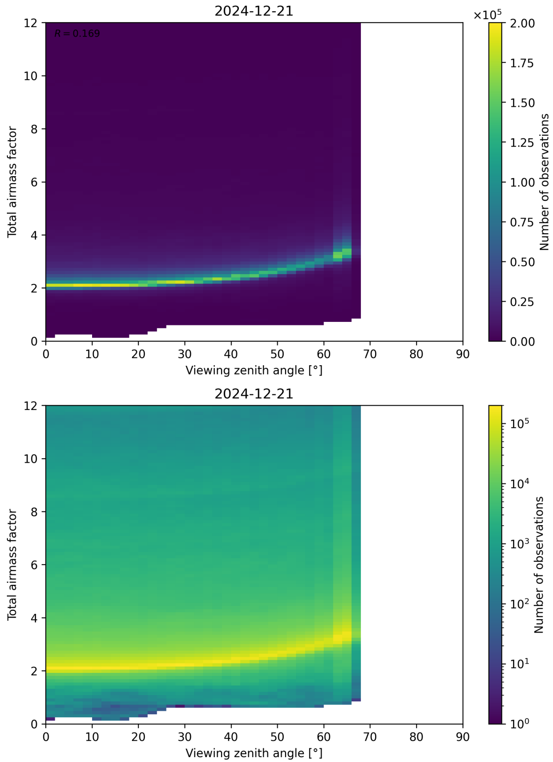
Figure 160: Scatter density plot of “Viewing zenith angle” against “Total airmass factor” for 2024-12-20 to 2024-12-22.
