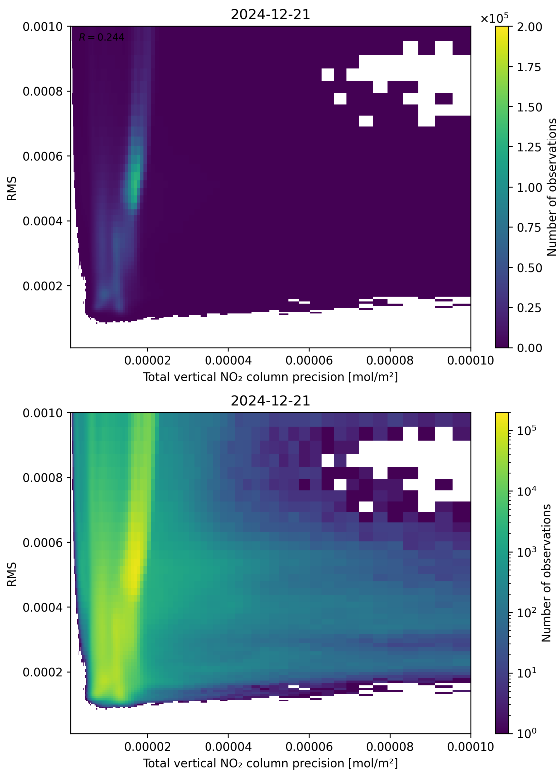
Figure 119: Scatter density plot of “Total vertical NO 2 column precision” against “RMS” for 2024-12-20 to 2024-12-22.
