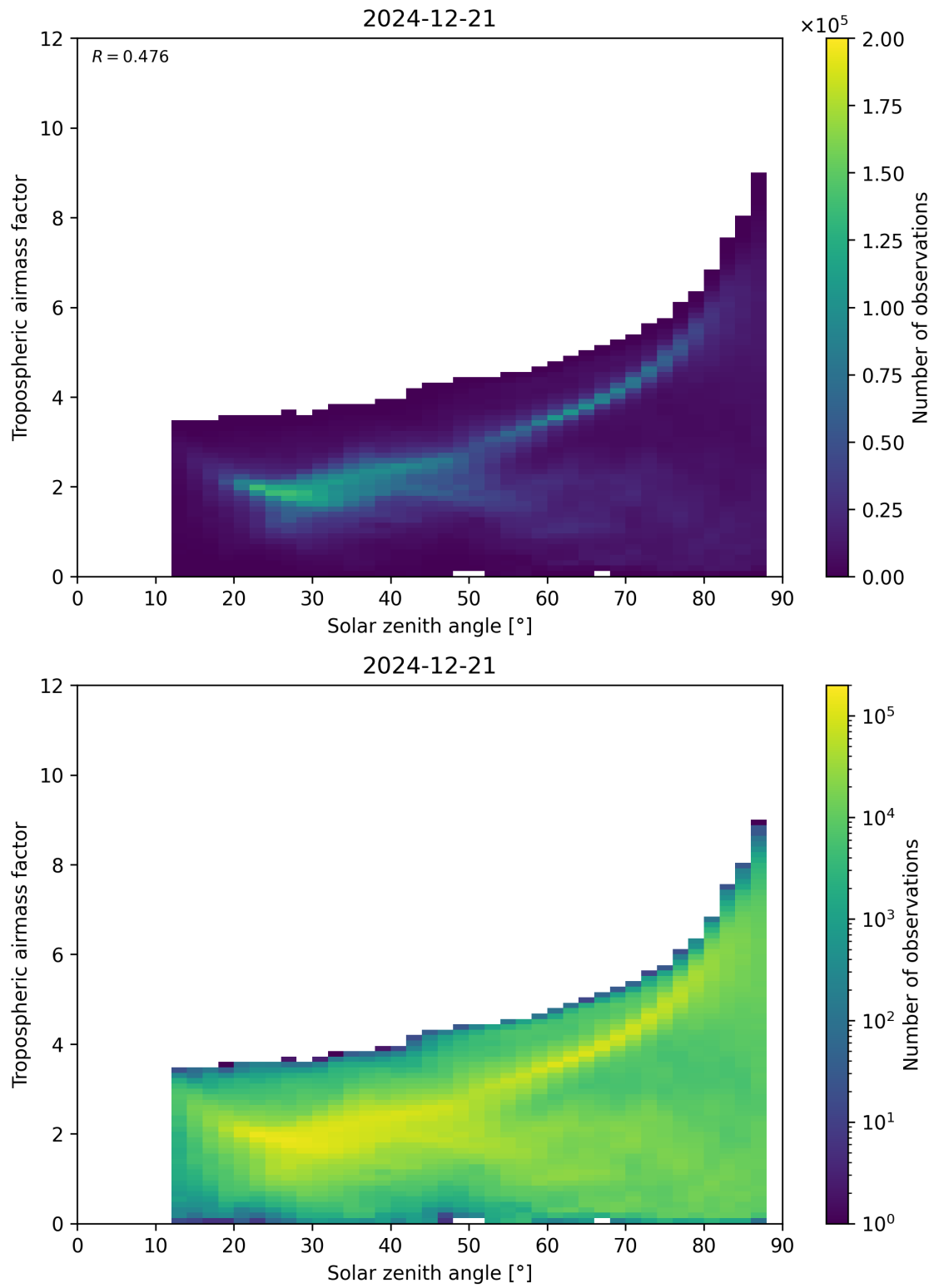
Figure 147: Scatter density plot of “Solar zenith angle” against “Tropospheric airmass factor” for 2024-12-20 to 2024-12-22.
