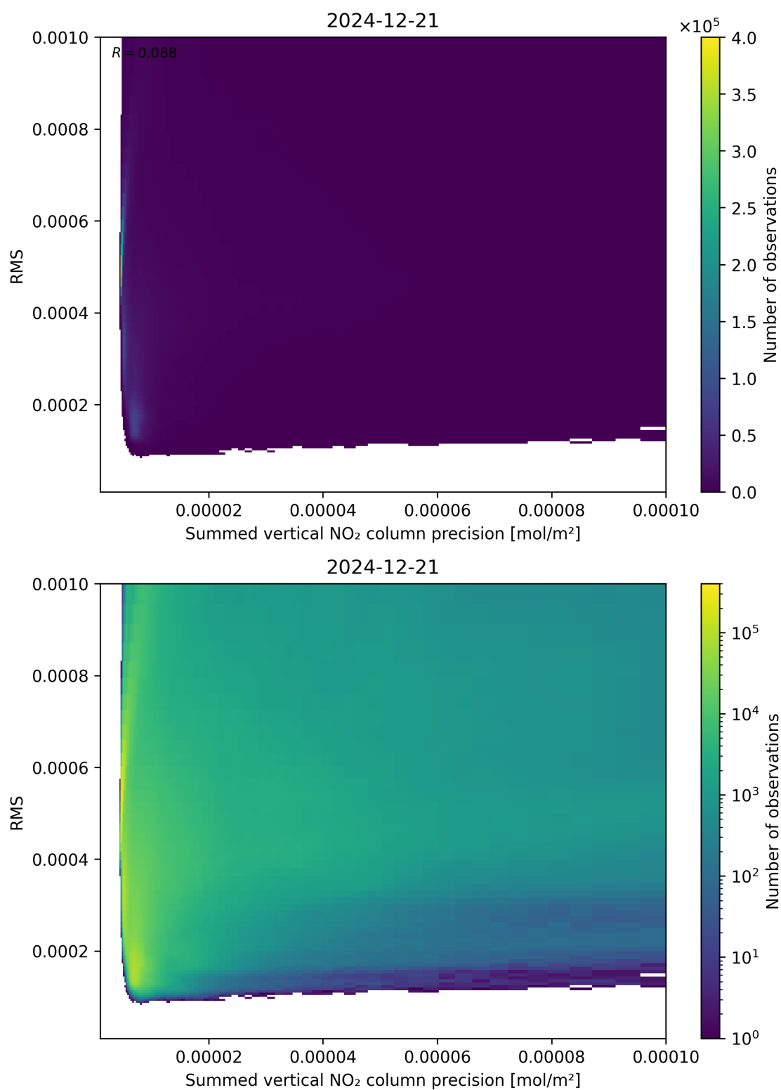
Figure 108: Scatter density plot of “Summed vertical NO 2 column precision” against “RMS” for 2024-12-20 to 2024-12-22.
