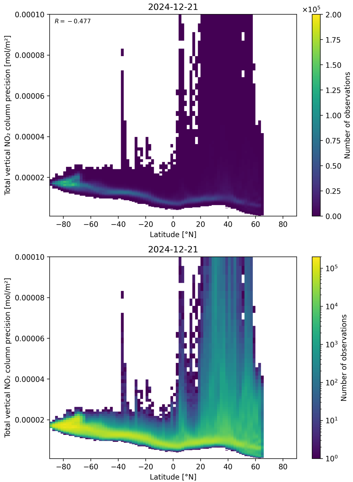
Figure 91: Scatter density plot of “Latitude” against “Total vertical NO 2 column precision” for 2024-12-20 to 2024-12-22.
