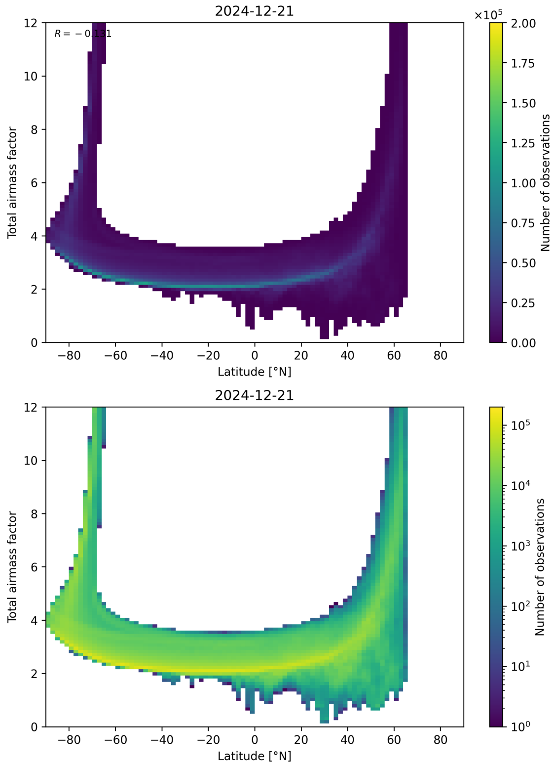
Figure 84: Scatter density plot of “Latitude” against “Total airmass factor” for 2024-12-20 to 2024-12-22.
