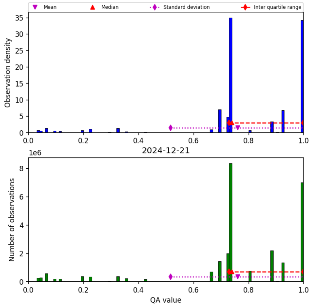
Figure 28: Histogram of “QA value” for 2024-12-20 to 2024-12-22
