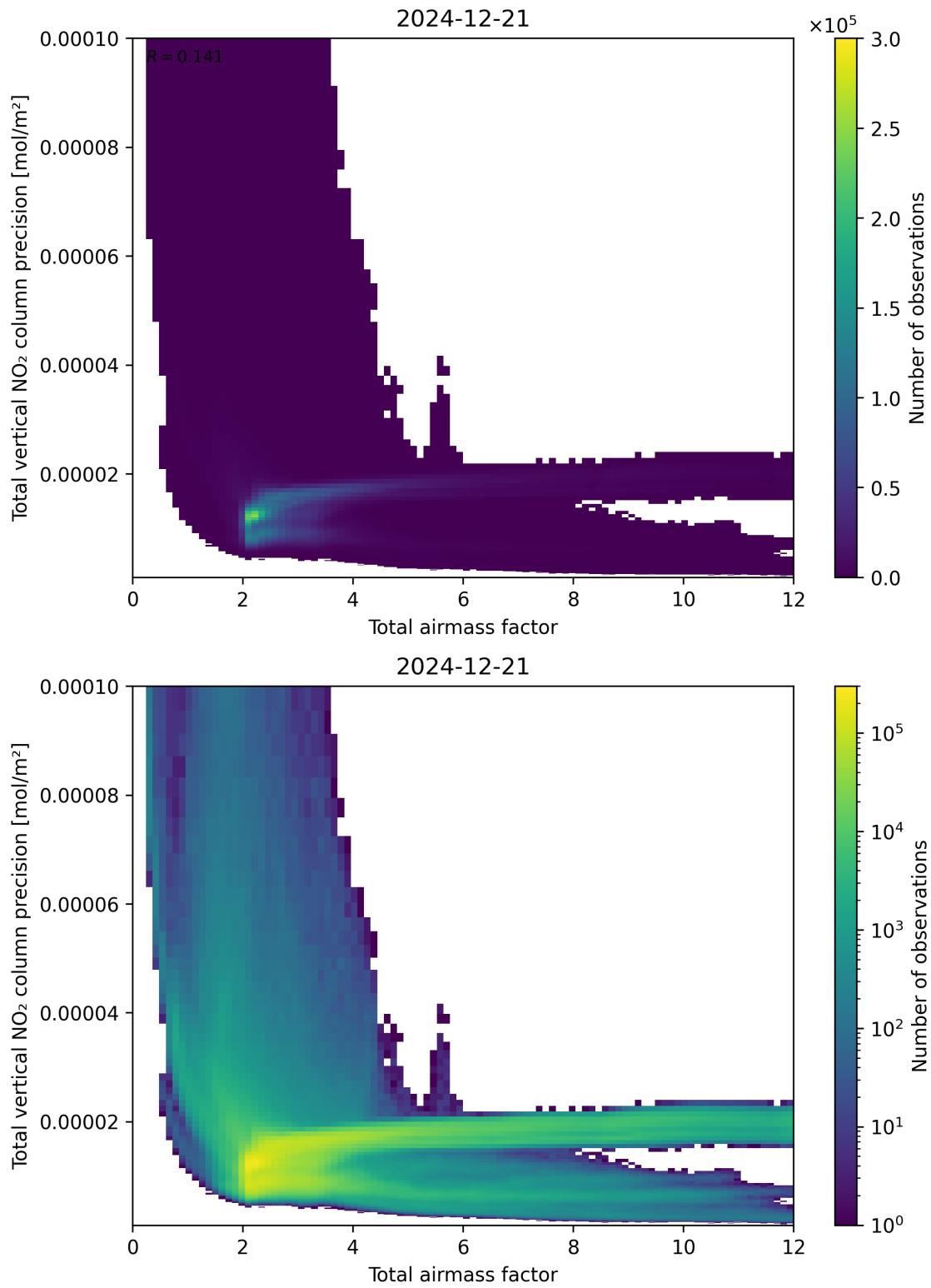
Figure 68: Scatter density plot of “Total airmass factor” against “Total vertical NO 2 column precision” for 2024-12-20 to 2024-12-22.
