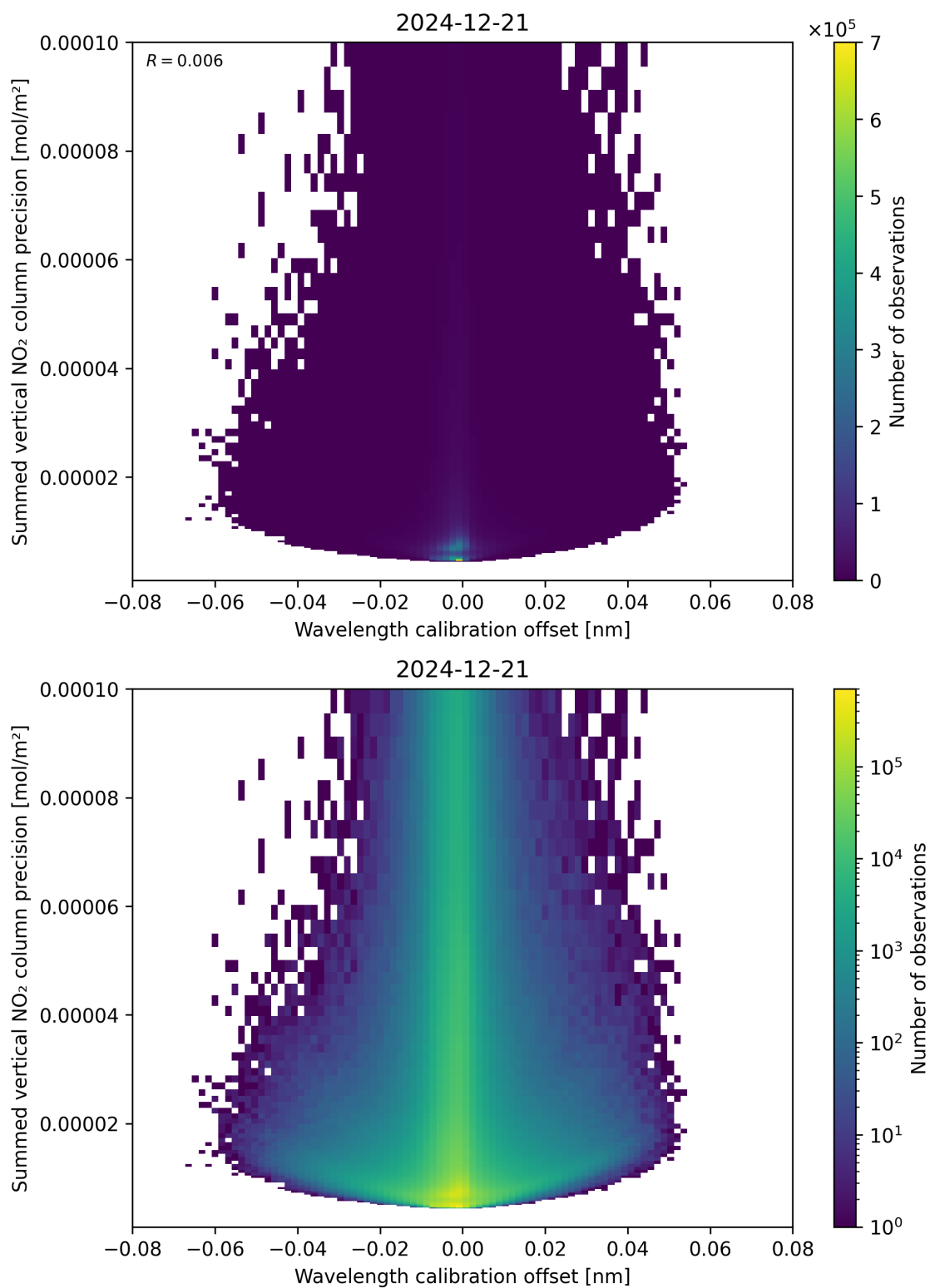
Figure 178: Scatter density plot of “Wavelength calibration offset” against “Summed vertical NO 2 column precision” for 2024-12-20 to 2024-12-22.
