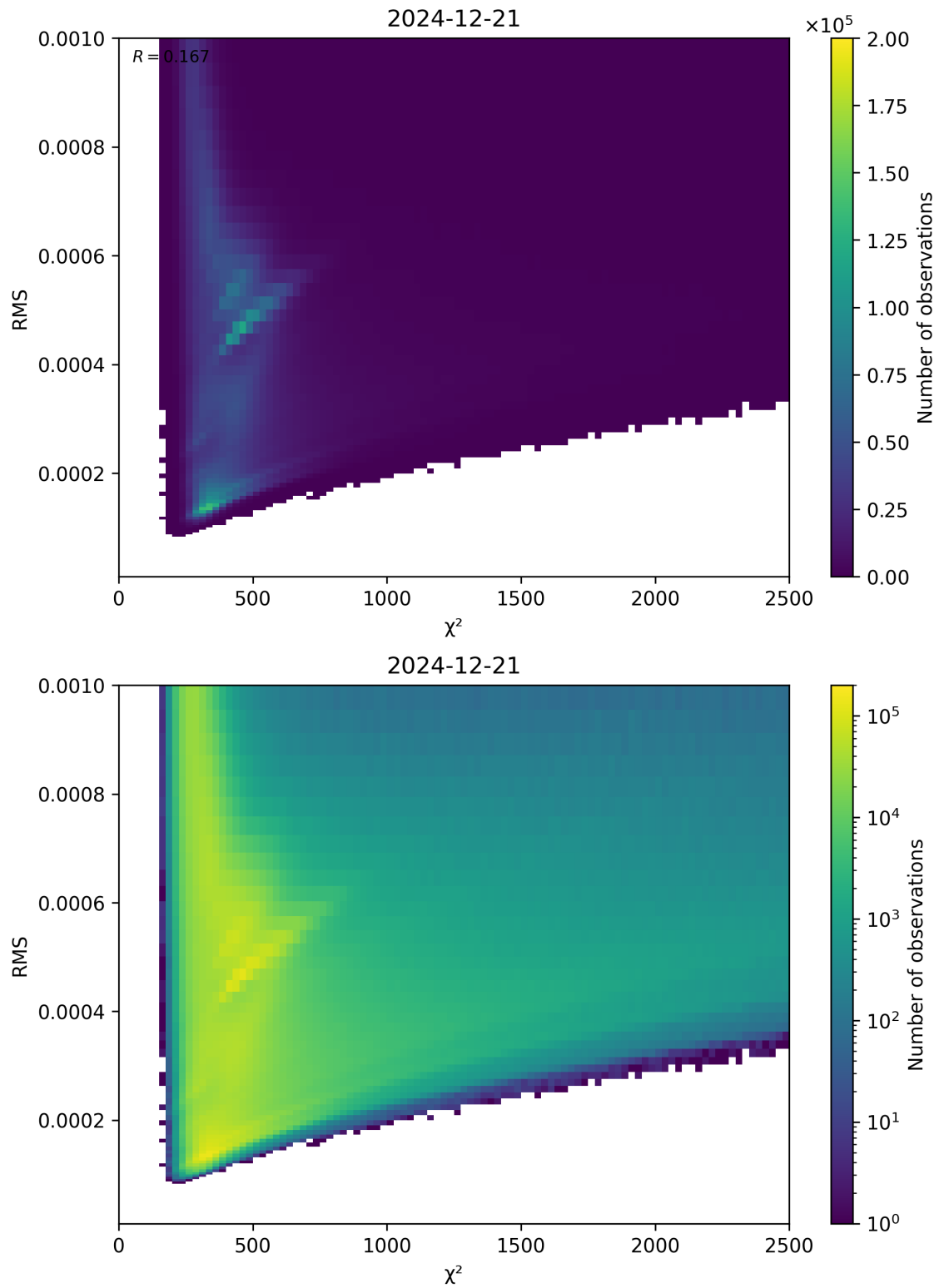
Figure 82: Scatter density plot of “ \chi^2 ” against “RMS” for 2024-12-20 to 2024-12-22.
