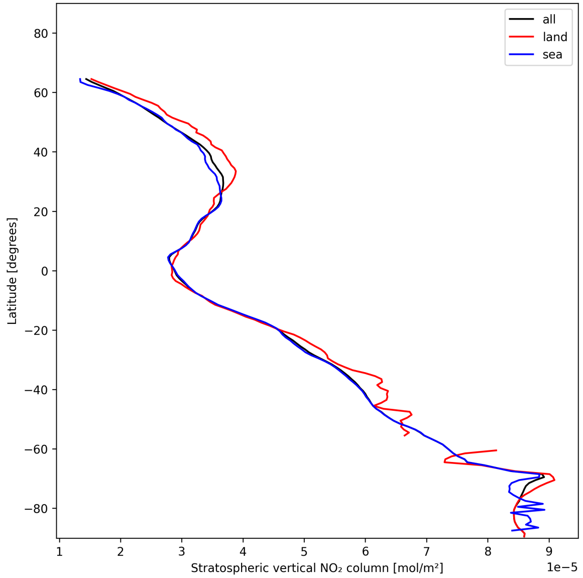
Figure 19: Zonal average of “Stratospheric vertical NO 2 column” for 2024-12-20 to 2024-12-22.
