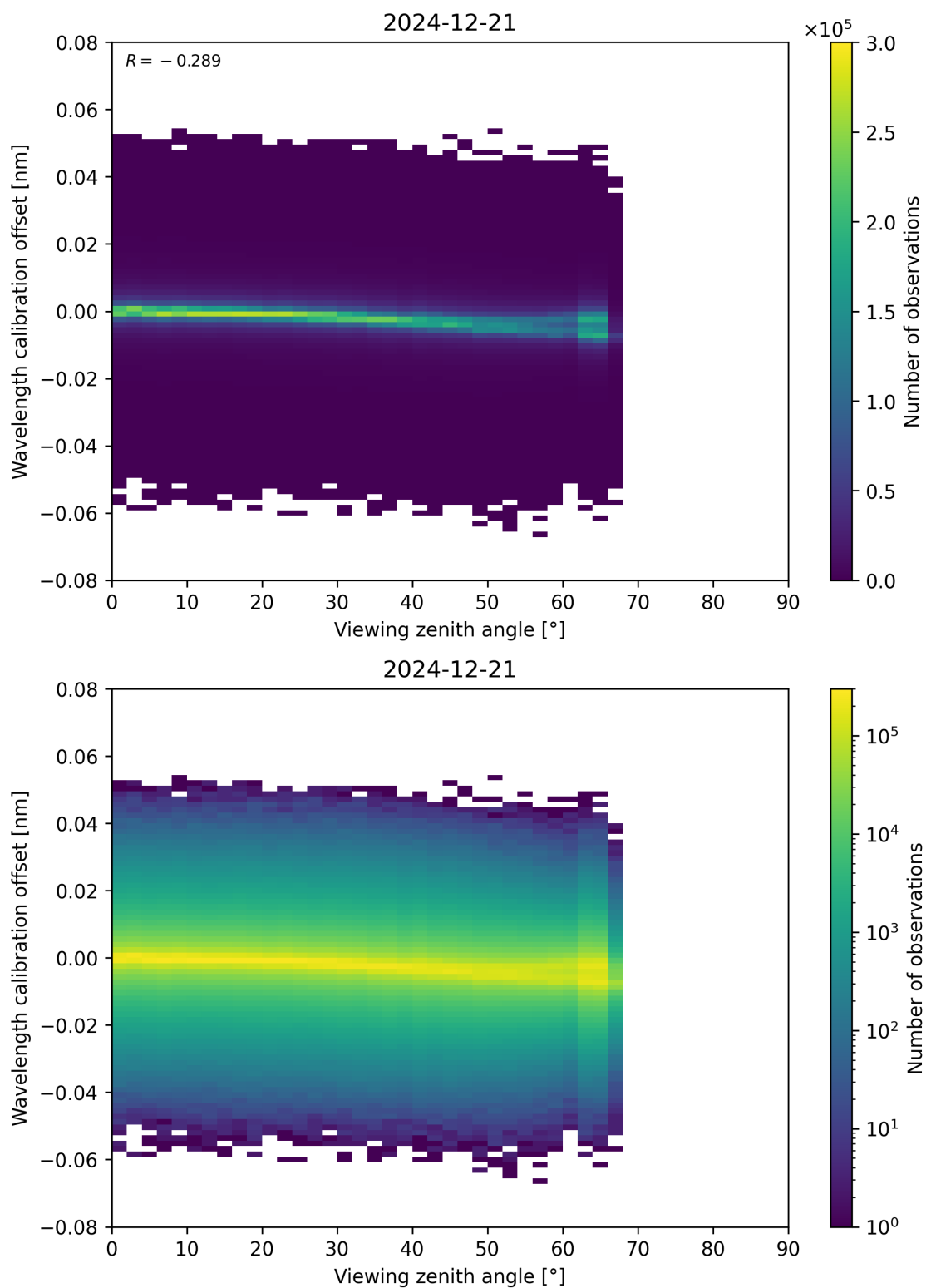
Figure 173: Scatter density plot of “Viewing zenith angle” against “Wavelength calibration offset” for 2024-12-20 to 2024-12-22.
