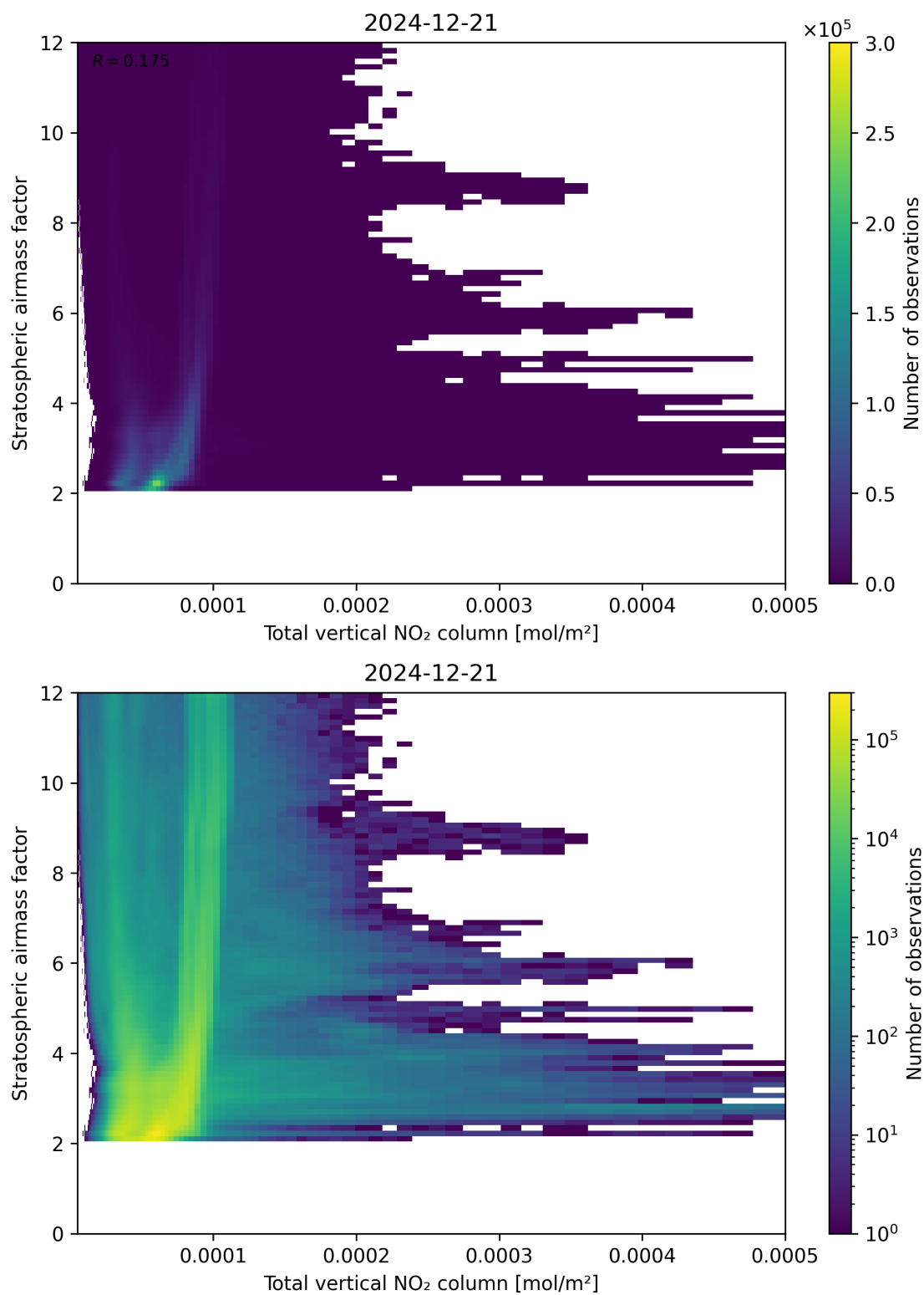
Figure 110: Scatter density plot of “Total vertical NO 2 column” against “Stratospheric airmass factor” for 2024-12-20 to 2024-12-22.
