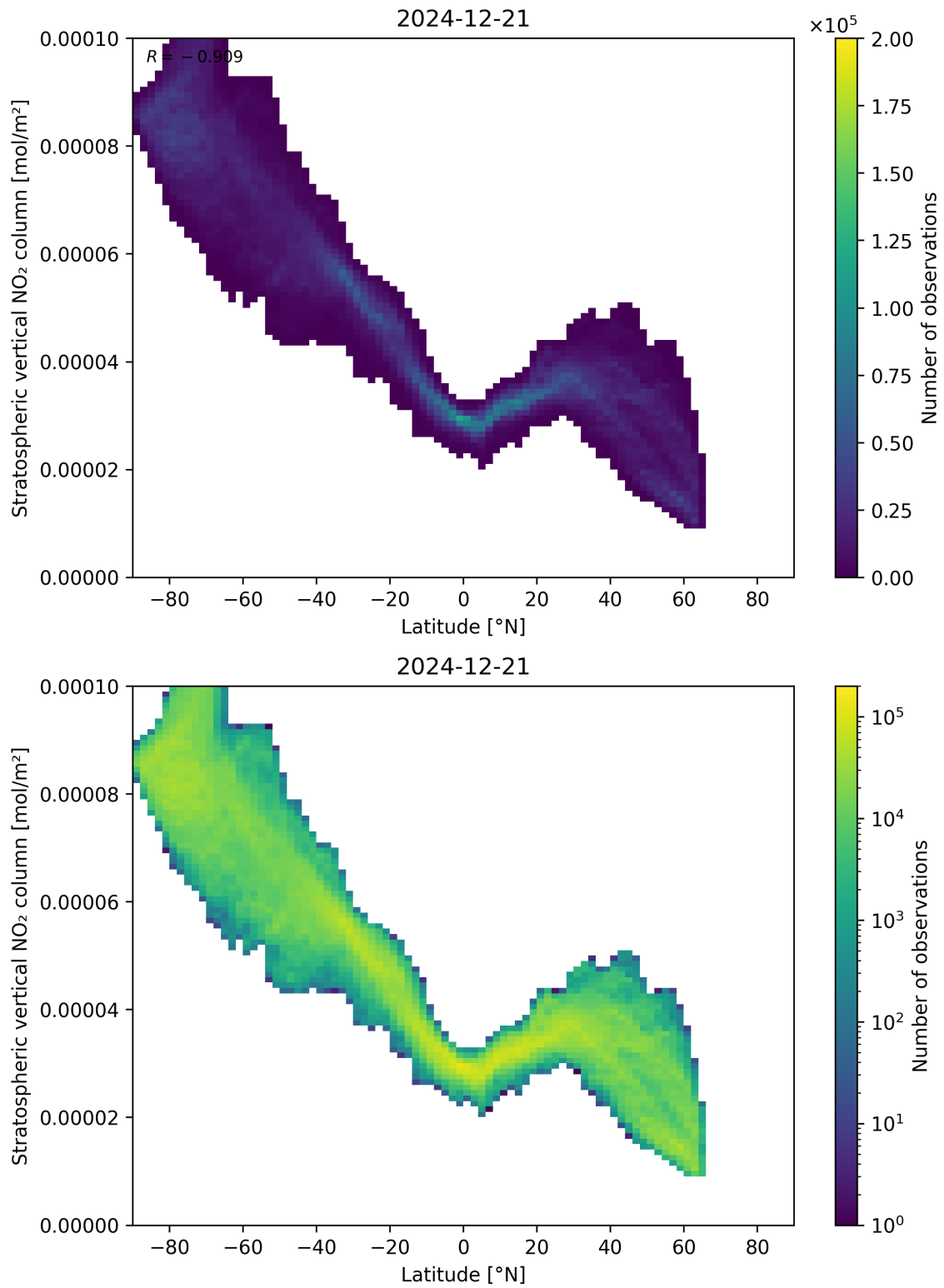
Figure 87: Scatter density plot of “Latitude” against “Stratospheric vertical NO 2 column” for 2024-12-20 to 2024-12-22.
