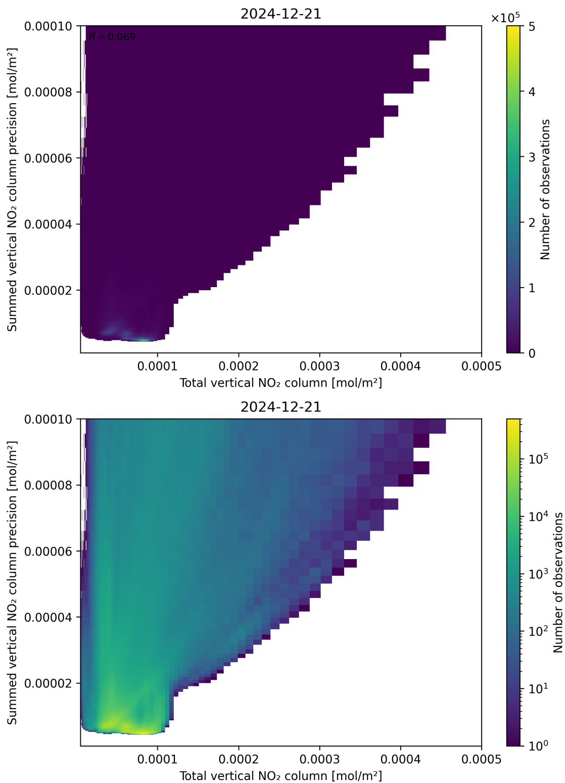
Figure 113: Scatter density plot of “Total vertical NO 2 column” against “Summed vertical NO 2 column precision” for 2024-12-20 to 2024-12-22.
