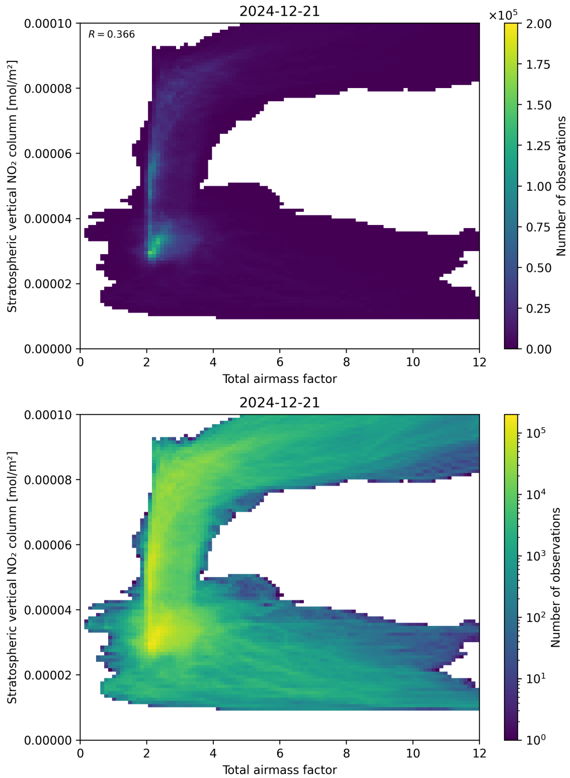
Figure 64: Scatter density plot of “Total airmass factor” against “Stratospheric vertical NO 2 column” for 2024-12-20 to 2024-12-22.
