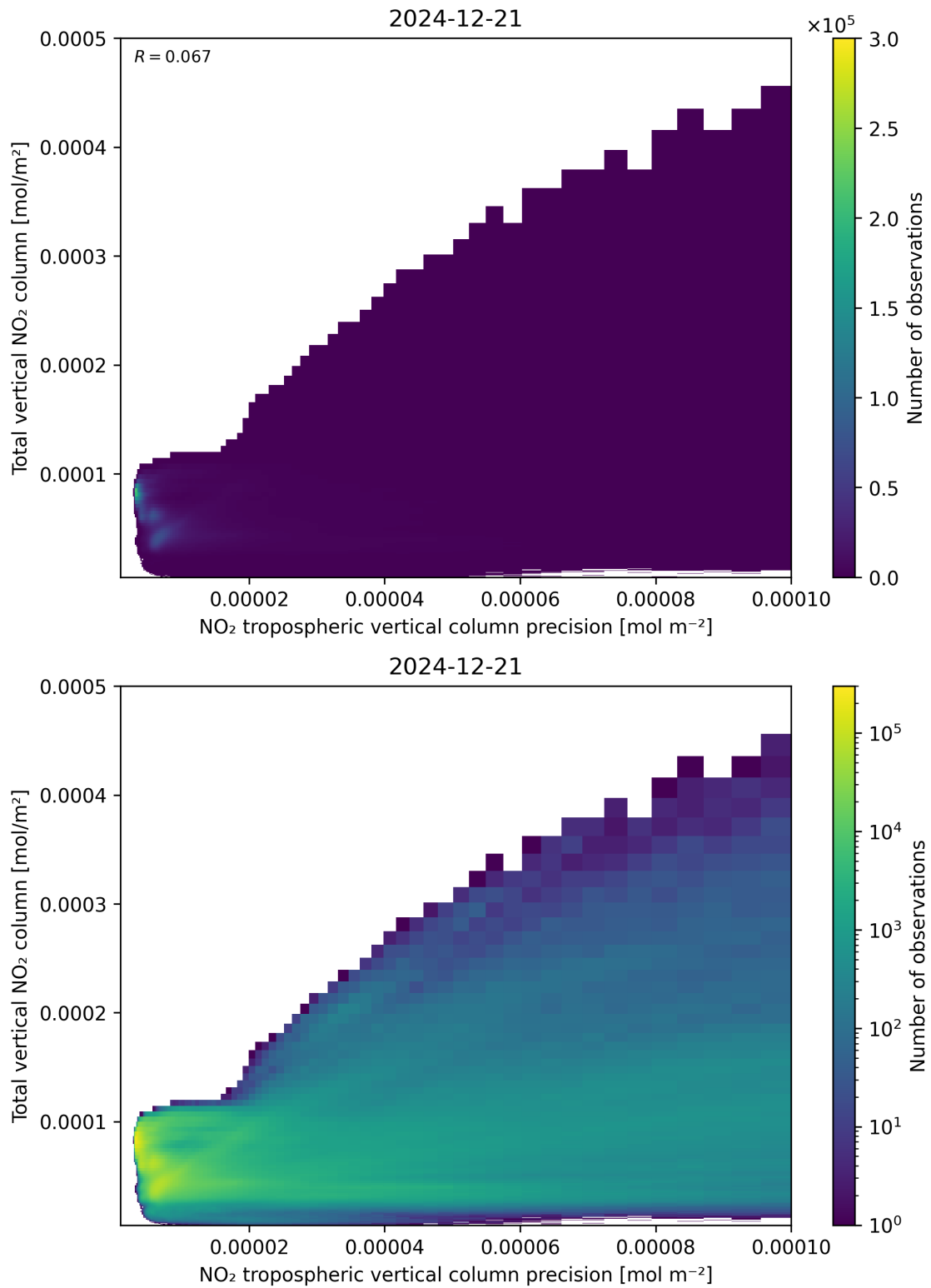
Figure 138: Scatter density plot of “NO 2 tropospheric vertical column precision” against “Total vertical NO 2 column” for 2024-12-20 to 2024-12-22.
