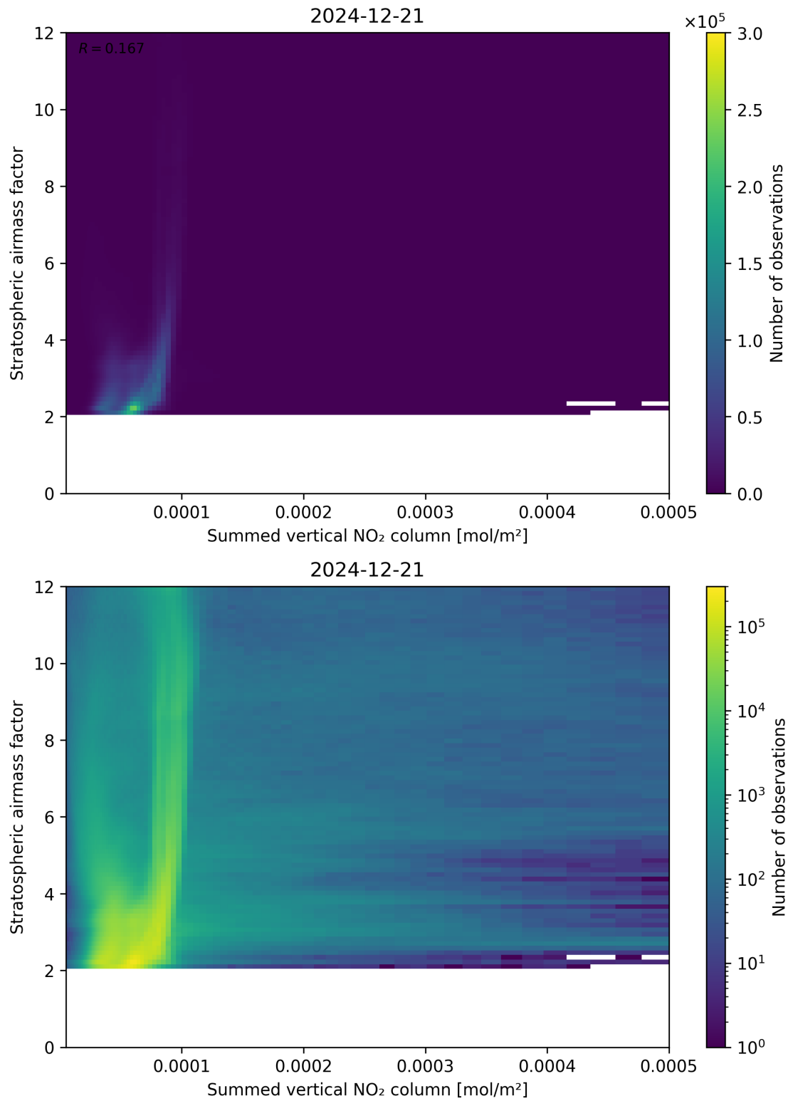
Figure 103: Scatter density plot of “Summed vertical NO 2 column” against “Stratospheric airmass factor” for 2024-12-20 to 2024-12-22.
