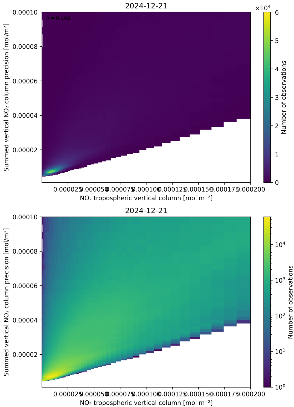
Figure 127: Scatter density plot of “NO 2 tropospheric vertical column” against “Summed vertical NO 2 column precision” for 2024-12-20 to 2024-12-22.
