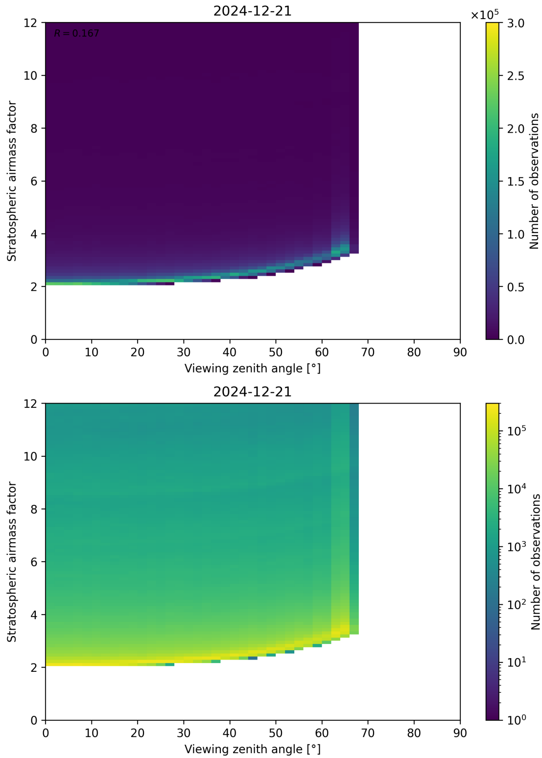
Figure 159: Scatter density plot of “Viewing zenith angle” against “Stratospheric airmass factor” for 2024-12-20 to 2024-12-22.
