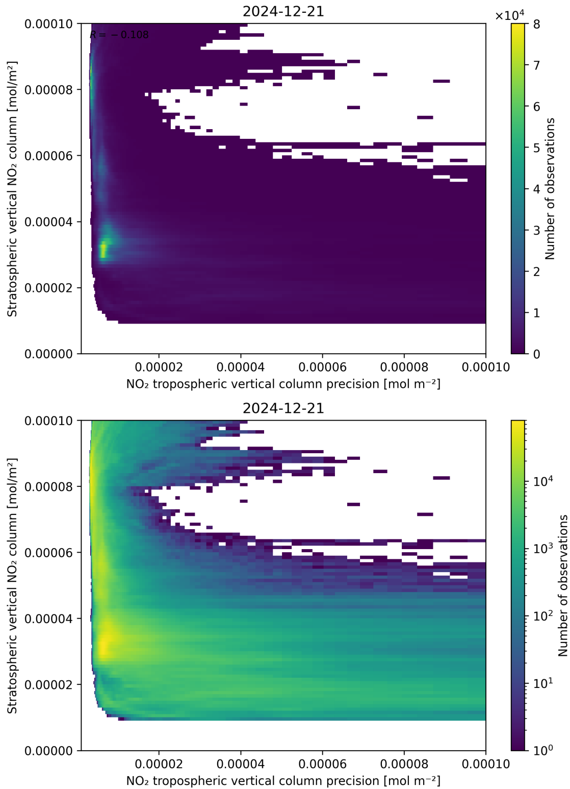
Figure 135: Scatter density plot of “NO 2 tropospheric vertical column precision” against “Stratospheric vertical NO 2 column” for 2024-12-20 to 2024-12-22.
