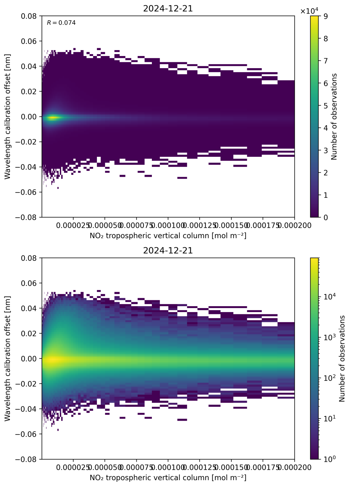
Figure 143: Scatter density plot of “NO 2 tropospheric vertical column” against “Wavelength calibration offset” for 2024-12-20 to 2024-12-22.
