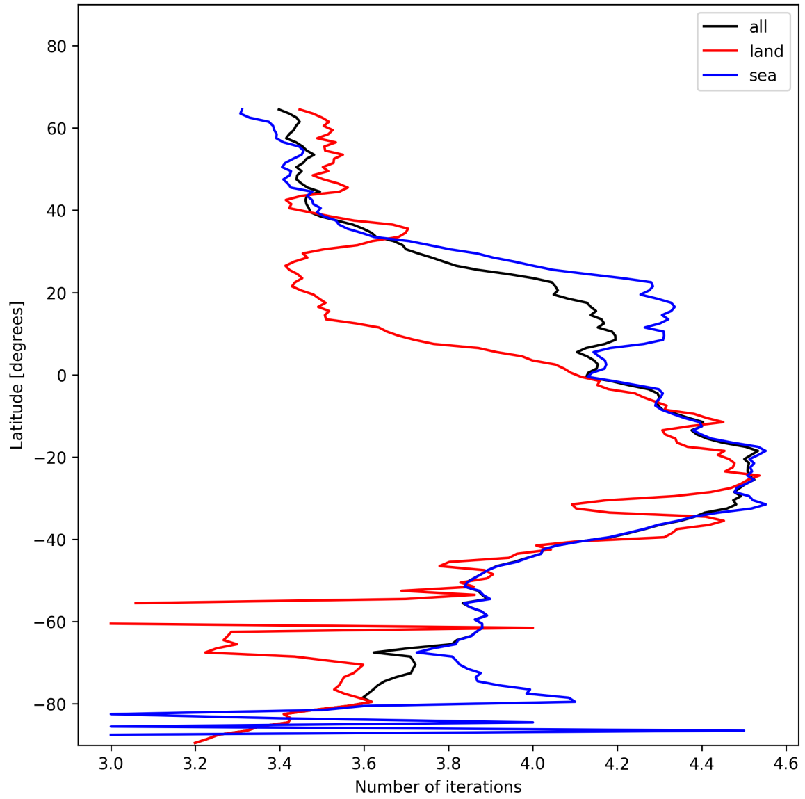
Figure 17: Zonal average of “Number of iterations” for 2024-12-20 to 2024-12-22.
