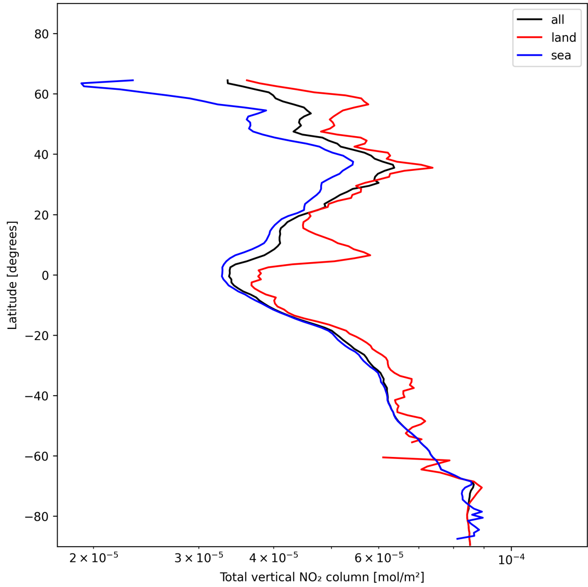
Figure 21: Zonal average of “Total vertical NO 2 column” for 2024-12-20 to 2024-12-22.
