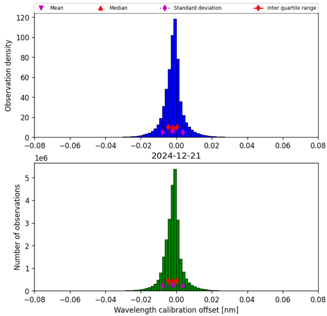
Figure 35: Histogram of “Wavelength calibration offset” for 2024-12-20 to 2024-12-22
