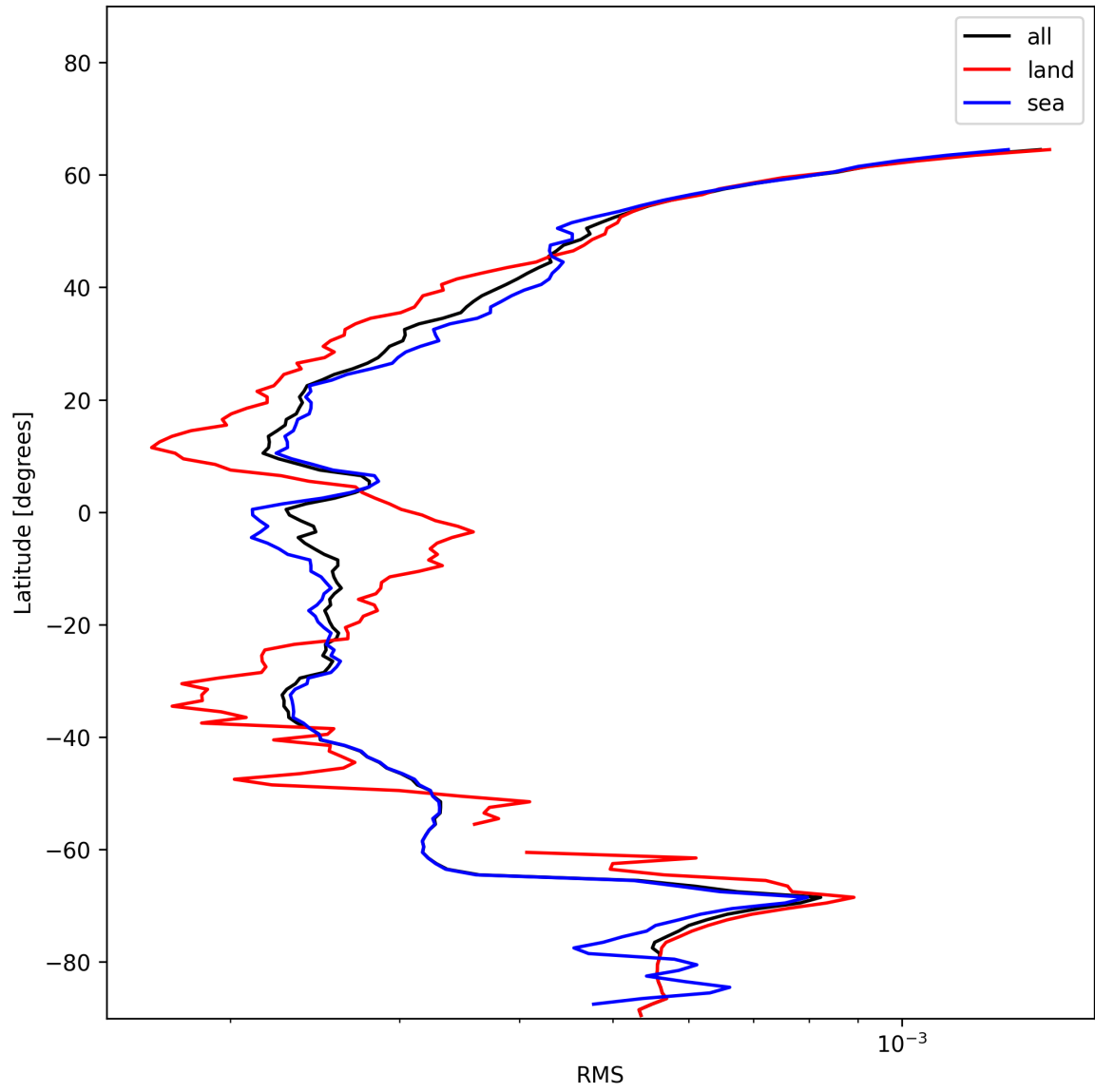
Figure 26: Zonal average of “RMS” for 2024-12-20 to 2024-12-22.
