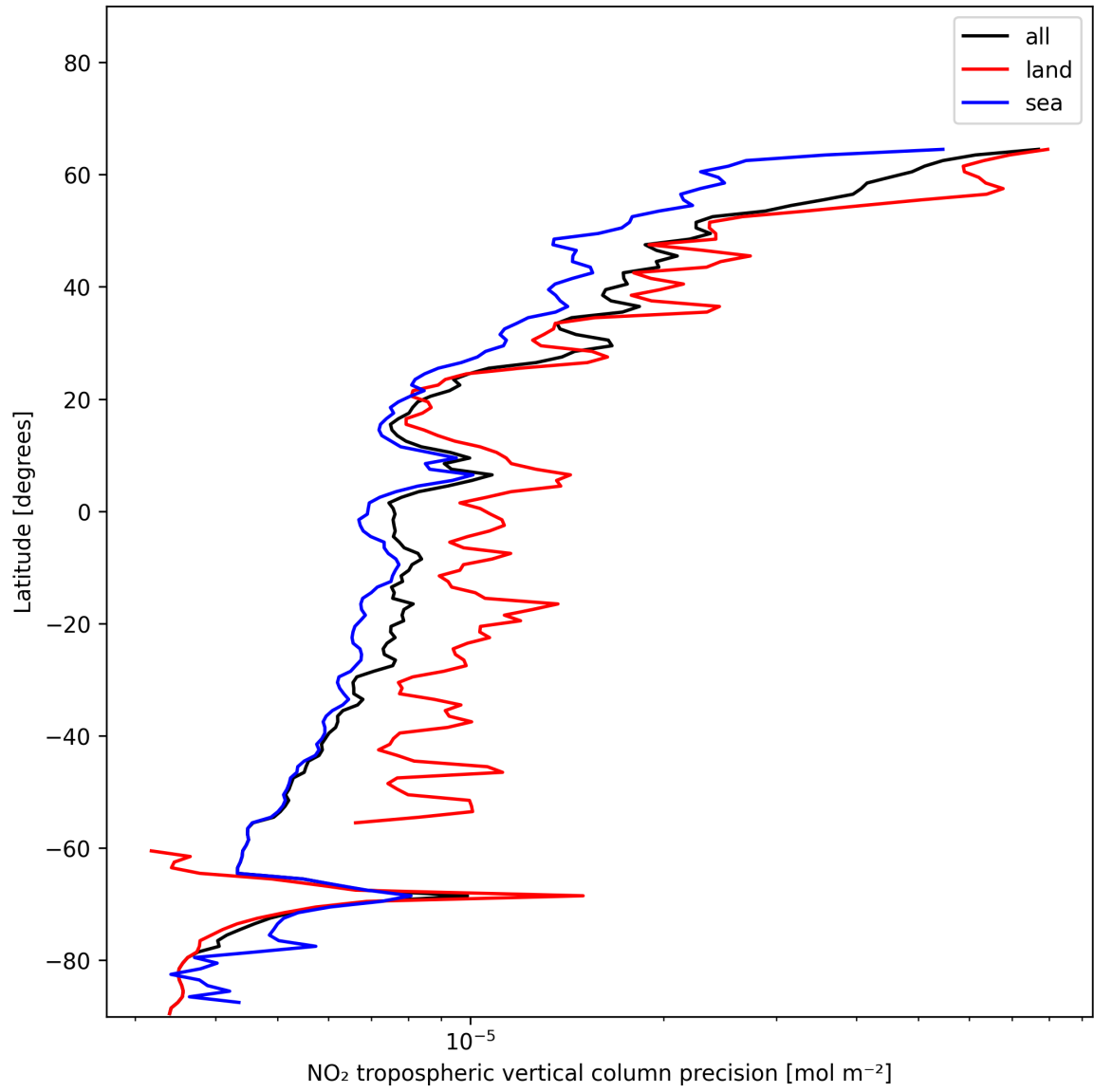
Figure 13: Zonal average of “NO 2 tropospheric vertical column precision” for 2024-12-20 to 2024-12-22.
