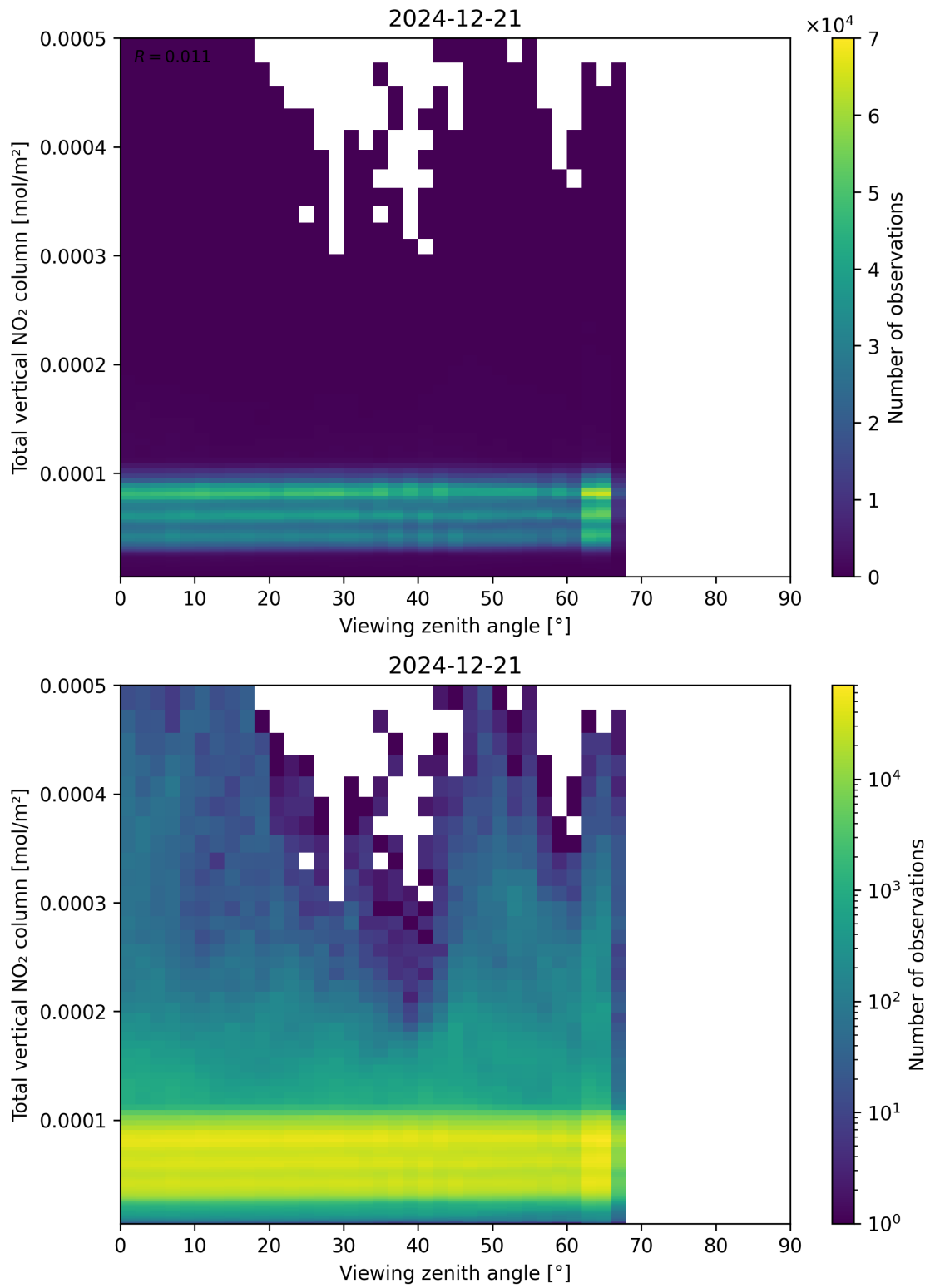
Figure 167: Scatter density plot of “Viewing zenith angle” against “Total vertical NO 2 column” for 2024-12-20 to 2024-12-22.
