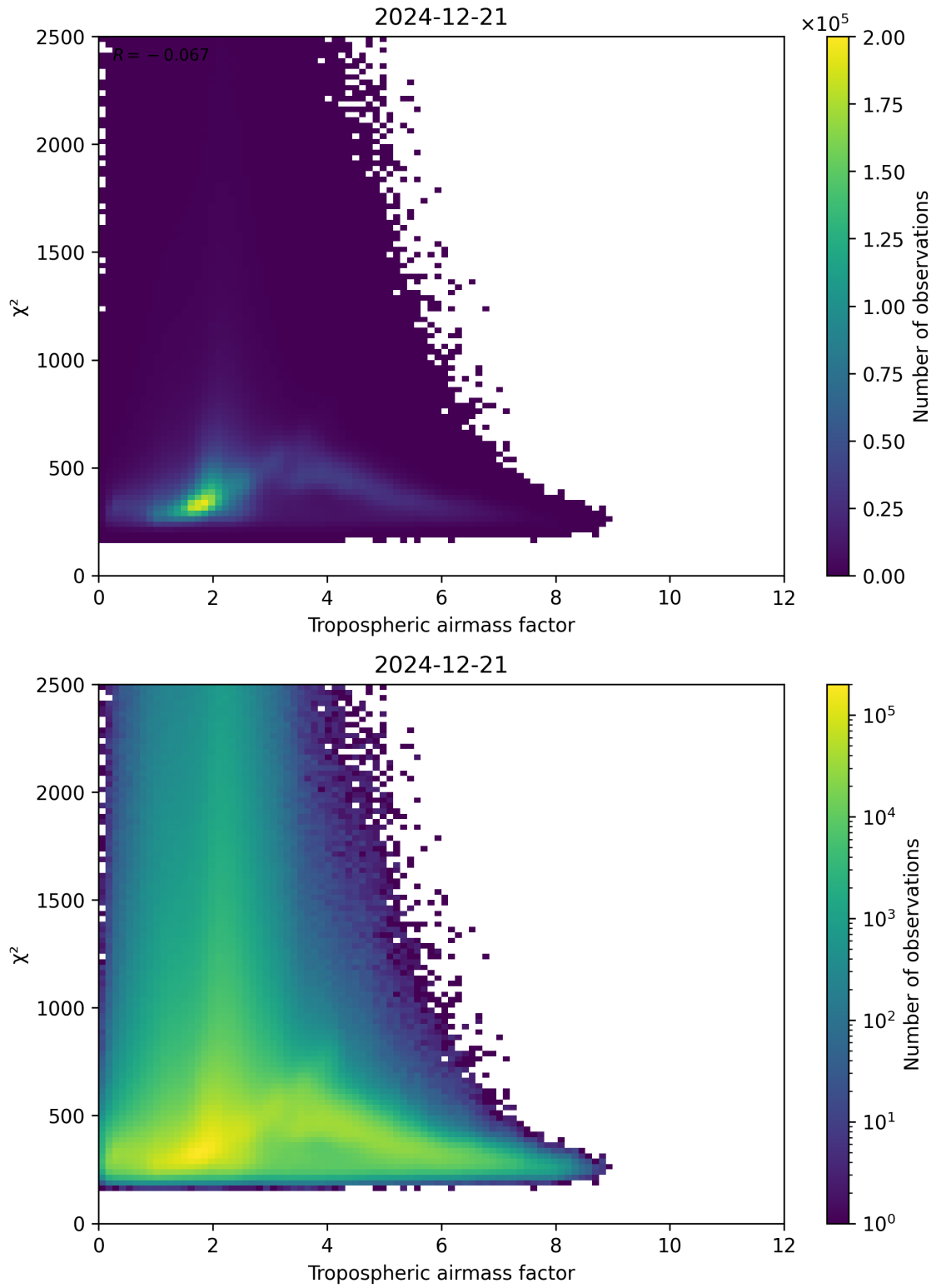
Figure 73: Scatter density plot of “Tropospheric airmass factor” against “ \chi^2 ” for 2024-12-20 to 2024-12-22.
