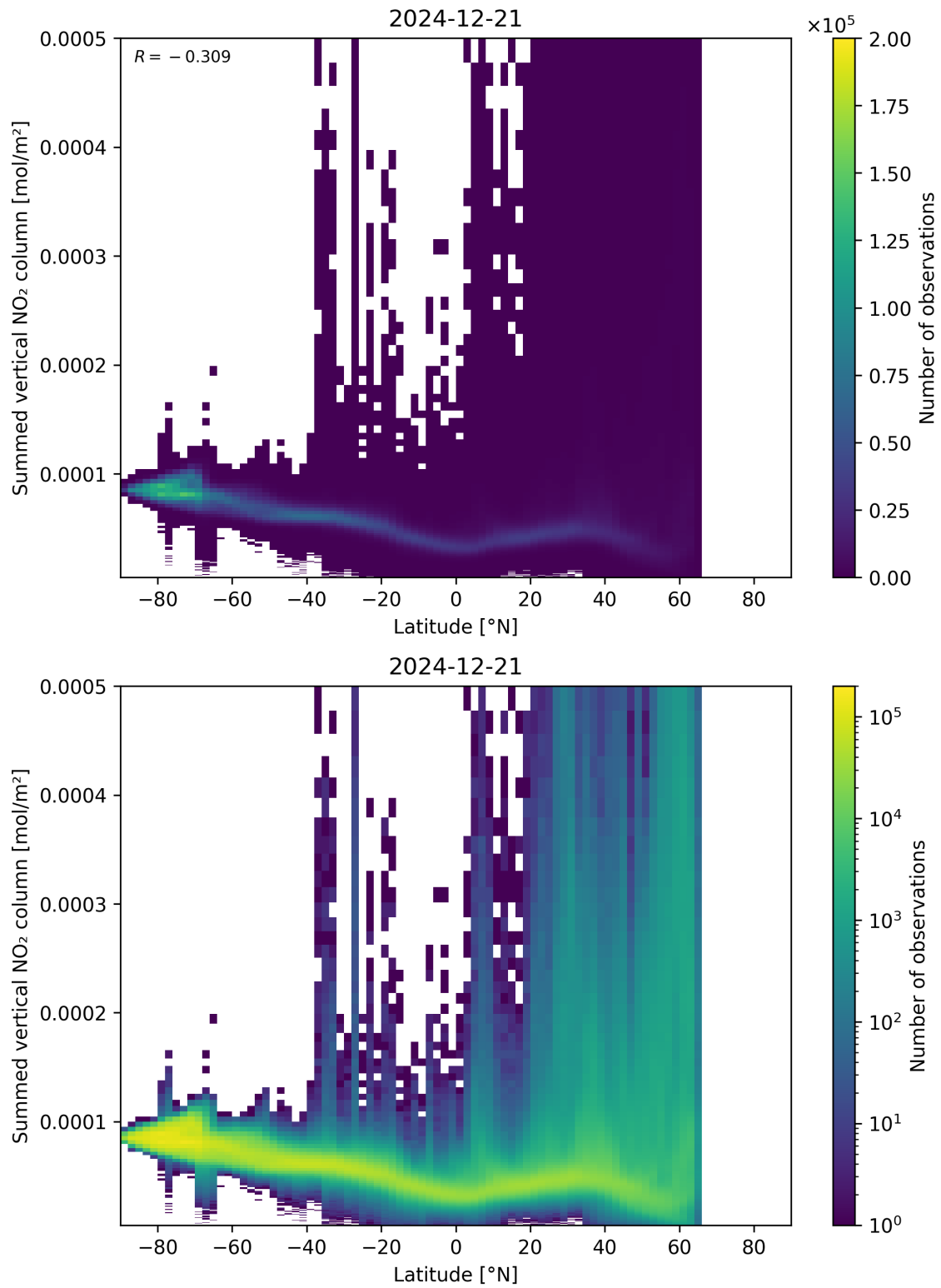
Figure 88: Scatter density plot of “Latitude” against “Summed vertical NO 2 column” for 2024-12-20 to 2024-12-22.
