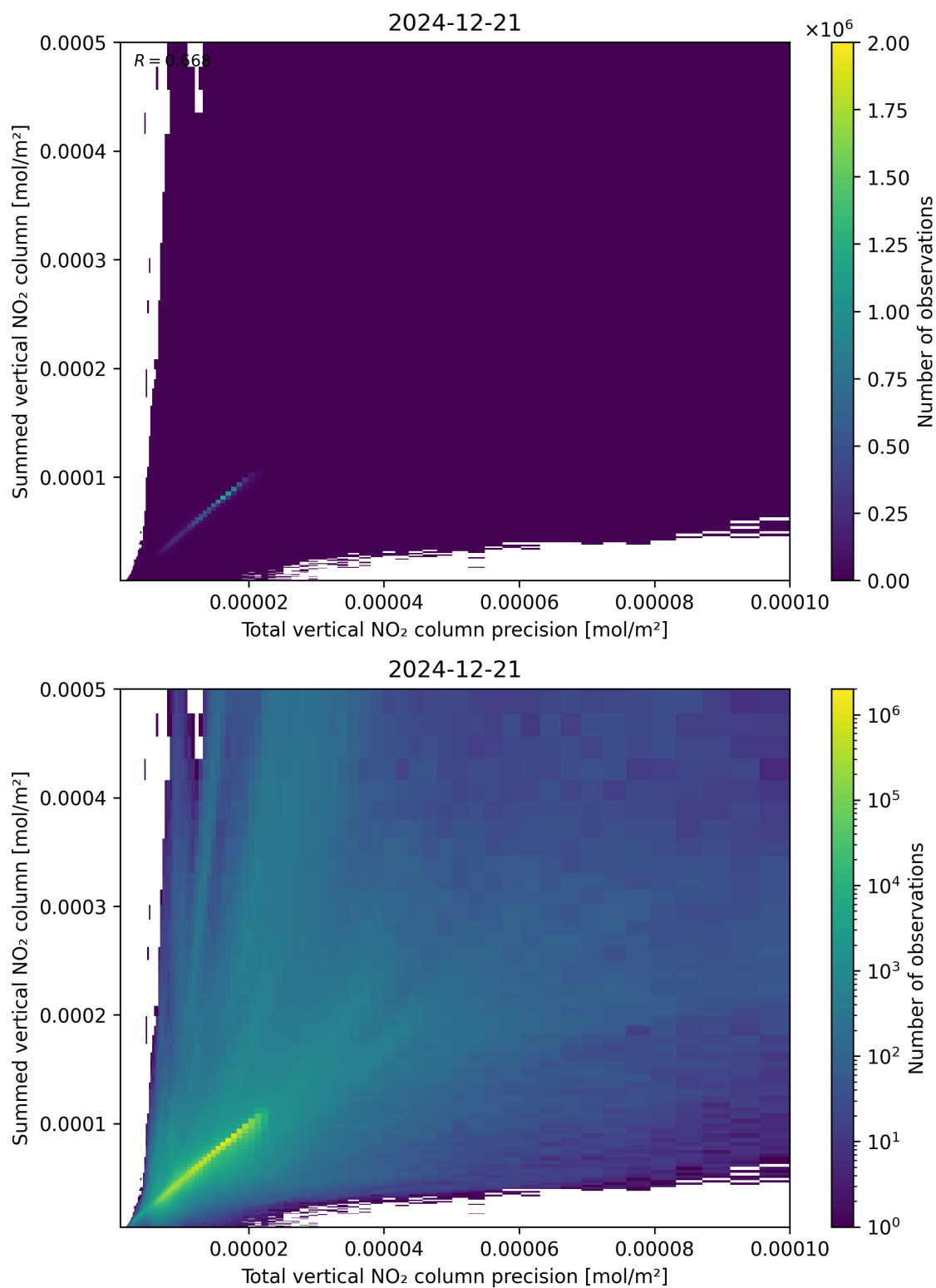
Figure 117: Scatter density plot of “Total vertical NO 2 column precision” against “Summed vertical NO 2 column” for 2024-12-20 to 2024-12-22.
