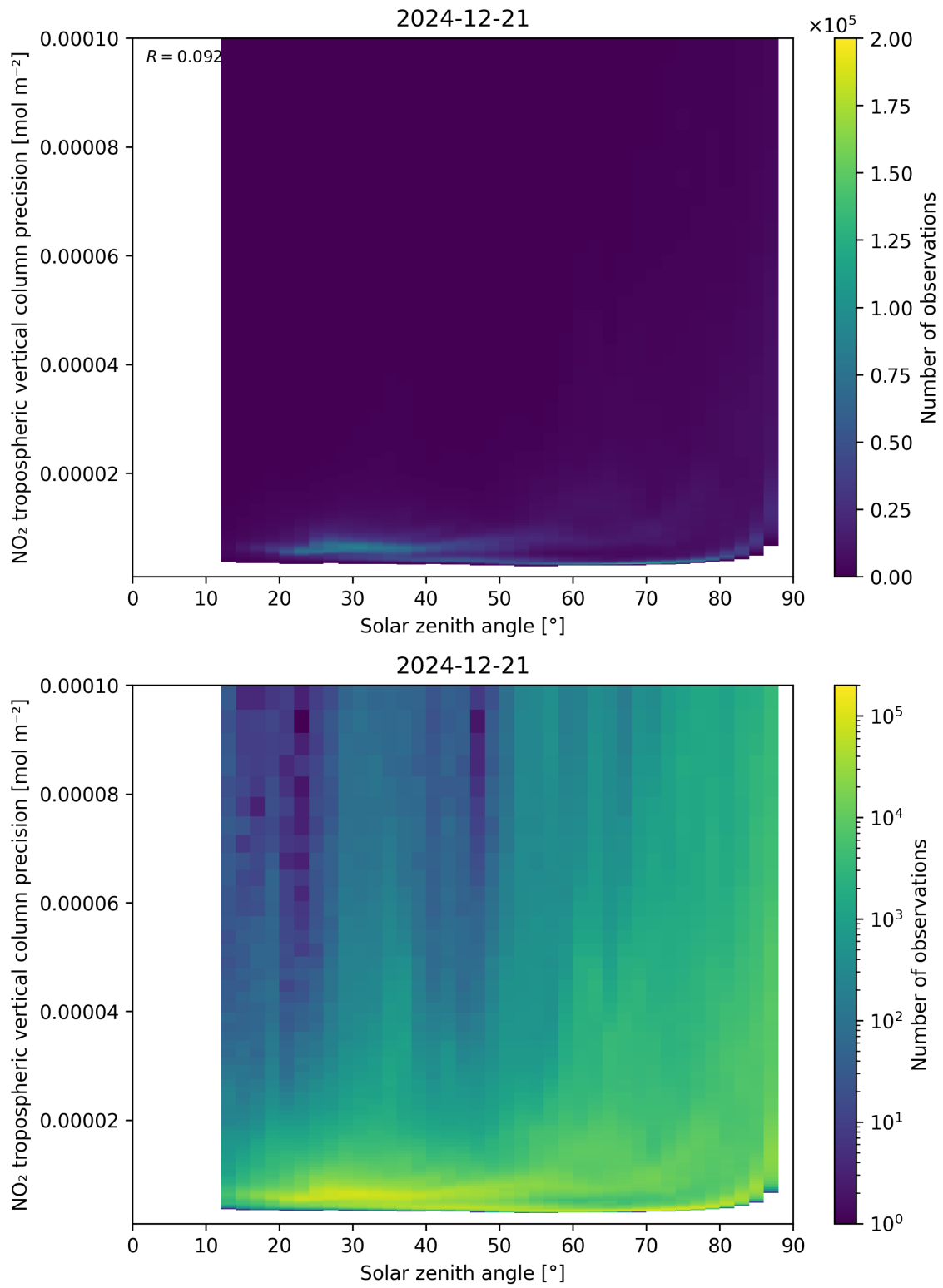
Figure 156: Scatter density plot of “Solar zenith angle” against “NO 2 tropospheric vertical column precision” for 2024-12-20 to 2024-12-22.
