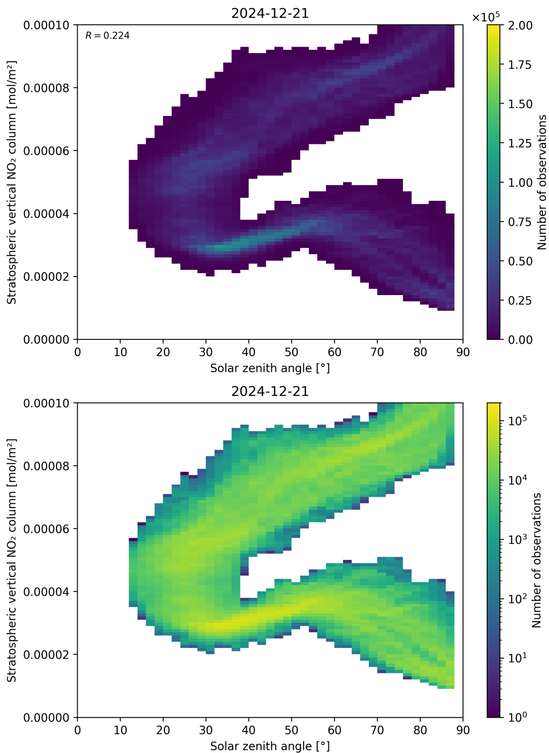
Figure 150: Scatter density plot of “Solar zenith angle” against “Stratospheric vertical NO 2 column” for 2024-12-20 to 2024-12-22.
