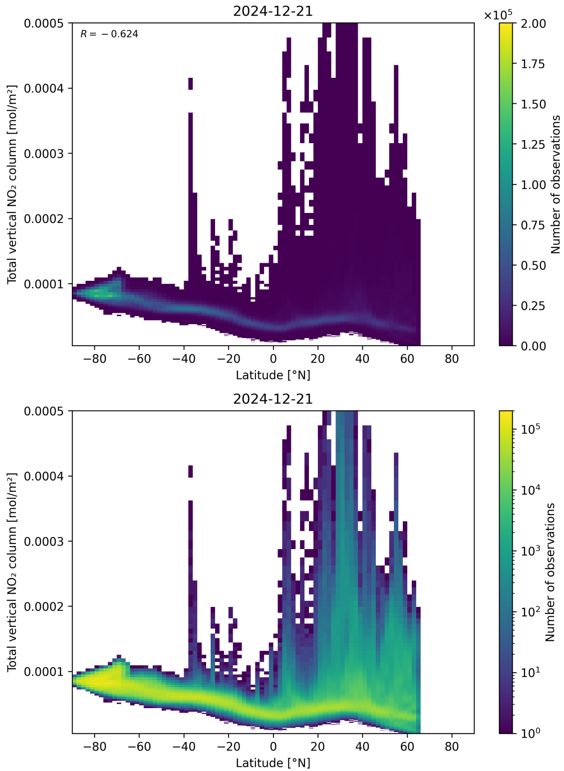
Figure 90: Scatter density plot of “Latitude” against “Total vertical NO 2 column” for 2024-12-20 to 2024-12-22.
