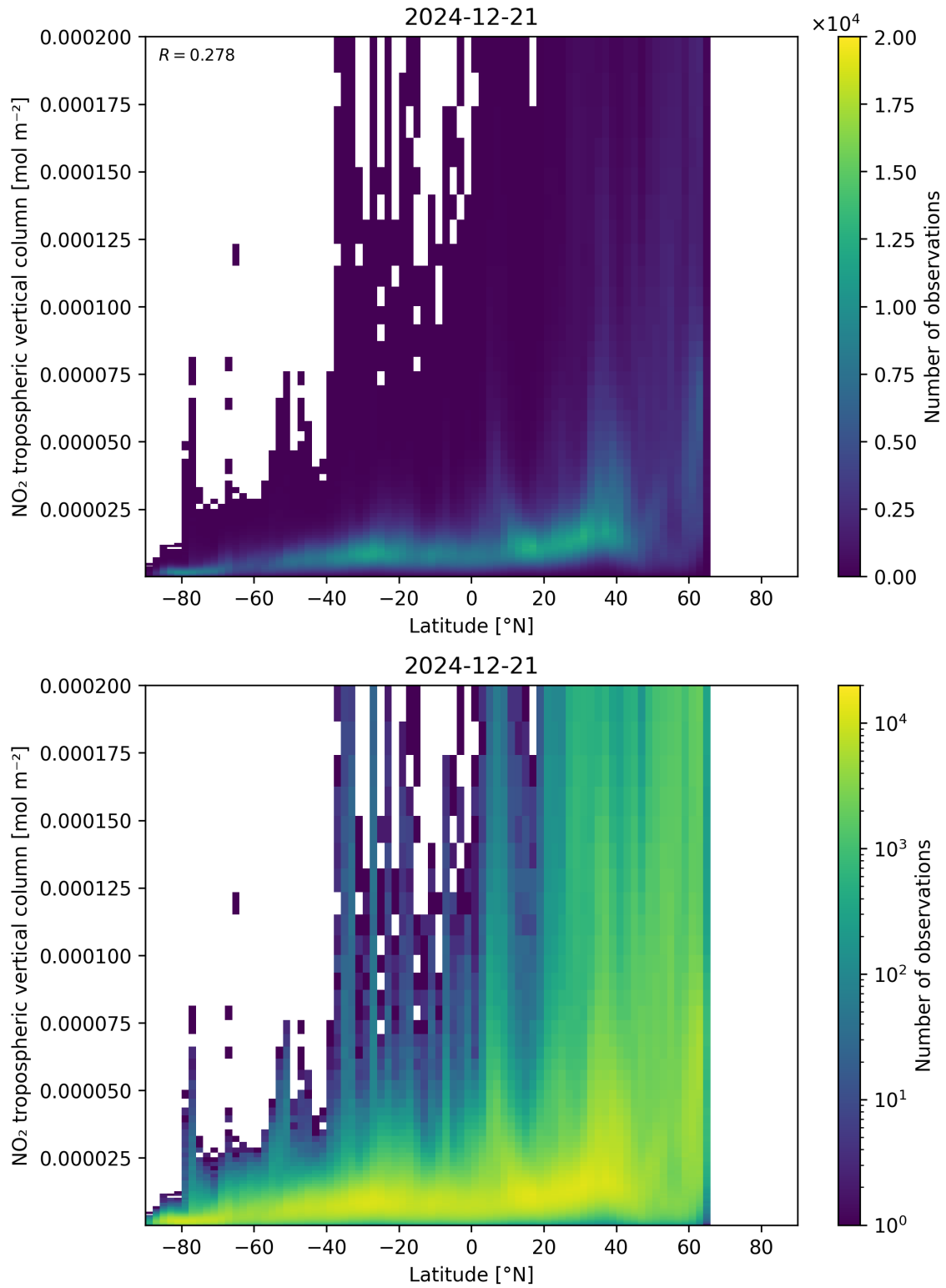
Figure 92: Scatter density plot of “Latitude” against “NO 2 tropospheric vertical column” for 2024-12-20 to 2024-12-22.
