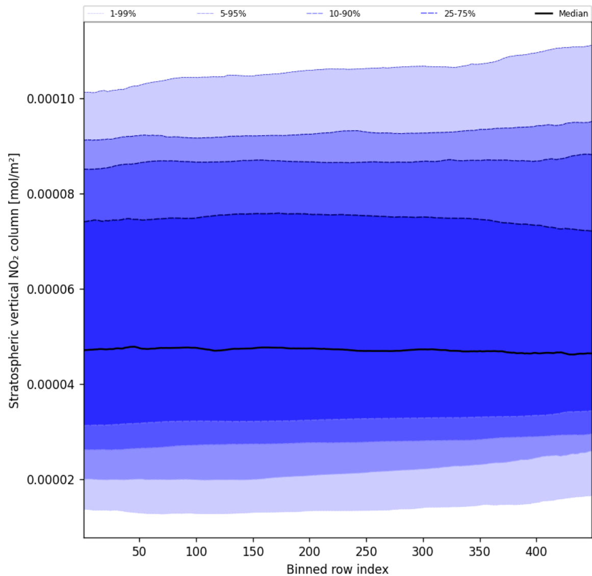
Figure 53: Along track statistics of “Stratospheric vertical NO 2 column” for 2024-12-20 to 2024-12-22
