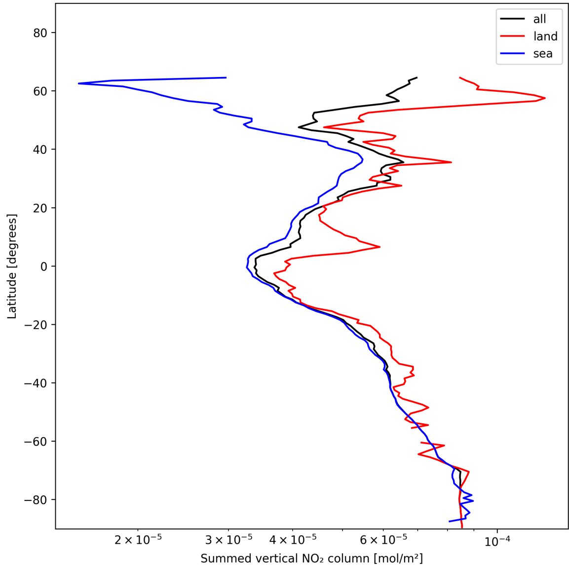
Figure 23: Zonal average of “Summed vertical NO 2 column” for 2024-12-20 to 2024-12-22.
