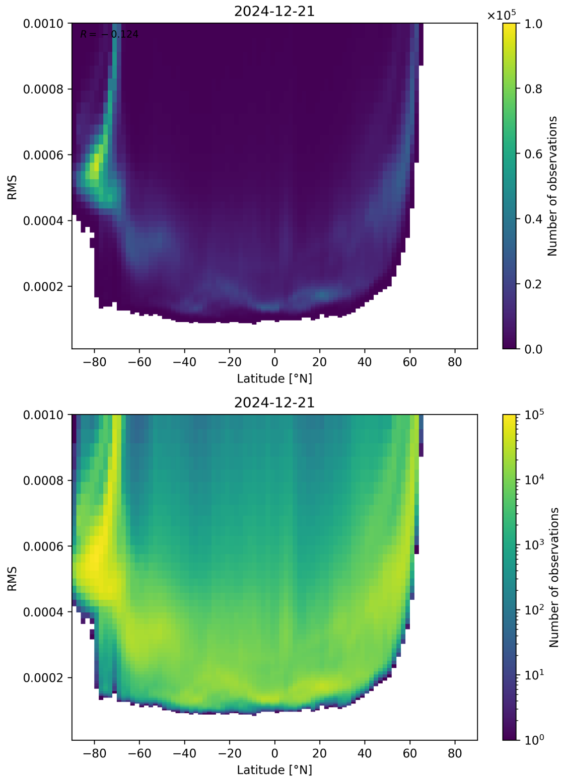
Figure 94: Scatter density plot of “Latitude” against “RMS” for 2024-12-20 to 2024-12-22.
