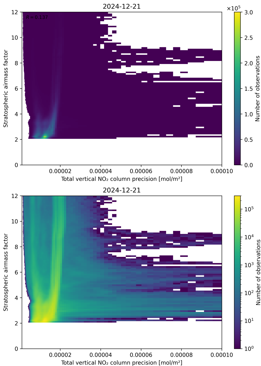
Figure 115: Scatter density plot of “Total vertical NO 2 column precision” against “Stratospheric air mass factor” for 2024-12-20 to 2024-12-22.
