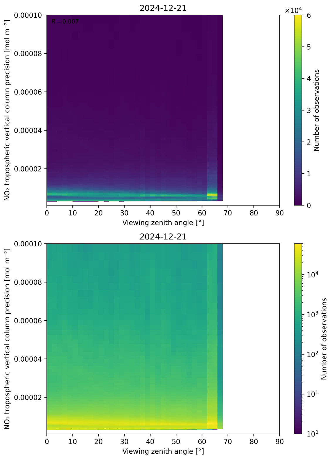
Figure 170: Scatter density plot of “Viewing zenith angle” against “NO 2 tropospheric vertical column precision” for 2024-12-20 to 2024-12-22.
