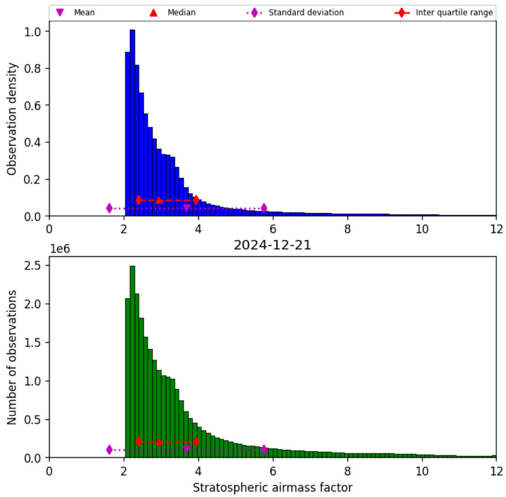
Figure 44: Histogram of “Stratospheric airmass factor” for 2024-12-20 to 2024-12-22
