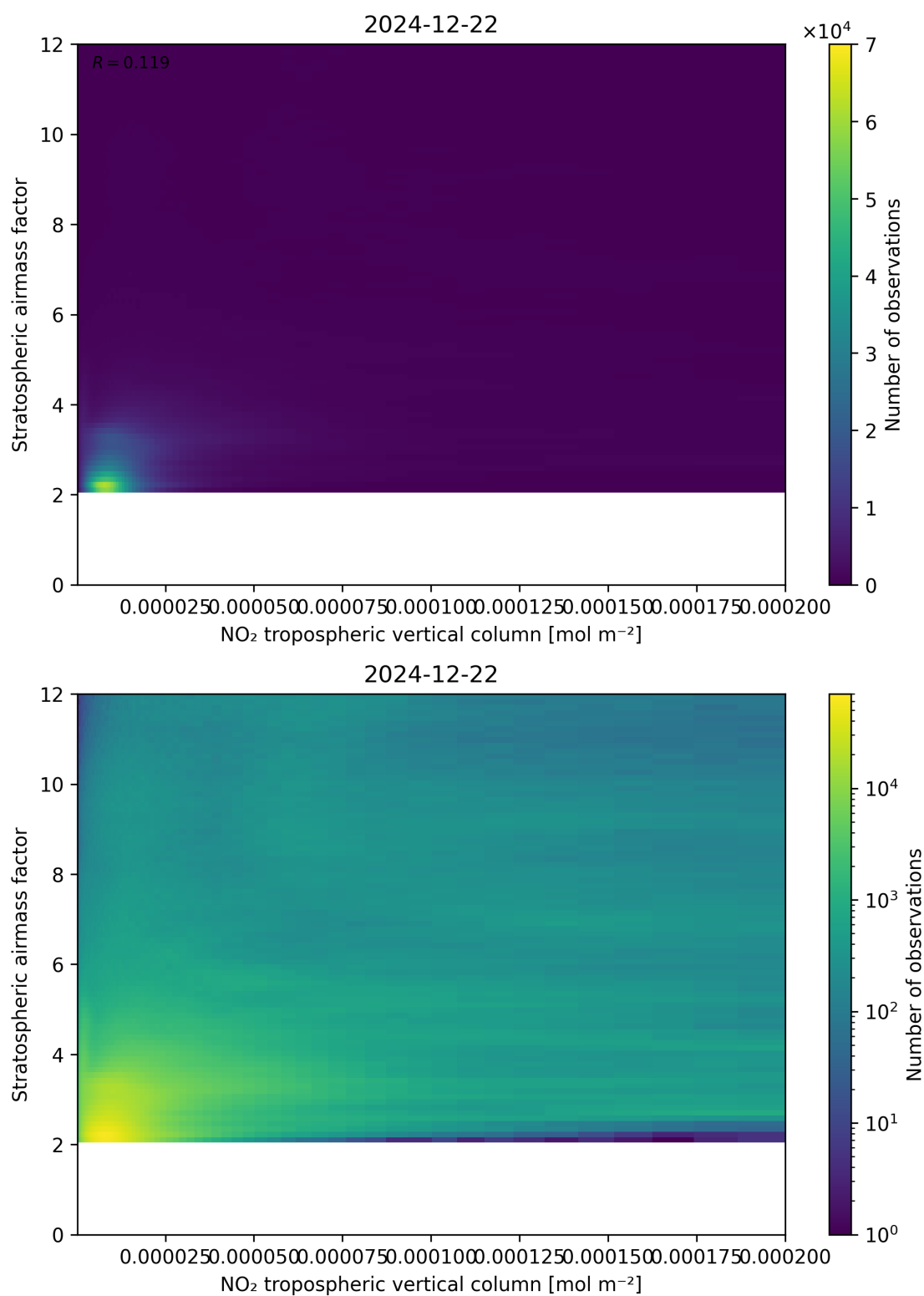
Figure 121: Scatter density plot of “NO 2 tropospheric vertical column” against “Stratospheric airmass factor” for 2024-12-22 to 2024-12-23.
