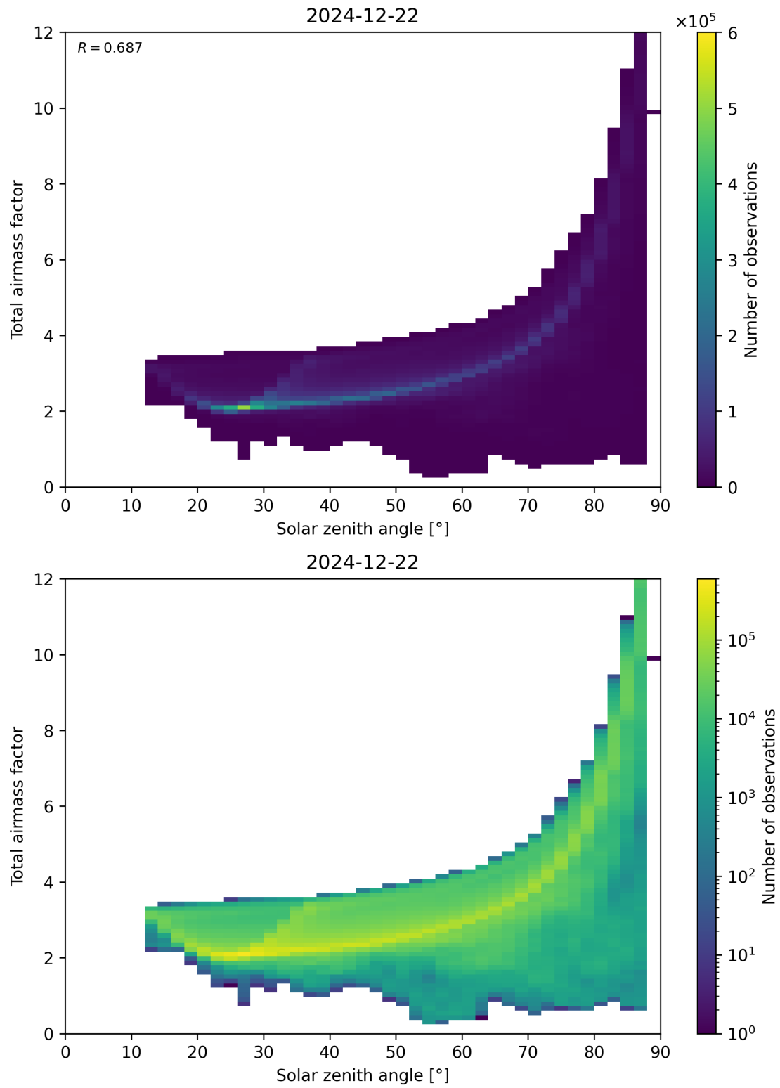
Figure 146: Scatter density plot of “Solar zenith angle” against “Total airmass factor” for 2024-12-22 to 2024-12-23.
