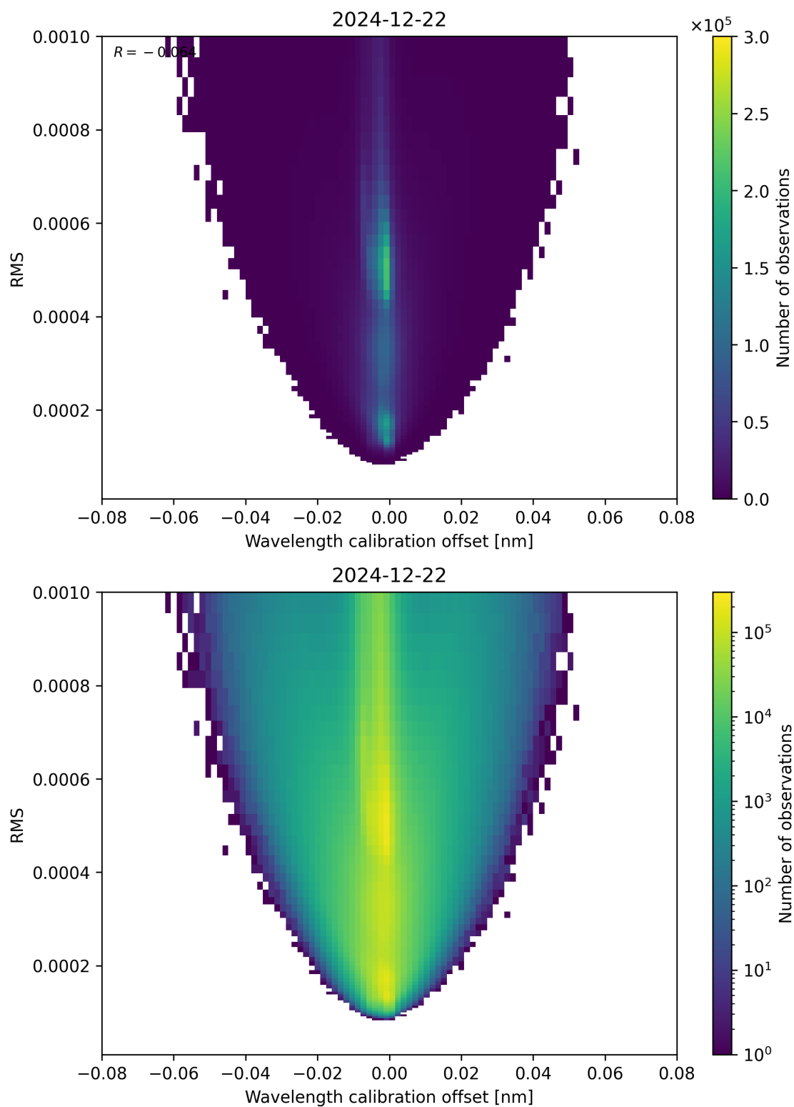
Figure 181: Scatter density plot of “Wavelength calibration offset” against “RMS” for 2024-12-22 to 2024-12-23.
