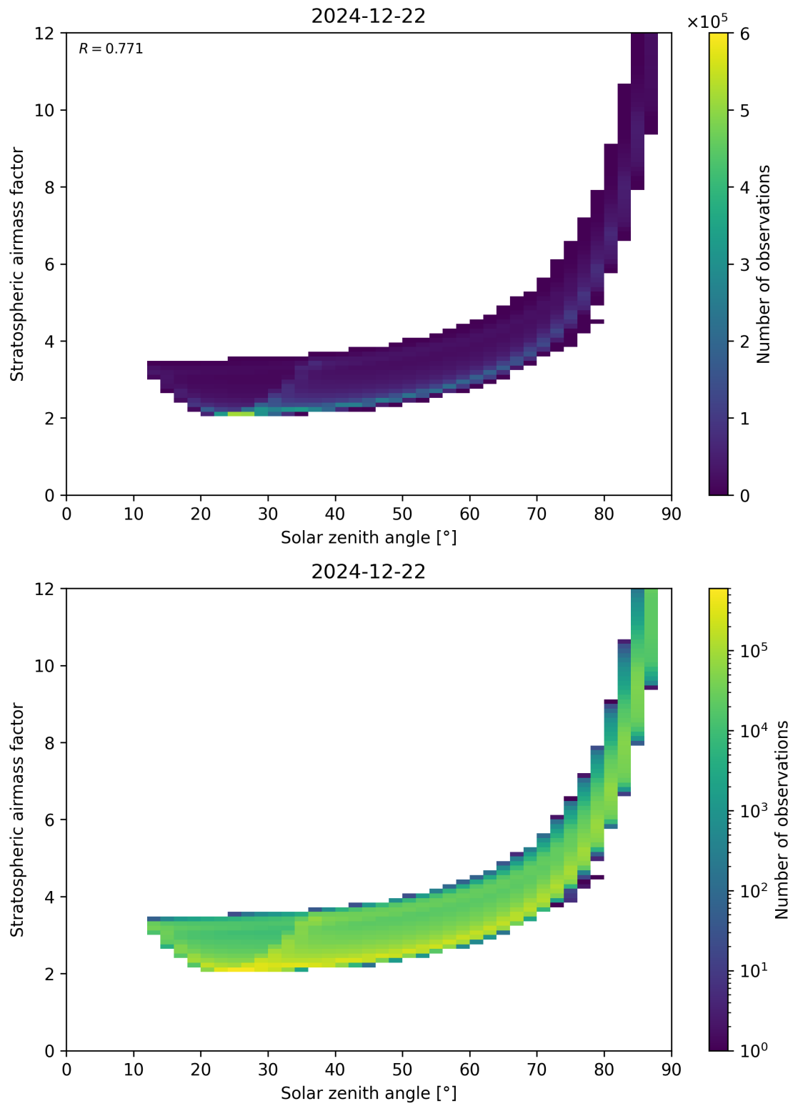
Figure 145: Scatter density plot of “Solar zenith angle” against “Stratospheric airmass factor” for 2024-12-22 to 2024-12-23.
