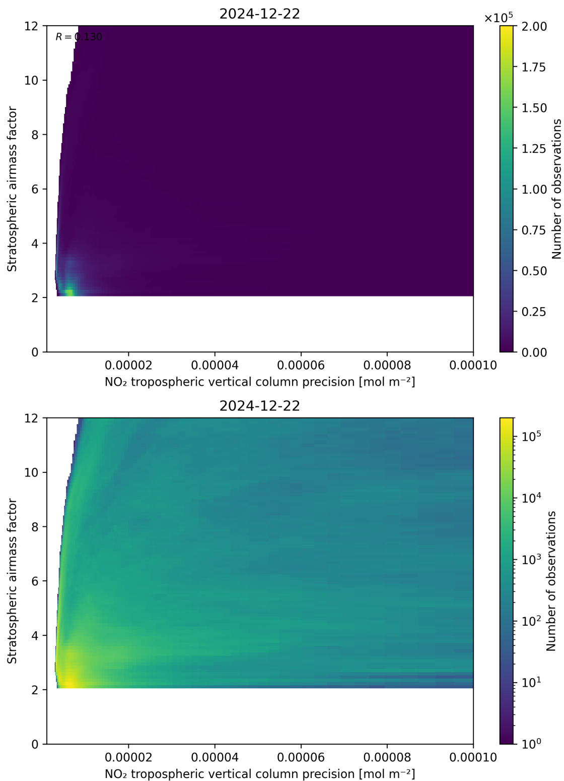
Figure 131: Scatter density plot of “NO 2 tropospheric vertical column precision” against “Stratospheric airmass factor” for 2024-12-22 to 2024-12-23.
