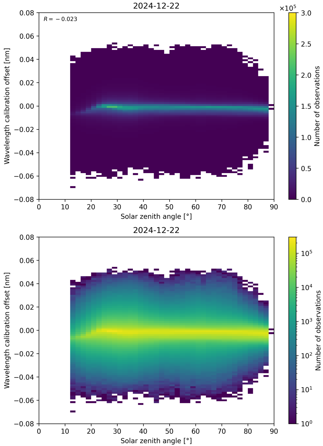
Figure 158: Scatter density plot of “Solar zenith angle” against “Wavelength calibration offset” for 2024-12-22 to 2024-12-23.
