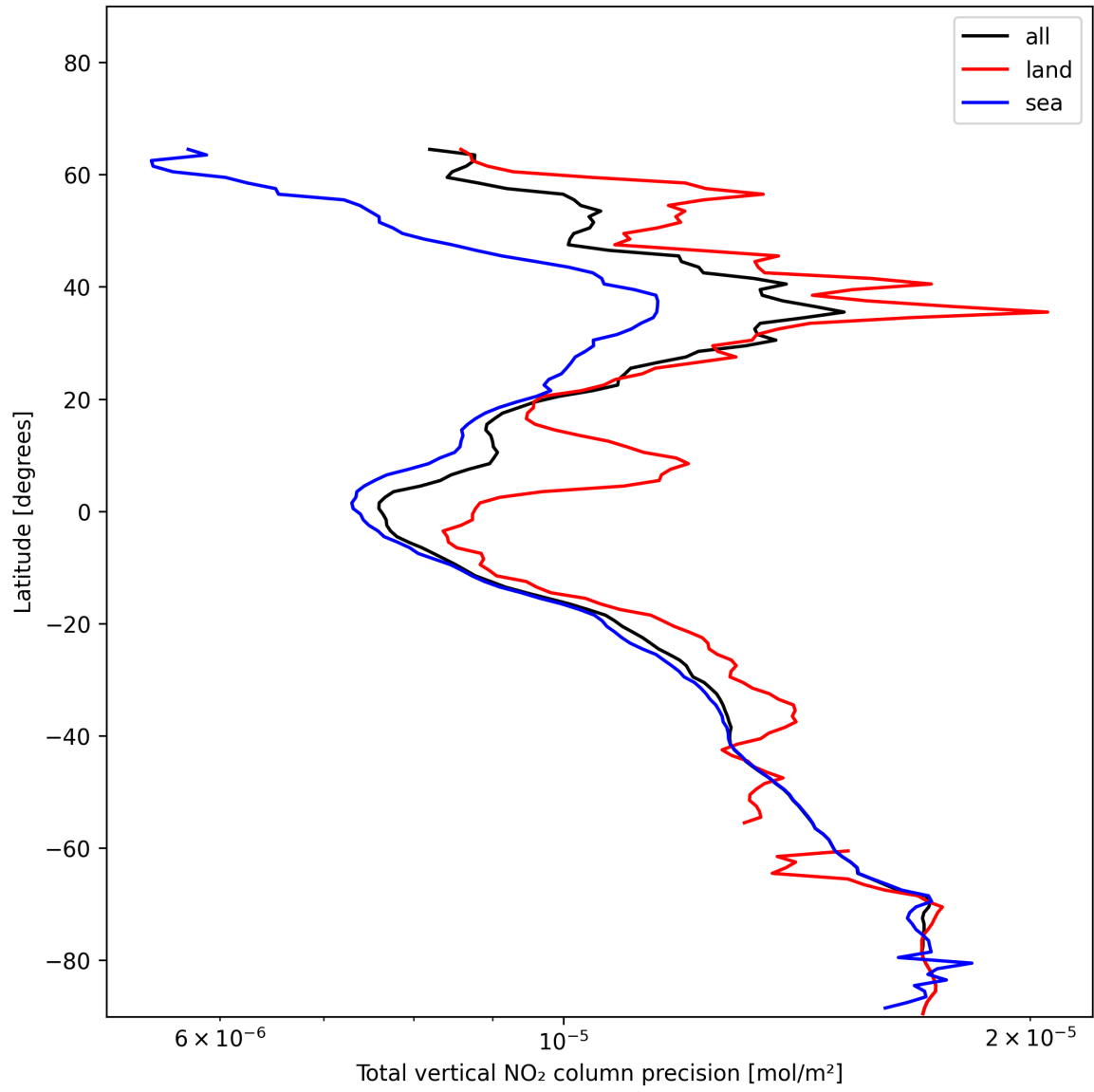
Figure 22: Zonal average of “Total vertical NO 2 column precision” for 2024-12-22 to 2024-12-23.
