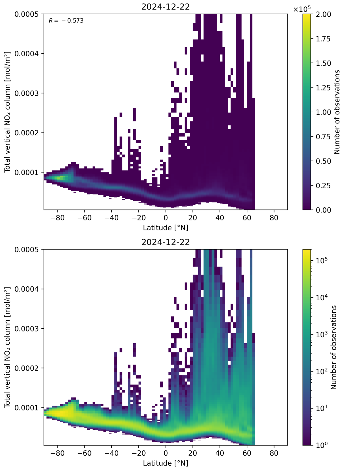
Figure 90: Scatter density plot of “Latitude” against “Total vertical NO 2 column” for 2024-12-22 to 2024-12-23.
