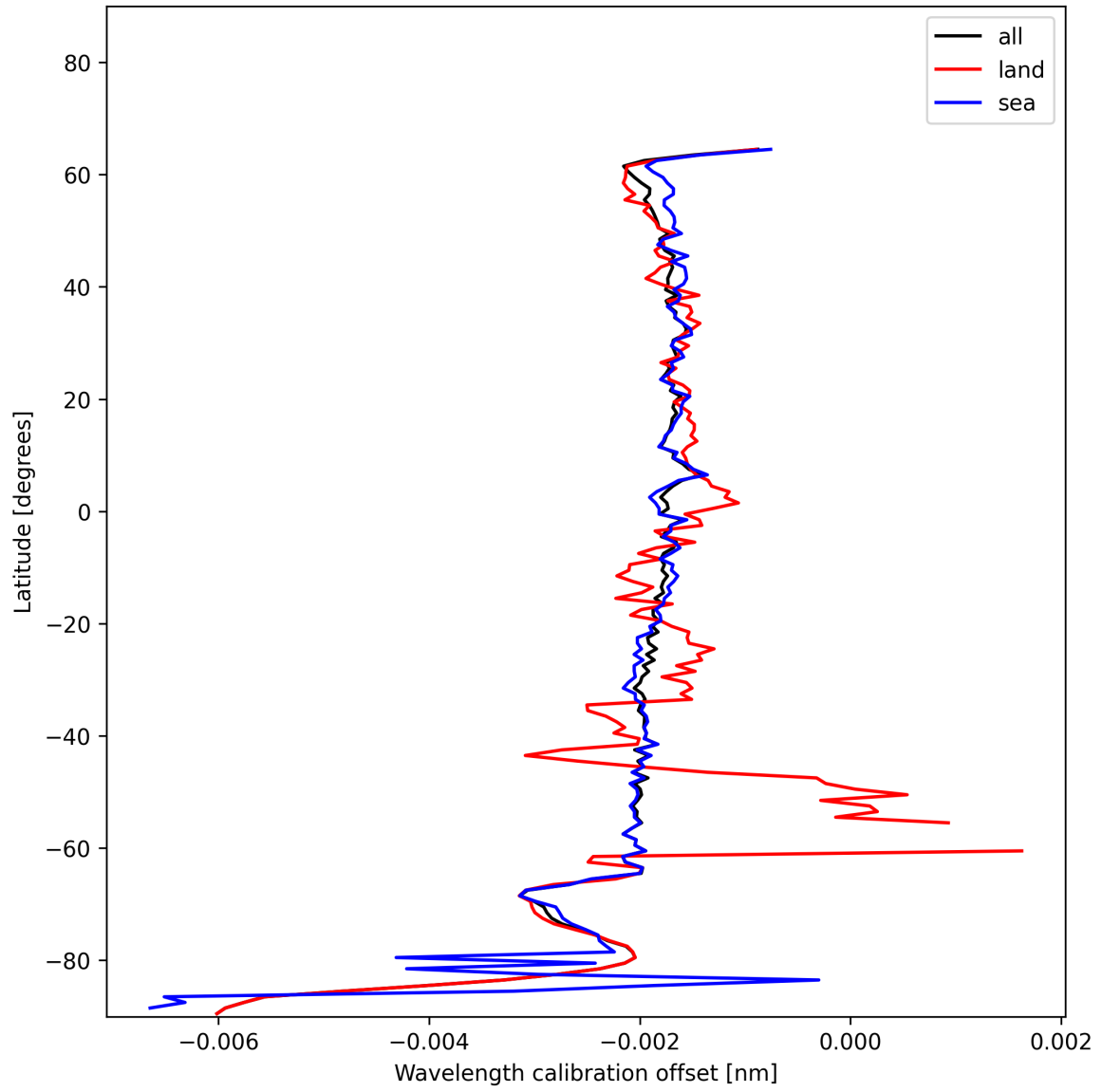
Figure 18: Zonal average of “Wavelength calibration offset” for 2024-12-22 to 2024-12-23.
