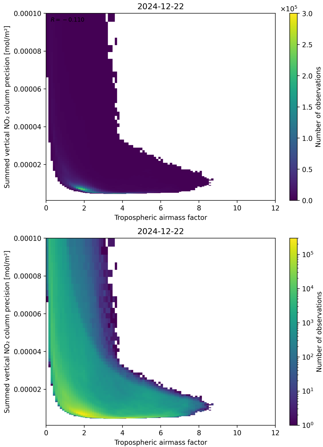
Figure 76: Scatter density plot of “Tropospheric air mass factor” against “Summed vertical NO 2 column precision” for 2024-12-22 to 2024-12-23.
