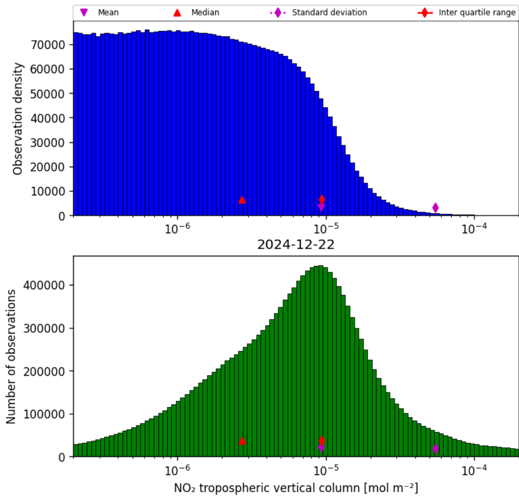
Figure 29: Histogram of “NO 2 tropospheric vertical column” for 2024-12-22 to 2024-12-23
