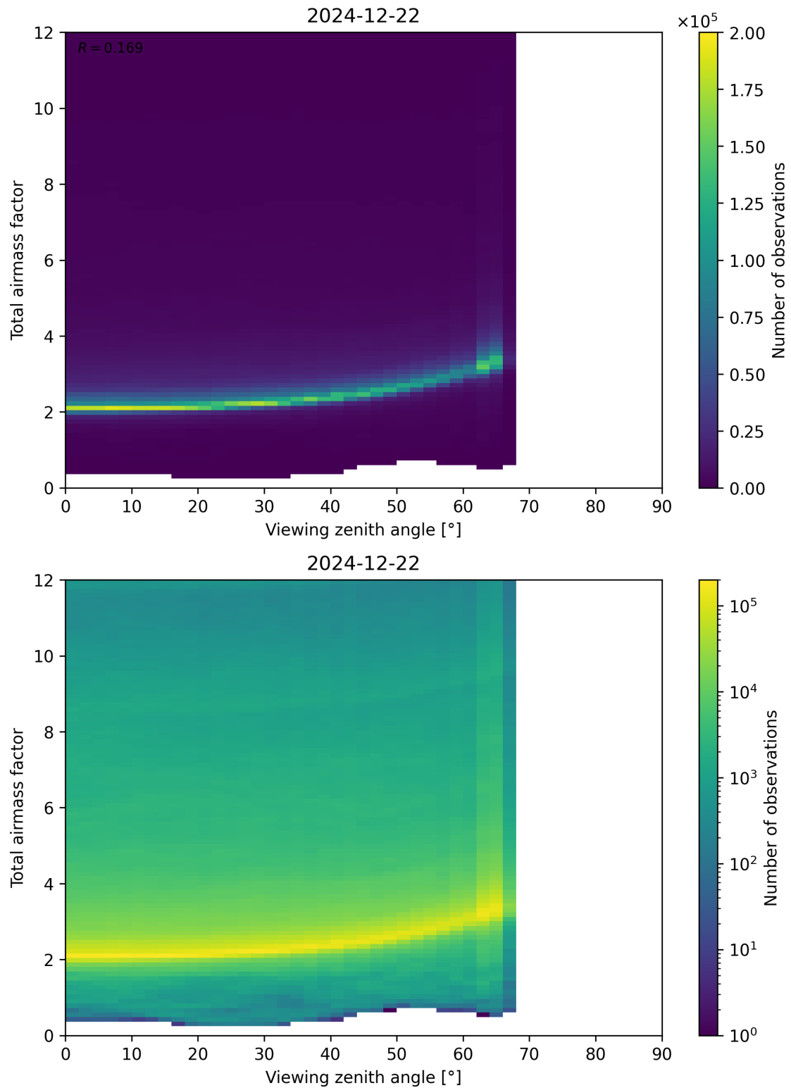
Figure 160: Scatter density plot of “Viewing zenith angle” against “Total airmass factor” for 2024-12-22 to 2024-12-23.
