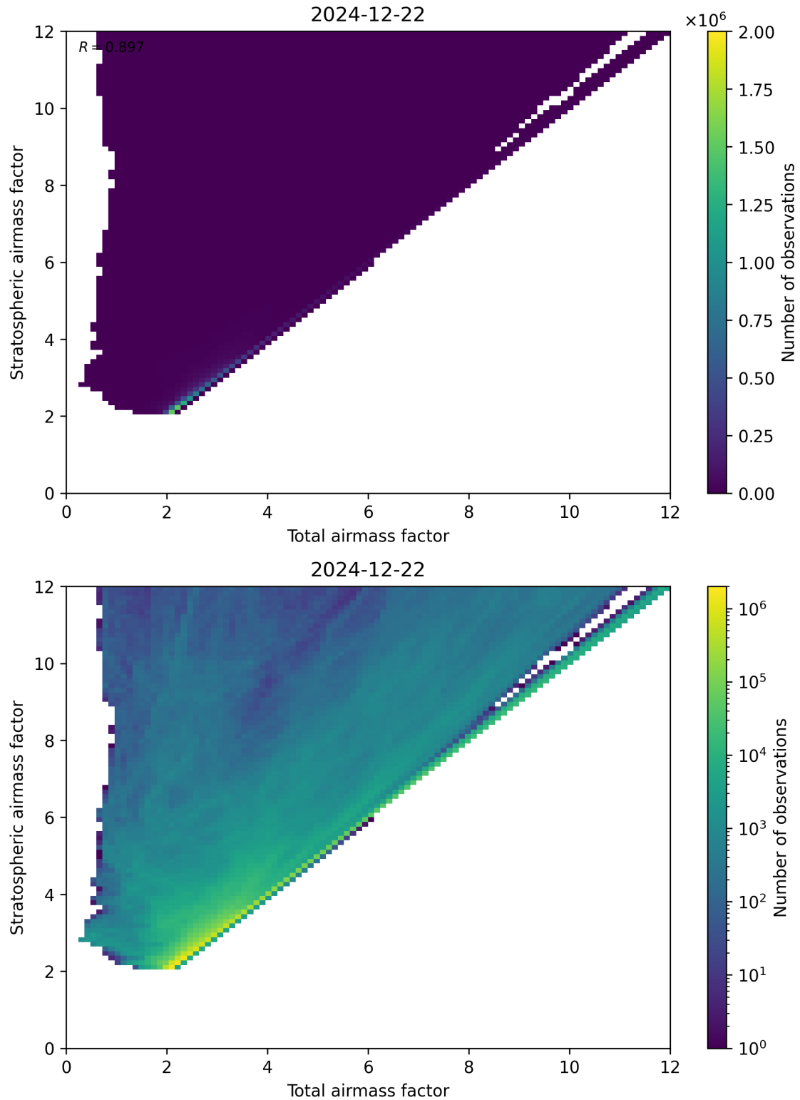
Figure 62: Scatter density plot of “Total airmass factor” against “Stratospheric airmass factor” for 2024-12-22 to 2024-12-23.
