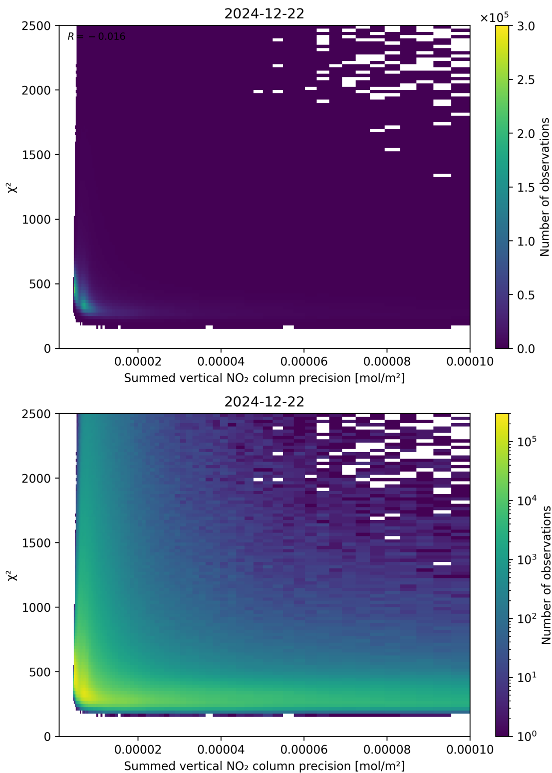
Figure 107: Scatter density plot of “Summed vertical NO 2 column precision” against “ \chi^2 ” for 2024-12-22 to 2024-12-23.
