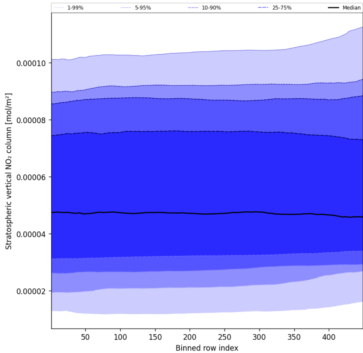
Figure 53: Along track statistics of “Stratospheric vertical NO 2 column” for 2024-12-22 to 2024-12-23
