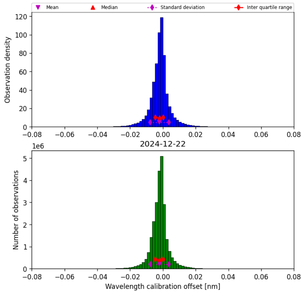
Figure 35: Histogram of “Wavelength calibration offset” for 2024-12-22 to 2024-12-23
