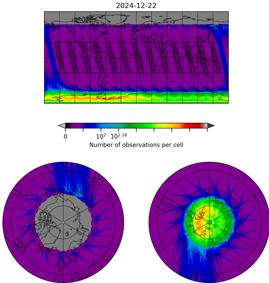
Figure 10: Map of the number of observations for 2024-12-22 to 2024-12-23
