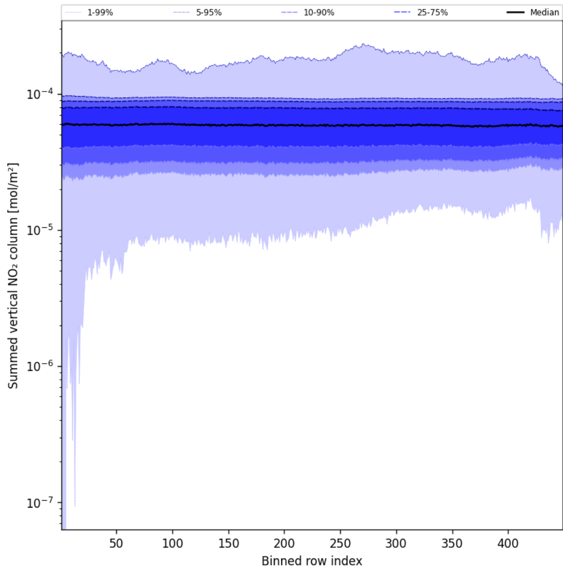
Figure 57: Along track statistics of “Summed vertical NO 2 column” for 2024-12-22 to 2024-12-23
