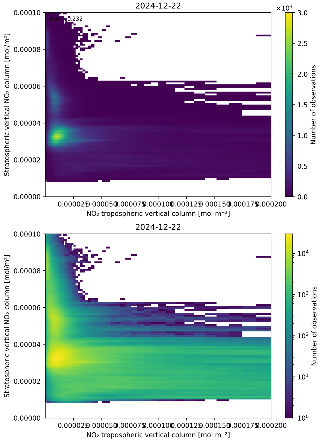
Figure 125: Scatter density plot of “NO 2 tropospheric vertical column” against “Stratospheric vertical NO 2 column” for 2024-12-22 to 2024-12-23.
