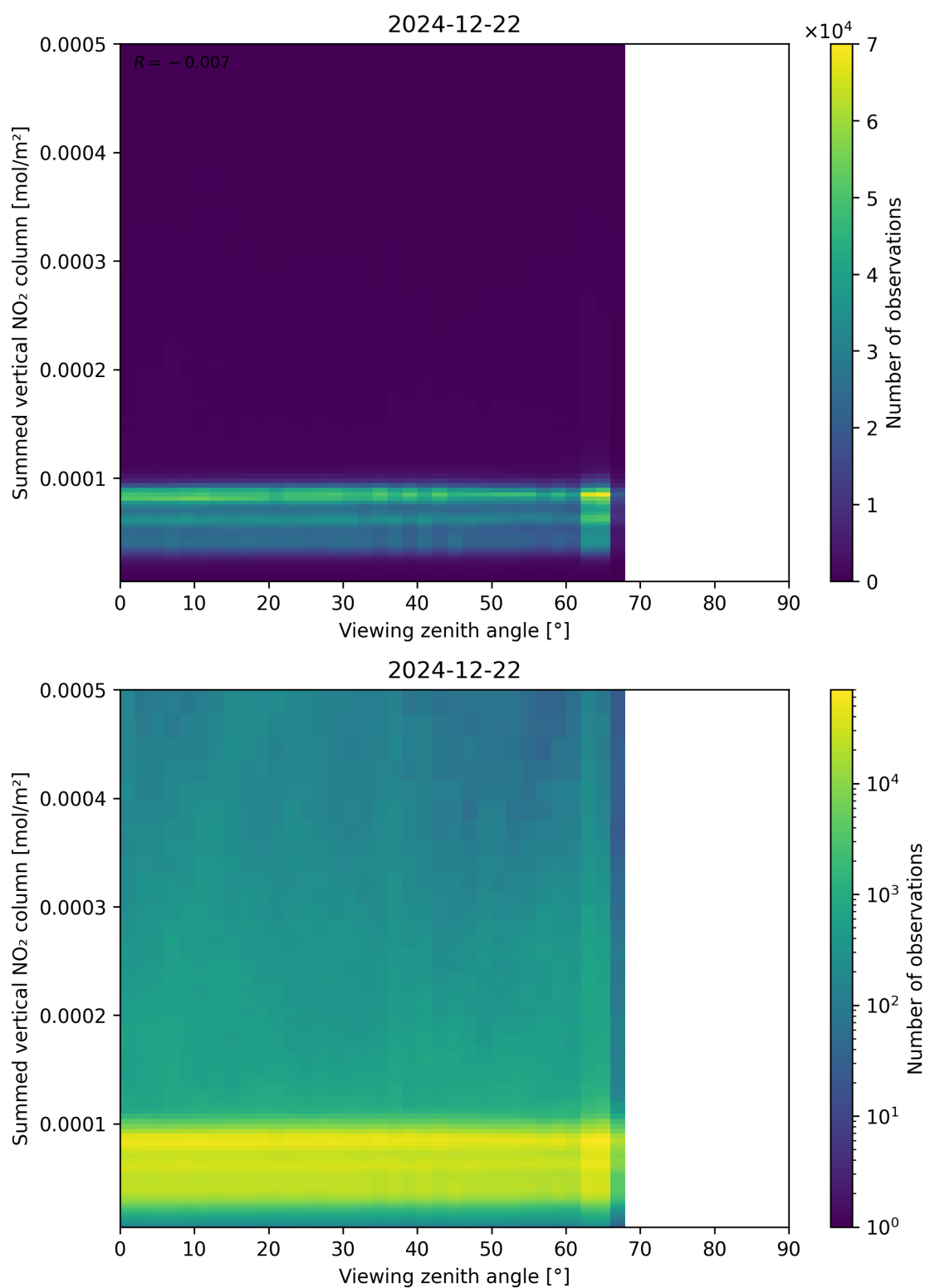
Figure 165: Scatter density plot of “Viewing zenith angle” against “Summed vertical NO 2 column” for 2024-12-22 to 2024-12-23.
