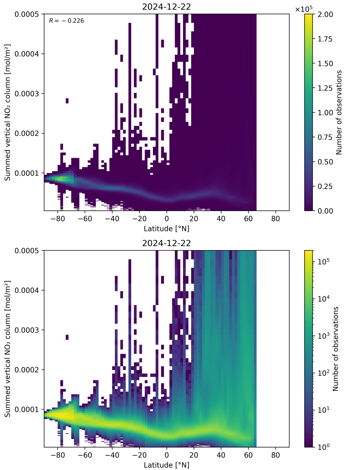
Figure 88: Scatter density plot of “Latitude” against “Summed vertical NO 2 column” for 2024-12-22 to 2024-12-23.
