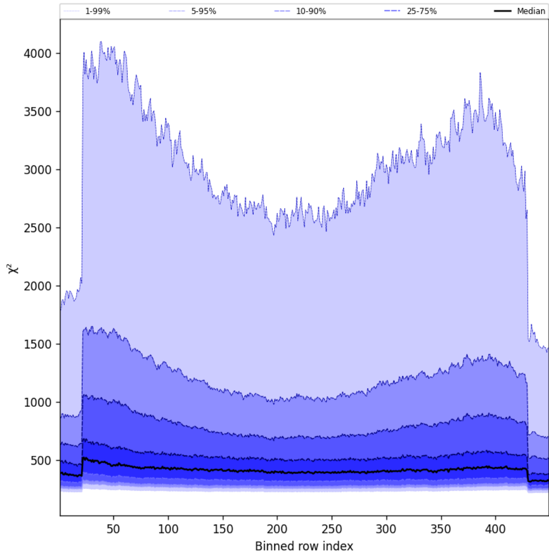
Figure 59: Along track statistics of “ \chi^2 ” for 2024-12-22 to 2024-12-23
