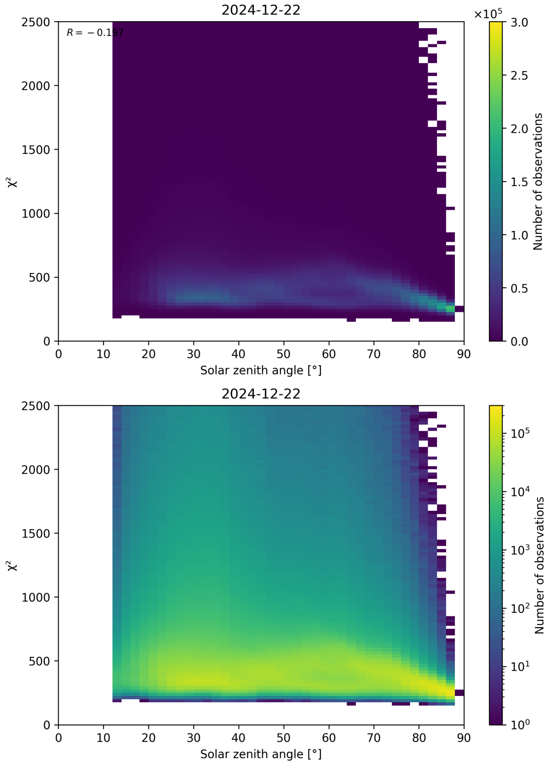
Figure 148: Scatter density plot of “Solar zenith angle” against “ \chi^2 ” for 2024-12-22 to 2024-12-23.
