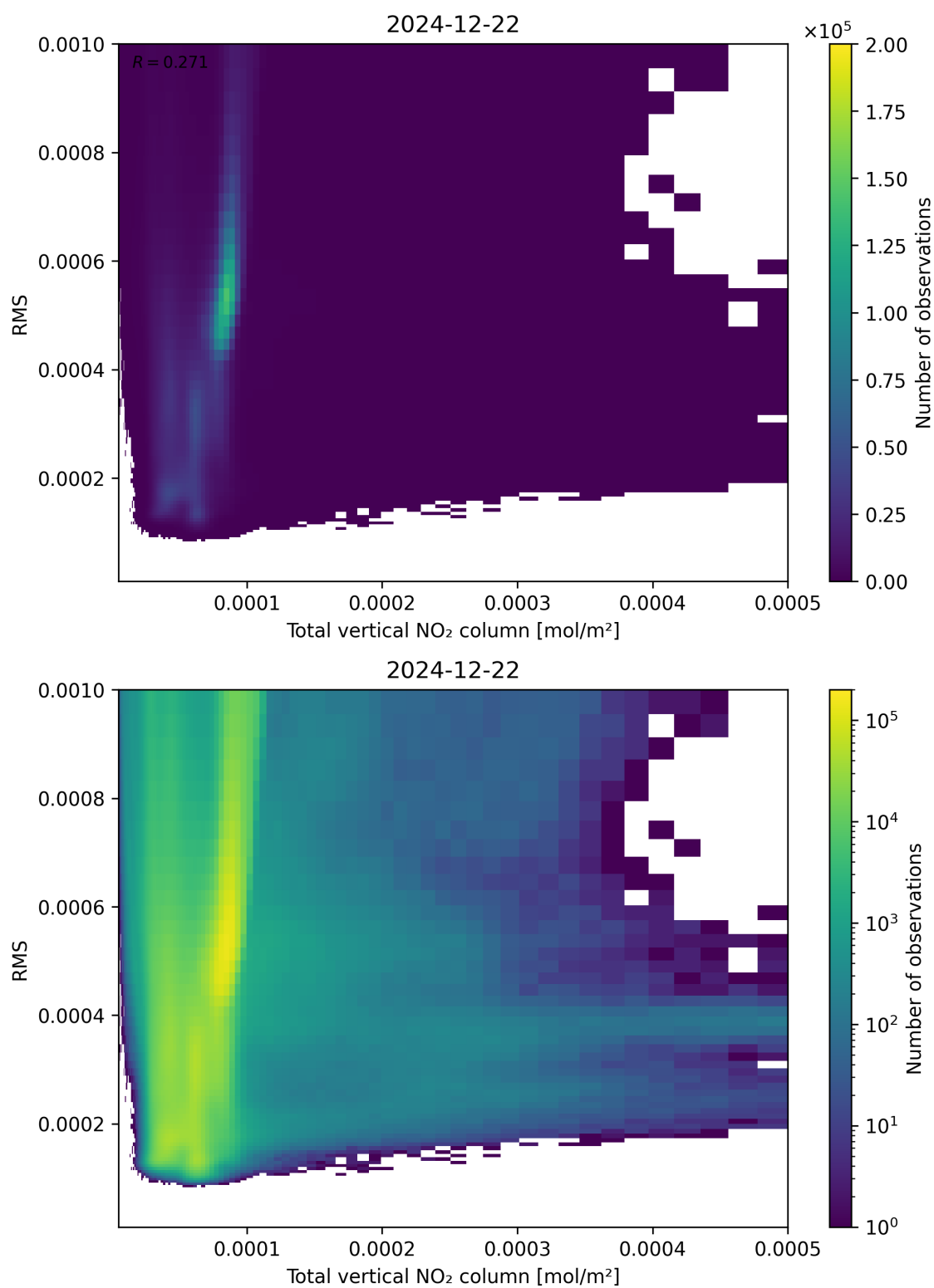
Figure 120: Scatter density plot of “Total vertical NO 2 column” against “RMS” for 2024-12-22 to 2024-12-23.
