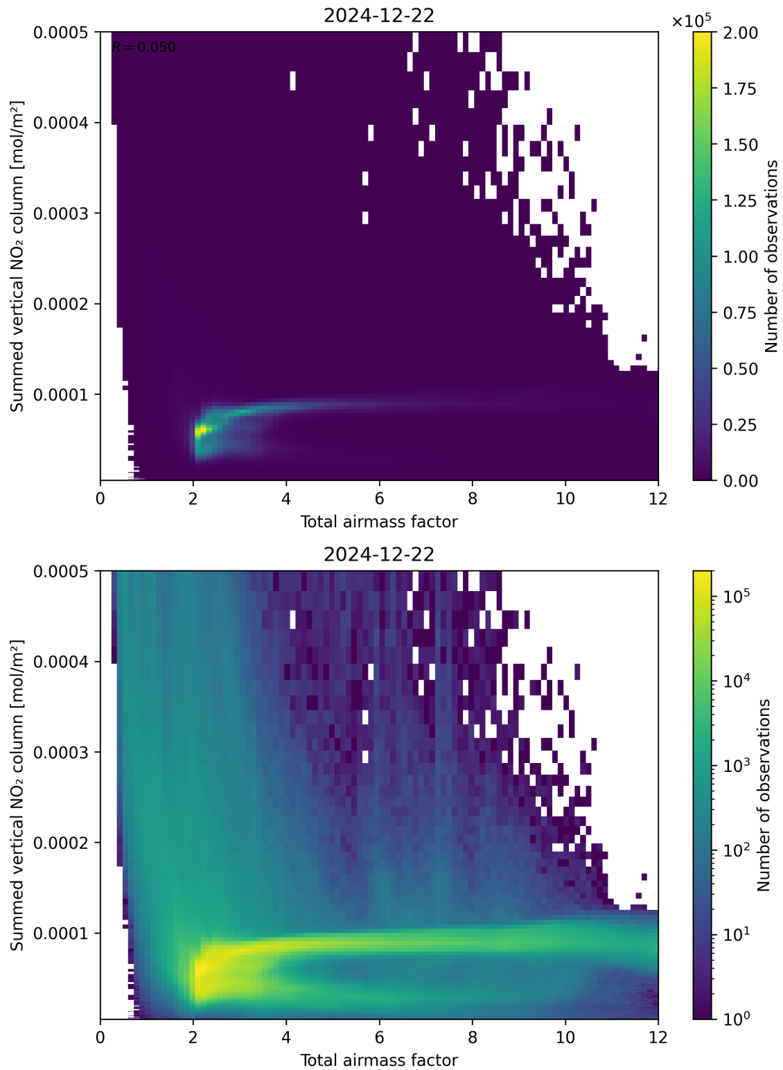
Figure 65: Scatter density plot of “Total air mass factor” against “Summed vertical NO 2 column” for 2024-12-22 to 2024-12-23.
