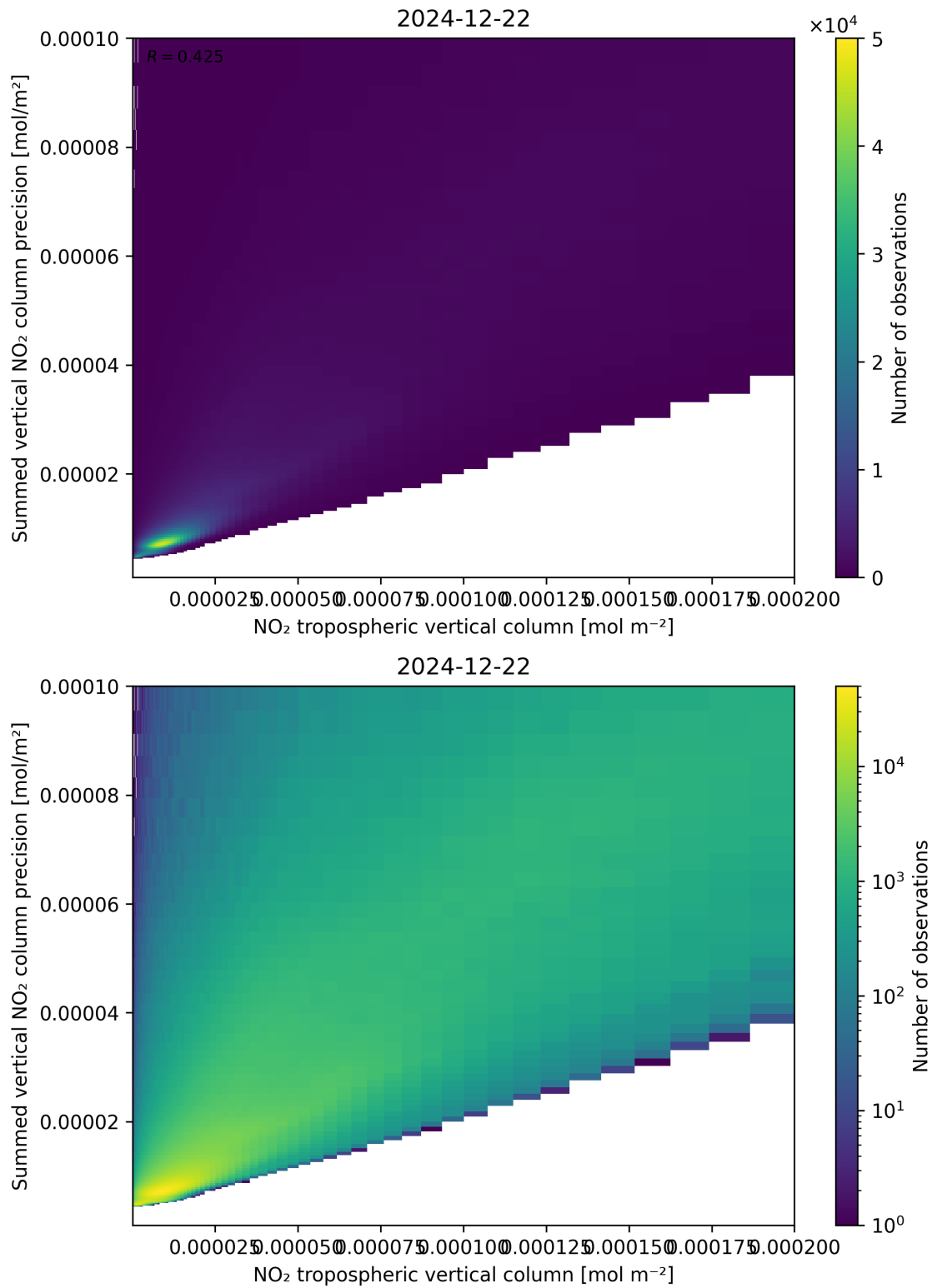
Figure 127: Scatter density plot of “NO 2 tropospheric vertical column” against “Summed vertical NO 2 column precision” for 2024-12-22 to 2024-12-23.
