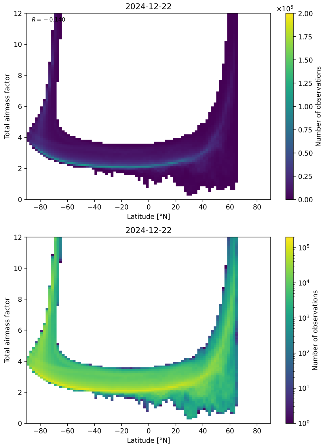
Figure 84: Scatter density plot of “Latitude” against “Total airmass factor” for 2024-12-22 to 2024-12-23.
