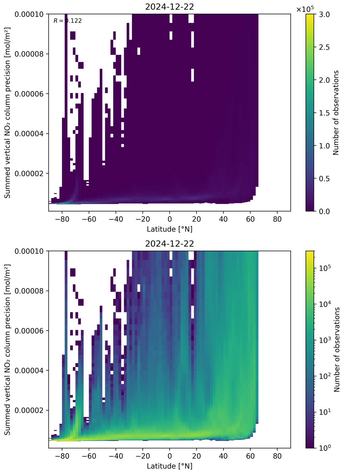
Figure 89: Scatter density plot of “Latitude” against “Summed vertical NO 2 column precision” for 2024-12-22 to 2024-12-23.
