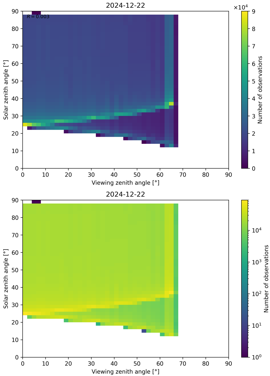
Figure 172: Scatter density plot of “Viewing zenith angle” against “Solar zenith angle” for 2024-12-22 to 2024-12-23.
