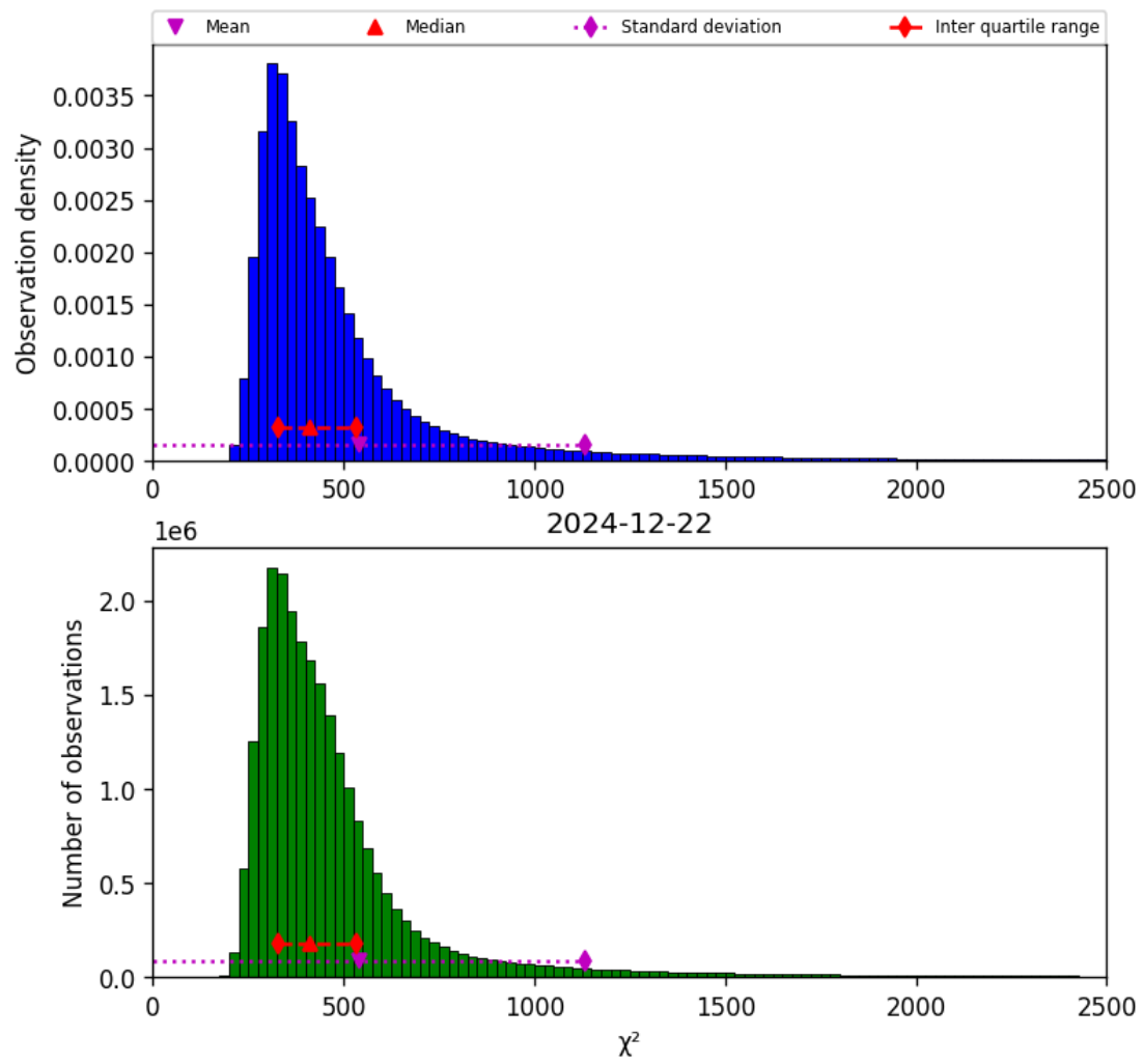
Figure 42: Histogram of “ \chi^2 ” for 2024-12-22 to 2024-12-23
