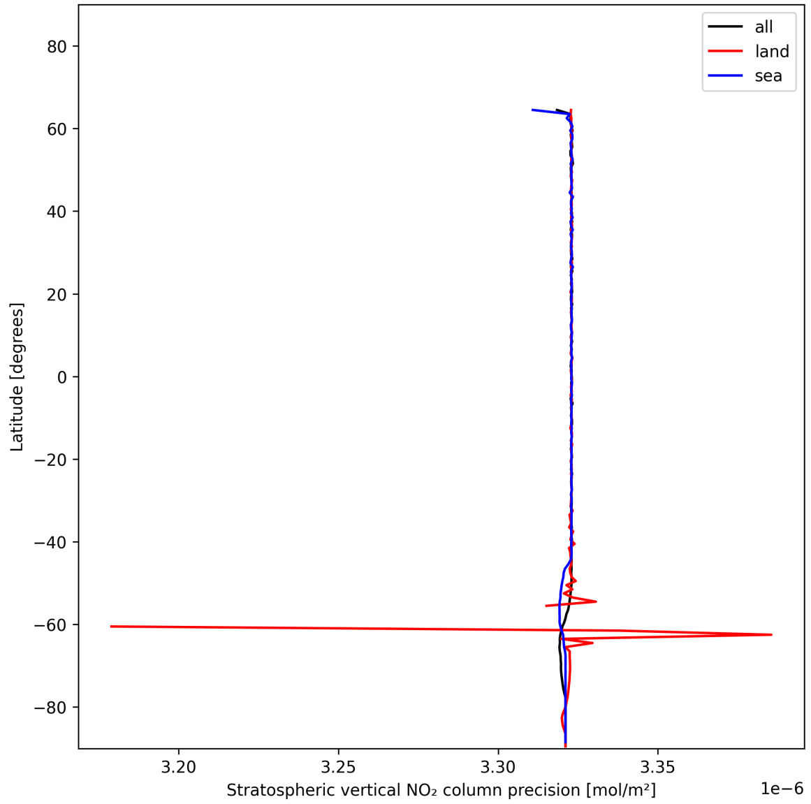
Figure 20: Zonal average of "Stratospheric vertical NO 2 column precision" for 2024-12-22 to 2024-12-23.
