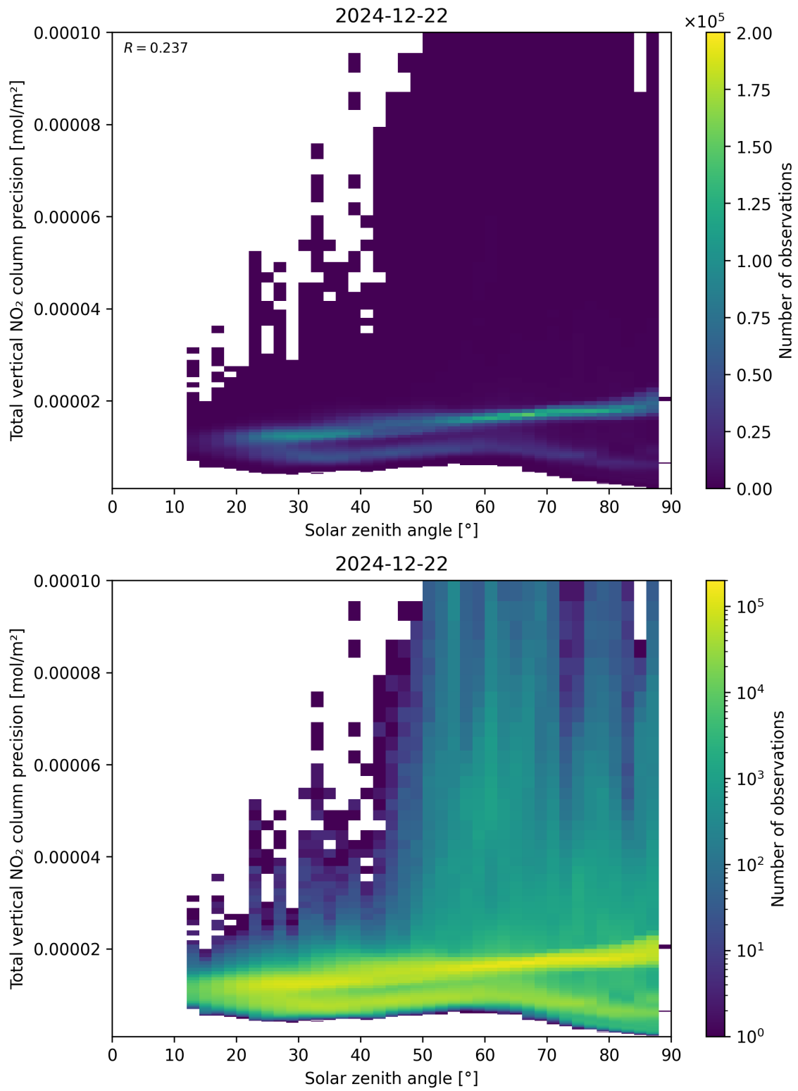
Figure 154: Scatter density plot of “Solar zenith angle” against “Total vertical NO 2 column precision” for 2024-12-22 to 2024-12-23.
