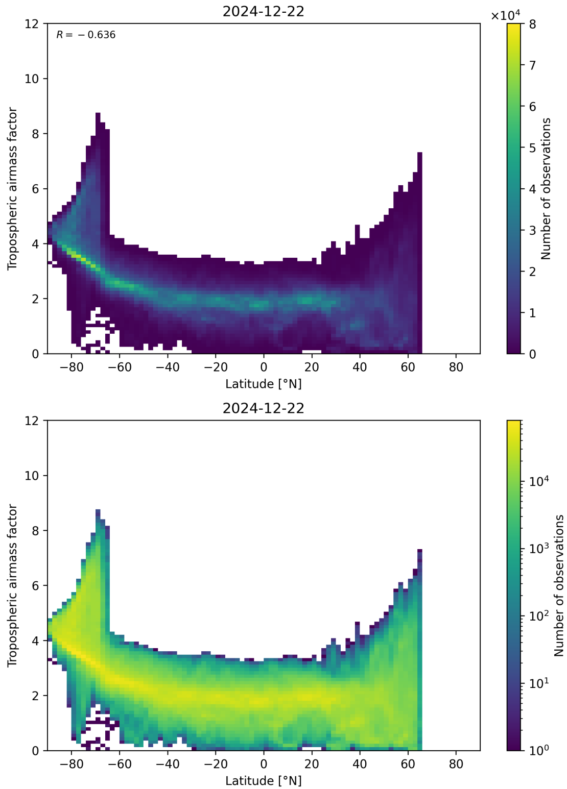
Figure 85: Scatter density plot of “Latitude” against “Tropospheric airmass factor” for 2024-12-22 to 2024-12-23.
