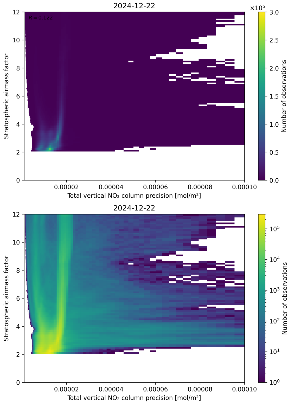
Figure 115: Scatter density plot of “Total vertical NO 2 column precision” against “Stratospheric air mass factor” for 2024-12-22 to 2024-12-23.
