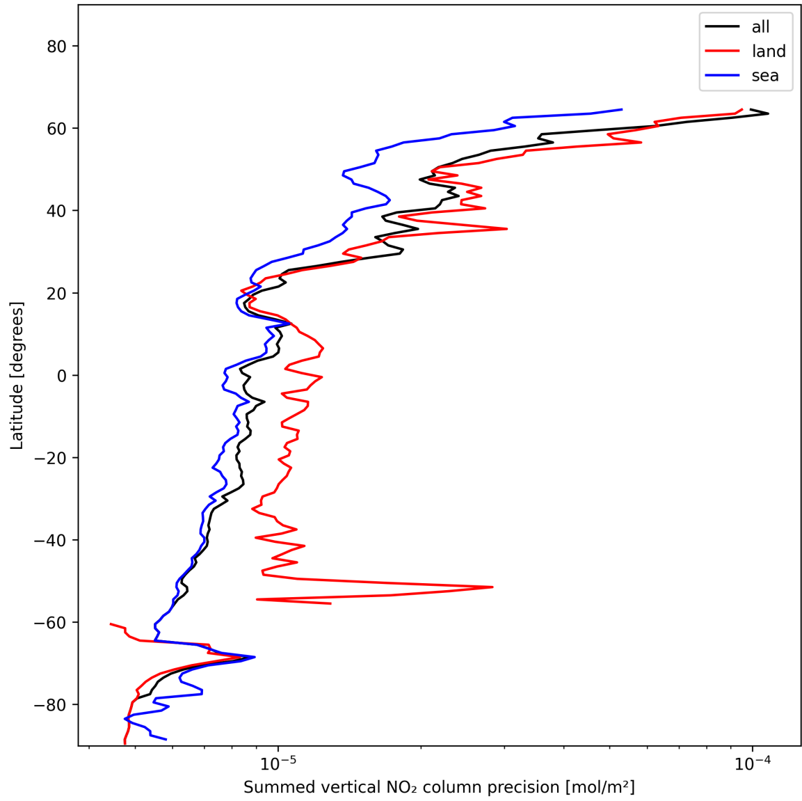
Figure 24: Zonal average of “Summed vertical NO 2 column precision” for 2024-12-22 to 2024-12-23.
