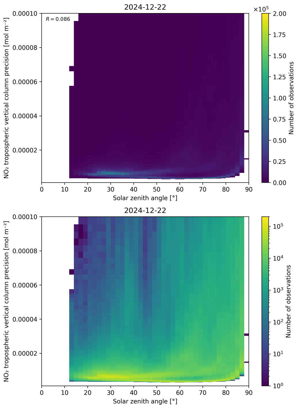
Figure 156: Scatter density plot of “Solar zenith angle” against “NO 2 tropospheric vertical column precision” for 2024-12-22 to 2024-12-23.
