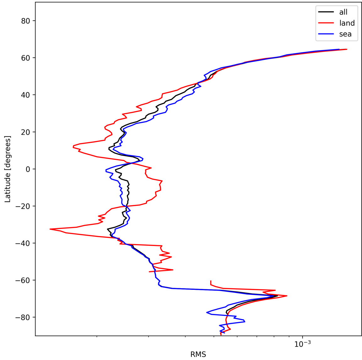
Figure 26: Zonal average of “RMS” for 2024-12-22 to 2024-12-23.
