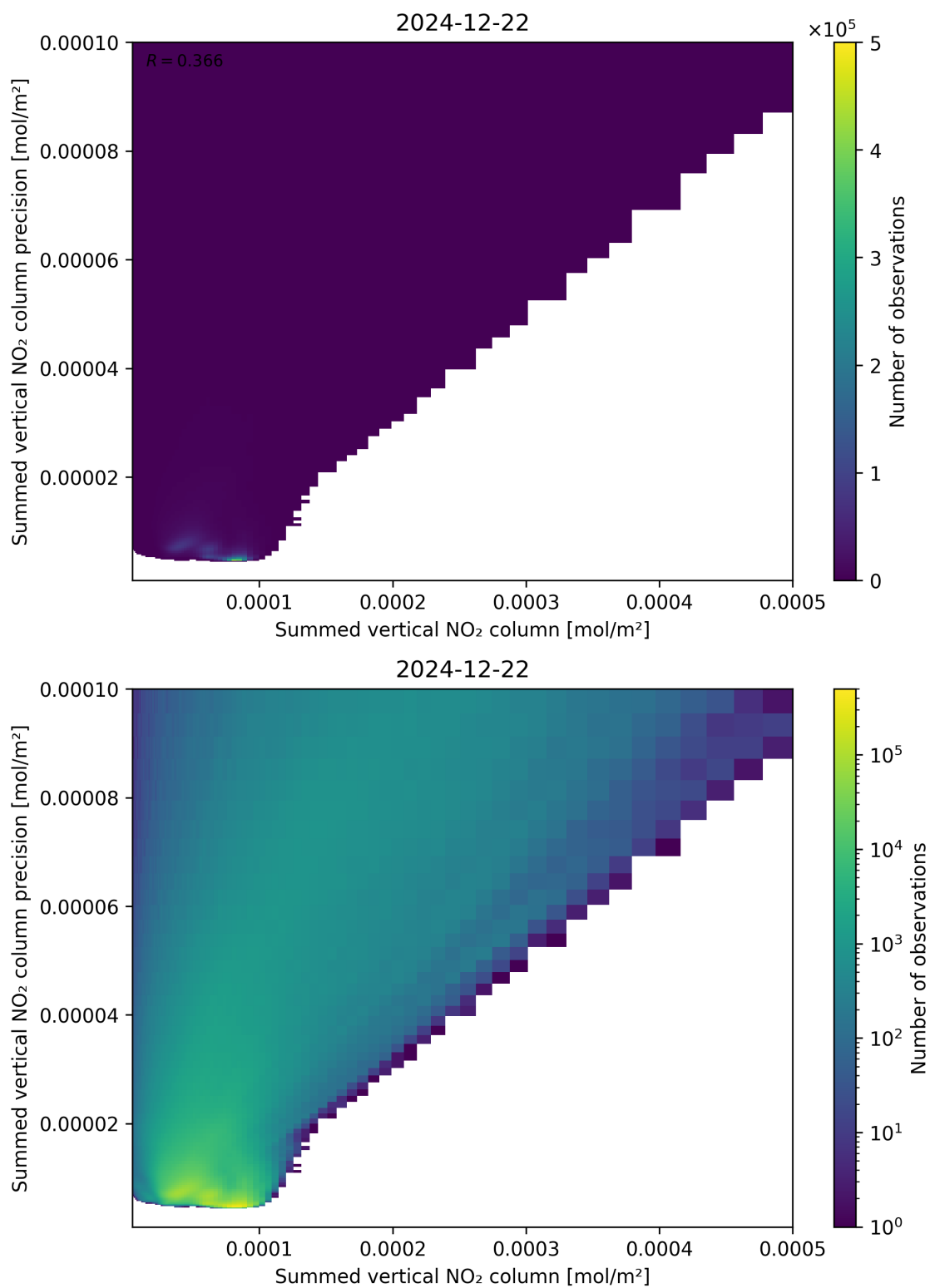
Figure 105: Scatter density plot of “Summed vertical NO 2 column” against “Summed vertical NO 2 column precision” for 2024-12-22 to 2024-12-23.
