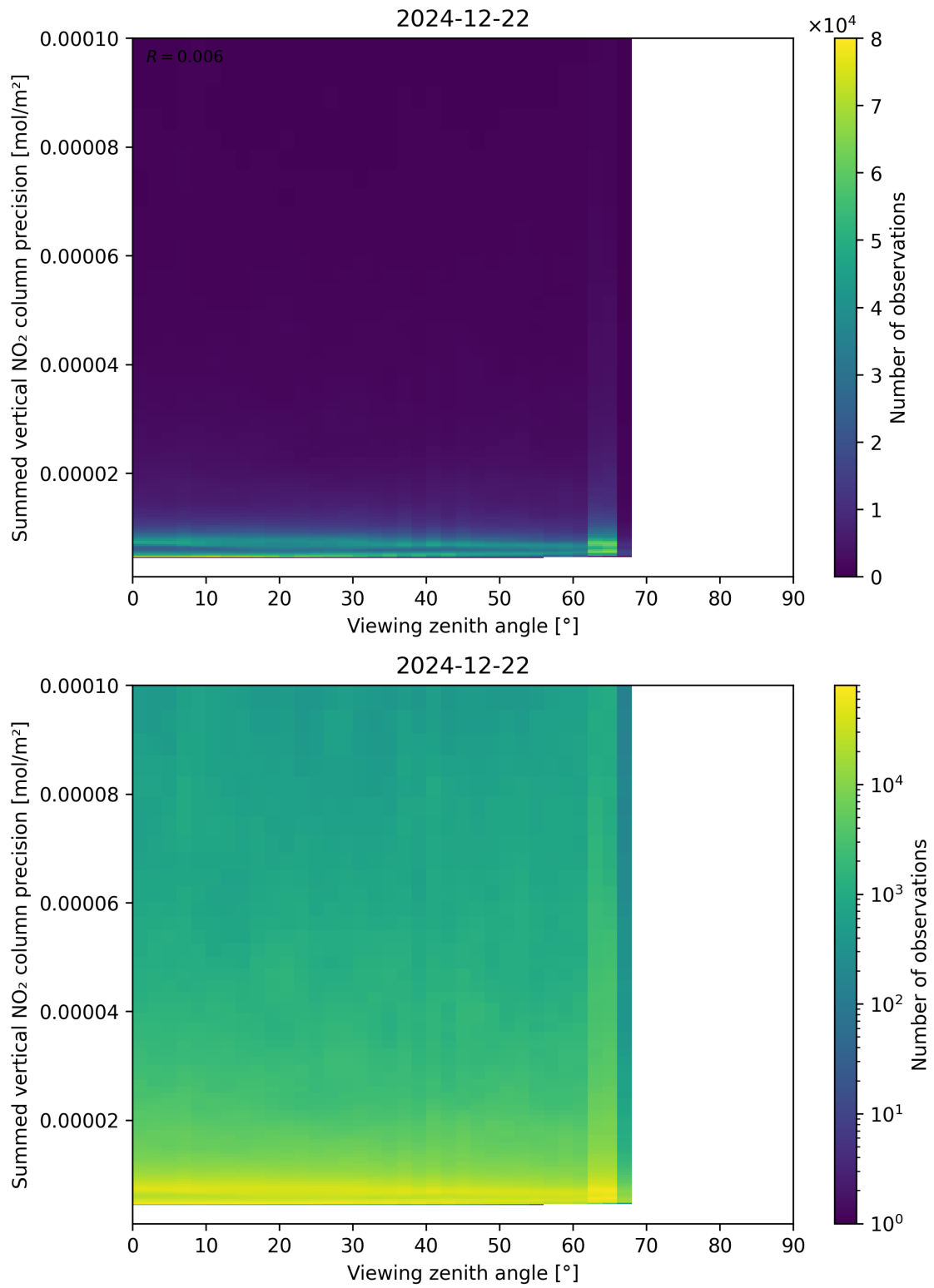
Figure 166: Scatter density plot of “Viewing zenith angle” against “Summed vertical NO 2 column precision” for 2024-12-22 to 2024-12-23.
