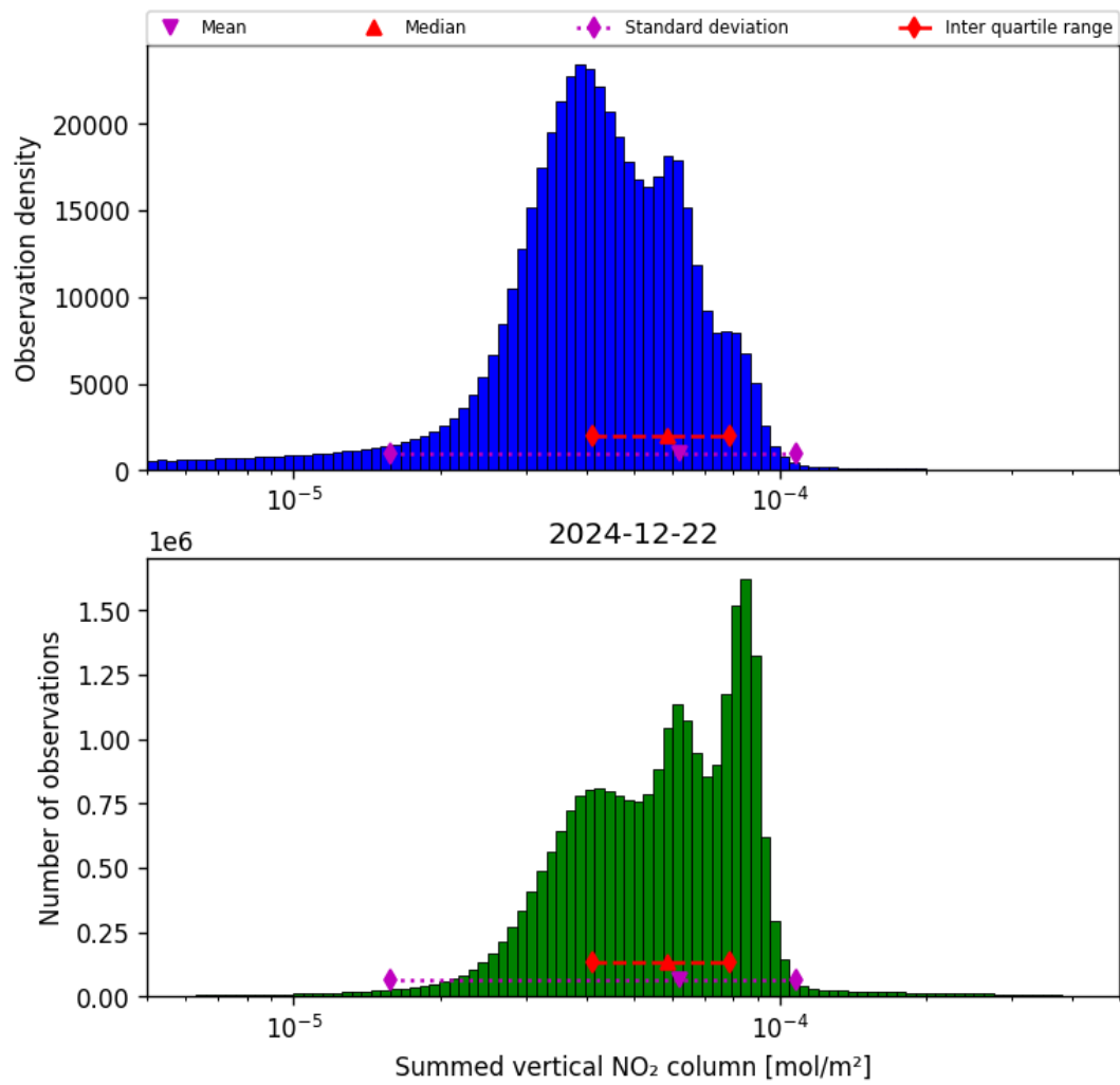
Figure 40: Histogram of “Summed vertical NO 2 column” for 2024-12-22 to 2024-12-23
