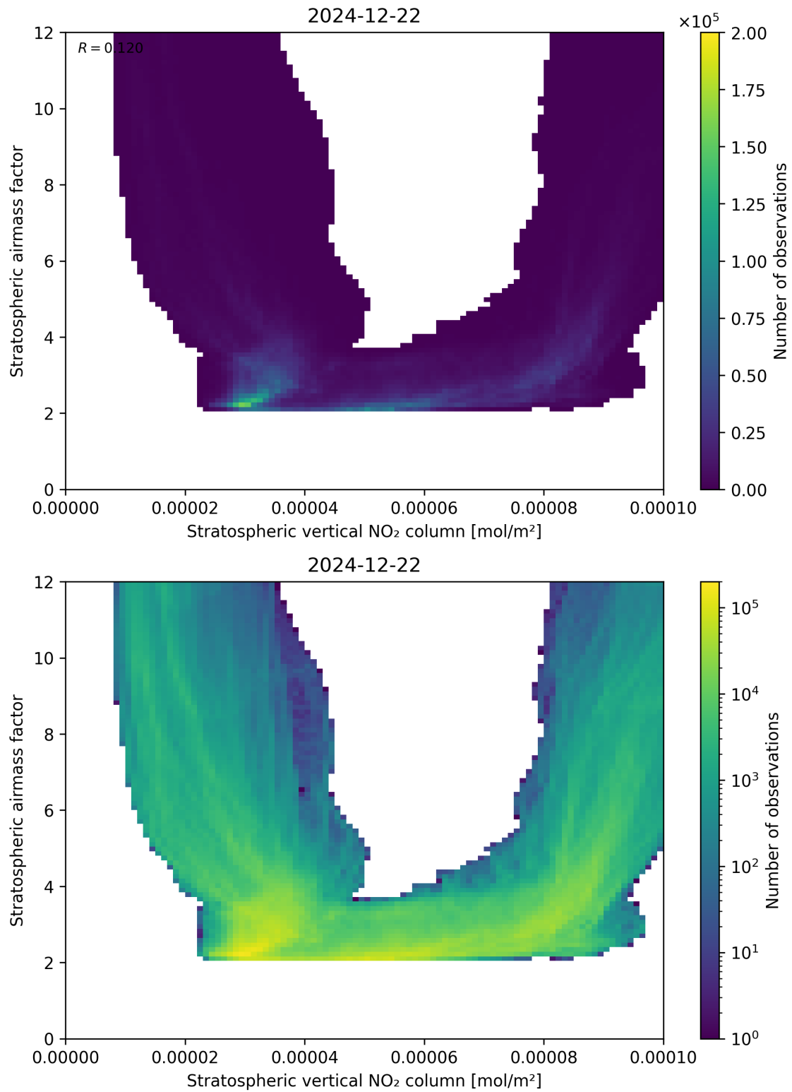
Figure 96: Scatter density plot of “Stratospheric vertical NO 2 column” against “Stratospheric airmass factor” for 2024-12-22 to 2024-12-23.
