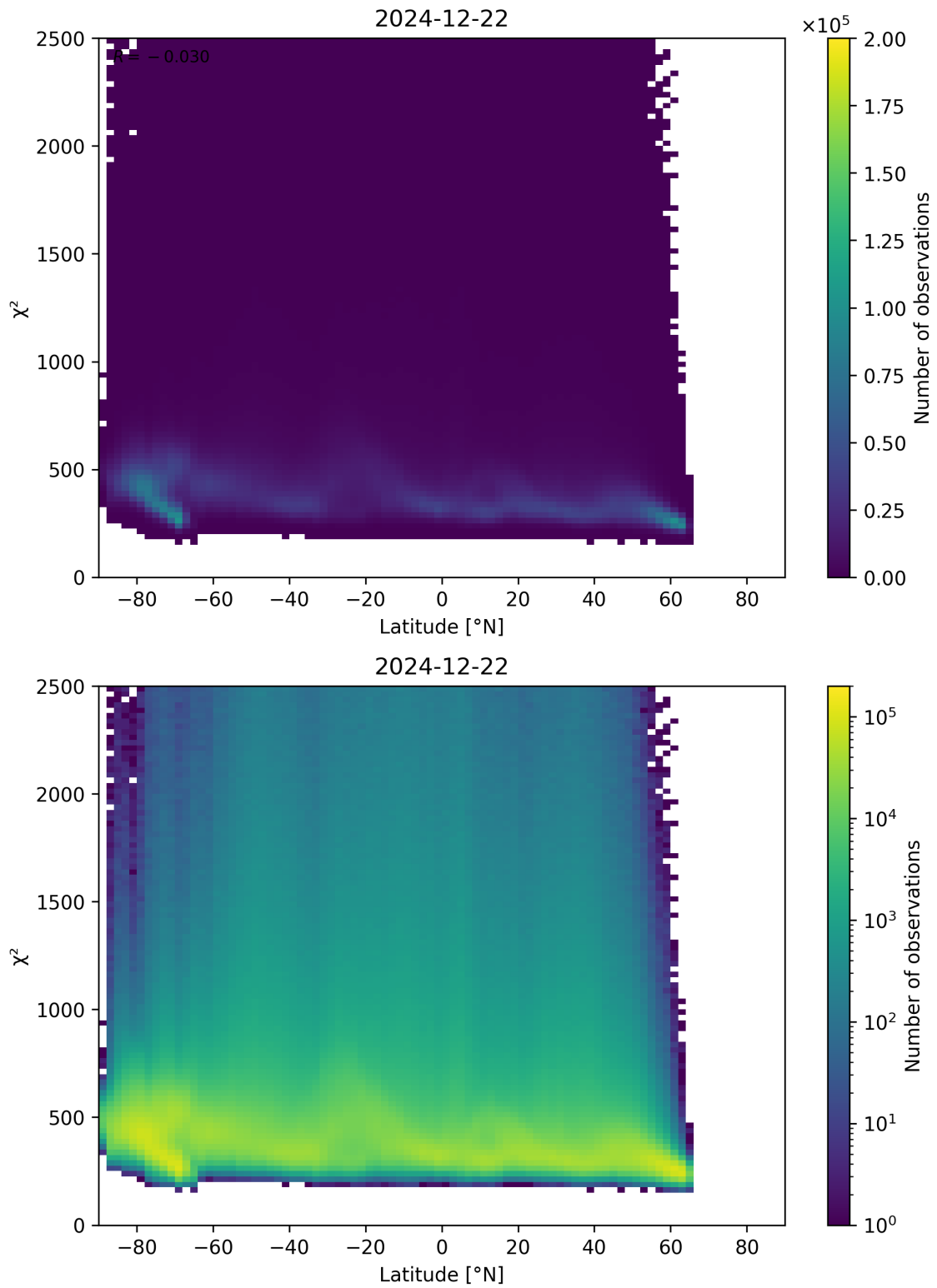
Figure 86: Scatter density plot of “Latitude” against “ \chi^2 ” for 2024-12-22 to 2024-12-23.
