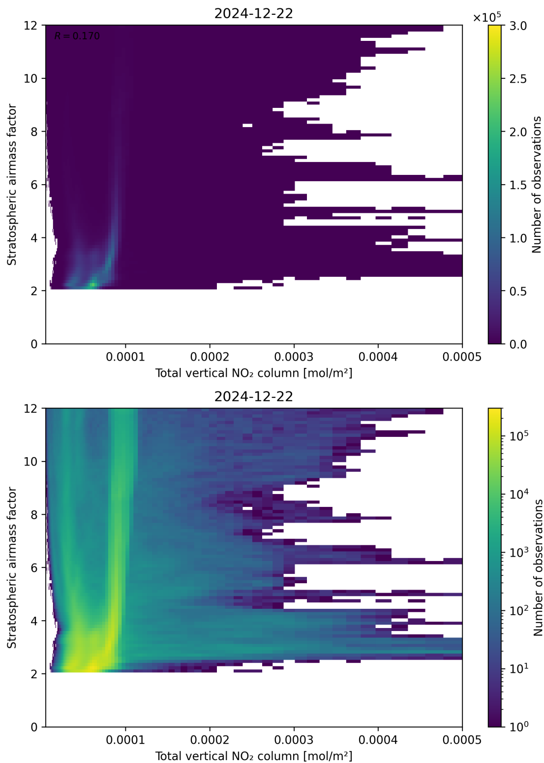
Figure 110: Scatter density plot of “Total vertical NO 2 column” against “Stratospheric airmass factor” for 2024-12-22 to 2024-12-23.
