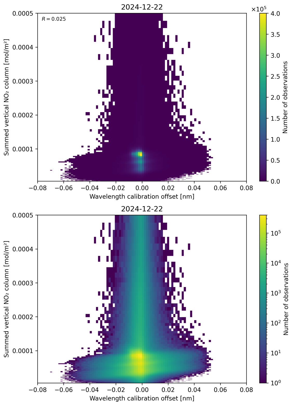
Figure 177: Scatter density plot of “Wavelength calibration offset” against “Summed vertical NO 2 column” for 2024-12-22 to 2024-12-23.
