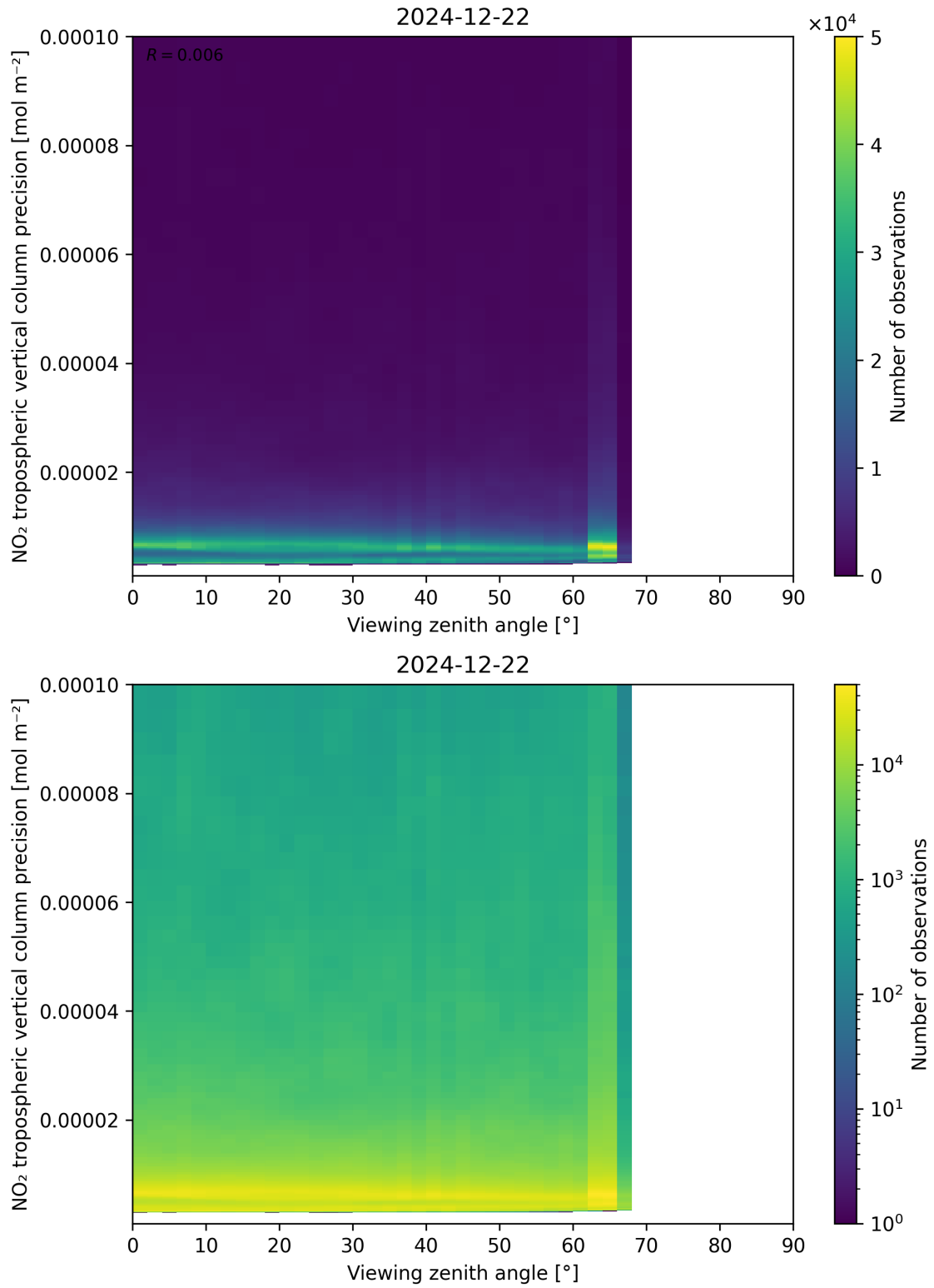
Figure 170: Scatter density plot of “Viewing zenith angle” against “NO 2 tropospheric vertical column precision” for 2024-12-22 to 2024-12-23.
