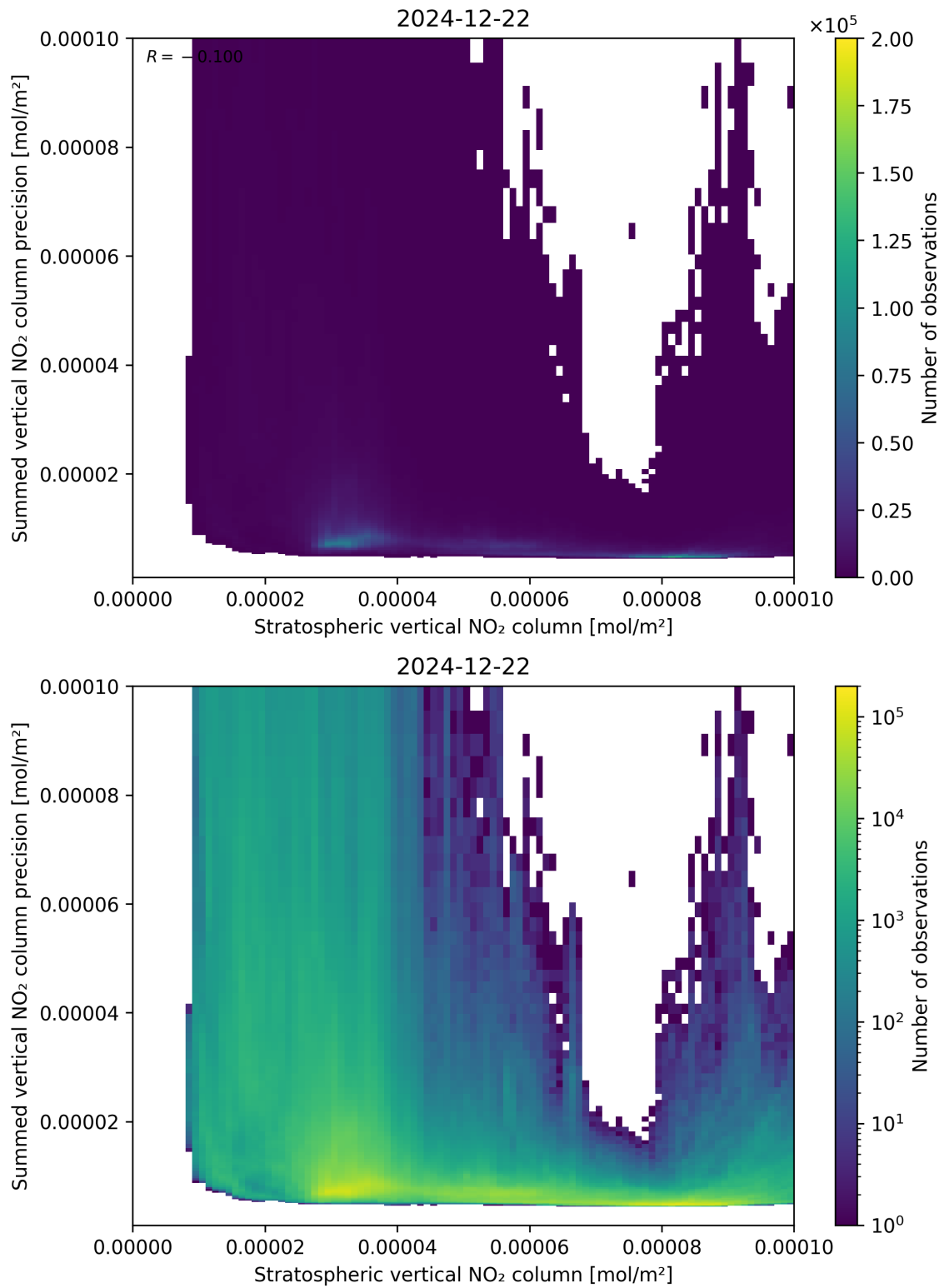
Figure 99: Scatter density plot of “Stratospheric vertical NO 2 column” against “Summed vertical NO 2 column precision” for 2024-12-22 to 2024-12-23.
