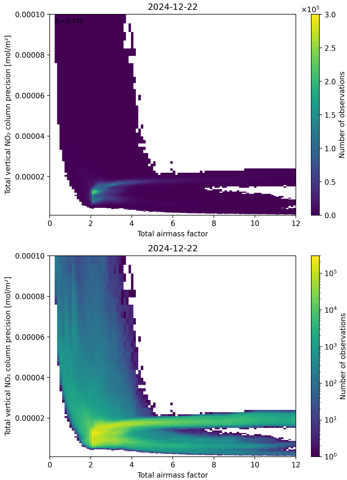
Figure 68: Scatter density plot of “Total airmass factor” against “Total vertical NO 2 column precision” for 2024-12-22 to 2024-12-23.
