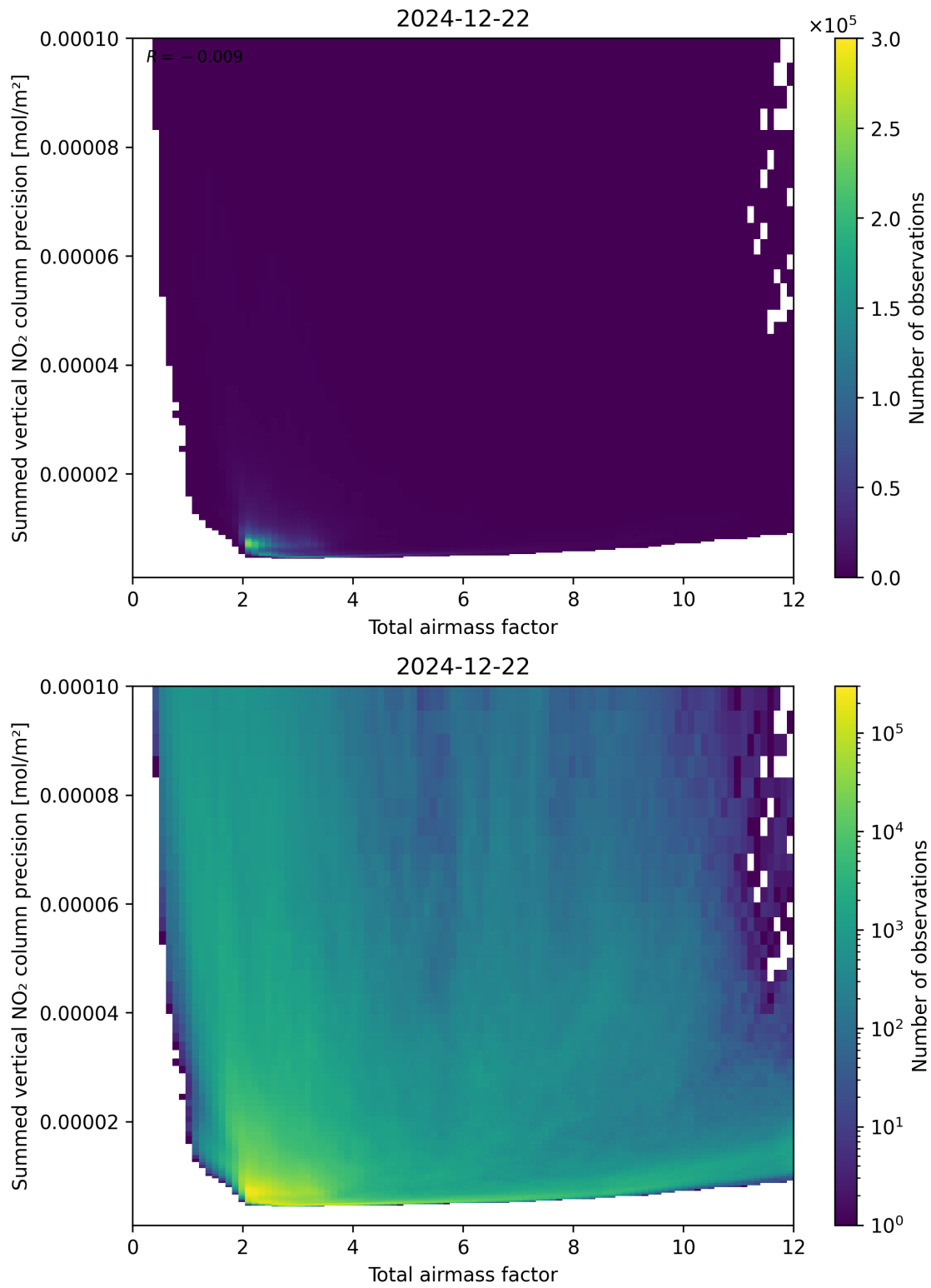
Figure 66: Scatter density plot of “Total airmass factor” against “Summed vertical NO 2 column precision” for 2024-12-22 to 2024-12-23.
