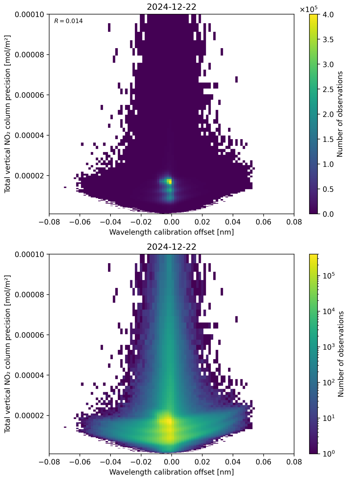
Figure 180: Scatter density plot of “Wavelength calibration offset” against “Total vertical NO 2 column precision” for 2024-12-22 to 2024-12-23.
