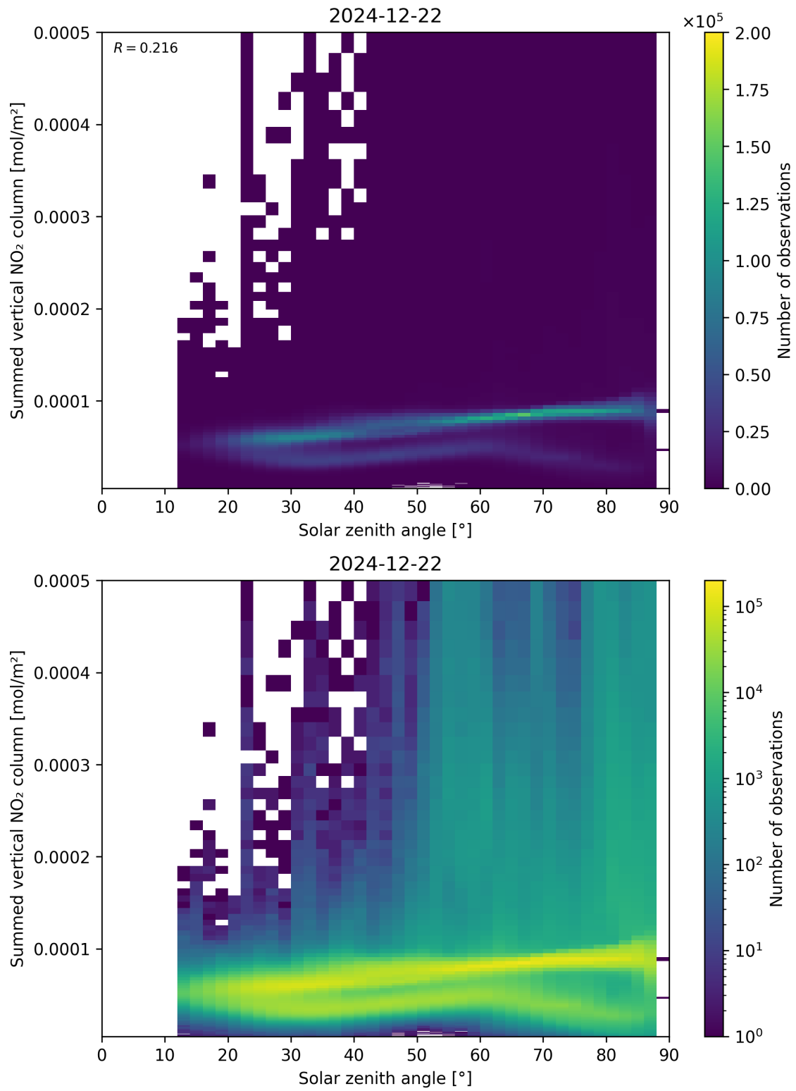
Figure 151: Scatter density plot of “Solar zenith angle” against “Summed vertical NO 2 column” for 2024-12-22 to 2024-12-23.
