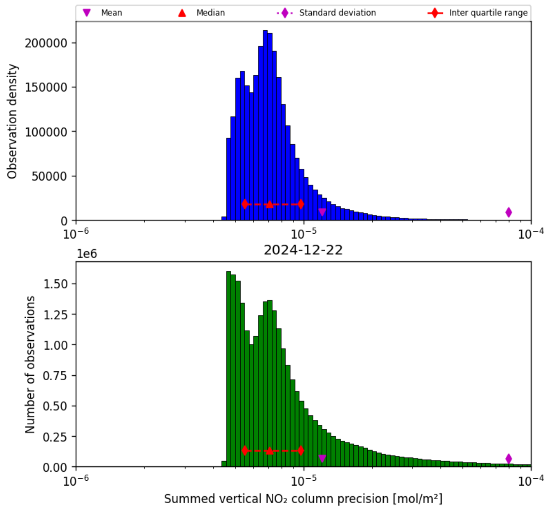
Figure 41: Histogram of “Summed vertical NO 2 column precision” for 2024-12-22 to 2024-12-23
