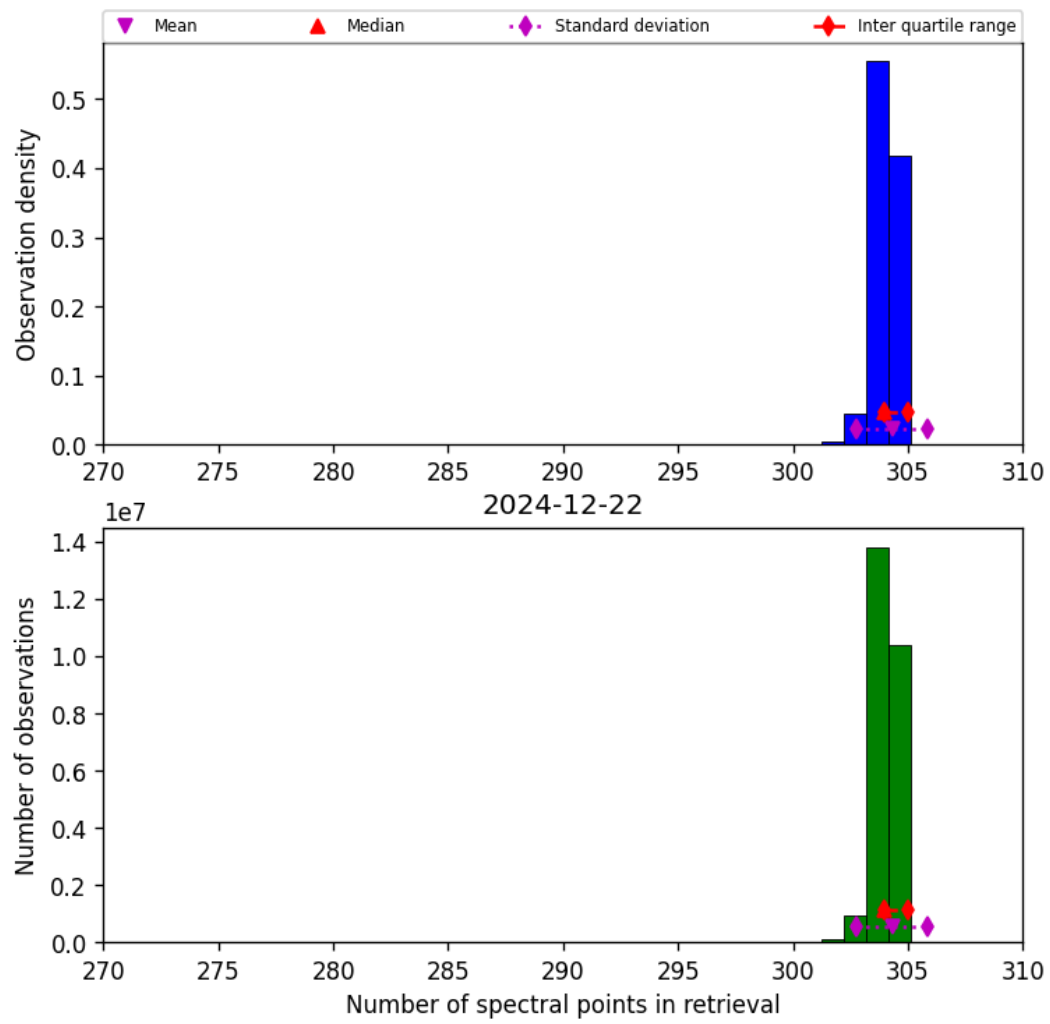
Figure 33: Histogram of “Number of spectral points in retrieval” for 2024-12-22 to 2024-12-23
