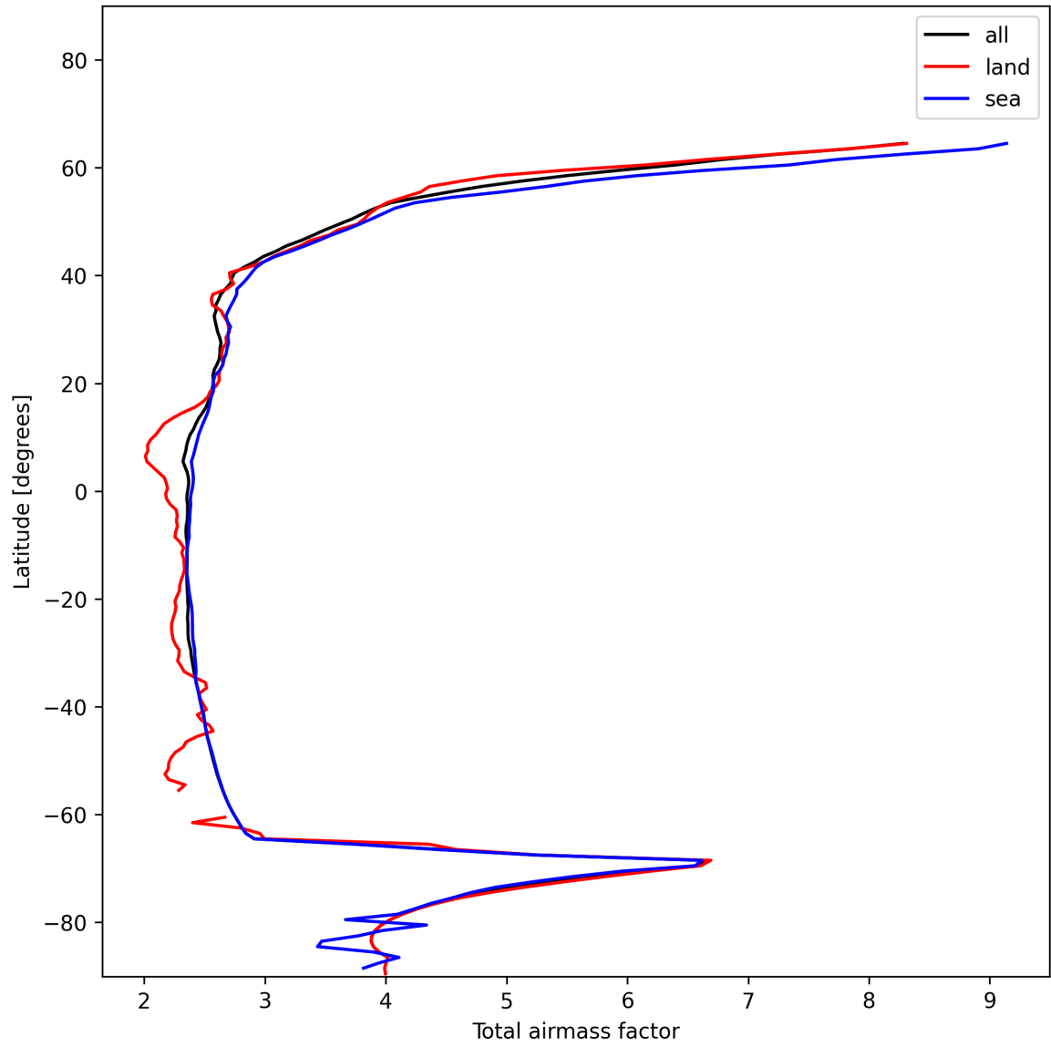
Figure 15: Zonal average of “Total airmass factor” for 2024-12-22 to 2024-12-23.
