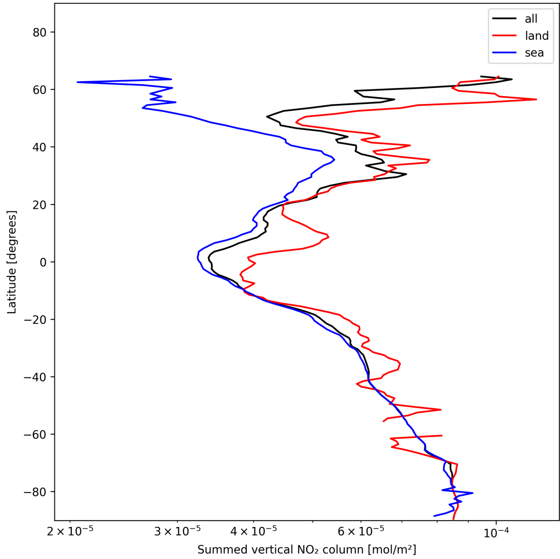
Figure 23: Zonal average of “Summed vertical NO 2 column” for 2024-12-22 to 2024-12-23.
