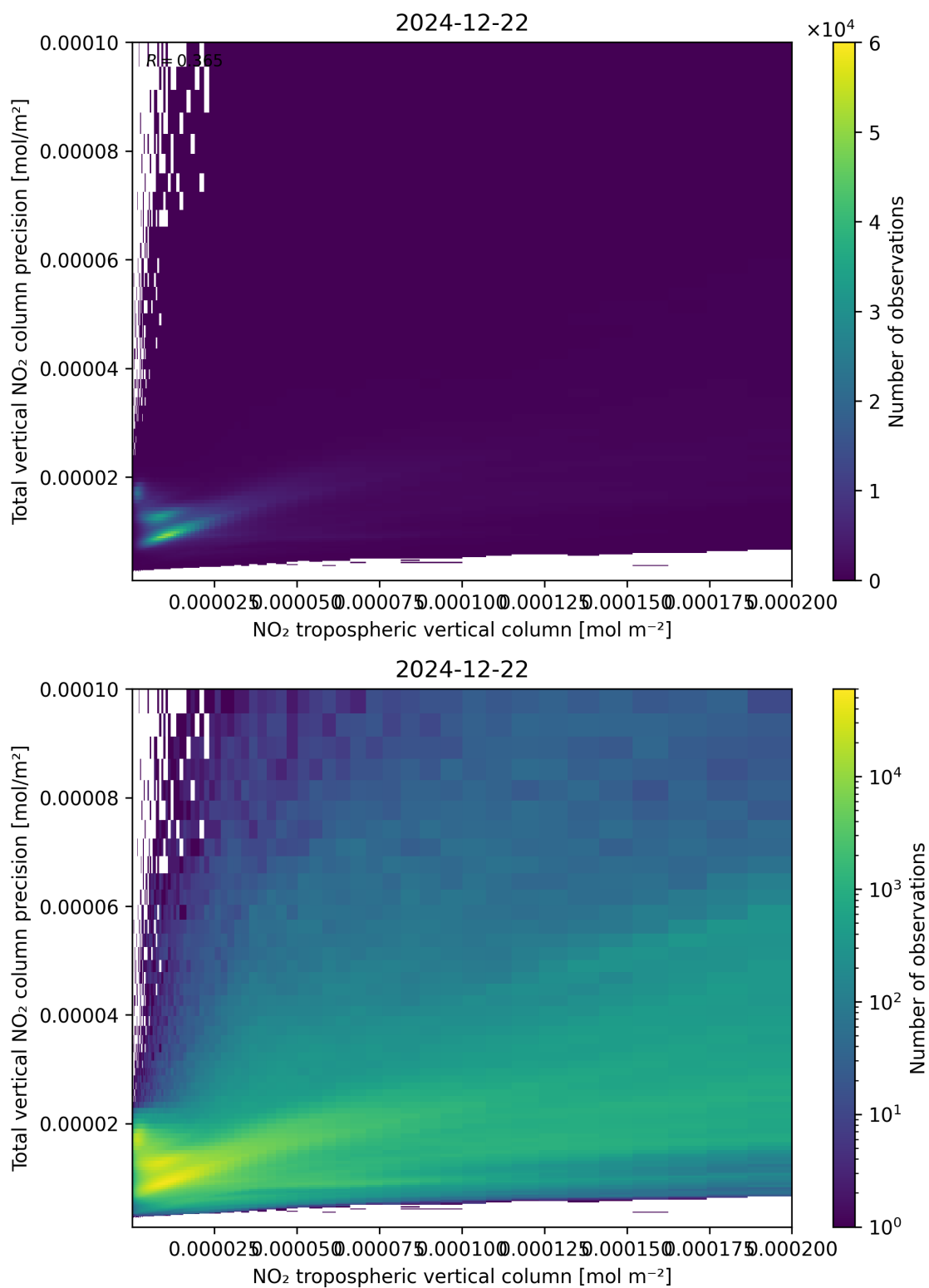
Figure 129: Scatter density plot of “NO 2 tropospheric vertical column” against “Total vertical NO 2 column precision” for 2024-12-22 to 2024-12-23.
