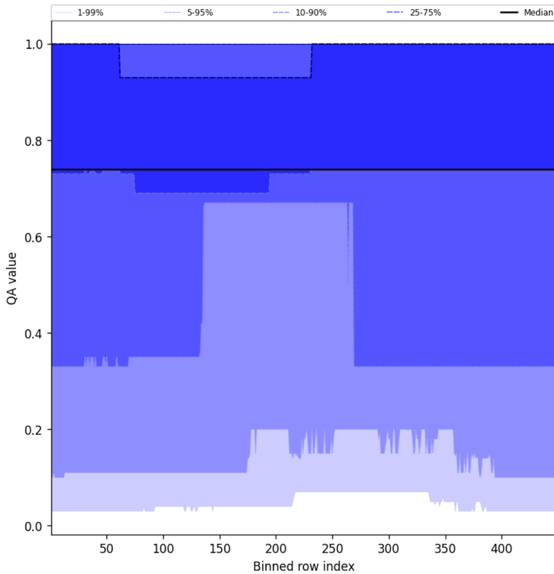
Figure 45: Along track statistics of “QA value” for 2024-12-22 to 2024-12-23
