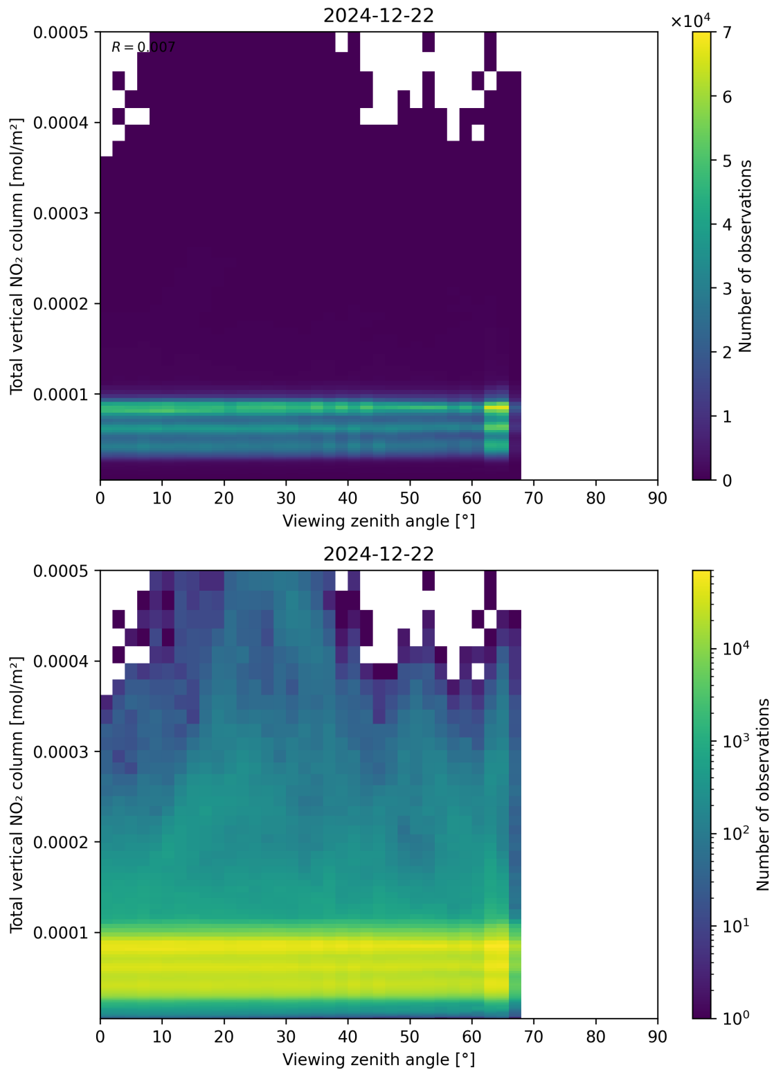
Figure 167: Scatter density plot of “Viewing zenith angle” against “Total vertical NO 2 column” for 2024-12-22 to 2024-12-23.
