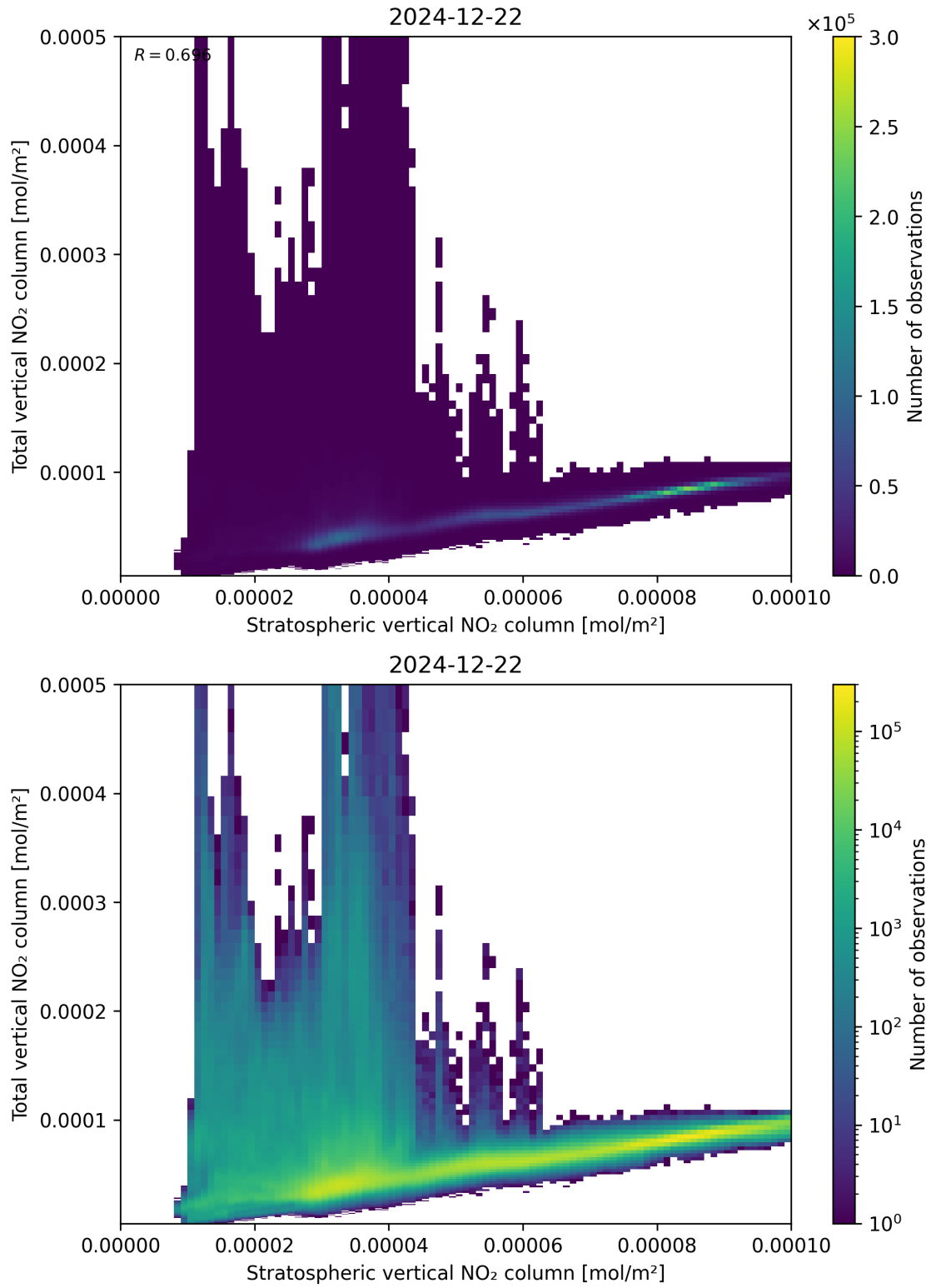
Figure 100: Scatter density plot of “Stratospheric vertical NO 2 column” against “Total vertical NO 2 column” for 2024-12-22 to 2024-12-23.
