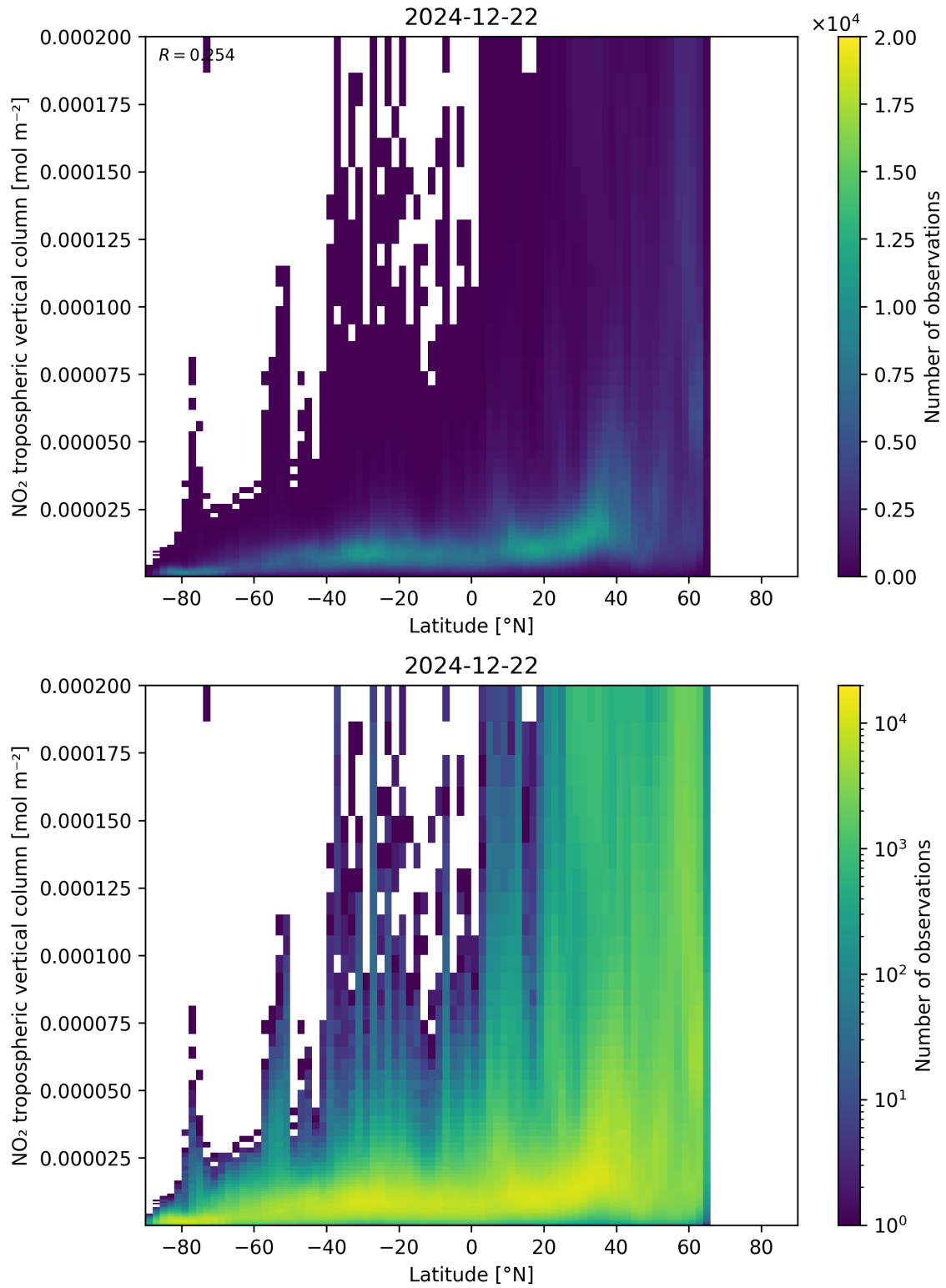
Figure 92: Scatter density plot of “Latitude” against “NO 2 tropospheric vertical column” for 2024-12-22 to 2024-12-23.
