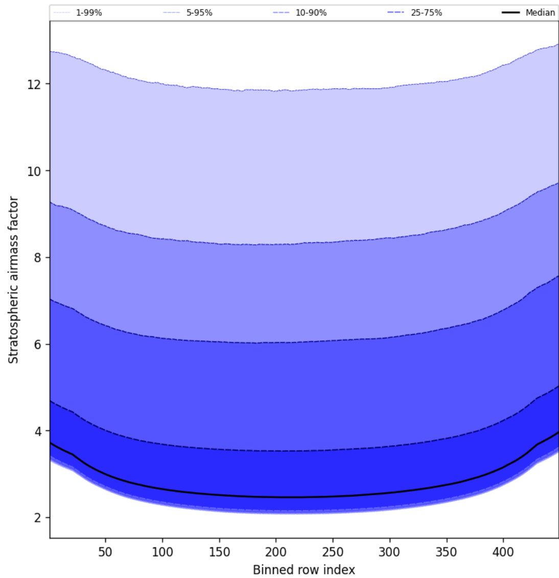
Figure 61: Along track statistics of “Stratospheric air mass factor” for 2024-12-22 to 2024-12-23
