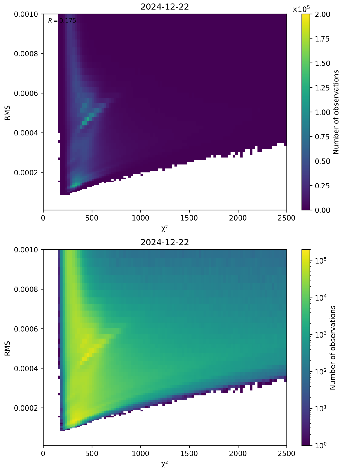
Figure 82: Scatter density plot of " \chi^2 " against "RMS" for 2024-12-22 to 2024-12-23.
