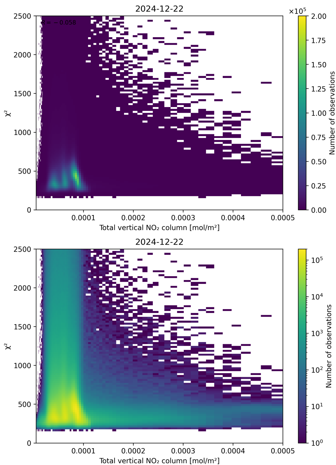
Figure 111: Scatter density plot of “Total vertical NO 2 column” against “ \chi^2 ” for 2024-12-22 to 2024-12-23.
