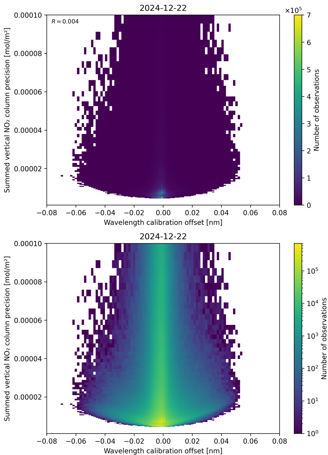
Figure 178: Scatter density plot of “Wavelength calibration offset” against “Summed vertical NO 2 column precision” for 2024-12-22 to 2024-12-23.
