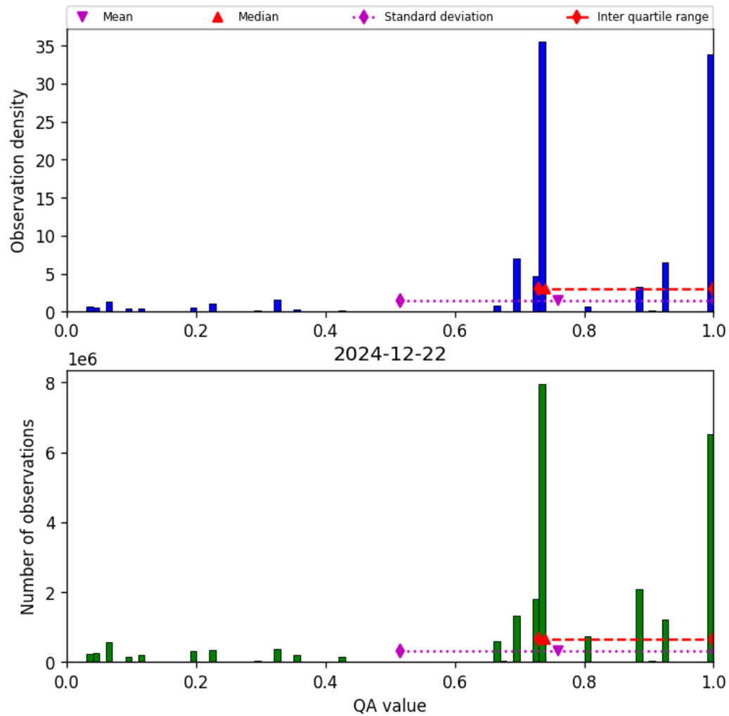
Figure 28: Histogram of “QA value” for 2024-12-22 to 2024-12-23
