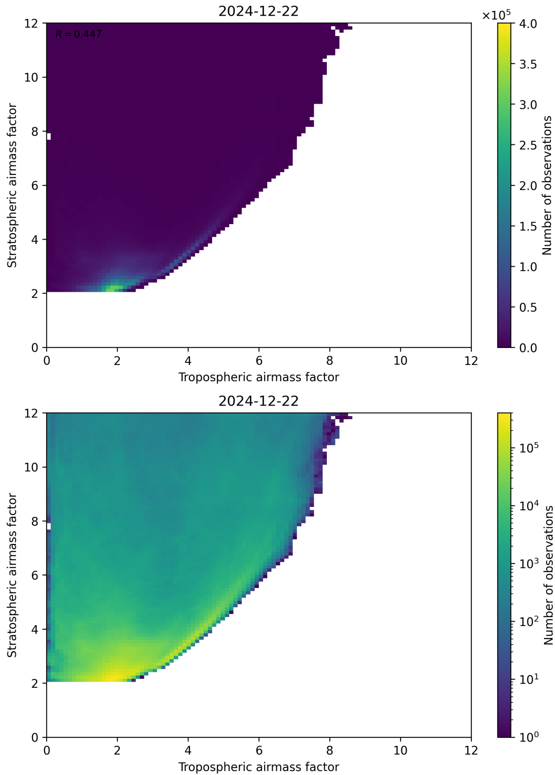
Figure 71: Scatter density plot of “Tropospheric airmass factor” against “Stratospheric airmass factor” for 2024-12-22 to 2024-12-23.
