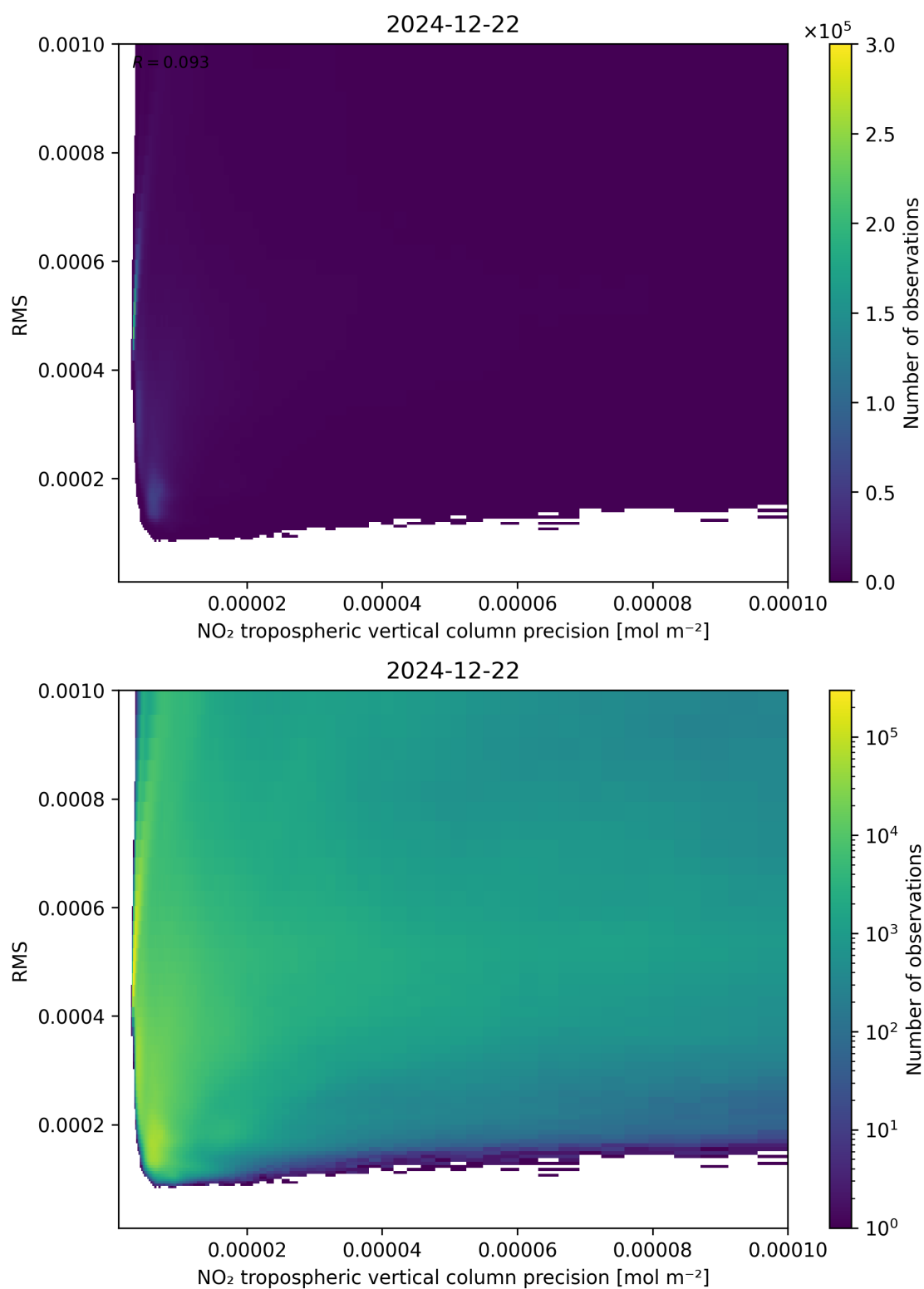
Figure 140: Scatter density plot of “NO 2 tropospheric vertical column precision” against “RMS” for 2024-12-22 to 2024-12-23.
