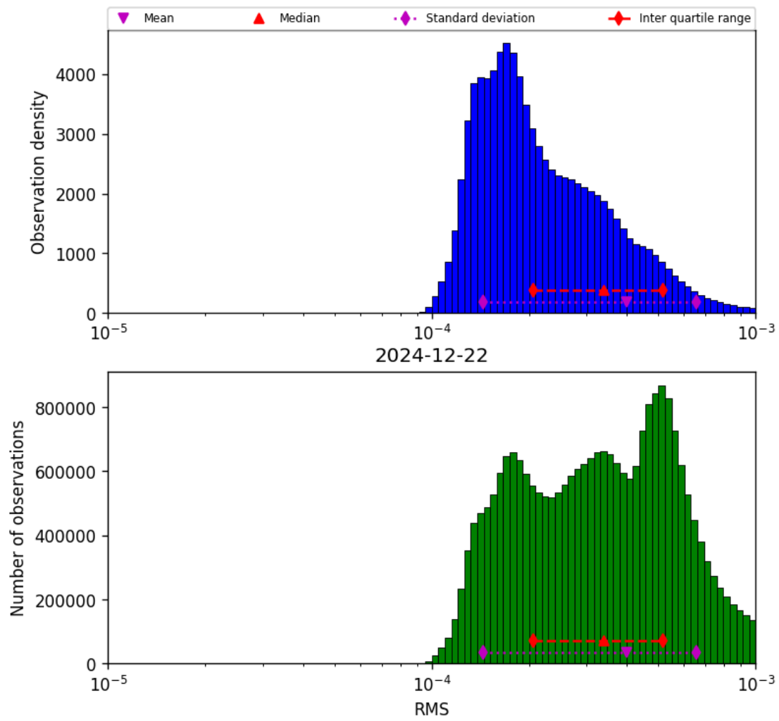
Figure 43: Histogram of “RMS” for 2024-12-22 to 2024-12-23
