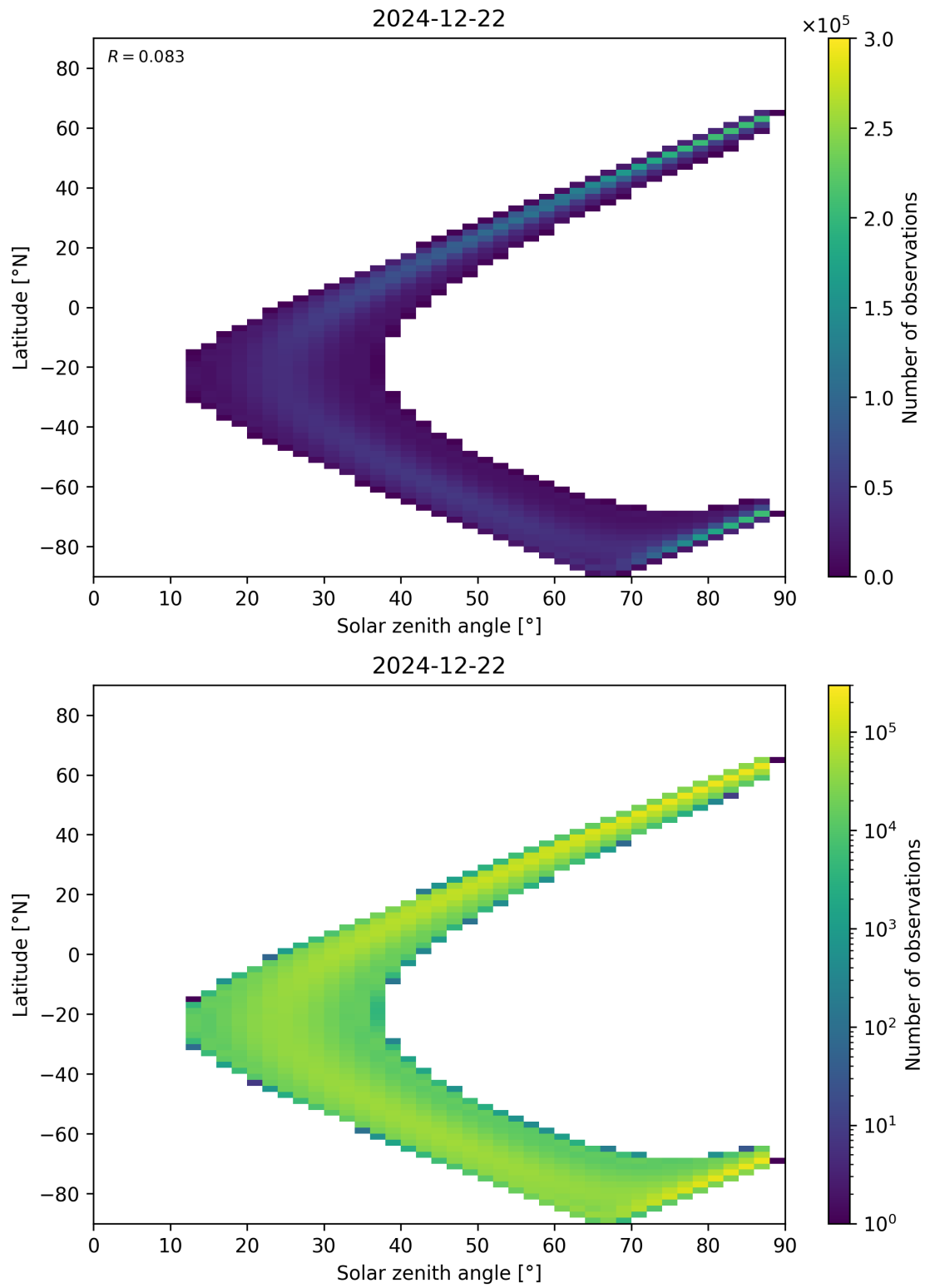
Figure 149: Scatter density plot of “Solar zenith angle” against “Latitude” for 2024-12-22 to 2024-12-23.
