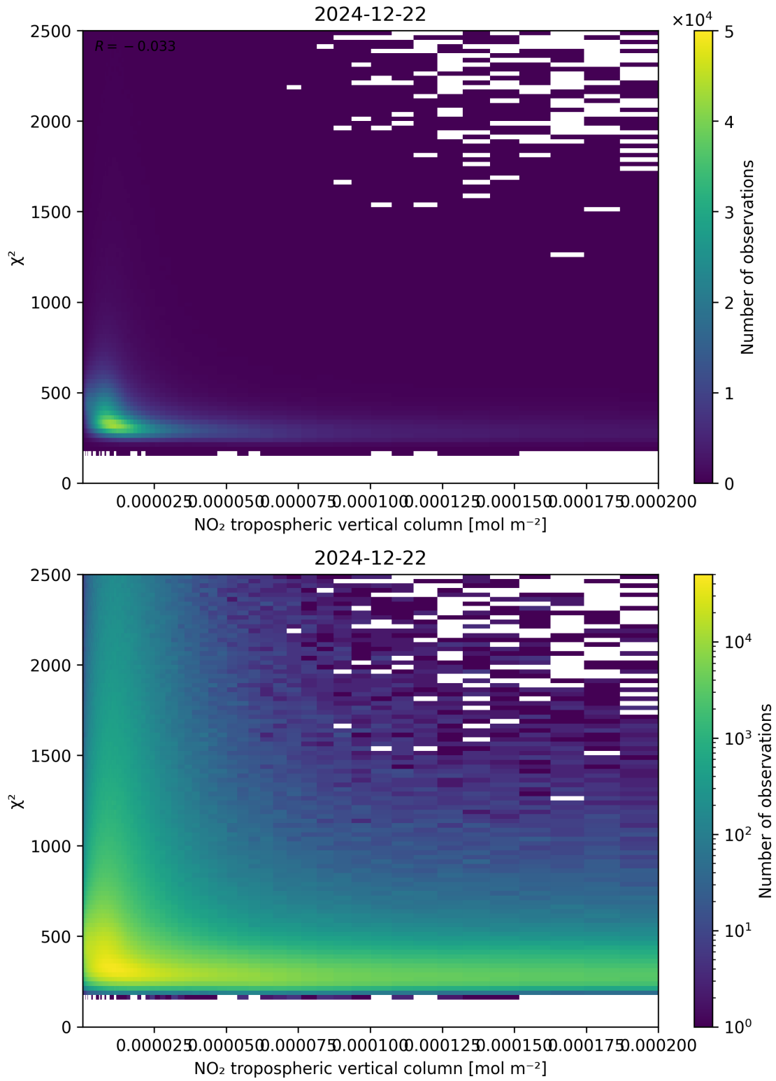
Figure 124: Scatter density plot of “NO 2 tropospheric vertical column” against “ \chi^2 ” for 2024-12-22 to 2024-12-23.
