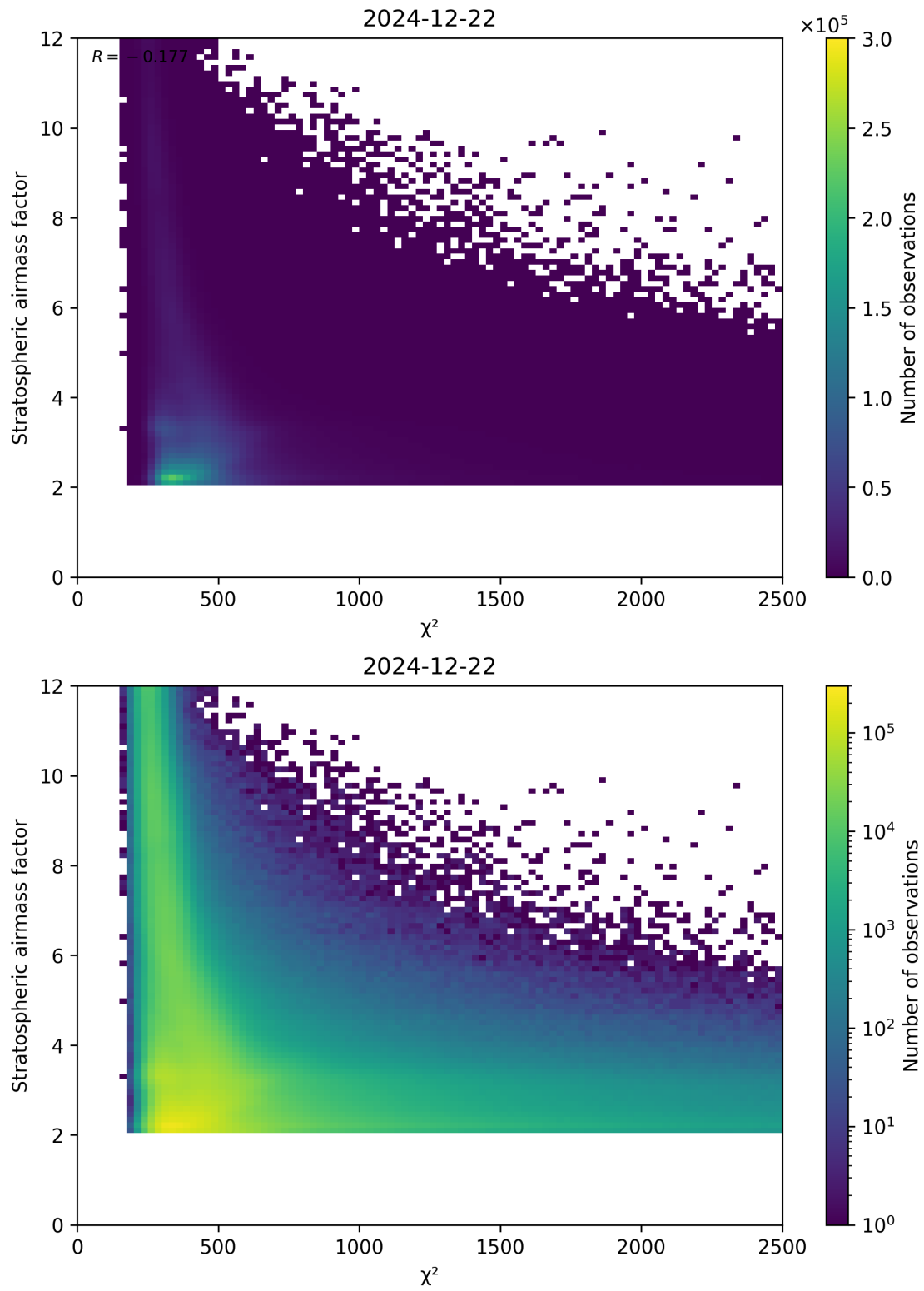
Figure 81: Scatter density plot of “ \chi^2 ” against “Stratospheric airmass factor” for 2024-12-22 to 2024-12-23.
