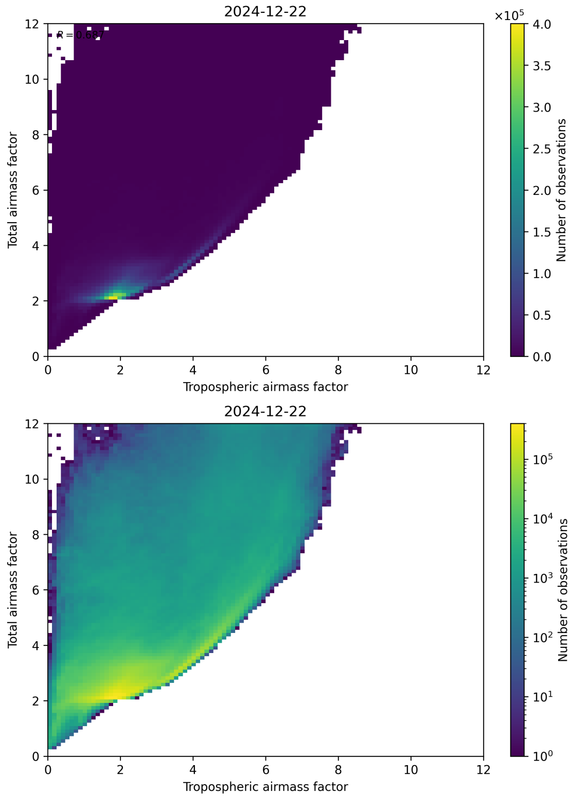
Figure 72: Scatter density plot of “Tropospheric airmass factor” against “Total airmass factor” for 2024-12-22 to 2024-12-23.
