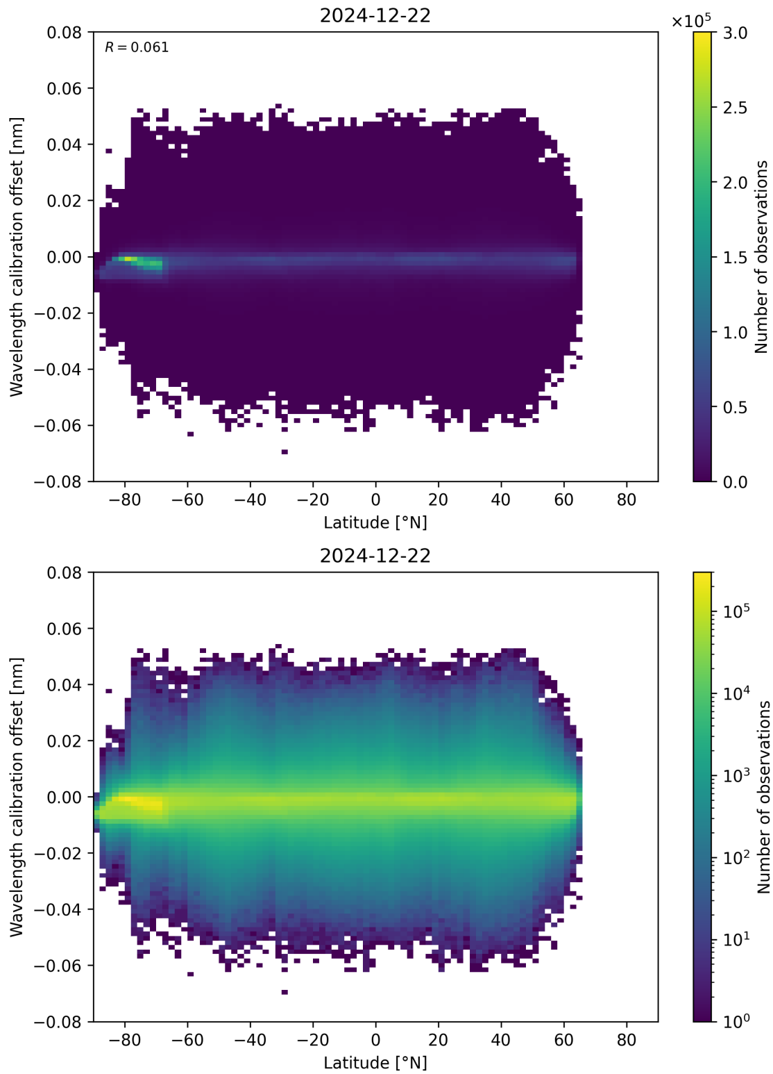
Figure 95: Scatter density plot of “Latitude” against “Wavelength calibration offset” for 2024-12-22 to 2024-12-23.
