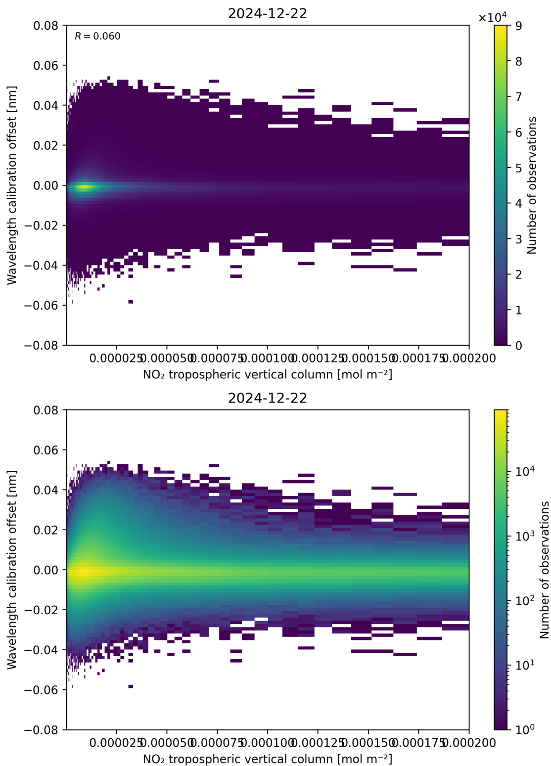
Figure 143: Scatter density plot of “NO 2 tropospheric vertical column” against “Wavelength calibration offset” for 2024-12-22 to 2024-12-23.
