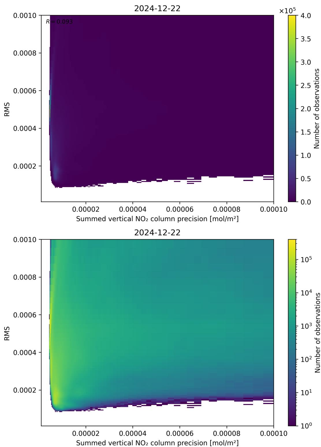
Figure 108: Scatter density plot of “Summed vertical NO 2 column precision” against “RMS” for 2024-12-22 to 2024-12-23.
