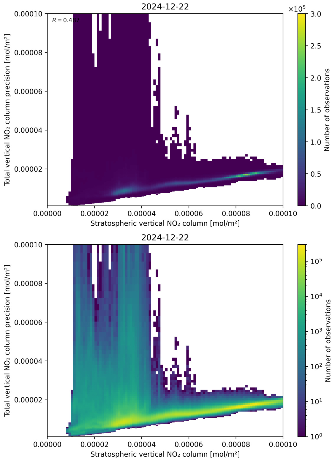
Figure 101: Scatter density plot of “Stratospheric vertical NO 2 column” against “Total vertical NO 2 column precision” for 2024-12-22 to 2024-12-23.
