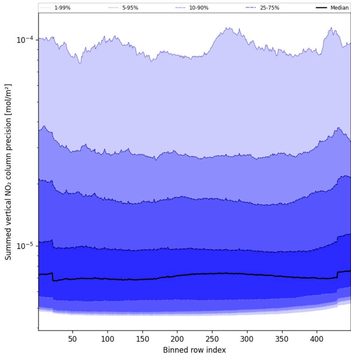
Figure 58: Along track statistics of “Summed vertical NO 2 column precision” for 2024-12-22 to 2024-12-23
