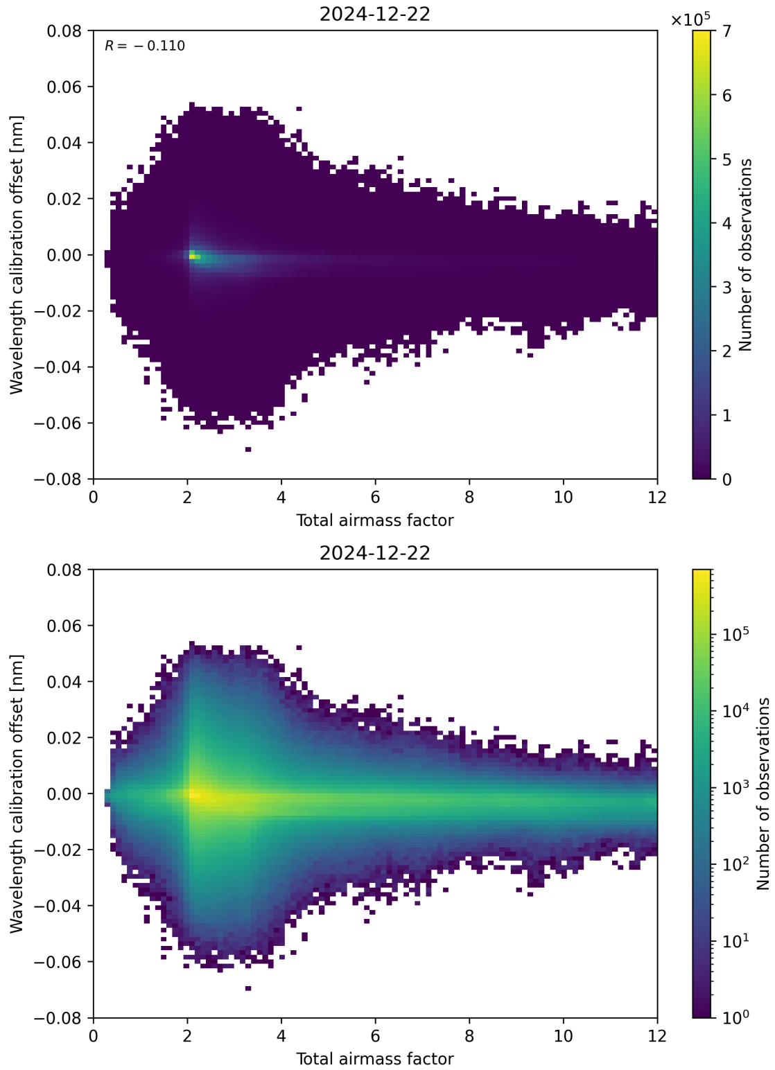
Figure 70: Scatter density plot of “Total airmass factor” against “Wavelength calibration offset” for 2024-12-22 to 2024-12-23.
