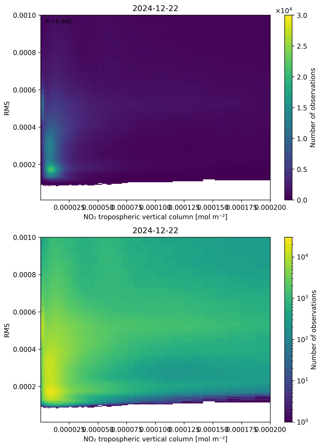
Figure 142: Scatter density plot of “NO 2 tropospheric vertical column” against “RMS” for 2024-12-22 to 2024-12-23.
