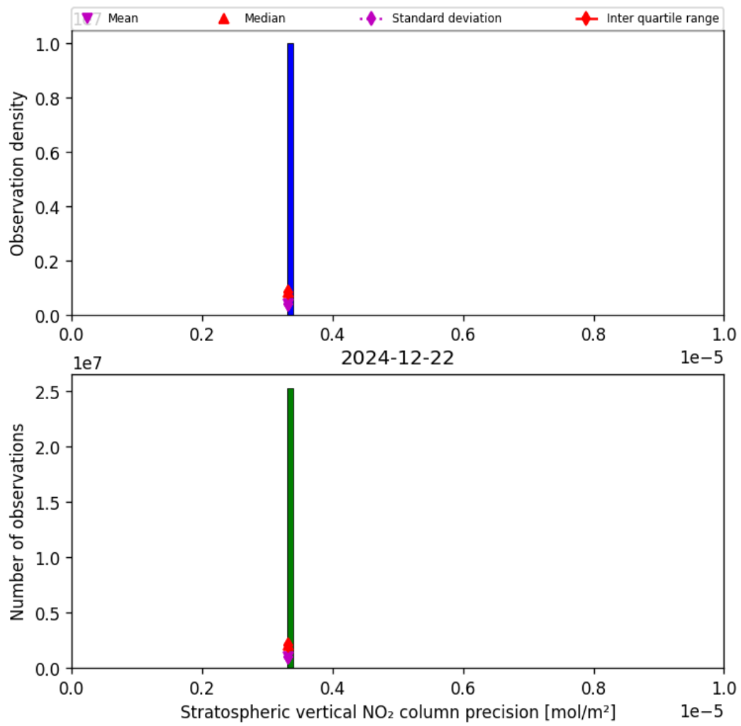
Figure 37: Histogram of “Stratospheric vertical NO 2 column precision” for 2024-12-22 to 2024-12-23
