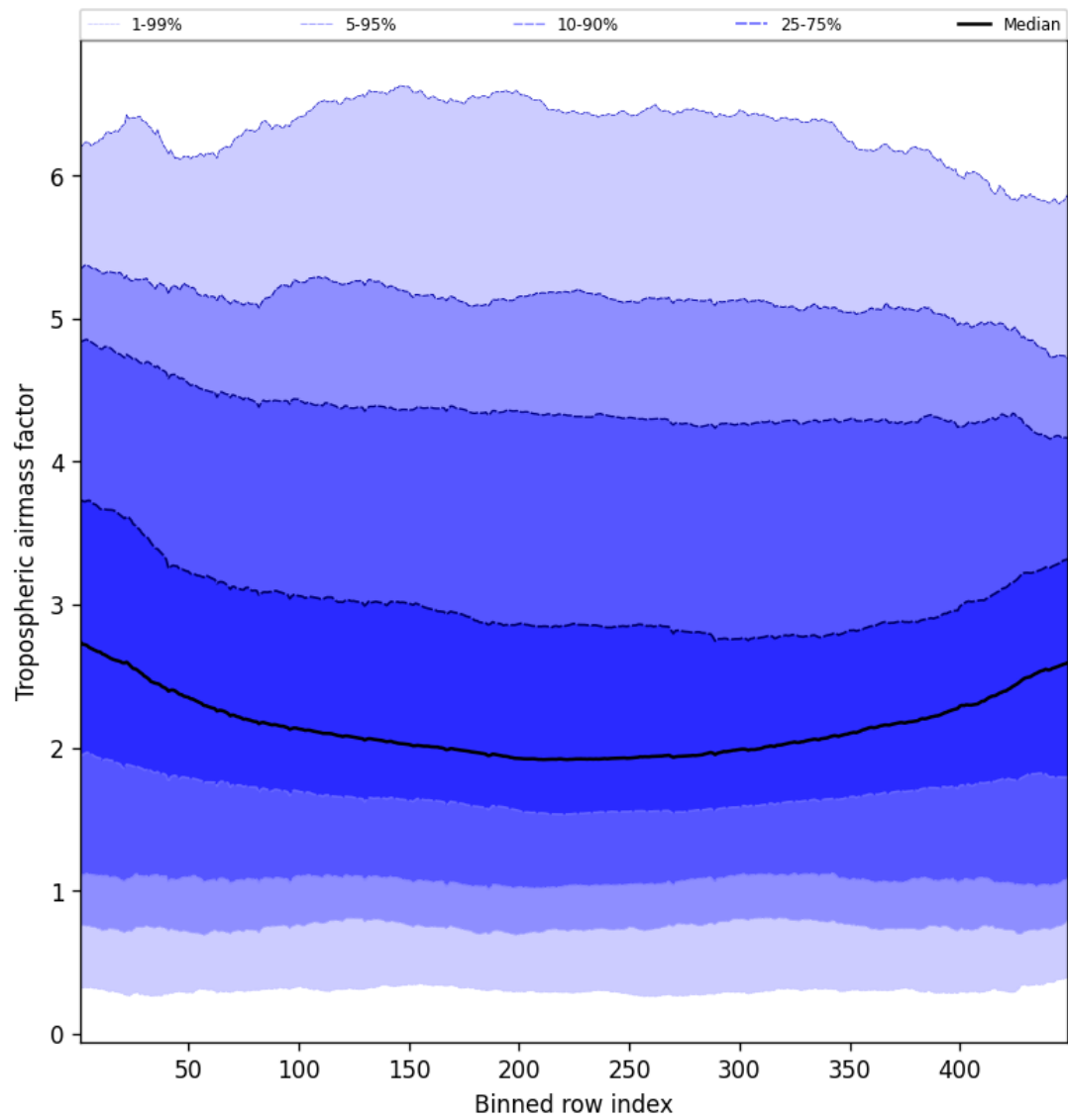
Figure 48: Along track statistics of “Tropospheric airmass factor” for 2024-12-22 to 2024-12-23
