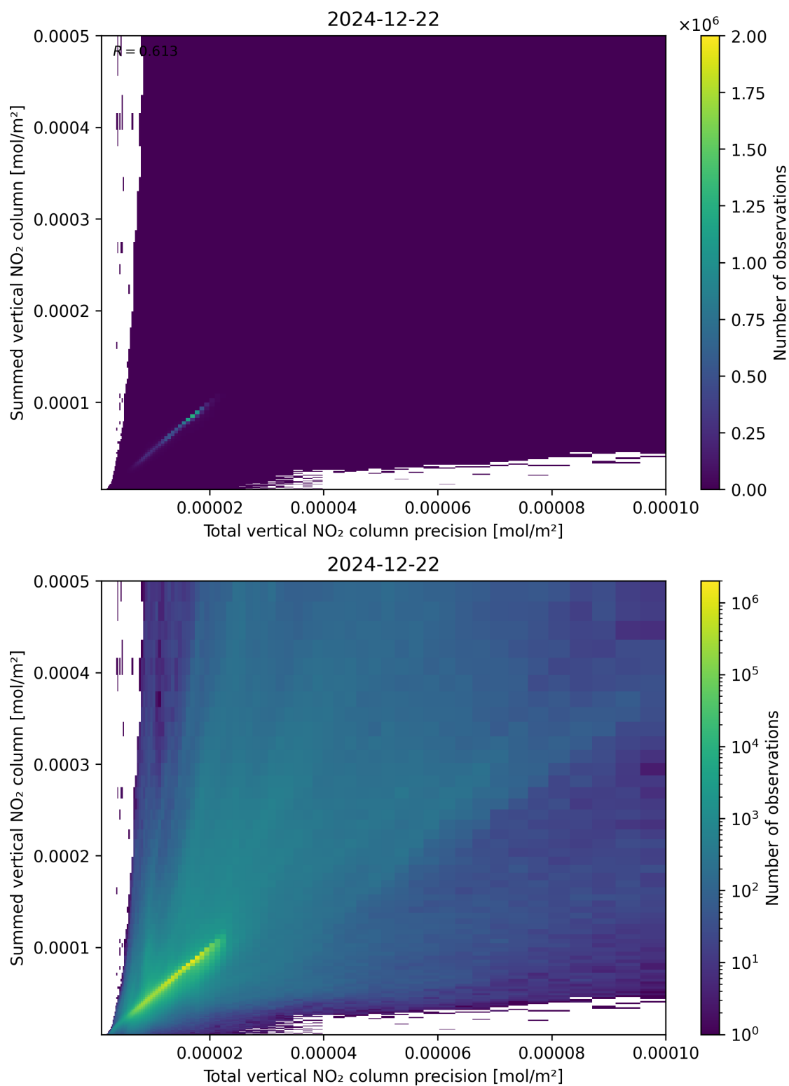
Figure 117: Scatter density plot of “Total vertical NO 2 column precision” against “Summed vertical NO 2 column” for 2024-12-22 to 2024-12-23.
