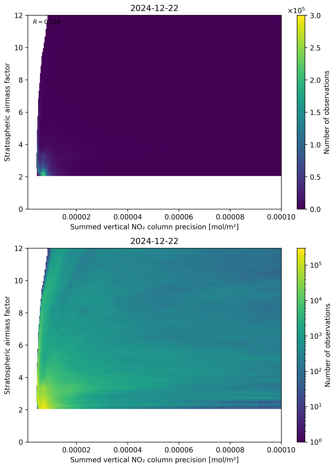
Figure 106: Scatter density plot of “Summed vertical NO 2 column precision” against “Stratospheric airmass factor” for 2024-12-22 to 2024-12-23.
