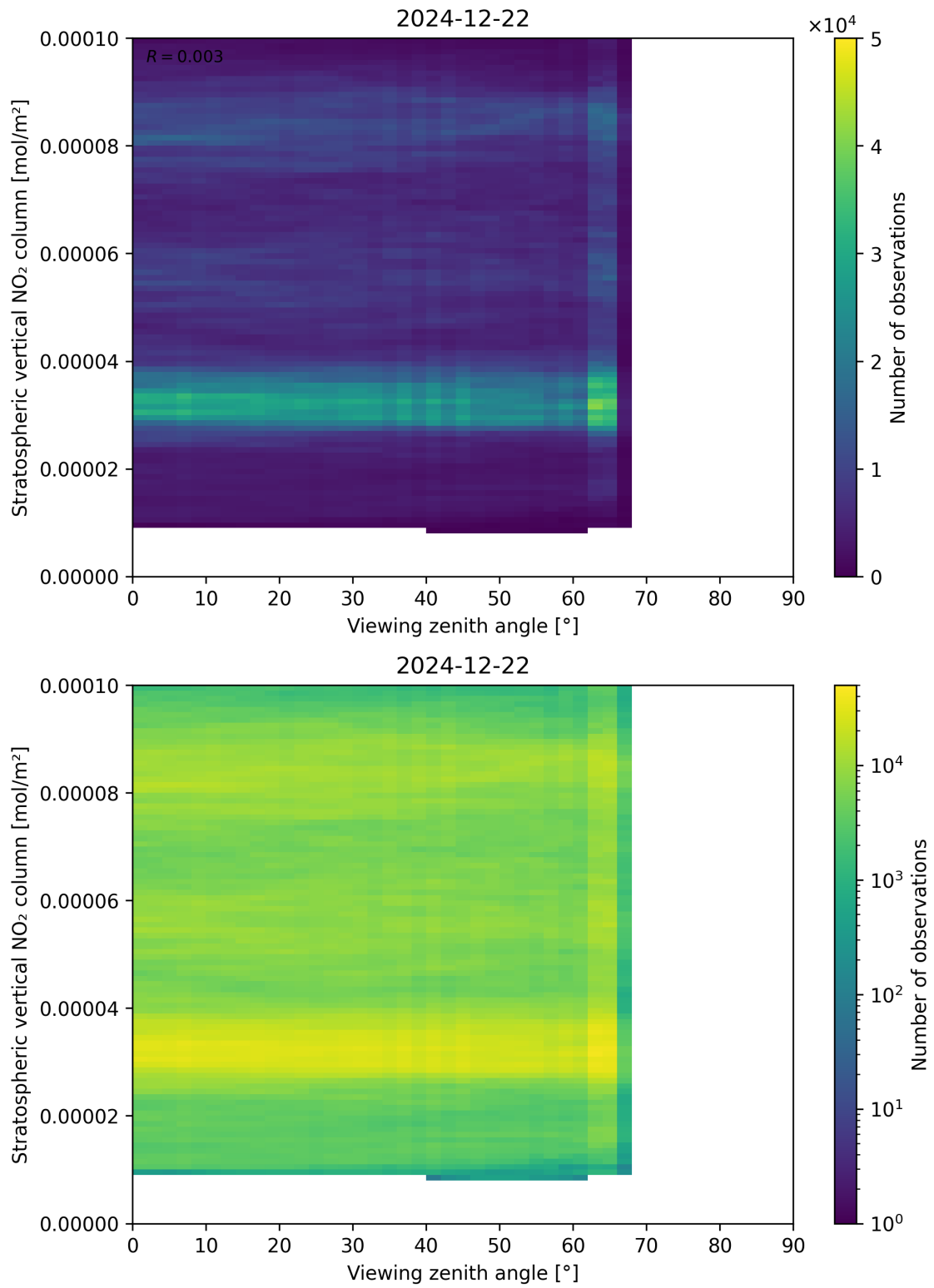
Figure 164: Scatter density plot of “Viewing zenith angle” against “Stratospheric vertical NO 2 column” for 2024-12-22 to 2024-12-23.
