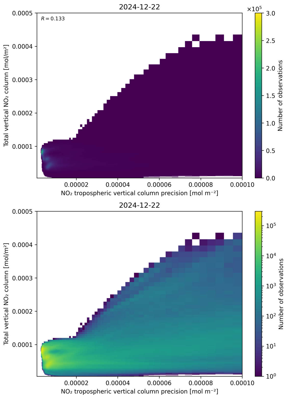
Figure 138: Scatter density plot of “NO 2 tropospheric vertical column precision” against “Total vertical NO 2 column” for 2024-12-22 to 2024-12-23.
