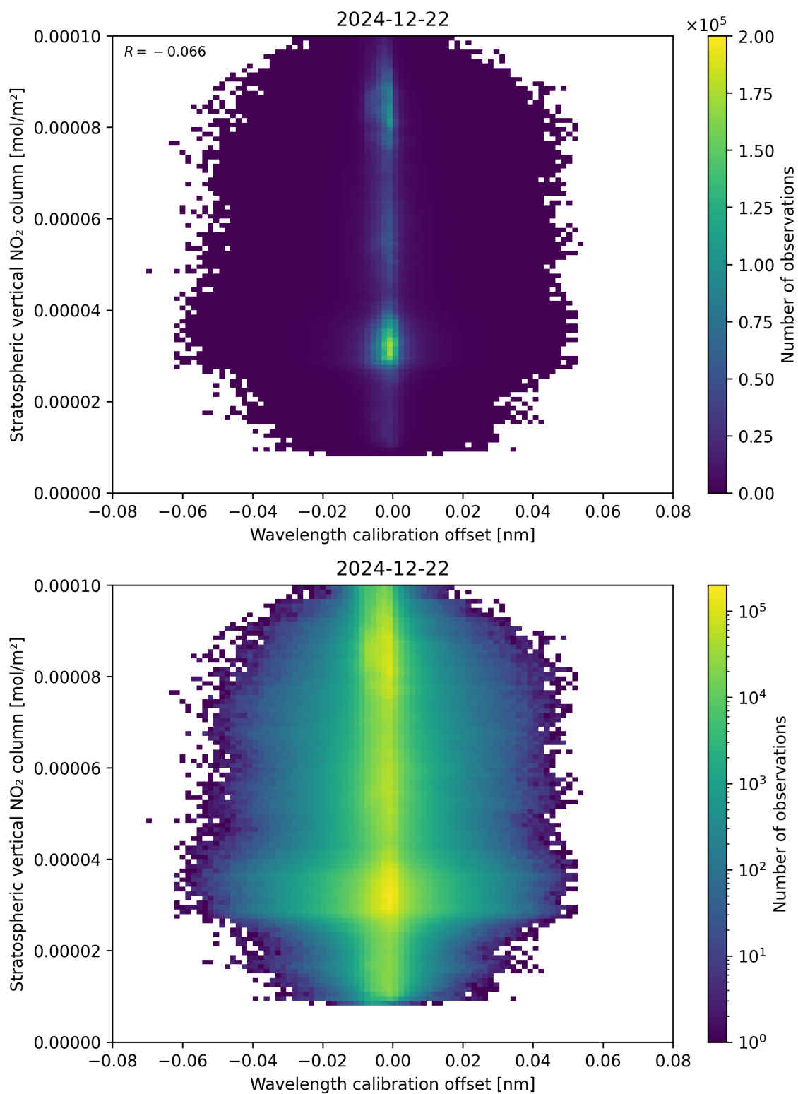
Figure 176: Scatter density plot of “Wavelength calibration offset” against “Stratospheric vertical NO 2 column” for 2024-12-22 to 2024-12-23.
