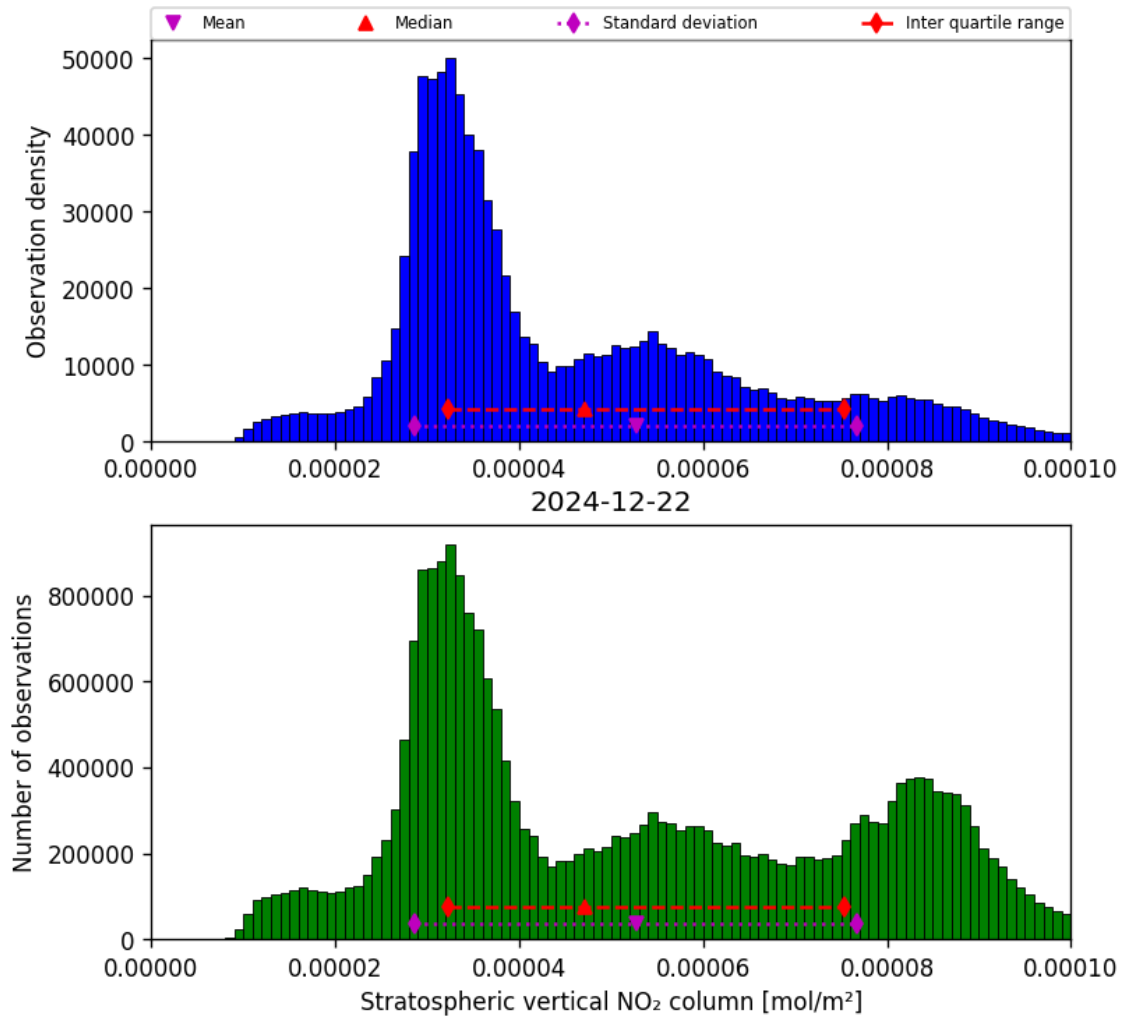
Figure 36: Histogram of “Stratospheric vertical NO 2 column” for 2024-12-22 to 2024-12-23
