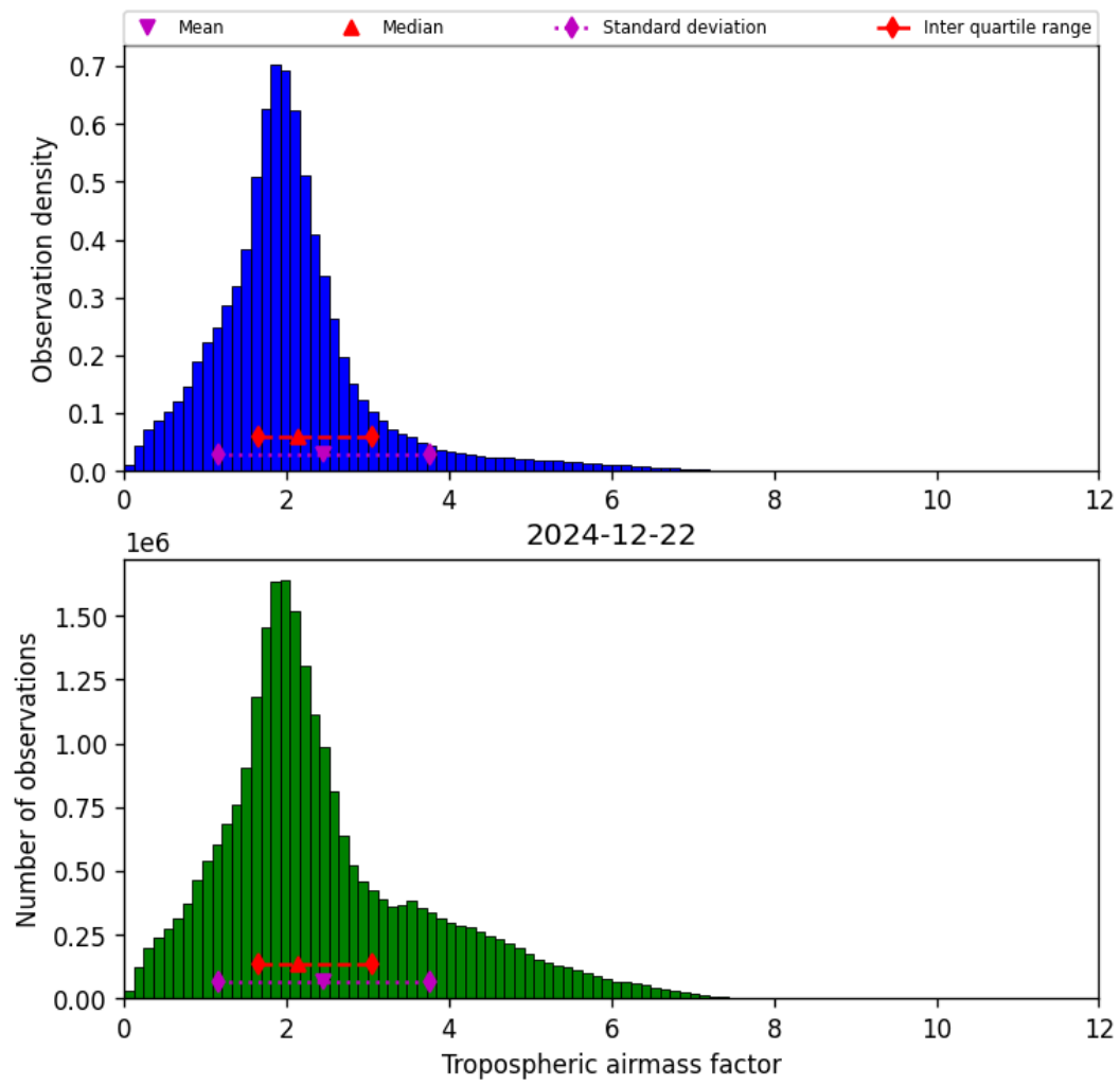
Figure 31: Histogram of “Tropospheric airmass factor” for 2024-12-22 to 2024-12-23
