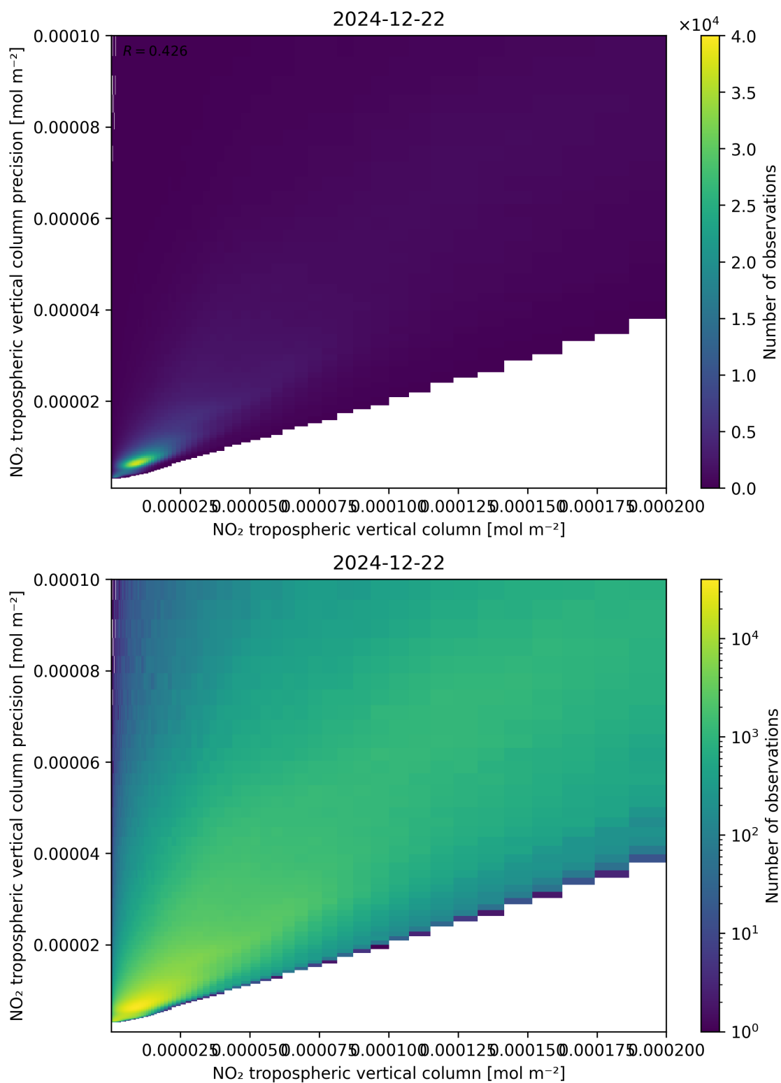
Figure 130: Scatter density plot of “NO 2 tropospheric vertical column” against “NO 2 tropospheric vertical column precision” for 2024-12-22 to 2024-12-23.
