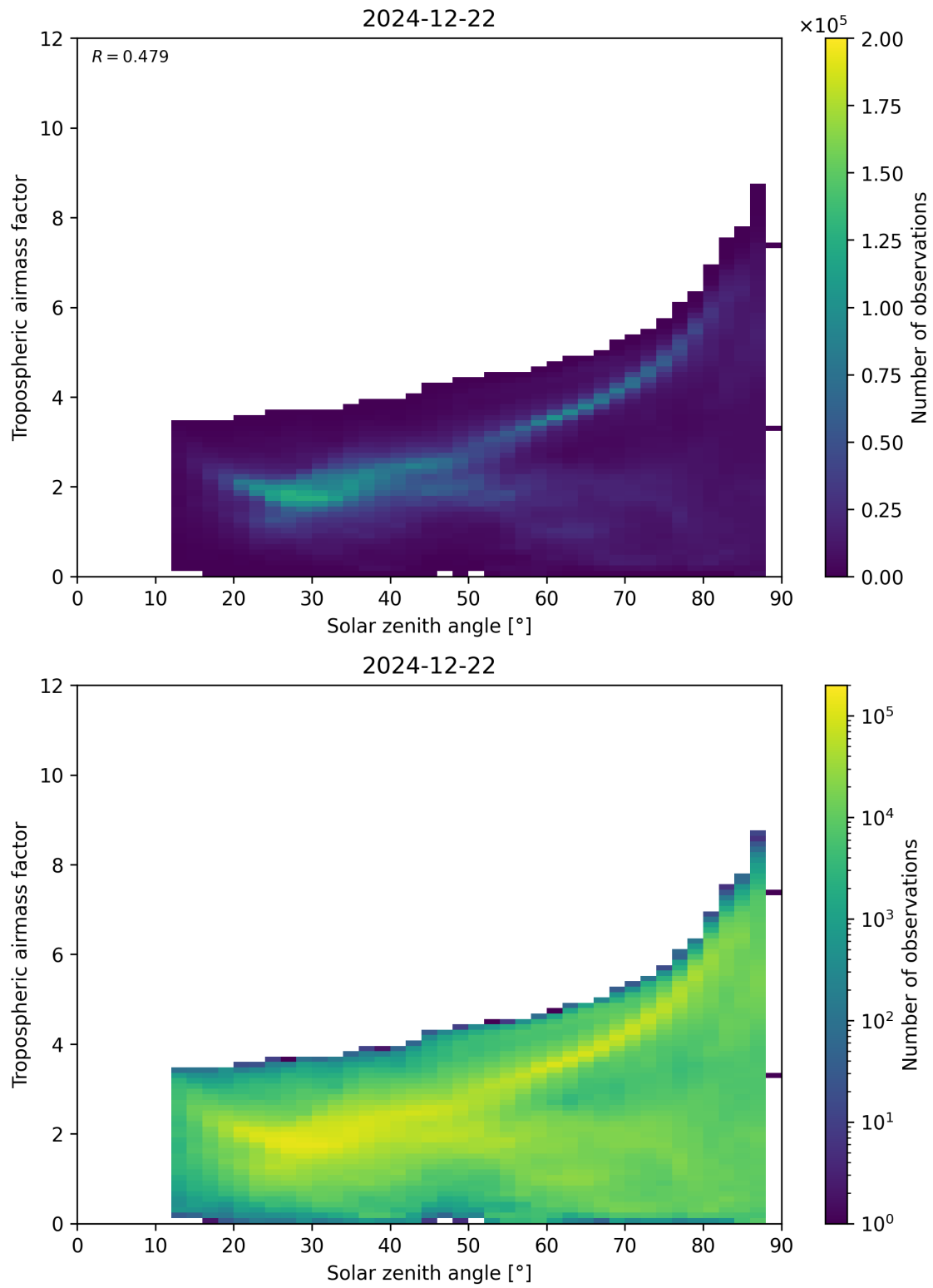
Figure 147: Scatter density plot of “Solar zenith angle” against “Tropospheric airmass factor” for 2024-12-22 to 2024-12-23.
