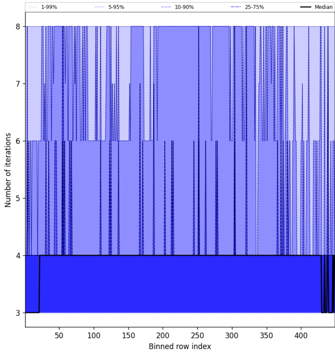
Figure 51: Along track statistics of “Number of iterations” for 2024-12-22 to 2024-12-23
