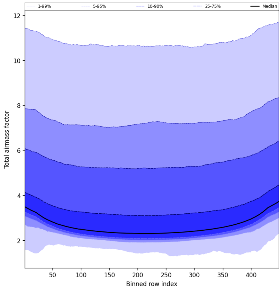
Figure 49: Along track statistics of “Total airmass factor” for 2024-12-22 to 2024-12-23
