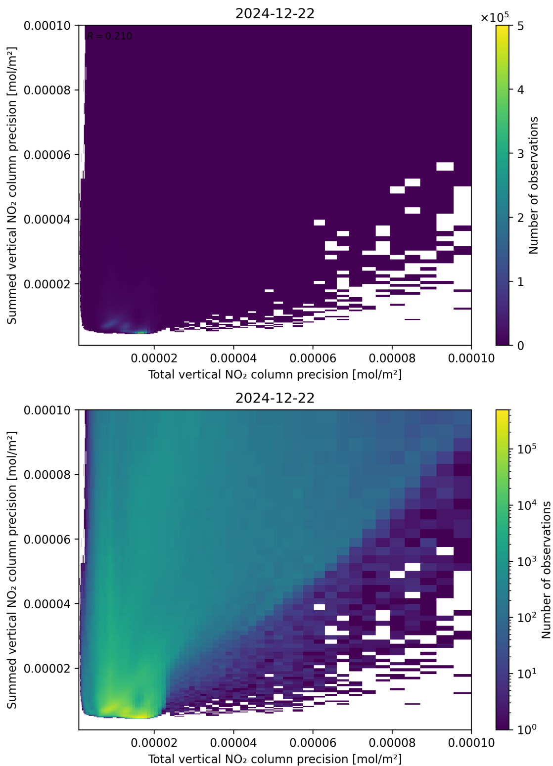
Figure 118: Scatter density plot of “Total vertical NO 2 column precision” against “Summed vertical NO 2 column precision” for 2024-12-22 to 2024-12-23.
