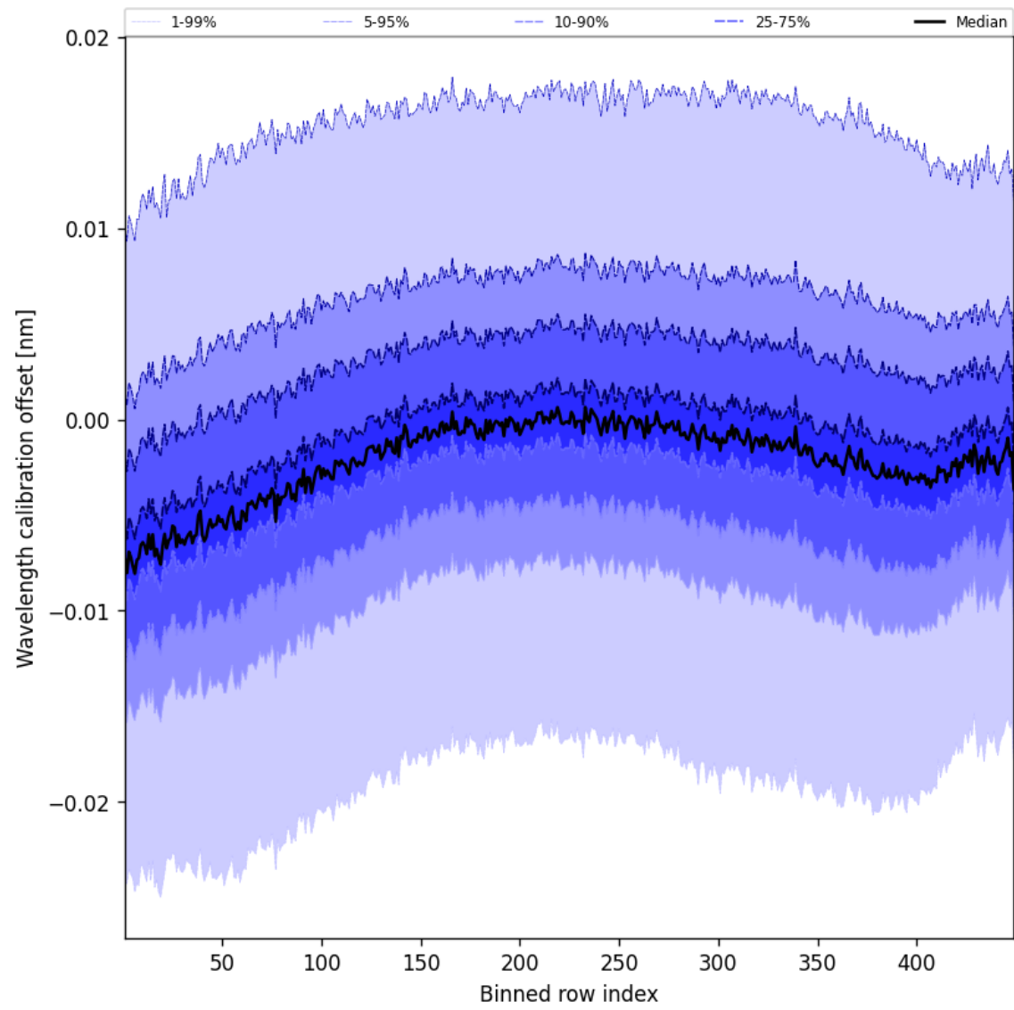
Figure 52: Along track statistics of “Wavelength calibration offset” for 2024-12-22 to 2024-12-23
