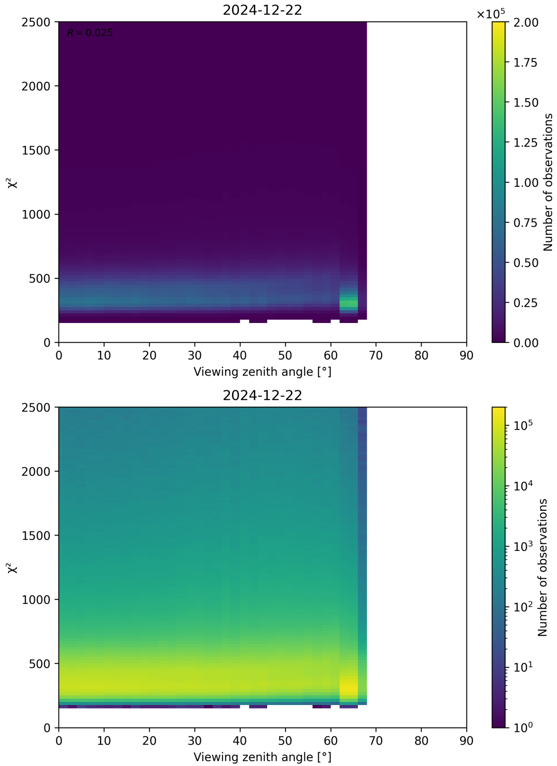
Figure 162: Scatter density plot of “Viewing zenith angle” against “ \chi^2 ” for 2024-12-22 to 2024-12-23.
