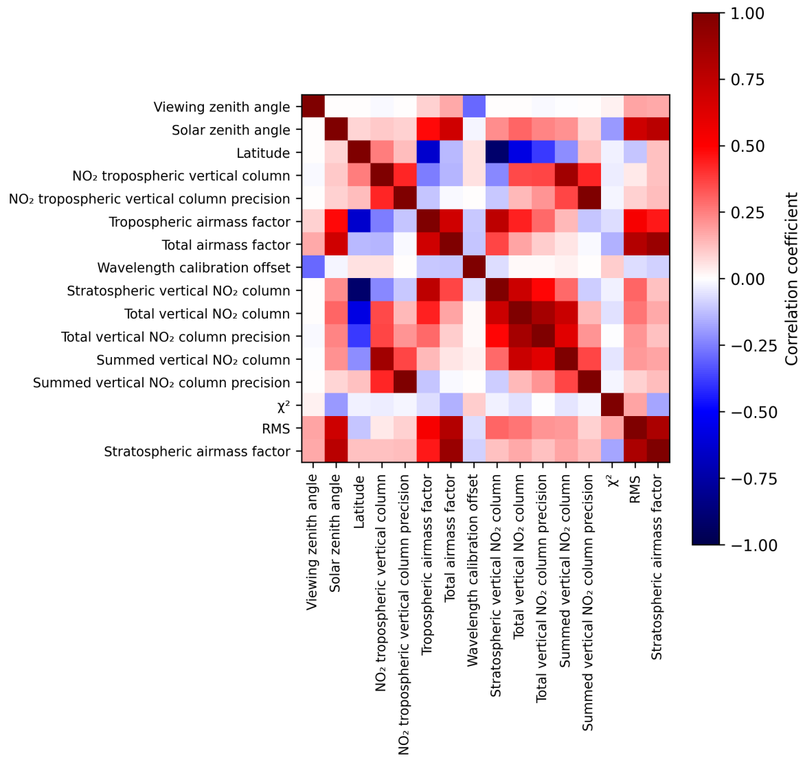
Figure 2: Map of correlation matrix for 2024-12-22 to 2024-12-23.
