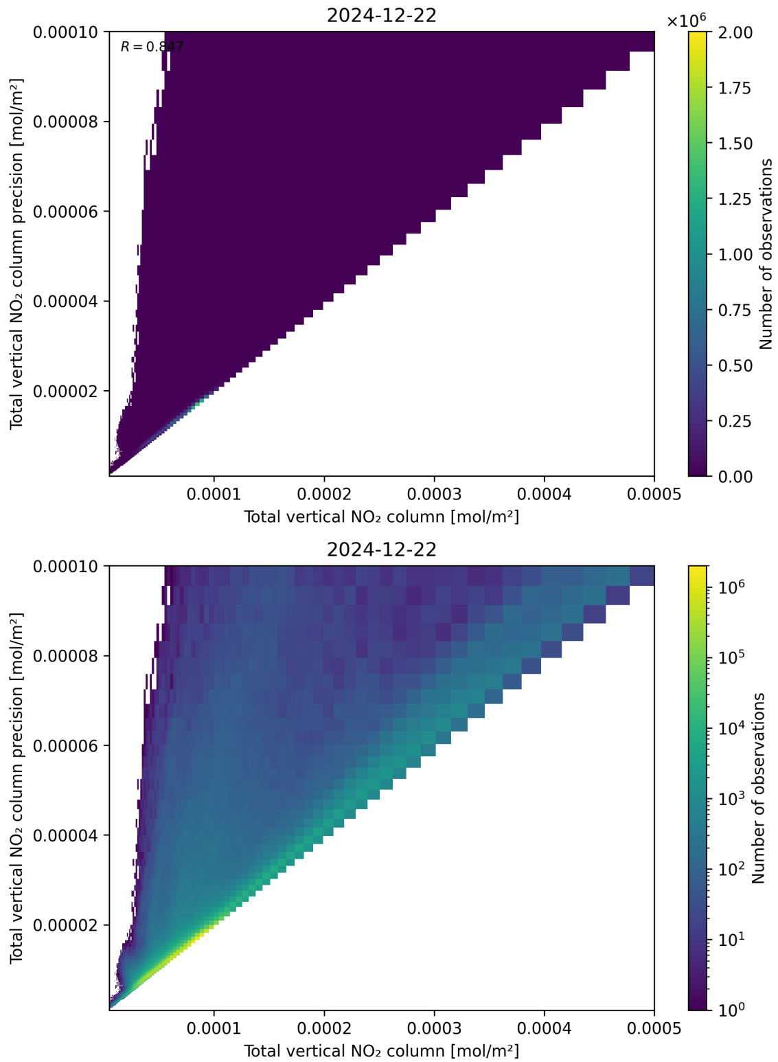
Figure 114: Scatter density plot of “Total vertical NO 2 column” against “Total vertical NO 2 column precision” for 2024-12-22 to 2024-12-23.
