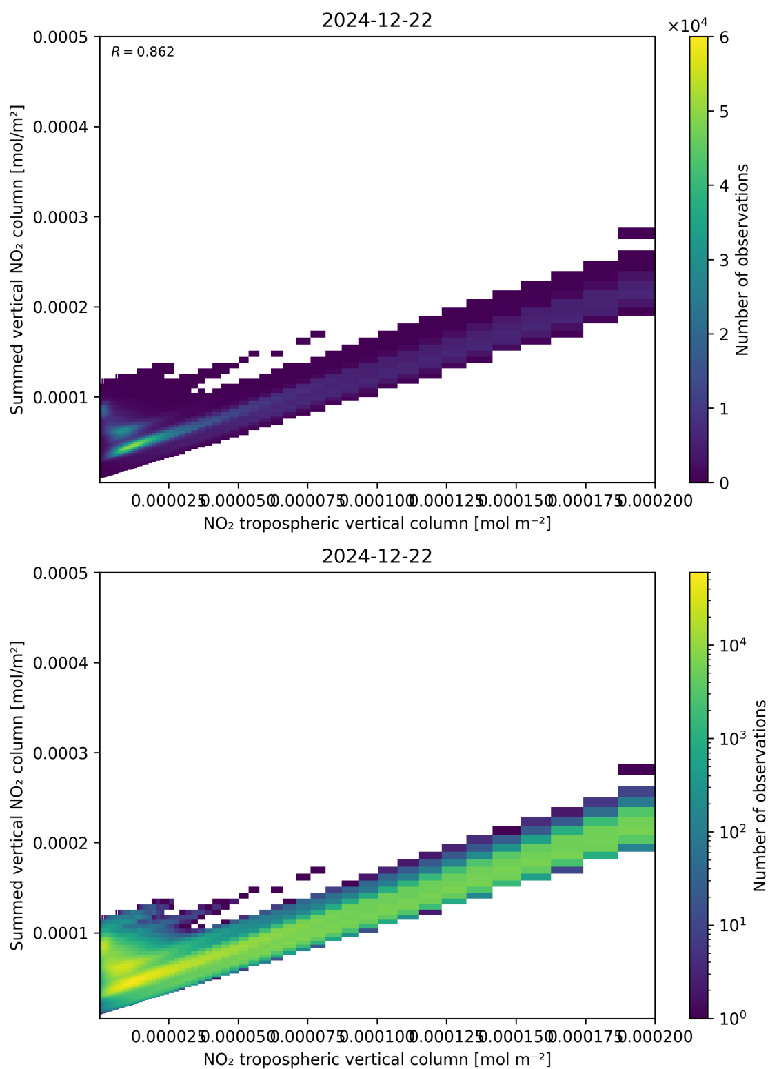
Figure 126: Scatter density plot of “NO 2 tropospheric vertical column” against “Summed vertical NO 2 column” for 2024-12-22 to 2024-12-23.
