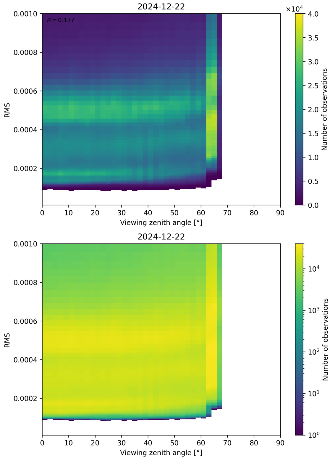
Figure 171: Scatter density plot of “Viewing zenith angle” against “RMS” for 2024-12-22 to 2024-12-23.
