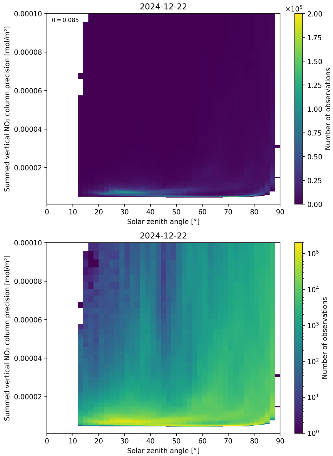
Figure 152: Scatter density plot of “Solar zenith angle” against “Summed vertical NO 2 column precision” for 2024-12-22 to 2024-12-23.
