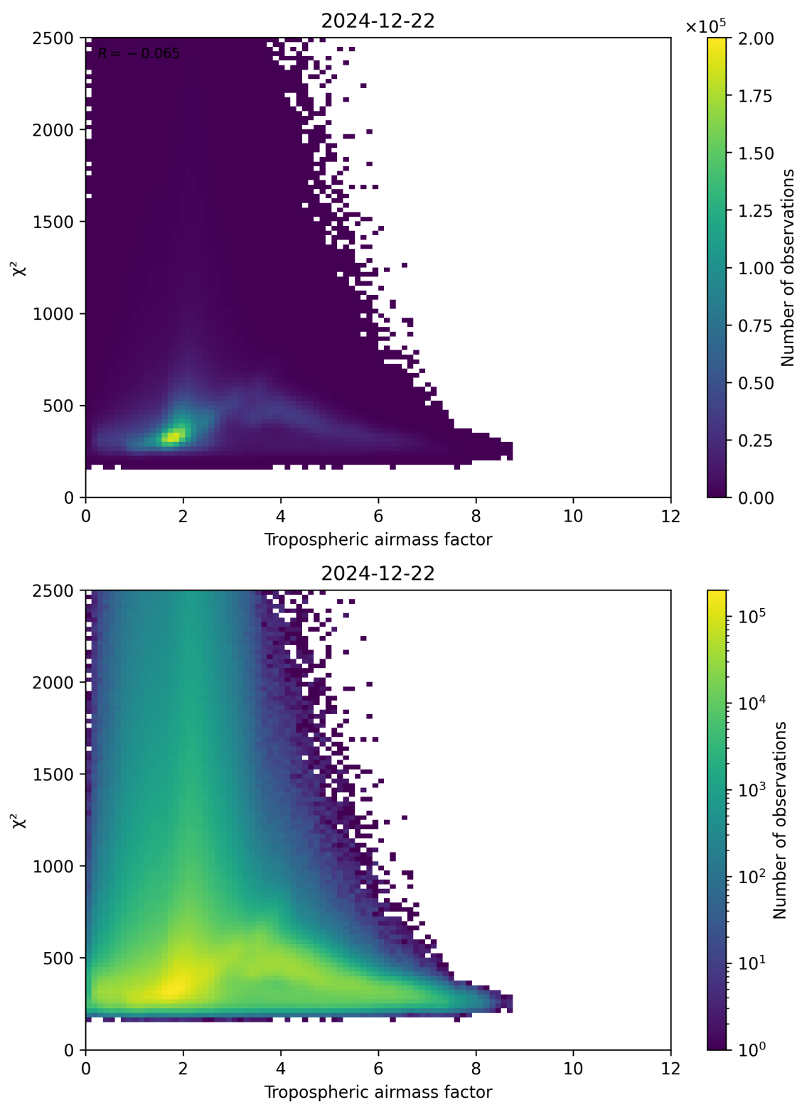
Figure 73: Scatter density plot of “Tropospheric airmass factor” against “ \chi^2 ” for 2024-12-22 to 2024-12-23.
