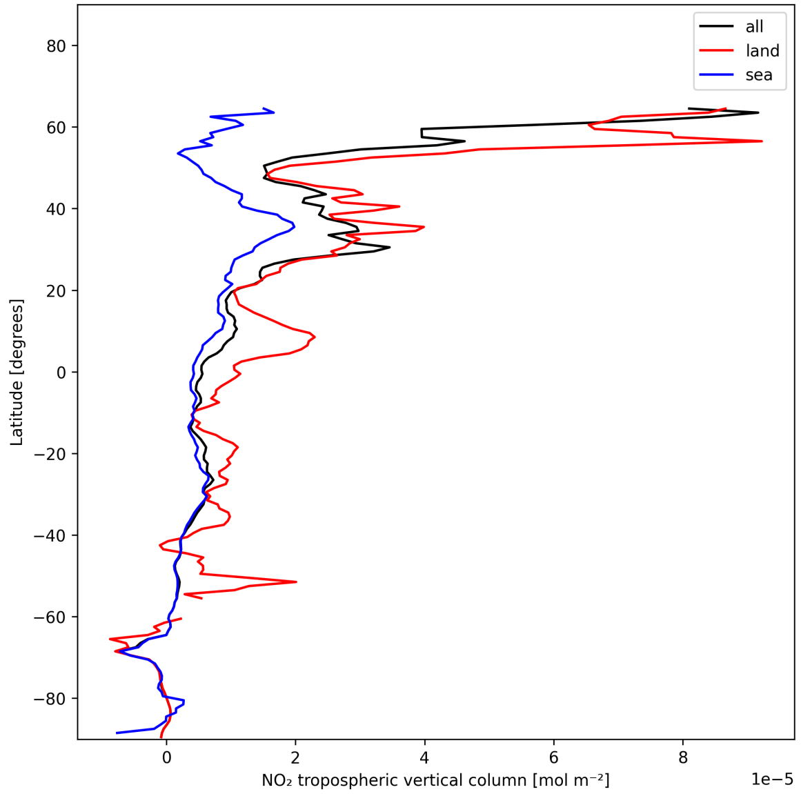
Figure 12: Zonal average of “NO 2 tropospheric vertical column” for 2024-12-22 to 2024-12-23.
