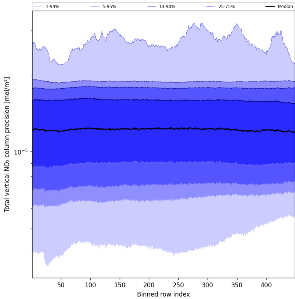
Figure 56: Along track statistics of “Total vertical NO 2 column precision” for 2024-12-22 to 2024-12-23
