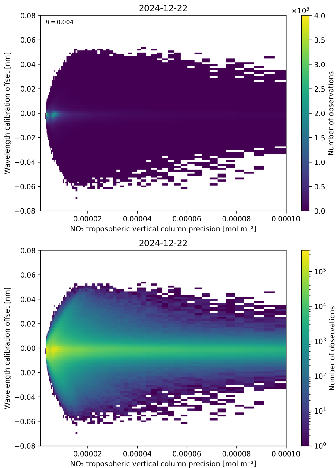
Figure 141: Scatter density plot of “NO 2 tropospheric vertical column precision” against “Wavelength calibration offset” for 2024-12-22 to 2024-12-23.
