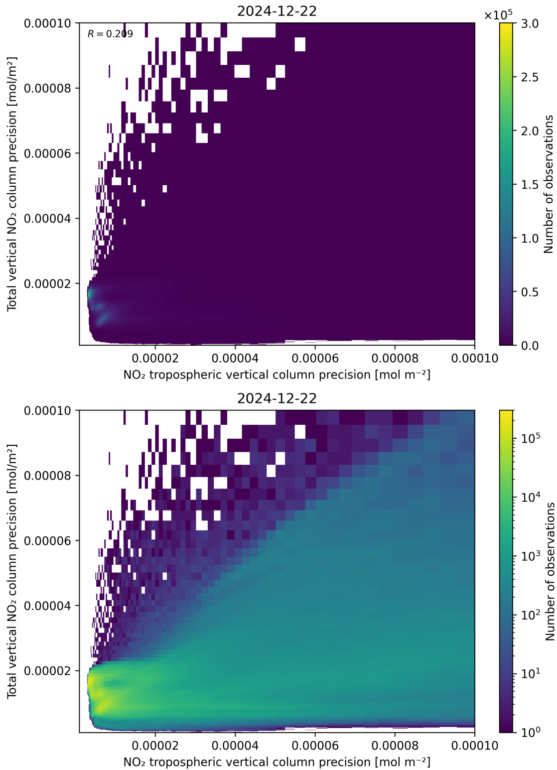
Figure 139: Scatter density plot of “NO 2 tropospheric vertical column precision” against “Total vertical NO 2 column precision” for 2024-12-22 to 2024-12-23.
