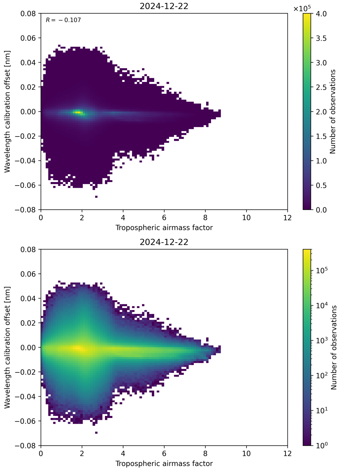
Figure 80: Scatter density plot of “Tropospheric airmass factor” against “Wavelength calibration offset” for 2024-12-22 to 2024-12-23.
