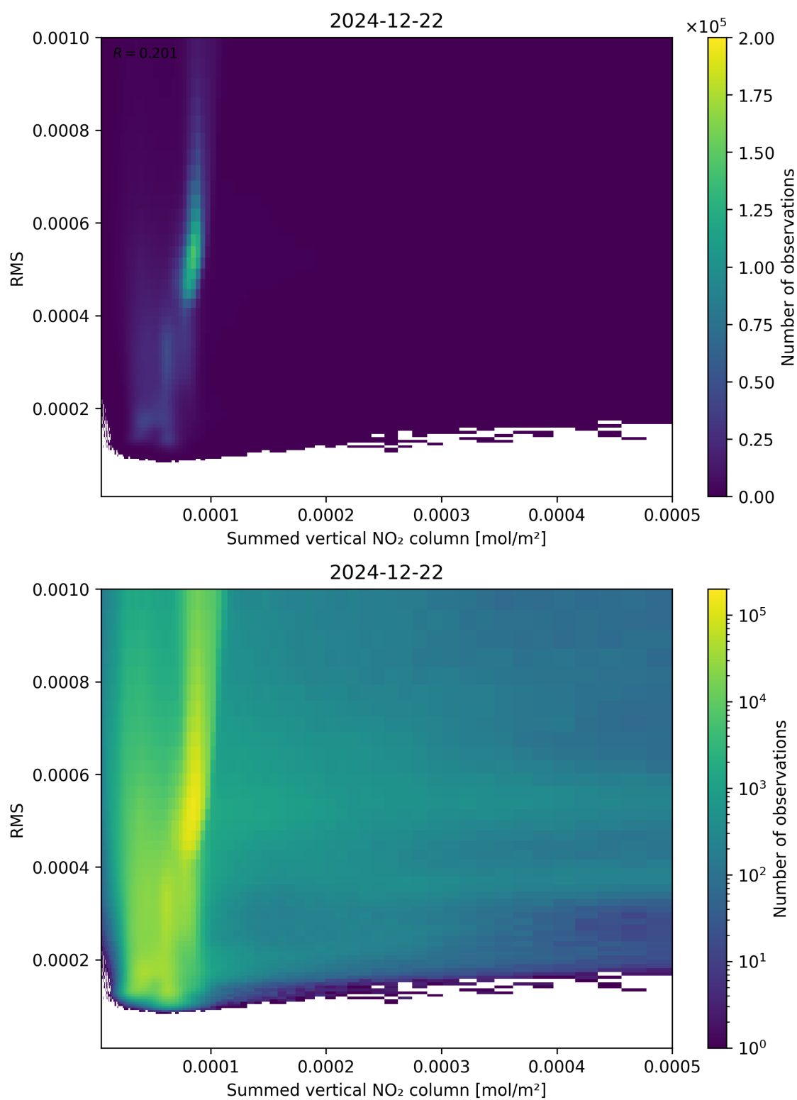
Figure 109: Scatter density plot of “Summed vertical NO 2 column” against “RMS” for 2024-12-22 to 2024-12-23.
