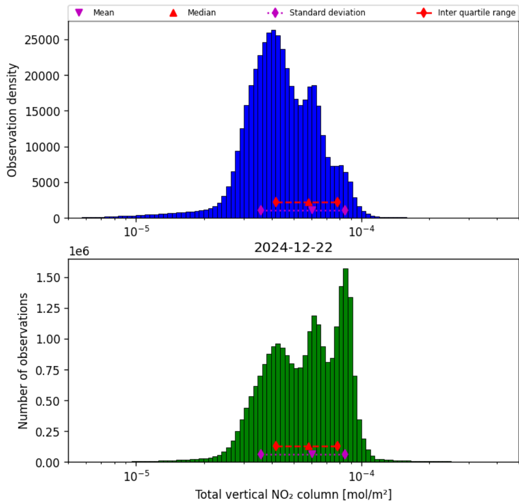
Figure 38: Histogram of “Total vertical NO 2 column” for 2024-12-22 to 2024-12-23
