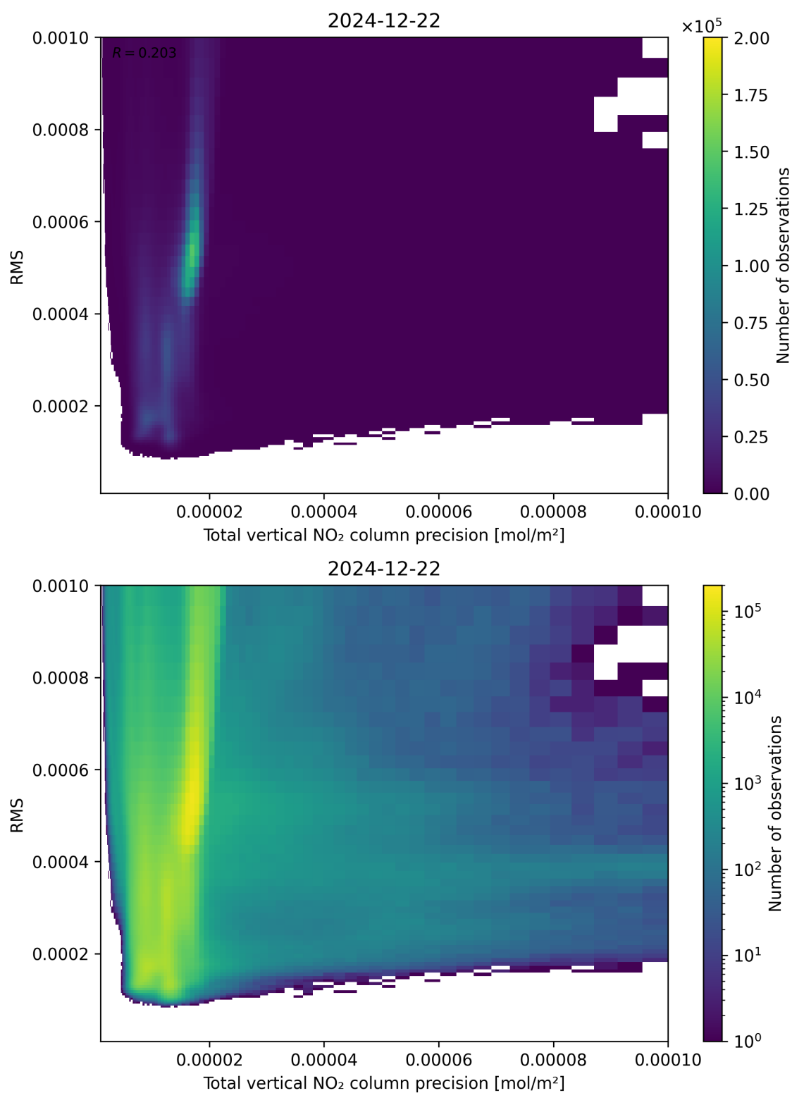
Figure 119: Scatter density plot of “Total vertical NO 2 column precision” against “RMS” for 2024-12-22 to 2024-12-23.
