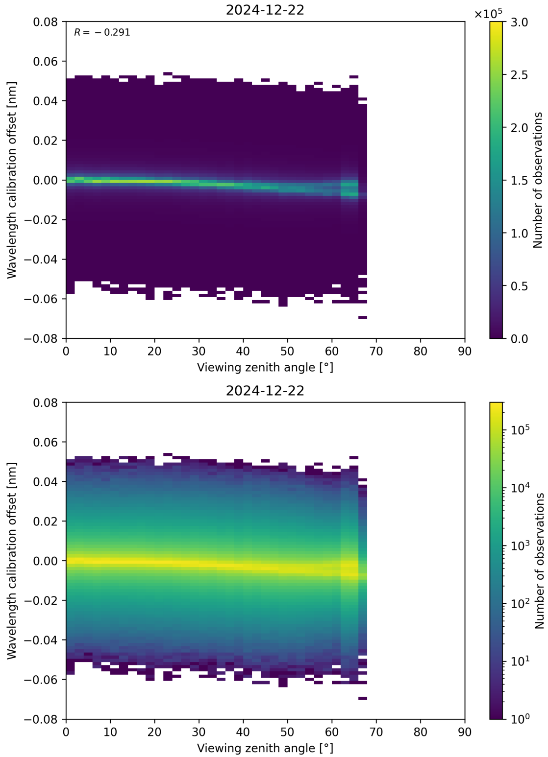
Figure 173: Scatter density plot of “Viewing zenith angle” against “Wavelength calibration offset” for 2024-12-22 to 2024-12-23.
