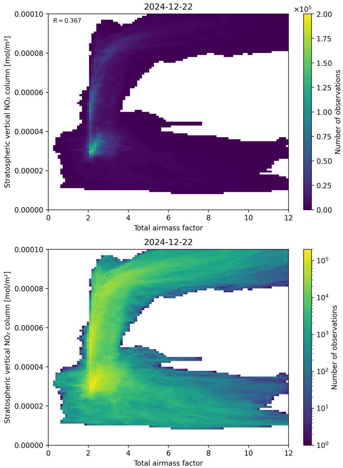
Figure 64: Scatter density plot of “Total airmass factor” against “Stratospheric vertical \text{NO}_2 column” for 2024-12-22 to 2024-12-23.
