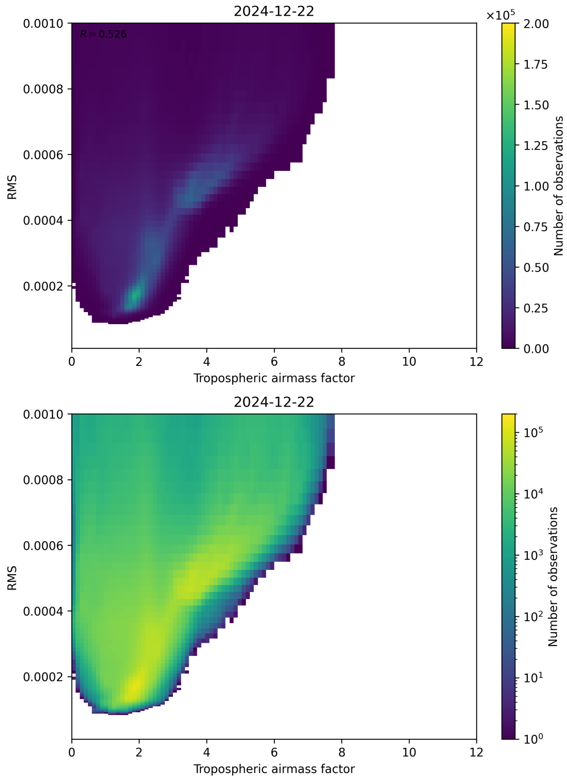
Figure 79: Scatter density plot of “Tropospheric airmass factor” against “RMS” for 2024-12-22 to 2024-12-23.
