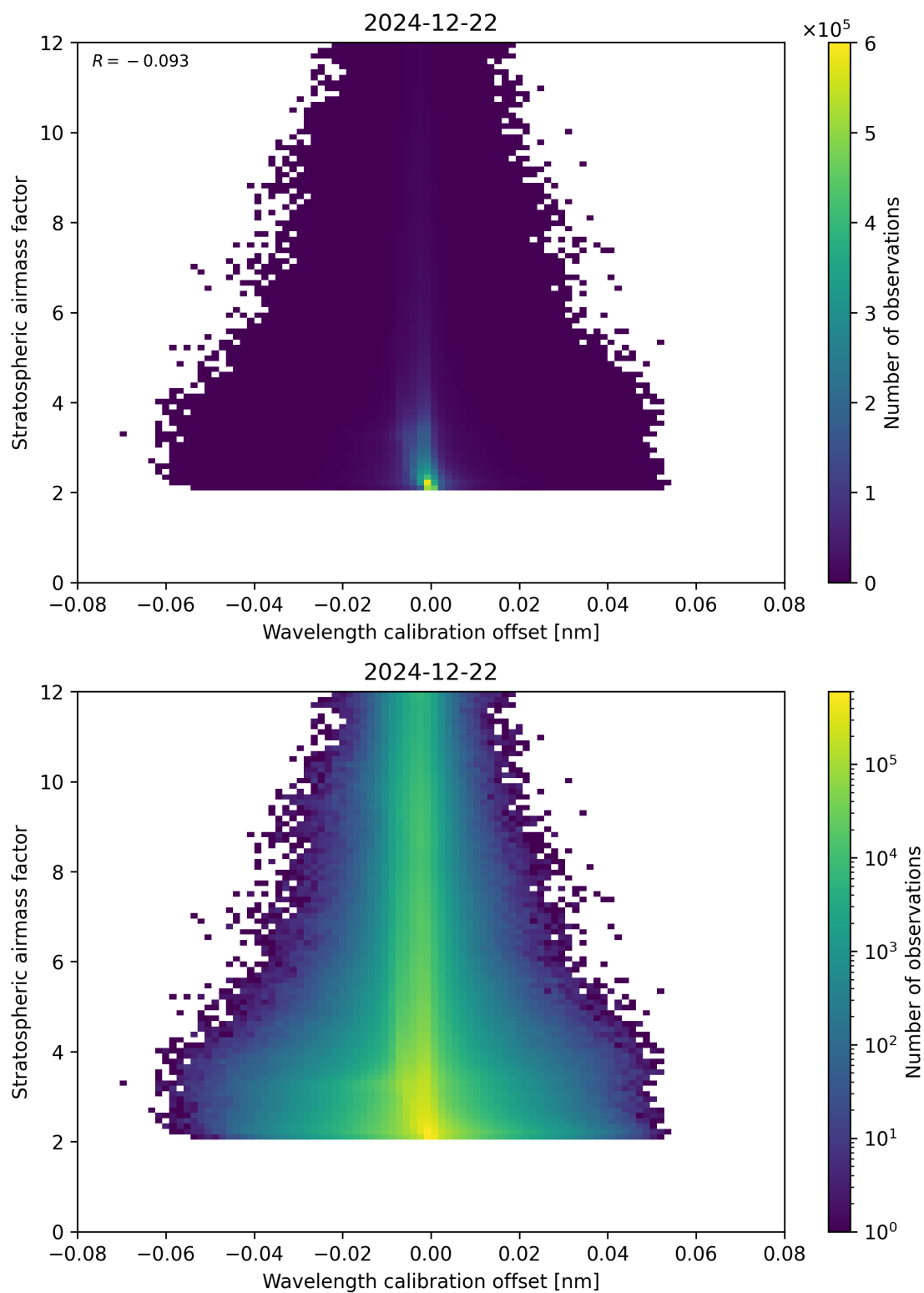
Figure 174: Scatter density plot of “Wavelength calibration offset” against “Stratospheric airmass factor” for 2024-12-22 to 2024-12-23.
