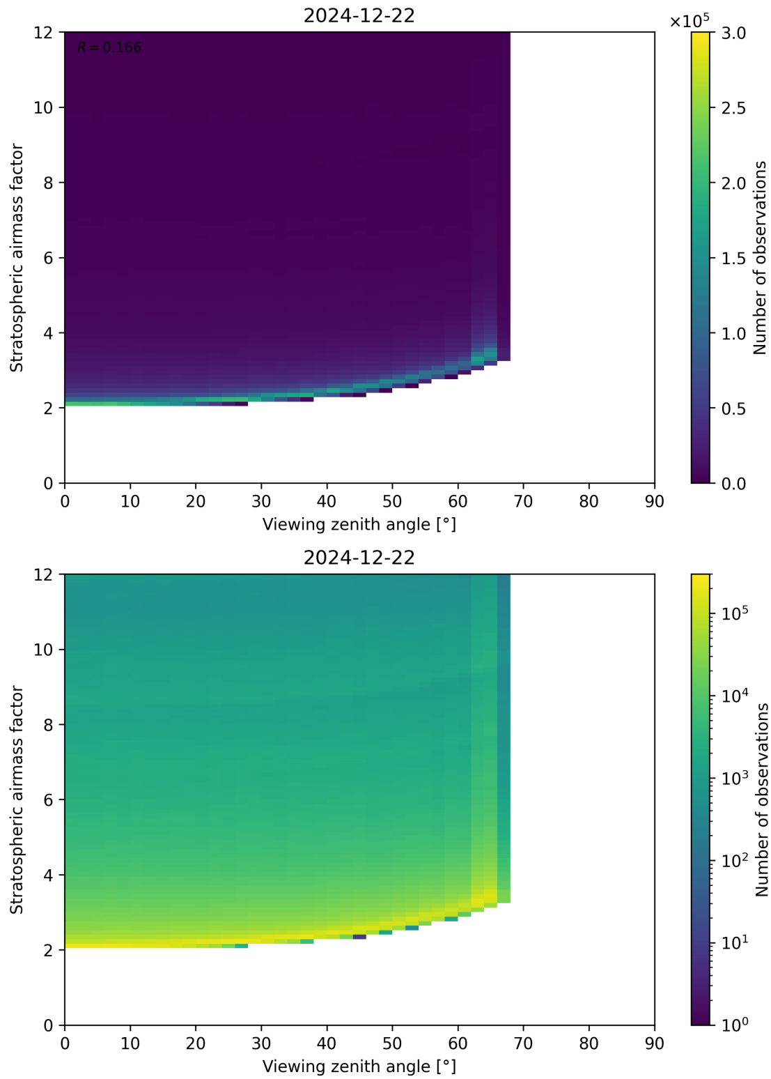
Figure 159: Scatter density plot of “Viewing zenith angle” against “Stratospheric airmass factor” for 2024-12-22 to 2024-12-23.
