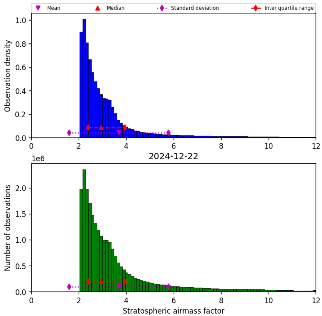
Figure 44: Histogram of “Stratospheric airmass factor” for 2024-12-22 to 2024-12-23
