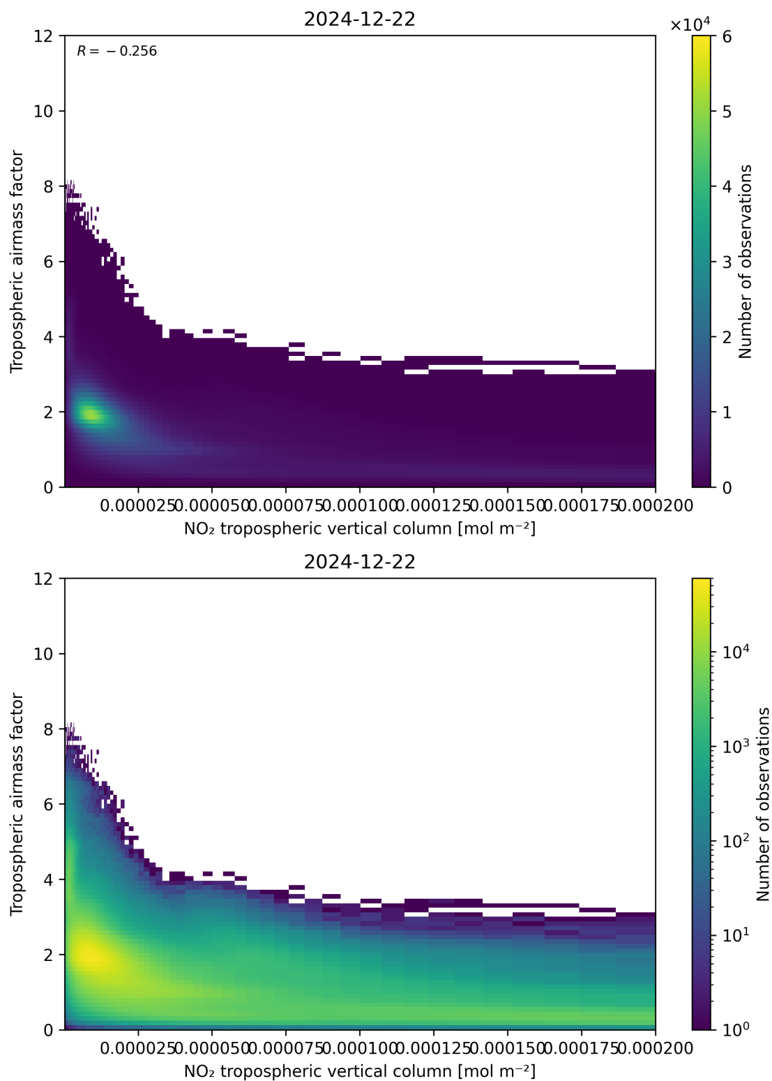
Figure 123: Scatter density plot of “NO 2 tropospheric vertical column” against “Tropospheric air mass factor” for 2024-12-22 to 2024-12-23.
