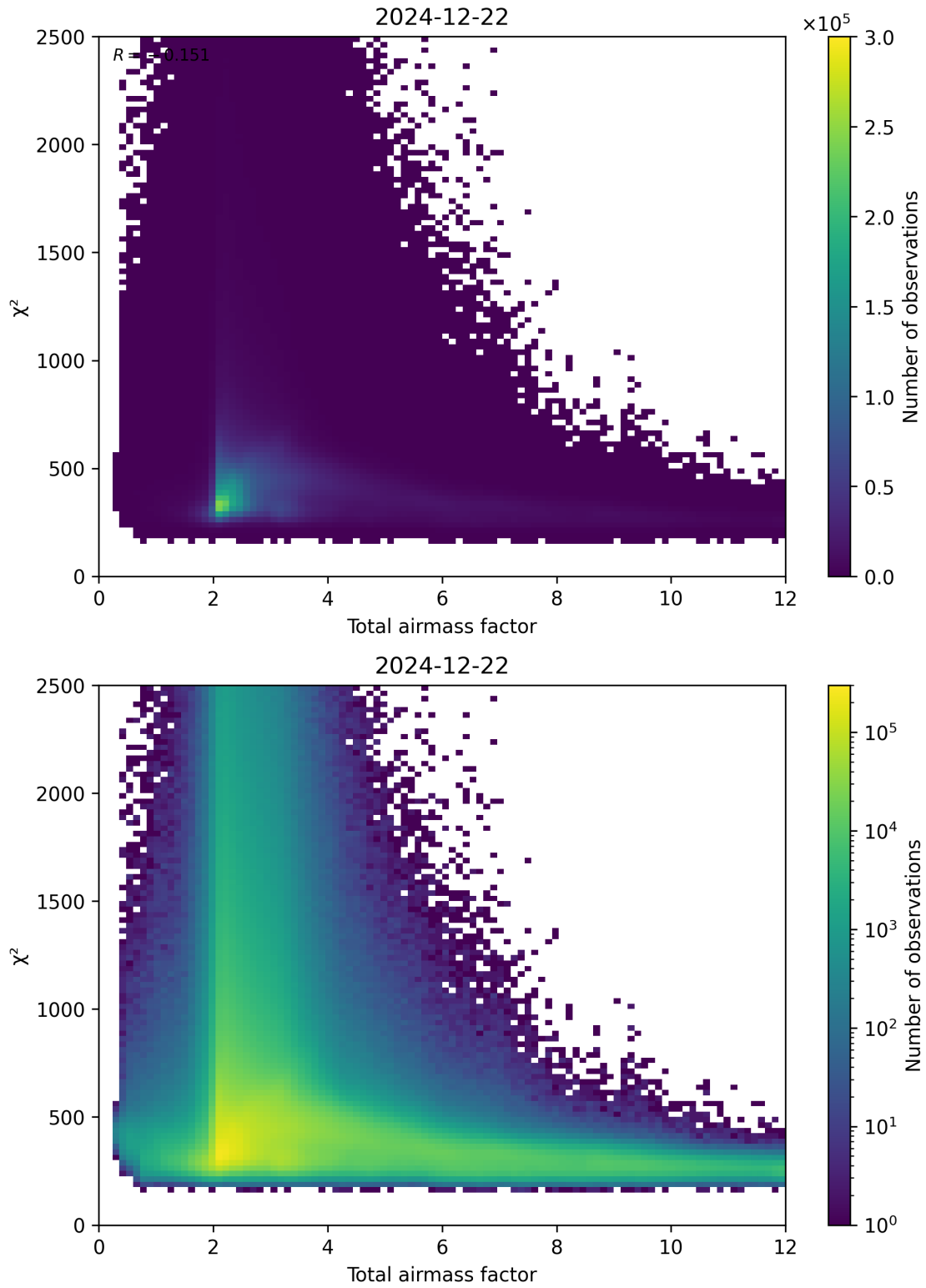
Figure 63: Scatter density plot of “Total airmass factor” against “ \chi^2 ” for 2024-12-22 to 2024-12-23.
