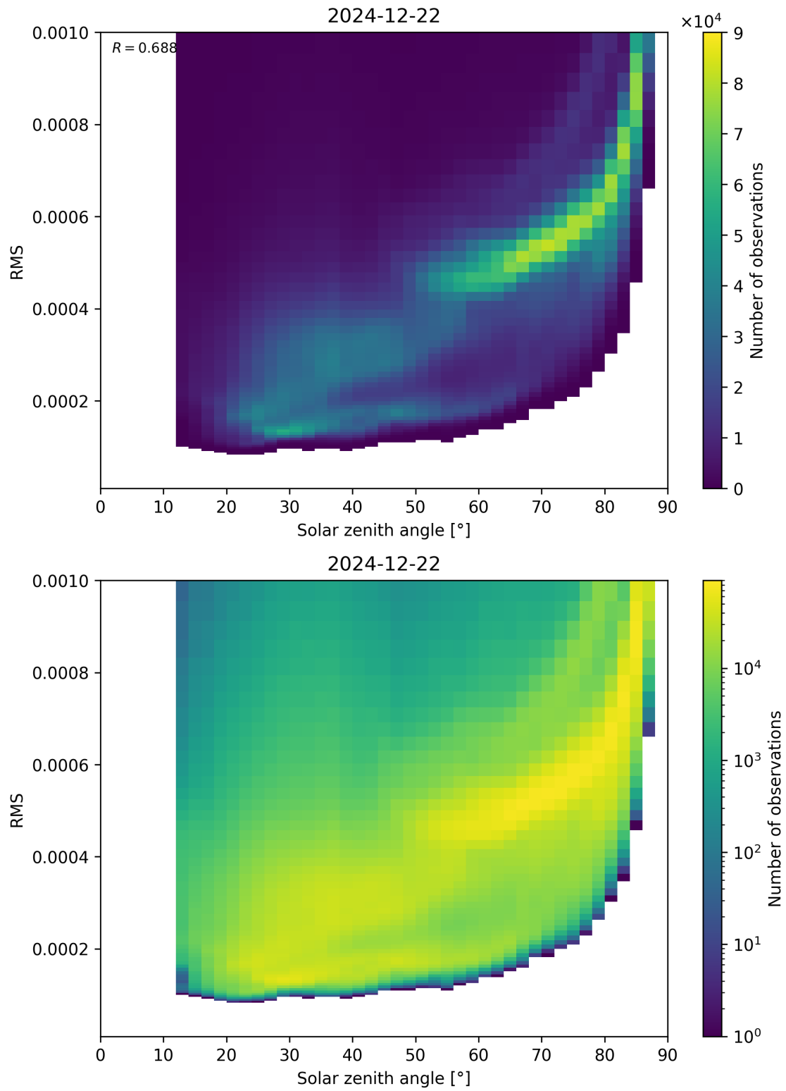
Figure 157: Scatter density plot of “Solar zenith angle” against “RMS” for 2024-12-22 to 2024-12-23.
