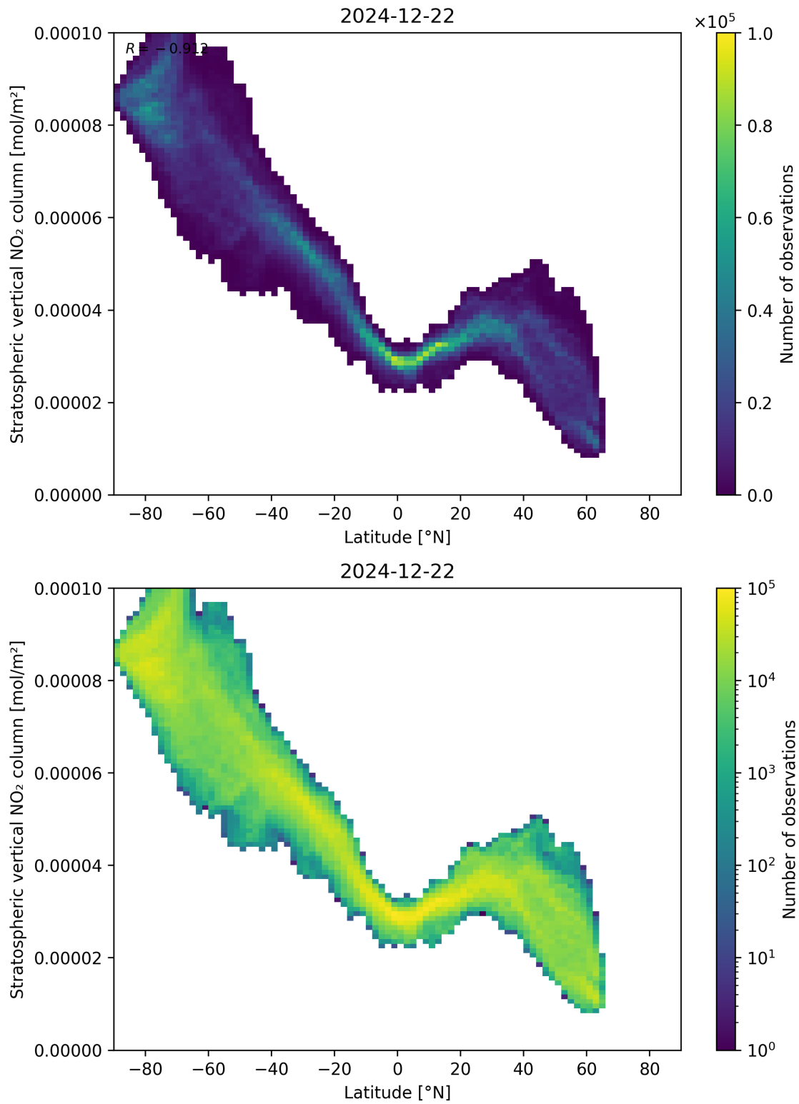
Figure 87: Scatter density plot of “Latitude” against “Stratospheric vertical NO 2 column” for 2024-12-22 to 2024-12-23.
