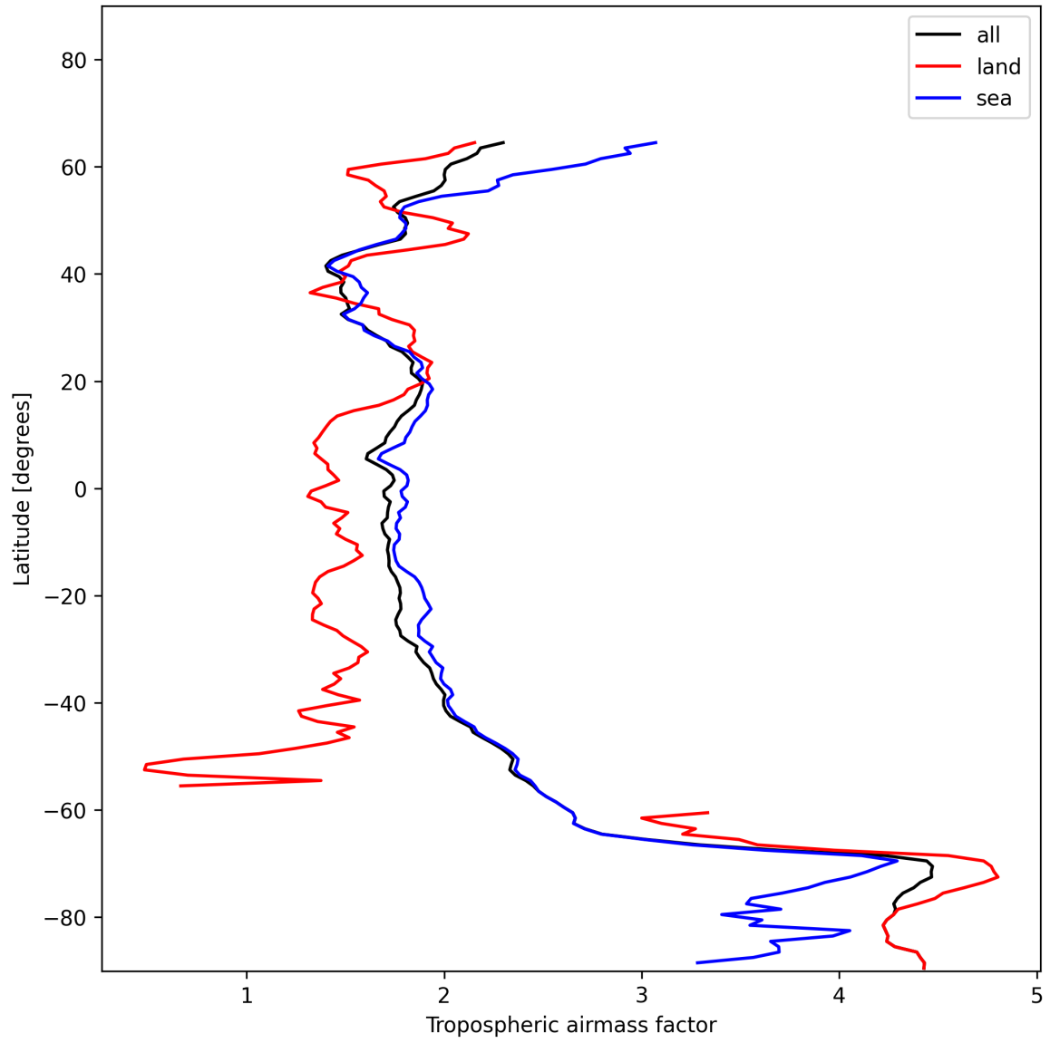
Figure 14: Zonal average of “Tropospheric airmass factor” for 2024-12-22 to 2024-12-23.
