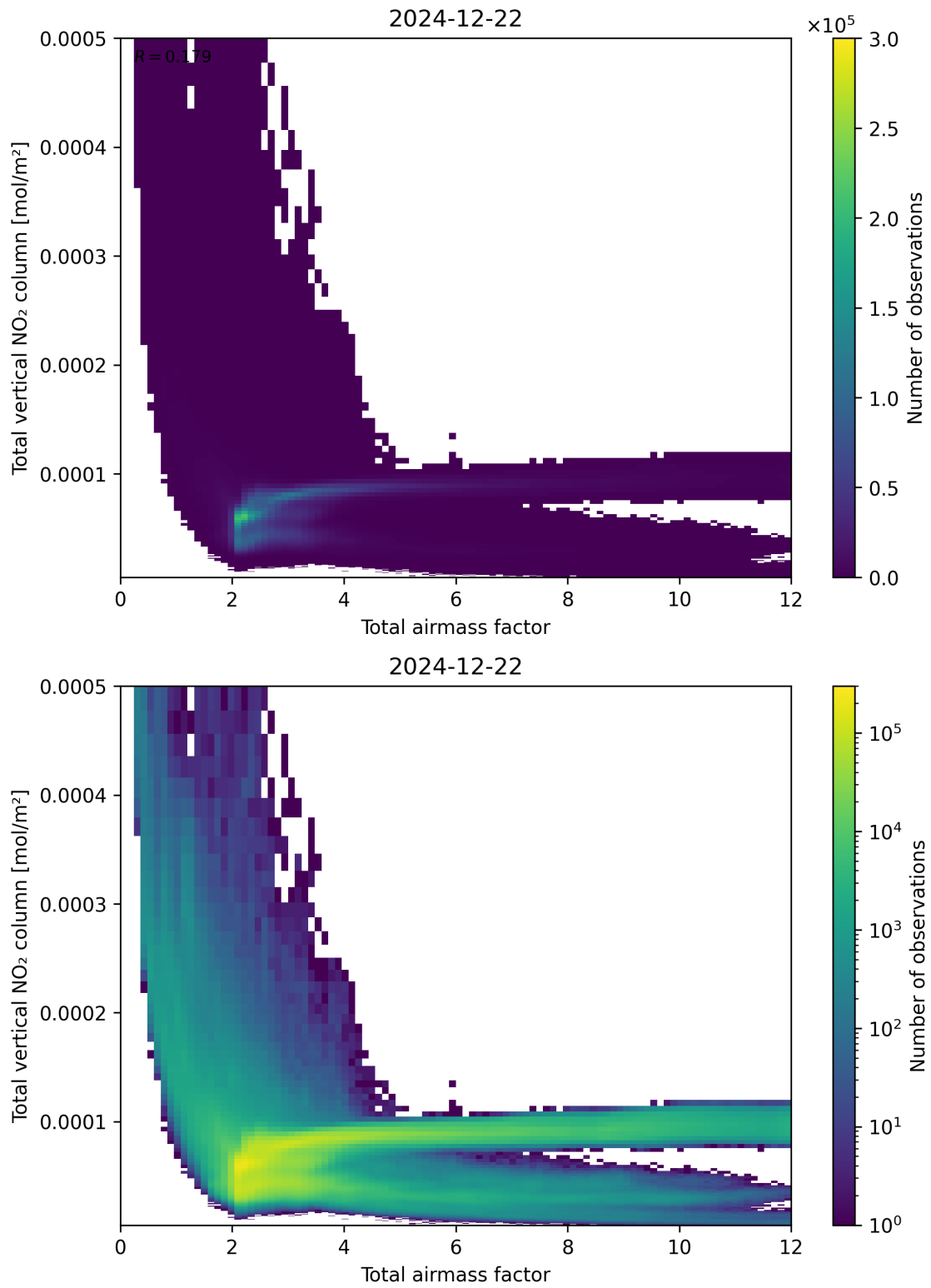
Figure 67: Scatter density plot of “Total airmass factor” against “Total vertical NO 2 column” for 2024-12-22 to 2024-12-23.
