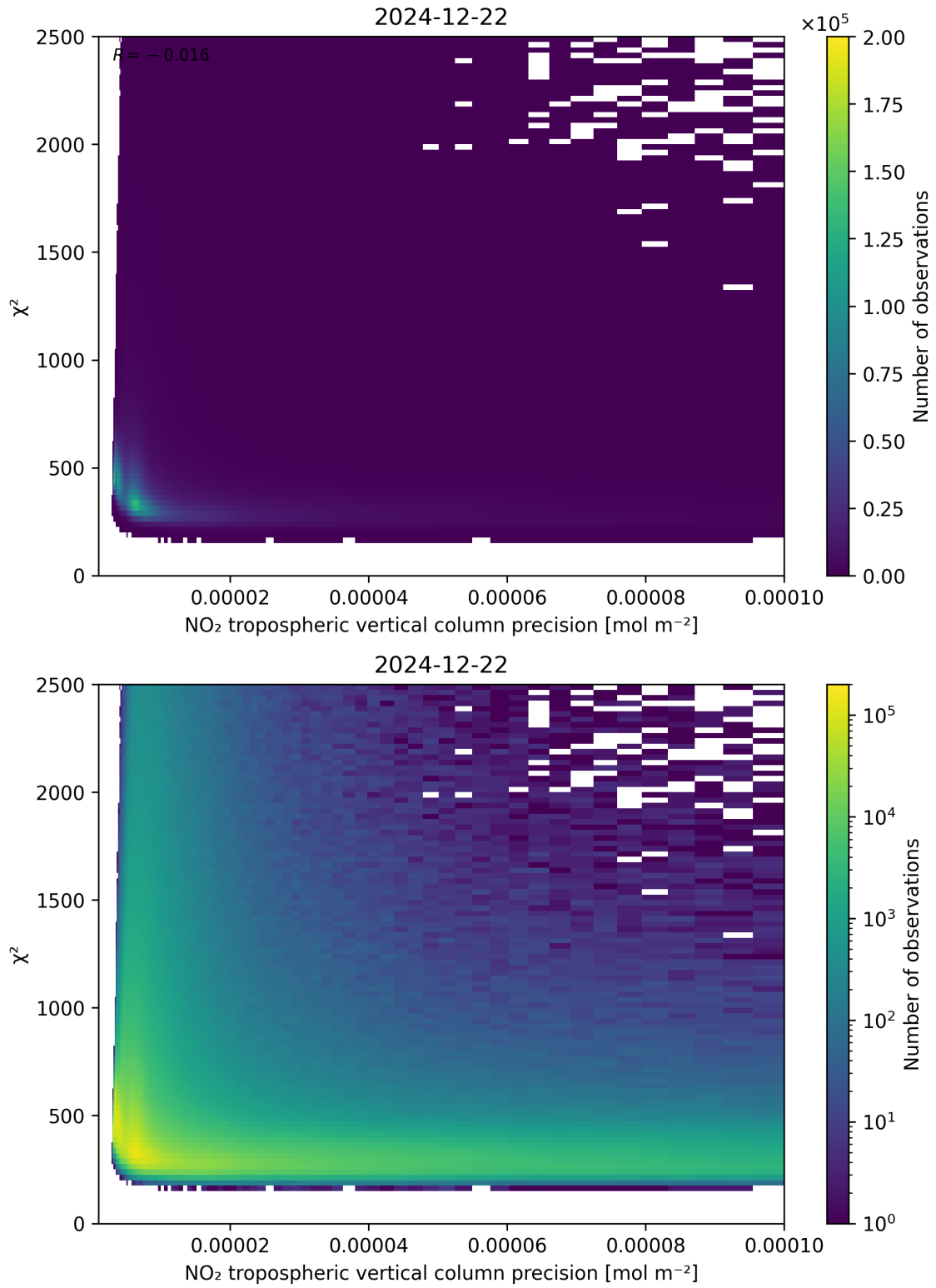
Figure 134: Scatter density plot of “NO 2 tropospheric vertical column precision” against “ \chi^2 ” for 2024-12-22 to 2024-12-23.
