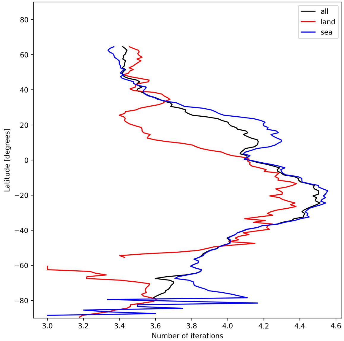
Figure 17: Zonal average of “Number of iterations” for 2024-12-22 to 2024-12-23.
