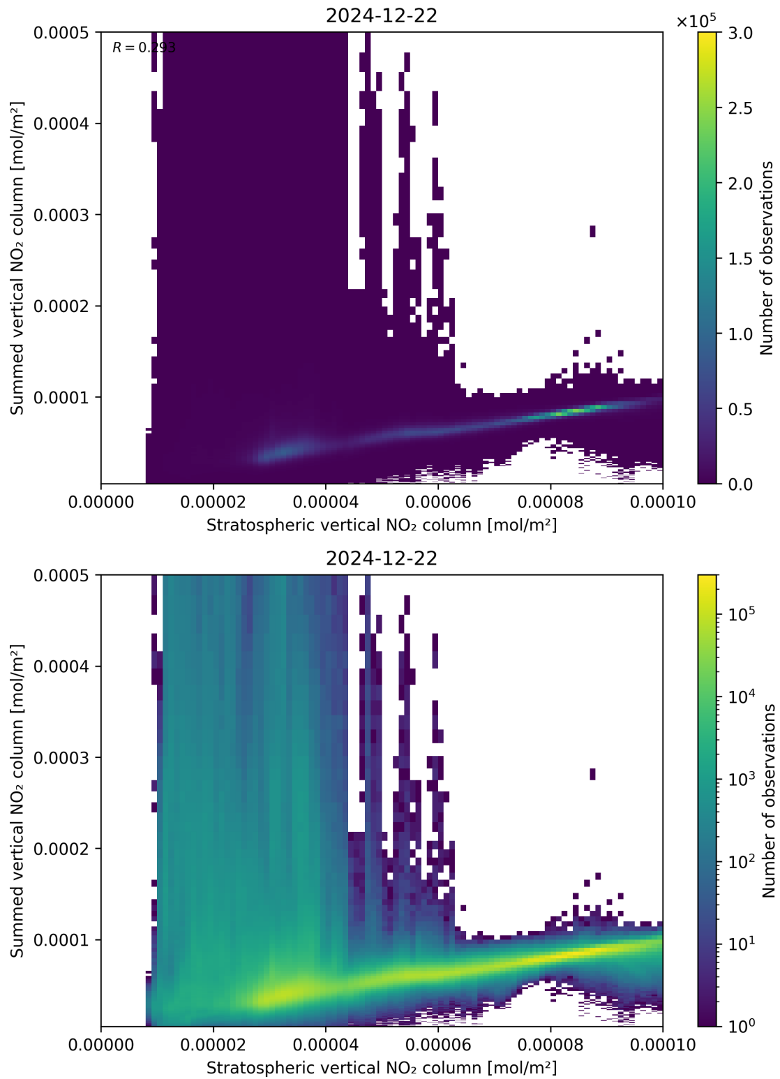
Figure 98: Scatter density plot of “Stratospheric vertical NO 2 column” against “Summed vertical NO 2 column” for 2024-12-22 to 2024-12-23.
