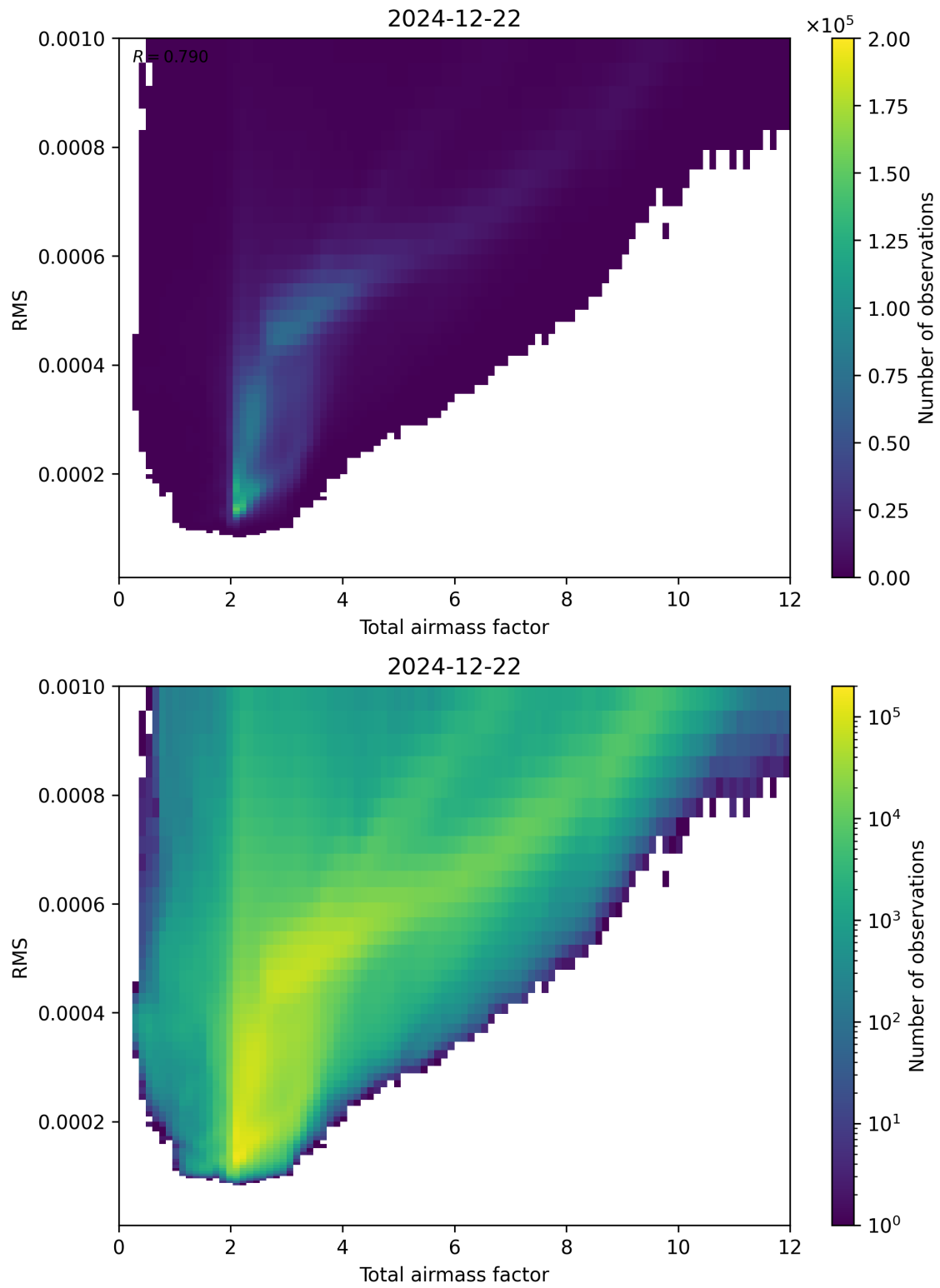
Figure 69: Scatter density plot of “Total airmass factor” against “RMS” for 2024-12-22 to 2024-12-23.
