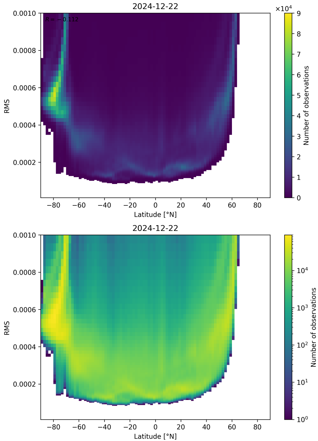
Figure 94: Scatter density plot of “Latitude” against “RMS” for 2024-12-22 to 2024-12-23.
