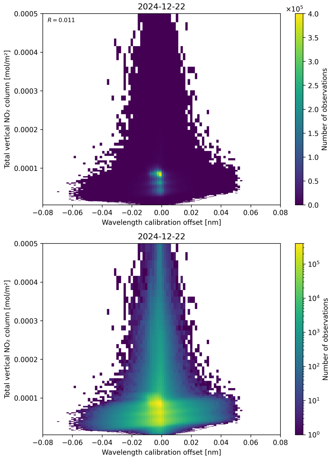
Figure 179: Scatter density plot of “Wavelength calibration offset” against “Total vertical NO 2 column” for 2024-12-22 to 2024-12-23.
