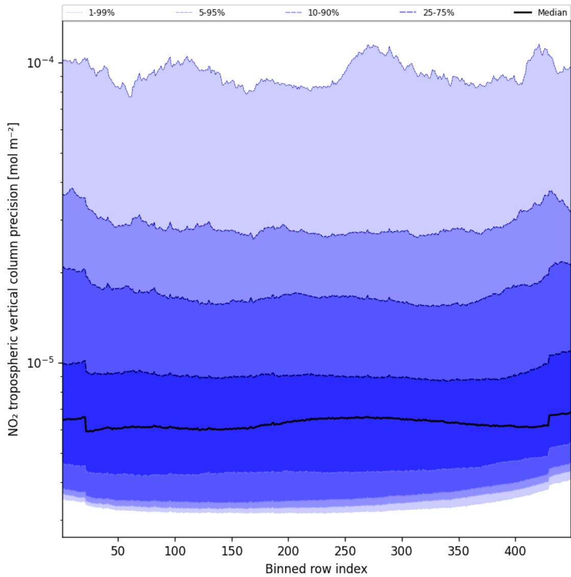
Figure 47: Along track statistics of “NO 2 tropospheric vertical column precision” for 2024-12-22 to 2024-12-23
