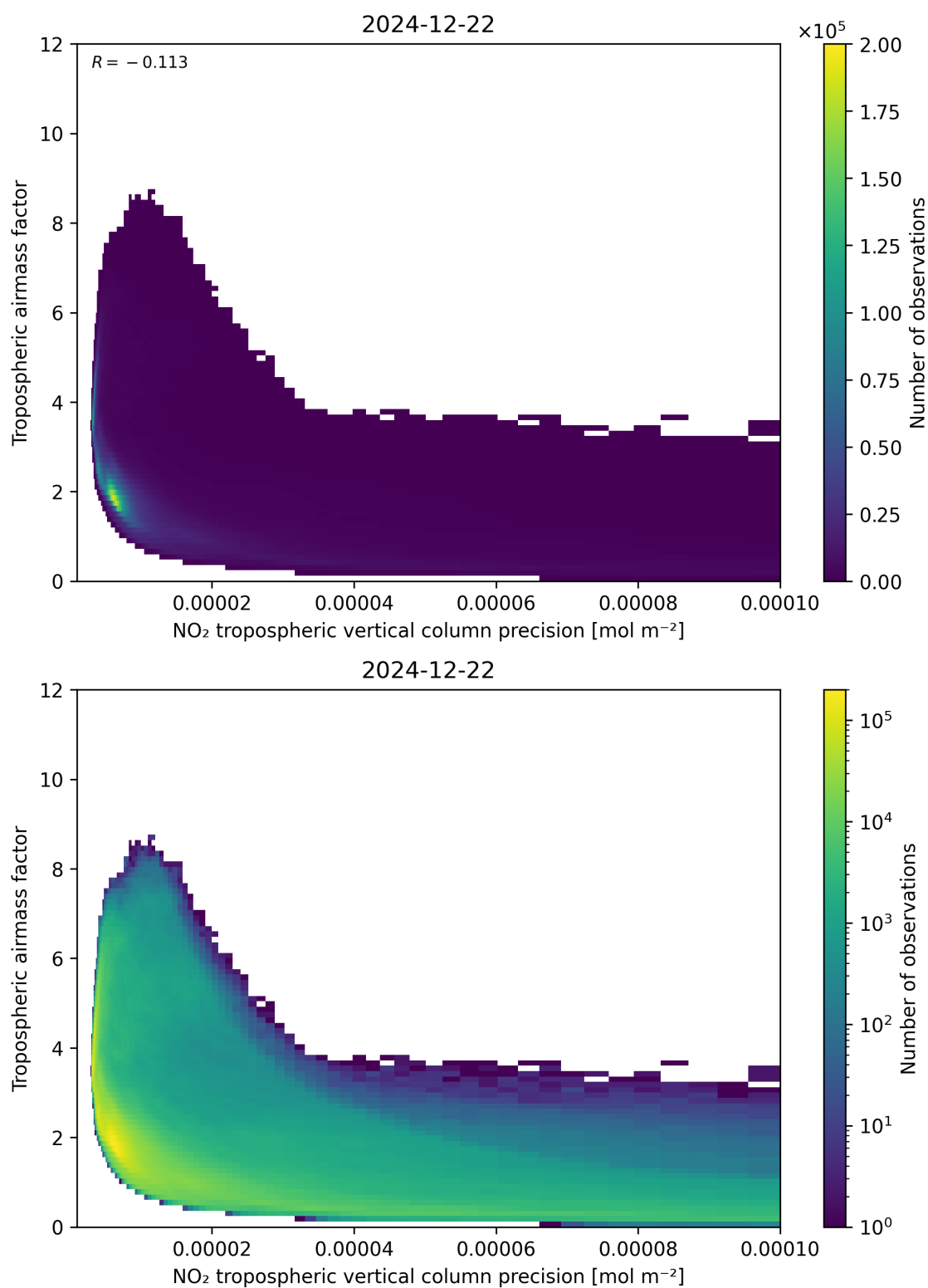
Figure 133: Scatter density plot of “NO 2 tropospheric vertical column precision” against “Tropospheric airmass factor” for 2024-12-22 to 2024-12-23.
