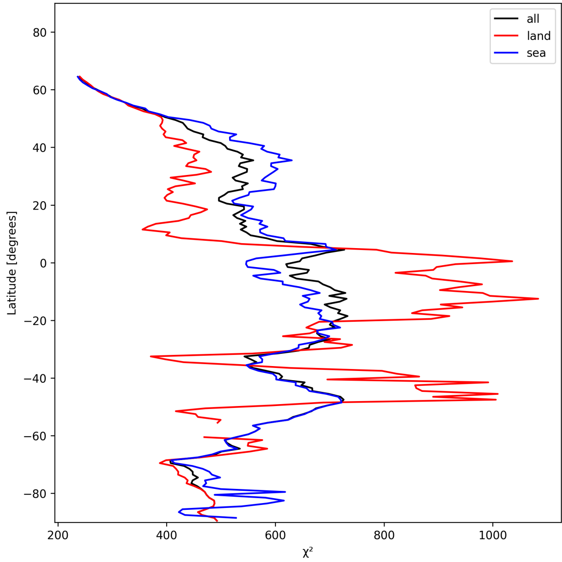
Figure 25: Zonal average of “ \chi^2 ” for 2024-12-22 to 2024-12-23.
