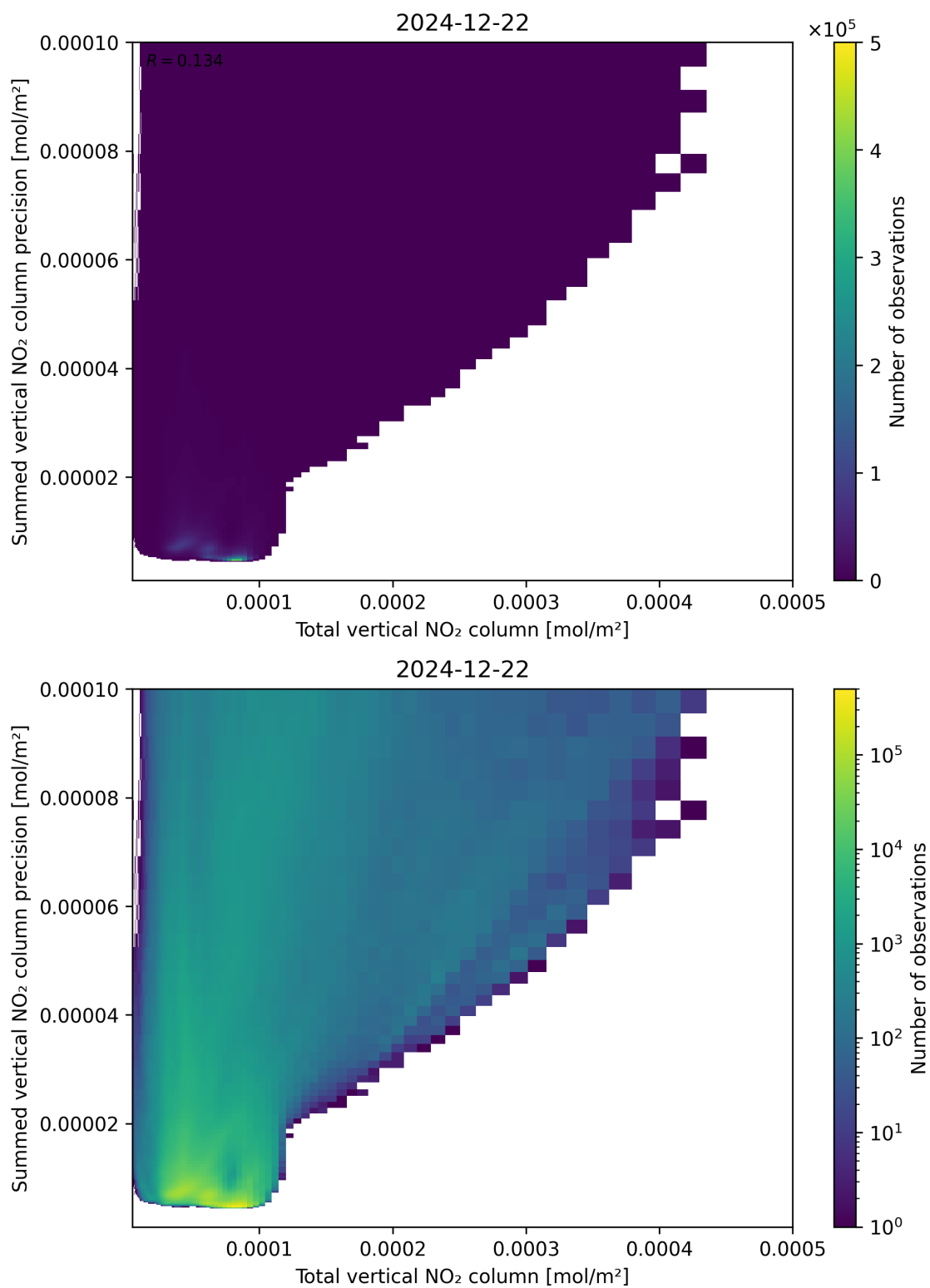
Figure 113: Scatter density plot of “Total vertical NO 2 column” against “Summed vertical NO 2 column precision” for 2024-12-22 to 2024-12-23.
