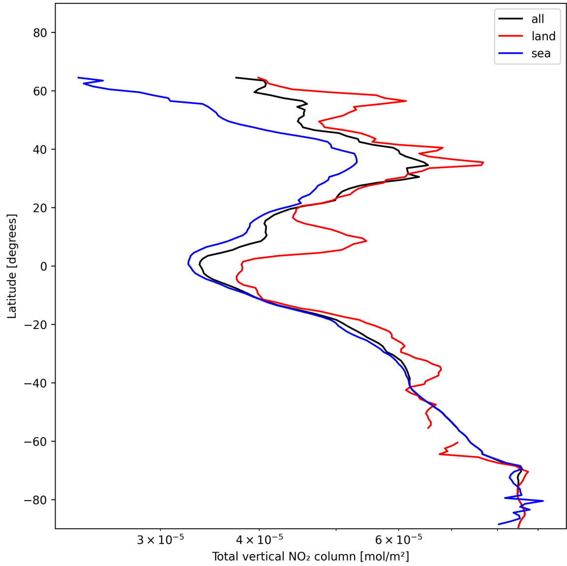
Figure 21: Zonal average of “Total vertical NO 2 column” for 2024-12-22 to 2024-12-23.
