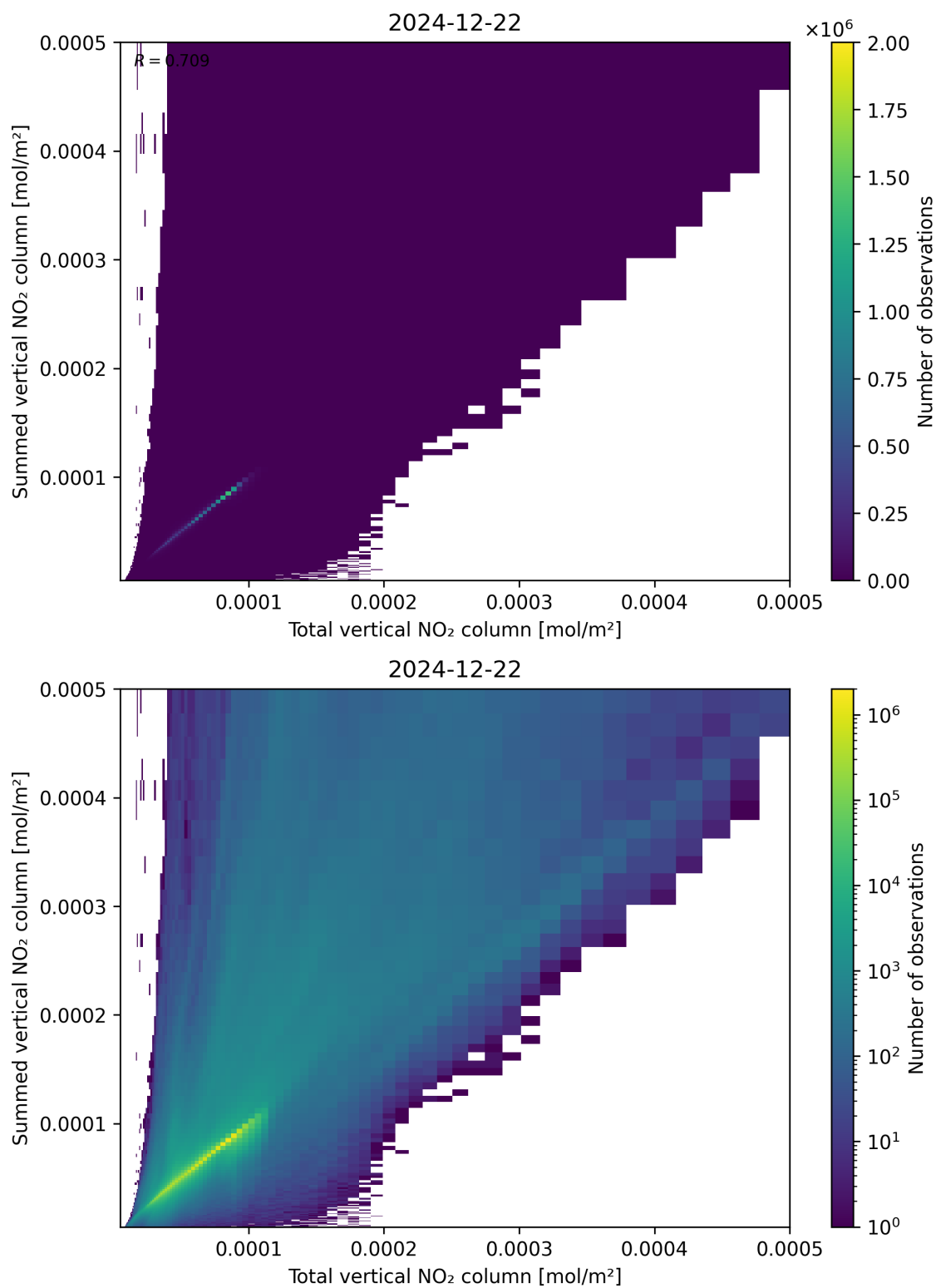
Figure 112: Scatter density plot of “Total vertical NO 2 column” against “Summed vertical NO 2 column” for 2024-12-22 to 2024-12-23.
