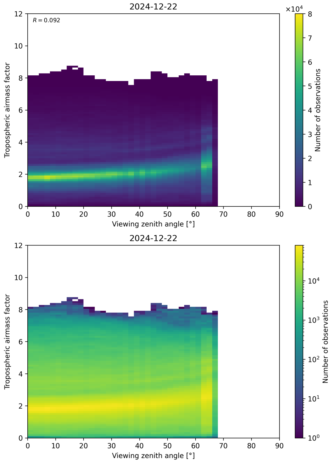
Figure 161: Scatter density plot of “Viewing zenith angle” against “Tropospheric airmass factor” for 2024-12-22 to 2024-12-23.
