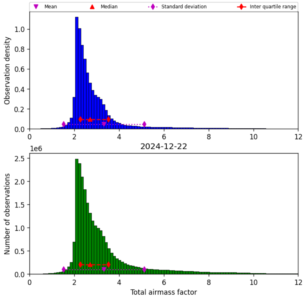
Figure 32: Histogram of “Total airmass factor” for 2024-12-22 to 2024-12-23
