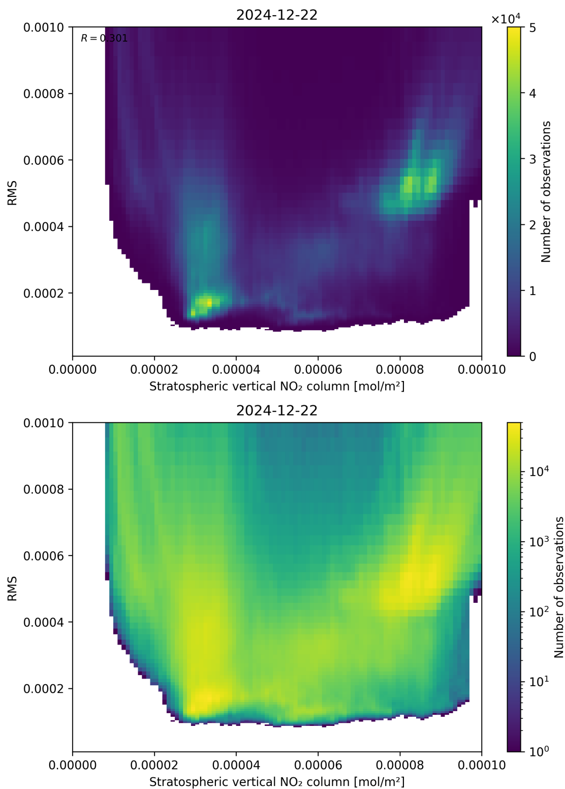
Figure 102: Scatter density plot of “Stratospheric vertical NO 2 column” against “RMS” for 2024-12-22 to 2024-12-23.
