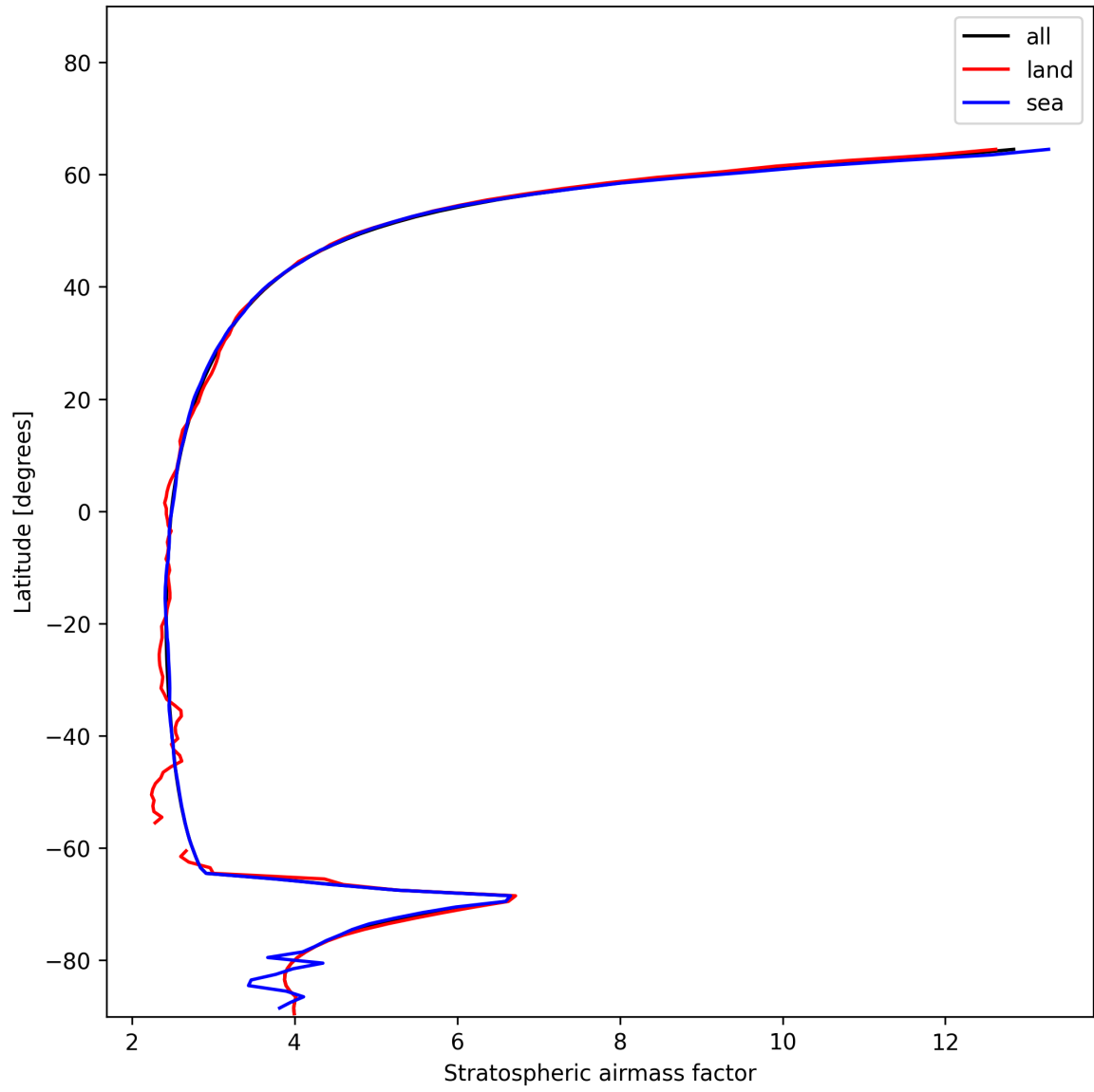
Figure 27: Zonal average of “Stratospheric air mass factor” for 2024-12-22 to 2024-12-23.
