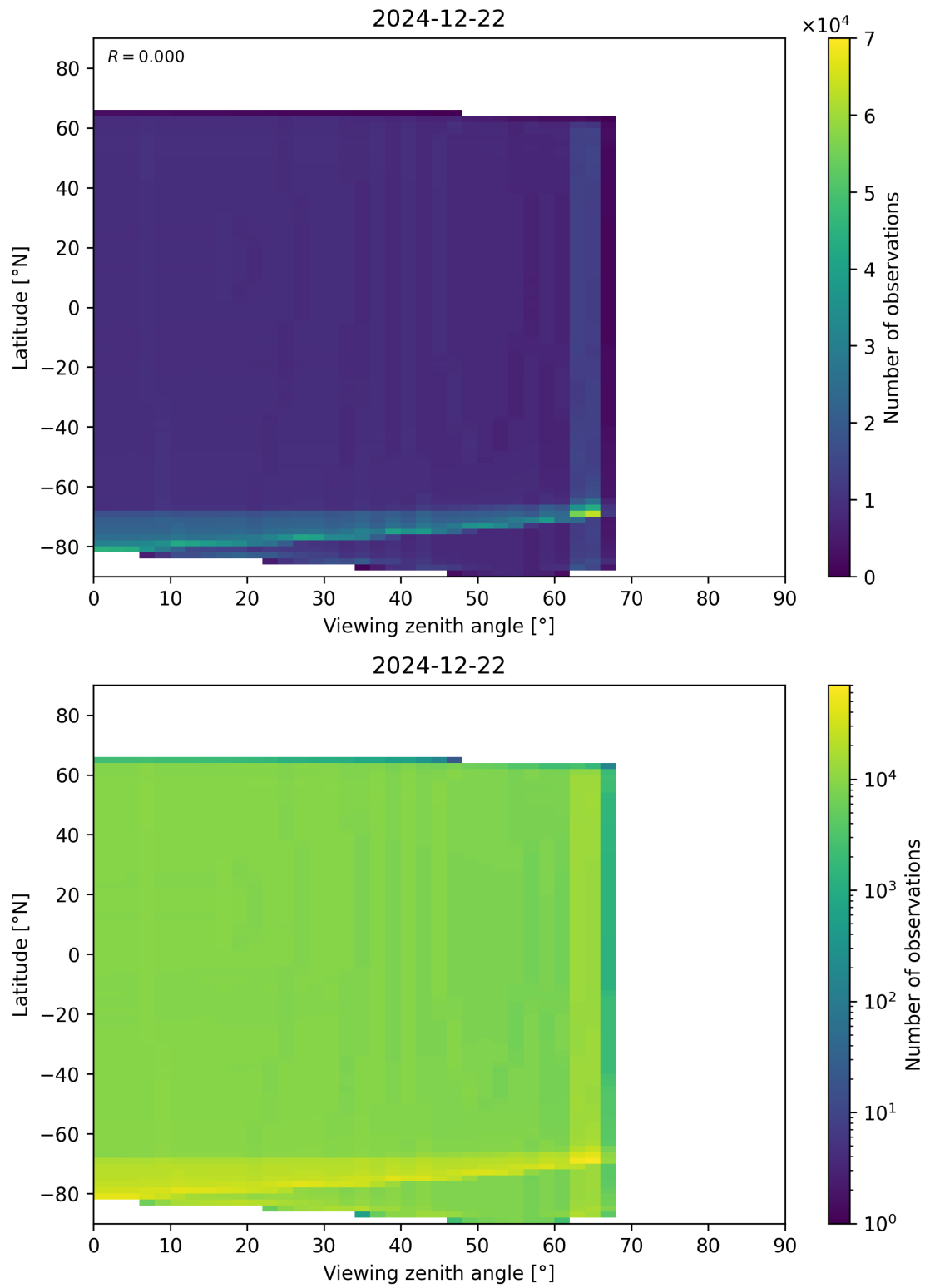
Figure 163: Scatter density plot of “Viewing zenith angle” against “Latitude” for 2024-12-22 to 2024-12-23.
