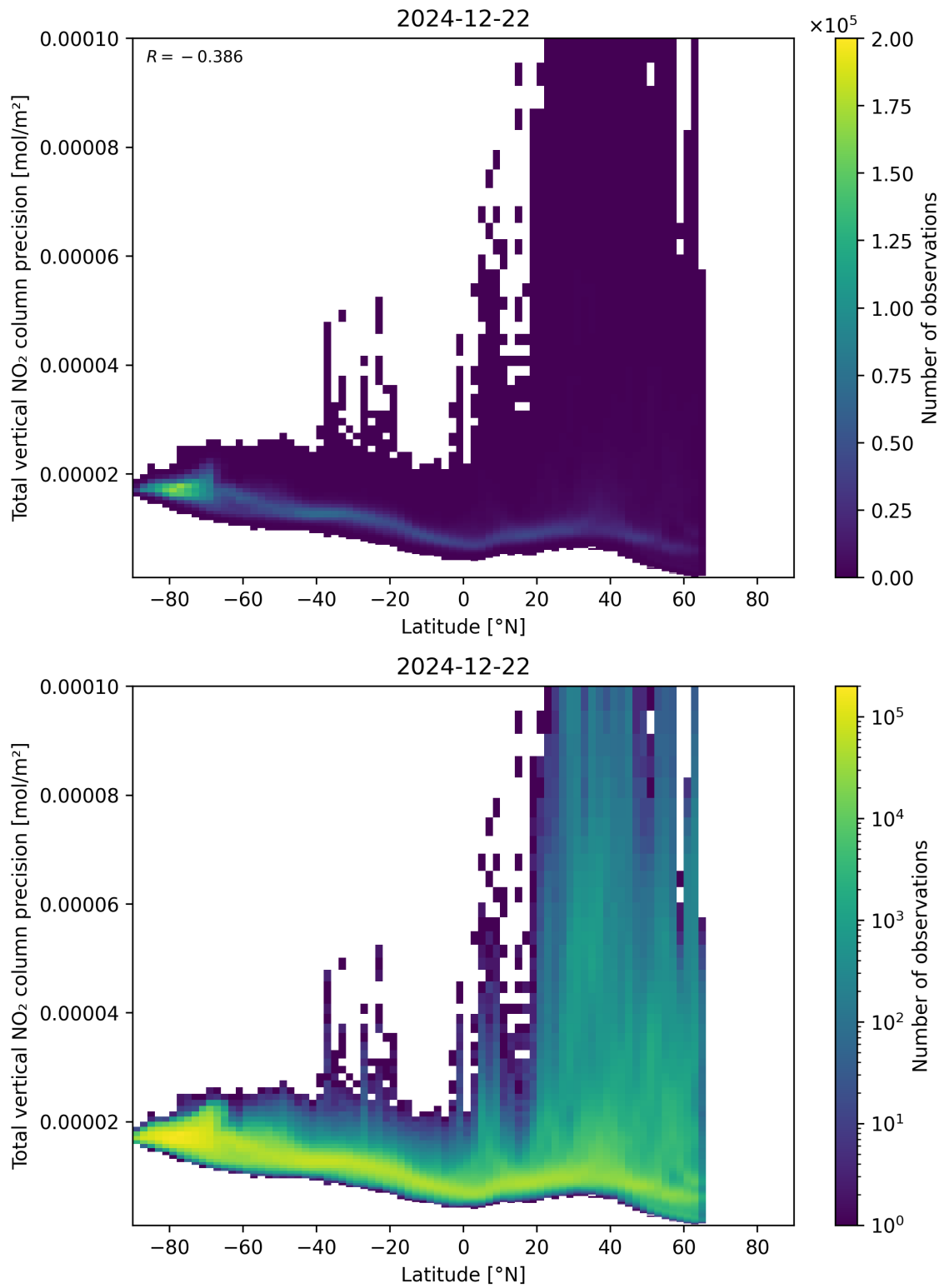
Figure 91: Scatter density plot of “Latitude” against “Total vertical NO 2 column precision” for 2024-12-22 to 2024-12-23.
