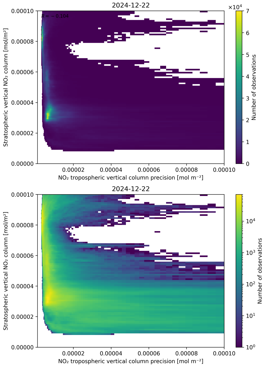
Figure 135: Scatter density plot of “NO 2 tropospheric vertical column precision” against “Stratospheric vertical NO 2 column” for 2024-12-22 to 2024-12-23.
