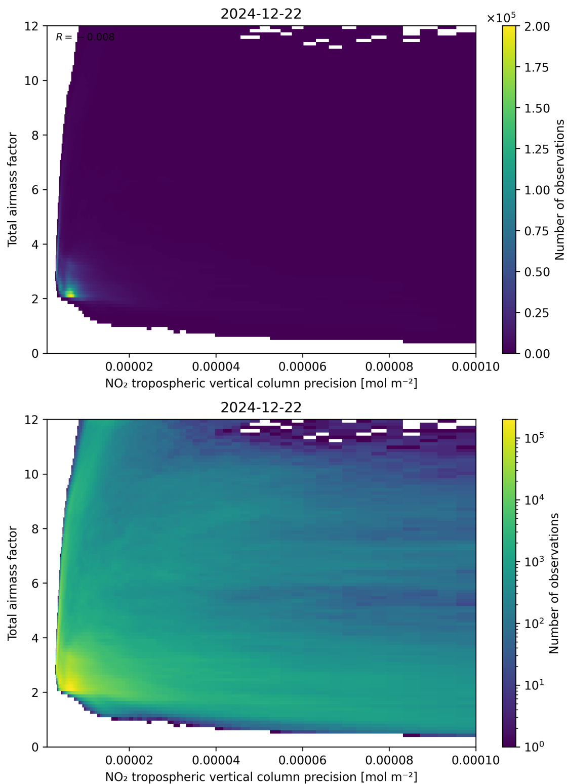
Figure 132: Scatter density plot of “NO 2 tropospheric vertical column precision” against “Total air mass factor” for 2024-12-22 to 2024-12-23.
