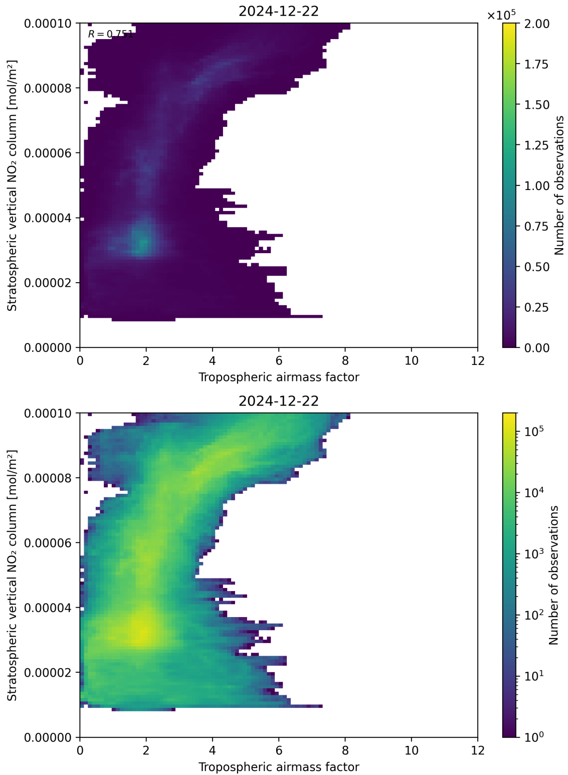
Figure 74: Scatter density plot of “Tropospheric air mass factor” against “Stratospheric vertical NO 2 column” for 2024-12-22 to 2024-12-23.
