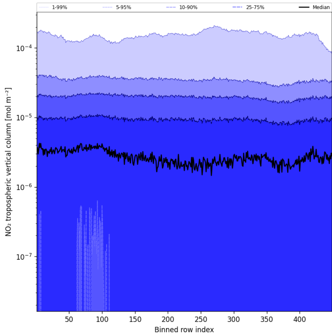
Figure 46: Along track statistics of “NO 2 tropospheric vertical column” for 2024-12-22 to 2024-12-23
