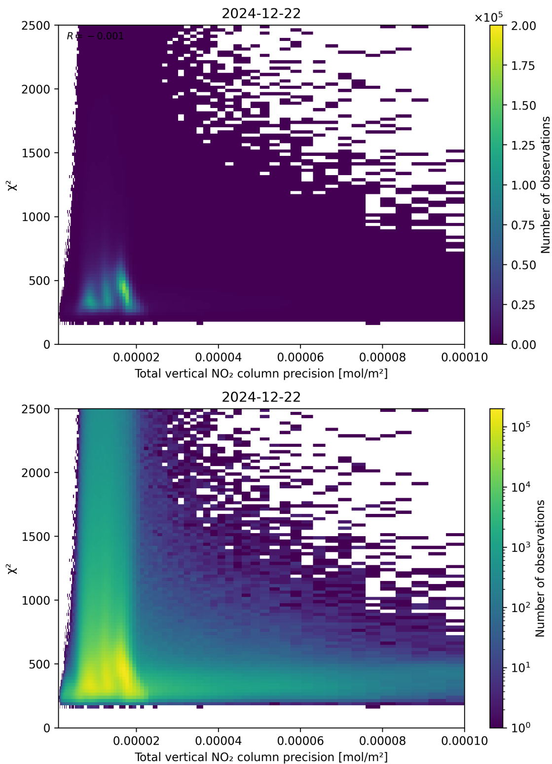
Figure 116: Scatter density plot of “Total vertical NO 2 column precision” against “ \chi^2 ” for 2024-12-22 to 2024-12-23.
