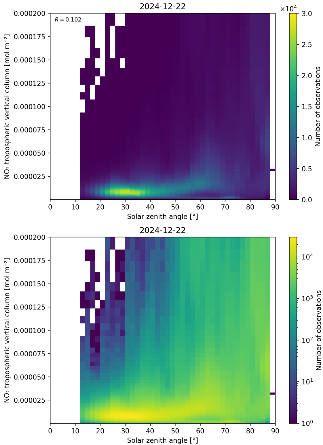
Figure 155: Scatter density plot of “Solar zenith angle” against “NO 2 tropospheric vertical column” for 2024-12-22 to 2024-12-23.
