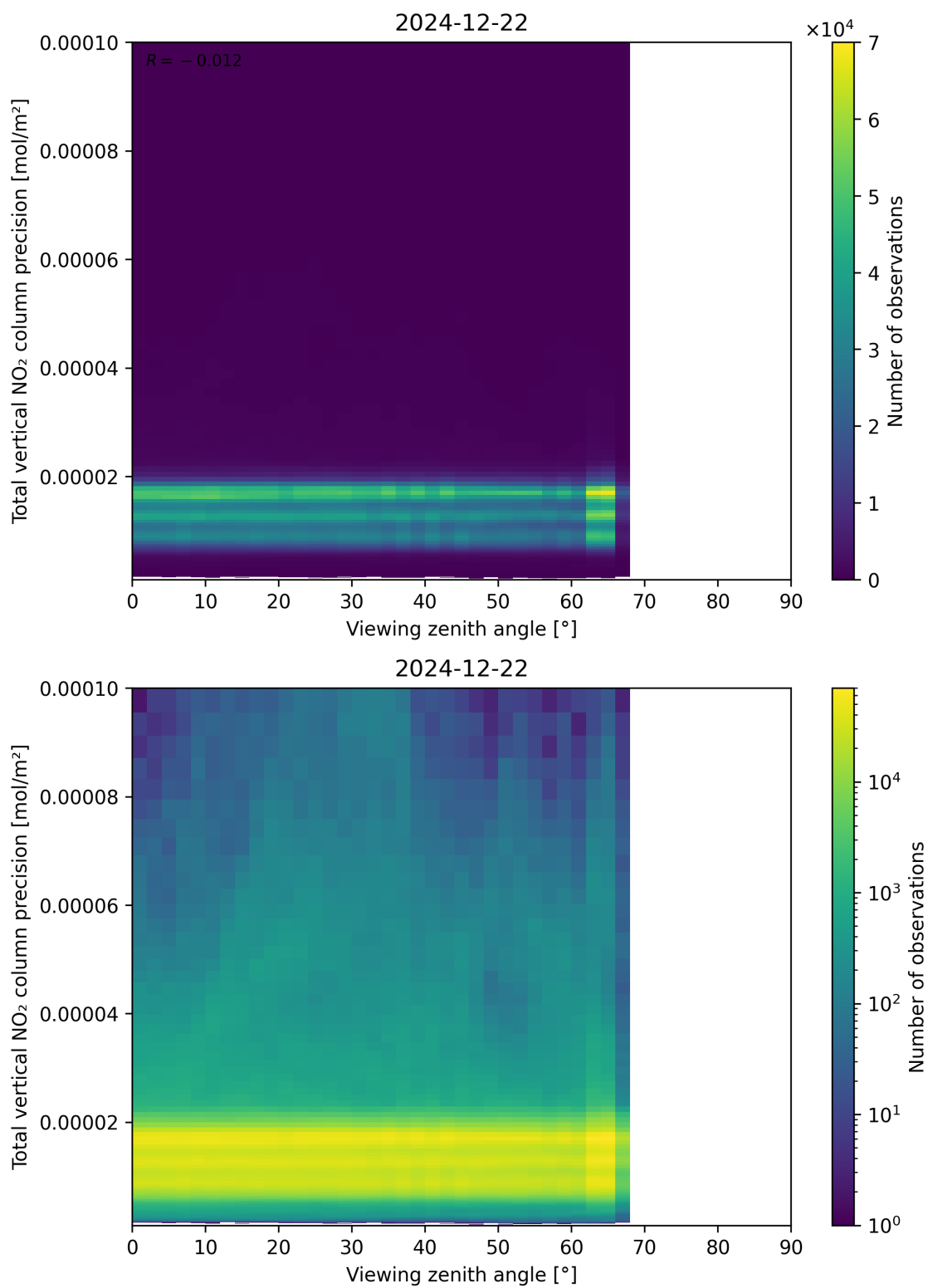
Figure 168: Scatter density plot of “Viewing zenith angle” against “Total vertical NO 2 column precision” for 2024-12-22 to 2024-12-23.
