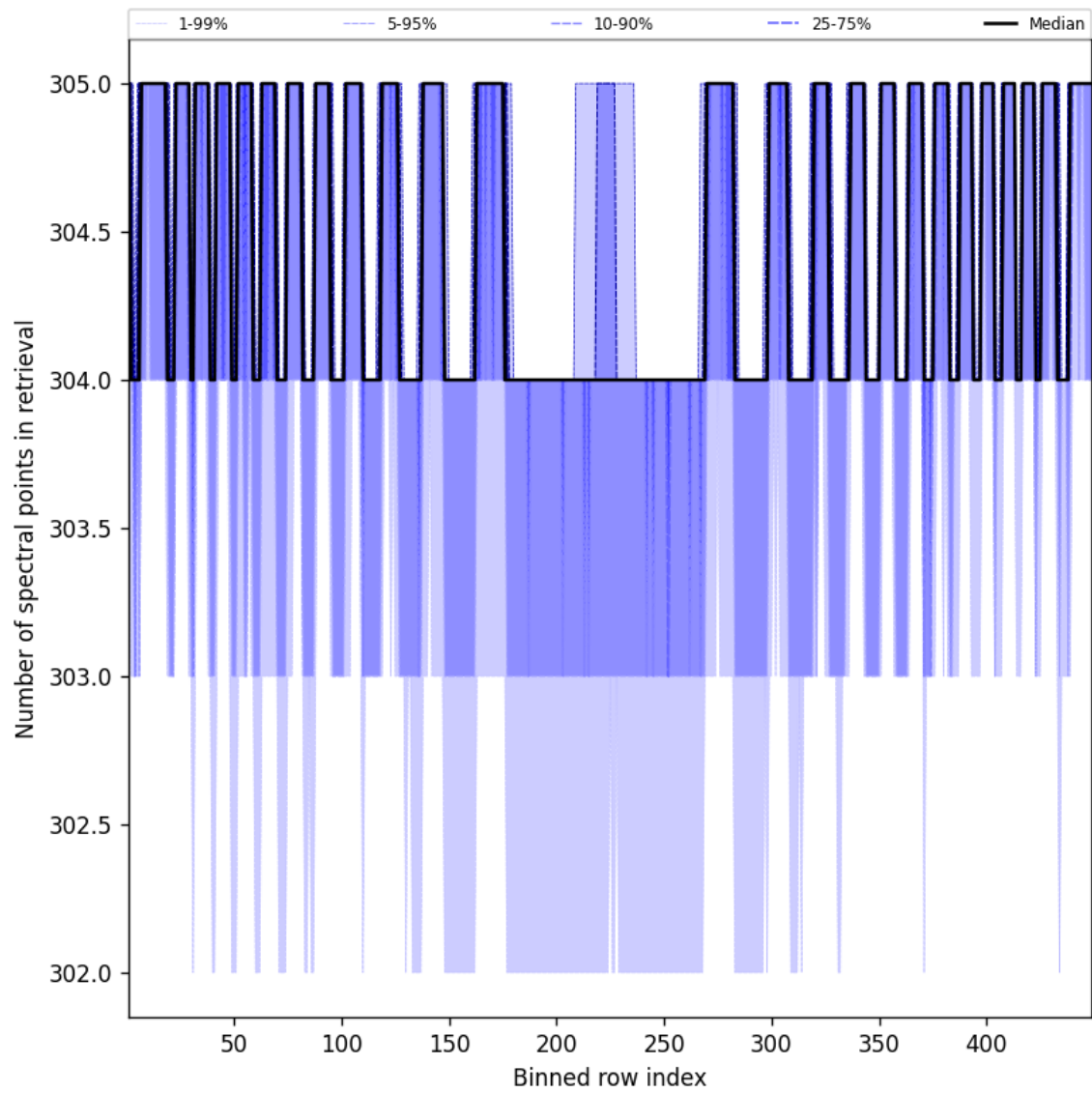
Figure 50: Along track statistics of “Number of spectral points in retrieval” for 2024-12-22 to 2024-12-23
