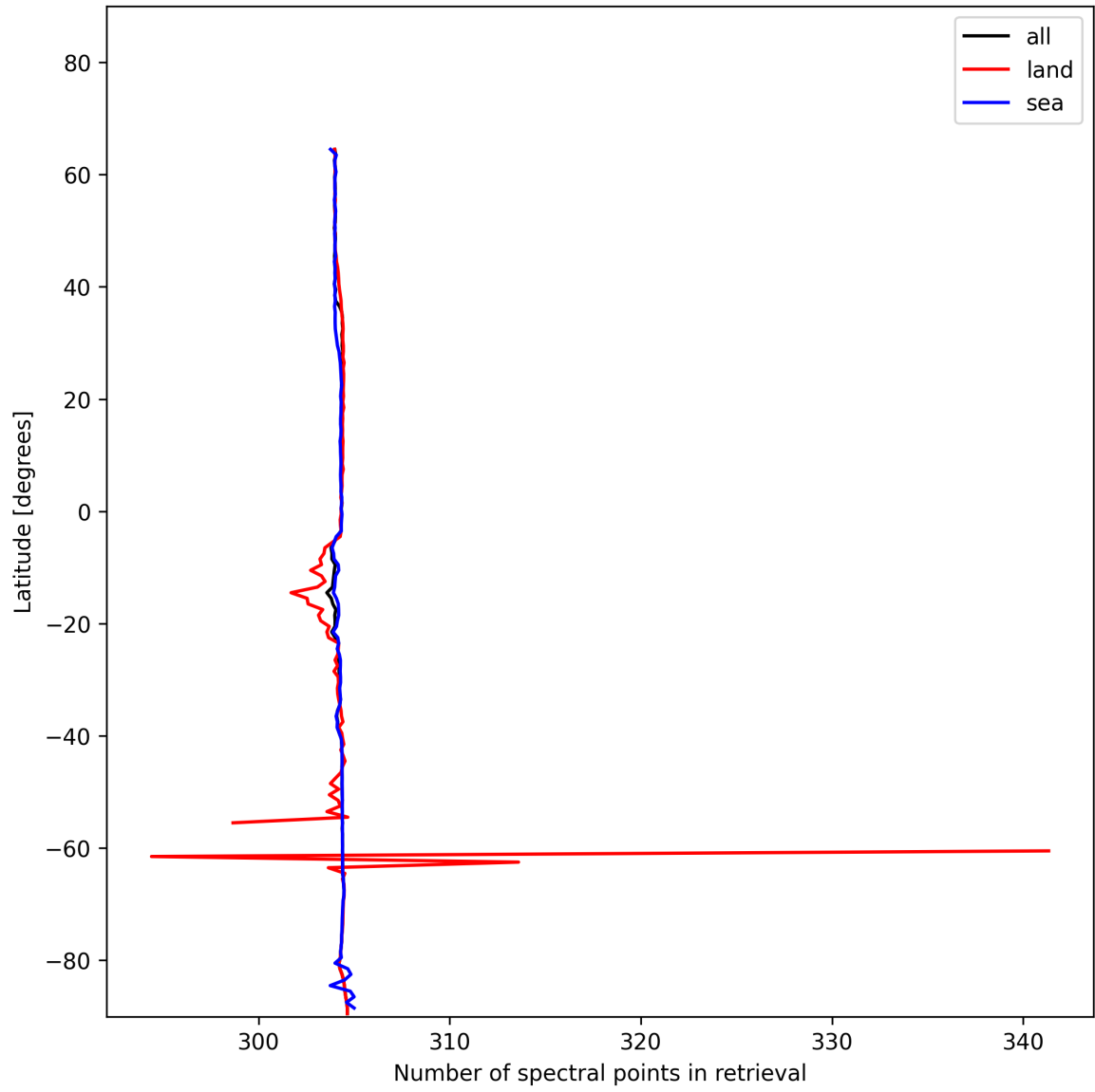
Figure 16: Zonal average of “Number of spectral points in retrieval” for 2024-12-22 to 2024-12-23.
