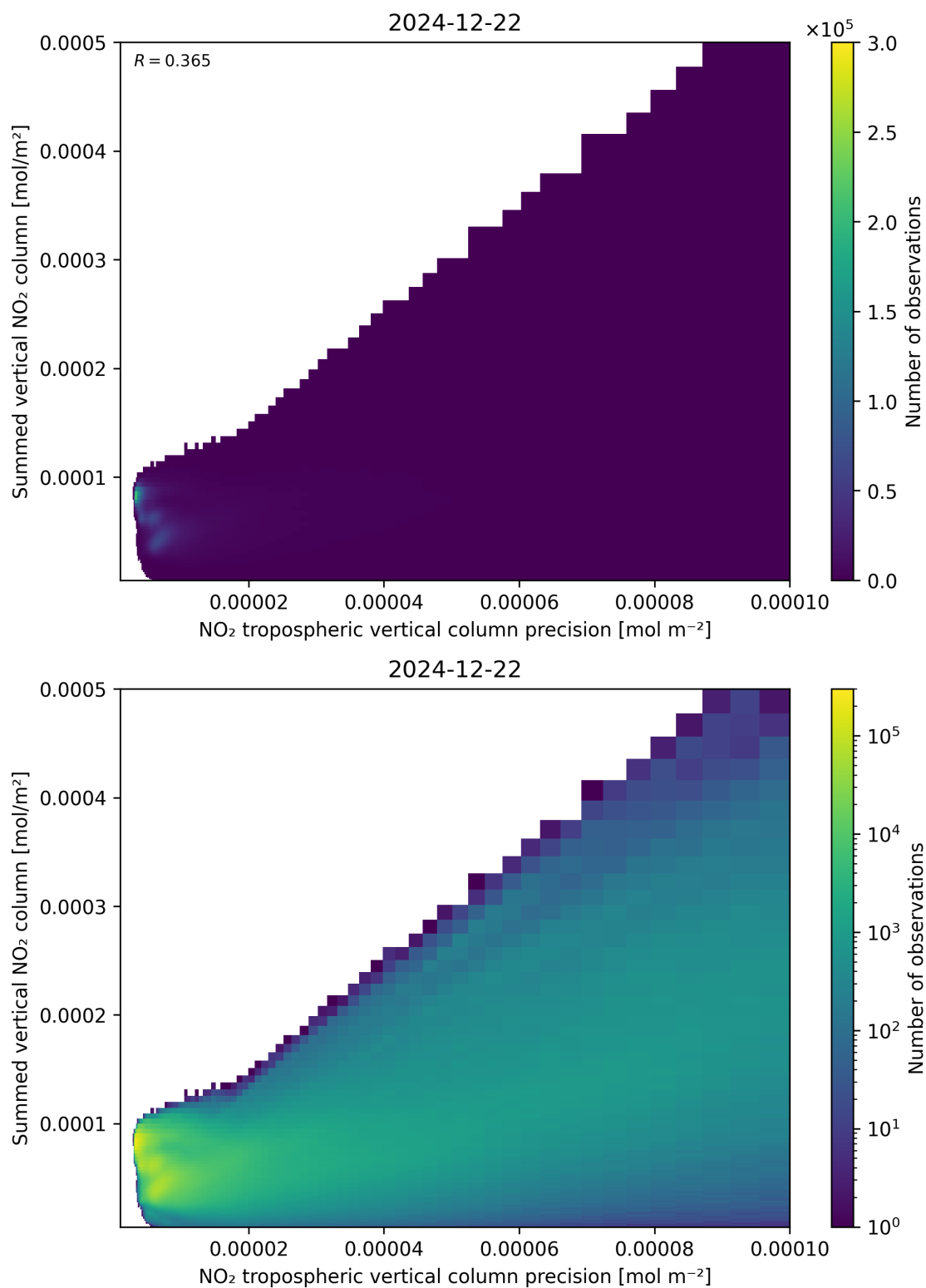
Figure 136: Scatter density plot of “NO 2 tropospheric vertical column precision” against “Summed vertical NO 2 column” for 2024-12-22 to 2024-12-23.
