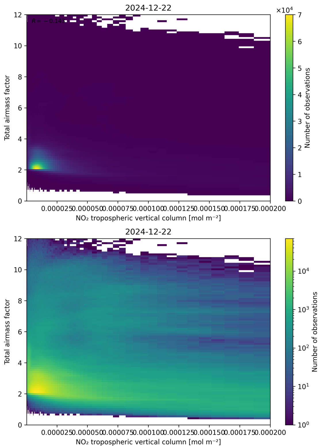
Figure 122: Scatter density plot of “NO 2 tropospheric vertical column” against “Total air mass factor” for 2024-12-22 to 2024-12-23.
