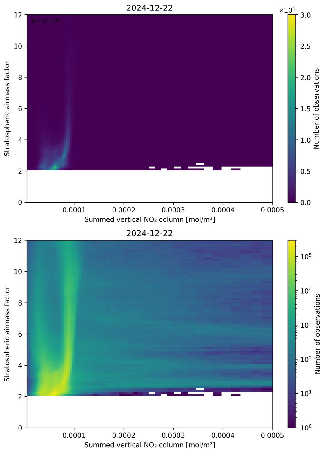
Figure 103: Scatter density plot of “Summed vertical NO 2 column” against “Stratospheric air mass factor” for 2024-12-22 to 2024-12-23.
