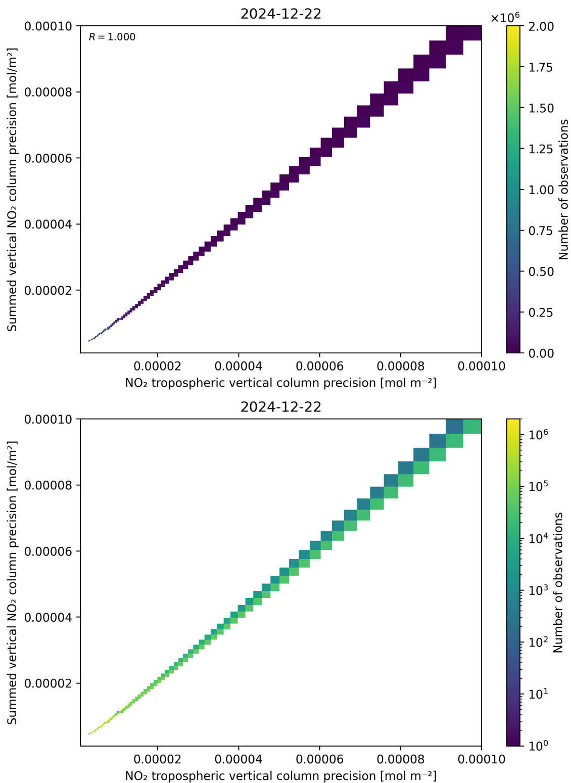
Figure 137: Scatter density plot of “NO 2 tropospheric vertical column precision” against “Summed vertical NO 2 column precision” for 2024-12-22 to 2024-12-23.
