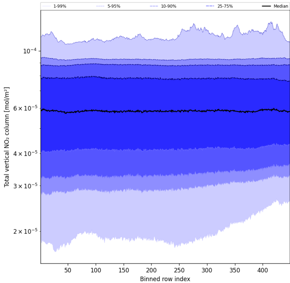
Figure 55: Along track statistics of “Total vertical NO 2 column” for 2024-12-22 to 2024-12-23
