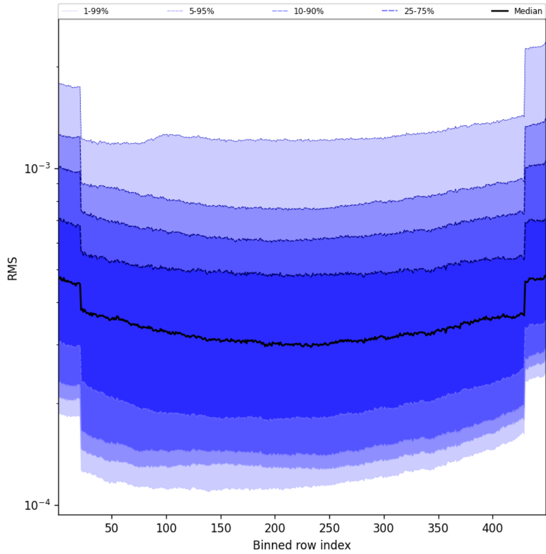
Figure 60: Along track statistics of “RMS” for 2024-12-22 to 2024-12-23
