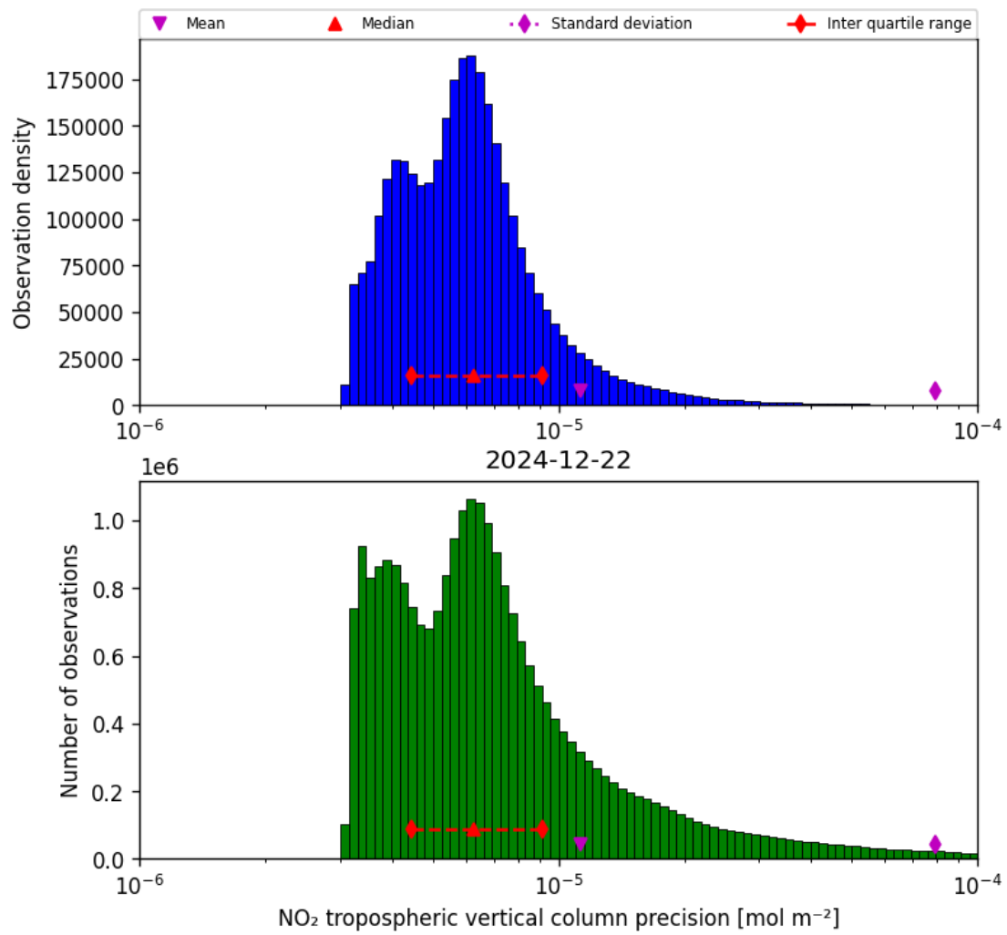
Figure 30: Histogram of “NO 2 tropospheric vertical column precision” for 2024-12-22 to 2024-12-23
