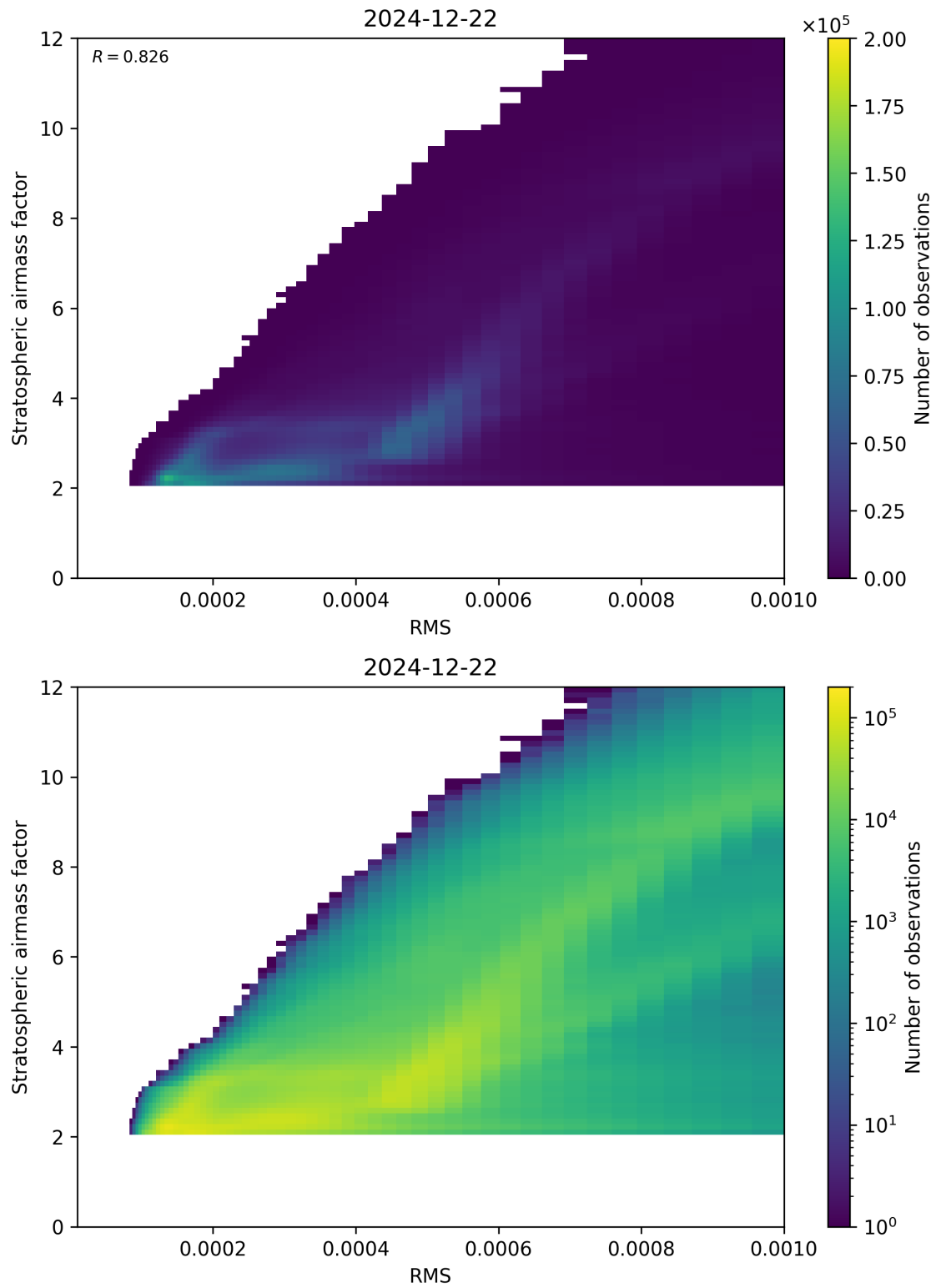
Figure 144: Scatter density plot of “RMS” against “Stratospheric airmass factor” for 2024-12-22 to 2024-12-23.
