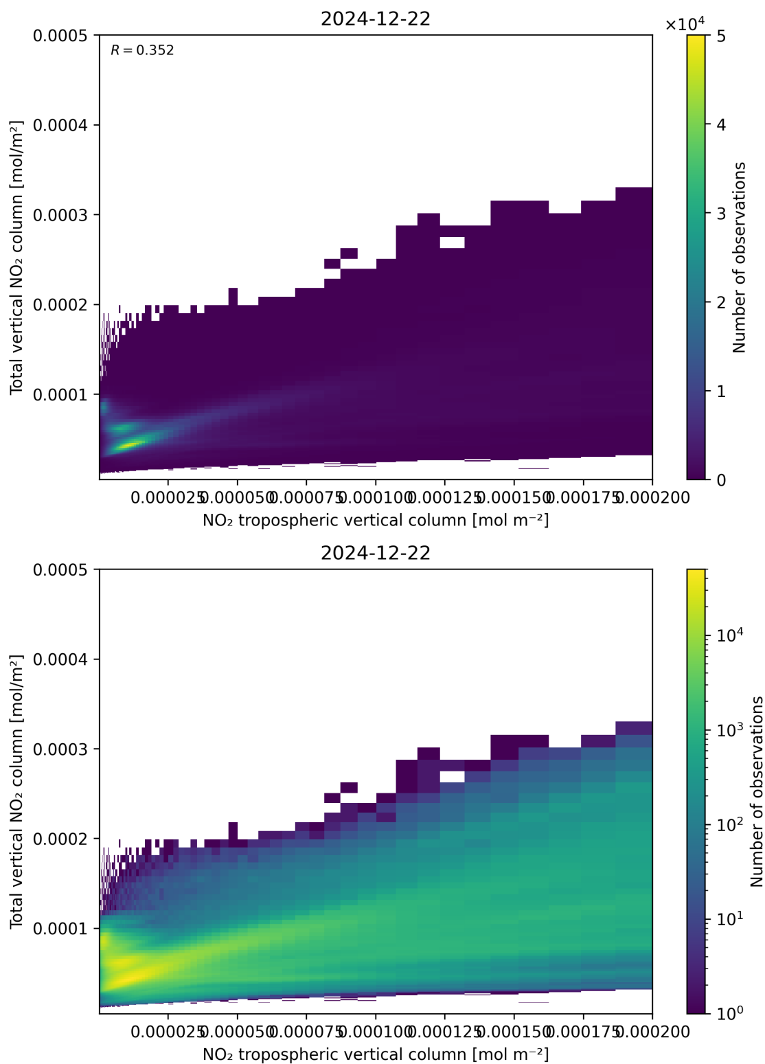
Figure 128: Scatter density plot of “NO 2 tropospheric vertical column” against “Total vertical NO 2 column” for 2024-12-22 to 2024-12-23.
