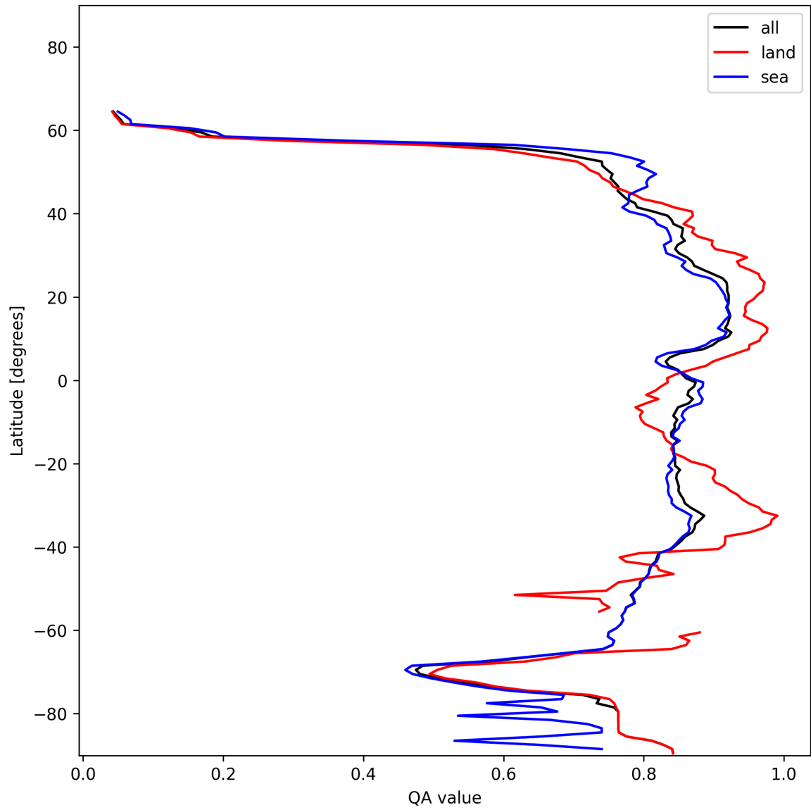
Figure 11: Zonal average of “QA value” for 2024-12-22 to 2024-12-23.
