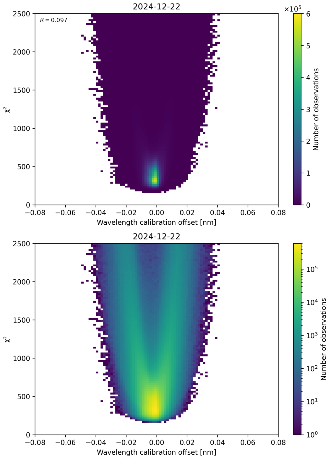
Figure 175: Scatter density plot of “Wavelength calibration offset” against “ \chi^2 ” for 2024-12-22 to 2024-12-23.
