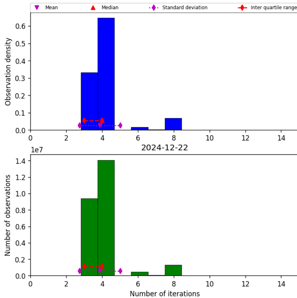
Figure 34: Histogram of “Number of iterations” for 2024-12-22 to 2024-12-23
