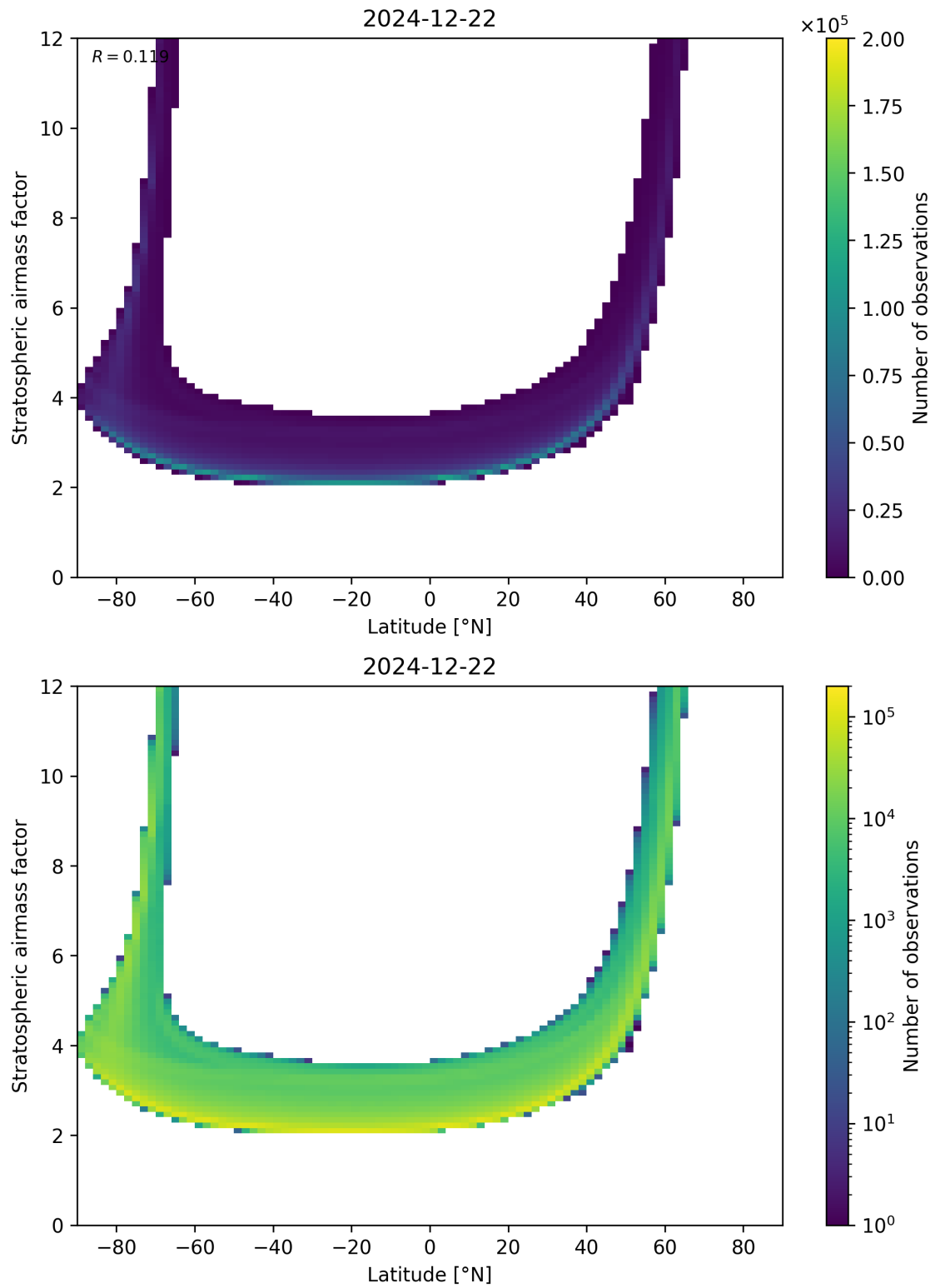
Figure 83: Scatter density plot of “Latitude” against “Stratospheric air mass factor” for 2024-12-22 to 2024-12-23.
