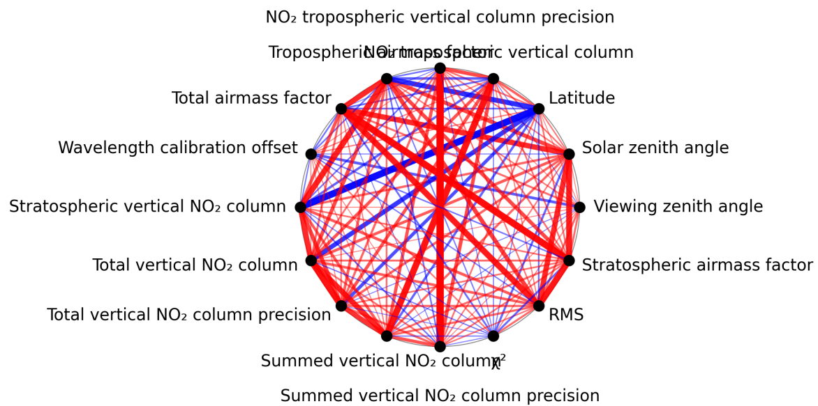
Figure 1: Map of correlation graph for 2024-12-22 to 2024-12-23.
