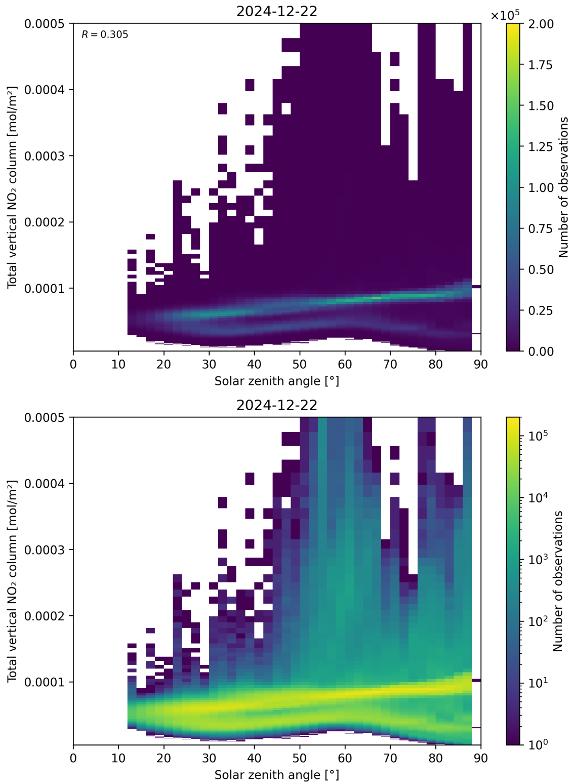
Figure 153: Scatter density plot of “Solar zenith angle” against “Total vertical NO 2 column” for 2024-12-22 to 2024-12-23.
