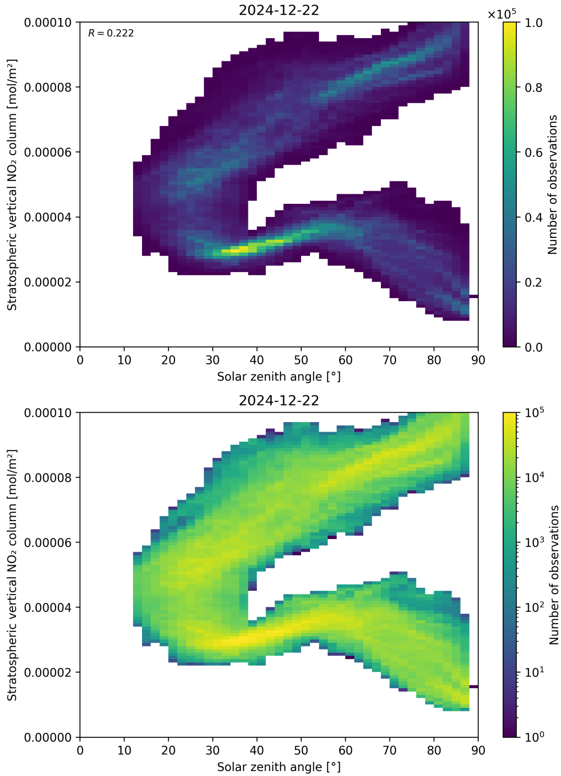
Figure 150: Scatter density plot of “Solar zenith angle” against “Stratospheric vertical NO 2 column” for 2024-12-22 to 2024-12-23.
