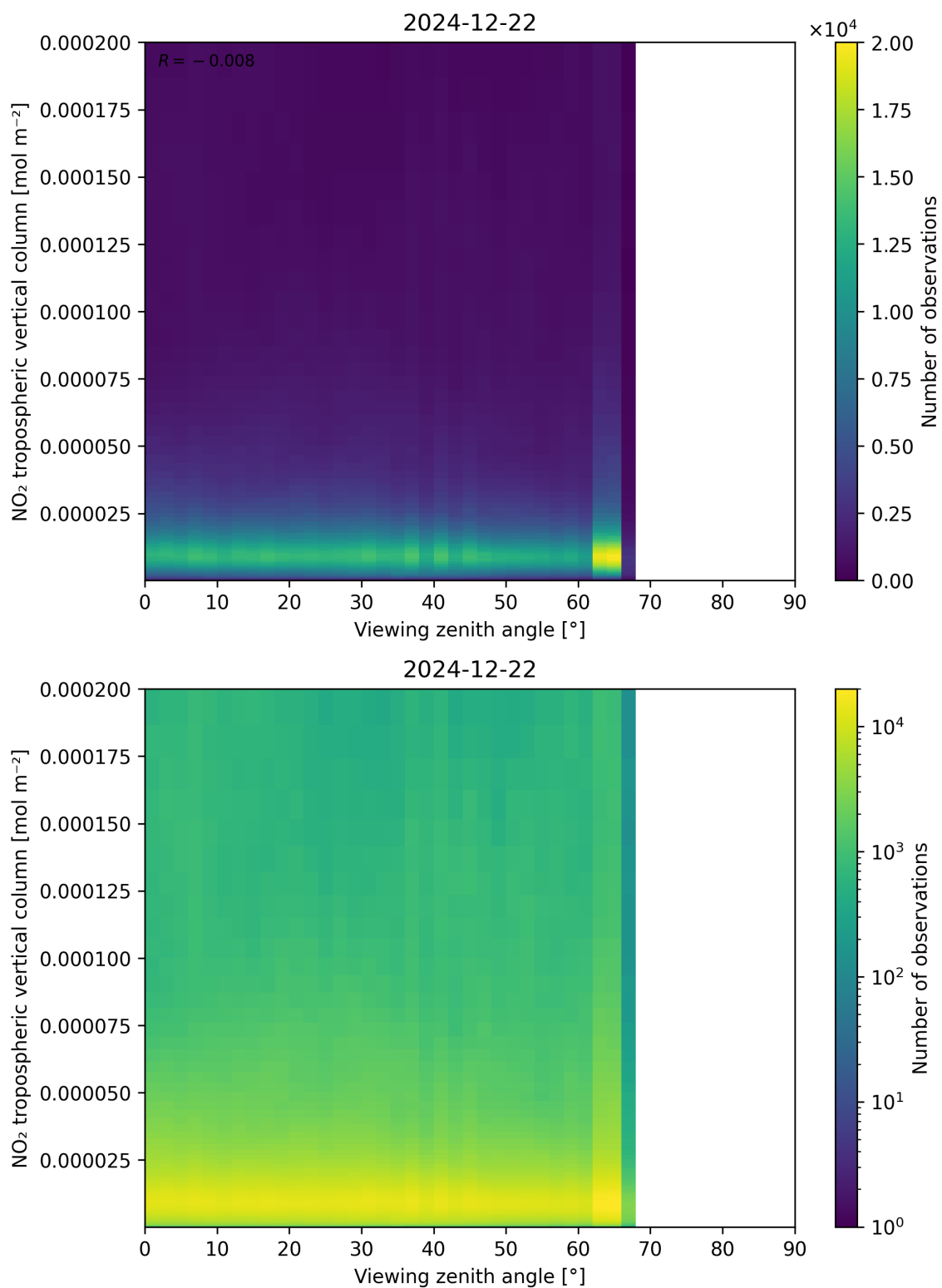
Figure 169: Scatter density plot of “Viewing zenith angle” against “NO 2 tropospheric vertical column” for 2024-12-22 to 2024-12-23.
