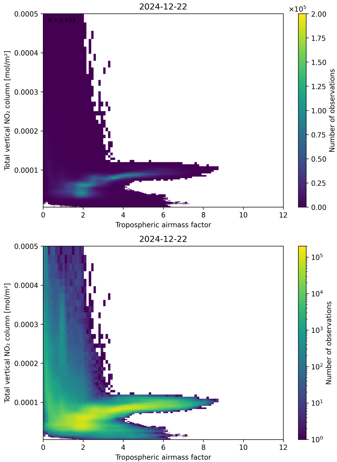
Figure 77: Scatter density plot of “Tropospheric airmass factor” against “Total vertical \text{NO}_2 column” for 2024-12-22 to 2024-12-23.
