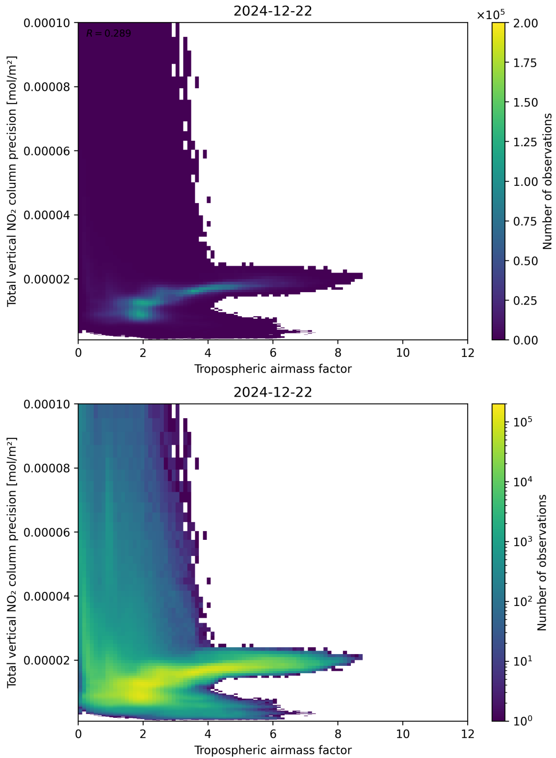
Figure 78: Scatter density plot of “Tropospheric air mass factor” against “Total vertical NO 2 column precision” for 2024-12-22 to 2024-12-23.
