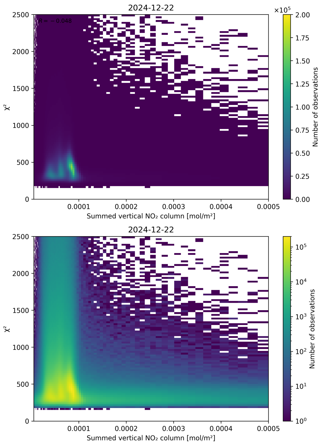
Figure 104: Scatter density plot of “Summed vertical NO 2 column” against “ \chi^2 ” for 2024-12-22 to 2024-12-23.
