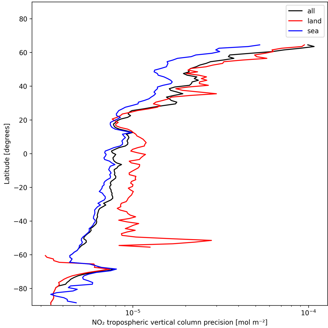
Figure 13: Zonal average of “NO 2 tropospheric vertical column precision” for 2024-12-22 to 2024-12-23.
