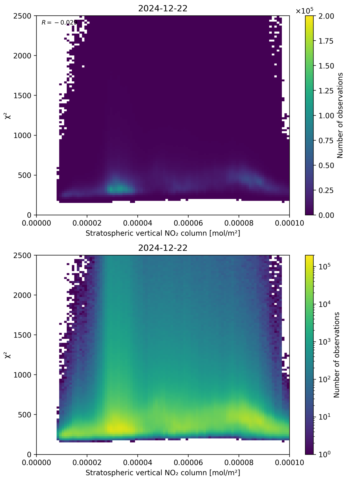
Figure 97: Scatter density plot of “Stratospheric vertical NO 2 column” against “ \chi^2 ” for 2024-12-22 to 2024-12-23.
