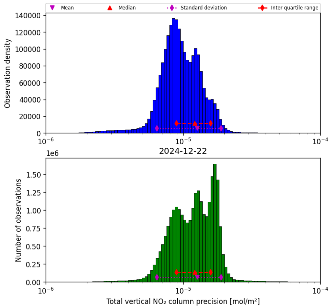
Figure 39: Histogram of “Total vertical NO 2 column precision” for 2024-12-22 to 2024-12-23
