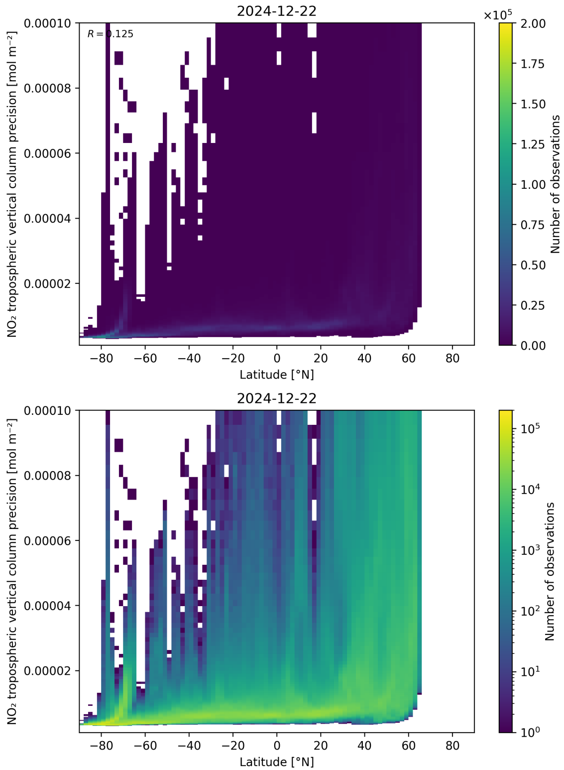
Figure 93: Scatter density plot of “Latitude” against “NO 2 tropospheric vertical column precision” for 2024-12-22 to 2024-12-23.
