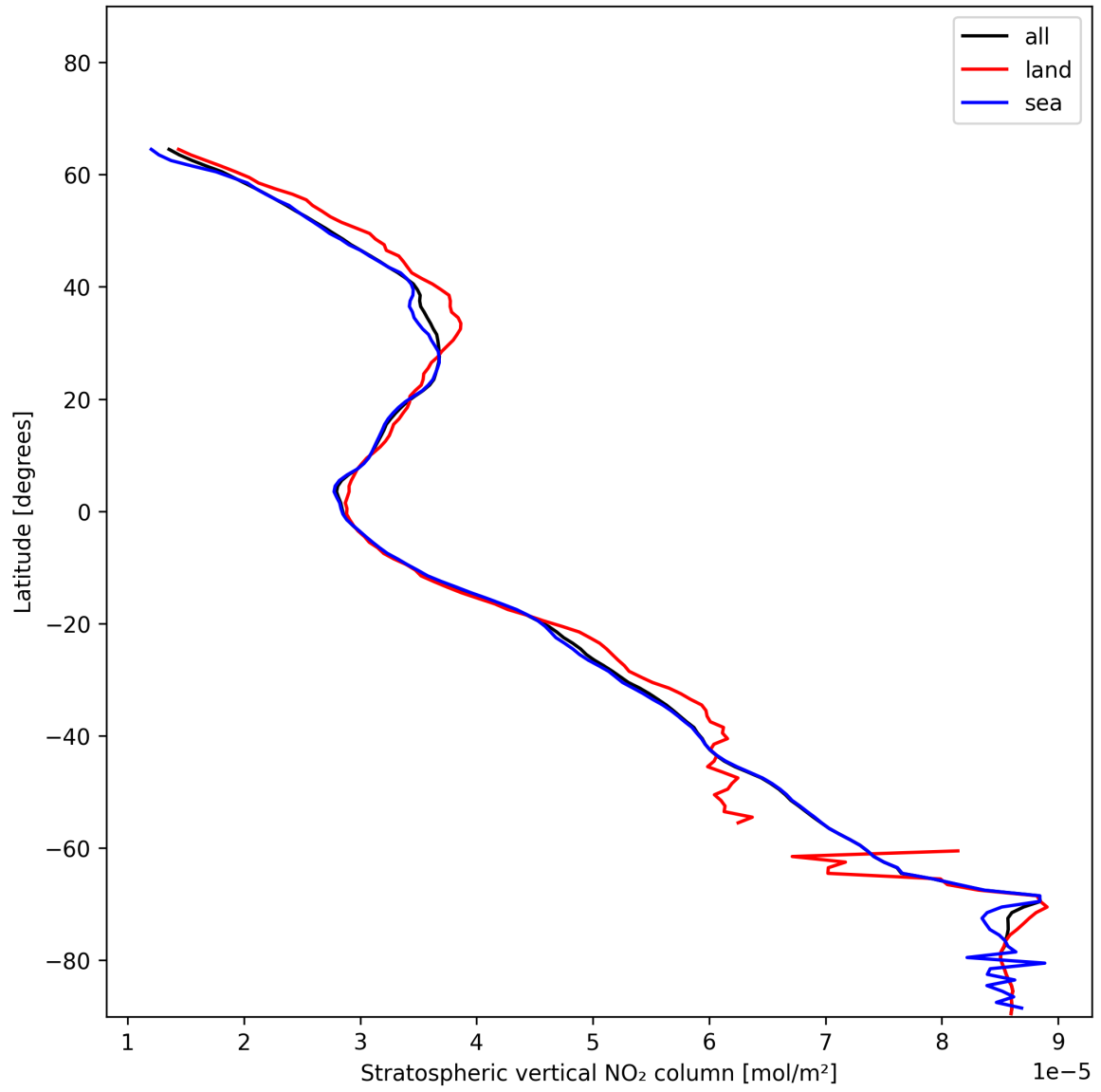
Figure 19: Zonal average of “Stratospheric vertical NO 2 column” for 2024-12-22 to 2024-12-23.
