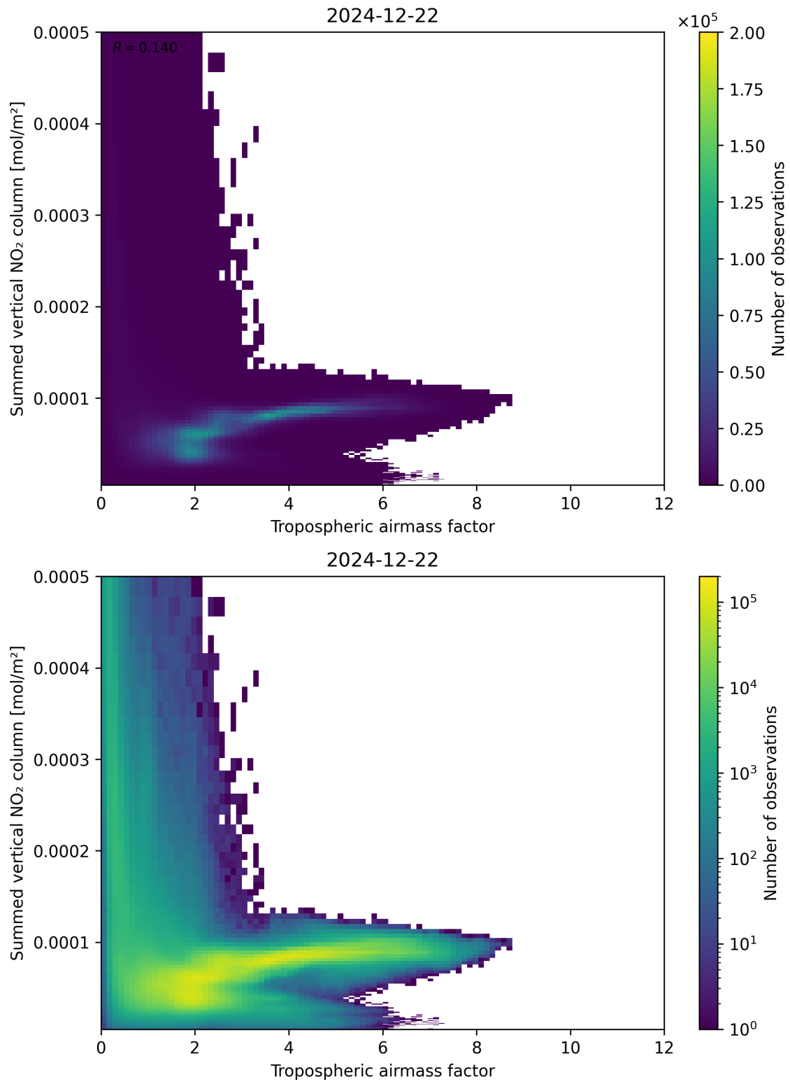
Figure 75: Scatter density plot of “Tropospheric airmass factor” against “Summed vertical NO 2 column” for 2024-12-22 to 2024-12-23.
