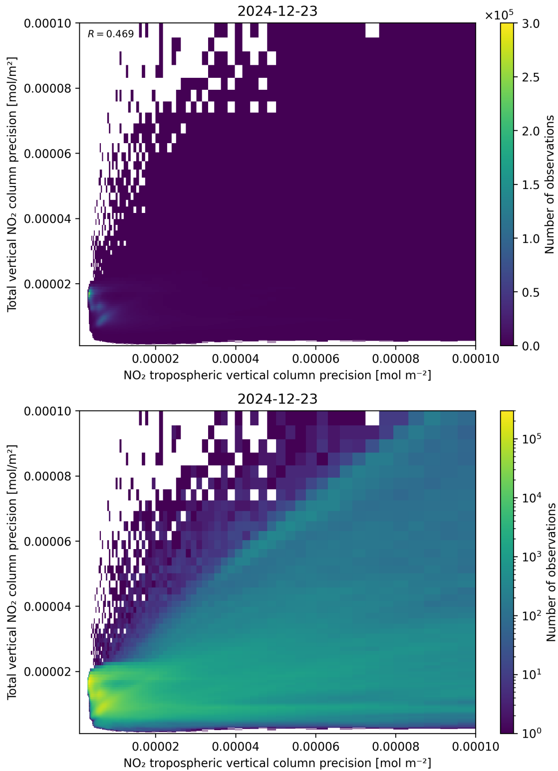
Figure 139: Scatter density plot of “NO 2 tropospheric vertical column precision” against “Total vertical NO 2 column precision” for 2024-12-22 to 2024-12-24.
