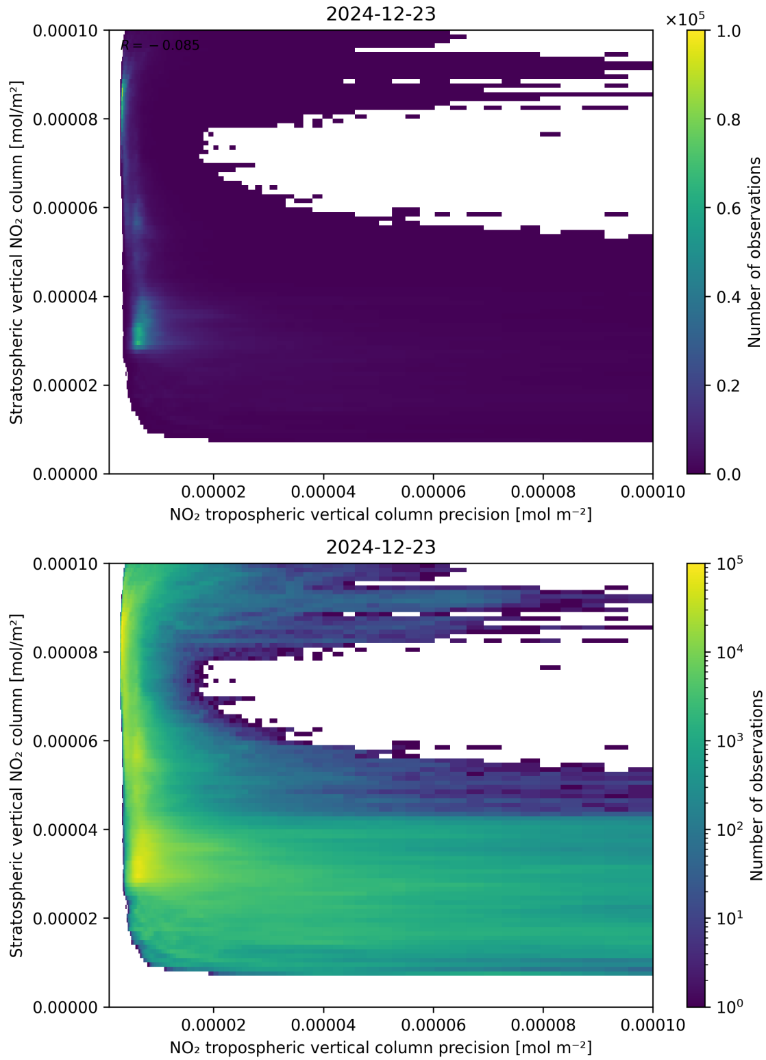
Figure 135: Scatter density plot of “NO 2 tropospheric vertical column precision” against “Stratospheric vertical NO 2 column” for 2024-12-22 to 2024-12-24.
