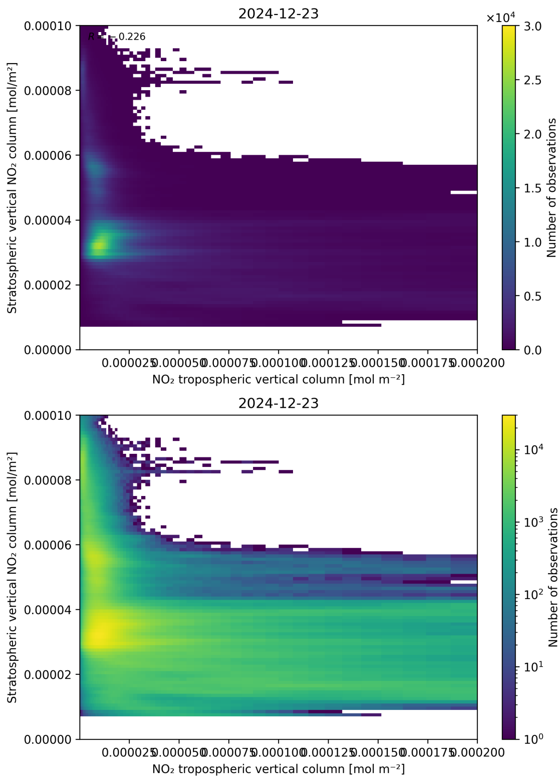
Figure 125: Scatter density plot of “NO 2 tropospheric vertical column” against “Stratospheric vertical NO 2 column” for 2024-12-22 to 2024-12-24.
