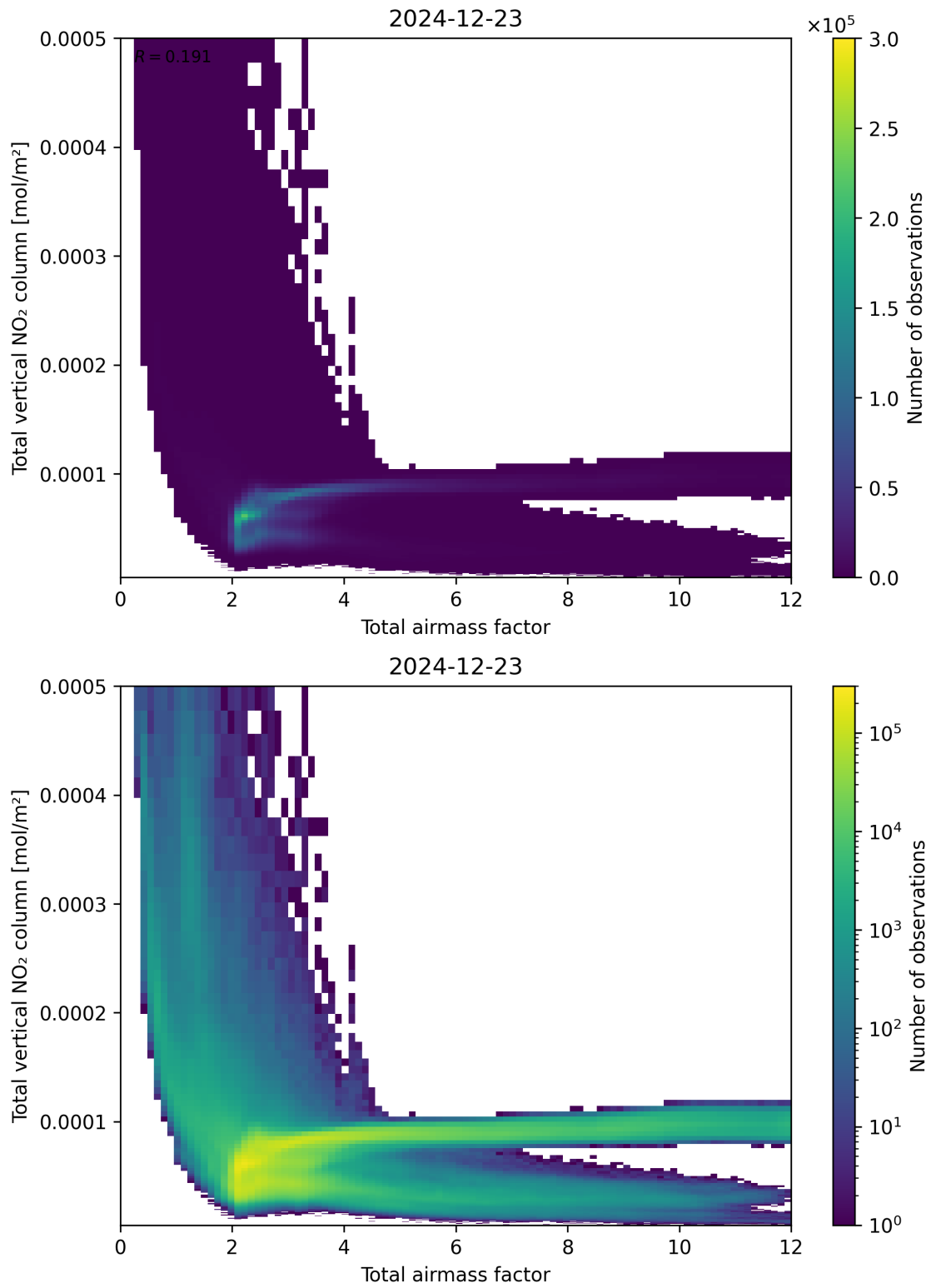
Figure 67: Scatter density plot of “Total airmass factor” against “Total vertical NO 2 column” for 2024-12-22 to 2024-12-24.
