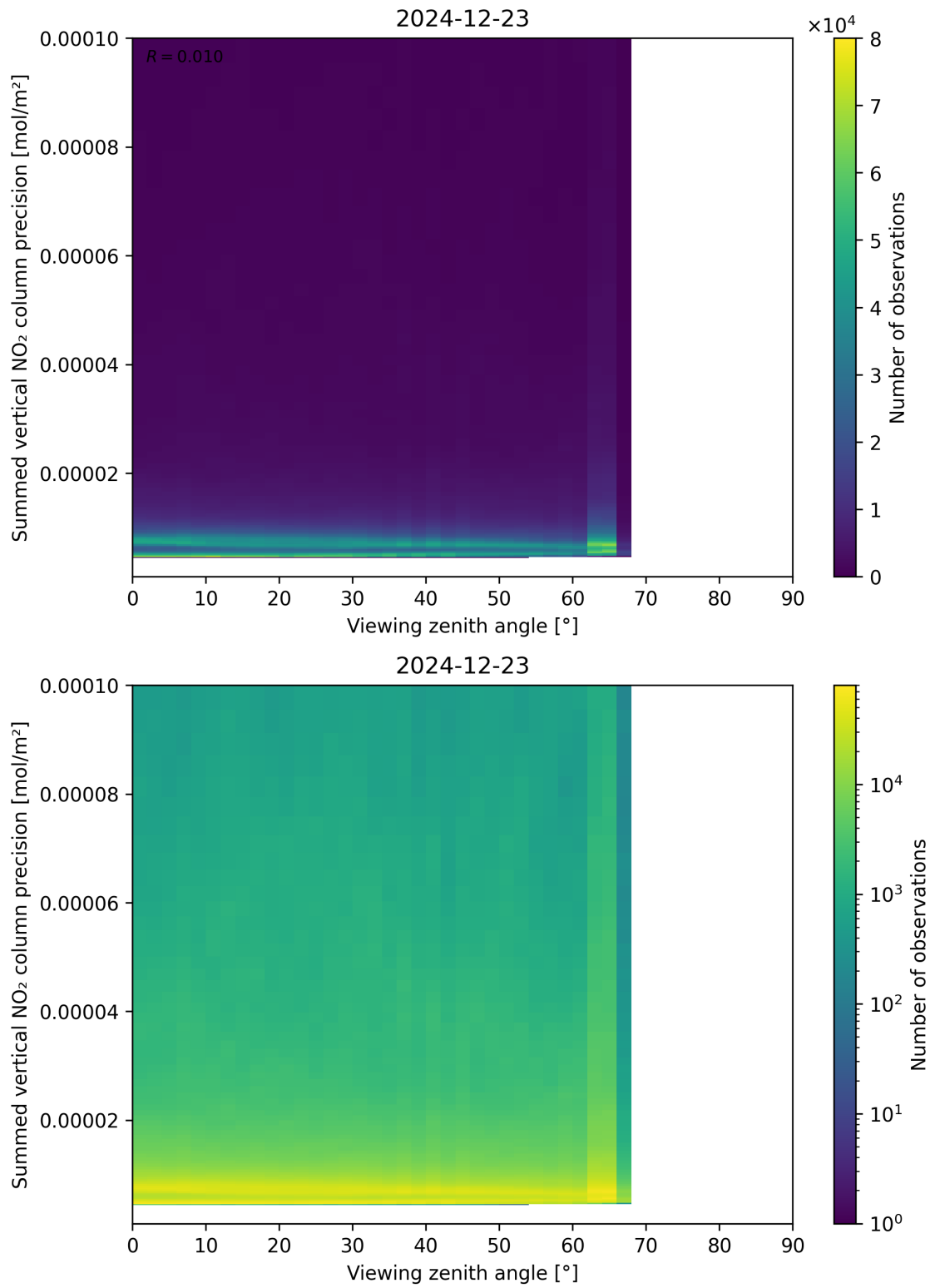
Figure 166: Scatter density plot of “Viewing zenith angle” against “Summed vertical NO 2 column precision” for 2024-12-22 to 2024-12-24.
