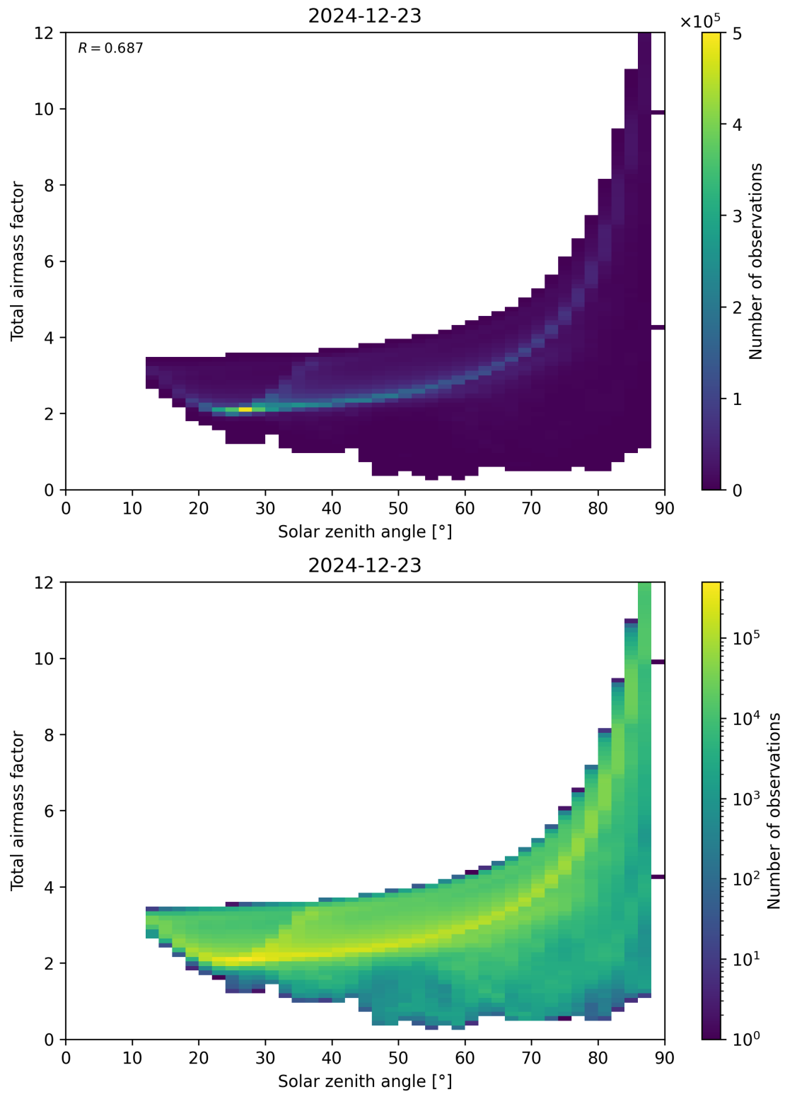
Figure 146: Scatter density plot of “Solar zenith angle” against “Total air mass factor” for 2024-12-22 to 2024-12-24.
