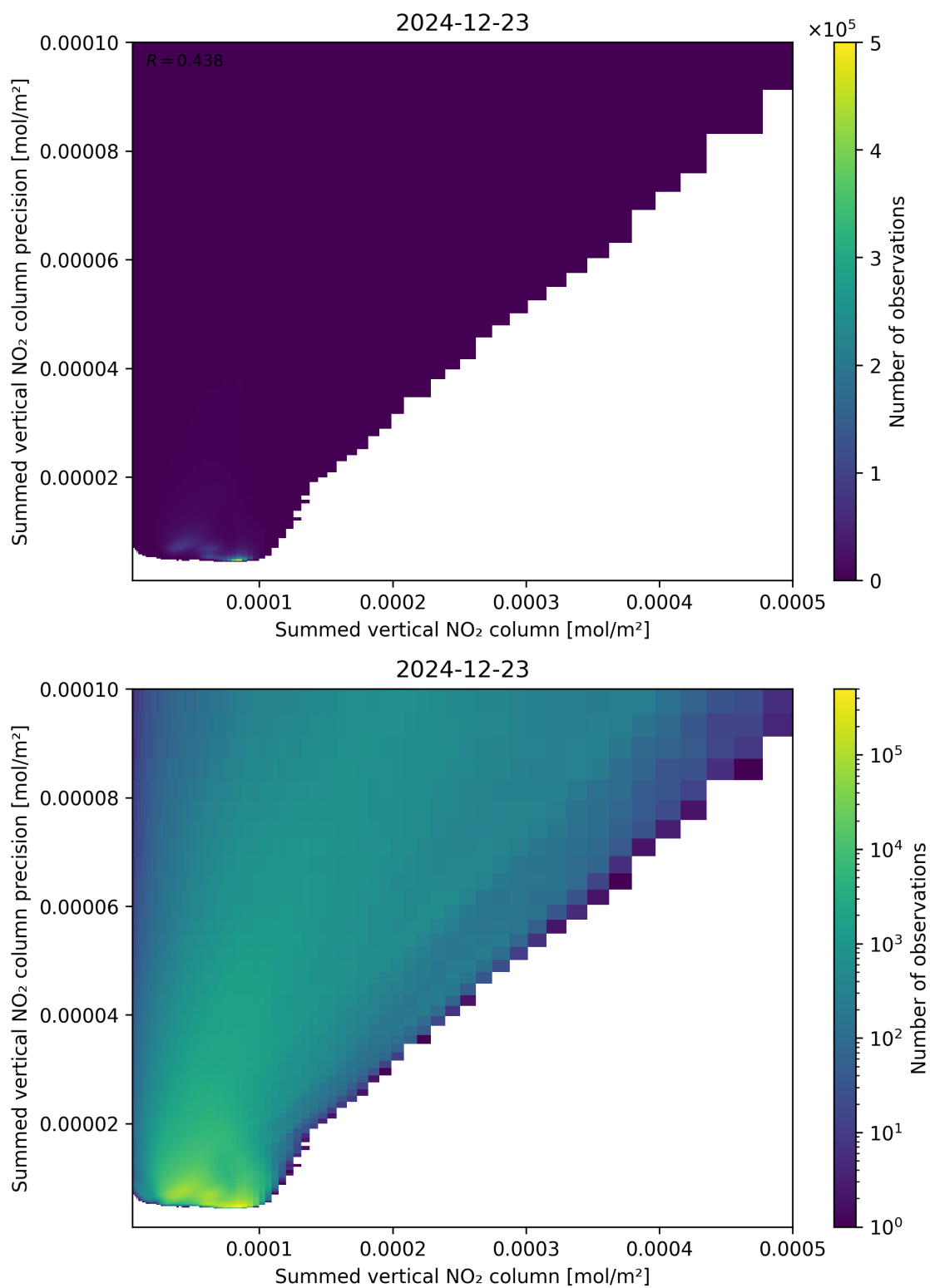
Figure 105: Scatter density plot of “Summed vertical NO 2 column” against “Summed vertical NO 2 column precision” for 2024-12-22 to 2024-12-24.
