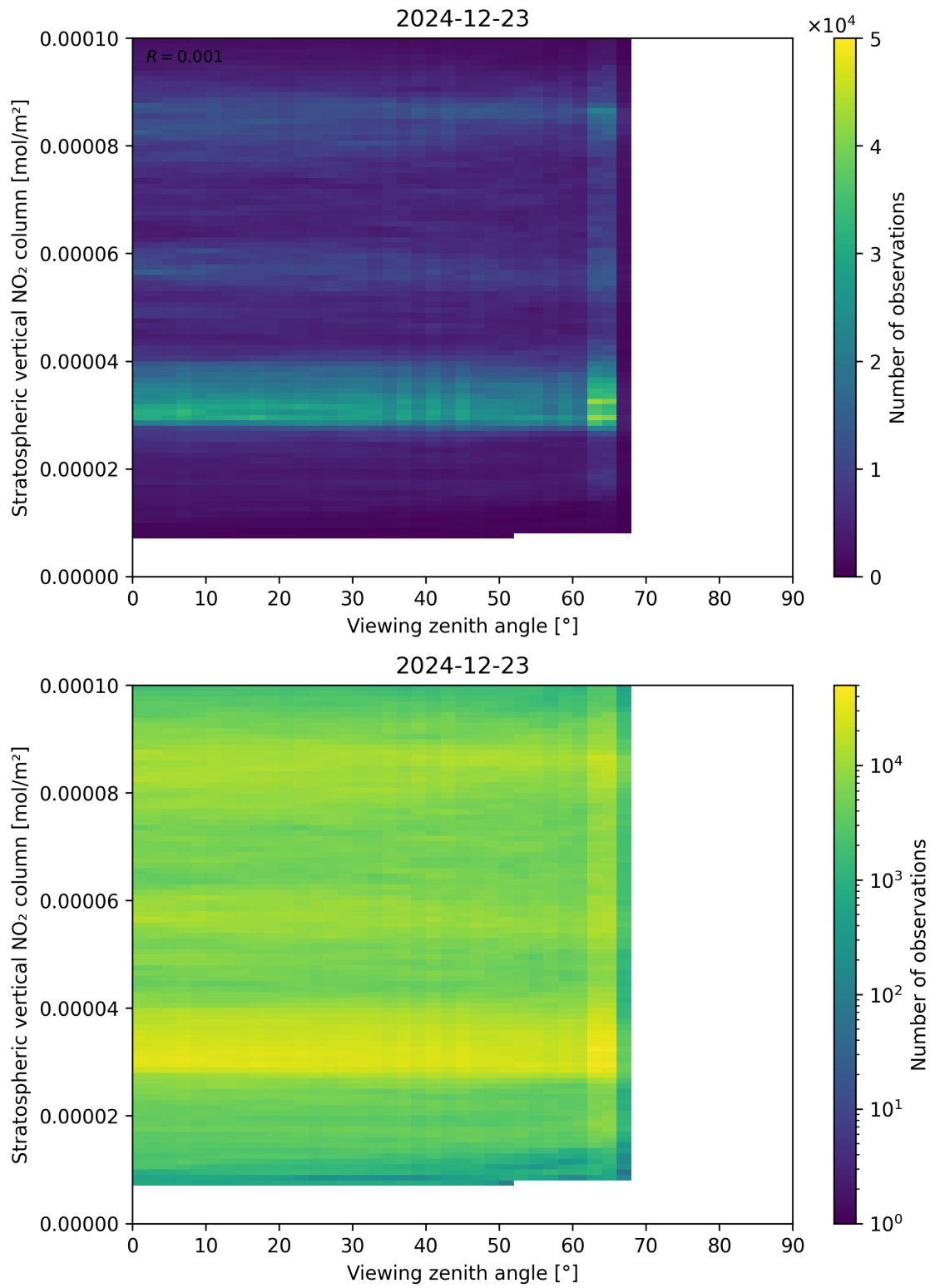
Figure 164: Scatter density plot of “Viewing zenith angle” against “Stratospheric vertical NO 2 column” for 2024-12-22 to 2024-12-24.
