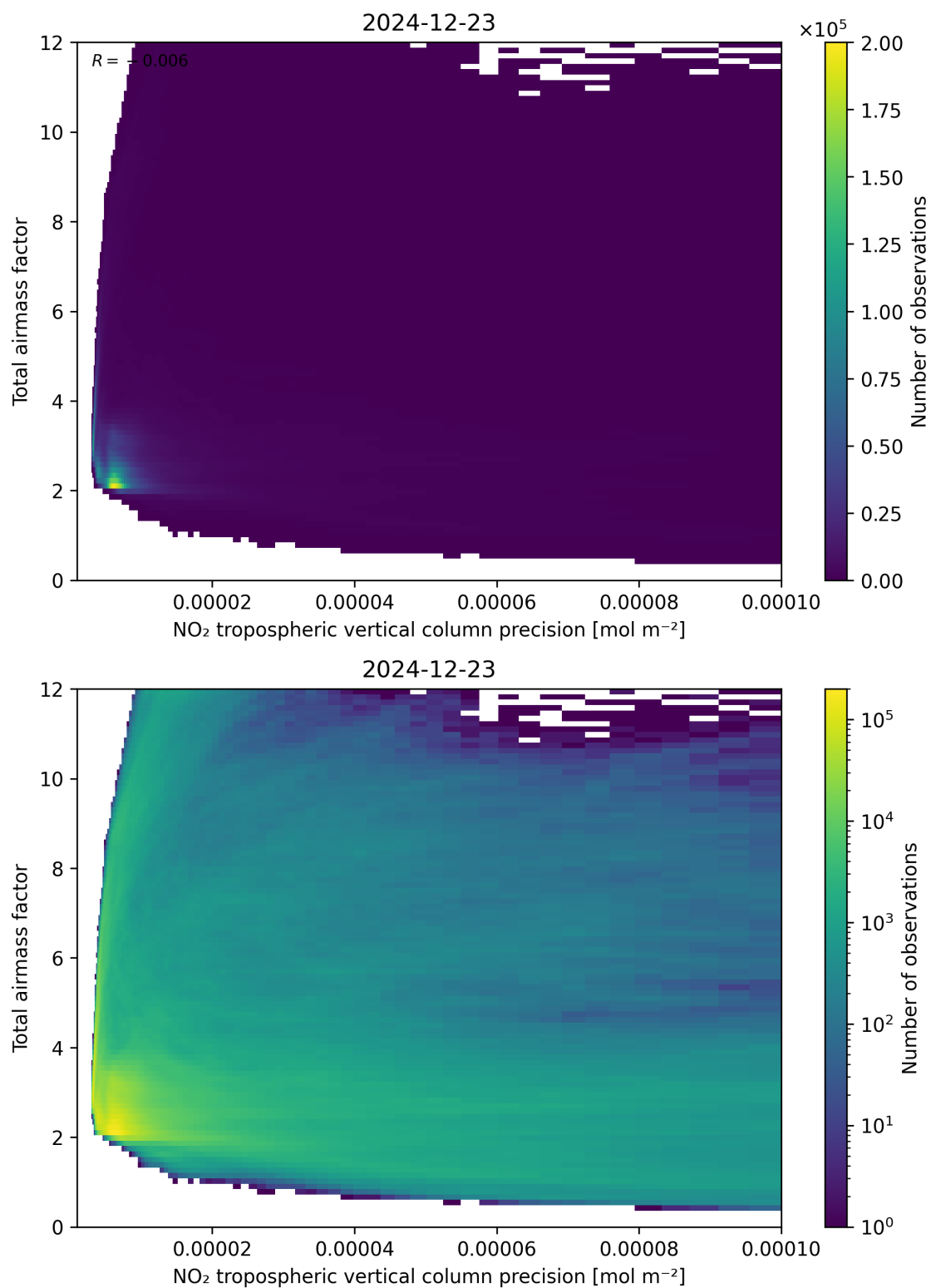
Figure 132: Scatter density plot of “NO 2 tropospheric vertical column precision” against “Total airmass factor” for 2024-12-22 to 2024-12-24.
