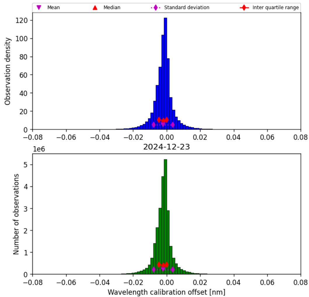
Figure 35: Histogram of “Wavelength calibration offset” for 2024-12-22 to 2024-12-24
