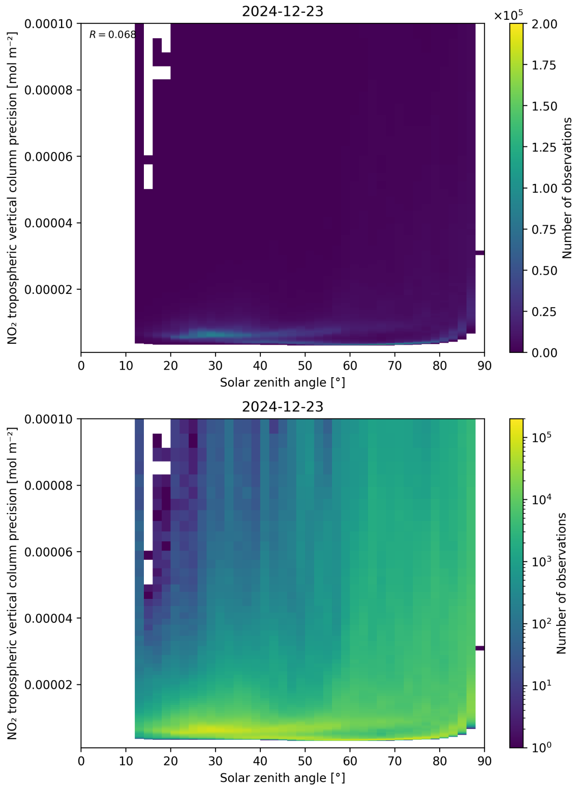
Figure 156: Scatter density plot of “Solar zenith angle” against “NO 2 tropospheric vertical column precision” for 2024-12-22 to 2024-12-24.
