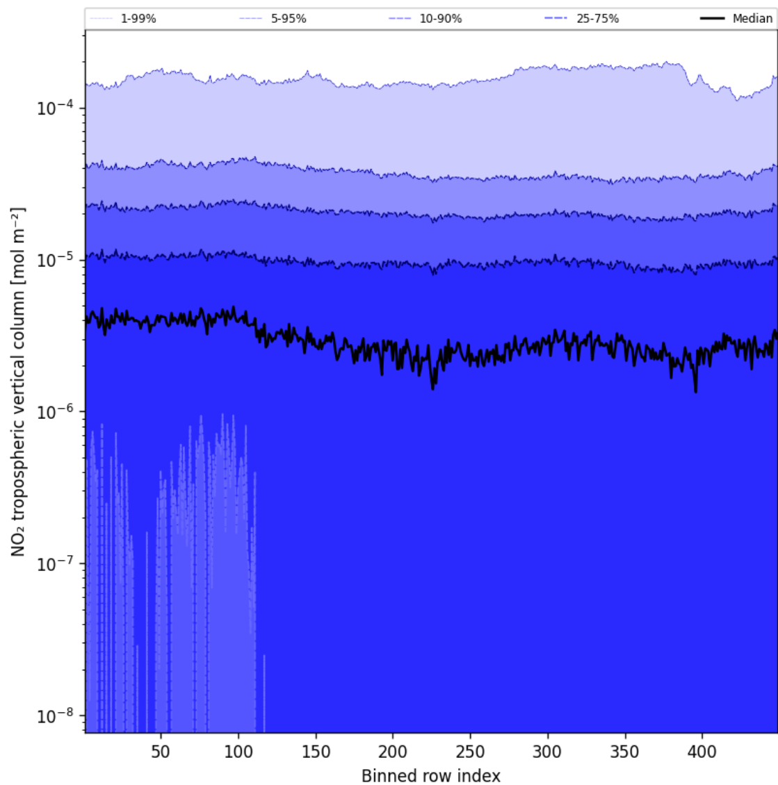
Figure 46: Along track statistics of “NO 2 tropospheric vertical column” for 2024-12-22 to 2024-12-24
