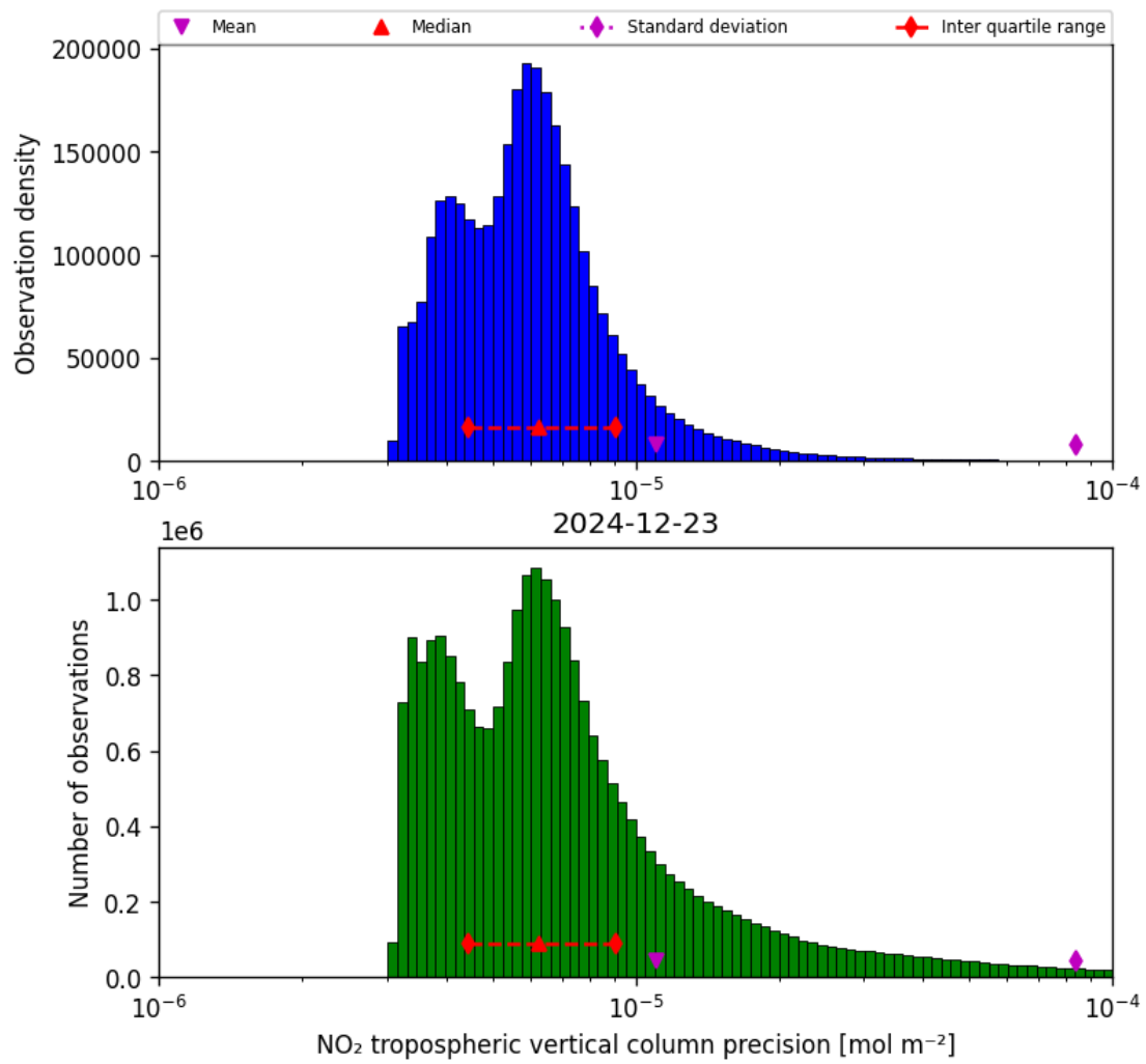
Figure 30: Histogram of “NO 2 tropospheric vertical column precision” for 2024-12-22 to 2024-12-24
