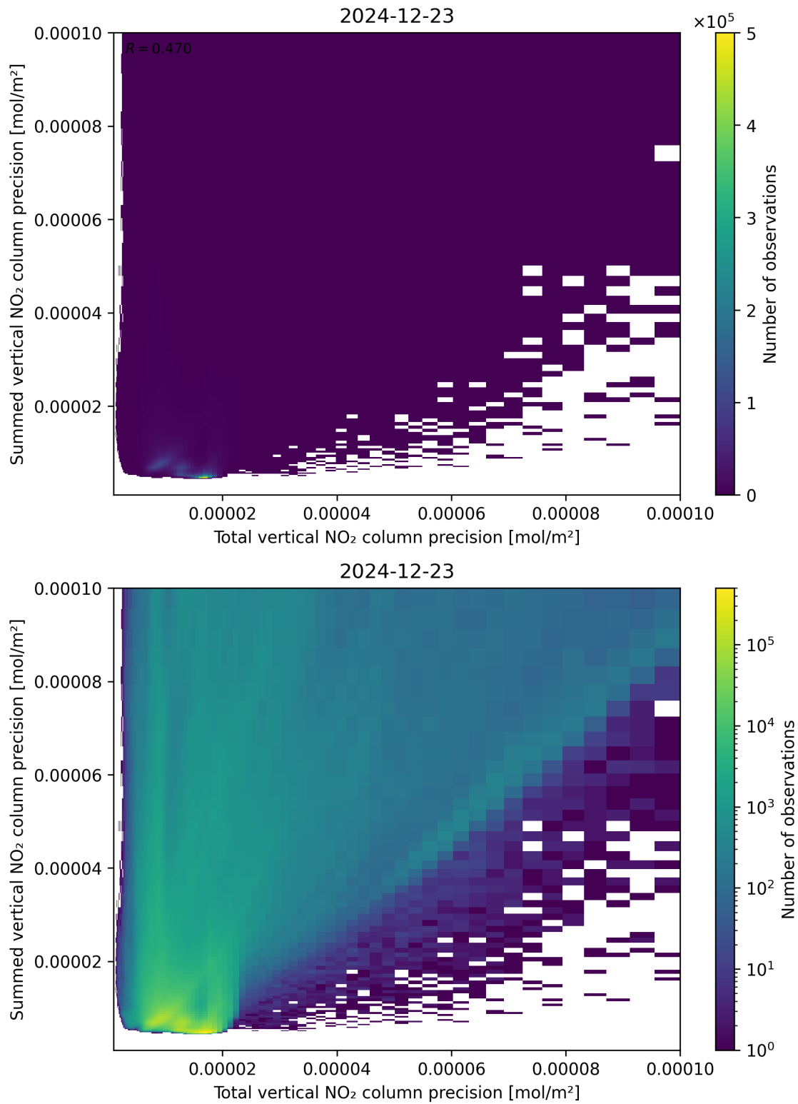
Figure 118: Scatter density plot of “Total vertical NO 2 column precision” against “Summed vertical NO 2 column precision” for 2024-12-22 to 2024-12-24.
