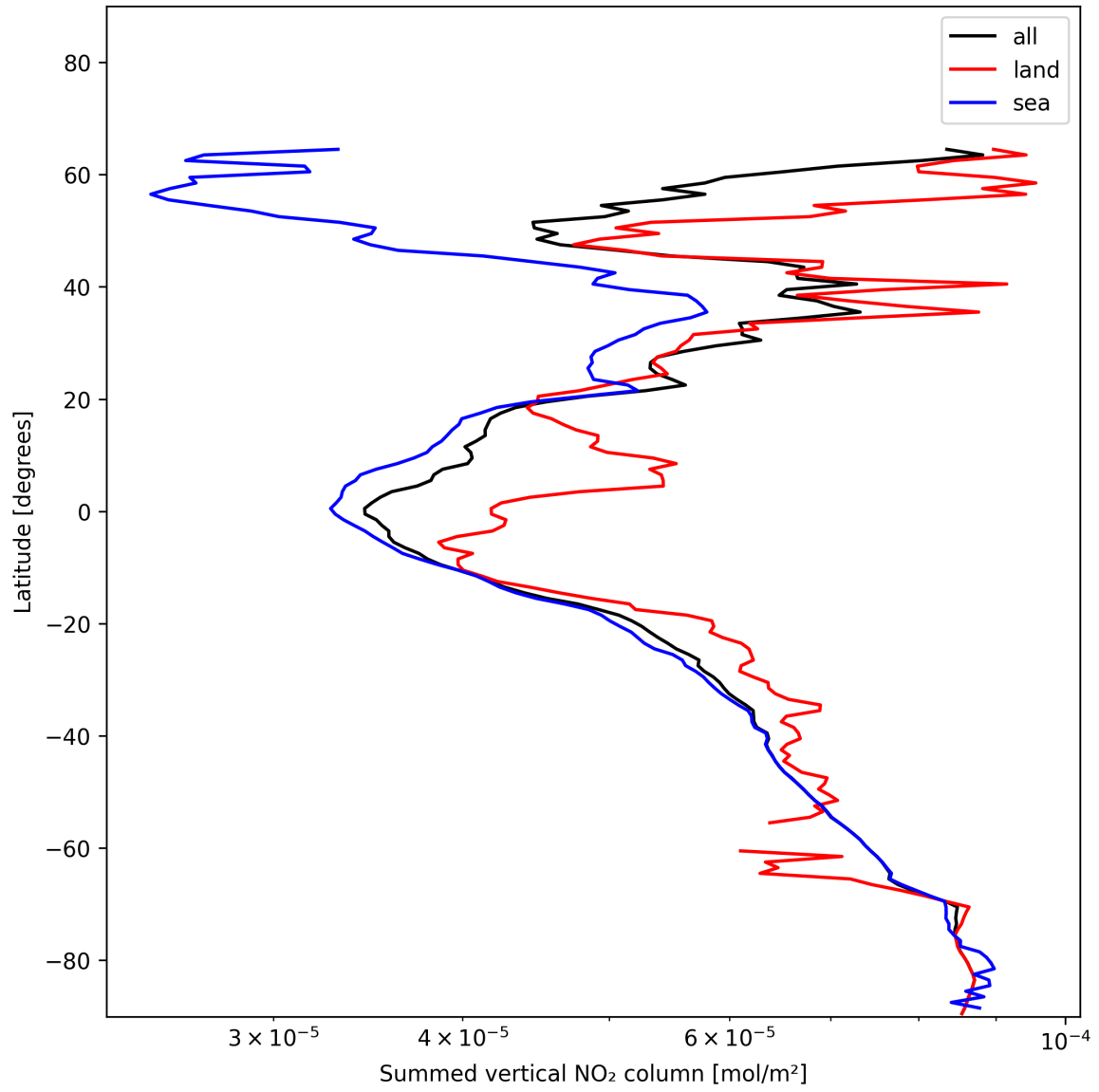
Figure 23: Zonal average of “Summed vertical NO 2 column” for 2024-12-22 to 2024-12-24.
