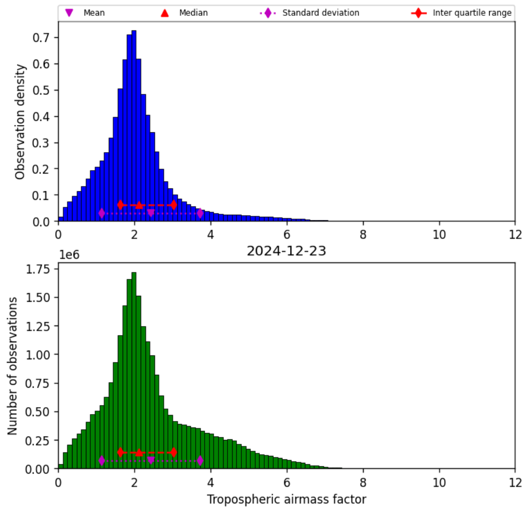
Figure 31: Histogram of “Tropospheric airmass factor” for 2024-12-22 to 2024-12-24
