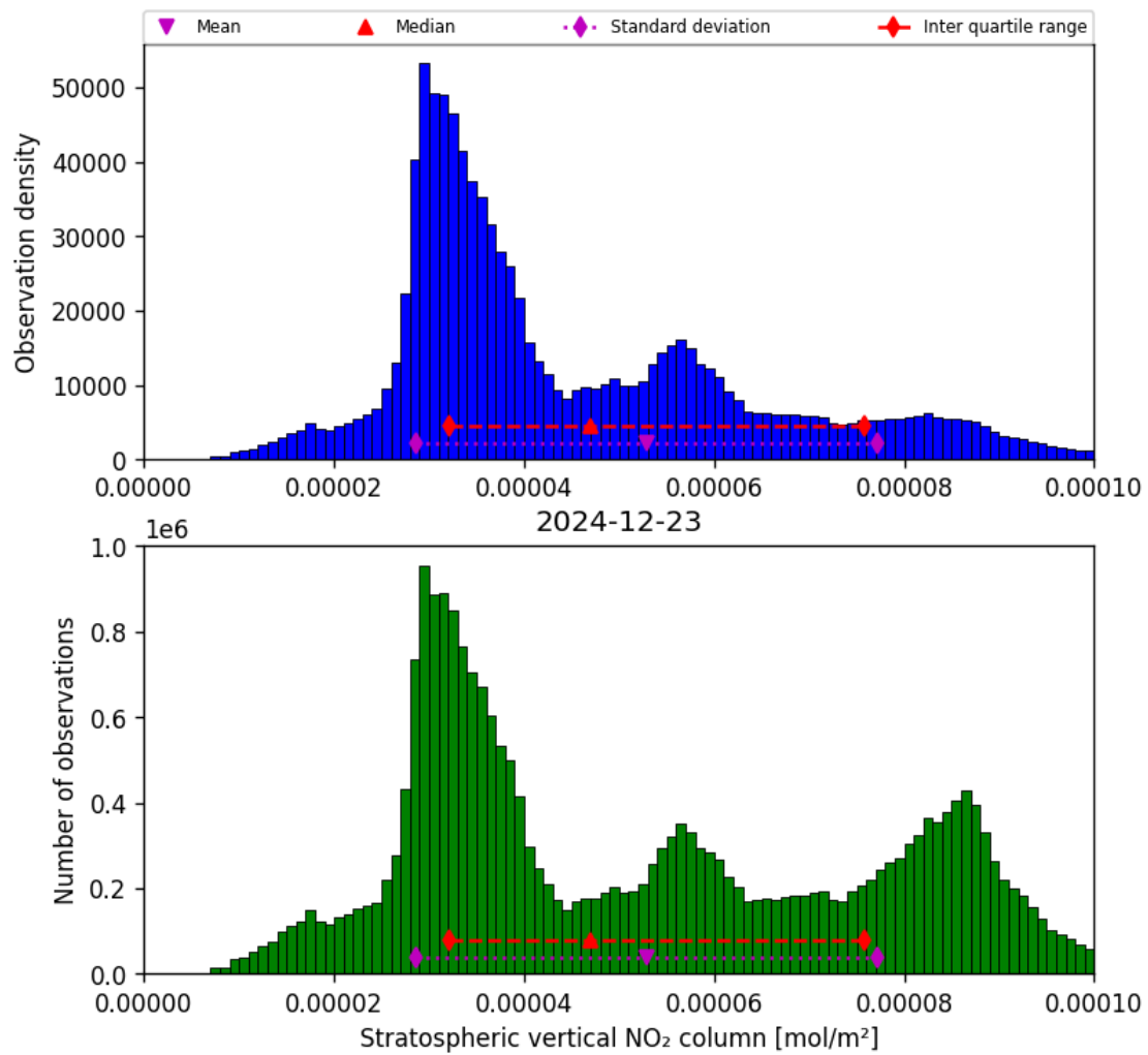
Figure 36: Histogram of “Stratospheric vertical NO 2 column” for 2024-12-22 to 2024-12-24
