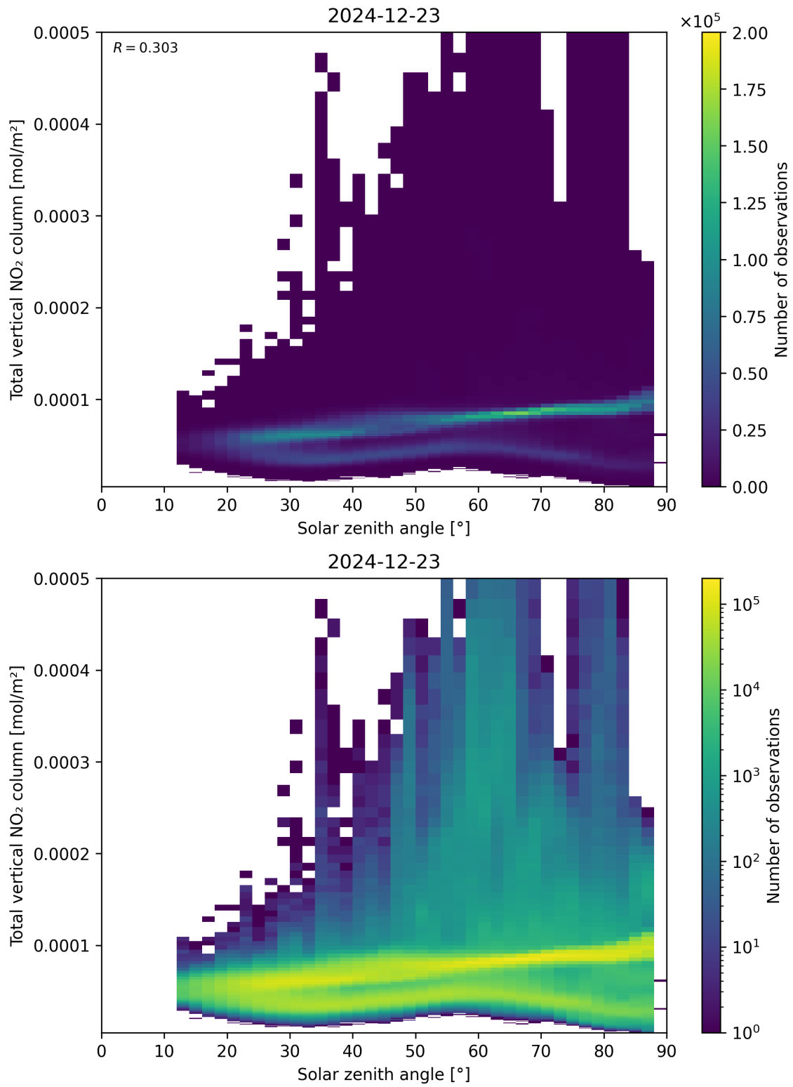
Figure 153: Scatter density plot of “Solar zenith angle” against “Total vertical NO 2 column” for 2024-12-22 to 2024-12-24.
