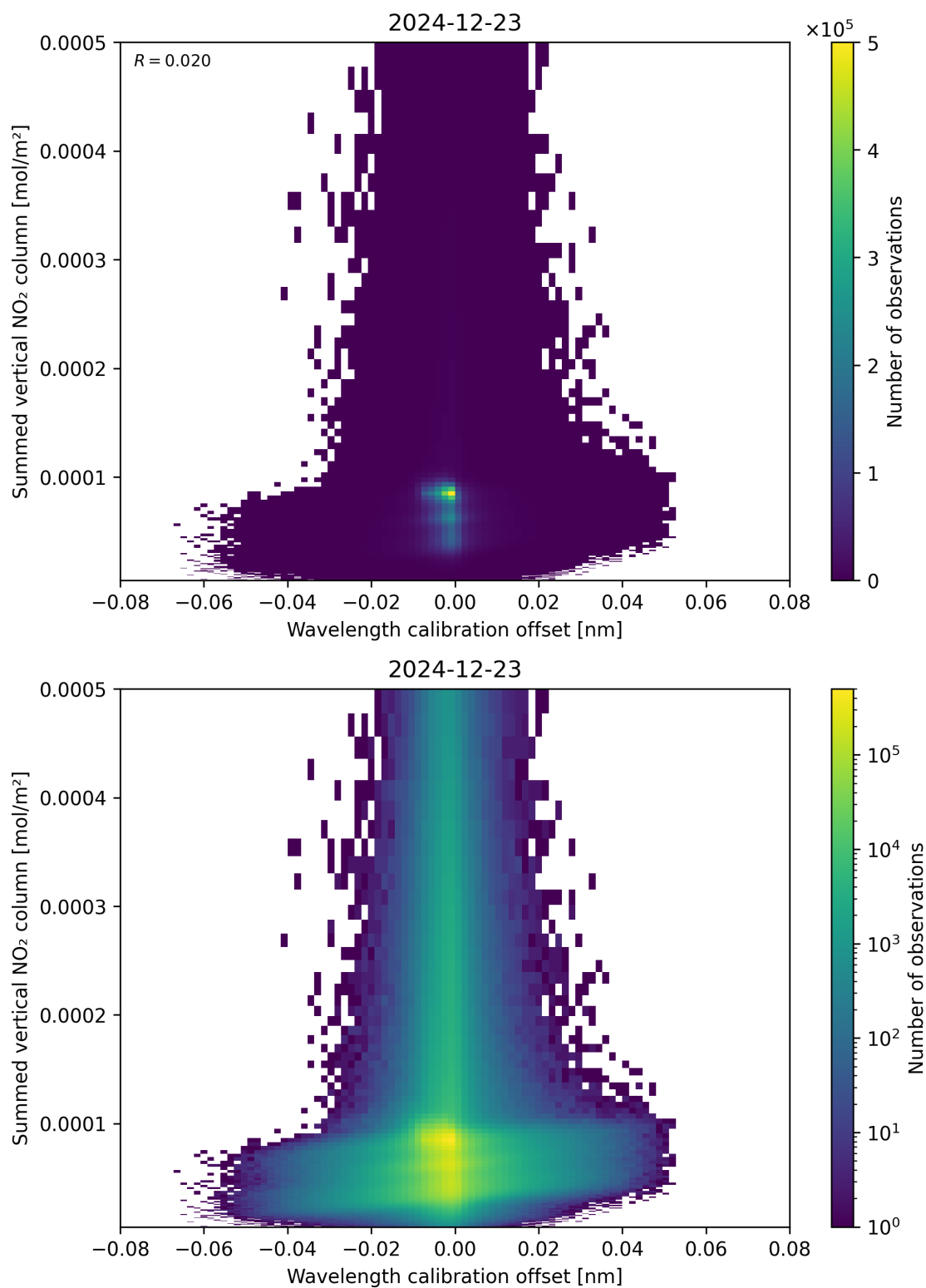
Figure 177: Scatter density plot of “Wavelength calibration offset” against “Summed vertical NO 2 column” for 2024-12-22 to 2024-12-24.
