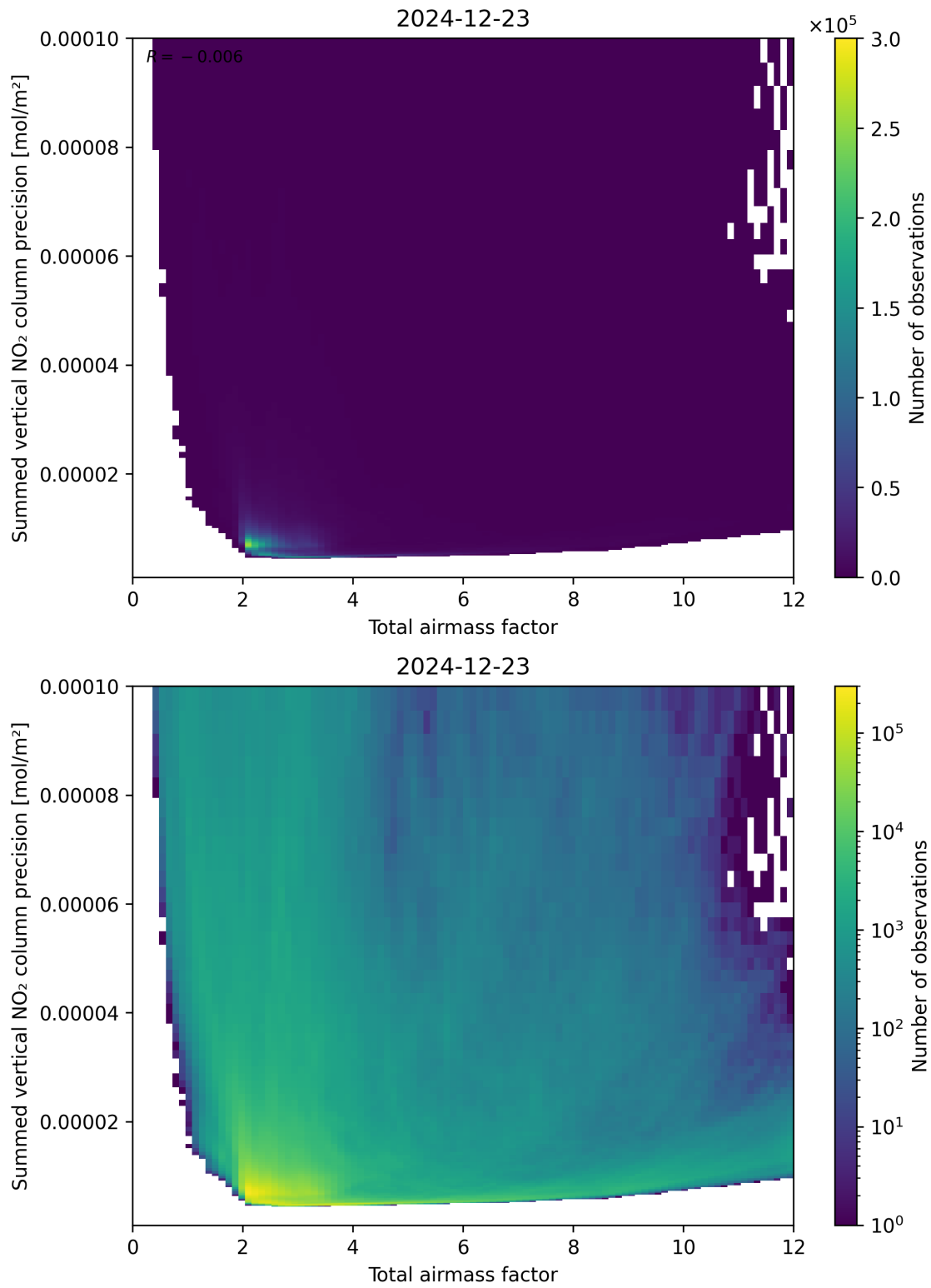
Figure 66: Scatter density plot of “Total airmass factor” against “Summed vertical NO 2 column precision” for 2024-12-22 to 2024-12-24.
