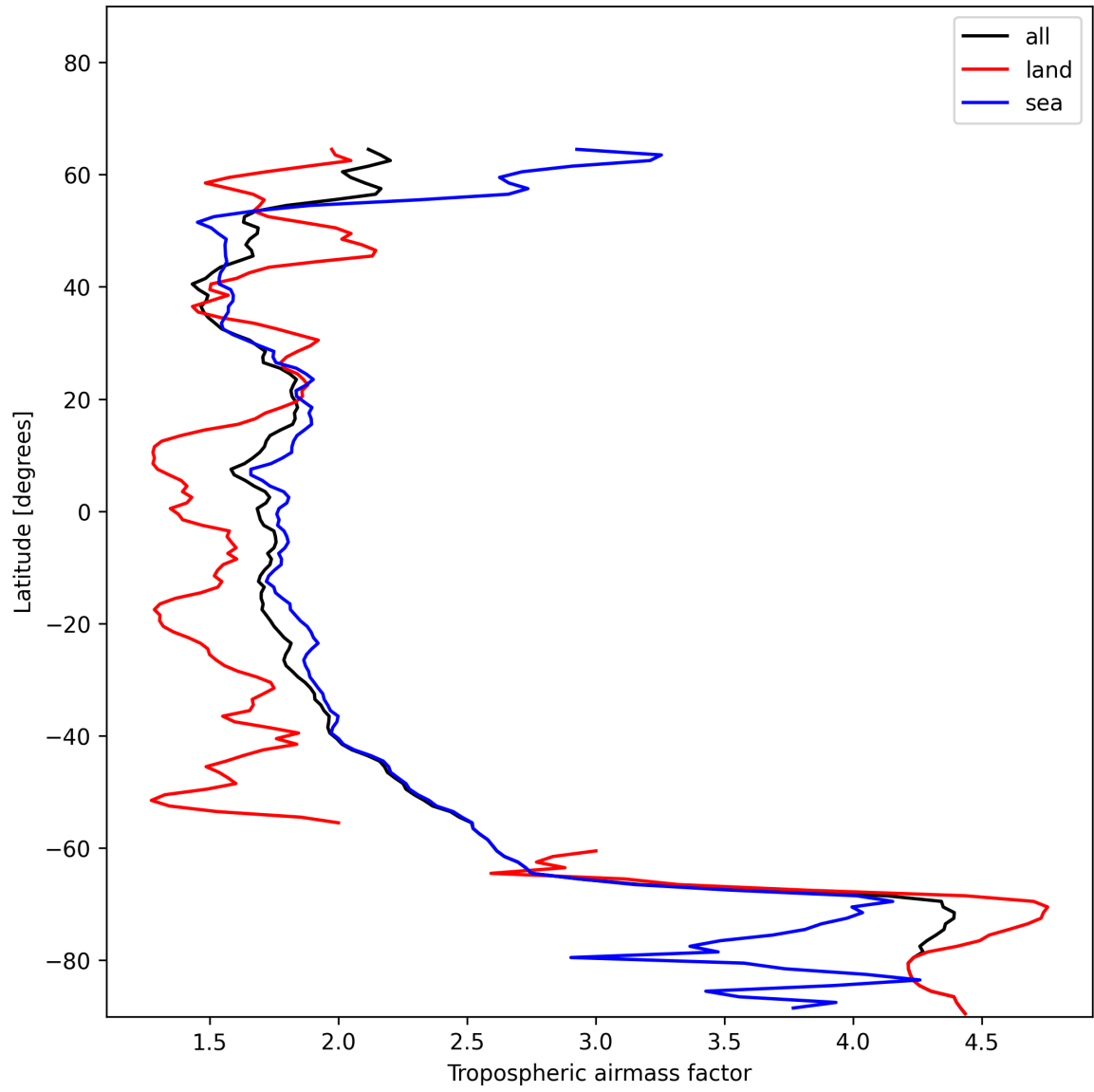
Figure 14: Zonal average of “Tropospheric airmass factor” for 2024-12-22 to 2024-12-24.
