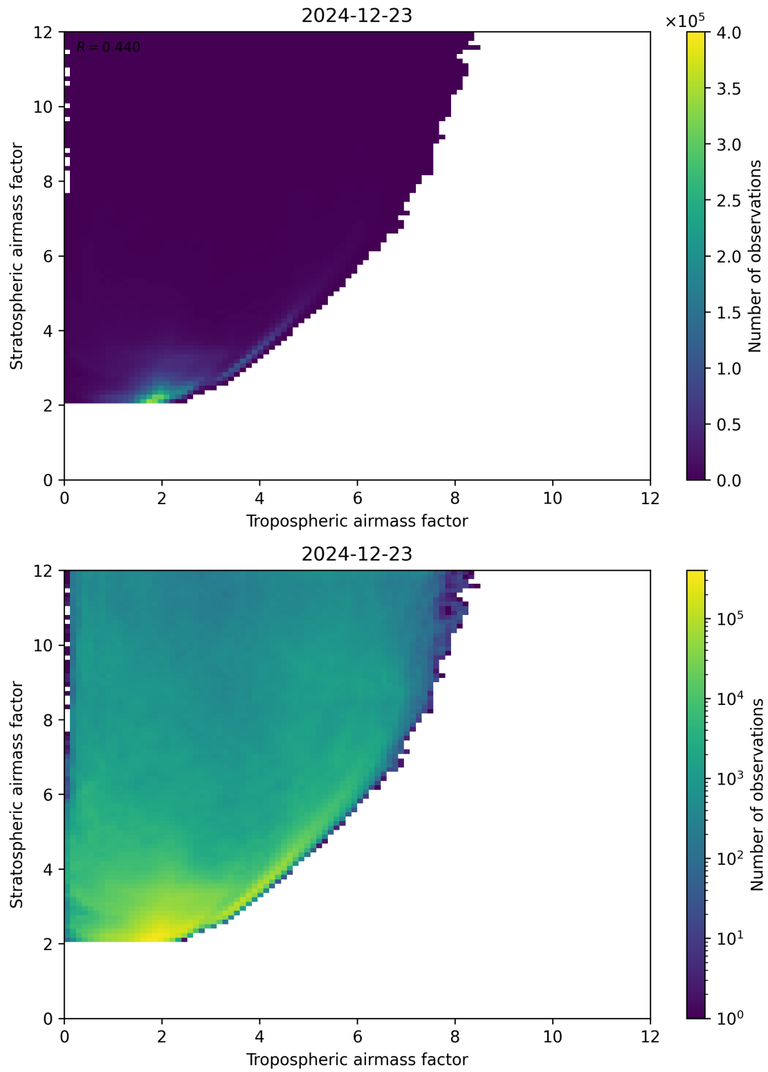
Figure 71: Scatter density plot of “Tropospheric airmass factor” against “Stratospheric airmass factor” for 2024-12-22 to 2024-12-24.
