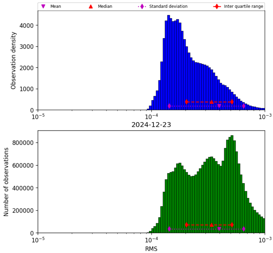
Figure 43: Histogram of “RMS” for 2024-12-22 to 2024-12-24
