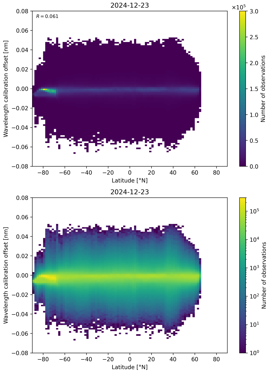
Figure 95: Scatter density plot of “Latitude” against “Wavelength calibration offset” for 2024-12-22 to 2024-12-24.
