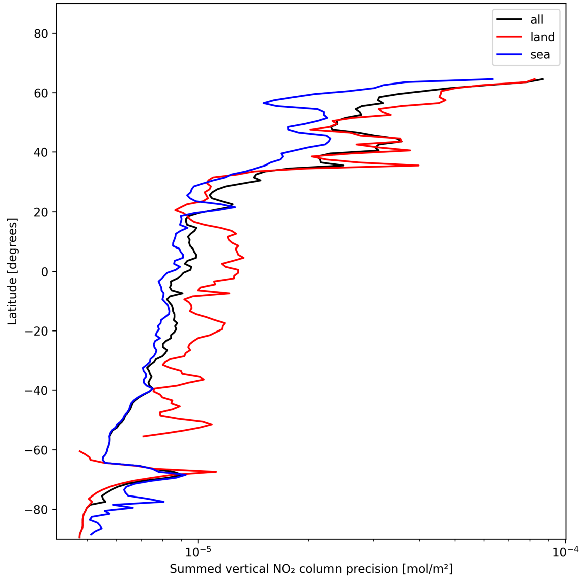
Figure 24: Zonal average of “Summed vertical NO 2 column precision” for 2024-12-22 to 2024-12-24.
