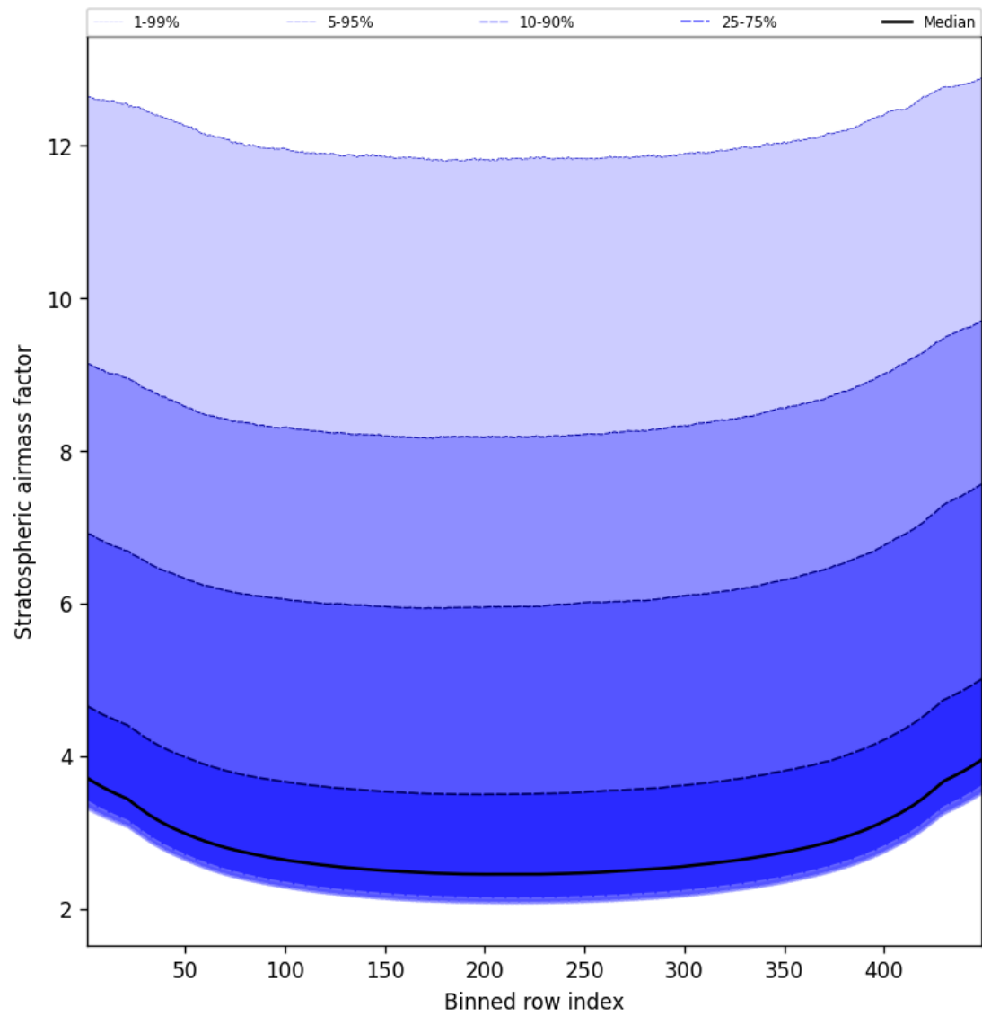
Figure 61: Along track statistics of “Stratospheric airmass factor” for 2024-12-22 to 2024-12-24
