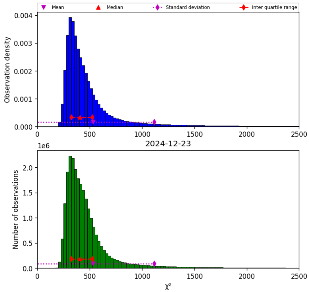
Figure 42: Histogram of " \chi^2 " for 2024-12-22 to 2024-12-24
