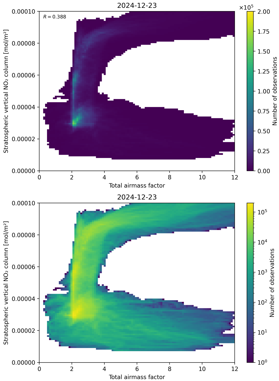
Figure 64: Scatter density plot of “Total airmass factor” against “Stratospheric vertical \text{NO}_2 column” for 2024-12-22 to 2024-12-24.
