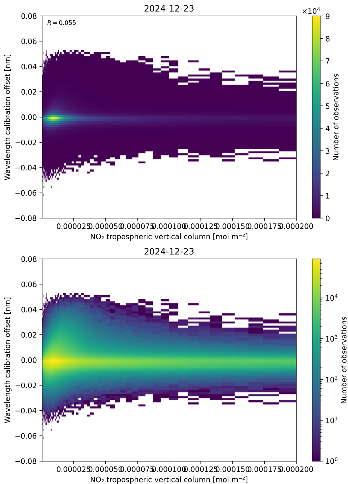
Figure 143: Scatter density plot of “NO 2 tropospheric vertical column” against “Wavelength calibration offset” for 2024-12-22 to 2024-12-24.
