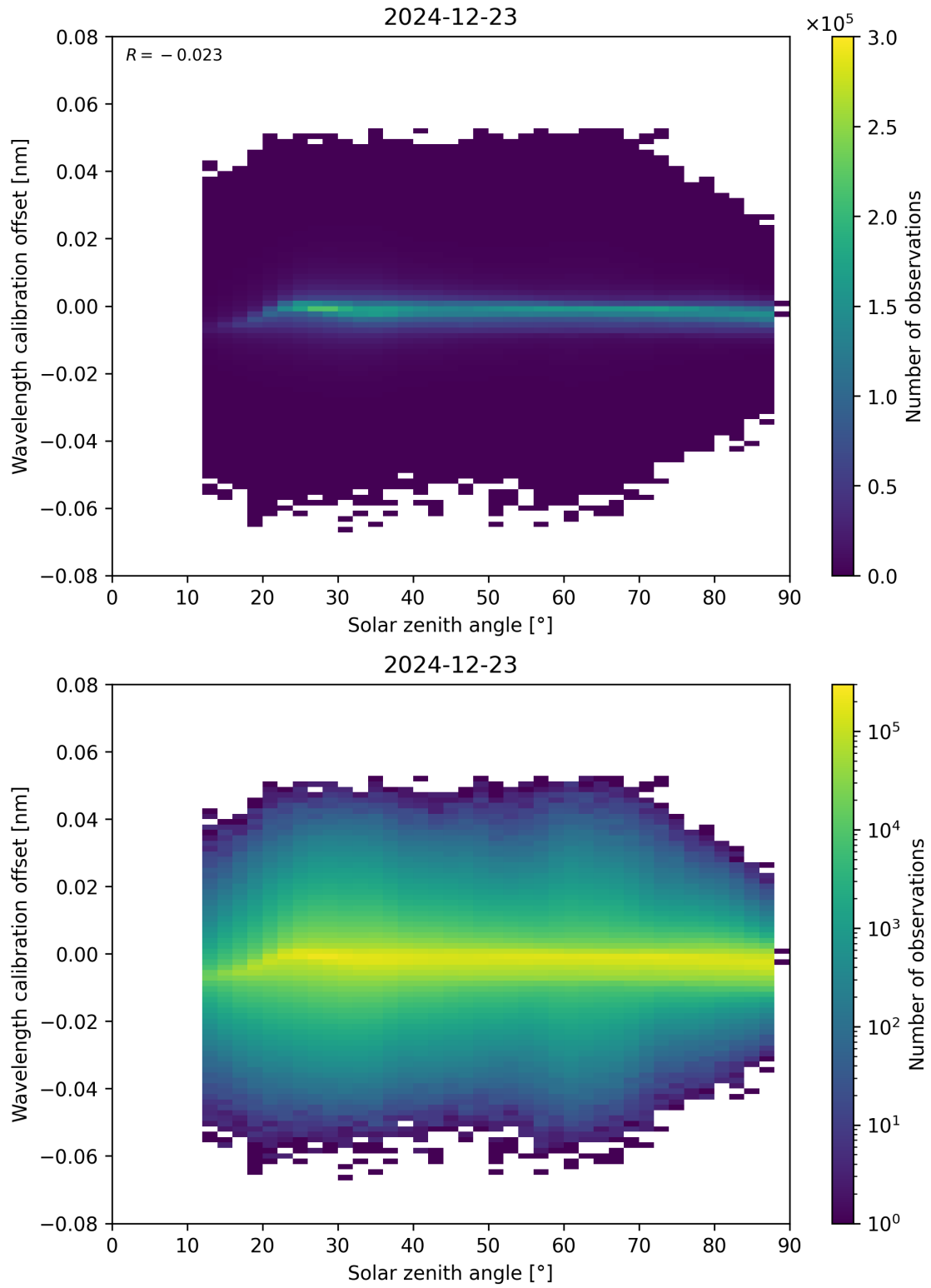
Figure 158: Scatter density plot of “Solar zenith angle” against “Wavelength calibration offset” for 2024-12-22 to 2024-12-24.
