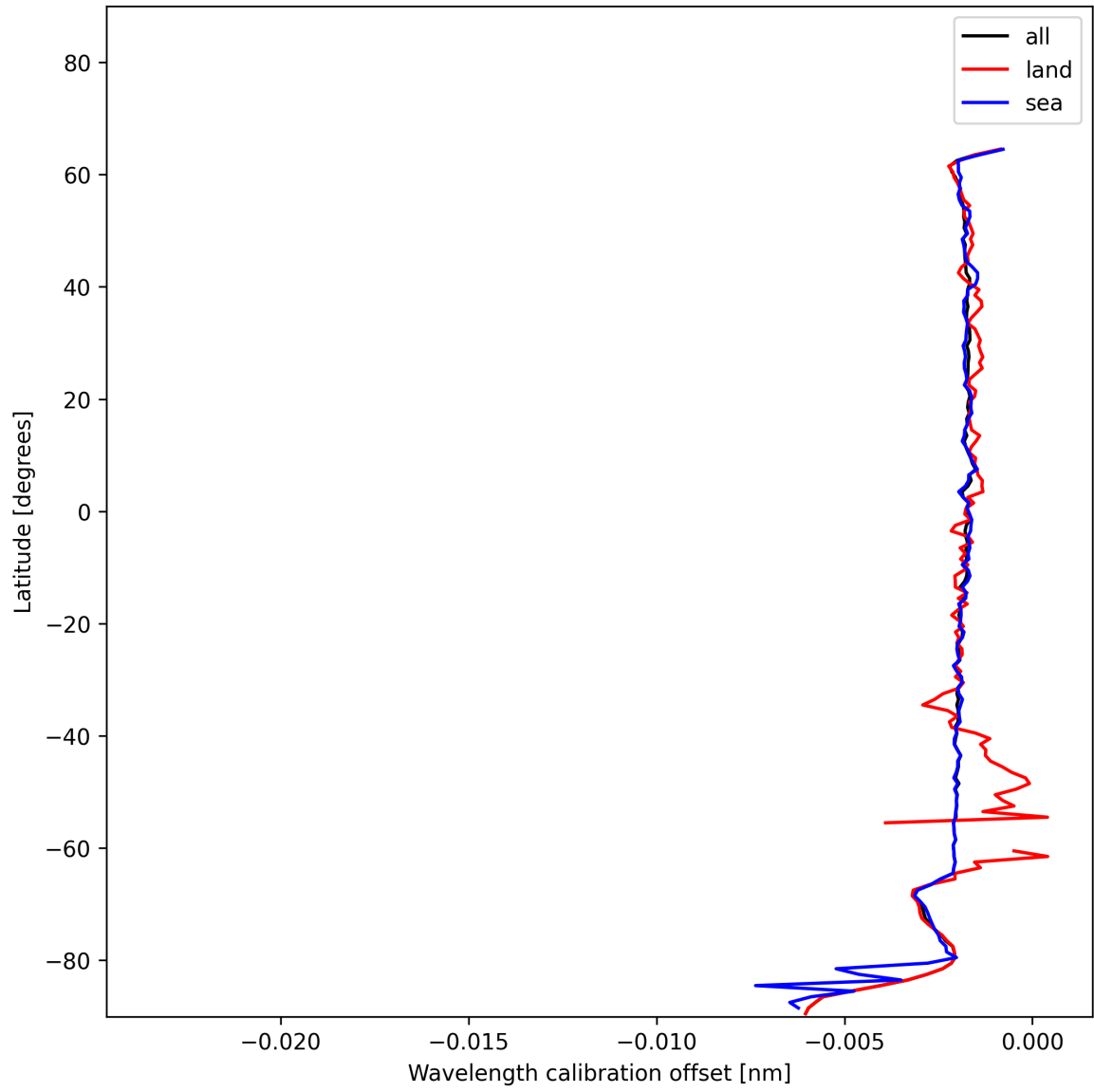
Figure 18: Zonal average of “Wavelength calibration offset” for 2024-12-22 to 2024-12-24.
