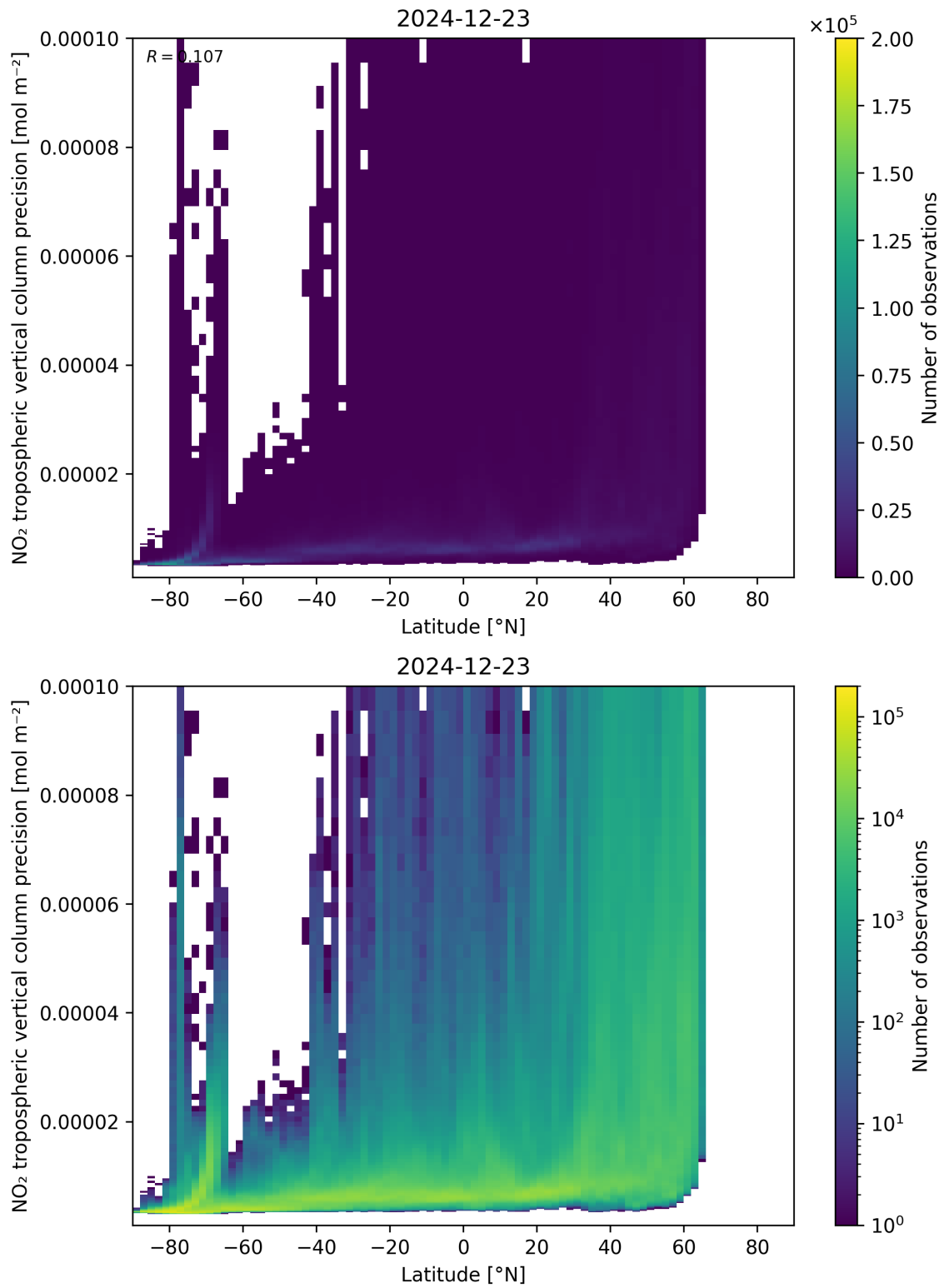
Figure 93: Scatter density plot of “Latitude” against “NO 2 tropospheric vertical column precision” for 2024-12-22 to 2024-12-24.
