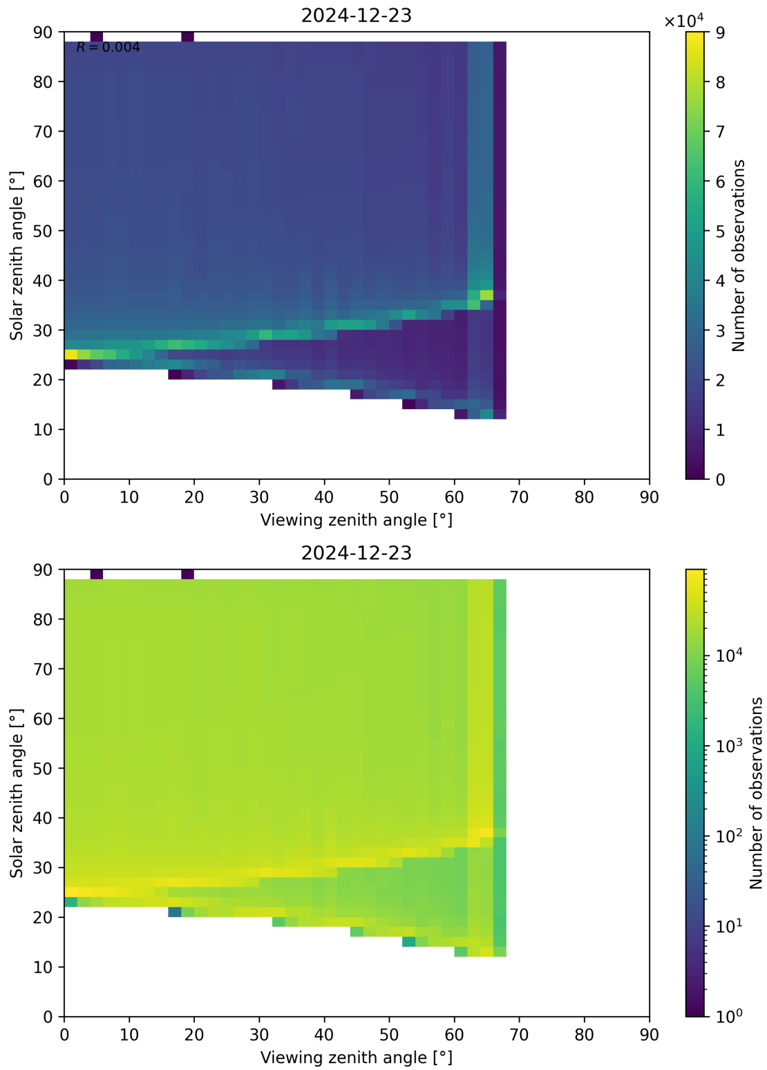
Figure 172: Scatter density plot of “Viewing zenith angle” against “Solar zenith angle” for 2024-12-22 to 2024-12-24.
