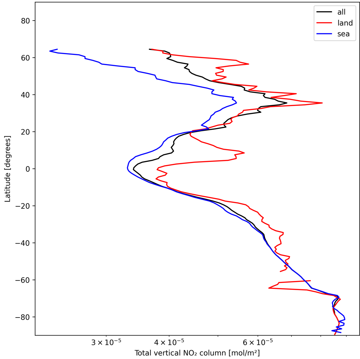
Figure 21: Zonal average of “Total vertical NO 2 column” for 2024-12-22 to 2024-12-24.
