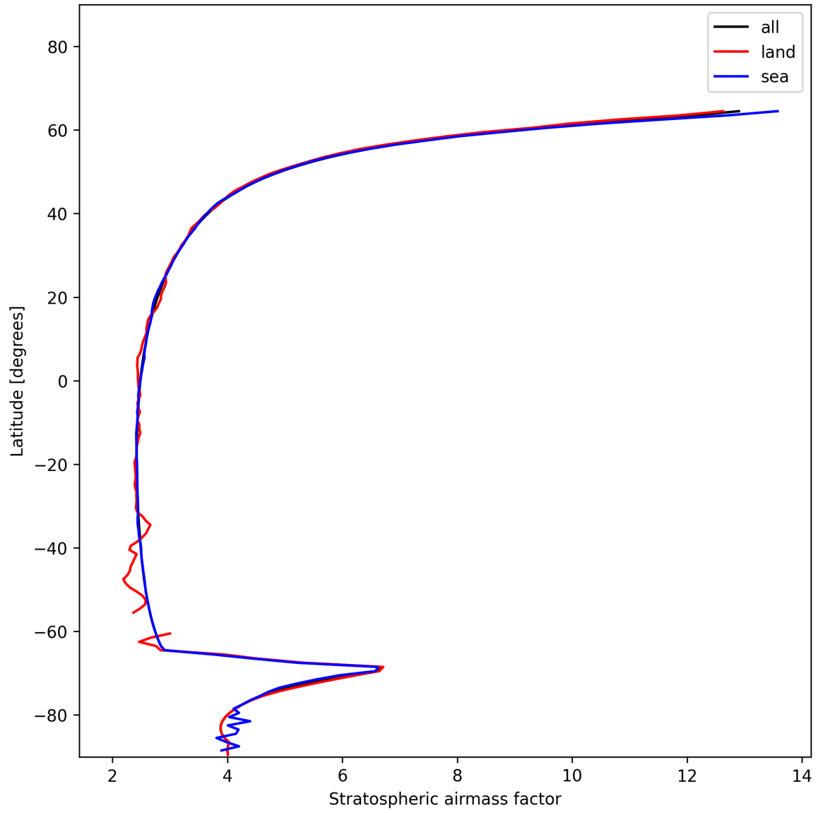
Figure 27: Zonal average of “Stratospheric airmass factor” for 2024-12-22 to 2024-12-24.
