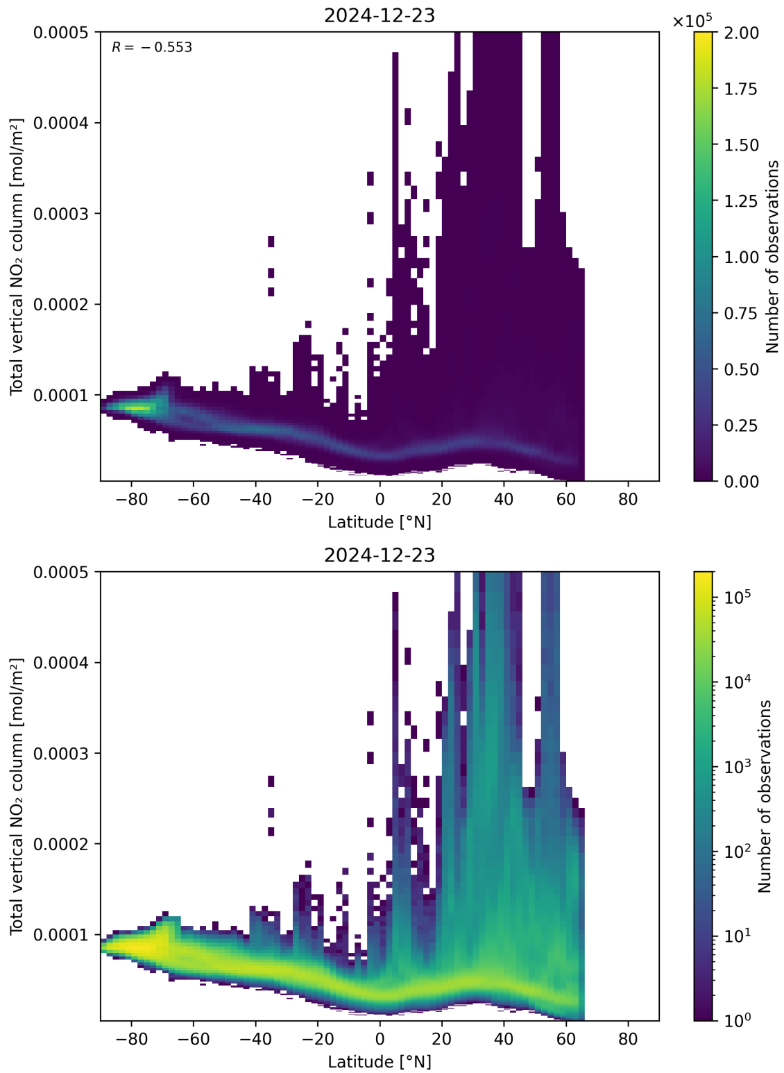
Figure 90: Scatter density plot of “Latitude” against “Total vertical NO 2 column” for 2024-12-22 to 2024-12-24.
