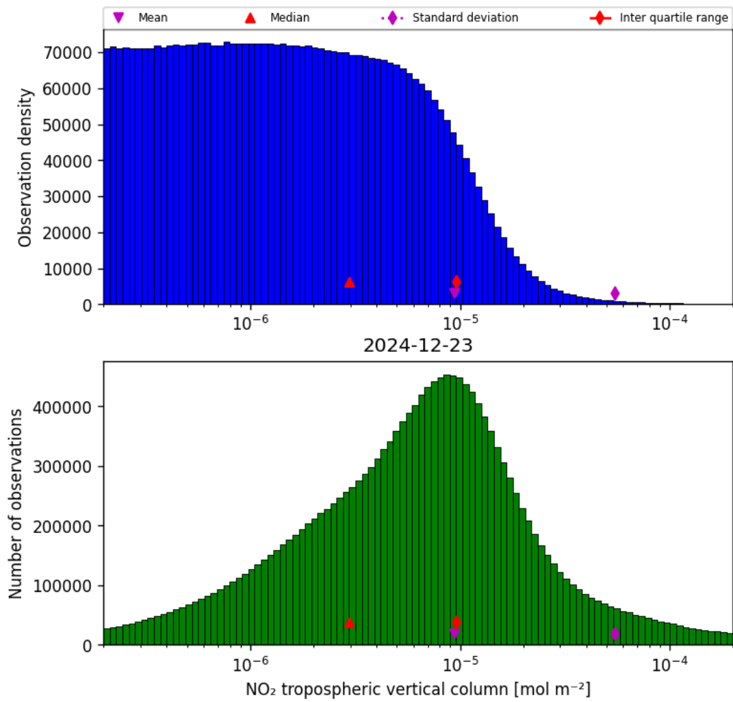
Figure 29: Histogram of “NO 2 tropospheric vertical column” for 2024-12-22 to 2024-12-24
