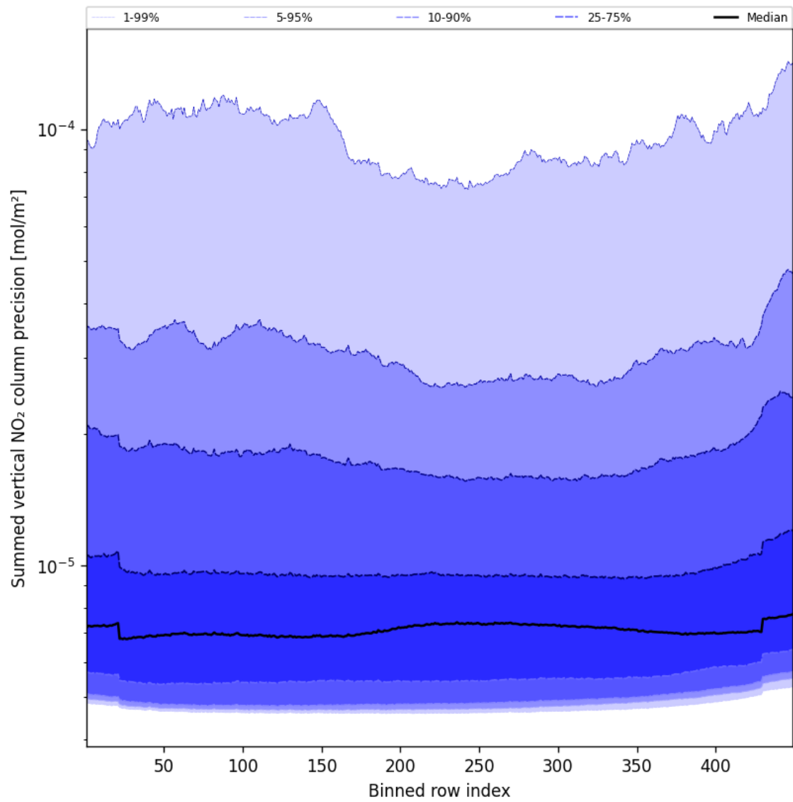
Figure 58: Along track statistics of “Summed vertical NO 2 column precision” for 2024-12-22 to 2024-12-24
