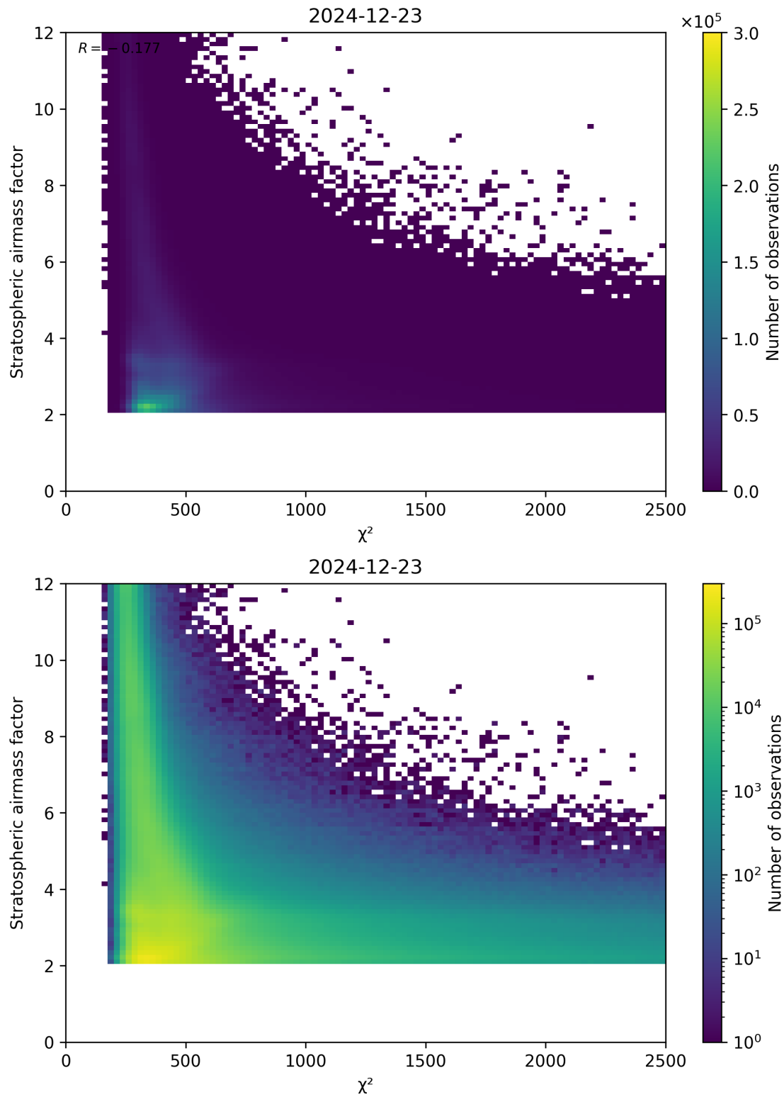
Figure 81: Scatter density plot of “ \chi^2 ” against “Stratospheric airmass factor” for 2024-12-22 to 2024-12-24.
