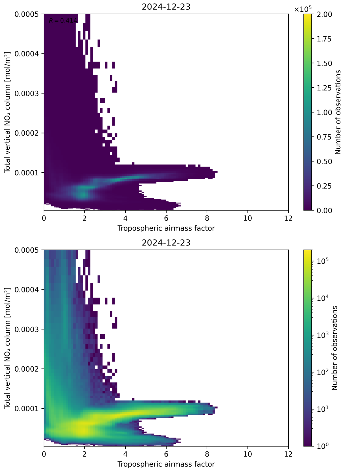
Figure 77: Scatter density plot of “Tropospheric airmass factor” against “Total vertical NO 2 column” for 2024-12-22 to 2024-12-24.
