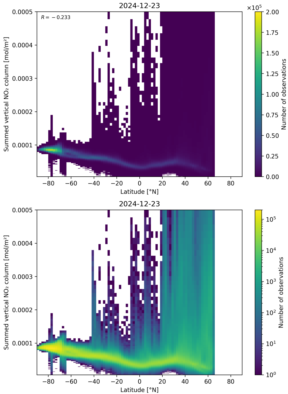
Figure 88: Scatter density plot of “Latitude” against “Summed vertical NO 2 column” for 2024-12-22 to 2024-12-24.
