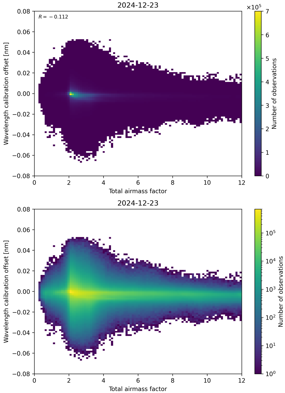
Figure 70: Scatter density plot of “Total airmass factor” against “Wavelength calibration offset” for 2024-12-22 to 2024-12-24.
