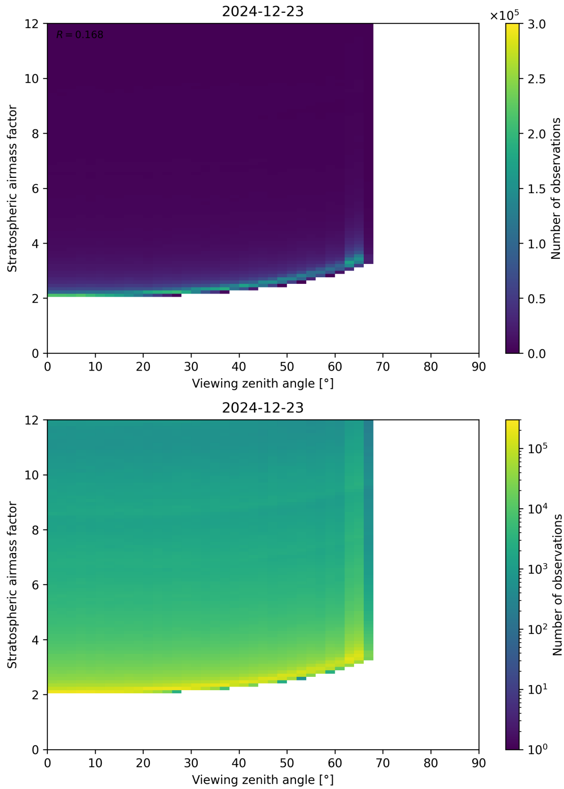
Figure 159: Scatter density plot of “Viewing zenith angle” against “Stratospheric airmass factor” for 2024-12-22 to 2024-12-24.
