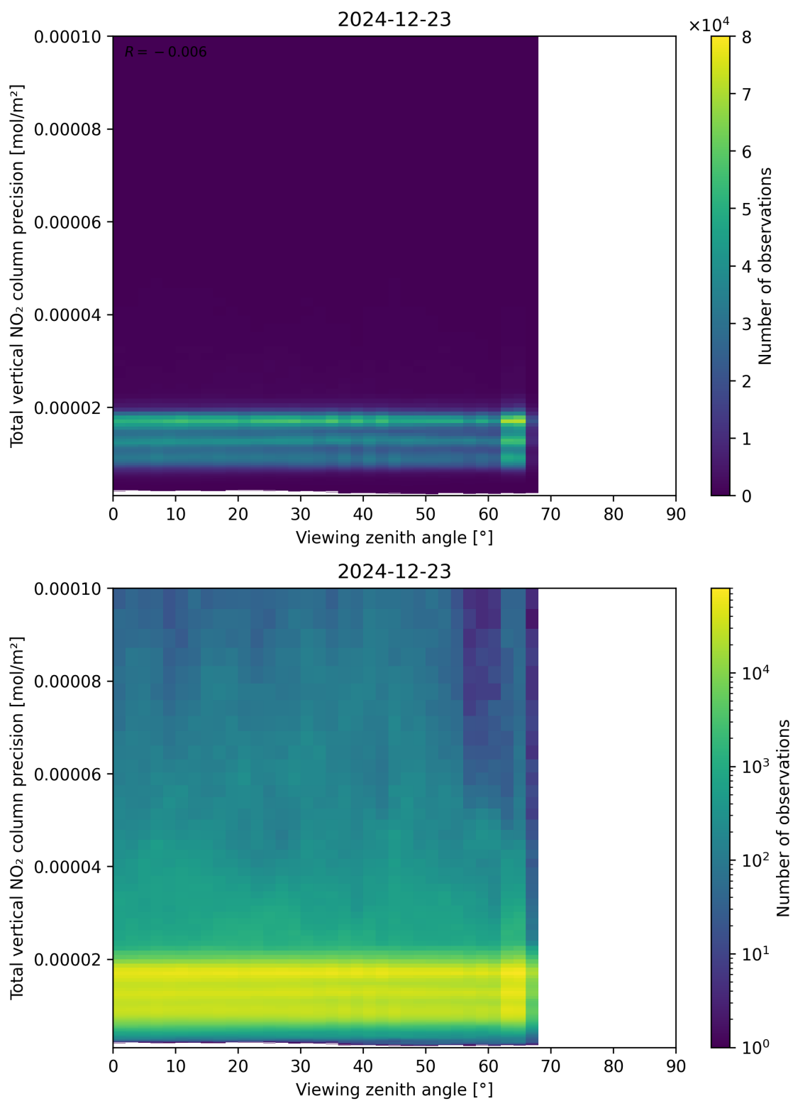
Figure 168: Scatter density plot of “Viewing zenith angle” against “Total vertical NO 2 column precision” for 2024-12-22 to 2024-12-24.
