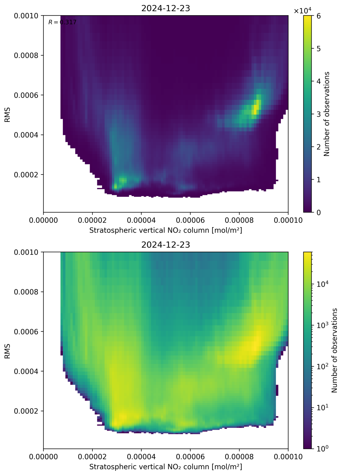
Figure 102: Scatter density plot of “Stratospheric vertical NO 2 column” against “RMS” for 2024-12-22 to 2024-12-24.
