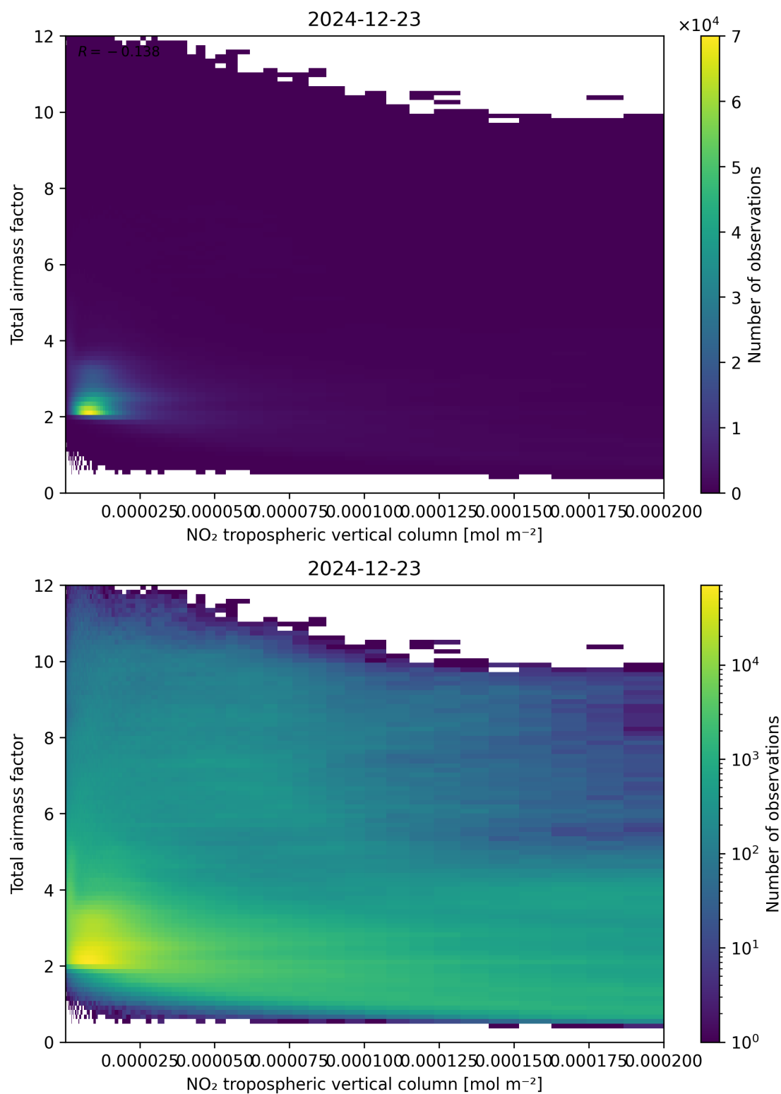
Figure 122: Scatter density plot of “NO 2 tropospheric vertical column” against “Total air mass factor” for 2024-12-22 to 2024-12-24.
