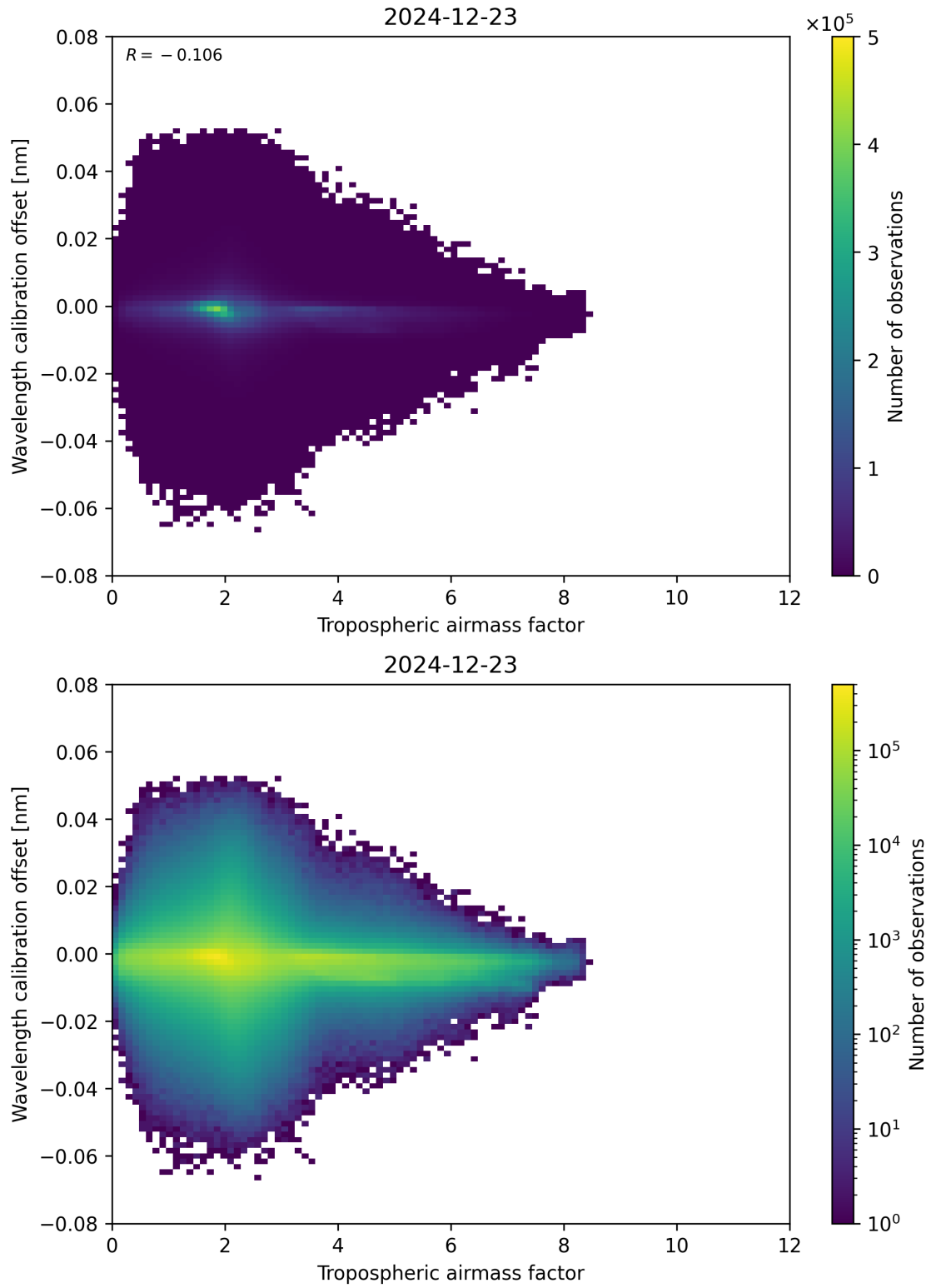
Figure 80: Scatter density plot of “Tropospheric airmass factor” against “Wavelength calibration offset” for 2024-12-22 to 2024-12-24.
