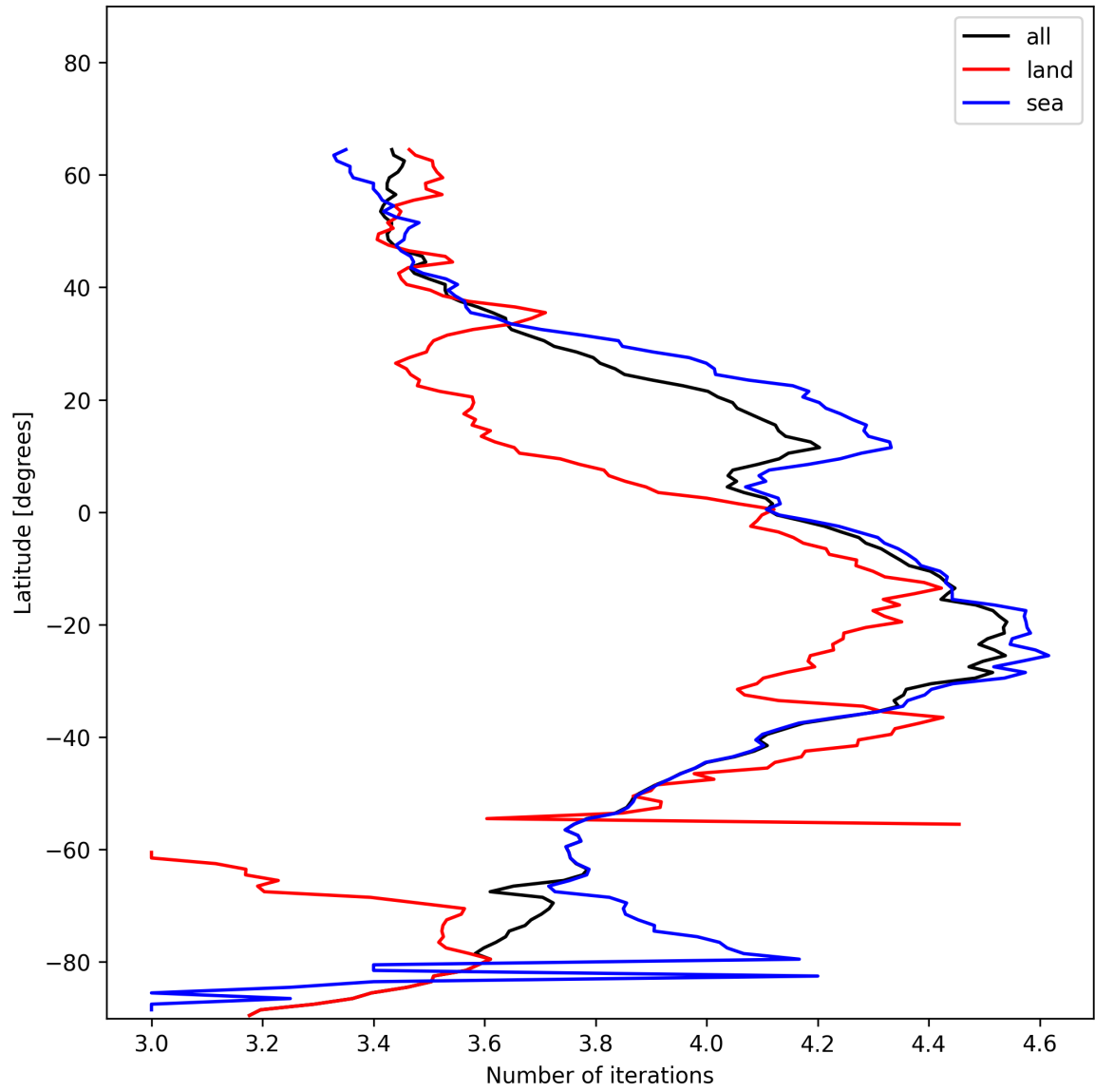
Figure 17: Zonal average of “Number of iterations” for 2024-12-22 to 2024-12-24.
