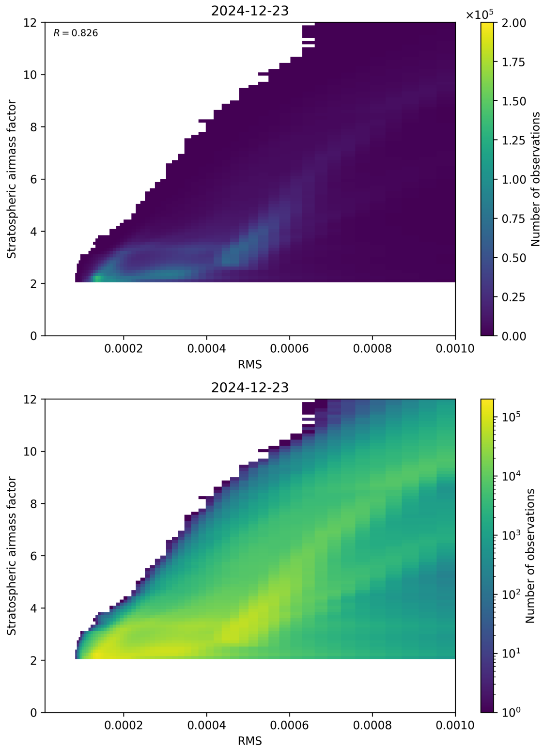
Figure 144: Scatter density plot of “RMS” against “Stratospheric airmass factor” for 2024-12-22 to 2024-12-24.
