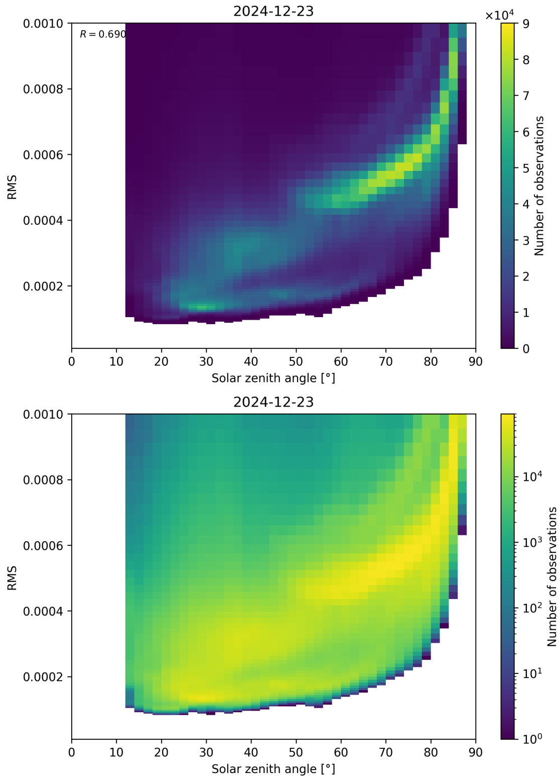
Figure 157: Scatter density plot of “Solar zenith angle” against “RMS” for 2024-12-22 to 2024-12-24.
