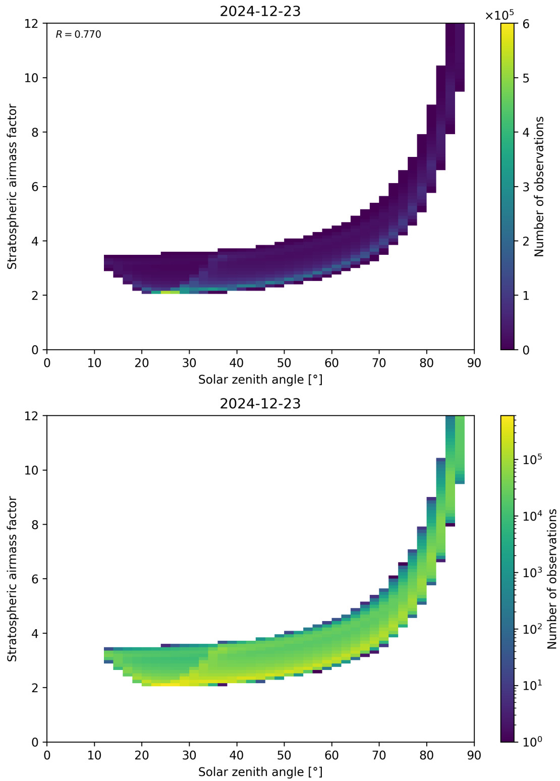
Figure 145: Scatter density plot of “Solar zenith angle” against “Stratospheric airmass factor” for 2024-12-22 to 2024-12-24.
