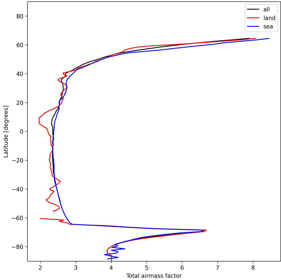
Figure 15: Zonal average of “Total airmass factor” for 2024-12-22 to 2024-12-24.
