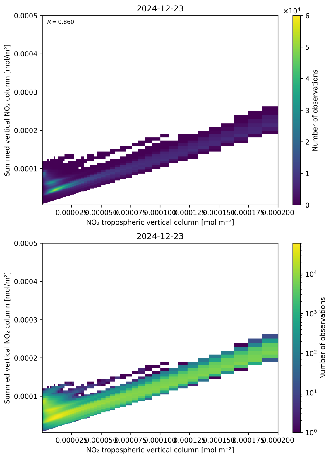
Figure 126: Scatter density plot of “NO 2 tropospheric vertical column” against “Summed vertical NO 2 column” for 2024-12-22 to 2024-12-24.
