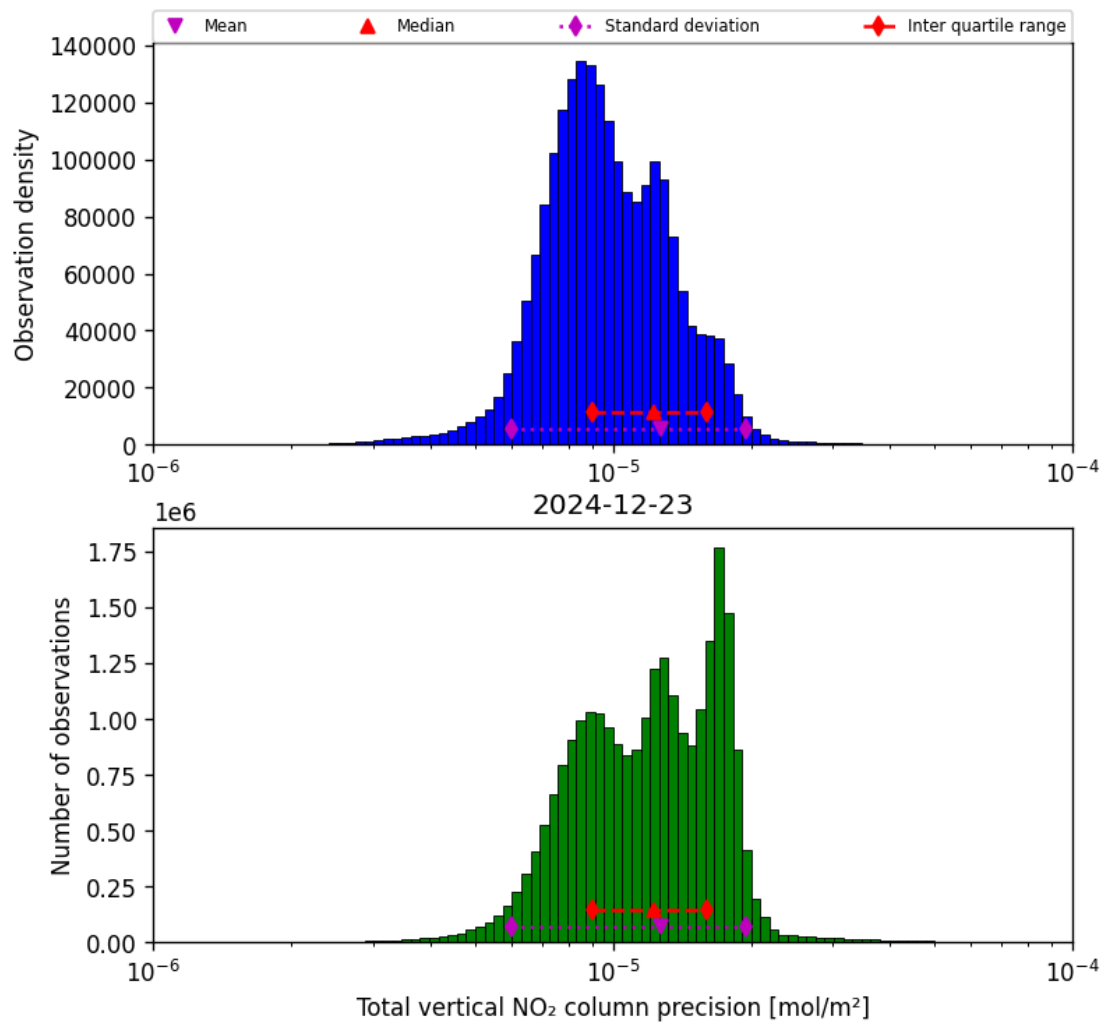
Figure 39: Histogram of “Total vertical NO 2 column precision” for 2024-12-22 to 2024-12-24
