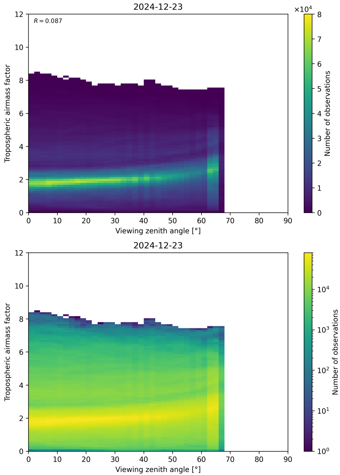
Figure 161: Scatter density plot of “Viewing zenith angle” against “Tropospheric airmass factor” for 2024-12-22 to 2024-12-24.
