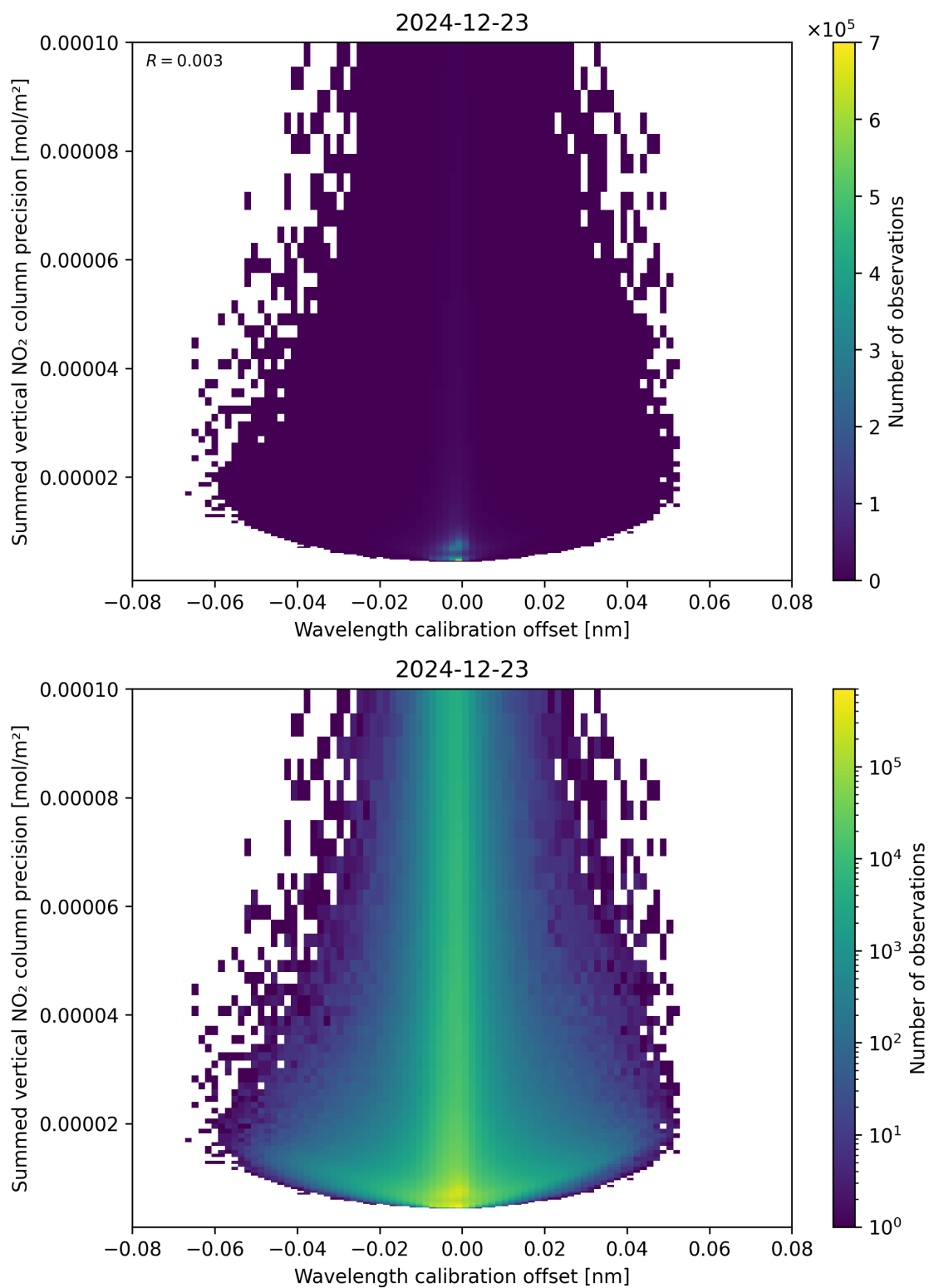
Figure 178: Scatter density plot of “Wavelength calibration offset” against “Summed vertical NO 2 column precision” for 2024-12-22 to 2024-12-24.
