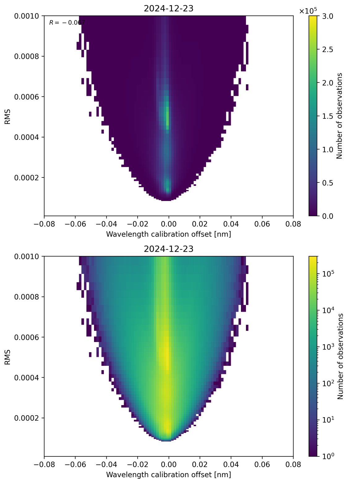
Figure 181: Scatter density plot of “Wavelength calibration offset” against “RMS” for 2024-12-22 to 2024-12-24.
