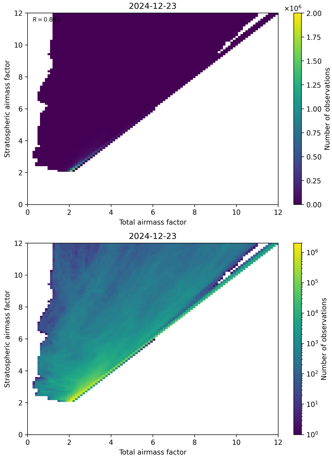
Figure 62: Scatter density plot of “Total airmass factor” against “Stratospheric airmass factor” for 2024-12-22 to 2024-12-24.
