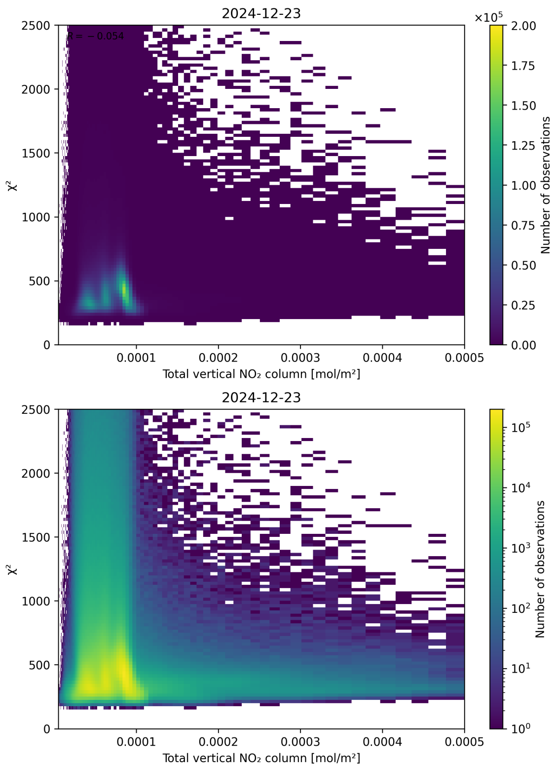
Figure 111: Scatter density plot of “Total vertical NO 2 column” against “ \chi^2 ” for 2024-12-22 to 2024-12-24.
