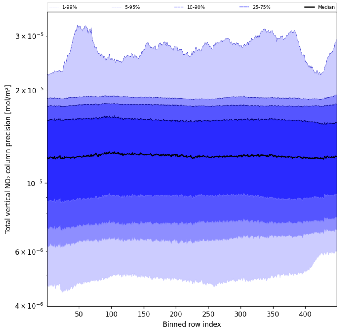
Figure 56: Along track statistics of “Total vertical NO 2 column precision” for 2024-12-22 to 2024-12-24
