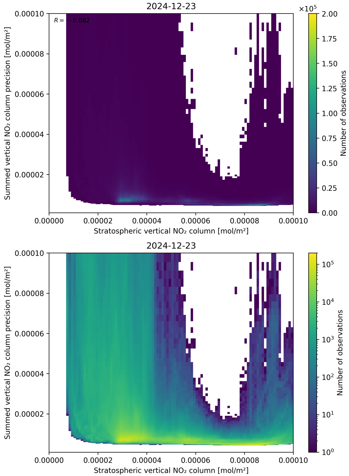
Figure 99: Scatter density plot of “Stratospheric vertical NO 2 column” against “Summed vertical NO 2 column precision” for 2024-12-22 to 2024-12-24.
