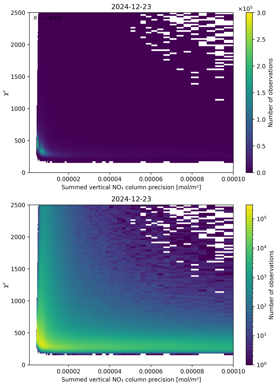
Figure 107: Scatter density plot of “Summed vertical NO 2 column precision” against “ \chi^2 ” for 2024-12-22 to 2024-12-24.
