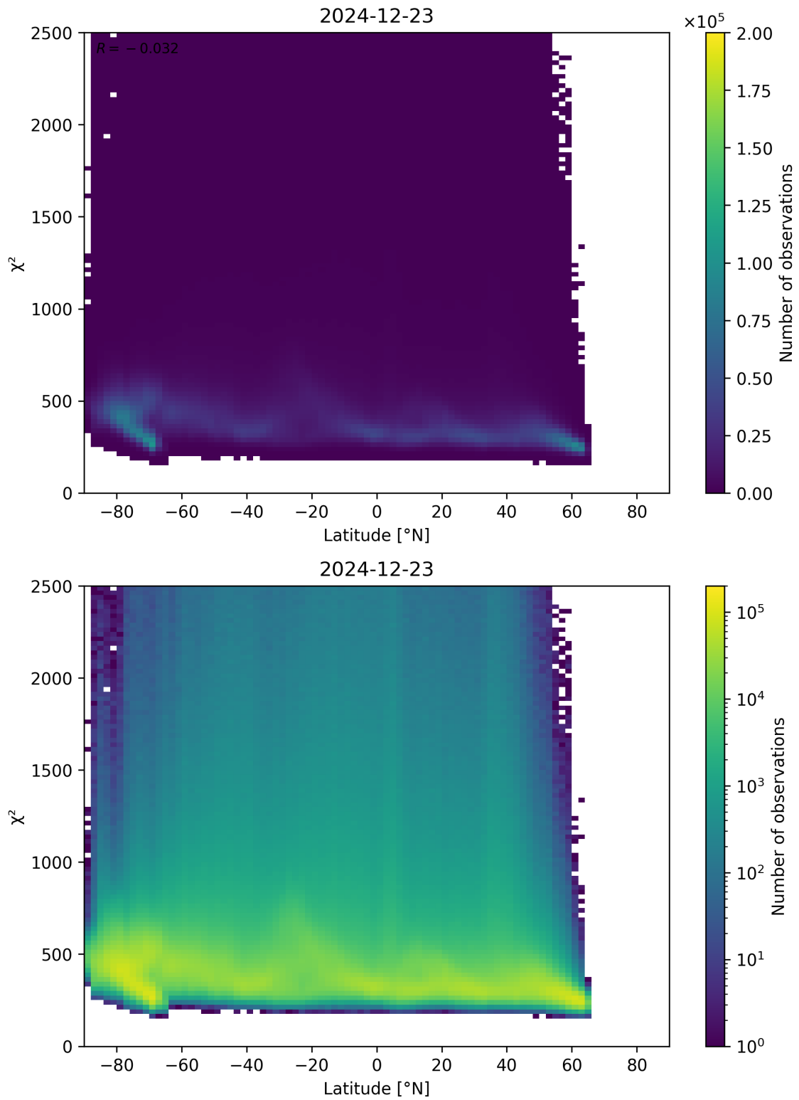
Figure 86: Scatter density plot of “Latitude” against “ \chi^2 ” for 2024-12-22 to 2024-12-24.
