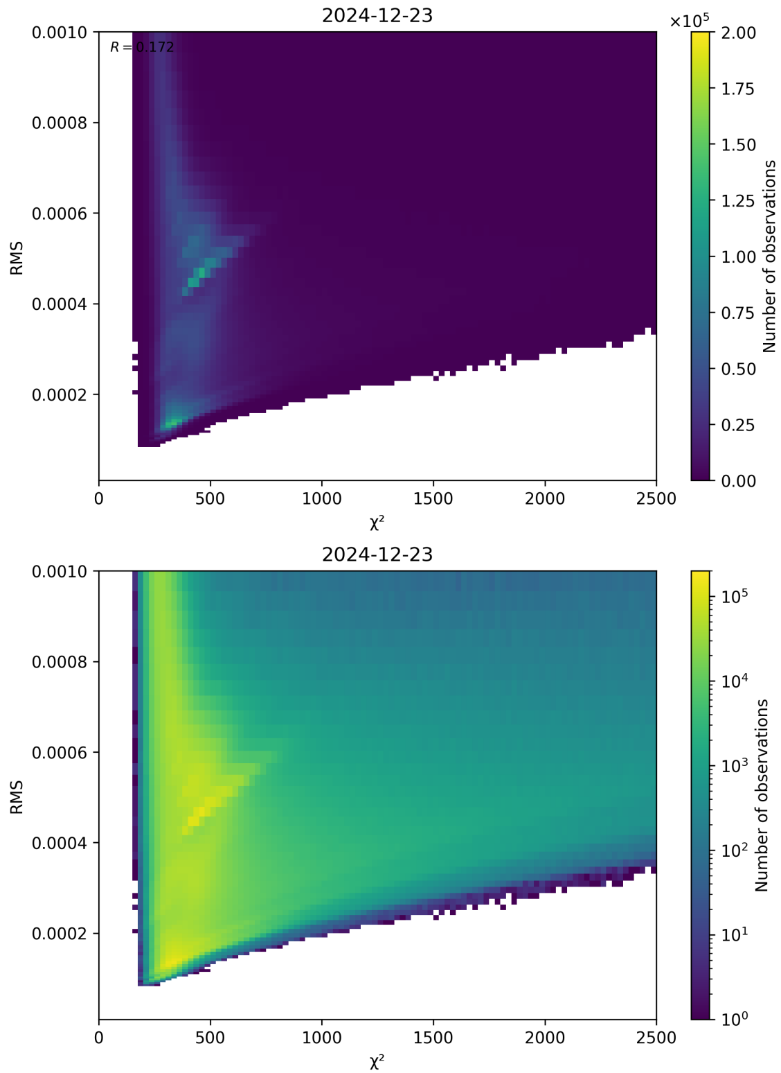
Figure 82: Scatter density plot of “ \chi^2 ” against “RMS” for 2024-12-22 to 2024-12-24.
