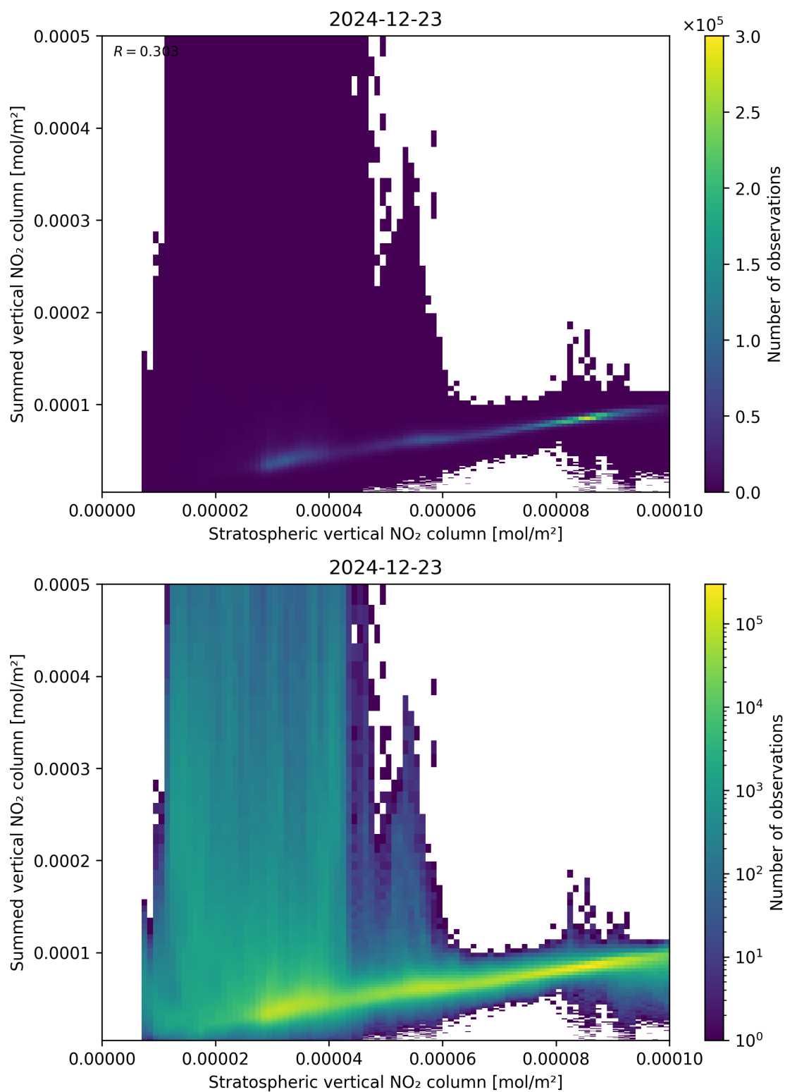
Figure 98: Scatter density plot of “Stratospheric vertical NO 2 column” against “Summed vertical NO 2 column” for 2024-12-22 to 2024-12-24.
