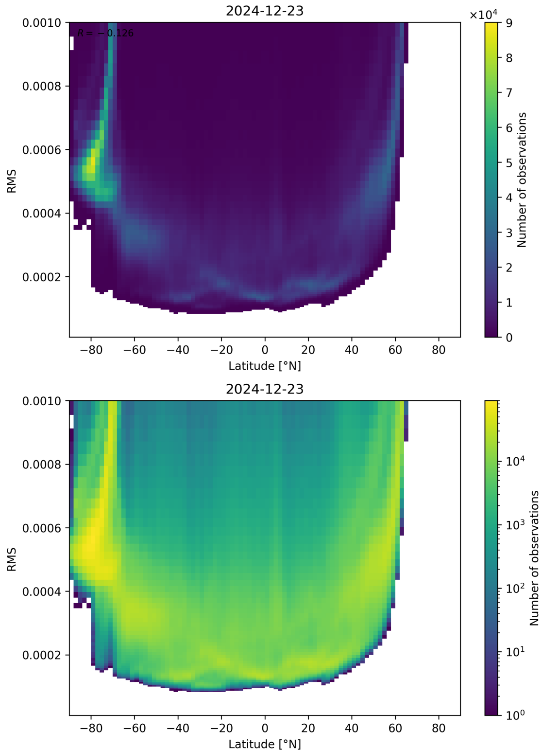
Figure 94: Scatter density plot of “Latitude” against “RMS” for 2024-12-22 to 2024-12-24.
