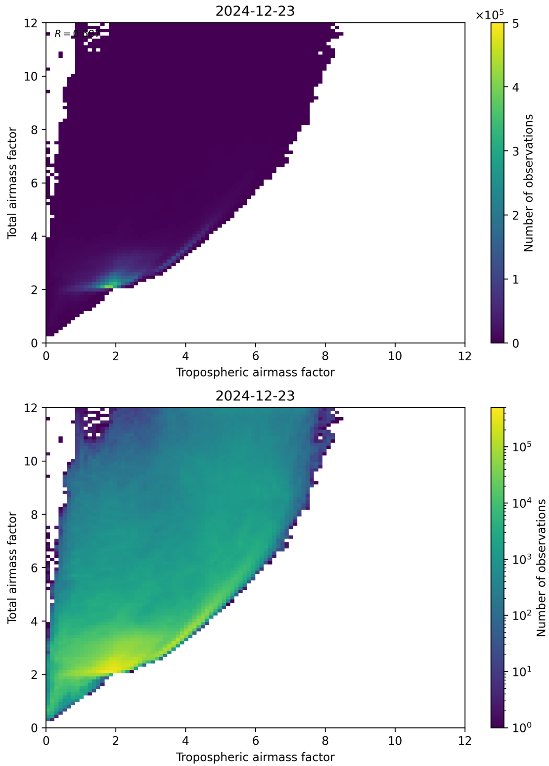
Figure 72: Scatter density plot of “Tropospheric airmass factor” against “Total airmass factor” for 2024-12-22 to 2024-12-24.
