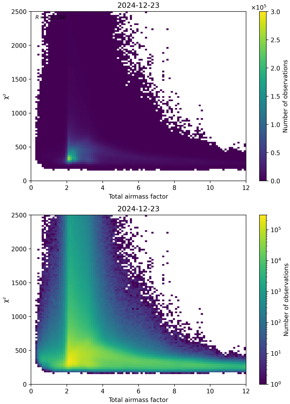
Figure 63: Scatter density plot of “Total airmass factor” against “ \chi^2 ” for 2024-12-22 to 2024-12-24.
