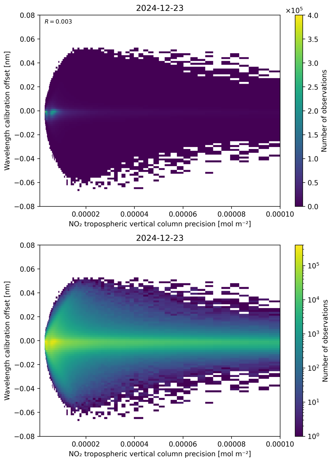
Figure 141: Scatter density plot of “NO 2 tropospheric vertical column precision” against “Wavelength calibration offset” for 2024-12-22 to 2024-12-24.
