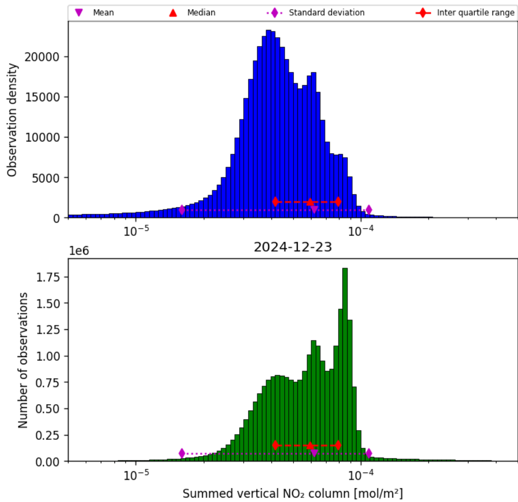
Figure 40: Histogram of “Summed vertical NO 2 column” for 2024-12-22 to 2024-12-24
