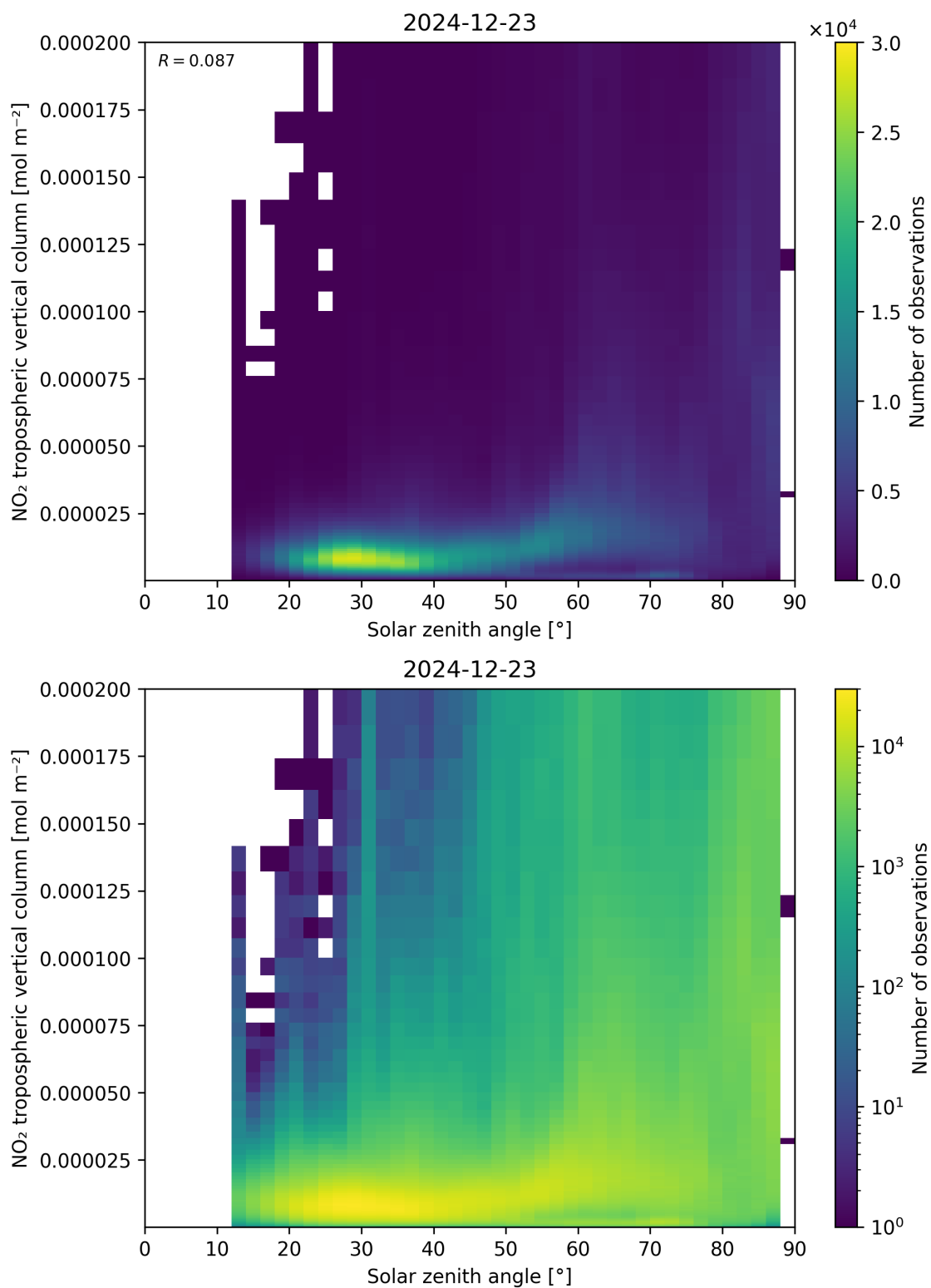
Figure 155: Scatter density plot of “Solar zenith angle” against “NO 2 tropospheric vertical column” for 2024-12-22 to 2024-12-24.
