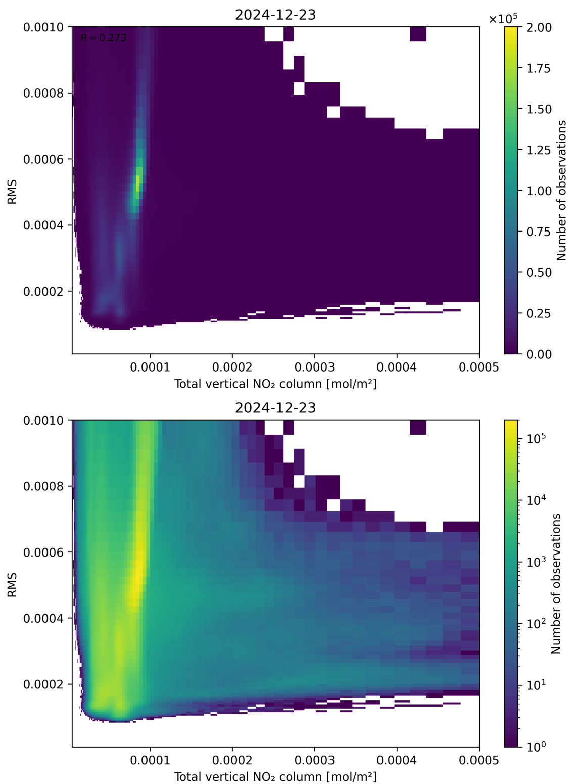
Figure 120: Scatter density plot of “Total vertical NO 2 column” against “RMS” for 2024-12-22 to 2024-12-24.
