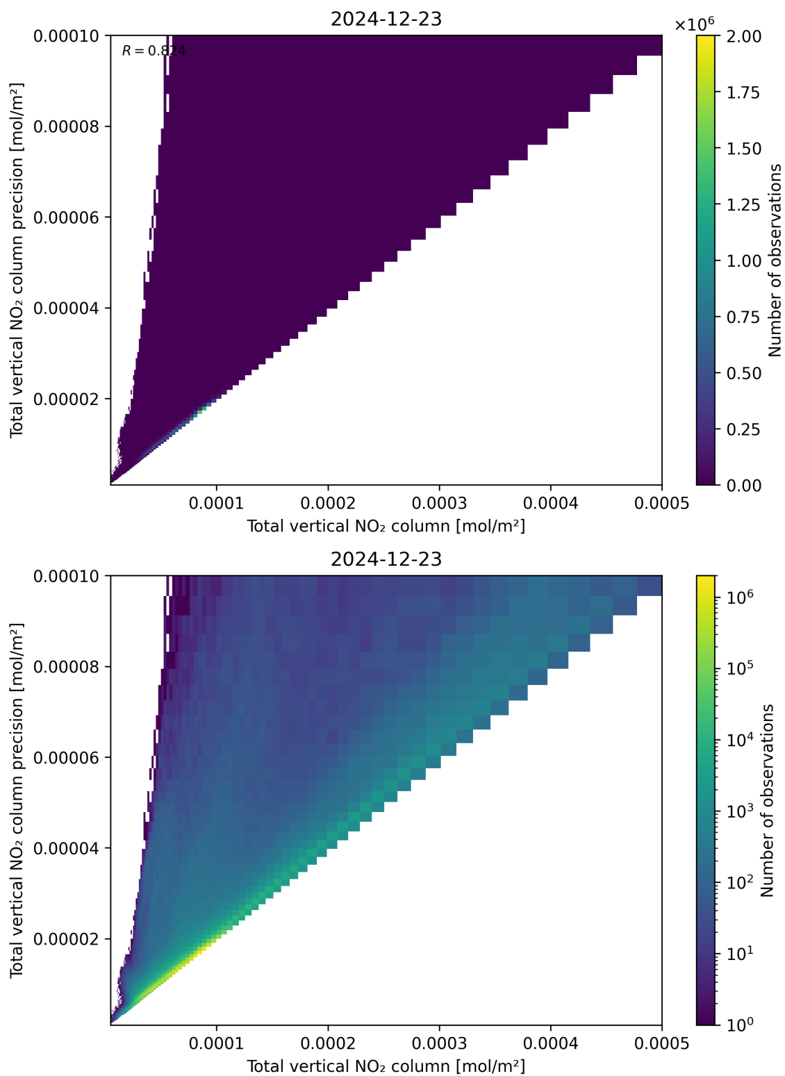
Figure 114: Scatter density plot of “Total vertical NO 2 column” against “Total vertical NO 2 column precision” for 2024-12-22 to 2024-12-24.
