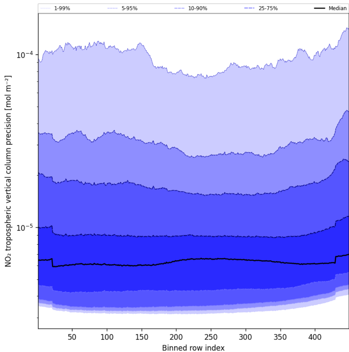
Figure 47: Along track statistics of “NO 2 tropospheric vertical column precision” for 2024-12-22 to 2024-12-24
