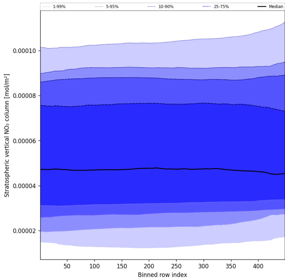
Figure 53: Along track statistics of “Stratospheric vertical NO 2 column” for 2024-12-22 to 2024-12-24
