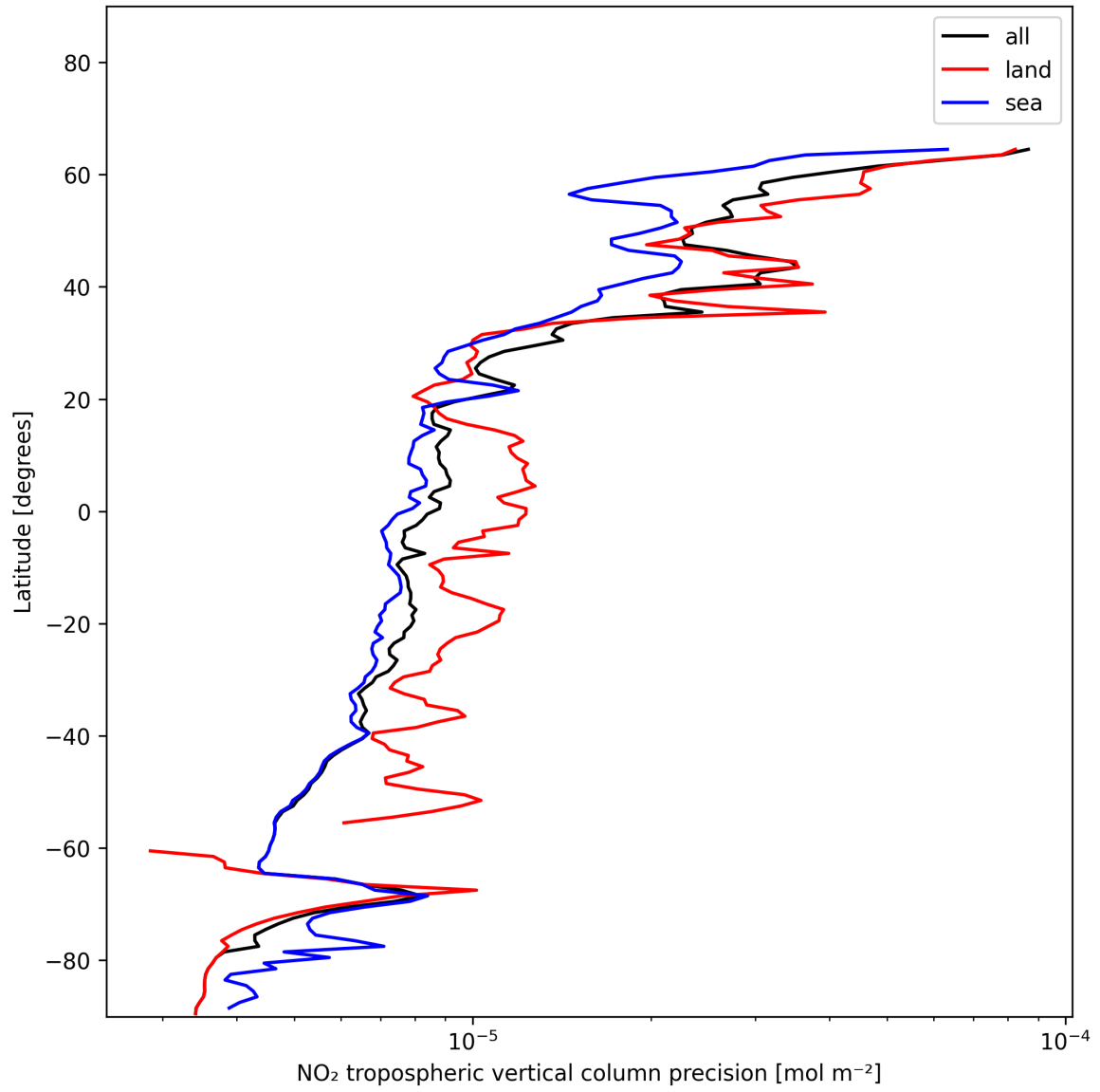
Figure 13: Zonal average of “NO 2 tropospheric vertical column precision” for 2024-12-22 to 2024-12-24.
