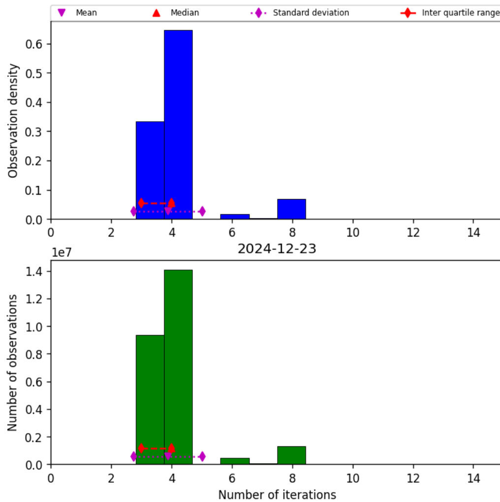
Figure 34: Histogram of “Number of iterations” for 2024-12-22 to 2024-12-24
