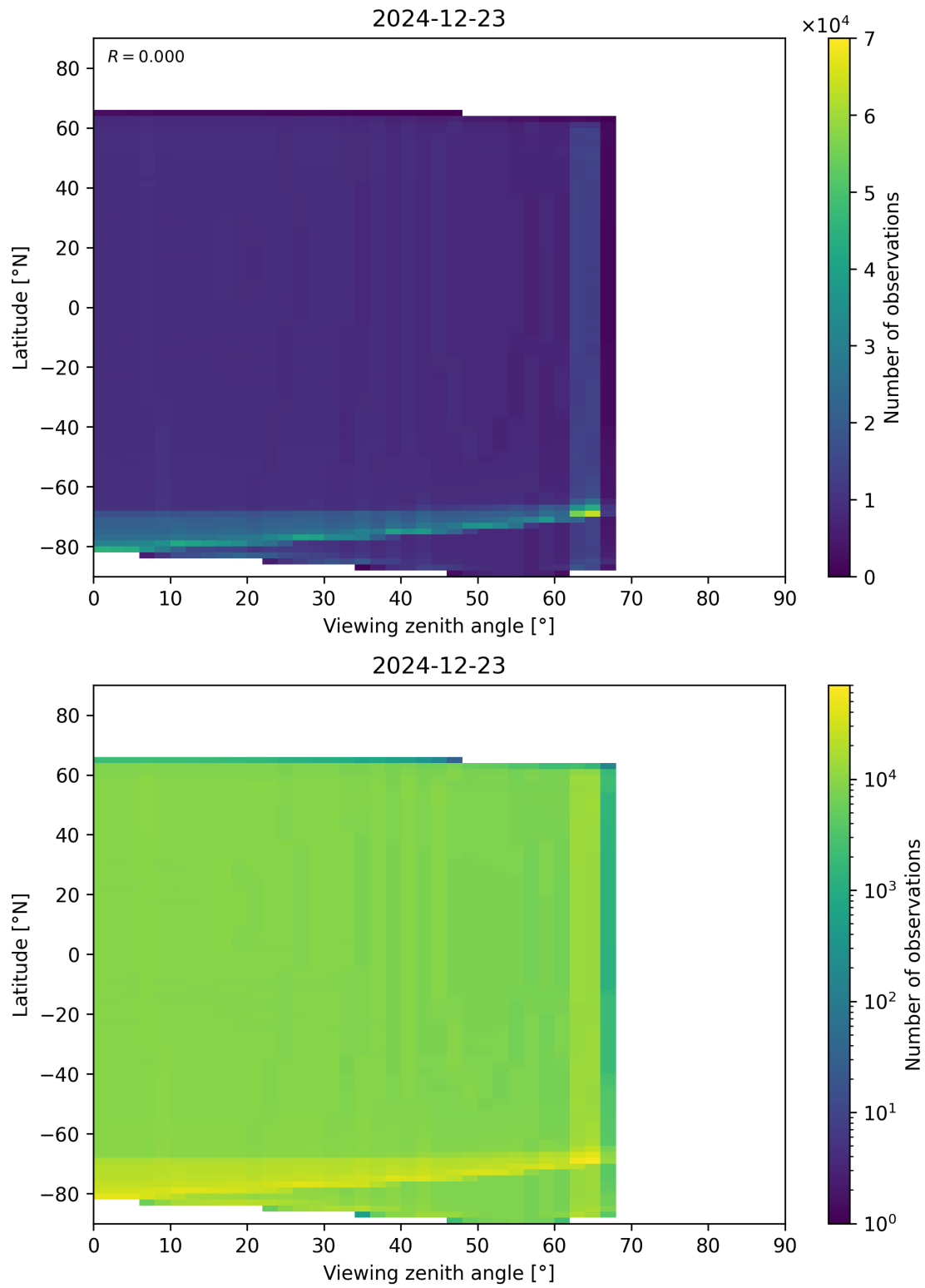
Figure 163: Scatter density plot of “Viewing zenith angle” against “Latitude” for 2024-12-22 to 2024-12-24.
