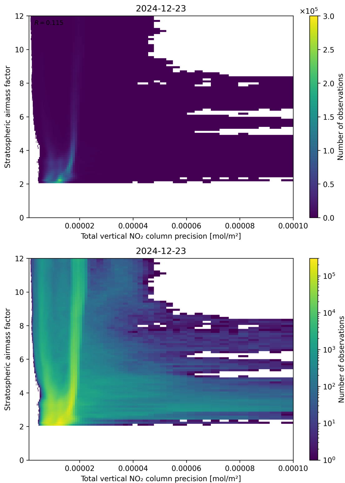
Figure 115: Scatter density plot of “Total vertical NO 2 column precision” against “Stratospheric air mass factor” for 2024-12-22 to 2024-12-24.
