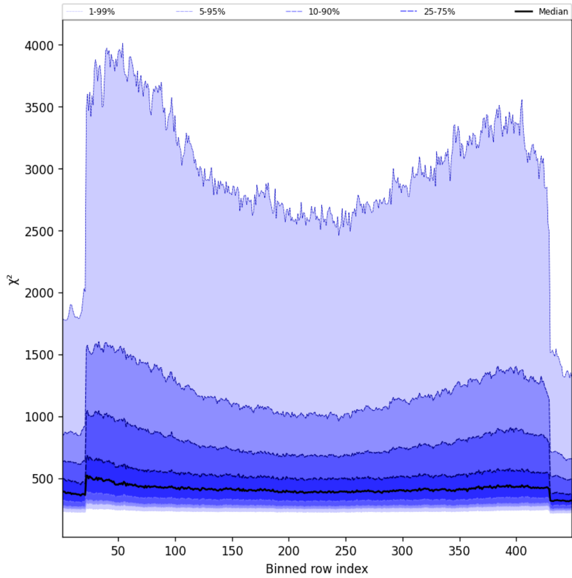
Figure 59: Along track statistics of “ \chi^2 ” for 2024-12-22 to 2024-12-24
