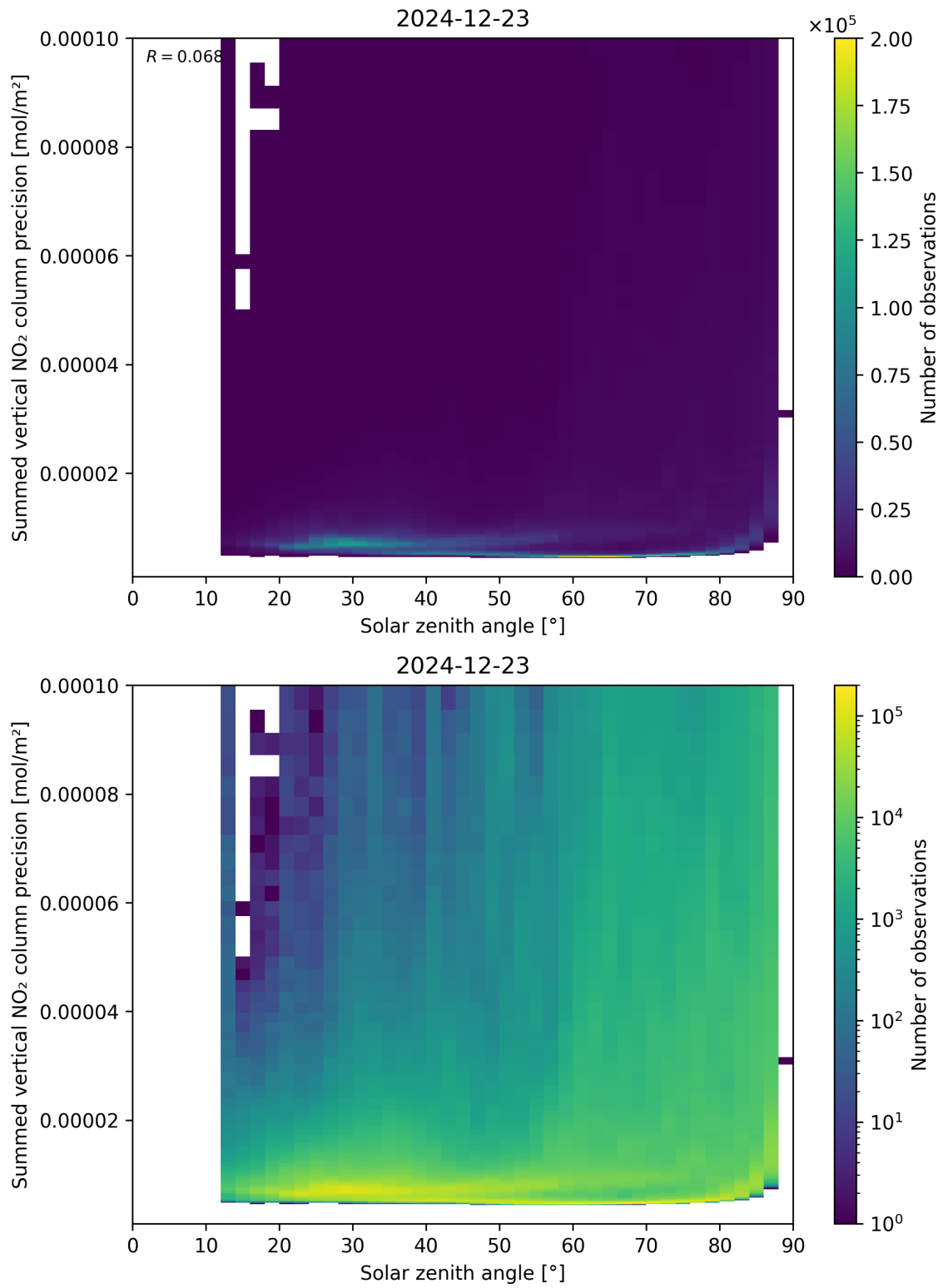
Figure 152: Scatter density plot of “Solar zenith angle” against “Summed vertical NO 2 column precision” for 2024-12-22 to 2024-12-24.
