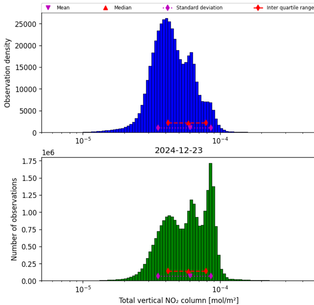
Figure 38: Histogram of “Total vertical NO 2 column” for 2024-12-22 to 2024-12-24
