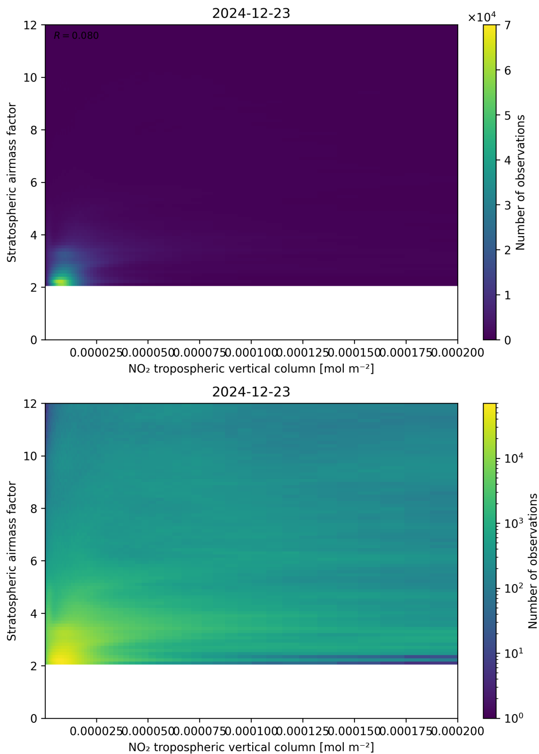
Figure 121: Scatter density plot of “NO 2 tropospheric vertical column” against “Stratospheric airmass factor” for 2024-12-22 to 2024-12-24.
