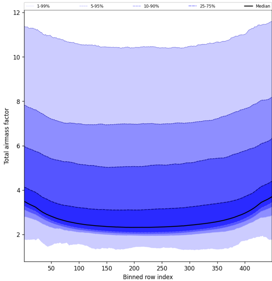
Figure 49: Along track statistics of “Total airmass factor” for 2024-12-22 to 2024-12-24
