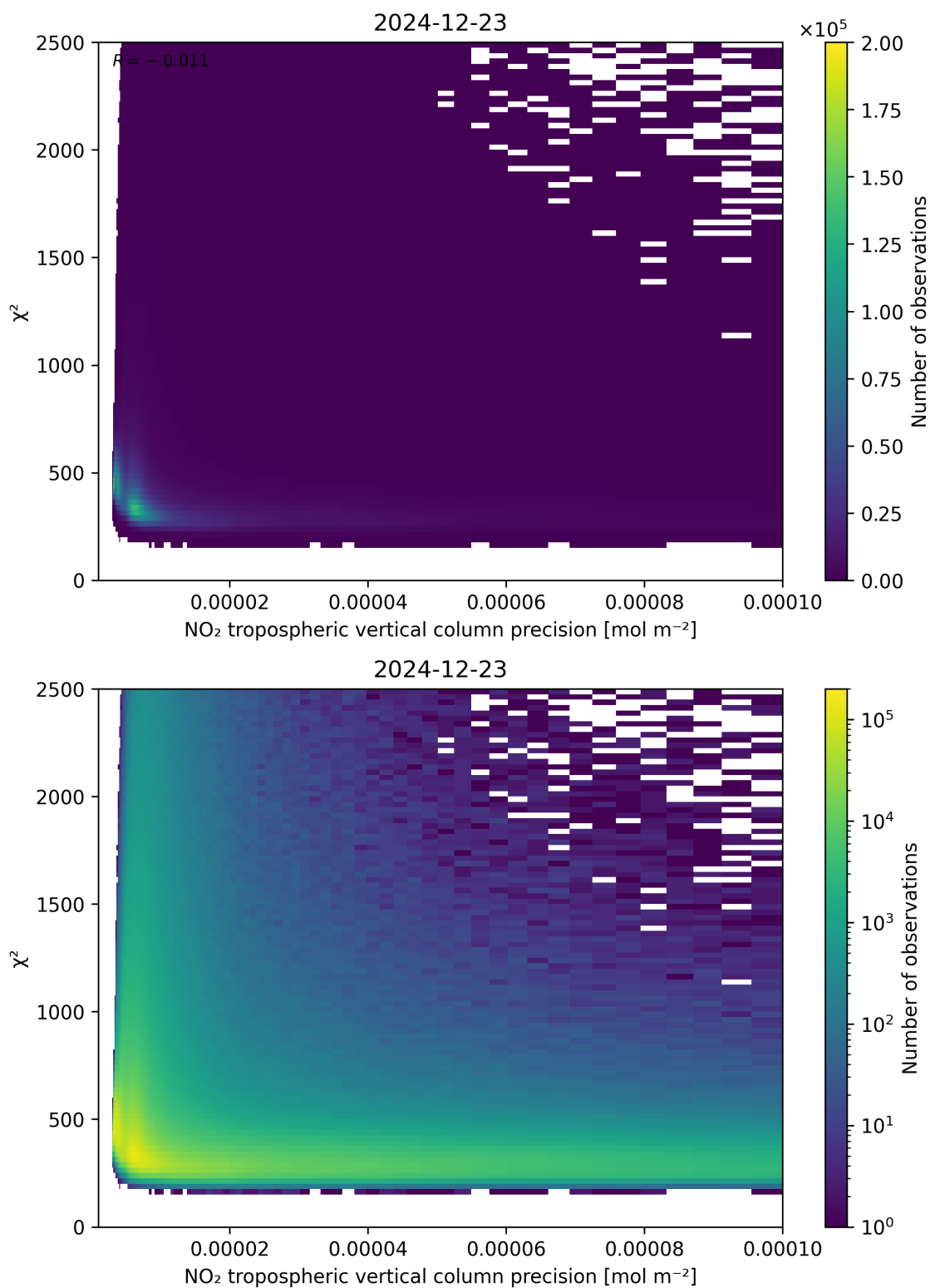
Figure 134: Scatter density plot of “NO 2 tropospheric vertical column precision” against “ \chi^2 ” for 2024-12-22 to 2024-12-24.
