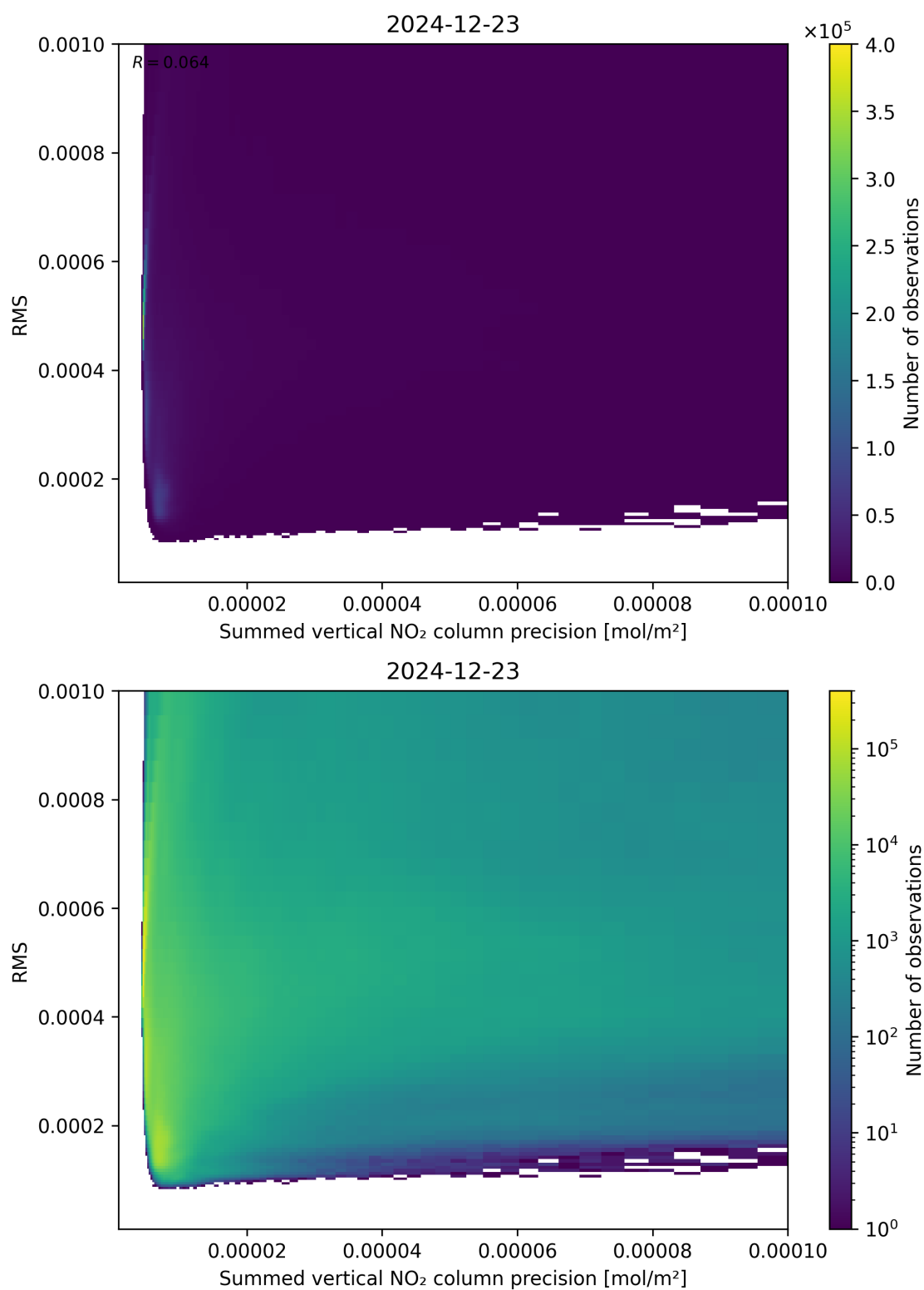
Figure 108: Scatter density plot of “Summed vertical NO 2 column precision” against “RMS” for 2024-12-22 to 2024-12-24.
