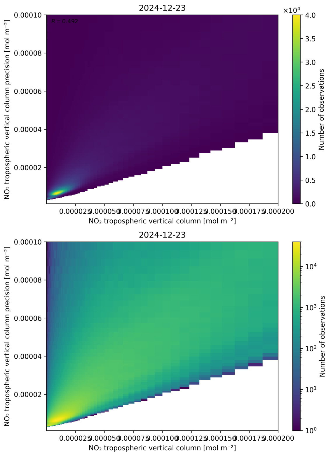
Figure 130: Scatter density plot of “NO 2 tropospheric vertical column” against “NO 2 tropospheric vertical column precision” for 2024-12-22 to 2024-12-24.
