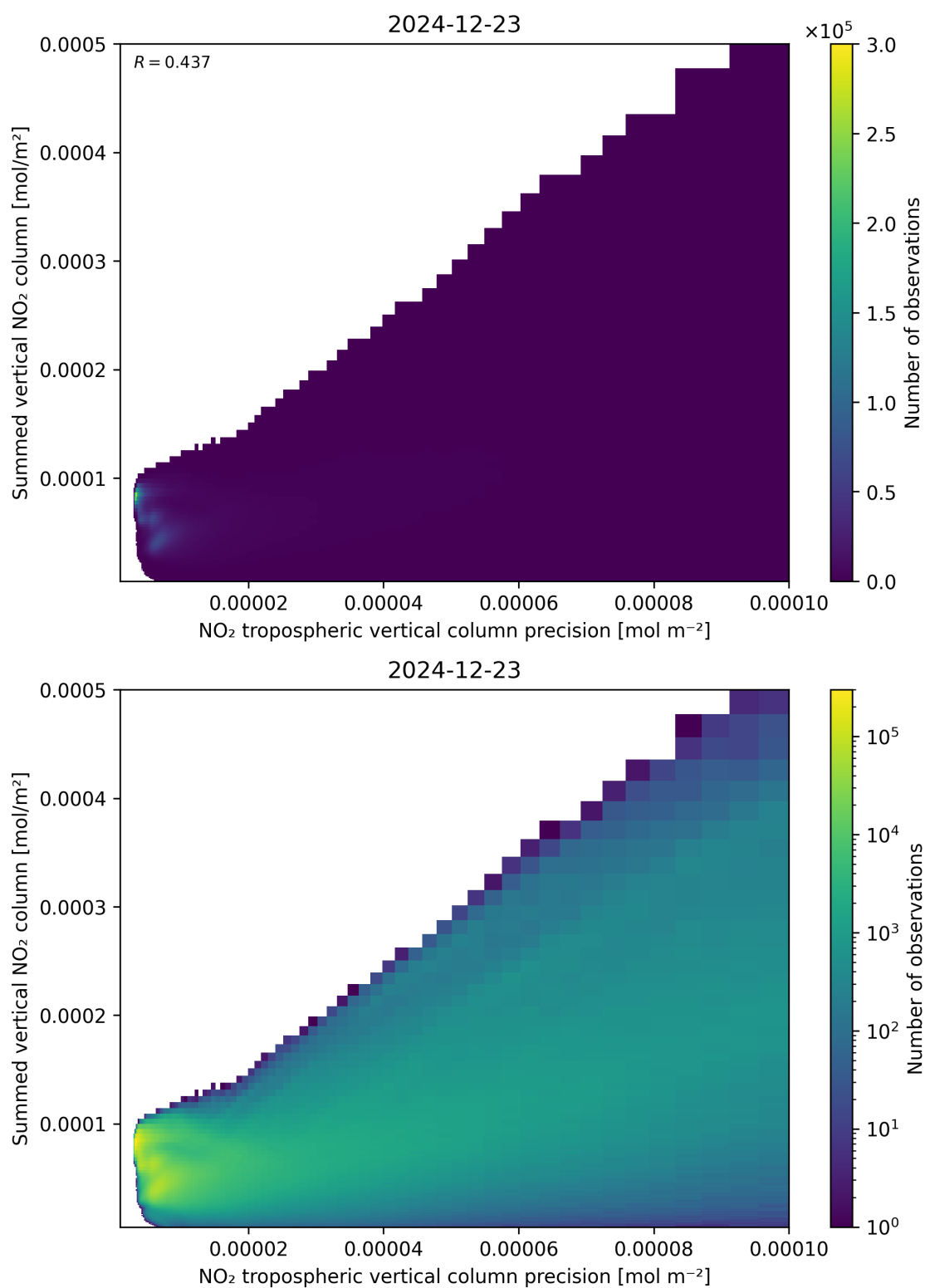
Figure 136: Scatter density plot of “NO 2 tropospheric vertical column precision” against “Summed vertical NO 2 column” for 2024-12-22 to 2024-12-24.
