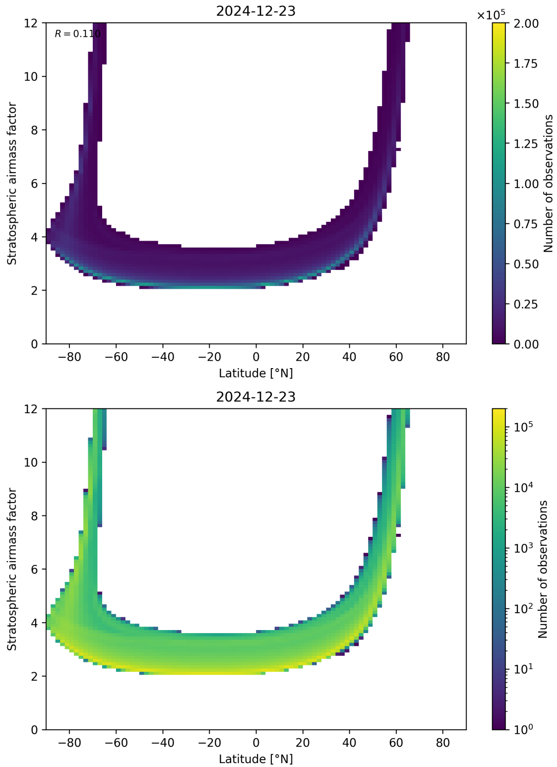
Figure 83: Scatter density plot of “Latitude” against “Stratospheric airmass factor” for 2024-12-22 to 2024-12-24.
