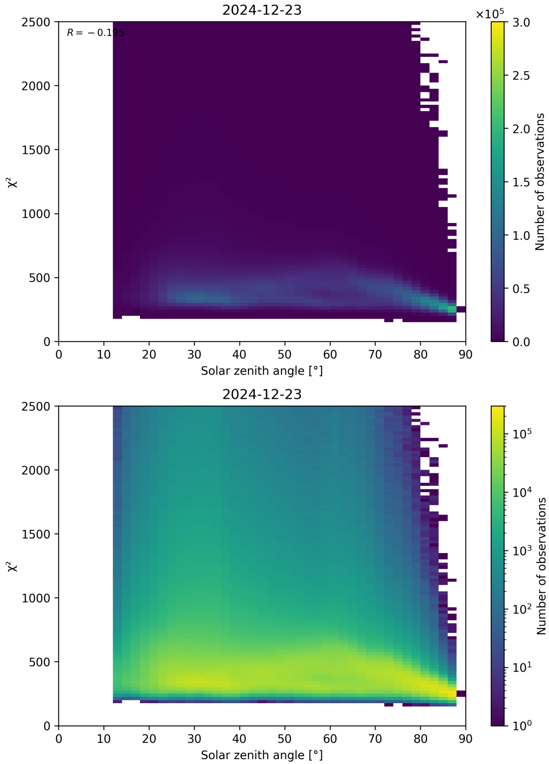
Figure 148: Scatter density plot of “Solar zenith angle” against “ \chi^2 ” for 2024-12-22 to 2024-12-24.
