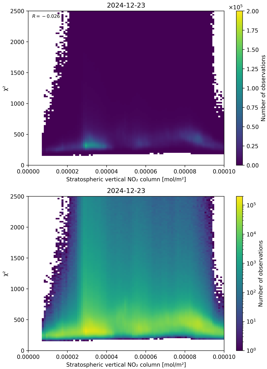
Figure 97: Scatter density plot of “Stratospheric vertical NO 2 column” against “ \chi^2 ” for 2024-12-22 to 2024-12-24.
