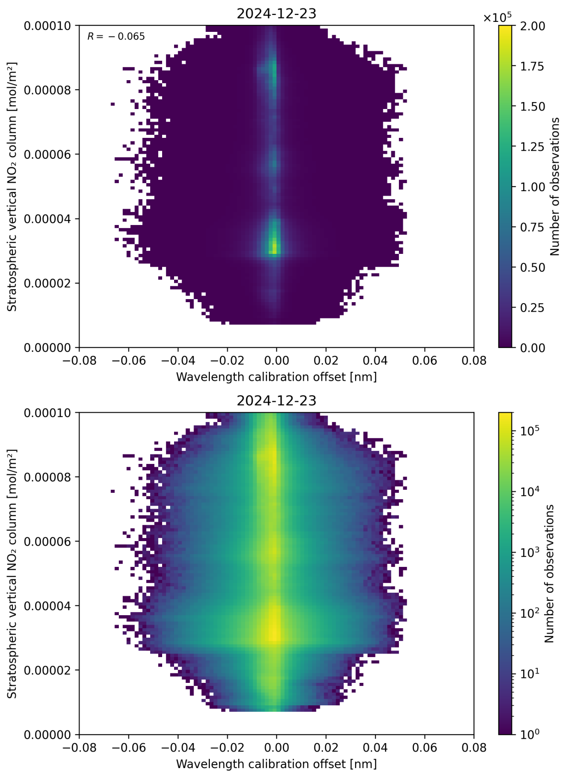
Figure 176: Scatter density plot of “Wavelength calibration offset” against “Stratospheric vertical NO 2 column” for 2024-12-22 to 2024-12-24.
