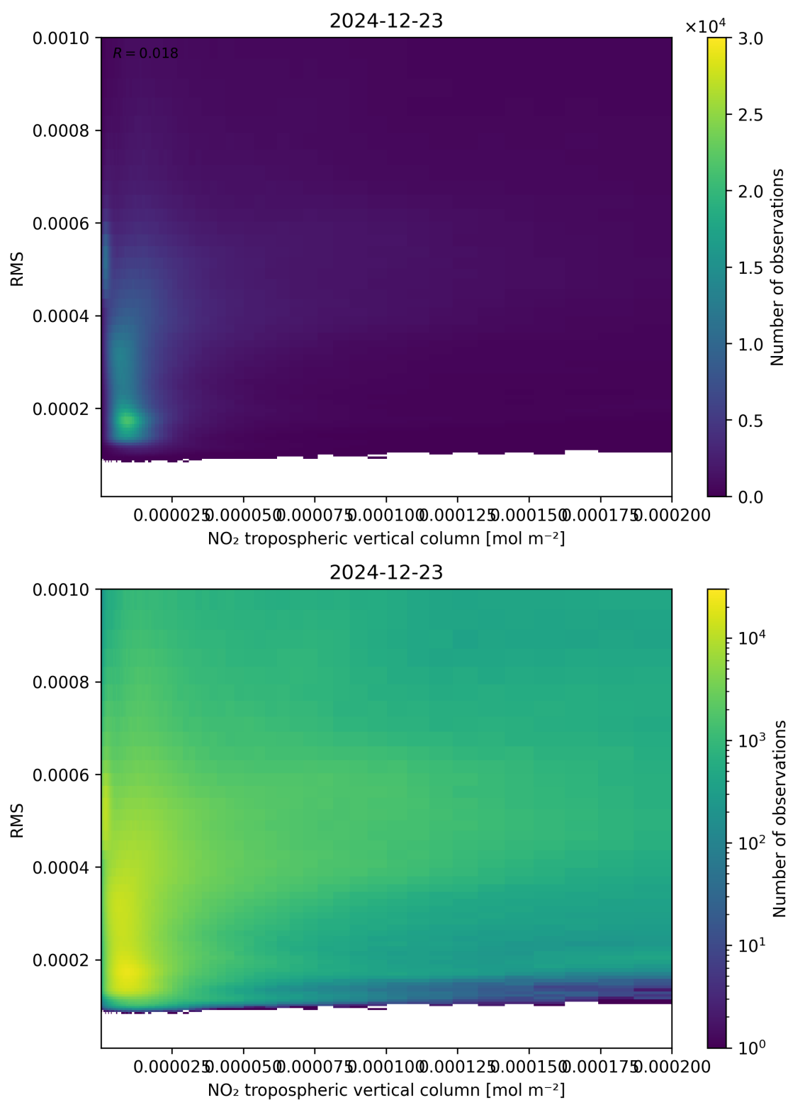
Figure 142: Scatter density plot of “NO 2 tropospheric vertical column” against “RMS” for 2024-12-22 to 2024-12-24.
