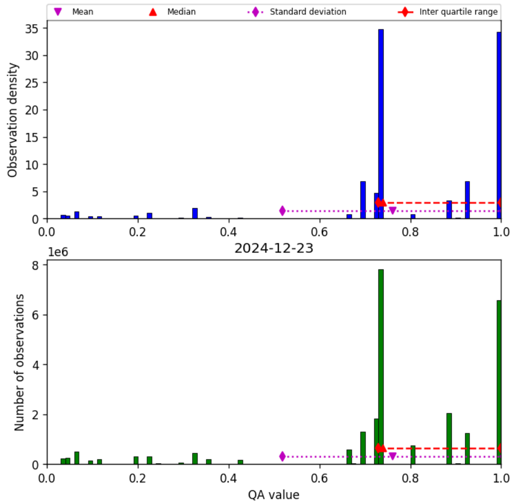
Figure 28: Histogram of “QA value” for 2024-12-22 to 2024-12-24
