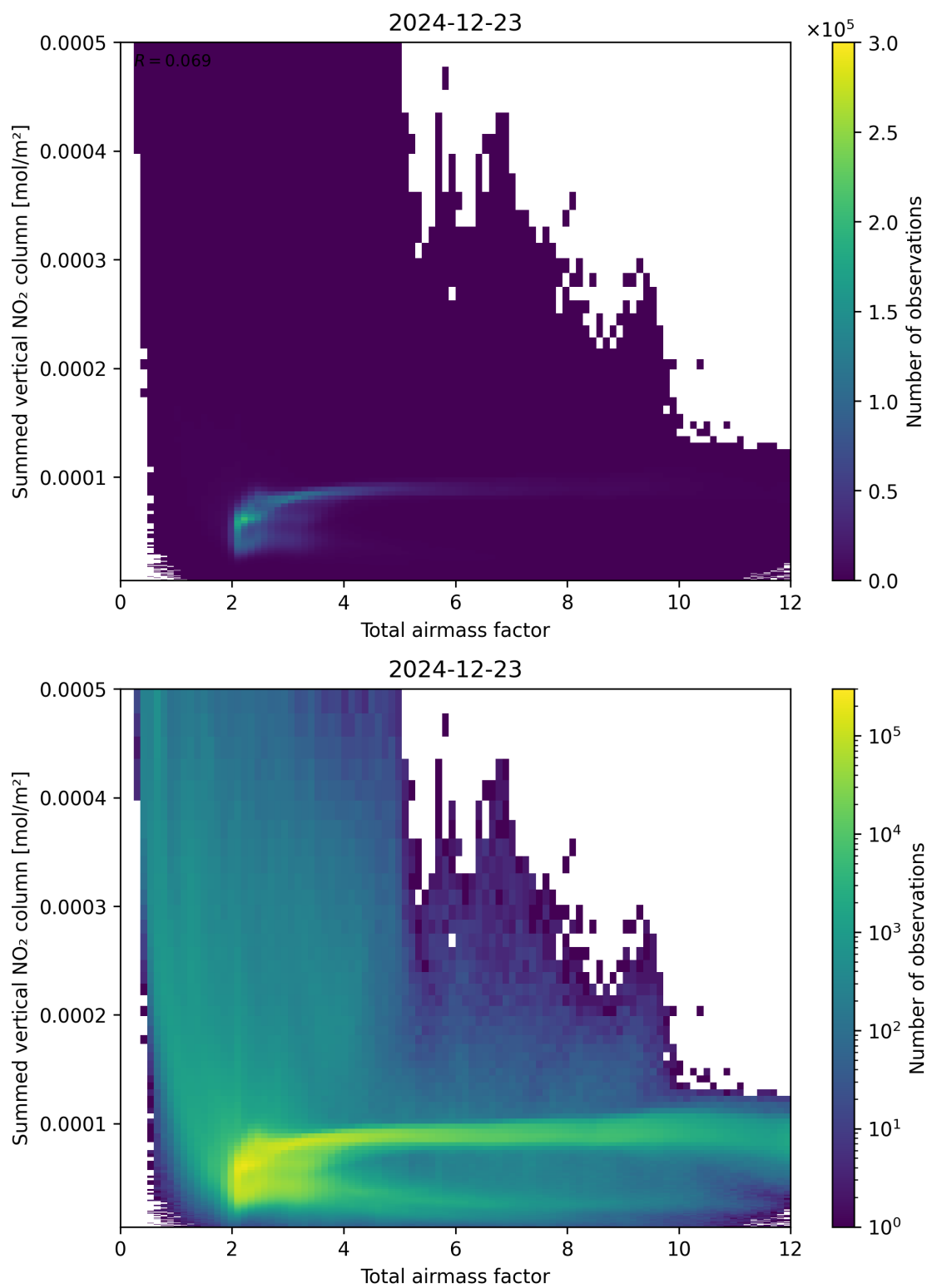
Figure 65: Scatter density plot of “Total airmass factor” against “Summed vertical NO 2 column” for 2024-12-22 to 2024-12-24.
