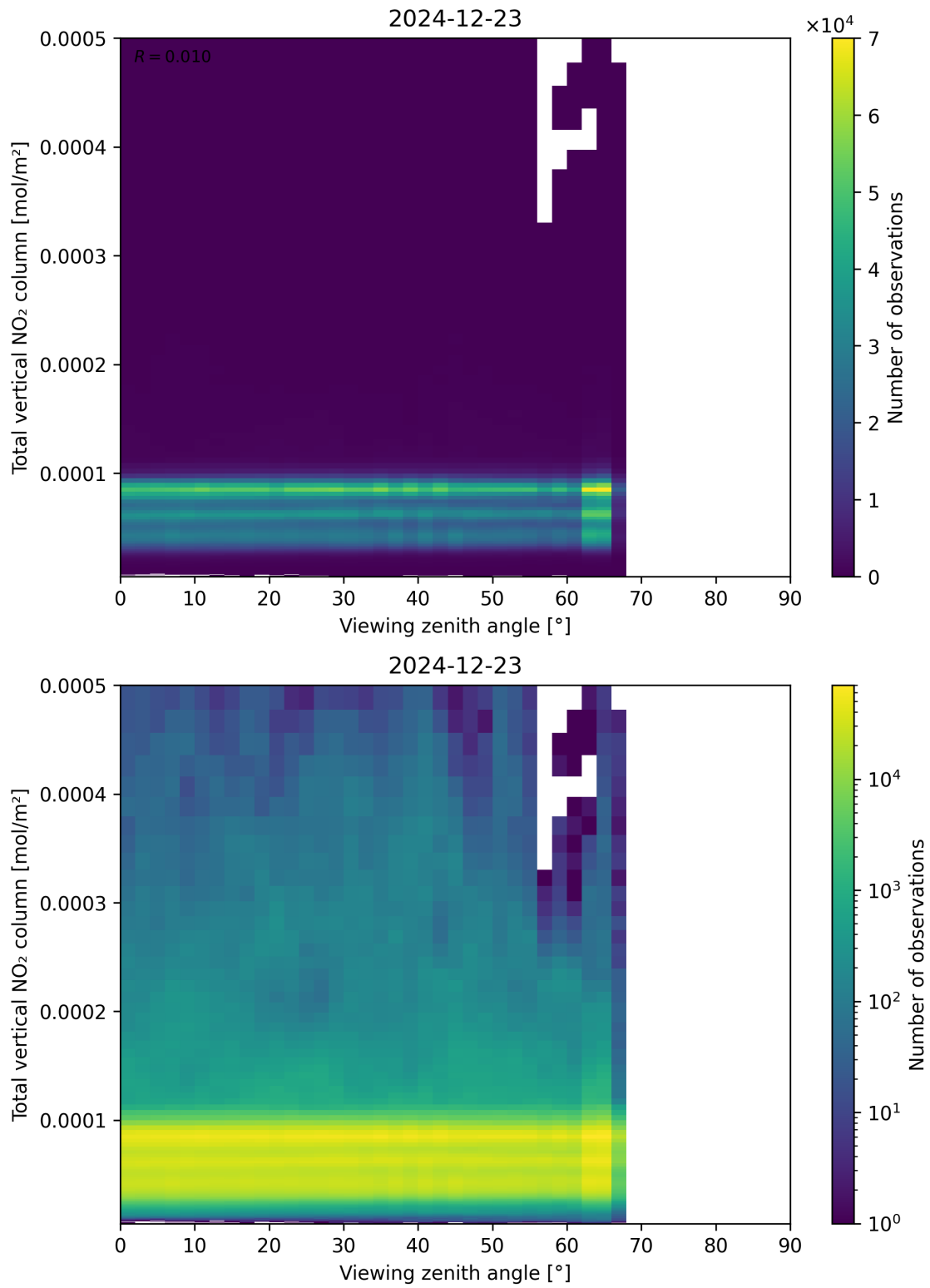
Figure 167: Scatter density plot of “Viewing zenith angle” against “Total vertical NO 2 column” for 2024-12-22 to 2024-12-24.
