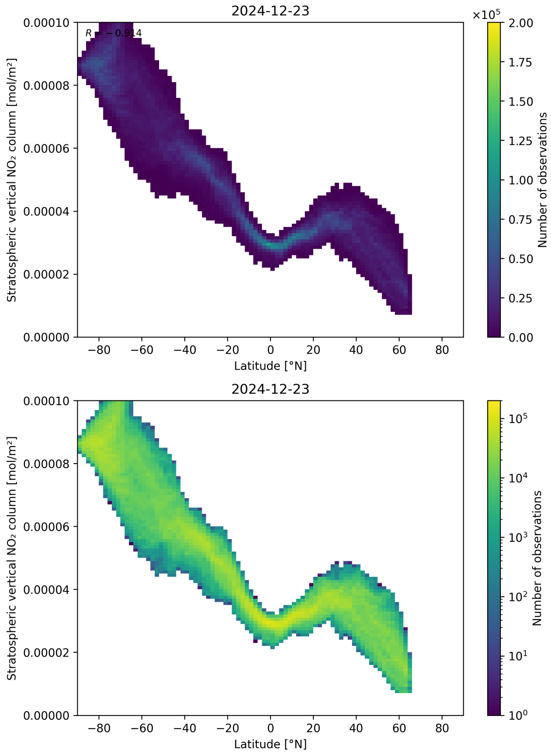
Figure 87: Scatter density plot of “Latitude” against “Stratospheric vertical NO 2 column” for 2024-12-22 to 2024-12-24.
