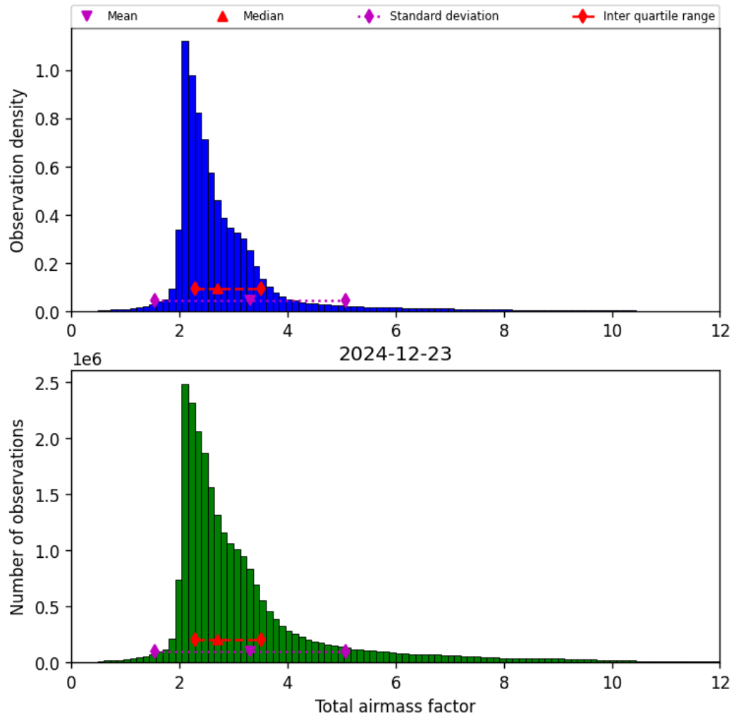
Figure 32: Histogram of “Total airmass factor” for 2024-12-22 to 2024-12-24
