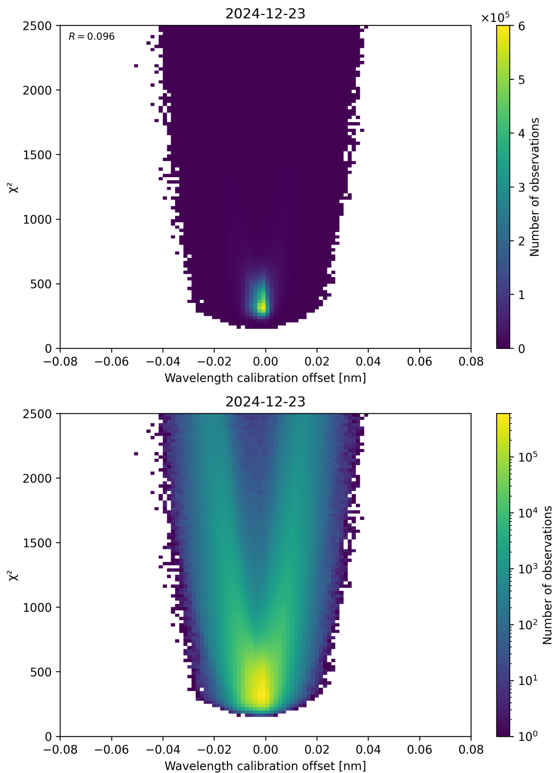
Figure 175: Scatter density plot of “Wavelength calibration offset” against “ \chi^2 ” for 2024-12-22 to 2024-12-24.
