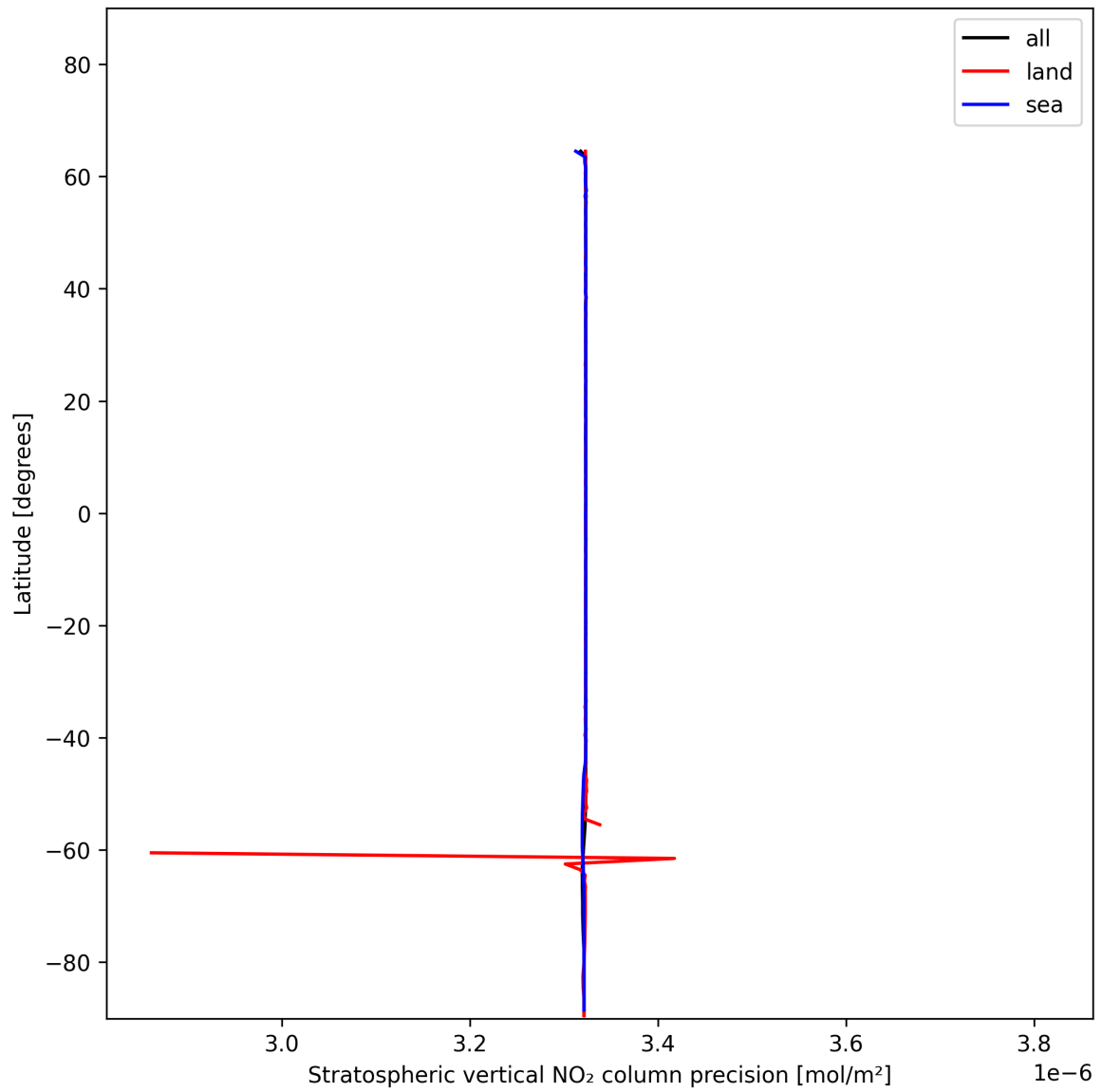
Figure 20: Zonal average of “Stratospheric vertical NO 2 column precision” for 2024-12-22 to 2024-12-24.
