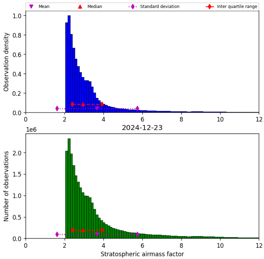
Figure 44: Histogram of “Stratospheric airmass factor” for 2024-12-22 to 2024-12-24
