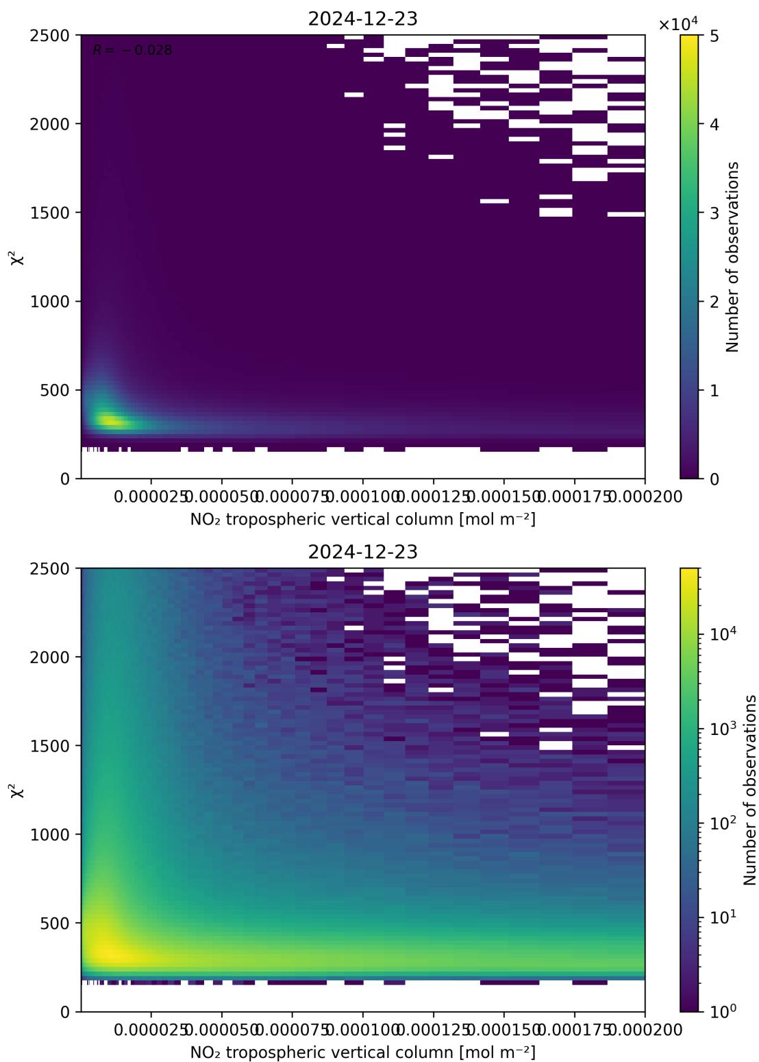
Figure 124: Scatter density plot of “NO 2 tropospheric vertical column” against “ \chi^2 ” for 2024-12-22 to 2024-12-24.
