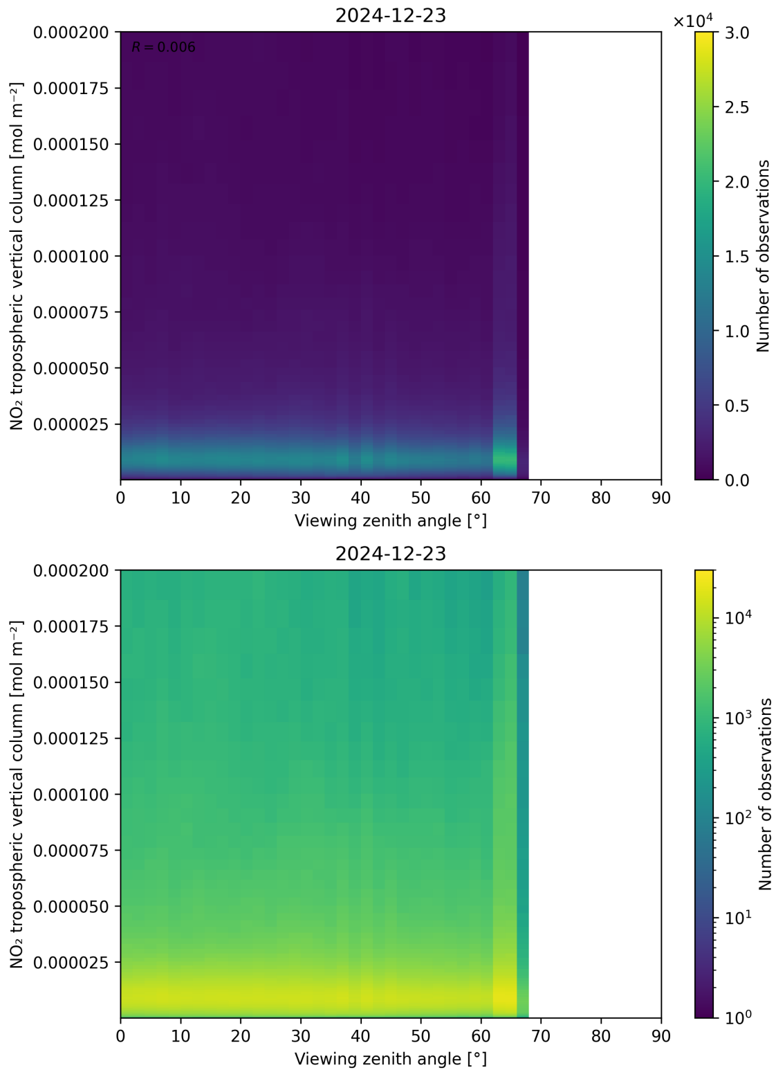
Figure 169: Scatter density plot of “Viewing zenith angle” against “NO 2 tropospheric vertical column” for 2024-12-22 to 2024-12-24.
