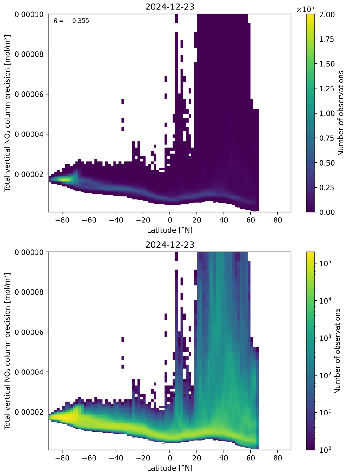
Figure 91: Scatter density plot of “Latitude” against “Total vertical NO 2 column precision” for 2024-12-22 to 2024-12-24.
