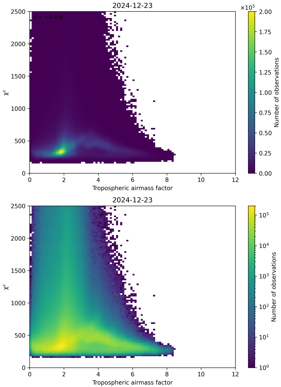
Figure 73: Scatter density plot of “Tropospheric airmass factor” against “ \chi^2 ” for 2024-12-22 to 2024-12-24.
