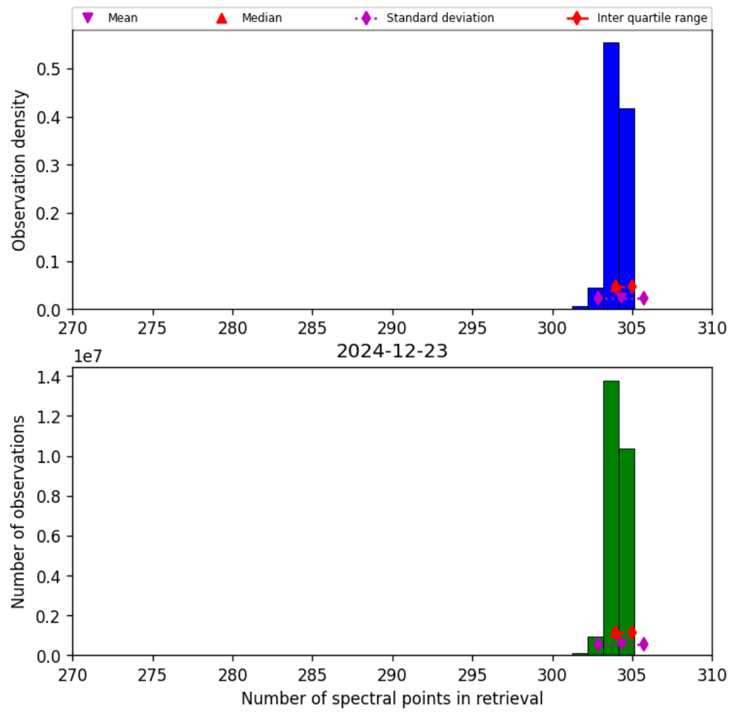
Figure 33: Histogram of “Number of spectral points in retrieval” for 2024-12-22 to 2024-12-24
