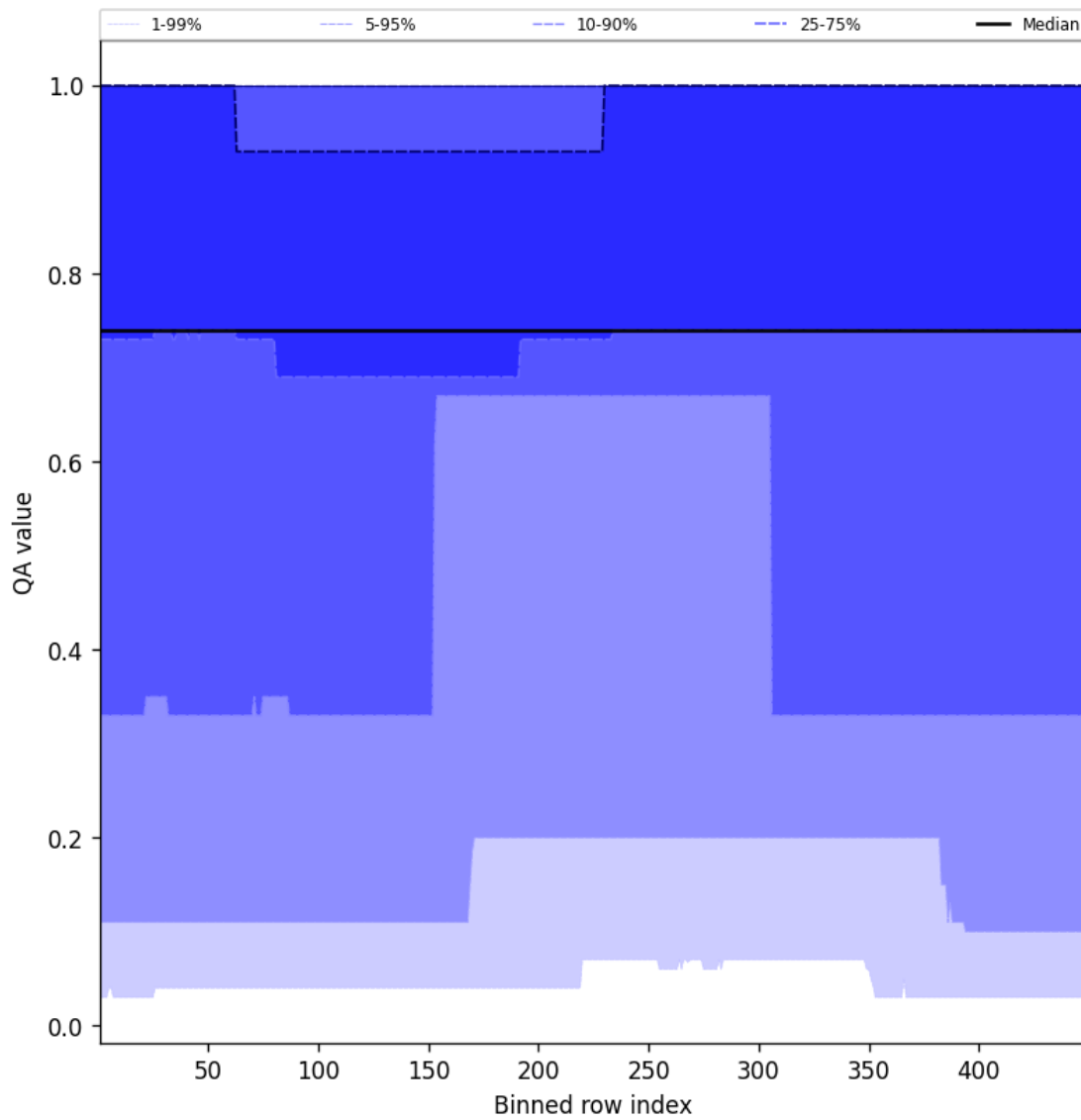
Figure 45: Along track statistics of “QA value” for 2024-12-22 to 2024-12-24
