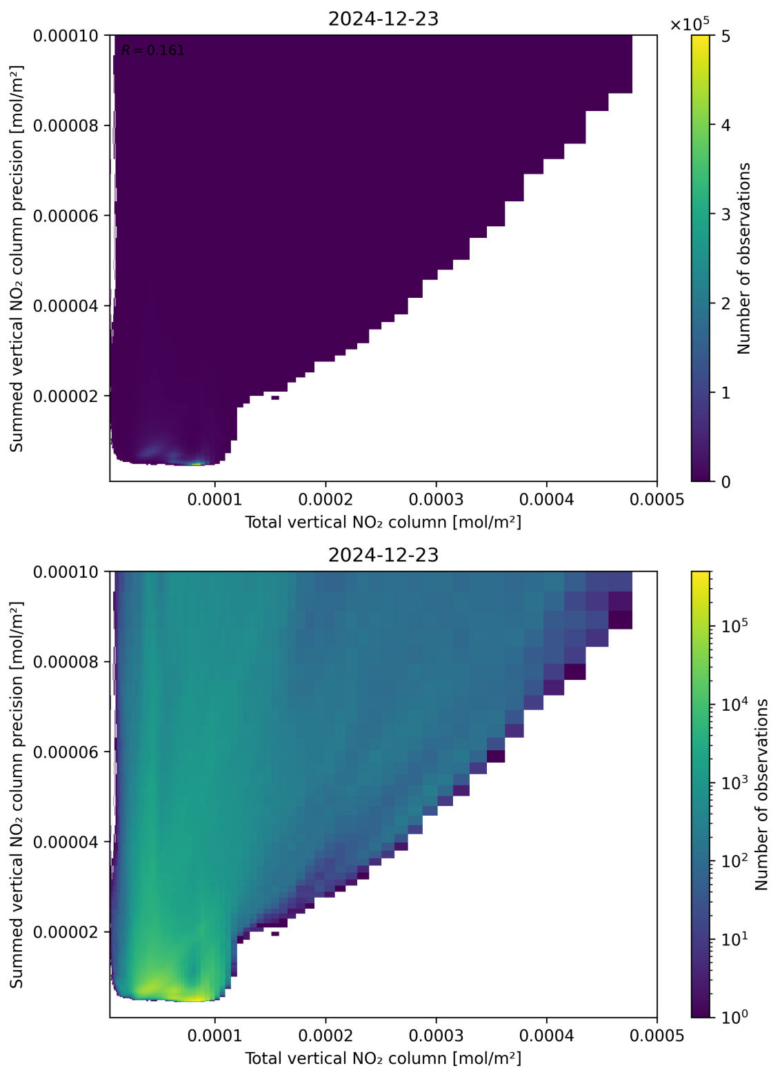
Figure 113: Scatter density plot of “Total vertical NO 2 column” against “Summed vertical NO 2 column precision” for 2024-12-22 to 2024-12-24.
