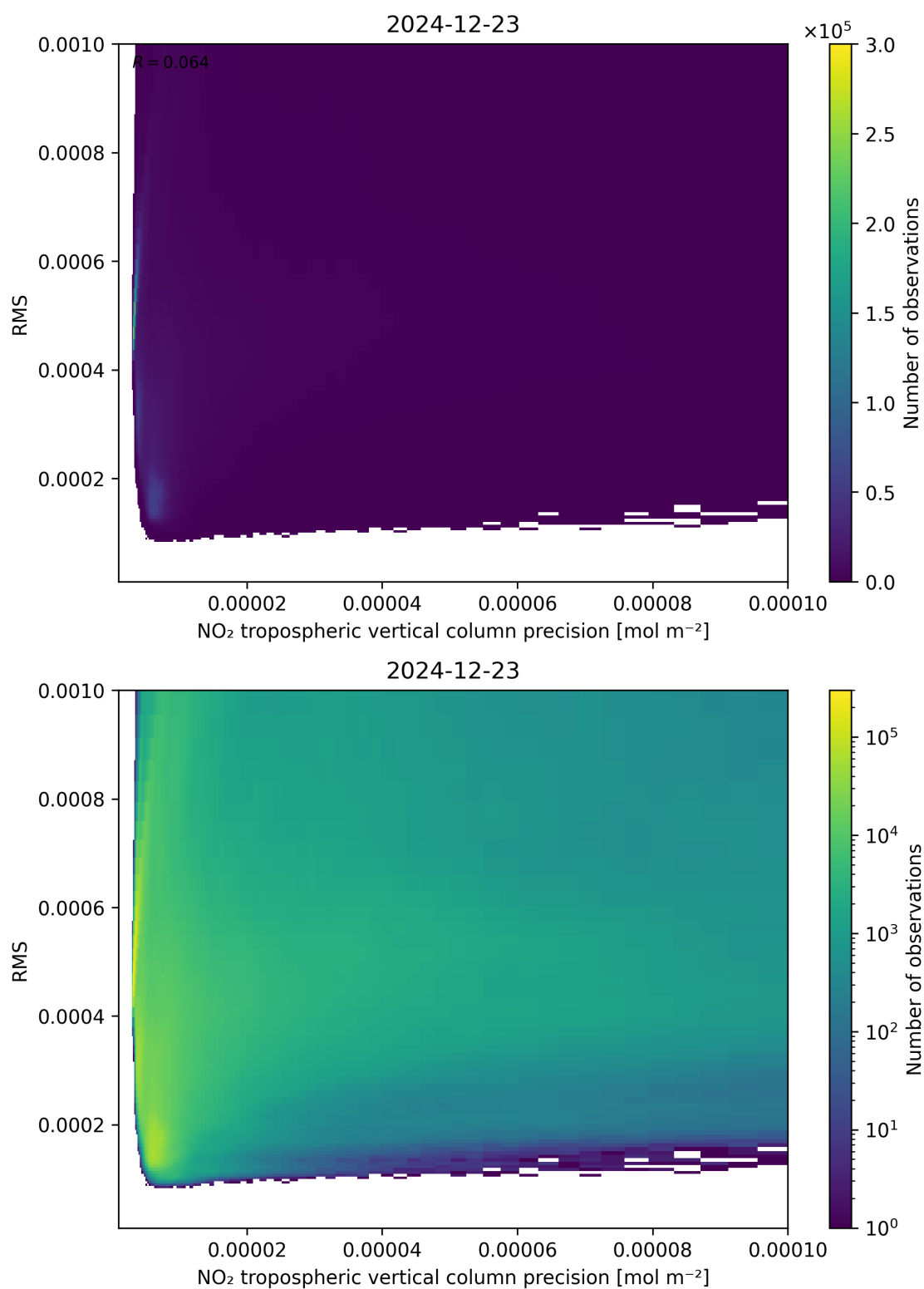
Figure 140: Scatter density plot of “NO 2 tropospheric vertical column precision” against “RMS” for 2024-12-22 to 2024-12-24.
