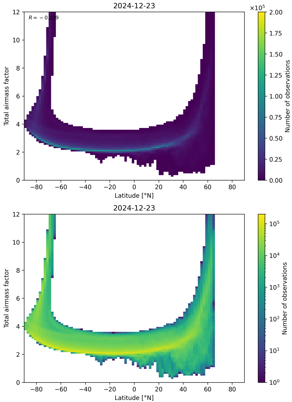
Figure 84: Scatter density plot of “Latitude” against “Total airmass factor” for 2024-12-22 to 2024-12-24.
