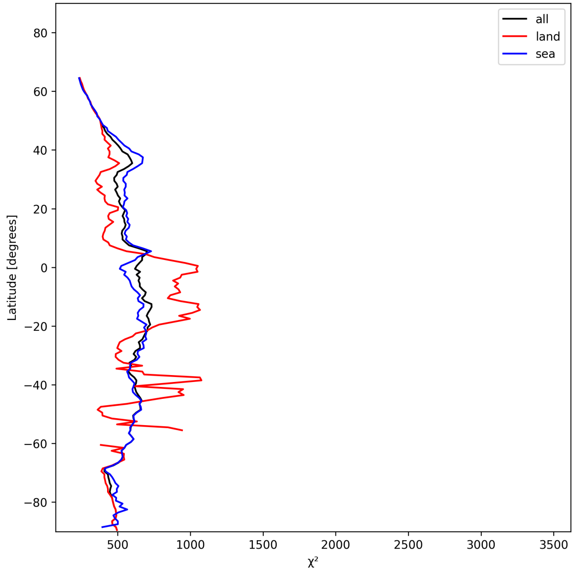
Figure 25: Zonal average of “ \chi^2 ” for 2024-12-22 to 2024-12-24.
