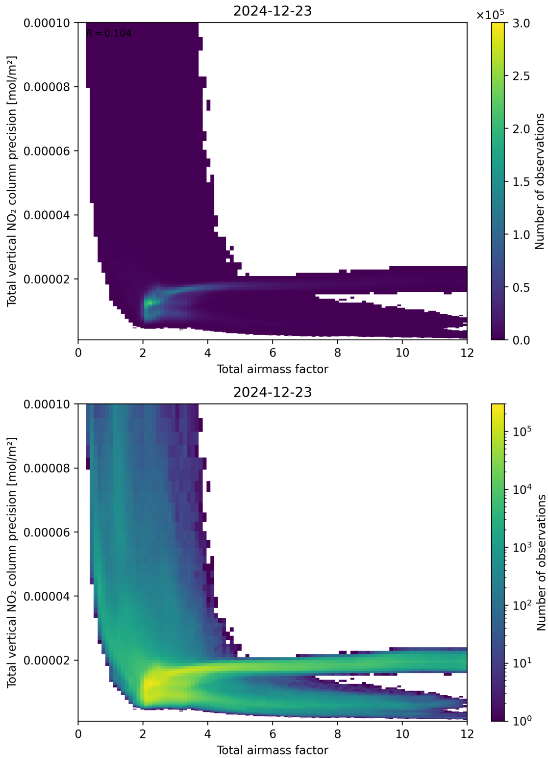
Figure 68: Scatter density plot of “Total airmass factor” against “Total vertical NO 2 column precision” for 2024-12-22 to 2024-12-24.
