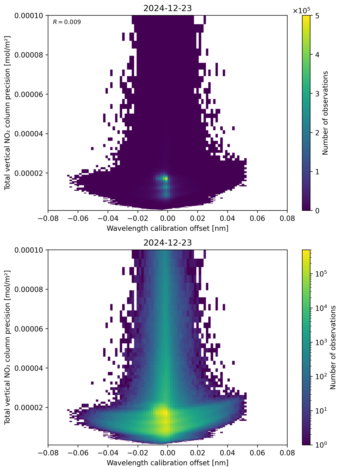
Figure 180: Scatter density plot of “Wavelength calibration offset” against “Total vertical NO 2 column precision” for 2024-12-22 to 2024-12-24.
