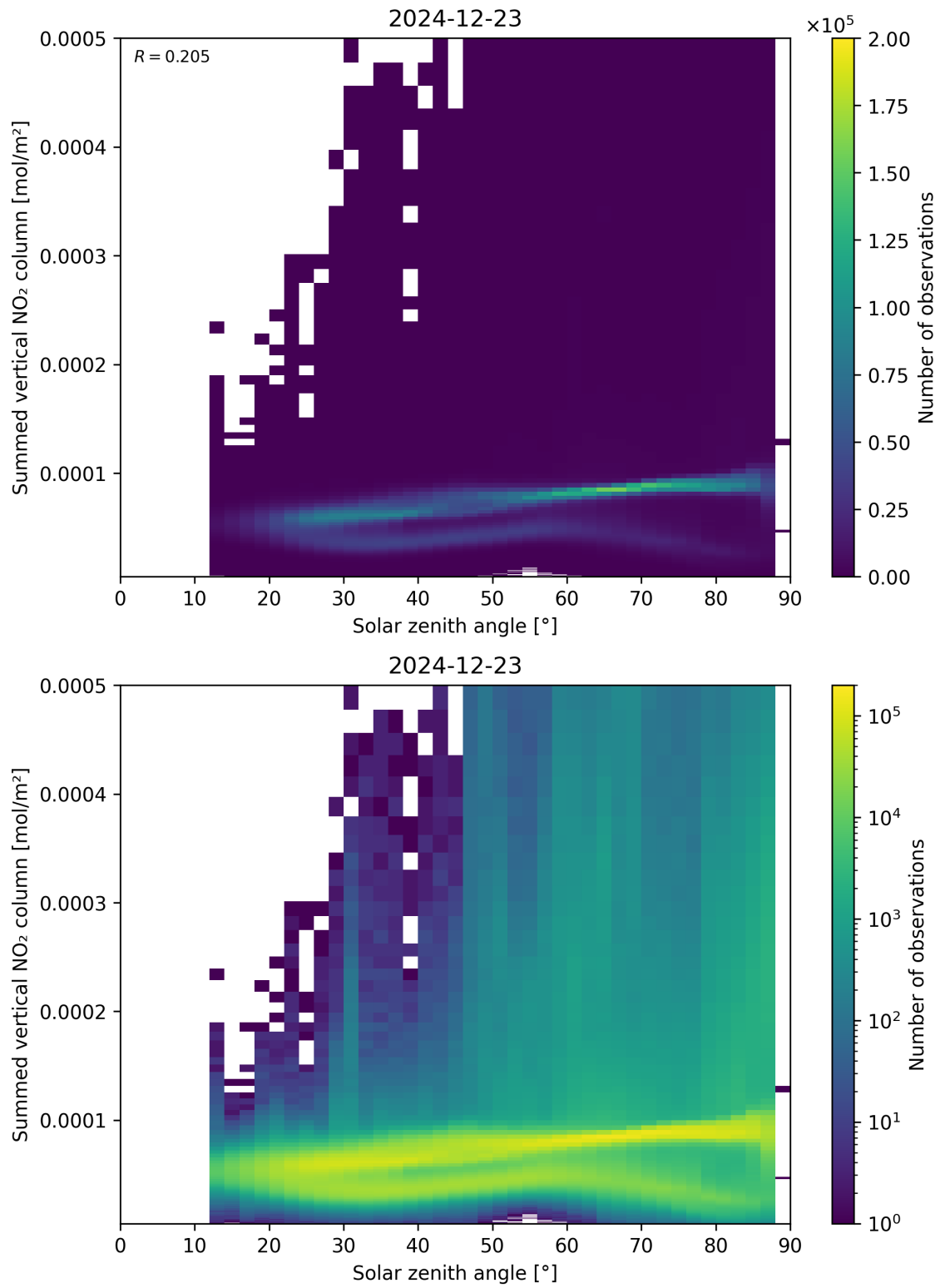
Figure 151: Scatter density plot of “Solar zenith angle” against “Summed vertical NO 2 column” for 2024-12-22 to 2024-12-24.
