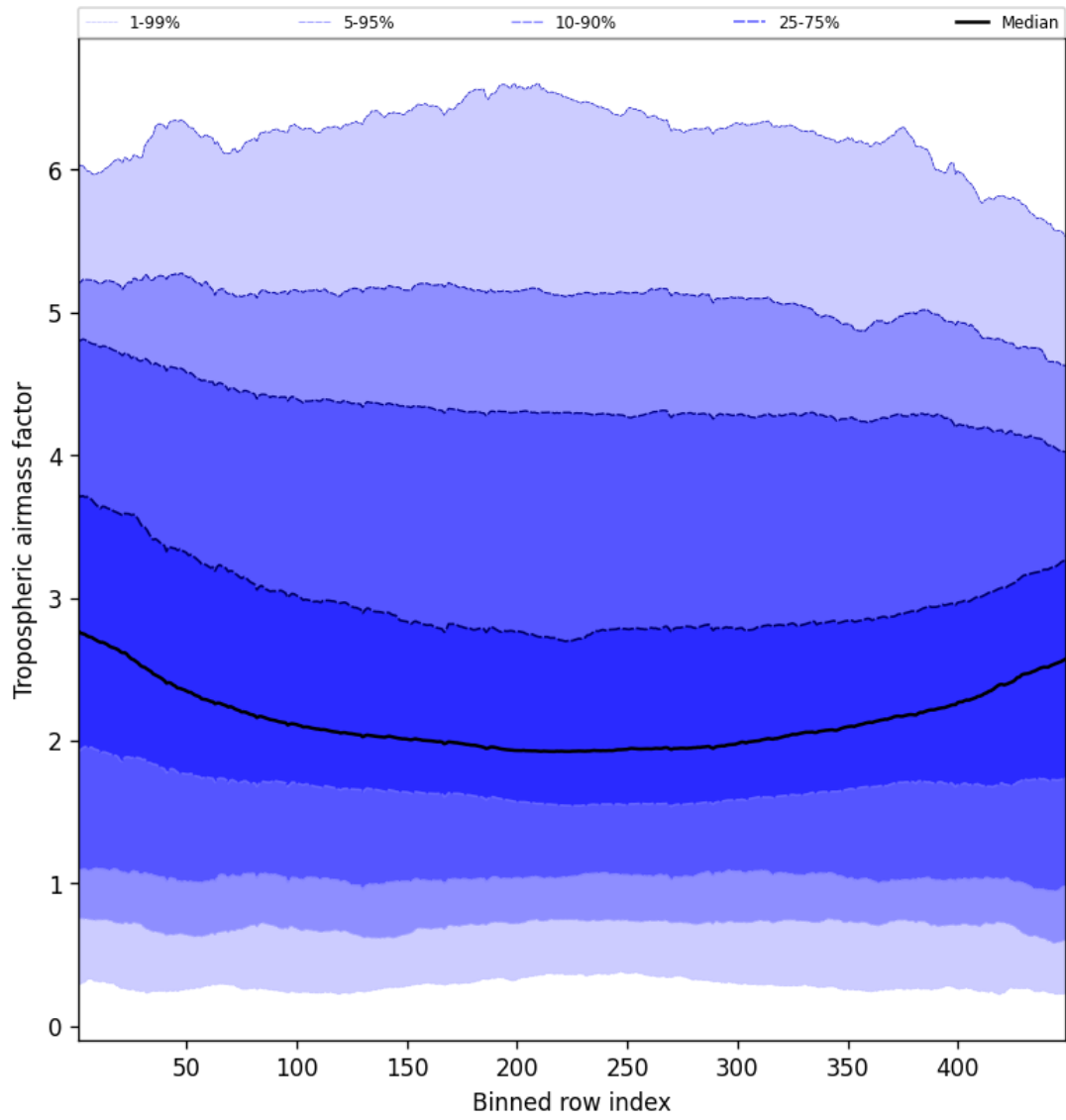
Figure 48: Along track statistics of “Tropospheric air mass factor” for 2024-12-22 to 2024-12-24
