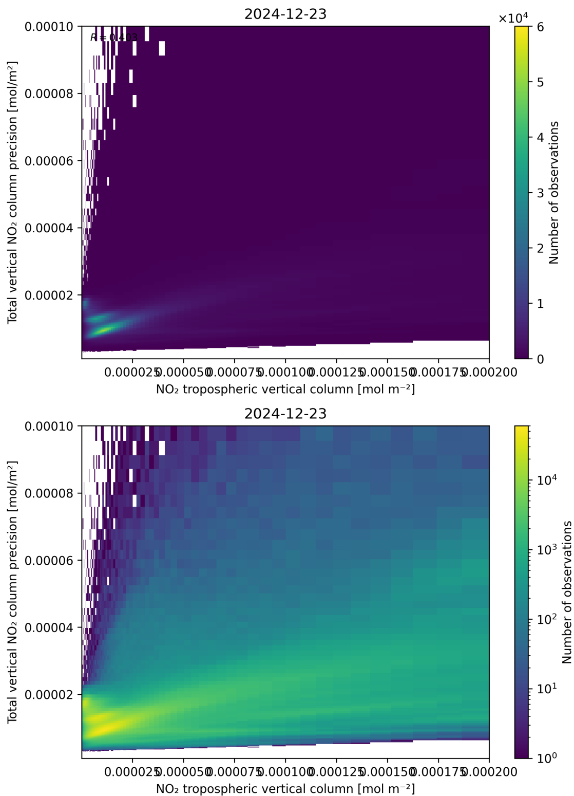
Figure 129: Scatter density plot of “NO 2 tropospheric vertical column” against “Total vertical NO 2 column precision” for 2024-12-22 to 2024-12-24.
