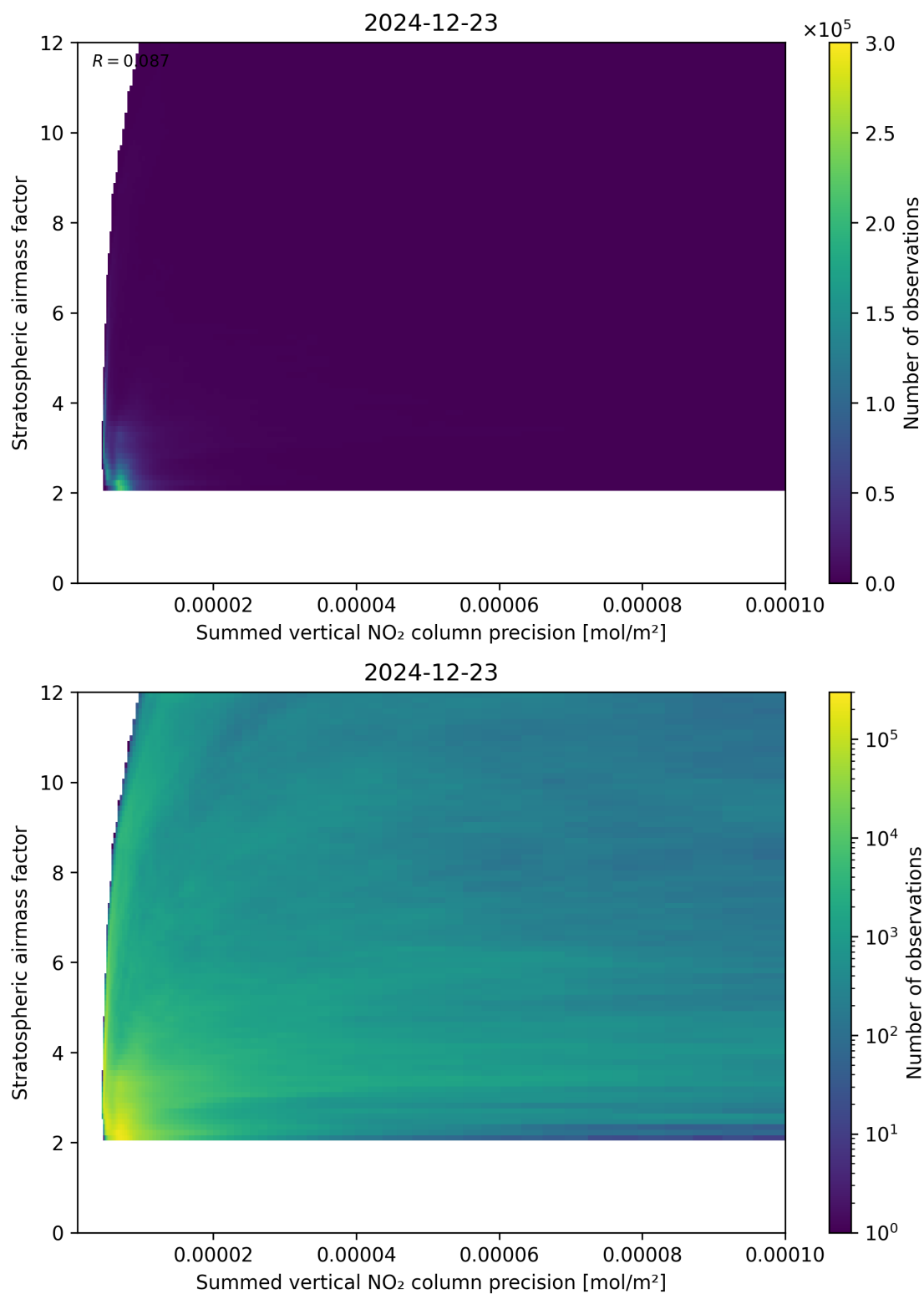
Figure 106: Scatter density plot of “Summed vertical NO 2 column precision” against “Stratospheric airmass factor” for 2024-12-22 to 2024-12-24.
