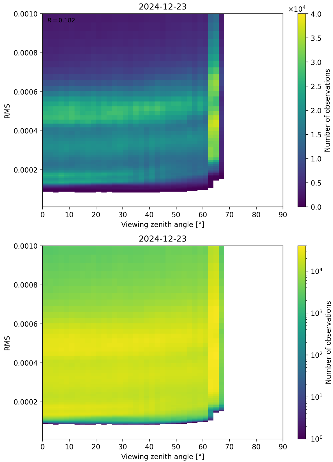
Figure 171: Scatter density plot of “Viewing zenith angle” against “RMS” for 2024-12-22 to 2024-12-24.
