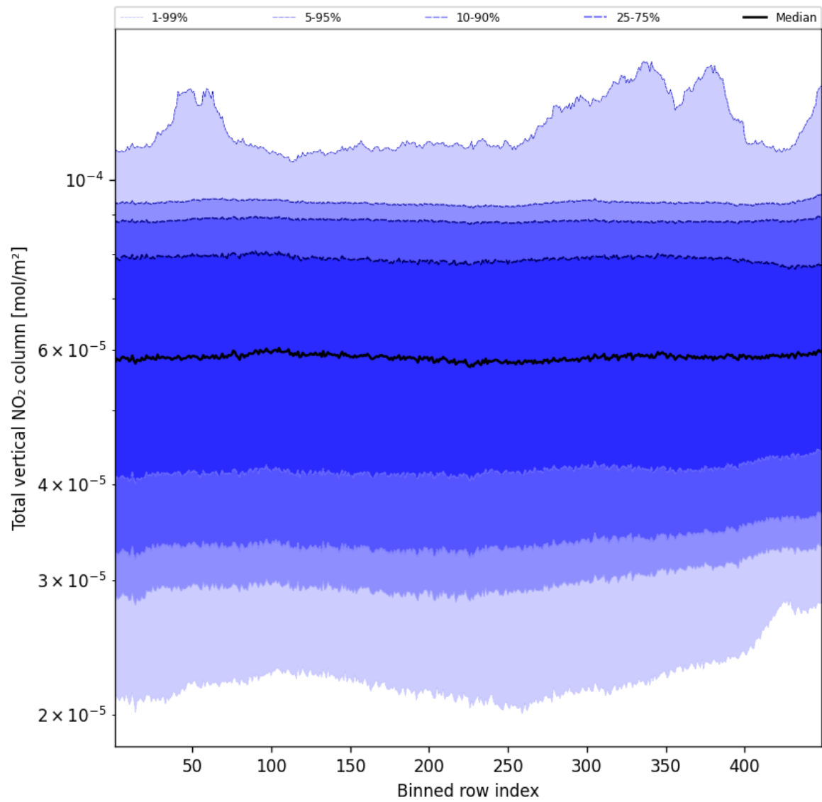
Figure 55: Along track statistics of “Total vertical NO 2 column” for 2024-12-22 to 2024-12-24
