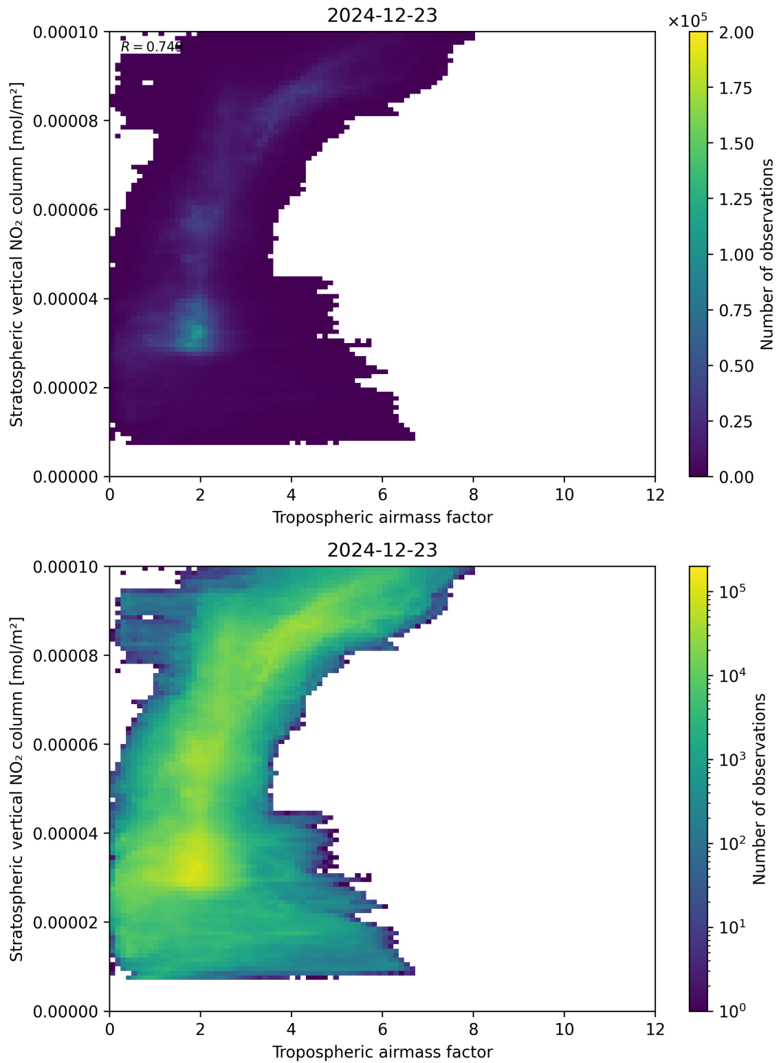
Figure 74: Scatter density plot of “Tropospheric air mass factor” against “Stratospheric vertical NO 2 column” for 2024-12-22 to 2024-12-24.
