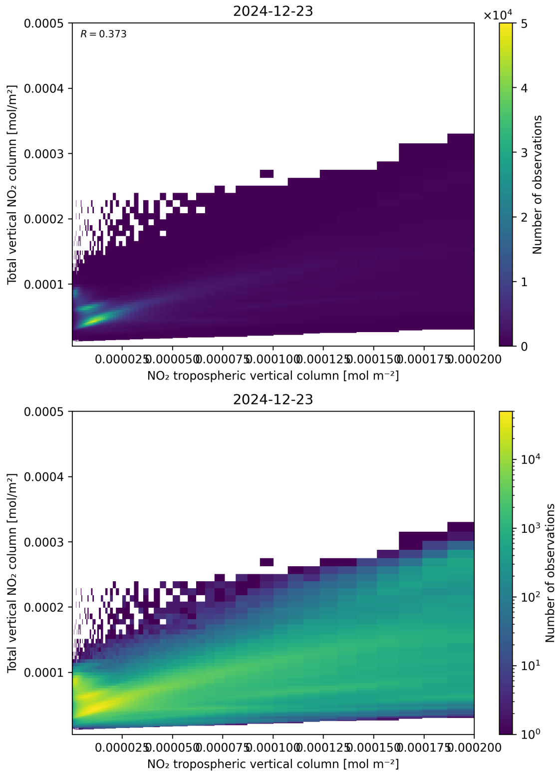
Figure 128: Scatter density plot of “NO 2 tropospheric vertical column” against “Total vertical NO 2 column” for 2024-12-22 to 2024-12-24.
