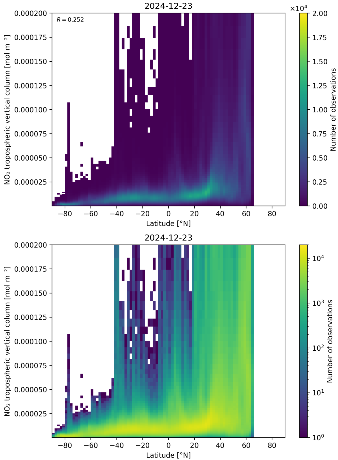
Figure 92: Scatter density plot of “Latitude” against “NO 2 tropospheric vertical column” for 2024-12-22 to 2024-12-24.
