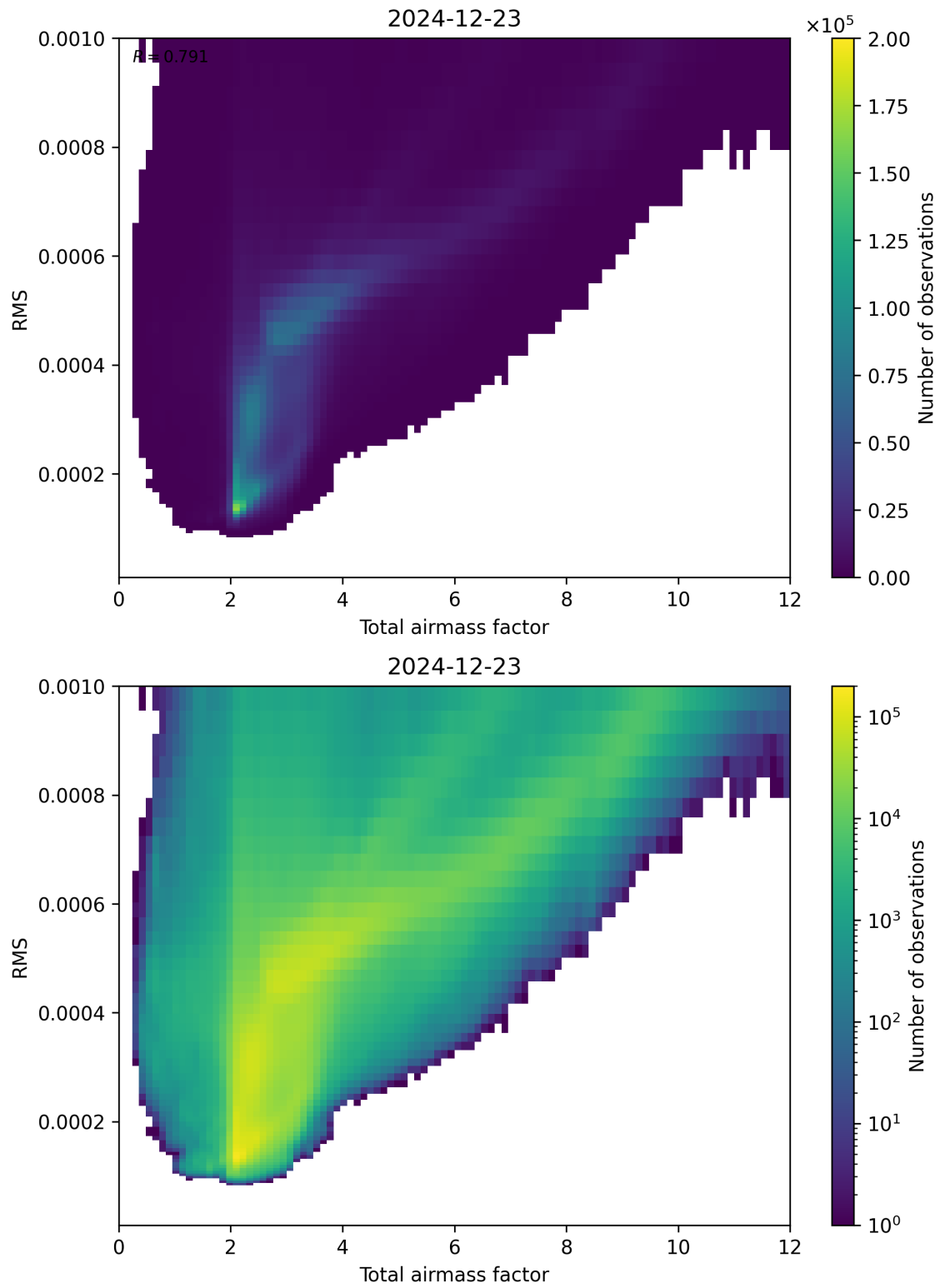
Figure 69: Scatter density plot of “Total airmass factor” against “RMS” for 2024-12-22 to 2024-12-24.
