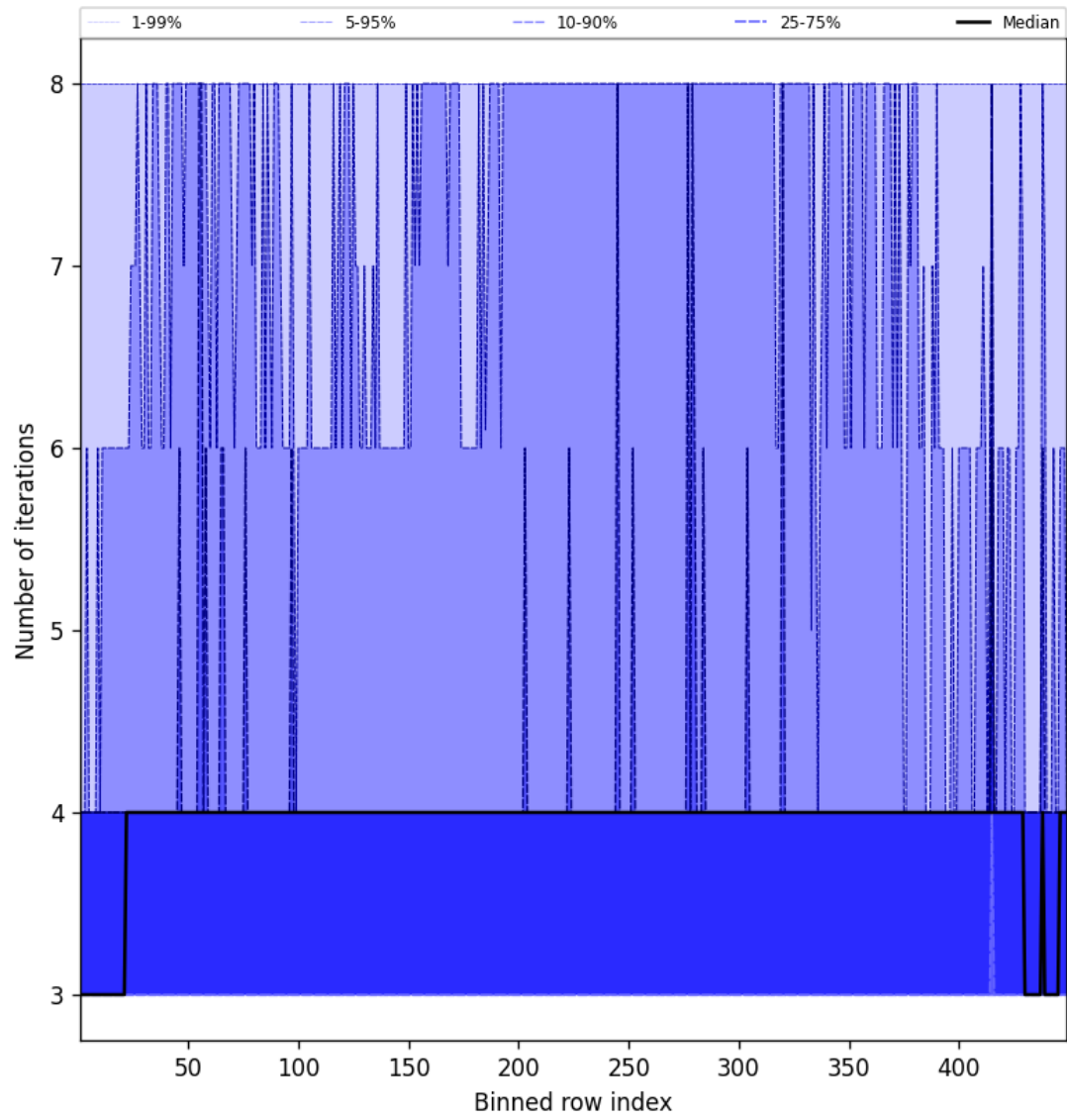
Figure 51: Along track statistics of “Number of iterations” for 2024-12-22 to 2024-12-24
