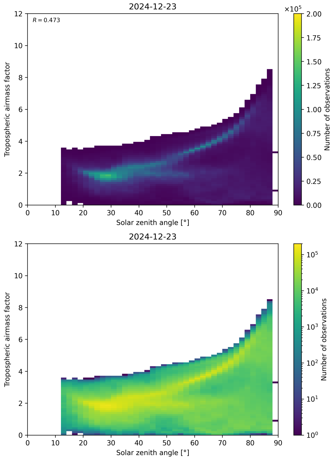
Figure 147: Scatter density plot of “Solar zenith angle” against “Tropospheric airmass factor” for 2024-12-22 to 2024-12-24.
