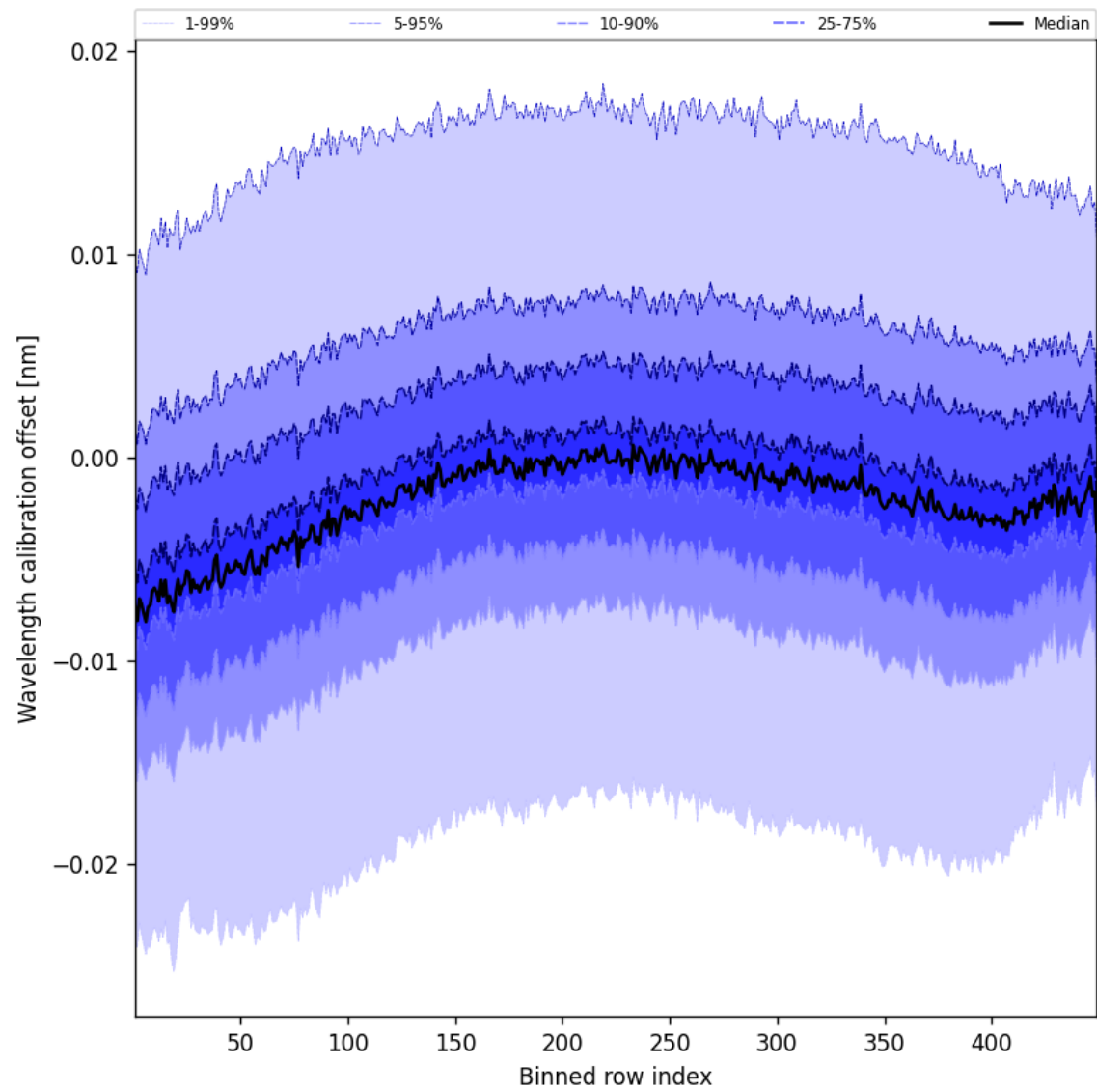
Figure 52: Along track statistics of “Wavelength calibration offset” for 2024-12-22 to 2024-12-24
