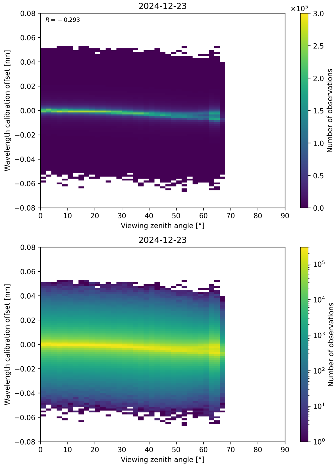
Figure 173: Scatter density plot of “Viewing zenith angle” against “Wavelength calibration offset” for 2024-12-22 to 2024-12-24.
