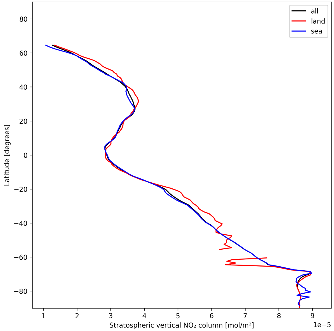
Figure 19: Zonal average of “Stratospheric vertical NO 2 column” for 2024-12-22 to 2024-12-24.
