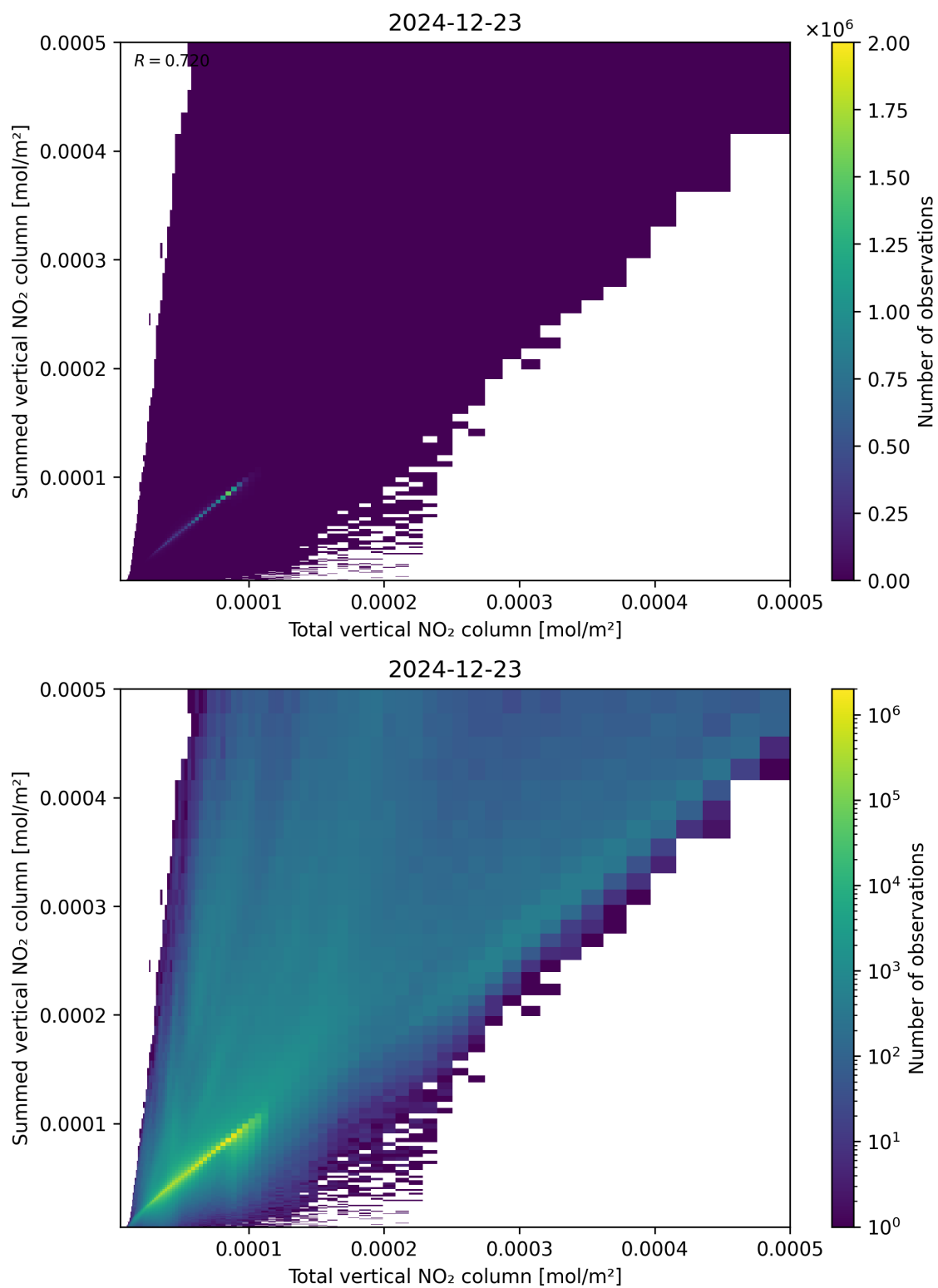
Figure 112: Scatter density plot of “Total vertical NO 2 column” against “Summed vertical NO 2 column” for 2024-12-22 to 2024-12-24.
