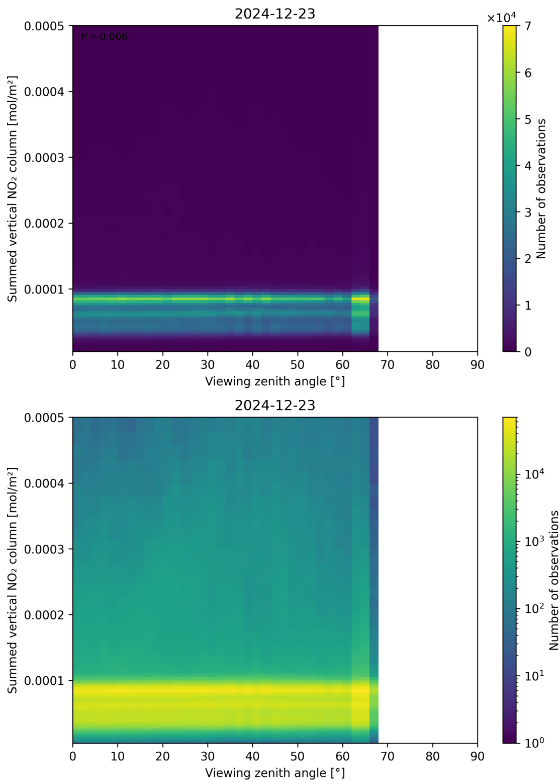
Figure 165: Scatter density plot of “Viewing zenith angle” against “Summed vertical NO 2 column” for 2024-12-22 to 2024-12-24.
