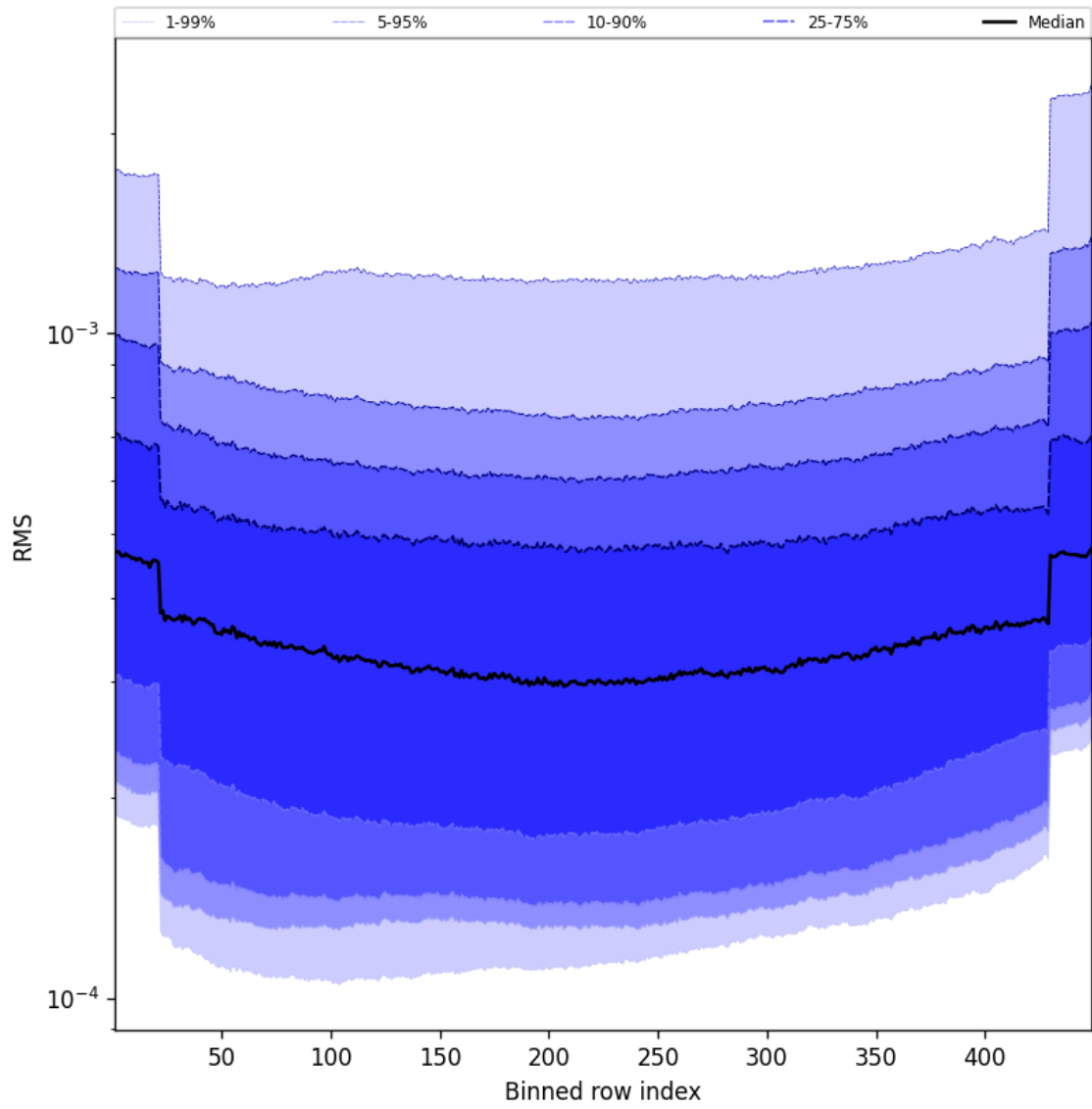
Figure 60: Along track statistics of “RMS” for 2024-12-22 to 2024-12-24
