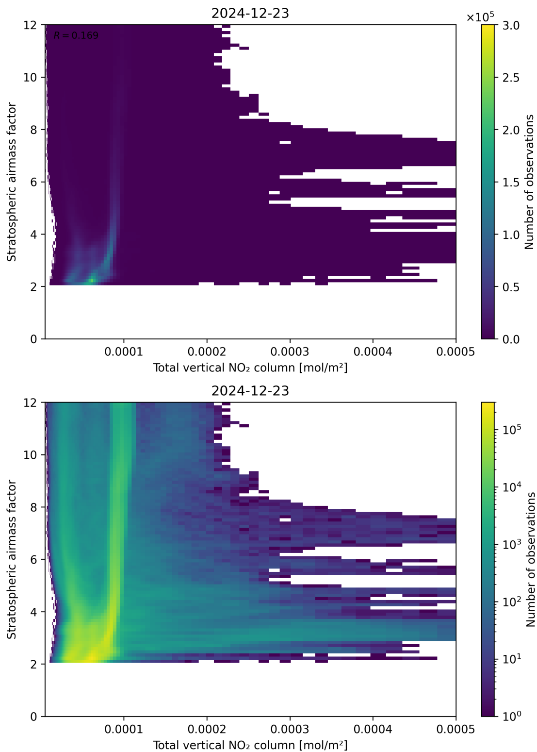
Figure 110: Scatter density plot of “Total vertical NO 2 column” against “Stratospheric air mass factor” for 2024-12-22 to 2024-12-24.
