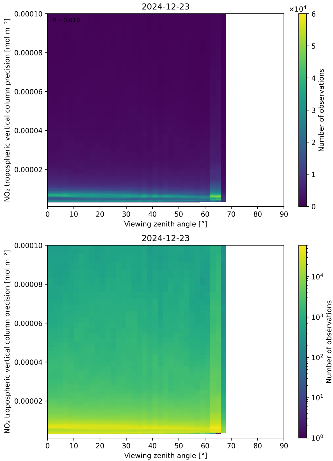
Figure 170: Scatter density plot of “Viewing zenith angle” against “NO 2 tropospheric vertical column precision” for 2024-12-22 to 2024-12-24.
