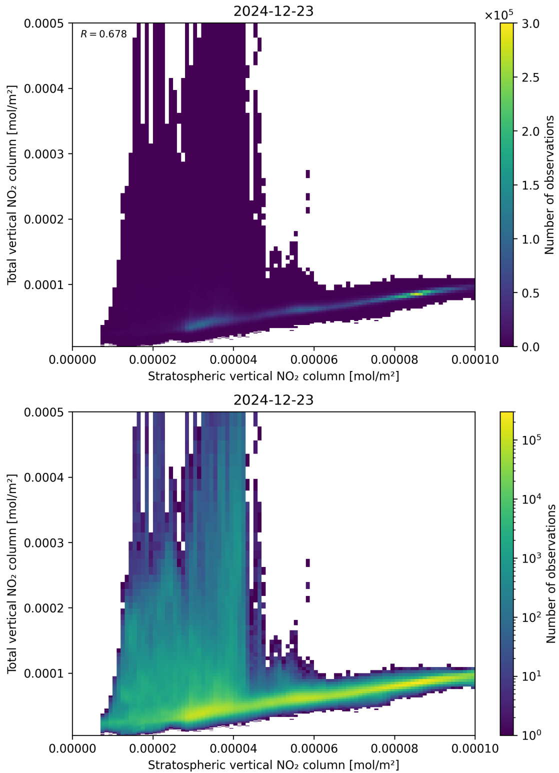
Figure 100: Scatter density plot of “Stratospheric vertical NO 2 column” against “Total vertical NO 2 column” for 2024-12-22 to 2024-12-24.
