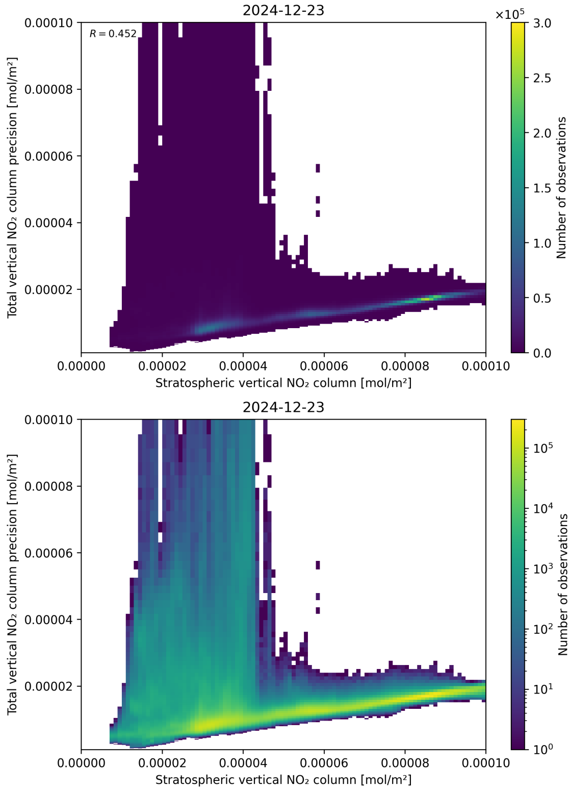
Figure 101: Scatter density plot of “Stratospheric vertical NO 2 column” against “Total vertical NO 2 column precision” for 2024-12-22 to 2024-12-24.
