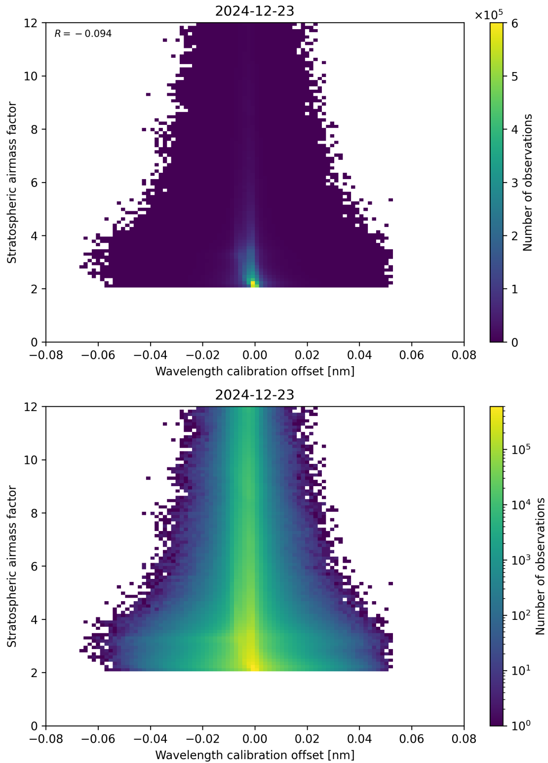
Figure 174: Scatter density plot of “Wavelength calibration offset” against “Stratospheric airmass factor” for 2024-12-22 to 2024-12-24.
