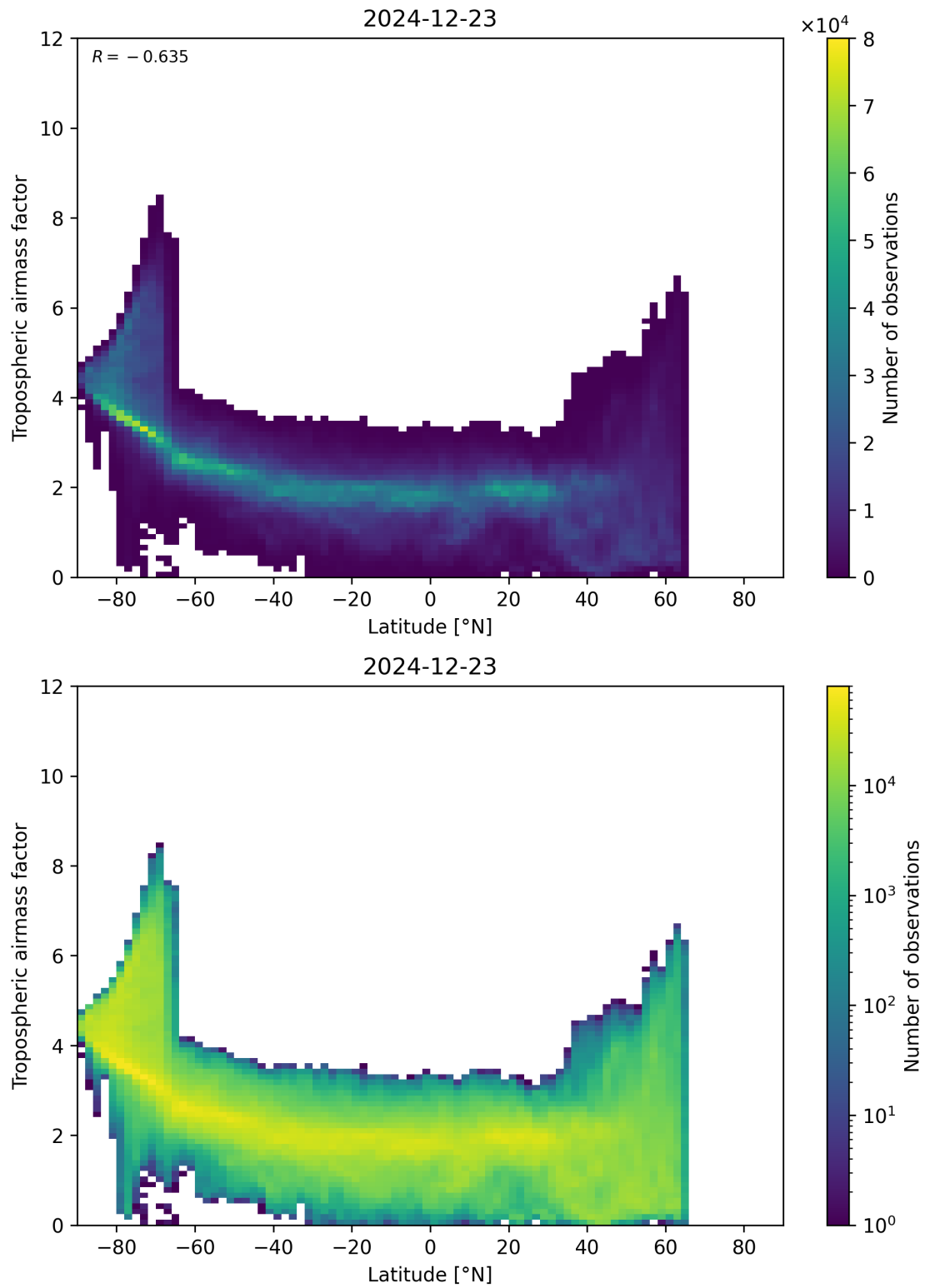
Figure 85: Scatter density plot of “Latitude” against “Tropospheric airmass factor” for 2024-12-22 to 2024-12-24.
