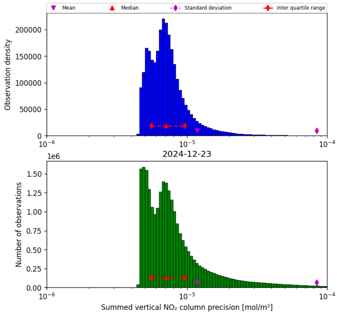
Figure 41: Histogram of “Summed vertical NO 2 column precision” for 2024-12-22 to 2024-12-24
