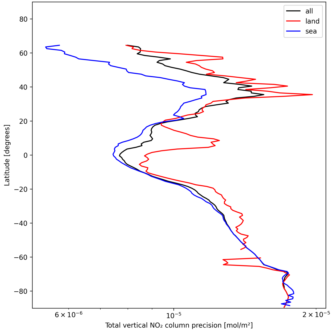
Figure 22: Zonal average of “Total vertical NO 2 column precision” for 2024-12-22 to 2024-12-24.
