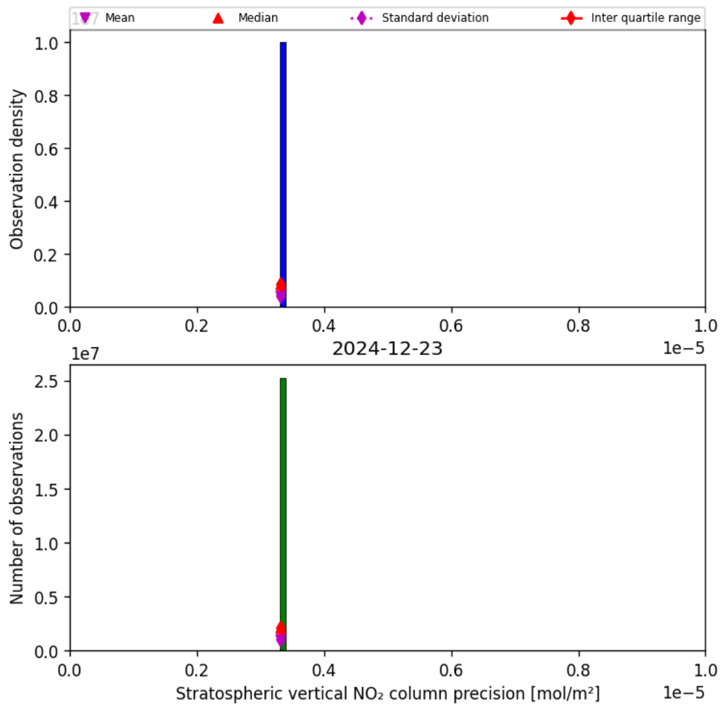
Figure 37: Histogram of “Stratospheric vertical NO 2 column precision” for 2024-12-22 to 2024-12-24
