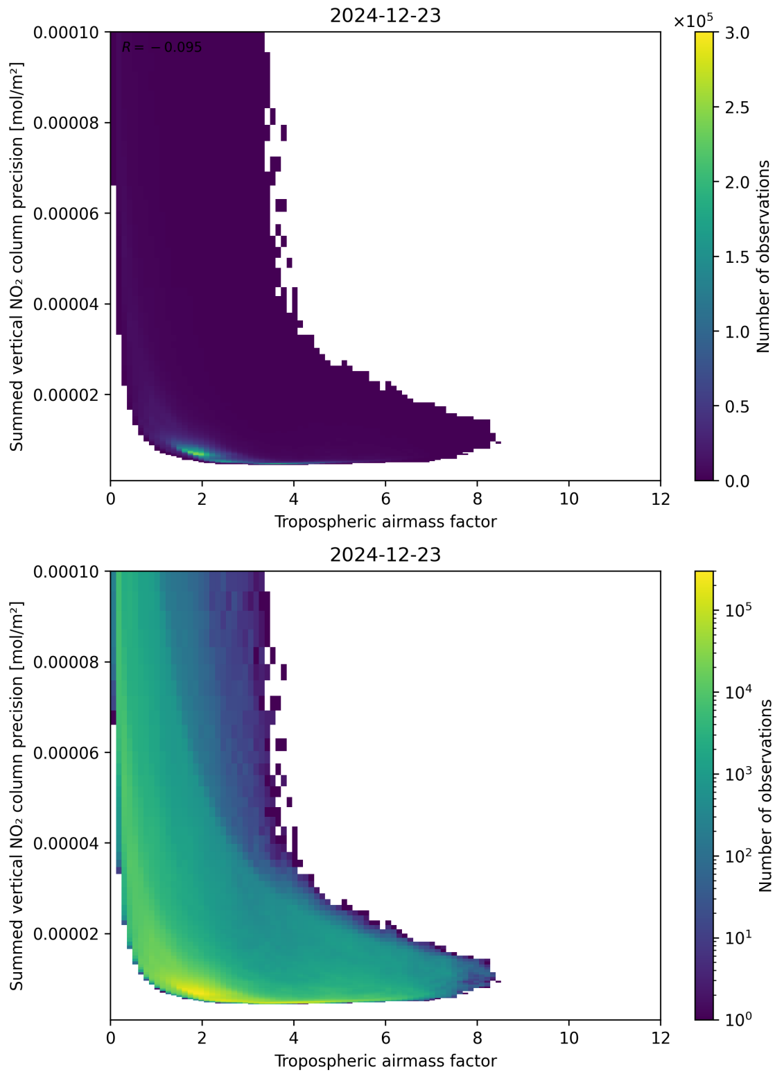
Figure 76: Scatter density plot of “Tropospheric air mass factor” against “Summed vertical NO 2 column precision” for 2024-12-22 to 2024-12-24.
