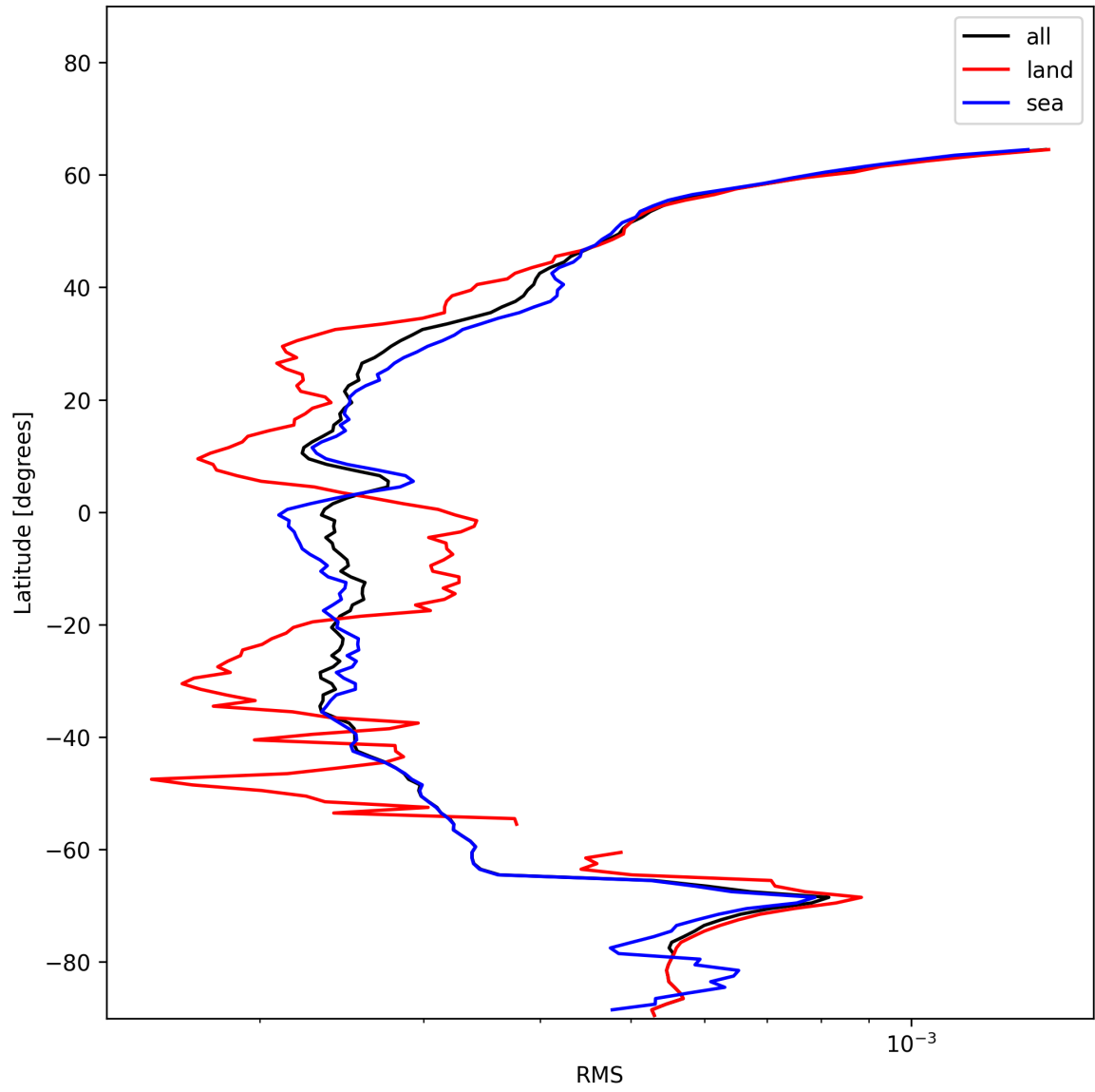
Figure 26: Zonal average of “RMS” for 2024-12-22 to 2024-12-24.
