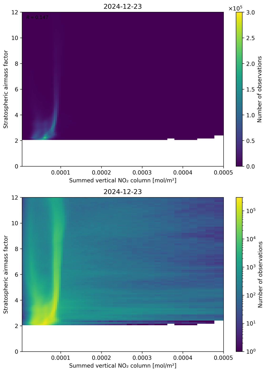
Figure 103: Scatter density plot of “Summed vertical NO 2 column” against “Stratospheric airmass factor” for 2024-12-22 to 2024-12-24.
