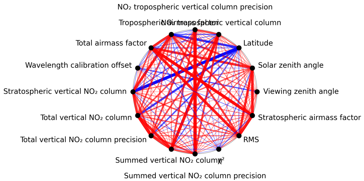
Figure 1: Map of correlation graph for 2024-12-22 to 2024-12-24.
