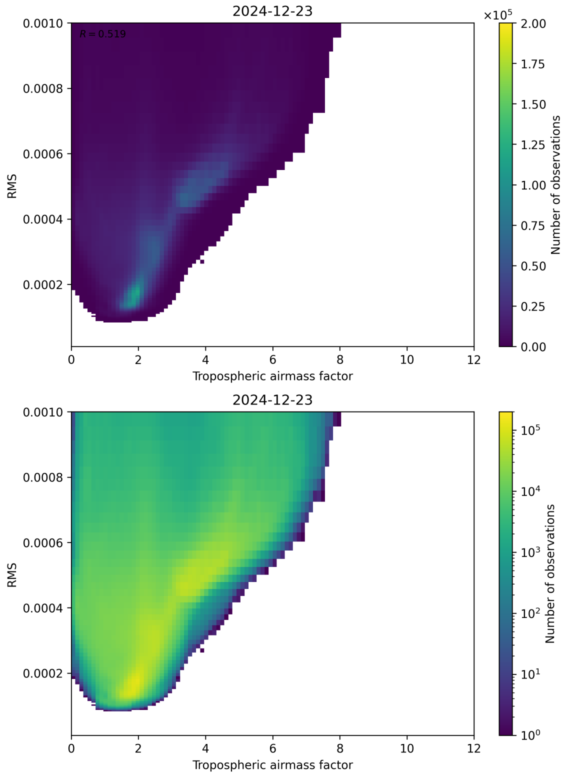
Figure 79: Scatter density plot of “Tropospheric airmass factor” against “RMS” for 2024-12-22 to 2024-12-24.
