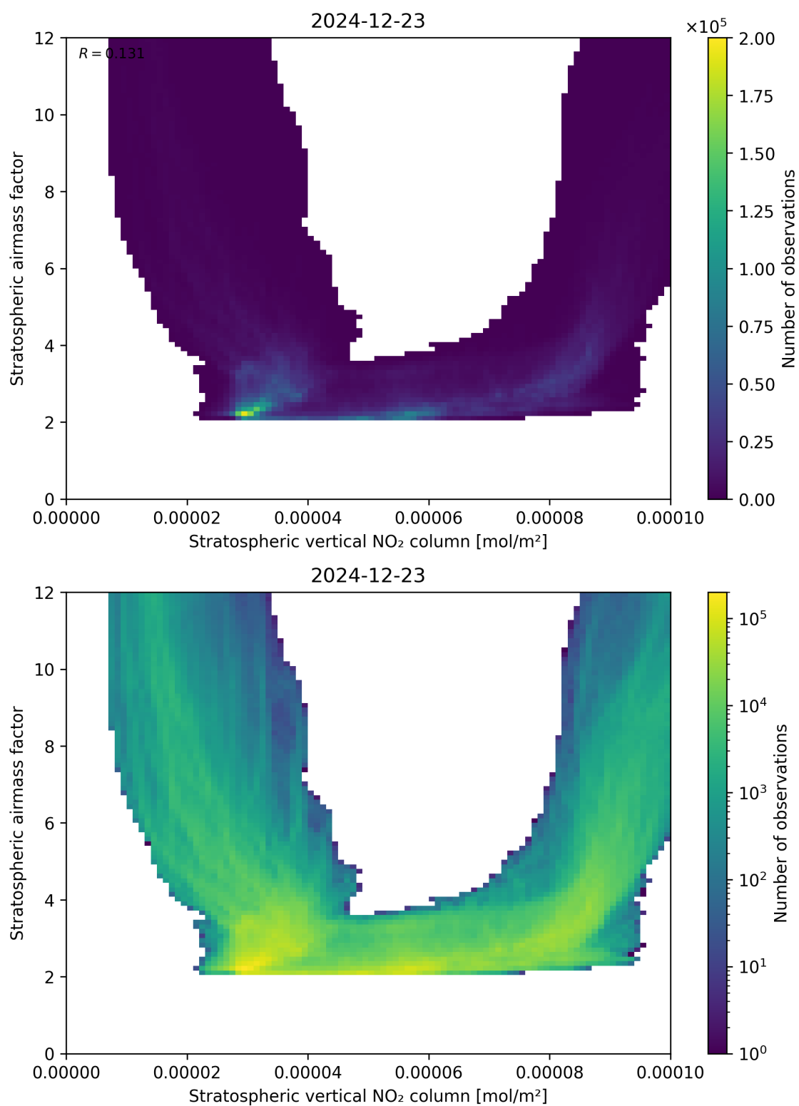
Figure 96: Scatter density plot of “Stratospheric vertical NO 2 column” against “Stratospheric airmass factor” for 2024-12-22 to 2024-12-24.
