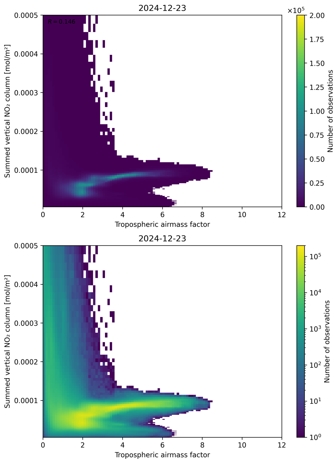
Figure 75: Scatter density plot of “Tropospheric air mass factor” against “Summed vertical NO 2 column” for 2024-12-22 to 2024-12-24.
