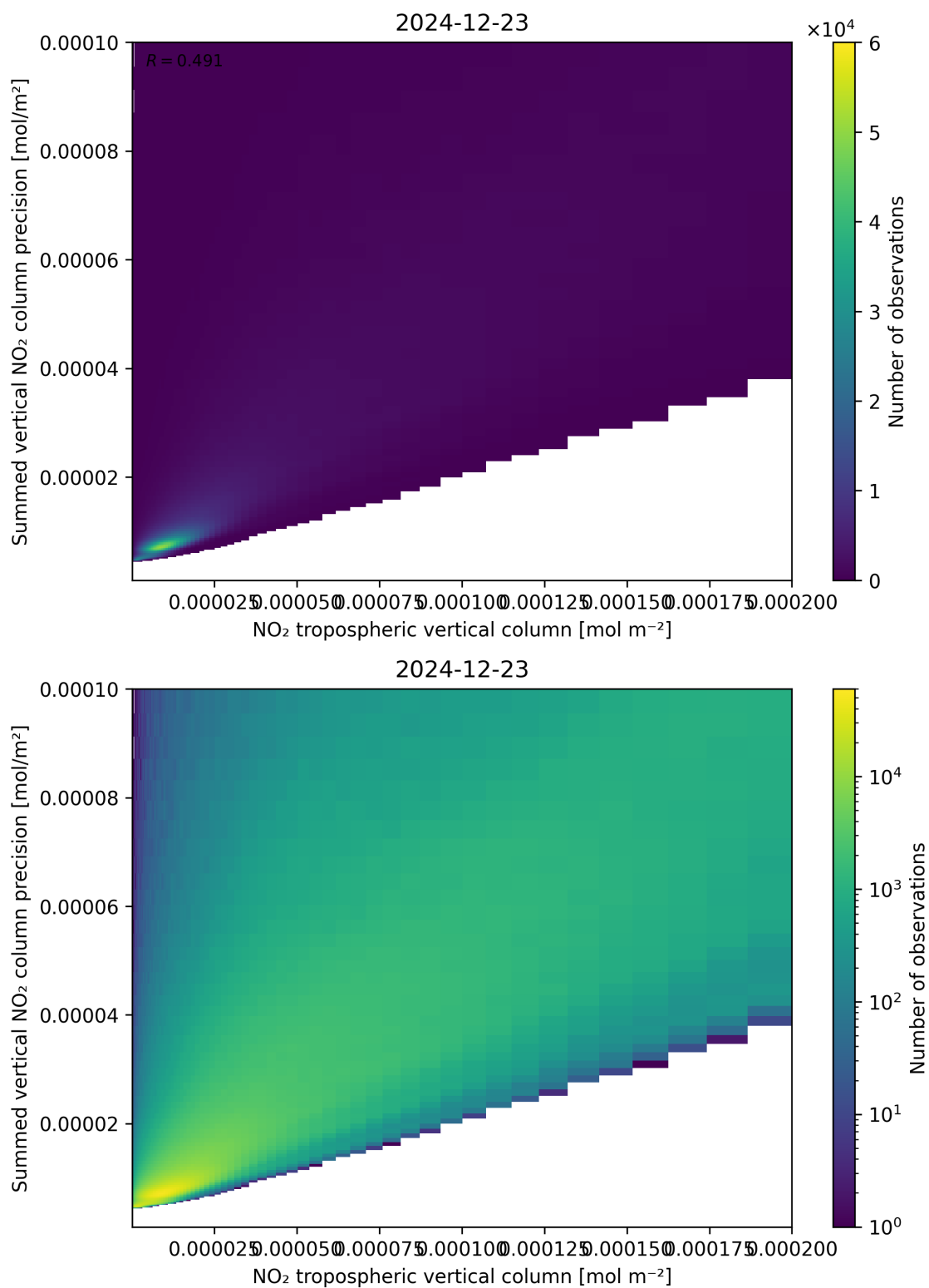
Figure 127: Scatter density plot of “NO 2 tropospheric vertical column” against “Summed vertical NO 2 column precision” for 2024-12-22 to 2024-12-24.
