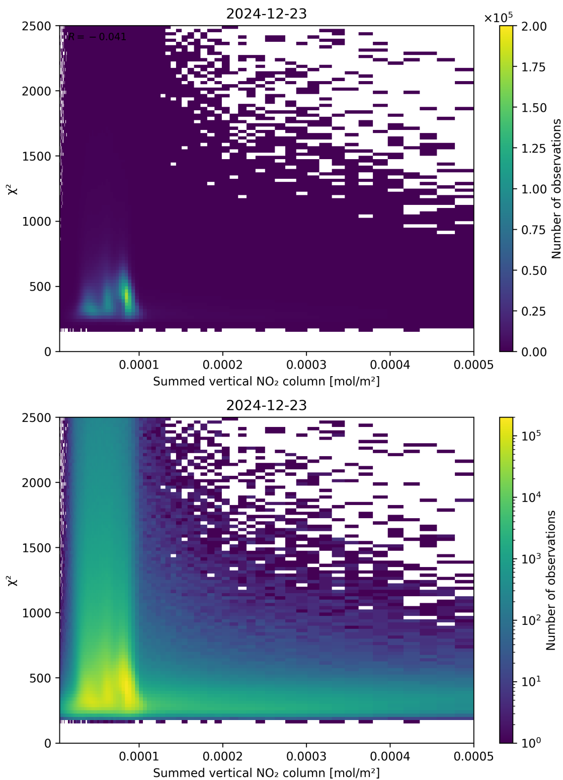
Figure 104: Scatter density plot of “Summed vertical NO 2 column” against “ \chi^2 ” for 2024-12-22 to 2024-12-24.
