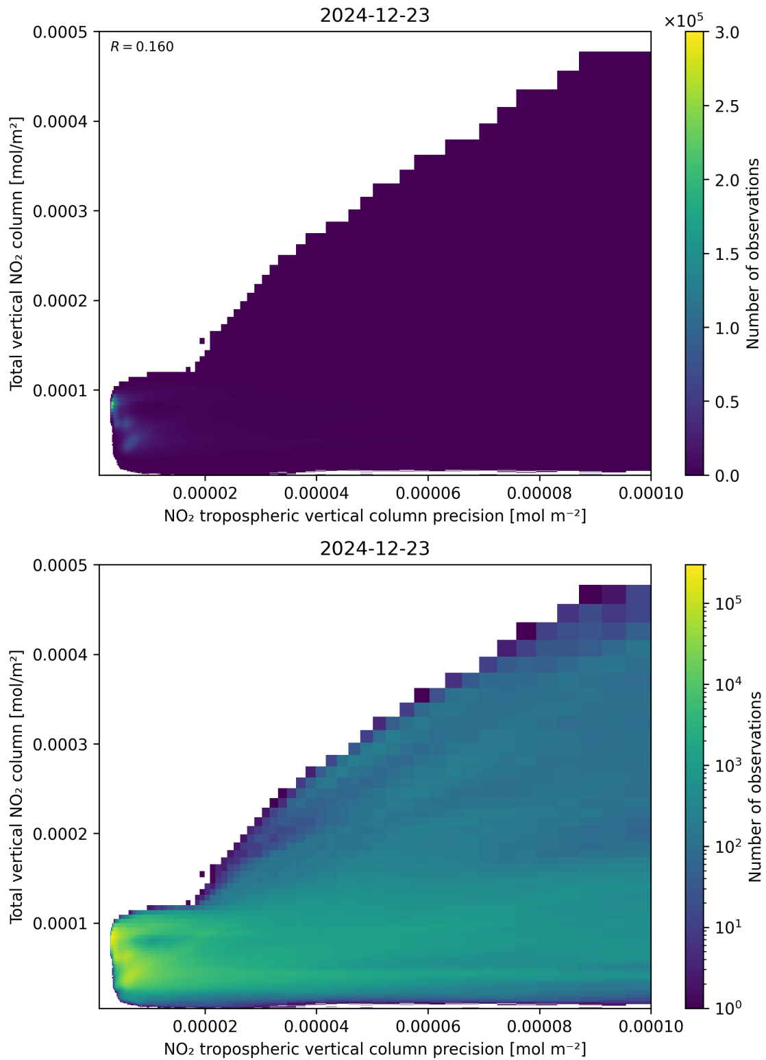
Figure 138: Scatter density plot of “NO 2 tropospheric vertical column precision” against “Total vertical NO 2 column” for 2024-12-22 to 2024-12-24.
