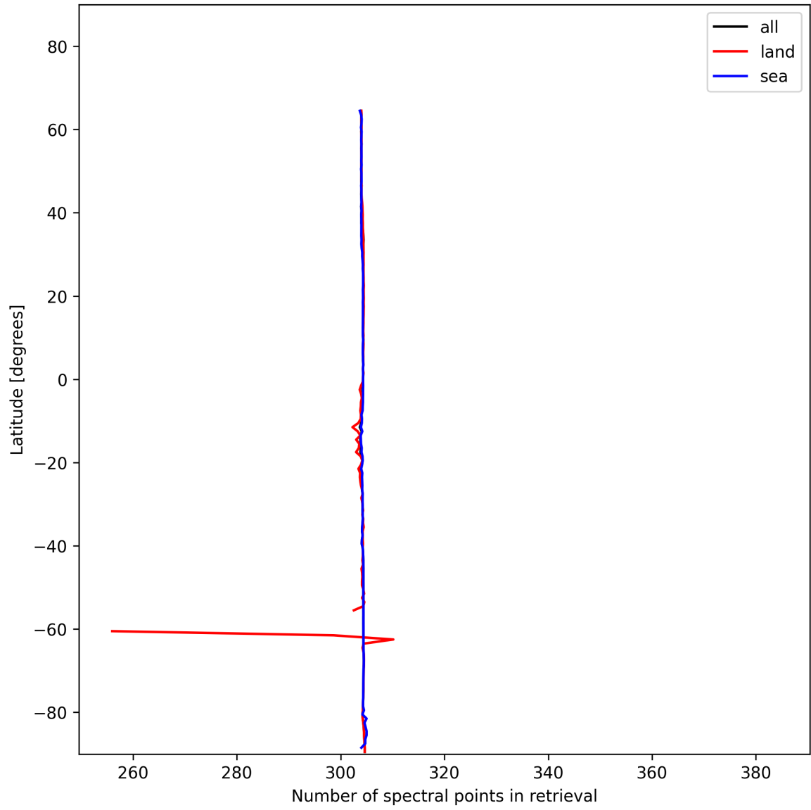
Figure 16: Zonal average of “Number of spectral points in retrieval” for 2024-12-22 to 2024-12-24.
