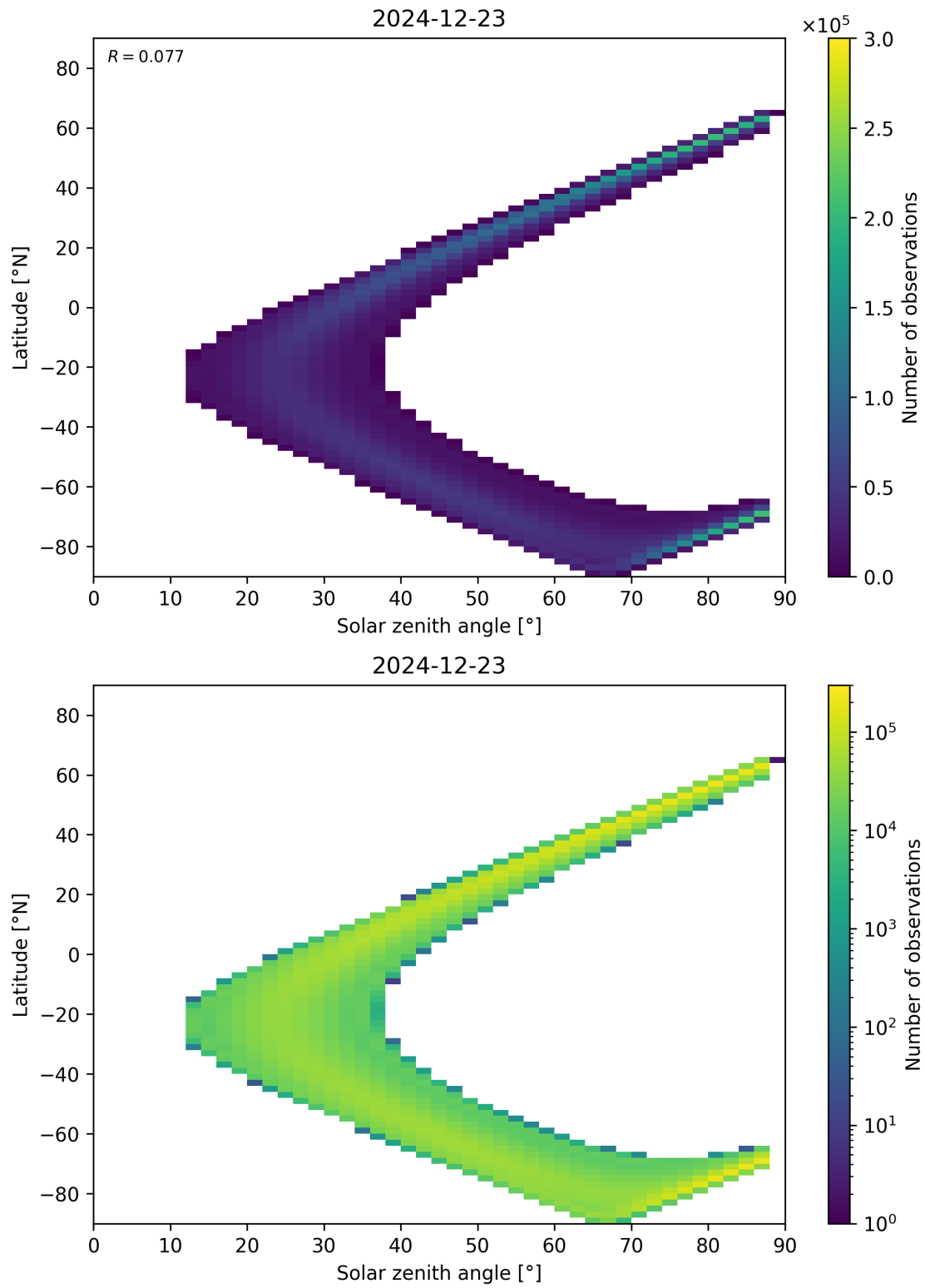
Figure 149: Scatter density plot of “Solar zenith angle” against “Latitude” for 2024-12-22 to 2024-12-24.
