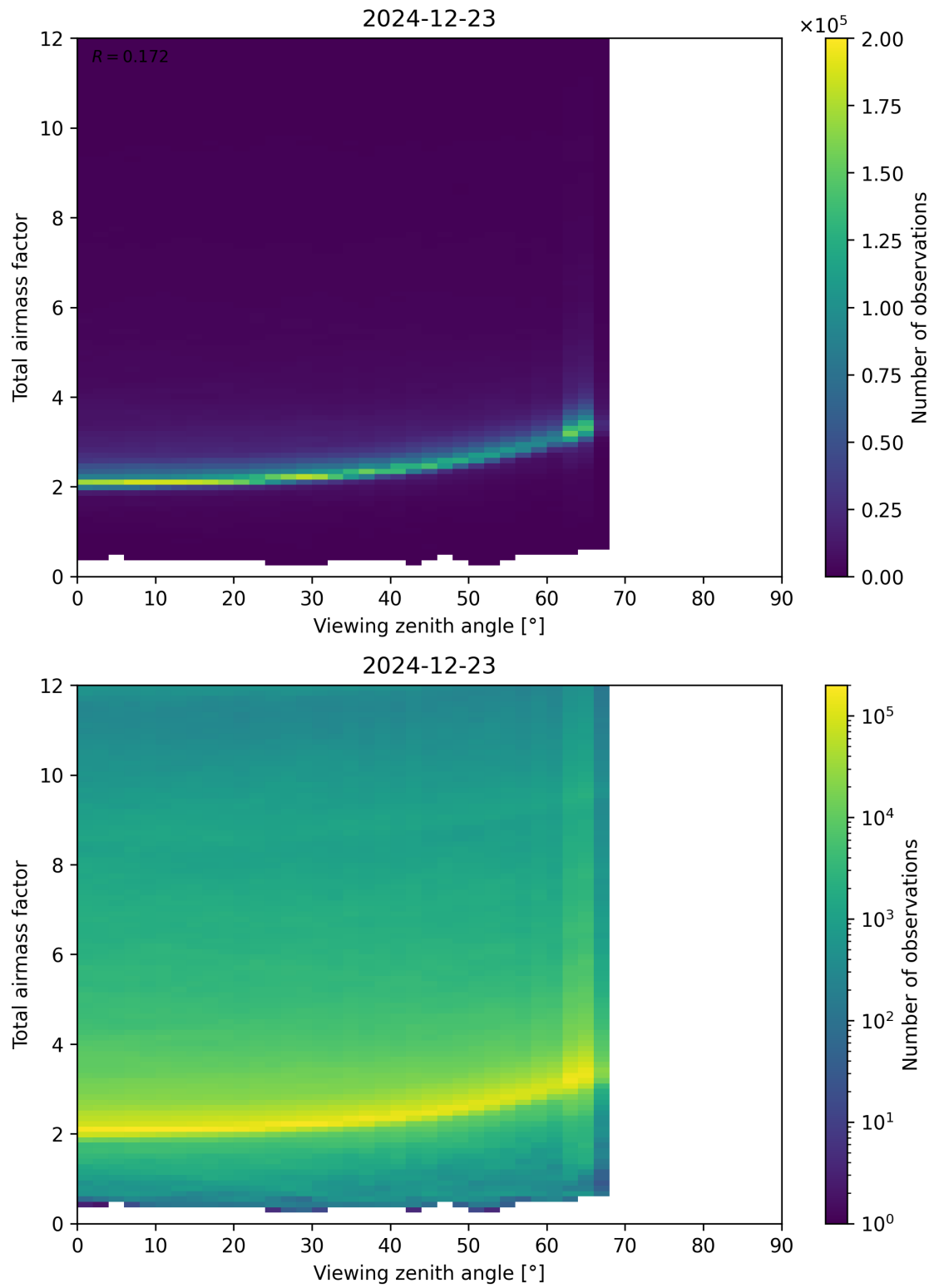
Figure 160: Scatter density plot of “Viewing zenith angle” against “Total airmass factor” for 2024-12-22 to 2024-12-24.
