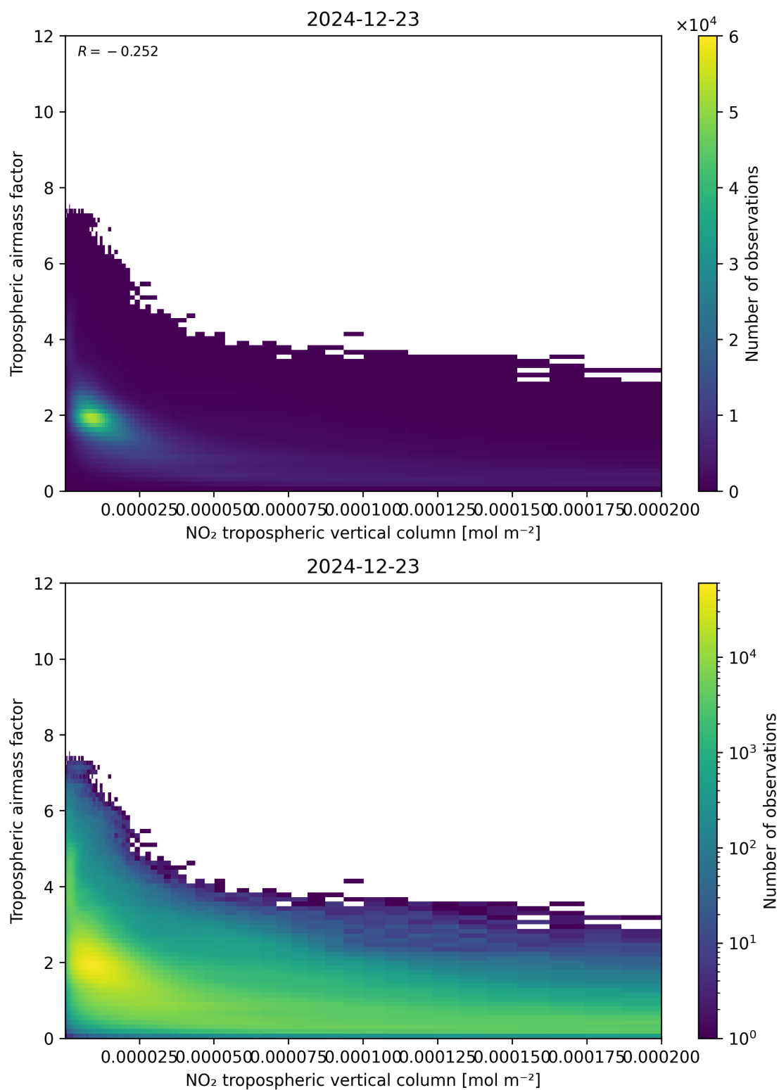
Figure 123: Scatter density plot of “NO 2 tropospheric vertical column” against “Tropospheric air mass factor” for 2024-12-22 to 2024-12-24.
