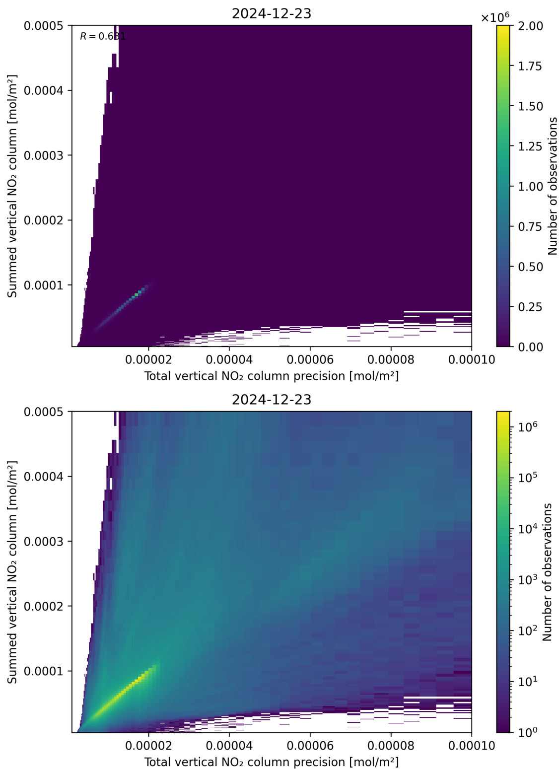
Figure 117: Scatter density plot of “Total vertical NO 2 column precision” against “Summed vertical NO 2 column” for 2024-12-22 to 2024-12-24.
