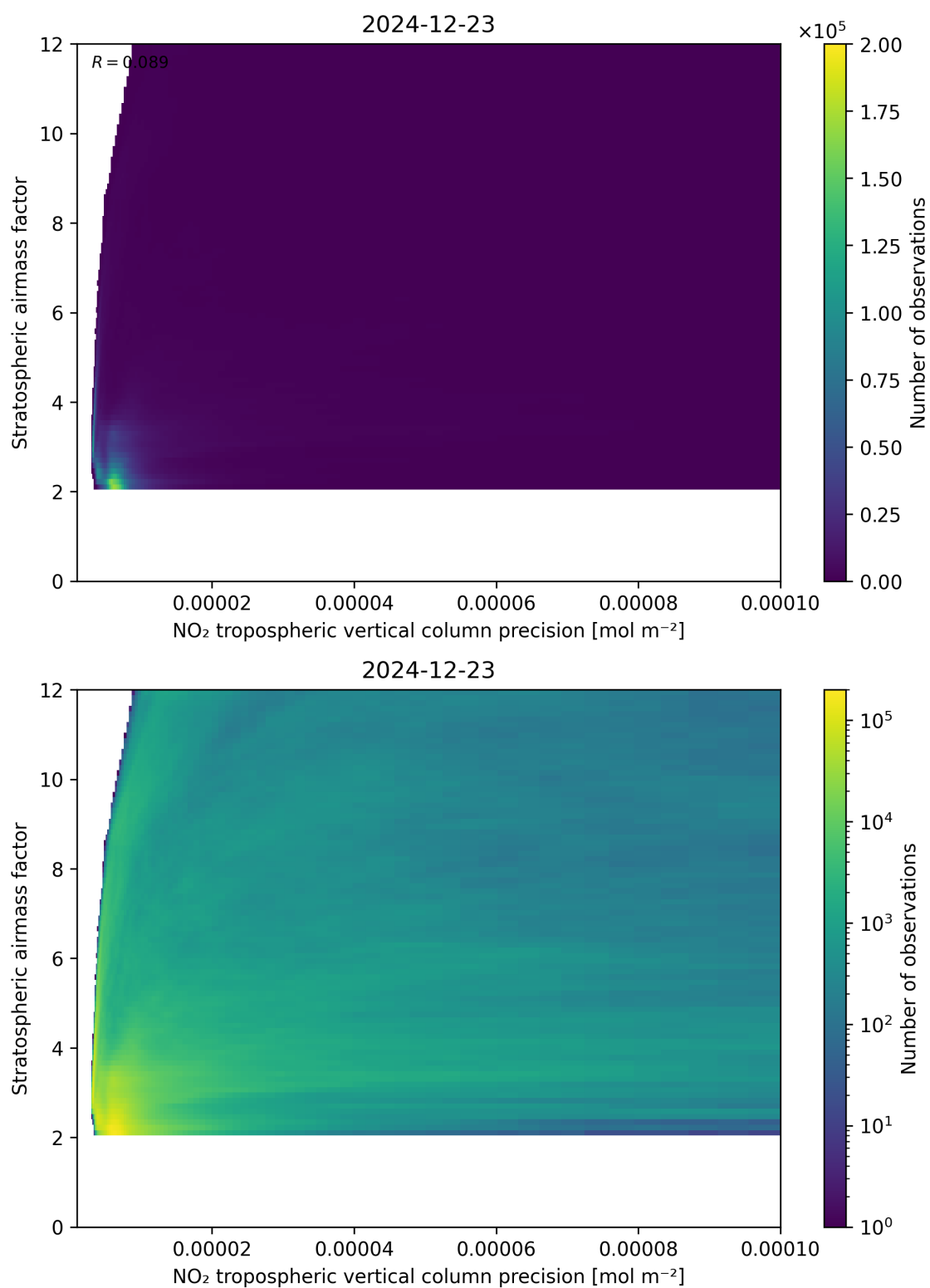
Figure 131: Scatter density plot of “NO 2 tropospheric vertical column precision” against “Stratospheric airmass factor” for 2024-12-22 to 2024-12-24.
