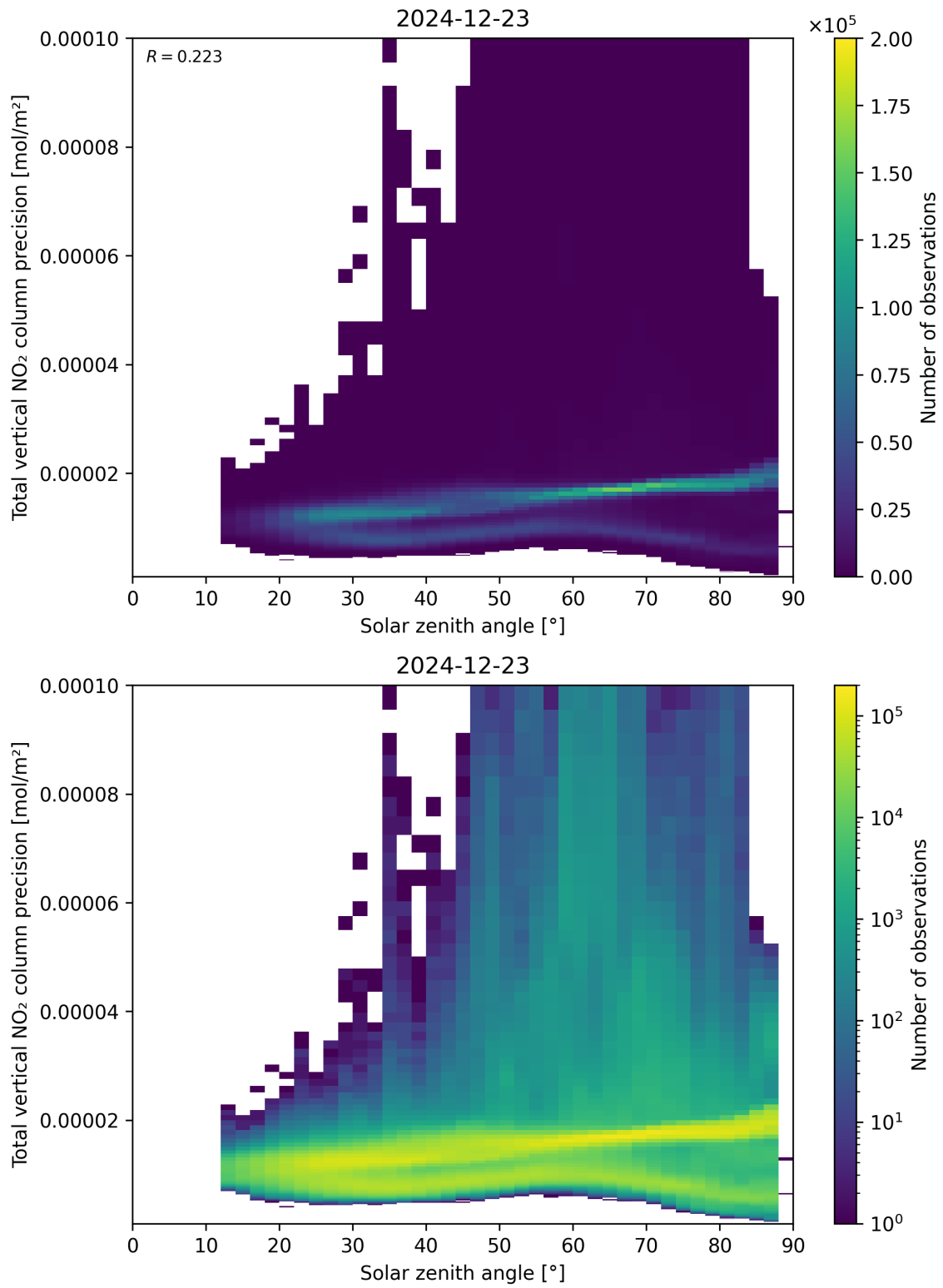
Figure 154: Scatter density plot of “Solar zenith angle” against “Total vertical NO 2 column precision” for 2024-12-22 to 2024-12-24.
