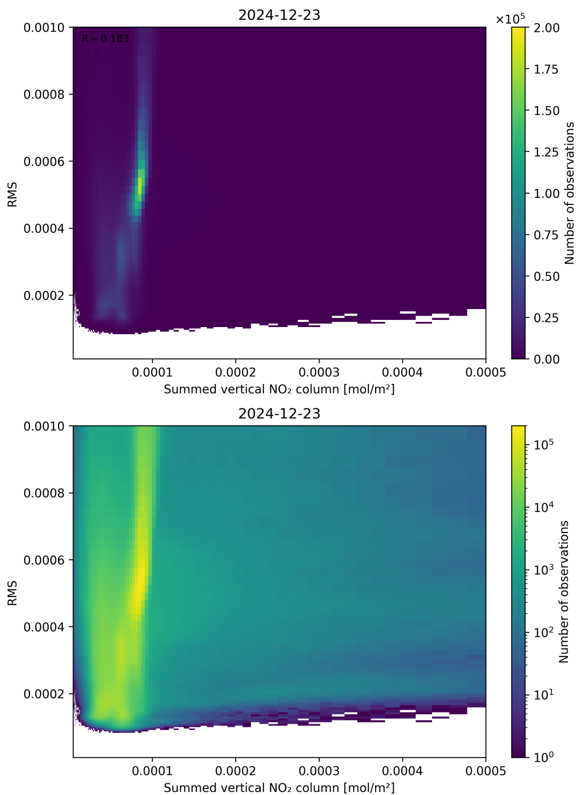
Figure 109: Scatter density plot of “Summed vertical NO 2 column” against “RMS” for 2024-12-22 to 2024-12-24.
