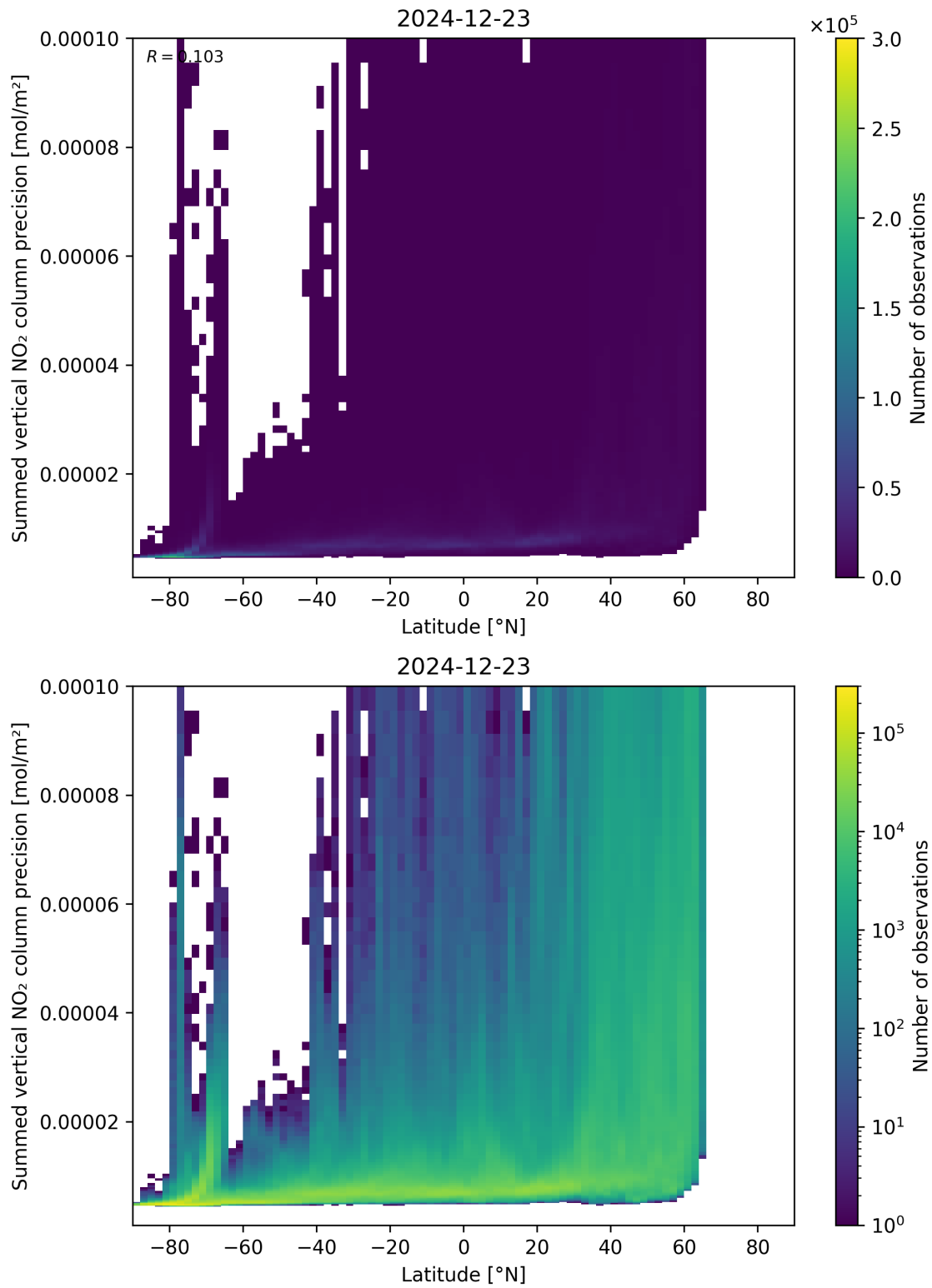
Figure 89: Scatter density plot of “Latitude” against “Summed vertical NO 2 column precision” for 2024-12-22 to 2024-12-24.
