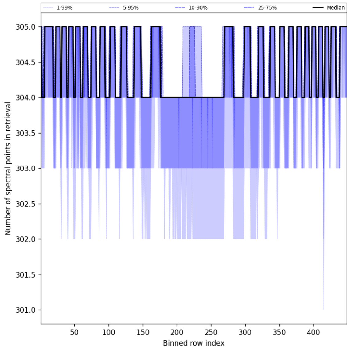
Figure 50: Along track statistics of “Number of spectral points in retrieval” for 2024-12-22 to 2024-12-24
