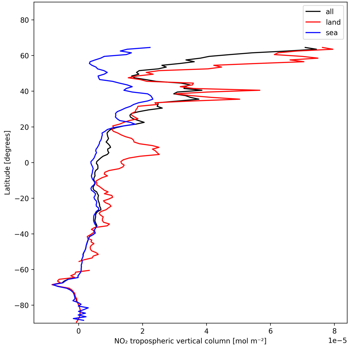
Figure 12: Zonal average of “NO 2 tropospheric vertical column” for 2024-12-22 to 2024-12-24.
