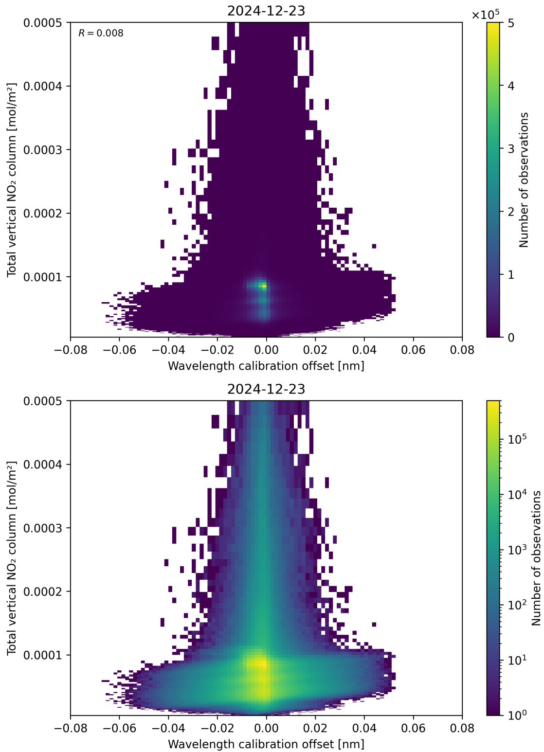
Figure 179: Scatter density plot of “Wavelength calibration offset” against “Total vertical NO 2 column” for 2024-12-22 to 2024-12-24.
