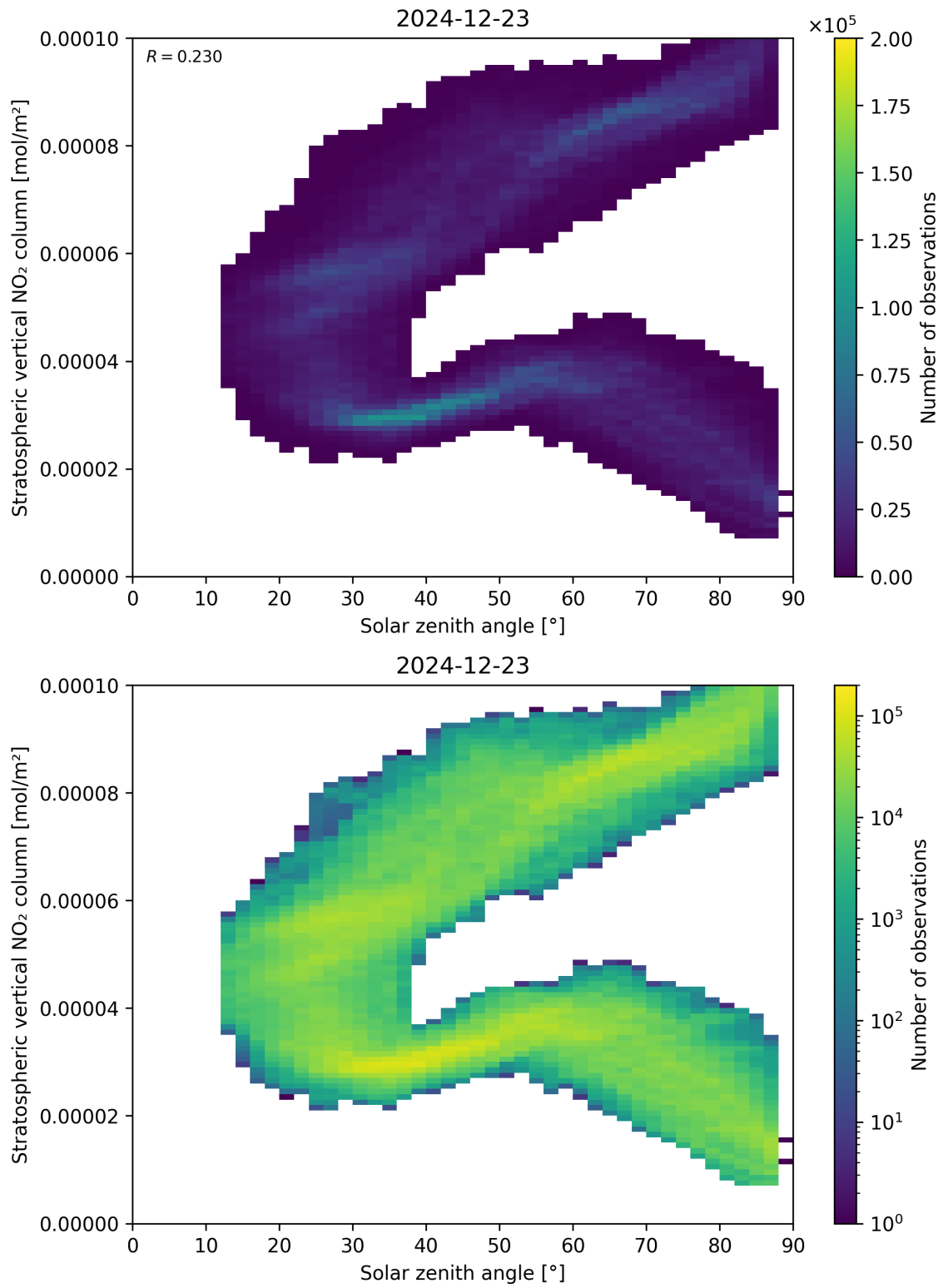
Figure 150: Scatter density plot of “Solar zenith angle” against “Stratospheric vertical NO 2 column” for 2024-12-22 to 2024-12-24.
