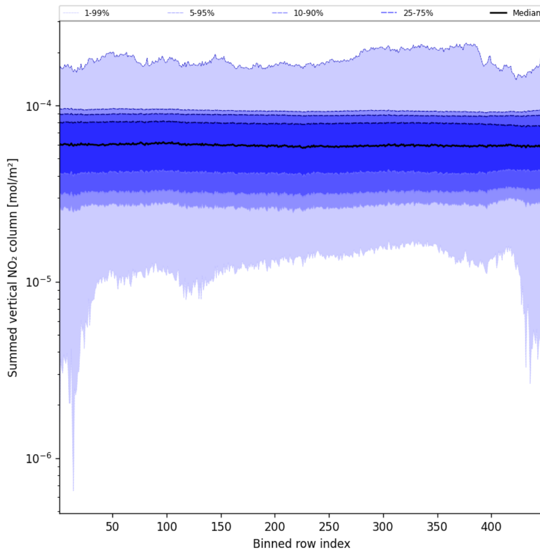
Figure 57: Along track statistics of “Summed vertical NO 2 column” for 2024-12-22 to 2024-12-24
