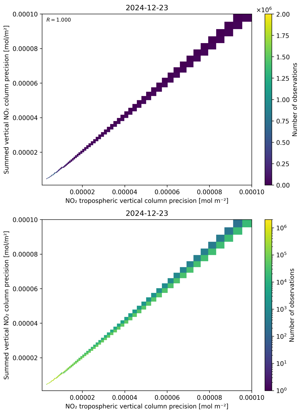
Figure 137: Scatter density plot of “NO 2 tropospheric vertical column precision” against “Summed vertical NO 2 column precision” for 2024-12-22 to 2024-12-24.
