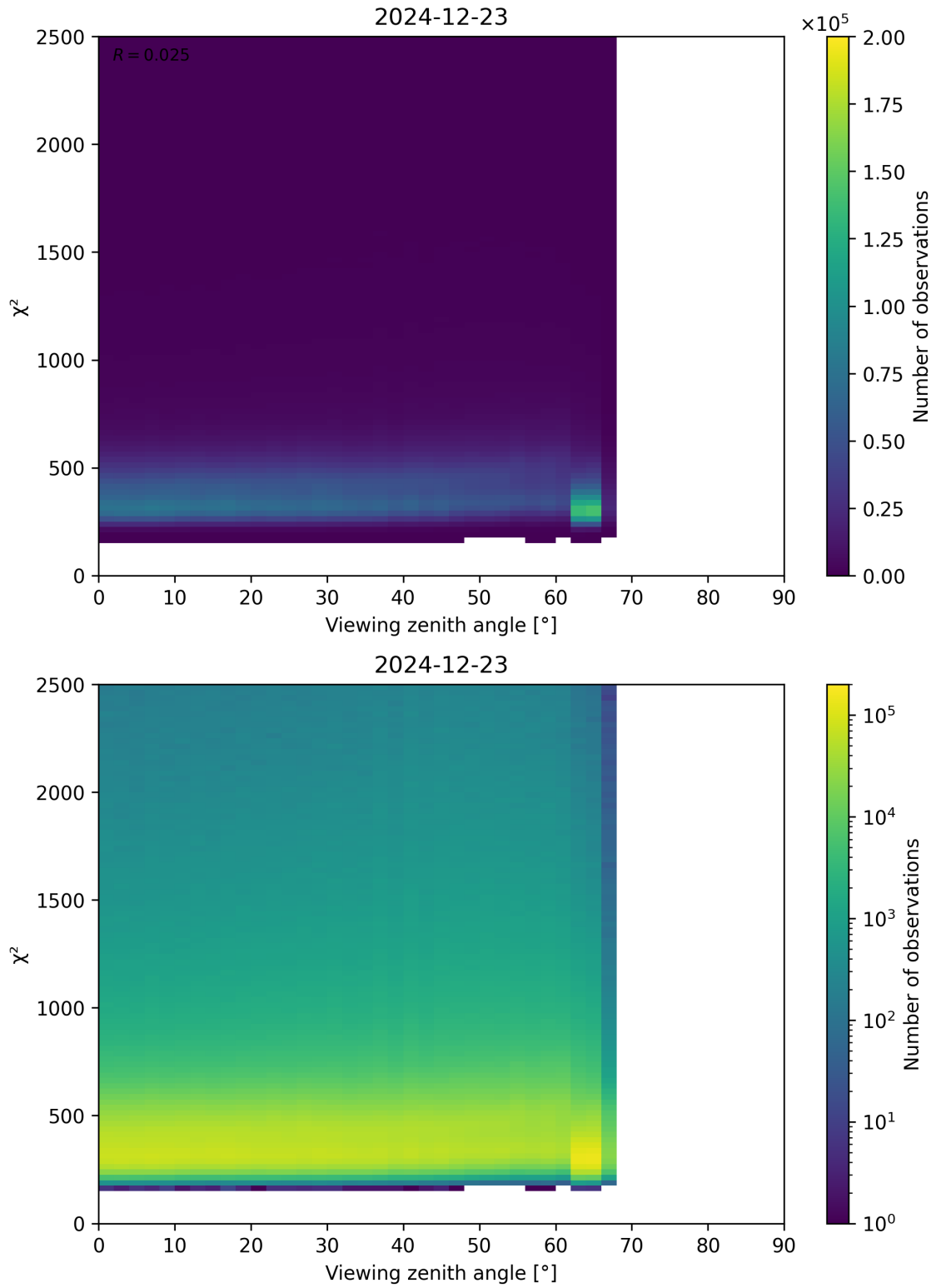
Figure 162: Scatter density plot of “Viewing zenith angle” against “ \chi^2 ” for 2024-12-22 to 2024-12-24.
