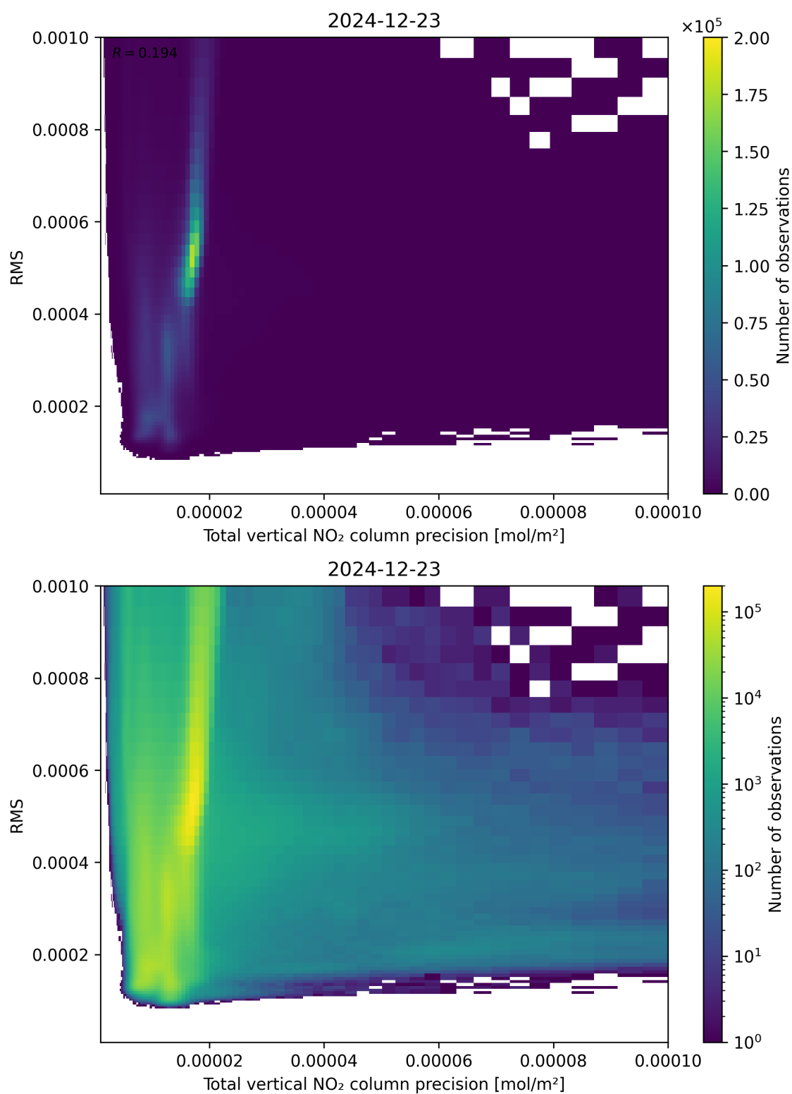
Figure 119: Scatter density plot of “Total vertical NO 2 column precision” against “RMS” for 2024-12-22 to 2024-12-24.
