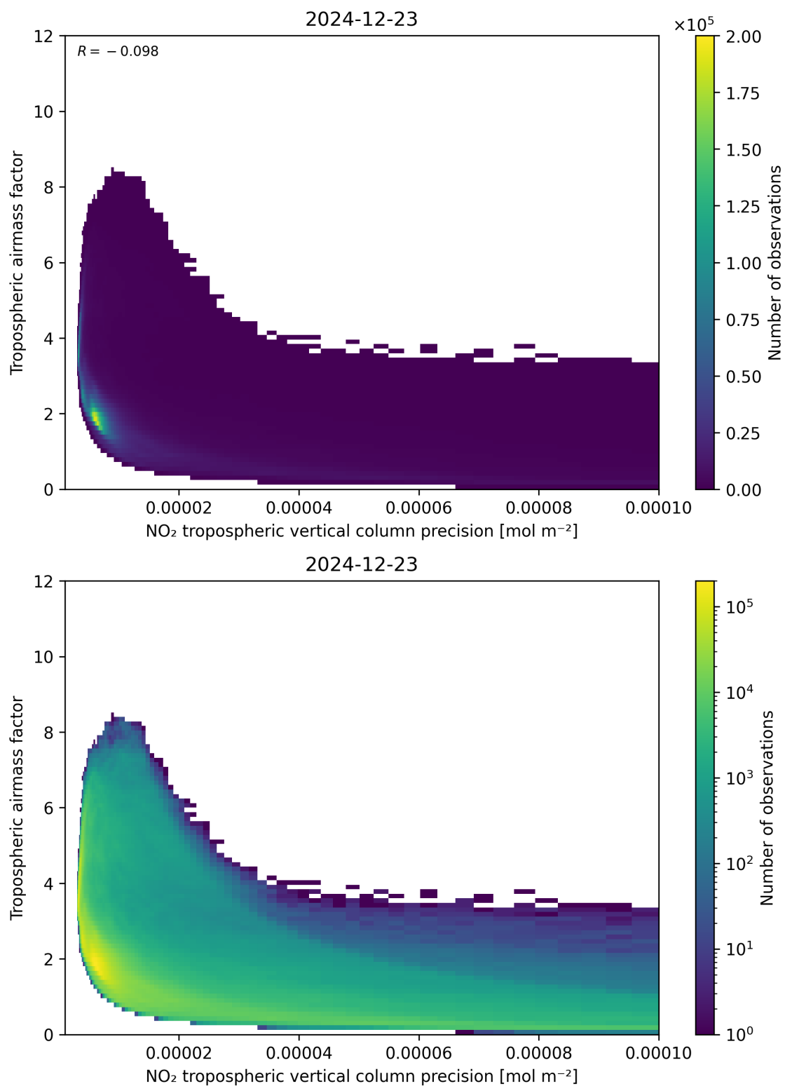
Figure 133: Scatter density plot of “NO 2 tropospheric vertical column precision” against “Tropospheric air mass factor” for 2024-12-22 to 2024-12-24.
