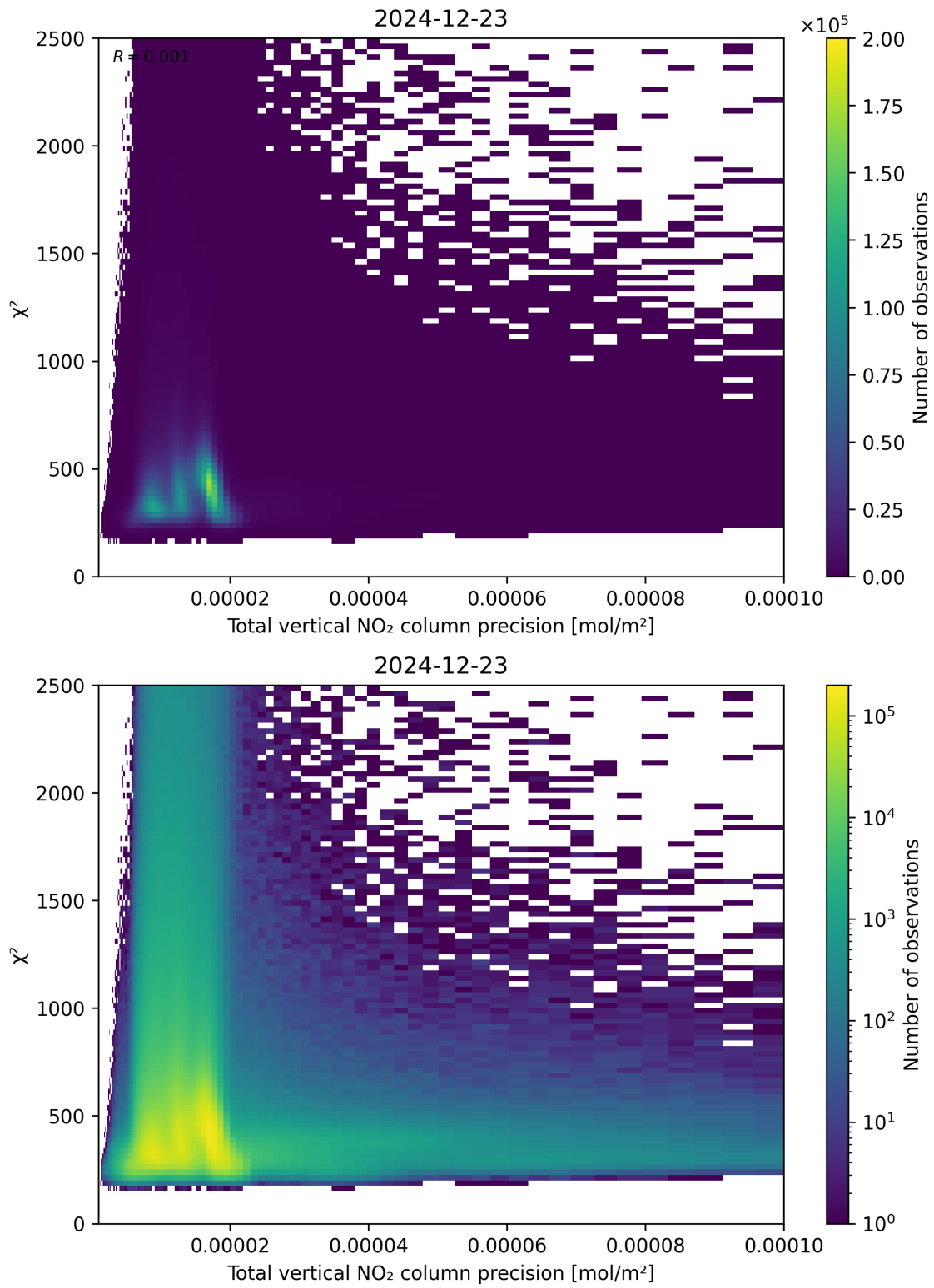
Figure 116: Scatter density plot of “Total vertical NO 2 column precision” against “ \chi^2 ” for 2024-12-22 to 2024-12-24.
