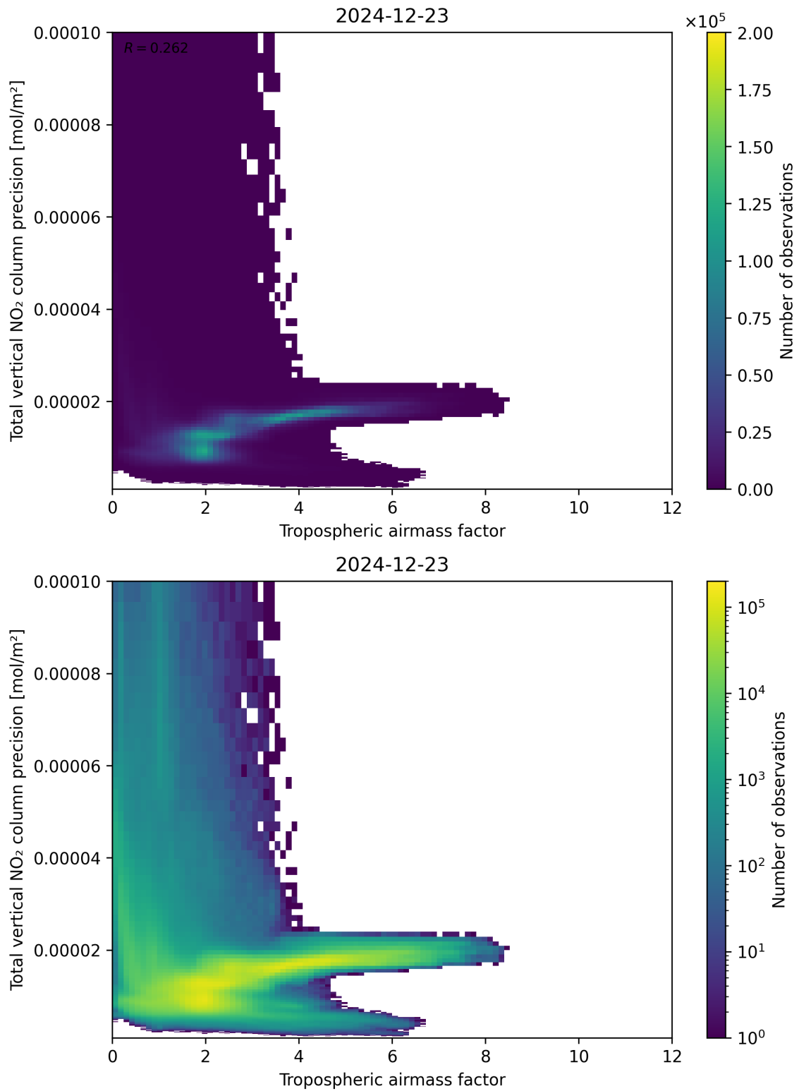
Figure 78: Scatter density plot of “Tropospheric air mass factor” against “Total vertical NO 2 column precision” for 2024-12-22 to 2024-12-24.
