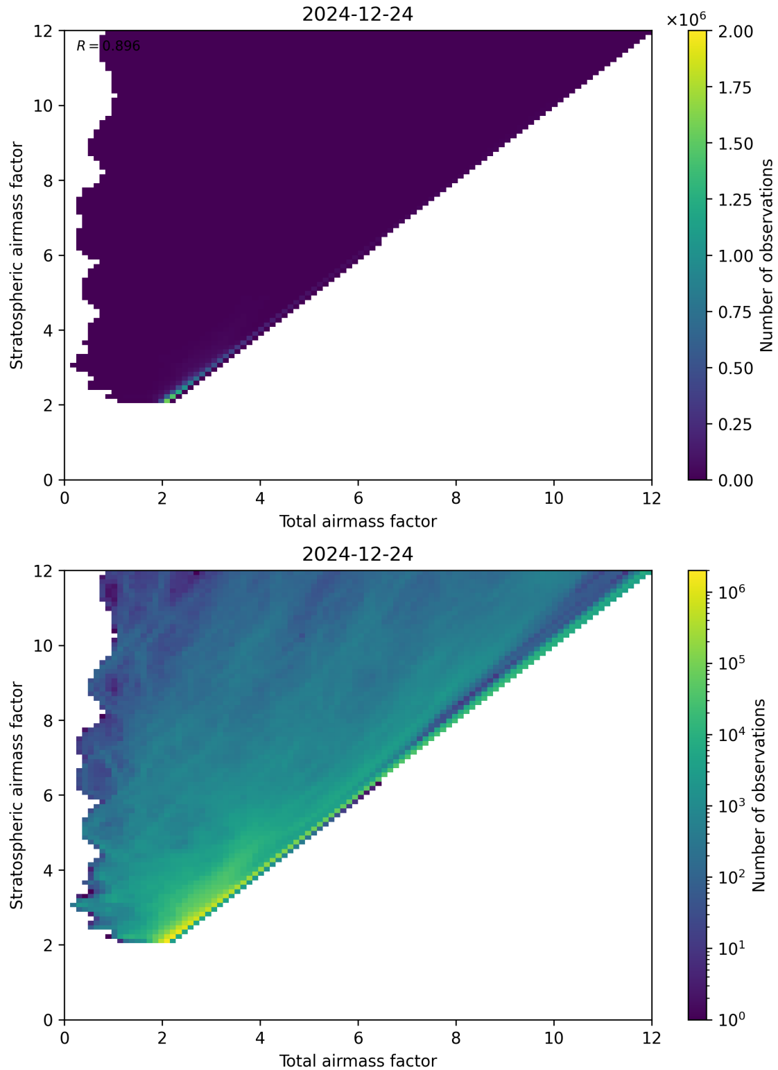
Figure 62: Scatter density plot of “Total airmass factor” against “Stratospheric airmass factor” for 2024-12-23 to 2024-12-25.
