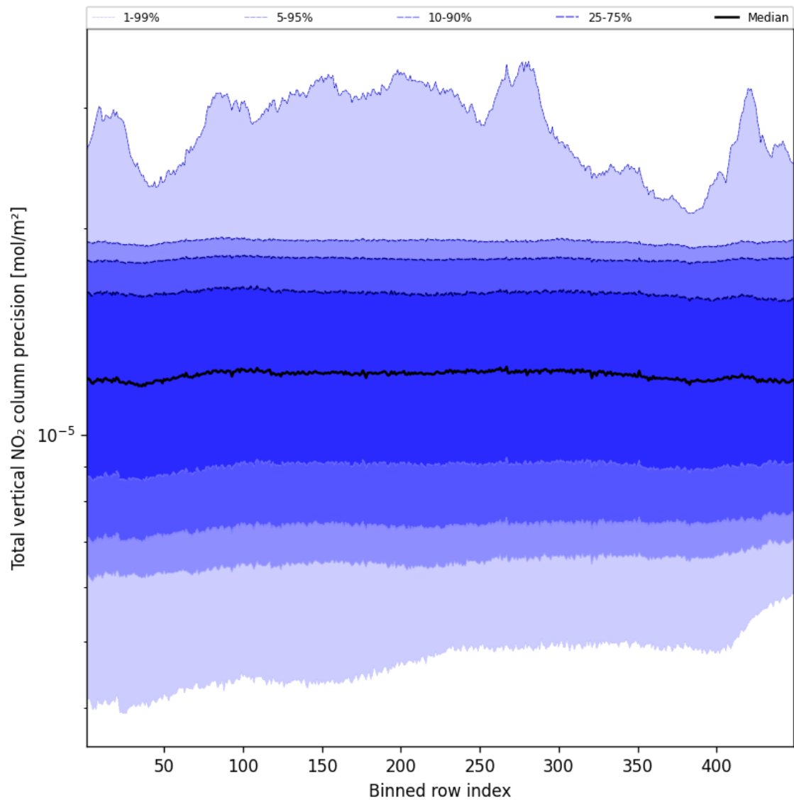
Figure 56: Along track statistics of “Total vertical NO 2 column precision” for 2024-12-23 to 2024-12-25
