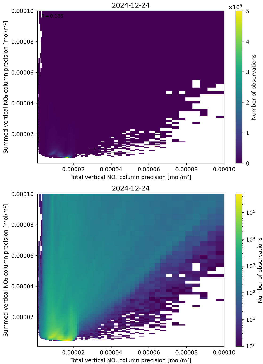
Figure 118: Scatter density plot of “Total vertical NO 2 column precision” against “Summed vertical NO 2 column precision” for 2024-12-23 to 2024-12-25.
