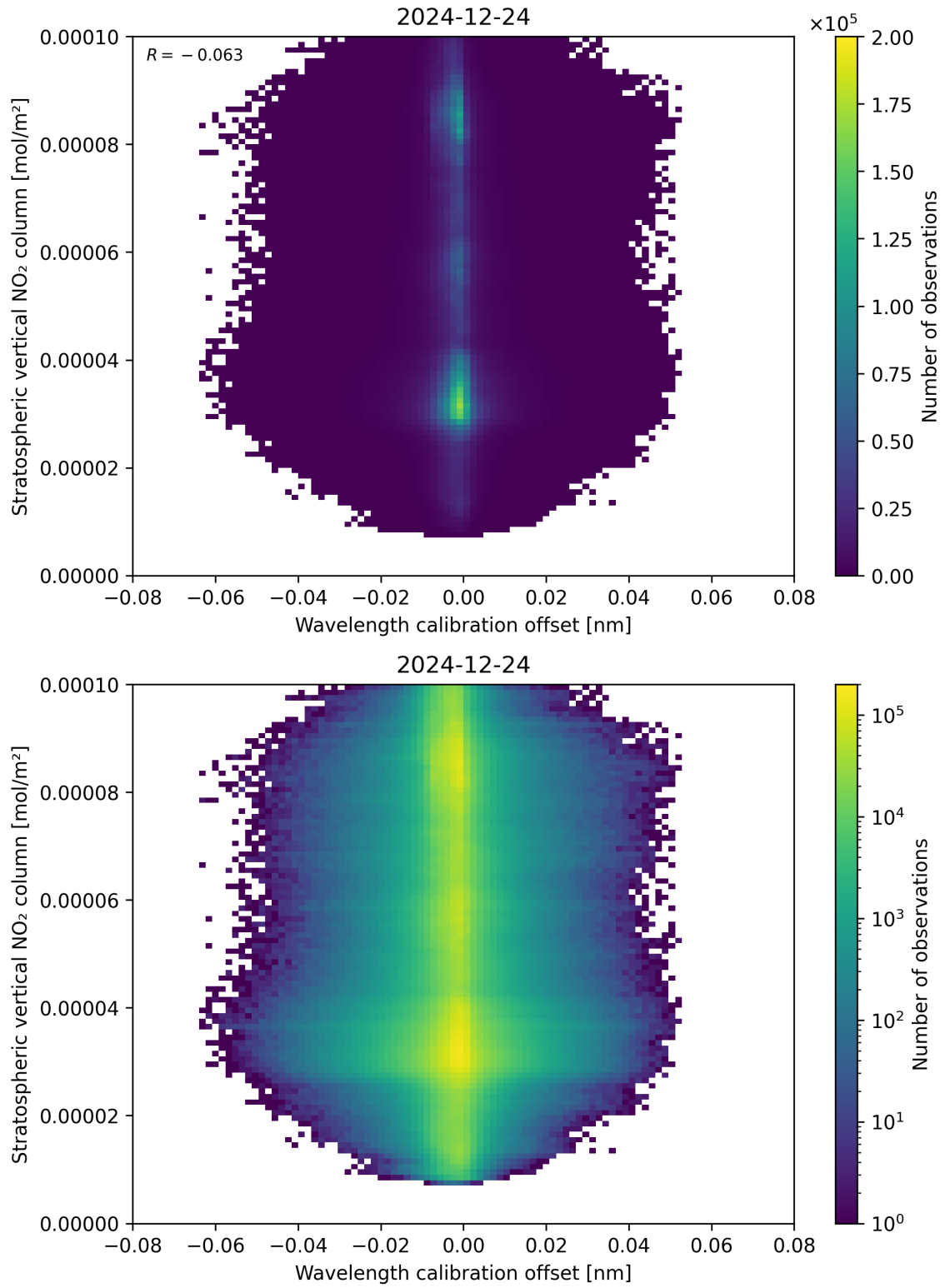
Figure 176: Scatter density plot of “Wavelength calibration offset” against “Stratospheric vertical NO 2 column” for 2024-12-23 to 2024-12-25.
