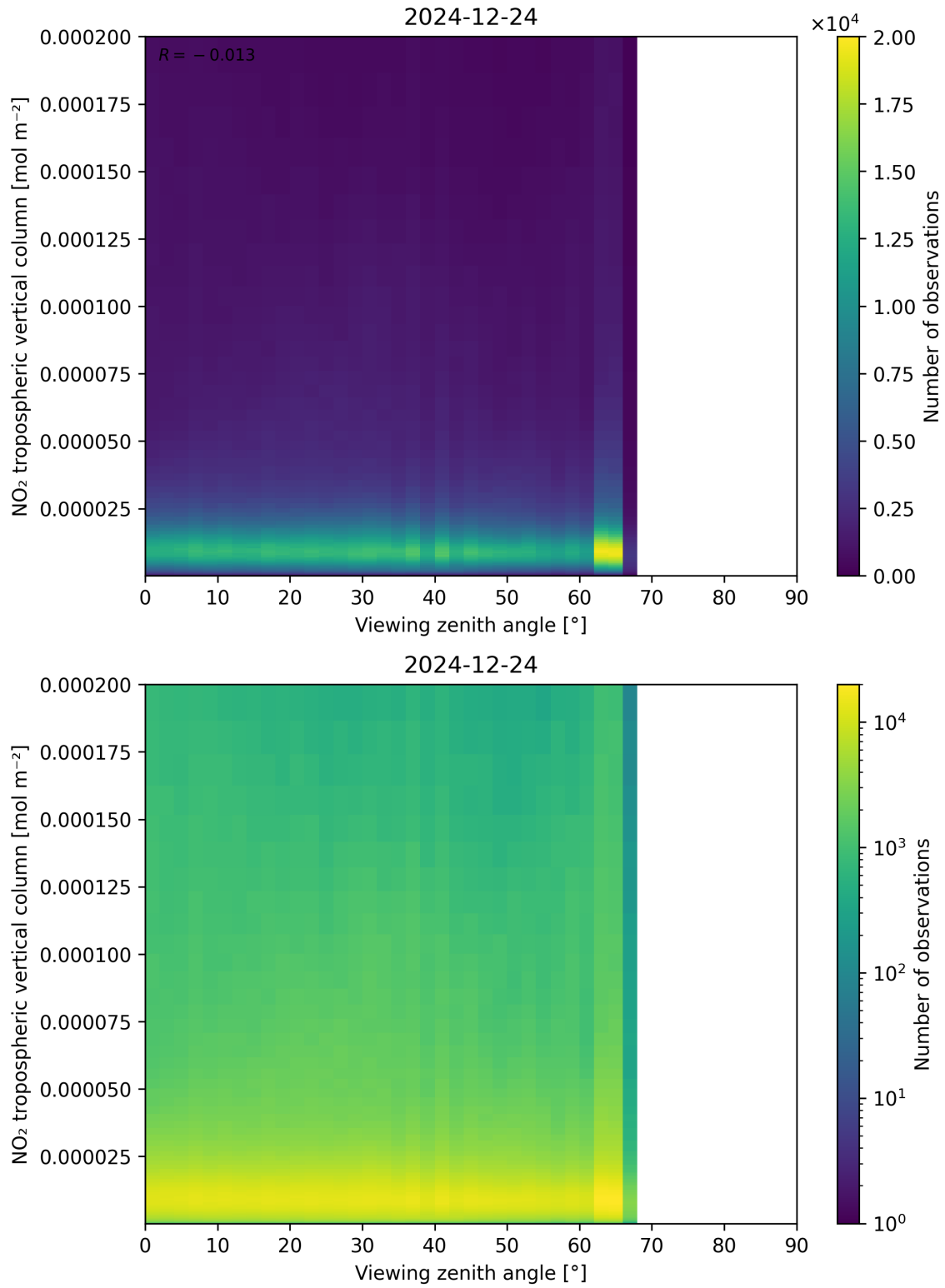
Figure 169: Scatter density plot of “Viewing zenith angle” against “NO 2 tropospheric vertical column” for 2024-12-23 to 2024-12-25.
