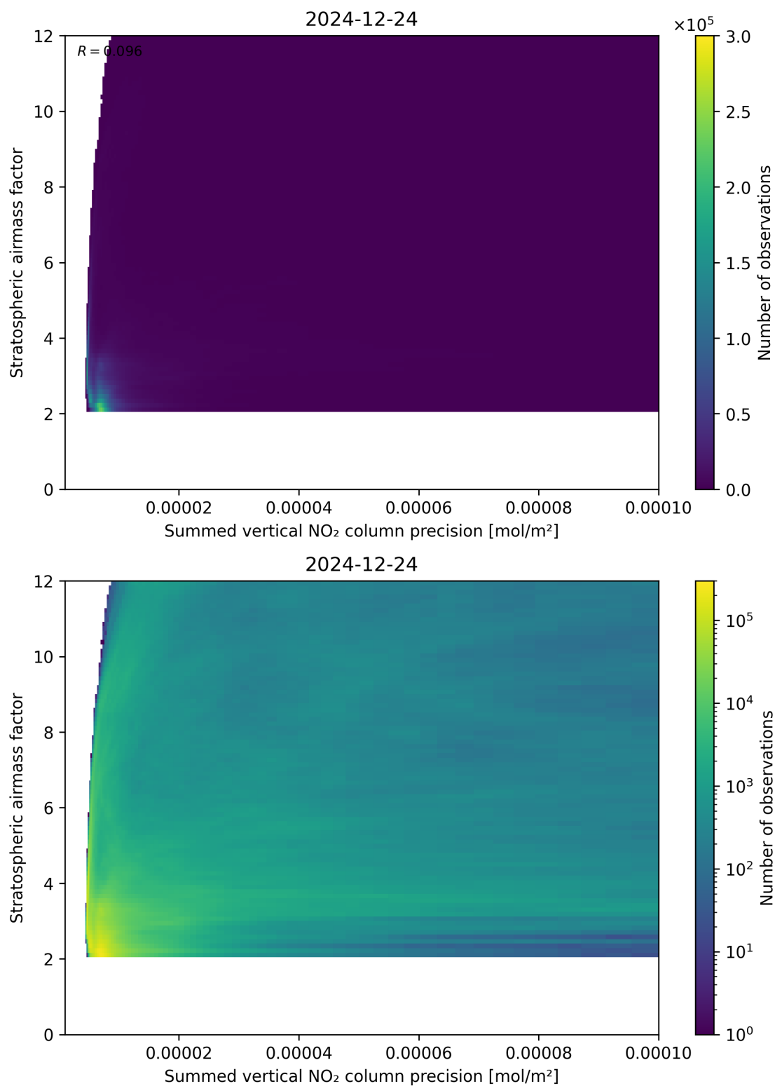
Figure 106: Scatter density plot of “Summed vertical NO 2 column precision” against “Stratospheric airmass factor” for 2024-12-23 to 2024-12-25.
