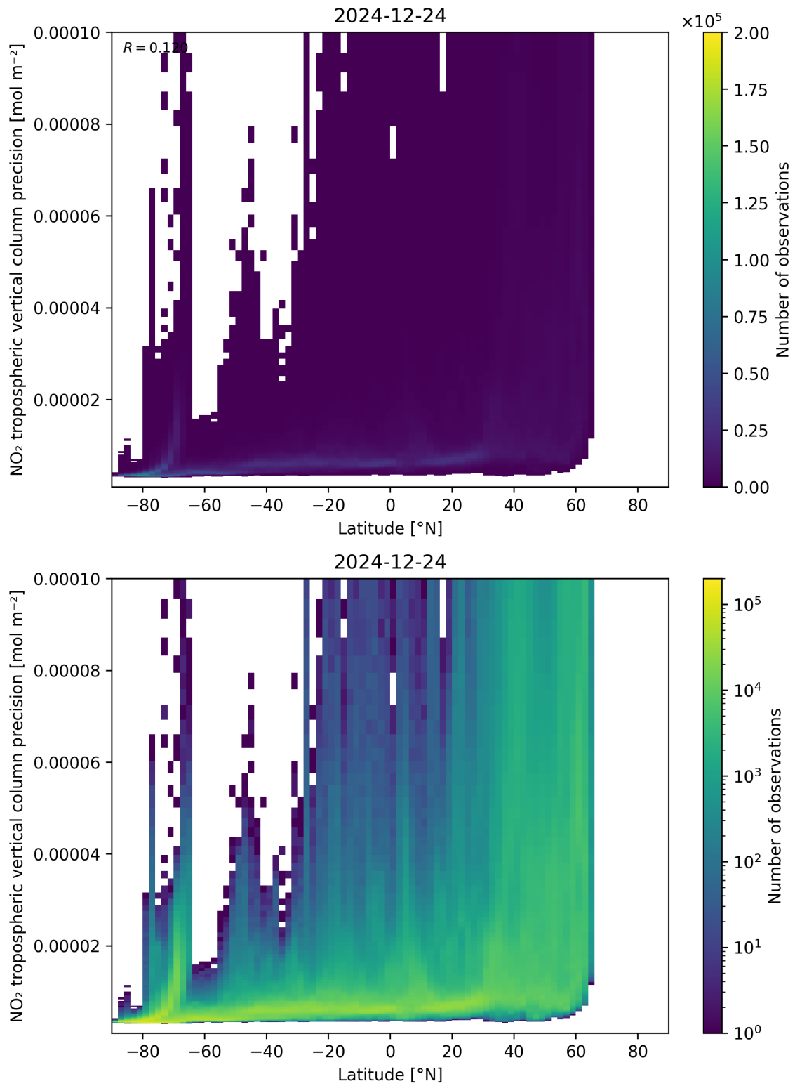
Figure 93: Scatter density plot of “Latitude” against “NO 2 tropospheric vertical column precision” for 2024-12-23 to 2024-12-25.
