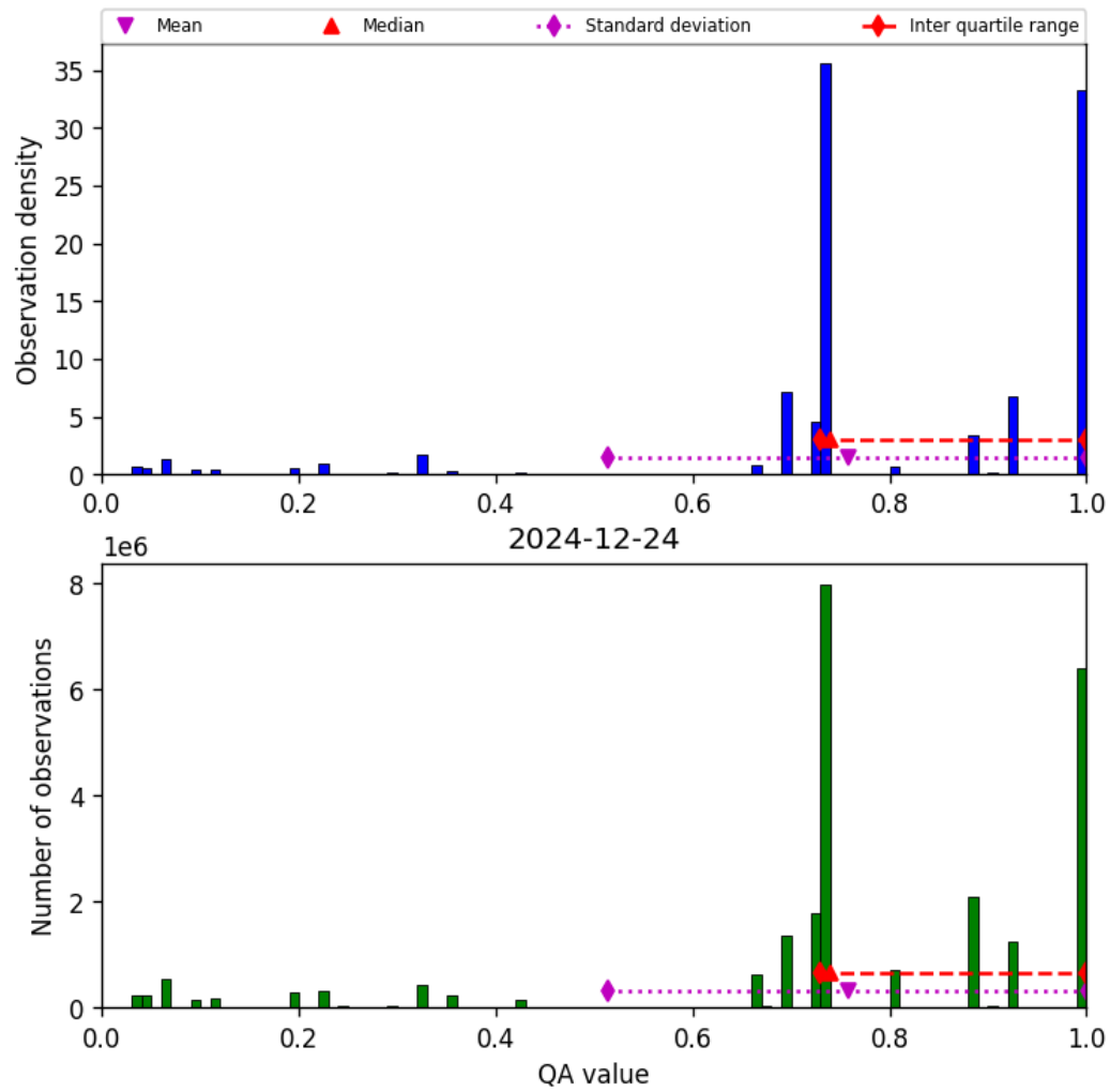
Figure 28: Histogram of “QA value” for 2024-12-23 to 2024-12-25
