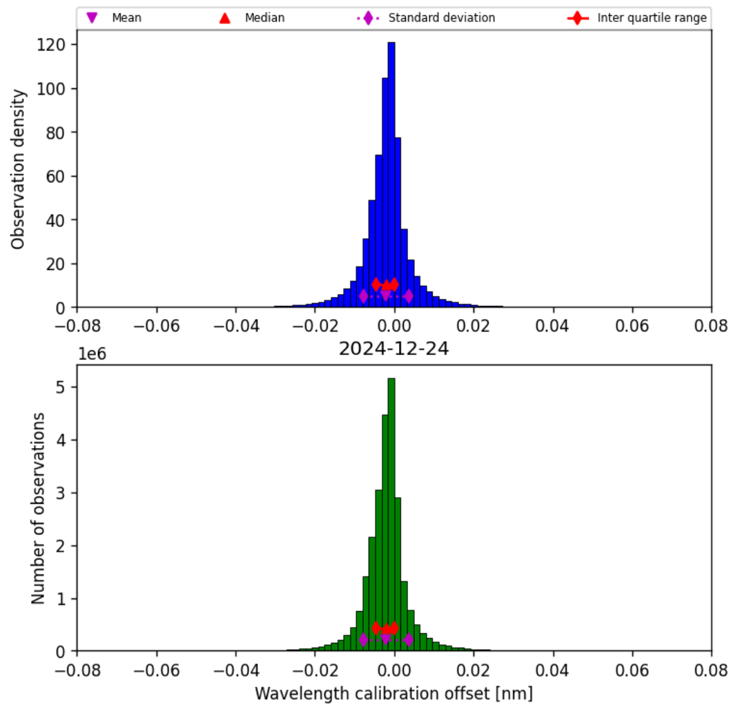
Figure 35: Histogram of “Wavelength calibration offset” for 2024-12-23 to 2024-12-25
