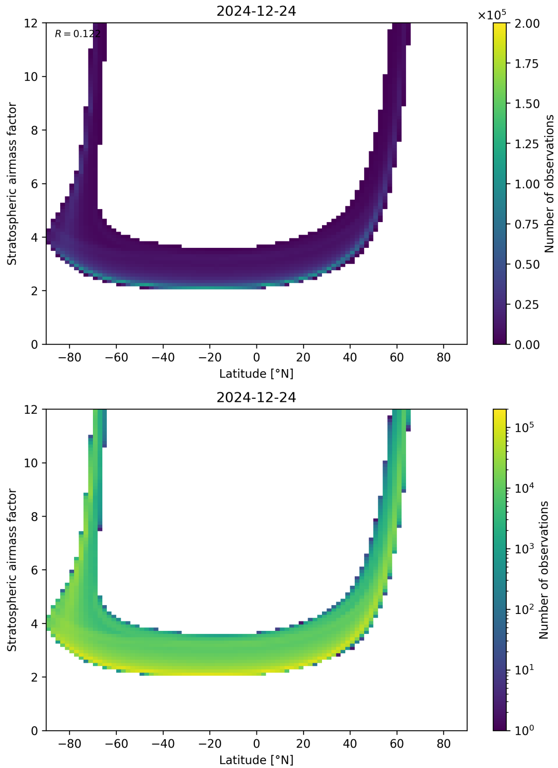
Figure 83: Scatter density plot of “Latitude” against “Stratospheric airmass factor” for 2024-12-23 to 2024-12-25.
