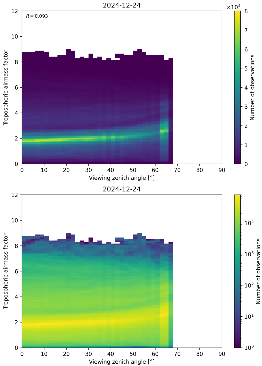
Figure 161: Scatter density plot of “Viewing zenith angle” against “Tropospheric airmass factor” for 2024-12-23 to 2024-12-25.
