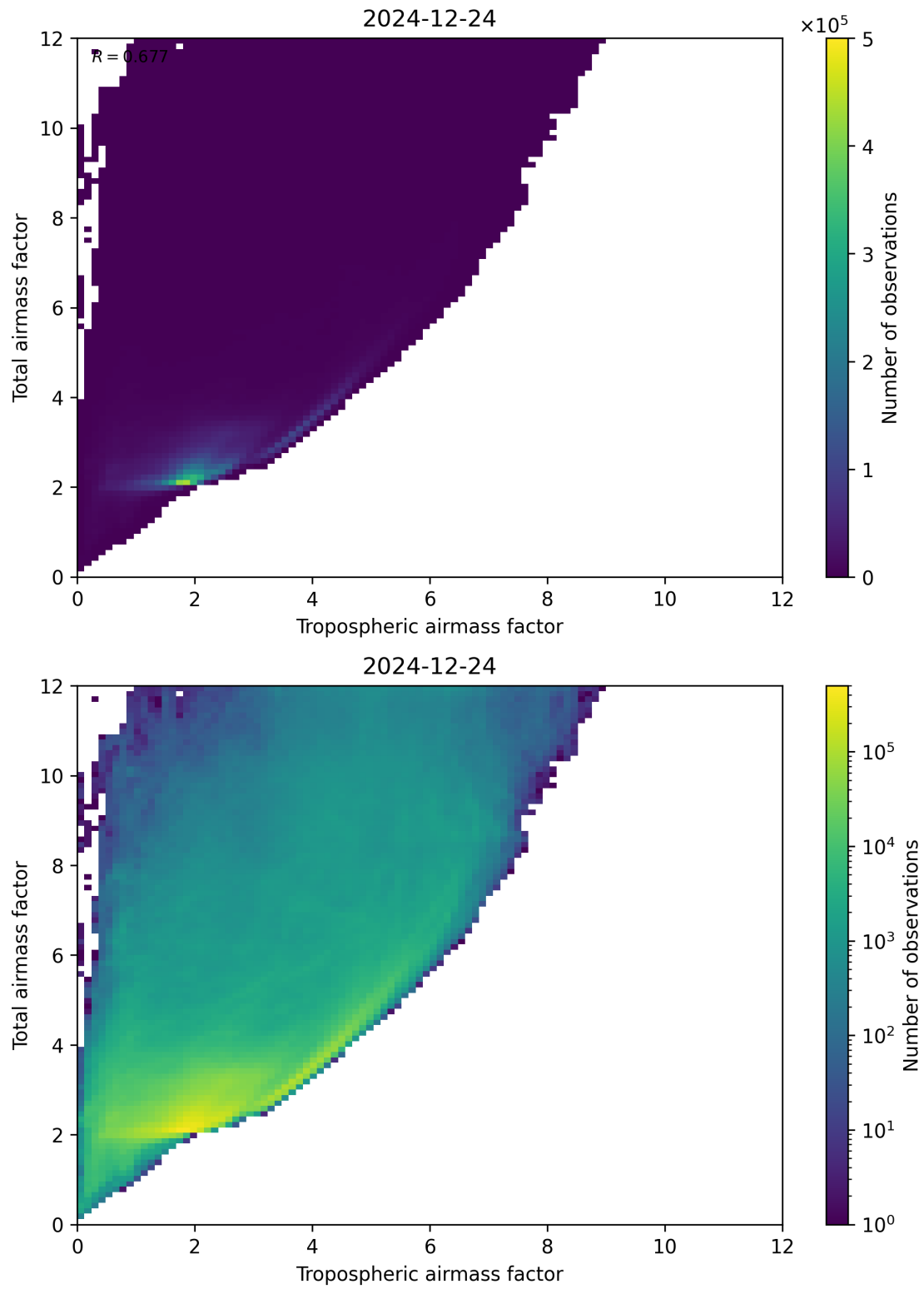
Figure 72: Scatter density plot of “Tropospheric airmass factor” against “Total airmass factor” for 2024-12-23 to 2024-12-25.
