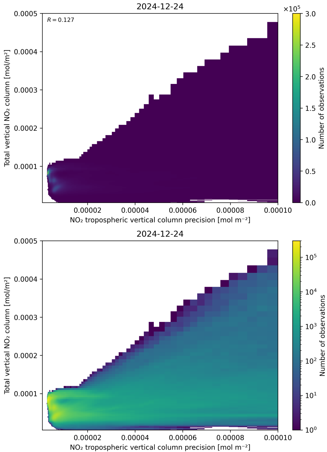
Figure 138: Scatter density plot of “NO 2 tropospheric vertical column precision” against “Total vertical NO 2 column” for 2024-12-23 to 2024-12-25.
