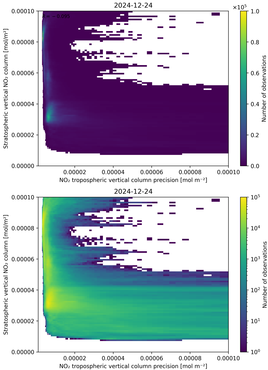
Figure 135: Scatter density plot of “NO 2 tropospheric vertical column precision” against “Stratospheric vertical NO 2 column” for 2024-12-23 to 2024-12-25.
