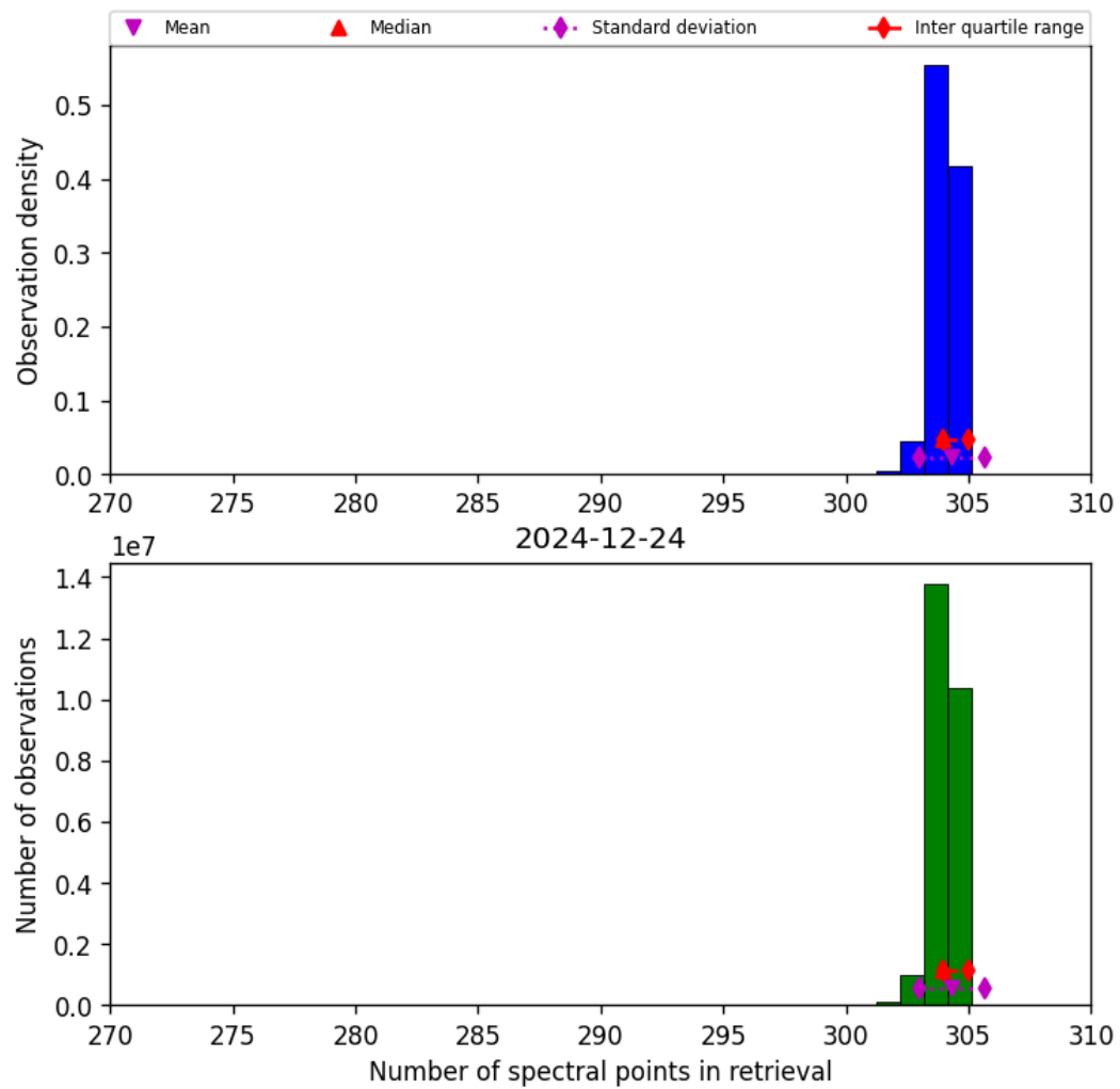
Figure 33: Histogram of “Number of spectral points in retrieval” for 2024-12-23 to 2024-12-25
