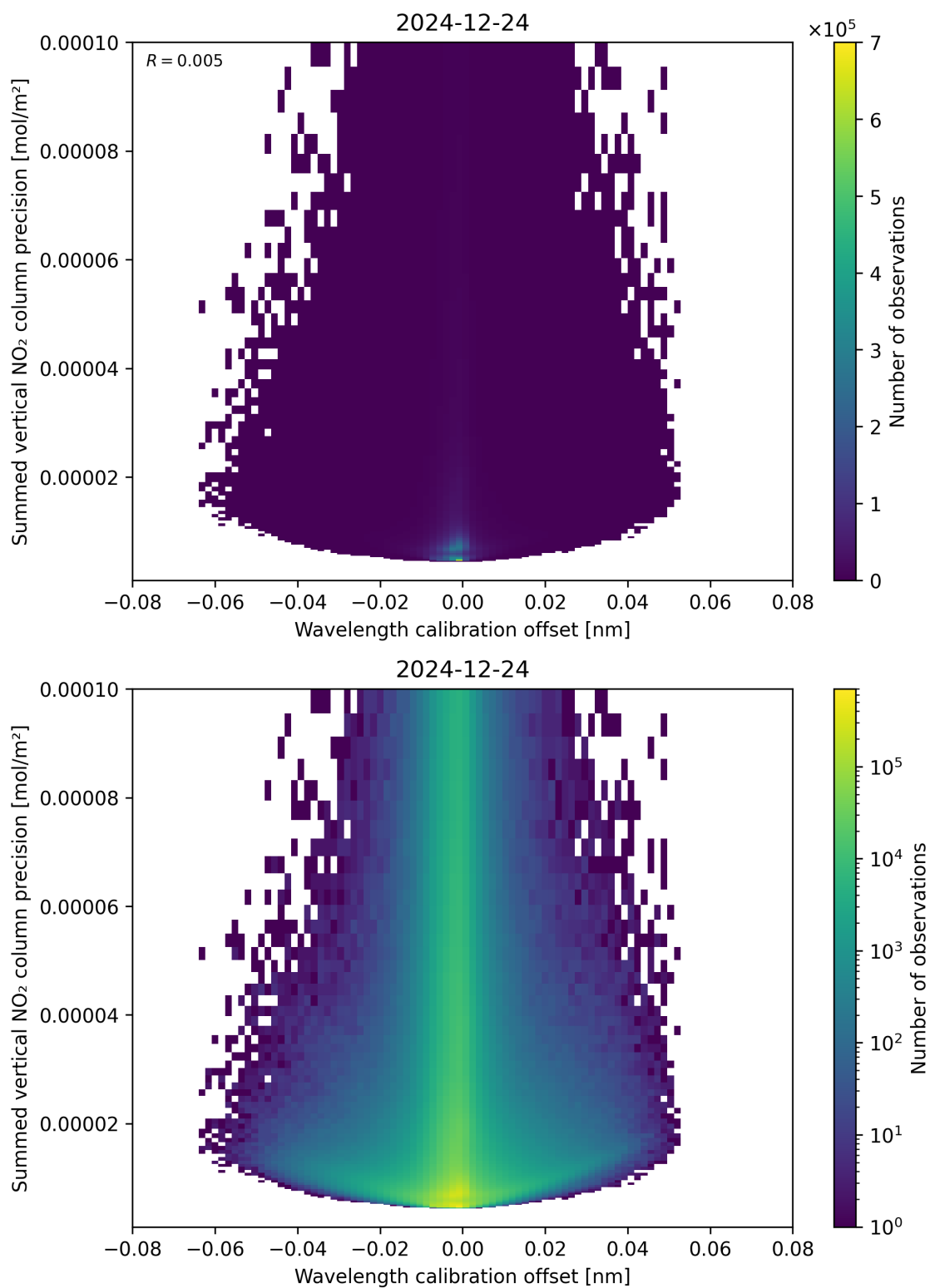
Figure 178: Scatter density plot of “Wavelength calibration offset” against “Summed vertical NO 2 column precision” for 2024-12-23 to 2024-12-25.
