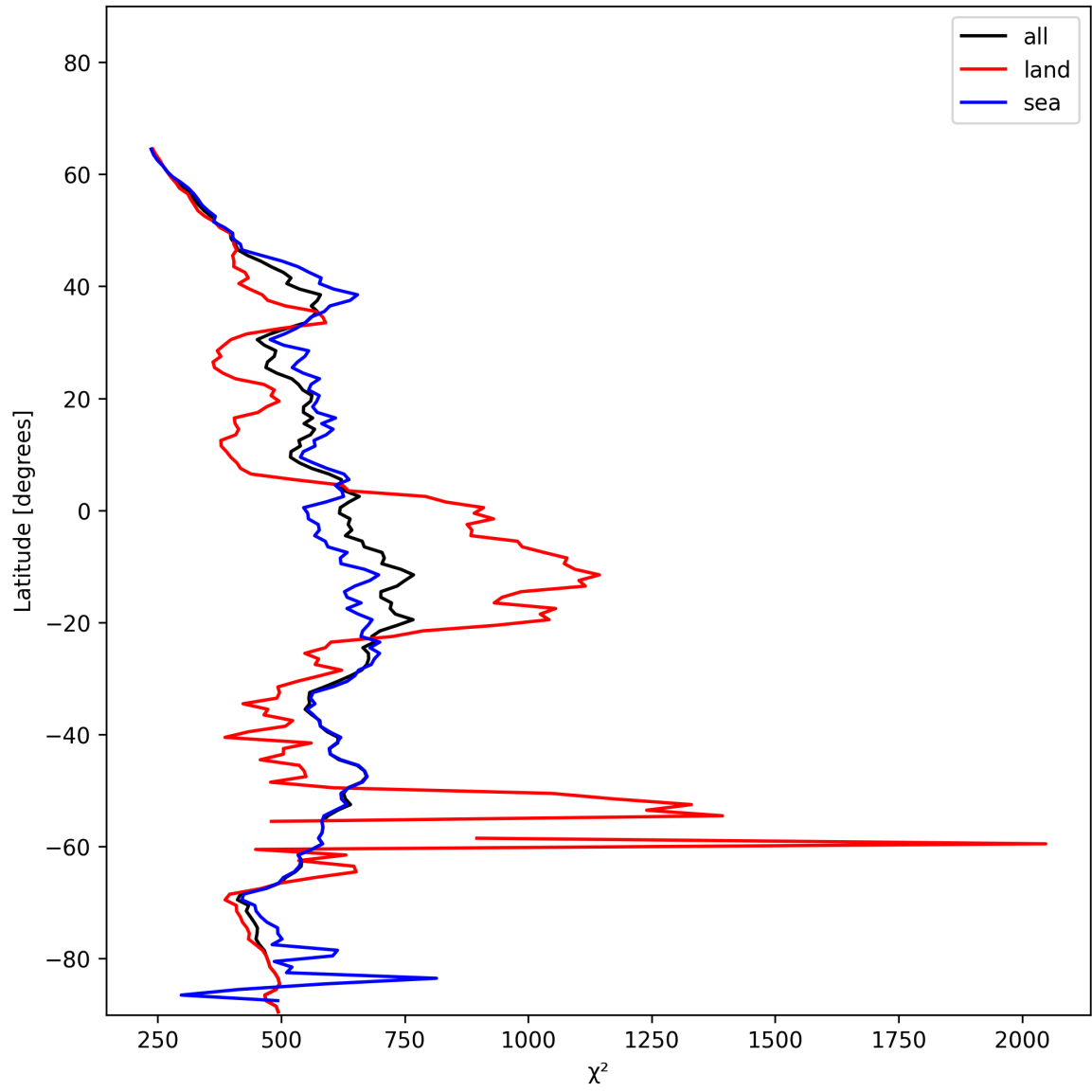
Figure 25: Zonal average of “ \chi^2 ” for 2024-12-23 to 2024-12-25.
