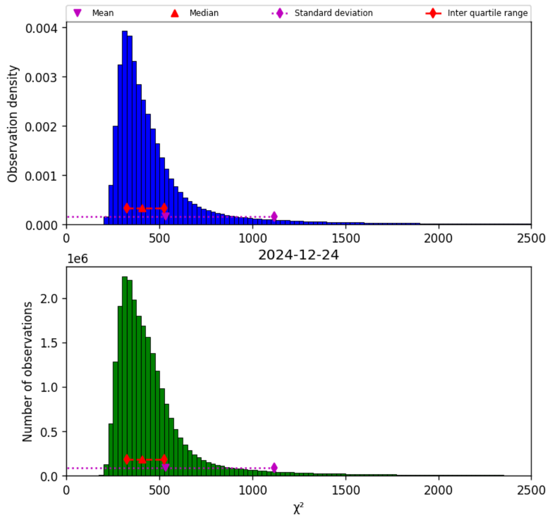
Figure 42: Histogram of “ \chi^2 ” for 2024-12-23 to 2024-12-25
