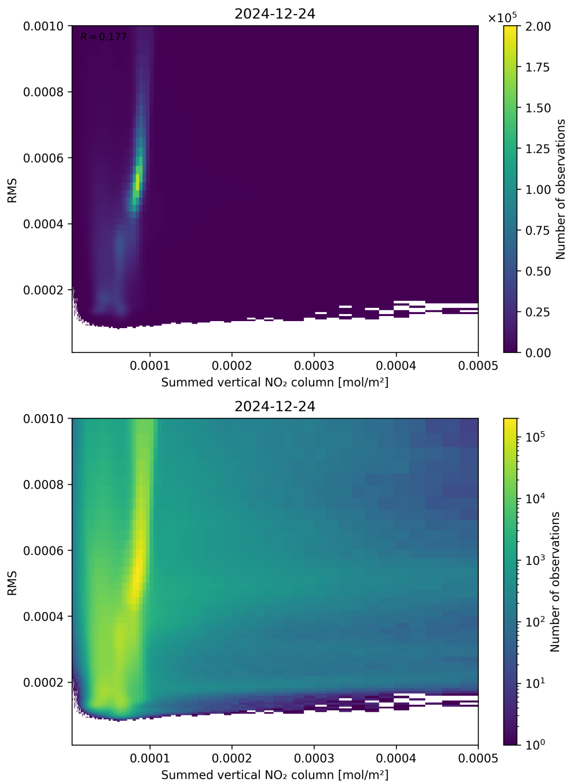
Figure 109: Scatter density plot of “Summed vertical NO 2 column” against “RMS” for 2024-12-23 to 2024-12-25.
