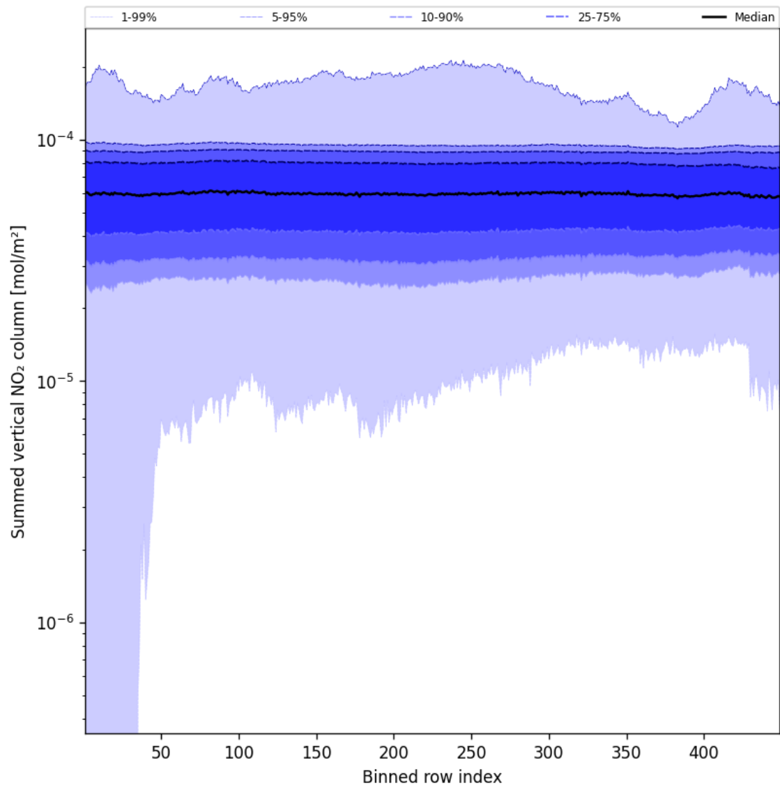
Figure 57: Along track statistics of “Summed vertical NO 2 column” for 2024-12-23 to 2024-12-25
