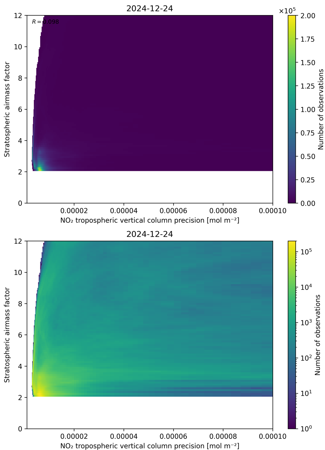
Figure 131: Scatter density plot of “NO 2 tropospheric vertical column precision” against “Stratospheric airmass factor” for 2024-12-23 to 2024-12-25.
