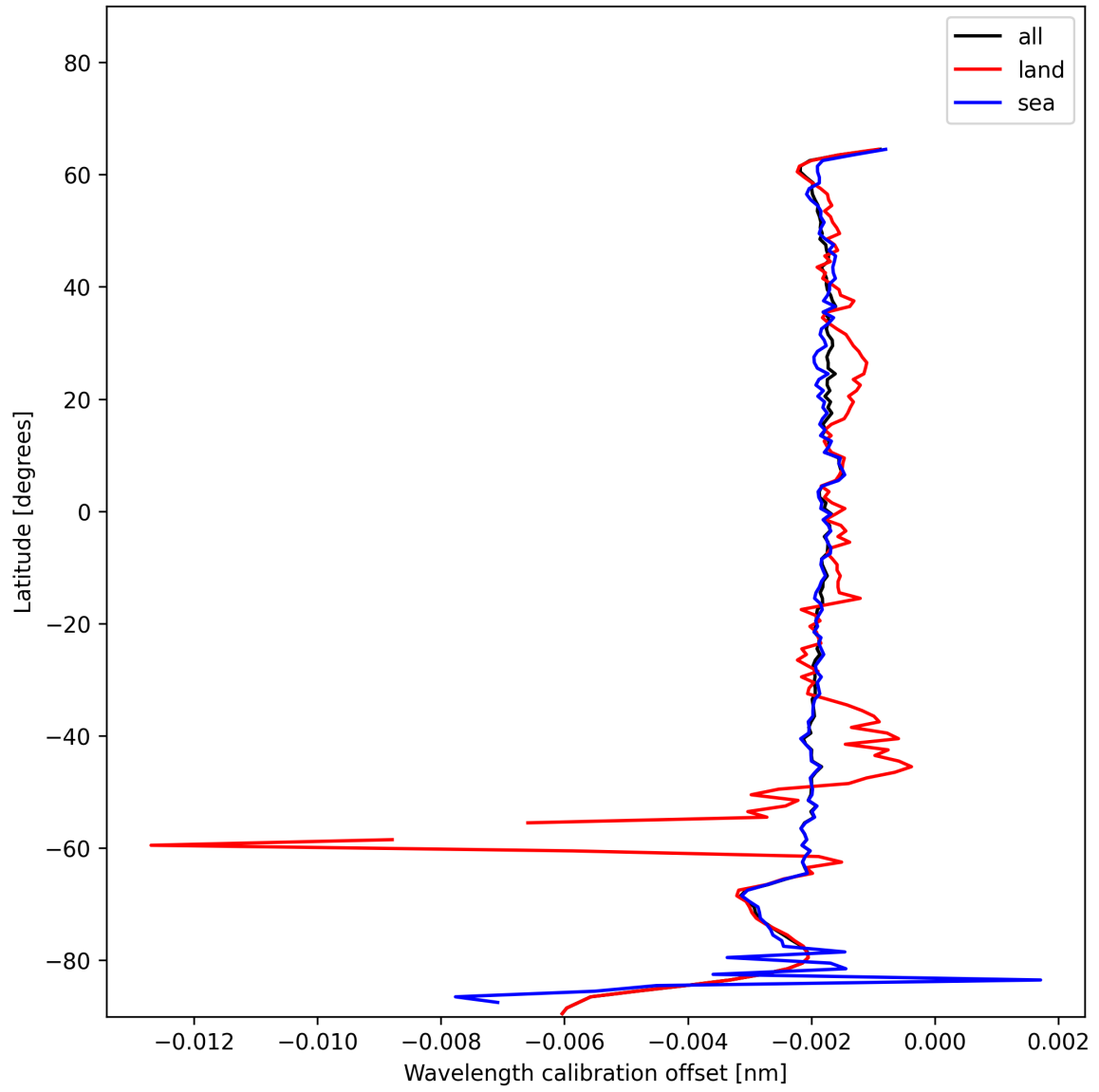
Figure 18: Zonal average of “Wavelength calibration offset” for 2024-12-23 to 2024-12-25.
