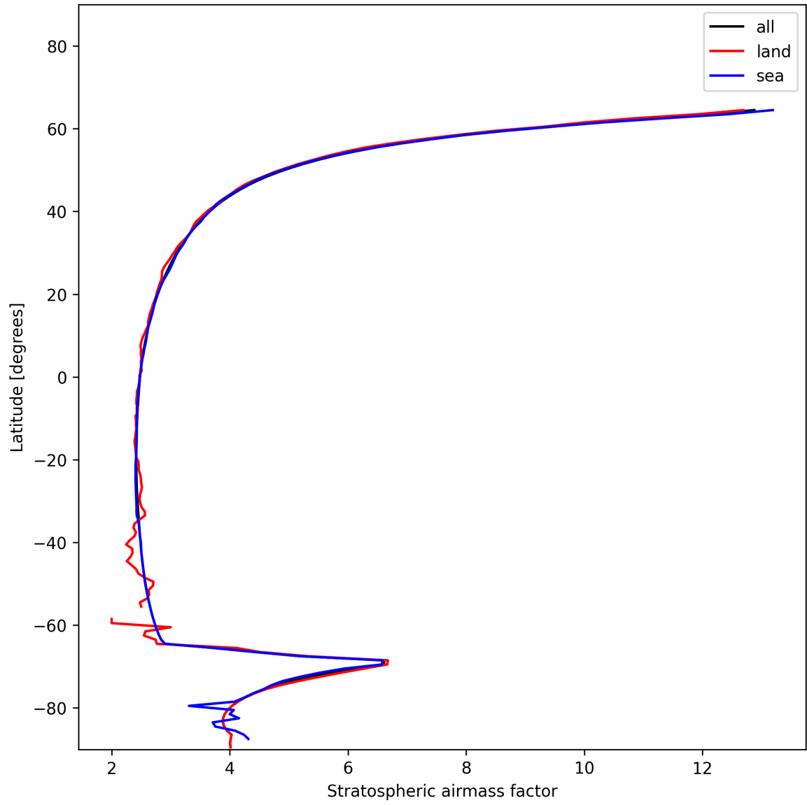
Figure 27: Zonal average of “Stratospheric airmass factor” for 2024-12-23 to 2024-12-25.
