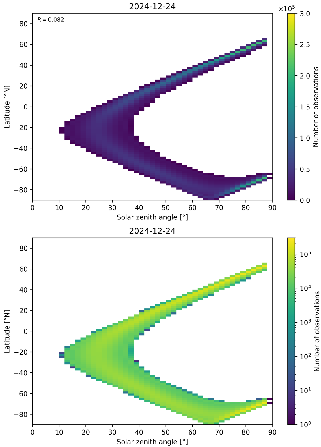
Figure 149: Scatter density plot of “Solar zenith angle” against “Latitude” for 2024-12-23 to 2024-12-25.
