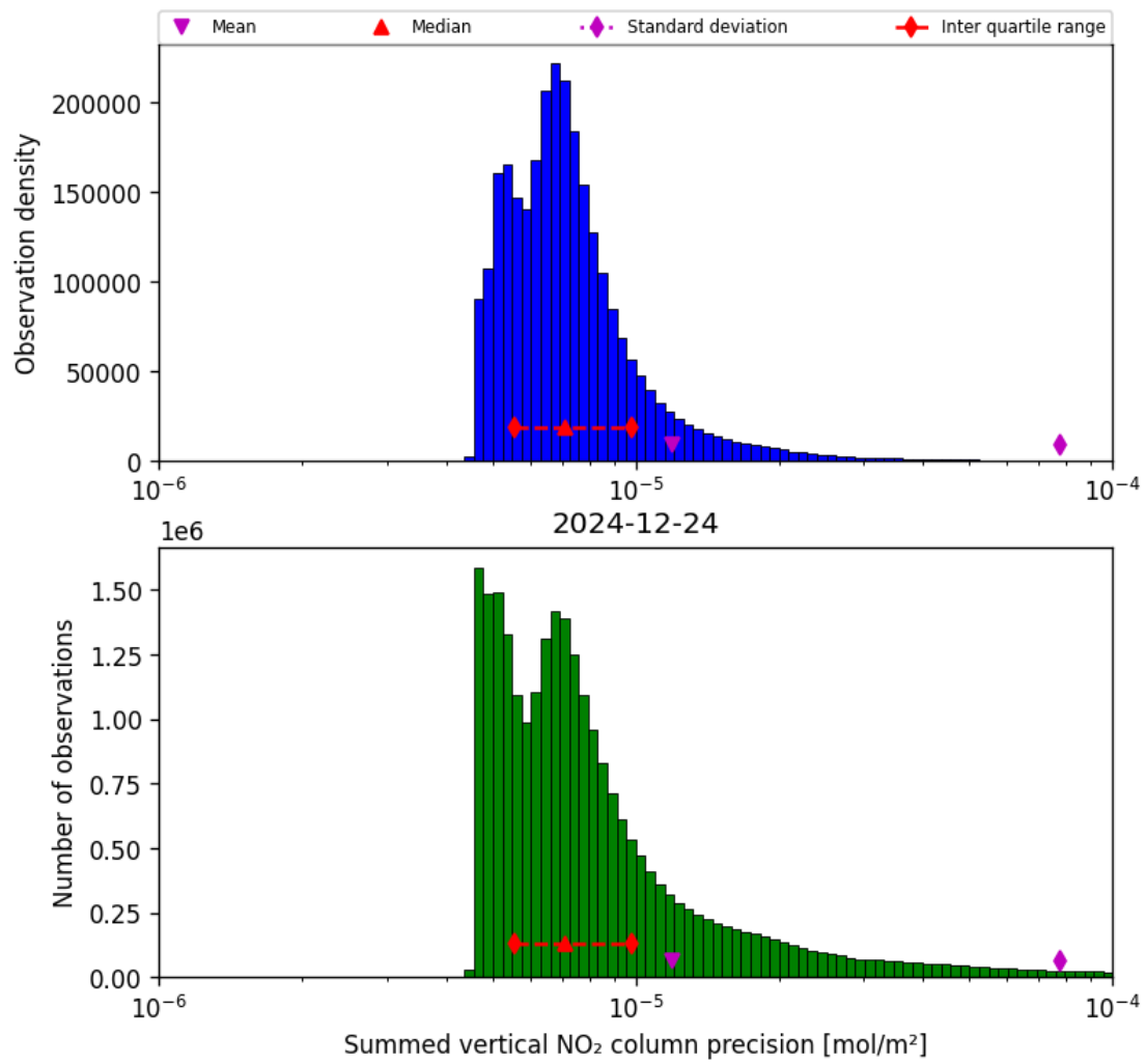
Figure 41: Histogram of "Summed vertical NO 2 column precision" for 2024-12-23 to 2024-12-25
