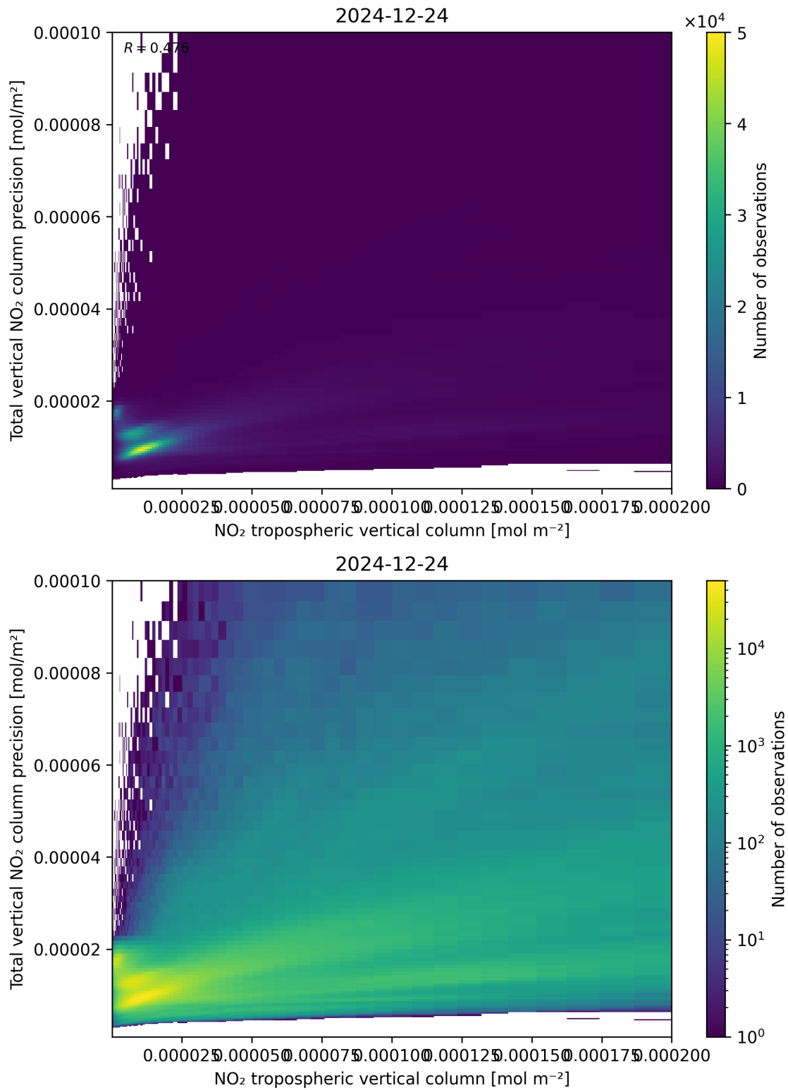
Figure 129: Scatter density plot of “NO 2 tropospheric vertical column” against “Total vertical NO 2 column precision” for 2024-12-23 to 2024-12-25.
