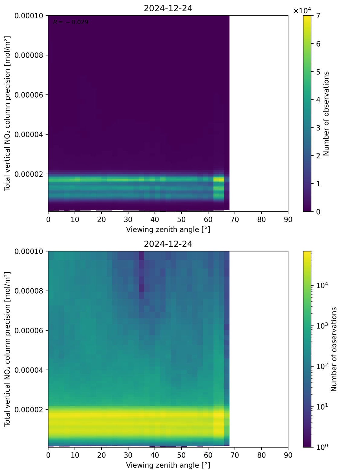
Figure 168: Scatter density plot of “Viewing zenith angle” against “Total vertical NO 2 column precision” for 2024-12-23 to 2024-12-25.
