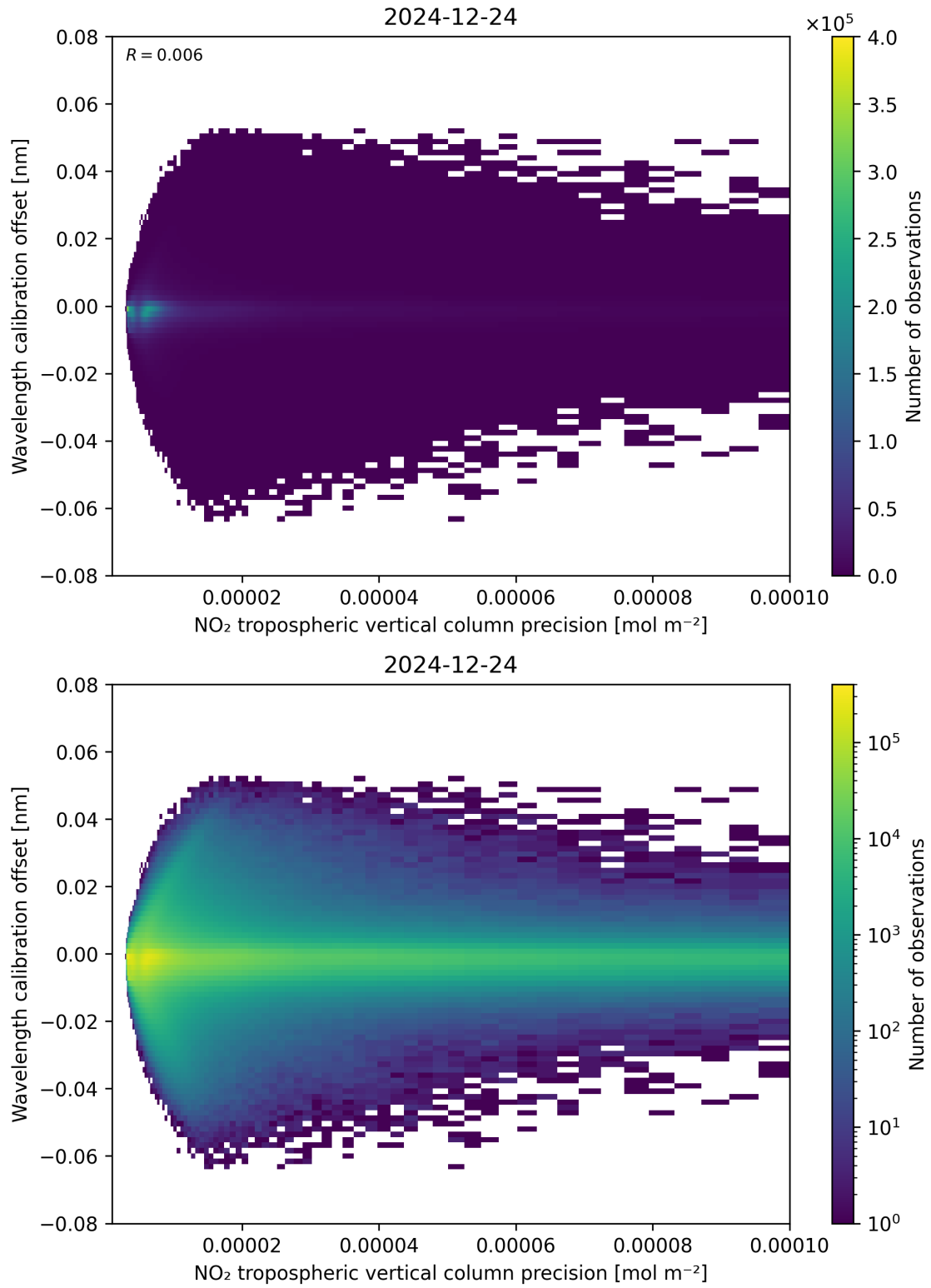
Figure 141: Scatter density plot of “NO 2 tropospheric vertical column precision” against “Wavelength calibration offset” for 2024-12-23 to 2024-12-25.
