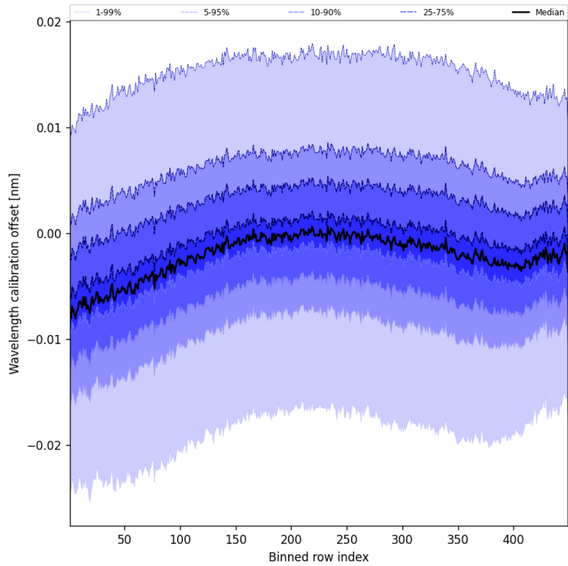
Figure 52: Along track statistics of “Wavelength calibration offset” for 2024-12-23 to 2024-12-25
