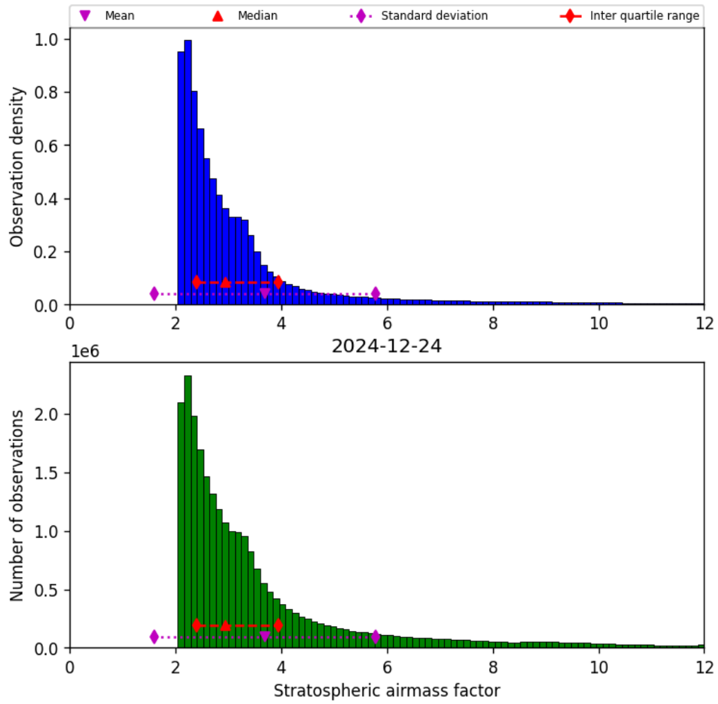
Figure 44: Histogram of “Stratospheric airmass factor” for 2024-12-23 to 2024-12-25
