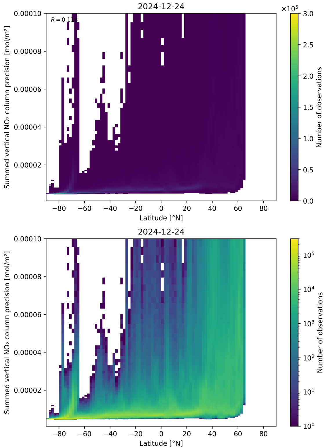
Figure 89: Scatter density plot of “Latitude” against “Summed vertical NO 2 column precision” for 2024-12-23 to 2024-12-25.
