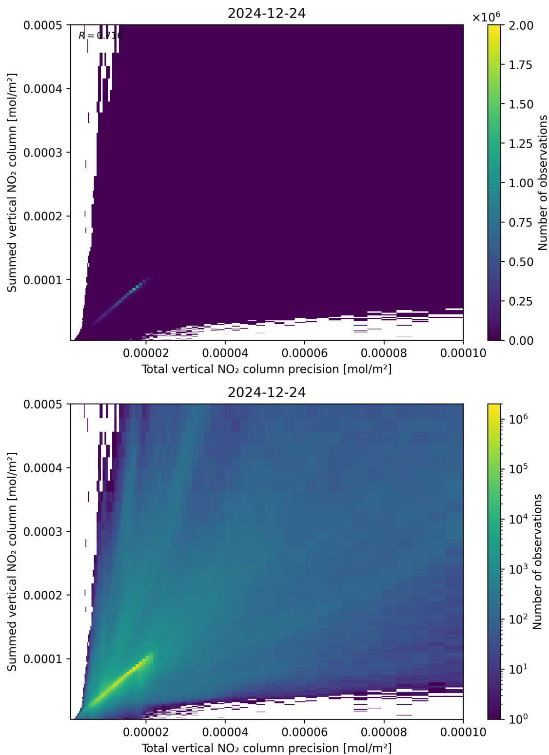
Figure 117: Scatter density plot of “Total vertical NO 2 column precision” against “Summed vertical NO 2 column” for 2024-12-23 to 2024-12-25.
