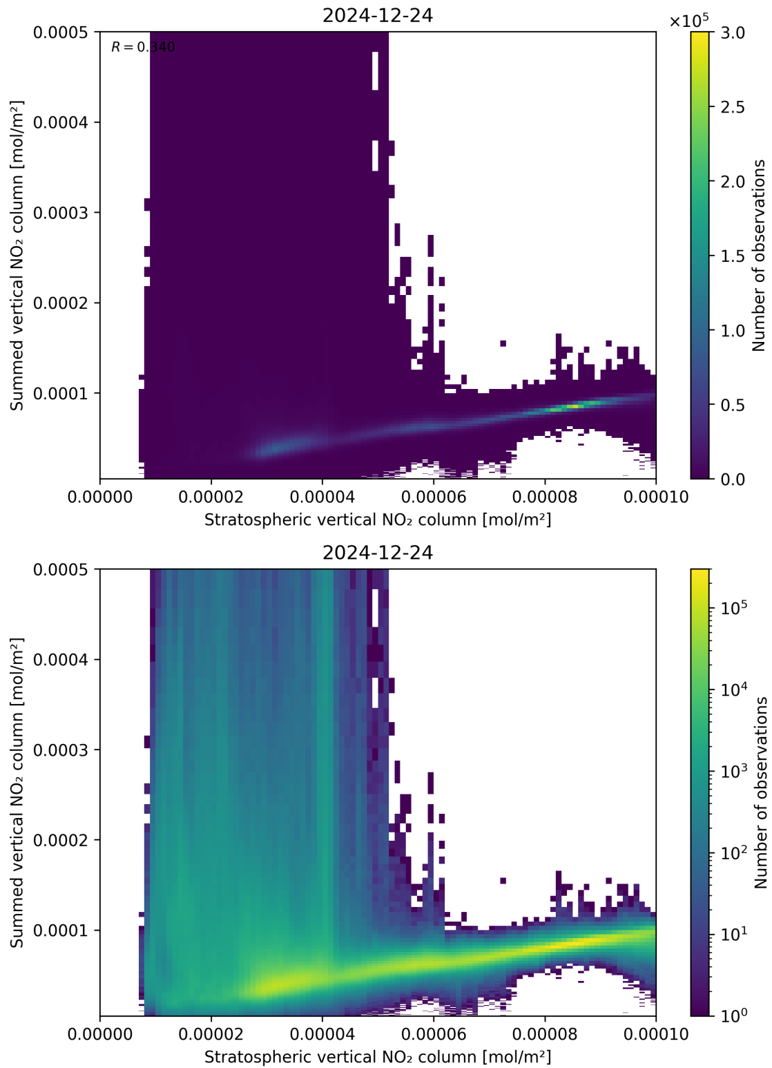
Figure 98: Scatter density plot of “Stratospheric vertical NO 2 column” against “Summed vertical NO 2 column” for 2024-12-23 to 2024-12-25.
