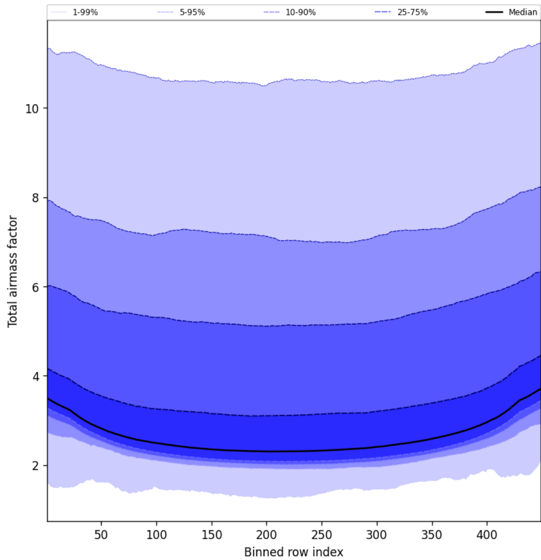
Figure 49: Along track statistics of “Total airmass factor” for 2024-12-23 to 2024-12-25
