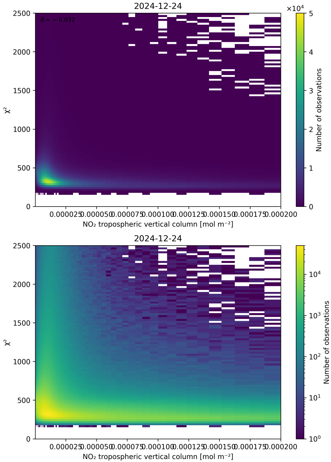
Figure 124: Scatter density plot of “NO 2 tropospheric vertical column” against “ \chi^2 ” for 2024-12-23 to 2024-12-25.
