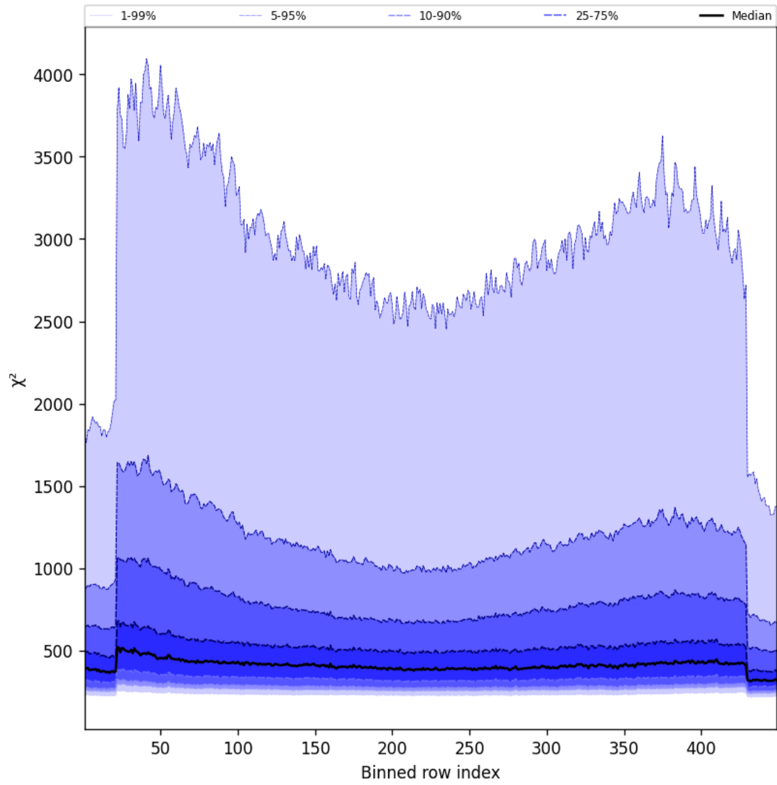
Figure 59: Along track statistics of “ \chi^2 ” for 2024-12-23 to 2024-12-25
