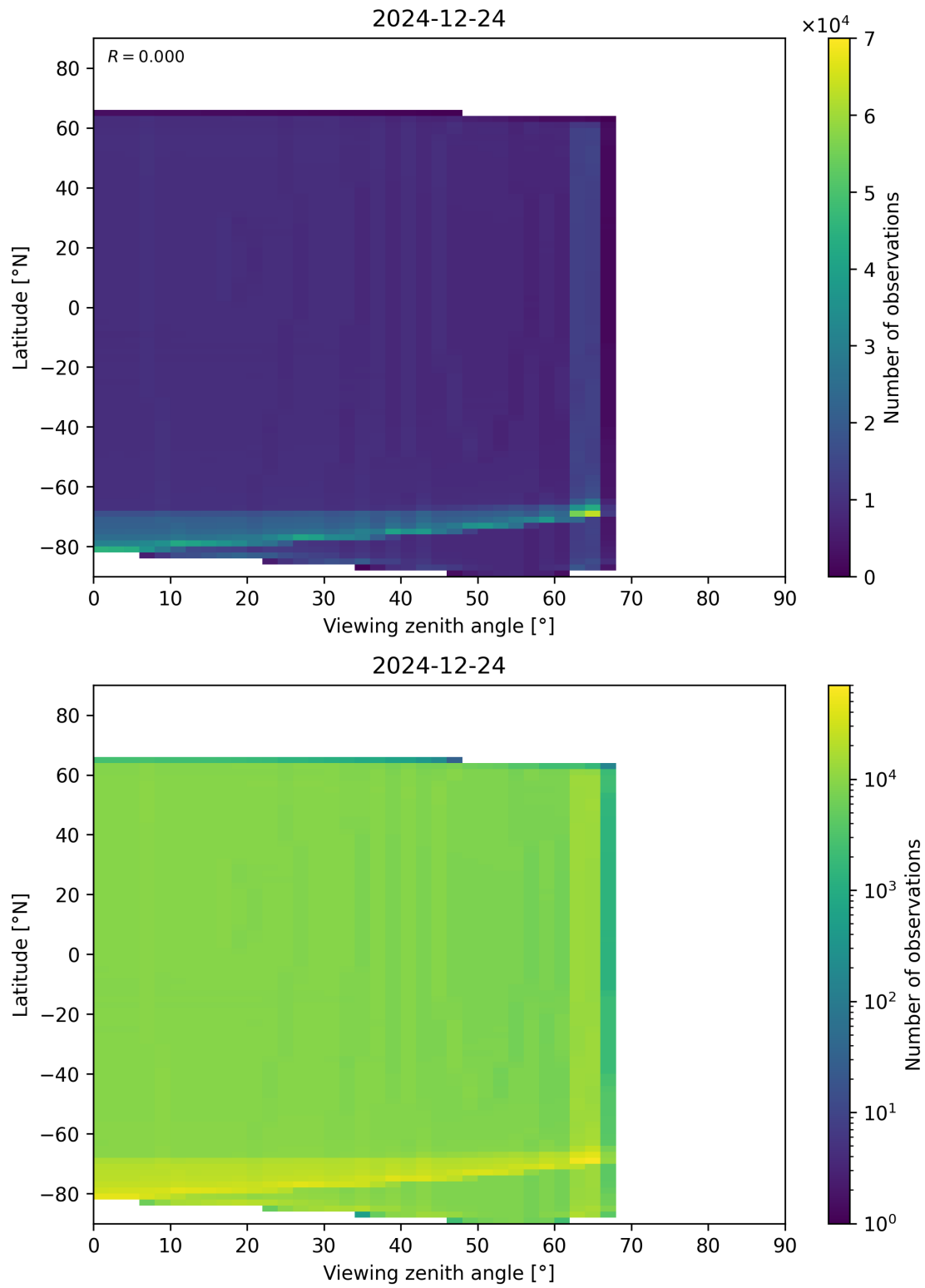
Figure 163: Scatter density plot of “Viewing zenith angle” against “Latitude” for 2024-12-23 to 2024-12-25.
