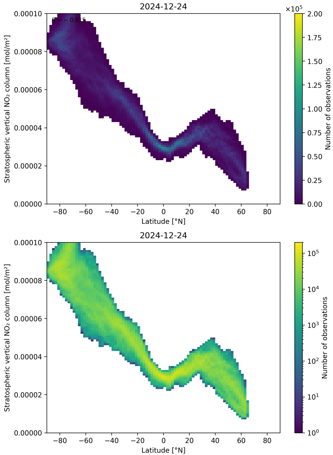
Figure 87: Scatter density plot of “Latitude” against “Stratospheric vertical NO 2 column” for 2024-12-23 to 2024-12-25.
