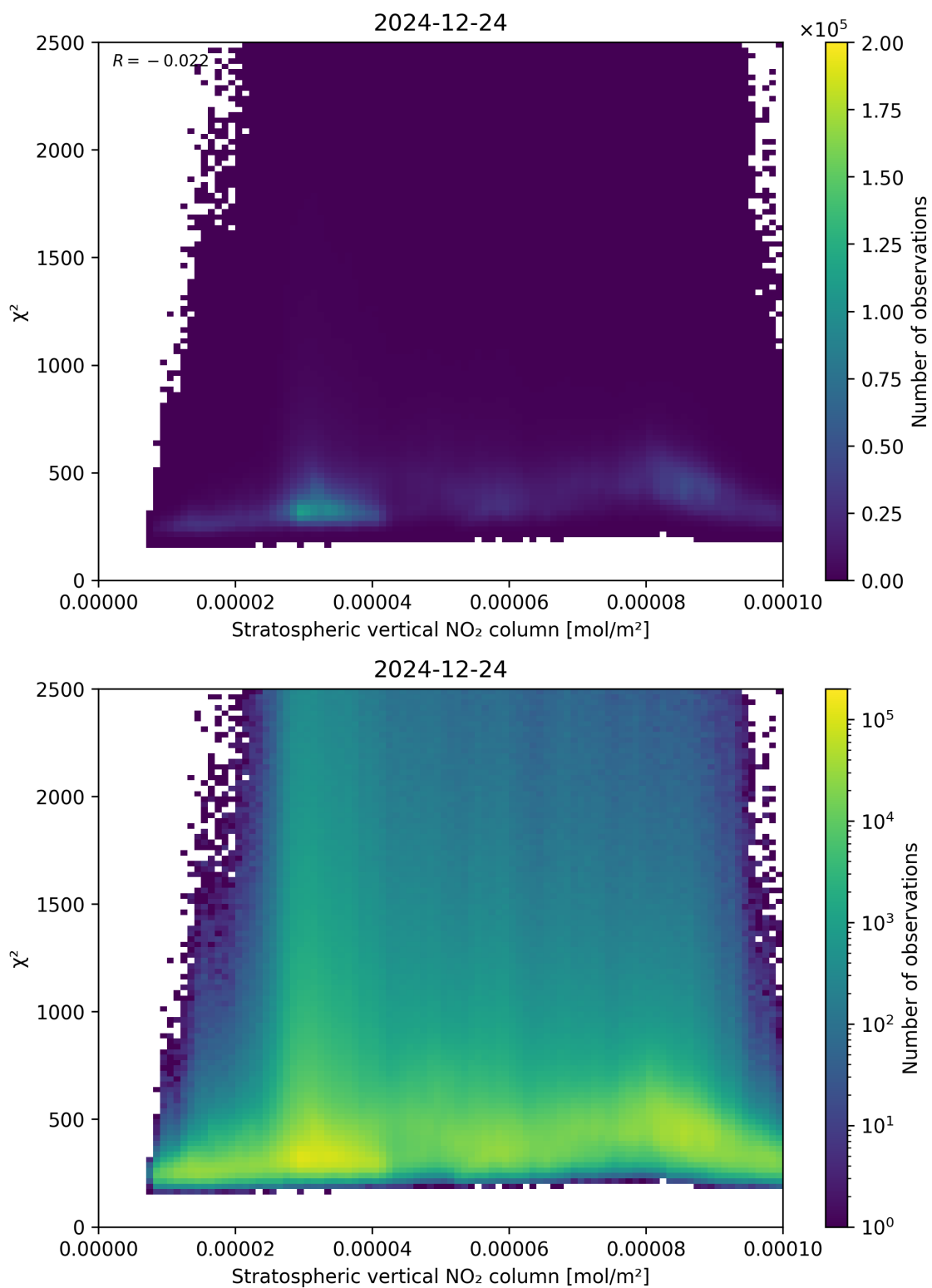
Figure 97: Scatter density plot of “Stratospheric vertical NO 2 column” against “ \chi^2 ” for 2024-12-23 to 2024-12-25.
