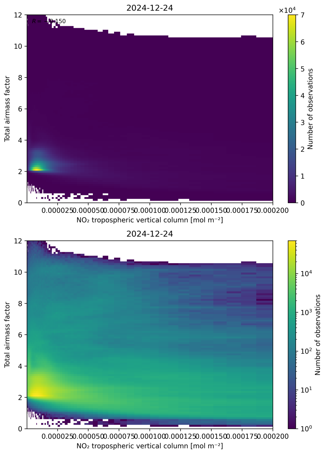
Figure 122: Scatter density plot of “NO 2 tropospheric vertical column” against “Total air mass factor” for 2024-12-23 to 2024-12-25.
