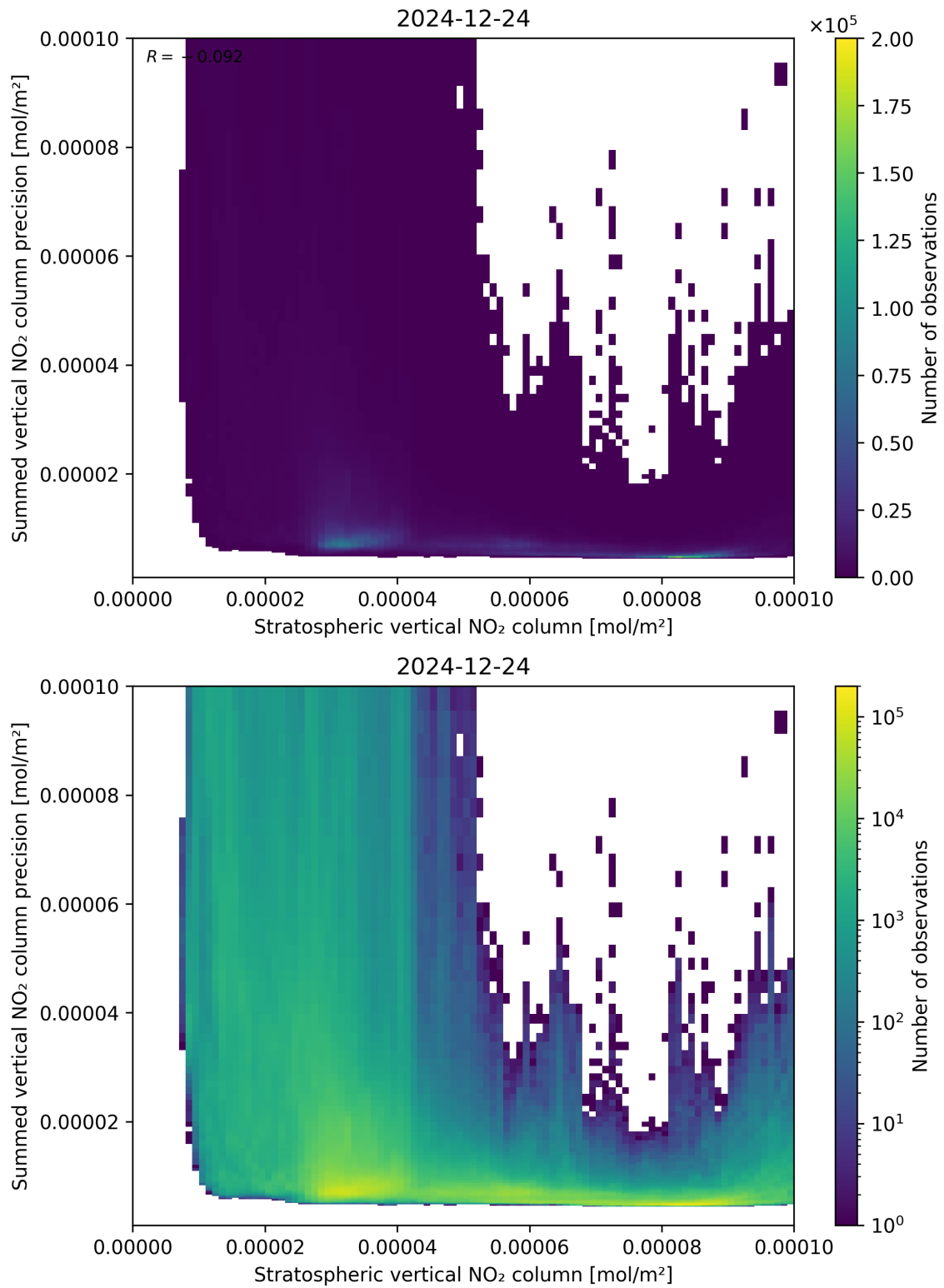
Figure 99: Scatter density plot of “Stratospheric vertical NO 2 column” against “Summed vertical NO 2 column precision” for 2024-12-23 to 2024-12-25.
