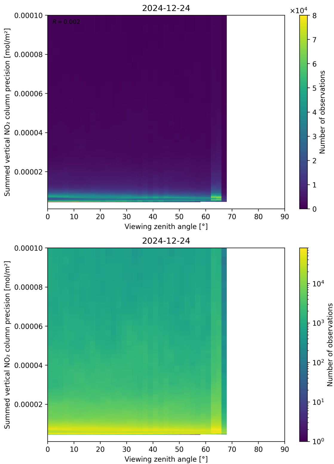
Figure 166: Scatter density plot of “Viewing zenith angle” against “Summed vertical NO 2 column precision” for 2024-12-23 to 2024-12-25.
