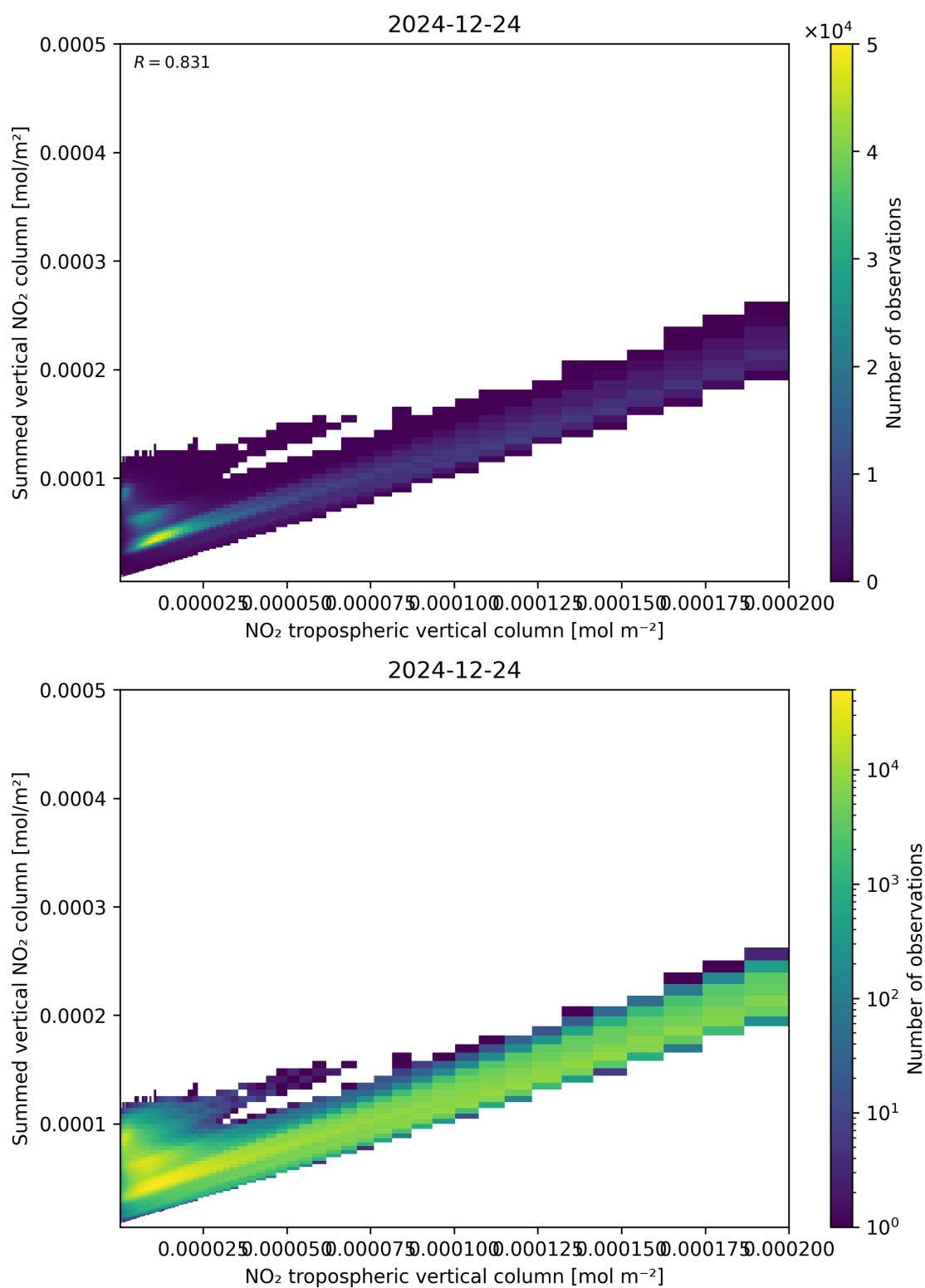
Figure 126: Scatter density plot of “NO 2 tropospheric vertical column” against “Summed vertical NO 2 column” for 2024-12-23 to 2024-12-25.
