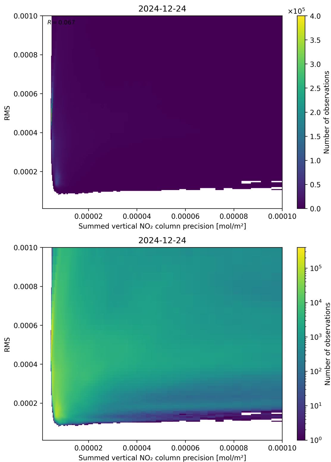
Figure 108: Scatter density plot of “Summed vertical NO 2 column precision” against “RMS” for 2024-12-23 to 2024-12-25.
