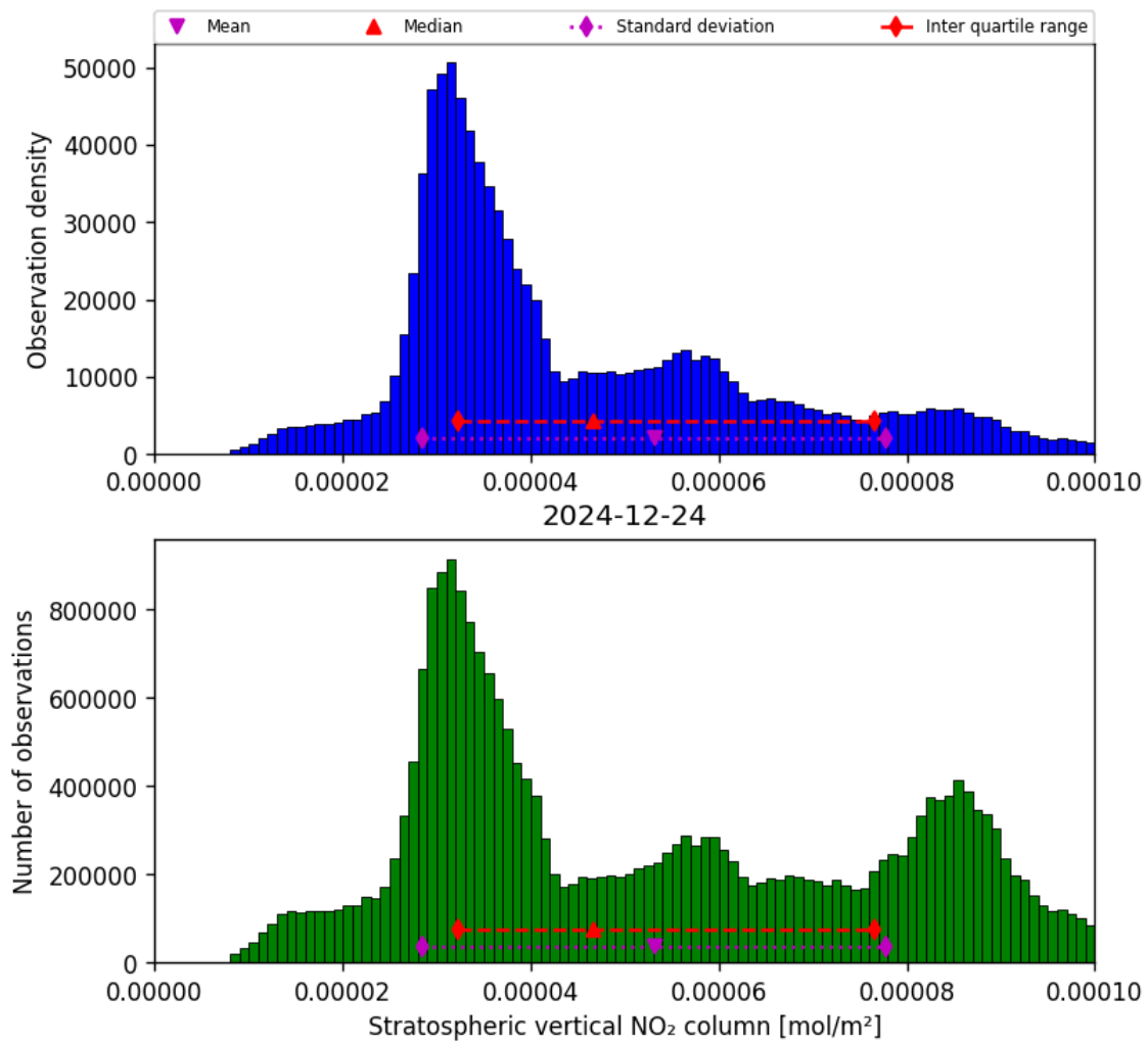
Figure 36: Histogram of “Stratospheric vertical NO 2 column” for 2024-12-23 to 2024-12-25
