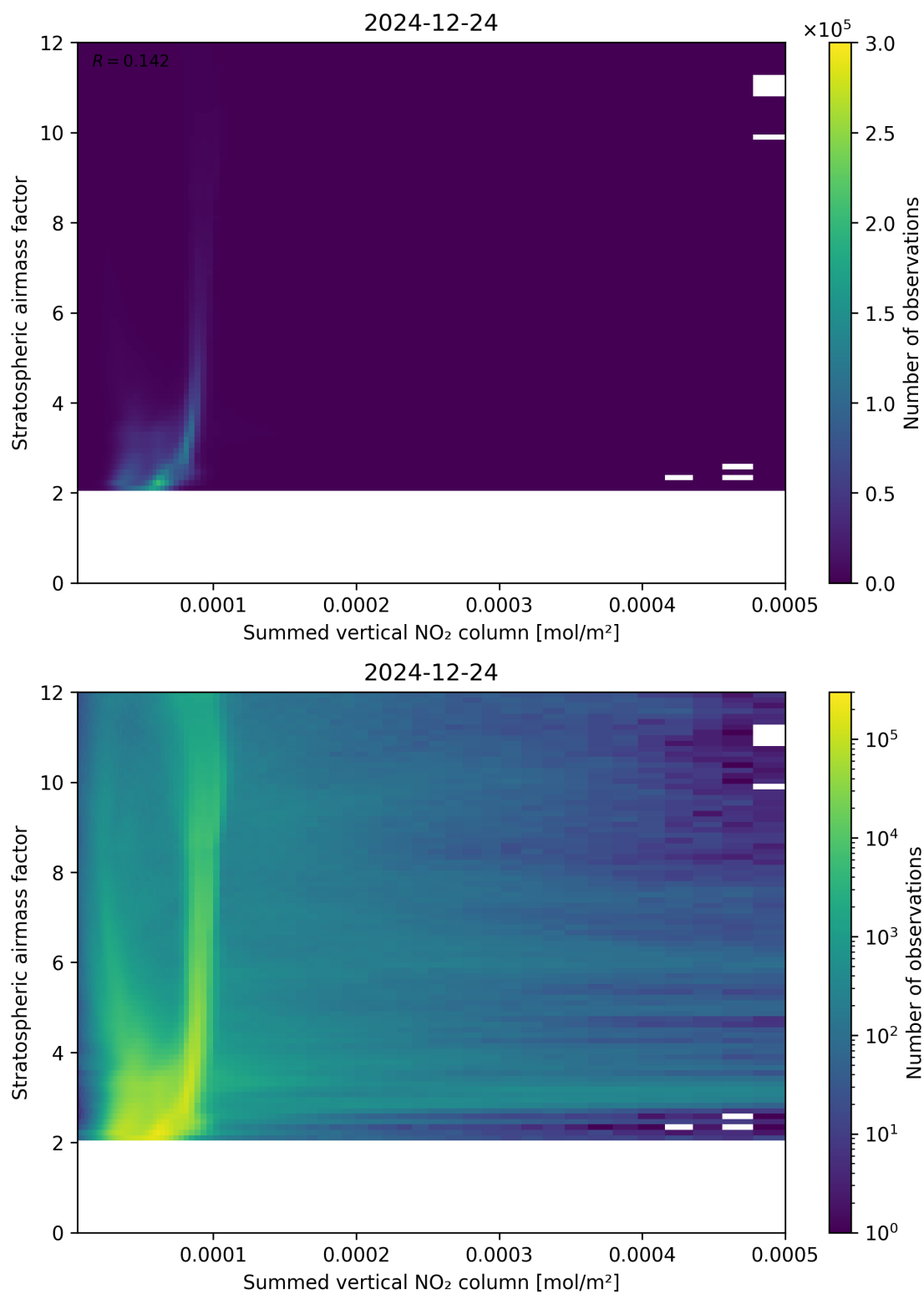
Figure 103: Scatter density plot of “Summed vertical NO 2 column” against “Stratospheric airmass factor” for 2024-12-23 to 2024-12-25.
