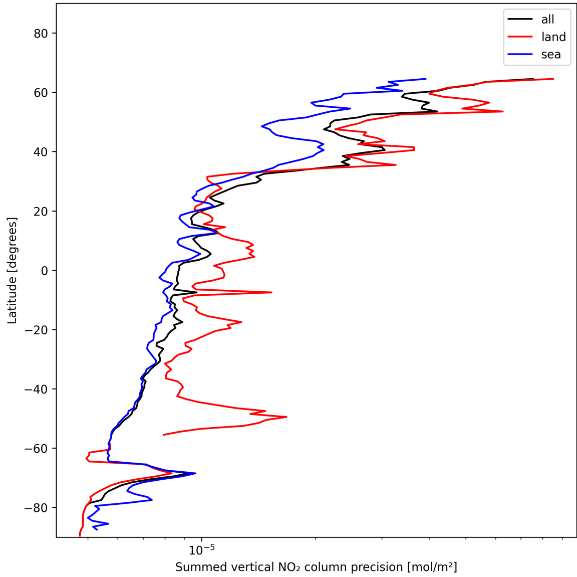
Figure 24: Zonal average of “Summed vertical NO 2 column precision” for 2024-12-23 to 2024-12-25.
