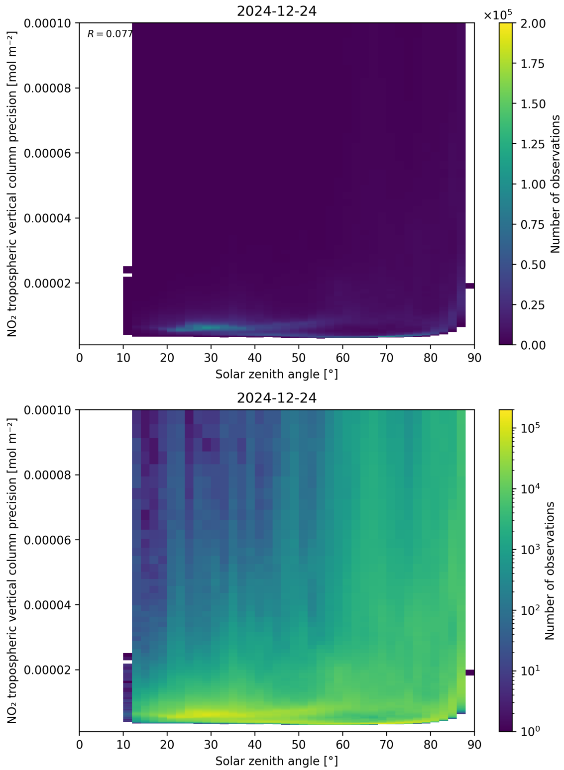
Figure 156: Scatter density plot of “Solar zenith angle” against “NO 2 tropospheric vertical column precision” for 2024-12-23 to 2024-12-25.
