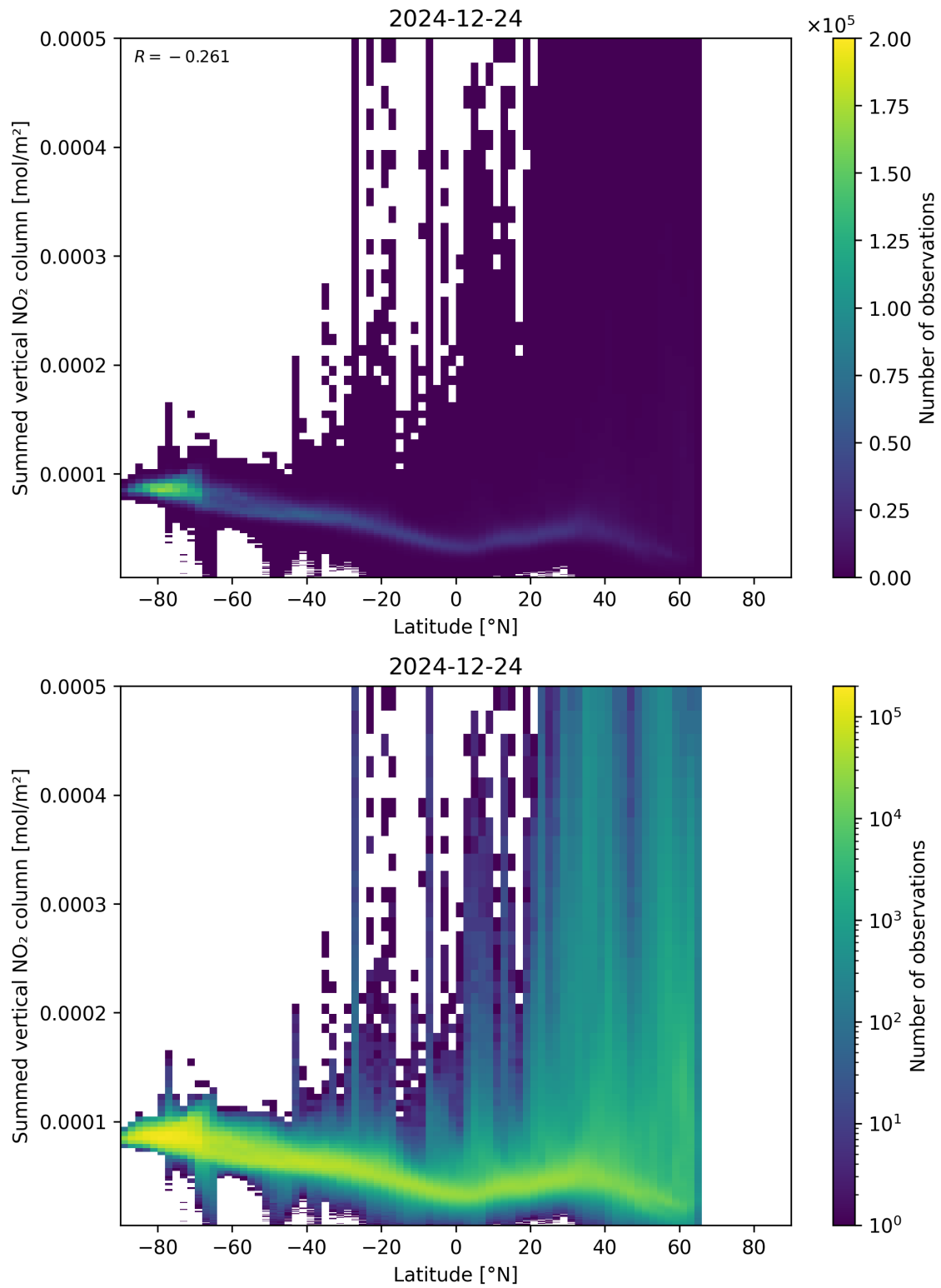
Figure 88: Scatter density plot of “Latitude” against “Summed vertical NO 2 column” for 2024-12-23 to 2024-12-25.
