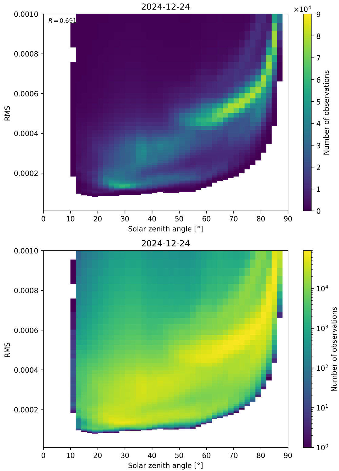
Figure 157: Scatter density plot of “Solar zenith angle” against “RMS” for 2024-12-23 to 2024-12-25.
