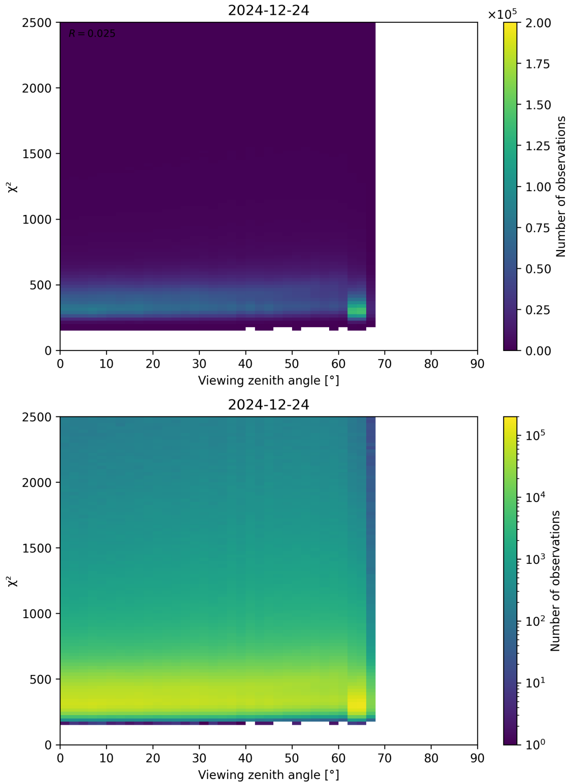
Figure 162: Scatter density plot of “Viewing zenith angle” against “ \chi^2 ” for 2024-12-23 to 2024-12-25.
