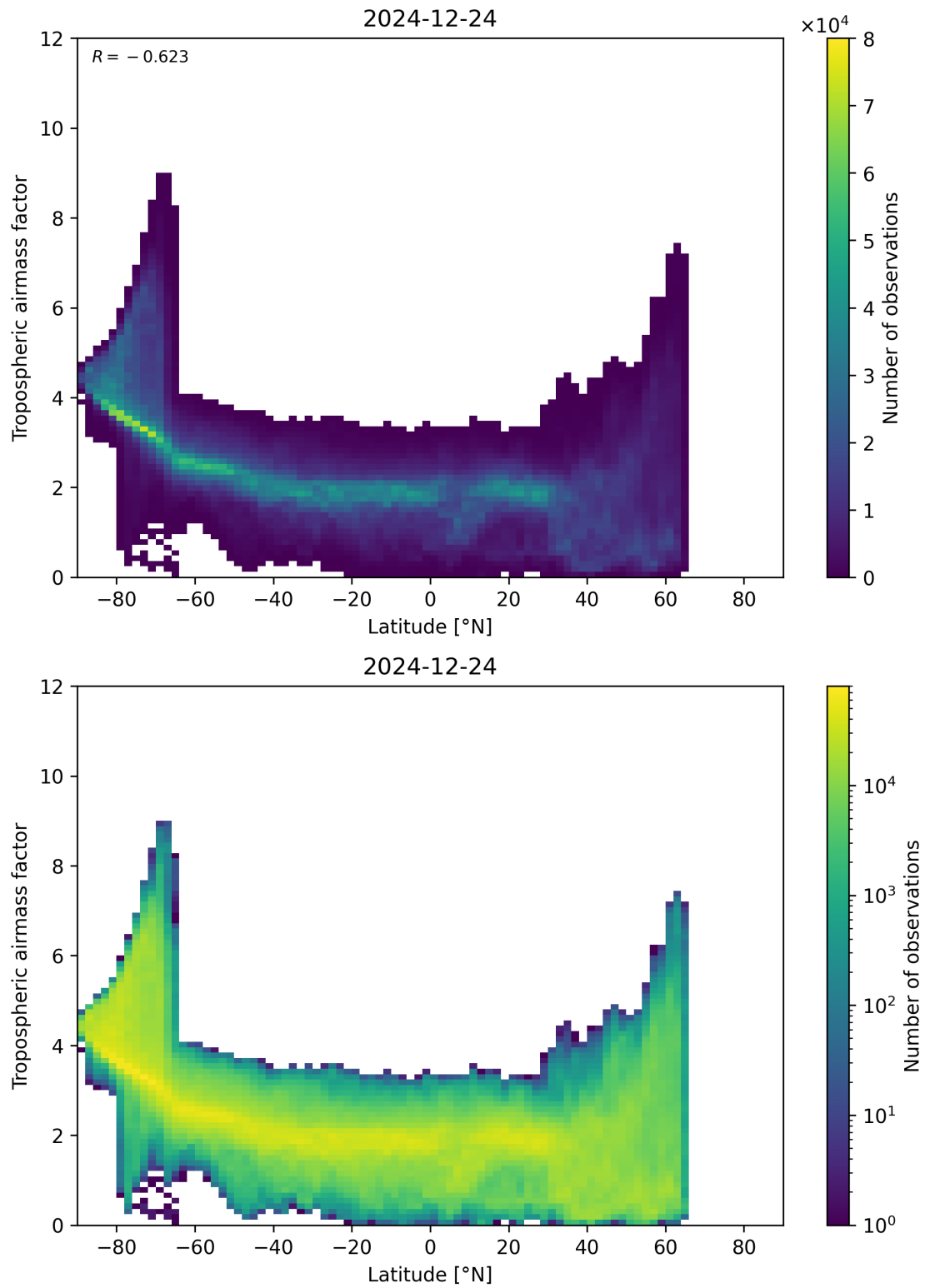
Figure 85: Scatter density plot of “Latitude” against “Tropospheric air mass factor” for 2024-12-23 to 2024-12-25.
