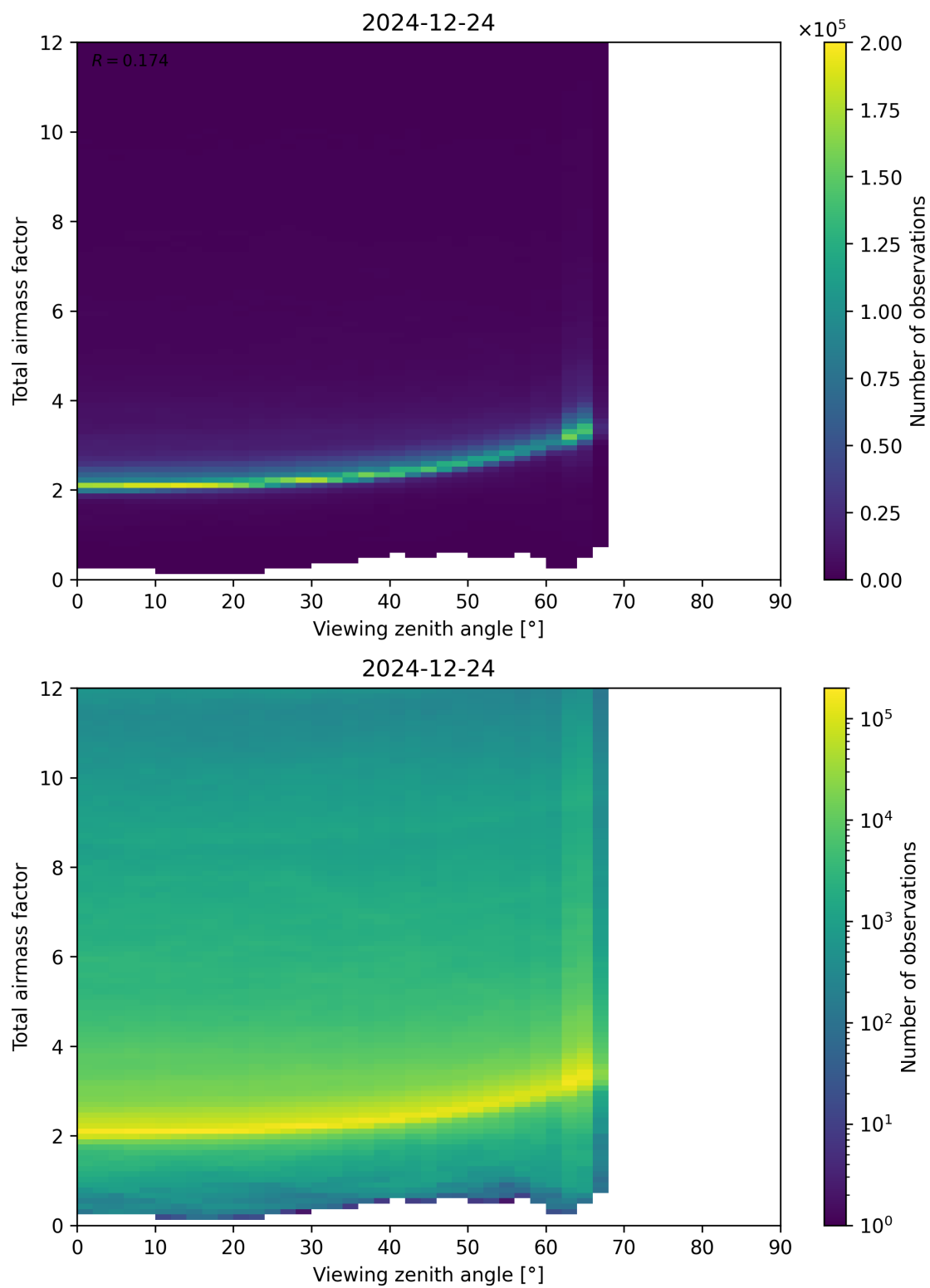
Figure 160: Scatter density plot of “Viewing zenith angle” against “Total airmass factor” for 2024-12-23 to 2024-12-25.
