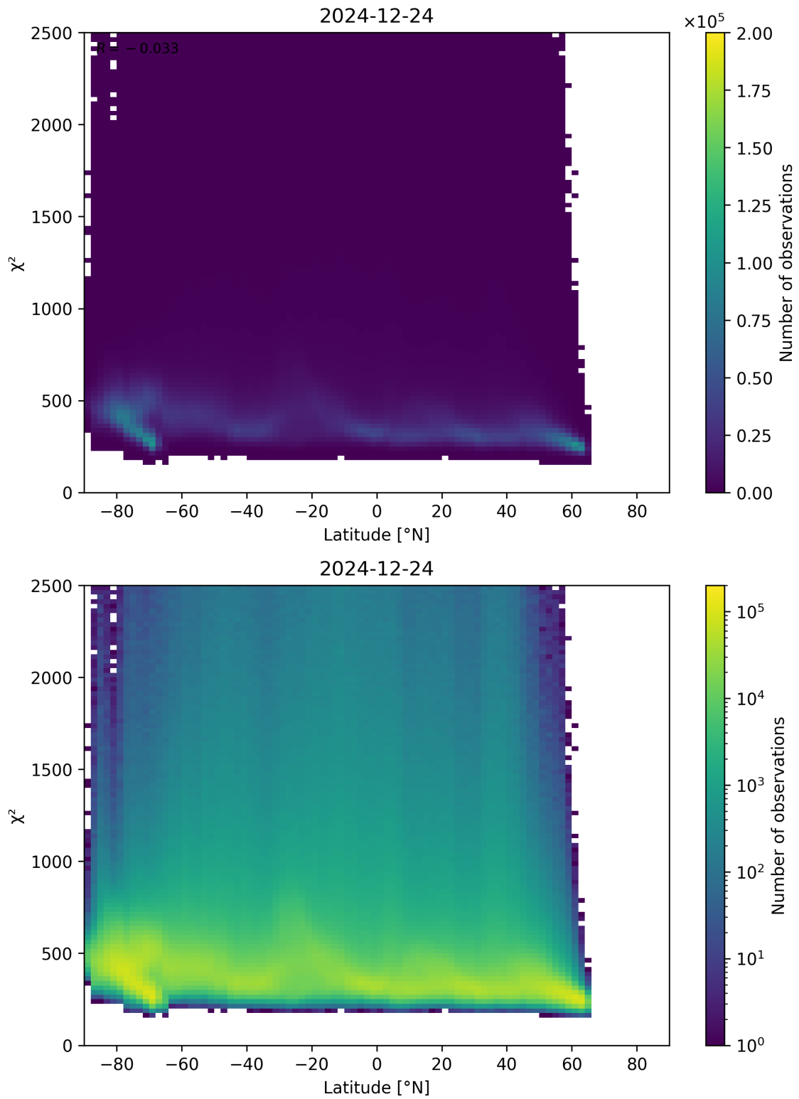
Figure 86: Scatter density plot of “Latitude” against “ \chi^2 ” for 2024-12-23 to 2024-12-25.
