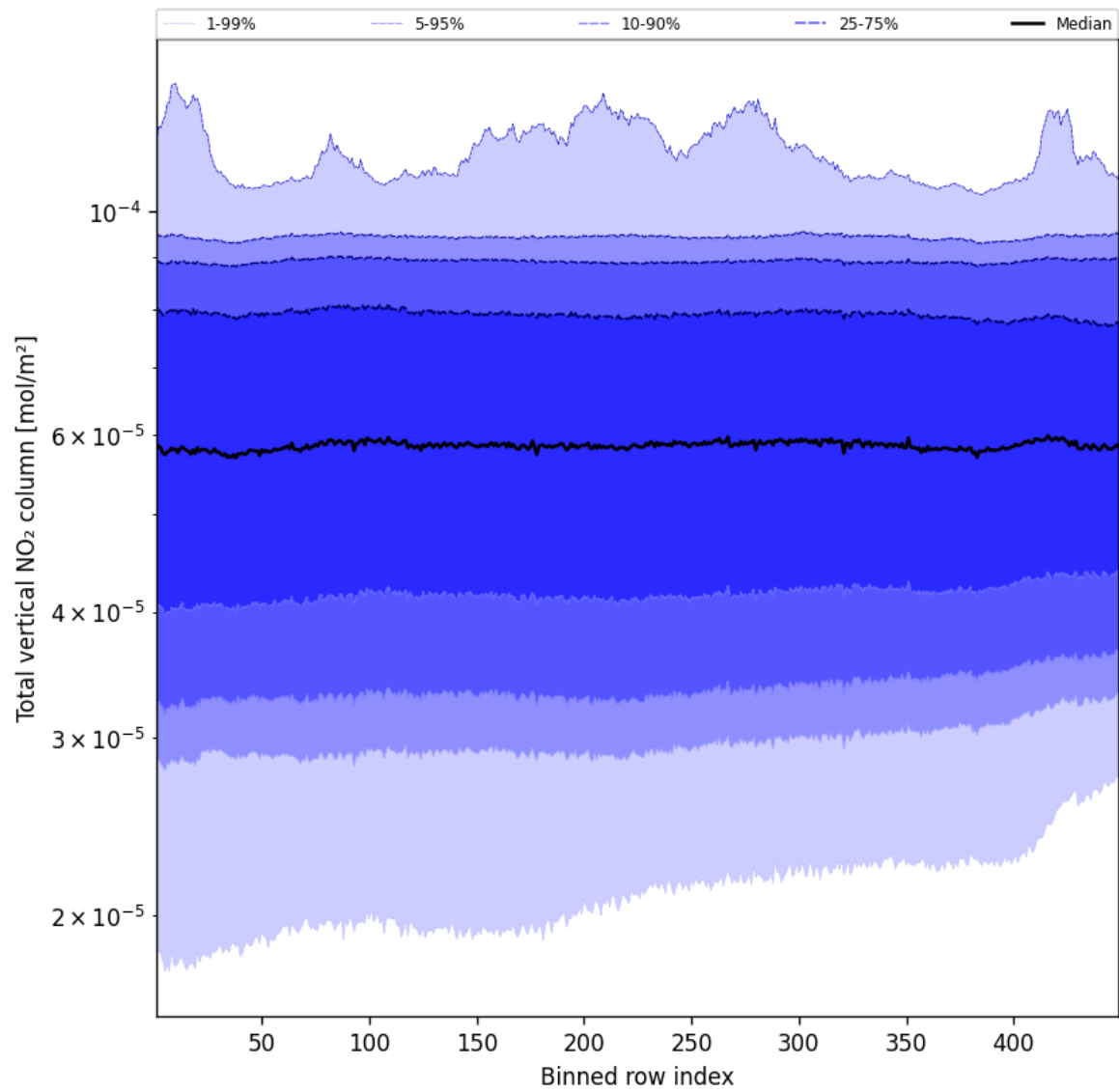
Figure 55: Along track statistics of “Total vertical NO 2 column” for 2024-12-23 to 2024-12-25
