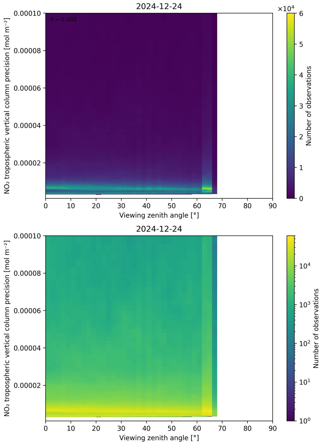
Figure 170: Scatter density plot of “Viewing zenith angle” against “NO 2 tropospheric vertical column precision” for 2024-12-23 to 2024-12-25.
