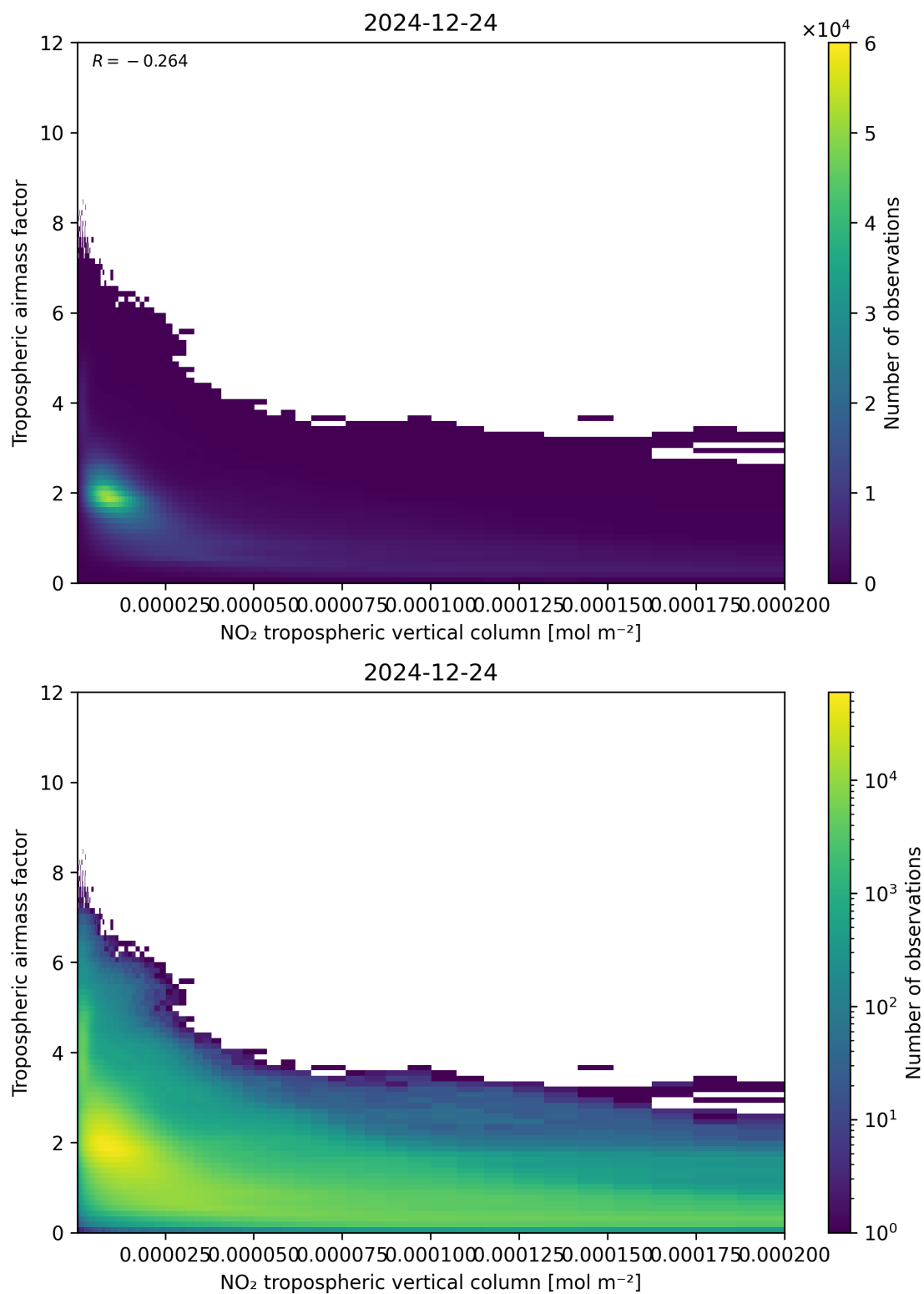
Figure 123: Scatter density plot of “NO 2 tropospheric vertical column” against “Tropospheric airmass factor” for 2024-12-23 to 2024-12-25.
