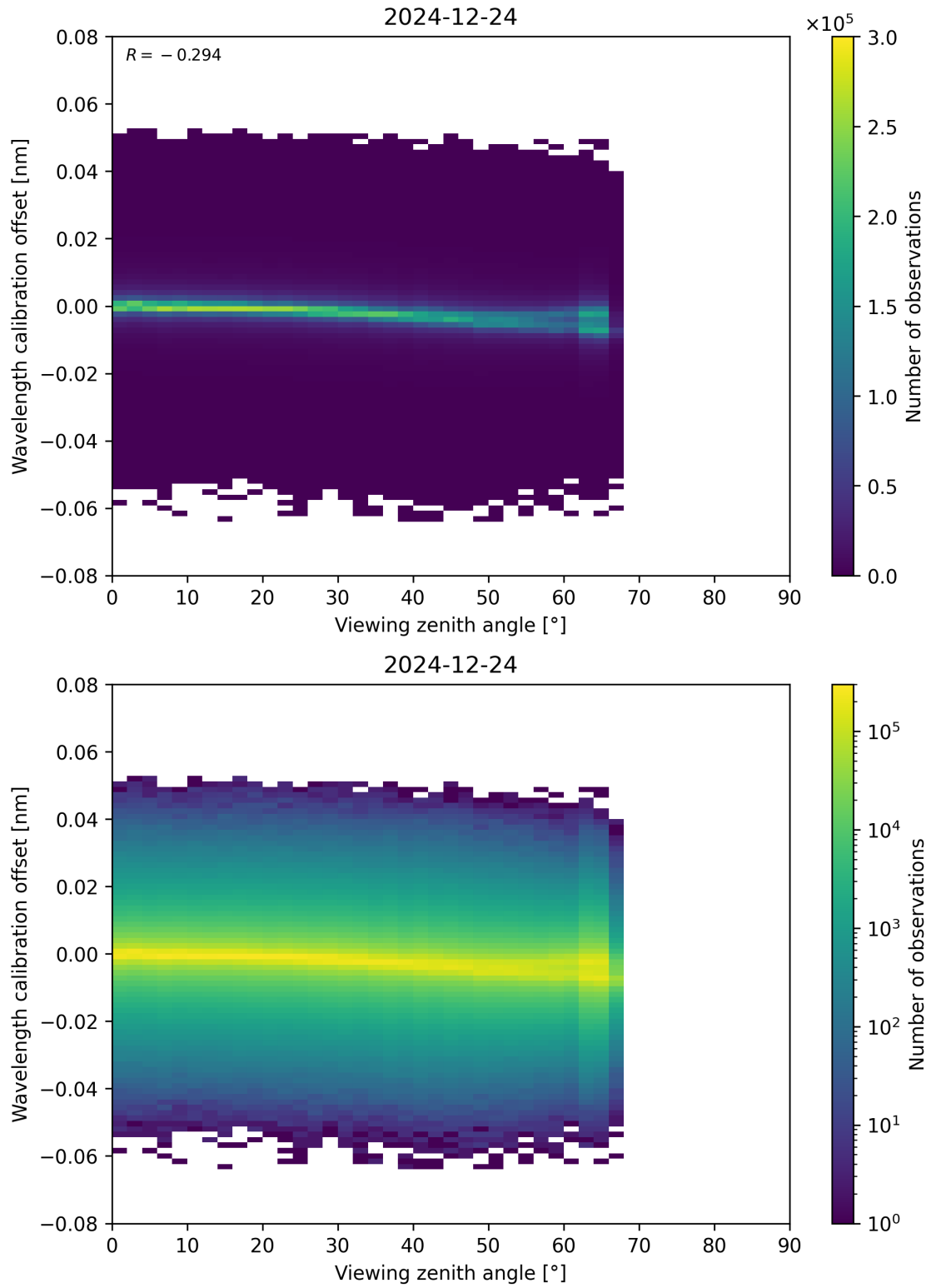
Figure 173: Scatter density plot of “Viewing zenith angle” against “Wavelength calibration offset” for 2024-12-23 to 2024-12-25.
