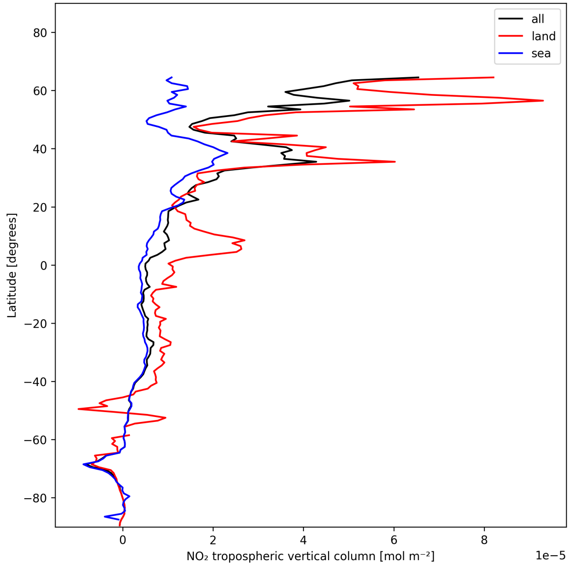
Figure 12: Zonal average of “NO 2 tropospheric vertical column” for 2024-12-23 to 2024-12-25.
