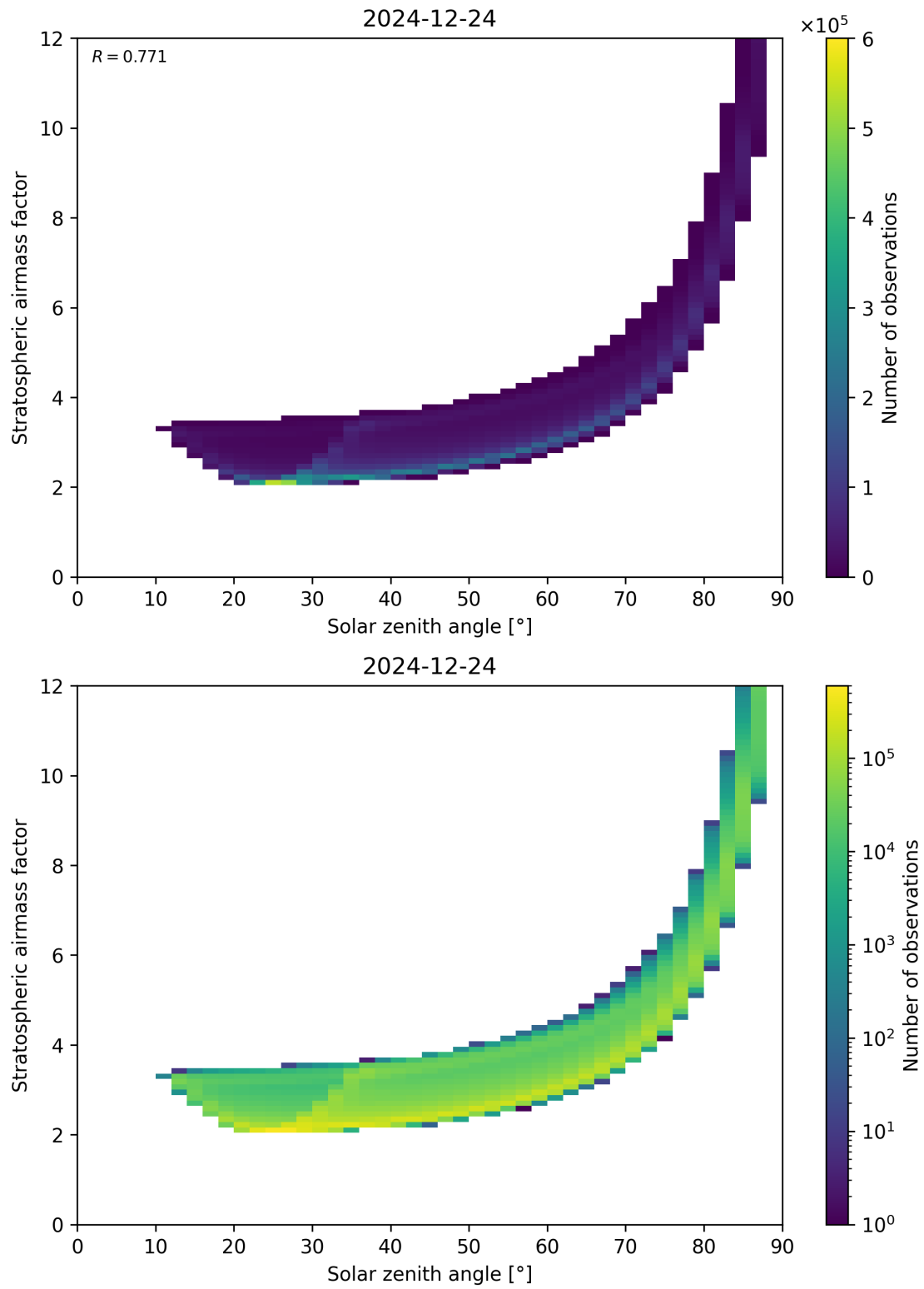
Figure 145: Scatter density plot of “Solar zenith angle” against “Stratospheric airmass factor” for 2024-12-23 to 2024-12-25.
