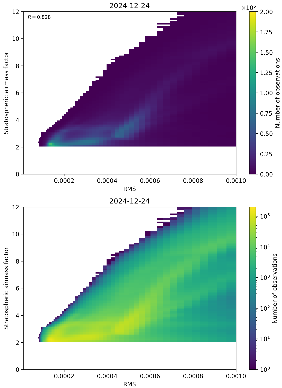
Figure 144: Scatter density plot of “RMS” against “Stratospheric airmass factor” for 2024-12-23 to 2024-12-25.
