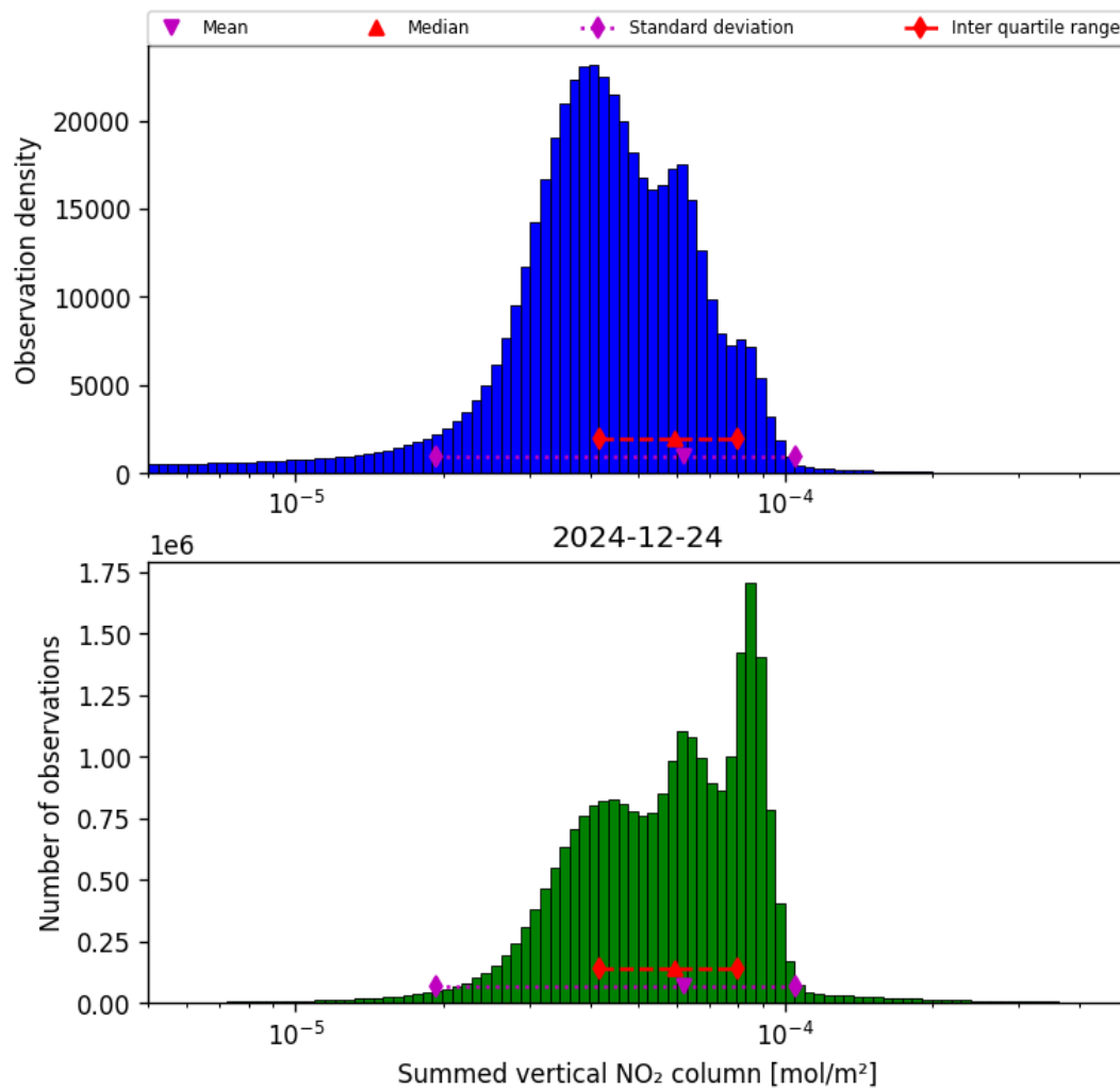
Figure 40: Histogram of “Summed vertical NO 2 column” for 2024-12-23 to 2024-12-25
