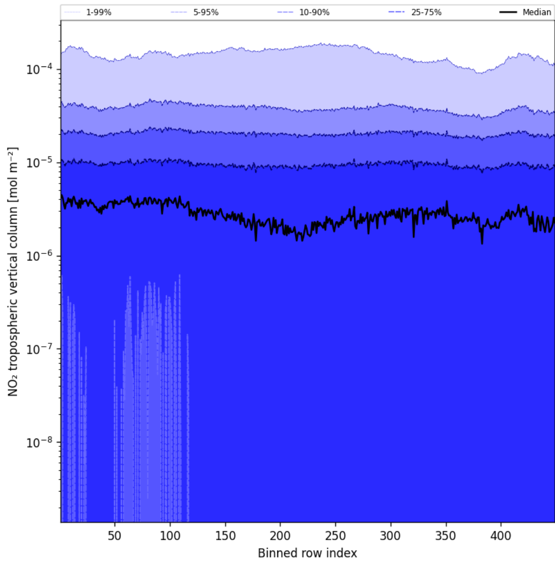
Figure 46: Along track statistics of “NO 2 tropospheric vertical column” for 2024-12-23 to 2024-12-25
