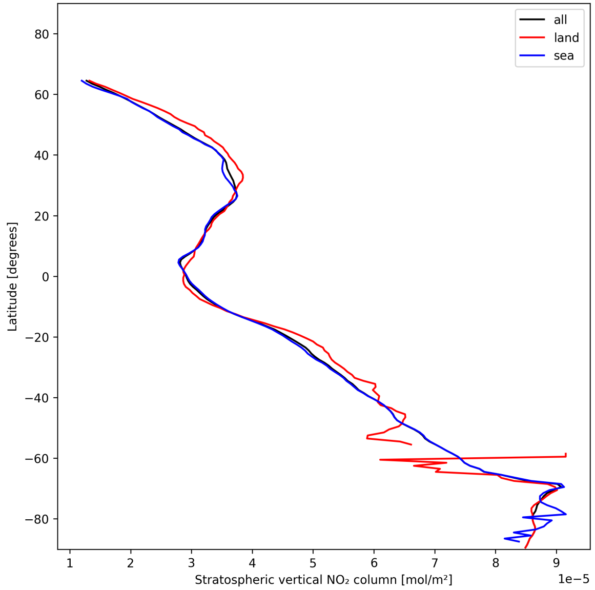
Figure 19: Zonal average of “Stratospheric vertical NO 2 column” for 2024-12-23 to 2024-12-25.
