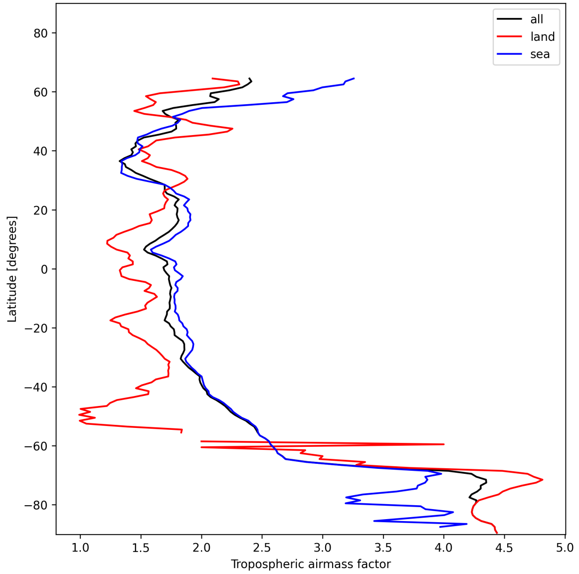
Figure 14: Zonal average of “Tropospheric airmass factor” for 2024-12-23 to 2024-12-25.
