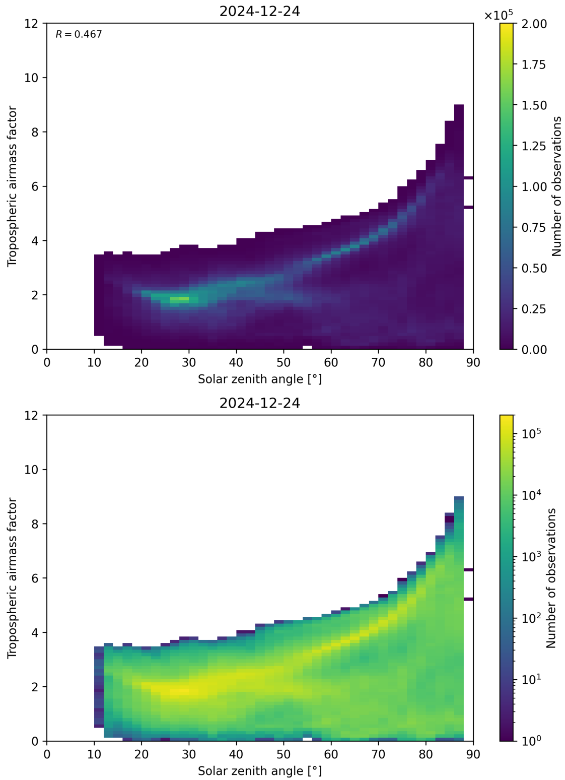
Figure 147: Scatter density plot of “Solar zenith angle” against “Tropospheric airmass factor” for 2024-12-23 to 2024-12-25.
