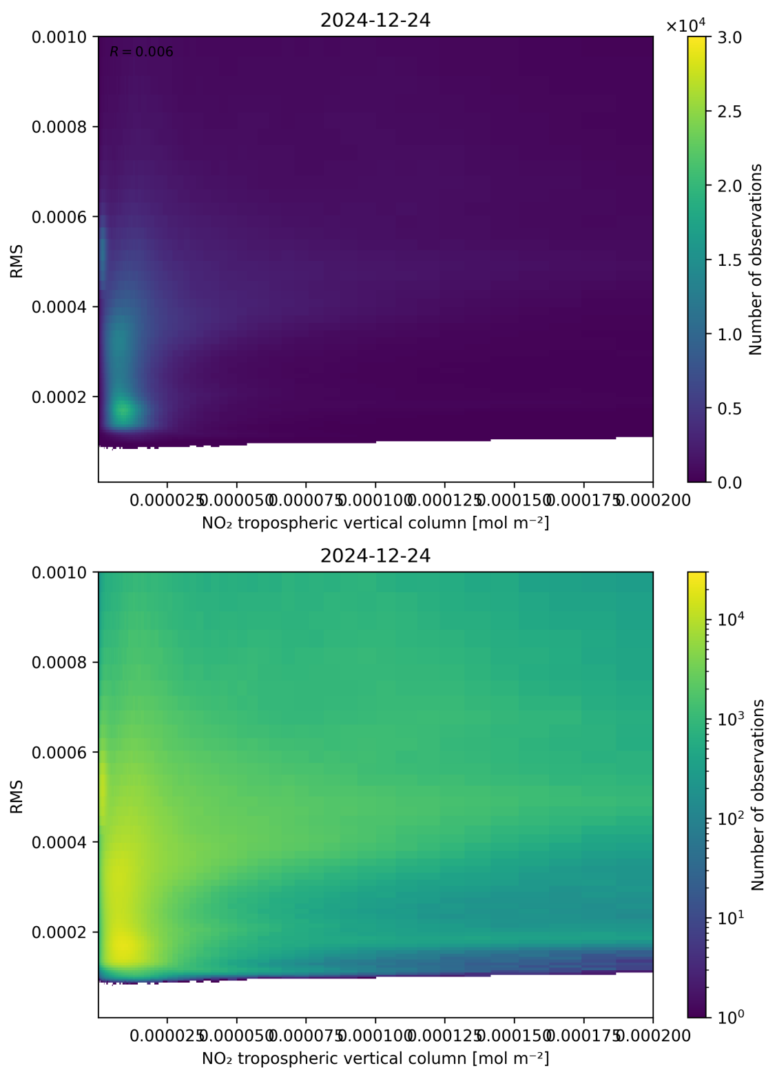
Figure 142: Scatter density plot of “NO 2 tropospheric vertical column” against “RMS” for 2024-12-23 to 2024-12-25.
