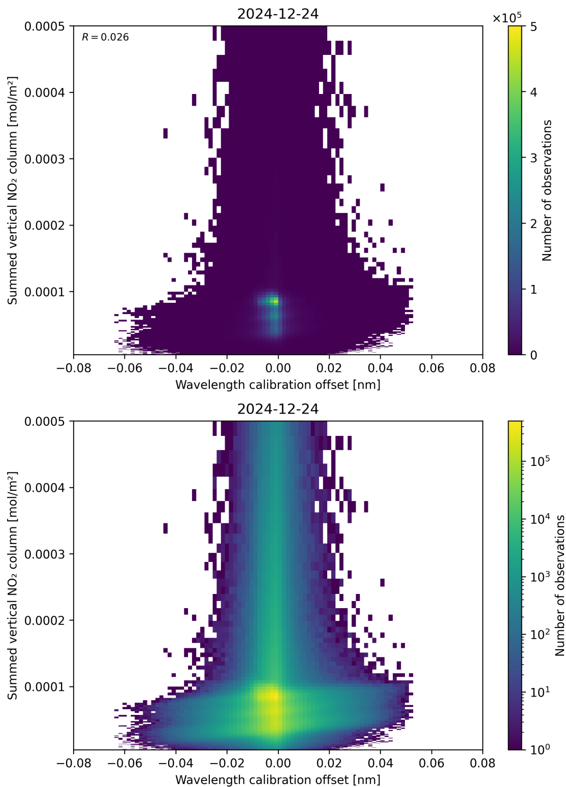
Figure 177: Scatter density plot of “Wavelength calibration offset” against “Summed vertical NO 2 column” for 2024-12-23 to 2024-12-25.
