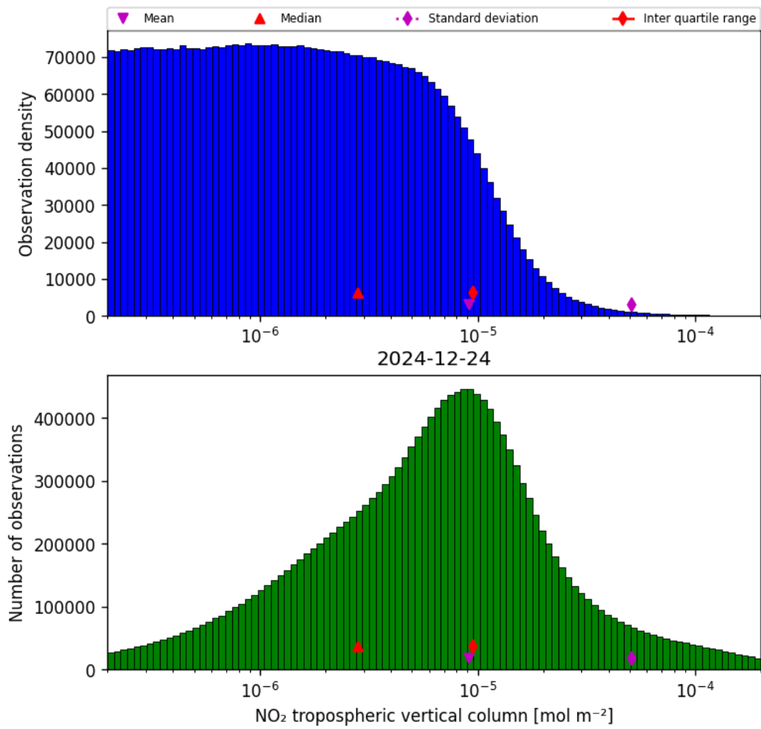
Figure 29: Histogram of “NO 2 tropospheric vertical column” for 2024-12-23 to 2024-12-25
