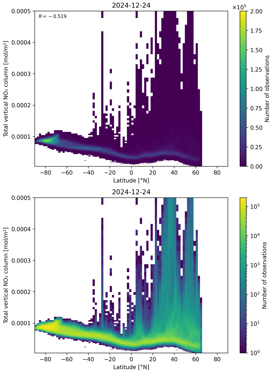
Figure 90: Scatter density plot of “Latitude” against “Total vertical NO 2 column” for 2024-12-23 to 2024-12-25.
