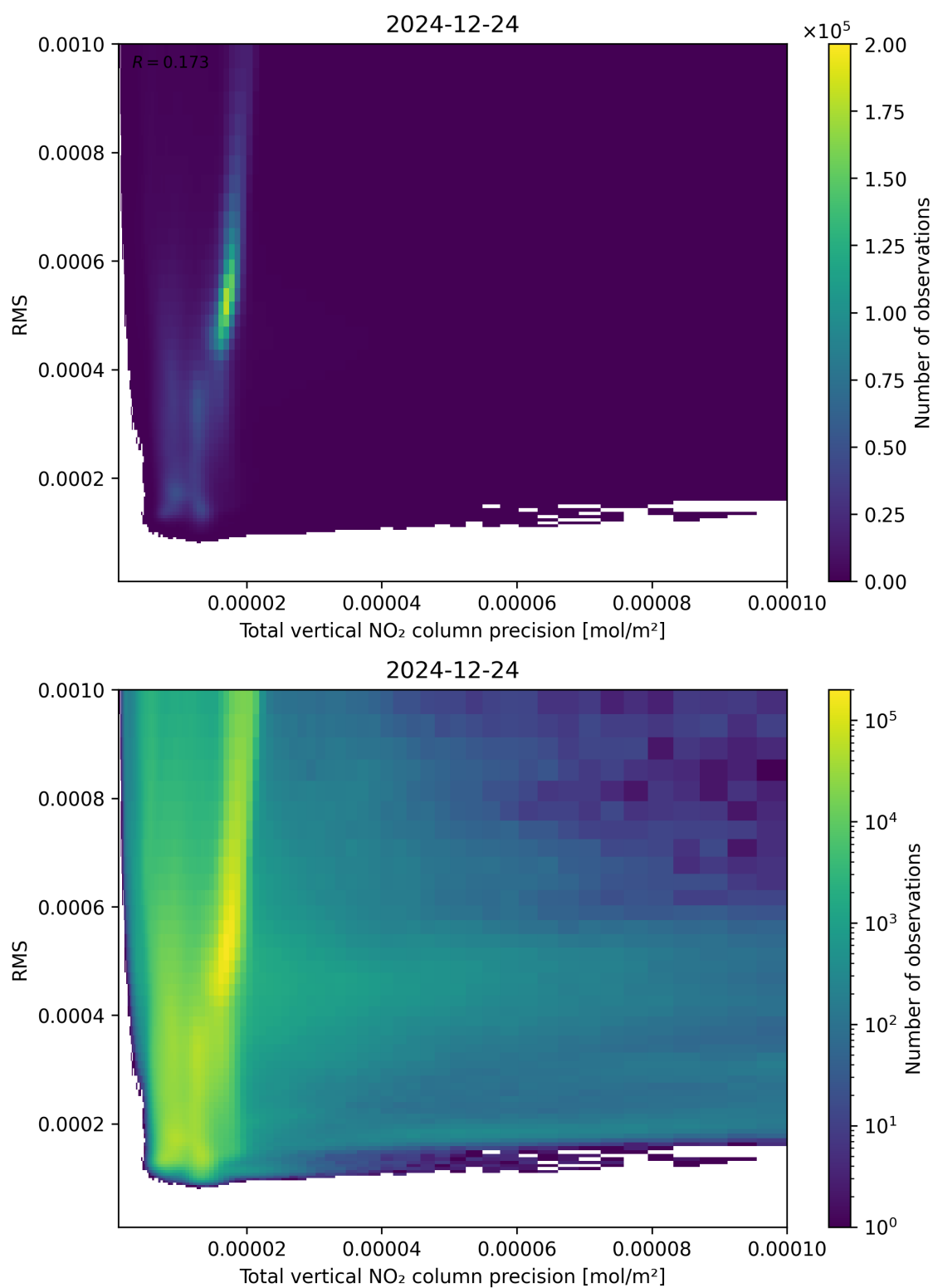
Figure 119: Scatter density plot of “Total vertical NO 2 column precision” against “RMS” for 2024-12-23 to 2024-12-25.
