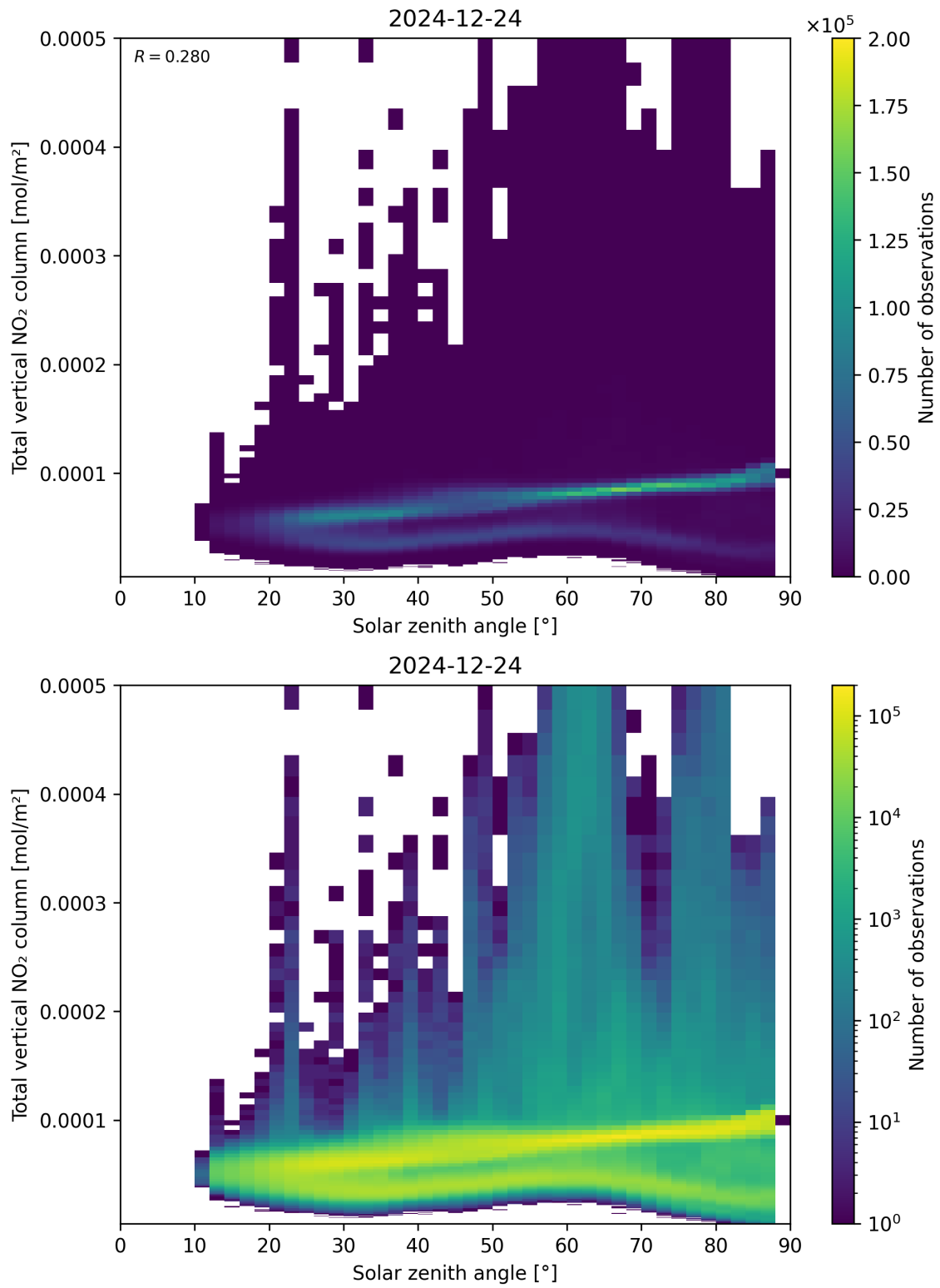
Figure 153: Scatter density plot of “Solar zenith angle” against “Total vertical NO 2 column” for 2024-12-23 to 2024-12-25.
