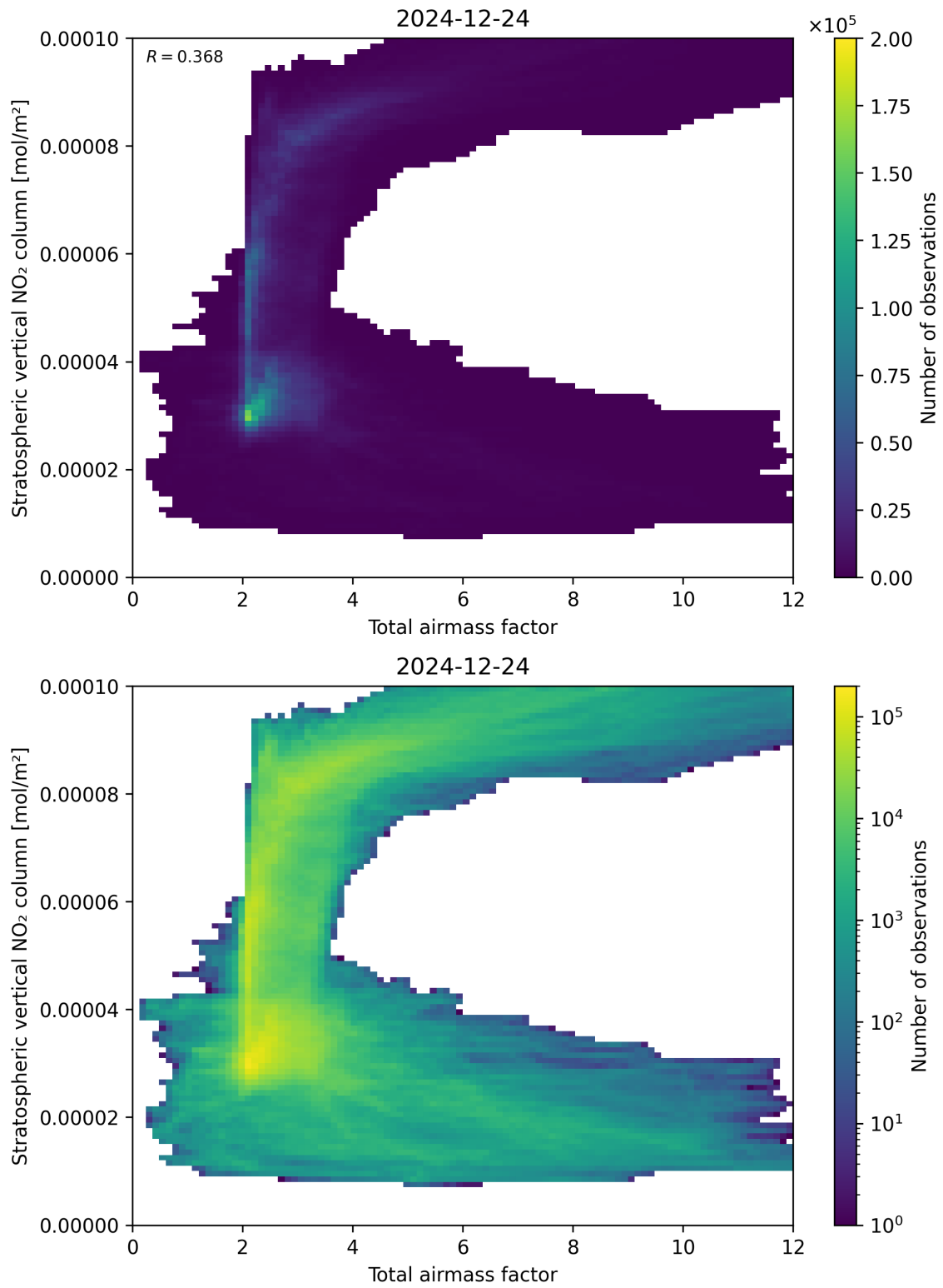
Figure 64: Scatter density plot of “Total airmass factor” against “Stratospheric vertical \text{NO}_2 column” for 2024-12-23 to 2024-12-25.
