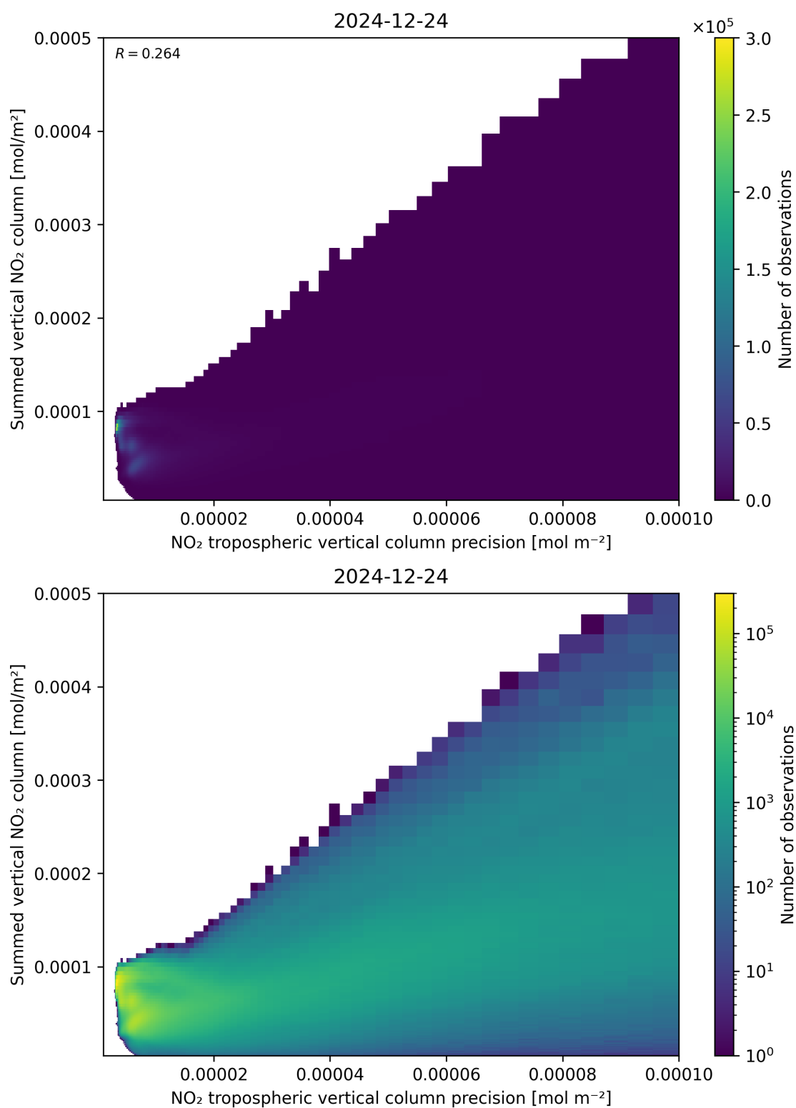
Figure 136: Scatter density plot of “NO 2 tropospheric vertical column precision” against “Summed vertical NO 2 column” for 2024-12-23 to 2024-12-25.
