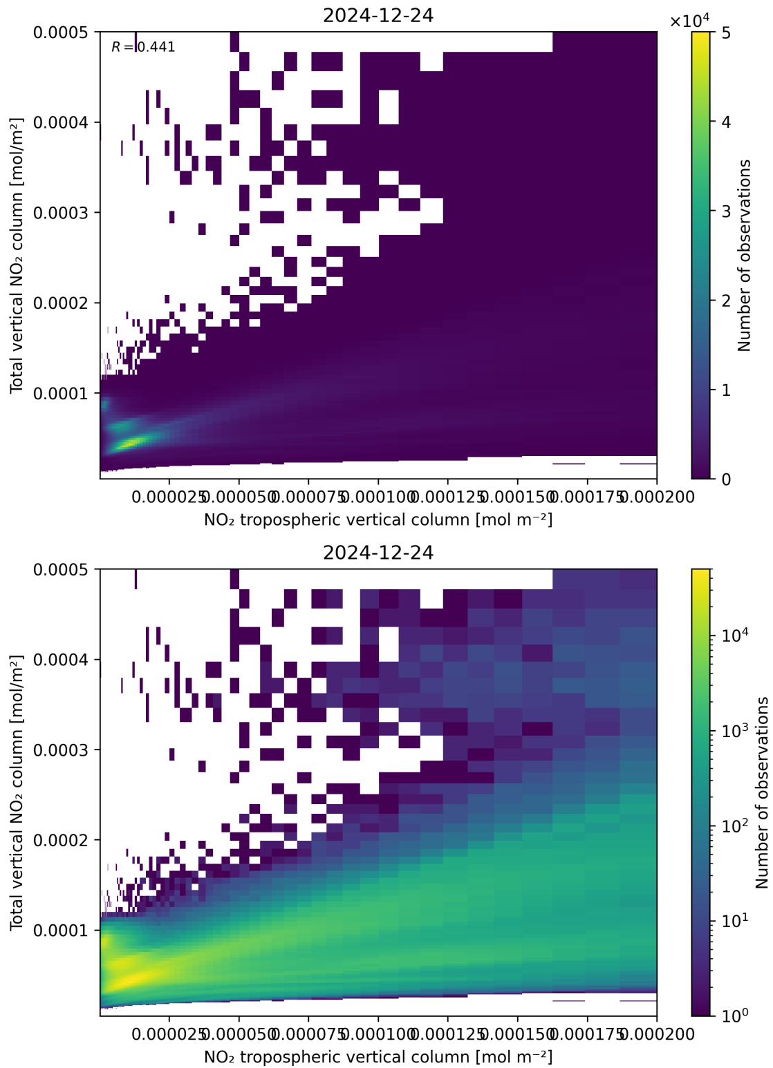
Figure 128: Scatter density plot of “NO 2 tropospheric vertical column” against “Total vertical NO 2 column” for 2024-12-23 to 2024-12-25.
