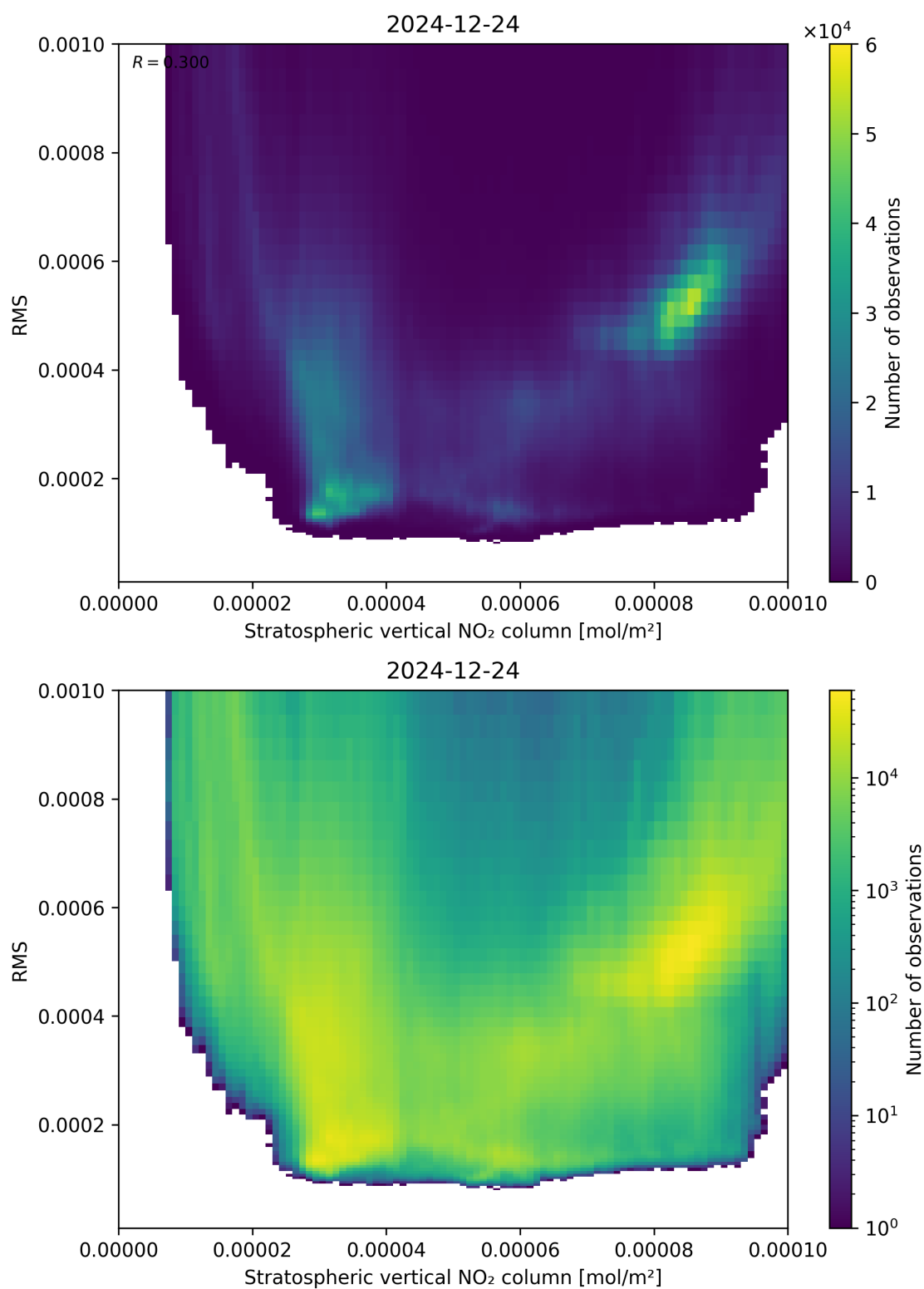
Figure 102: Scatter density plot of “Stratospheric vertical NO 2 column” against “RMS” for 2024-12-23 to 2024-12-25.
