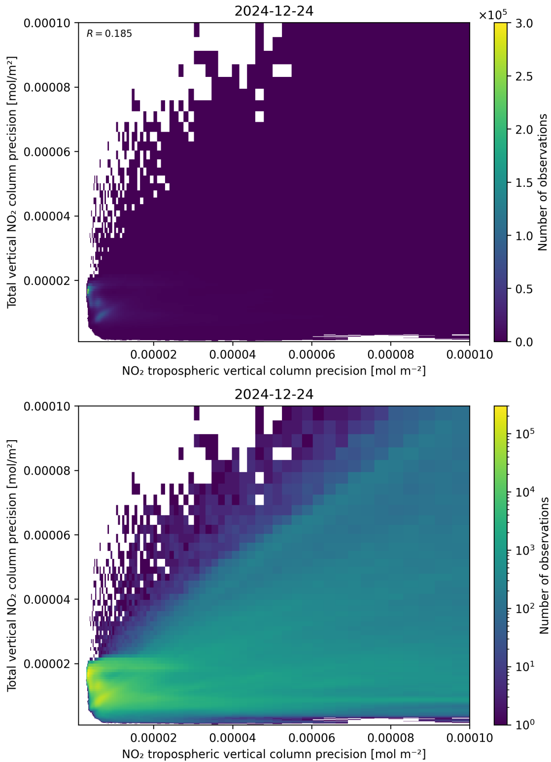
Figure 139: Scatter density plot of “NO 2 tropospheric vertical column precision” against “Total vertical NO 2 column precision” for 2024-12-23 to 2024-12-25.
