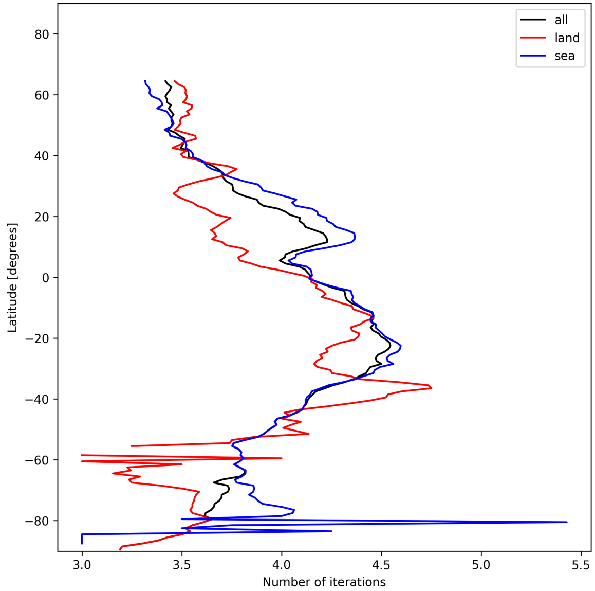
Figure 17: Zonal average of “Number of iterations” for 2024-12-23 to 2024-12-25.
