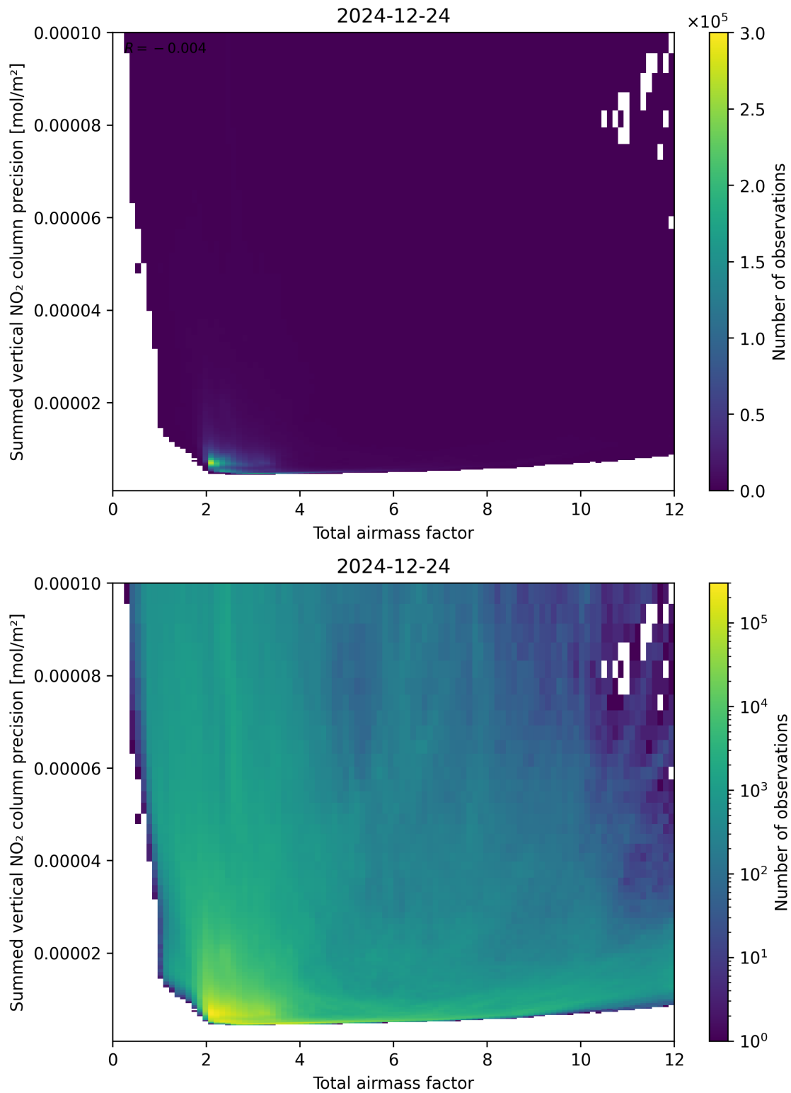
Figure 66: Scatter density plot of “Total airmass factor” against “Summed vertical NO 2 column precision” for 2024-12-23 to 2024-12-25.
