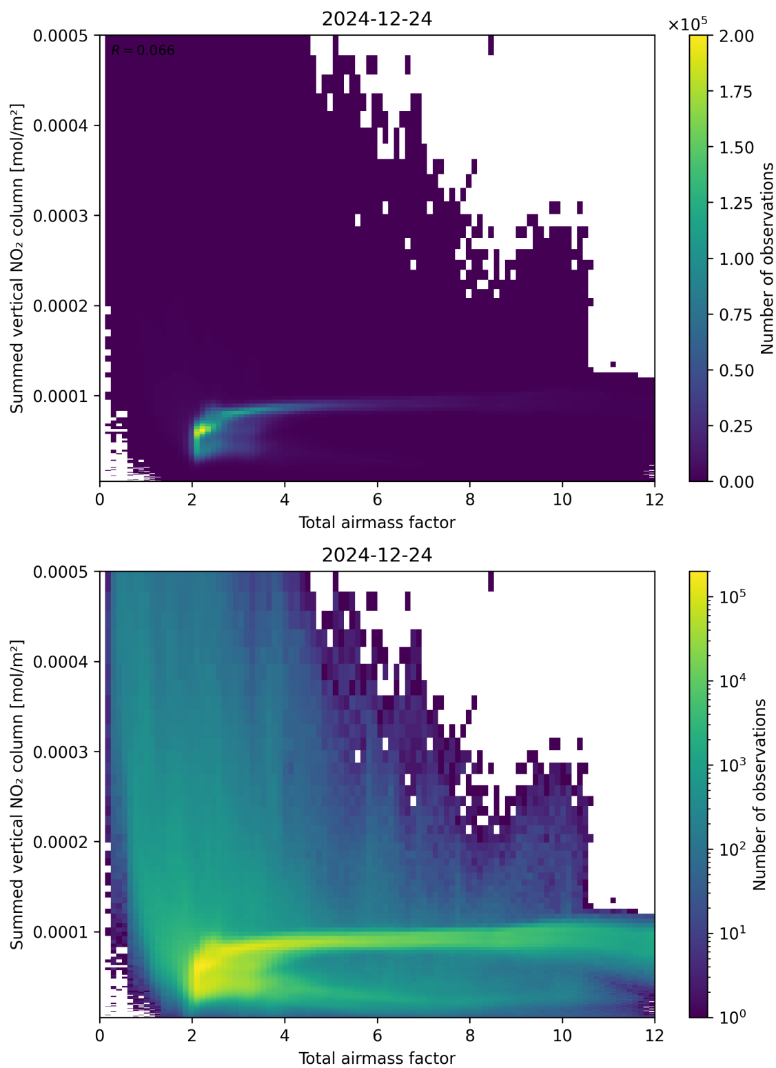
Figure 65: Scatter density plot of “Total airmass factor” against “Summed vertical NO 2 column” for 2024-12-23 to 2024-12-25.
