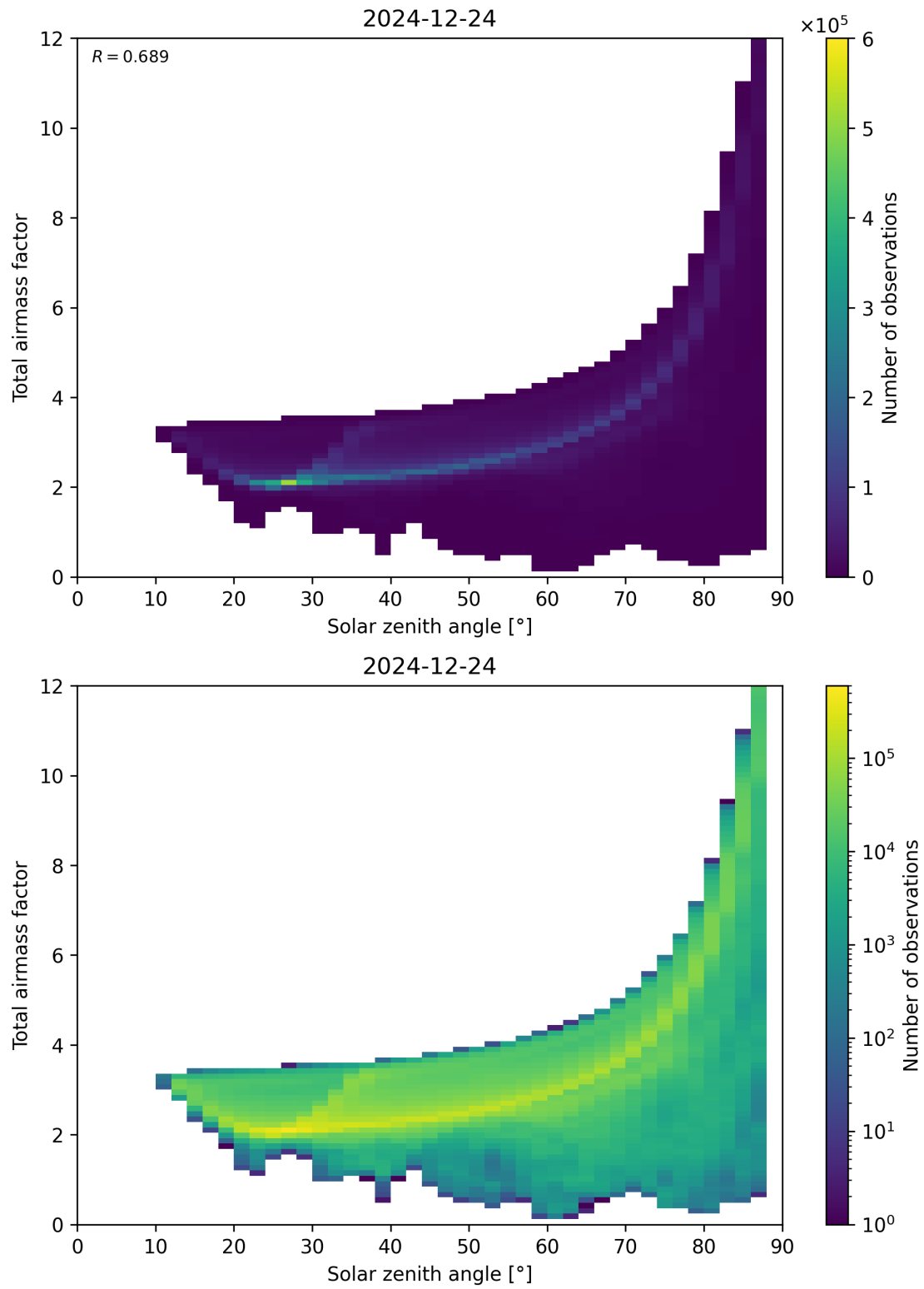
Figure 146: Scatter density plot of “Solar zenith angle” against “Total airmass factor” for 2024-12-23 to 2024-12-25.
