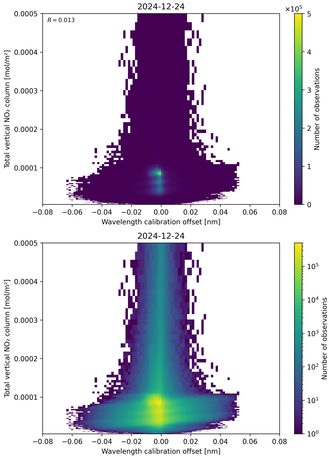
Figure 179: Scatter density plot of “Wavelength calibration offset” against “Total vertical NO 2 column” for 2024-12-23 to 2024-12-25.
