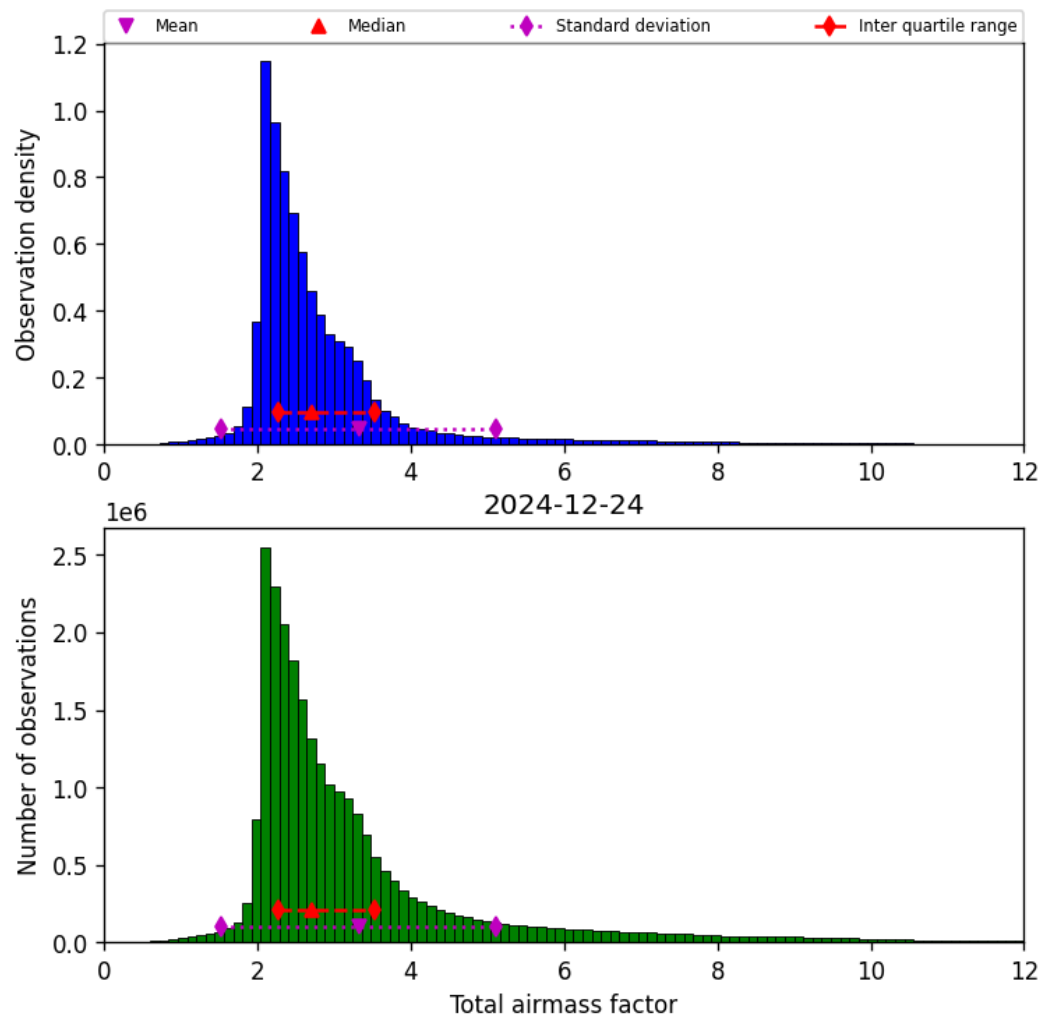
Figure 32: Histogram of “Total airmass factor” for 2024-12-23 to 2024-12-25
