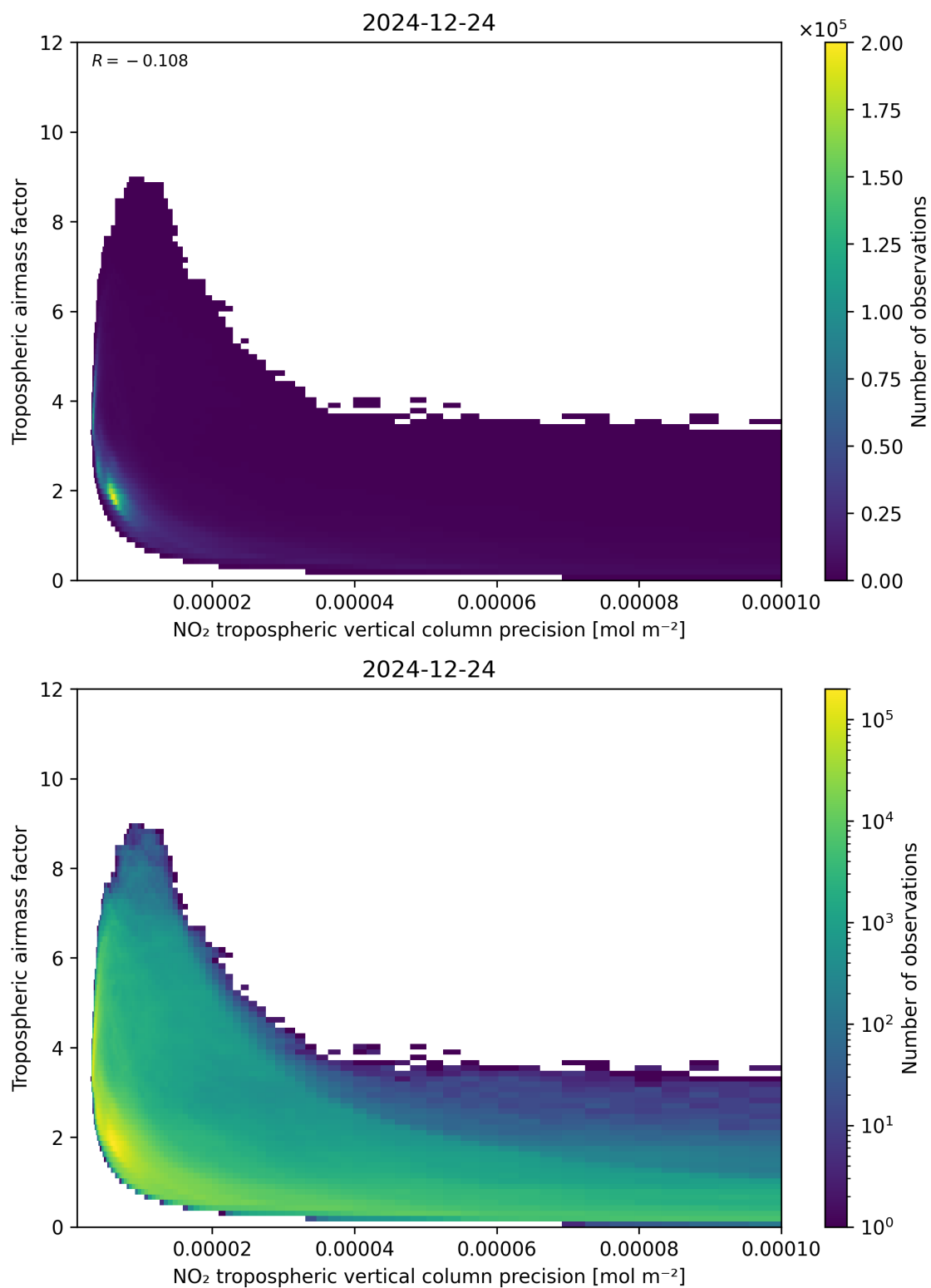
Figure 133: Scatter density plot of “NO 2 tropospheric vertical column precision” against “Tropospheric air mass factor” for 2024-12-23 to 2024-12-25.
