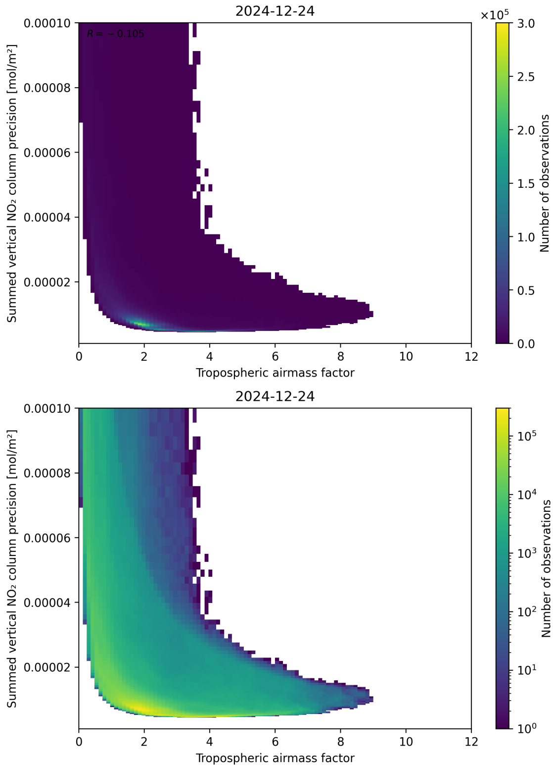
Figure 76: Scatter density plot of “Tropospheric air mass factor” against “Summed vertical NO 2 column precision” for 2024-12-23 to 2024-12-25.
