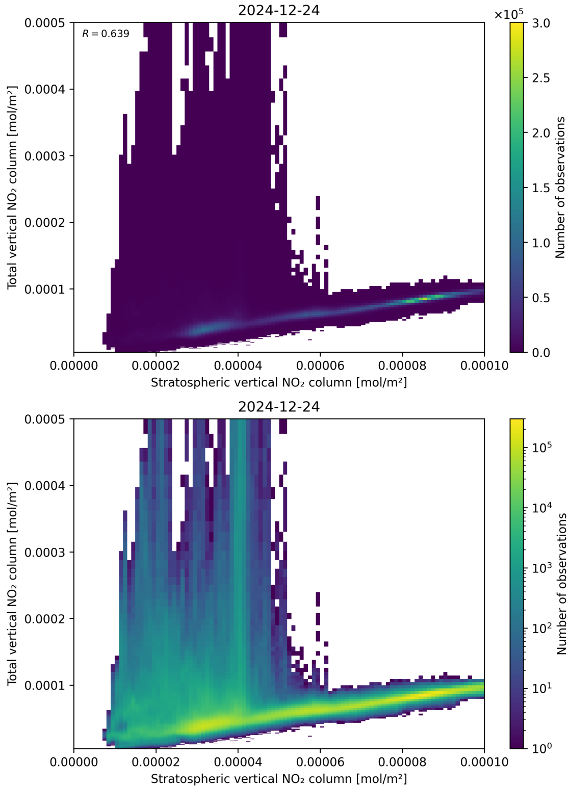
Figure 100: Scatter density plot of “Stratospheric vertical NO 2 column” against “Total vertical NO 2 column” for 2024-12-23 to 2024-12-25.
