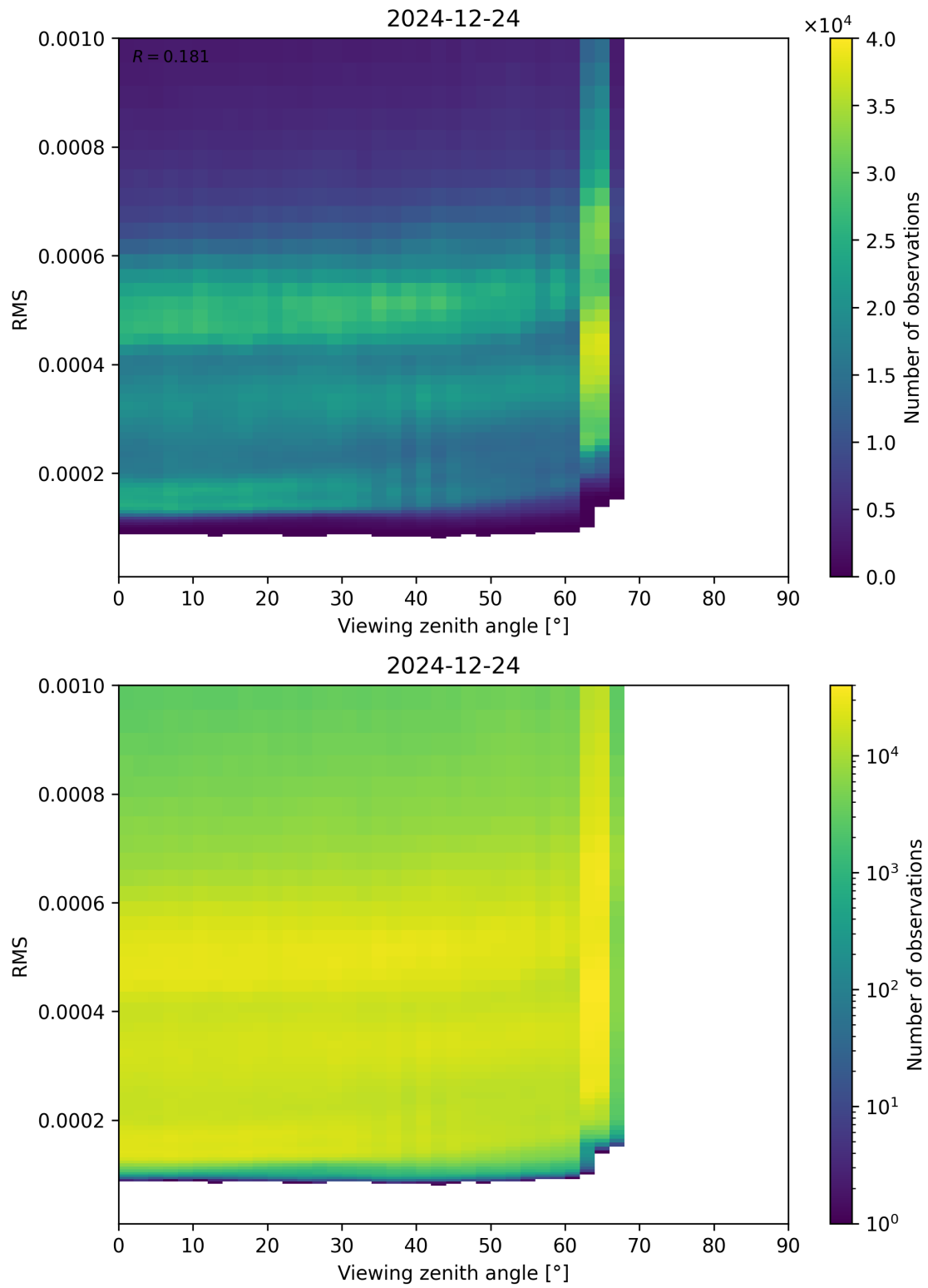
Figure 171: Scatter density plot of “Viewing zenith angle” against “RMS” for 2024-12-23 to 2024-12-25.
