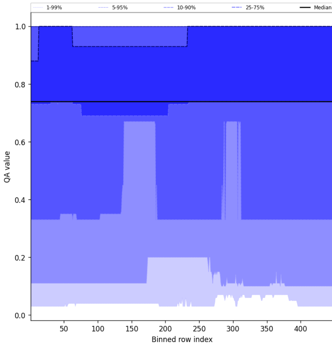
Figure 45: Along track statistics of “QA value” for 2024-12-23 to 2024-12-25
