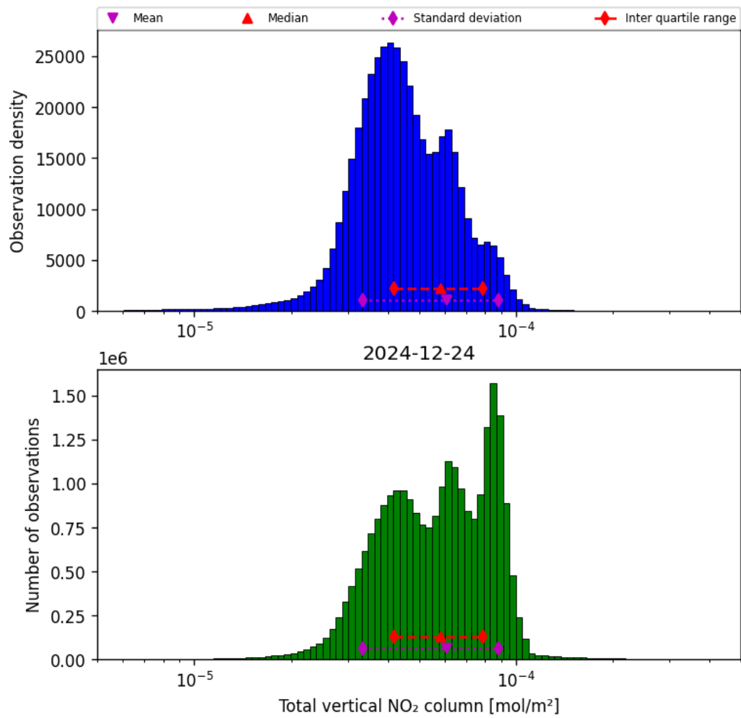
Figure 38: Histogram of “Total vertical NO 2 column” for 2024-12-23 to 2024-12-25
