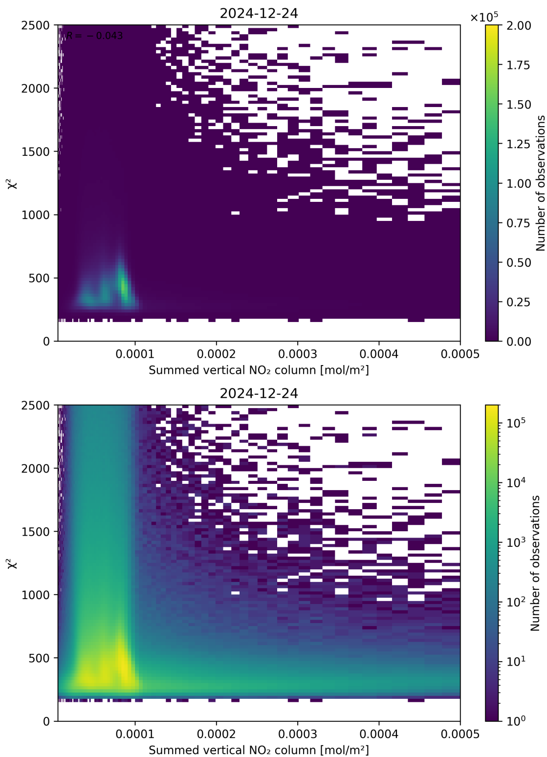
Figure 104: Scatter density plot of “Summed vertical NO 2 column” against “ \chi^2 ” for 2024-12-23 to 2024-12-25.
