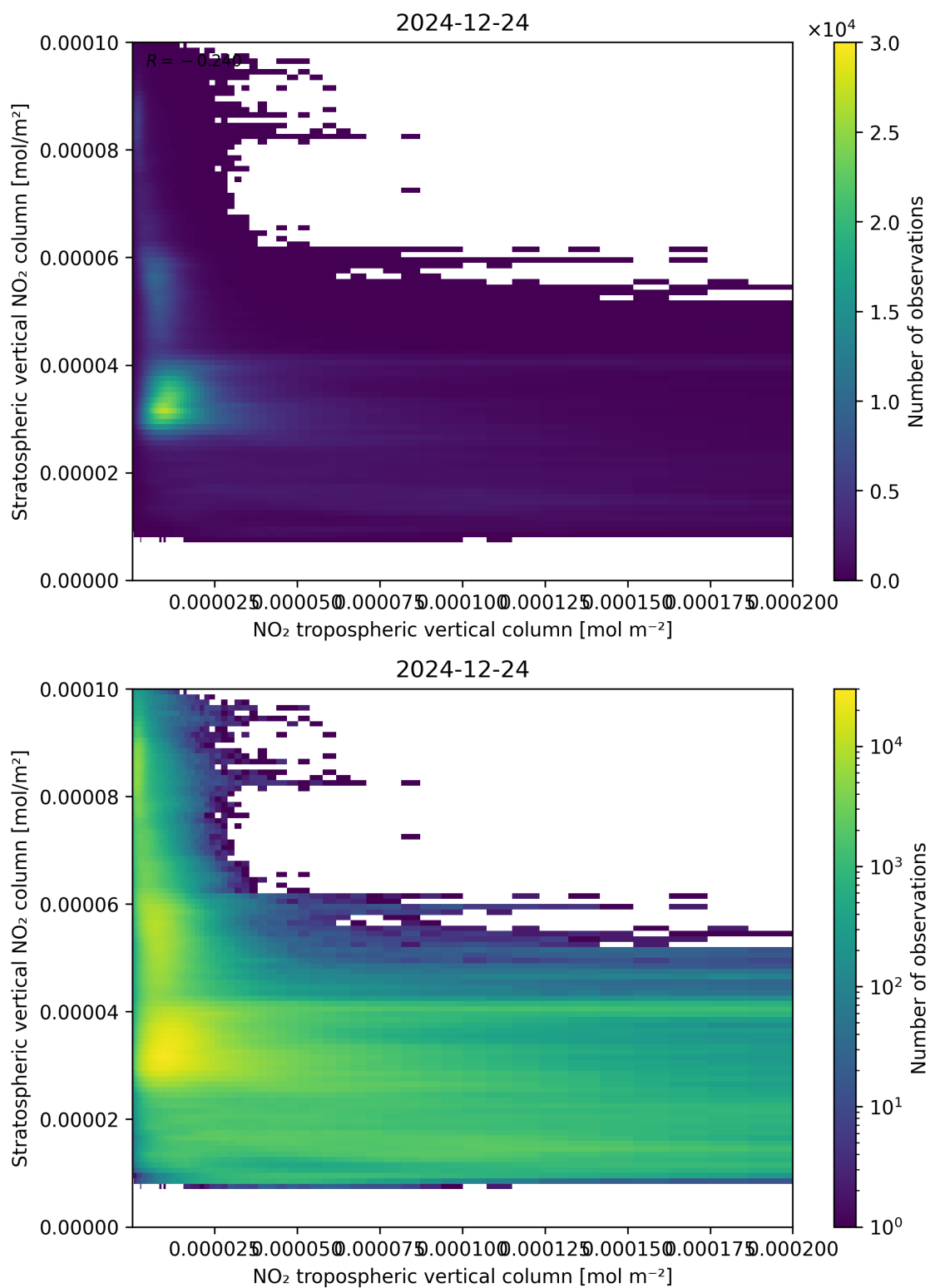
Figure 125: Scatter density plot of “NO 2 tropospheric vertical column” against “Stratospheric vertical NO 2 column” for 2024-12-23 to 2024-12-25.
