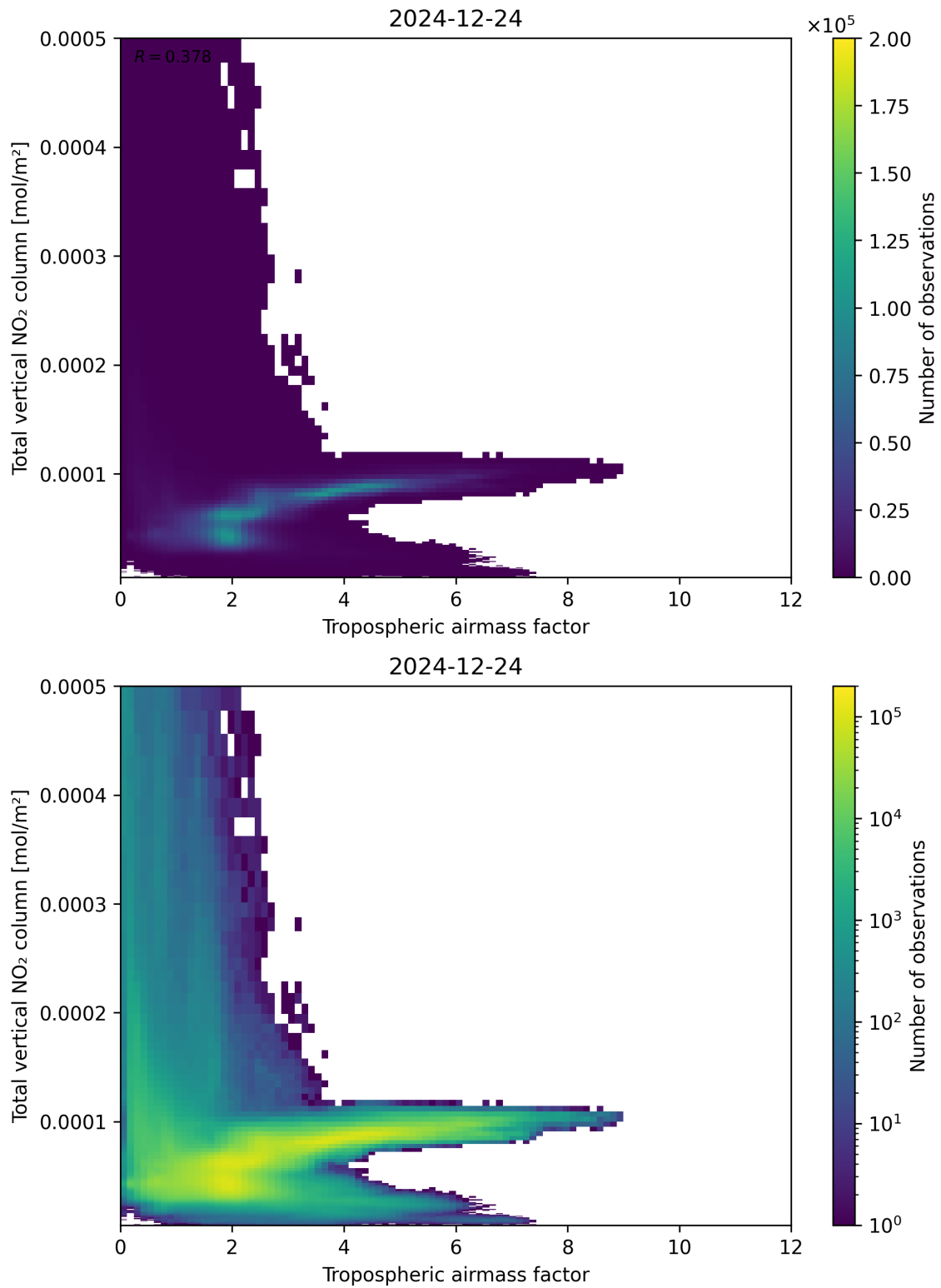
Figure 77: Scatter density plot of “Tropospheric airmass factor” against “Total vertical NO 2 column” for 2024-12-23 to 2024-12-25.
