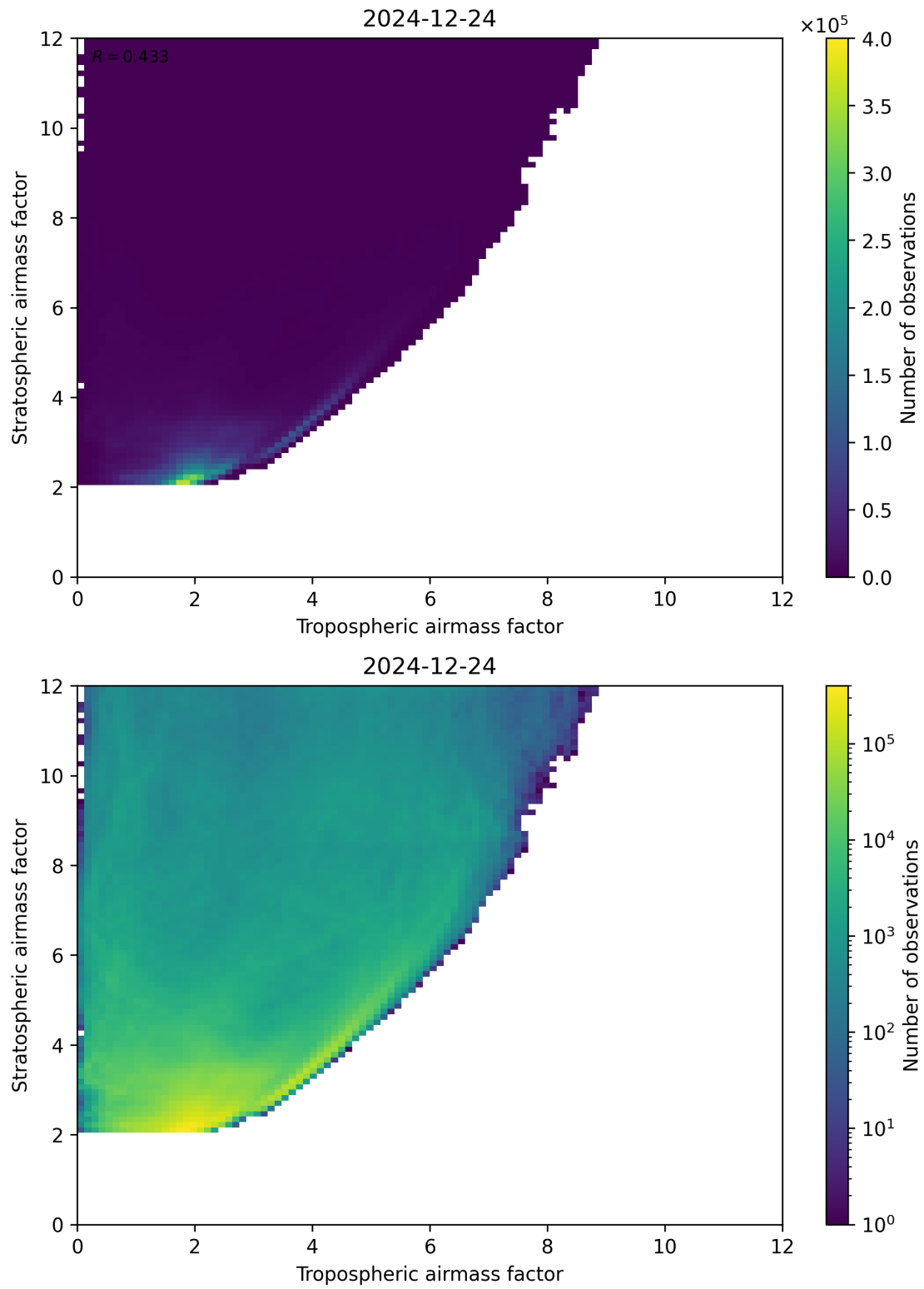
Figure 71: Scatter density plot of “Tropospheric airmass factor” against “Stratospheric airmass factor” for 2024-12-23 to 2024-12-25.
