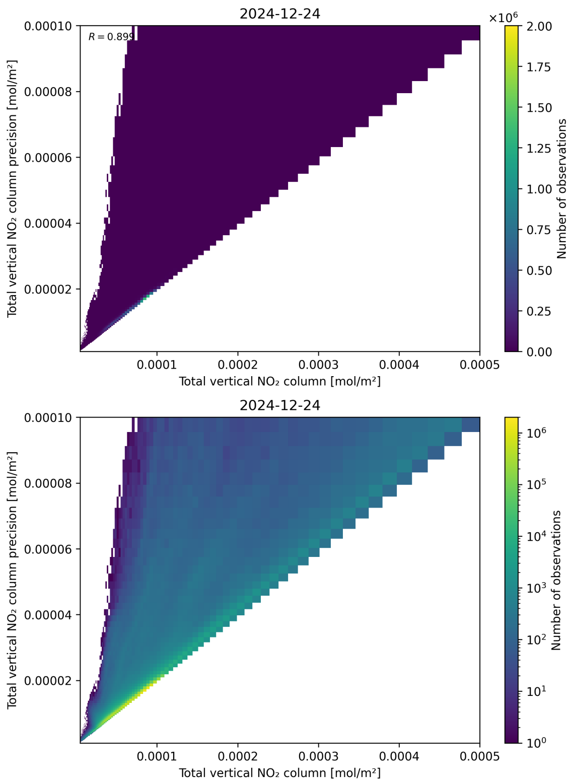
Figure 114: Scatter density plot of “Total vertical NO 2 column” against “Total vertical NO 2 column precision” for 2024-12-23 to 2024-12-25.
