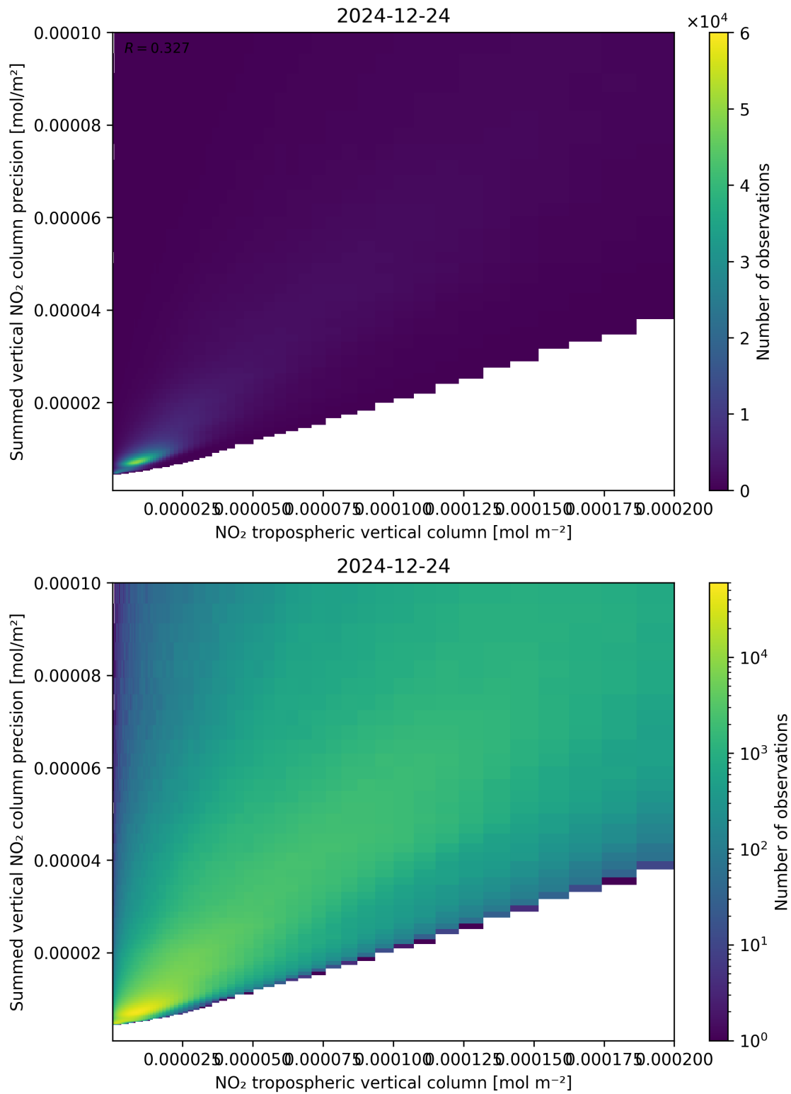
Figure 127: Scatter density plot of “NO 2 tropospheric vertical column” against “Summed vertical NO 2 column precision” for 2024-12-23 to 2024-12-25.
