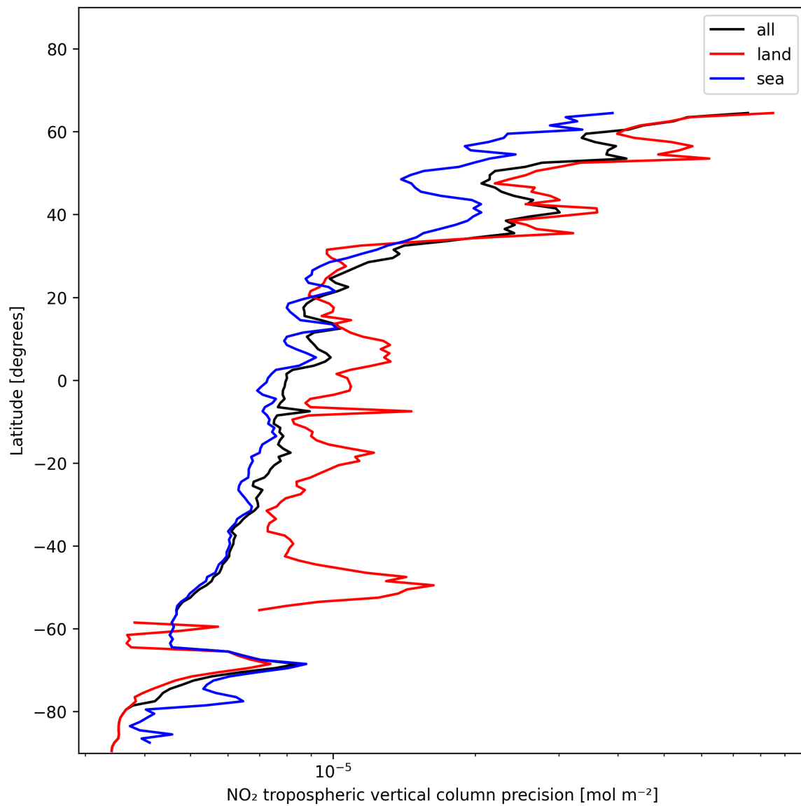
Figure 13: Zonal average of “NO 2 tropospheric vertical column precision” for 2024-12-23 to 2024-12-25.
