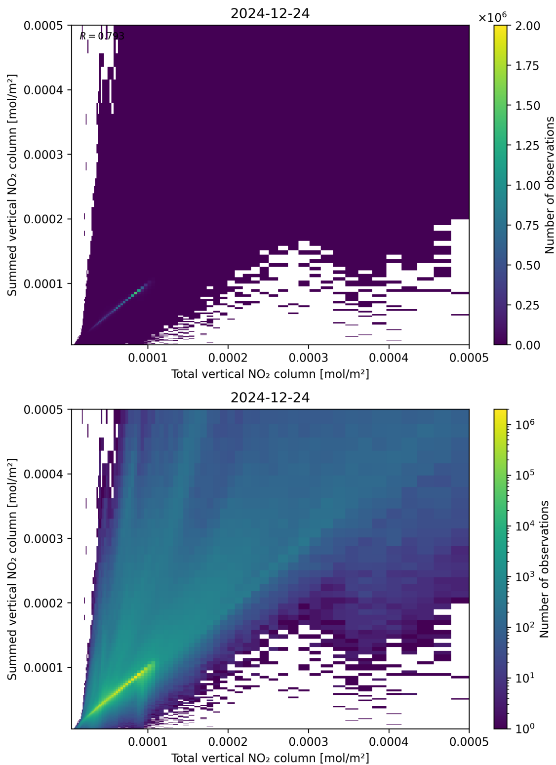
Figure 112: Scatter density plot of “Total vertical NO 2 column” against “Summed vertical NO 2 column” for 2024-12-23 to 2024-12-25.
