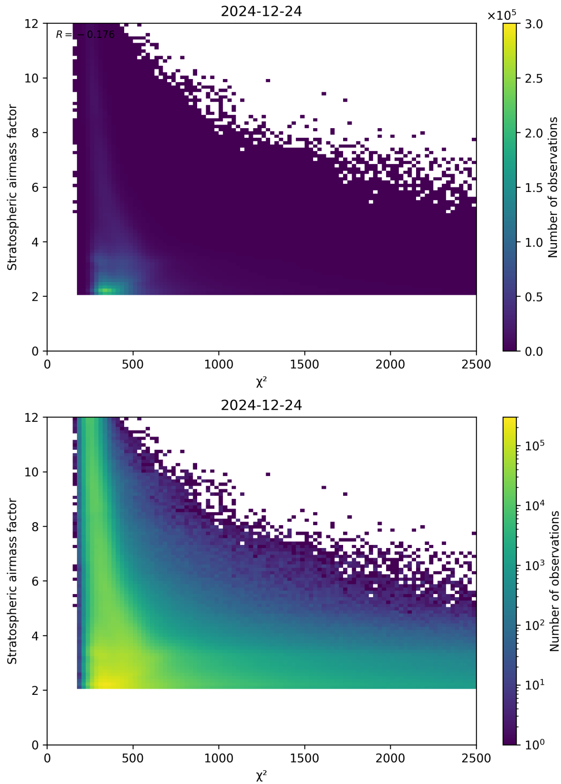
Figure 81: Scatter density plot of “ \chi^2 ” against “Stratospheric airmass factor” for 2024-12-23 to 2024-12-25.
