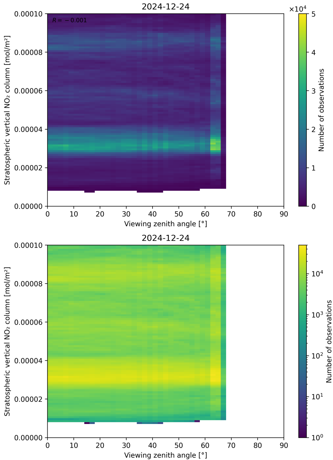
Figure 164: Scatter density plot of “Viewing zenith angle” against “Stratospheric vertical NO 2 column” for 2024-12-23 to 2024-12-25.
