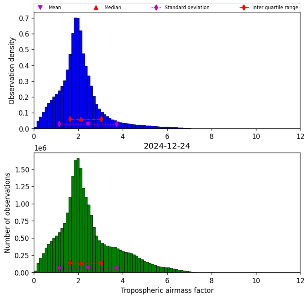
Figure 31: Histogram of “Tropospheric airmass factor” for 2024-12-23 to 2024-12-25
