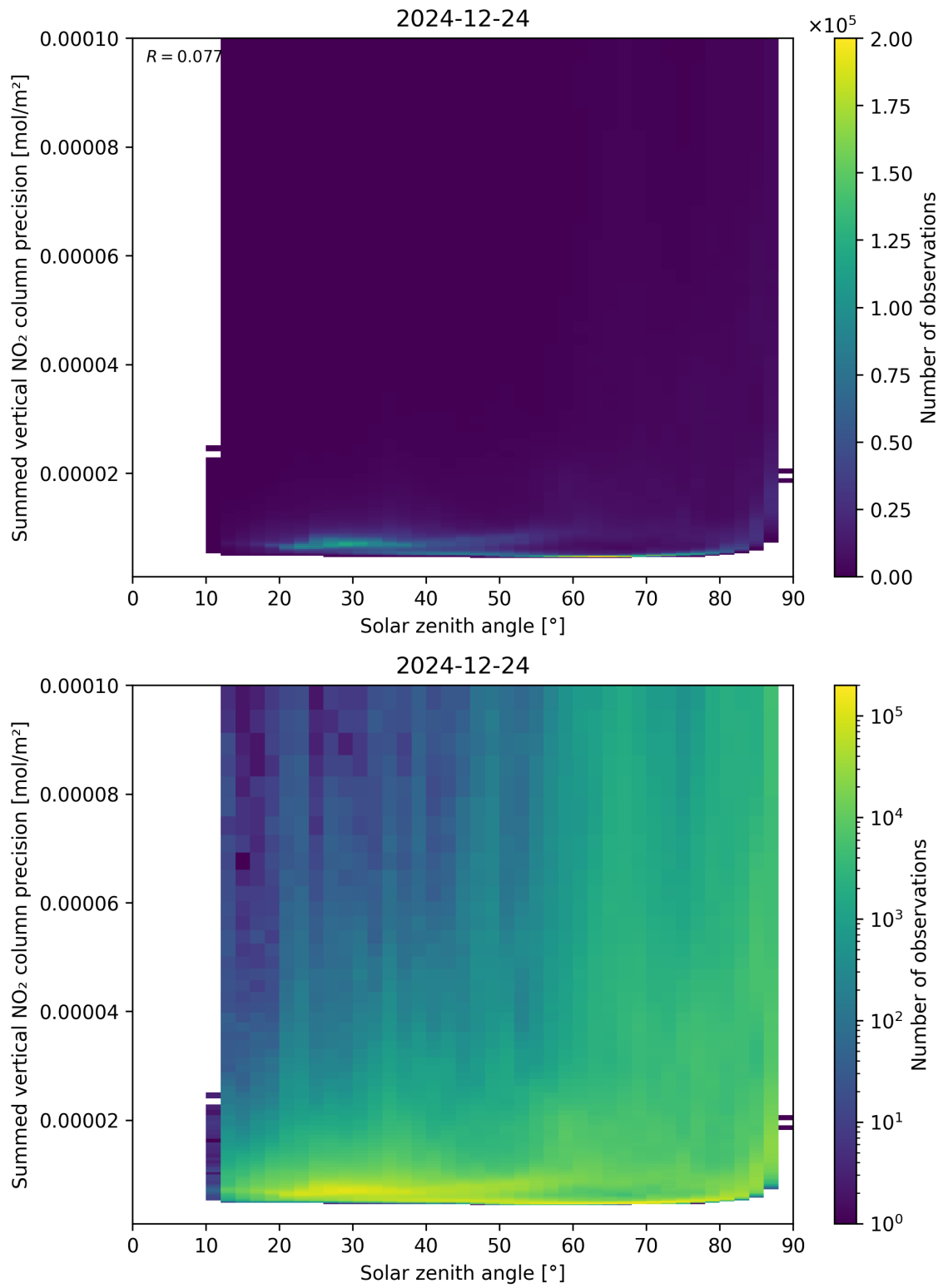
Figure 152: Scatter density plot of “Solar zenith angle” against “Summed vertical NO 2 column precision” for 2024-12-23 to 2024-12-25.
