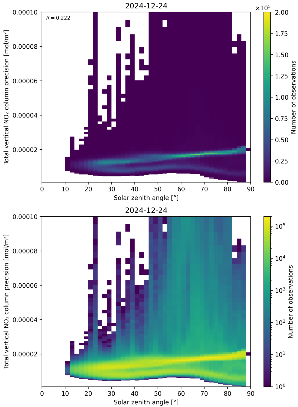
Figure 154: Scatter density plot of “Solar zenith angle” against “Total vertical NO 2 column precision” for 2024-12-23 to 2024-12-25.
