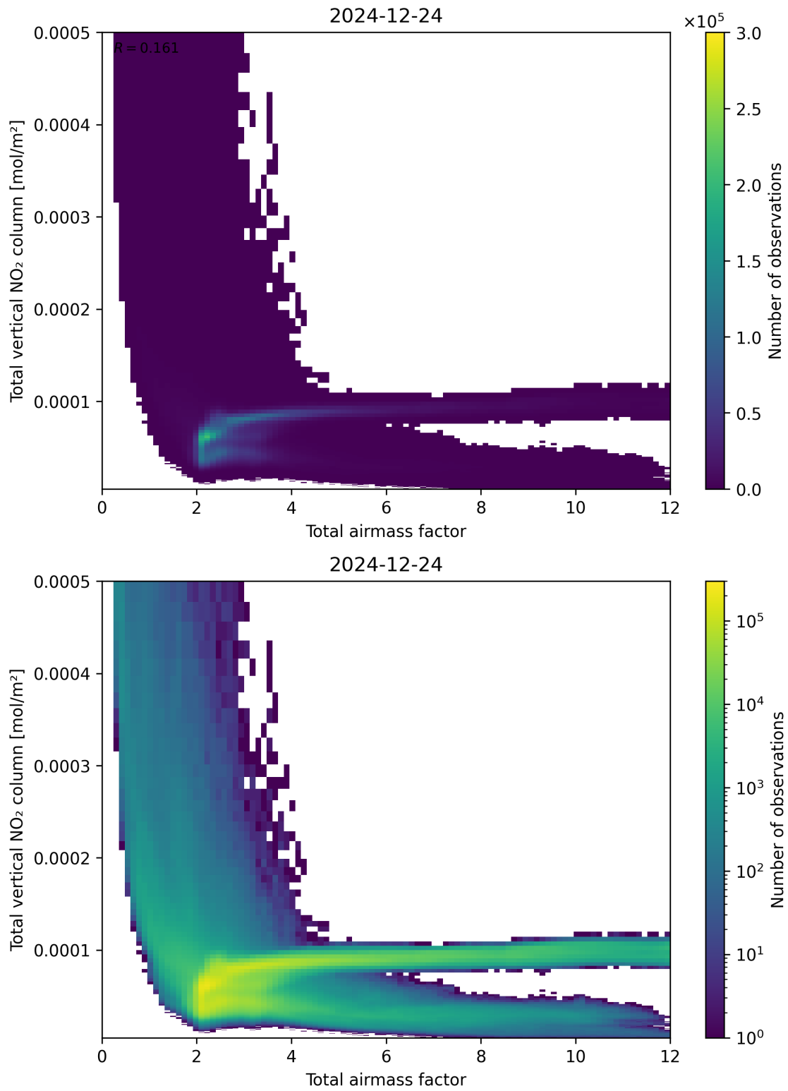
Figure 67: Scatter density plot of “Total airmass factor” against “Total vertical NO 2 column” for 2024-12-23 to 2024-12-25.
