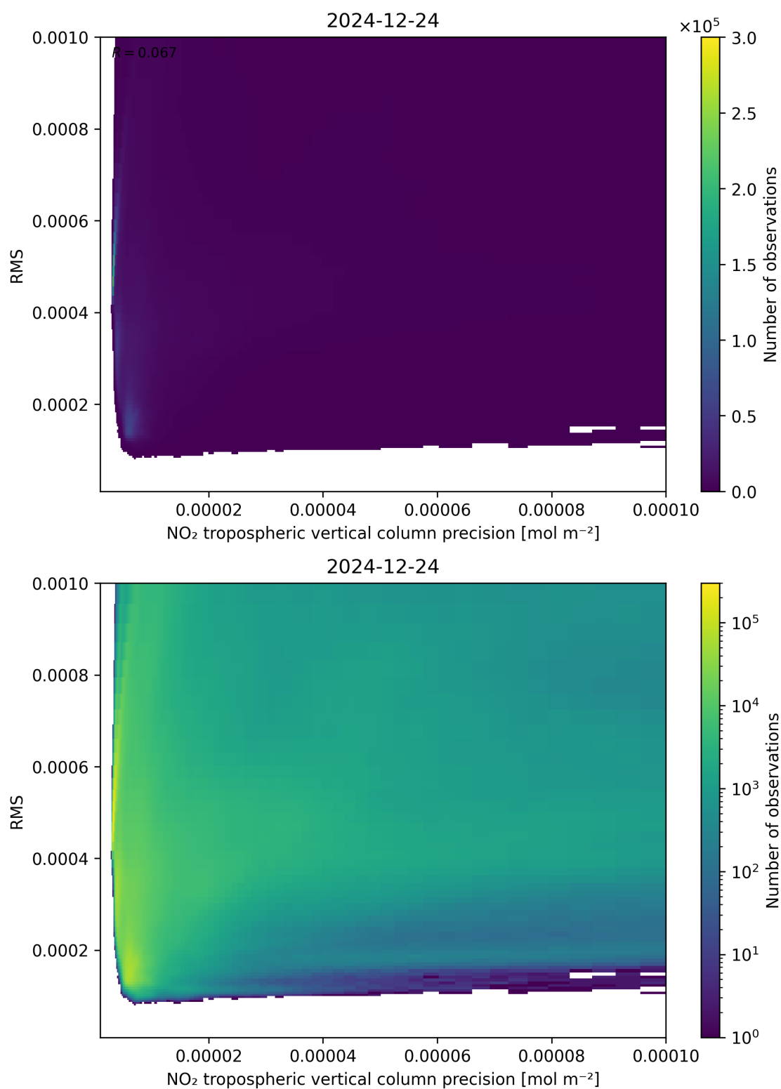
Figure 140: Scatter density plot of “NO 2 tropospheric vertical column precision” against “RMS” for 2024-12-23 to 2024-12-25.
