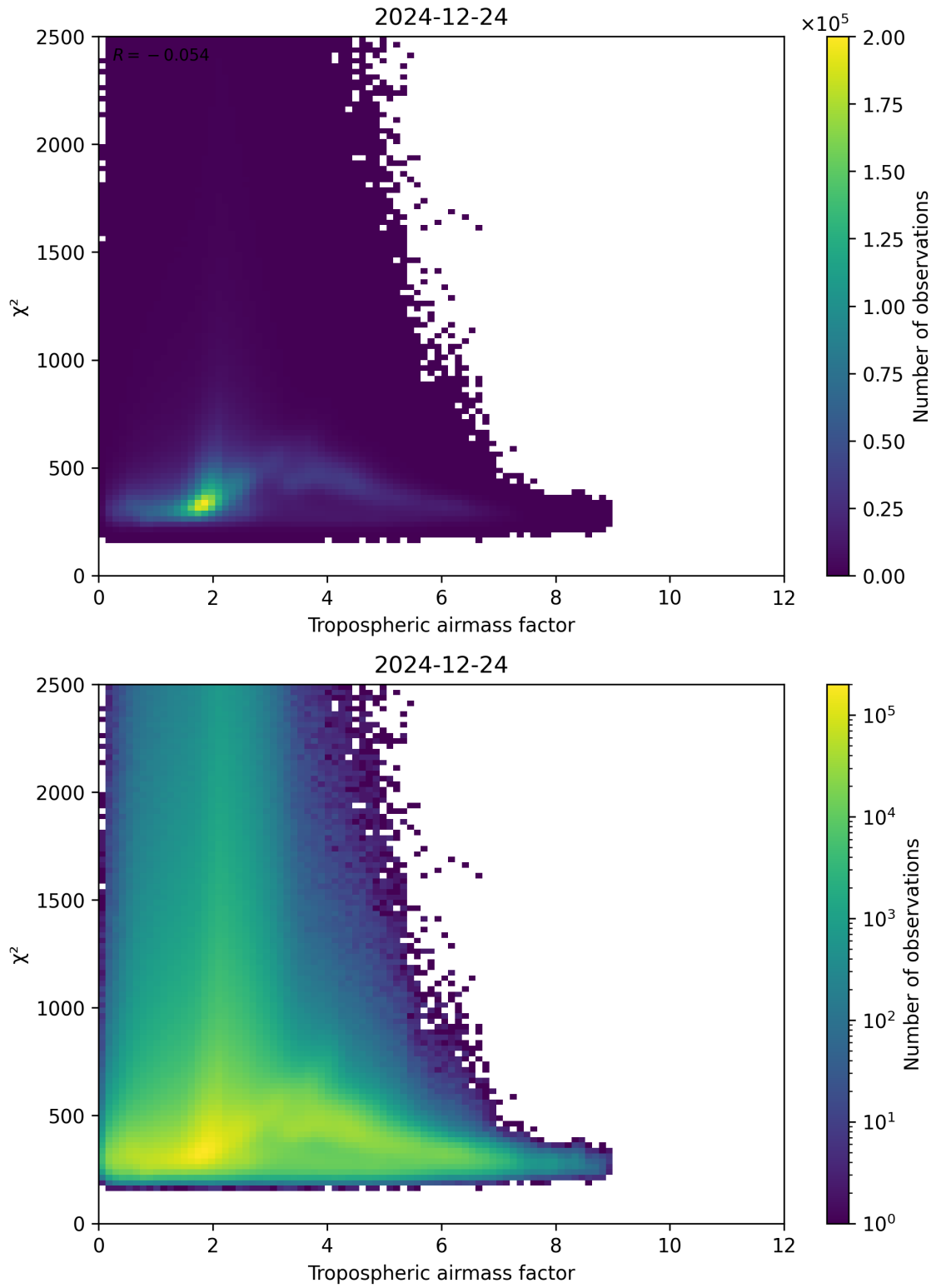
Figure 73: Scatter density plot of “Tropospheric airmass factor” against “ \chi^2 ” for 2024-12-23 to 2024-12-25.
