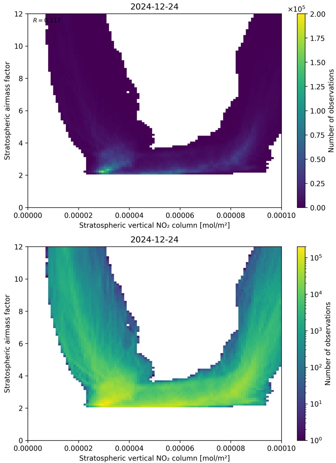
Figure 96: Scatter density plot of “Stratospheric vertical NO 2 column” against “Stratospheric airmass factor” for 2024-12-23 to 2024-12-25.
