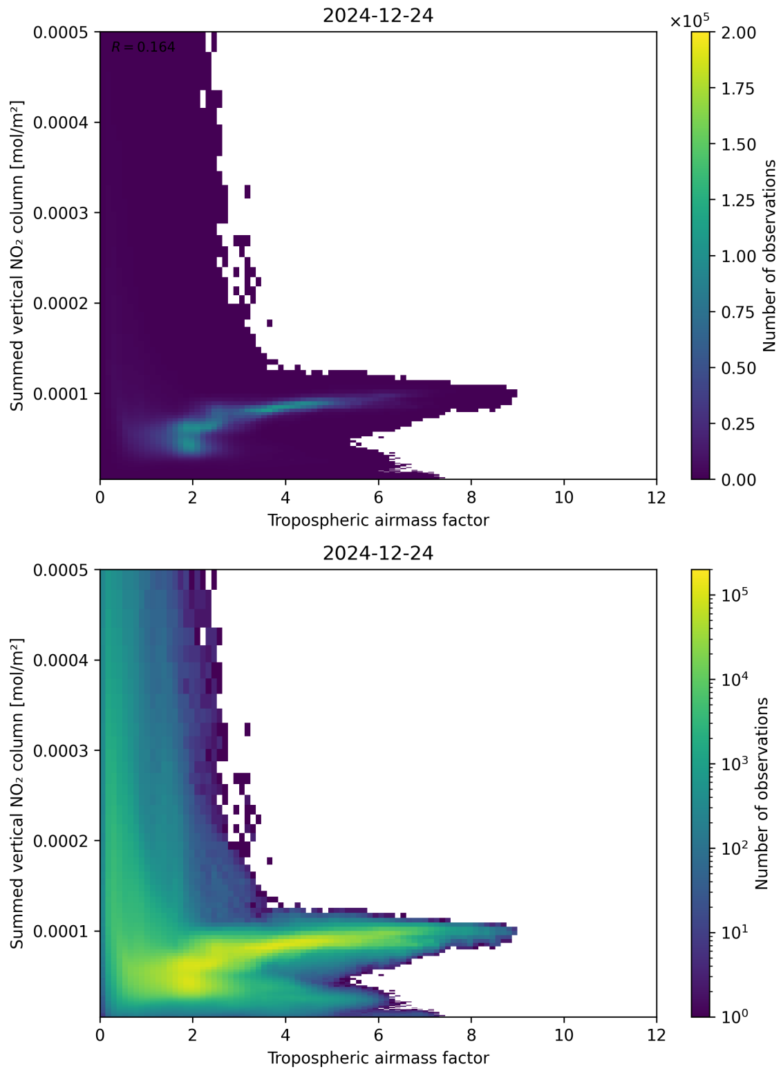
Figure 75: Scatter density plot of “Tropospheric air mass factor” against “Summed vertical NO 2 column” for 2024-12-23 to 2024-12-25.
