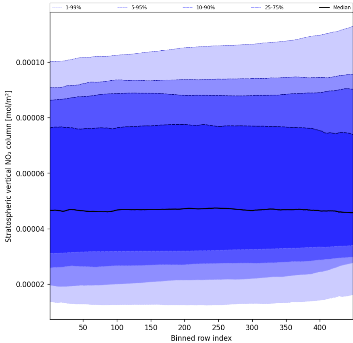
Figure 53: Along track statistics of “Stratospheric vertical NO 2 column” for 2024-12-23 to 2024-12-25
