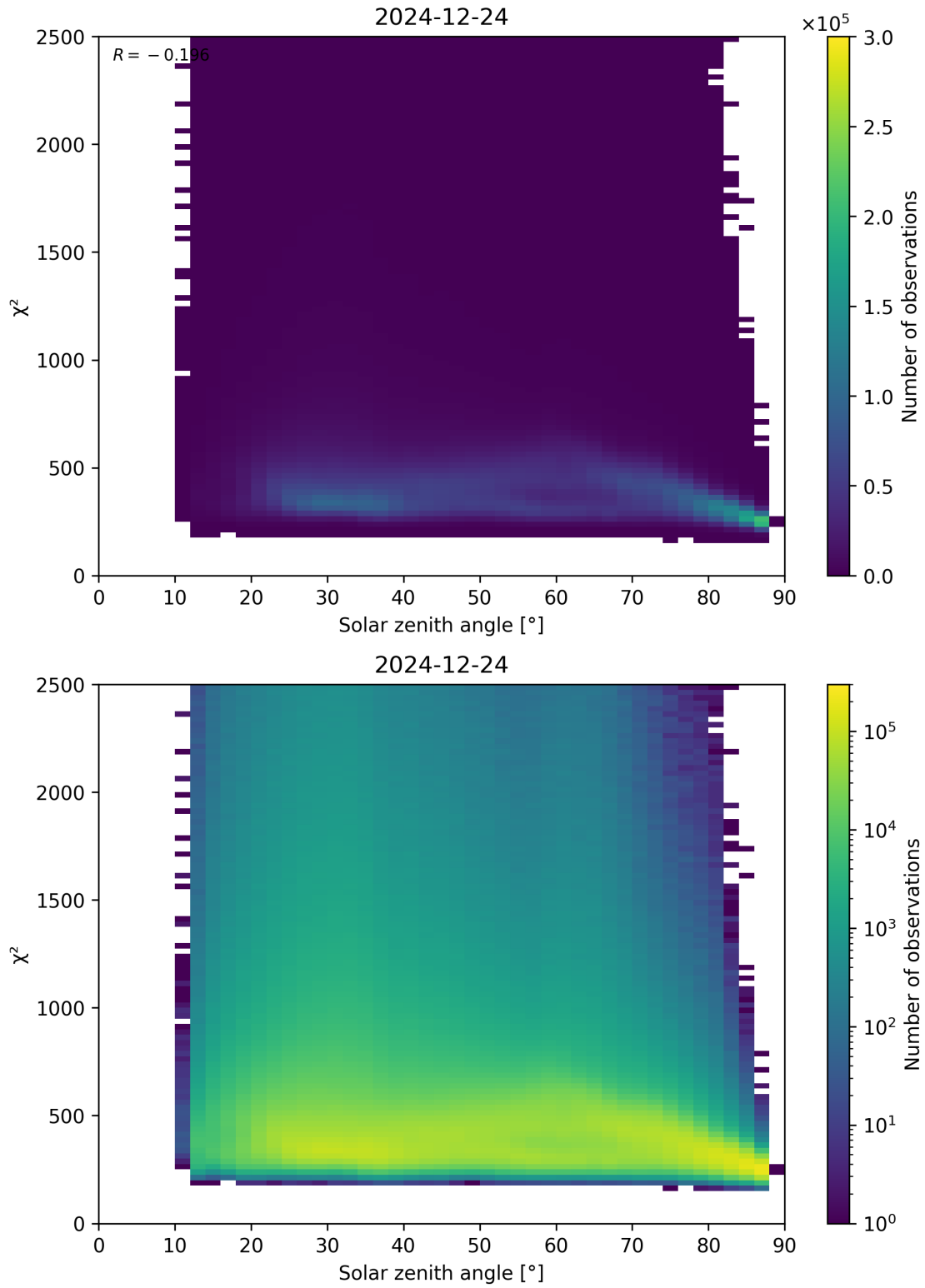
Figure 148: Scatter density plot of “Solar zenith angle” against “ \chi^2 ” for 2024-12-23 to 2024-12-25.
