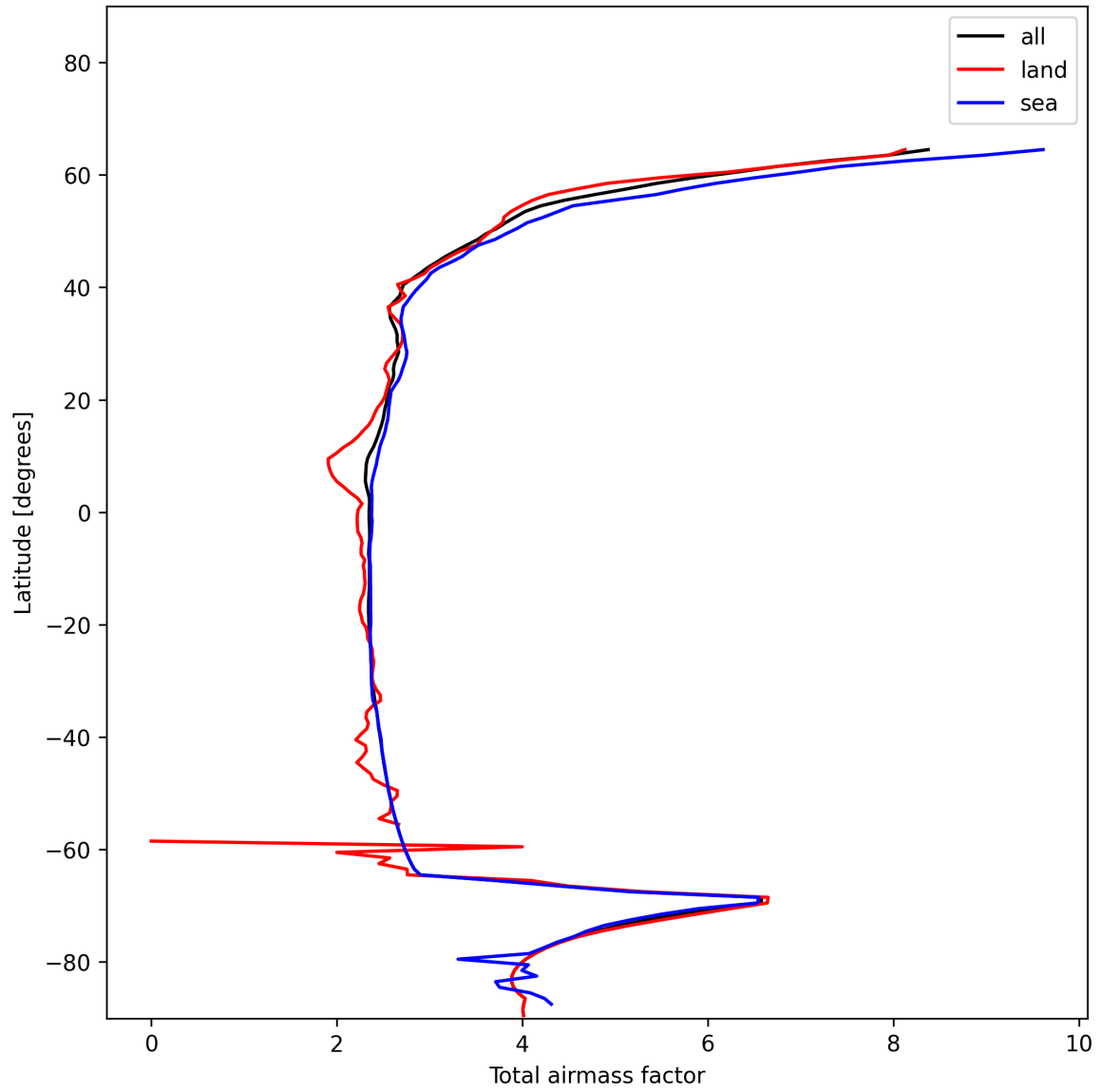
Figure 15: Zonal average of “Total airmass factor” for 2024-12-23 to 2024-12-25.
