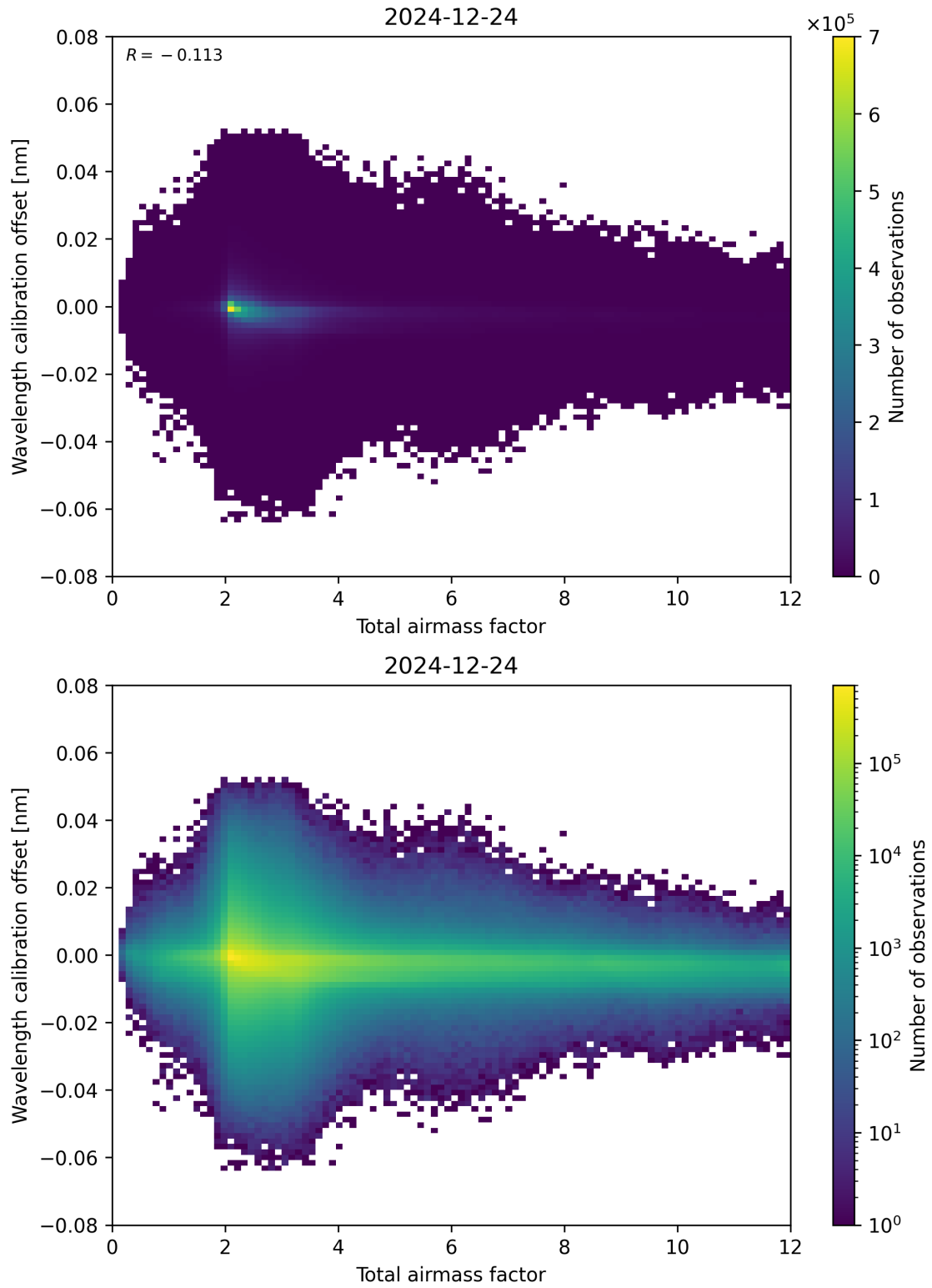
Figure 70: Scatter density plot of “Total airmass factor” against “Wavelength calibration offset” for 2024-12-23 to 2024-12-25.
