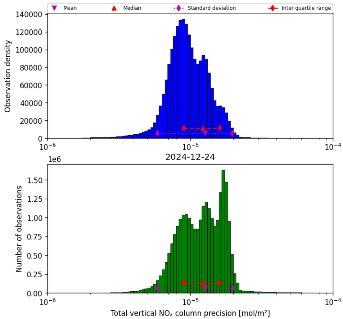
Figure 39: Histogram of “Total vertical NO 2 column precision” for 2024-12-23 to 2024-12-25
