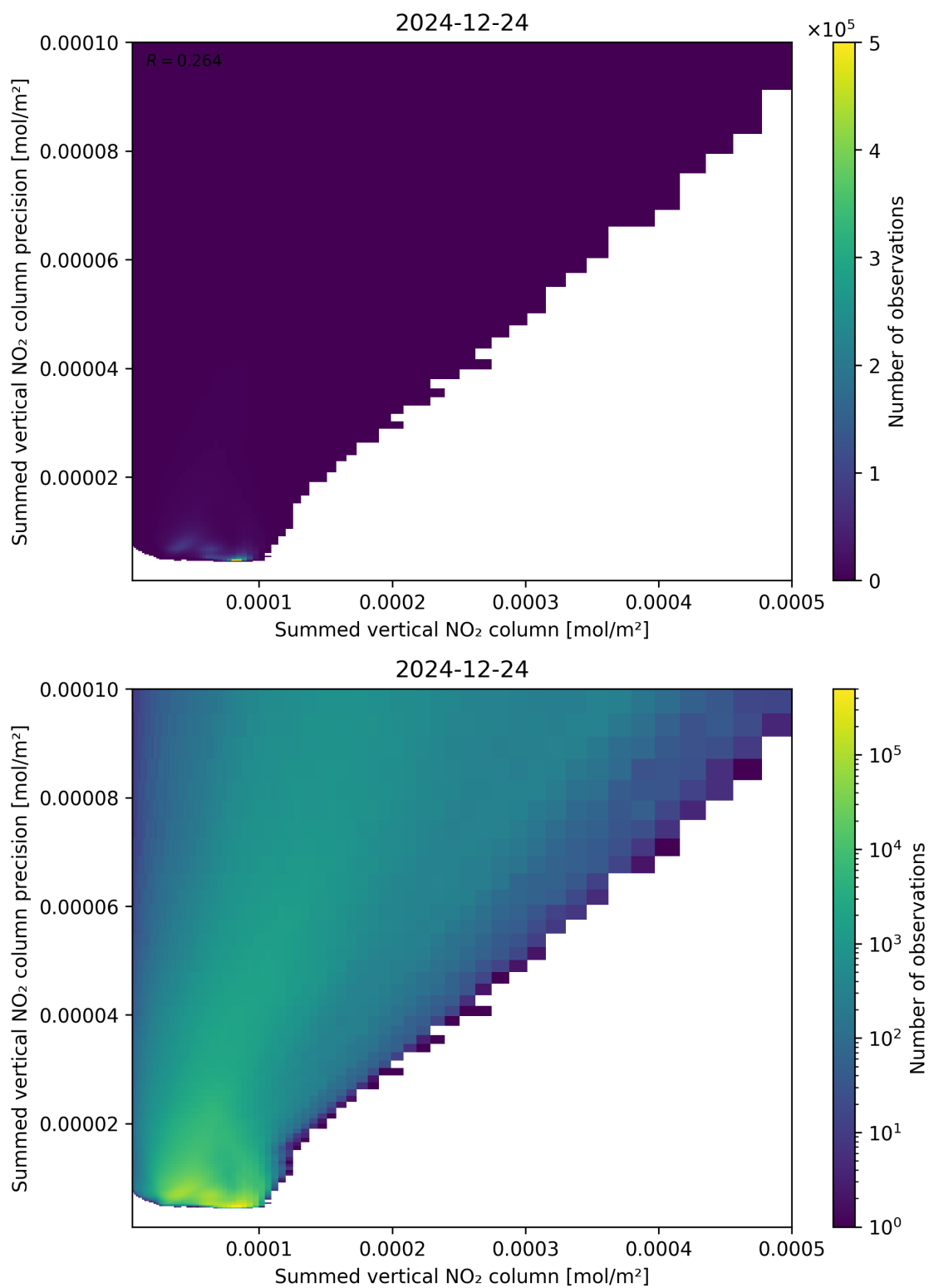
Figure 105: Scatter density plot of “Summed vertical NO 2 column” against “Summed vertical NO 2 column precision” for 2024-12-23 to 2024-12-25.
