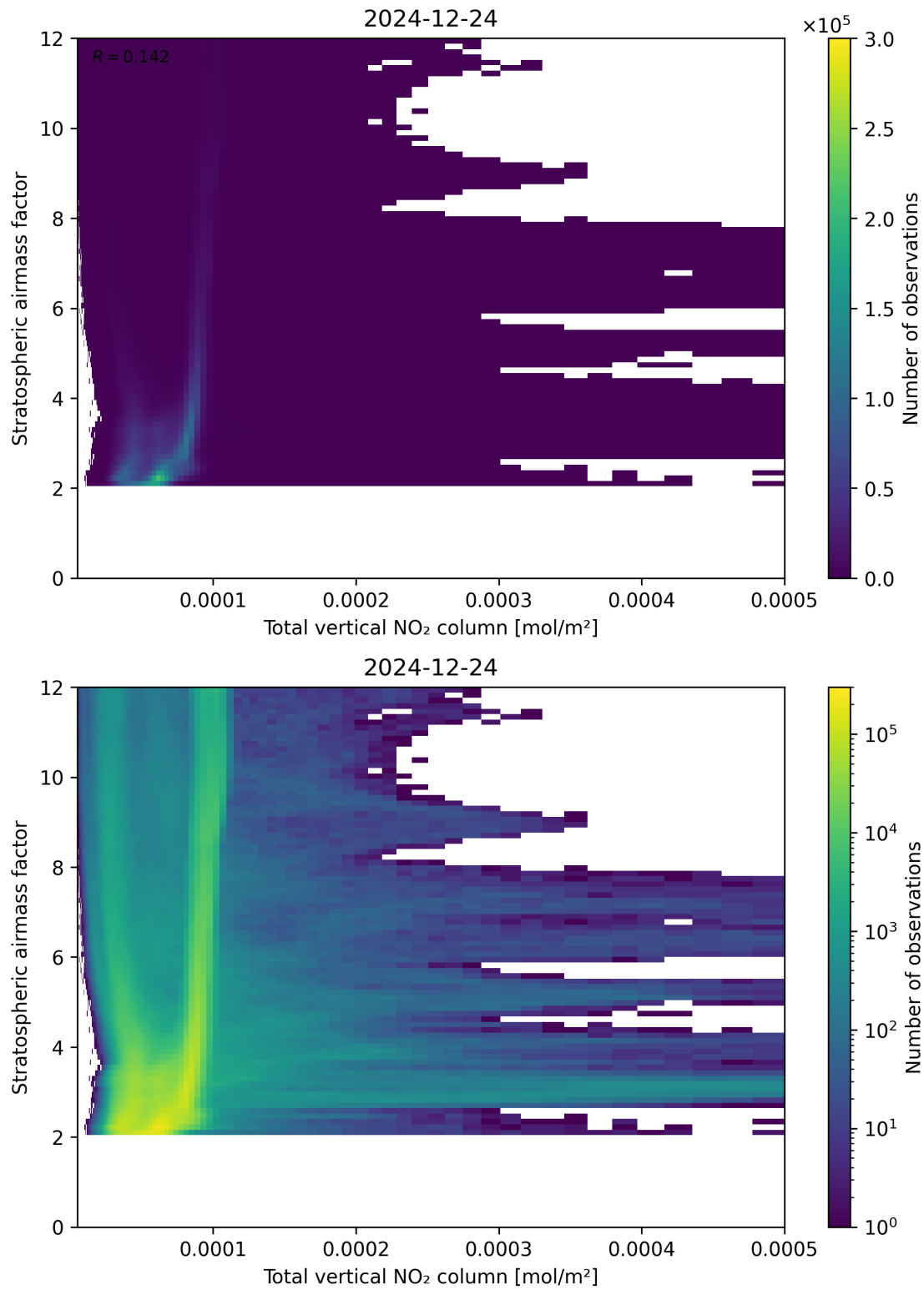
Figure 110: Scatter density plot of “Total vertical NO 2 column” against “Stratospheric airmass factor” for 2024-12-23 to 2024-12-25.
