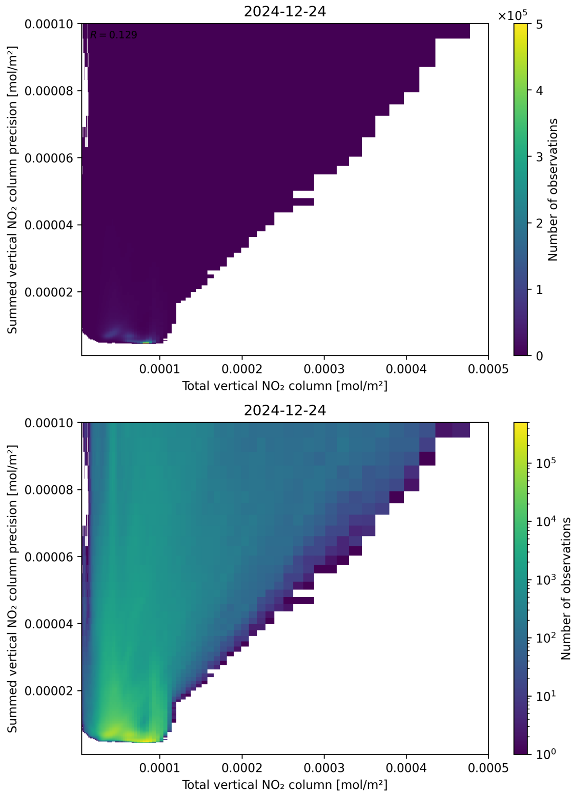
Figure 113: Scatter density plot of “Total vertical NO 2 column” against “Summed vertical NO 2 column precision” for 2024-12-23 to 2024-12-25.
