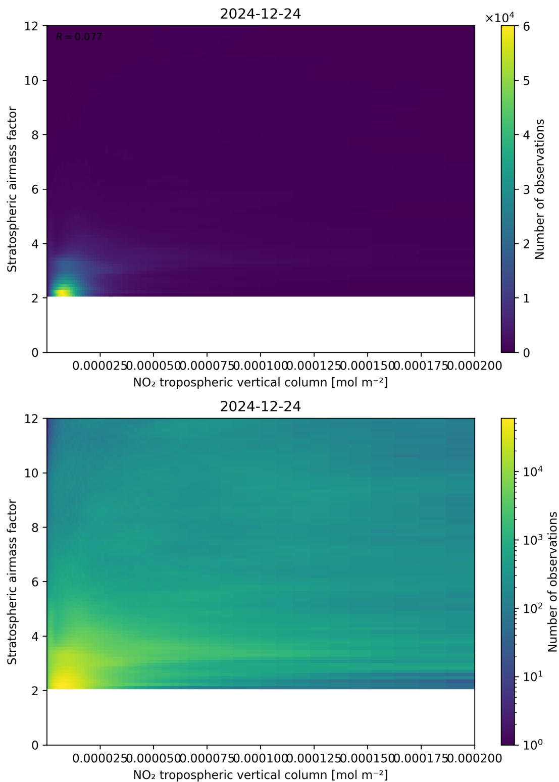
Figure 121: Scatter density plot of “NO 2 tropospheric vertical column” against “Stratospheric airmass factor” for 2024-12-23 to 2024-12-25.
