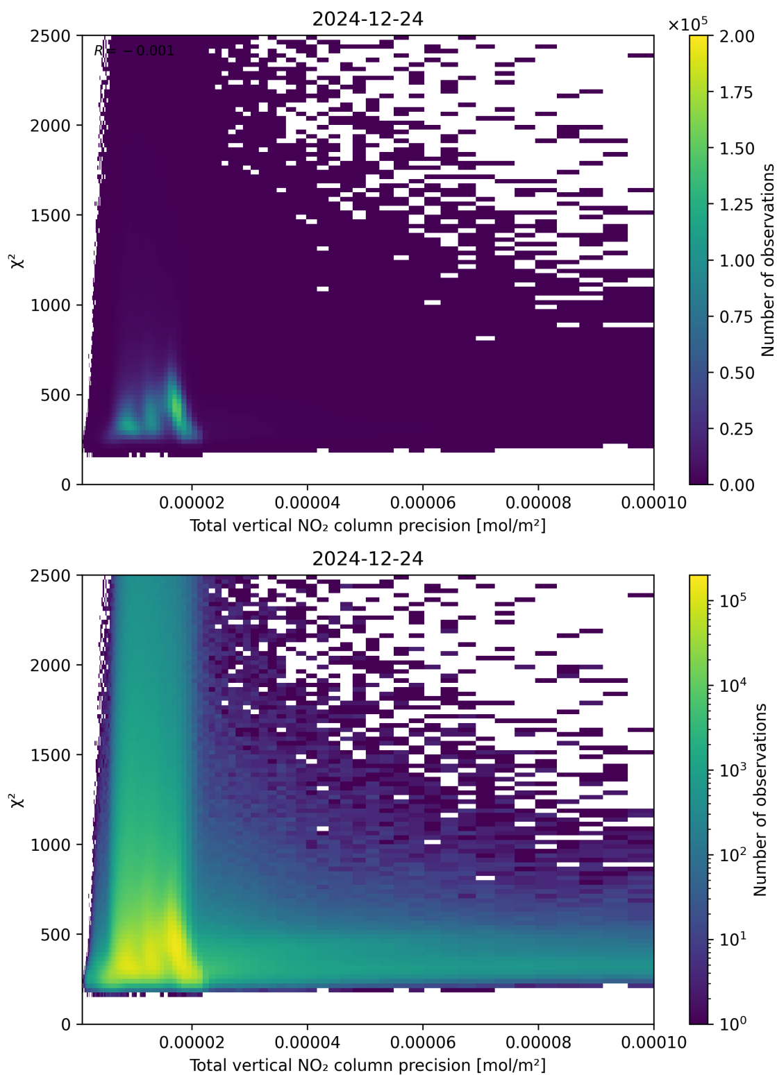
Figure 116: Scatter density plot of “Total vertical NO 2 column precision” against “ \chi^2 ” for 2024-12-23 to 2024-12-25.
