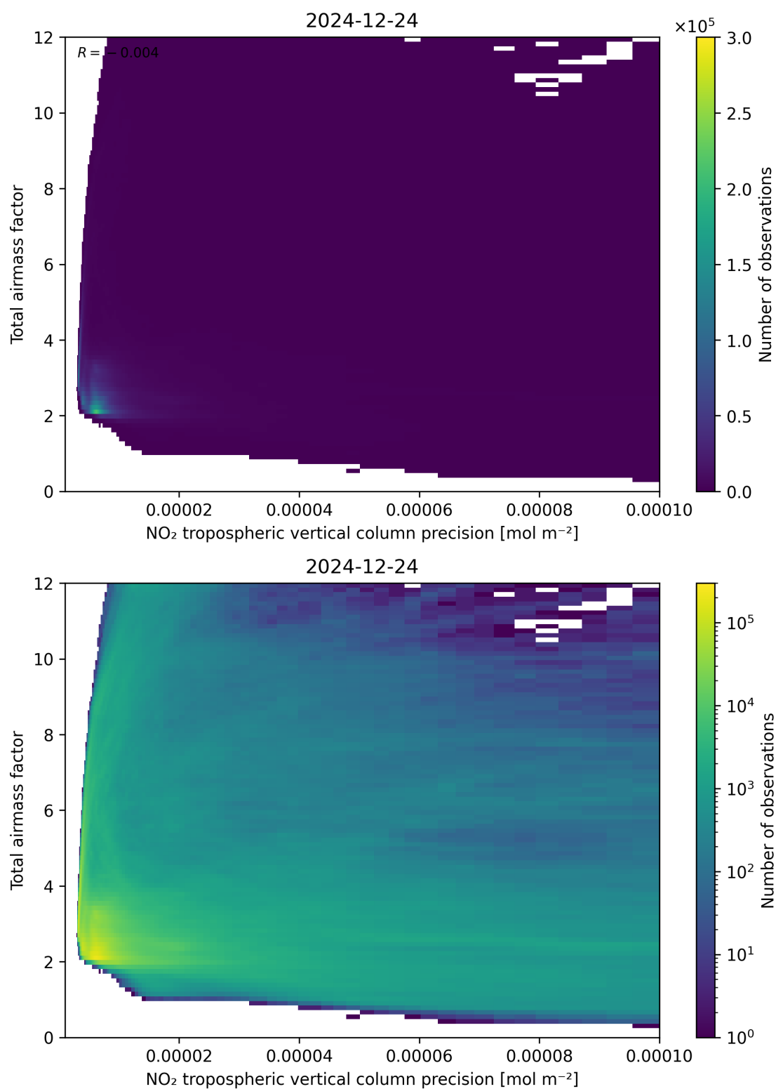
Figure 132: Scatter density plot of “NO 2 tropospheric vertical column precision” against “Total air mass factor” for 2024-12-23 to 2024-12-25.
