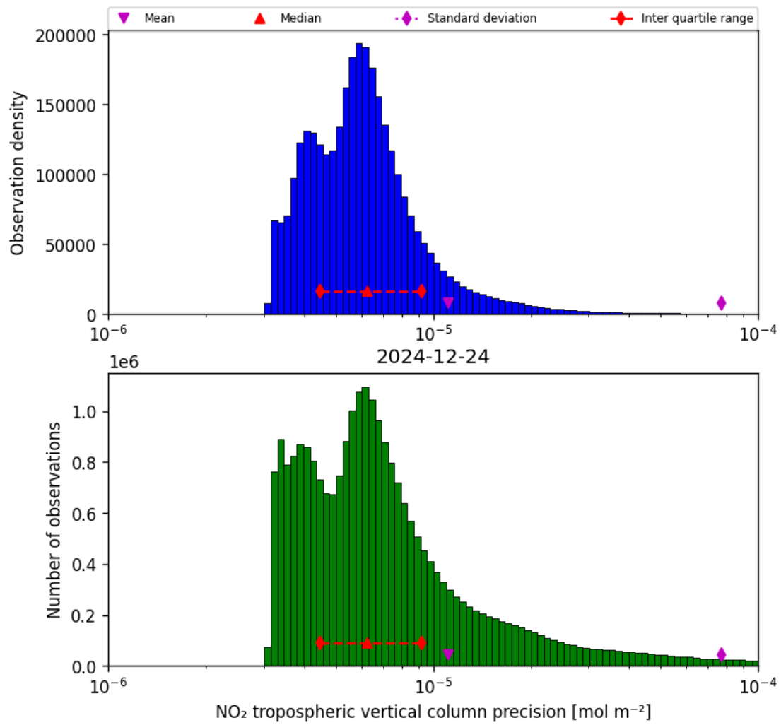
Figure 30: Histogram of “NO 2 tropospheric vertical column precision” for 2024-12-23 to 2024-12-25
