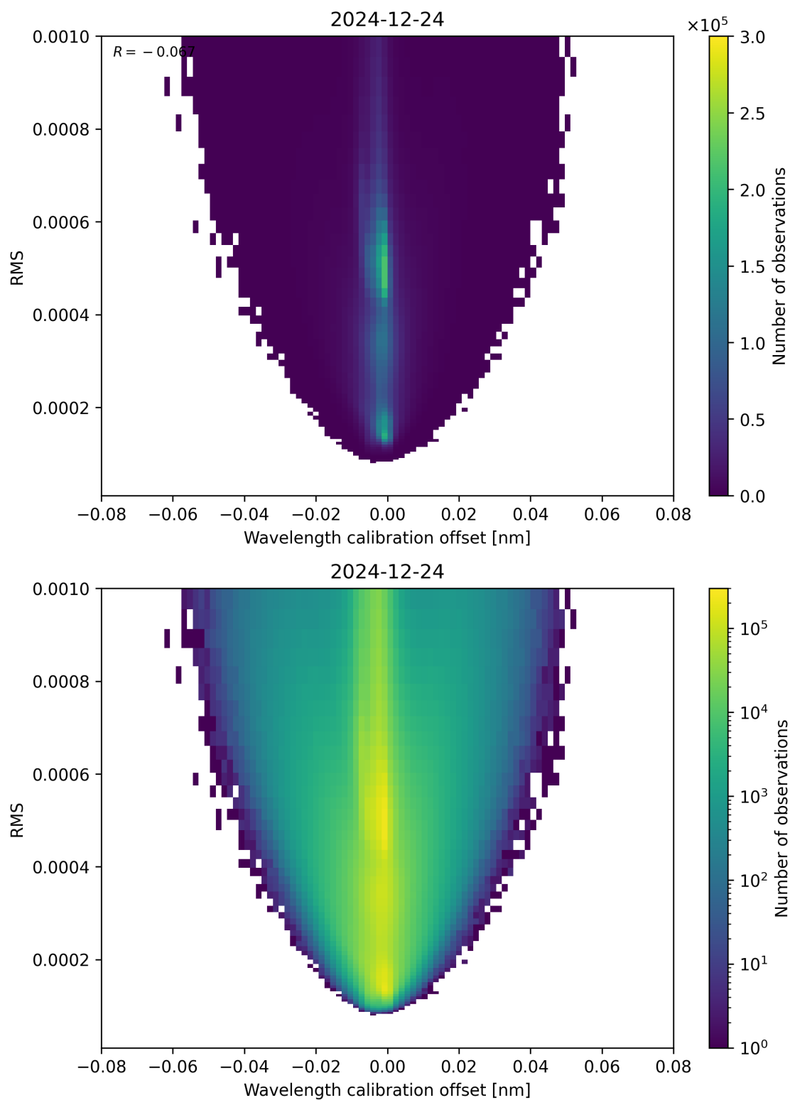
Figure 181: Scatter density plot of “Wavelength calibration offset” against “RMS” for 2024-12-23 to 2024-12-25.
