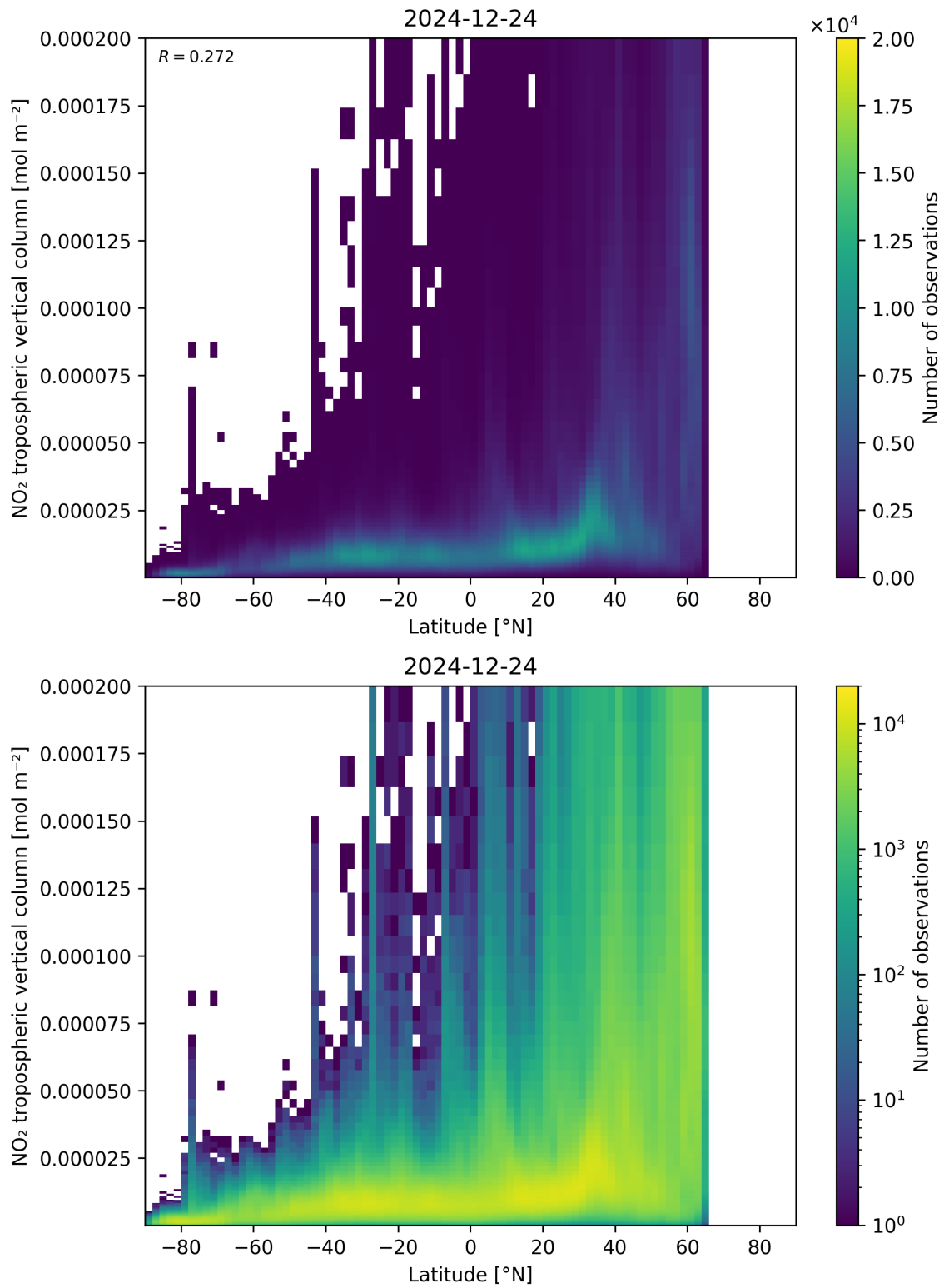
Figure 92: Scatter density plot of “Latitude” against “NO 2 tropospheric vertical column” for 2024-12-23 to 2024-12-25.
