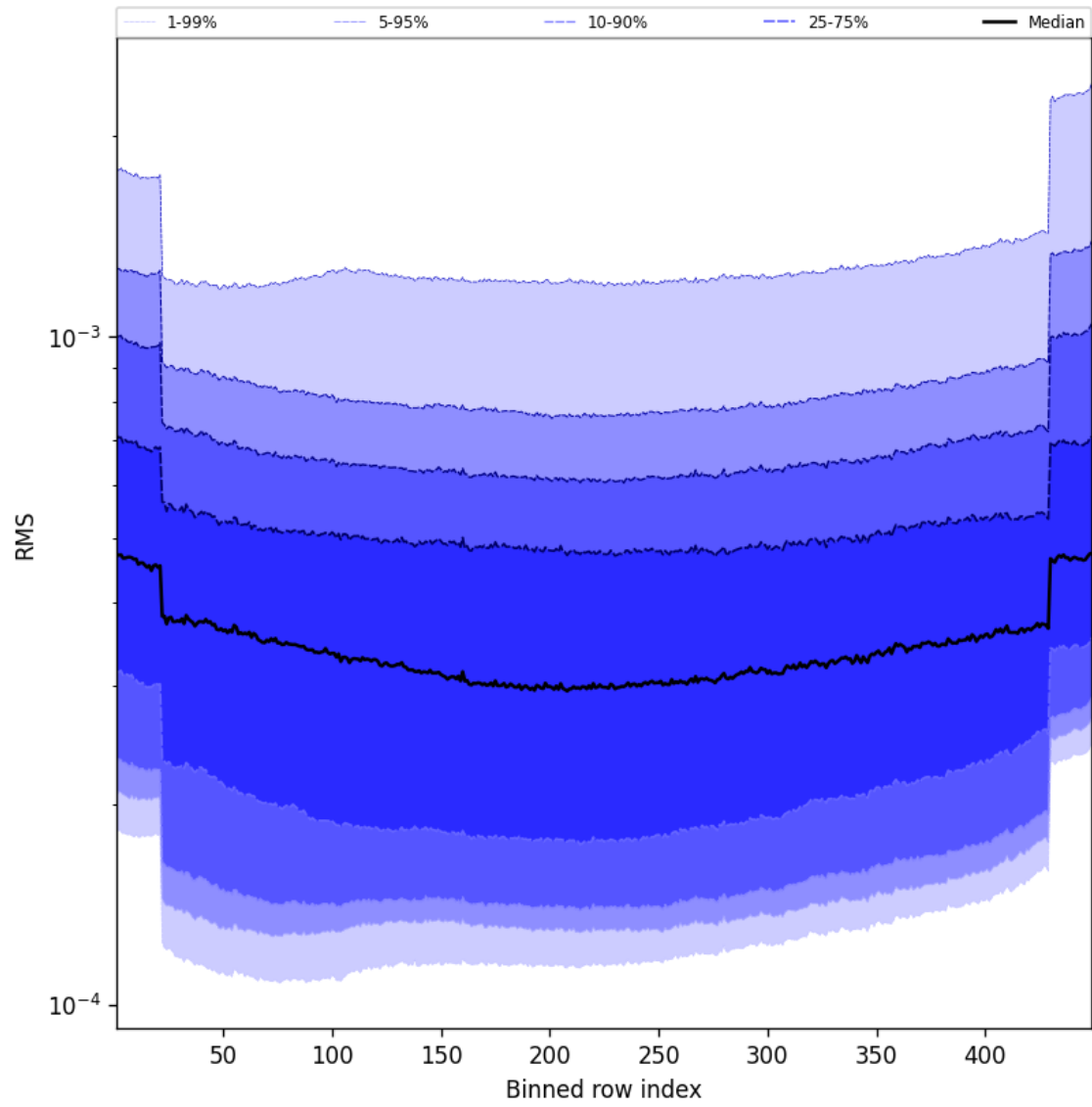
Figure 60: Along track statistics of “RMS” for 2024-12-23 to 2024-12-25
