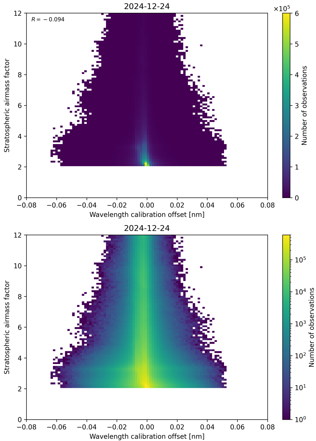
Figure 174: Scatter density plot of “Wavelength calibration offset” against “Stratospheric airmass factor” for 2024-12-23 to 2024-12-25.
