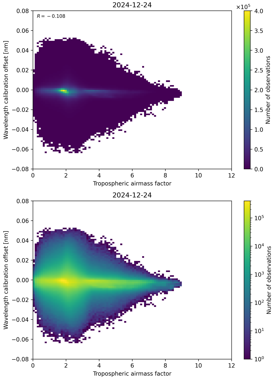
Figure 80: Scatter density plot of “Tropospheric airmass factor” against “Wavelength calibration offset” for 2024-12-23 to 2024-12-25.
