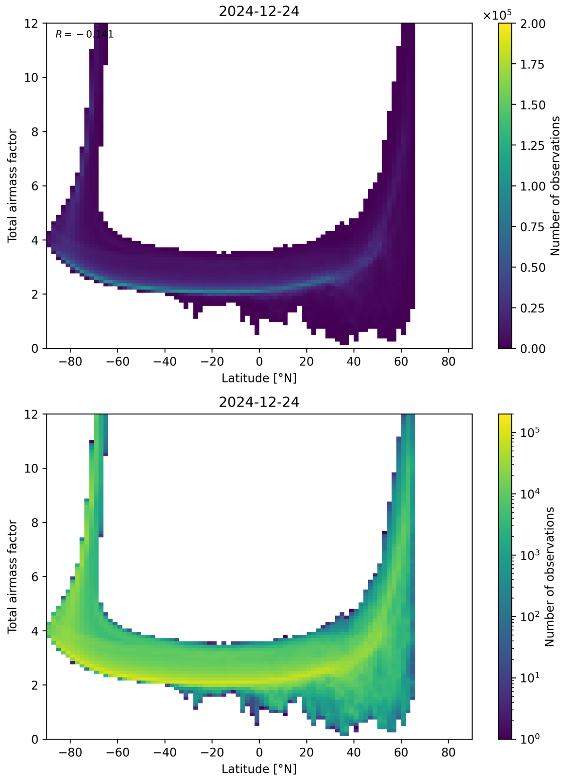
Figure 84: Scatter density plot of “Latitude” against “Total airmass factor” for 2024-12-23 to 2024-12-25.
