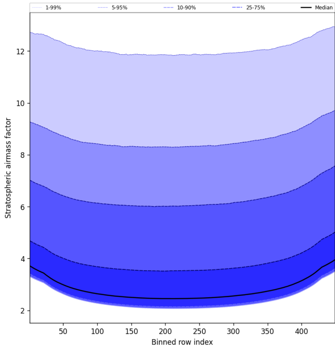
Figure 61: Along track statistics of “Stratospheric airmass factor” for 2024-12-23 to 2024-12-25
