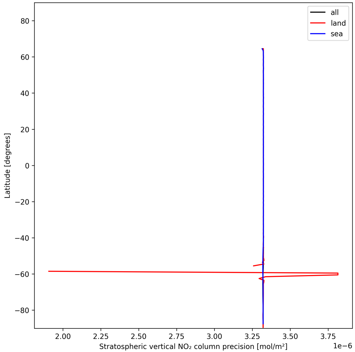
Figure 20: Zonal average of “Stratospheric vertical NO 2 column precision” for 2024-12-23 to 2024-12-25.
