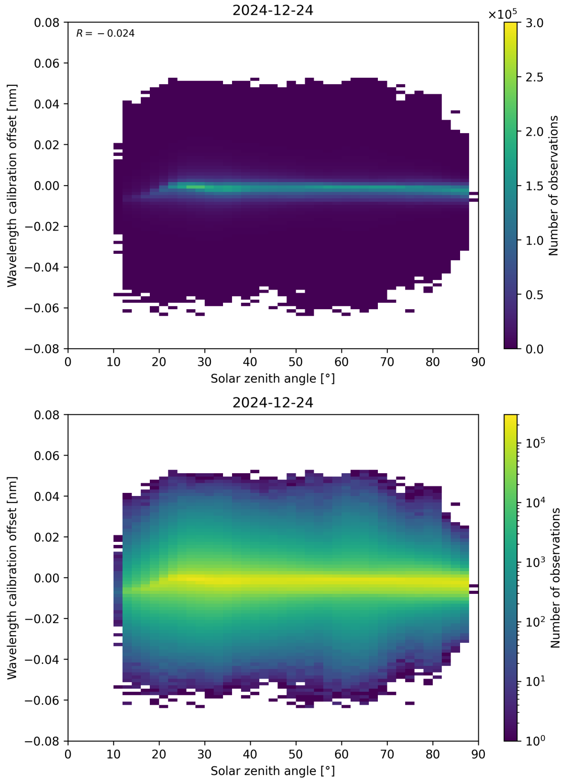
Figure 158: Scatter density plot of “Solar zenith angle” against “Wavelength calibration offset” for 2024-12-23 to 2024-12-25.
