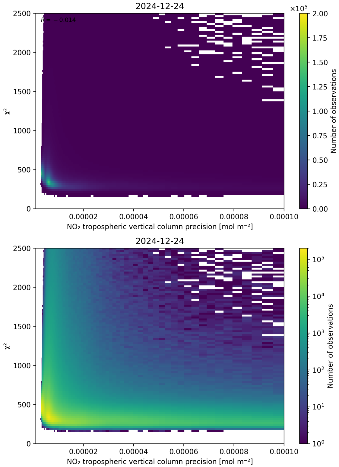
Figure 134: Scatter density plot of “NO 2 tropospheric vertical column precision” against “ \chi^2 ” for 2024-12-23 to 2024-12-25.
