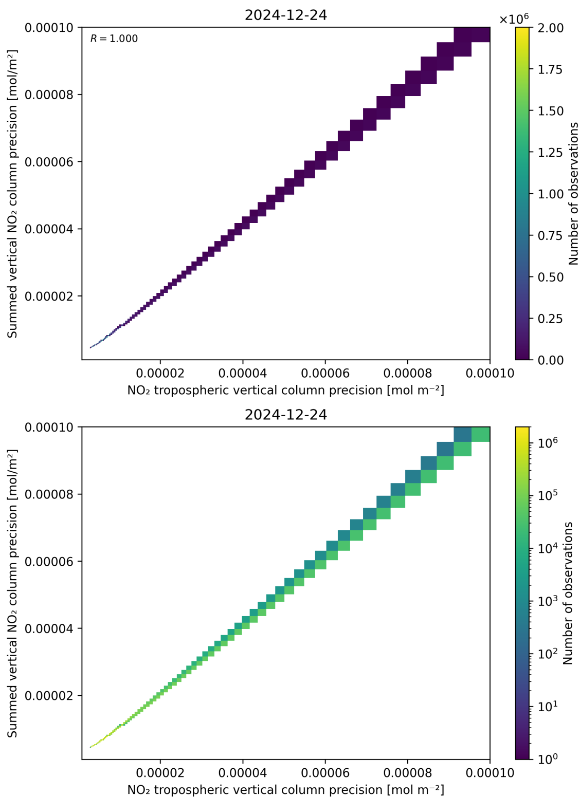
Figure 137: Scatter density plot of “NO 2 tropospheric vertical column precision” against “Summed vertical NO 2 column precision” for 2024-12-23 to 2024-12-25.
