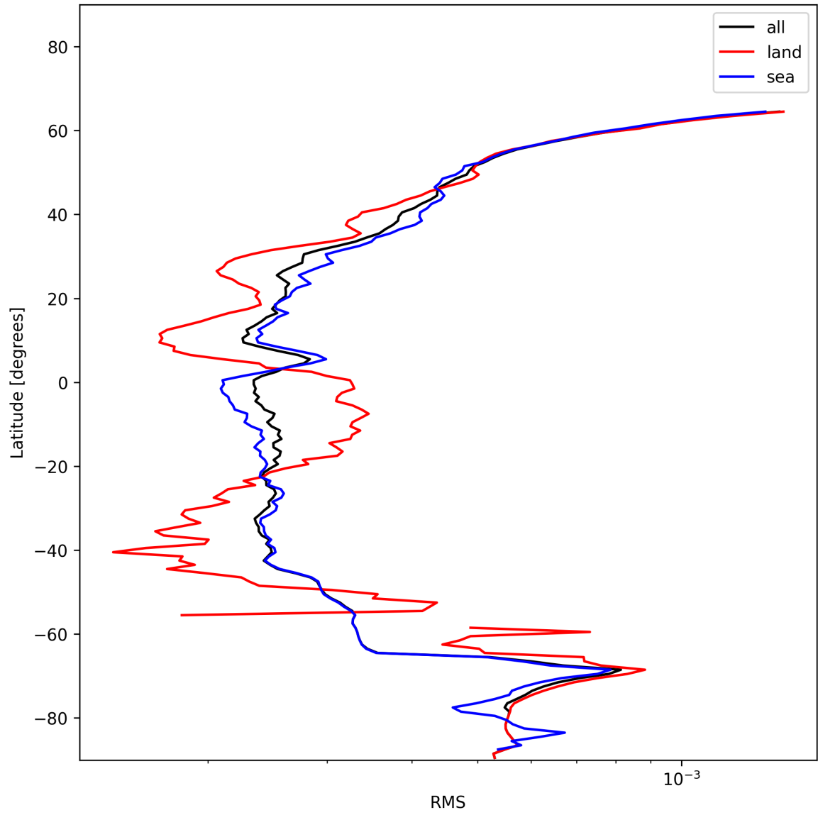
Figure 26: Zonal average of “RMS” for 2024-12-23 to 2024-12-25.
