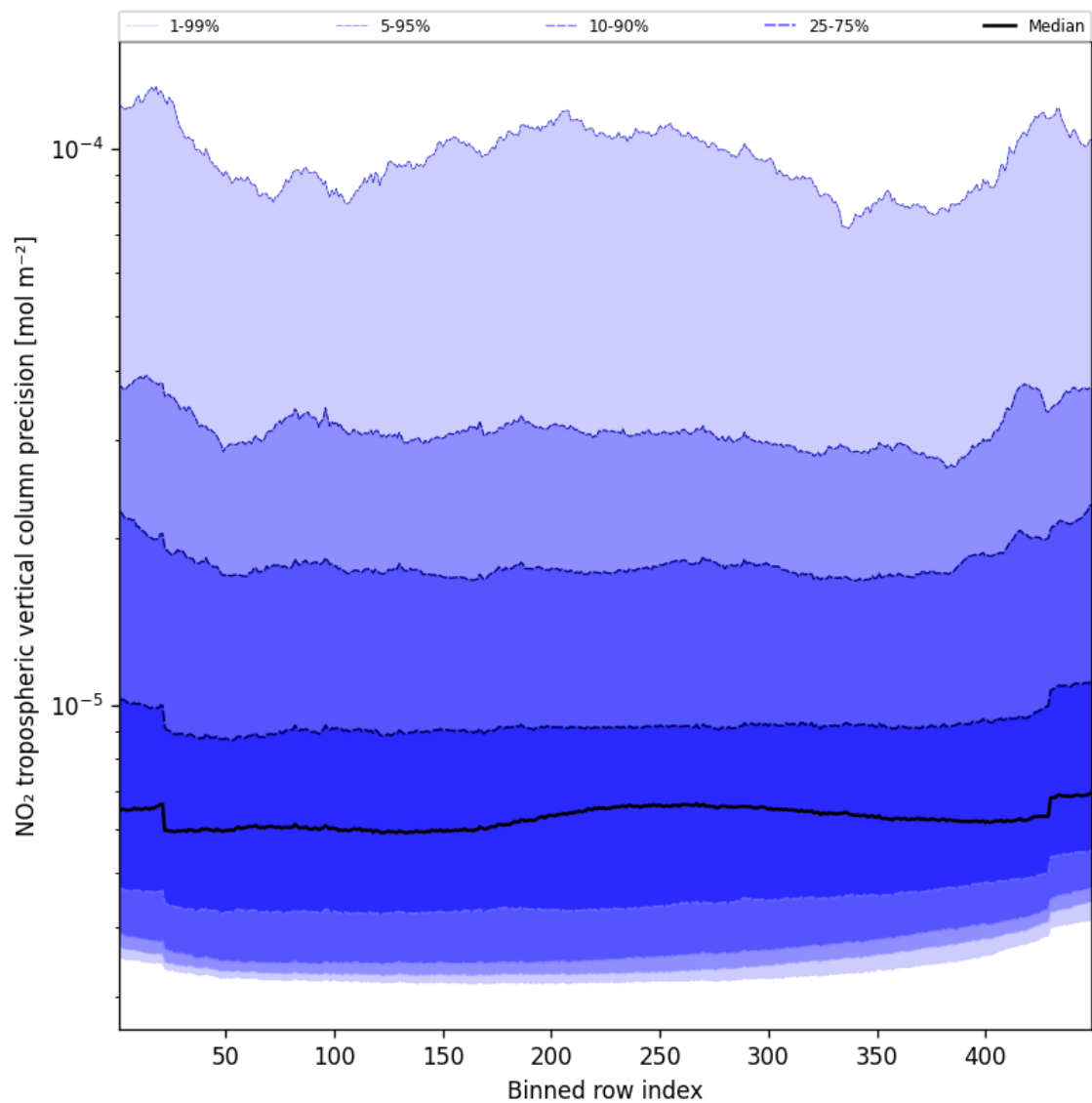
Figure 47: Along track statistics of “NO 2 tropospheric vertical column precision” for 2024-12-23 to 2024-12-25
