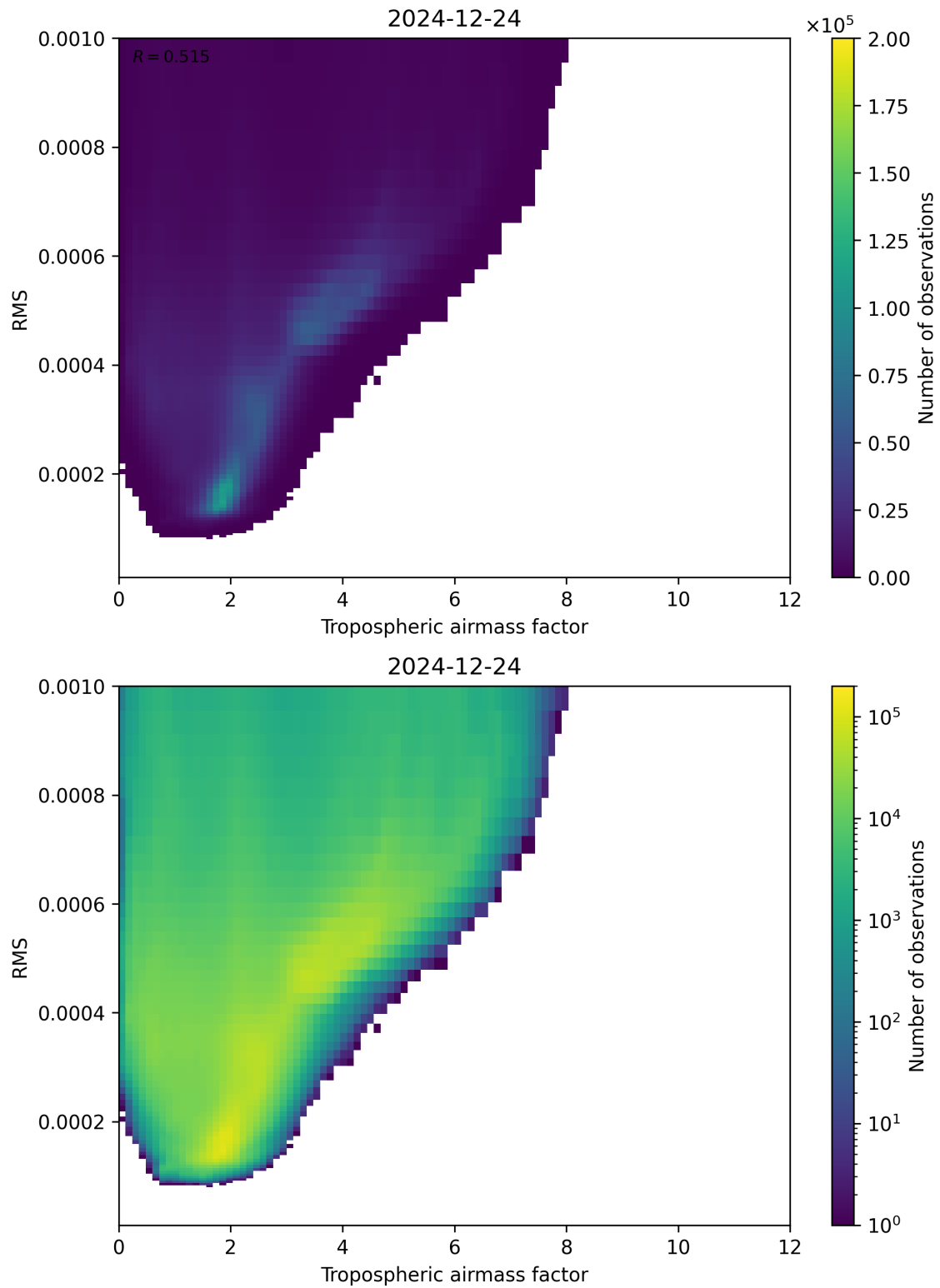
Figure 79: Scatter density plot of “Tropospheric airmass factor” against “RMS” for 2024-12-23 to 2024-12-25.
