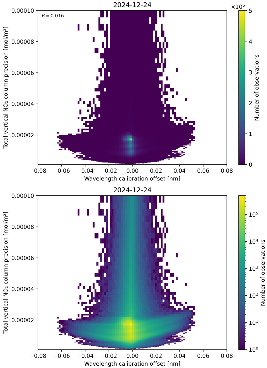
Figure 180: Scatter density plot of “Wavelength calibration offset” against “Total vertical NO 2 column precision” for 2024-12-23 to 2024-12-25.
