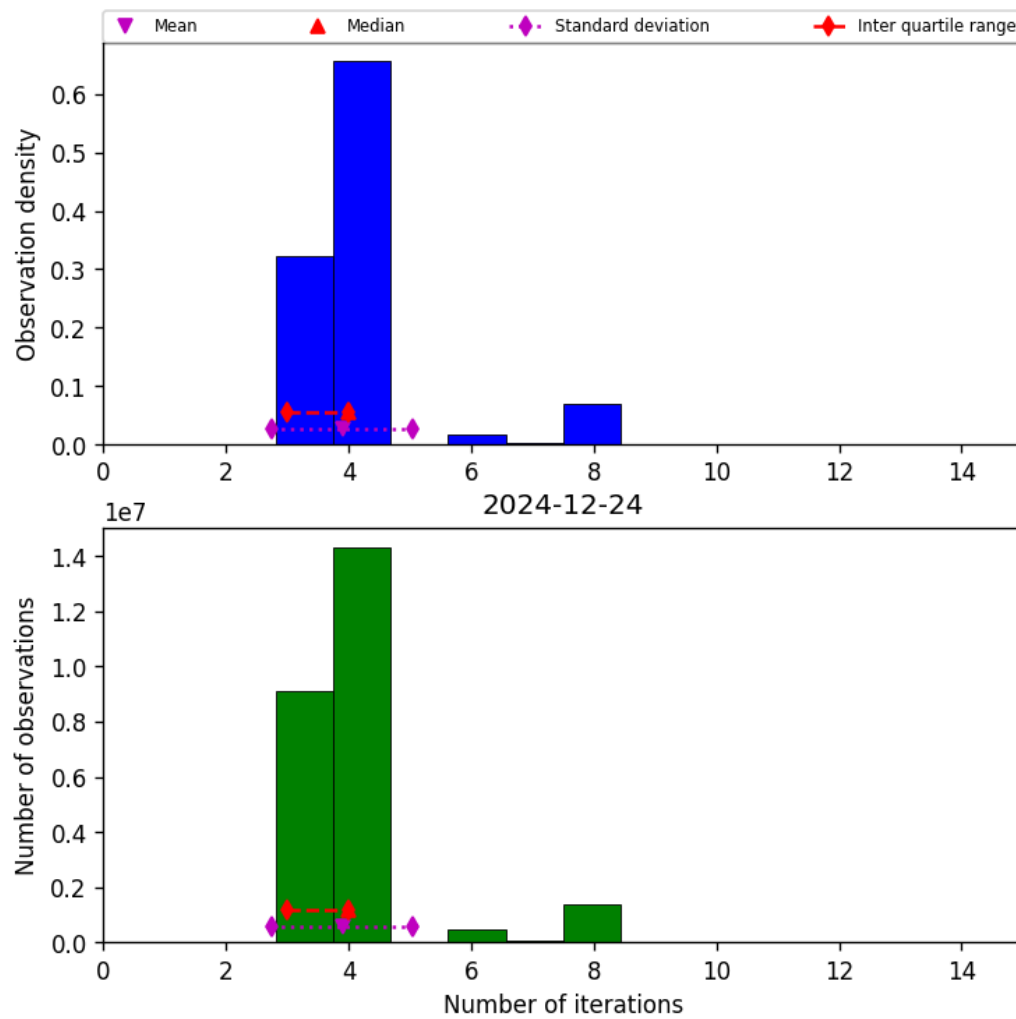
Figure 34: Histogram of “Number of iterations” for 2024-12-23 to 2024-12-25
