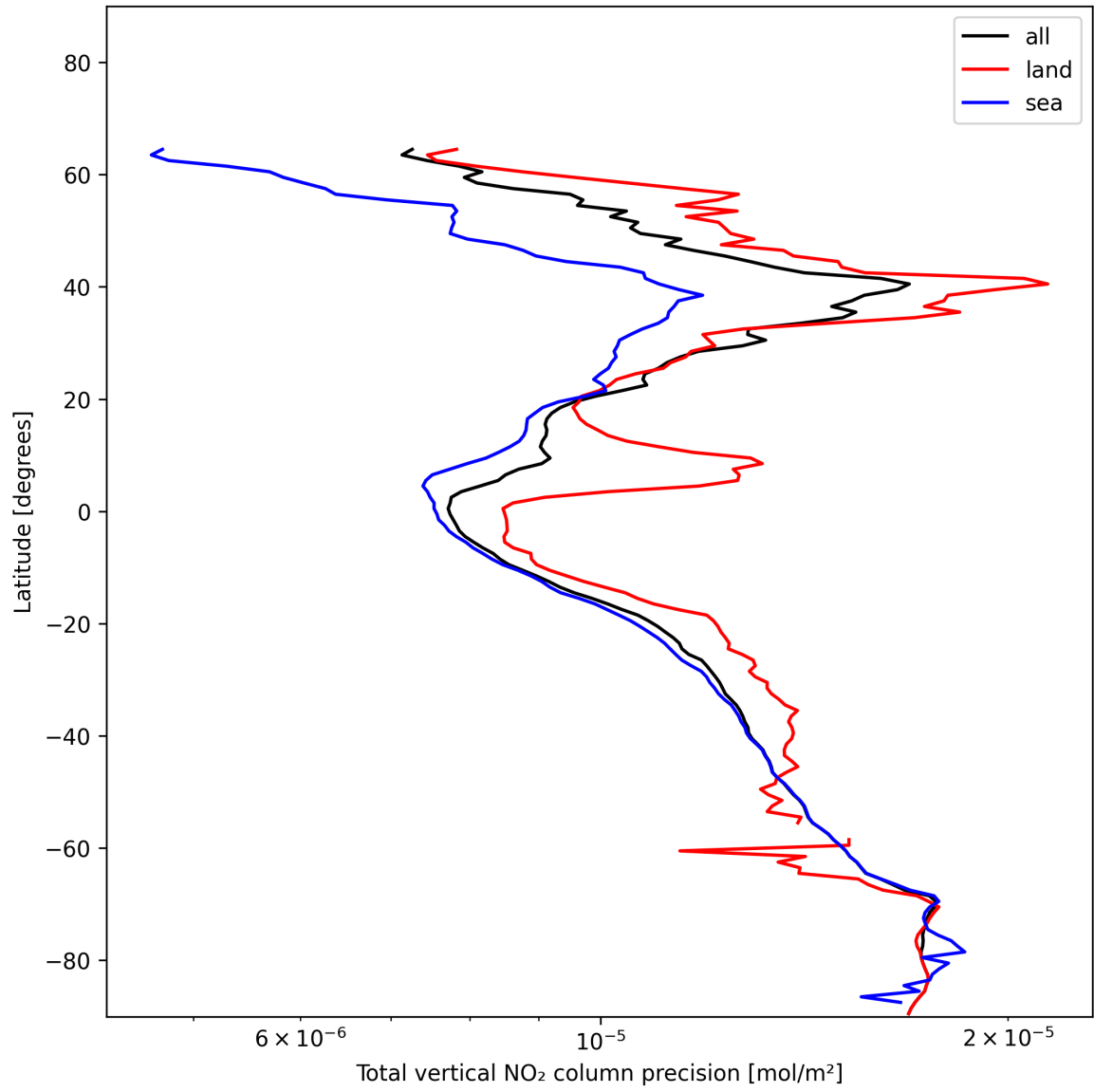
Figure 22: Zonal average of “Total vertical NO 2 column precision” for 2024-12-23 to 2024-12-25.
