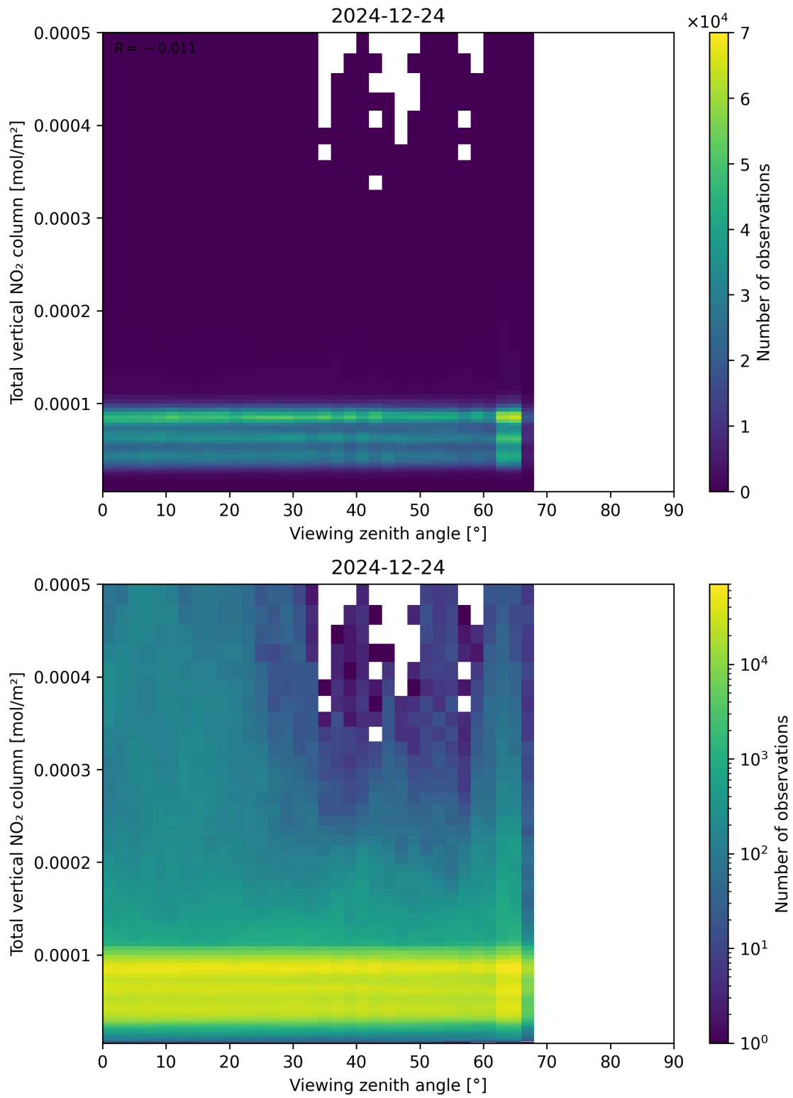
Figure 167: Scatter density plot of “Viewing zenith angle” against “Total vertical NO 2 column” for 2024-12-23 to 2024-12-25.
