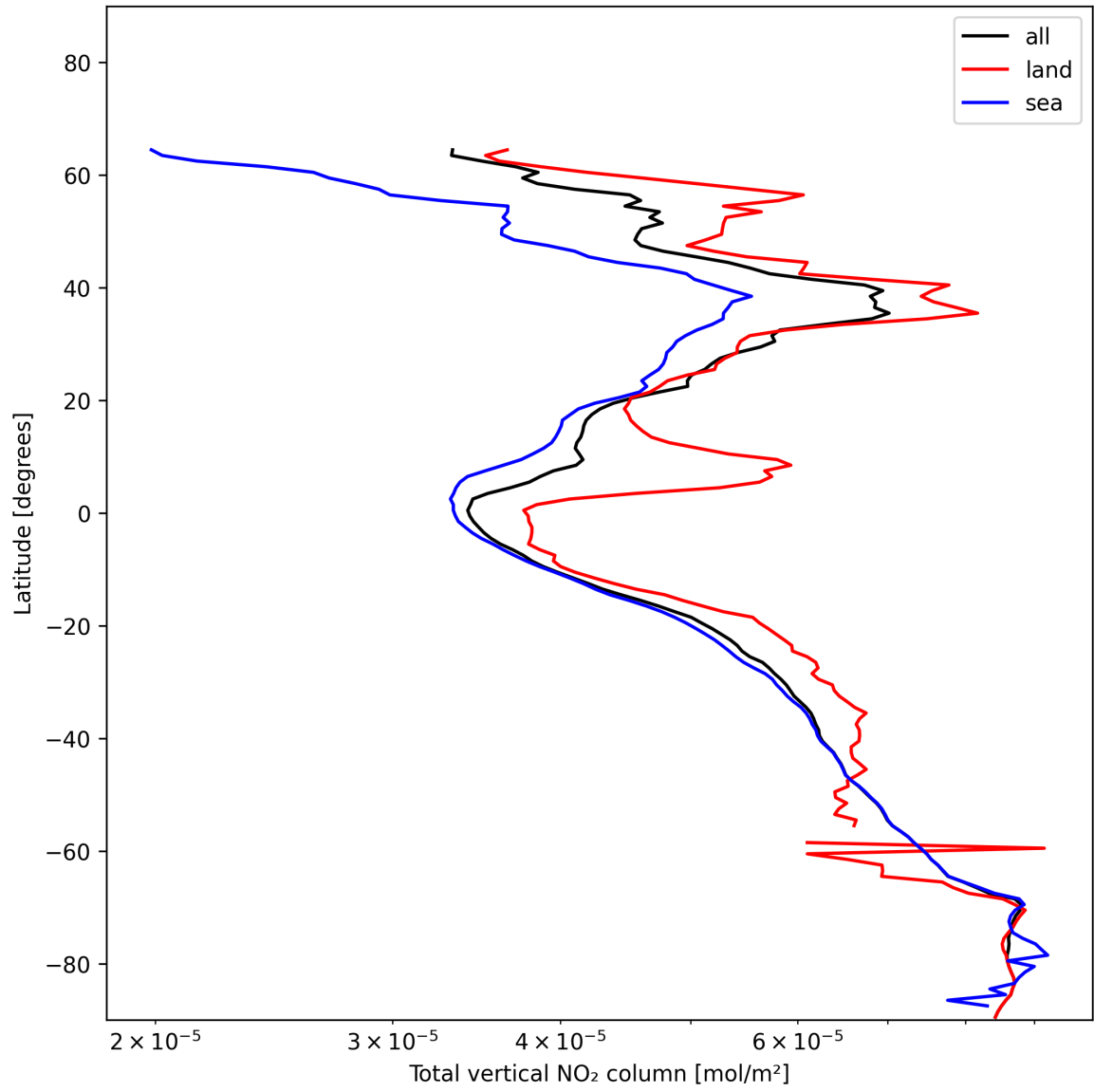
Figure 21: Zonal average of “Total vertical NO 2 column” for 2024-12-23 to 2024-12-25.
