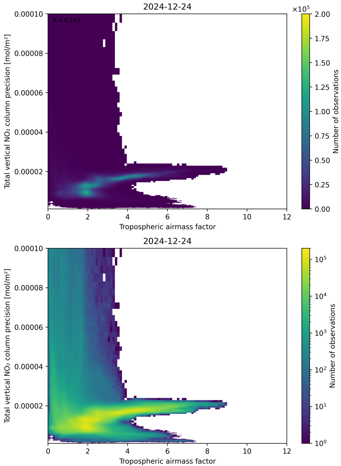
Figure 78: Scatter density plot of “Tropospheric air mass factor” against “Total vertical NO 2 column precision” for 2024-12-23 to 2024-12-25.
