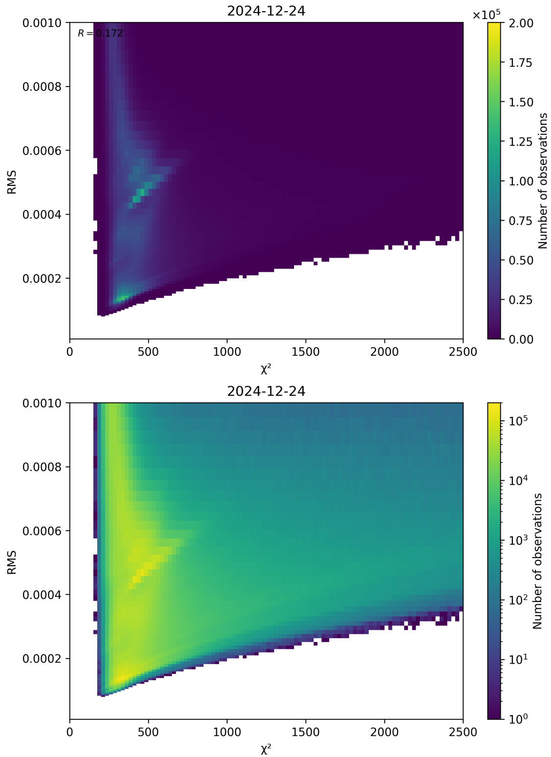
Figure 82: Scatter density plot of “ \chi^2 ” against “RMS” for 2024-12-23 to 2024-12-25.
