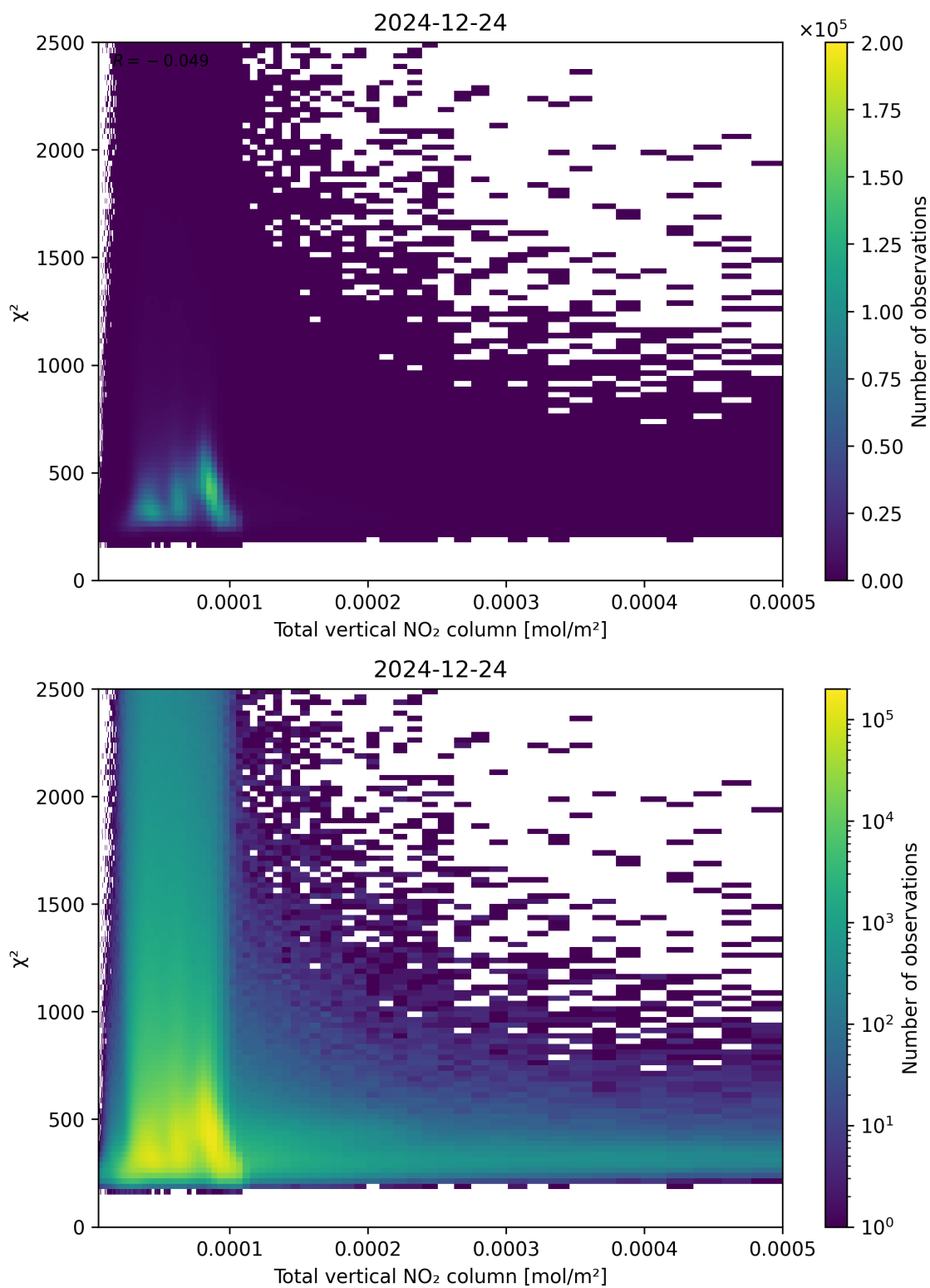
Figure 111: Scatter density plot of “Total vertical NO 2 column” against “ \chi^2 ” for 2024-12-23 to 2024-12-25.
