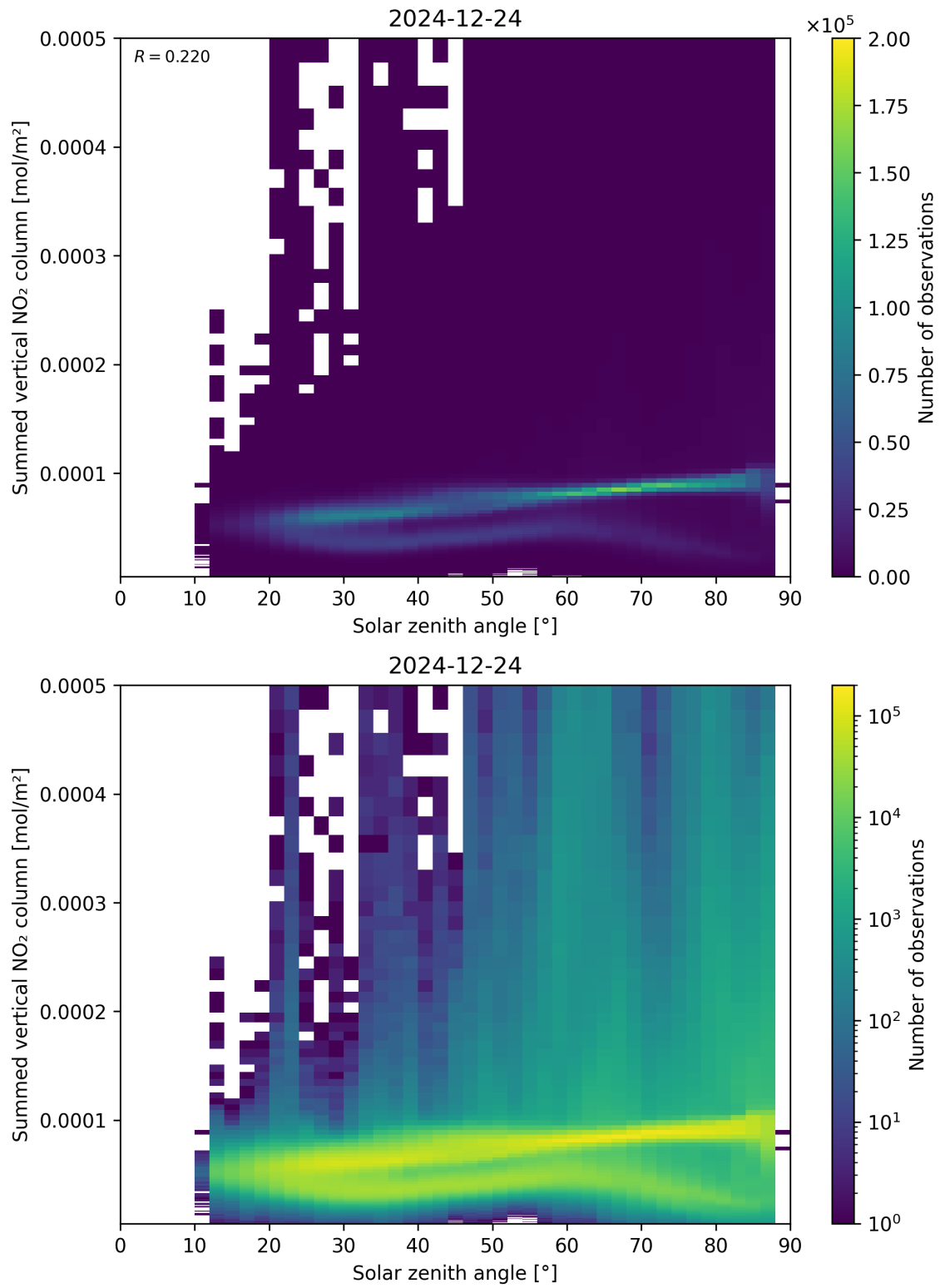
Figure 151: Scatter density plot of “Solar zenith angle” against “Summed vertical NO 2 column” for 2024-12-23 to 2024-12-25.
