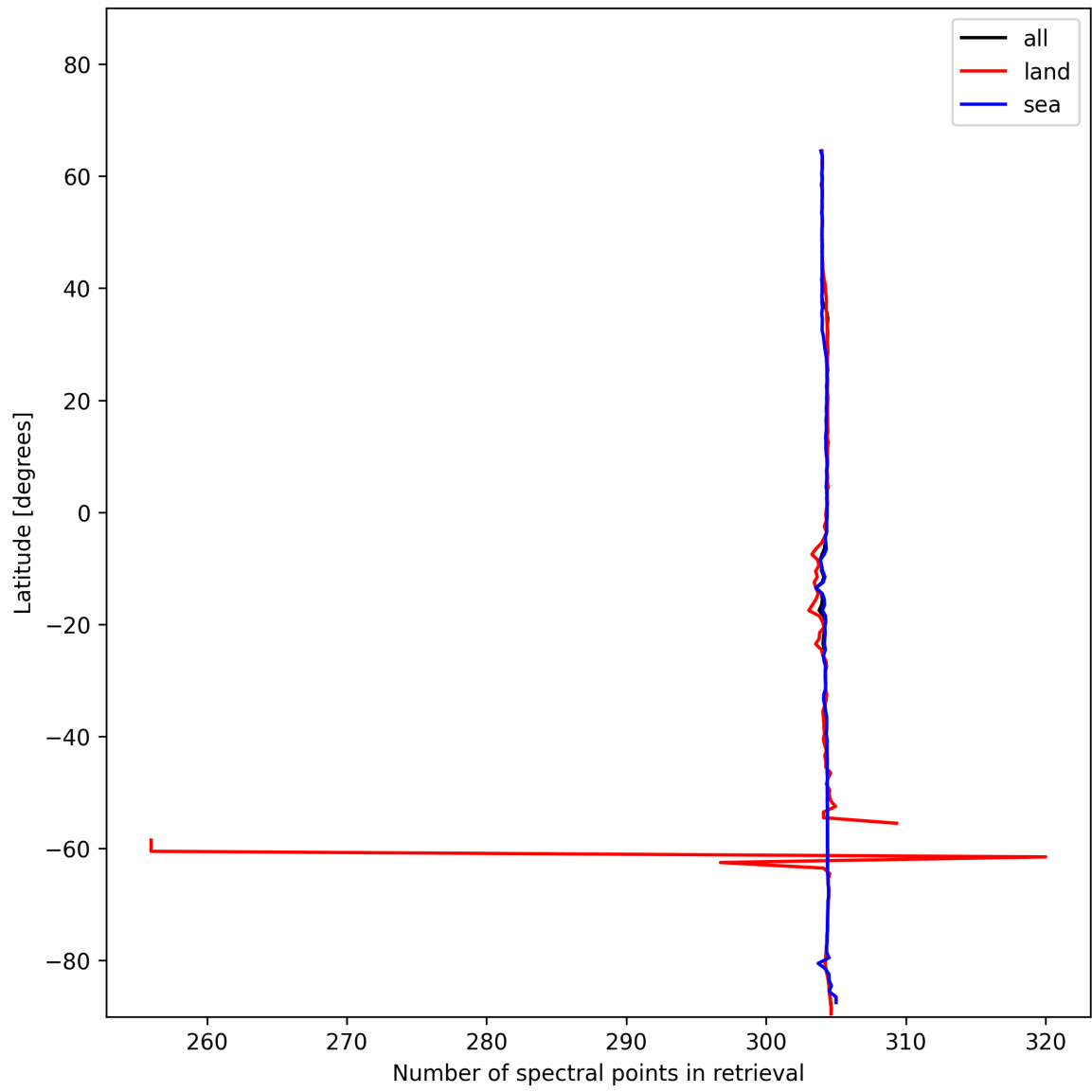
Figure 16: Zonal average of “Number of spectral points in retrieval” for 2024-12-23 to 2024-12-25.
