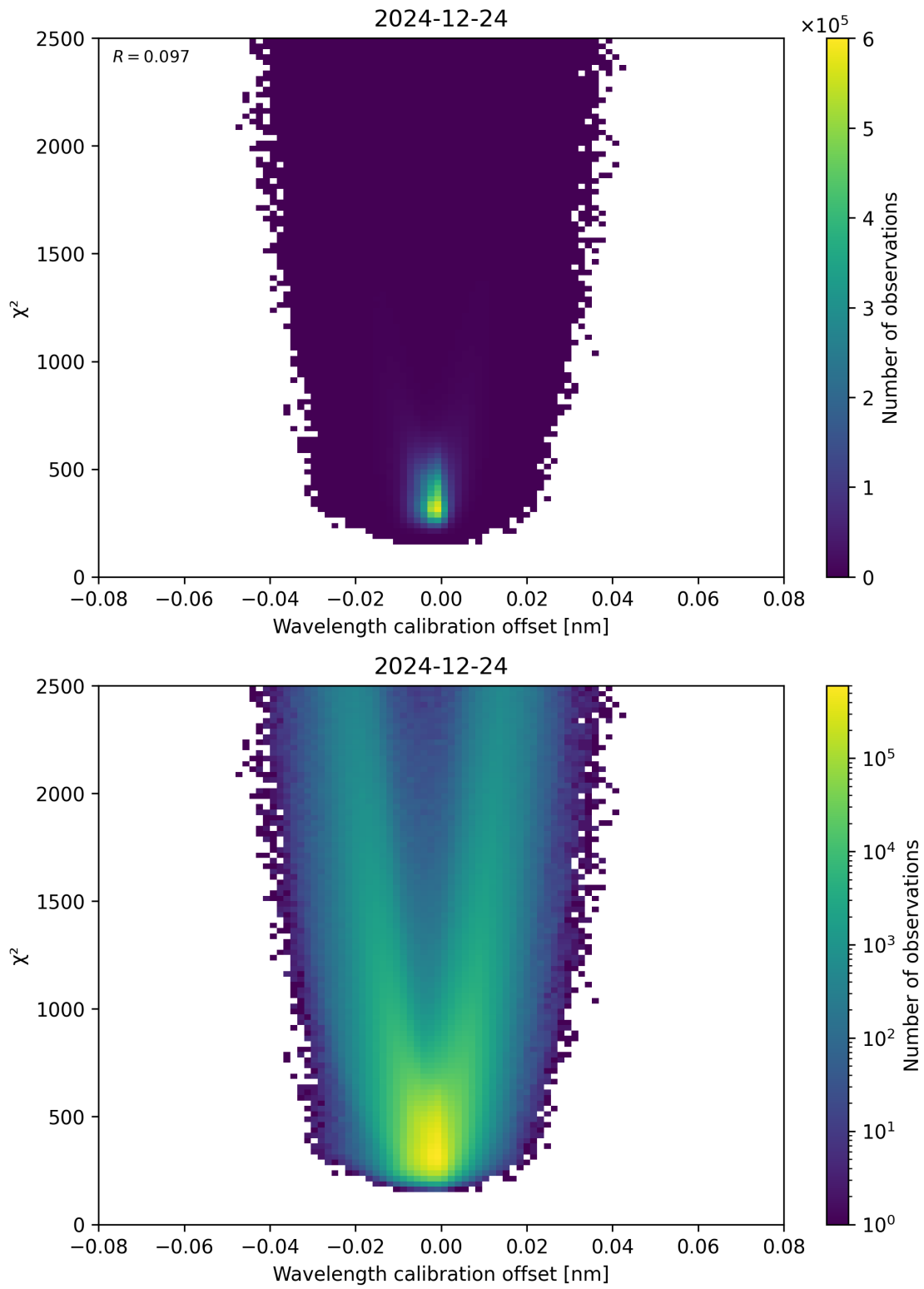
Figure 175: Scatter density plot of “Wavelength calibration offset” against “ \chi^2 ” for 2024-12-23 to 2024-12-25.
