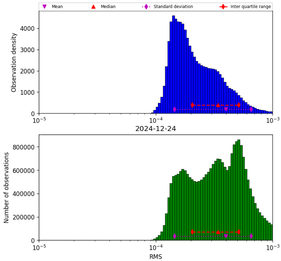
Figure 43: Histogram of “RMS” for 2024-12-23 to 2024-12-25
