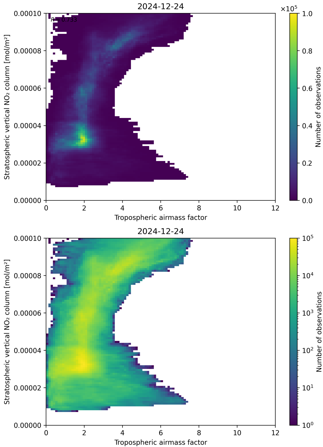
Figure 74: Scatter density plot of “Tropospheric air mass factor” against “Stratospheric vertical NO 2 column” for 2024-12-23 to 2024-12-25.
