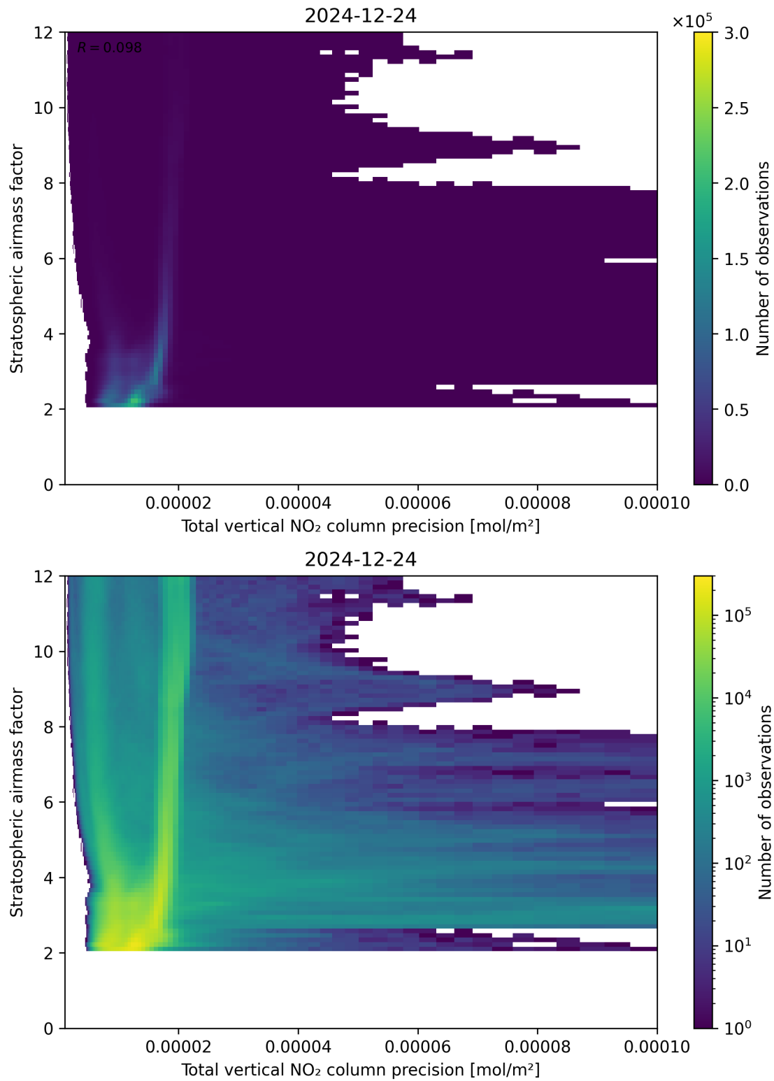
Figure 115: Scatter density plot of “Total vertical NO 2 column precision” against “Stratospheric air mass factor” for 2024-12-23 to 2024-12-25.
