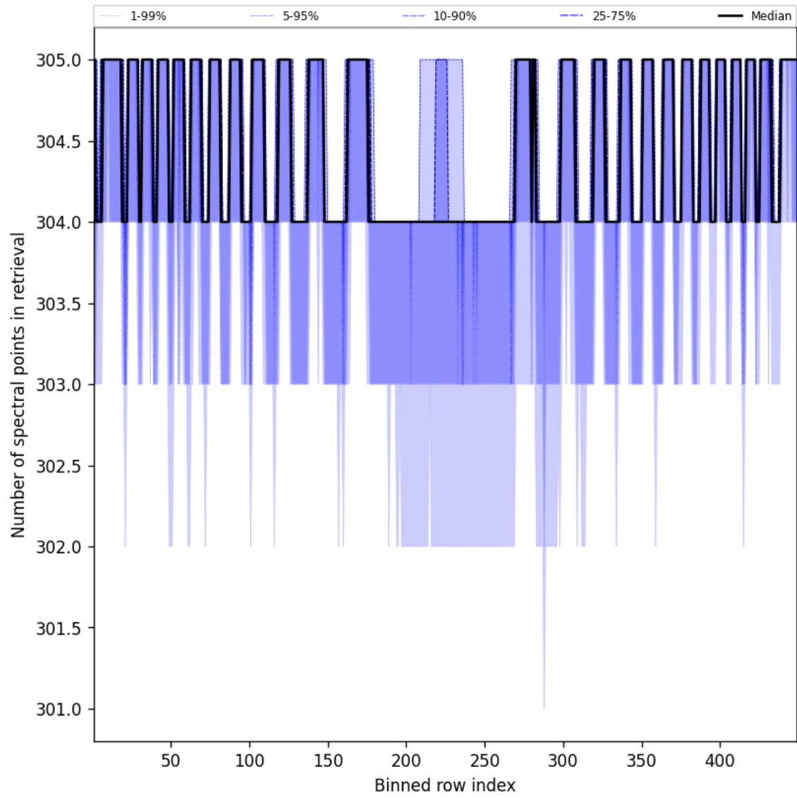
Figure 50: Along track statistics of “Number of spectral points in retrieval” for 2024-12-23 to 2024-12-25
