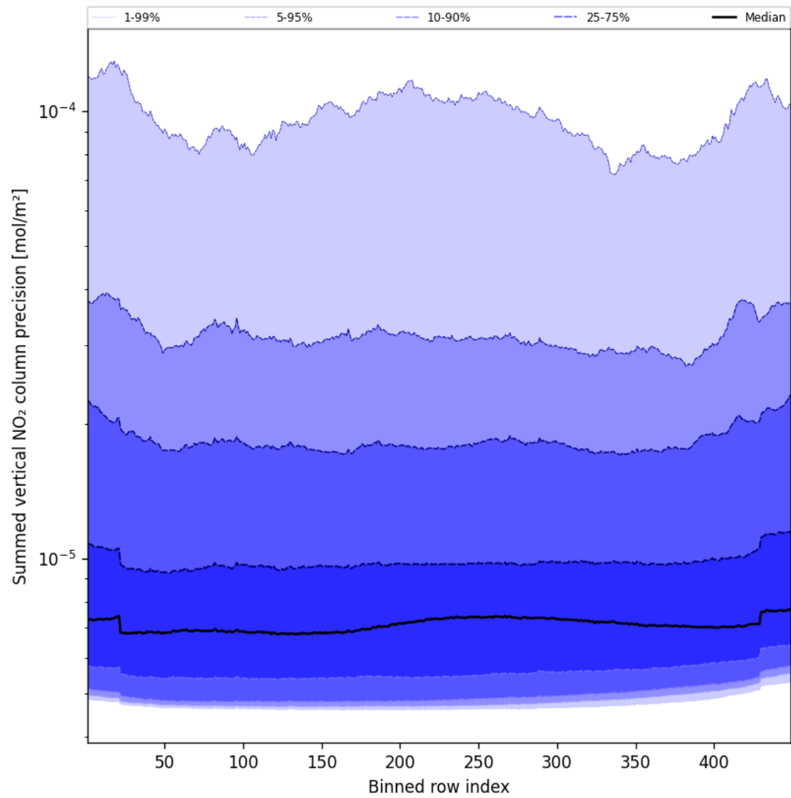
Figure 58: Along track statistics of “Summed vertical NO 2 column precision” for 2024-12-23 to 2024-12-25
