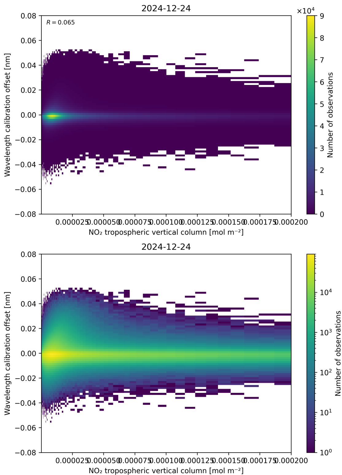
Figure 143: Scatter density plot of “NO 2 tropospheric vertical column” against “Wavelength calibration offset” for 2024-12-23 to 2024-12-25.
