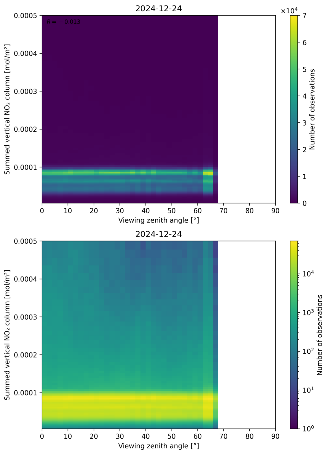
Figure 165: Scatter density plot of “Viewing zenith angle” against “Summed vertical NO 2 column” for 2024-12-23 to 2024-12-25.
