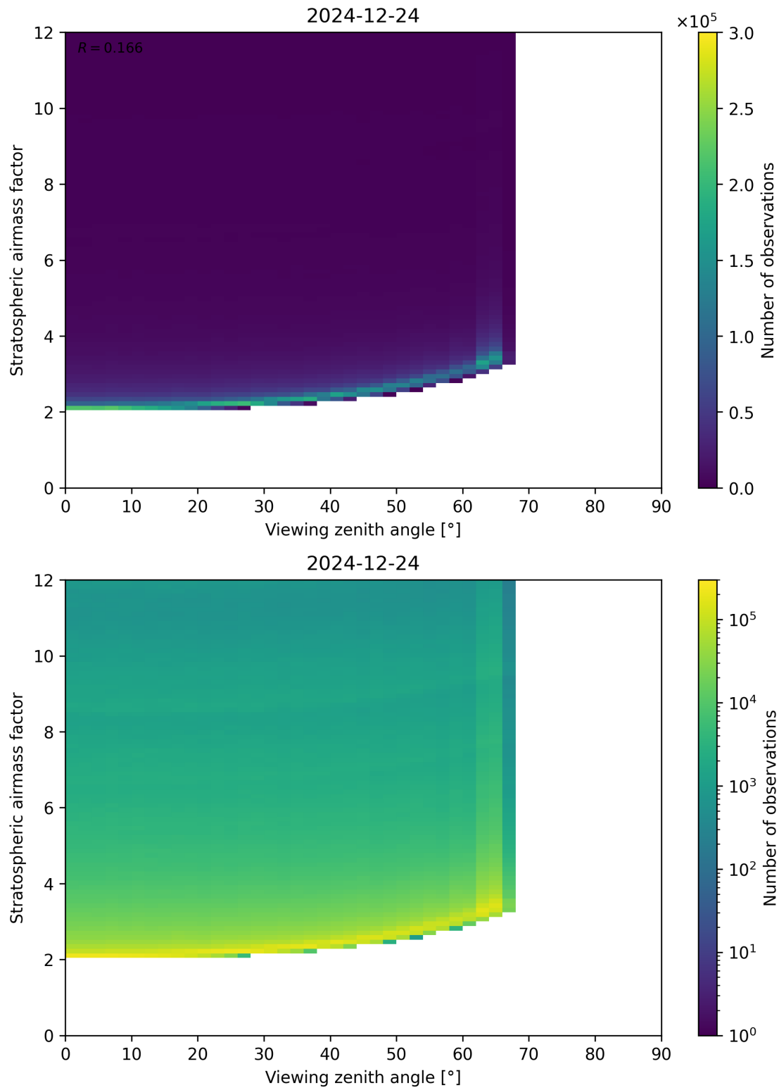
Figure 159: Scatter density plot of “Viewing zenith angle” against “Stratospheric airmass factor” for 2024-12-23 to 2024-12-25.
