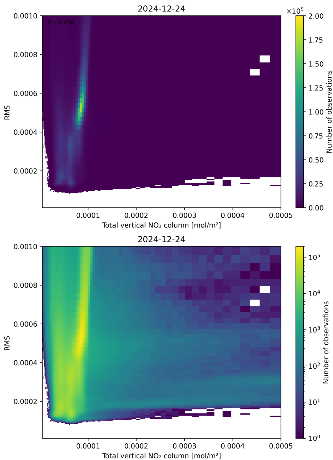
Figure 120: Scatter density plot of “Total vertical NO 2 column” against “RMS” for 2024-12-23 to 2024-12-25.
