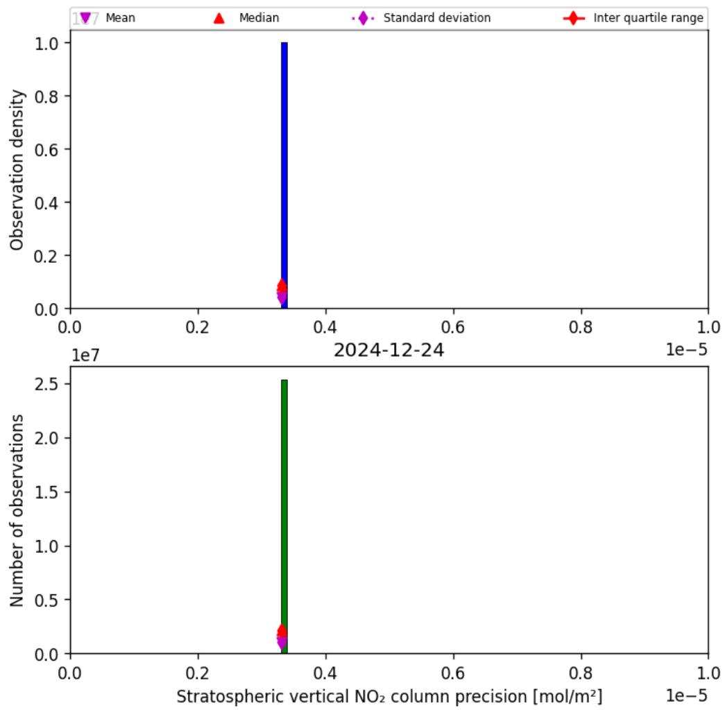
Figure 37: Histogram of “Stratospheric vertical NO 2 column precision” for 2024-12-23 to 2024-12-25
