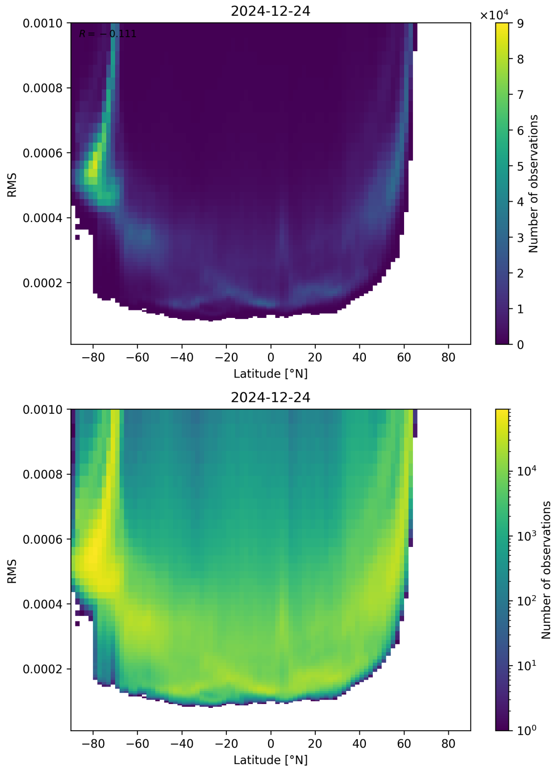
Figure 94: Scatter density plot of “Latitude” against “RMS” for 2024-12-23 to 2024-12-25.
