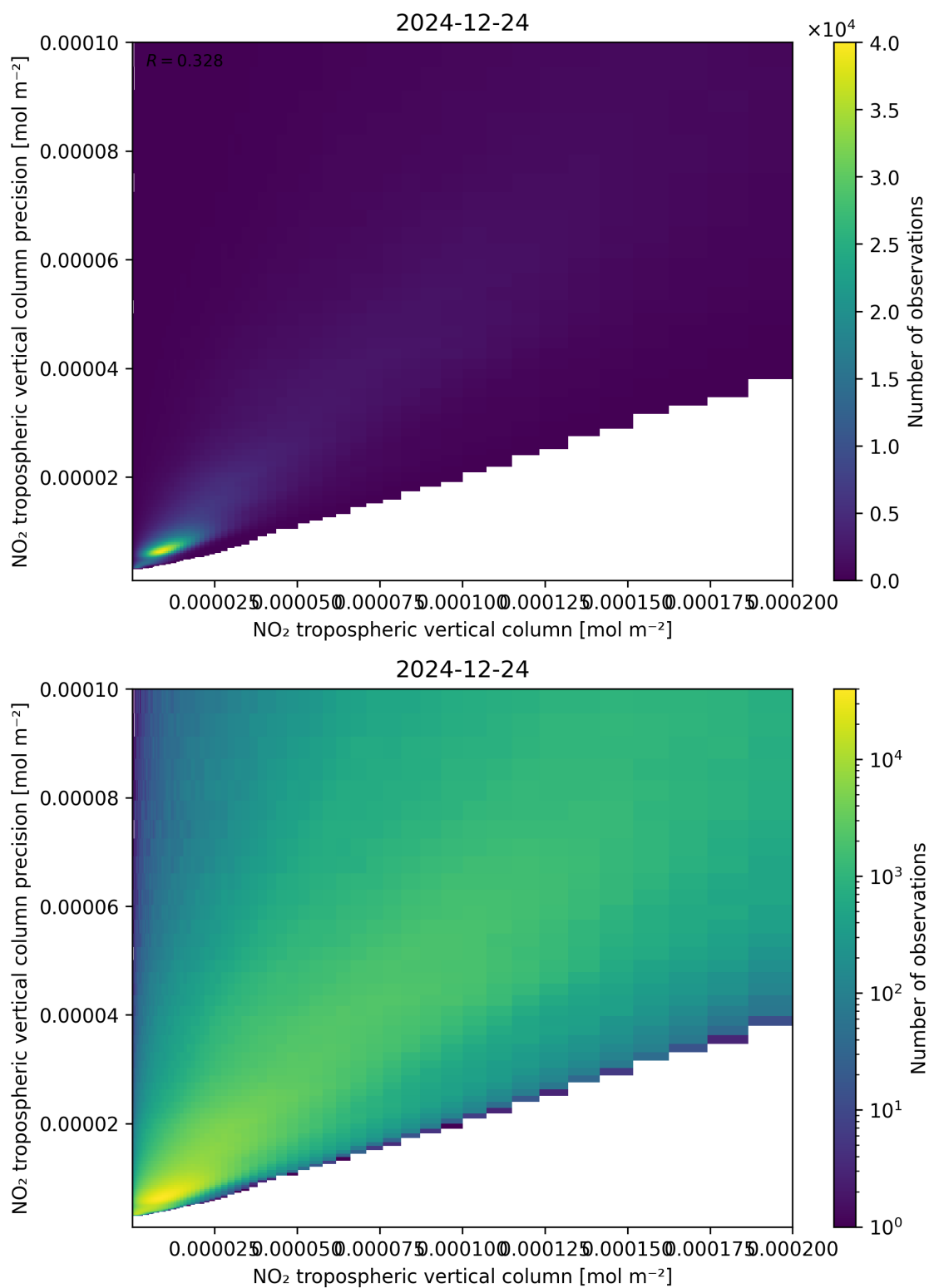
Figure 130: Scatter density plot of “NO 2 tropospheric vertical column” against “NO 2 tropospheric vertical column precision” for 2024-12-23 to 2024-12-25.
