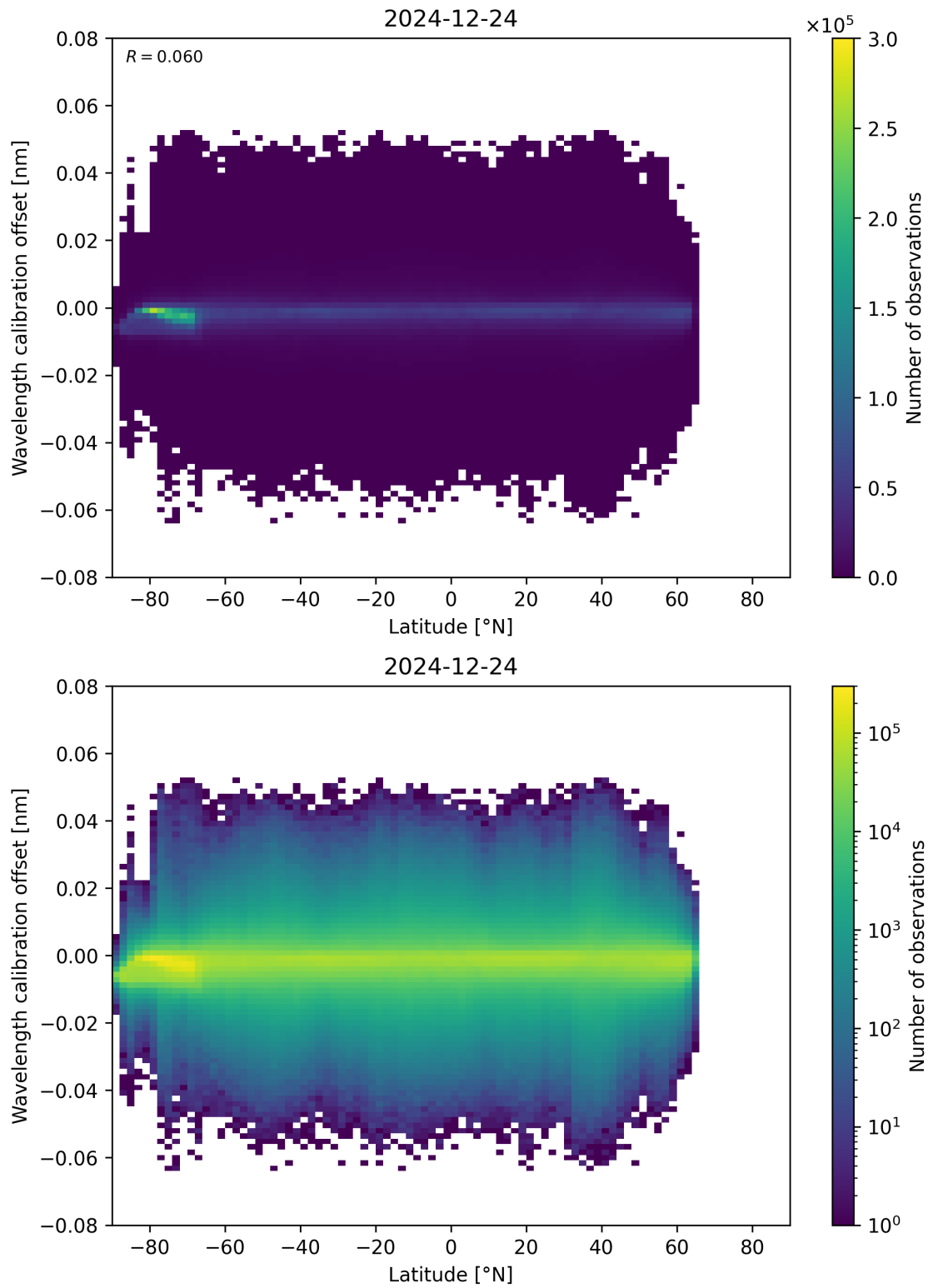
Figure 95: Scatter density plot of “Latitude” against “Wavelength calibration offset” for 2024-12-23 to 2024-12-25.
