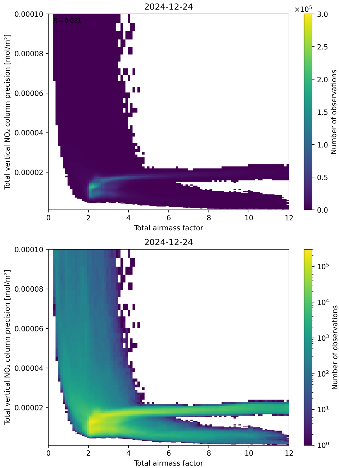
Figure 68: Scatter density plot of “Total airmass factor” against “Total vertical NO 2 column precision” for 2024-12-23 to 2024-12-25.
