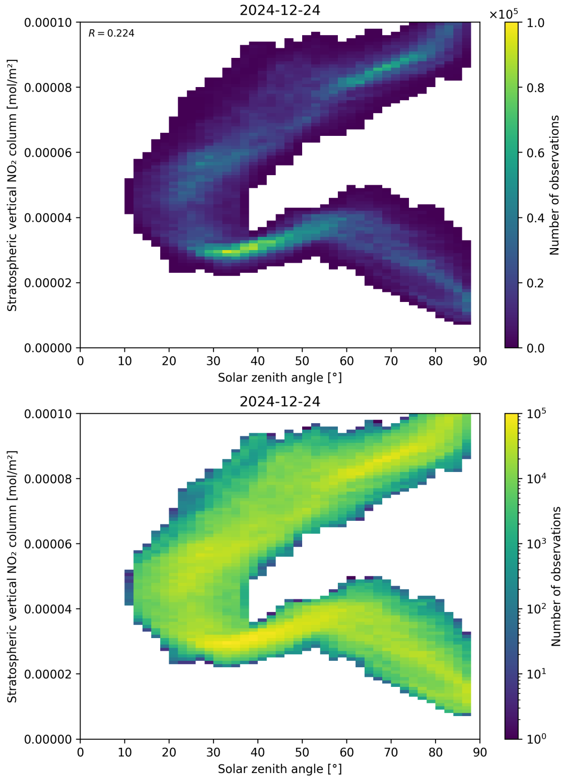
Figure 150: Scatter density plot of “Solar zenith angle” against “Stratospheric vertical NO 2 column” for 2024-12-23 to 2024-12-25.
