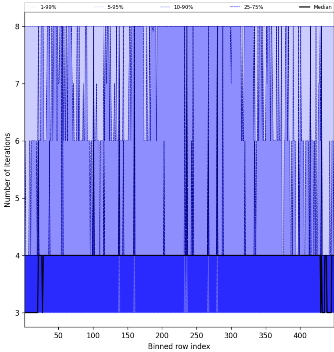
Figure 51: Along track statistics of “Number of iterations” for 2024-12-23 to 2024-12-25
