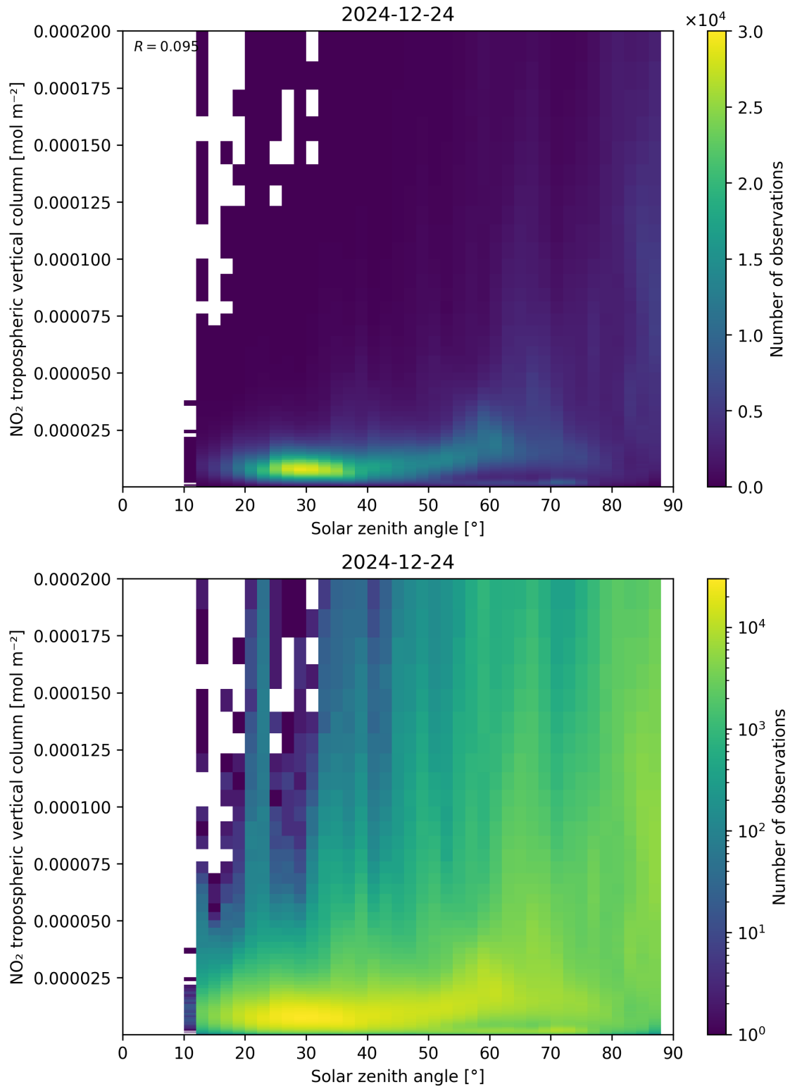
Figure 155: Scatter density plot of “Solar zenith angle” against “NO 2 tropospheric vertical column” for 2024-12-23 to 2024-12-25.
