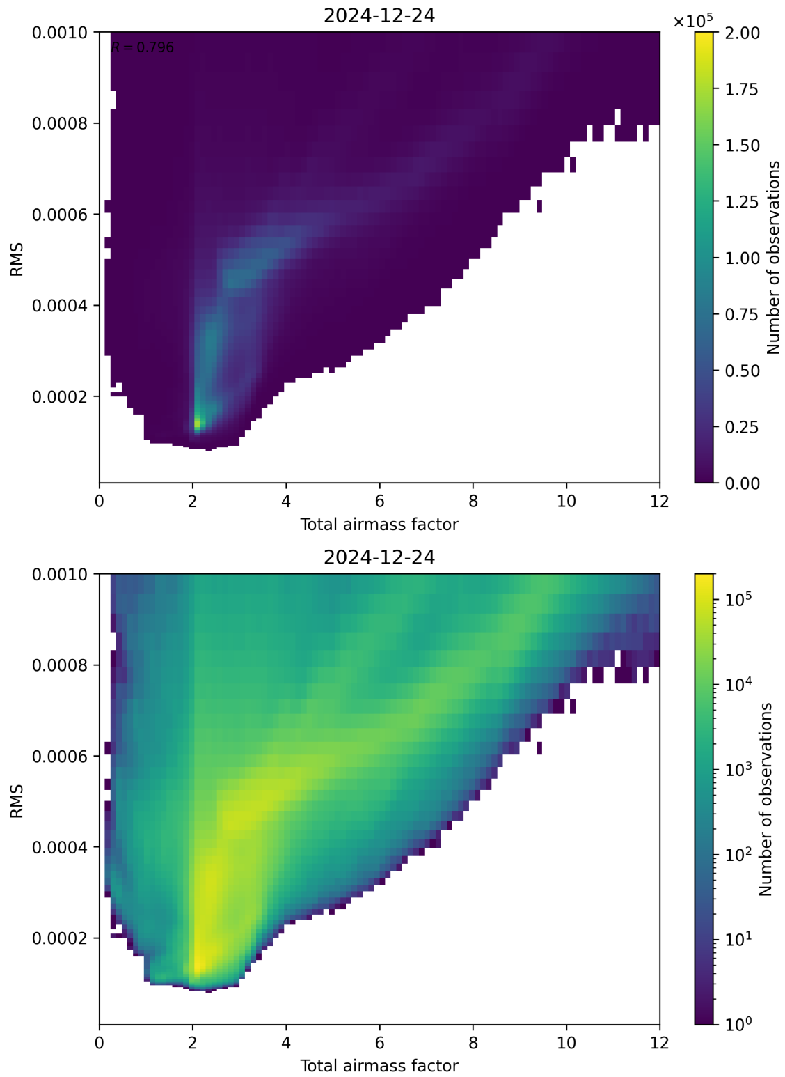
Figure 69: Scatter density plot of “Total airmass factor” against “RMS” for 2024-12-23 to 2024-12-25.
