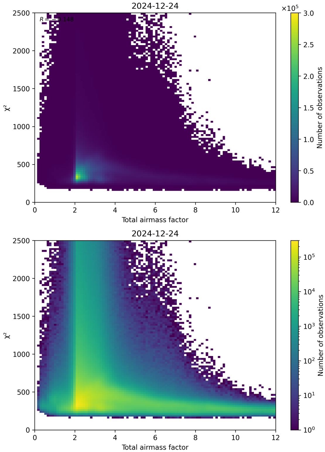
Figure 63: Scatter density plot of “Total airmass factor” against “ \chi^2 ” for 2024-12-23 to 2024-12-25.
