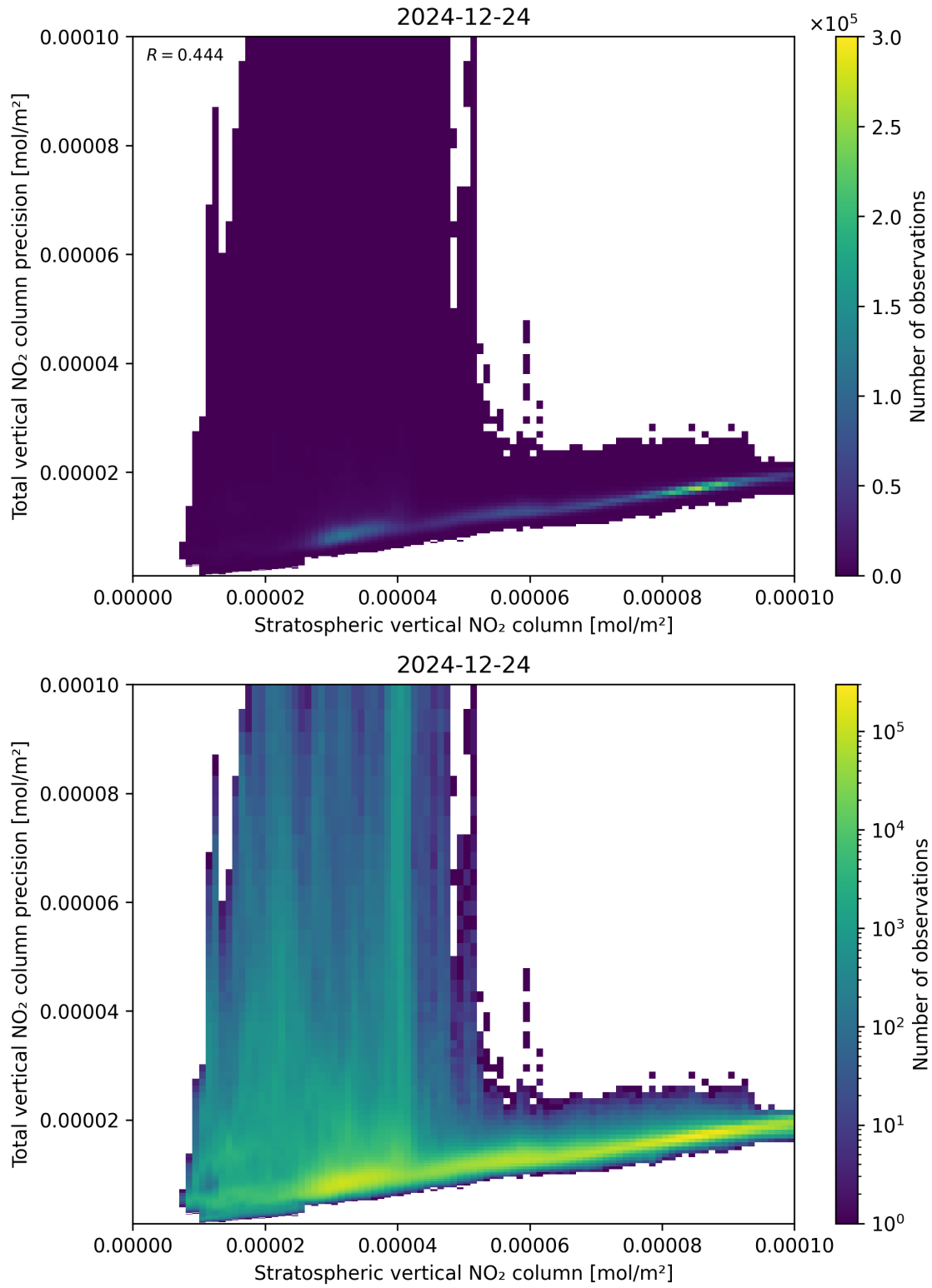
Figure 101: Scatter density plot of “Stratospheric vertical NO 2 column” against “Total vertical NO 2 column precision” for 2024-12-23 to 2024-12-25.
