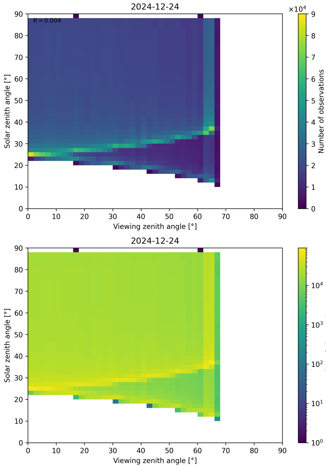
Figure 172: Scatter density plot of “Viewing zenith angle” against “Solar zenith angle” for 2024-12-23 to 2024-12-25.
