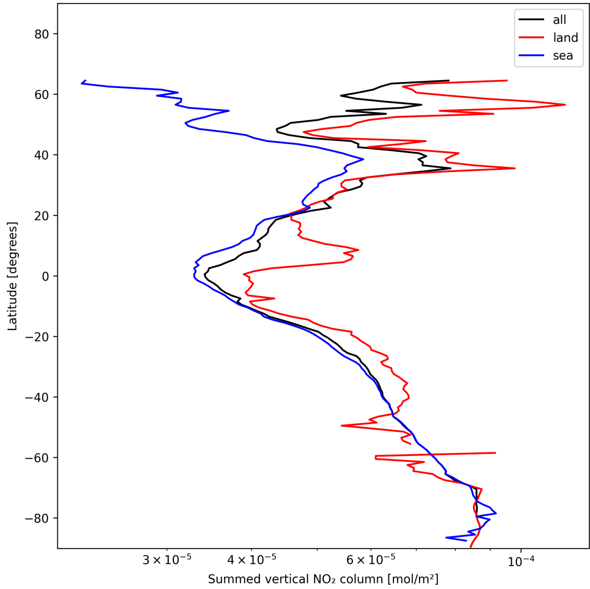
Figure 23: Zonal average of “Summed vertical NO 2 column” for 2024-12-23 to 2024-12-25.
