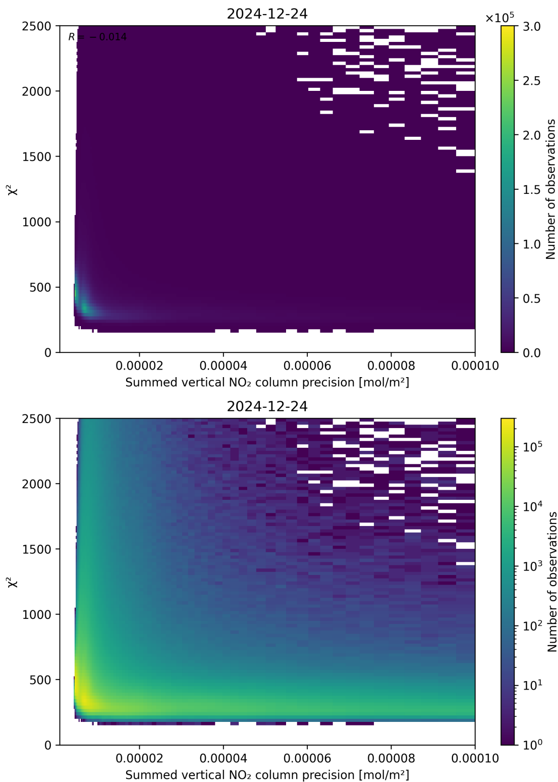
Figure 107: Scatter density plot of “Summed vertical NO 2 column precision” against “ \chi^2 ” for 2024-12-23 to 2024-12-25.
