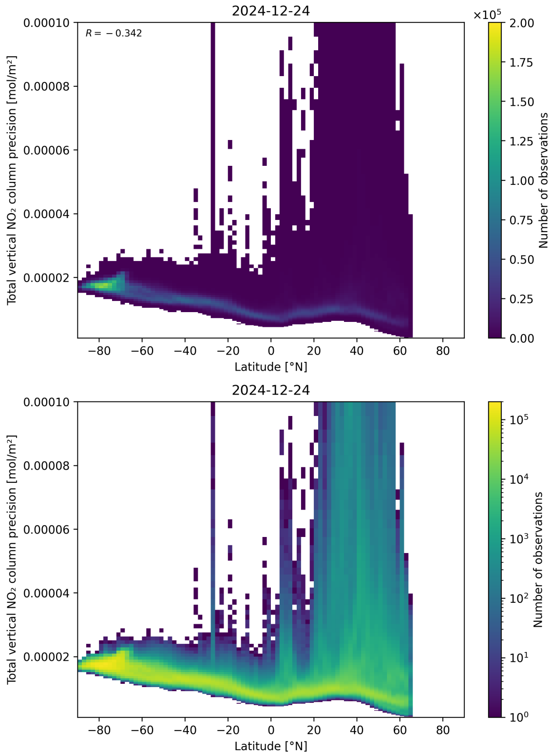
Figure 91: Scatter density plot of “Latitude” against “Total vertical NO 2 column precision” for 2024-12-23 to 2024-12-25.
