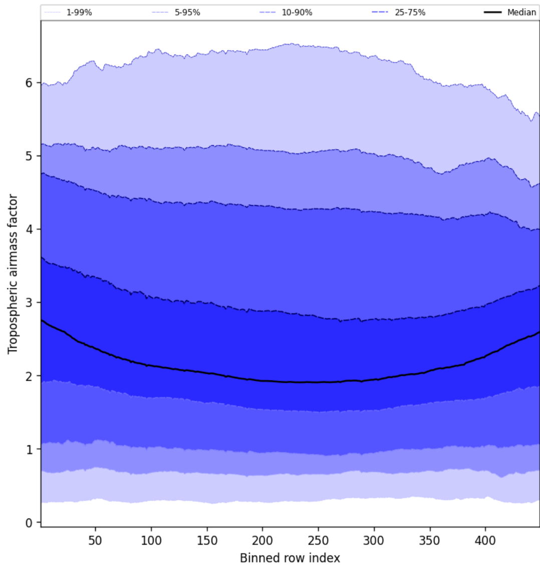
Figure 48: Along track statistics of “Tropospheric air mass factor” for 2024-12-23 to 2024-12-25
