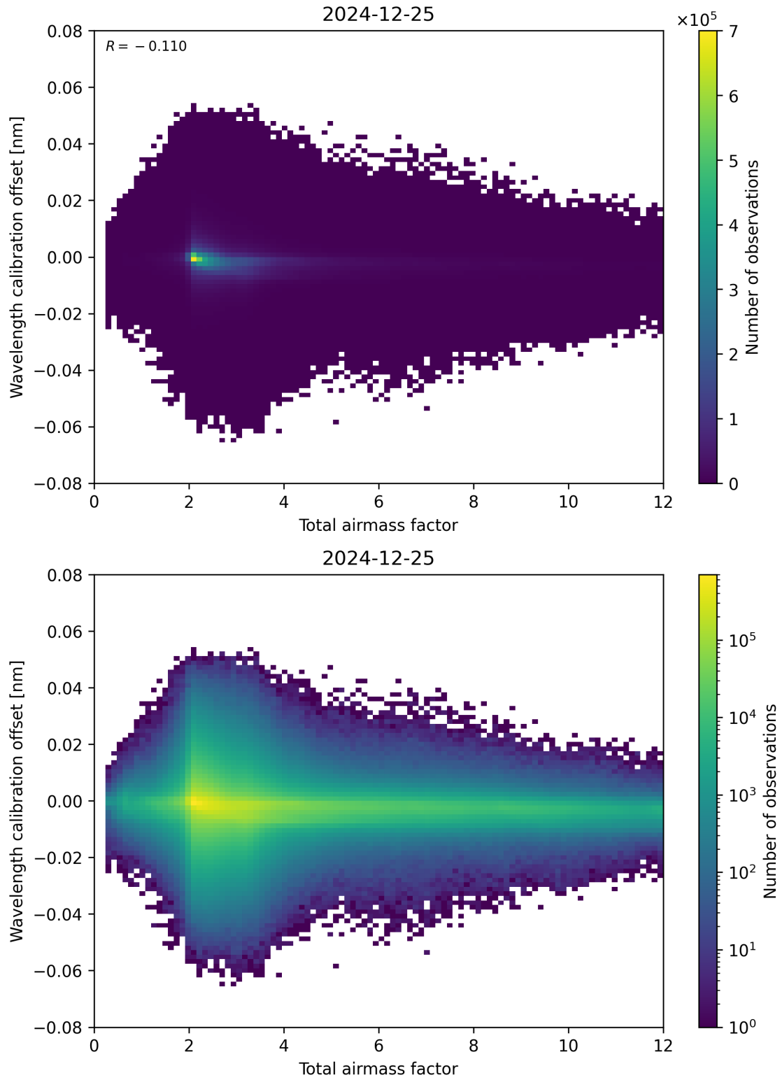
Figure 70: Scatter density plot of “Total airmass factor” against “Wavelength calibration offset” for 2024-12-24 to 2024-12-26.
