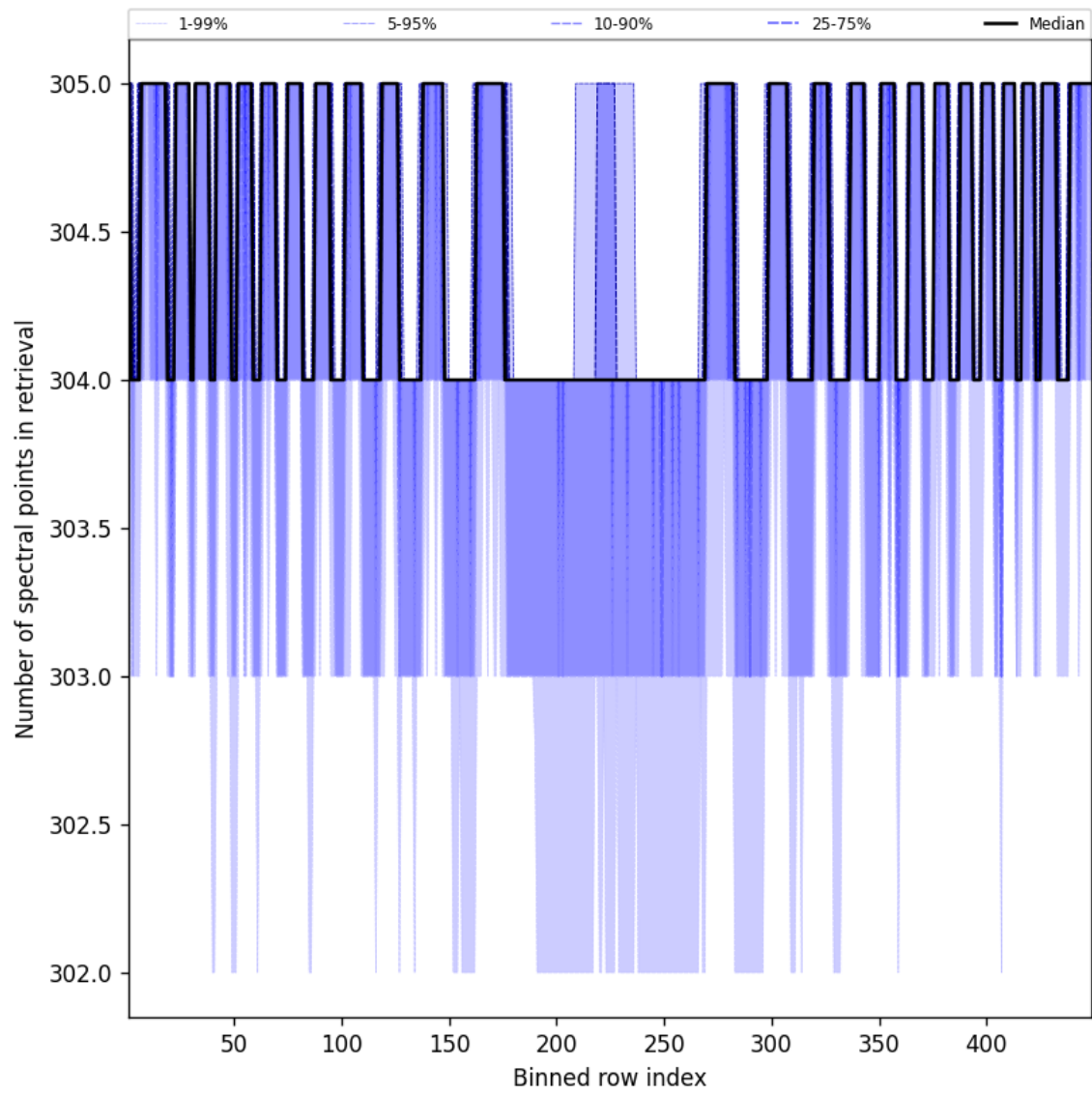
Figure 50: Along track statistics of “Number of spectral points in retrieval” for 2024-12-24 to 2024-12-26
