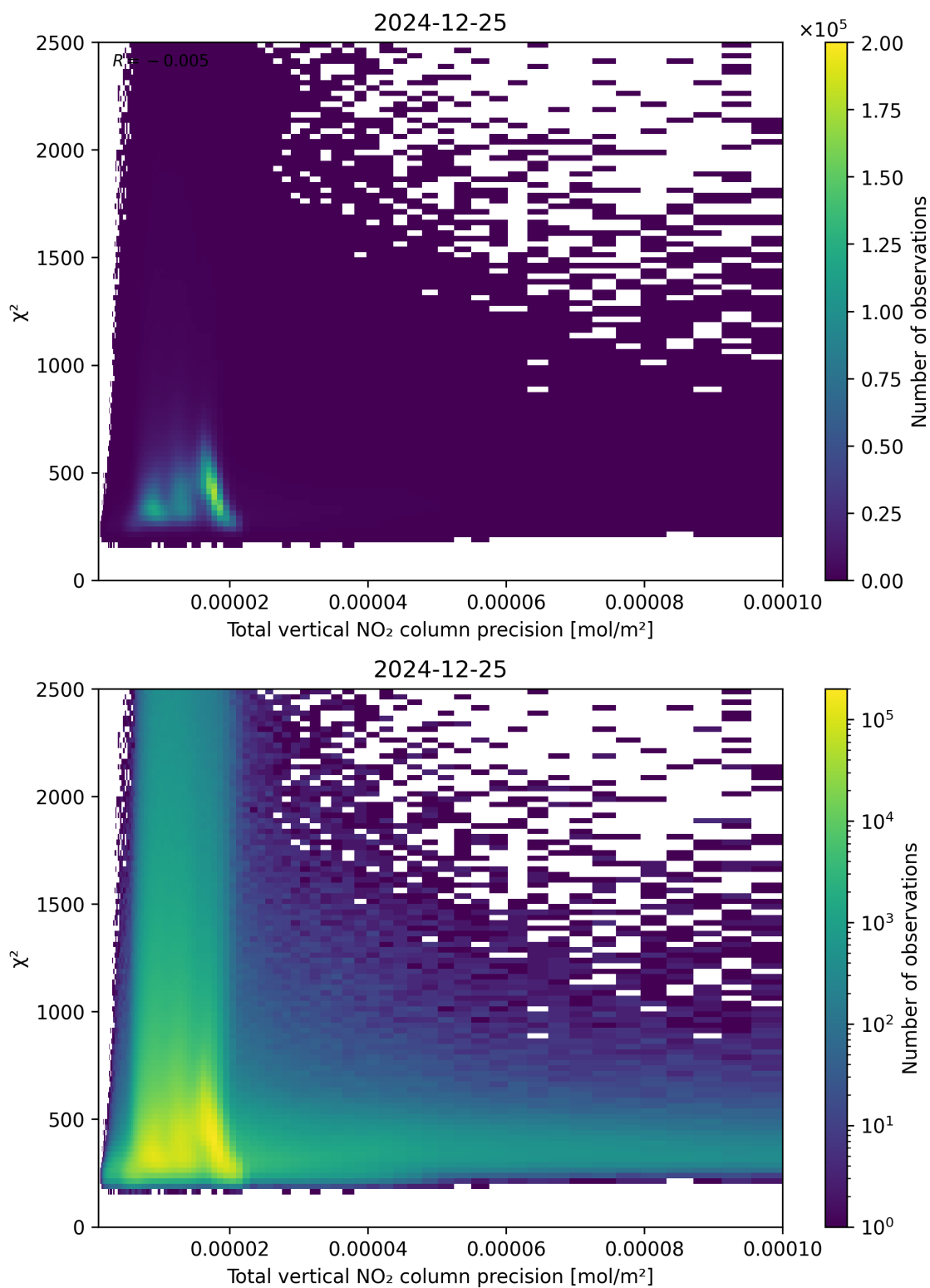
Figure 116: Scatter density plot of “Total vertical NO 2 column precision” against “ \chi^2 ” for 2024-12-24 to 2024-12-26.
