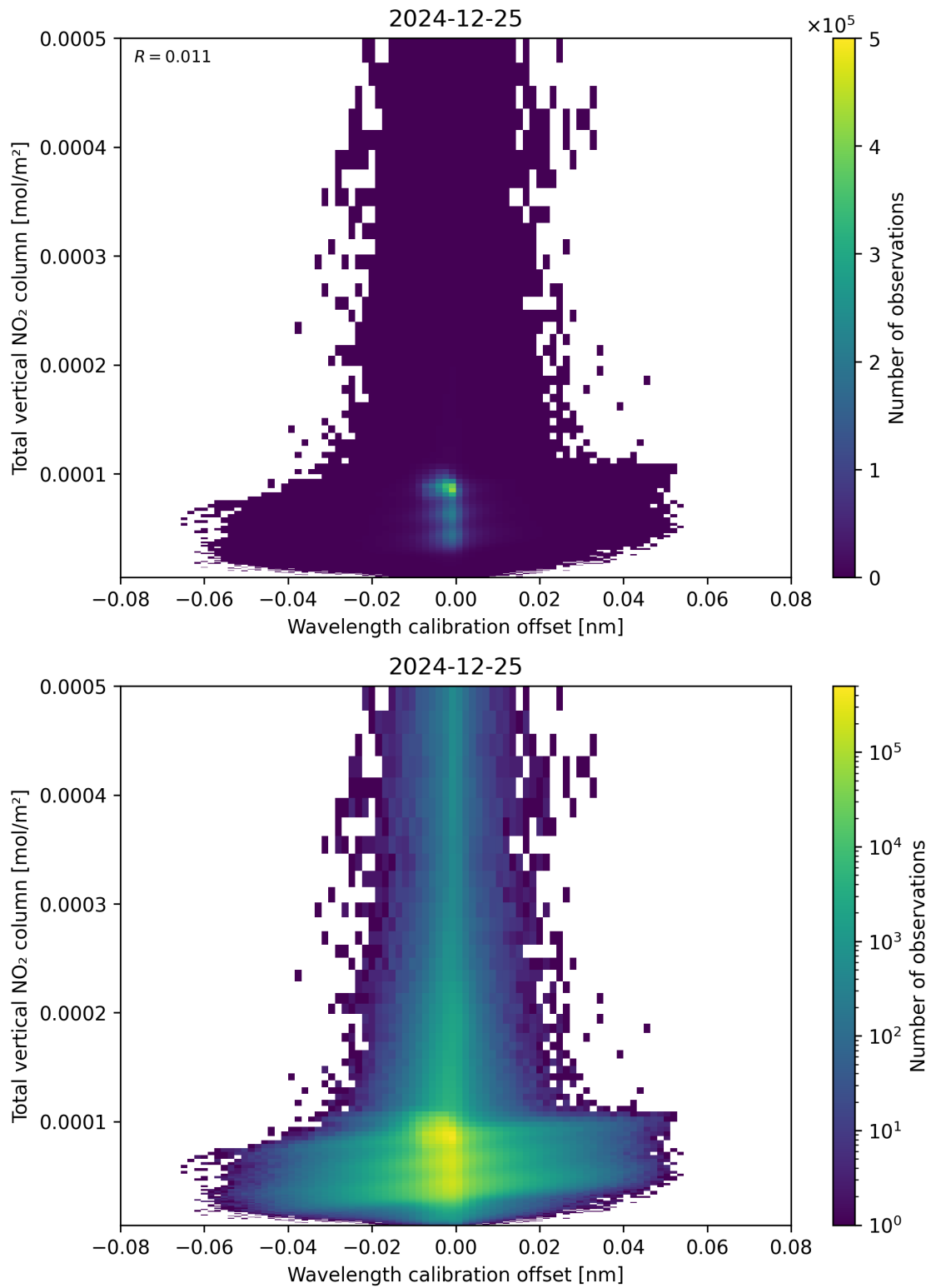
Figure 179: Scatter density plot of “Wavelength calibration offset” against “Total vertical NO 2 column” for 2024-12-24 to 2024-12-26.
