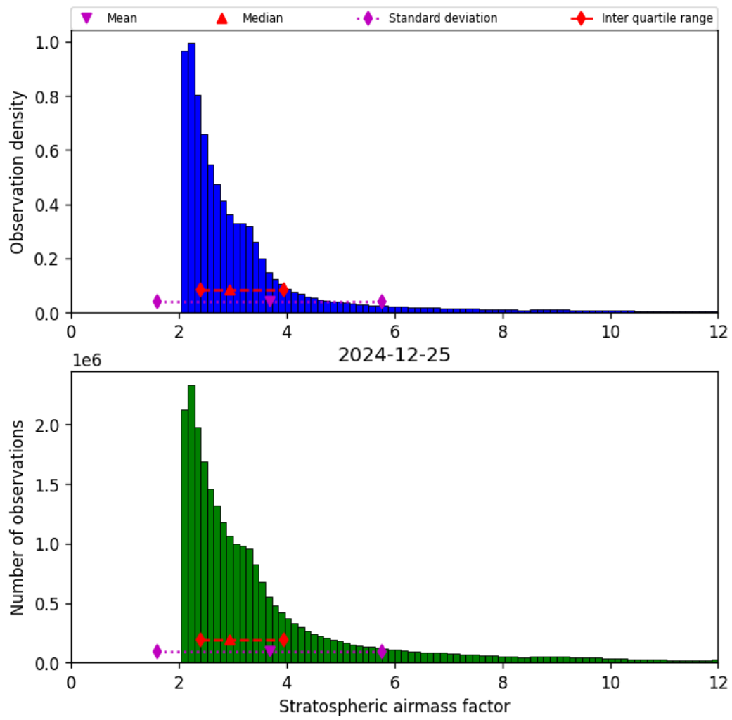
Figure 44: Histogram of “Stratospheric airmass factor” for 2024-12-24 to 2024-12-26
