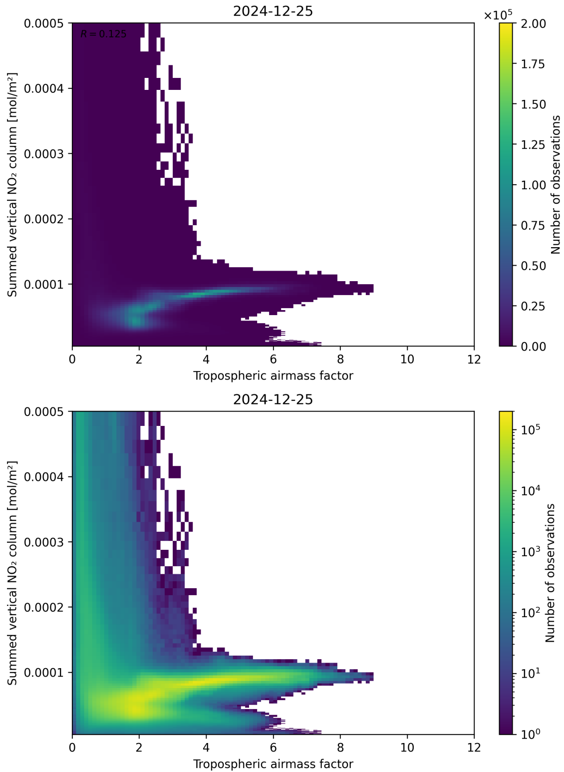
Figure 75: Scatter density plot of “Tropospheric air mass factor” against “Summed vertical NO 2 column” for 2024-12-24 to 2024-12-26.
