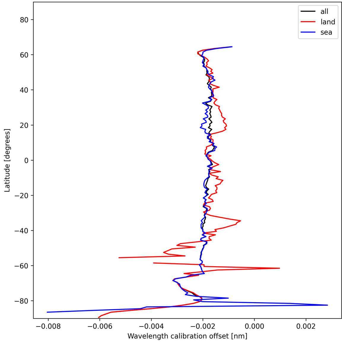
Figure 18: Zonal average of “Wavelength calibration offset” for 2024-12-24 to 2024-12-26.
