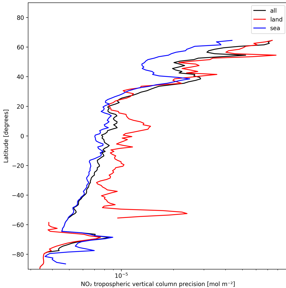
Figure 13: Zonal average of “NO 2 tropospheric vertical column precision” for 2024-12-24 to 2024-12-26.
