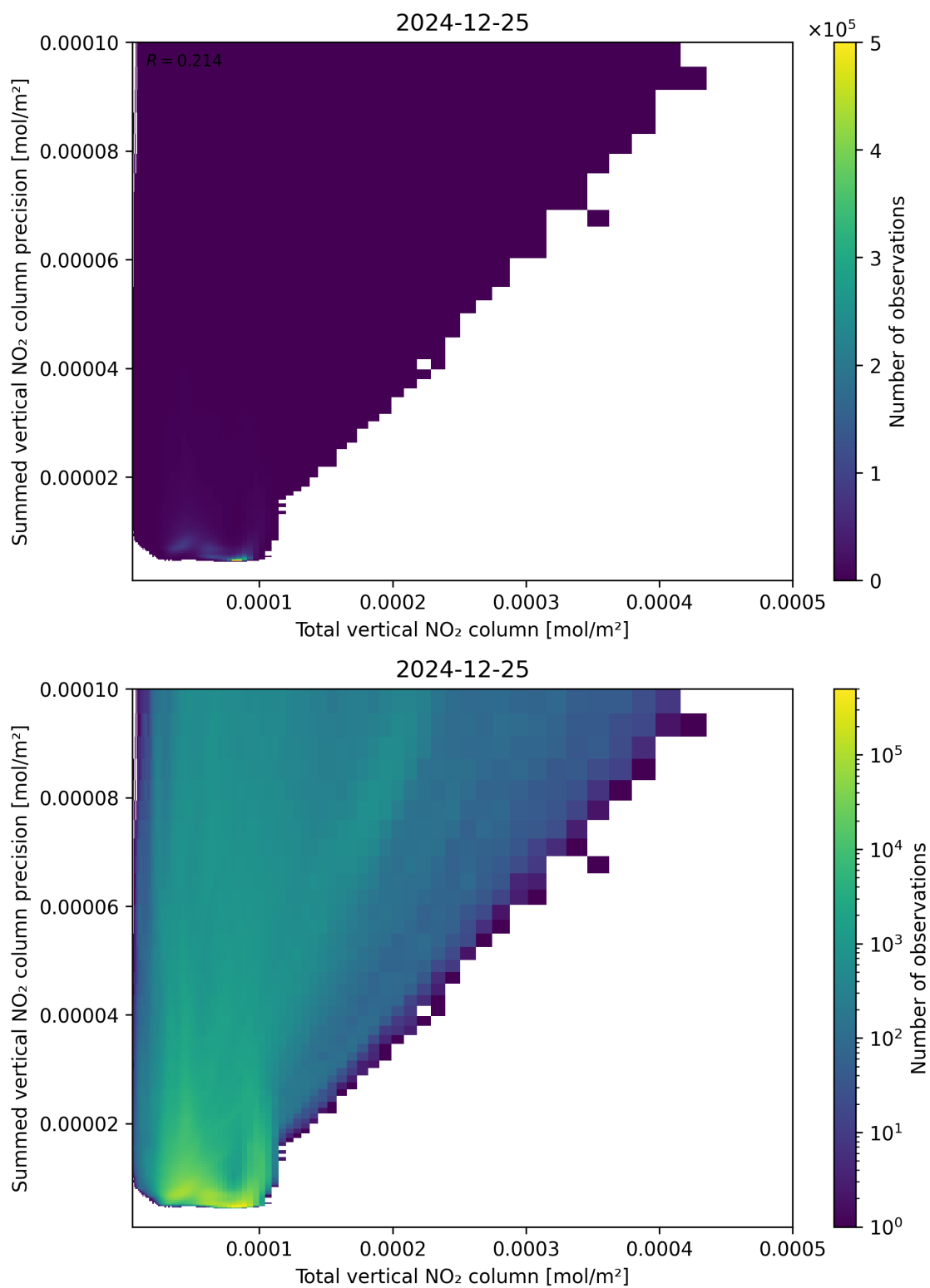
Figure 113: Scatter density plot of “Total vertical NO 2 column” against “Summed vertical NO 2 column precision” for 2024-12-24 to 2024-12-26.
