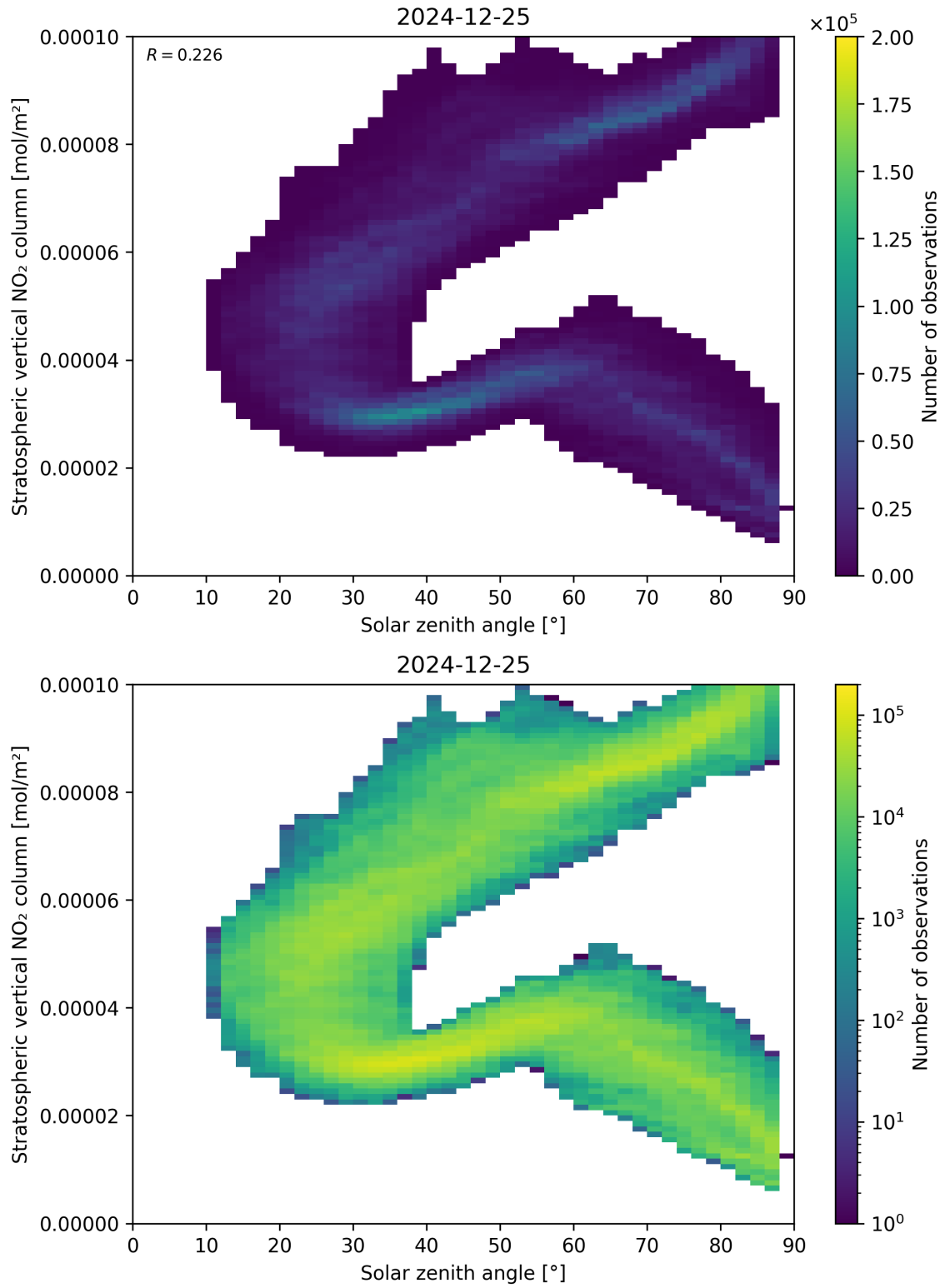
Figure 150: Scatter density plot of “Solar zenith angle” against “Stratospheric vertical NO 2 column” for 2024-12-24 to 2024-12-26.
