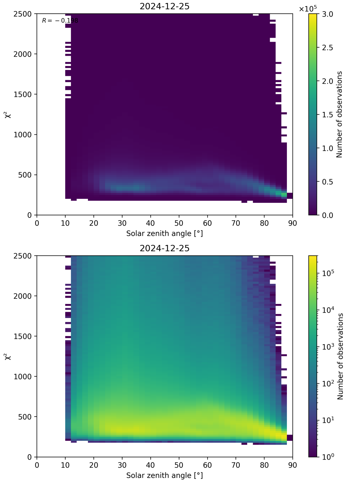
Figure 148: Scatter density plot of “Solar zenith angle” against “ \chi^2 ” for 2024-12-24 to 2024-12-26.
