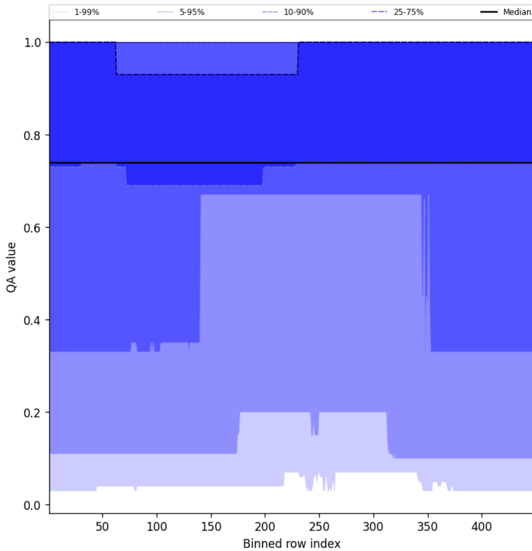
Figure 45: Along track statistics of "QA value" for 2024-12-24 to 2024-12-26
