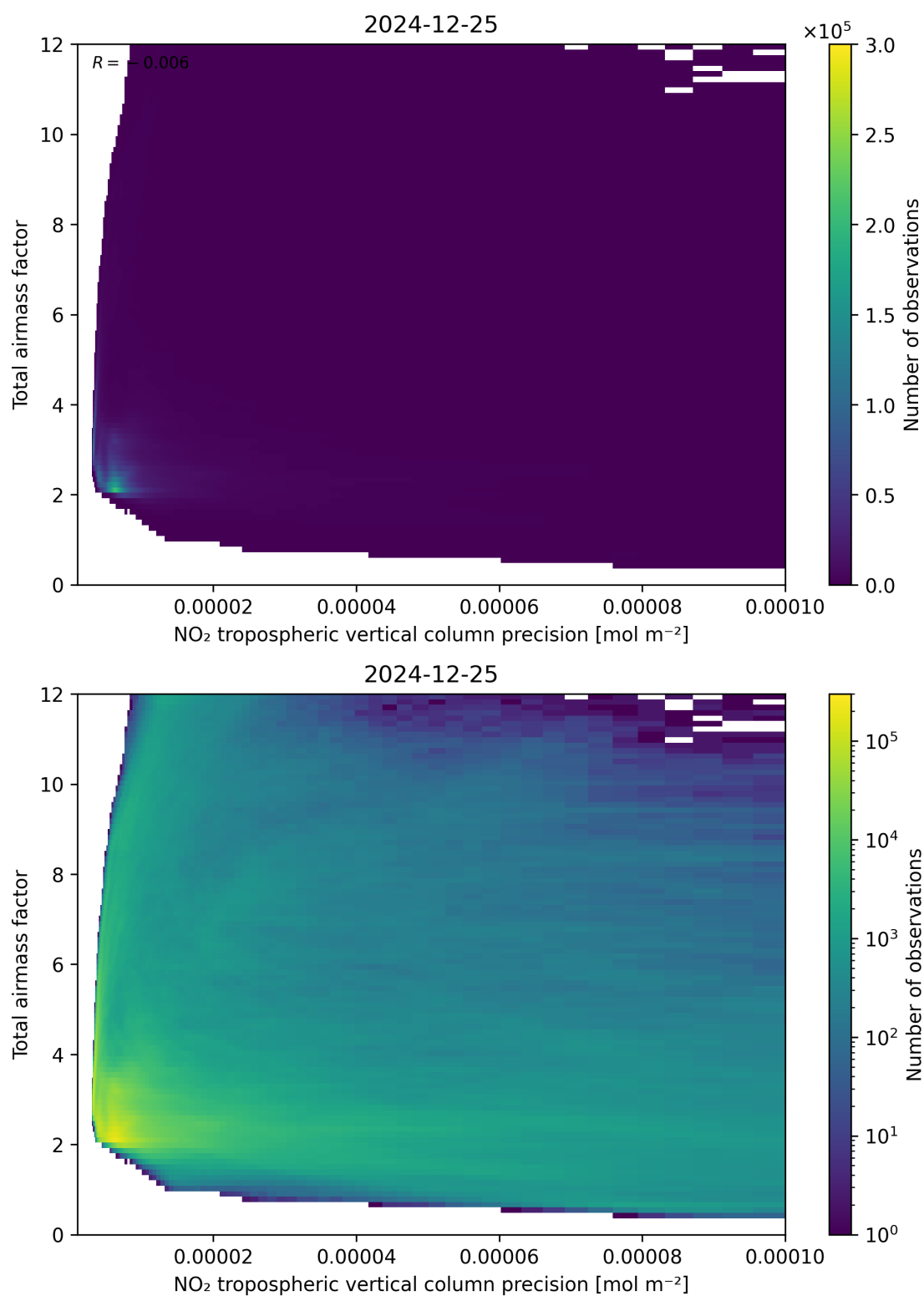
Figure 132: Scatter density plot of “NO 2 tropospheric vertical column precision” against “Total airmass factor” for 2024-12-24 to 2024-12-26.
