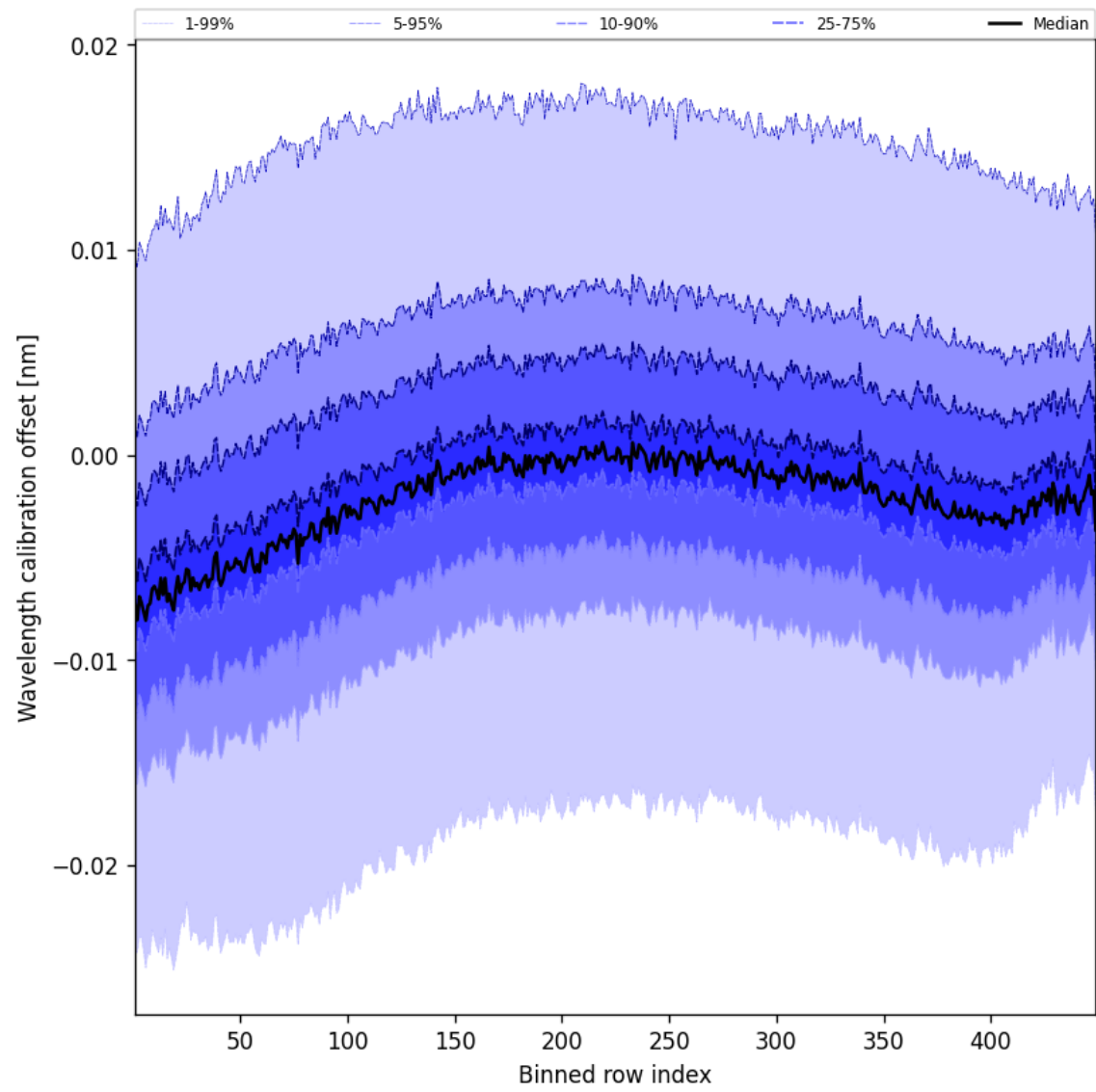
Figure 52: Along track statistics of “Wavelength calibration offset” for 2024-12-24 to 2024-12-26
