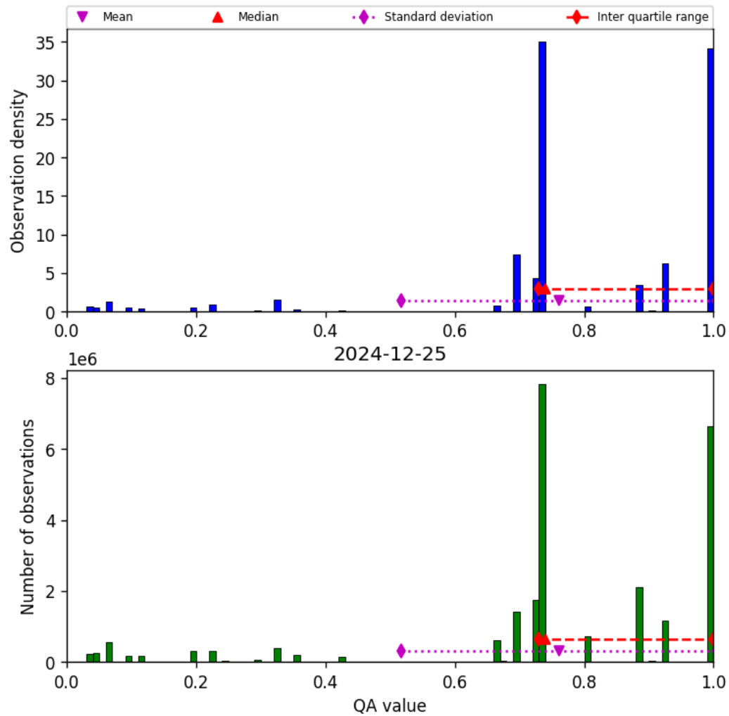
Figure 28: Histogram of “QA value” for 2024-12-24 to 2024-12-26
