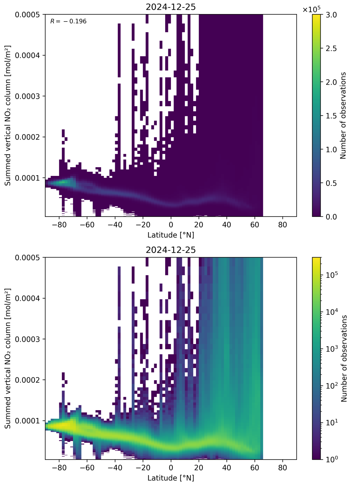
Figure 88: Scatter density plot of “Latitude” against “Summed vertical NO 2 column” for 2024-12-24 to 2024-12-26.
