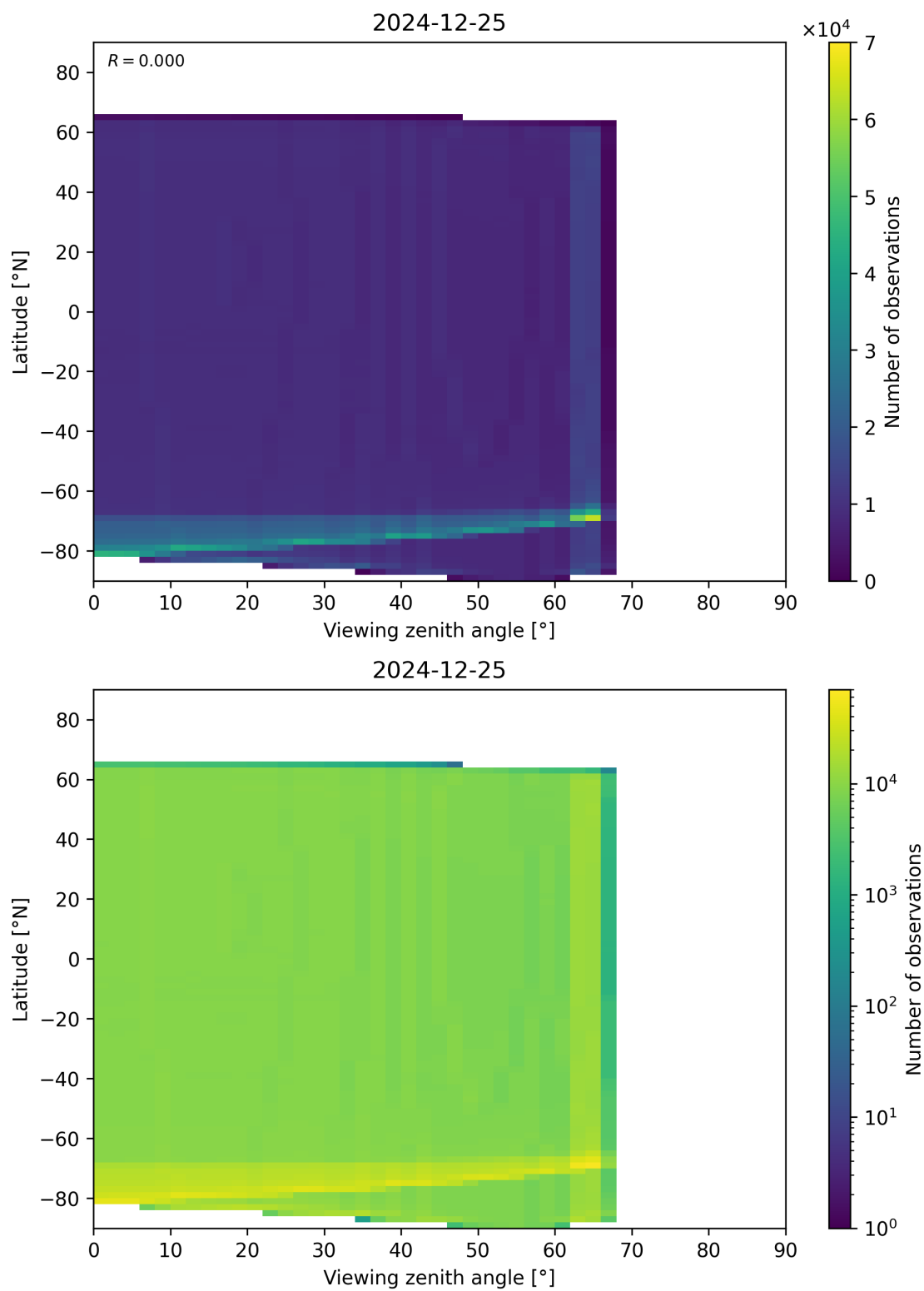
Figure 163: Scatter density plot of “Viewing zenith angle” against “Latitude” for 2024-12-24 to 2024-12-26.
