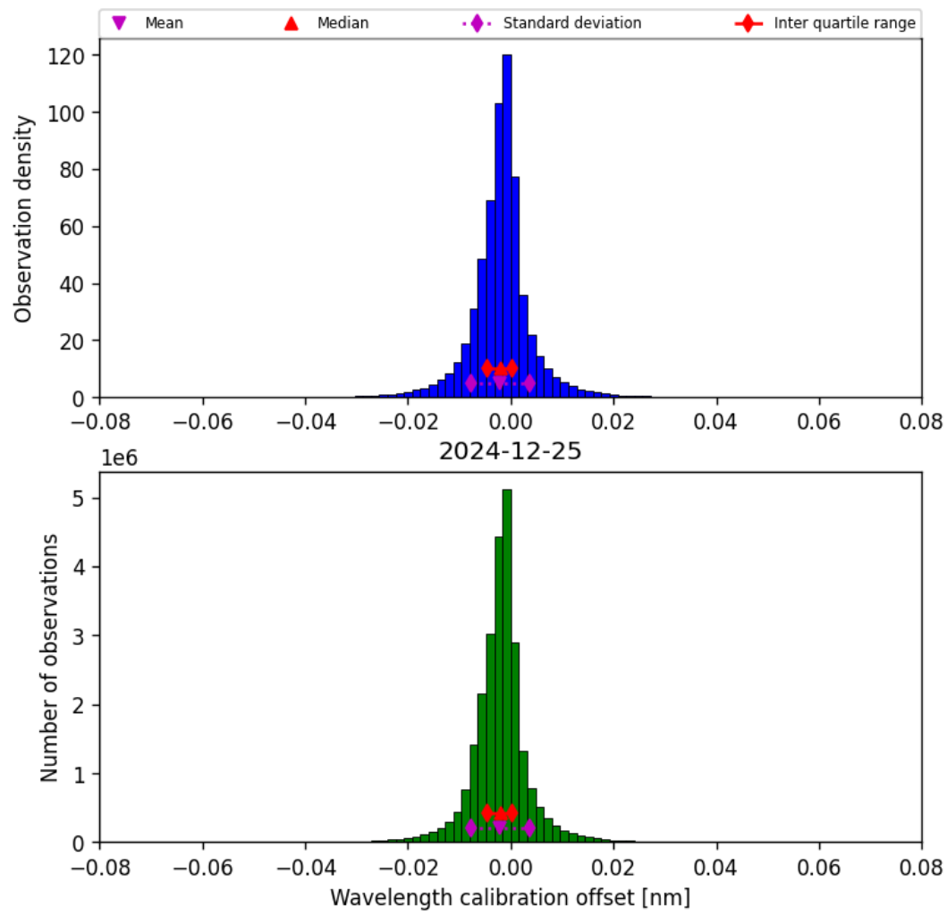
Figure 35: Histogram of “Wavelength calibration offset” for 2024-12-24 to 2024-12-26
