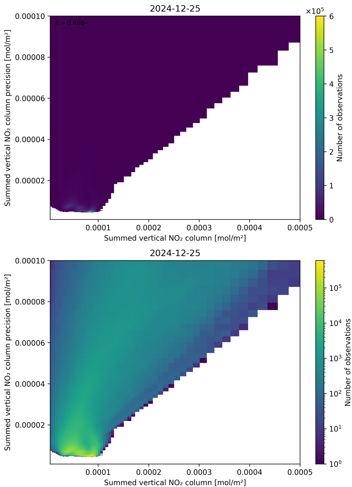
Figure 105: Scatter density plot of “Summed vertical NO 2 column” against “Summed vertical NO 2 column precision” for 2024-12-24 to 2024-12-26.
