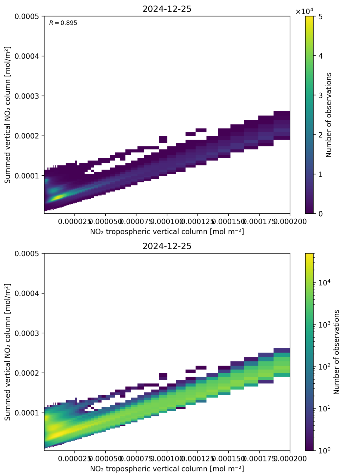
Figure 126: Scatter density plot of “NO 2 tropospheric vertical column” against “Summed vertical NO 2 column” for 2024-12-24 to 2024-12-26.
