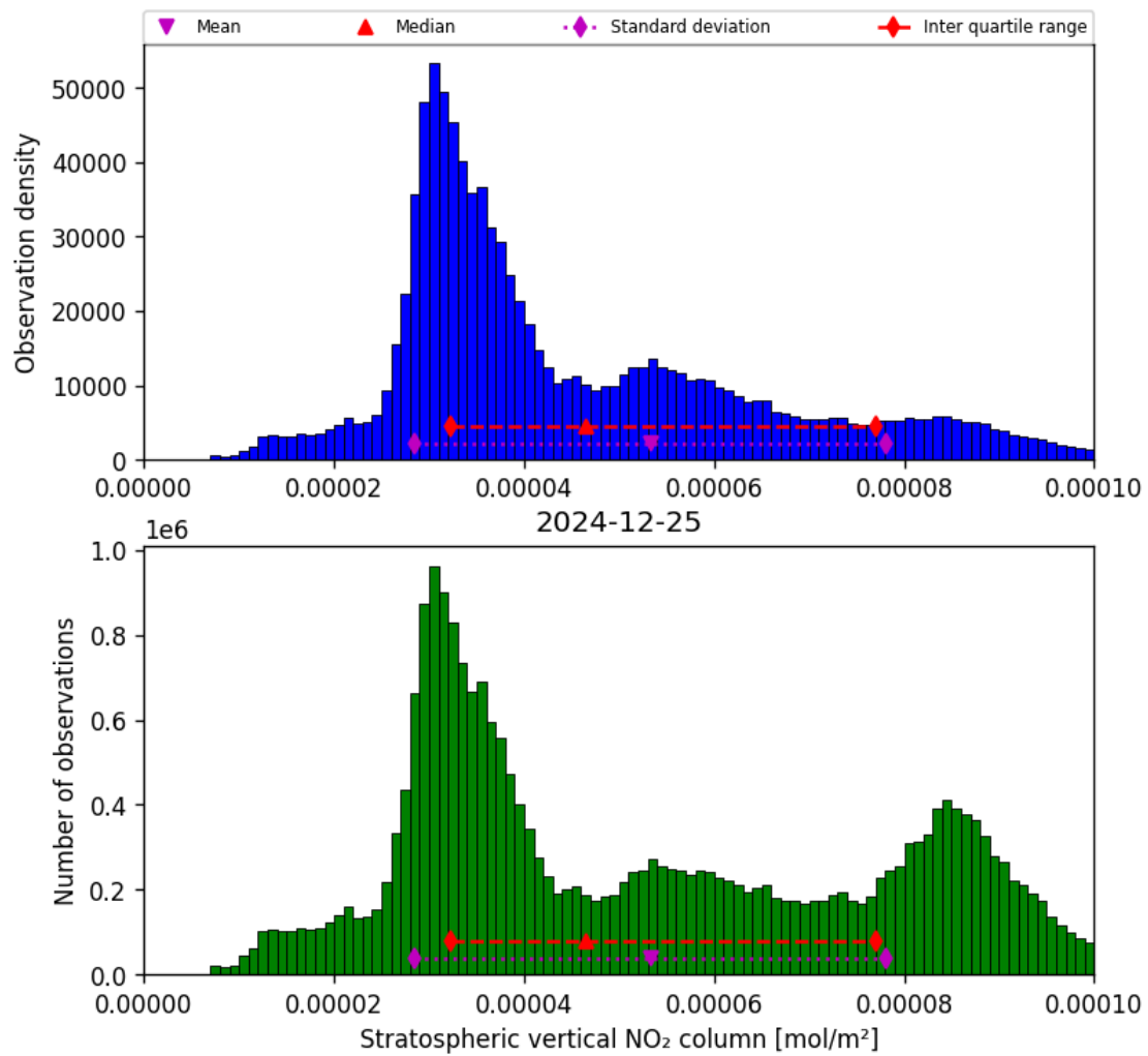
Figure 36: Histogram of “Stratospheric vertical NO 2 column” for 2024-12-24 to 2024-12-26
