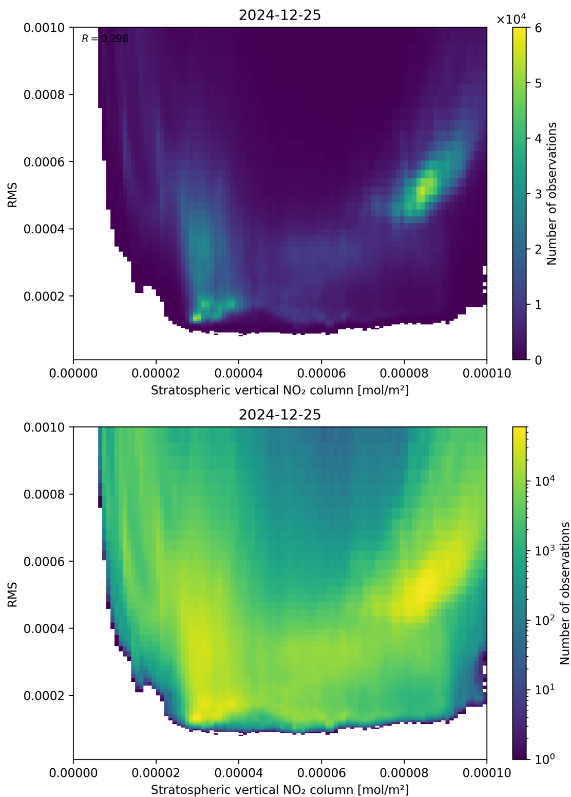
Figure 102: Scatter density plot of “Stratospheric vertical NO 2 column” against “RMS” for 2024-12-24 to 2024-12-26.
