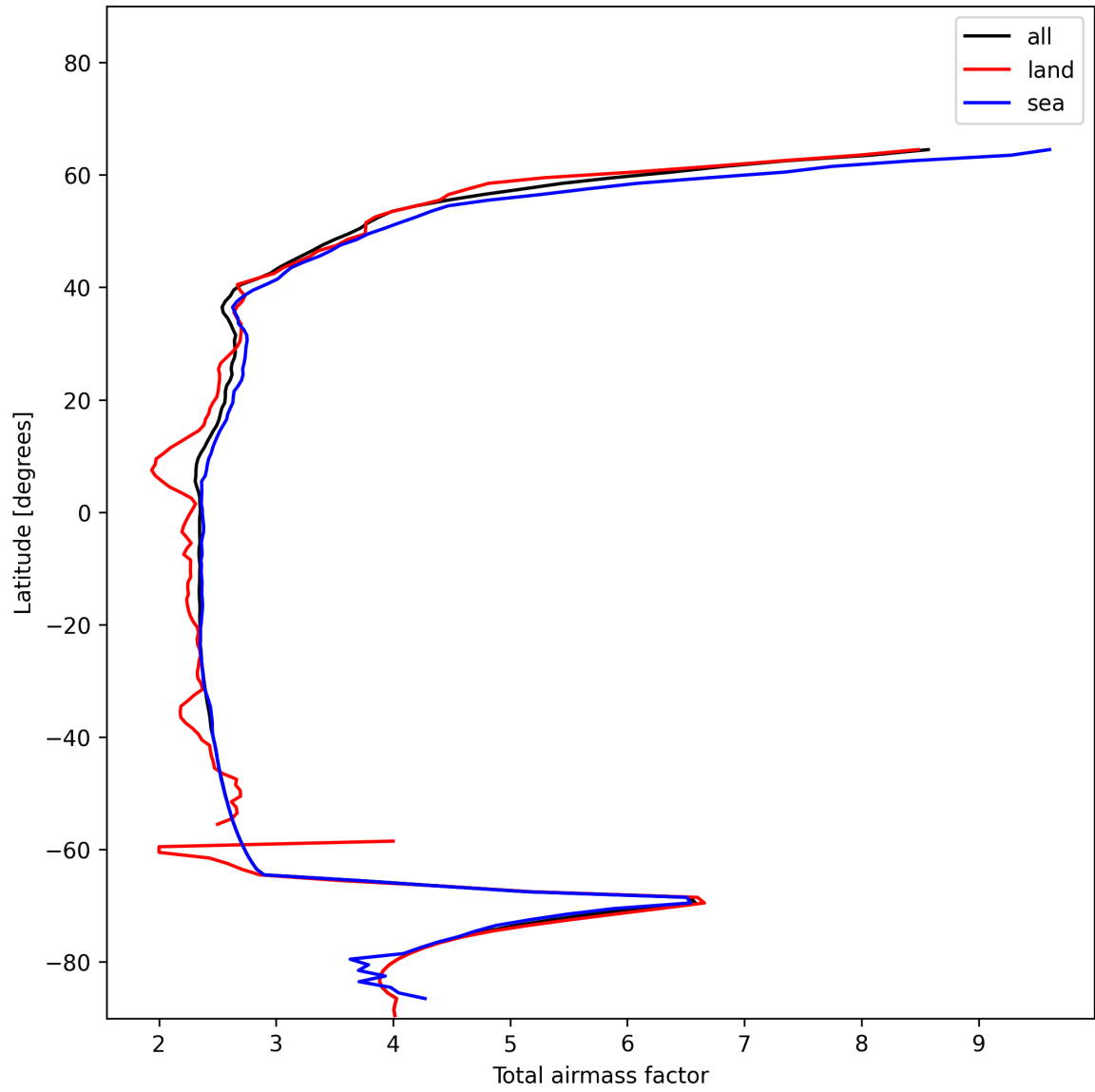
Figure 15: Zonal average of “Total airmass factor” for 2024-12-24 to 2024-12-26.
