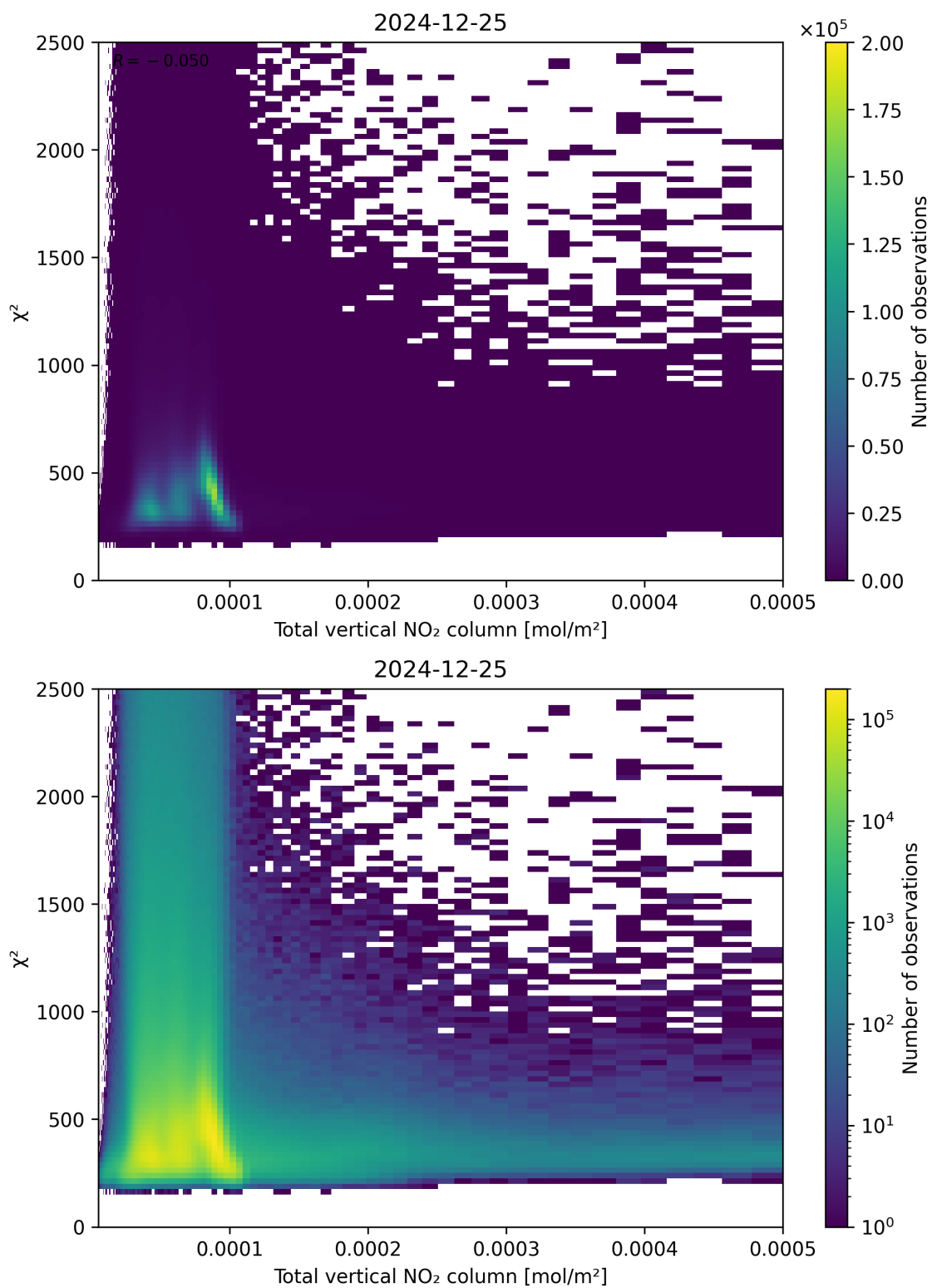
Figure 111: Scatter density plot of “Total vertical NO 2 column” against “ \chi^2 ” for 2024-12-24 to 2024-12-26.
