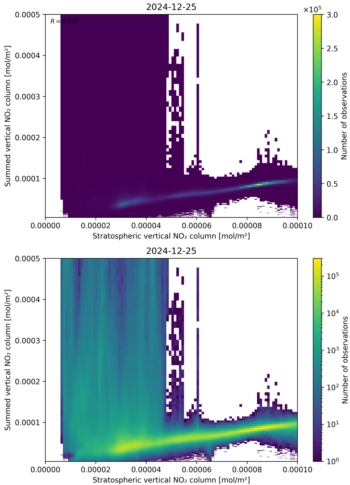
Figure 98: Scatter density plot of “Stratospheric vertical NO 2 column” against “Summed vertical NO 2 column” for 2024-12-24 to 2024-12-26.
