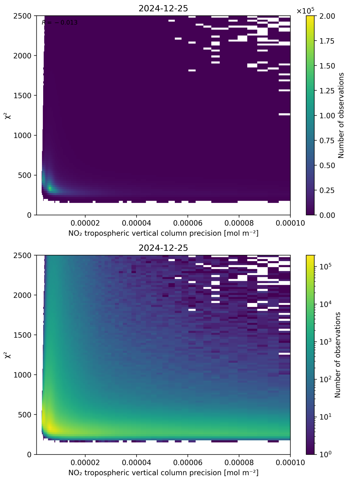
Figure 134: Scatter density plot of “NO 2 tropospheric vertical column precision” against “ \chi^2 ” for 2024-12-24 to 2024-12-26.
