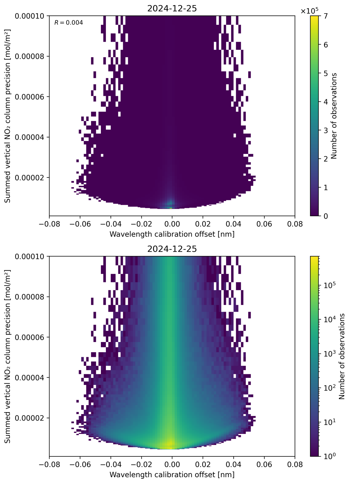
Figure 178: Scatter density plot of “Wavelength calibration offset” against “Summed vertical NO 2 column precision” for 2024-12-24 to 2024-12-26.
