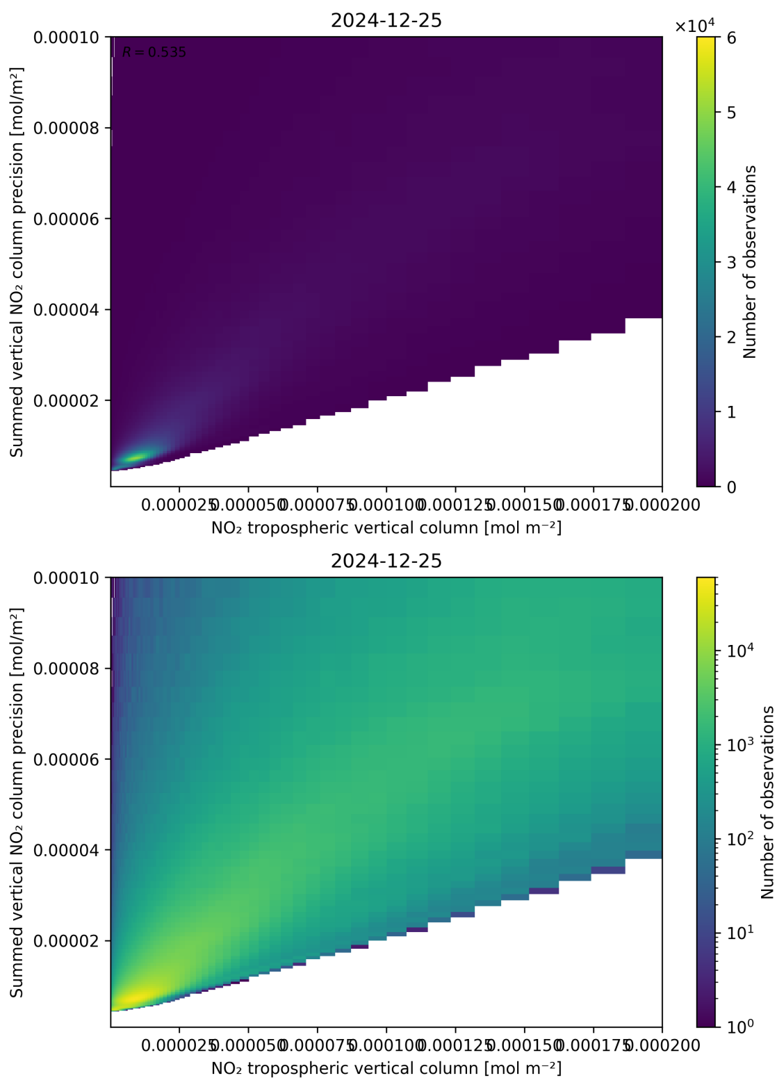
Figure 127: Scatter density plot of “NO 2 tropospheric vertical column” against “Summed vertical NO 2 column precision” for 2024-12-24 to 2024-12-26.
