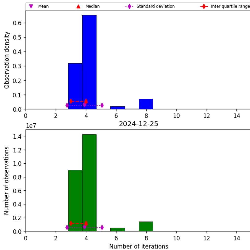
Figure 34: Histogram of “Number of iterations” for 2024-12-24 to 2024-12-26
