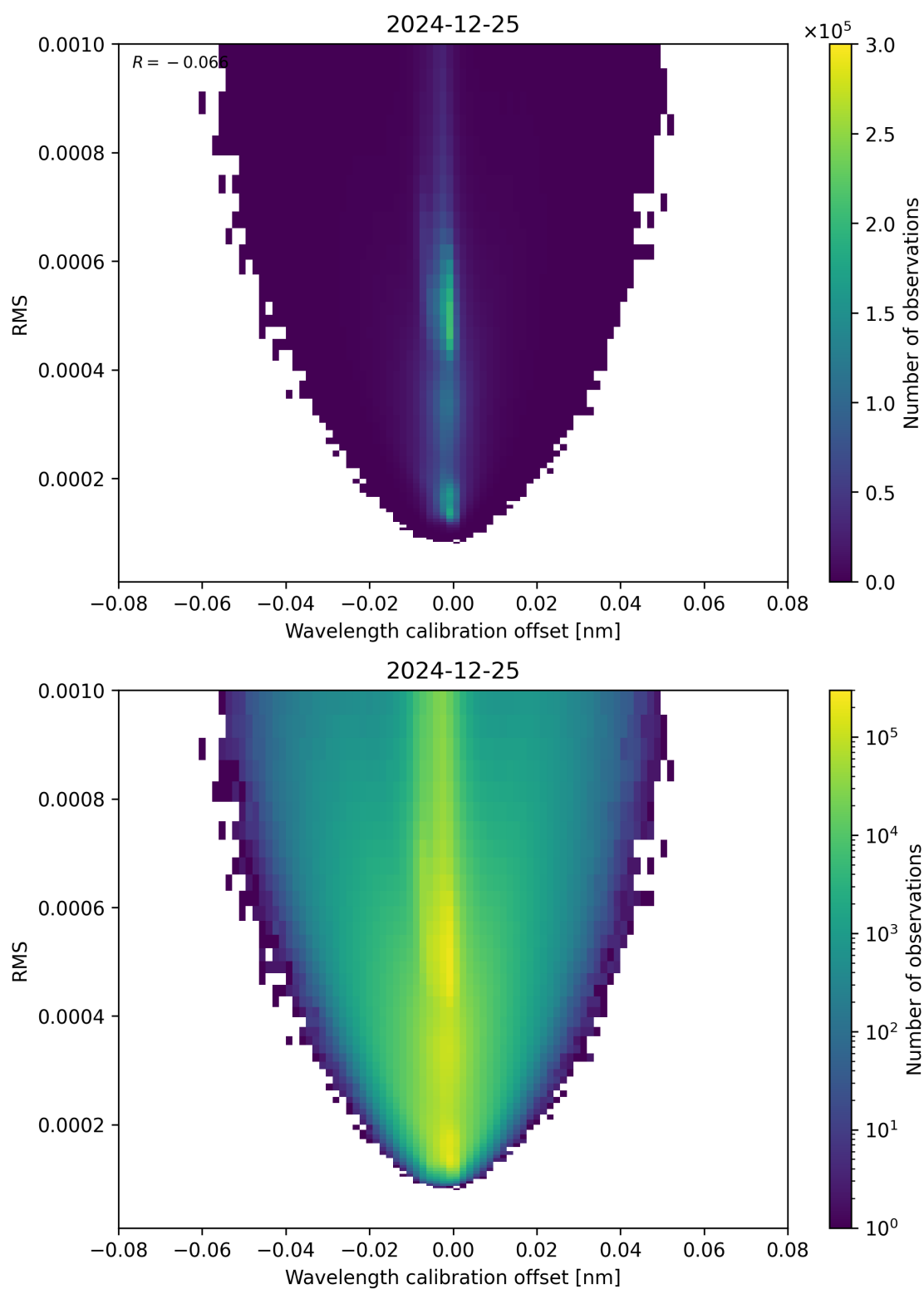
Figure 181: Scatter density plot of “Wavelength calibration offset” against “RMS” for 2024-12-24 to 2024-12-26.
