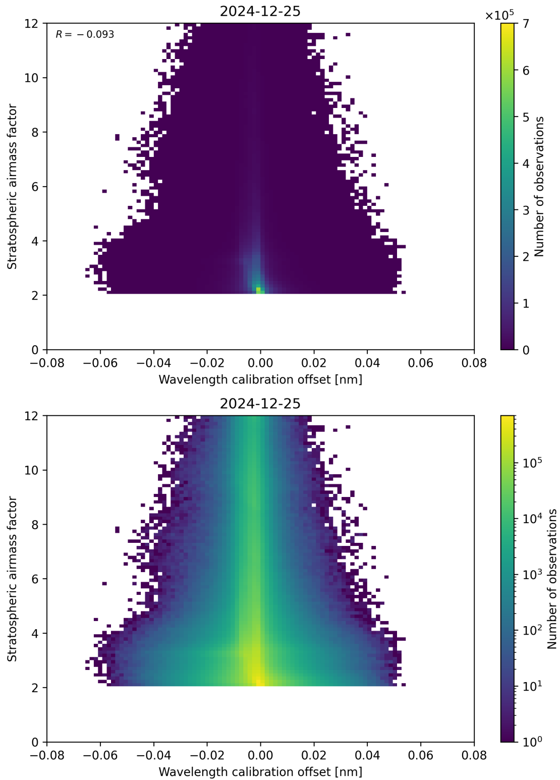
Figure 174: Scatter density plot of “Wavelength calibration offset” against “Stratospheric airmass factor” for 2024-12-24 to 2024-12-26.
