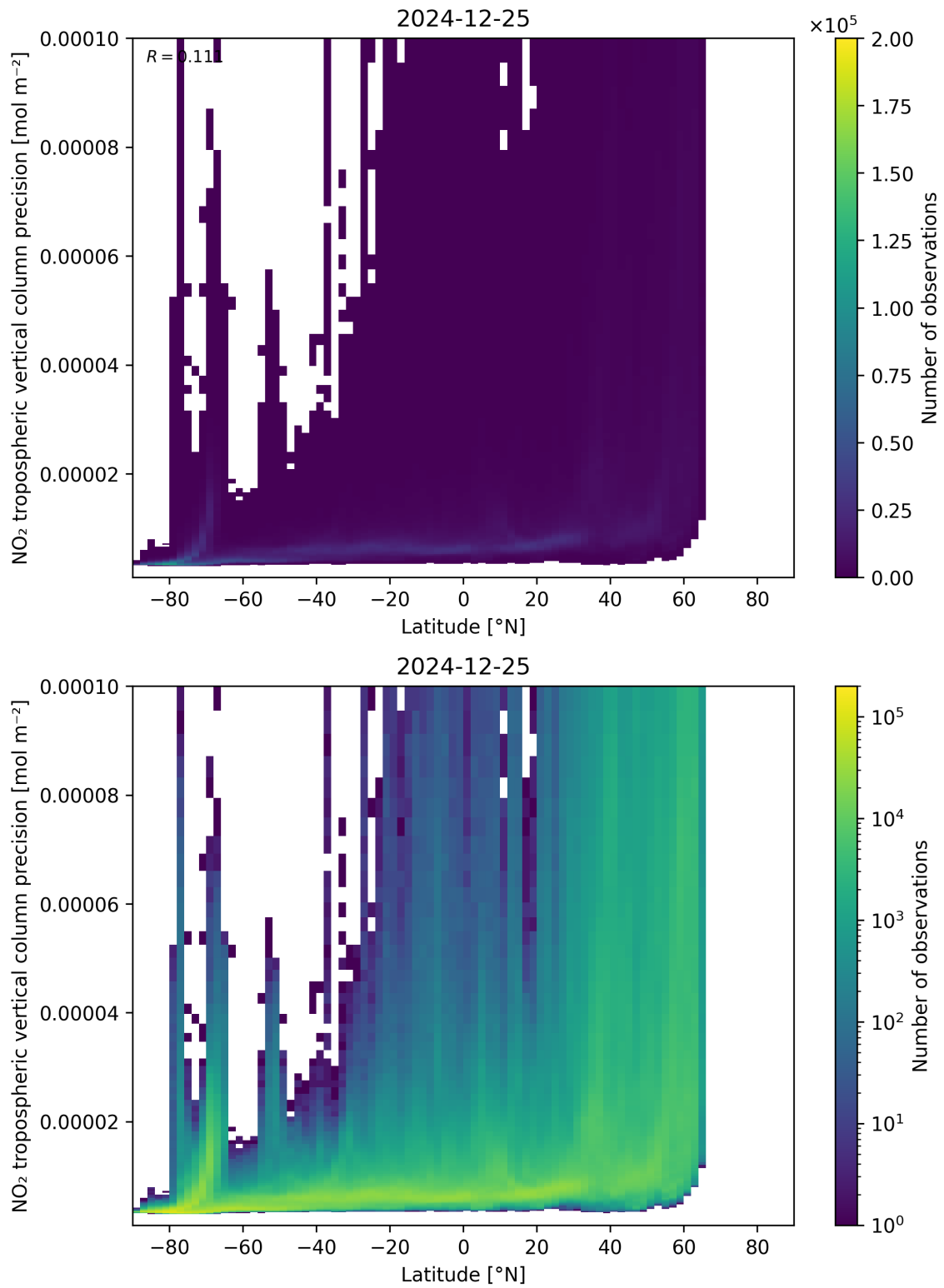
Figure 93: Scatter density plot of “Latitude” against “NO 2 tropospheric vertical column precision” for 2024-12-24 to 2024-12-26.
