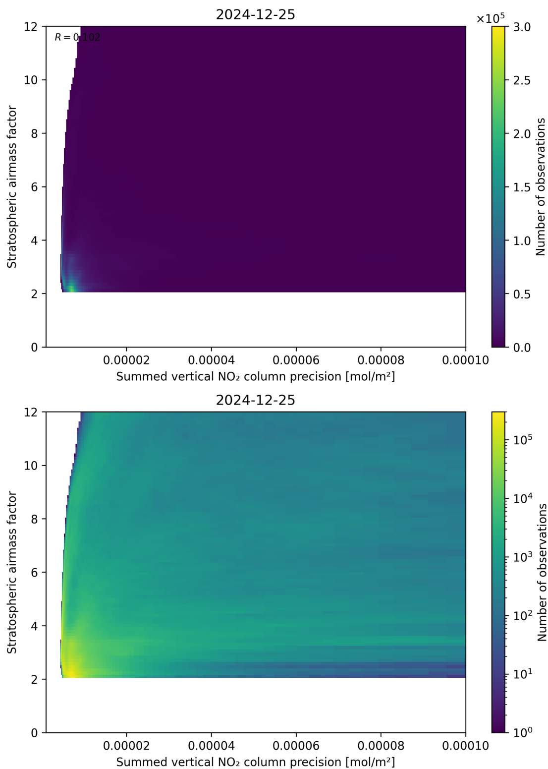
Figure 106: Scatter density plot of “Summed vertical NO 2 column precision” against “Stratospheric airmass factor” for 2024-12-24 to 2024-12-26.
