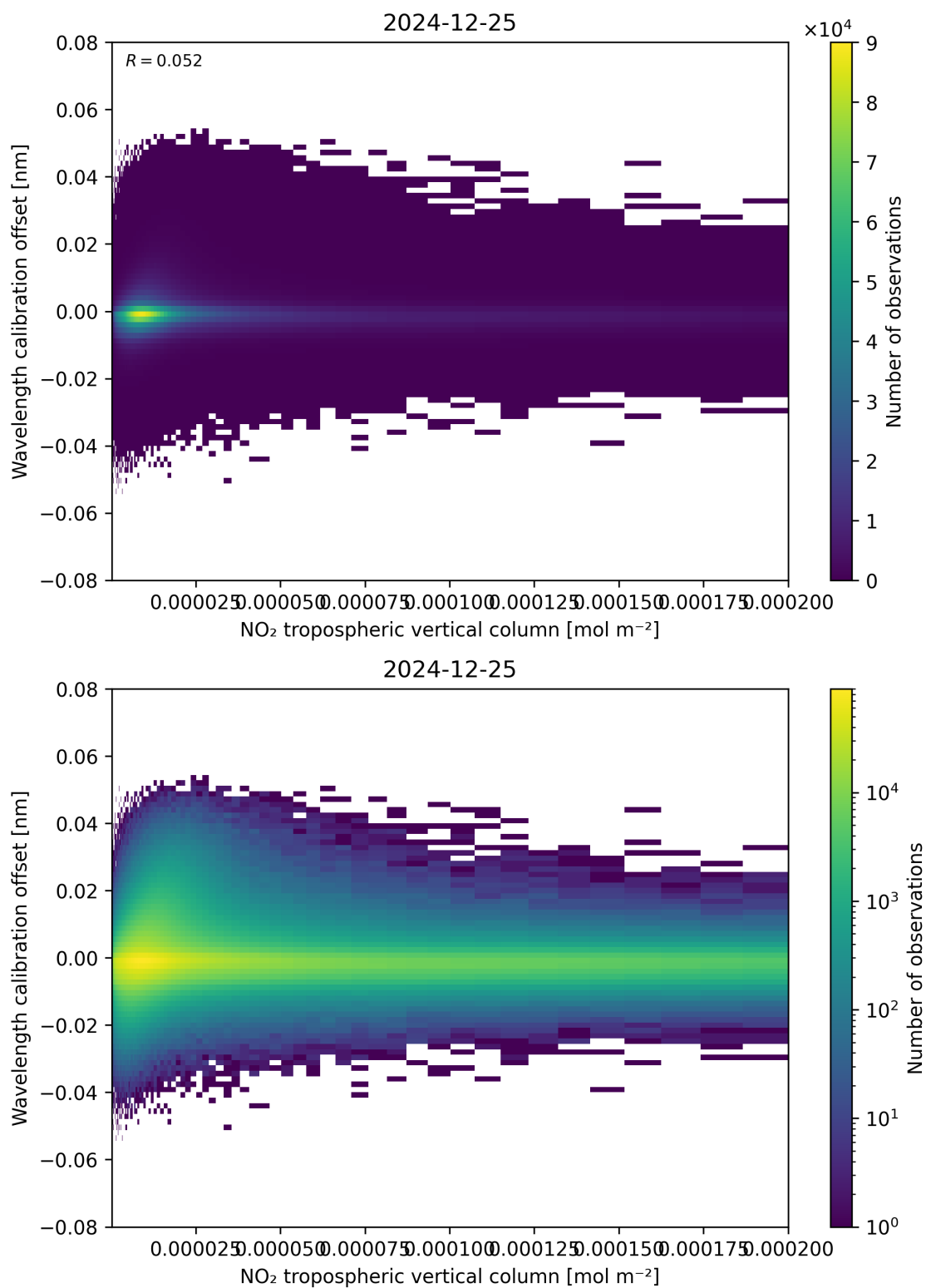
Figure 143: Scatter density plot of “NO 2 tropospheric vertical column” against “Wavelength calibration offset” for 2024-12-24 to 2024-12-26.
