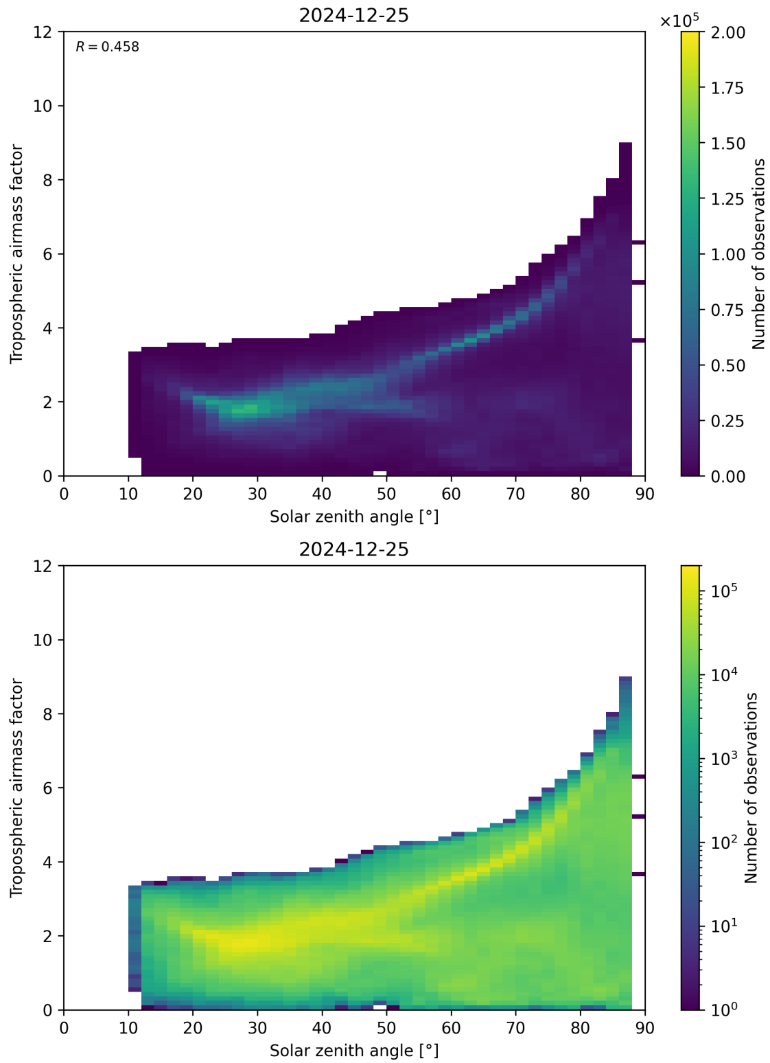
Figure 147: Scatter density plot of “Solar zenith angle” against “Tropospheric airmass factor” for 2024-12-24 to 2024-12-26.
