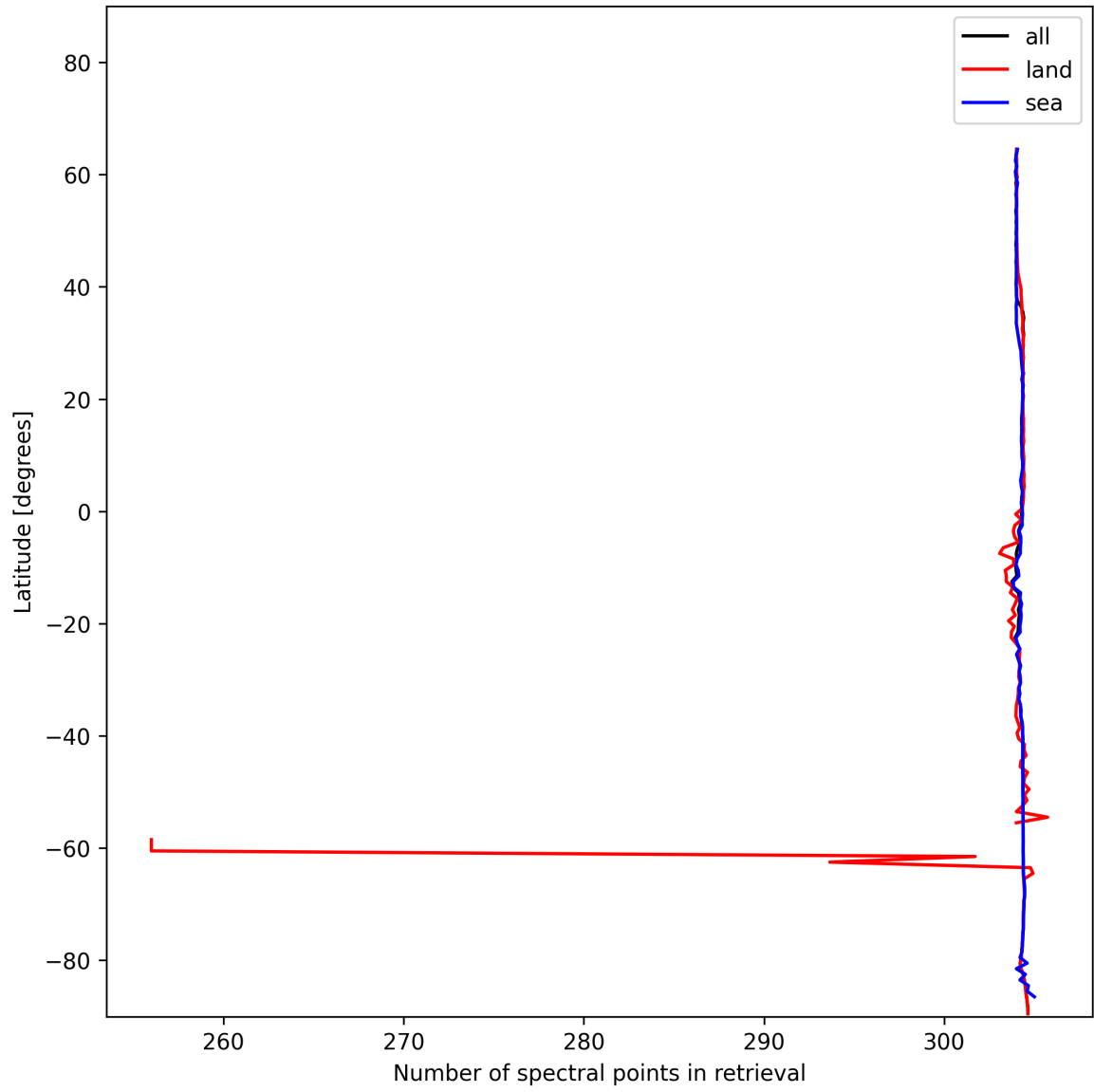
Figure 16: Zonal average of “Number of spectral points in retrieval” for 2024-12-24 to 2024-12-26.
