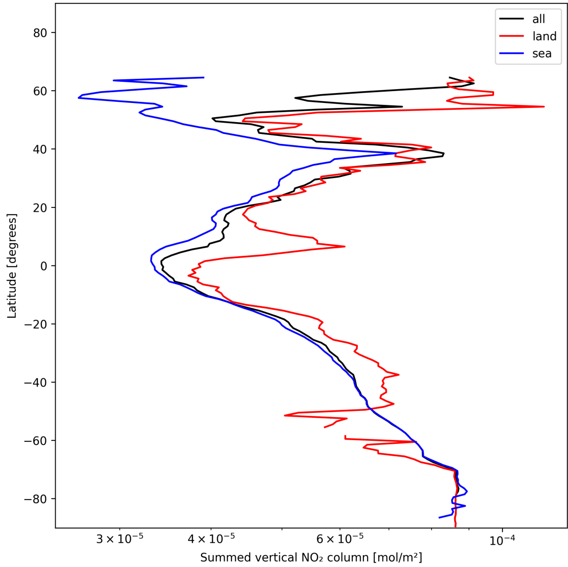
Figure 23: Zonal average of “Summed vertical NO 2 column” for 2024-12-24 to 2024-12-26.
