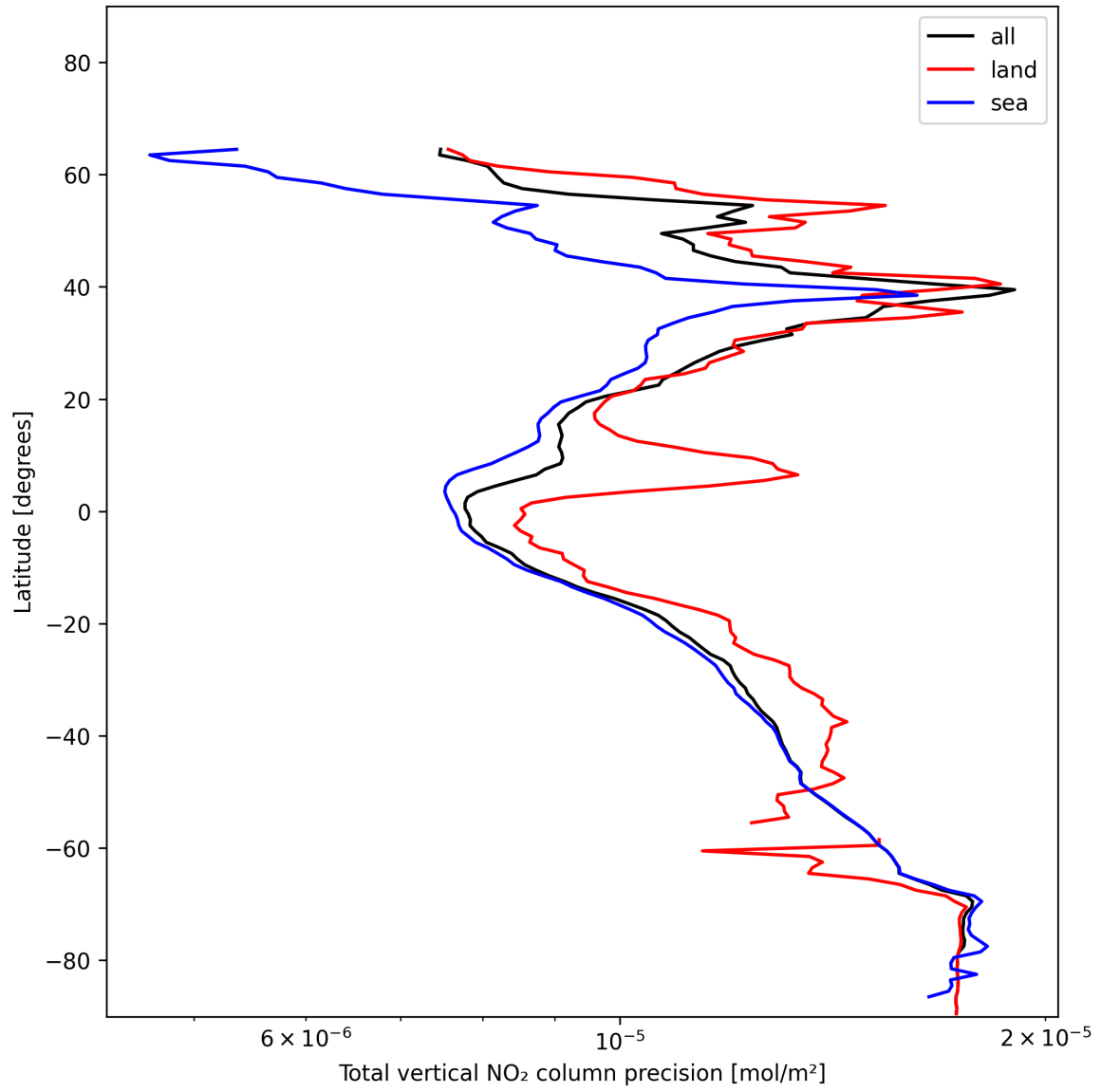
Figure 22: Zonal average of “Total vertical NO 2 column precision” for 2024-12-24 to 2024-12-26.
