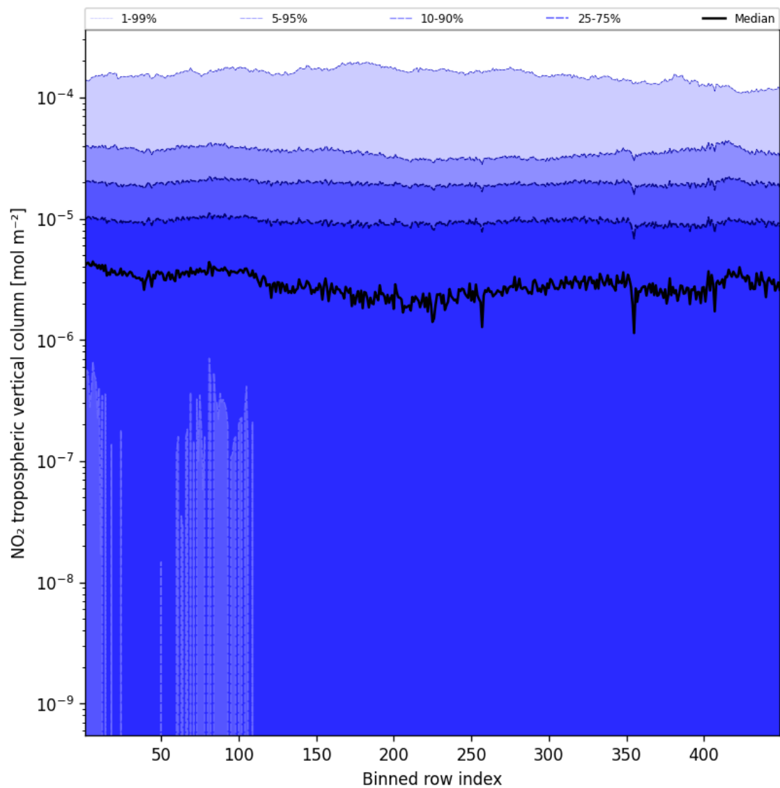
Figure 46: Along track statistics of “NO 2 tropospheric vertical column” for 2024-12-24 to 2024-12-26
