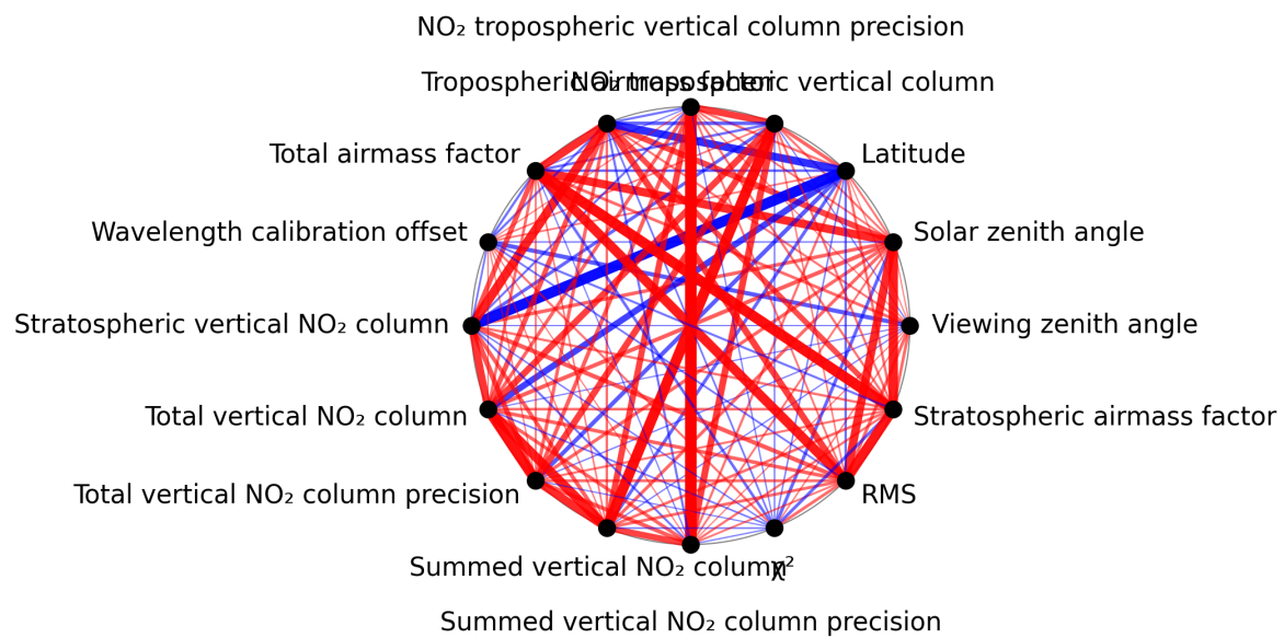
Figure 1: Map of correlation graph for 2024-12-24 to 2024-12-26.
