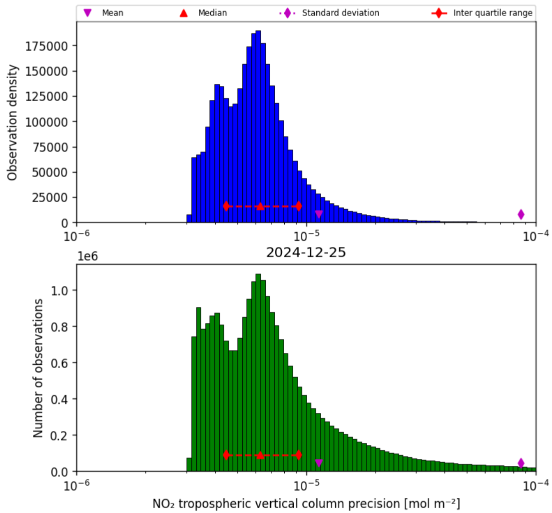
Figure 30: Histogram of “NO 2 tropospheric vertical column precision” for 2024-12-24 to 2024-12-26
