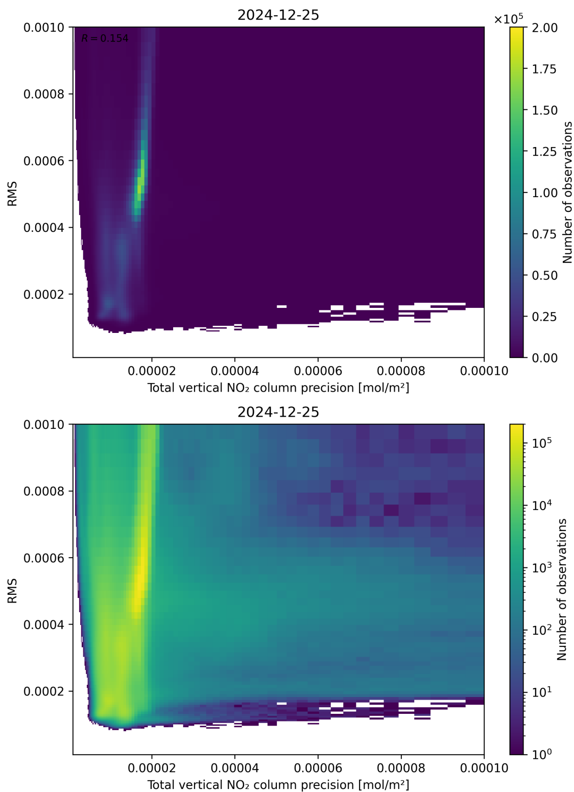
Figure 119: Scatter density plot of “Total vertical NO 2 column precision” against “RMS” for 2024-12-24 to 2024-12-26.
