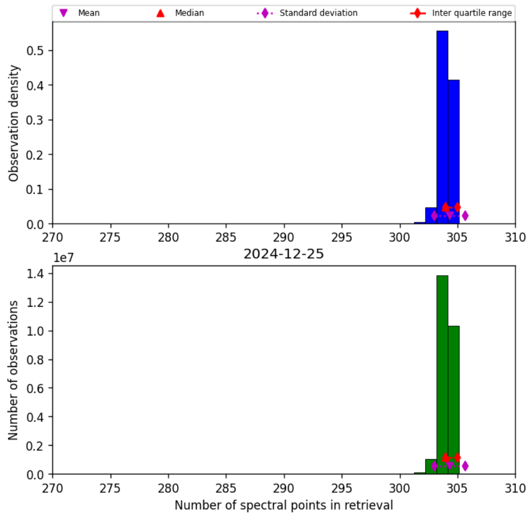
Figure 33: Histogram of “Number of spectral points in retrieval” for 2024-12-24 to 2024-12-26
