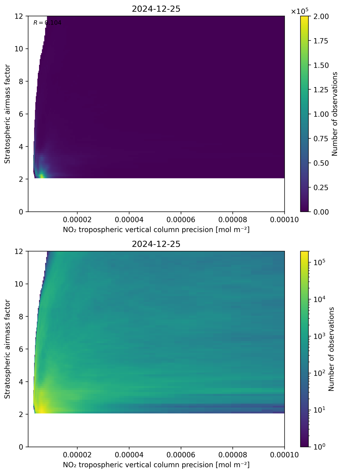
Figure 131: Scatter density plot of “NO 2 tropospheric vertical column precision” against “Stratospheric airmass factor” for 2024-12-24 to 2024-12-26.
