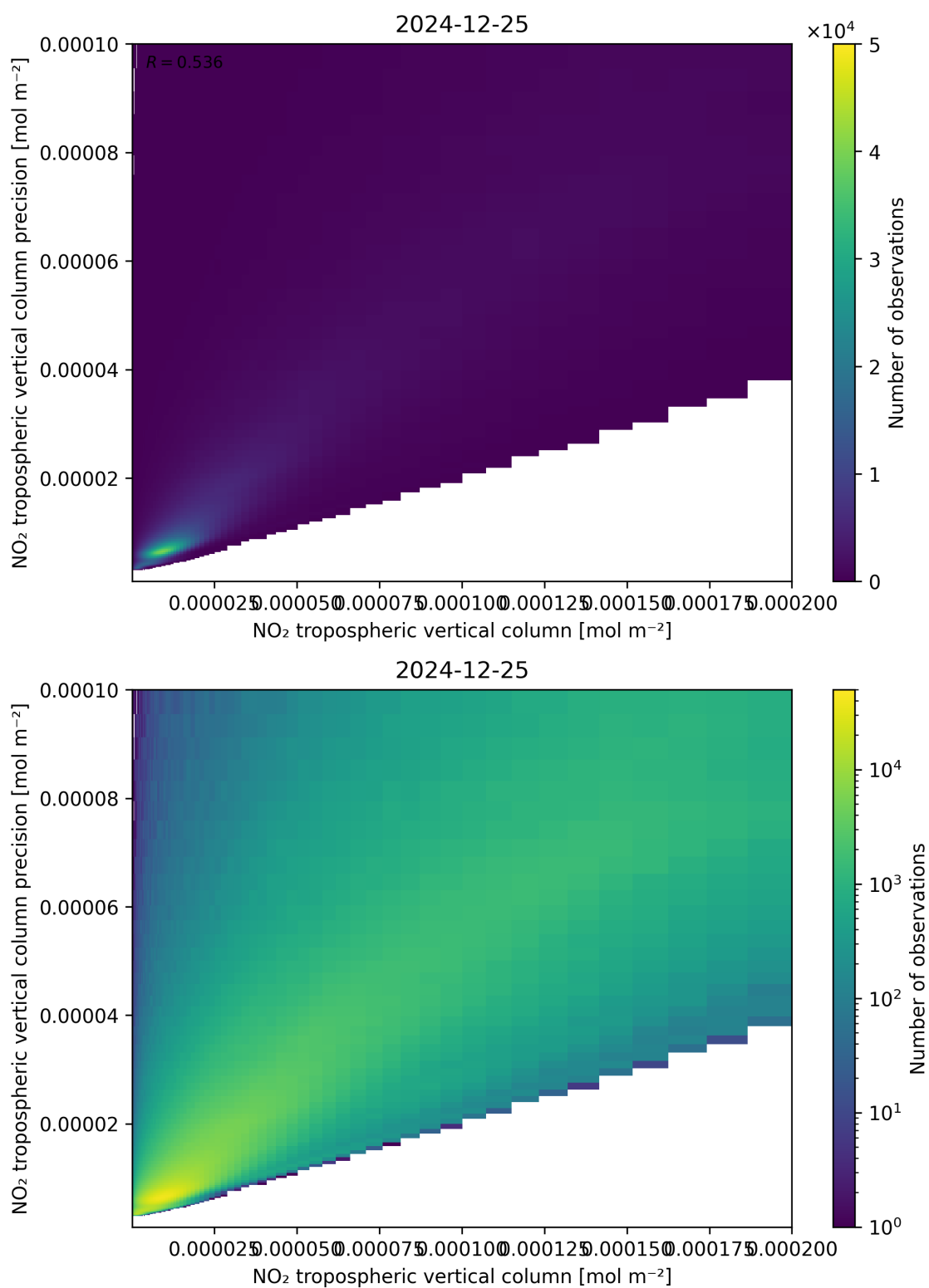
Figure 130: Scatter density plot of “NO 2 tropospheric vertical column” against “NO 2 tropospheric vertical column precision” for 2024-12-24 to 2024-12-26.
