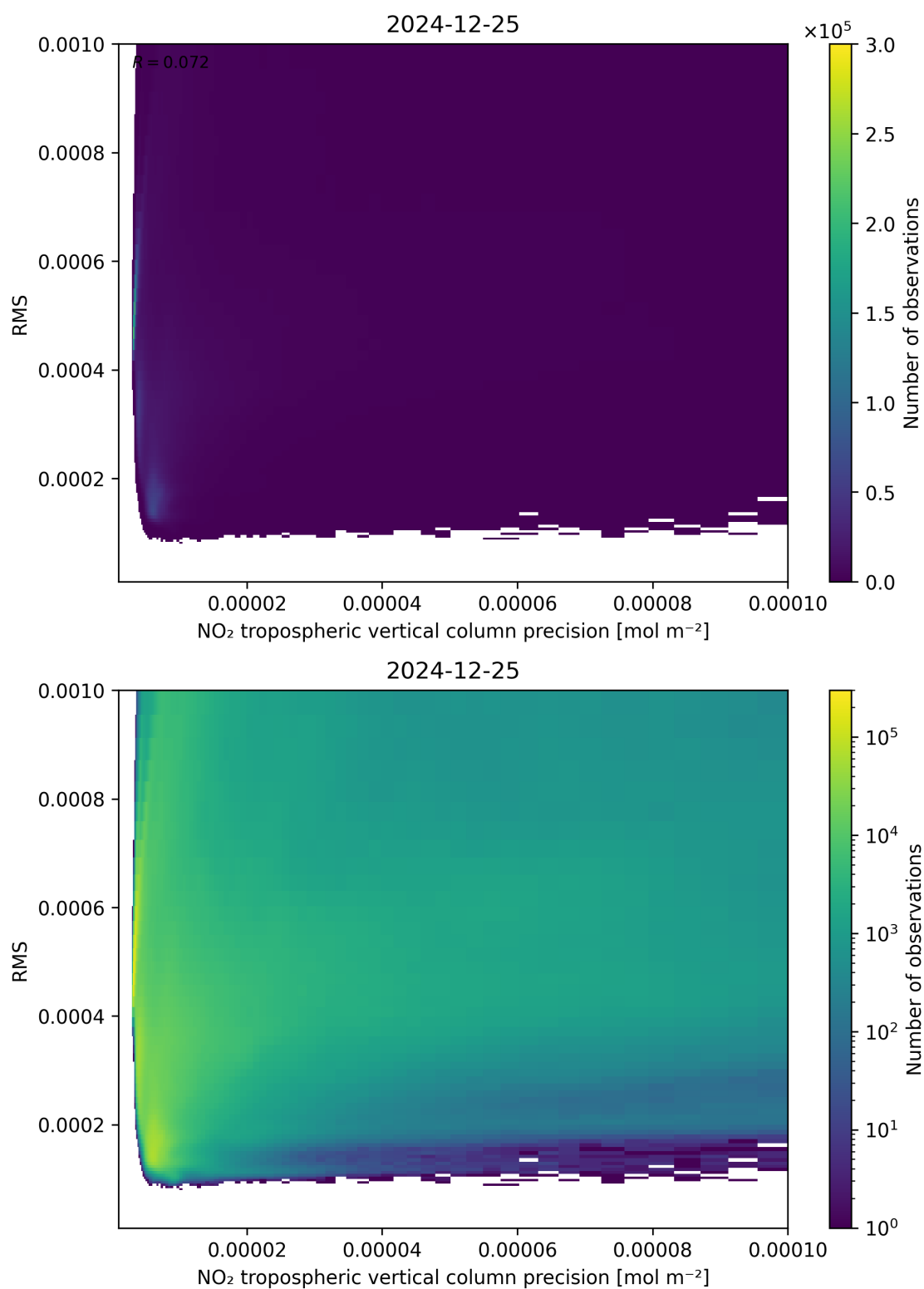
Figure 140: Scatter density plot of “NO 2 tropospheric vertical column precision” against “RMS” for 2024-12-24 to 2024-12-26.
