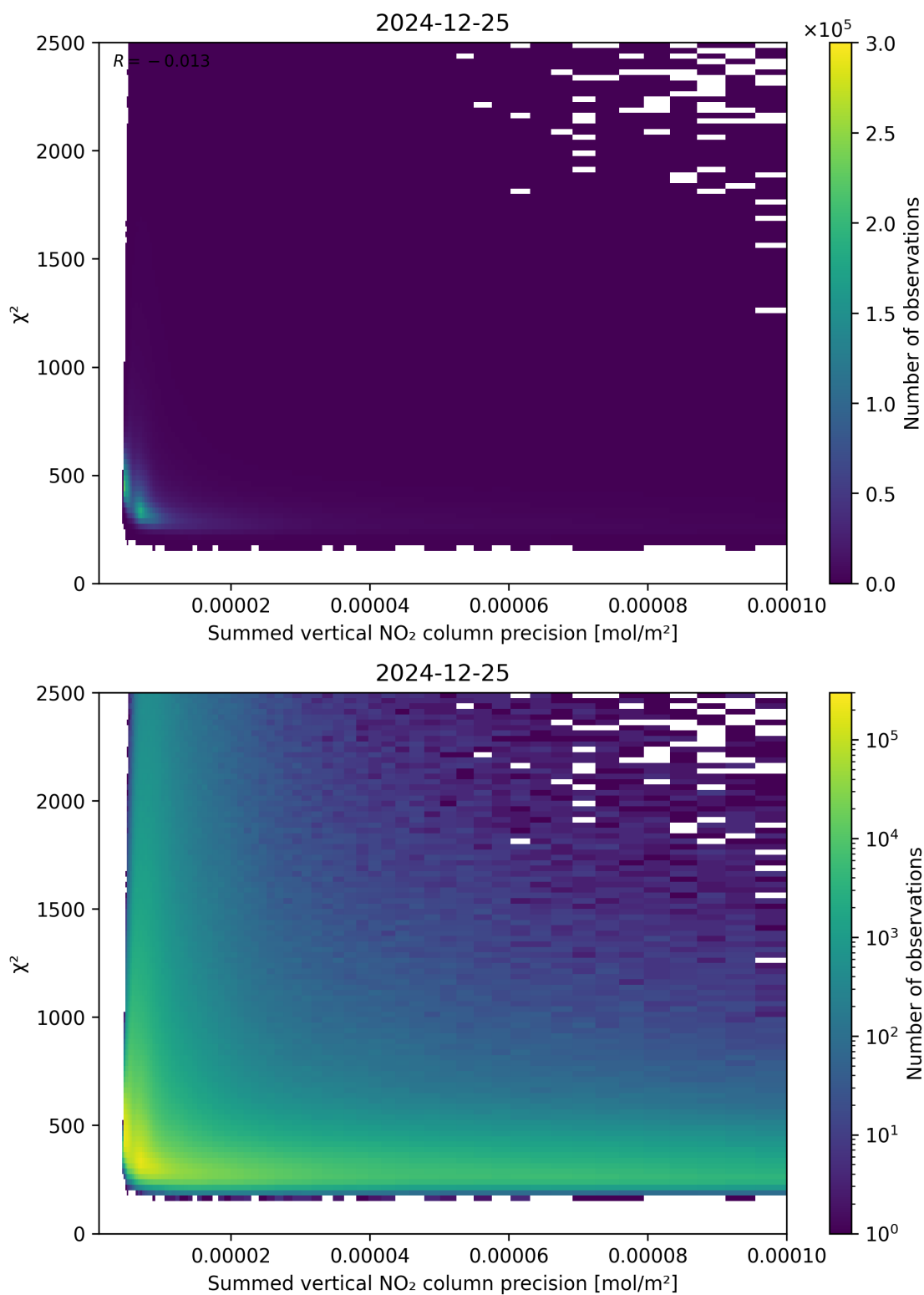
Figure 107: Scatter density plot of “Summed vertical NO 2 column precision” against “ \chi^2 ” for 2024-12-24 to 2024-12-26.
