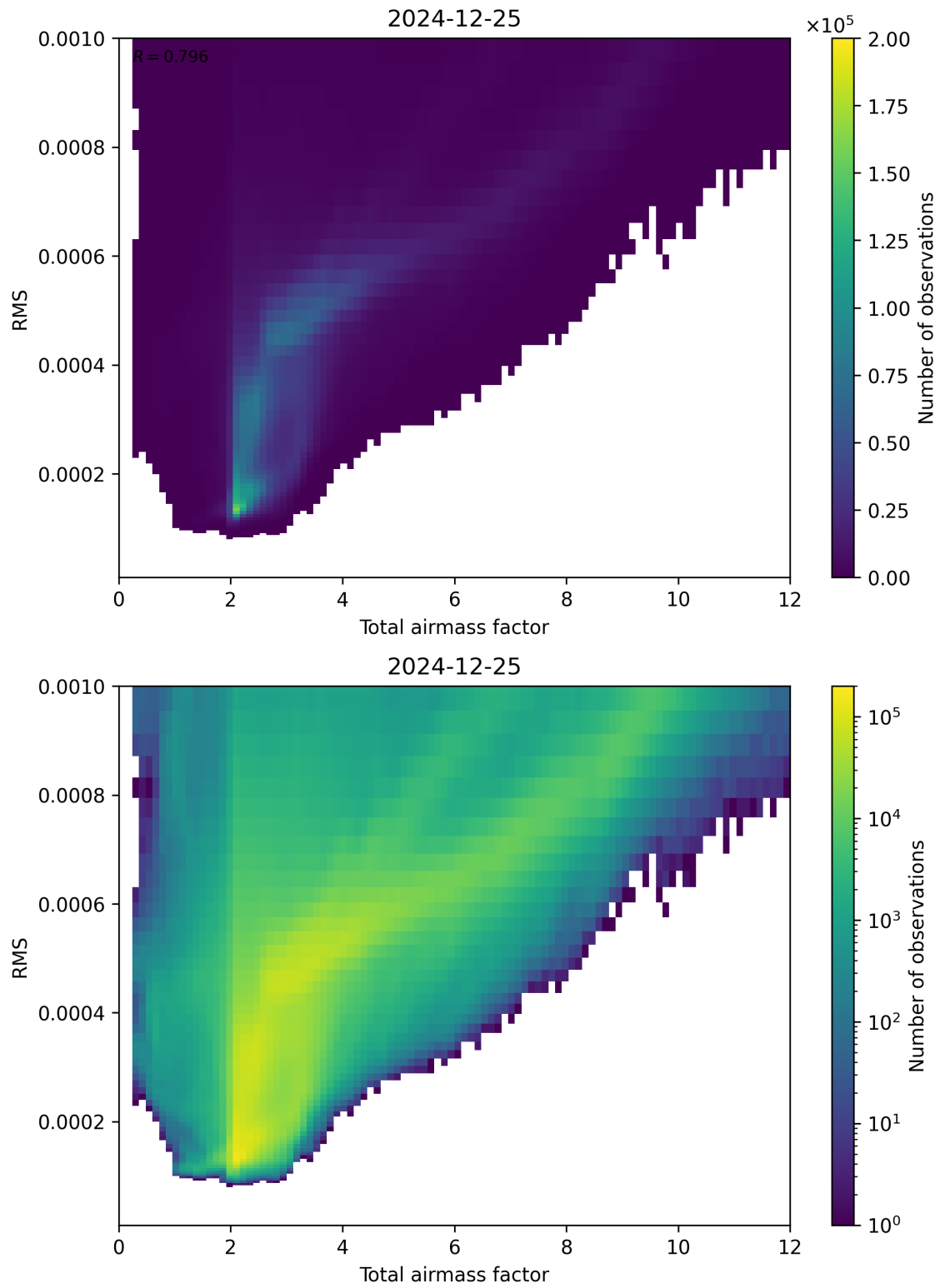
Figure 69: Scatter density plot of “Total airmass factor” against “RMS” for 2024-12-24 to 2024-12-26.
