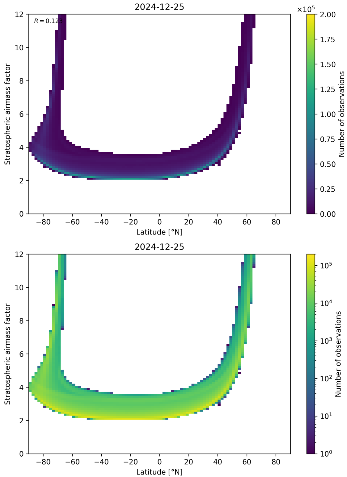
Figure 83: Scatter density plot of “Latitude” against “Stratospheric air mass factor” for 2024-12-24 to 2024-12-26.
