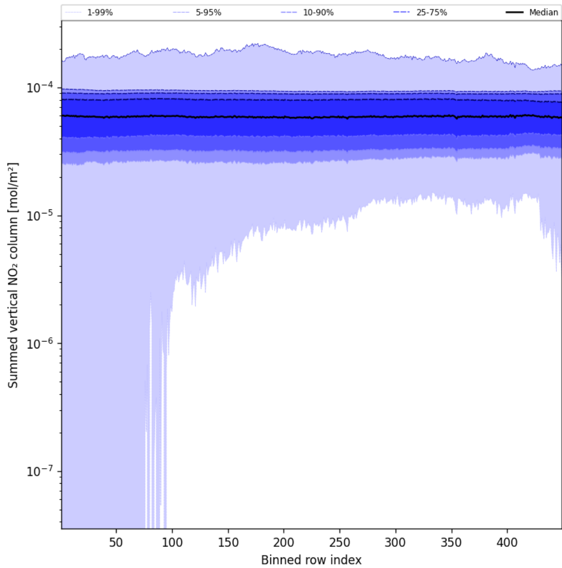
Figure 57: Along track statistics of “Summed vertical NO 2 column” for 2024-12-24 to 2024-12-26
