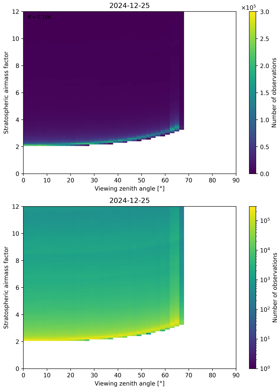
Figure 159: Scatter density plot of “Viewing zenith angle” against “Stratospheric airmass factor” for 2024-12-24 to 2024-12-26.
