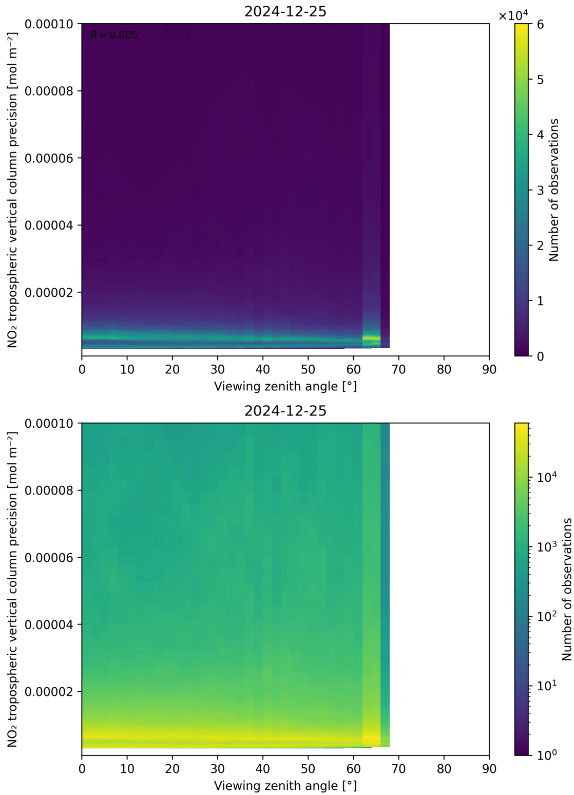
Figure 170: Scatter density plot of “Viewing zenith angle” against “NO 2 tropospheric vertical column precision” for 2024-12-24 to 2024-12-26.
