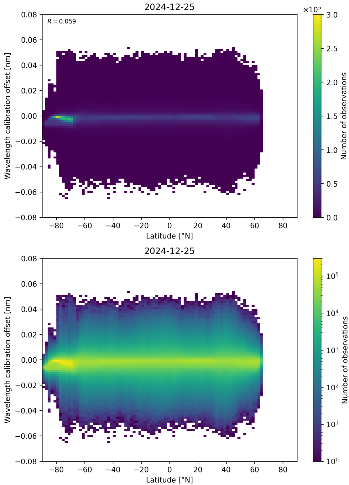
Figure 95: Scatter density plot of “Latitude” against “Wavelength calibration offset” for 2024-12-24 to 2024-12-26.
