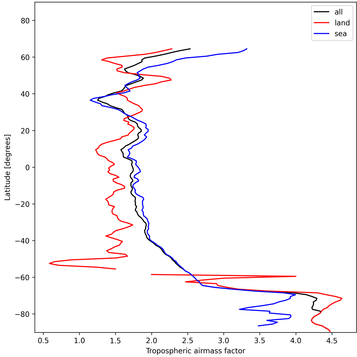
Figure 14: Zonal average of “Tropospheric airmass factor” for 2024-12-24 to 2024-12-26.
