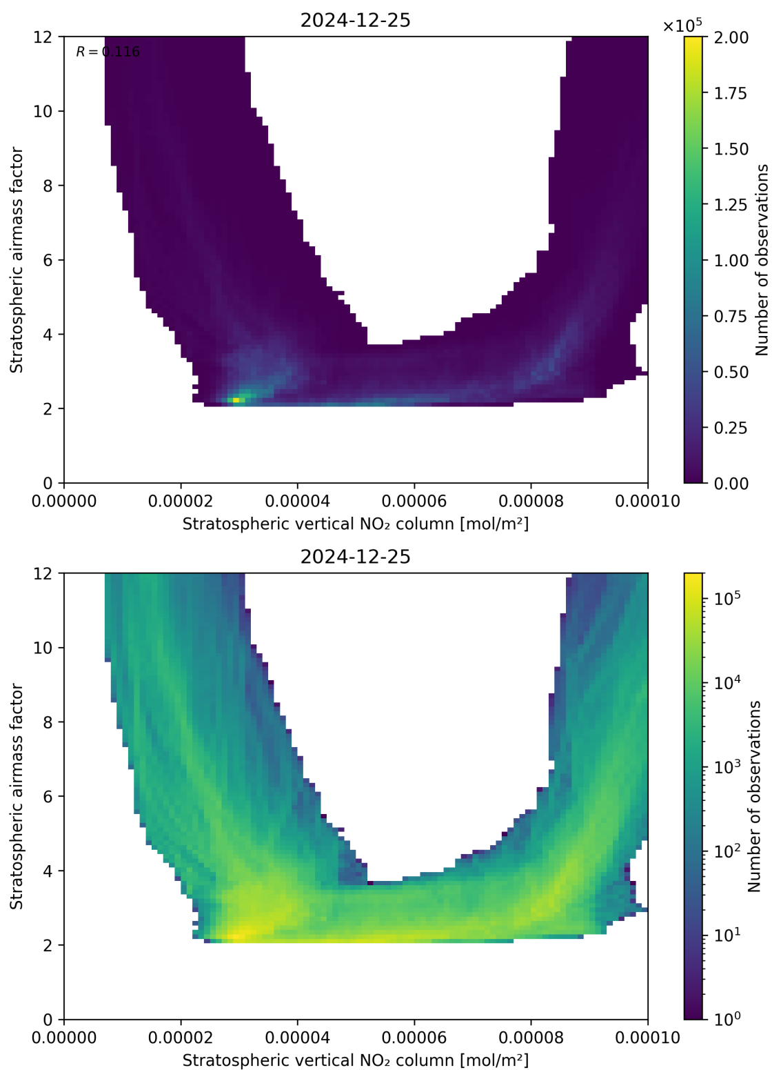
Figure 96: Scatter density plot of “Stratospheric vertical NO 2 column” against “Stratospheric airmass factor” for 2024-12-24 to 2024-12-26.
