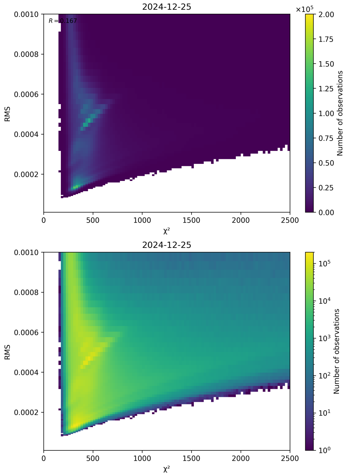
Figure 82: Scatter density plot of “ \chi^2 ” against “RMS” for 2024-12-24 to 2024-12-26.
