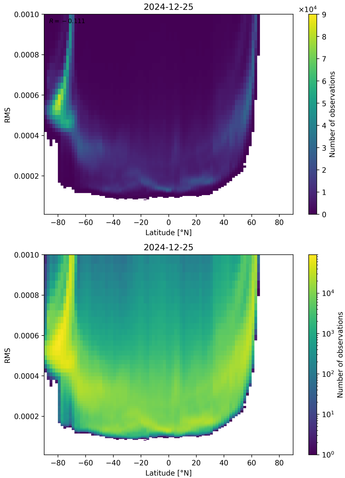
Figure 94: Scatter density plot of “Latitude” against “RMS” for 2024-12-24 to 2024-12-26.
