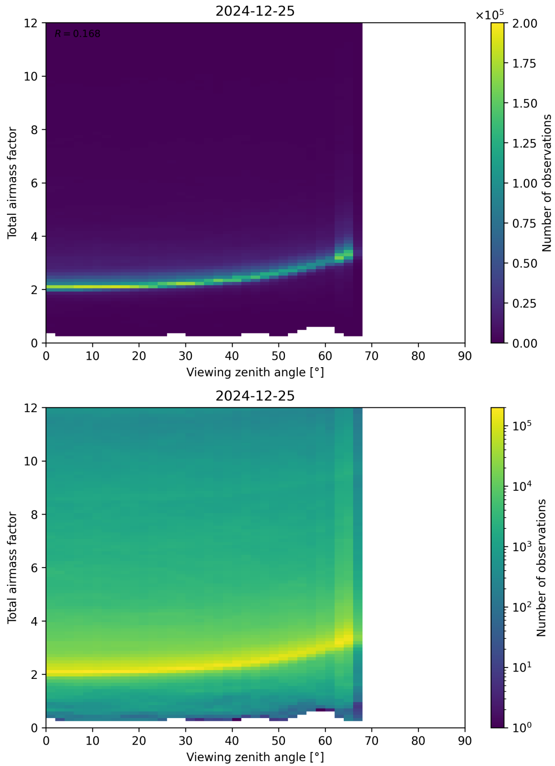
Figure 160: Scatter density plot of “Viewing zenith angle” against “Total airmass factor” for 2024-12-24 to 2024-12-26.
