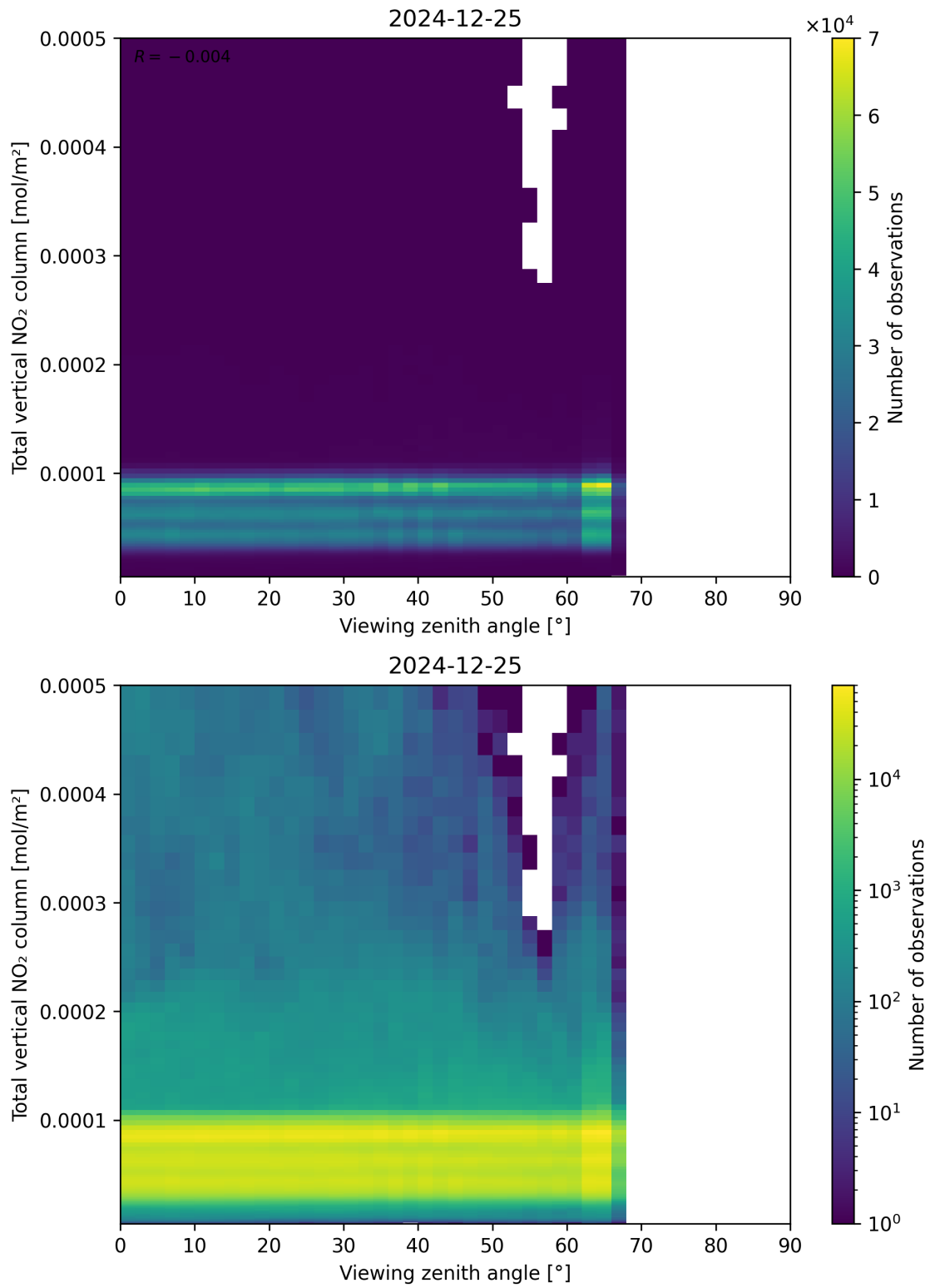
Figure 167: Scatter density plot of “Viewing zenith angle” against “Total vertical NO 2 column” for 2024-12-24 to 2024-12-26.
