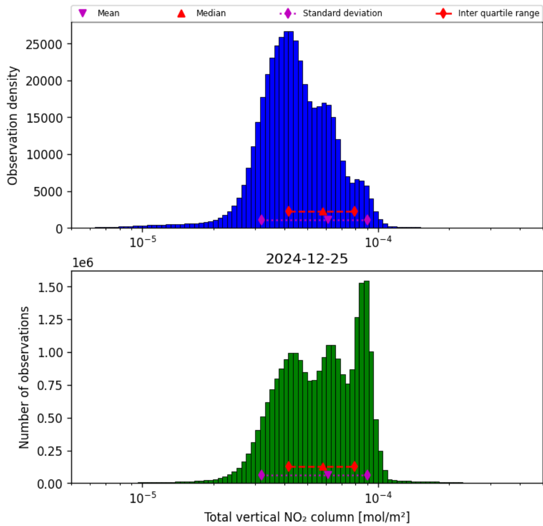
Figure 38: Histogram of “Total vertical NO 2 column” for 2024-12-24 to 2024-12-26
