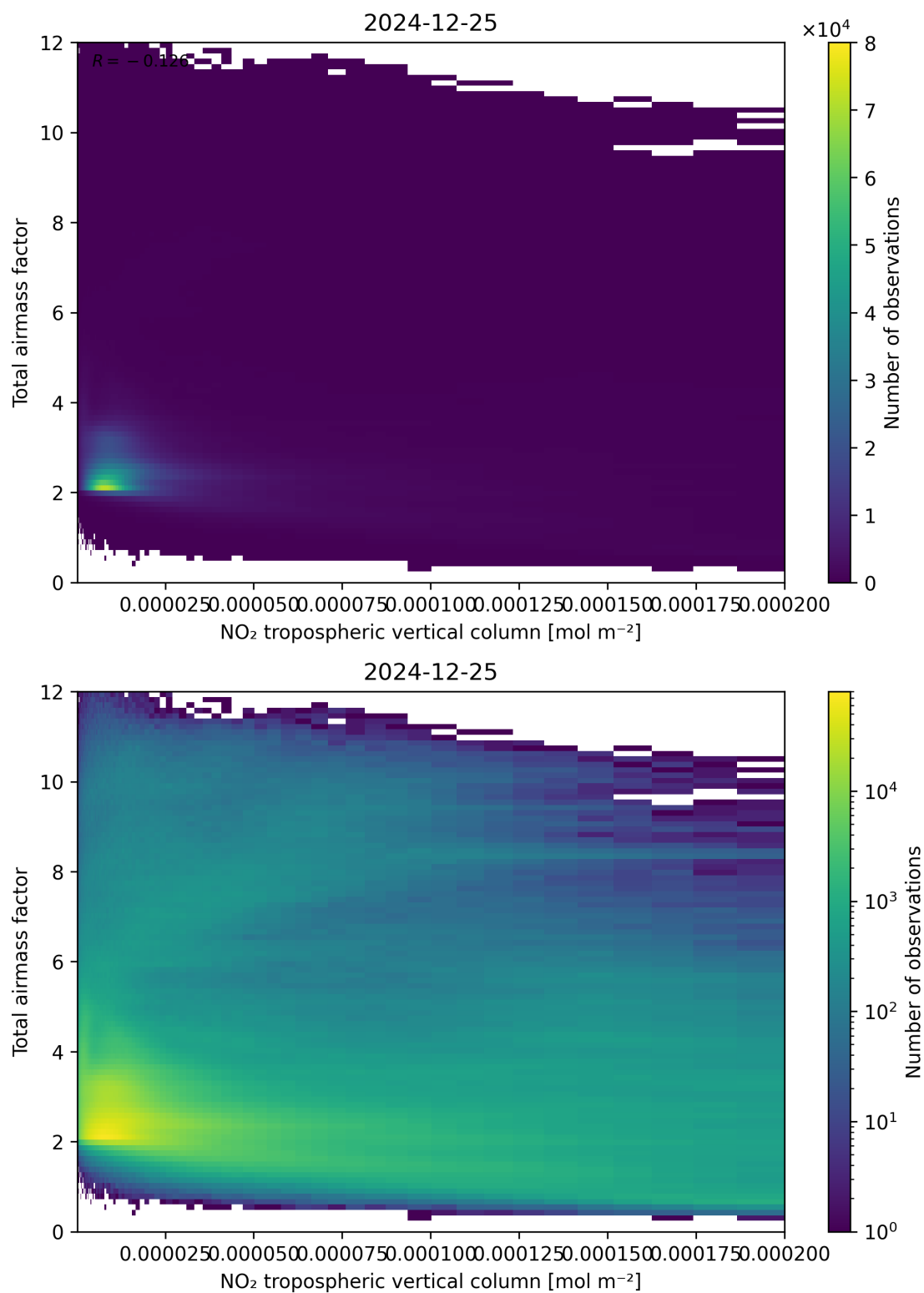
Figure 122: Scatter density plot of “NO 2 tropospheric vertical column” against “Total air mass factor” for 2024-12-24 to 2024-12-26.
