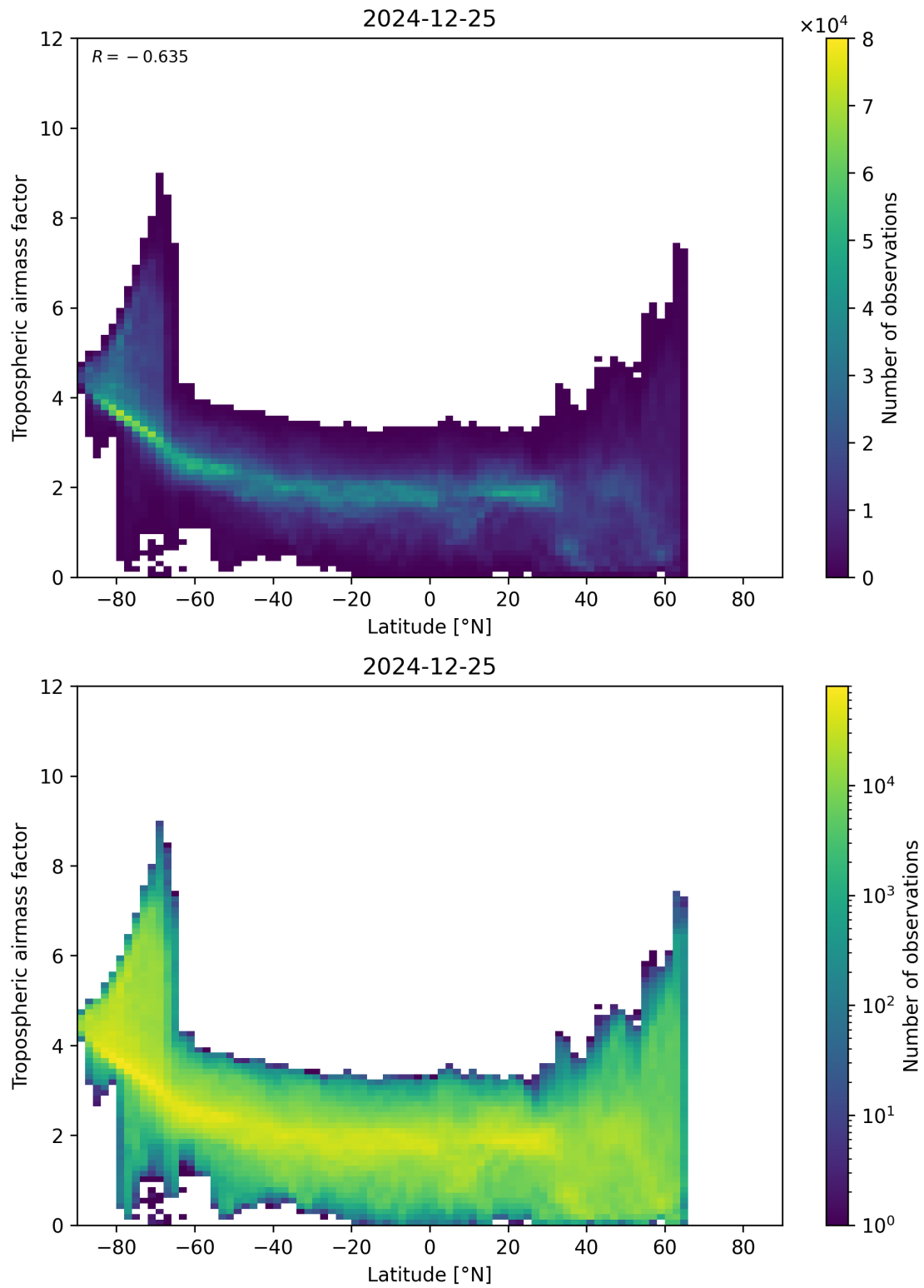
Figure 85: Scatter density plot of “Latitude” against “Tropospheric airmass factor” for 2024-12-24 to 2024-12-26.
