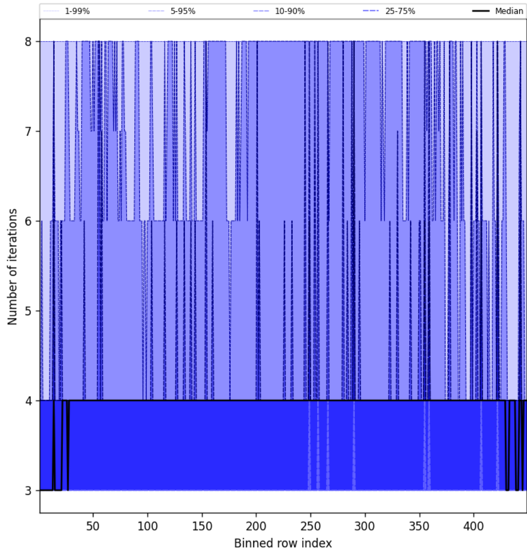
Figure 51: Along track statistics of “Number of iterations” for 2024-12-24 to 2024-12-26
