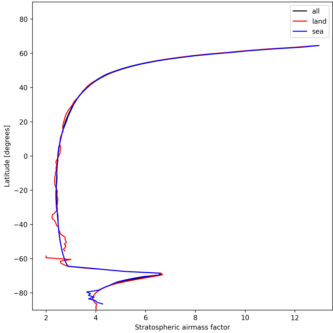
Figure 27: Zonal average of “Stratospheric airmass factor” for 2024-12-24 to 2024-12-26.
