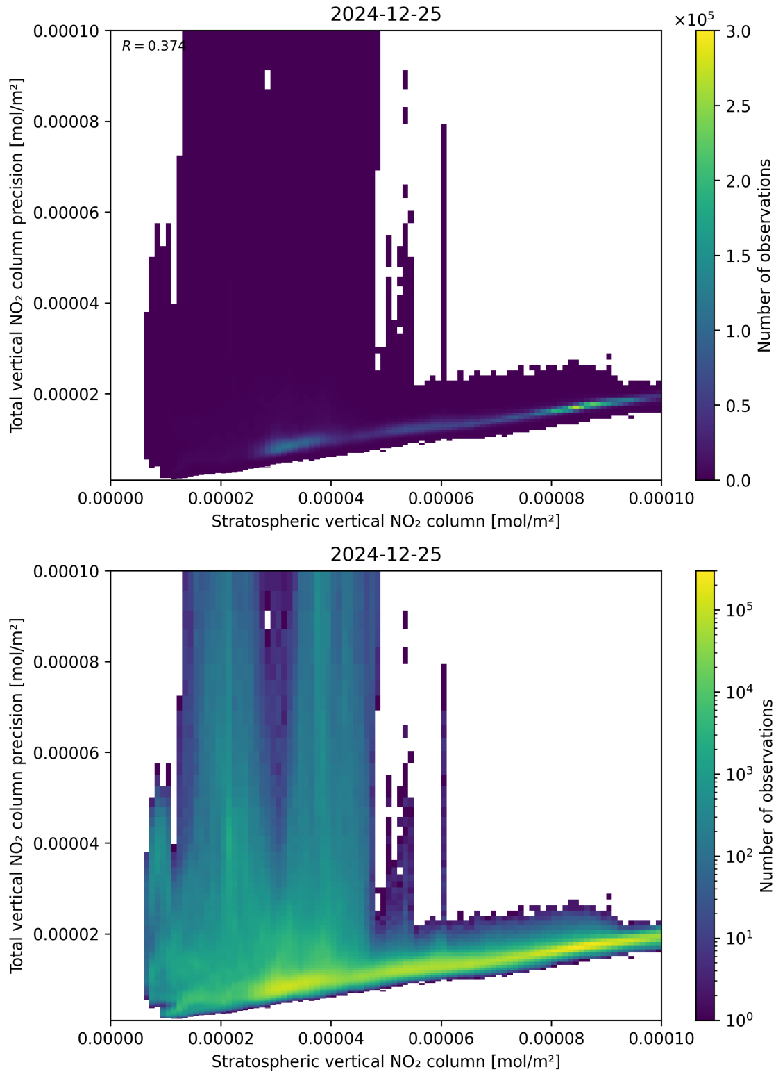
Figure 101: Scatter density plot of “Stratospheric vertical NO 2 column” against “Total vertical NO 2 column precision” for 2024-12-24 to 2024-12-26.
