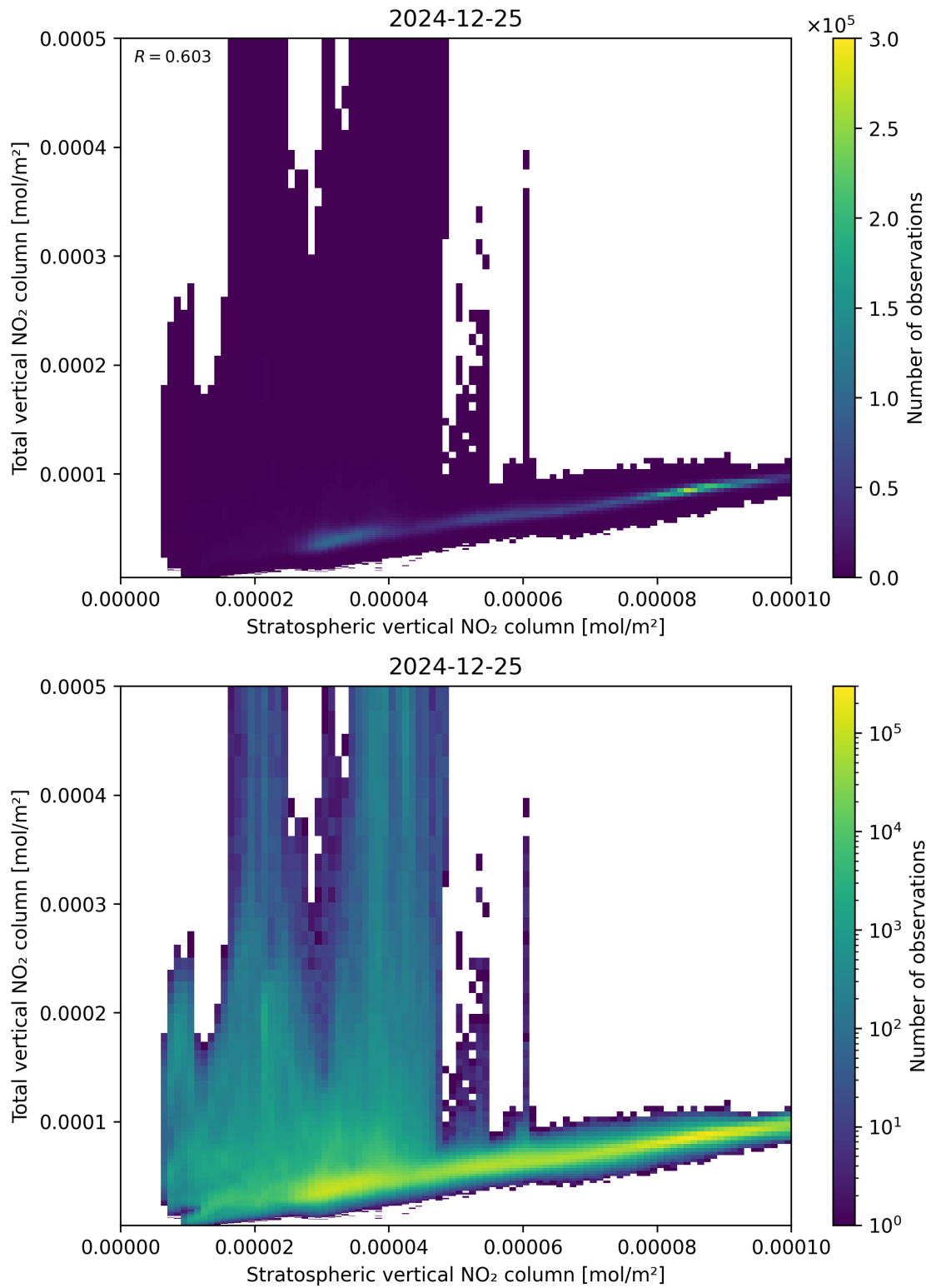
Figure 100: Scatter density plot of “Stratospheric vertical NO 2 column” against “Total vertical NO 2 column” for 2024-12-24 to 2024-12-26.
