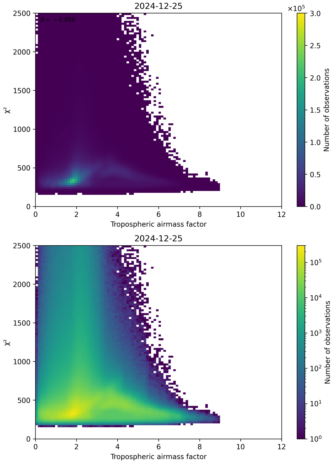
Figure 73: Scatter density plot of “Tropospheric airmass factor” against “ \chi^2 ” for 2024-12-24 to 2024-12-26.
