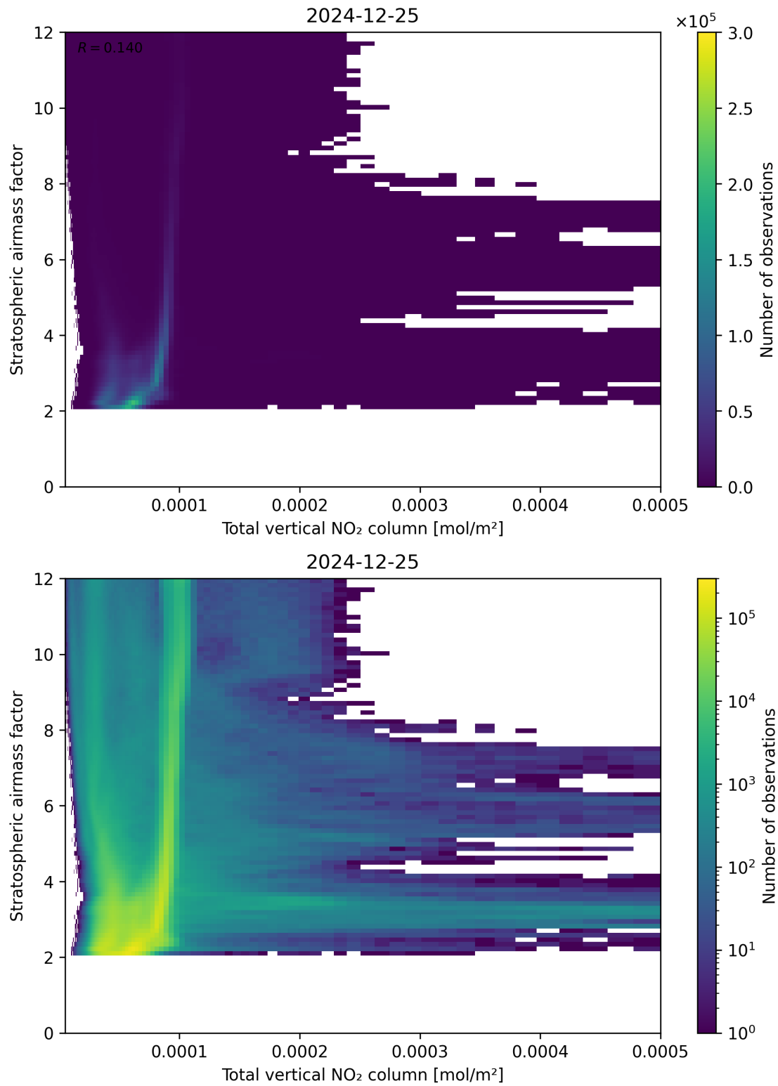
Figure 110: Scatter density plot of “Total vertical NO 2 column” against “Stratospheric airmass factor” for 2024-12-24 to 2024-12-26.
