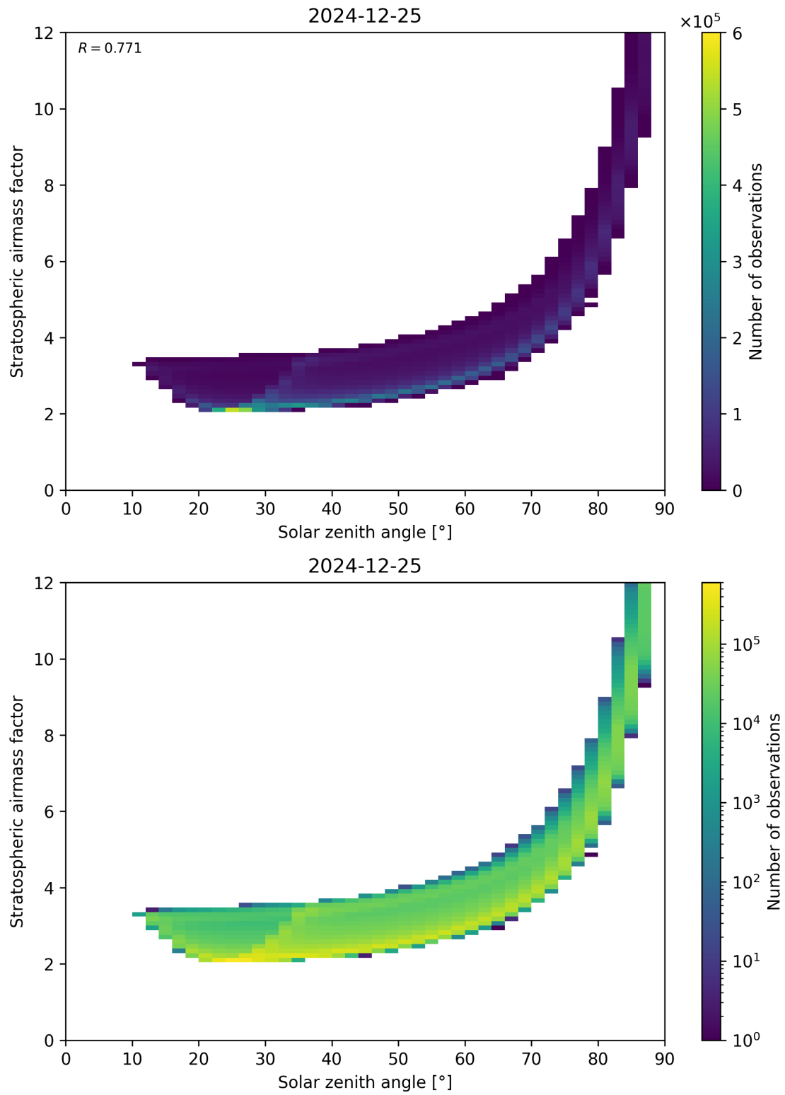
Figure 145: Scatter density plot of “Solar zenith angle” against “Stratospheric airmass factor” for 2024-12-24 to 2024-12-26.
