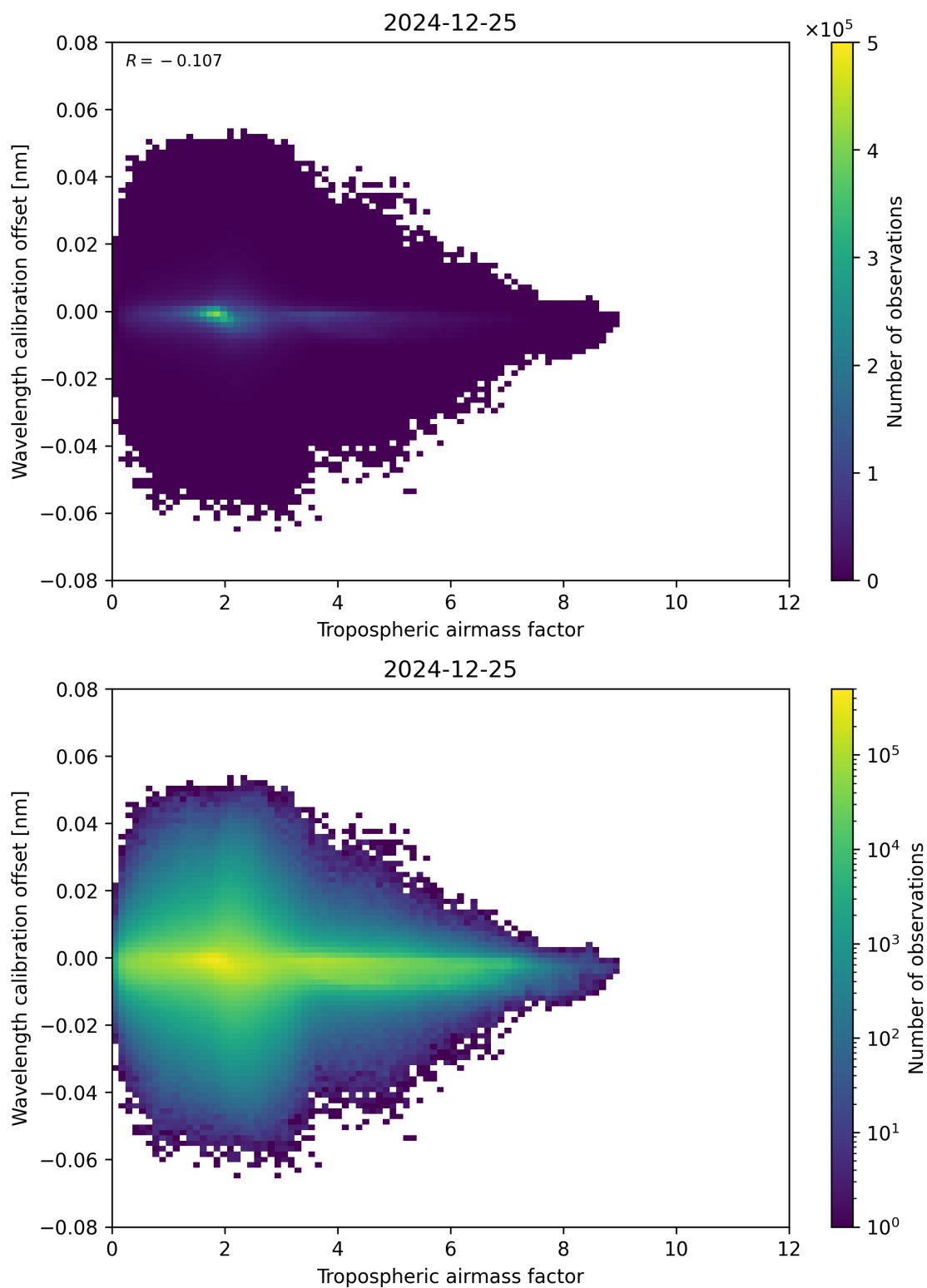
Figure 80: Scatter density plot of “Tropospheric airmass factor” against “Wavelength calibration offset” for 2024-12-24 to 2024-12-26.
