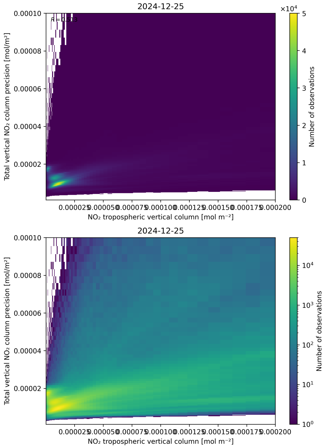
Figure 129: Scatter density plot of “NO 2 tropospheric vertical column” against “Total vertical NO 2 column precision” for 2024-12-24 to 2024-12-26.
