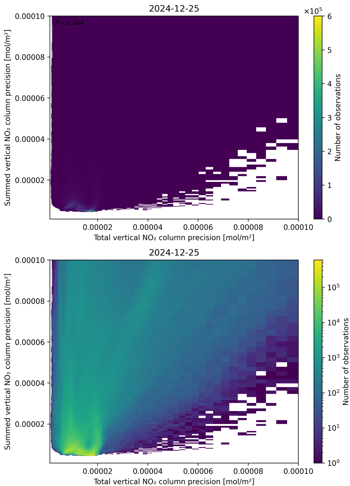
Figure 118: Scatter density plot of “Total vertical NO 2 column precision” against “Summed vertical NO 2 column precision” for 2024-12-24 to 2024-12-26.
