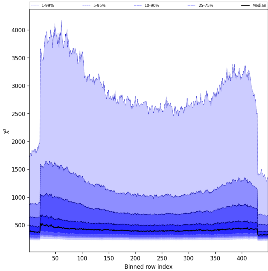
Figure 59: Along track statistics of “ \chi^2 ” for 2024-12-24 to 2024-12-26
