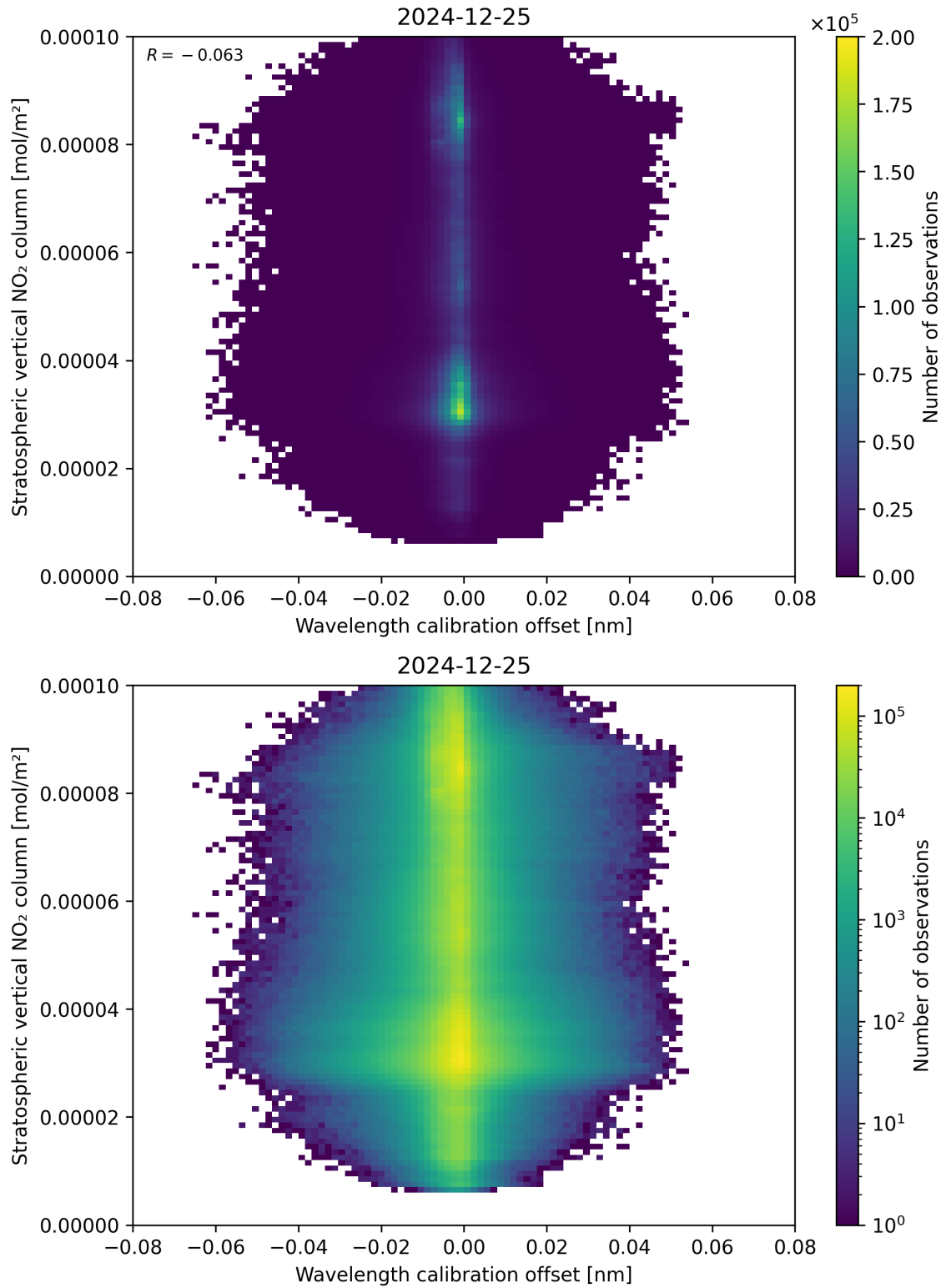
Figure 176: Scatter density plot of “Wavelength calibration offset” against “Stratospheric vertical NO 2 column” for 2024-12-24 to 2024-12-26.
