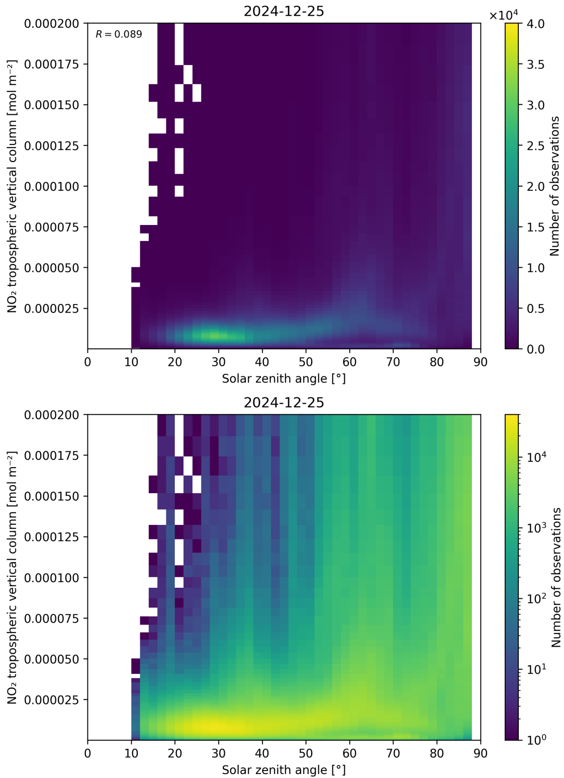
Figure 155: Scatter density plot of “Solar zenith angle” against “NO 2 tropospheric vertical column” for 2024-12-24 to 2024-12-26.
