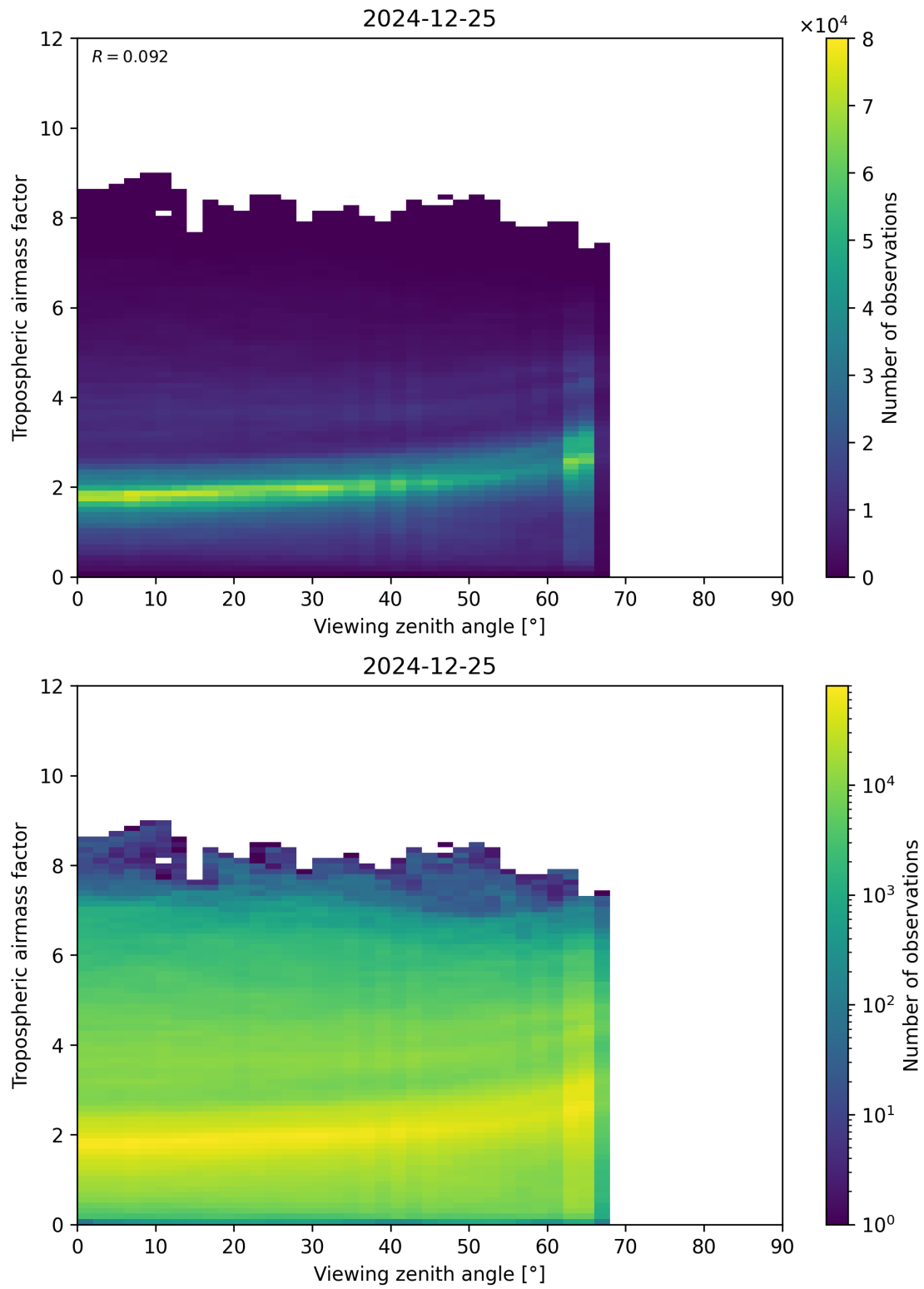
Figure 161: Scatter density plot of “Viewing zenith angle” against “Tropospheric airmass factor” for 2024-12-24 to 2024-12-26.
