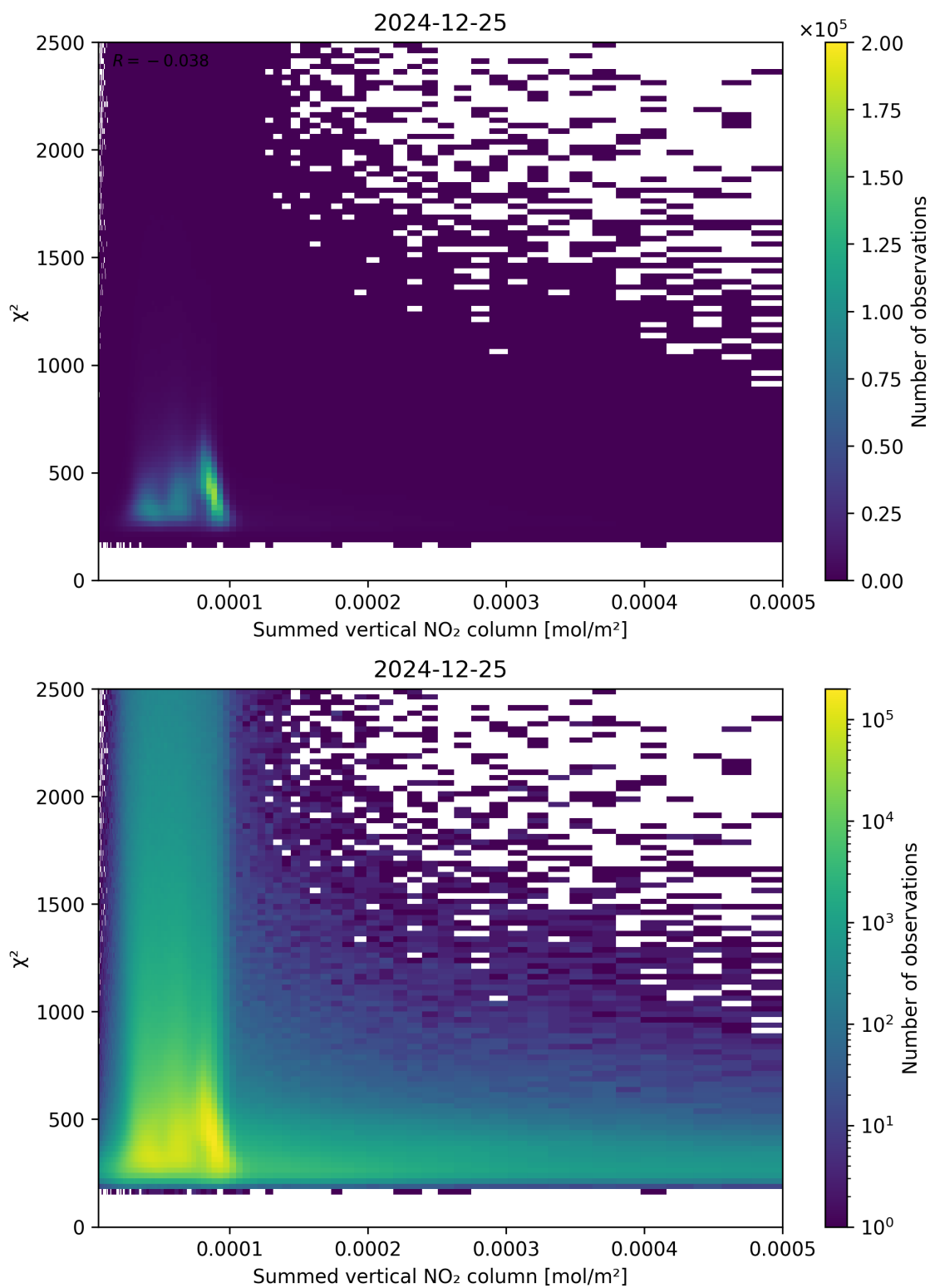
Figure 104: Scatter density plot of “Summed vertical NO 2 column” against “ \chi^2 ” for 2024-12-24 to 2024-12-26.
