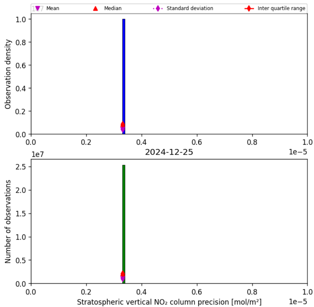
Figure 37: Histogram of “Stratospheric vertical NO 2 column precision” for 2024-12-24 to 2024-12-26
