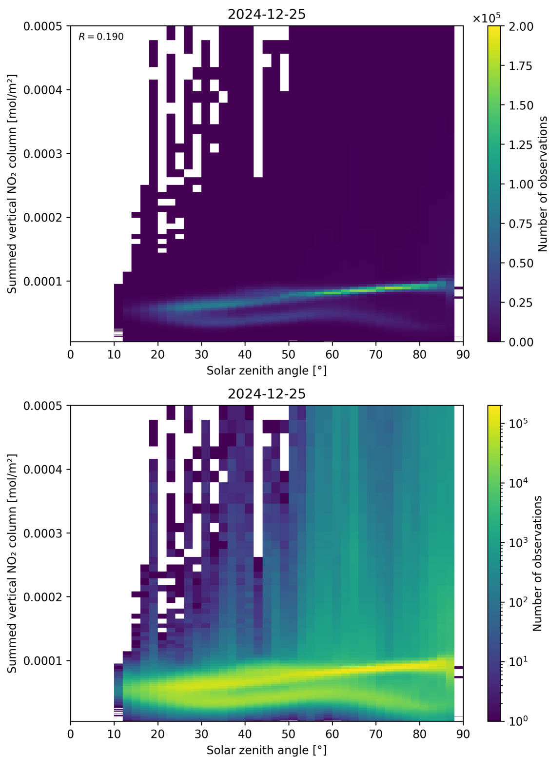
Figure 151: Scatter density plot of “Solar zenith angle” against “Summed vertical NO 2 column” for 2024-12-24 to 2024-12-26.
