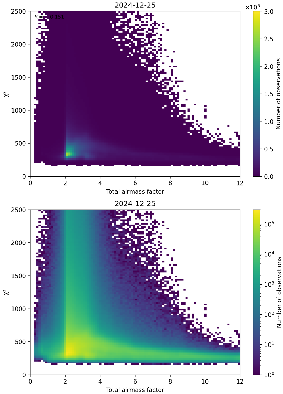
Figure 63: Scatter density plot of “Total airmass factor” against “ \chi^2 ” for 2024-12-24 to 2024-12-26.
