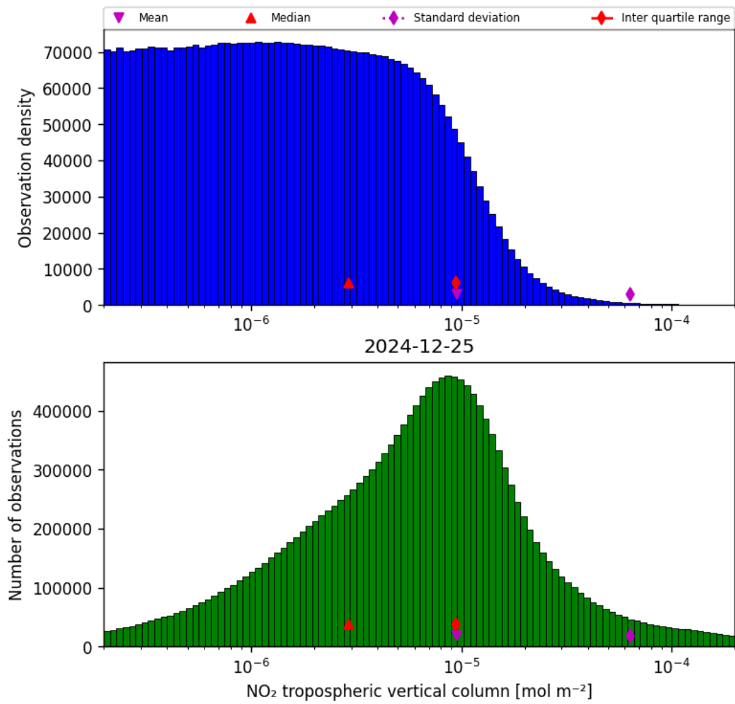
Figure 29: Histogram of “NO 2 tropospheric vertical column” for 2024-12-24 to 2024-12-26
