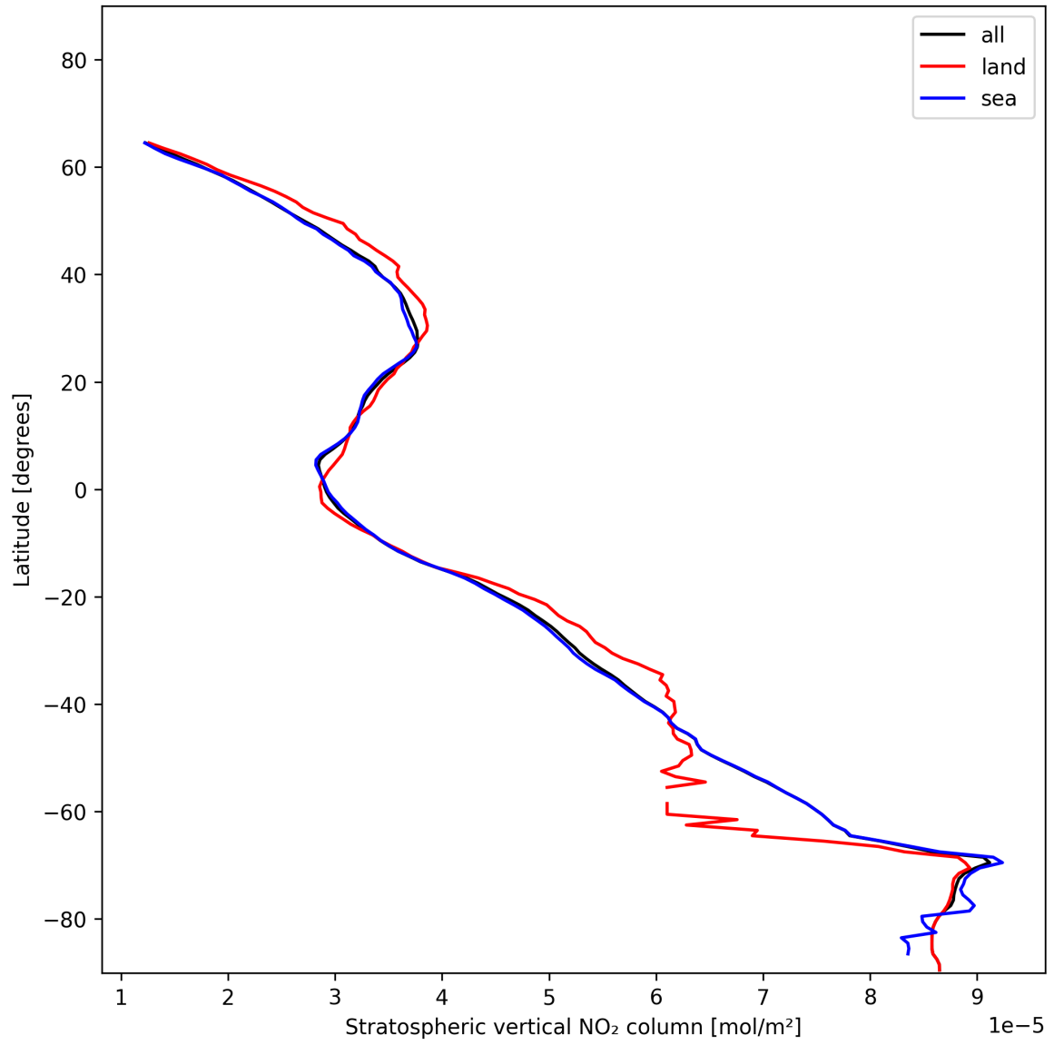
Figure 19: Zonal average of “Stratospheric vertical NO 2 column” for 2024-12-24 to 2024-12-26.
