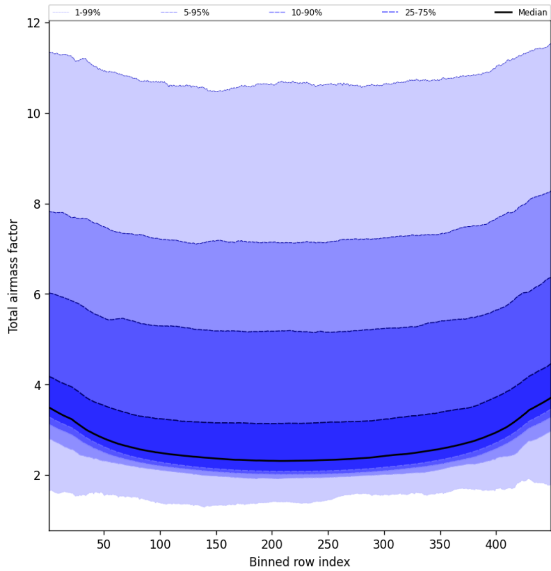
Figure 49: Along track statistics of “Total airmass factor” for 2024-12-24 to 2024-12-26
