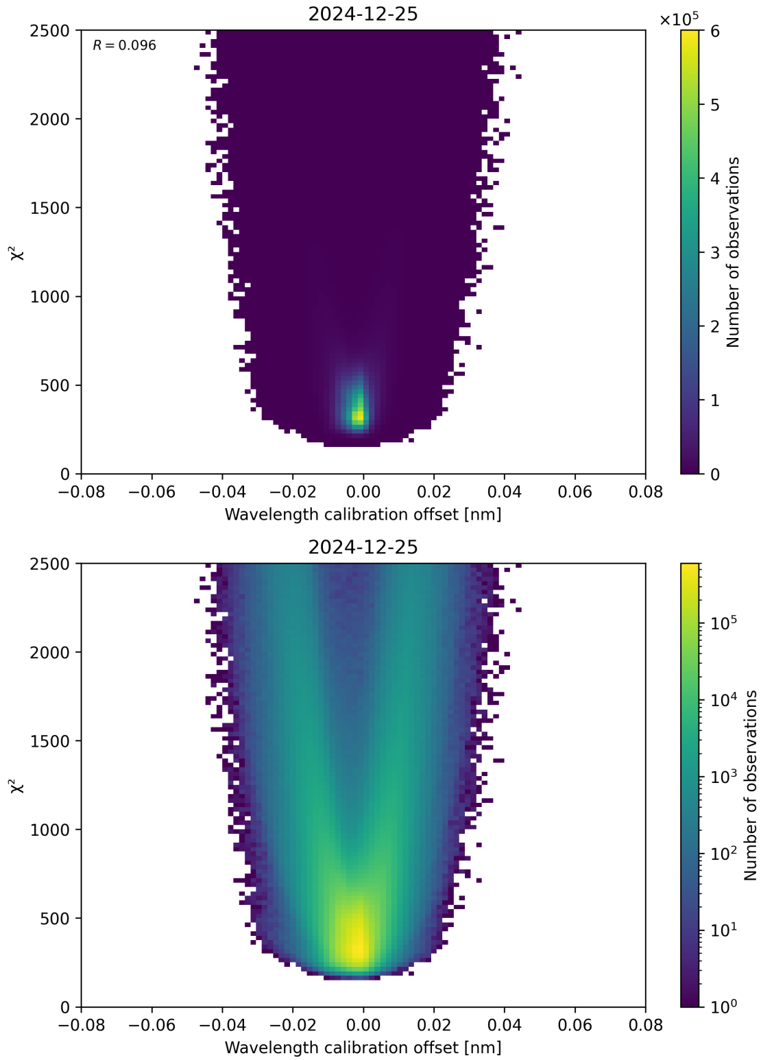
Figure 175: Scatter density plot of “Wavelength calibration offset” against “ \chi^2 ” for 2024-12-24 to 2024-12-26.
