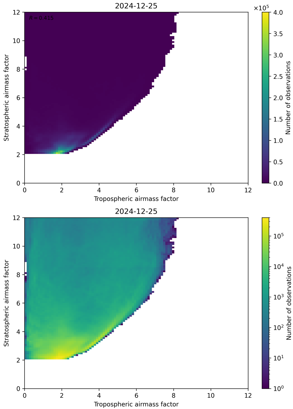
Figure 71: Scatter density plot of “Tropospheric airmass factor” against “Stratospheric airmass factor” for 2024-12-24 to 2024-12-26.
