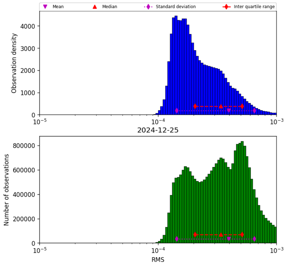
Figure 43: Histogram of “RMS” for 2024-12-24 to 2024-12-26
