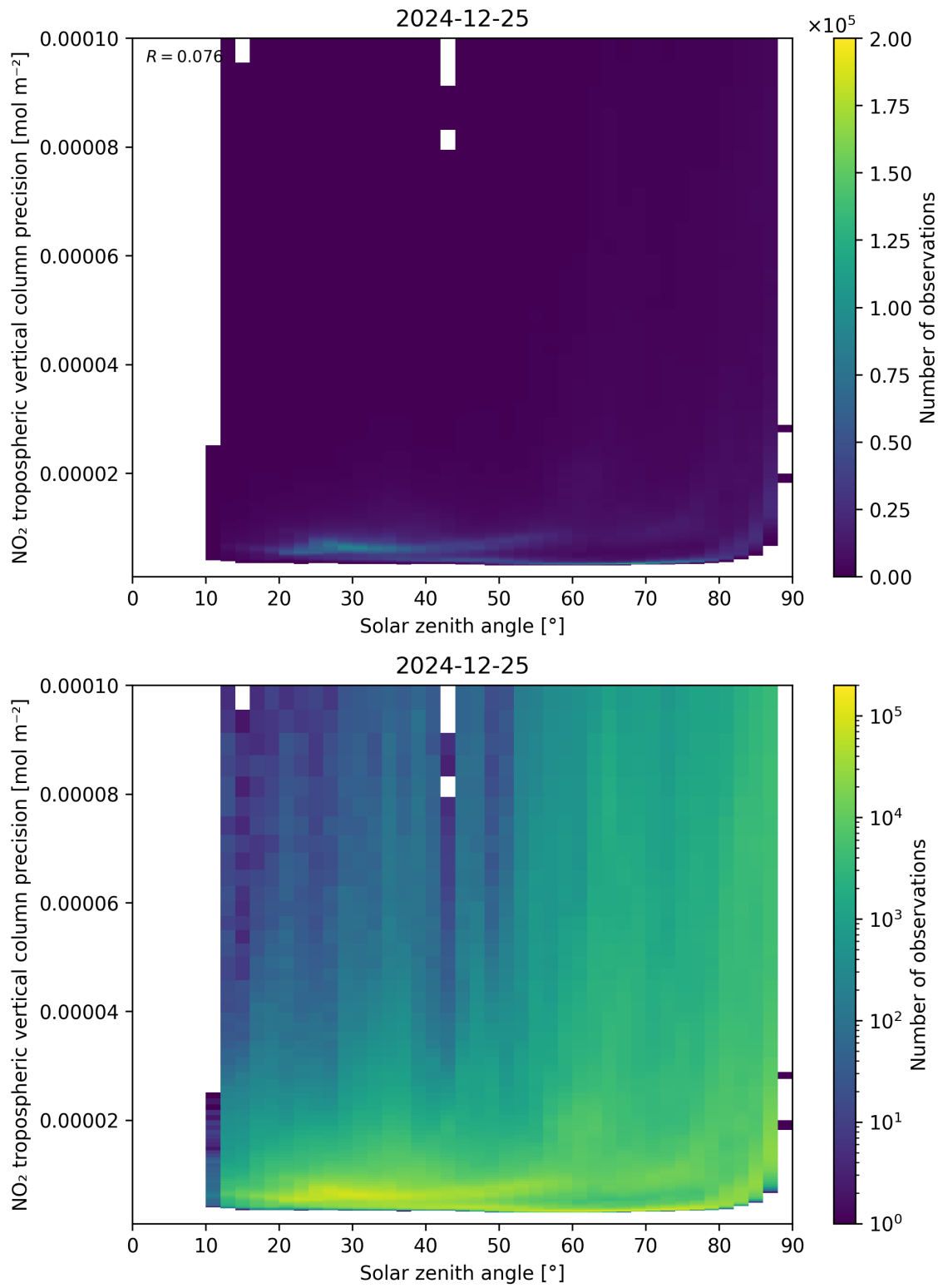
Figure 156: Scatter density plot of “Solar zenith angle” against “NO 2 tropospheric vertical column precision” for 2024-12-24 to 2024-12-26.
