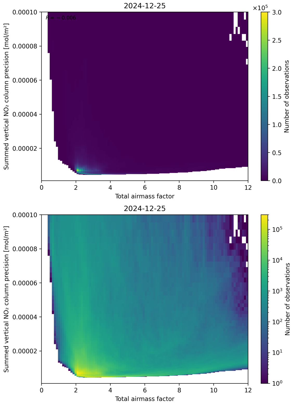
Figure 66: Scatter density plot of “Total airmass factor” against “Summed vertical NO 2 column precision” for 2024-12-24 to 2024-12-26.
