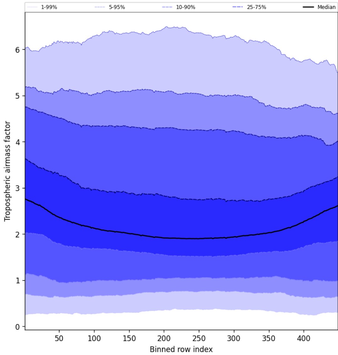
Figure 48: Along track statistics of “Tropospheric airmass factor” for 2024-12-24 to 2024-12-26
