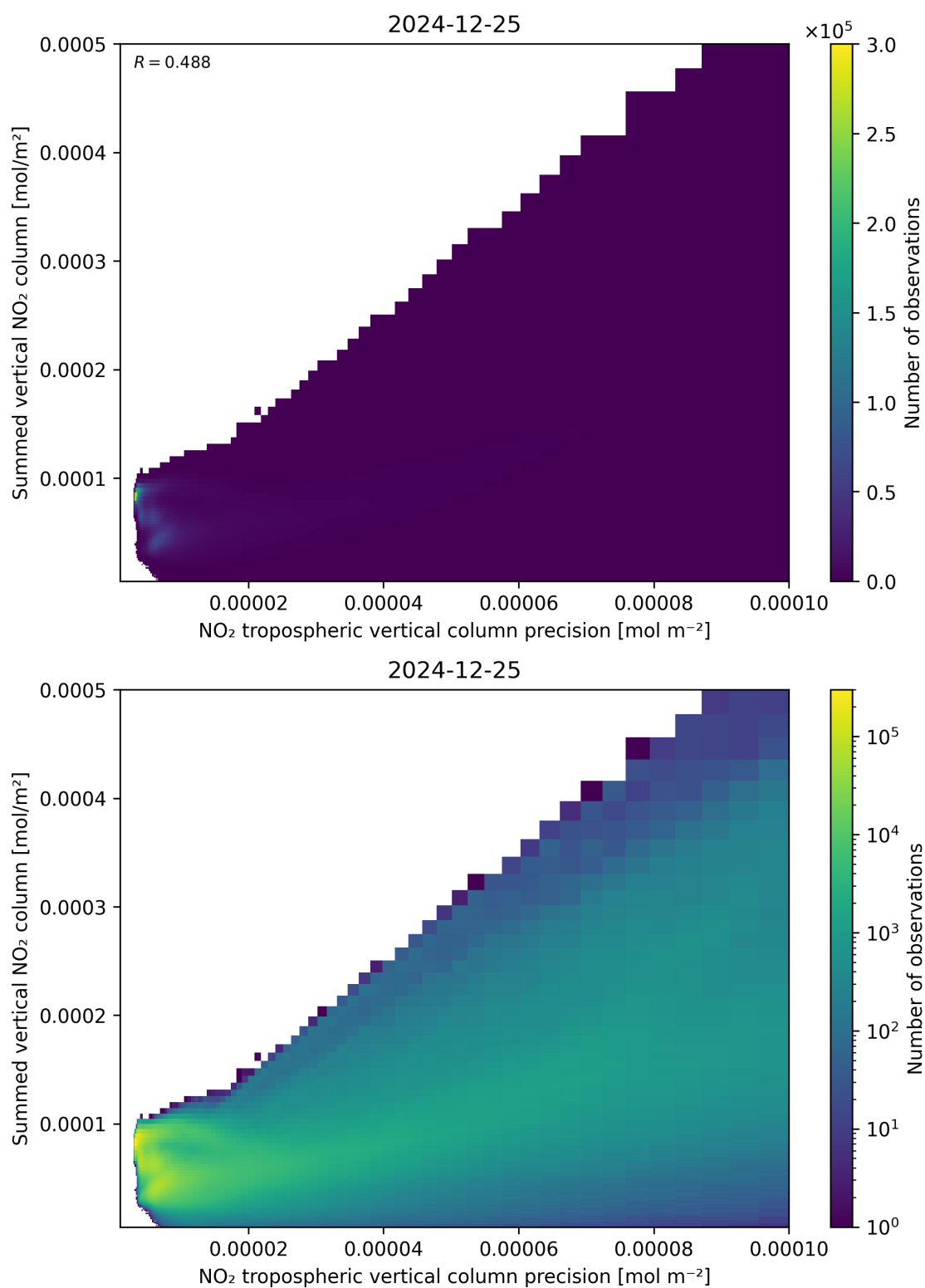
Figure 136: Scatter density plot of “NO 2 tropospheric vertical column precision” against “Summed vertical NO 2 column” for 2024-12-24 to 2024-12-26.
