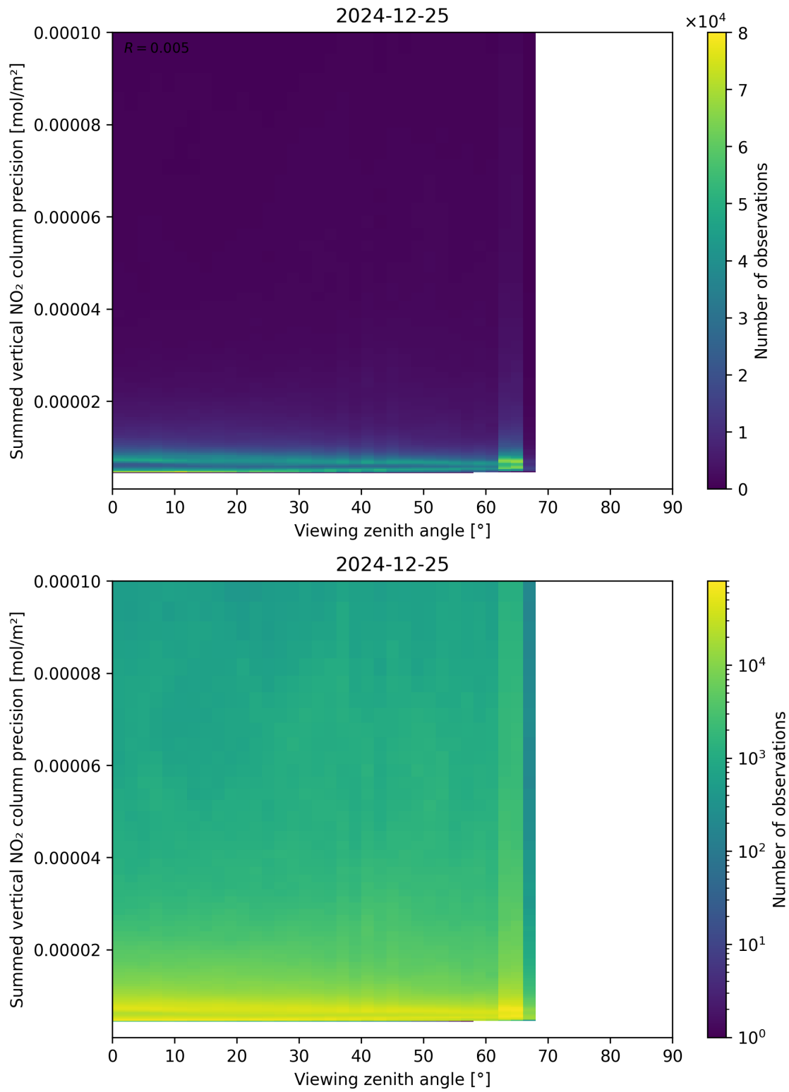
Figure 166: Scatter density plot of “Viewing zenith angle” against “Summed vertical NO 2 column precision” for 2024-12-24 to 2024-12-26.
