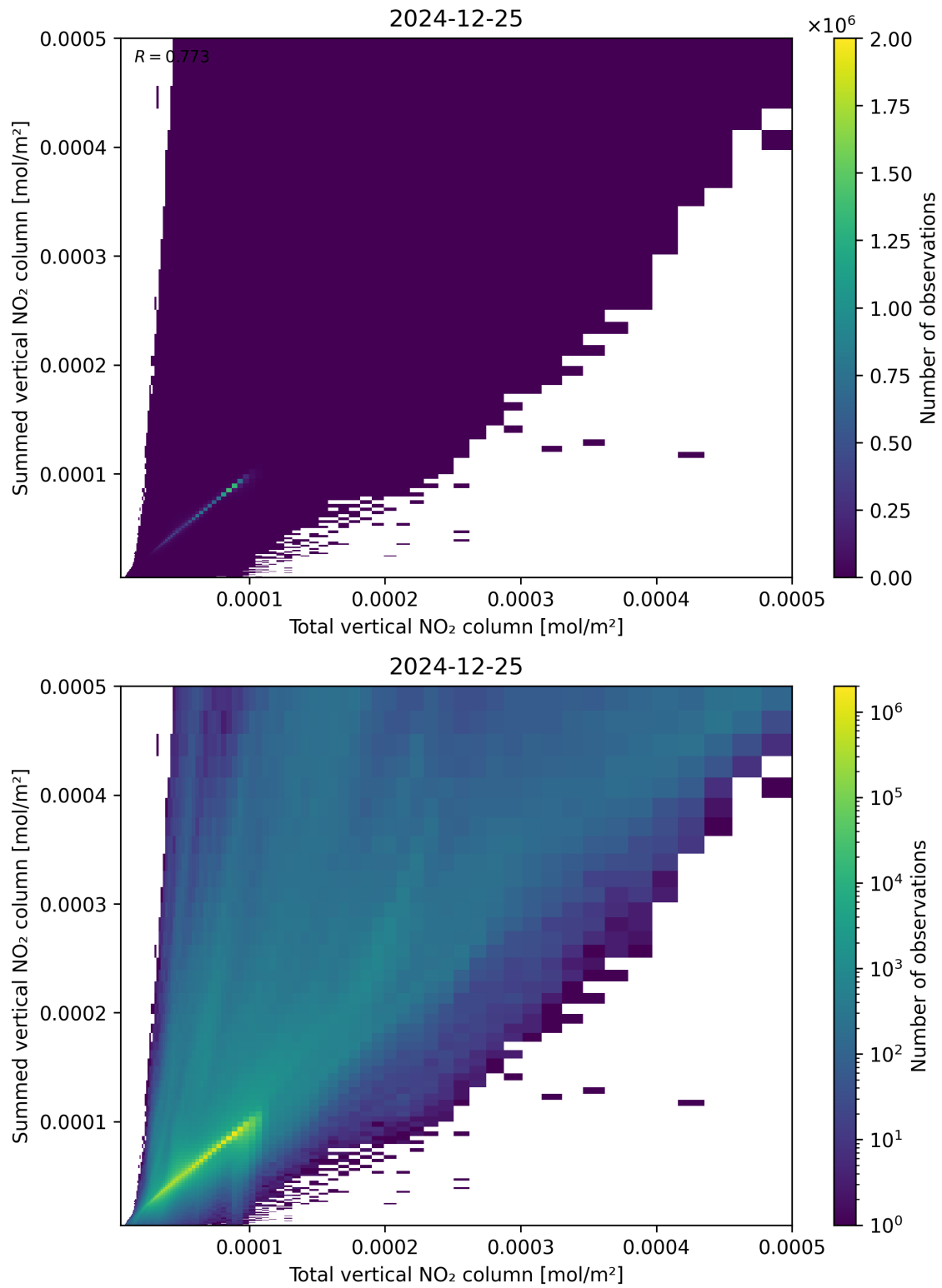
Figure 112: Scatter density plot of “Total vertical NO 2 column” against “Summed vertical NO 2 column” for 2024-12-24 to 2024-12-26.
