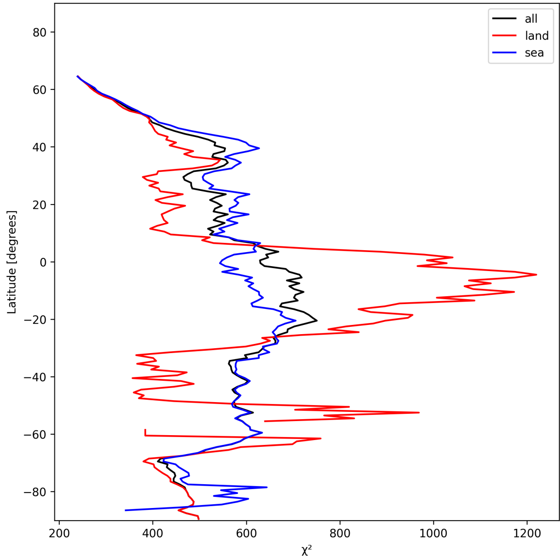
Figure 25: Zonal average of “ \chi^2 ” for 2024-12-24 to 2024-12-26.
