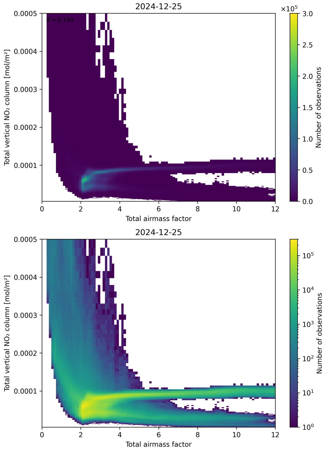
Figure 67: Scatter density plot of “Total airmass factor” against “Total vertical NO 2 column” for 2024-12-24 to 2024-12-26.
