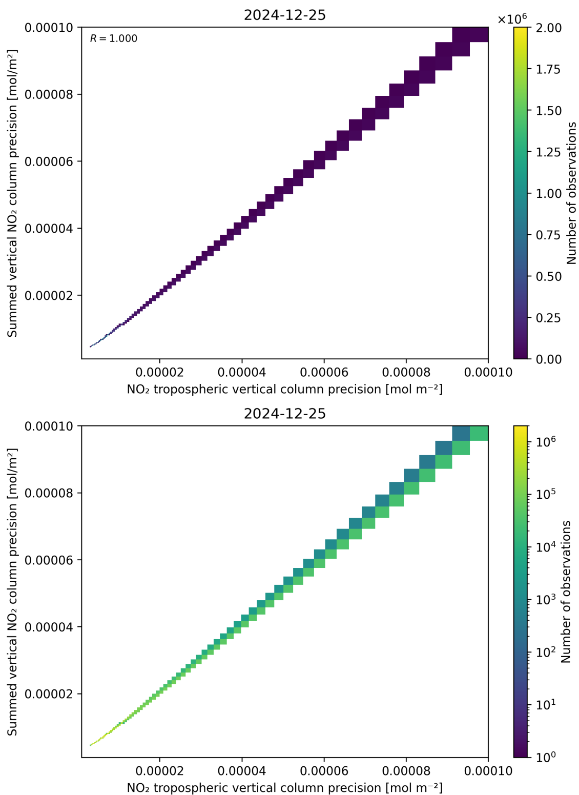
Figure 137: Scatter density plot of “NO 2 tropospheric vertical column precision” against “Summed vertical NO 2 column precision” for 2024-12-24 to 2024-12-26.
