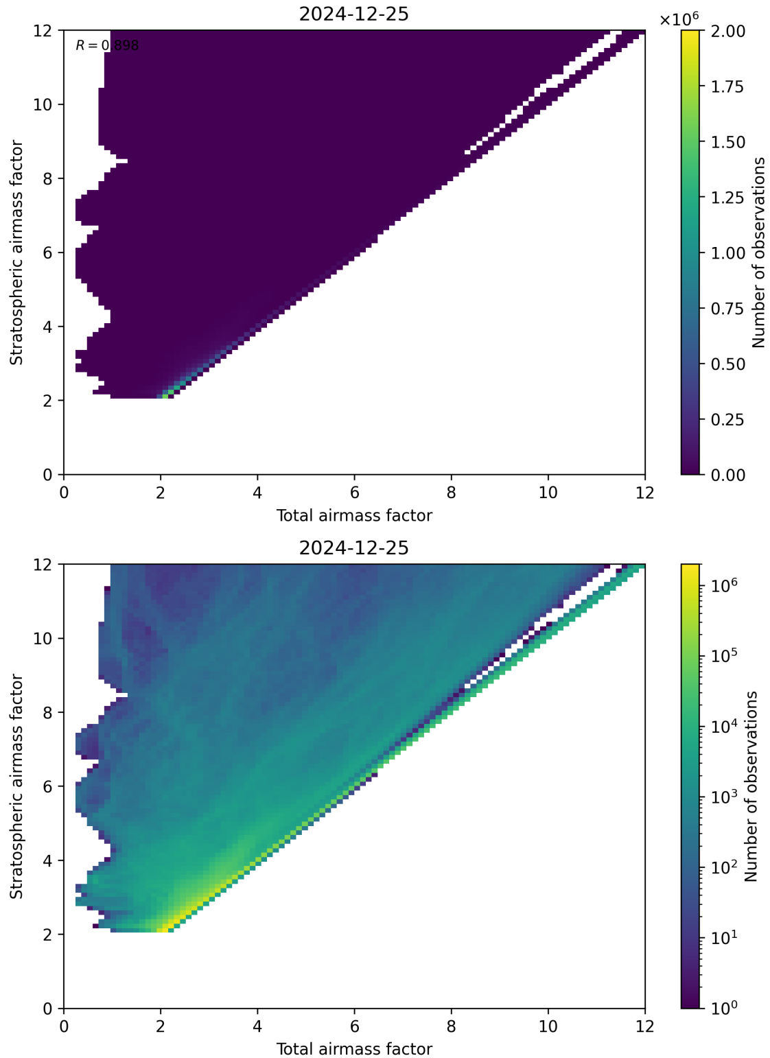
Figure 62: Scatter density plot of “Total airmass factor” against “Stratospheric airmass factor” for 2024-12-24 to 2024-12-26.
