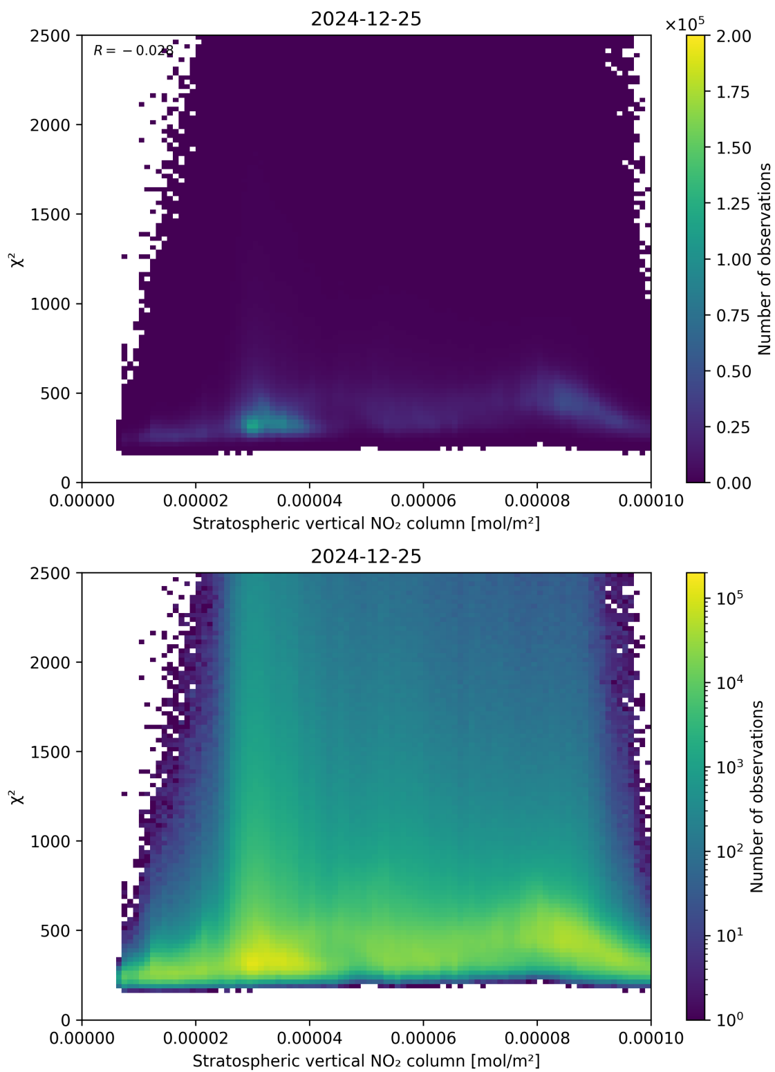
Figure 97: Scatter density plot of “Stratospheric vertical NO 2 column” against “ \chi^2 ” for 2024-12-24 to 2024-12-26.
