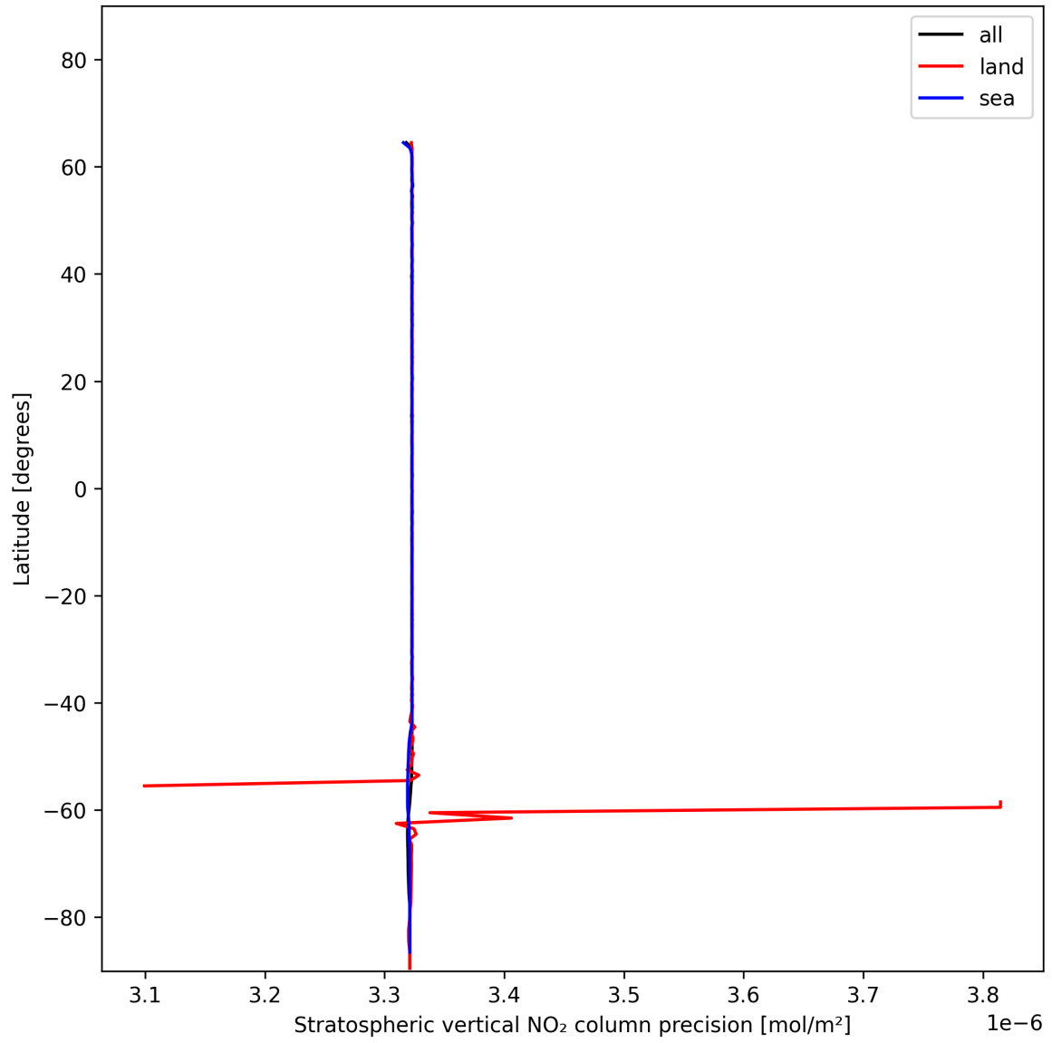
Figure 20: Zonal average of “Stratospheric vertical NO 2 column precision” for 2024-12-24 to 2024-12-26.
