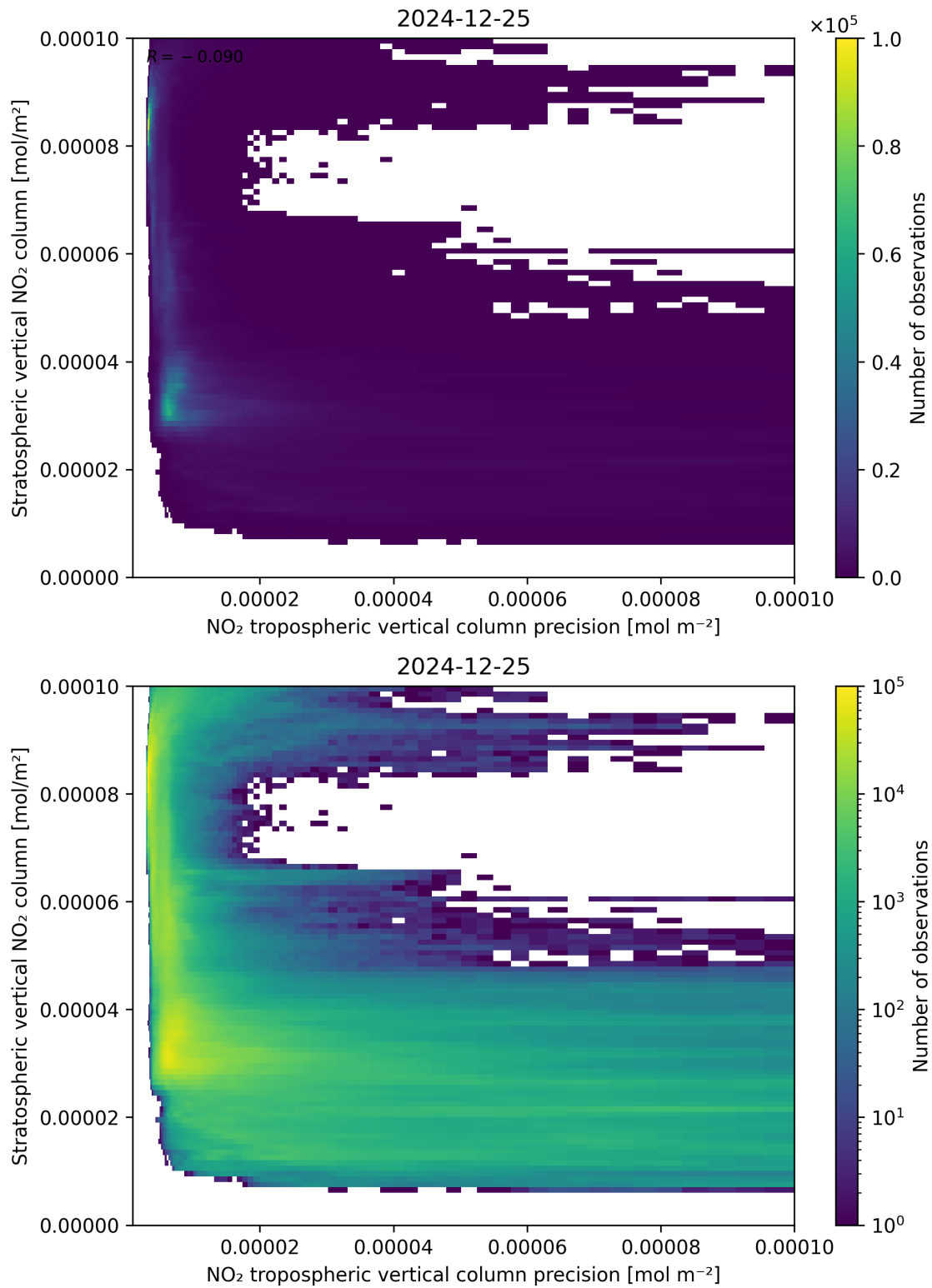
Figure 135: Scatter density plot of “NO 2 tropospheric vertical column precision” against “Stratospheric vertical NO 2 column” for 2024-12-24 to 2024-12-26.
