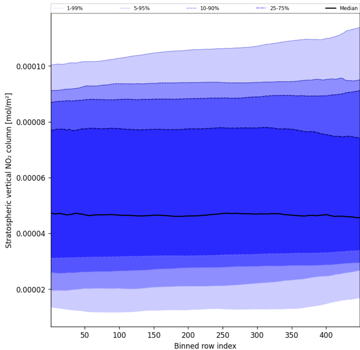
Figure 53: Along track statistics of “Stratospheric vertical NO 2 column” for 2024-12-24 to 2024-12-26
