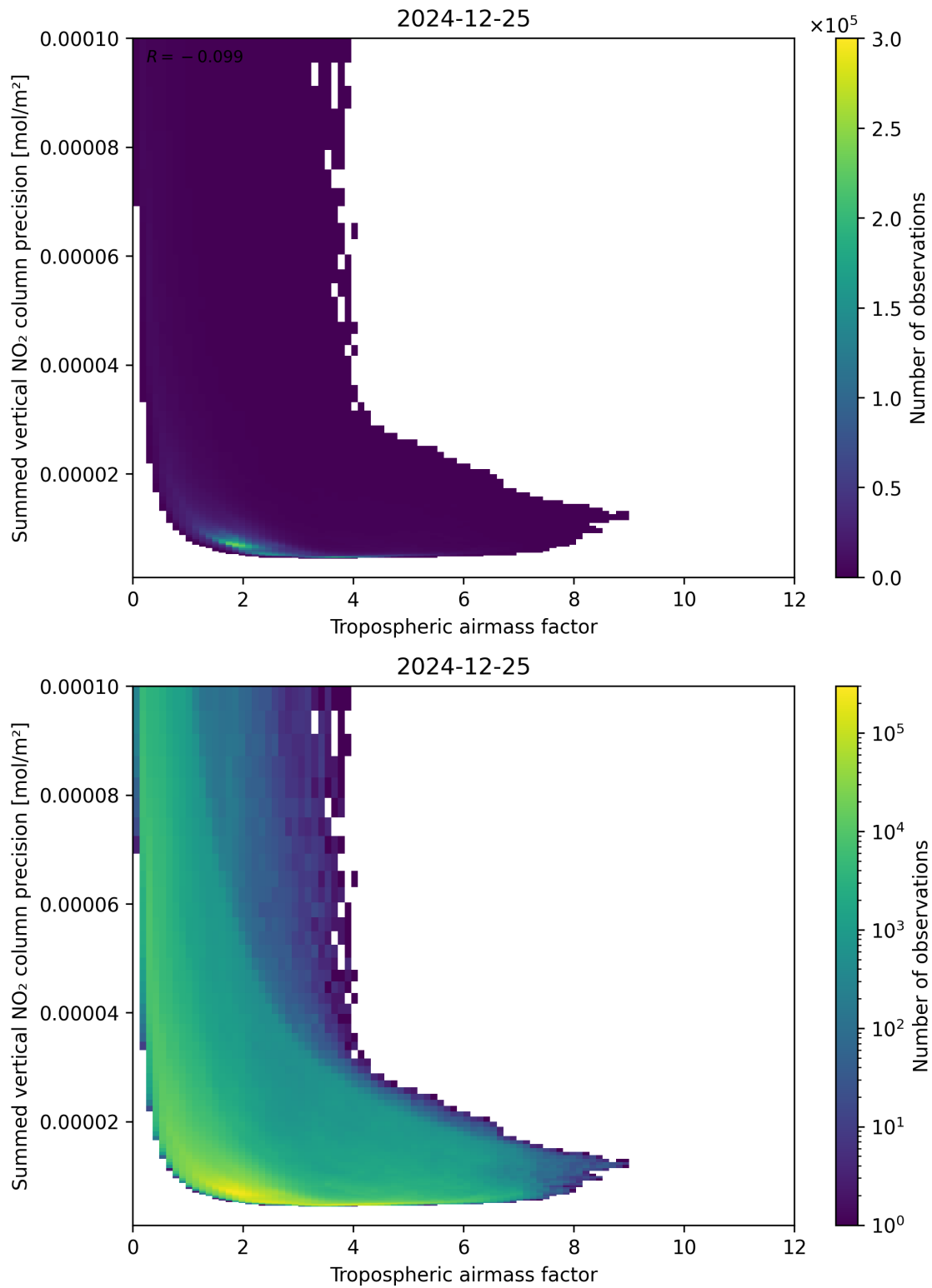
Figure 76: Scatter density plot of “Tropospheric air mass factor” against “Summed vertical NO 2 column precision” for 2024-12-24 to 2024-12-26.
