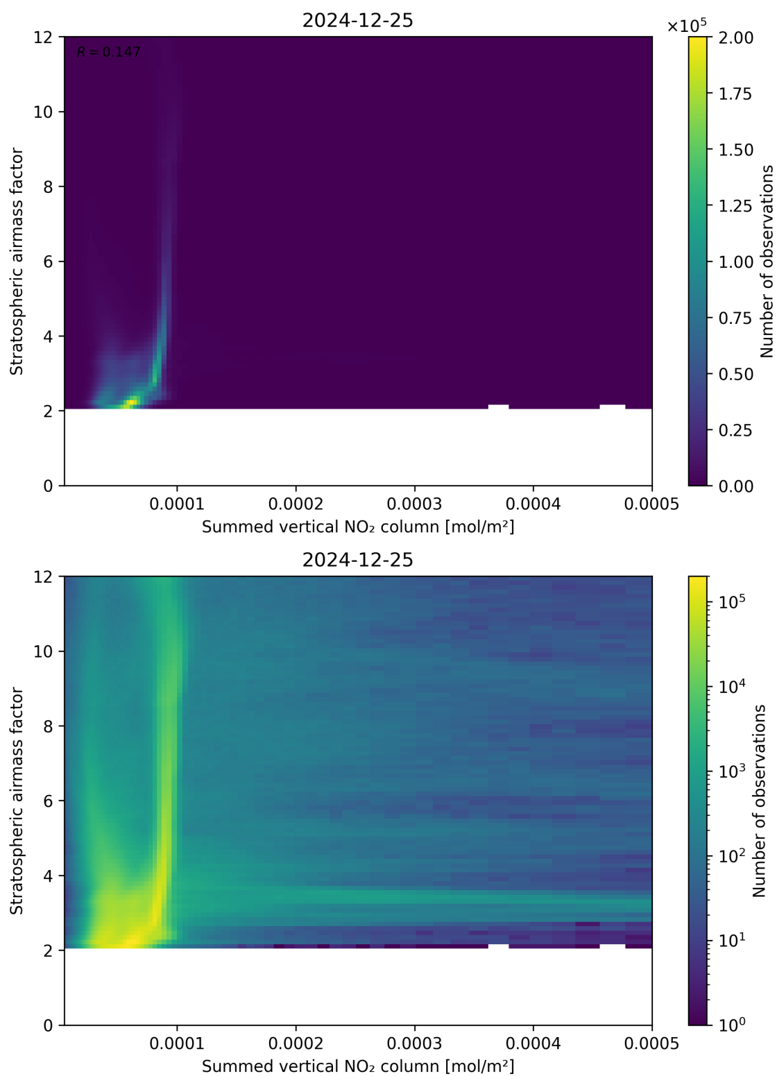
Figure 103: Scatter density plot of “Summed vertical NO 2 column” against “Stratospheric airmass factor” for 2024-12-24 to 2024-12-26.
