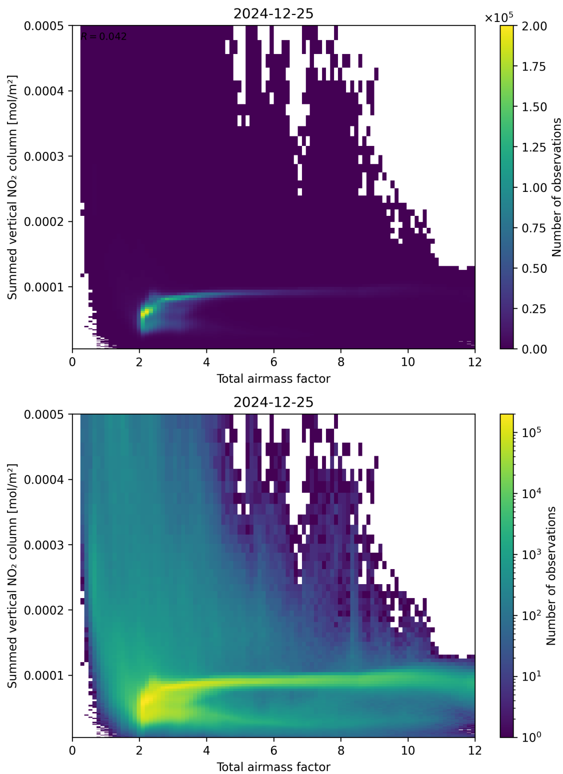
Figure 65: Scatter density plot of “Total airmass factor” against “Summed vertical NO 2 column” for 2024-12-24 to 2024-12-26.
