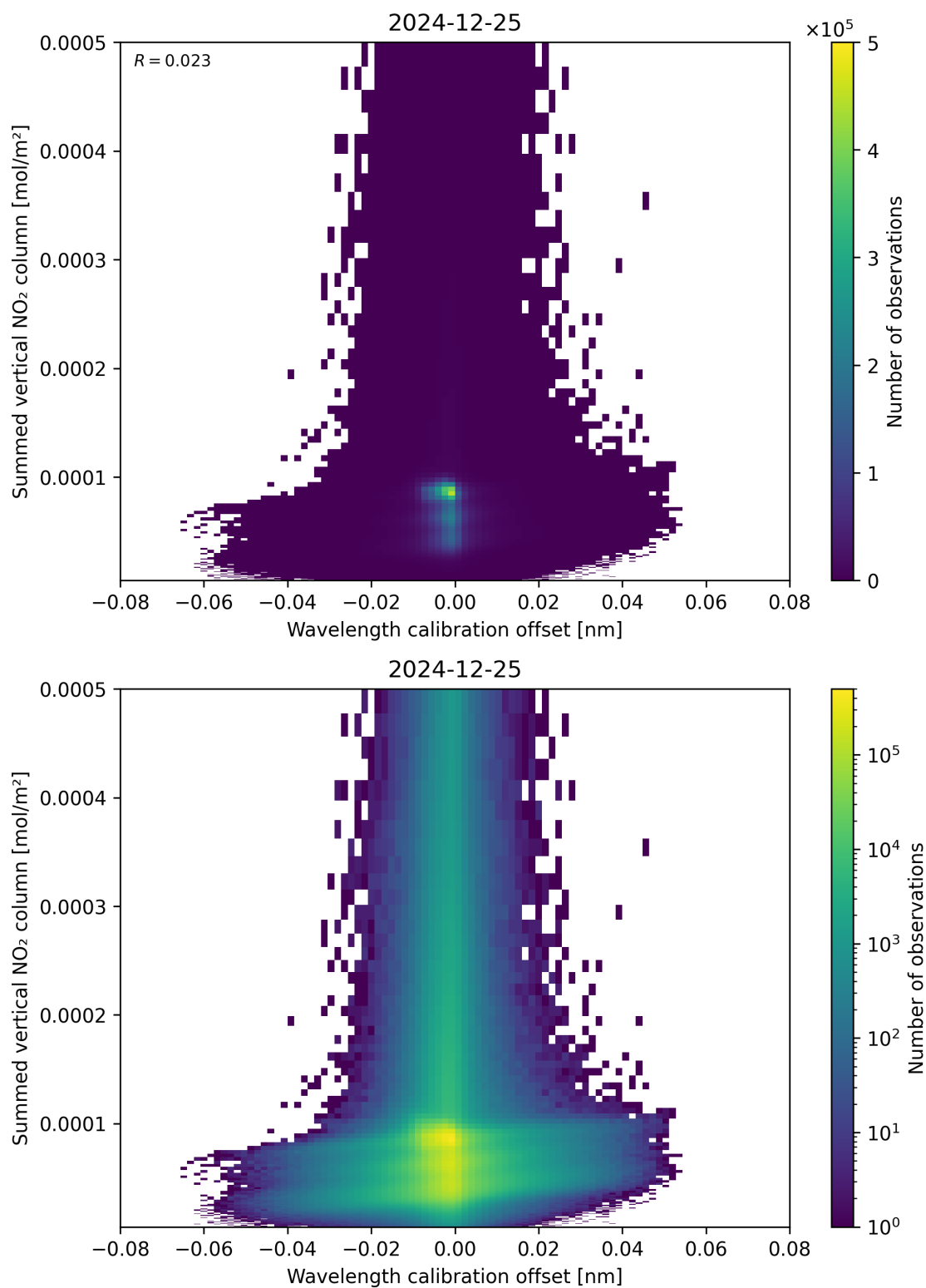
Figure 177: Scatter density plot of “Wavelength calibration offset” against “Summed vertical NO 2 column” for 2024-12-24 to 2024-12-26.
