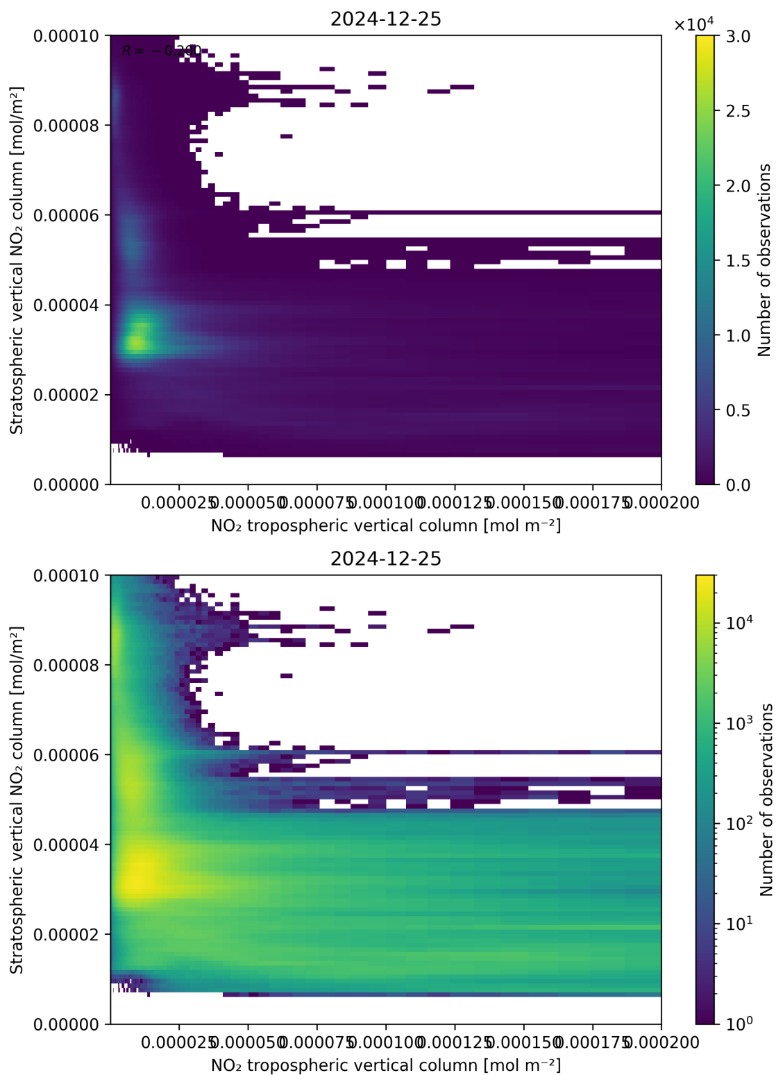
Figure 125: Scatter density plot of “NO 2 tropospheric vertical column” against “Stratospheric vertical NO 2 column” for 2024-12-24 to 2024-12-26.
