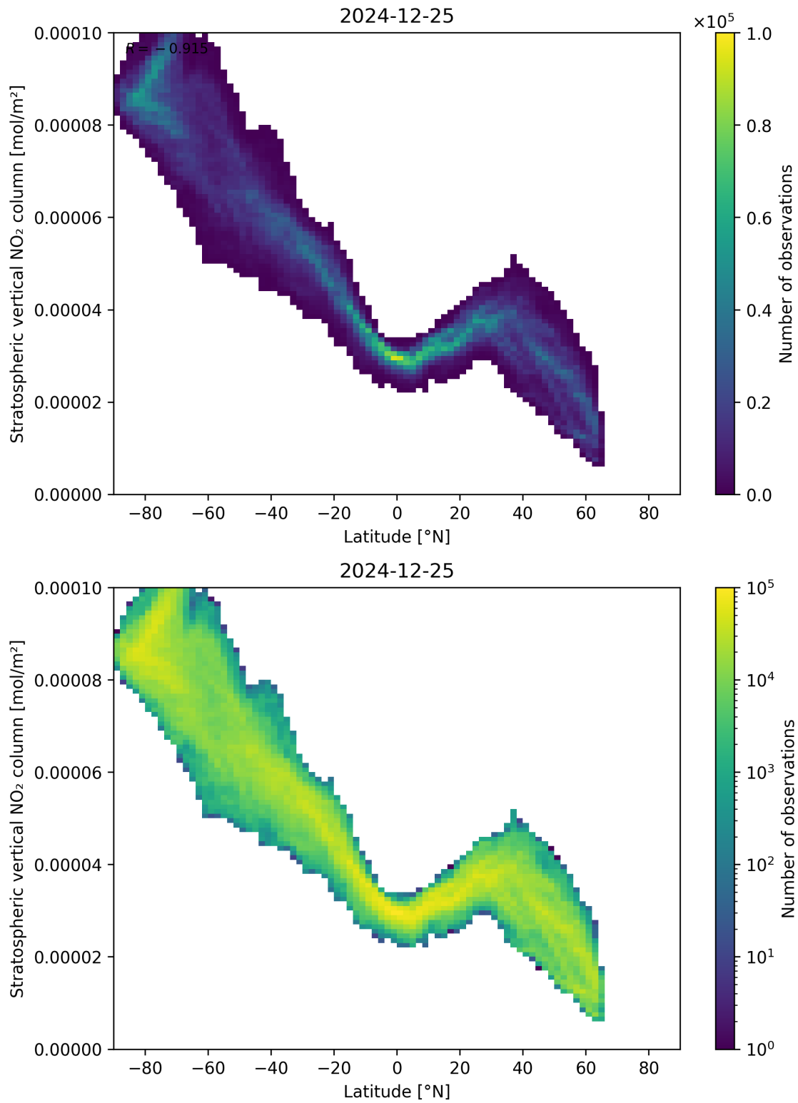
Figure 87: Scatter density plot of “Latitude” against “Stratospheric vertical NO 2 column” for 2024-12-24 to 2024-12-26.
