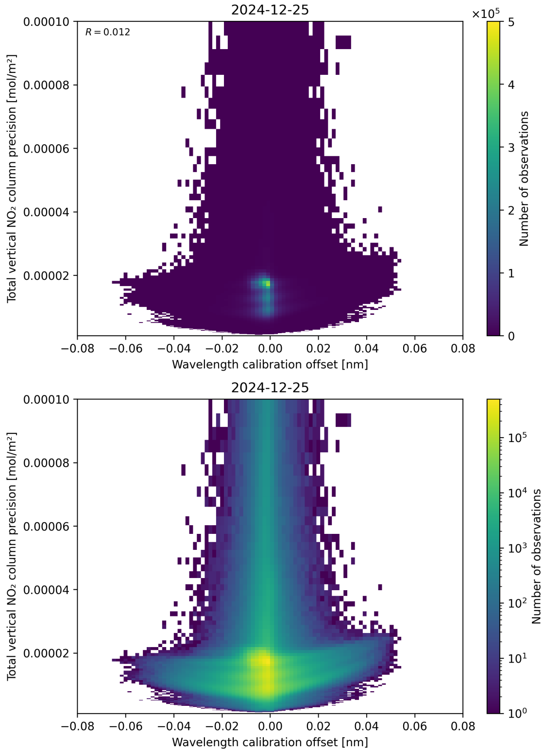
Figure 180: Scatter density plot of “Wavelength calibration offset” against “Total vertical NO 2 column precision” for 2024-12-24 to 2024-12-26.
