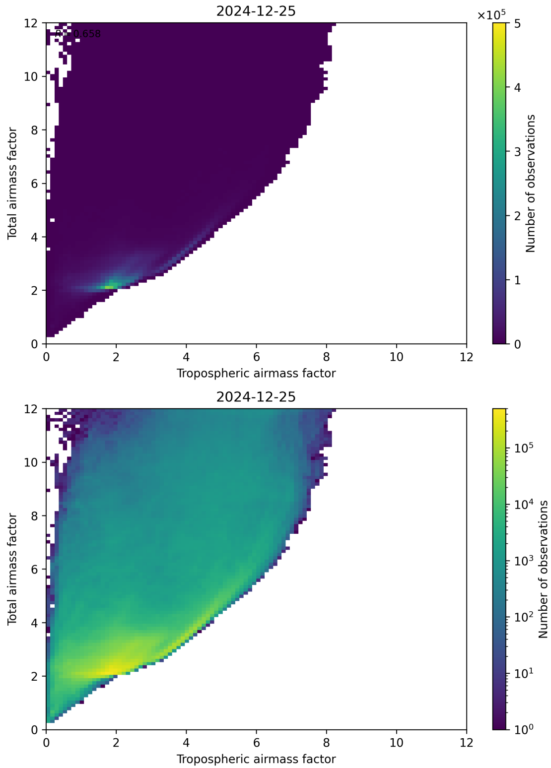
Figure 72: Scatter density plot of “Tropospheric airmass factor” against “Total airmass factor” for 2024-12-24 to 2024-12-26.
