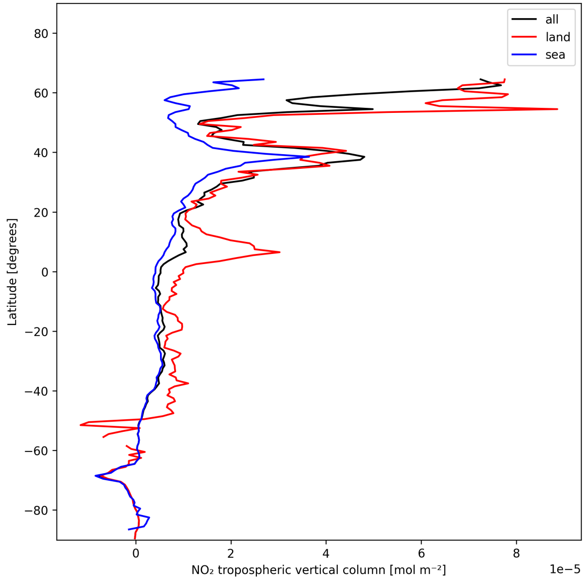
Figure 12: Zonal average of “NO 2 tropospheric vertical column” for 2024-12-24 to 2024-12-26.
