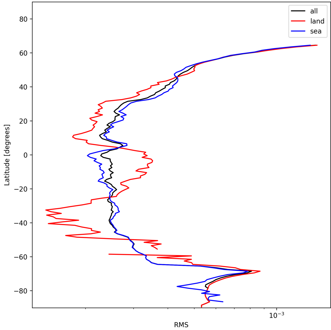
Figure 26: Zonal average of “RMS” for 2024-12-24 to 2024-12-26.
