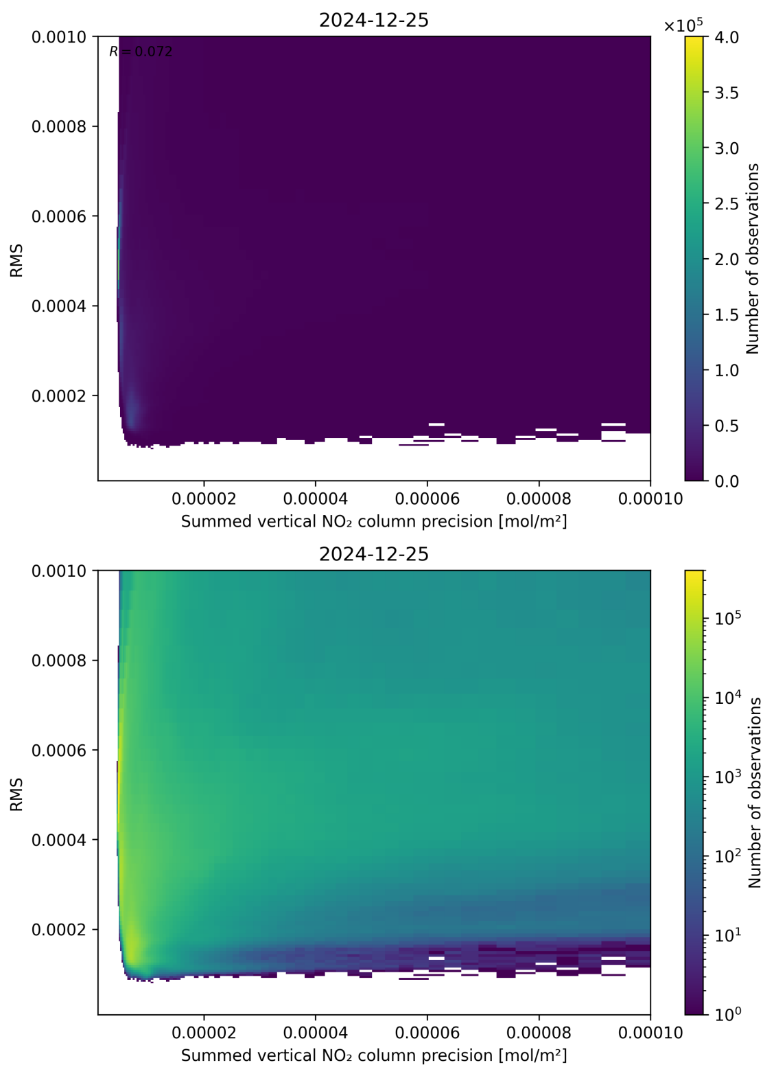
Figure 108: Scatter density plot of “Summed vertical NO 2 column precision” against “RMS” for 2024-12-24 to 2024-12-26.
