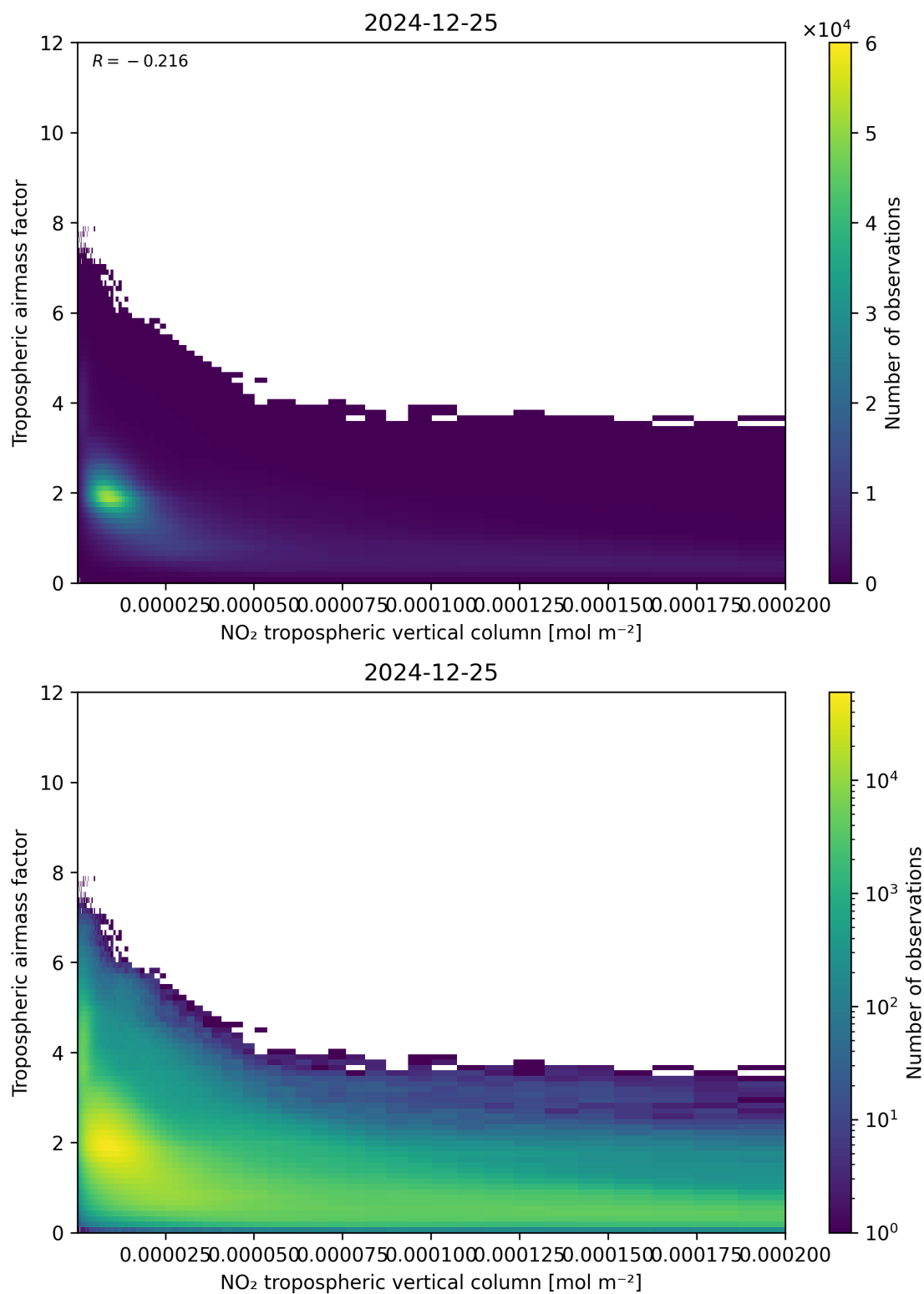
Figure 123: Scatter density plot of “NO 2 tropospheric vertical column” against “Tropospheric air mass factor” for 2024-12-24 to 2024-12-26.
