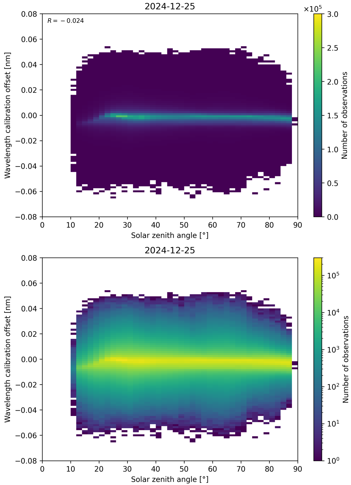
Figure 158: Scatter density plot of “Solar zenith angle” against “Wavelength calibration offset” for 2024-12-24 to 2024-12-26.
