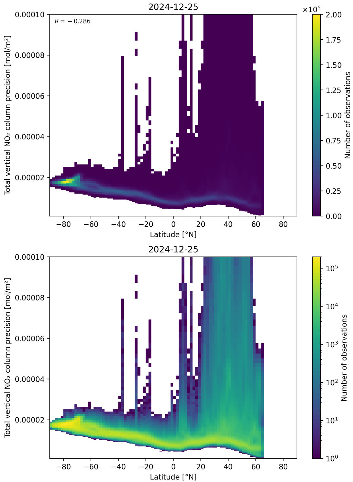
Figure 91: Scatter density plot of “Latitude” against “Total vertical NO 2 column precision” for 2024-12-24 to 2024-12-26.
