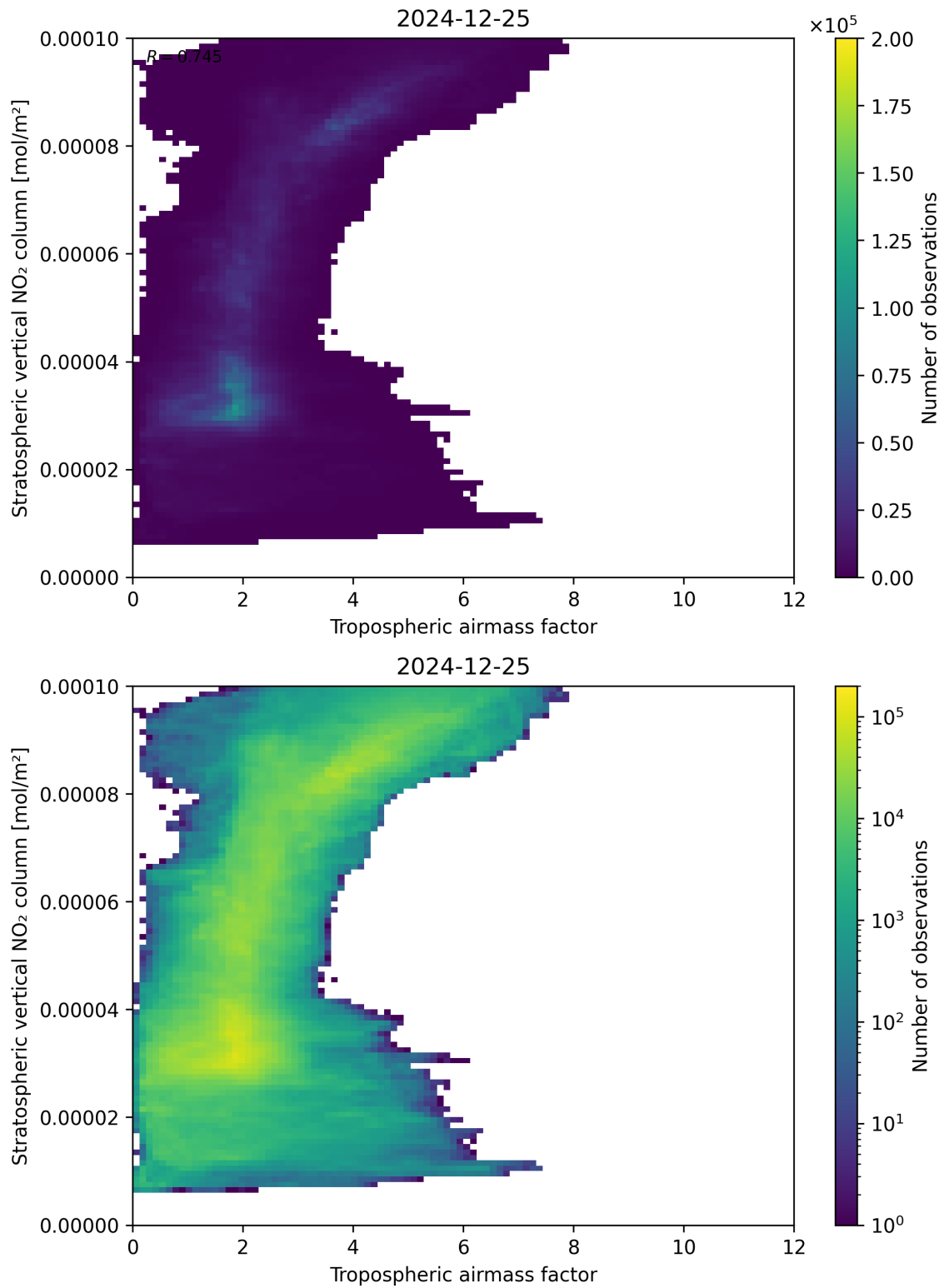
Figure 74: Scatter density plot of “Tropospheric airmass factor” against “Stratospheric vertical NO 2 column” for 2024-12-24 to 2024-12-26.
