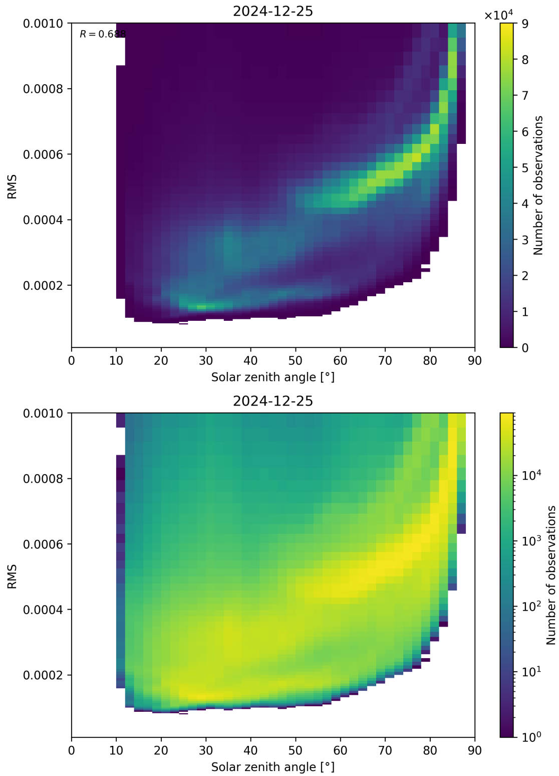
Figure 157: Scatter density plot of “Solar zenith angle” against “RMS” for 2024-12-24 to 2024-12-26.
