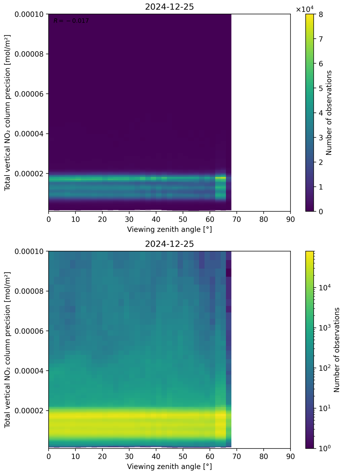
Figure 168: Scatter density plot of “Viewing zenith angle” against “Total vertical NO 2 column precision” for 2024-12-24 to 2024-12-26.
