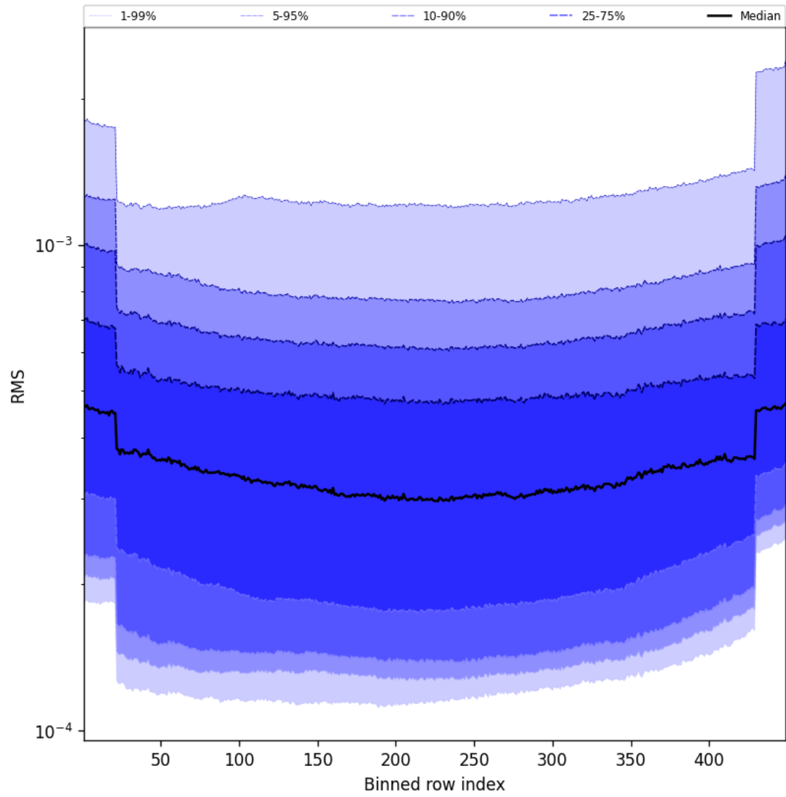
Figure 60: Along track statistics of “RMS” for 2024-12-24 to 2024-12-26
