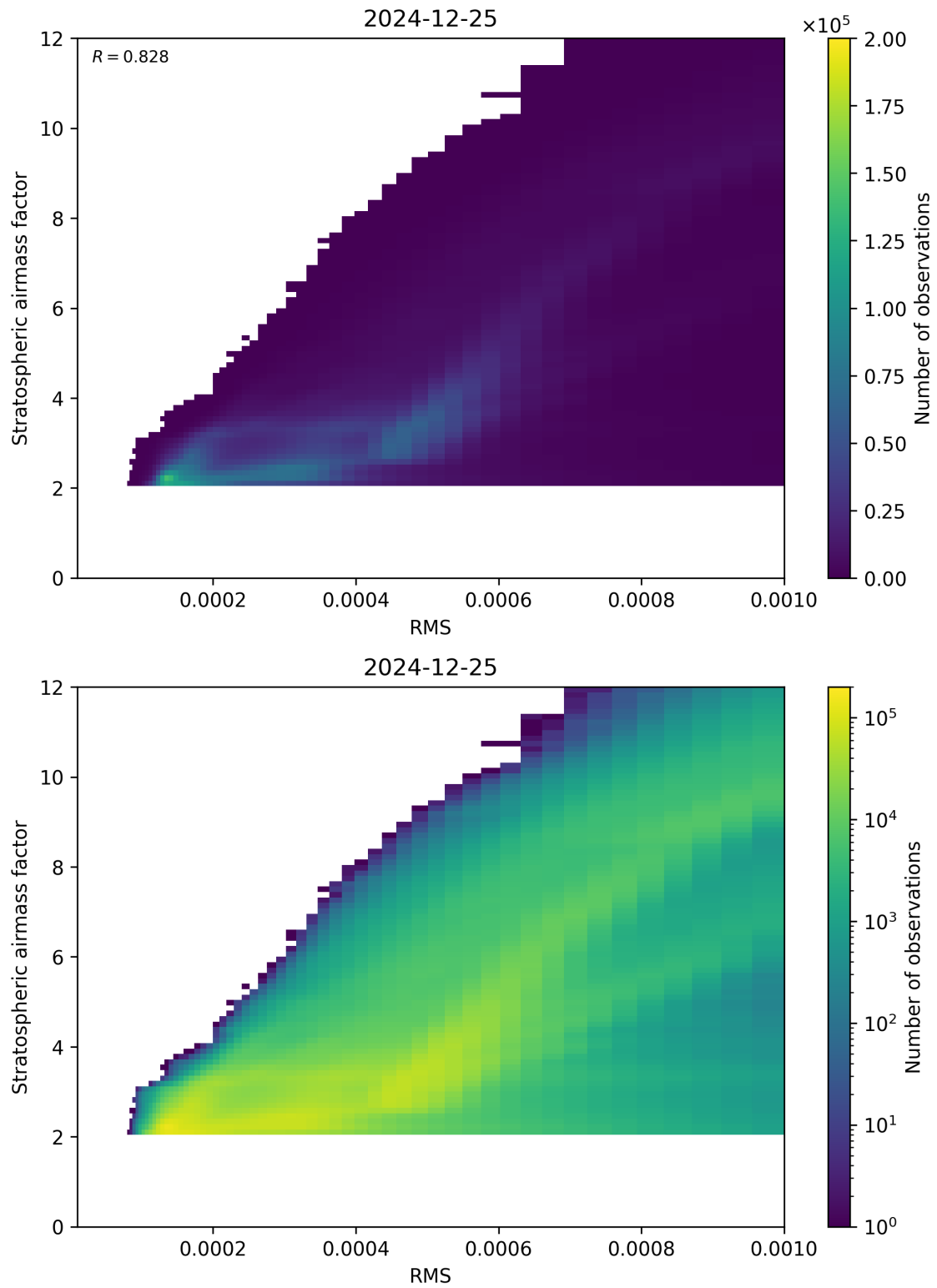
Figure 144: Scatter density plot of “RMS” against “Stratospheric airmass factor” for 2024-12-24 to 2024-12-26.
