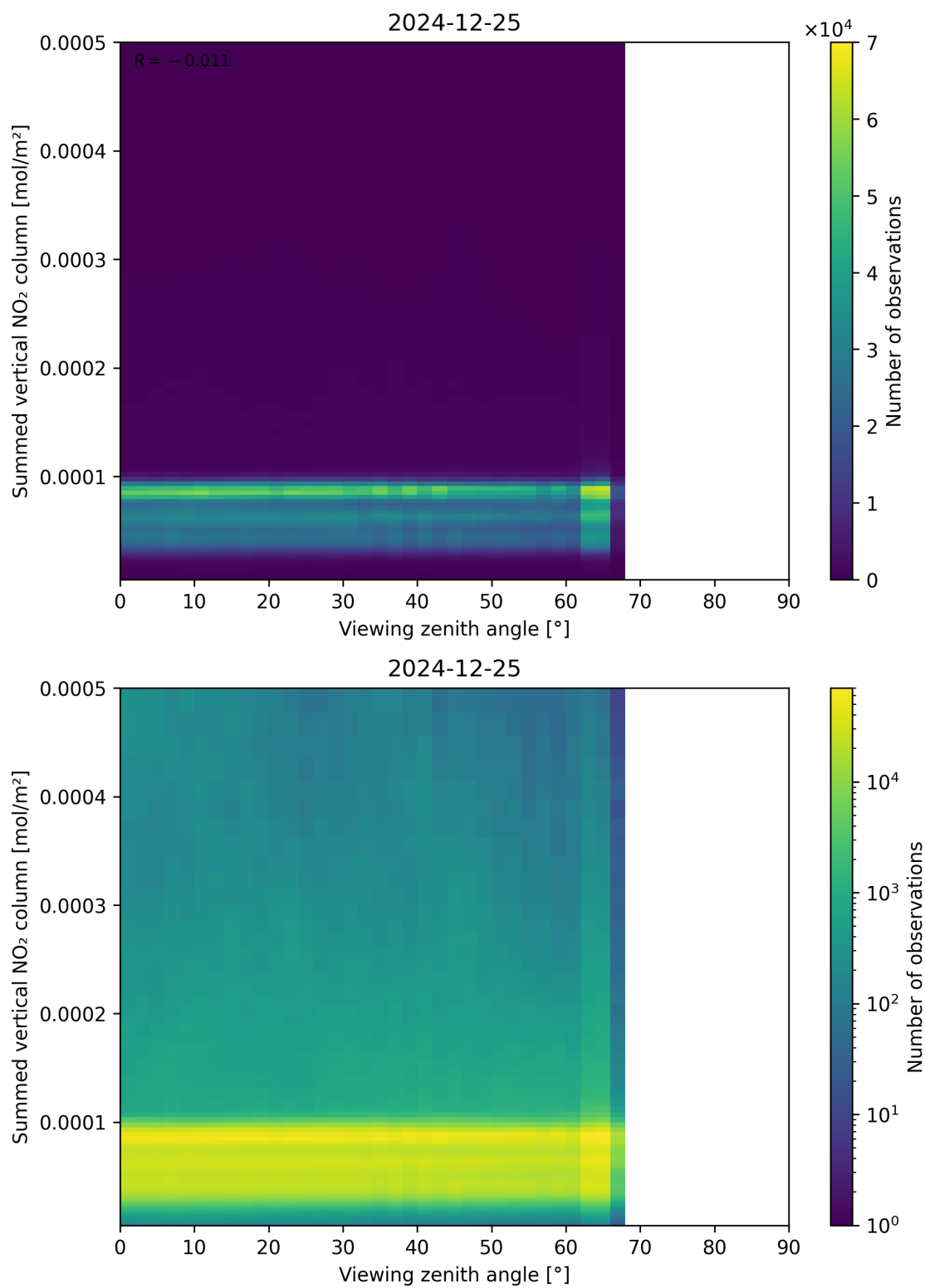
Figure 165: Scatter density plot of “Viewing zenith angle” against “Summed vertical NO 2 column” for 2024-12-24 to 2024-12-26.
