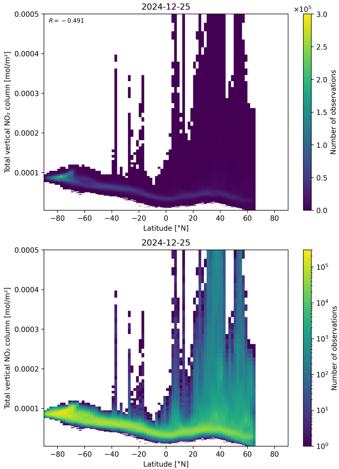
Figure 90: Scatter density plot of “Latitude” against “Total vertical NO 2 column” for 2024-12-24 to 2024-12-26.
