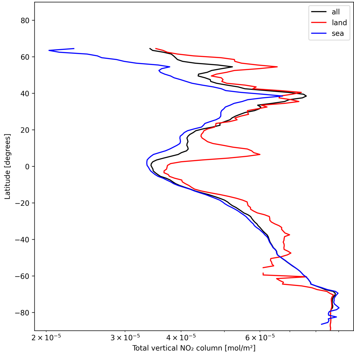
Figure 21: Zonal average of “Total vertical NO 2 column” for 2024-12-24 to 2024-12-26.
