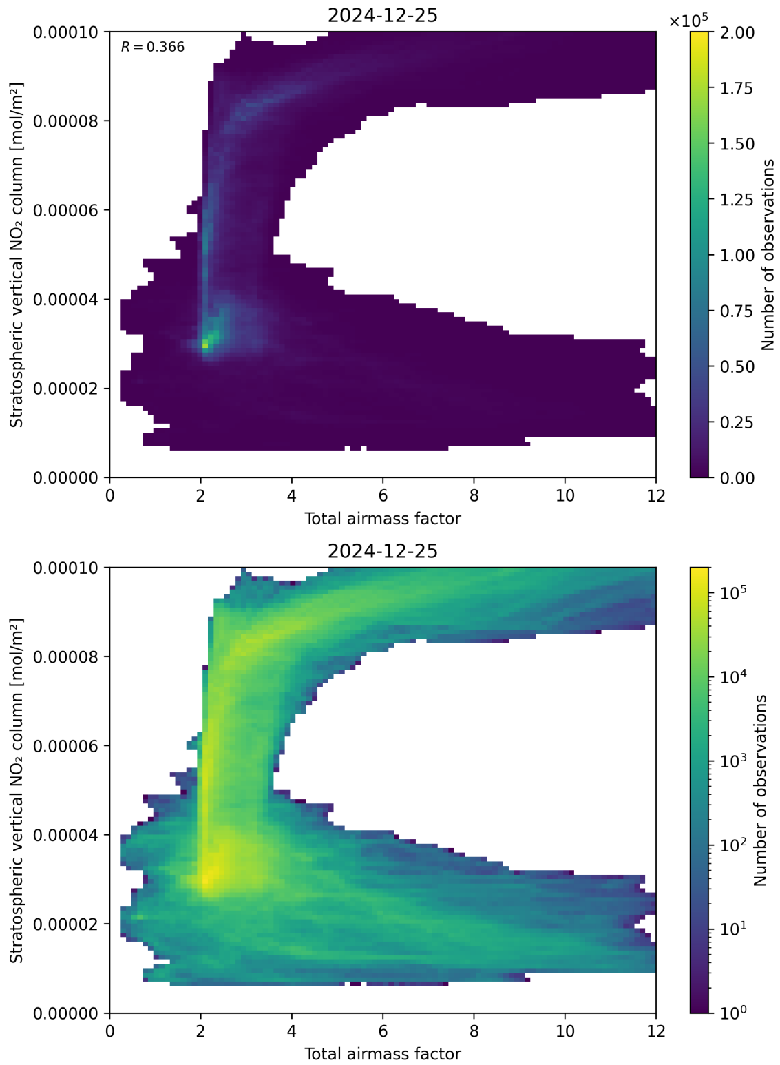
Figure 64: Scatter density plot of “Total airmass factor” against “Stratospheric vertical \text{NO}_2 column” for 2024-12-24 to 2024-12-26.
