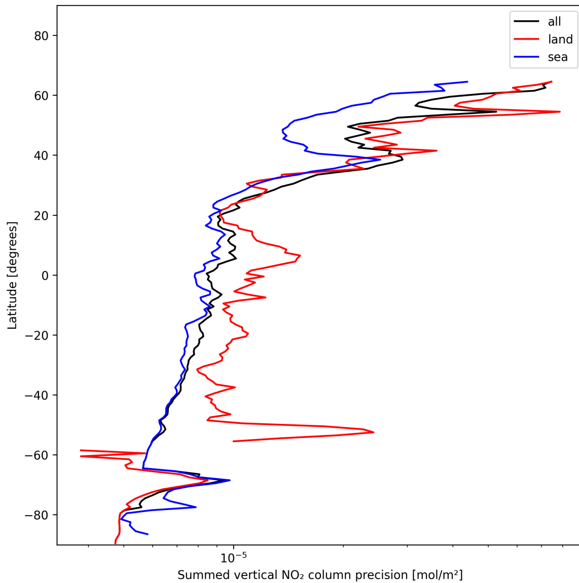
Figure 24: Zonal average of “Summed vertical NO 2 column precision” for 2024-12-24 to 2024-12-26.
