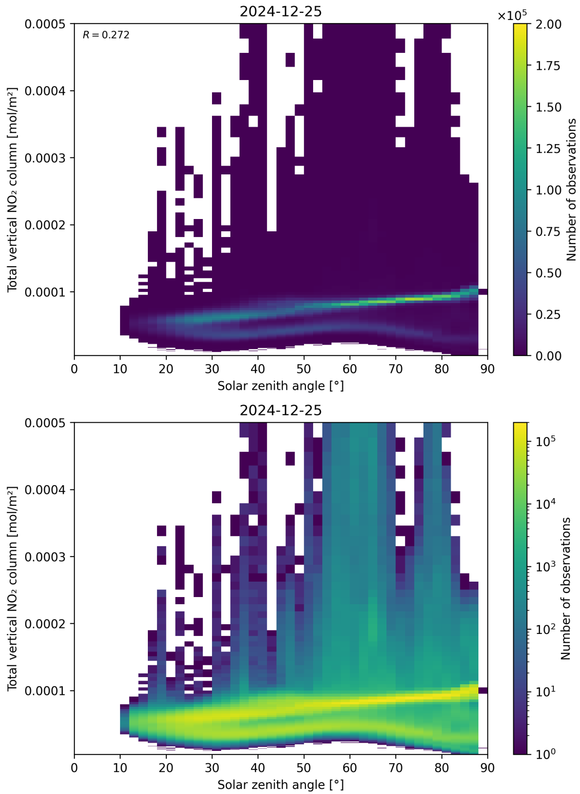
Figure 153: Scatter density plot of “Solar zenith angle” against “Total vertical NO 2 column” for 2024-12-24 to 2024-12-26.
