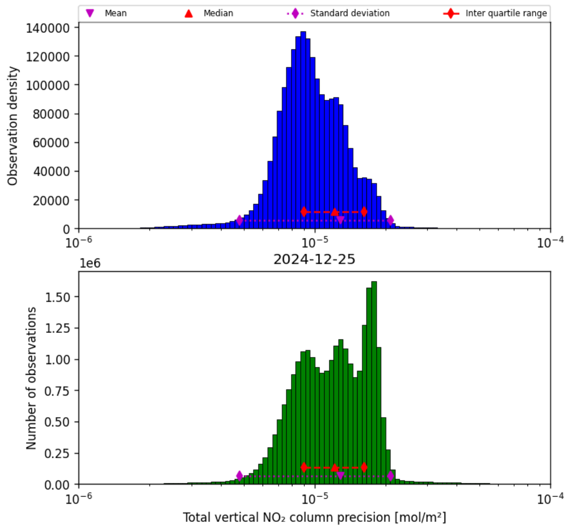
Figure 39: Histogram of “Total vertical NO 2 column precision” for 2024-12-24 to 2024-12-26
