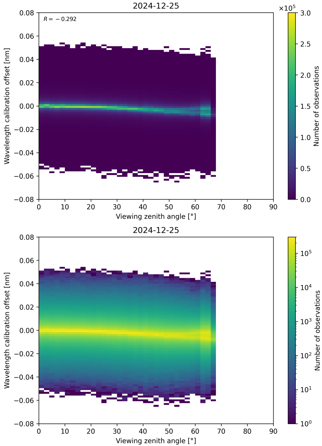
Figure 173: Scatter density plot of “Viewing zenith angle” against “Wavelength calibration offset” for 2024-12-24 to 2024-12-26.
