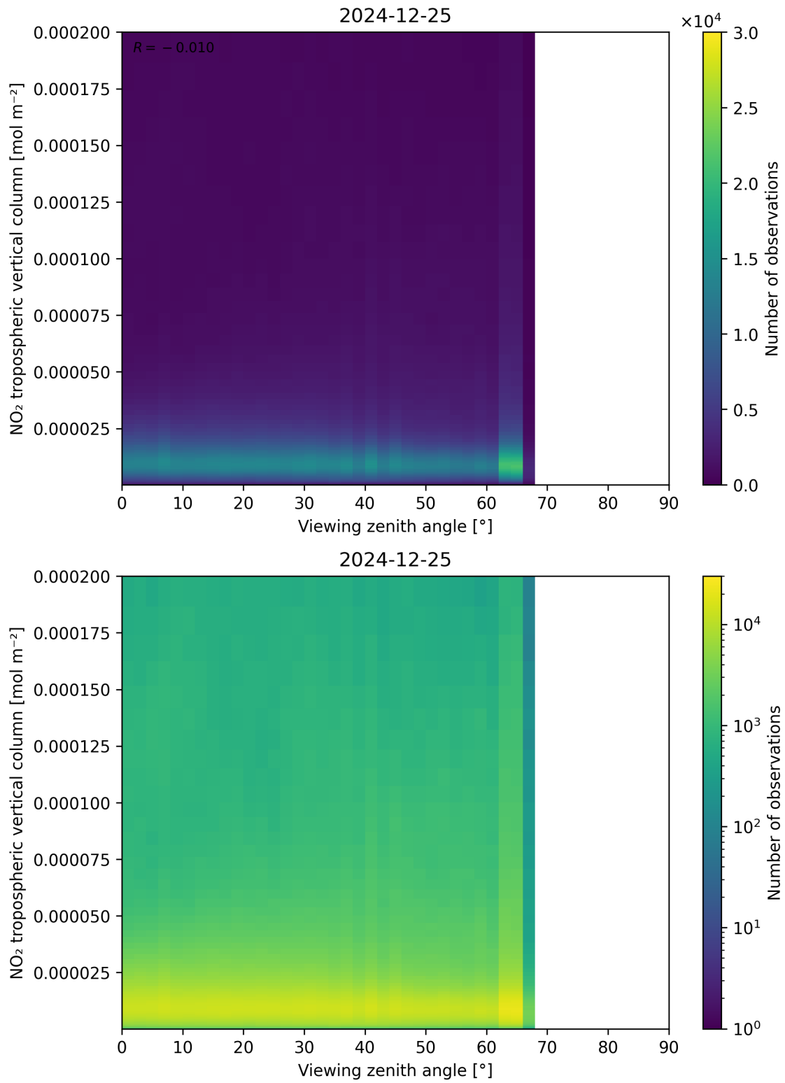
Figure 169: Scatter density plot of “Viewing zenith angle” against “NO 2 tropospheric vertical column” for 2024-12-24 to 2024-12-26.
