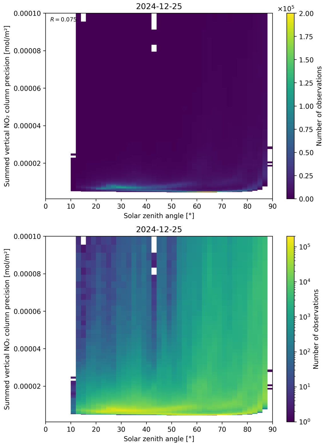
Figure 152: Scatter density plot of “Solar zenith angle” against “Summed vertical NO 2 column precision” for 2024-12-24 to 2024-12-26.
