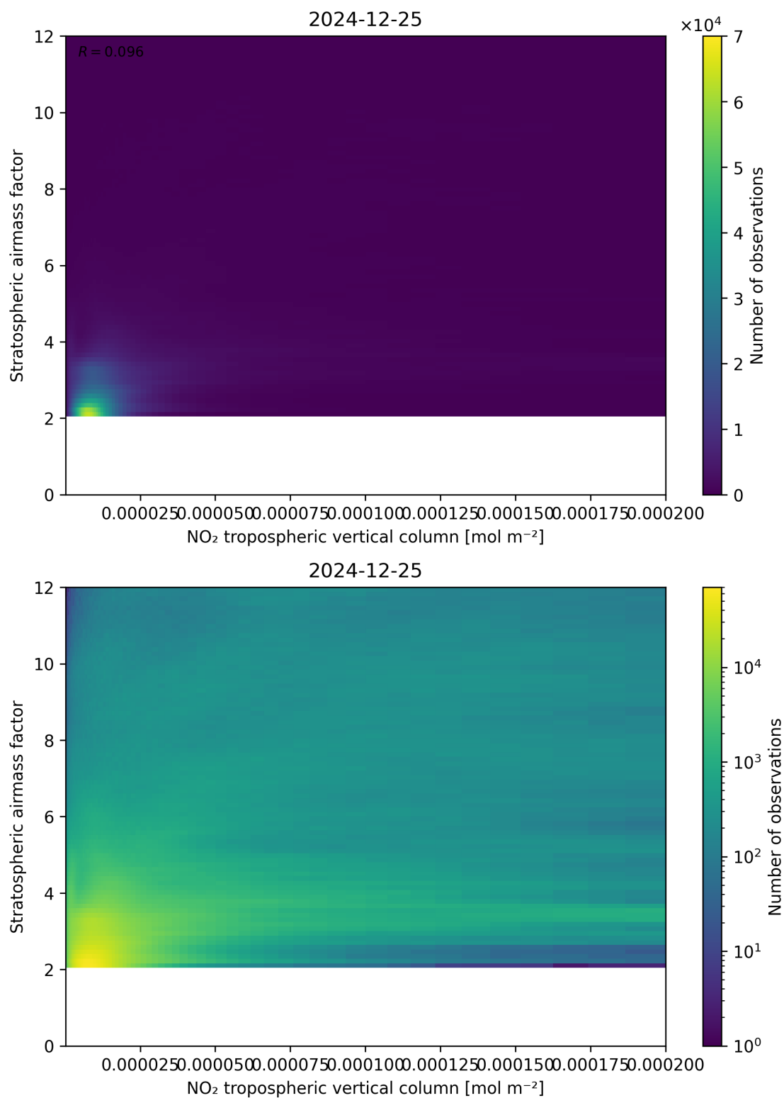
Figure 121: Scatter density plot of “NO 2 tropospheric vertical column” against “Stratospheric airmass factor” for 2024-12-24 to 2024-12-26.
