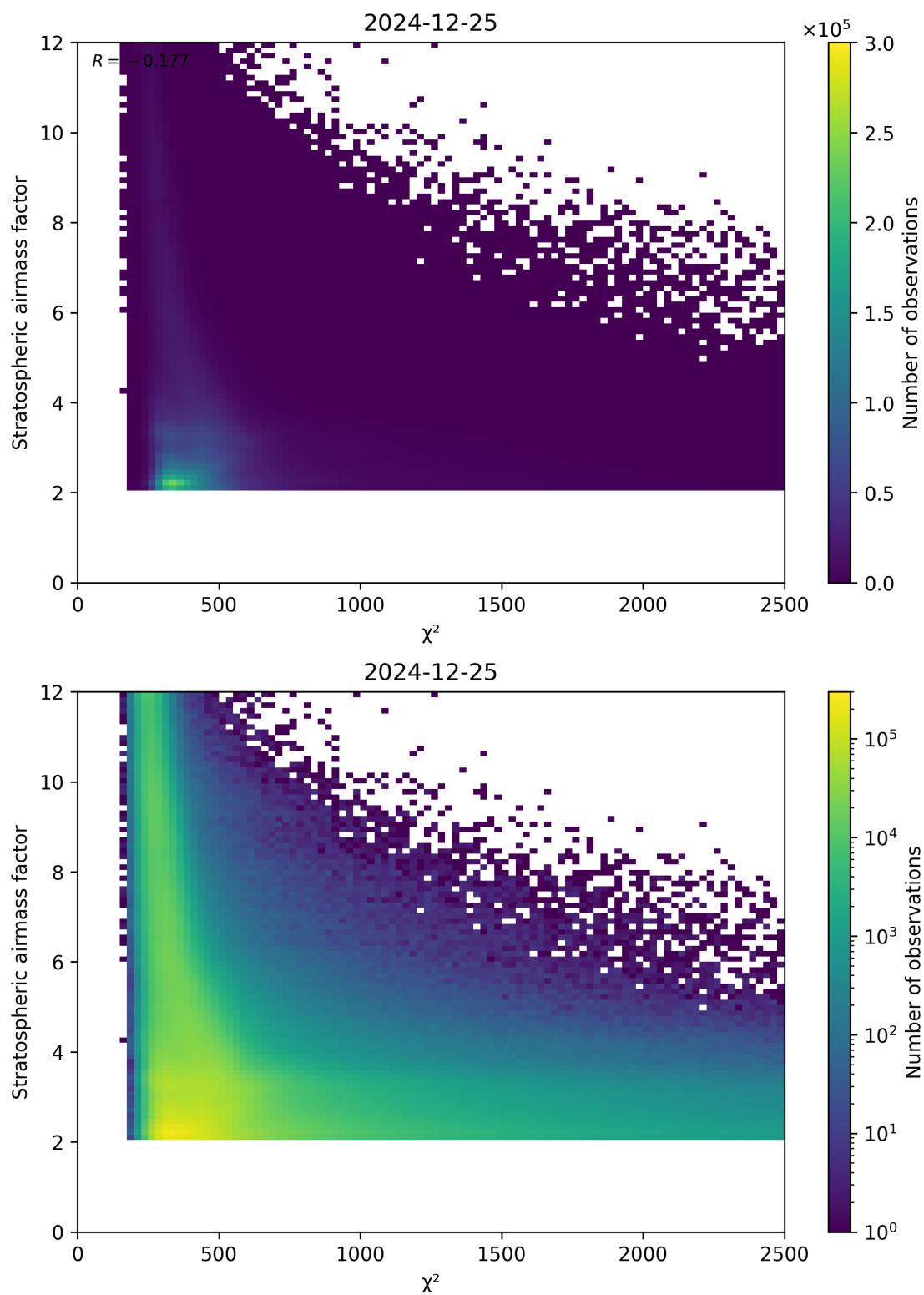
Figure 81: Scatter density plot of “ \chi^2 ” against “Stratospheric air mass factor” for 2024-12-24 to 2024-12-26.
