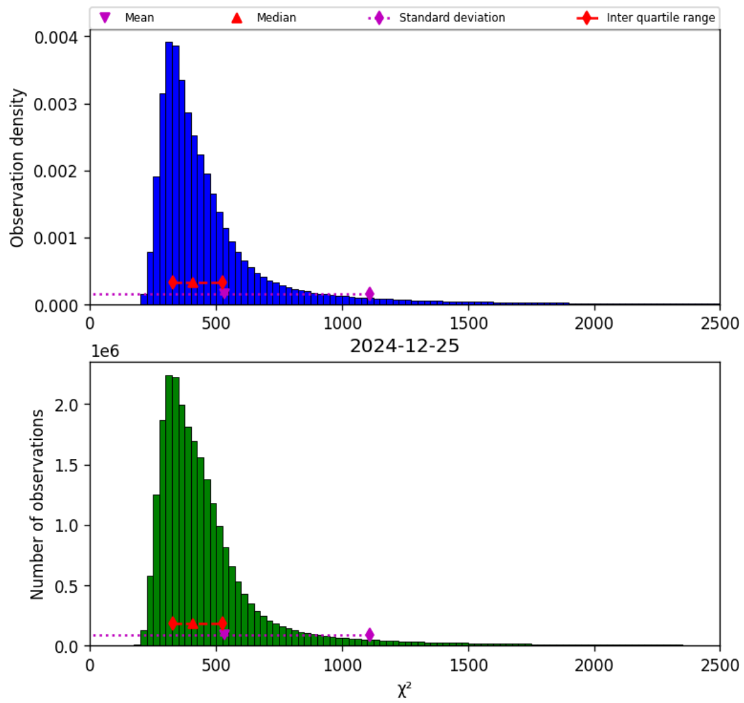
Figure 42: Histogram of " \chi^2 " for 2024-12-24 to 2024-12-26
