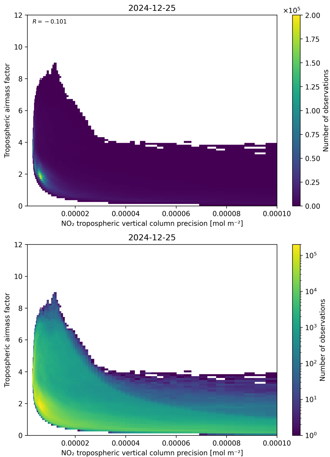
Figure 133: Scatter density plot of “NO 2 tropospheric vertical column precision” against “Tropospheric airmass factor” for 2024-12-24 to 2024-12-26.
