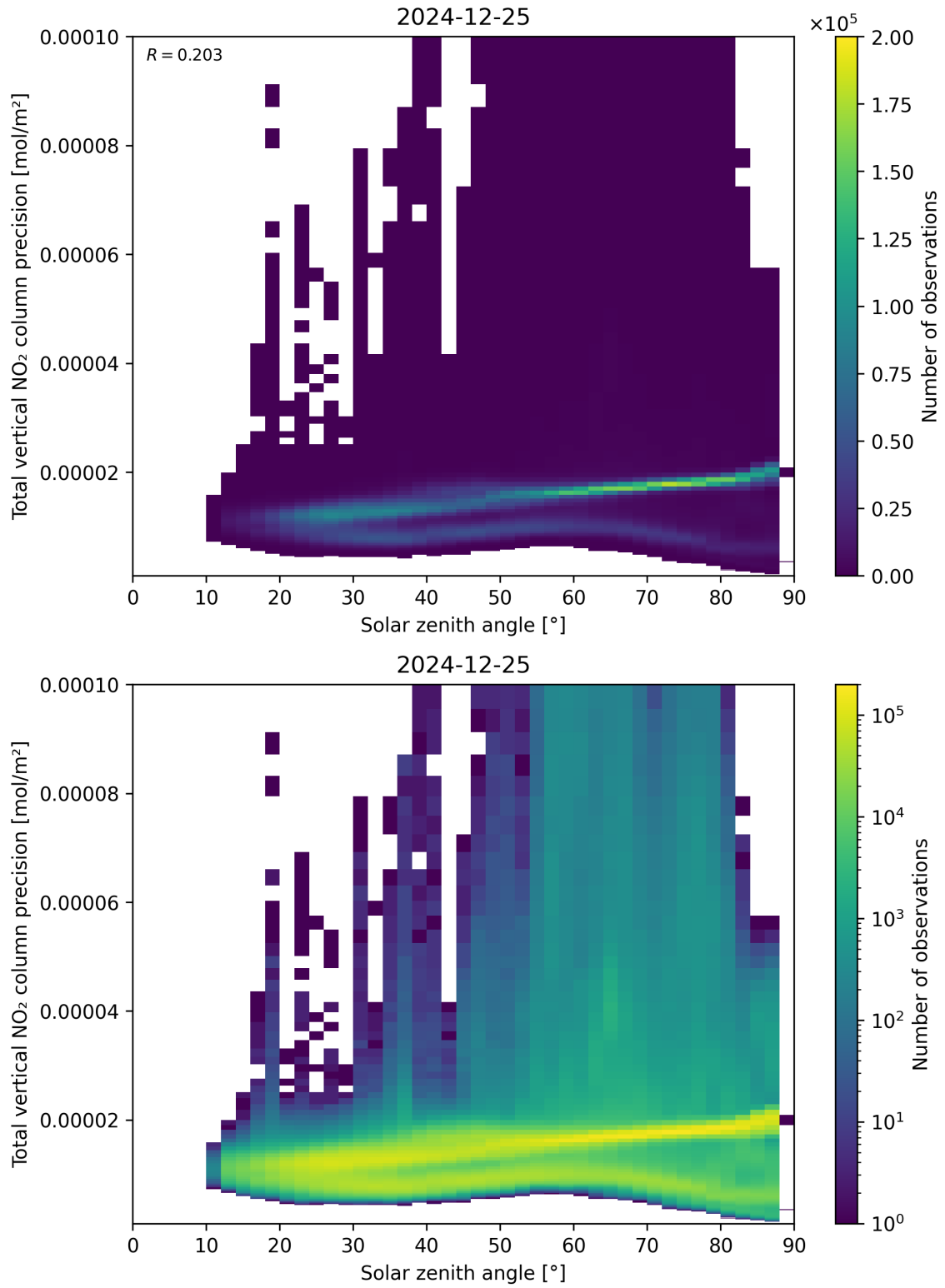
Figure 154: Scatter density plot of “Solar zenith angle” against “Total vertical NO 2 column precision” for 2024-12-24 to 2024-12-26.
