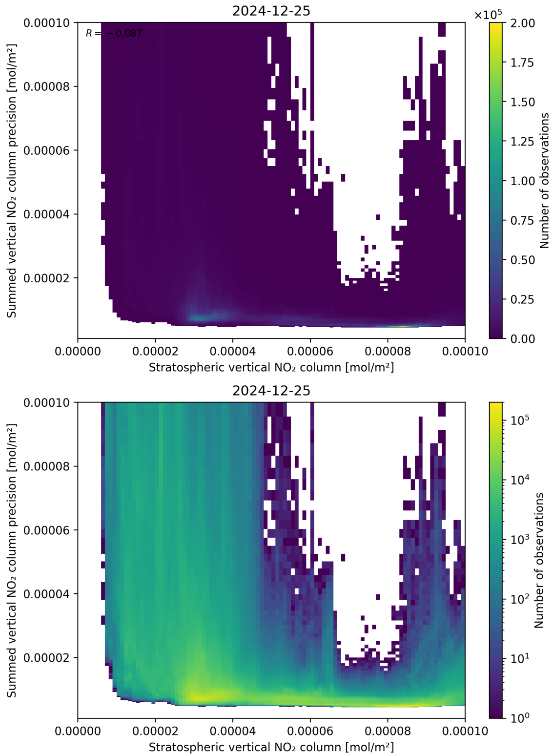
Figure 99: Scatter density plot of “Stratospheric vertical NO 2 column” against “Summed vertical NO 2 column precision” for 2024-12-24 to 2024-12-26.
