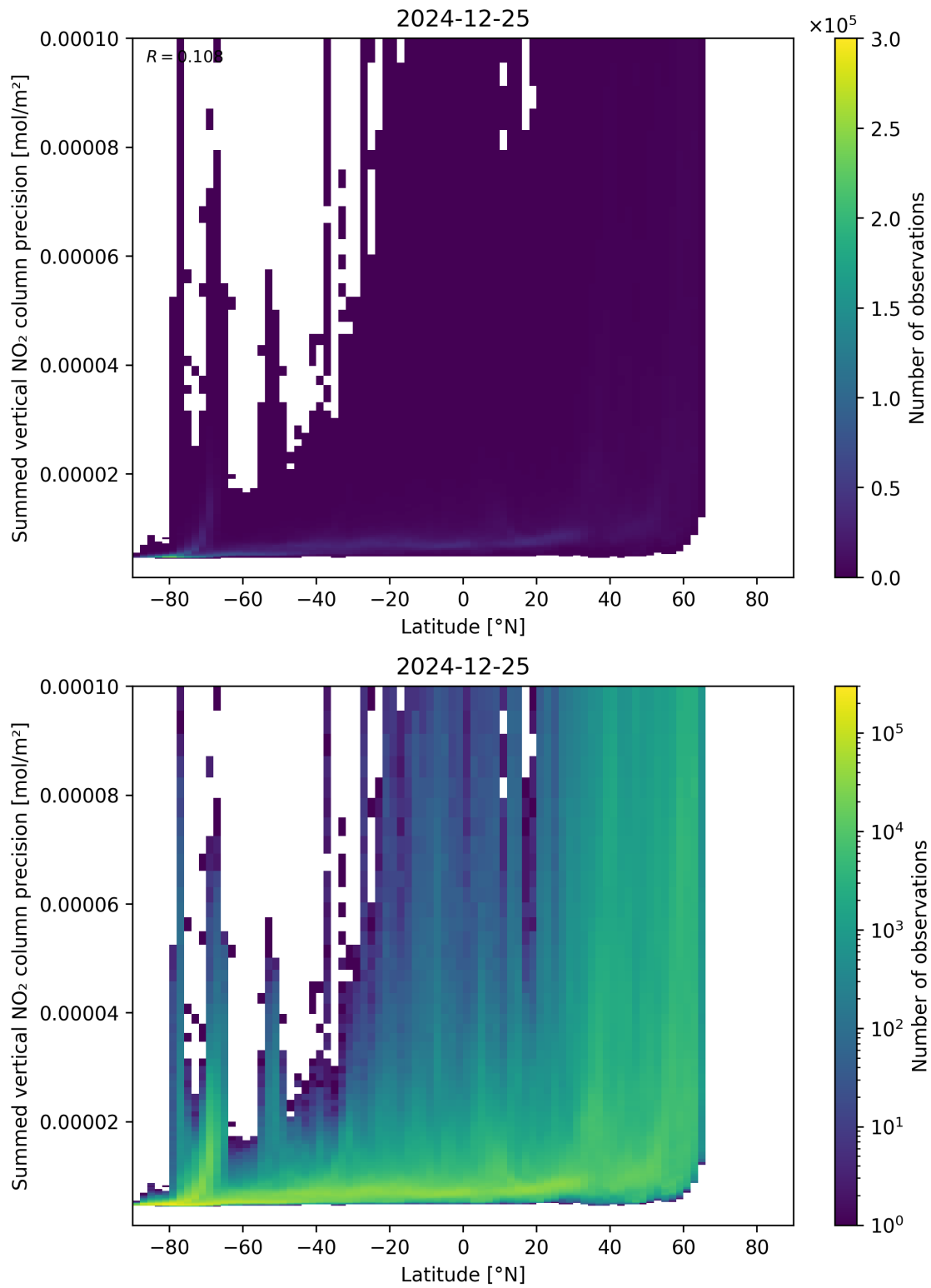
Figure 89: Scatter density plot of “Latitude” against “Summed vertical NO 2 column precision” for 2024-12-24 to 2024-12-26.
