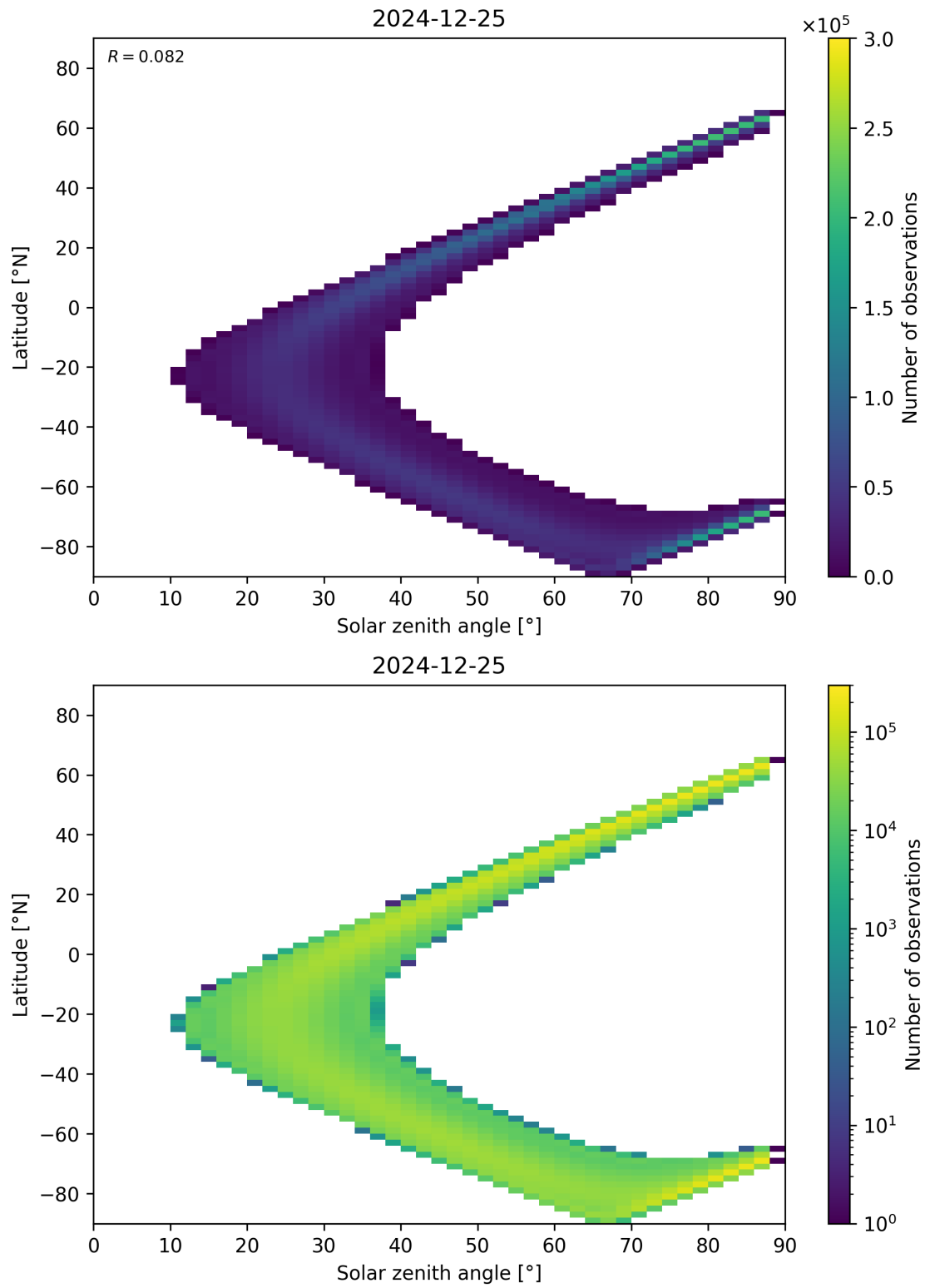
Figure 149: Scatter density plot of “Solar zenith angle” against “Latitude” for 2024-12-24 to 2024-12-26.
