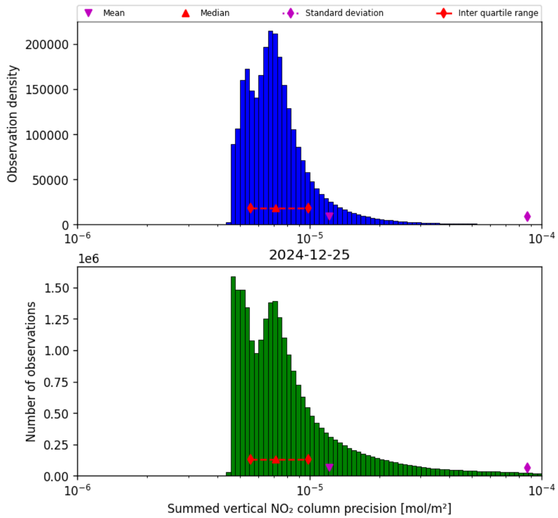
Figure 41: Histogram of “Summed vertical NO 2 column precision” for 2024-12-24 to 2024-12-26
