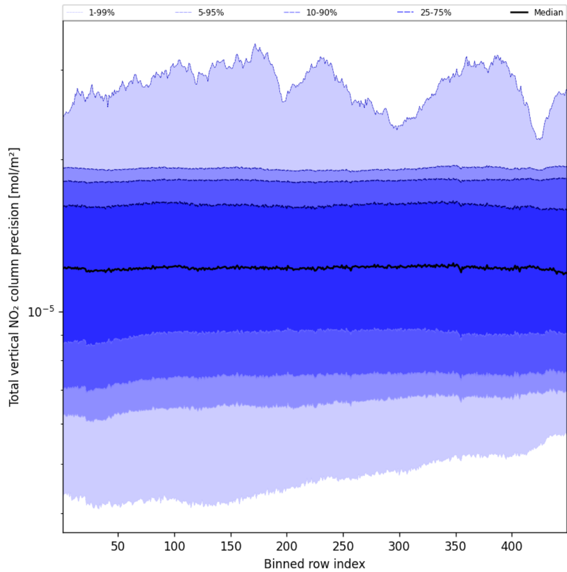
Figure 56: Along track statistics of “Total vertical NO 2 column precision” for 2024-12-24 to 2024-12-26
