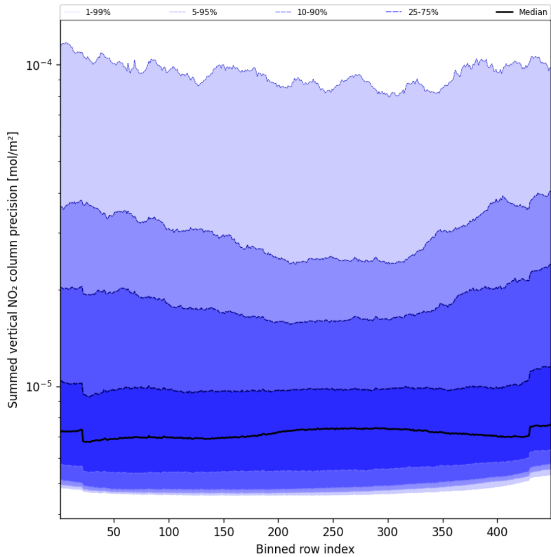
Figure 58: Along track statistics of “Summed vertical NO 2 column precision” for 2024-12-24 to 2024-12-26
