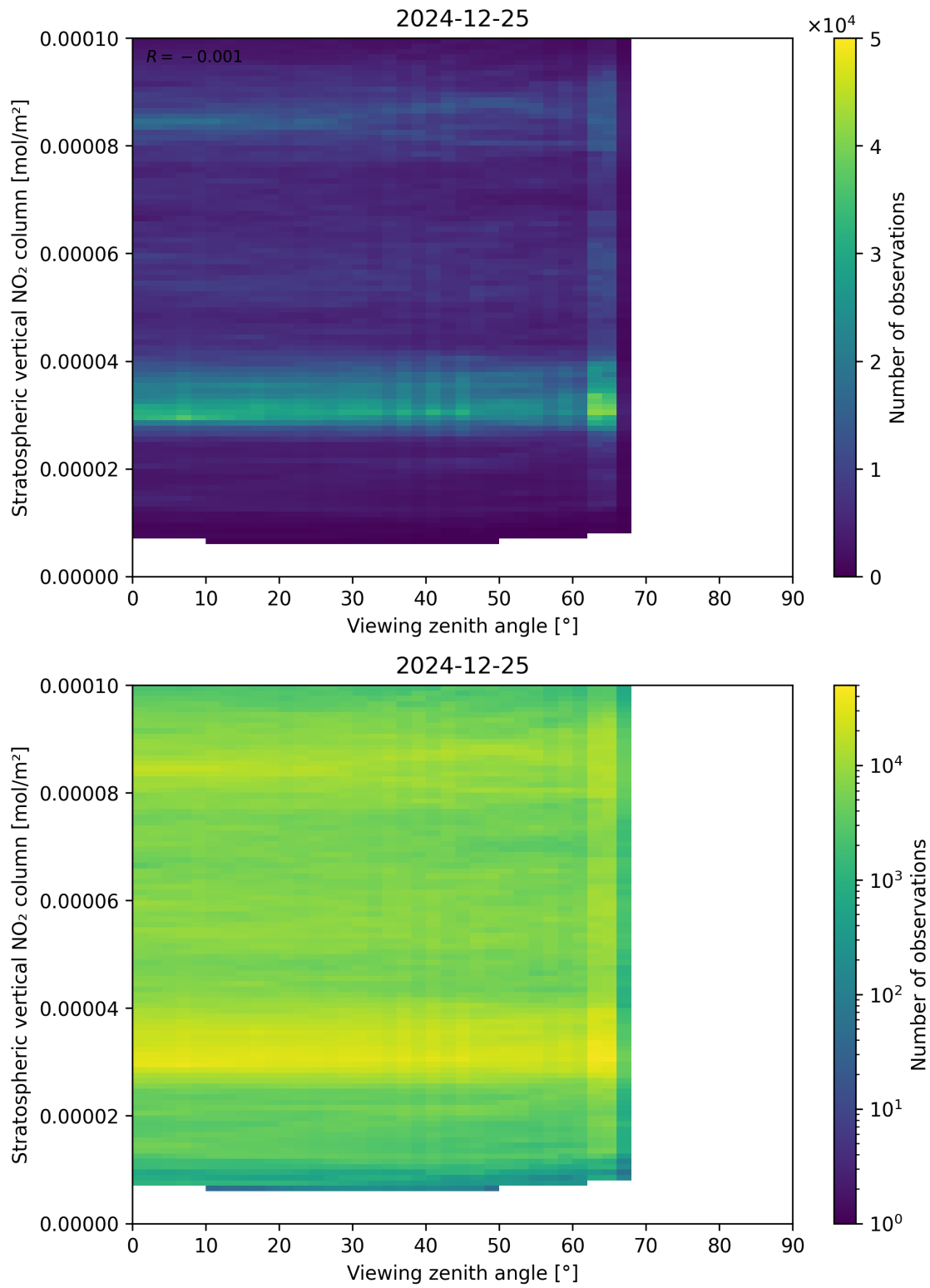
Figure 164: Scatter density plot of “Viewing zenith angle” against “Stratospheric vertical NO 2 column” for 2024-12-24 to 2024-12-26.
