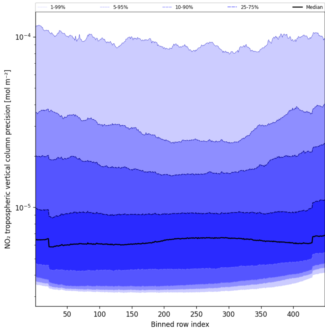
Figure 47: Along track statistics of “NO 2 tropospheric vertical column precision” for 2024-12-24 to 2024-12-26
