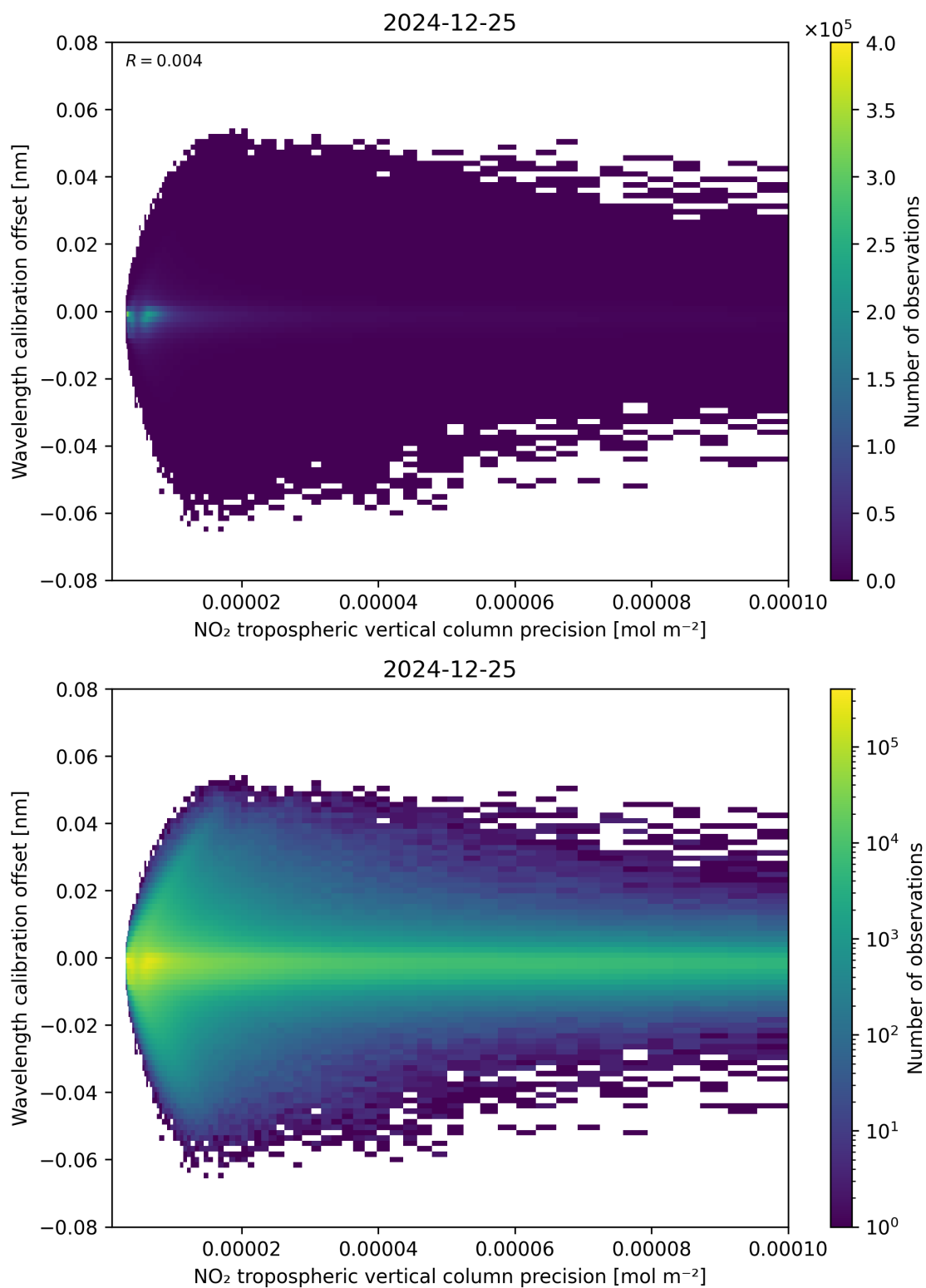
Figure 141: Scatter density plot of “NO 2 tropospheric vertical column precision” against “Wavelength calibration offset” for 2024-12-24 to 2024-12-26.
