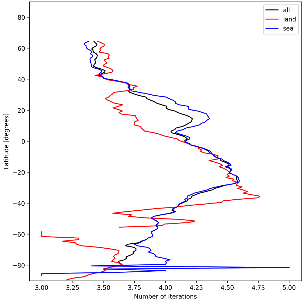
Figure 17: Zonal average of “Number of iterations” for 2024-12-24 to 2024-12-26.
