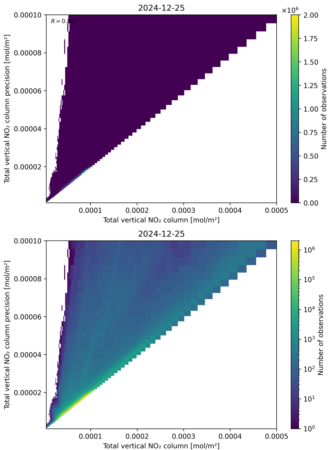
Figure 114: Scatter density plot of “Total vertical NO 2 column” against “Total vertical NO 2 column precision” for 2024-12-24 to 2024-12-26.
