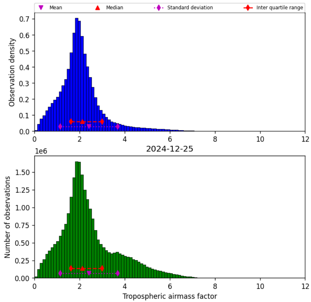
Figure 31: Histogram of “Tropospheric airmass factor” for 2024-12-24 to 2024-12-26
