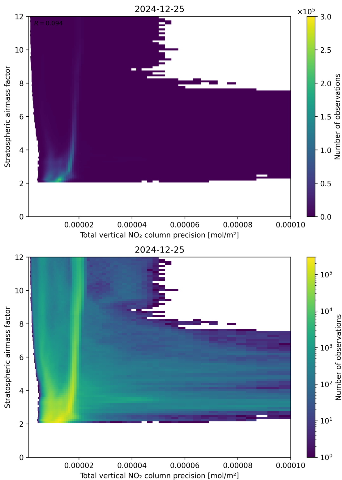
Figure 115: Scatter density plot of “Total vertical NO 2 column precision” against “Stratospheric airmass factor” for 2024-12-24 to 2024-12-26.
