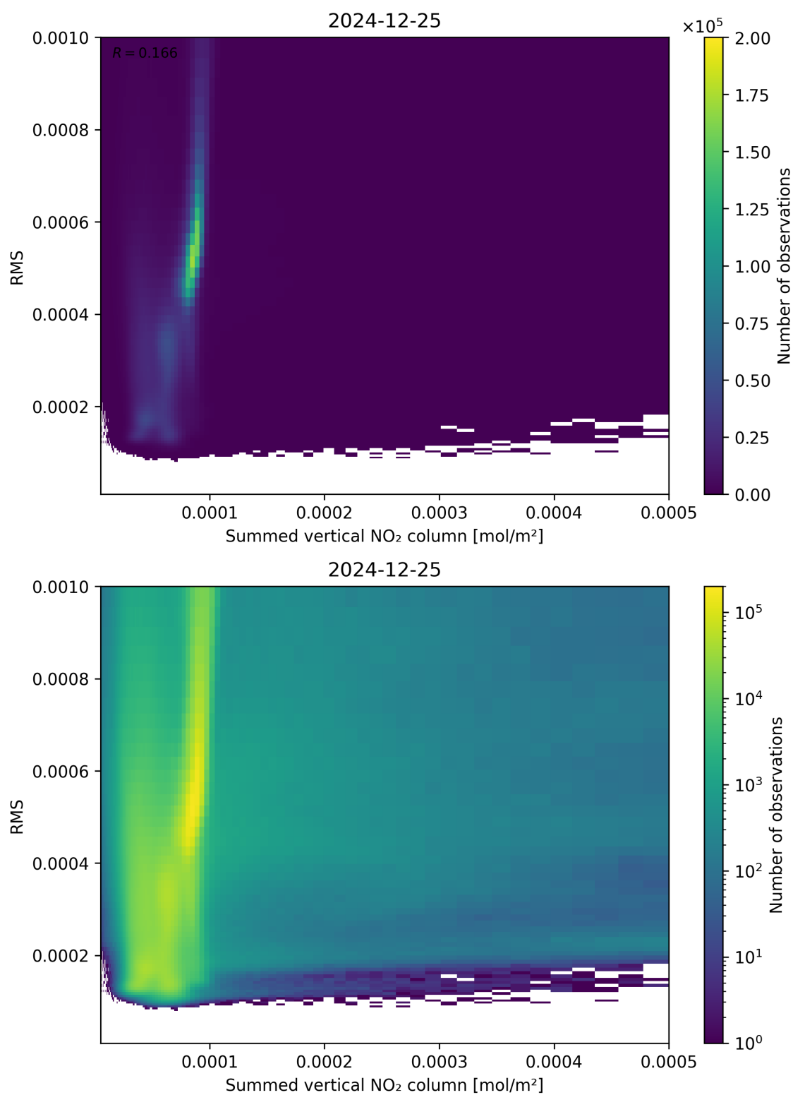
Figure 109: Scatter density plot of “Summed vertical NO 2 column” against “RMS” for 2024-12-24 to 2024-12-26.
