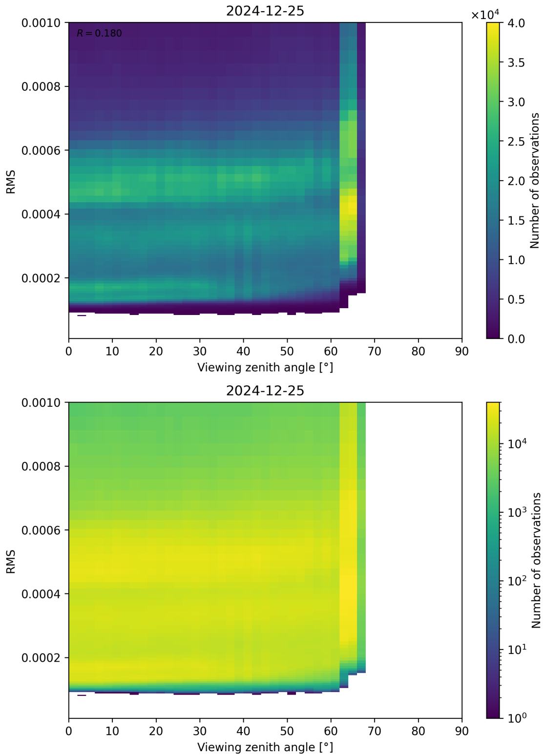
Figure 171: Scatter density plot of “Viewing zenith angle” against “RMS” for 2024-12-24 to 2024-12-26.
