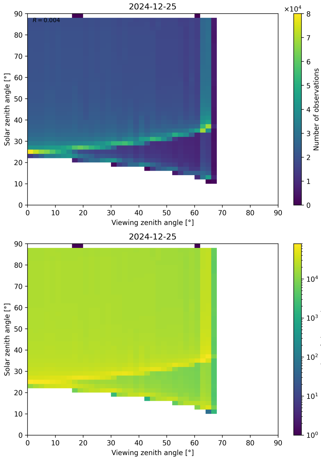
Figure 172: Scatter density plot of “Viewing zenith angle” against “Solar zenith angle” for 2024-12-24 to 2024-12-26.
