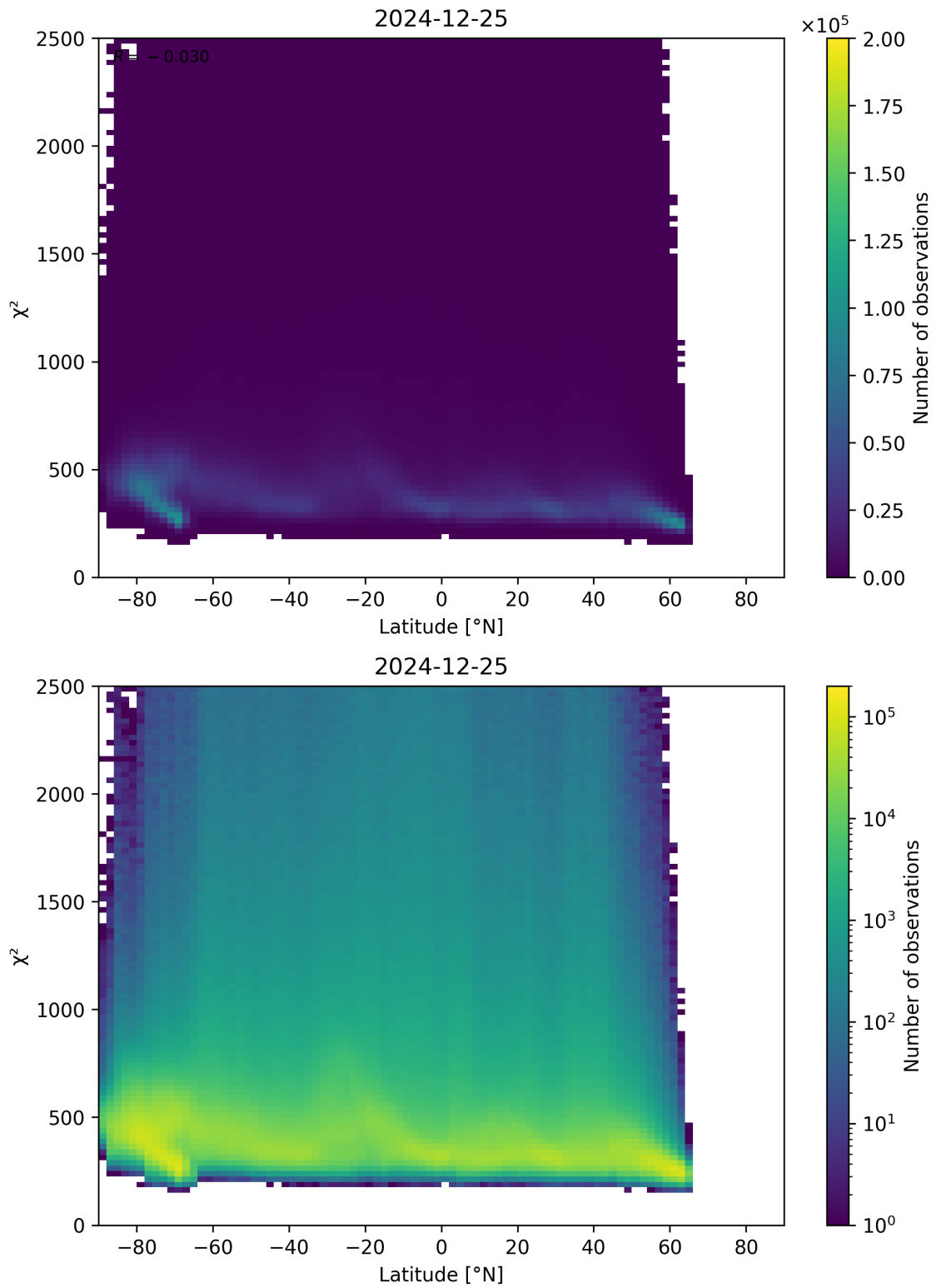
Figure 86: Scatter density plot of “Latitude” against “ \chi^2 ” for 2024-12-24 to 2024-12-26.
