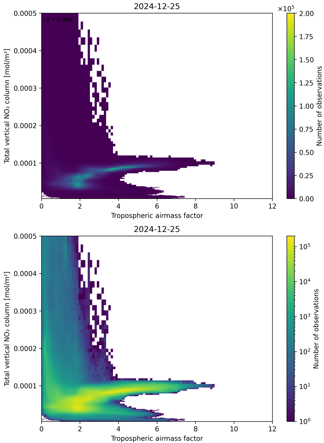
Figure 77: Scatter density plot of “Tropospheric airmass factor” against “Total vertical \text{NO}_2 column” for 2024-12-24 to 2024-12-26.
