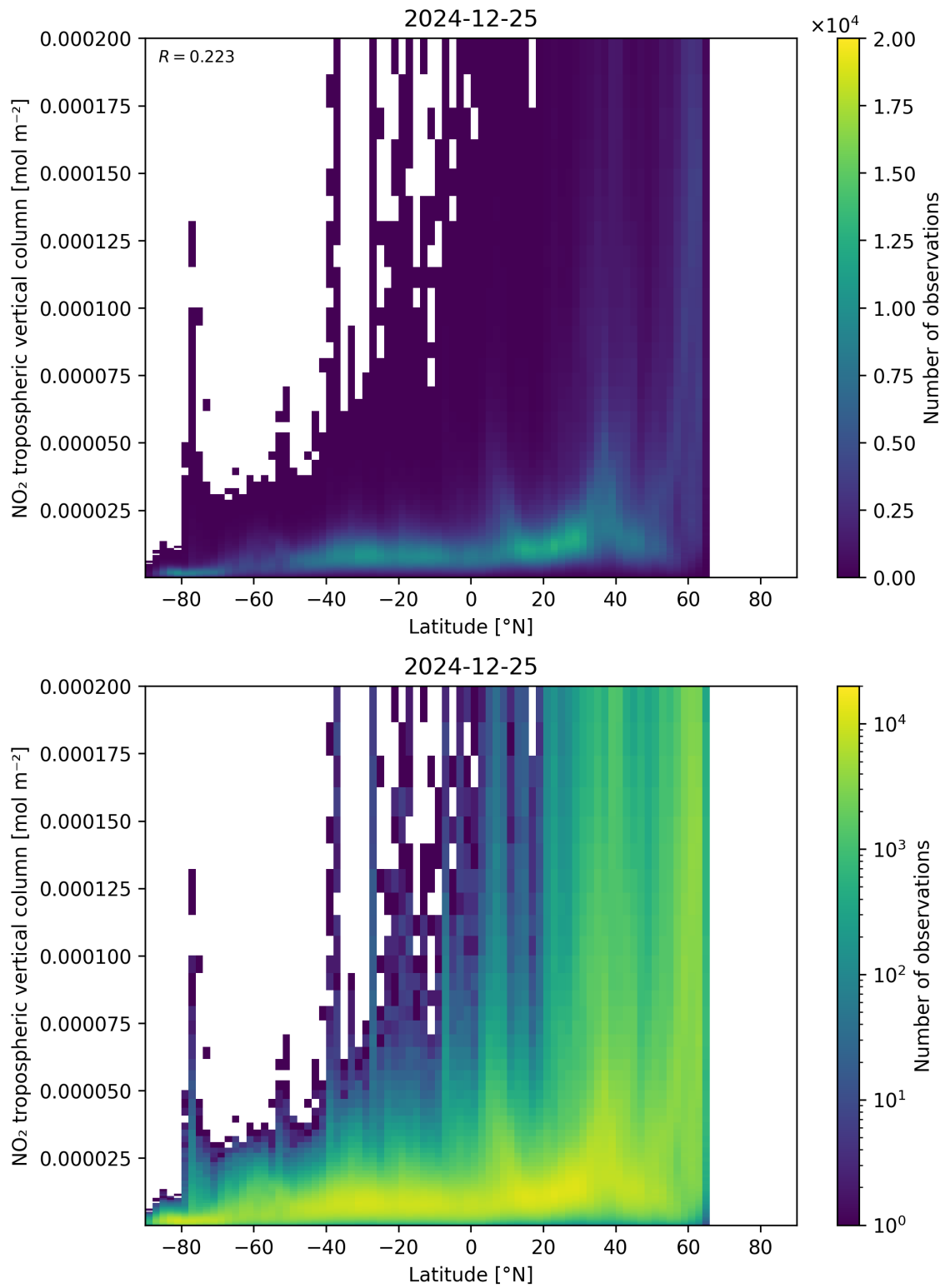
Figure 92: Scatter density plot of “Latitude” against “NO 2 tropospheric vertical column” for 2024-12-24 to 2024-12-26.
