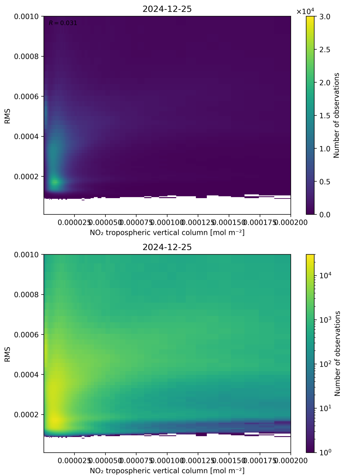
Figure 142: Scatter density plot of “NO 2 tropospheric vertical column” against “RMS” for 2024-12-24 to 2024-12-26.
