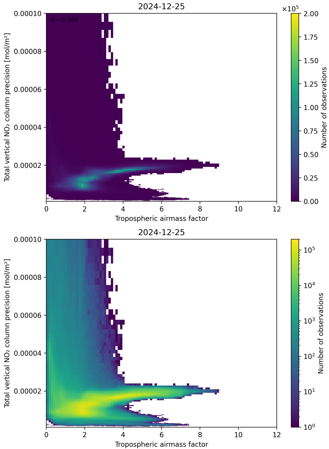
Figure 78: Scatter density plot of “Tropospheric air mass factor” against “Total vertical NO 2 column precision” for 2024-12-24 to 2024-12-26.
