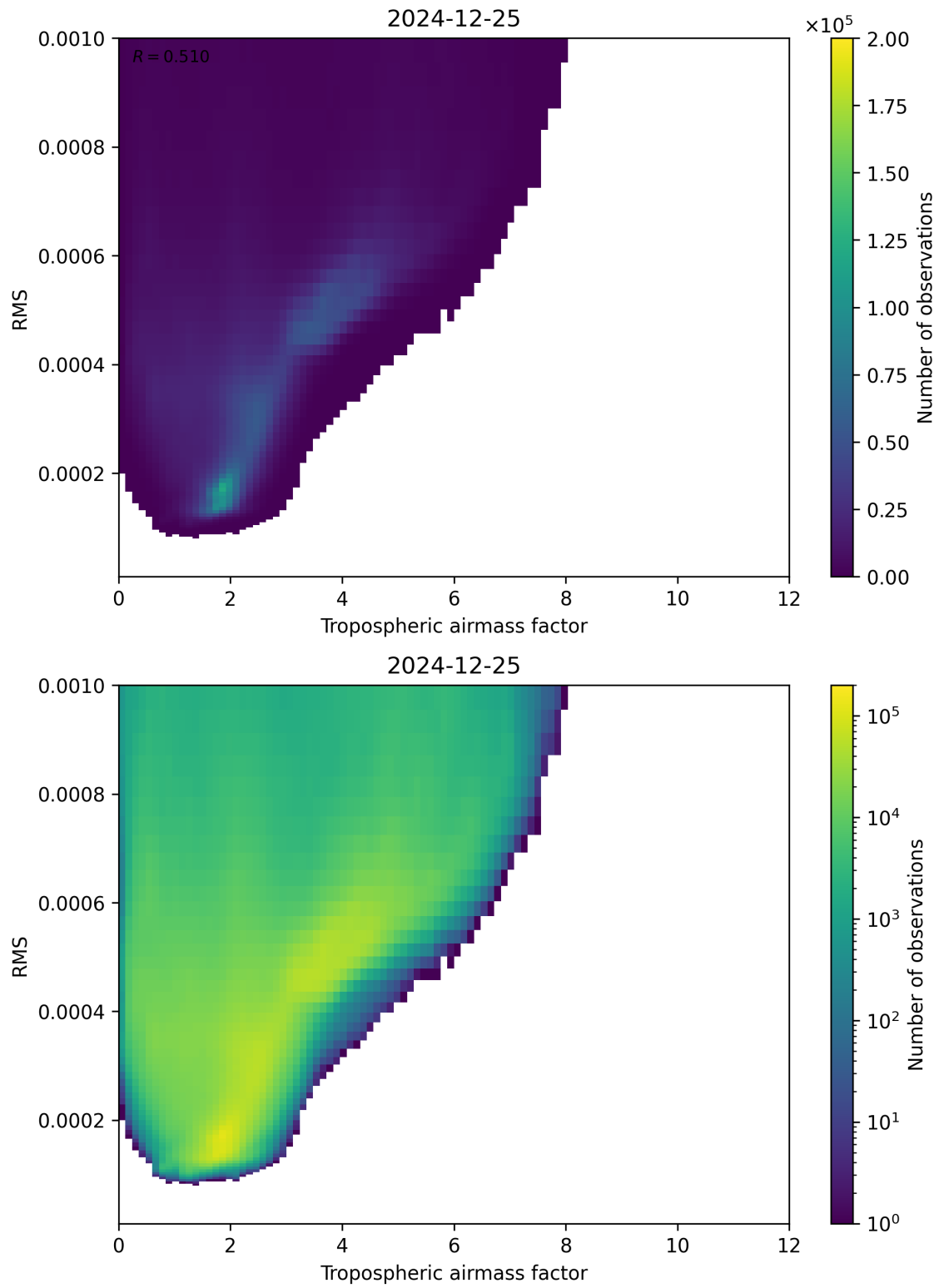
Figure 79: Scatter density plot of “Tropospheric airmass factor” against “RMS” for 2024-12-24 to 2024-12-26.
