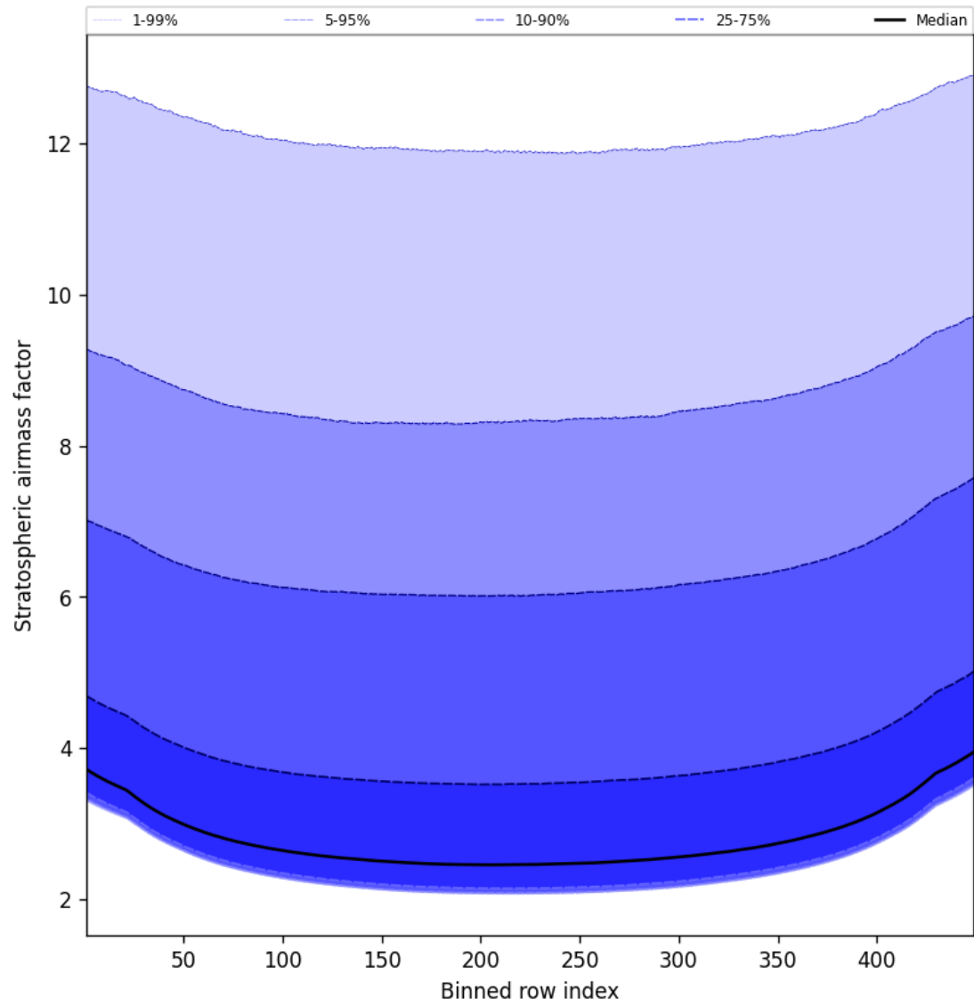
Figure 61: Along track statistics of “Stratospheric airmass factor” for 2024-12-24 to 2024-12-26
