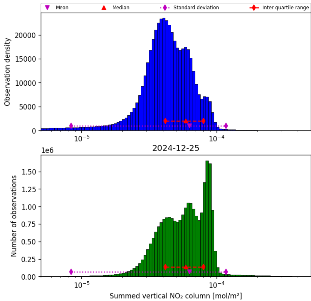
Figure 40: Histogram of “Summed vertical NO 2 column” for 2024-12-24 to 2024-12-26
