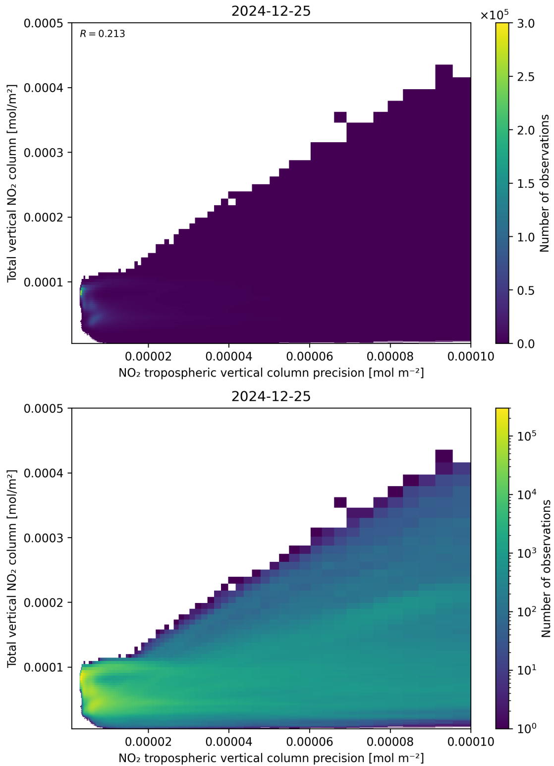
Figure 138: Scatter density plot of “NO 2 tropospheric vertical column precision” against “Total vertical NO 2 column” for 2024-12-24 to 2024-12-26.
