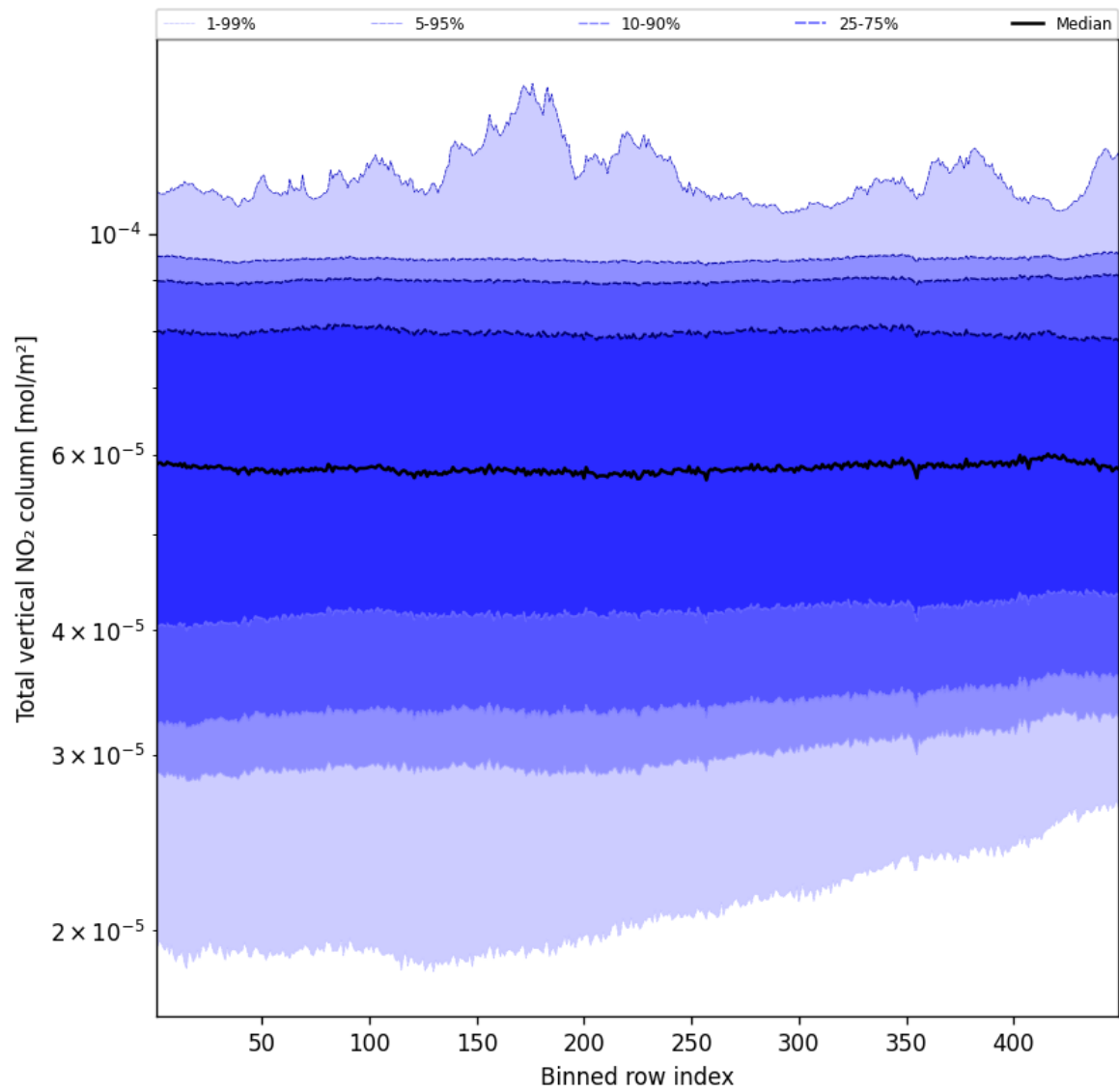
Figure 55: Along track statistics of “Total vertical NO 2 column” for 2024-12-24 to 2024-12-26
