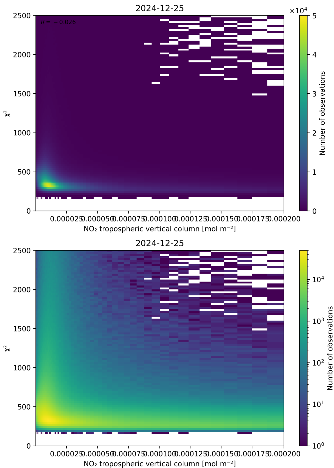
Figure 124: Scatter density plot of “NO 2 tropospheric vertical column” against “ \chi^2 ” for 2024-12-24 to 2024-12-26.
