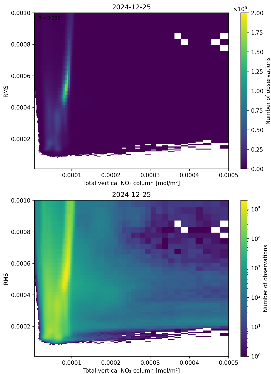
Figure 120: Scatter density plot of “Total vertical NO 2 column” against “RMS” for 2024-12-24 to 2024-12-26.
