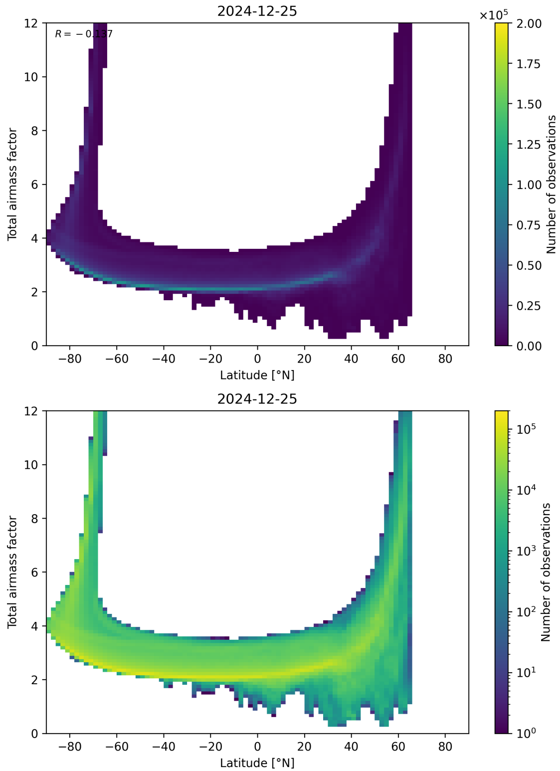
Figure 84: Scatter density plot of “Latitude” against “Total airmass factor” for 2024-12-24 to 2024-12-26.
