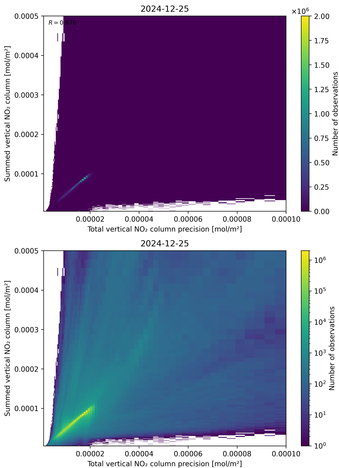
Figure 117: Scatter density plot of “Total vertical NO 2 column precision” against “Summed vertical NO 2 column” for 2024-12-24 to 2024-12-26.
