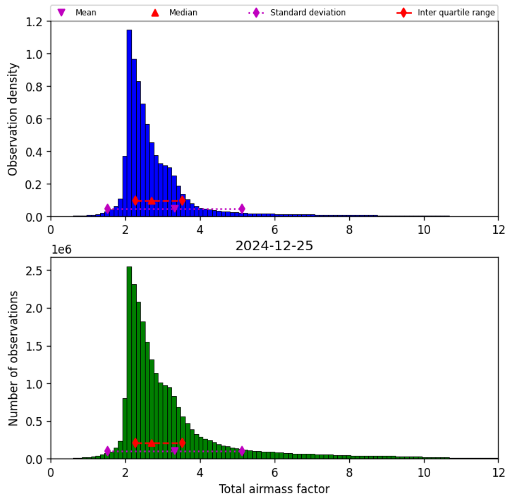
Figure 32: Histogram of “Total airmass factor” for 2024-12-24 to 2024-12-26
