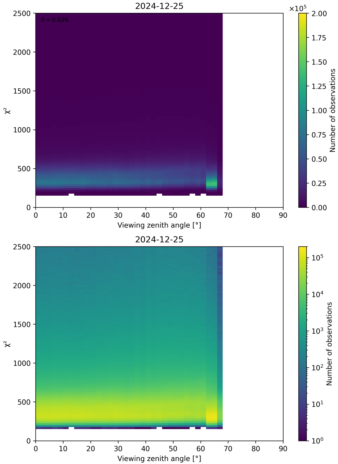
Figure 162: Scatter density plot of “Viewing zenith angle” against “ \chi^2 ” for 2024-12-24 to 2024-12-26.
