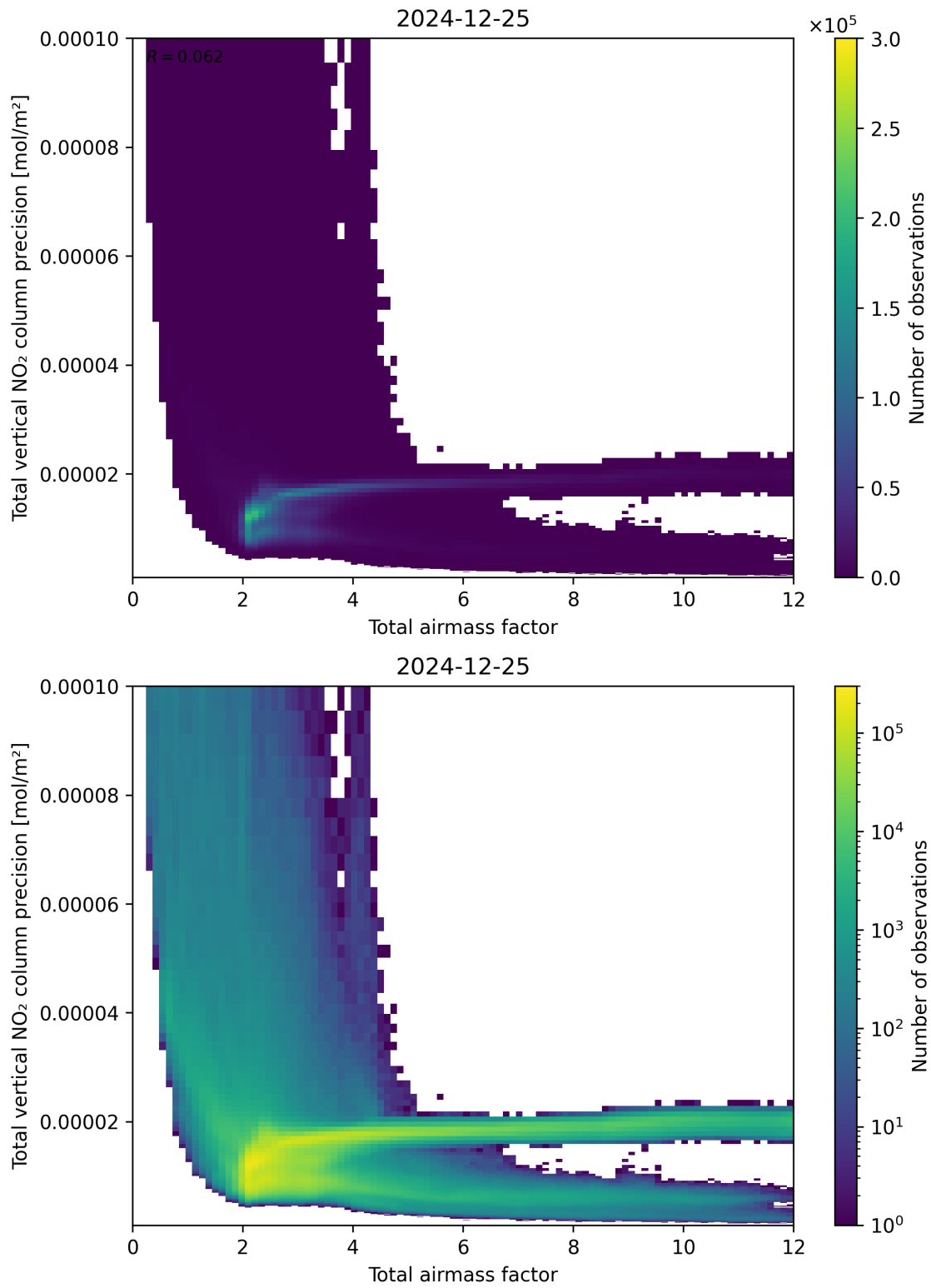
Figure 68: Scatter density plot of “Total airmass factor” against “Total vertical NO 2 column precision” for 2024-12-24 to 2024-12-26.
