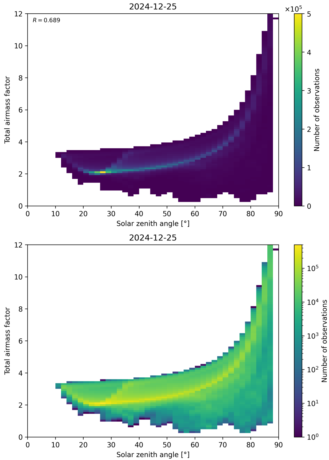
Figure 146: Scatter density plot of “Solar zenith angle” against “Total air mass factor” for 2024-12-24 to 2024-12-26.
