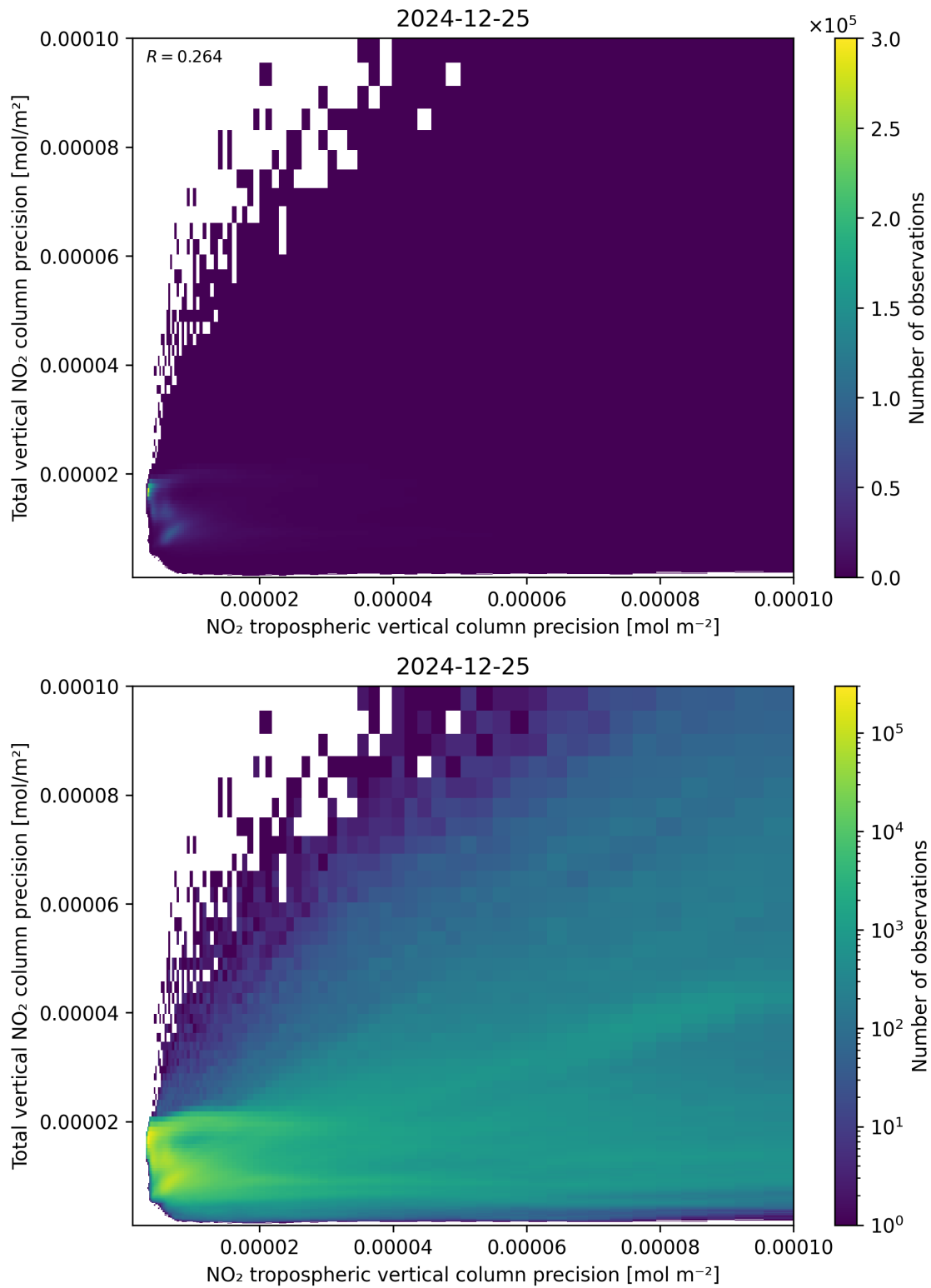
Figure 139: Scatter density plot of “NO 2 tropospheric vertical column precision” against “Total vertical NO 2 column precision” for 2024-12-24 to 2024-12-26.
