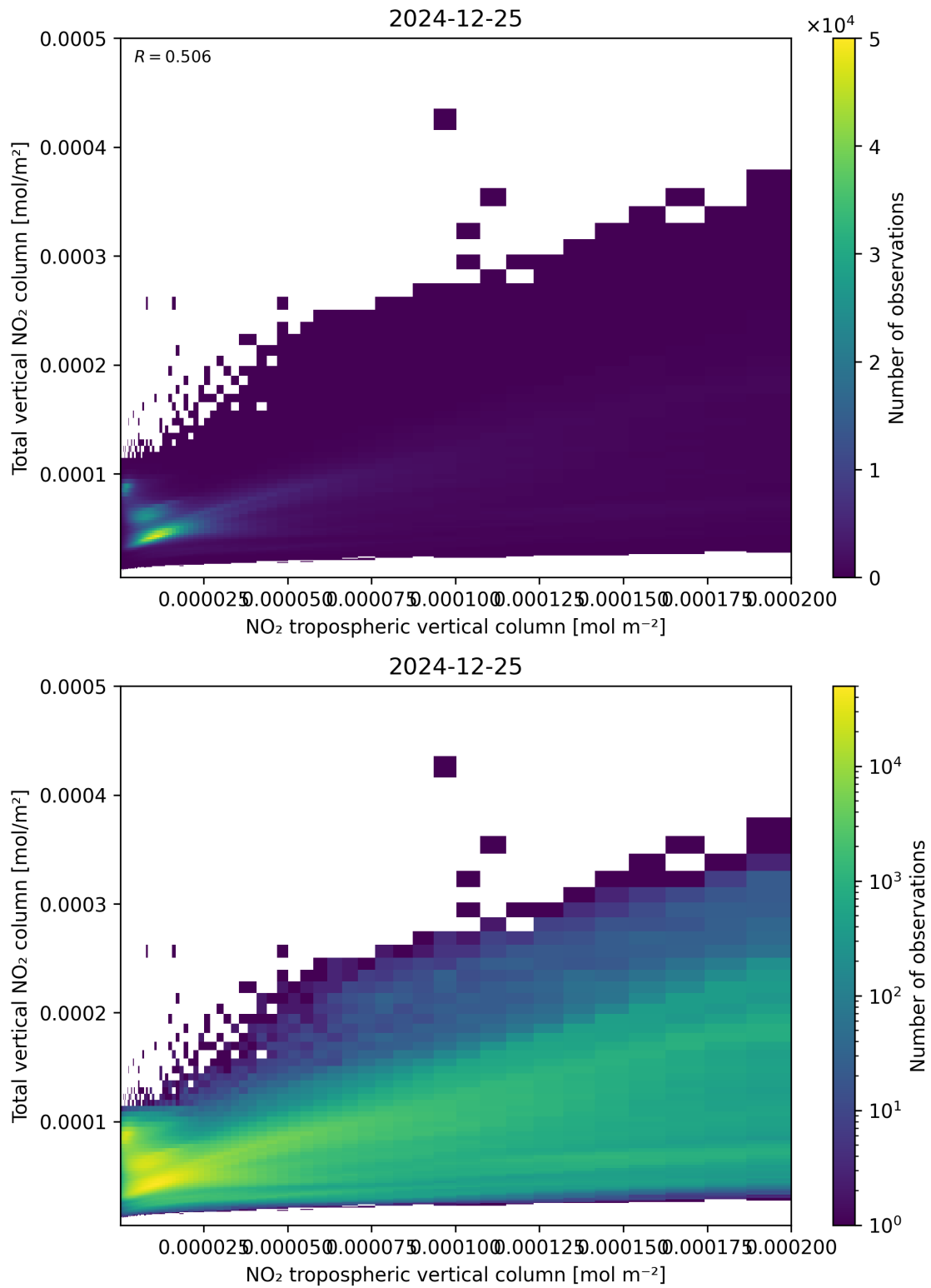
Figure 128: Scatter density plot of “NO 2 tropospheric vertical column” against “Total vertical NO 2 column” for 2024-12-24 to 2024-12-26.
