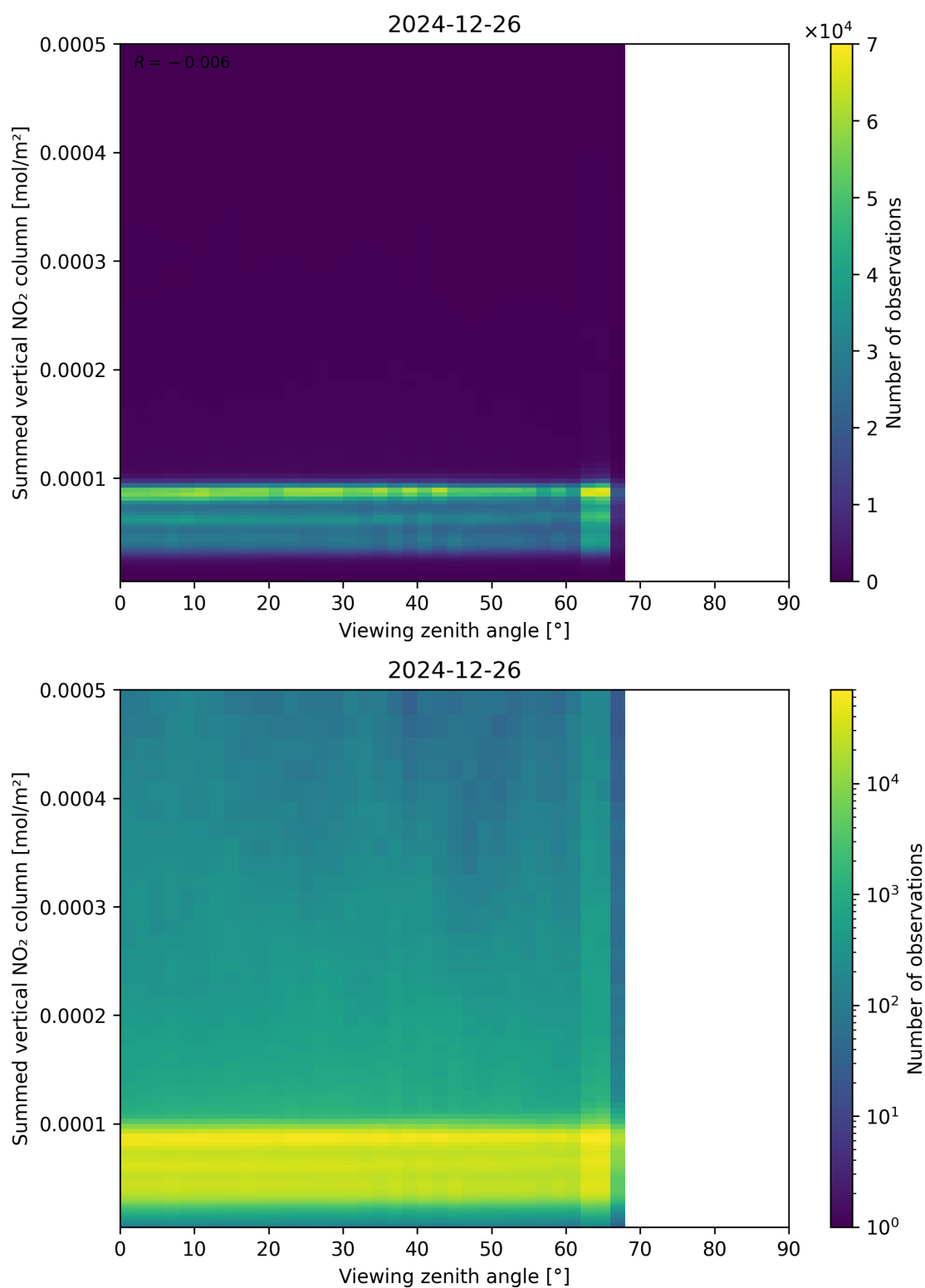
Figure 165: Scatter density plot of “Viewing zenith angle” against “Summed vertical NO 2 column” for 2024-12-25 to 2024-12-27.
