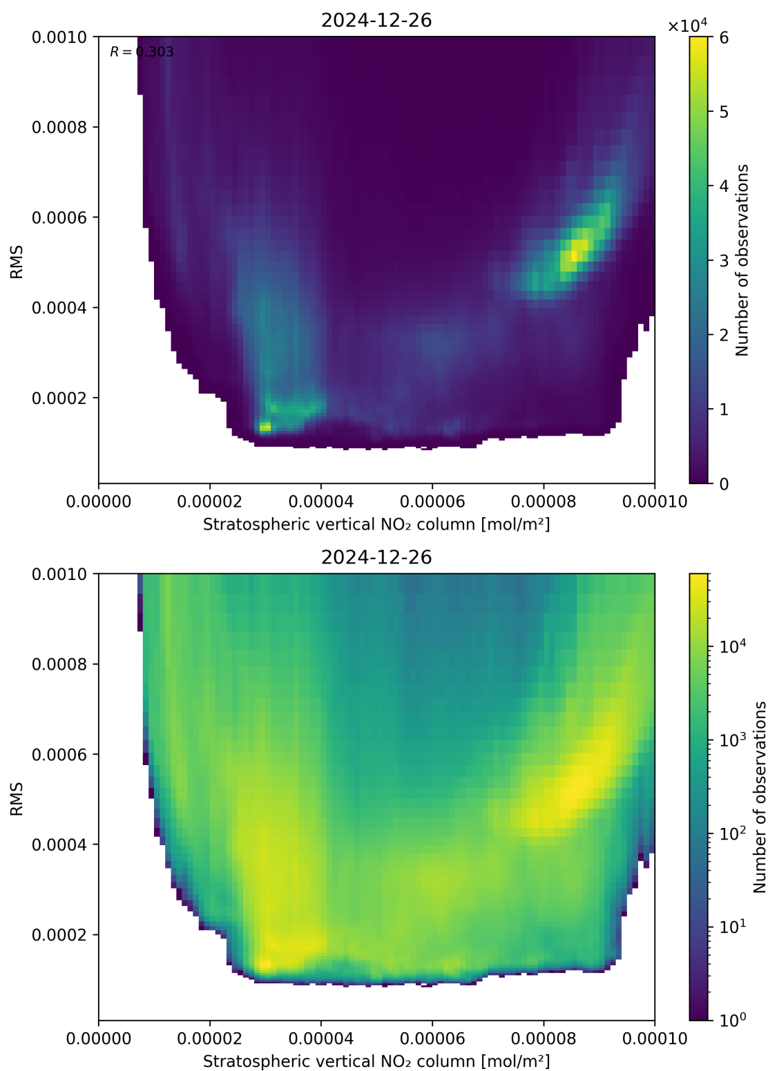
Figure 102: Scatter density plot of “Stratospheric vertical NO 2 column” against “RMS” for 2024-12-25 to 2024-12-27.
