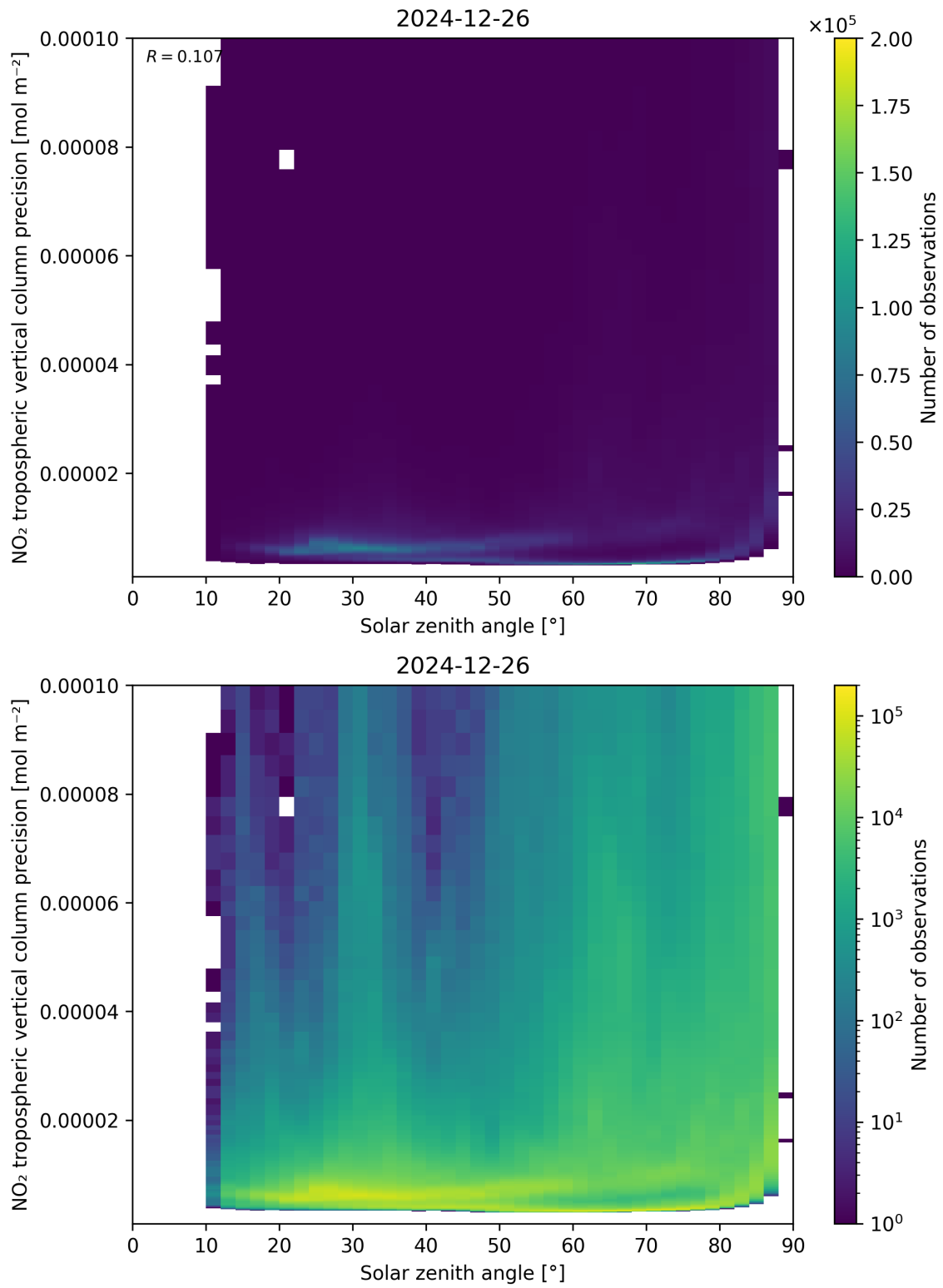
Figure 156: Scatter density plot of “Solar zenith angle” against “NO 2 tropospheric vertical column precision” for 2024-12-25 to 2024-12-27.
