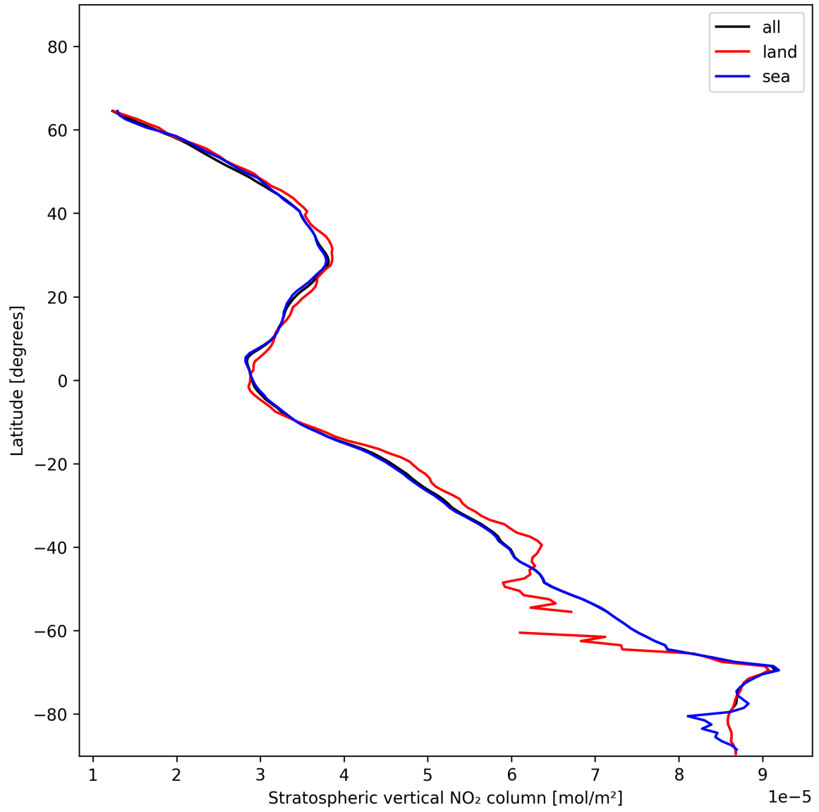
Figure 19: Zonal average of “Stratospheric vertical NO 2 column” for 2024-12-25 to 2024-12-27.
