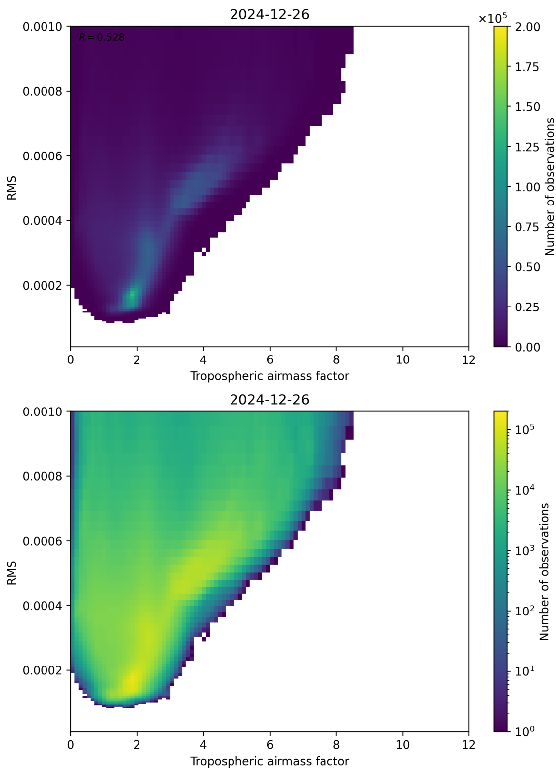
Figure 79: Scatter density plot of “Tropospheric airmass factor” against “RMS” for 2024-12-25 to 2024-12-27.
