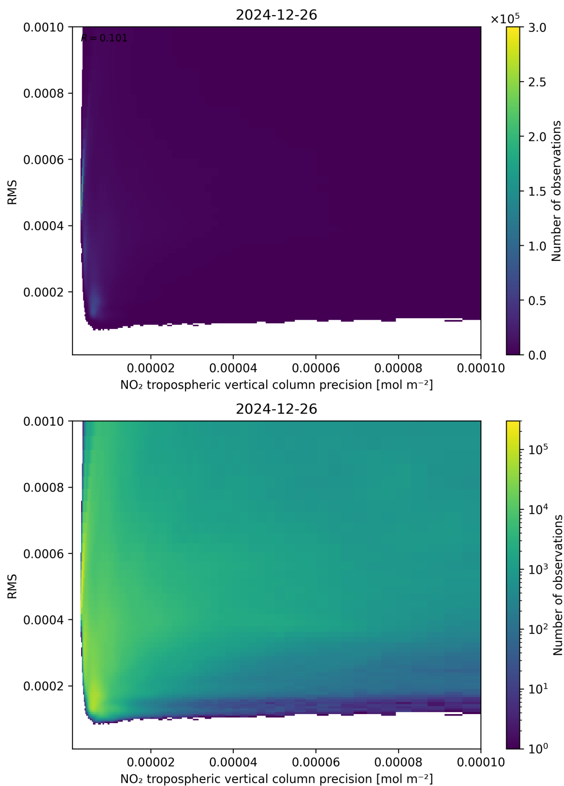
Figure 140: Scatter density plot of “NO 2 tropospheric vertical column precision” against “RMS” for 2024-12-25 to 2024-12-27.
