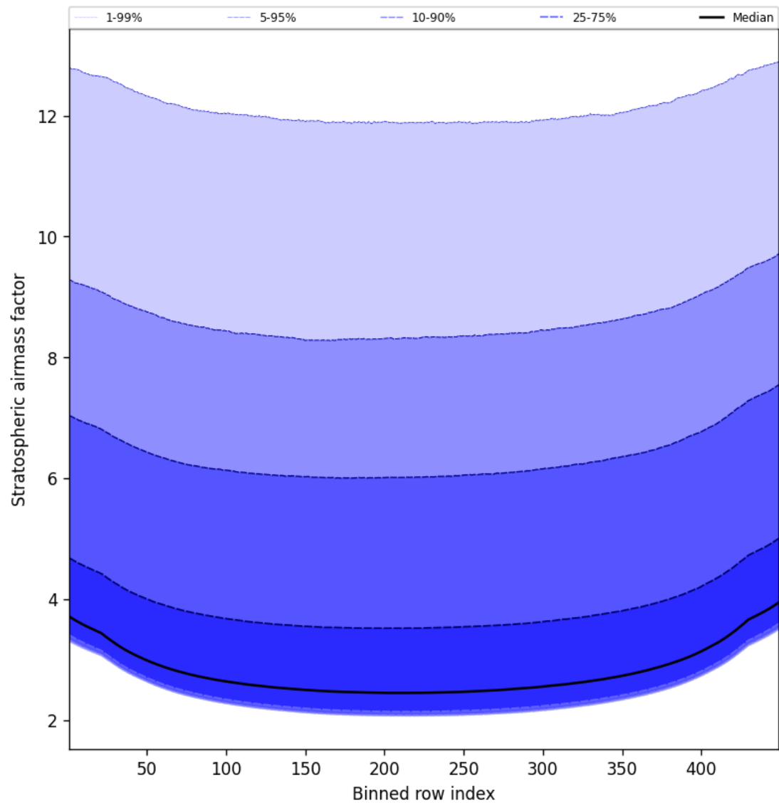
Figure 61: Along track statistics of “Stratospheric air mass factor” for 2024-12-25 to 2024-12-27
