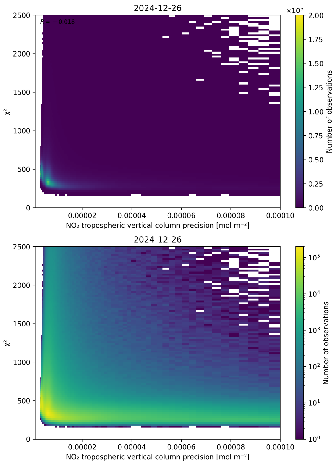
Figure 134: Scatter density plot of “NO 2 tropospheric vertical column precision” against “ \chi^2 ” for 2024-12-25 to 2024-12-27.
