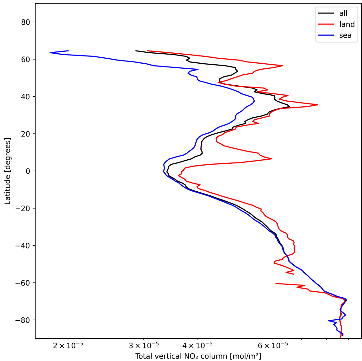
Figure 21: Zonal average of “Total vertical NO 2 column” for 2024-12-25 to 2024-12-27.
