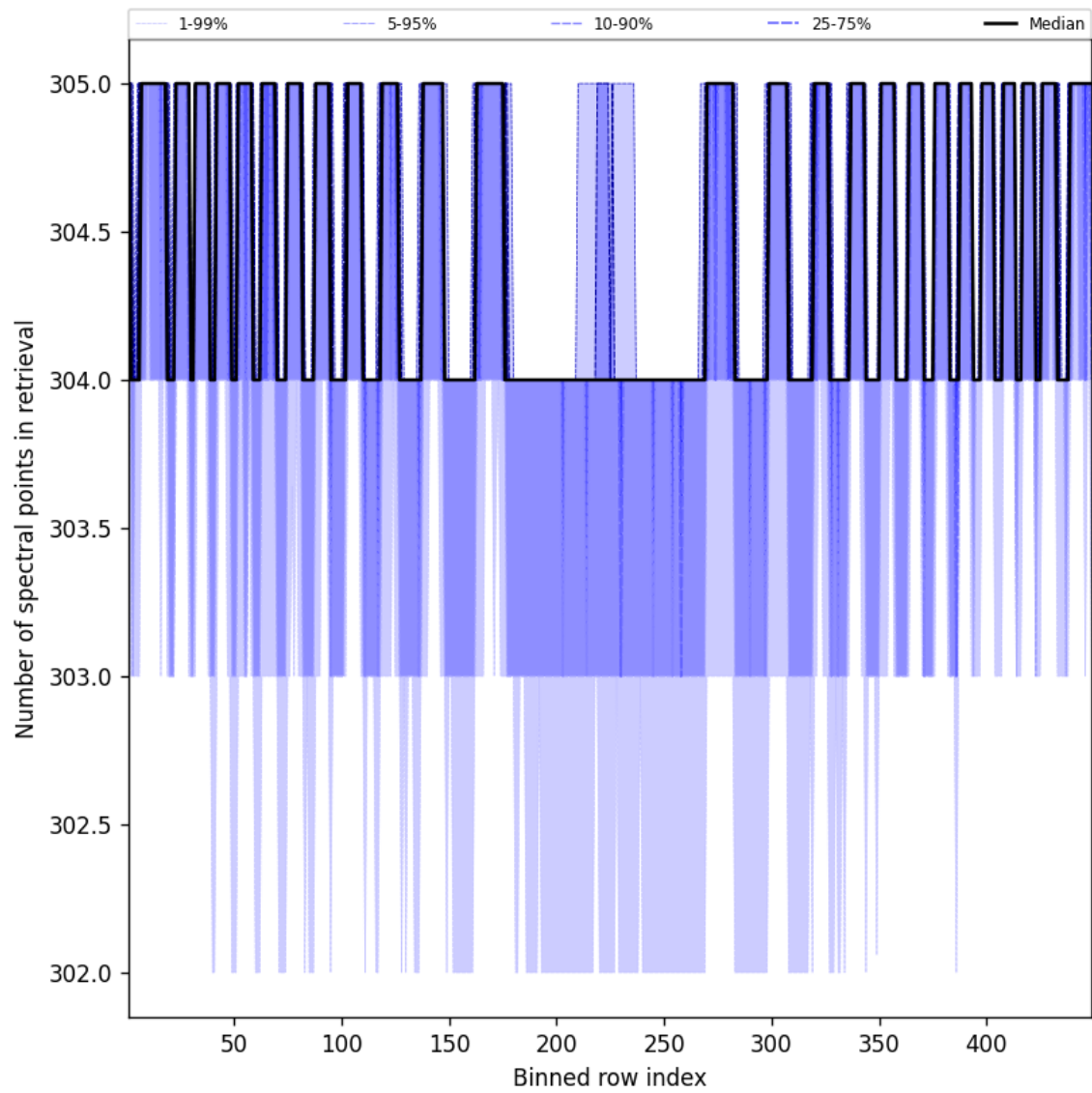
Figure 50: Along track statistics of “Number of spectral points in retrieval” for 2024-12-25 to 2024-12-27
