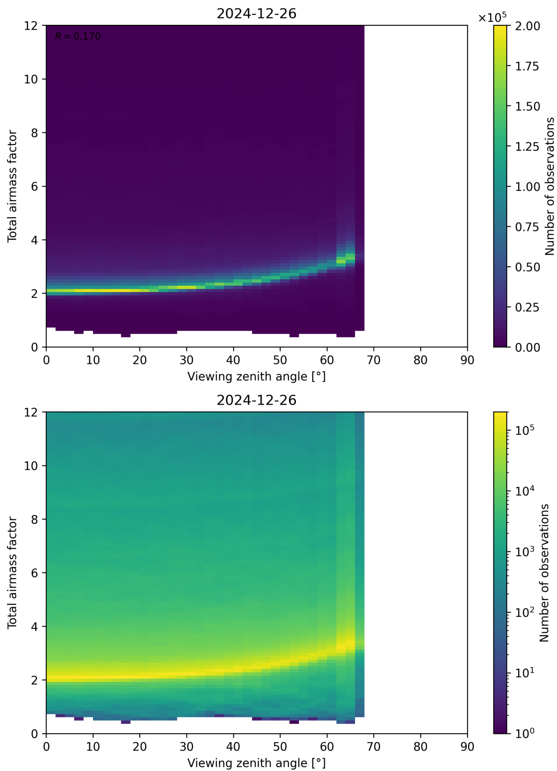
Figure 160: Scatter density plot of “Viewing zenith angle” against “Total airmass factor” for 2024-12-25 to 2024-12-27.
