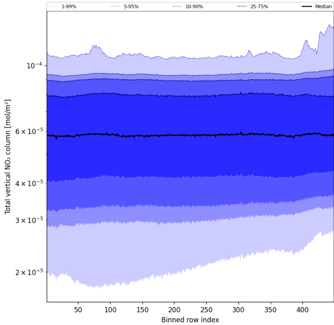
Figure 55: Along track statistics of “Total vertical NO 2 column” for 2024-12-25 to 2024-12-27
