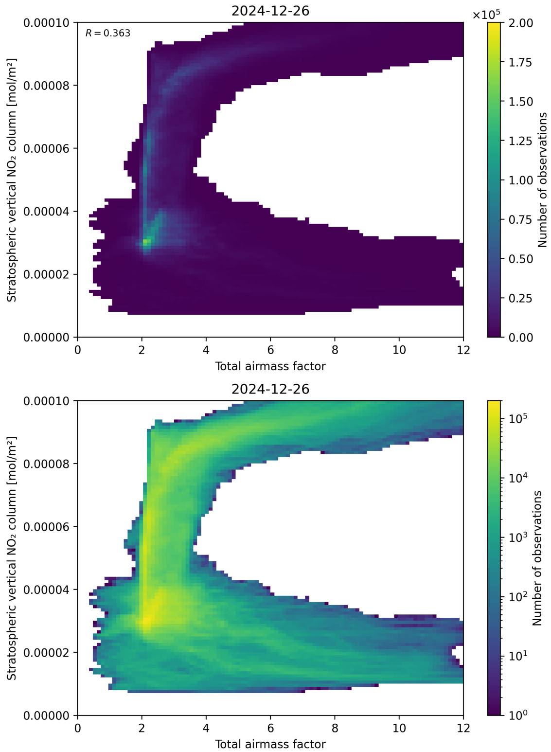
Figure 64: Scatter density plot of “Total airmass factor” against “Stratospheric vertical \text{NO}_2 column” for 2024-12-25 to 2024-12-27.
