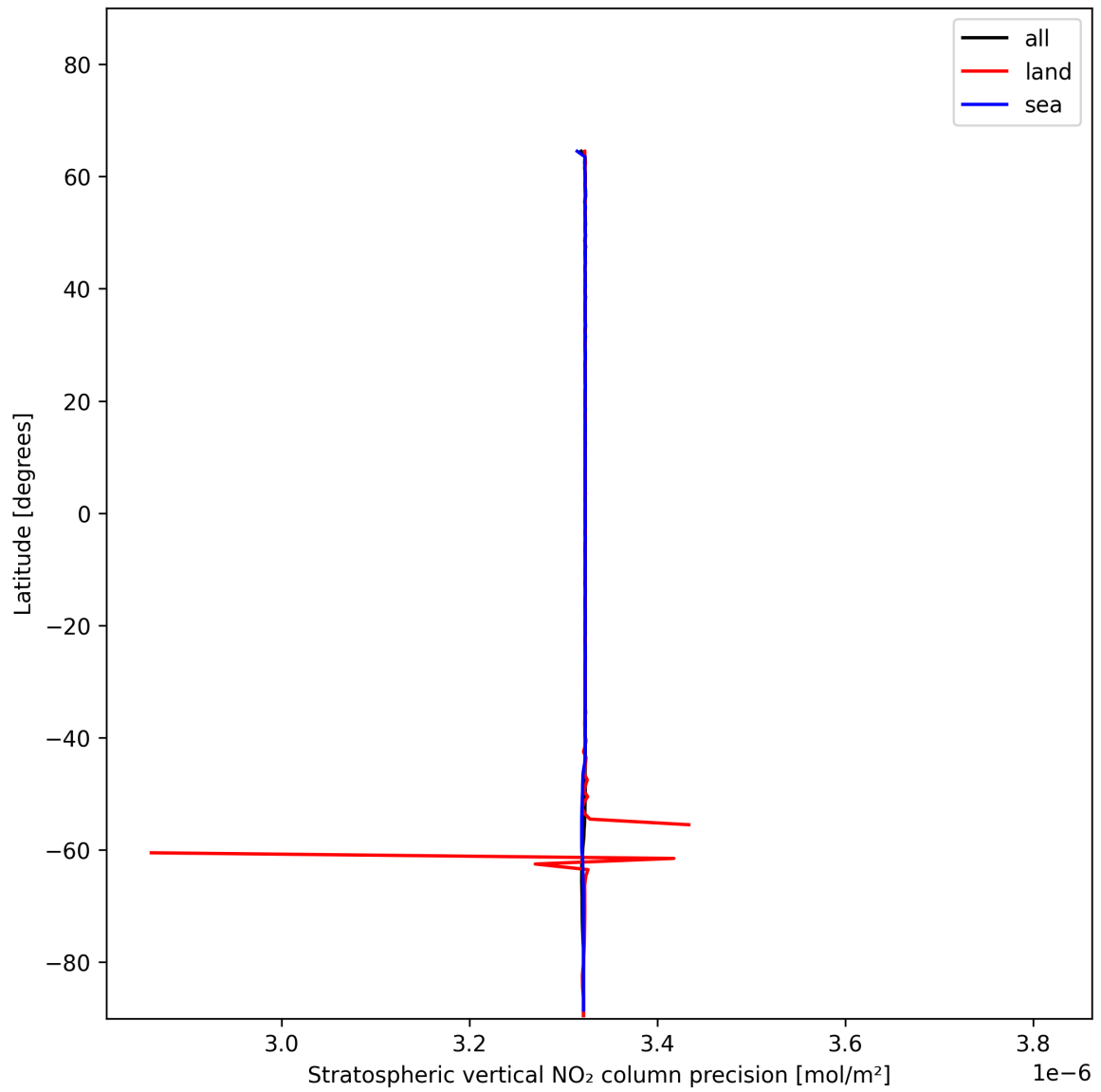
Figure 20: Zonal average of “Stratospheric vertical NO 2 column precision” for 2024-12-25 to 2024-12-27.
