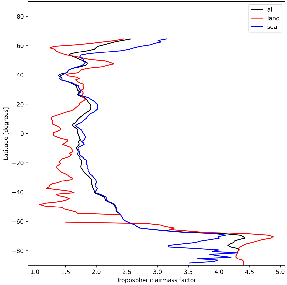
Figure 14: Zonal average of “Tropospheric airmass factor” for 2024-12-25 to 2024-12-27.
