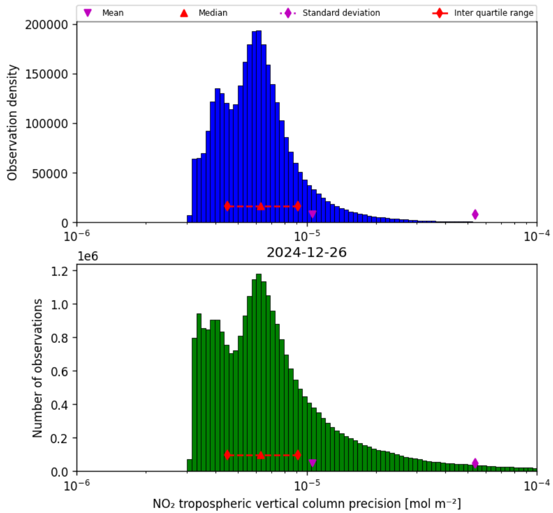
Figure 30: Histogram of “NO 2 tropospheric vertical column precision” for 2024-12-25 to 2024-12-27
