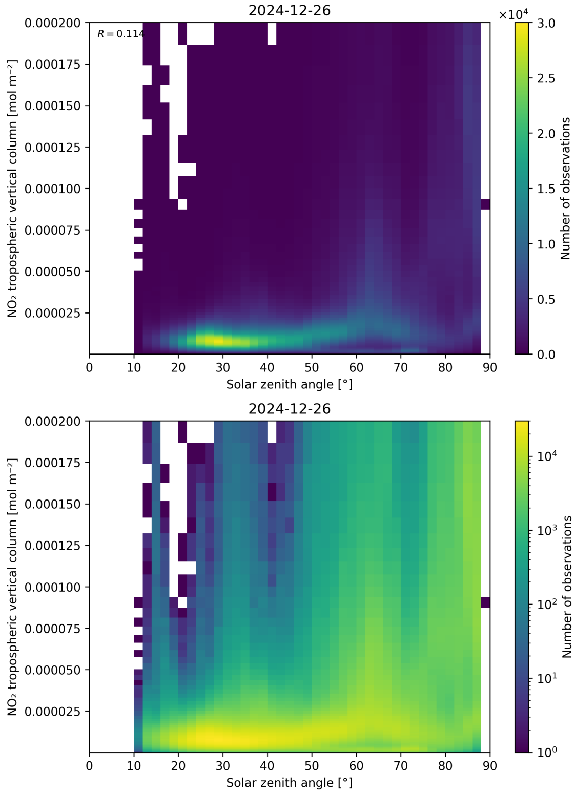
Figure 155: Scatter density plot of “Solar zenith angle” against “NO 2 tropospheric vertical column” for 2024-12-25 to 2024-12-27.
