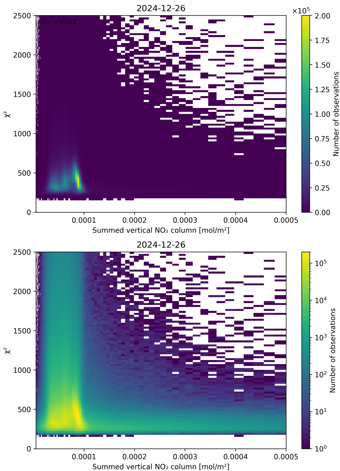
Figure 104: Scatter density plot of “Summed vertical NO 2 column” against “ \chi^2 ” for 2024-12-25 to 2024-12-27.
