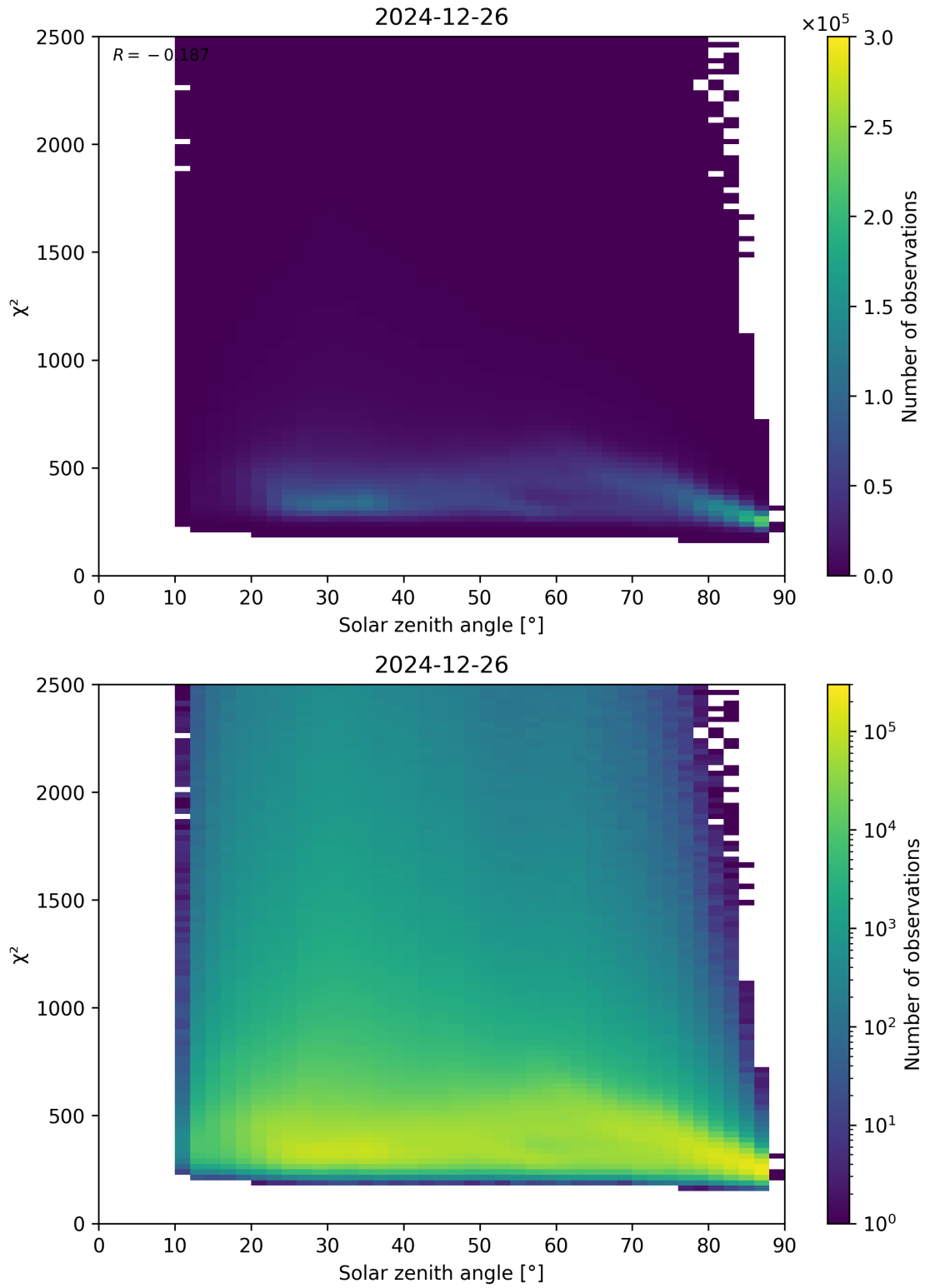
Figure 148: Scatter density plot of “Solar zenith angle” against “ \chi^2 ” for 2024-12-25 to 2024-12-27.
