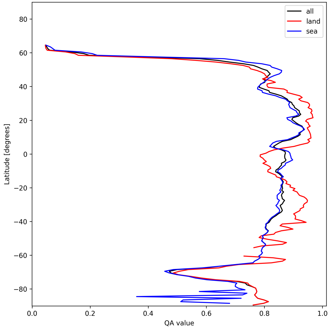
Figure 11: Zonal average of “QA value” for 2024-12-25 to 2024-12-27.
