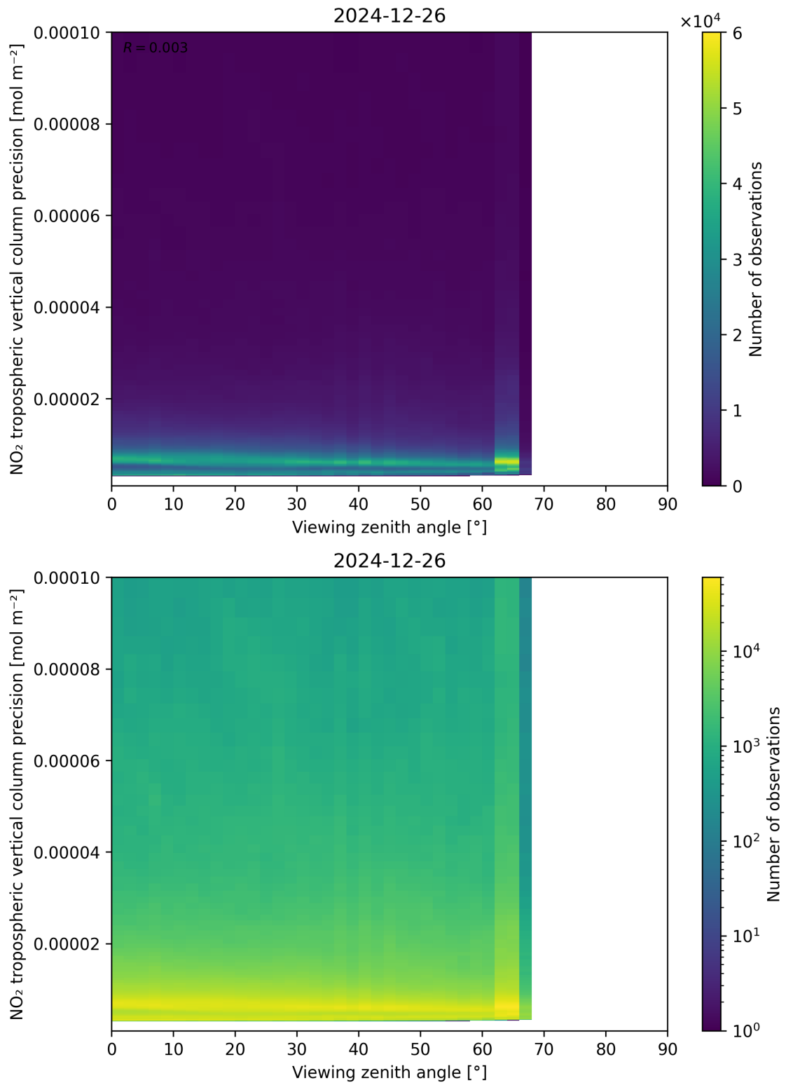
Figure 170: Scatter density plot of “Viewing zenith angle” against “NO 2 tropospheric vertical column precision” for 2024-12-25 to 2024-12-27.
