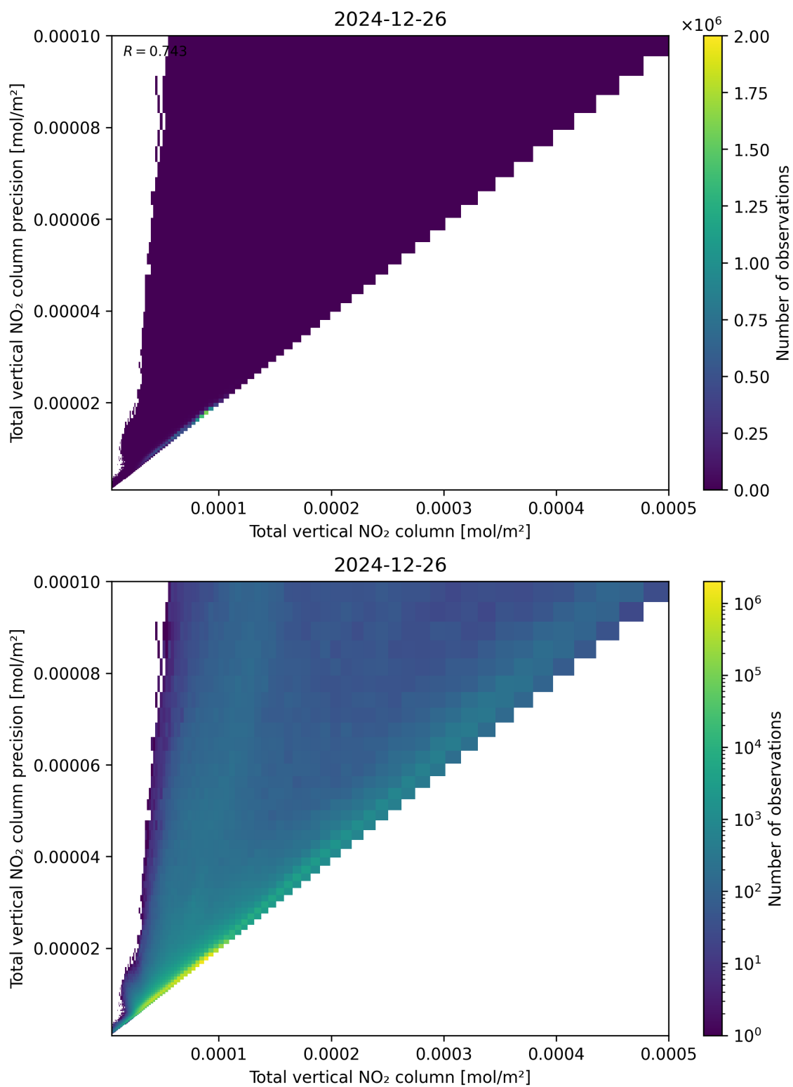
Figure 114: Scatter density plot of “Total vertical NO 2 column” against “Total vertical NO 2 column precision” for 2024-12-25 to 2024-12-27.
