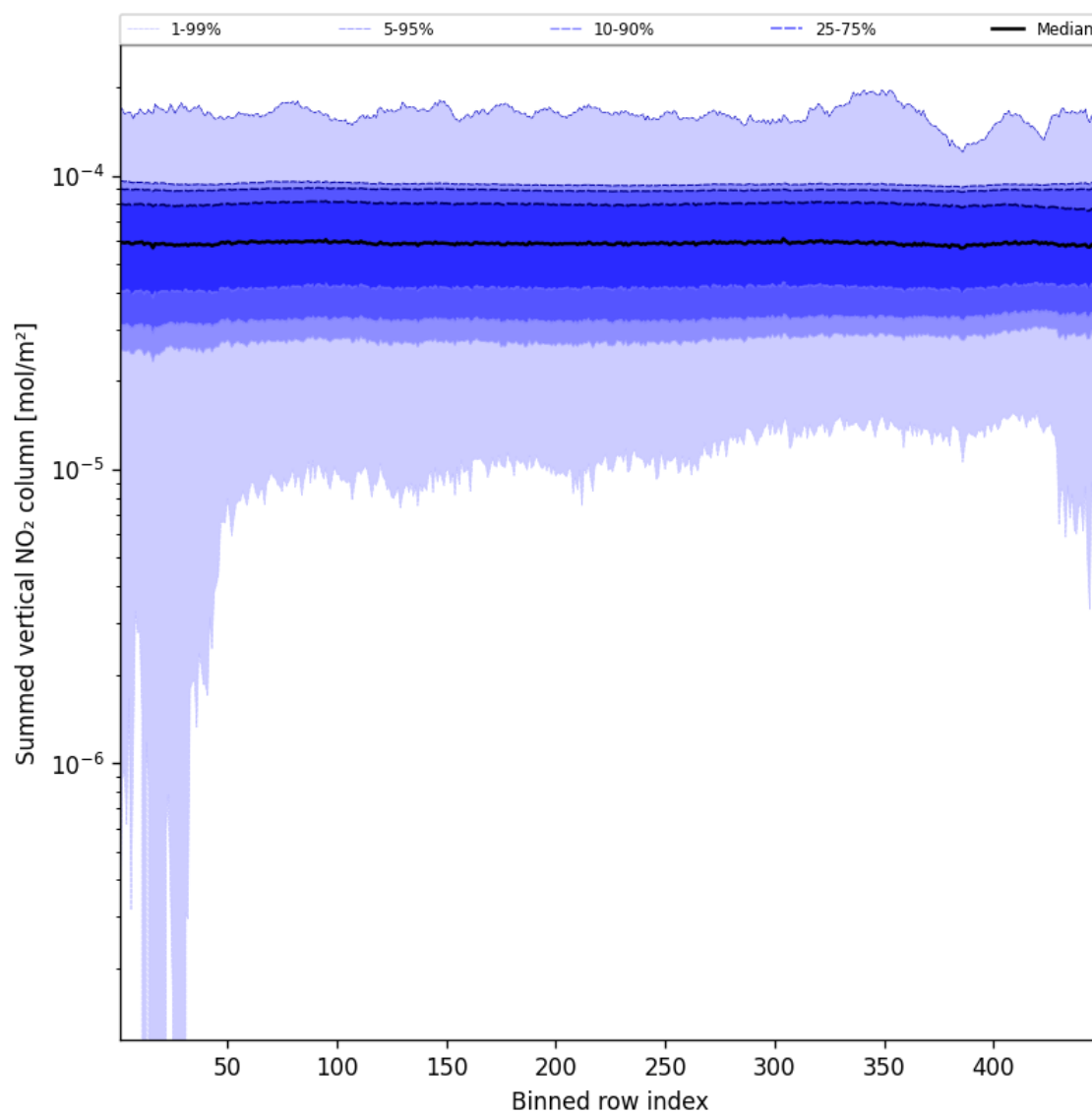
Figure 57: Along track statistics of “Summed vertical NO 2 column” for 2024-12-25 to 2024-12-27
