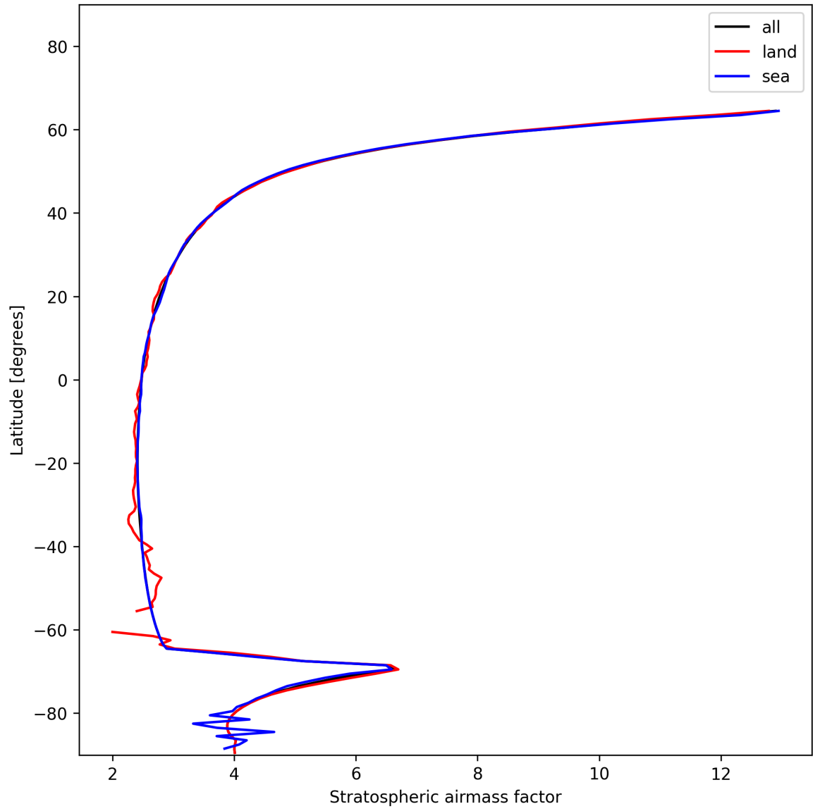
Figure 27: Zonal average of “Stratospheric airmass factor” for 2024-12-25 to 2024-12-27.
