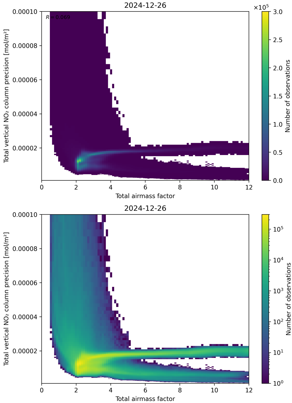
Figure 68: Scatter density plot of “Total airmass factor” against “Total vertical NO 2 column precision” for 2024-12-25 to 2024-12-27.
