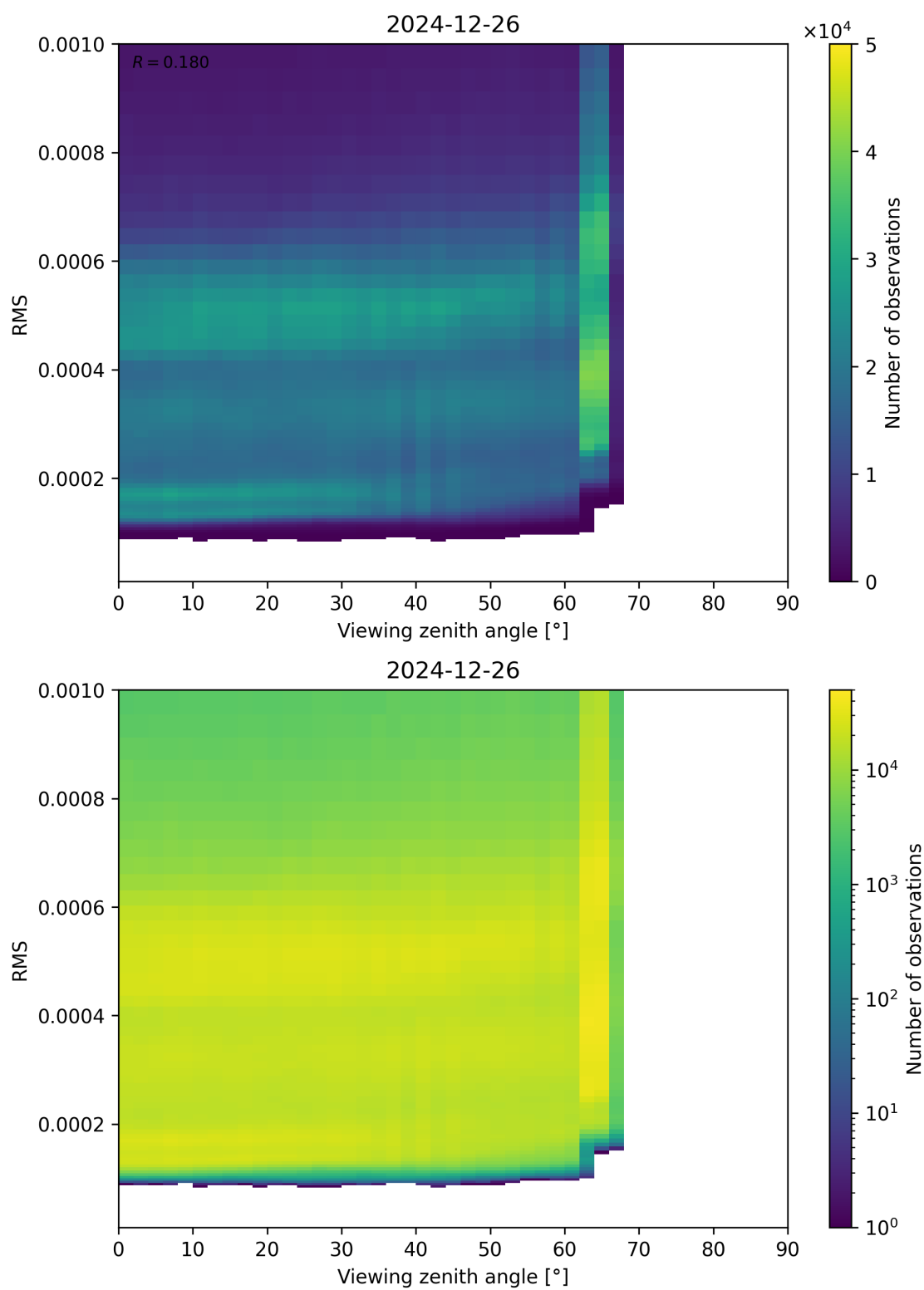
Figure 171: Scatter density plot of “Viewing zenith angle” against “RMS” for 2024-12-25 to 2024-12-27.
