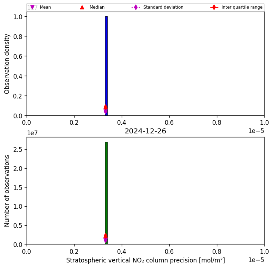
Figure 37: Histogram of “Stratospheric vertical NO 2 column precision” for 2024-12-25 to 2024-12-27
