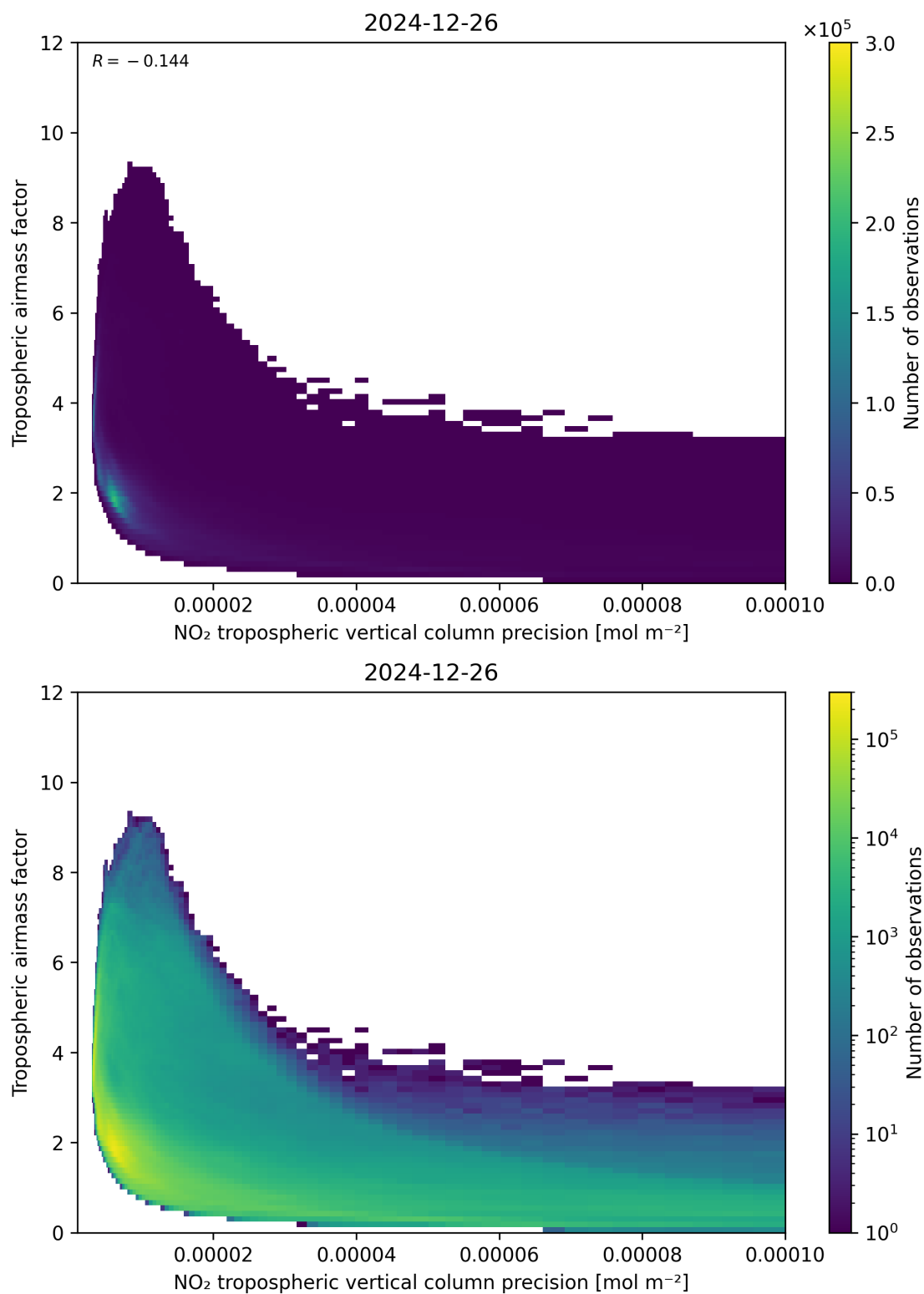
Figure 133: Scatter density plot of “NO 2 tropospheric vertical column precision” against “Tropospheric air mass factor” for 2024-12-25 to 2024-12-27.
