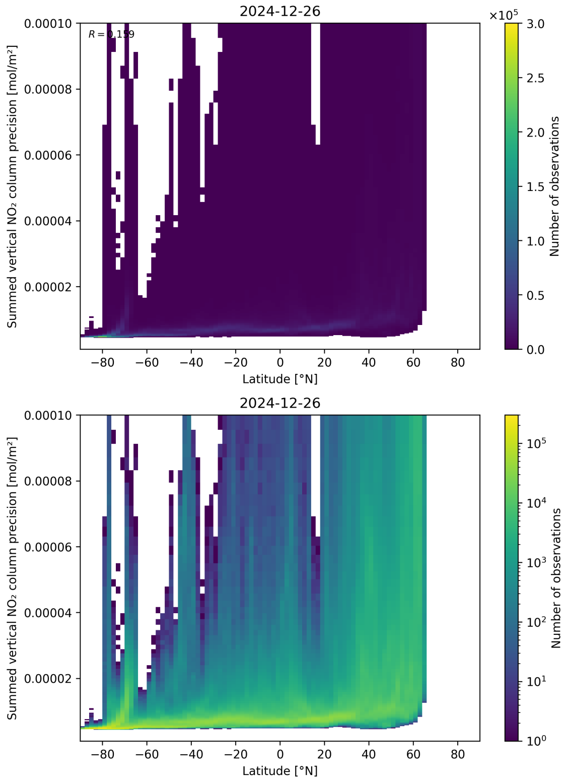
Figure 89: Scatter density plot of “Latitude” against “Summed vertical NO 2 column precision” for 2024-12-25 to 2024-12-27.
