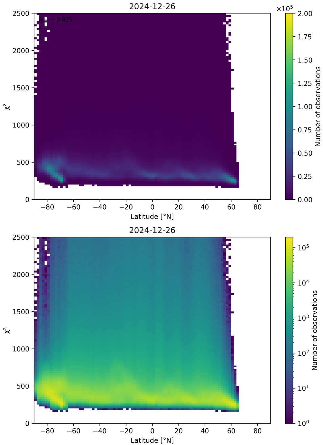
Figure 86: Scatter density plot of “Latitude” against “ \chi^2 ” for 2024-12-25 to 2024-12-27.
