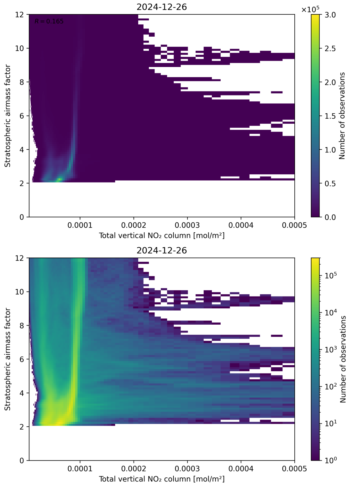
Figure 110: Scatter density plot of “Total vertical NO 2 column” against “Stratospheric airmass factor” for 2024-12-25 to 2024-12-27.
