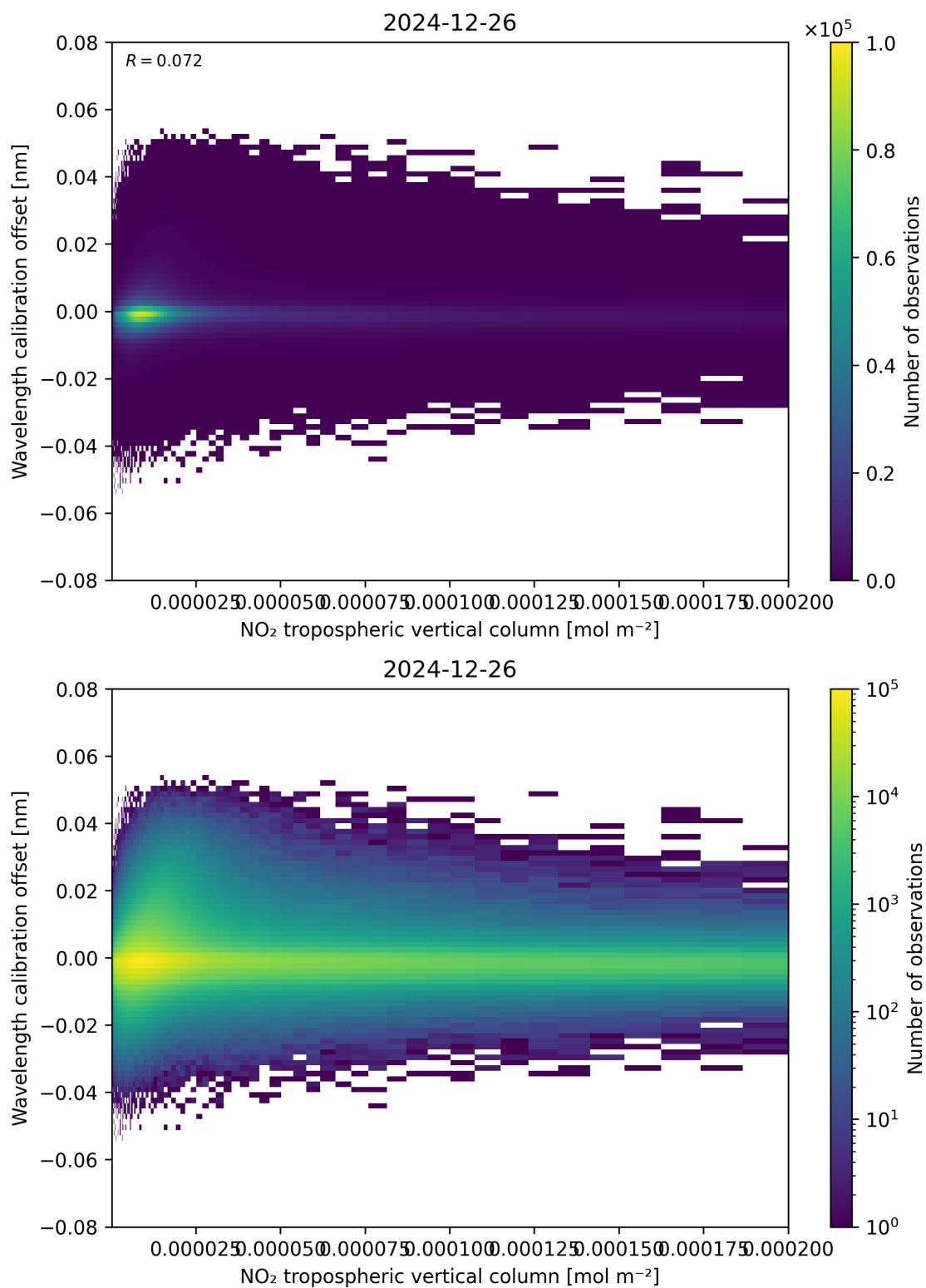
Figure 143: Scatter density plot of “NO 2 tropospheric vertical column” against “Wavelength calibration offset” for 2024-12-25 to 2024-12-27.
