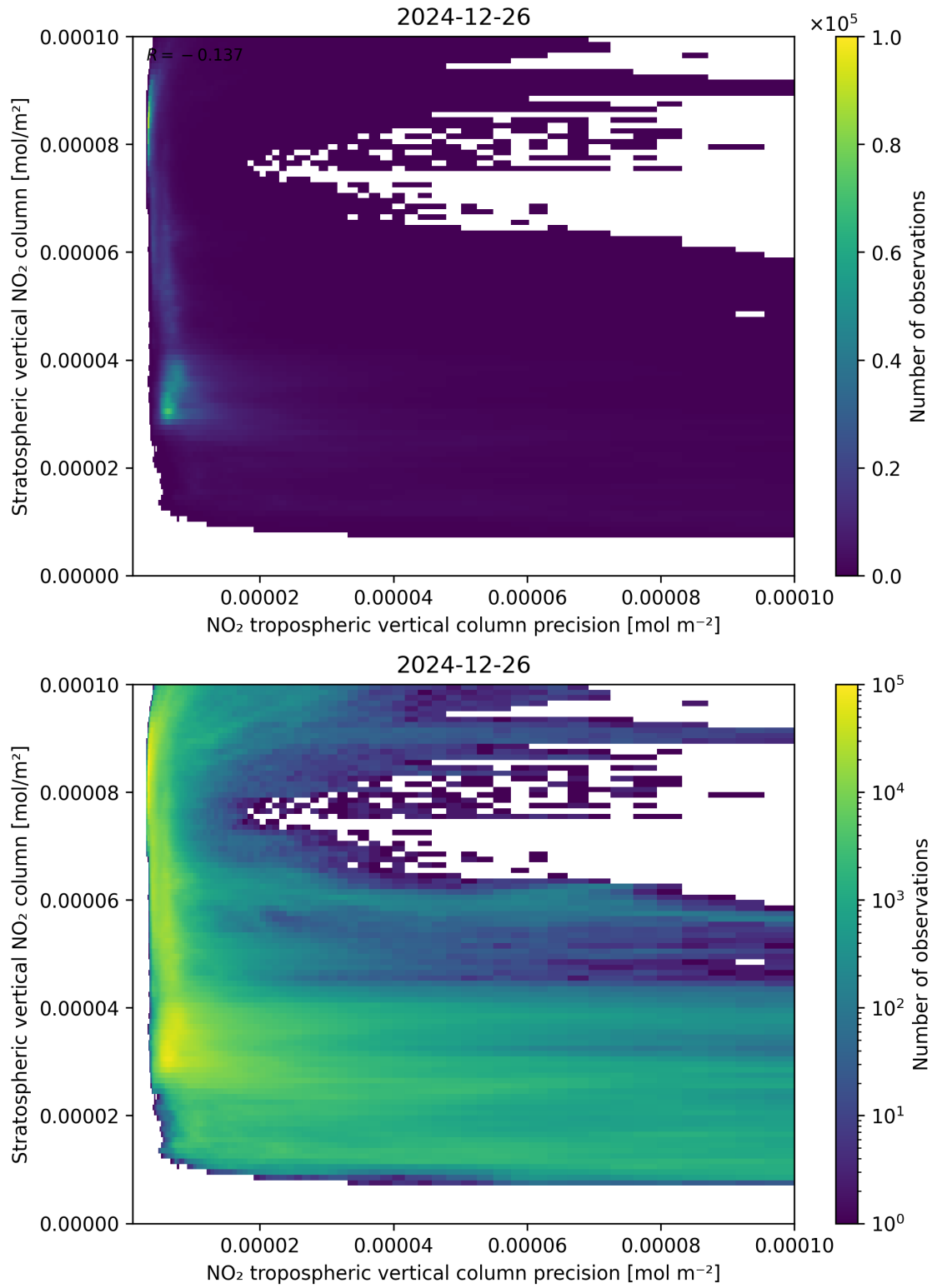
Figure 135: Scatter density plot of “NO 2 tropospheric vertical column precision” against “Stratospheric vertical NO 2 column” for 2024-12-25 to 2024-12-27.
