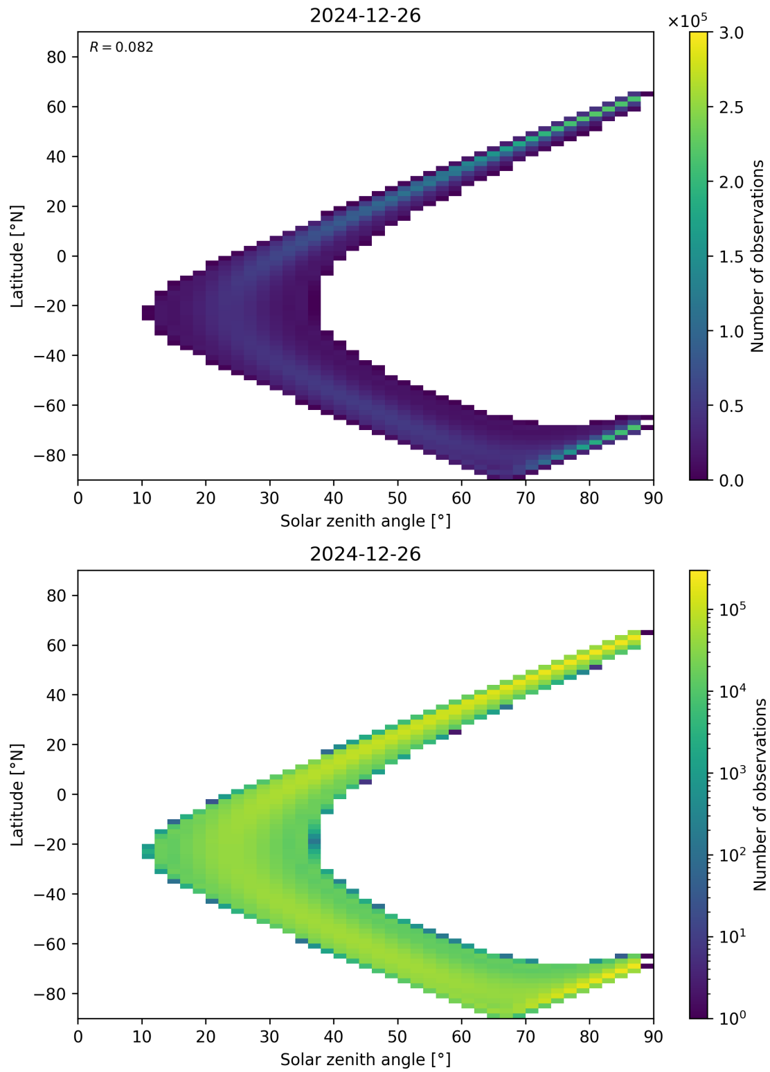
Figure 149: Scatter density plot of “Solar zenith angle” against “Latitude” for 2024-12-25 to 2024-12-27.
