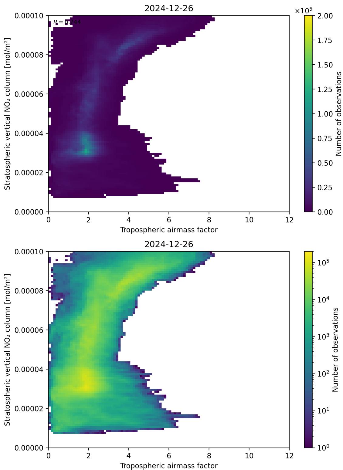
Figure 74: Scatter density plot of “Tropospheric airmass factor” against “Stratospheric vertical NO 2 column” for 2024-12-25 to 2024-12-27.
