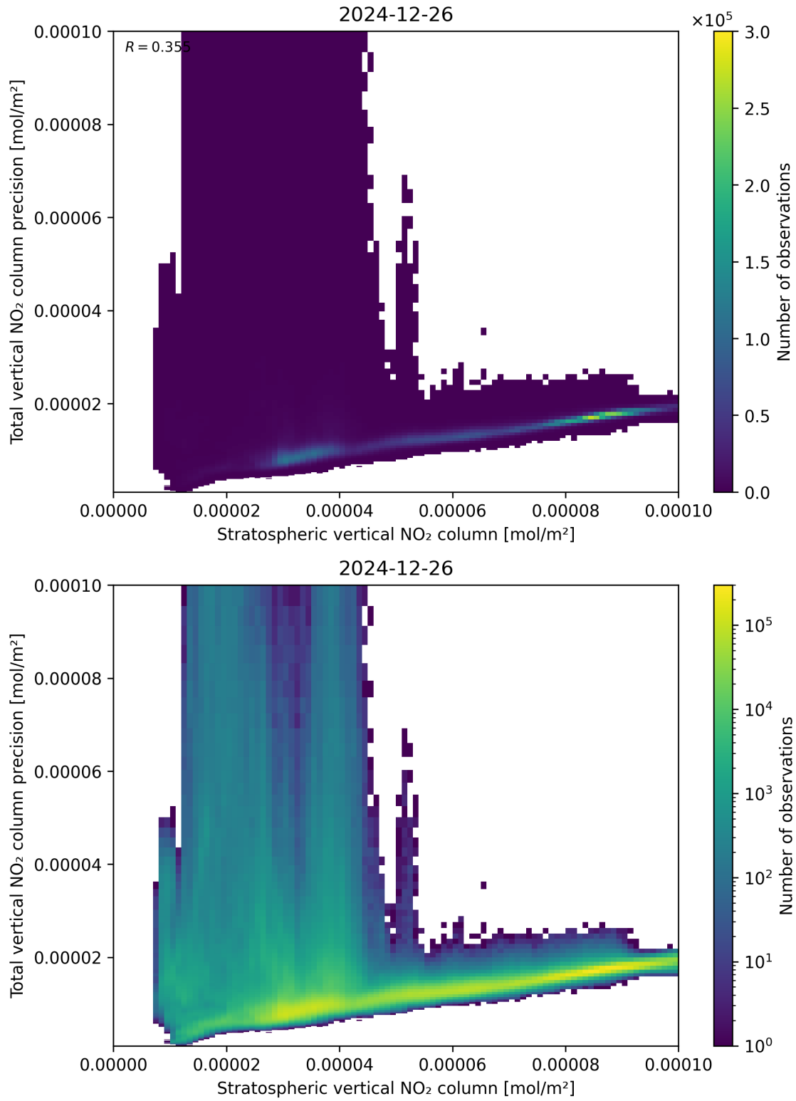
Figure 101: Scatter density plot of “Stratospheric vertical NO 2 column” against “Total vertical NO 2 column precision” for 2024-12-25 to 2024-12-27.
