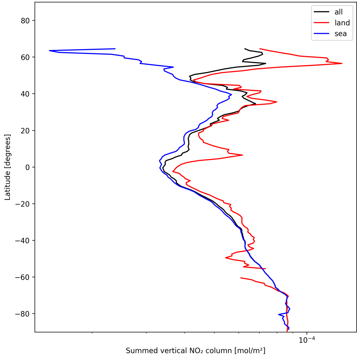
Figure 23: Zonal average of “Summed vertical NO 2 column” for 2024-12-25 to 2024-12-27.
