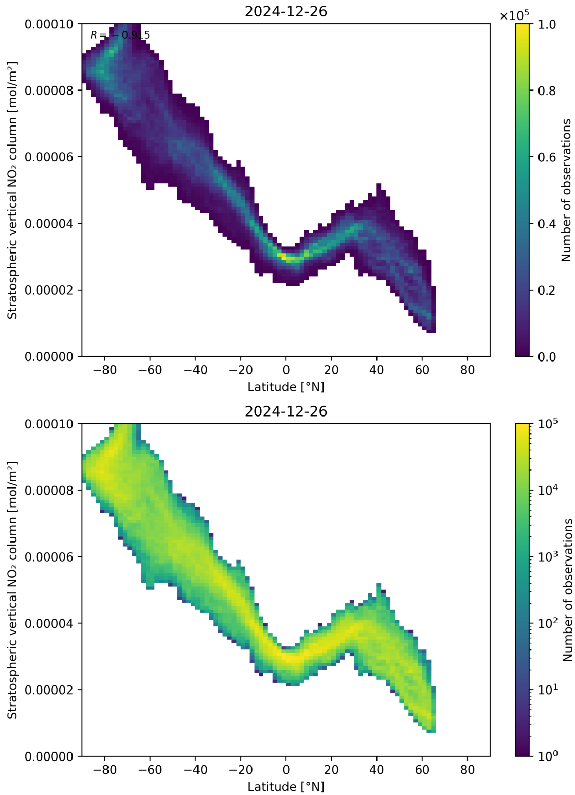
Figure 87: Scatter density plot of “Latitude” against “Stratospheric vertical NO 2 column” for 2024-12-25 to 2024-12-27.
