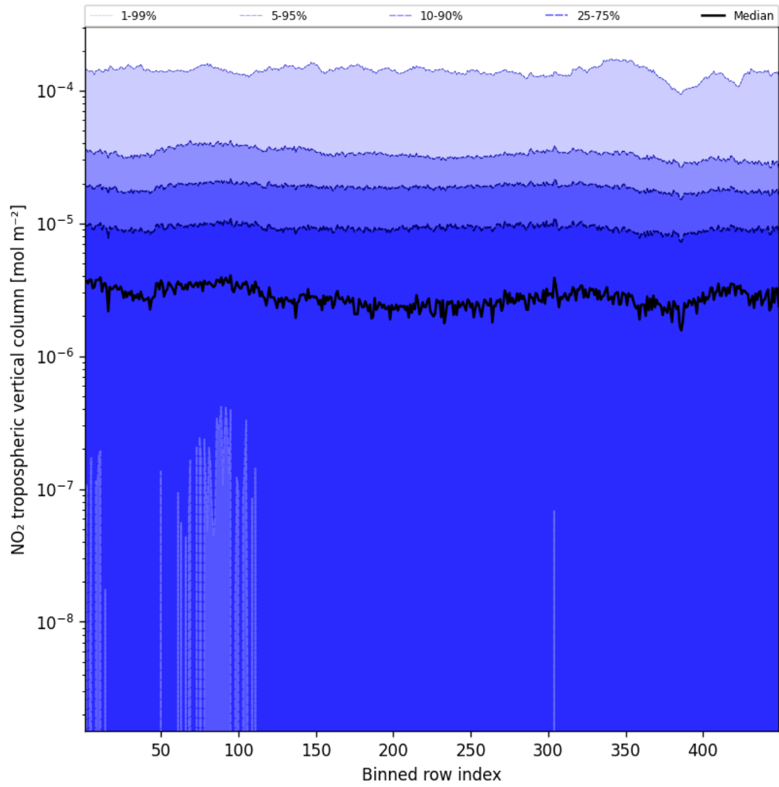
Figure 46: Along track statistics of “ \text{NO}_2 tropospheric vertical column” for 2024-12-25 to 2024-12-27
