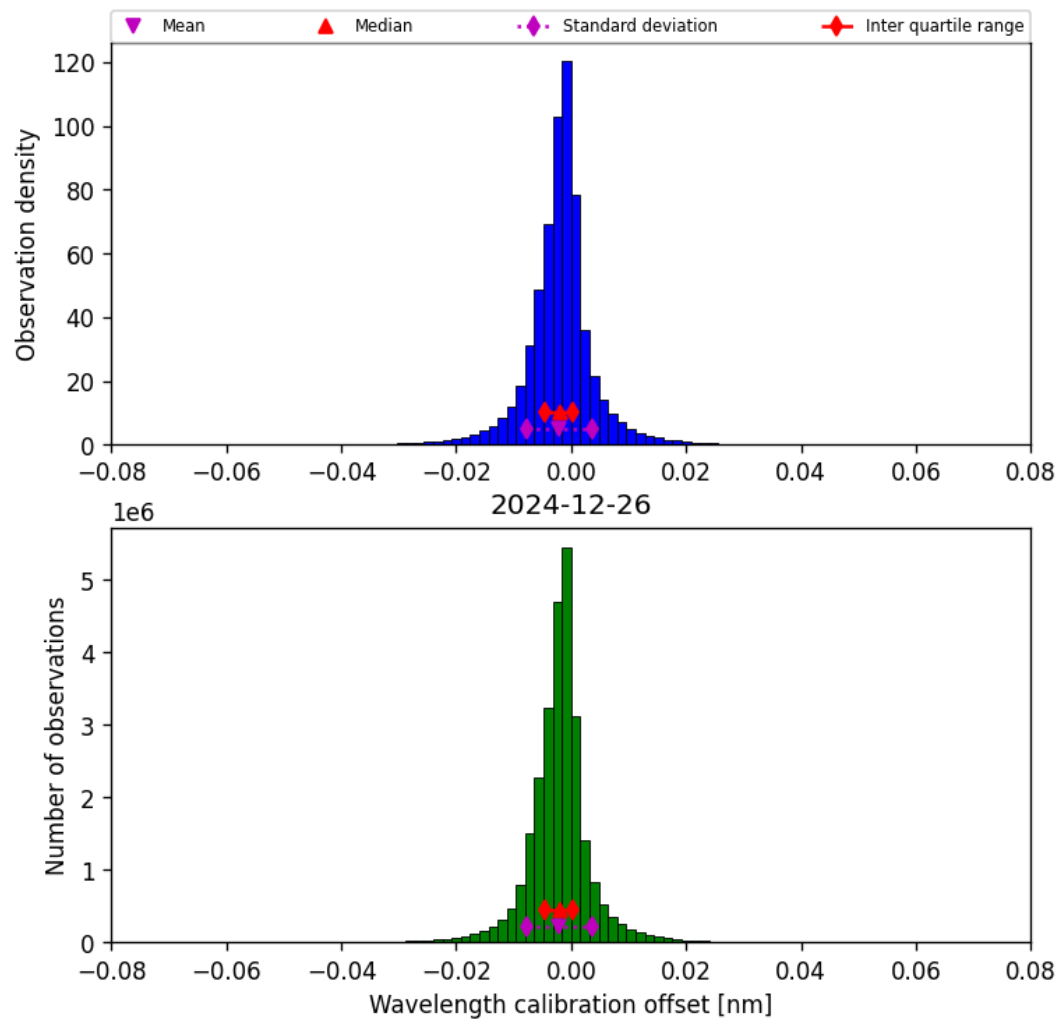
Figure 35: Histogram of “Wavelength calibration offset” for 2024-12-25 to 2024-12-27
