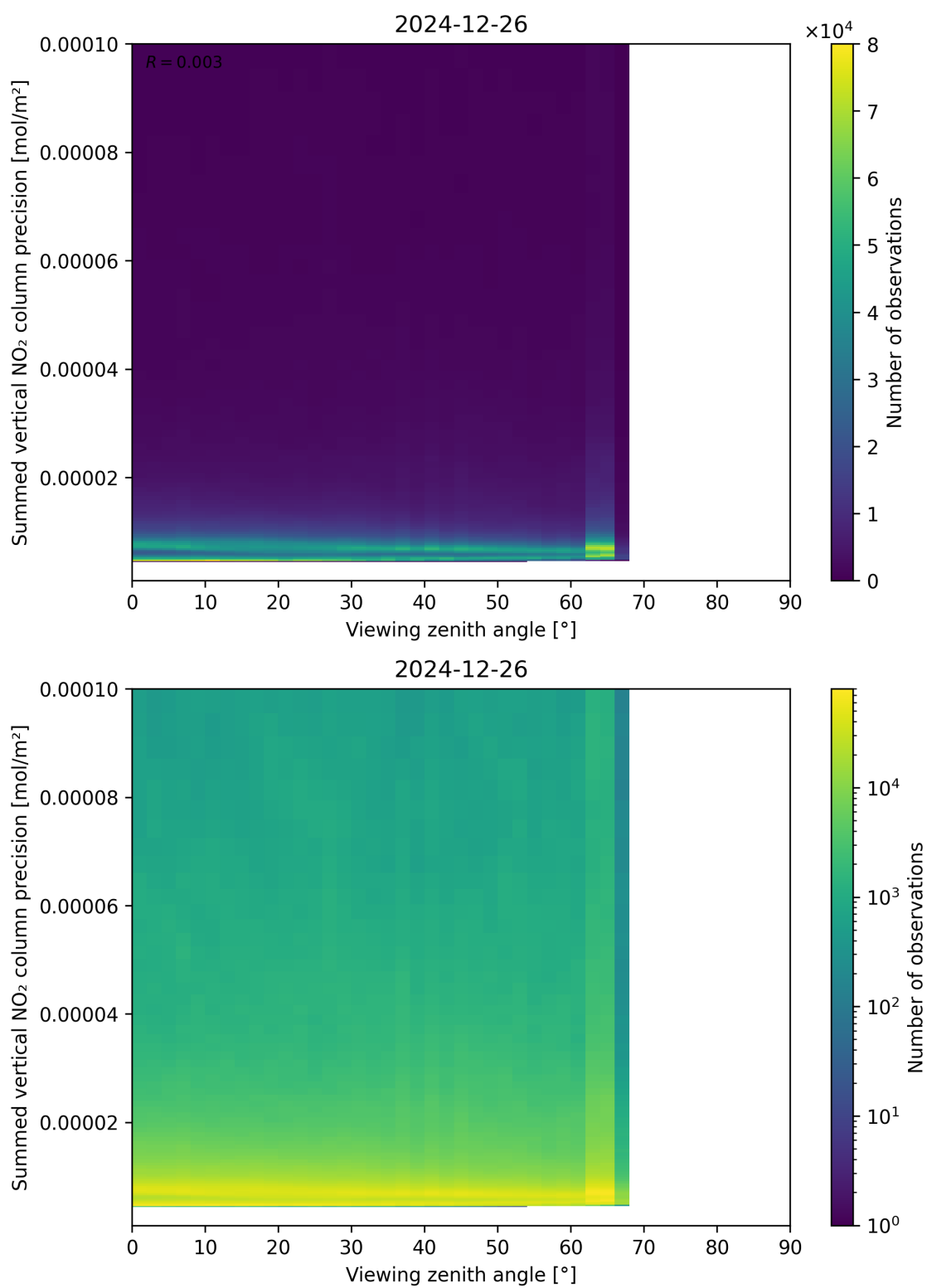
Figure 166: Scatter density plot of “Viewing zenith angle” against “Summed vertical NO 2 column precision” for 2024-12-25 to 2024-12-27.
