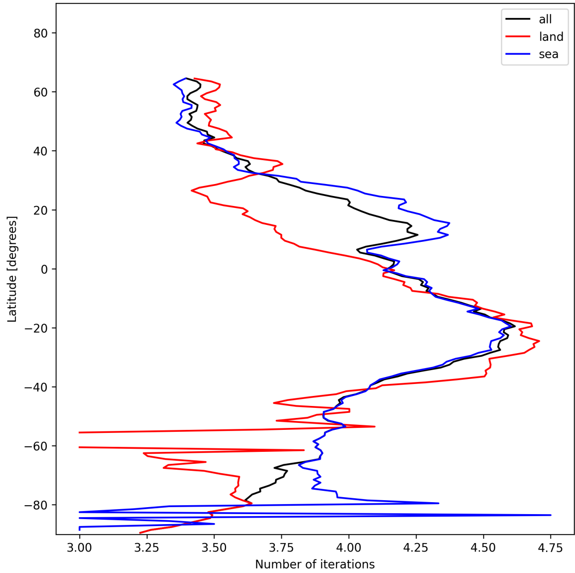
Figure 17: Zonal average of “Number of iterations” for 2024-12-25 to 2024-12-27.
