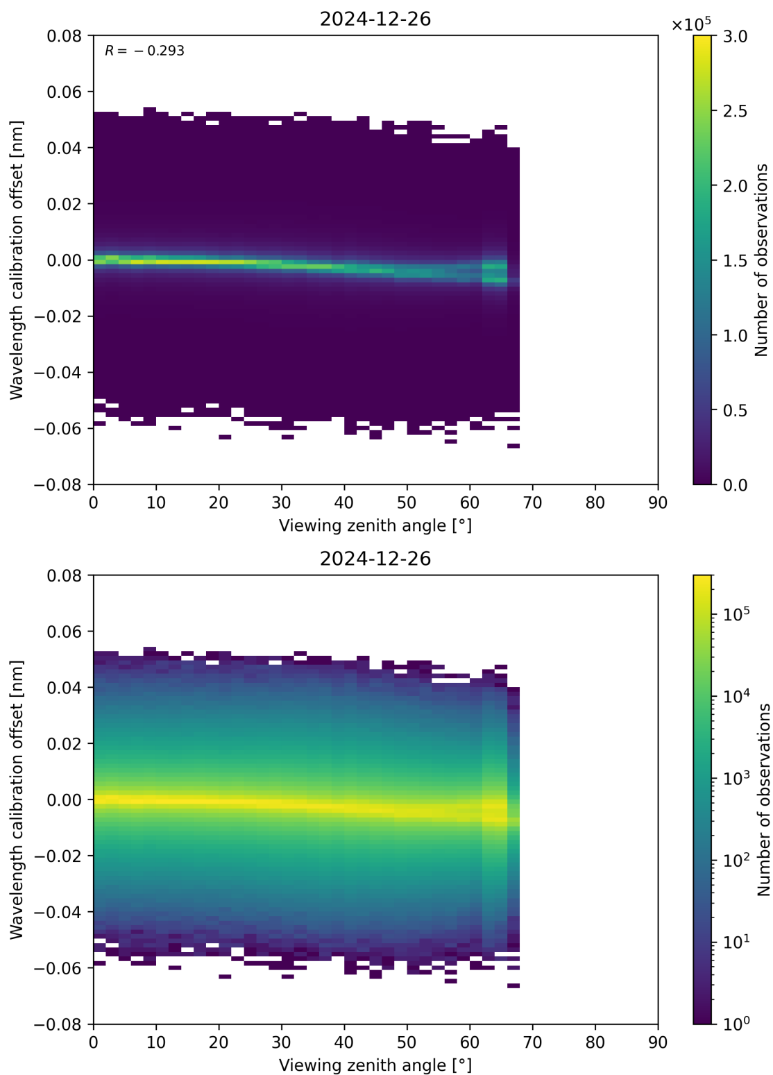
Figure 173: Scatter density plot of “Viewing zenith angle” against “Wavelength calibration offset” for 2024-12-25 to 2024-12-27.
