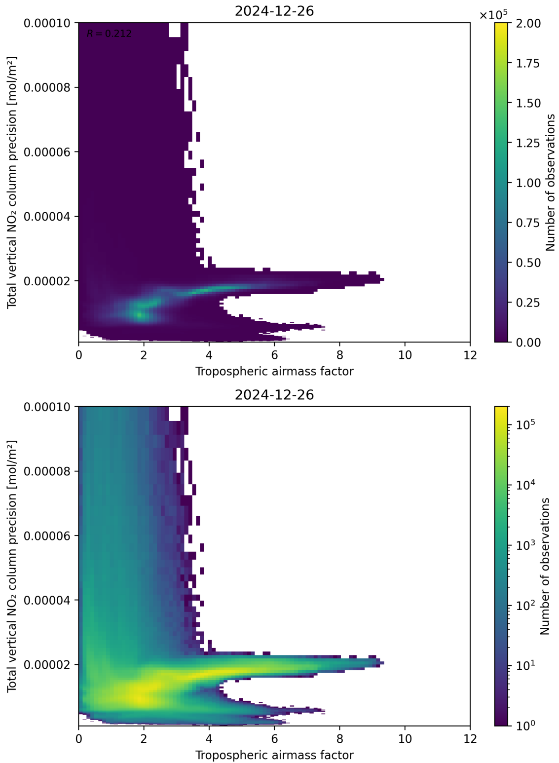
Figure 78: Scatter density plot of “Tropospheric air mass factor” against “Total vertical NO 2 column precision” for 2024-12-25 to 2024-12-27.
