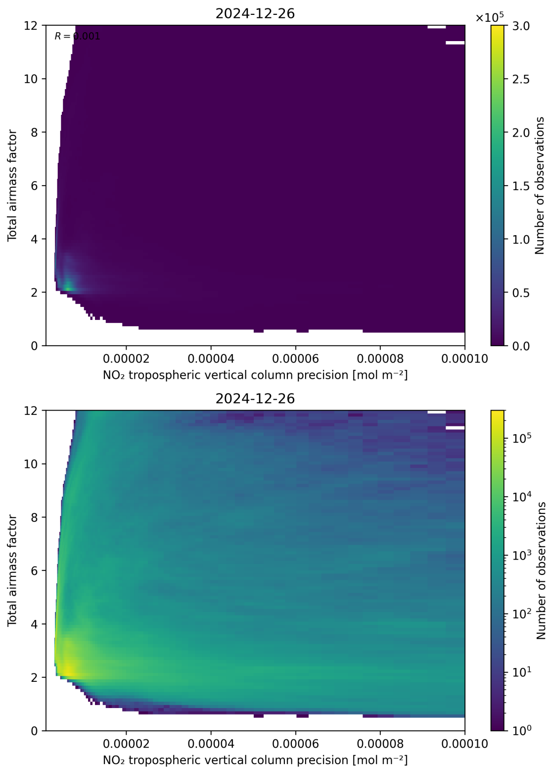
Figure 132: Scatter density plot of “NO 2 tropospheric vertical column precision” against “Total air mass factor” for 2024-12-25 to 2024-12-27.
