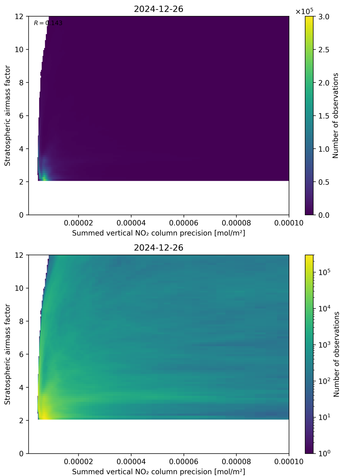
Figure 106: Scatter density plot of “Summed vertical NO 2 column precision” against “Stratospheric airmass factor” for 2024-12-25 to 2024-12-27.
