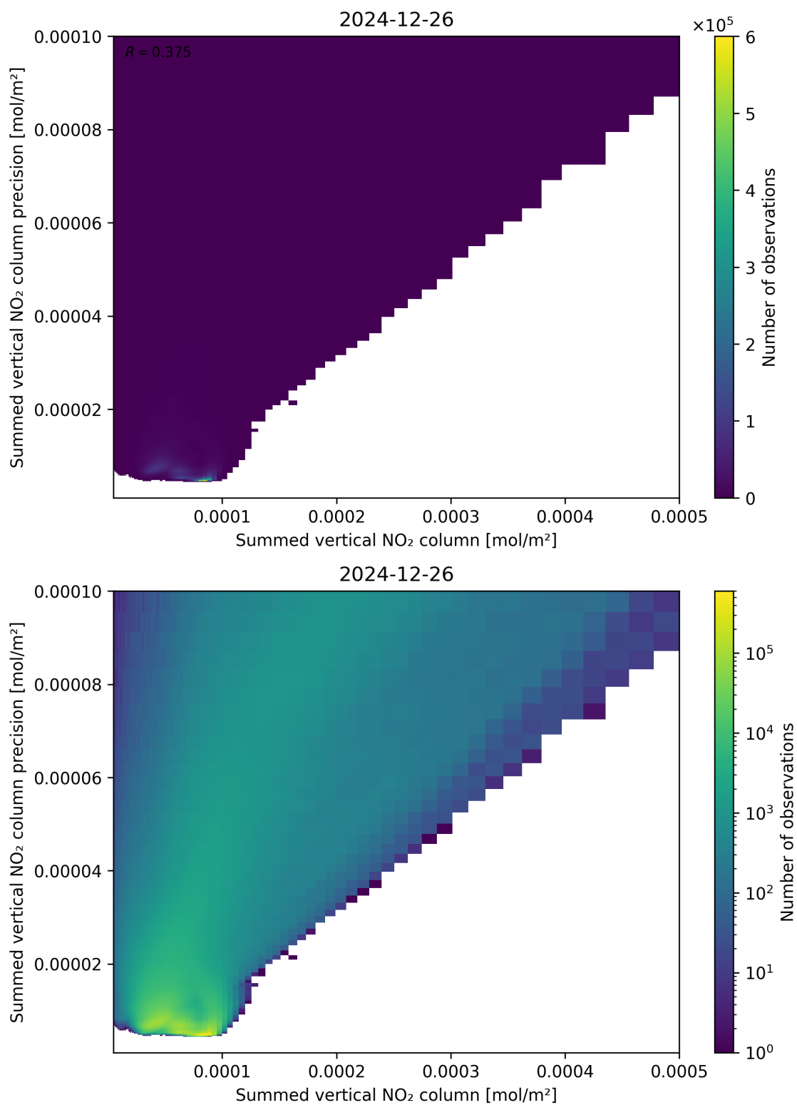
Figure 105: Scatter density plot of “Summed vertical NO 2 column” against “Summed vertical NO 2 column precision” for 2024-12-25 to 2024-12-27.
