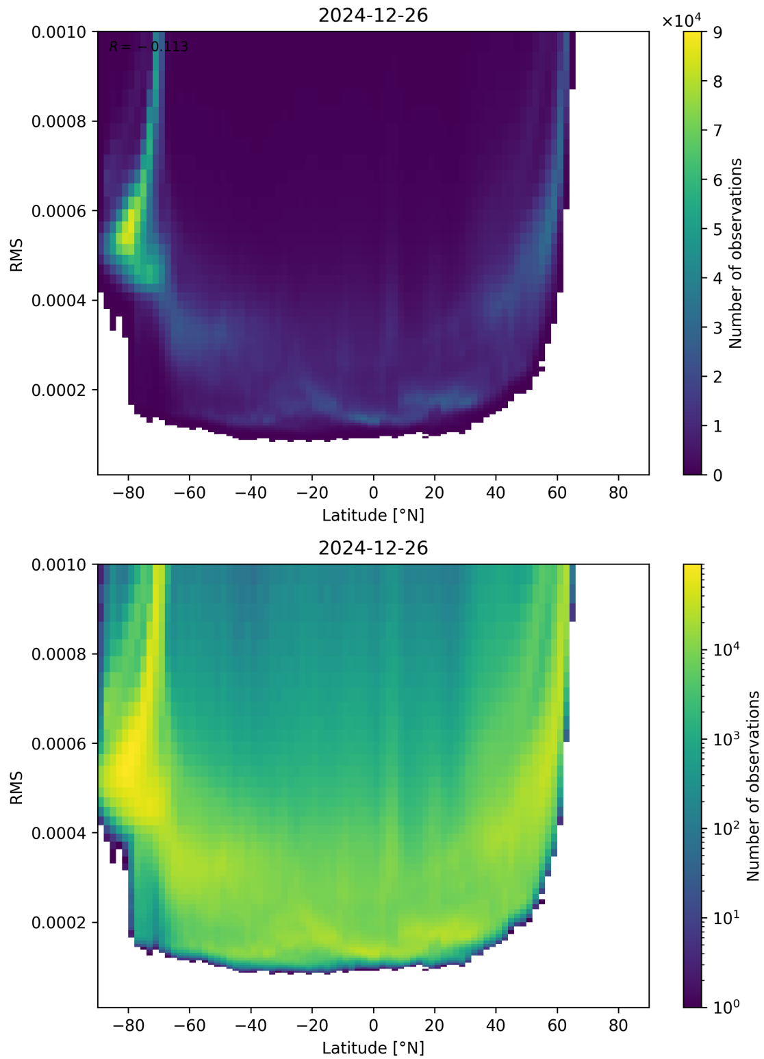
Figure 94: Scatter density plot of “Latitude” against “RMS” for 2024-12-25 to 2024-12-27.
