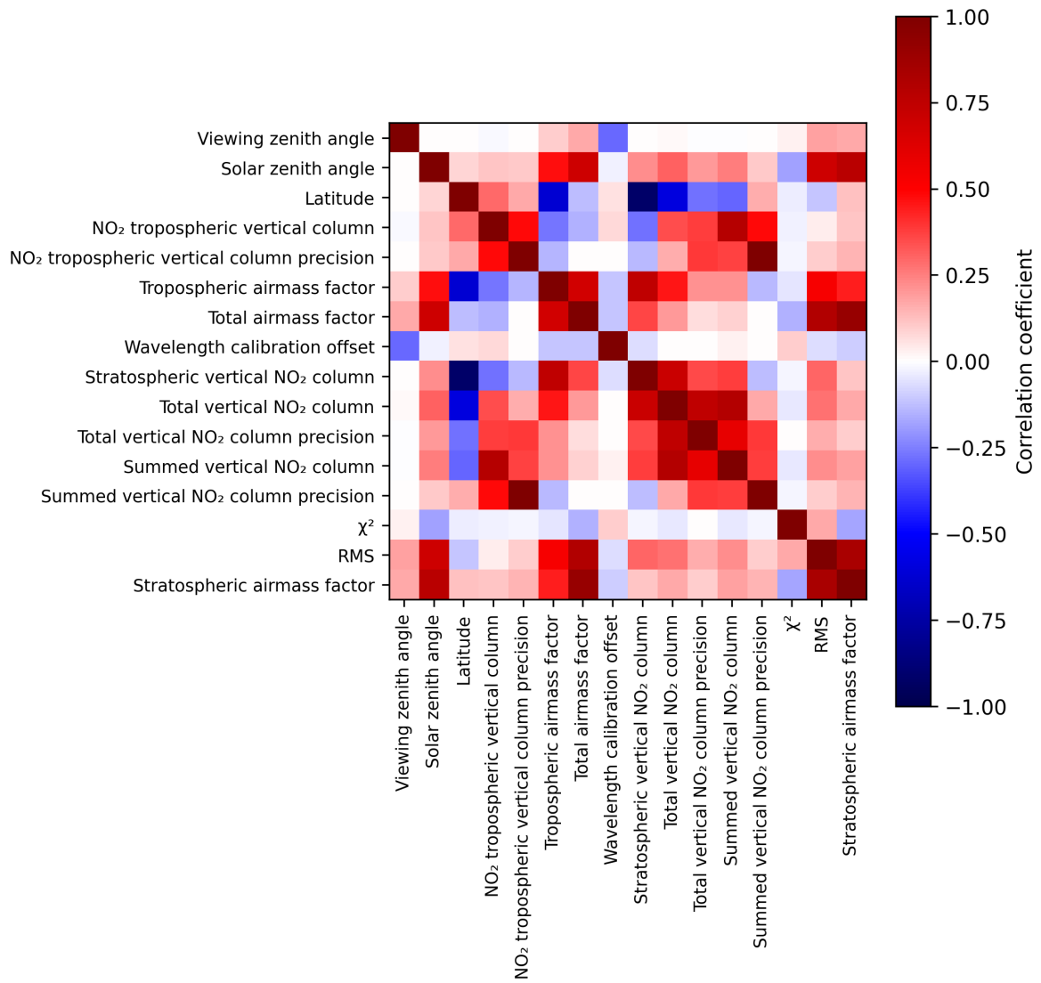
Figure 2: Map of correlation matrix for 2024-12-25 to 2024-12-27.
