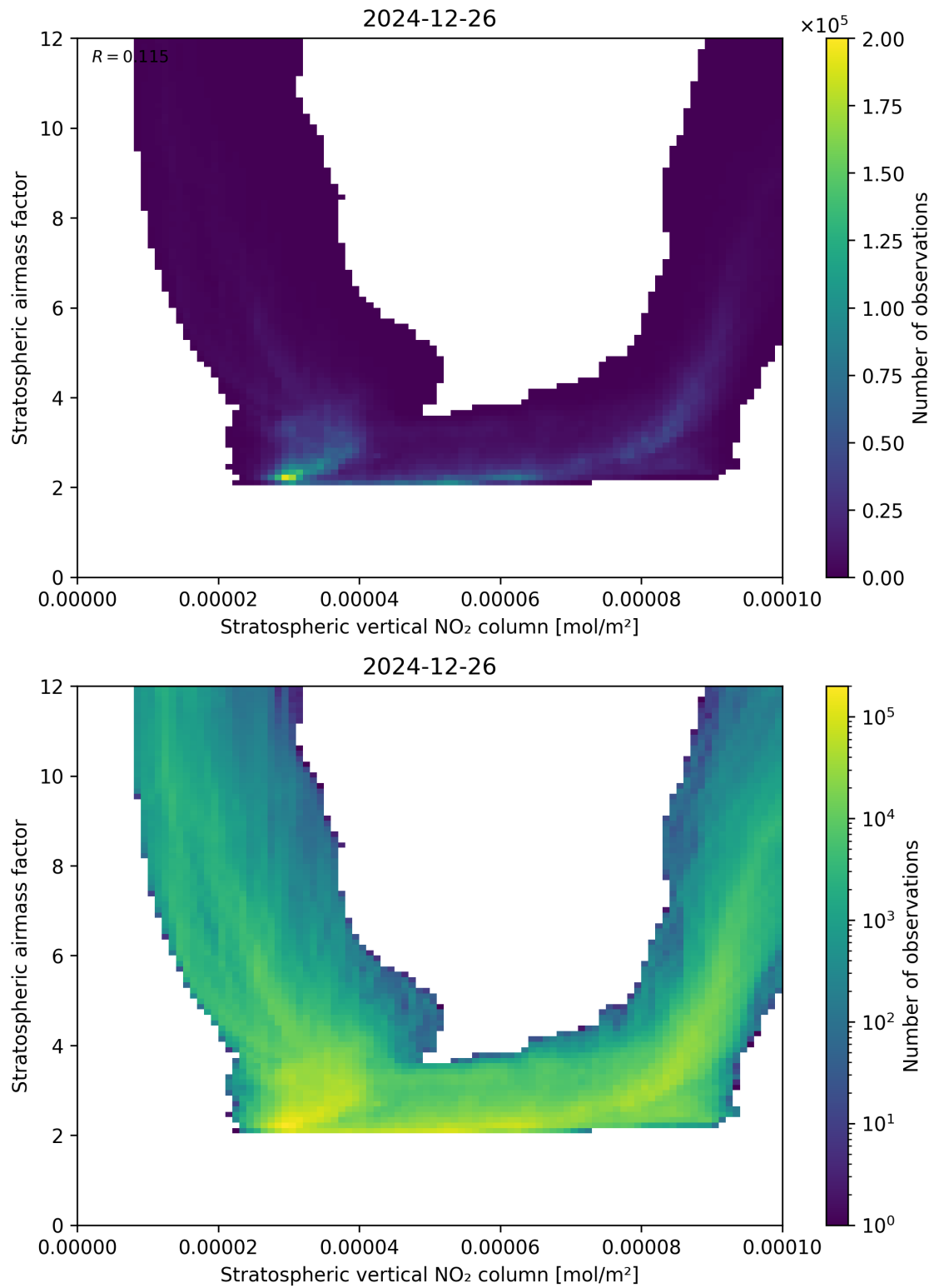
Figure 96: Scatter density plot of “Stratospheric vertical NO 2 column” against “Stratospheric airmass factor” for 2024-12-25 to 2024-12-27.
