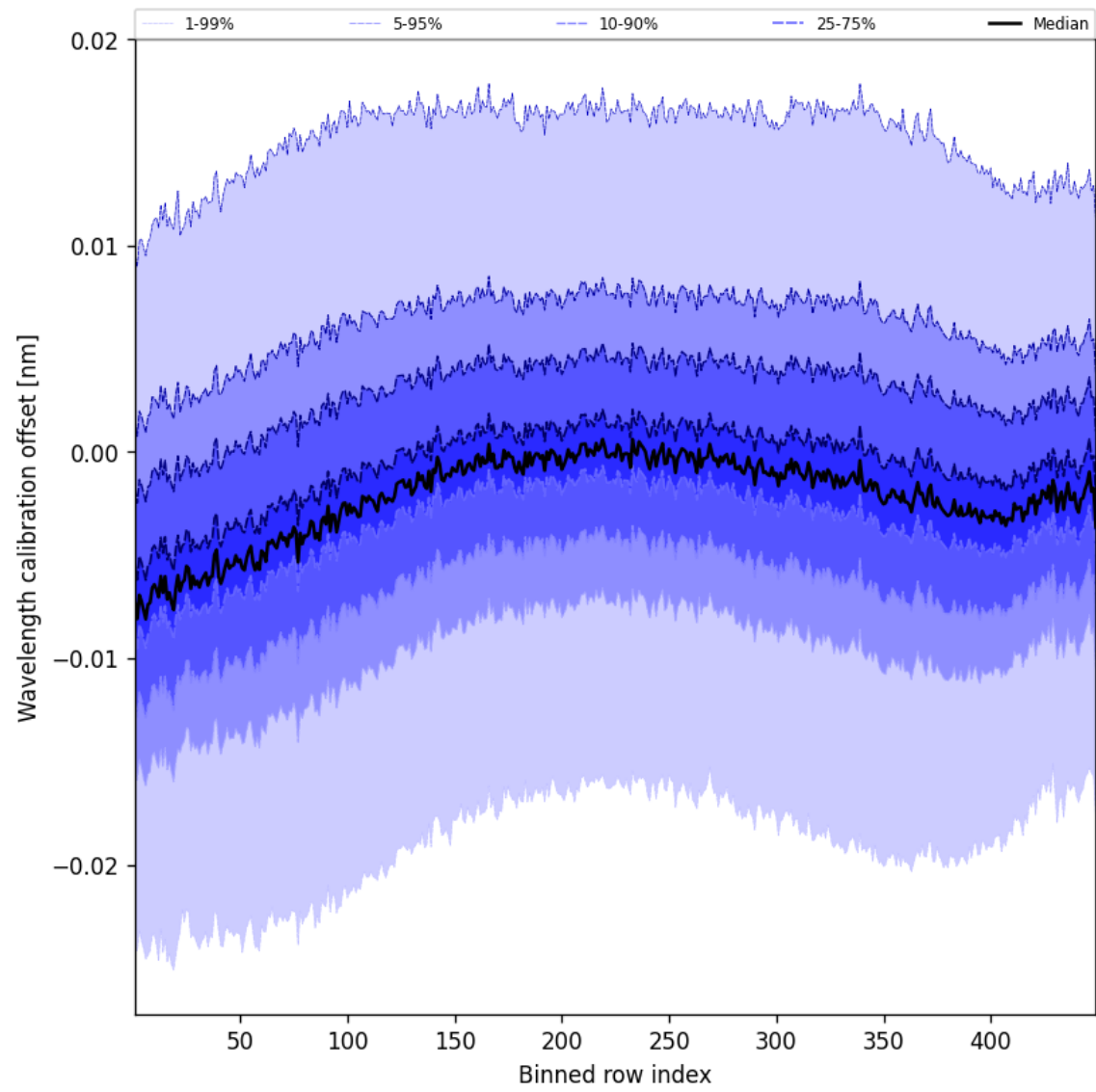
Figure 52: Along track statistics of “Wavelength calibration offset” for 2024-12-25 to 2024-12-27
