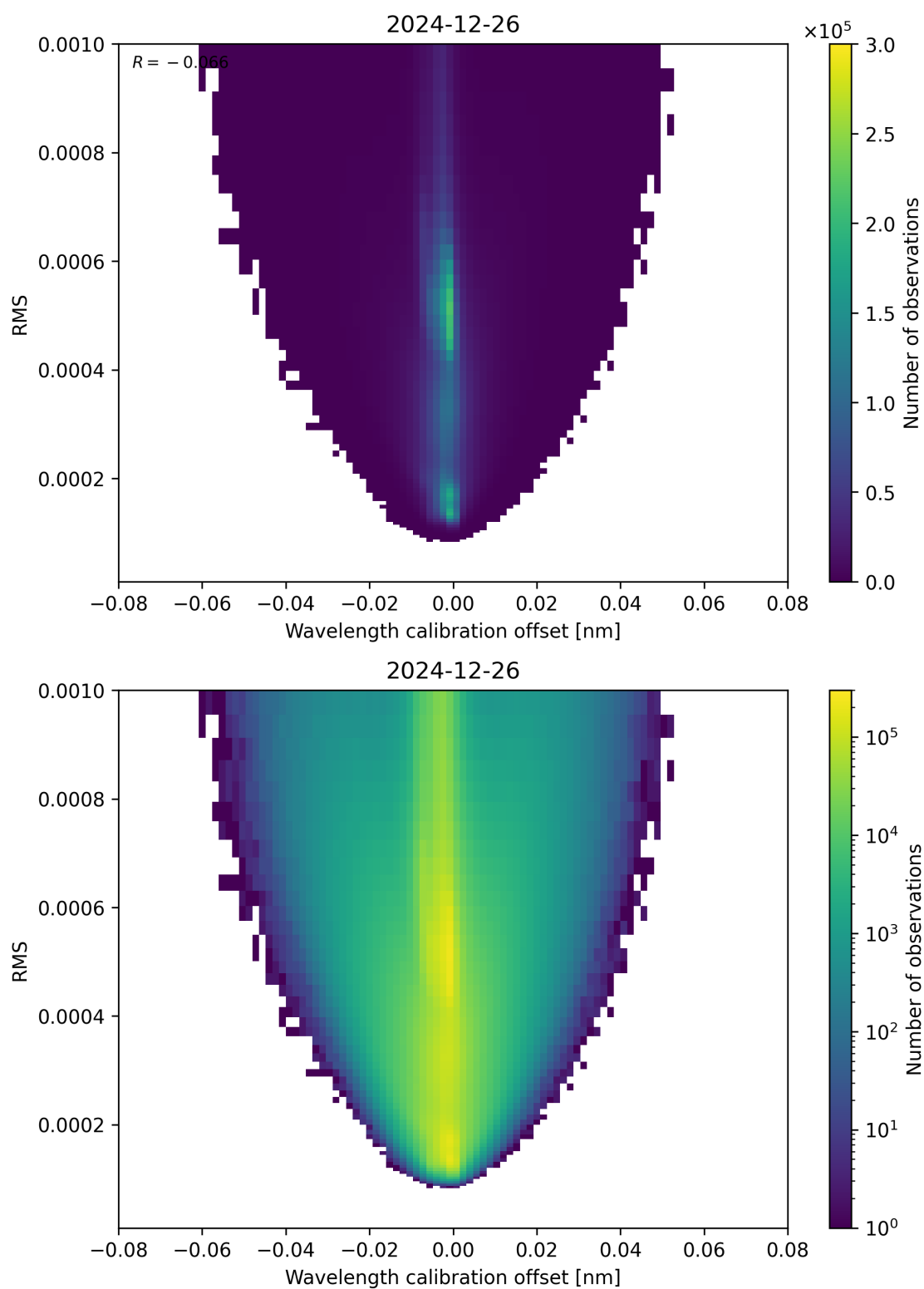
Figure 181: Scatter density plot of “Wavelength calibration offset” against “RMS” for 2024-12-25 to 2024-12-27.
