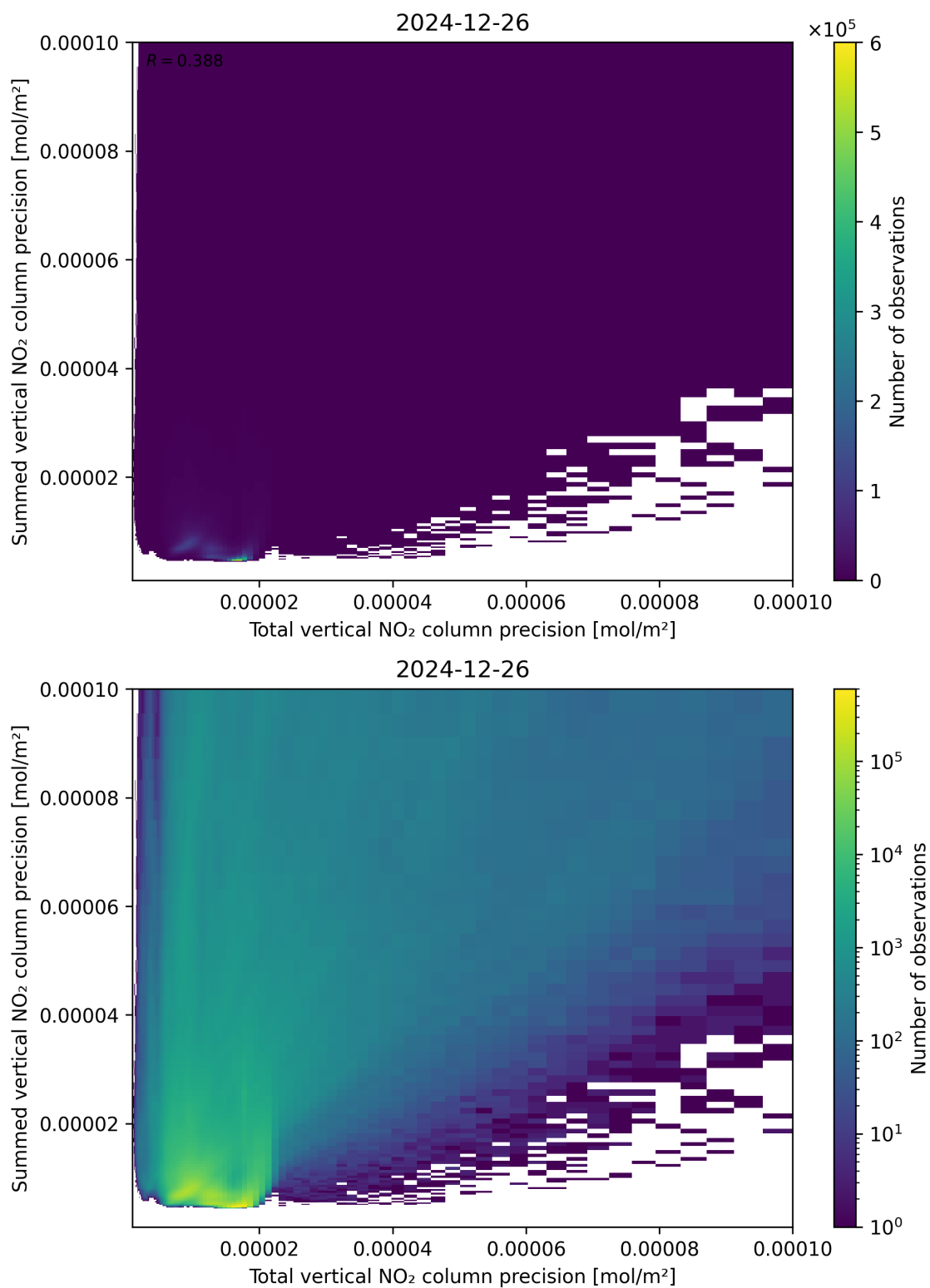
Figure 118: Scatter density plot of “Total vertical NO 2 column precision” against “Summed vertical NO 2 column precision” for 2024-12-25 to 2024-12-27.
