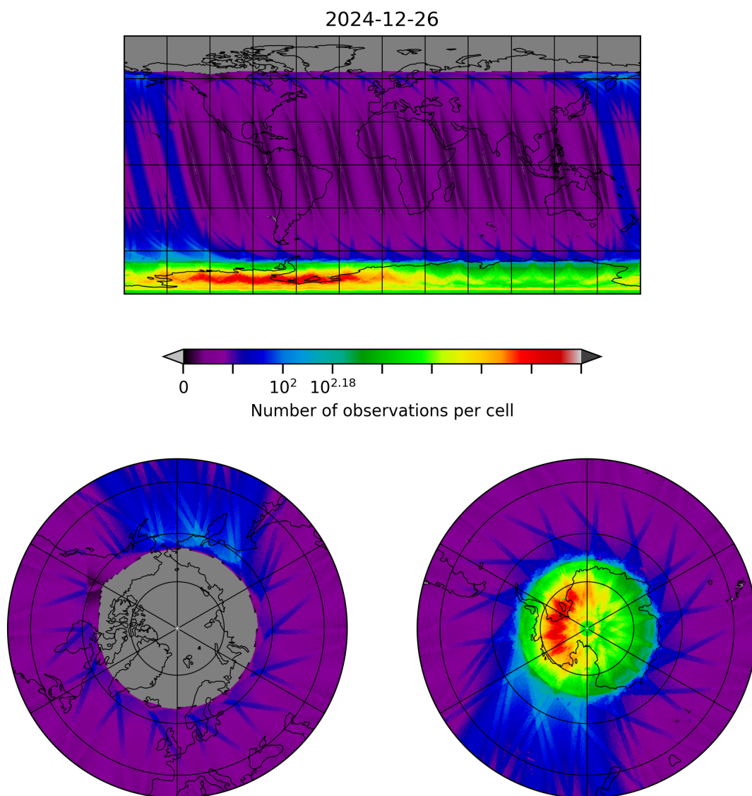
Figure 10: Map of the number of observations for 2024-12-25 to 2024-12-27
