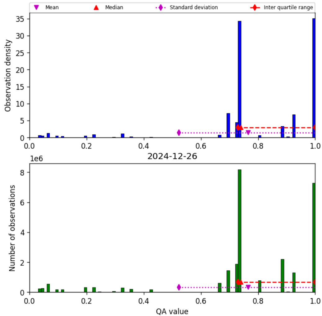
Figure 28: Histogram of “QA value” for 2024-12-25 to 2024-12-27
