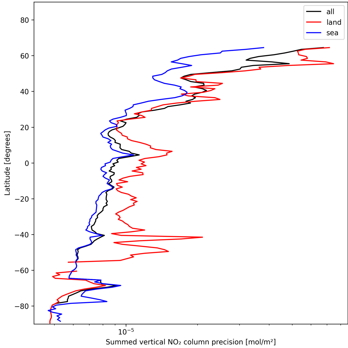
Figure 24: Zonal average of “Summed vertical NO 2 column precision” for 2024-12-25 to 2024-12-27.
