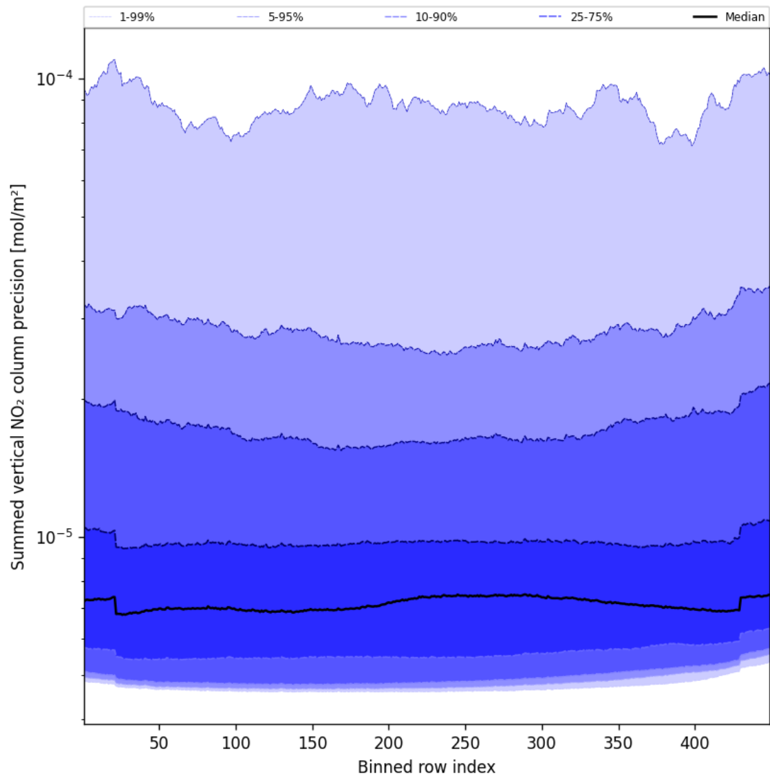
Figure 58: Along track statistics of “Summed vertical NO 2 column precision” for 2024-12-25 to 2024-12-27
