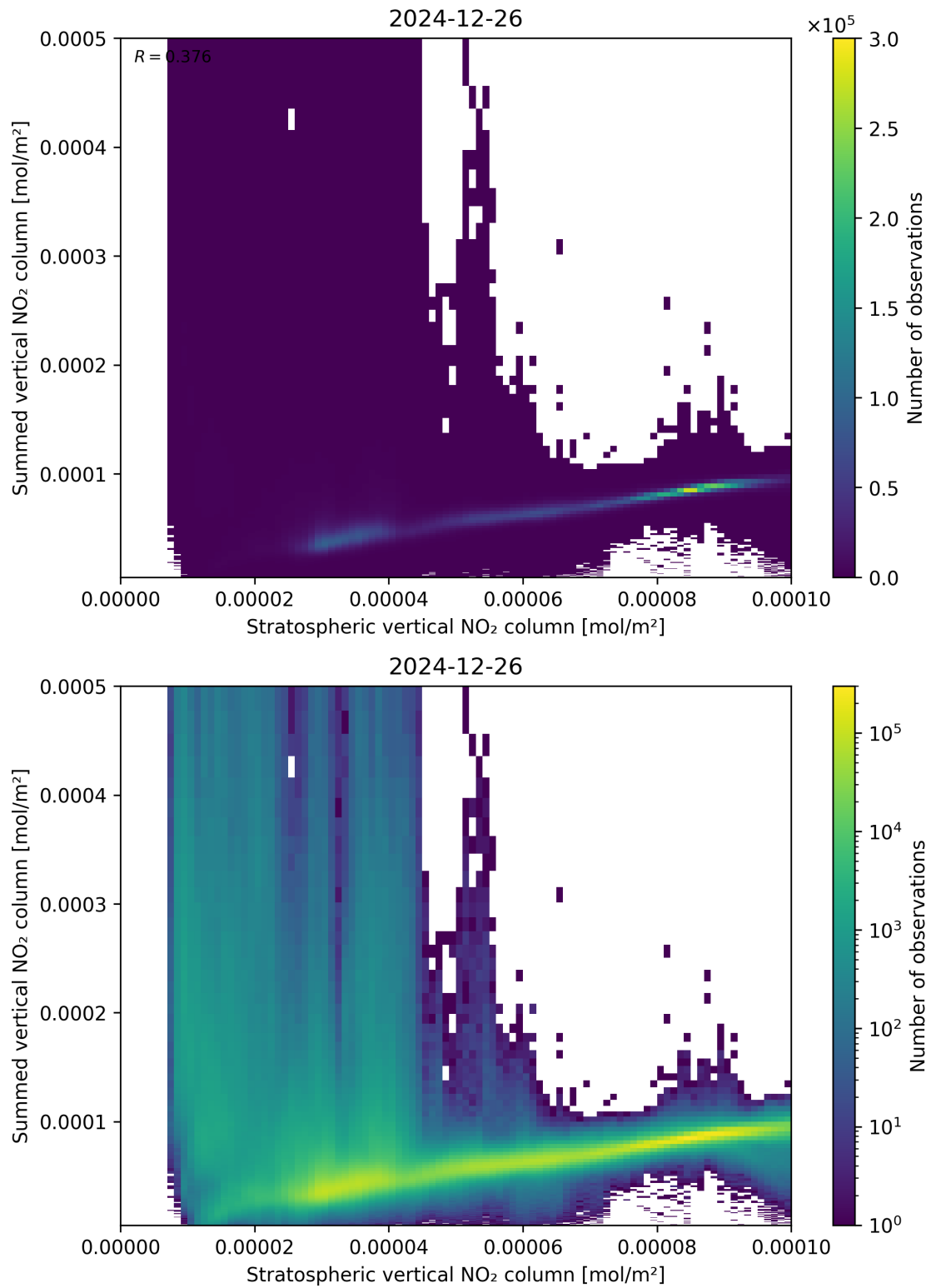
Figure 98: Scatter density plot of “Stratospheric vertical NO 2 column” against “Summed vertical NO 2 column” for 2024-12-25 to 2024-12-27.
