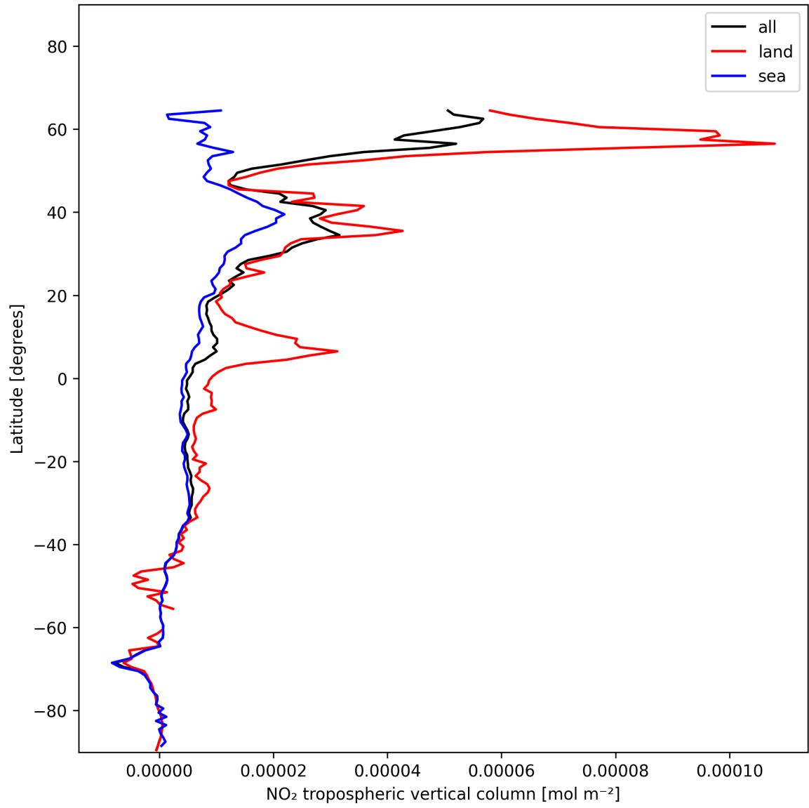
Figure 12: Zonal average of “NO 2 tropospheric vertical column” for 2024-12-25 to 2024-12-27.
