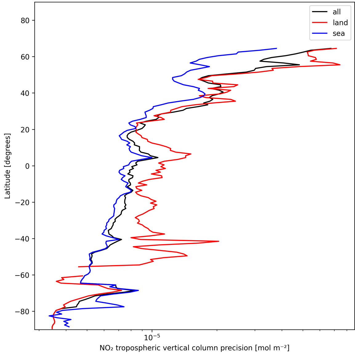
Figure 13: Zonal average of “NO 2 tropospheric vertical column precision” for 2024-12-25 to 2024-12-27.
