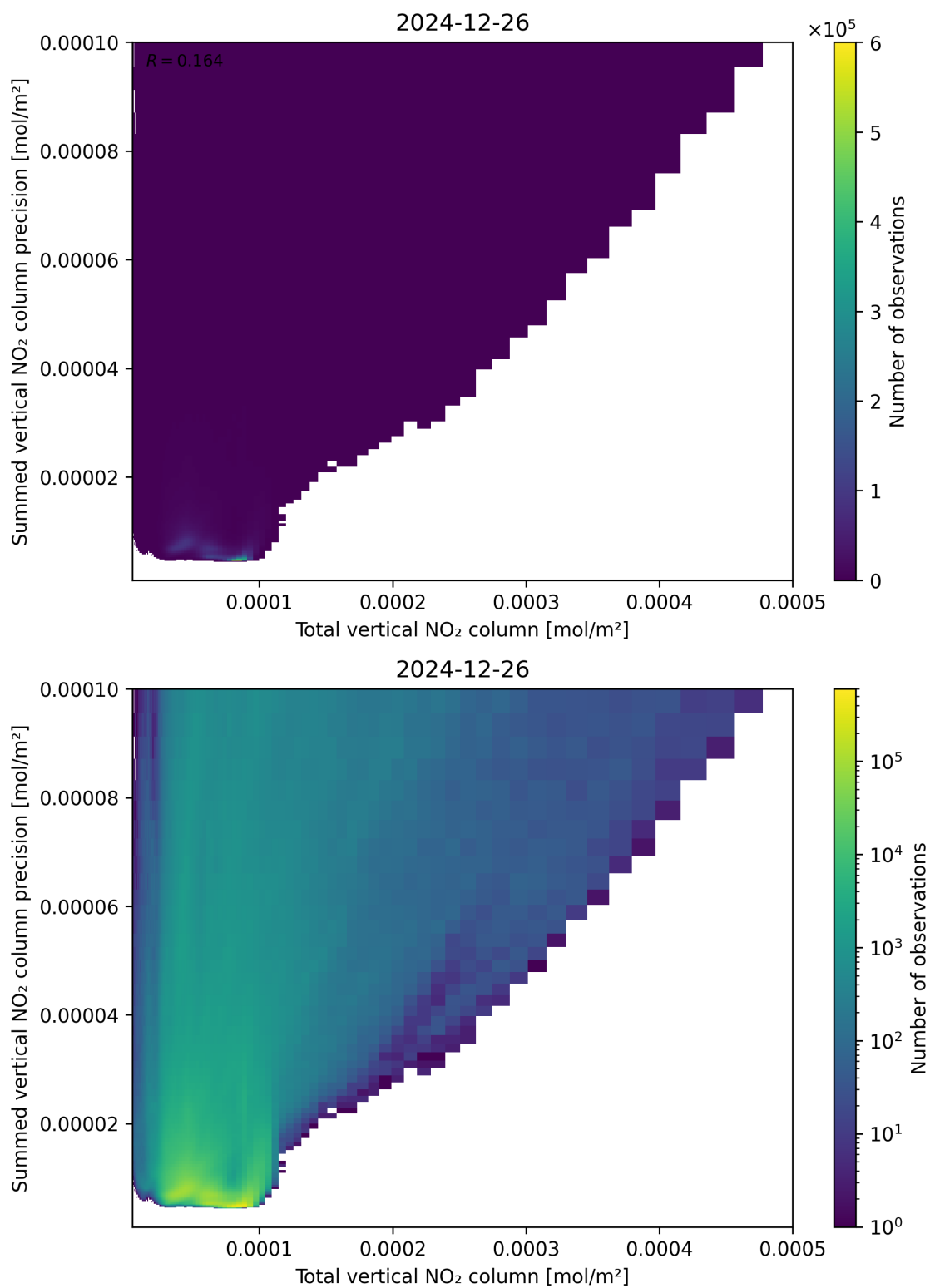
Figure 113: Scatter density plot of “Total vertical NO 2 column” against “Summed vertical NO 2 column precision” for 2024-12-25 to 2024-12-27.
