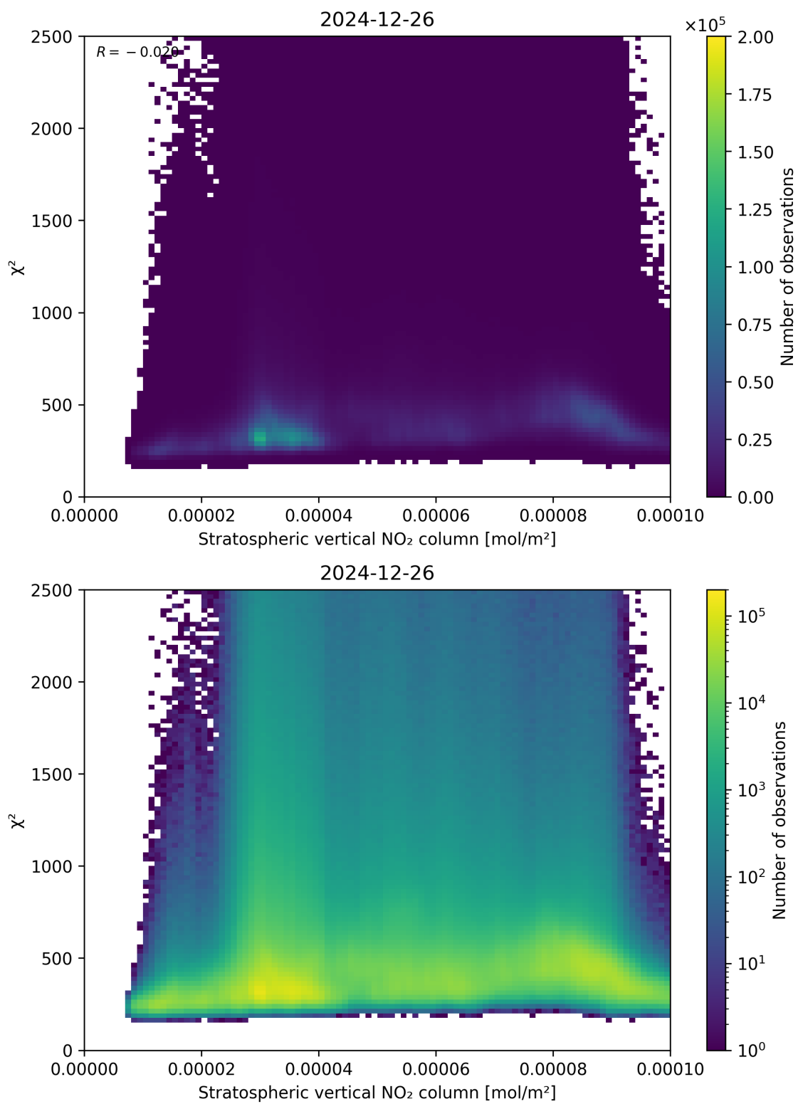
Figure 97: Scatter density plot of “Stratospheric vertical NO 2 column” against “ \chi^2 ” for 2024-12-25 to 2024-12-27.
