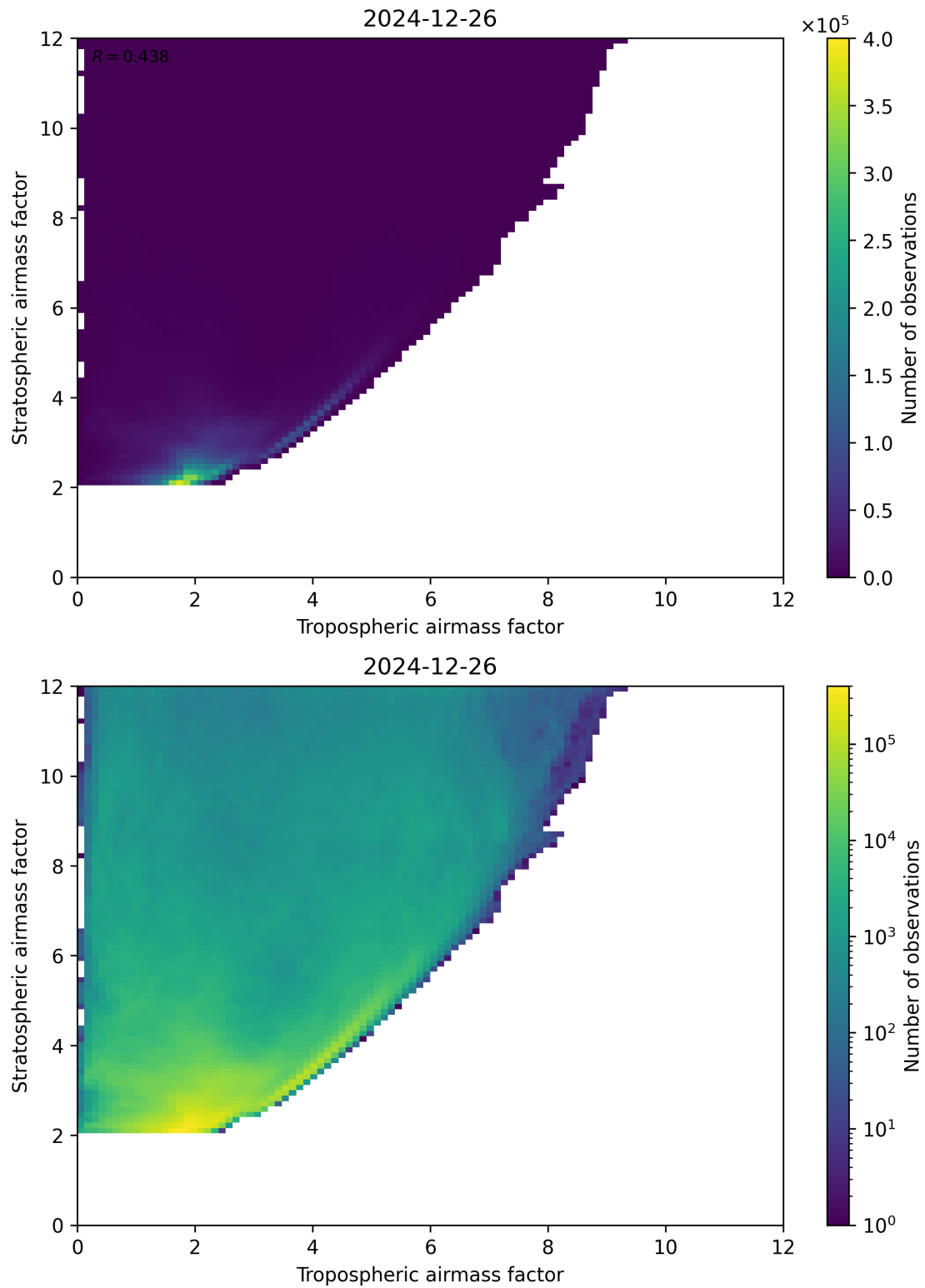
Figure 71: Scatter density plot of “Tropospheric airmass factor” against “Stratospheric airmass factor” for 2024-12-25 to 2024-12-27.
