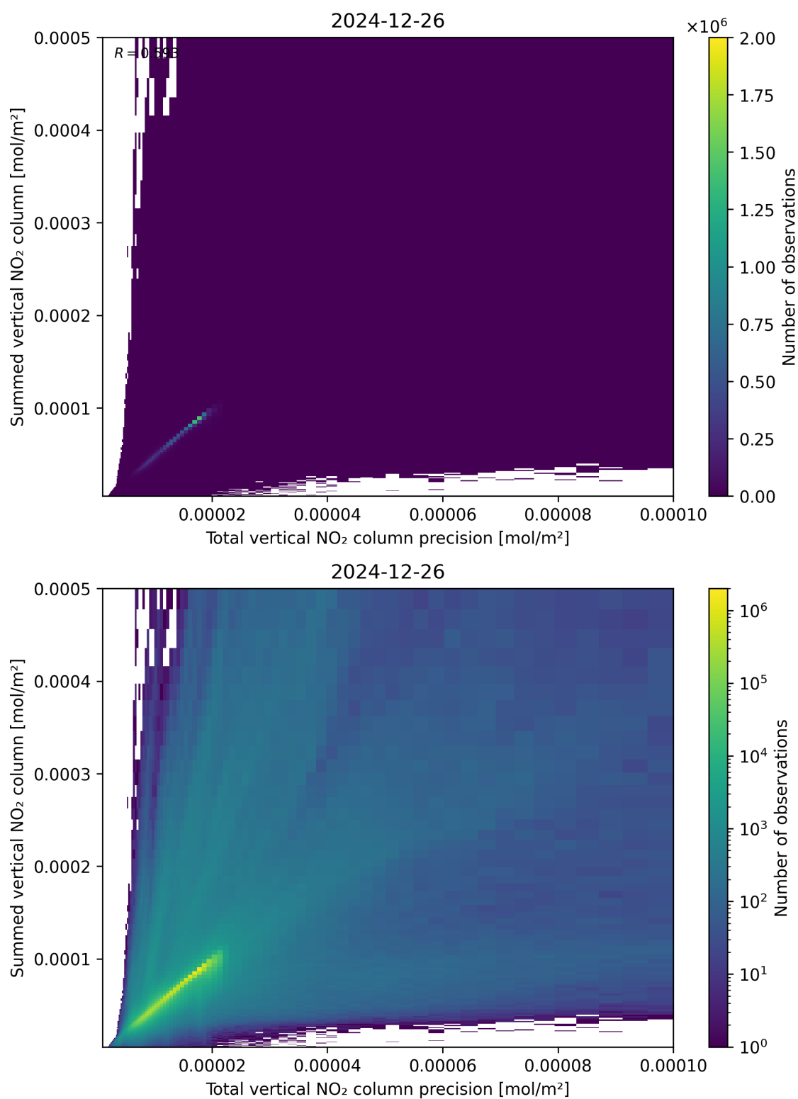
Figure 117: Scatter density plot of “Total vertical NO 2 column precision” against “Summed vertical NO 2 column” for 2024-12-25 to 2024-12-27.
