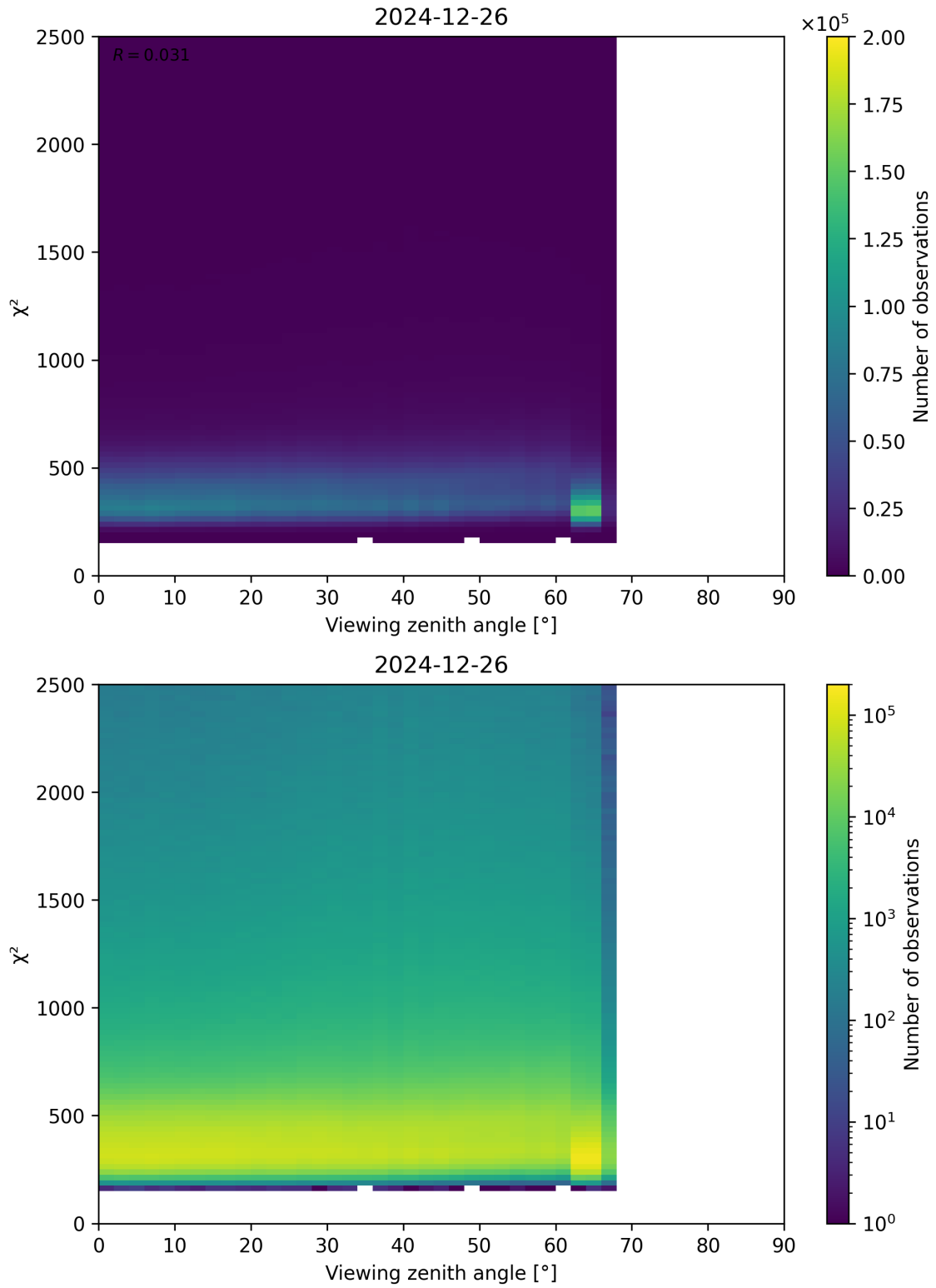
Figure 162: Scatter density plot of “Viewing zenith angle” against “ \chi^2 ” for 2024-12-25 to 2024-12-27.
