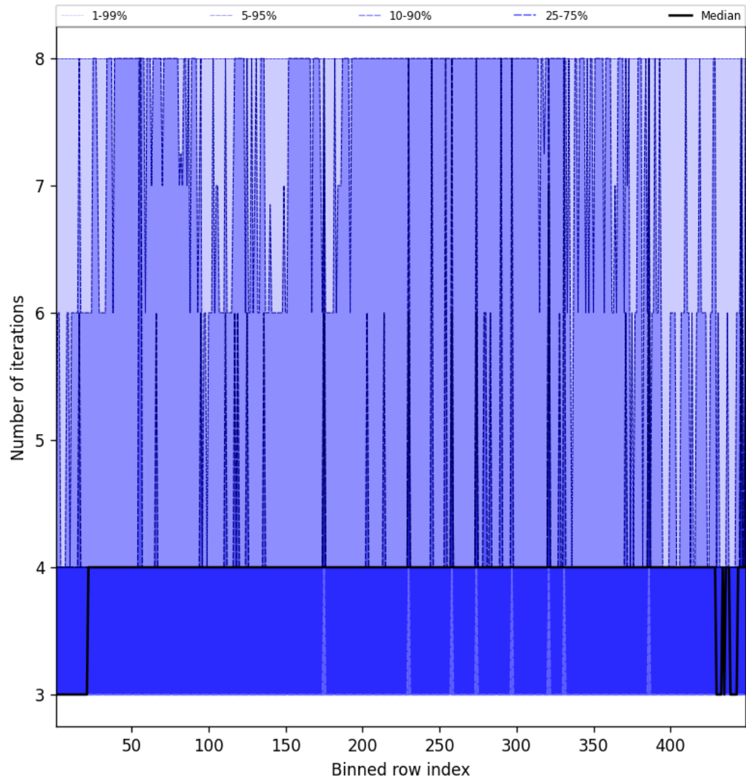
Figure 51: Along track statistics of “Number of iterations” for 2024-12-25 to 2024-12-27
