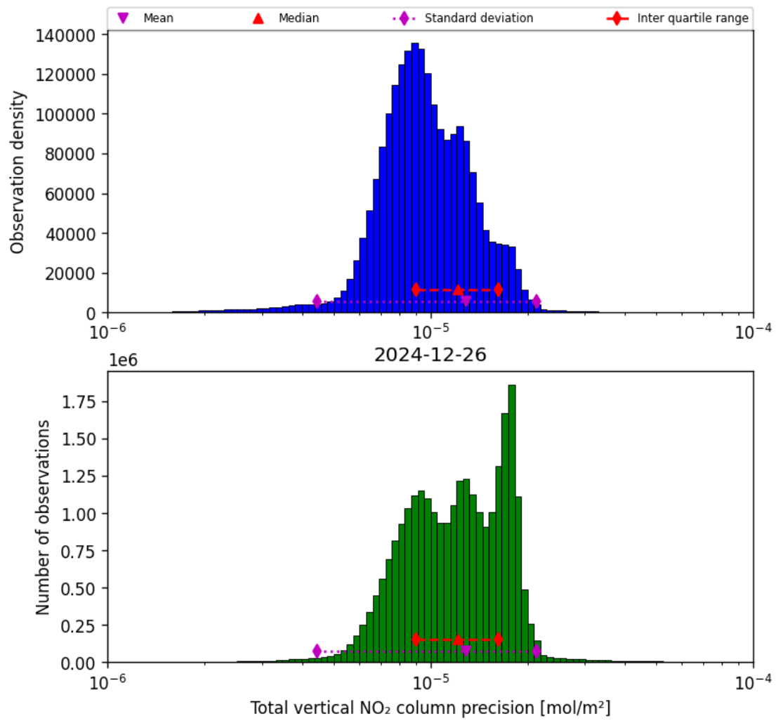
Figure 39: Histogram of "Total vertical NO 2 column precision" for 2024-12-25 to 2024-12-27
