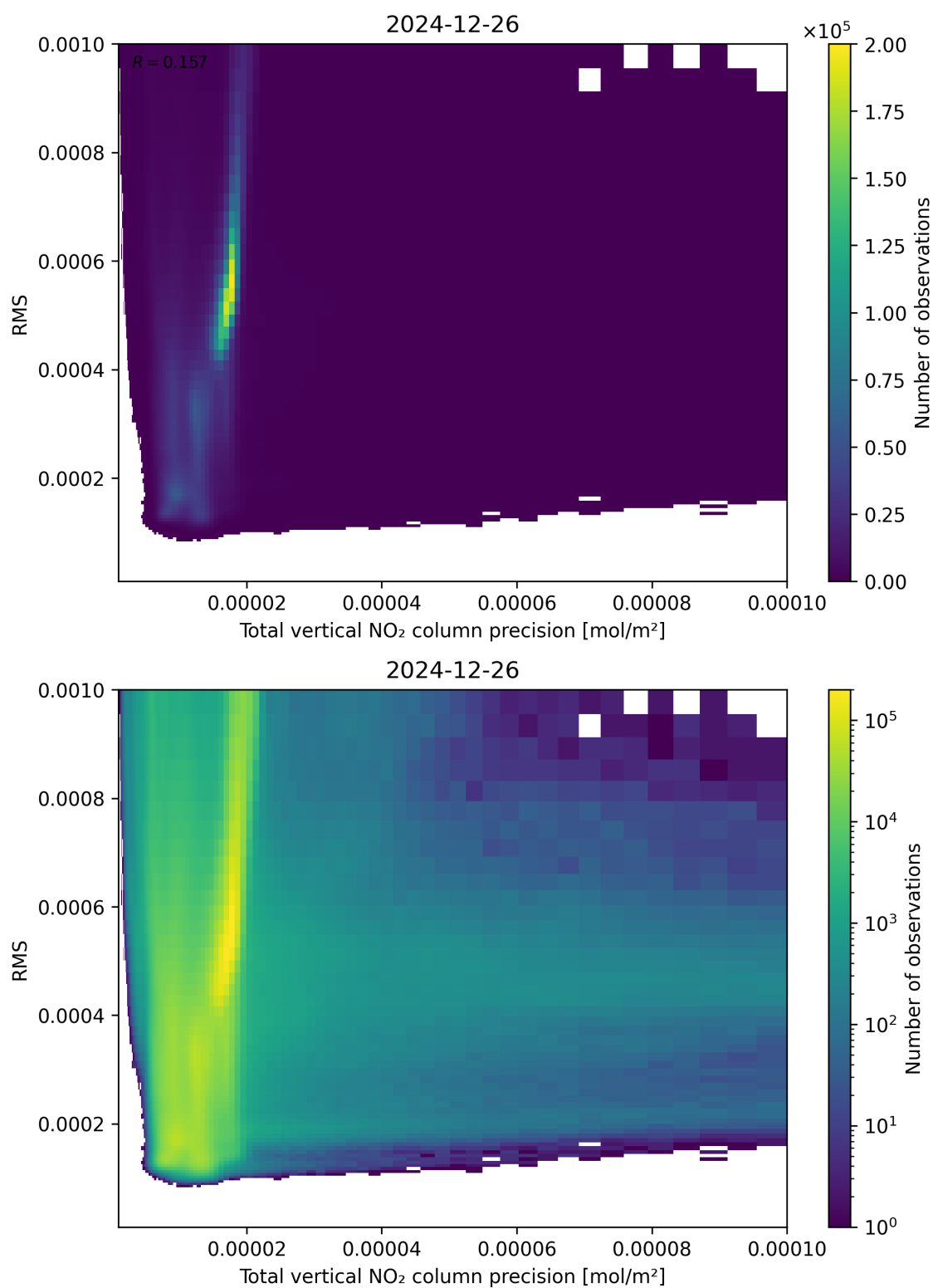
Figure 119: Scatter density plot of “Total vertical NO 2 column precision” against “RMS” for 2024-12-25 to 2024-12-27.
