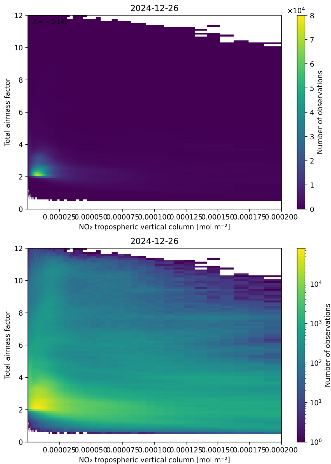
Figure 122: Scatter density plot of “NO 2 tropospheric vertical column” against “Total air mass factor” for 2024-12-25 to 2024-12-27.
