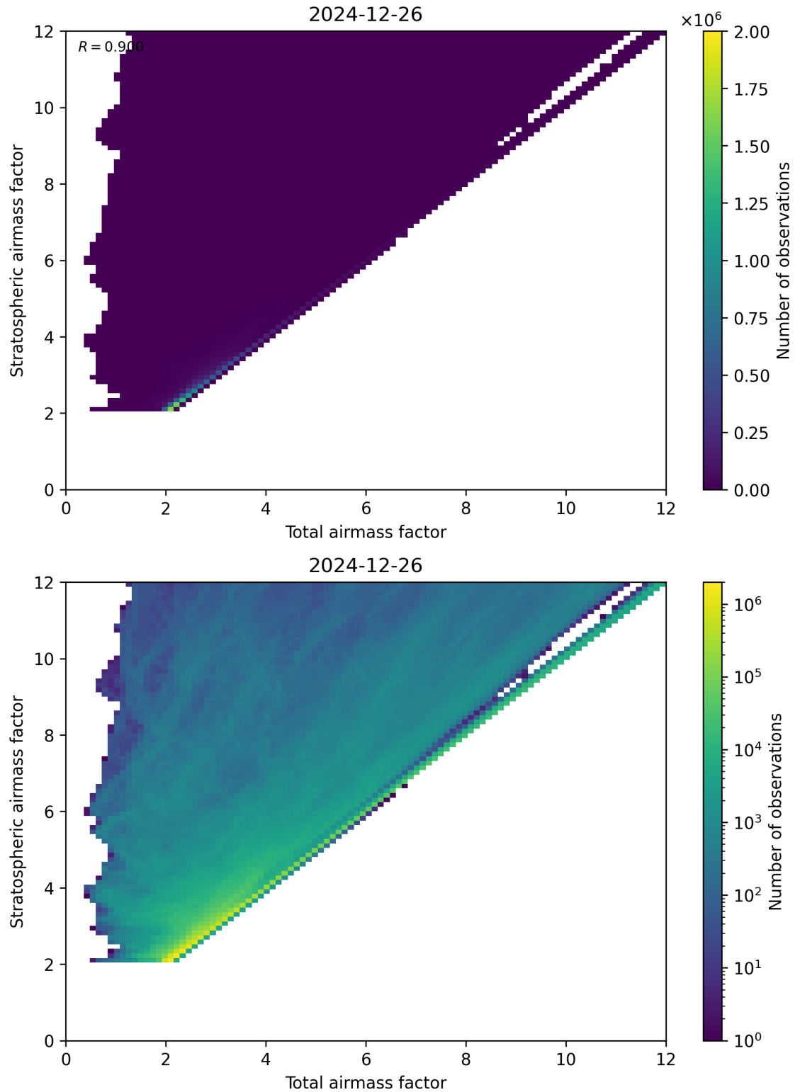
Figure 62: Scatter density plot of “Total airmass factor” against “Stratospheric airmass factor” for 2024-12-25 to 2024-12-27.
