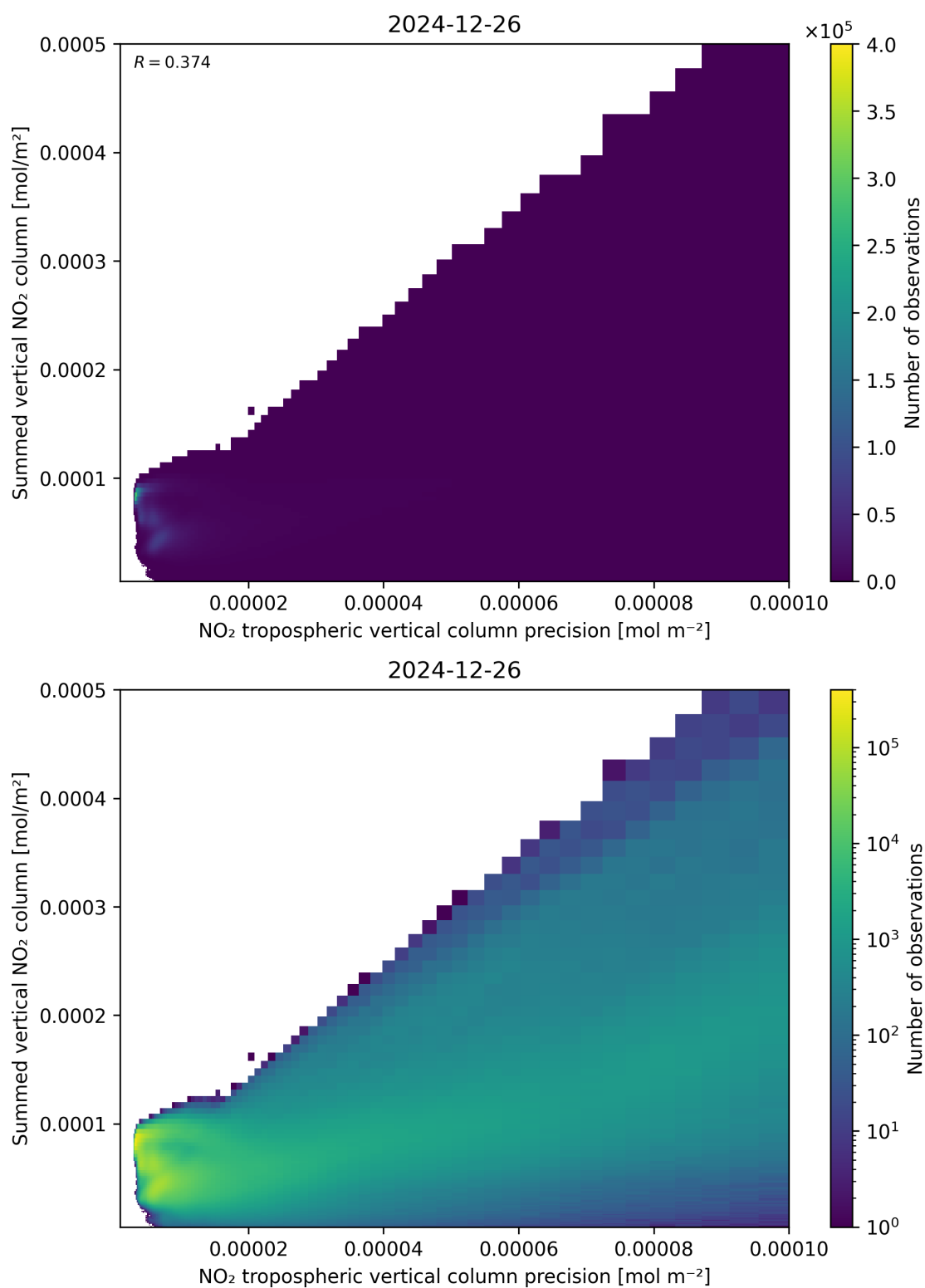
Figure 136: Scatter density plot of “NO 2 tropospheric vertical column precision” against “Summed vertical NO 2 column” for 2024-12-25 to 2024-12-27.
