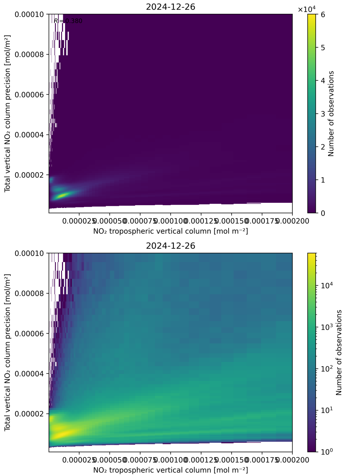
Figure 129: Scatter density plot of “NO 2 tropospheric vertical column” against “Total vertical NO 2 column precision” for 2024-12-25 to 2024-12-27.
