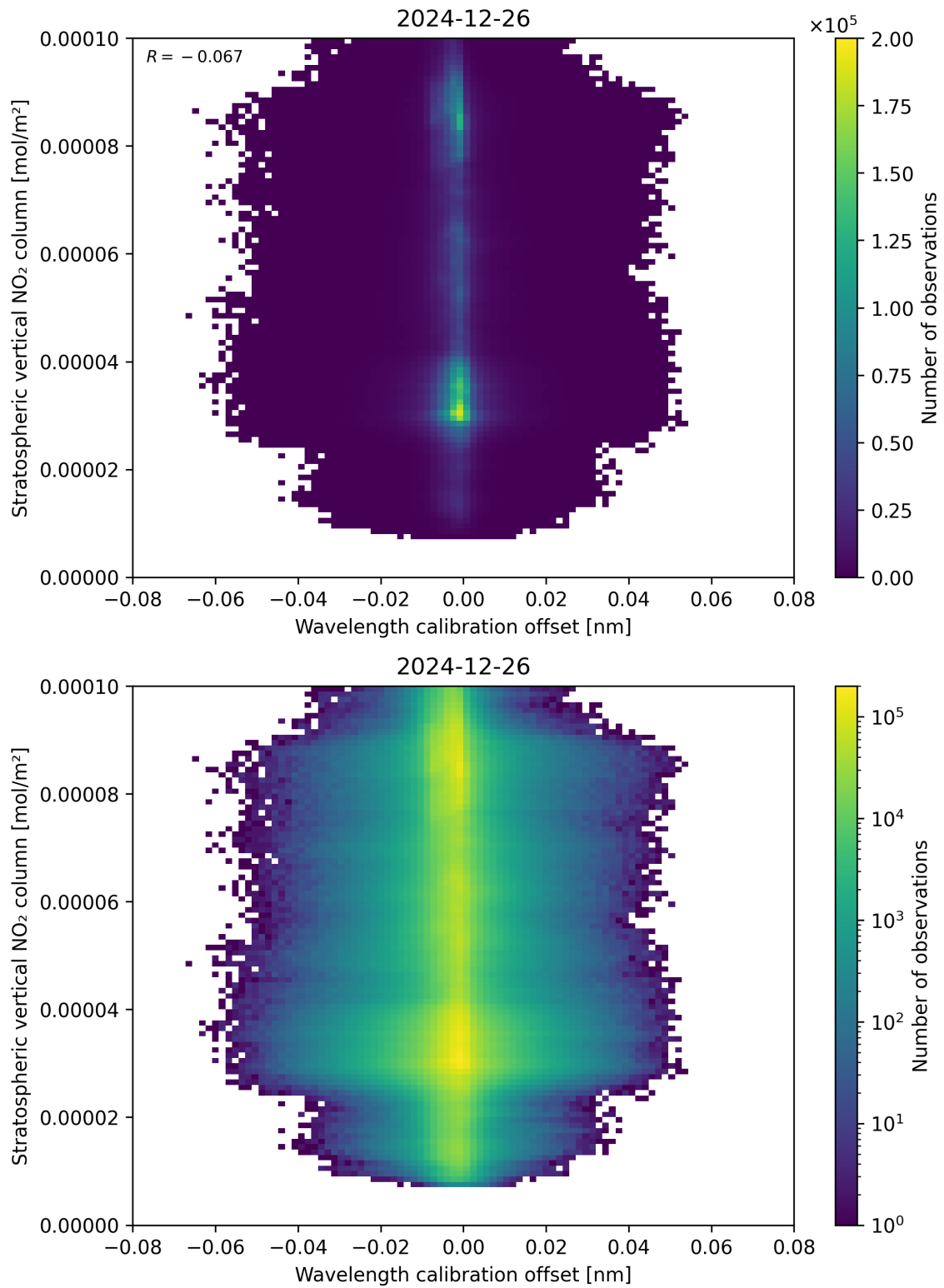
Figure 176: Scatter density plot of “Wavelength calibration offset” against “Stratospheric vertical NO 2 column” for 2024-12-25 to 2024-12-27.
