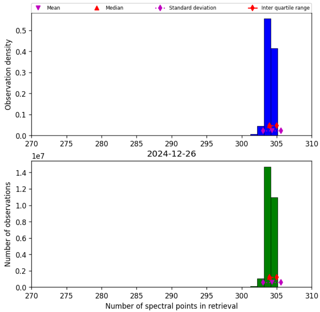
Figure 33: Histogram of “Number of spectral points in retrieval” for 2024-12-25 to 2024-12-27
