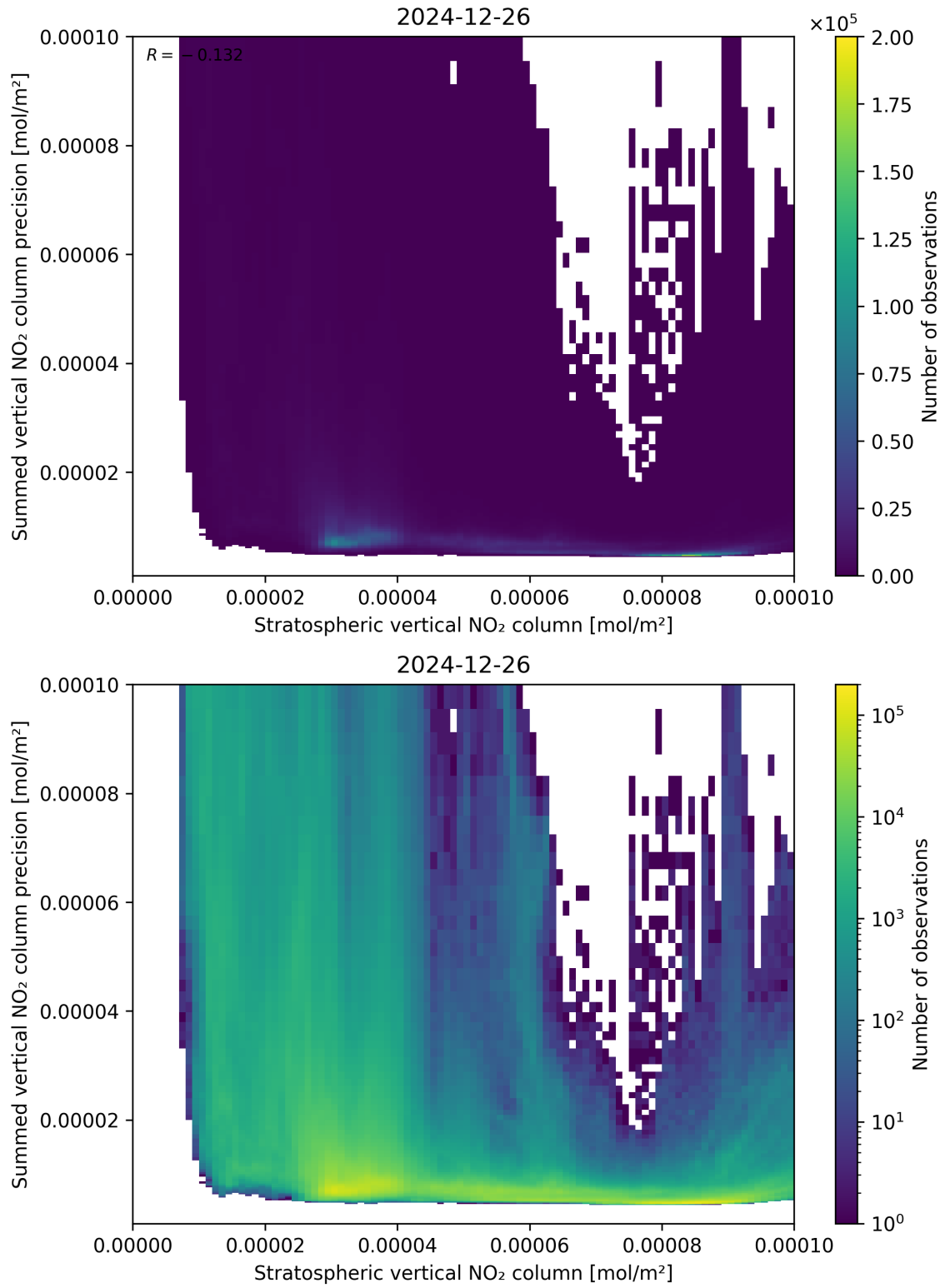
Figure 99: Scatter density plot of “Stratospheric vertical NO 2 column” against “Summed vertical NO 2 column precision” for 2024-12-25 to 2024-12-27.
