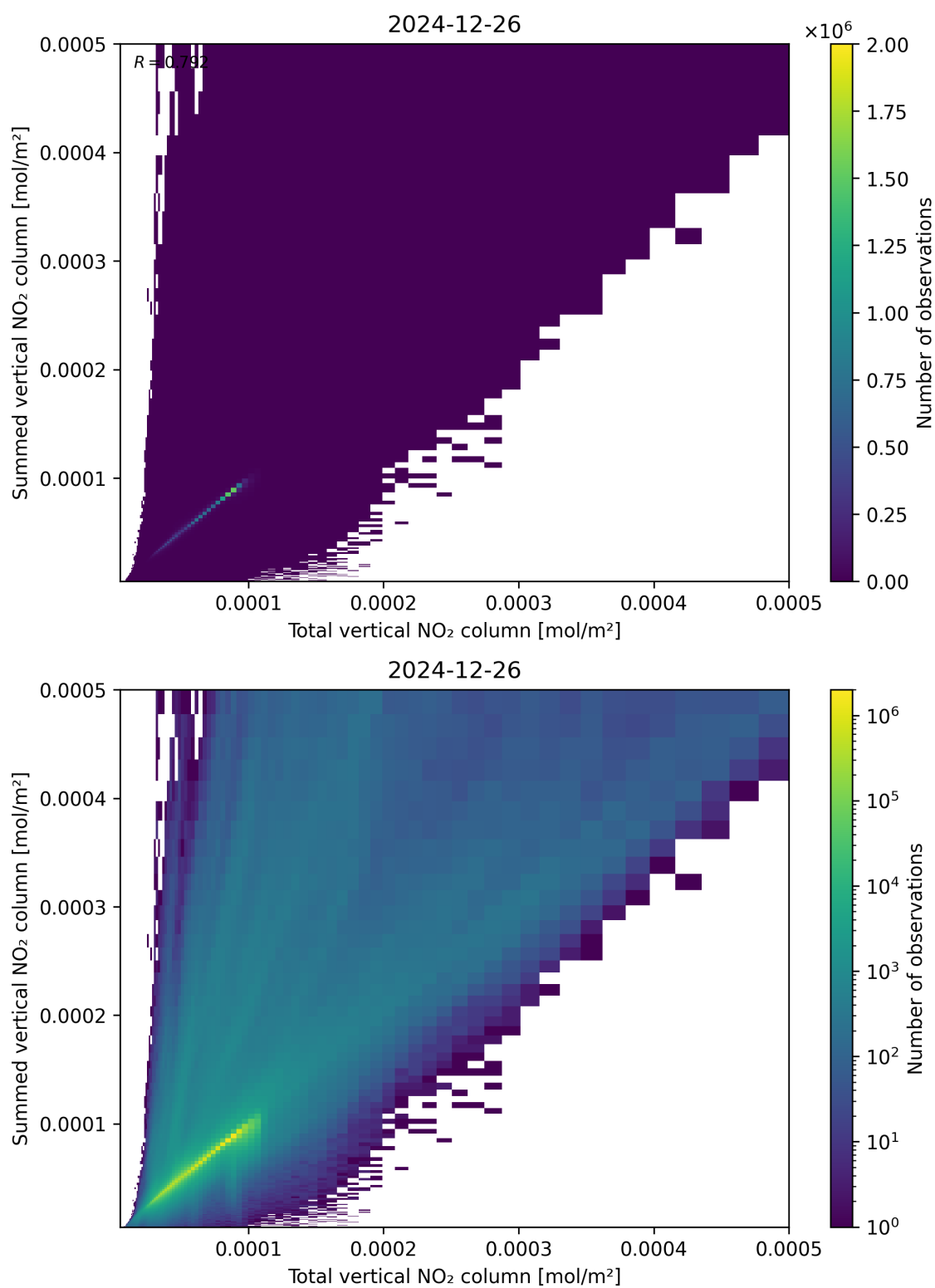
Figure 112: Scatter density plot of “Total vertical NO 2 column” against “Summed vertical NO 2 column” for 2024-12-25 to 2024-12-27.
