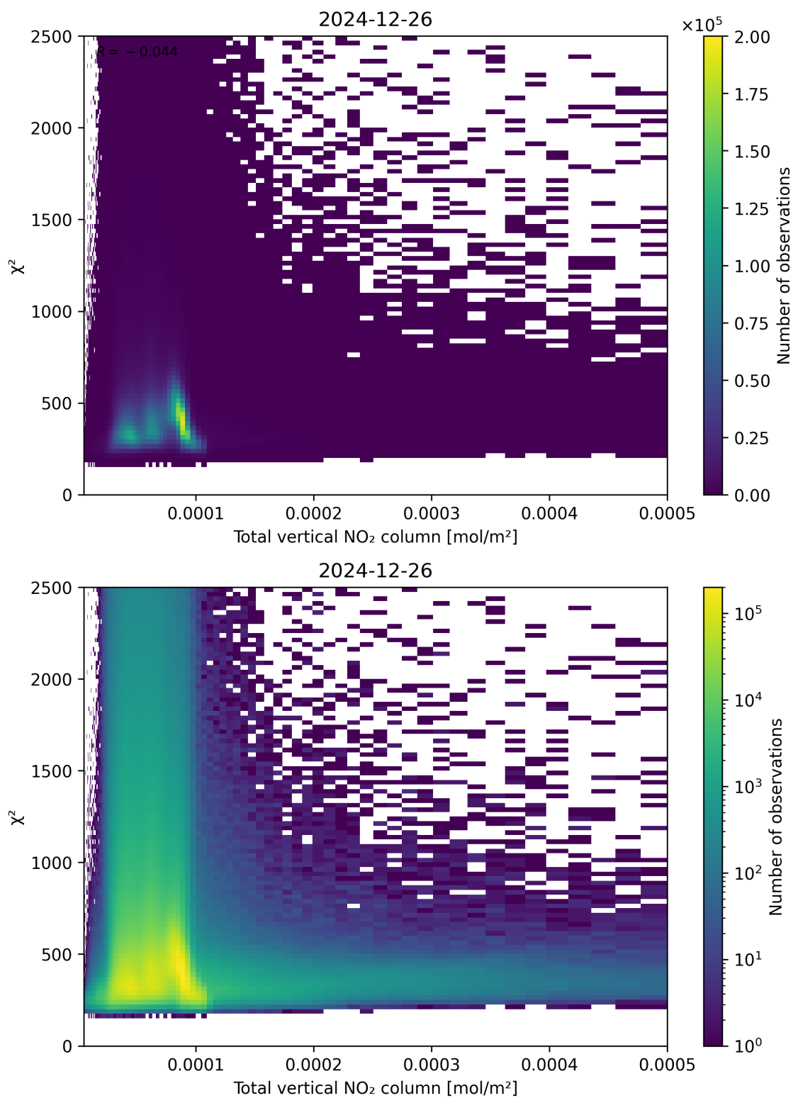
Figure 111: Scatter density plot of “Total vertical NO 2 column” against “ \chi^2 ” for 2024-12-25 to 2024-12-27.
