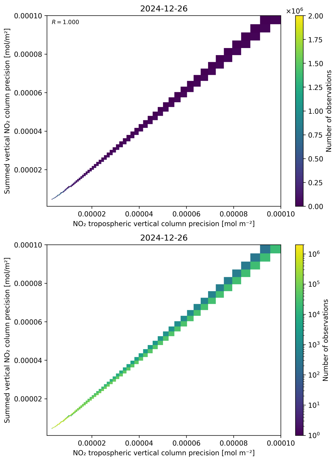
Figure 137: Scatter density plot of “NO 2 tropospheric vertical column precision” against “Summed vertical NO 2 column precision” for 2024-12-25 to 2024-12-27.
