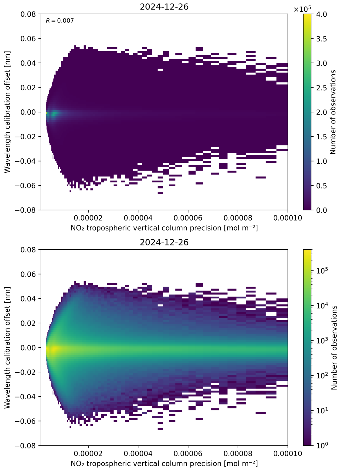
Figure 141: Scatter density plot of “NO 2 tropospheric vertical column precision” against “Wavelength calibration offset” for 2024-12-25 to 2024-12-27.
