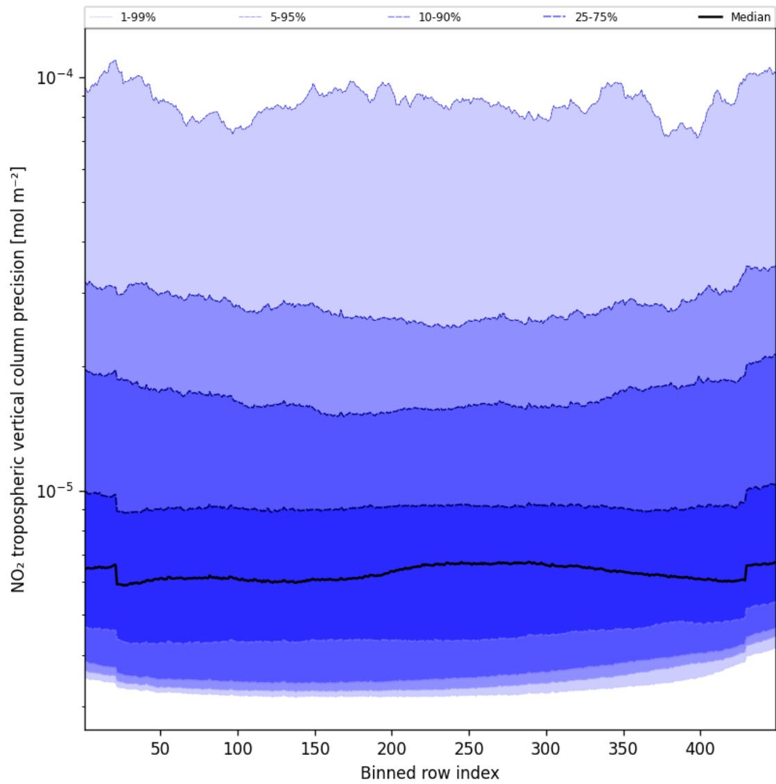
Figure 47: Along track statistics of “NO 2 tropospheric vertical column precision” for 2024-12-25 to 2024-12-27
