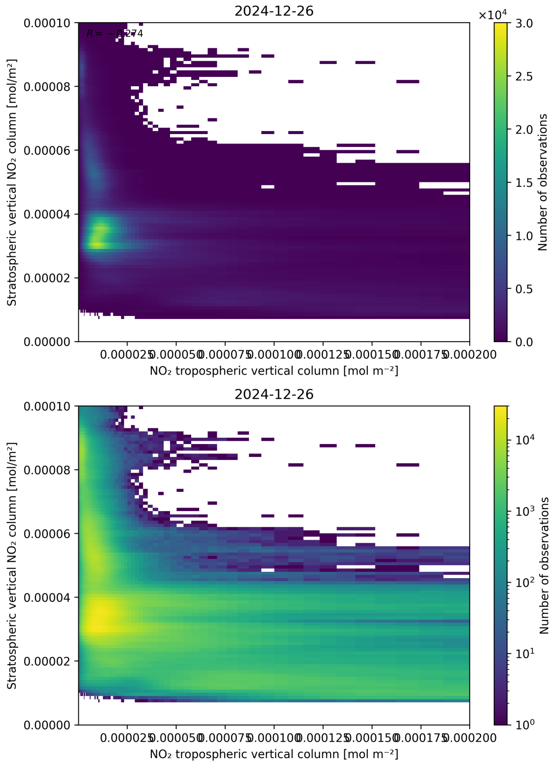
Figure 125: Scatter density plot of “NO 2 tropospheric vertical column” against “Stratospheric vertical NO 2 column” for 2024-12-25 to 2024-12-27.
