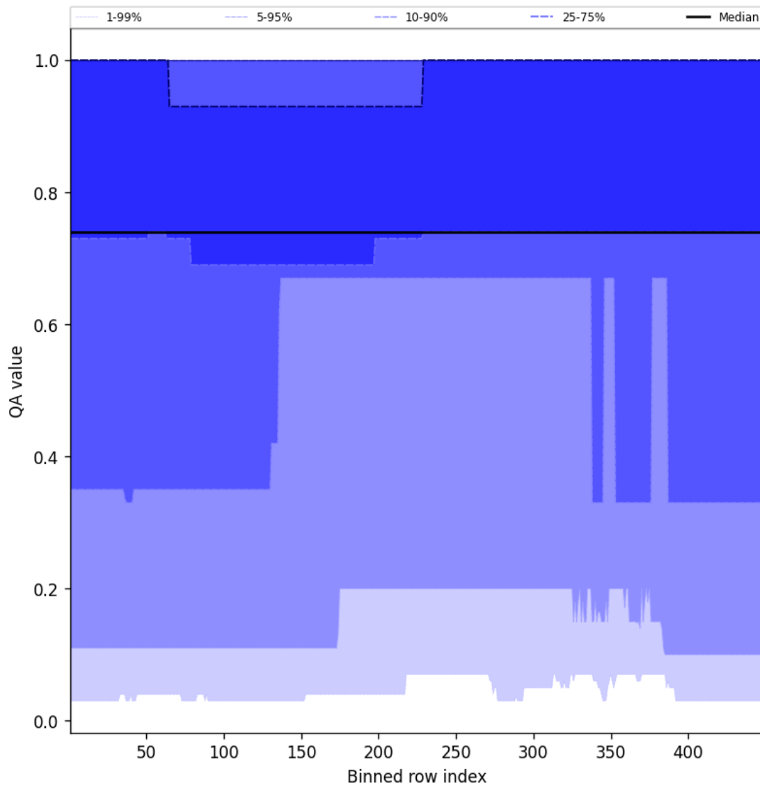
Figure 45: Along track statistics of "QA value" for 2024-12-25 to 2024-12-27
