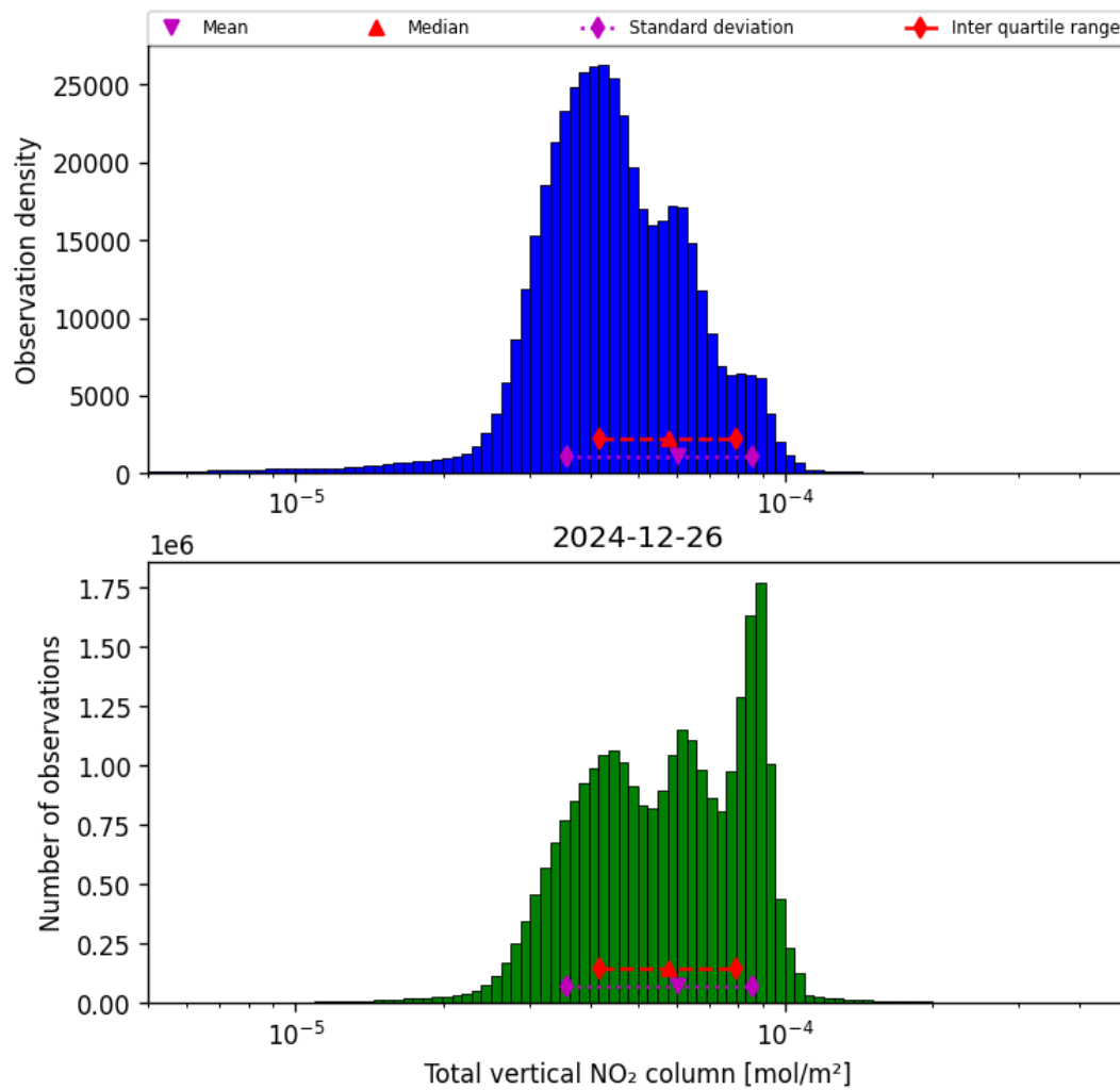
Figure 38: Histogram of “Total vertical NO 2 column” for 2024-12-25 to 2024-12-27
