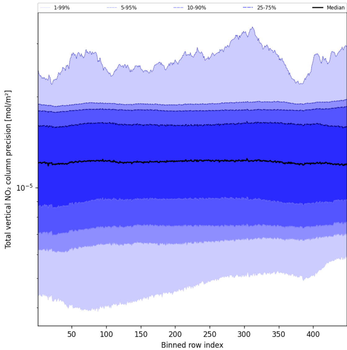
Figure 56: Along track statistics of “Total vertical NO 2 column precision” for 2024-12-25 to 2024-12-27
