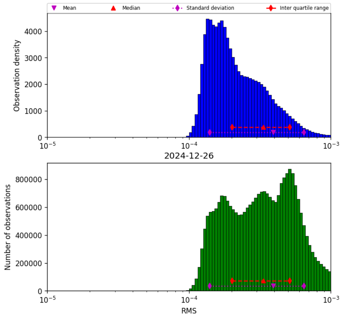
Figure 43: Histogram of “RMS” for 2024-12-25 to 2024-12-27
