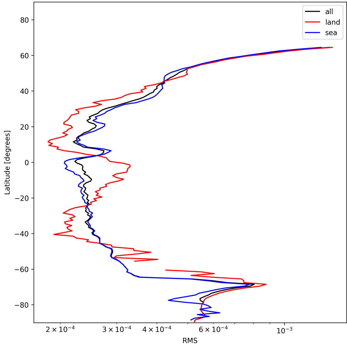
Figure 26: Zonal average of “RMS” for 2024-12-25 to 2024-12-27.
