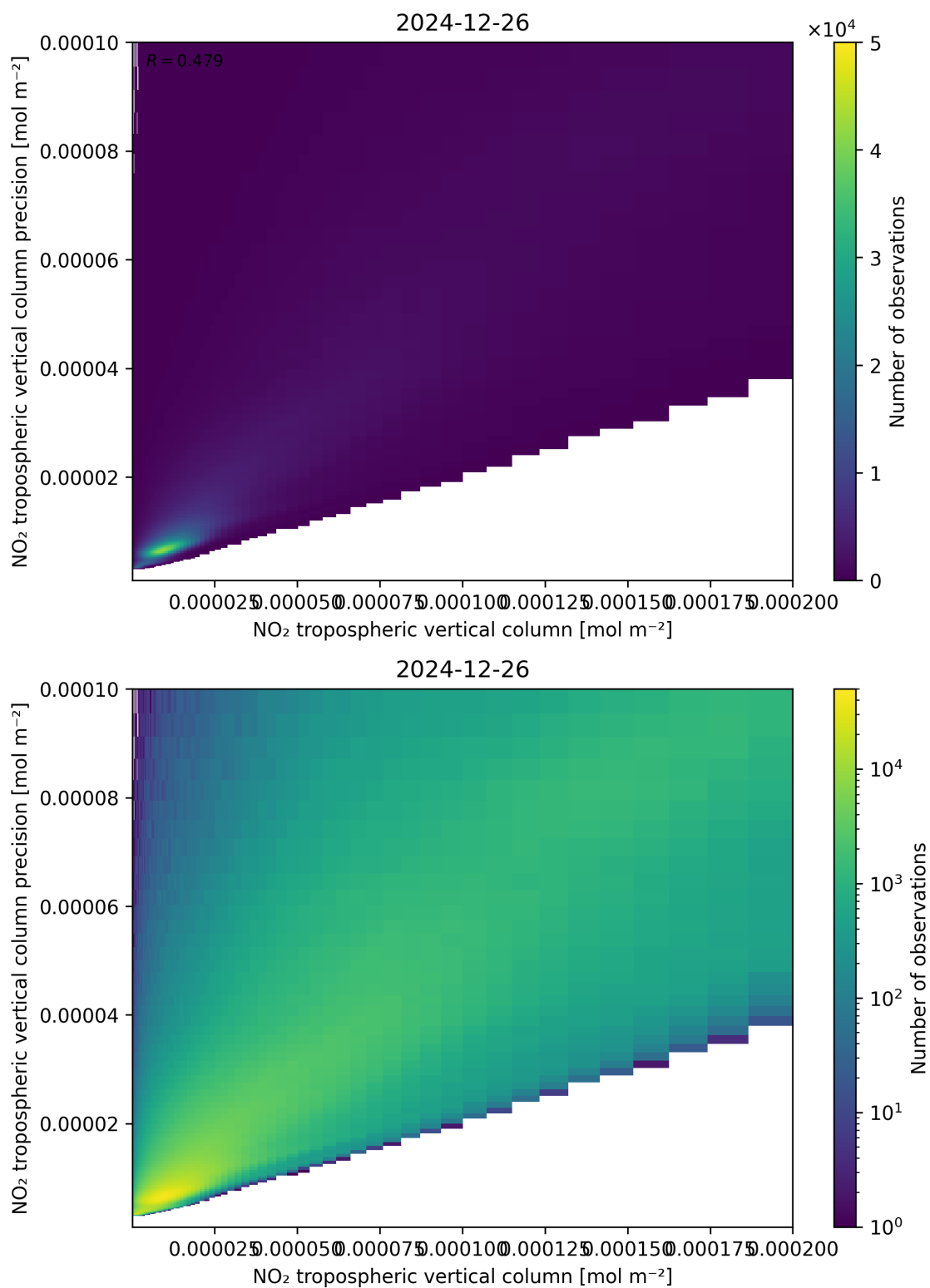
Figure 130: Scatter density plot of “NO 2 tropospheric vertical column” against “NO 2 tropospheric vertical column precision” for 2024-12-25 to 2024-12-27.
