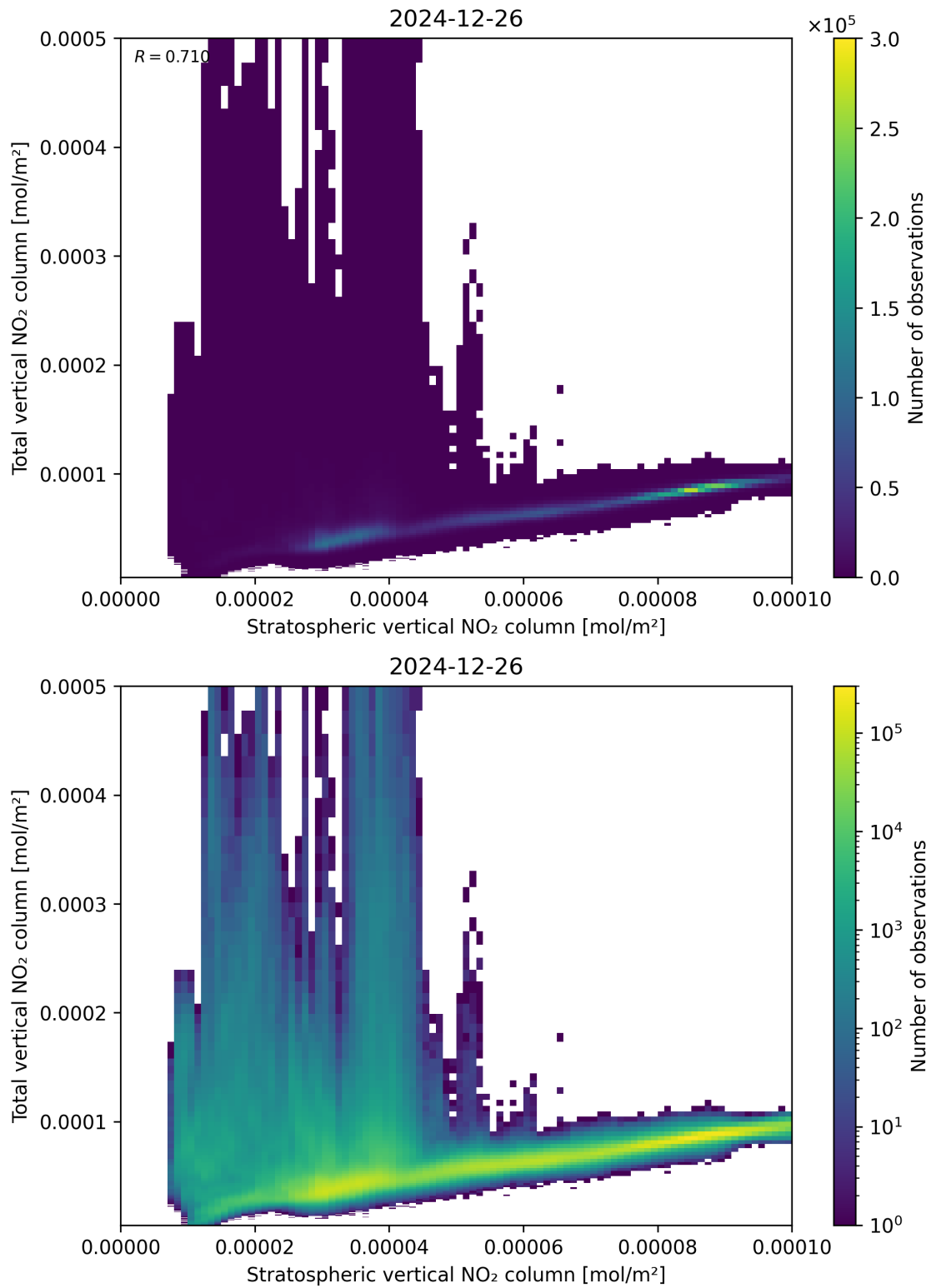
Figure 100: Scatter density plot of “Stratospheric vertical NO 2 column” against “Total vertical NO 2 column” for 2024-12-25 to 2024-12-27.
