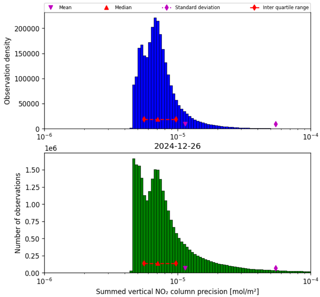
Figure 41: Histogram of “Summed vertical NO 2 column precision” for 2024-12-25 to 2024-12-27
