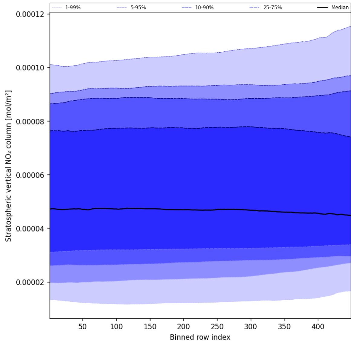
Figure 53: Along track statistics of “Stratospheric vertical NO 2 column” for 2024-12-25 to 2024-12-27
