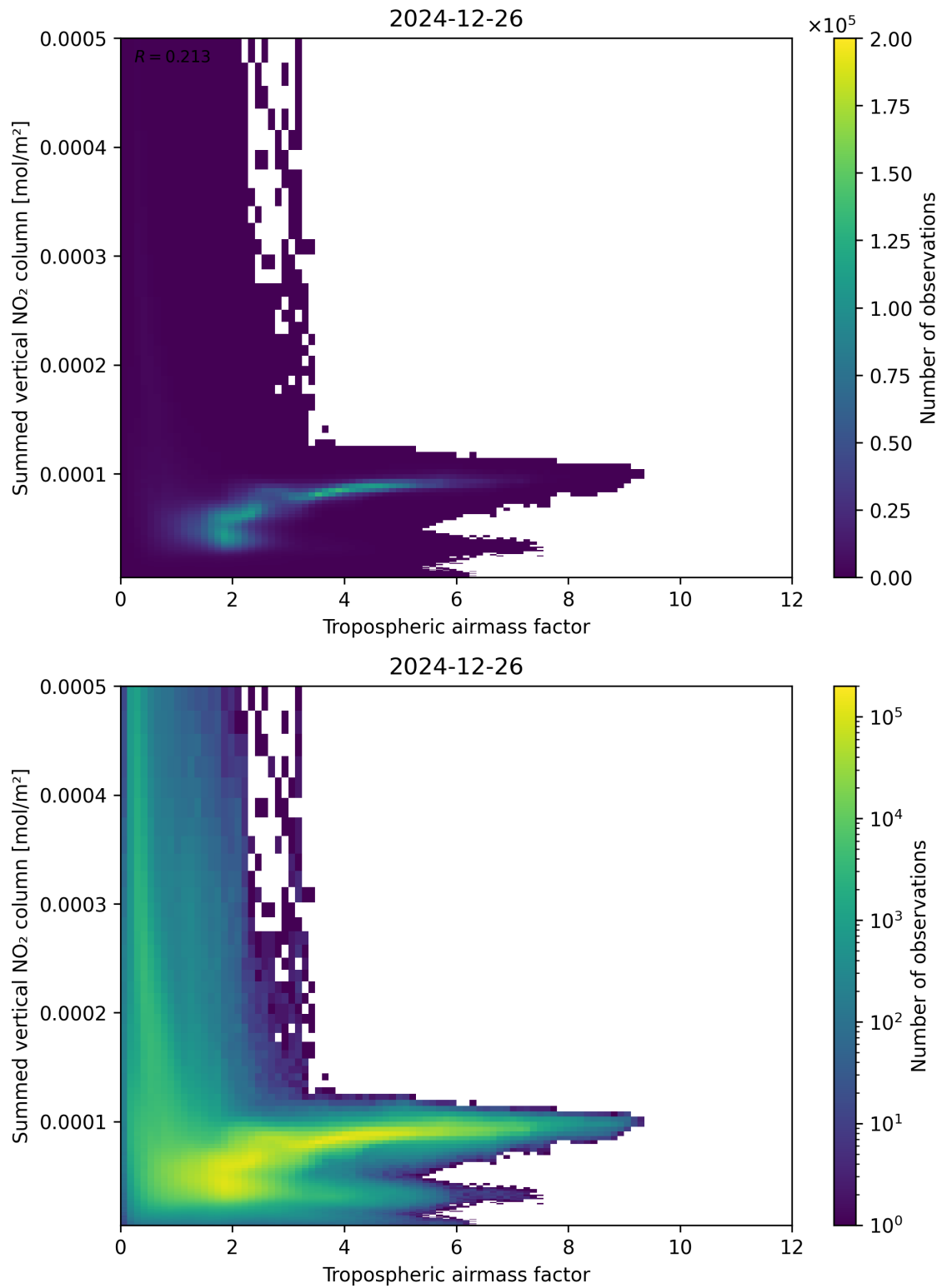
Figure 75: Scatter density plot of “Tropospheric airmass factor” against “Summed vertical NO 2 column” for 2024-12-25 to 2024-12-27.
