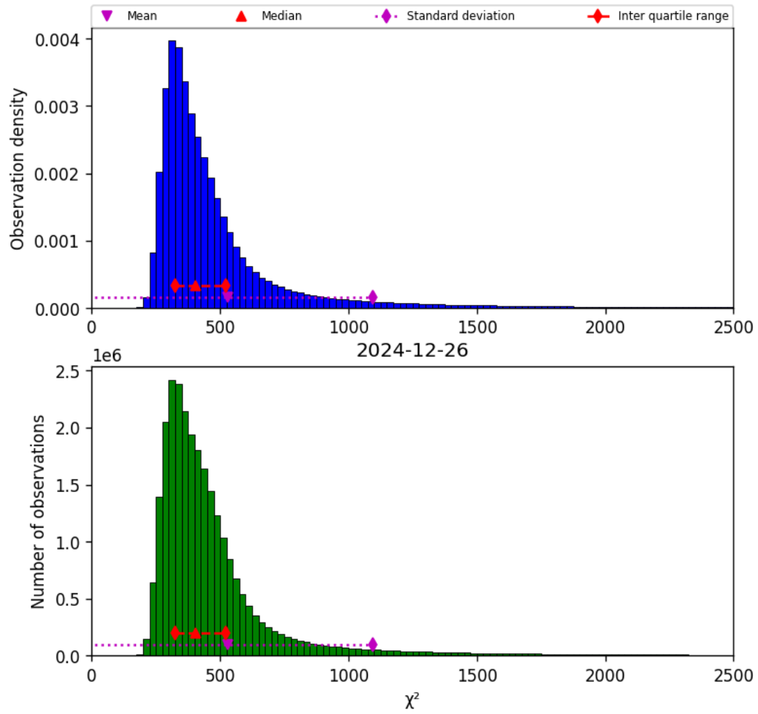
Figure 42: Histogram of “ \chi^2 ” for 2024-12-25 to 2024-12-27
