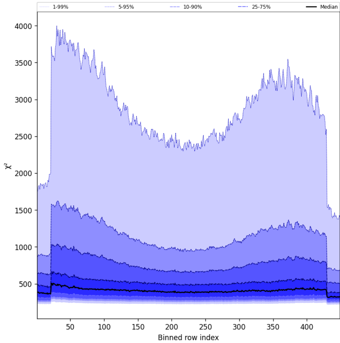
Figure 59: Along track statistics of “ \chi^2 ” for 2024-12-25 to 2024-12-27
