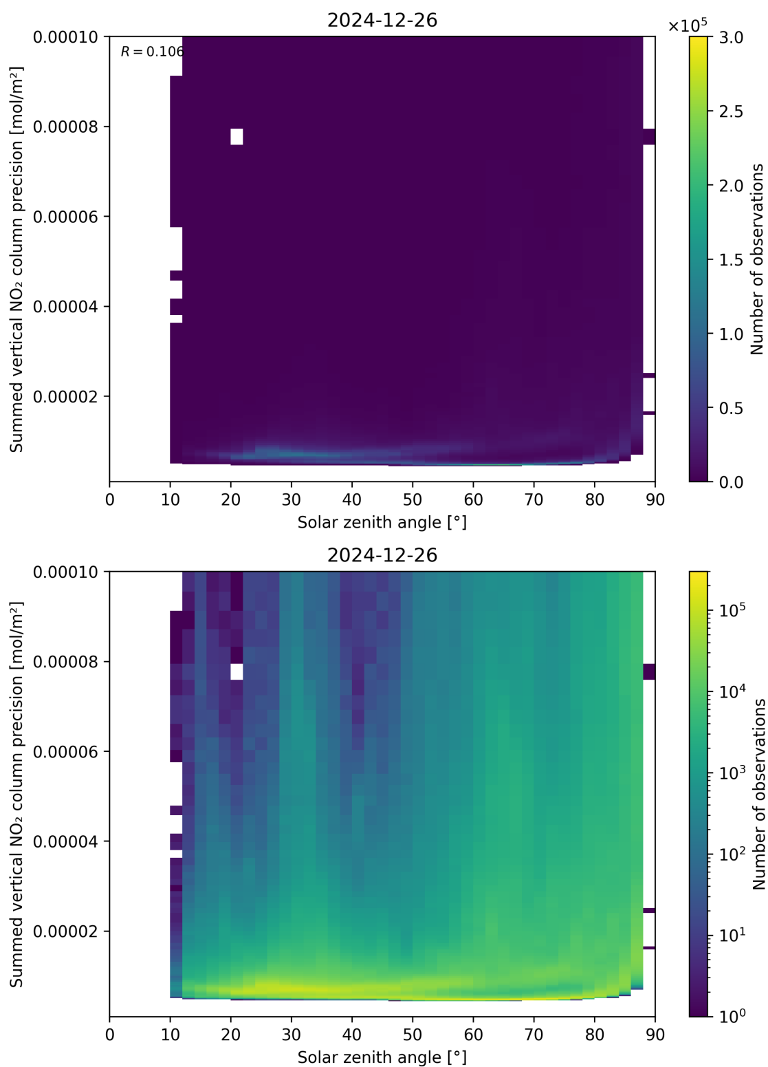
Figure 152: Scatter density plot of “Solar zenith angle” against “Summed vertical NO 2 column precision” for 2024-12-25 to 2024-12-27.
