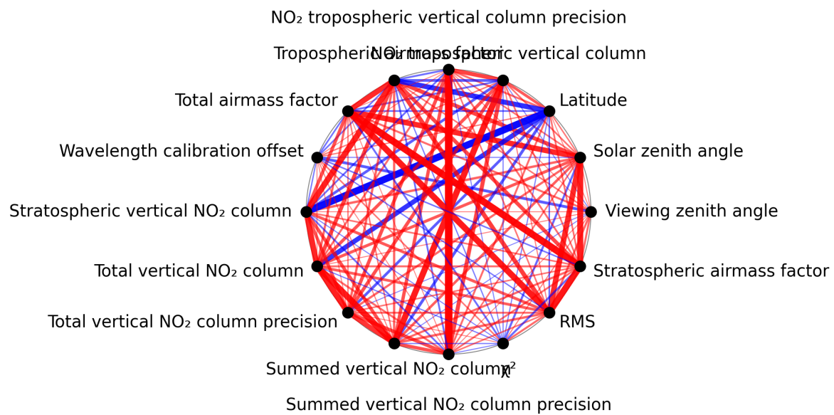
Figure 1: Map of correlation graph for 2024-12-25 to 2024-12-27.
