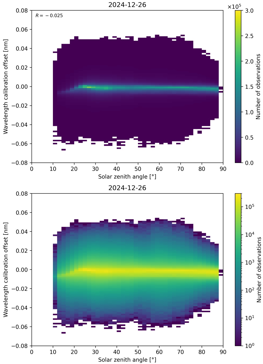
Figure 158: Scatter density plot of “Solar zenith angle” against “Wavelength calibration offset” for 2024-12-25 to 2024-12-27.
