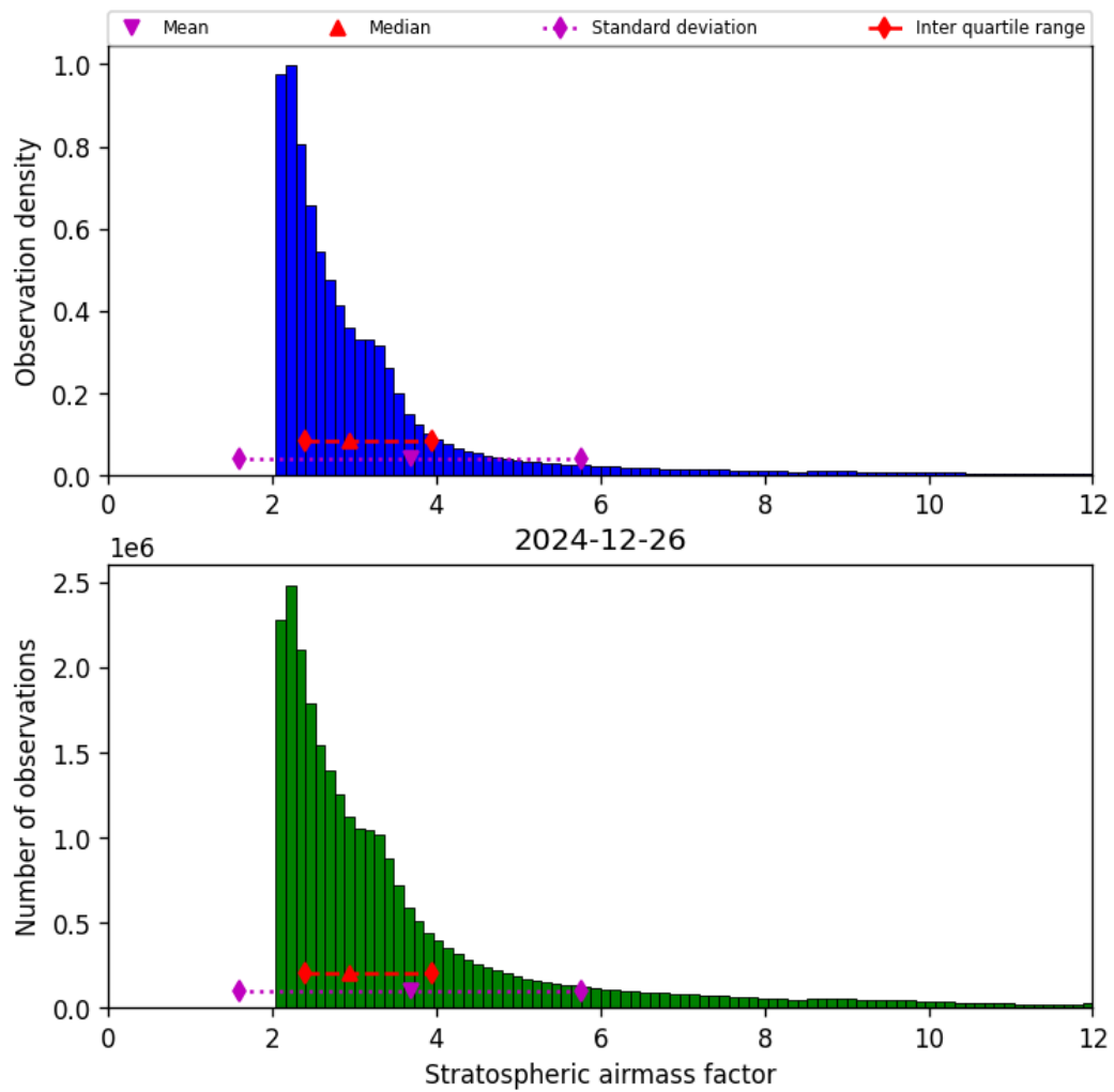
Figure 44: Histogram of “Stratospheric airmass factor” for 2024-12-25 to 2024-12-27
