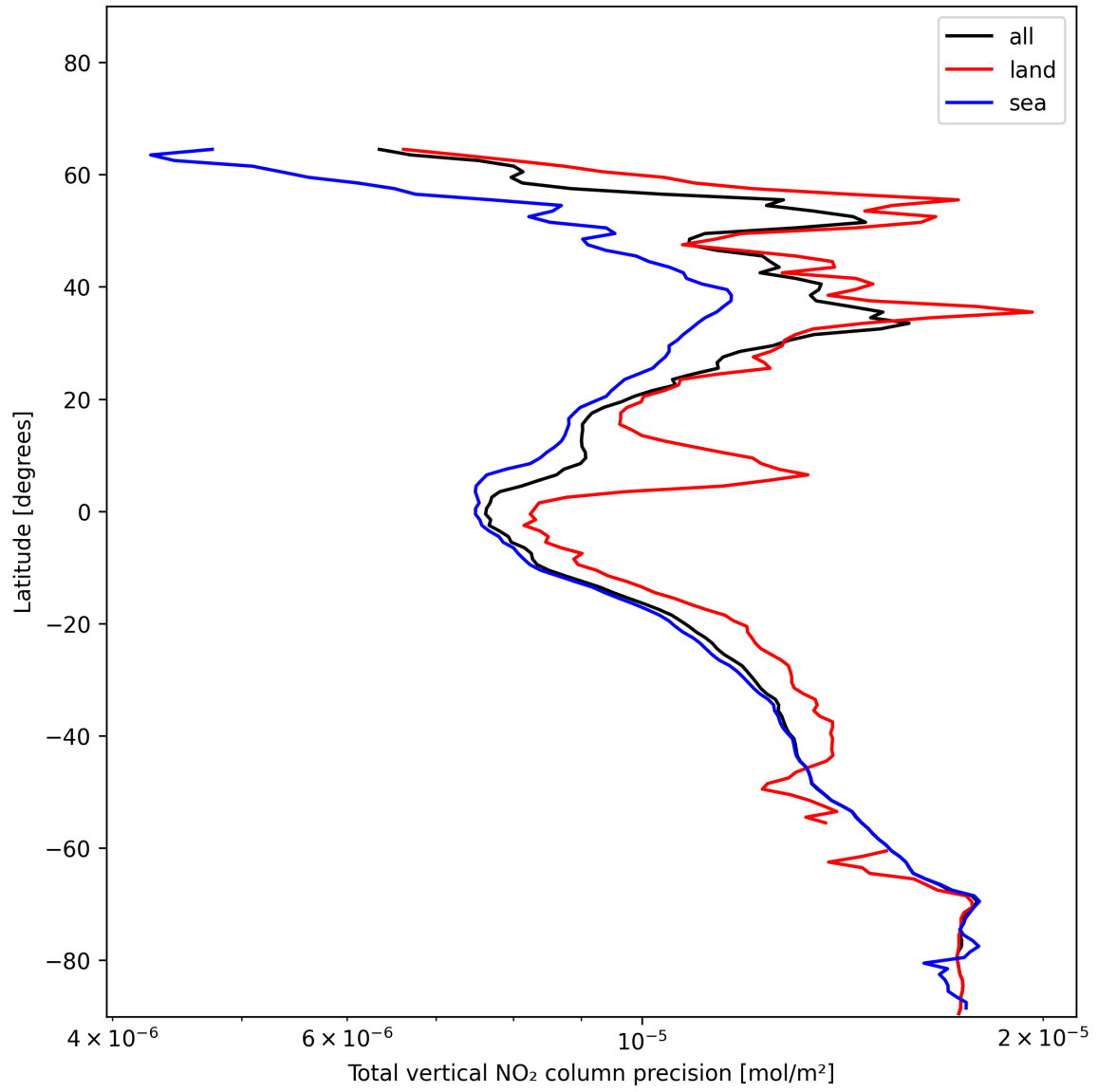
Figure 22: Zonal average of “Total vertical NO 2 column precision” for 2024-12-25 to 2024-12-27.
