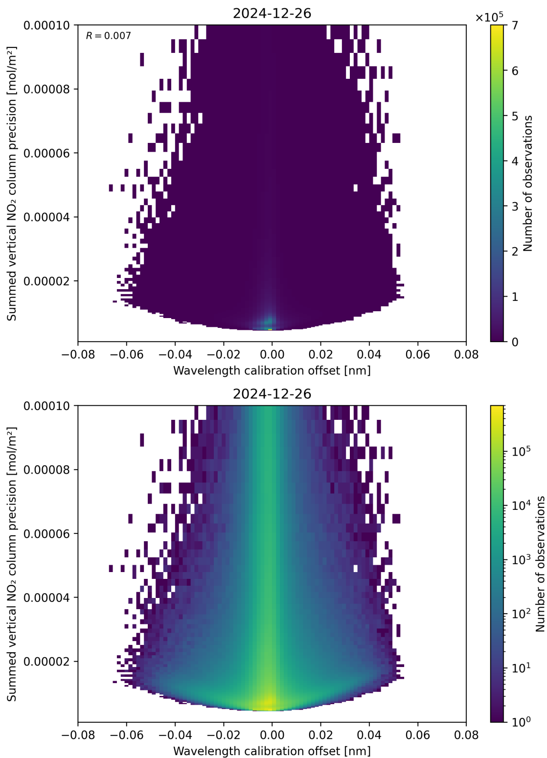
Figure 178: Scatter density plot of “Wavelength calibration offset” against “Summed vertical NO 2 column precision” for 2024-12-25 to 2024-12-27.
