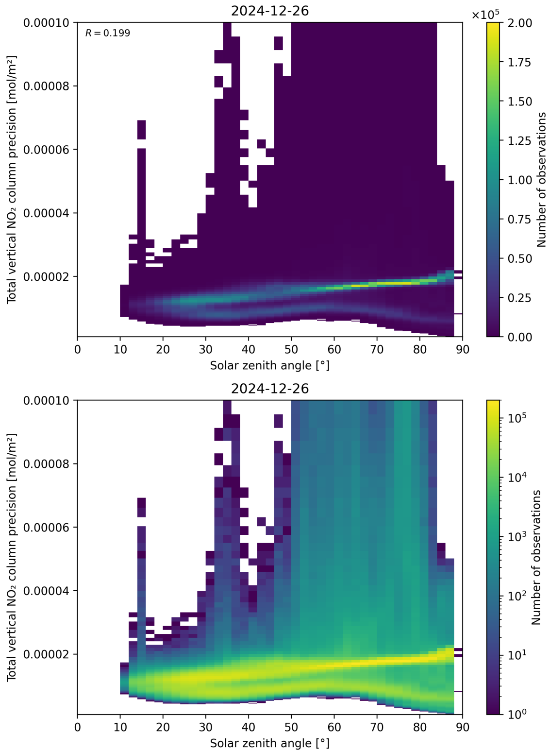
Figure 154: Scatter density plot of “Solar zenith angle” against “Total vertical NO 2 column precision” for 2024-12-25 to 2024-12-27.
