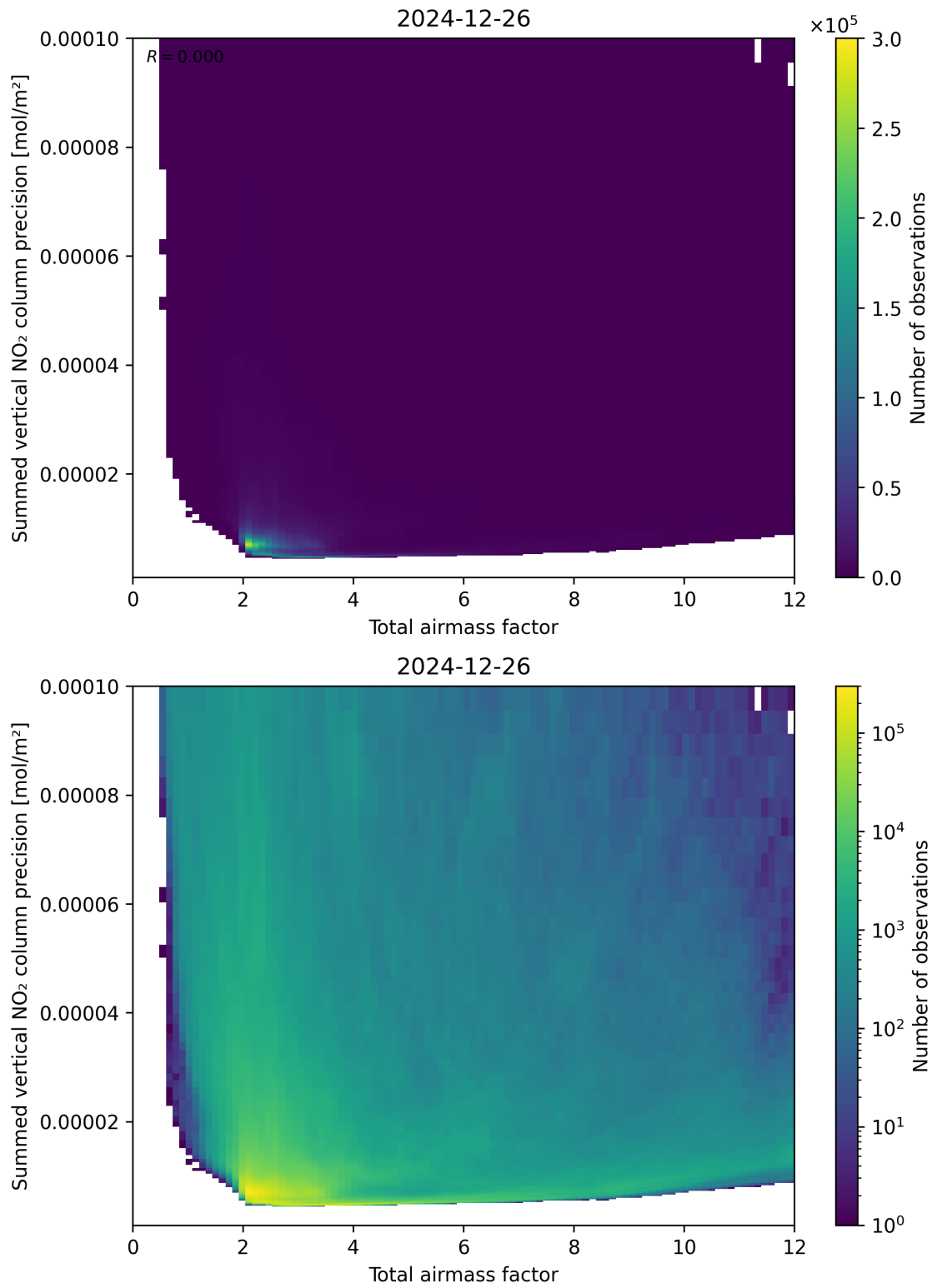
Figure 66: Scatter density plot of “Total airmass factor” against “Summed vertical NO 2 column precision” for 2024-12-25 to 2024-12-27.
