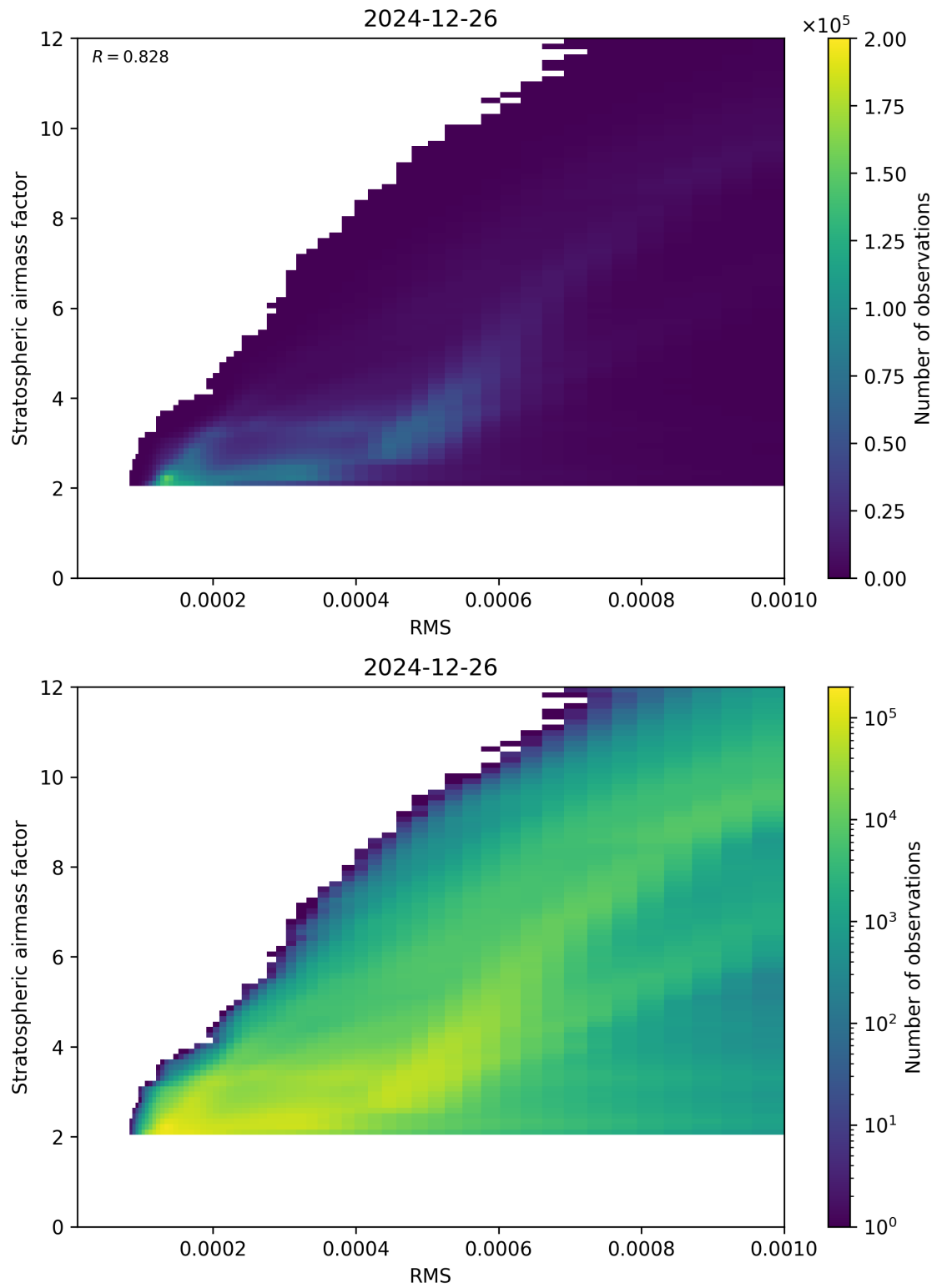
Figure 144: Scatter density plot of “RMS” against “Stratospheric airmass factor” for 2024-12-25 to 2024-12-27.
