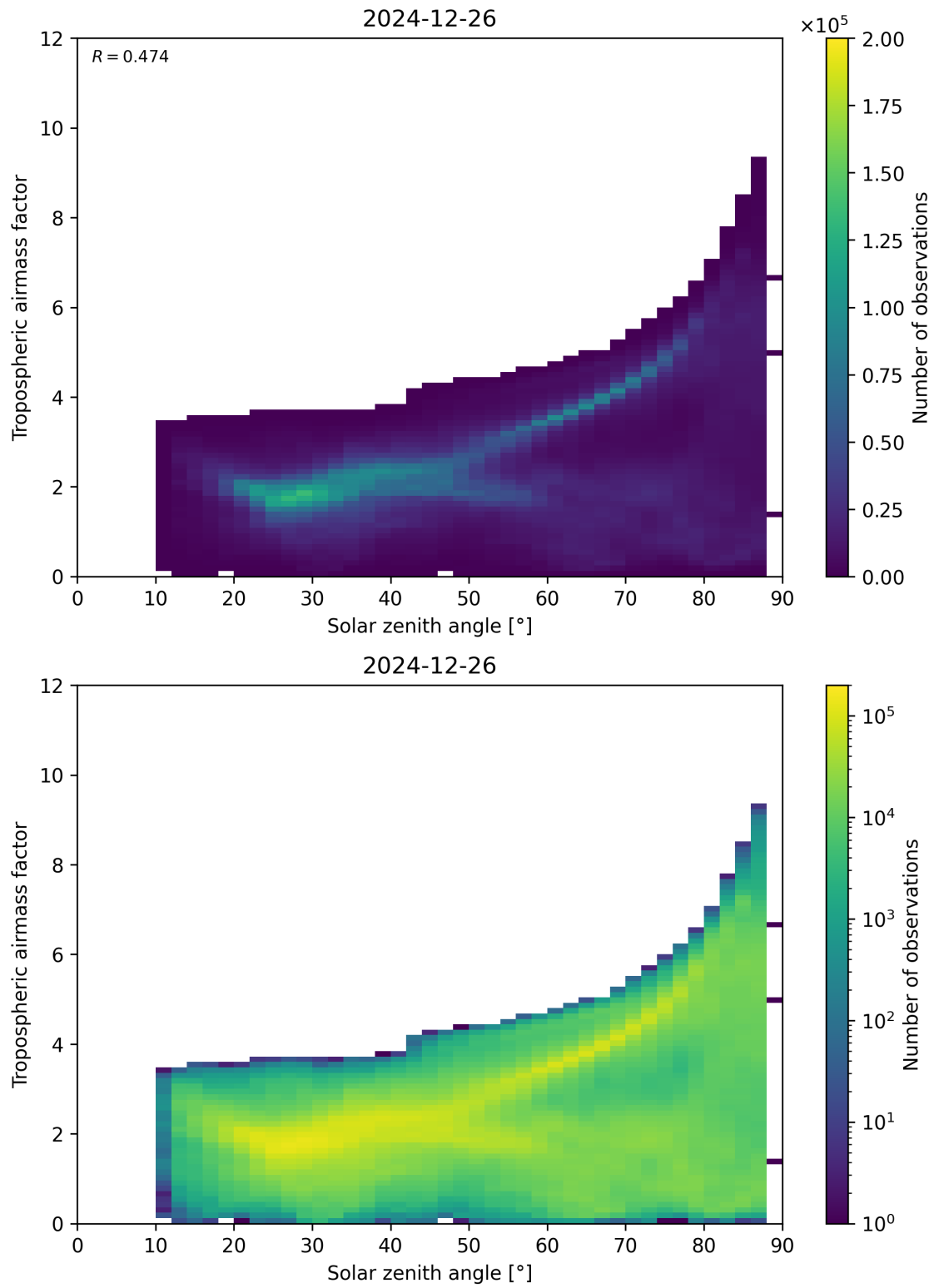
Figure 147: Scatter density plot of “Solar zenith angle” against “Tropospheric airmass factor” for 2024-12-25 to 2024-12-27.
