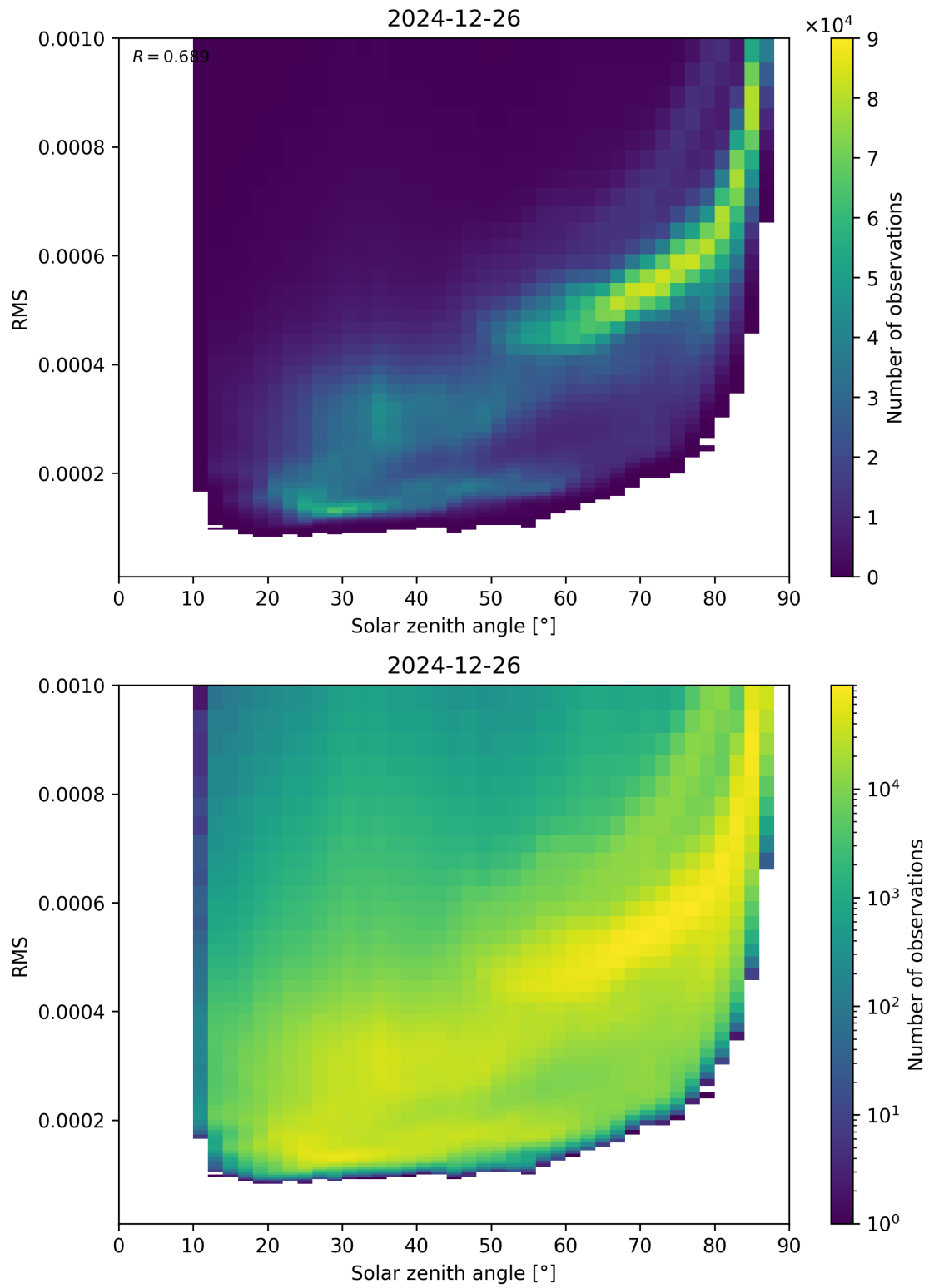
Figure 157: Scatter density plot of “Solar zenith angle” against “RMS” for 2024-12-25 to 2024-12-27.
