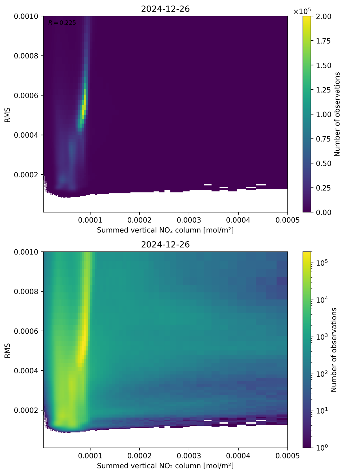
Figure 109: Scatter density plot of “Summed vertical NO 2 column” against “RMS” for 2024-12-25 to 2024-12-27.
