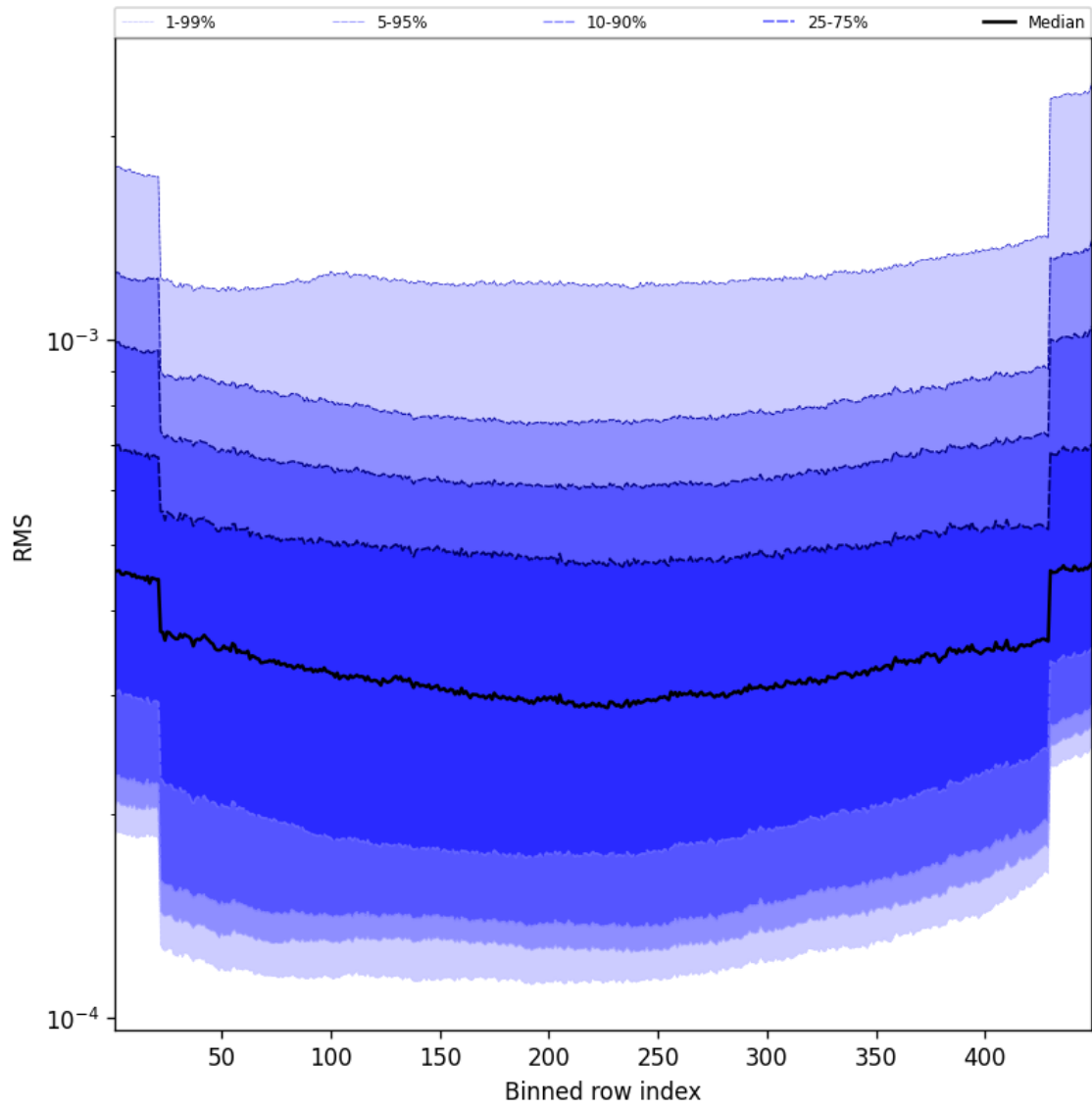
Figure 60: Along track statistics of “RMS” for 2024-12-25 to 2024-12-27
