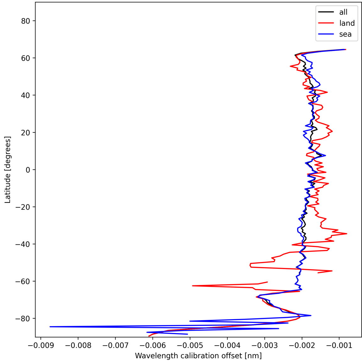
Figure 18: Zonal average of “Wavelength calibration offset” for 2024-12-25 to 2024-12-27.
