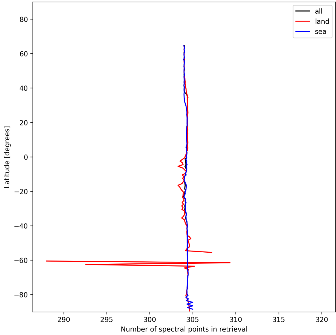
Figure 16: Zonal average of “Number of spectral points in retrieval” for 2024-12-25 to 2024-12-27.
