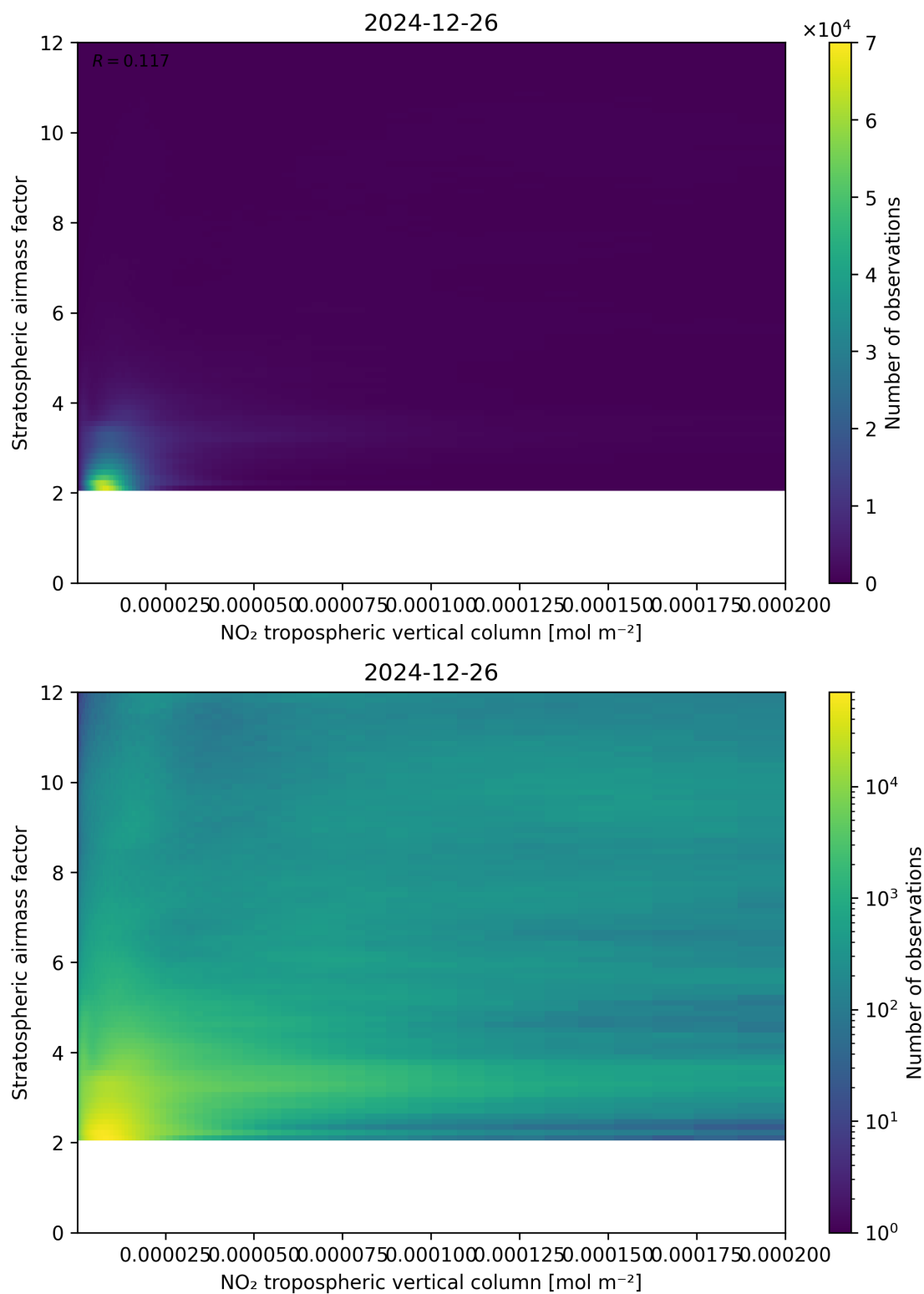
Figure 121: Scatter density plot of “NO 2 tropospheric vertical column” against “Stratospheric airmass factor” for 2024-12-25 to 2024-12-27.
