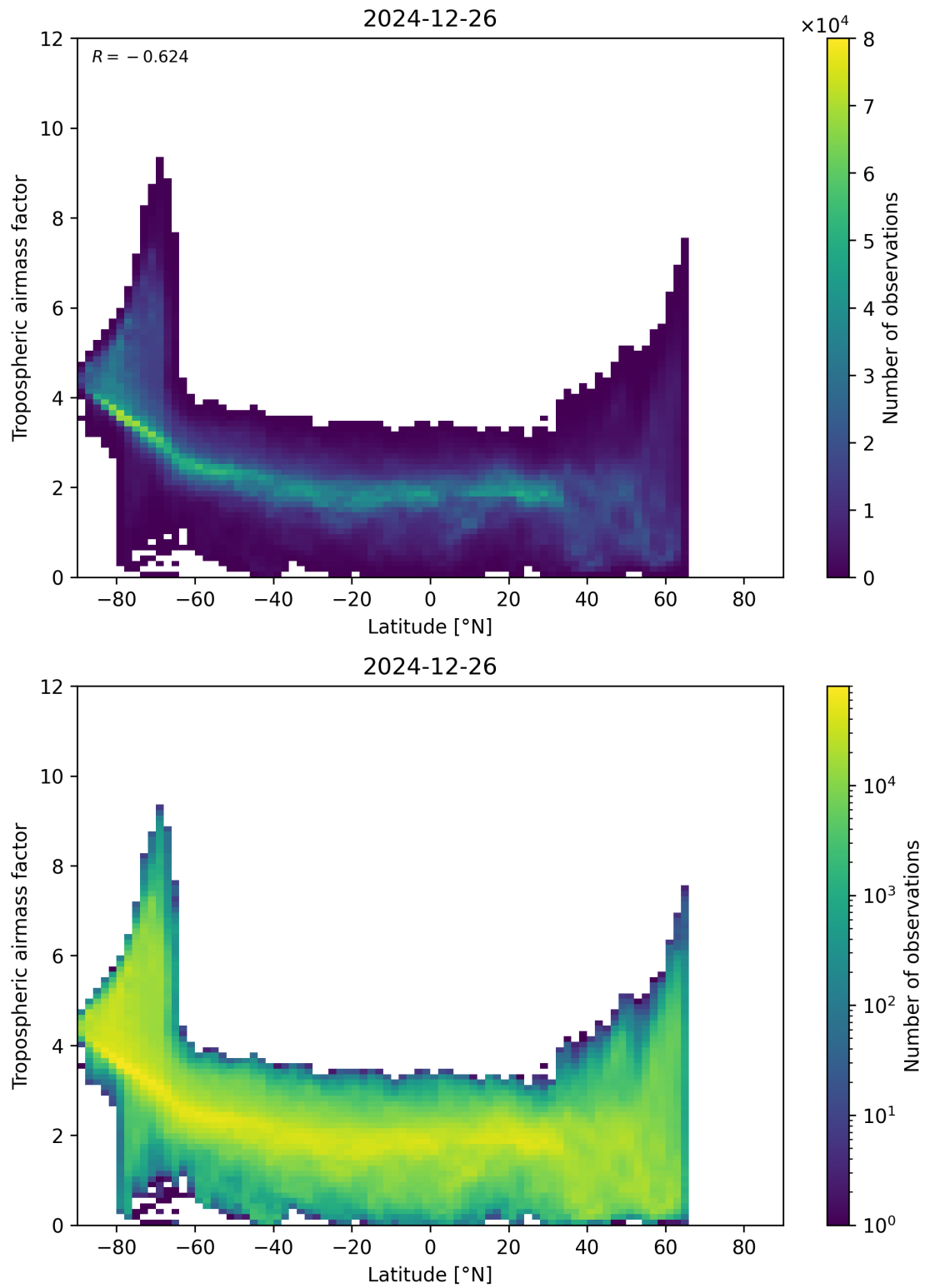
Figure 85: Scatter density plot of “Latitude” against “Tropospheric air mass factor” for 2024-12-25 to 2024-12-27.
