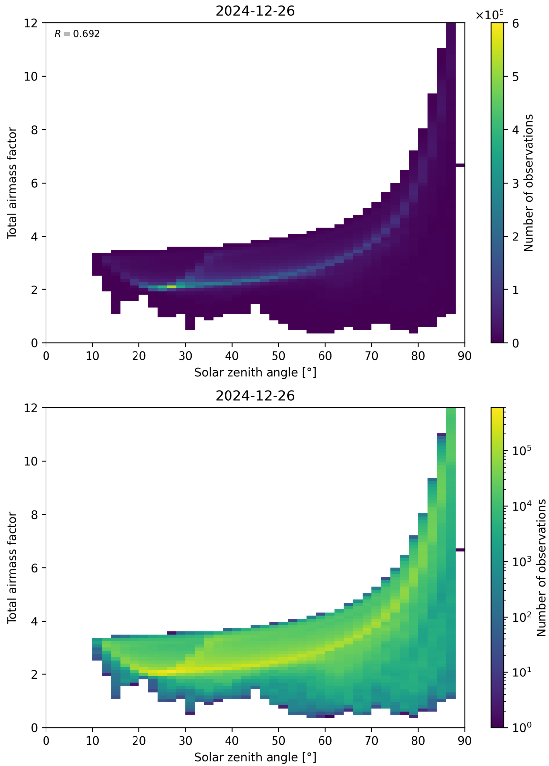
Figure 146: Scatter density plot of “Solar zenith angle” against “Total air mass factor” for 2024-12-25 to 2024-12-27.
