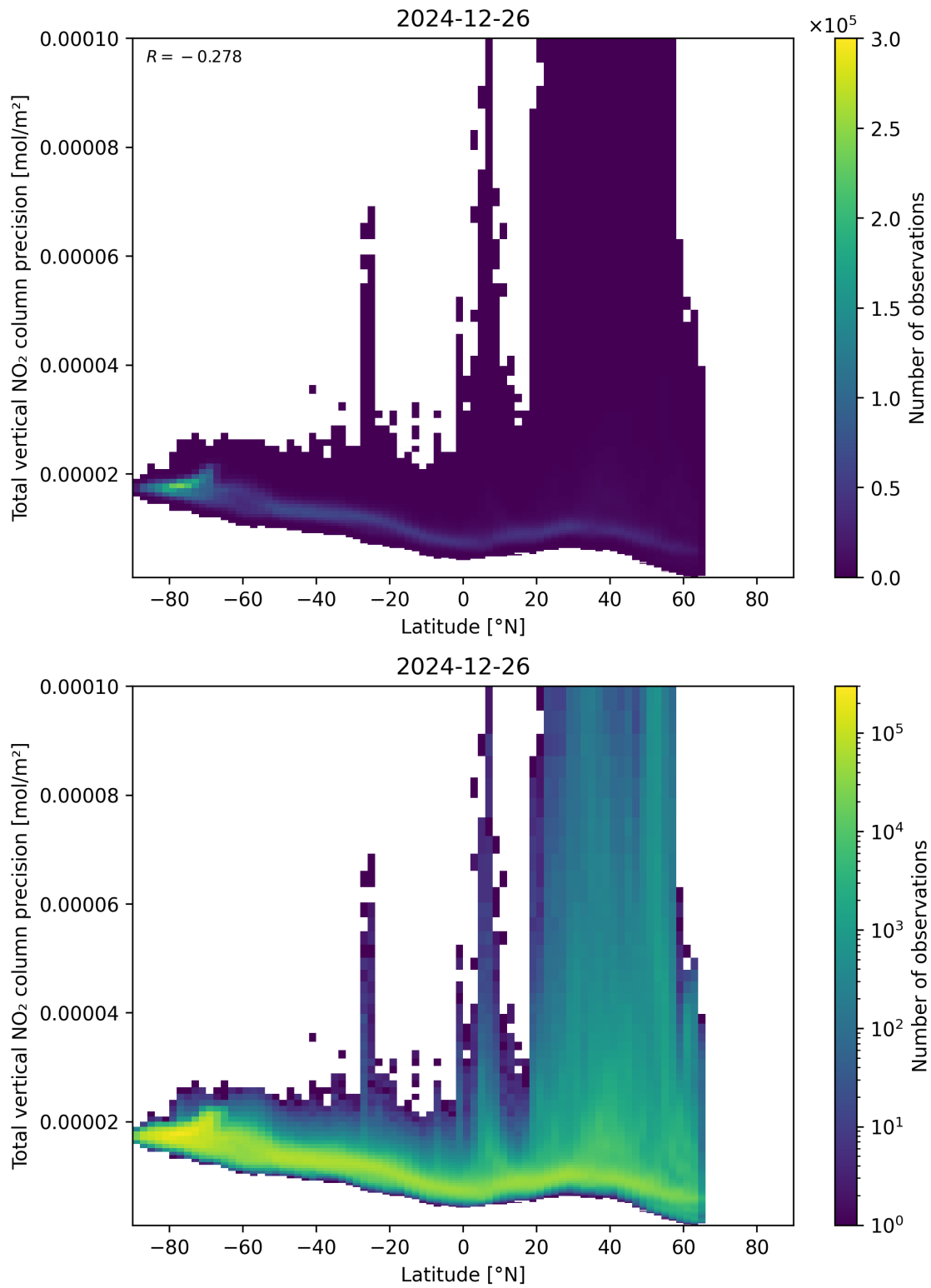
Figure 91: Scatter density plot of “Latitude” against “Total vertical NO 2 column precision” for 2024-12-25 to 2024-12-27.
