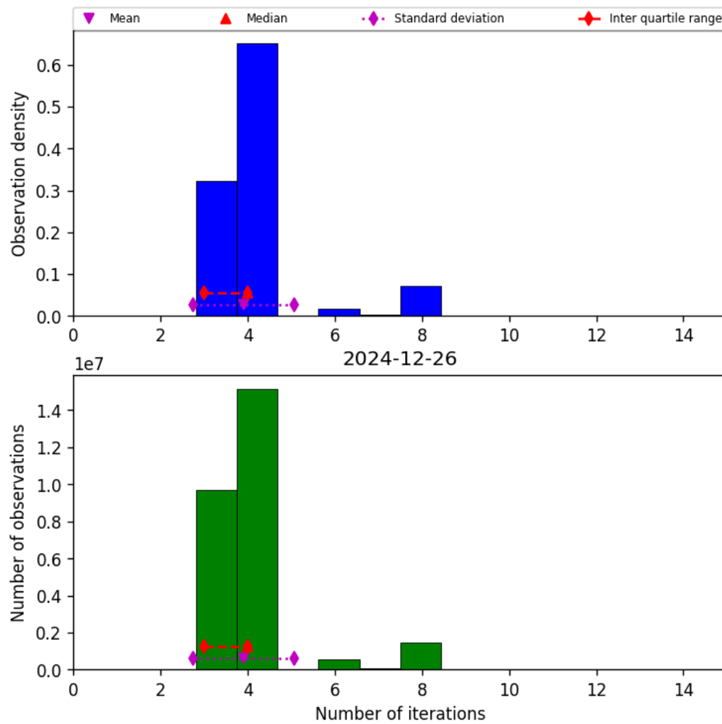
Figure 34: Histogram of “Number of iterations” for 2024-12-25 to 2024-12-27
