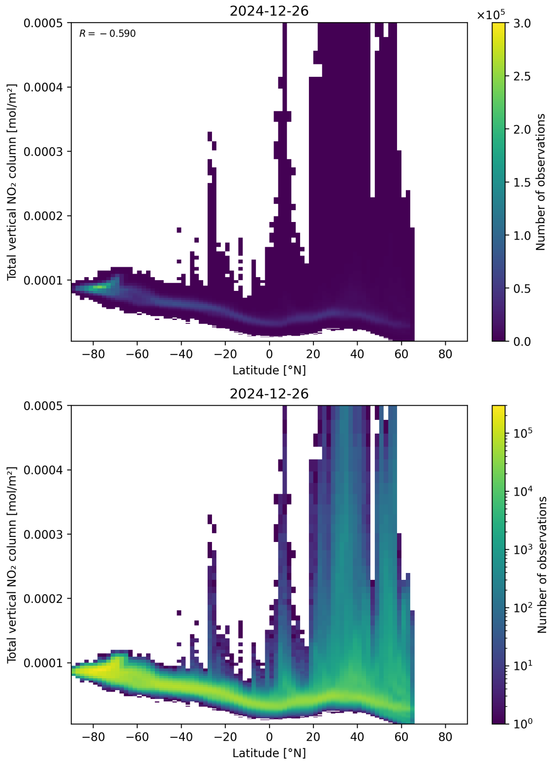
Figure 90: Scatter density plot of “Latitude” against “Total vertical NO 2 column” for 2024-12-25 to 2024-12-27.
