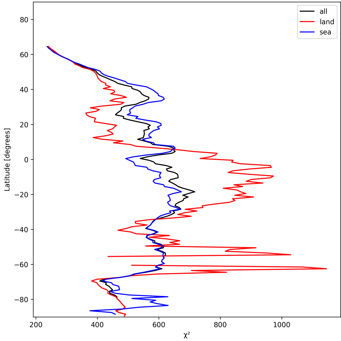
Figure 25: Zonal average of “ \chi^2 ” for 2024-12-25 to 2024-12-27.
