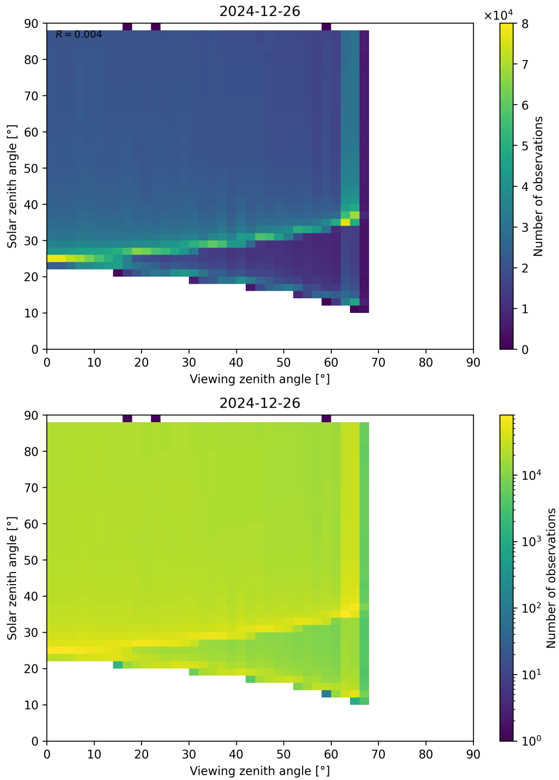
Figure 172: Scatter density plot of “Viewing zenith angle” against “Solar zenith angle” for 2024-12-25 to 2024-12-27.
