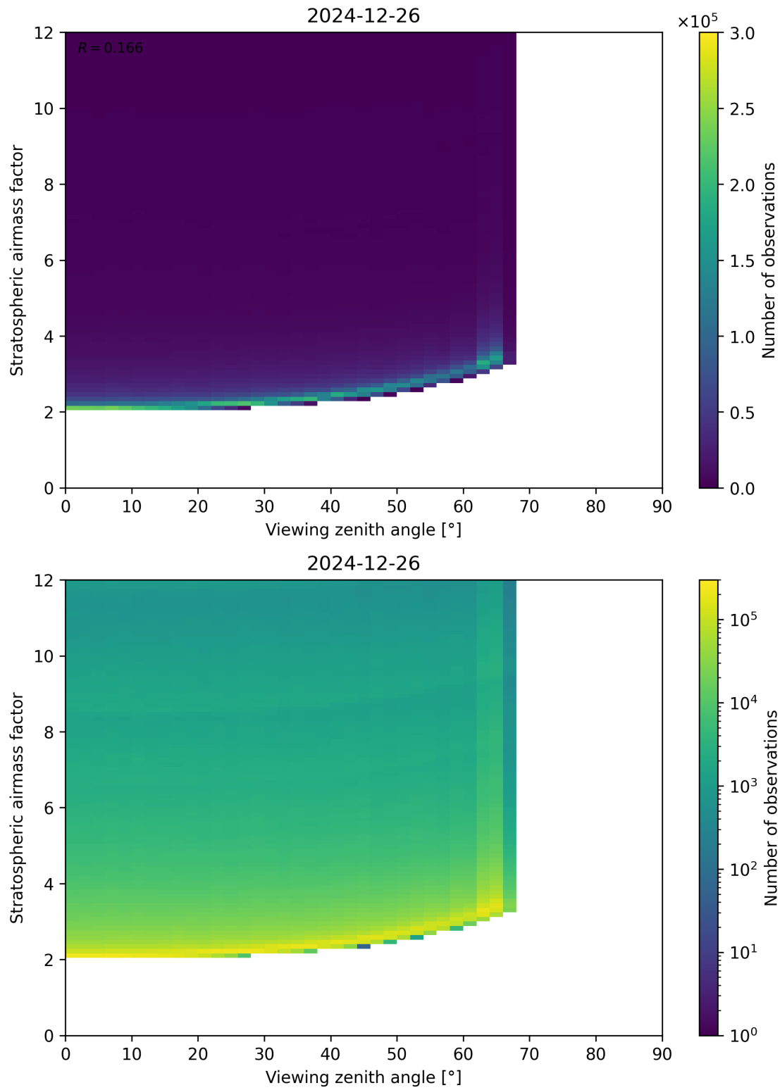
Figure 159: Scatter density plot of “Viewing zenith angle” against “Stratospheric airmass factor” for 2024-12-25 to 2024-12-27.
