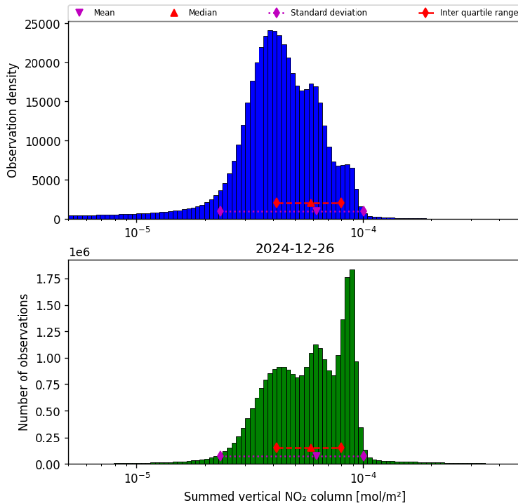
Figure 40: Histogram of “Summed vertical NO 2 column” for 2024-12-25 to 2024-12-27
