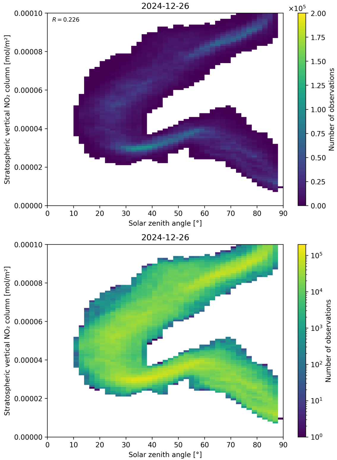
Figure 150: Scatter density plot of “Solar zenith angle” against “Stratospheric vertical NO 2 column” for 2024-12-25 to 2024-12-27.
