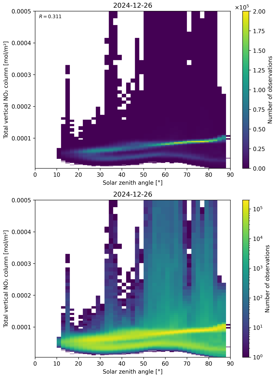
Figure 153: Scatter density plot of “Solar zenith angle” against “Total vertical \text{NO}_2 column” for 2024-12-25 to 2024-12-27.
