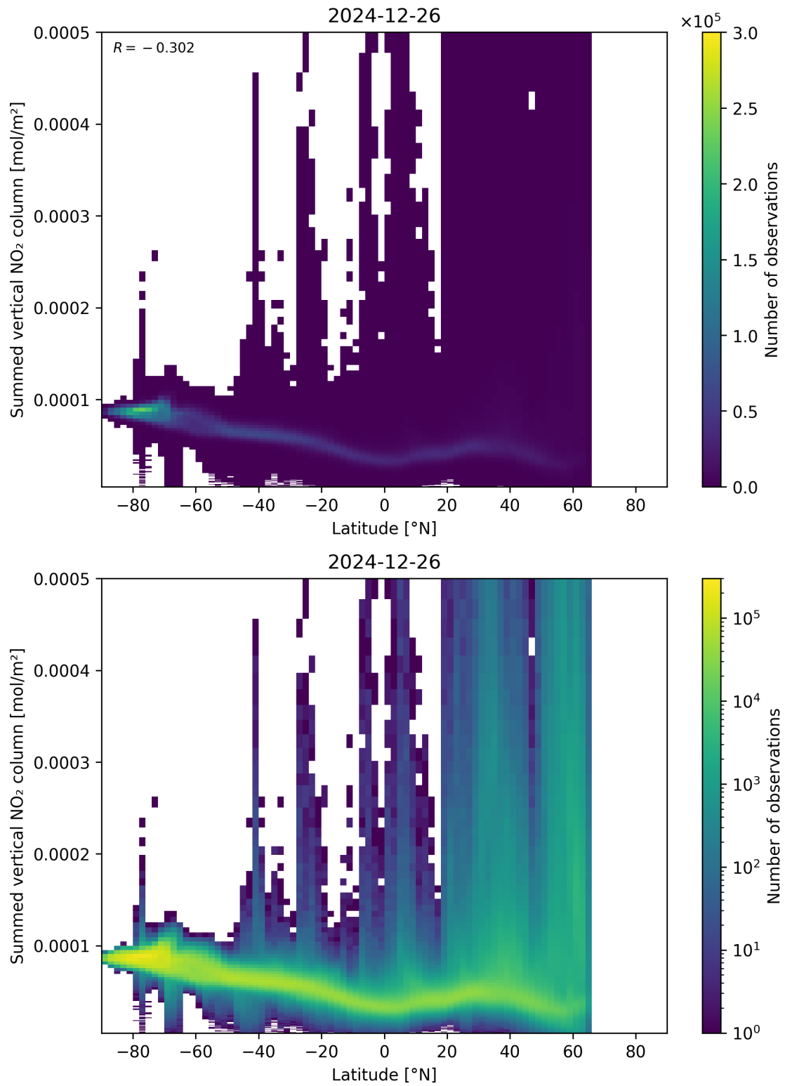
Figure 88: Scatter density plot of “Latitude” against “Summed vertical NO 2 column” for 2024-12-25 to 2024-12-27.
