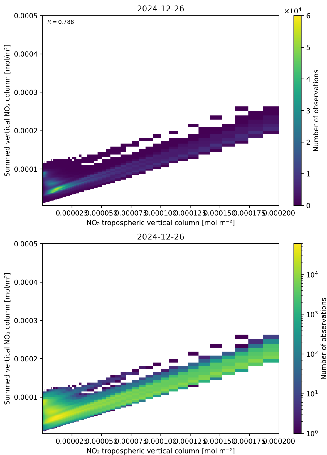
Figure 126: Scatter density plot of “NO 2 tropospheric vertical column” against “Summed vertical NO 2 column” for 2024-12-25 to 2024-12-27.
