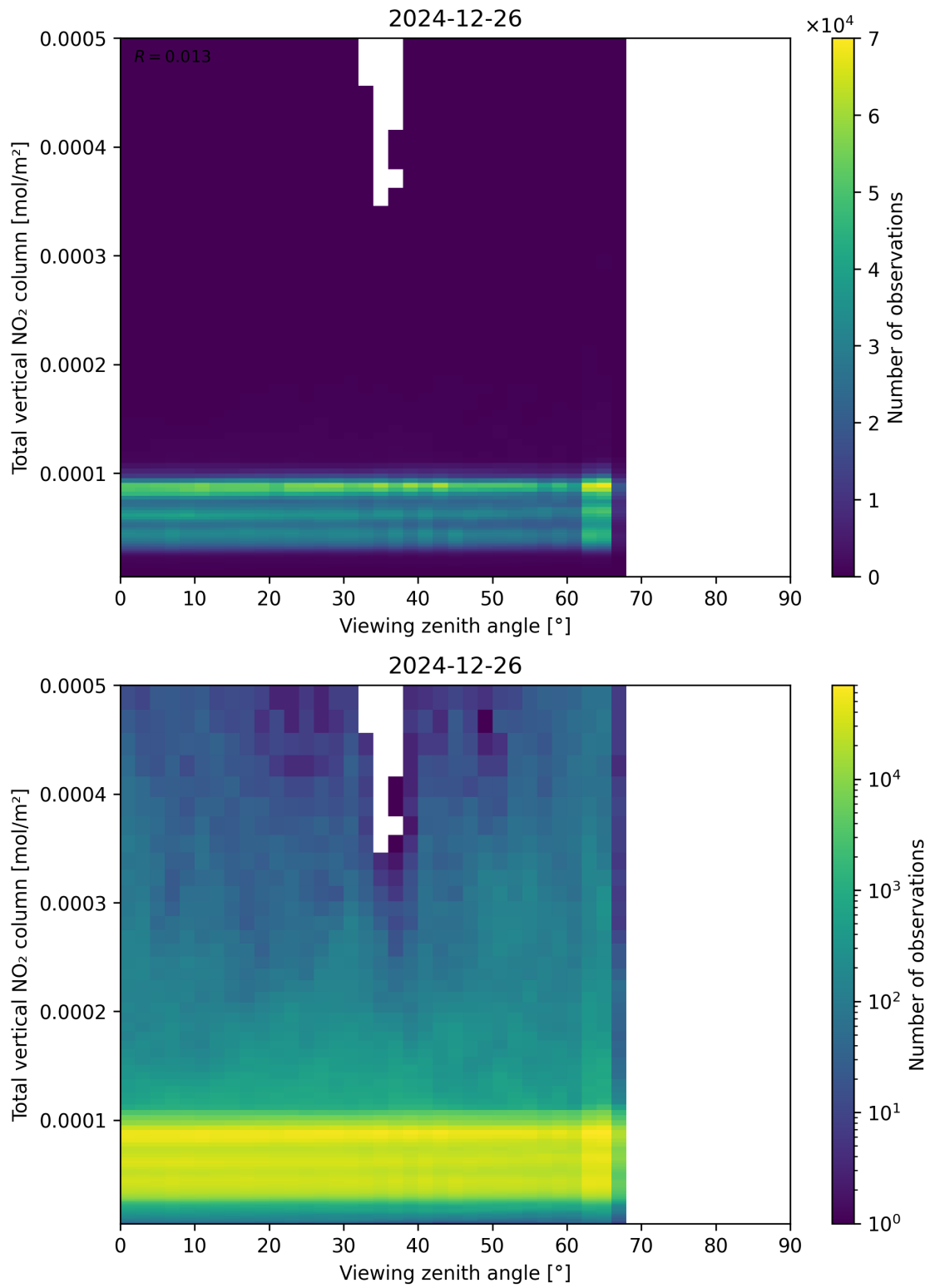
Figure 167: Scatter density plot of “Viewing zenith angle” against “Total vertical NO 2 column” for 2024-12-25 to 2024-12-27.
