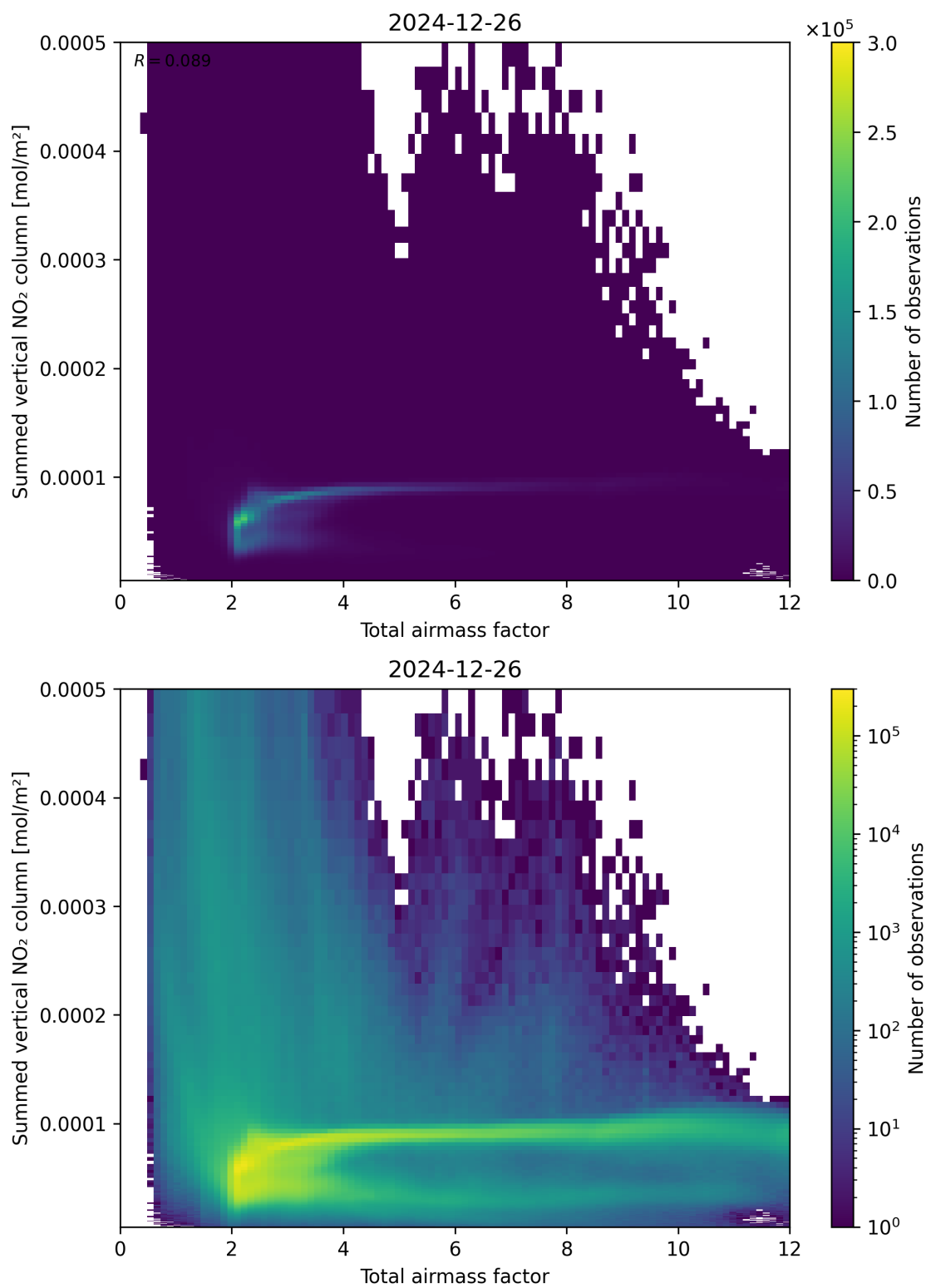
Figure 65: Scatter density plot of “Total airmass factor” against “Summed vertical NO 2 column” for 2024-12-25 to 2024-12-27.
