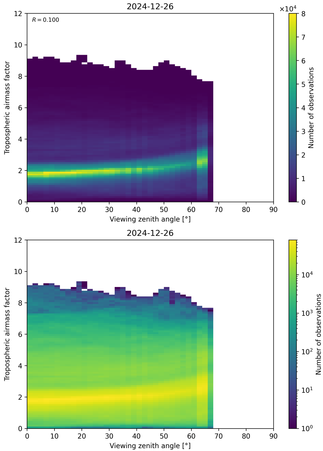
Figure 161: Scatter density plot of “Viewing zenith angle” against “Tropospheric airmass factor” for 2024-12-25 to 2024-12-27.
