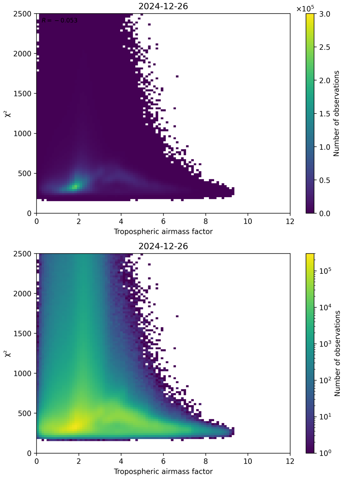
Figure 73: Scatter density plot of “Tropospheric airmass factor” against “ \chi^2 ” for 2024-12-25 to 2024-12-27.
