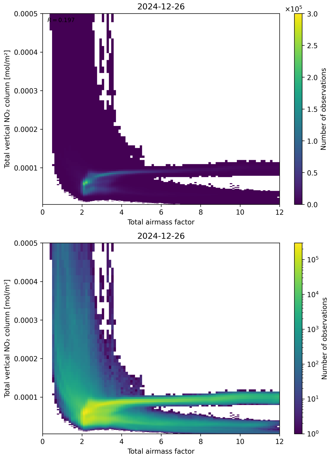
Figure 67: Scatter density plot of “Total air mass factor” against “Total vertical NO 2 column” for 2024-12-25 to 2024-12-27.
