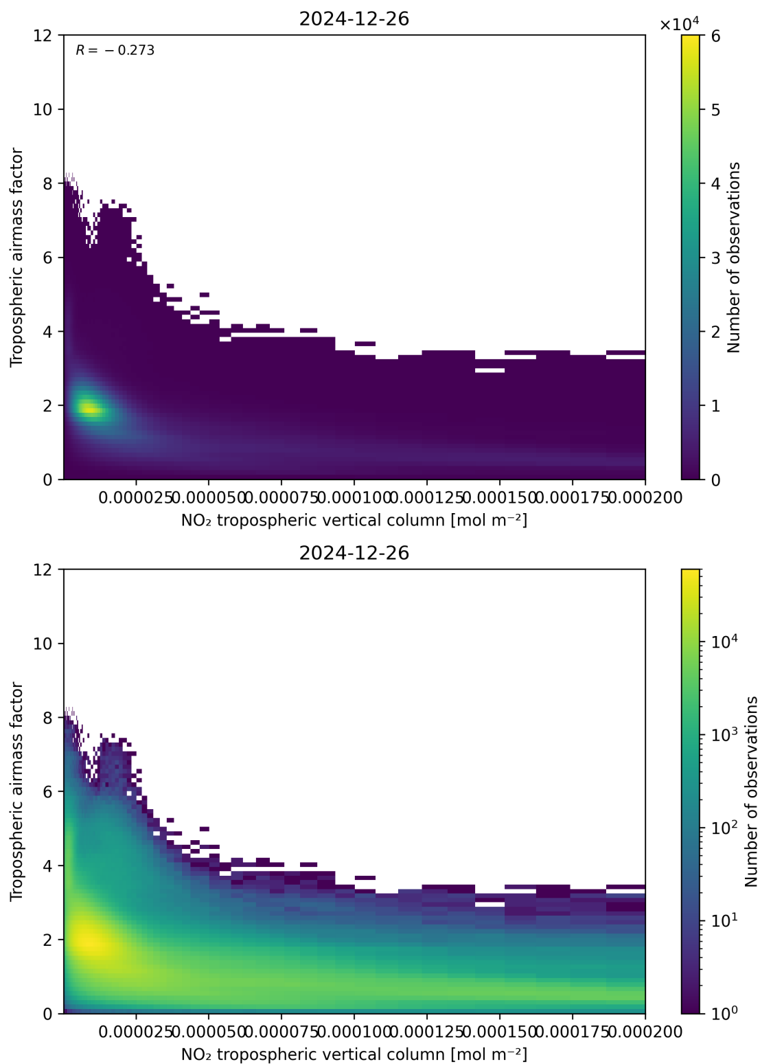
Figure 123: Scatter density plot of “NO 2 tropospheric vertical column” against “Tropospheric air mass factor” for 2024-12-25 to 2024-12-27.
