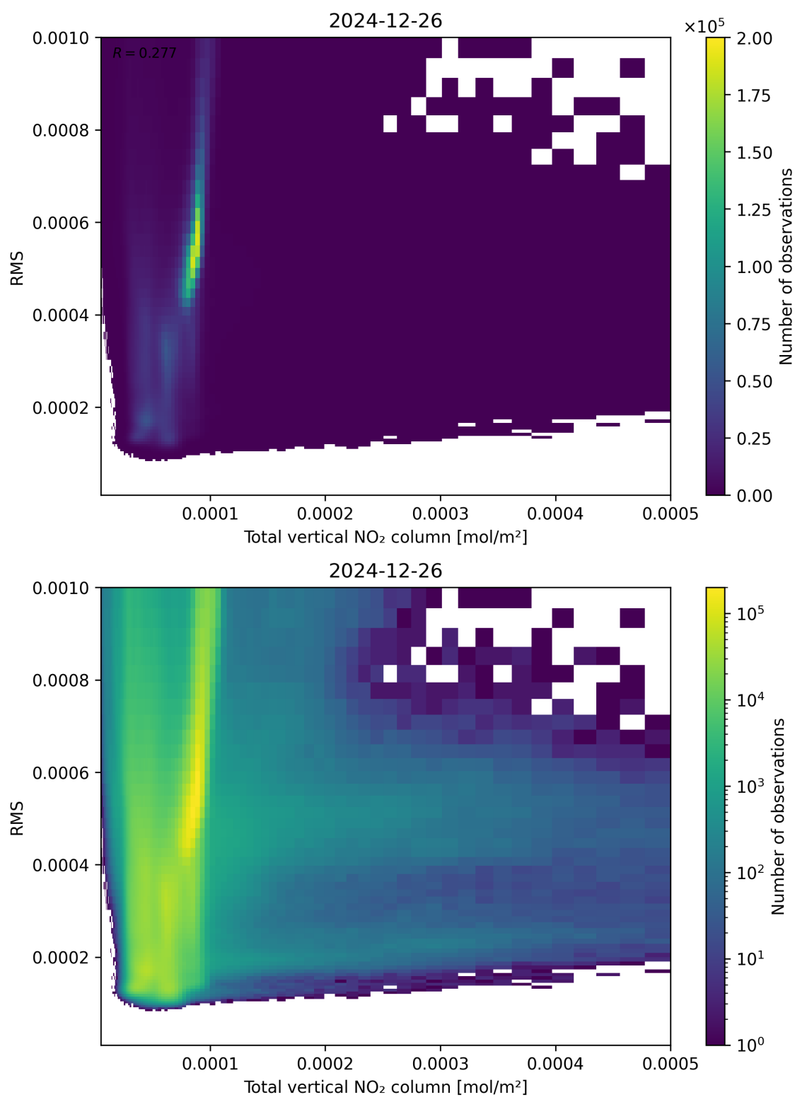
Figure 120: Scatter density plot of “Total vertical NO 2 column” against “RMS” for 2024-12-25 to 2024-12-27.
