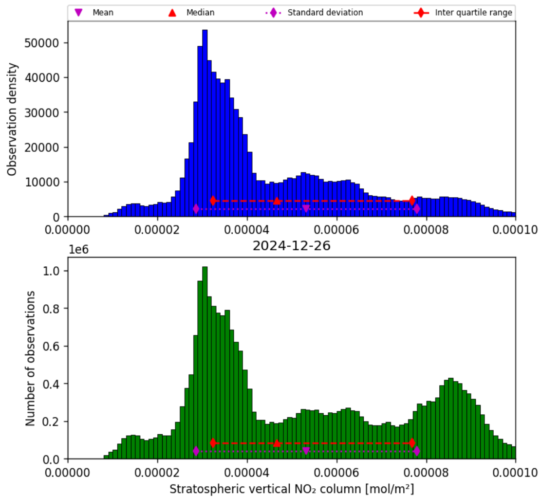
Figure 36: Histogram of “Stratospheric vertical NO 2 column” for 2024-12-25 to 2024-12-27
