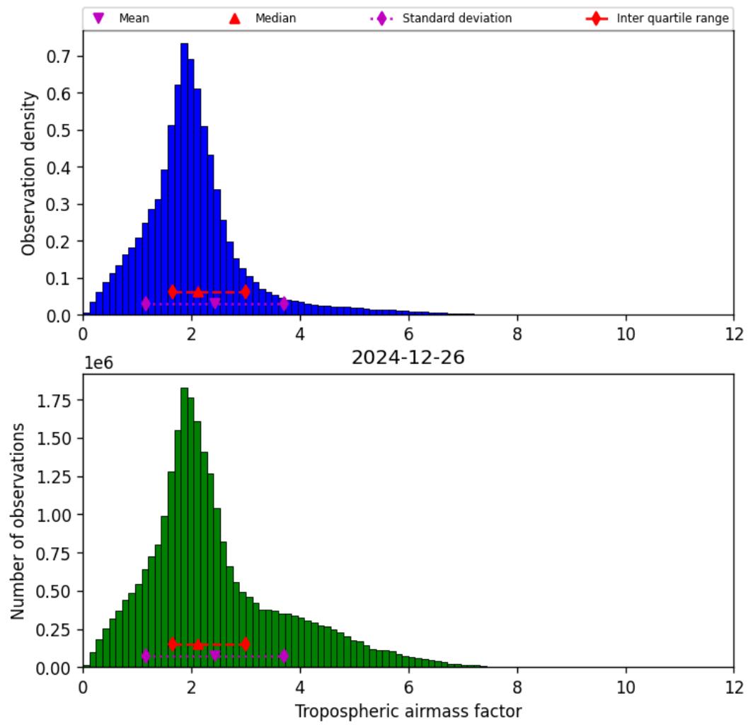
Figure 31: Histogram of “Tropospheric airmass factor” for 2024-12-25 to 2024-12-27
