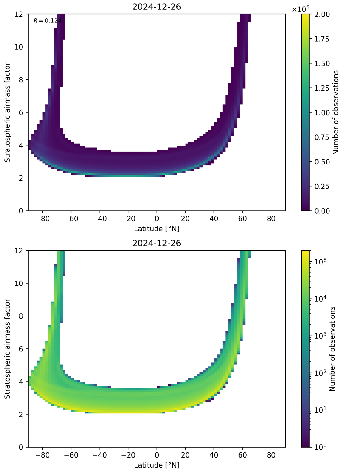
Figure 83: Scatter density plot of “Latitude” against “Stratospheric airmass factor” for 2024-12-25 to 2024-12-27.
