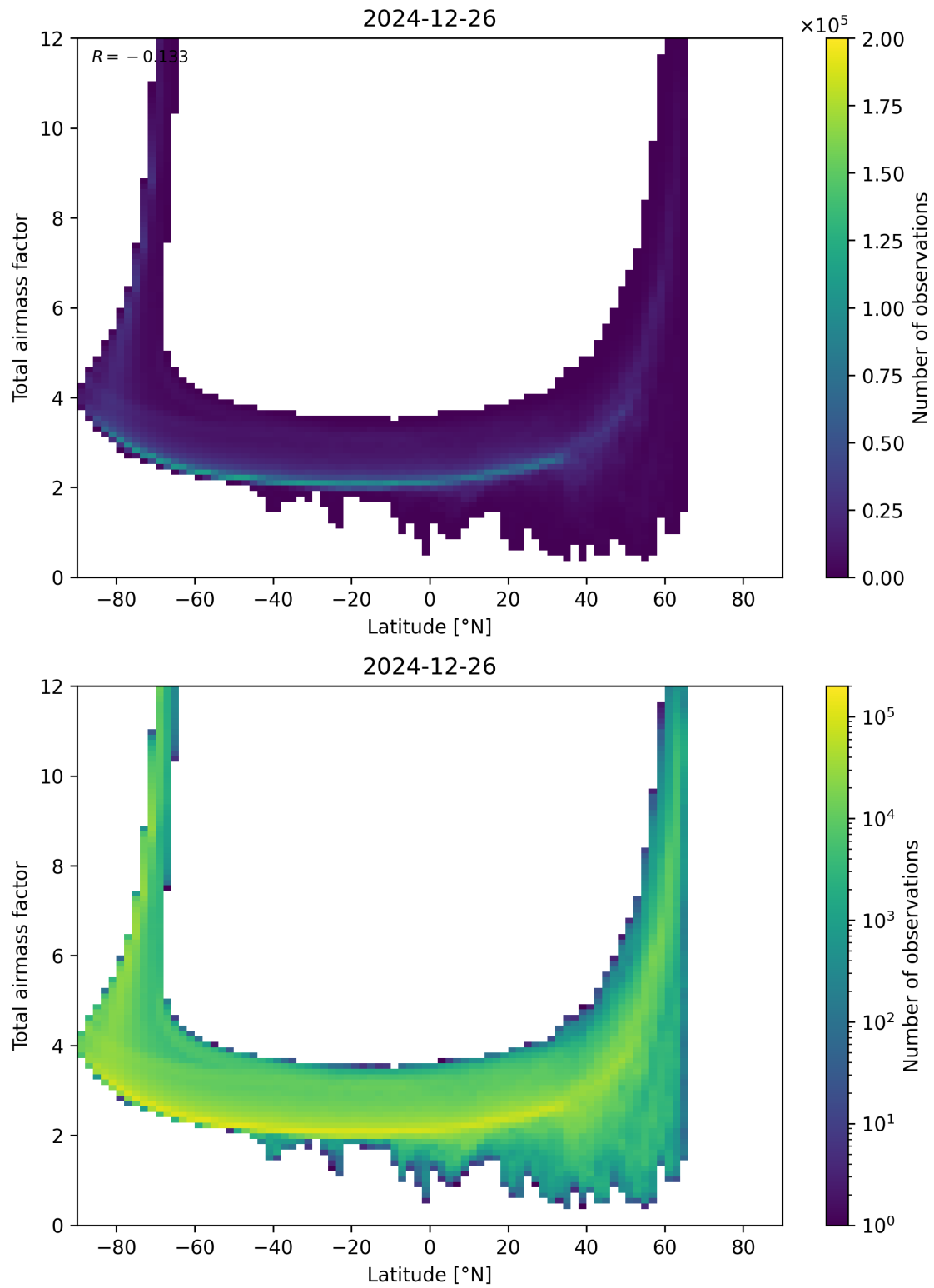
Figure 84: Scatter density plot of “Latitude” against “Total airmass factor” for 2024-12-25 to 2024-12-27.
