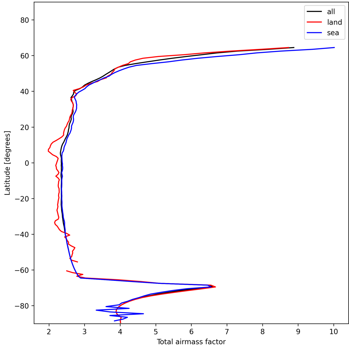
Figure 15: Zonal average of “Total airmass factor” for 2024-12-25 to 2024-12-27.
