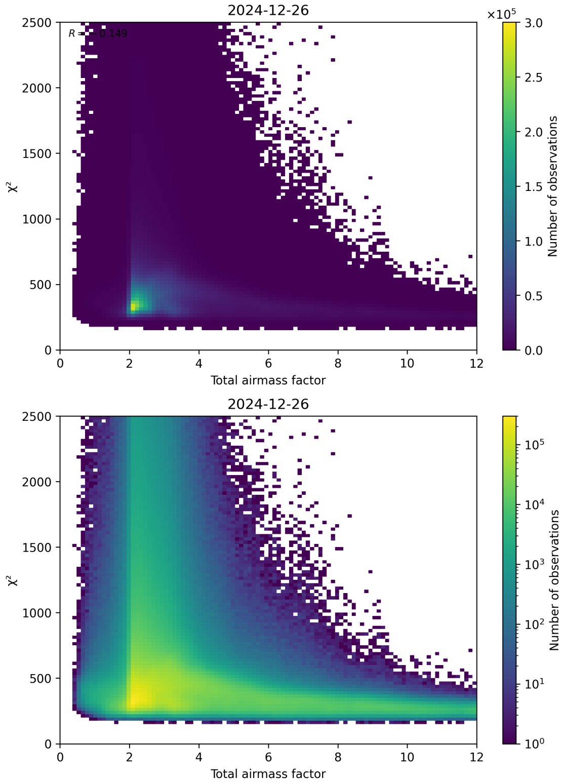
Figure 63: Scatter density plot of “Total airmass factor” against “ \chi^2 ” for 2024-12-25 to 2024-12-27.
