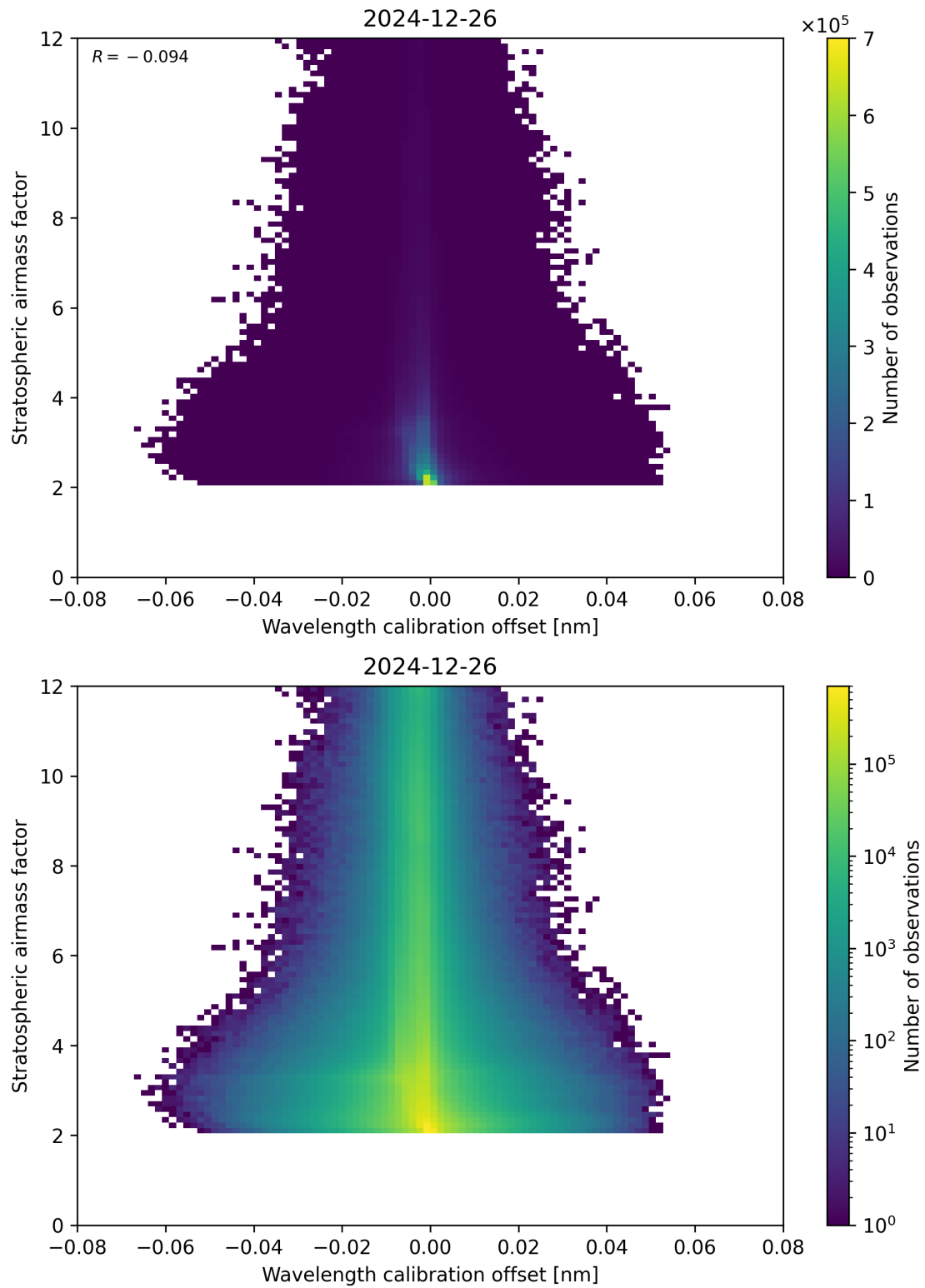
Figure 174: Scatter density plot of “Wavelength calibration offset” against “Stratospheric airmass factor” for 2024-12-25 to 2024-12-27.
