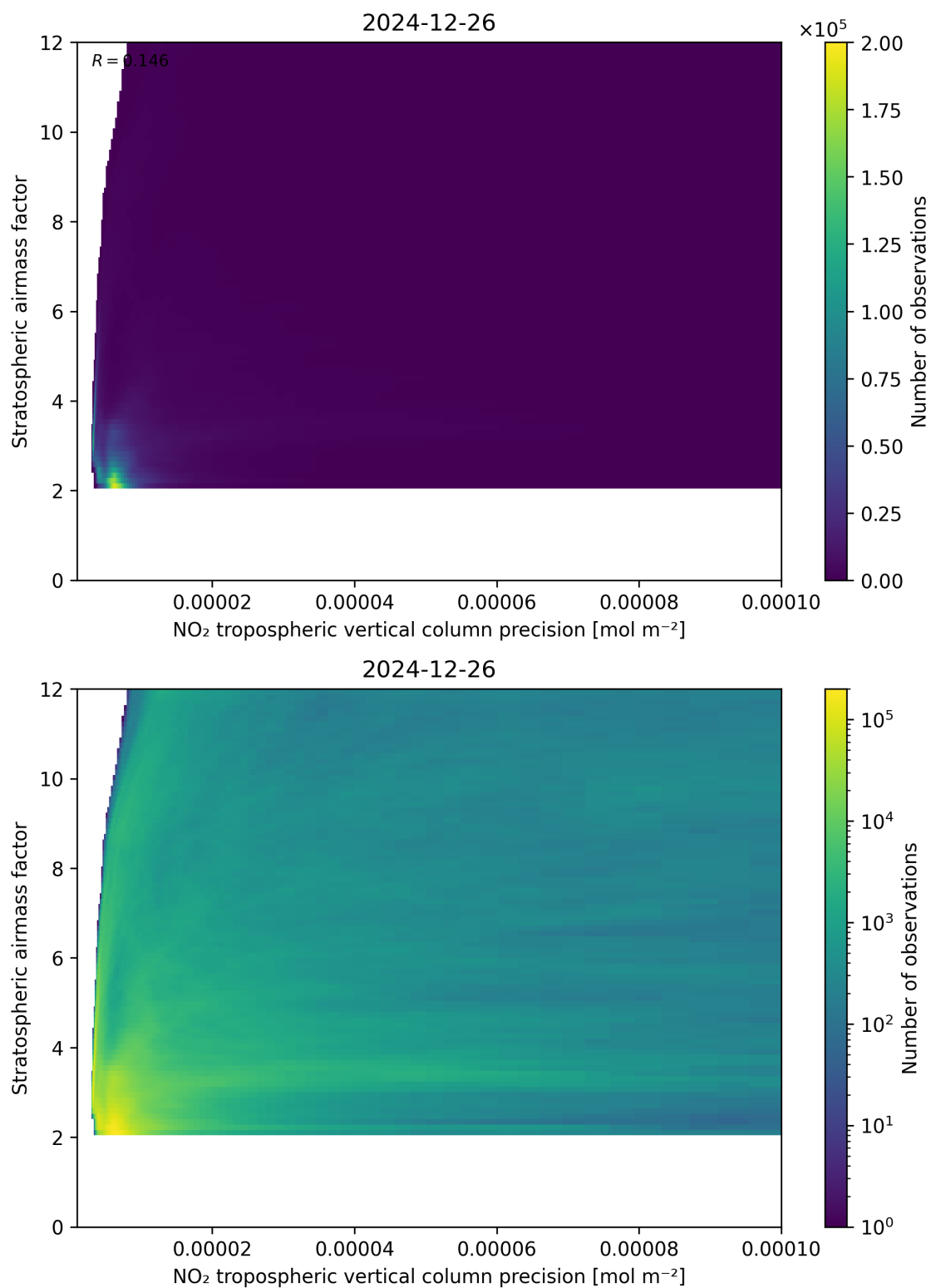
Figure 131: Scatter density plot of “NO 2 tropospheric vertical column precision” against “Stratospheric airmass factor” for 2024-12-25 to 2024-12-27.
