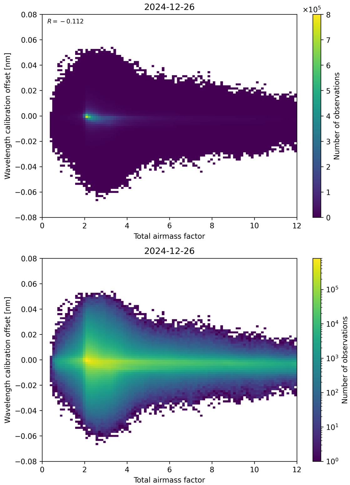
Figure 70: Scatter density plot of “Total airmass factor” against “Wavelength calibration offset” for 2024-12-25 to 2024-12-27.
