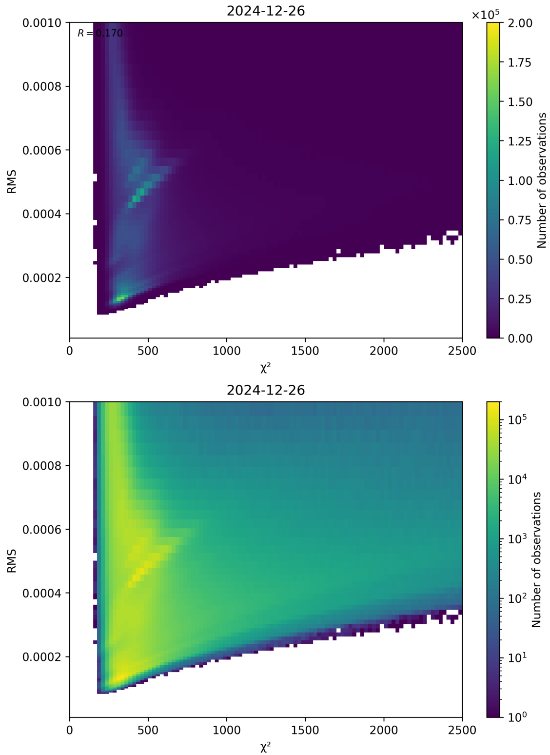
Figure 82: Scatter density plot of “ \chi^2 ” against “RMS” for 2024-12-25 to 2024-12-27.
