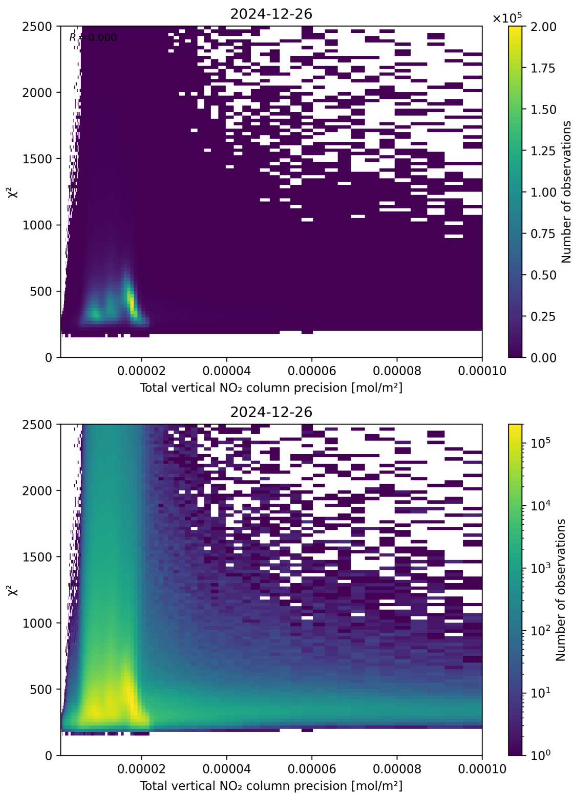
Figure 116: Scatter density plot of “Total vertical NO 2 column precision” against “ \chi^2 ” for 2024-12-25 to 2024-12-27.
