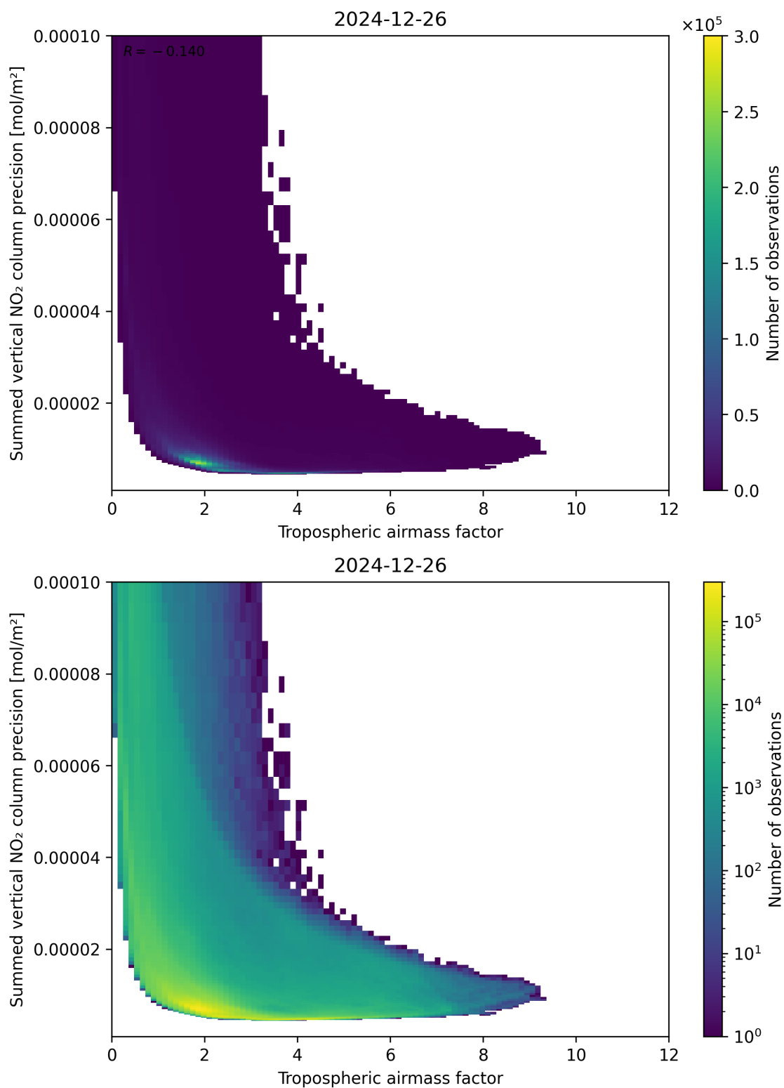
Figure 76: Scatter density plot of “Tropospheric air mass factor” against “Summed vertical NO 2 column precision” for 2024-12-25 to 2024-12-27.
