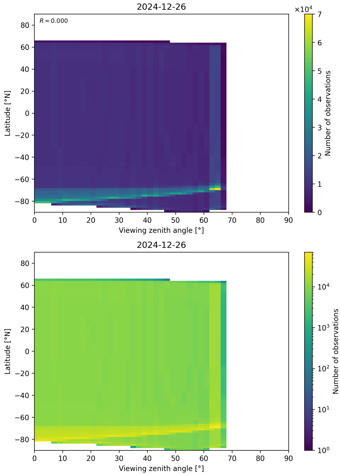
Figure 163: Scatter density plot of “Viewing zenith angle” against “Latitude” for 2024-12-25 to 2024-12-27.
