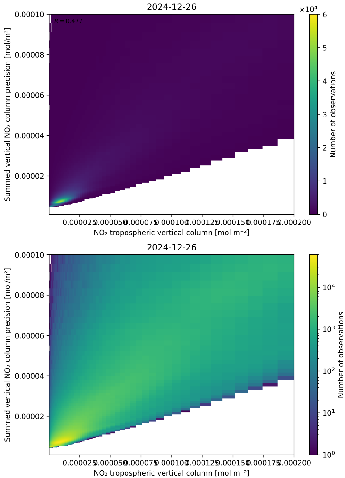
Figure 127: Scatter density plot of “NO 2 tropospheric vertical column” against “Summed vertical NO 2 column precision” for 2024-12-25 to 2024-12-27.
