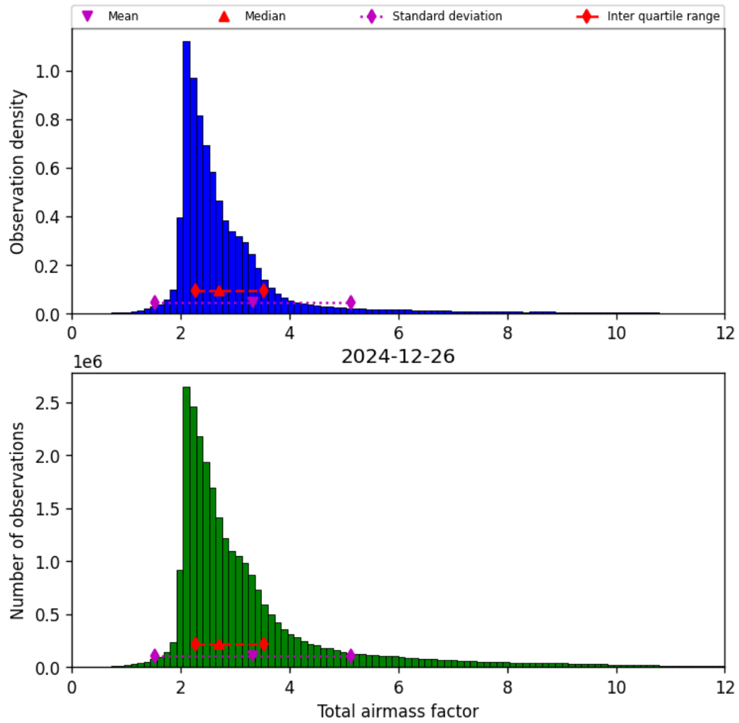
Figure 32: Histogram of “Total airmass factor” for 2024-12-25 to 2024-12-27
