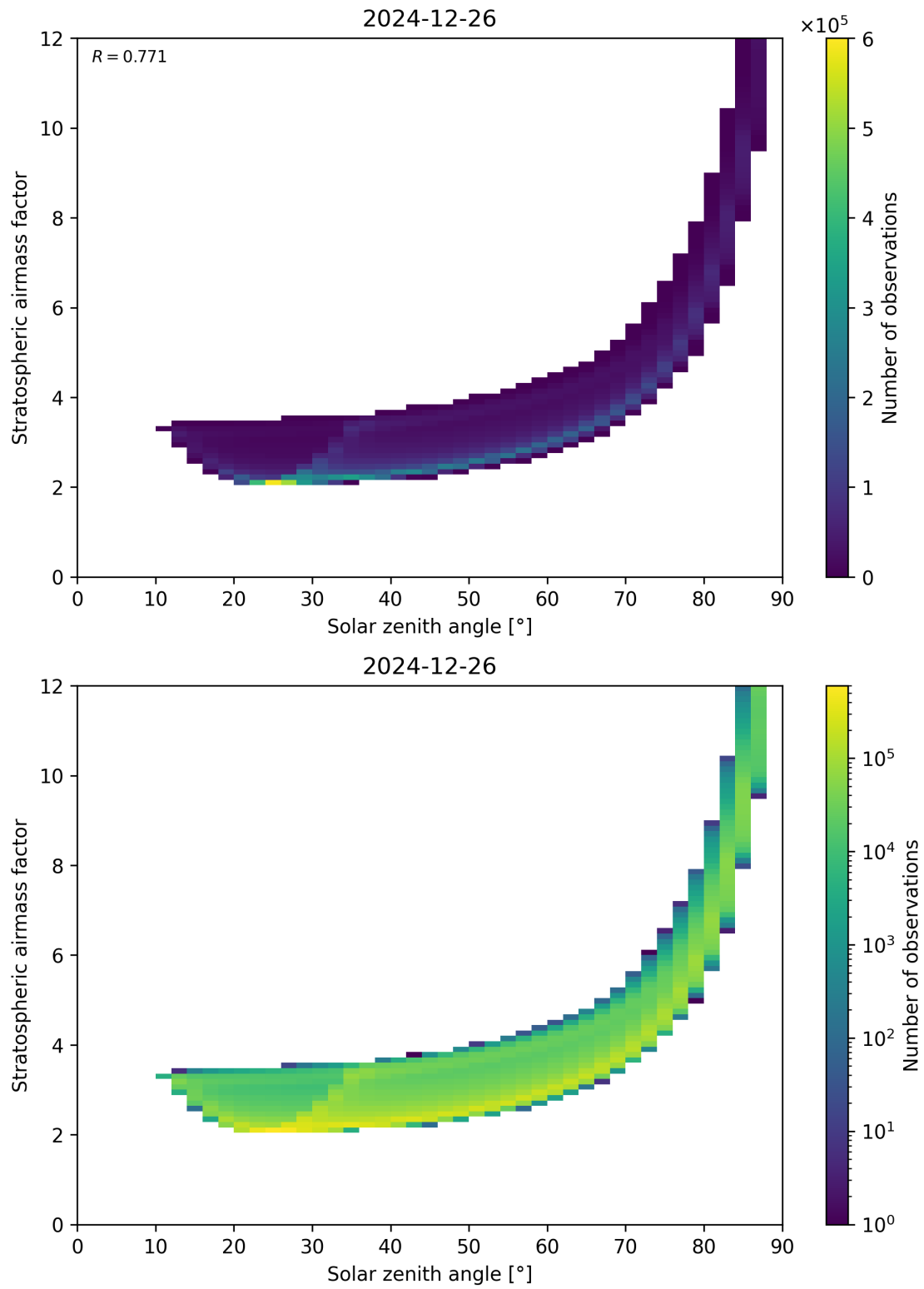
Figure 145: Scatter density plot of “Solar zenith angle” against “Stratospheric airmass factor” for 2024-12-25 to 2024-12-27.
