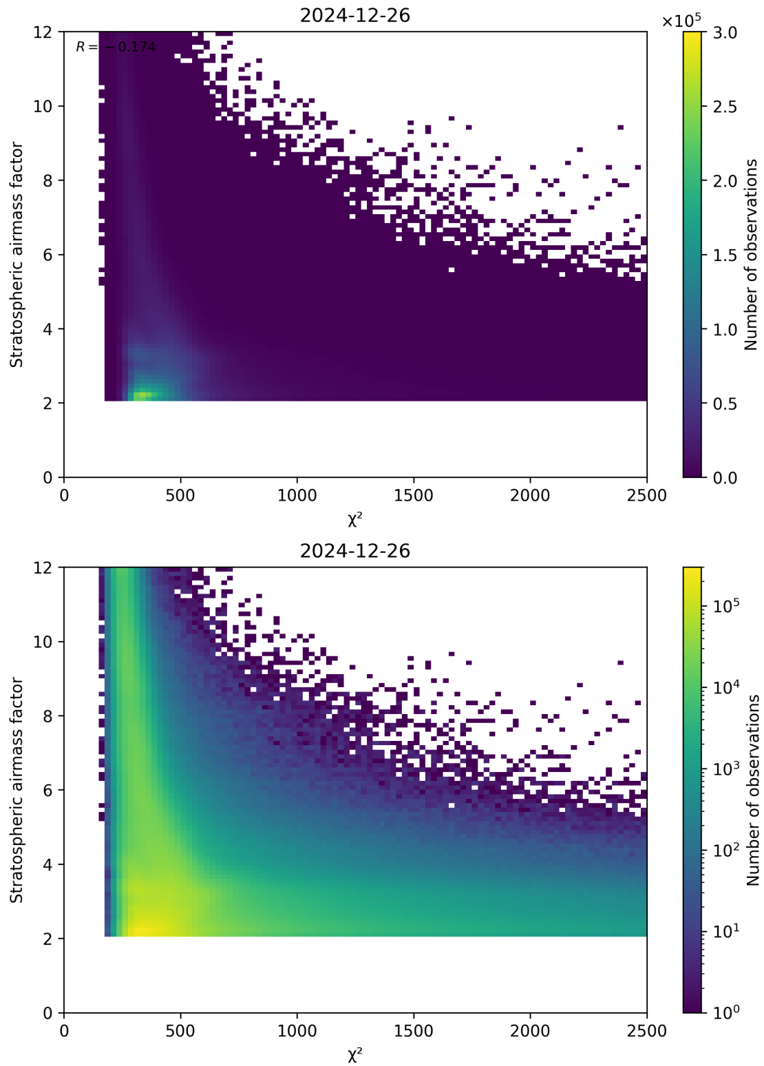
Figure 81: Scatter density plot of “ \chi^2 ” against “Stratospheric airmass factor” for 2024-12-25 to 2024-12-27.
