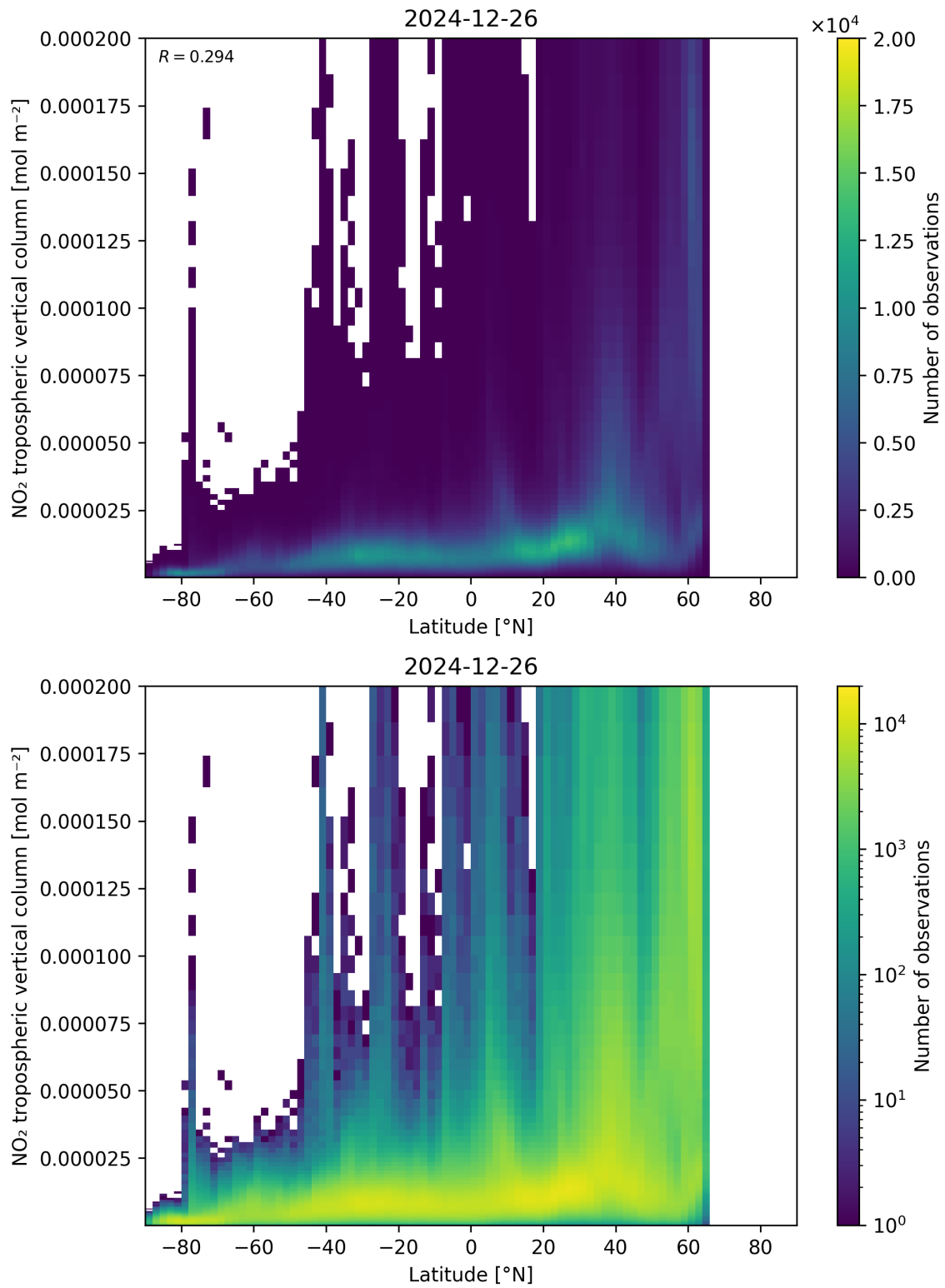
Figure 92: Scatter density plot of “Latitude” against “NO 2 tropospheric vertical column” for 2024-12-25 to 2024-12-27.
