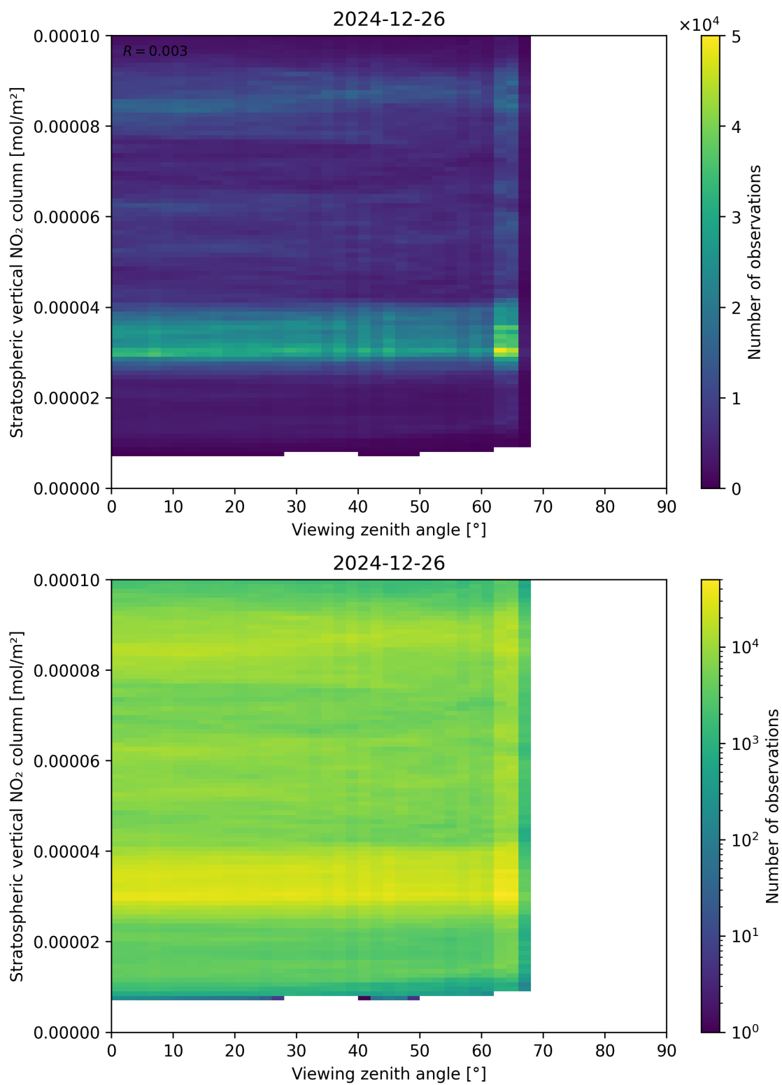
Figure 164: Scatter density plot of “Viewing zenith angle” against “Stratospheric vertical NO 2 column” for 2024-12-25 to 2024-12-27.
