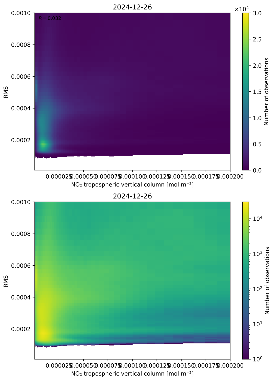
Figure 142: Scatter density plot of “NO 2 tropospheric vertical column” against “RMS” for 2024-12-25 to 2024-12-27.
