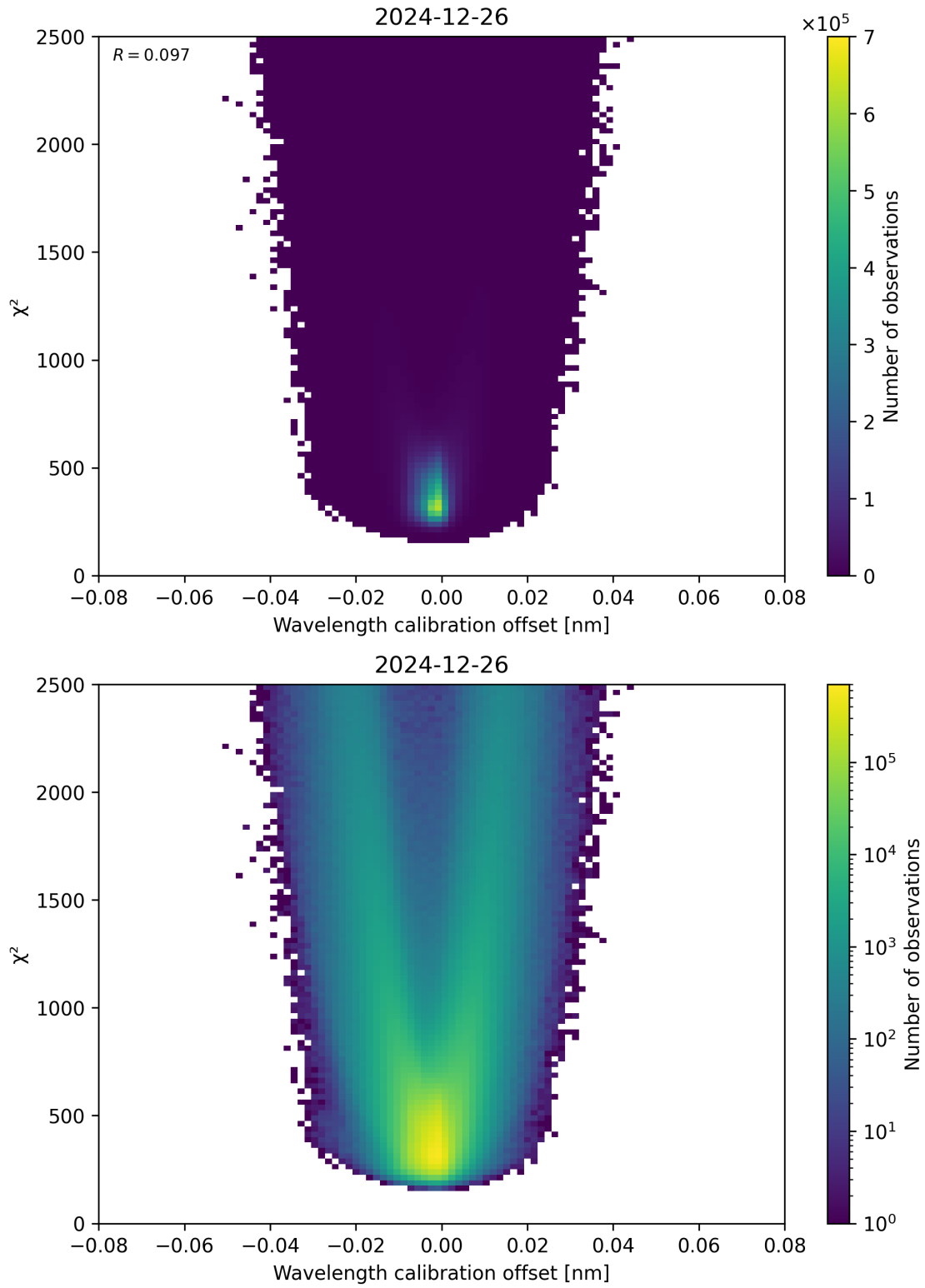
Figure 175: Scatter density plot of “Wavelength calibration offset” against “ \chi^2 ” for 2024-12-25 to 2024-12-27.
