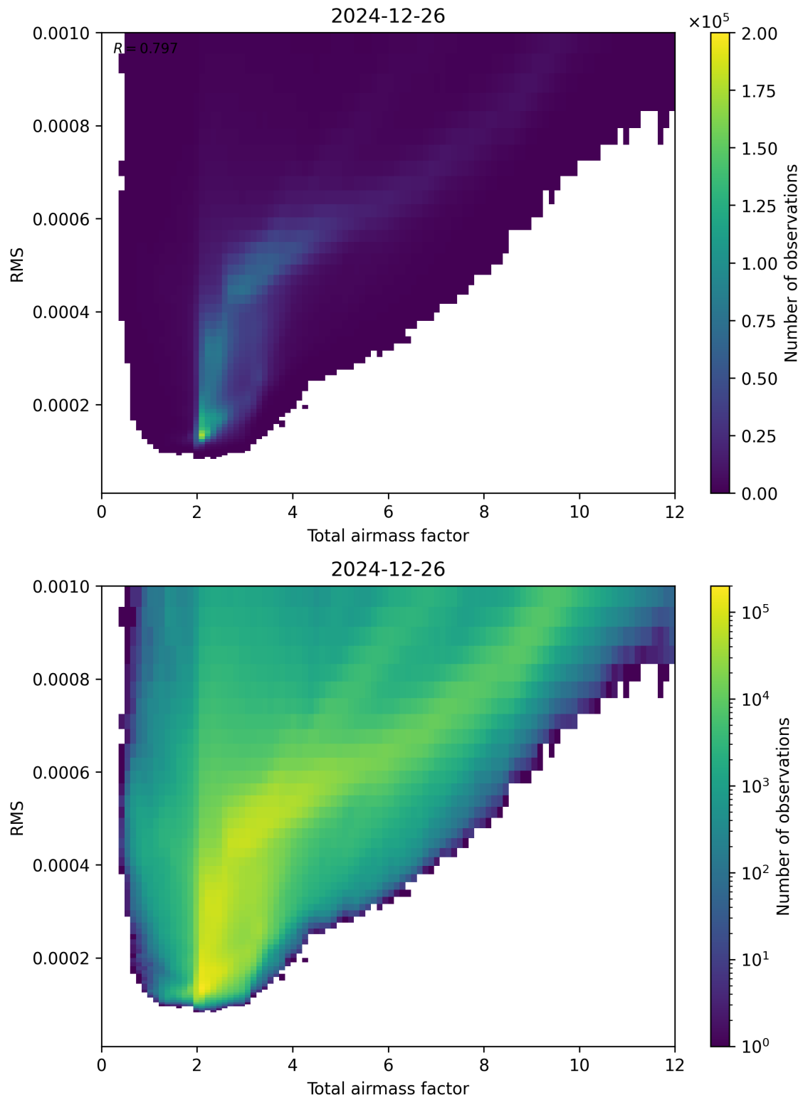
Figure 69: Scatter density plot of “Total airmass factor” against “RMS” for 2024-12-25 to 2024-12-27.
