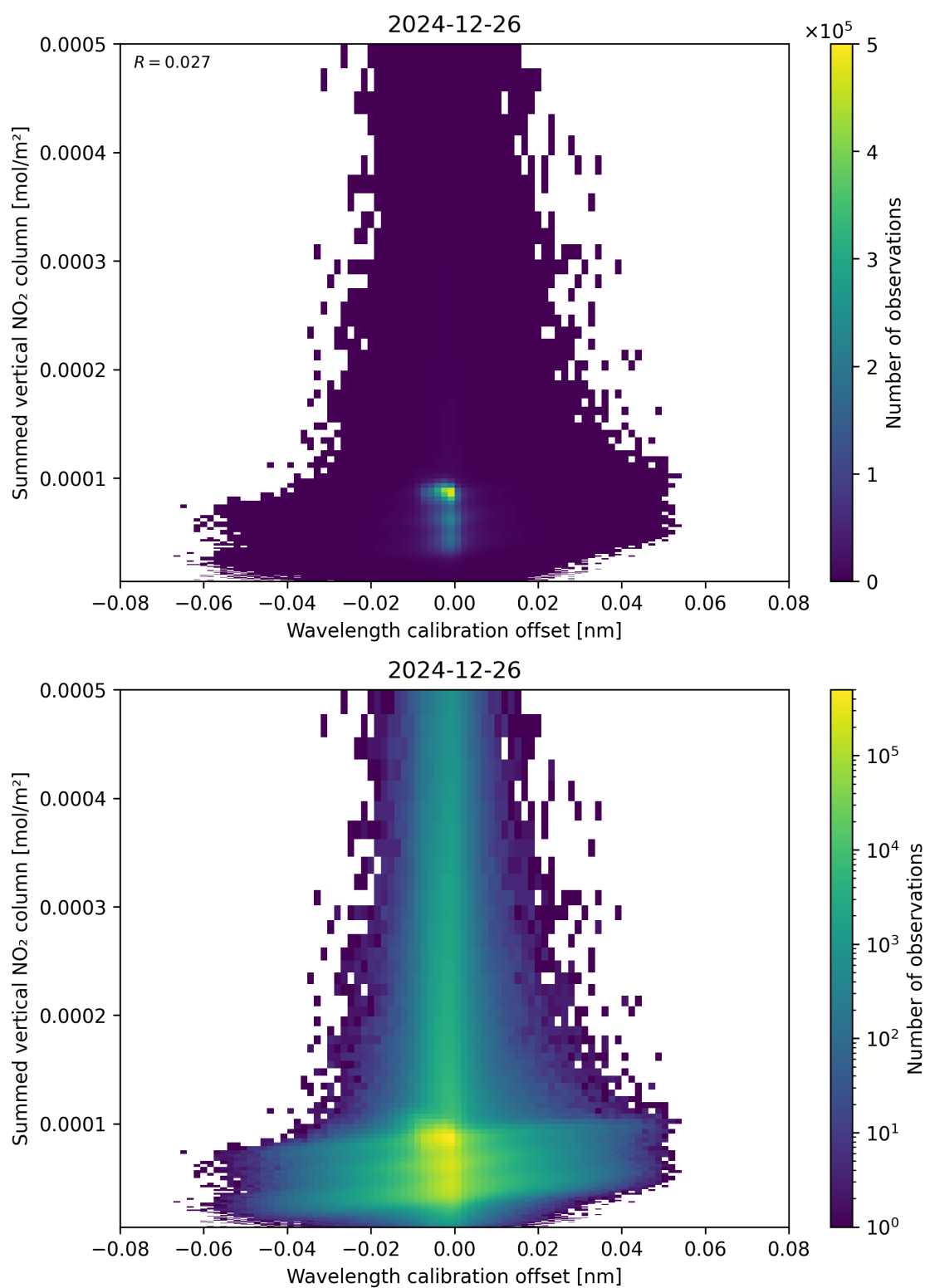
Figure 177: Scatter density plot of “Wavelength calibration offset” against “Summed vertical NO 2 column” for 2024-12-25 to 2024-12-27.
