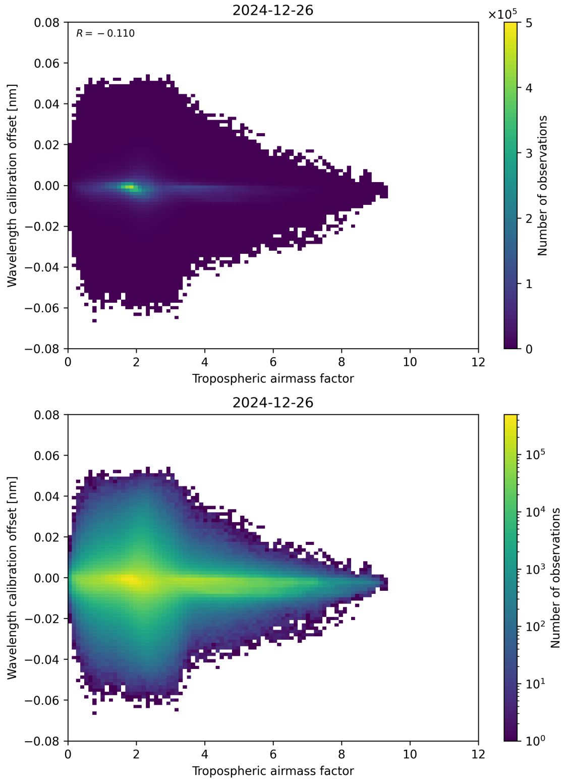
Figure 80: Scatter density plot of “Tropospheric airmass factor” against “Wavelength calibration offset” for 2024-12-25 to 2024-12-27.
