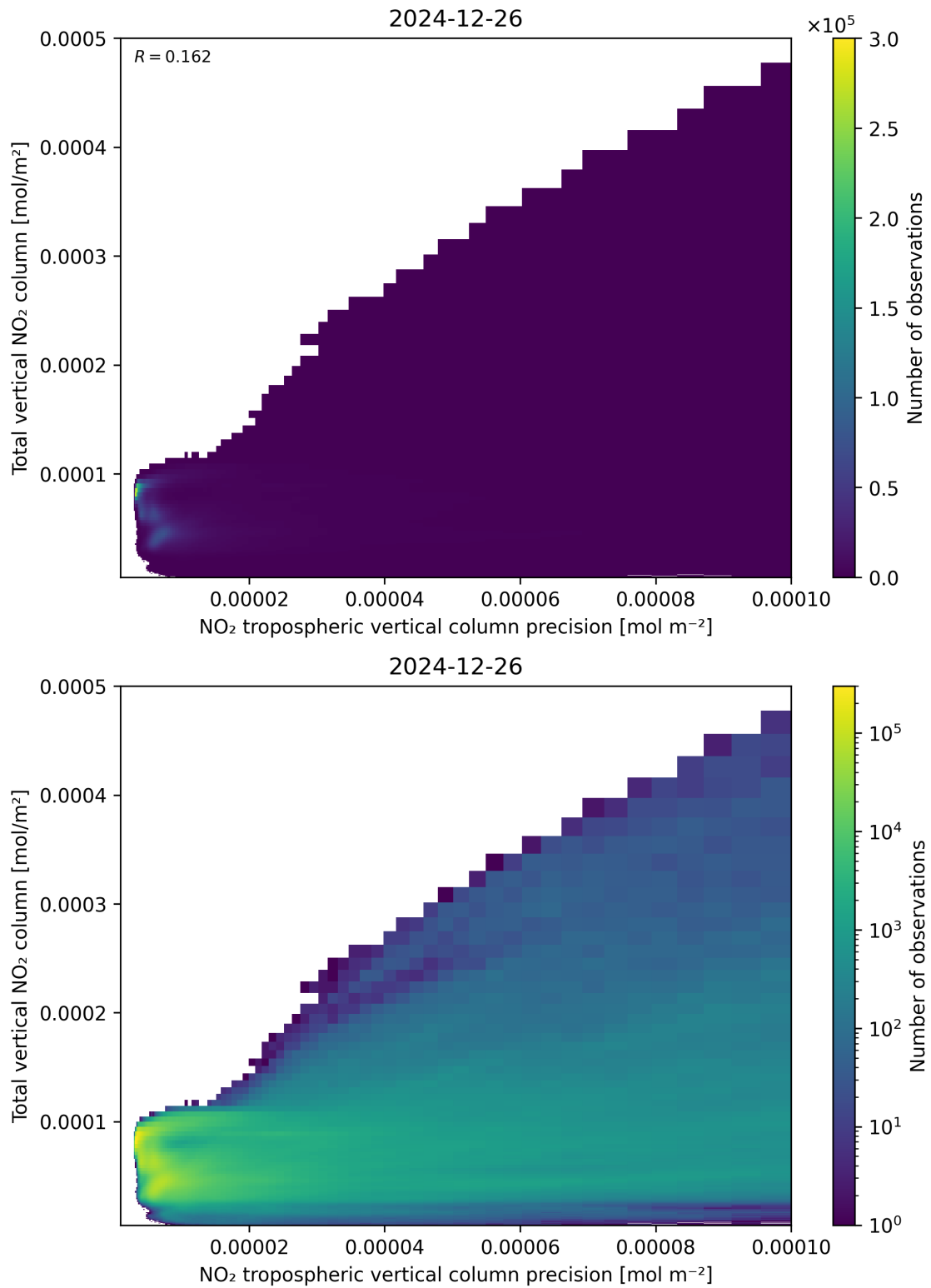
Figure 138: Scatter density plot of “NO 2 tropospheric vertical column precision” against “Total vertical NO 2 column” for 2024-12-25 to 2024-12-27.
