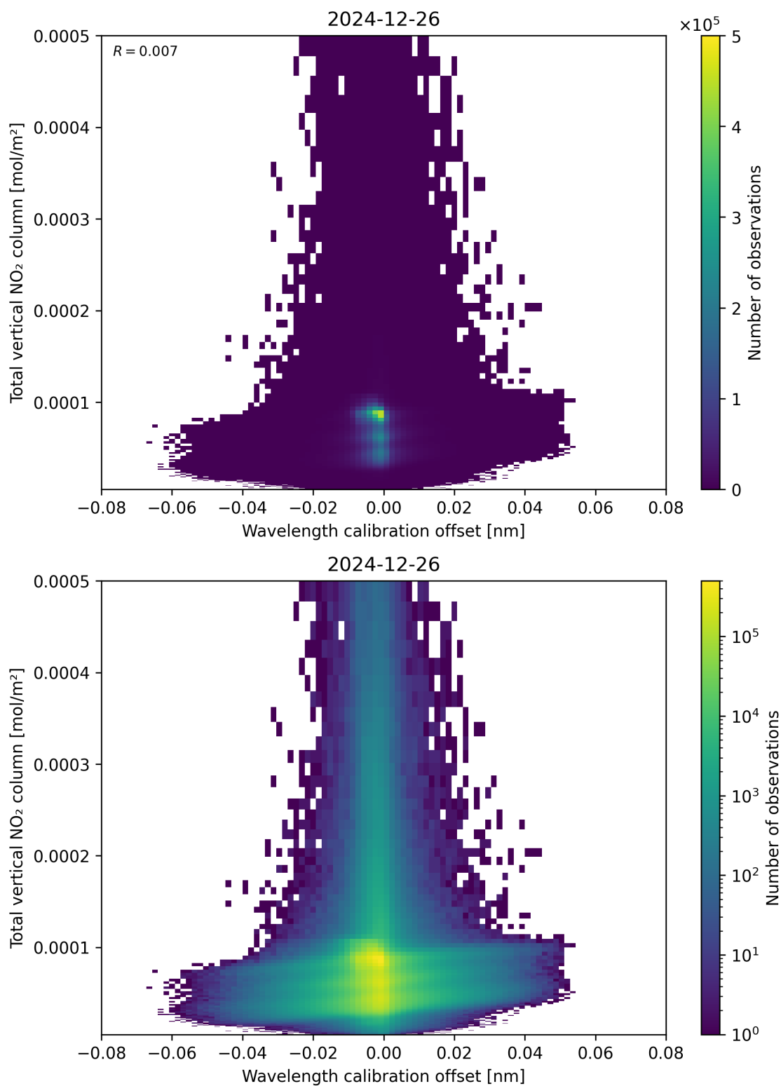
Figure 179: Scatter density plot of “Wavelength calibration offset” against “Total vertical NO 2 column” for 2024-12-25 to 2024-12-27.
