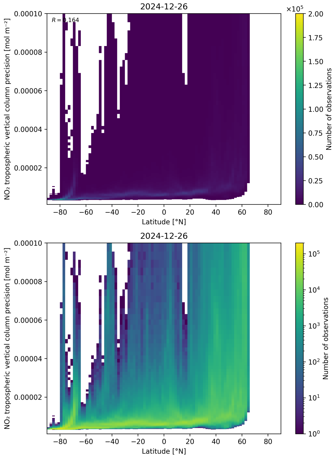
Figure 93: Scatter density plot of “Latitude” against “NO 2 tropospheric vertical column precision” for 2024-12-25 to 2024-12-27.
