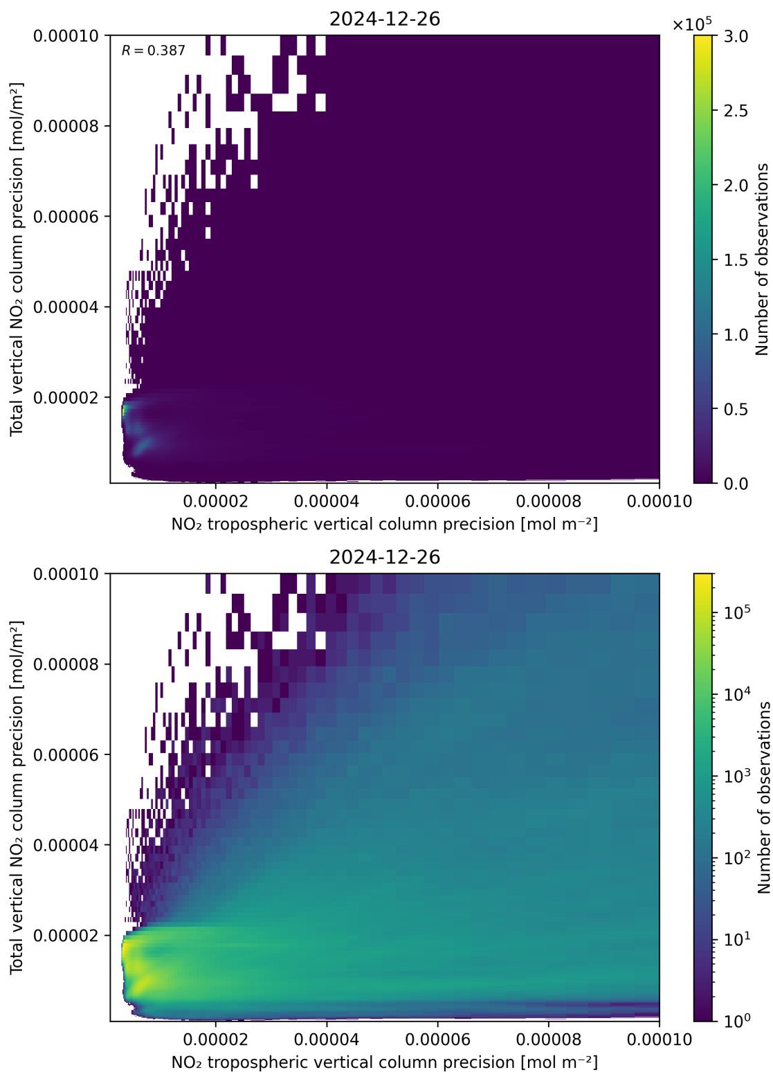
Figure 139: Scatter density plot of “NO 2 tropospheric vertical column precision” against “Total vertical NO 2 column precision” for 2024-12-25 to 2024-12-27.
