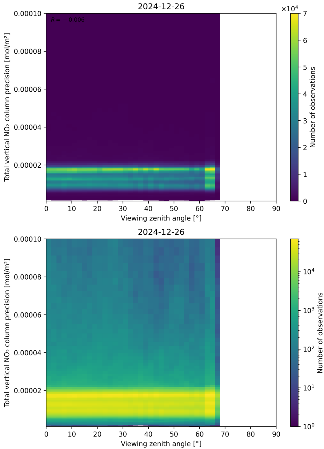
Figure 168: Scatter density plot of “Viewing zenith angle” against “Total vertical NO 2 column precision” for 2024-12-25 to 2024-12-27.
