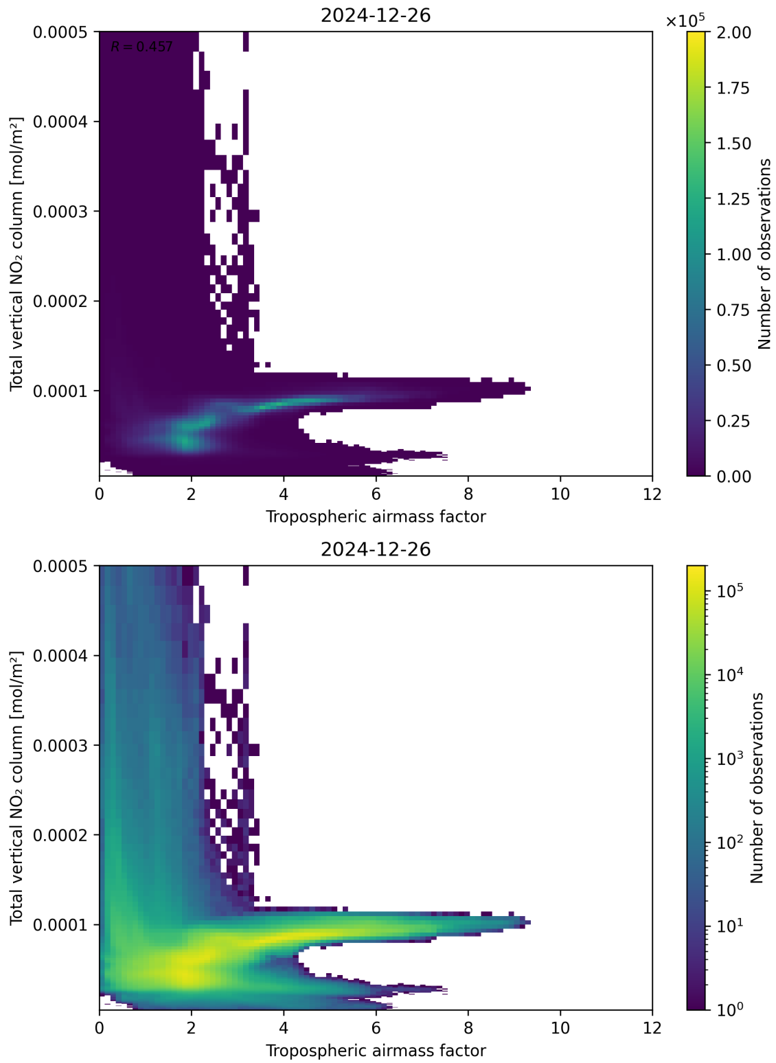
Figure 77: Scatter density plot of “Tropospheric airmass factor” against “Total vertical NO 2 column” for 2024-12-25 to 2024-12-27.
