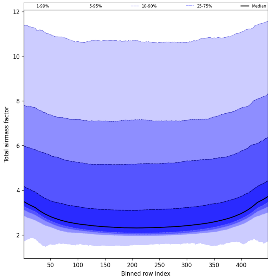
Figure 49: Along track statistics of “Total airmass factor” for 2024-12-25 to 2024-12-27
