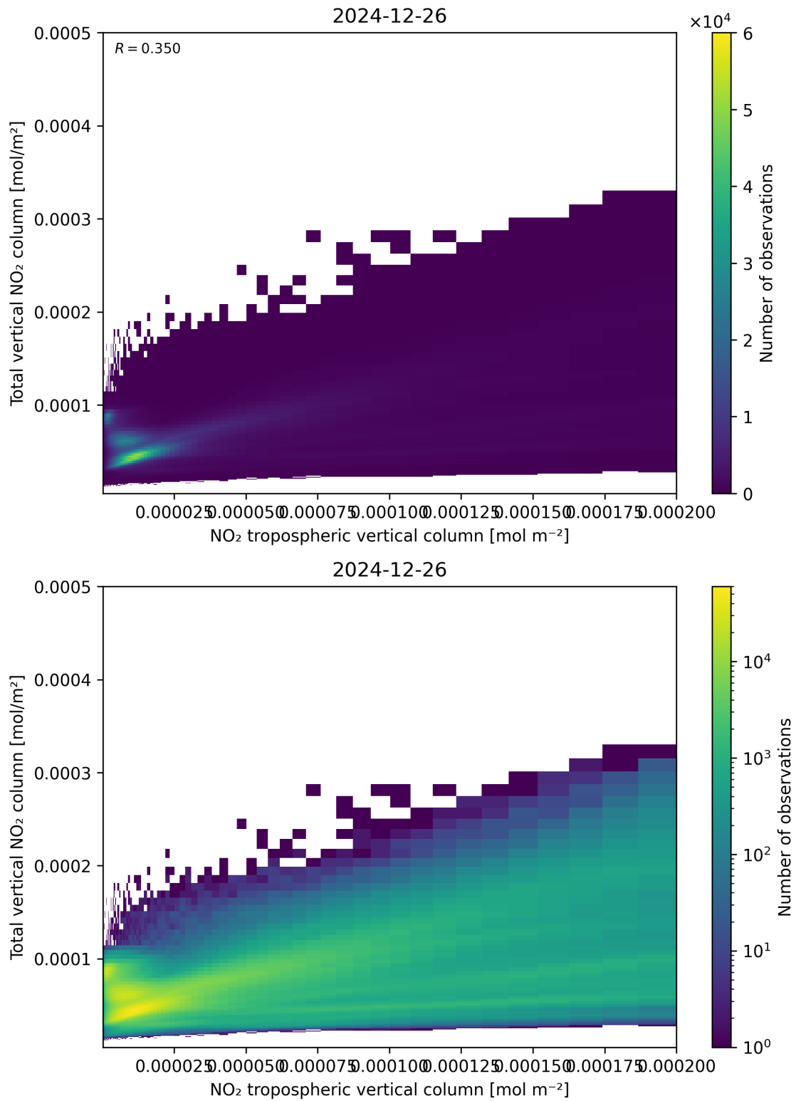
Figure 128: Scatter density plot of “NO 2 tropospheric vertical column” against “Total vertical NO 2 column” for 2024-12-25 to 2024-12-27.
