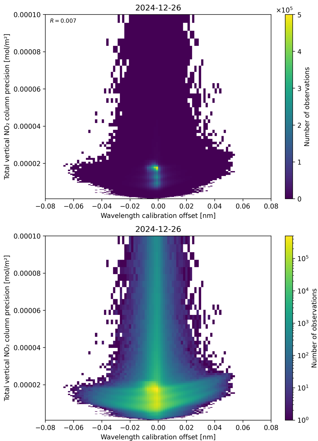
Figure 180: Scatter density plot of “Wavelength calibration offset” against “Total vertical NO 2 column precision” for 2024-12-25 to 2024-12-27.
