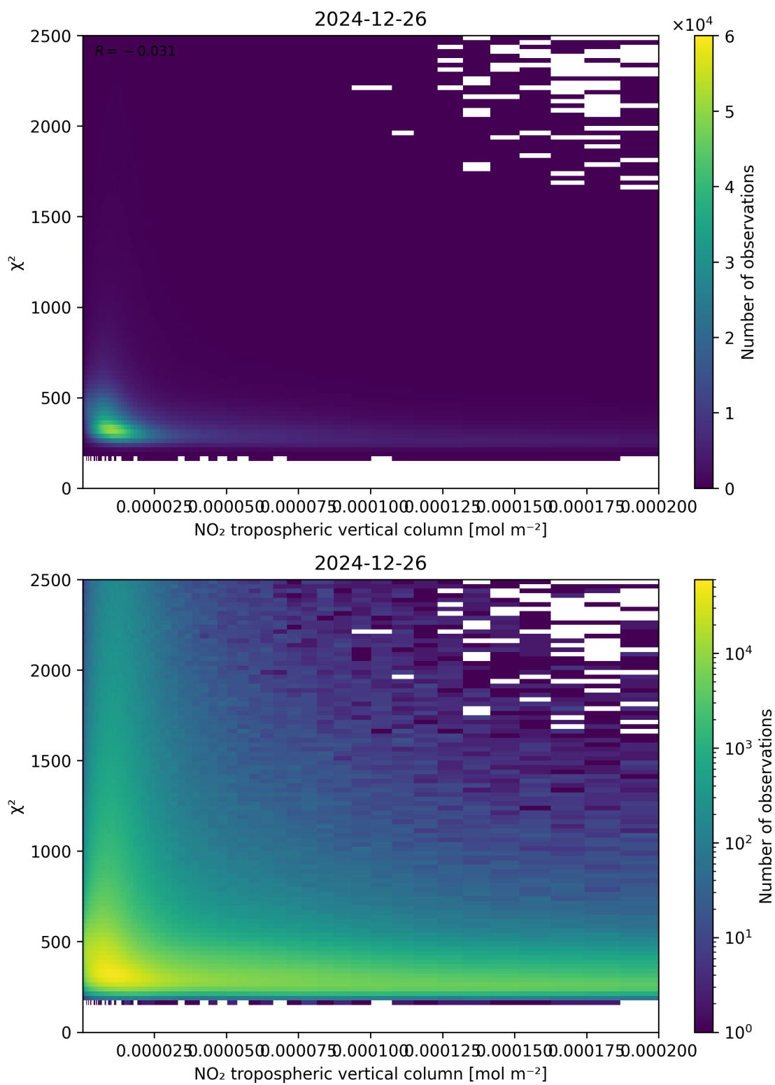
Figure 124: Scatter density plot of “NO 2 tropospheric vertical column” against “ \chi^2 ” for 2024-12-25 to 2024-12-27.
