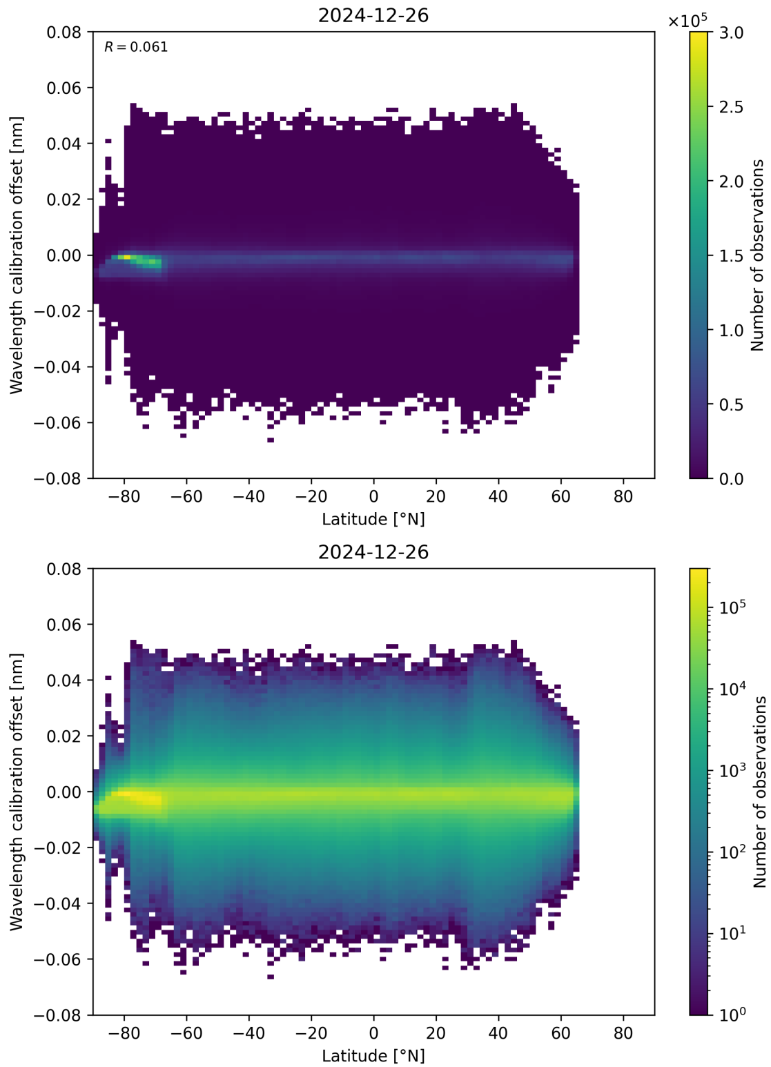
Figure 95: Scatter density plot of “Latitude” against “Wavelength calibration offset” for 2024-12-25 to 2024-12-27.
