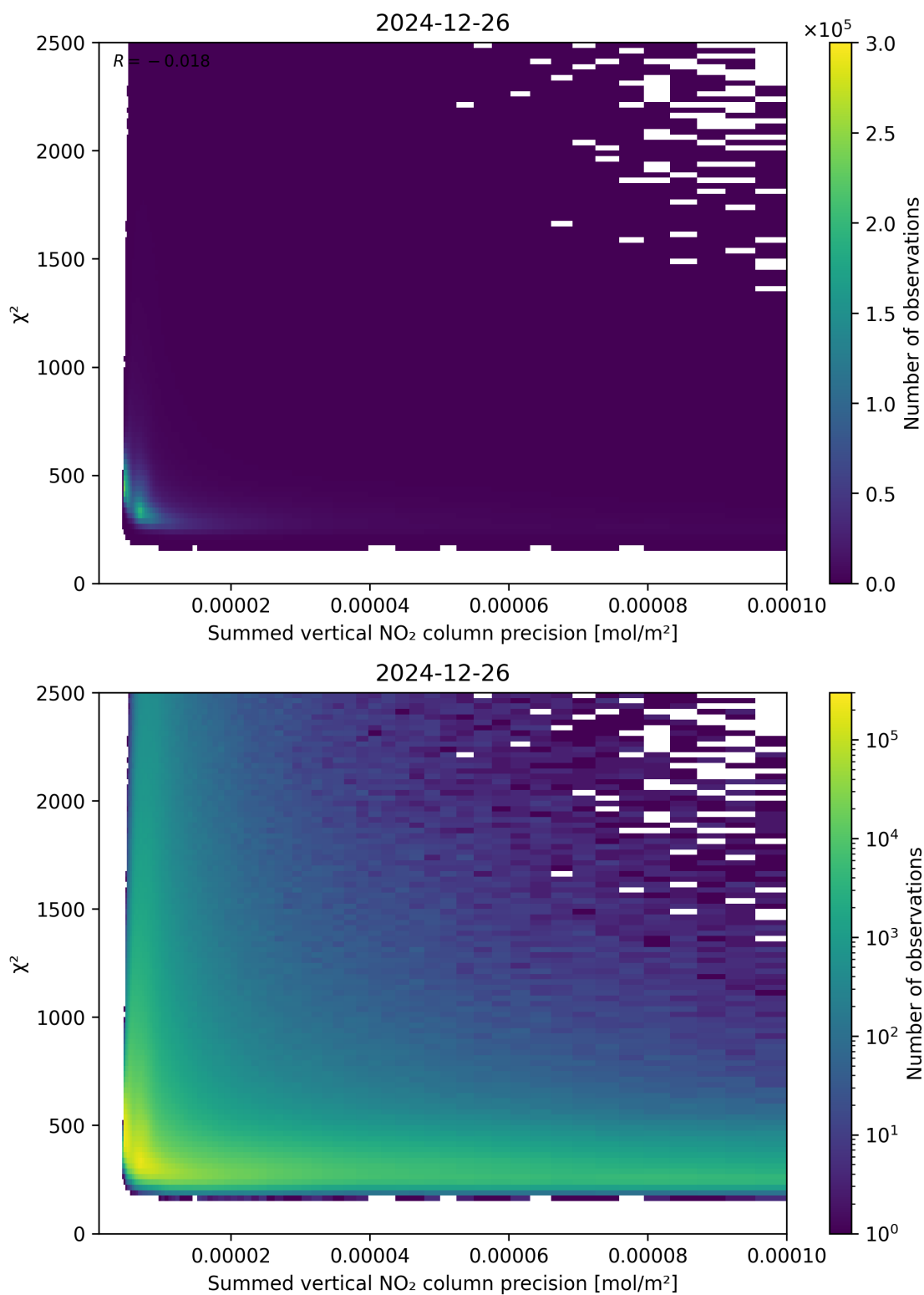
Figure 107: Scatter density plot of “Summed vertical NO 2 column precision” against “ \chi^2 ” for 2024-12-25 to 2024-12-27.
