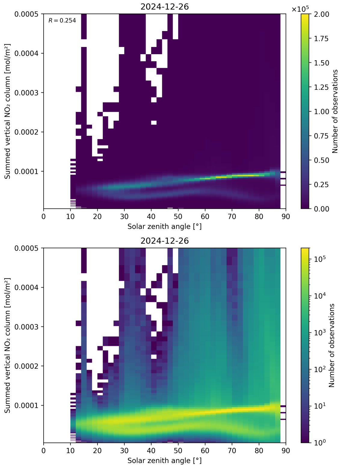
Figure 151: Scatter density plot of “Solar zenith angle” against “Summed vertical NO 2 column” for 2024-12-25 to 2024-12-27.
