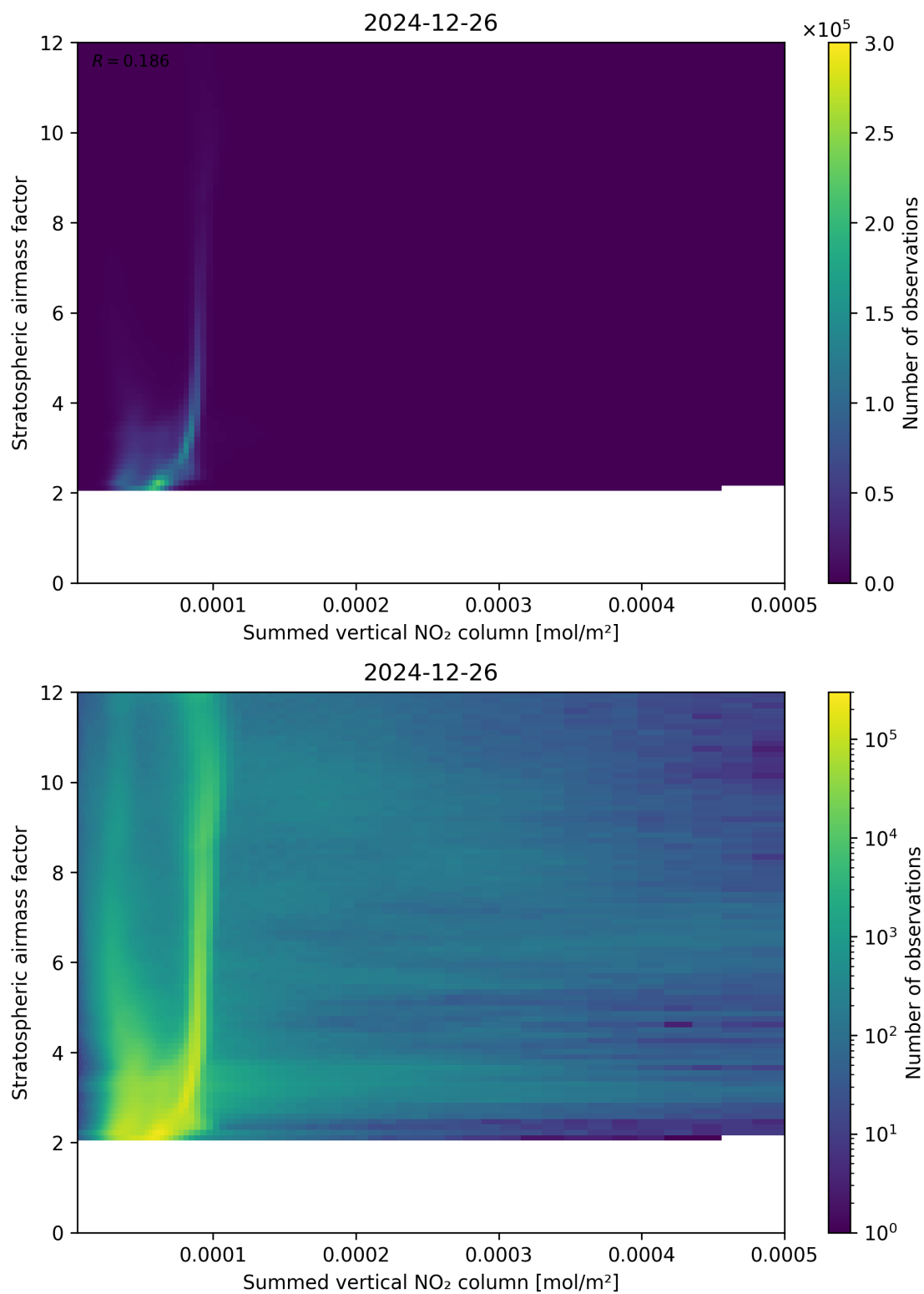
Figure 103: Scatter density plot of “Summed vertical NO 2 column” against “Stratospheric air mass factor” for 2024-12-25 to 2024-12-27.
