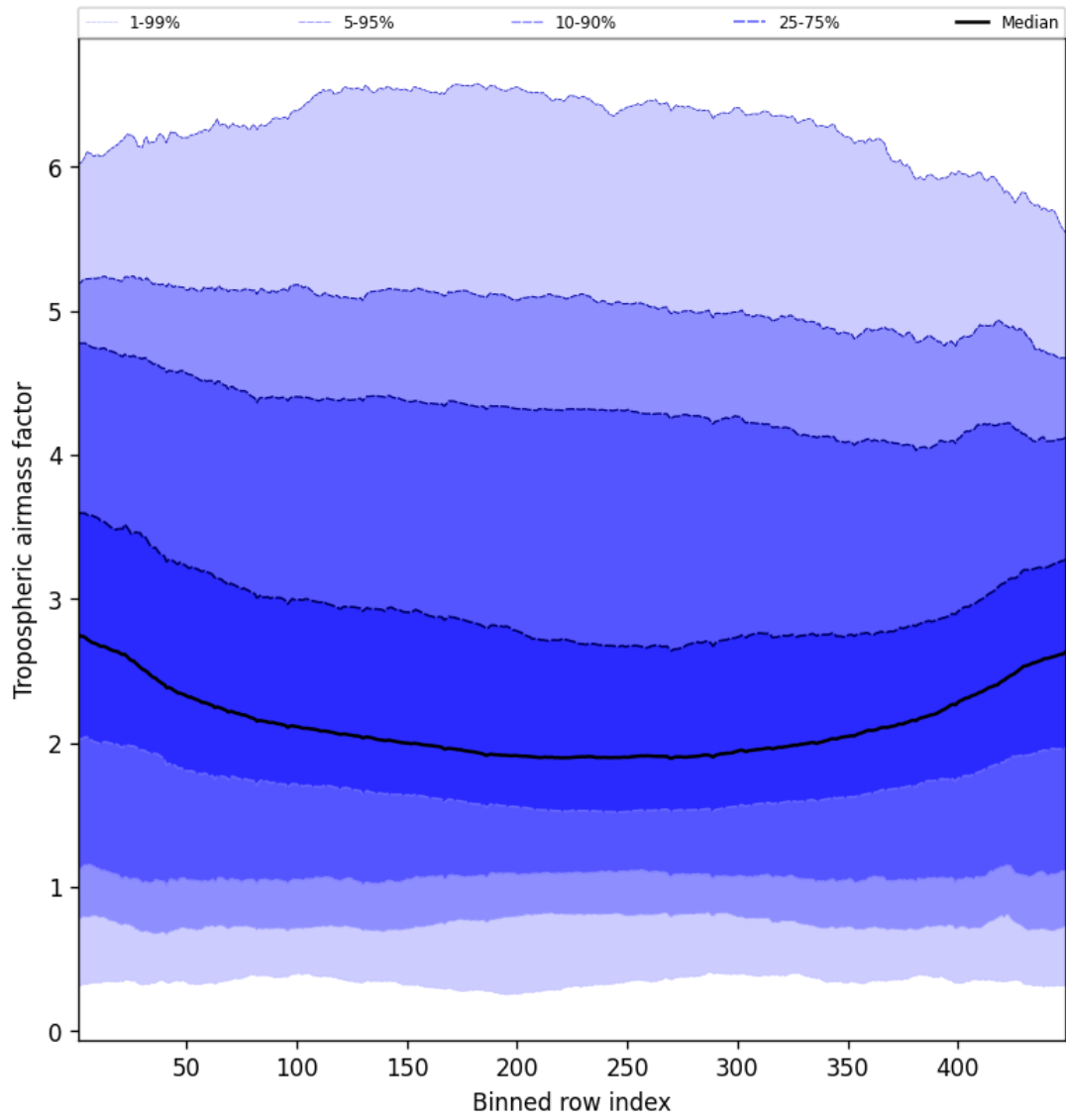
Figure 48: Along track statistics of “Tropospheric air mass factor” for 2024-12-25 to 2024-12-27
