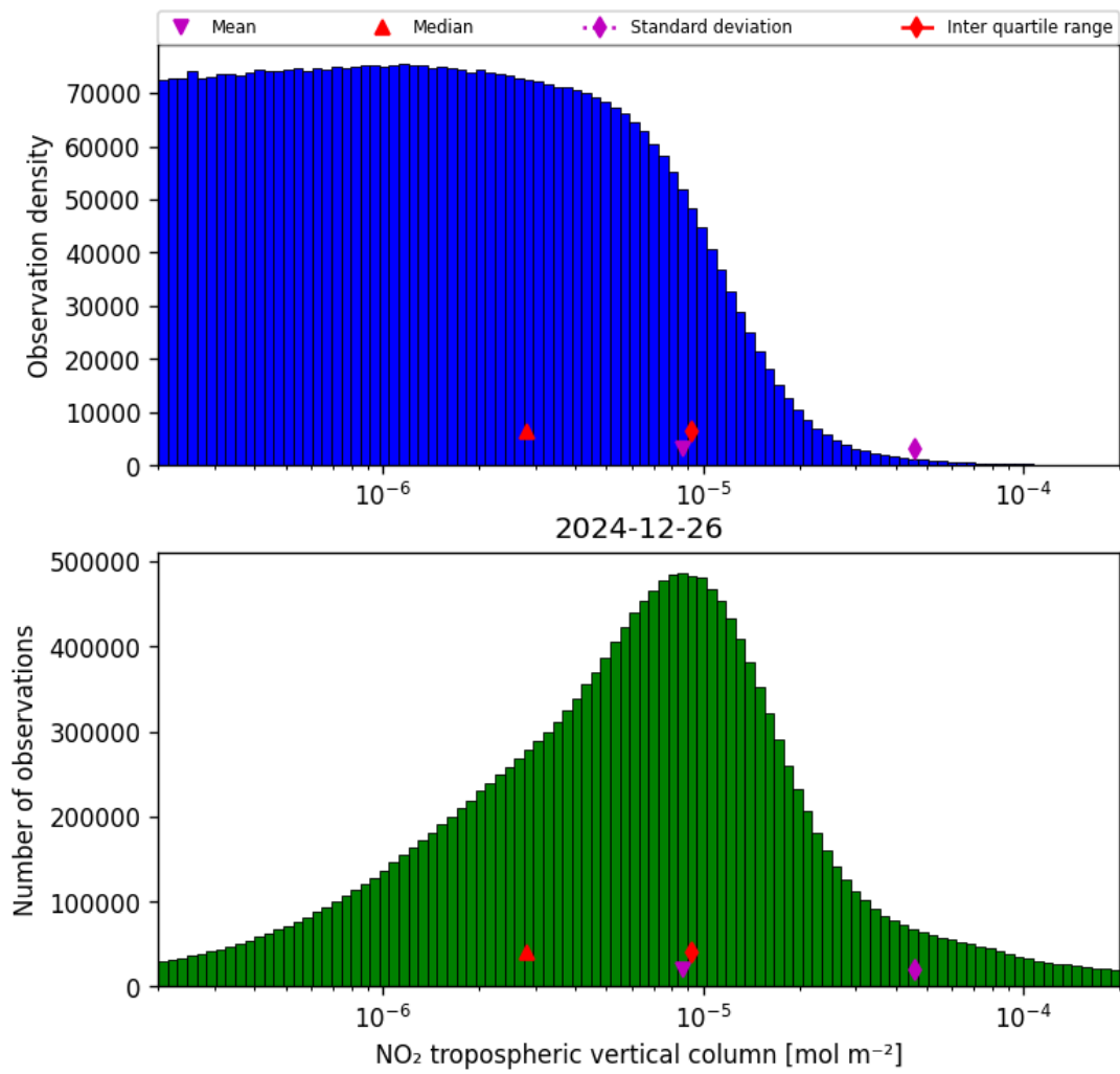
Figure 29: Histogram of “NO 2 tropospheric vertical column” for 2024-12-25 to 2024-12-27
