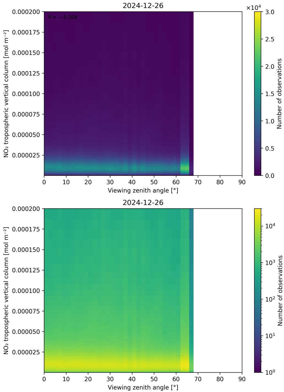
Figure 169: Scatter density plot of “Viewing zenith angle” against “NO 2 tropospheric vertical column” for 2024-12-25 to 2024-12-27.
