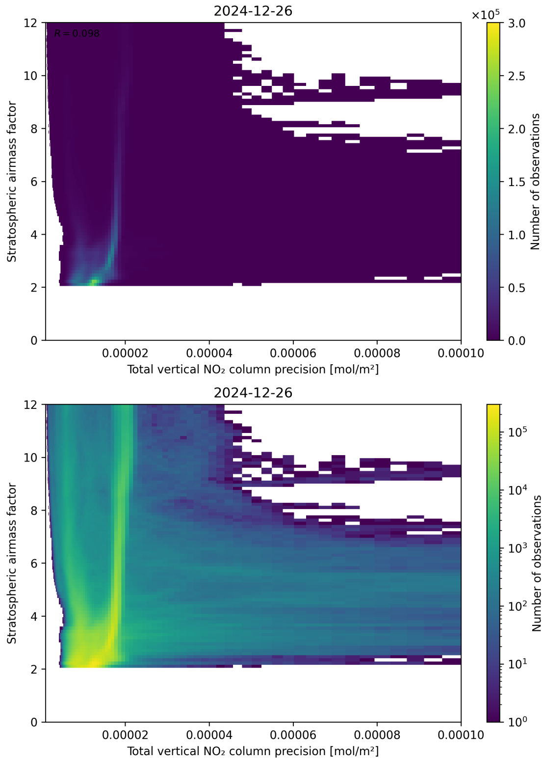
Figure 115: Scatter density plot of “Total vertical NO 2 column precision” against “Stratospheric air mass factor” for 2024-12-25 to 2024-12-27.
