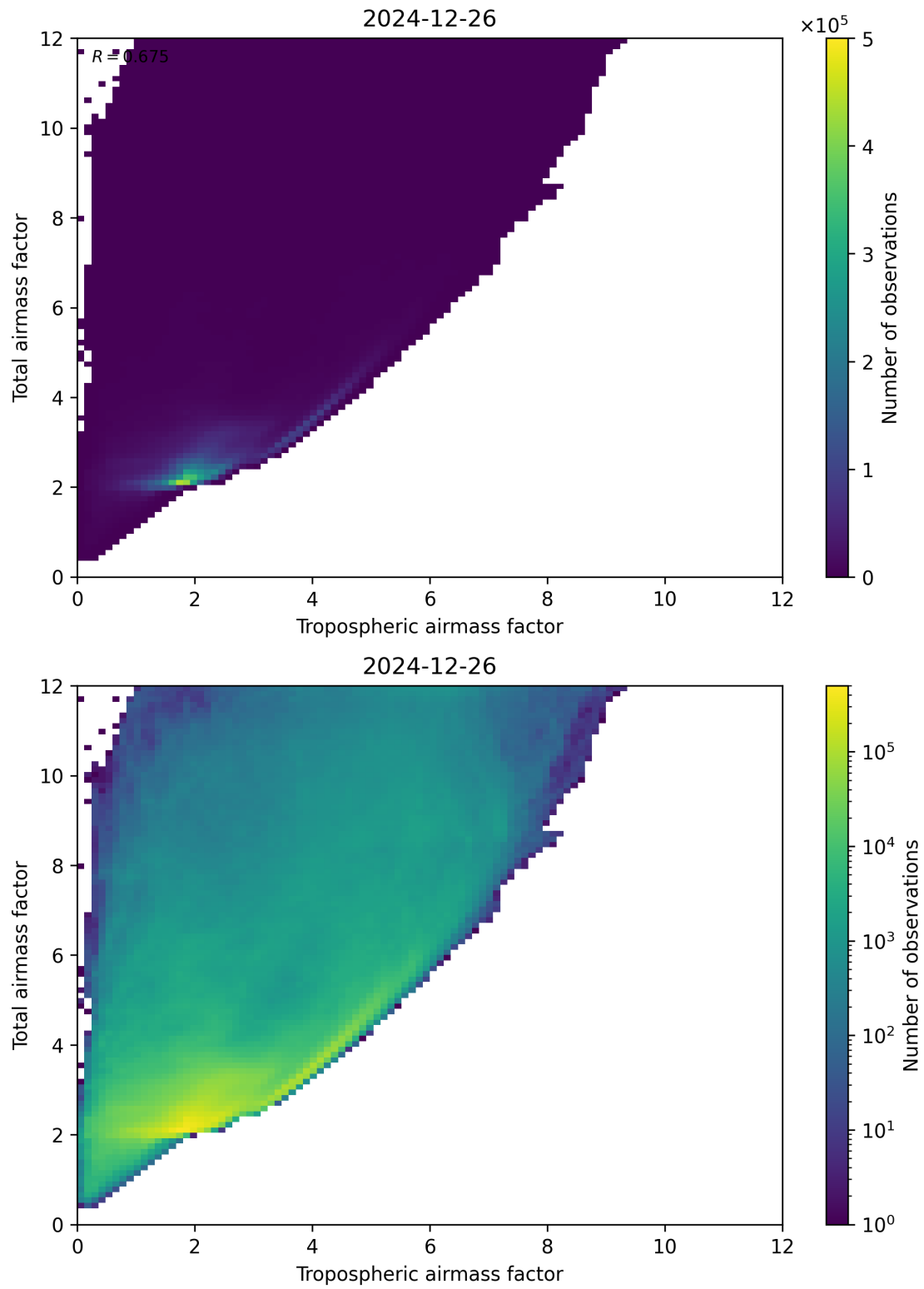
Figure 72: Scatter density plot of “Tropospheric airmass factor” against “Total airmass factor” for 2024-12-25 to 2024-12-27.
