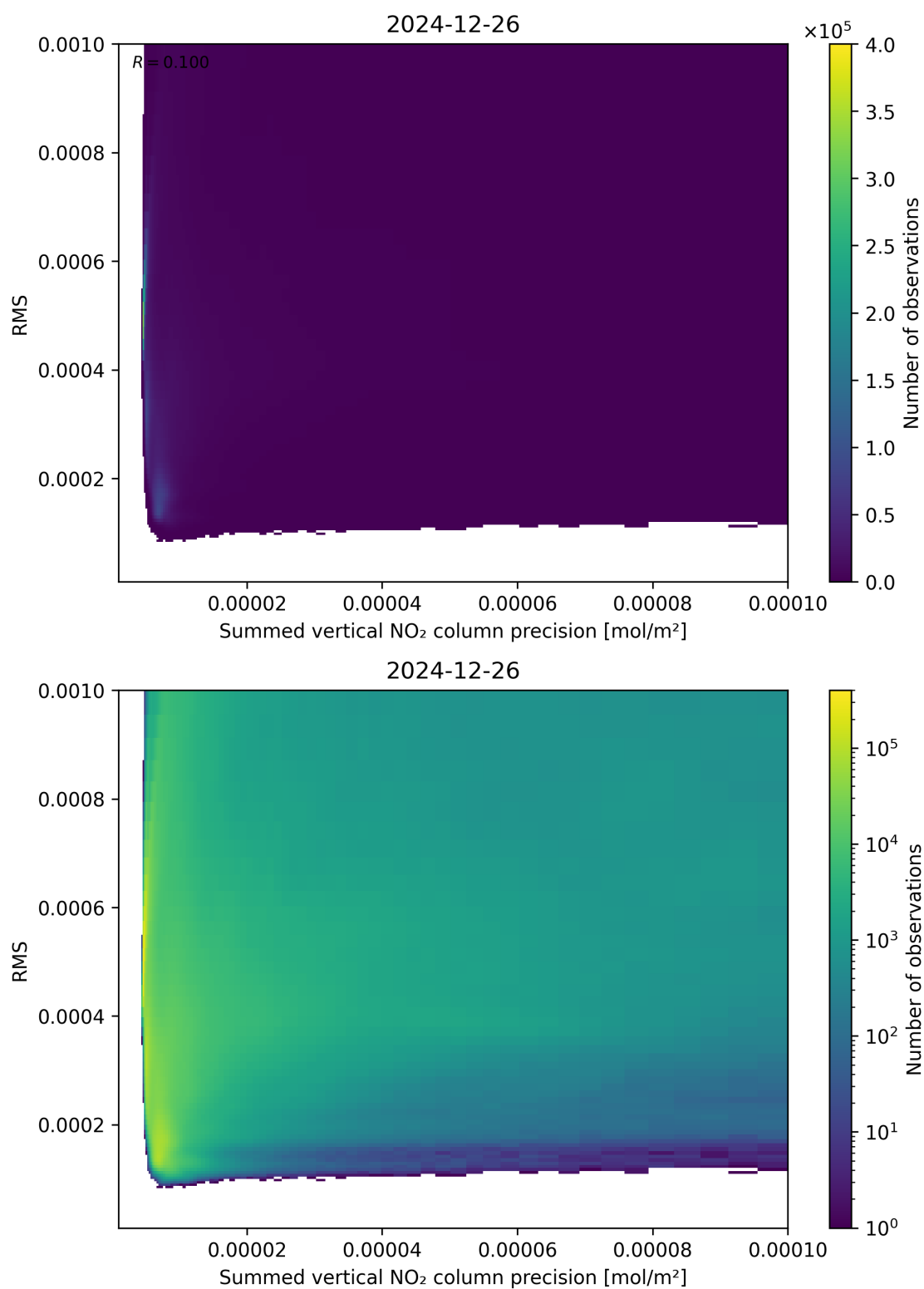
Figure 108: Scatter density plot of “Summed vertical NO 2 column precision” against “RMS” for 2024-12-25 to 2024-12-27.
