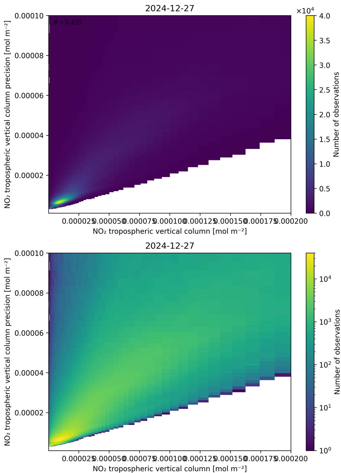
Figure 130: Scatter density plot of “NO 2 tropospheric vertical column” against “NO 2 tropospheric vertical column precision” for 2024-12-27 to 2024-12-28.
