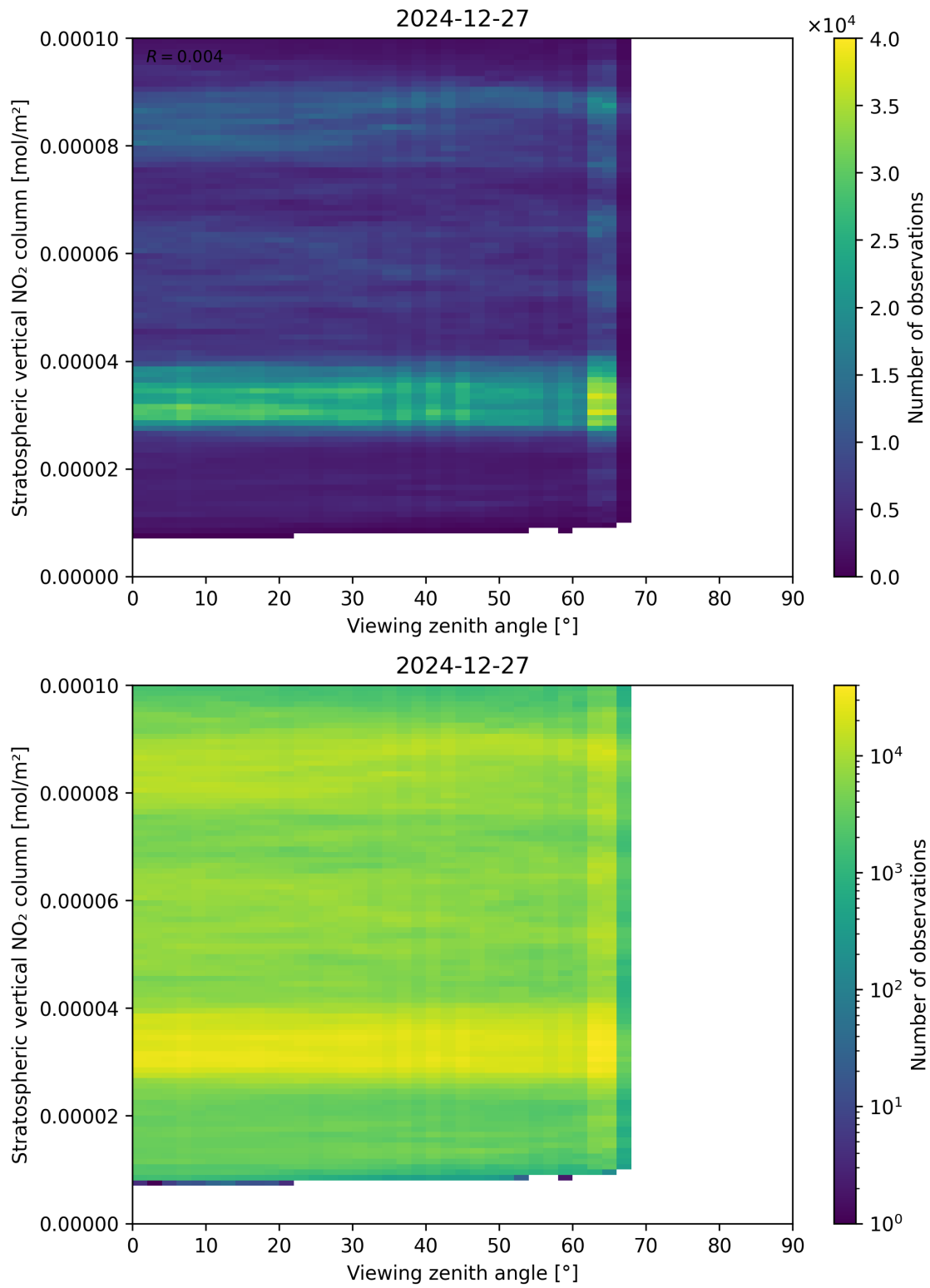
Figure 164: Scatter density plot of “Viewing zenith angle” against “Stratospheric vertical NO 2 column” for 2024-12-27 to 2024-12-28.
