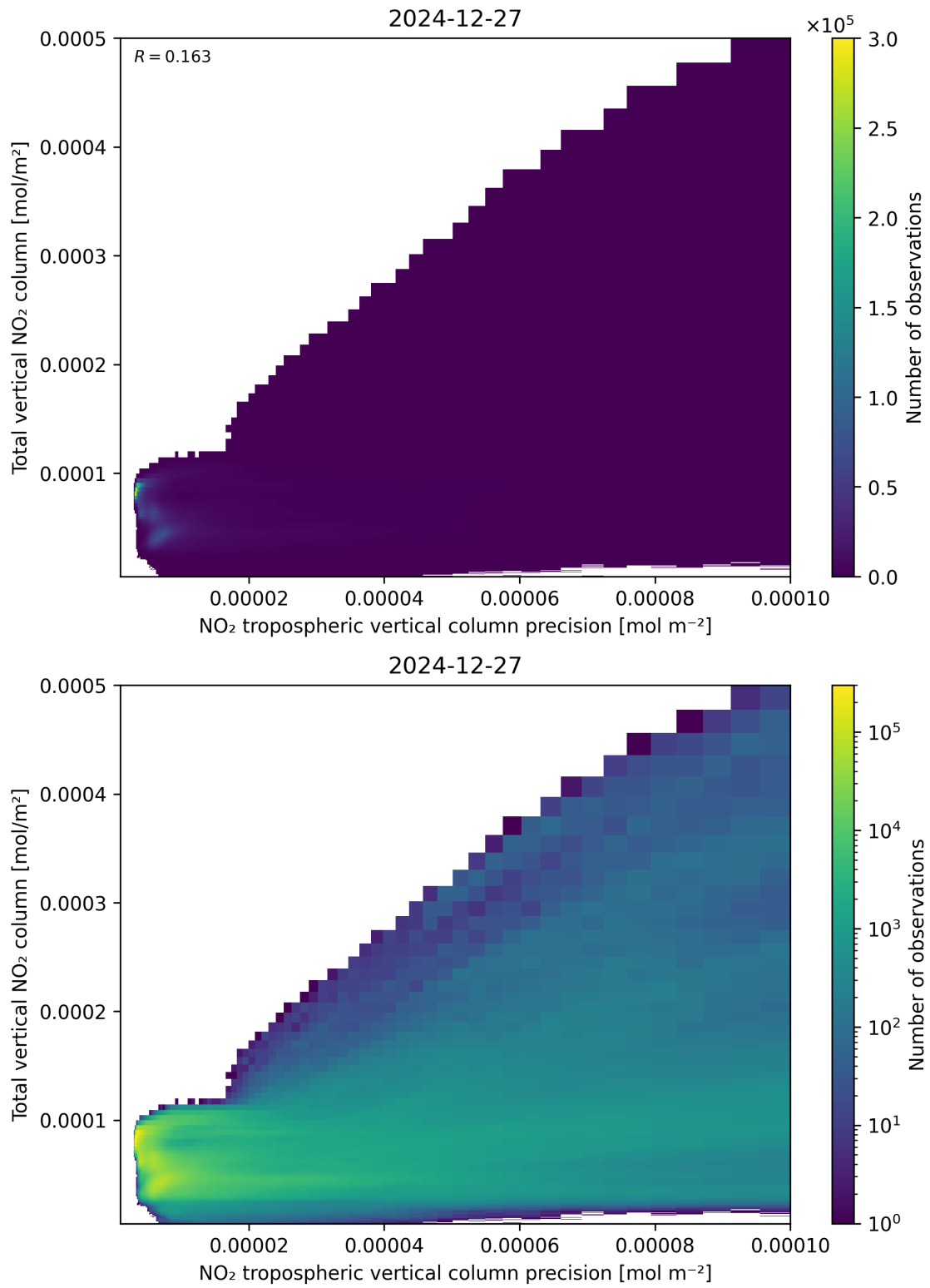
Figure 138: Scatter density plot of “NO 2 tropospheric vertical column precision” against “Total vertical NO 2 column” for 2024-12-27 to 2024-12-28.
