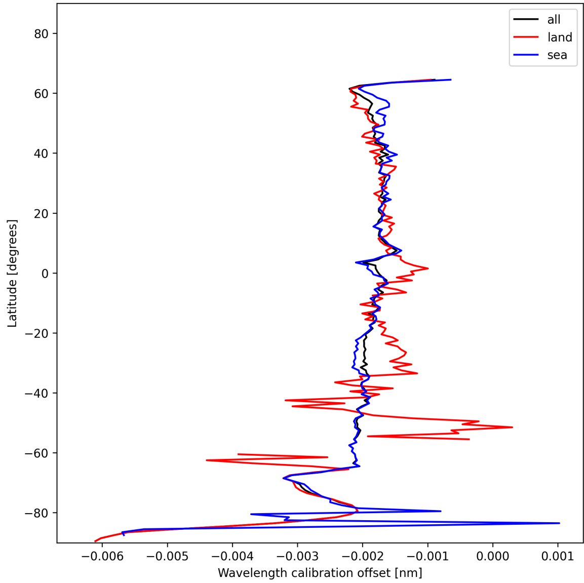
Figure 18: Zonal average of “Wavelength calibration offset” for 2024-12-27 to 2024-12-28.
