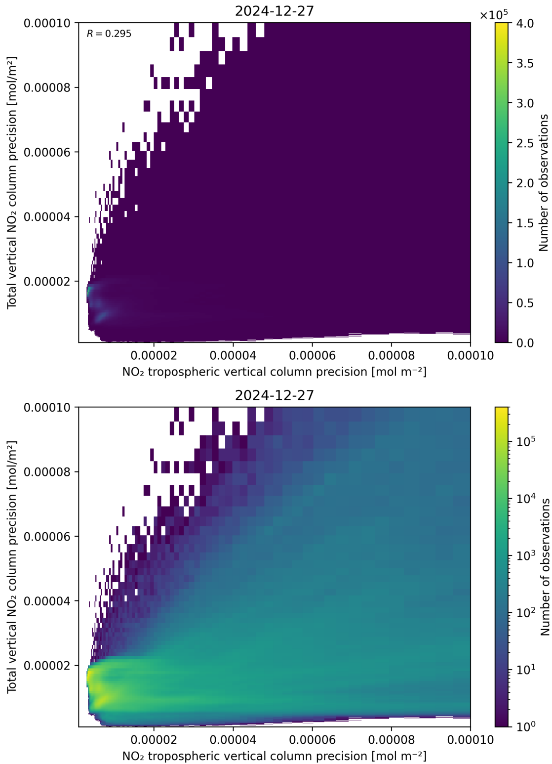
Figure 139: Scatter density plot of “NO 2 tropospheric vertical column precision” against “Total vertical NO 2 column precision” for 2024-12-27 to 2024-12-28.
