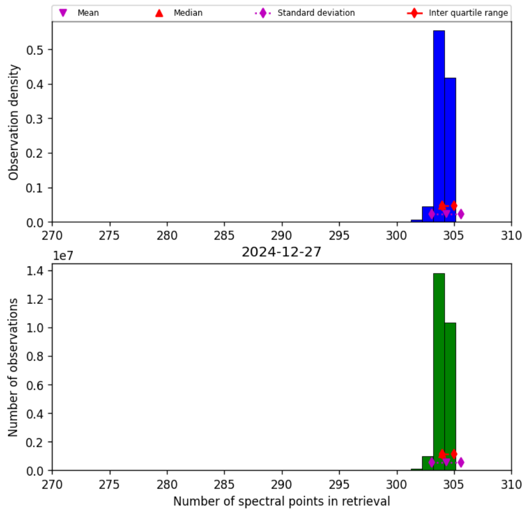
Figure 33: Histogram of “Number of spectral points in retrieval” for 2024-12-27 to 2024-12-28
