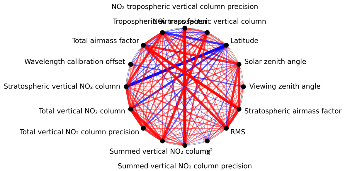
Figure 1: Map of correlation graph for 2024-12-27 to 2024-12-28.
