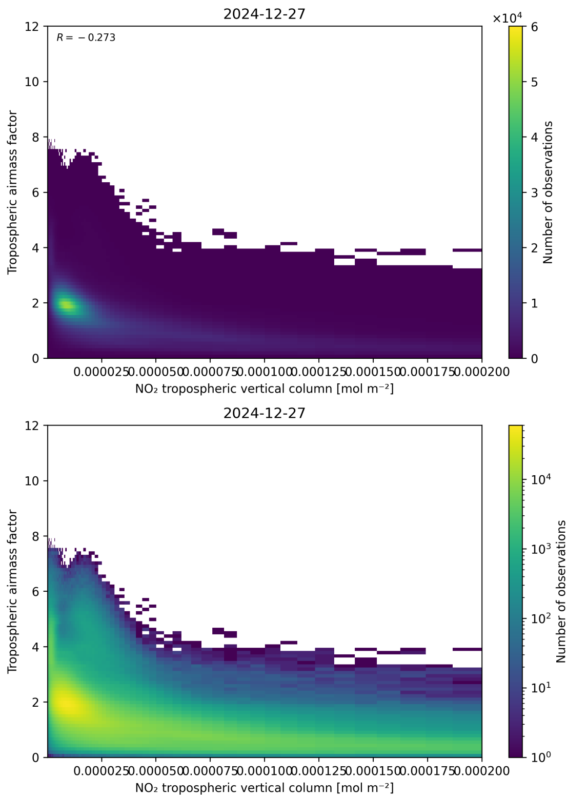
Figure 123: Scatter density plot of “NO 2 tropospheric vertical column” against “Tropospheric air mass factor” for 2024-12-27 to 2024-12-28.
