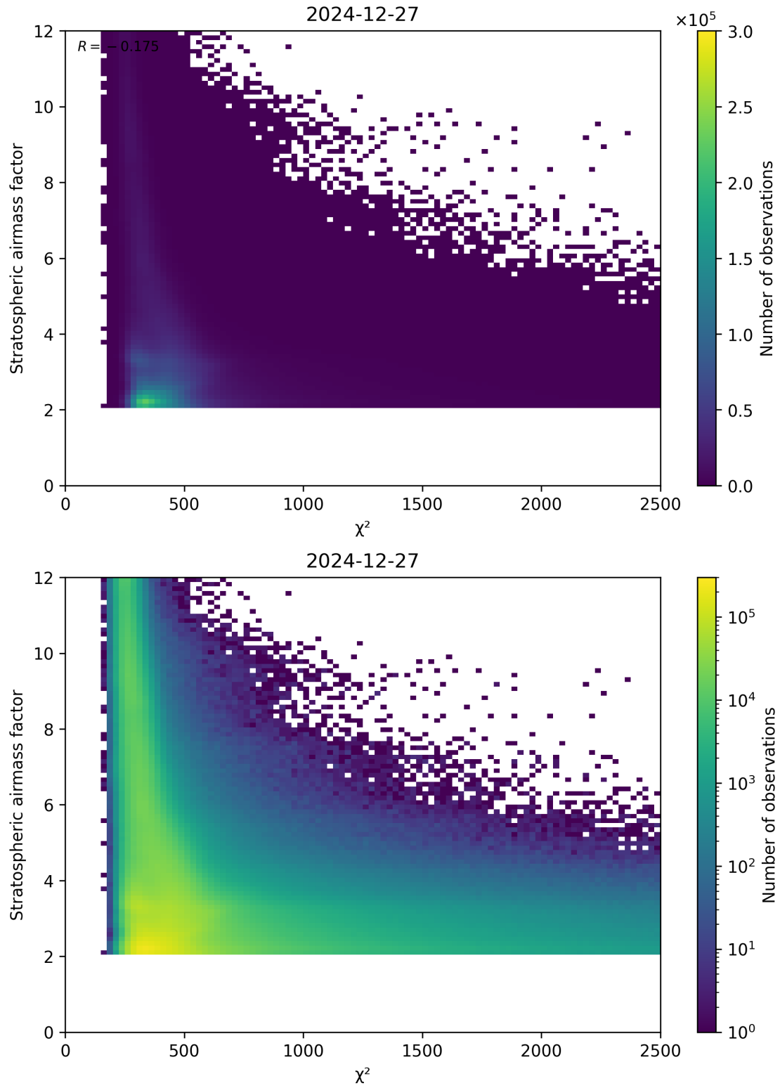
Figure 81: Scatter density plot of “ \chi^2 ” against “Stratospheric airmass factor” for 2024-12-27 to 2024-12-28.
