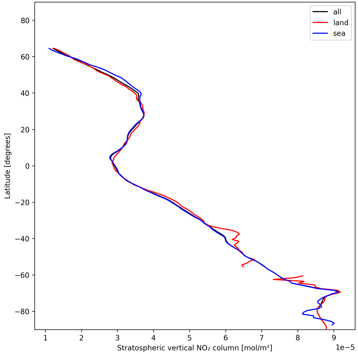
Figure 19: Zonal average of “Stratospheric vertical NO 2 column” for 2024-12-27 to 2024-12-28.
