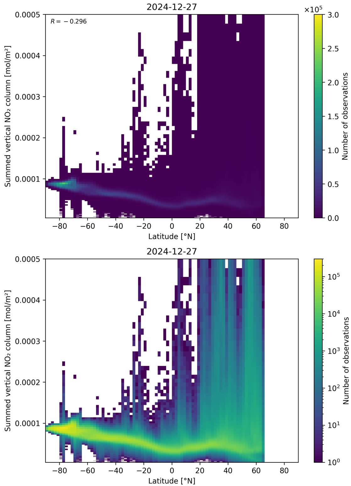
Figure 88: Scatter density plot of “Latitude” against “Summed vertical NO 2 column” for 2024-12-27 to 2024-12-28.
