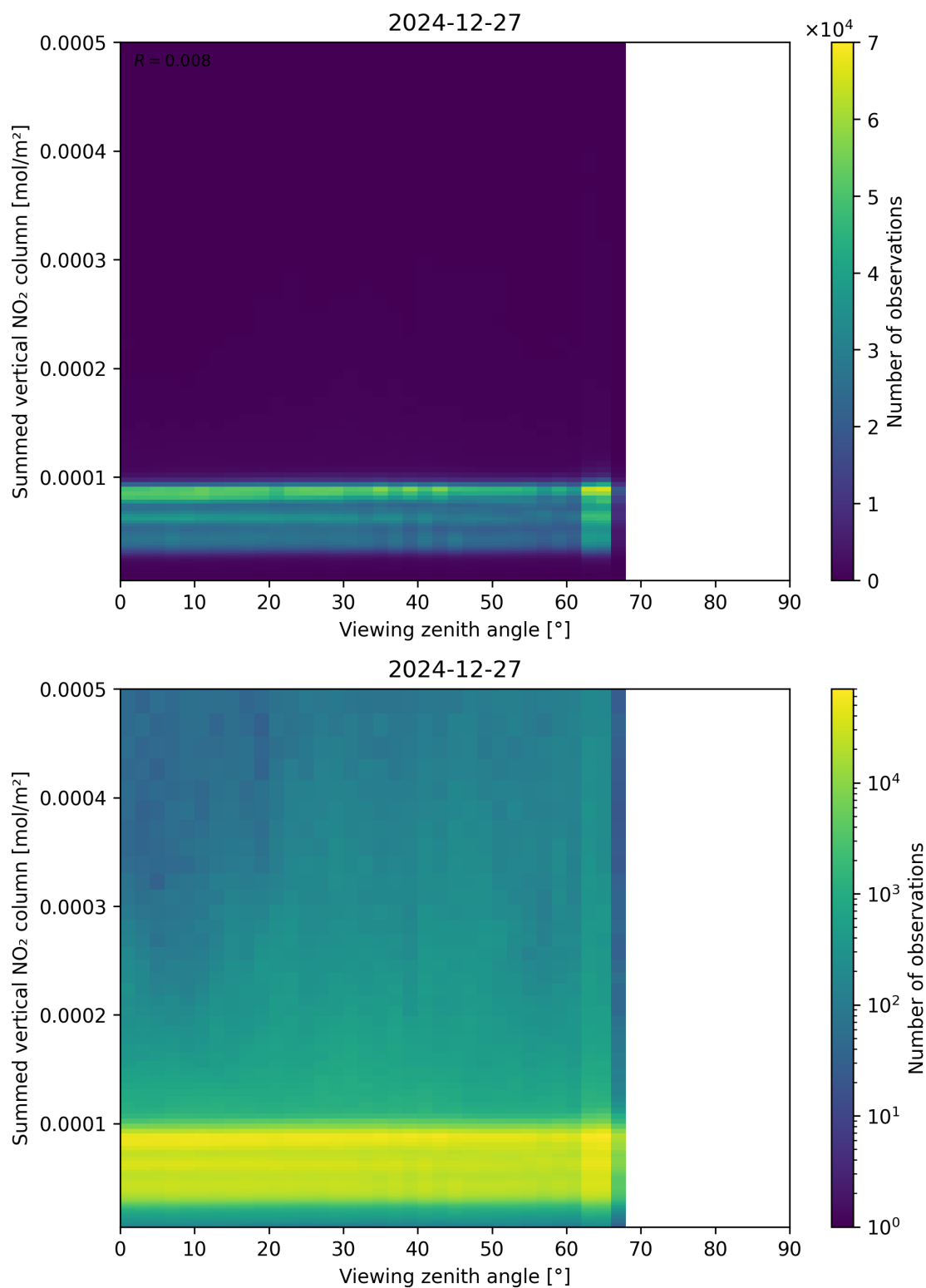
Figure 165: Scatter density plot of “Viewing zenith angle” against “Summed vertical NO 2 column” for 2024-12-27 to 2024-12-28.
