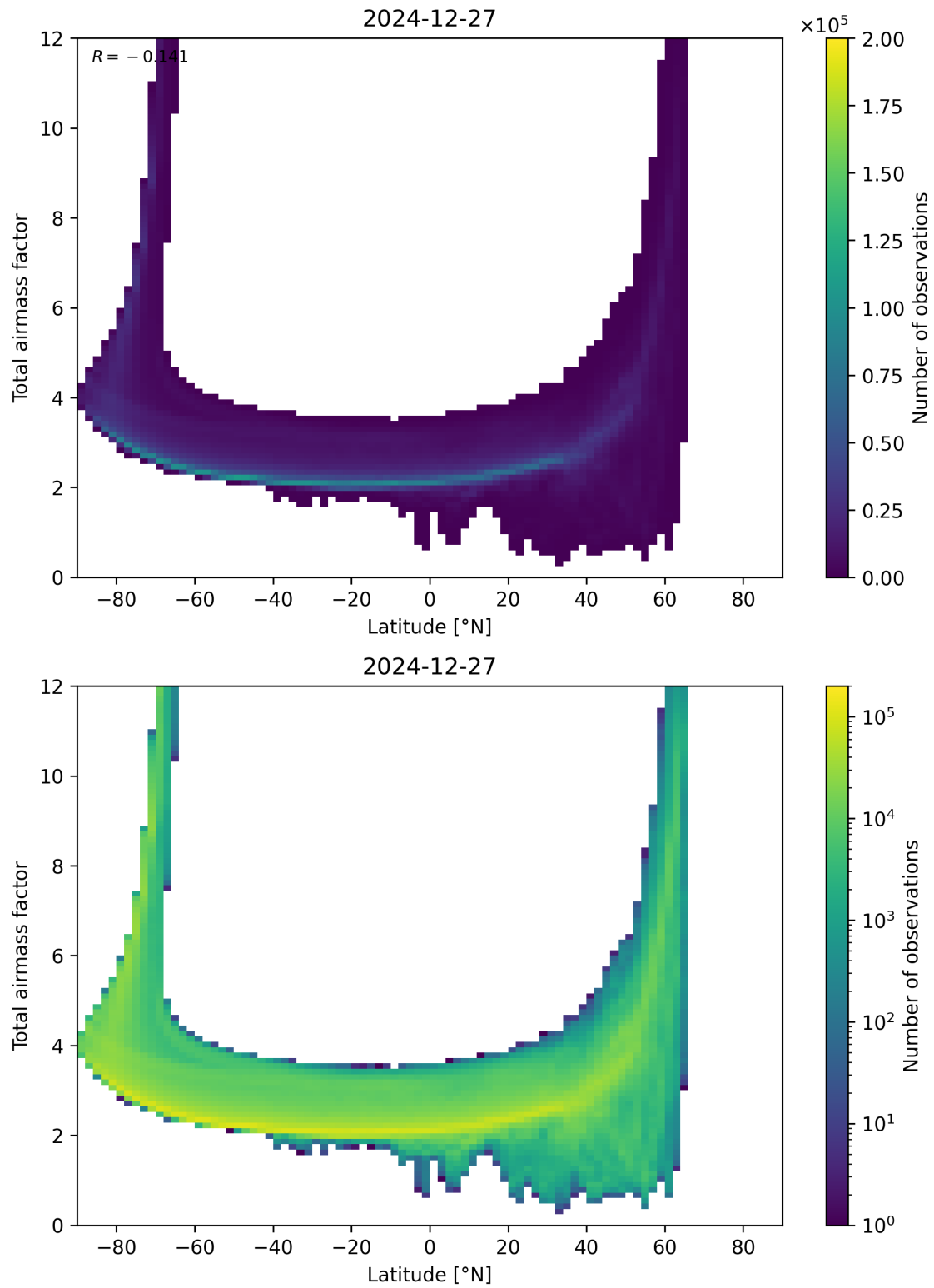
Figure 84: Scatter density plot of “Latitude” against “Total airmass factor” for 2024-12-27 to 2024-12-28.
