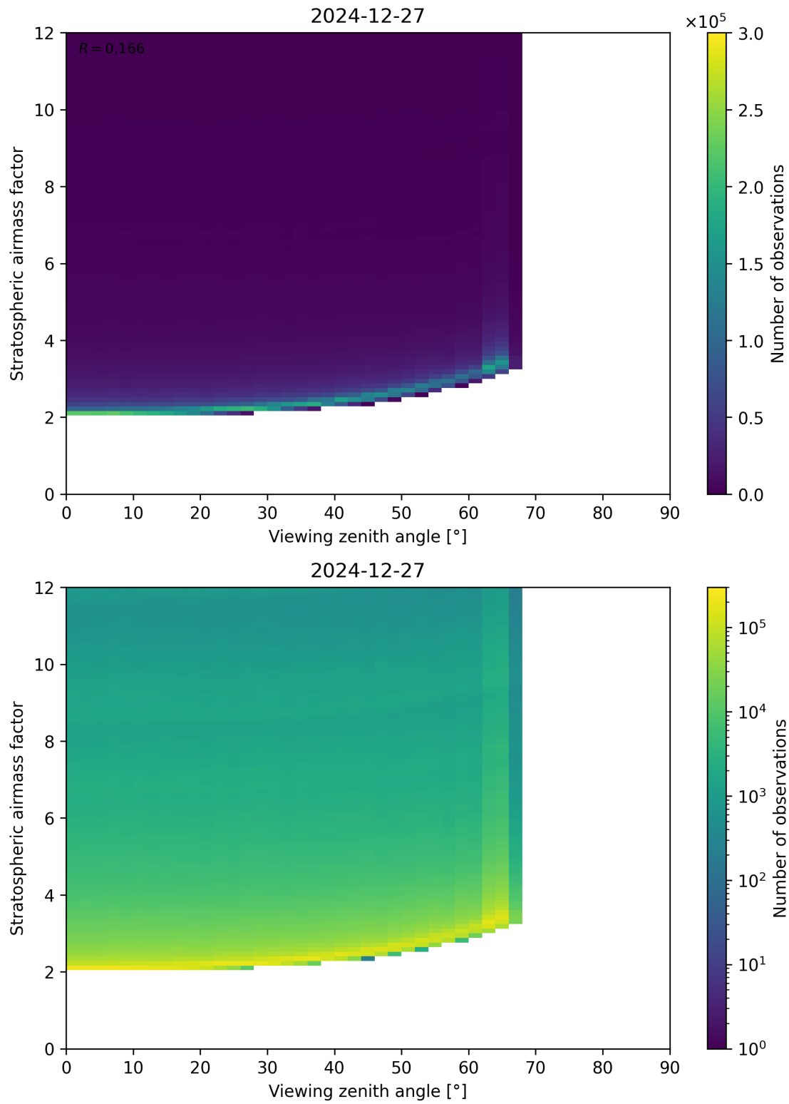
Figure 159: Scatter density plot of “Viewing zenith angle” against “Stratospheric airmass factor” for 2024-12-27 to 2024-12-28.
