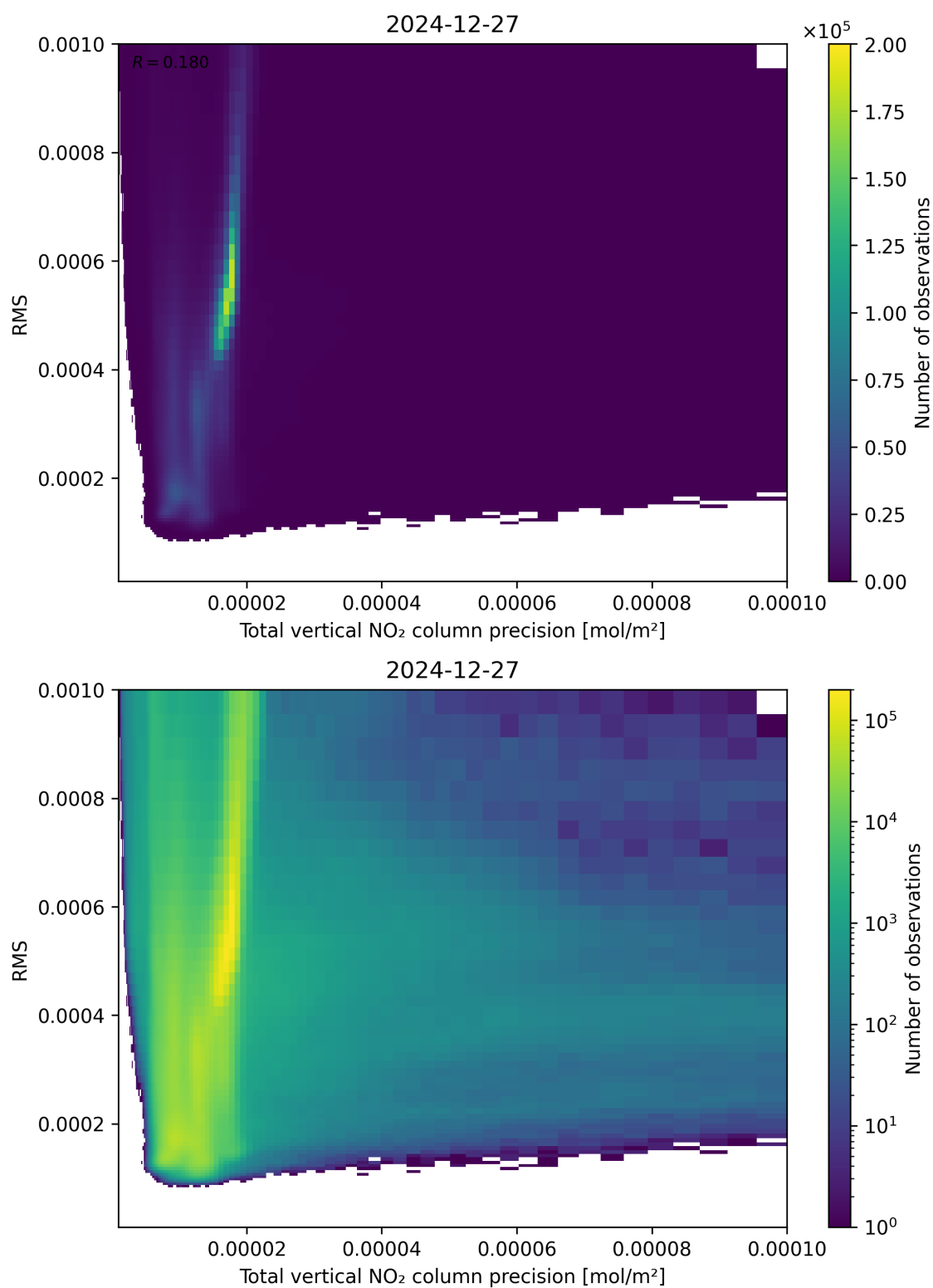
Figure 119: Scatter density plot of “Total vertical NO 2 column precision” against “RMS” for 2024-12-27 to 2024-12-28.
