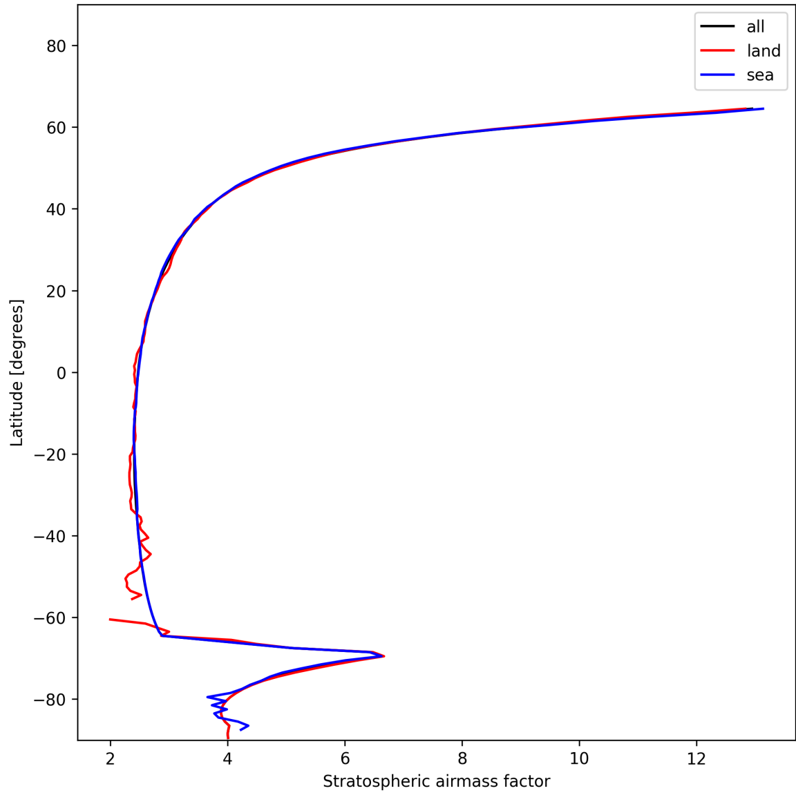
Figure 27: Zonal average of “Stratospheric airmass factor” for 2024-12-27 to 2024-12-28.
