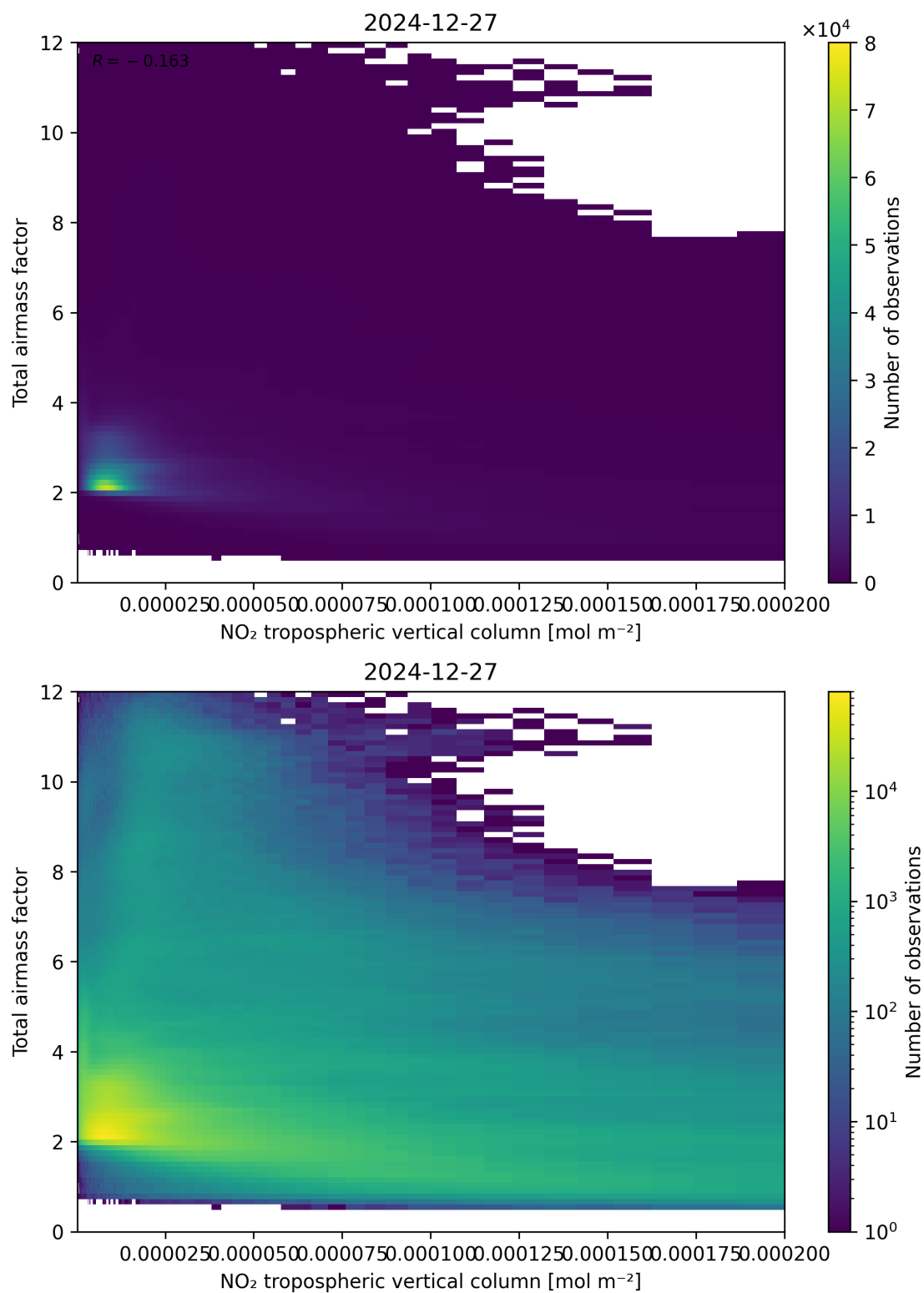
Figure 122: Scatter density plot of “NO 2 tropospheric vertical column” against “Total air mass factor” for 2024-12-27 to 2024-12-28.
