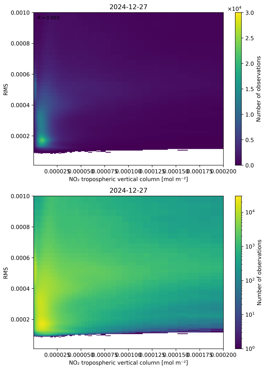
Figure 142: Scatter density plot of “NO 2 tropospheric vertical column” against “RMS” for 2024-12-27 to 2024-12-28.
