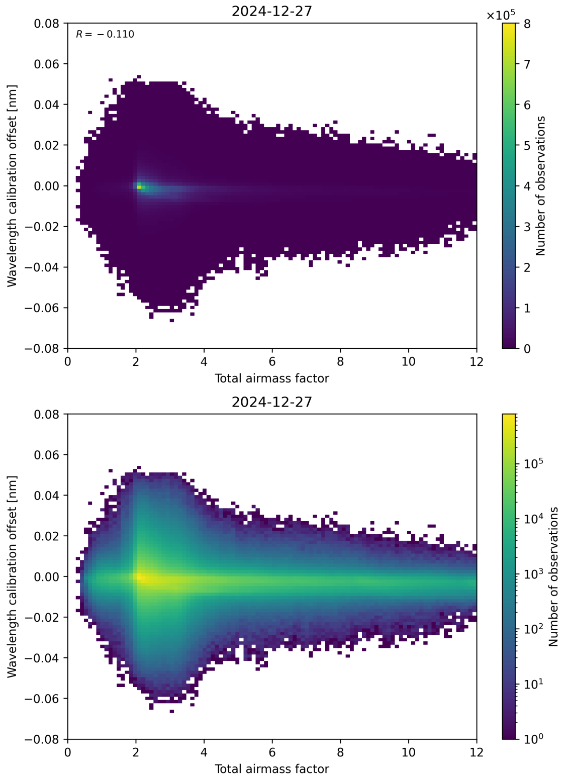
Figure 70: Scatter density plot of “Total airmass factor” against “Wavelength calibration offset” for 2024-12-27 to 2024-12-28.
