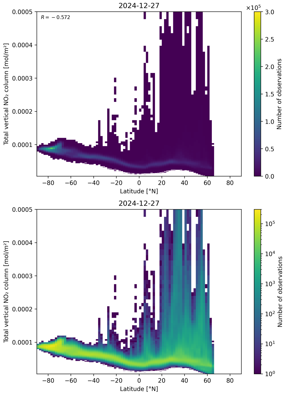
Figure 90: Scatter density plot of “Latitude” against “Total vertical NO 2 column” for 2024-12-27 to 2024-12-28.
