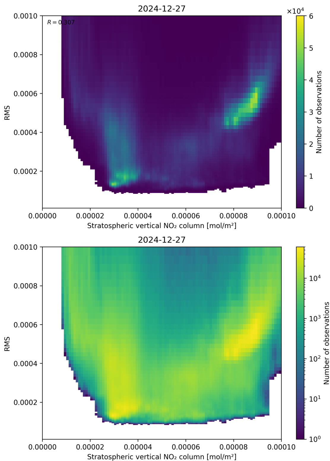
Figure 102: Scatter density plot of “Stratospheric vertical NO 2 column” against “RMS” for 2024-12-27 to 2024-12-28.
