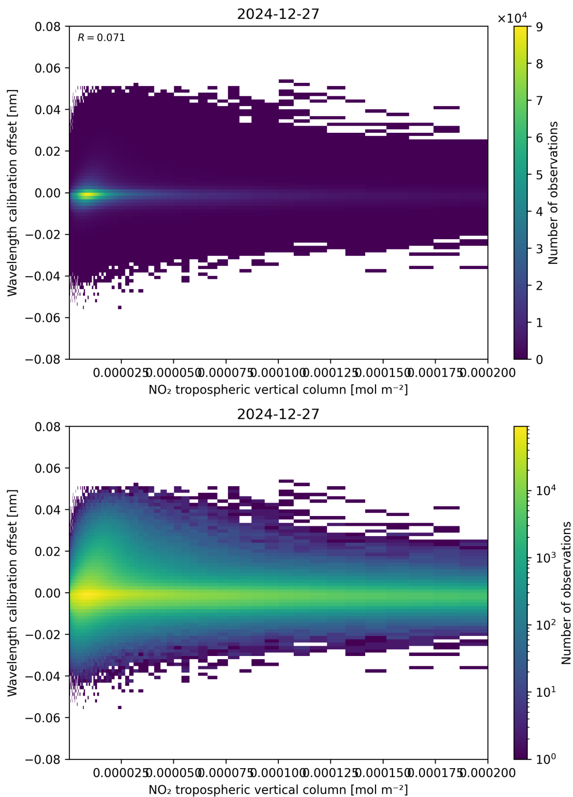
Figure 143: Scatter density plot of “NO 2 tropospheric vertical column” against “Wavelength calibration offset” for 2024-12-27 to 2024-12-28.
