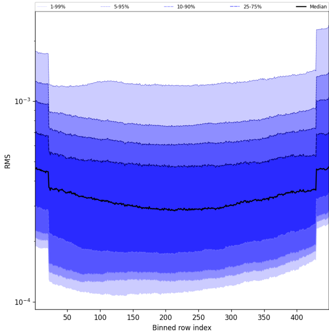
Figure 60: Along track statistics of “RMS” for 2024-12-27 to 2024-12-28
