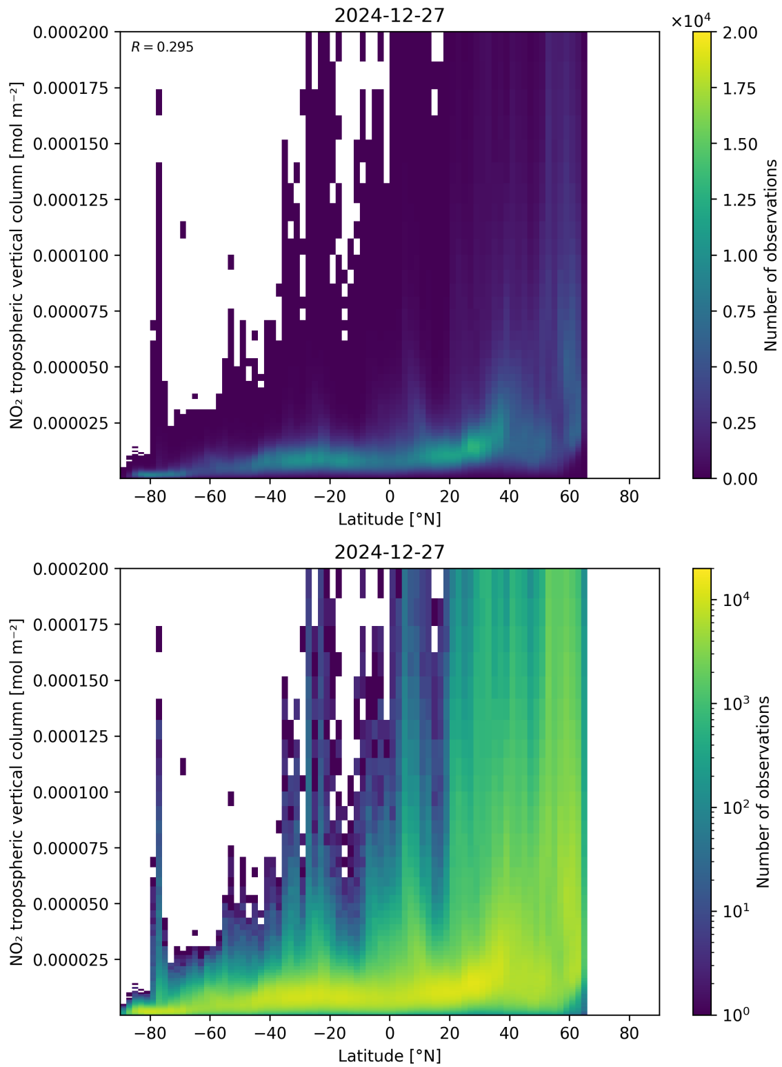
Figure 92: Scatter density plot of “Latitude” against “NO 2 tropospheric vertical column” for 2024-12-27 to 2024-12-28.
