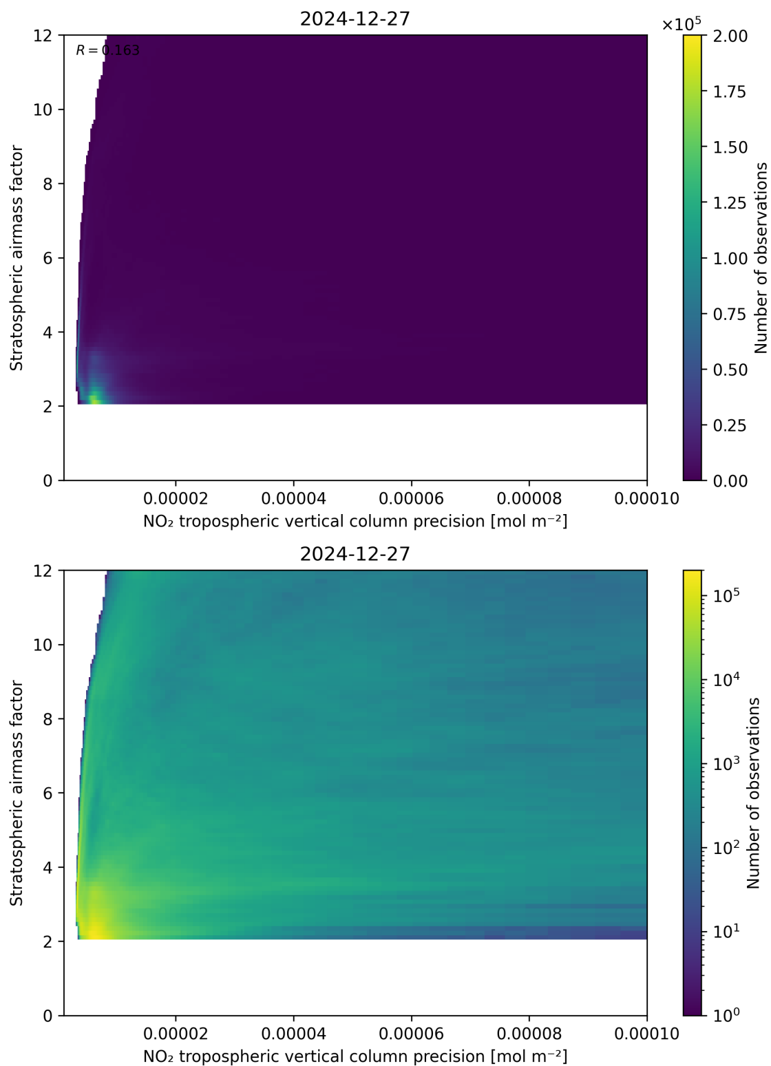
Figure 131: Scatter density plot of “NO 2 tropospheric vertical column precision” against “Stratospheric airmass factor” for 2024-12-27 to 2024-12-28.
