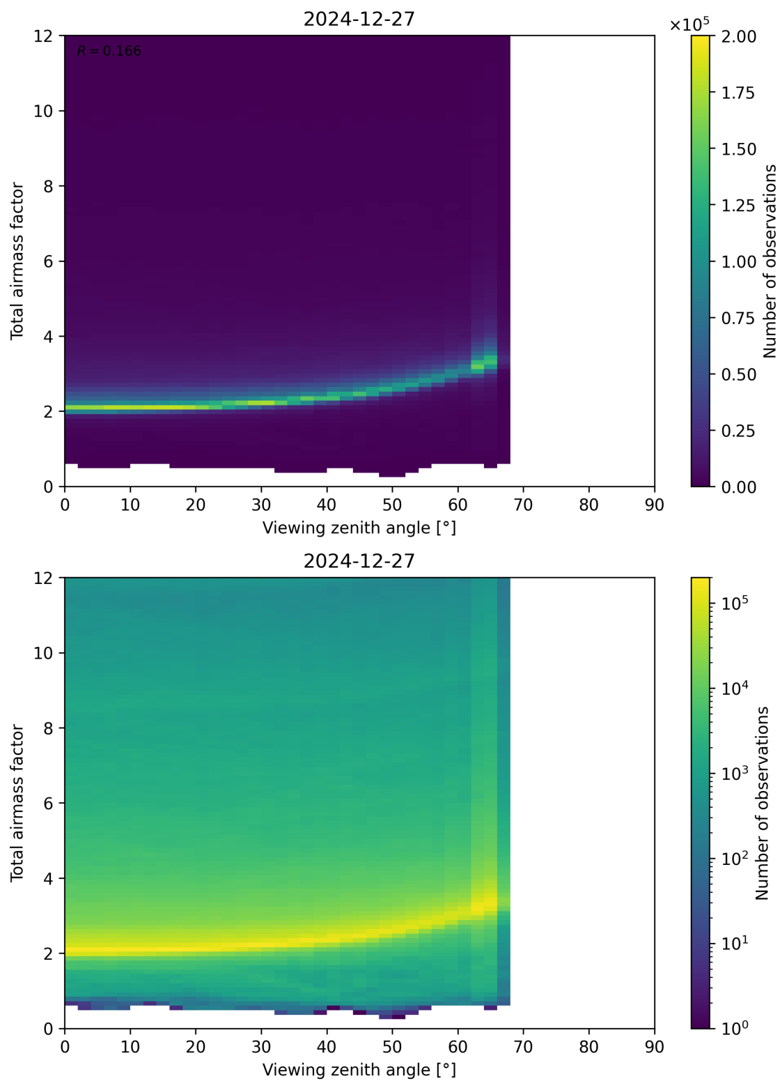
Figure 160: Scatter density plot of “Viewing zenith angle” against “Total airmass factor” for 2024-12-27 to 2024-12-28.
