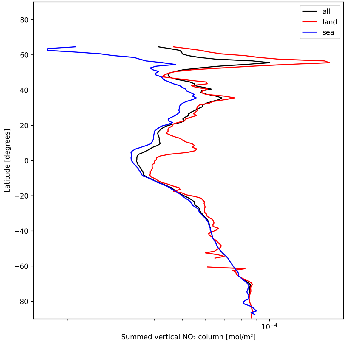
Figure 23: Zonal average of “Summed vertical NO 2 column” for 2024-12-27 to 2024-12-28.
