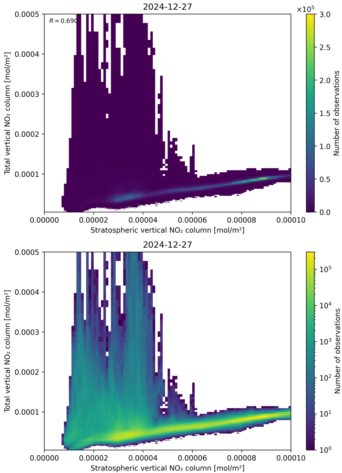
Figure 100: Scatter density plot of “Stratospheric vertical NO 2 column” against “Total vertical NO 2 column” for 2024-12-27 to 2024-12-28.
