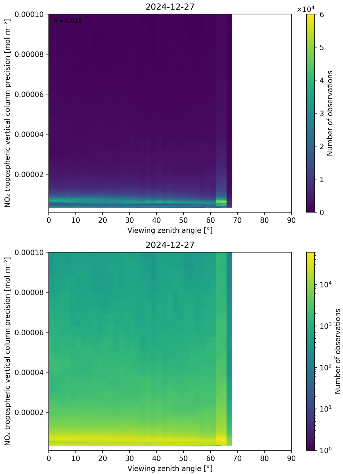
Figure 170: Scatter density plot of “Viewing zenith angle” against “NO 2 tropospheric vertical column precision” for 2024-12-27 to 2024-12-28.
