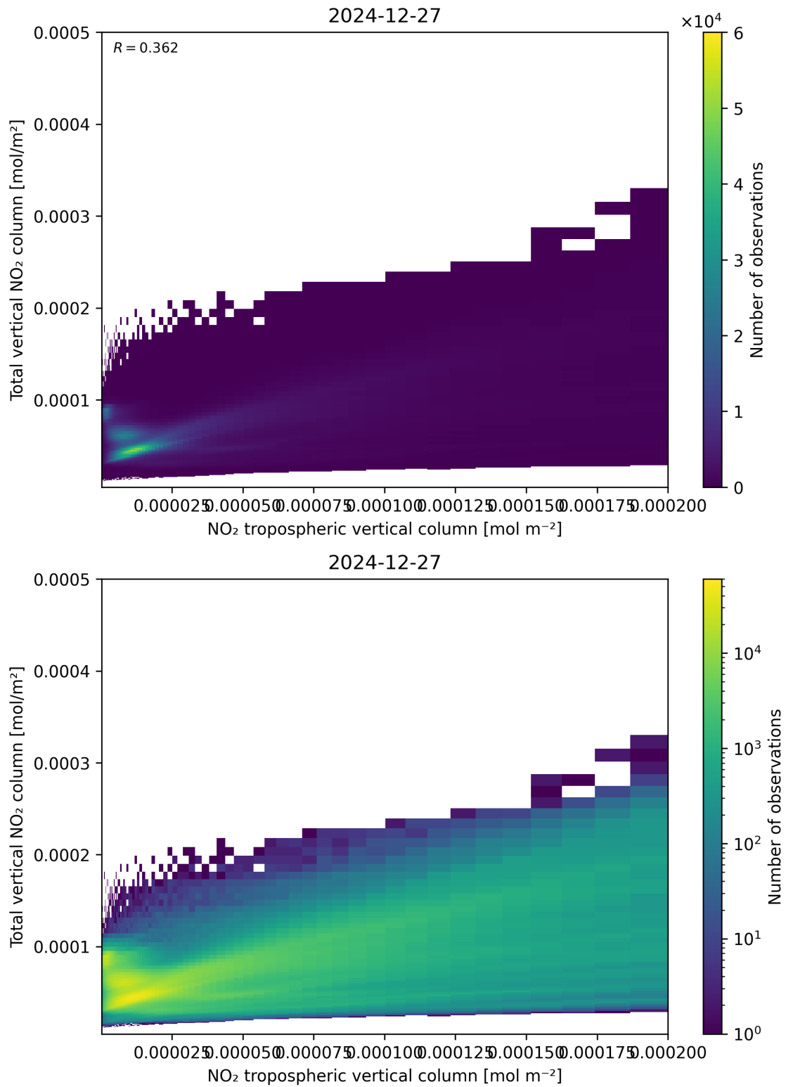
Figure 128: Scatter density plot of “NO 2 tropospheric vertical column” against “Total vertical NO 2 column” for 2024-12-27 to 2024-12-28.
