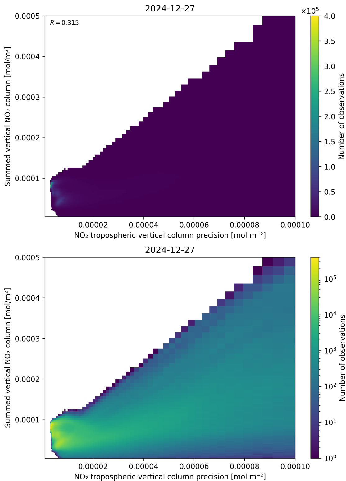
Figure 136: Scatter density plot of “NO 2 tropospheric vertical column precision” against “Summed vertical NO 2 column” for 2024-12-27 to 2024-12-28.
