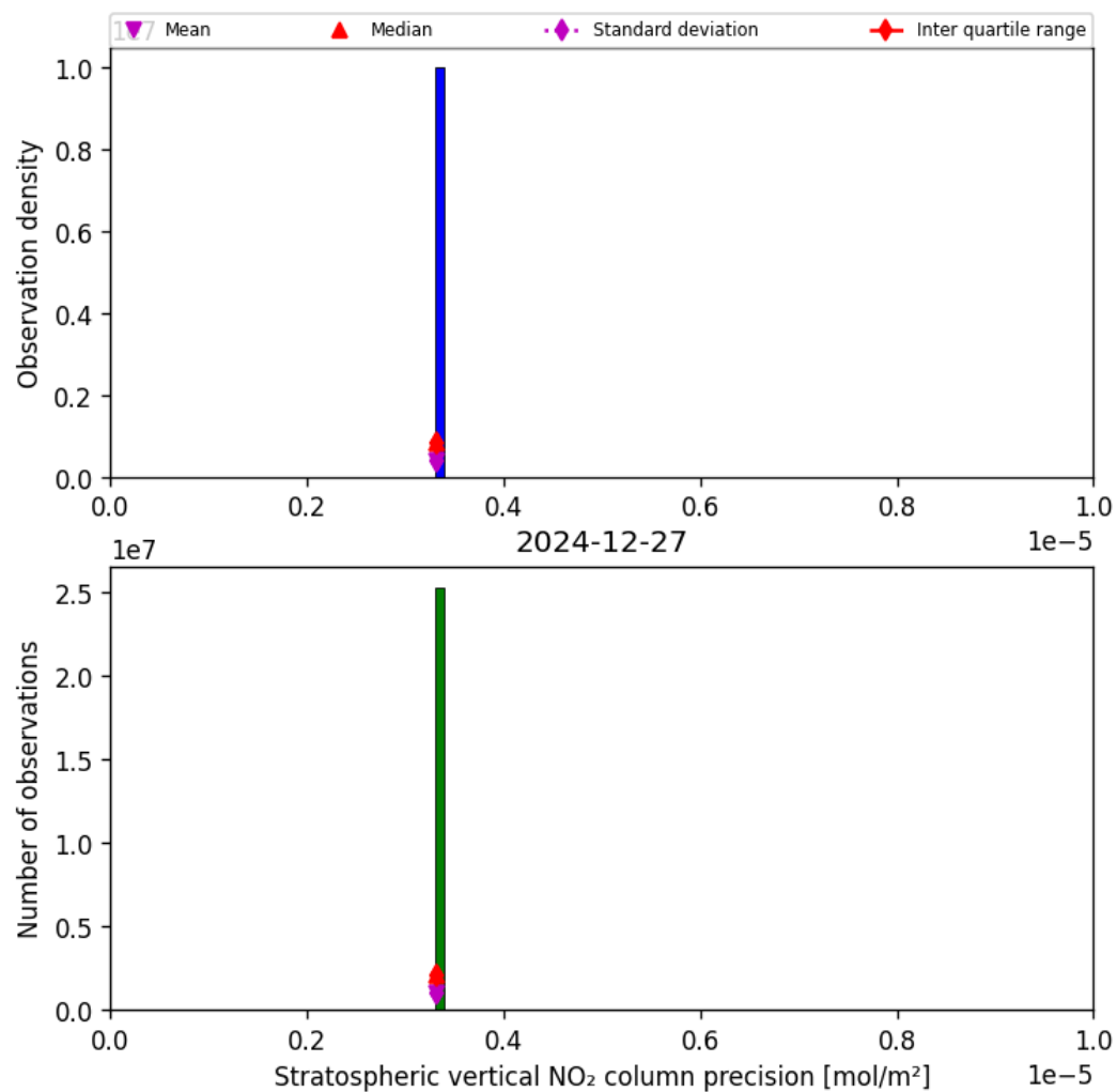
Figure 37: Histogram of “Stratospheric vertical NO 2 column precision” for 2024-12-27 to 2024-12-28
