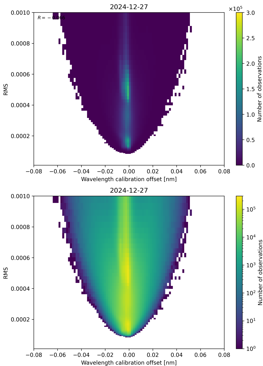
Figure 181: Scatter density plot of “Wavelength calibration offset” against “RMS” for 2024-12-27 to 2024-12-28.
