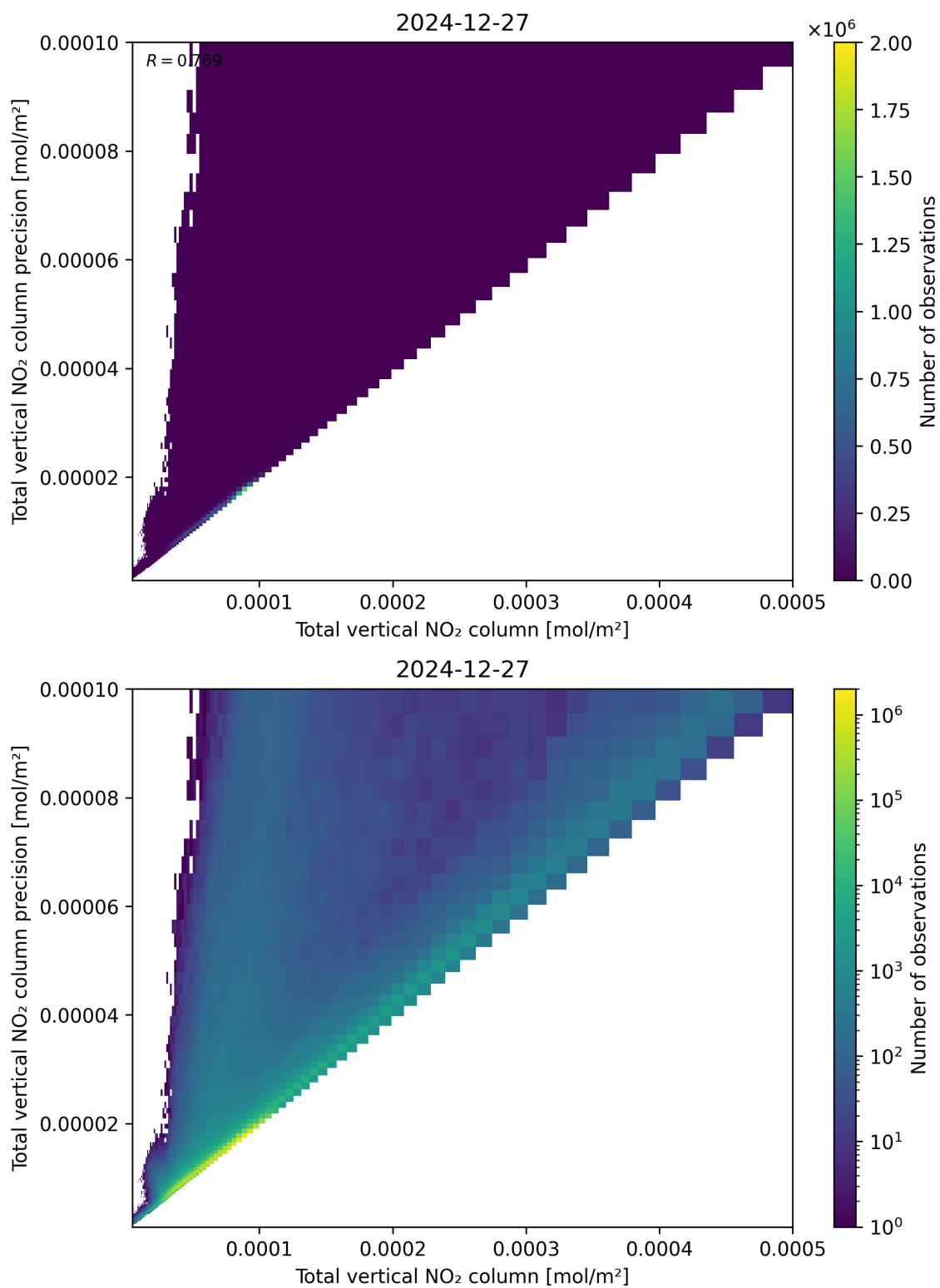
Figure 114: Scatter density plot of “Total vertical NO 2 column” against “Total vertical NO 2 column precision” for 2024-12-27 to 2024-12-28.
