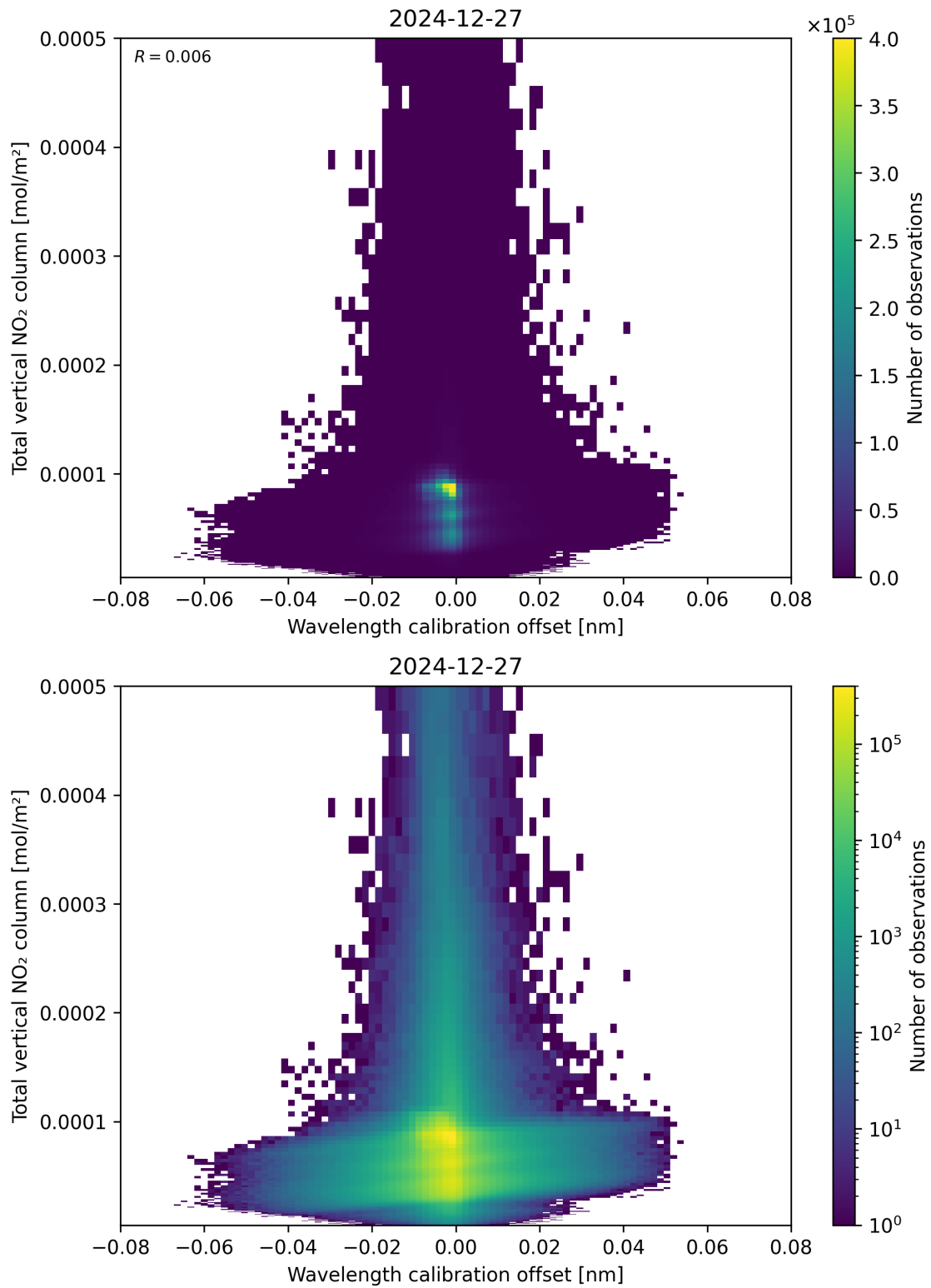
Figure 179: Scatter density plot of “Wavelength calibration offset” against “Total vertical NO 2 column” for 2024-12-27 to 2024-12-28.
