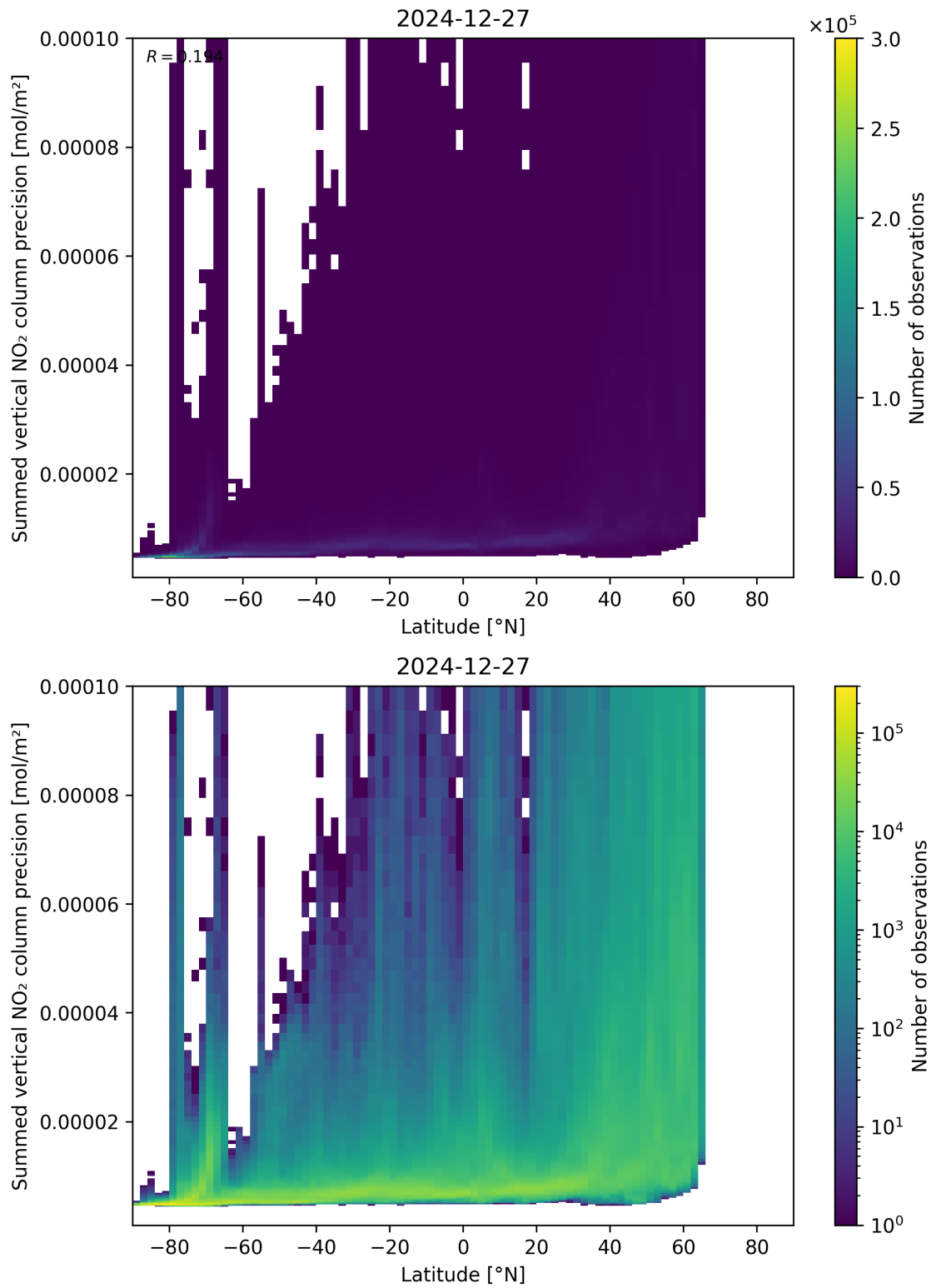
Figure 89: Scatter density plot of “Latitude” against “Summed vertical NO 2 column precision” for 2024-12-27 to 2024-12-28.
