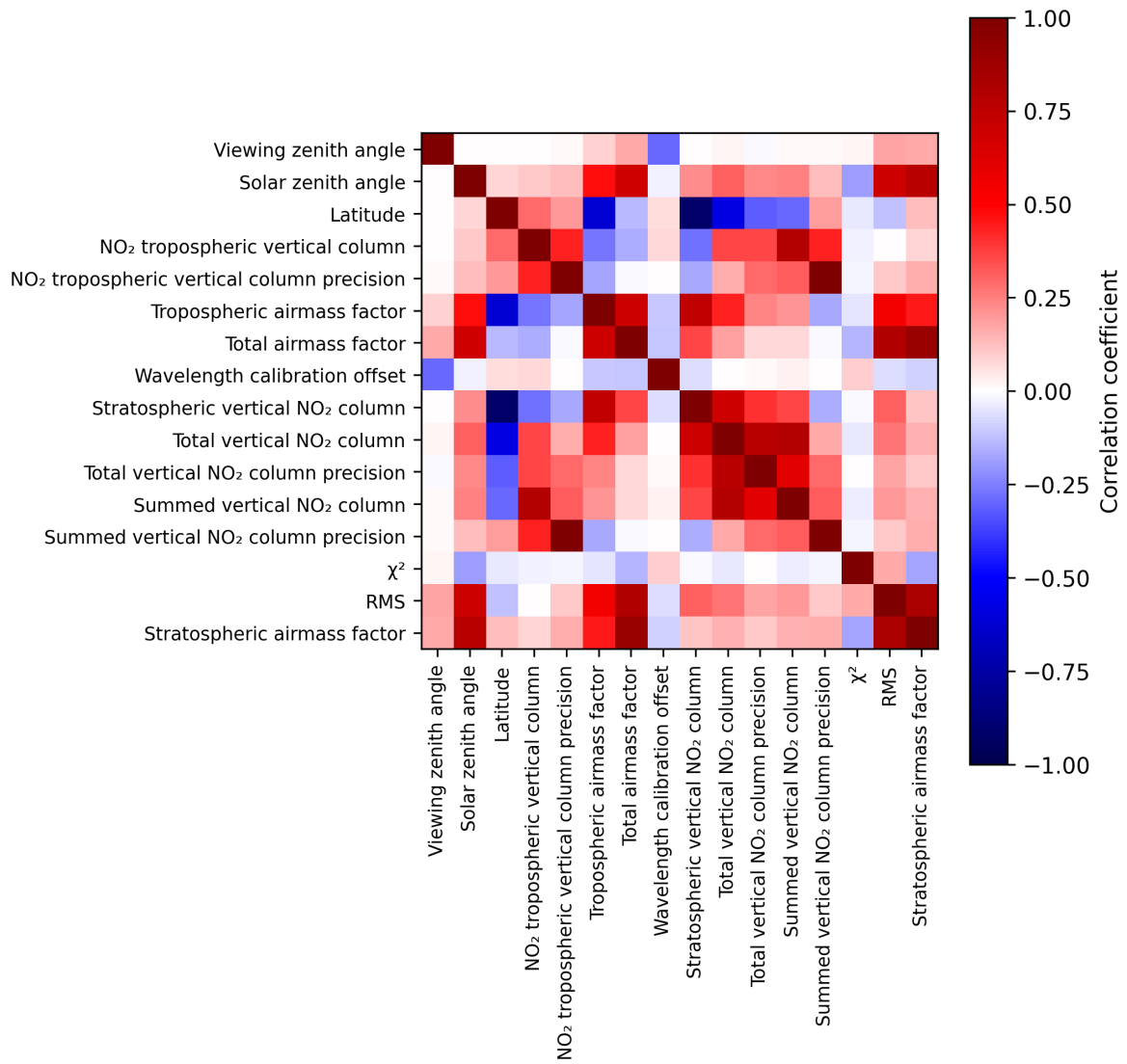
Figure 2: Map of correlation matrix for 2024-12-27 to 2024-12-28.
