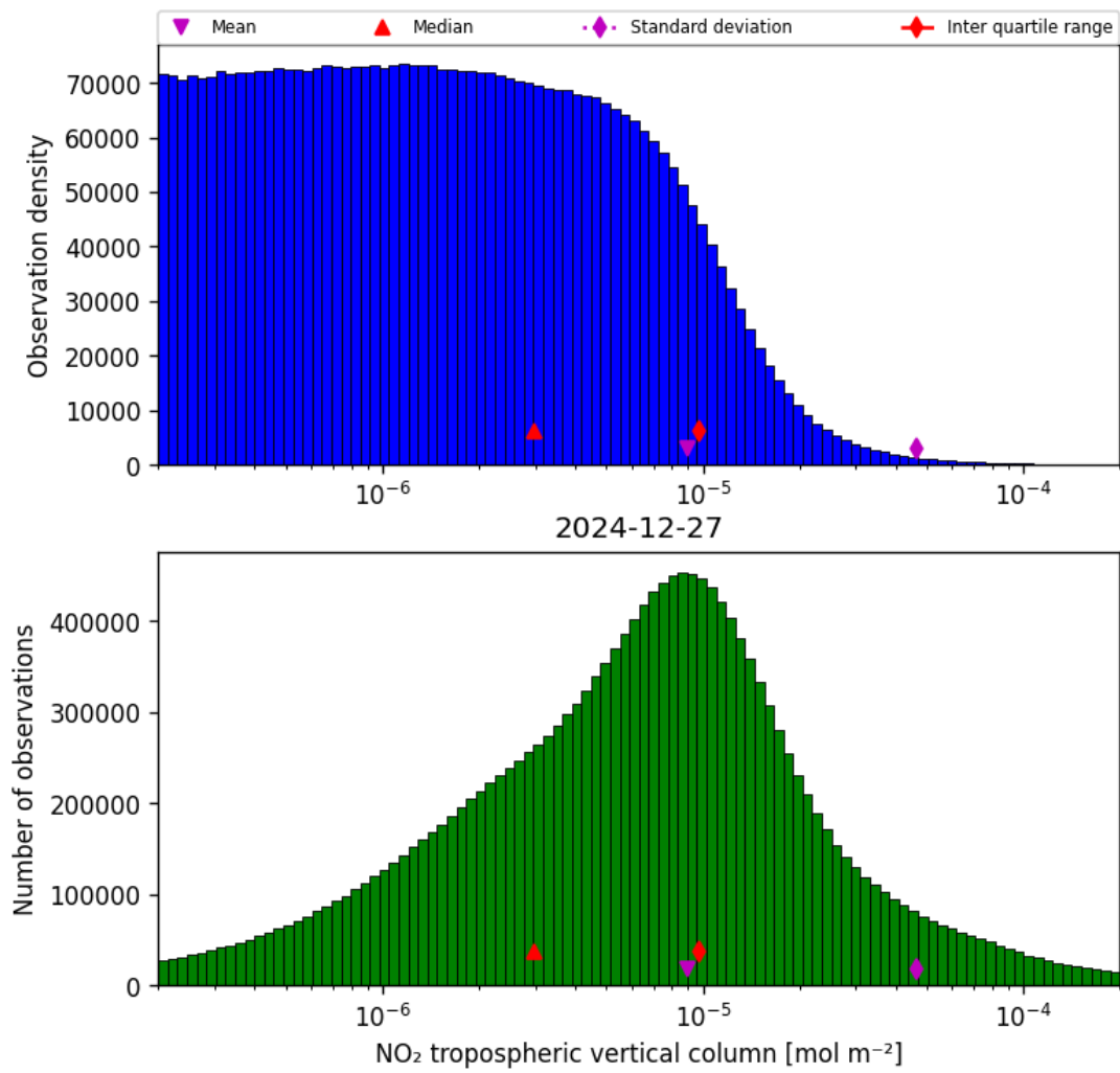
Figure 29: Histogram of “NO 2 tropospheric vertical column” for 2024-12-27 to 2024-12-28
