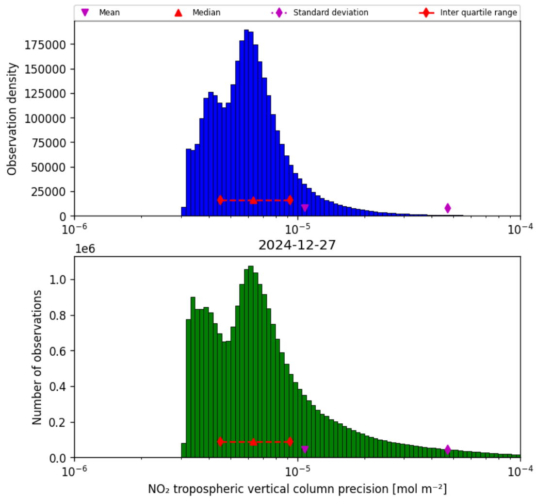
Figure 30: Histogram of “NO 2 tropospheric vertical column precision” for 2024-12-27 to 2024-12-28
