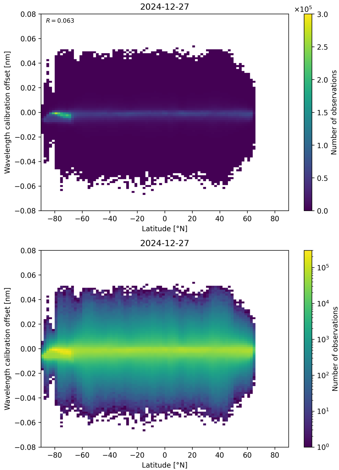
Figure 95: Scatter density plot of “Latitude” against “Wavelength calibration offset” for 2024-12-27 to 2024-12-28.
