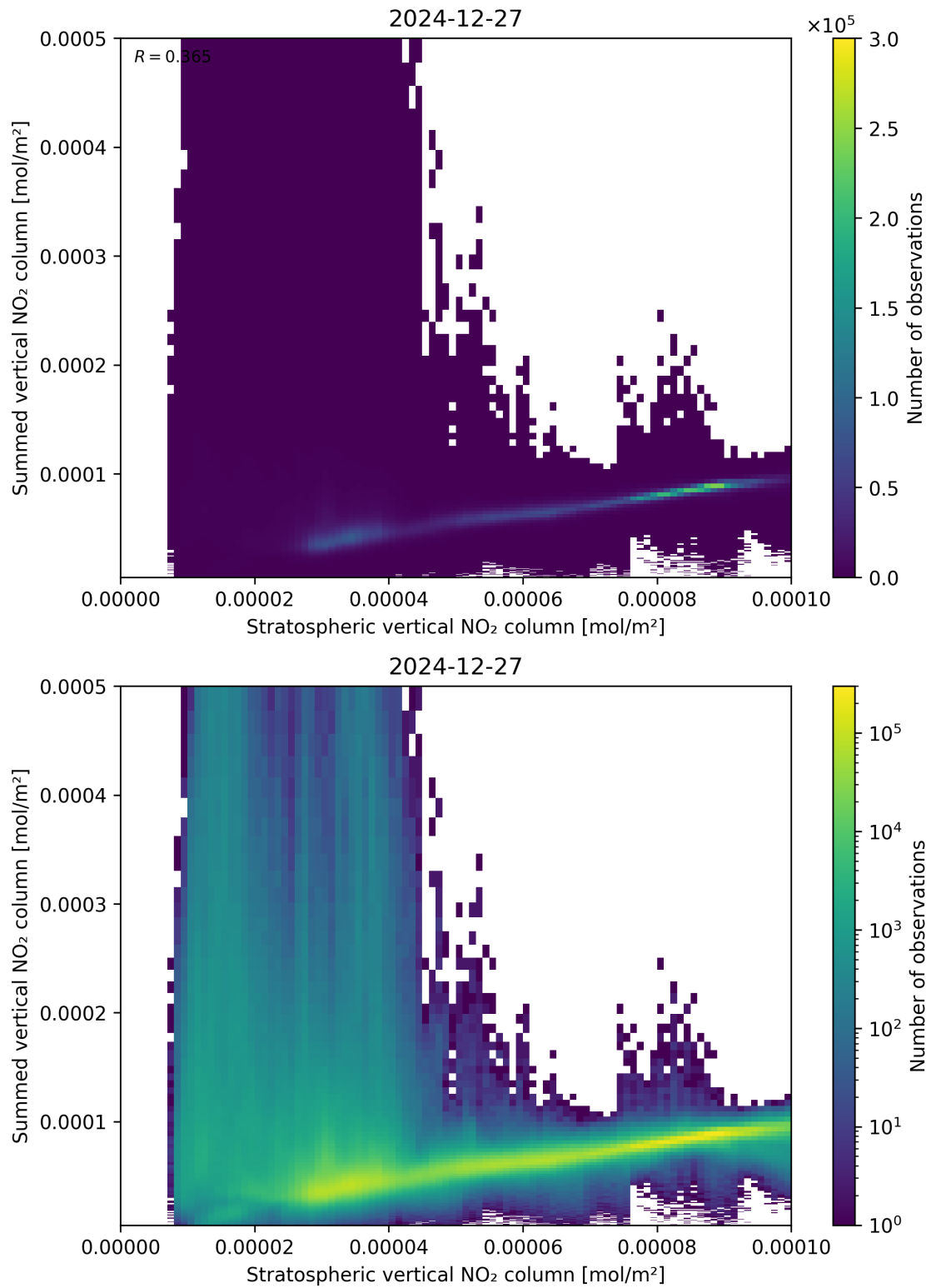
Figure 98: Scatter density plot of “Stratospheric vertical NO 2 column” against “Summed vertical NO 2 column” for 2024-12-27 to 2024-12-28.
