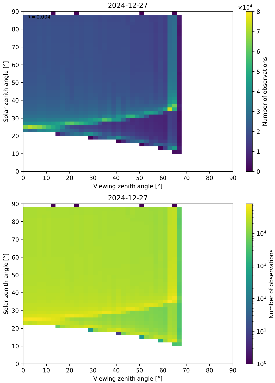
Figure 172: Scatter density plot of “Viewing zenith angle” against “Solar zenith angle” for 2024-12-27 to 2024-12-28.
