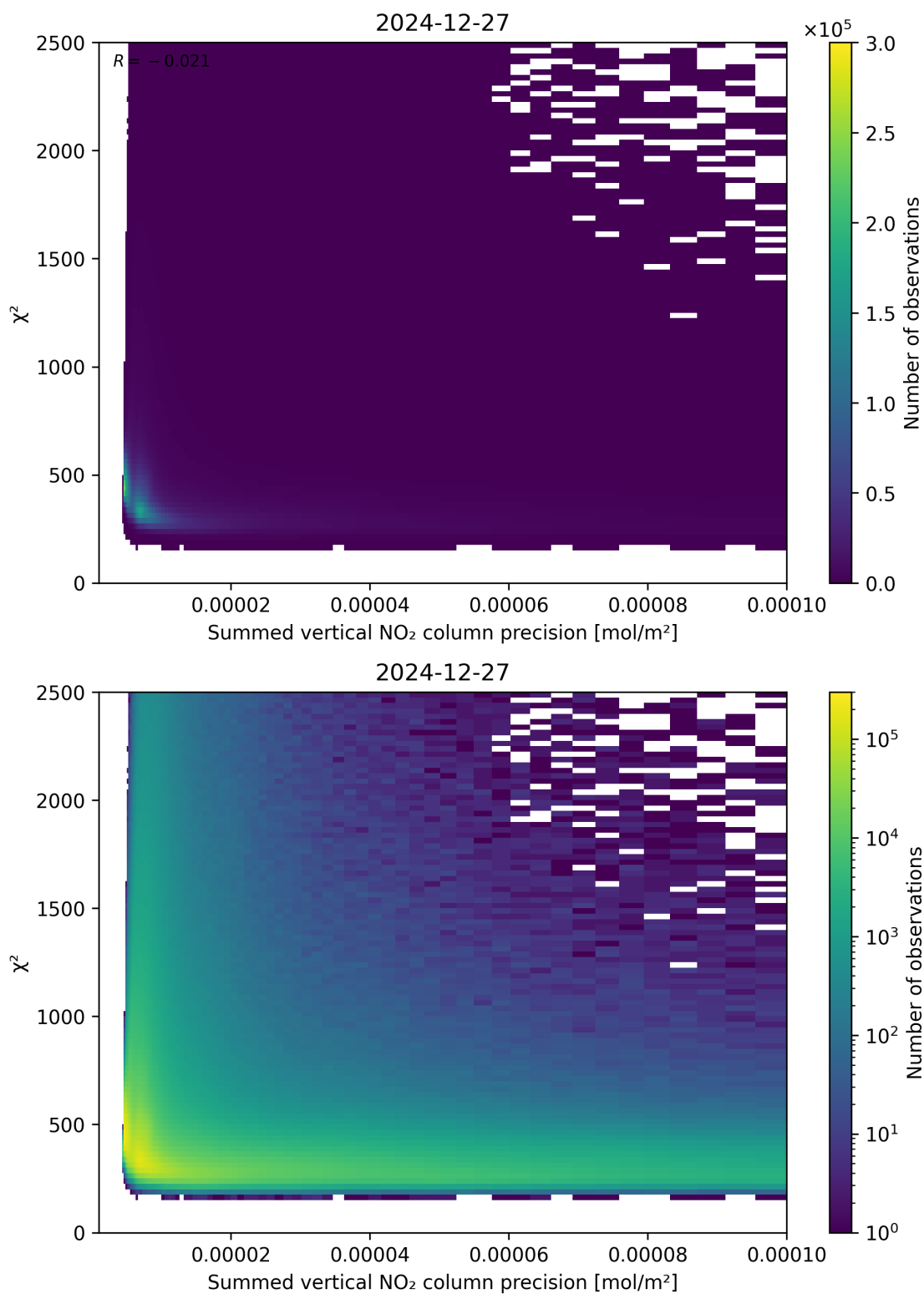
Figure 107: Scatter density plot of “Summed vertical NO 2 column precision” against “ \chi^2 ” for 2024-12-27 to 2024-12-28.
