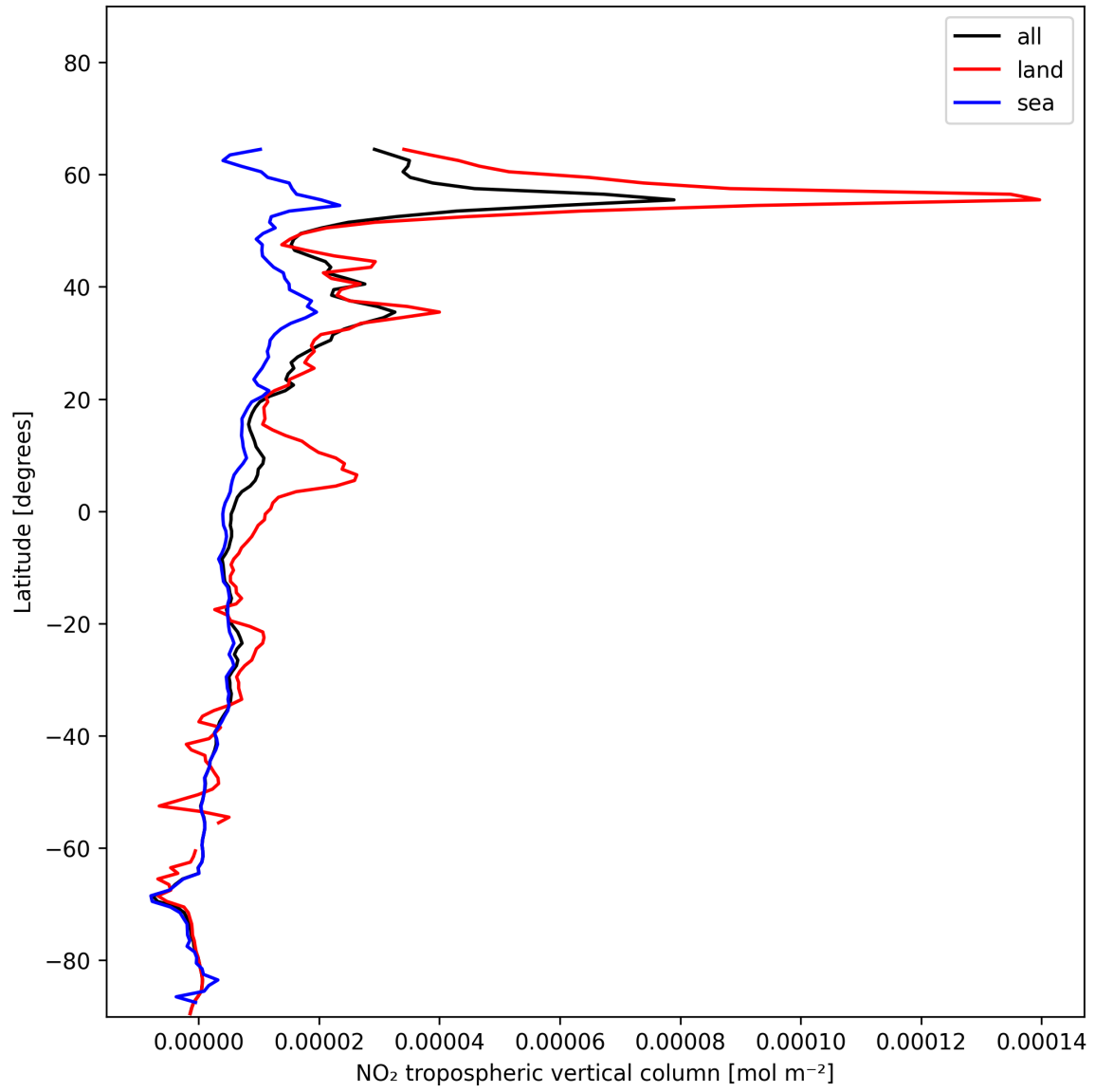
Figure 12: Zonal average of “NO 2 tropospheric vertical column” for 2024-12-27 to 2024-12-28.
