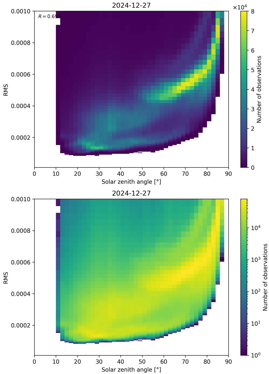
Figure 157: Scatter density plot of “Solar zenith angle” against “RMS” for 2024-12-27 to 2024-12-28.
