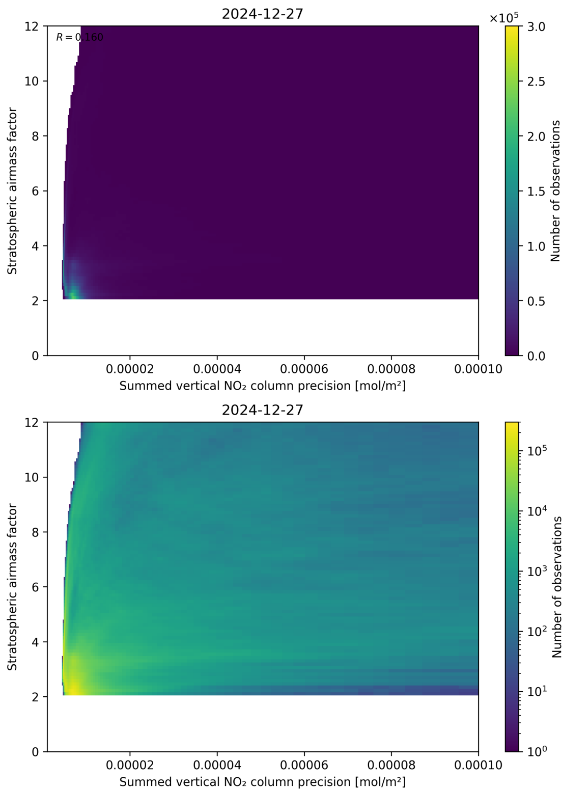
Figure 106: Scatter density plot of “Summed vertical NO 2 column precision” against “Stratospheric airmass factor” for 2024-12-27 to 2024-12-28.
