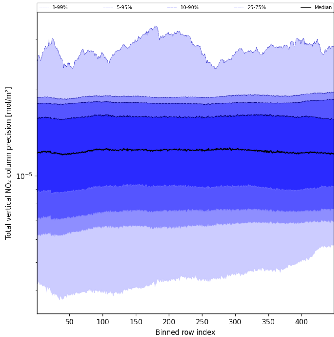
Figure 56: Along track statistics of “Total vertical NO 2 column precision” for 2024-12-27 to 2024-12-28
