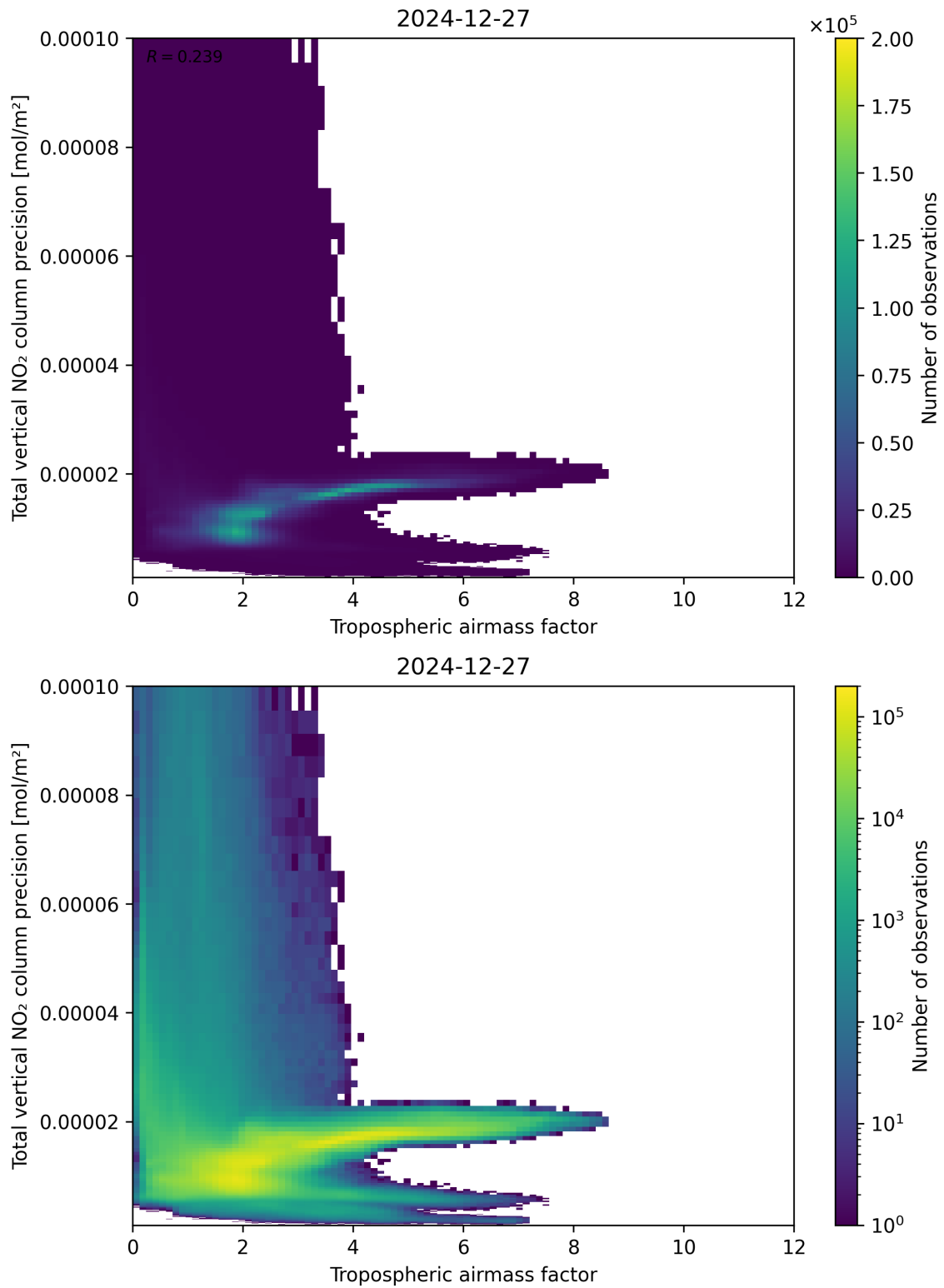
Figure 78: Scatter density plot of “Tropospheric airmass factor” against “Total vertical NO 2 column precision” for 2024-12-27 to 2024-12-28.
