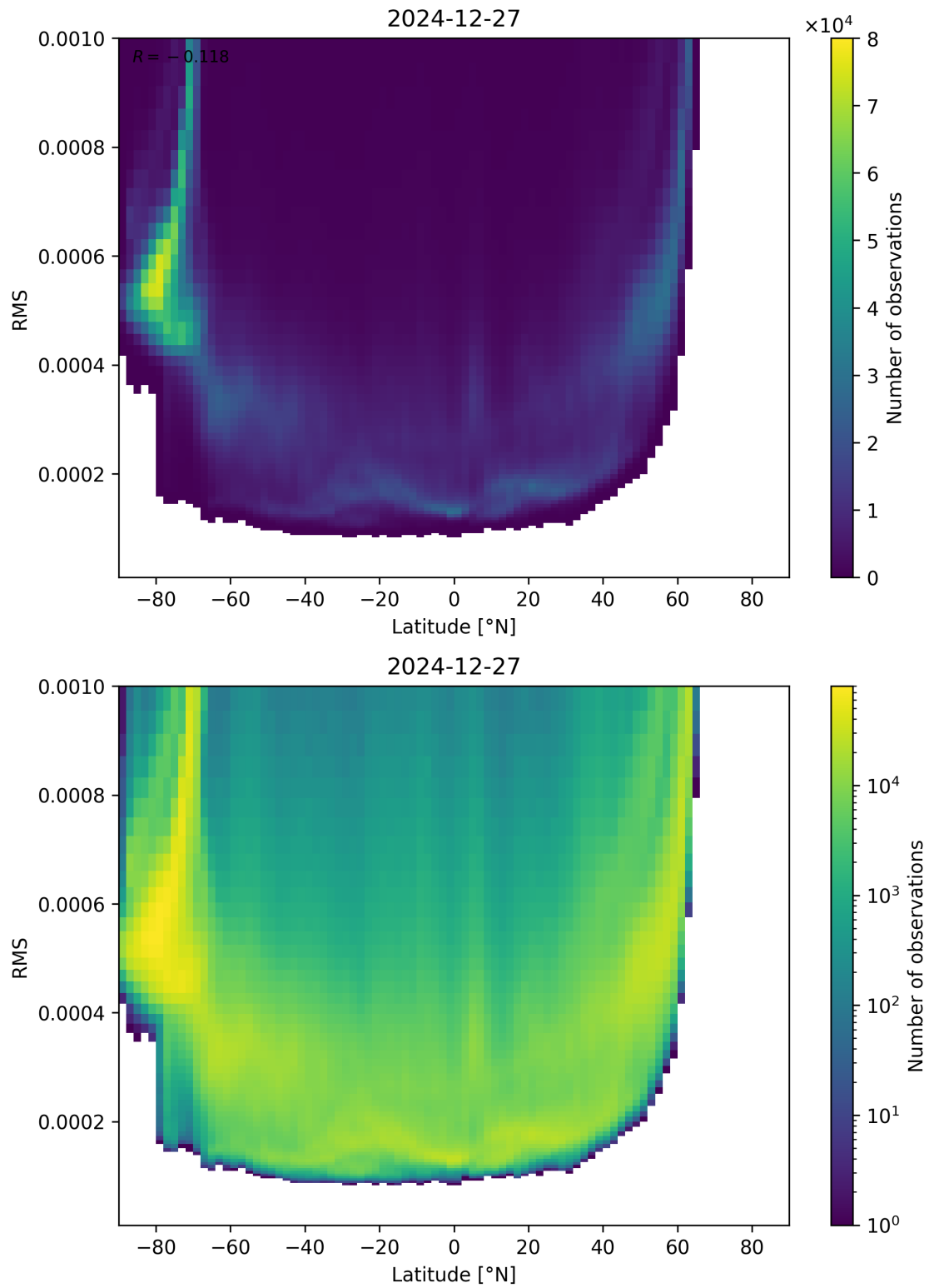
Figure 94: Scatter density plot of “Latitude” against “RMS” for 2024-12-27 to 2024-12-28.
