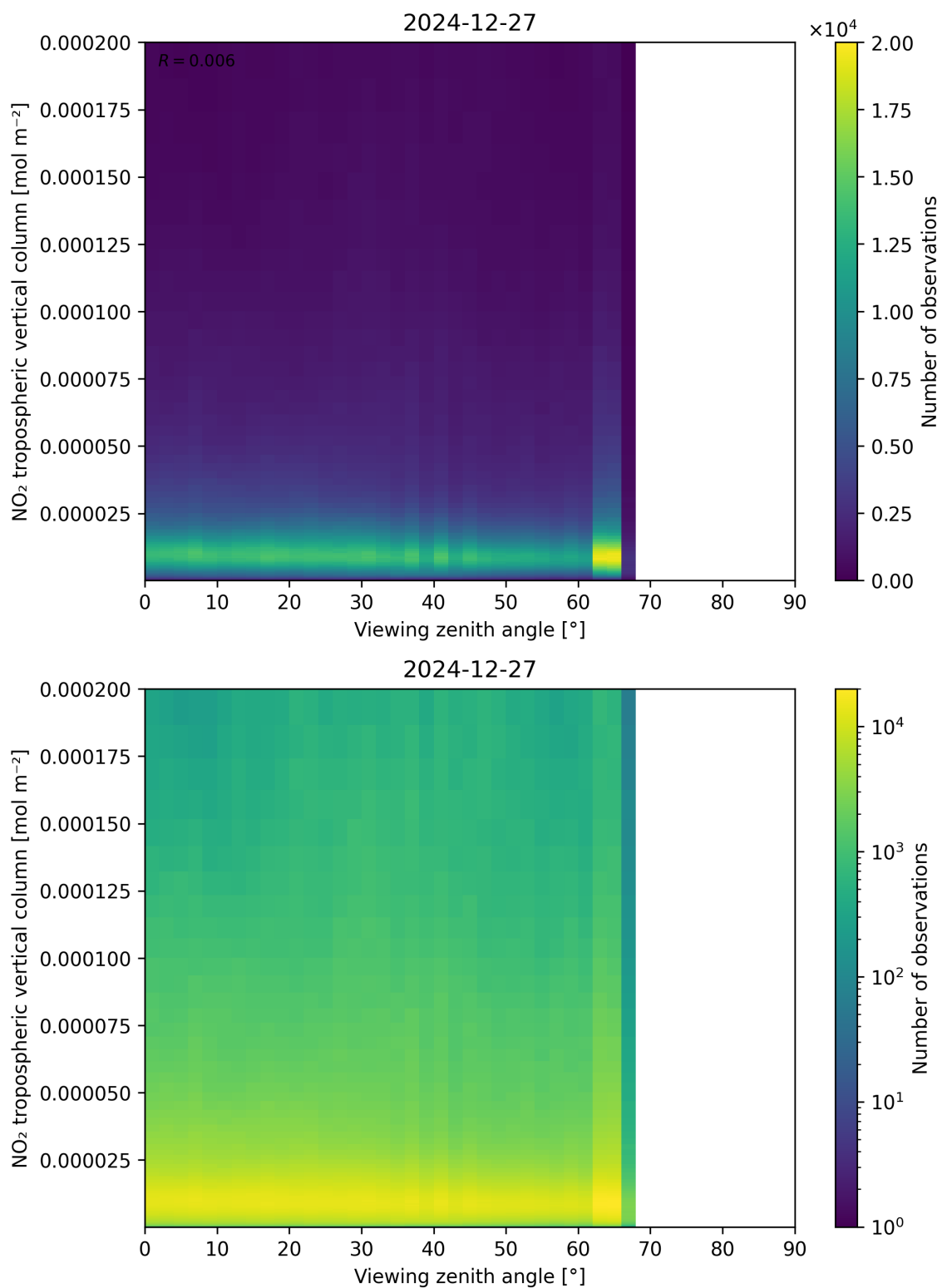
Figure 169: Scatter density plot of “Viewing zenith angle” against “NO 2 tropospheric vertical column” for 2024-12-27 to 2024-12-28.
