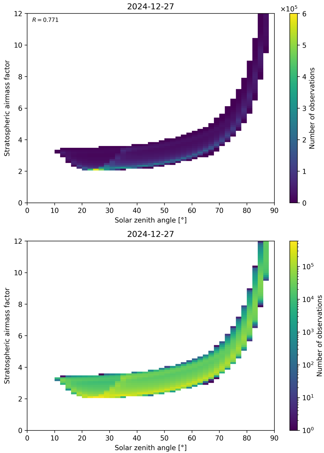
Figure 145: Scatter density plot of “Solar zenith angle” against “Stratospheric airmass factor” for 2024-12-27 to 2024-12-28.
