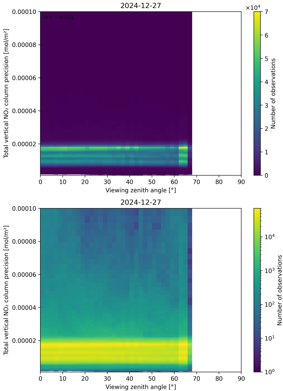
Figure 168: Scatter density plot of “Viewing zenith angle” against “Total vertical NO 2 column precision” for 2024-12-27 to 2024-12-28.
