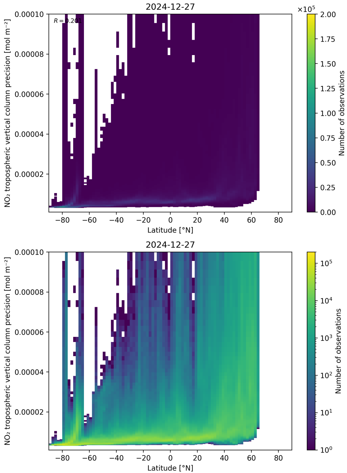
Figure 93: Scatter density plot of “Latitude” against “NO 2 tropospheric vertical column precision” for 2024-12-27 to 2024-12-28.
