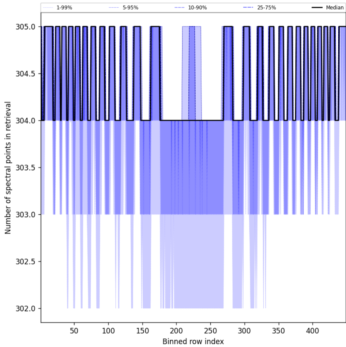
Figure 50: Along track statistics of “Number of spectral points in retrieval” for 2024-12-27 to 2024-12-28
