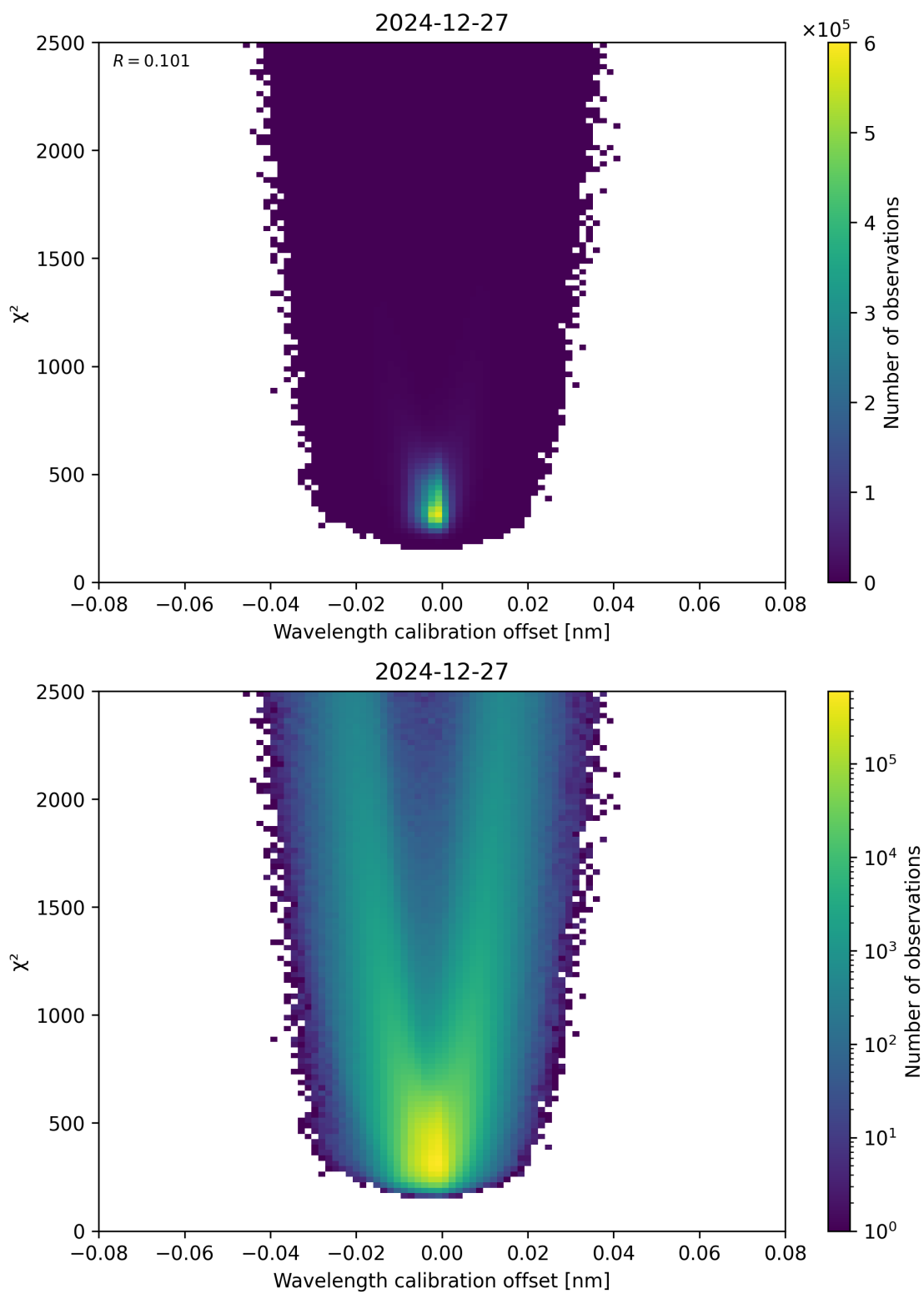
Figure 175: Scatter density plot of “Wavelength calibration offset” against “ \chi^2 ” for 2024-12-27 to 2024-12-28.
