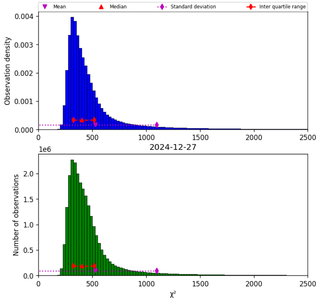
Figure 42: Histogram of “ \chi^2 ” for 2024-12-27 to 2024-12-28
