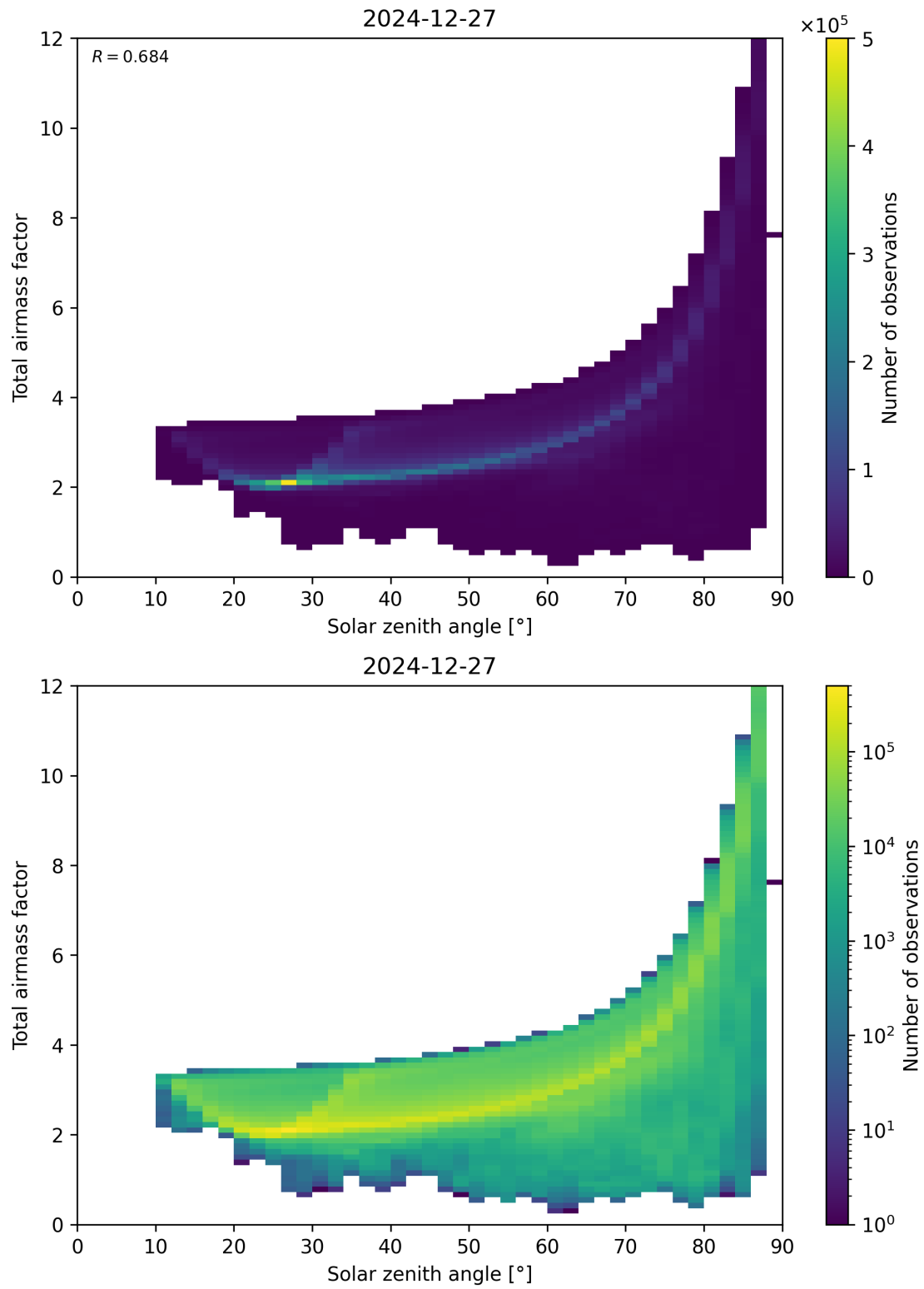
Figure 146: Scatter density plot of “Solar zenith angle” against “Total airmass factor” for 2024-12-27 to 2024-12-28.
