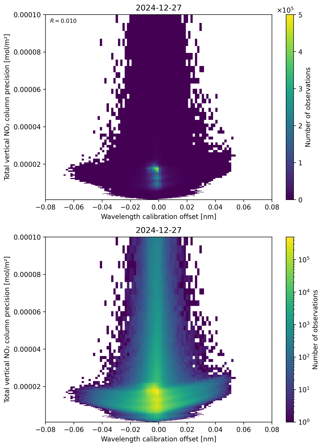
Figure 180: Scatter density plot of “Wavelength calibration offset” against “Total vertical NO 2 column precision” for 2024-12-27 to 2024-12-28.
