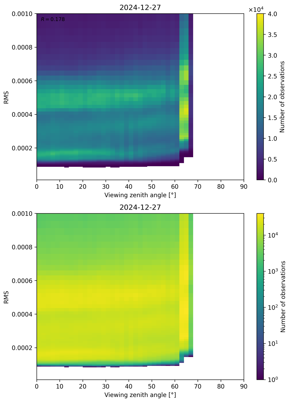
Figure 171: Scatter density plot of “Viewing zenith angle” against “RMS” for 2024-12-27 to 2024-12-28.
