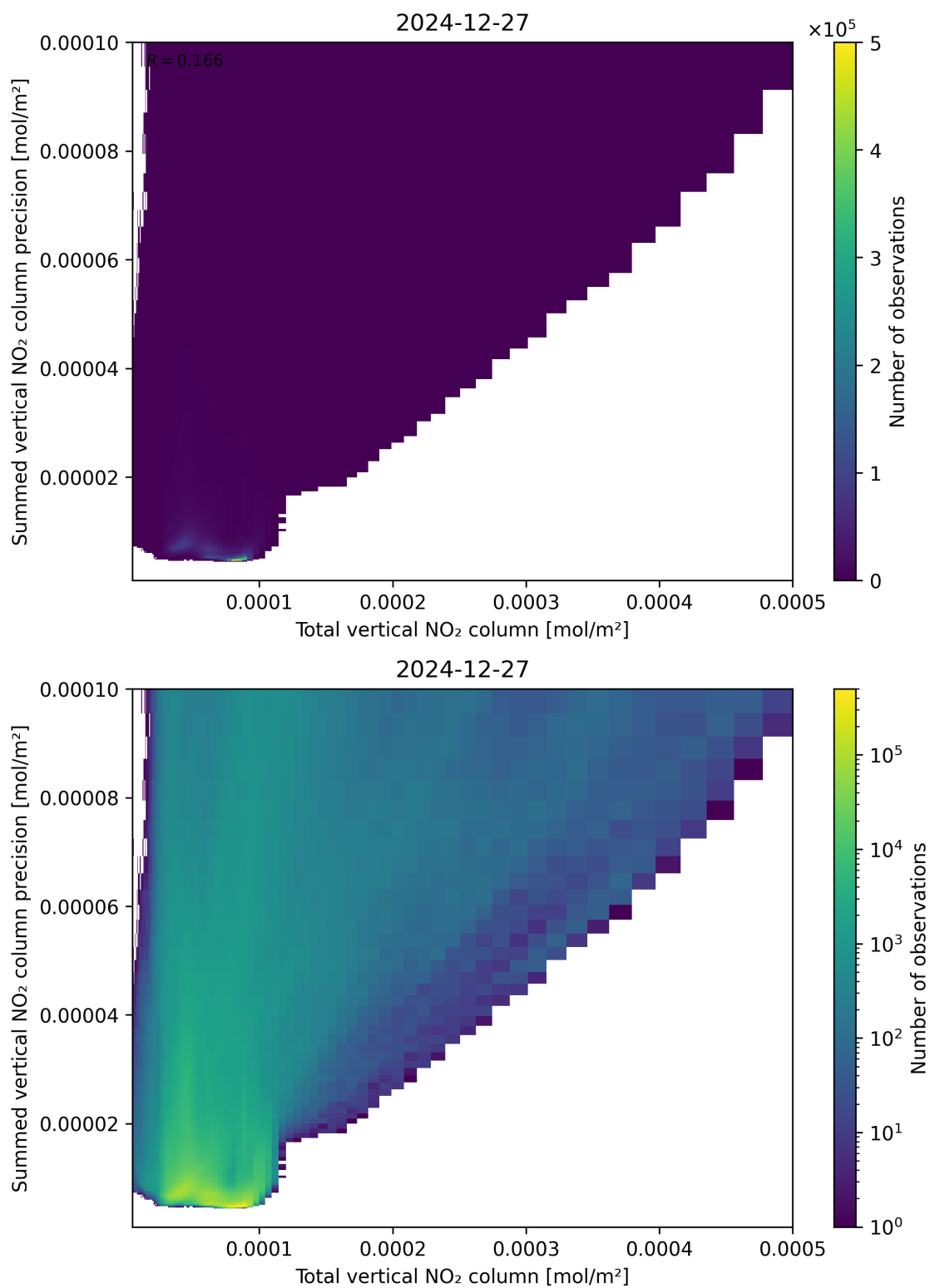
Figure 113: Scatter density plot of “Total vertical NO 2 column” against “Summed vertical NO 2 column precision” for 2024-12-27 to 2024-12-28.
