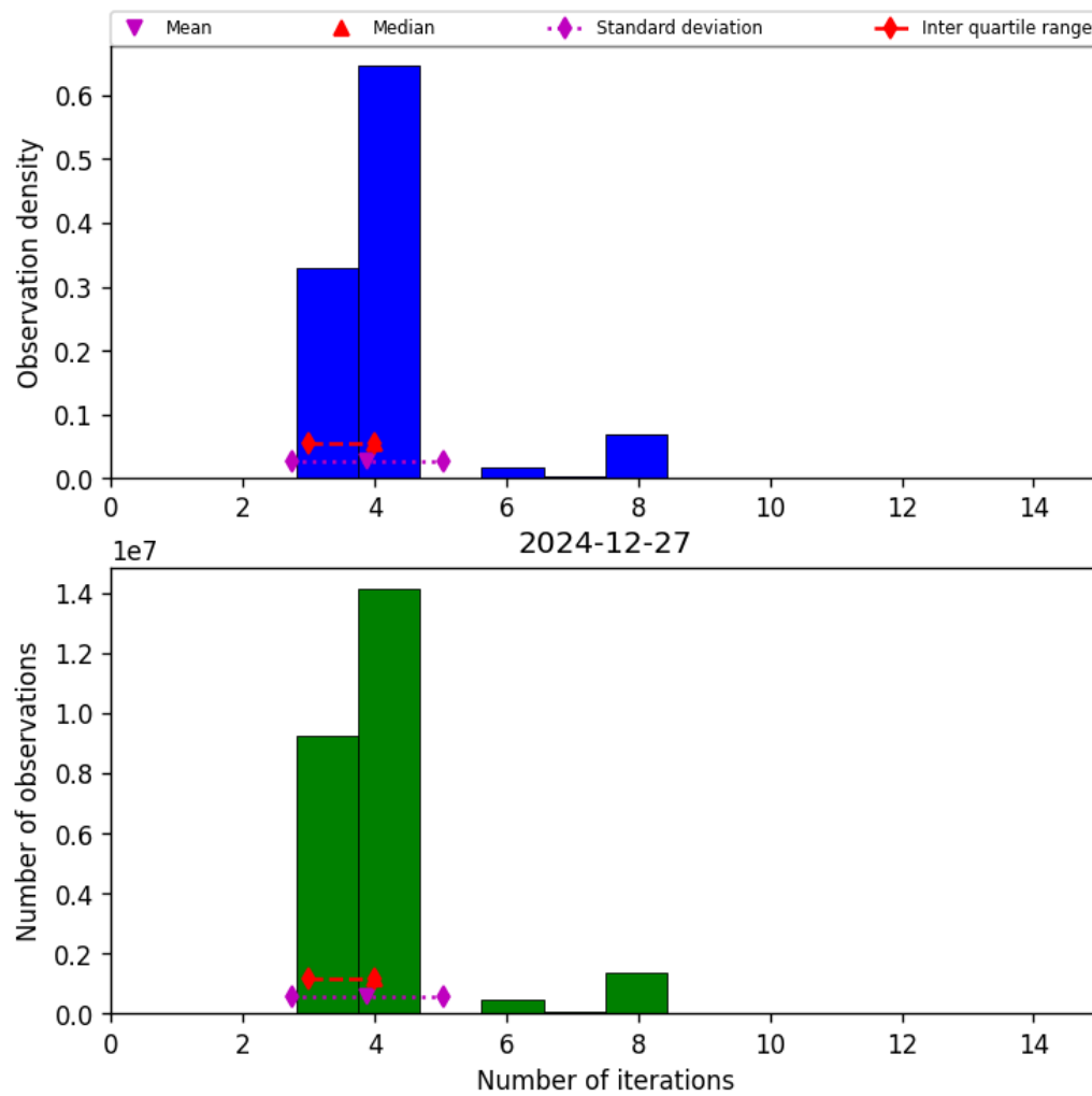
Figure 34: Histogram of “Number of iterations” for 2024-12-27 to 2024-12-28
