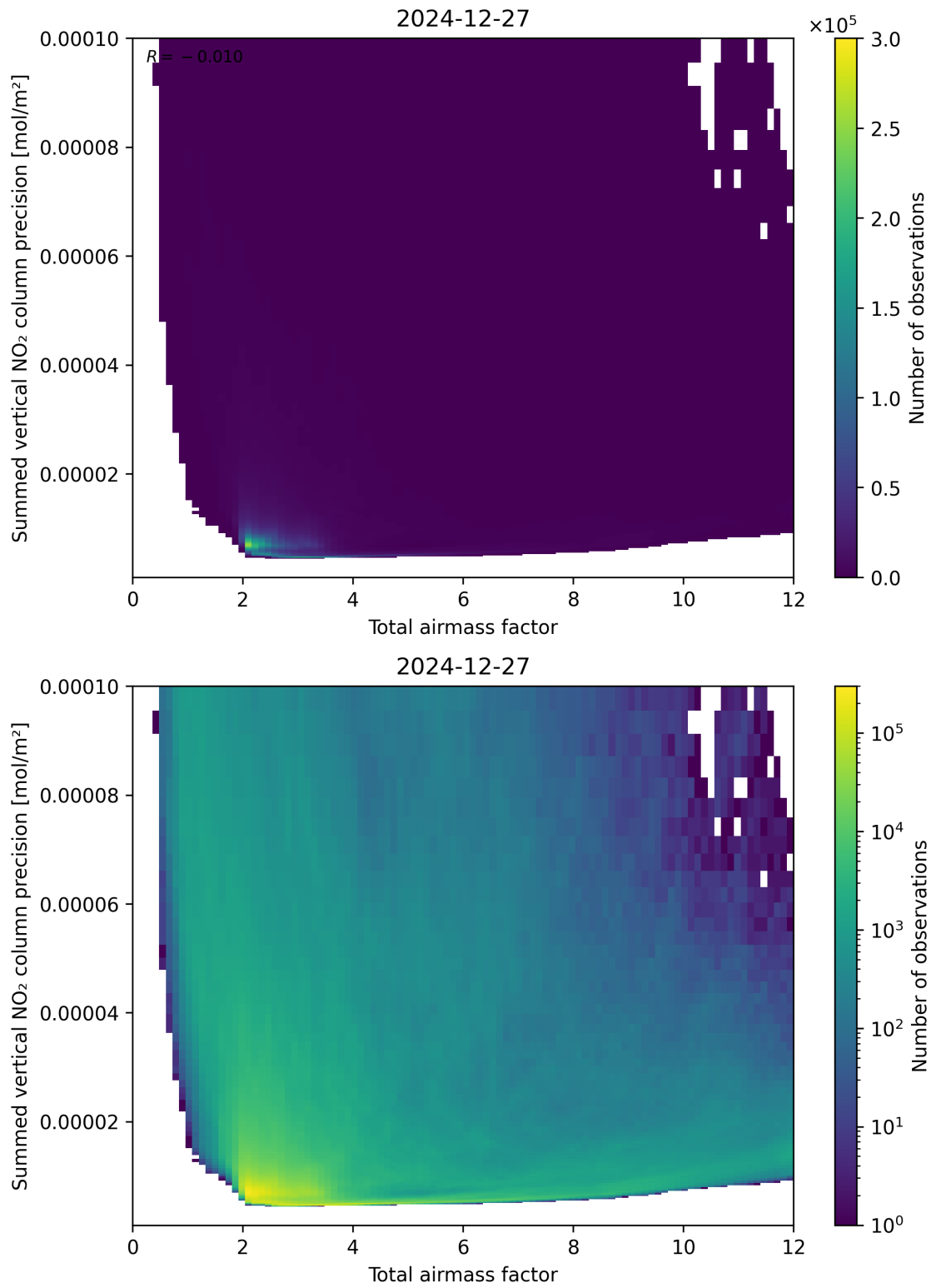
Figure 66: Scatter density plot of “Total airmass factor” against “Summed vertical NO 2 column precision” for 2024-12-27 to 2024-12-28.
