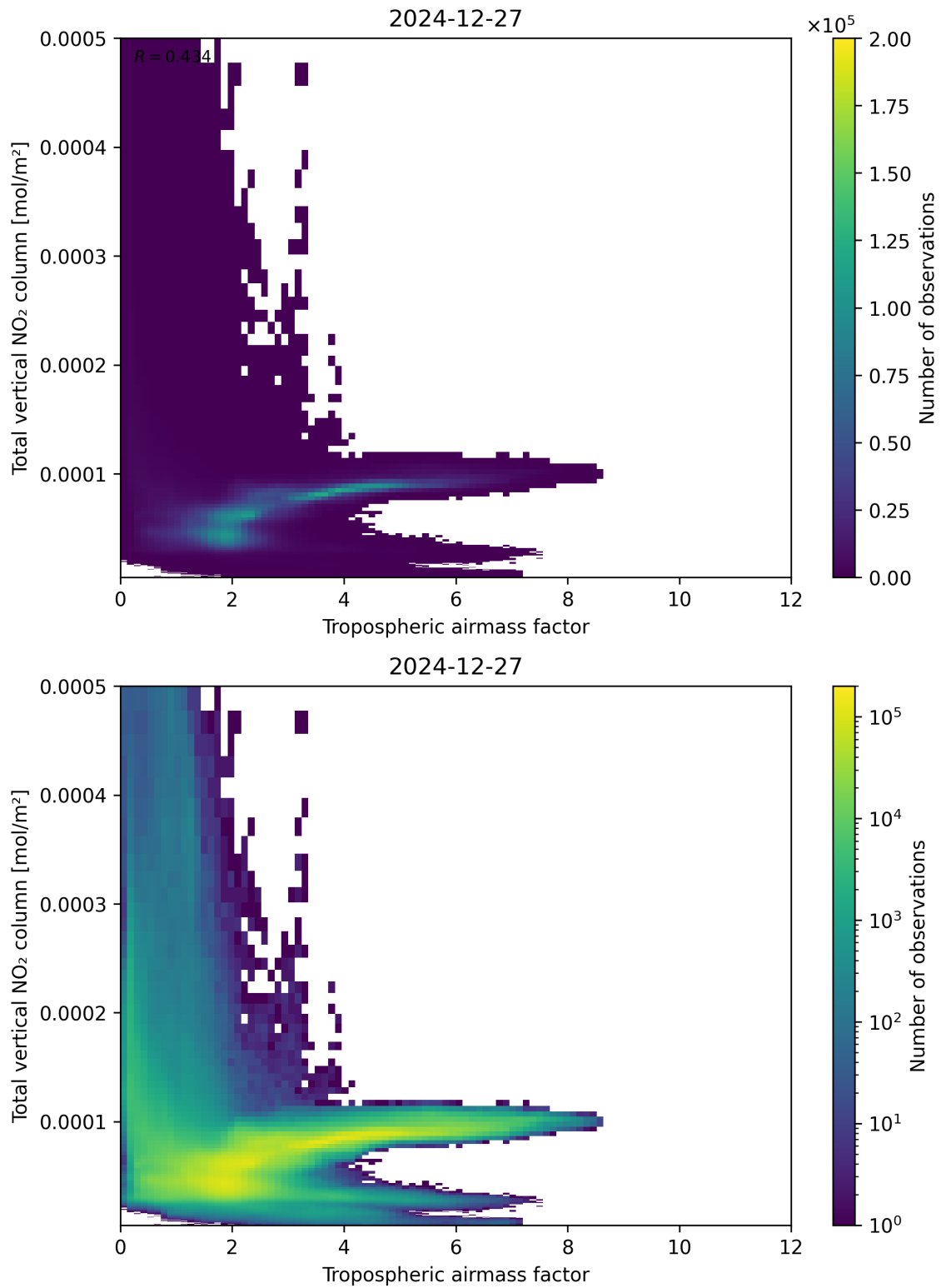
Figure 77: Scatter density plot of “Tropospheric airmass factor” against “Total vertical \text{NO}_2 column” for 2024-12-27 to 2024-12-28.
