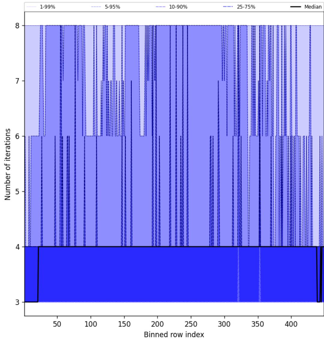
Figure 51: Along track statistics of “Number of iterations” for 2024-12-27 to 2024-12-28
