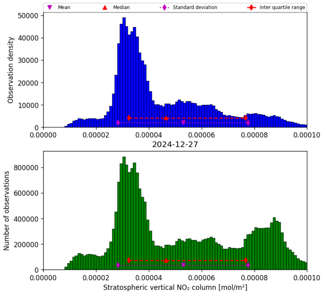
Figure 36: Histogram of “Stratospheric vertical NO 2 column” for 2024-12-27 to 2024-12-28
