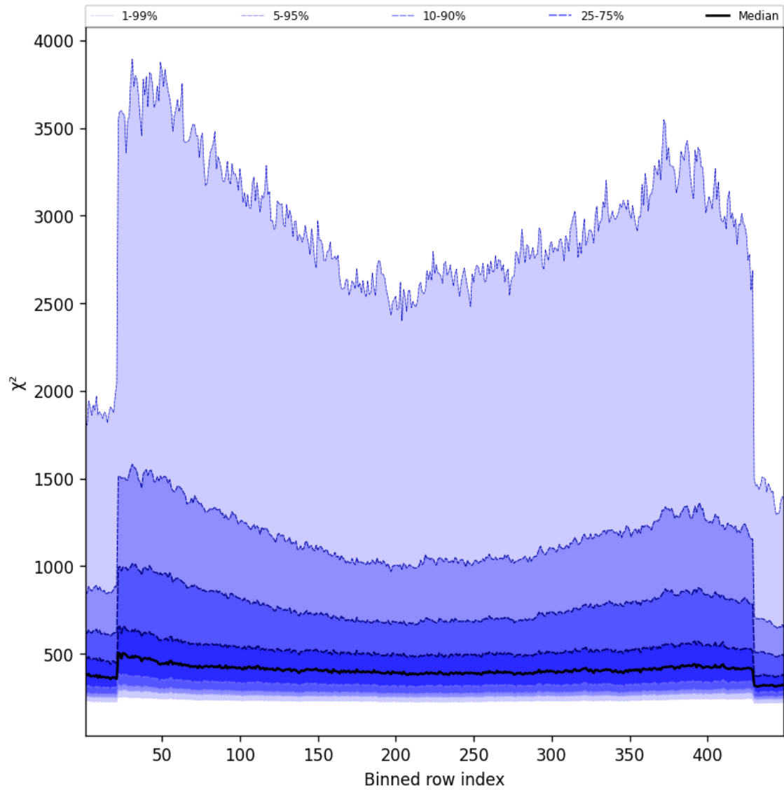
Figure 59: Along track statistics of “ \chi^2 ” for 2024-12-27 to 2024-12-28
