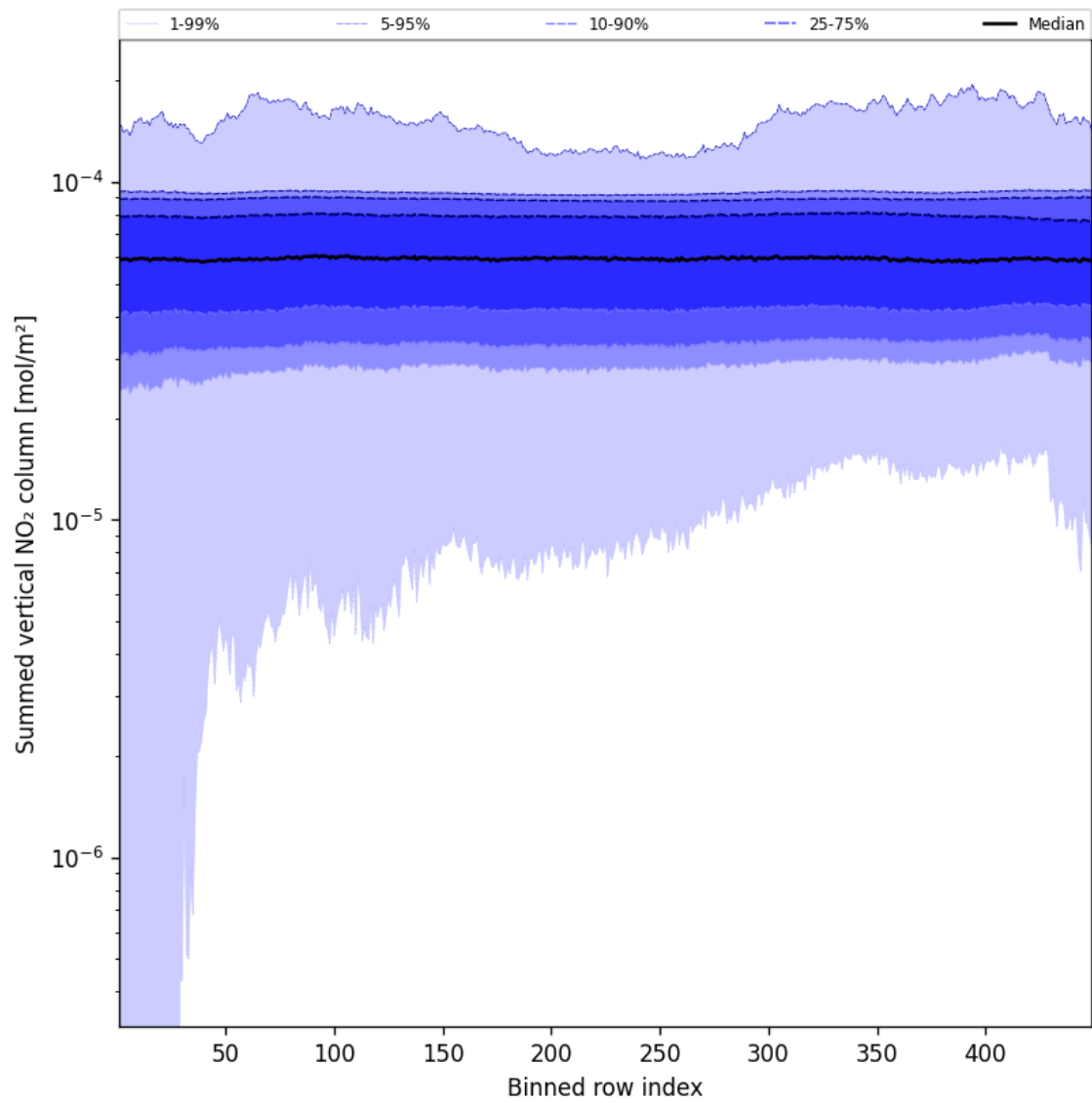
Figure 57: Along track statistics of “Summed vertical NO 2 column” for 2024-12-27 to 2024-12-28
