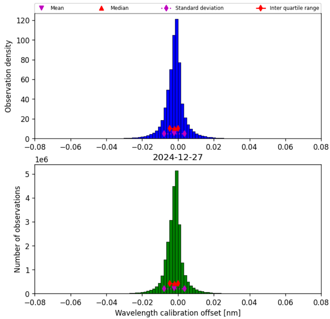
Figure 35: Histogram of “Wavelength calibration offset” for 2024-12-27 to 2024-12-28
