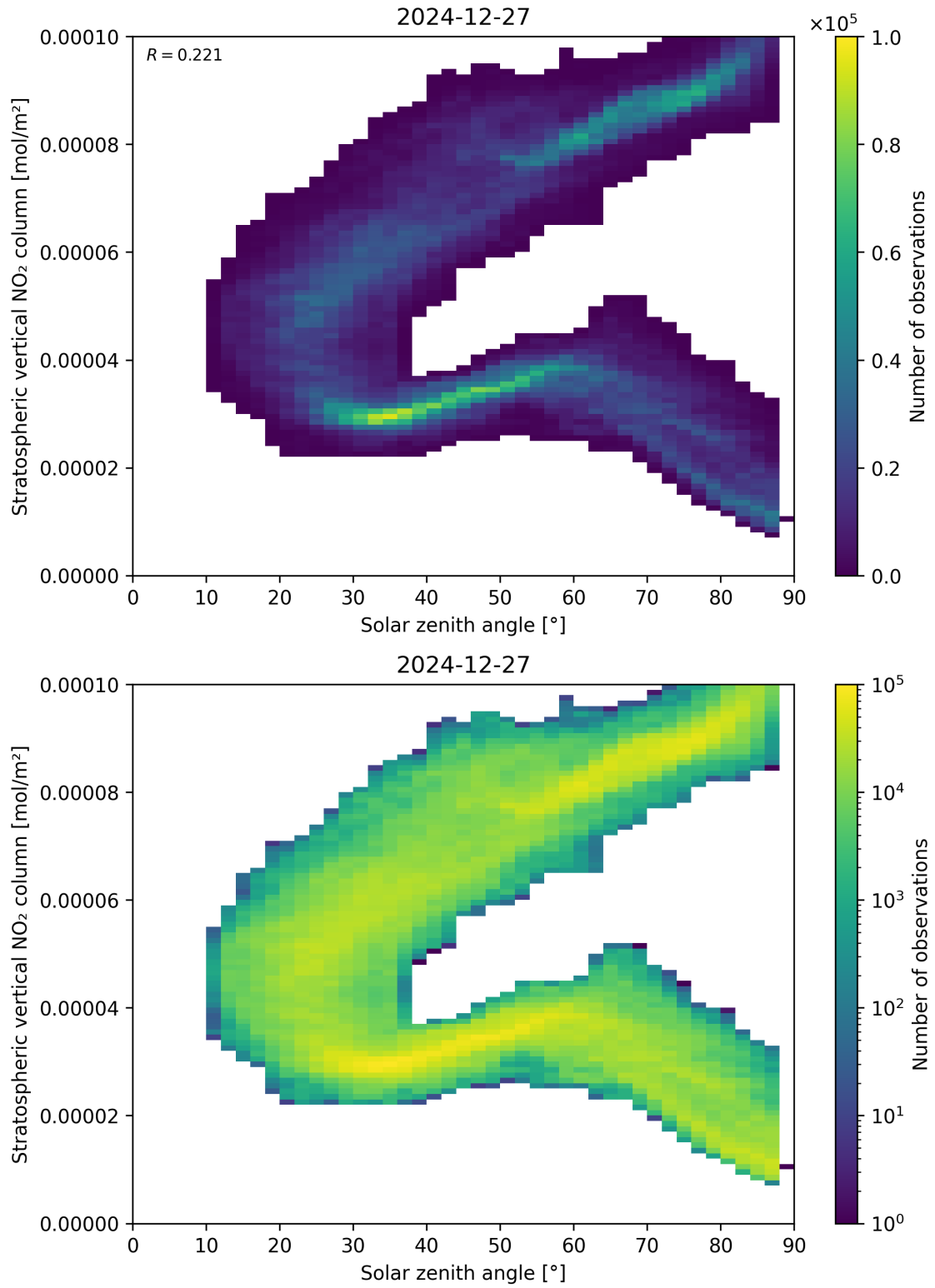
Figure 150: Scatter density plot of “Solar zenith angle” against “Stratospheric vertical \text{NO}_2 column” for 2024-12-27 to 2024-12-28.
