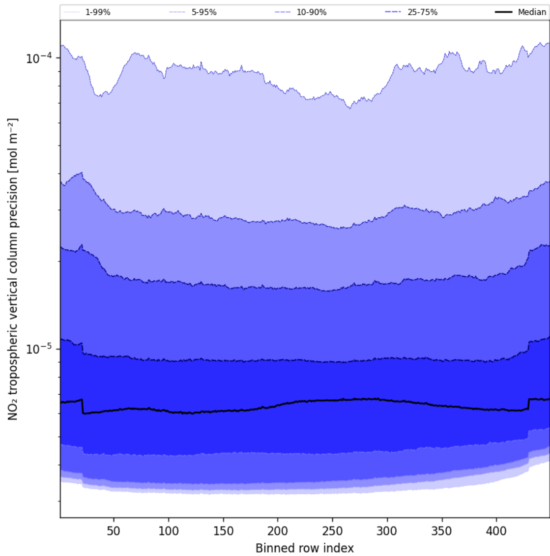
Figure 47: Along track statistics of “NO 2 tropospheric vertical column precision” for 2024-12-27 to 2024-12-28
