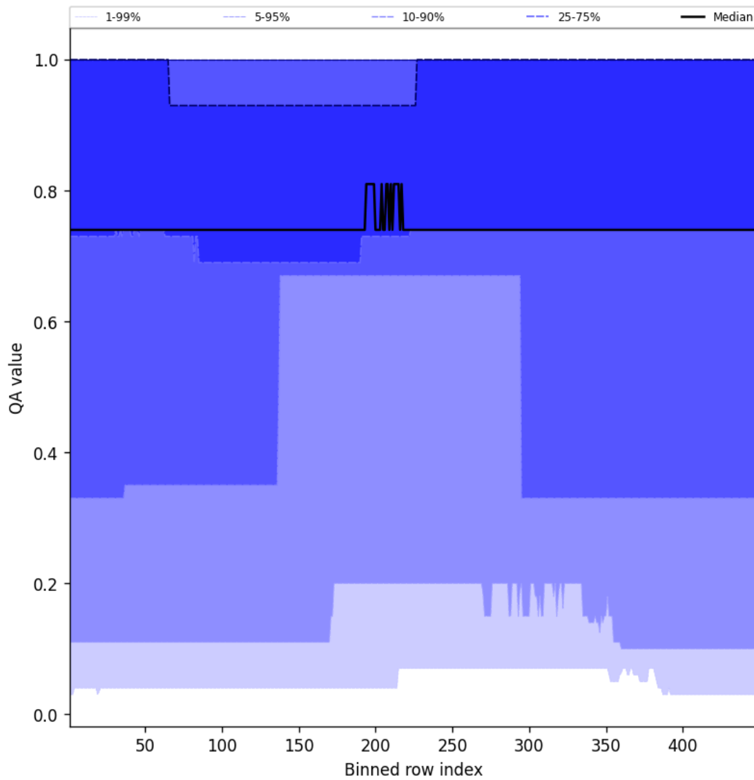
Figure 45: Along track statistics of "QA value" for 2024-12-27 to 2024-12-28
