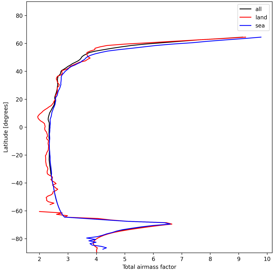
Figure 15: Zonal average of “Total airmass factor” for 2024-12-27 to 2024-12-28.
