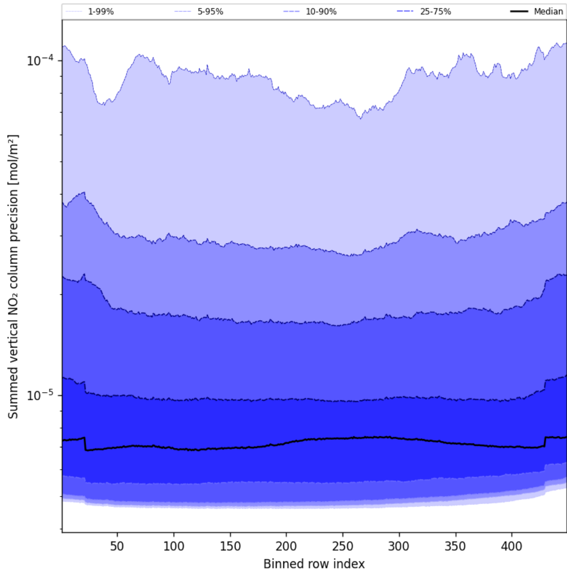
Figure 58: Along track statistics of “Summed vertical NO 2 column precision” for 2024-12-27 to 2024-12-28
