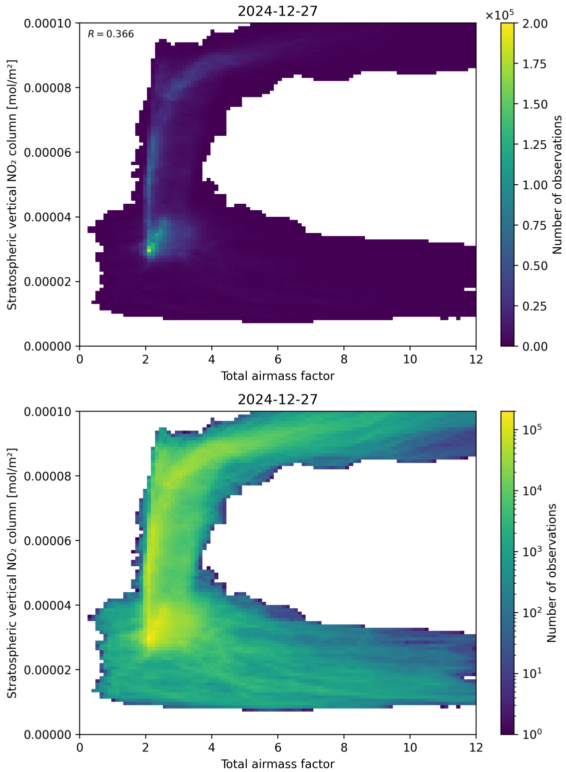
Figure 64: Scatter density plot of “Total airmass factor” against “Stratospheric vertical \text{NO}_2 column” for 2024-12-27 to 2024-12-28.
