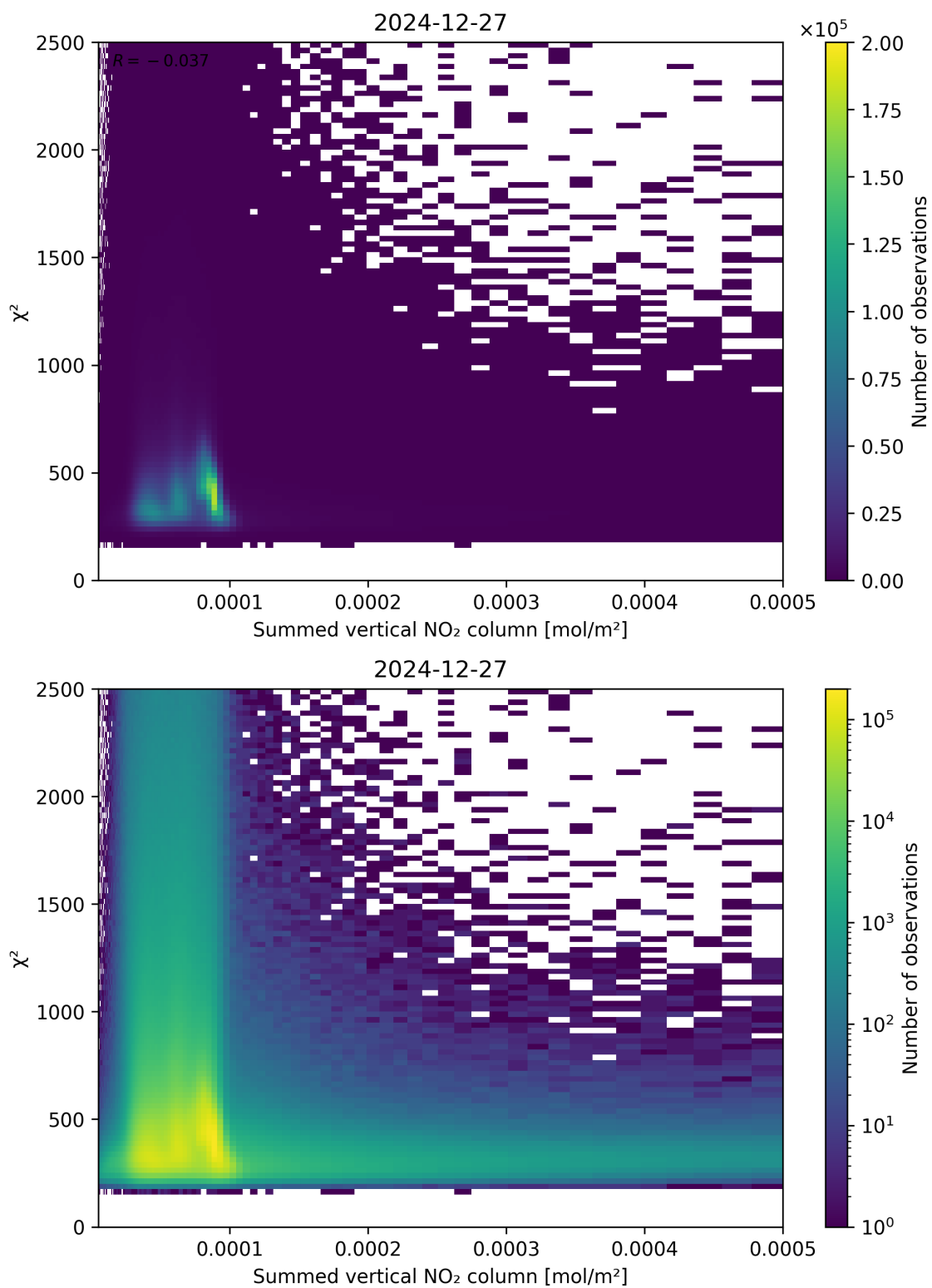
Figure 104: Scatter density plot of “Summed vertical NO 2 column” against “ \chi^2 ” for 2024-12-27 to 2024-12-28.
