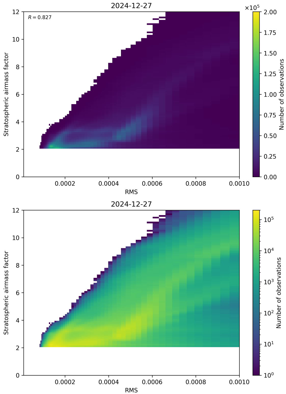
Figure 144: Scatter density plot of “RMS” against “Stratospheric airmass factor” for 2024-12-27 to 2024-12-28.
