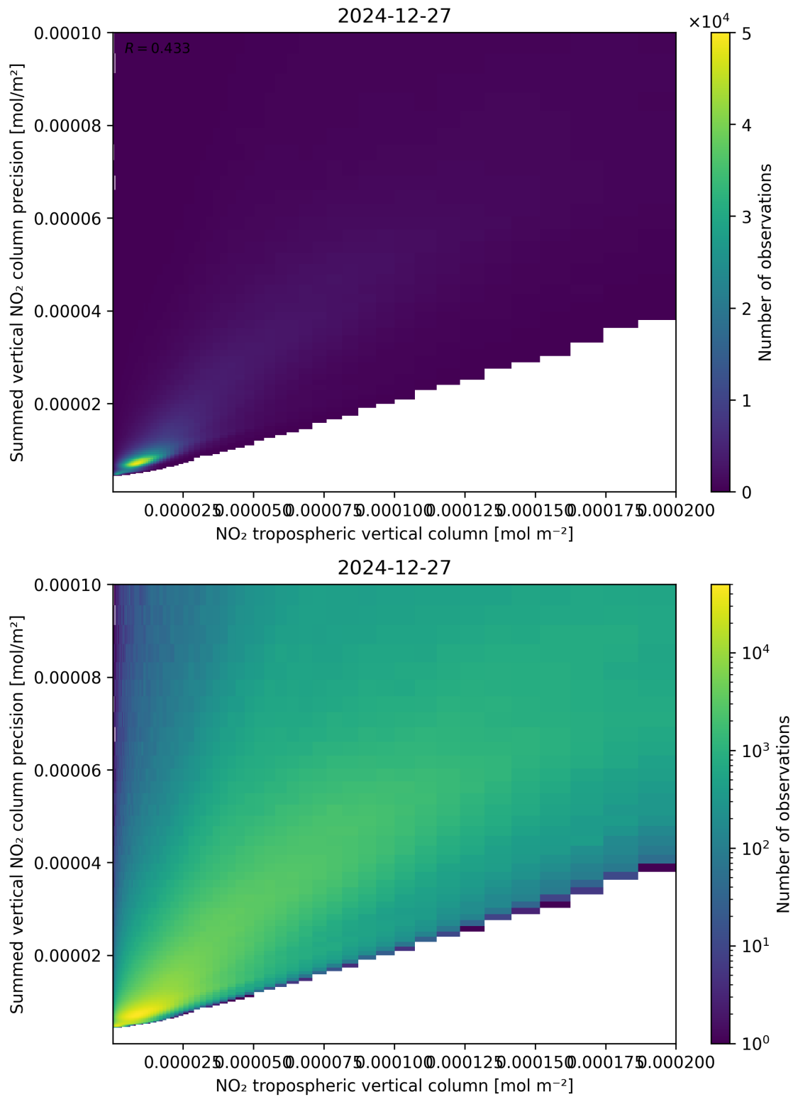
Figure 127: Scatter density plot of “NO 2 tropospheric vertical column” against “Summed vertical NO 2 column precision” for 2024-12-27 to 2024-12-28.
