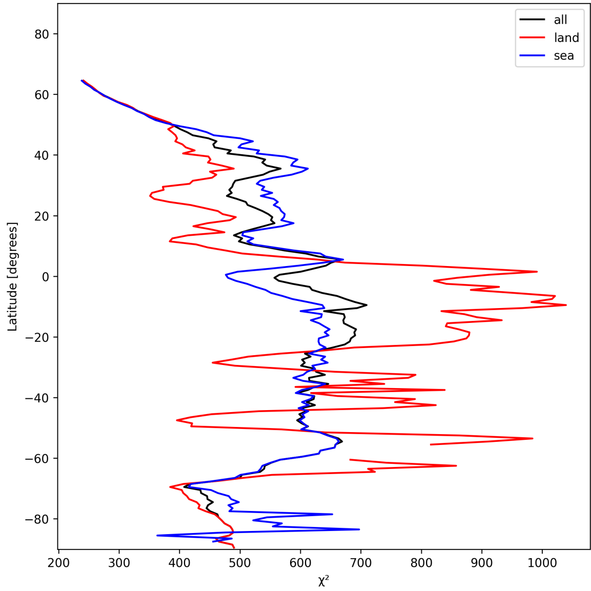
Figure 25: Zonal average of “ \chi^2 ” for 2024-12-27 to 2024-12-28.
