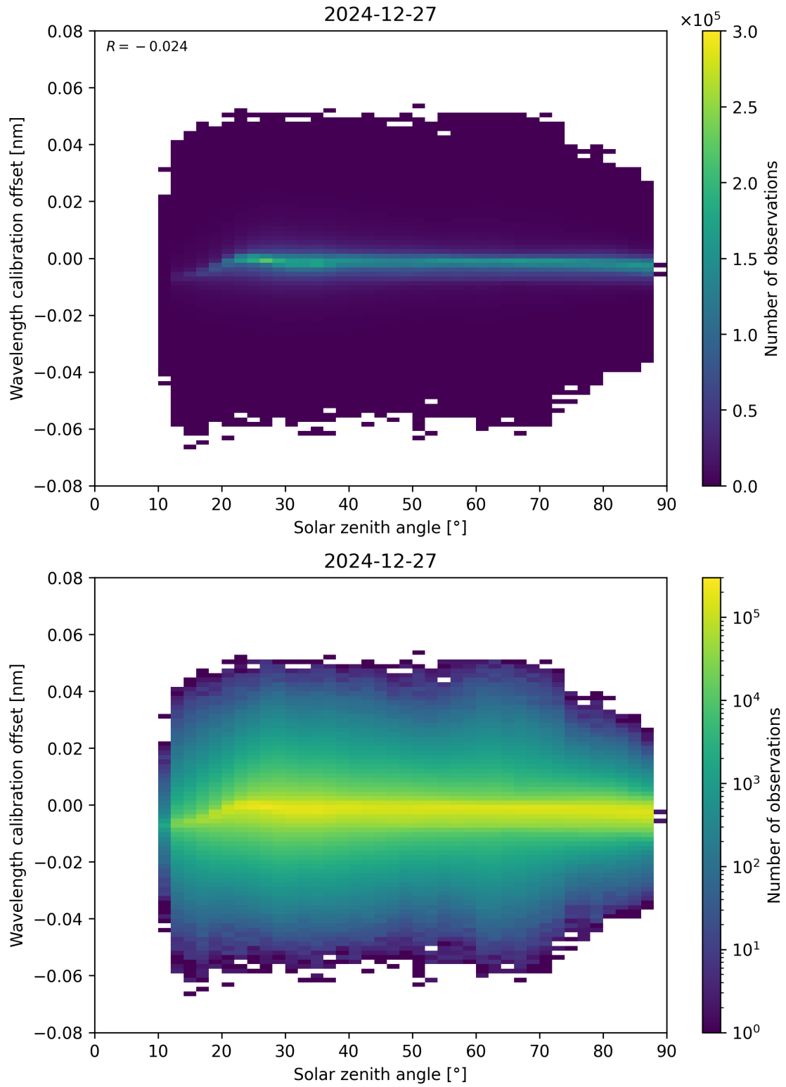
Figure 158: Scatter density plot of “Solar zenith angle” against “Wavelength calibration offset” for 2024-12-27 to 2024-12-28.
