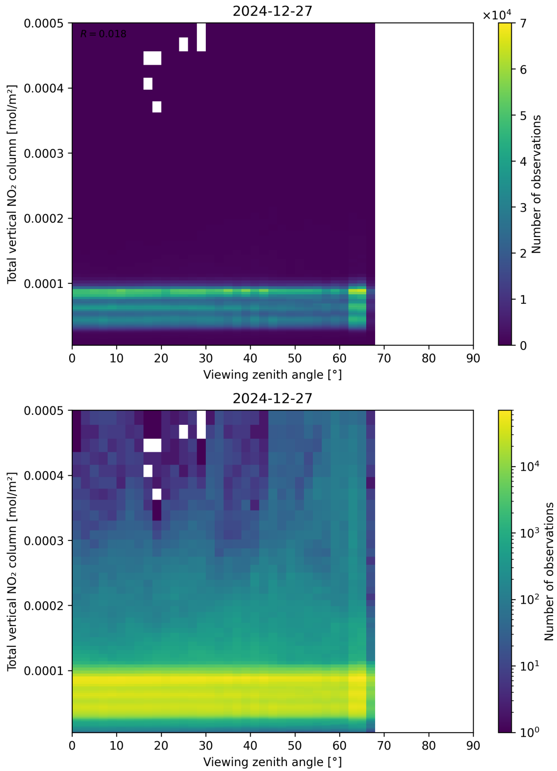
Figure 167: Scatter density plot of “Viewing zenith angle” against “Total vertical NO 2 column” for 2024-12-27 to 2024-12-28.
