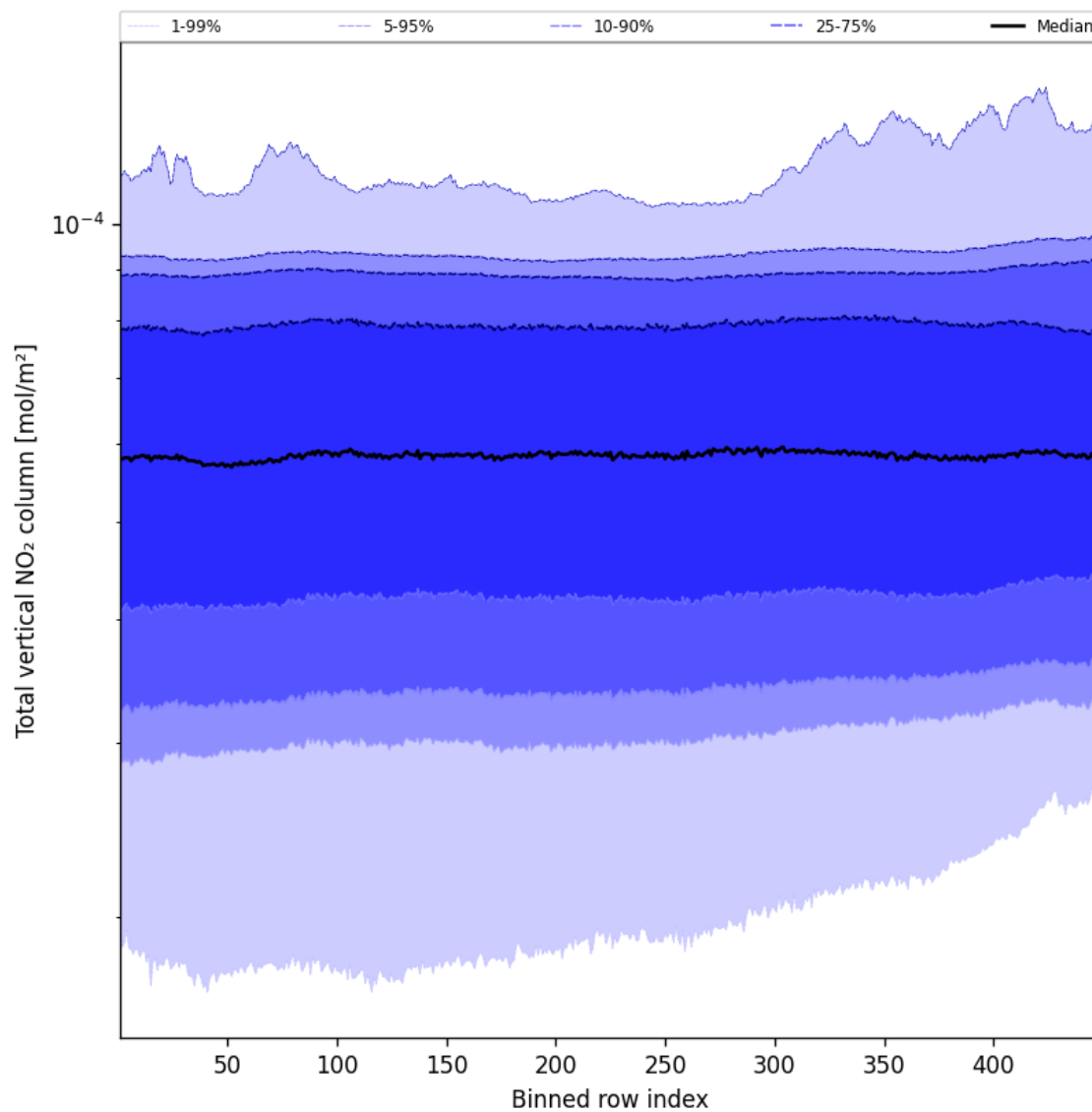
Figure 55: Along track statistics of “Total vertical NO 2 column” for 2024-12-27 to 2024-12-28
