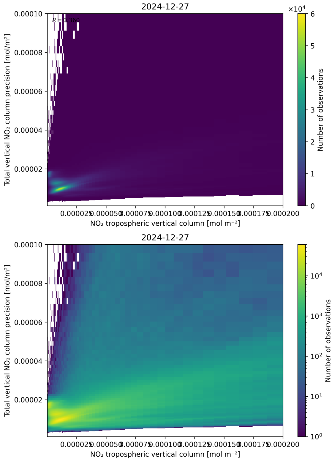
Figure 129: Scatter density plot of “NO 2 tropospheric vertical column” against “Total vertical NO 2 column precision” for 2024-12-27 to 2024-12-28.
