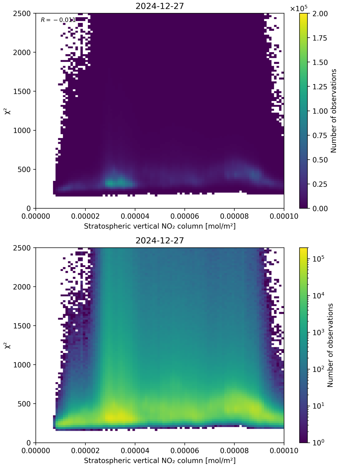
Figure 97: Scatter density plot of “Stratospheric vertical NO 2 column” against “ \chi^2 ” for 2024-12-27 to 2024-12-28.
