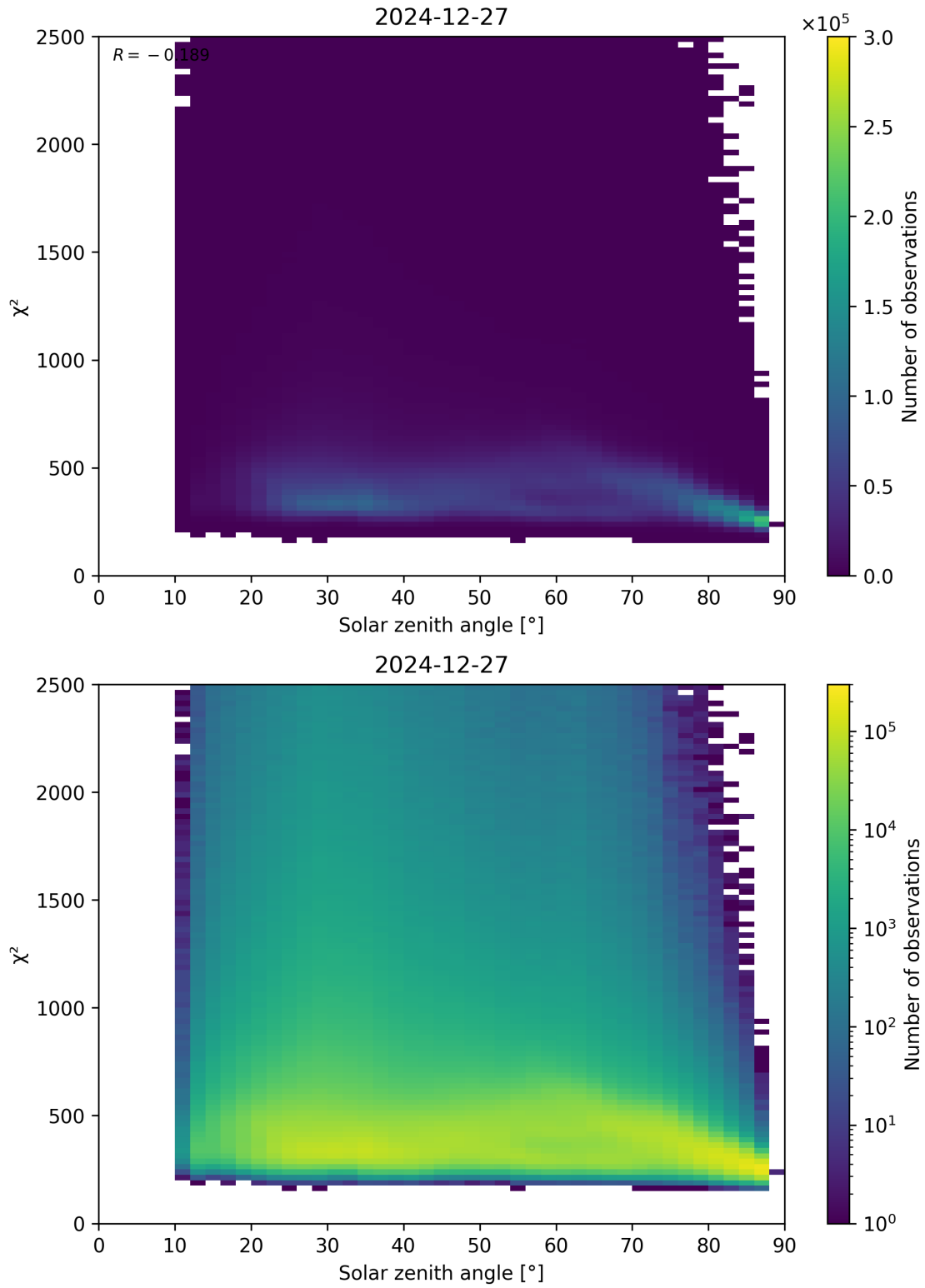
Figure 148: Scatter density plot of “Solar zenith angle” against “ \chi^2 ” for 2024-12-27 to 2024-12-28.
