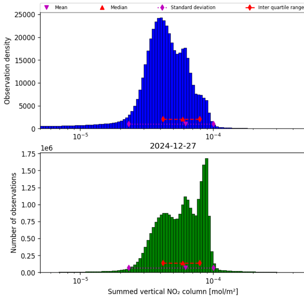
Figure 40: Histogram of “Summed vertical NO 2 column” for 2024-12-27 to 2024-12-28
