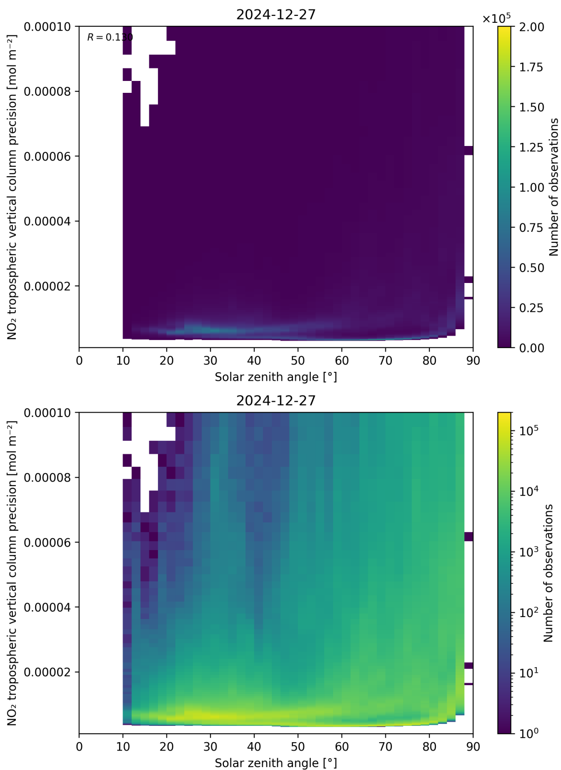
Figure 156: Scatter density plot of “Solar zenith angle” against “NO 2 tropospheric vertical column precision” for 2024-12-27 to 2024-12-28.
