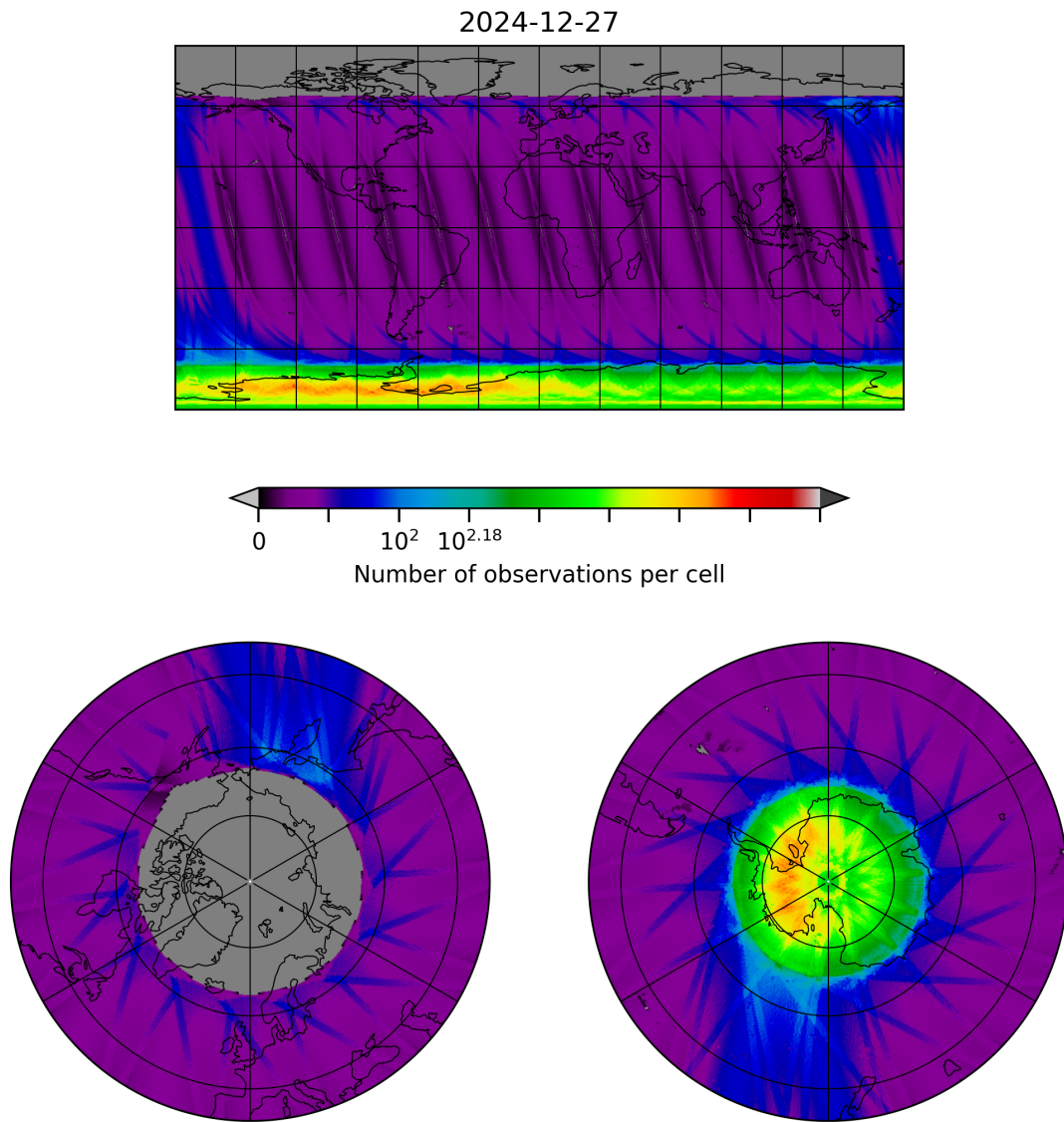
Figure 10: Map of the number of observations for 2024-12-27 to 2024-12-28
