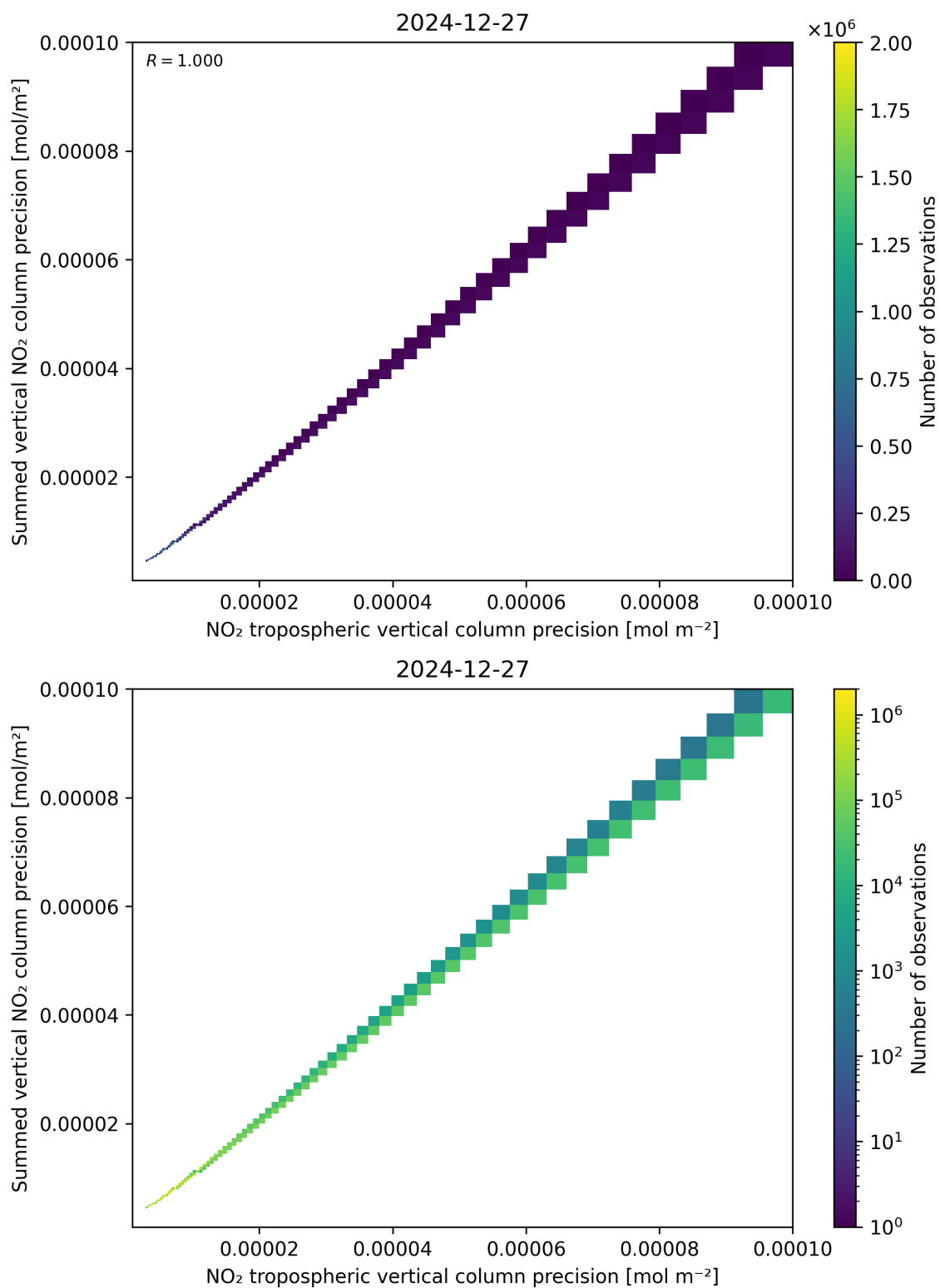
Figure 137: Scatter density plot of “NO 2 tropospheric vertical column precision” against “Summed vertical NO 2 column precision” for 2024-12-27 to 2024-12-28.
