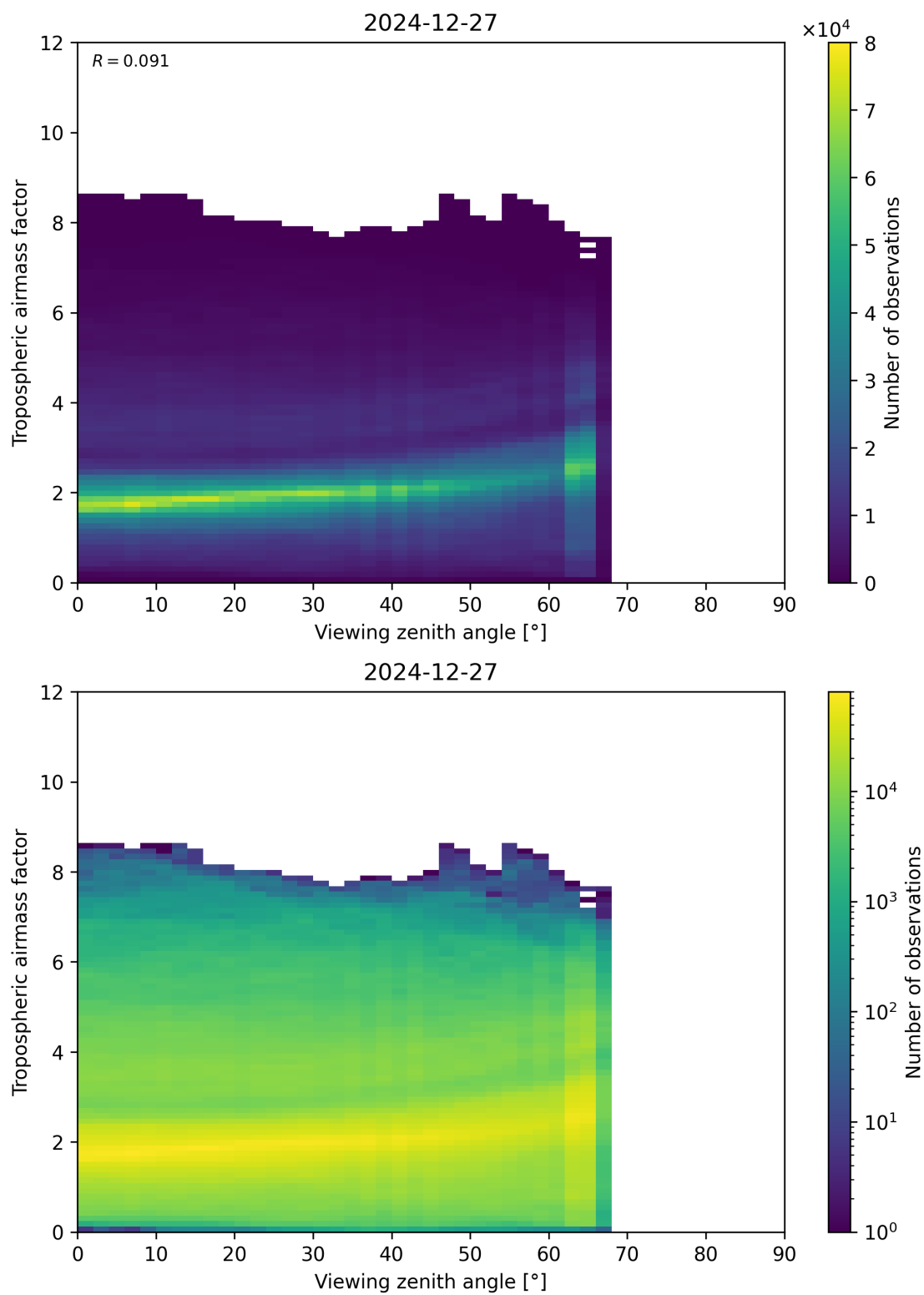
Figure 161: Scatter density plot of “Viewing zenith angle” against “Tropospheric airmass factor” for 2024-12-27 to 2024-12-28.
