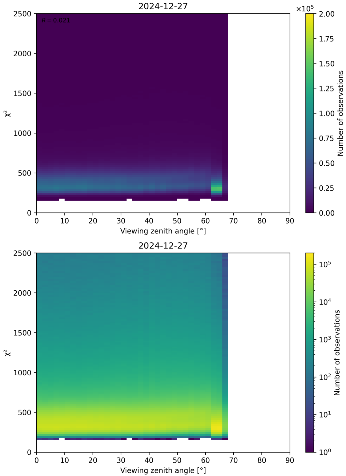
Figure 162: Scatter density plot of “Viewing zenith angle” against “ \chi^2 ” for 2024-12-27 to 2024-12-28.
