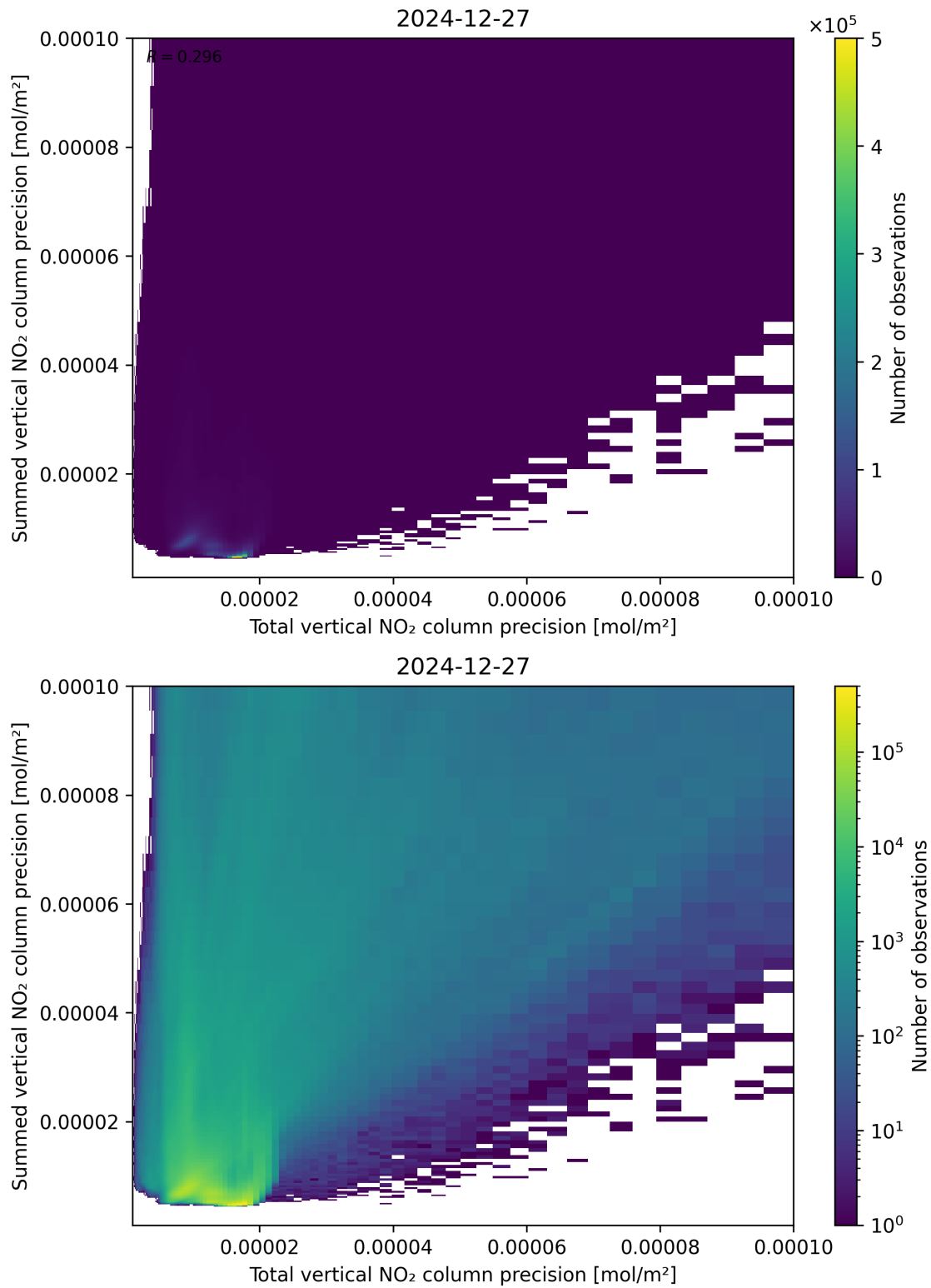
Figure 118: Scatter density plot of “Total vertical NO 2 column precision” against “Summed vertical NO 2 column precision” for 2024-12-27 to 2024-12-28.
