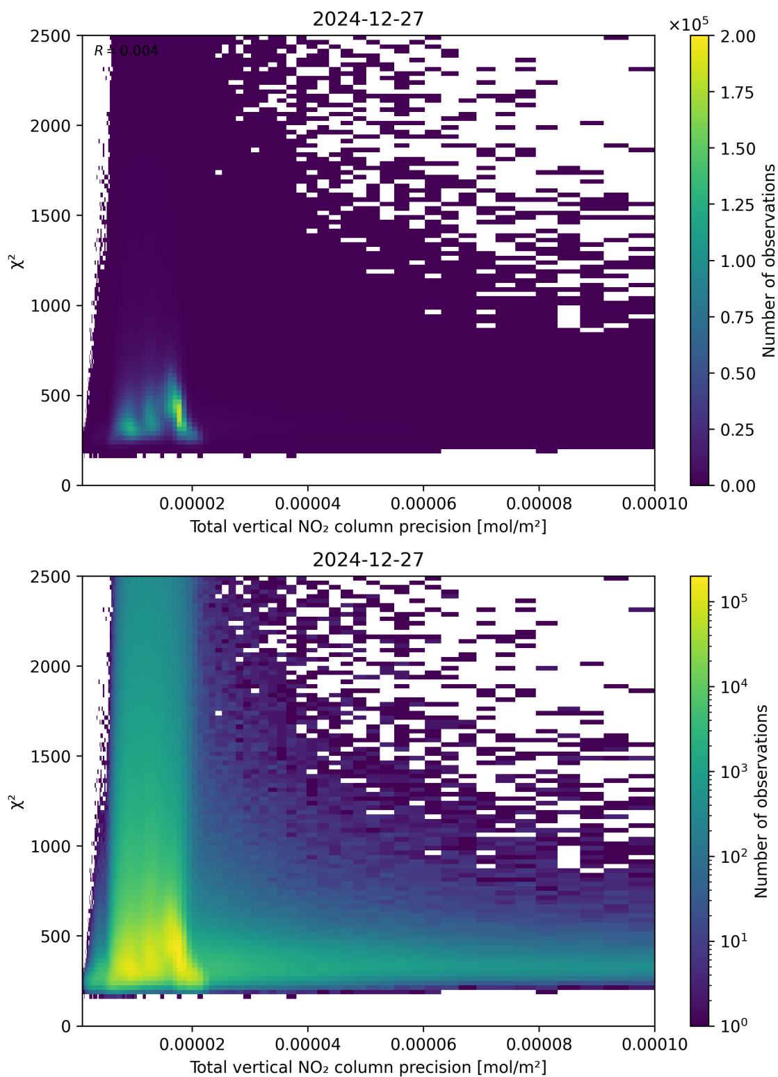
Figure 116: Scatter density plot of “Total vertical NO 2 column precision” against “ \chi^2 ” for 2024-12-27 to 2024-12-28.
