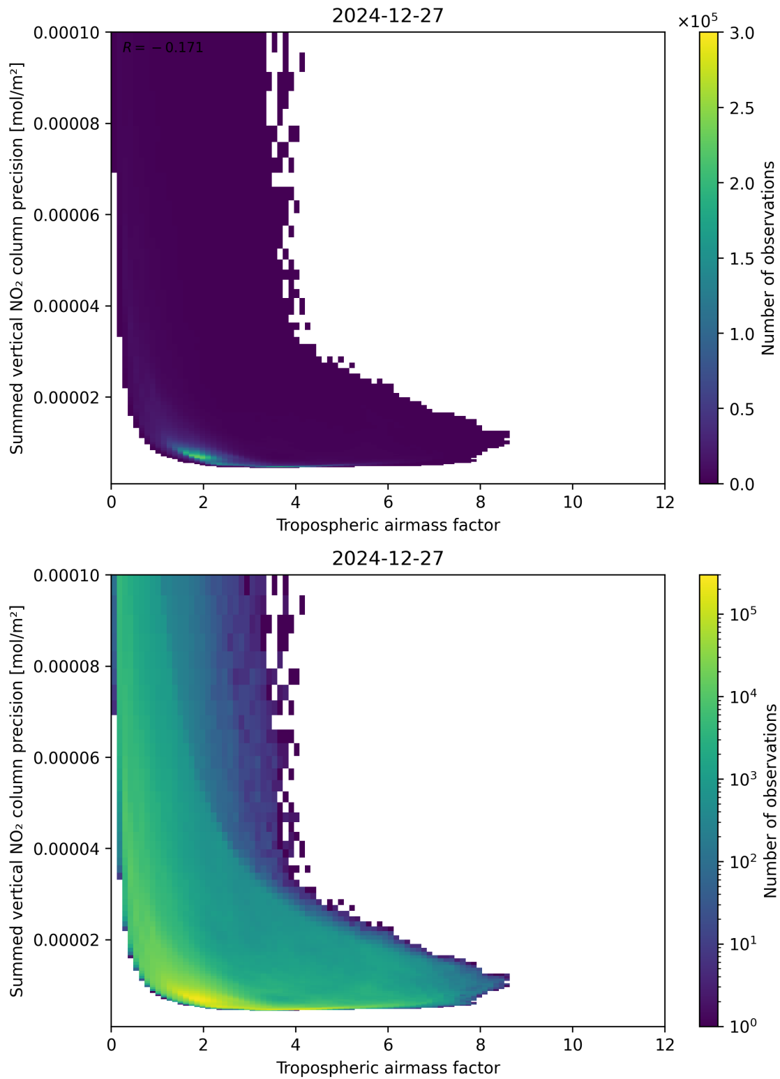
Figure 76: Scatter density plot of “Tropospheric air mass factor” against “Summed vertical NO 2 column precision” for 2024-12-27 to 2024-12-28.
