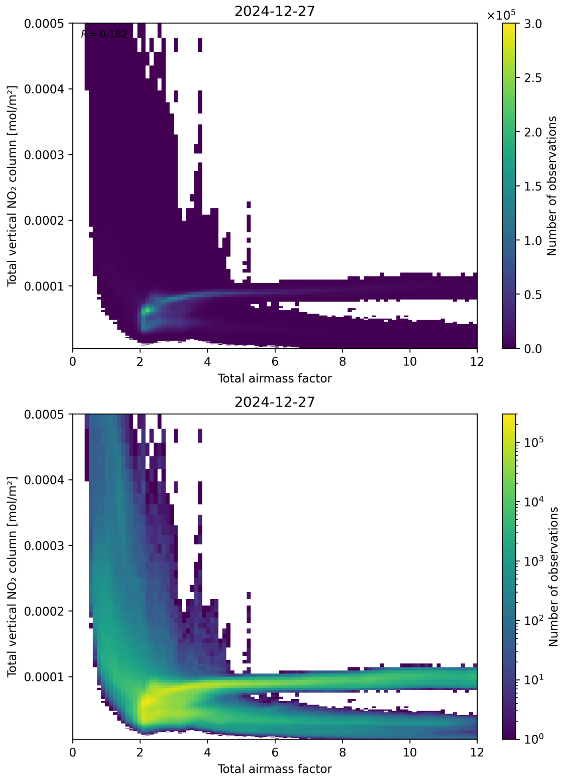
Figure 67: Scatter density plot of “Total airmass factor” against “Total vertical NO 2 column” for 2024-12-27 to 2024-12-28.
