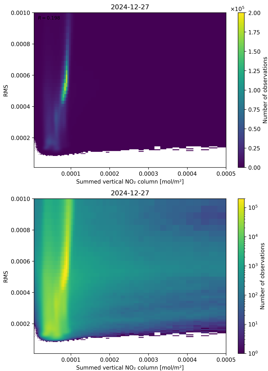
Figure 109: Scatter density plot of “Summed vertical NO 2 column” against “RMS” for 2024-12-27 to 2024-12-28.
