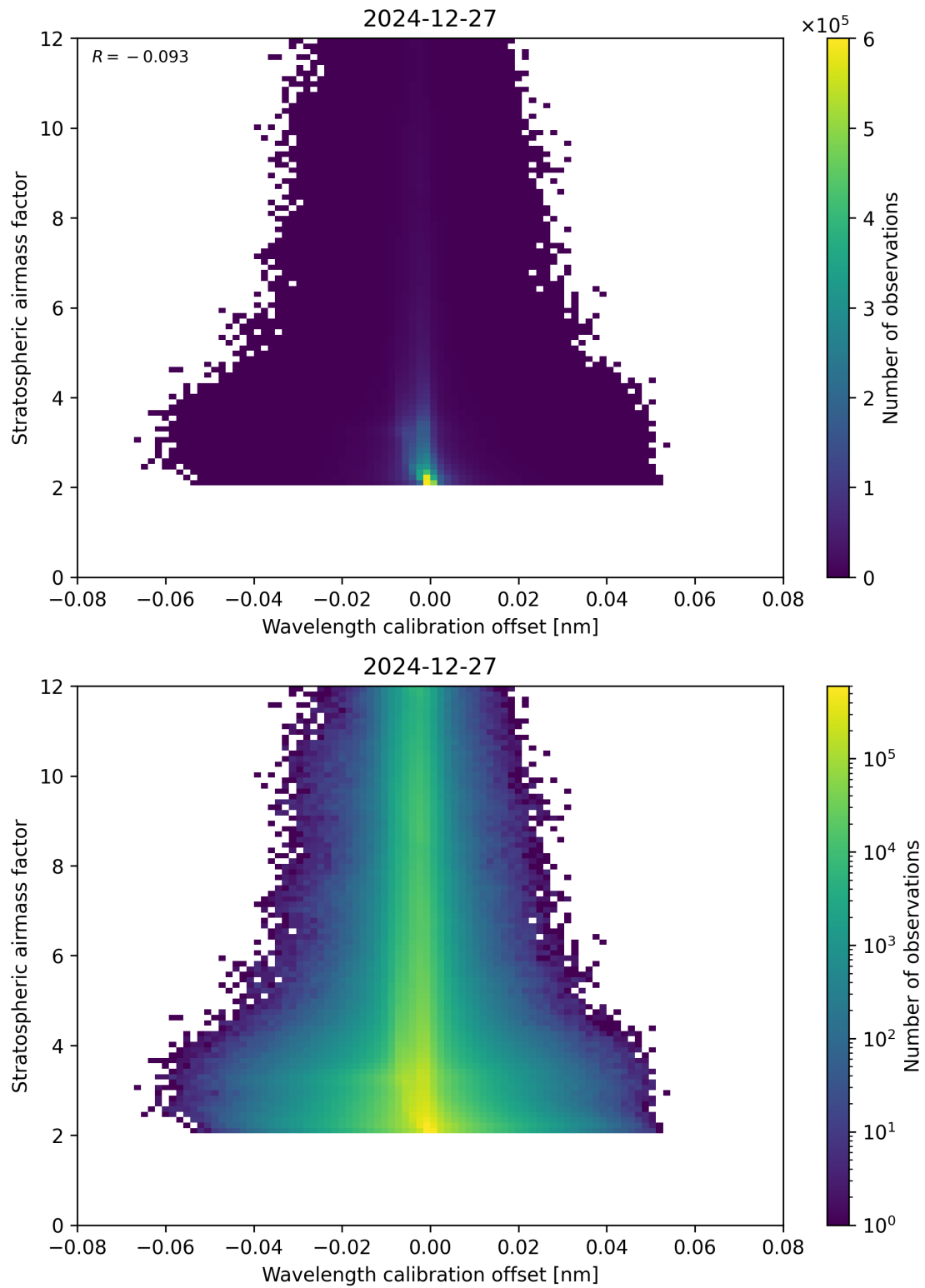
Figure 174: Scatter density plot of “Wavelength calibration offset” against “Stratospheric airmass factor” for 2024-12-27 to 2024-12-28.
