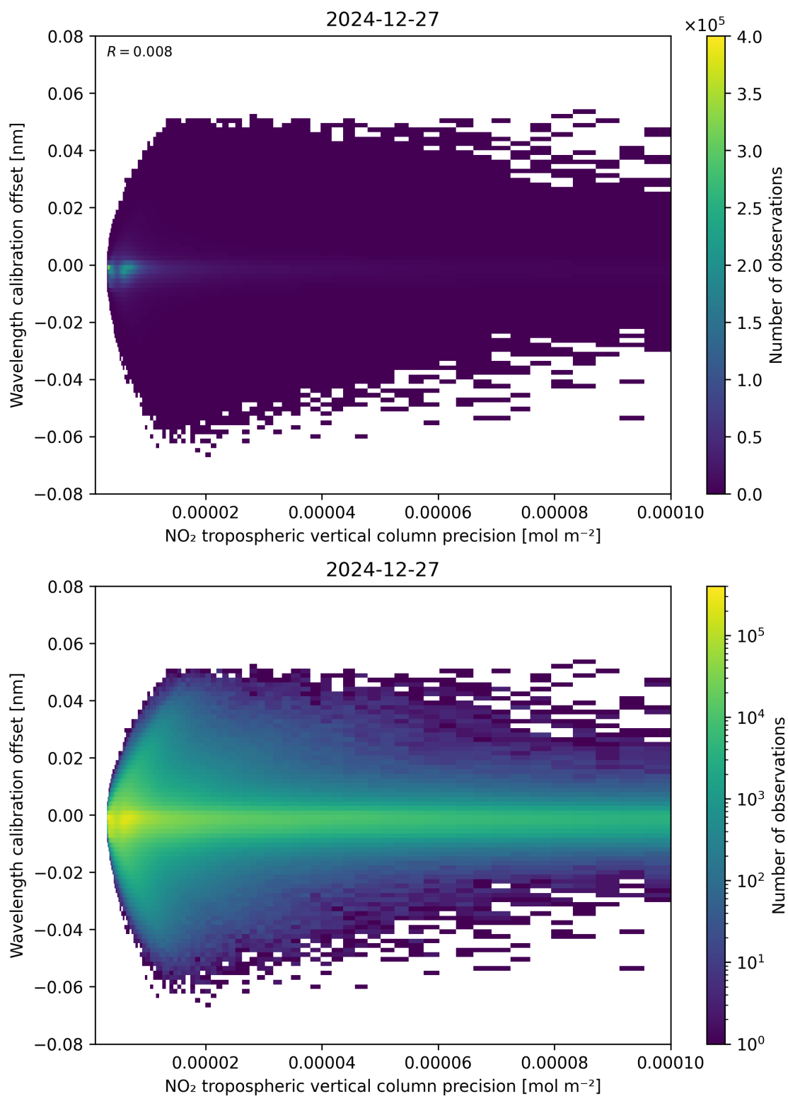
Figure 141: Scatter density plot of “NO 2 tropospheric vertical column precision” against “Wavelength calibration offset” for 2024-12-27 to 2024-12-28.
