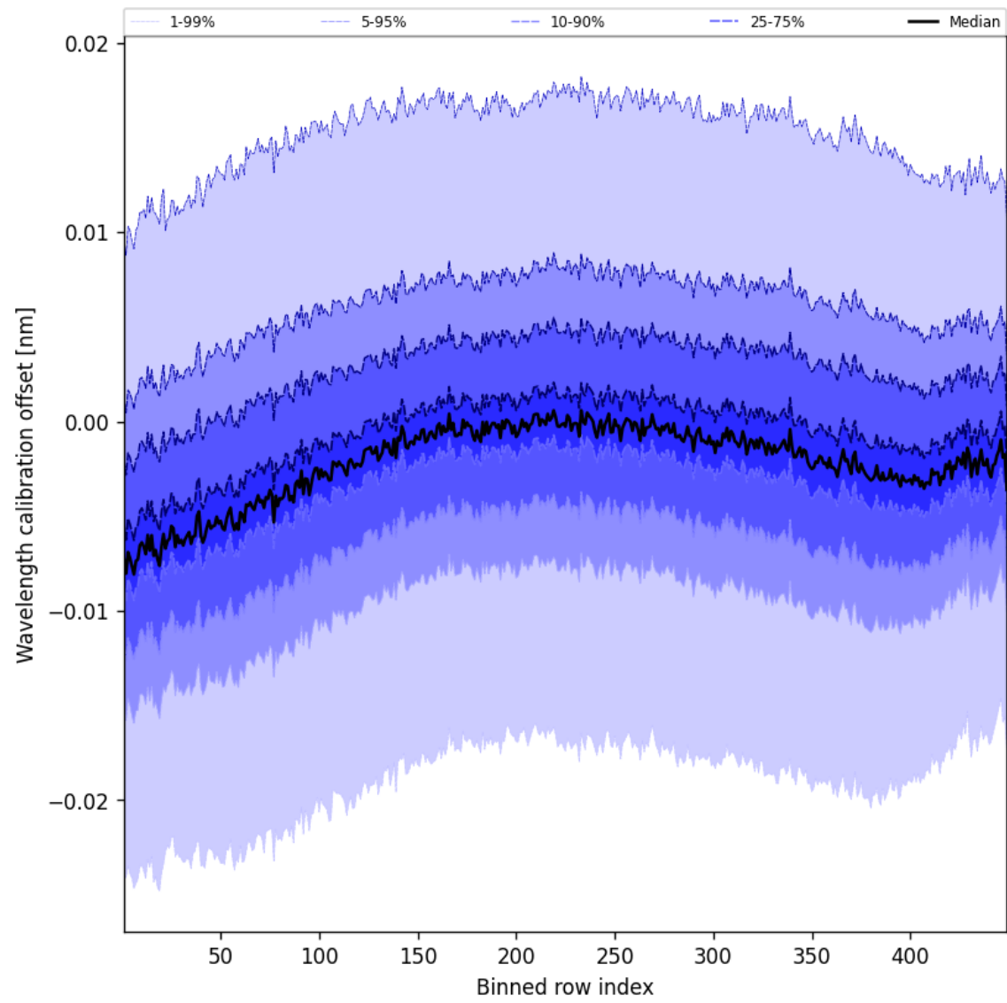
Figure 52: Along track statistics of “Wavelength calibration offset” for 2024-12-27 to 2024-12-28
