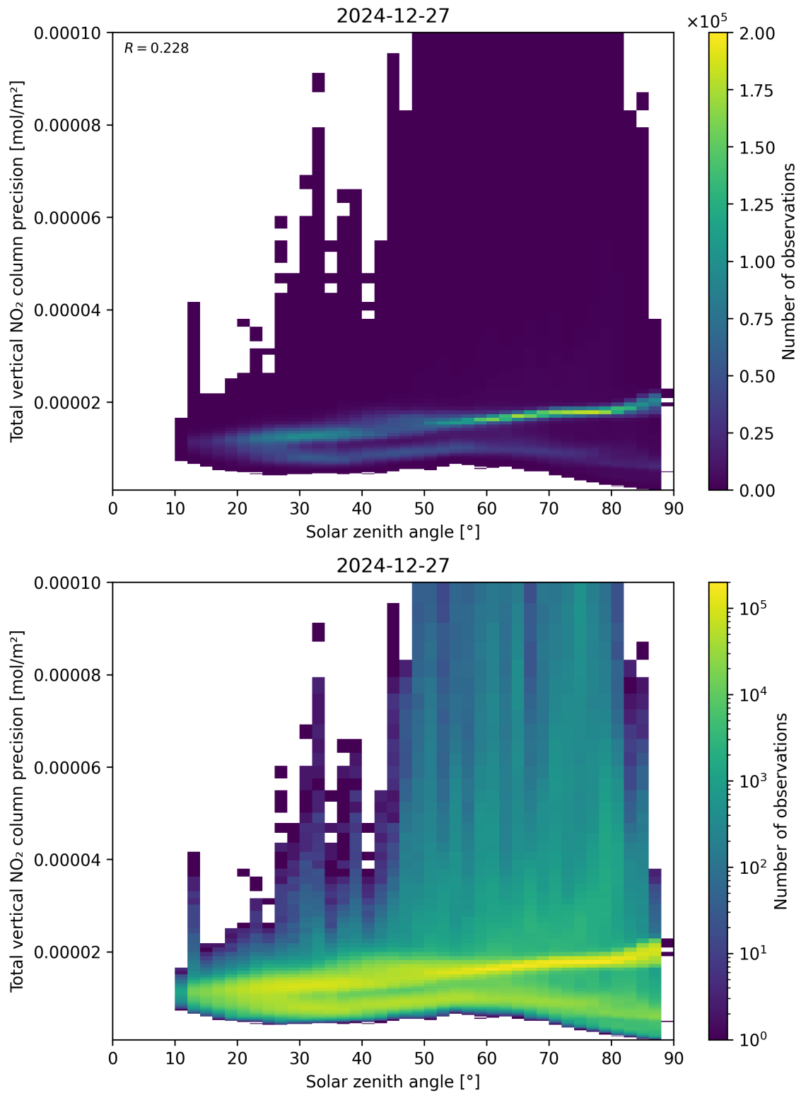
Figure 154: Scatter density plot of “Solar zenith angle” against “Total vertical NO 2 column precision” for 2024-12-27 to 2024-12-28.
