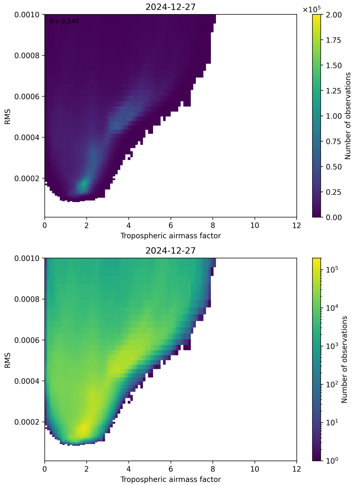
Figure 79: Scatter density plot of “Tropospheric airmass factor” against “RMS” for 2024-12-27 to 2024-12-28.
