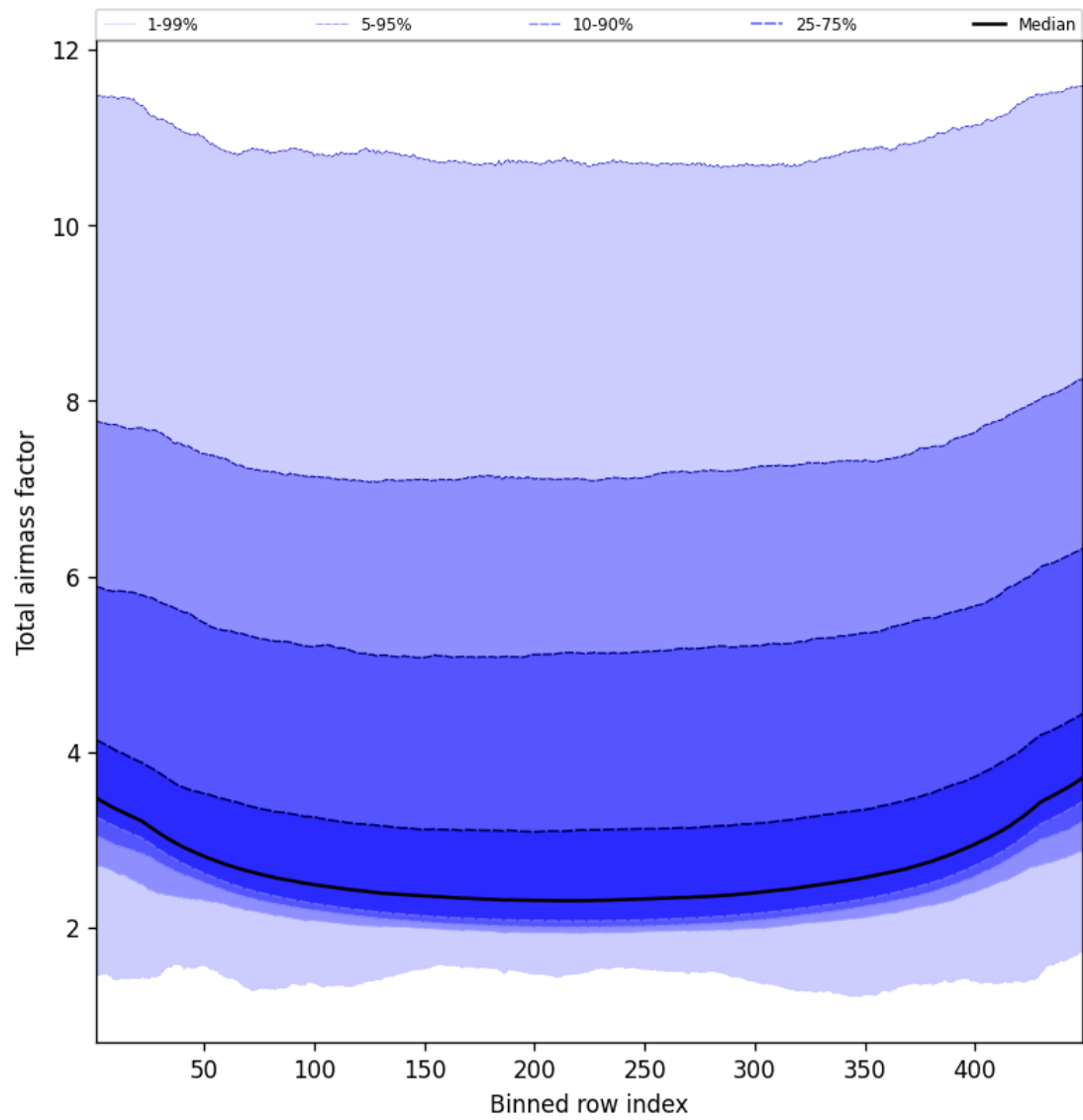
Figure 49: Along track statistics of “Total airmass factor” for 2024-12-27 to 2024-12-28
