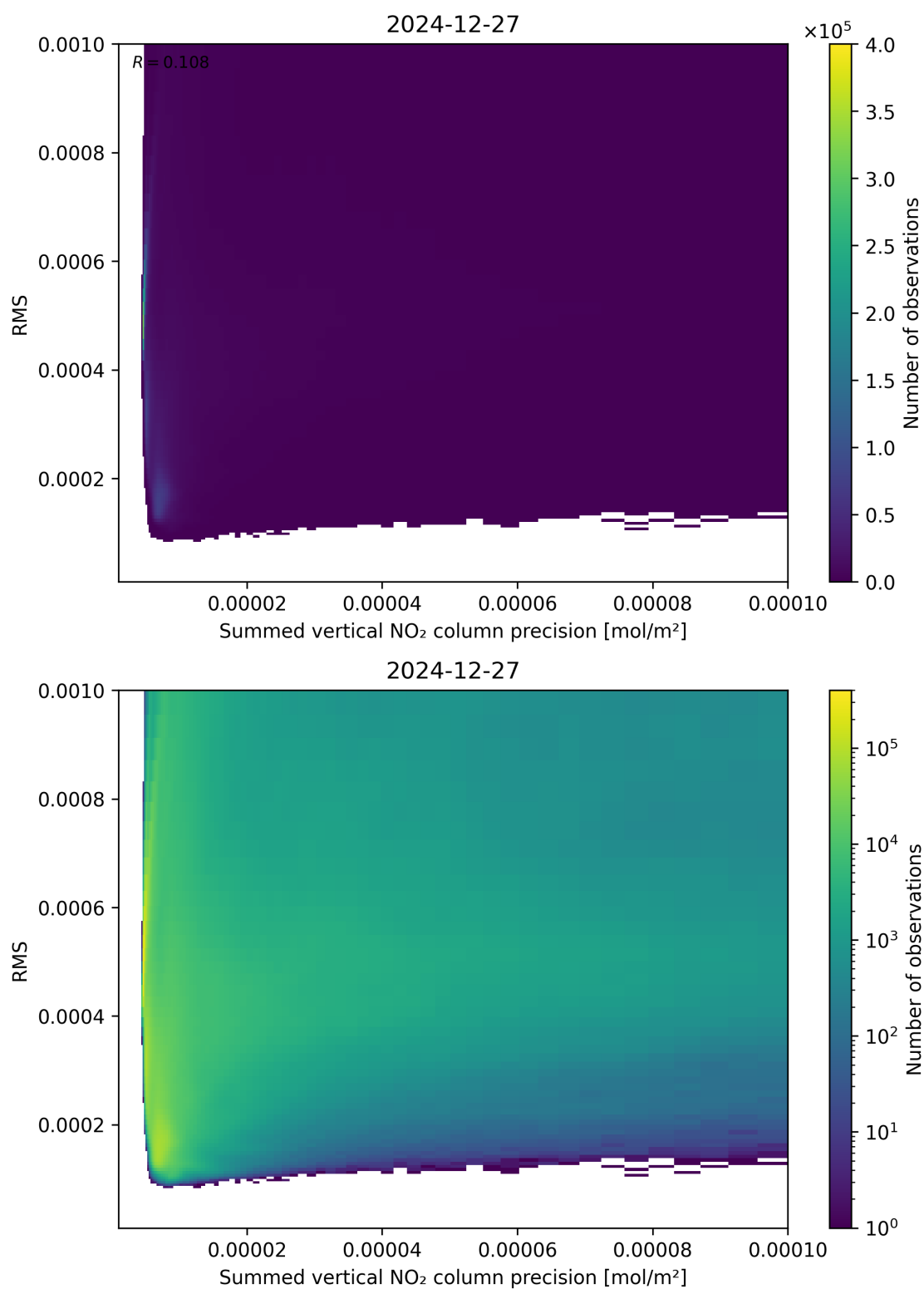
Figure 108: Scatter density plot of “Summed vertical NO 2 column precision” against “RMS” for 2024-12-27 to 2024-12-28.
