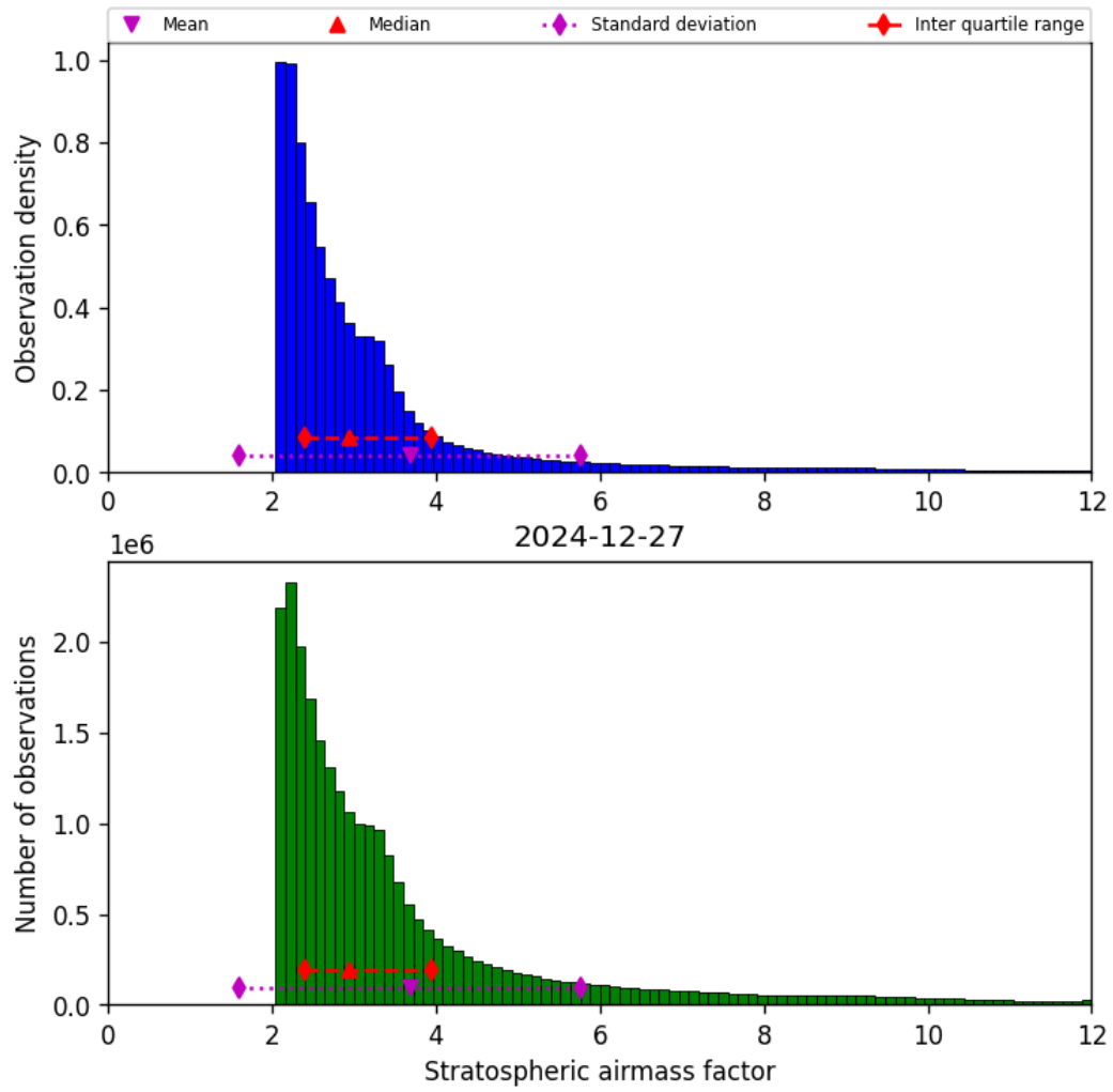
Figure 44: Histogram of “Stratospheric airmass factor” for 2024-12-27 to 2024-12-28
