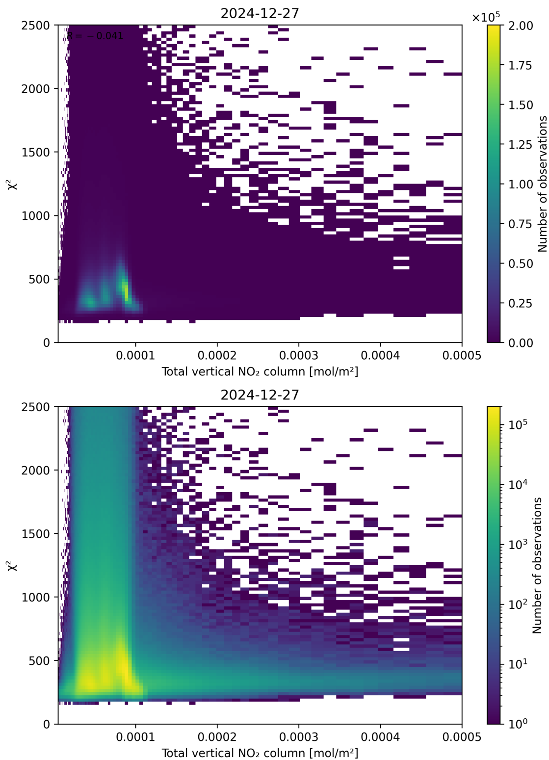
Figure 111: Scatter density plot of “Total vertical NO 2 column” against “ \chi^2 ” for 2024-12-27 to 2024-12-28.
