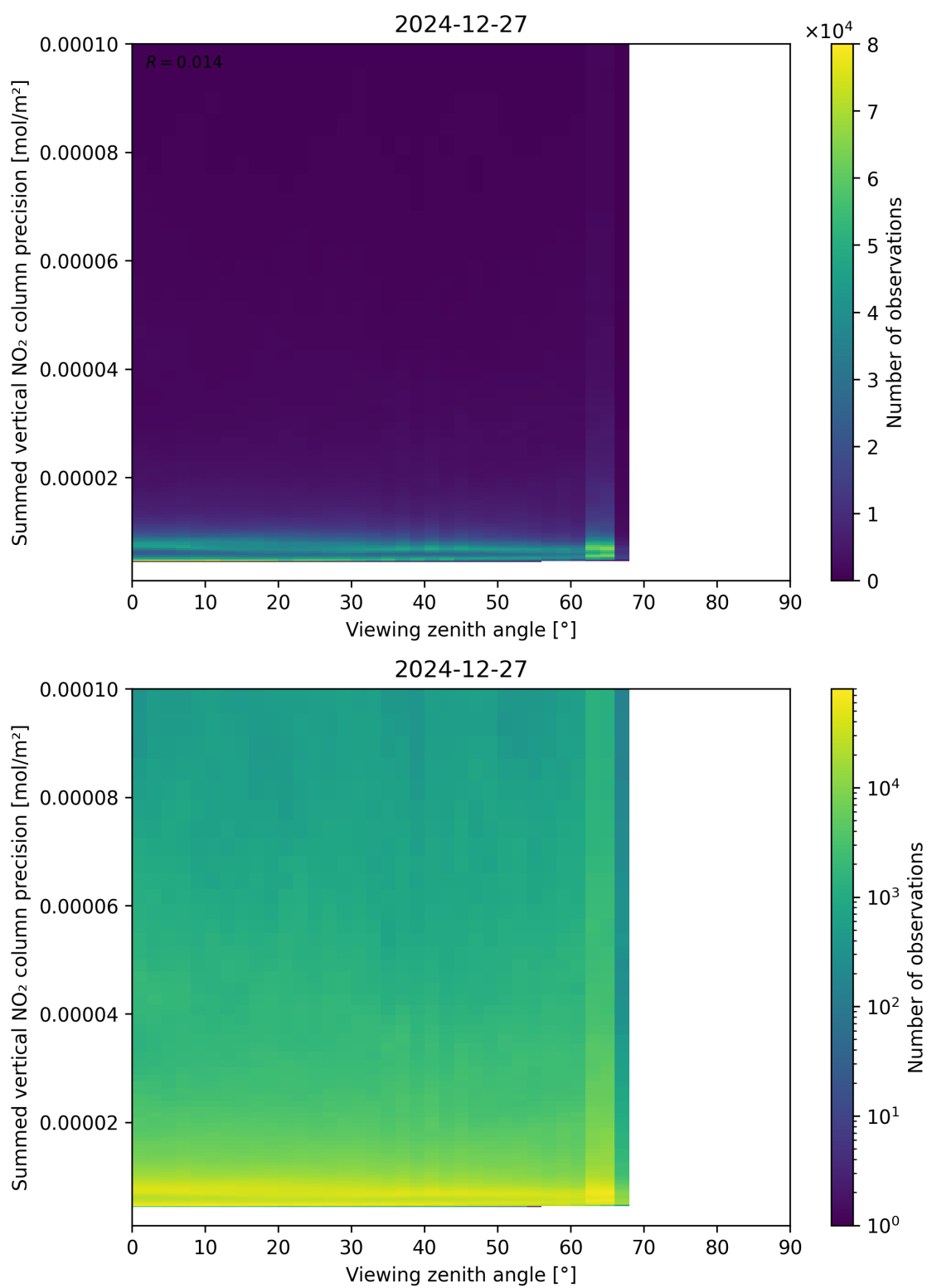
Figure 166: Scatter density plot of “Viewing zenith angle” against “Summed vertical NO 2 column precision” for 2024-12-27 to 2024-12-28.
