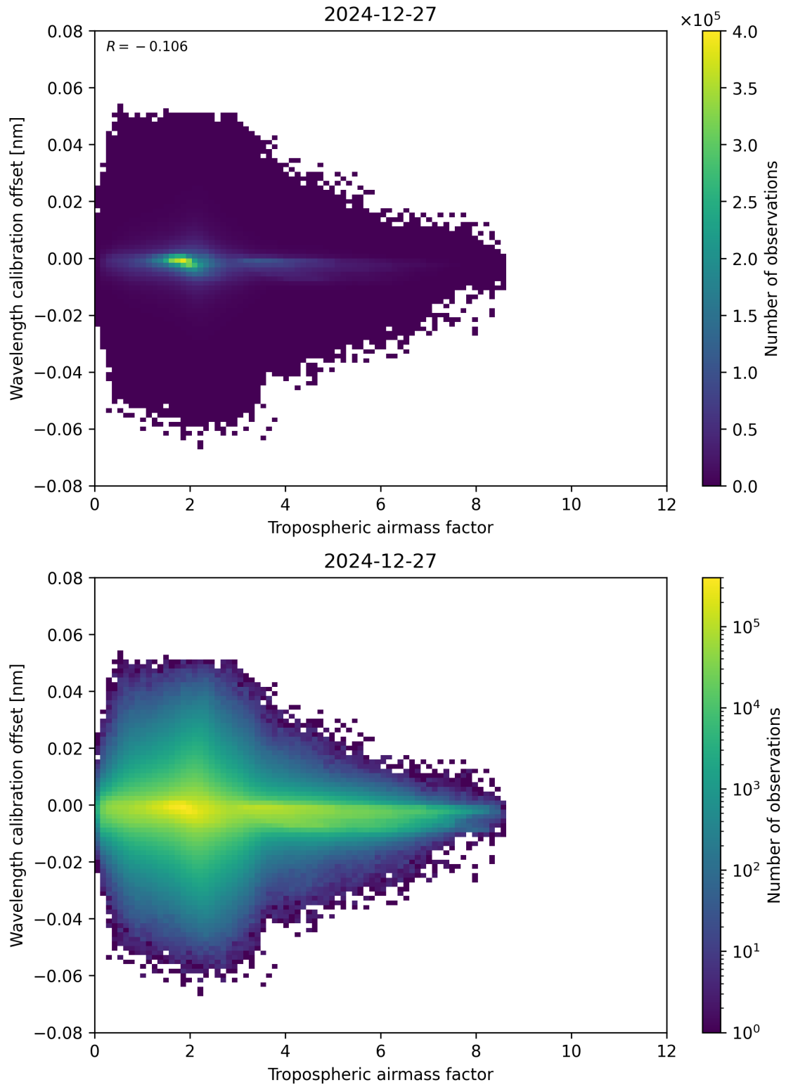
Figure 80: Scatter density plot of “Tropospheric airmass factor” against “Wavelength calibration offset” for 2024-12-27 to 2024-12-28.
