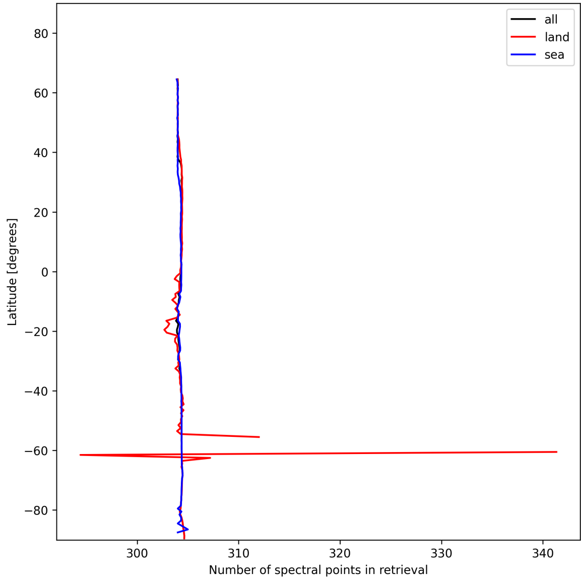
Figure 16: Zonal average of “Number of spectral points in retrieval” for 2024-12-27 to 2024-12-28.
