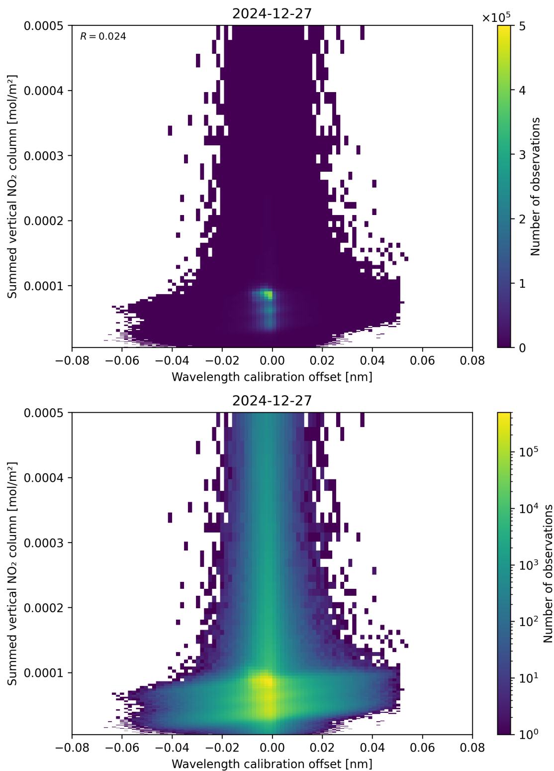
Figure 177: Scatter density plot of “Wavelength calibration offset” against “Summed vertical NO 2 column” for 2024-12-27 to 2024-12-28.
