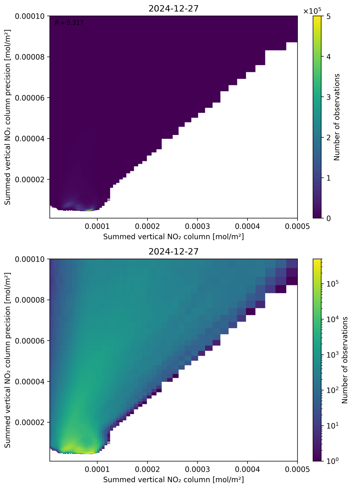
Figure 105: Scatter density plot of “Summed vertical NO 2 column” against “Summed vertical NO 2 column precision” for 2024-12-27 to 2024-12-28.
