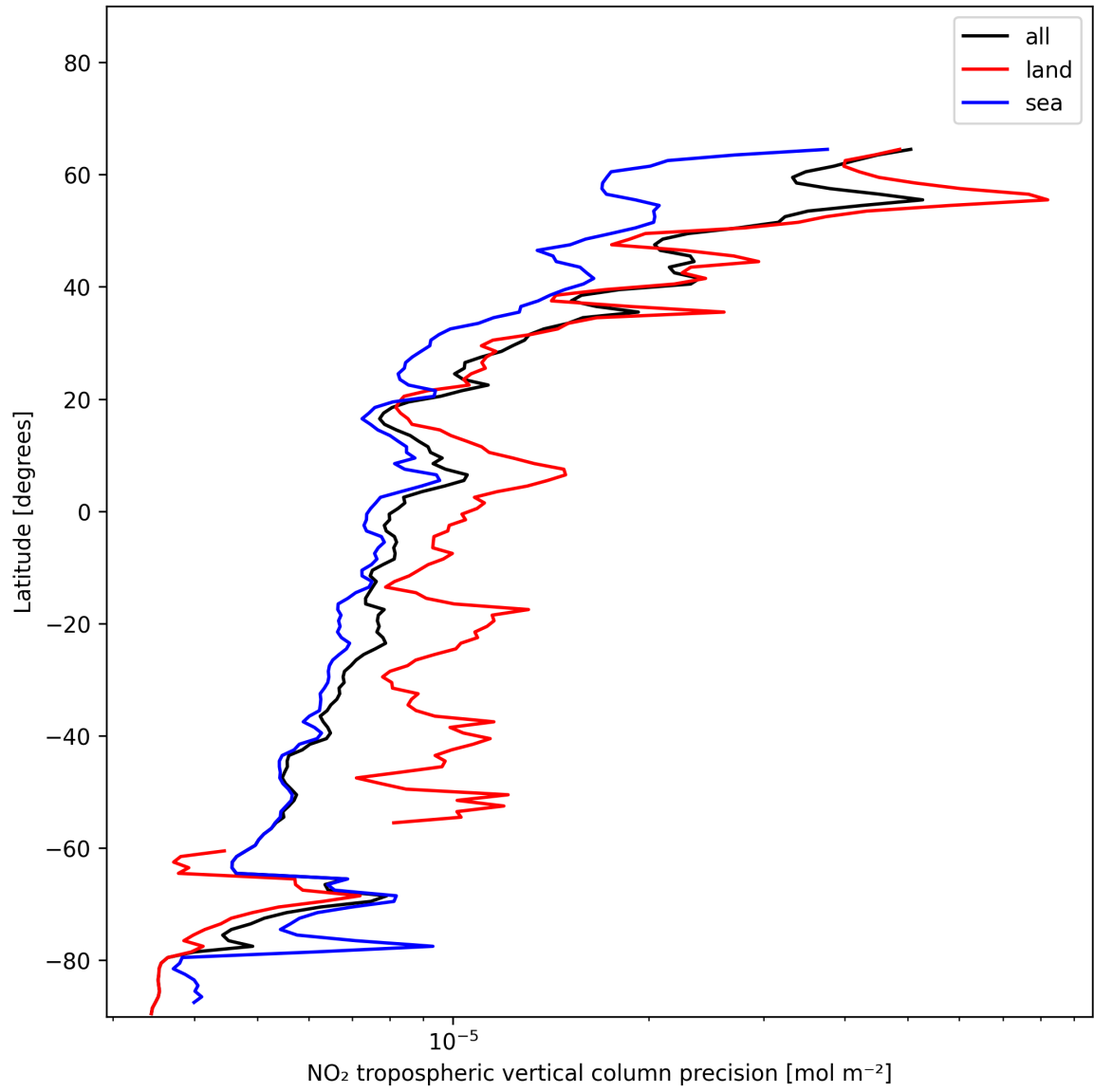
Figure 13: Zonal average of “NO 2 tropospheric vertical column precision” for 2024-12-27 to 2024-12-28.
