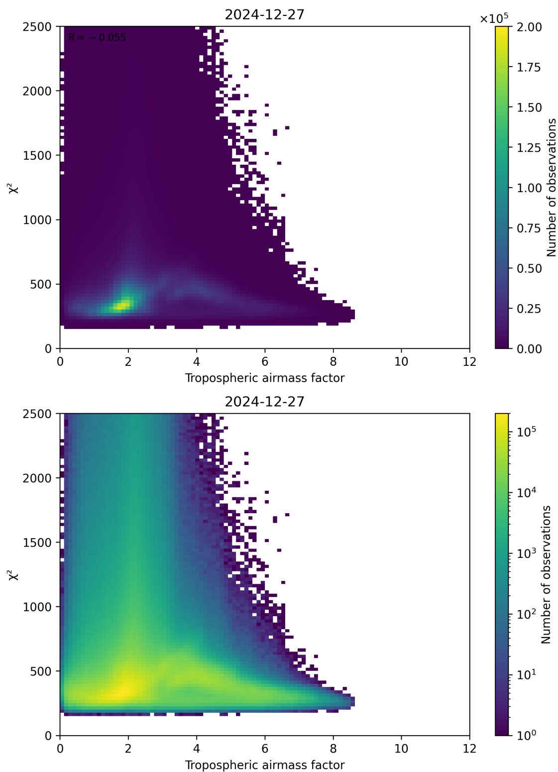
Figure 73: Scatter density plot of “Tropospheric airmass factor” against “ \chi^2 ” for 2024-12-27 to 2024-12-28.
