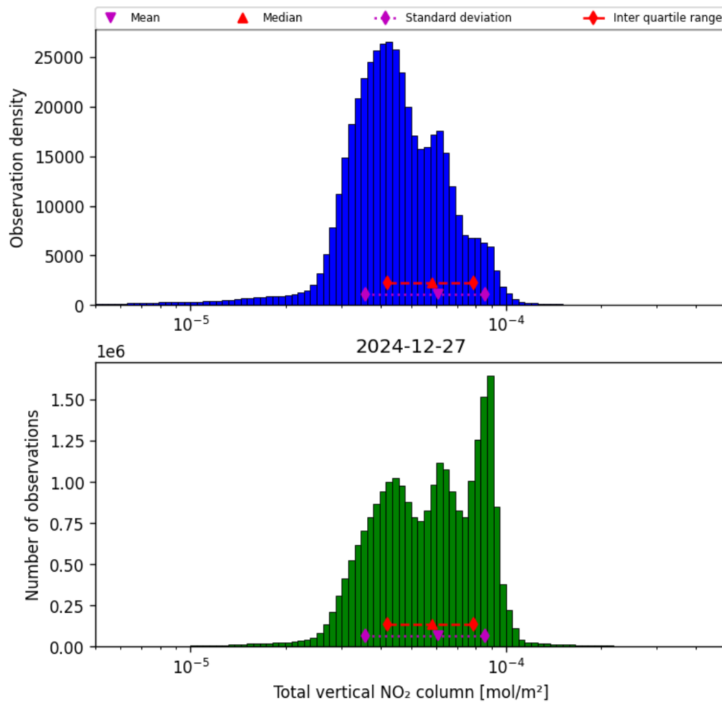
Figure 38: Histogram of “Total vertical NO 2 column” for 2024-12-27 to 2024-12-28
