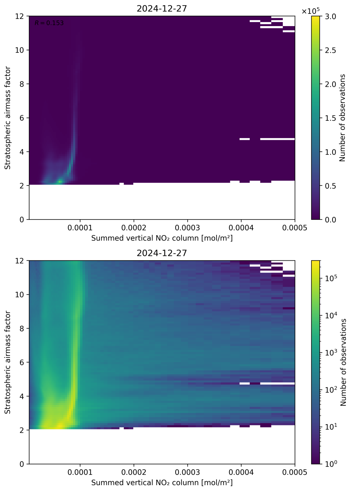
Figure 103: Scatter density plot of “Summed vertical NO 2 column” against “Stratospheric air mass factor” for 2024-12-27 to 2024-12-28.
