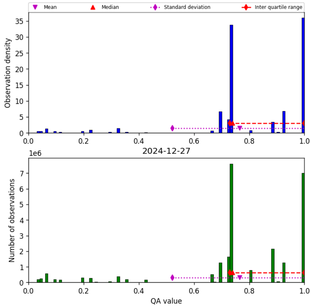
Figure 28: Histogram of “QA value” for 2024-12-27 to 2024-12-28
