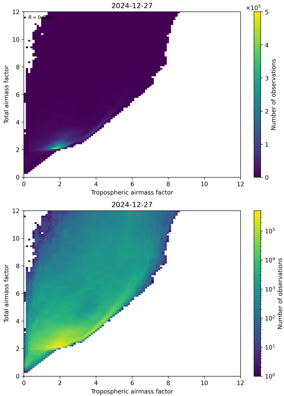
Figure 72: Scatter density plot of “Tropospheric airmass factor” against “Total airmass factor” for 2024-12-27 to 2024-12-28.
