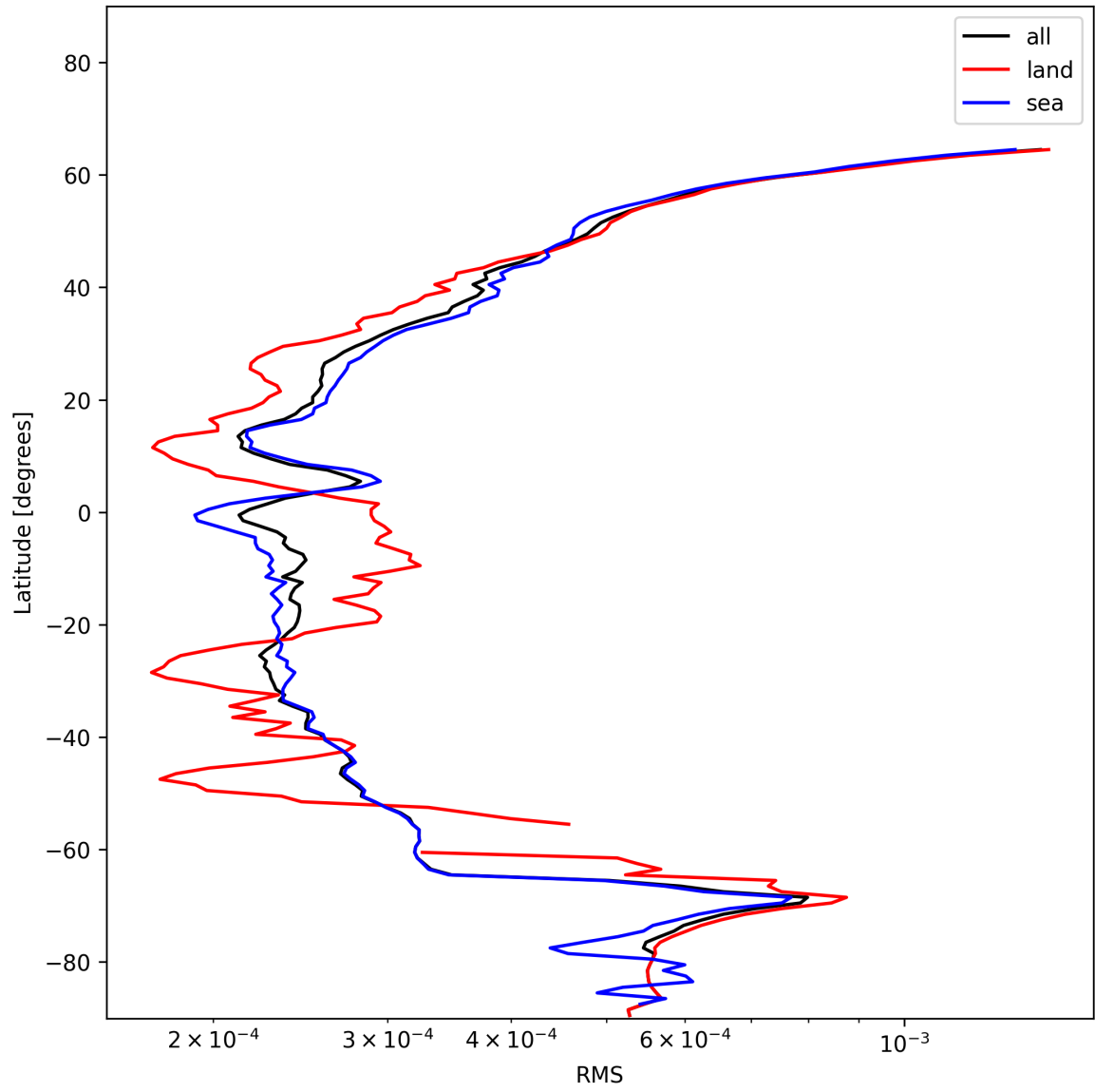
Figure 26: Zonal average of “RMS” for 2024-12-27 to 2024-12-28.
