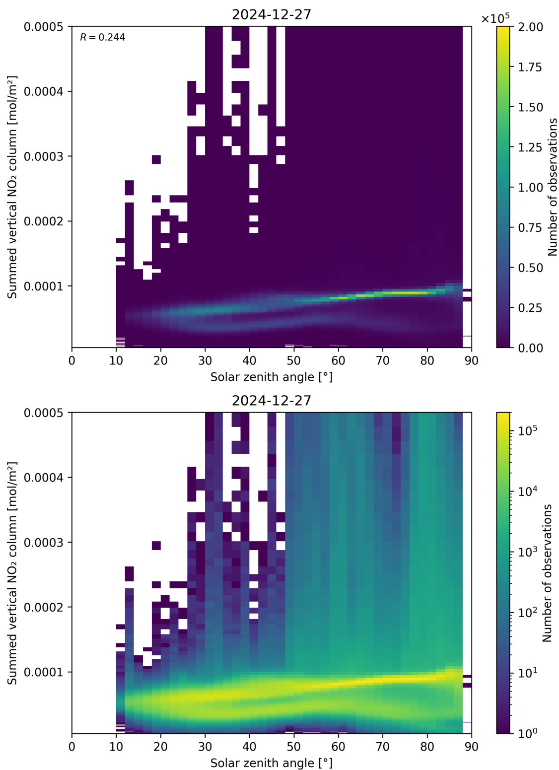
Figure 151: Scatter density plot of “Solar zenith angle” against “Summed vertical NO 2 column” for 2024-12-27 to 2024-12-28.
