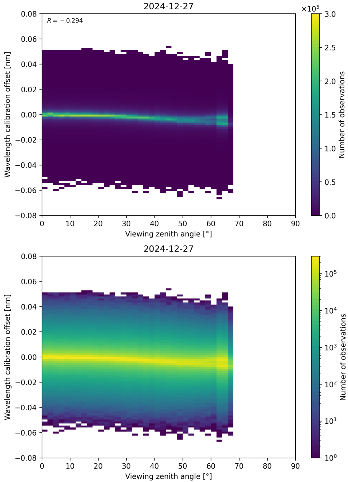
Figure 173: Scatter density plot of “Viewing zenith angle” against “Wavelength calibration offset” for 2024-12-27 to 2024-12-28.
