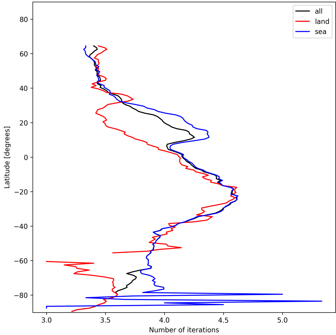
Figure 17: Zonal average of “Number of iterations” for 2024-12-27 to 2024-12-28.
