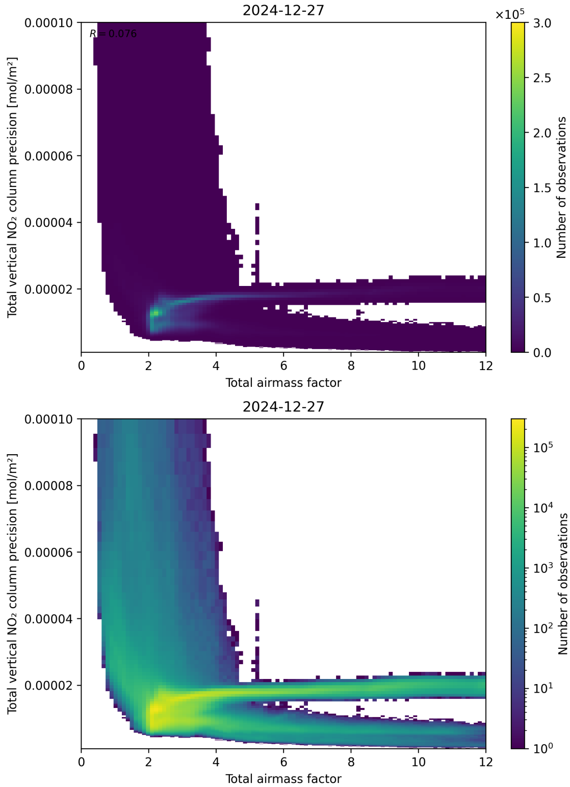
Figure 68: Scatter density plot of “Total airmass factor” against “Total vertical NO 2 column precision” for 2024-12-27 to 2024-12-28.
