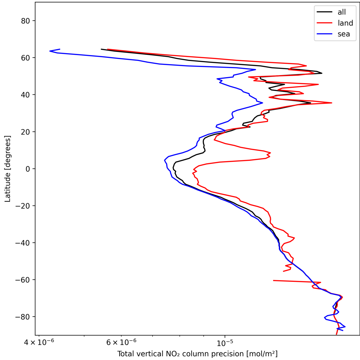
Figure 22: Zonal average of “Total vertical NO 2 column precision” for 2024-12-27 to 2024-12-28.
