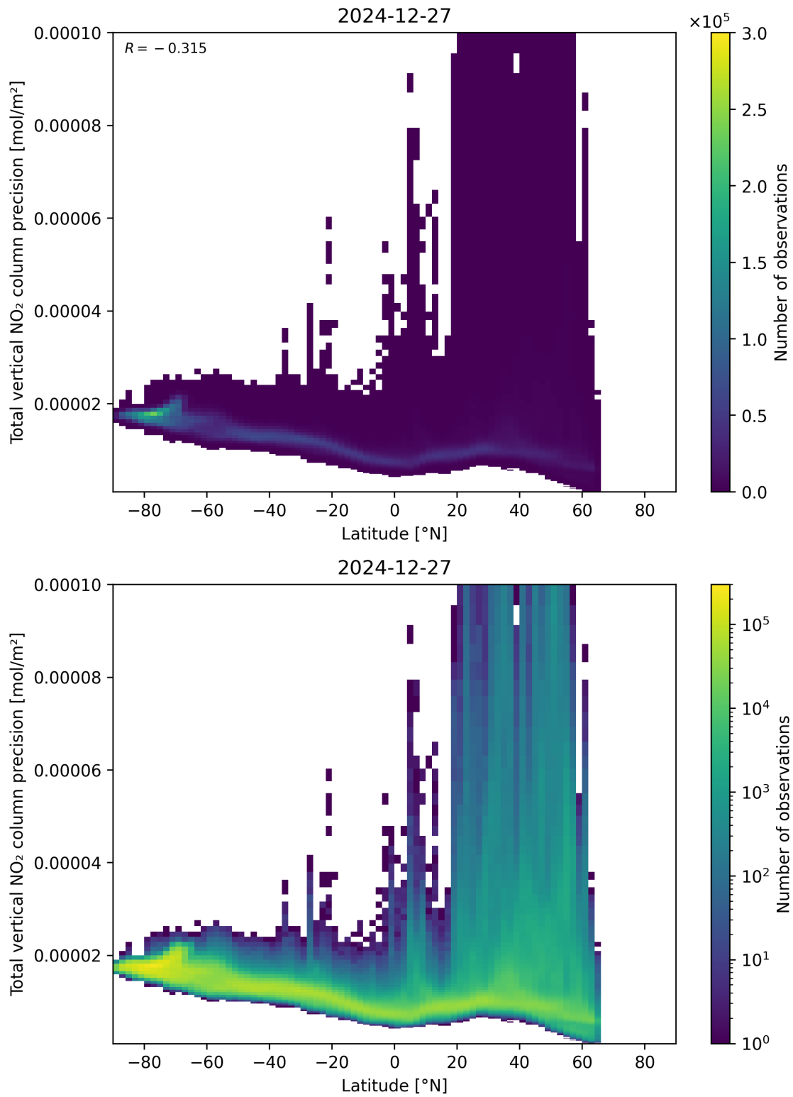
Figure 91: Scatter density plot of “Latitude” against “Total vertical NO 2 column precision” for 2024-12-27 to 2024-12-28.
