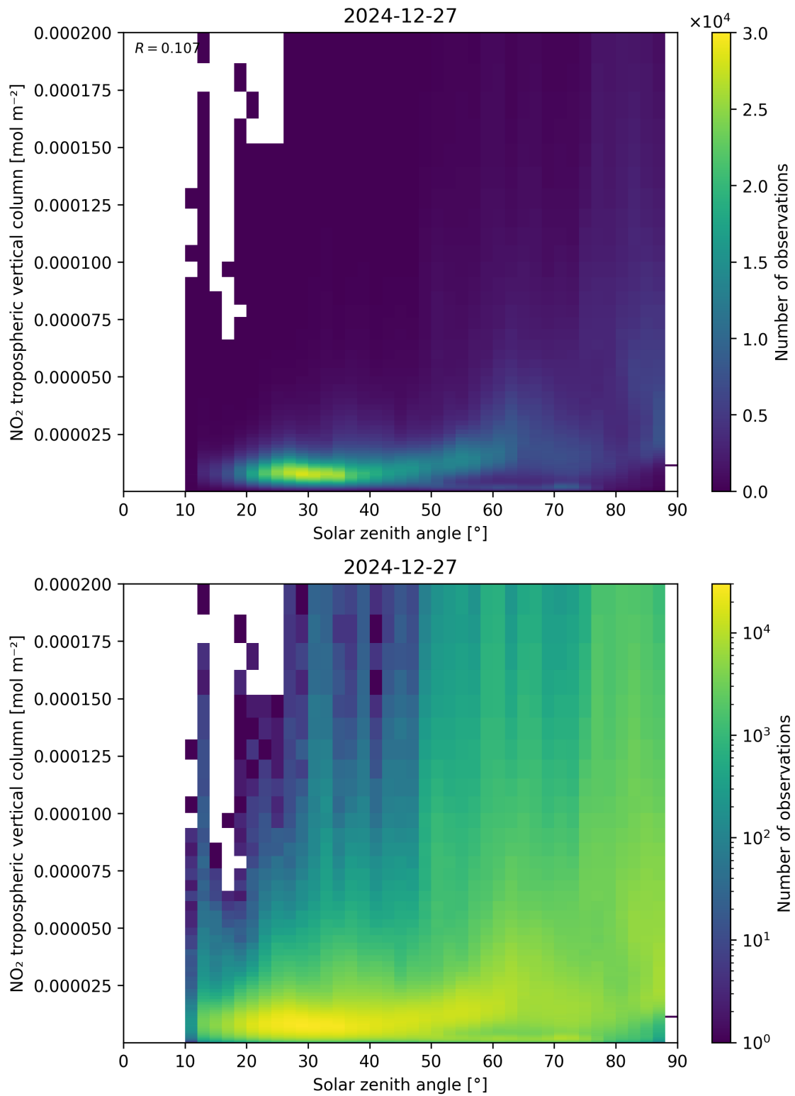
Figure 155: Scatter density plot of “Solar zenith angle” against “NO 2 tropospheric vertical column” for 2024-12-27 to 2024-12-28.
