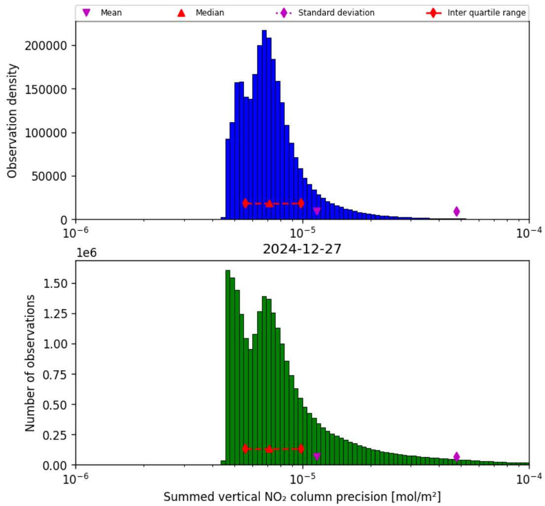
Figure 41: Histogram of “Summed vertical NO 2 column precision” for 2024-12-27 to 2024-12-28
