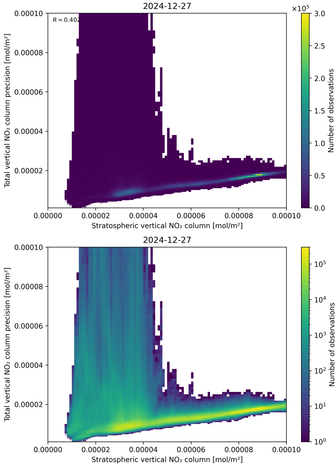
Figure 101: Scatter density plot of “Stratospheric vertical NO 2 column” against “Total vertical NO 2 column precision” for 2024-12-27 to 2024-12-28.
