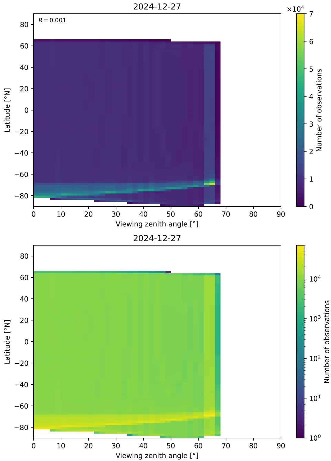
Figure 163: Scatter density plot of “Viewing zenith angle” against “Latitude” for 2024-12-27 to 2024-12-28.
