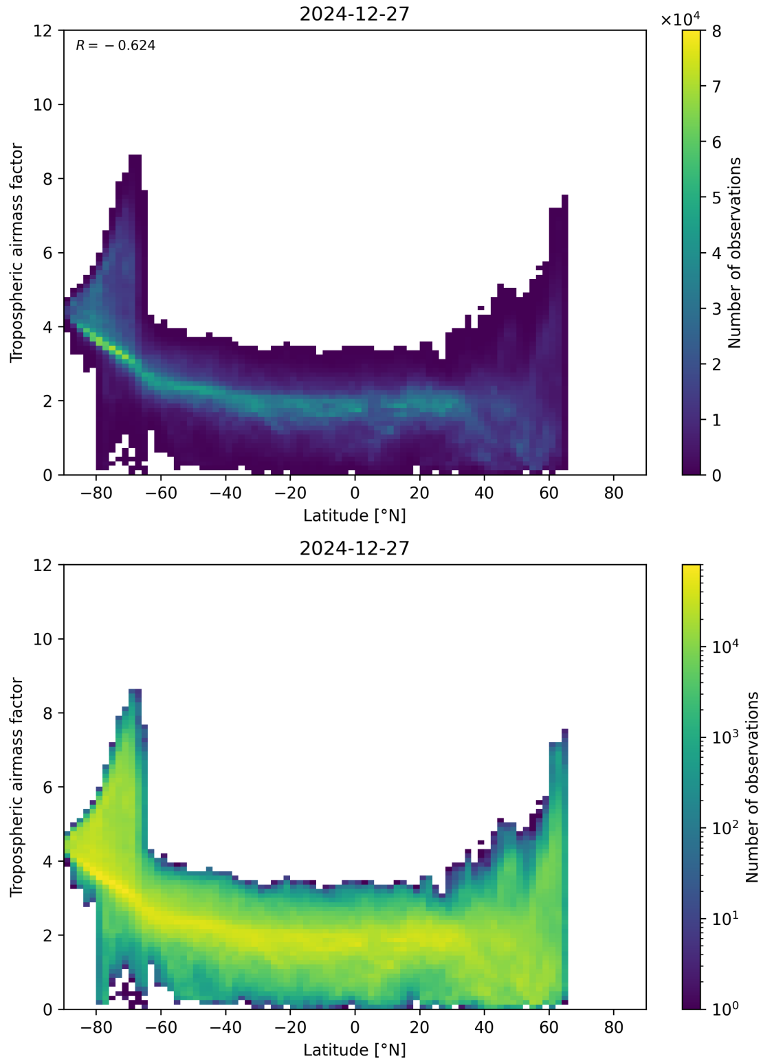
Figure 85: Scatter density plot of “Latitude” against “Tropospheric air mass factor” for 2024-12-27 to 2024-12-28.
