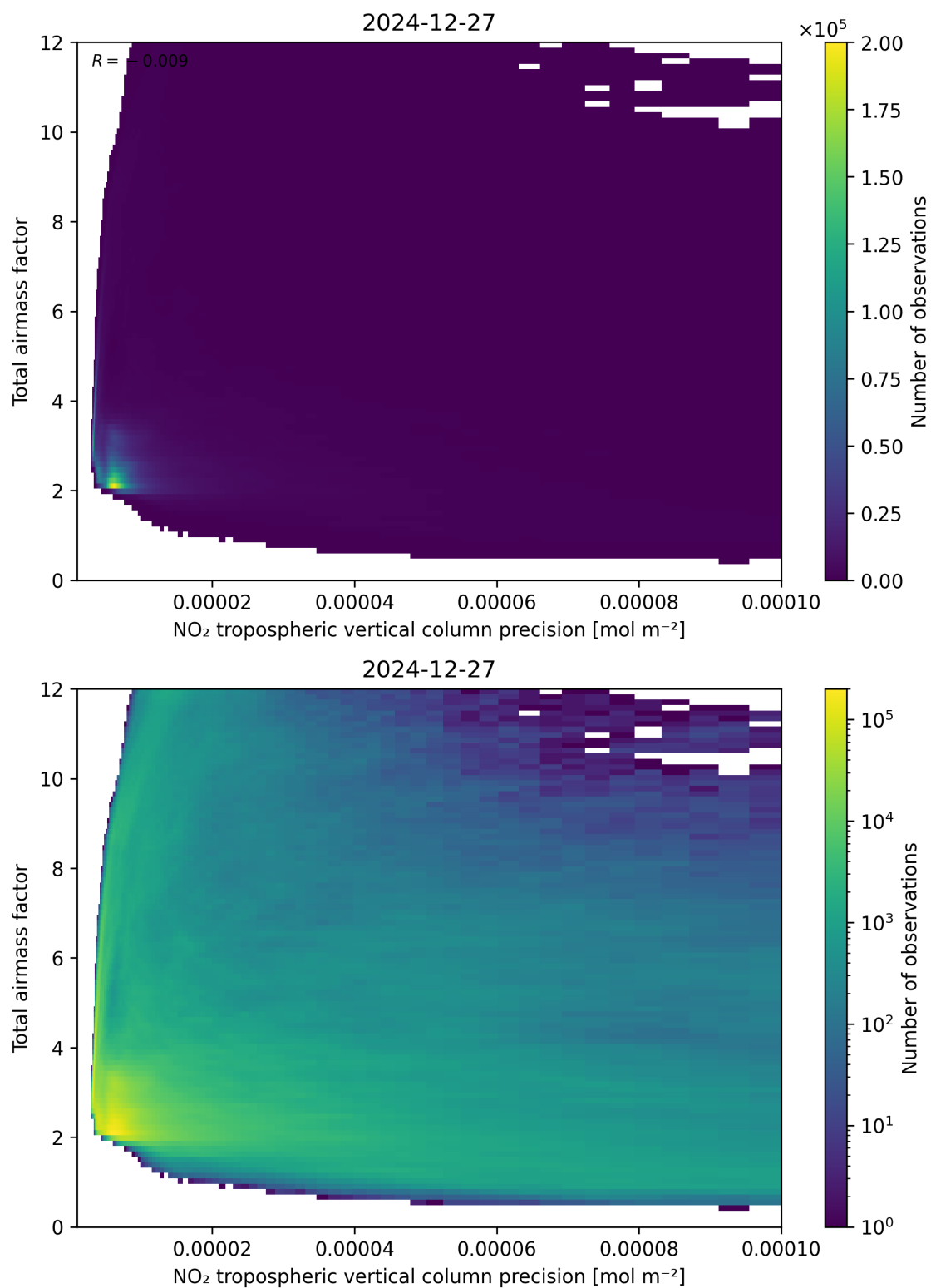
Figure 132: Scatter density plot of “NO 2 tropospheric vertical column precision” against “Total air mass factor” for 2024-12-27 to 2024-12-28.
