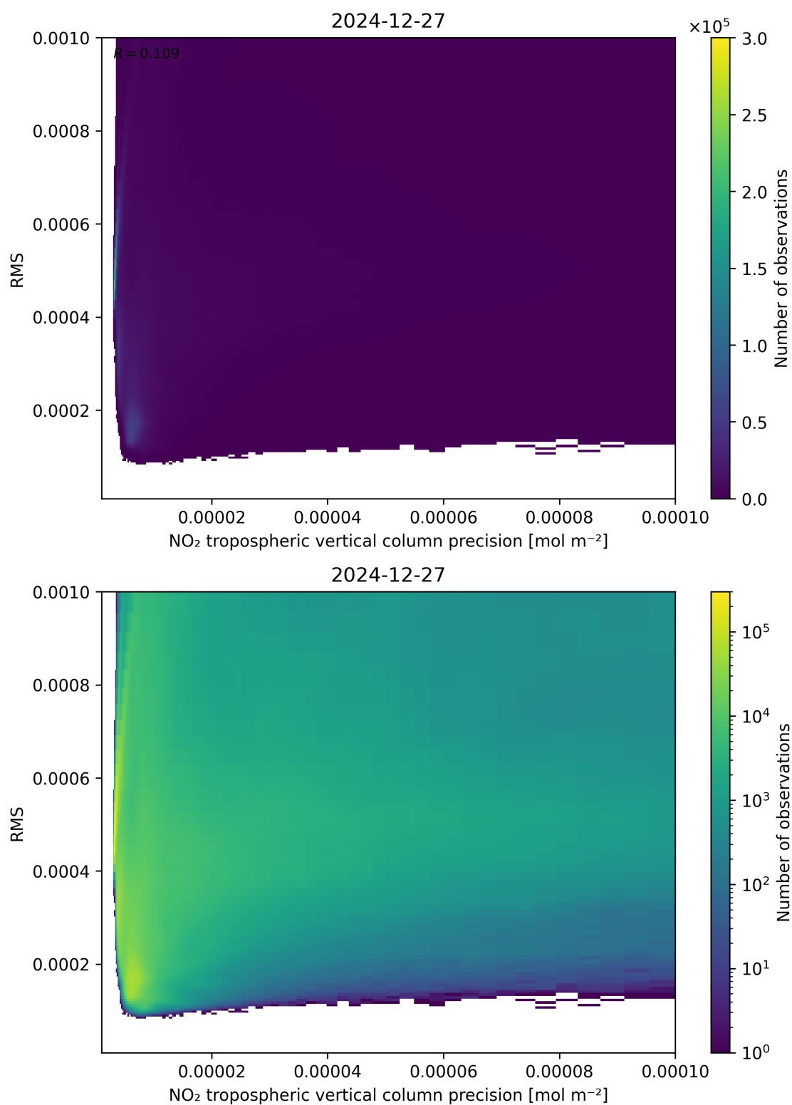
Figure 140: Scatter density plot of “NO 2 tropospheric vertical column precision” against “RMS” for 2024-12-27 to 2024-12-28.
