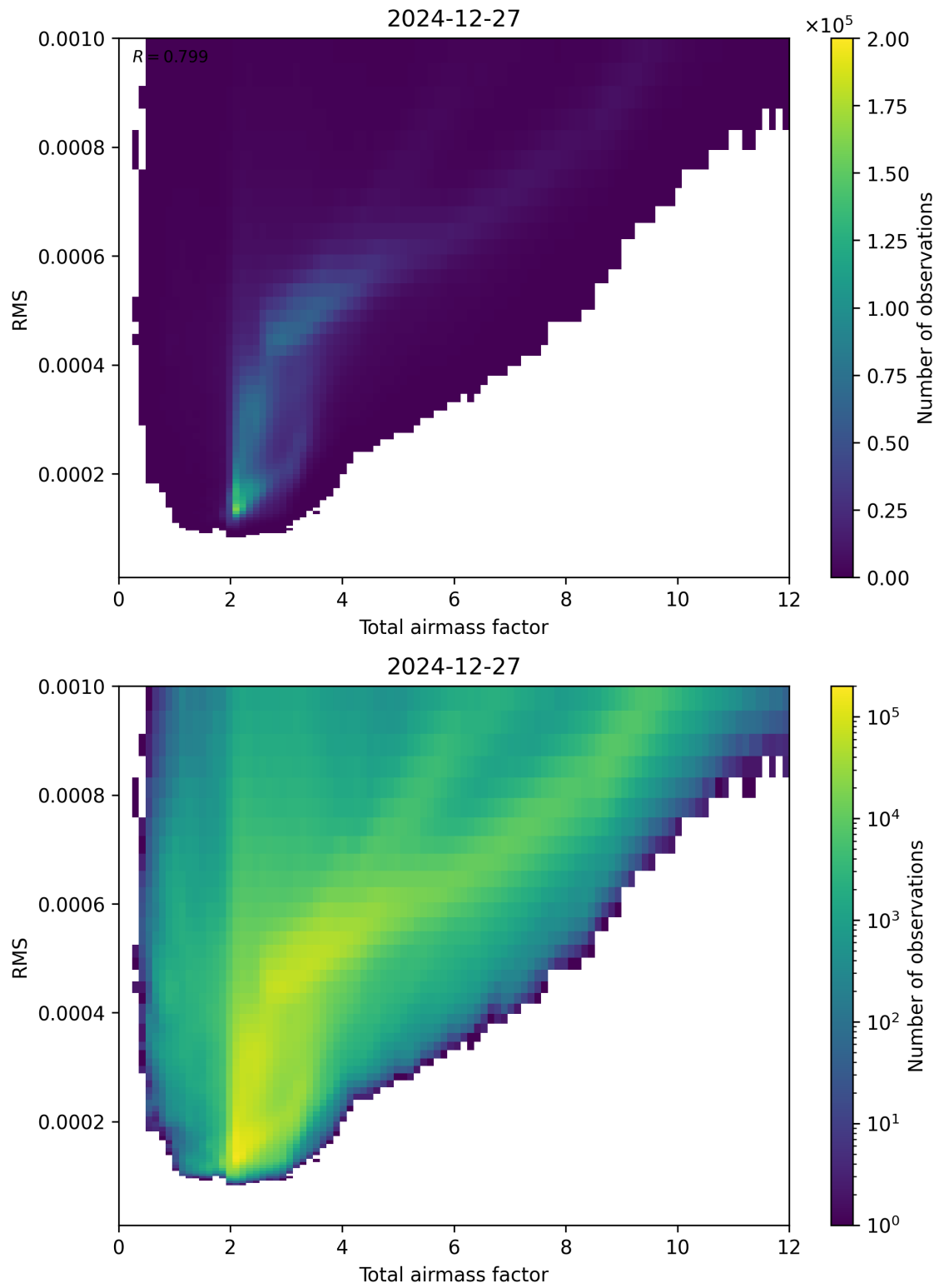
Figure 69: Scatter density plot of “Total airmass factor” against “RMS” for 2024-12-27 to 2024-12-28.
