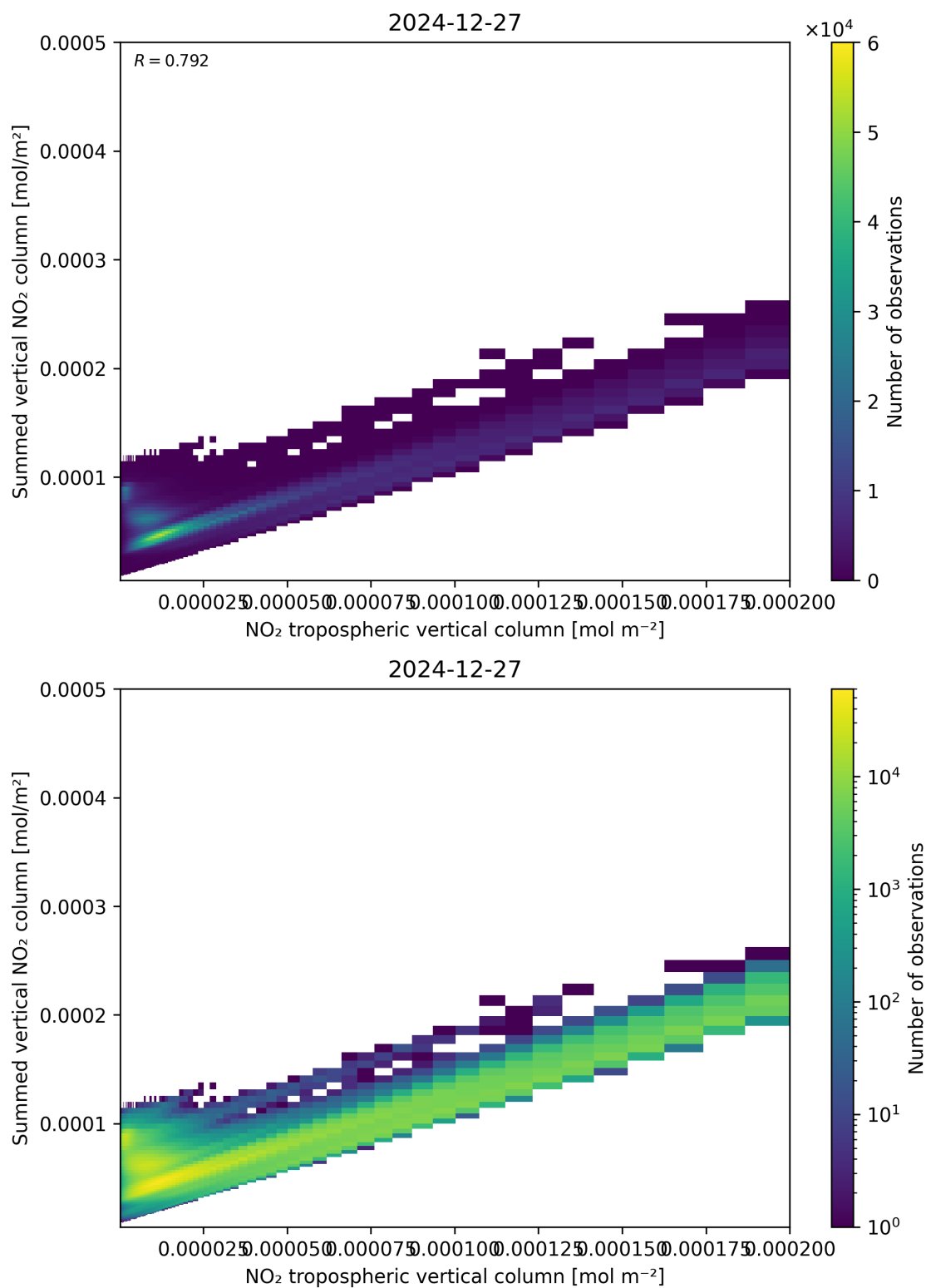
Figure 126: Scatter density plot of “NO 2 tropospheric vertical column” against “Summed vertical NO 2 column” for 2024-12-27 to 2024-12-28.
