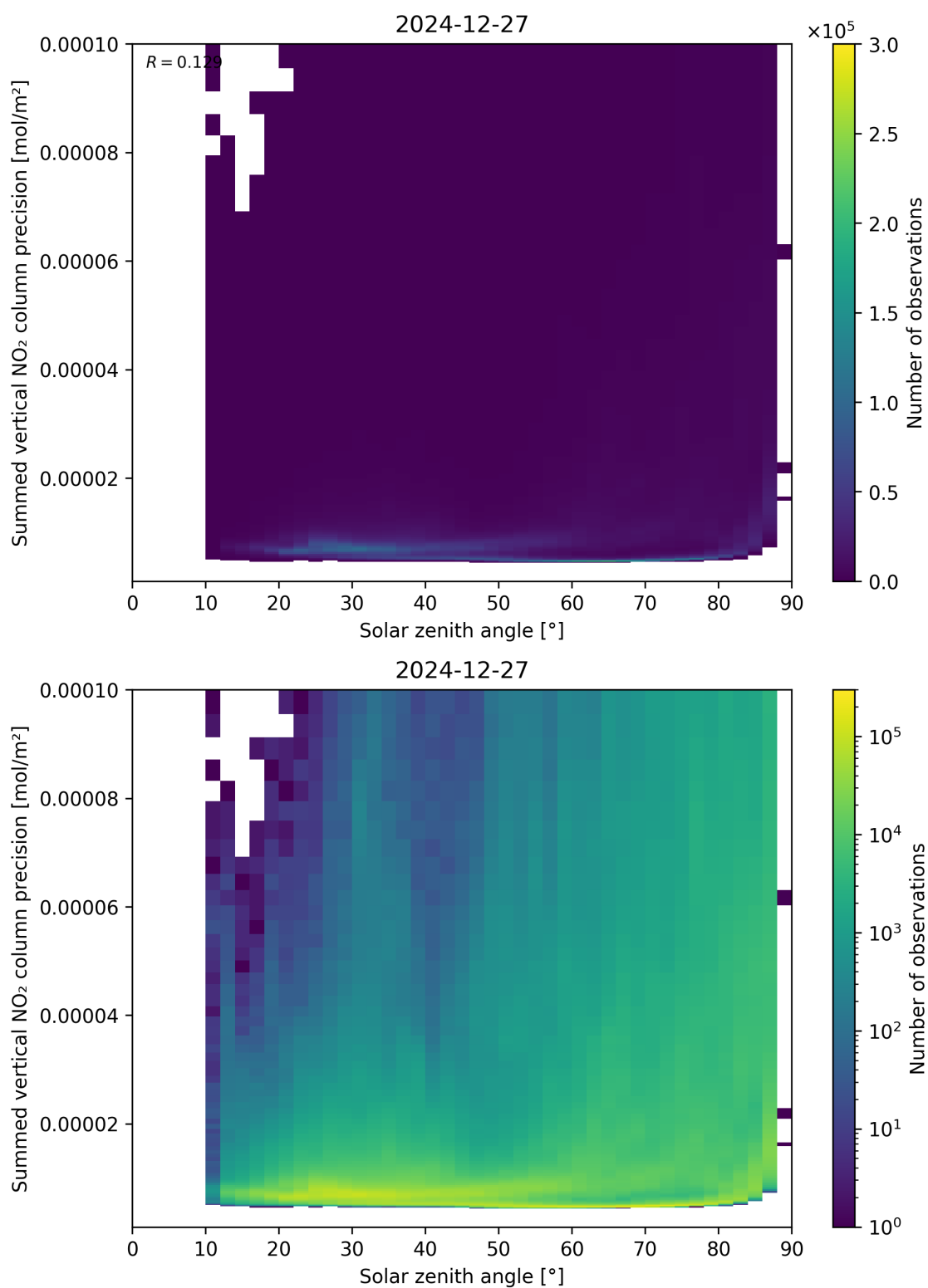
Figure 152: Scatter density plot of “Solar zenith angle” against “Summed vertical NO 2 column precision” for 2024-12-27 to 2024-12-28.
