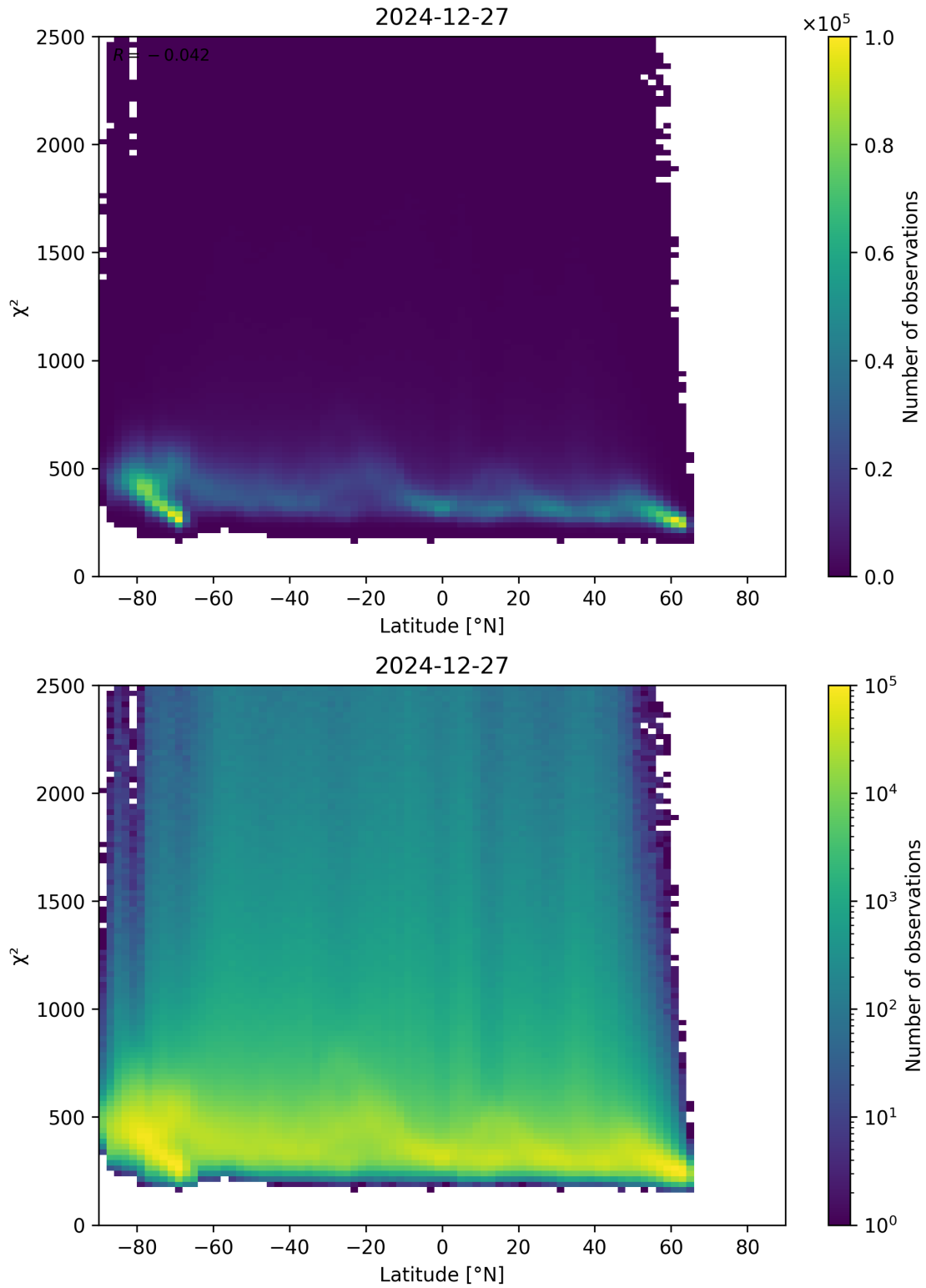
Figure 86: Scatter density plot of “Latitude” against “ \chi^2 ” for 2024-12-27 to 2024-12-28.
