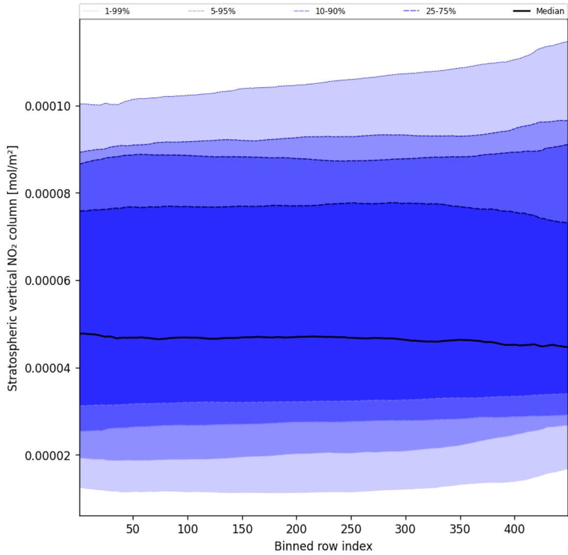
Figure 53: Along track statistics of “Stratospheric vertical NO 2 column” for 2024-12-27 to 2024-12-28
