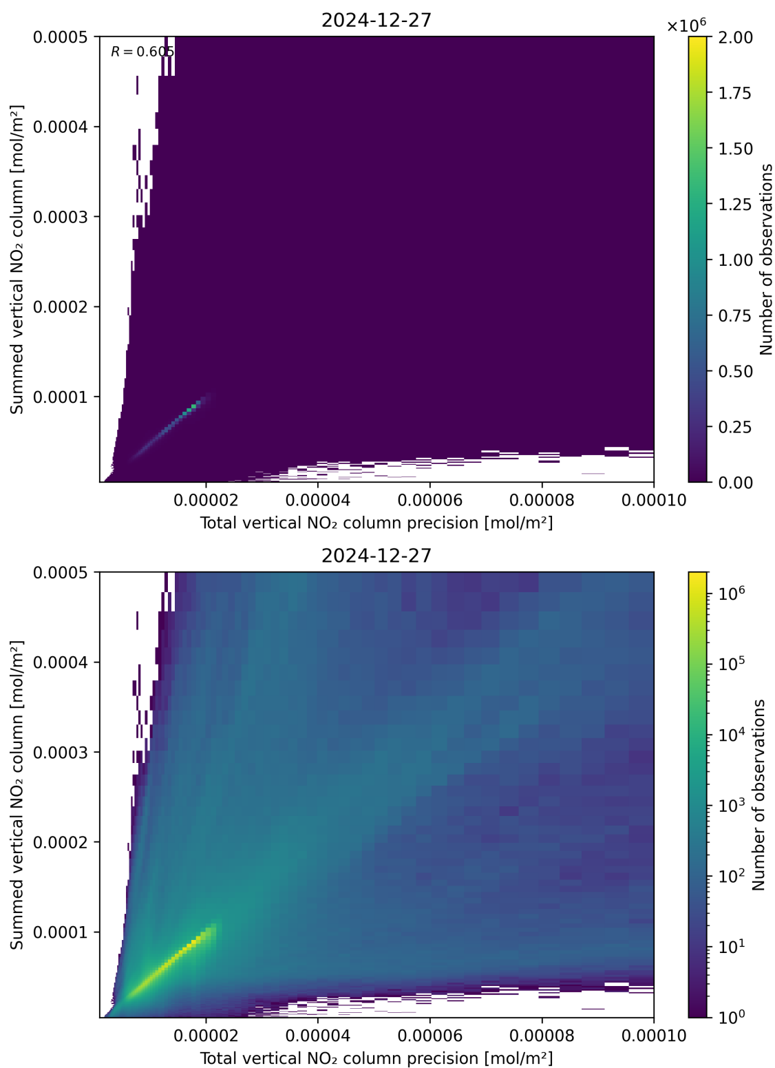
Figure 117: Scatter density plot of “Total vertical NO 2 column precision” against “Summed vertical NO 2 column” for 2024-12-27 to 2024-12-28.
