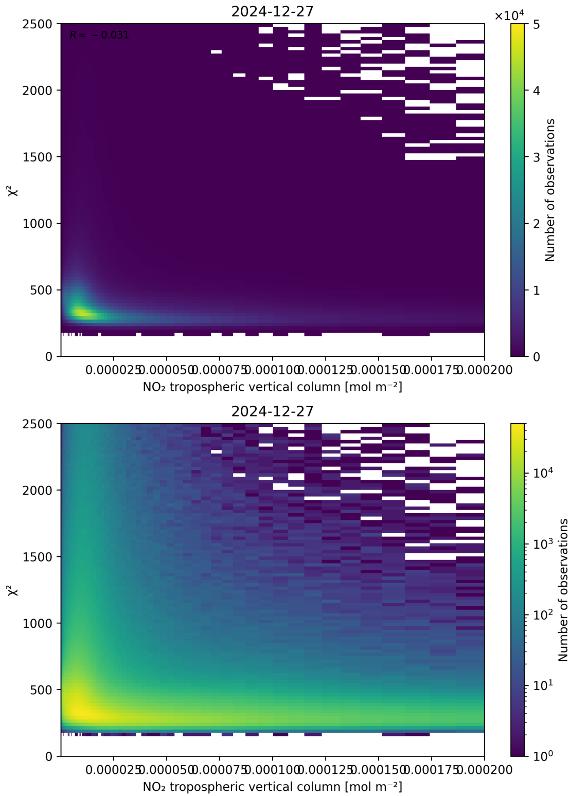
Figure 124: Scatter density plot of “NO 2 tropospheric vertical column” against “ \chi^2 ” for 2024-12-27 to 2024-12-28.
