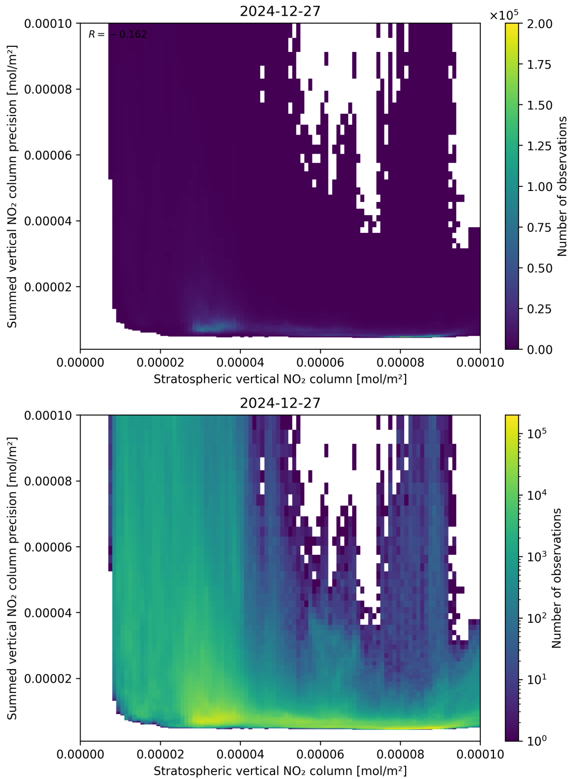
Figure 99: Scatter density plot of “Stratospheric vertical NO 2 column” against “Summed vertical NO 2 column precision” for 2024-12-27 to 2024-12-28.
