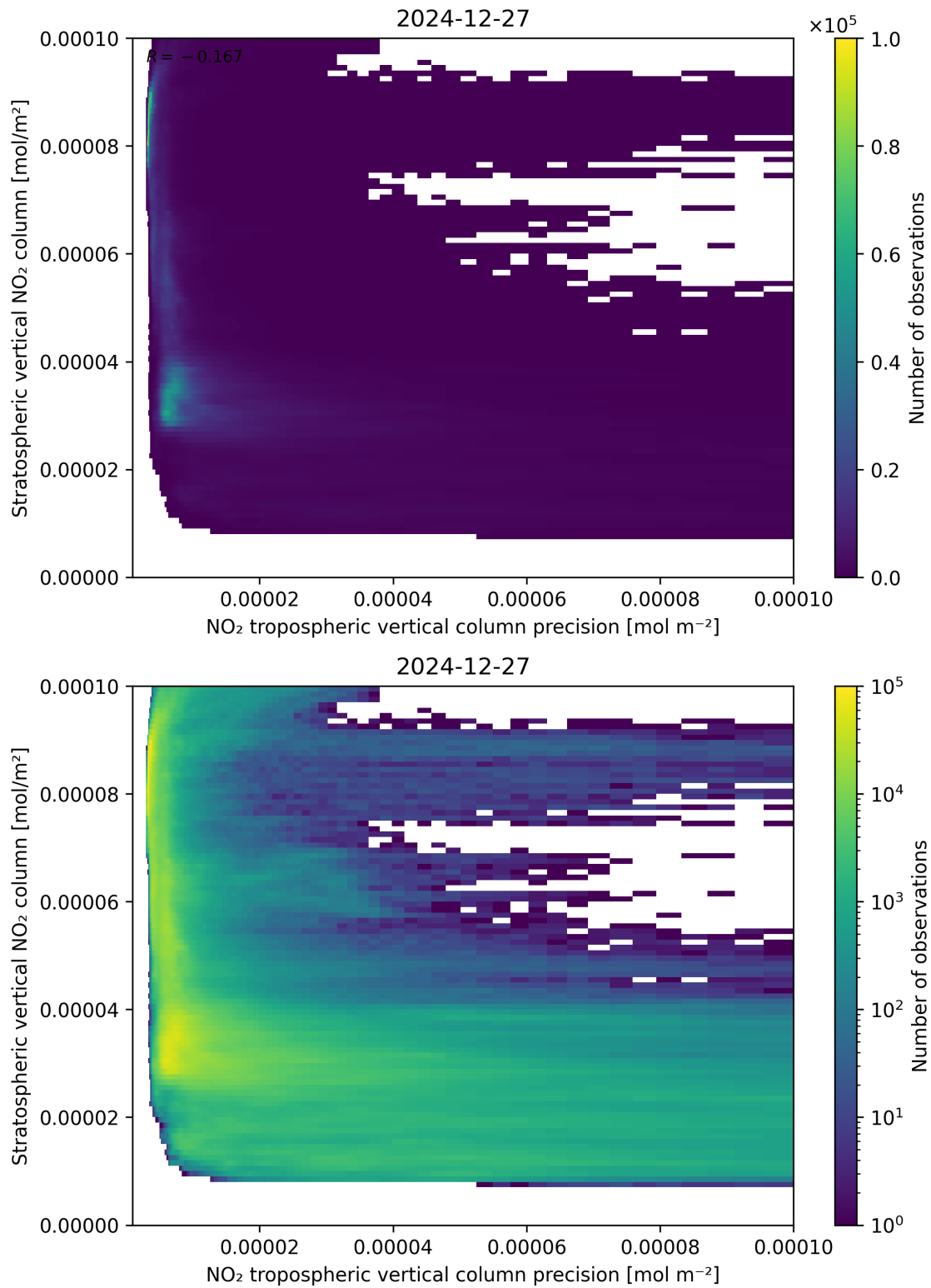
Figure 135: Scatter density plot of “NO 2 tropospheric vertical column precision” against “Stratospheric vertical NO 2 column” for 2024-12-27 to 2024-12-28.
