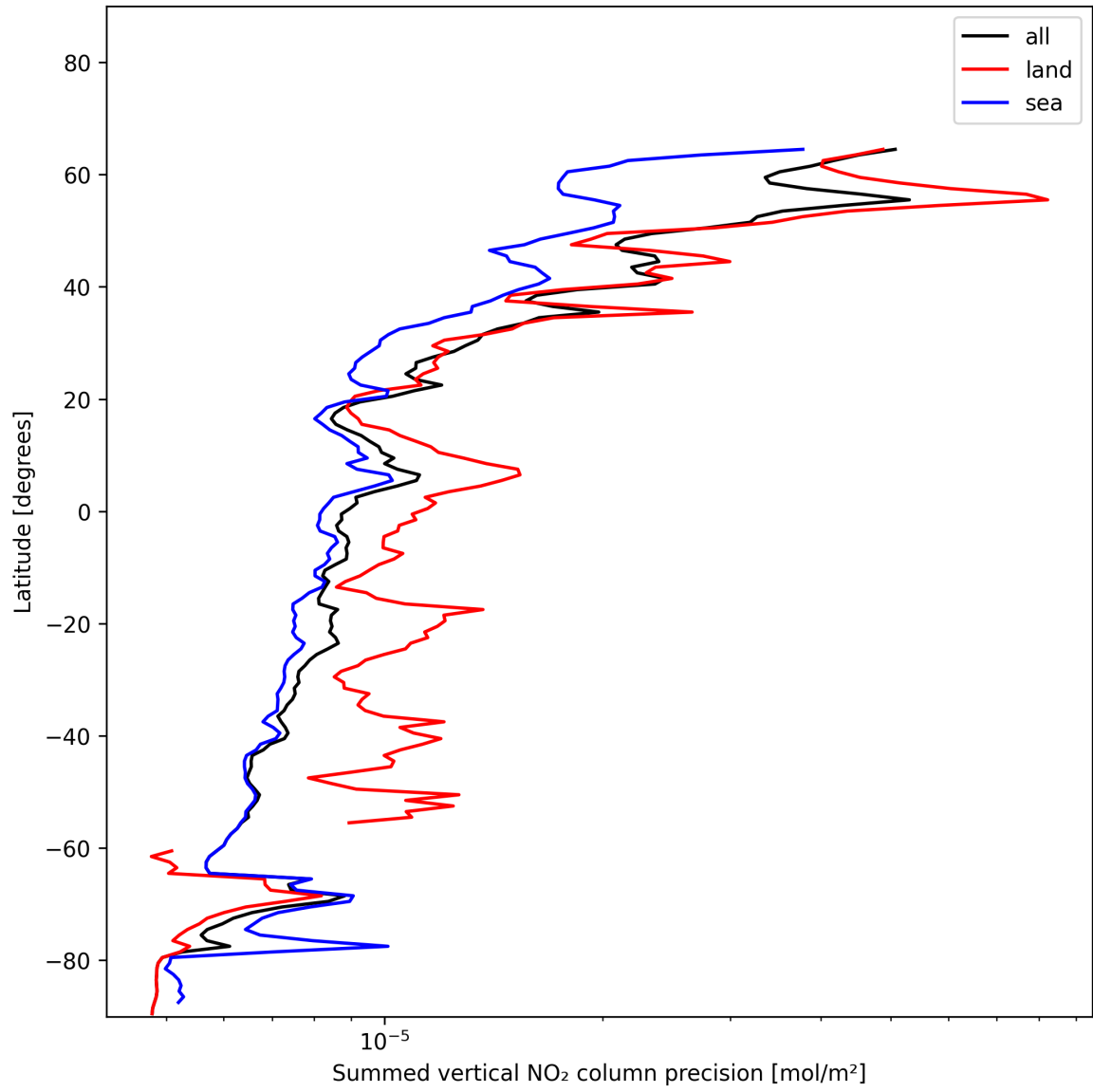
Figure 24: Zonal average of “Summed vertical NO 2 column precision” for 2024-12-27 to 2024-12-28.
