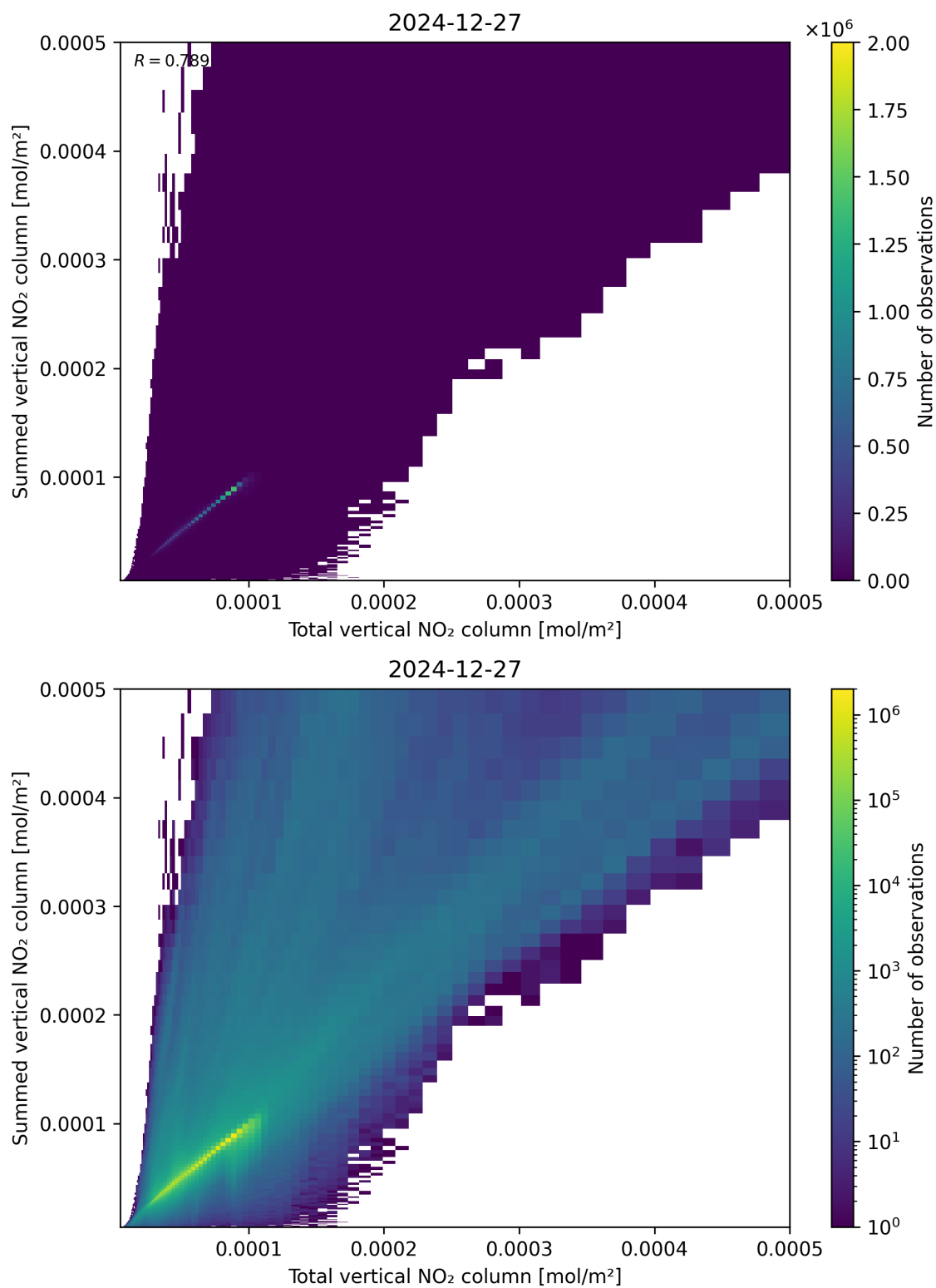
Figure 112: Scatter density plot of “Total vertical NO 2 column” against “Summed vertical NO 2 column” for 2024-12-27 to 2024-12-28.
