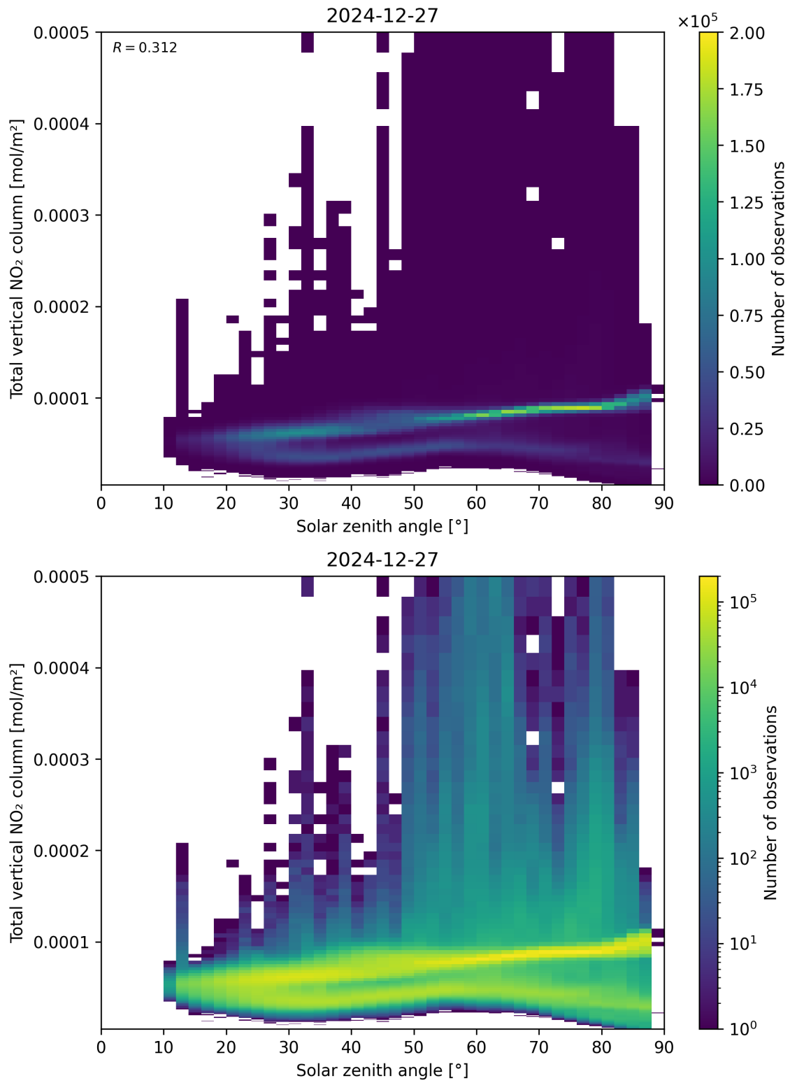
Figure 153: Scatter density plot of “Solar zenith angle” against “Total vertical \text{NO}_2 column” for 2024-12-27 to 2024-12-28.
