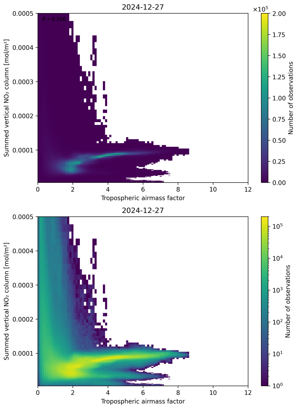
Figure 75: Scatter density plot of “Tropospheric air mass factor” against “Summed vertical NO 2 column” for 2024-12-27 to 2024-12-28.
