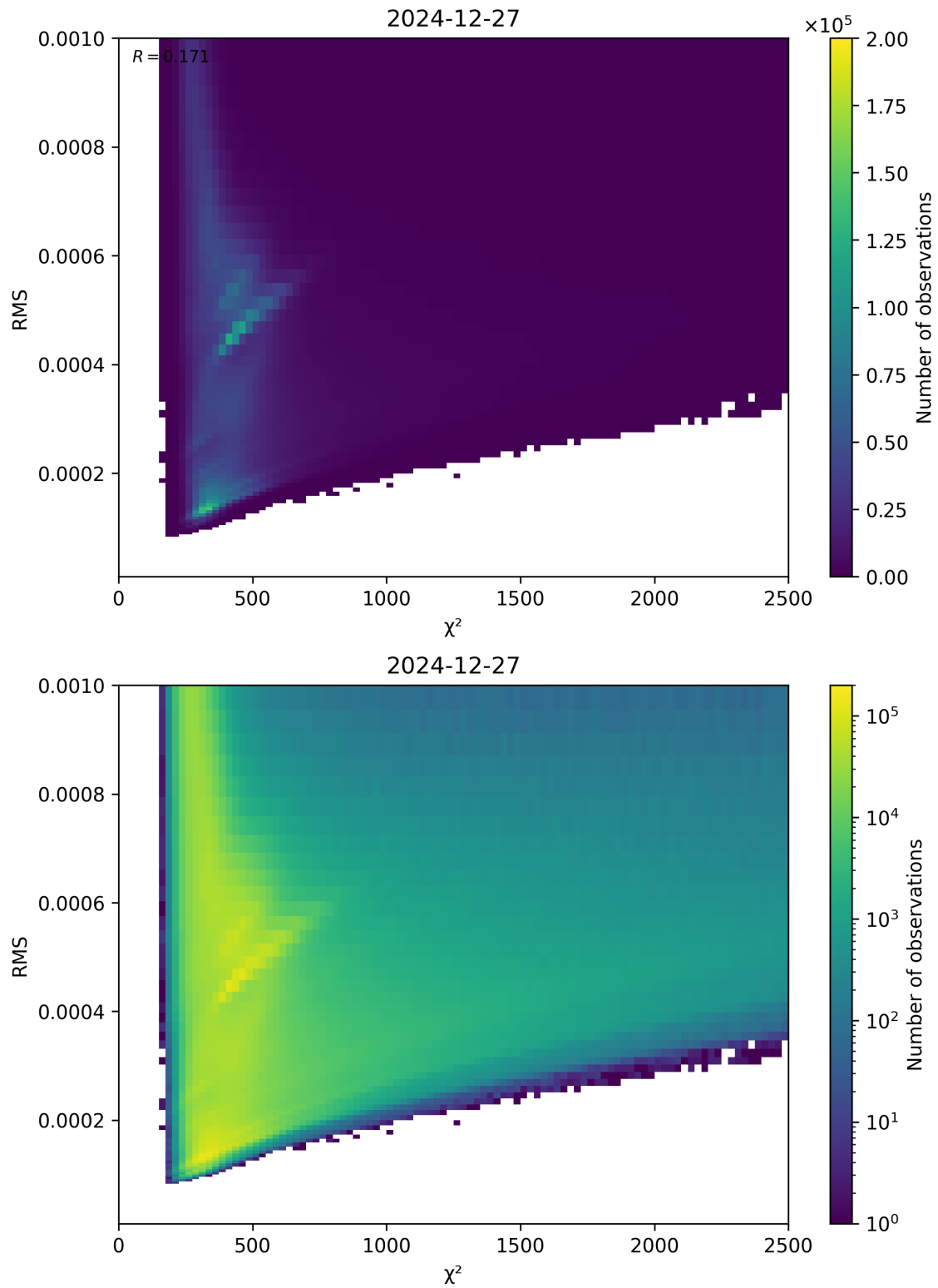
Figure 82: Scatter density plot of “ \chi^2 ” against “RMS” for 2024-12-27 to 2024-12-28.
