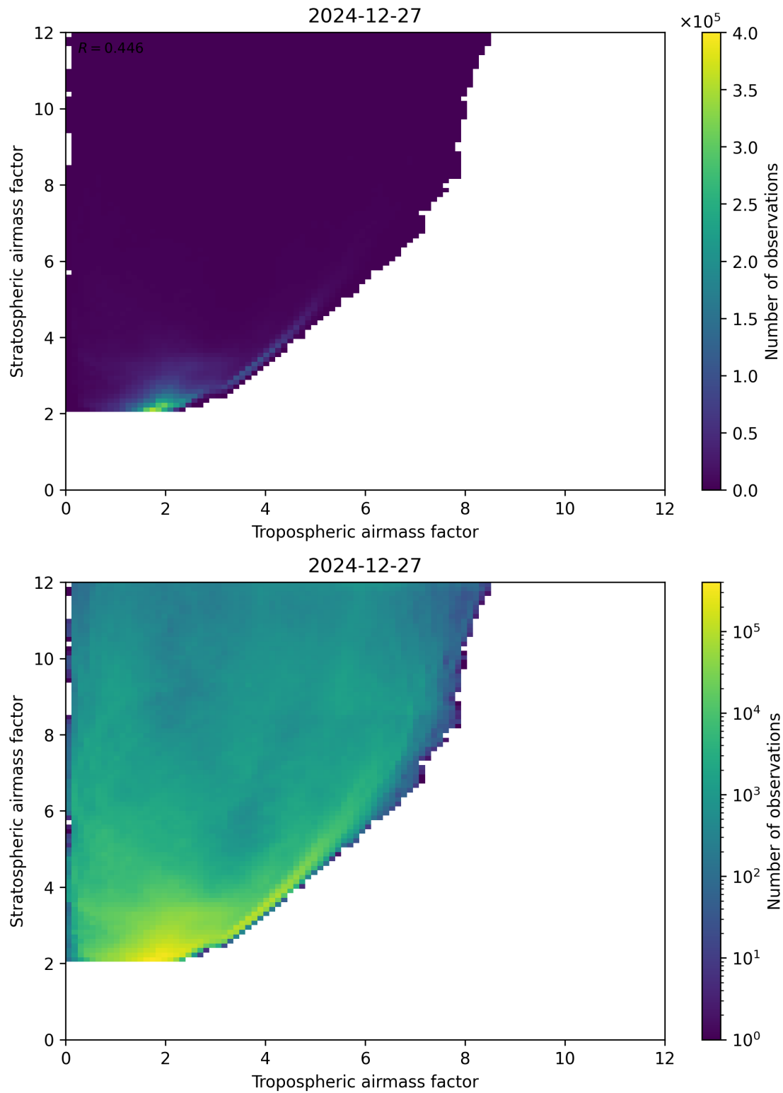
Figure 71: Scatter density plot of “Tropospheric airmass factor” against “Stratospheric airmass factor” for 2024-12-27 to 2024-12-28.
