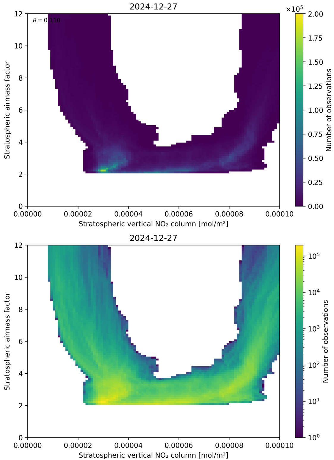
Figure 96: Scatter density plot of “Stratospheric vertical NO 2 column” against “Stratospheric airmass factor” for 2024-12-27 to 2024-12-28.
