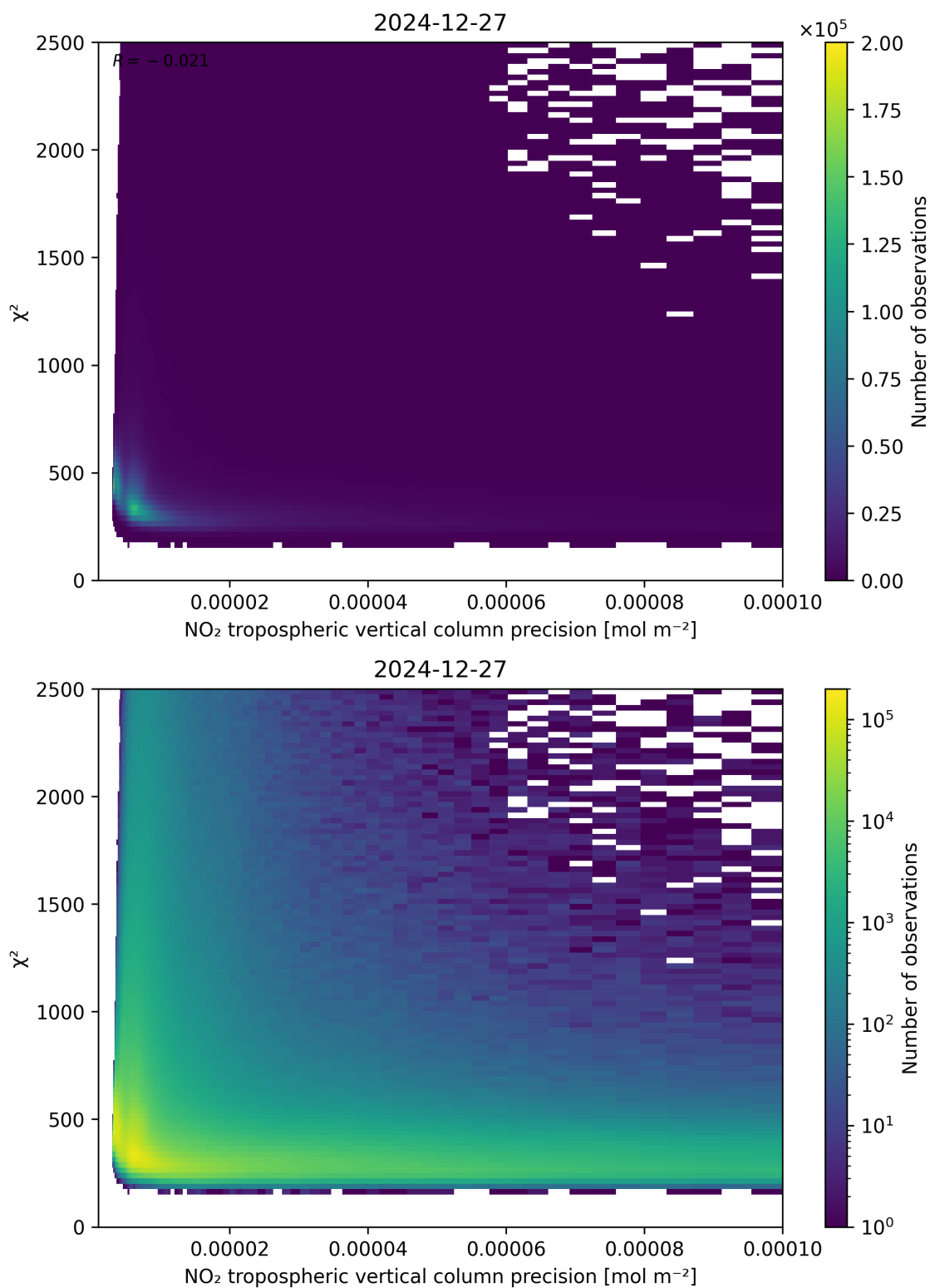
Figure 134: Scatter density plot of “NO 2 tropospheric vertical column precision” against “ \chi^2 ” for 2024-12-27 to 2024-12-28.
