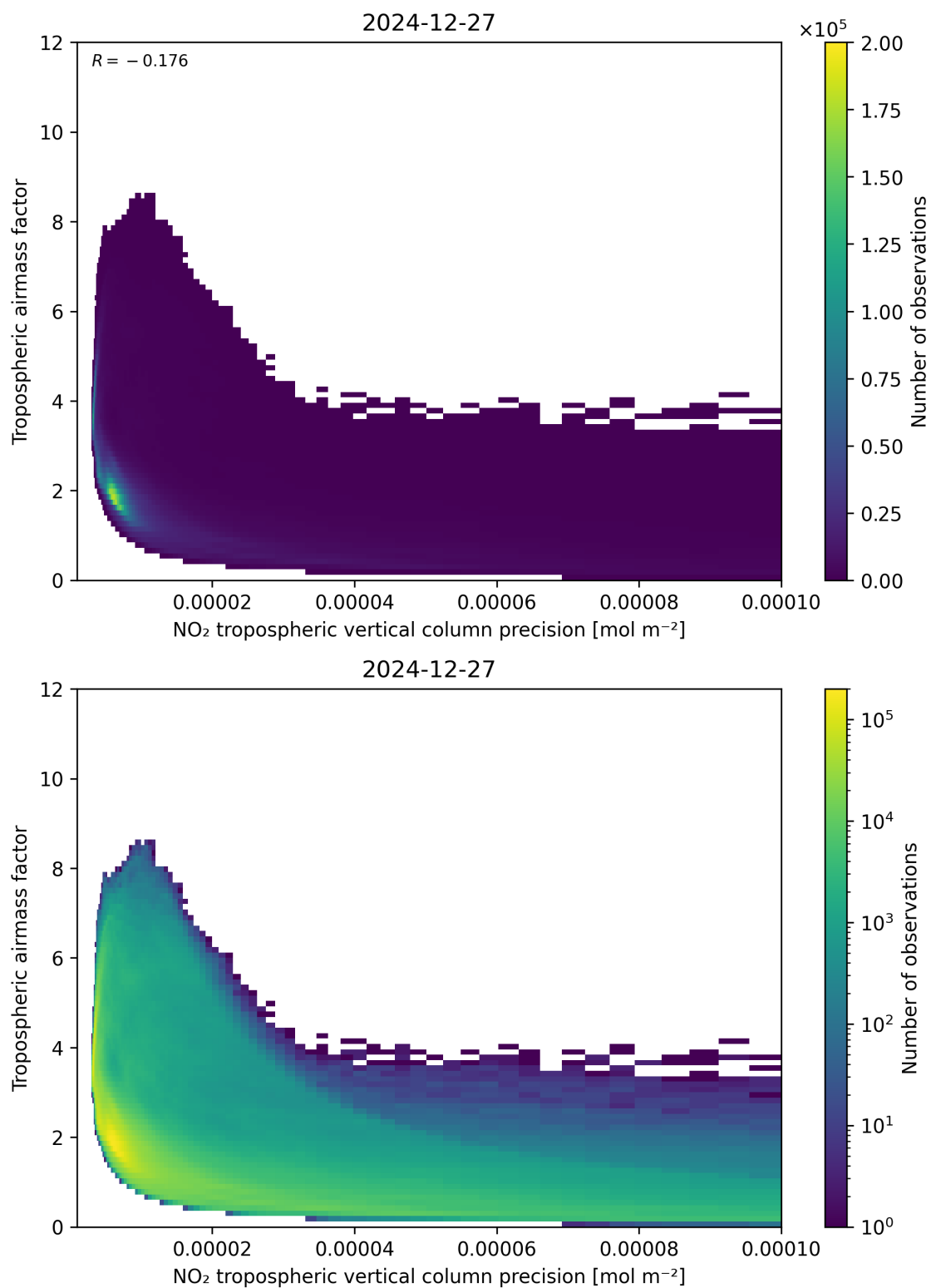
Figure 133: Scatter density plot of “NO 2 tropospheric vertical column precision” against “Tropospheric airmass factor” for 2024-12-27 to 2024-12-28.
