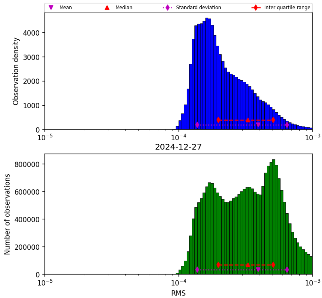
Figure 43: Histogram of “RMS” for 2024-12-27 to 2024-12-28
