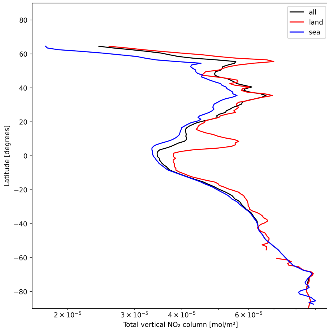
Figure 21: Zonal average of “Total vertical NO 2 column” for 2024-12-27 to 2024-12-28.
