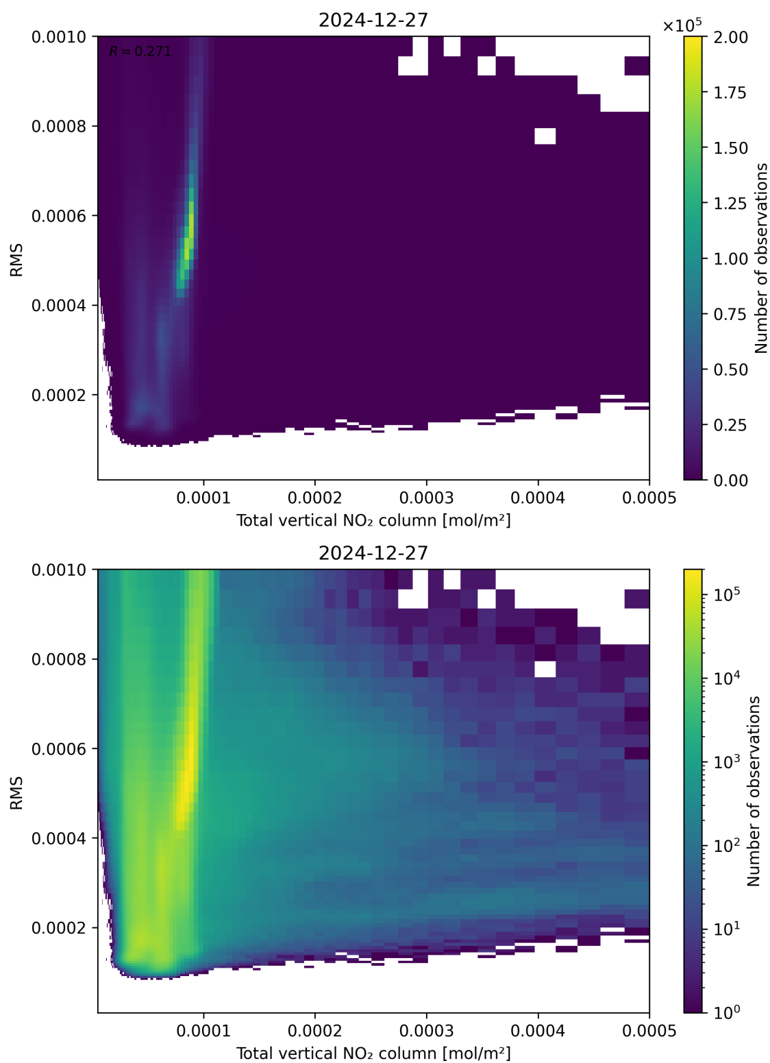
Figure 120: Scatter density plot of “Total vertical NO 2 column” against “RMS” for 2024-12-27 to 2024-12-28.
