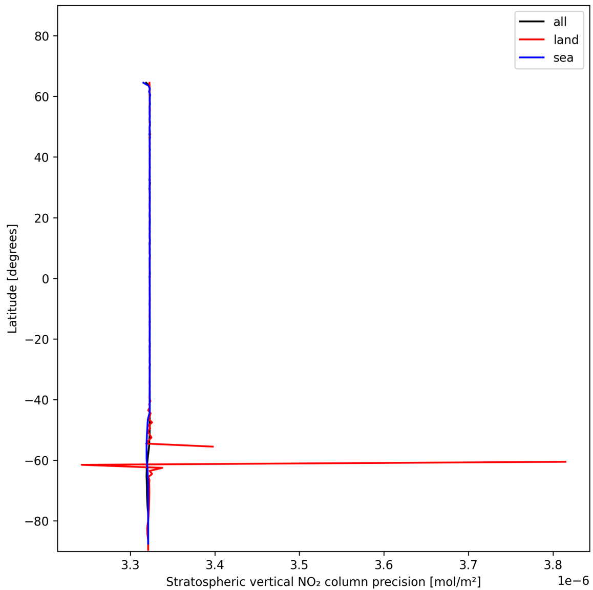
Figure 20: Zonal average of “Stratospheric vertical NO 2 column precision” for 2024-12-27 to 2024-12-28.
