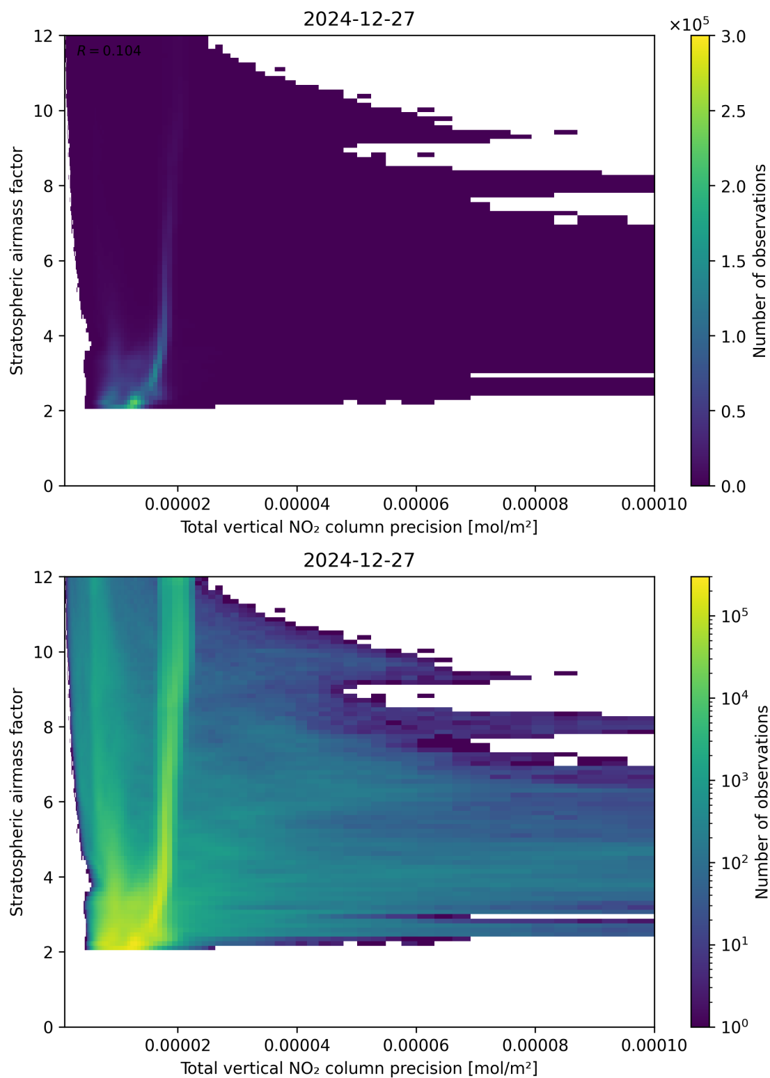
Figure 115: Scatter density plot of “Total vertical NO 2 column precision” against “Stratospheric air mass factor” for 2024-12-27 to 2024-12-28.
