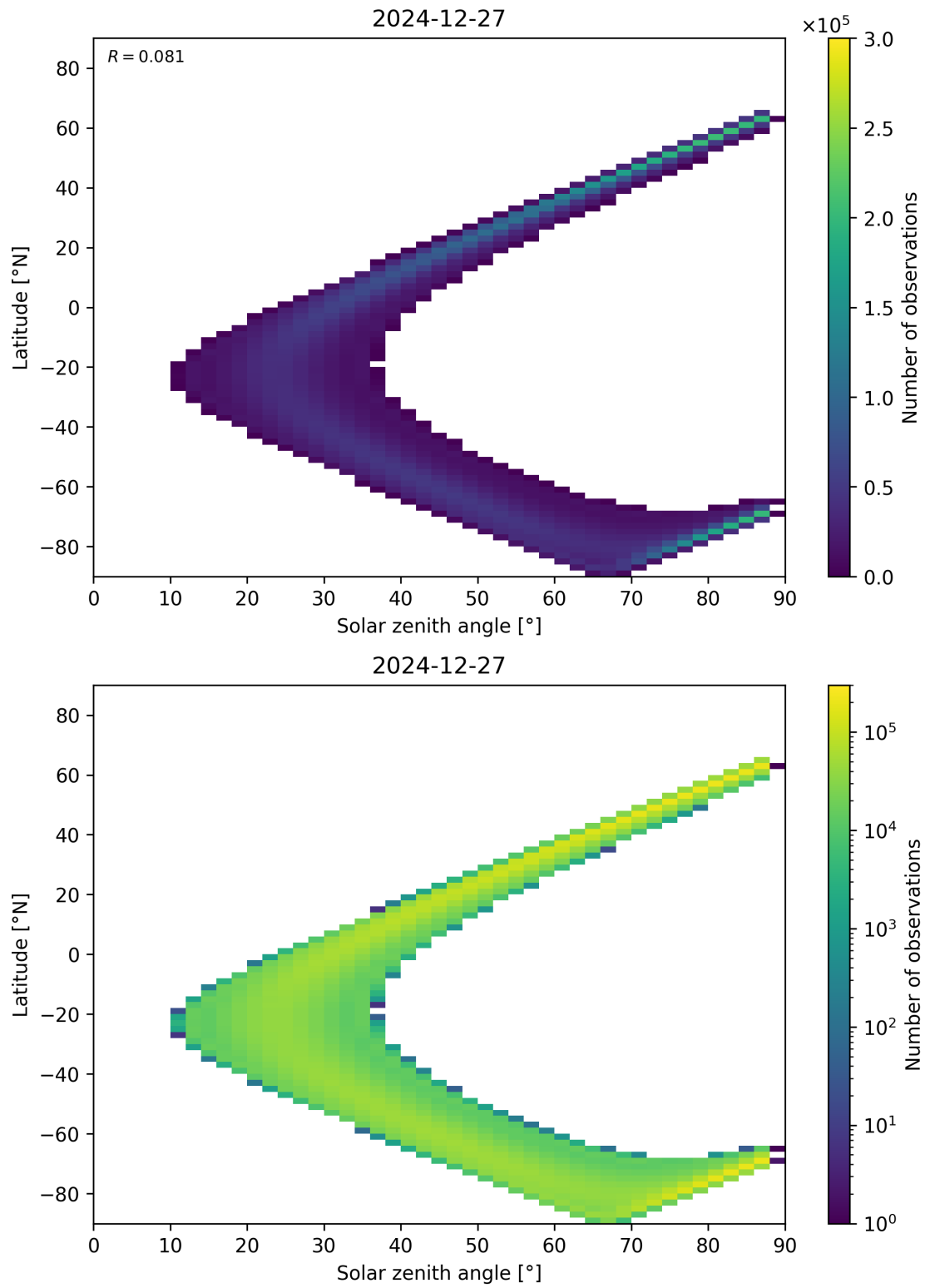
Figure 149: Scatter density plot of “Solar zenith angle” against “Latitude” for 2024-12-27 to 2024-12-28.
