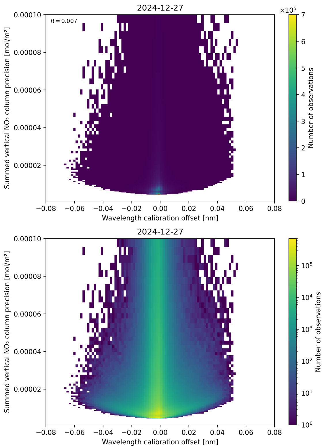
Figure 178: Scatter density plot of “Wavelength calibration offset” against “Summed vertical NO 2 column precision” for 2024-12-27 to 2024-12-28.
