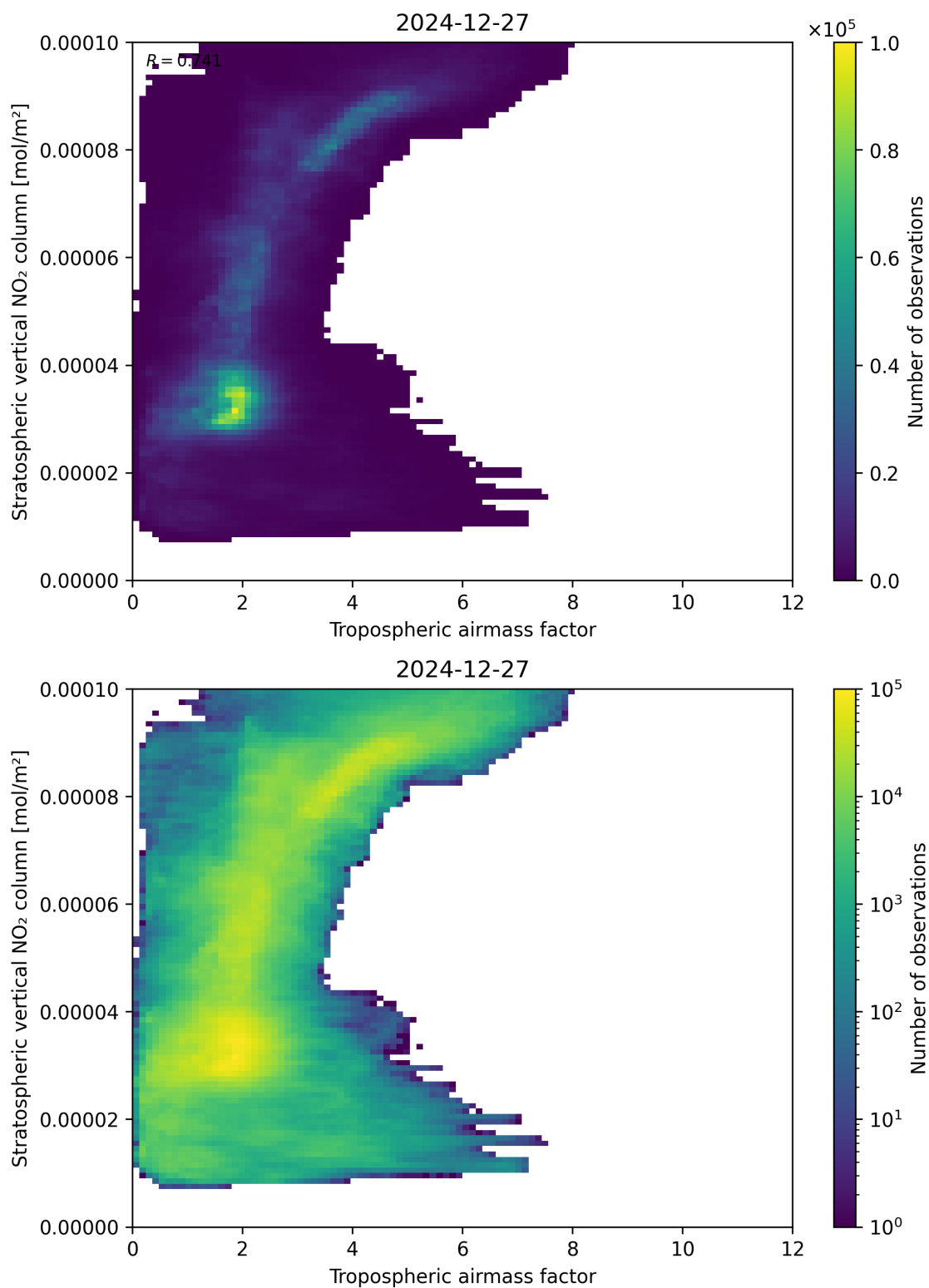
Figure 74: Scatter density plot of “Tropospheric air mass factor” against “Stratospheric vertical NO 2 column” for 2024-12-27 to 2024-12-28.
