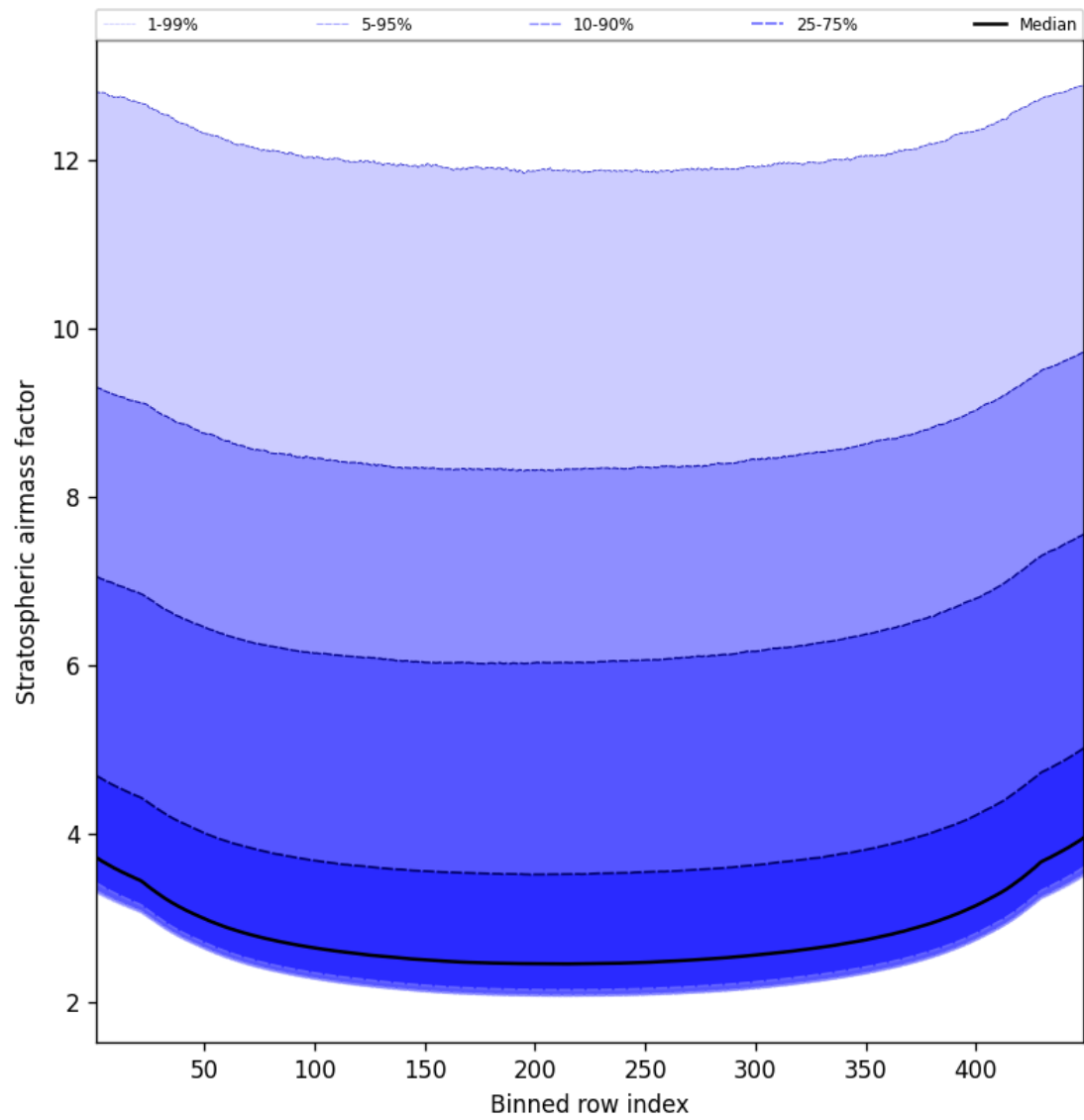
Figure 61: Along track statistics of “Stratospheric airmass factor” for 2024-12-27 to 2024-12-28
