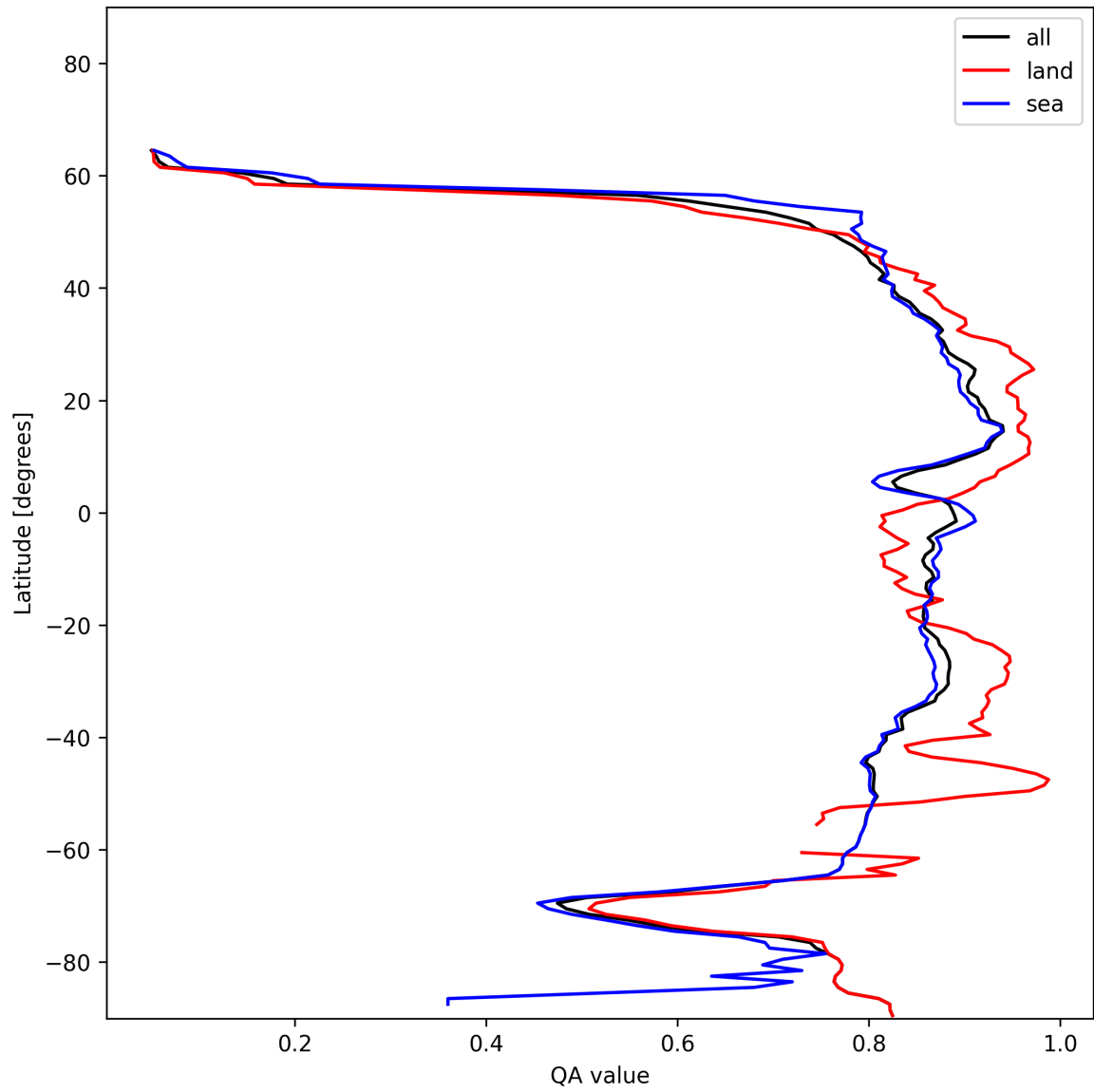
Figure 11: Zonal average of “QA value” for 2024-12-27 to 2024-12-28.
