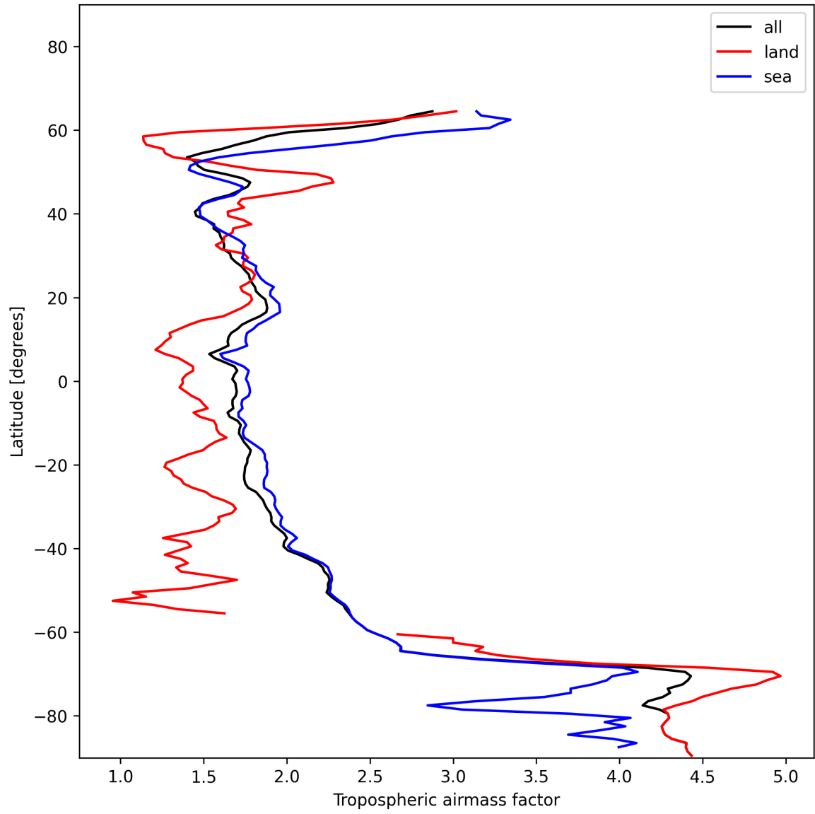
Figure 14: Zonal average of “Tropospheric airmass factor” for 2024-12-27 to 2024-12-28.
