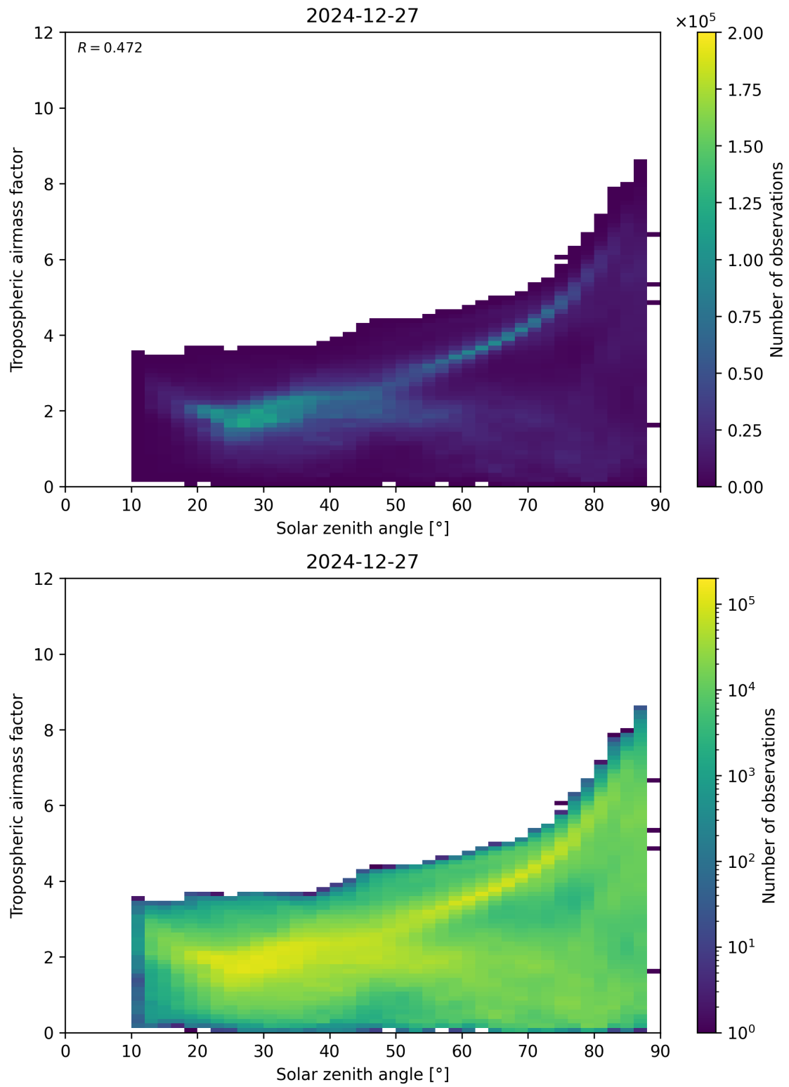
Figure 147: Scatter density plot of “Solar zenith angle” against “Tropospheric airmass factor” for 2024-12-27 to 2024-12-28.
