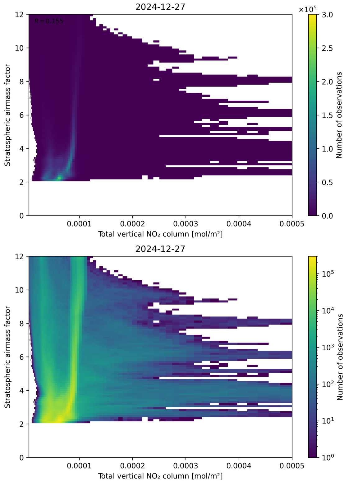
Figure 110: Scatter density plot of “Total vertical NO 2 column” against “Stratospheric airmass factor” for 2024-12-27 to 2024-12-28.
