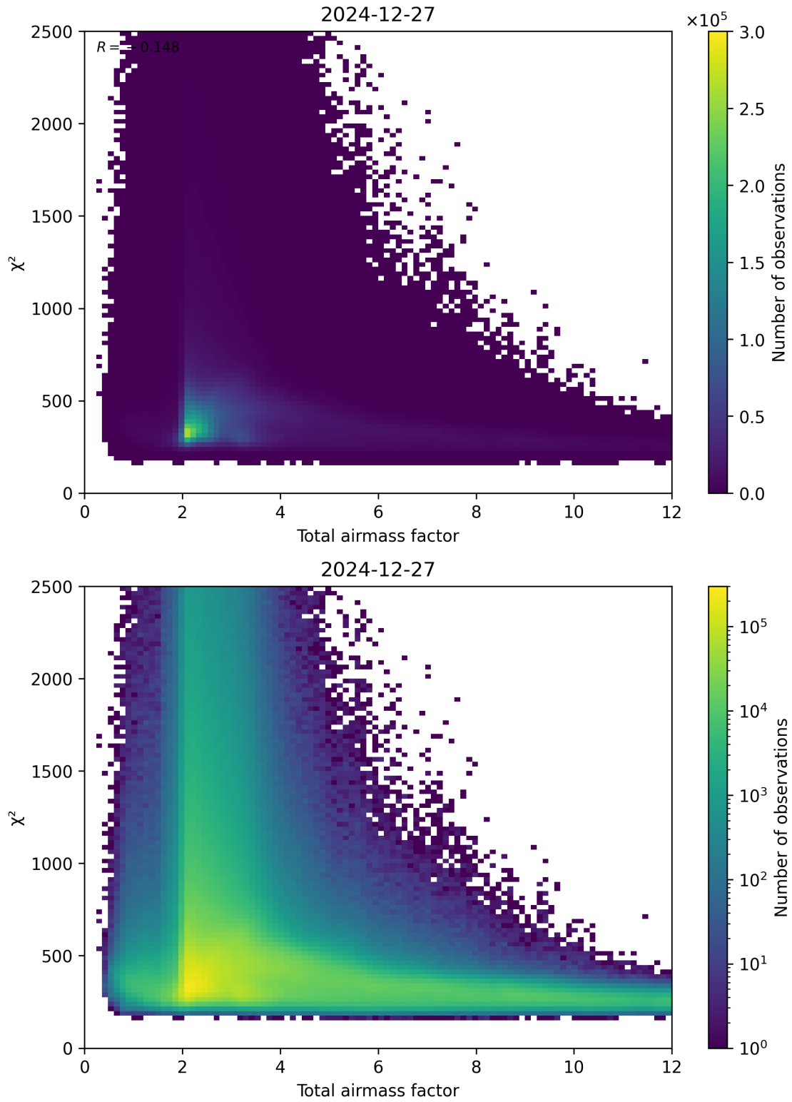
Figure 63: Scatter density plot of “Total airmass factor” against “ \chi^2 ” for 2024-12-27 to 2024-12-28.
