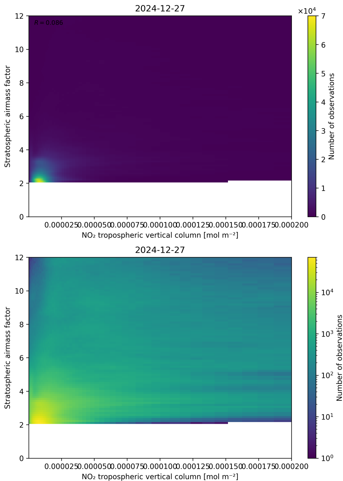
Figure 121: Scatter density plot of “NO 2 tropospheric vertical column” against “Stratospheric air mass factor” for 2024-12-27 to 2024-12-28.
