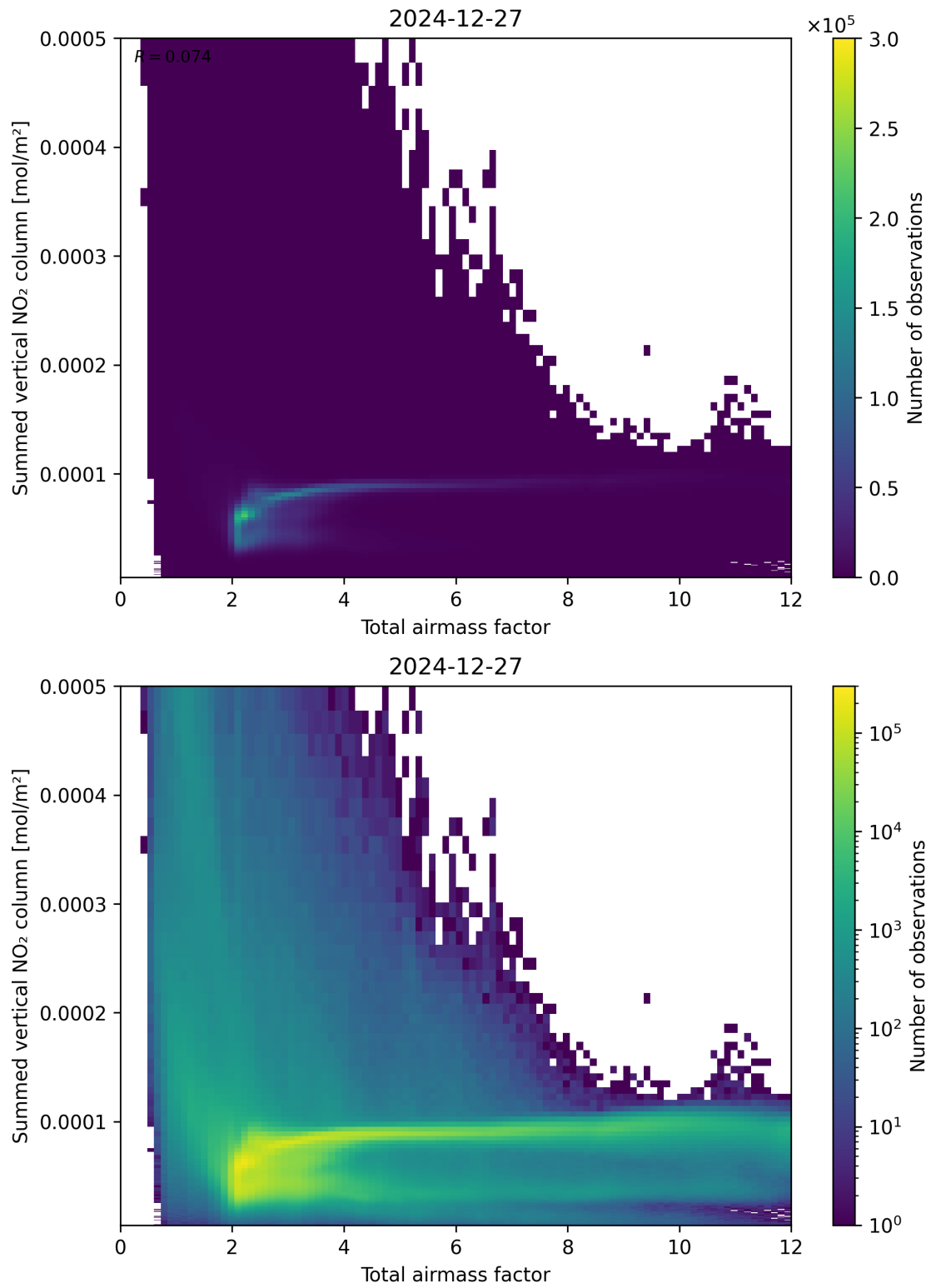
Figure 65: Scatter density plot of “Total airmass factor” against “Summed vertical NO 2 column” for 2024-12-27 to 2024-12-28.
