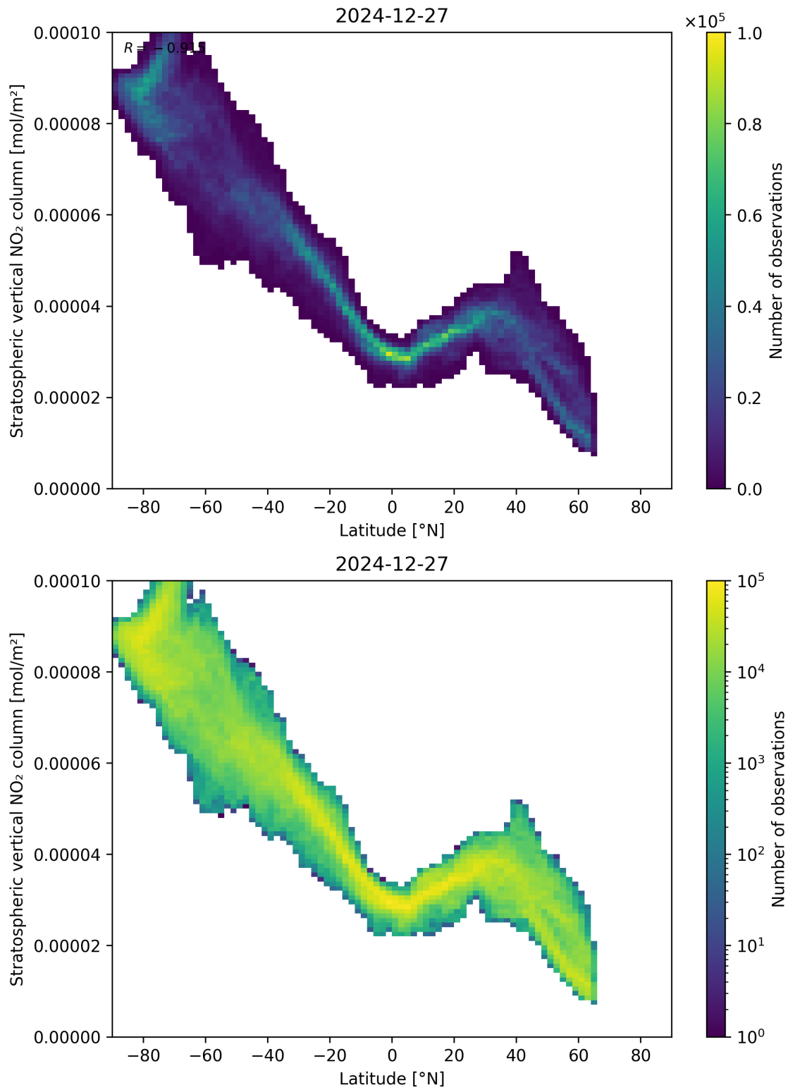
Figure 87: Scatter density plot of “Latitude” against “Stratospheric vertical NO 2 column” for 2024-12-27 to 2024-12-28.
