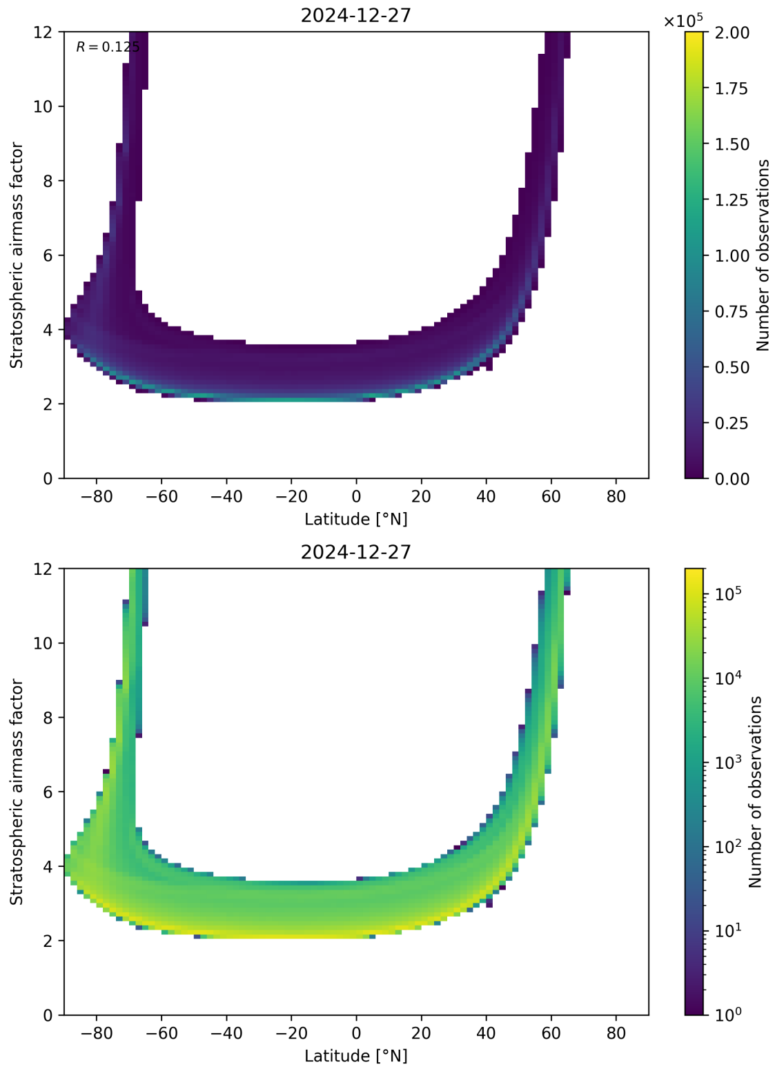
Figure 83: Scatter density plot of “Latitude” against “Stratospheric air mass factor” for 2024-12-27 to 2024-12-28.
