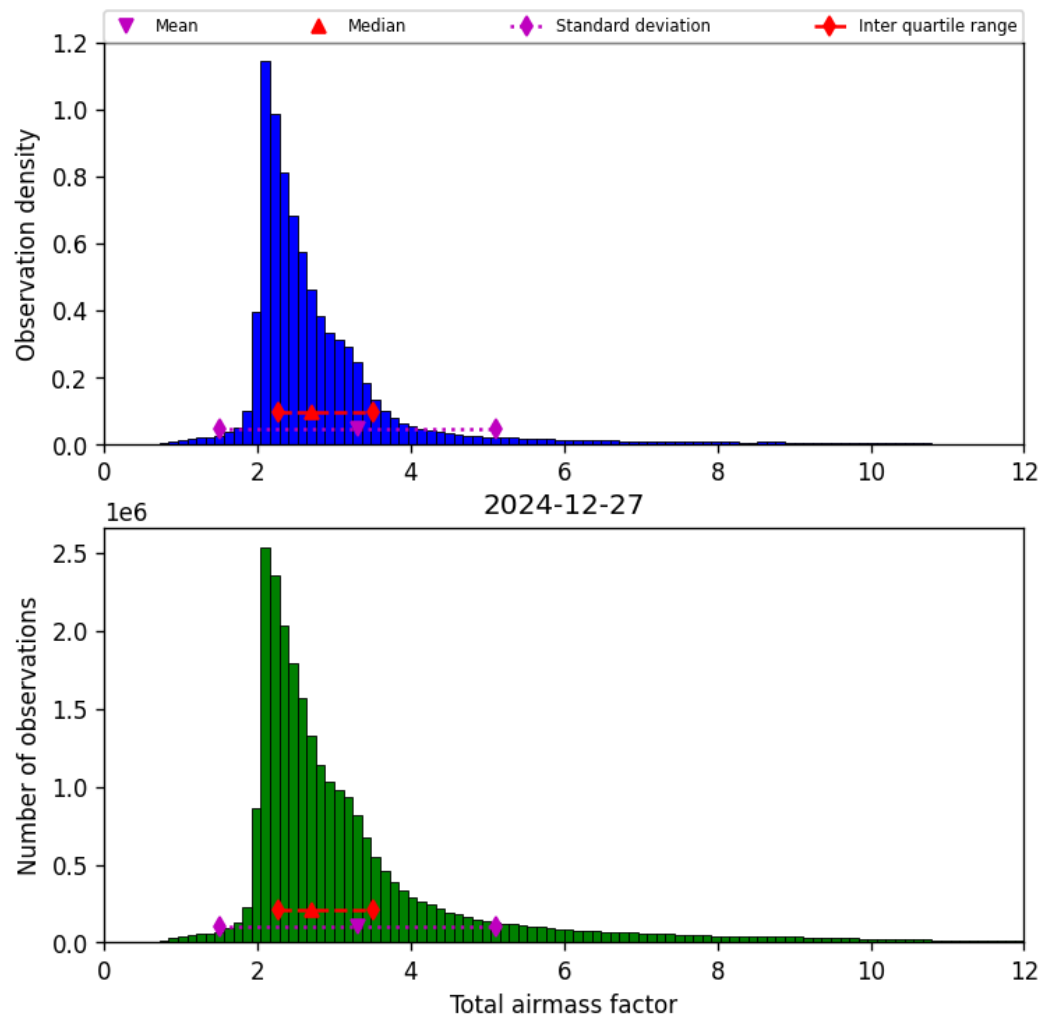
Figure 32: Histogram of “Total airmass factor” for 2024-12-27 to 2024-12-28
