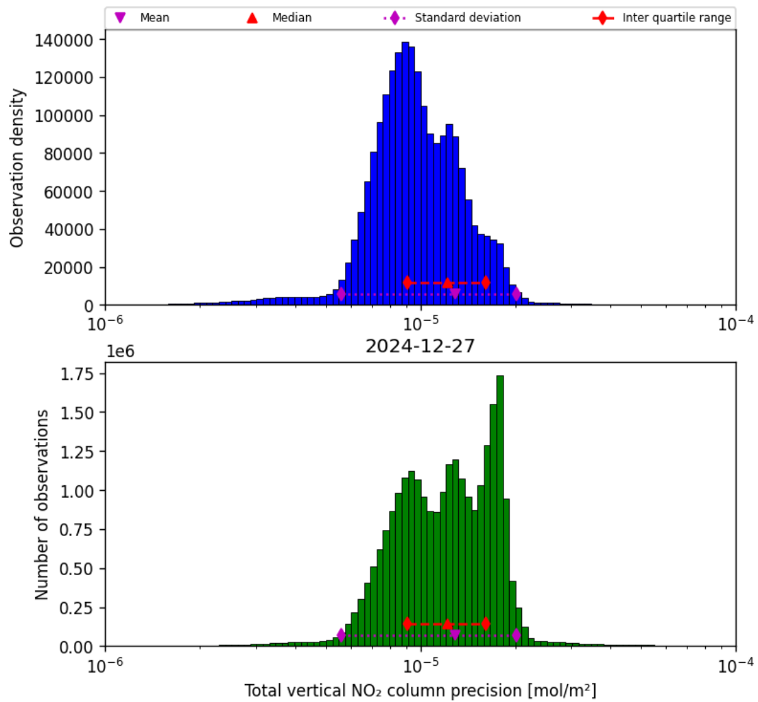
Figure 39: Histogram of “Total vertical NO 2 column precision” for 2024-12-27 to 2024-12-28
