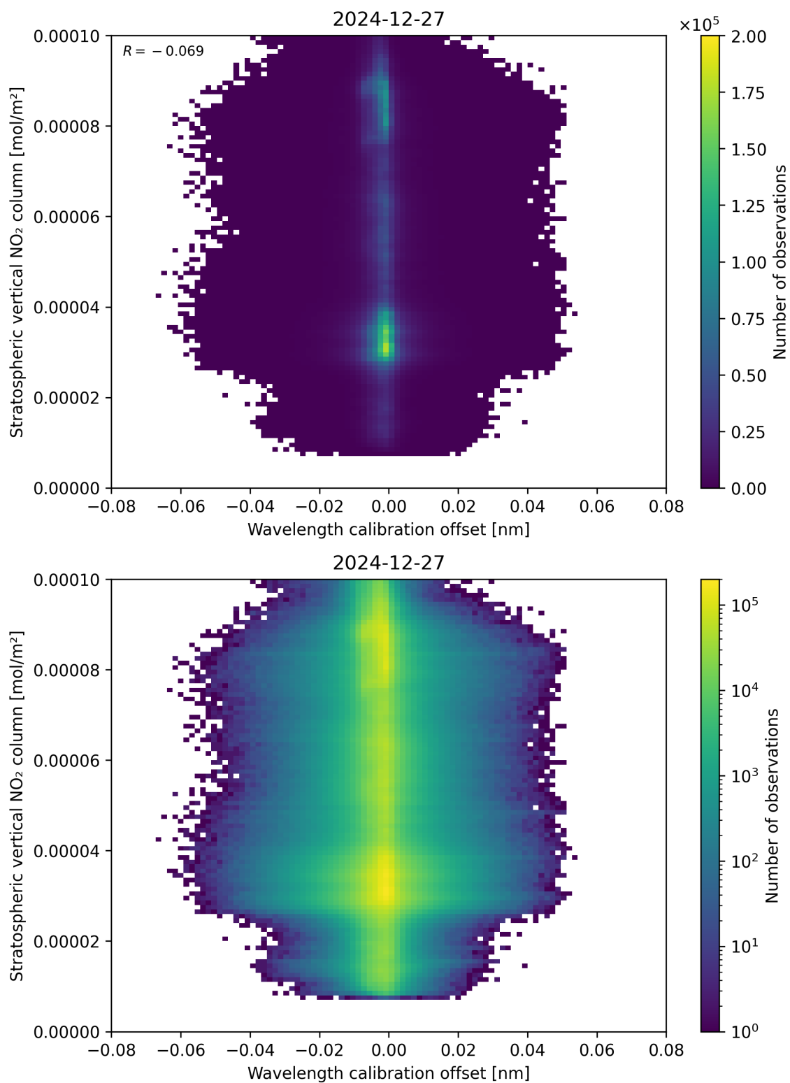
Figure 176: Scatter density plot of “Wavelength calibration offset” against “Stratospheric vertical NO 2 column” for 2024-12-27 to 2024-12-28.
