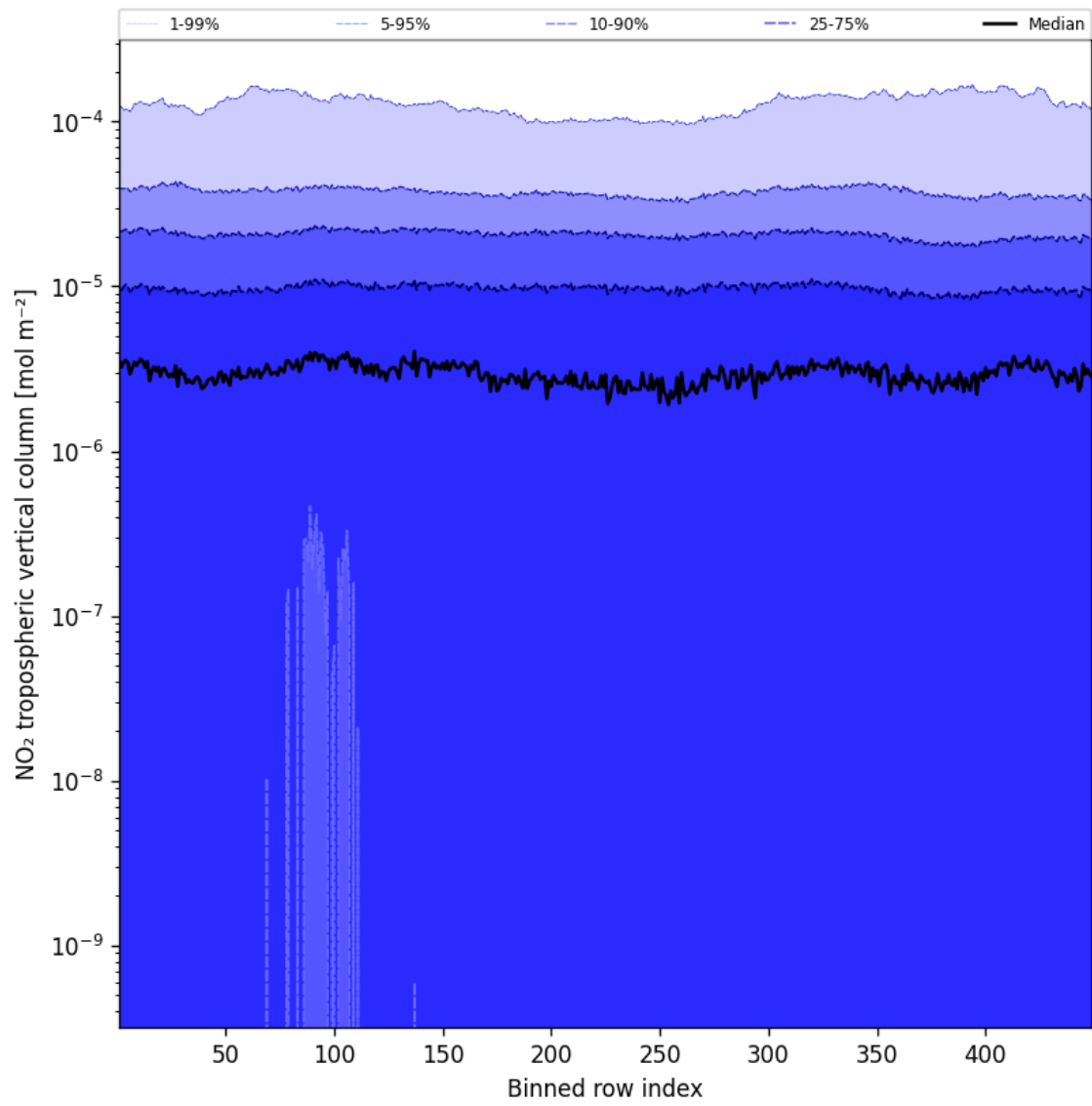
Figure 46: Along track statistics of “NO 2 tropospheric vertical column” for 2024-12-27 to 2024-12-28
