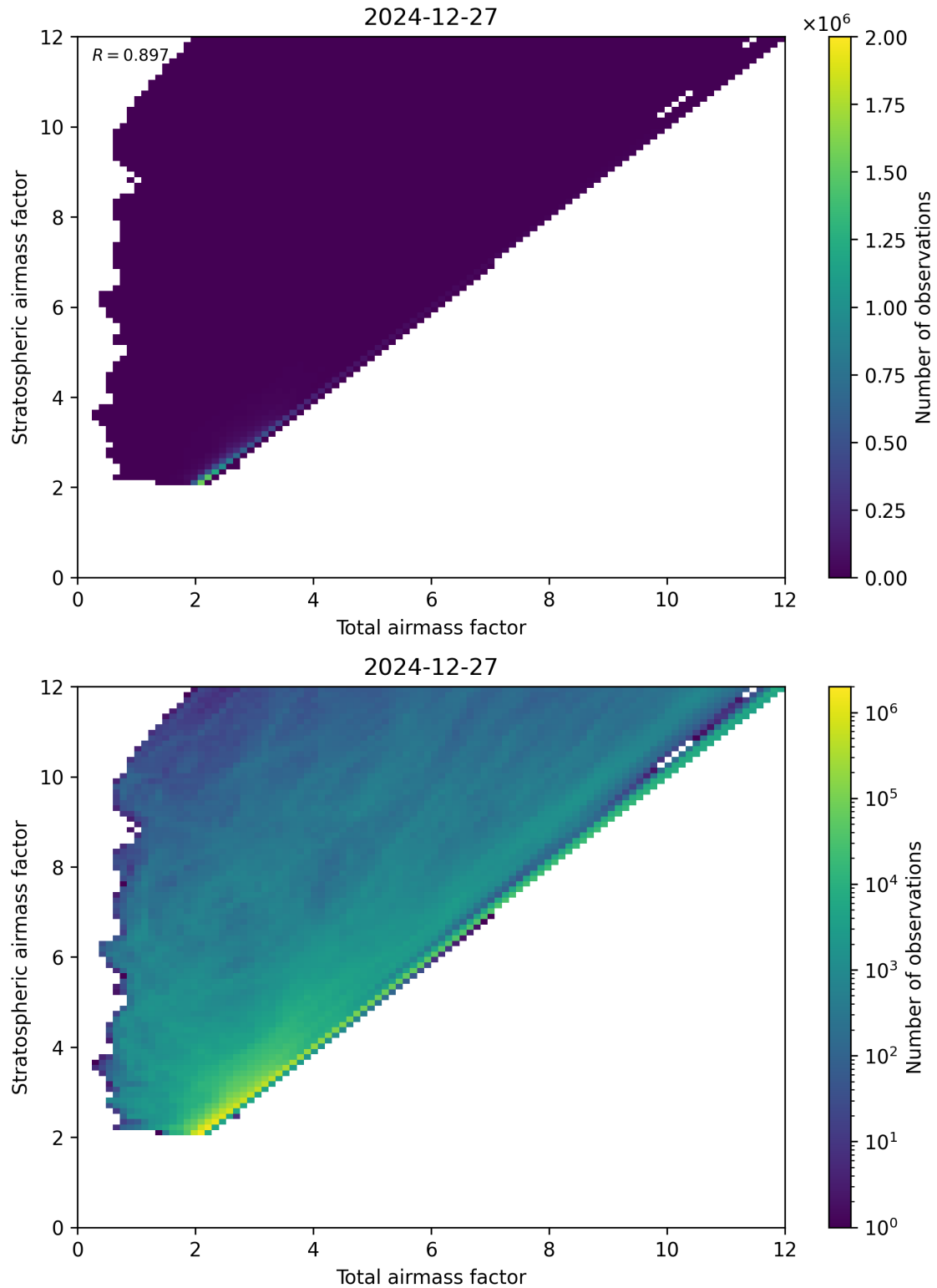
Figure 62: Scatter density plot of “Total airmass factor” against “Stratospheric airmass factor” for 2024-12-27 to 2024-12-28.
