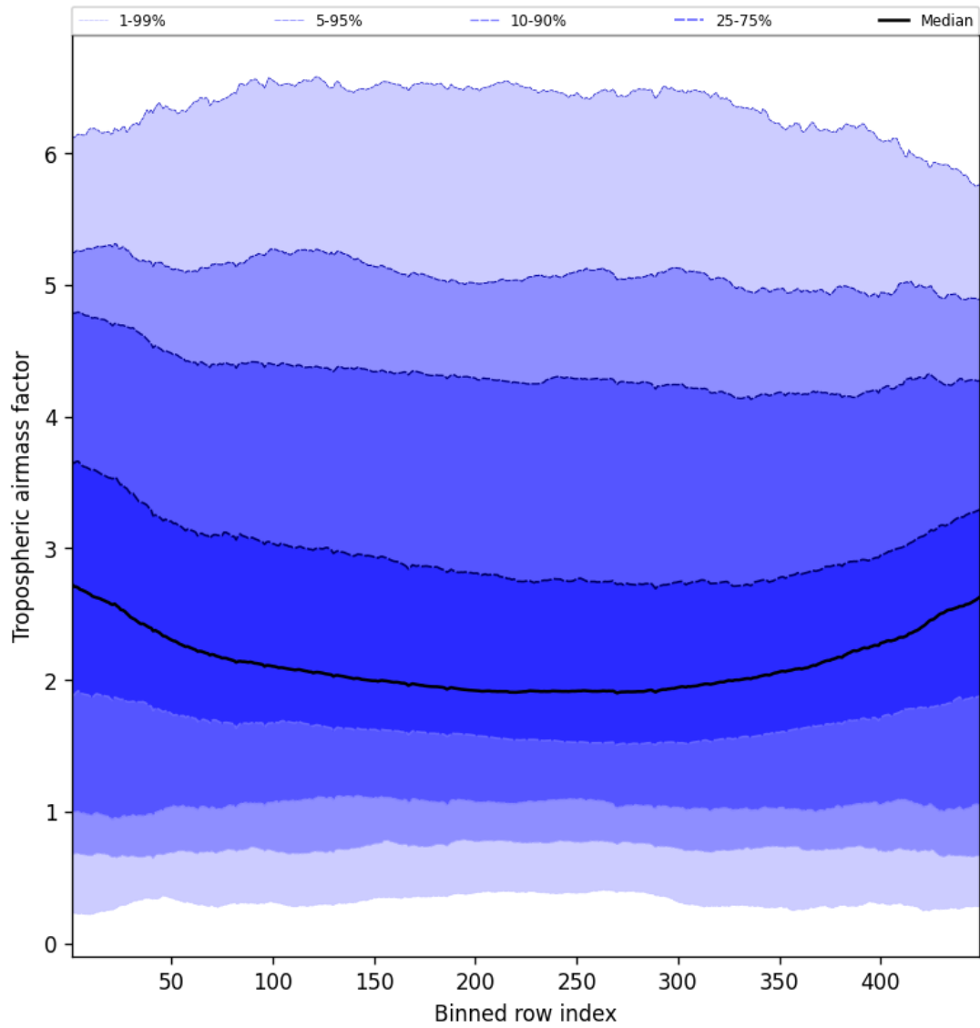
Figure 48: Along track statistics of “Tropospheric airmass factor” for 2024-12-27 to 2024-12-28
