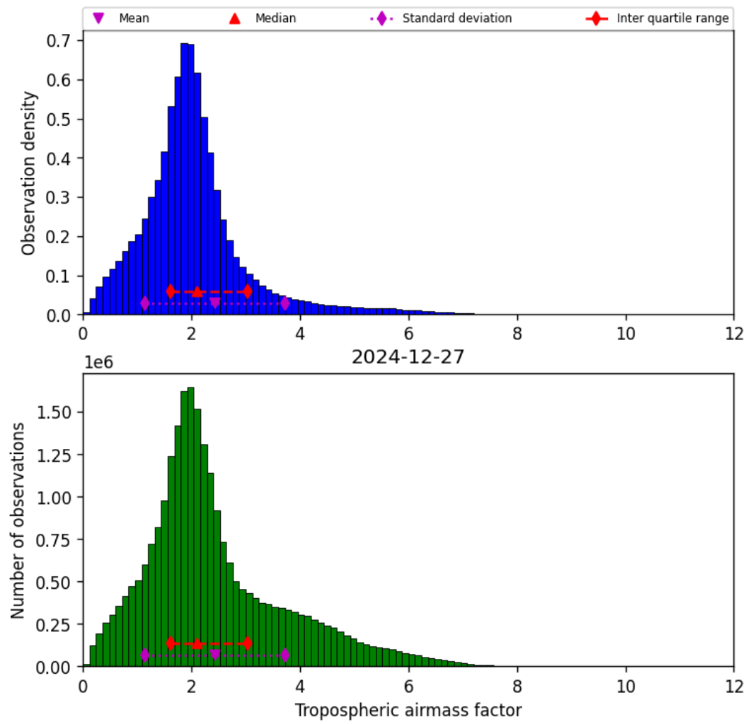
Figure 31: Histogram of “Tropospheric airmass factor” for 2024-12-27 to 2024-12-28
