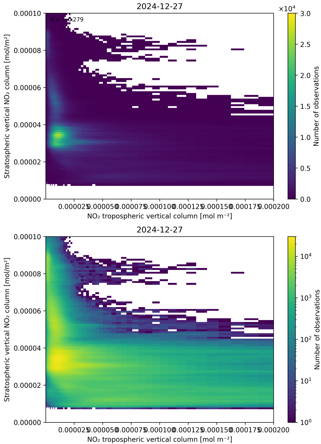
Figure 125: Scatter density plot of “NO 2 tropospheric vertical column” against “Stratospheric vertical NO 2 column” for 2024-12-27 to 2024-12-28.
