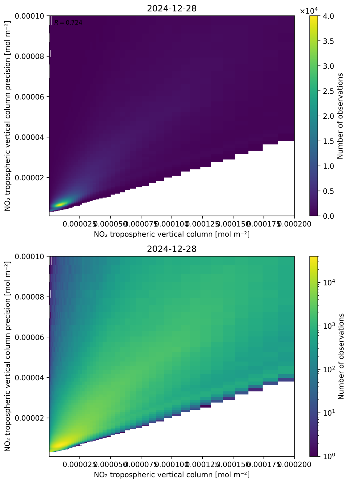
Figure 130: Scatter density plot of “NO 2 tropospheric vertical column” against “NO 2 tropospheric vertical column precision” for 2024-12-27 to 2024-12-29.
