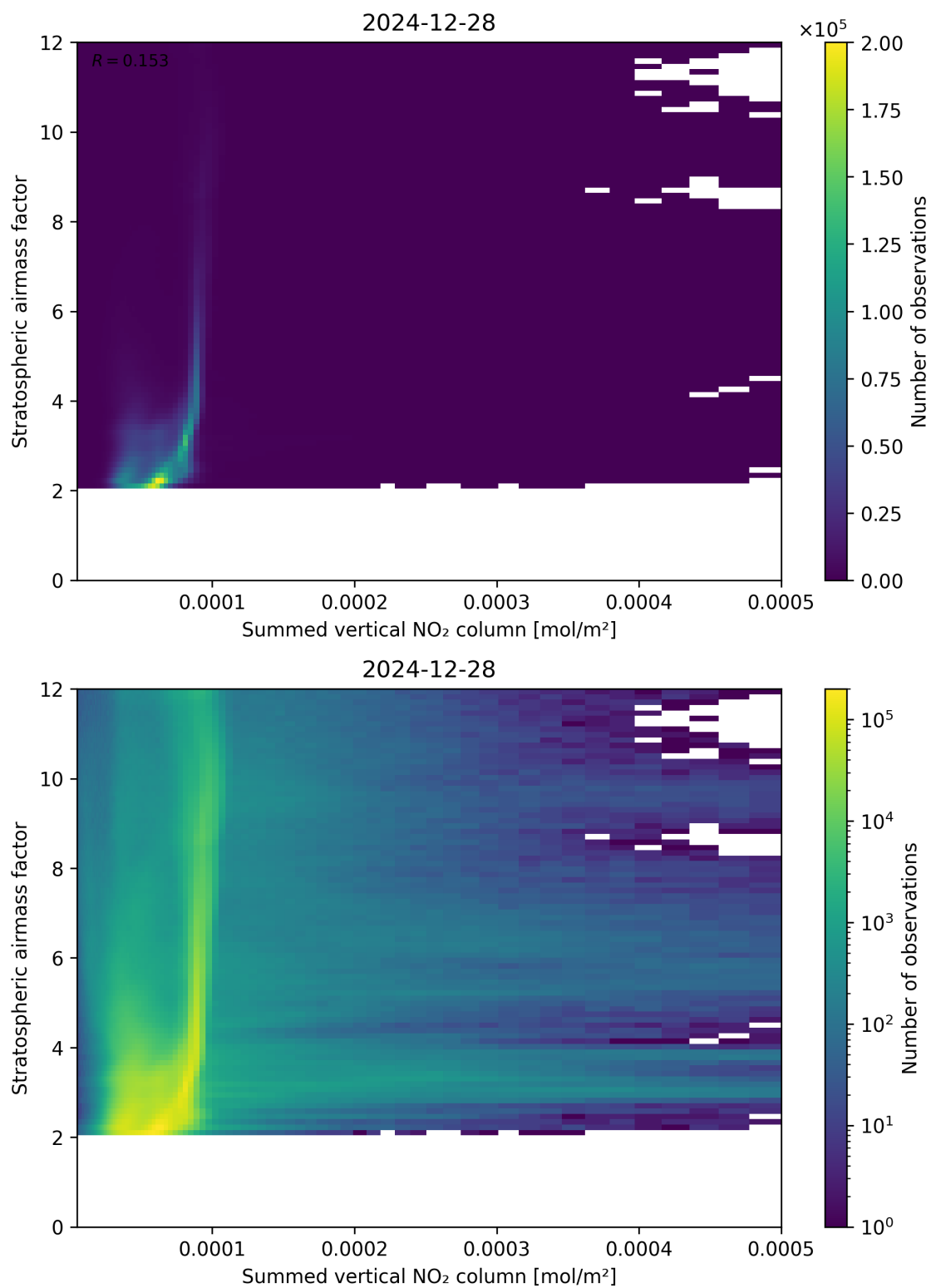
Figure 103: Scatter density plot of “Summed vertical NO 2 column” against “Stratospheric air mass factor” for 2024-12-27 to 2024-12-29.
