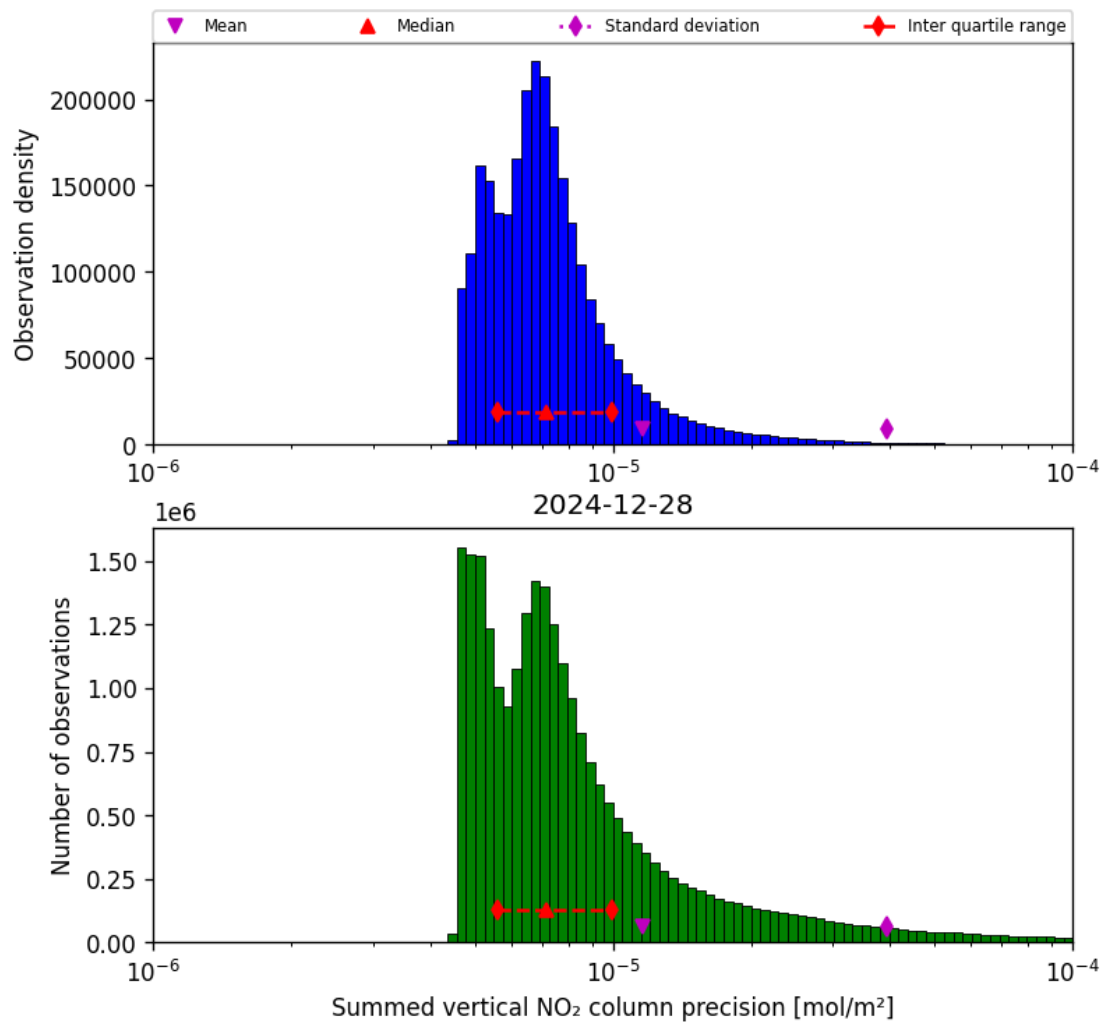
Figure 41: Histogram of "Summed vertical NO 2 column precision" for 2024-12-27 to 2024-12-29
