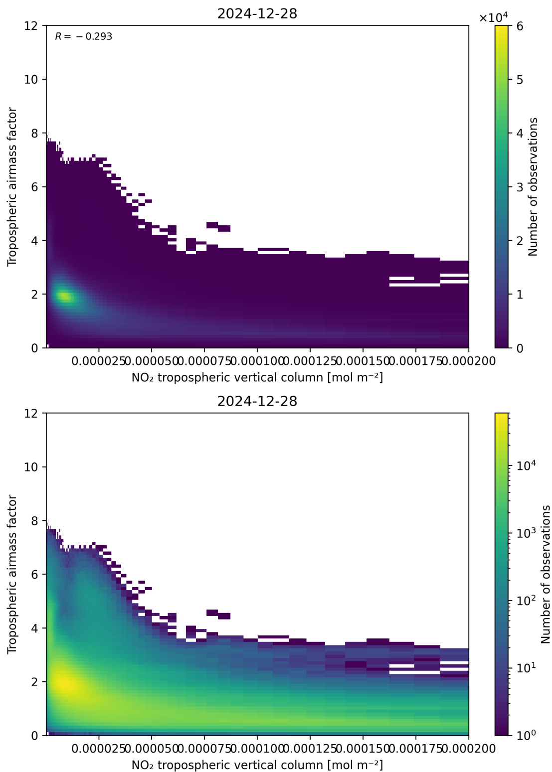
Figure 123: Scatter density plot of “NO 2 tropospheric vertical column” against “Tropospheric air mass factor” for 2024-12-27 to 2024-12-29.
