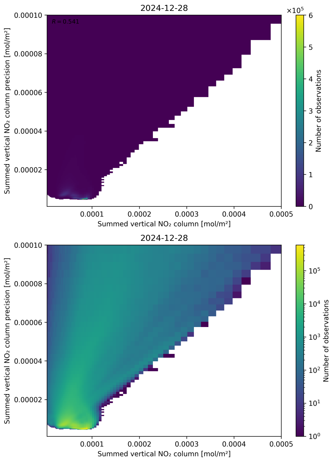
Figure 105: Scatter density plot of “Summed vertical NO 2 column” against “Summed vertical NO 2 column precision” for 2024-12-27 to 2024-12-29.
