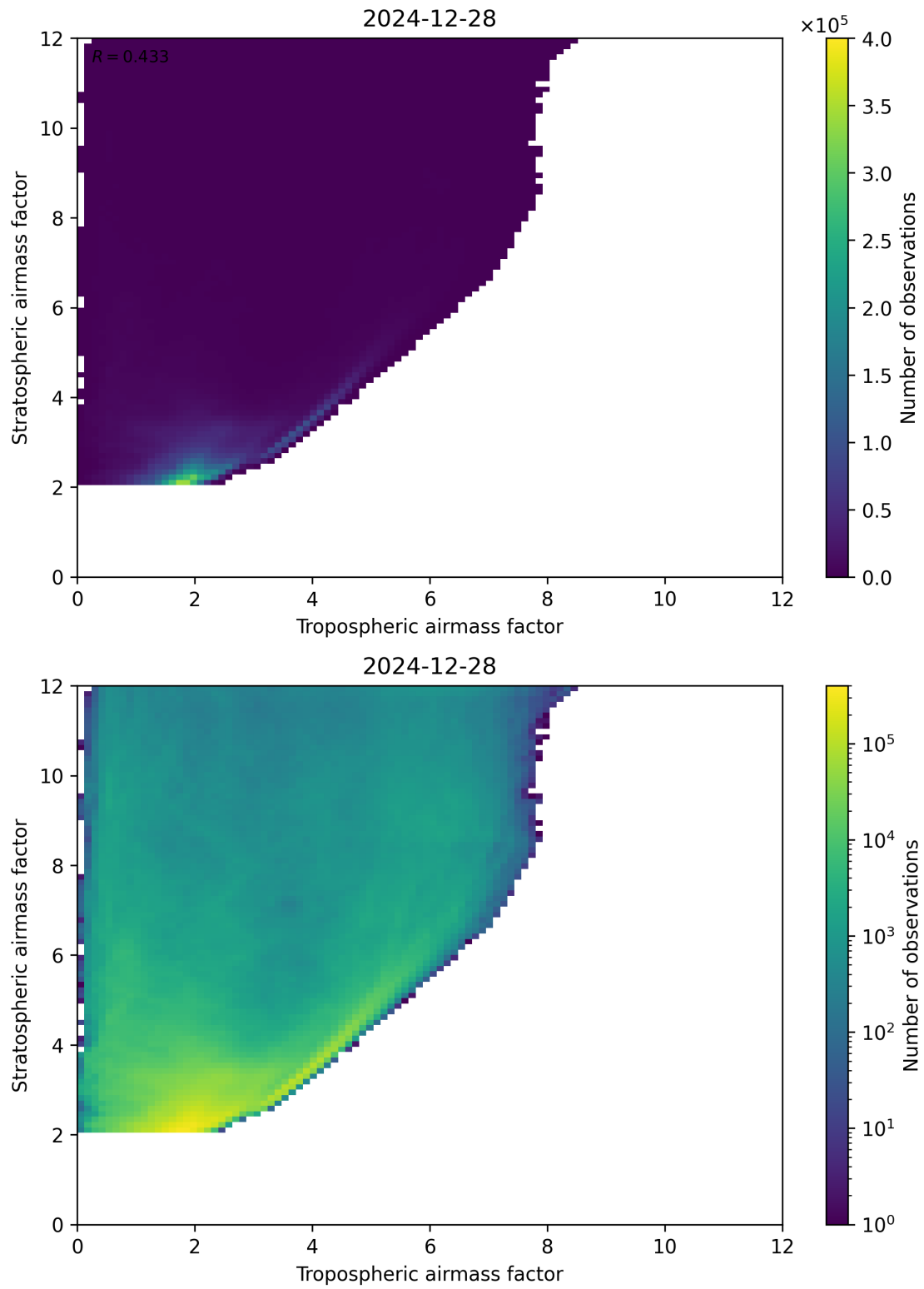
Figure 71: Scatter density plot of “Tropospheric airmass factor” against “Stratospheric airmass factor” for 2024-12-27 to 2024-12-29.
