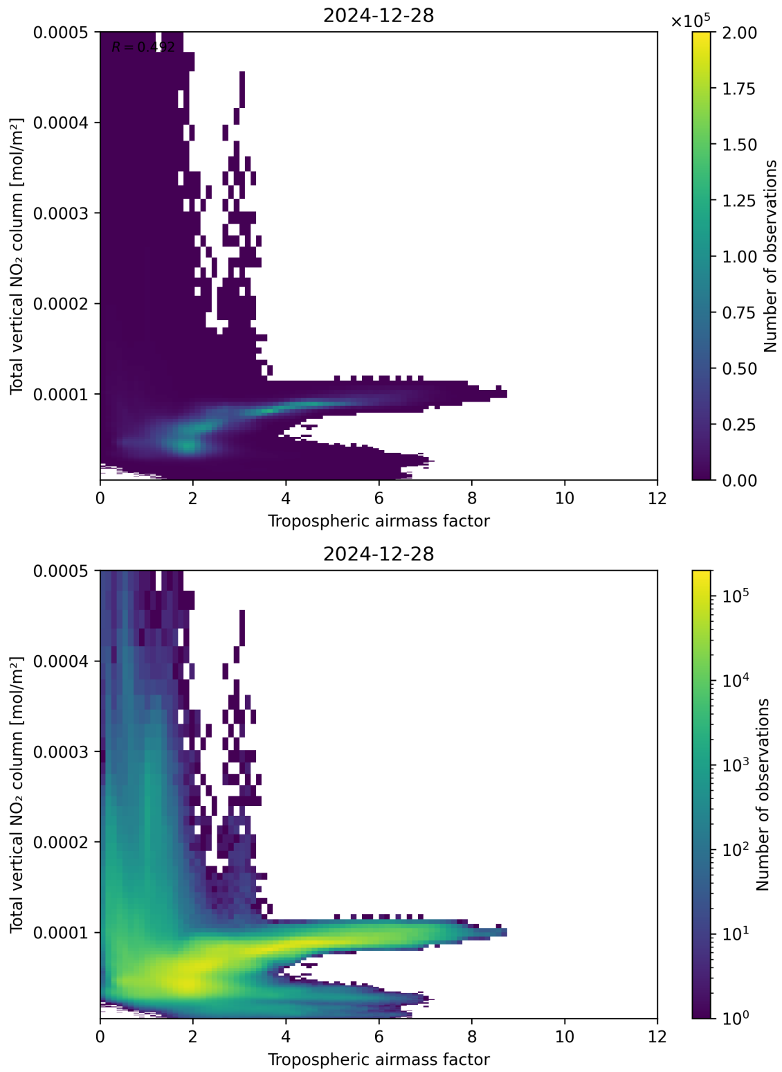
Figure 77: Scatter density plot of “Tropospheric airmass factor” against “Total vertical NO 2 column” for 2024-12-27 to 2024-12-29.
