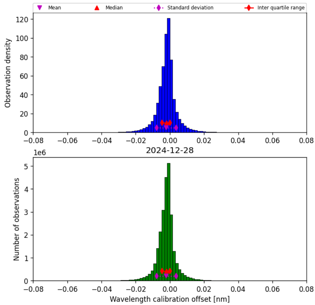
Figure 35: Histogram of “Wavelength calibration offset” for 2024-12-27 to 2024-12-29
