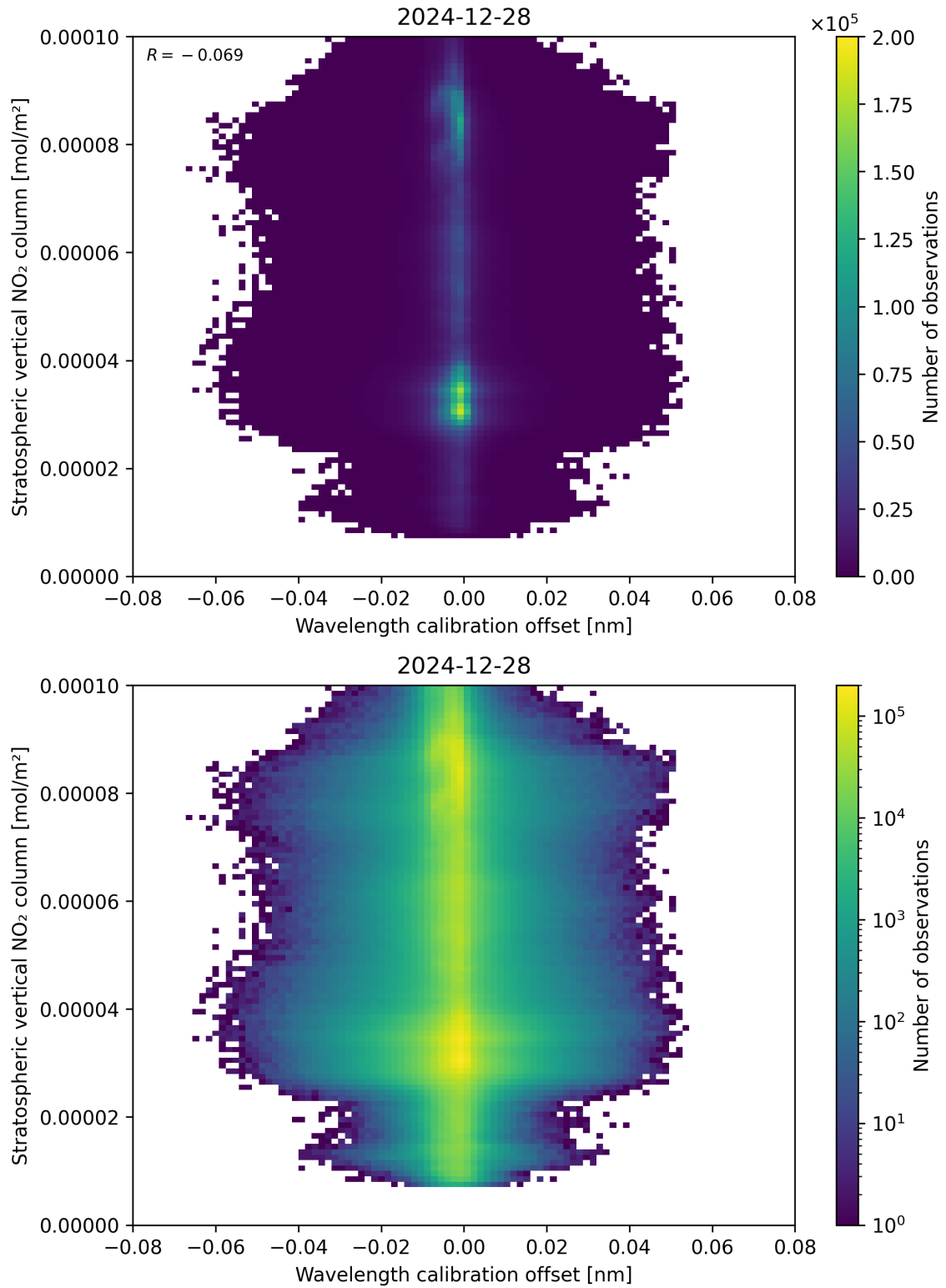
Figure 176: Scatter density plot of “Wavelength calibration offset” against “Stratospheric vertical NO 2 column” for 2024-12-27 to 2024-12-29.
