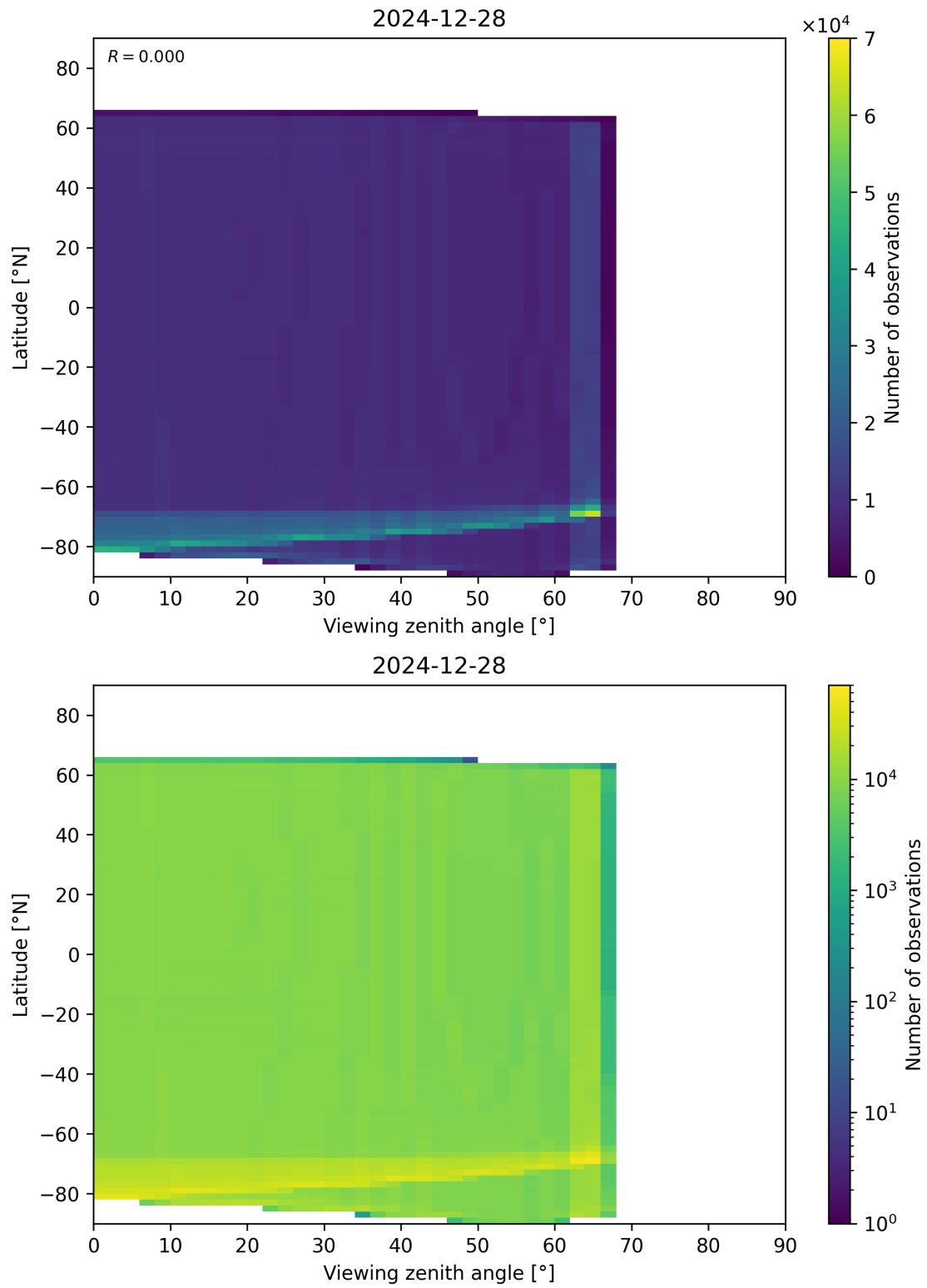
Figure 163: Scatter density plot of “Viewing zenith angle” against “Latitude” for 2024-12-27 to 2024-12-29.
