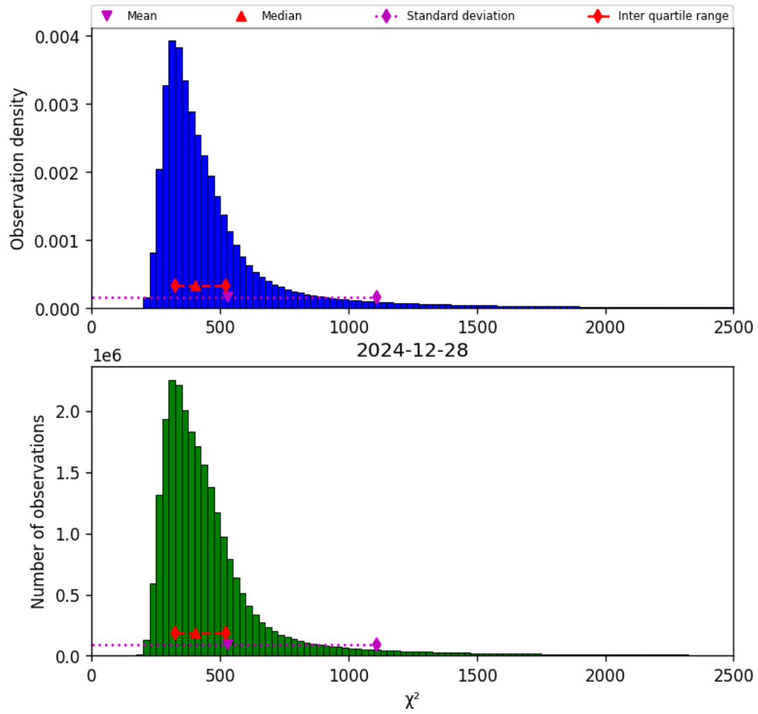
Figure 42: Histogram of “ \chi^2 ” for 2024-12-27 to 2024-12-29
