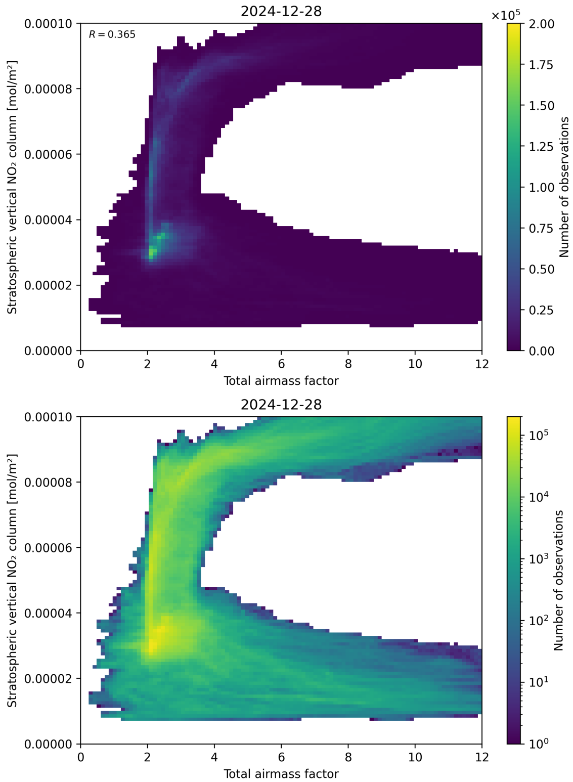
Figure 64: Scatter density plot of “Total airmass factor” against “Stratospheric vertical NO 2 column” for 2024-12-27 to 2024-12-29.
