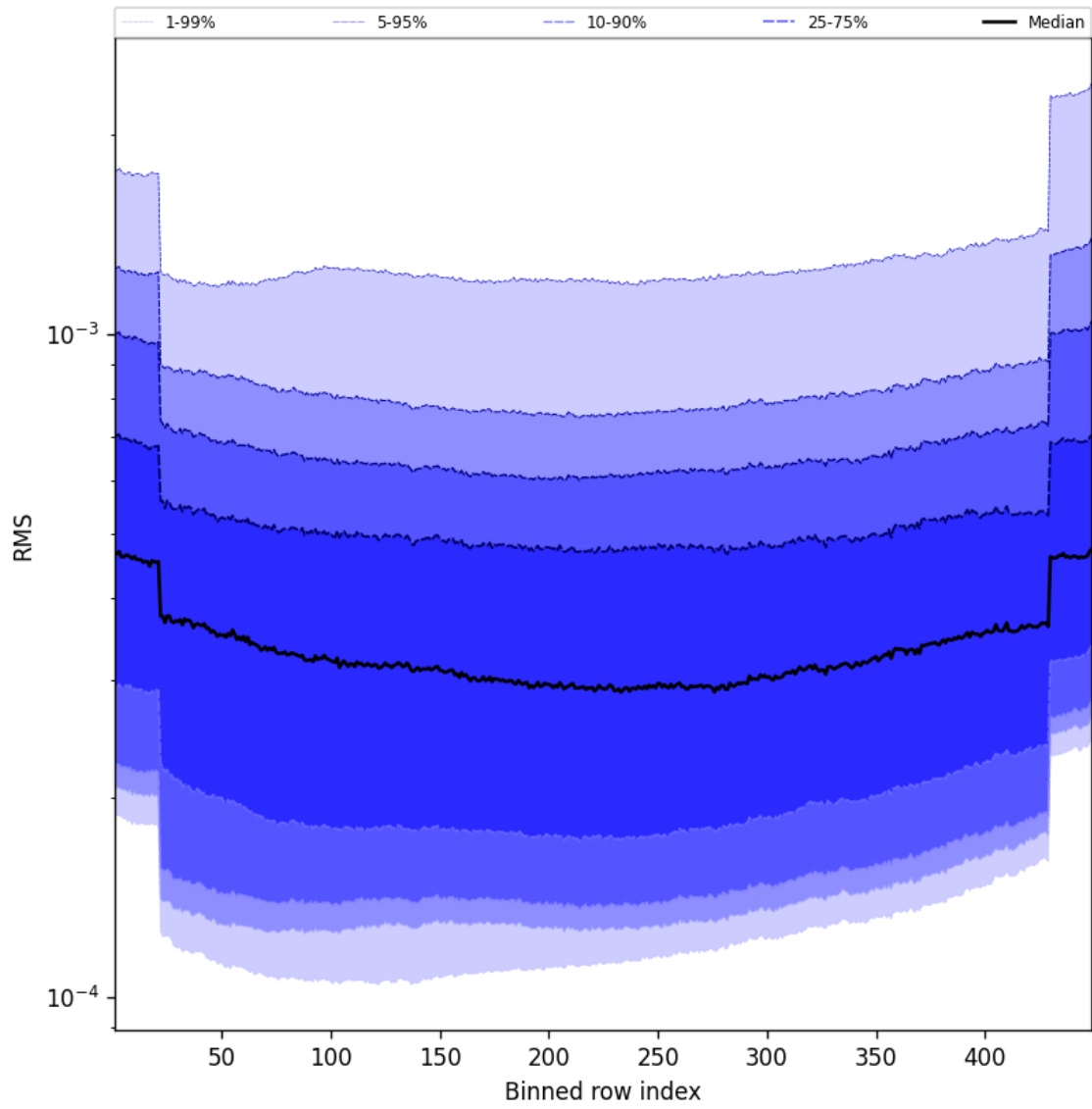
Figure 60: Along track statistics of “RMS” for 2024-12-27 to 2024-12-29
