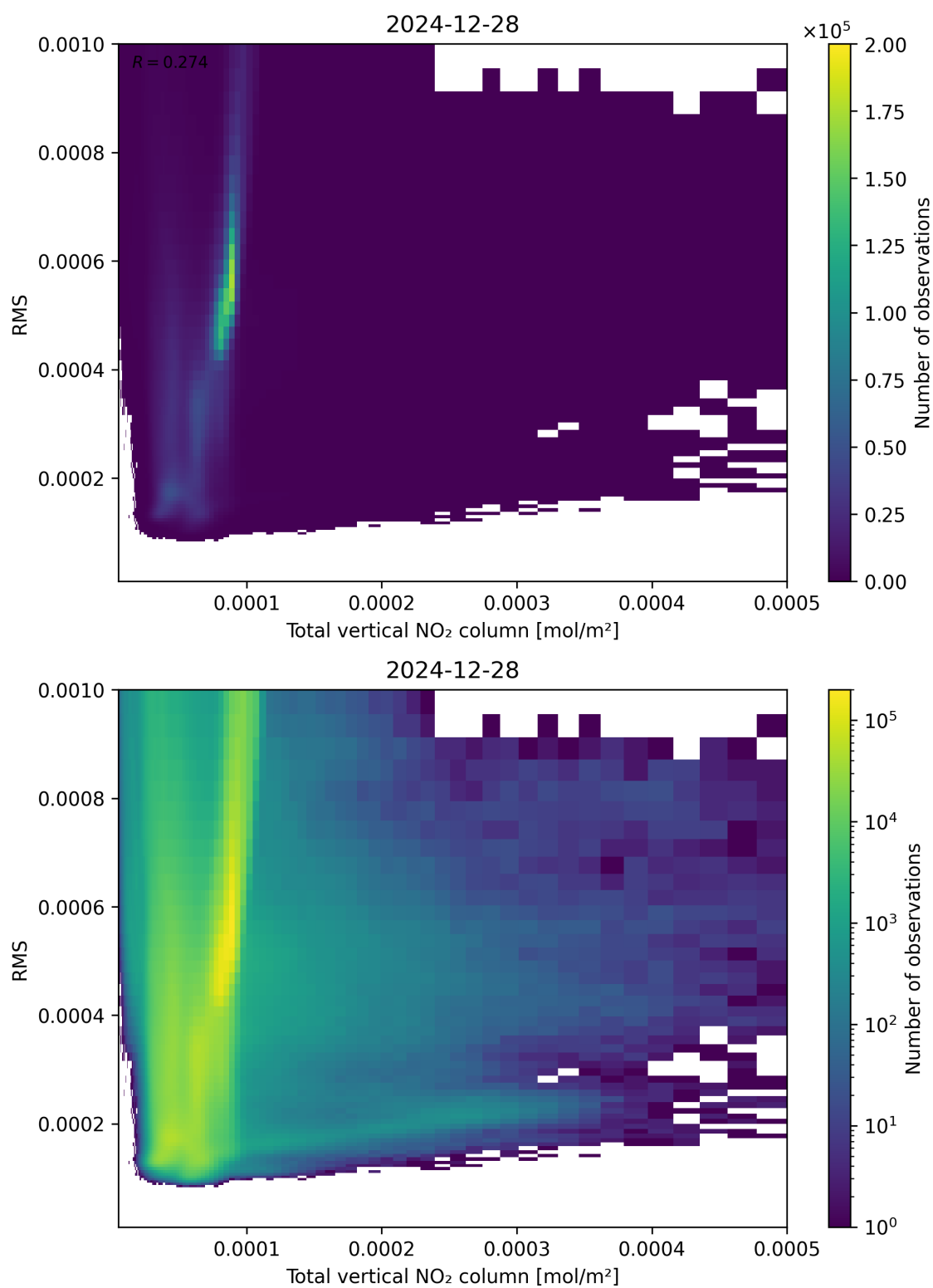
Figure 120: Scatter density plot of “Total vertical NO 2 column” against “RMS” for 2024-12-27 to 2024-12-29.
