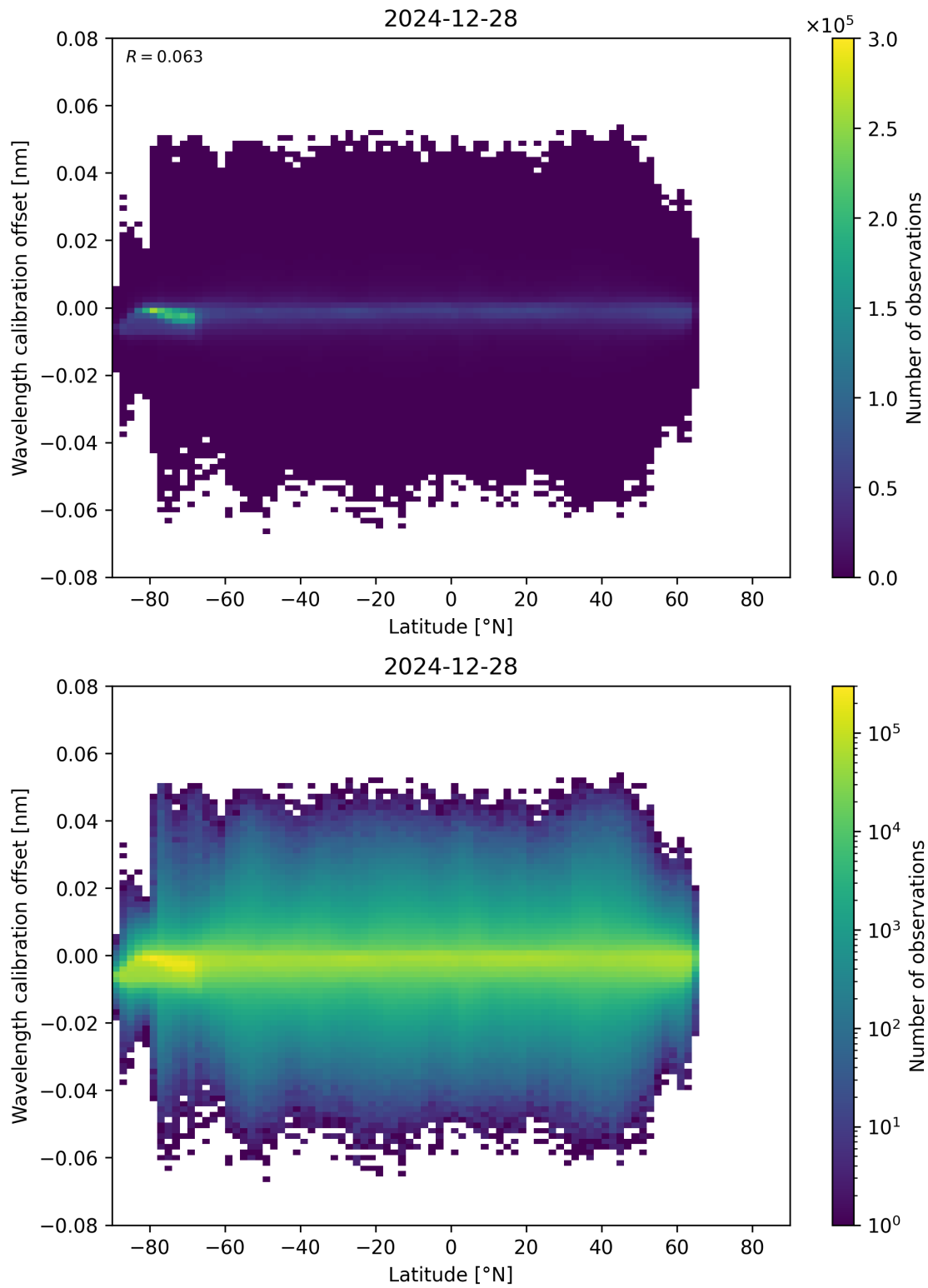
Figure 95: Scatter density plot of “Latitude” against “Wavelength calibration offset” for 2024-12-27 to 2024-12-29.
