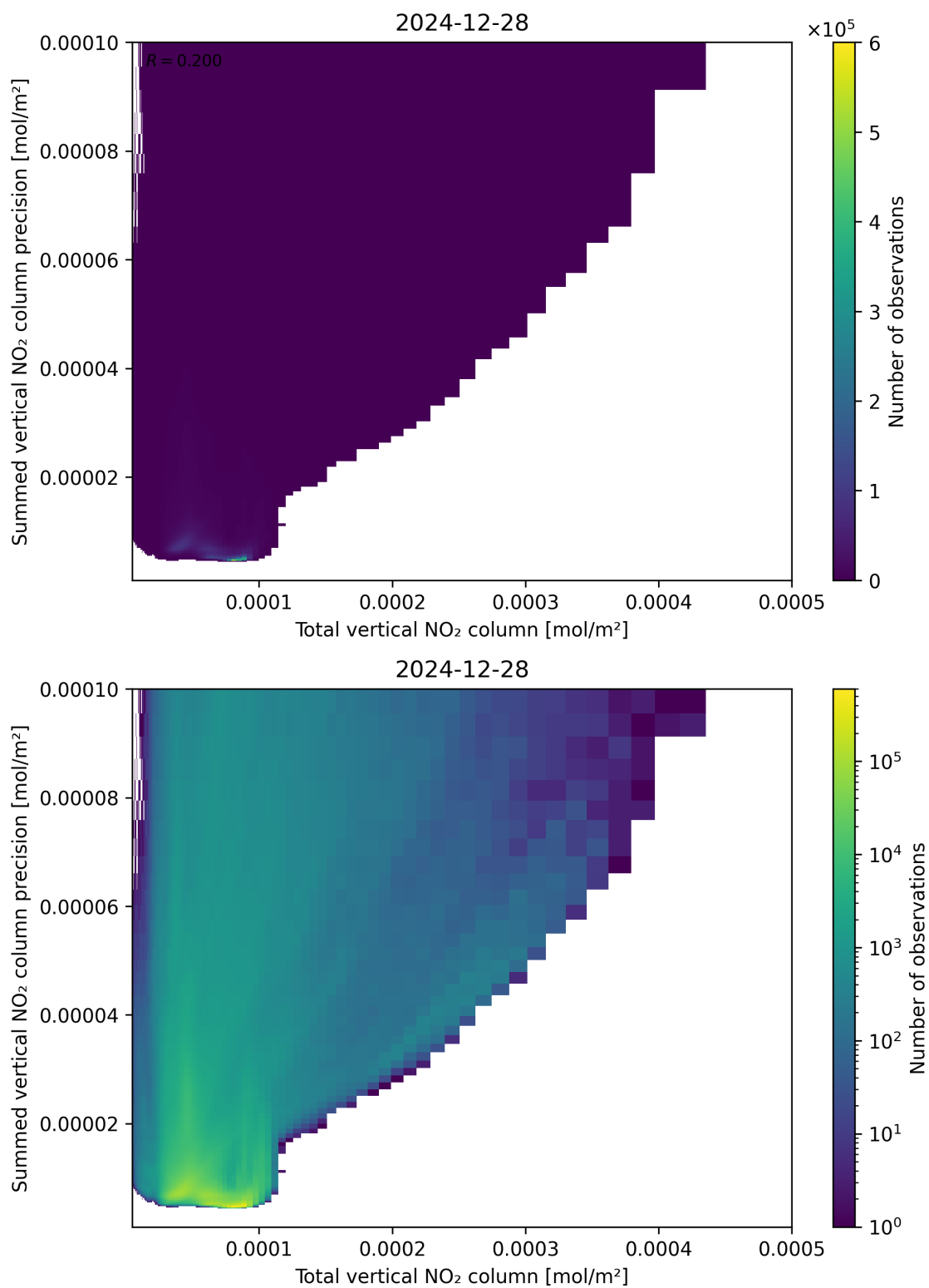
Figure 113: Scatter density plot of “Total vertical NO 2 column” against “Summed vertical NO 2 column precision” for 2024-12-27 to 2024-12-29.
