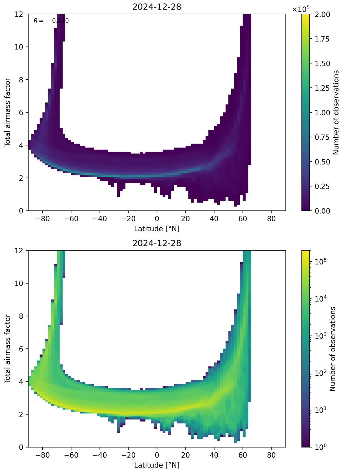
Figure 84: Scatter density plot of “Latitude” against “Total airmass factor” for 2024-12-27 to 2024-12-29.
