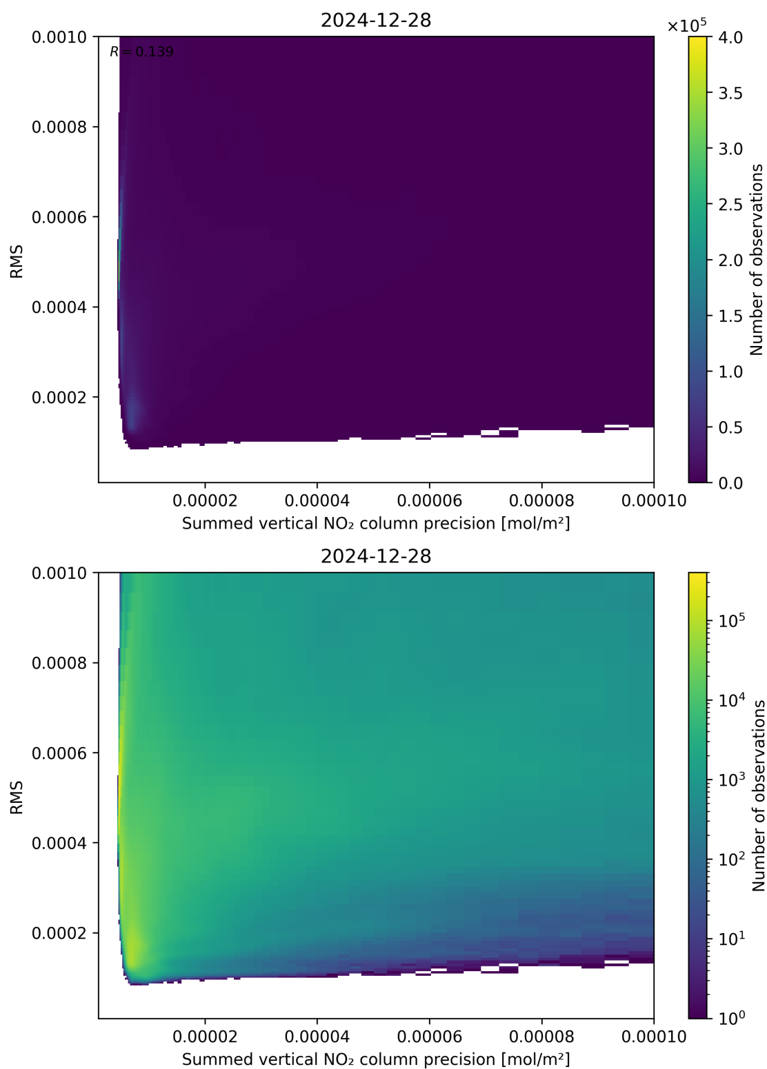
Figure 108: Scatter density plot of “Summed vertical NO 2 column precision” against “RMS” for 2024-12-27 to 2024-12-29.
