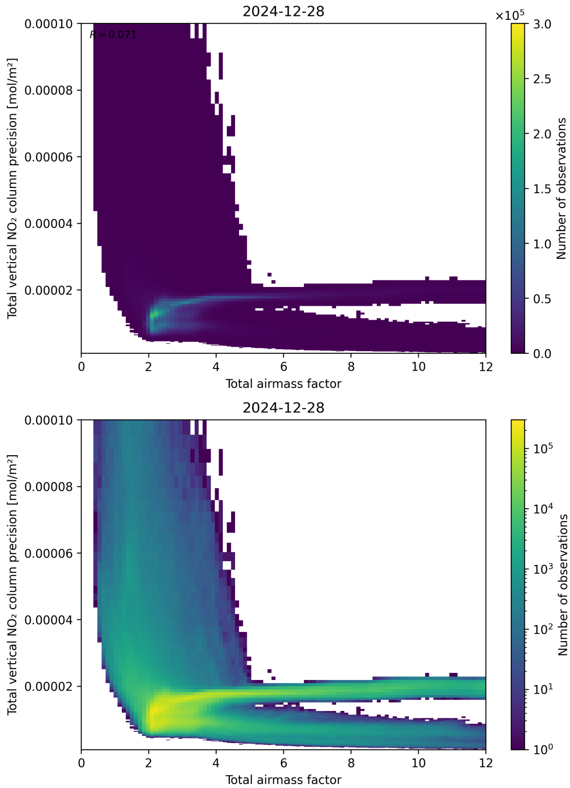
Figure 68: Scatter density plot of “Total airmass factor” against “Total vertical NO 2 column precision” for 2024-12-27 to 2024-12-29.
