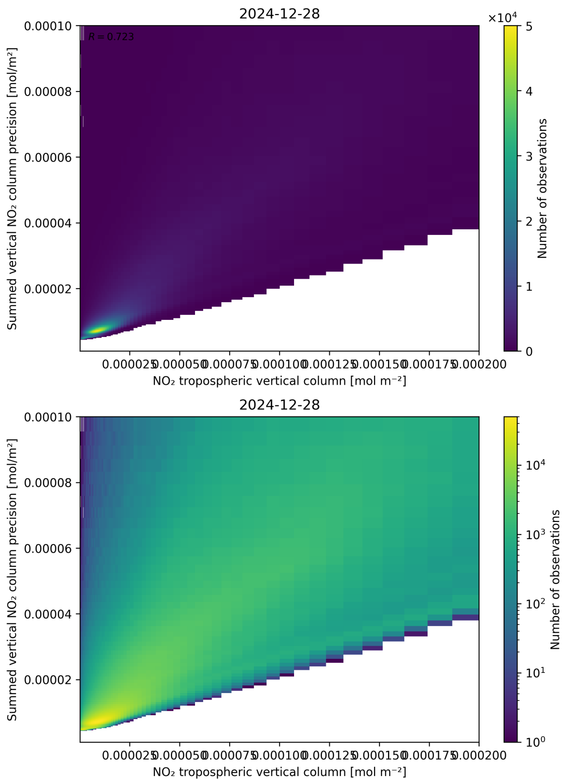
Figure 127: Scatter density plot of “NO 2 tropospheric vertical column” against “Summed vertical NO 2 column precision” for 2024-12-27 to 2024-12-29.
