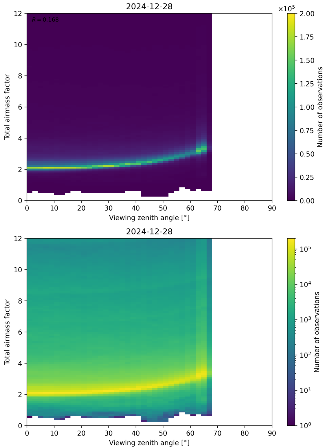
Figure 160: Scatter density plot of “Viewing zenith angle” against “Total airmass factor” for 2024-12-27 to 2024-12-29.
