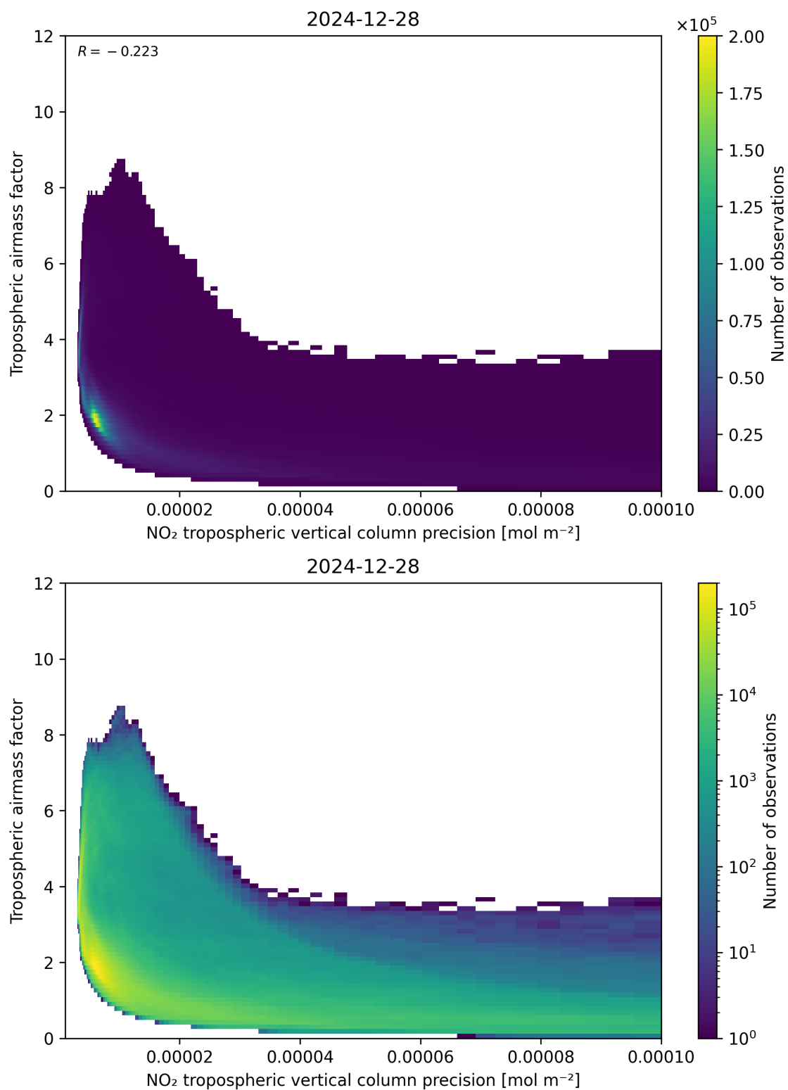
Figure 133: Scatter density plot of “NO 2 tropospheric vertical column precision” against “Tropospheric airmass factor” for 2024-12-27 to 2024-12-29.
