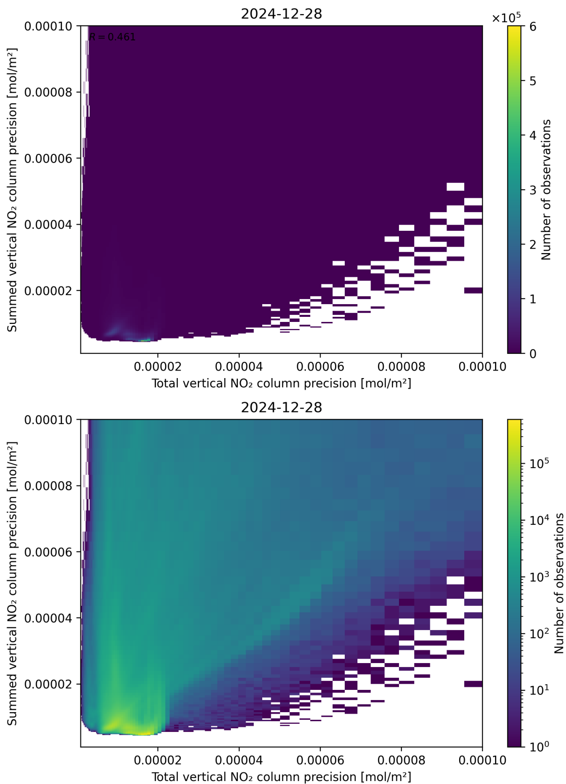
Figure 118: Scatter density plot of “Total vertical NO 2 column precision” against “Summed vertical NO 2 column precision” for 2024-12-27 to 2024-12-29.
