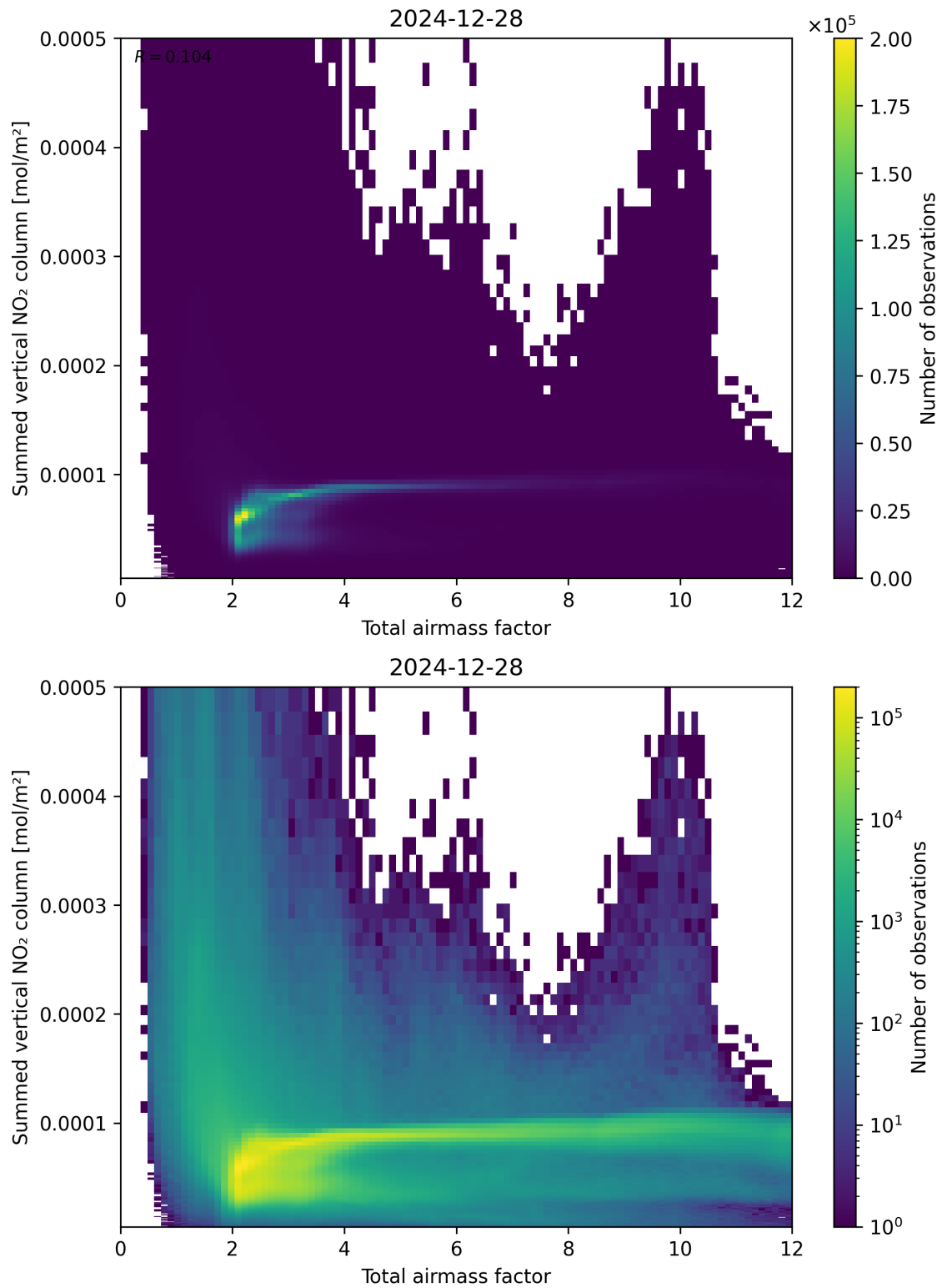
Figure 65: Scatter density plot of “Total airmass factor” against “Summed vertical NO 2 column” for 2024-12-27 to 2024-12-29.
