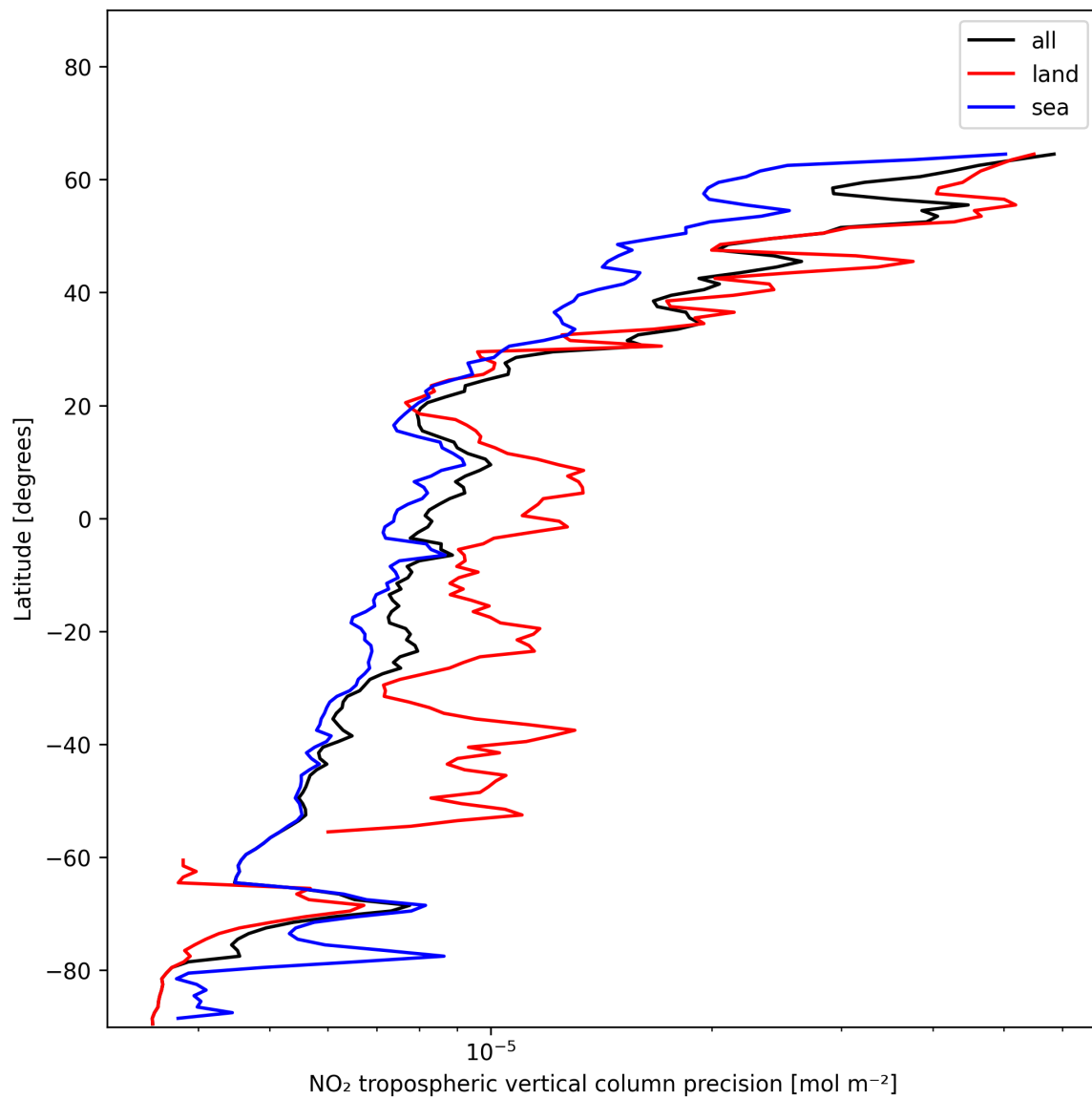
Figure 13: Zonal average of “NO 2 tropospheric vertical column precision” for 2024-12-27 to 2024-12-29.
