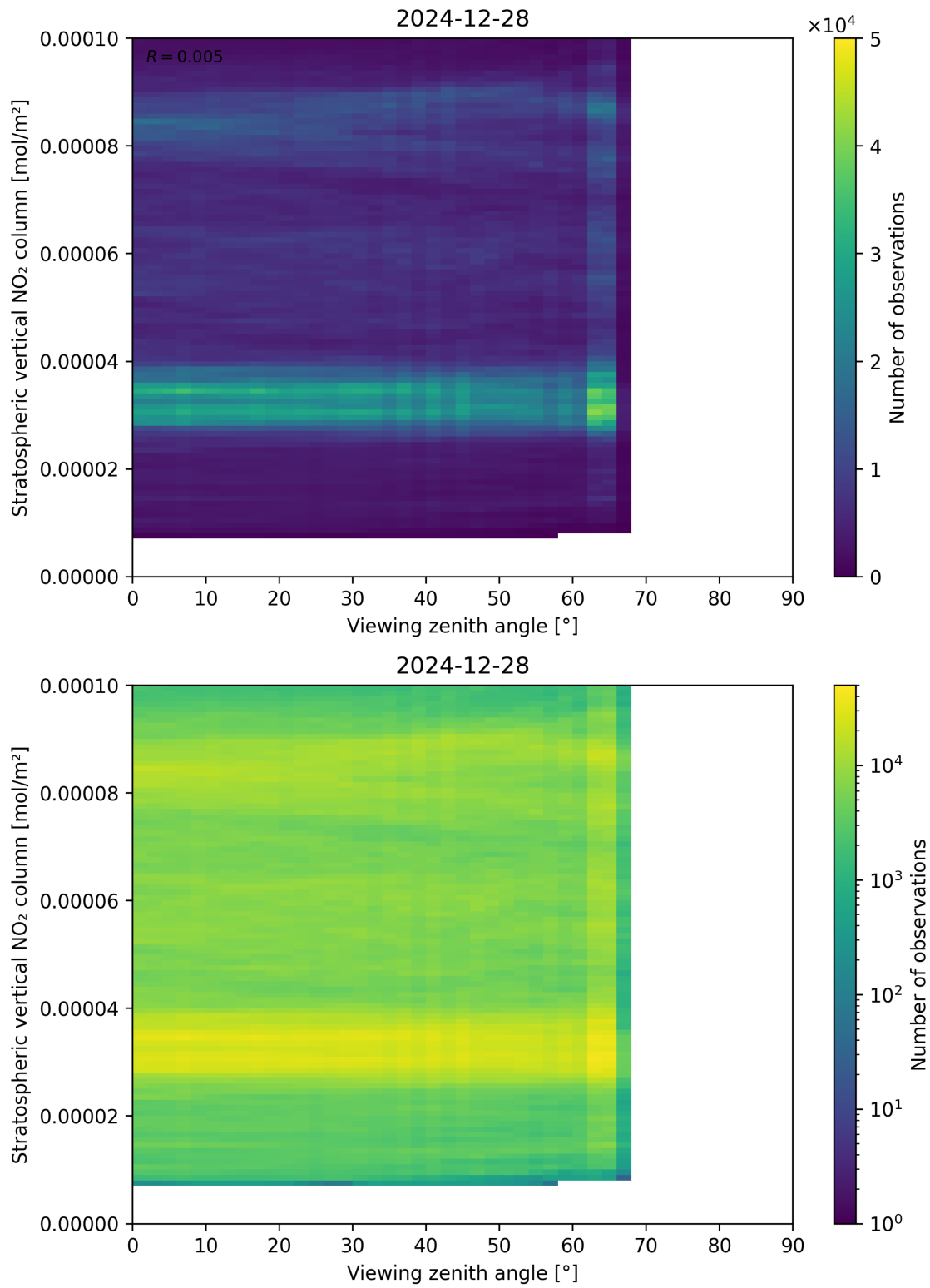
Figure 164: Scatter density plot of “Viewing zenith angle” against “Stratospheric vertical NO 2 column” for 2024-12-27 to 2024-12-29.
