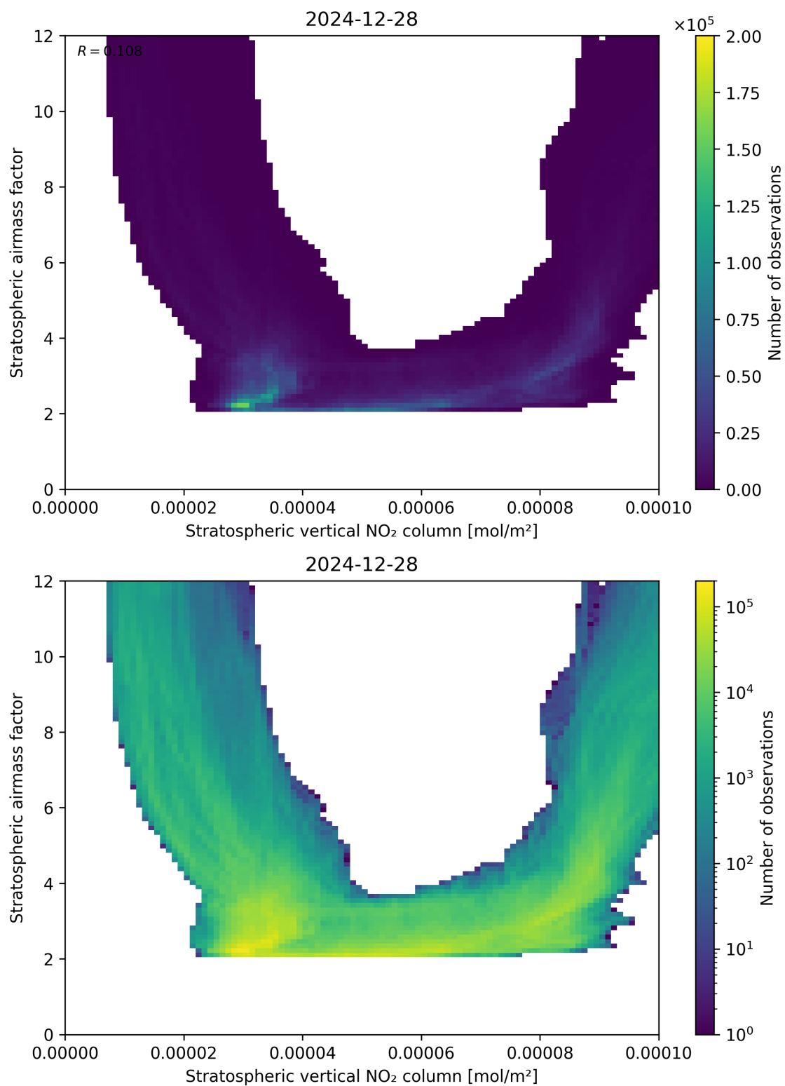
Figure 96: Scatter density plot of “Stratospheric vertical NO 2 column” against “Stratospheric airmass factor” for 2024-12-27 to 2024-12-29.
