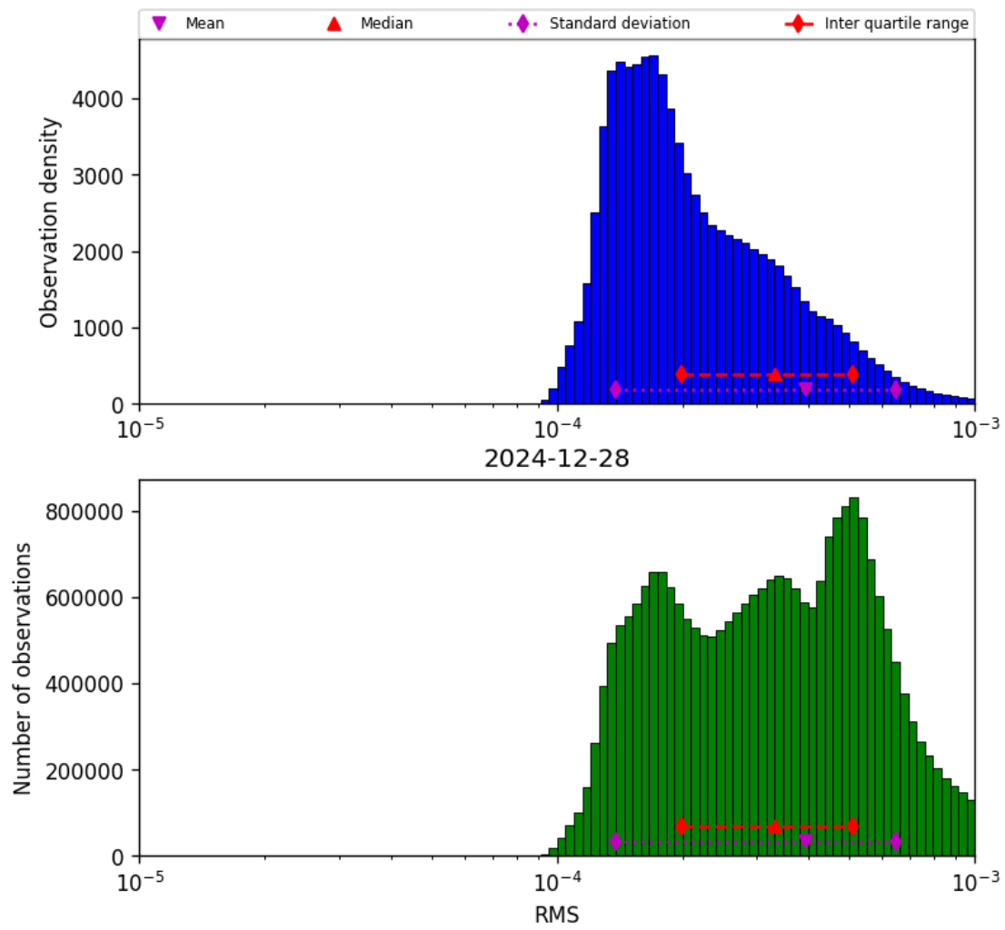
Figure 43: Histogram of “RMS” for 2024-12-27 to 2024-12-29
