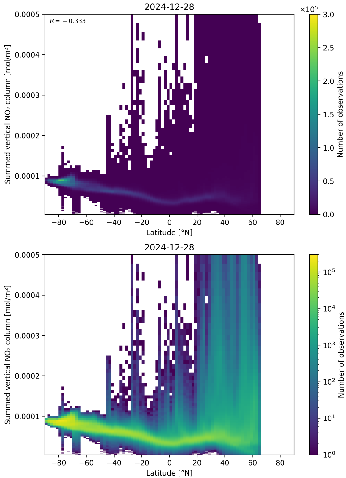
Figure 88: Scatter density plot of “Latitude” against “Summed vertical NO 2 column” for 2024-12-27 to 2024-12-29.
