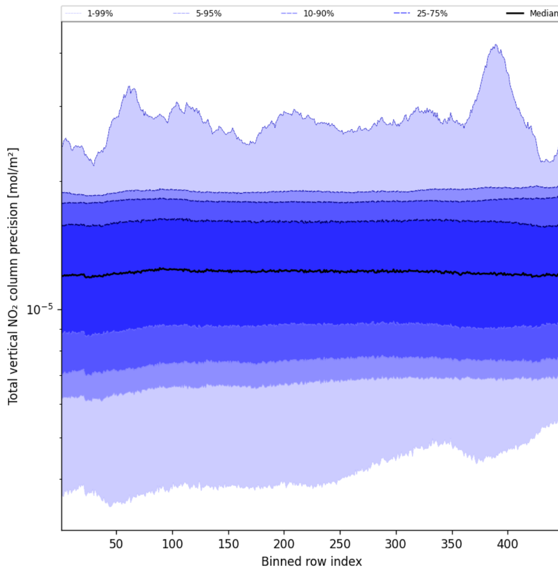
Figure 56: Along track statistics of “Total vertical NO 2 column precision” for 2024-12-27 to 2024-12-29
