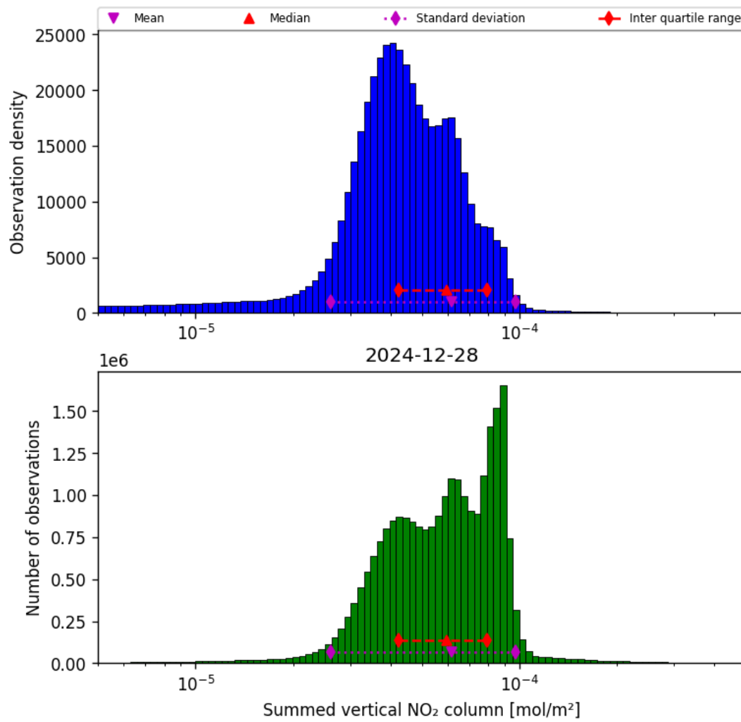
Figure 40: Histogram of “Summed vertical NO 2 column” for 2024-12-27 to 2024-12-29
