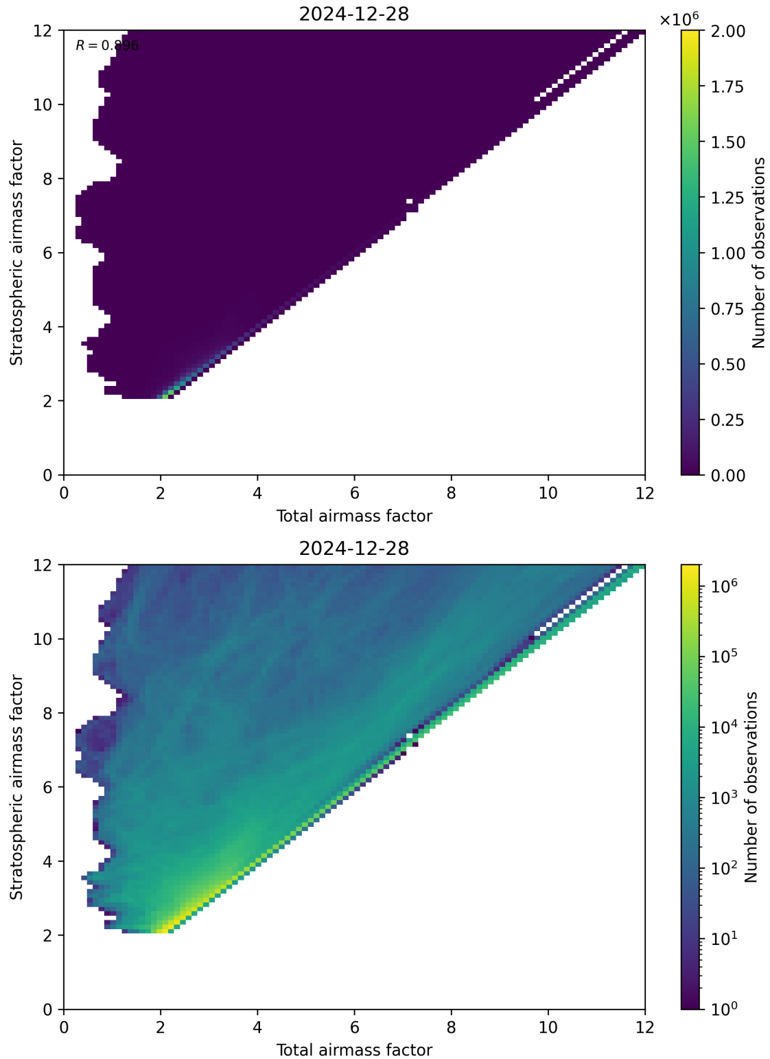
Figure 62: Scatter density plot of “Total airmass factor” against “Stratospheric airmass factor” for 2024-12-27 to 2024-12-29.
