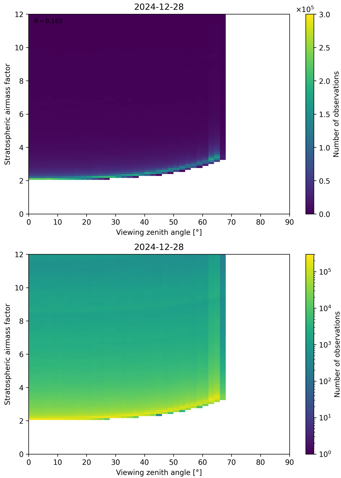
Figure 159: Scatter density plot of “Viewing zenith angle” against “Stratospheric airmass factor” for 2024-12-27 to 2024-12-29.
