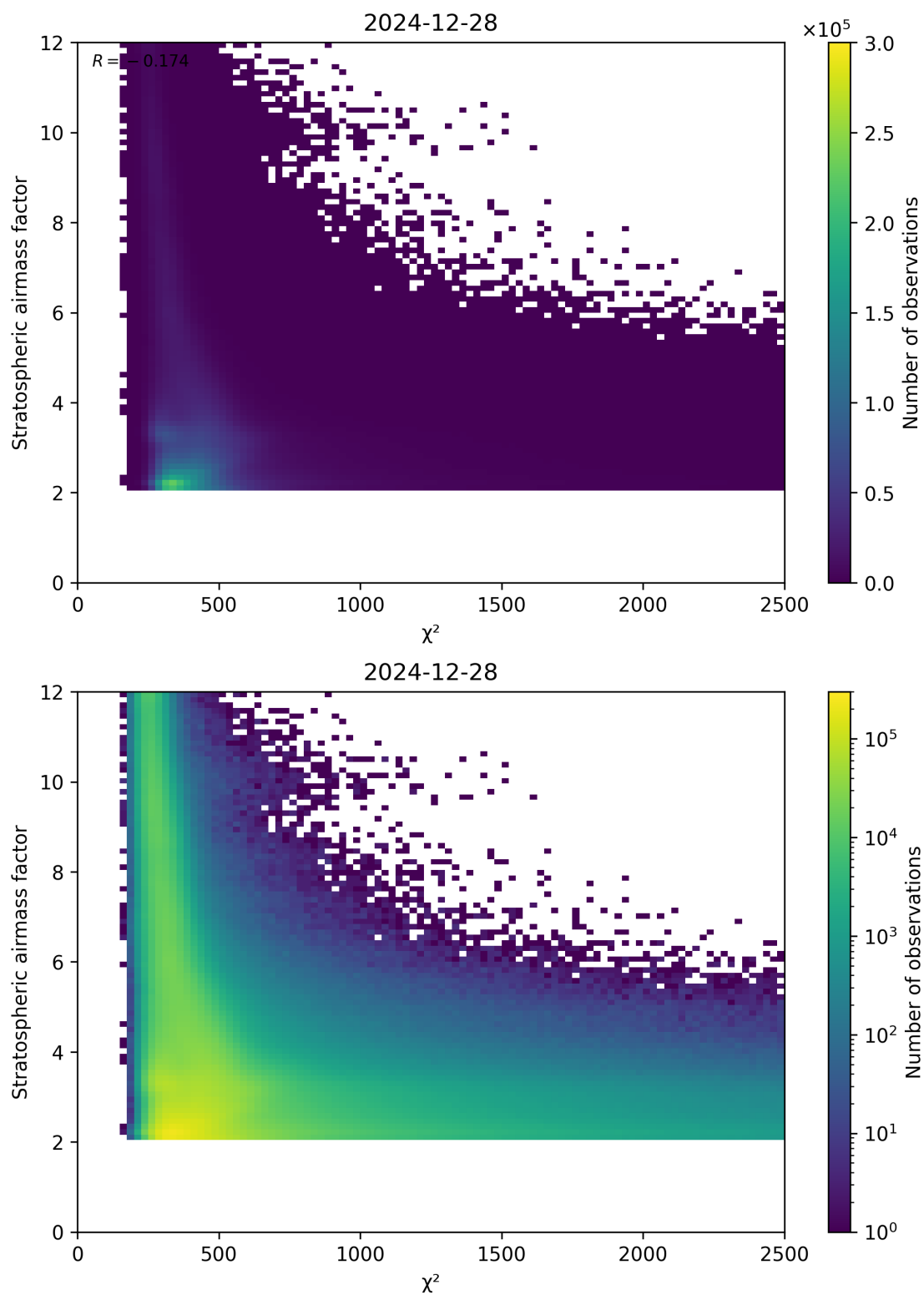
Figure 81: Scatter density plot of “ \chi^2 ” against “Stratospheric airmass factor” for 2024-12-27 to 2024-12-29.
