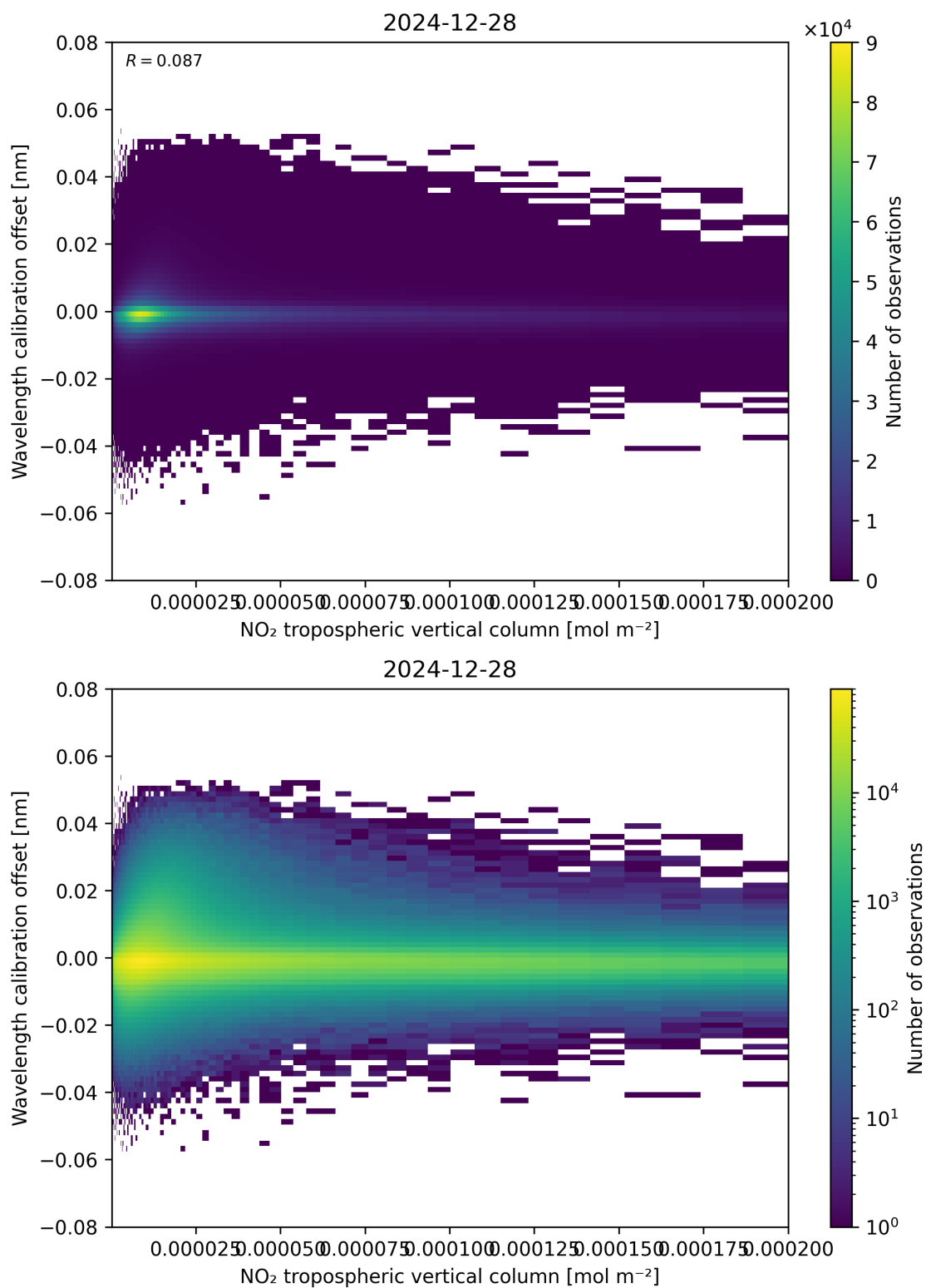
Figure 143: Scatter density plot of “NO 2 tropospheric vertical column” against “Wavelength calibration offset” for 2024-12-27 to 2024-12-29.
