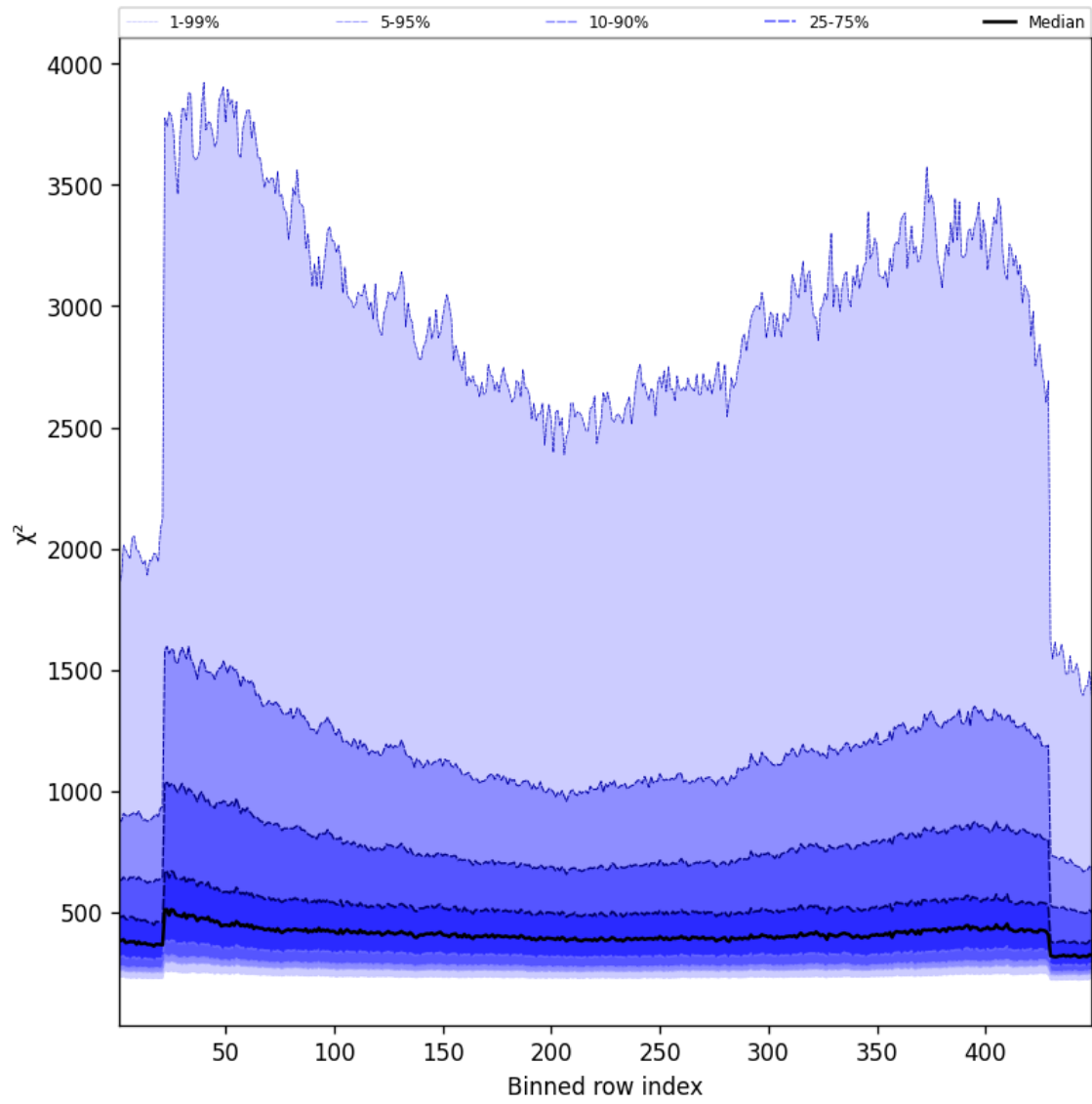
Figure 59: Along track statistics of “ \chi^2 ” for 2024-12-27 to 2024-12-29
