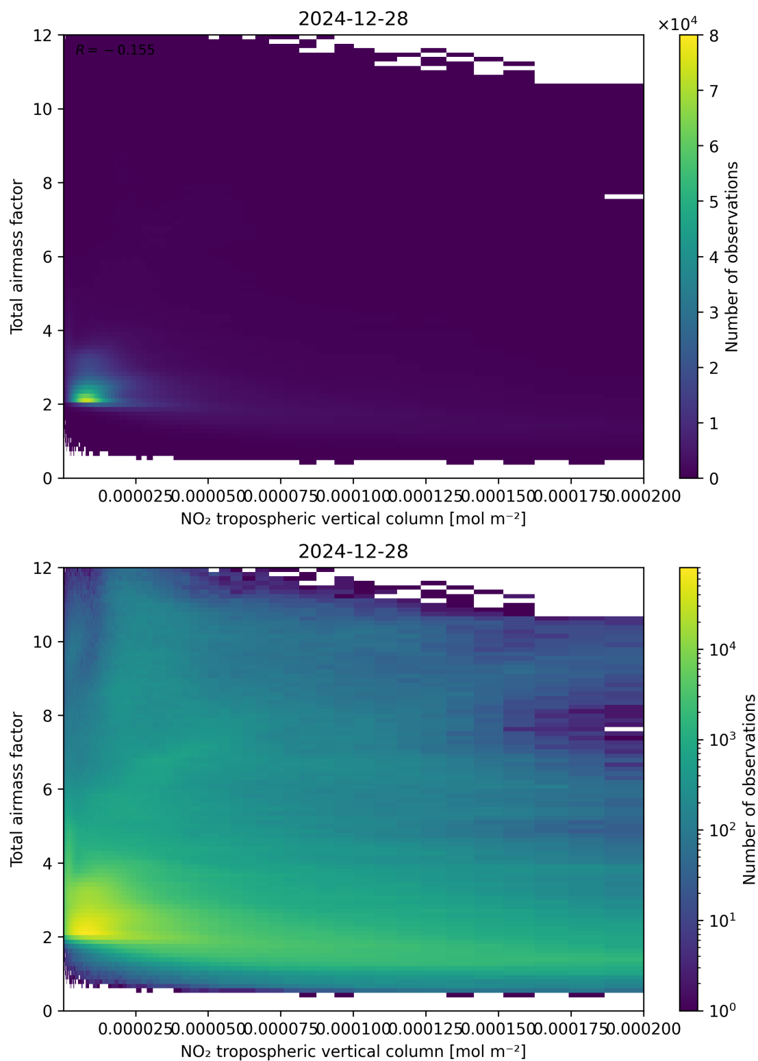
Figure 122: Scatter density plot of “NO 2 tropospheric vertical column” against “Total air mass factor” for 2024-12-27 to 2024-12-29.
