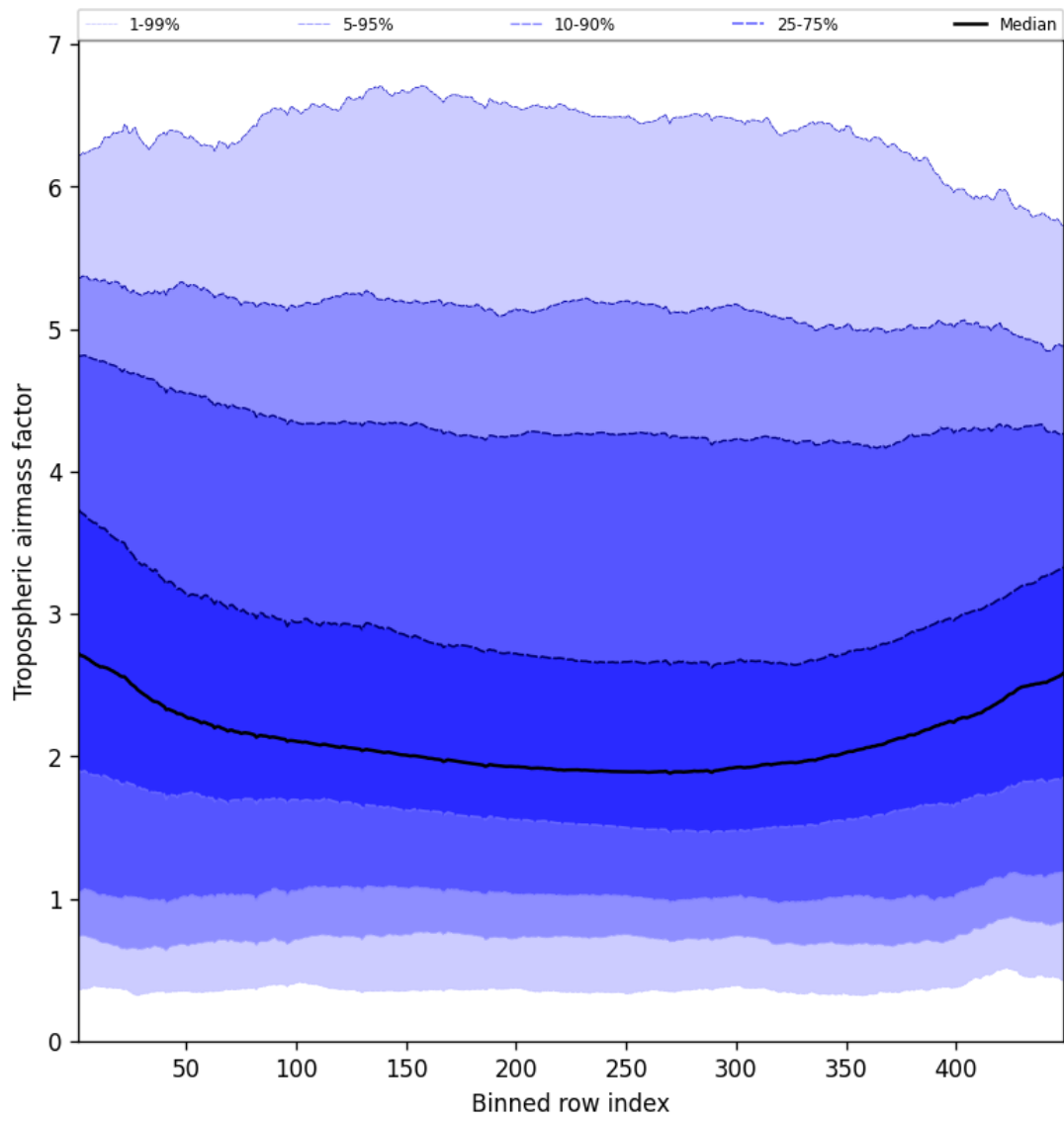
Figure 48: Along track statistics of “Tropospheric airmass factor” for 2024-12-27 to 2024-12-29
