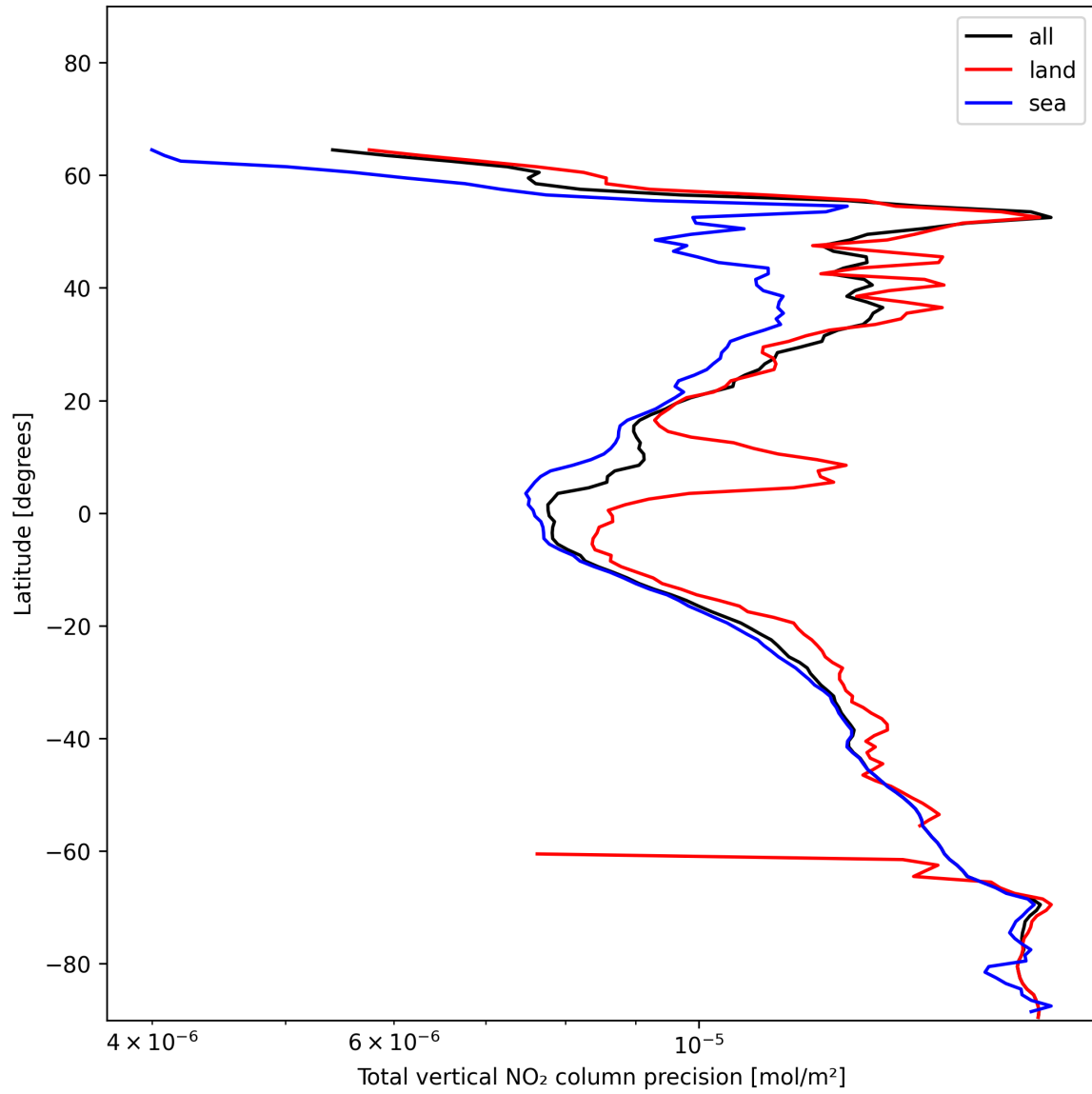
Figure 22: Zonal average of “Total vertical NO 2 column precision” for 2024-12-27 to 2024-12-29.
