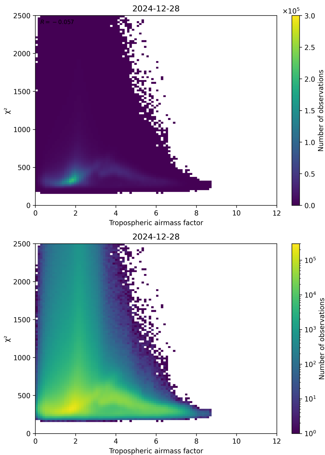
Figure 73: Scatter density plot of “Tropospheric airmass factor” against “ \chi^2 ” for 2024-12-27 to 2024-12-29.
