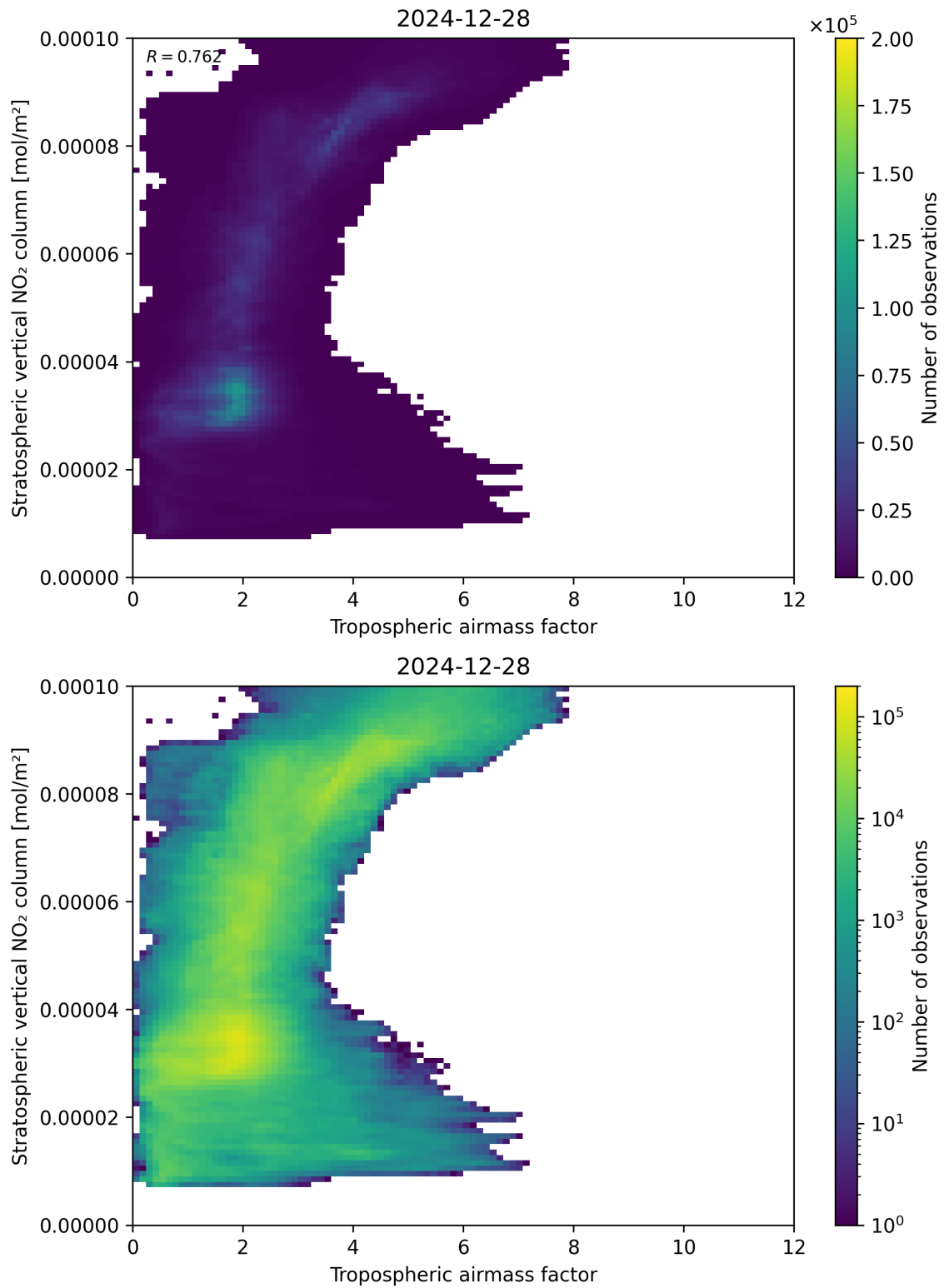
Figure 74: Scatter density plot of “Tropospheric air mass factor” against “Stratospheric vertical NO 2 column” for 2024-12-27 to 2024-12-29.
