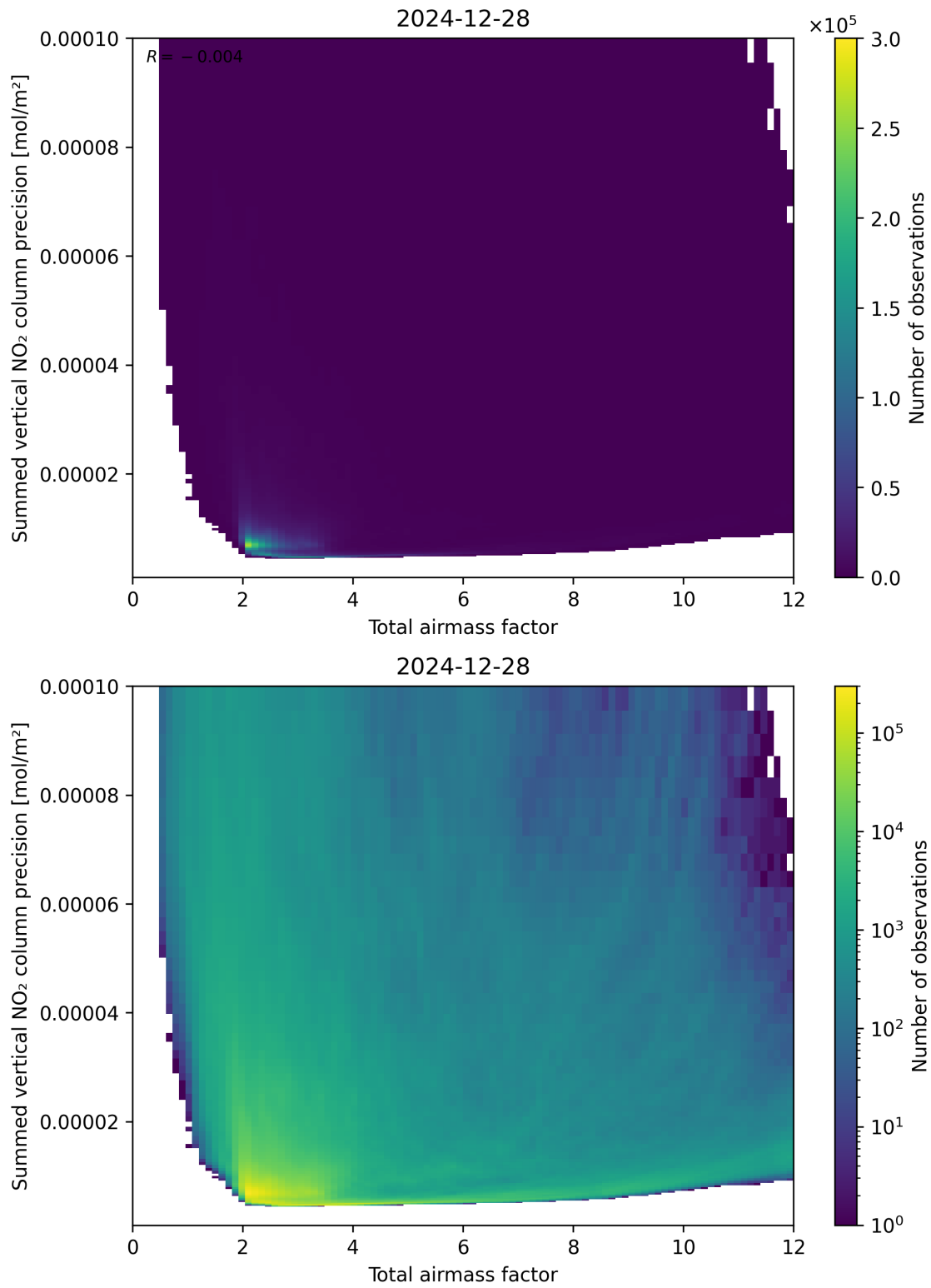
Figure 66: Scatter density plot of “Total airmass factor” against “Summed vertical NO 2 column precision” for 2024-12-27 to 2024-12-29.
