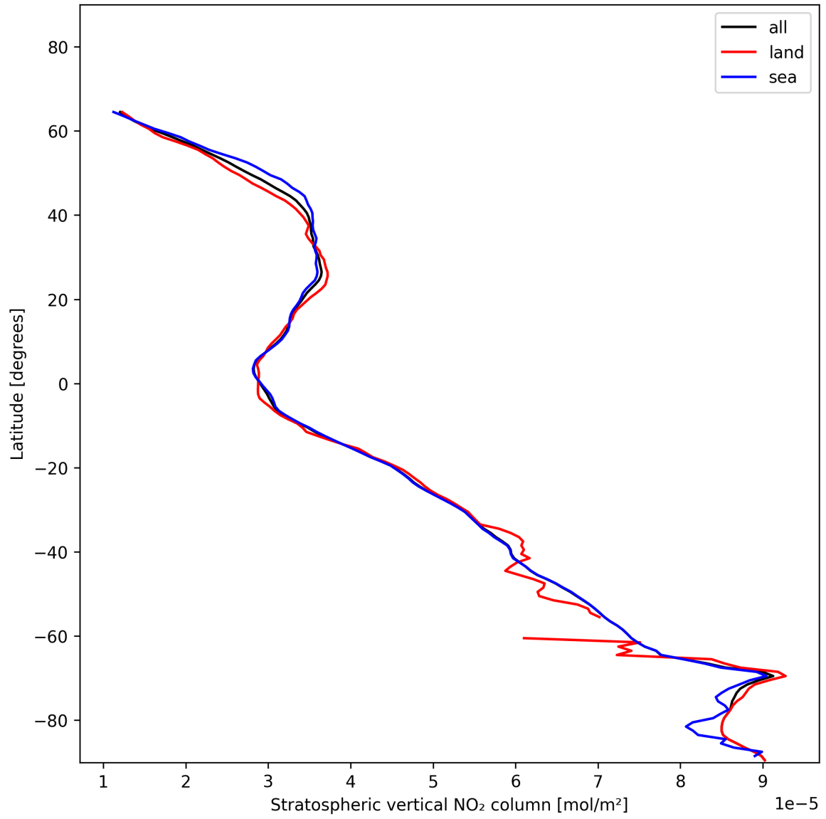
Figure 19: Zonal average of “Stratospheric vertical NO 2 column” for 2024-12-27 to 2024-12-29.
