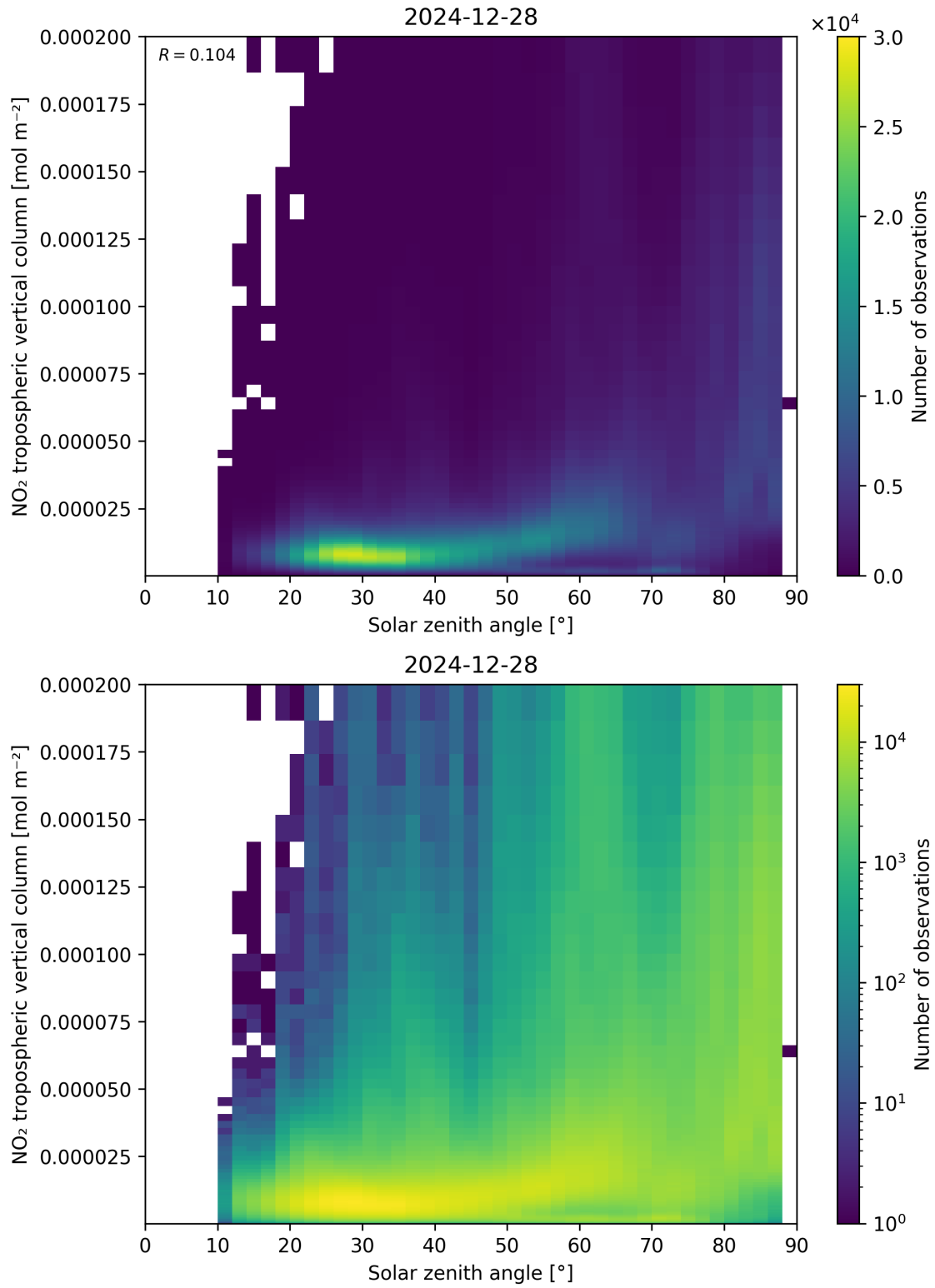
Figure 155: Scatter density plot of “Solar zenith angle” against “NO 2 tropospheric vertical column” for 2024-12-27 to 2024-12-29.
