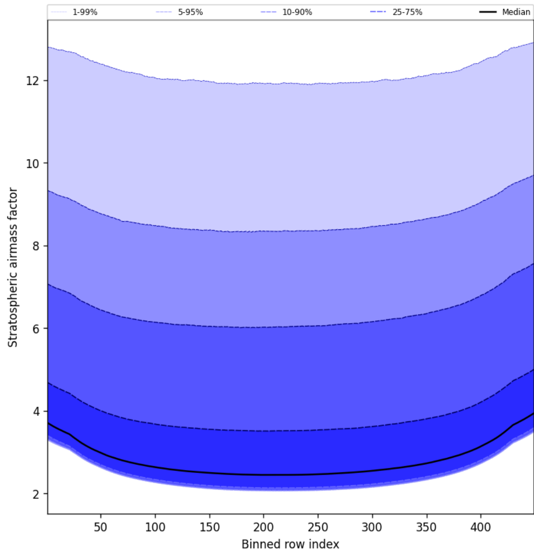
Figure 61: Along track statistics of “Stratospheric airmass factor” for 2024-12-27 to 2024-12-29
