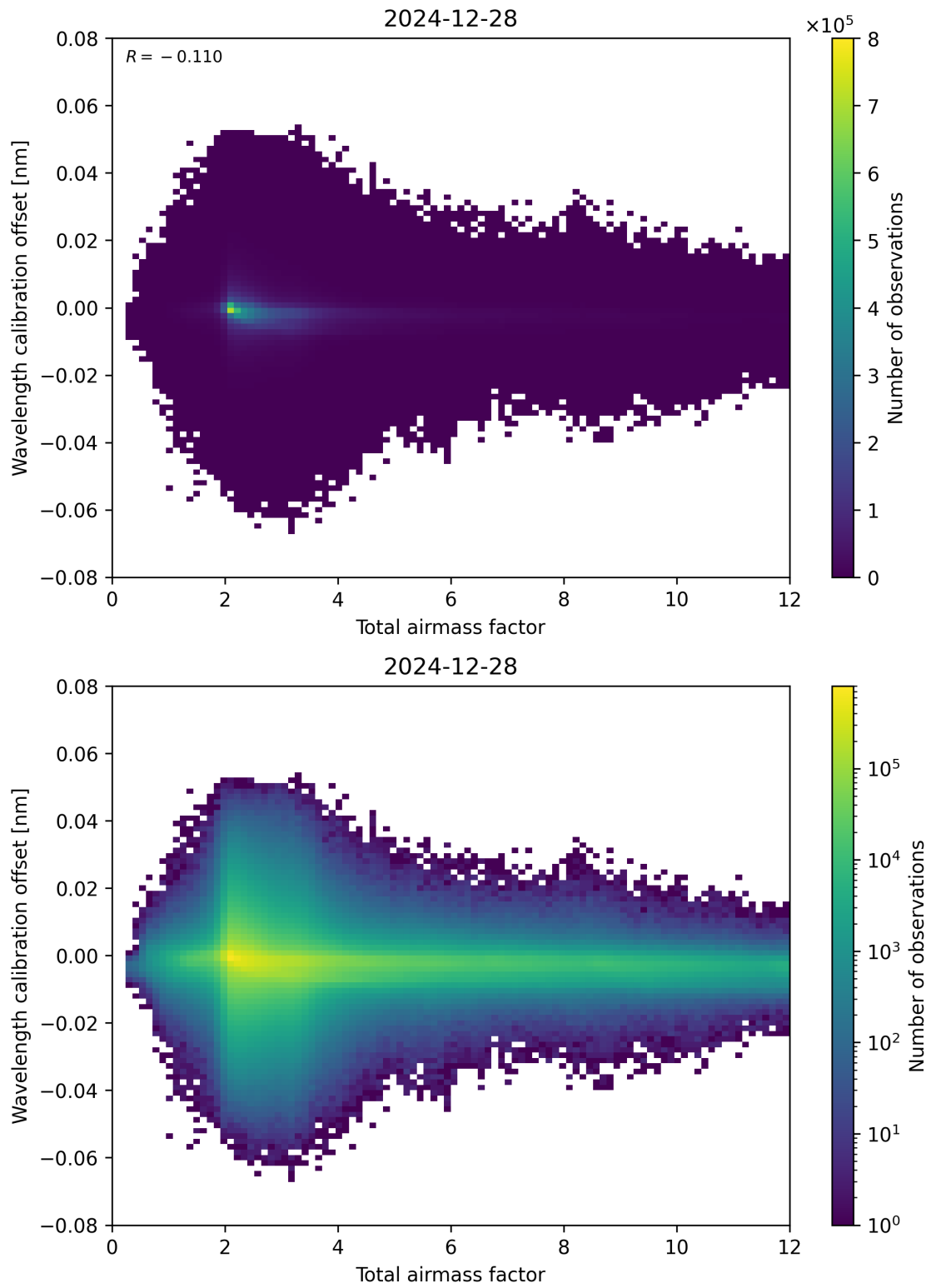
Figure 70: Scatter density plot of “Total airmass factor” against “Wavelength calibration offset” for 2024-12-27 to 2024-12-29.
