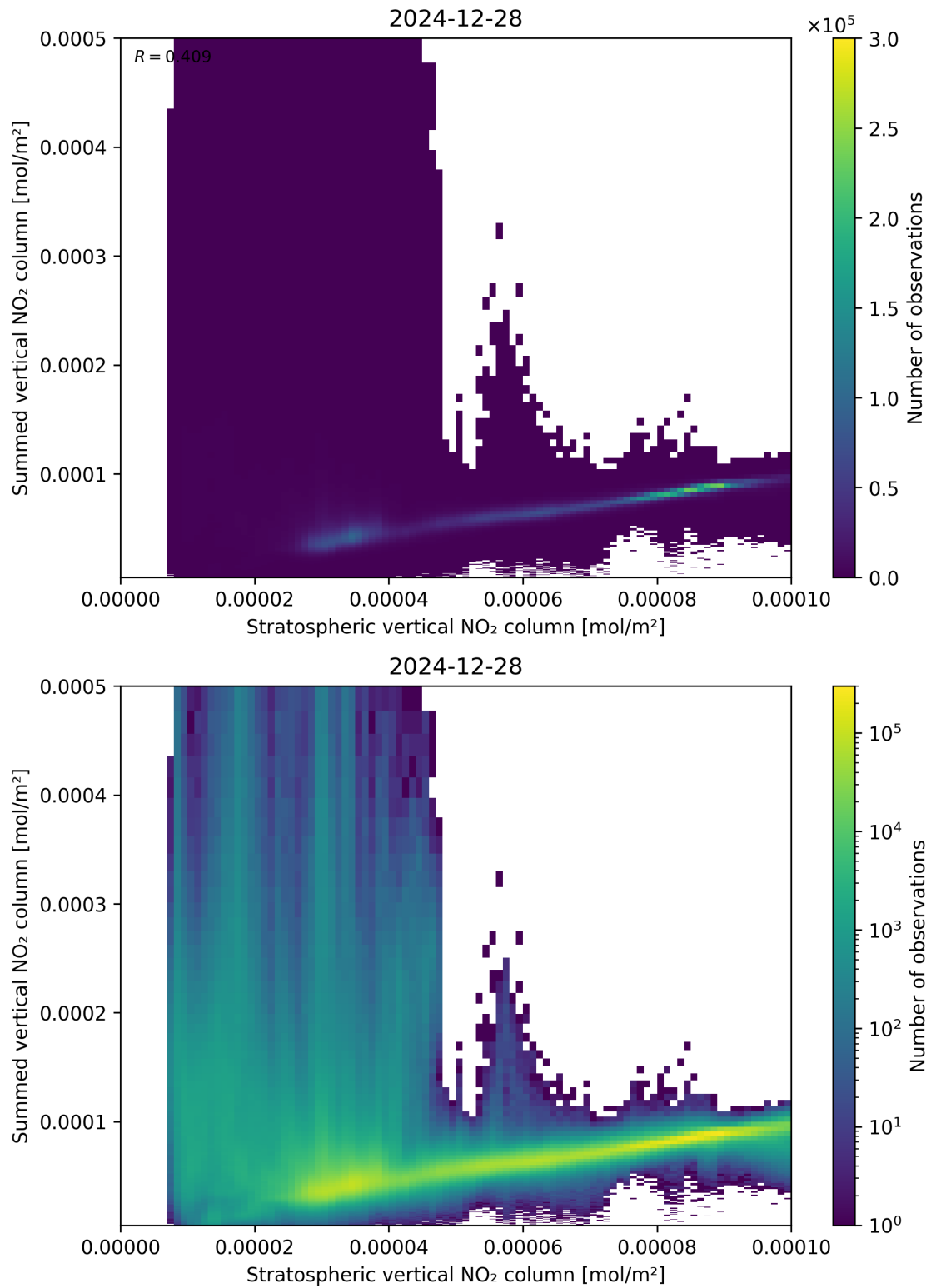
Figure 98: Scatter density plot of “Stratospheric vertical NO 2 column” against “Summed vertical NO 2 column” for 2024-12-27 to 2024-12-29.
