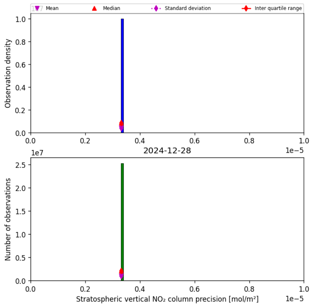
Figure 37: Histogram of “Stratospheric vertical NO 2 column precision” for 2024-12-27 to 2024-12-29
