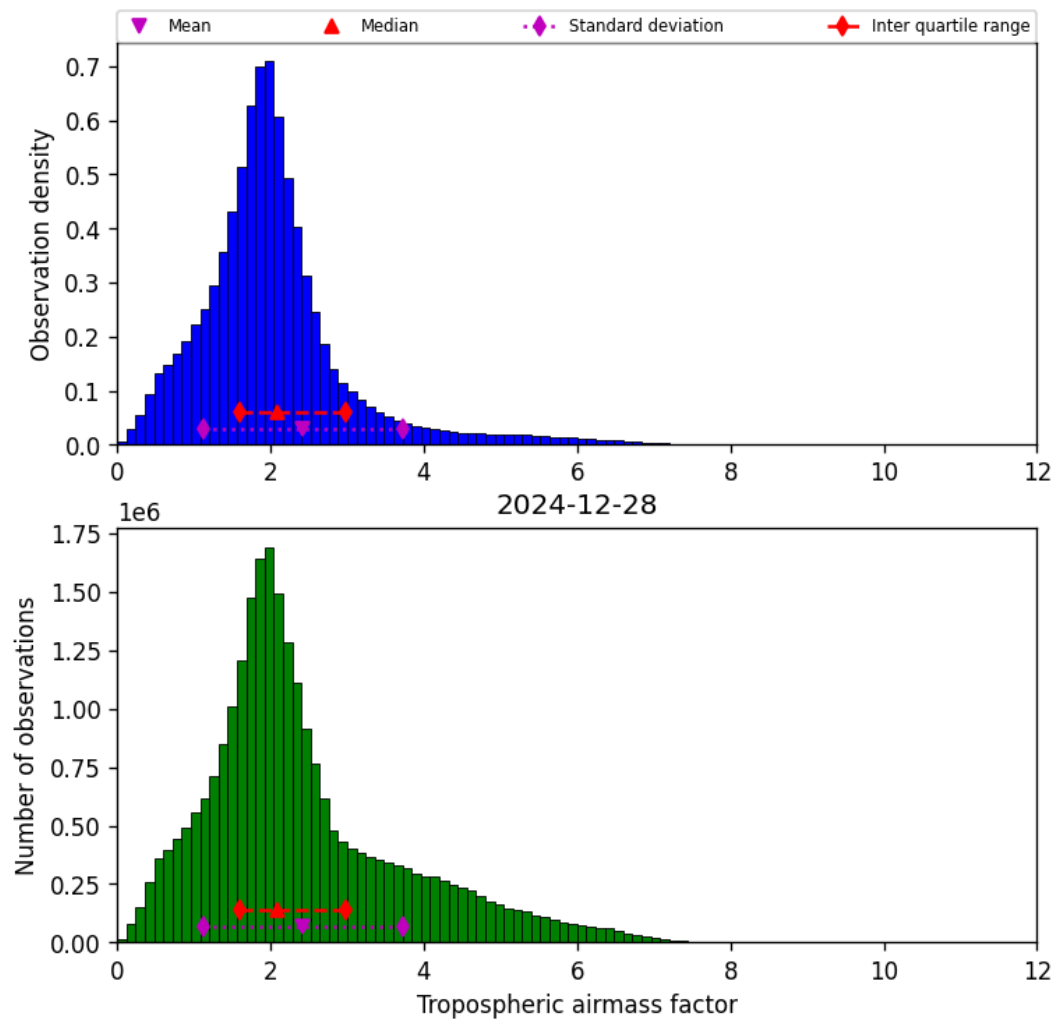
Figure 31: Histogram of “Tropospheric airmass factor” for 2024-12-27 to 2024-12-29
