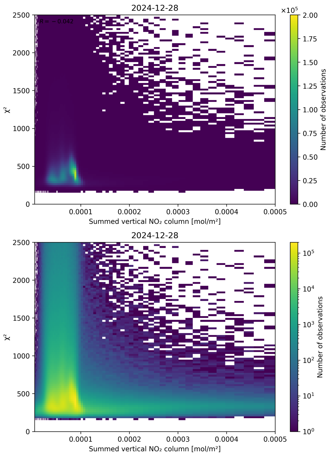
Figure 104: Scatter density plot of “Summed vertical NO 2 column” against “ \chi^2 ” for 2024-12-27 to 2024-12-29.
