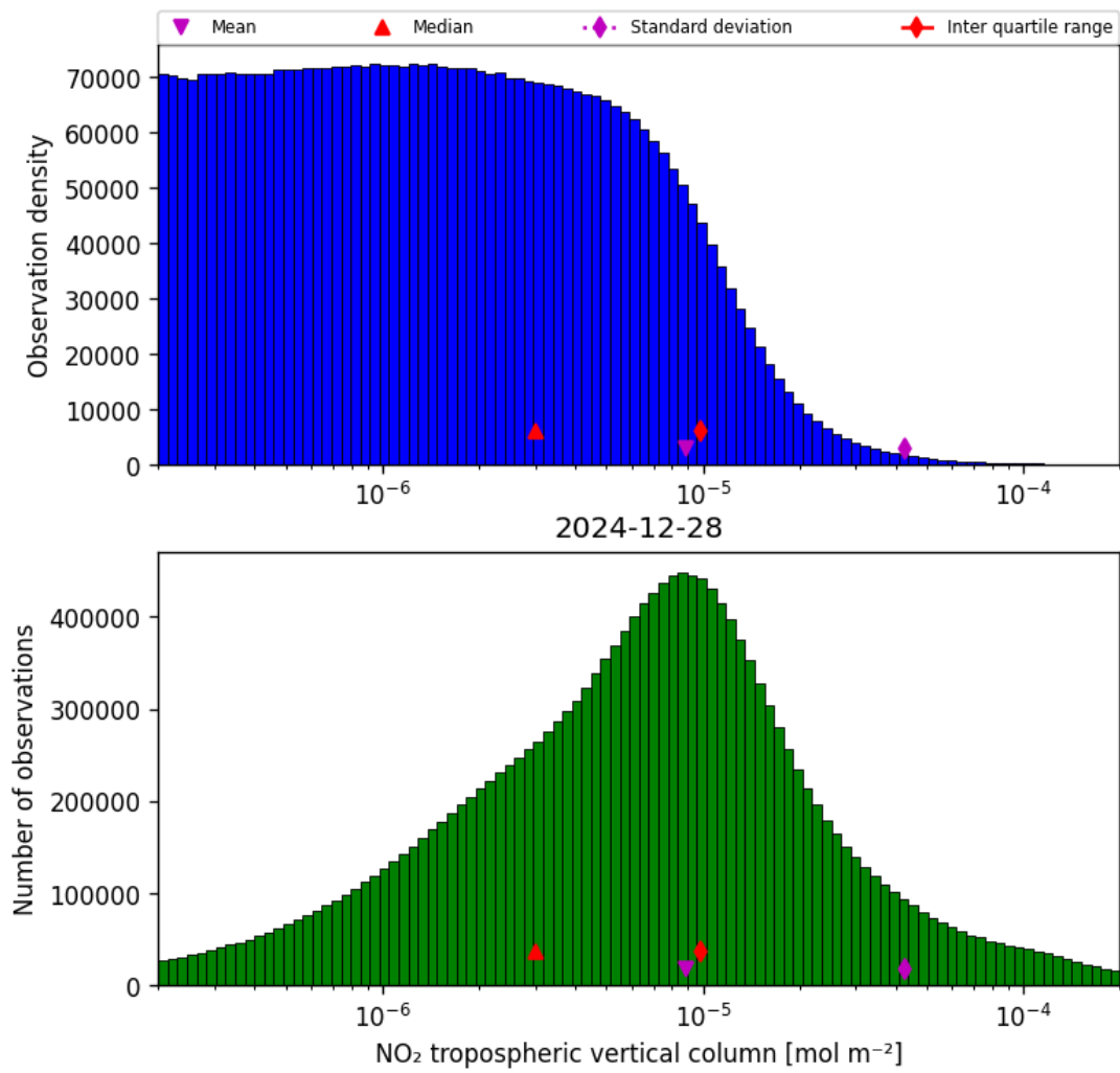
Figure 29: Histogram of “NO 2 tropospheric vertical column” for 2024-12-27 to 2024-12-29
