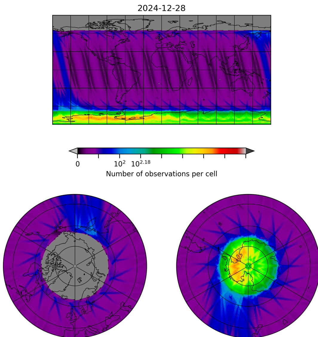
Figure 10: Map of the number of observations for 2024-12-27 to 2024-12-29
