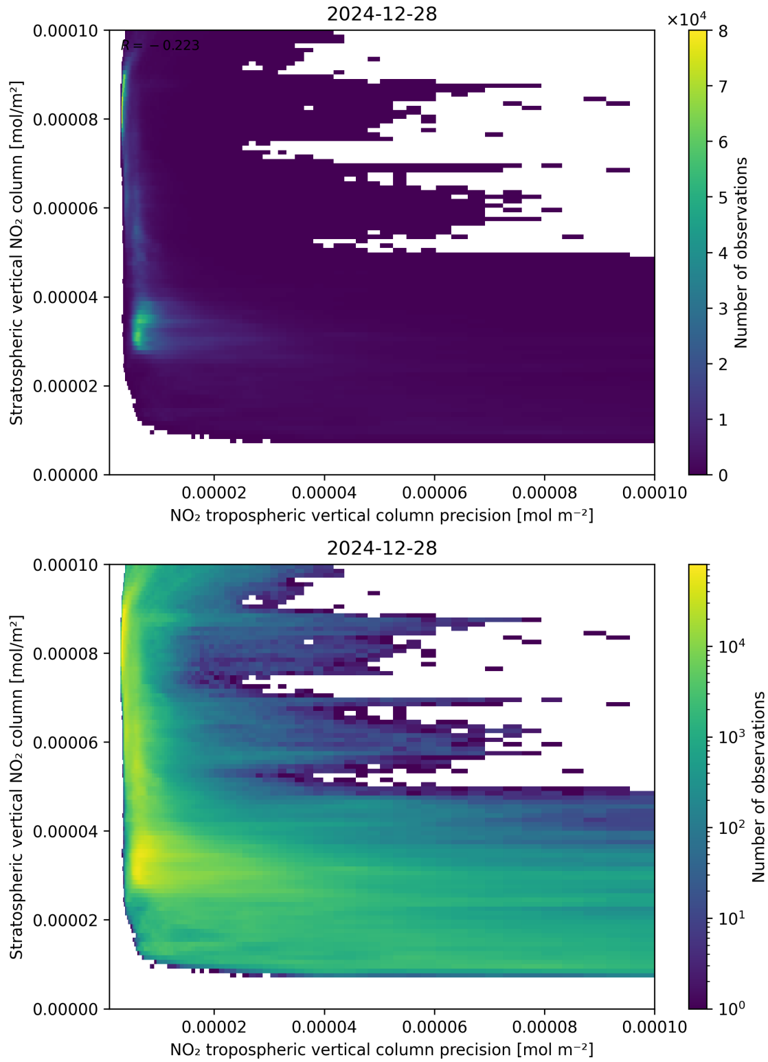
Figure 135: Scatter density plot of “NO 2 tropospheric vertical column precision” against “Stratospheric vertical NO 2 column” for 2024-12-27 to 2024-12-29.
