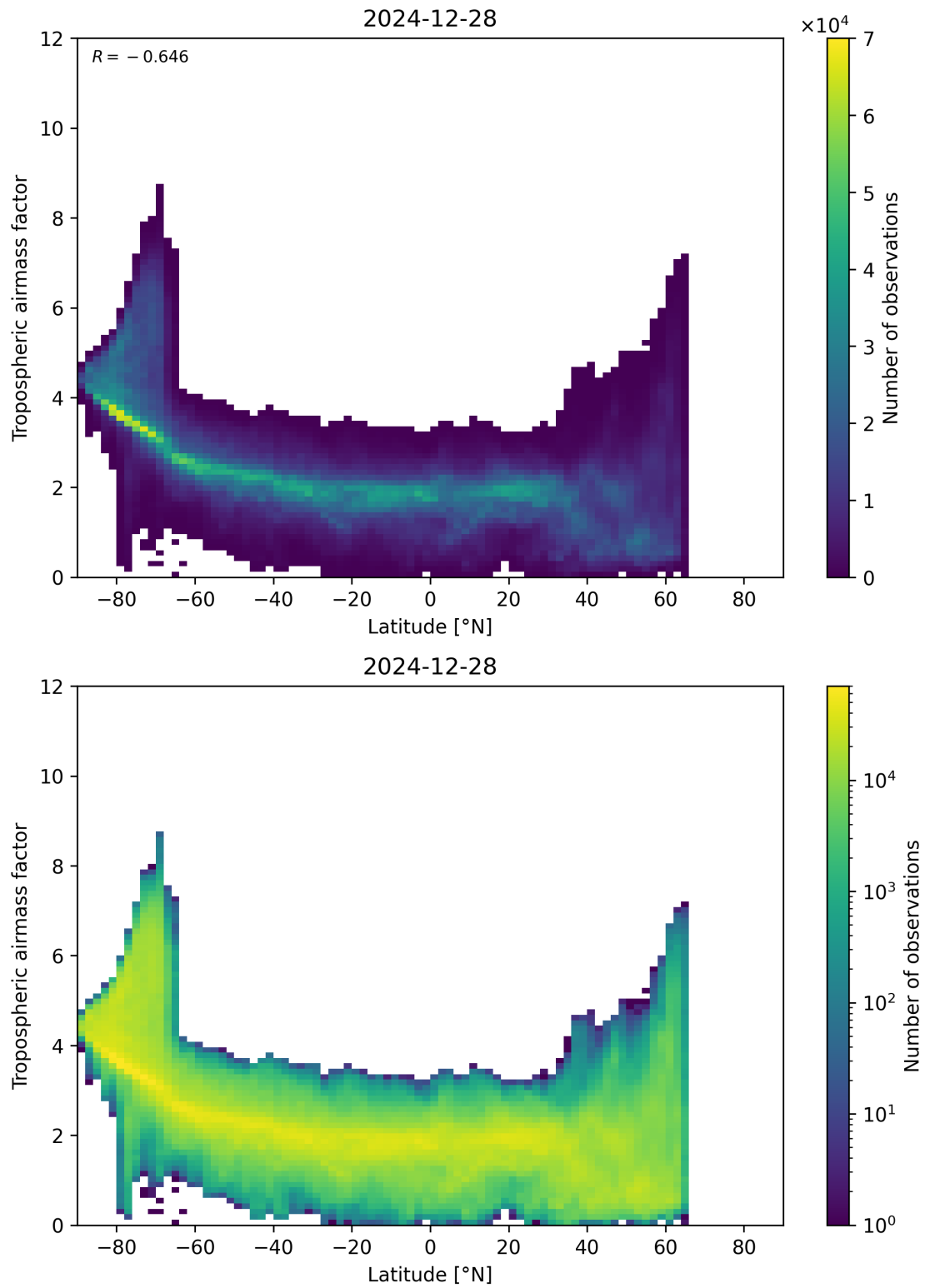
Figure 85: Scatter density plot of “Latitude” against “Tropospheric airmass factor” for 2024-12-27 to 2024-12-29.
