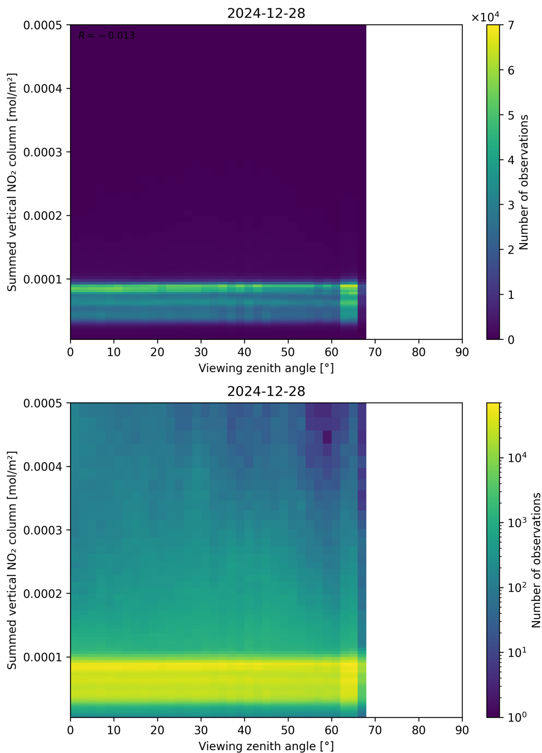
Figure 165: Scatter density plot of “Viewing zenith angle” against “Summed vertical NO 2 column” for 2024-12-27 to 2024-12-29.
