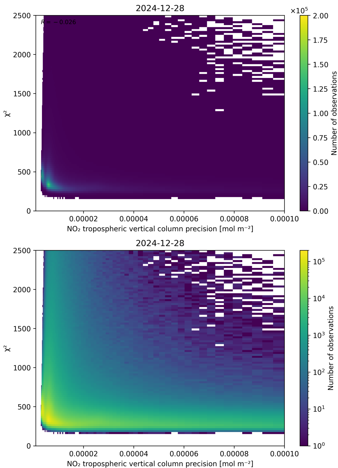
Figure 134: Scatter density plot of “NO 2 tropospheric vertical column precision” against “ \chi^2 ” for 2024-12-27 to 2024-12-29.
