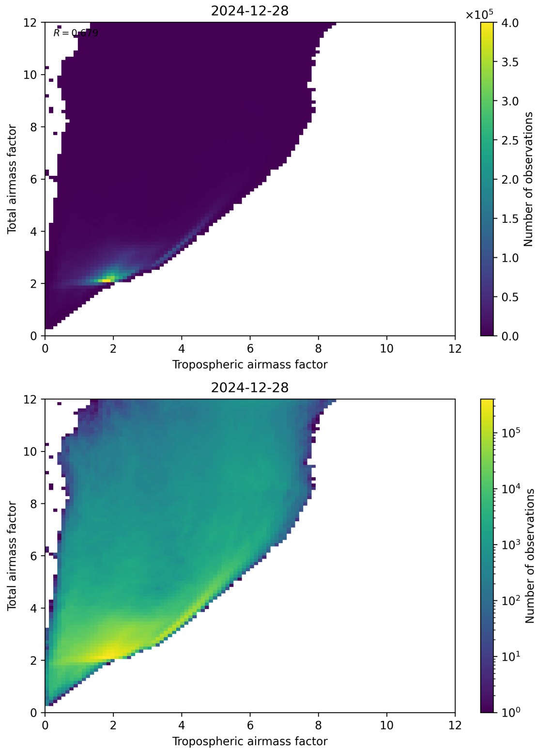
Figure 72: Scatter density plot of “Tropospheric airmass factor” against “Total airmass factor” for 2024-12-27 to 2024-12-29.
