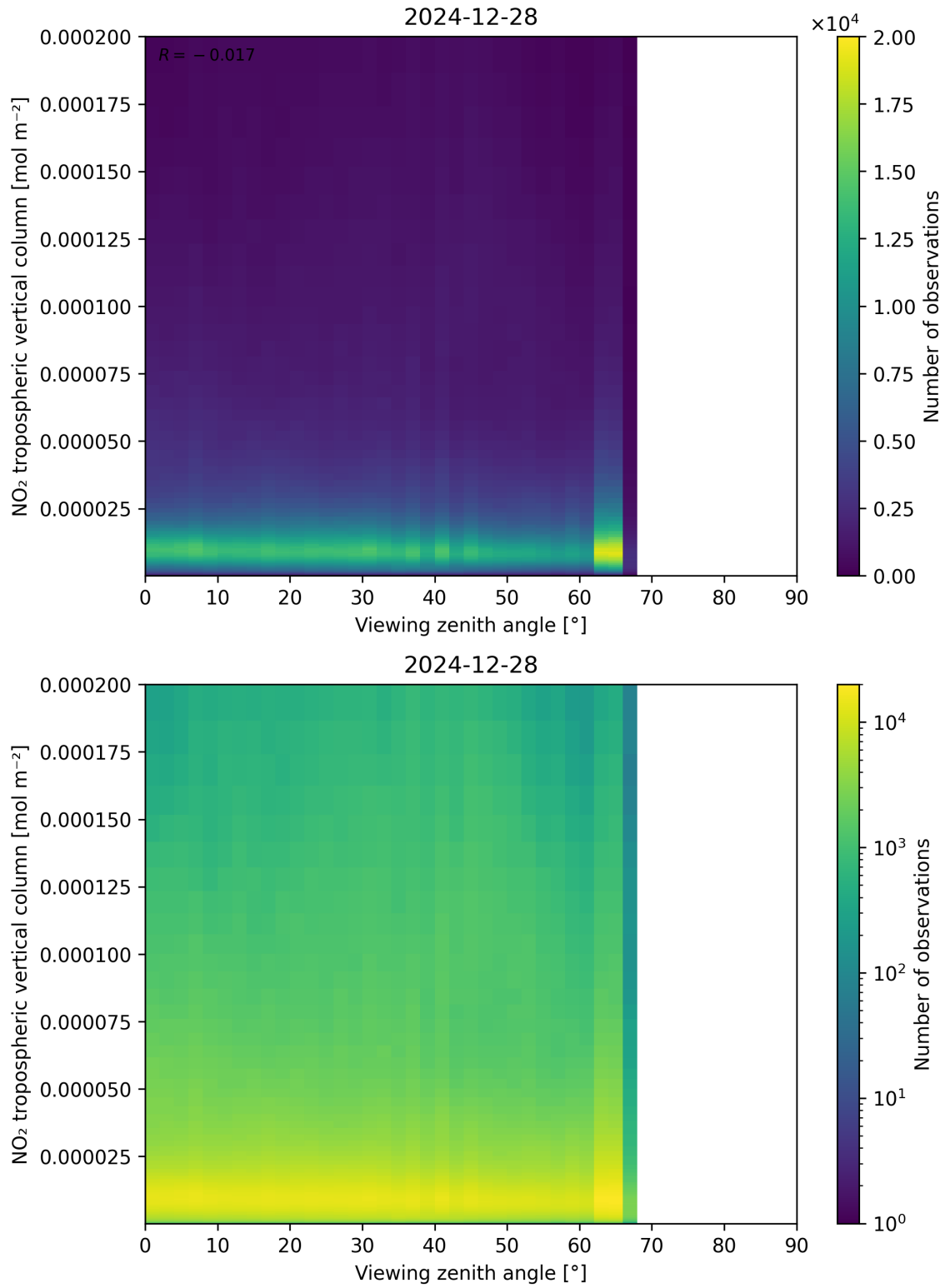
Figure 169: Scatter density plot of “Viewing zenith angle” against “NO 2 tropospheric vertical column” for 2024-12-27 to 2024-12-29.
