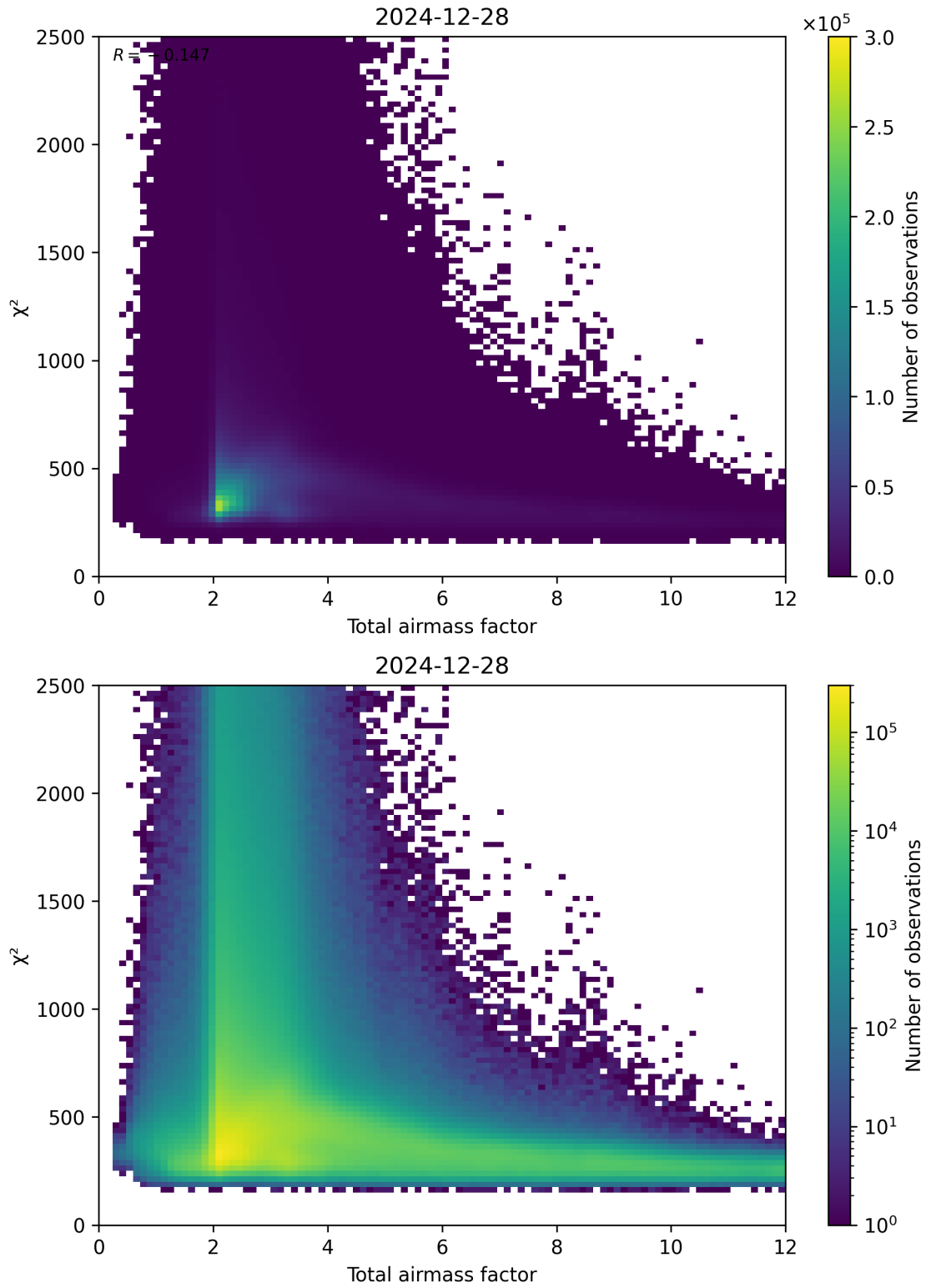
Figure 63: Scatter density plot of “Total airmass factor” against “ \chi^2 ” for 2024-12-27 to 2024-12-29.
