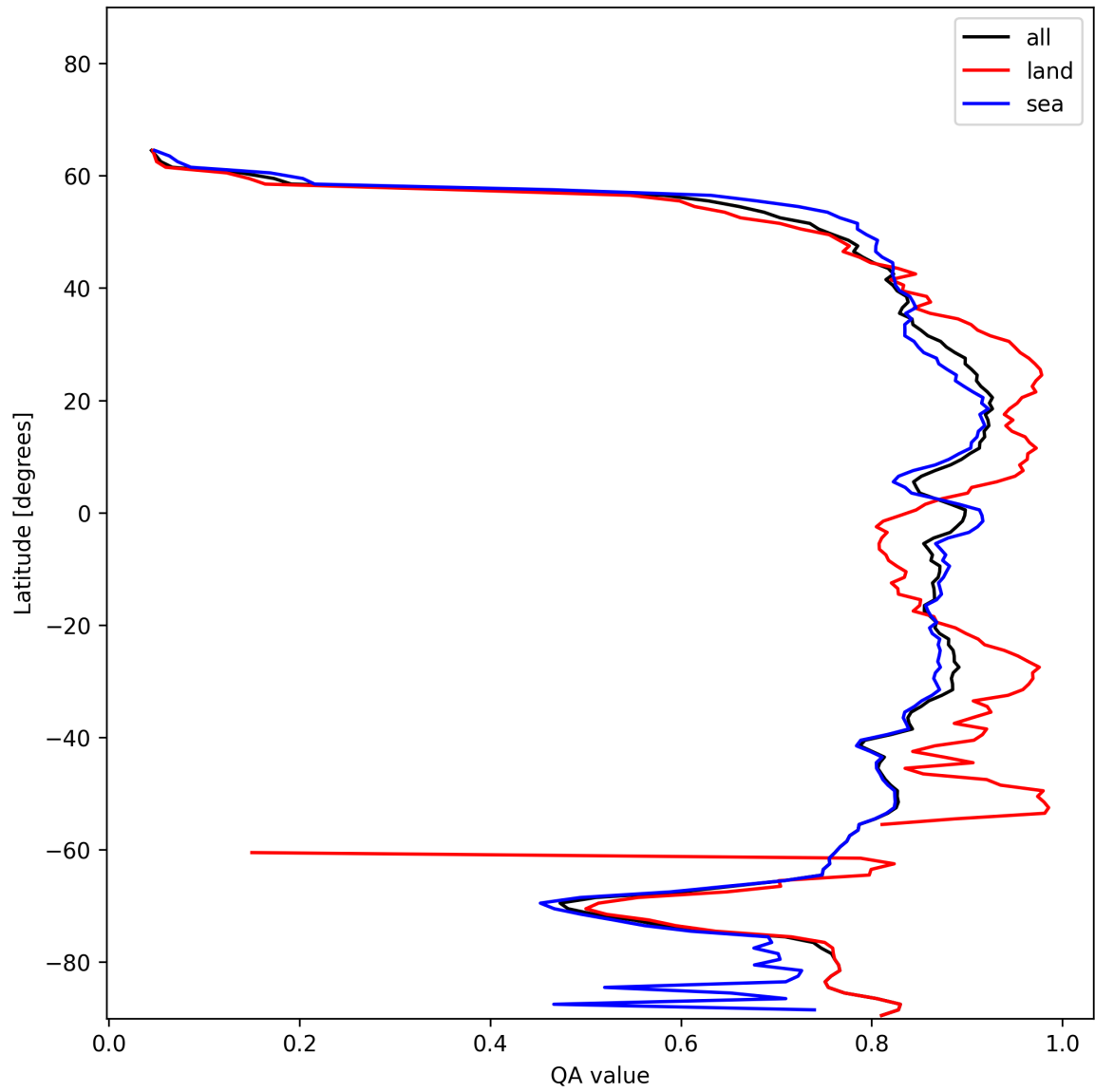
Figure 11: Zonal average of “QA value” for 2024-12-27 to 2024-12-29.
