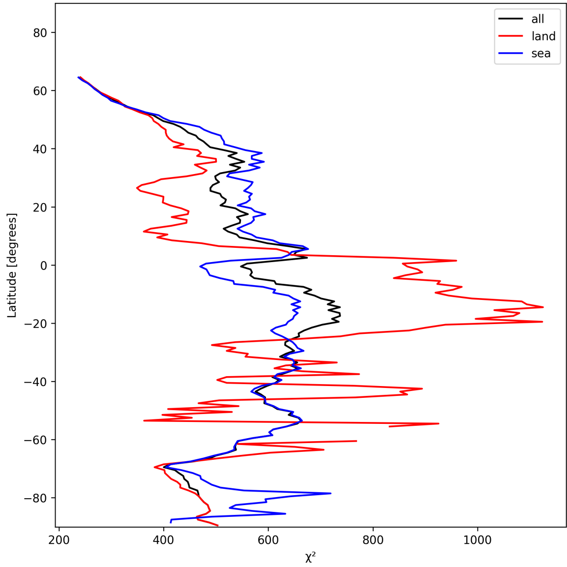
Figure 25: Zonal average of “ \chi^2 ” for 2024-12-27 to 2024-12-29.
