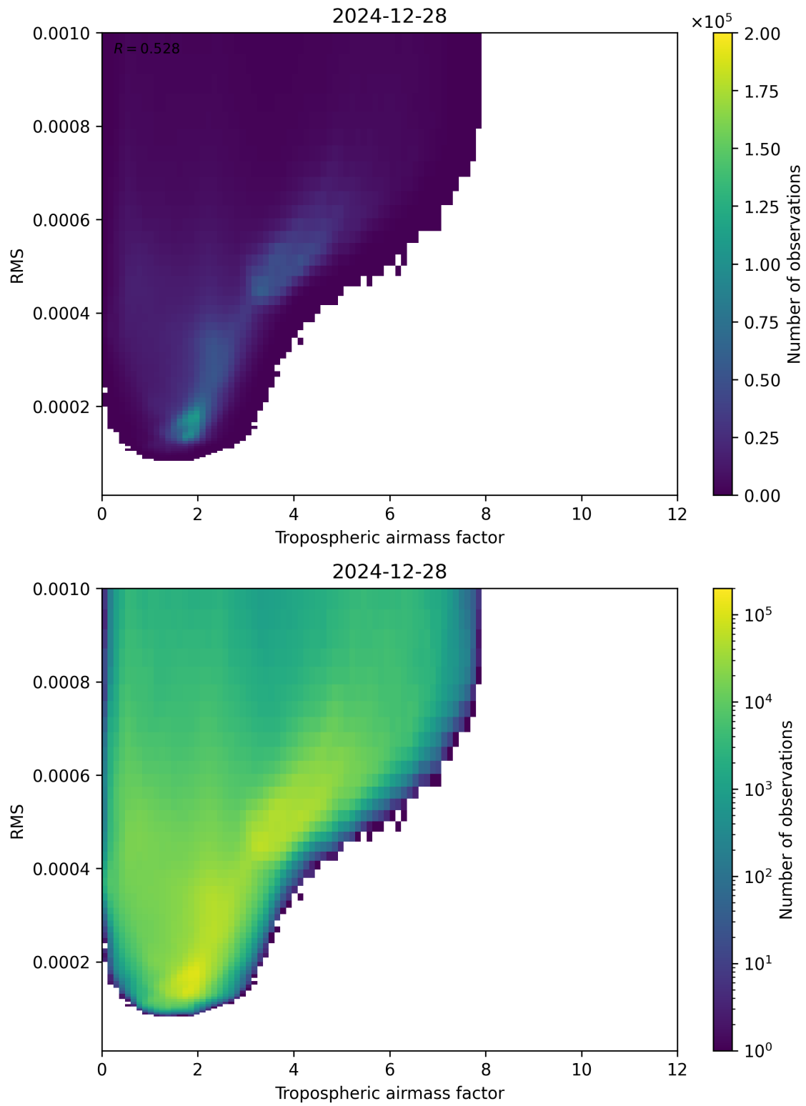
Figure 79: Scatter density plot of “Tropospheric airmass factor” against “RMS” for 2024-12-27 to 2024-12-29.
