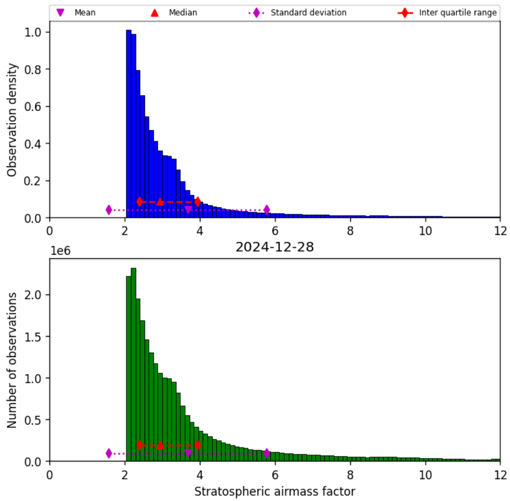
Figure 44: Histogram of “Stratospheric airmass factor” for 2024-12-27 to 2024-12-29
