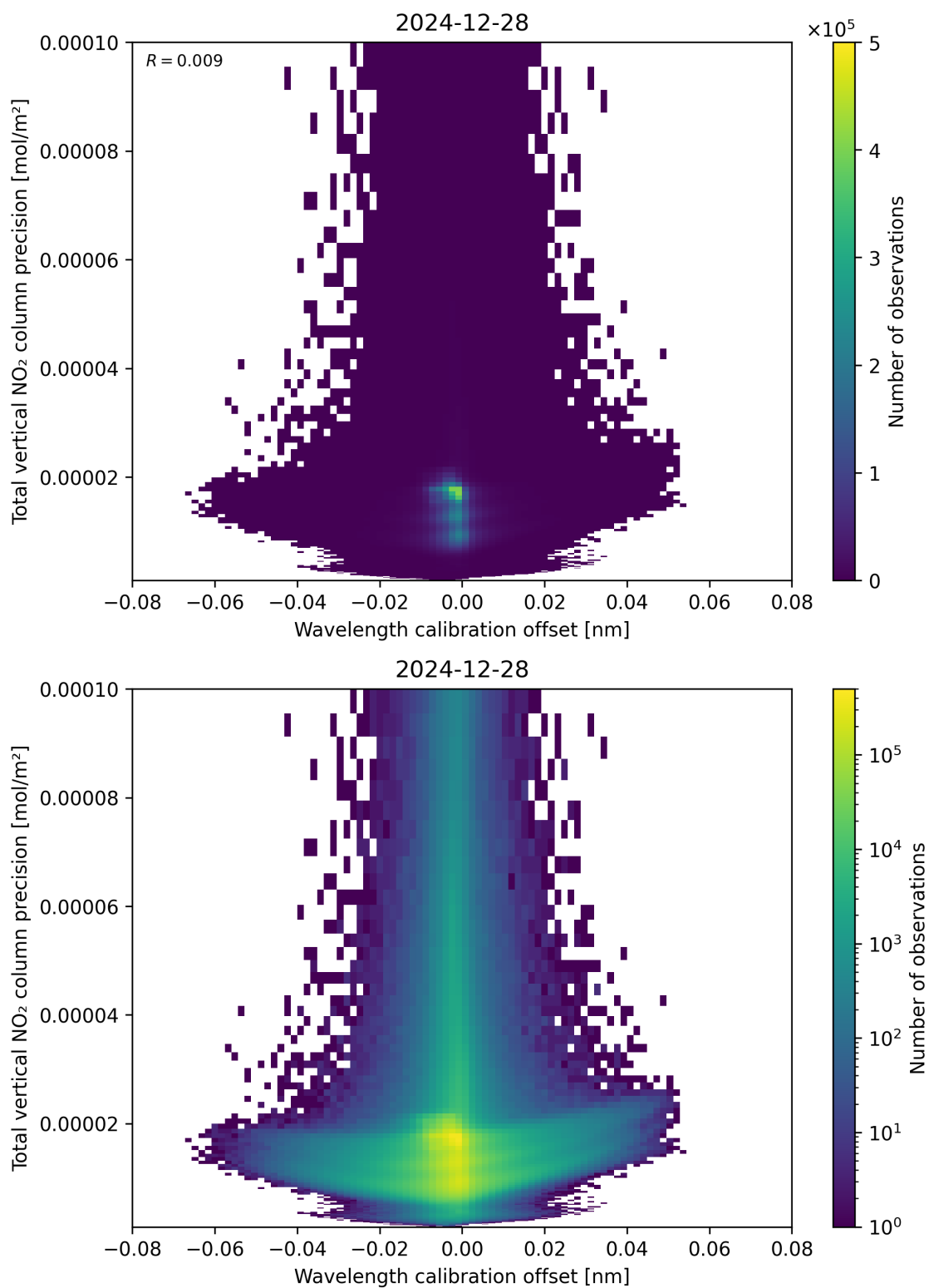
Figure 180: Scatter density plot of “Wavelength calibration offset” against “Total vertical NO 2 column precision” for 2024-12-27 to 2024-12-29.
