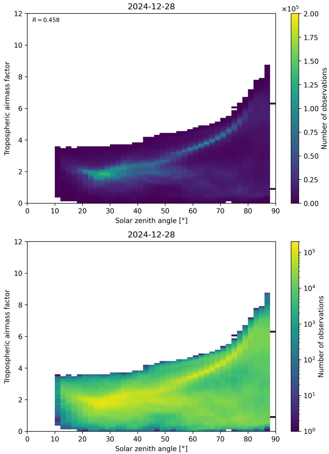
Figure 147: Scatter density plot of “Solar zenith angle” against “Tropospheric airmass factor” for 2024-12-27 to 2024-12-29.
