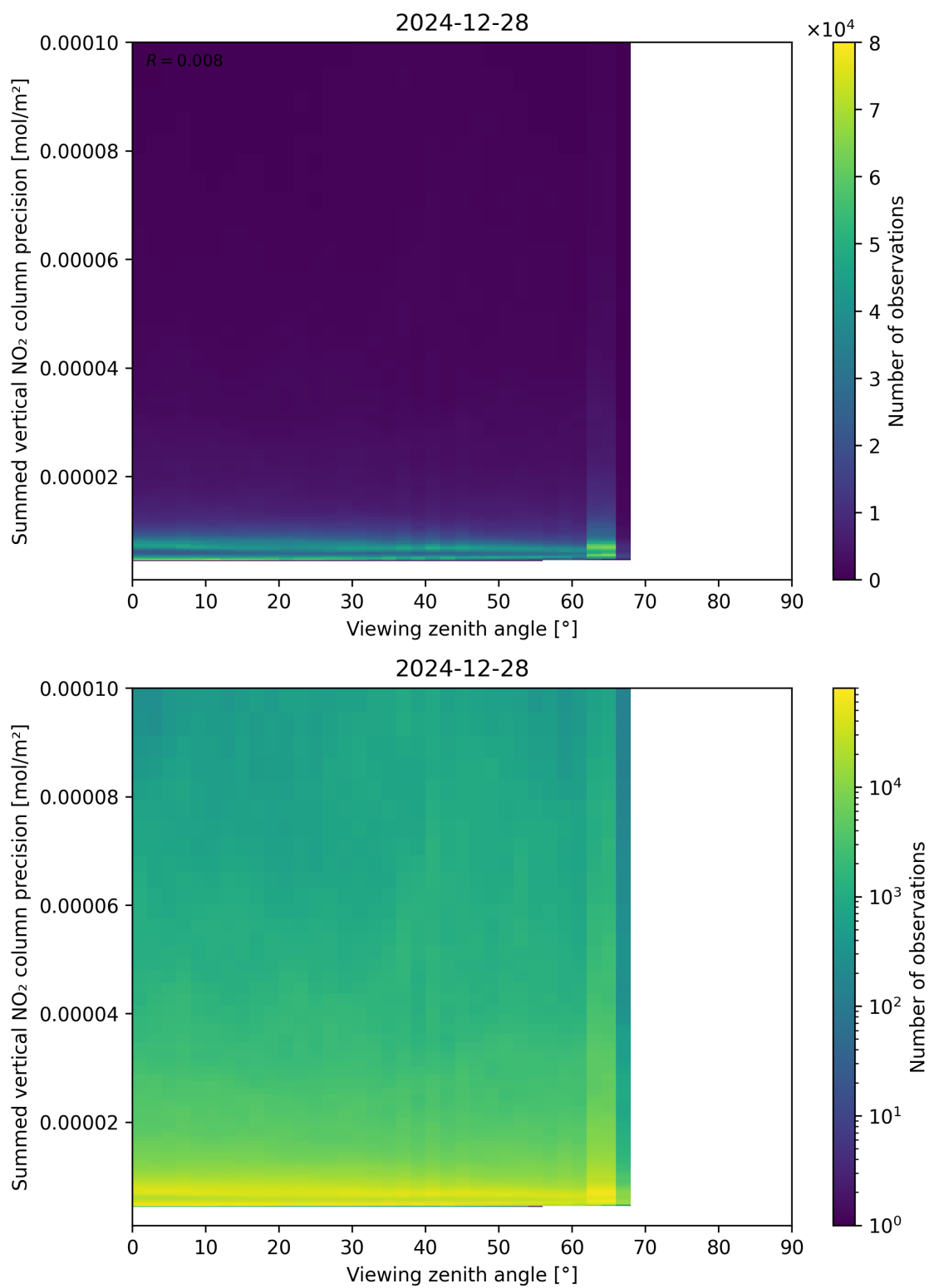
Figure 166: Scatter density plot of “Viewing zenith angle” against “Summed vertical NO 2 column precision” for 2024-12-27 to 2024-12-29.
