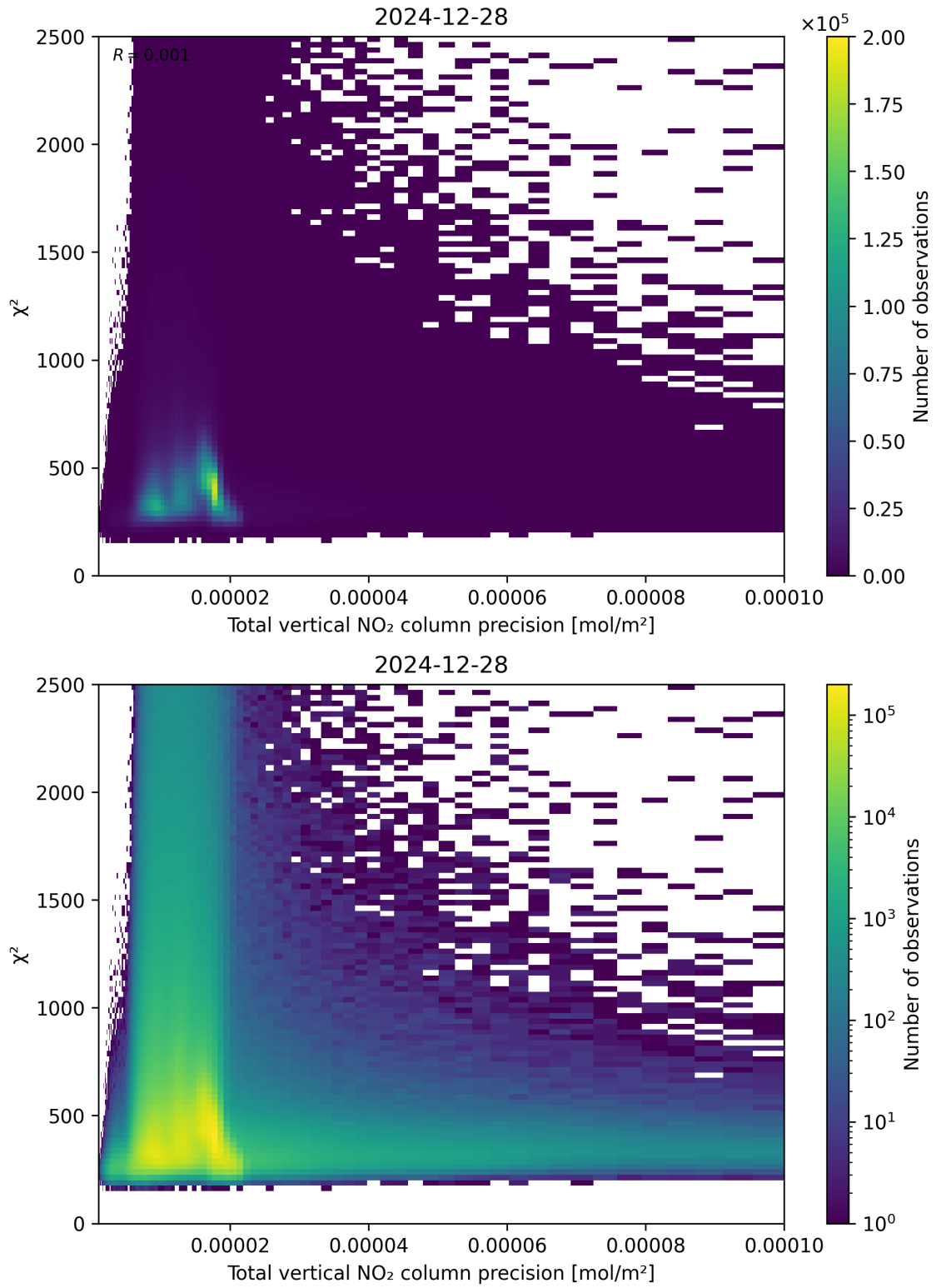
Figure 116: Scatter density plot of “Total vertical NO 2 column precision” against “ \chi^2 ” for 2024-12-27 to 2024-12-29.
