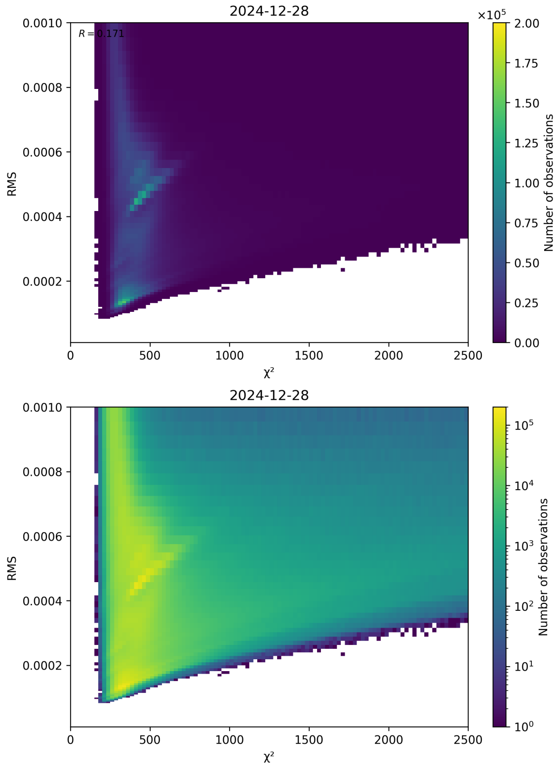
Figure 82: Scatter density plot of “ \chi^2 ” against “RMS” for 2024-12-27 to 2024-12-29.
