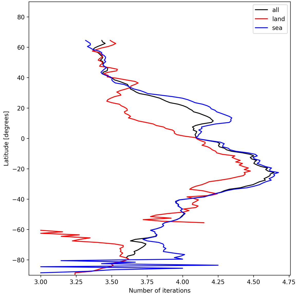
Figure 17: Zonal average of “Number of iterations” for 2024-12-27 to 2024-12-29.
