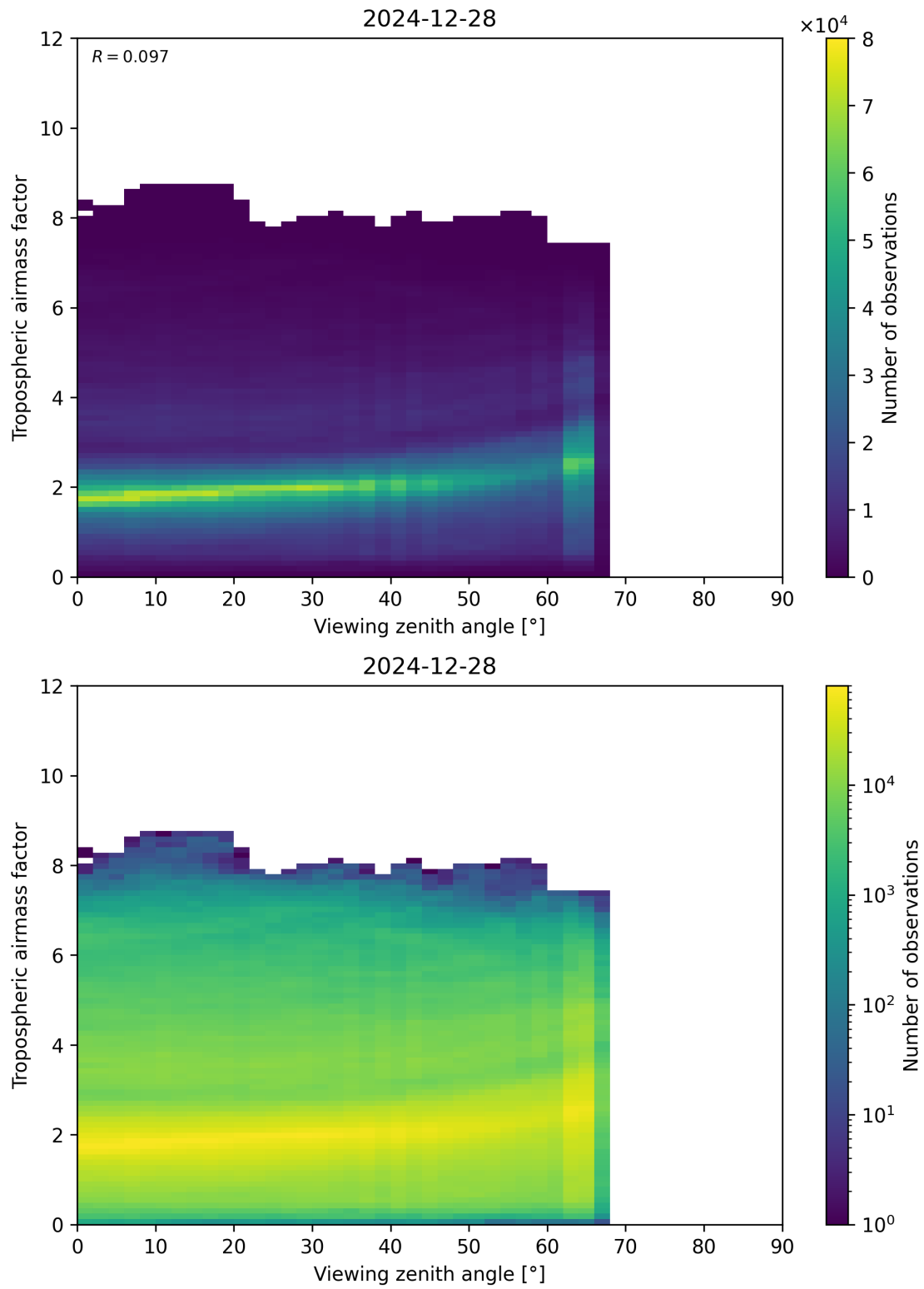
Figure 161: Scatter density plot of “Viewing zenith angle” against “Tropospheric airmass factor” for 2024-12-27 to 2024-12-29.
