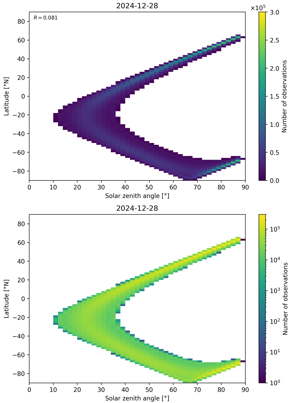
Figure 149: Scatter density plot of “Solar zenith angle” against “Latitude” for 2024-12-27 to 2024-12-29.
