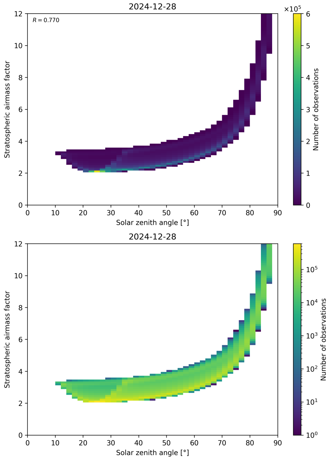
Figure 145: Scatter density plot of “Solar zenith angle” against “Stratospheric airmass factor” for 2024-12-27 to 2024-12-29.
