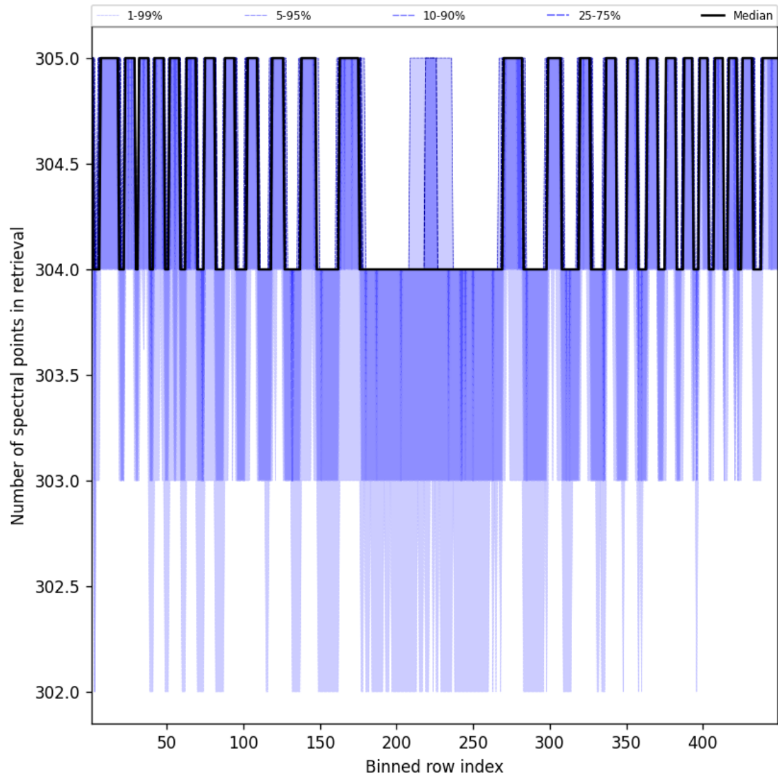
Figure 50: Along track statistics of “Number of spectral points in retrieval” for 2024-12-27 to 2024-12-29
