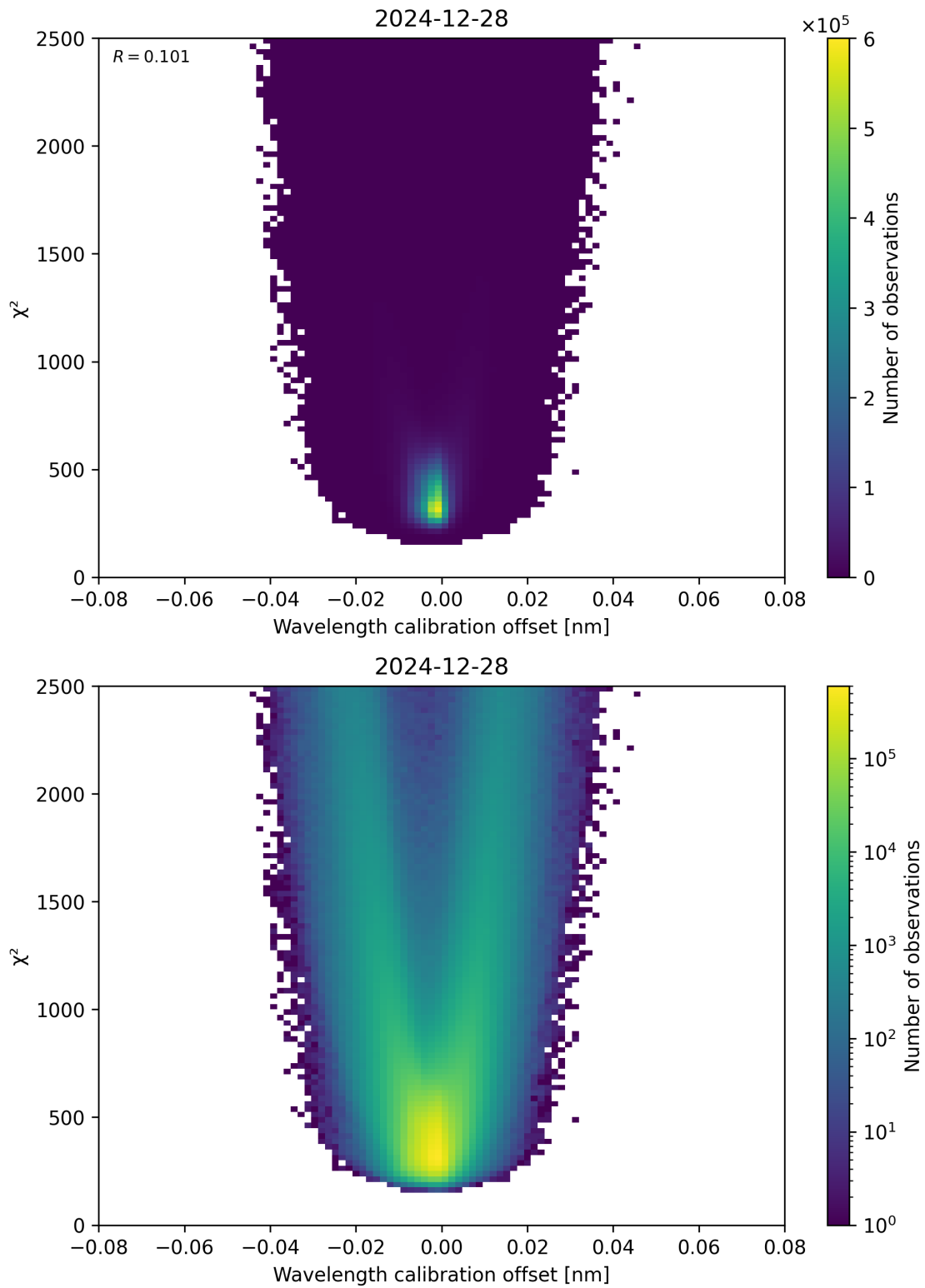
Figure 175: Scatter density plot of “Wavelength calibration offset” against “ \chi^2 ” for 2024-12-27 to 2024-12-29.
