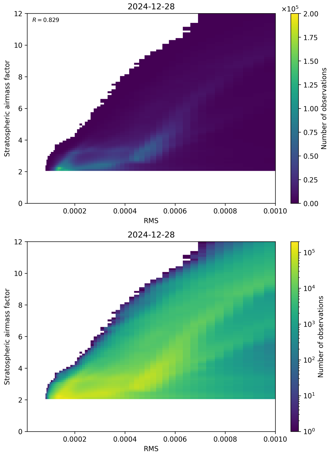
Figure 144: Scatter density plot of “RMS” against “Stratospheric airmass factor” for 2024-12-27 to 2024-12-29.
