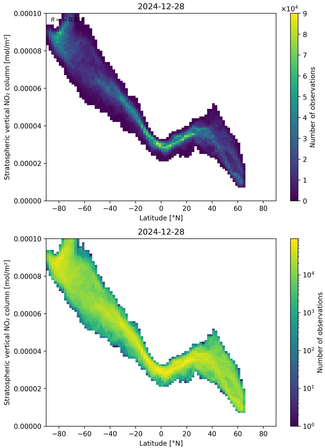
Figure 87: Scatter density plot of “Latitude” against “Stratospheric vertical NO 2 column” for 2024-12-27 to 2024-12-29.
