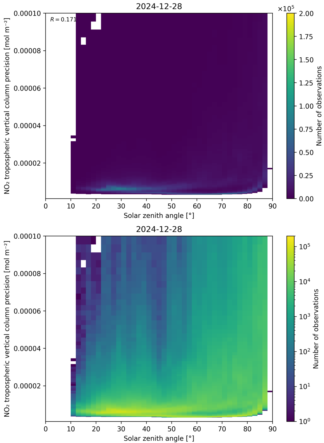
Figure 156: Scatter density plot of “Solar zenith angle” against “NO 2 tropospheric vertical column precision” for 2024-12-27 to 2024-12-29.
