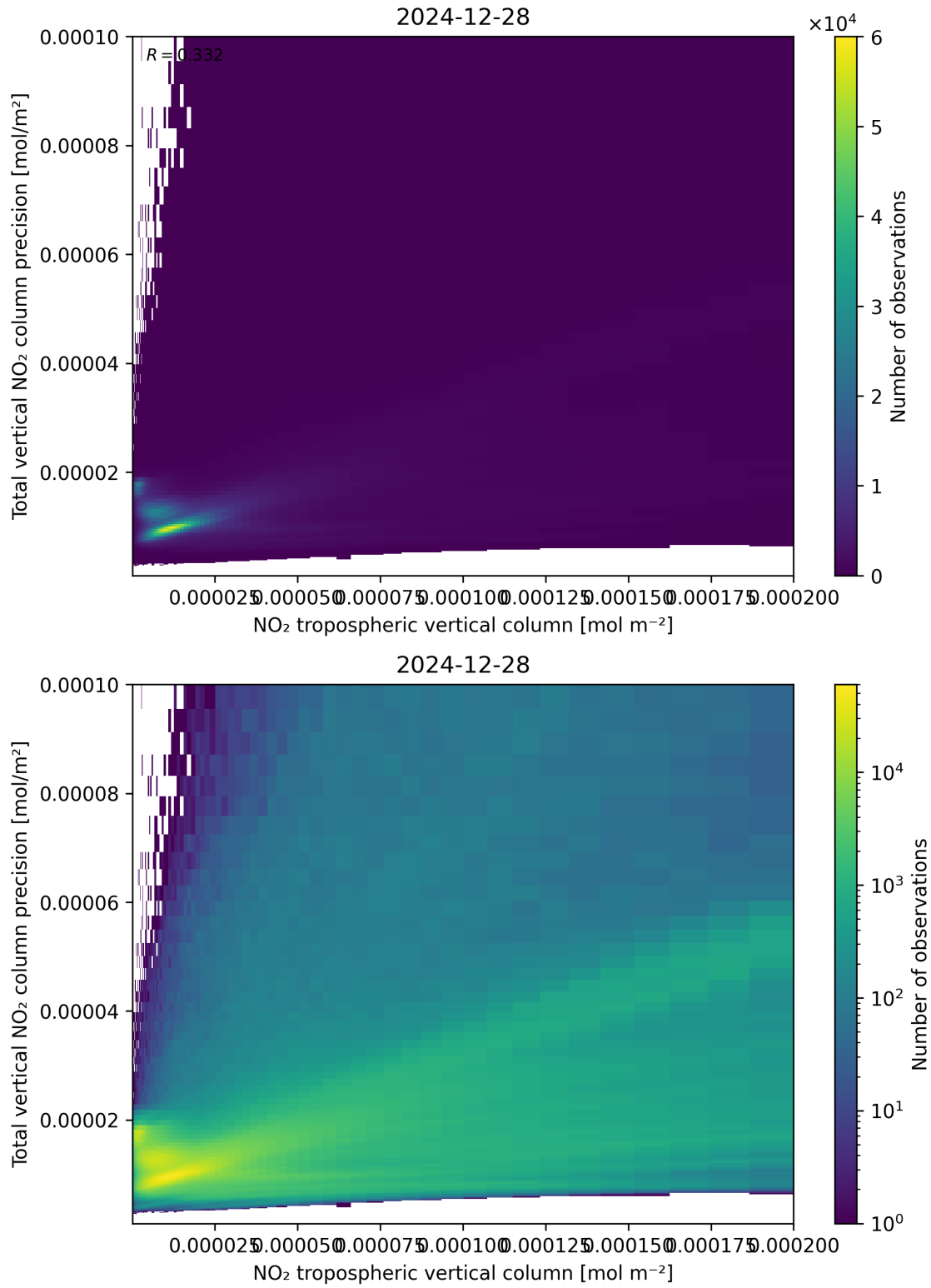
Figure 129: Scatter density plot of “NO 2 tropospheric vertical column” against “Total vertical NO 2 column precision” for 2024-12-27 to 2024-12-29.
