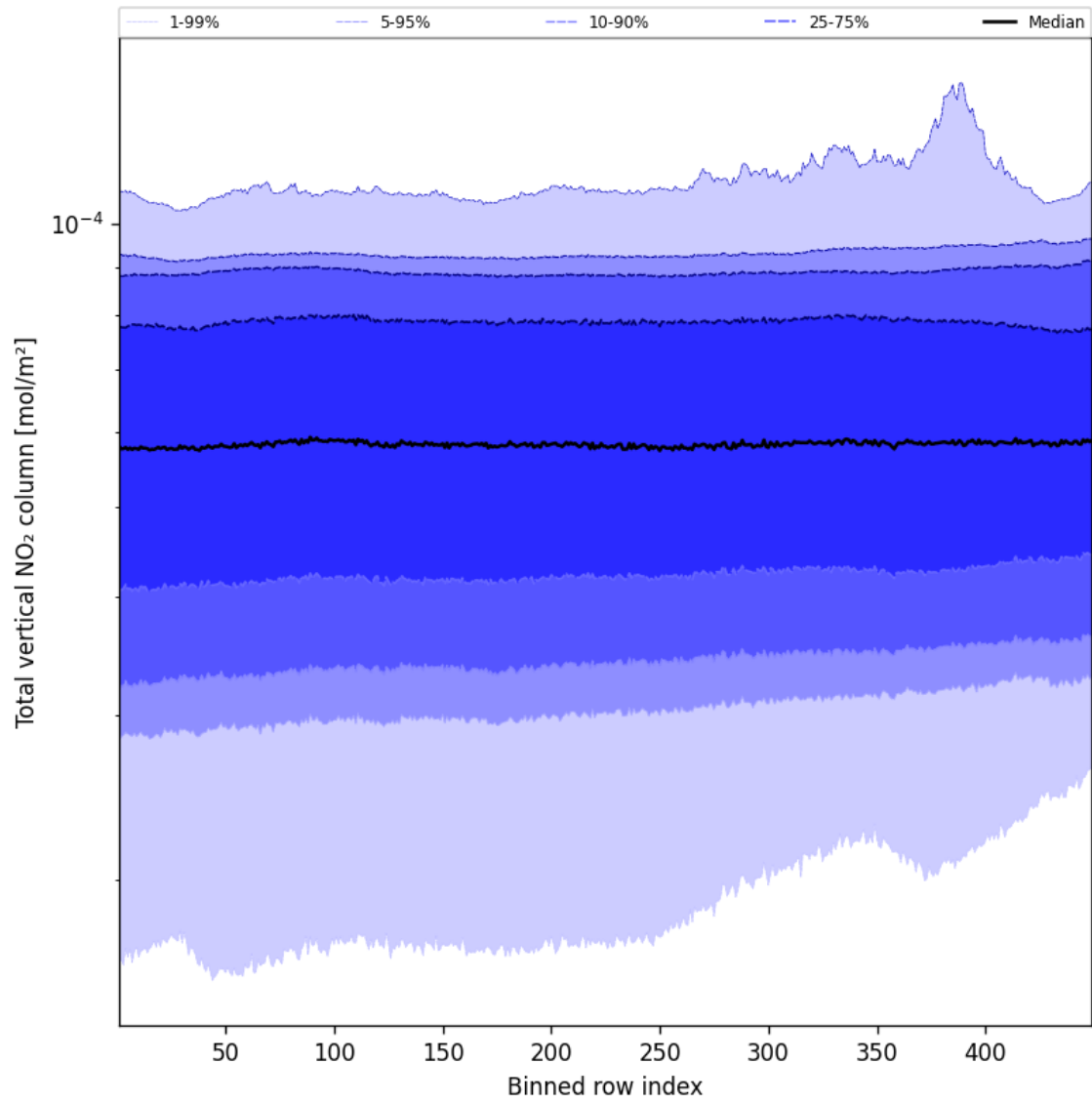
Figure 55: Along track statistics of “Total vertical NO 2 column” for 2024-12-27 to 2024-12-29
