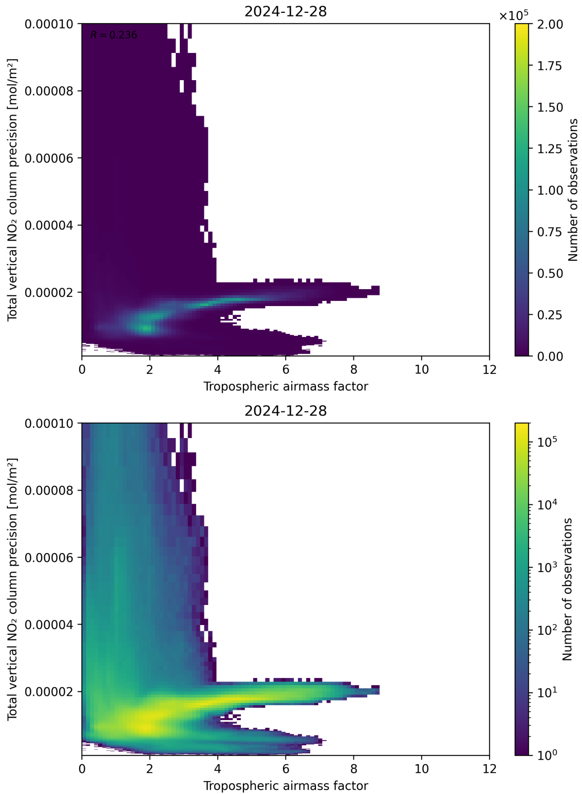
Figure 78: Scatter density plot of “Tropospheric air mass factor” against “Total vertical NO 2 column precision” for 2024-12-27 to 2024-12-29.
