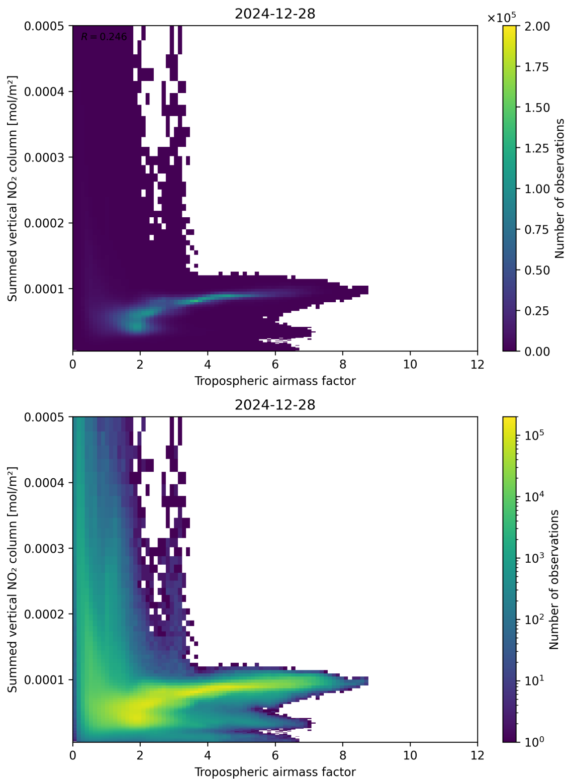
Figure 75: Scatter density plot of “Tropospheric air mass factor” against “Summed vertical NO 2 column” for 2024-12-27 to 2024-12-29.
