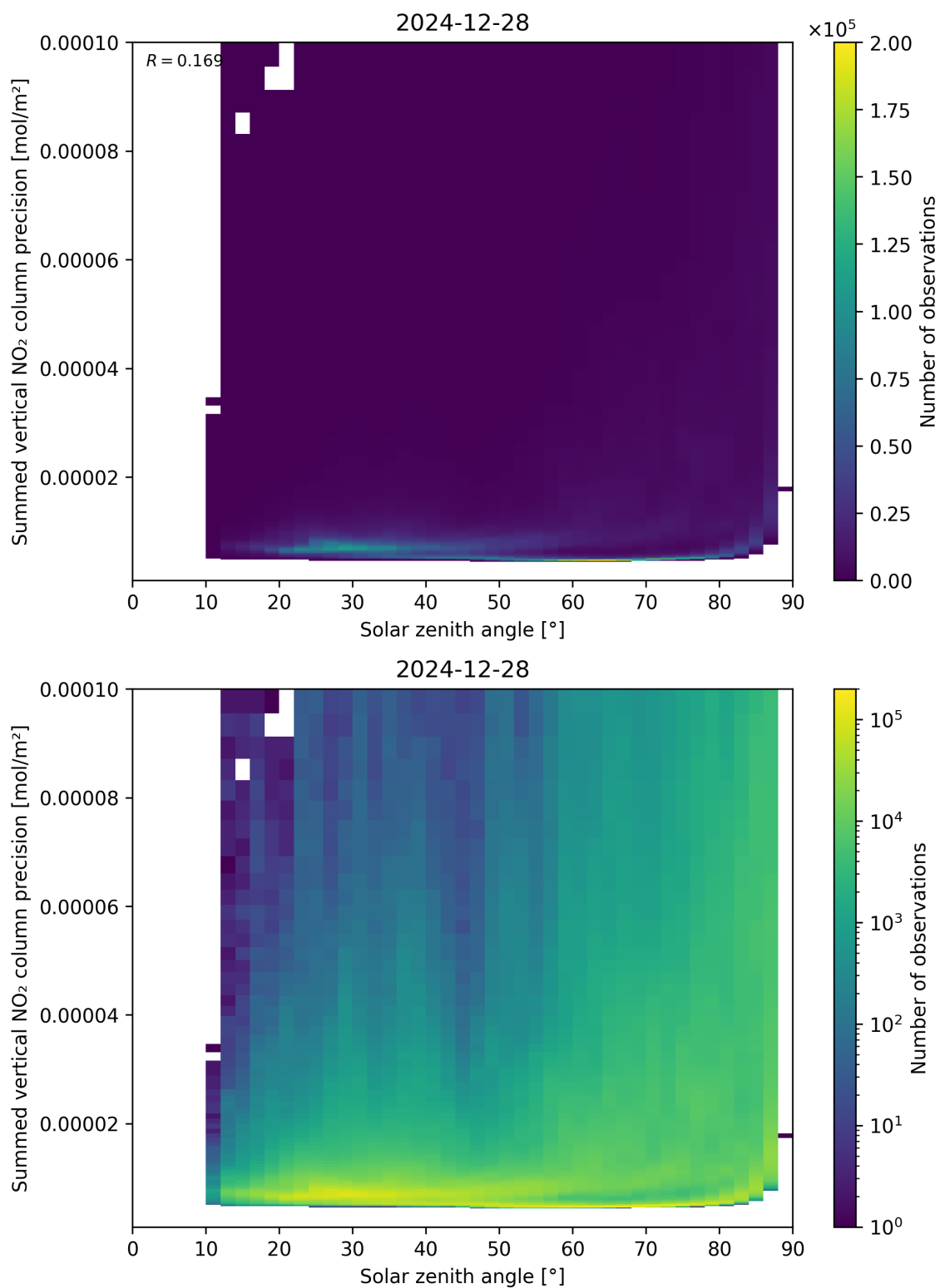
Figure 152: Scatter density plot of “Solar zenith angle” against “Summed vertical NO 2 column precision” for 2024-12-27 to 2024-12-29.
