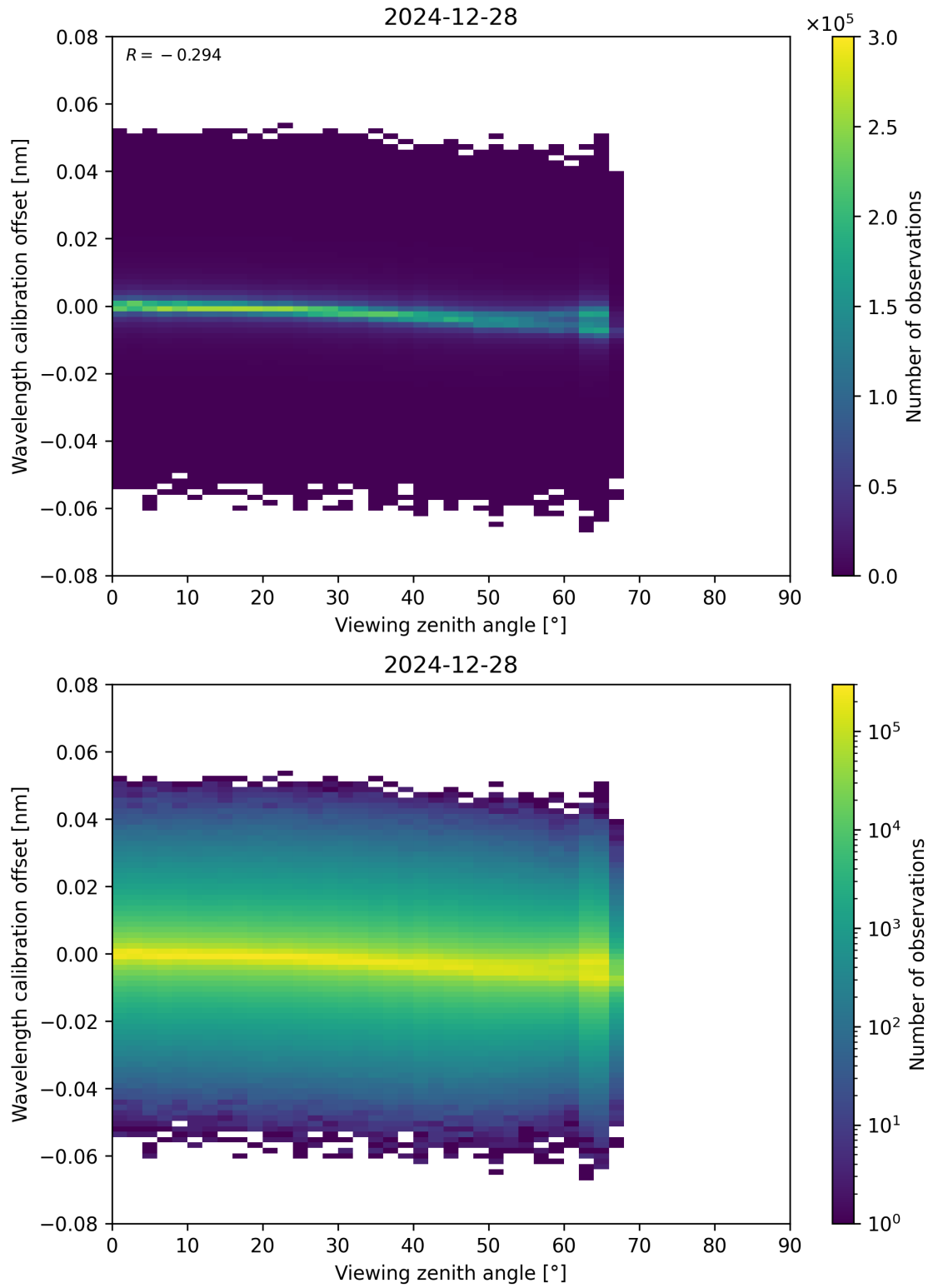
Figure 173: Scatter density plot of “Viewing zenith angle” against “Wavelength calibration offset” for 2024-12-27 to 2024-12-29.
