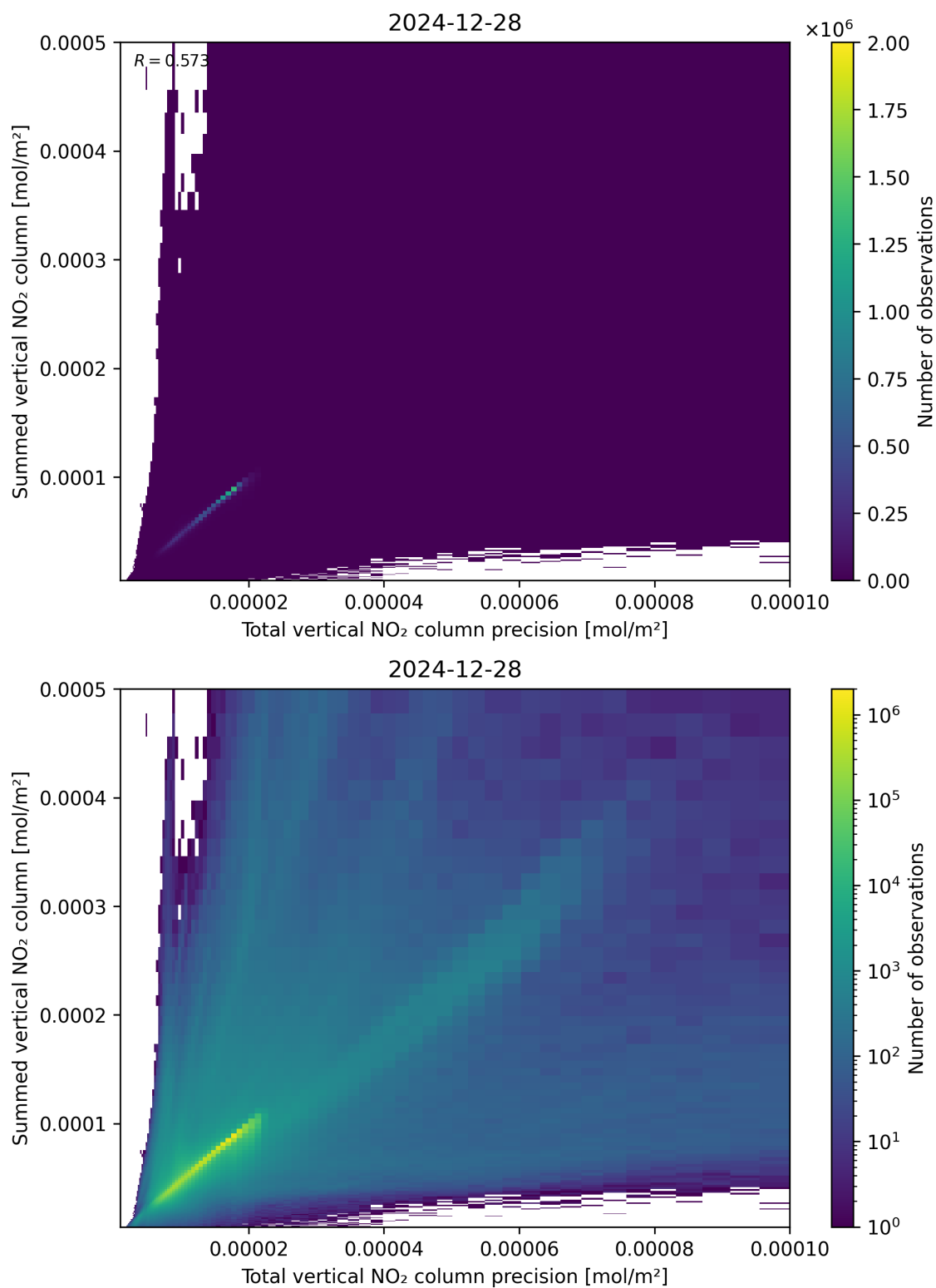
Figure 117: Scatter density plot of “Total vertical NO 2 column precision” against “Summed vertical NO 2 column” for 2024-12-27 to 2024-12-29.
