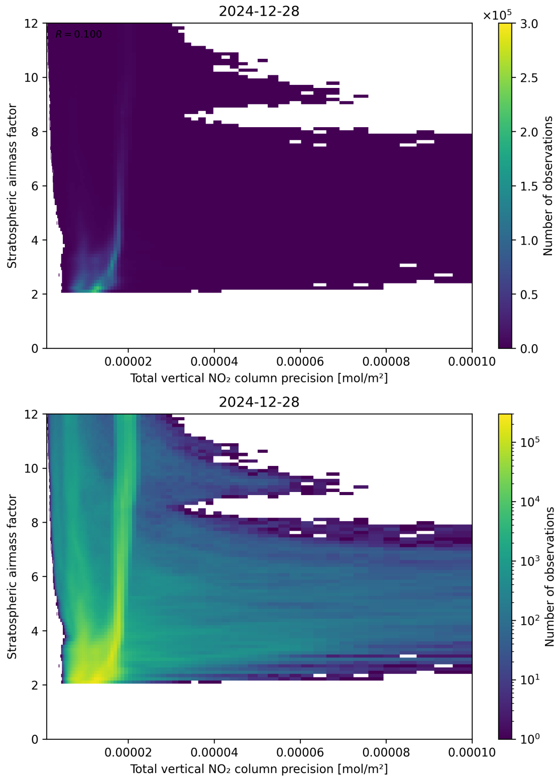
Figure 115: Scatter density plot of “Total vertical NO 2 column precision” against “Stratospheric air mass factor” for 2024-12-27 to 2024-12-29.
