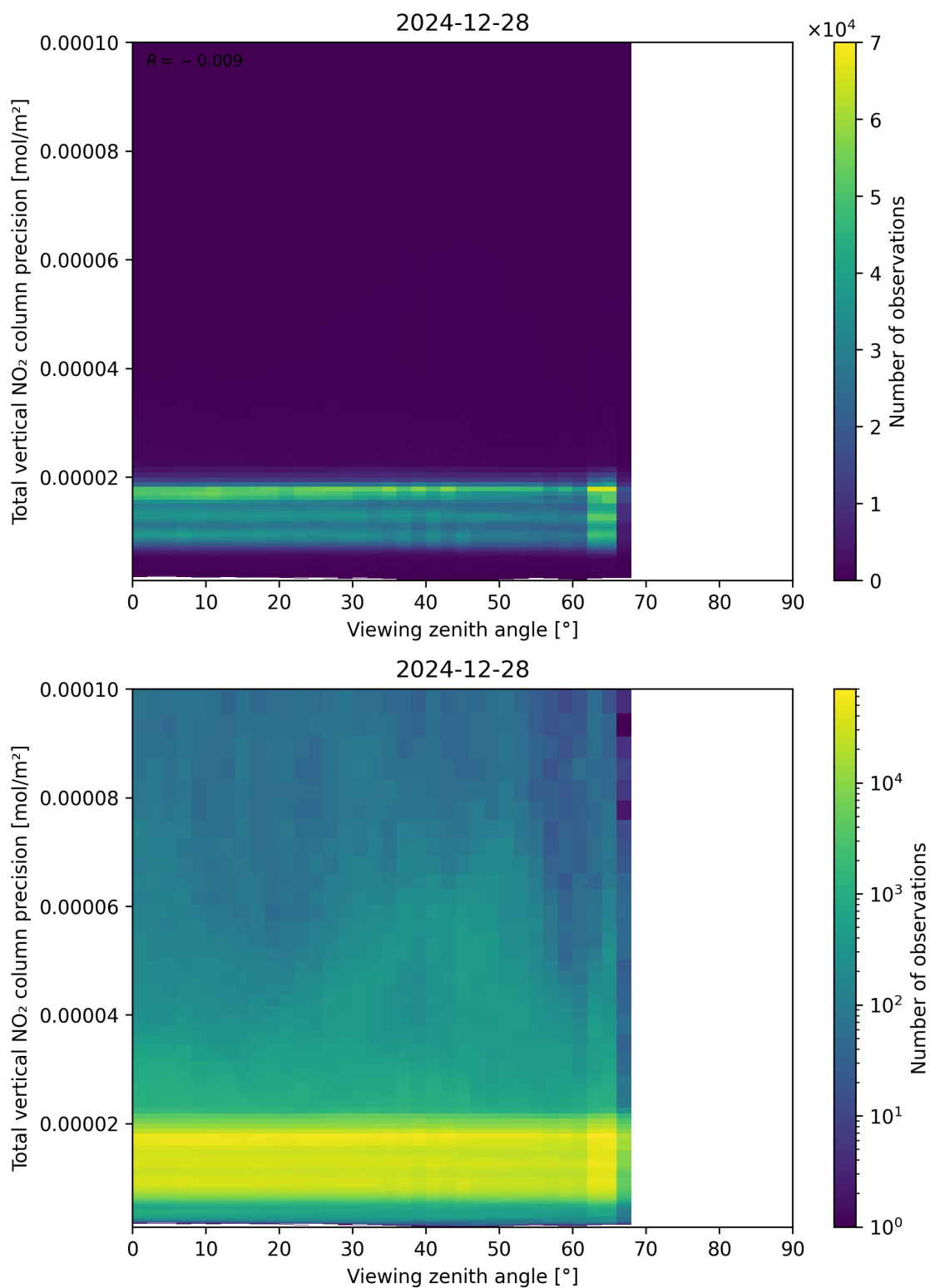
Figure 168: Scatter density plot of “Viewing zenith angle” against “Total vertical NO 2 column precision” for 2024-12-27 to 2024-12-29.
