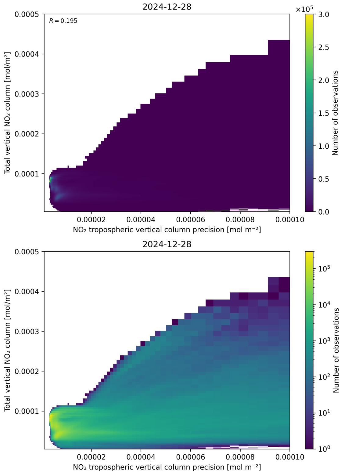
Figure 138: Scatter density plot of “NO 2 tropospheric vertical column precision” against “Total vertical NO 2 column” for 2024-12-27 to 2024-12-29.
