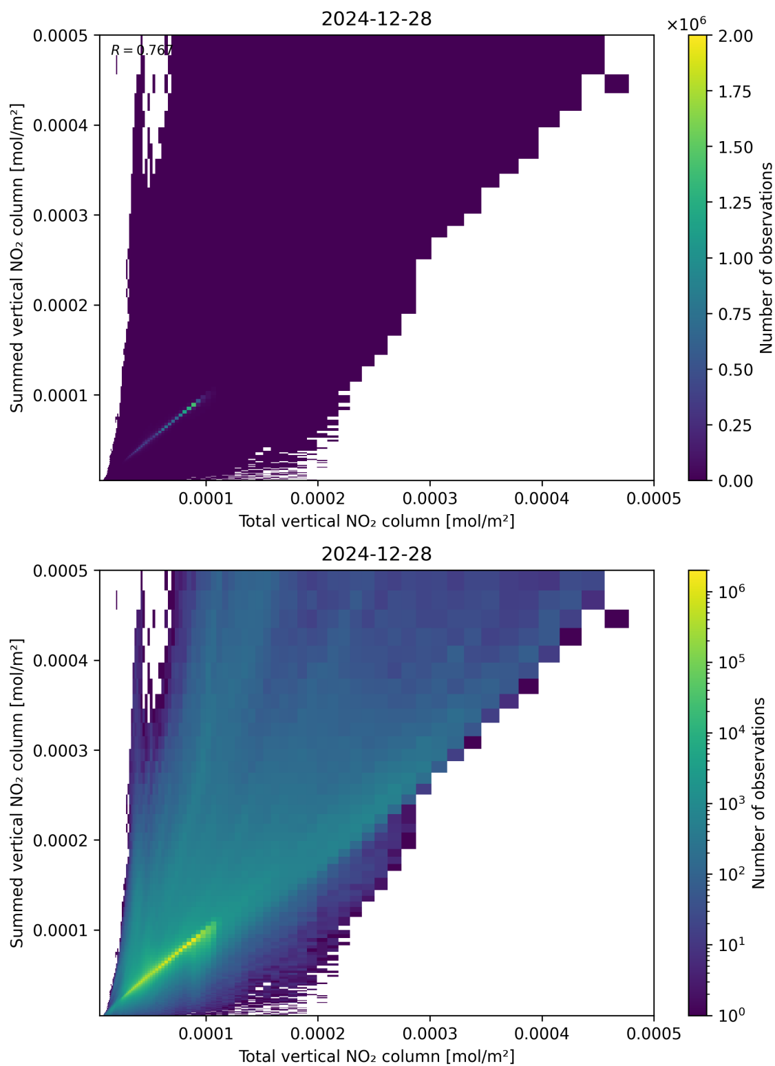
Figure 112: Scatter density plot of “Total vertical NO 2 column” against “Summed vertical NO 2 column” for 2024-12-27 to 2024-12-29.
