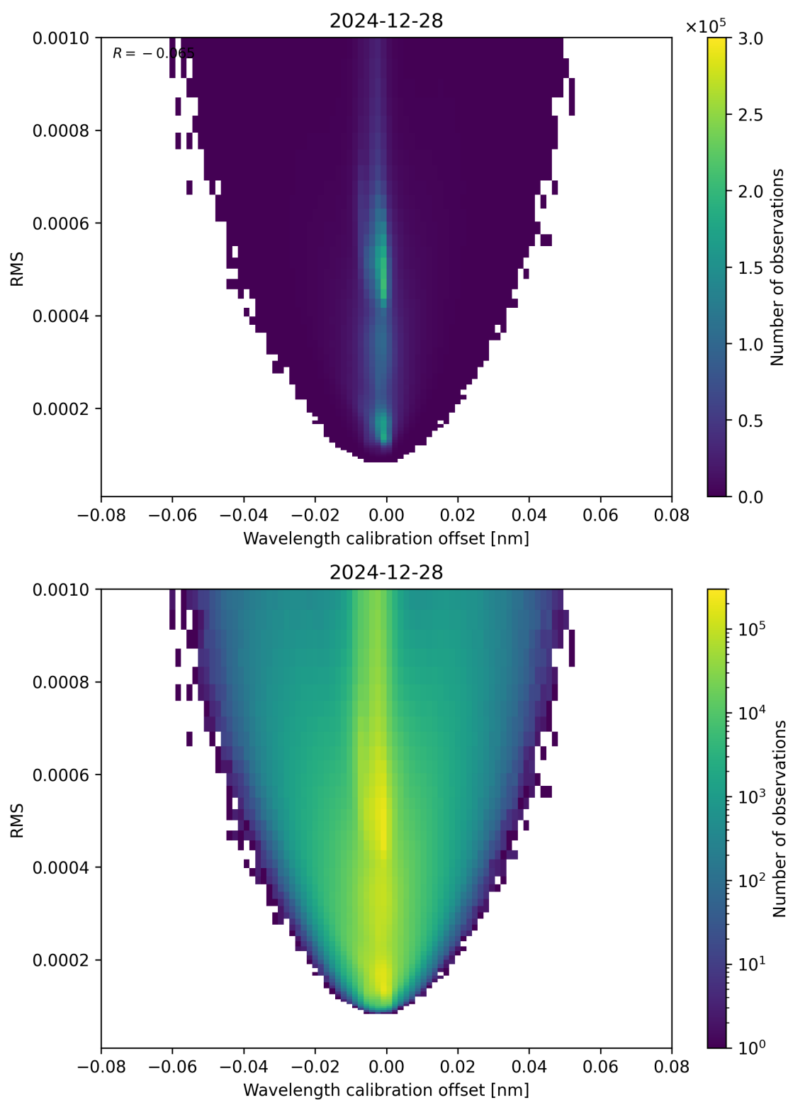
Figure 181: Scatter density plot of “Wavelength calibration offset” against “RMS” for 2024-12-27 to 2024-12-29.
