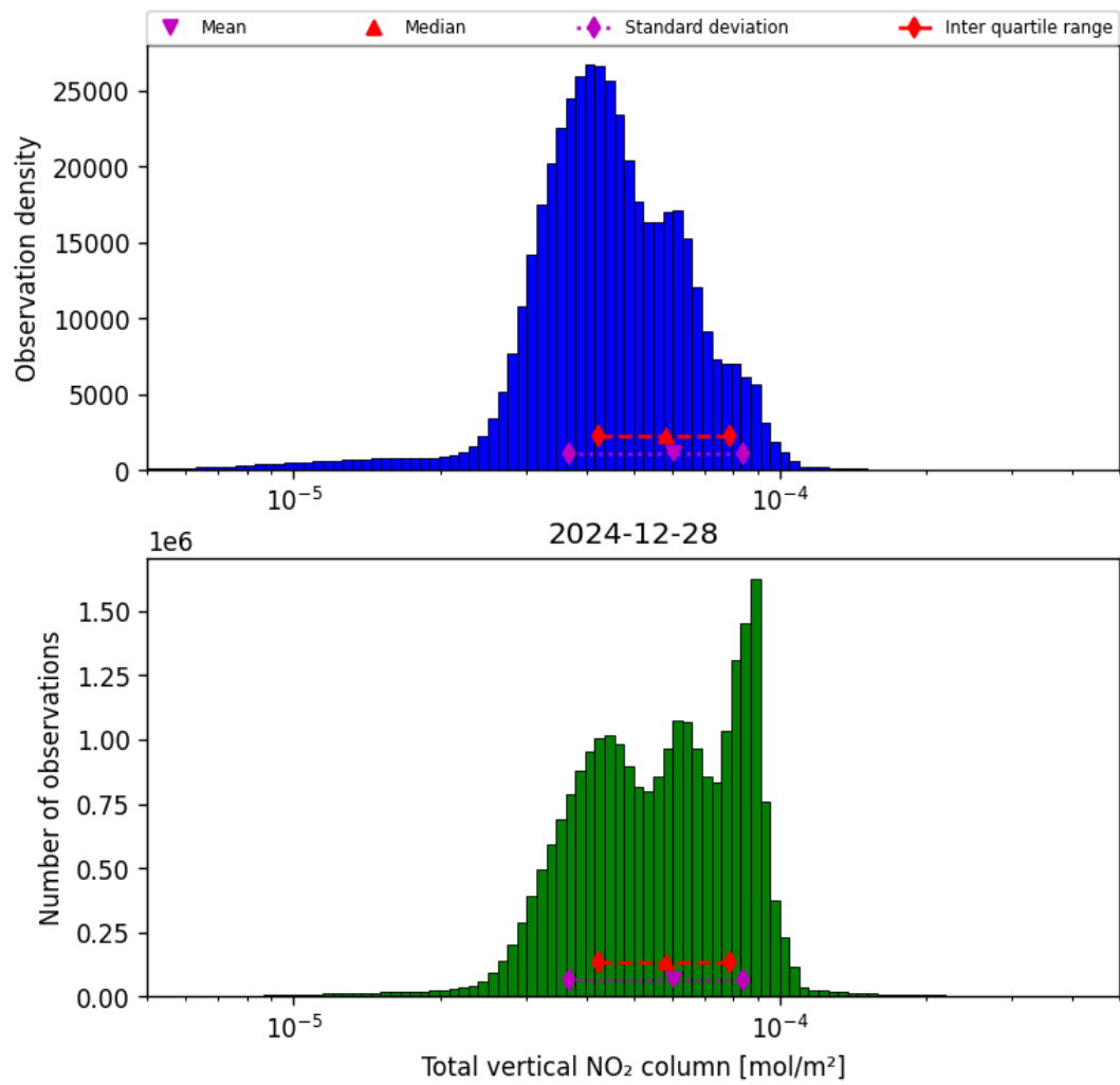
Figure 38: Histogram of “Total vertical NO 2 column” for 2024-12-27 to 2024-12-29
