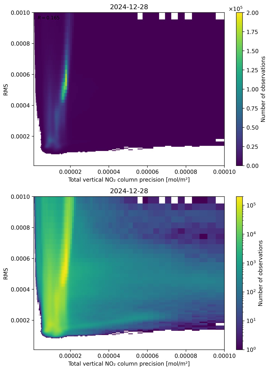
Figure 119: Scatter density plot of “Total vertical NO 2 column precision” against “RMS” for 2024-12-27 to 2024-12-29.
