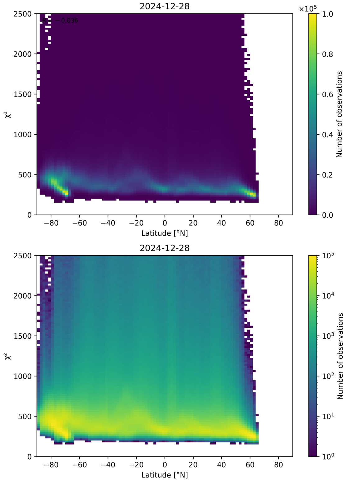
Figure 86: Scatter density plot of “Latitude” against “ \chi^2 ” for 2024-12-27 to 2024-12-29.
