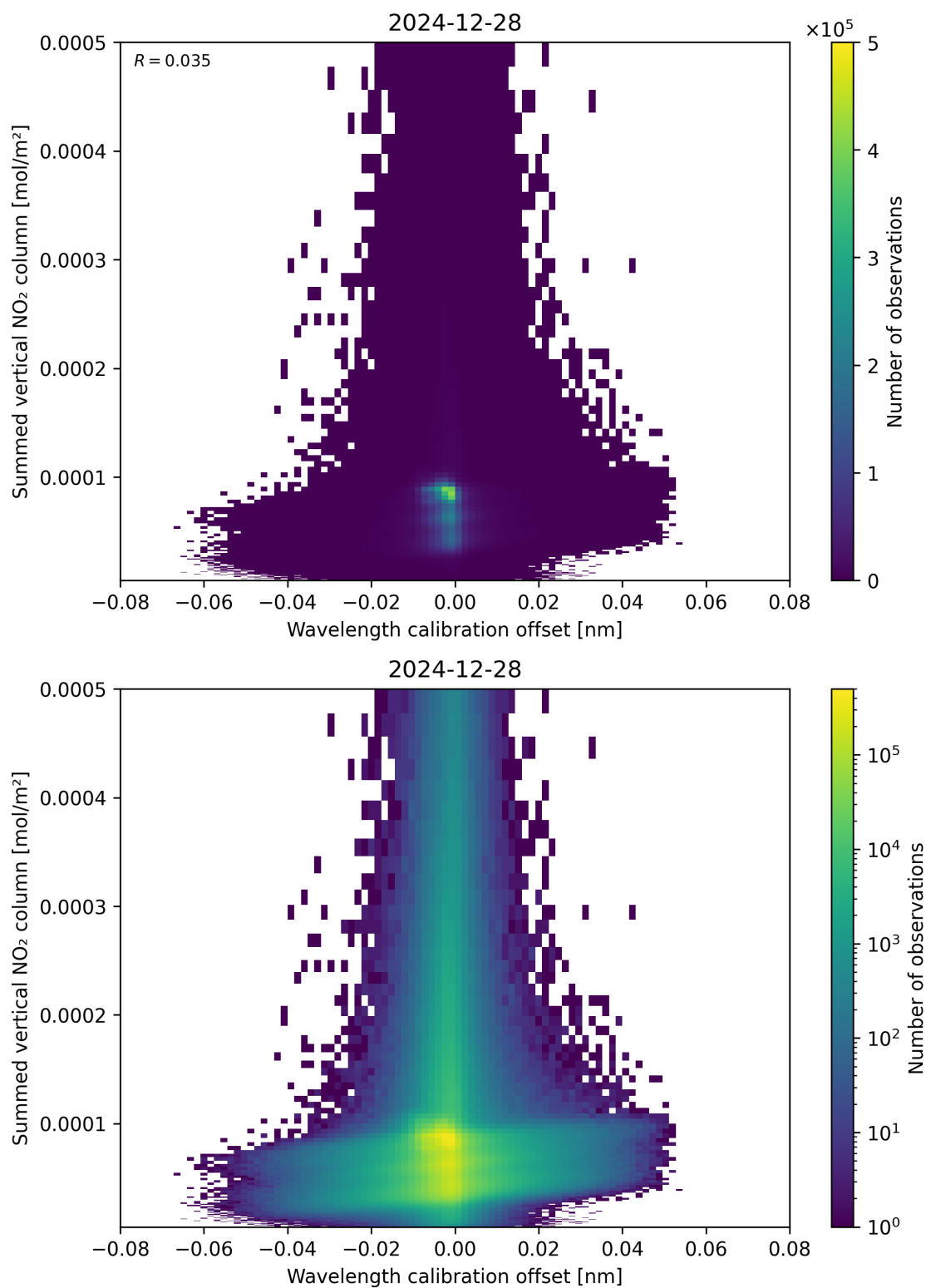
Figure 177: Scatter density plot of “Wavelength calibration offset” against “Summed vertical NO 2 column” for 2024-12-27 to 2024-12-29.
