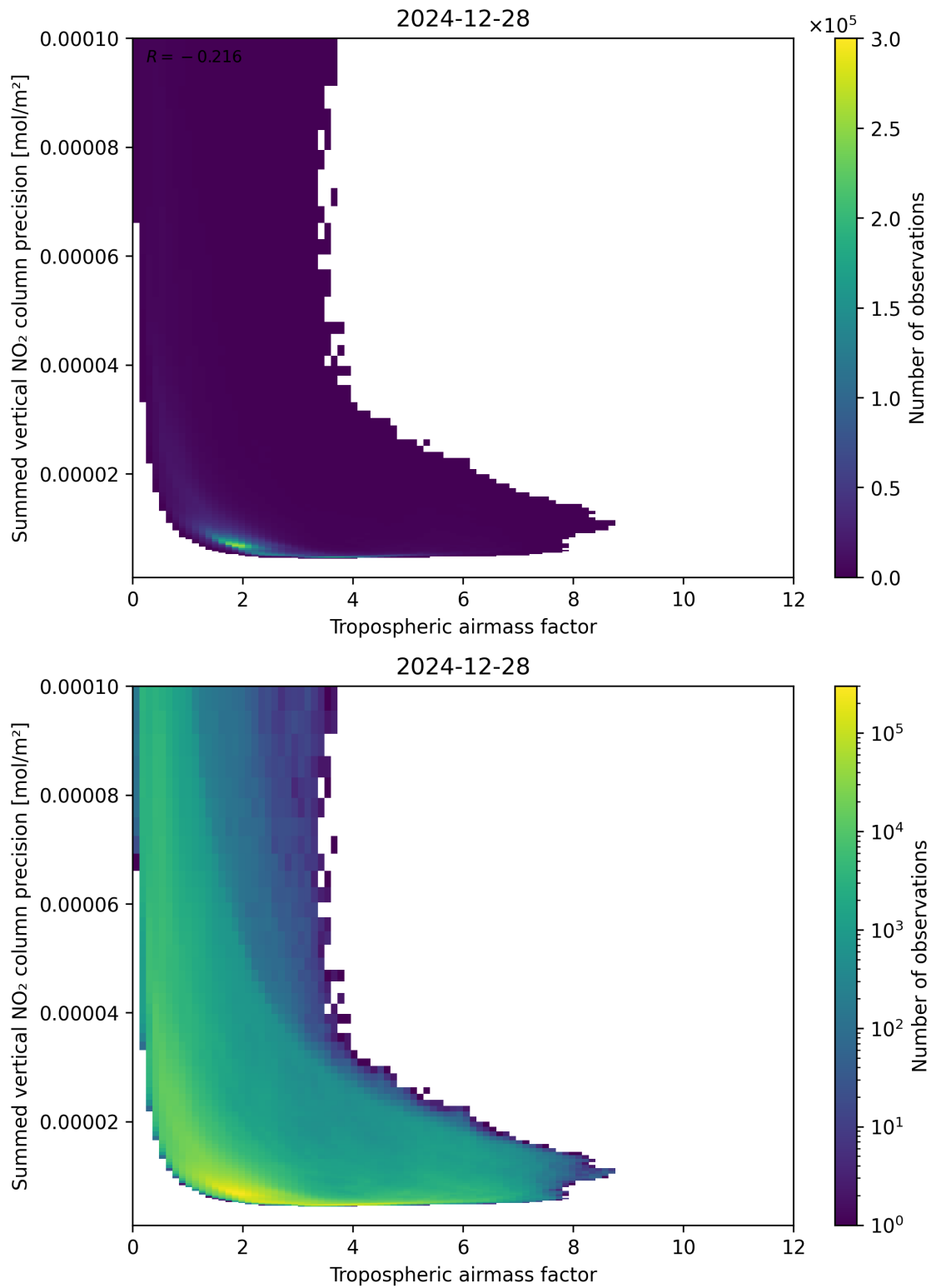
Figure 76: Scatter density plot of “Tropospheric air mass factor” against “Summed vertical NO 2 column precision” for 2024-12-27 to 2024-12-29.
