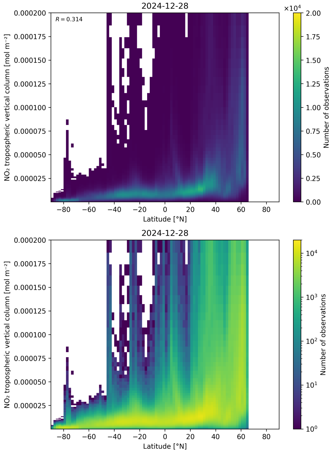
Figure 92: Scatter density plot of “Latitude” against “NO 2 tropospheric vertical column” for 2024-12-27 to 2024-12-29.
