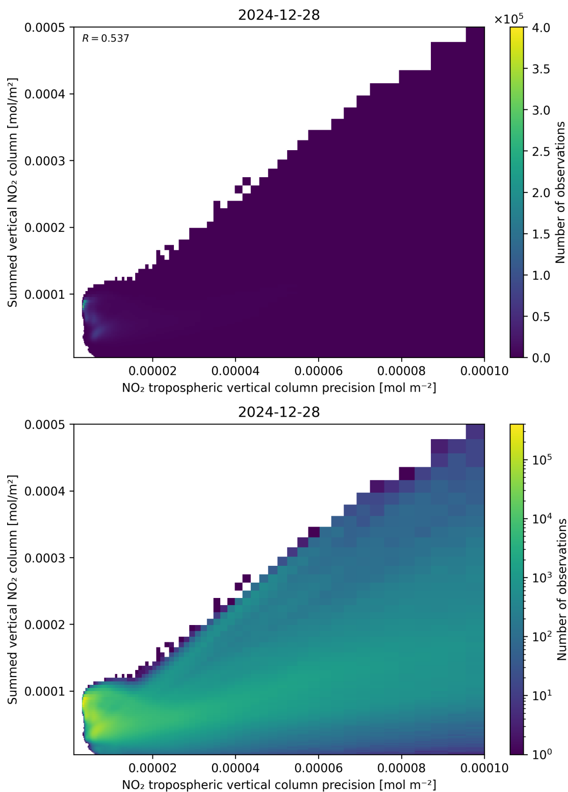
Figure 136: Scatter density plot of “NO 2 tropospheric vertical column precision” against “Summed vertical NO 2 column” for 2024-12-27 to 2024-12-29.
