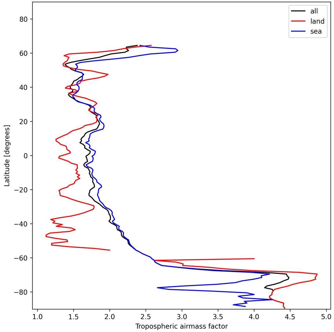
Figure 14: Zonal average of “Tropospheric airmass factor” for 2024-12-27 to 2024-12-29.
