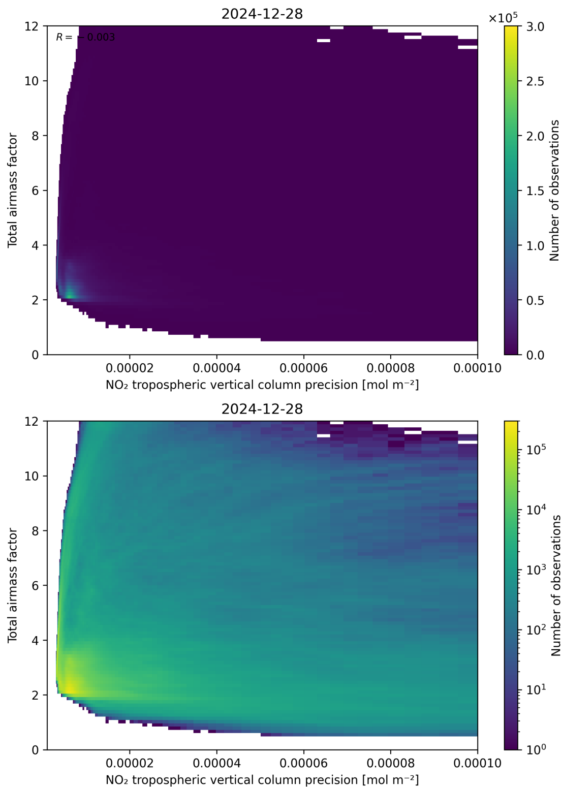
Figure 132: Scatter density plot of “NO 2 tropospheric vertical column precision” against “Total airmass factor” for 2024-12-27 to 2024-12-29.
