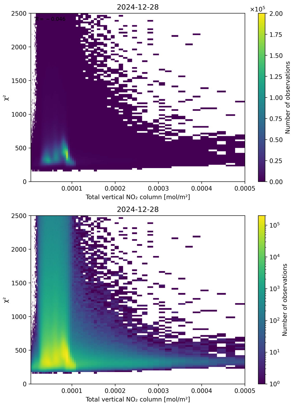
Figure 111: Scatter density plot of “Total vertical NO 2 column” against “ \chi^2 ” for 2024-12-27 to 2024-12-29.
