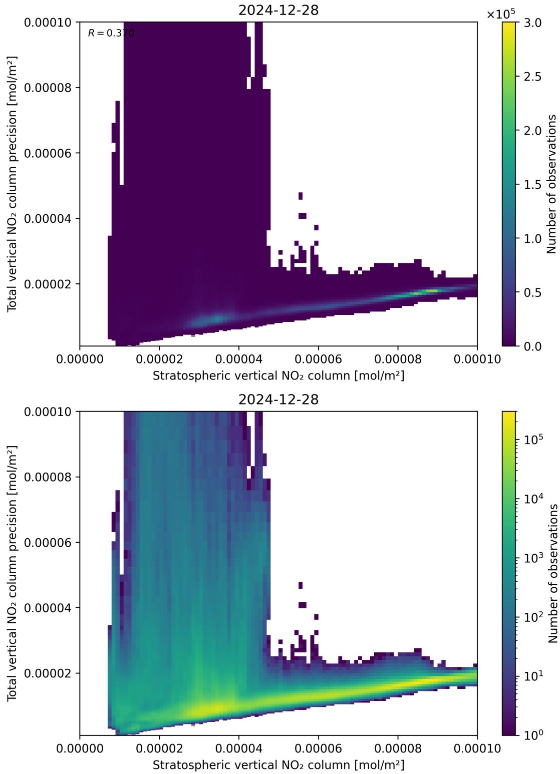
Figure 101: Scatter density plot of “Stratospheric vertical NO 2 column” against “Total vertical NO 2 column precision” for 2024-12-27 to 2024-12-29.
