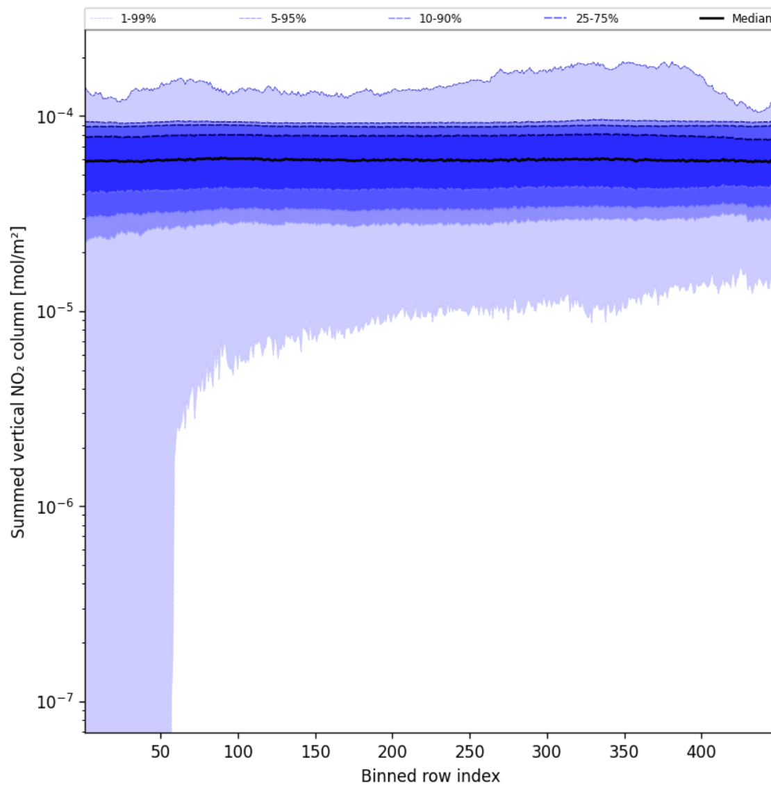
Figure 57: Along track statistics of “Summed vertical NO 2 column” for 2024-12-27 to 2024-12-29
