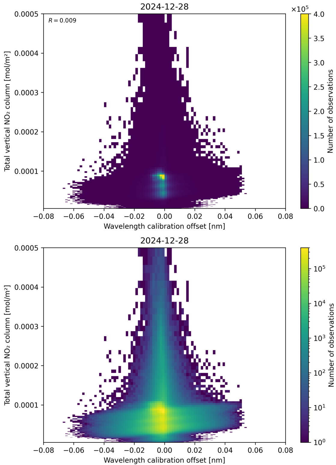
Figure 179: Scatter density plot of “Wavelength calibration offset” against “Total vertical NO 2 column” for 2024-12-27 to 2024-12-29.
