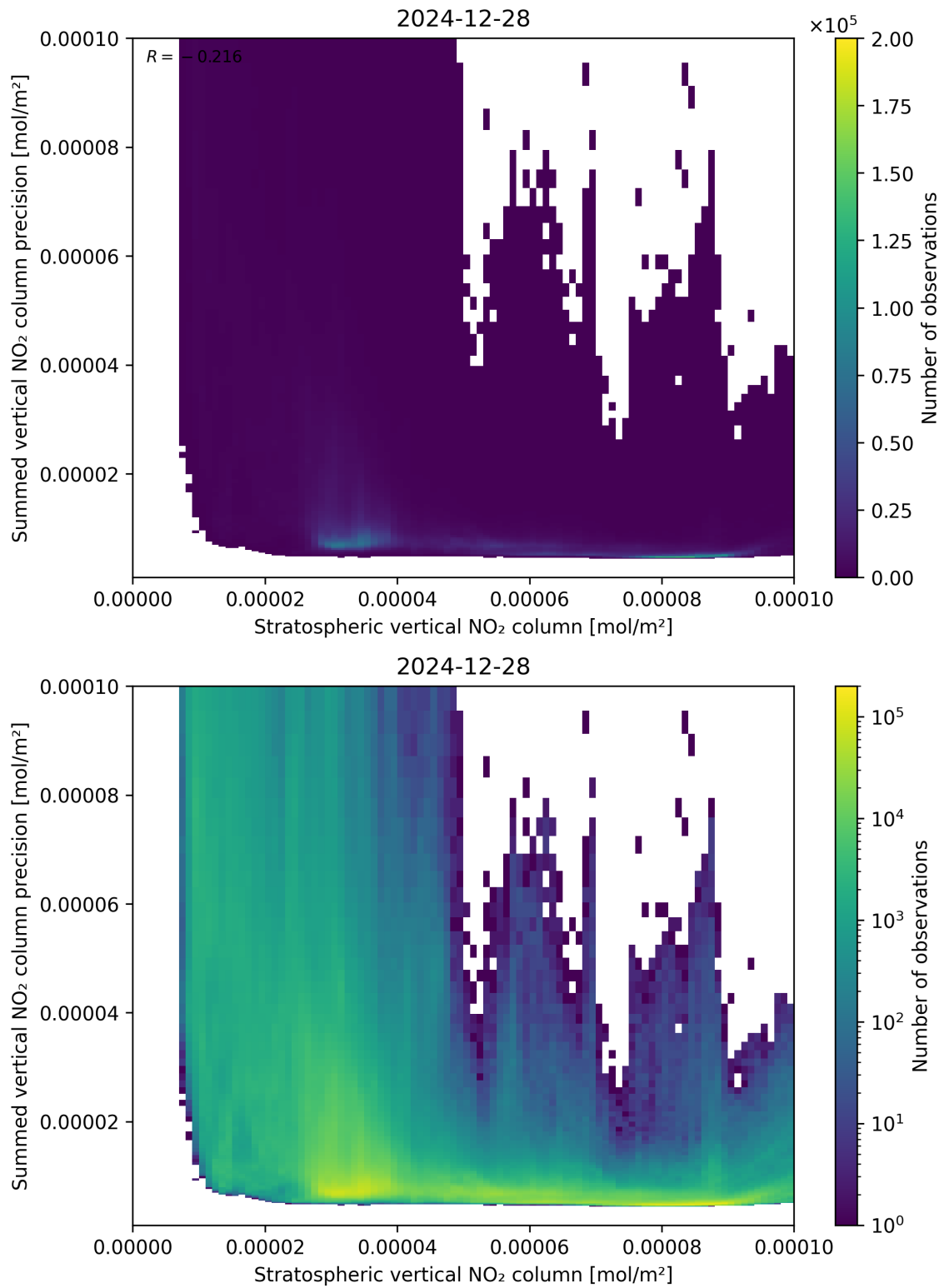
Figure 99: Scatter density plot of “Stratospheric vertical NO 2 column” against “Summed vertical NO 2 column precision” for 2024-12-27 to 2024-12-29.
