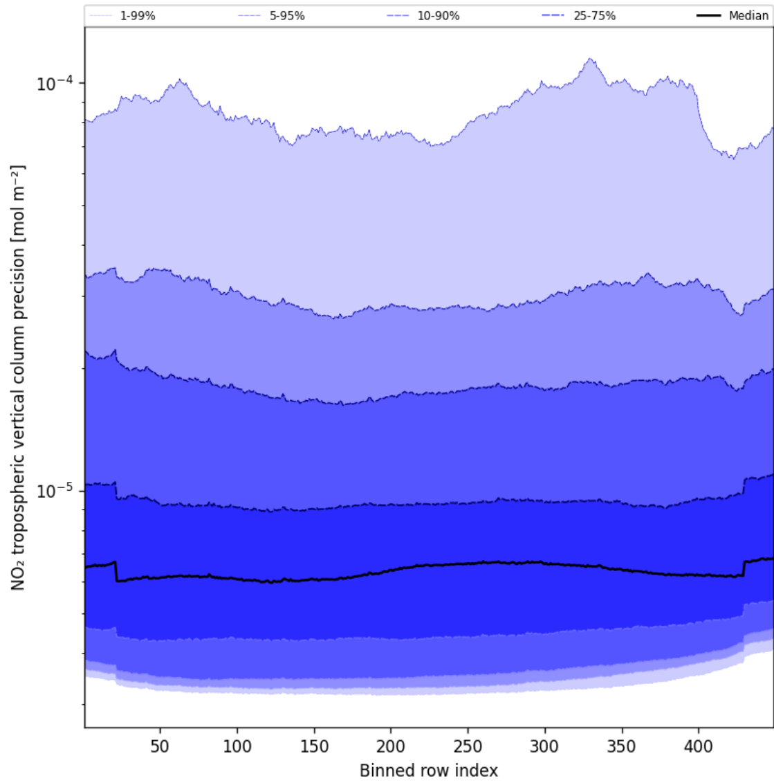
Figure 47: Along track statistics of “NO 2 tropospheric vertical column precision” for 2024-12-27 to 2024-12-29
