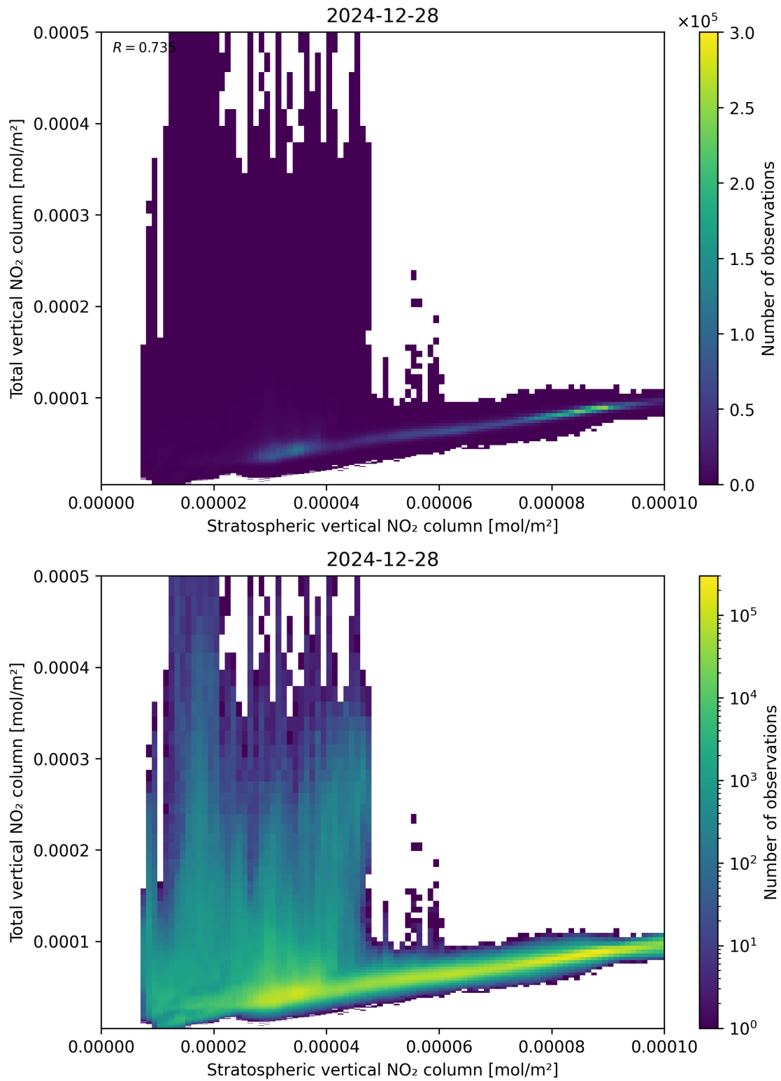
Figure 100: Scatter density plot of “Stratospheric vertical NO 2 column” against “Total vertical NO 2 column” for 2024-12-27 to 2024-12-29.
