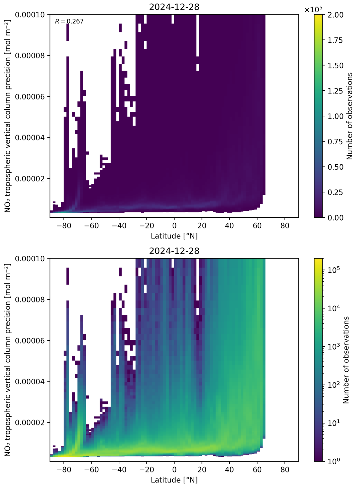
Figure 93: Scatter density plot of “Latitude” against “NO 2 tropospheric vertical column precision” for 2024-12-27 to 2024-12-29.
