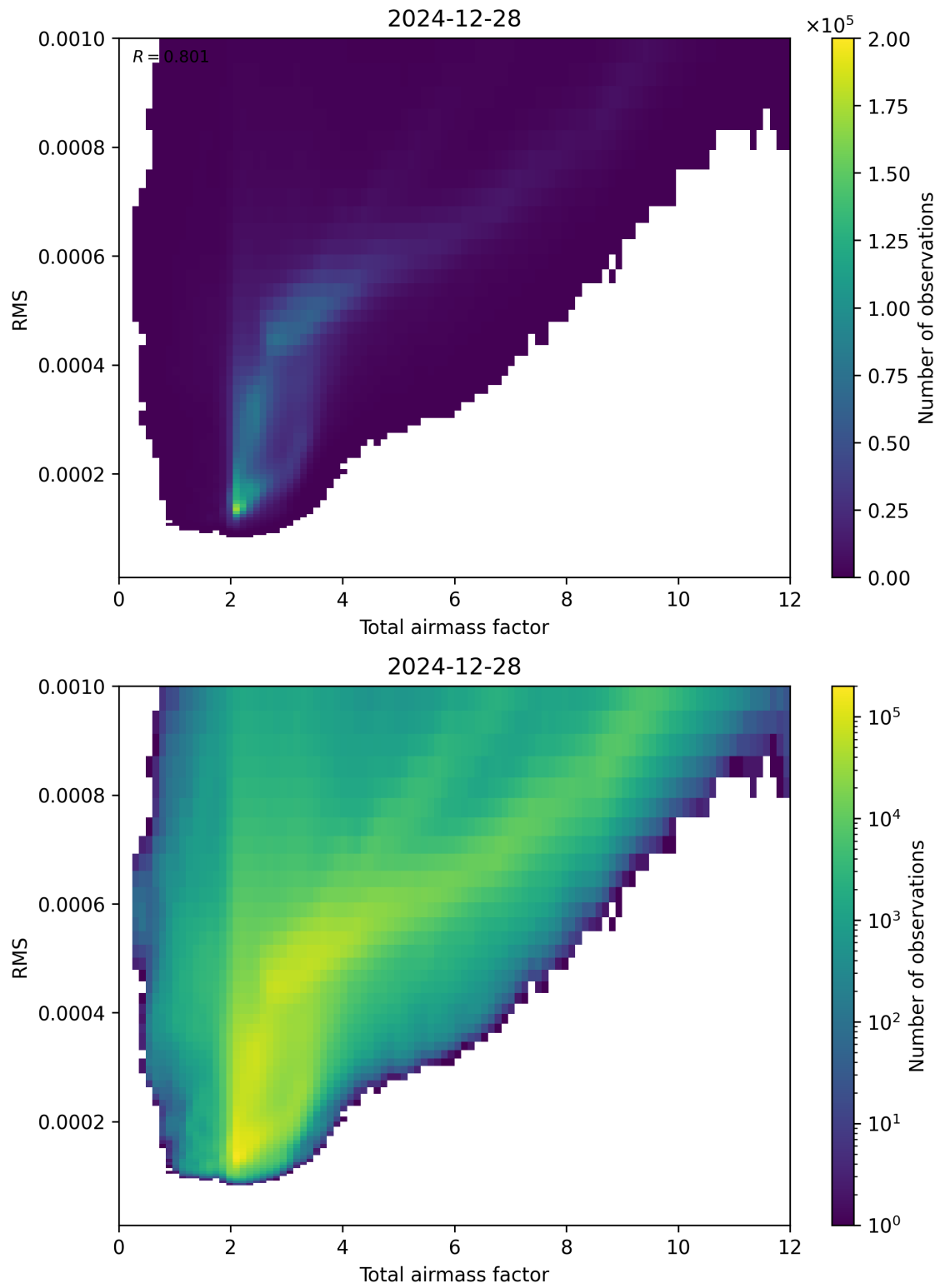
Figure 69: Scatter density plot of “Total airmass factor” against “RMS” for 2024-12-27 to 2024-12-29.
