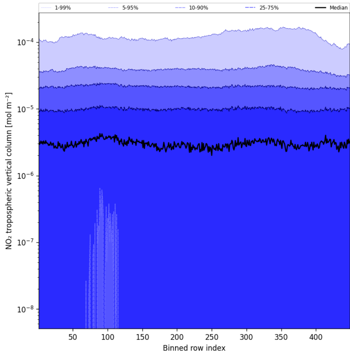
Figure 46: Along track statistics of “NO 2 tropospheric vertical column” for 2024-12-27 to 2024-12-29
