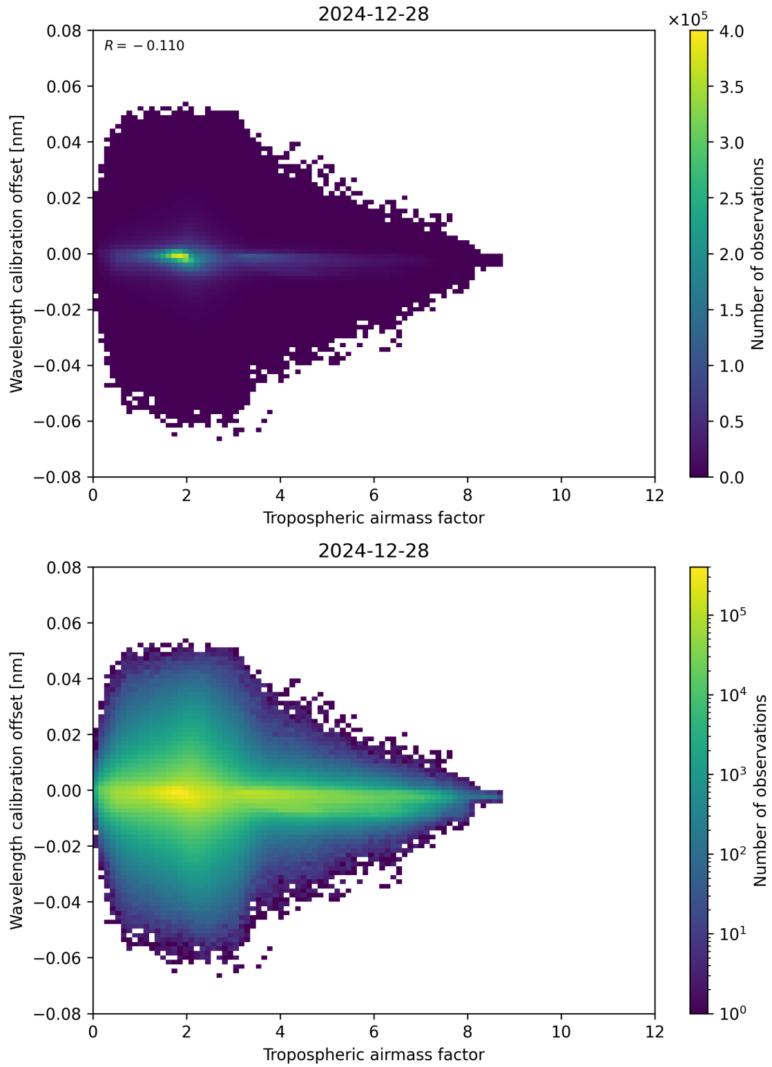
Figure 80: Scatter density plot of “Tropospheric airmass factor” against “Wavelength calibration offset” for 2024-12-27 to 2024-12-29.
