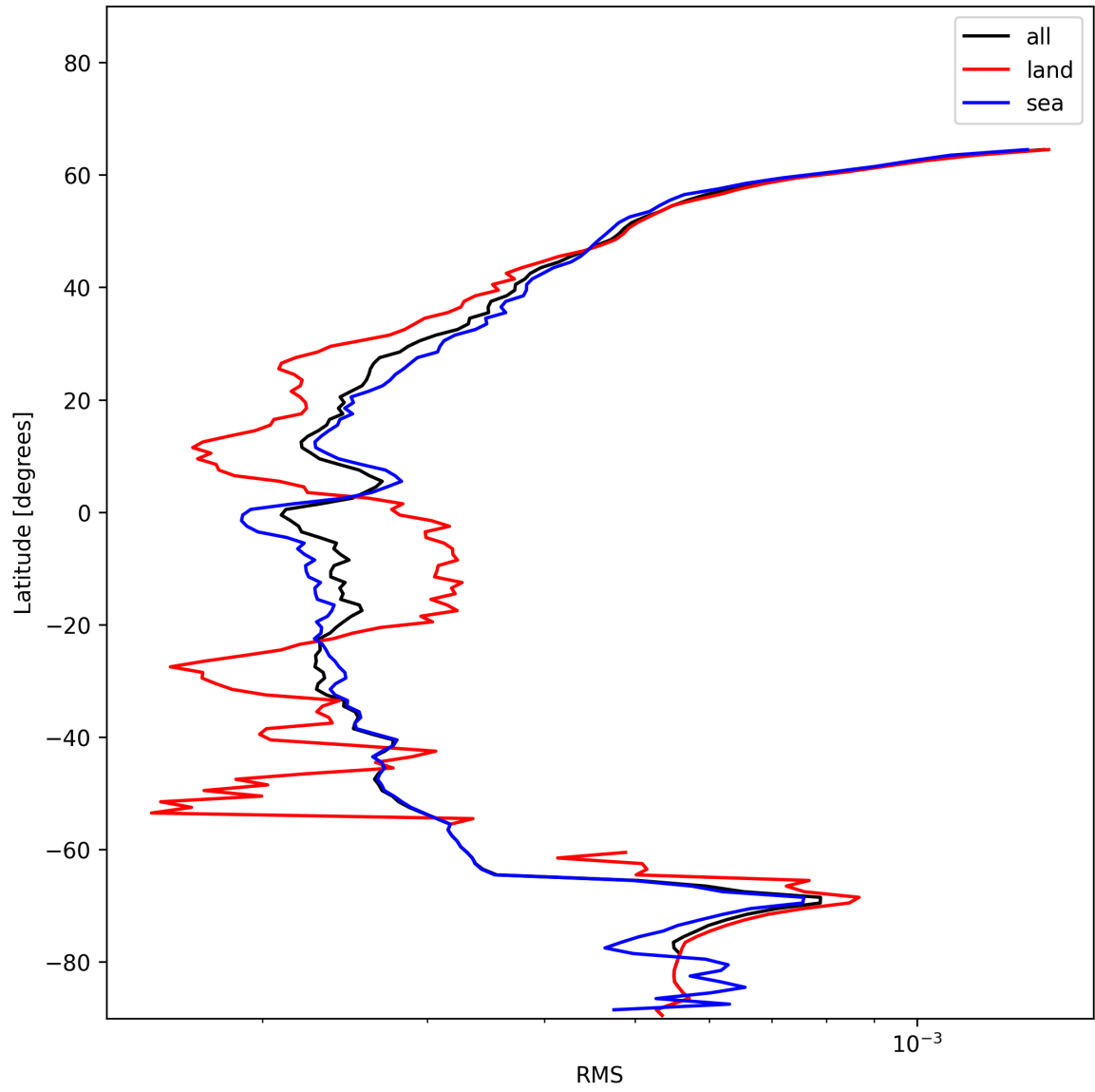
Figure 26: Zonal average of “RMS” for 2024-12-27 to 2024-12-29.
