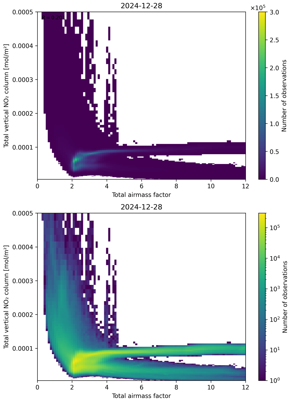
Figure 67: Scatter density plot of “Total airmass factor” against “Total vertical NO 2 column” for 2024-12-27 to 2024-12-29.
