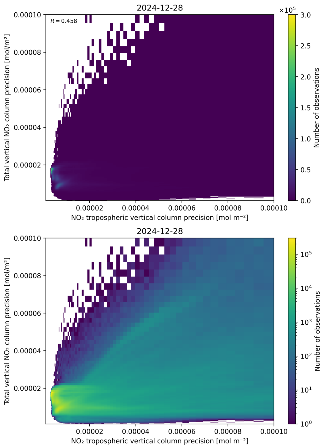
Figure 139: Scatter density plot of “NO 2 tropospheric vertical column precision” against “Total vertical NO 2 column precision” for 2024-12-27 to 2024-12-29.
