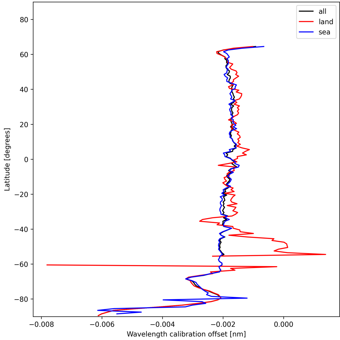
Figure 18: Zonal average of “Wavelength calibration offset” for 2024-12-27 to 2024-12-29.
