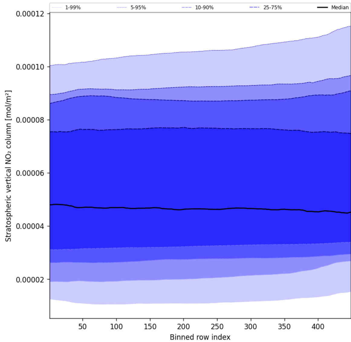
Figure 53: Along track statistics of “Stratospheric vertical NO 2 column” for 2024-12-27 to 2024-12-29
