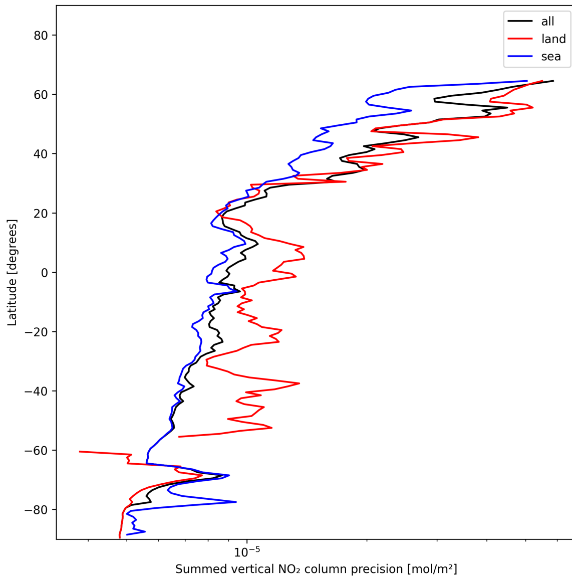
Figure 24: Zonal average of “Summed vertical NO 2 column precision” for 2024-12-27 to 2024-12-29.
