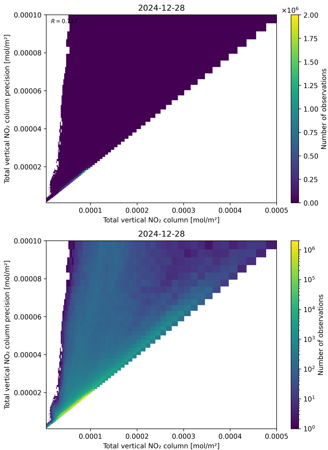
Figure 114: Scatter density plot of “Total vertical NO 2 column” against “Total vertical NO 2 column precision” for 2024-12-27 to 2024-12-29.
