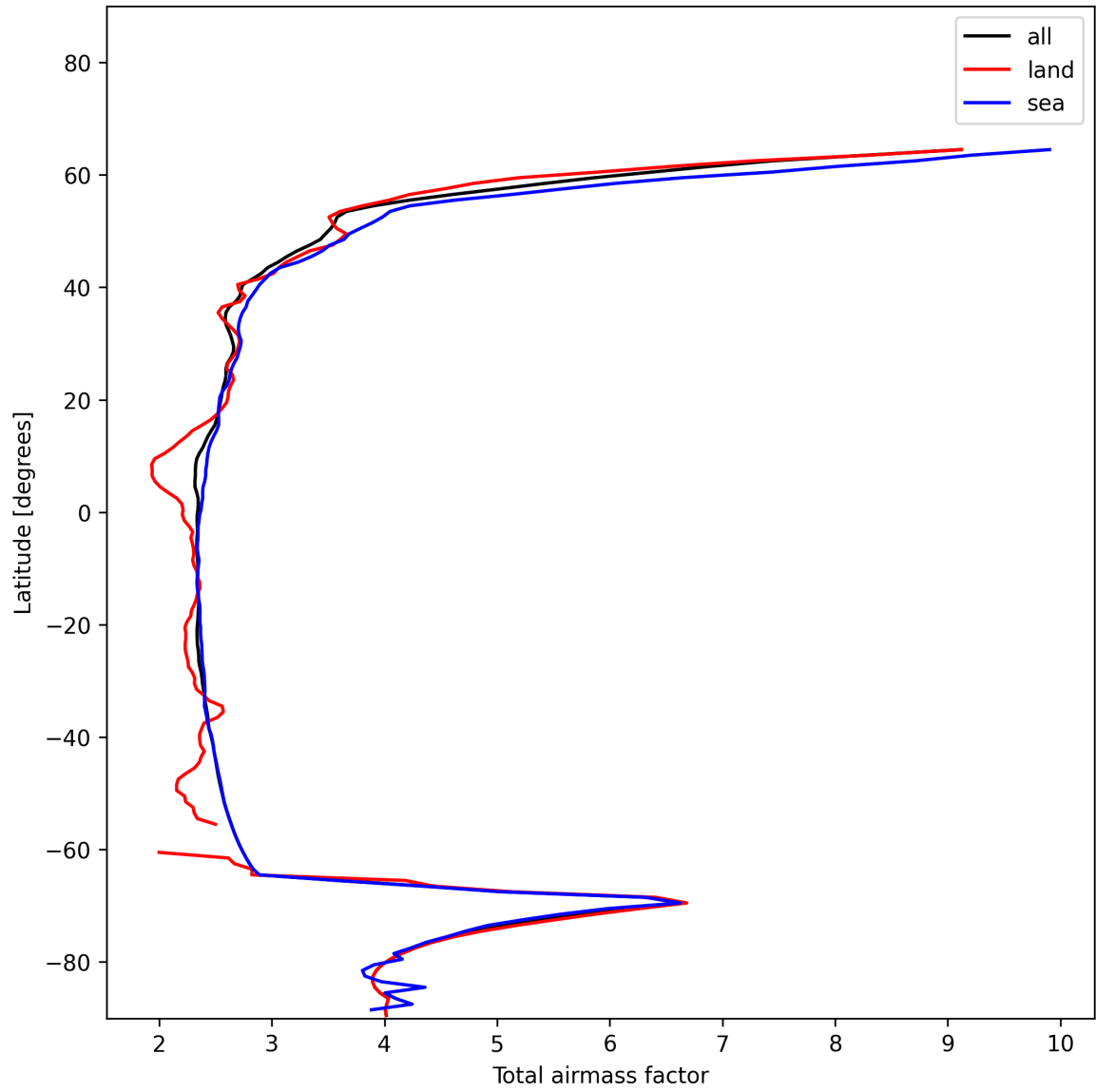
Figure 15: Zonal average of “Total airmass factor” for 2024-12-27 to 2024-12-29.
