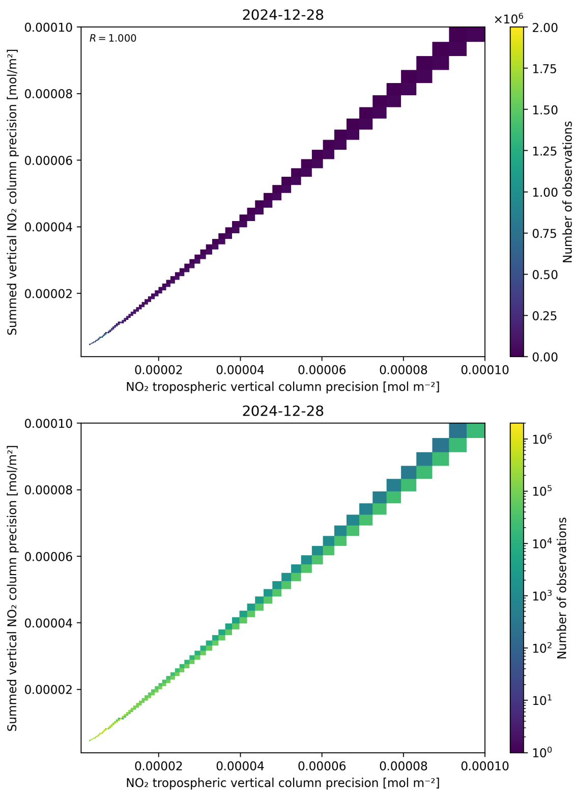
Figure 137: Scatter density plot of “NO 2 tropospheric vertical column precision” against “Summed vertical NO 2 column precision” for 2024-12-27 to 2024-12-29.
