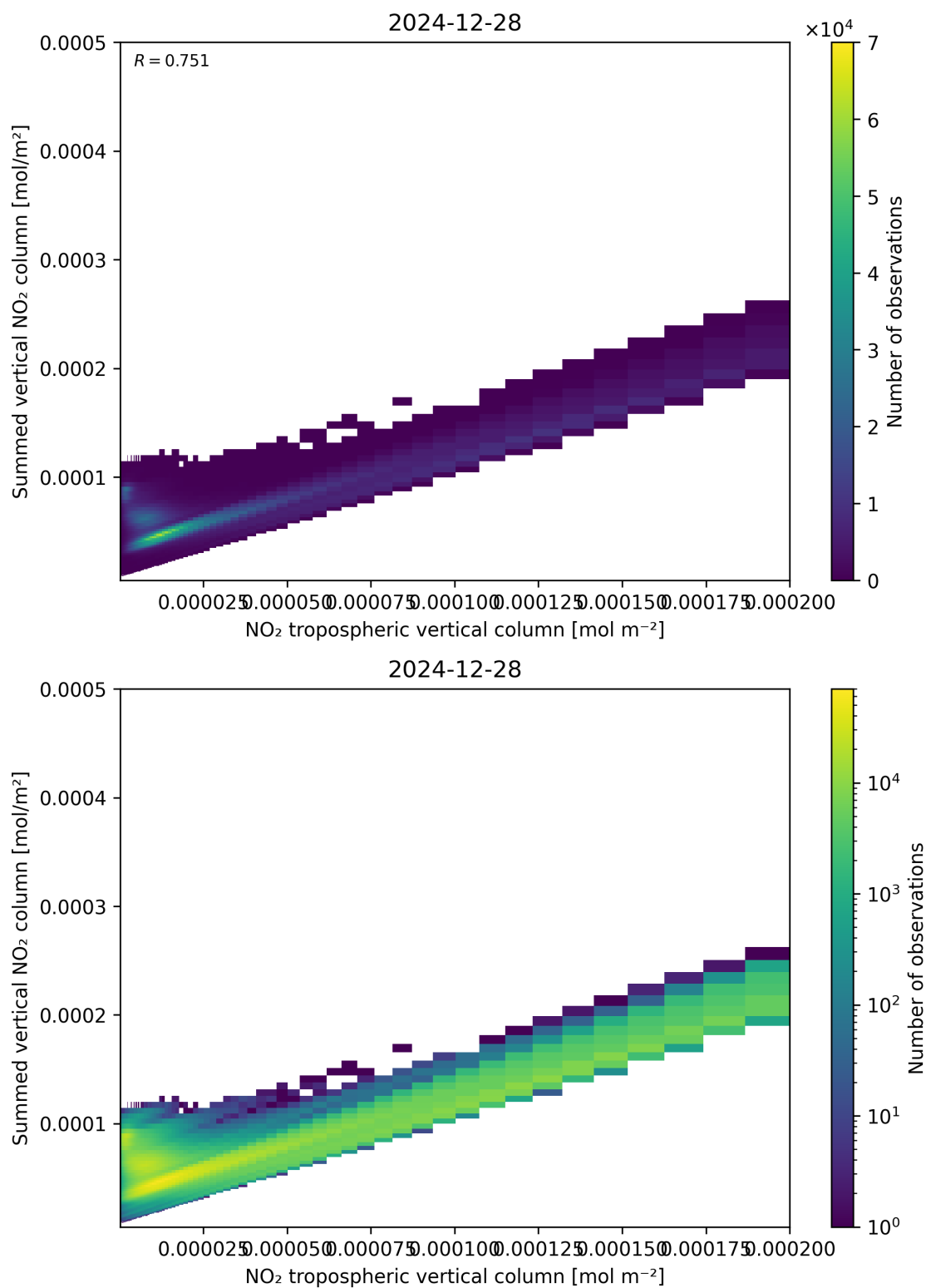
Figure 126: Scatter density plot of “NO 2 tropospheric vertical column” against “Summed vertical NO 2 column” for 2024-12-27 to 2024-12-29.
