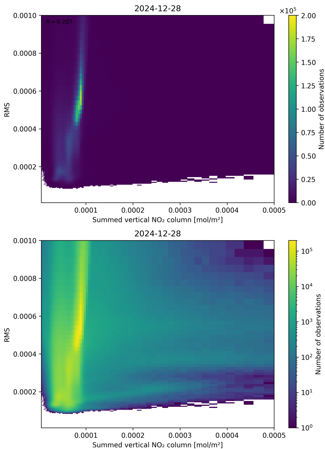
Figure 109: Scatter density plot of “Summed vertical NO 2 column” against “RMS” for 2024-12-27 to 2024-12-29.
