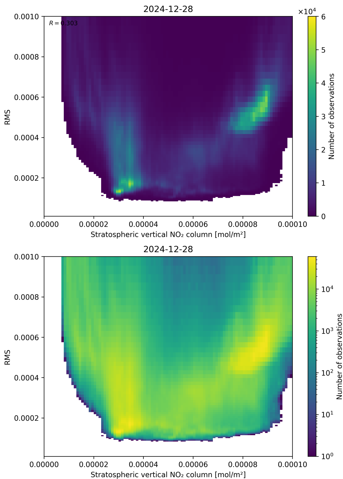
Figure 102: Scatter density plot of “Stratospheric vertical NO 2 column” against “RMS” for 2024-12-27 to 2024-12-29.
