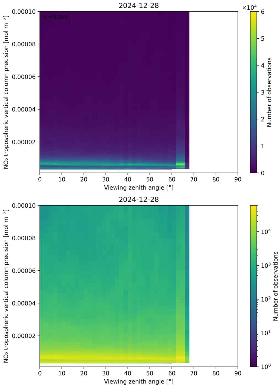
Figure 170: Scatter density plot of “Viewing zenith angle” against “NO 2 tropospheric vertical column precision” for 2024-12-27 to 2024-12-29.
