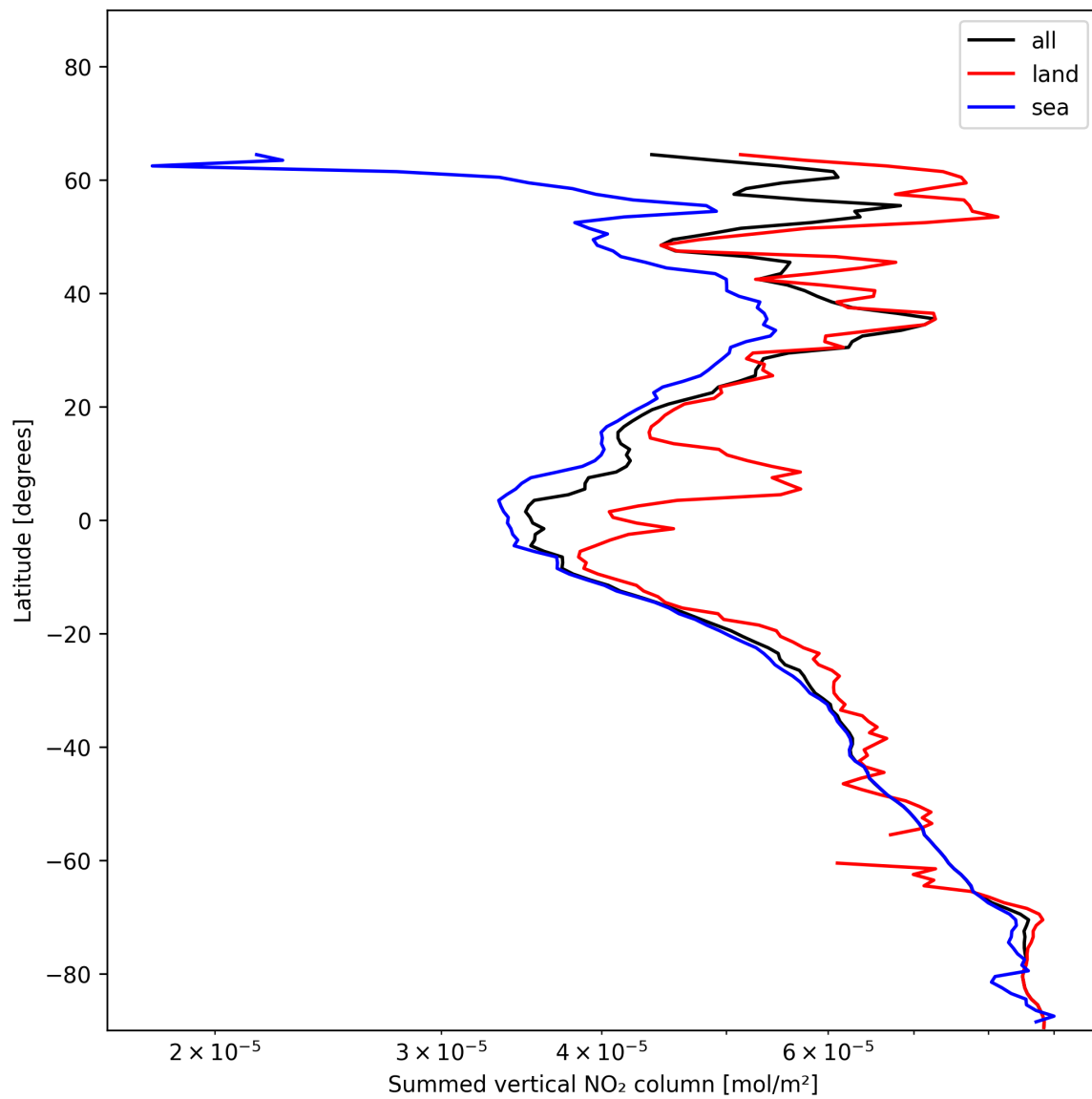
Figure 23: Zonal average of “Summed vertical NO 2 column” for 2024-12-27 to 2024-12-29.
