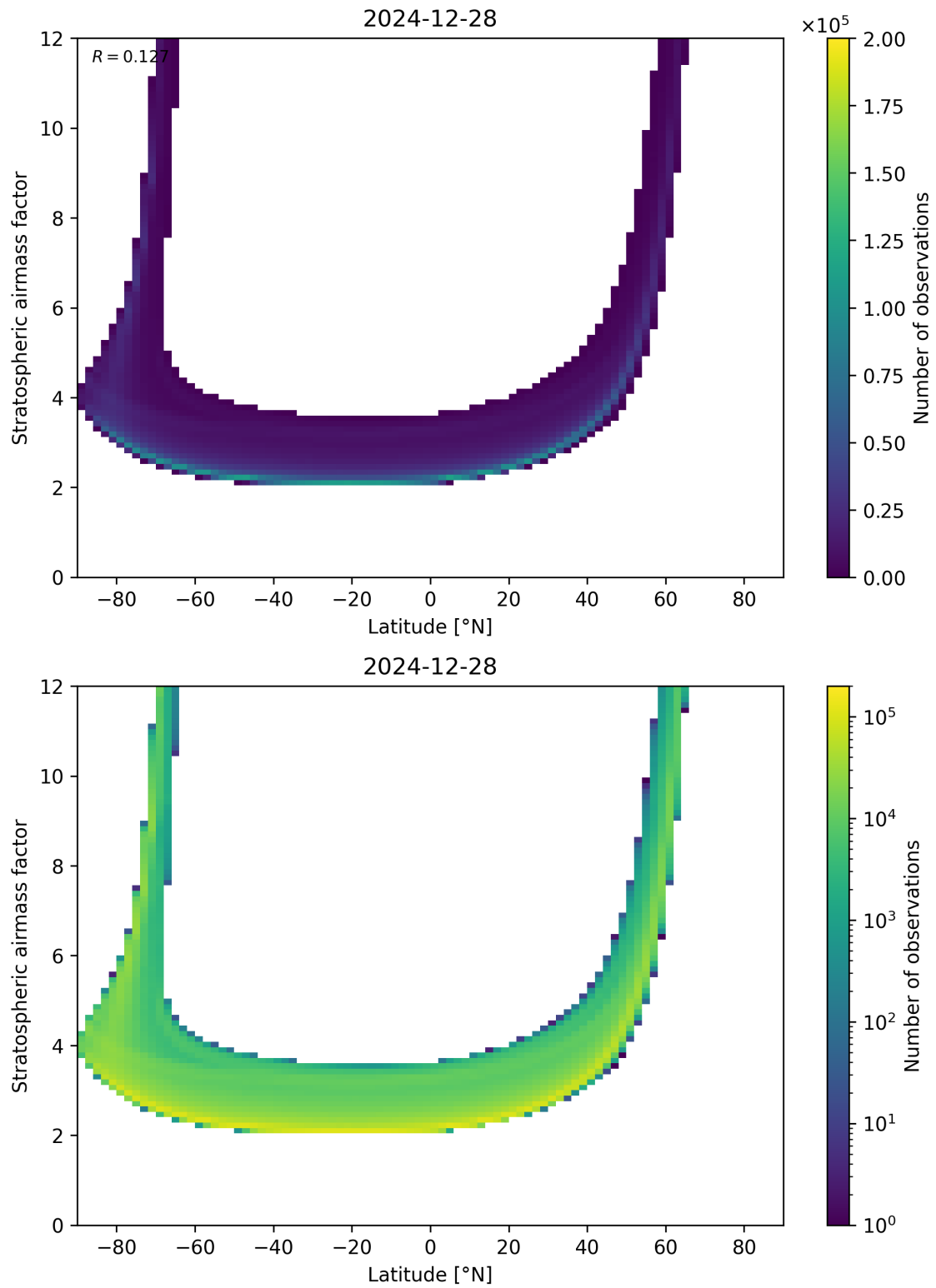
Figure 83: Scatter density plot of “Latitude” against “Stratospheric air mass factor” for 2024-12-27 to 2024-12-29.
