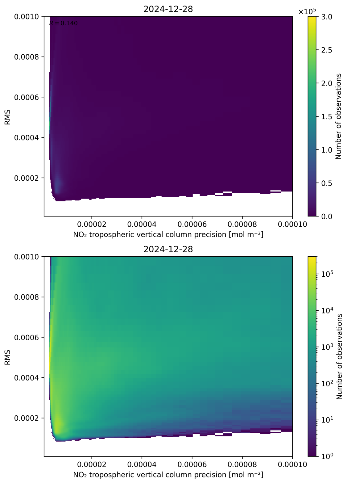
Figure 140: Scatter density plot of “NO 2 tropospheric vertical column precision” against “RMS” for 2024-12-27 to 2024-12-29.
