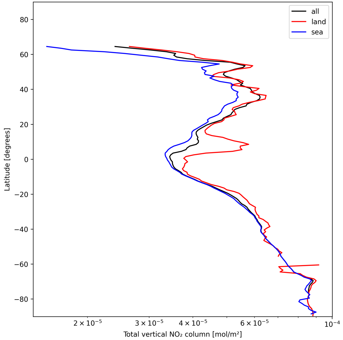
Figure 21: Zonal average of “Total vertical NO 2 column” for 2024-12-27 to 2024-12-29.
