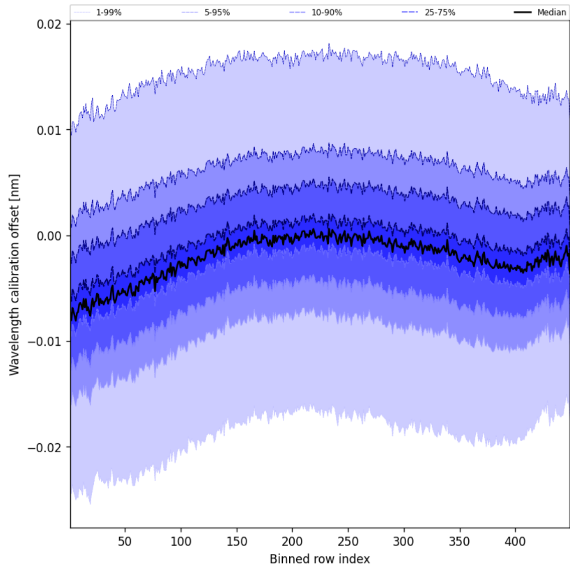
Figure 52: Along track statistics of “Wavelength calibration offset” for 2024-12-27 to 2024-12-29
