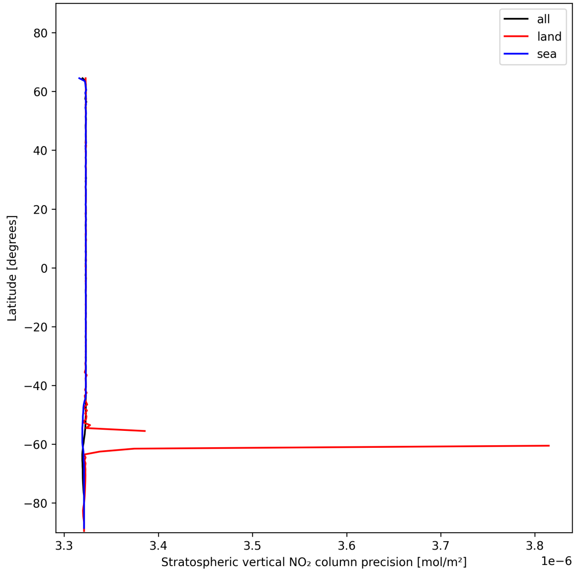
Figure 20: Zonal average of “Stratospheric vertical NO 2 column precision” for 2024-12-27 to 2024-12-29.
