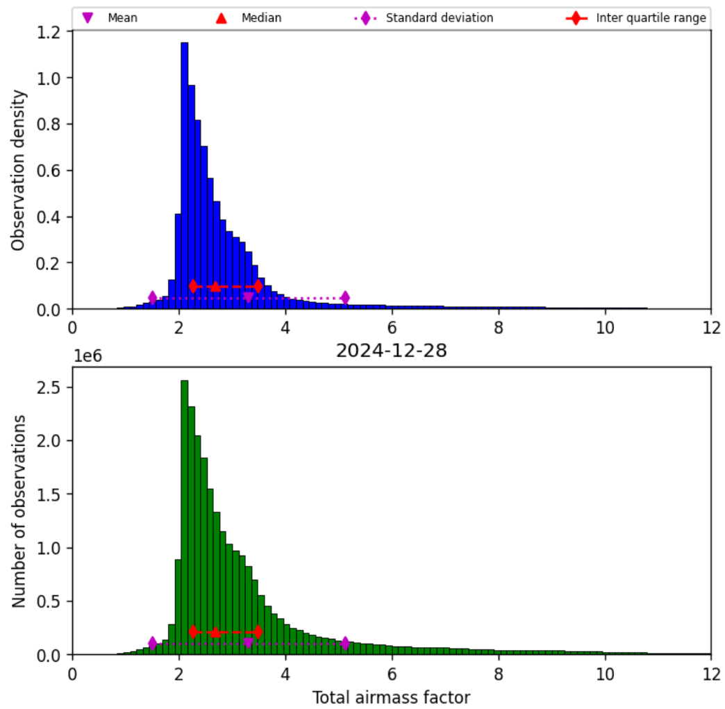
Figure 32: Histogram of “Total airmass factor” for 2024-12-27 to 2024-12-29
