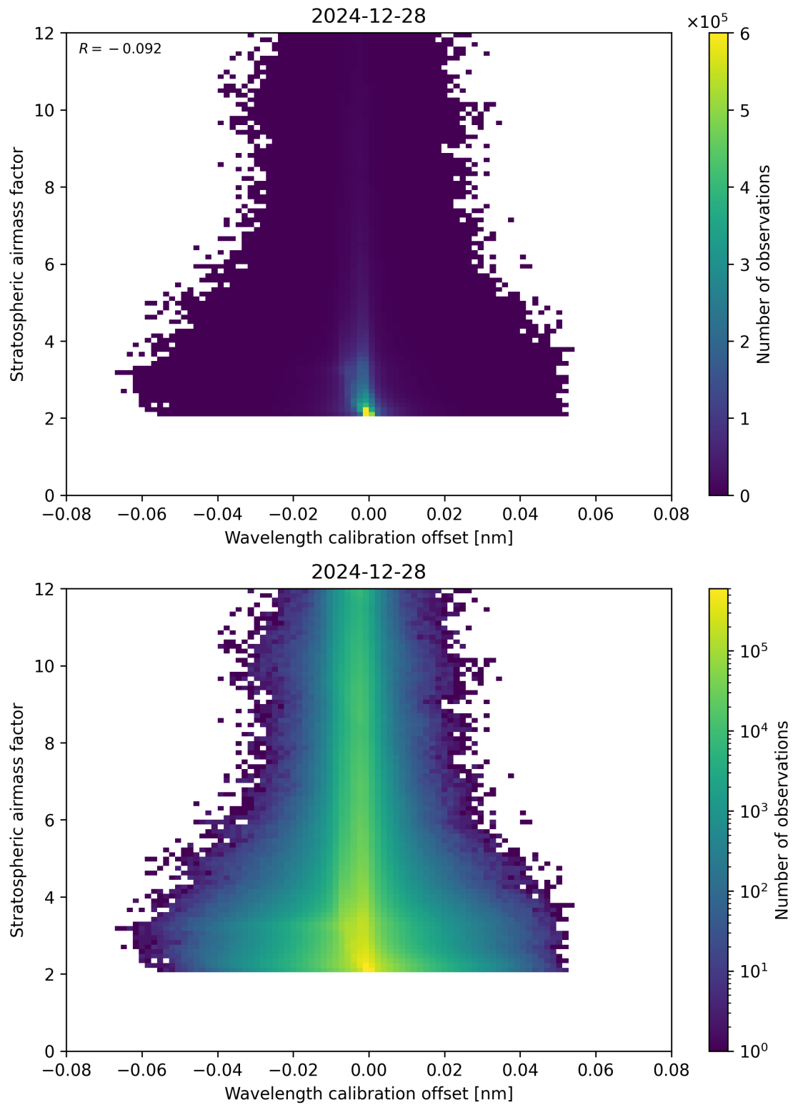
Figure 174: Scatter density plot of “Wavelength calibration offset” against “Stratospheric airmass factor” for 2024-12-27 to 2024-12-29.
