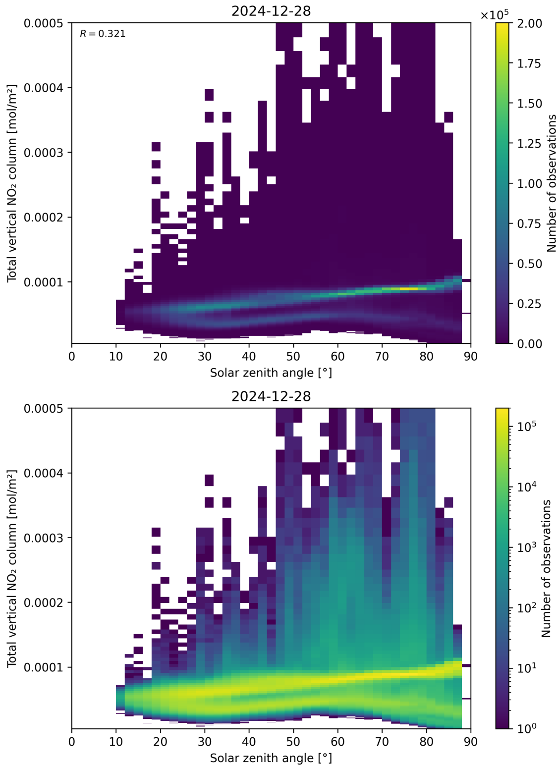
Figure 153: Scatter density plot of “Solar zenith angle” against “Total vertical NO 2 column” for 2024-12-27 to 2024-12-29.
