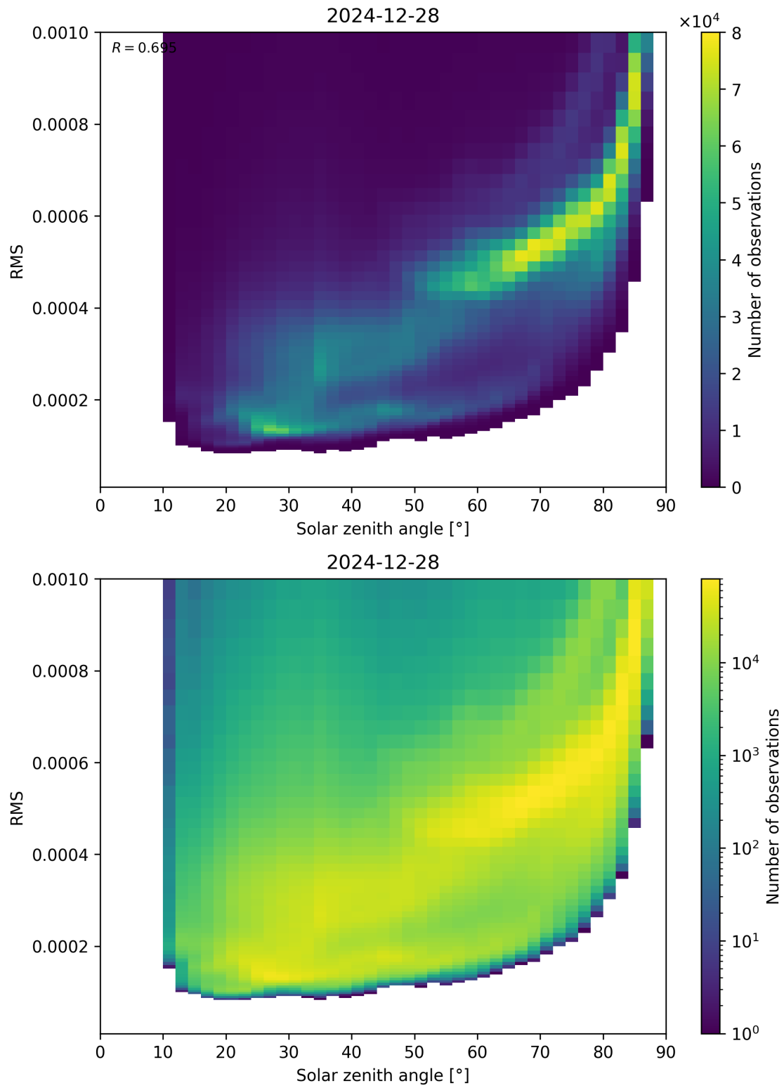
Figure 157: Scatter density plot of “Solar zenith angle” against “RMS” for 2024-12-27 to 2024-12-29.
