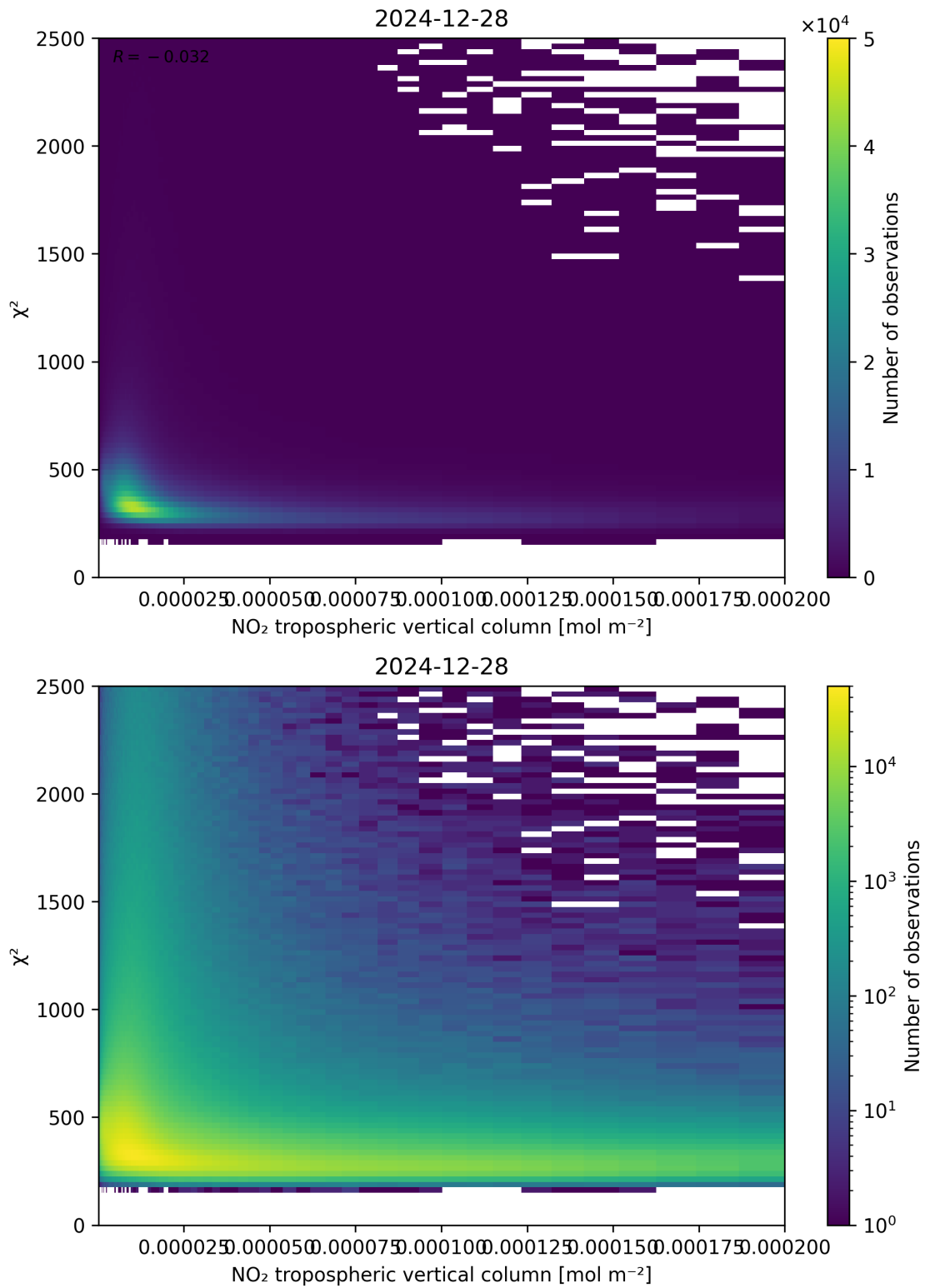
Figure 124: Scatter density plot of “NO 2 tropospheric vertical column” against “ \chi^2 ” for 2024-12-27 to 2024-12-29.
