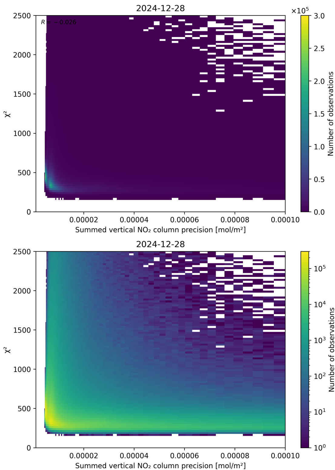
Figure 107: Scatter density plot of “Summed vertical NO 2 column precision” against “ \chi^2 ” for 2024-12-27 to 2024-12-29.
