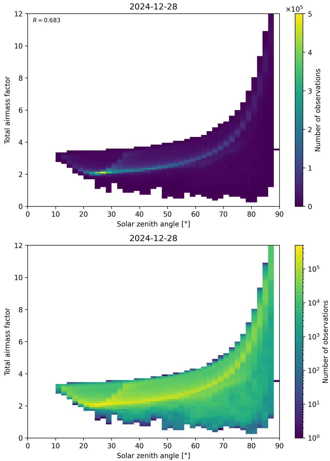
Figure 146: Scatter density plot of “Solar zenith angle” against “Total air mass factor” for 2024-12-27 to 2024-12-29.
