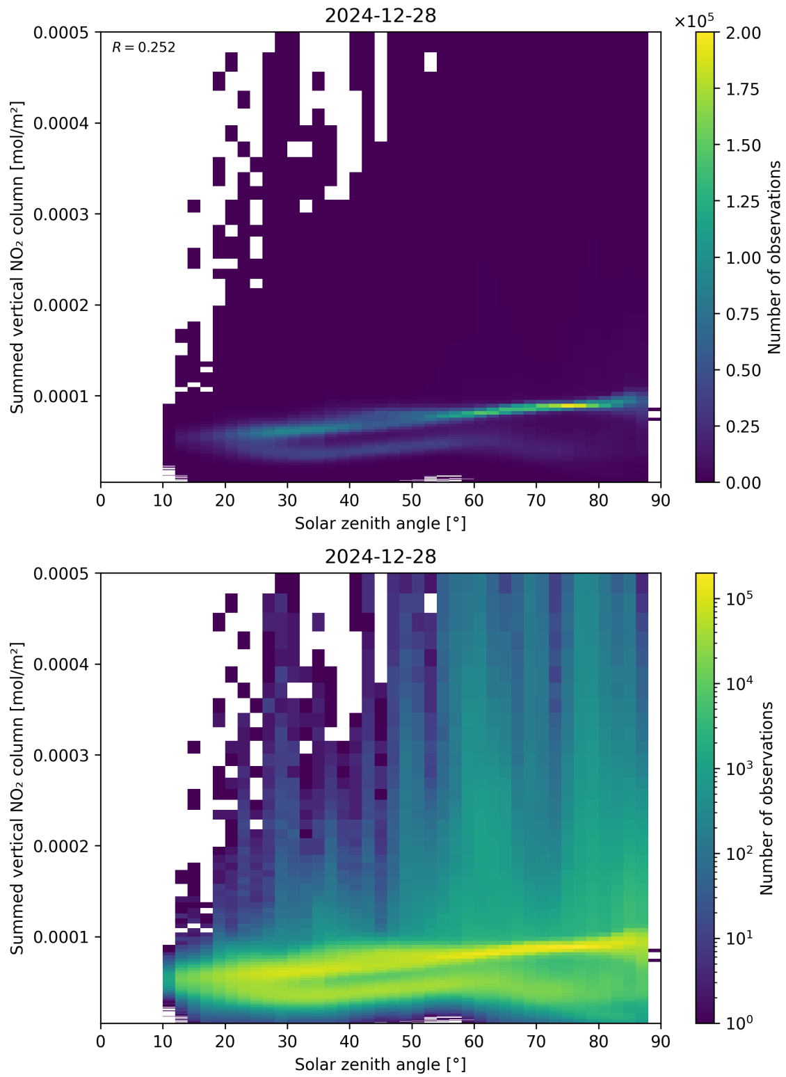
Figure 151: Scatter density plot of “Solar zenith angle” against “Summed vertical NO 2 column” for 2024-12-27 to 2024-12-29.
