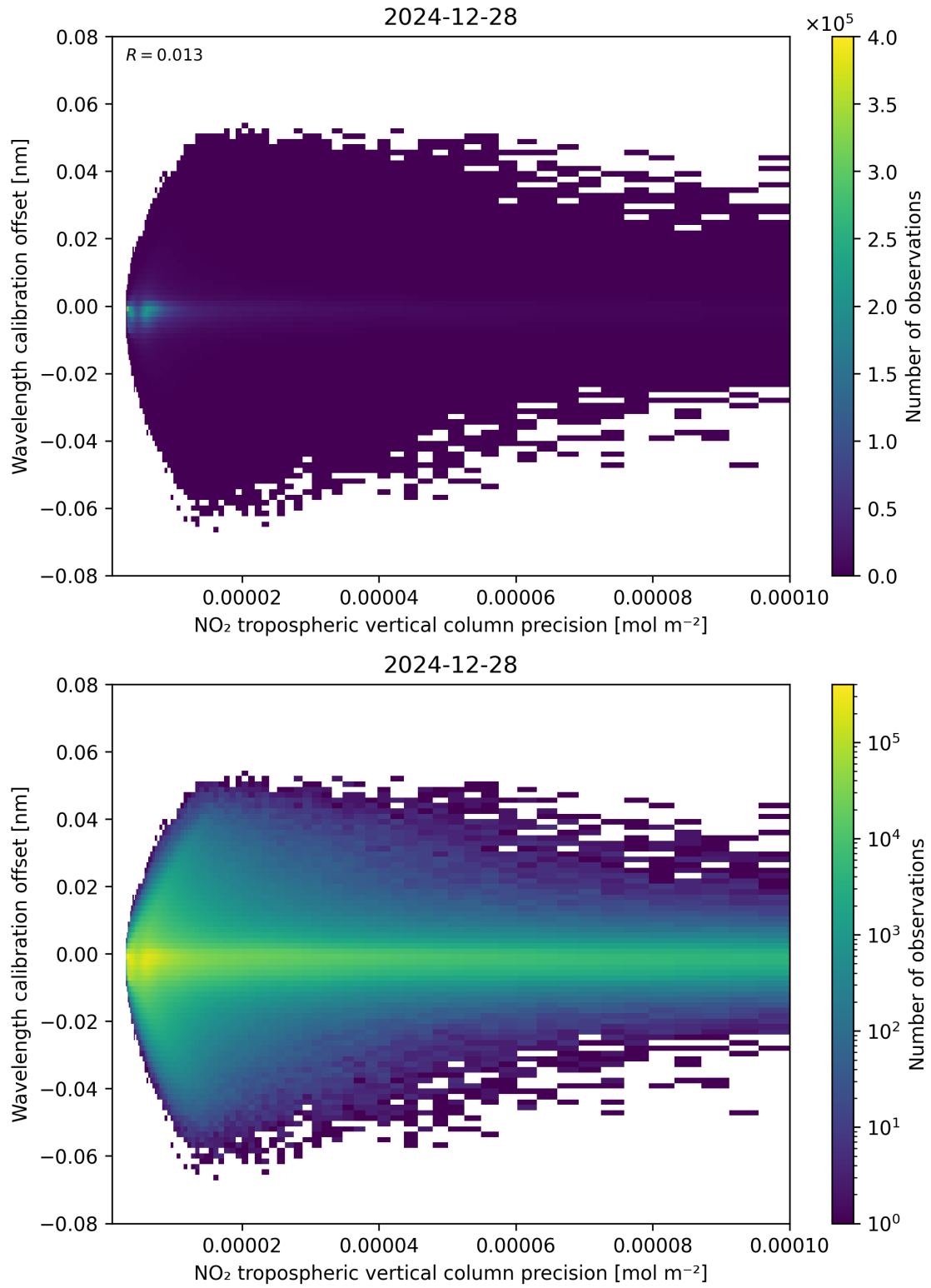
Figure 141: Scatter density plot of “NO 2 tropospheric vertical column precision” against “Wavelength calibration offset” for 2024-12-27 to 2024-12-29.
