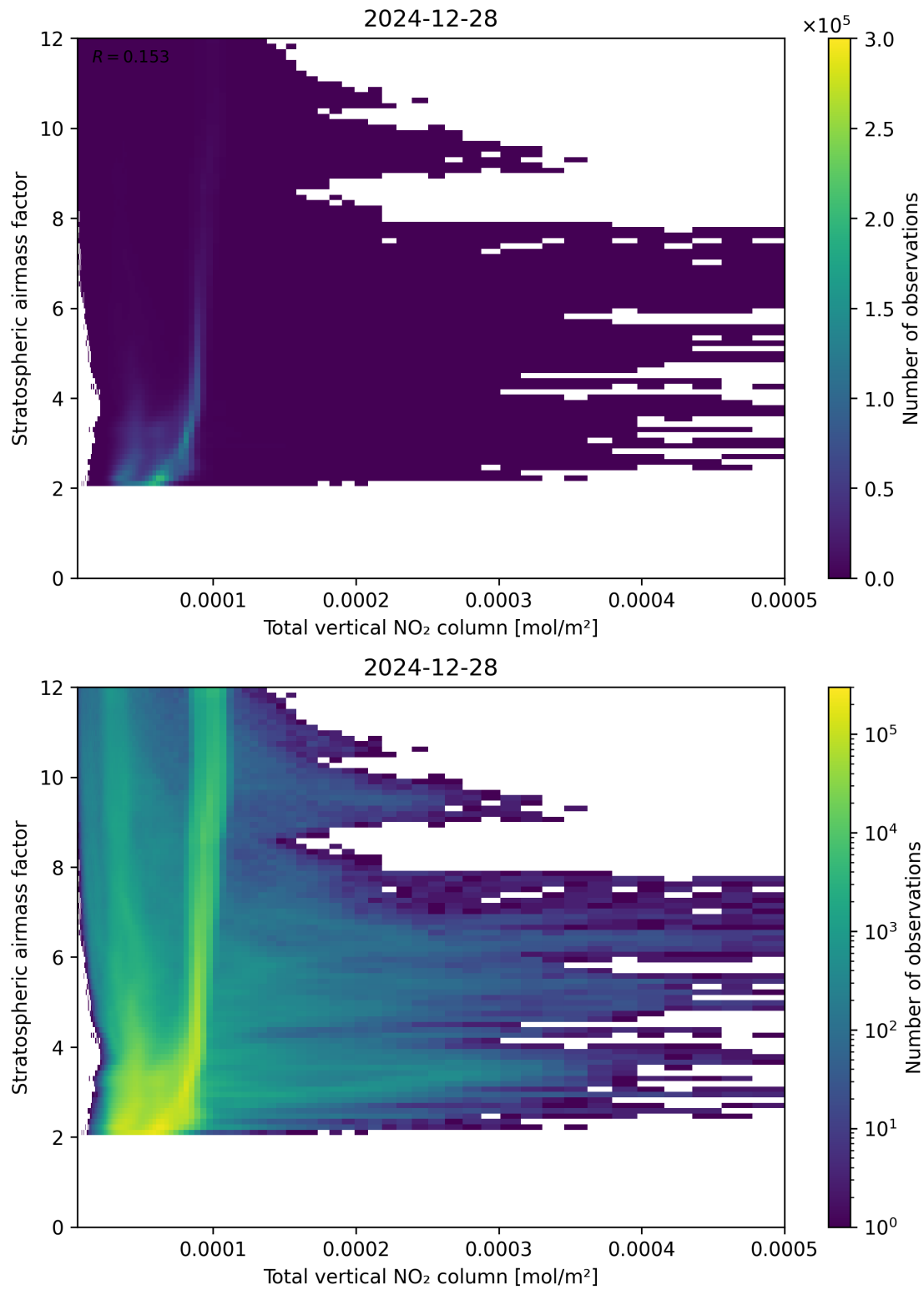
Figure 110: Scatter density plot of “Total vertical NO 2 column” against “Stratospheric airmass factor” for 2024-12-27 to 2024-12-29.
