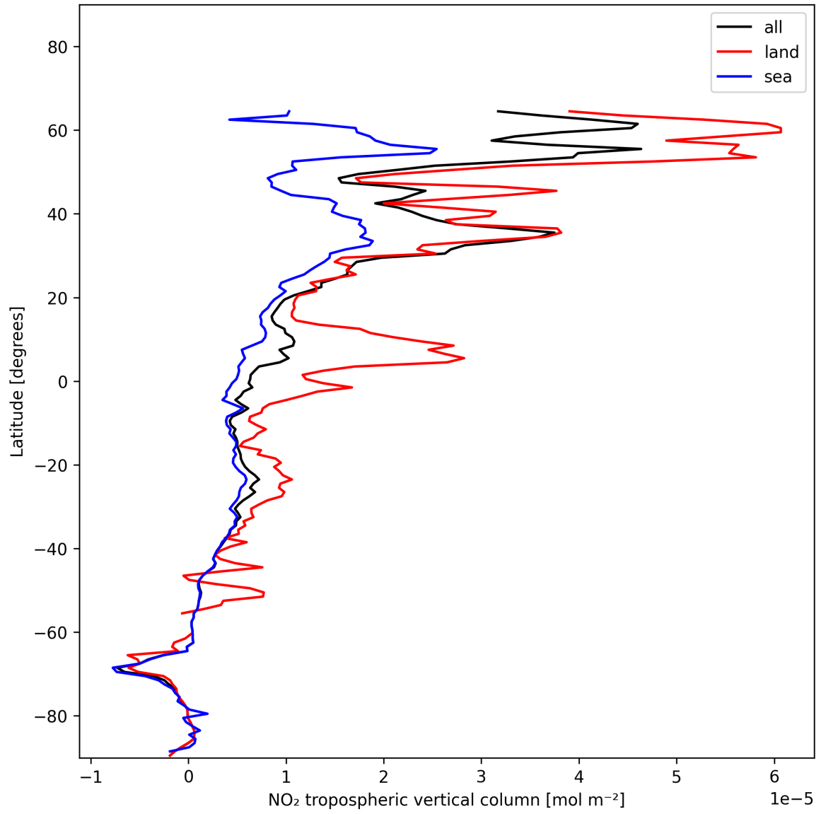
Figure 12: Zonal average of “NO 2 tropospheric vertical column” for 2024-12-27 to 2024-12-29.
