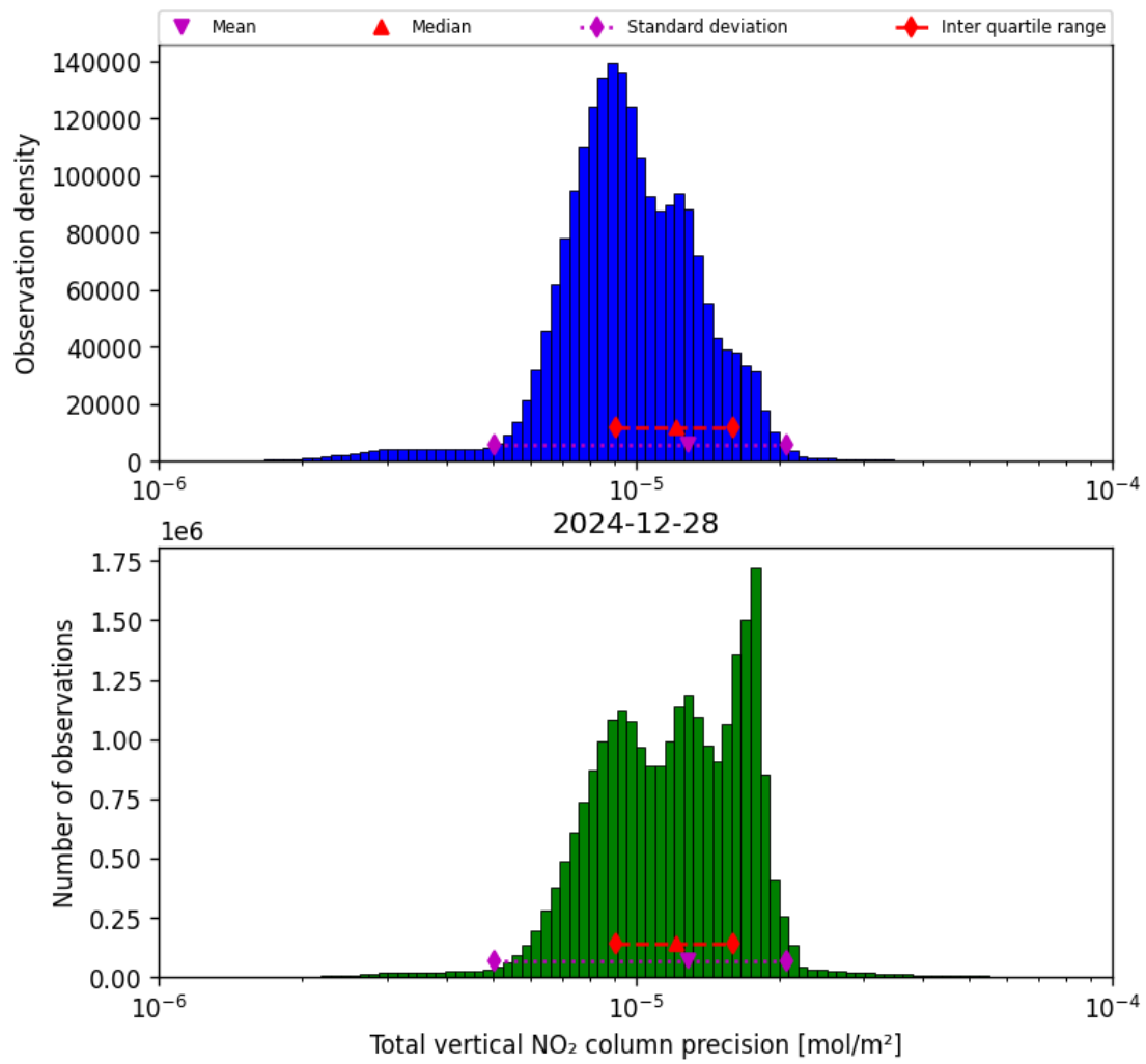
Figure 39: Histogram of “Total vertical NO 2 column precision” for 2024-12-27 to 2024-12-29
