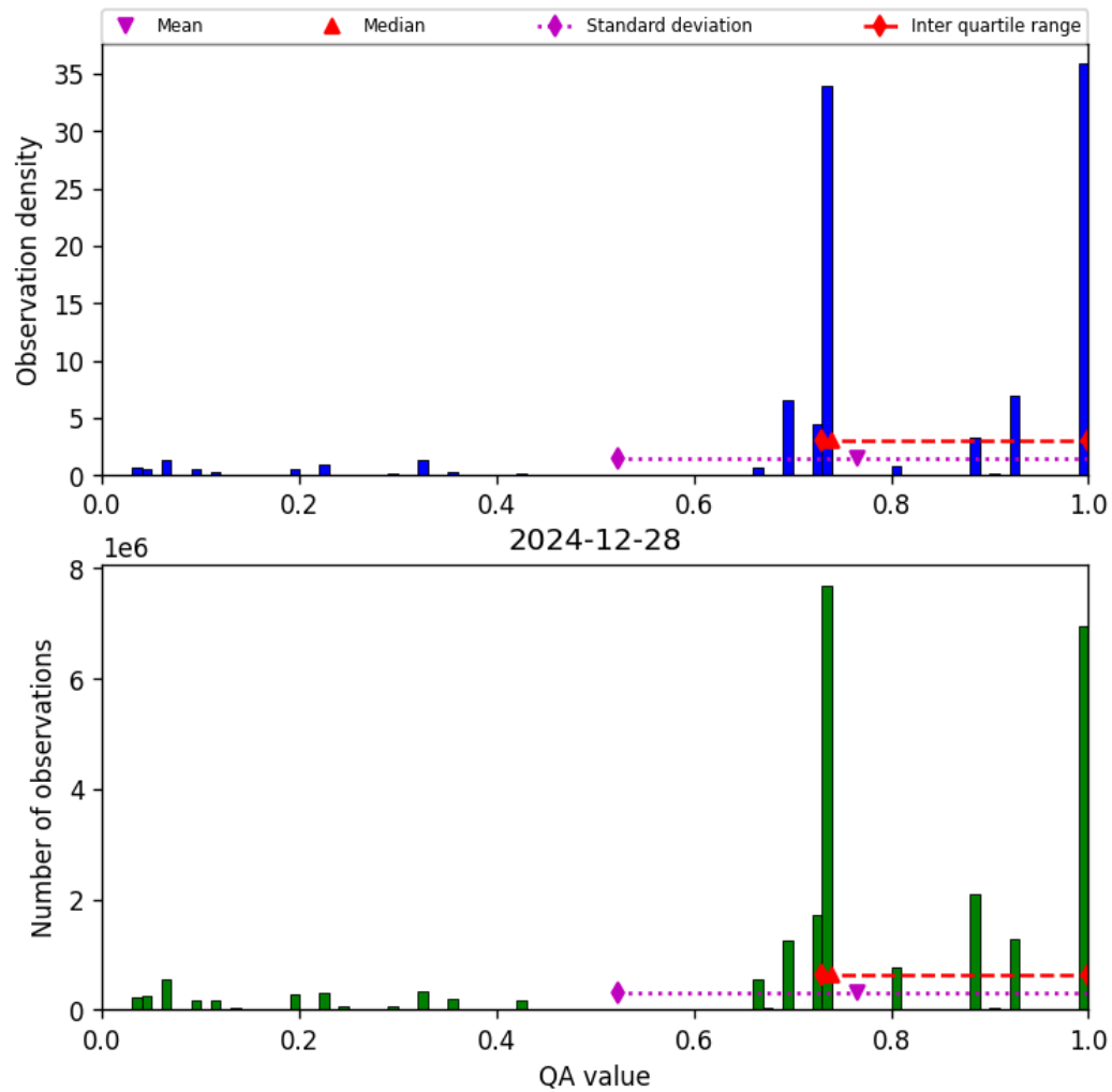
Figure 28: Histogram of “QA value” for 2024-12-27 to 2024-12-29
