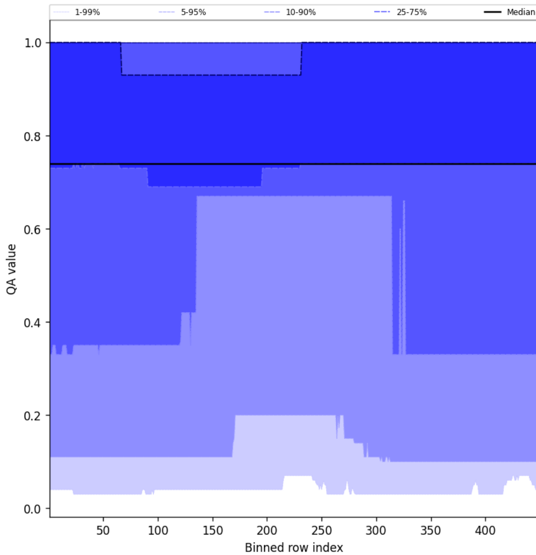
Figure 45: Along track statistics of “QA value” for 2024-12-27 to 2024-12-29
