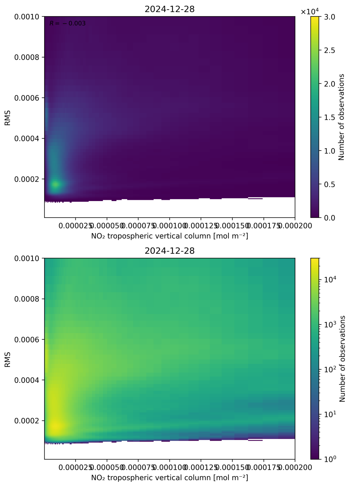
Figure 142: Scatter density plot of “NO 2 tropospheric vertical column” against “RMS” for 2024-12-27 to 2024-12-29.
