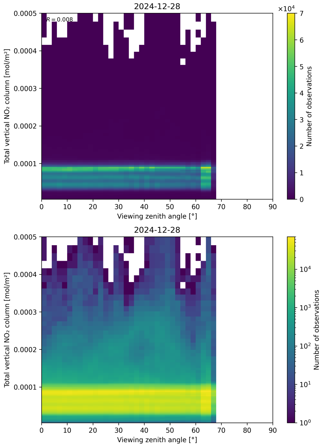
Figure 167: Scatter density plot of “Viewing zenith angle” against “Total vertical NO 2 column” for 2024-12-27 to 2024-12-29.
