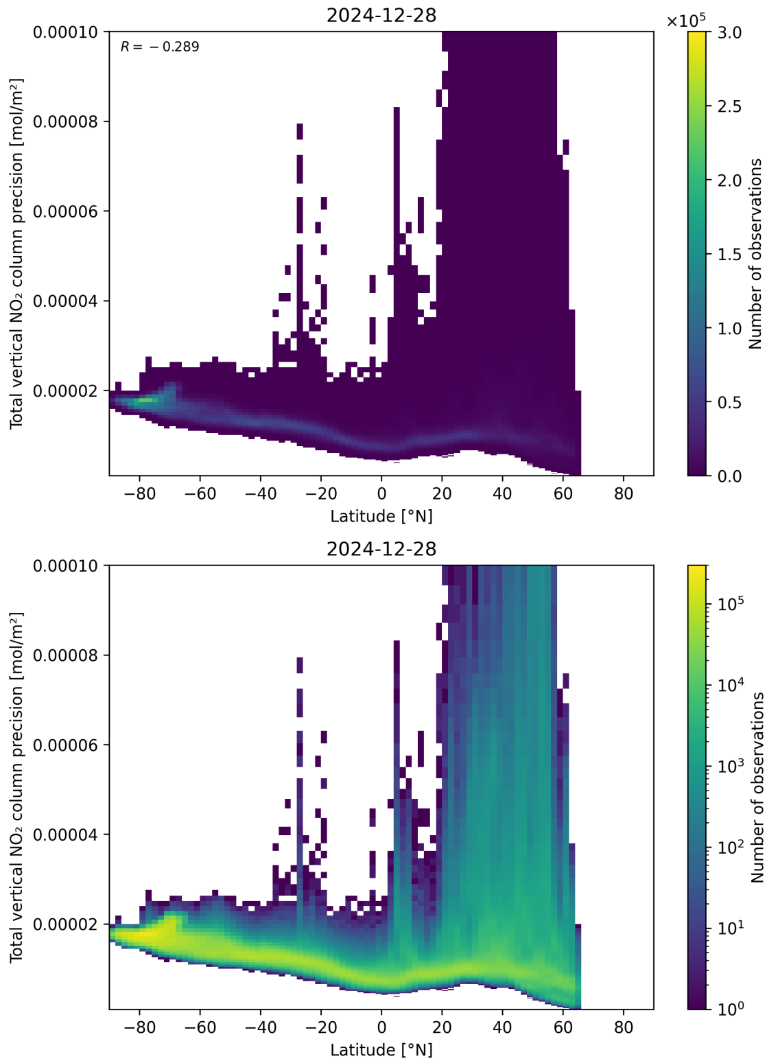
Figure 91: Scatter density plot of “Latitude” against “Total vertical NO 2 column precision” for 2024-12-27 to 2024-12-29.
