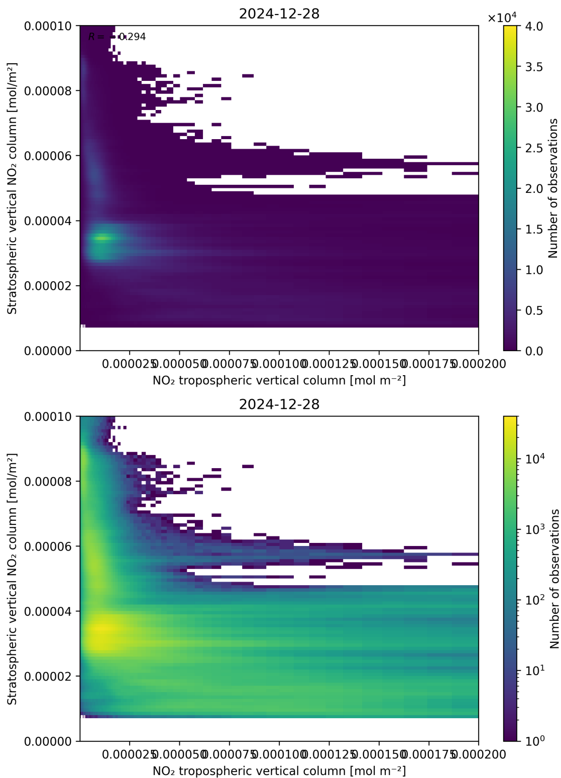
Figure 125: Scatter density plot of “NO 2 tropospheric vertical column” against “Stratospheric vertical NO 2 column” for 2024-12-27 to 2024-12-29.
