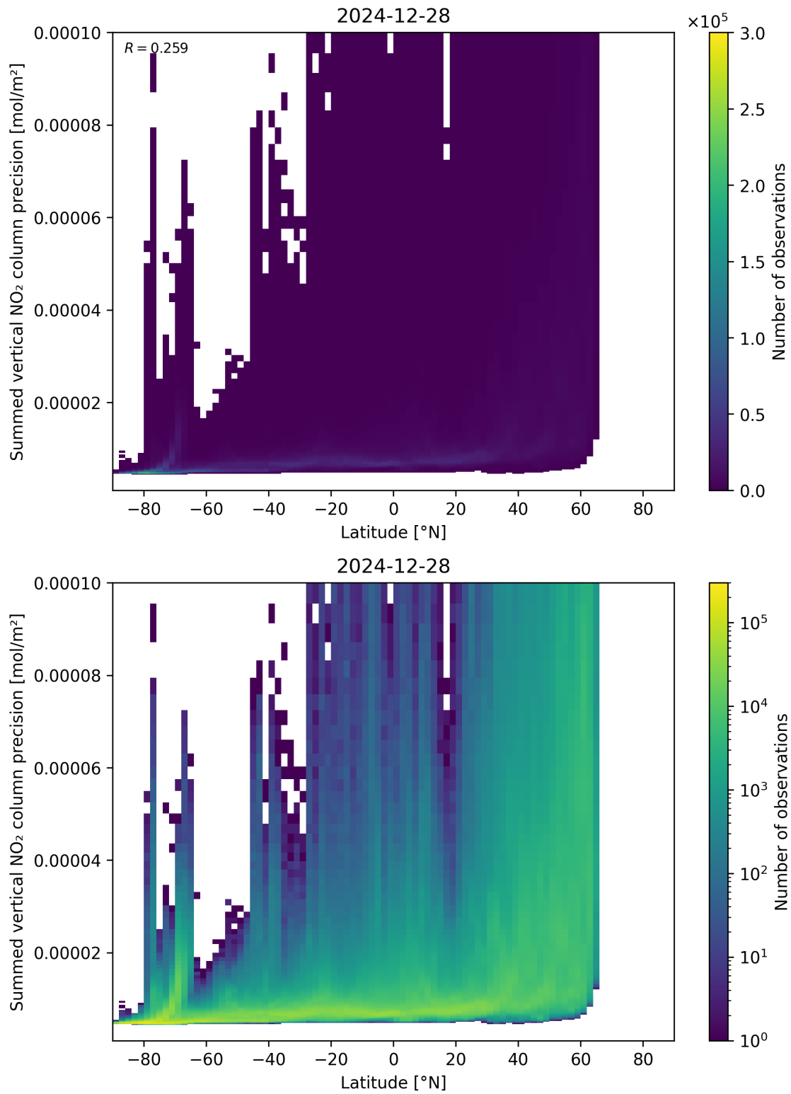
Figure 89: Scatter density plot of “Latitude” against “Summed vertical NO 2 column precision” for 2024-12-27 to 2024-12-29.
