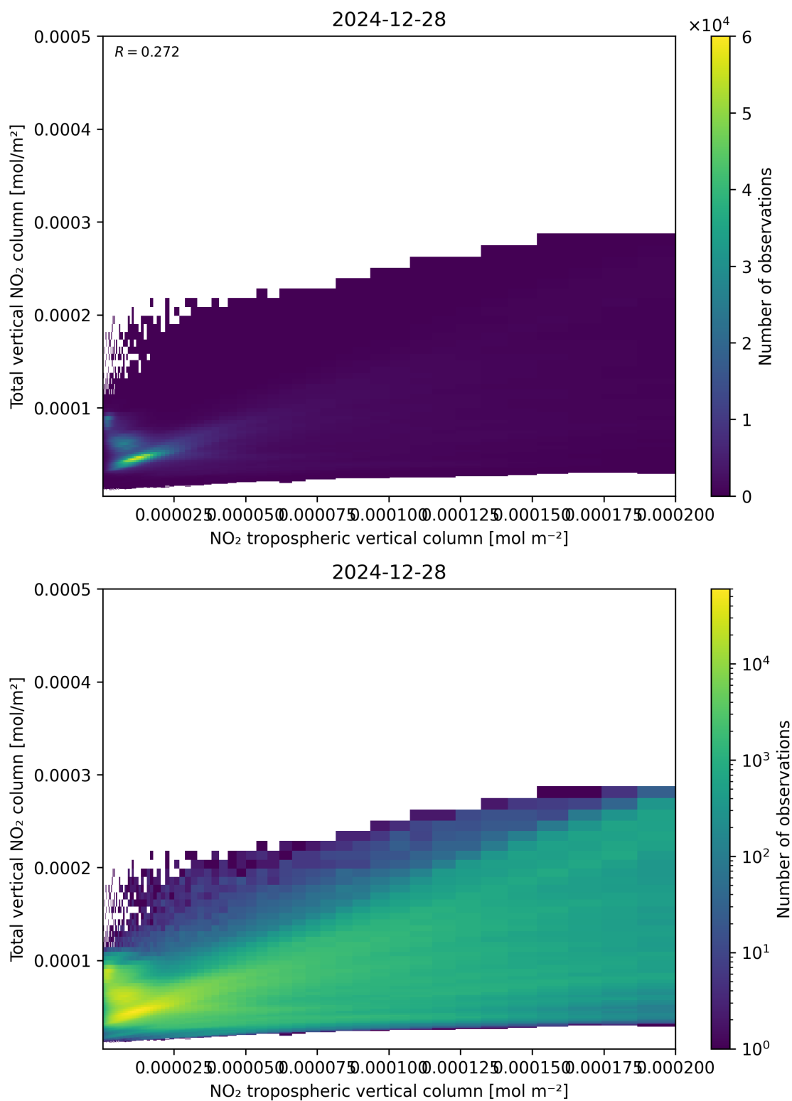
Figure 128: Scatter density plot of “NO 2 tropospheric vertical column” against “Total vertical NO 2 column” for 2024-12-27 to 2024-12-29.
