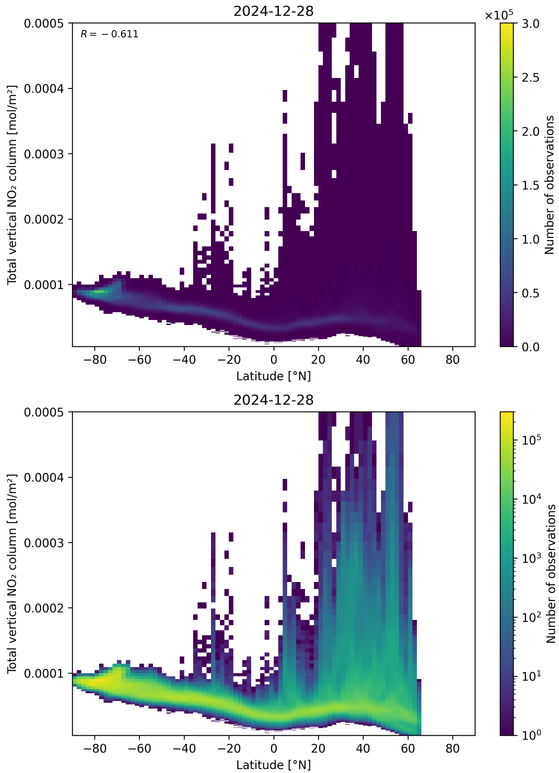
Figure 90: Scatter density plot of “Latitude” against “Total vertical NO 2 column” for 2024-12-27 to 2024-12-29.
