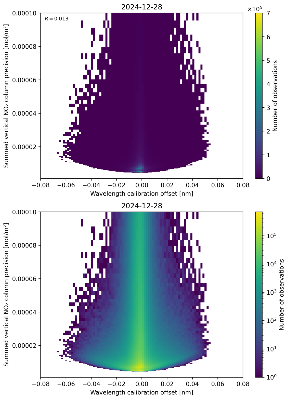
Figure 178: Scatter density plot of “Wavelength calibration offset” against “Summed vertical NO 2 column precision” for 2024-12-27 to 2024-12-29.
