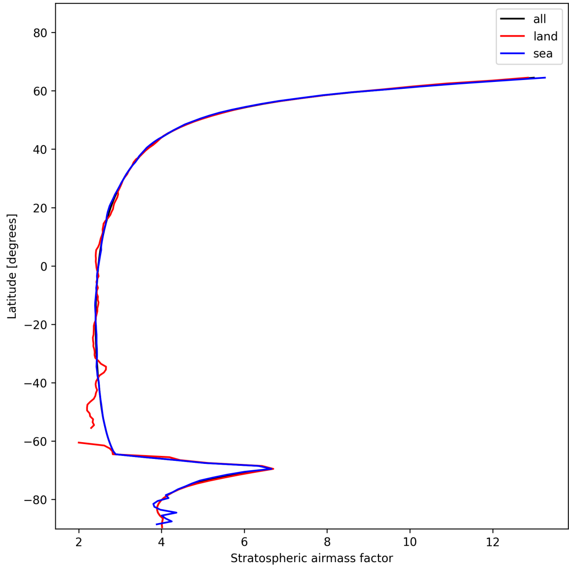
Figure 27: Zonal average of “Stratospheric air mass factor” for 2024-12-27 to 2024-12-29.
