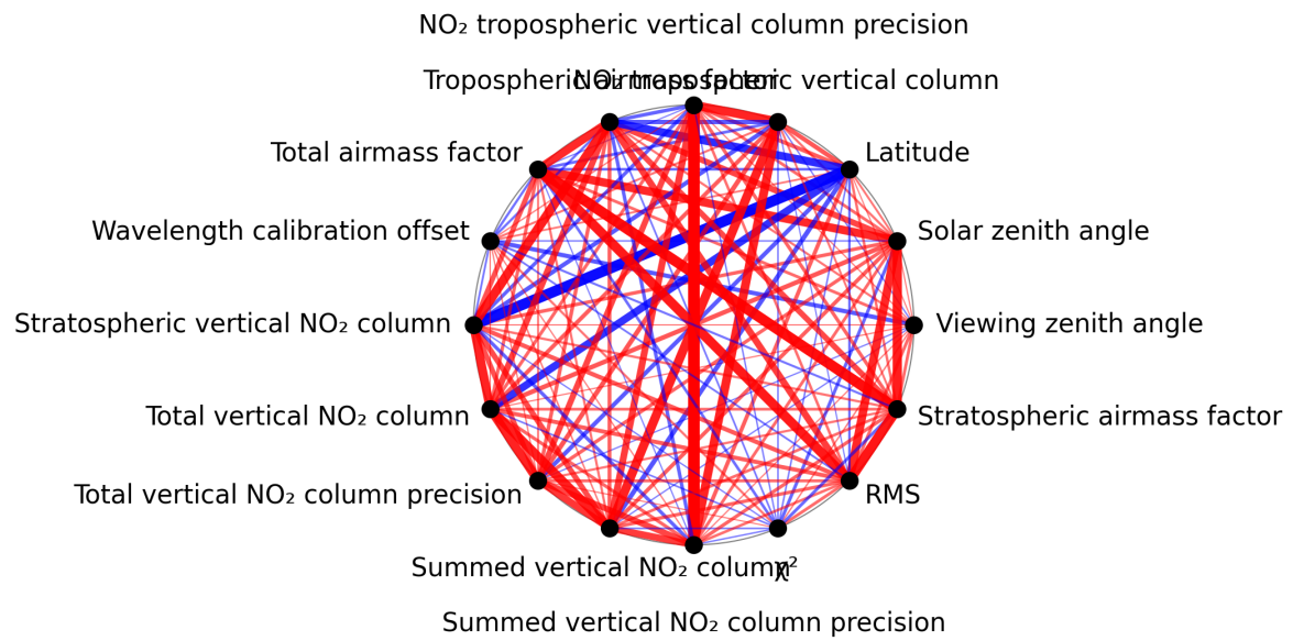
Figure 1: Map of correlation graph for 2024-12-27 to 2024-12-29.
