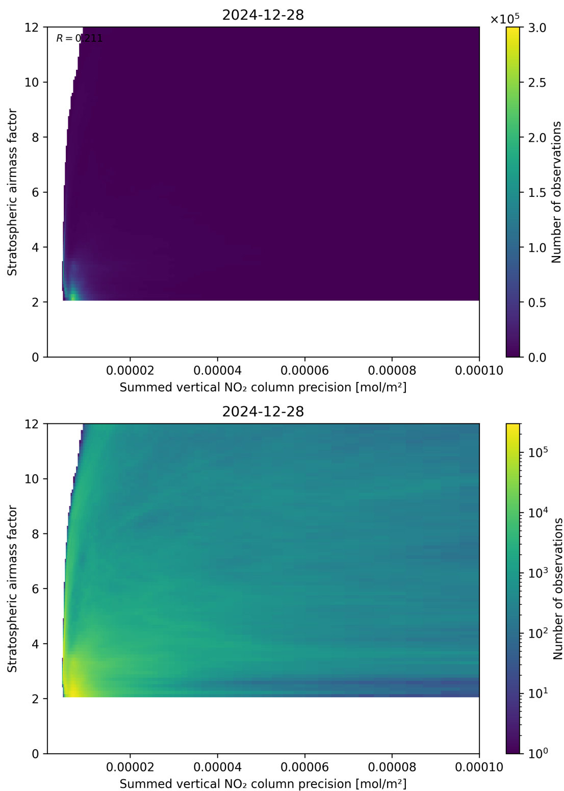
Figure 106: Scatter density plot of “Summed vertical NO 2 column precision” against “Stratospheric airmass factor” for 2024-12-27 to 2024-12-29.
