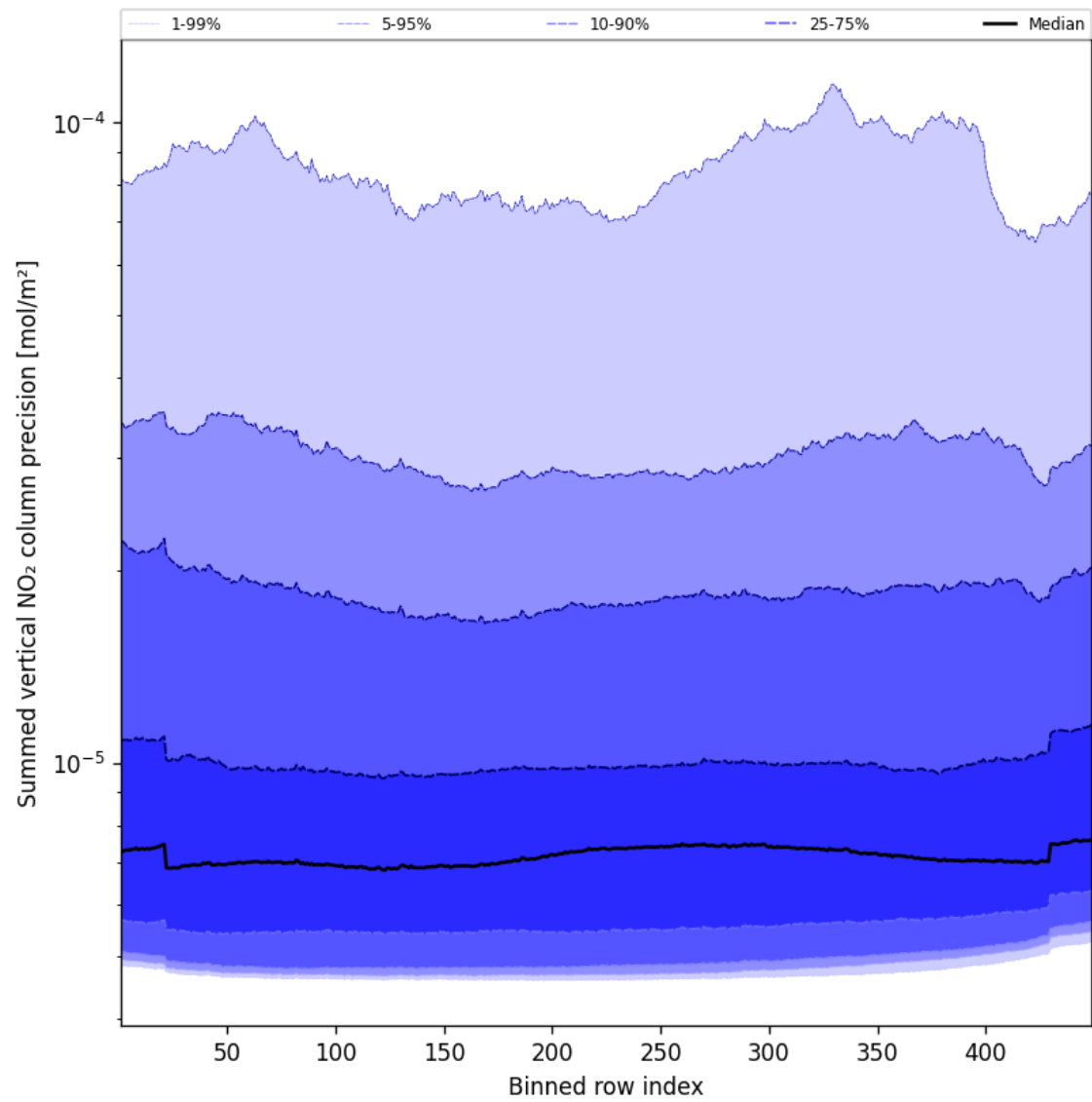
Figure 58: Along track statistics of “Summed vertical NO 2 column precision” for 2024-12-27 to 2024-12-29
