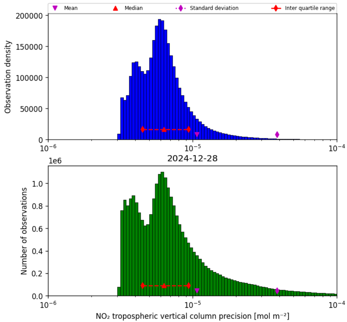
Figure 30: Histogram of “NO 2 tropospheric vertical column precision” for 2024-12-27 to 2024-12-29
