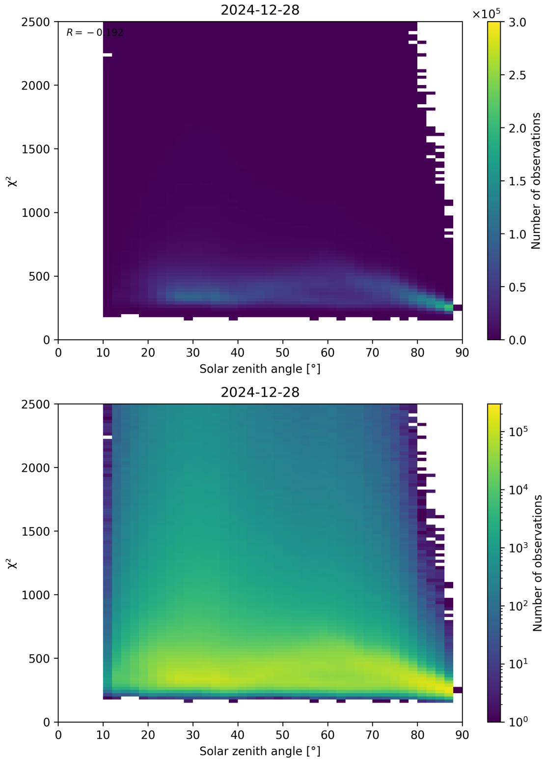
Figure 148: Scatter density plot of “Solar zenith angle” against “ \chi^2 ” for 2024-12-27 to 2024-12-29.
