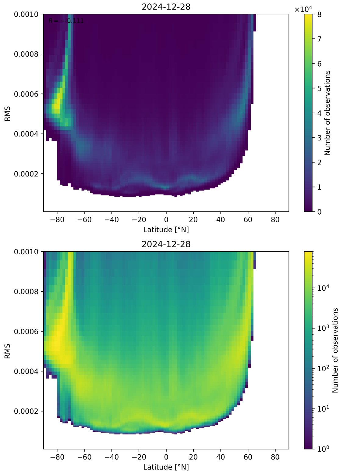
Figure 94: Scatter density plot of “Latitude” against “RMS” for 2024-12-27 to 2024-12-29.
