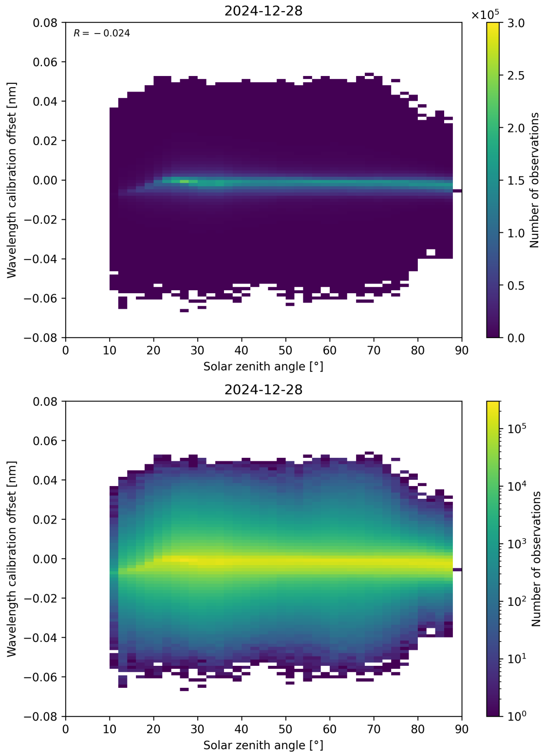
Figure 158: Scatter density plot of “Solar zenith angle” against “Wavelength calibration offset” for 2024-12-27 to 2024-12-29.
