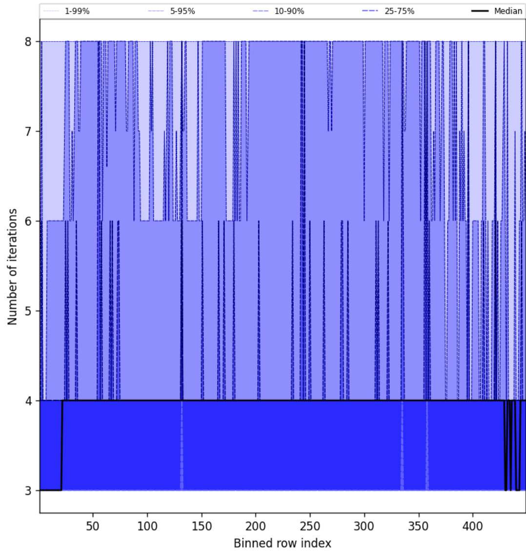
Figure 51: Along track statistics of “Number of iterations” for 2024-12-27 to 2024-12-29
