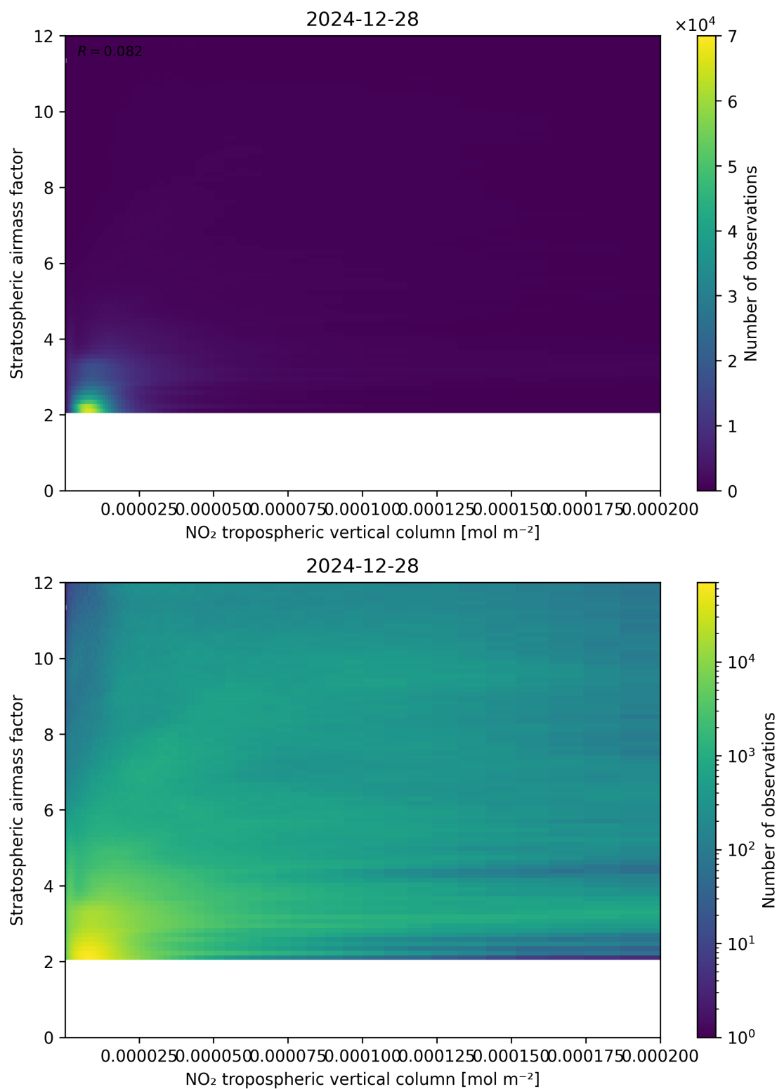
Figure 121: Scatter density plot of “NO 2 tropospheric vertical column” against “Stratospheric airmass factor” for 2024-12-27 to 2024-12-29.
