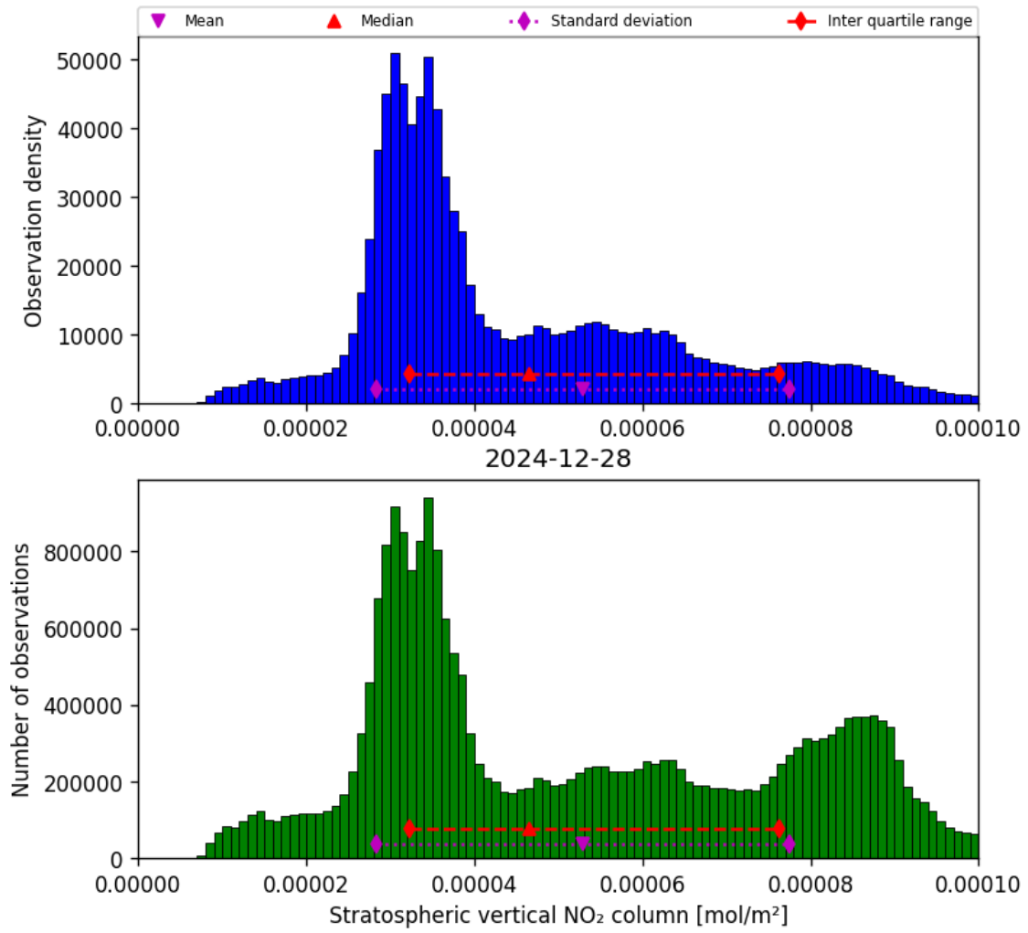
Figure 36: Histogram of “Stratospheric vertical NO 2 column” for 2024-12-27 to 2024-12-29
