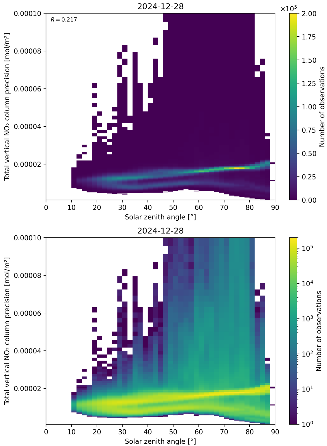
Figure 154: Scatter density plot of “Solar zenith angle” against “Total vertical NO 2 column precision” for 2024-12-27 to 2024-12-29.
