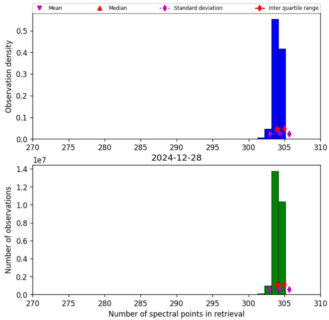
Figure 33: Histogram of “Number of spectral points in retrieval” for 2024-12-27 to 2024-12-29
