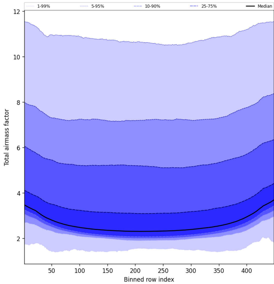
Figure 49: Along track statistics of “Total airmass factor” for 2024-12-27 to 2024-12-29
