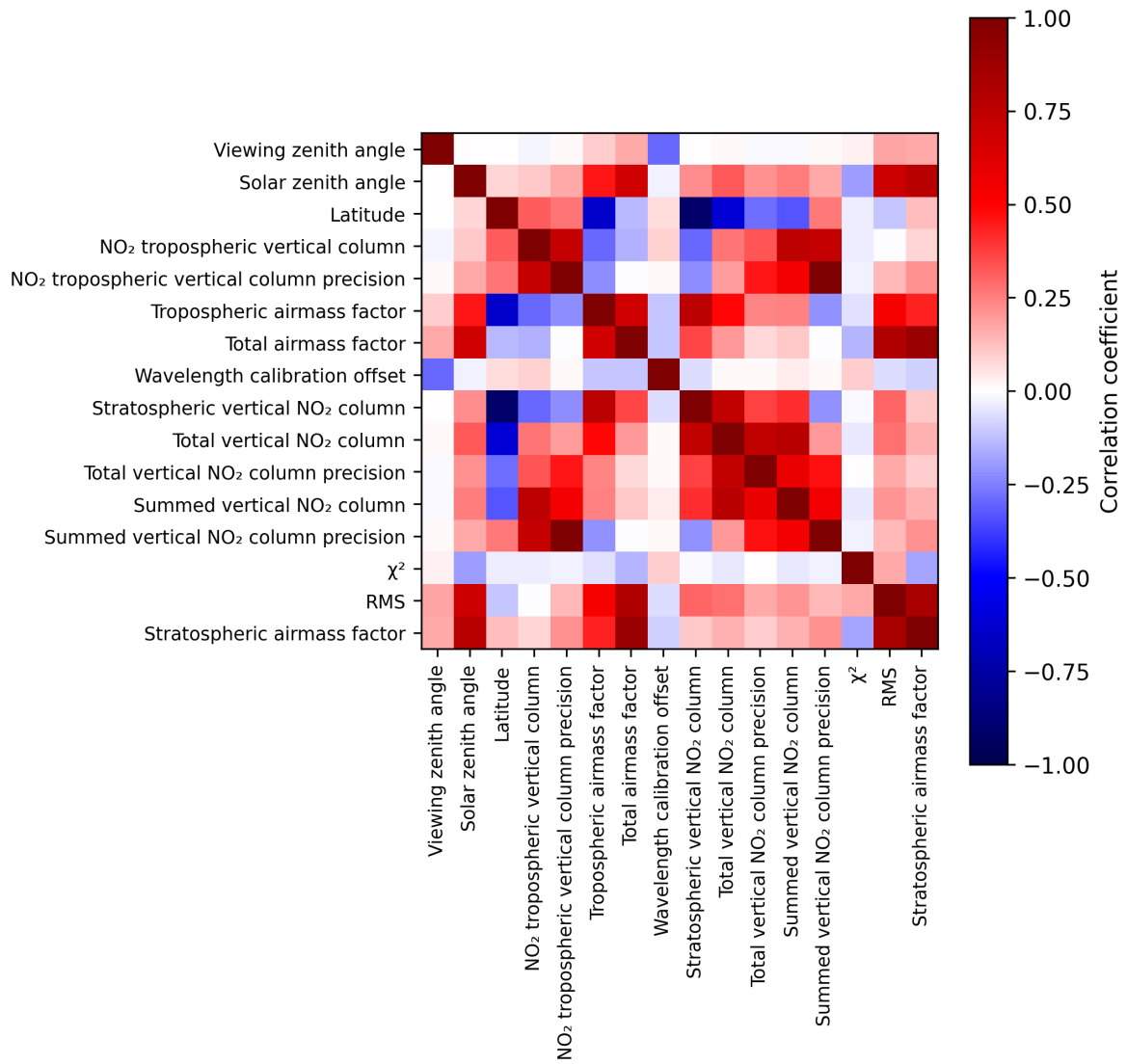
Figure 2: Map of correlation matrix for 2024-12-27 to 2024-12-29.
