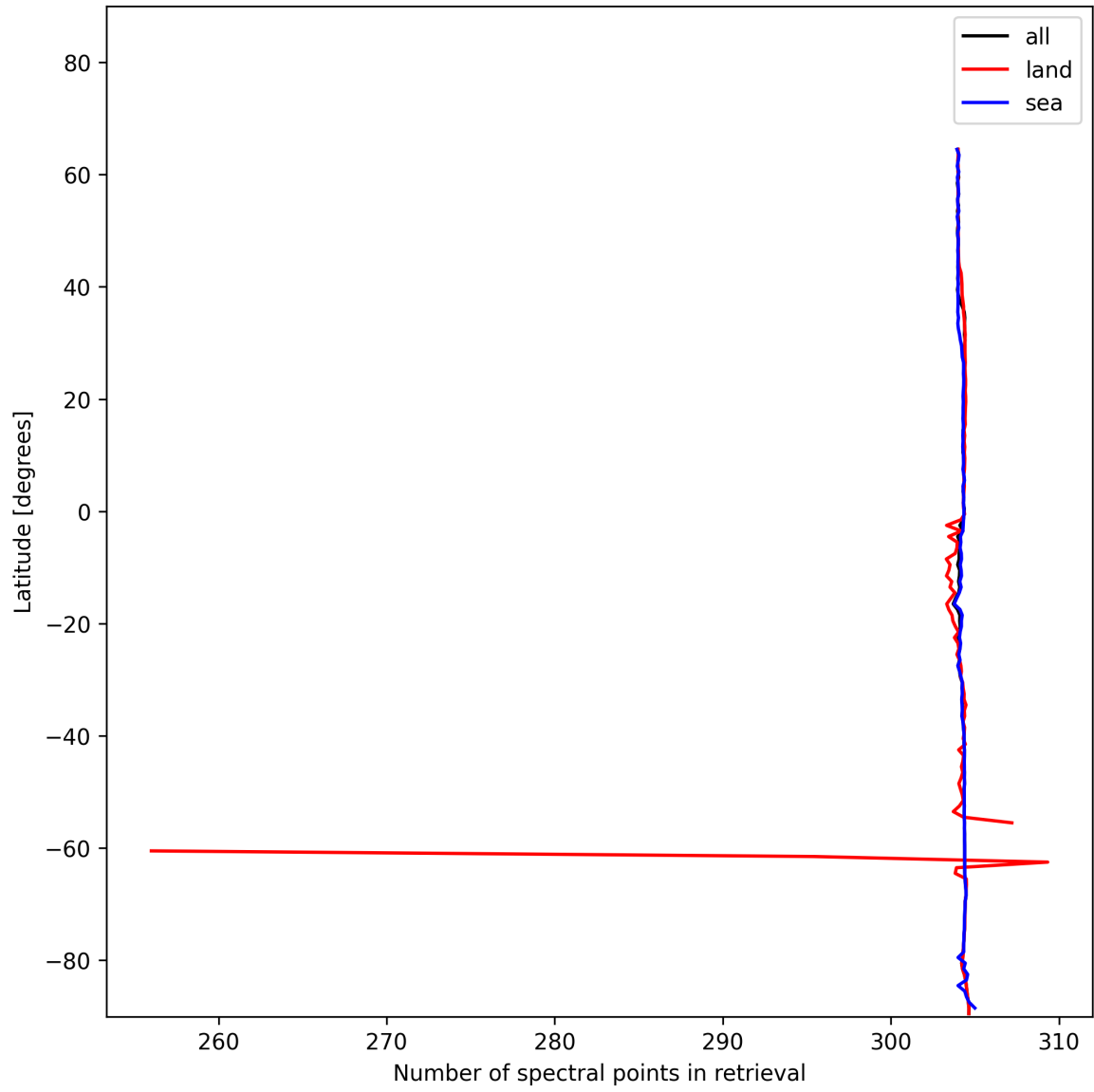
Figure 16: Zonal average of “Number of spectral points in retrieval” for 2024-12-27 to 2024-12-29.
