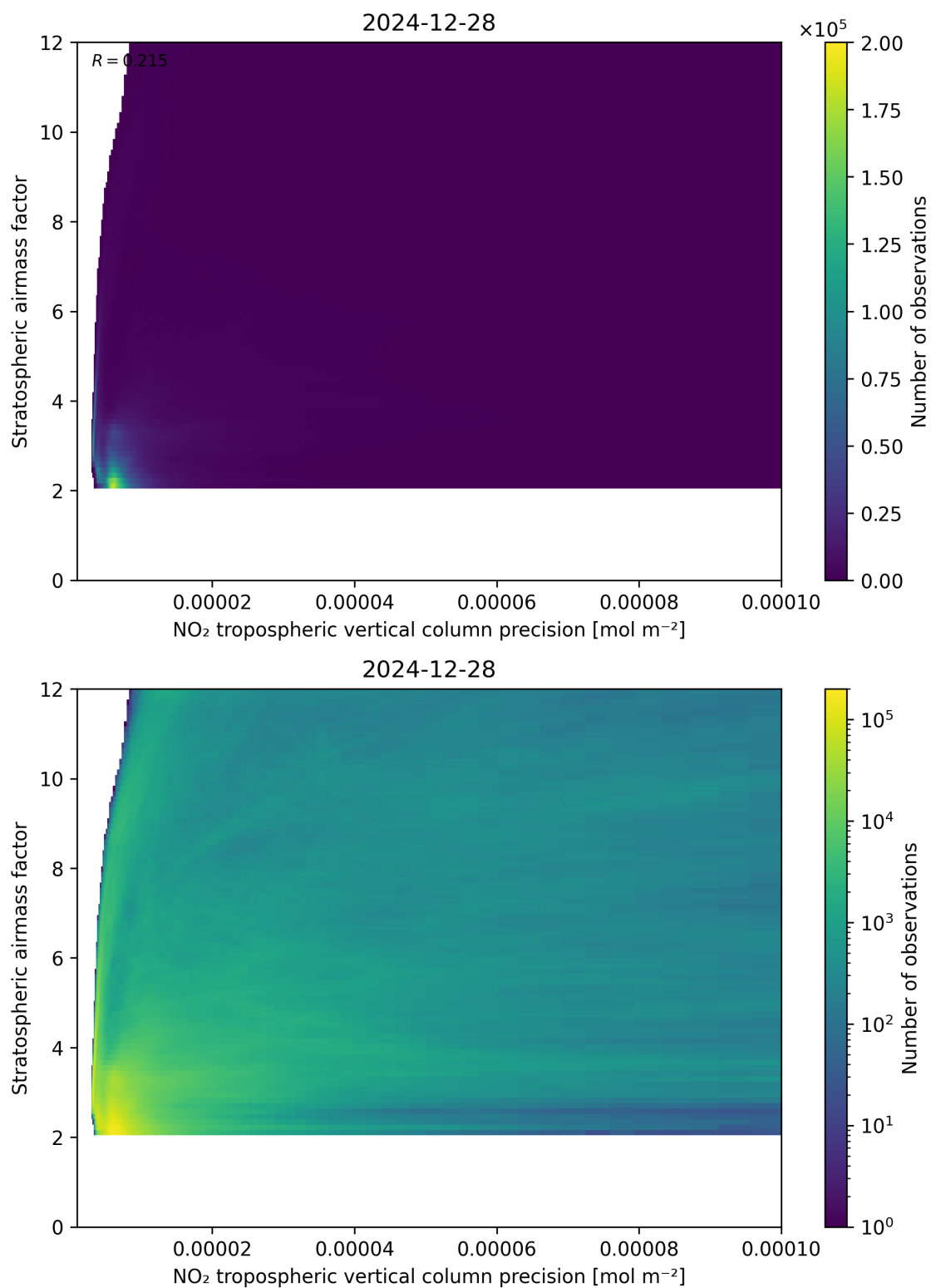
Figure 131: Scatter density plot of “NO 2 tropospheric vertical column precision” against “Stratospheric airmass factor” for 2024-12-27 to 2024-12-29.
