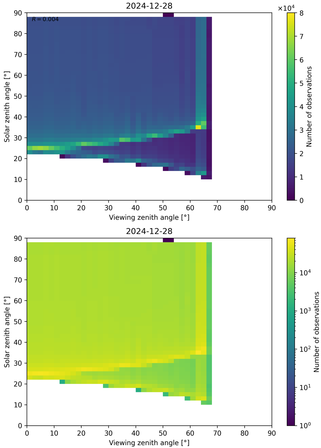
Figure 172: Scatter density plot of “Viewing zenith angle” against “Solar zenith angle” for 2024-12-27 to 2024-12-29.
