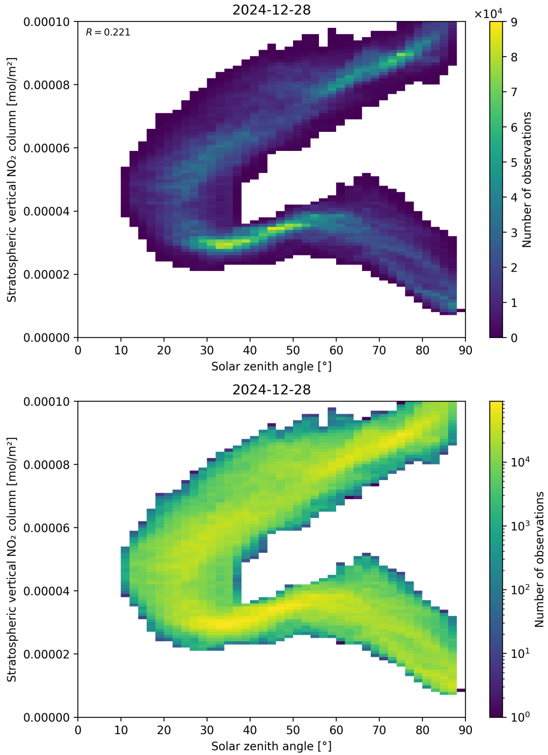
Figure 150: Scatter density plot of “Solar zenith angle” against “Stratospheric vertical NO 2 column” for 2024-12-27 to 2024-12-29.
