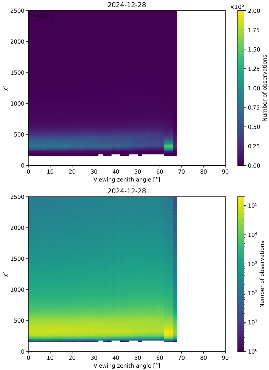
Figure 162: Scatter density plot of “Viewing zenith angle” against “ \chi^2 ” for 2024-12-27 to 2024-12-29.
