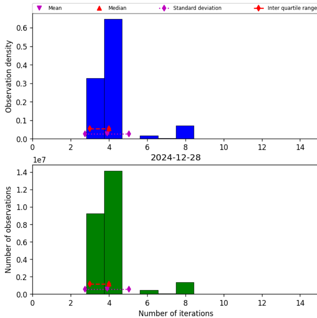
Figure 34: Histogram of “Number of iterations” for 2024-12-27 to 2024-12-29
