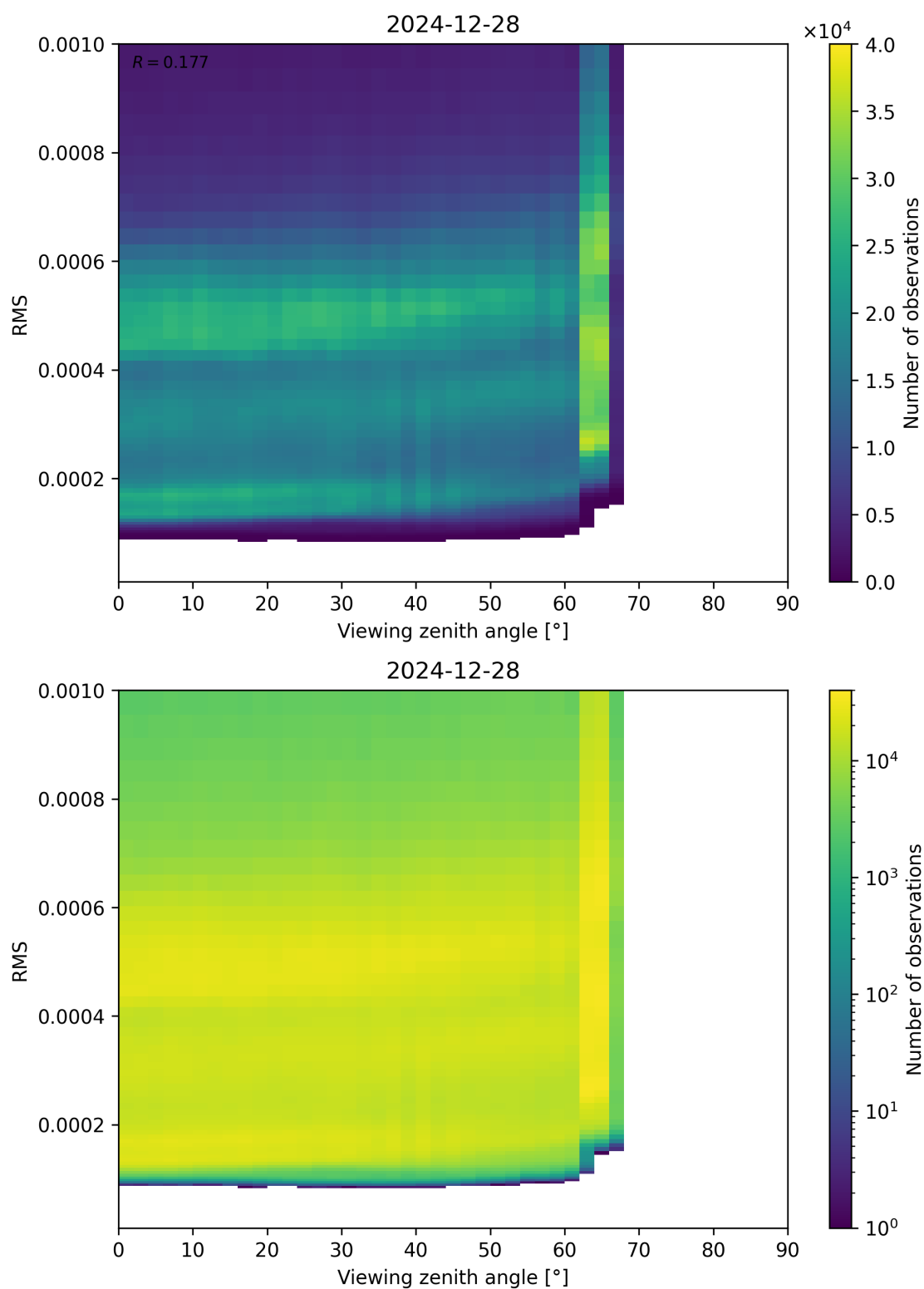
Figure 171: Scatter density plot of “Viewing zenith angle” against “RMS” for 2024-12-27 to 2024-12-29.
