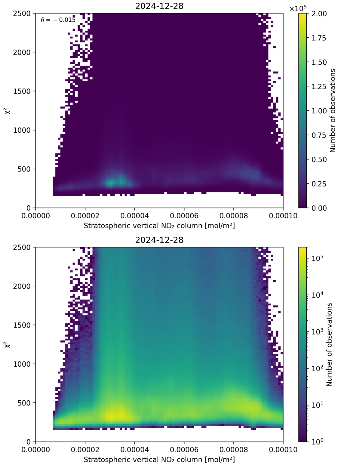
Figure 97: Scatter density plot of “Stratospheric vertical NO 2 column” against “ \chi^2 ” for 2024-12-27 to 2024-12-29.
