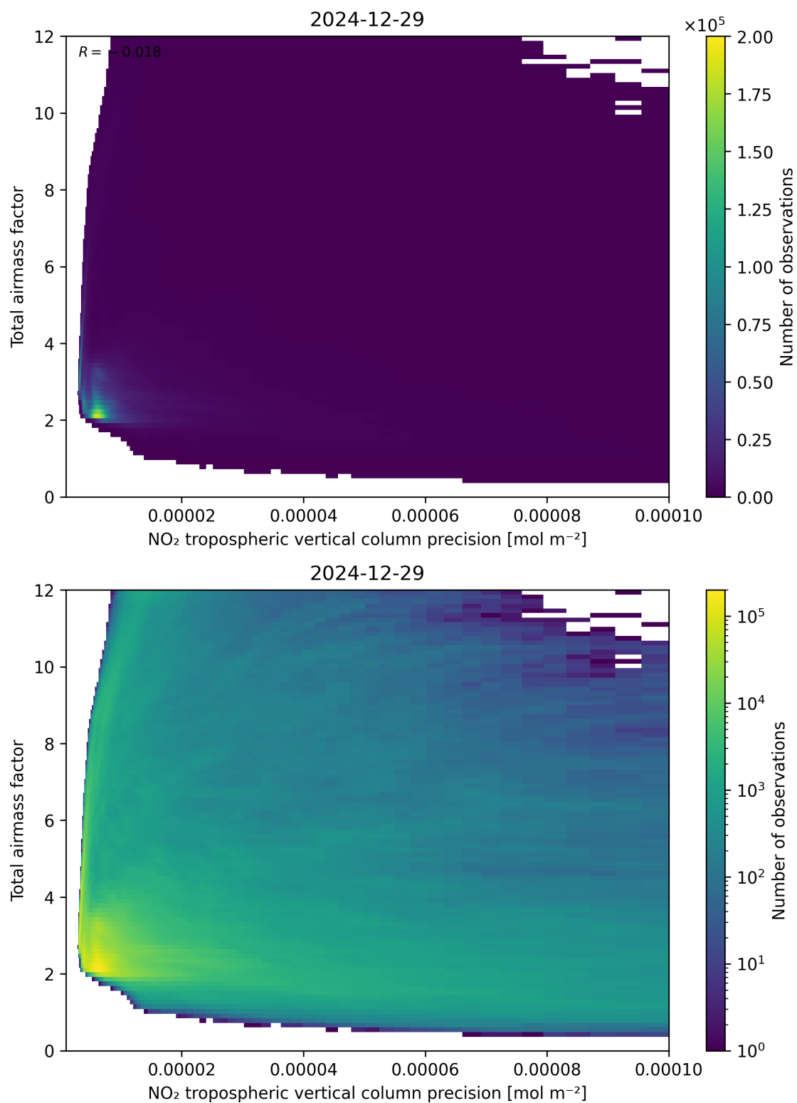
Figure 132: Scatter density plot of “NO 2 tropospheric vertical column precision” against “Total air mass factor” for 2024-12-28 to 2024-12-30.
