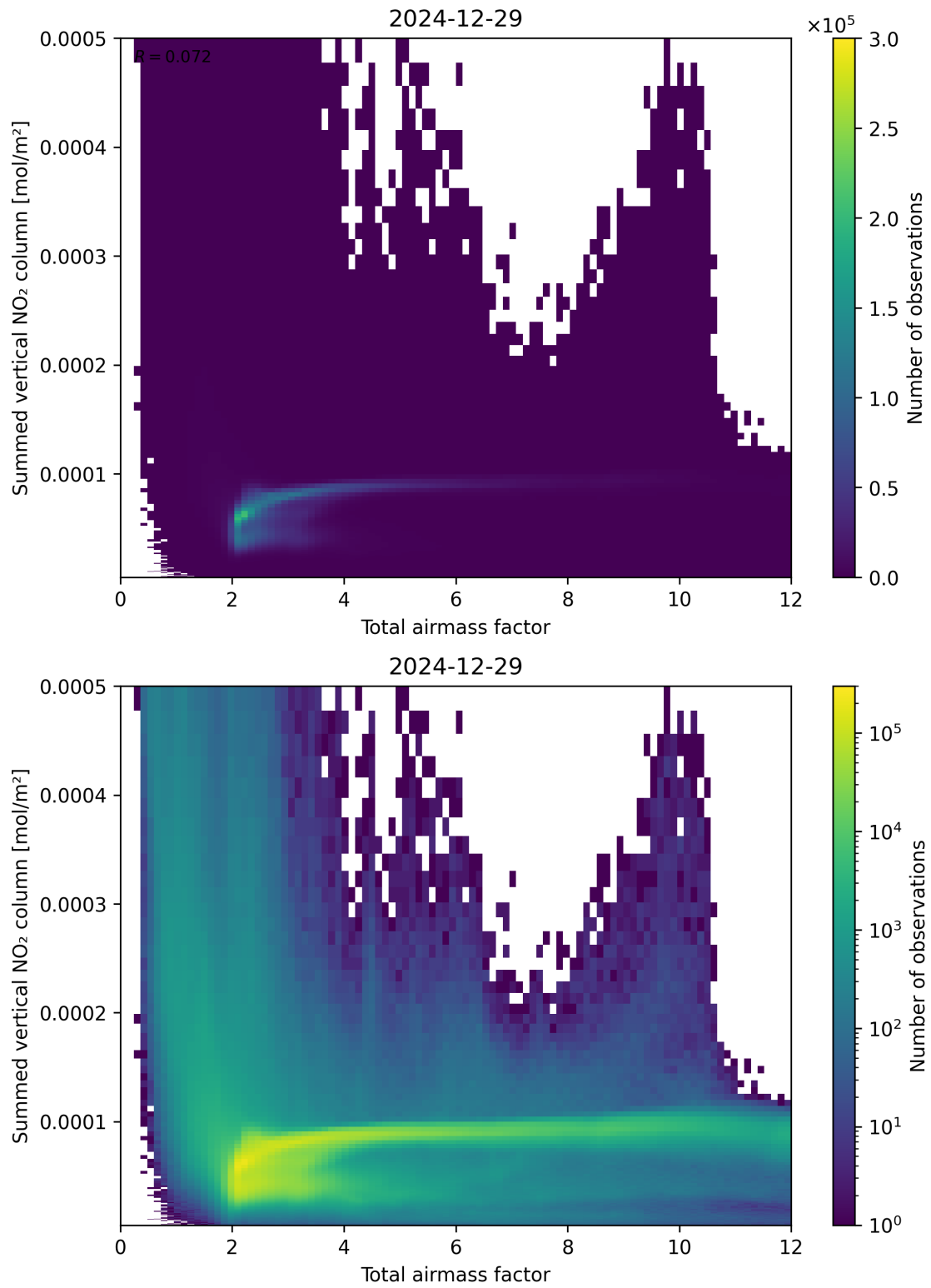
Figure 65: Scatter density plot of “Total airmass factor” against “Summed vertical NO 2 column” for 2024-12-28 to 2024-12-30.
