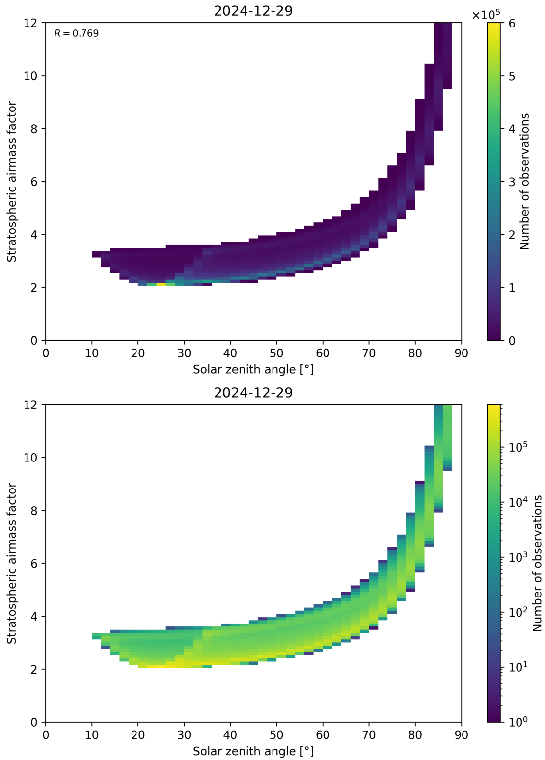
Figure 145: Scatter density plot of “Solar zenith angle” against “Stratospheric airmass factor” for 2024-12-28 to 2024-12-30.
