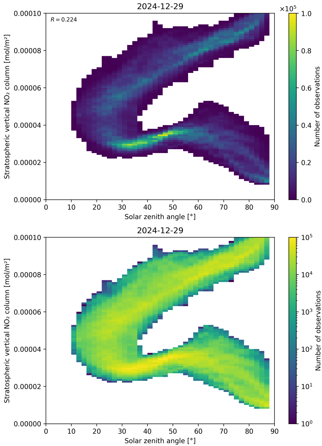
Figure 150: Scatter density plot of “Solar zenith angle” against “Stratospheric vertical NO 2 column” for 2024-12-28 to 2024-12-30.
