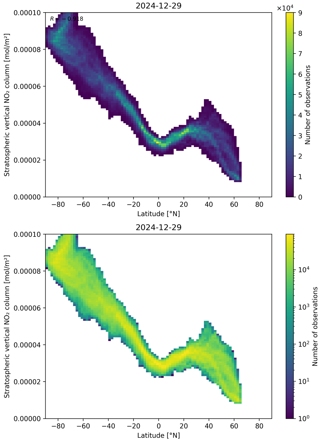
Figure 87: Scatter density plot of “Latitude” against “Stratospheric vertical NO 2 column” for 2024-12-28 to 2024-12-30.
