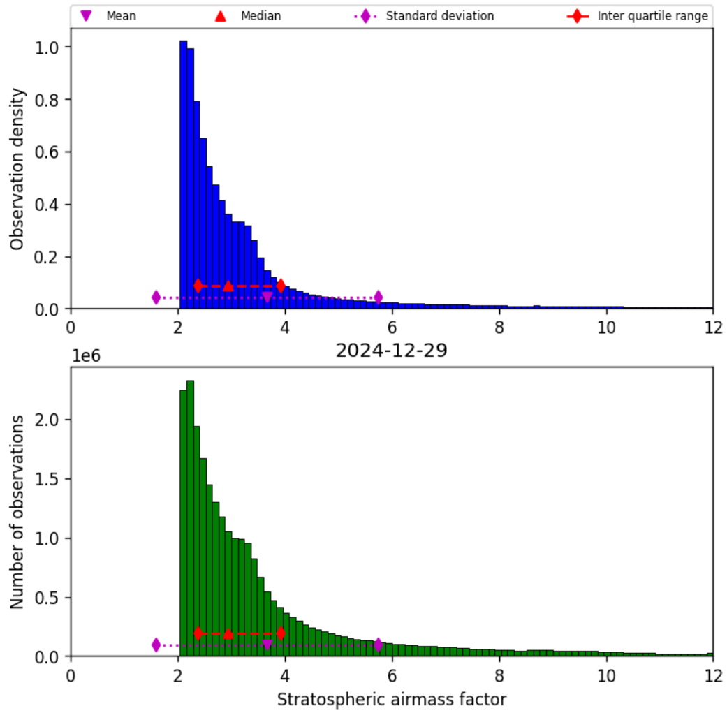
Figure 44: Histogram of “Stratospheric airmass factor” for 2024-12-28 to 2024-12-30
