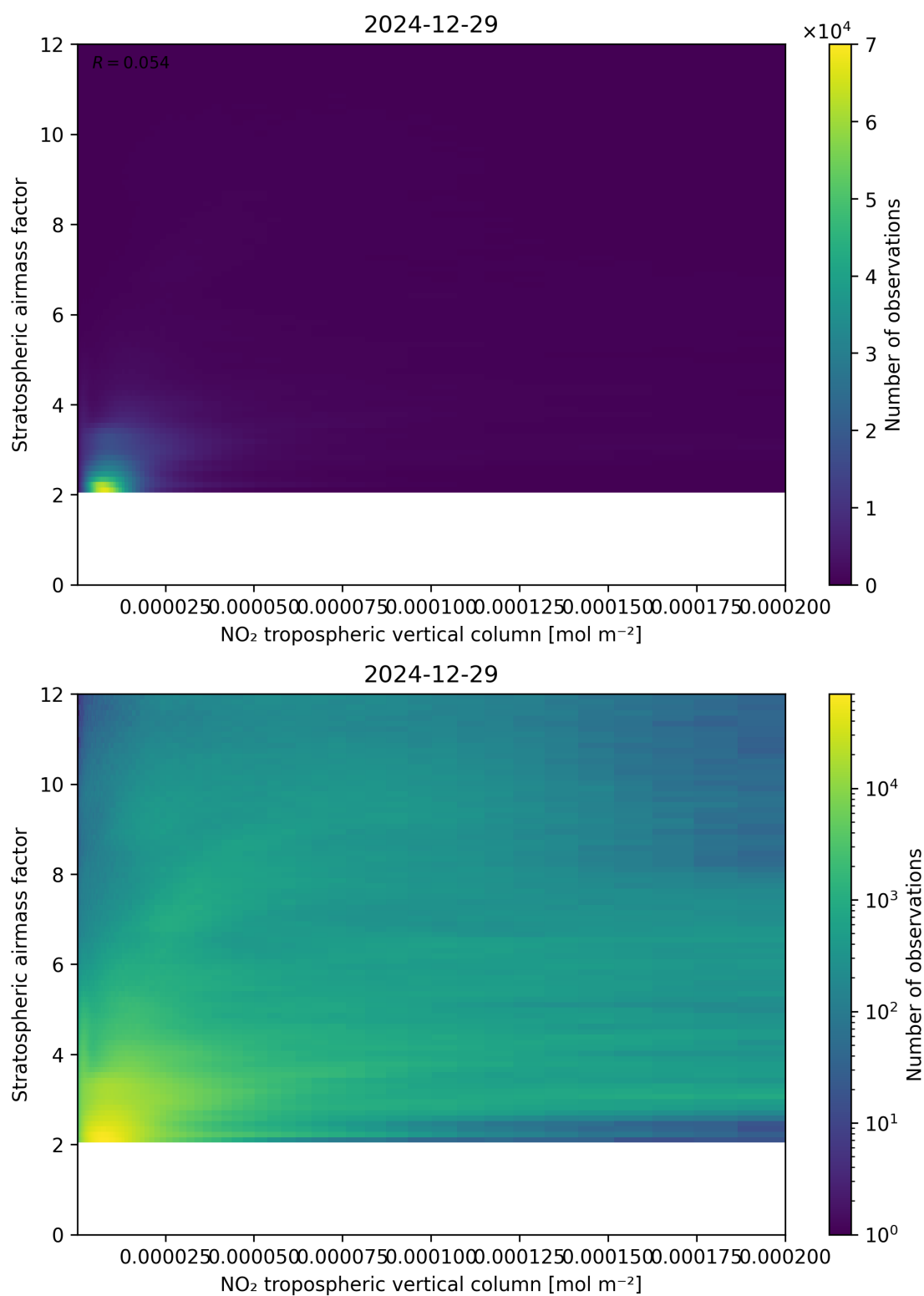
Figure 121: Scatter density plot of “NO 2 tropospheric vertical column” against “Stratospheric airmass factor” for 2024-12-28 to 2024-12-30.
