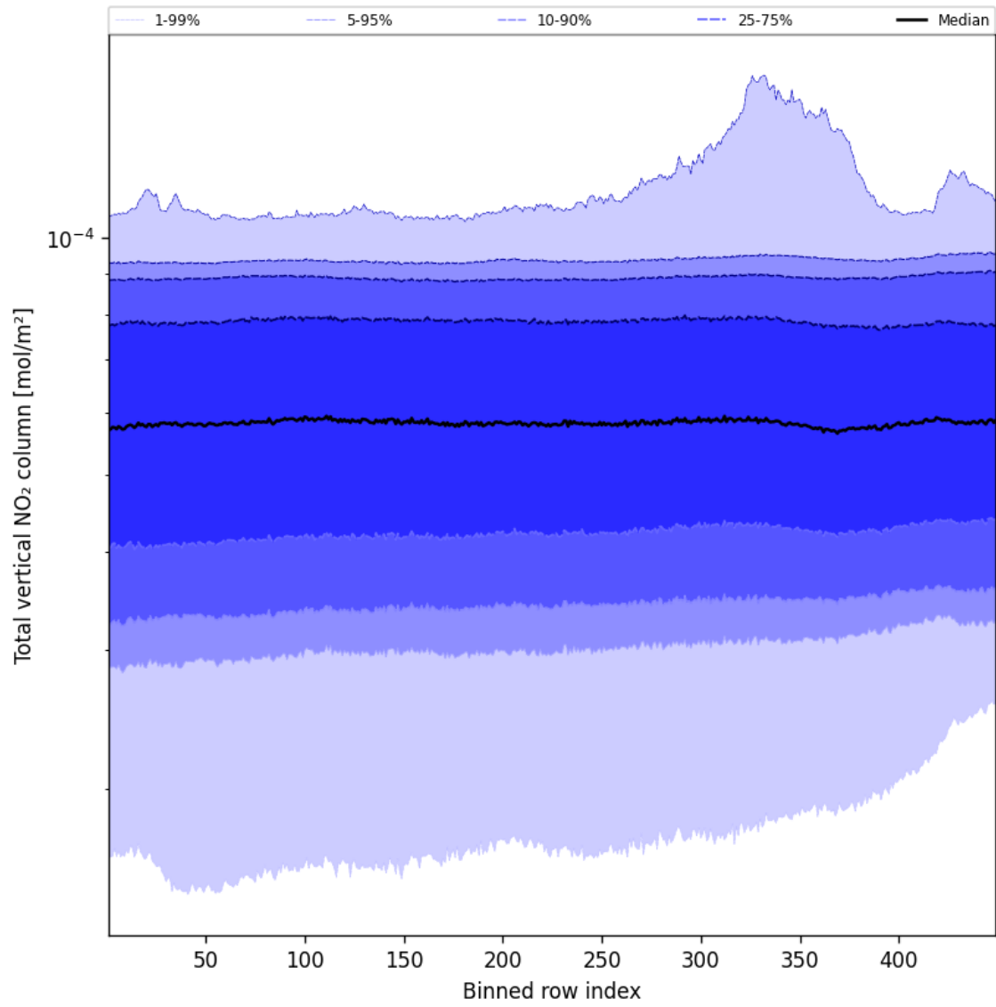
Figure 55: Along track statistics of “Total vertical NO 2 column” for 2024-12-28 to 2024-12-30
