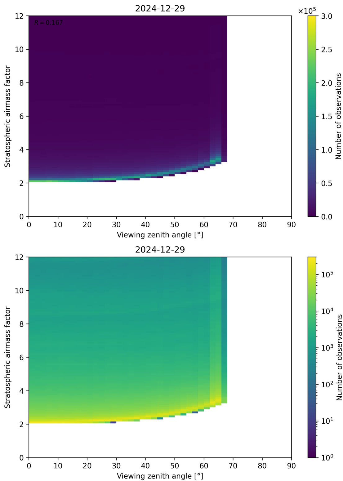
Figure 159: Scatter density plot of “Viewing zenith angle” against “Stratospheric airmass factor” for 2024-12-28 to 2024-12-30.
