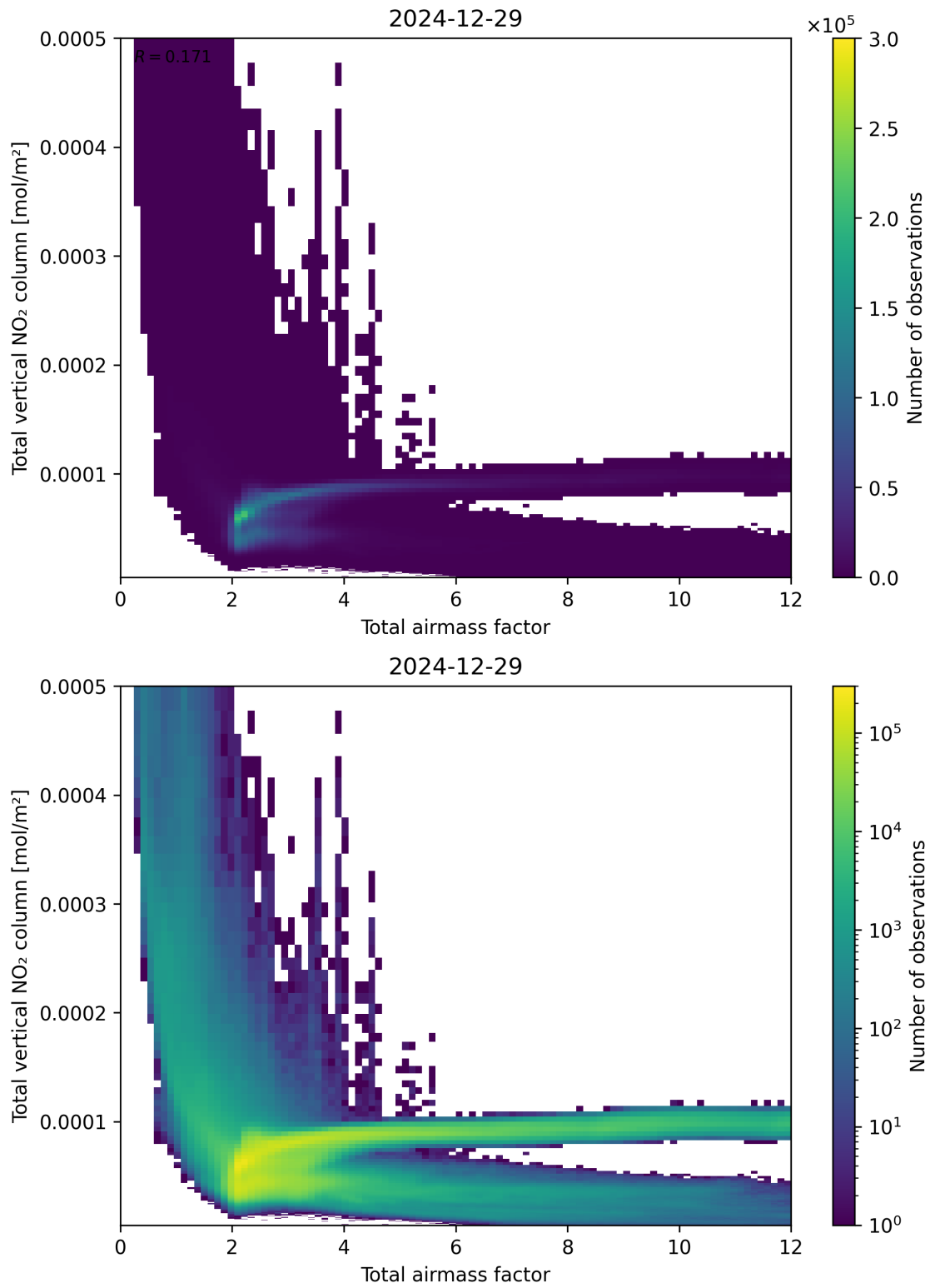
Figure 67: Scatter density plot of “Total airmass factor” against “Total vertical NO 2 column” for 2024-12-28 to 2024-12-30.
