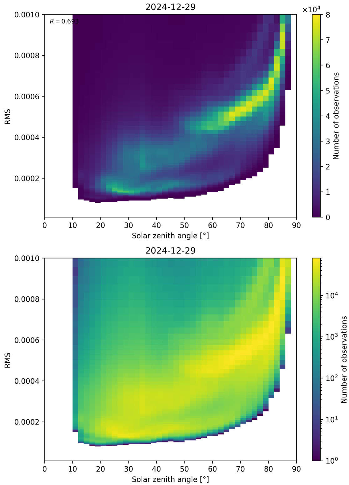
Figure 157: Scatter density plot of “Solar zenith angle” against “RMS” for 2024-12-28 to 2024-12-30.
