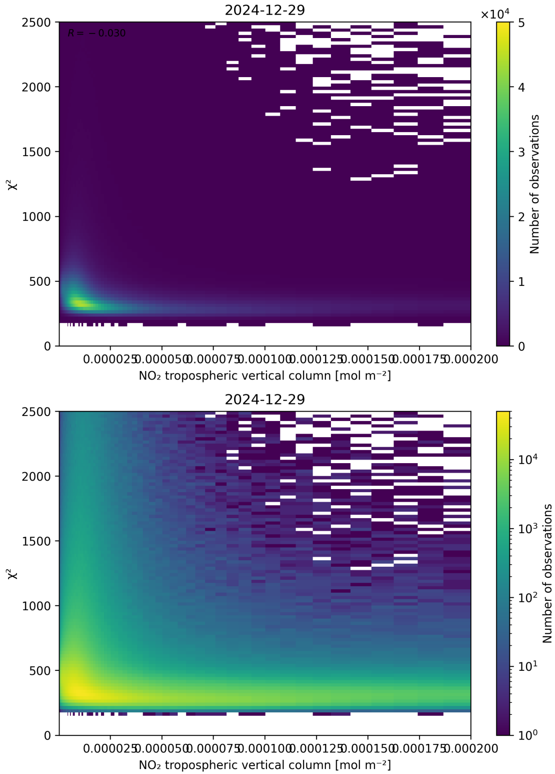
Figure 124: Scatter density plot of “NO 2 tropospheric vertical column” against “ \chi^2 ” for 2024-12-28 to 2024-12-30.
