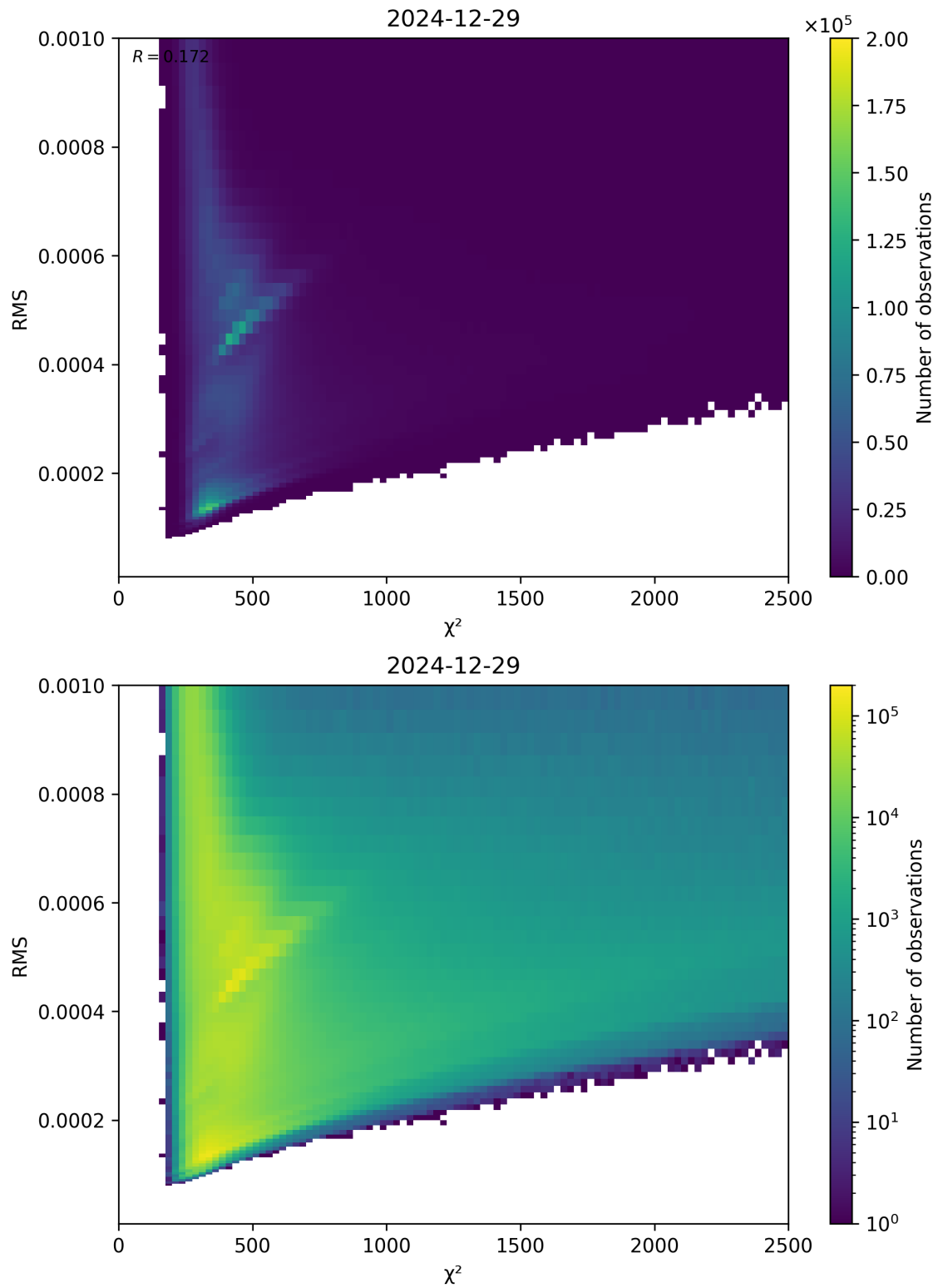
Figure 82: Scatter density plot of “ \chi^2 ” against “RMS” for 2024-12-28 to 2024-12-30.
