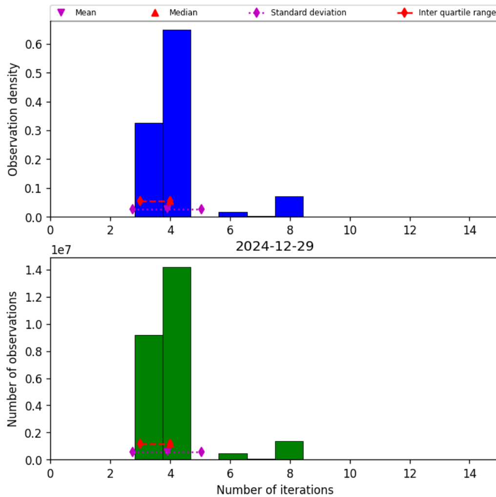
Figure 34: Histogram of “Number of iterations” for 2024-12-28 to 2024-12-30
