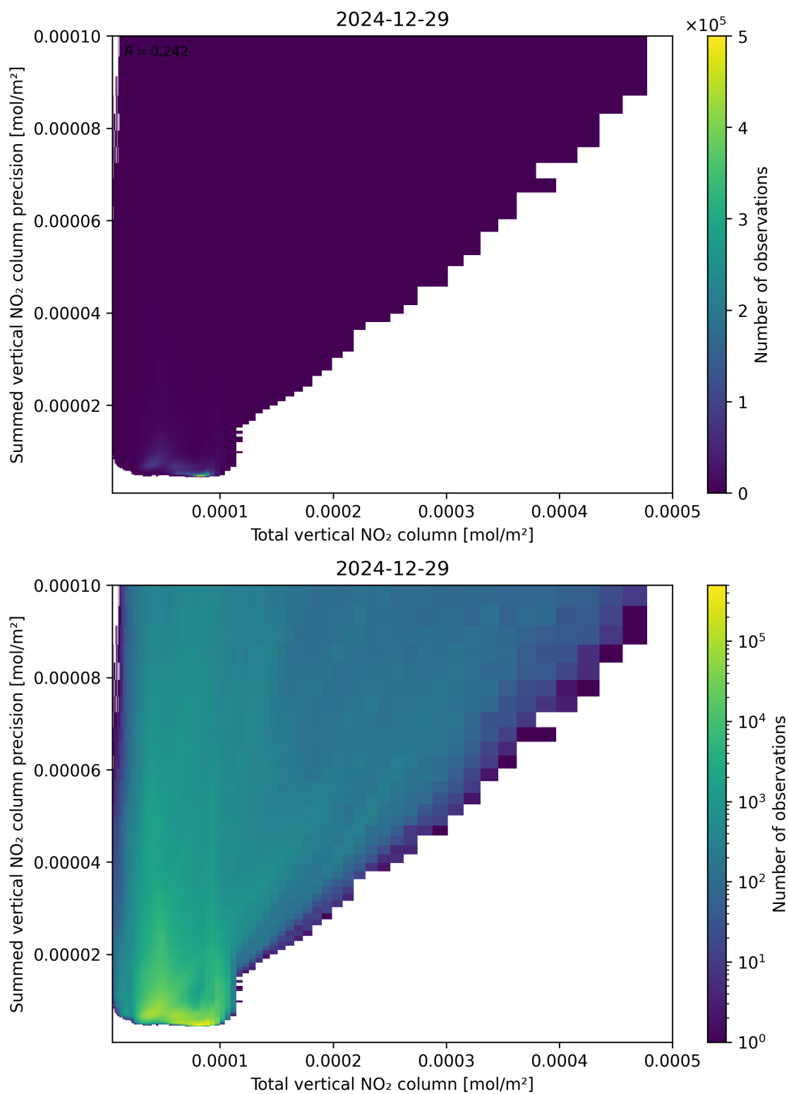
Figure 113: Scatter density plot of “Total vertical NO 2 column” against “Summed vertical NO 2 column precision” for 2024-12-28 to 2024-12-30.
