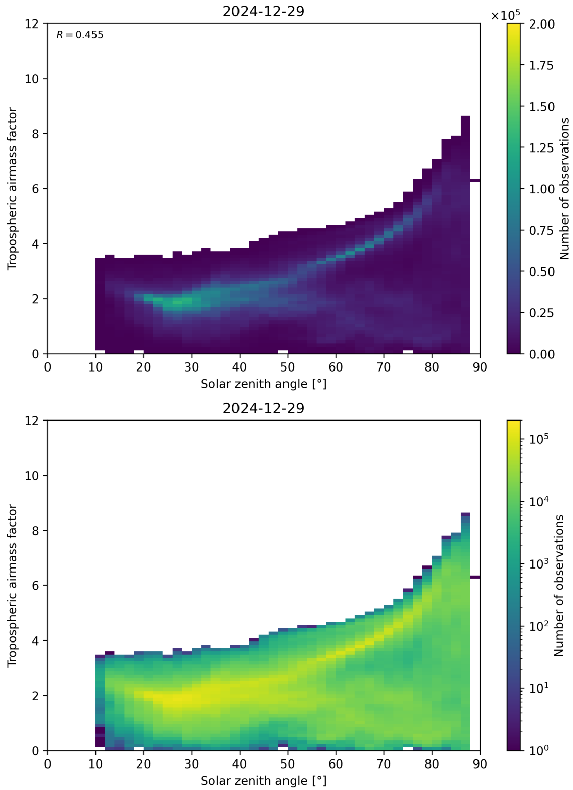
Figure 147: Scatter density plot of “Solar zenith angle” against “Tropospheric airmass factor” for 2024-12-28 to 2024-12-30.
