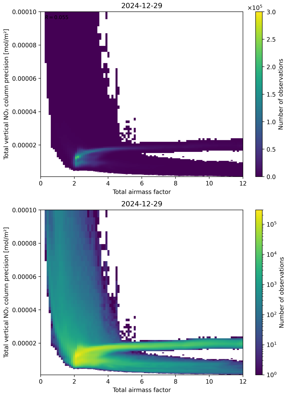
Figure 68: Scatter density plot of “Total airmass factor” against “Total vertical NO 2 column precision” for 2024-12-28 to 2024-12-30.
