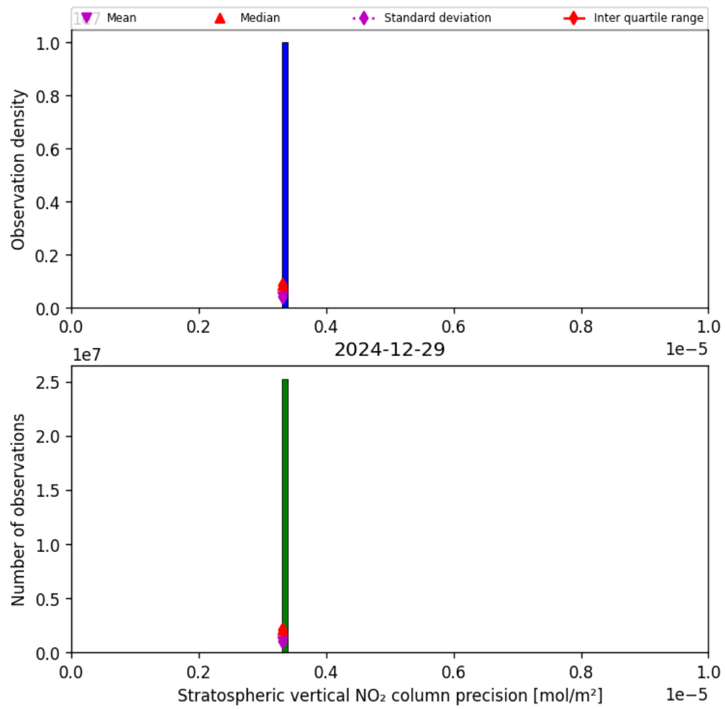
Figure 37: Histogram of “Stratospheric vertical NO 2 column precision” for 2024-12-28 to 2024-12-30
