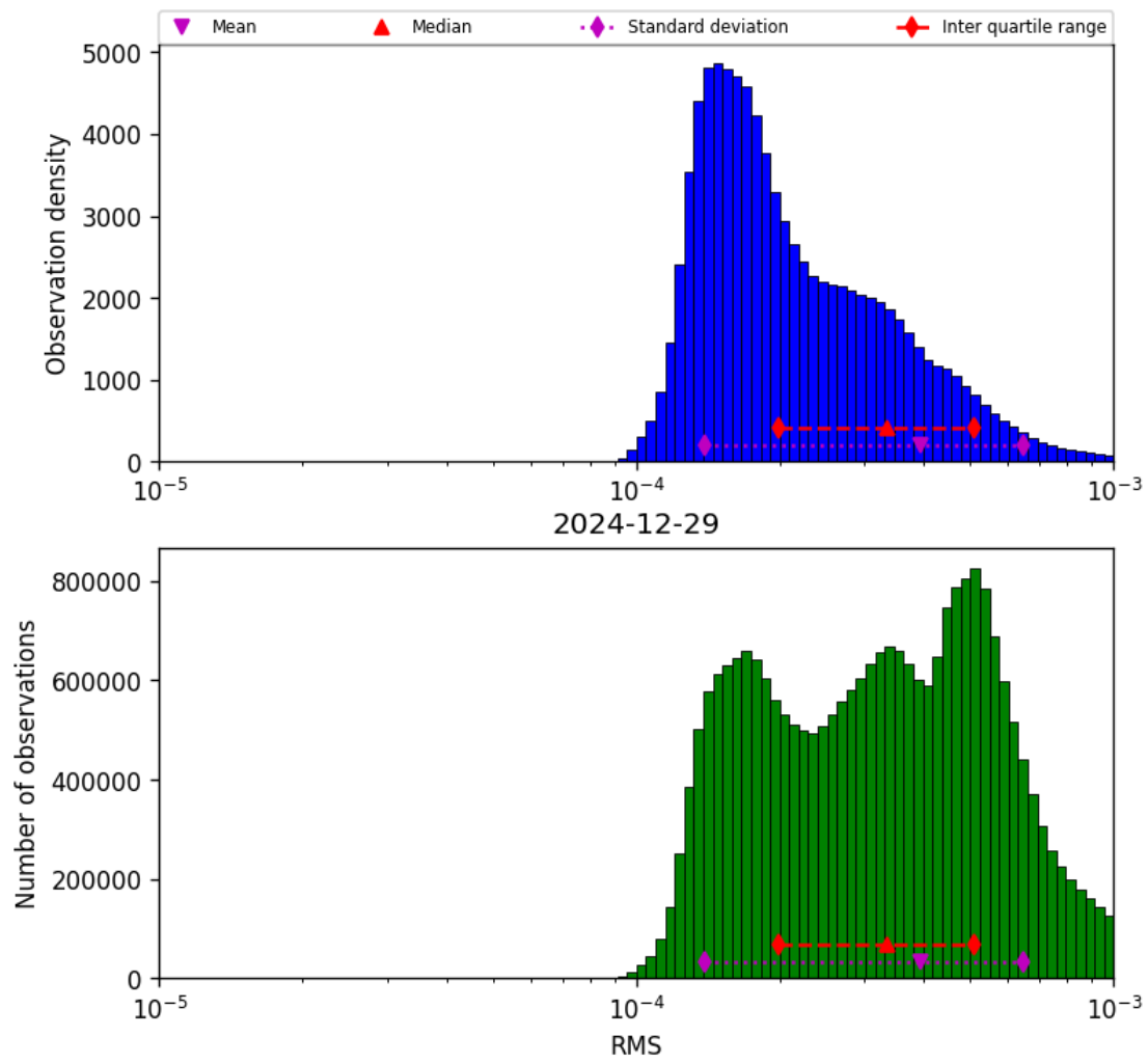
Figure 43: Histogram of “RMS” for 2024-12-28 to 2024-12-30
