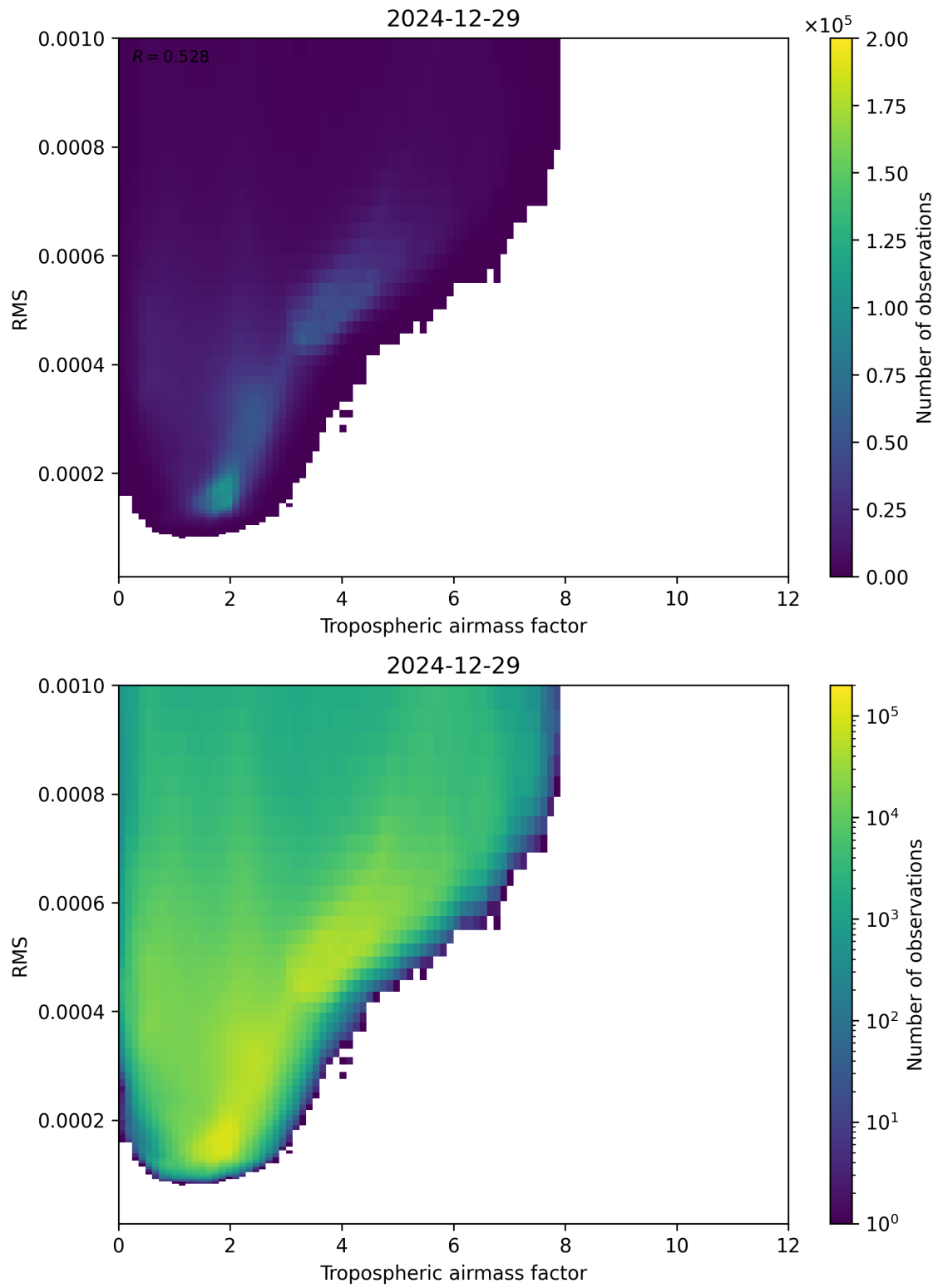
Figure 79: Scatter density plot of “Tropospheric airmass factor” against “RMS” for 2024-12-28 to 2024-12-30.
