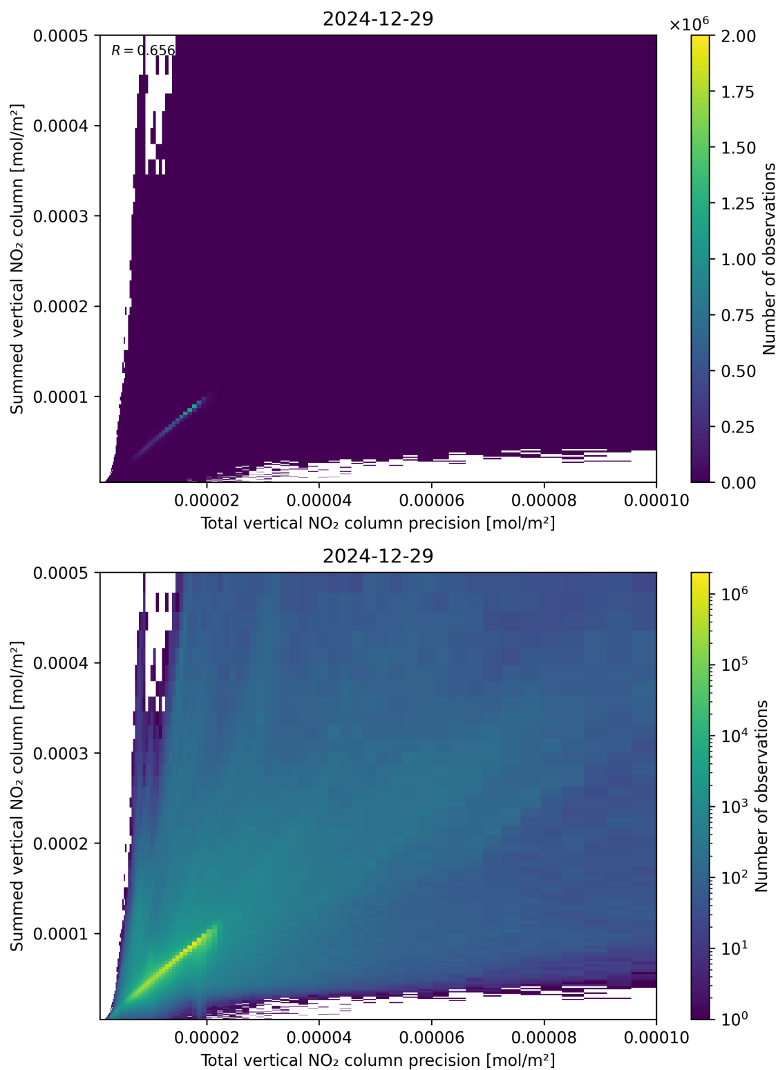
Figure 117: Scatter density plot of “Total vertical NO 2 column precision” against “Summed vertical NO 2 column” for 2024-12-28 to 2024-12-30.
