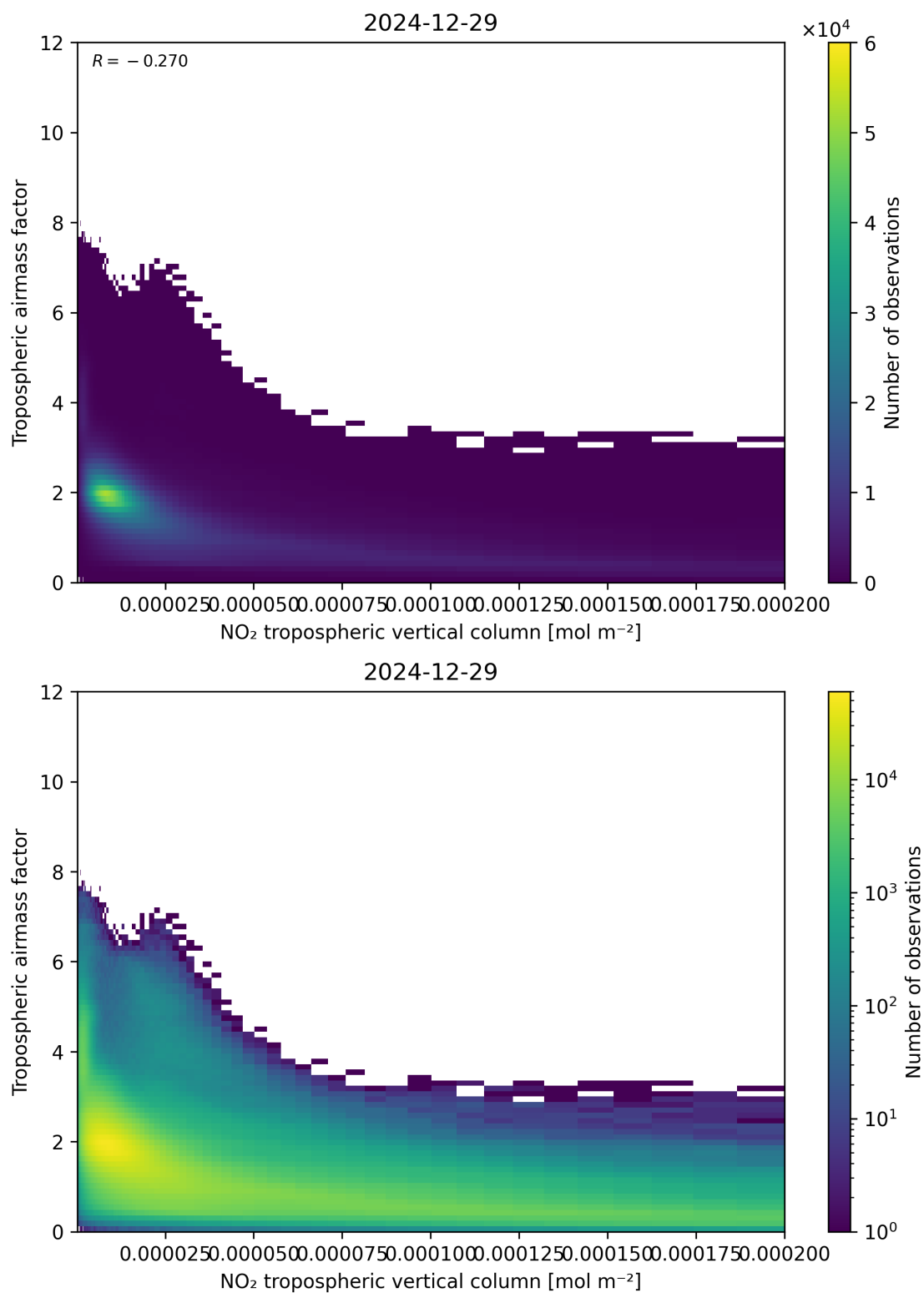
Figure 123: Scatter density plot of “NO 2 tropospheric vertical column” against “Tropospheric air mass factor” for 2024-12-28 to 2024-12-30.
