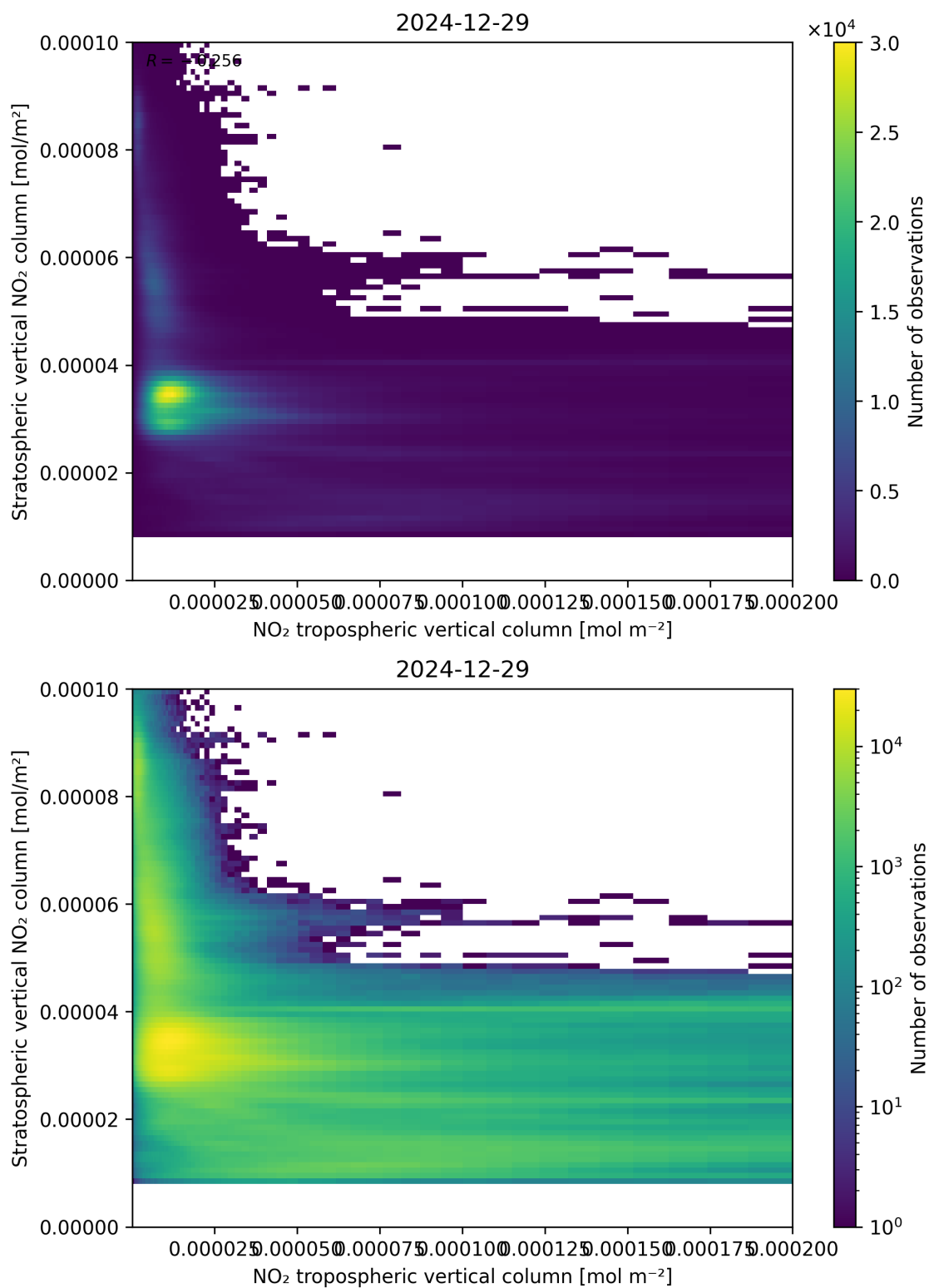
Figure 125: Scatter density plot of “NO 2 tropospheric vertical column” against “Stratospheric vertical NO 2 column” for 2024-12-28 to 2024-12-30.
