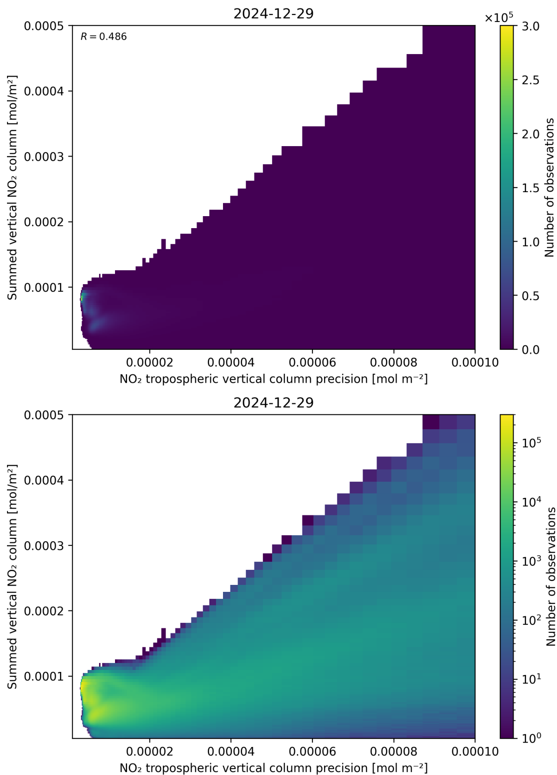
Figure 136: Scatter density plot of “NO 2 tropospheric vertical column precision” against “Summed vertical NO 2 column” for 2024-12-28 to 2024-12-30.
