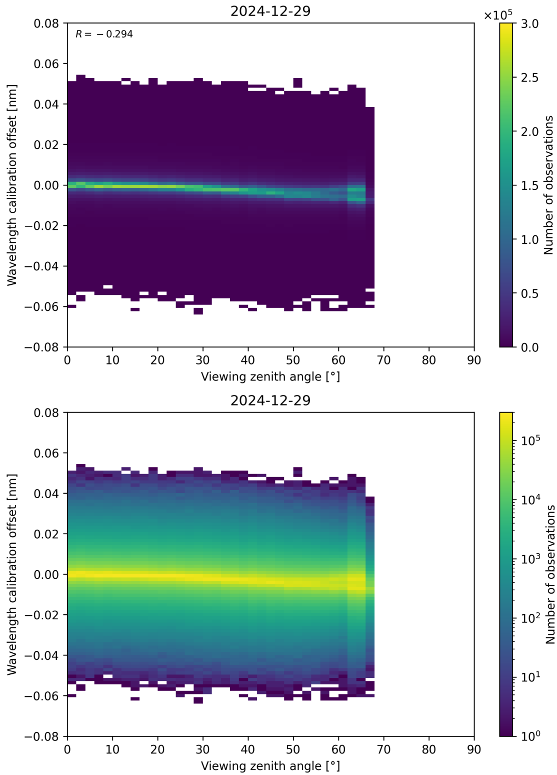
Figure 173: Scatter density plot of “Viewing zenith angle” against “Wavelength calibration offset” for 2024-12-28 to 2024-12-30.
