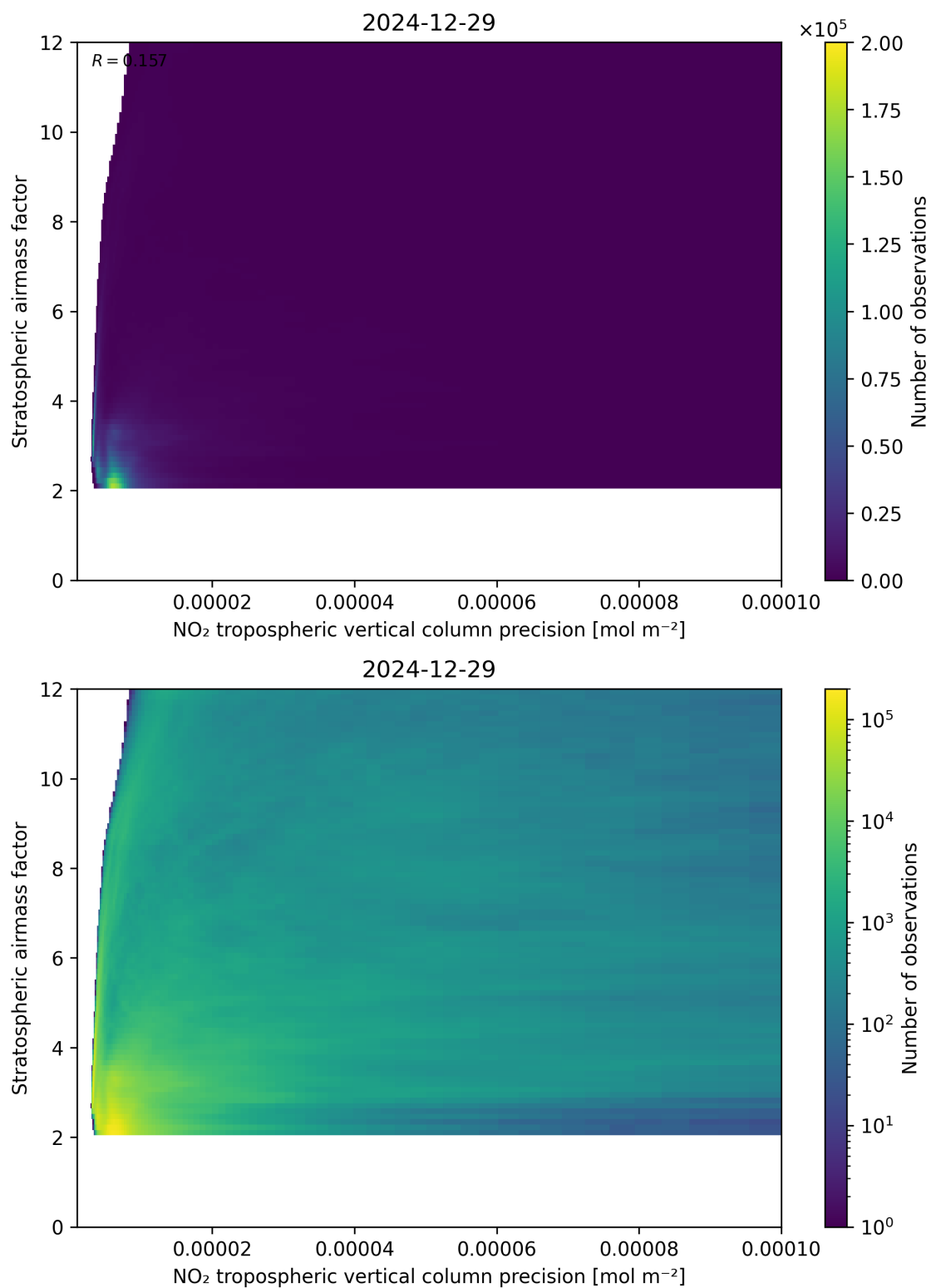
Figure 131: Scatter density plot of “NO 2 tropospheric vertical column precision” against “Stratospheric airmass factor” for 2024-12-28 to 2024-12-30.
