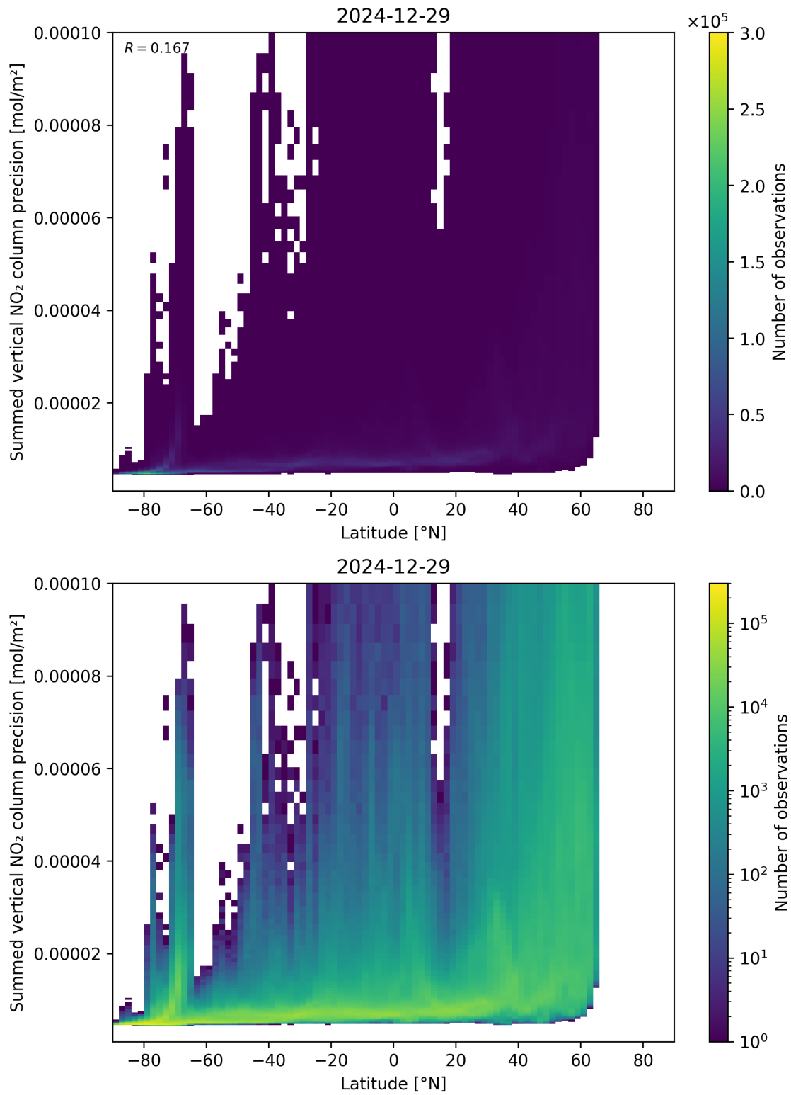
Figure 89: Scatter density plot of “Latitude” against “Summed vertical NO 2 column precision” for 2024-12-28 to 2024-12-30.
