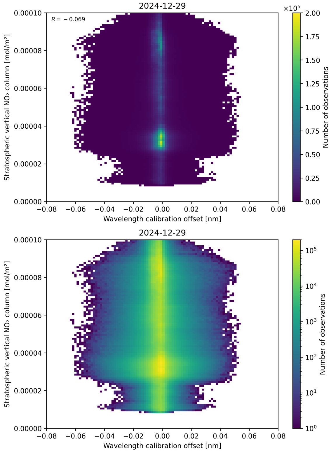
Figure 176: Scatter density plot of “Wavelength calibration offset” against “Stratospheric vertical NO 2 column” for 2024-12-28 to 2024-12-30.
