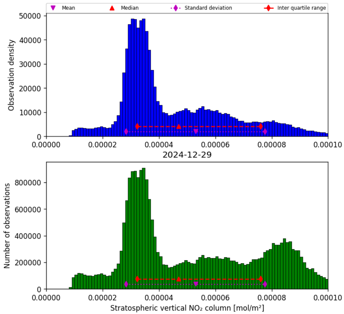
Figure 36: Histogram of “Stratospheric vertical NO 2 column” for 2024-12-28 to 2024-12-30
