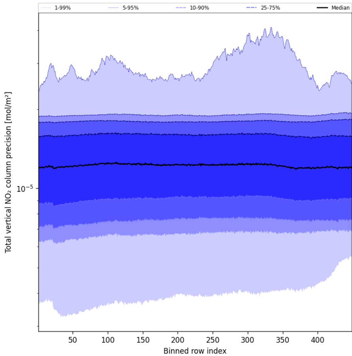
Figure 56: Along track statistics of “Total vertical NO 2 column precision” for 2024-12-28 to 2024-12-30
