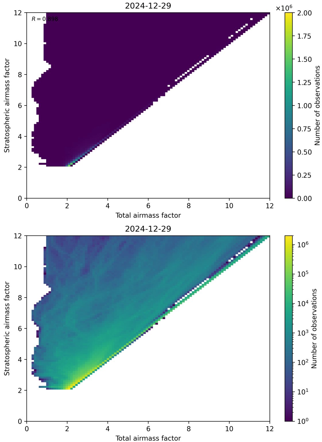
Figure 62: Scatter density plot of “Total airmass factor” against “Stratospheric airmass factor” for 2024-12-28 to 2024-12-30.
