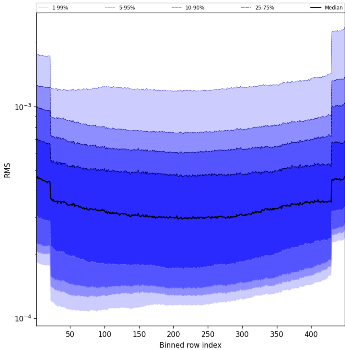
Figure 60: Along track statistics of “RMS” for 2024-12-28 to 2024-12-30
