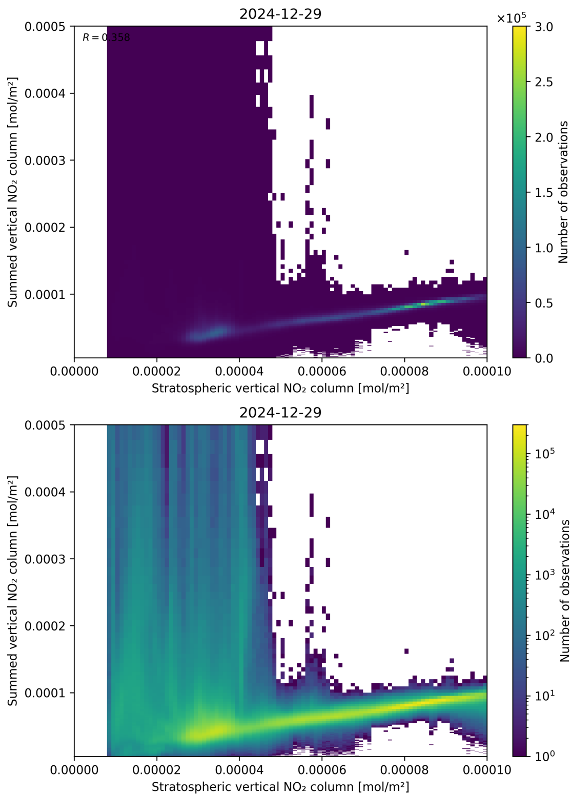
Figure 98: Scatter density plot of “Stratospheric vertical NO 2 column” against “Summed vertical NO 2 column” for 2024-12-28 to 2024-12-30.
