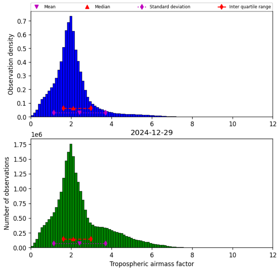
Figure 31: Histogram of “Tropospheric airmass factor” for 2024-12-28 to 2024-12-30
