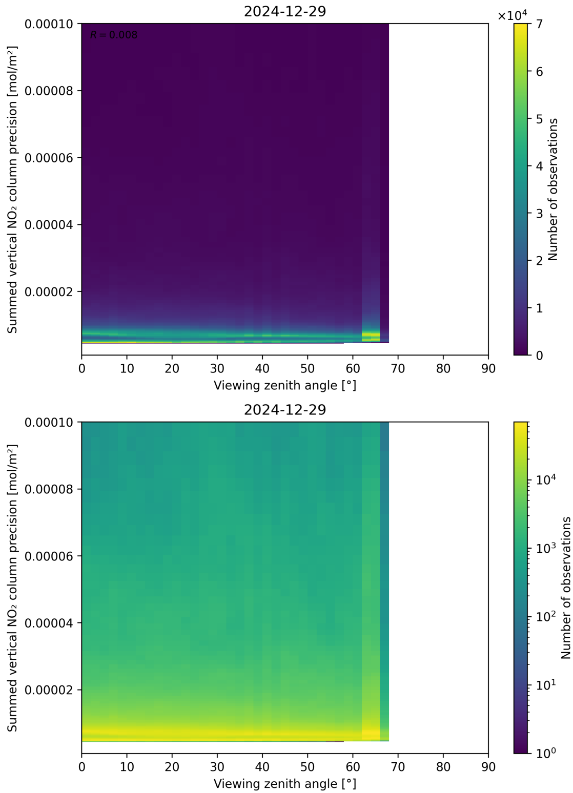
Figure 166: Scatter density plot of “Viewing zenith angle” against “Summed vertical NO 2 column precision” for 2024-12-28 to 2024-12-30.
