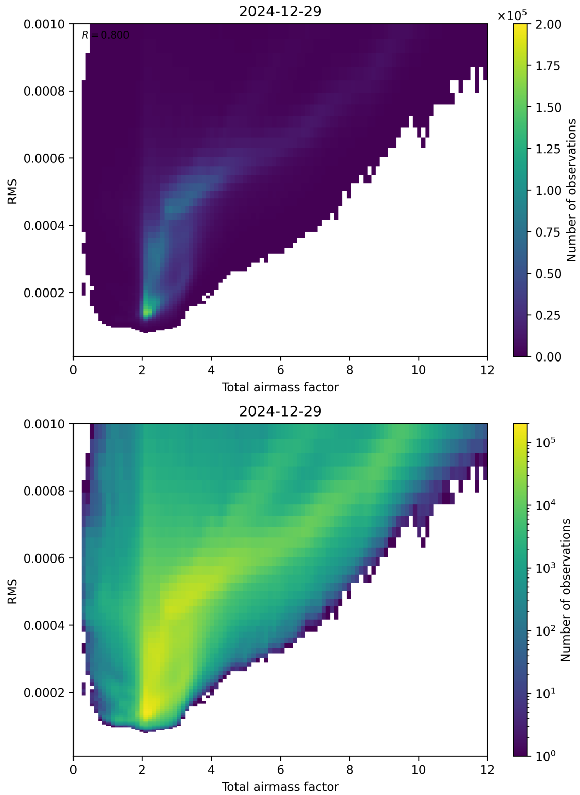
Figure 69: Scatter density plot of “Total airmass factor” against “RMS” for 2024-12-28 to 2024-12-30.
