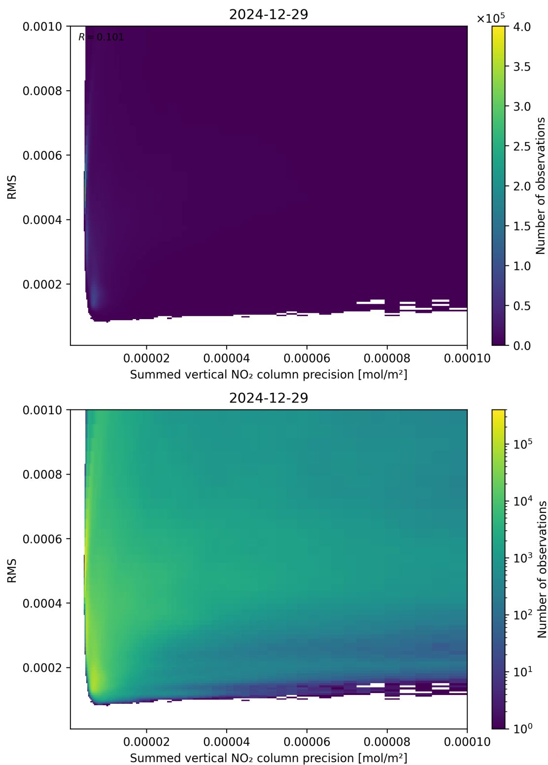
Figure 108: Scatter density plot of “Summed vertical NO 2 column precision” against “RMS” for 2024-12-28 to 2024-12-30.
