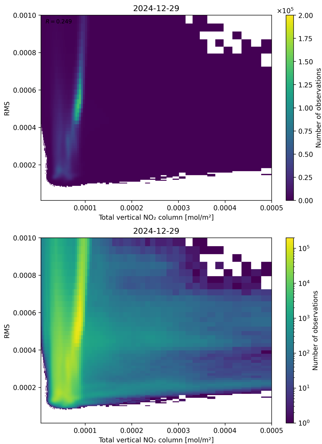
Figure 120: Scatter density plot of “Total vertical NO 2 column” against “RMS” for 2024-12-28 to 2024-12-30.
