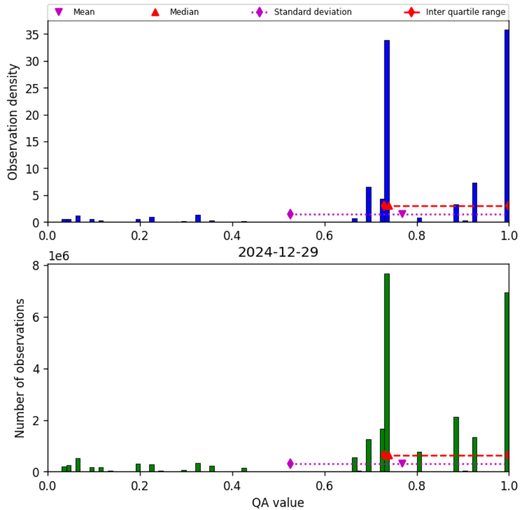
Figure 28: Histogram of “QA value” for 2024-12-28 to 2024-12-30
