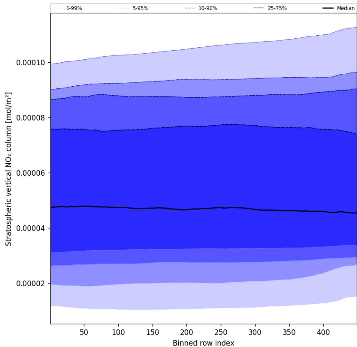
Figure 53: Along track statistics of “Stratospheric vertical NO 2 column” for 2024-12-28 to 2024-12-30
