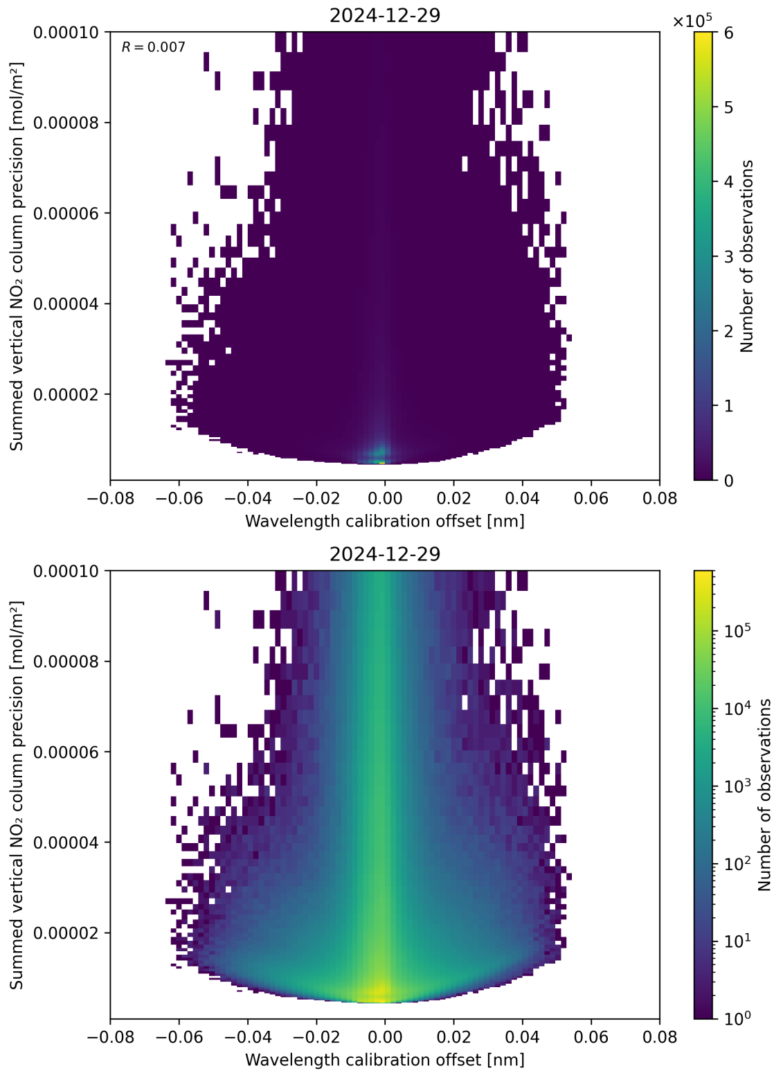
Figure 178: Scatter density plot of “Wavelength calibration offset” against “Summed vertical NO 2 column precision” for 2024-12-28 to 2024-12-30.
