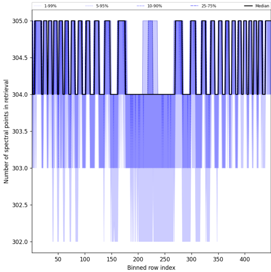
Figure 50: Along track statistics of “Number of spectral points in retrieval” for 2024-12-28 to 2024-12-30
