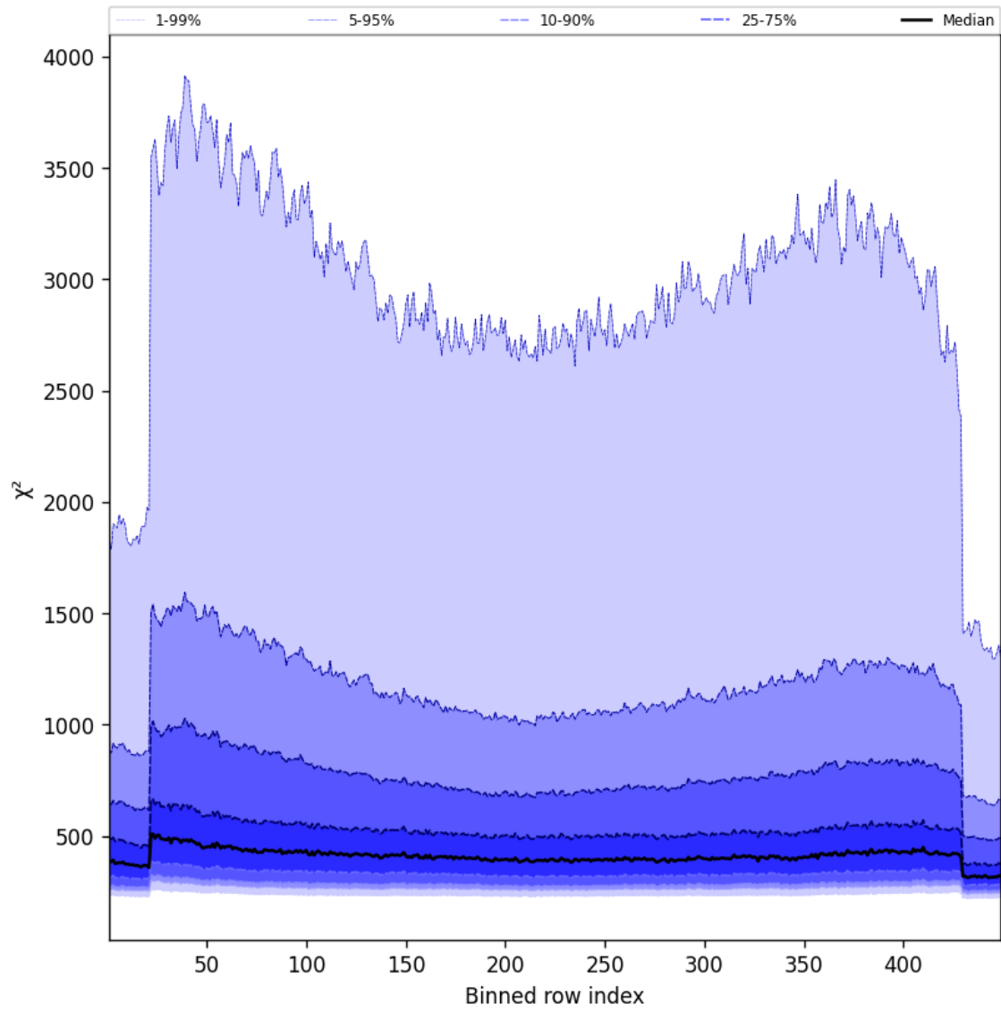
Figure 59: Along track statistics of “ \chi^2 ” for 2024-12-28 to 2024-12-30
