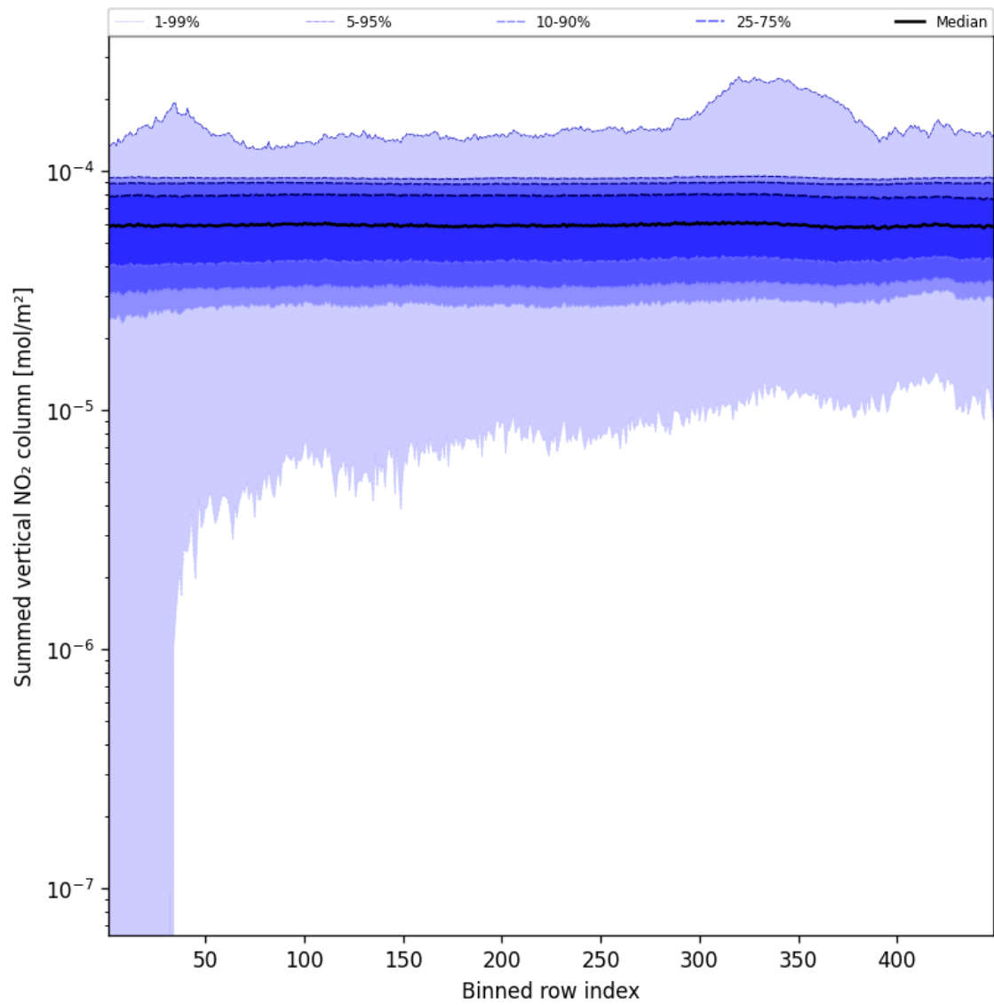
Figure 57: Along track statistics of “Summed vertical NO 2 column” for 2024-12-28 to 2024-12-30
