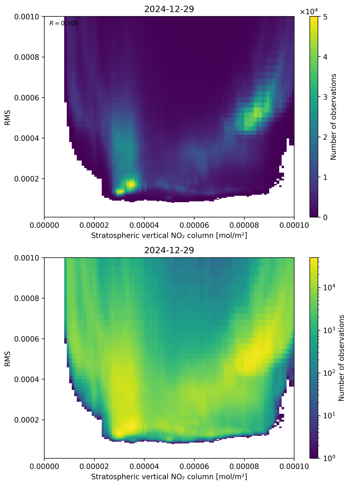
Figure 102: Scatter density plot of “Stratospheric vertical NO 2 column” against “RMS” for 2024-12-28 to 2024-12-30.
