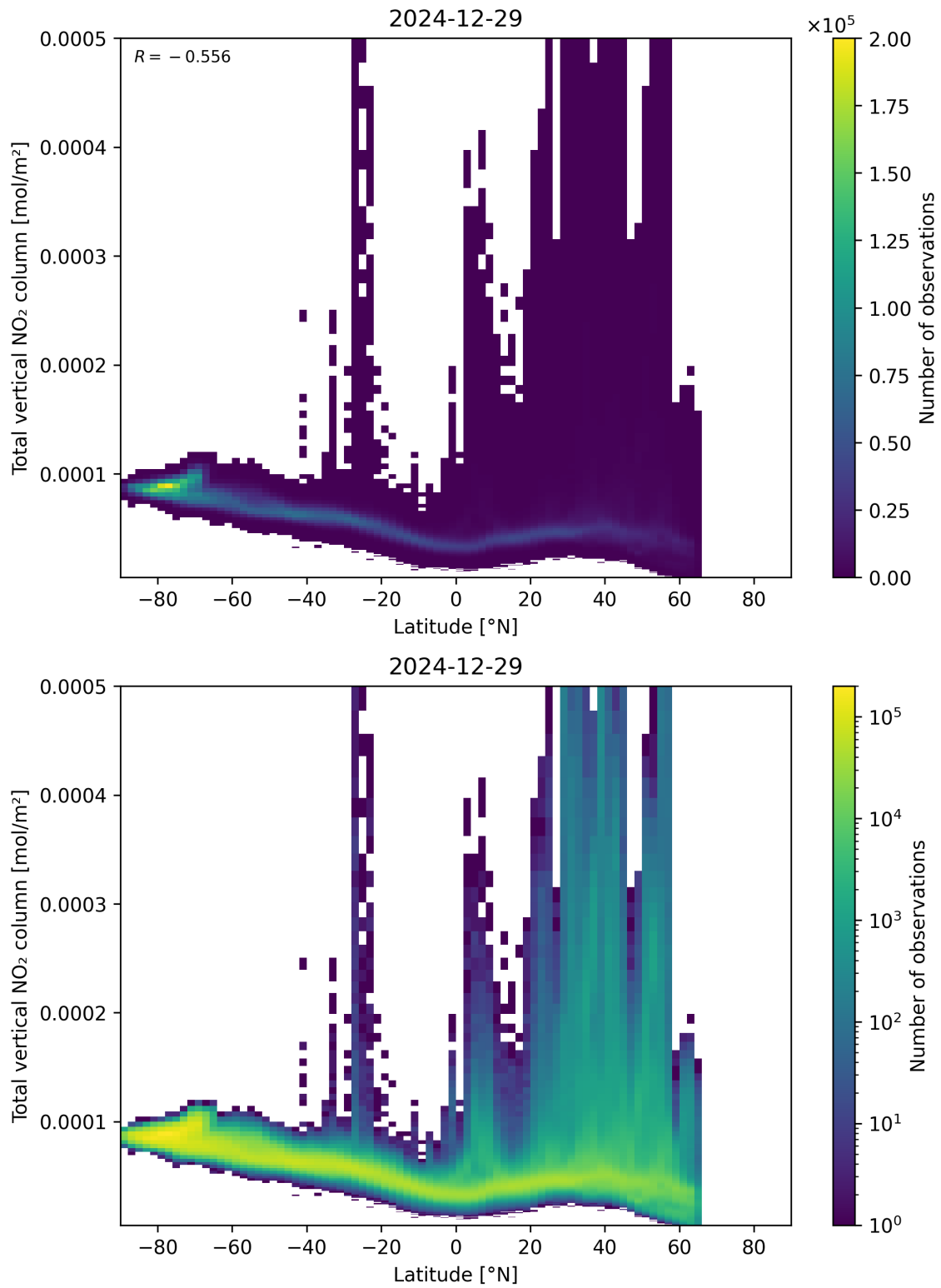
Figure 90: Scatter density plot of “Latitude” against “Total vertical NO 2 column” for 2024-12-28 to 2024-12-30.
