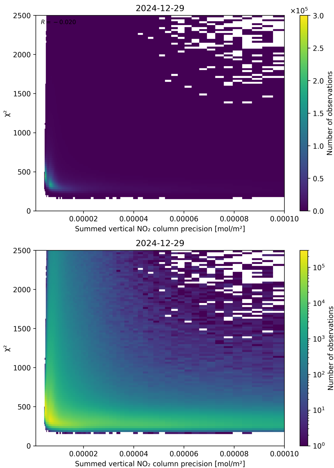
Figure 107: Scatter density plot of “Summed vertical NO 2 column precision” against “ \chi^2 ” for 2024-12-28 to 2024-12-30.
