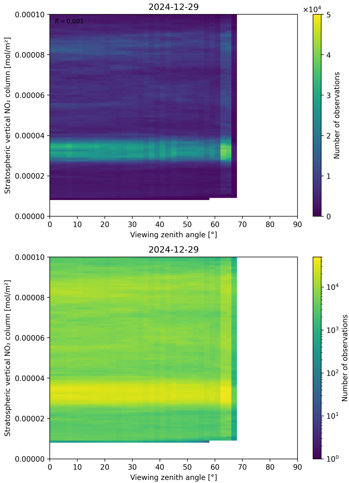
Figure 164: Scatter density plot of “Viewing zenith angle” against “Stratospheric vertical NO 2 column” for 2024-12-28 to 2024-12-30.
