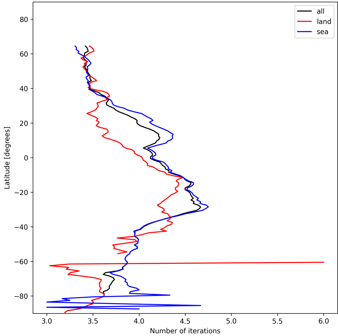
Figure 17: Zonal average of “Number of iterations” for 2024-12-28 to 2024-12-30.
