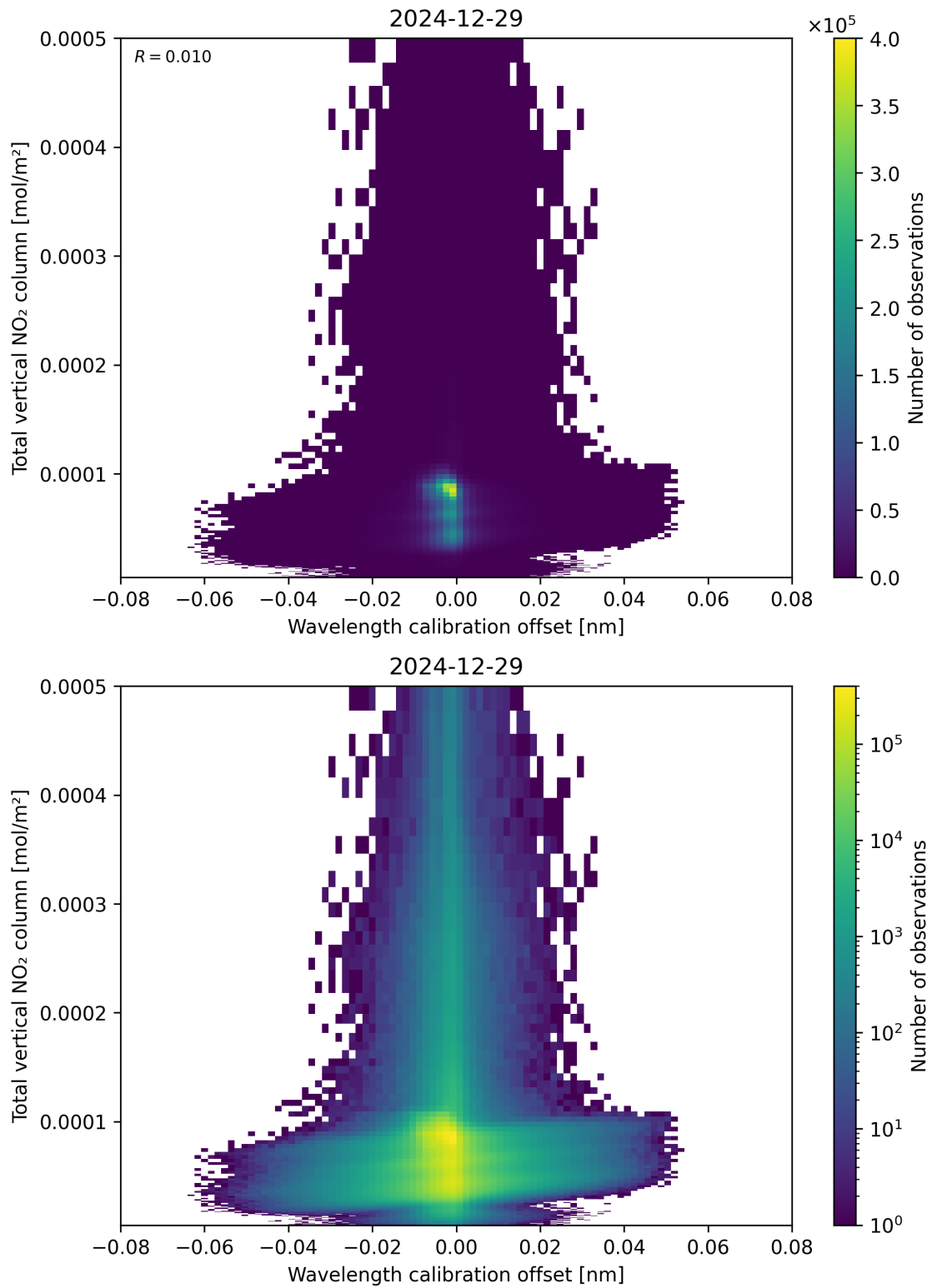
Figure 179: Scatter density plot of “Wavelength calibration offset” against “Total vertical NO 2 column” for 2024-12-28 to 2024-12-30.
