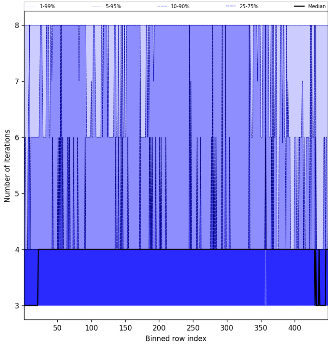
Figure 51: Along track statistics of “Number of iterations” for 2024-12-28 to 2024-12-30
