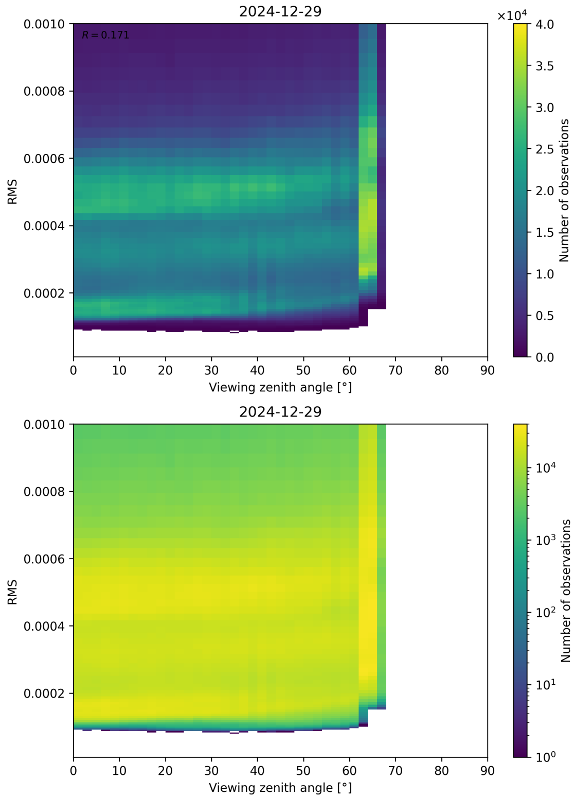
Figure 171: Scatter density plot of “Viewing zenith angle” against “RMS” for 2024-12-28 to 2024-12-30.
