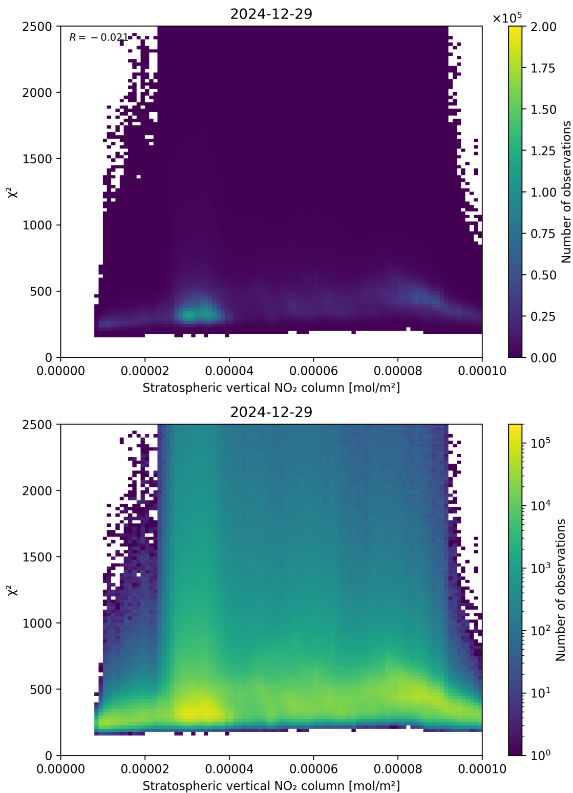
Figure 97: Scatter density plot of “Stratospheric vertical NO 2 column” against “ \chi^2 ” for 2024-12-28 to 2024-12-30.
