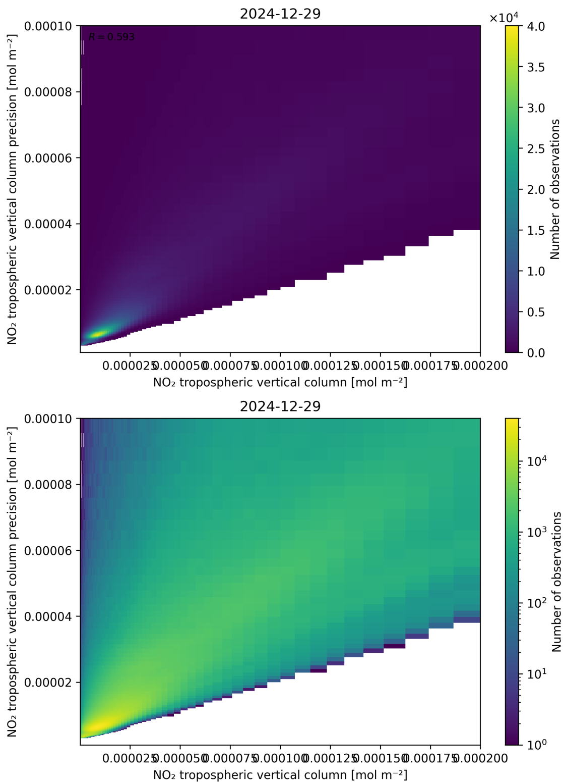
Figure 130: Scatter density plot of “NO 2 tropospheric vertical column” against “NO 2 tropospheric vertical column precision” for 2024-12-28 to 2024-12-30.
