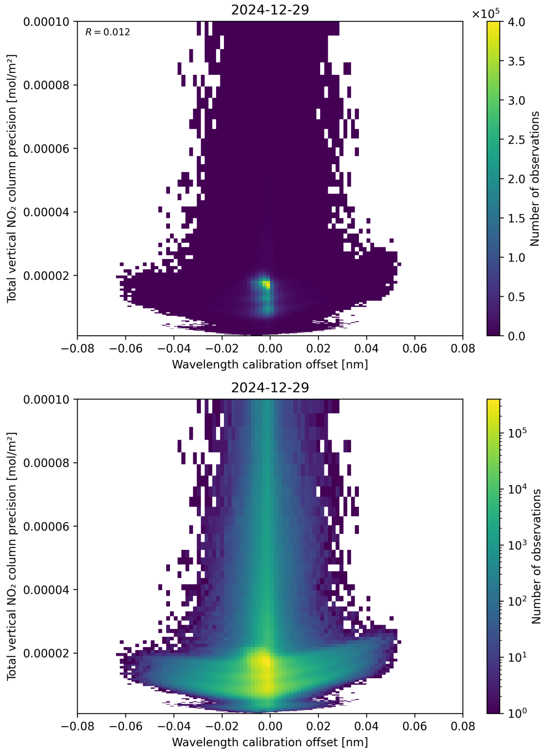
Figure 180: Scatter density plot of “Wavelength calibration offset” against “Total vertical NO 2 column precision” for 2024-12-28 to 2024-12-30.
