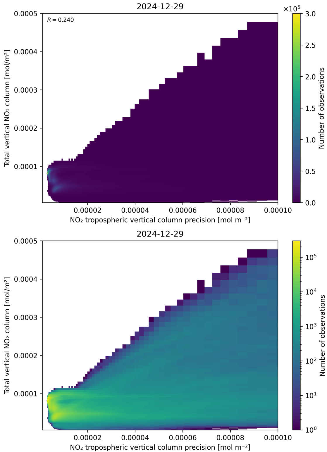
Figure 138: Scatter density plot of “NO 2 tropospheric vertical column precision” against “Total vertical NO 2 column” for 2024-12-28 to 2024-12-30.
