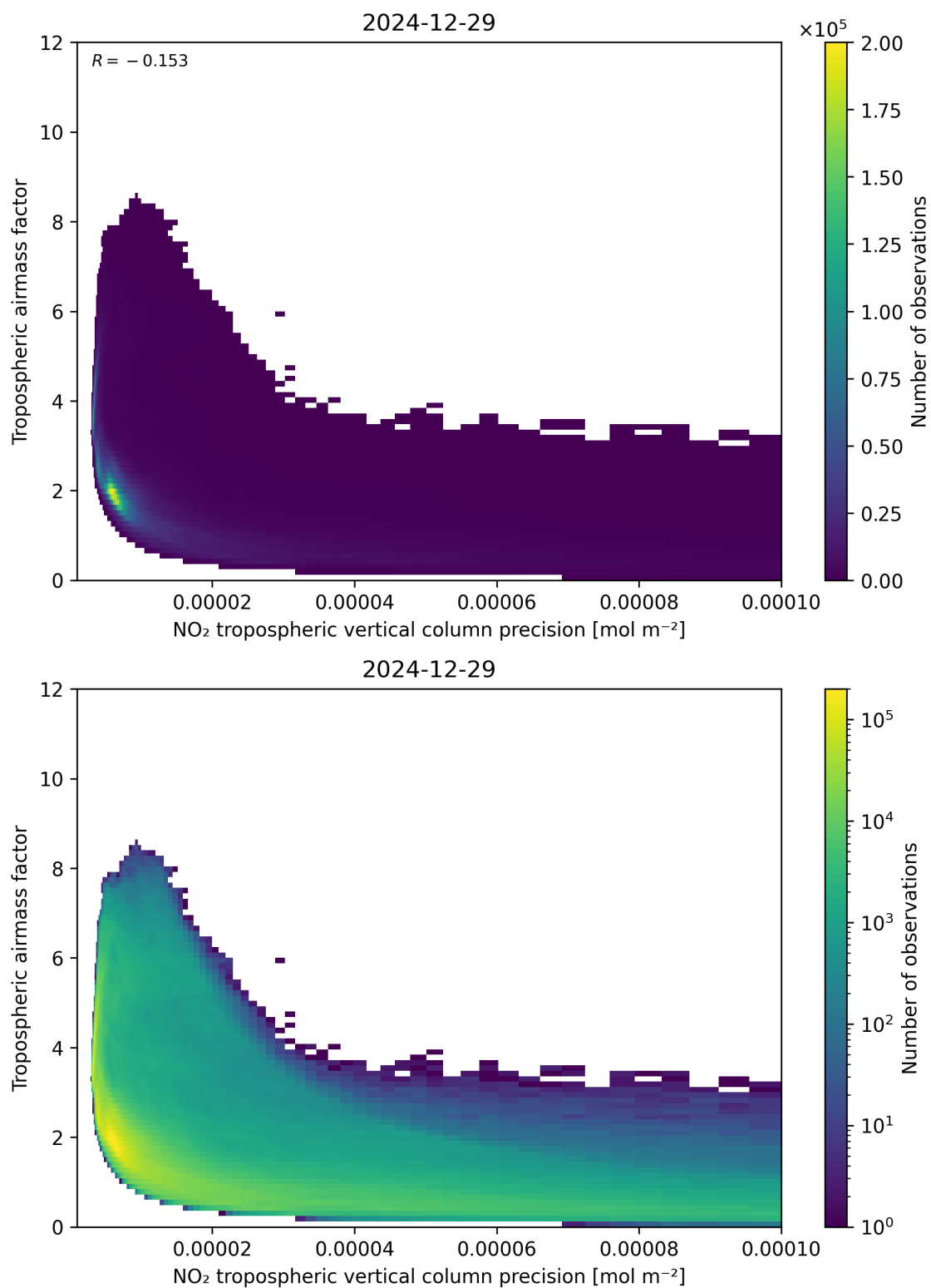
Figure 133: Scatter density plot of “NO 2 tropospheric vertical column precision” against “Tropospheric airmass factor” for 2024-12-28 to 2024-12-30.
