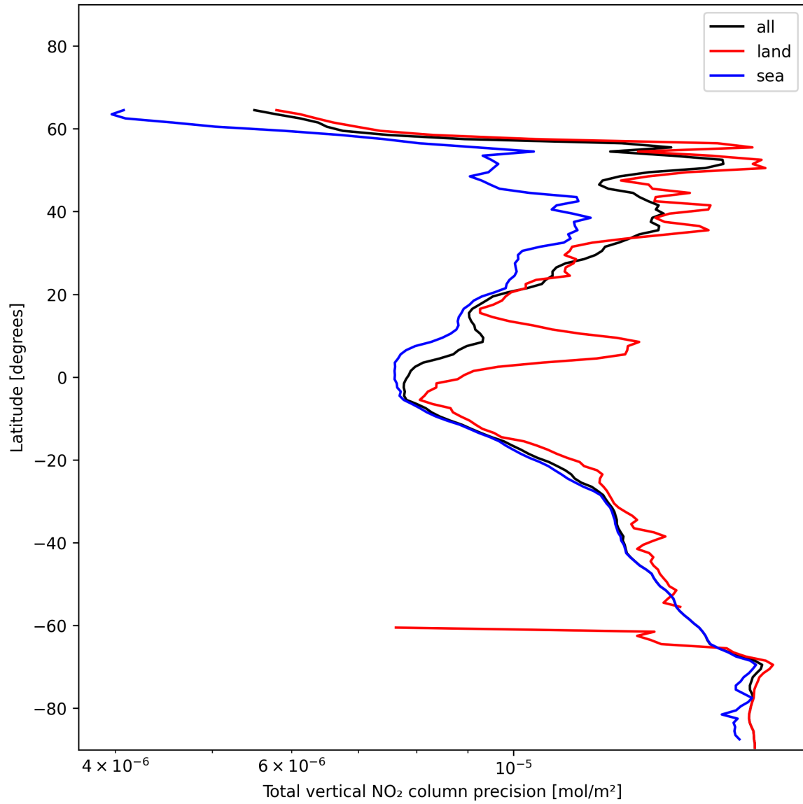
Figure 22: Zonal average of “Total vertical NO 2 column precision” for 2024-12-28 to 2024-12-30.
