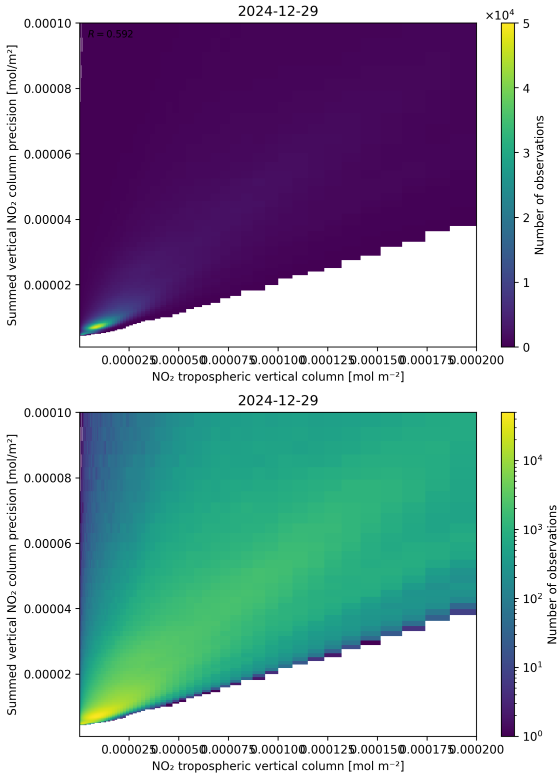
Figure 127: Scatter density plot of “NO 2 tropospheric vertical column” against “Summed vertical NO 2 column precision” for 2024-12-28 to 2024-12-30.
