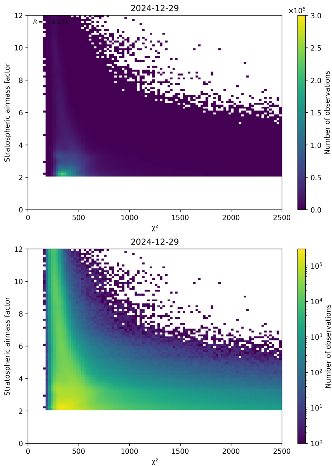
Figure 81: Scatter density plot of “ \chi^2 ” against “Stratospheric airmass factor” for 2024-12-28 to 2024-12-30.
