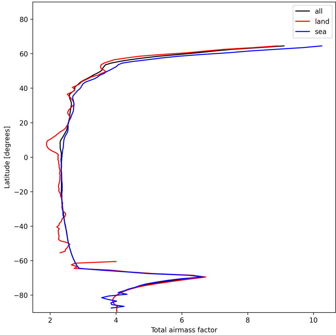
Figure 15: Zonal average of “Total airmass factor” for 2024-12-28 to 2024-12-30.
