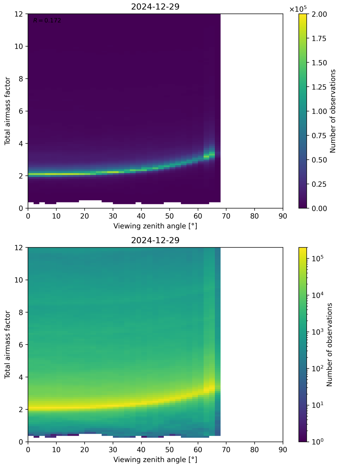
Figure 160: Scatter density plot of “Viewing zenith angle” against “Total airmass factor” for 2024-12-28 to 2024-12-30.
