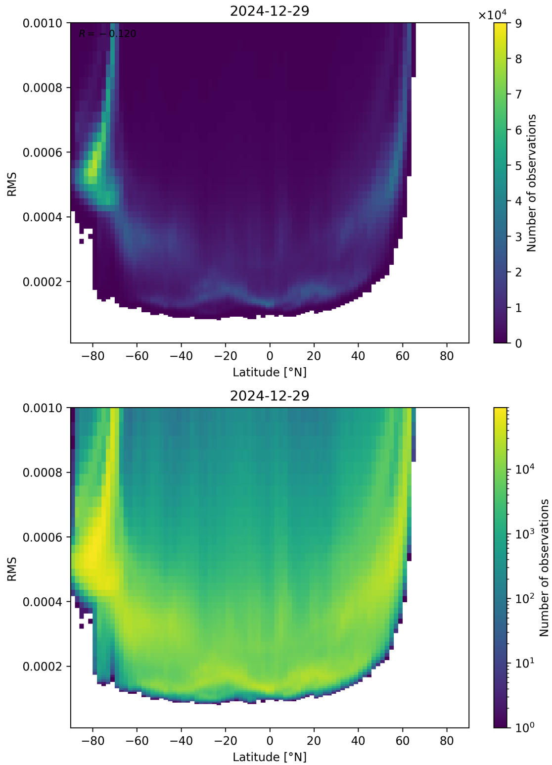
Figure 94: Scatter density plot of “Latitude” against “RMS” for 2024-12-28 to 2024-12-30.
