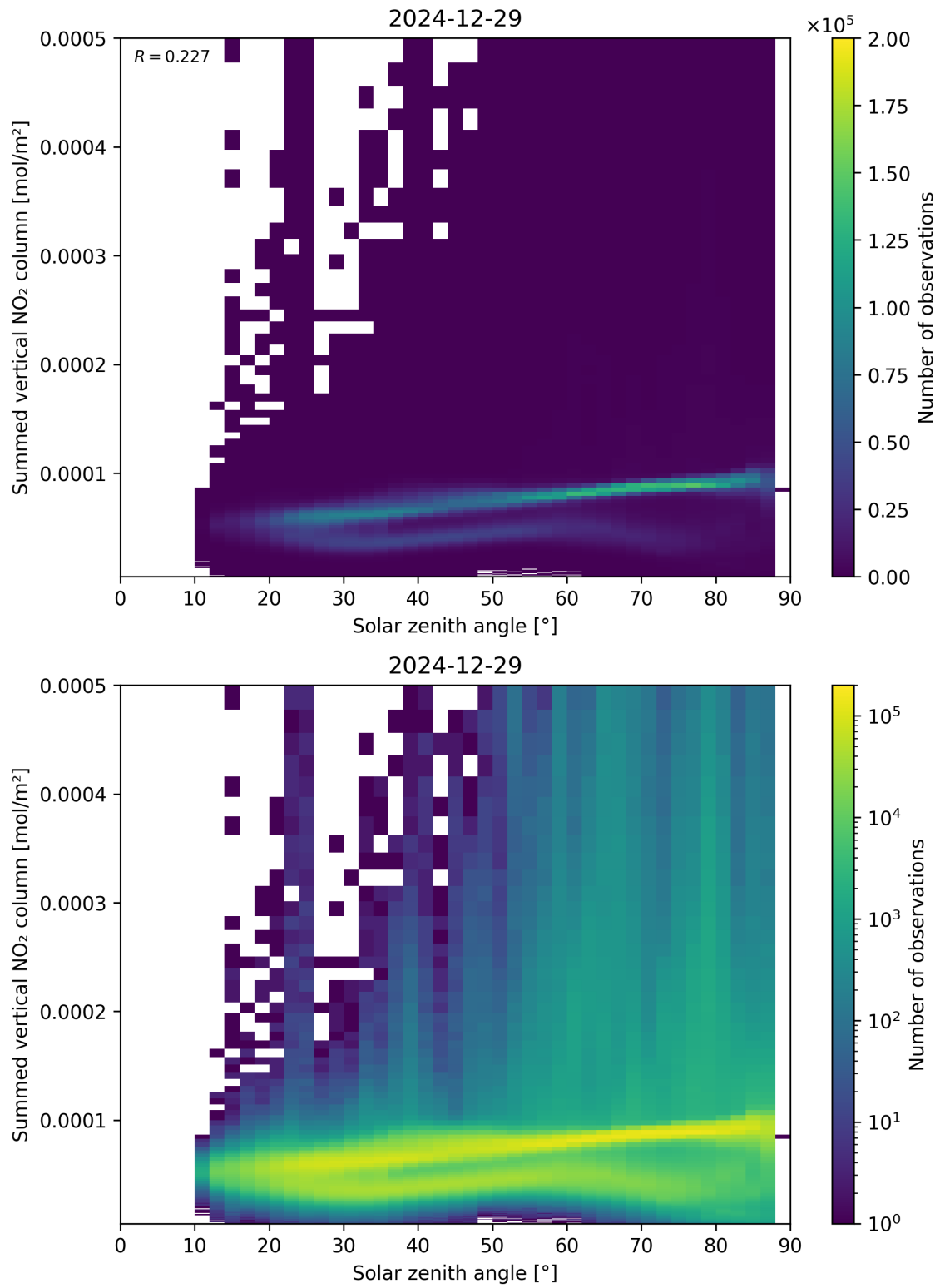
Figure 151: Scatter density plot of “Solar zenith angle” against “Summed vertical NO 2 column” for 2024-12-28 to 2024-12-30.
