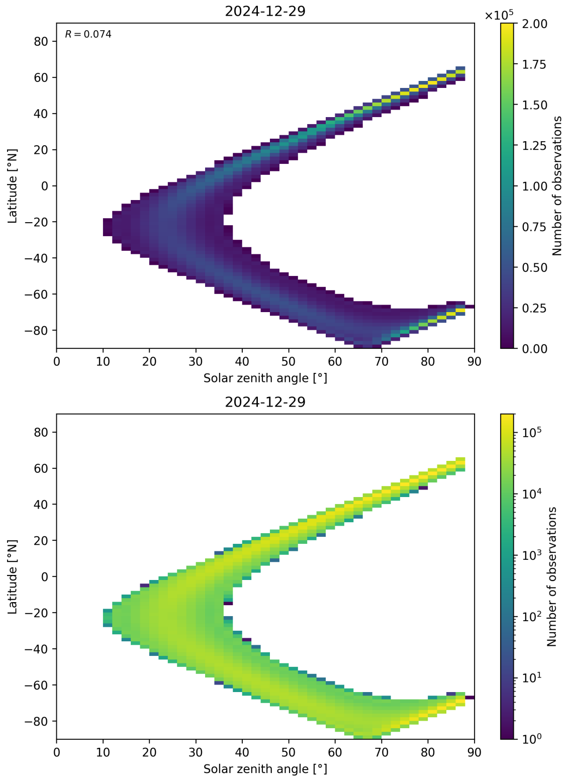
Figure 149: Scatter density plot of “Solar zenith angle” against “Latitude” for 2024-12-28 to 2024-12-30.
