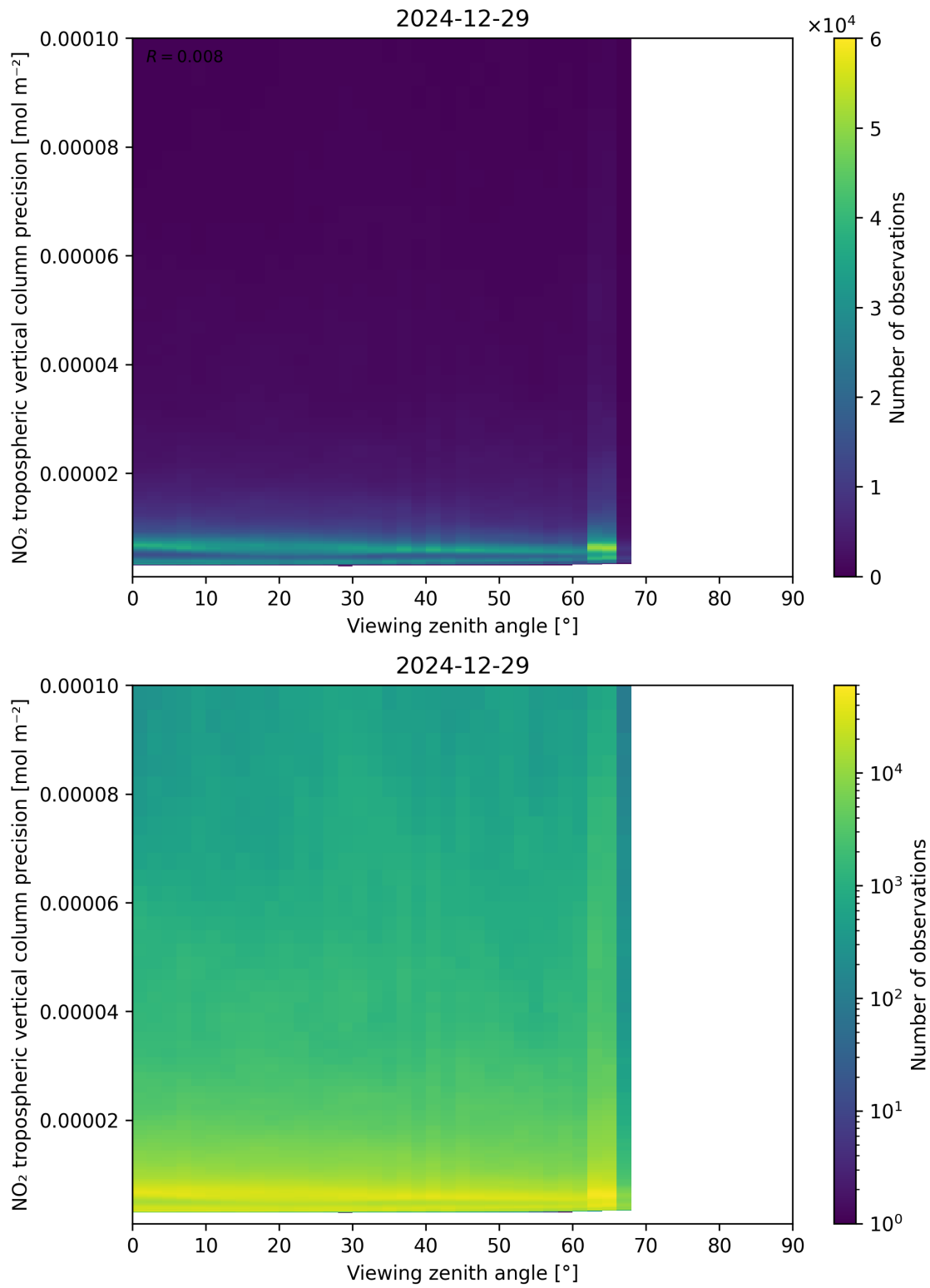
Figure 170: Scatter density plot of “Viewing zenith angle” against “NO 2 tropospheric vertical column precision” for 2024-12-28 to 2024-12-30.
