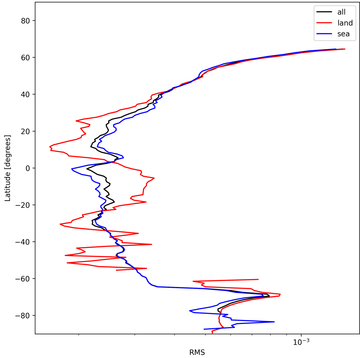
Figure 26: Zonal average of “RMS” for 2024-12-28 to 2024-12-30.
