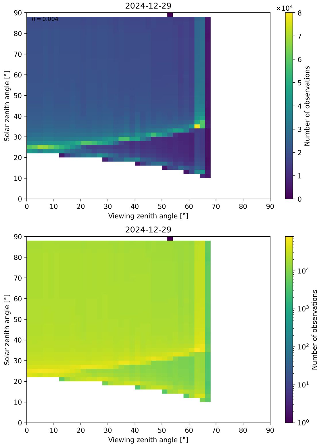
Figure 172: Scatter density plot of “Viewing zenith angle” against “Solar zenith angle” for 2024-12-28 to 2024-12-30.
