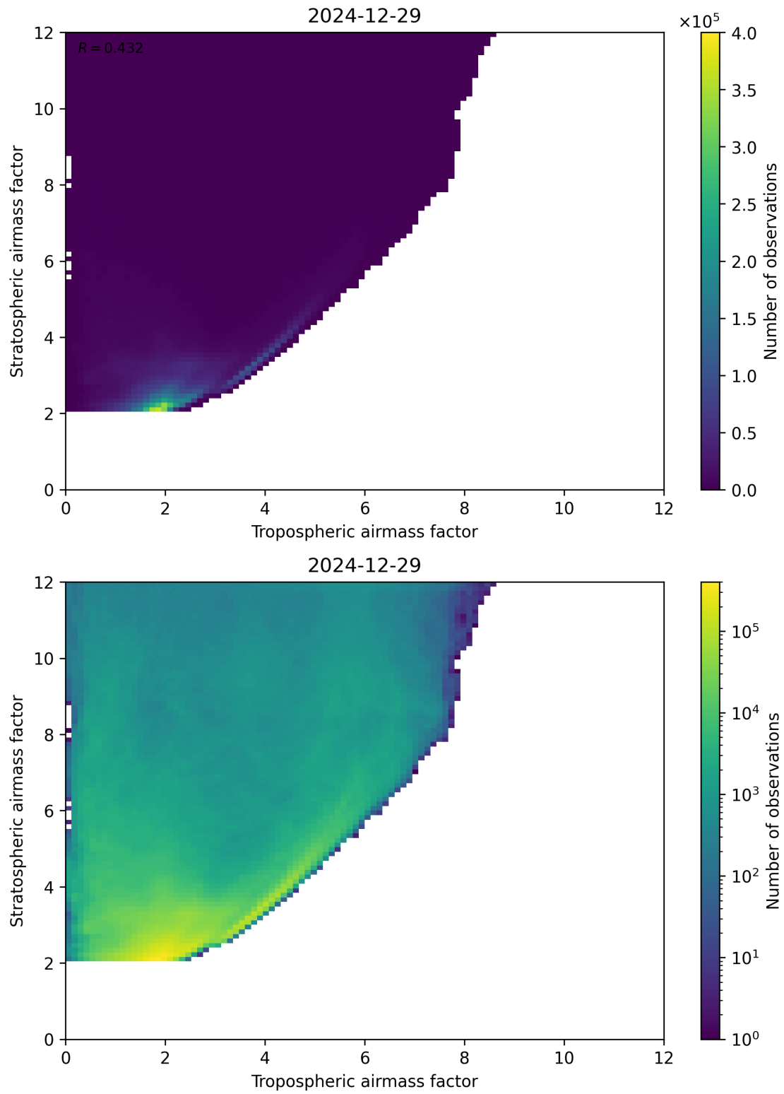
Figure 71: Scatter density plot of “Tropospheric airmass factor” against “Stratospheric airmass factor” for 2024-12-28 to 2024-12-30.
