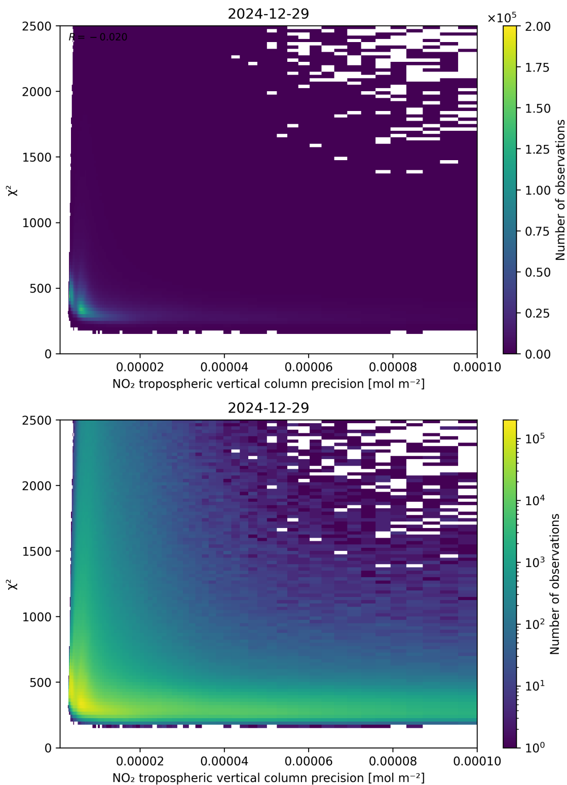
Figure 134: Scatter density plot of “NO 2 tropospheric vertical column precision” against “ \chi^2 ” for 2024-12-28 to 2024-12-30.
