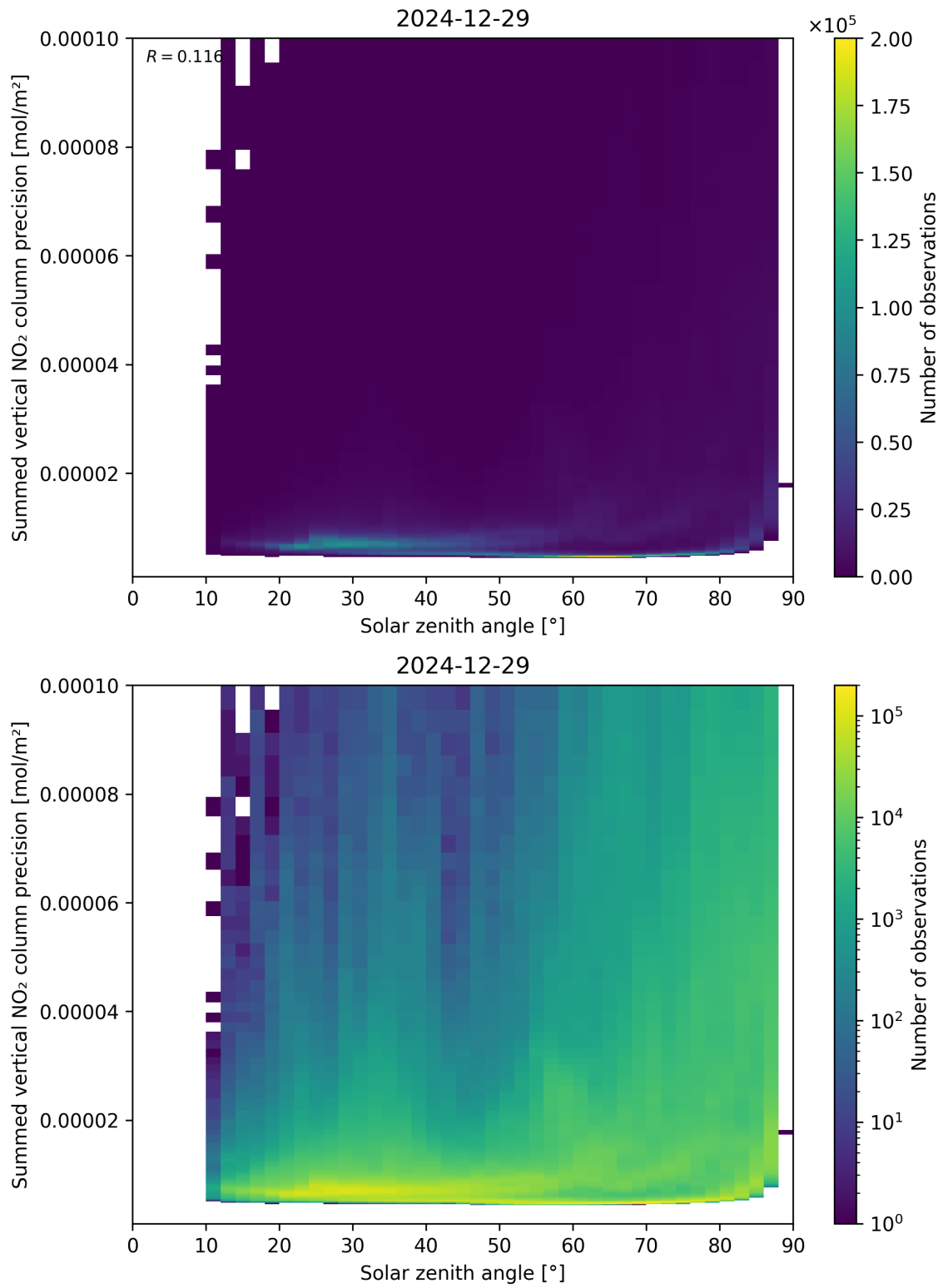
Figure 152: Scatter density plot of “Solar zenith angle” against “Summed vertical NO 2 column precision” for 2024-12-28 to 2024-12-30.
