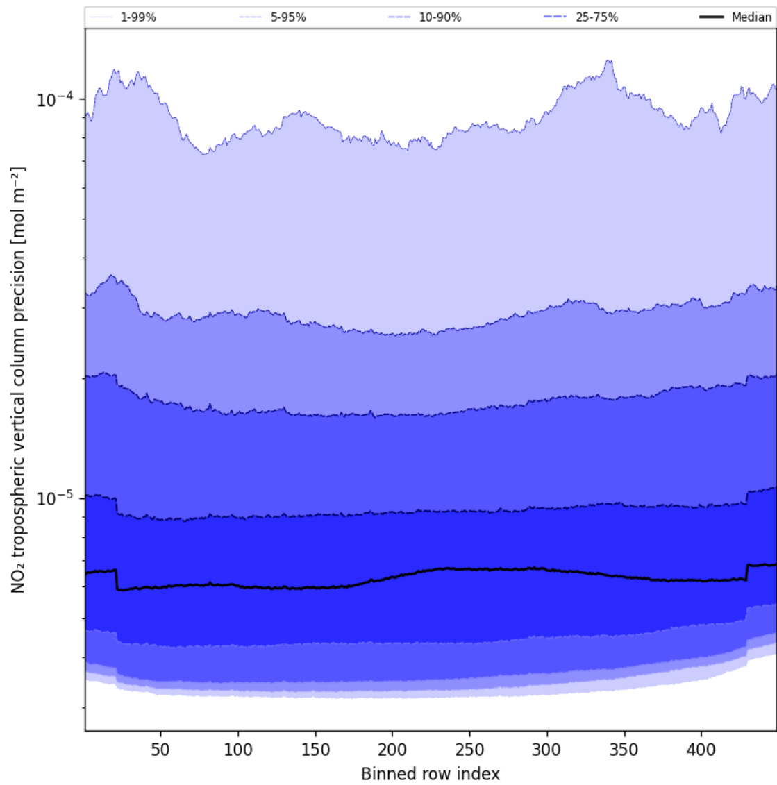
Figure 47: Along track statistics of “NO 2 tropospheric vertical column precision” for 2024-12-28 to 2024-12-30
