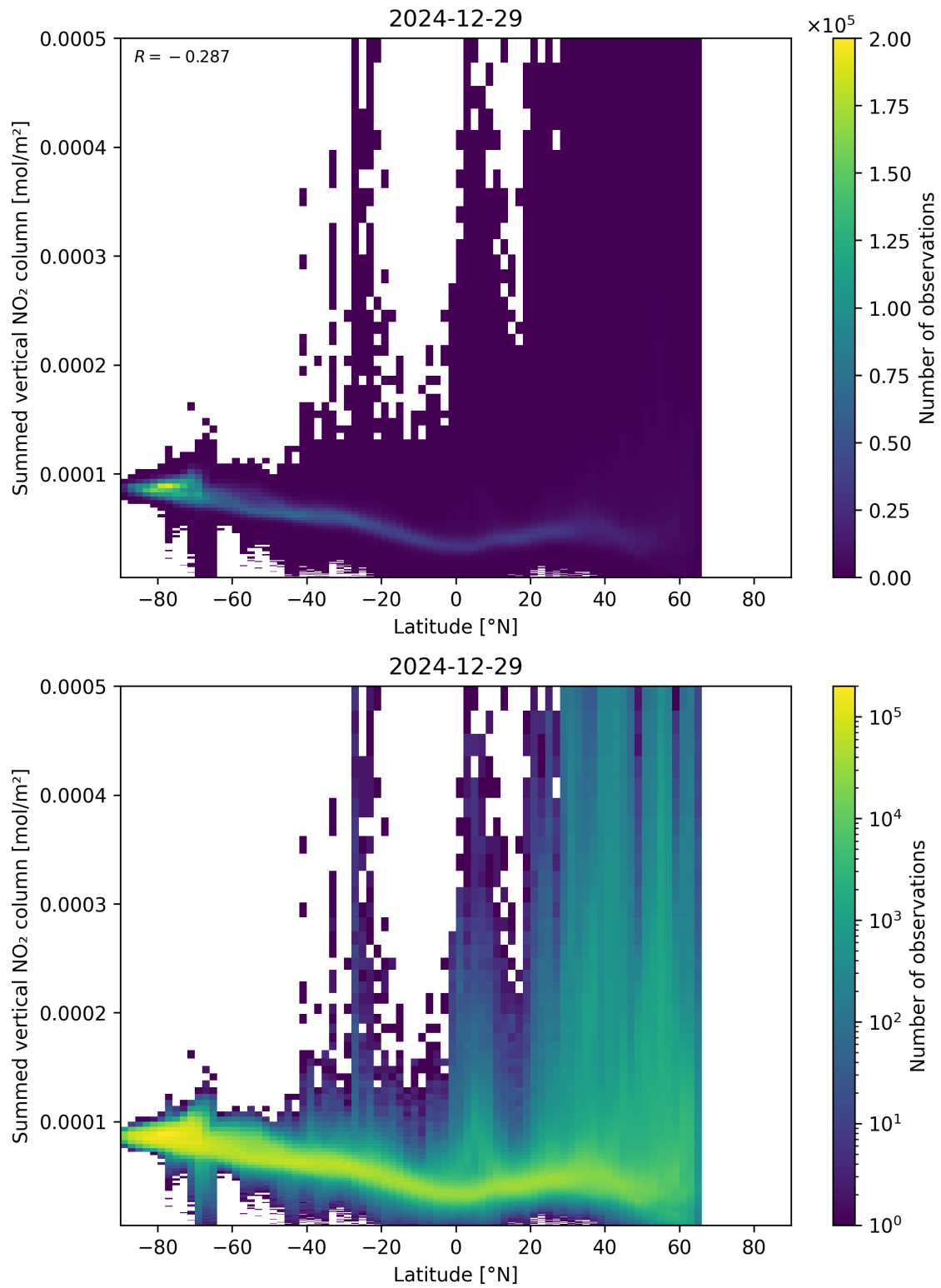
Figure 88: Scatter density plot of “Latitude” against “Summed vertical NO 2 column” for 2024-12-28 to 2024-12-30.
