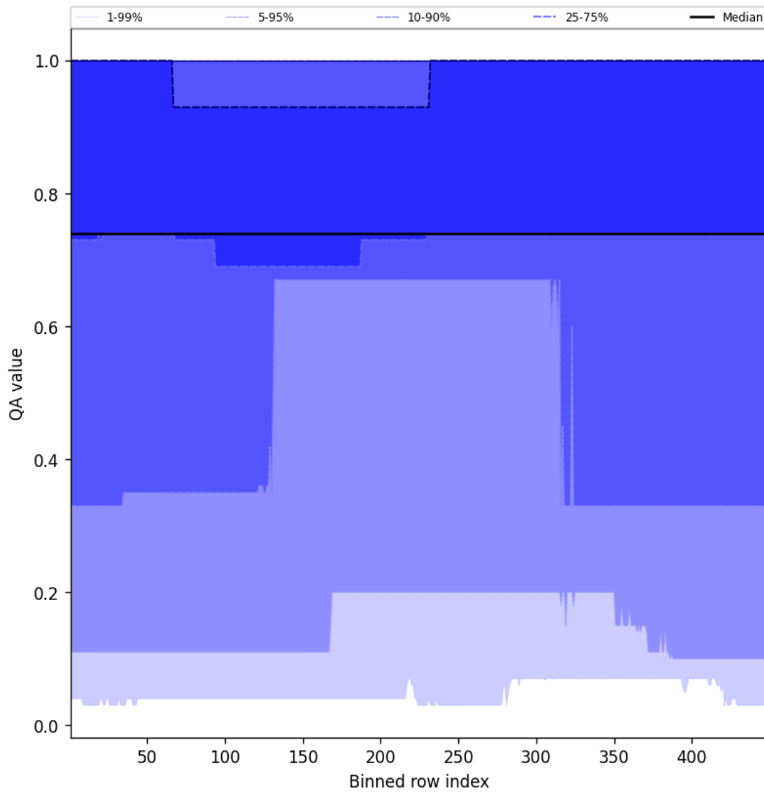
Figure 45: Along track statistics of “QA value” for 2024-12-28 to 2024-12-30
