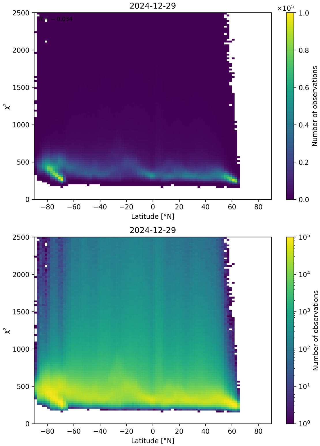
Figure 86: Scatter density plot of “Latitude” against “ \chi^2 ” for 2024-12-28 to 2024-12-30.
