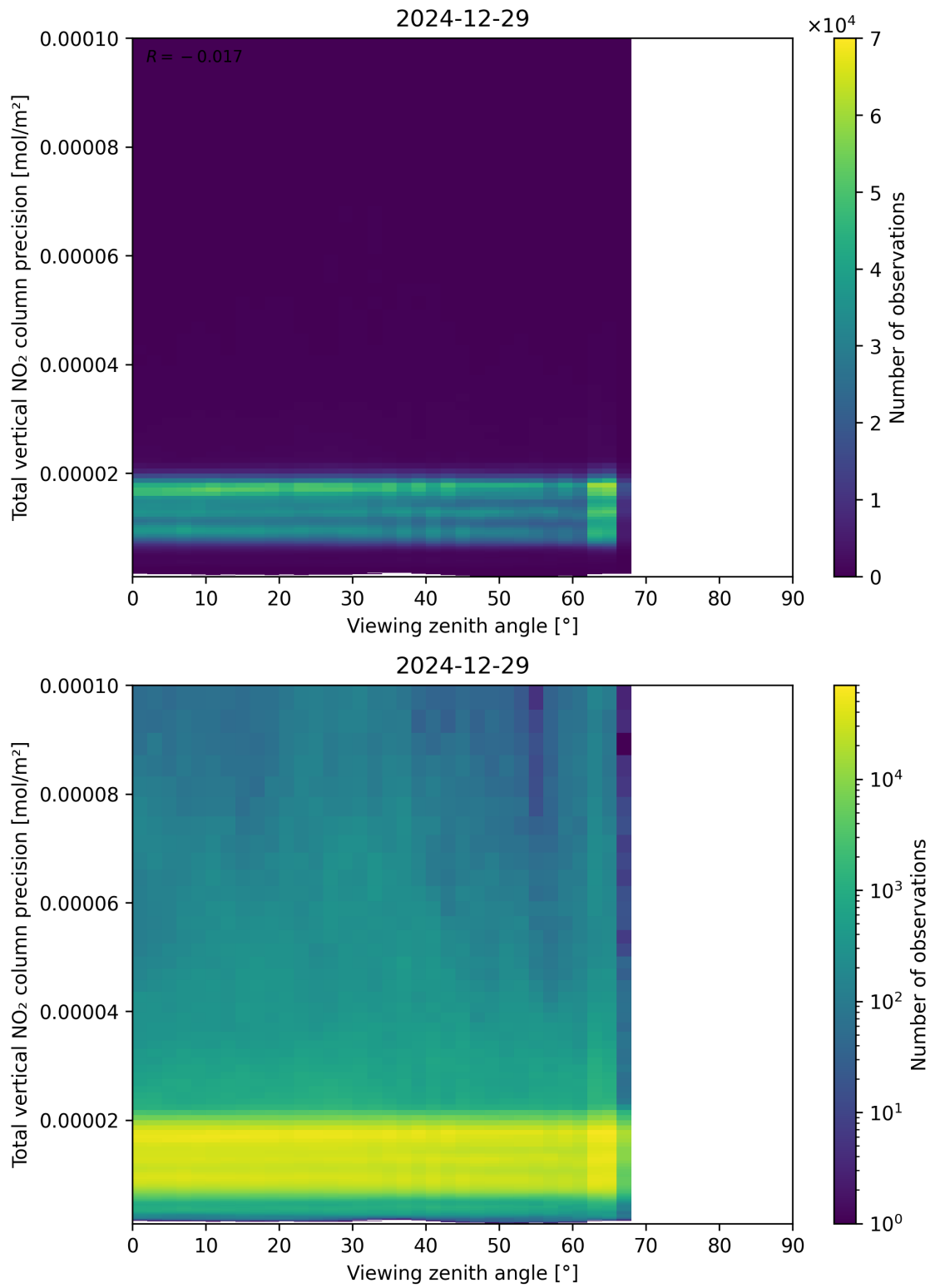
Figure 168: Scatter density plot of “Viewing zenith angle” against “Total vertical NO 2 column precision” for 2024-12-28 to 2024-12-30.
