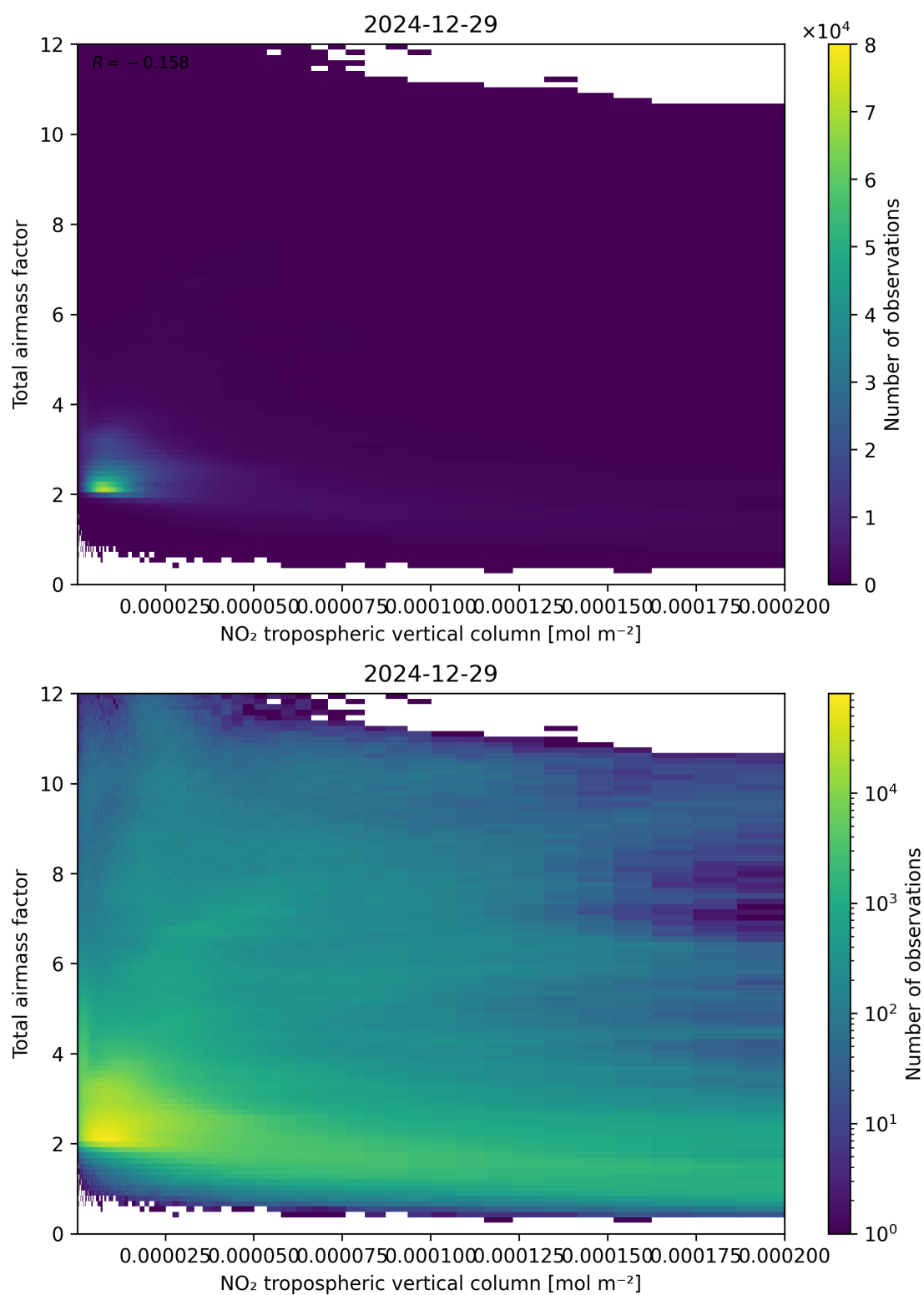
Figure 122: Scatter density plot of “NO 2 tropospheric vertical column” against “Total air mass factor” for 2024-12-28 to 2024-12-30.
