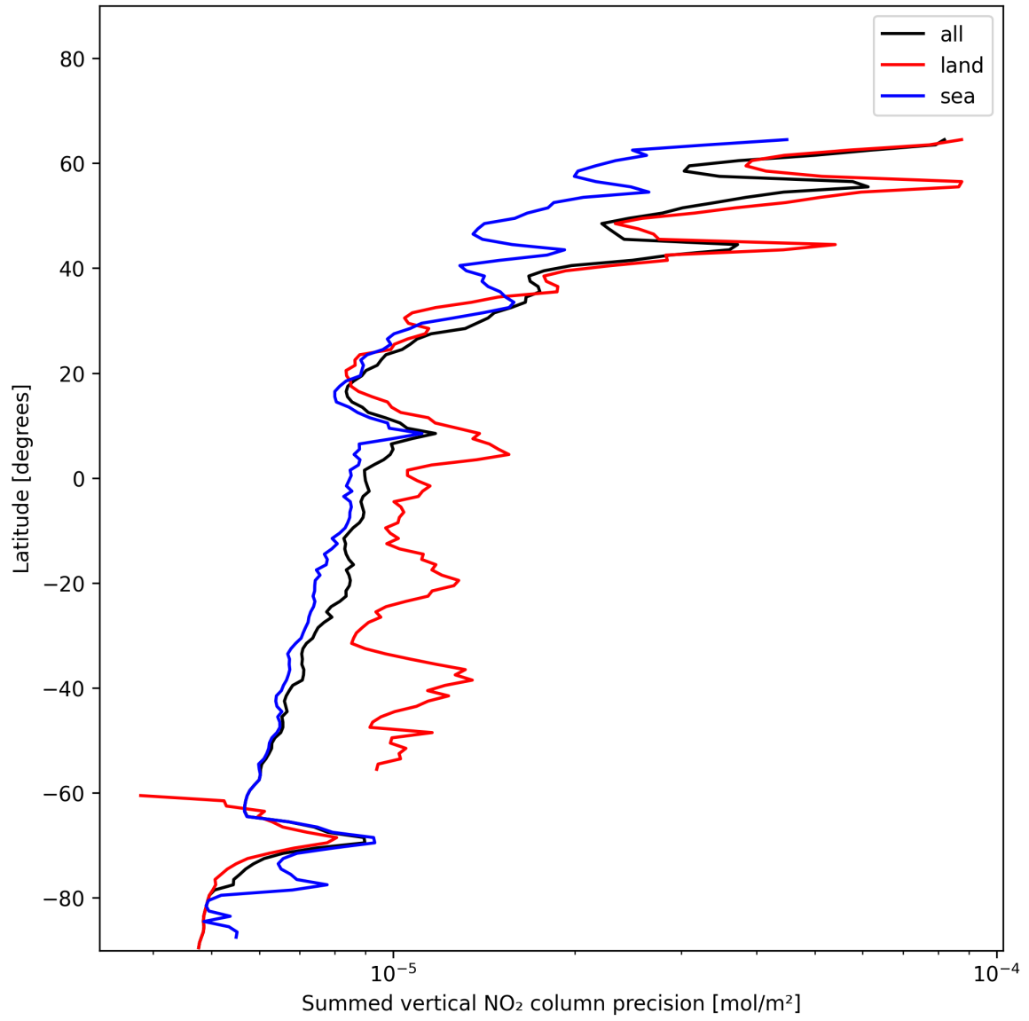
Figure 24: Zonal average of “Summed vertical NO 2 column precision” for 2024-12-28 to 2024-12-30.
