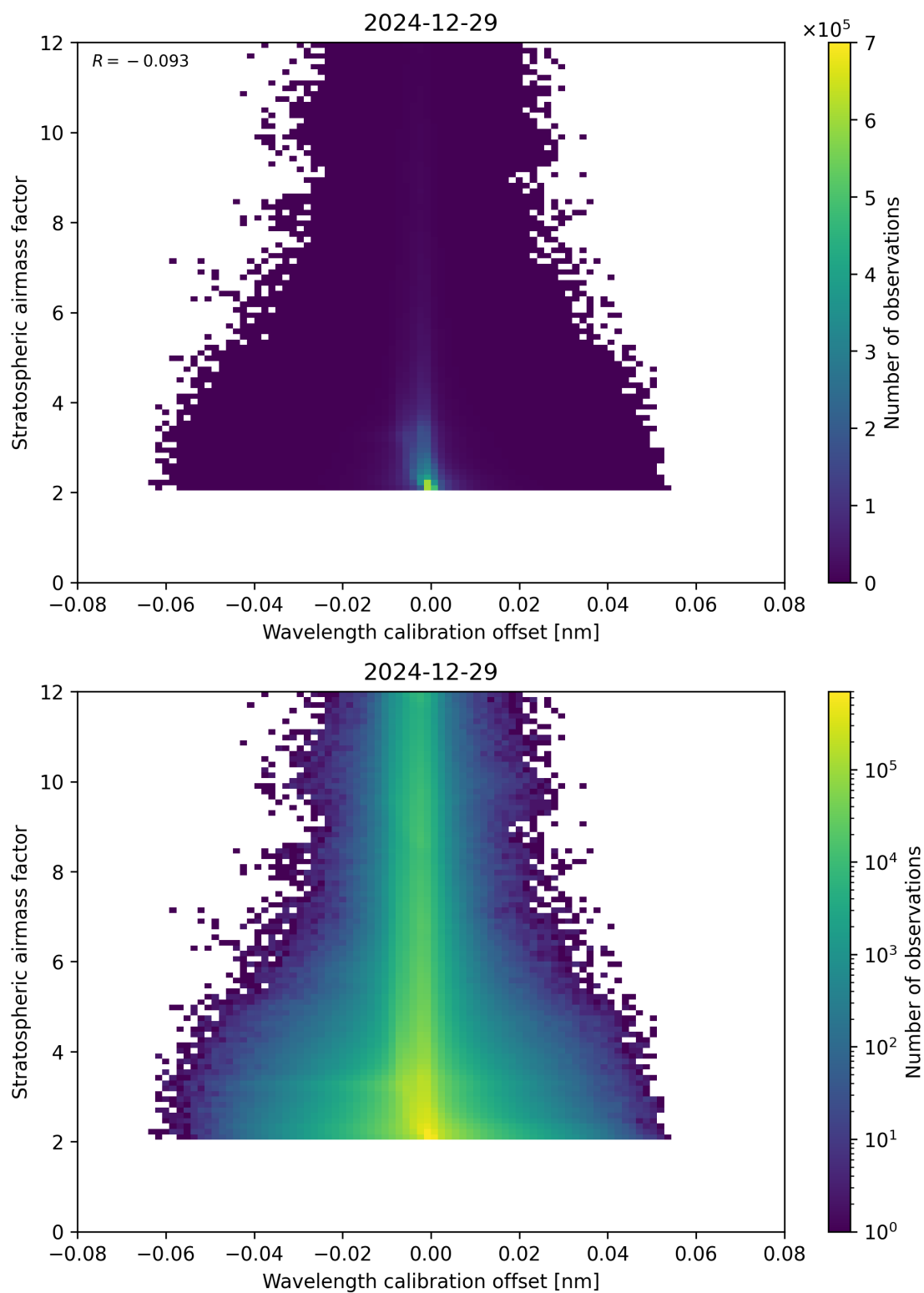
Figure 174: Scatter density plot of “Wavelength calibration offset” against “Stratospheric airmass factor” for 2024-12-28 to 2024-12-30.
