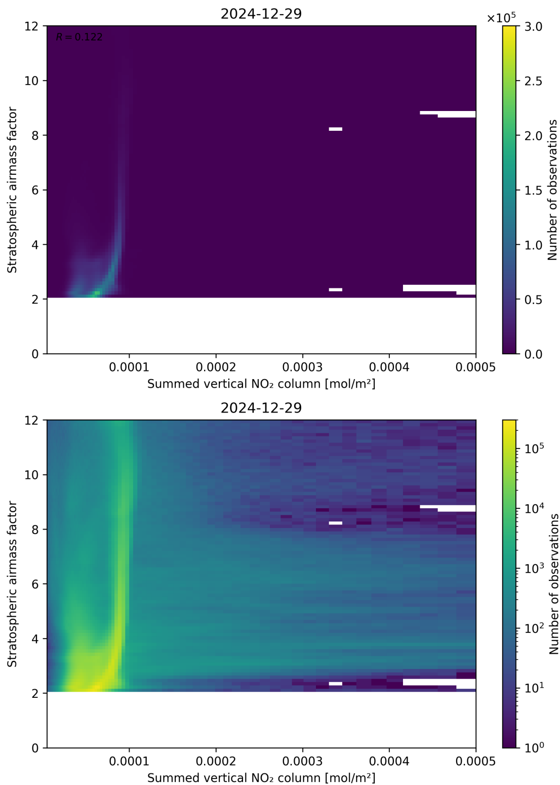
Figure 103: Scatter density plot of “Summed vertical NO 2 column” against “Stratospheric airmass factor” for 2024-12-28 to 2024-12-30.
