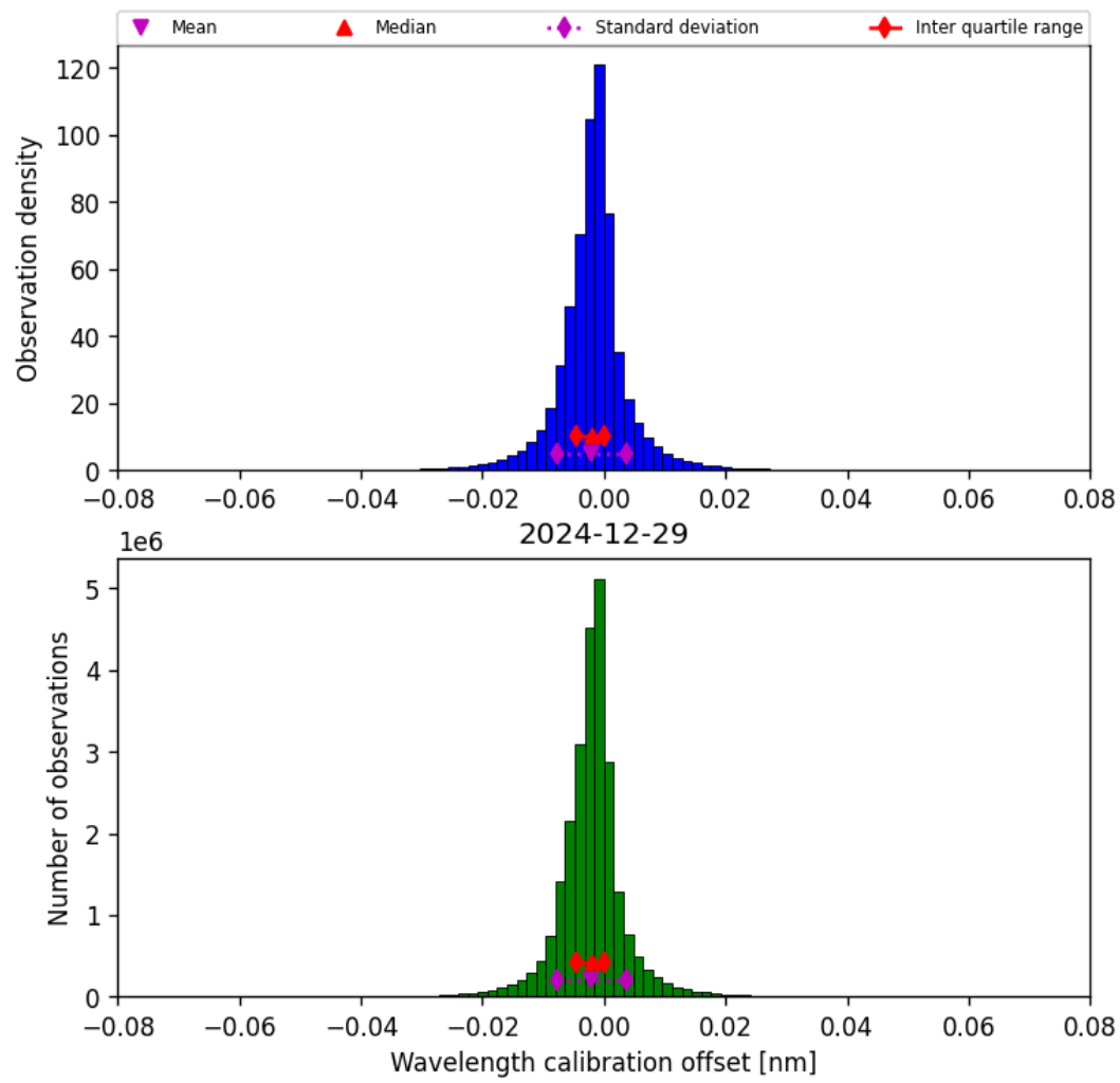
Figure 35: Histogram of “Wavelength calibration offset” for 2024-12-28 to 2024-12-30
