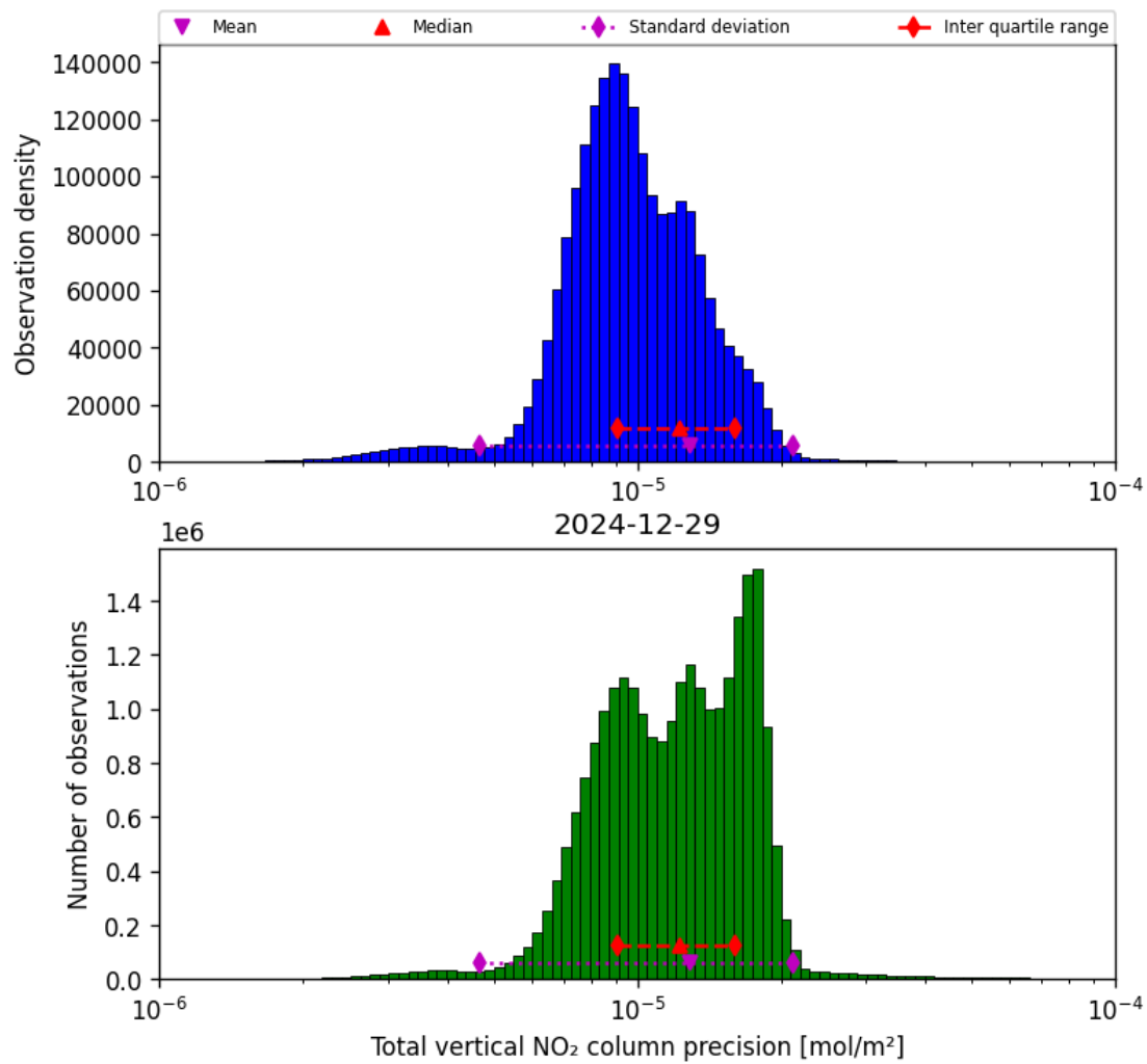
Figure 39: Histogram of “Total vertical NO 2 column precision” for 2024-12-28 to 2024-12-30
