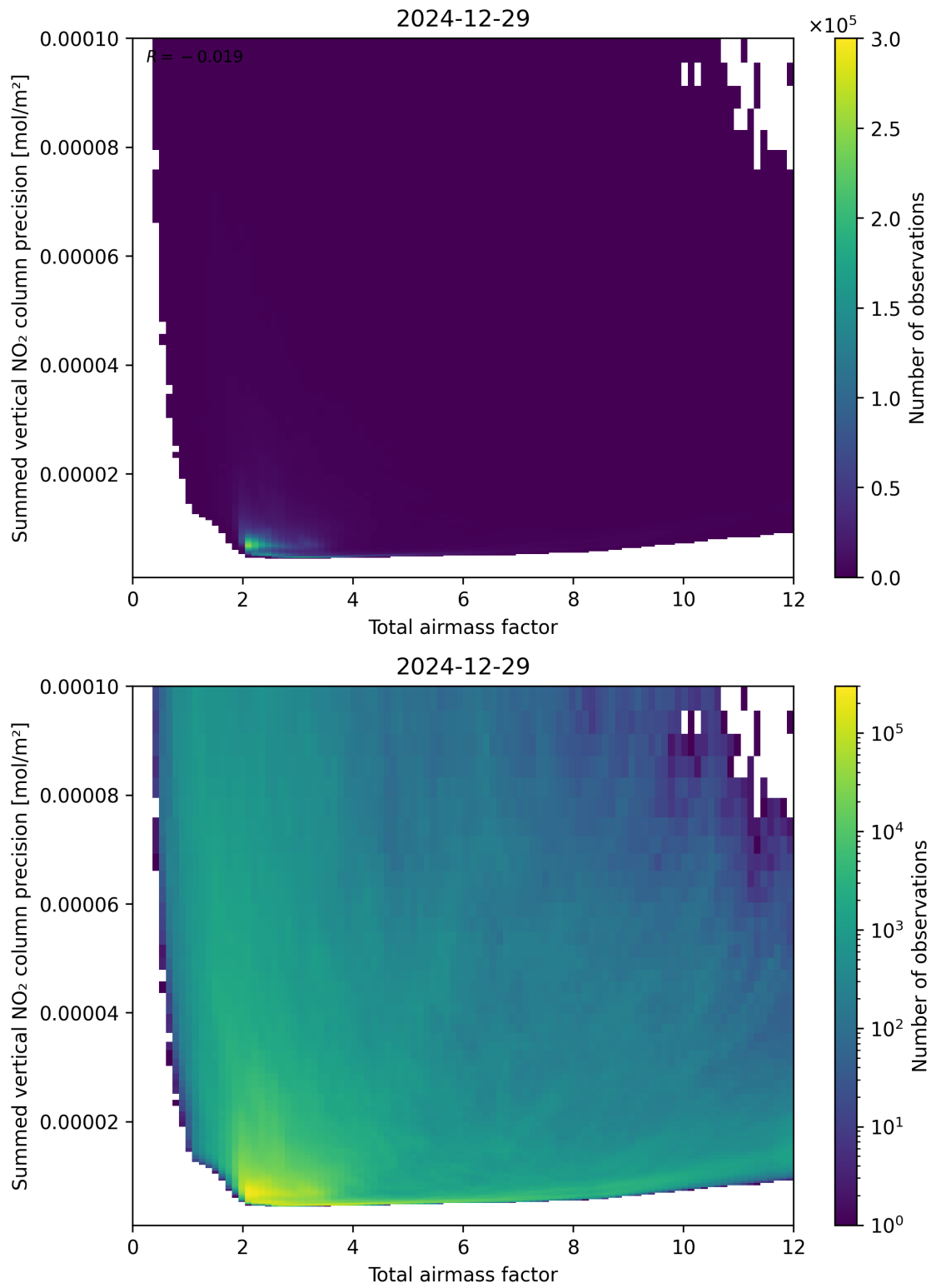
Figure 66: Scatter density plot of “Total airmass factor” against “Summed vertical NO 2 column precision” for 2024-12-28 to 2024-12-30.
