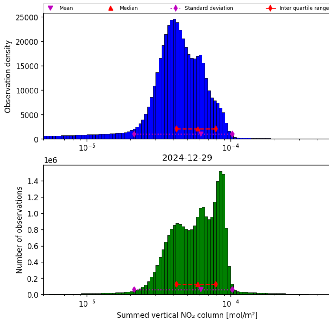
Figure 40: Histogram of “Summed vertical NO 2 column” for 2024-12-28 to 2024-12-30
