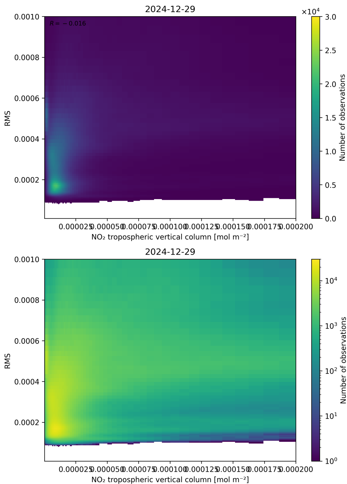
Figure 142: Scatter density plot of “NO 2 tropospheric vertical column” against “RMS” for 2024-12-28 to 2024-12-30.
