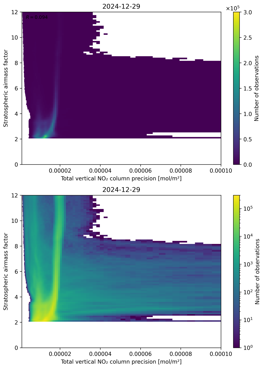
Figure 115: Scatter density plot of “Total vertical NO 2 column precision” against “Stratospheric air mass factor” for 2024-12-28 to 2024-12-30.
