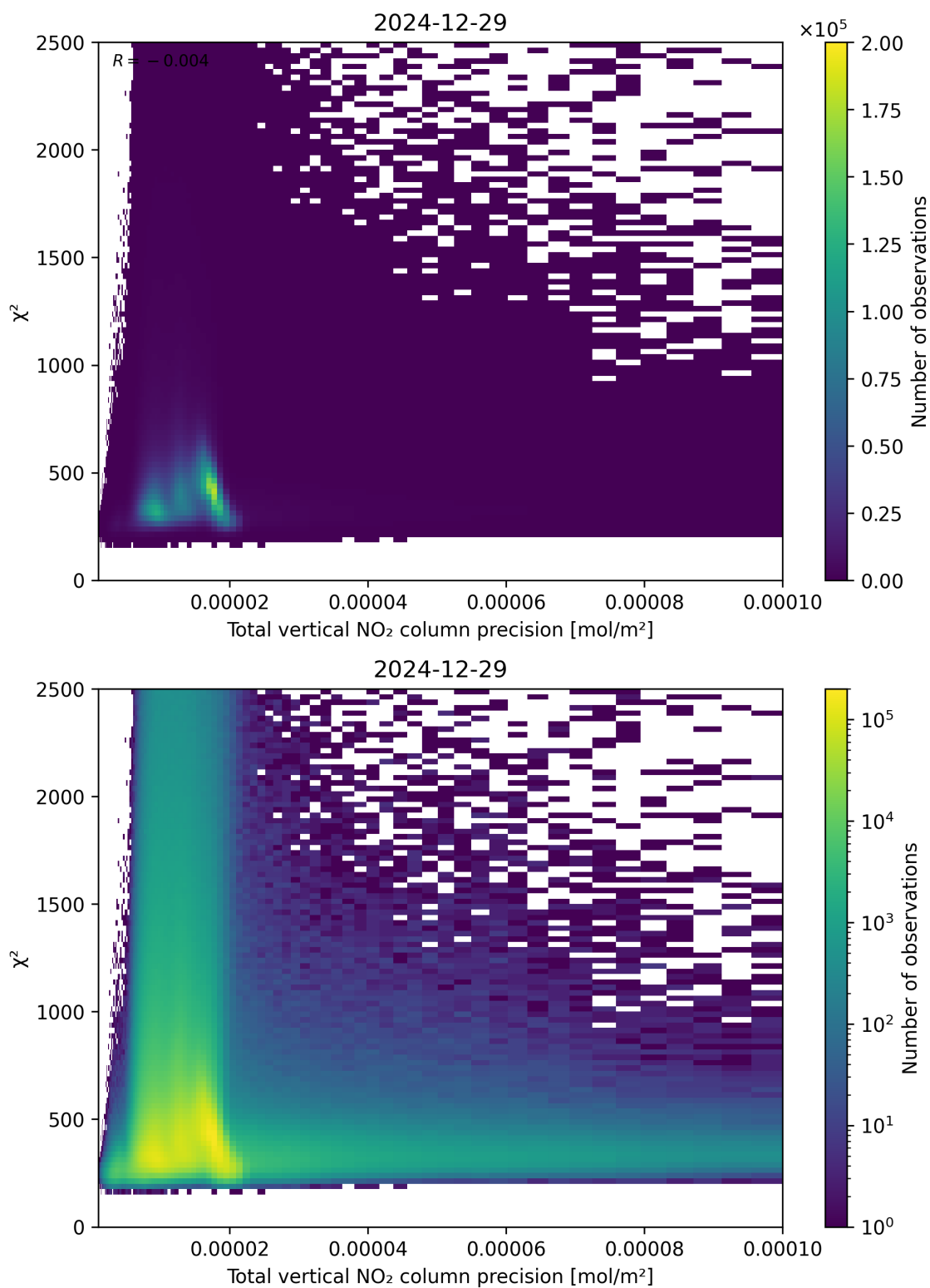
Figure 116: Scatter density plot of “Total vertical NO 2 column precision” against “ \chi^2 ” for 2024-12-28 to 2024-12-30.
