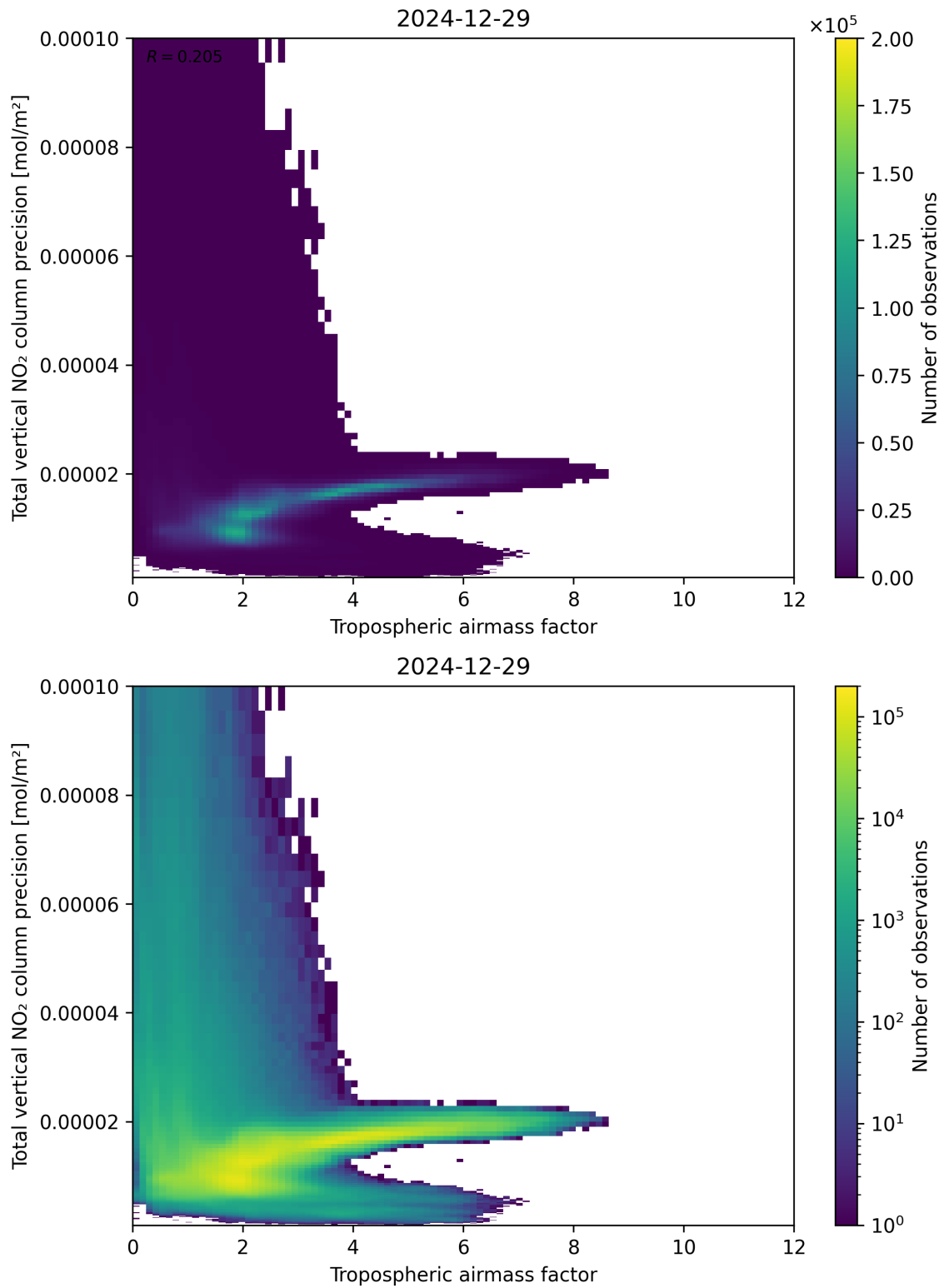
Figure 78: Scatter density plot of “Tropospheric air mass factor” against “Total vertical NO 2 column precision” for 2024-12-28 to 2024-12-30.
