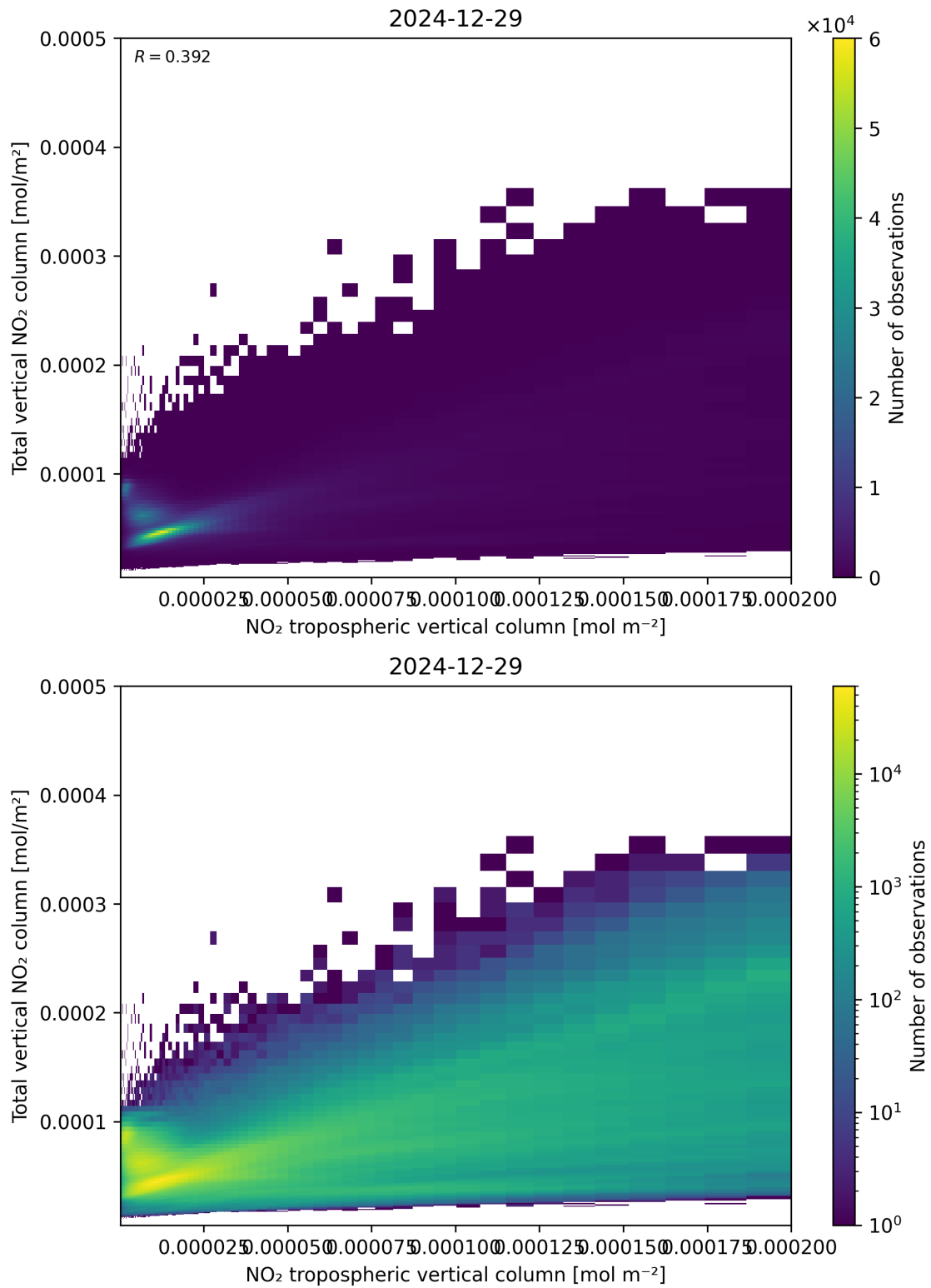
Figure 128: Scatter density plot of “NO 2 tropospheric vertical column” against “Total vertical NO 2 column” for 2024-12-28 to 2024-12-30.
