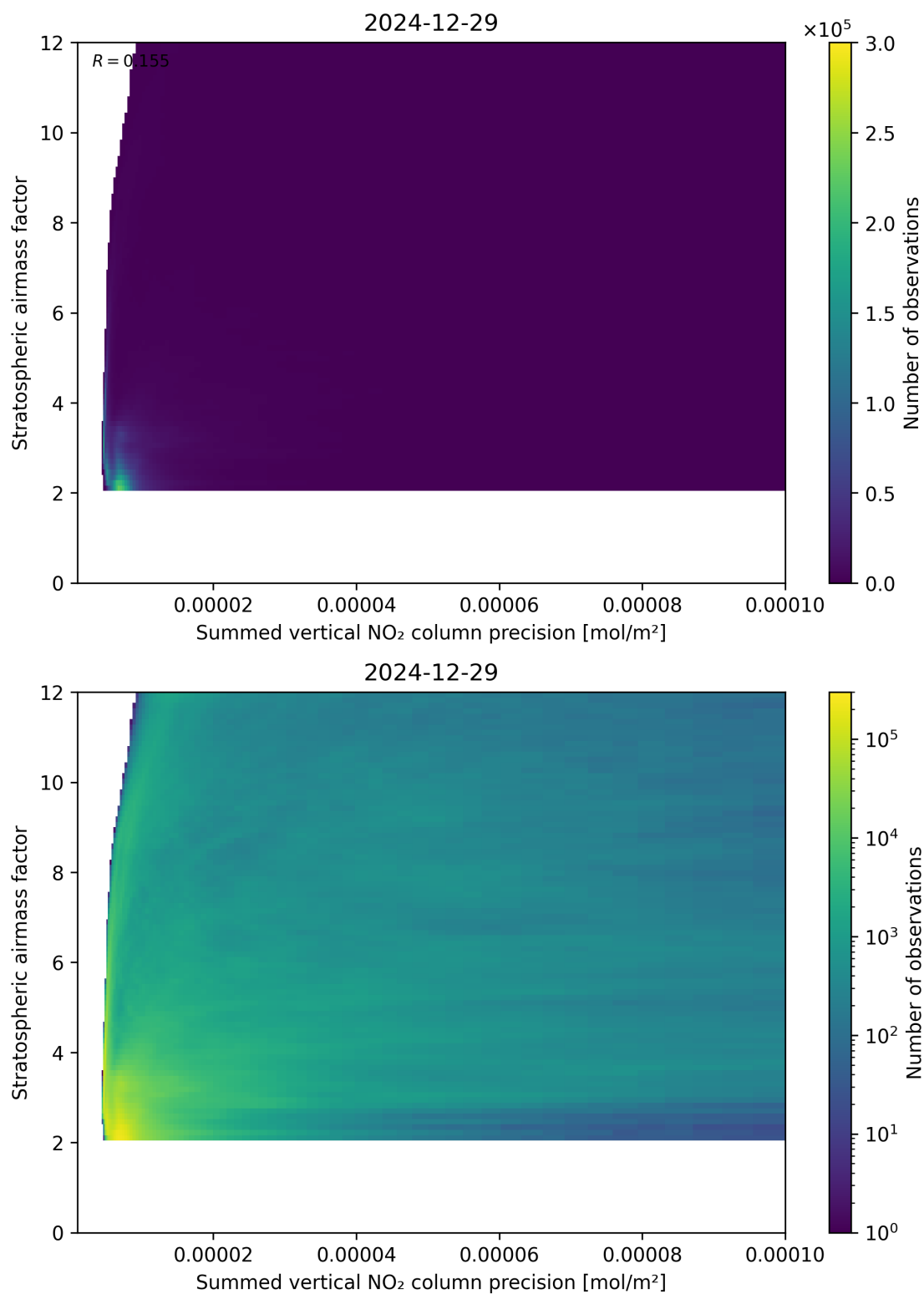
Figure 106: Scatter density plot of “Summed vertical NO 2 column precision” against “Stratospheric airmass factor” for 2024-12-28 to 2024-12-30.
