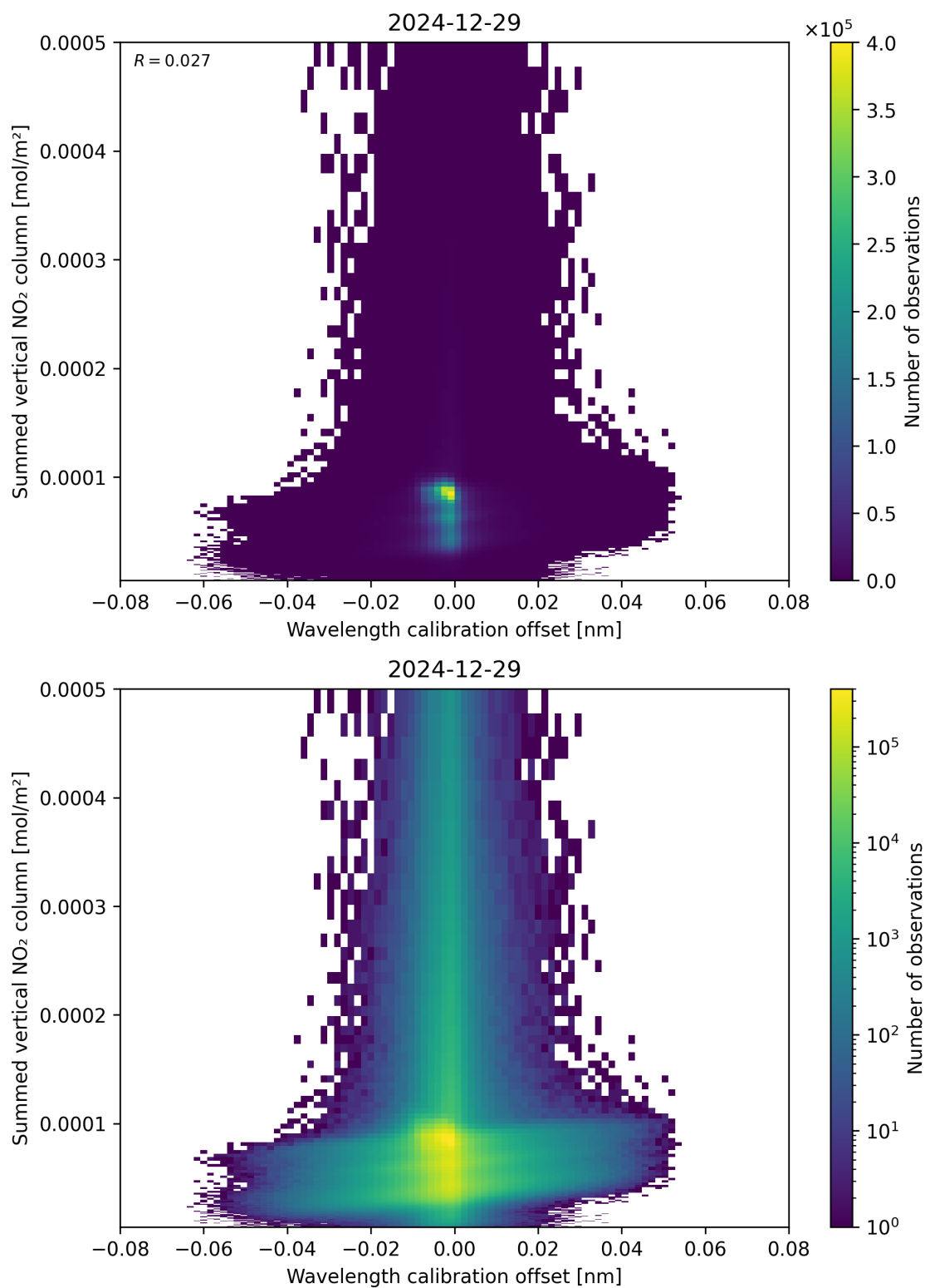
Figure 177: Scatter density plot of “Wavelength calibration offset” against “Summed vertical NO 2 column” for 2024-12-28 to 2024-12-30.
