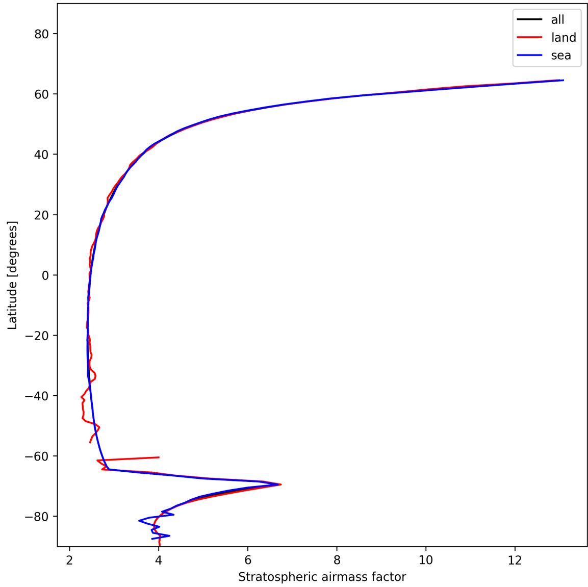
Figure 27: Zonal average of “Stratospheric air mass factor” for 2024-12-28 to 2024-12-30.
