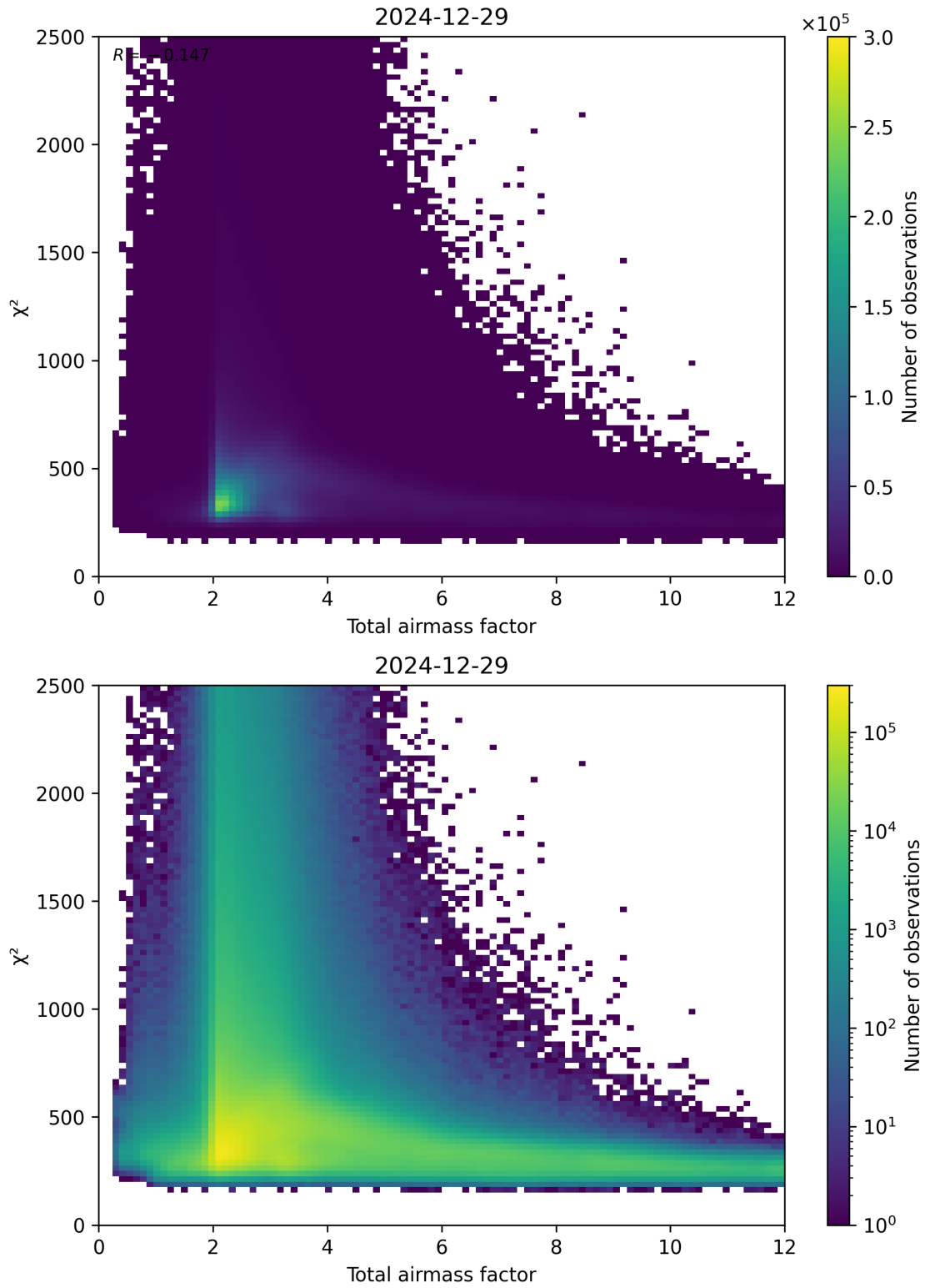
Figure 63: Scatter density plot of “Total airmass factor” against “ \chi^2 ” for 2024-12-28 to 2024-12-30.
