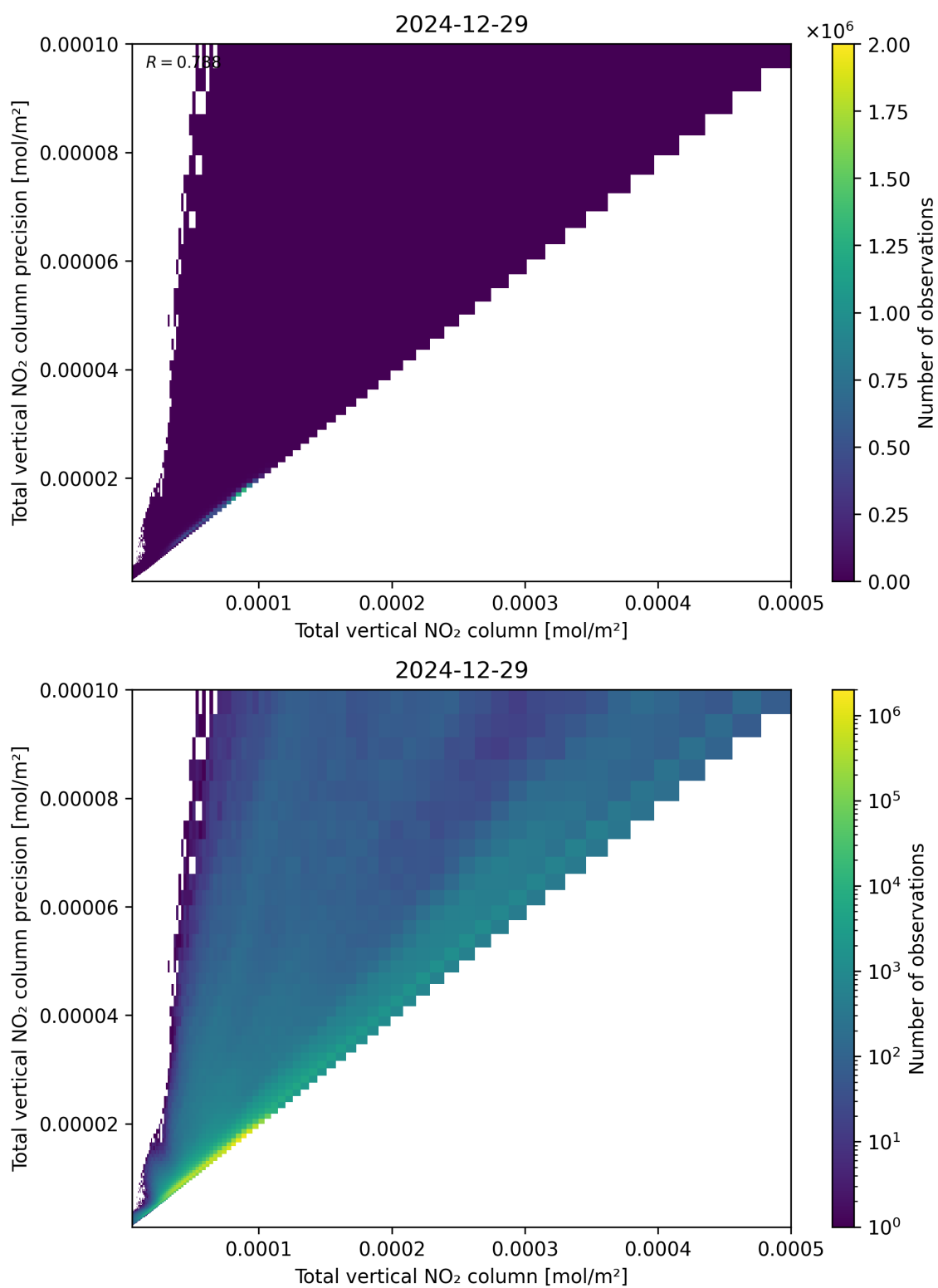
Figure 114: Scatter density plot of “Total vertical NO 2 column” against “Total vertical NO 2 column precision” for 2024-12-28 to 2024-12-30.
