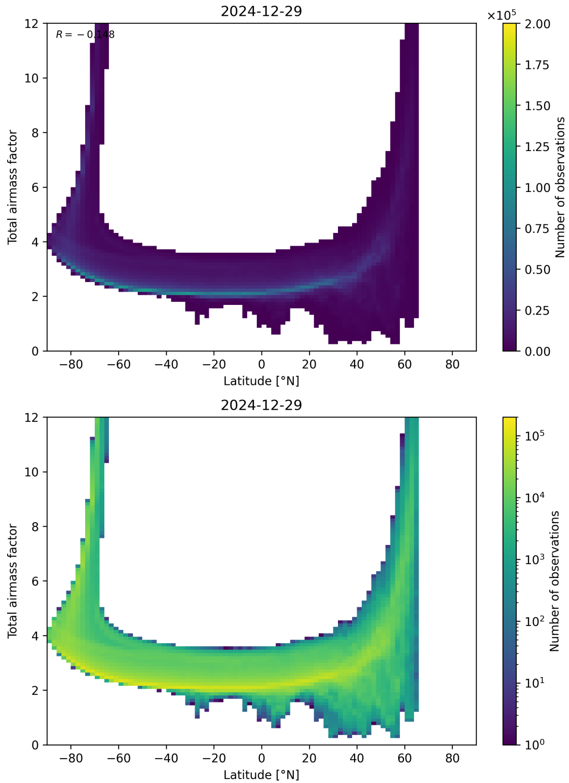
Figure 84: Scatter density plot of “Latitude” against “Total airmass factor” for 2024-12-28 to 2024-12-30.
