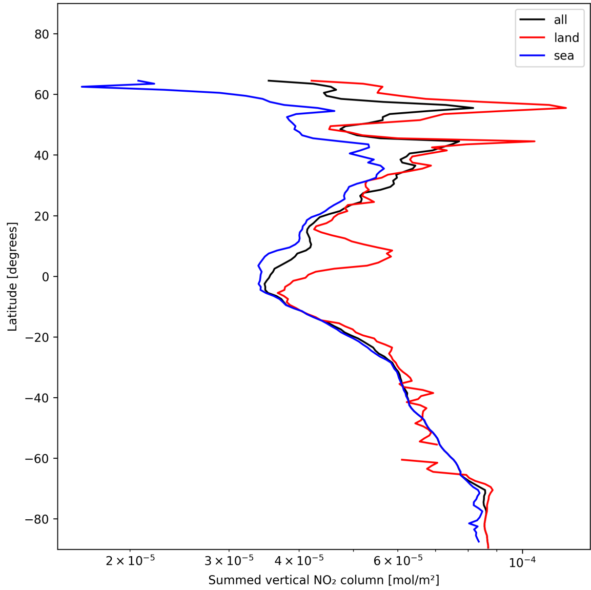
Figure 23: Zonal average of “Summed vertical NO 2 column” for 2024-12-28 to 2024-12-30.
