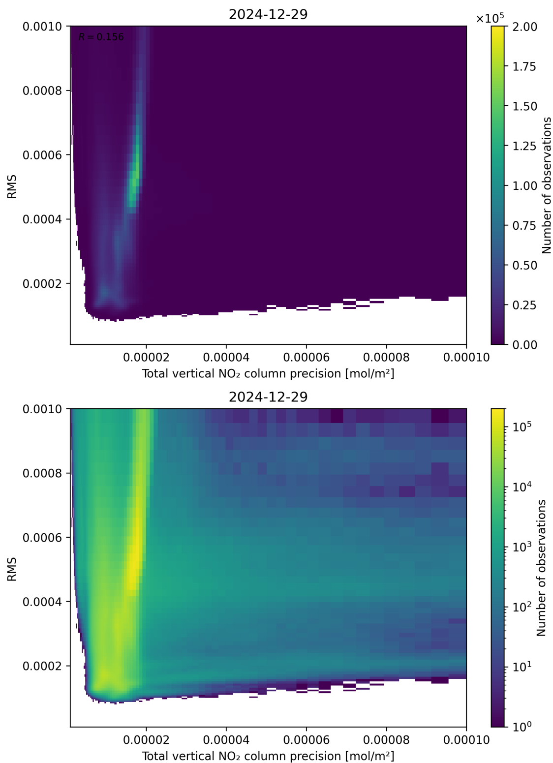
Figure 119: Scatter density plot of “Total vertical NO 2 column precision” against “RMS” for 2024-12-28 to 2024-12-30.
