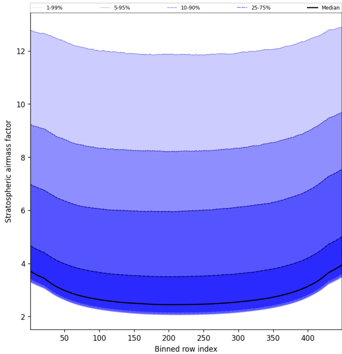
Figure 61: Along track statistics of “Stratospheric air mass factor” for 2024-12-28 to 2024-12-30
