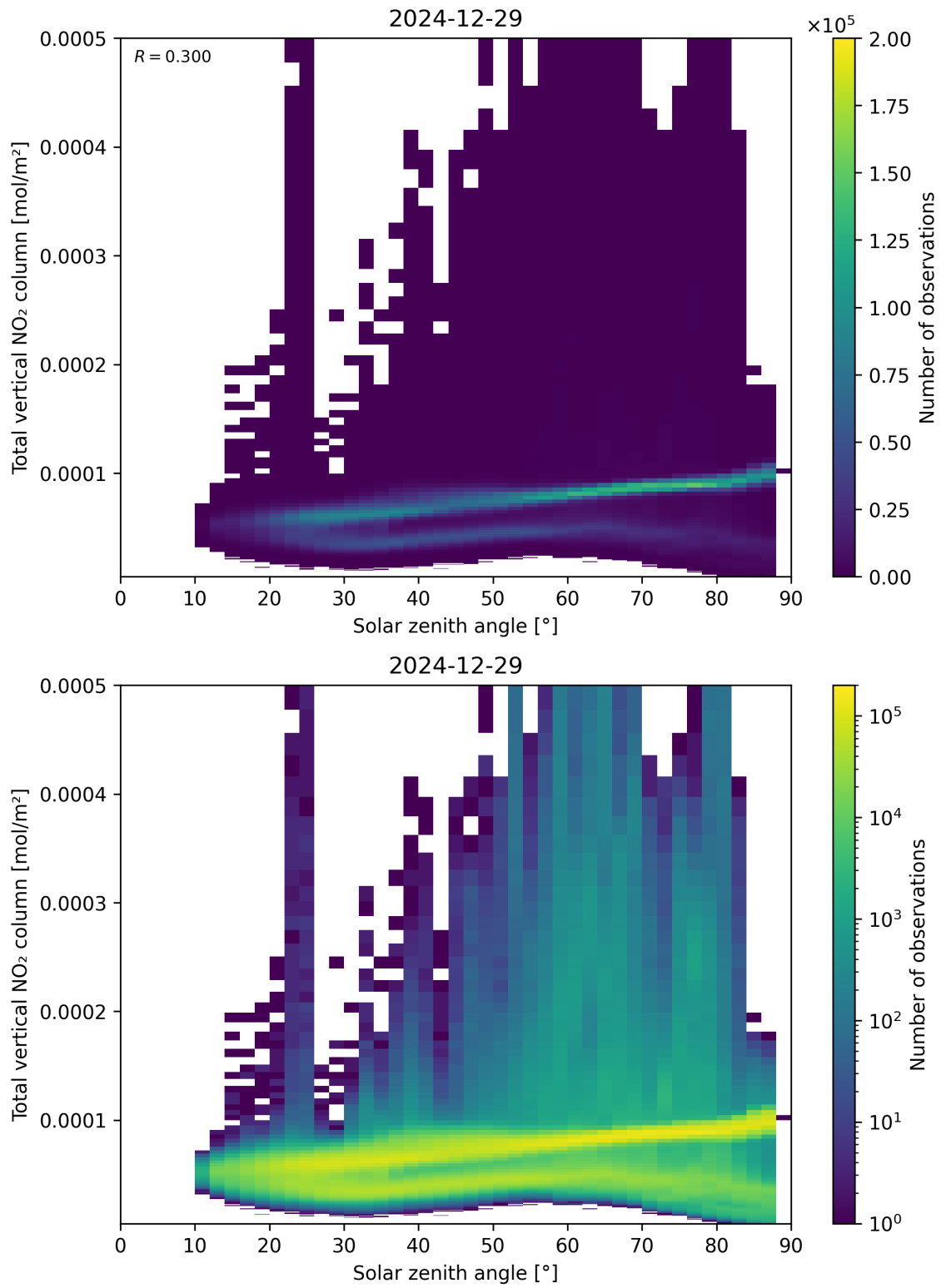
Figure 153: Scatter density plot of “Solar zenith angle” against “Total vertical NO 2 column” for 2024-12-28 to 2024-12-30.
