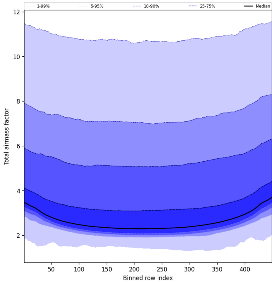
Figure 49: Along track statistics of “Total airmass factor” for 2024-12-28 to 2024-12-30
