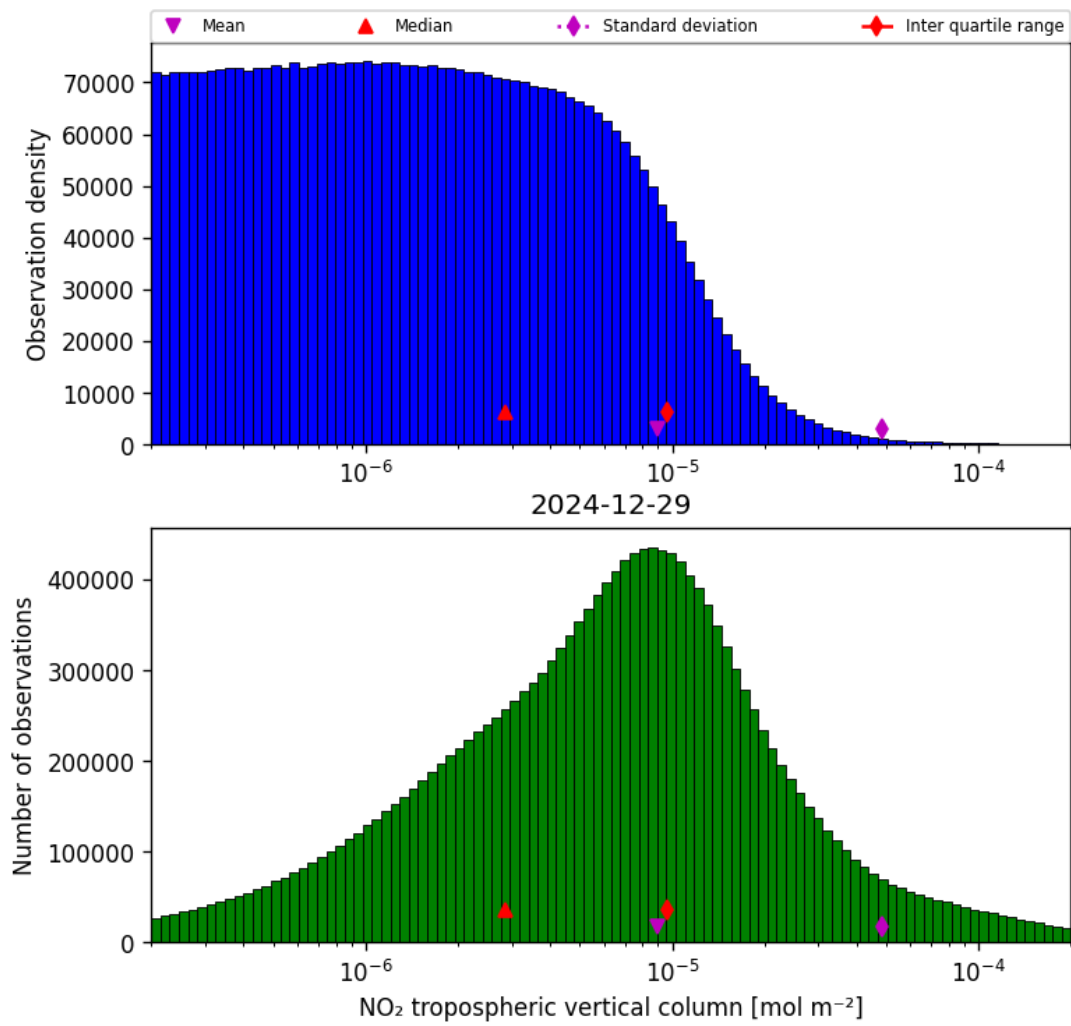
Figure 29: Histogram of “NO 2 tropospheric vertical column” for 2024-12-28 to 2024-12-30
