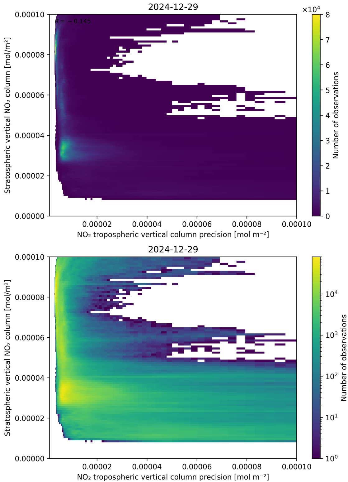
Figure 135: Scatter density plot of “NO 2 tropospheric vertical column precision” against “Stratospheric vertical NO 2 column” for 2024-12-28 to 2024-12-30.
