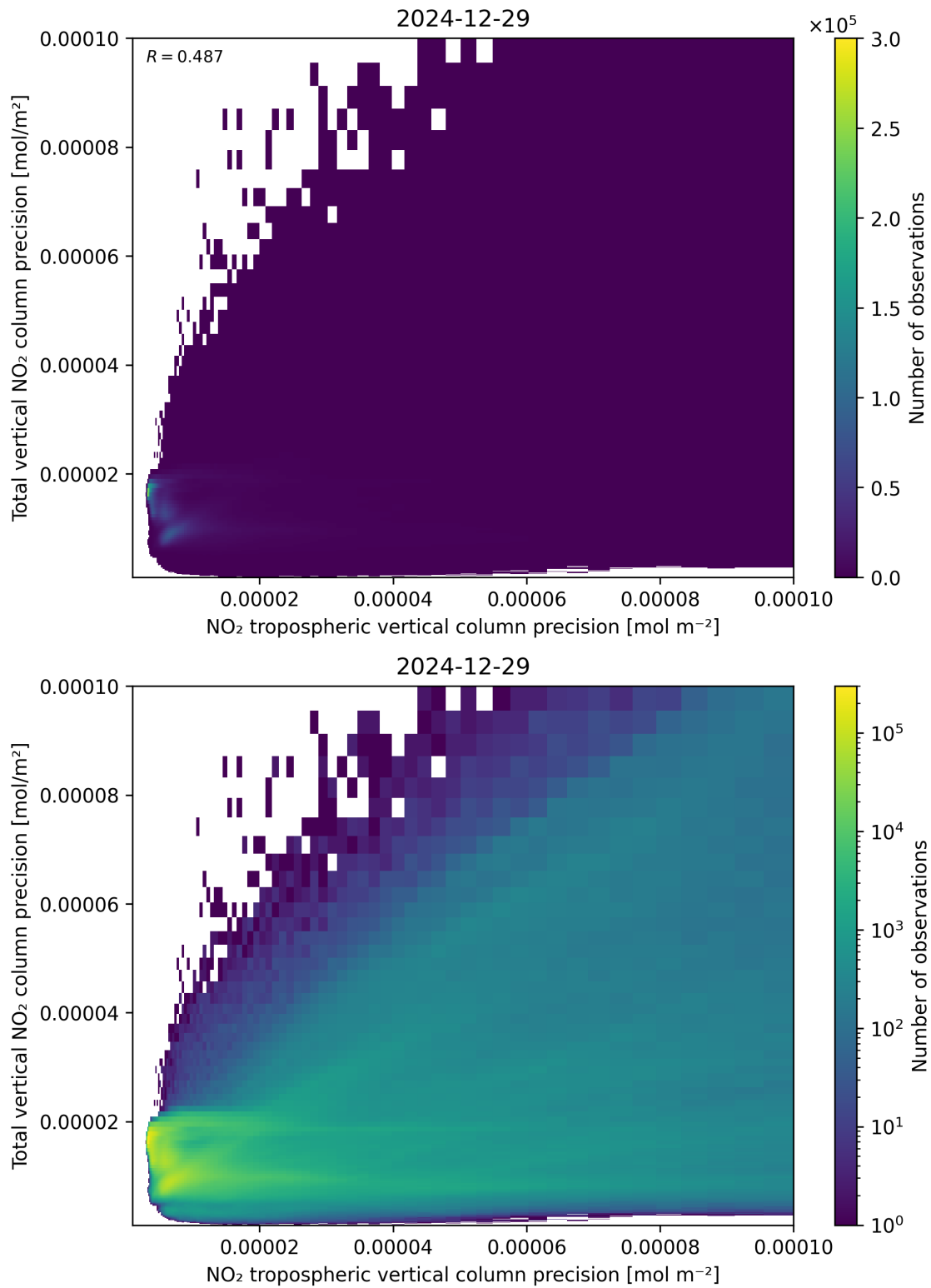
Figure 139: Scatter density plot of “NO 2 tropospheric vertical column precision” against “Total vertical NO 2 column precision” for 2024-12-28 to 2024-12-30.
