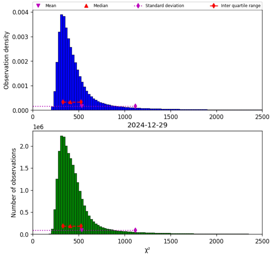
Figure 42: Histogram of “ \chi^2 ” for 2024-12-28 to 2024-12-30
