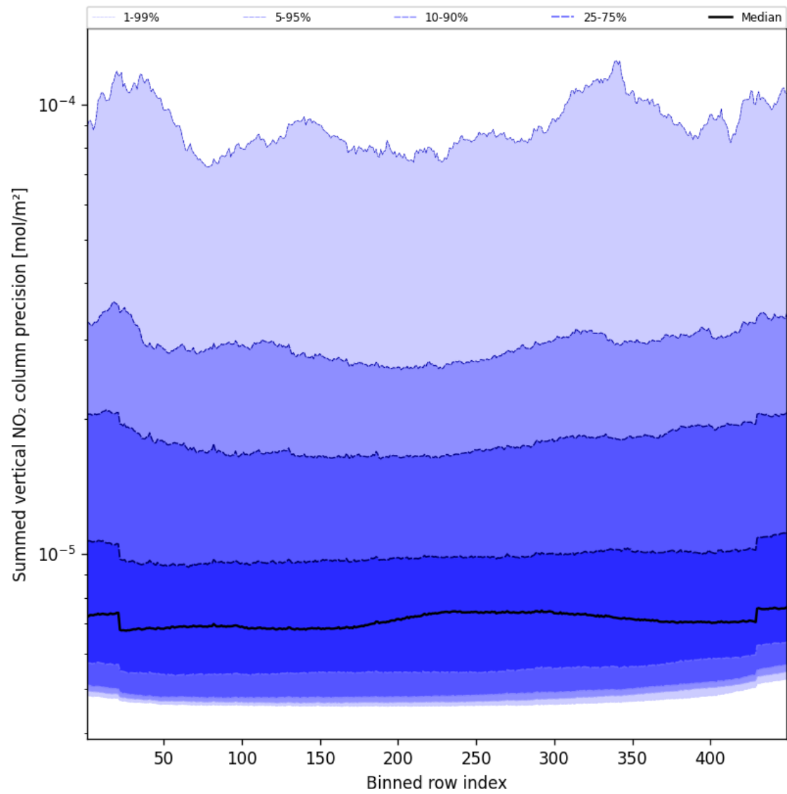
Figure 58: Along track statistics of “Summed vertical NO 2 column precision” for 2024-12-28 to 2024-12-30
