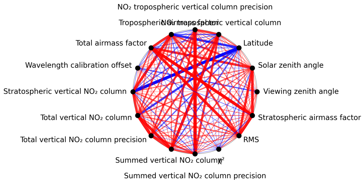
Figure 1: Map of correlation graph for 2024-12-28 to 2024-12-30.
