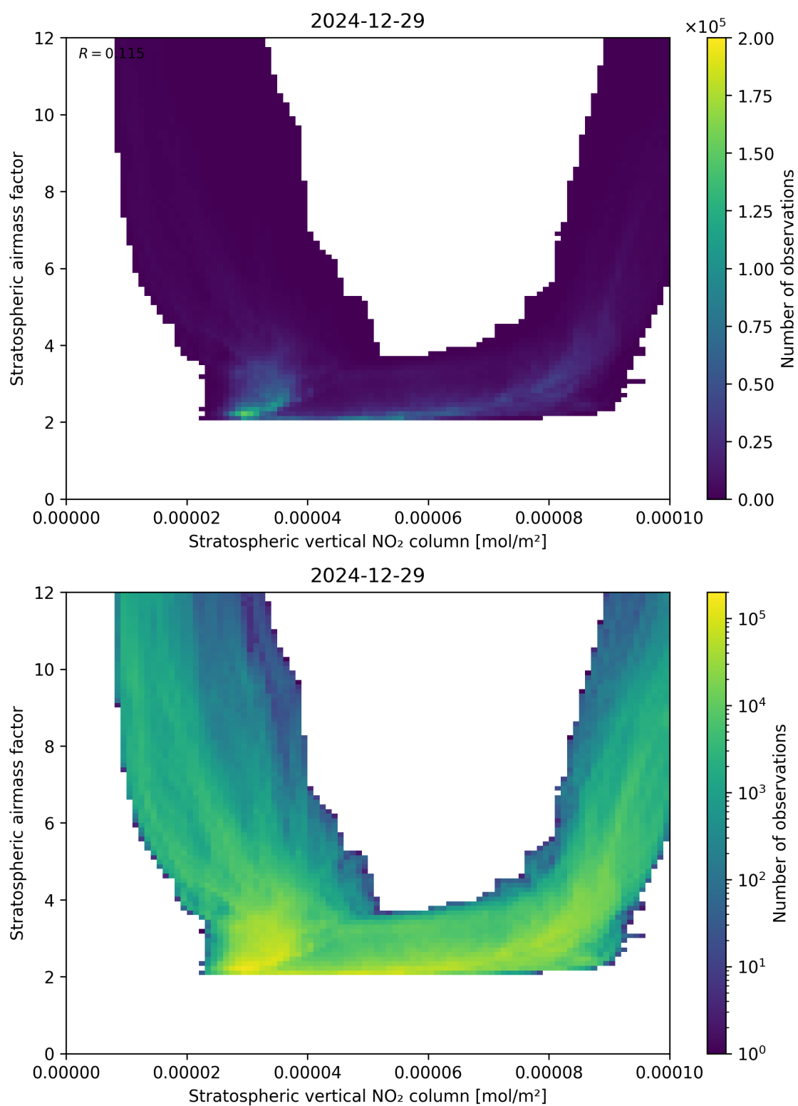
Figure 96: Scatter density plot of “Stratospheric vertical NO 2 column” against “Stratospheric airmass factor” for 2024-12-28 to 2024-12-30.
