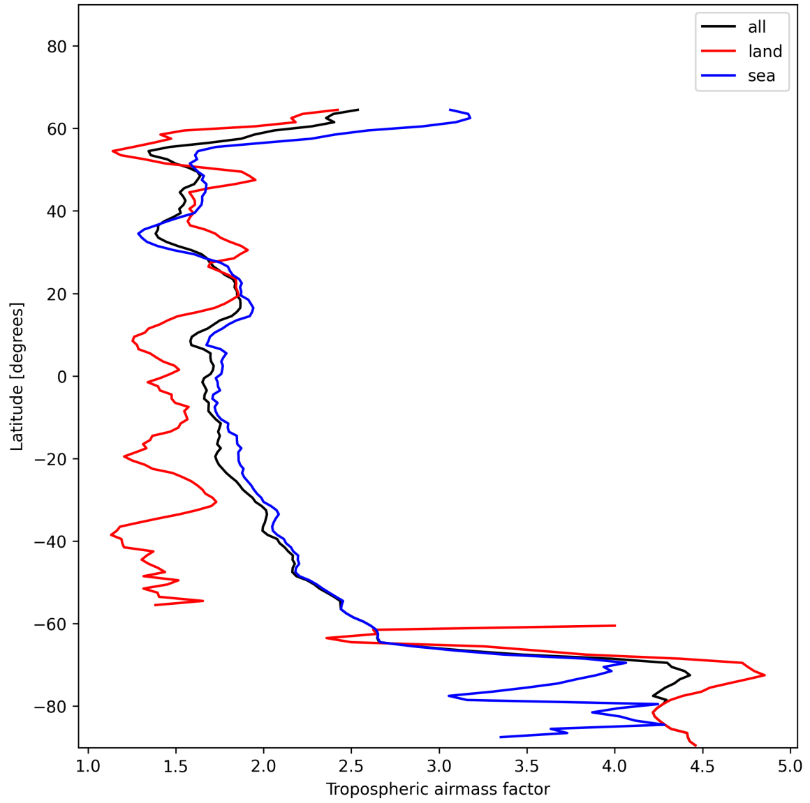
Figure 14: Zonal average of “Tropospheric airmass factor” for 2024-12-28 to 2024-12-30.
