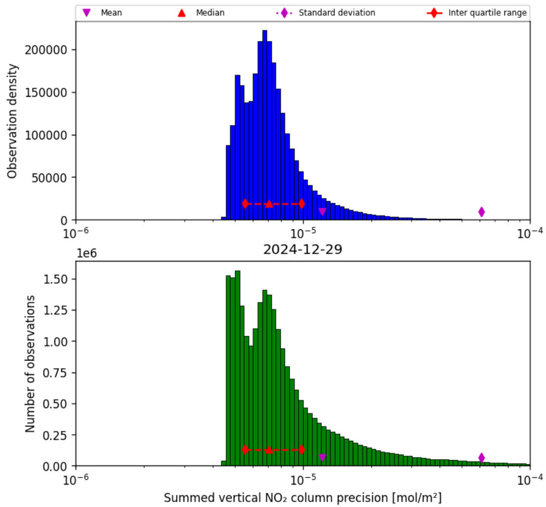
Figure 41: Histogram of “Summed vertical NO 2 column precision” for 2024-12-28 to 2024-12-30
