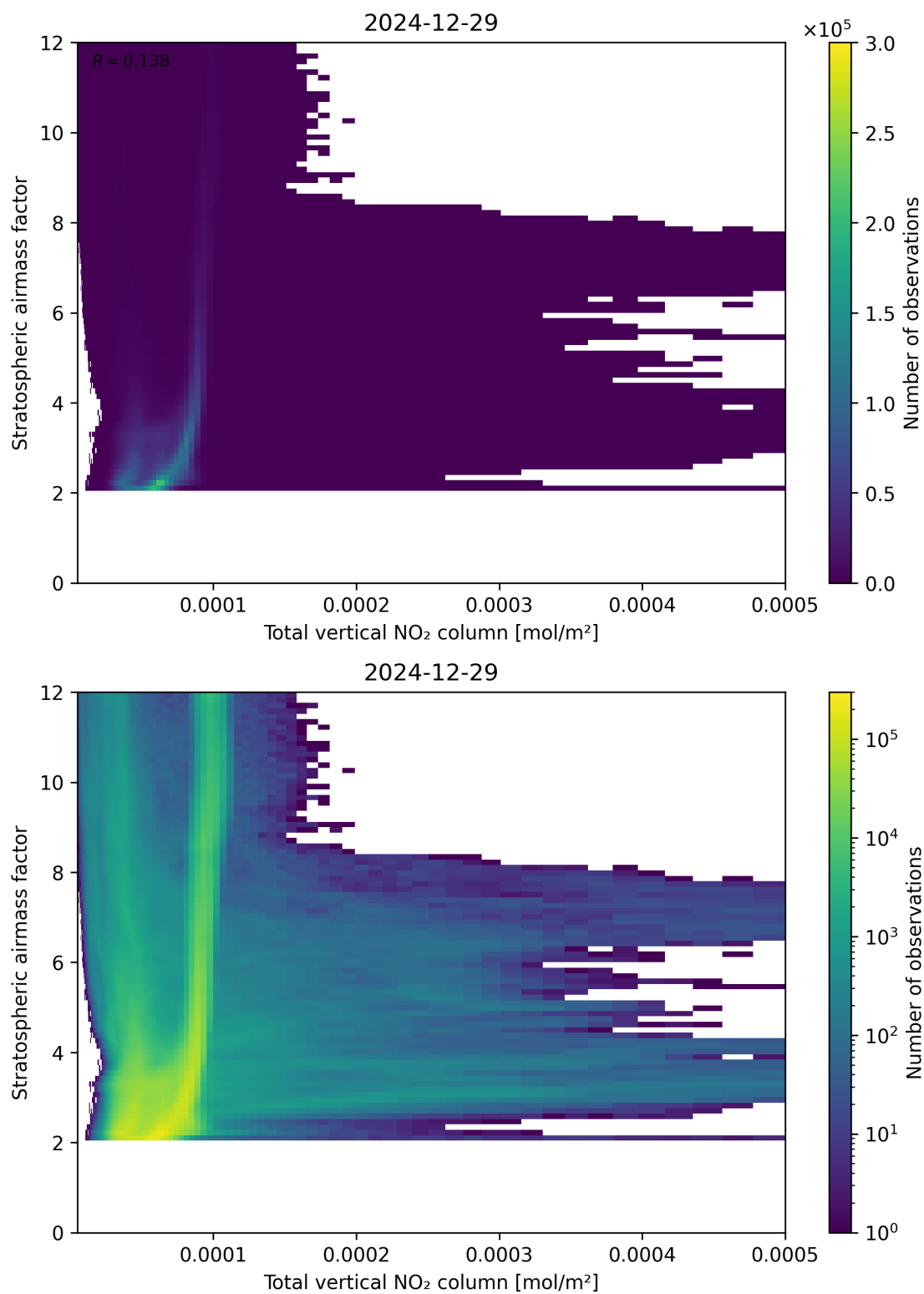
Figure 110: Scatter density plot of “Total vertical NO 2 column” against “Stratospheric air mass factor” for 2024-12-28 to 2024-12-30.
