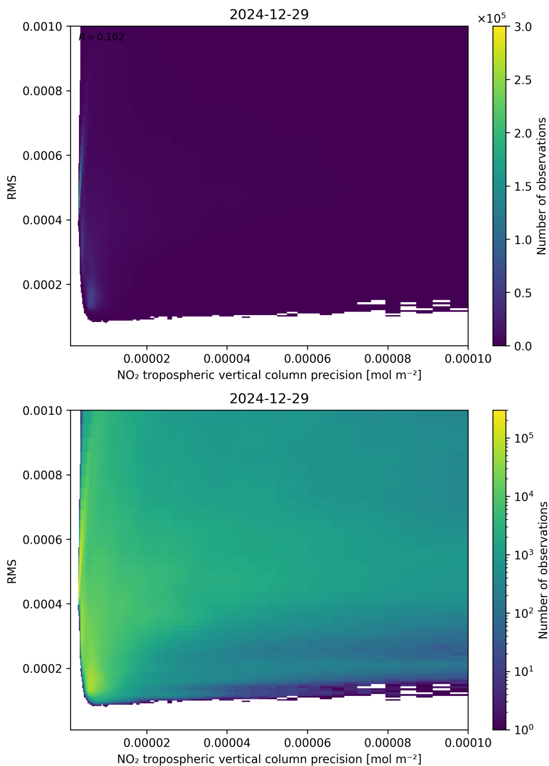
Figure 140: Scatter density plot of “NO 2 tropospheric vertical column precision” against “RMS” for 2024-12-28 to 2024-12-30.
