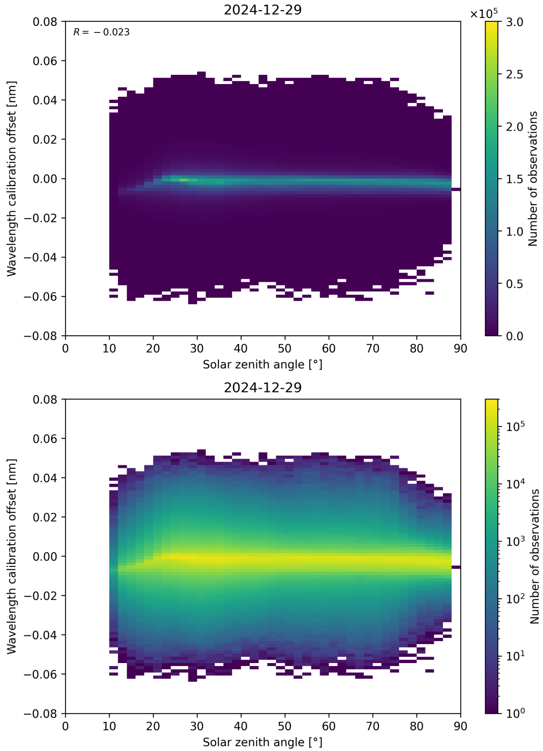
Figure 158: Scatter density plot of “Solar zenith angle” against “Wavelength calibration offset” for 2024-12-28 to 2024-12-30.
