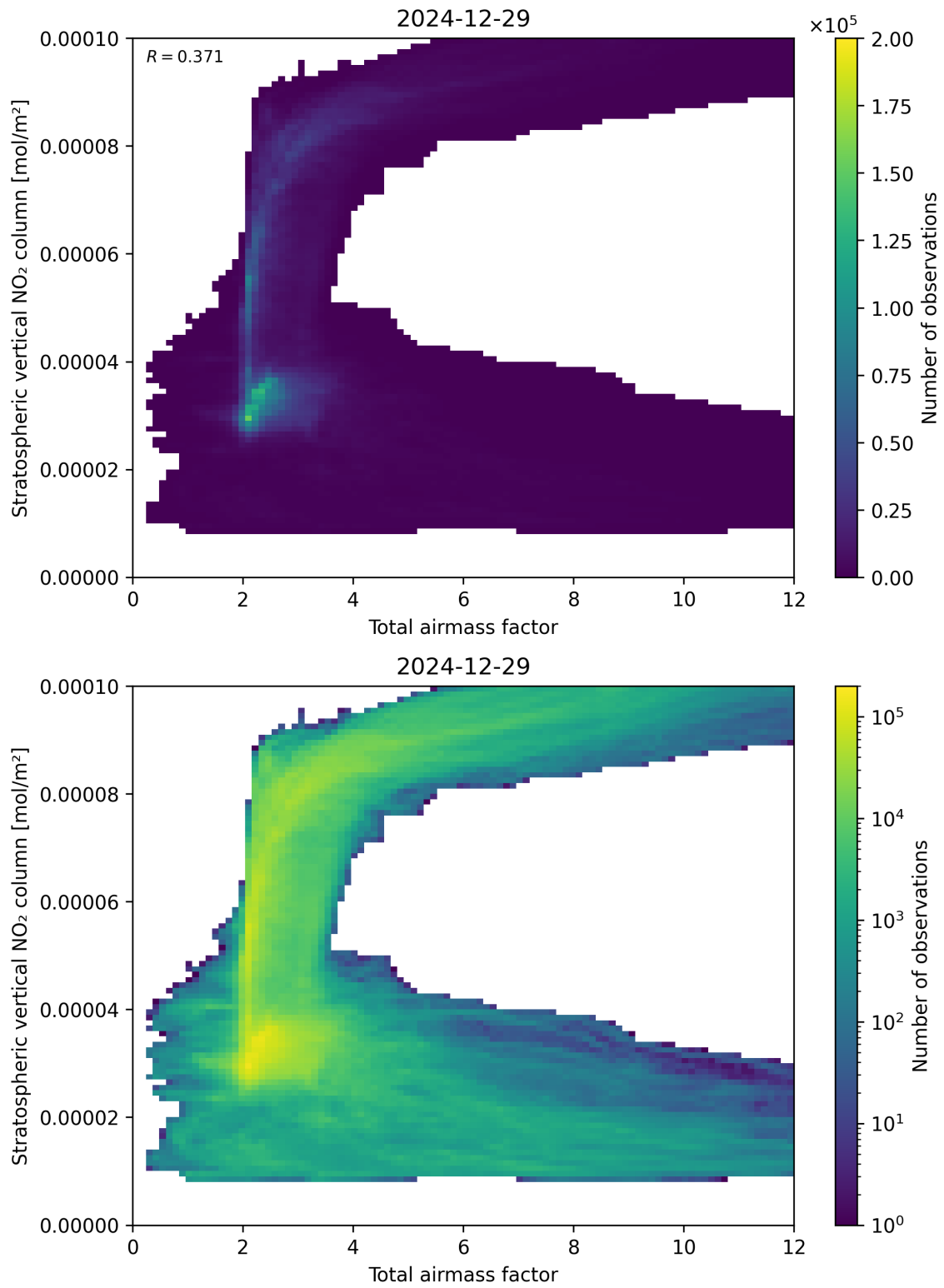
Figure 64: Scatter density plot of “Total airmass factor” against “Stratospheric vertical NO 2 column” for 2024-12-28 to 2024-12-30.
