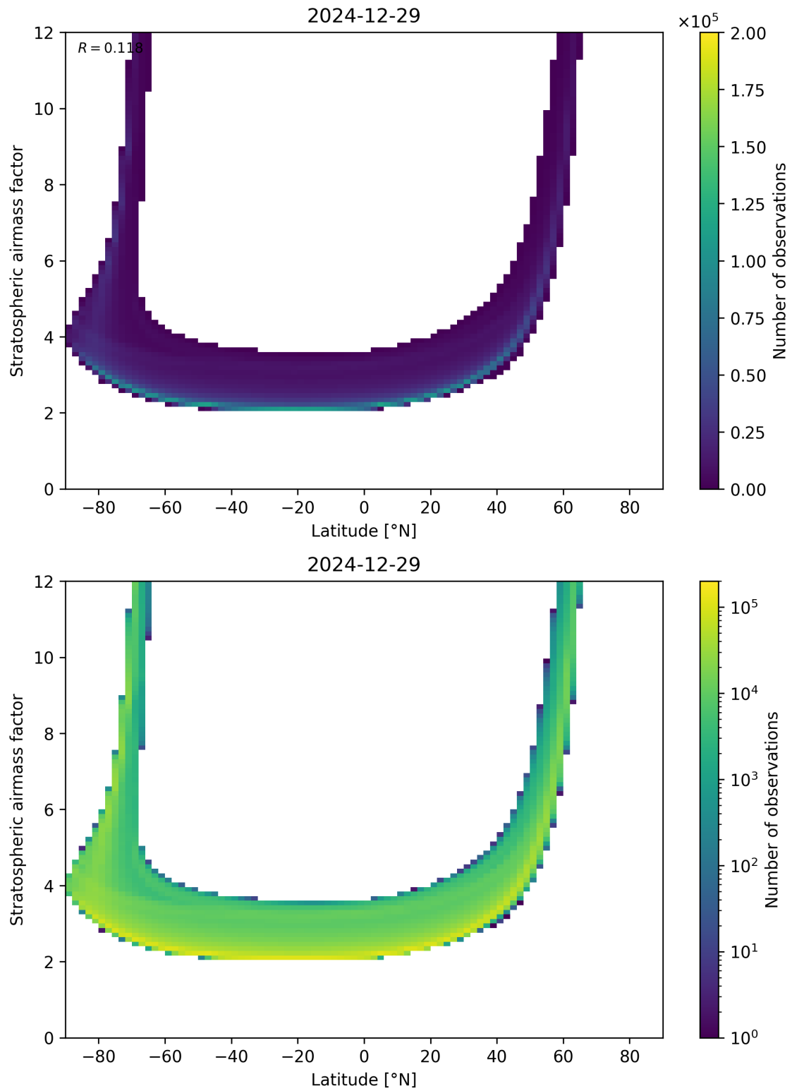
Figure 83: Scatter density plot of “Latitude” against “Stratospheric air mass factor” for 2024-12-28 to 2024-12-30.
