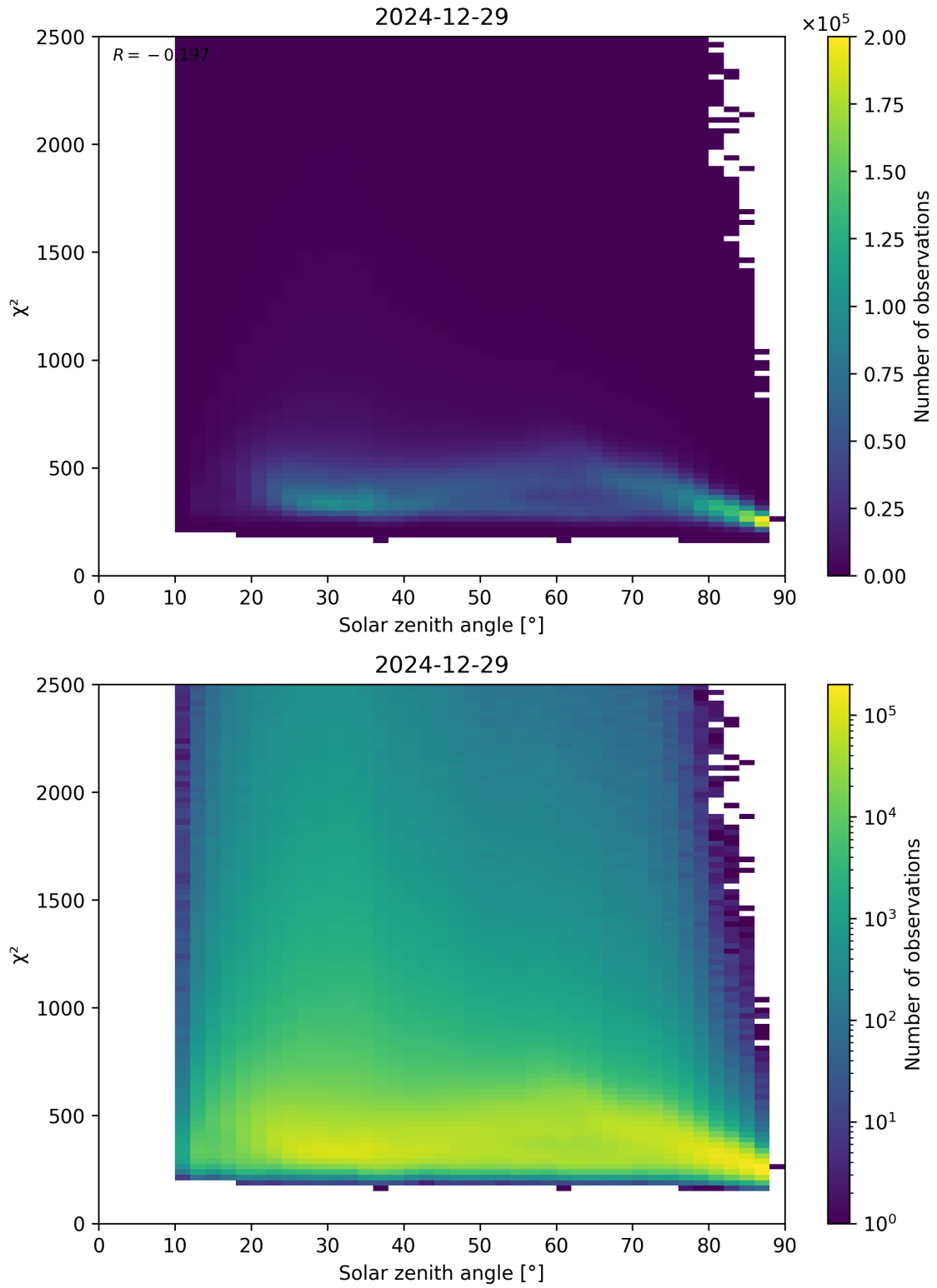
Figure 148: Scatter density plot of “Solar zenith angle” against “ \chi^2 ” for 2024-12-28 to 2024-12-30.
