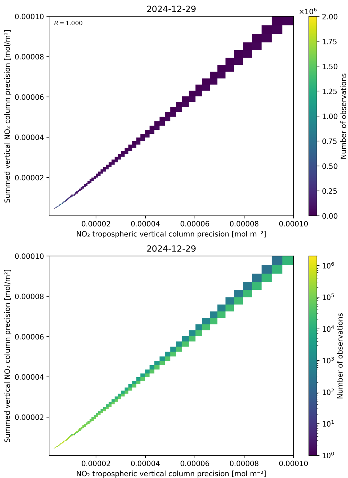
Figure 137: Scatter density plot of “NO 2 tropospheric vertical column precision” against “Summed vertical NO 2 column precision” for 2024-12-28 to 2024-12-30.
