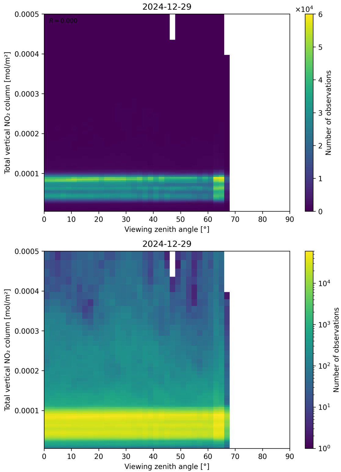
Figure 167: Scatter density plot of “Viewing zenith angle” against “Total vertical NO 2 column” for 2024-12-28 to 2024-12-30.
