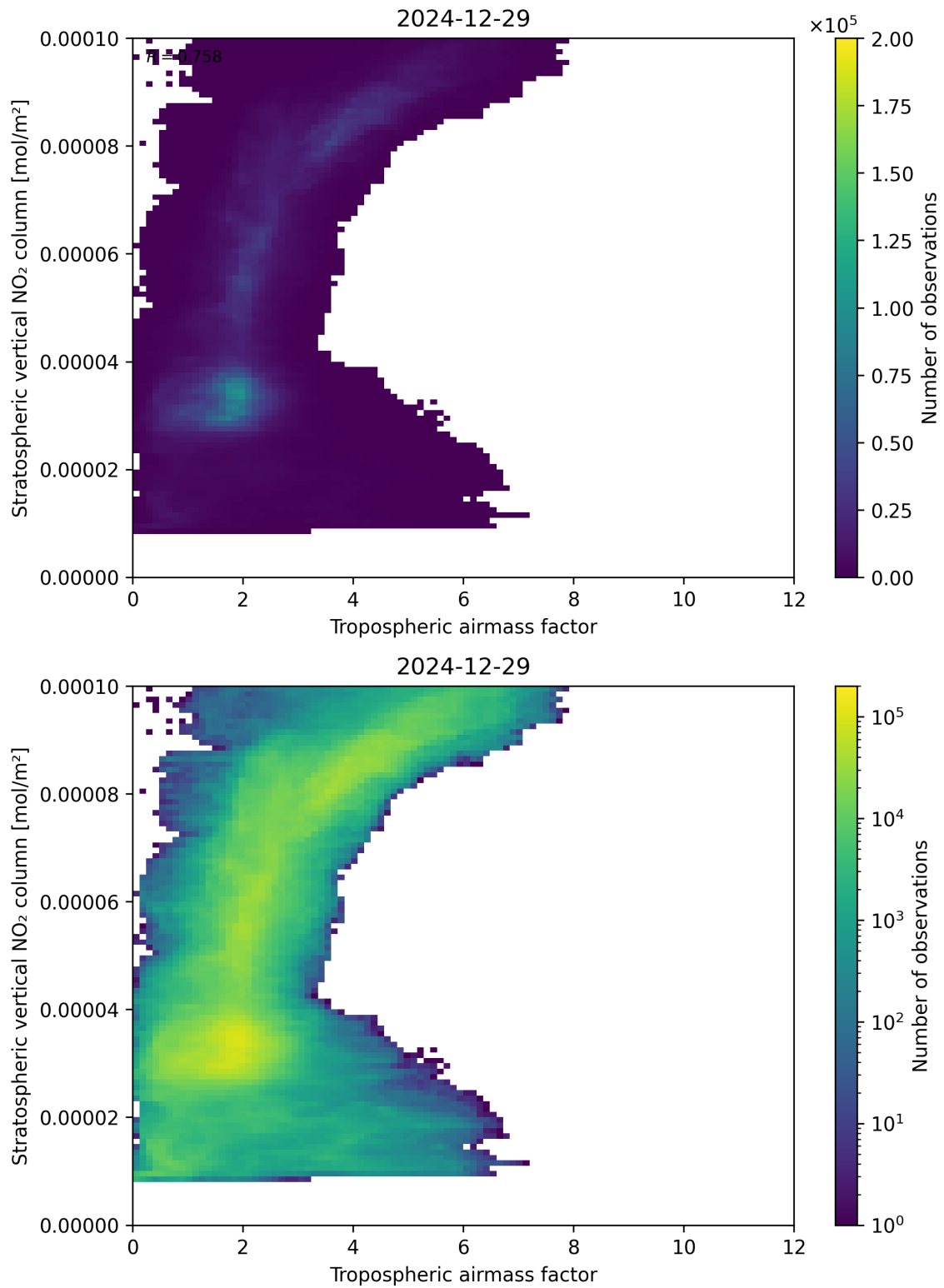
Figure 74: Scatter density plot of “Tropospheric airmass factor” against “Stratospheric vertical NO 2 column” for 2024-12-28 to 2024-12-30.
