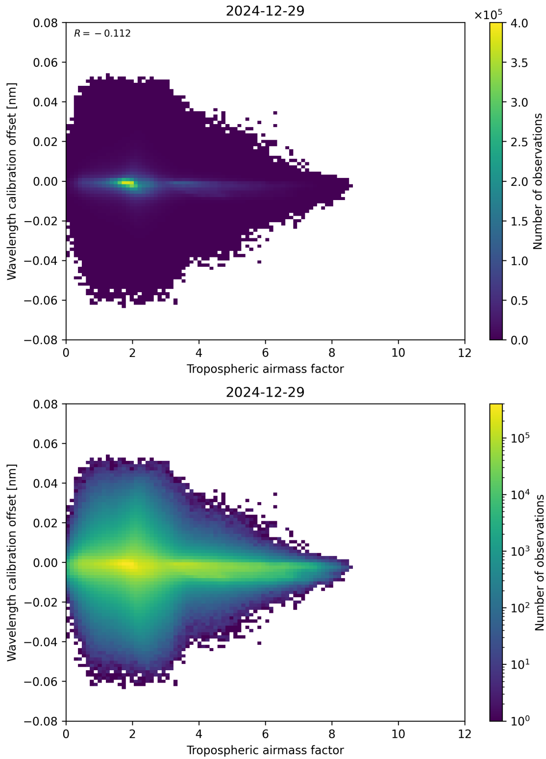
Figure 80: Scatter density plot of “Tropospheric airmass factor” against “Wavelength calibration offset” for 2024-12-28 to 2024-12-30.
