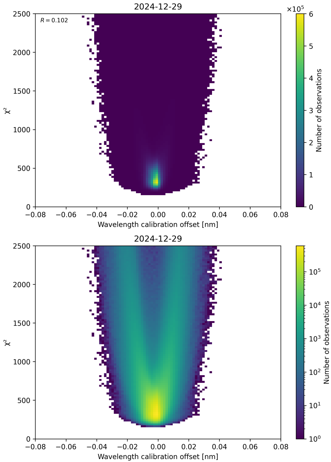
Figure 175: Scatter density plot of “Wavelength calibration offset” against “ \chi^2 ” for 2024-12-28 to 2024-12-30.
