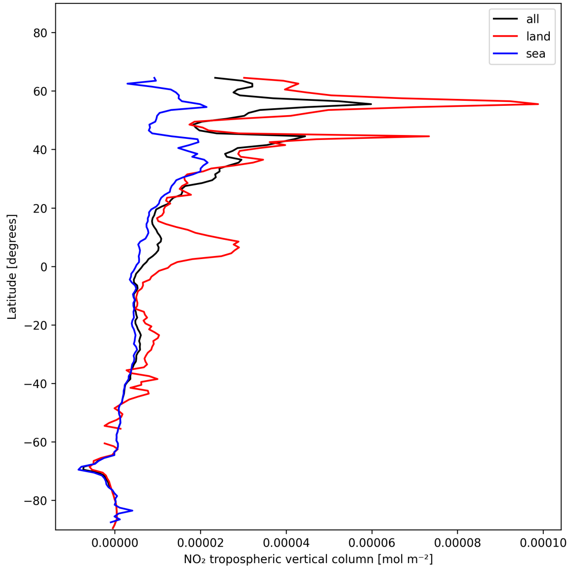
Figure 12: Zonal average of “NO 2 tropospheric vertical column” for 2024-12-28 to 2024-12-30.
