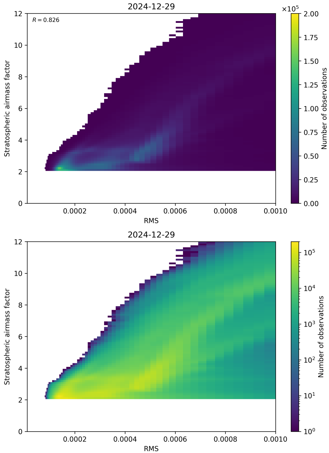
Figure 144: Scatter density plot of “RMS” against “Stratospheric airmass factor” for 2024-12-28 to 2024-12-30.
