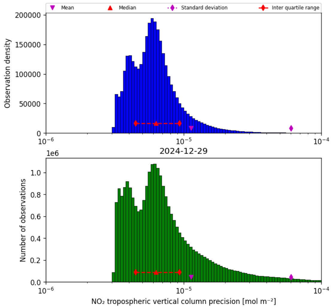
Figure 30: Histogram of “NO 2 tropospheric vertical column precision” for 2024-12-28 to 2024-12-30
