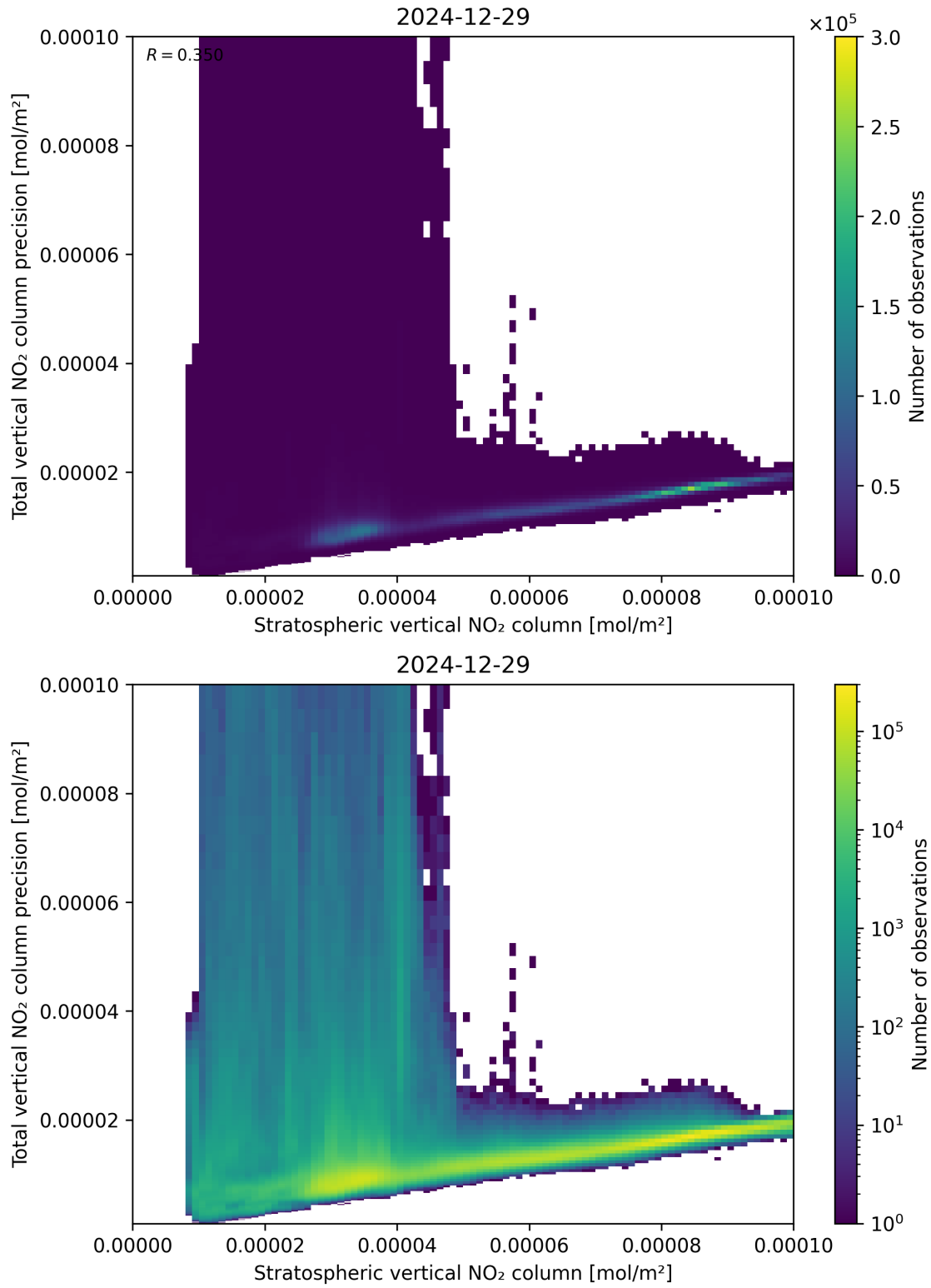
Figure 101: Scatter density plot of “Stratospheric vertical NO 2 column” against “Total vertical NO 2 column precision” for 2024-12-28 to 2024-12-30.
