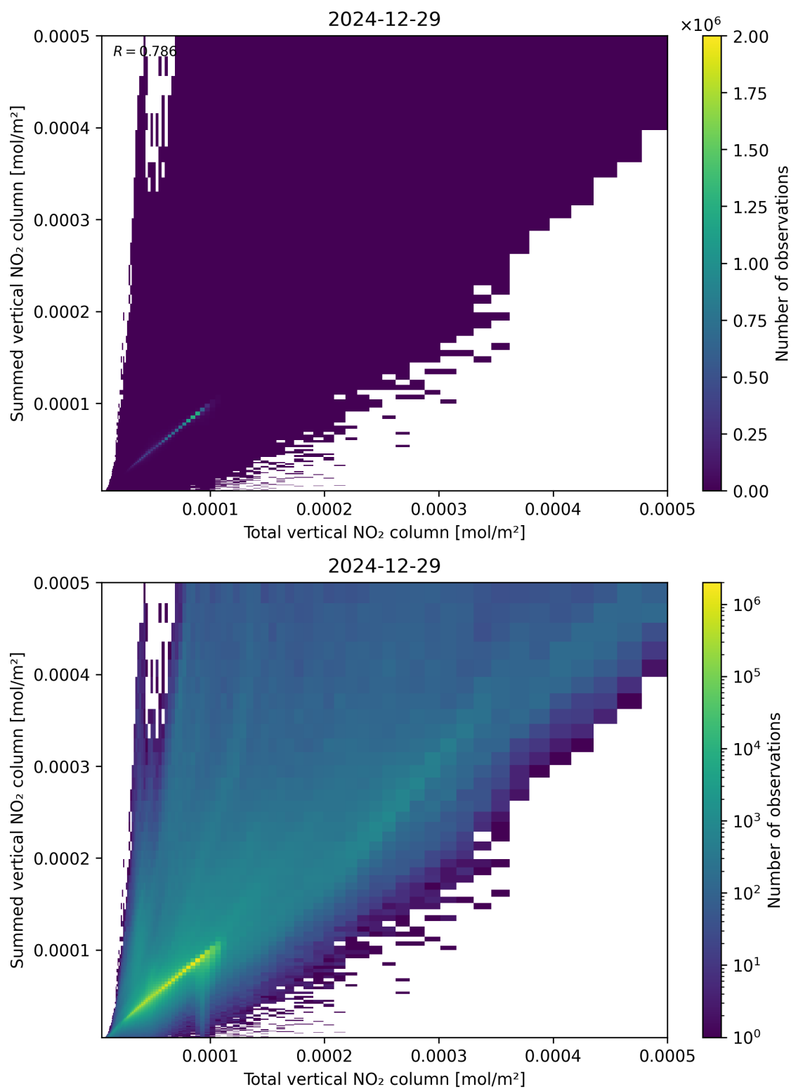
Figure 112: Scatter density plot of “Total vertical NO 2 column” against “Summed vertical NO 2 column” for 2024-12-28 to 2024-12-30.
