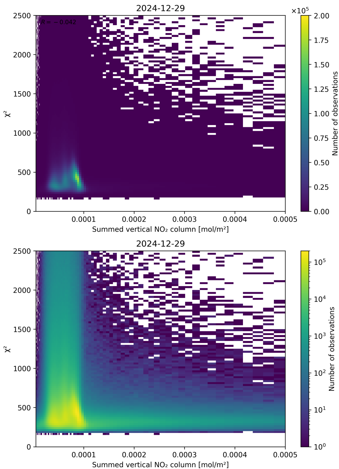
Figure 104: Scatter density plot of “Summed vertical NO 2 column” against “ \chi^2 ” for 2024-12-28 to 2024-12-30.
