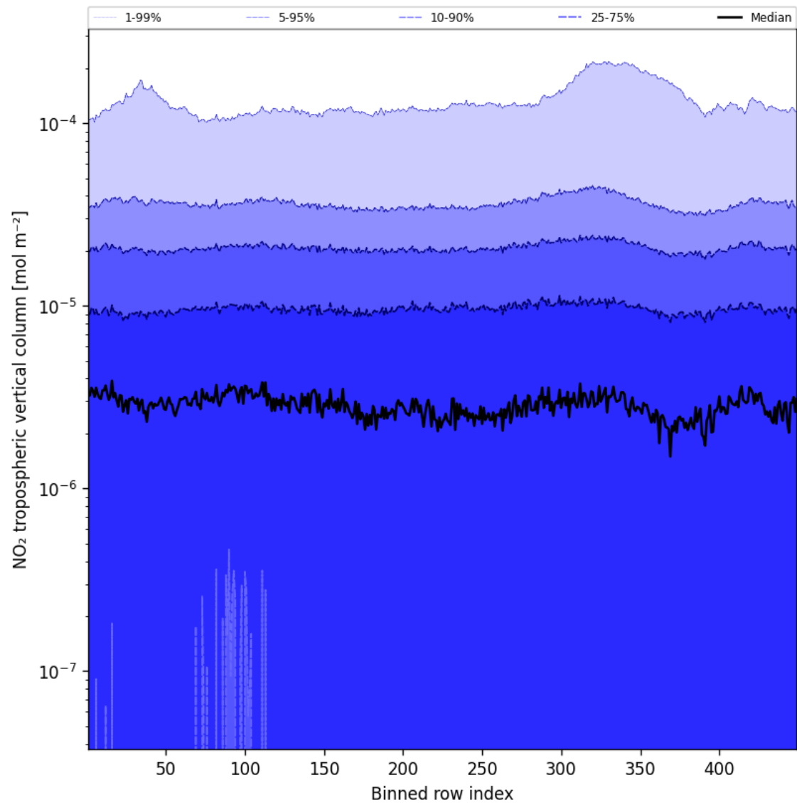
Figure 46: Along track statistics of “NO 2 tropospheric vertical column” for 2024-12-28 to 2024-12-30
