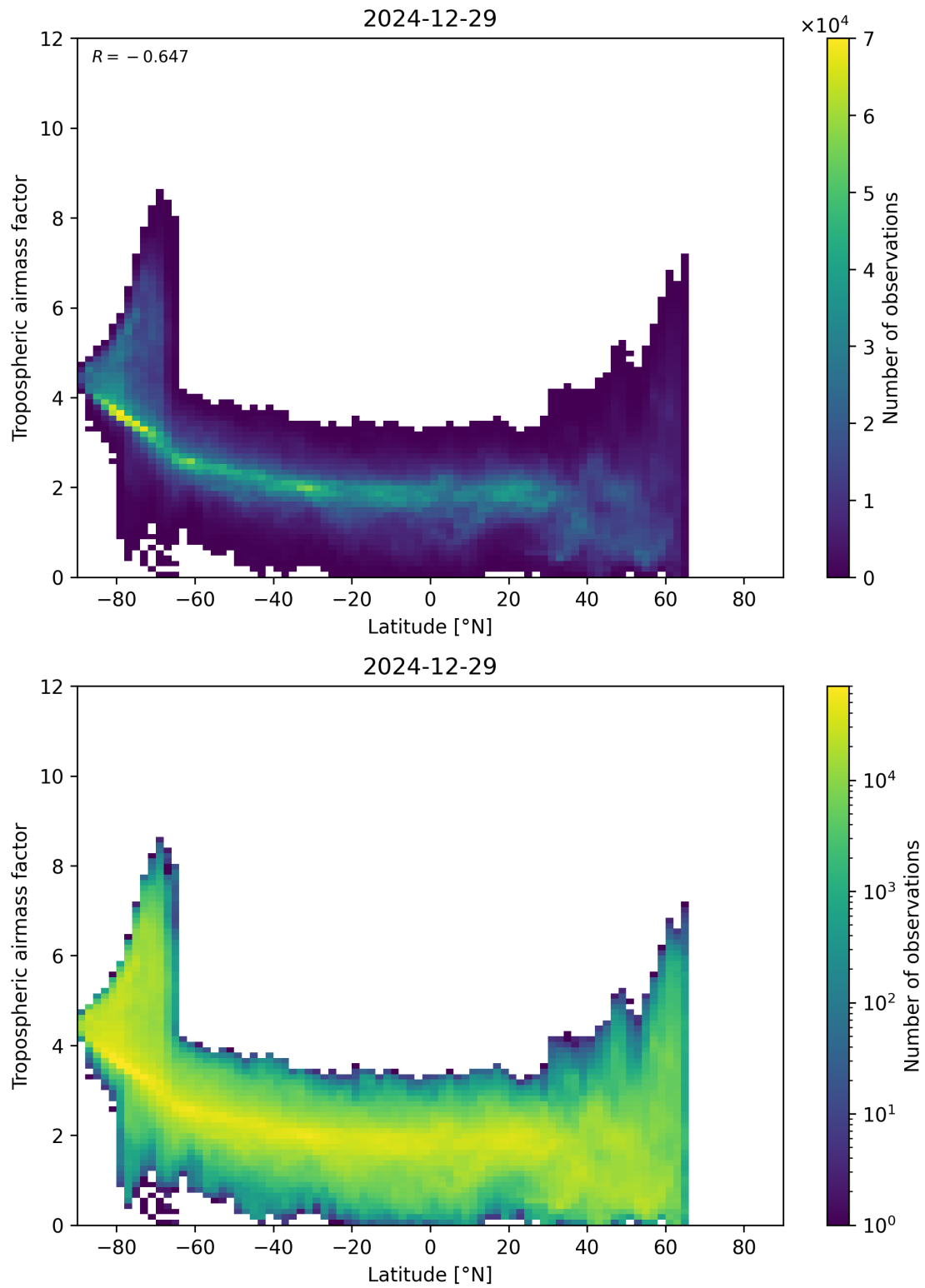
Figure 85: Scatter density plot of “Latitude” against “Tropospheric airmass factor” for 2024-12-28 to 2024-12-30.
