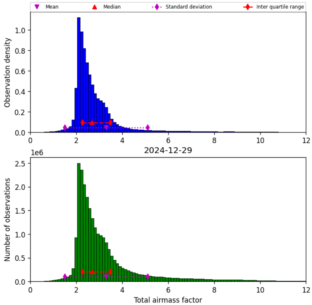
Figure 32: Histogram of “Total airmass factor” for 2024-12-28 to 2024-12-30
