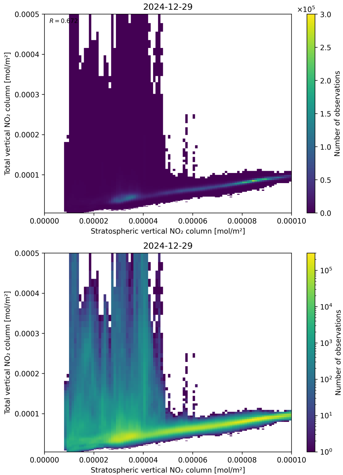
Figure 100: Scatter density plot of “Stratospheric vertical NO 2 column” against “Total vertical NO 2 column” for 2024-12-28 to 2024-12-30.
