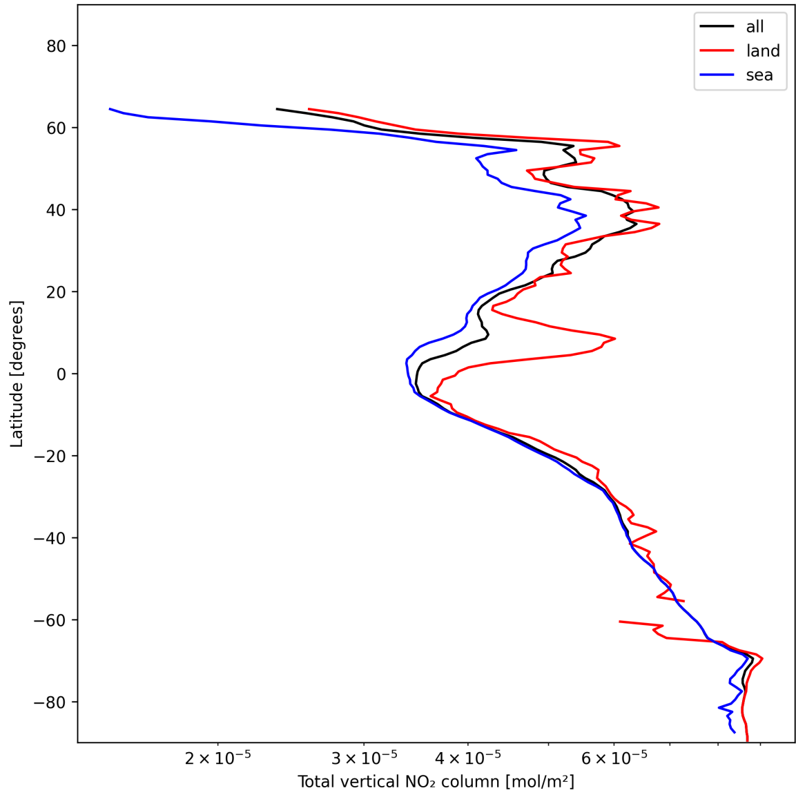
Figure 21: Zonal average of “Total vertical NO 2 column” for 2024-12-28 to 2024-12-30.
