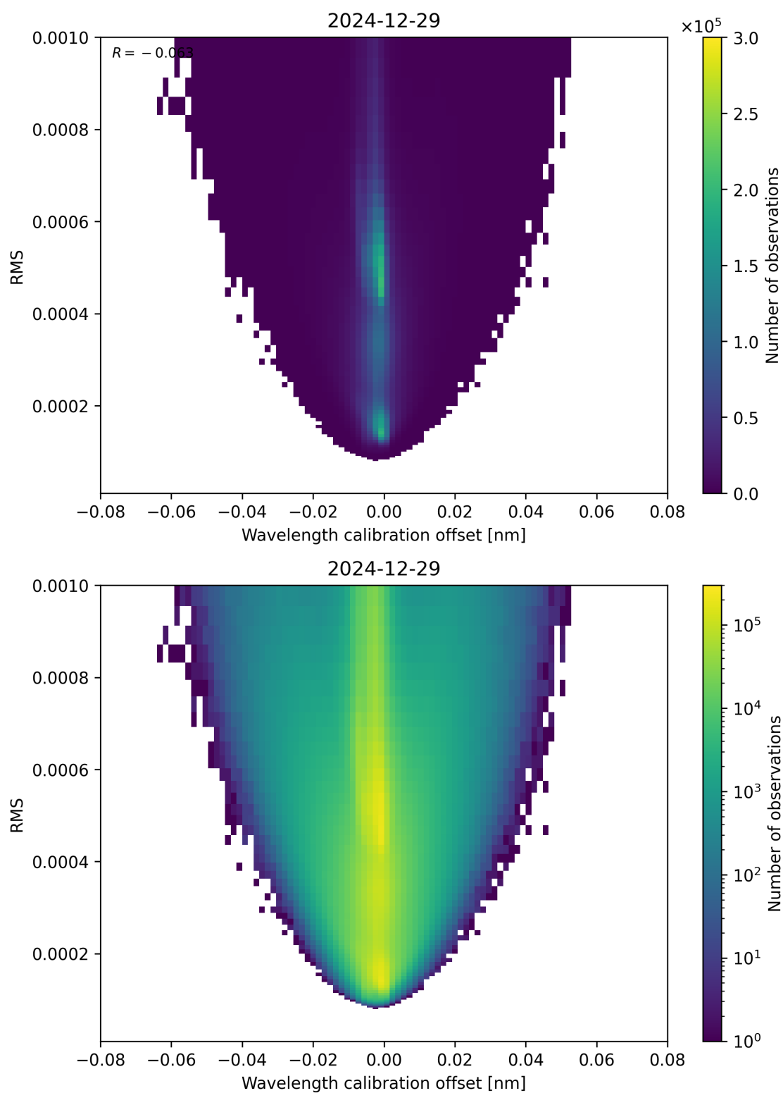
Figure 181: Scatter density plot of “Wavelength calibration offset” against “RMS” for 2024-12-28 to 2024-12-30.
