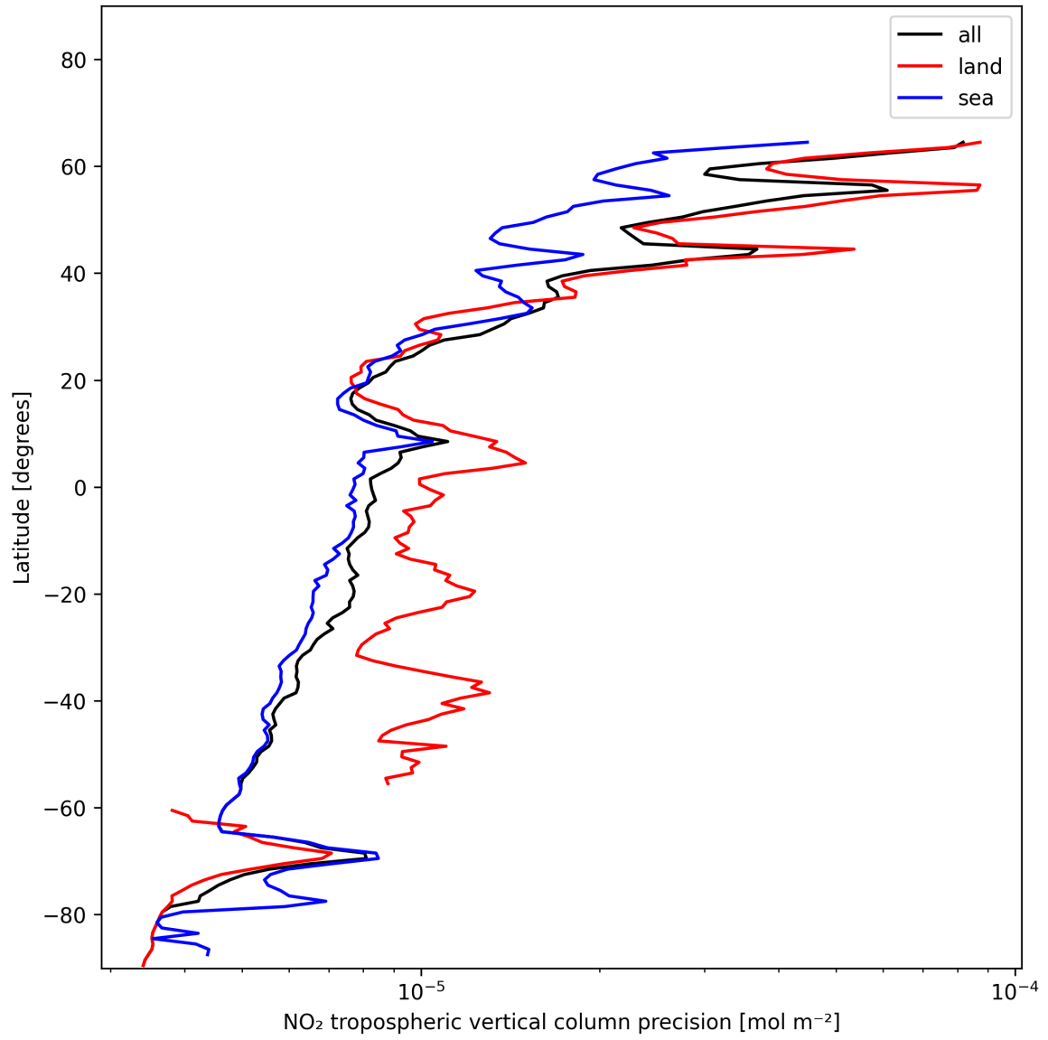
Figure 13: Zonal average of “NO 2 tropospheric vertical column precision” for 2024-12-28 to 2024-12-30.
