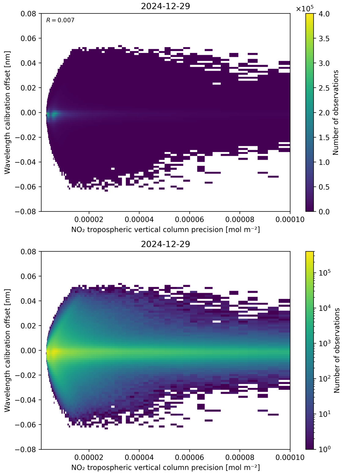
Figure 141: Scatter density plot of “NO 2 tropospheric vertical column precision” against “Wavelength calibration offset” for 2024-12-28 to 2024-12-30.
