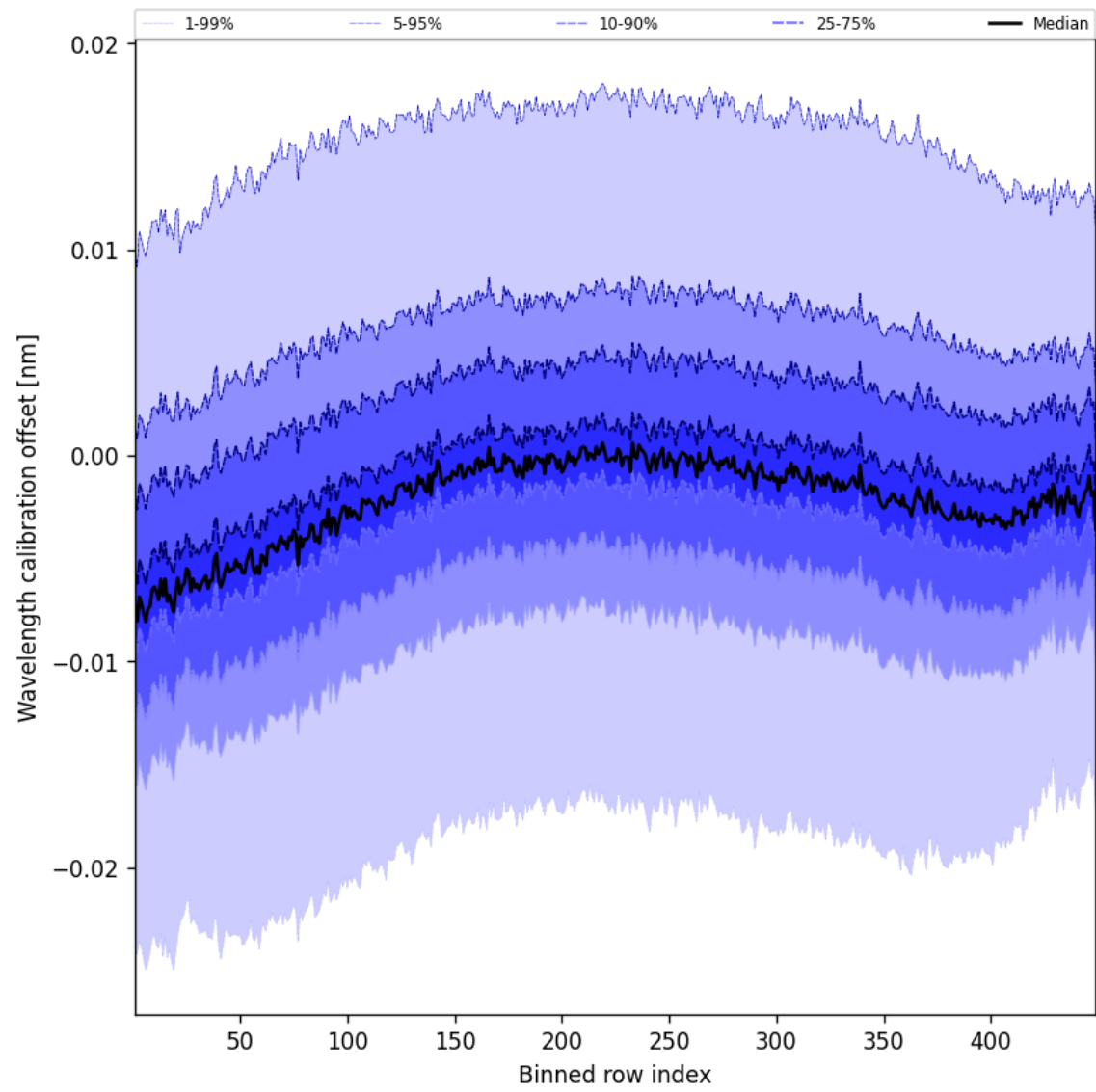
Figure 52: Along track statistics of “Wavelength calibration offset” for 2024-12-28 to 2024-12-30
