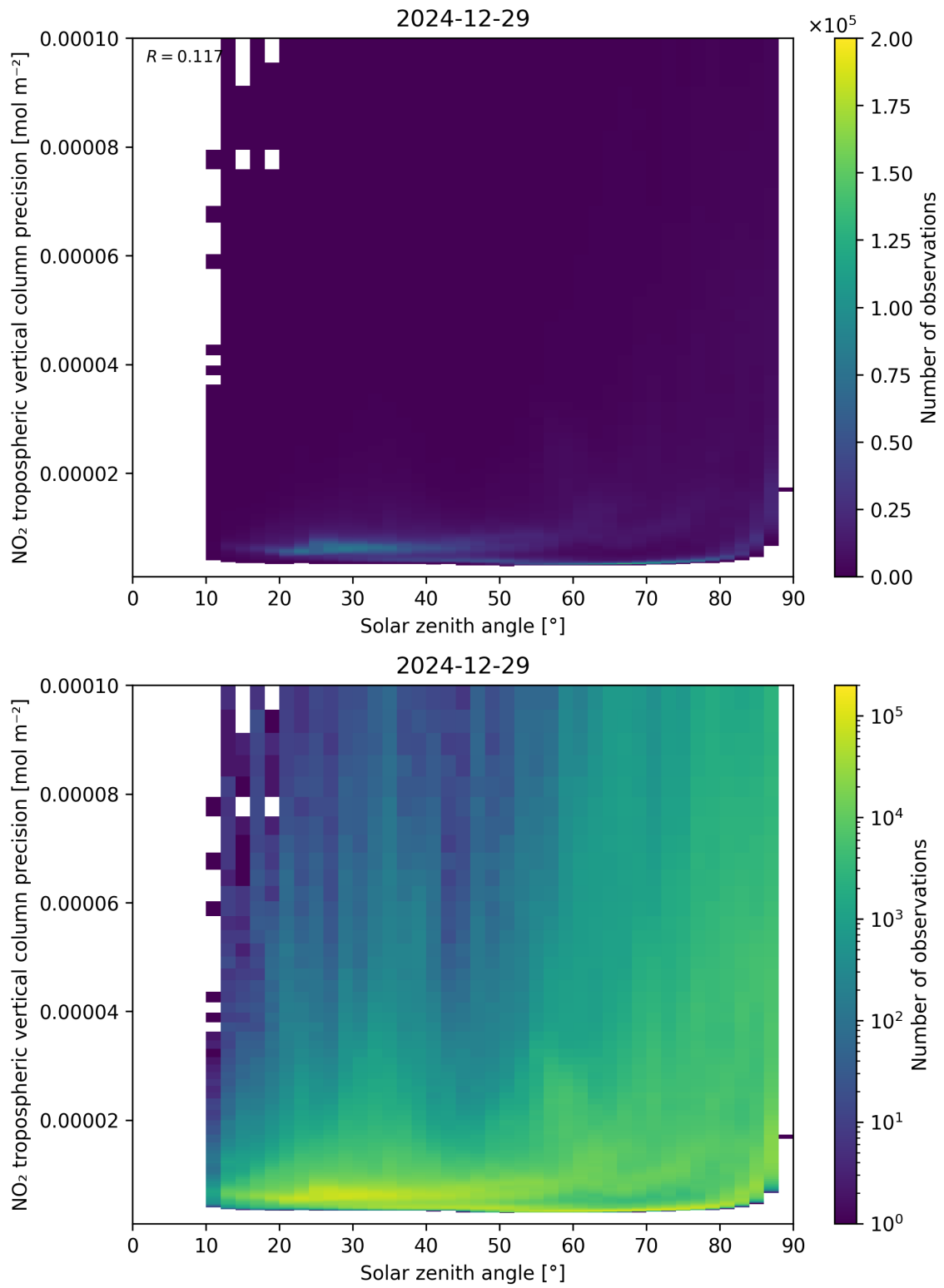
Figure 156: Scatter density plot of “Solar zenith angle” against “NO 2 tropospheric vertical column precision” for 2024-12-28 to 2024-12-30.
