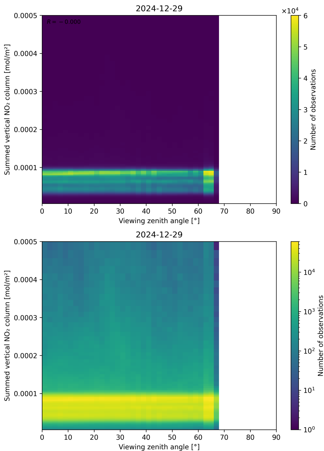
Figure 165: Scatter density plot of “Viewing zenith angle” against “Summed vertical NO 2 column” for 2024-12-28 to 2024-12-30.
