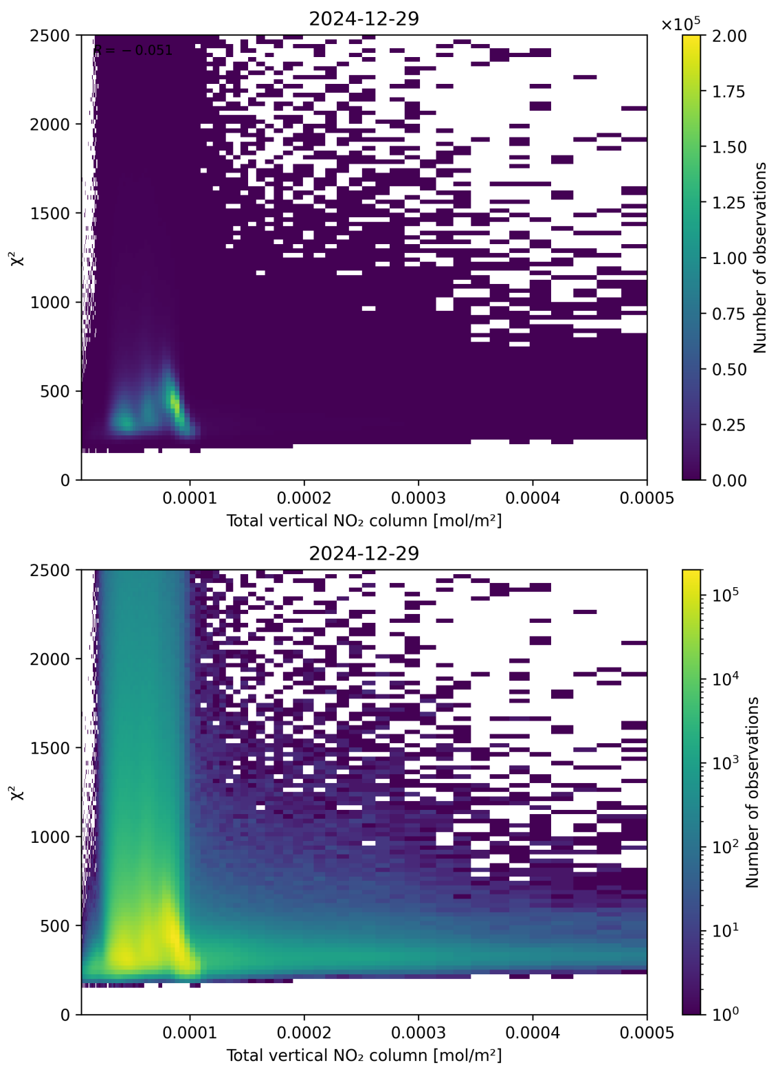
Figure 111: Scatter density plot of “Total vertical NO 2 column” against “ \chi^2 ” for 2024-12-28 to 2024-12-30.
