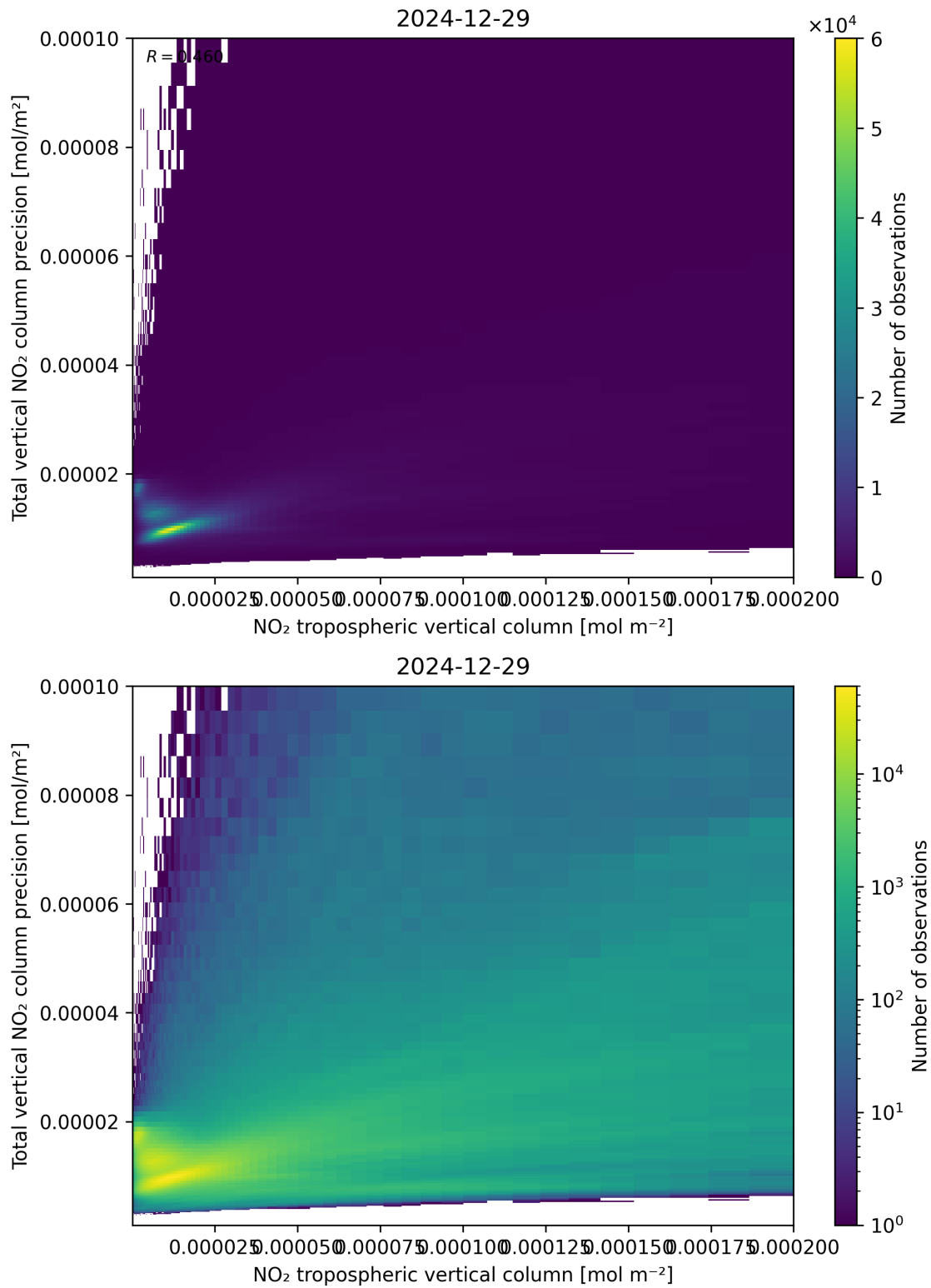
Figure 129: Scatter density plot of “NO 2 tropospheric vertical column” against “Total vertical NO 2 column precision” for 2024-12-28 to 2024-12-30.
