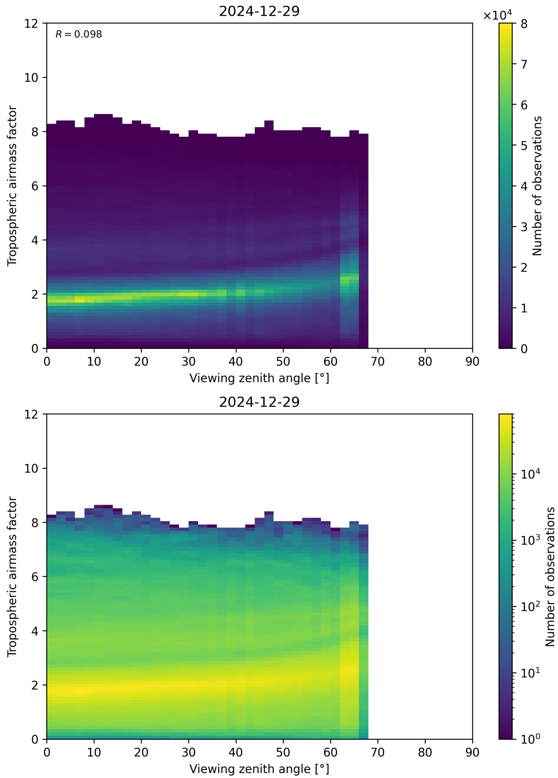
Figure 161: Scatter density plot of “Viewing zenith angle” against “Tropospheric airmass factor” for 2024-12-28 to 2024-12-30.
