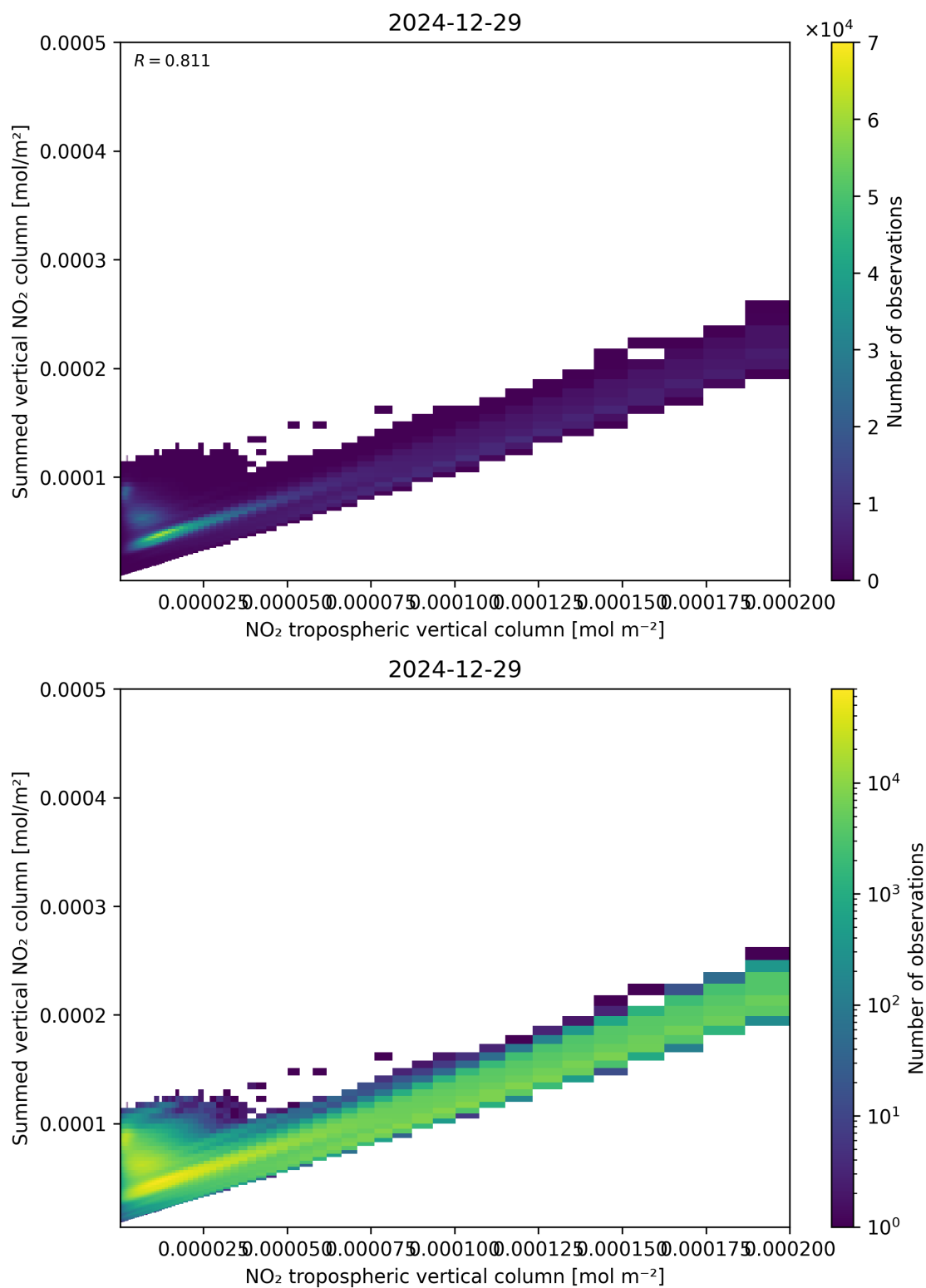
Figure 126: Scatter density plot of “NO 2 tropospheric vertical column” against “Summed vertical NO 2 column” for 2024-12-28 to 2024-12-30.
