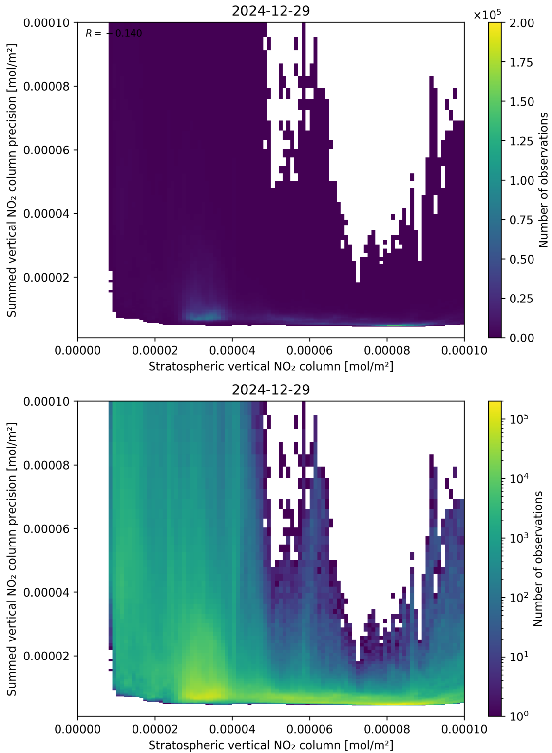
Figure 99: Scatter density plot of “Stratospheric vertical NO 2 column” against “Summed vertical NO 2 column precision” for 2024-12-28 to 2024-12-30.
