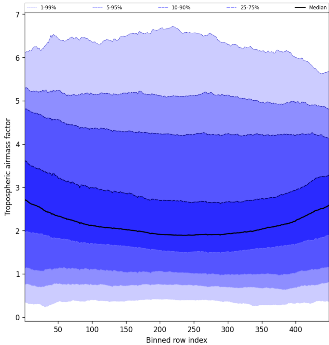
Figure 48: Along track statistics of “Tropospheric air mass factor” for 2024-12-28 to 2024-12-30
