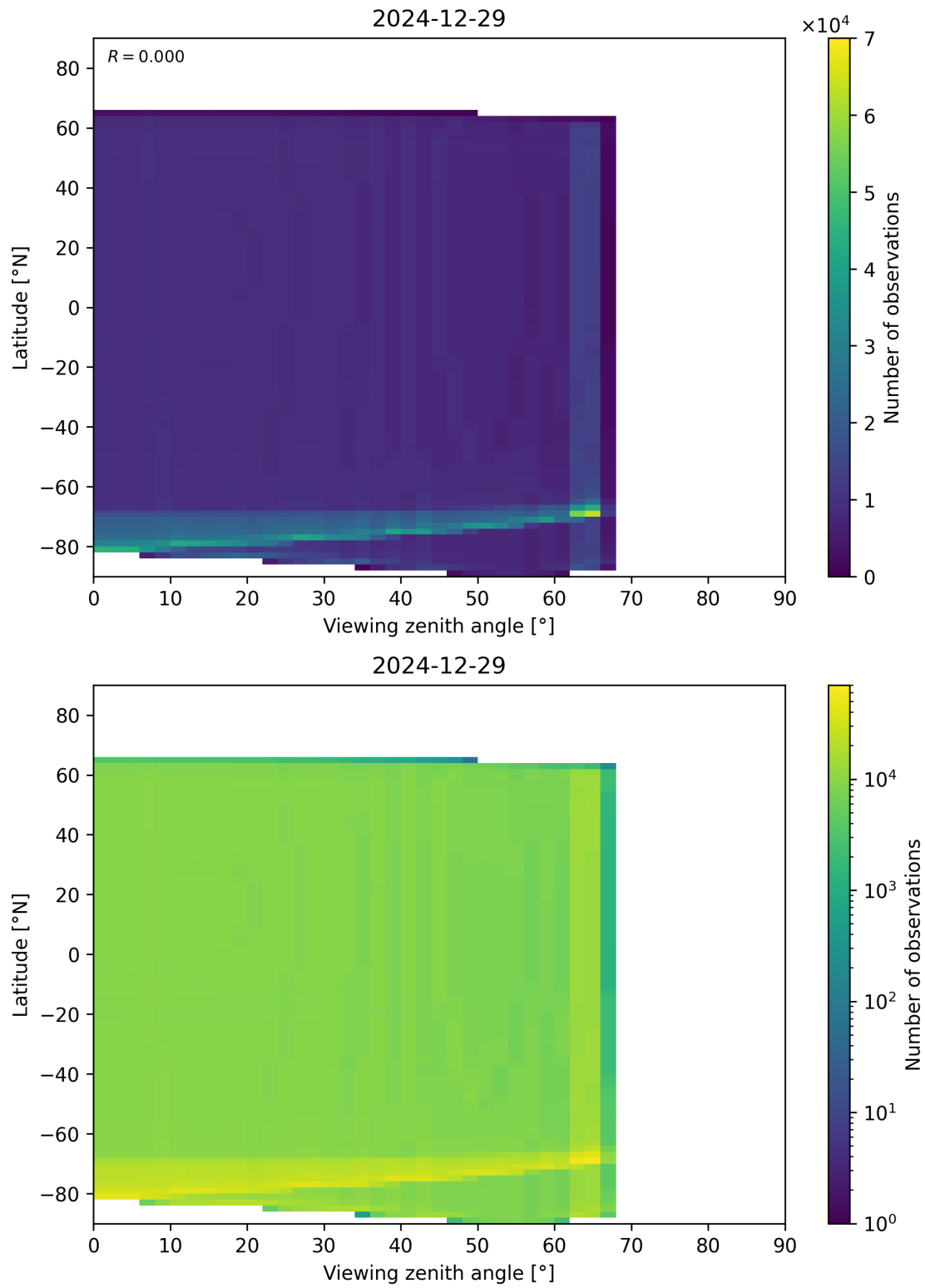
Figure 163: Scatter density plot of “Viewing zenith angle” against “Latitude” for 2024-12-28 to 2024-12-30.
