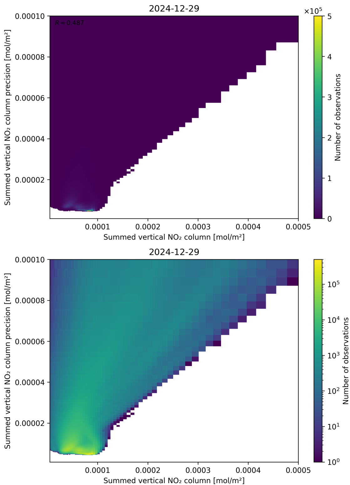
Figure 105: Scatter density plot of “Summed vertical NO 2 column” against “Summed vertical NO 2 column precision” for 2024-12-28 to 2024-12-30.
