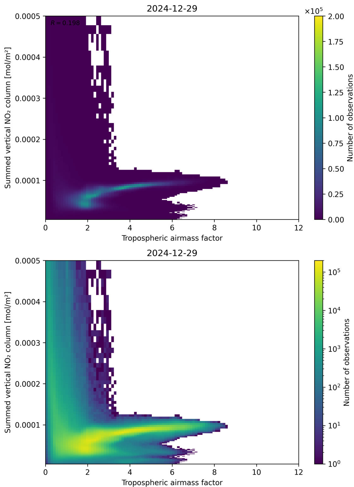
Figure 75: Scatter density plot of “Tropospheric air mass factor” against “Summed vertical NO 2 column” for 2024-12-28 to 2024-12-30.
