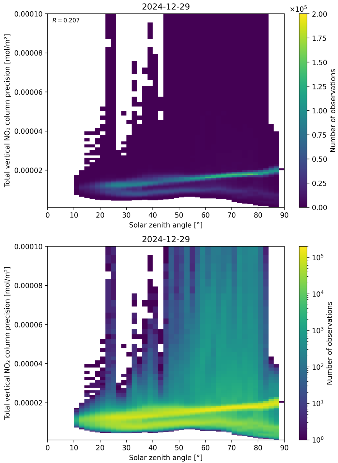
Figure 154: Scatter density plot of “Solar zenith angle” against “Total vertical NO 2 column precision” for 2024-12-28 to 2024-12-30.
