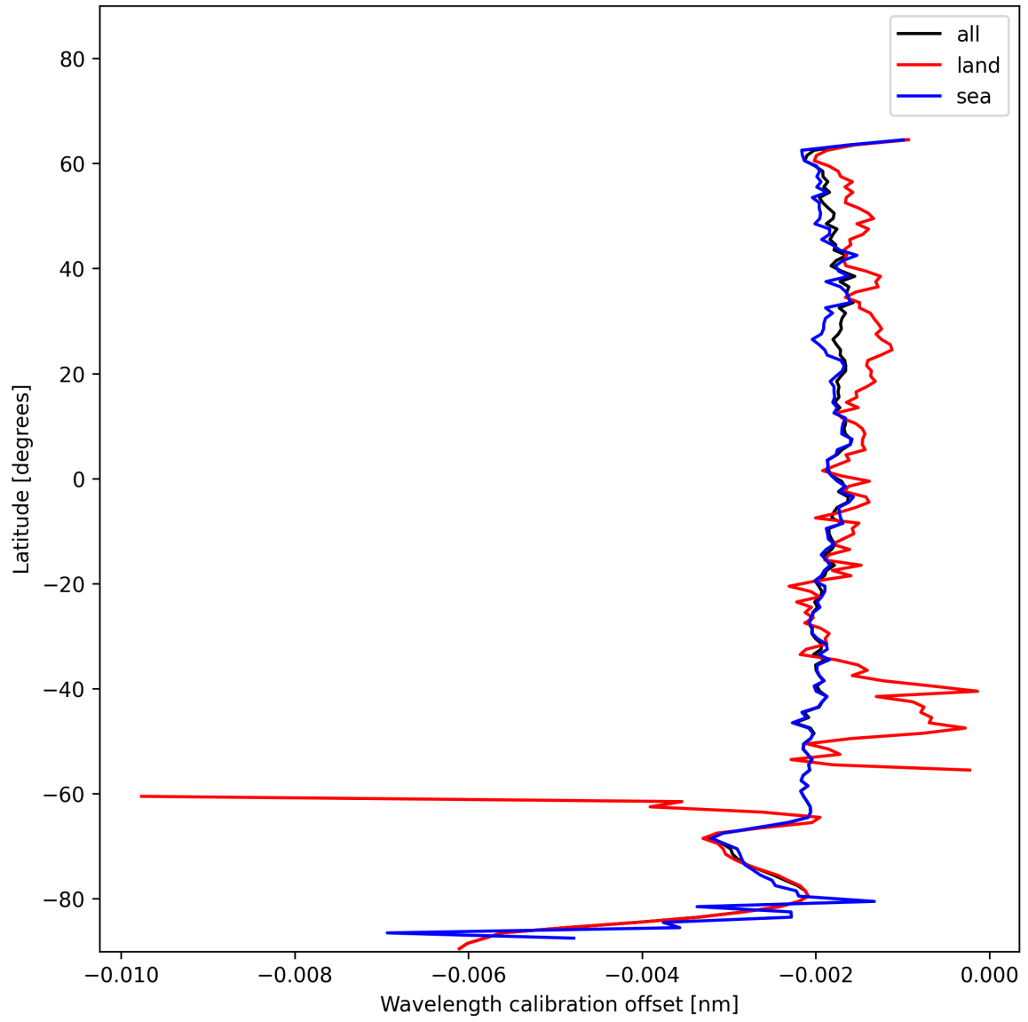
Figure 18: Zonal average of “Wavelength calibration offset” for 2024-12-28 to 2024-12-30.
