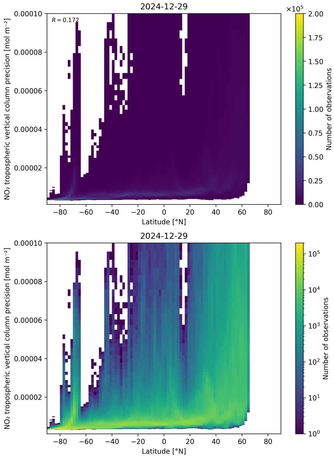
Figure 93: Scatter density plot of “Latitude” against “NO 2 tropospheric vertical column precision” for 2024-12-28 to 2024-12-30.
