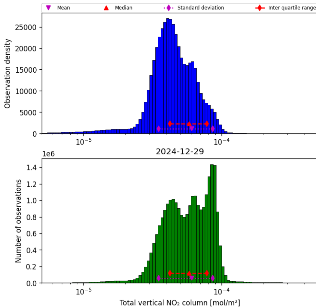
Figure 38: Histogram of “Total vertical NO 2 column” for 2024-12-28 to 2024-12-30
