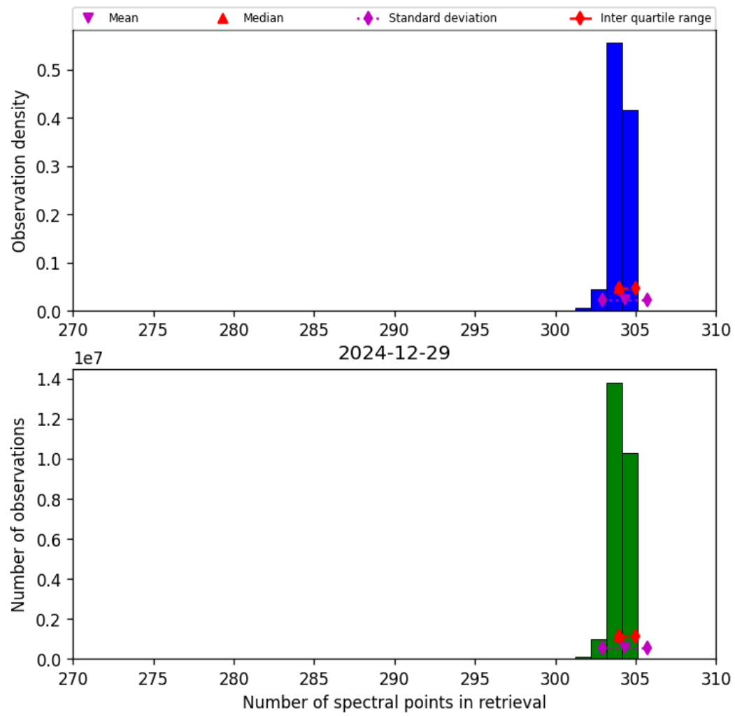
Figure 33: Histogram of “Number of spectral points in retrieval” for 2024-12-28 to 2024-12-30
