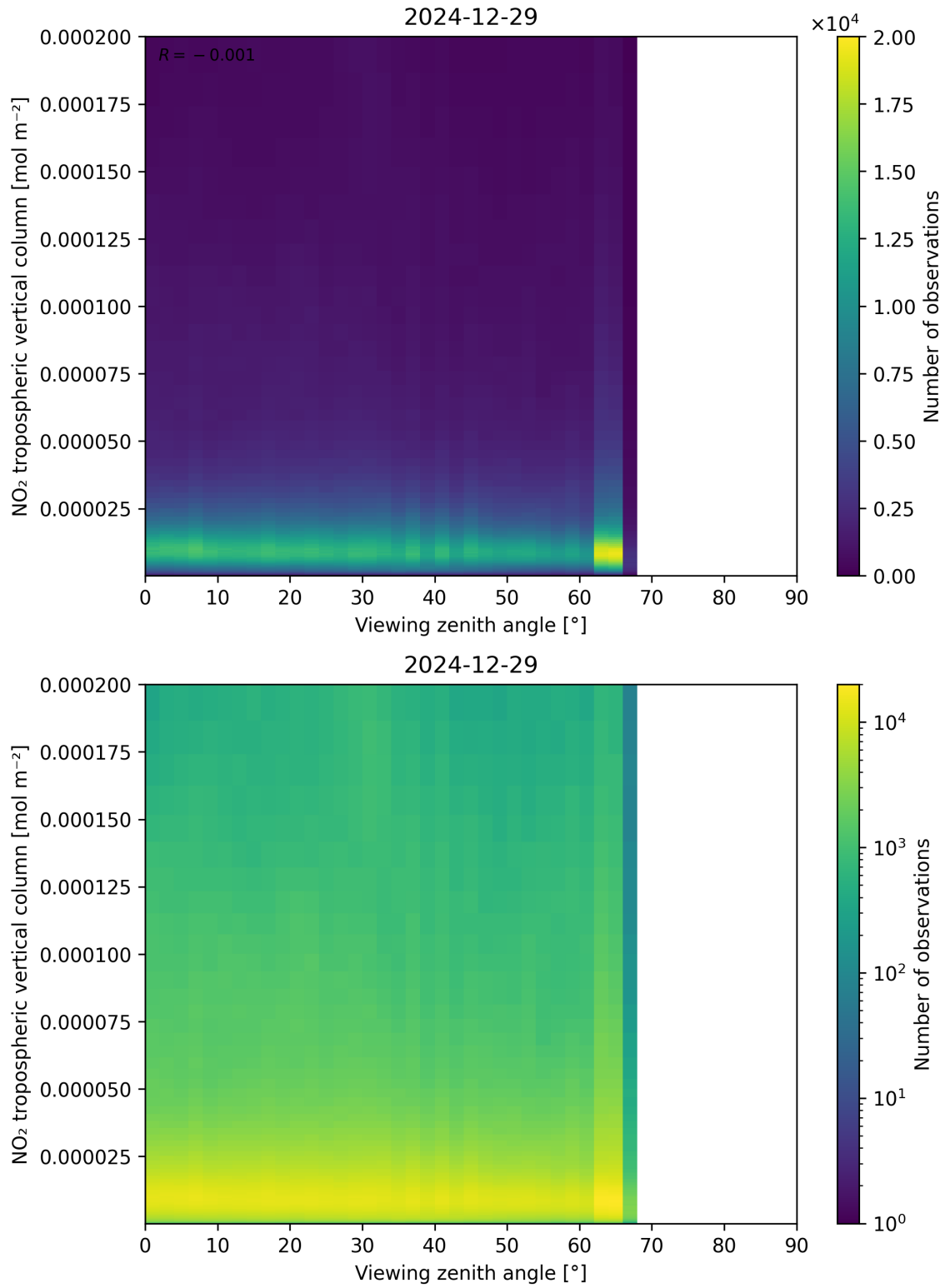
Figure 169: Scatter density plot of “Viewing zenith angle” against “NO 2 tropospheric vertical column” for 2024-12-28 to 2024-12-30.
