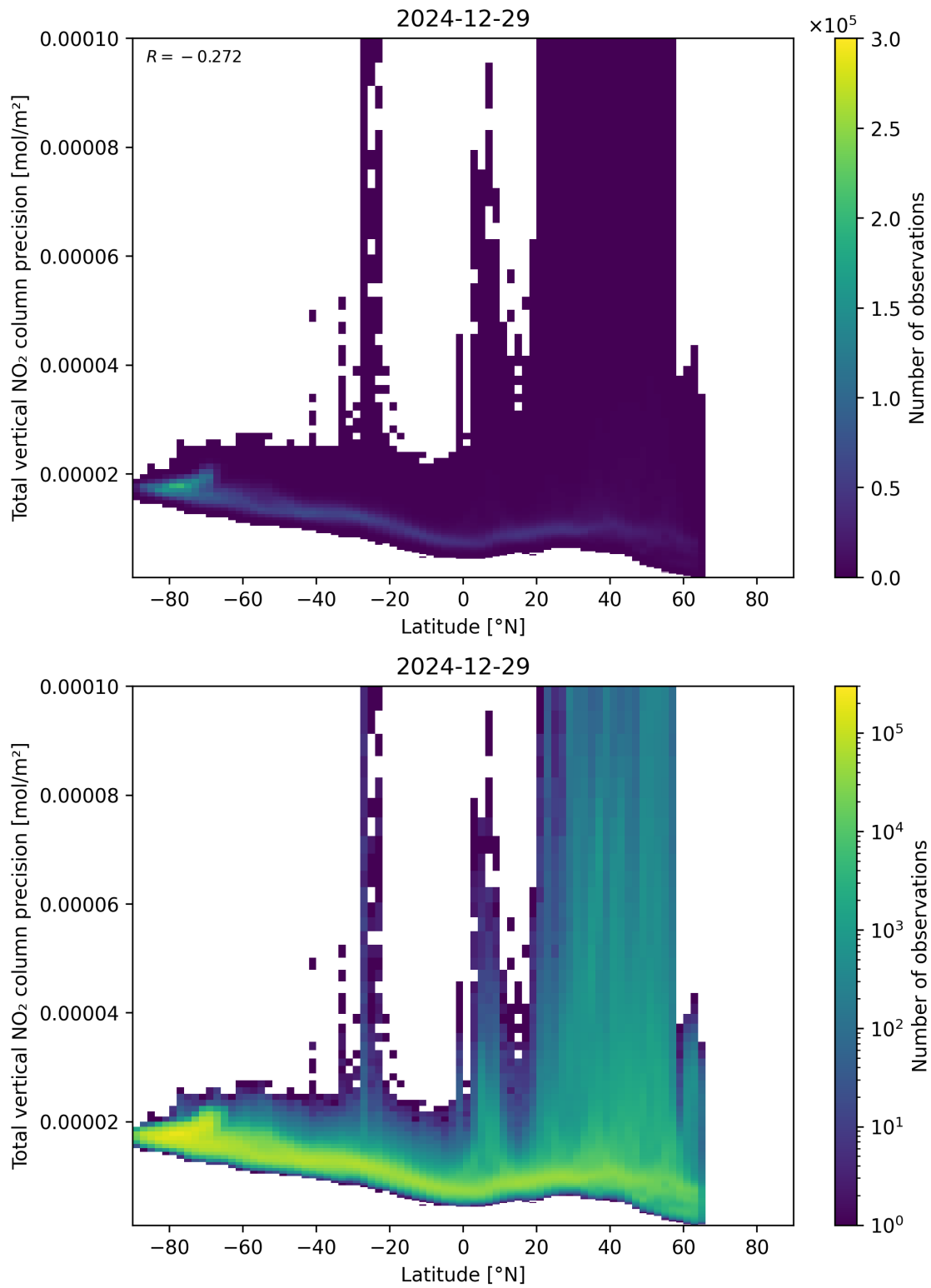
Figure 91: Scatter density plot of “Latitude” against “Total vertical NO 2 column precision” for 2024-12-28 to 2024-12-30.
