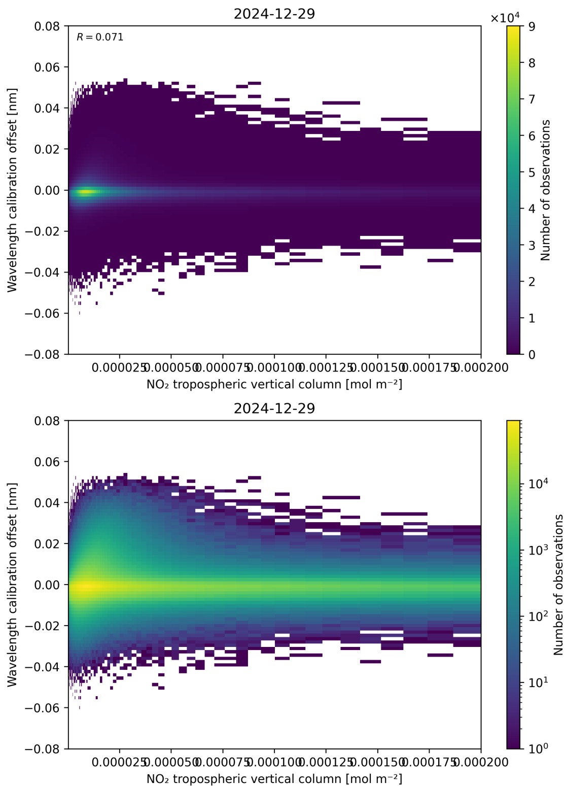
Figure 143: Scatter density plot of “NO 2 tropospheric vertical column” against “Wavelength calibration offset” for 2024-12-28 to 2024-12-30.
