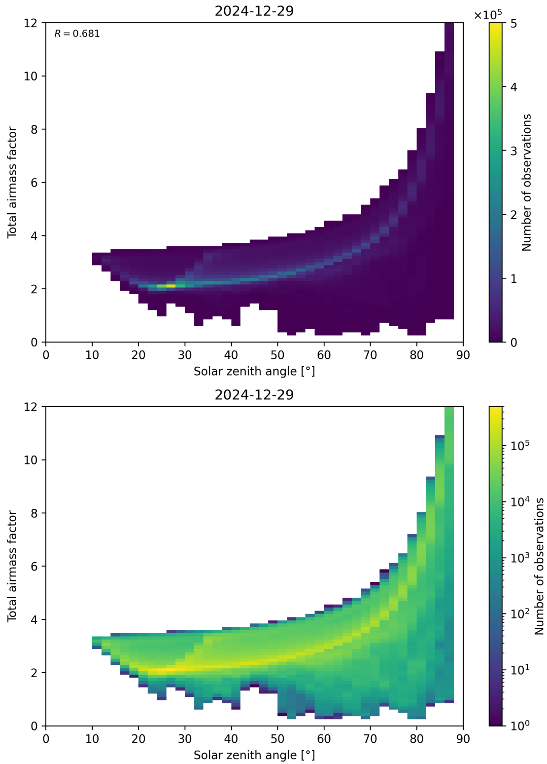
Figure 146: Scatter density plot of “Solar zenith angle” against “Total airmass factor” for 2024-12-28 to 2024-12-30.
