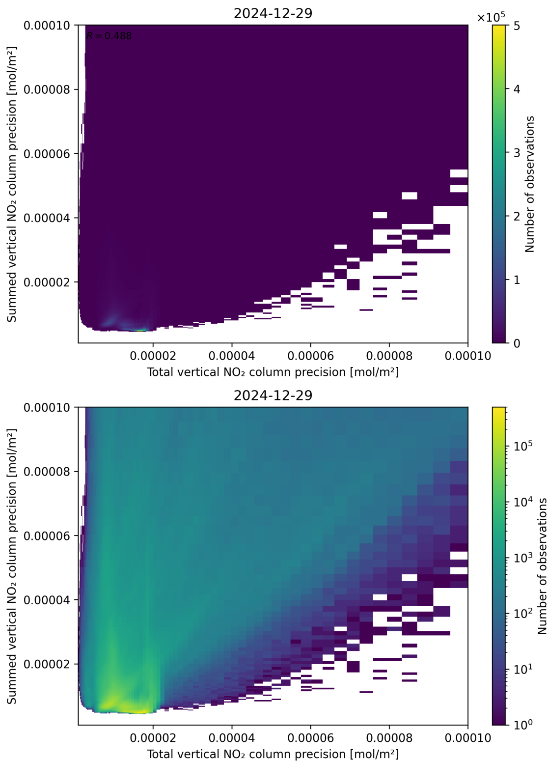
Figure 118: Scatter density plot of “Total vertical NO 2 column precision” against “Summed vertical NO 2 column precision” for 2024-12-28 to 2024-12-30.
