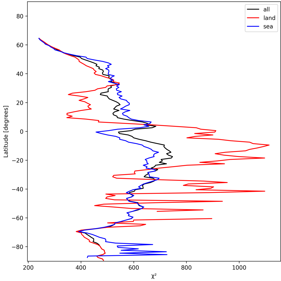
Figure 25: Zonal average of “ \chi^2 ” for 2024-12-28 to 2024-12-30.
