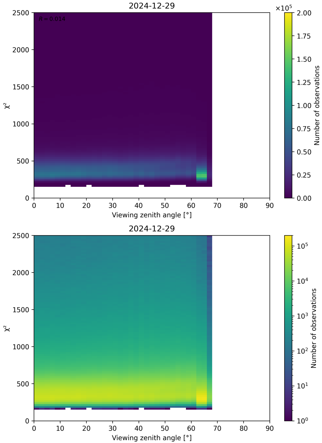
Figure 162: Scatter density plot of “Viewing zenith angle” against “ \chi^2 ” for 2024-12-28 to 2024-12-30.
