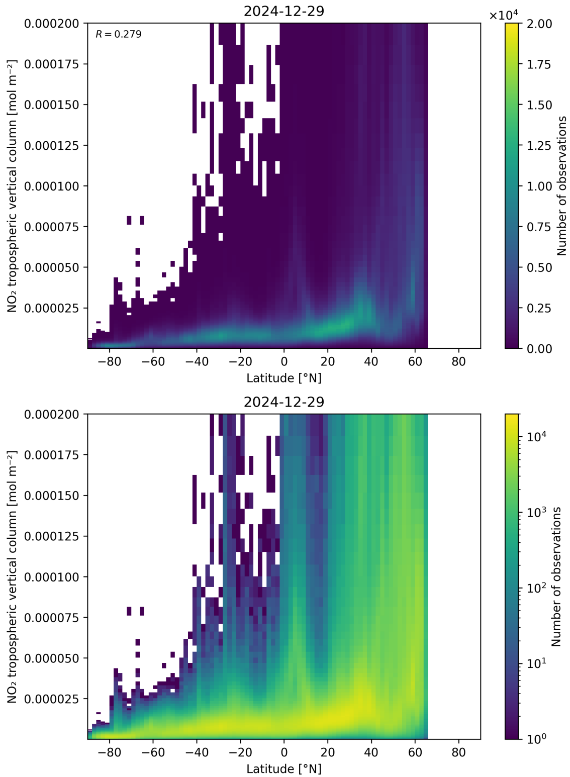
Figure 92: Scatter density plot of “Latitude” against “NO 2 tropospheric vertical column” for 2024-12-28 to 2024-12-30.
