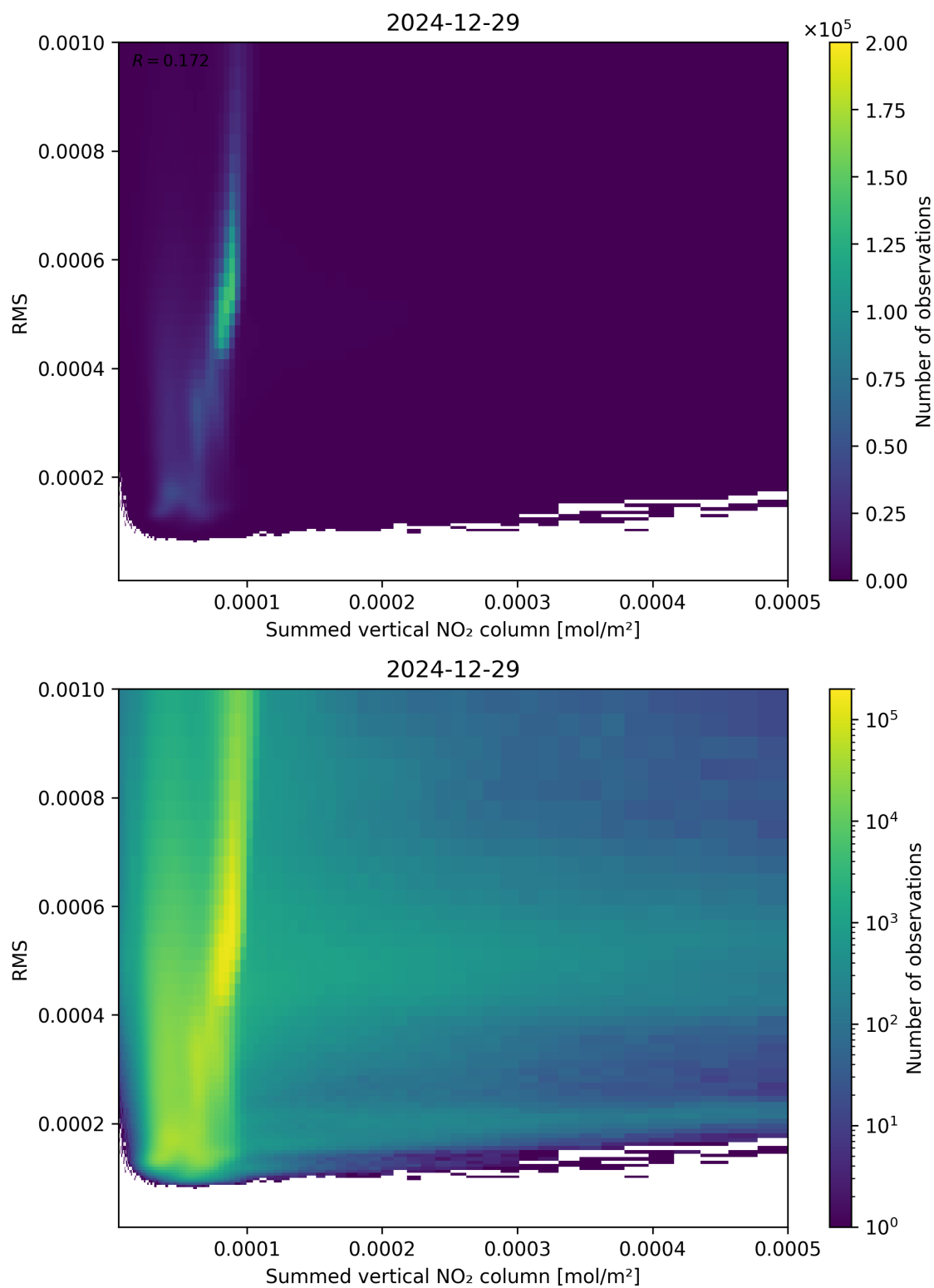
Figure 109: Scatter density plot of “Summed vertical NO 2 column” against “RMS” for 2024-12-28 to 2024-12-30.
