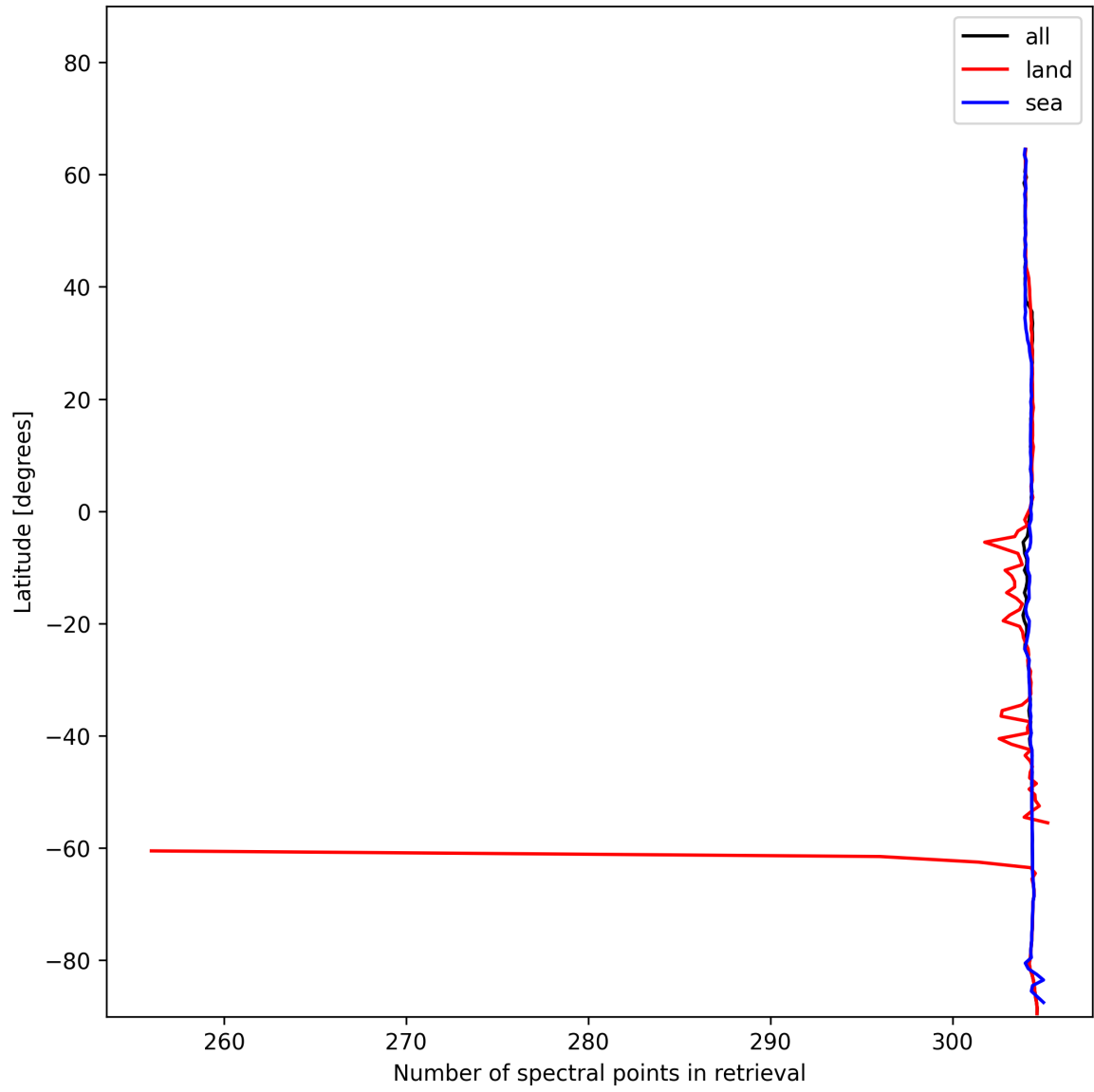
Figure 16: Zonal average of “Number of spectral points in retrieval” for 2024-12-28 to 2024-12-30.
