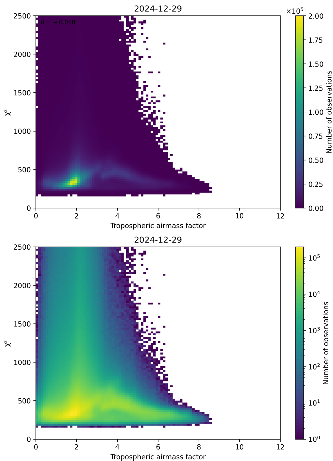
Figure 73: Scatter density plot of “Tropospheric airmass factor” against “ \chi^2 ” for 2024-12-28 to 2024-12-30.
