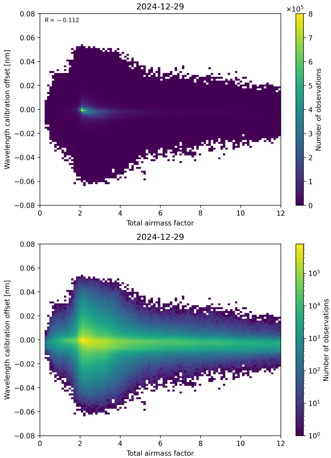
Figure 70: Scatter density plot of “Total airmass factor” against “Wavelength calibration offset” for 2024-12-28 to 2024-12-30.
