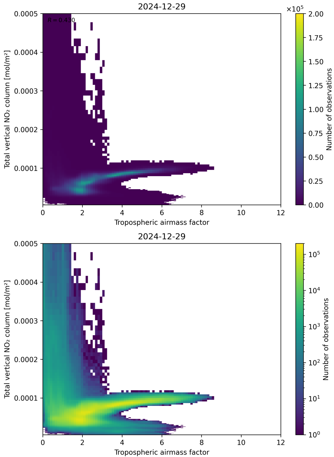
Figure 77: Scatter density plot of “Tropospheric air mass factor” against “Total vertical NO 2 column” for 2024-12-28 to 2024-12-30.
