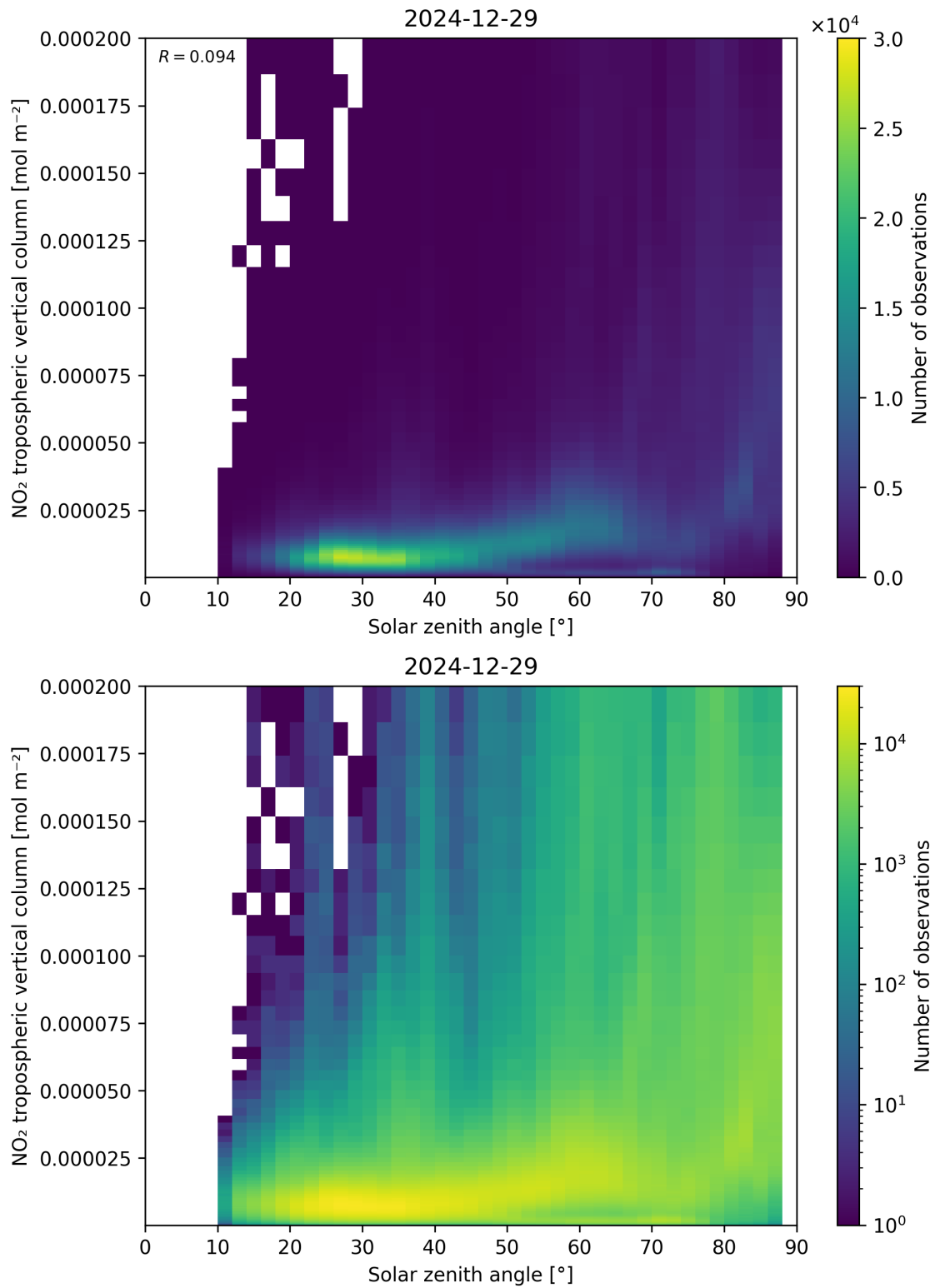
Figure 155: Scatter density plot of “Solar zenith angle” against “NO 2 tropospheric vertical column” for 2024-12-28 to 2024-12-30.
