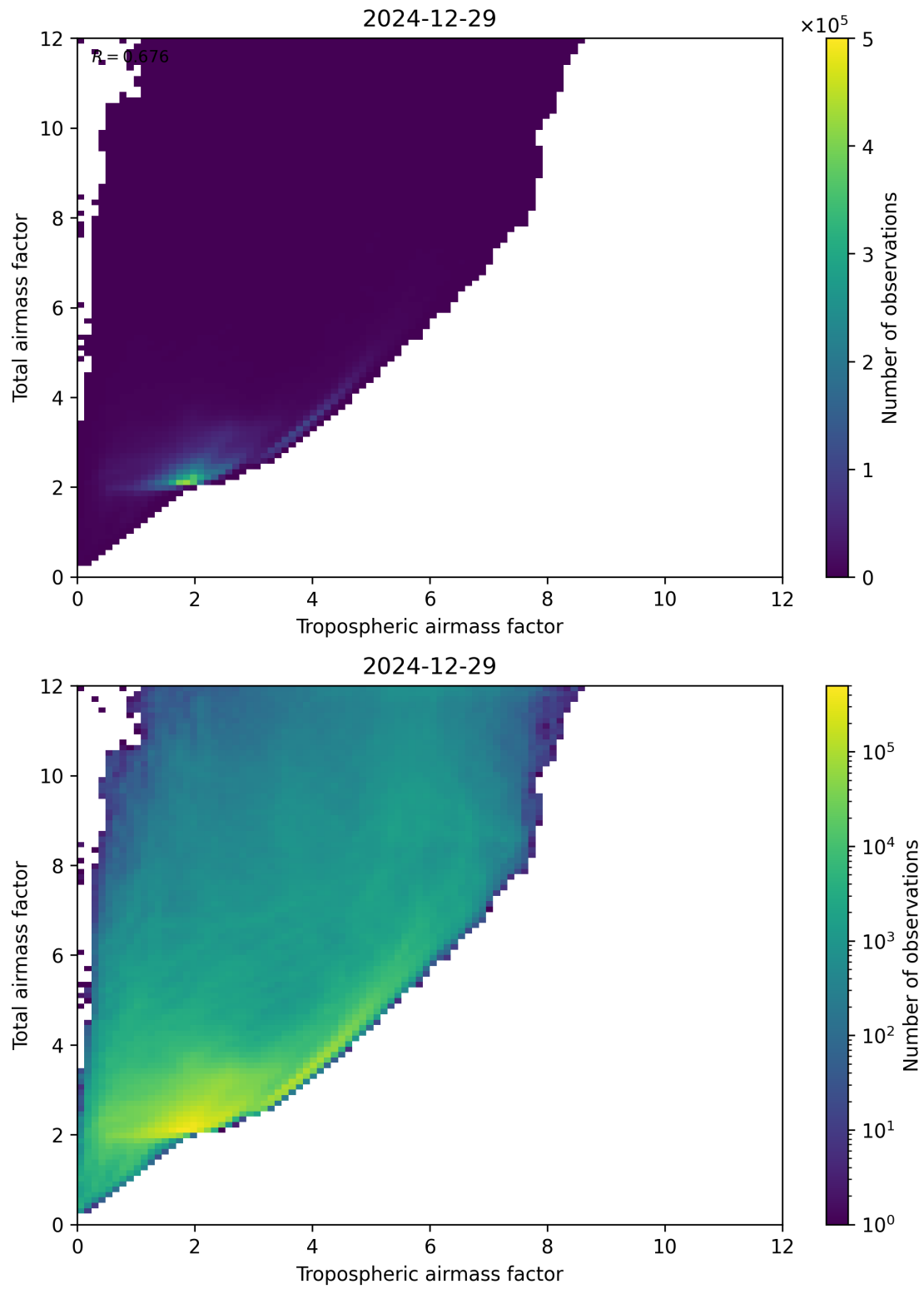
Figure 72: Scatter density plot of “Tropospheric airmass factor” against “Total airmass factor” for 2024-12-28 to 2024-12-30.
