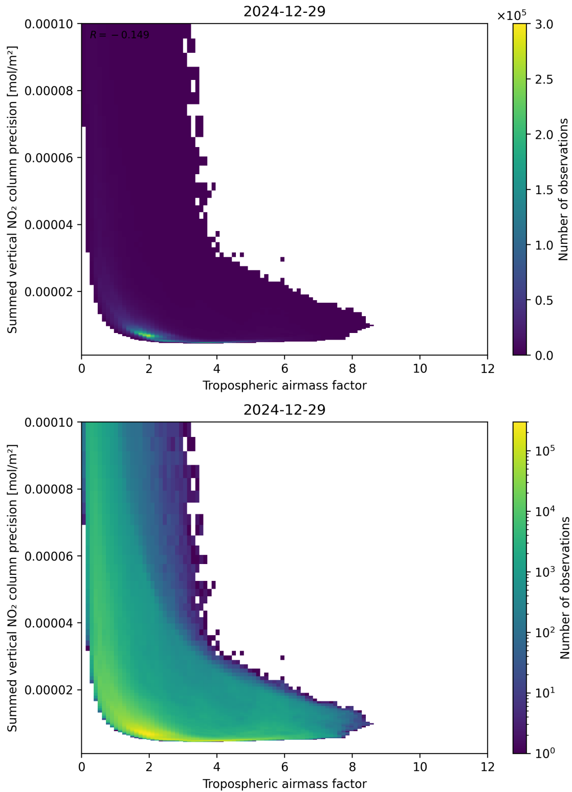
Figure 76: Scatter density plot of “Tropospheric air mass factor” against “Summed vertical NO 2 column precision” for 2024-12-28 to 2024-12-30.
