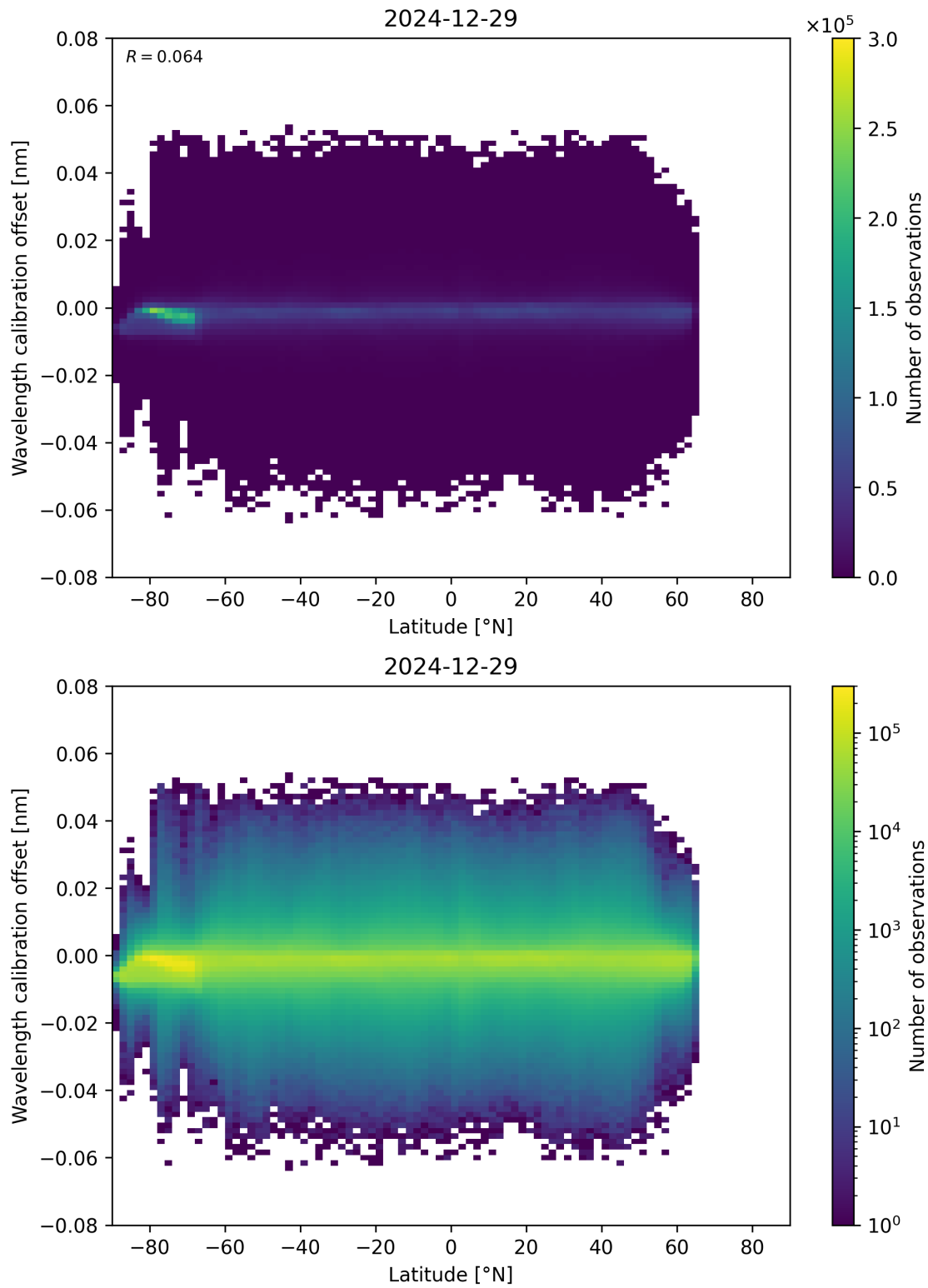
Figure 95: Scatter density plot of “Latitude” against “Wavelength calibration offset” for 2024-12-28 to 2024-12-30.
