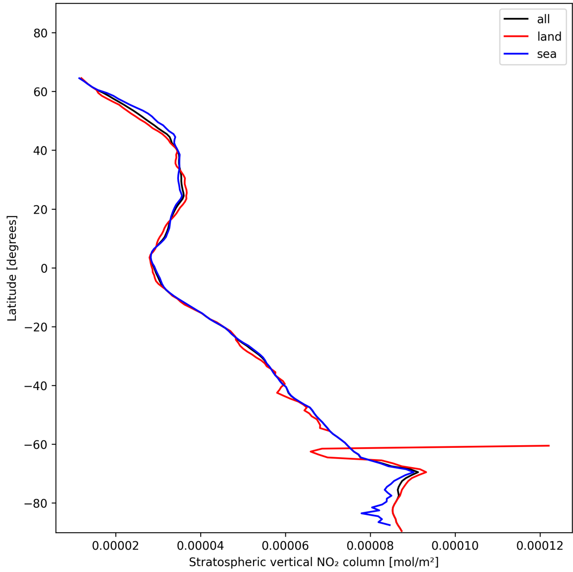
Figure 19: Zonal average of “Stratospheric vertical NO 2 column” for 2024-12-28 to 2024-12-30.
