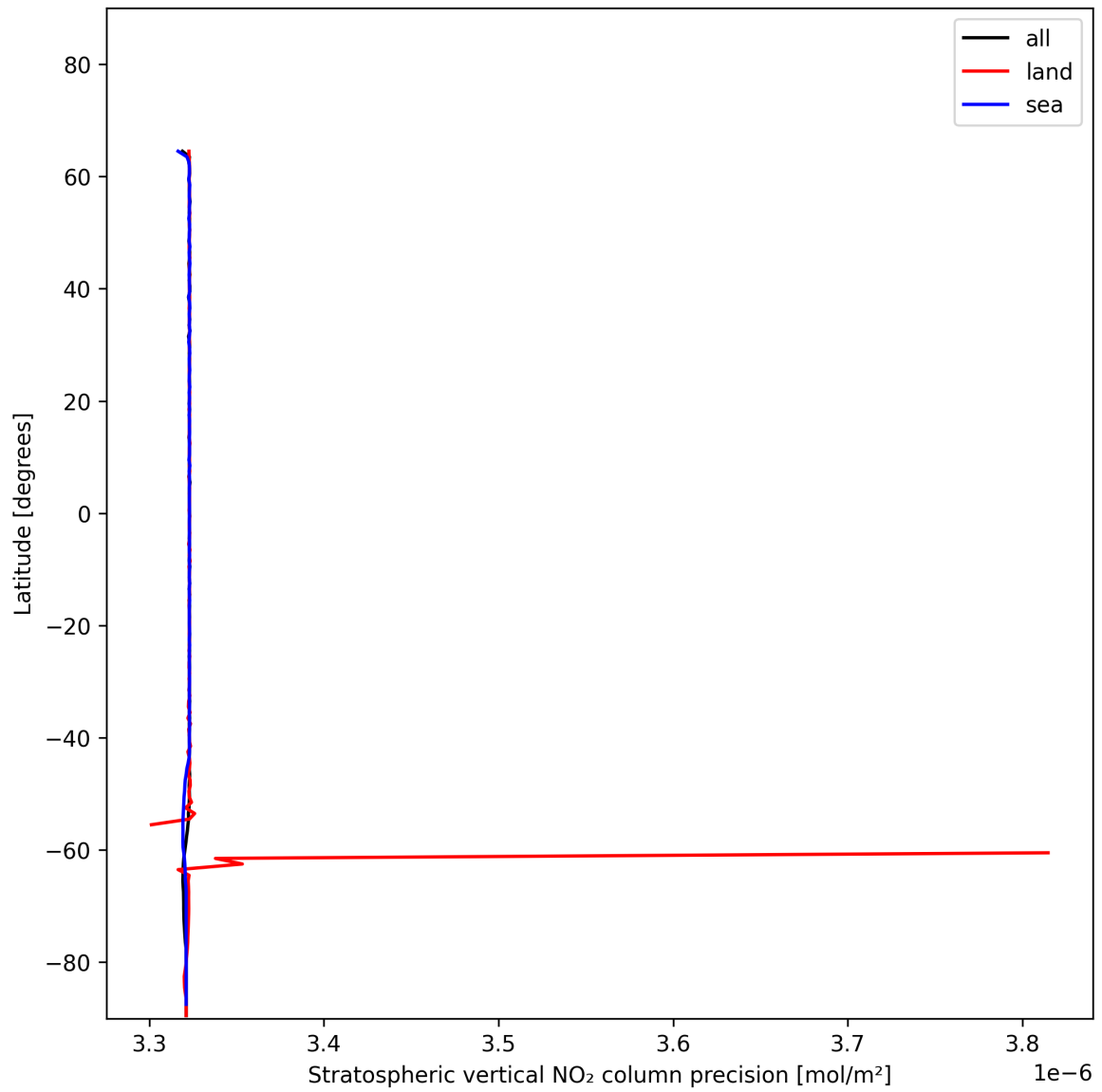
Figure 20: Zonal average of “Stratospheric vertical NO 2 column precision” for 2024-12-28 to 2024-12-30.
