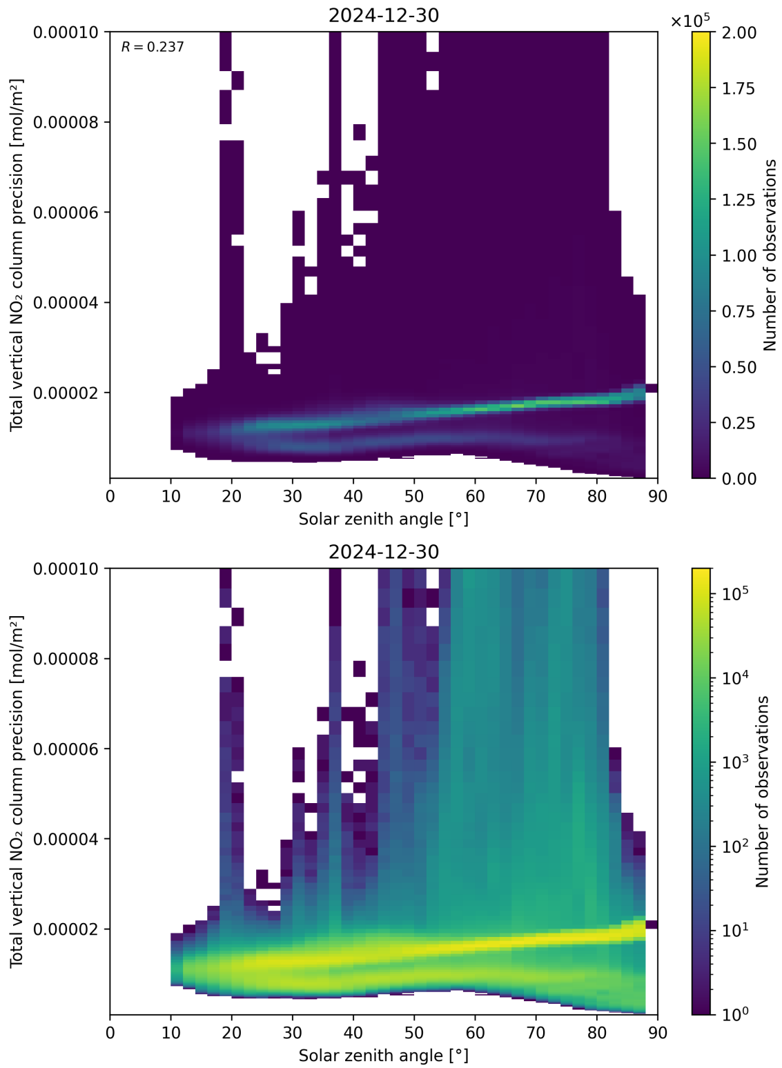
Figure 154: Scatter density plot of “Solar zenith angle” against “Total vertical NO 2 column precision” for 2024-12-29 to 2024-12-31.
