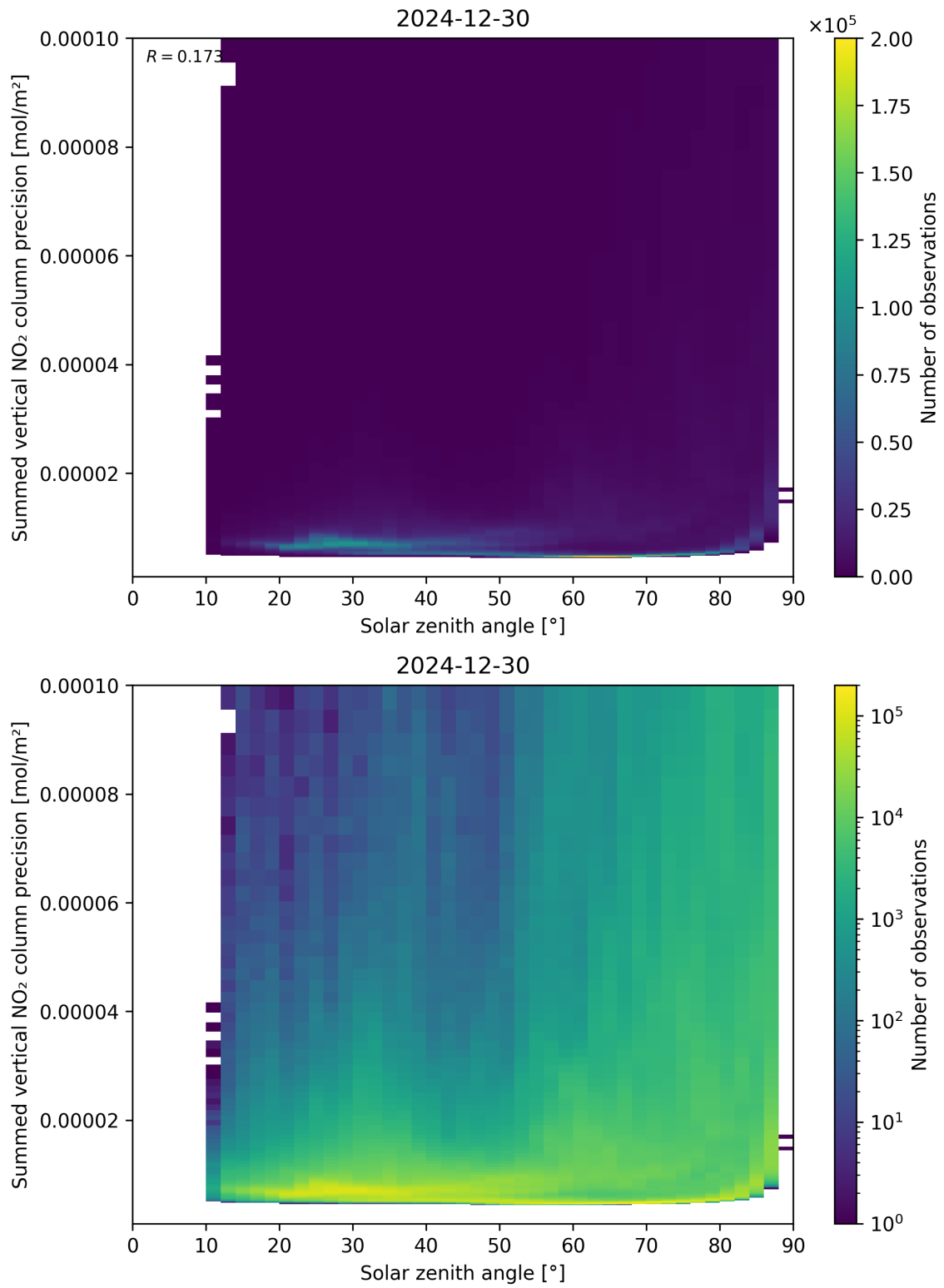
Figure 152: Scatter density plot of “Solar zenith angle” against “Summed vertical NO 2 column precision” for 2024-12-29 to 2024-12-31.
