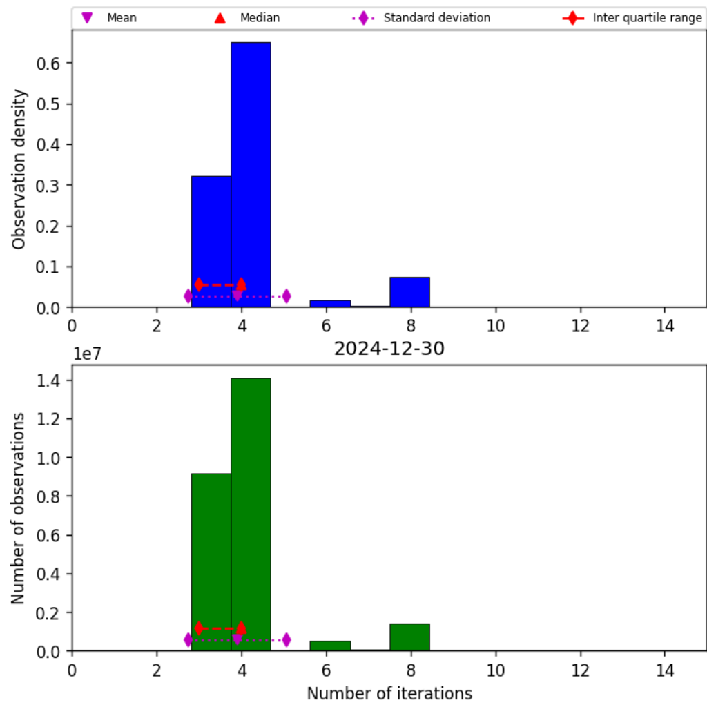
Figure 34: Histogram of “Number of iterations” for 2024-12-29 to 2024-12-31
