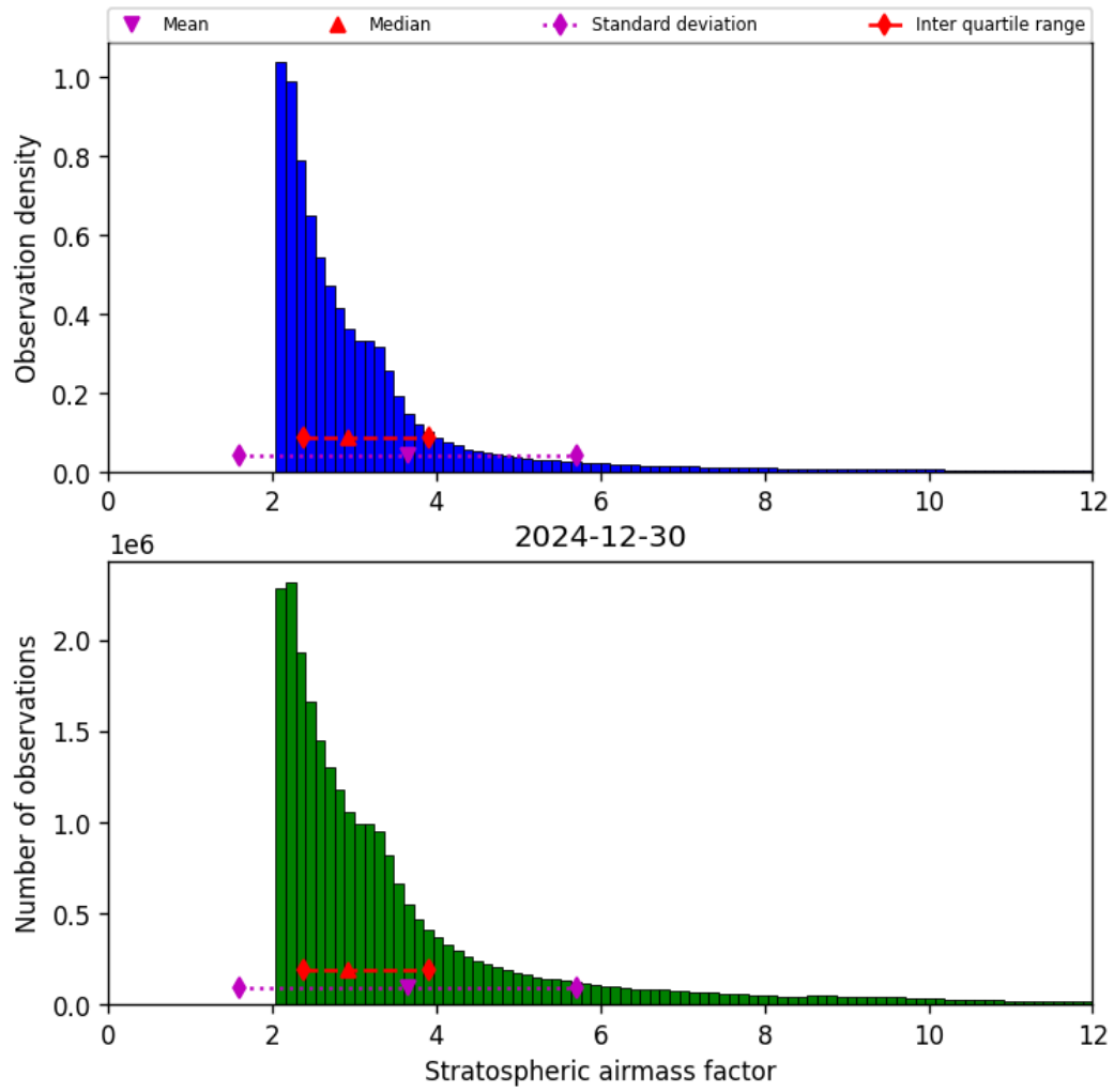
Figure 44: Histogram of “Stratospheric airmass factor” for 2024-12-29 to 2024-12-31
