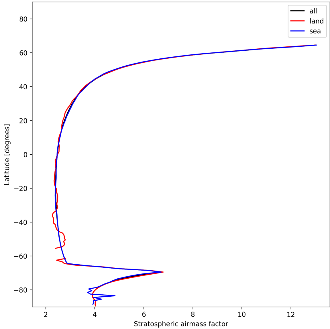
Figure 27: Zonal average of “Stratospheric air mass factor” for 2024-12-29 to 2024-12-31.
