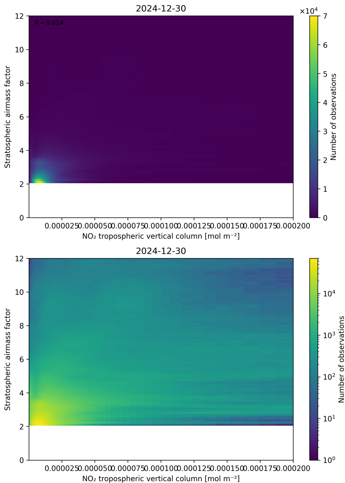
Figure 121: Scatter density plot of “NO 2 tropospheric vertical column” against “Stratospheric airmass factor” for 2024-12-29 to 2024-12-31.
