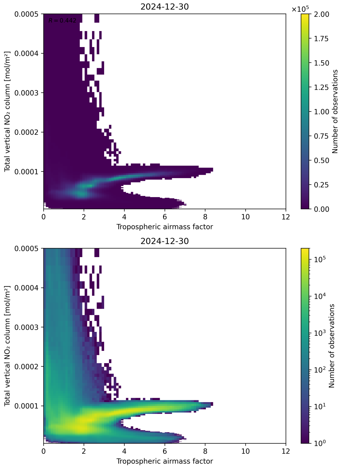
Figure 77: Scatter density plot of “Tropospheric airmass factor” against “Total vertical NO 2 column” for 2024-12-29 to 2024-12-31.
