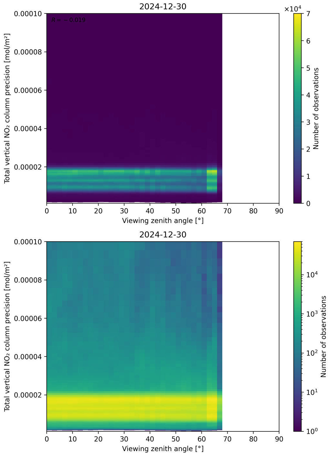
Figure 168: Scatter density plot of “Viewing zenith angle” against “Total vertical NO 2 column precision” for 2024-12-29 to 2024-12-31.
