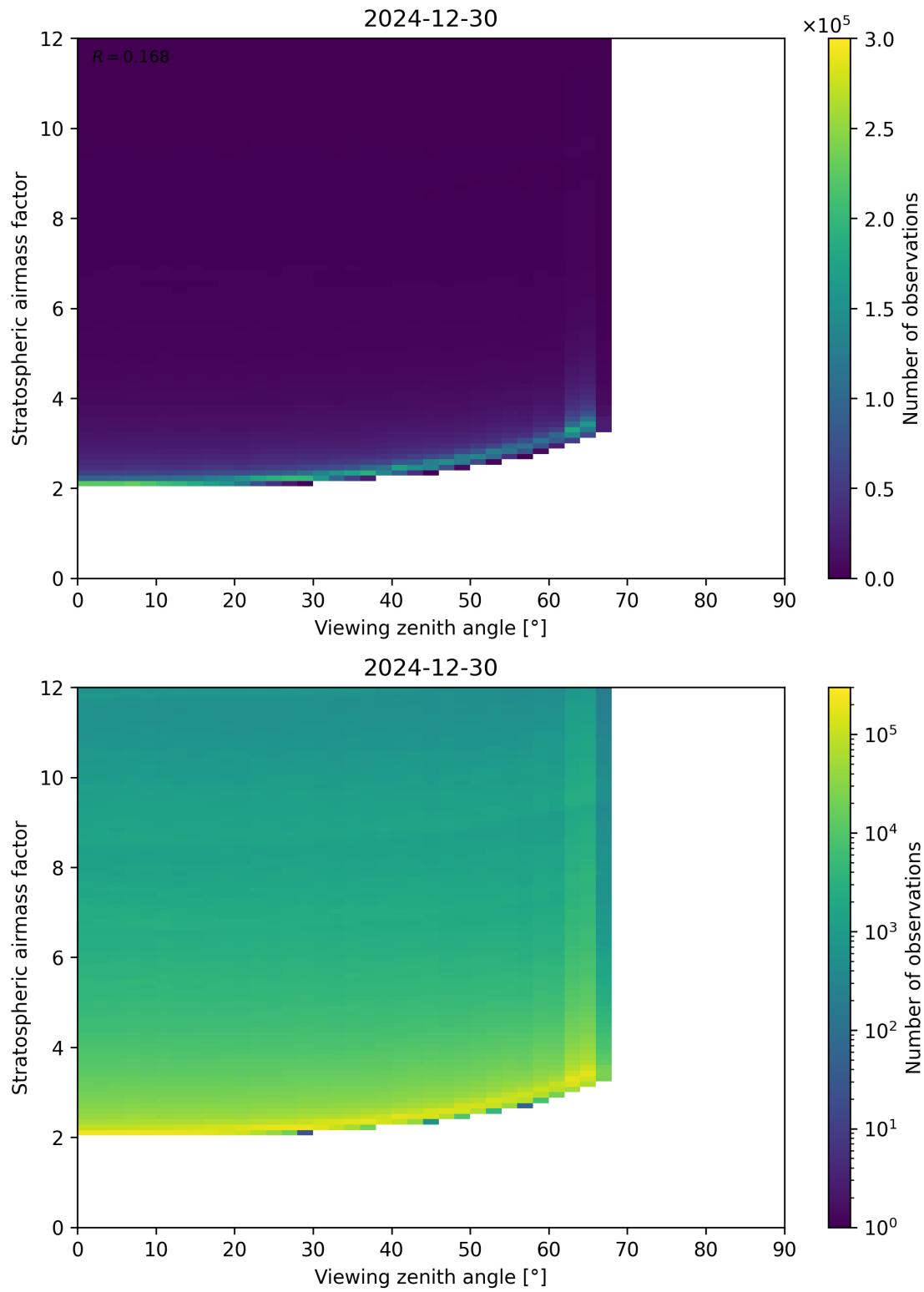
Figure 159: Scatter density plot of “Viewing zenith angle” against “Stratospheric airmass factor” for 2024-12-29 to 2024-12-31.
