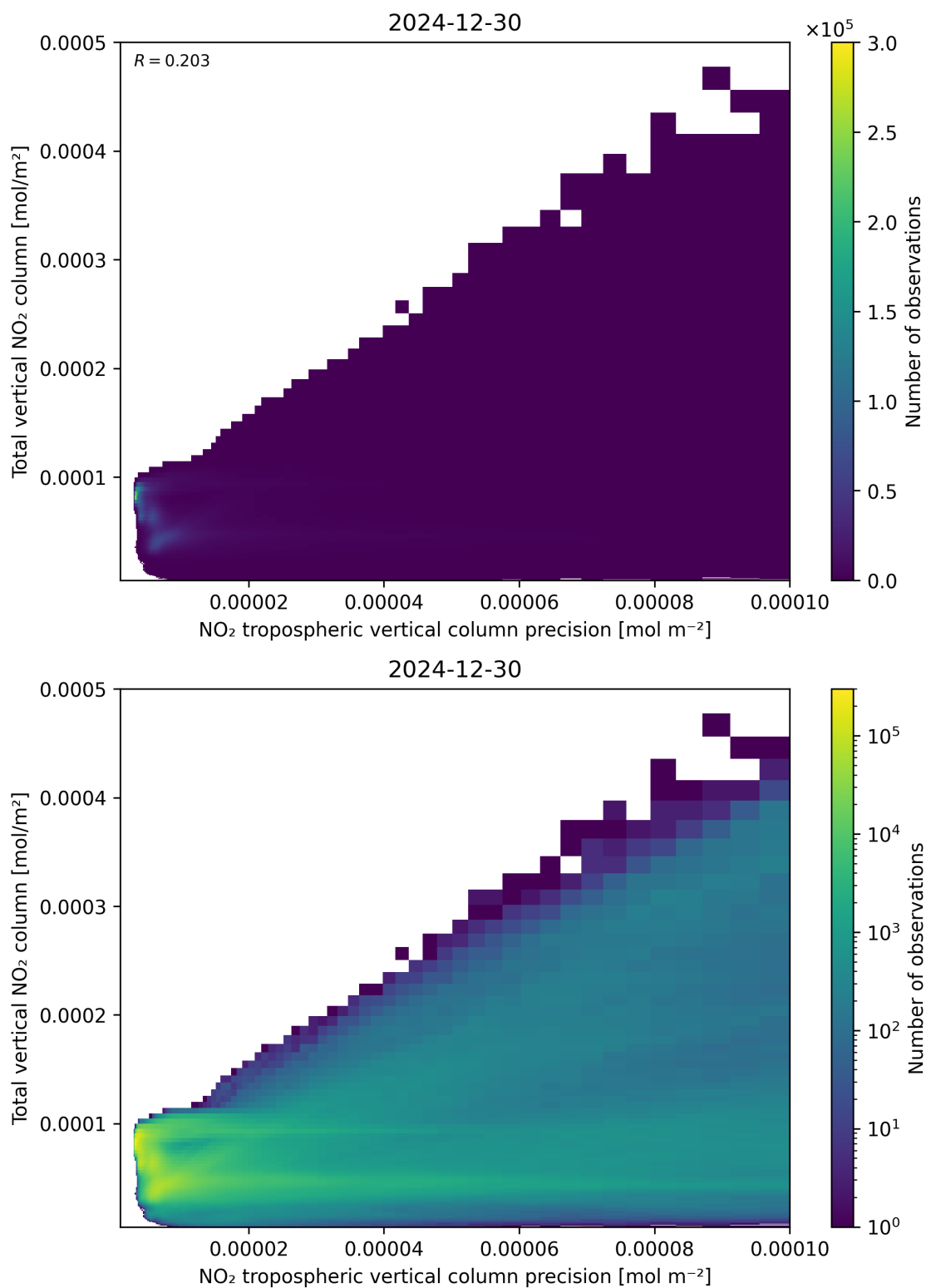
Figure 138: Scatter density plot of “NO 2 tropospheric vertical column precision” against “Total vertical NO 2 column” for 2024-12-29 to 2024-12-31.
