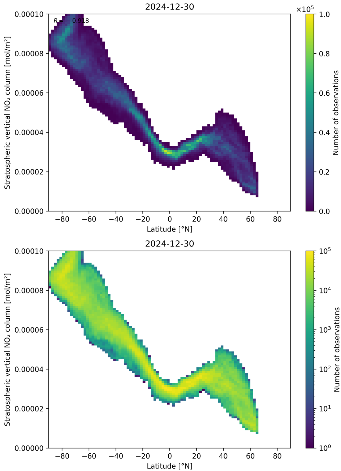
Figure 87: Scatter density plot of “Latitude” against “Stratospheric vertical NO 2 column” for 2024-12-29 to 2024-12-31.
