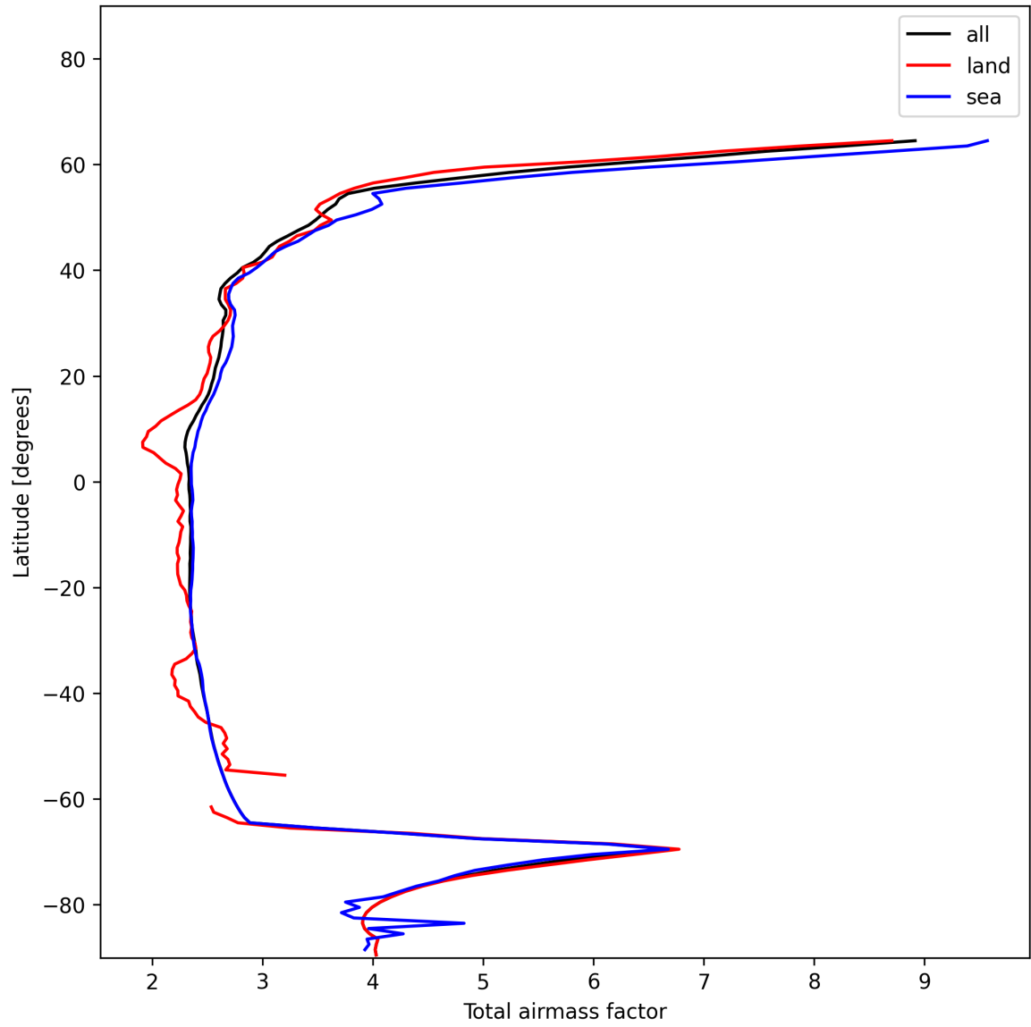
Figure 15: Zonal average of “Total airmass factor” for 2024-12-29 to 2024-12-31.
