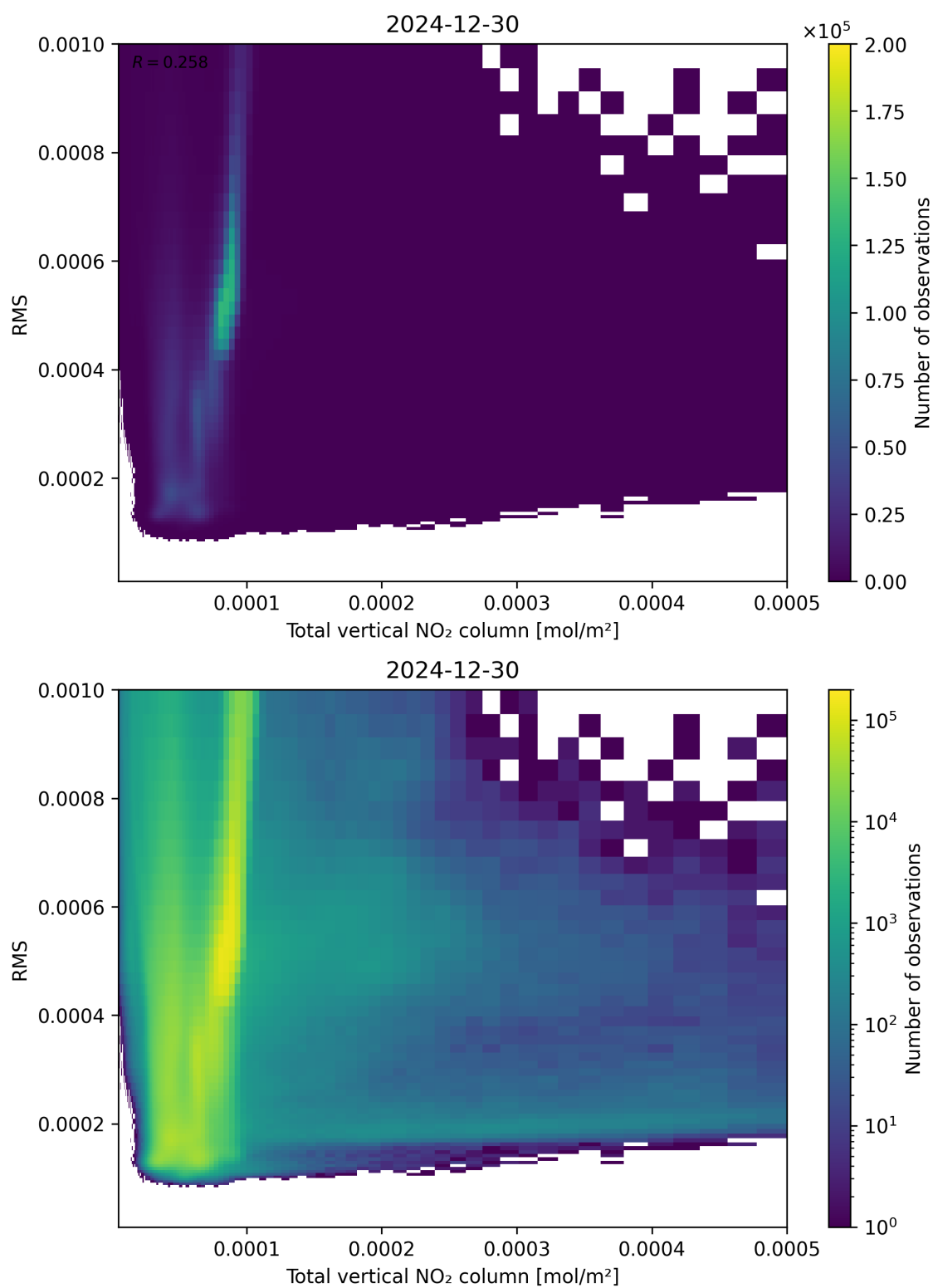
Figure 120: Scatter density plot of “Total vertical NO 2 column” against “RMS” for 2024-12-29 to 2024-12-31.
