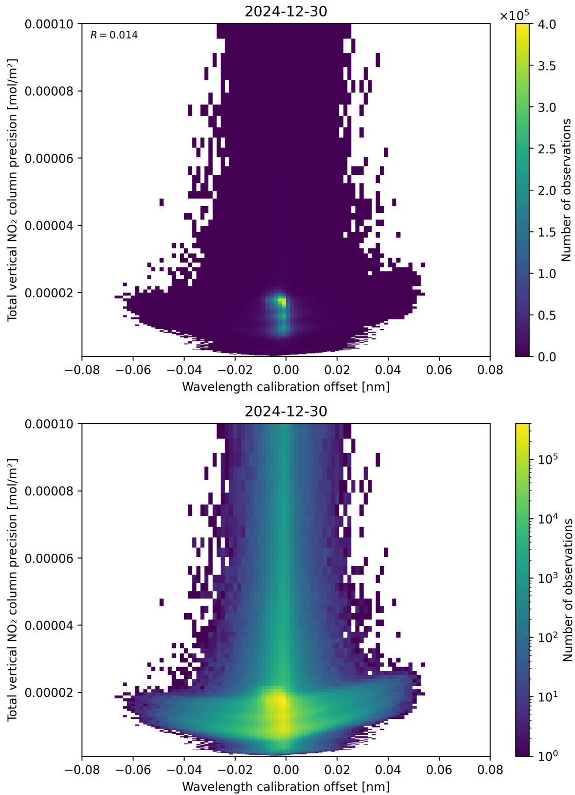
Figure 180: Scatter density plot of “Wavelength calibration offset” against “Total vertical NO 2 column precision” for 2024-12-29 to 2024-12-31.
