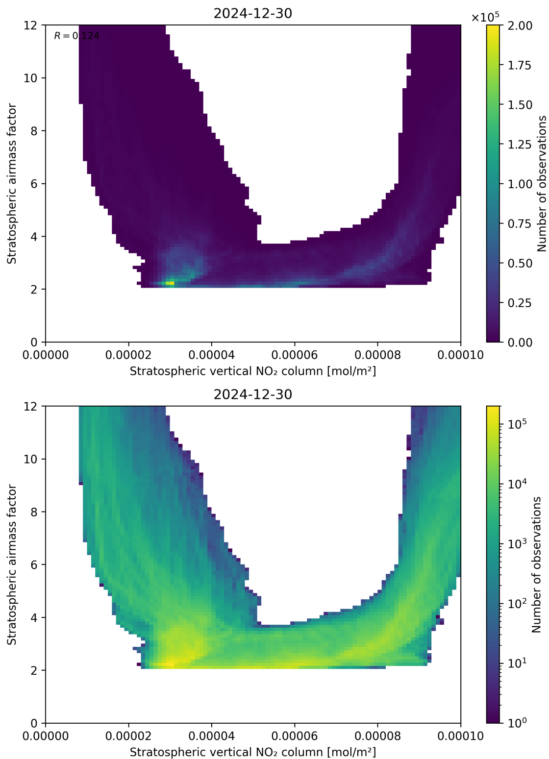
Figure 96: Scatter density plot of “Stratospheric vertical NO 2 column” against “Stratospheric airmass factor” for 2024-12-29 to 2024-12-31.
