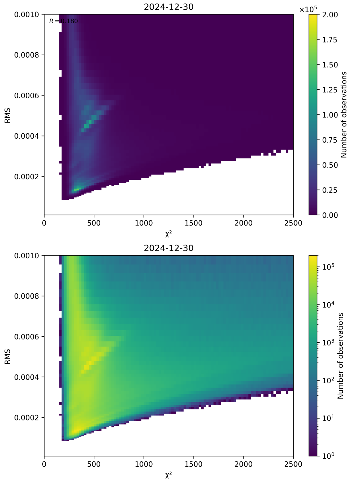
Figure 82: Scatter density plot of “ \chi^2 ” against “RMS” for 2024-12-29 to 2024-12-31.
