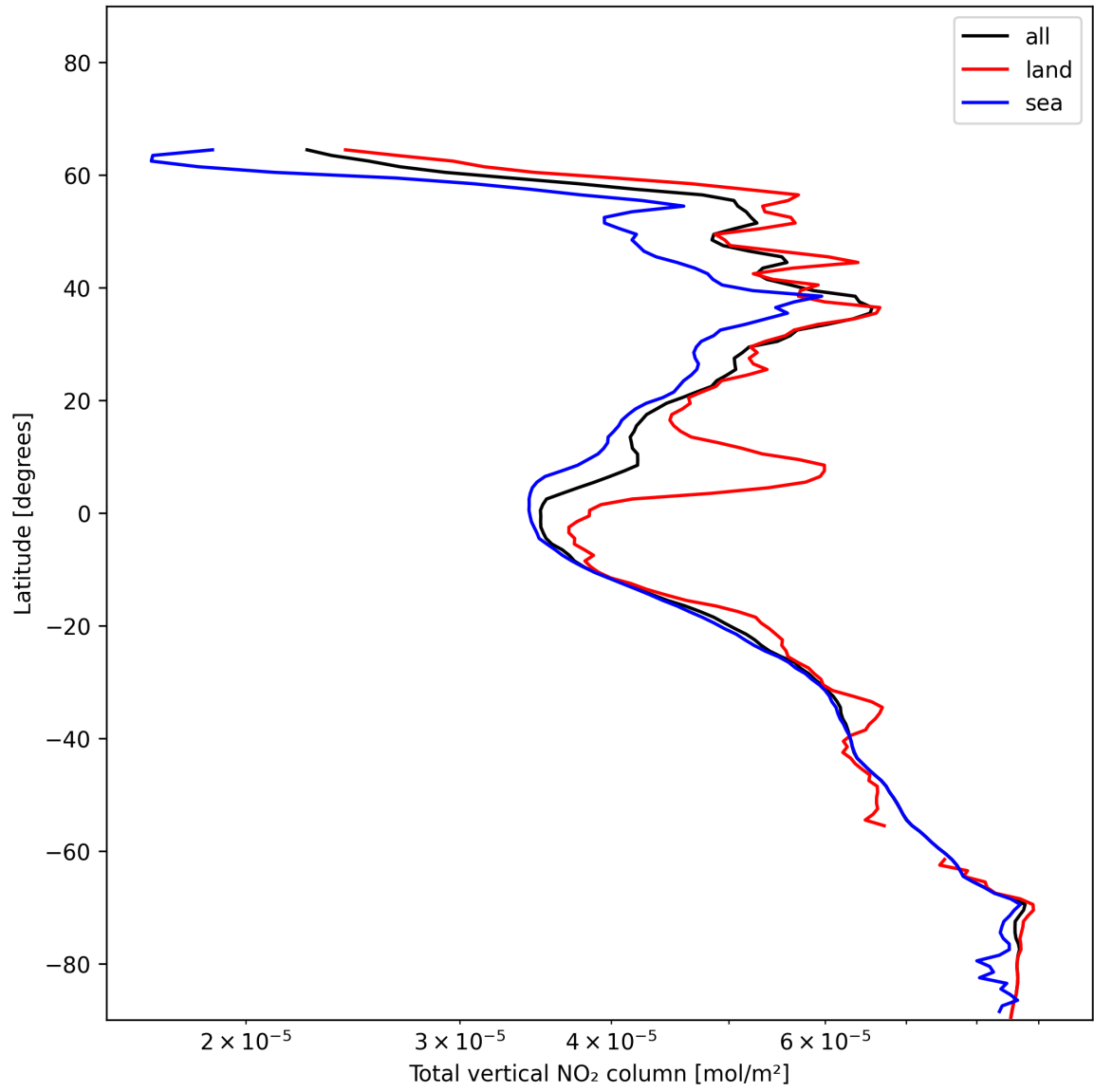
Figure 21: Zonal average of “Total vertical NO 2 column” for 2024-12-29 to 2024-12-31.
