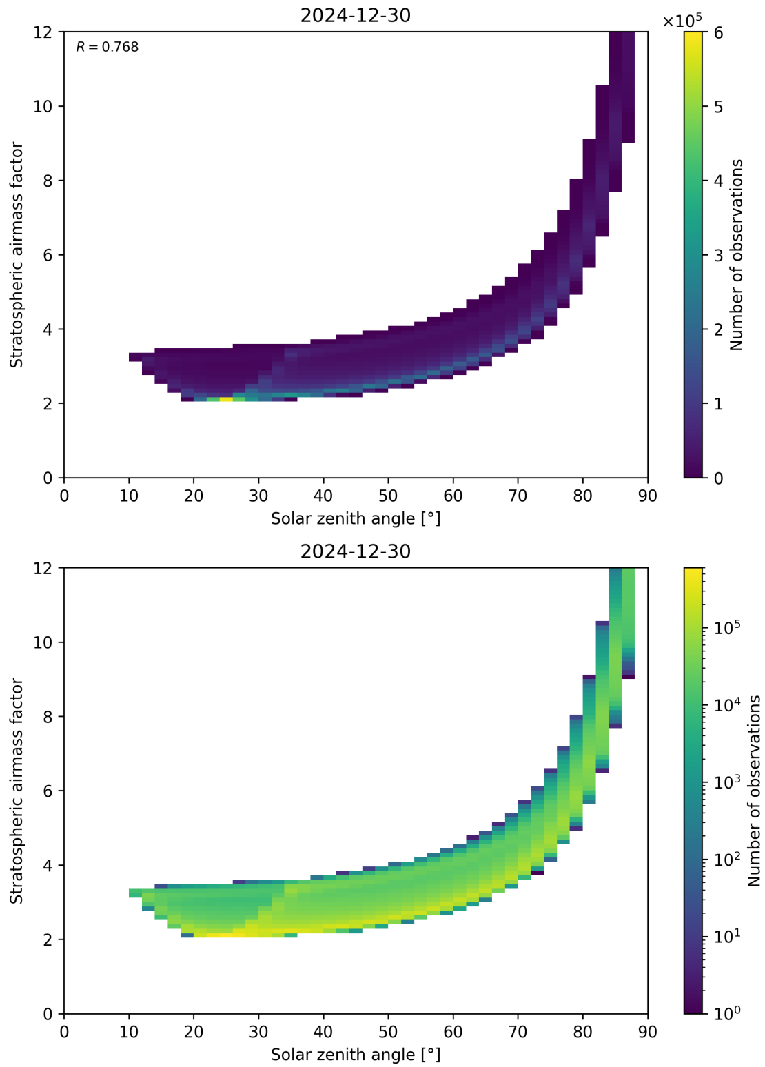
Figure 145: Scatter density plot of “Solar zenith angle” against “Stratospheric airmass factor” for 2024-12-29 to 2024-12-31.
