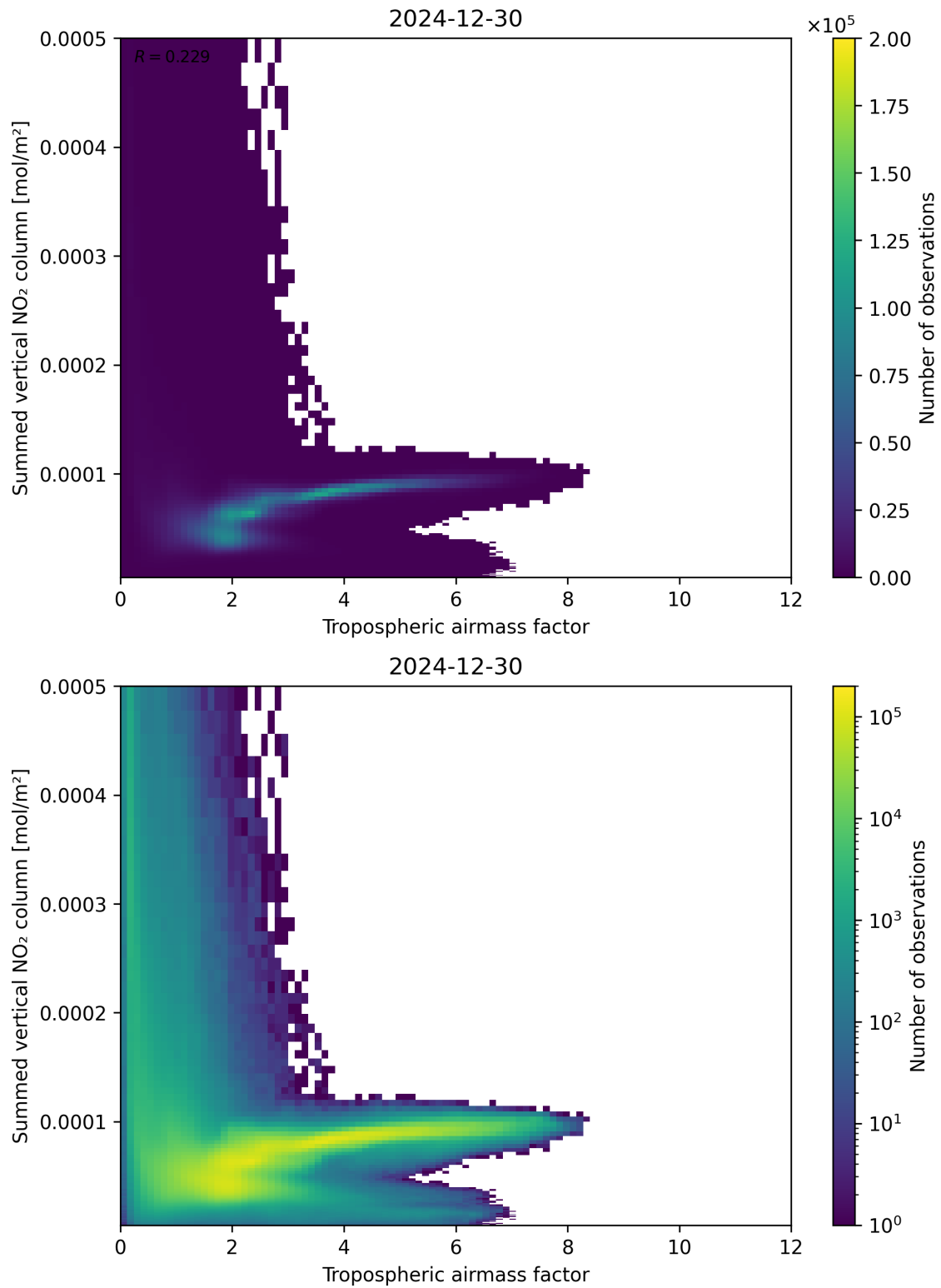
Figure 75: Scatter density plot of “Tropospheric air mass factor” against “Summed vertical NO 2 column” for 2024-12-29 to 2024-12-31.
