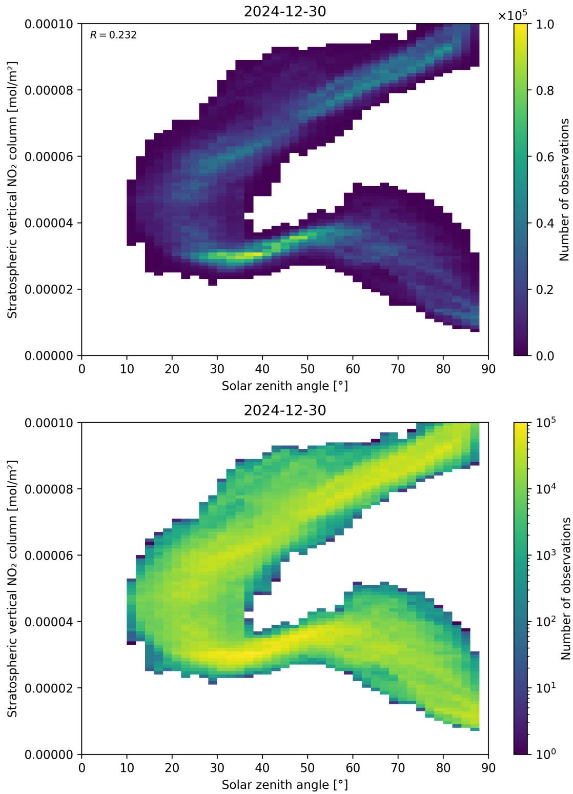
Figure 150: Scatter density plot of “Solar zenith angle” against “Stratospheric vertical NO 2 column” for 2024-12-29 to 2024-12-31.
