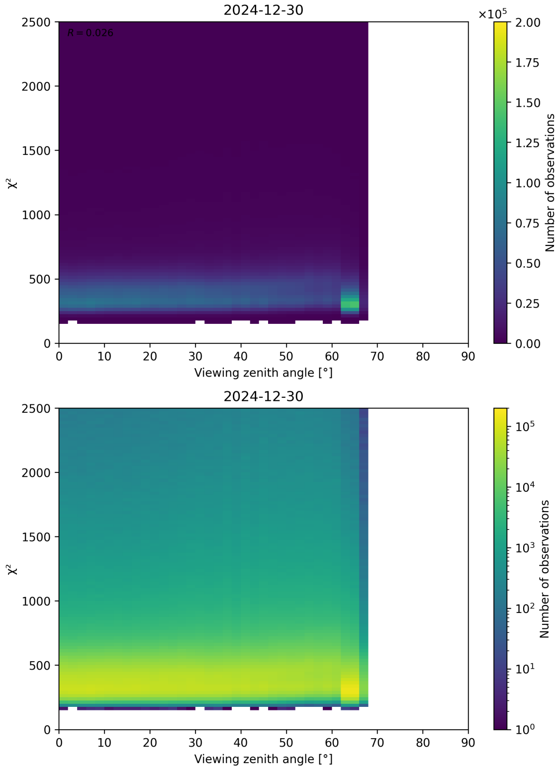
Figure 162: Scatter density plot of “Viewing zenith angle” against “ \chi^2 ” for 2024-12-29 to 2024-12-31.
