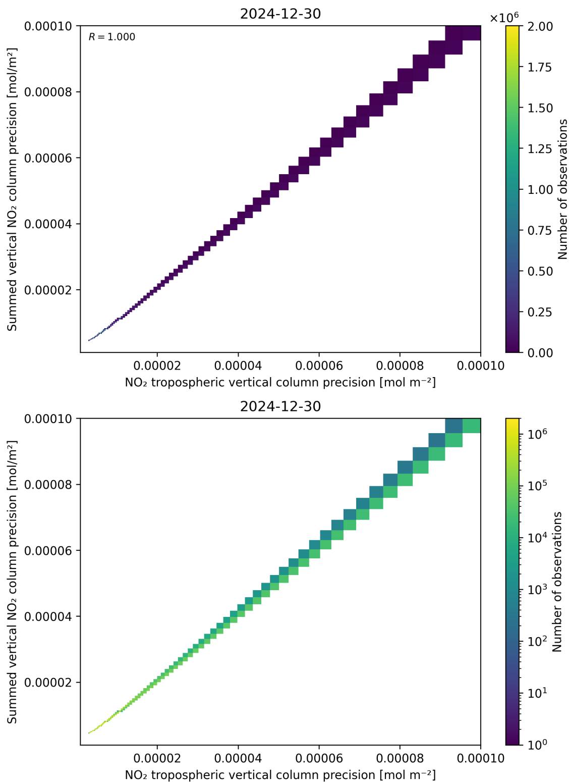
Figure 137: Scatter density plot of “NO 2 tropospheric vertical column precision” against “Summed vertical NO 2 column precision” for 2024-12-29 to 2024-12-31.
