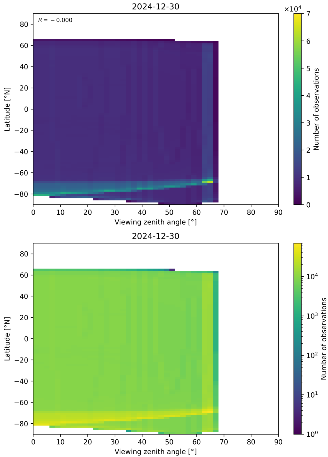
Figure 163: Scatter density plot of “Viewing zenith angle” against “Latitude” for 2024-12-29 to 2024-12-31.
