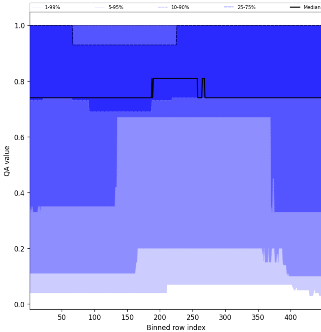
Figure 45: Along track statistics of “QA value” for 2024-12-29 to 2024-12-31
