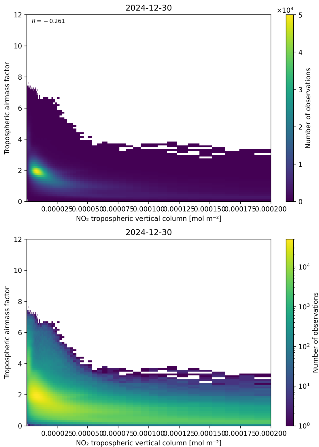
Figure 123: Scatter density plot of “NO 2 tropospheric vertical column” against “Tropospheric air mass factor” for 2024-12-29 to 2024-12-31.
