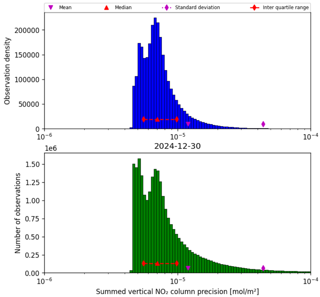
Figure 41: Histogram of "Summed vertical NO 2 column precision" for 2024-12-29 to 2024-12-31
