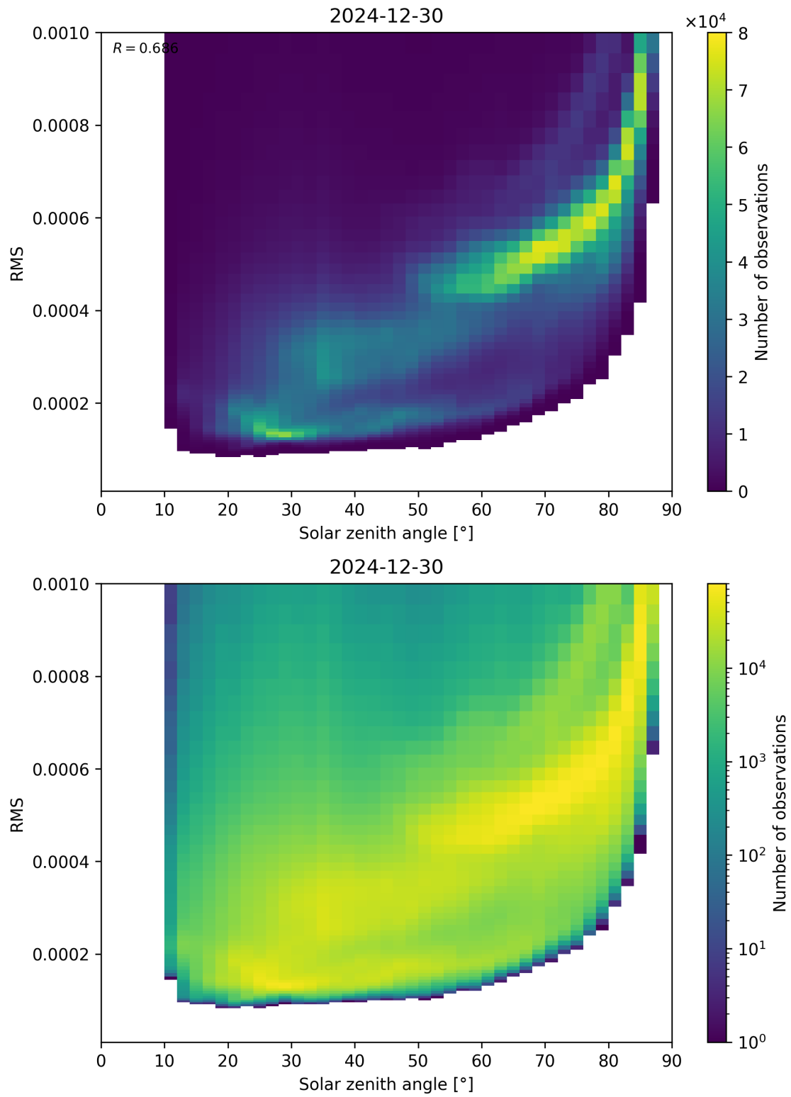
Figure 157: Scatter density plot of “Solar zenith angle” against “RMS” for 2024-12-29 to 2024-12-31.
