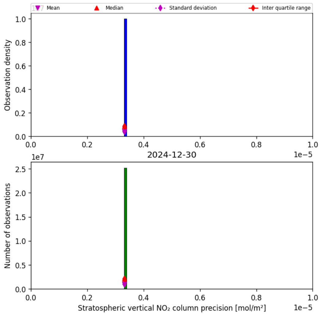
Figure 37: Histogram of “Stratospheric vertical NO 2 column precision” for 2024-12-29 to 2024-12-31
