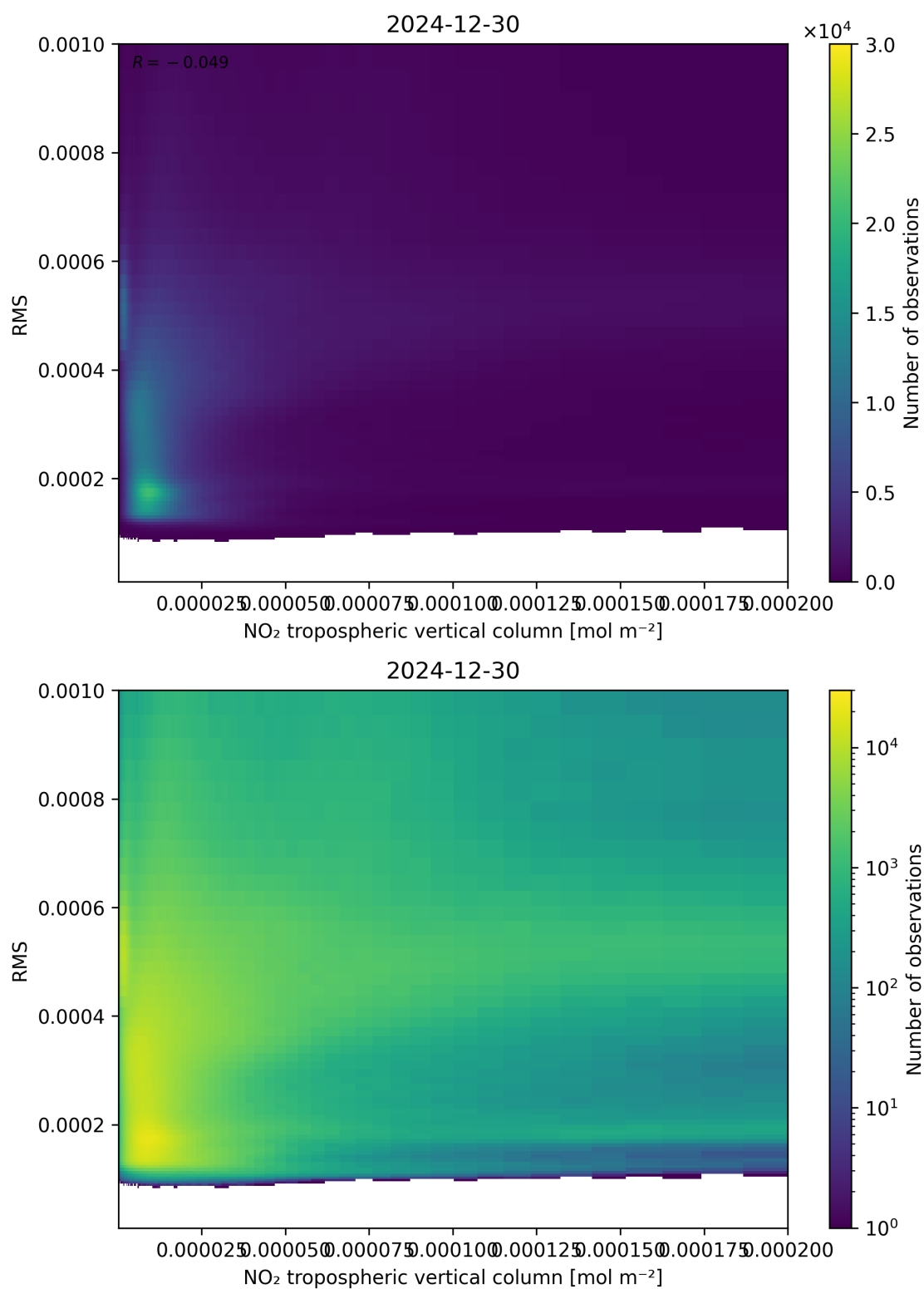
Figure 142: Scatter density plot of “NO 2 tropospheric vertical column” against “RMS” for 2024-12-29 to 2024-12-31.
