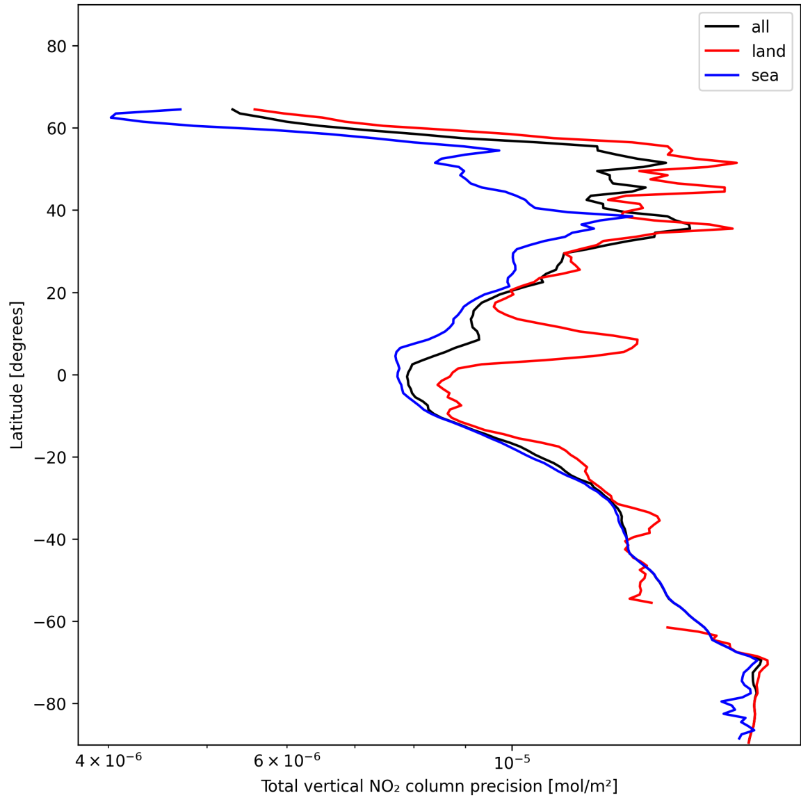
Figure 22: Zonal average of “Total vertical NO 2 column precision” for 2024-12-29 to 2024-12-31.
