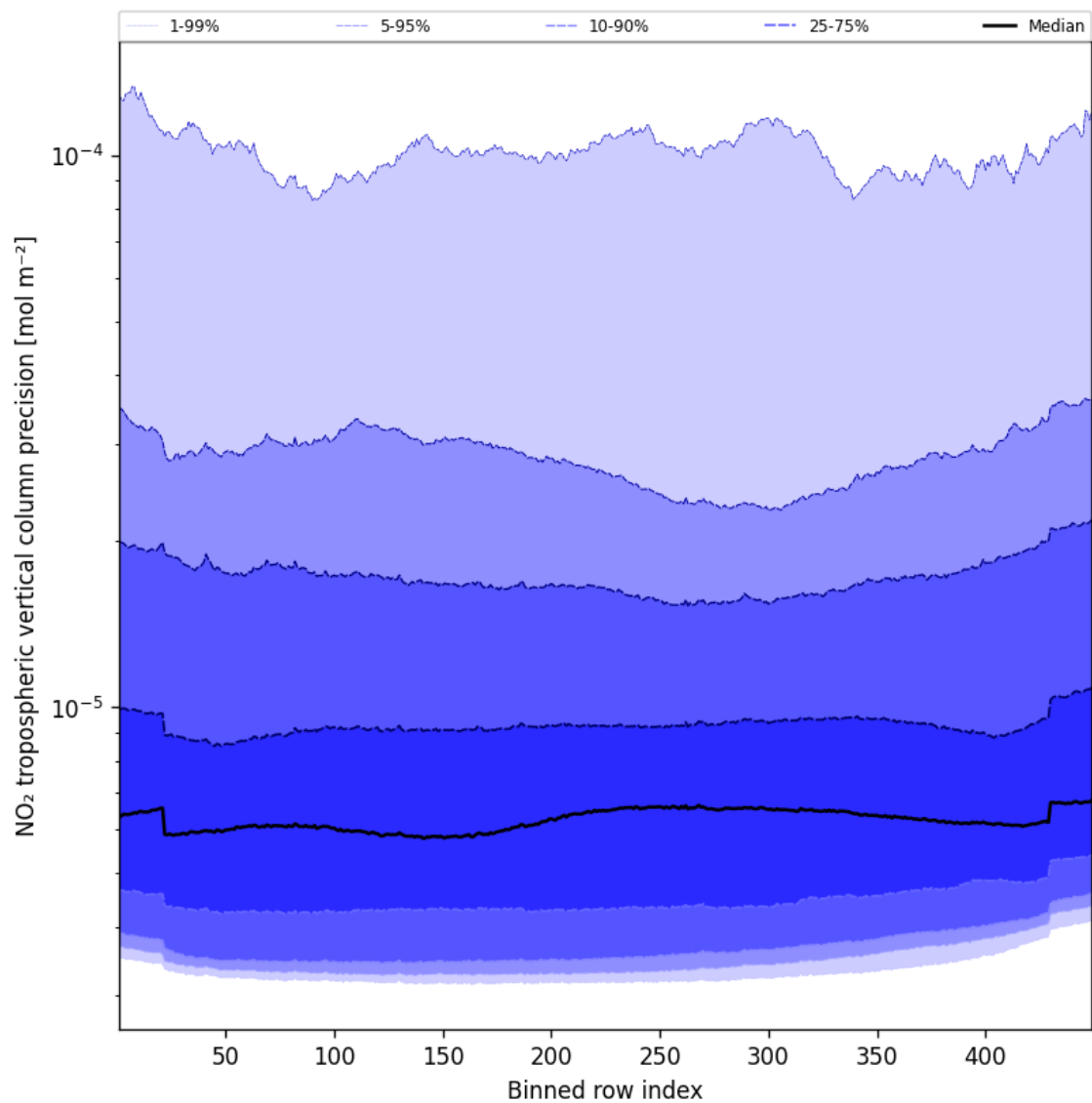
Figure 47: Along track statistics of “NO 2 tropospheric vertical column precision” for 2024-12-29 to 2024-12-31
