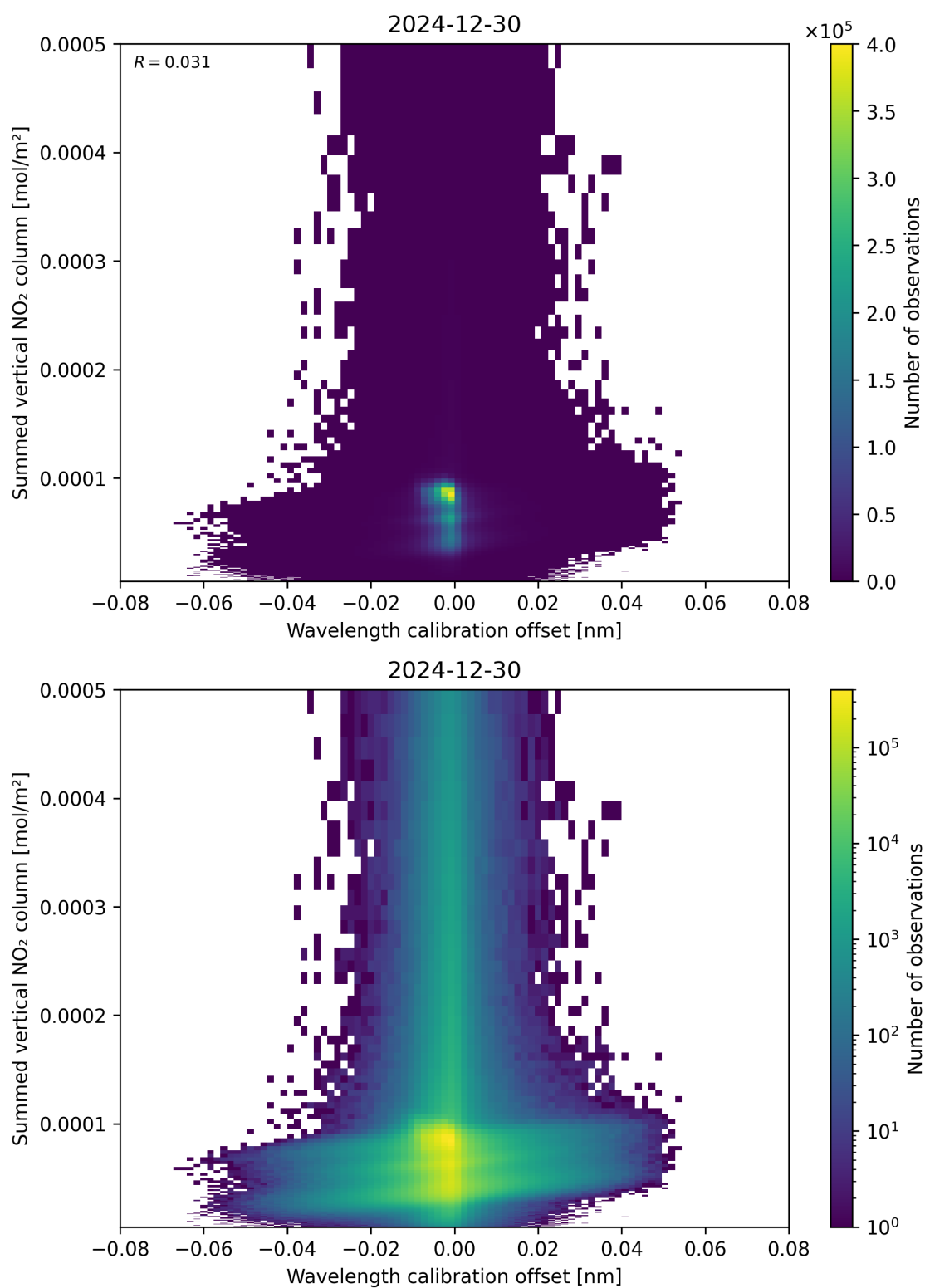
Figure 177: Scatter density plot of “Wavelength calibration offset” against “Summed vertical NO 2 column” for 2024-12-29 to 2024-12-31.
