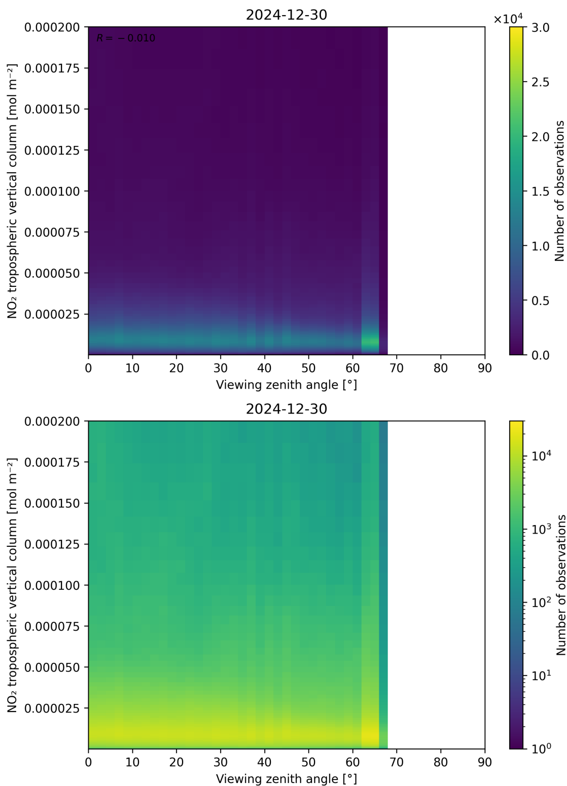
Figure 169: Scatter density plot of “Viewing zenith angle” against “NO 2 tropospheric vertical column” for 2024-12-29 to 2024-12-31.
