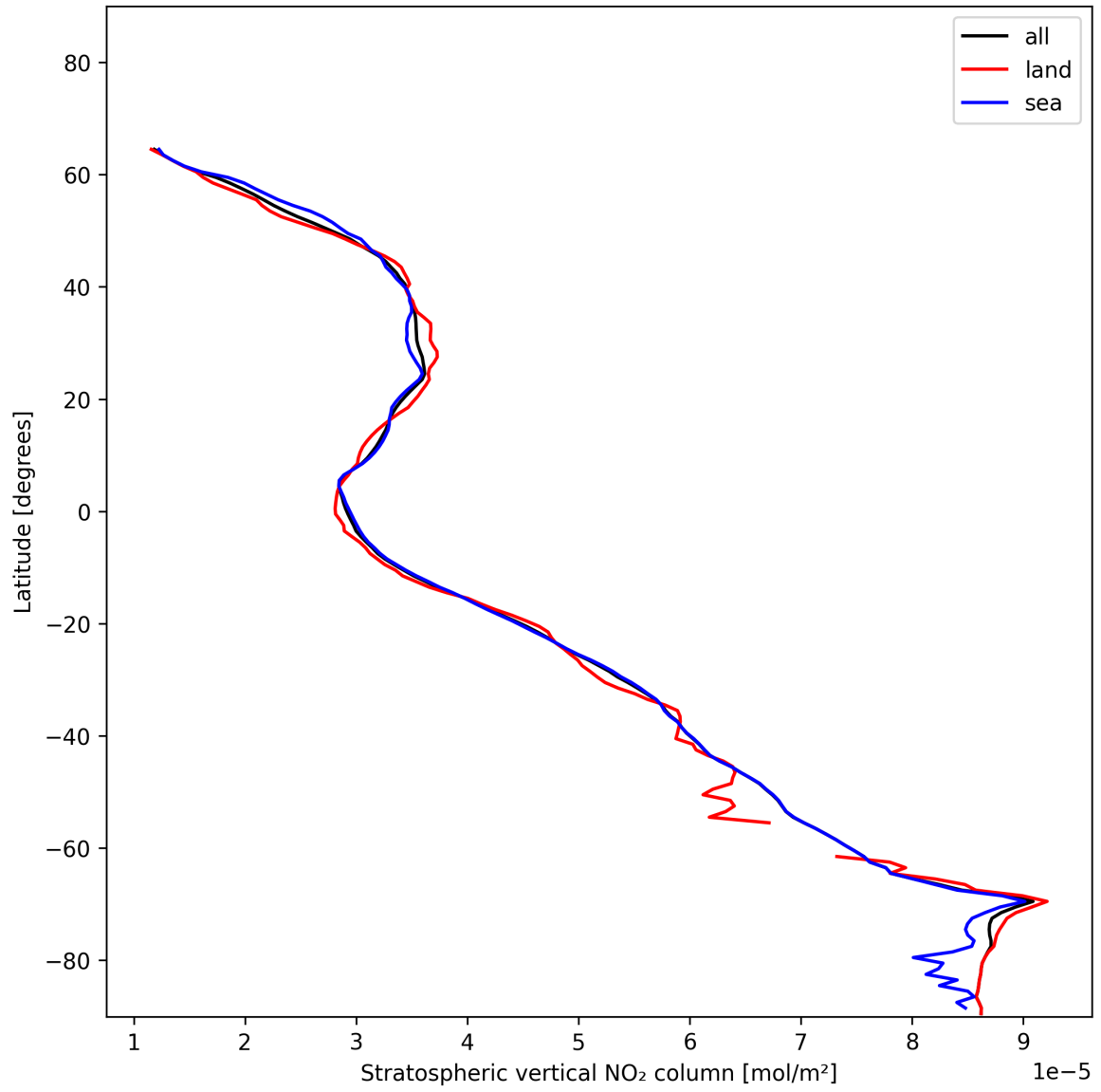
Figure 19: Zonal average of “Stratospheric vertical NO 2 column” for 2024-12-29 to 2024-12-31.
