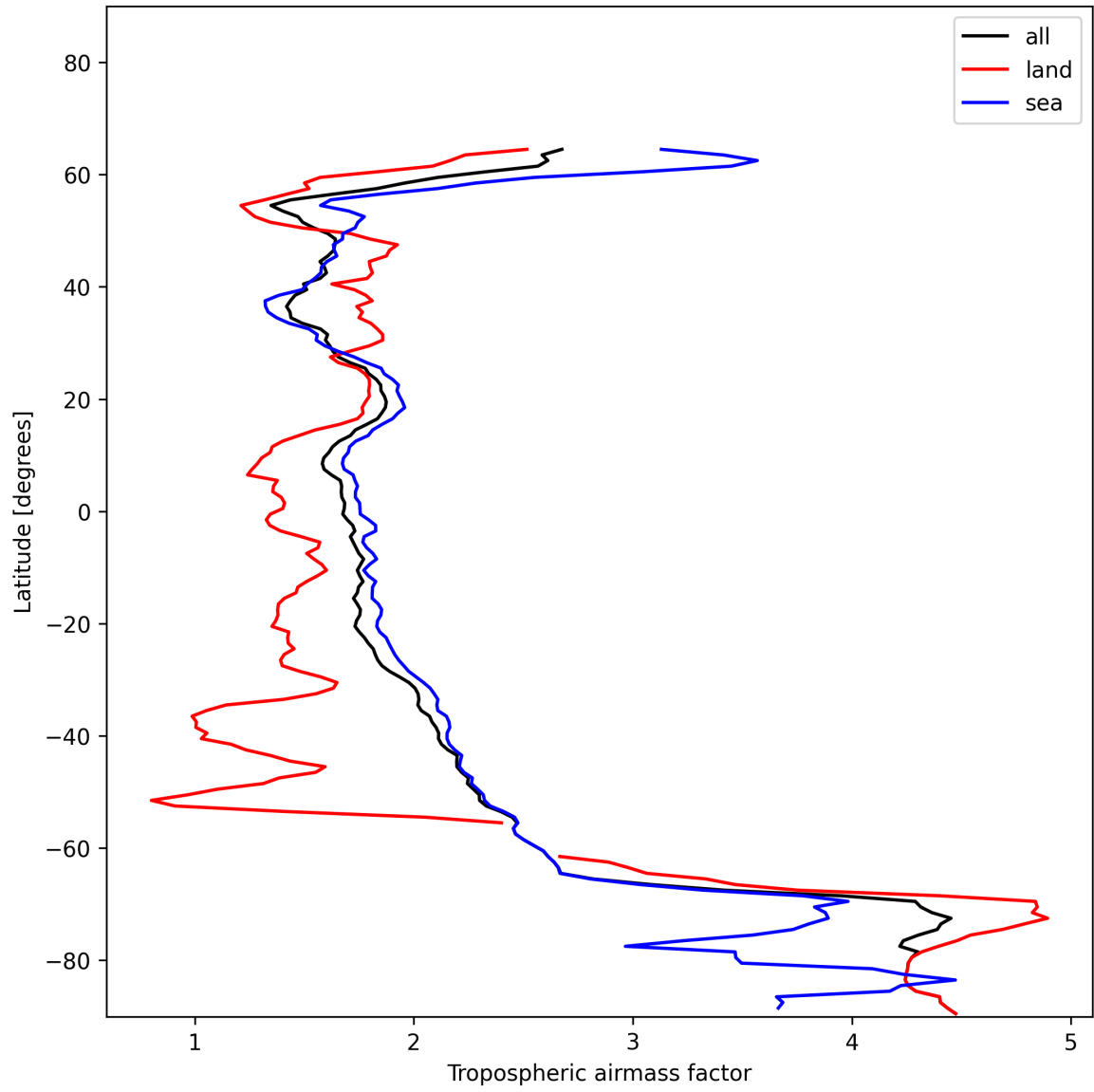
Figure 14: Zonal average of “Tropospheric airmass factor” for 2024-12-29 to 2024-12-31.
