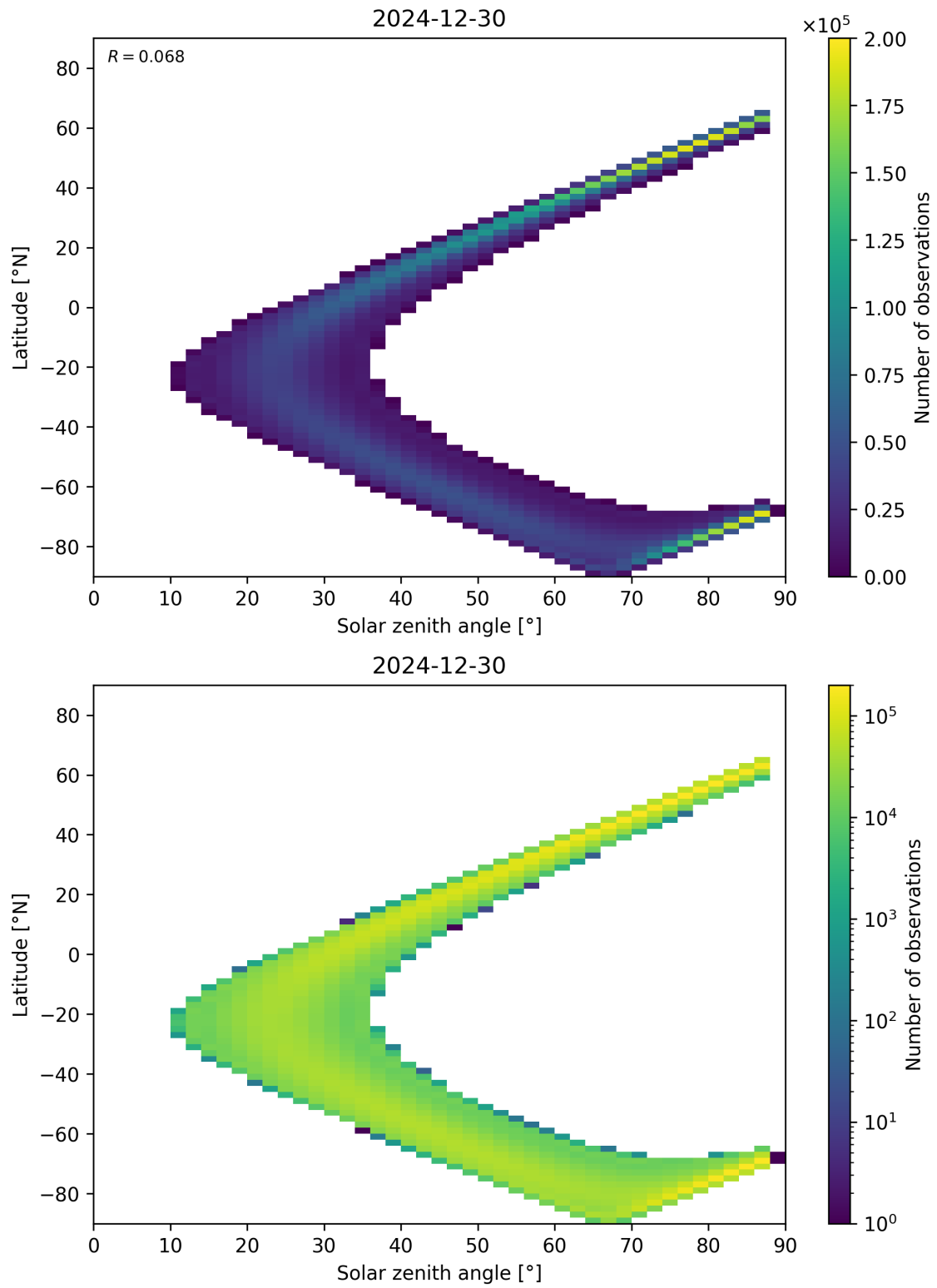
Figure 149: Scatter density plot of “Solar zenith angle” against “Latitude” for 2024-12-29 to 2024-12-31.
