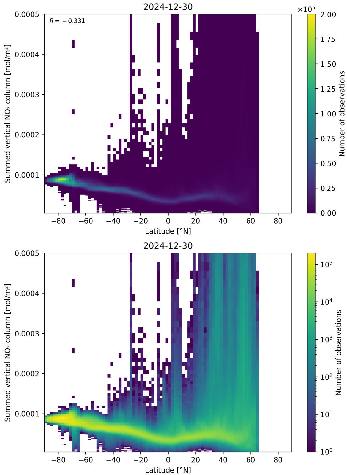
Figure 88: Scatter density plot of “Latitude” against “Summed vertical NO 2 column” for 2024-12-29 to 2024-12-31.
