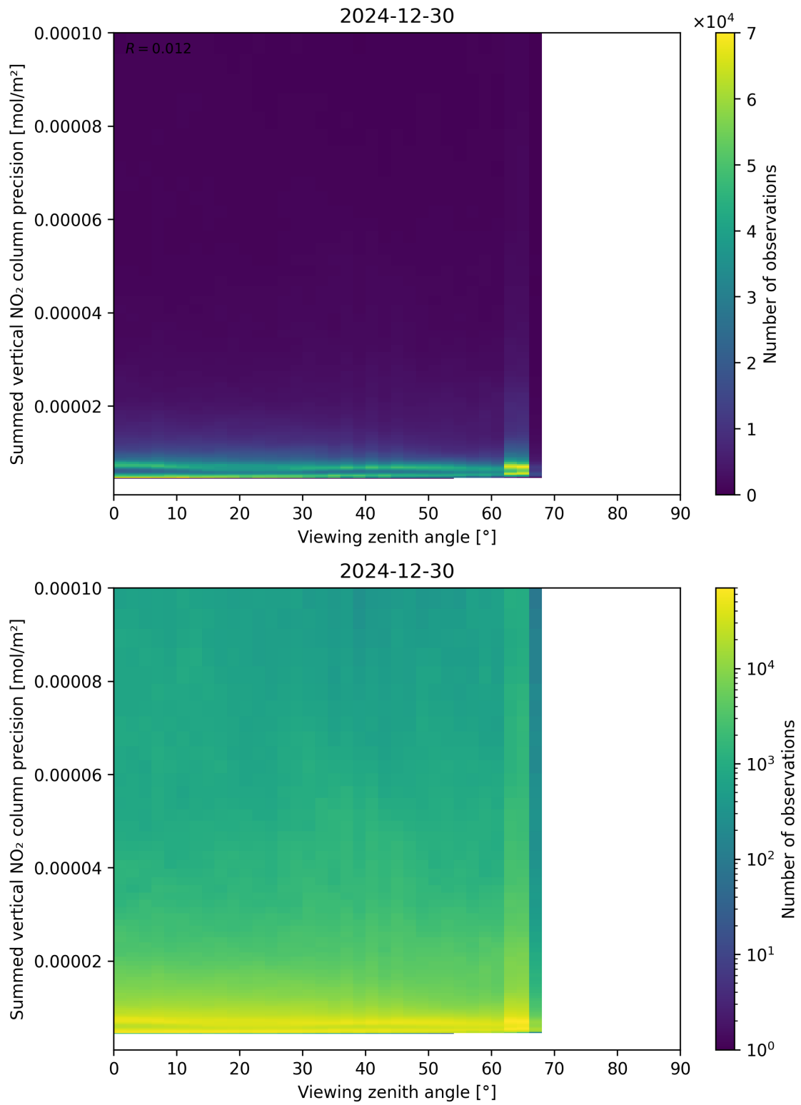
Figure 166: Scatter density plot of “Viewing zenith angle” against “Summed vertical NO 2 column precision” for 2024-12-29 to 2024-12-31.
