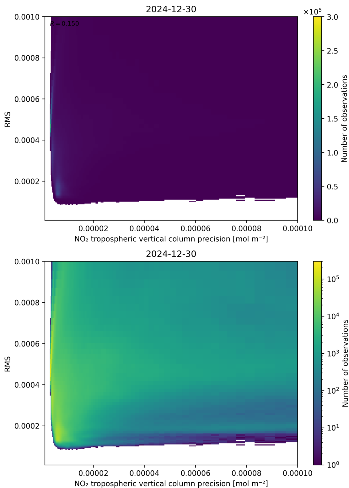
Figure 140: Scatter density plot of “NO 2 tropospheric vertical column precision” against “RMS” for 2024-12-29 to 2024-12-31.
