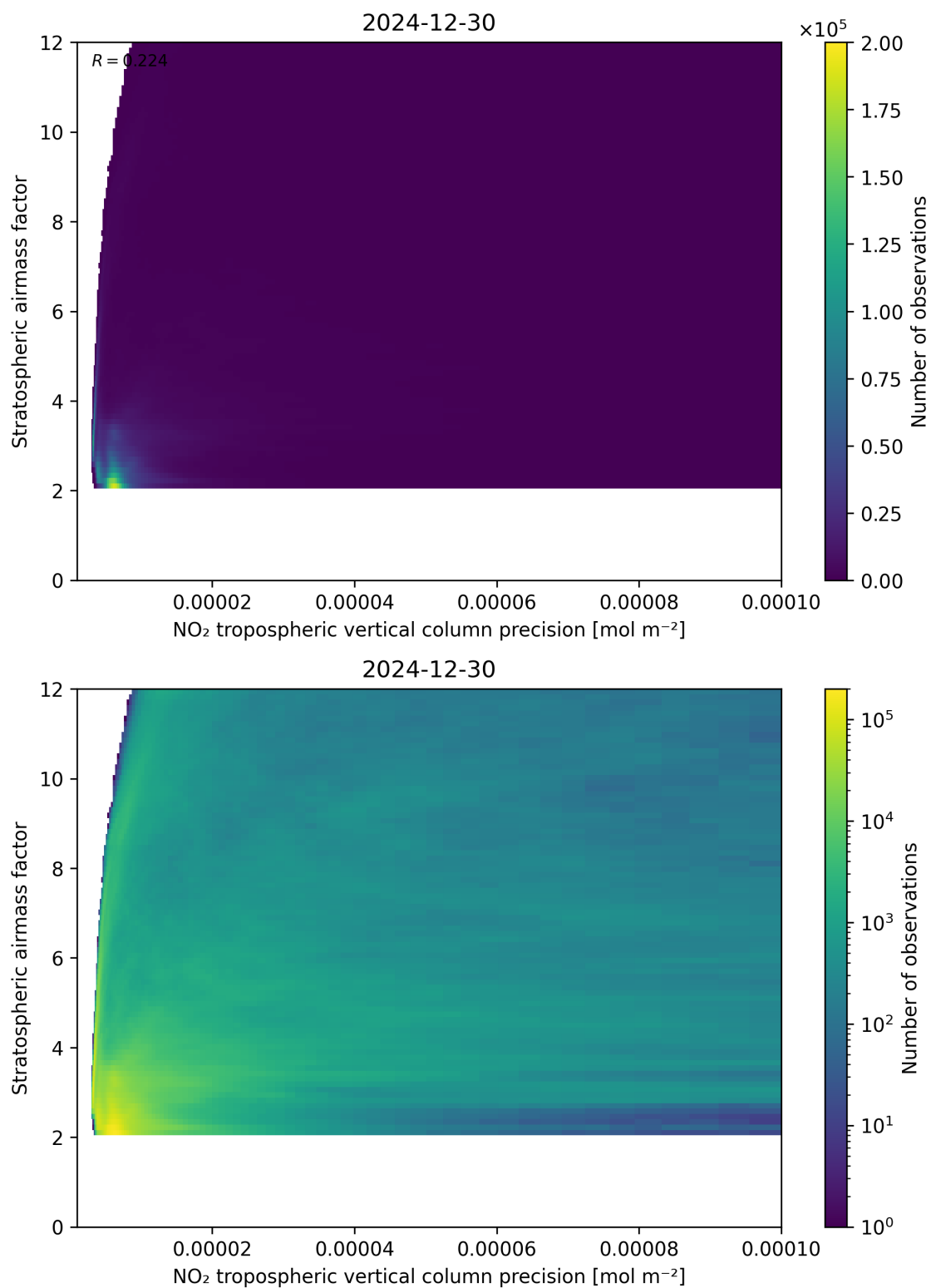
Figure 131: Scatter density plot of “NO 2 tropospheric vertical column precision” against “Stratospheric airmass factor” for 2024-12-29 to 2024-12-31.
