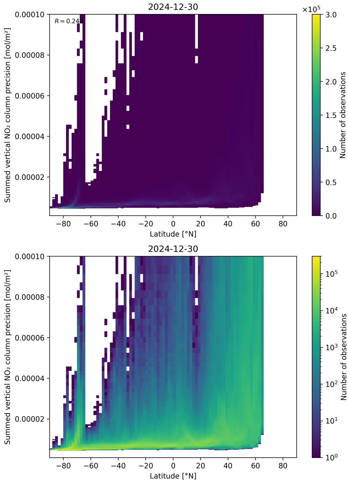
Figure 89: Scatter density plot of “Latitude” against “Summed vertical NO 2 column precision” for 2024-12-29 to 2024-12-31.
