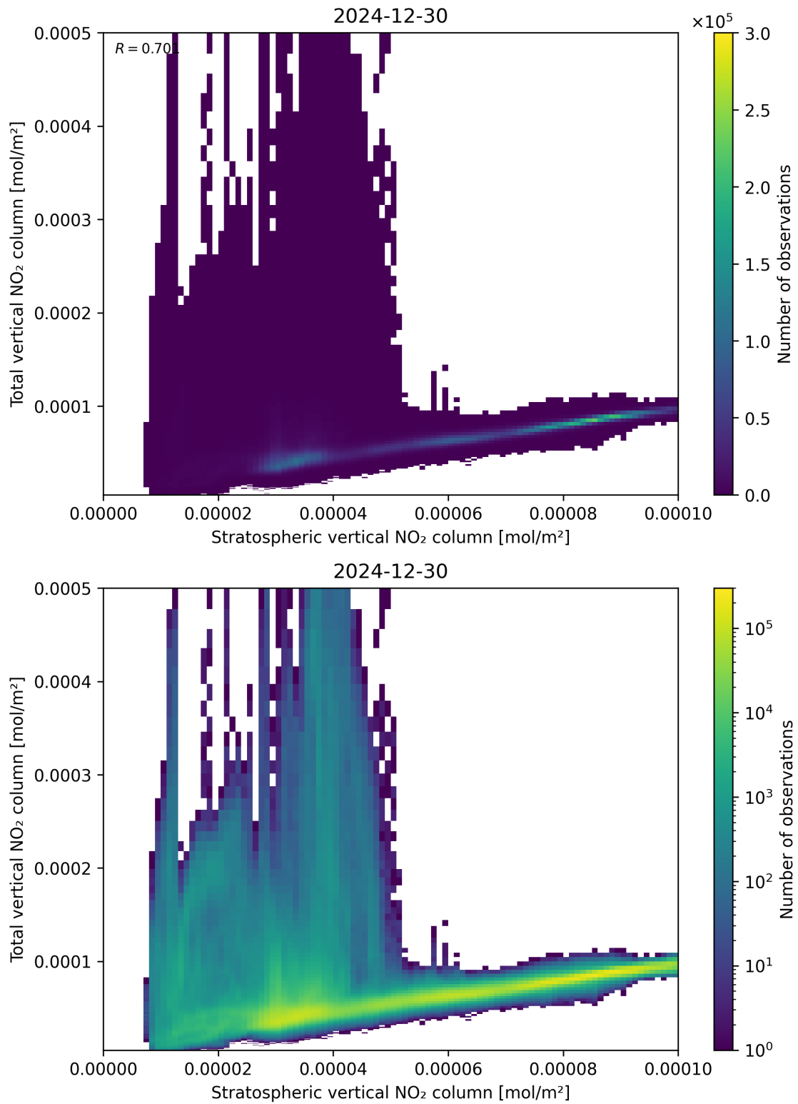
Figure 100: Scatter density plot of “Stratospheric vertical NO 2 column” against “Total vertical NO 2 column” for 2024-12-29 to 2024-12-31.
