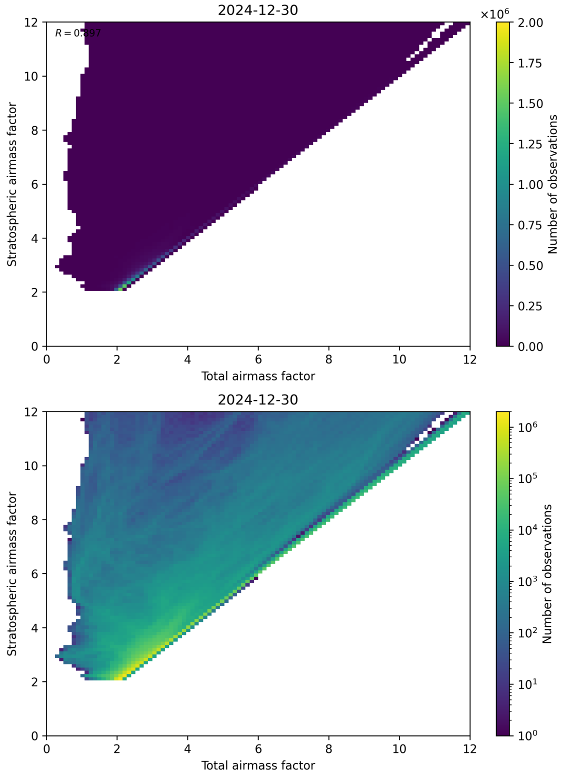
Figure 62: Scatter density plot of “Total airmass factor” against “Stratospheric airmass factor” for 2024-12-29 to 2024-12-31.
