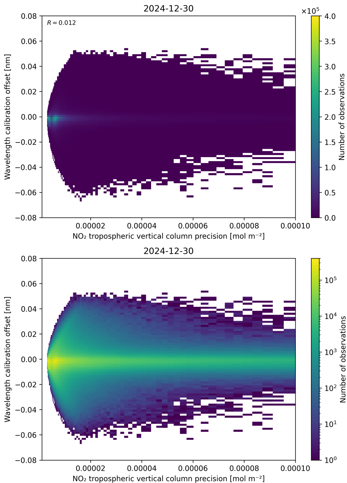
Figure 141: Scatter density plot of “NO 2 tropospheric vertical column precision” against “Wavelength calibration offset” for 2024-12-29 to 2024-12-31.
