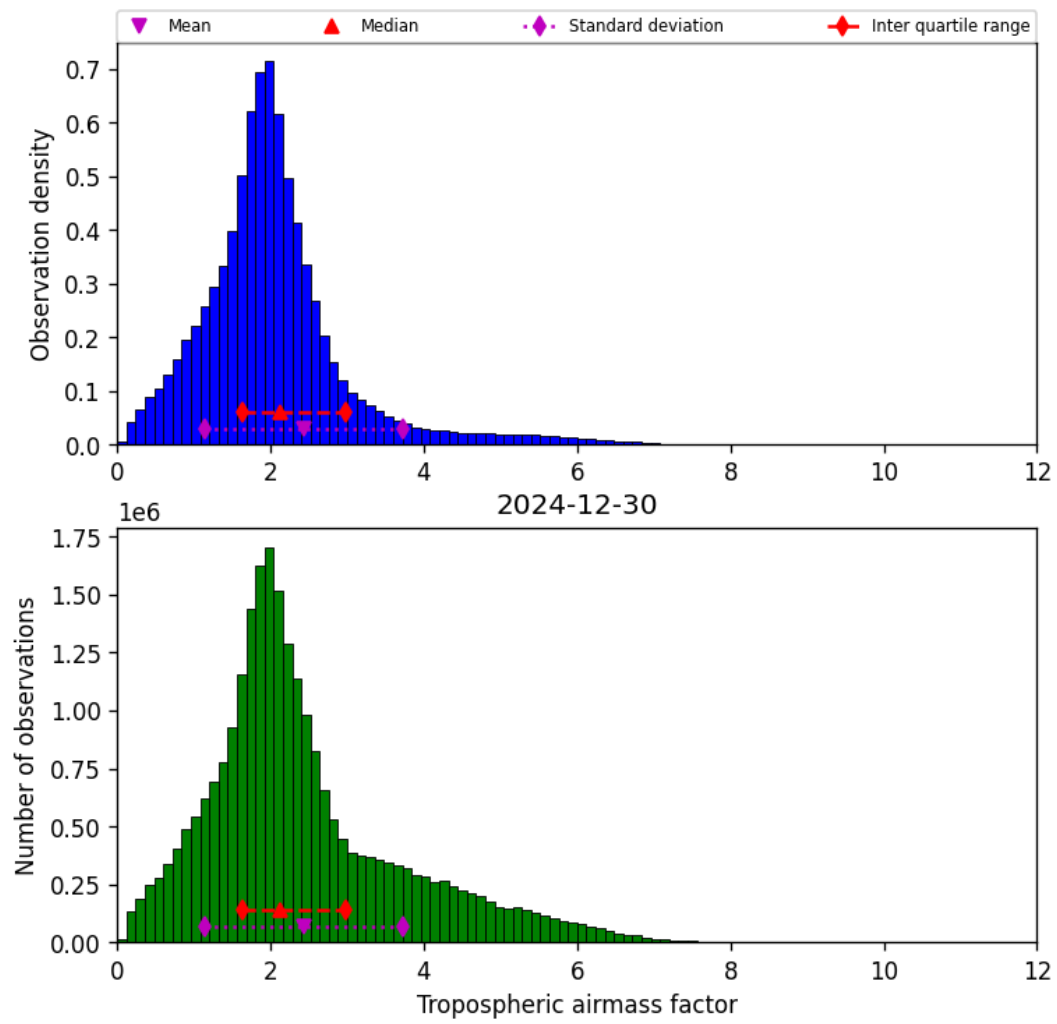
Figure 31: Histogram of “Tropospheric airmass factor” for 2024-12-29 to 2024-12-31
