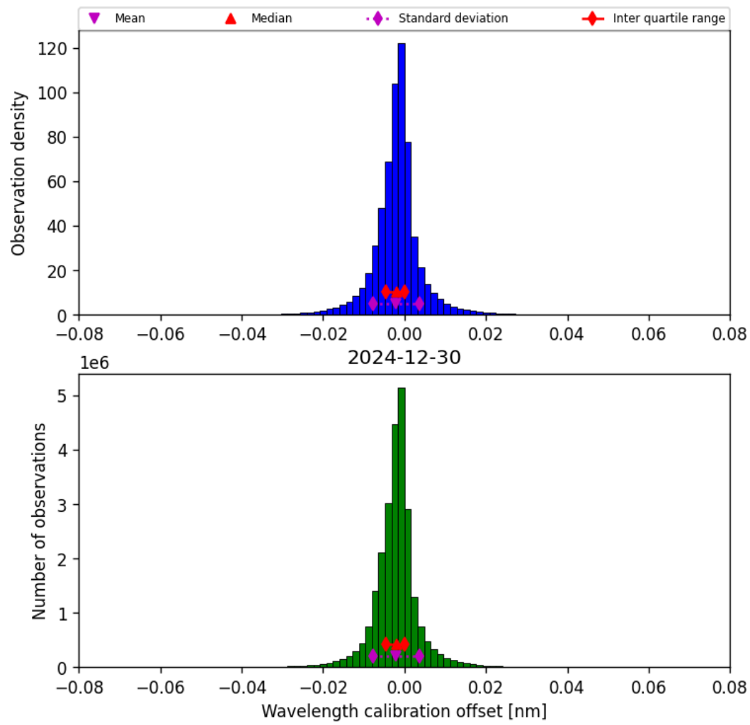
Figure 35: Histogram of “Wavelength calibration offset” for 2024-12-29 to 2024-12-31
