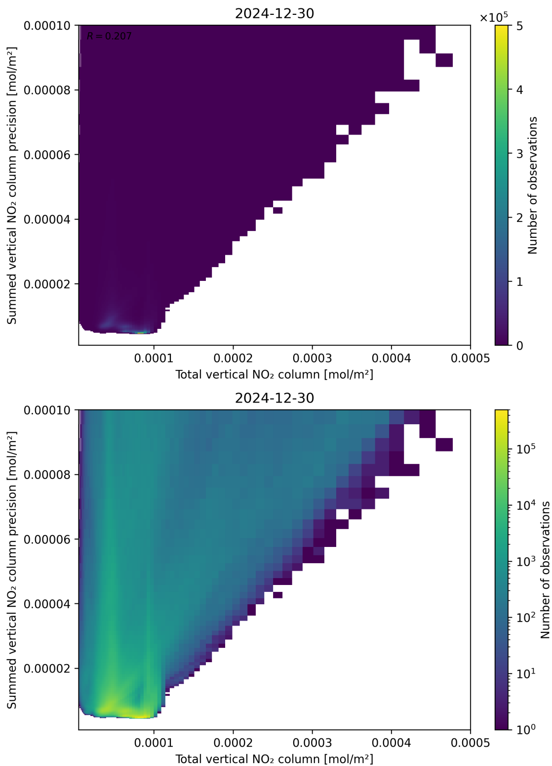
Figure 113: Scatter density plot of “Total vertical NO 2 column” against “Summed vertical NO 2 column precision” for 2024-12-29 to 2024-12-31.
