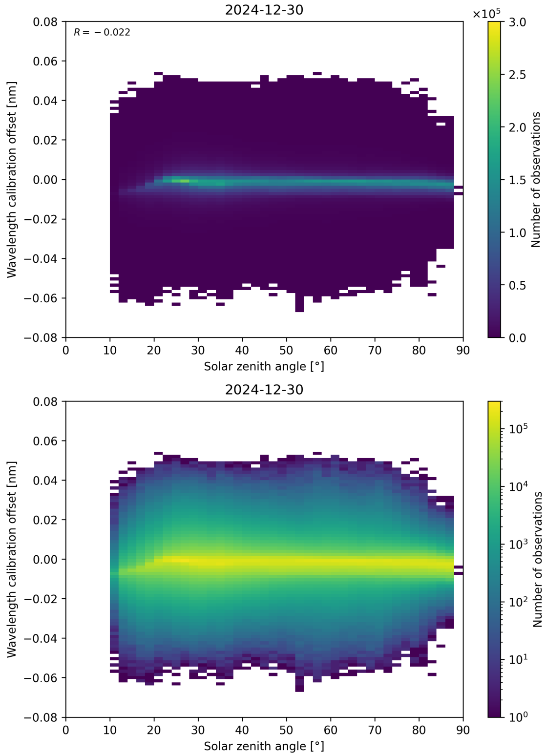
Figure 158: Scatter density plot of “Solar zenith angle” against “Wavelength calibration offset” for 2024-12-29 to 2024-12-31.
