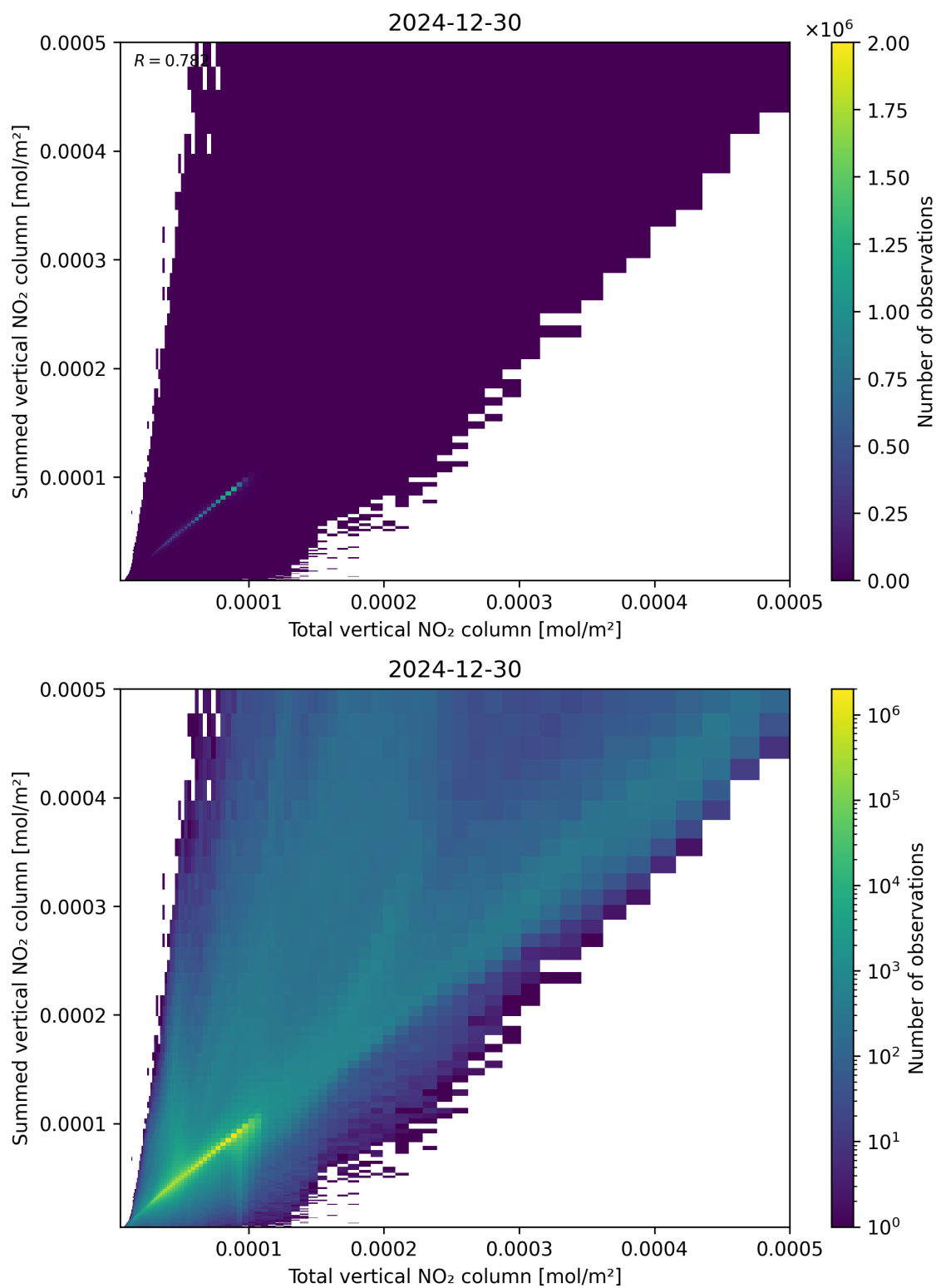
Figure 112: Scatter density plot of “Total vertical NO 2 column” against “Summed vertical NO 2 column” for 2024-12-29 to 2024-12-31.
