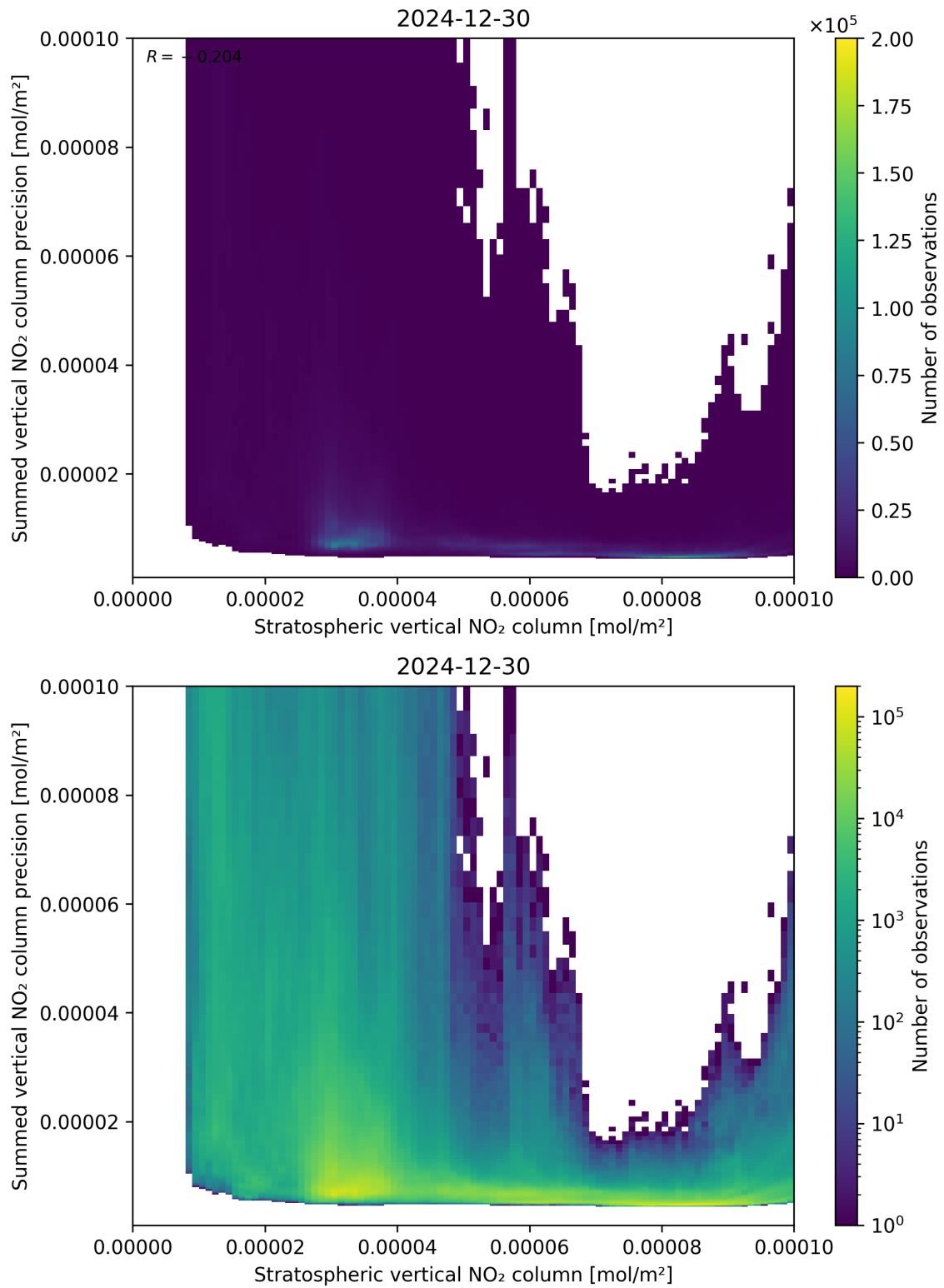
Figure 99: Scatter density plot of “Stratospheric vertical NO 2 column” against “Summed vertical NO 2 column precision” for 2024-12-29 to 2024-12-31.
