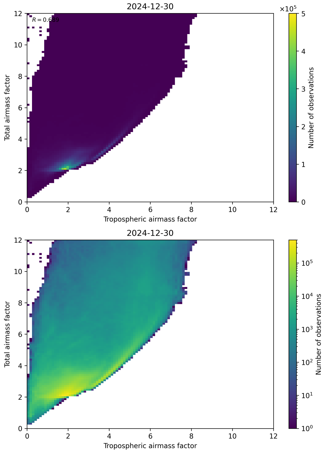
Figure 72: Scatter density plot of “Tropospheric airmass factor” against “Total airmass factor” for 2024-12-29 to 2024-12-31.
