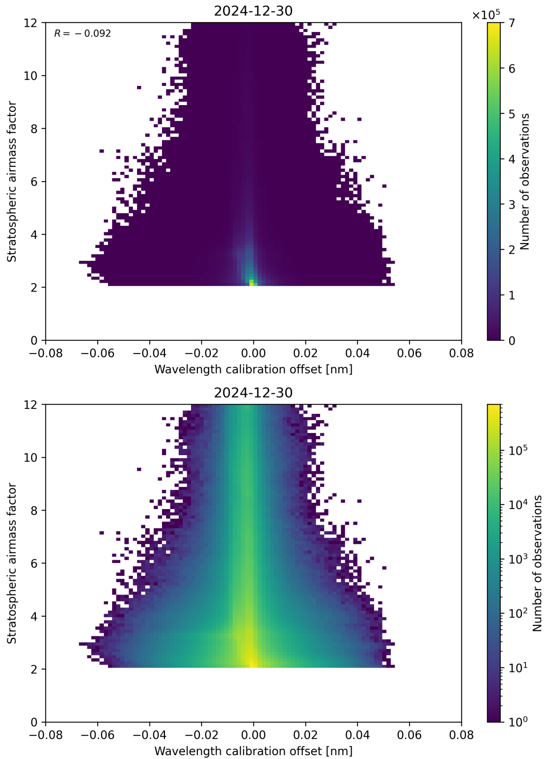
Figure 174: Scatter density plot of “Wavelength calibration offset” against “Stratospheric airmass factor” for 2024-12-29 to 2024-12-31.
