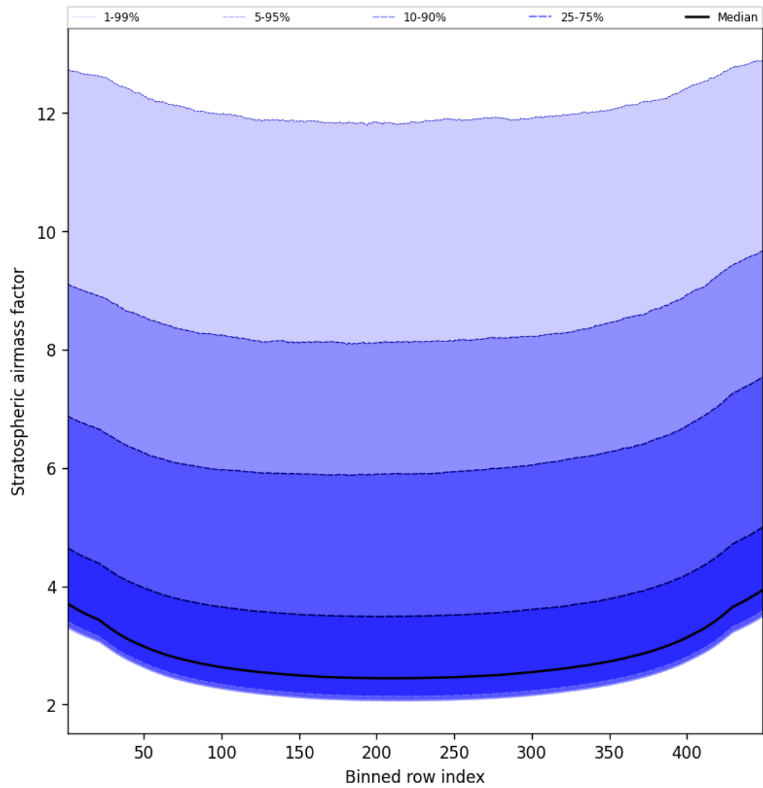
Figure 61: Along track statistics of “Stratospheric airmass factor” for 2024-12-29 to 2024-12-31
