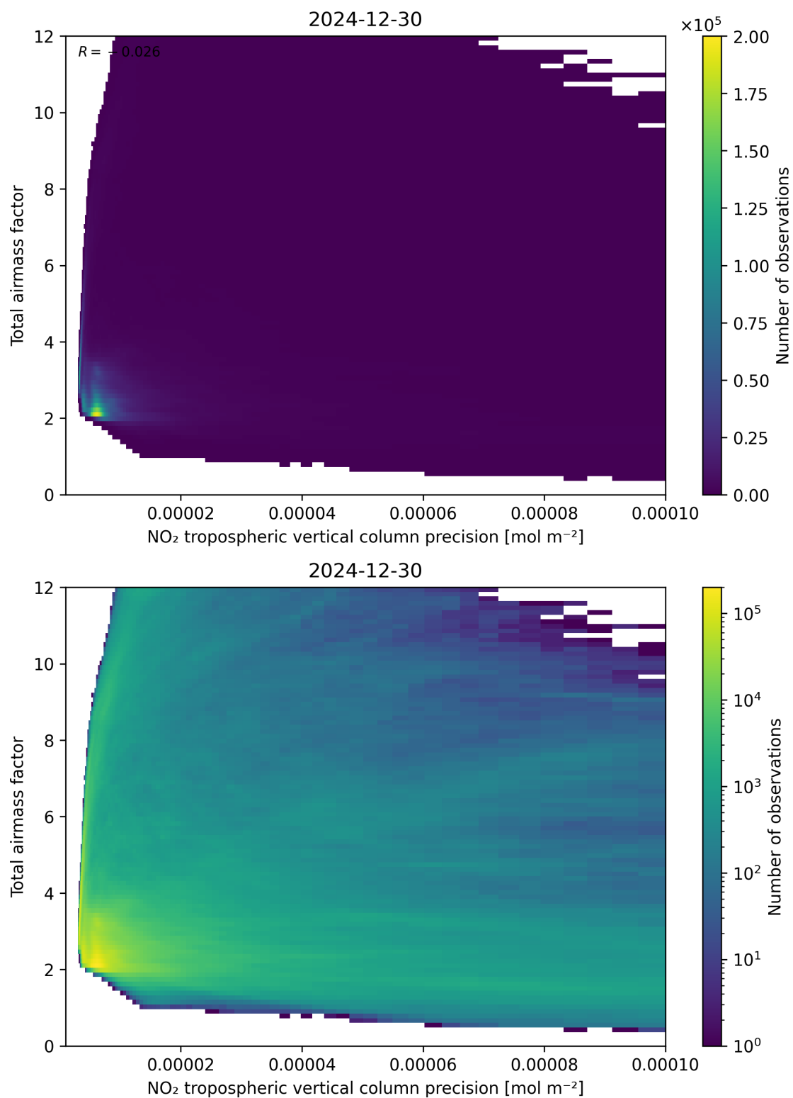
Figure 132: Scatter density plot of “NO 2 tropospheric vertical column precision” against “Total air mass factor” for 2024-12-29 to 2024-12-31.
