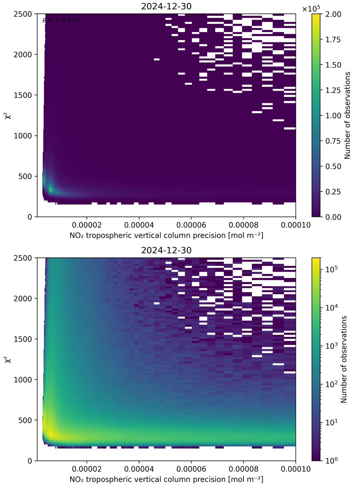
Figure 134: Scatter density plot of “NO 2 tropospheric vertical column precision” against “ \chi^2 ” for 2024-12-29 to 2024-12-31.
