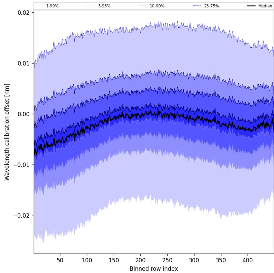
Figure 52: Along track statistics of “Wavelength calibration offset” for 2024-12-29 to 2024-12-31
