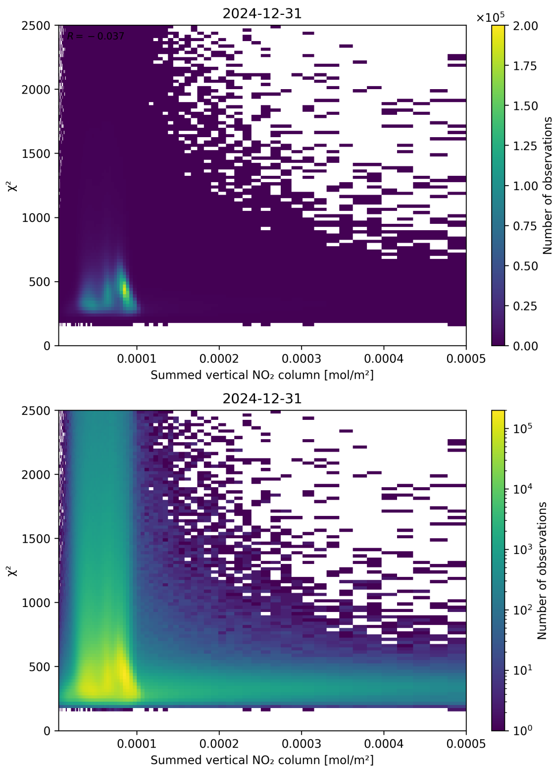
Figure 104: Scatter density plot of “Summed vertical NO 2 column” against “ \chi^2 ” for 2024-12-30 to 2025-01-01.
