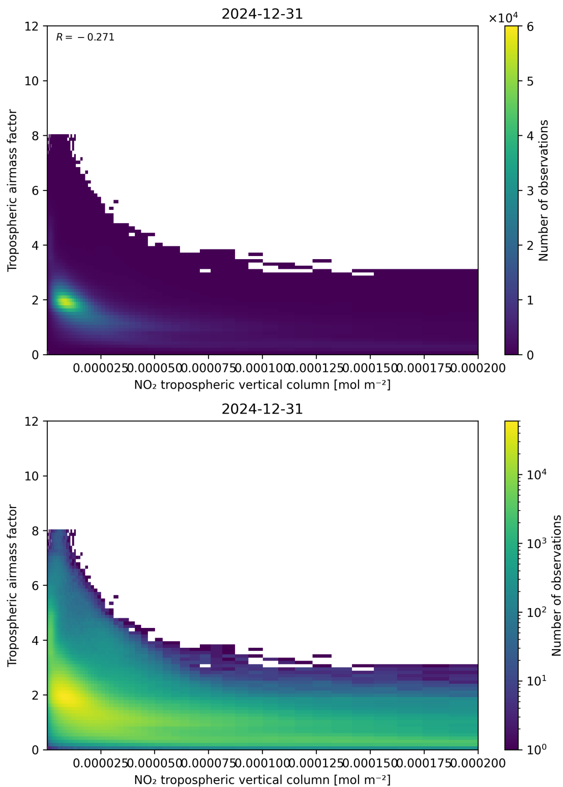
Figure 123: Scatter density plot of “NO 2 tropospheric vertical column” against “Tropospheric air mass factor” for 2024-12-30 to 2025-01-01.
