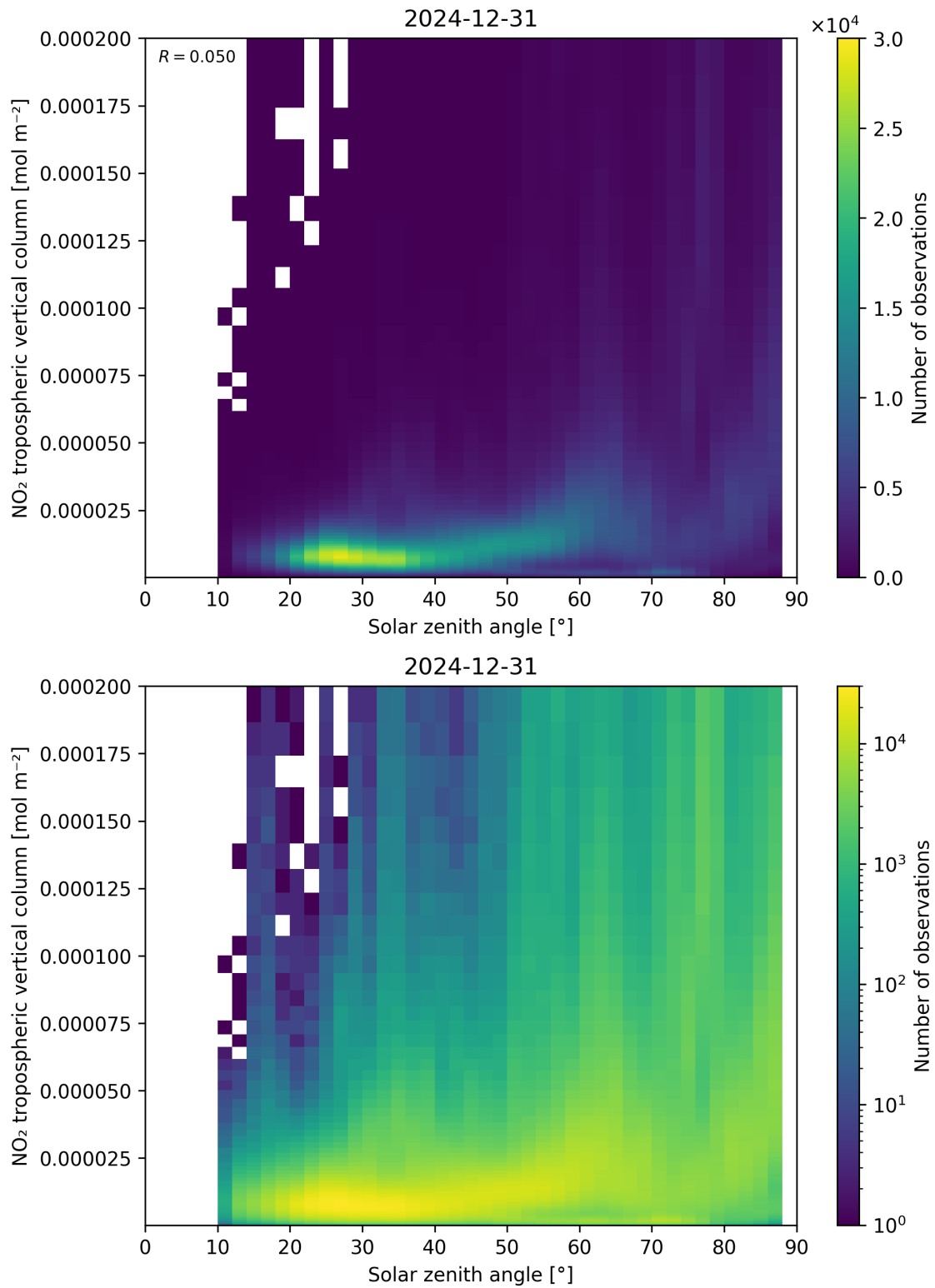
Figure 155: Scatter density plot of “Solar zenith angle” against “NO 2 tropospheric vertical column” for 2024-12-30 to 2025-01-01.
