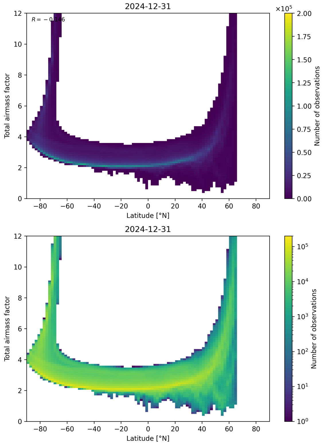
Figure 84: Scatter density plot of “Latitude” against “Total airmass factor” for 2024-12-30 to 2025-01-01.
