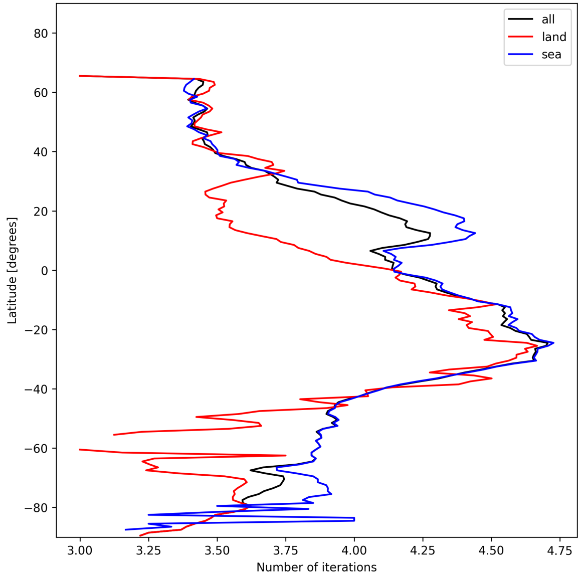
Figure 17: Zonal average of “Number of iterations” for 2024-12-30 to 2025-01-01.
