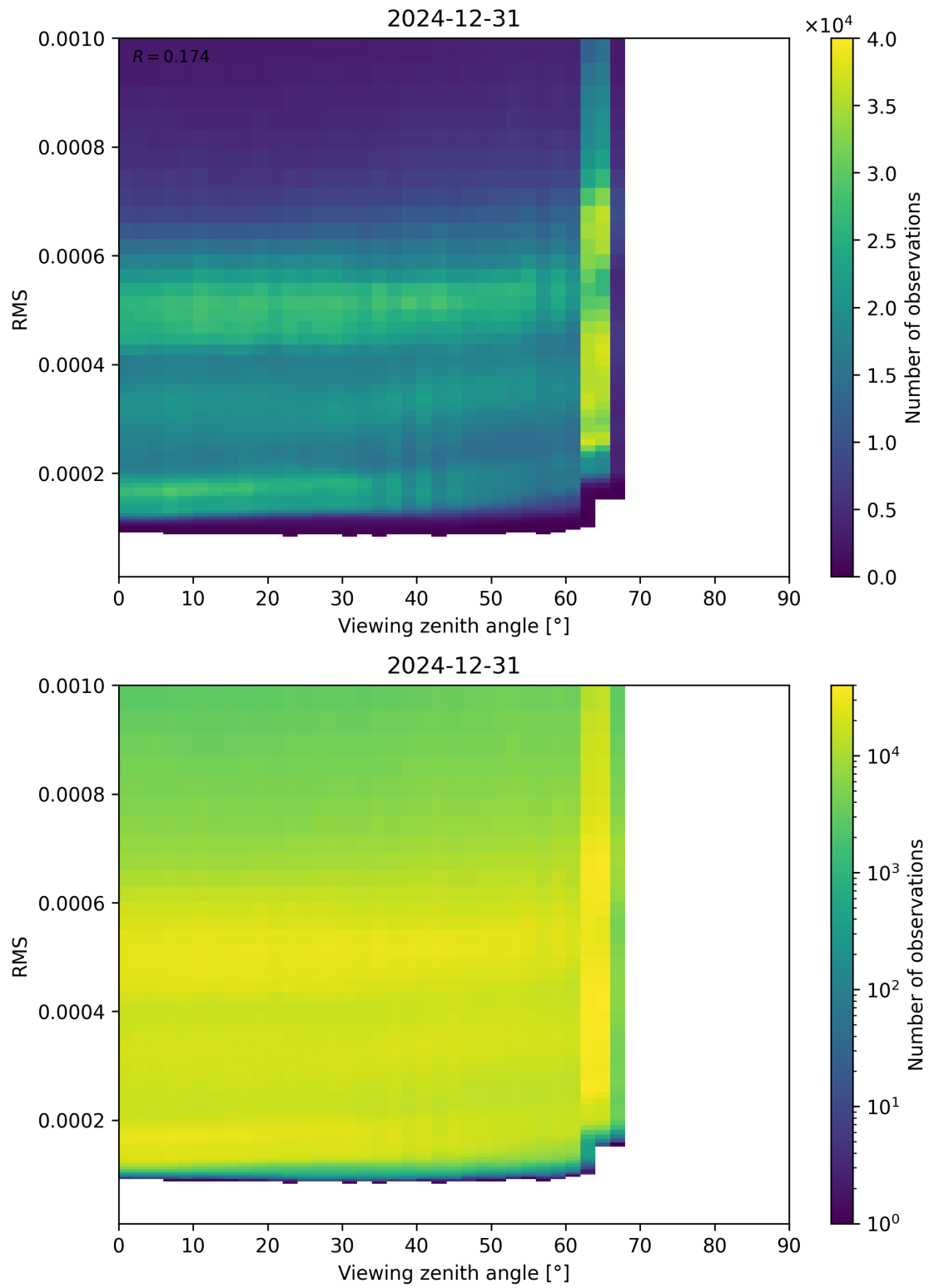
Figure 171: Scatter density plot of “Viewing zenith angle” against “RMS” for 2024-12-30 to 2025-01-01.
