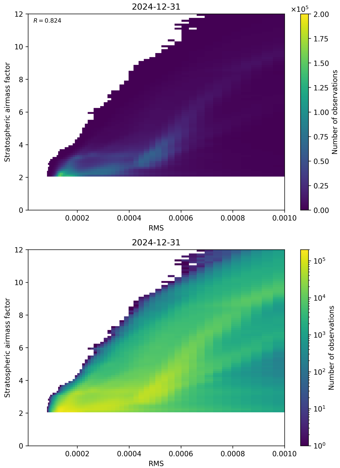
Figure 144: Scatter density plot of “RMS” against “Stratospheric airmass factor” for 2024-12-30 to 2025-01-01.
