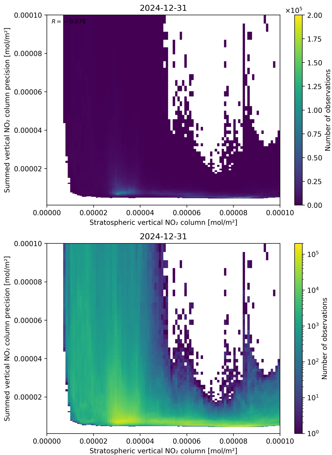
Figure 99: Scatter density plot of “Stratospheric vertical NO 2 column” against “Summed vertical NO 2 column precision” for 2024-12-30 to 2025-01-01.
