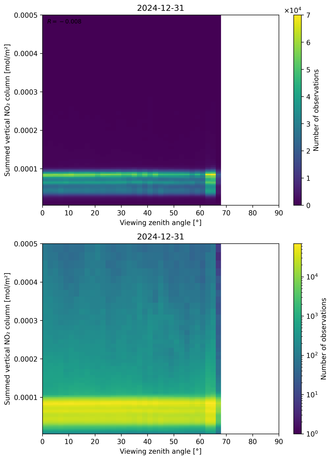
Figure 165: Scatter density plot of “Viewing zenith angle” against “Summed vertical NO 2 column” for 2024-12-30 to 2025-01-01.
