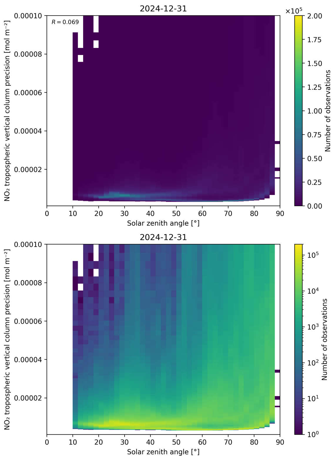
Figure 156: Scatter density plot of “Solar zenith angle” against “NO 2 tropospheric vertical column precision” for 2024-12-30 to 2025-01-01.
