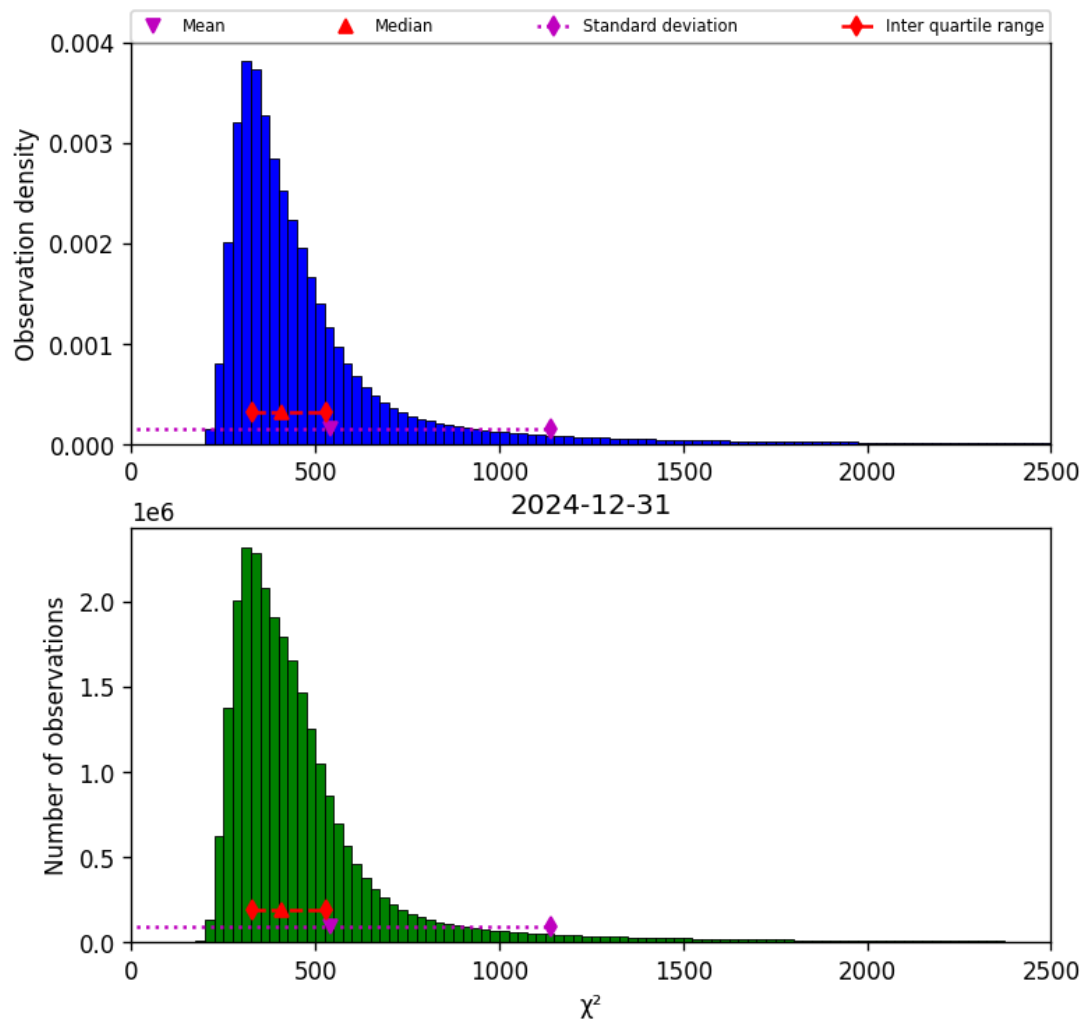
Figure 42: Histogram of " \chi^2 " for 2024-12-30 to 2025-01-01
