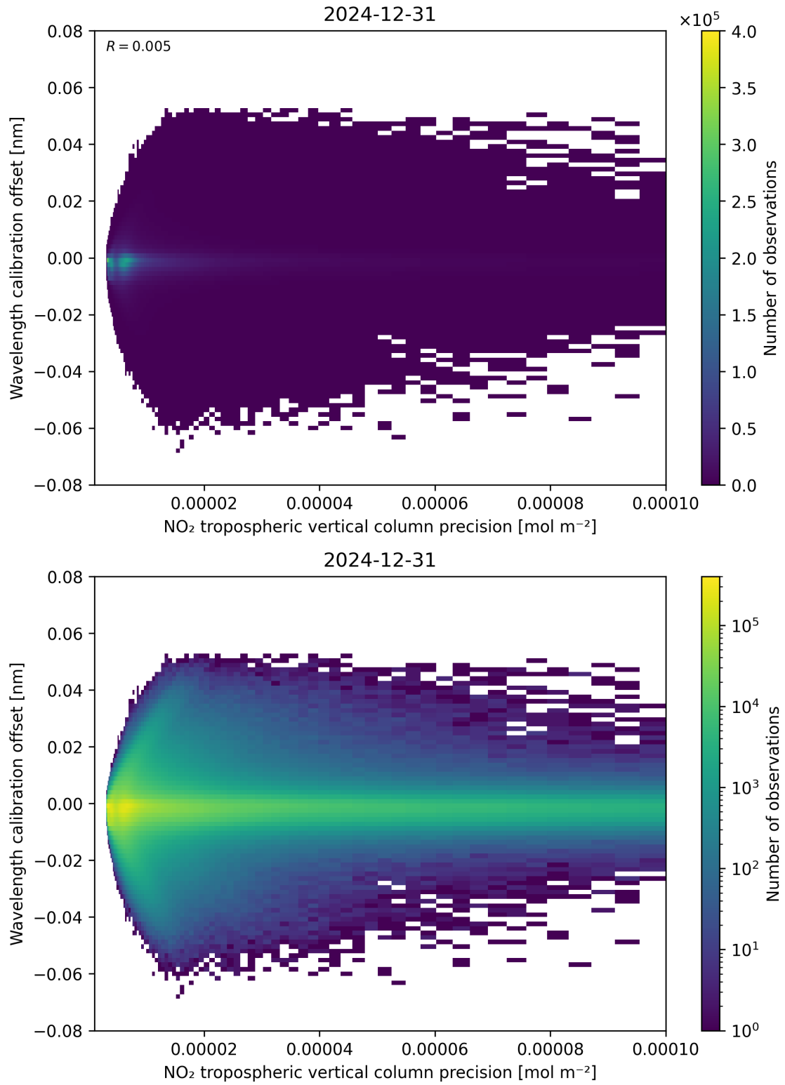
Figure 141: Scatter density plot of “NO 2 tropospheric vertical column precision” against “Wavelength calibration offset” for 2024-12-30 to 2025-01-01.
