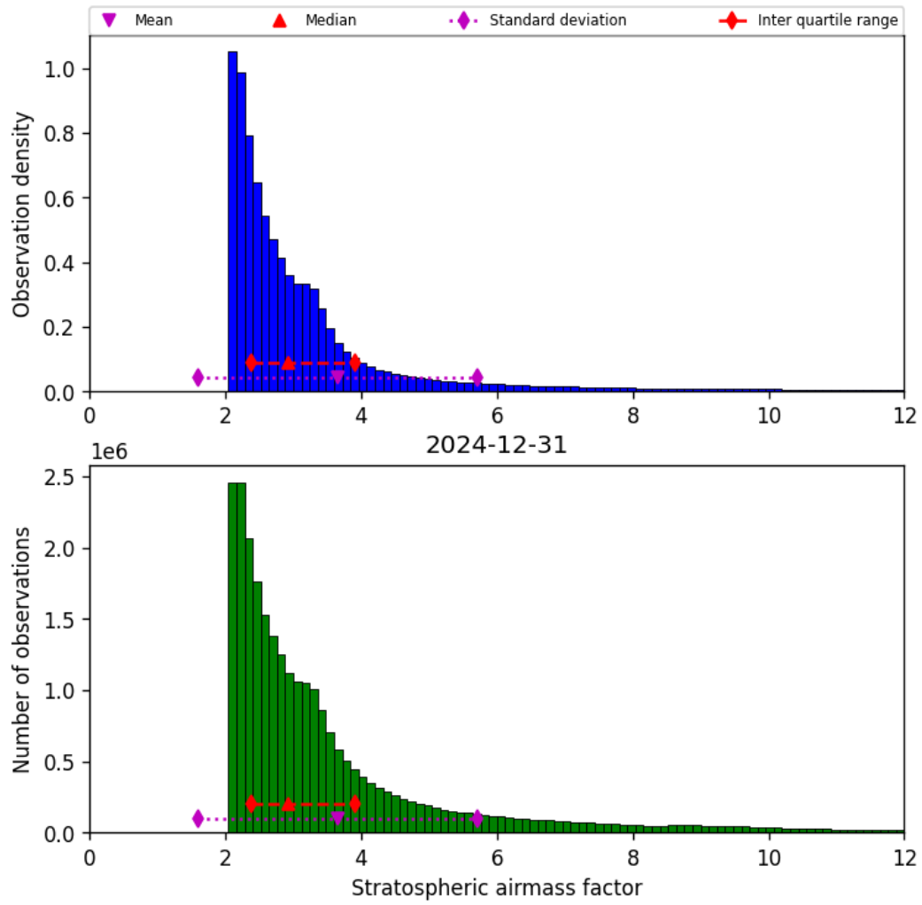
Figure 44: Histogram of “Stratospheric airmass factor” for 2024-12-30 to 2025-01-01
