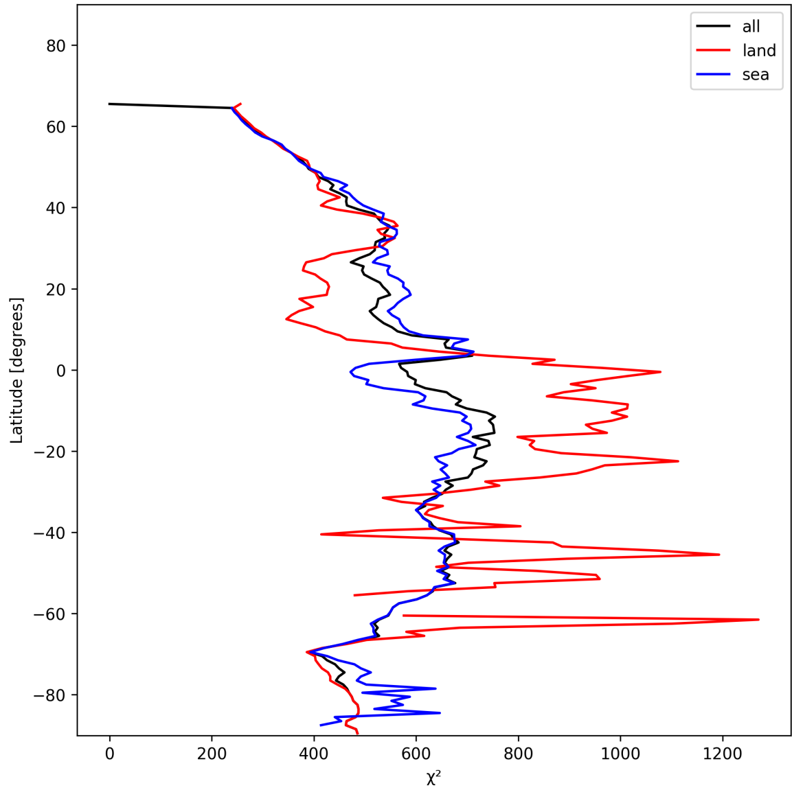
Figure 25: Zonal average of “ \chi^2 ” for 2024-12-30 to 2025-01-01.
