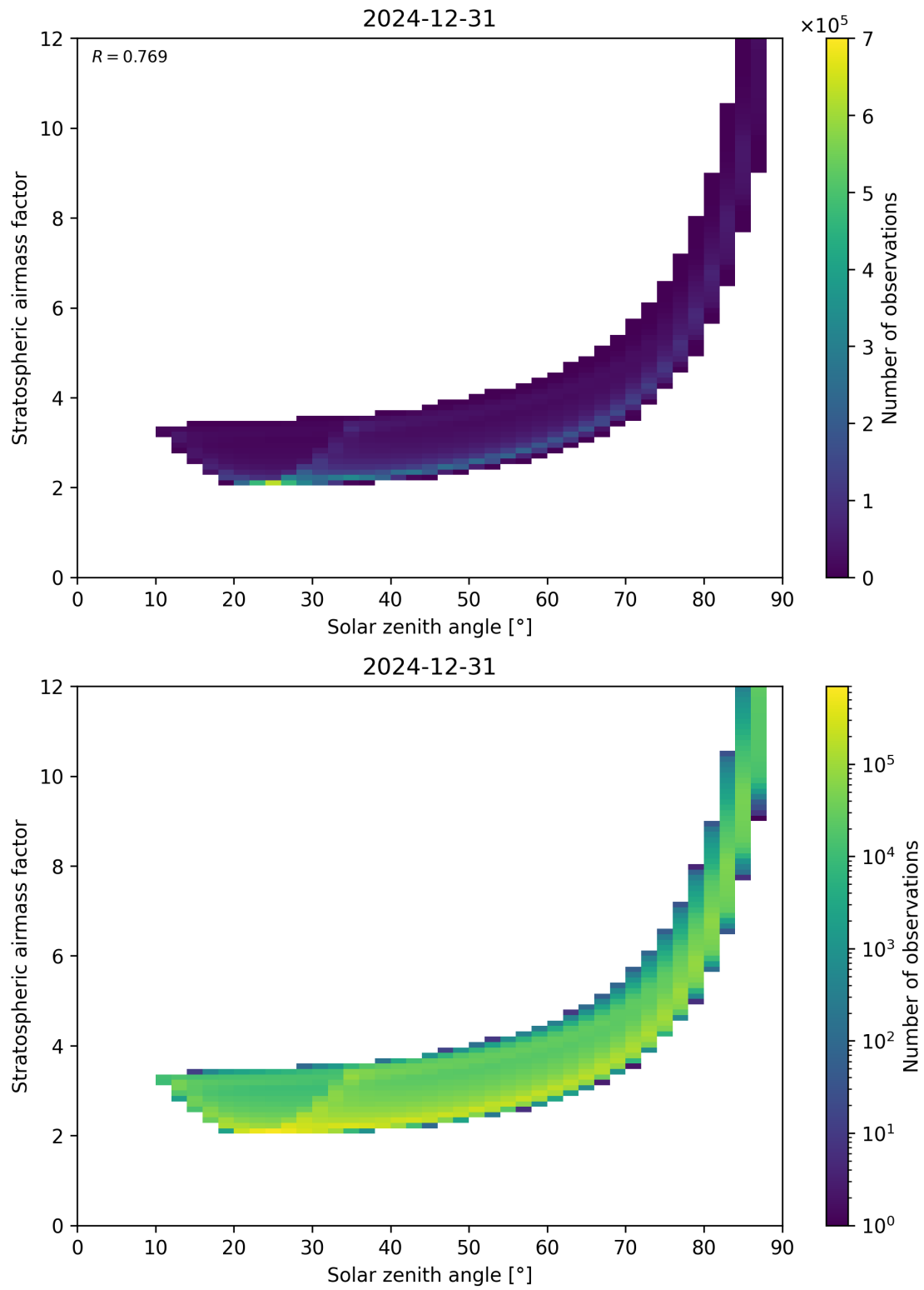
Figure 145: Scatter density plot of “Solar zenith angle” against “Stratospheric airmass factor” for 2024-12-30 to 2025-01-01.
