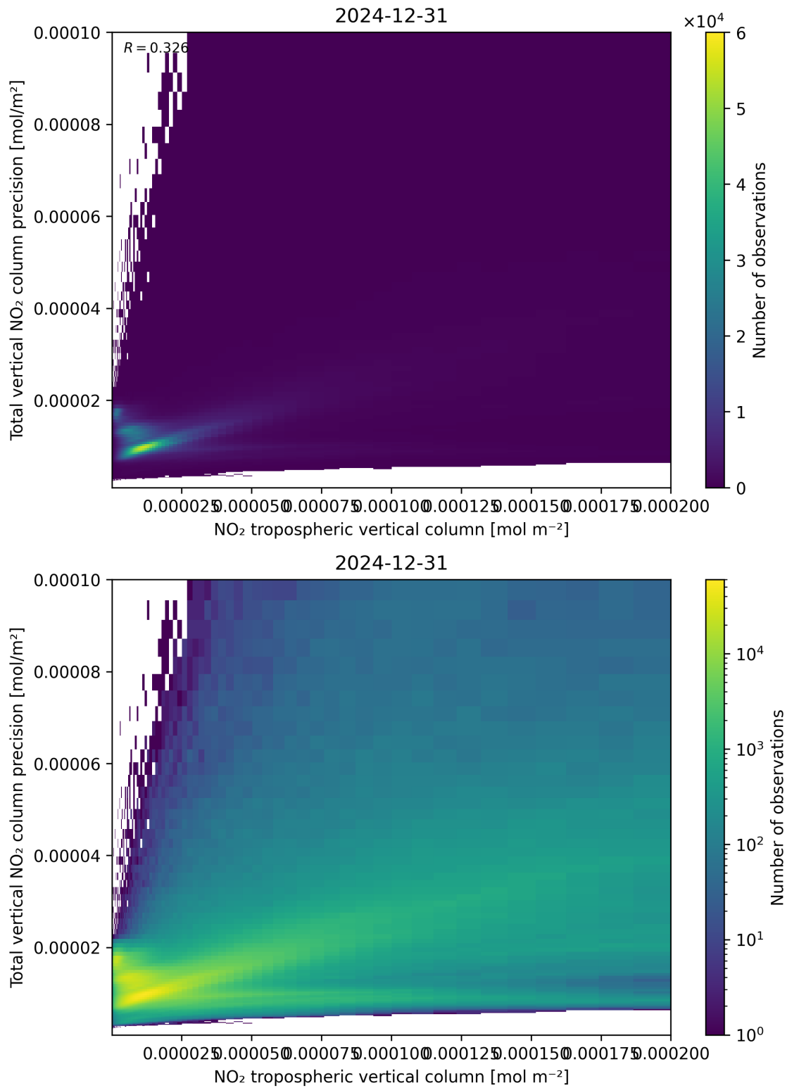
Figure 129: Scatter density plot of “NO 2 tropospheric vertical column” against “Total vertical NO 2 column precision” for 2024-12-30 to 2025-01-01.
