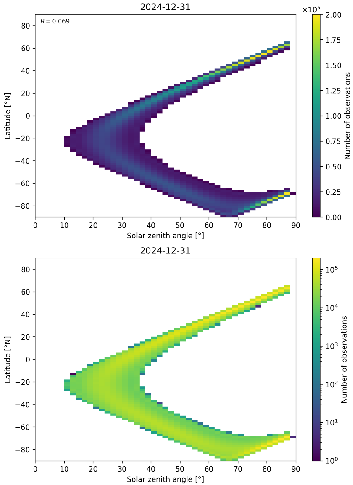
Figure 149: Scatter density plot of “Solar zenith angle” against “Latitude” for 2024-12-30 to 2025-01-01.
