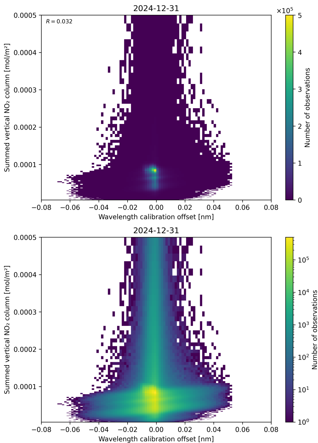
Figure 177: Scatter density plot of “Wavelength calibration offset” against “Summed vertical NO 2 column” for 2024-12-30 to 2025-01-01.
