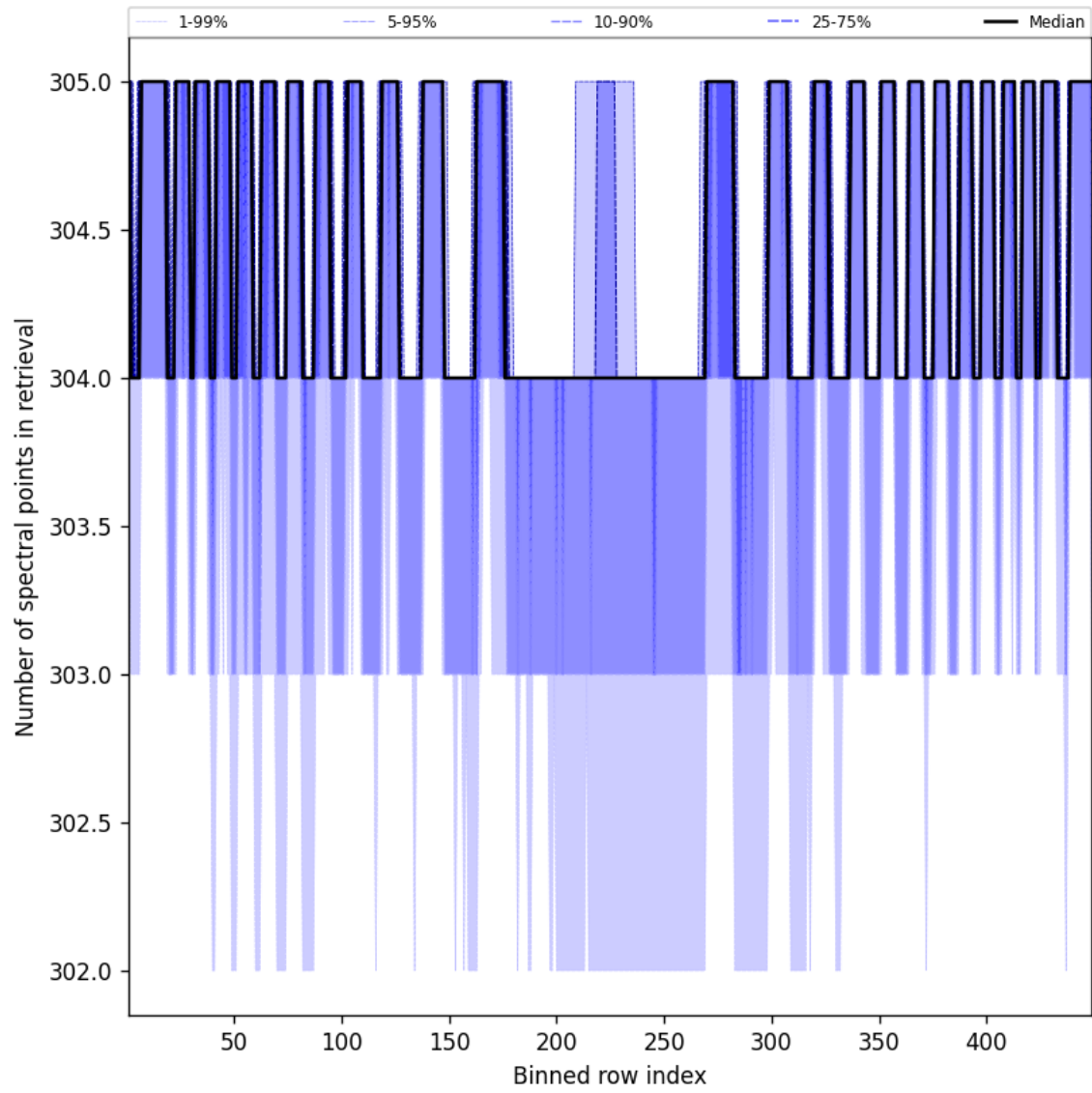
Figure 50: Along track statistics of “Number of spectral points in retrieval” for 2024-12-30 to 2025-01-01
