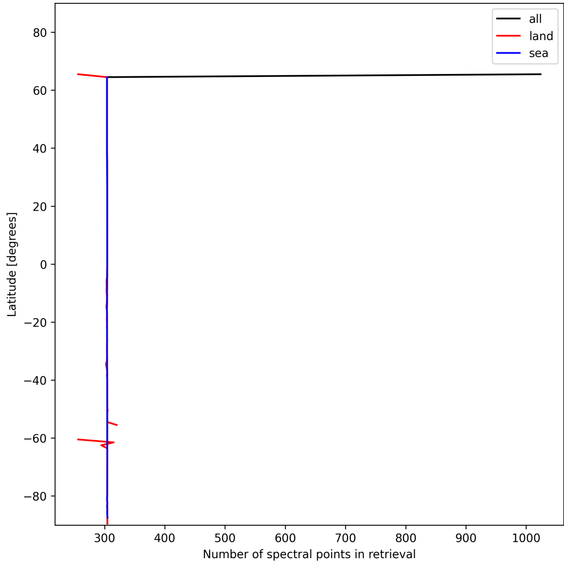
Figure 16: Zonal average of “Number of spectral points in retrieval” for 2024-12-30 to 2025-01-01.
