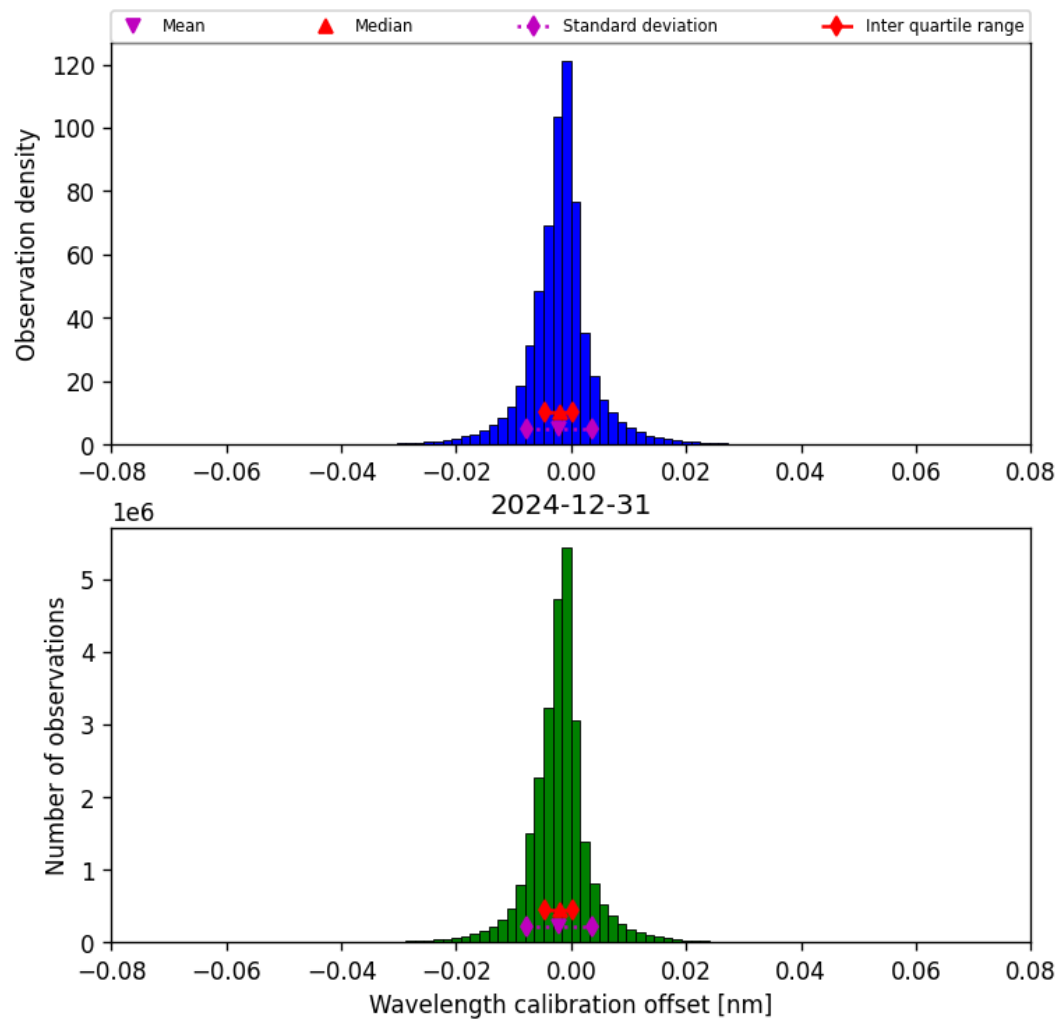
Figure 35: Histogram of “Wavelength calibration offset” for 2024-12-30 to 2025-01-01
