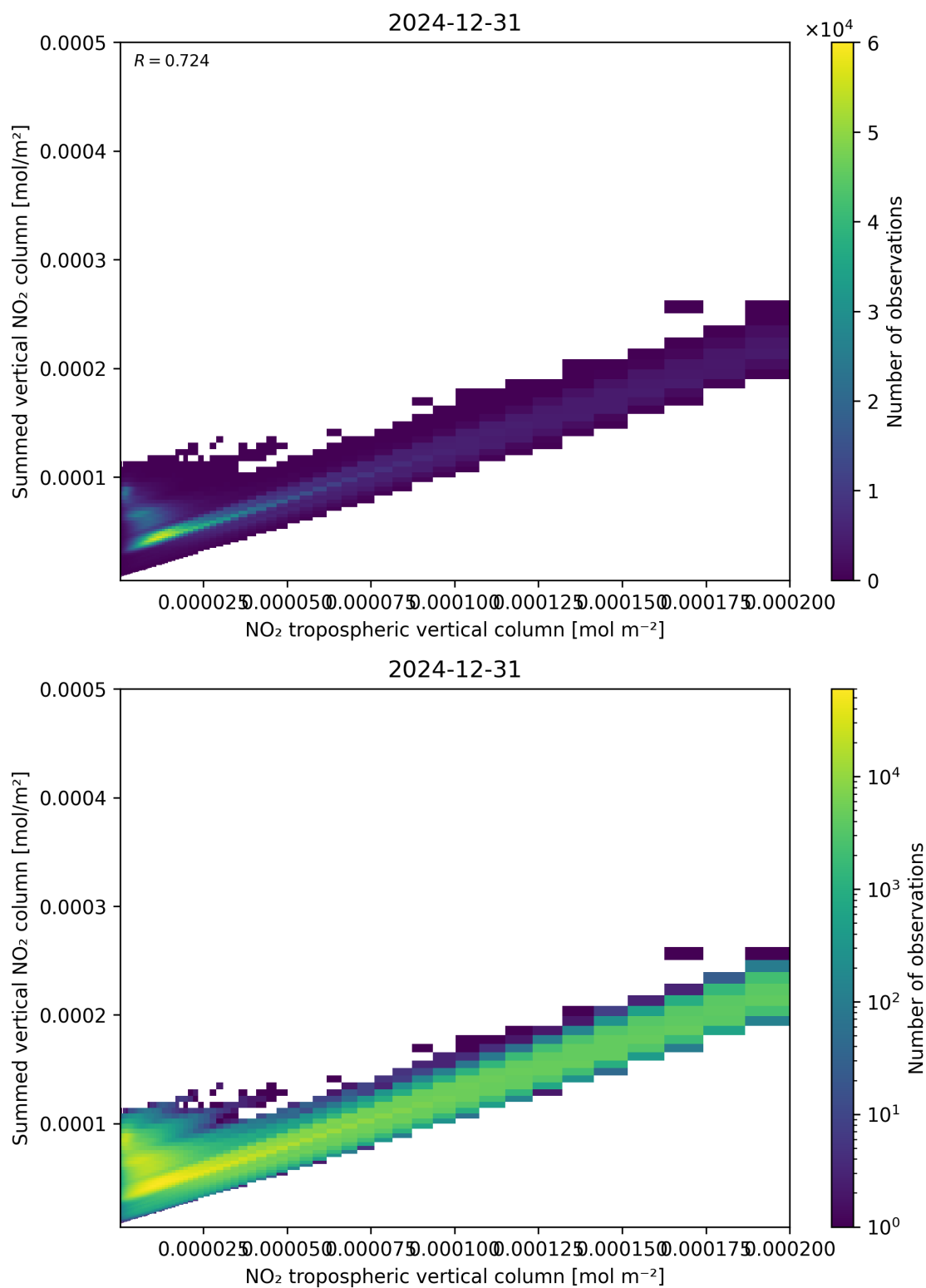
Figure 126: Scatter density plot of “NO 2 tropospheric vertical column” against “Summed vertical NO 2 column” for 2024-12-30 to 2025-01-01.
