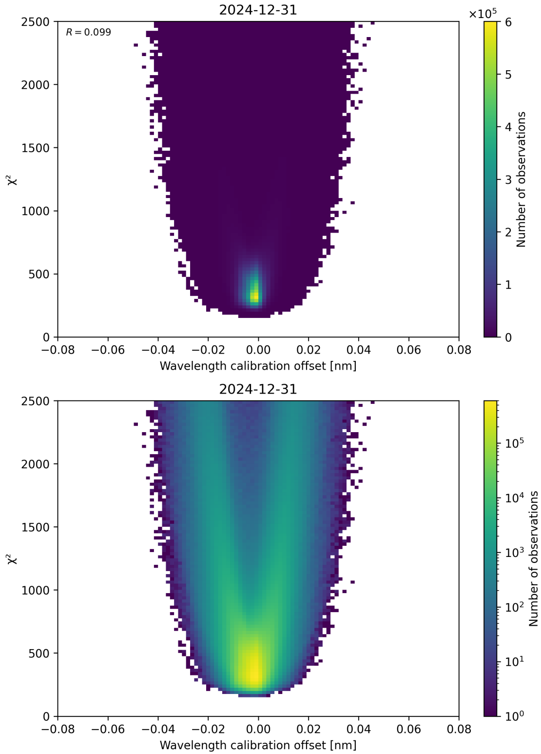
Figure 175: Scatter density plot of “Wavelength calibration offset” against “ \chi^2 ” for 2024-12-30 to 2025-01-01.
