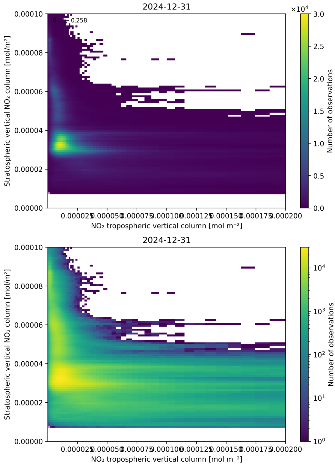
Figure 125: Scatter density plot of “NO 2 tropospheric vertical column” against “Stratospheric vertical NO 2 column” for 2024-12-30 to 2025-01-01.
