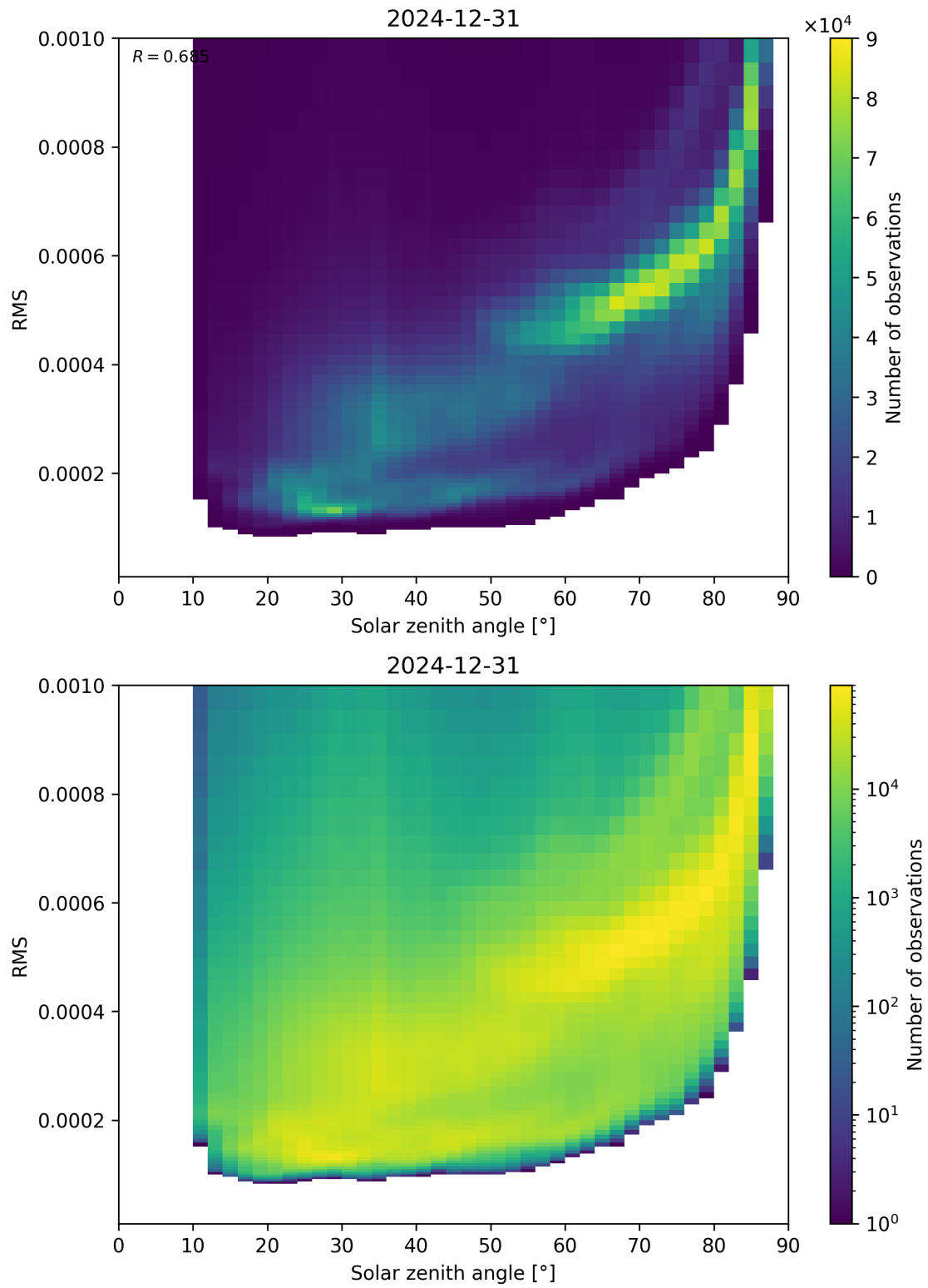
Figure 157: Scatter density plot of “Solar zenith angle” against “RMS” for 2024-12-30 to 2025-01-01.
