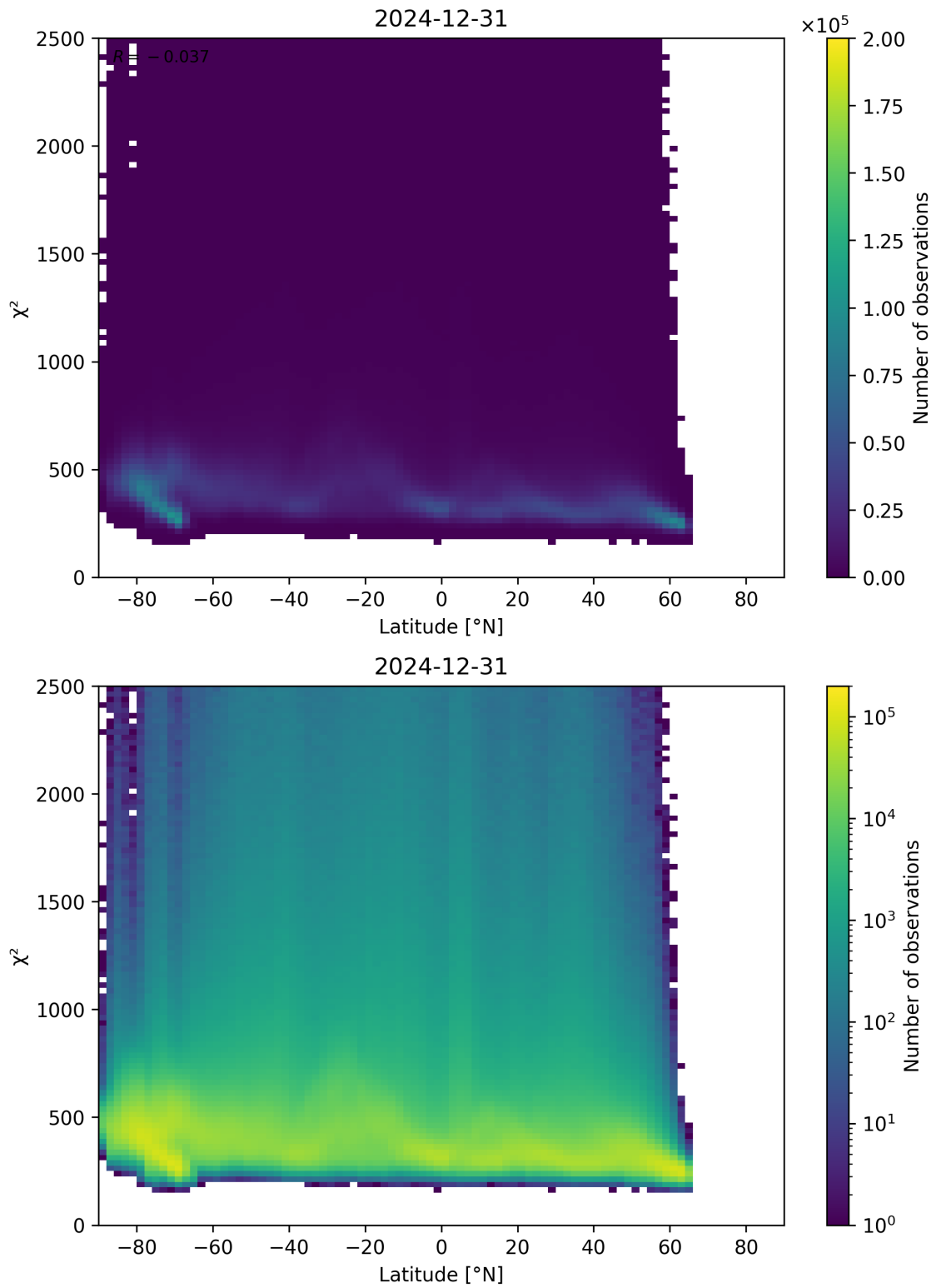
Figure 86: Scatter density plot of “Latitude” against “ \chi^2 ” for 2024-12-30 to 2025-01-01.
