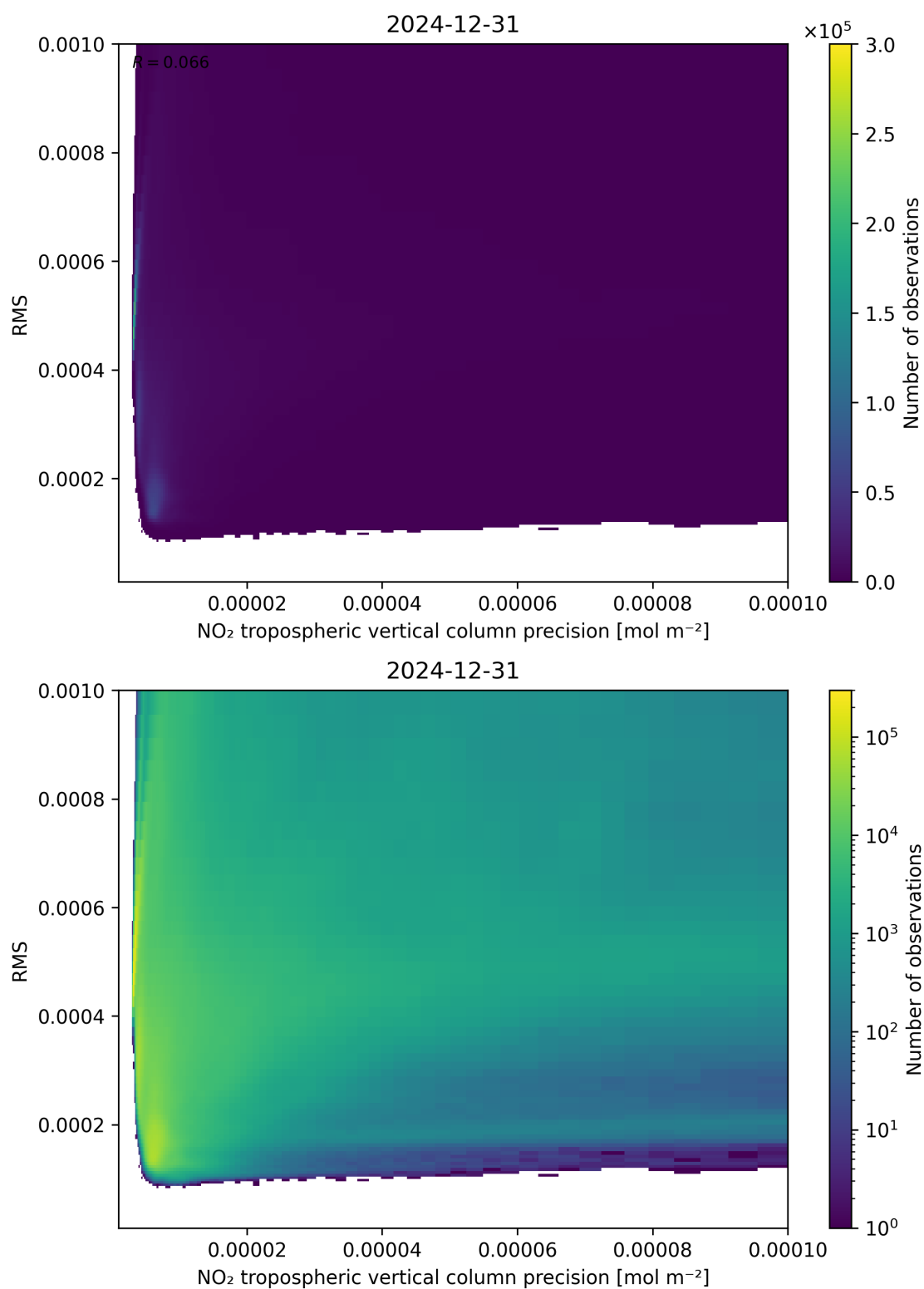
Figure 140: Scatter density plot of “NO 2 tropospheric vertical column precision” against “RMS” for 2024-12-30 to 2025-01-01.
