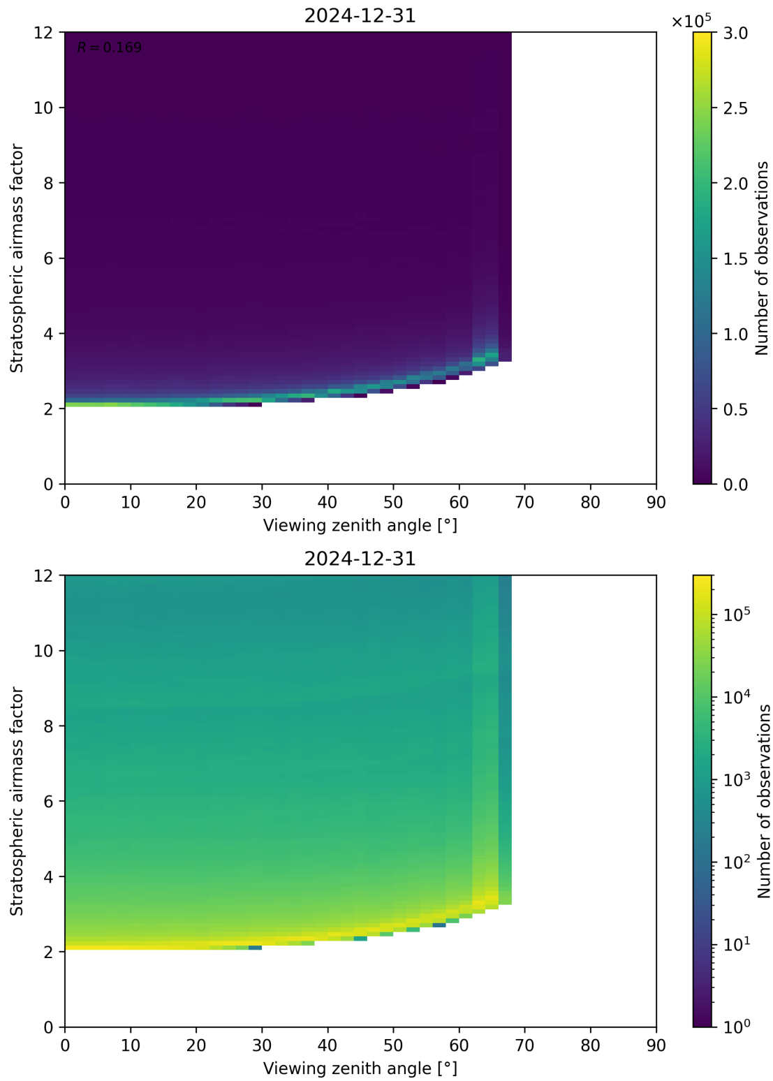
Figure 159: Scatter density plot of “Viewing zenith angle” against “Stratospheric airmass factor” for 2024-12-30 to 2025-01-01.
