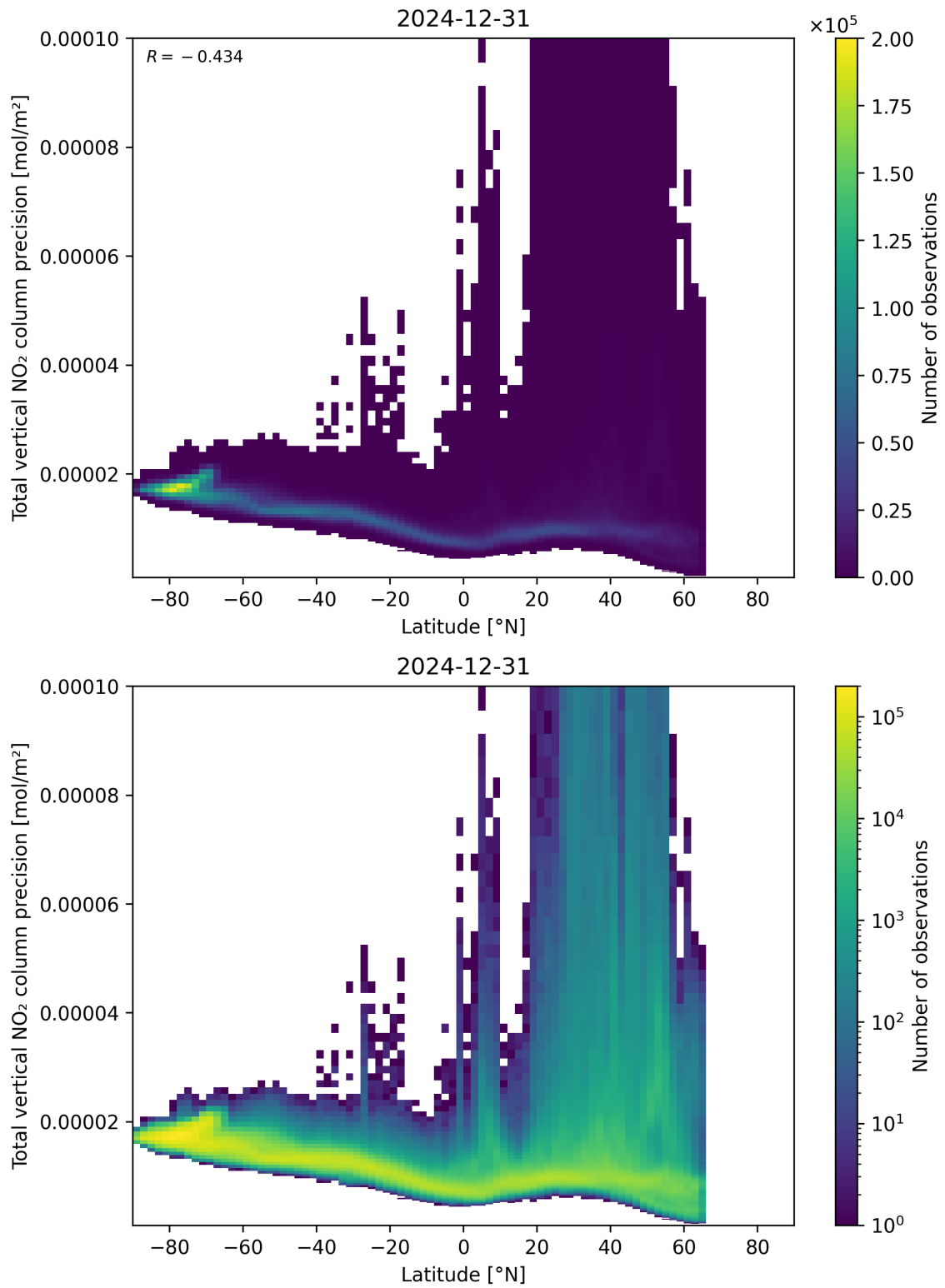
Figure 91: Scatter density plot of “Latitude” against “Total vertical NO 2 column precision” for 2024-12-30 to 2025-01-01.
