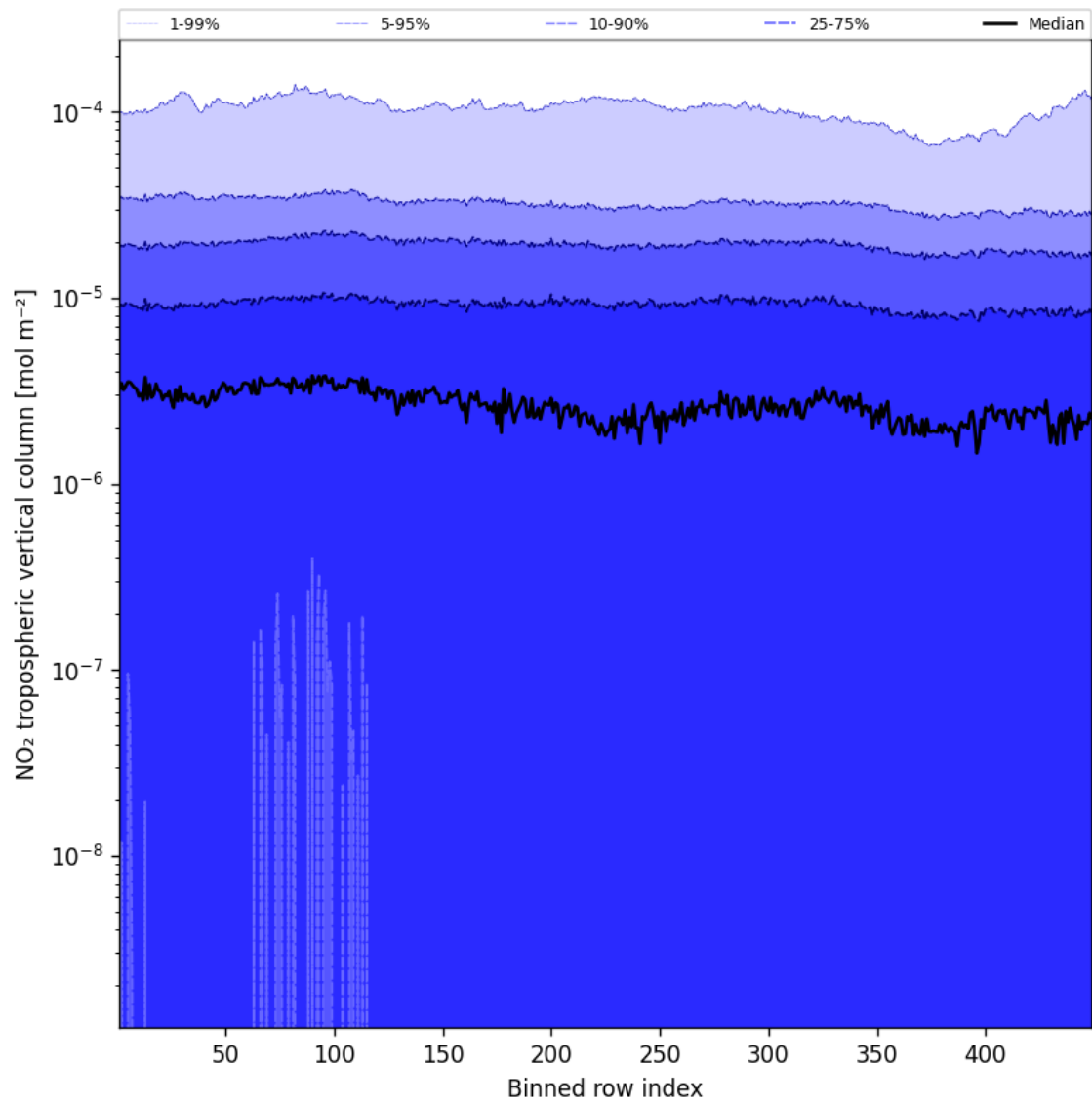
Figure 46: Along track statistics of “NO 2 tropospheric vertical column” for 2024-12-30 to 2025-01-01
