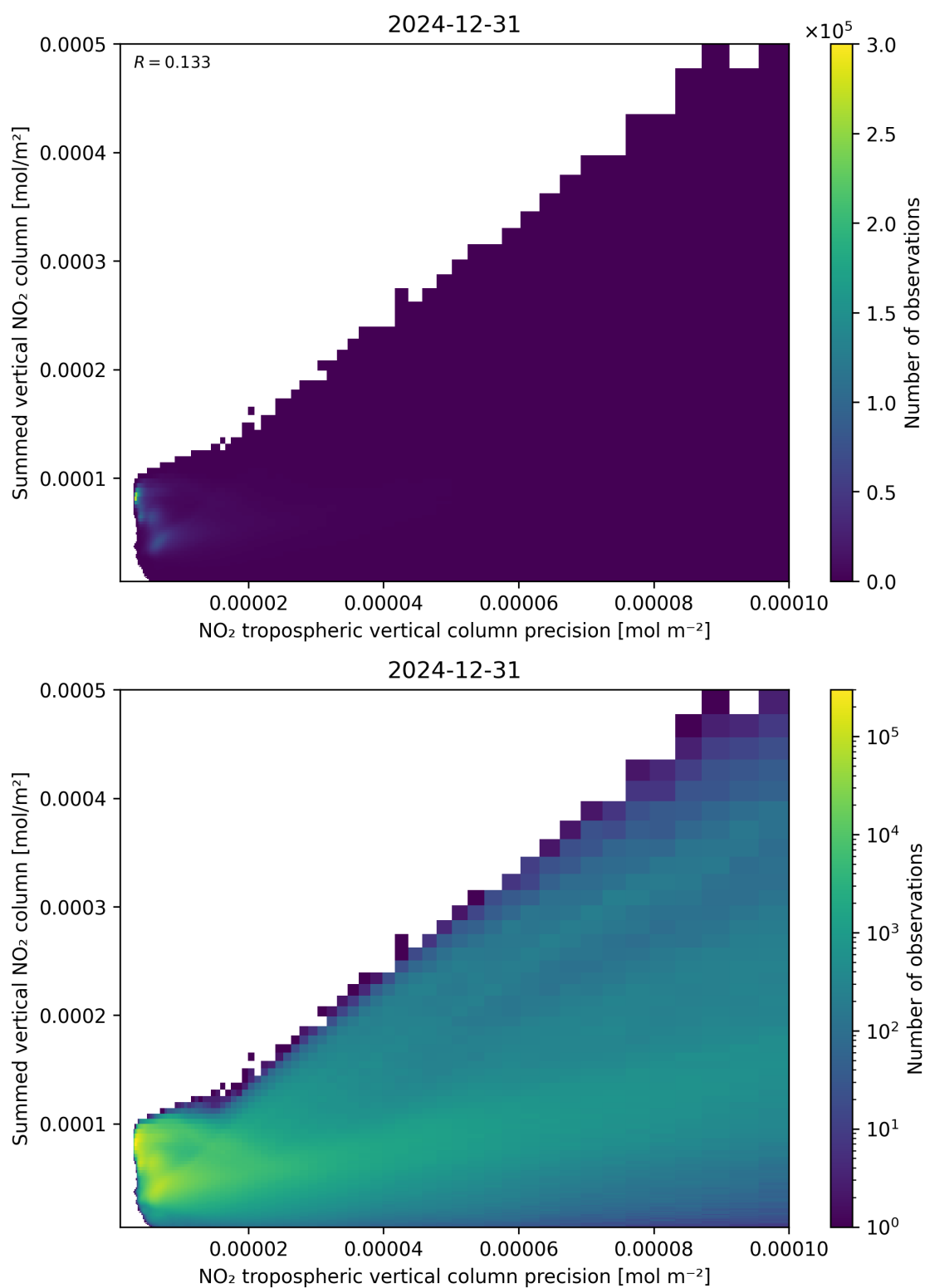
Figure 136: Scatter density plot of “NO 2 tropospheric vertical column precision” against “Summed vertical NO 2 column” for 2024-12-30 to 2025-01-01.
