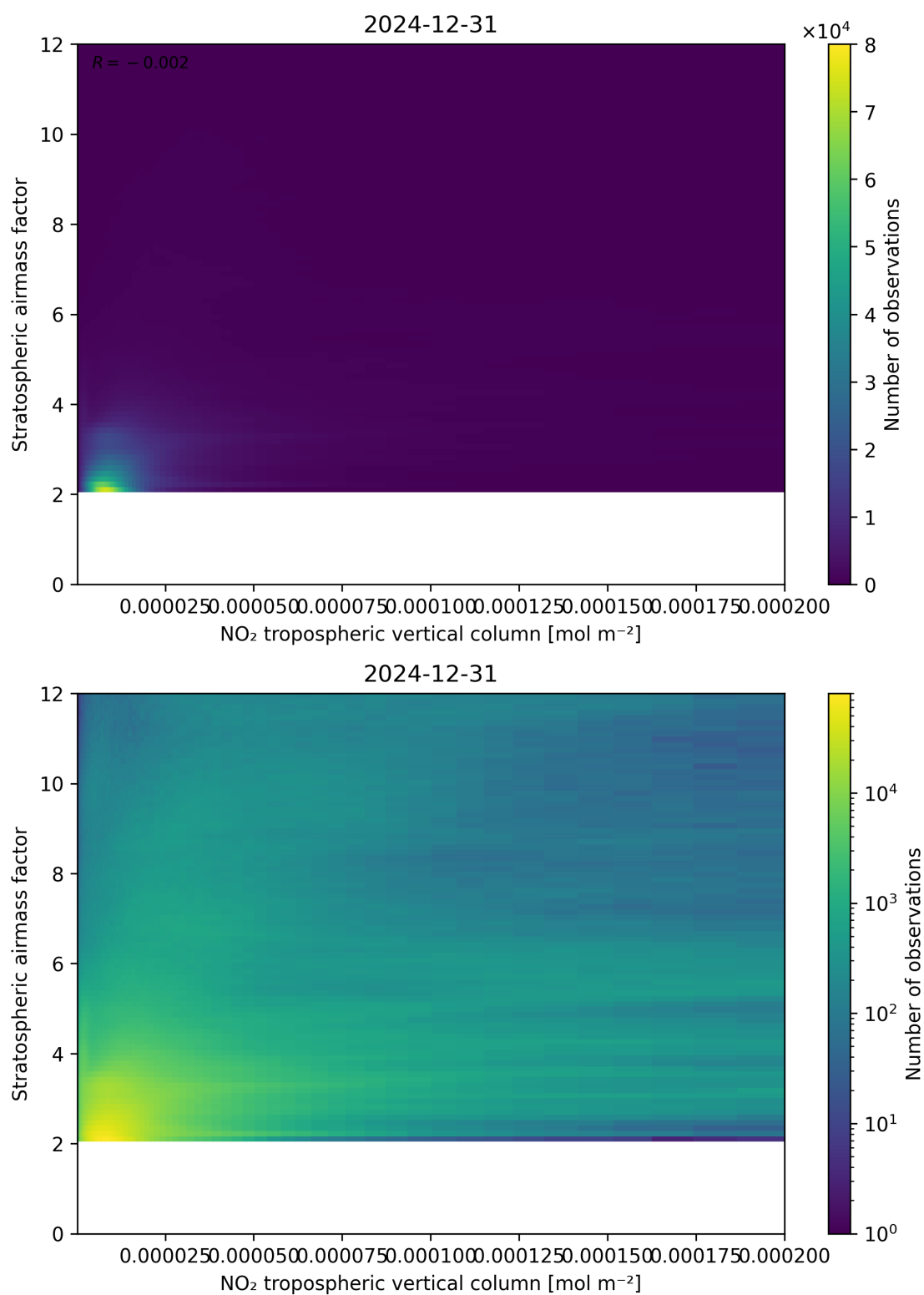
Figure 121: Scatter density plot of “NO 2 tropospheric vertical column” against “Stratospheric air mass factor” for 2024-12-30 to 2025-01-01.
