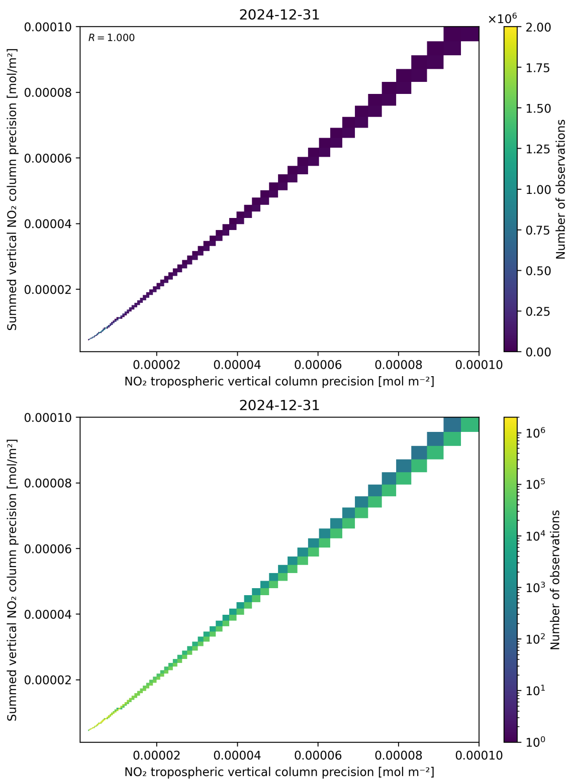
Figure 137: Scatter density plot of “NO 2 tropospheric vertical column precision” against “Summed vertical NO 2 column precision” for 2024-12-30 to 2025-01-01.
