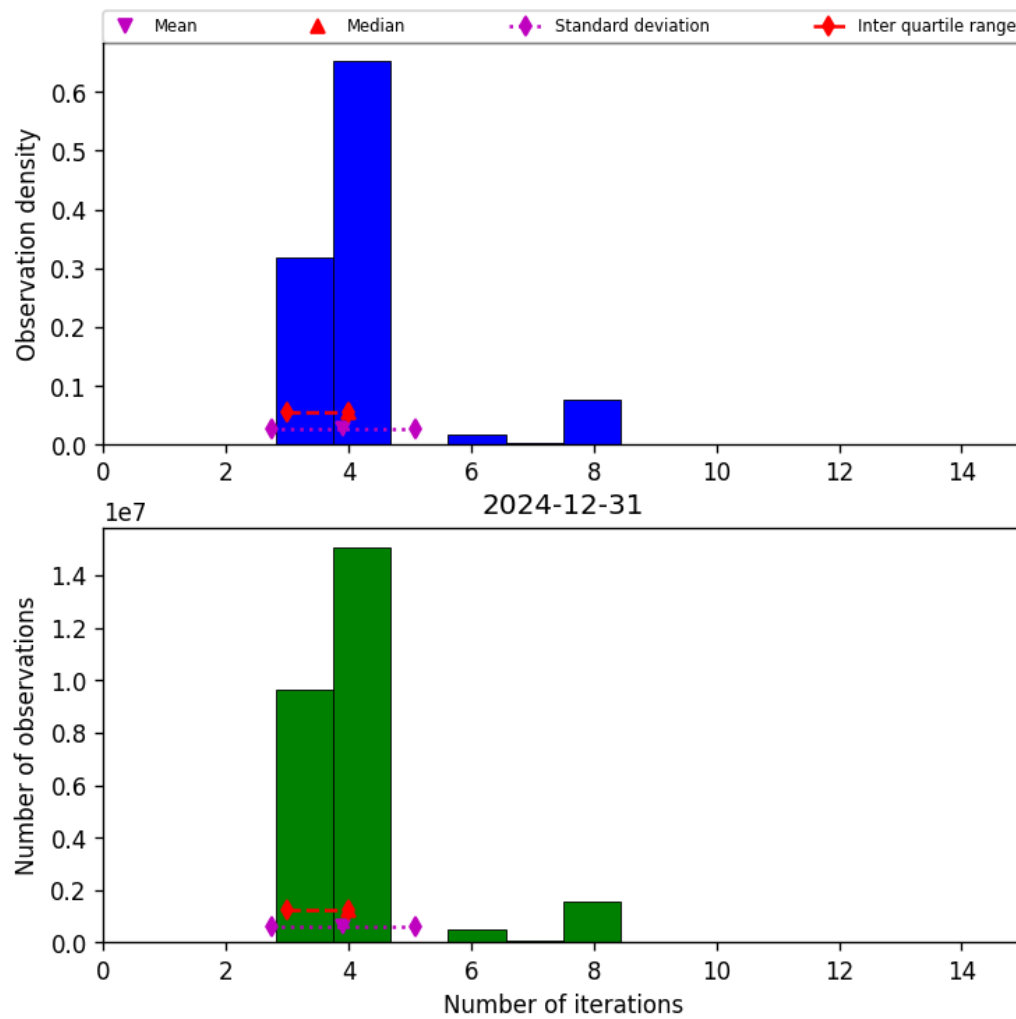
Figure 34: Histogram of “Number of iterations” for 2024-12-30 to 2025-01-01
