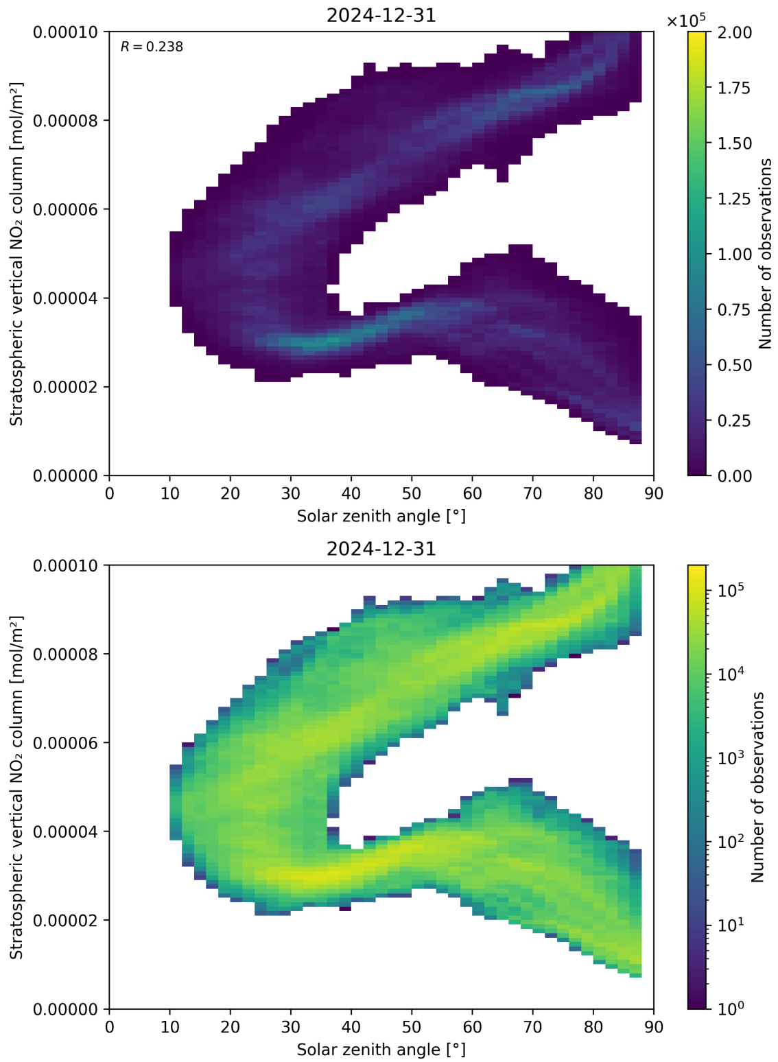
Figure 150: Scatter density plot of “Solar zenith angle” against “Stratospheric vertical NO 2 column” for 2024-12-30 to 2025-01-01.
