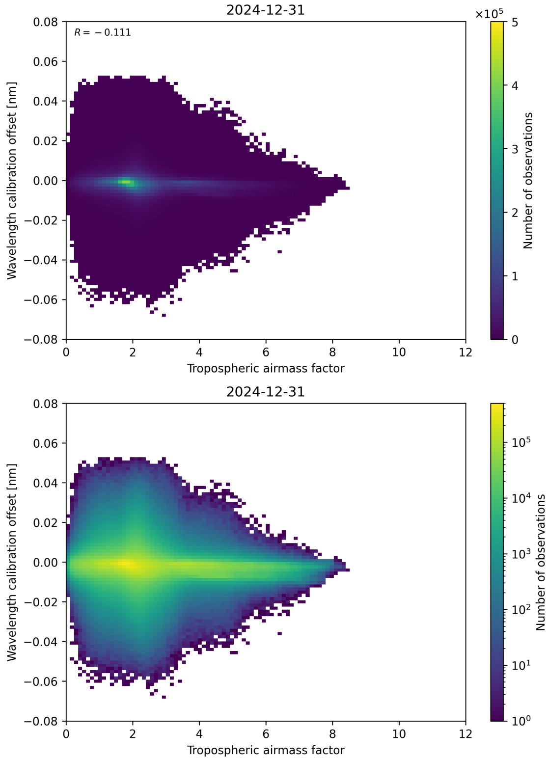
Figure 80: Scatter density plot of “Tropospheric airmass factor” against “Wavelength calibration offset” for 2024-12-30 to 2025-01-01.
