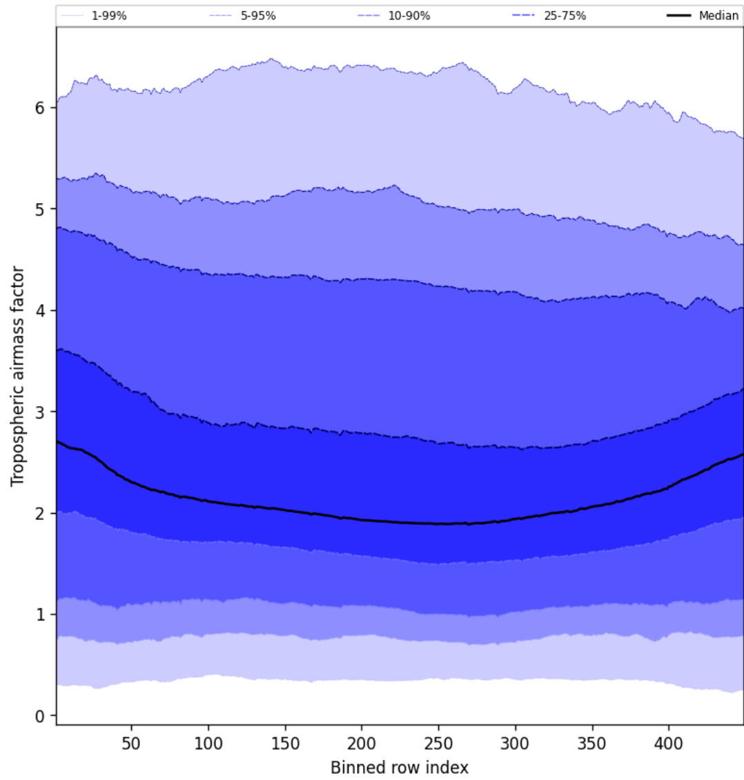
Figure 48: Along track statistics of “Tropospheric air mass factor” for 2024-12-30 to 2025-01-01
