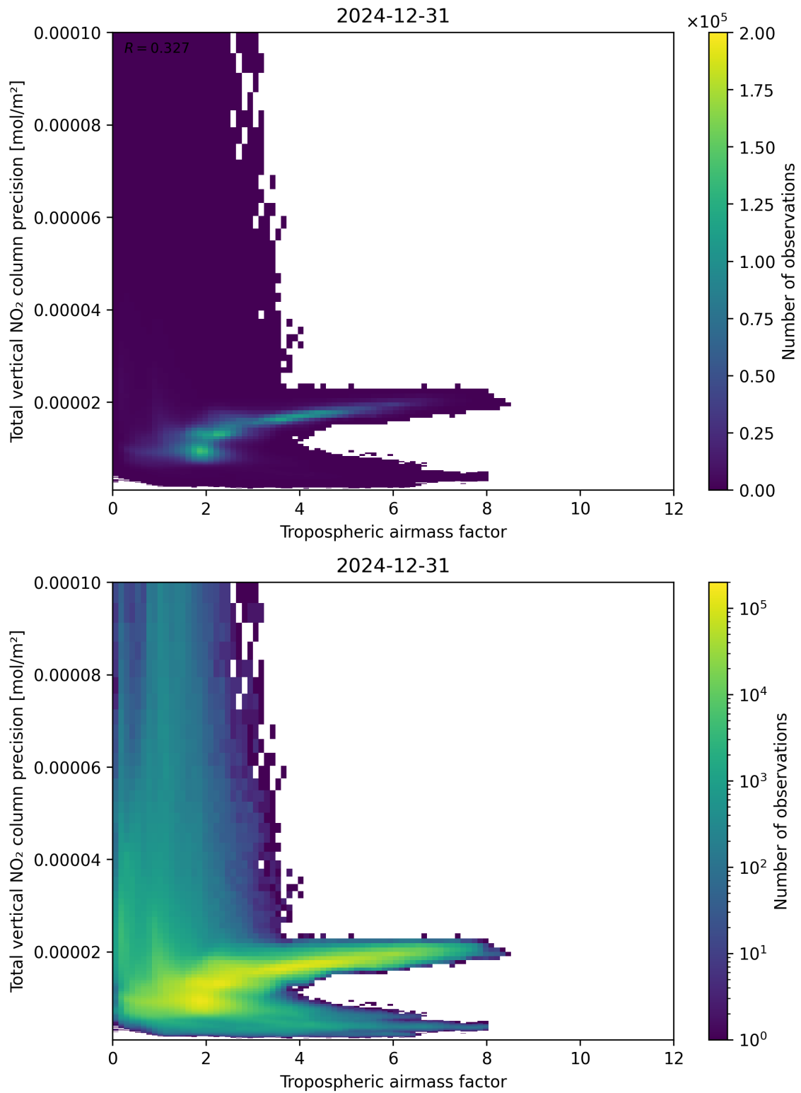
Figure 78: Scatter density plot of “Tropospheric air mass factor” against “Total vertical NO 2 column precision” for 2024-12-30 to 2025-01-01.
