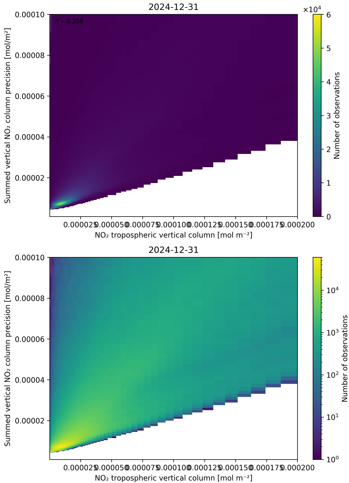
Figure 127: Scatter density plot of “NO 2 tropospheric vertical column” against “Summed vertical NO 2 column precision” for 2024-12-30 to 2025-01-01.
