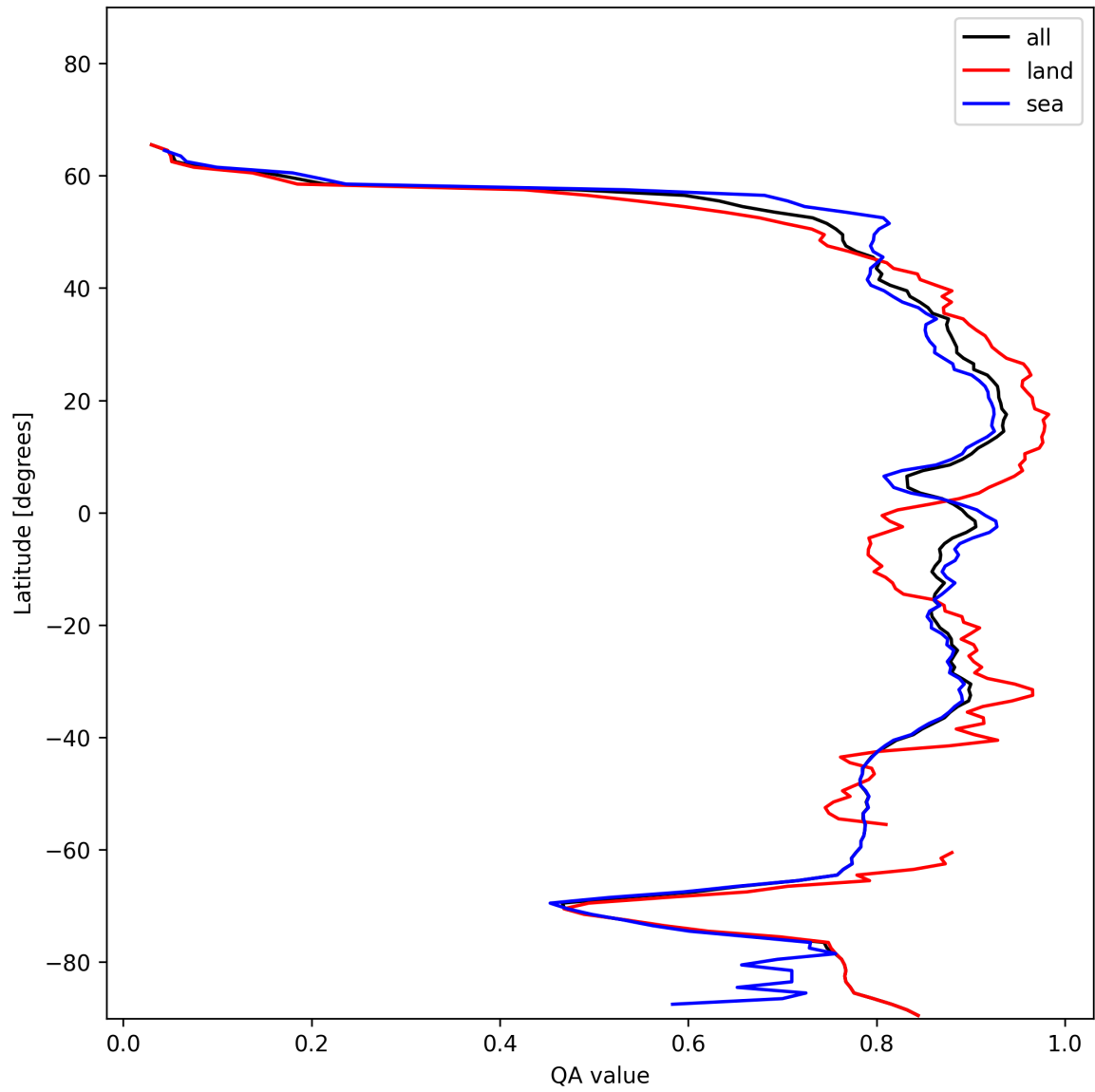
Figure 11: Zonal average of “QA value” for 2024-12-30 to 2025-01-01.
