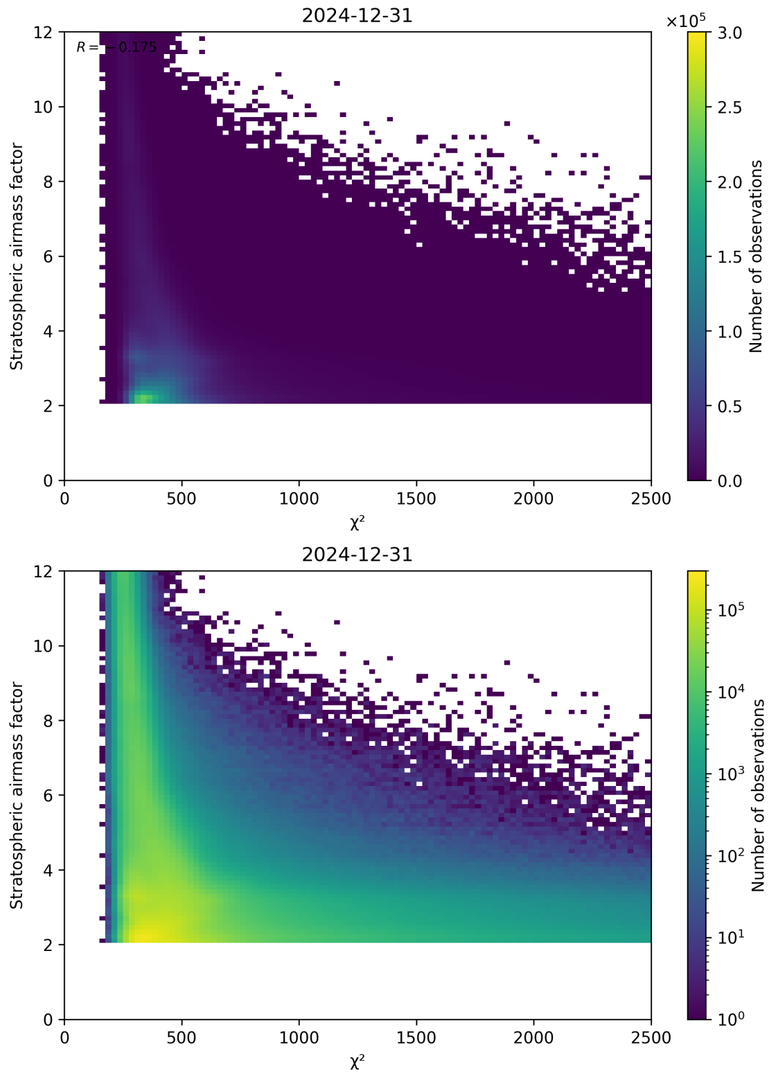
Figure 81: Scatter density plot of “ \chi^2 ” against “Stratospheric airmass factor” for 2024-12-30 to 2025-01-01.
