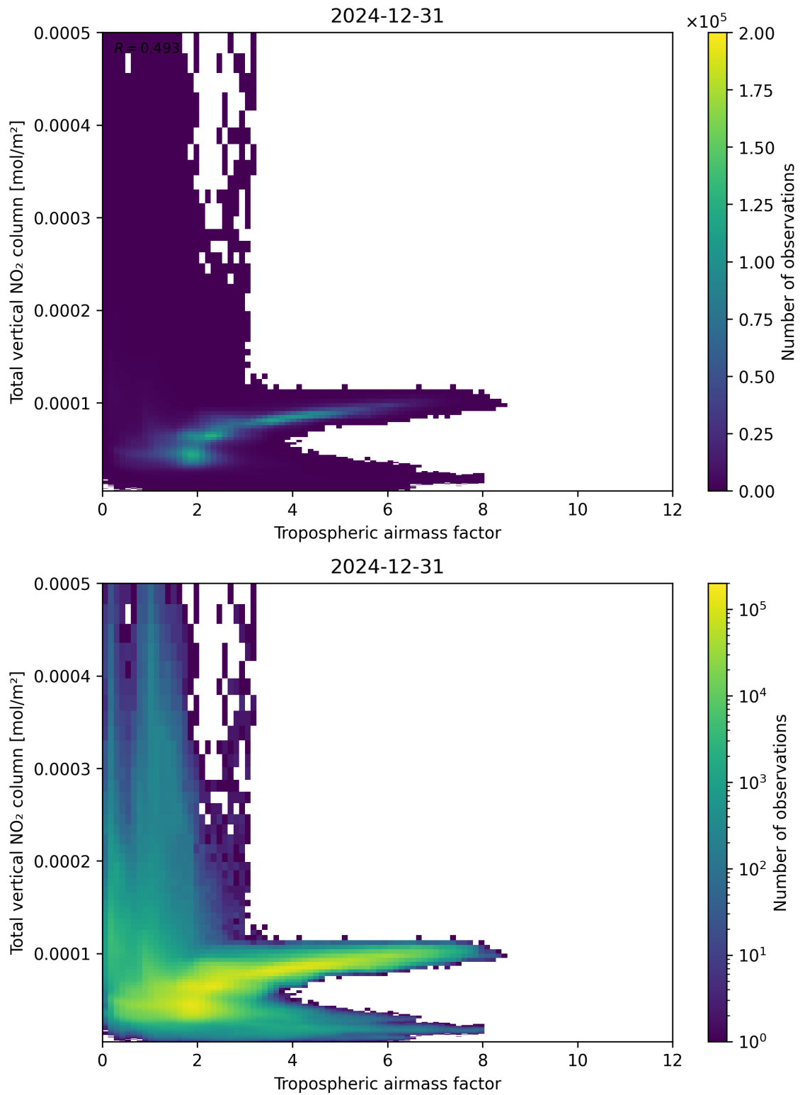
Figure 77: Scatter density plot of “Tropospheric airmass factor” against “Total vertical NO 2 column” for 2024-12-30 to 2025-01-01.
