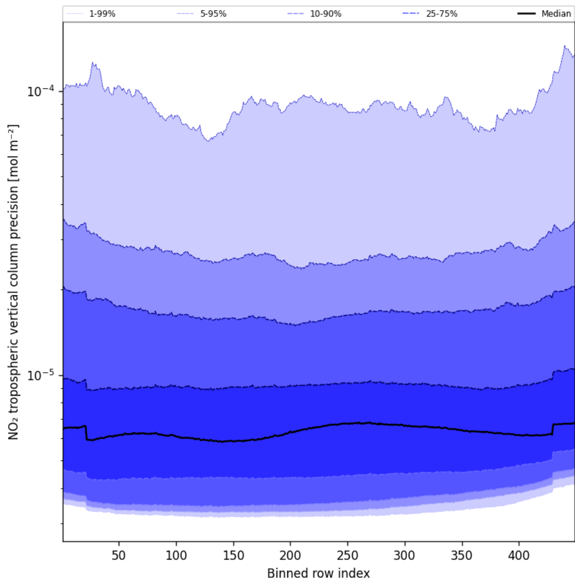
Figure 47: Along track statistics of “NO 2 tropospheric vertical column precision” for 2024-12-30 to 2025-01-01
