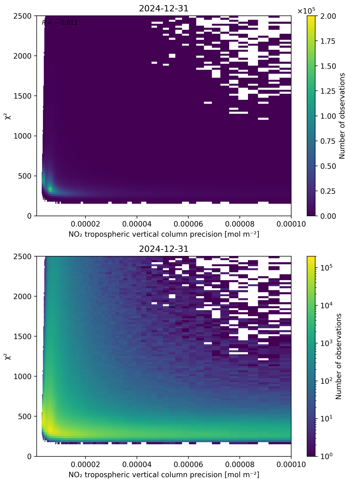
Figure 134: Scatter density plot of “NO 2 tropospheric vertical column precision” against “ \chi^2 ” for 2024-12-30 to 2025-01-01.
