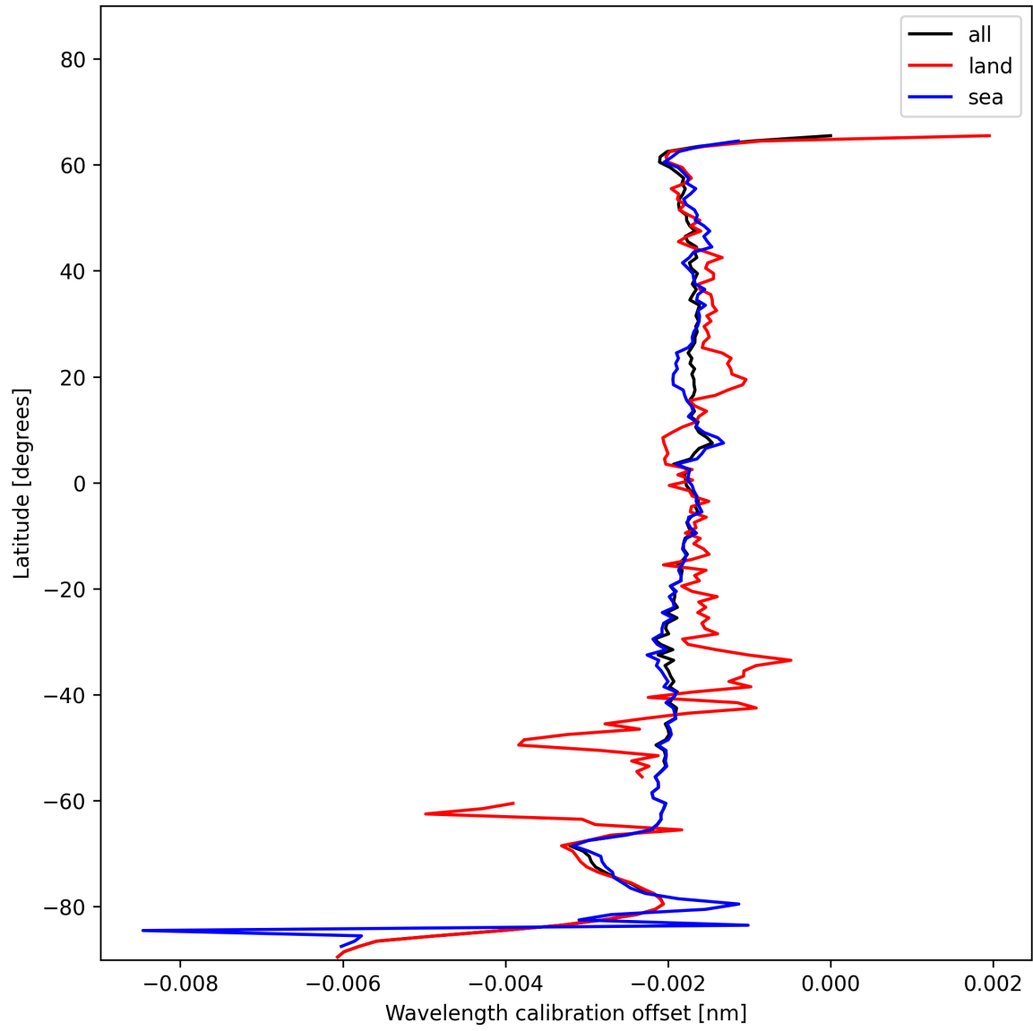
Figure 18: Zonal average of “Wavelength calibration offset” for 2024-12-30 to 2025-01-01.
