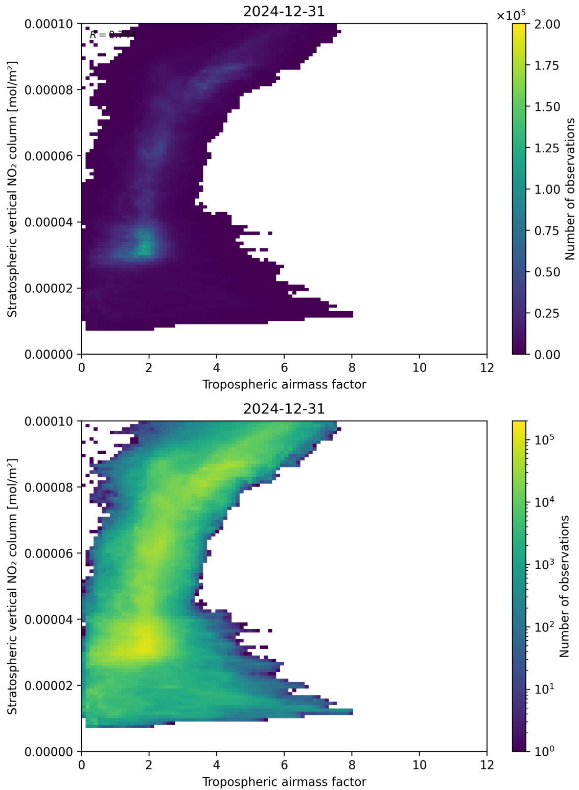
Figure 74: Scatter density plot of “Tropospheric air mass factor” against “Stratospheric vertical NO 2 column” for 2024-12-30 to 2025-01-01.
