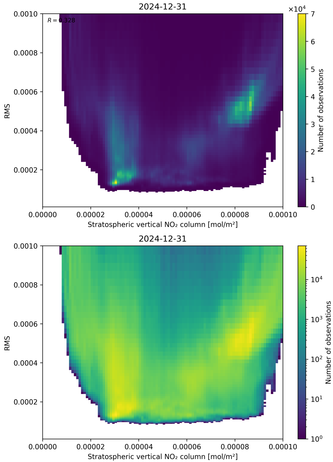
Figure 102: Scatter density plot of “Stratospheric vertical NO 2 column” against “RMS” for 2024-12-30 to 2025-01-01.
