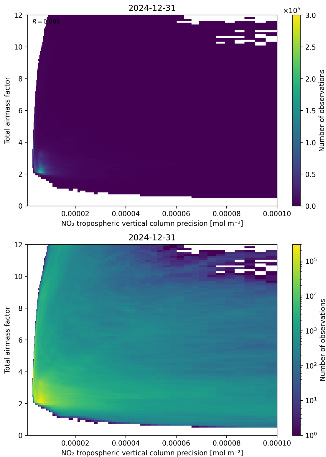
Figure 132: Scatter density plot of “NO 2 tropospheric vertical column precision” against “Total airmass factor” for 2024-12-30 to 2025-01-01.
