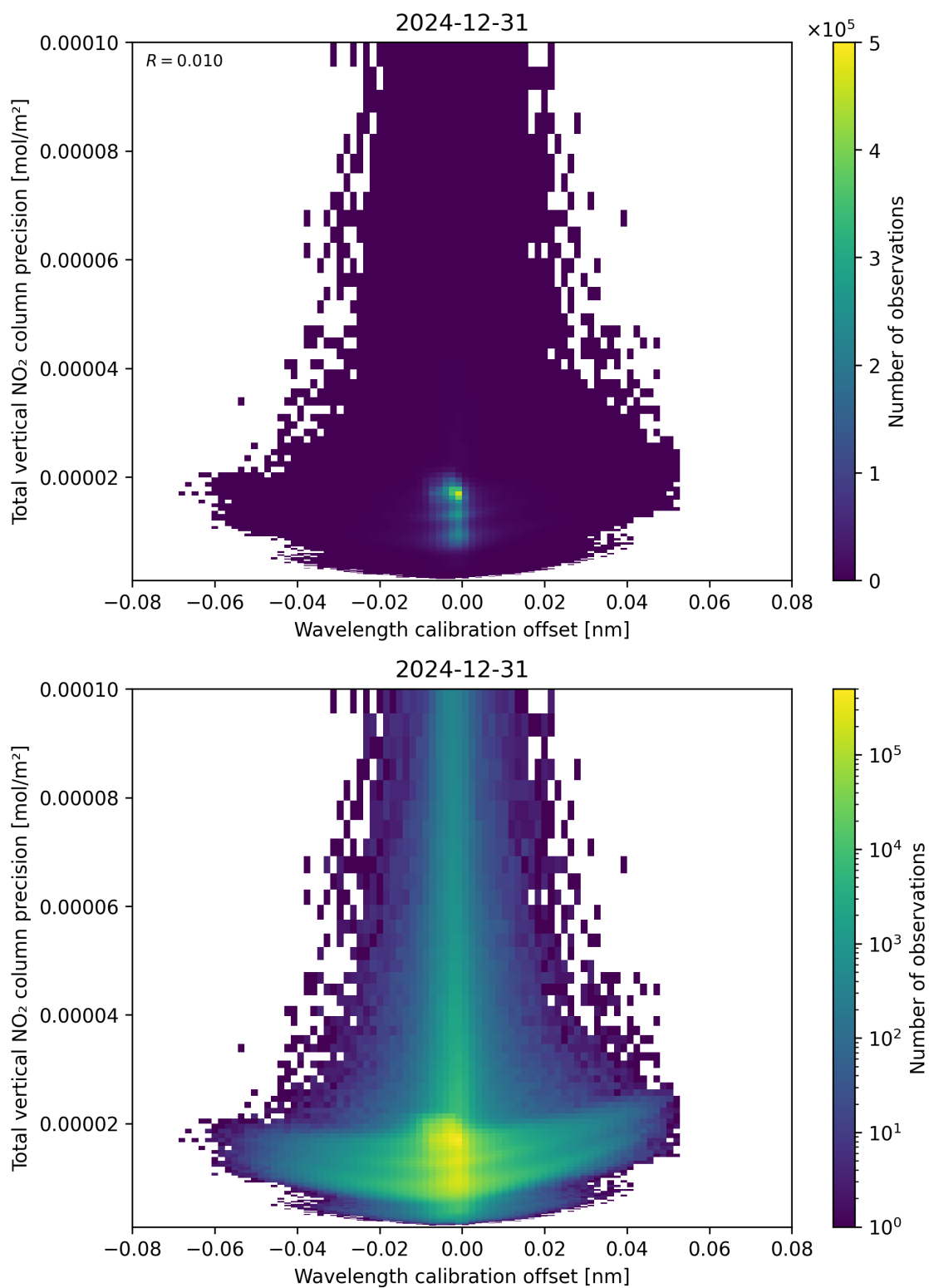
Figure 180: Scatter density plot of “Wavelength calibration offset” against “Total vertical NO 2 column precision” for 2024-12-30 to 2025-01-01.
