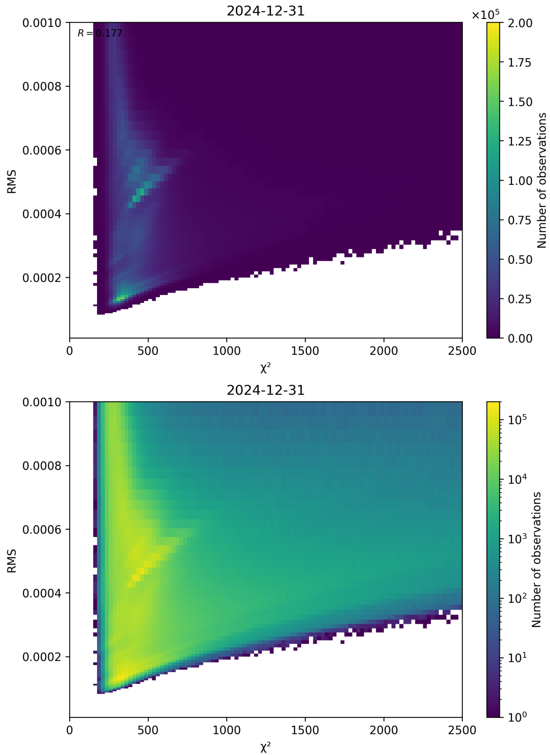
Figure 82: Scatter density plot of “ \chi^2 ” against “RMS” for 2024-12-30 to 2025-01-01.
