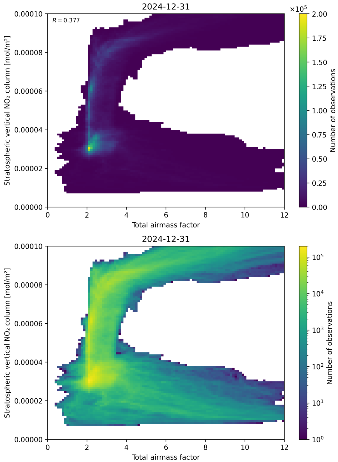
Figure 64: Scatter density plot of “Total airmass factor” against “Stratospheric vertical NO 2 column” for 2024-12-30 to 2025-01-01.
