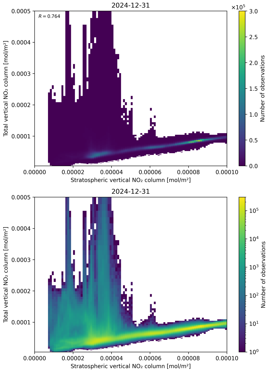
Figure 100: Scatter density plot of “Stratospheric vertical NO 2 column” against “Total vertical NO 2 column” for 2024-12-30 to 2025-01-01.
