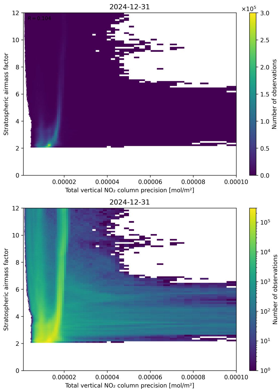
Figure 115: Scatter density plot of “Total vertical NO 2 column precision” against “Stratospheric air mass factor” for 2024-12-30 to 2025-01-01.
