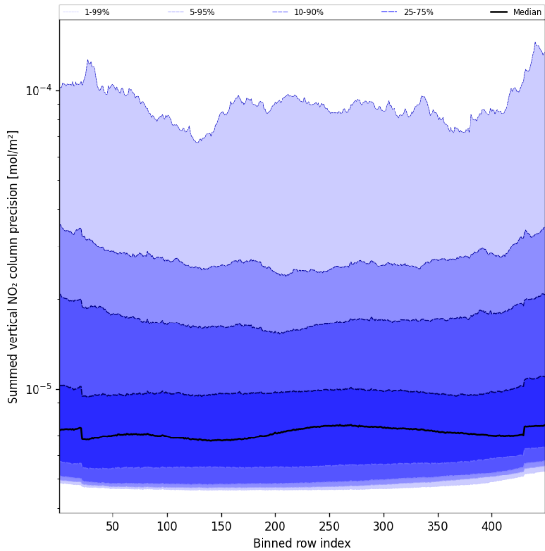
Figure 58: Along track statistics of “Summed vertical NO 2 column precision” for 2024-12-30 to 2025-01-01
