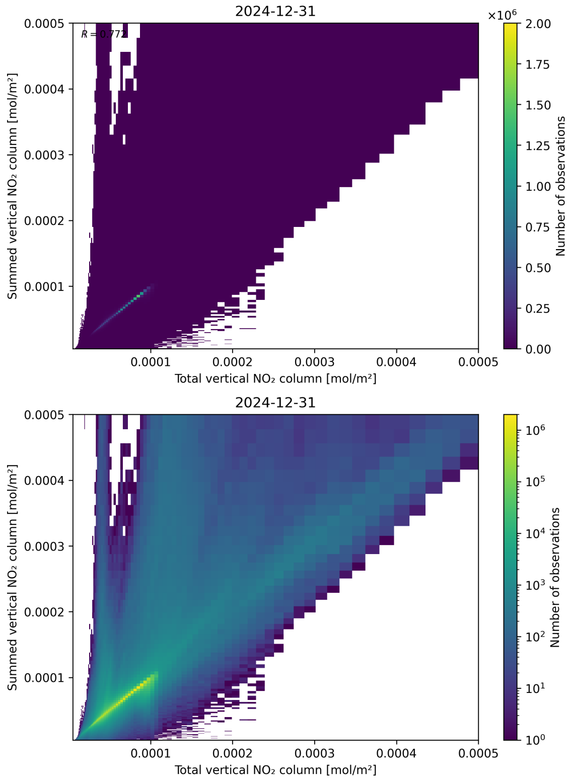
Figure 112: Scatter density plot of “Total vertical NO 2 column” against “Summed vertical NO 2 column” for 2024-12-30 to 2025-01-01.
