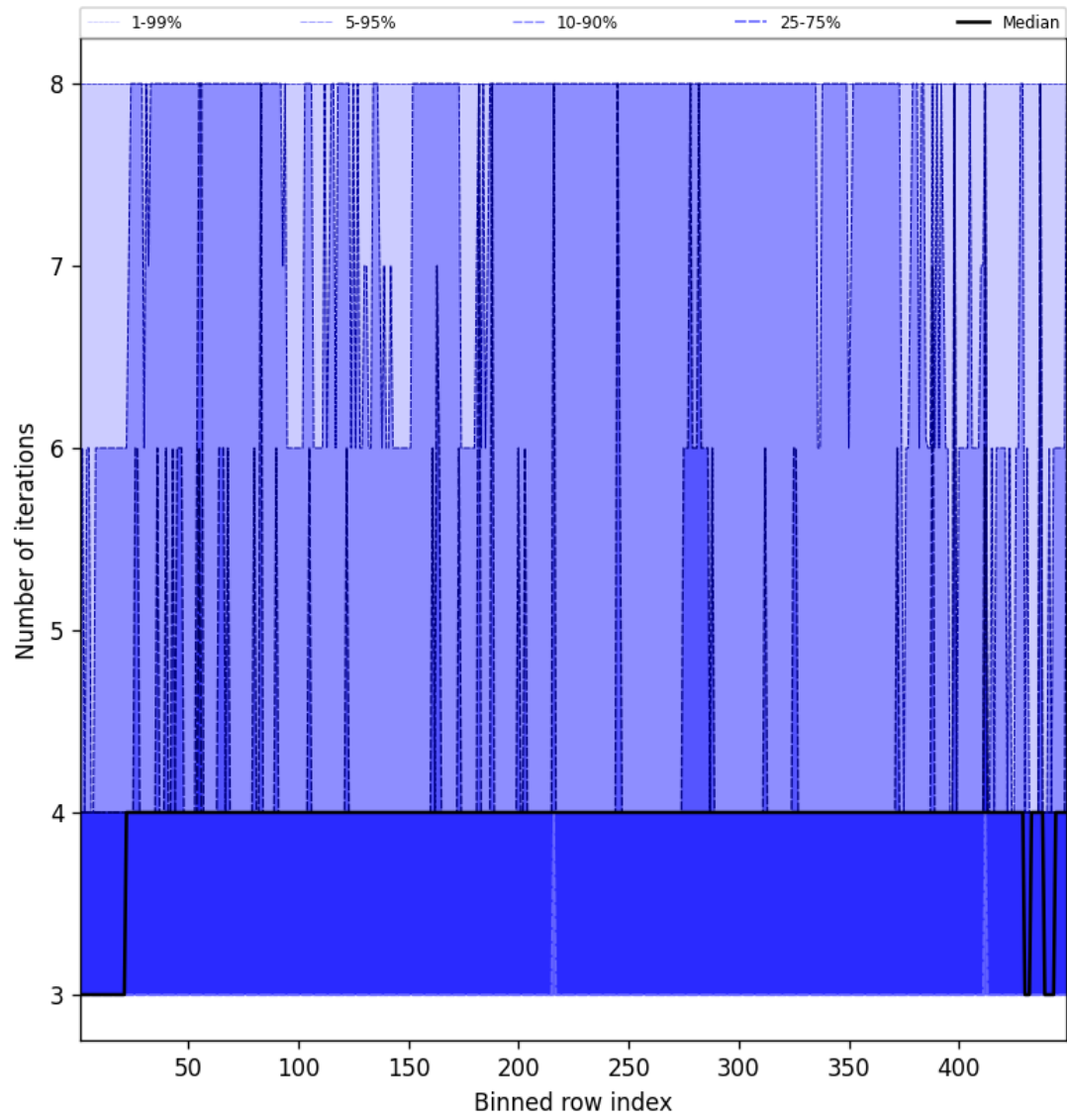
Figure 51: Along track statistics of “Number of iterations” for 2024-12-30 to 2025-01-01
