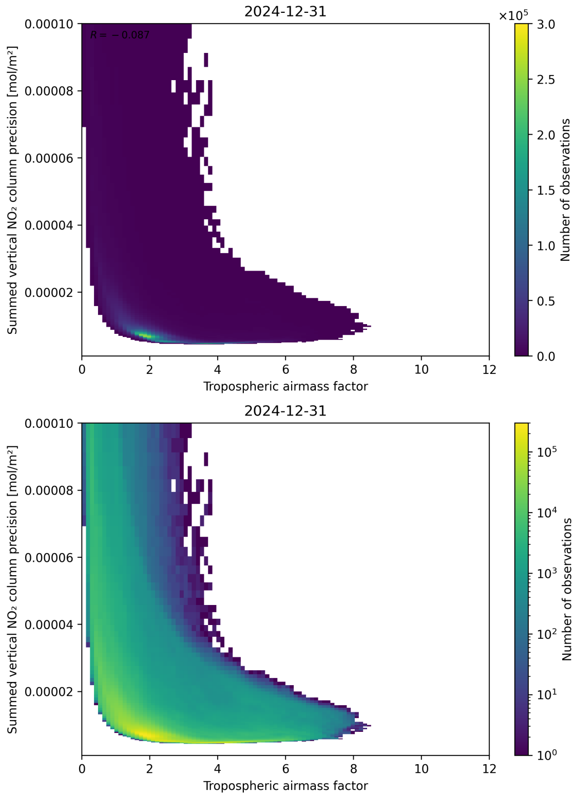
Figure 76: Scatter density plot of “Tropospheric air mass factor” against “Summed vertical NO 2 column precision” for 2024-12-30 to 2025-01-01.
