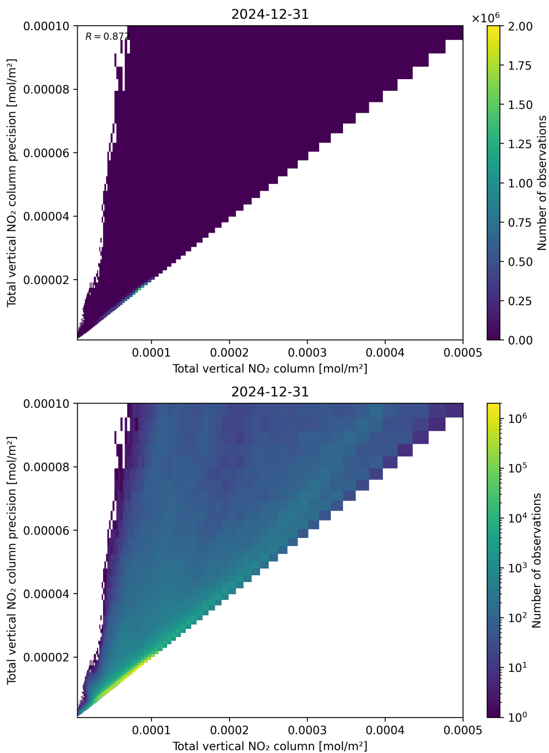
Figure 114: Scatter density plot of “Total vertical NO 2 column” against “Total vertical NO 2 column precision” for 2024-12-30 to 2025-01-01.
