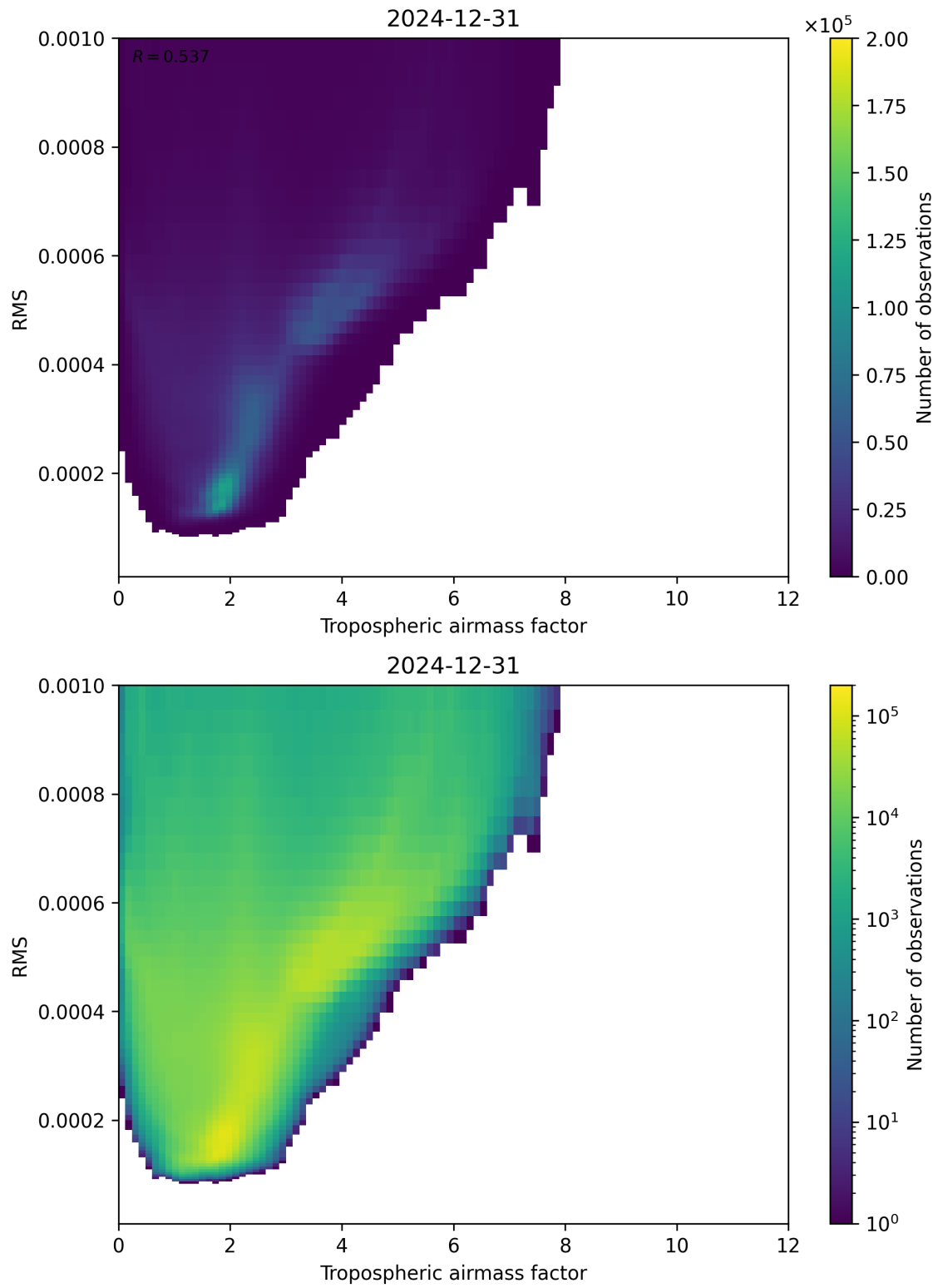
Figure 79: Scatter density plot of “Tropospheric airmass factor” against “RMS” for 2024-12-30 to 2025-01-01.
