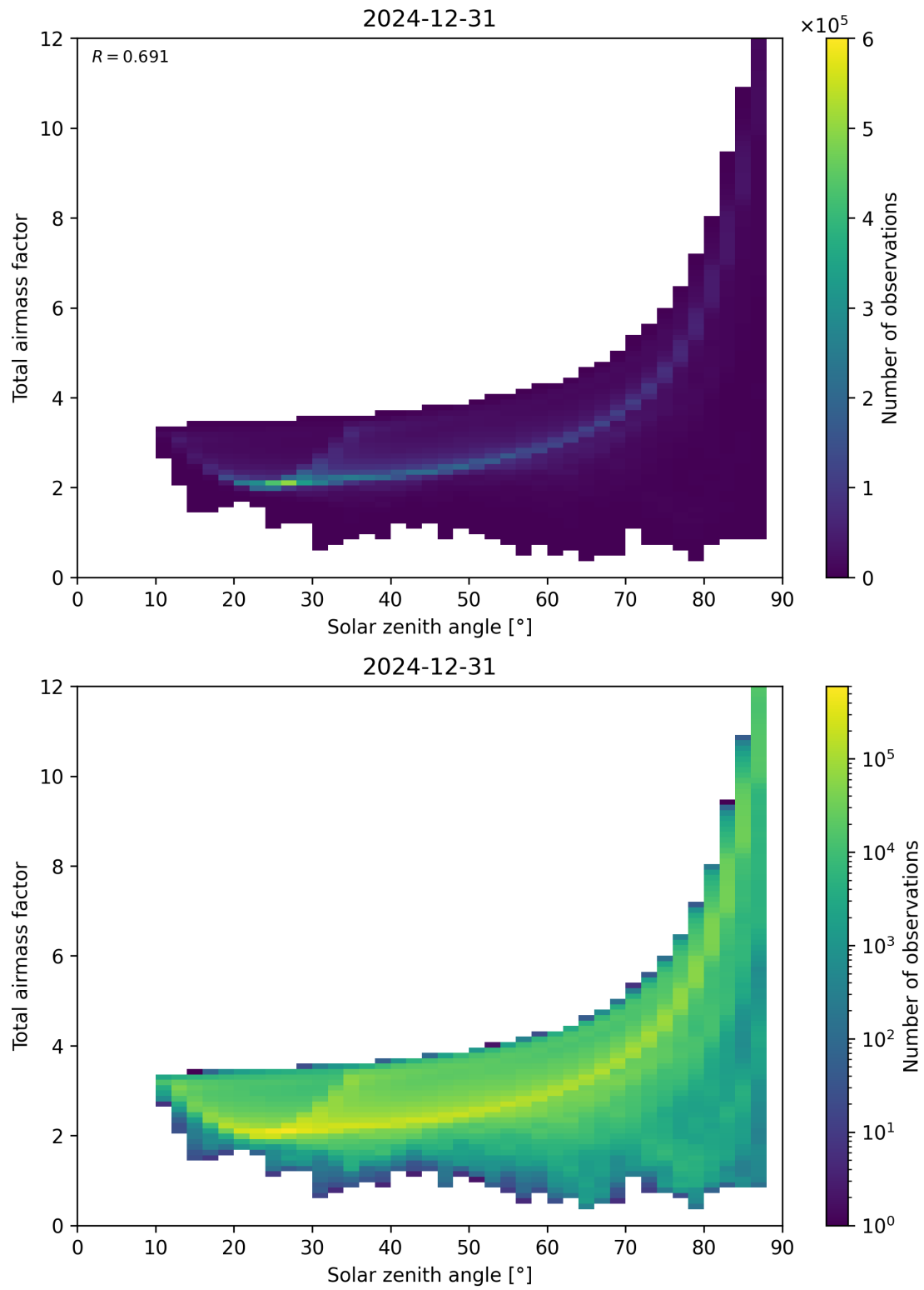
Figure 146: Scatter density plot of “Solar zenith angle” against “Total airmass factor” for 2024-12-30 to 2025-01-01.
