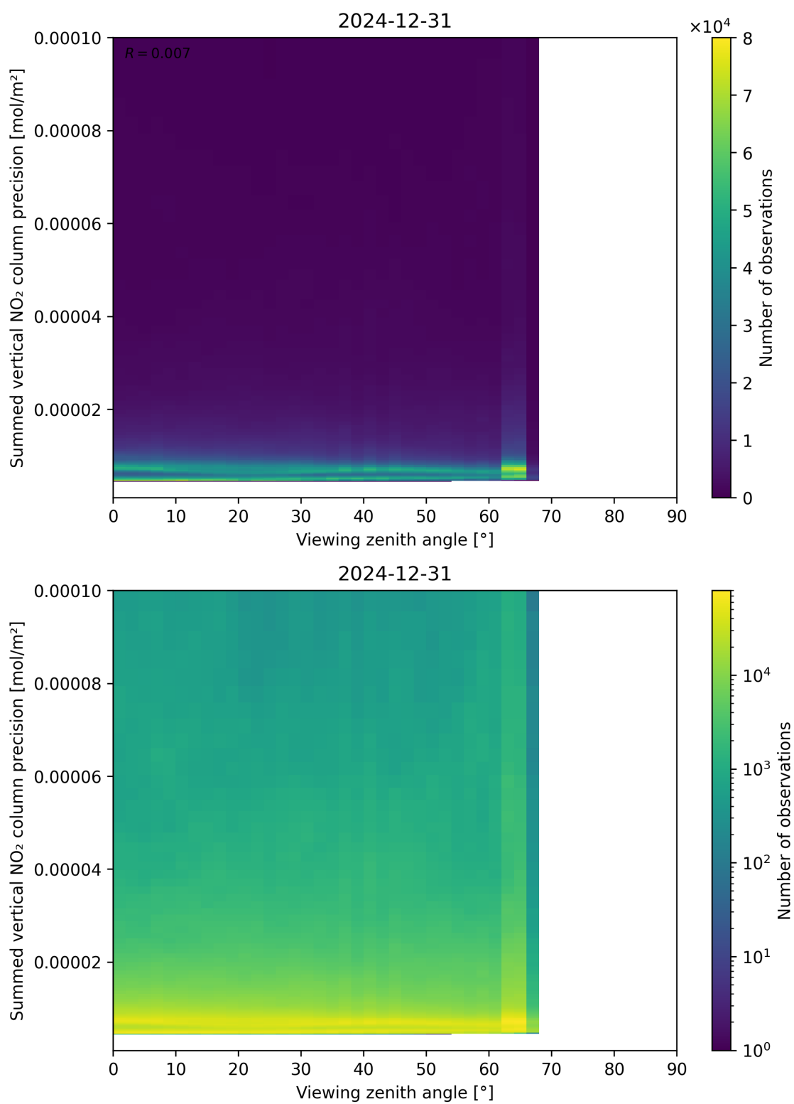
Figure 166: Scatter density plot of “Viewing zenith angle” against “Summed vertical NO 2 column precision” for 2024-12-30 to 2025-01-01.
