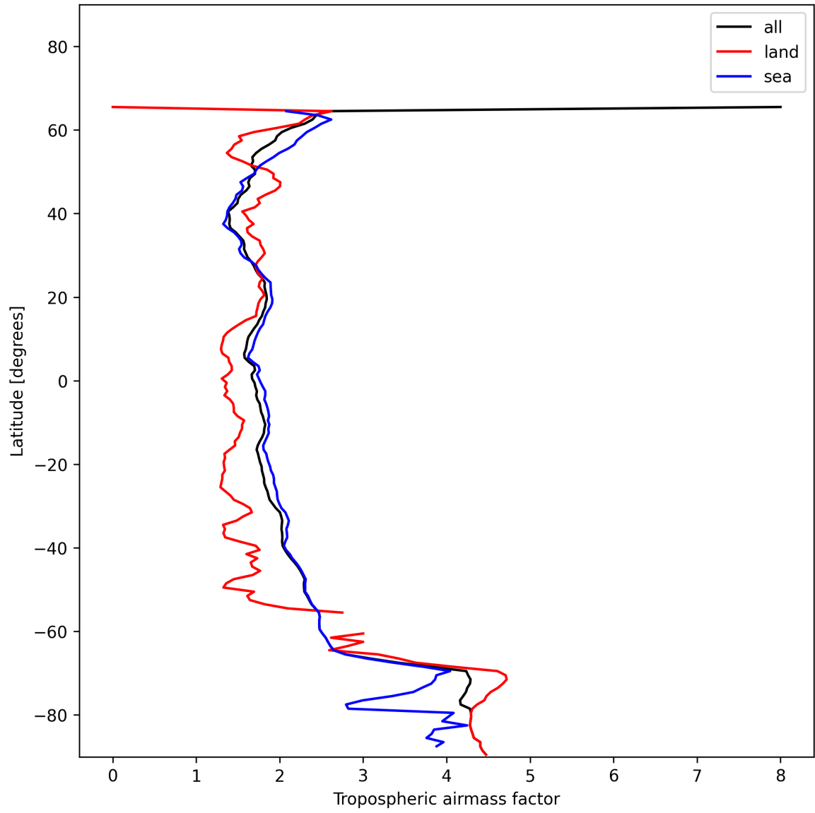
Figure 14: Zonal average of “Tropospheric airmass factor” for 2024-12-30 to 2025-01-01.
