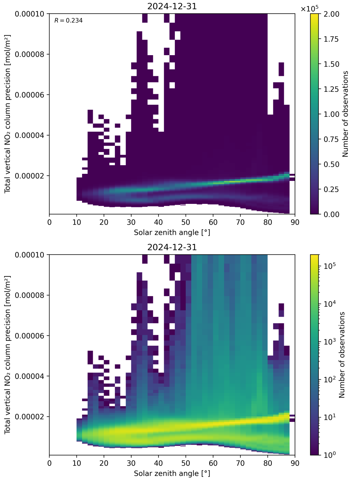
Figure 154: Scatter density plot of “Solar zenith angle” against “Total vertical NO 2 column precision” for 2024-12-30 to 2025-01-01.
