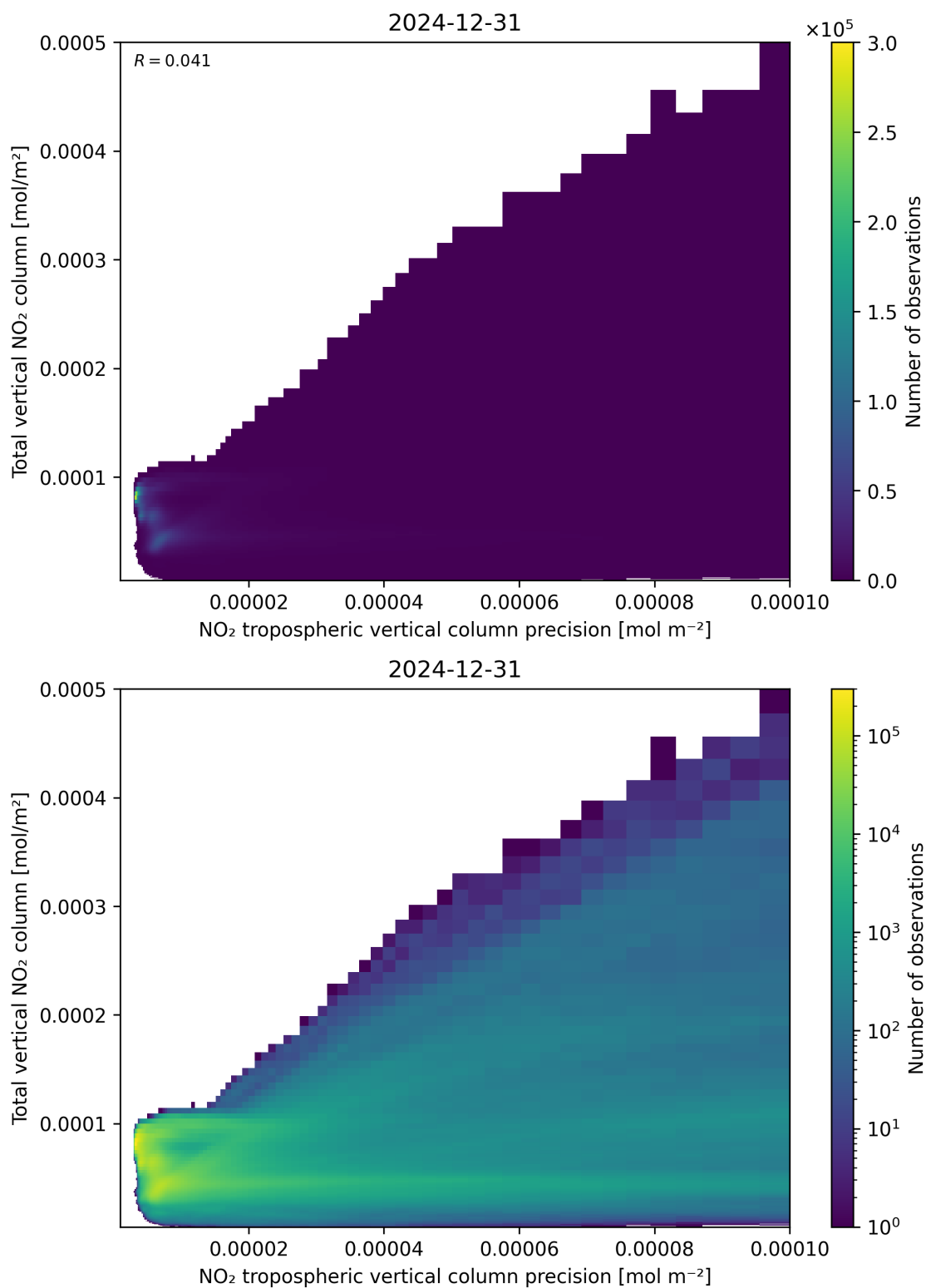
Figure 138: Scatter density plot of “NO 2 tropospheric vertical column precision” against “Total vertical NO 2 column” for 2024-12-30 to 2025-01-01.
