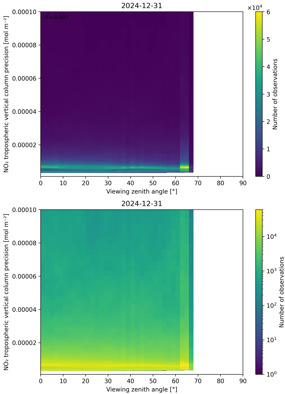
Figure 170: Scatter density plot of “Viewing zenith angle” against “NO 2 tropospheric vertical column precision” for 2024-12-30 to 2025-01-01.
