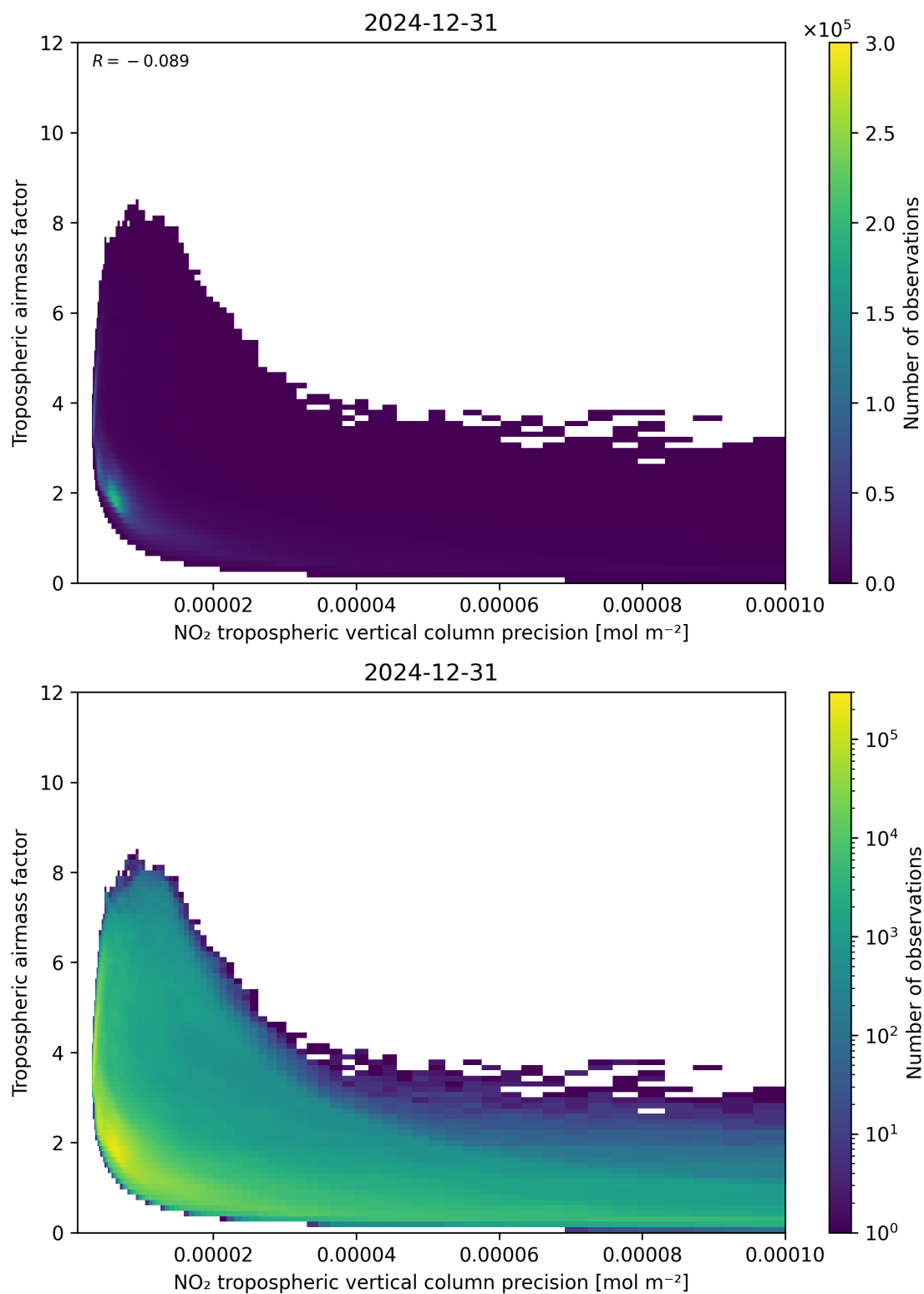
Figure 133: Scatter density plot of “NO 2 tropospheric vertical column precision” against “Tropospheric air mass factor” for 2024-12-30 to 2025-01-01.
