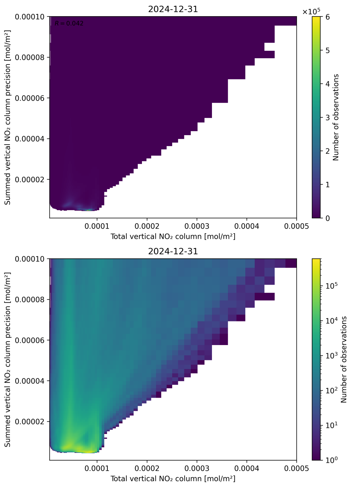
Figure 113: Scatter density plot of “Total vertical NO 2 column” against “Summed vertical NO 2 column precision” for 2024-12-30 to 2025-01-01.
