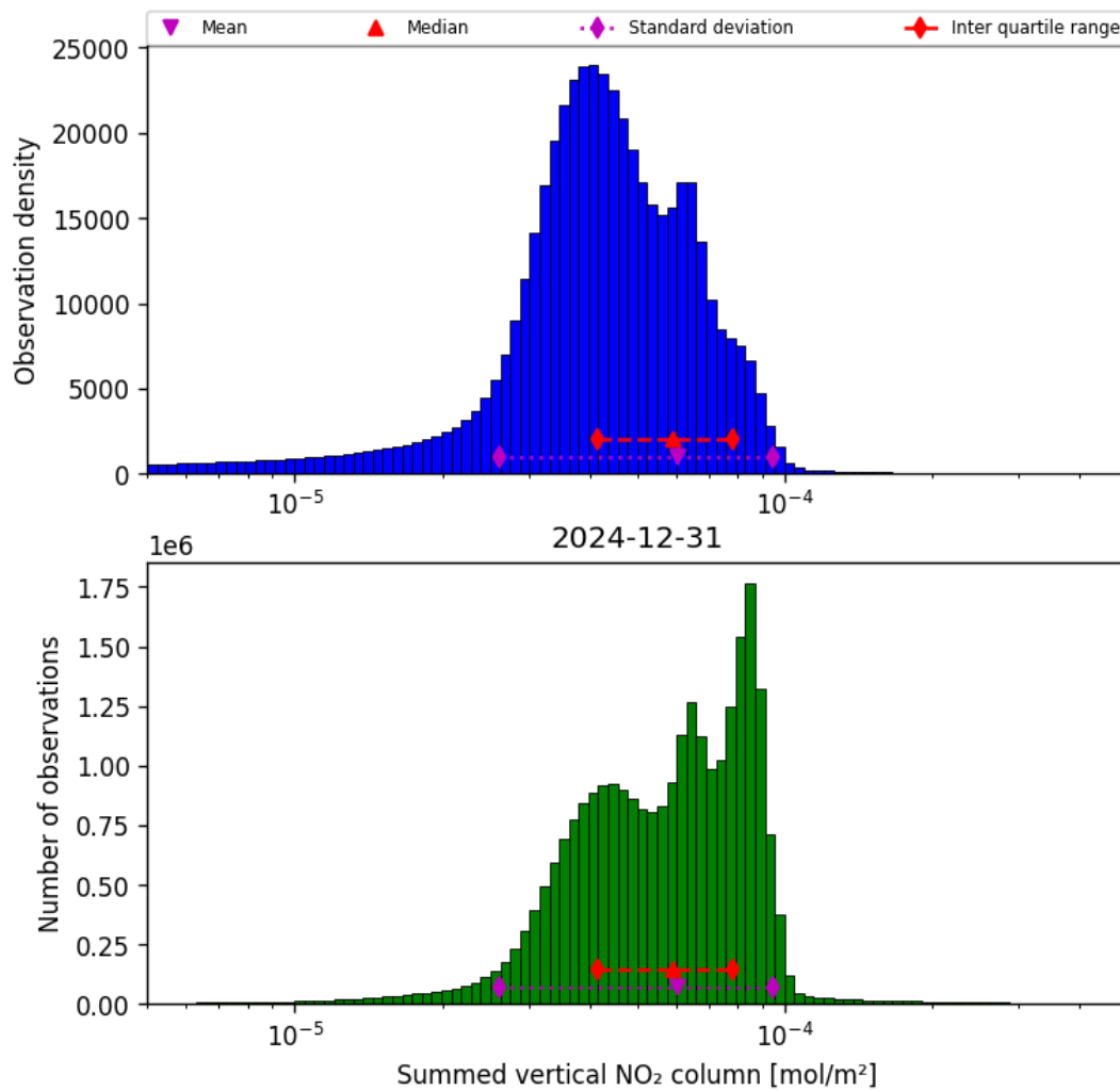
Figure 40: Histogram of “Summed vertical NO 2 column” for 2024-12-30 to 2025-01-01
