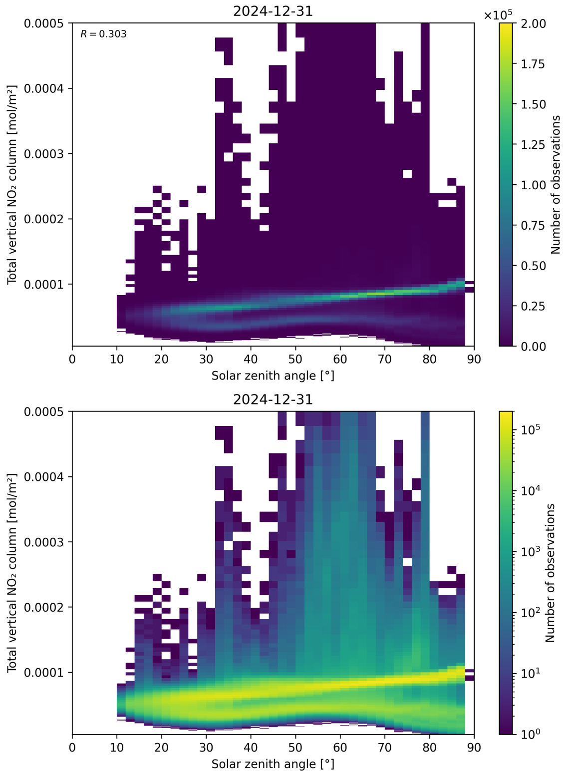
Figure 153: Scatter density plot of “Solar zenith angle” against “Total vertical NO 2 column” for 2024-12-30 to 2025-01-01.
