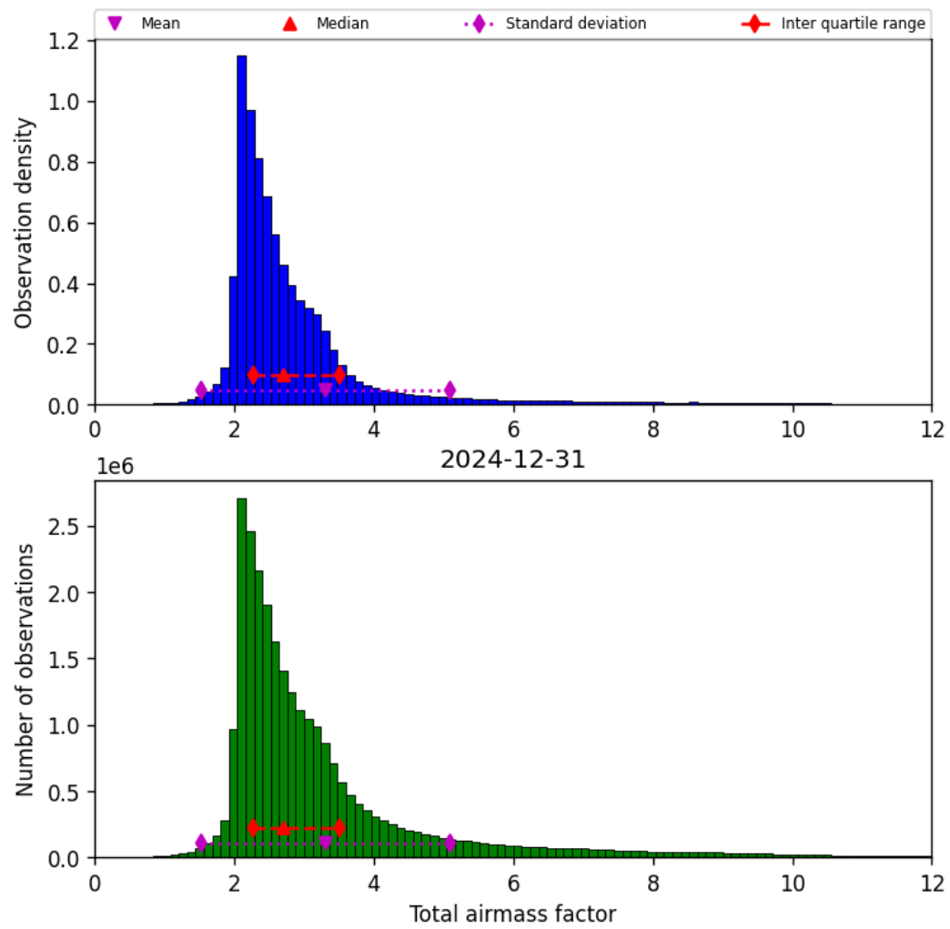
Figure 32: Histogram of “Total airmass factor” for 2024-12-30 to 2025-01-01
