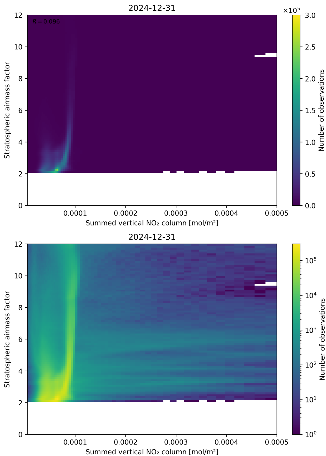
Figure 103: Scatter density plot of “Summed vertical NO 2 column” against “Stratospheric airmass factor” for 2024-12-30 to 2025-01-01.
