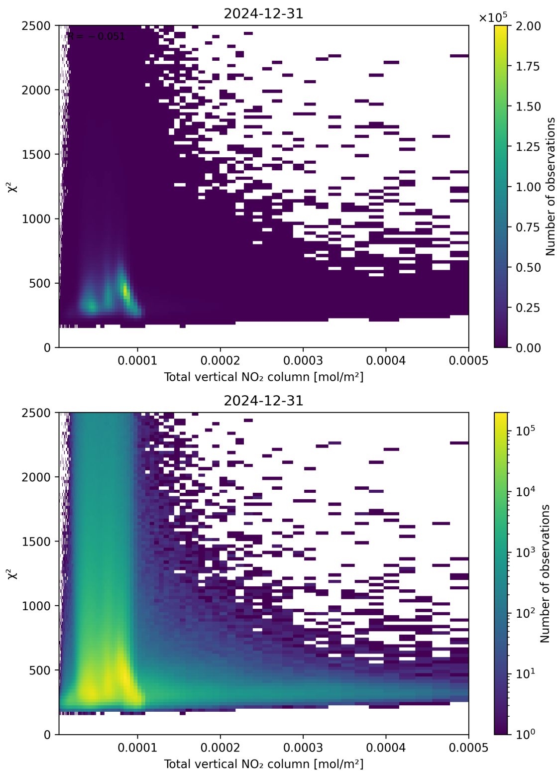
Figure 111: Scatter density plot of “Total vertical NO 2 column” against “ \chi^2 ” for 2024-12-30 to 2025-01-01.
