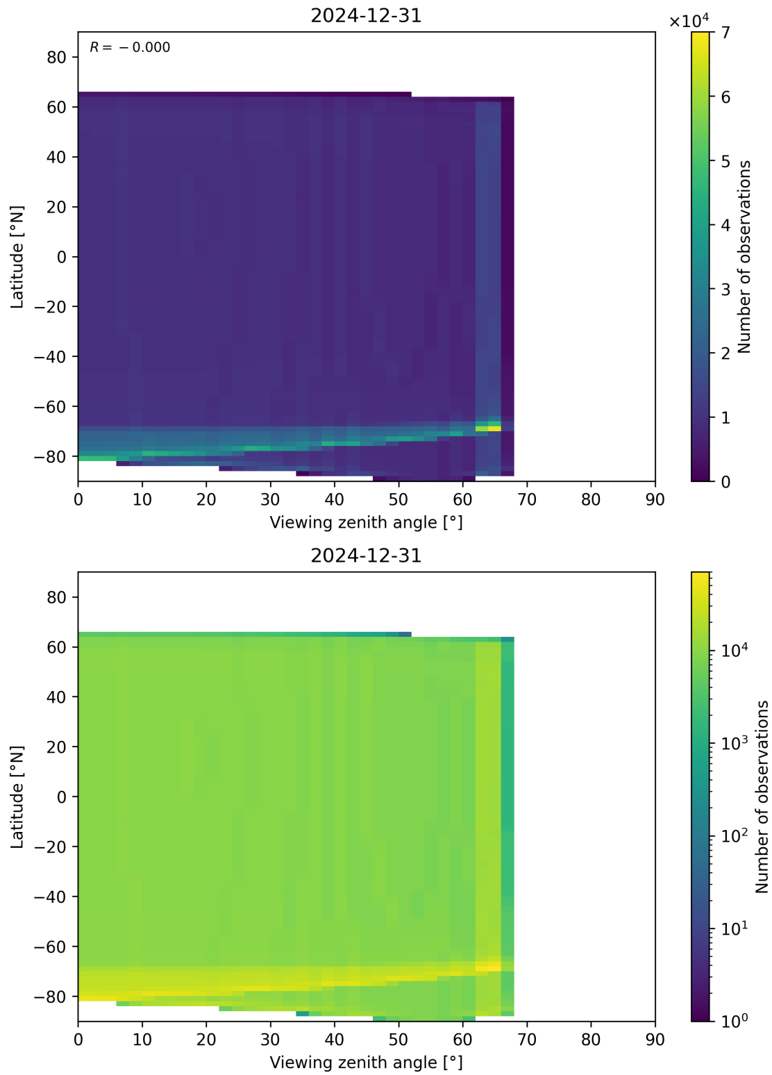
Figure 163: Scatter density plot of “Viewing zenith angle” against “Latitude” for 2024-12-30 to 2025-01-01.
