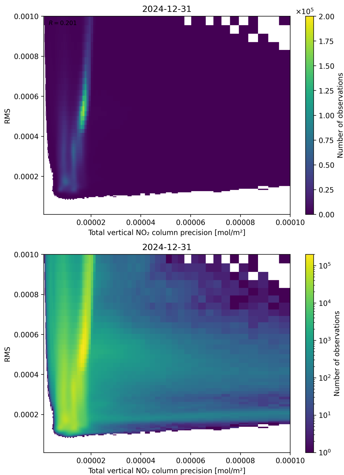
Figure 119: Scatter density plot of “Total vertical NO 2 column precision” against “RMS” for 2024-12-30 to 2025-01-01.
