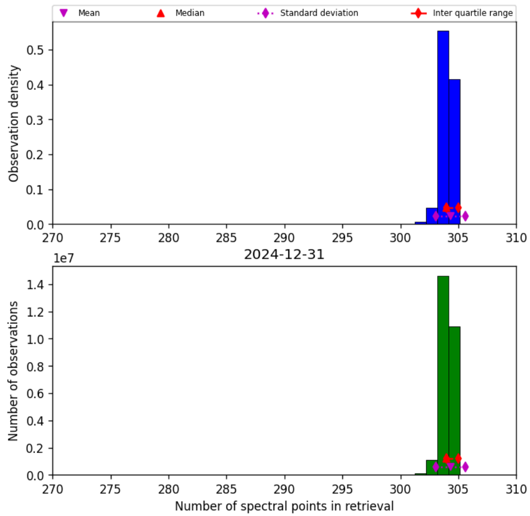
Figure 33: Histogram of “Number of spectral points in retrieval” for 2024-12-30 to 2025-01-01
