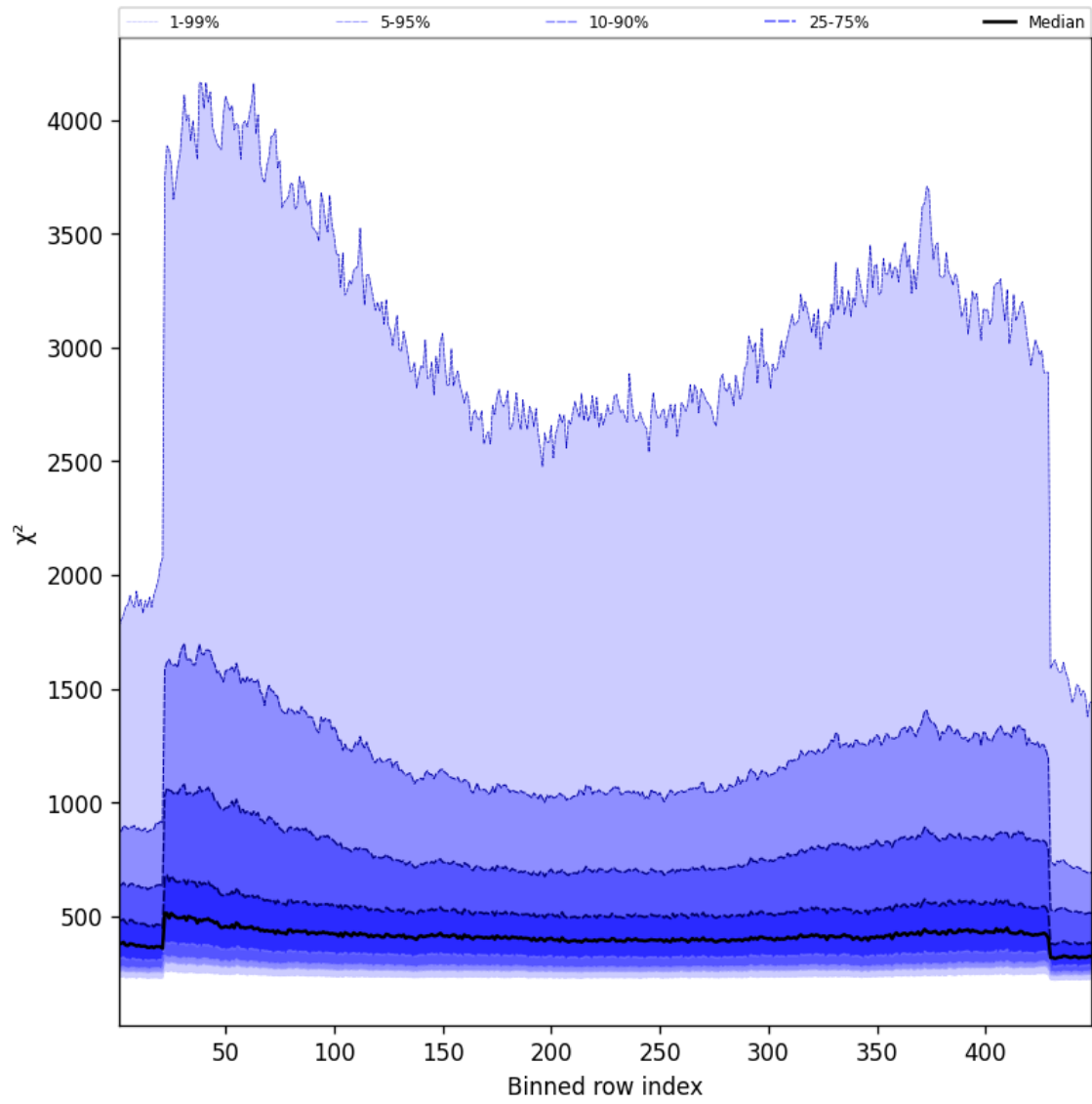
Figure 59: Along track statistics of “ \chi^2 ” for 2024-12-30 to 2025-01-01
