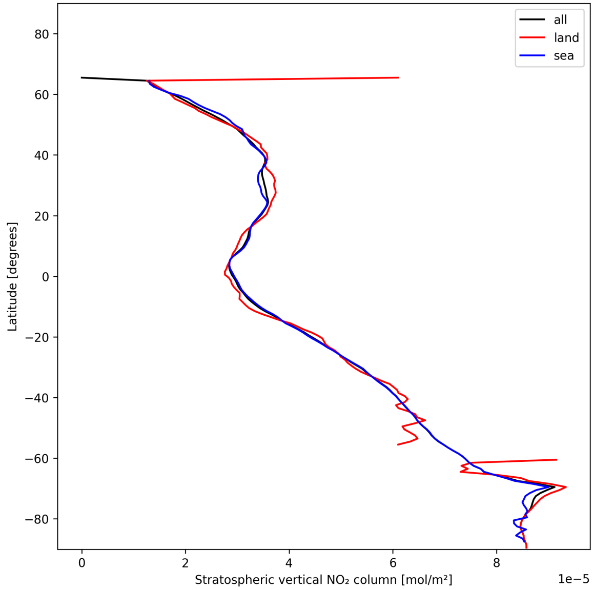
Figure 19: Zonal average of “Stratospheric vertical NO 2 column” for 2024-12-30 to 2025-01-01.
