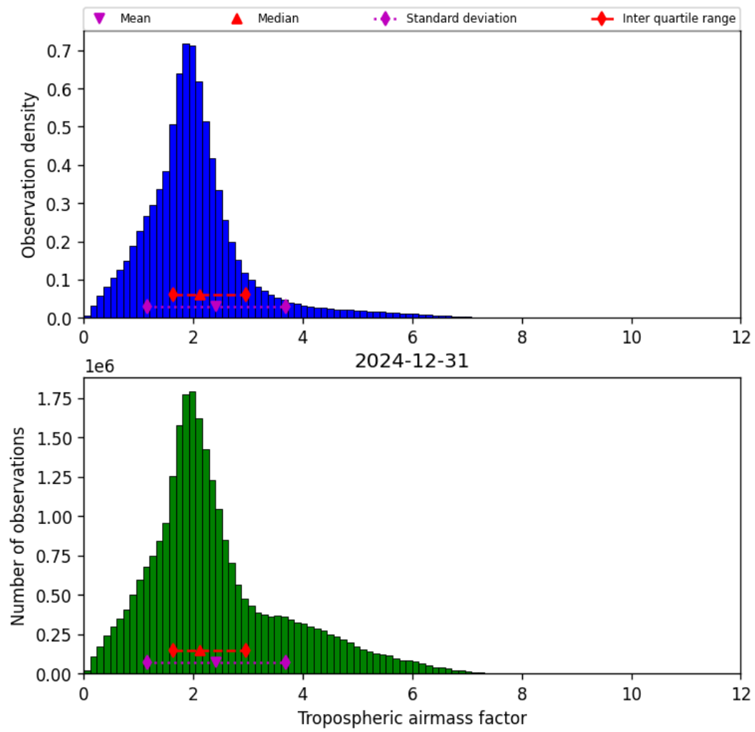
Figure 31: Histogram of “Tropospheric airmass factor” for 2024-12-30 to 2025-01-01
