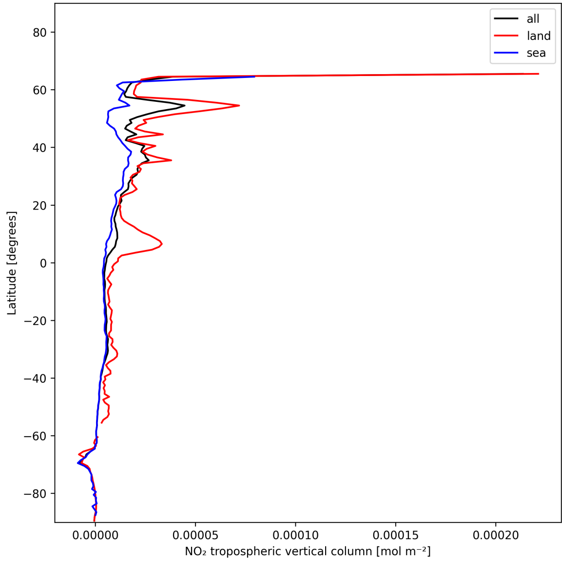
Figure 12: Zonal average of “NO 2 tropospheric vertical column” for 2024-12-30 to 2025-01-01.
