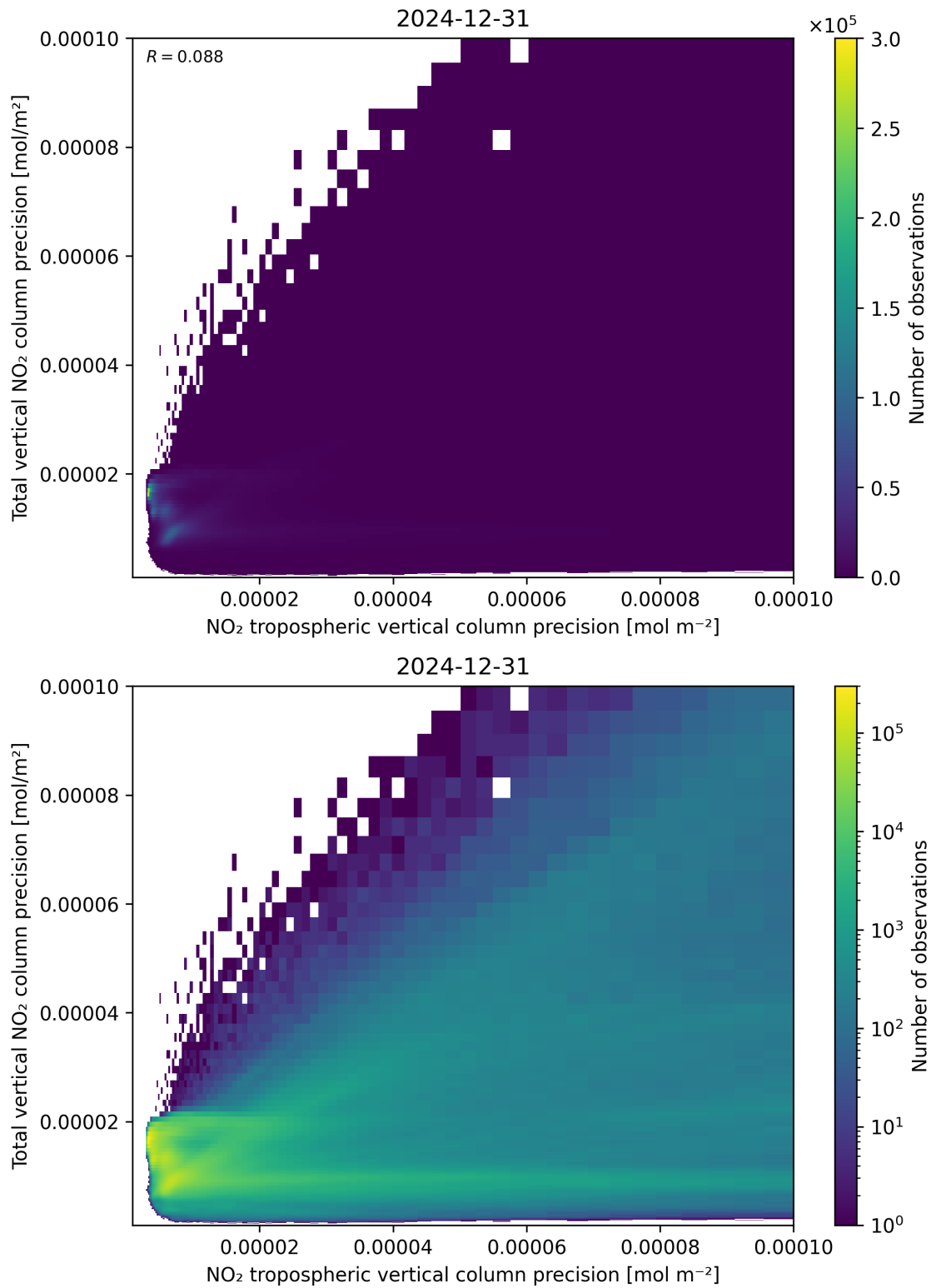
Figure 139: Scatter density plot of “NO 2 tropospheric vertical column precision” against “Total vertical NO 2 column precision” for 2024-12-30 to 2025-01-01.
