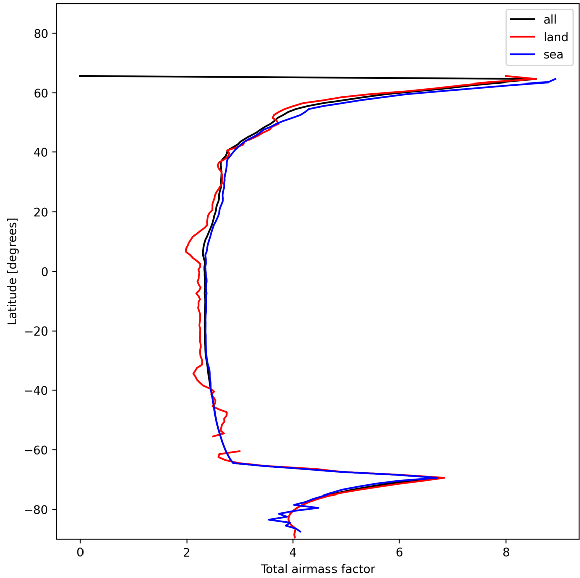
Figure 15: Zonal average of “Total airmass factor” for 2024-12-30 to 2025-01-01.
