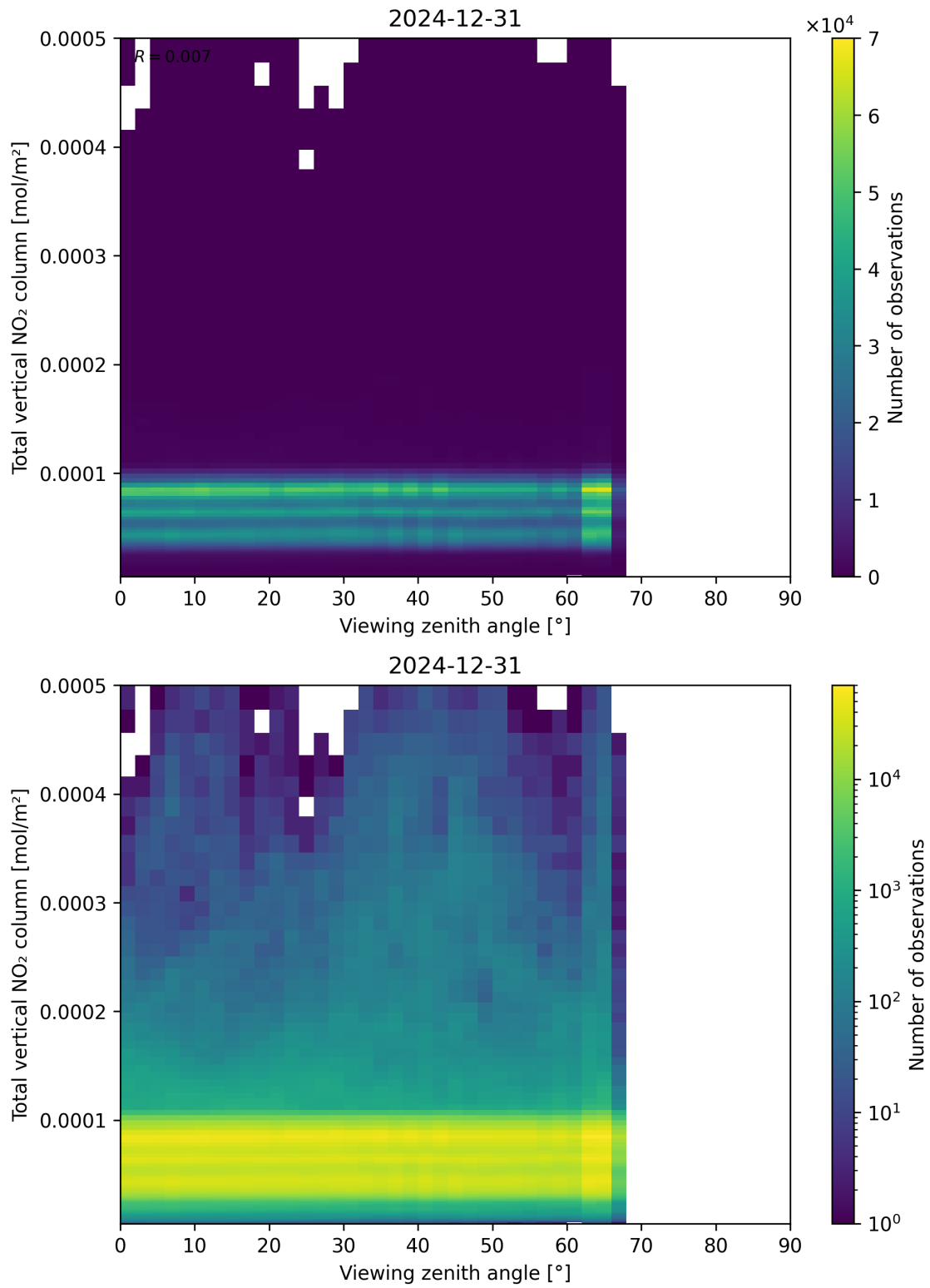
Figure 167: Scatter density plot of “Viewing zenith angle” against “Total vertical NO 2 column” for 2024-12-30 to 2025-01-01.
