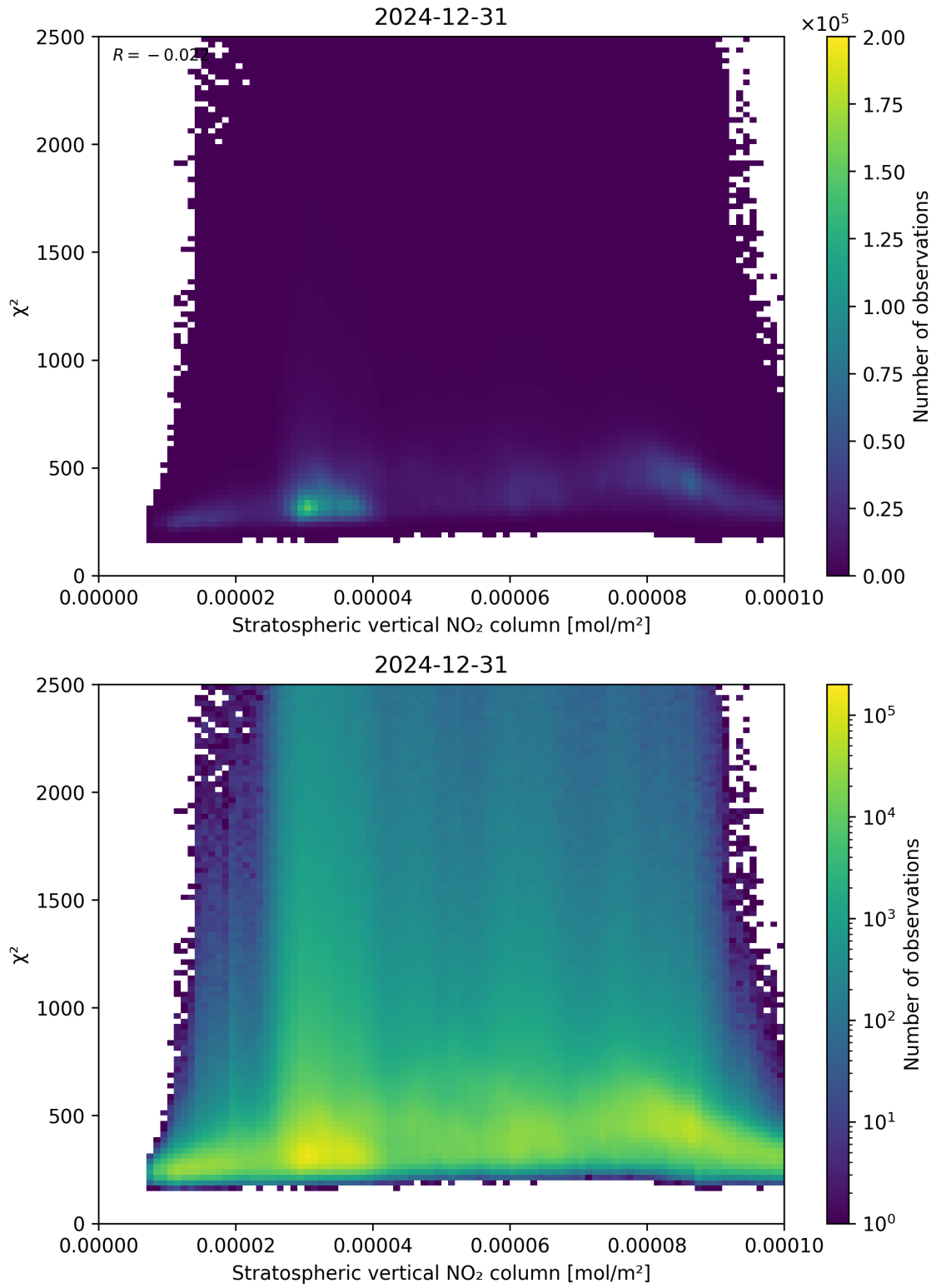
Figure 97: Scatter density plot of “Stratospheric vertical NO 2 column” against “ \chi^2 ” for 2024-12-30 to 2025-01-01.
