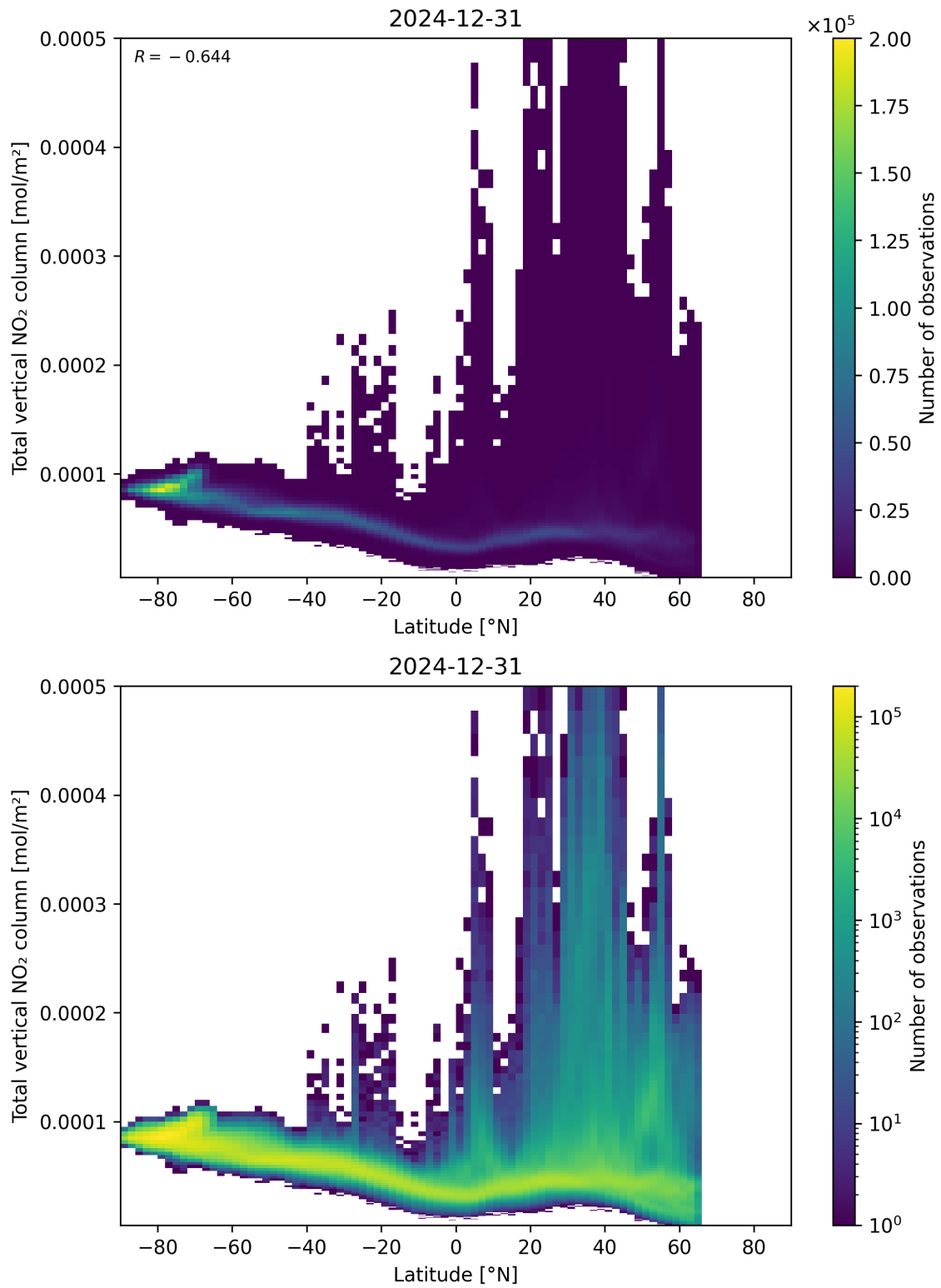
Figure 90: Scatter density plot of “Latitude” against “Total vertical NO 2 column” for 2024-12-30 to 2025-01-01.
