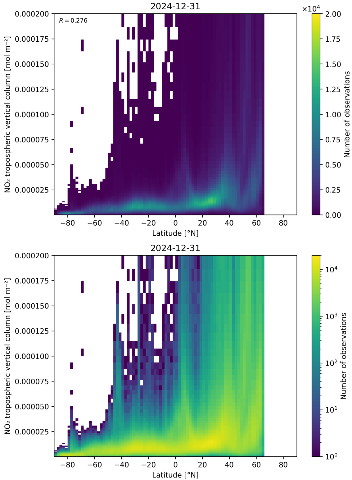
Figure 92: Scatter density plot of “Latitude” against “NO 2 tropospheric vertical column” for 2024-12-30 to 2025-01-01.
