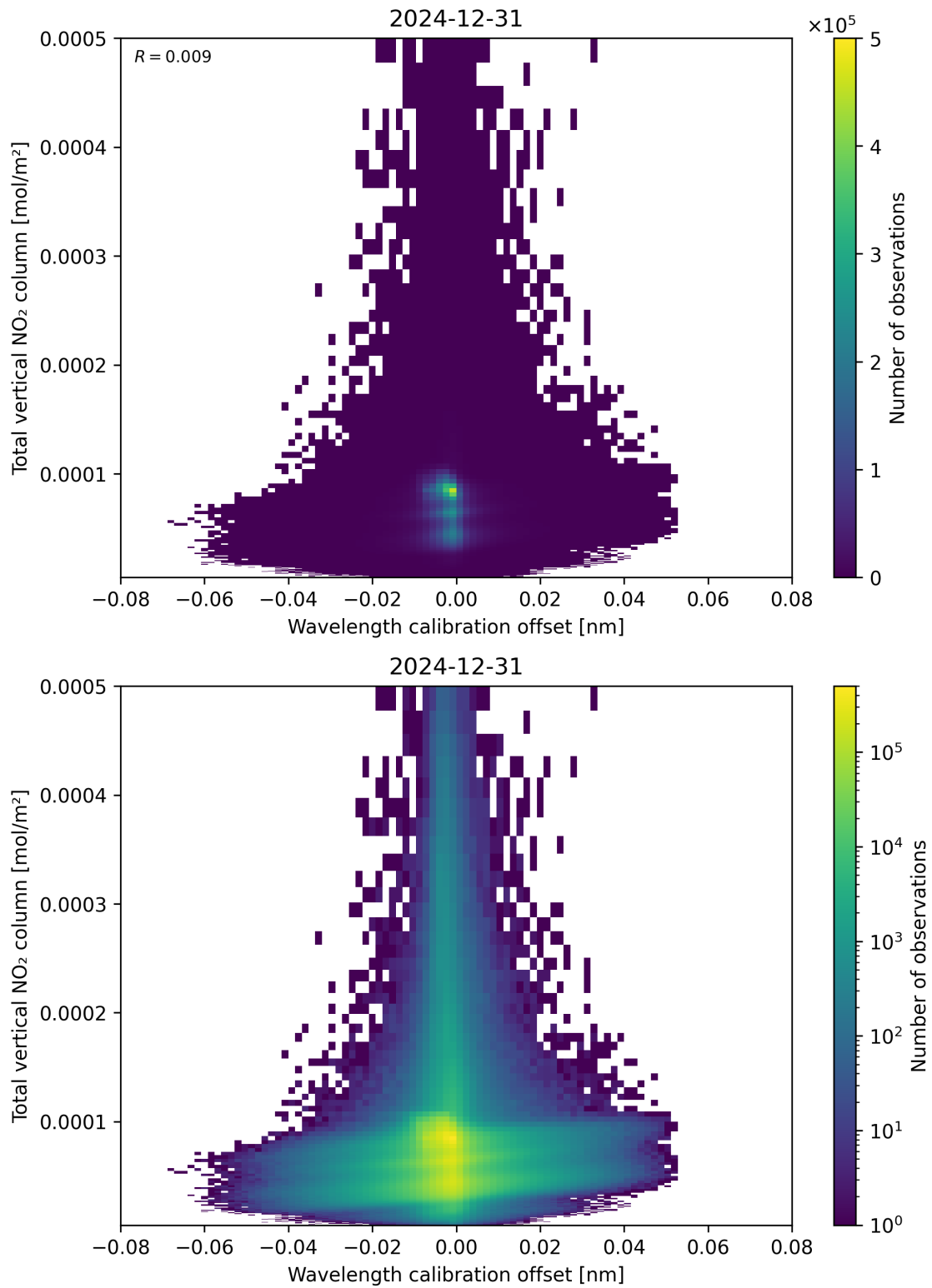
Figure 179: Scatter density plot of “Wavelength calibration offset” against “Total vertical NO 2 column” for 2024-12-30 to 2025-01-01.
