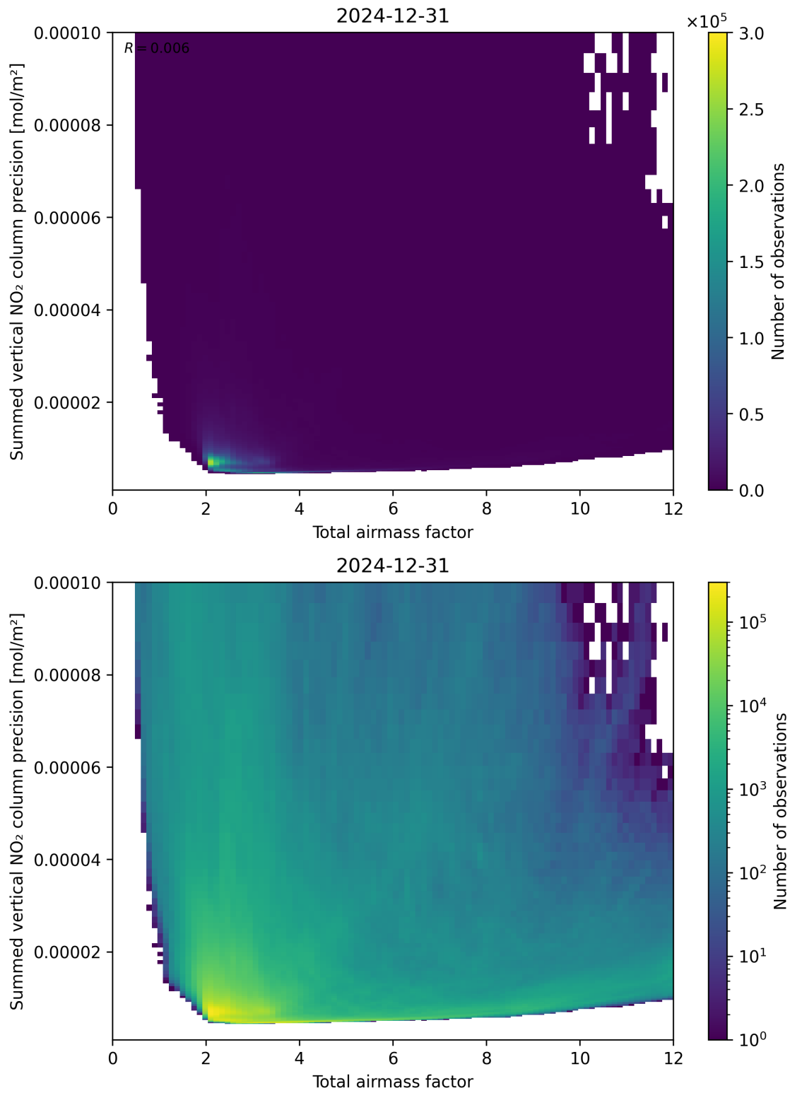
Figure 66: Scatter density plot of “Total airmass factor” against “Summed vertical NO 2 column precision” for 2024-12-30 to 2025-01-01.
