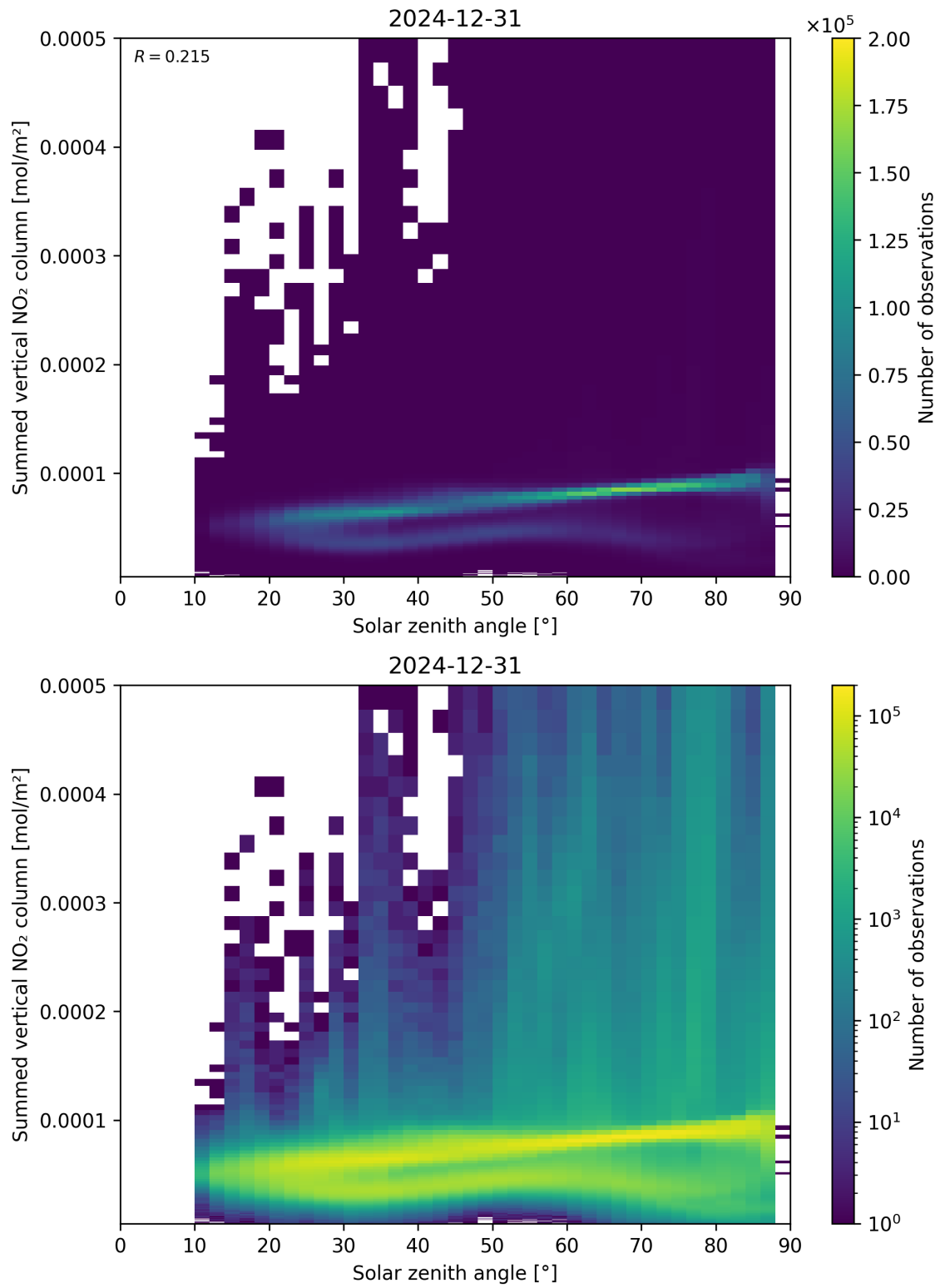
Figure 151: Scatter density plot of “Solar zenith angle” against “Summed vertical NO 2 column” for 2024-12-30 to 2025-01-01.
