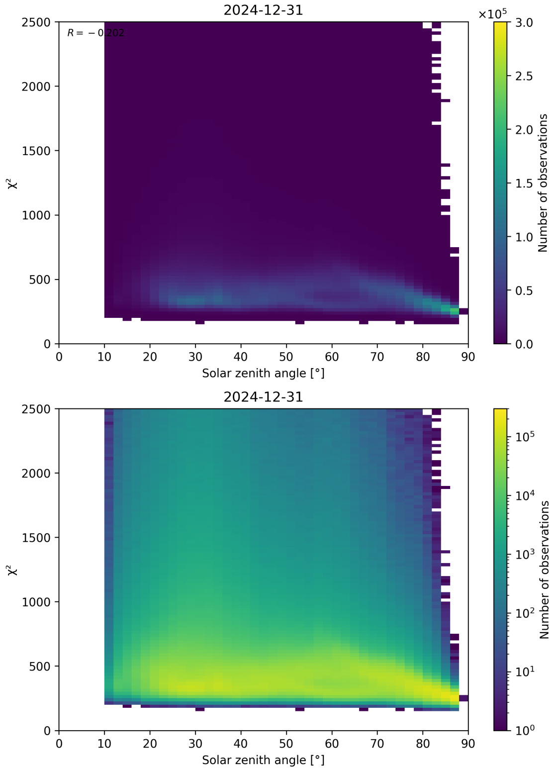
Figure 148: Scatter density plot of “Solar zenith angle” against “ \chi^2 ” for 2024-12-30 to 2025-01-01.
