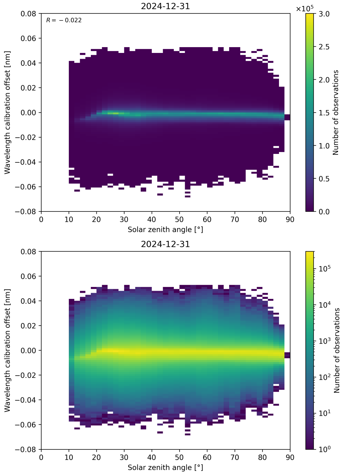
Figure 158: Scatter density plot of “Solar zenith angle” against “Wavelength calibration offset” for 2024-12-30 to 2025-01-01.
