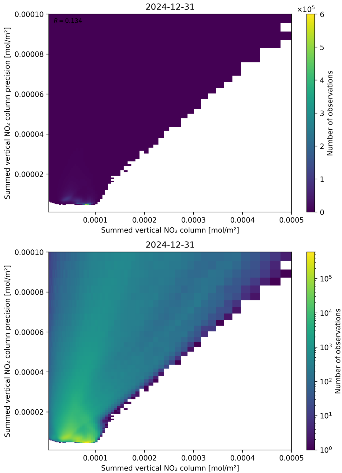
Figure 105: Scatter density plot of “Summed vertical NO 2 column” against “Summed vertical NO 2 column precision” for 2024-12-30 to 2025-01-01.
