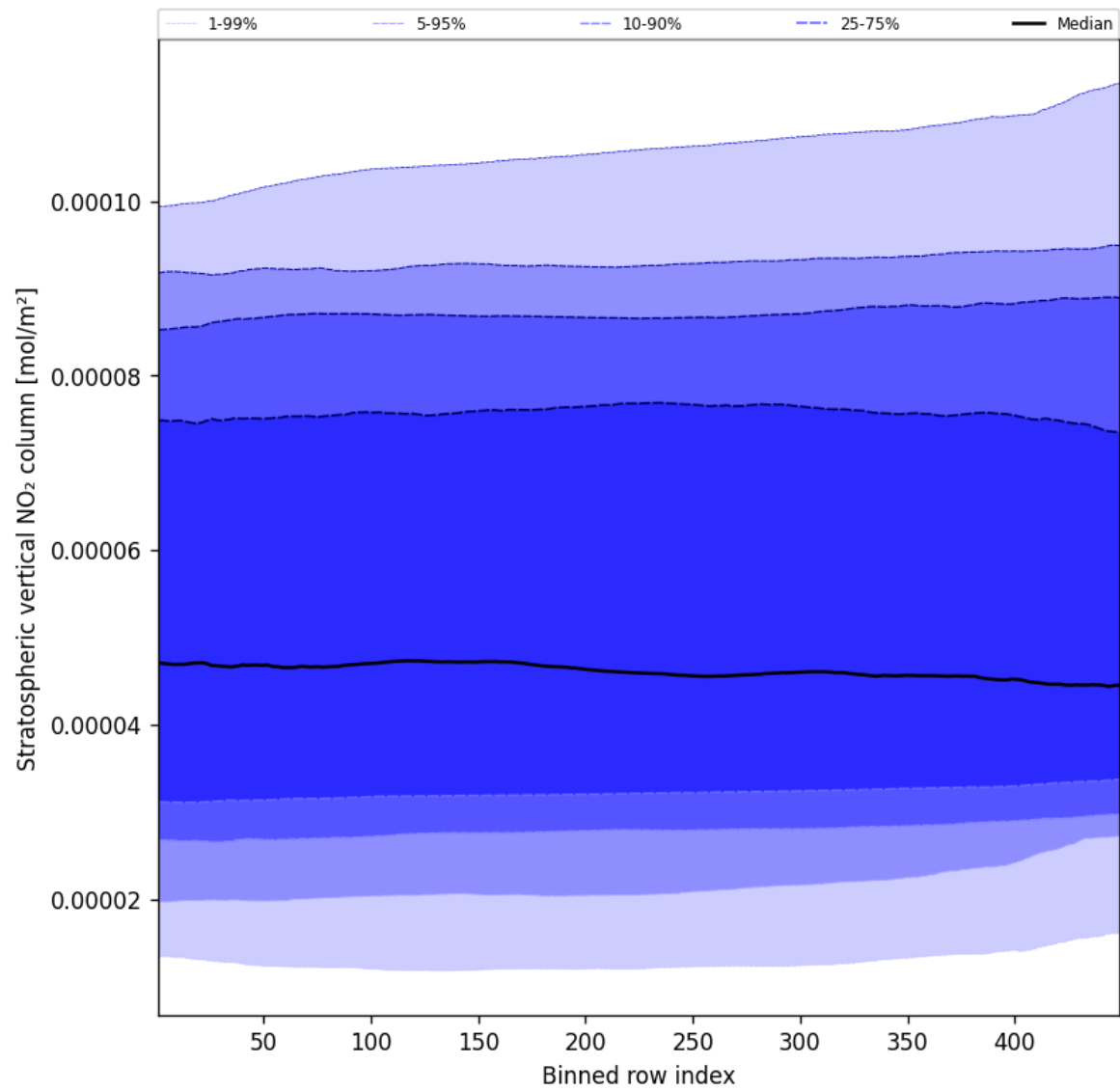
Figure 53: Along track statistics of “Stratospheric vertical NO 2 column” for 2024-12-30 to 2025-01-01
