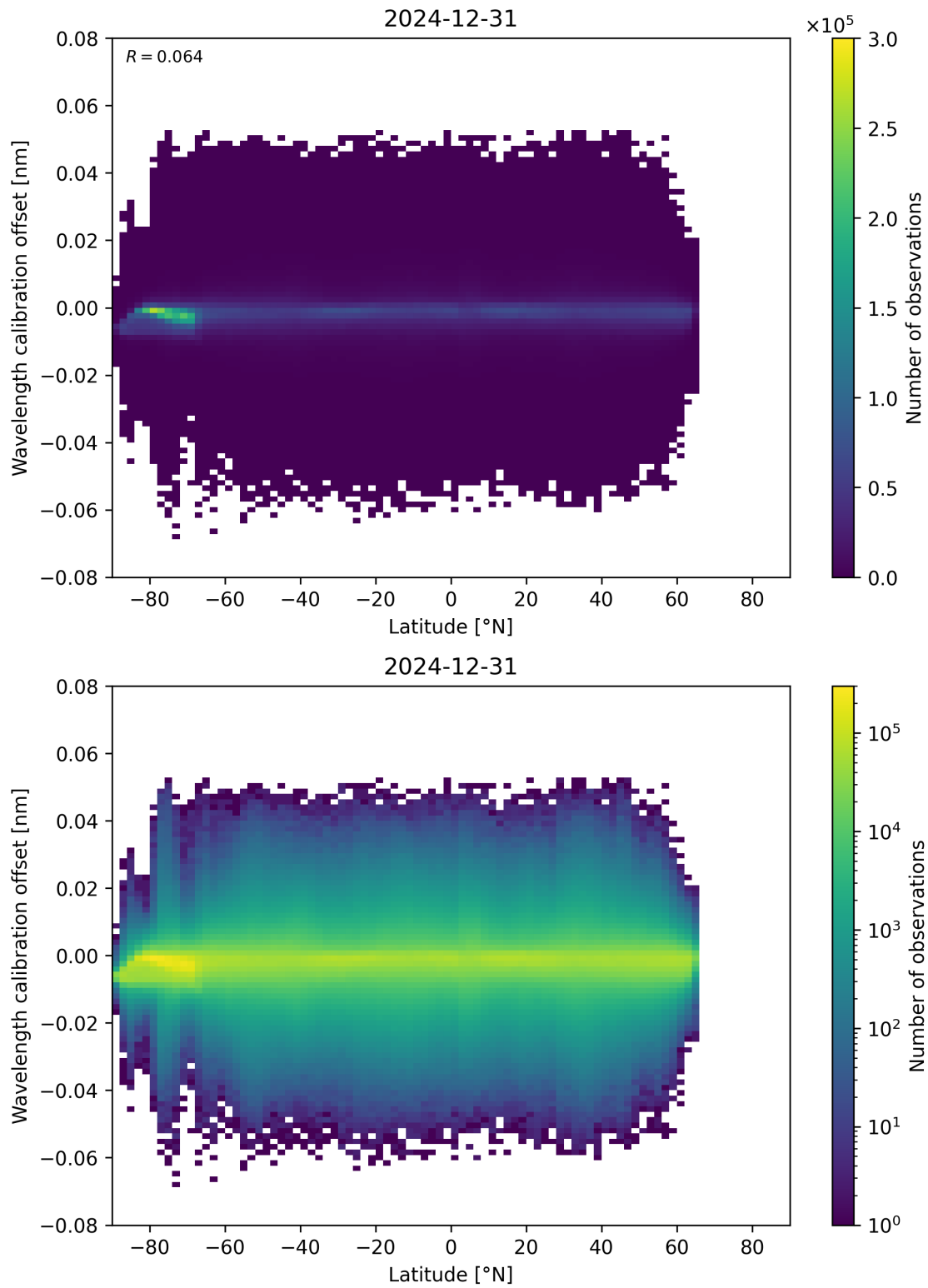
Figure 95: Scatter density plot of “Latitude” against “Wavelength calibration offset” for 2024-12-30 to 2025-01-01.
