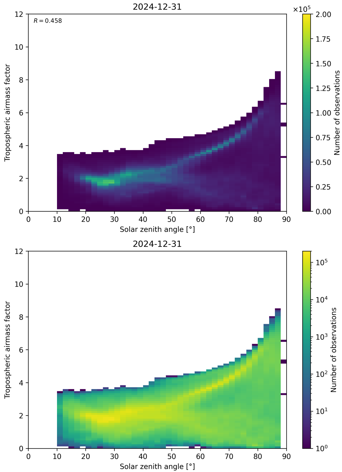
Figure 147: Scatter density plot of “Solar zenith angle” against “Tropospheric airmass factor” for 2024-12-30 to 2025-01-01.
