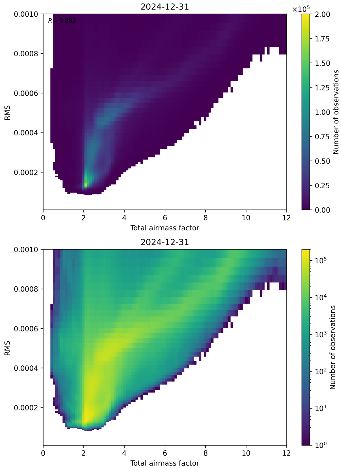
Figure 69: Scatter density plot of “Total airmass factor” against “RMS” for 2024-12-30 to 2025-01-01.
