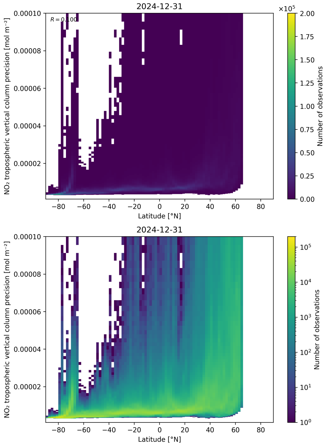
Figure 93: Scatter density plot of “Latitude” against “NO 2 tropospheric vertical column precision” for 2024-12-30 to 2025-01-01.
