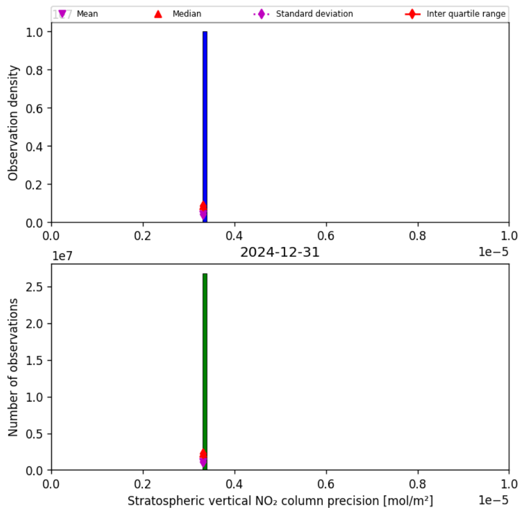
Figure 37: Histogram of “Stratospheric vertical NO 2 column precision” for 2024-12-30 to 2025-01-01
