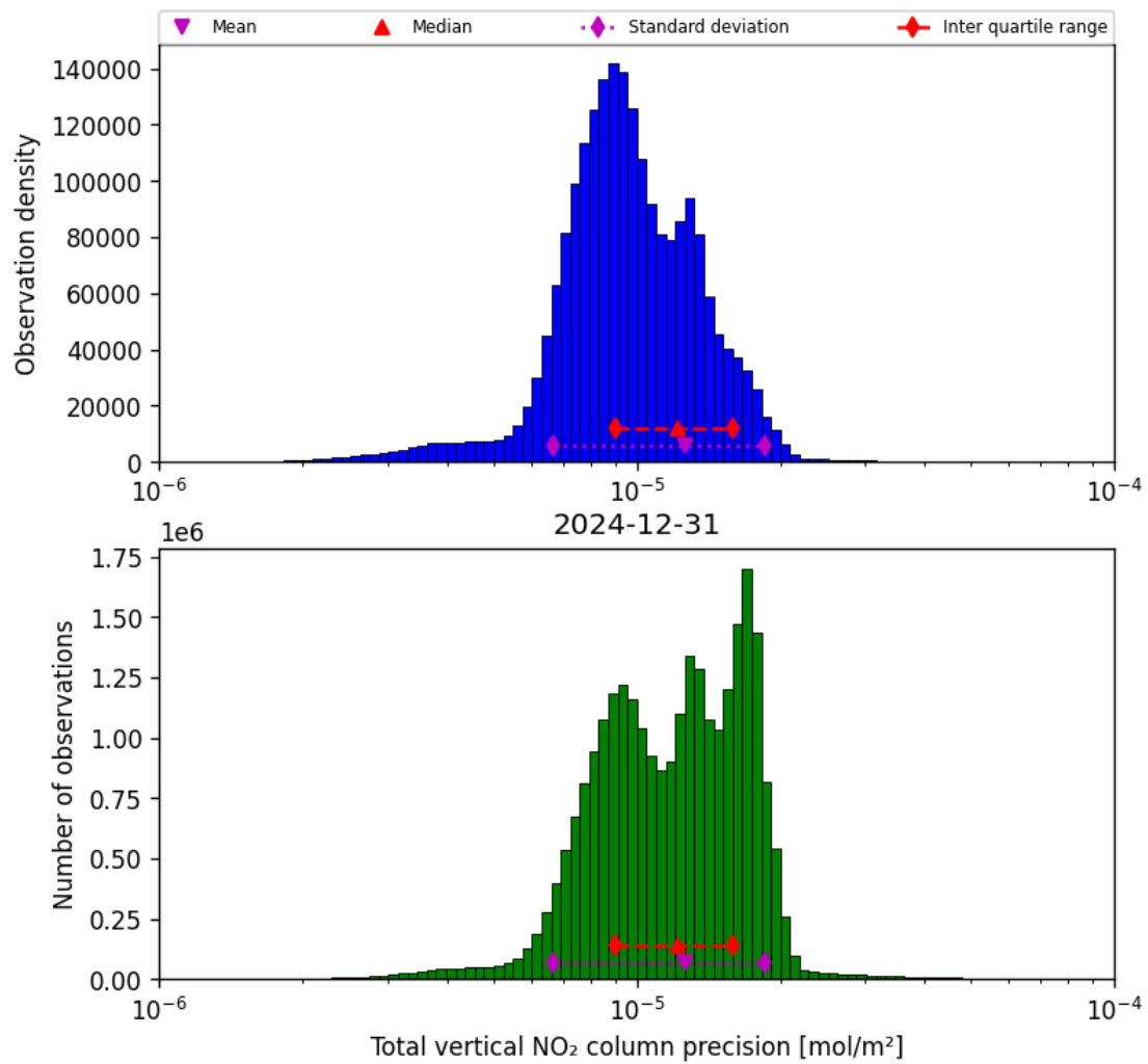
Figure 39: Histogram of “Total vertical NO 2 column precision” for 2024-12-30 to 2025-01-01
