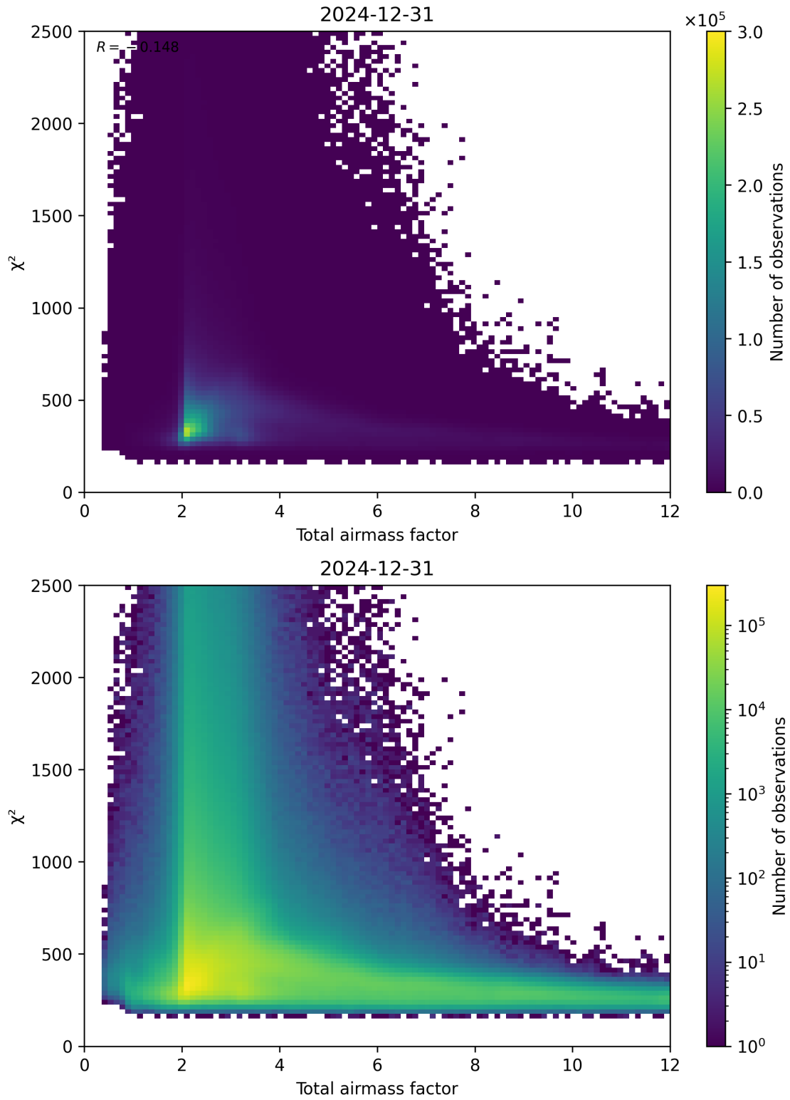
Figure 63: Scatter density plot of “Total airmass factor” against “ \chi^2 ” for 2024-12-30 to 2025-01-01.
