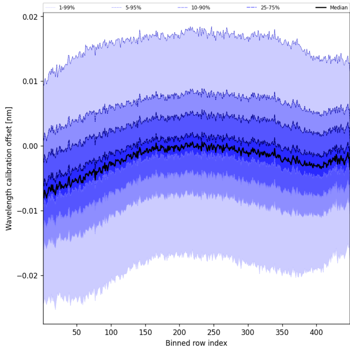
Figure 52: Along track statistics of “Wavelength calibration offset” for 2024-12-30 to 2025-01-01
