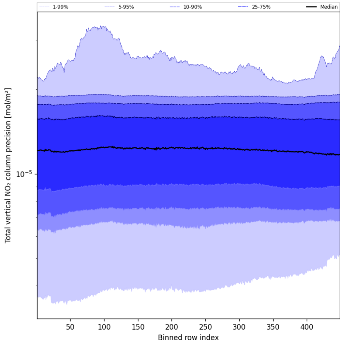
Figure 56: Along track statistics of “Total vertical NO 2 column precision” for 2024-12-30 to 2025-01-01
