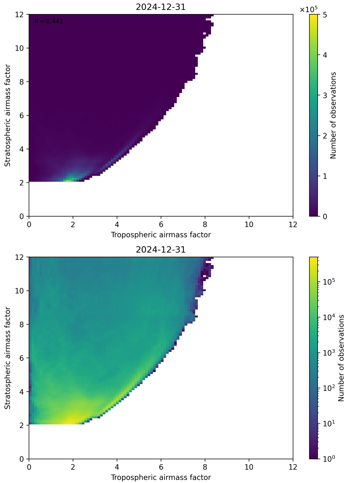
Figure 71: Scatter density plot of “Tropospheric airmass factor” against “Stratospheric airmass factor” for 2024-12-30 to 2025-01-01.
