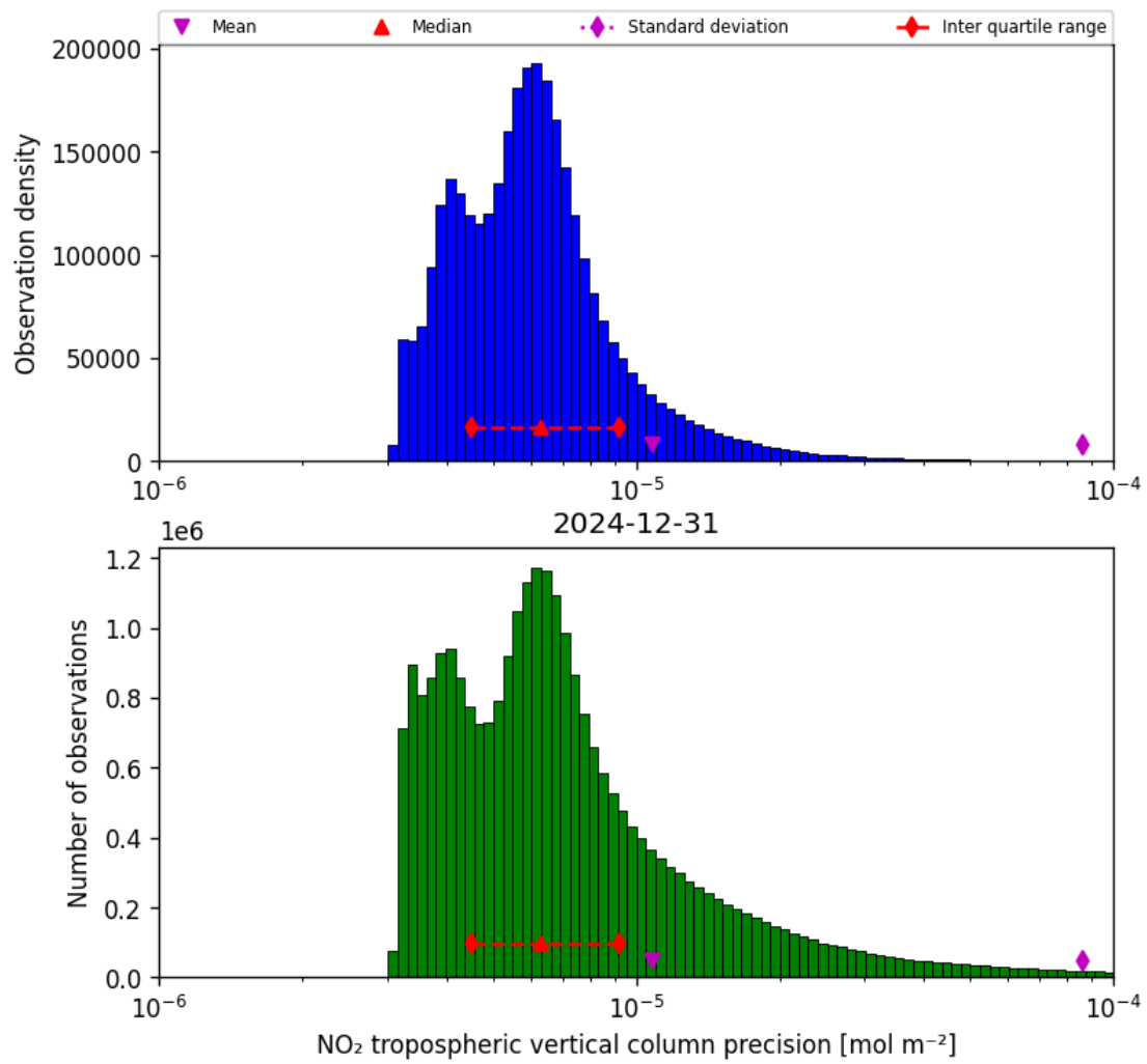
Figure 30: Histogram of “NO 2 tropospheric vertical column precision” for 2024-12-30 to 2025-01-01
