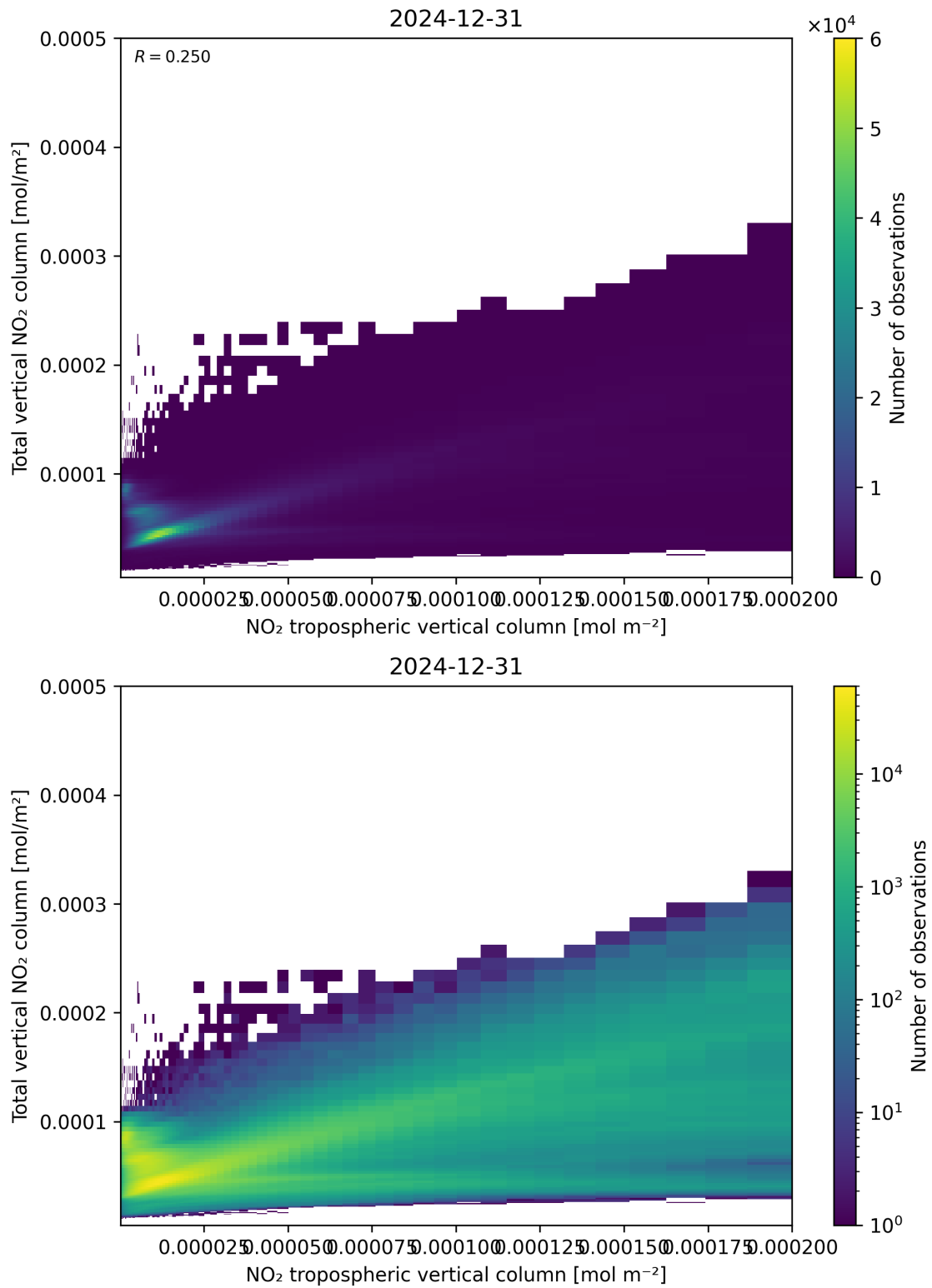
Figure 128: Scatter density plot of “NO 2 tropospheric vertical column” against “Total vertical NO 2 column” for 2024-12-30 to 2025-01-01.
