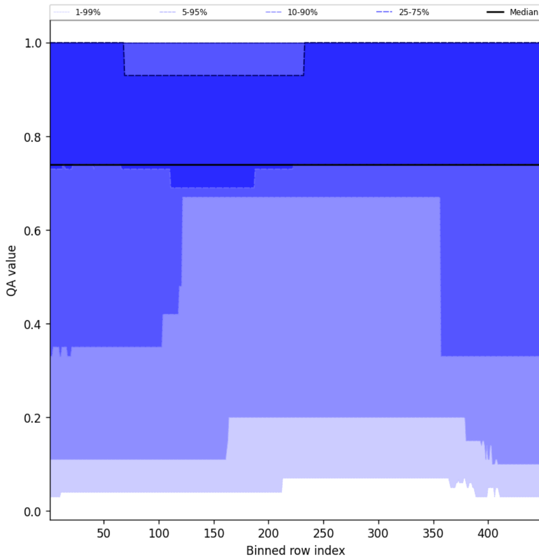
Figure 45: Along track statistics of “QA value” for 2024-12-30 to 2025-01-01
