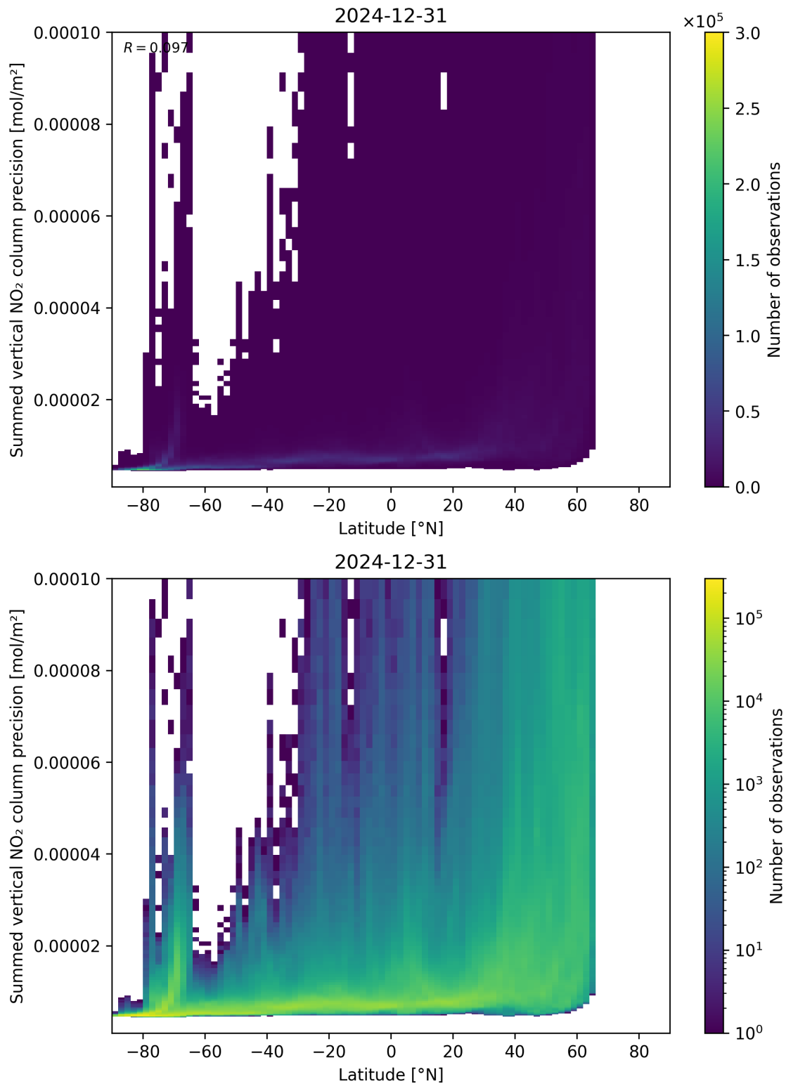
Figure 89: Scatter density plot of “Latitude” against “Summed vertical NO 2 column precision” for 2024-12-30 to 2025-01-01.
