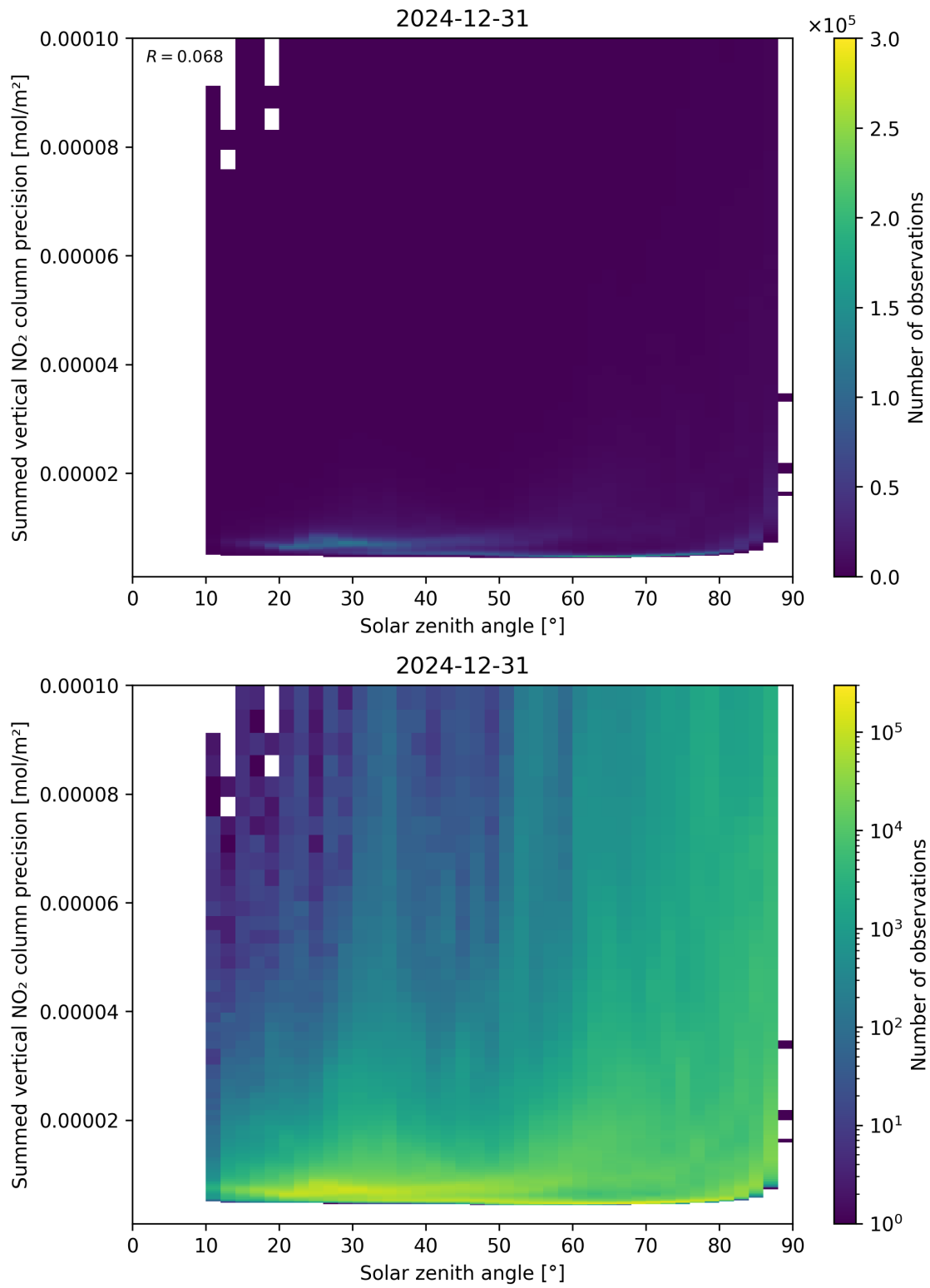
Figure 152: Scatter density plot of “Solar zenith angle” against “Summed vertical NO 2 column precision” for 2024-12-30 to 2025-01-01.
