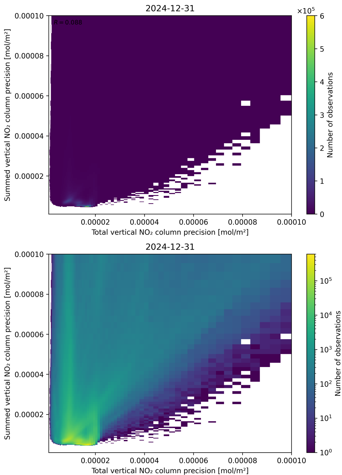
Figure 118: Scatter density plot of “Total vertical NO 2 column precision” against “Summed vertical NO 2 column precision” for 2024-12-30 to 2025-01-01.
