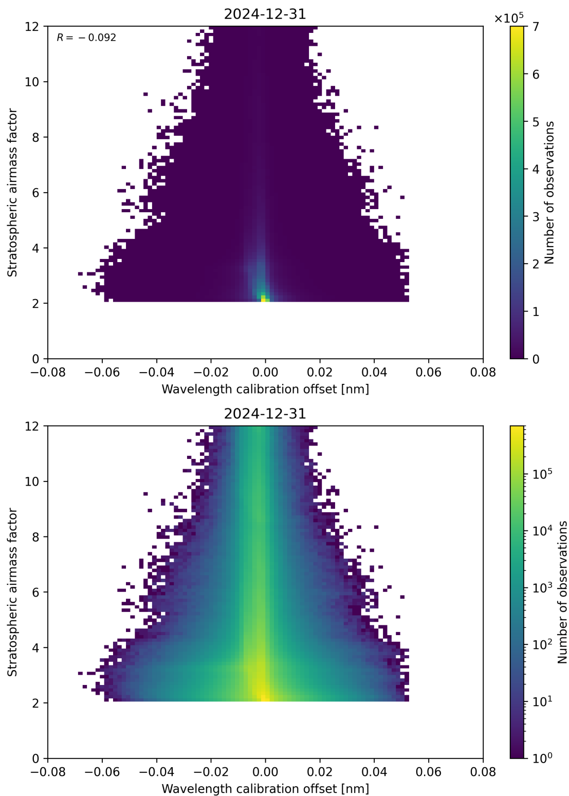
Figure 174: Scatter density plot of “Wavelength calibration offset” against “Stratospheric airmass factor” for 2024-12-30 to 2025-01-01.
