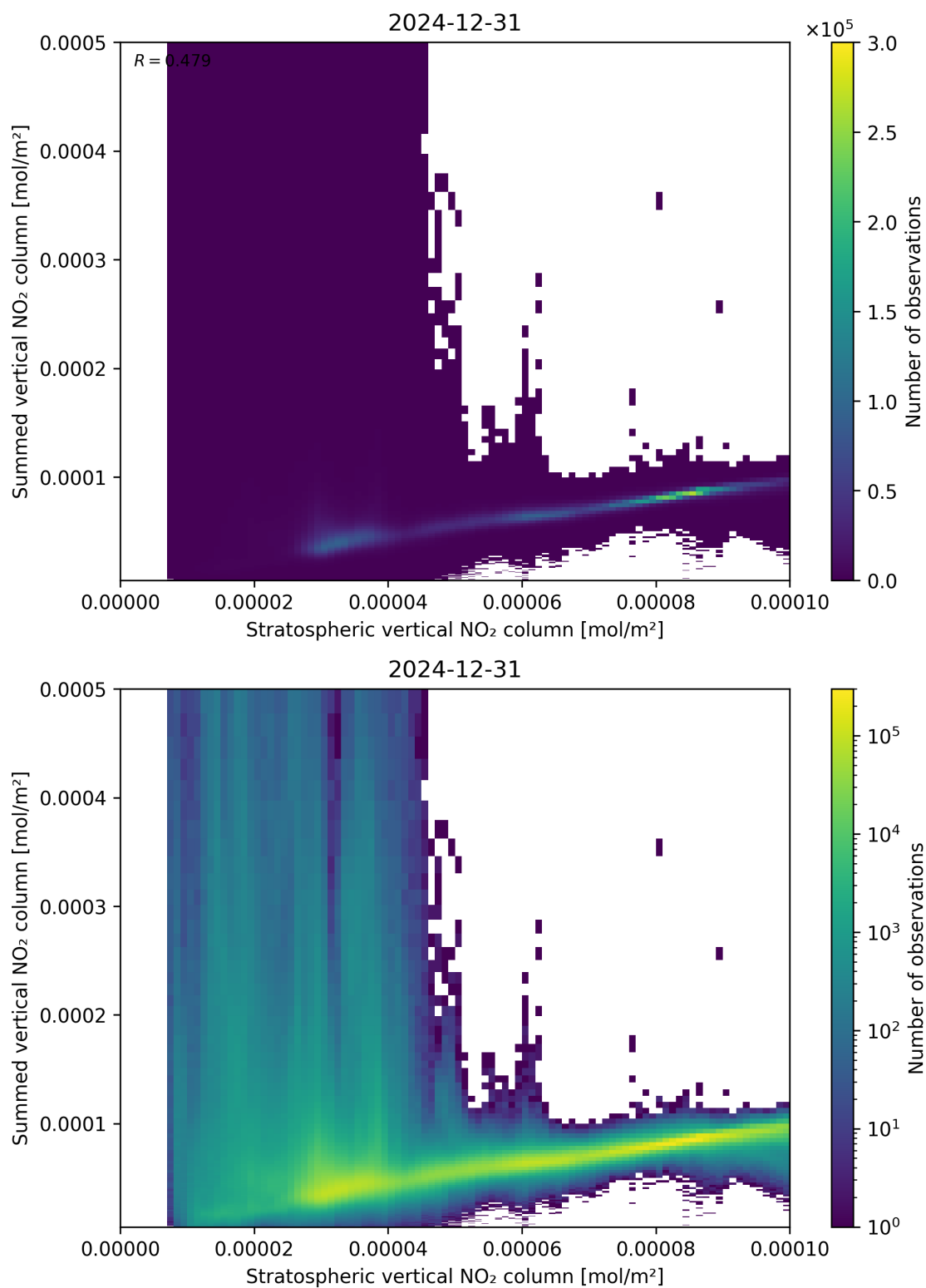
Figure 98: Scatter density plot of “Stratospheric vertical NO 2 column” against “Summed vertical NO 2 column” for 2024-12-30 to 2025-01-01.
