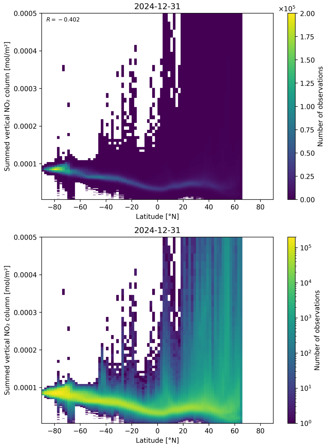
Figure 88: Scatter density plot of “Latitude” against “Summed vertical NO 2 column” for 2024-12-30 to 2025-01-01.
