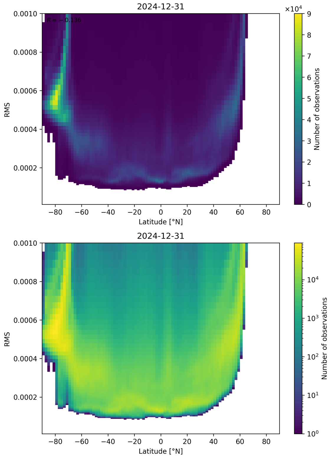
Figure 94: Scatter density plot of “Latitude” against “RMS” for 2024-12-30 to 2025-01-01.
