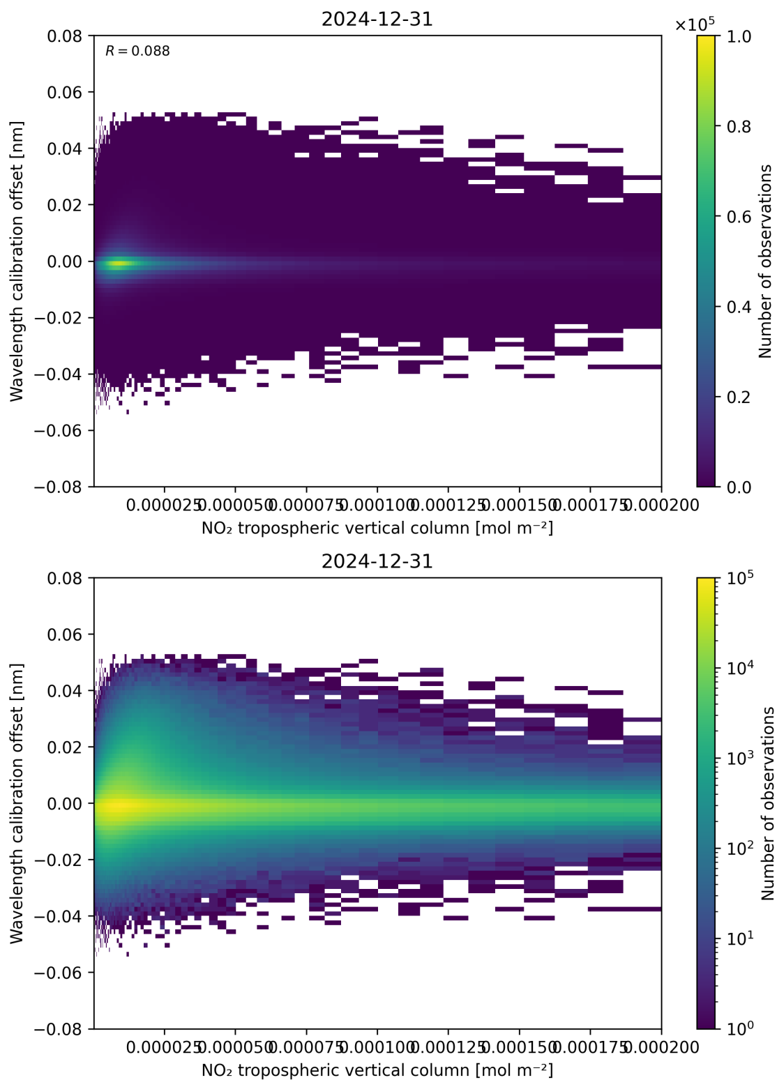
Figure 143: Scatter density plot of “NO 2 tropospheric vertical column” against “Wavelength calibration offset” for 2024-12-30 to 2025-01-01.
