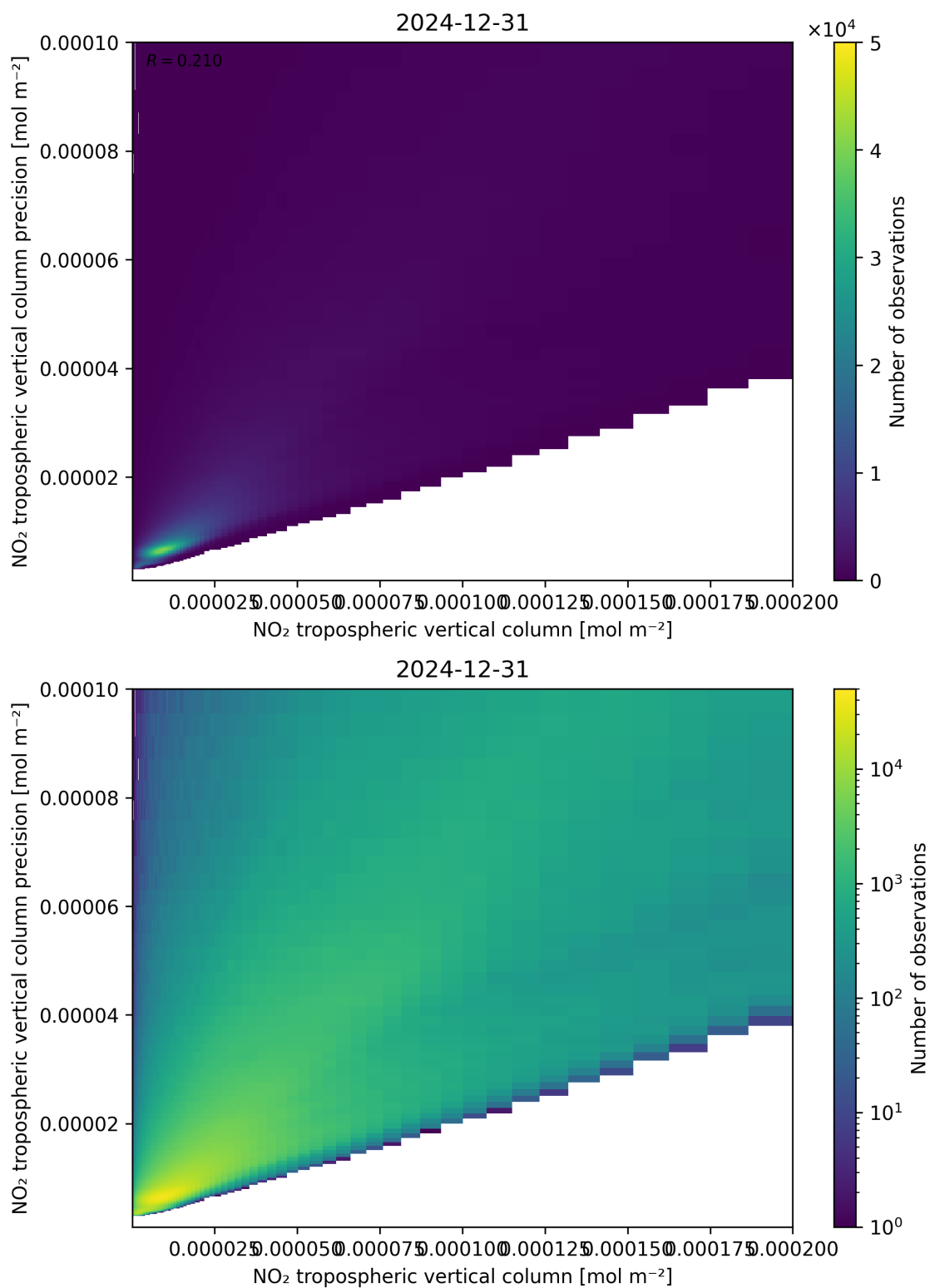
Figure 130: Scatter density plot of “NO 2 tropospheric vertical column” against “NO 2 tropospheric vertical column precision” for 2024-12-30 to 2025-01-01.
