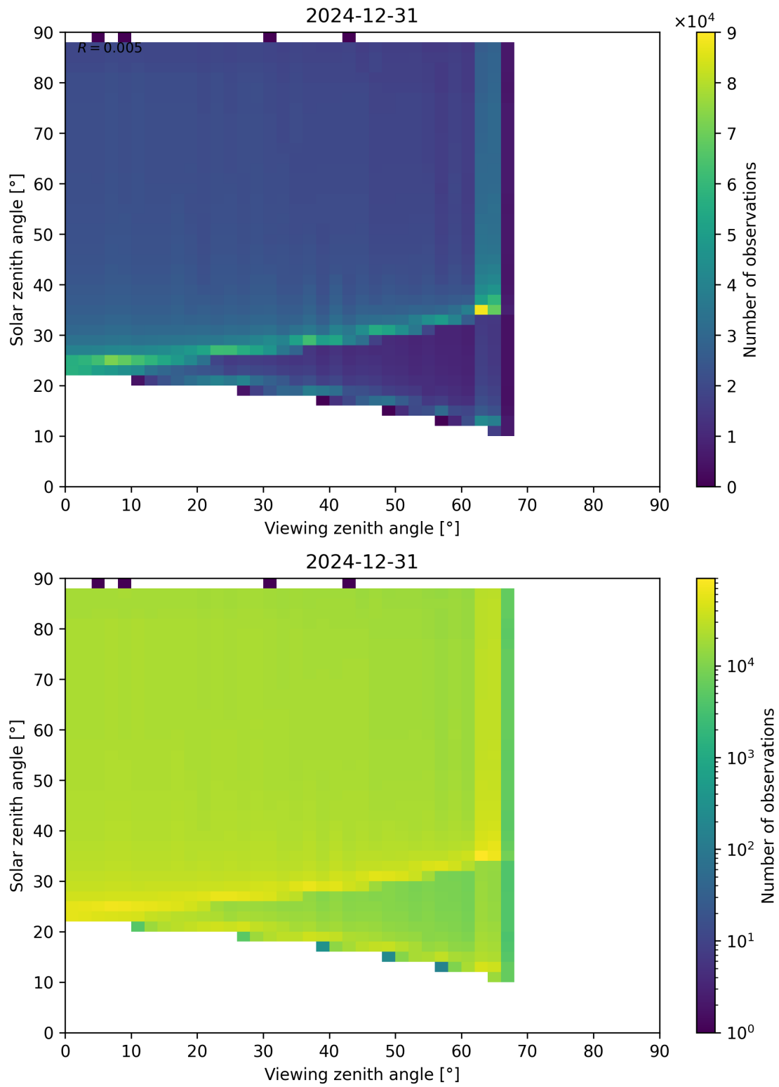
Figure 172: Scatter density plot of “Viewing zenith angle” against “Solar zenith angle” for 2024-12-30 to 2025-01-01.
