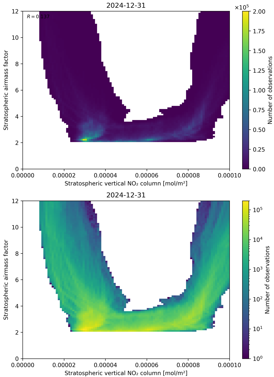
Figure 96: Scatter density plot of “Stratospheric vertical NO 2 column” against “Stratospheric airmass factor” for 2024-12-30 to 2025-01-01.
