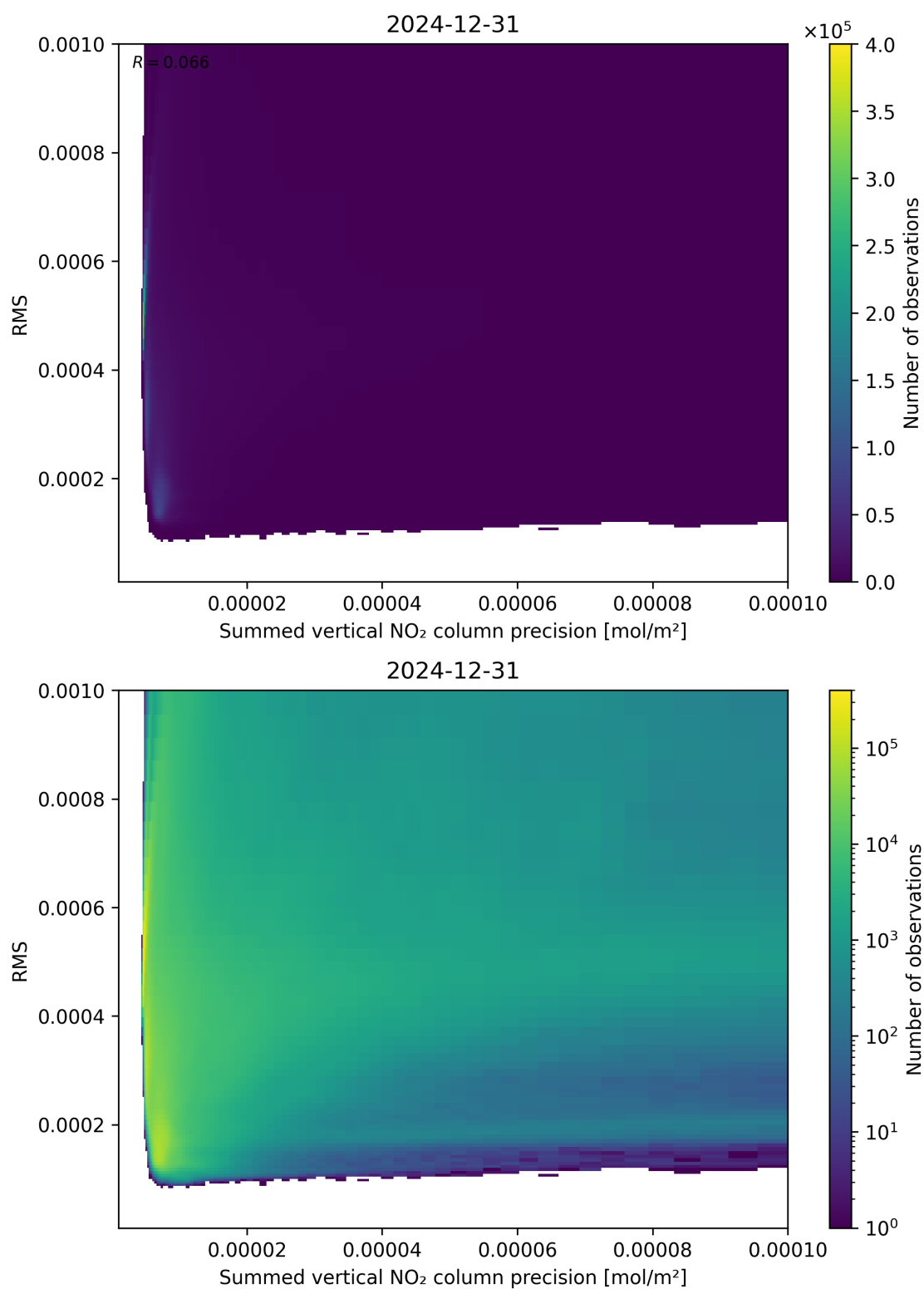
Figure 108: Scatter density plot of “Summed vertical NO 2 column precision” against “RMS” for 2024-12-30 to 2025-01-01.
