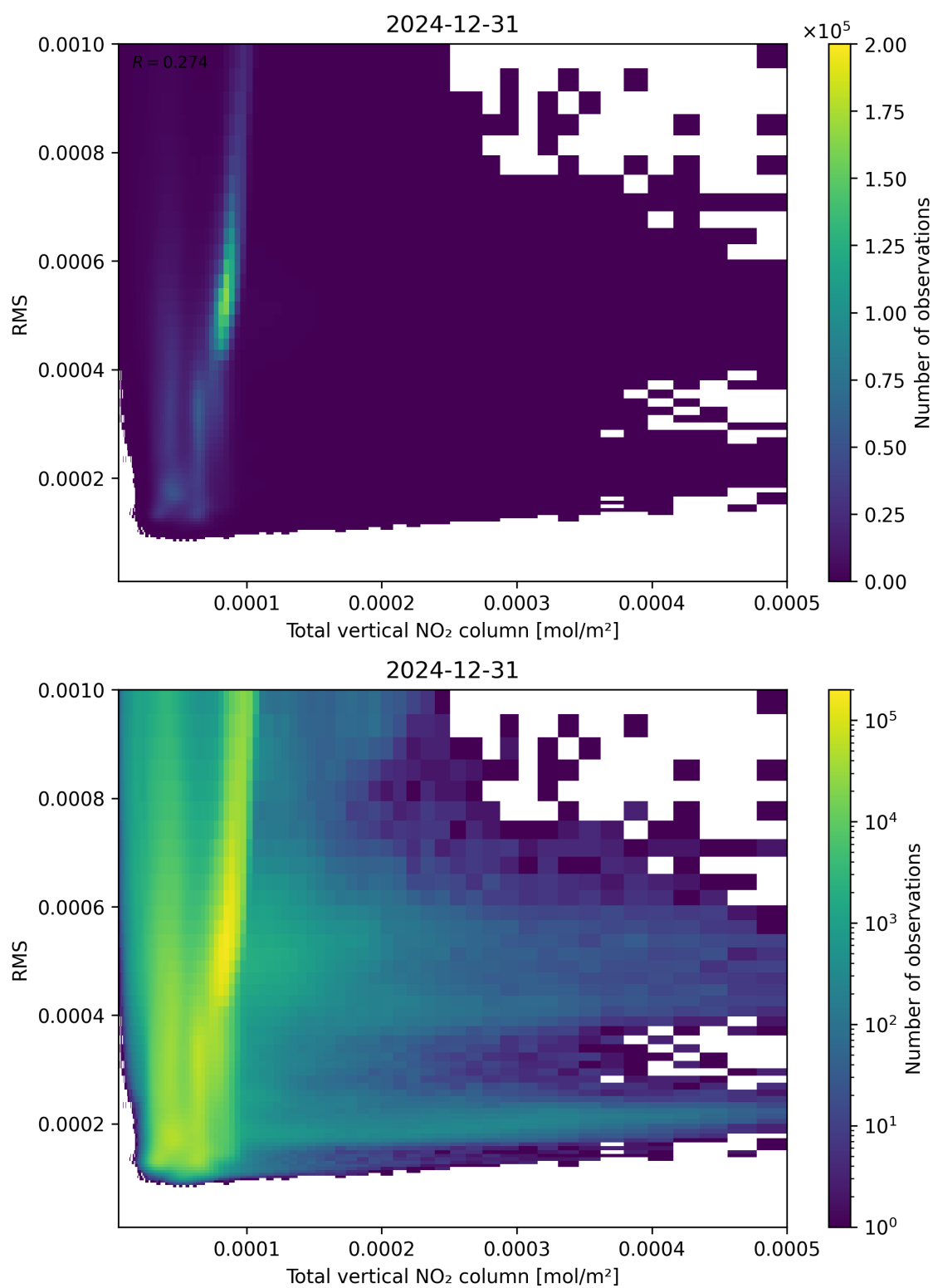
Figure 120: Scatter density plot of “Total vertical NO 2 column” against “RMS” for 2024-12-30 to 2025-01-01.
