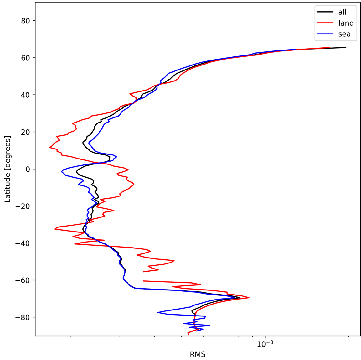
Figure 26: Zonal average of “RMS” for 2024-12-30 to 2025-01-01.
