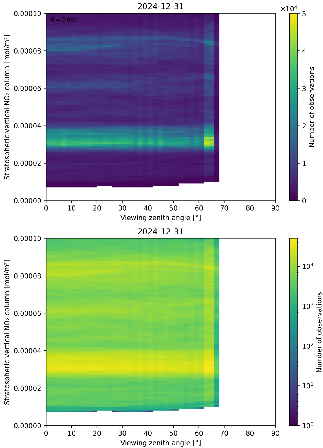
Figure 164: Scatter density plot of “Viewing zenith angle” against “Stratospheric vertical NO 2 column” for 2024-12-30 to 2025-01-01.
