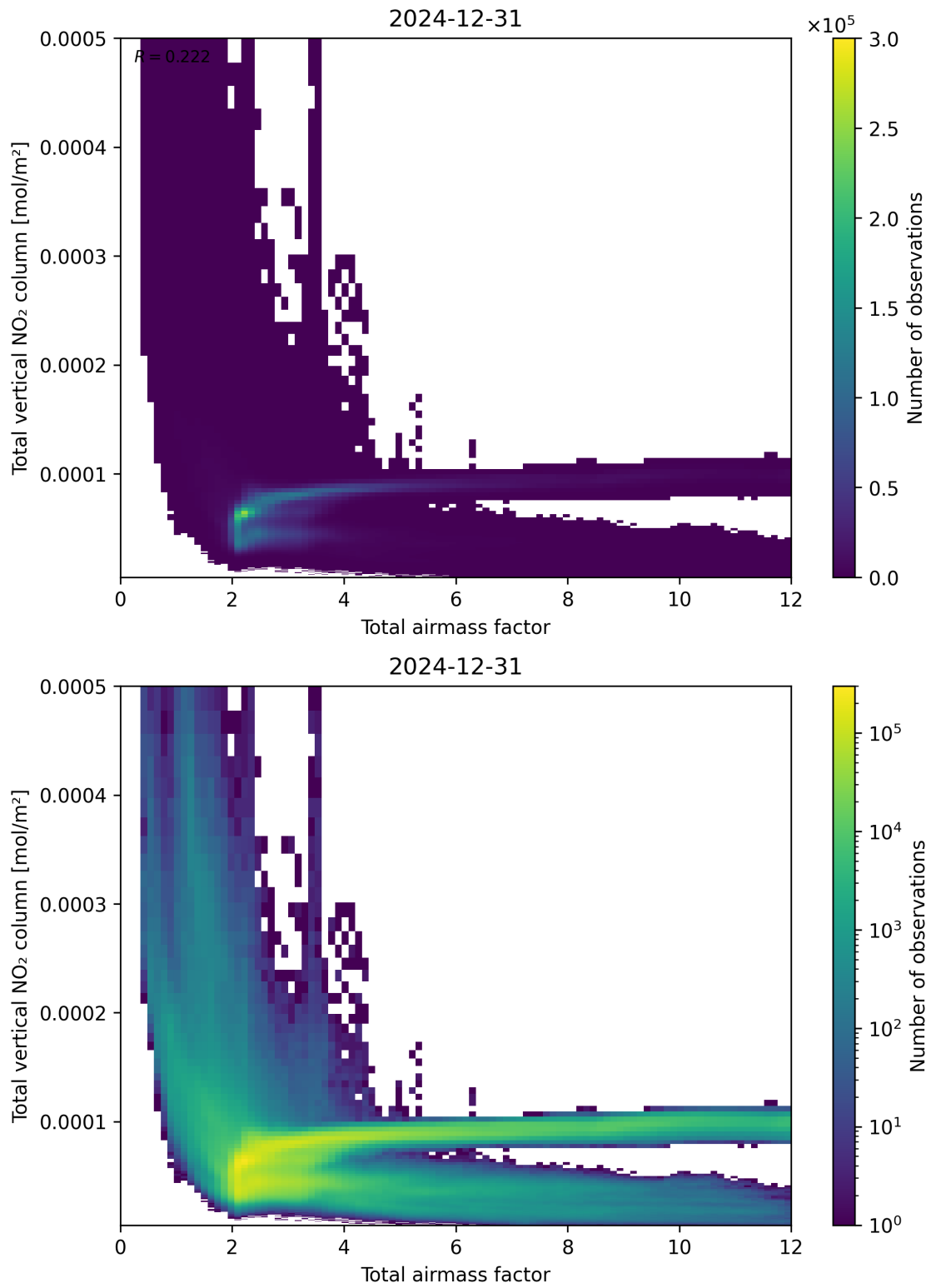
Figure 67: Scatter density plot of “Total airmass factor” against “Total vertical NO 2 column” for 2024-12-30 to 2025-01-01.
