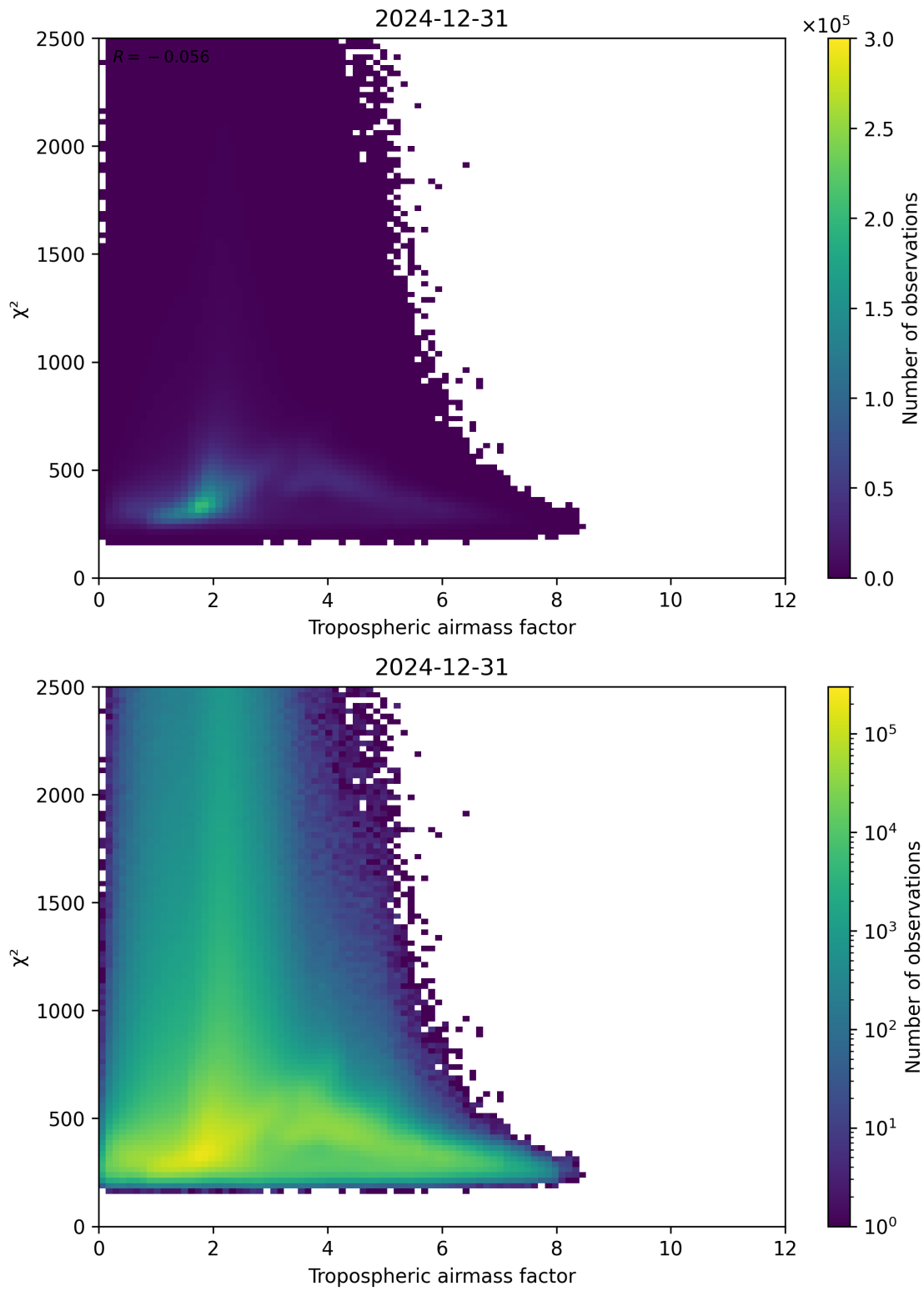
Figure 73: Scatter density plot of “Tropospheric airmass factor” against “ \chi^2 ” for 2024-12-30 to 2025-01-01.
