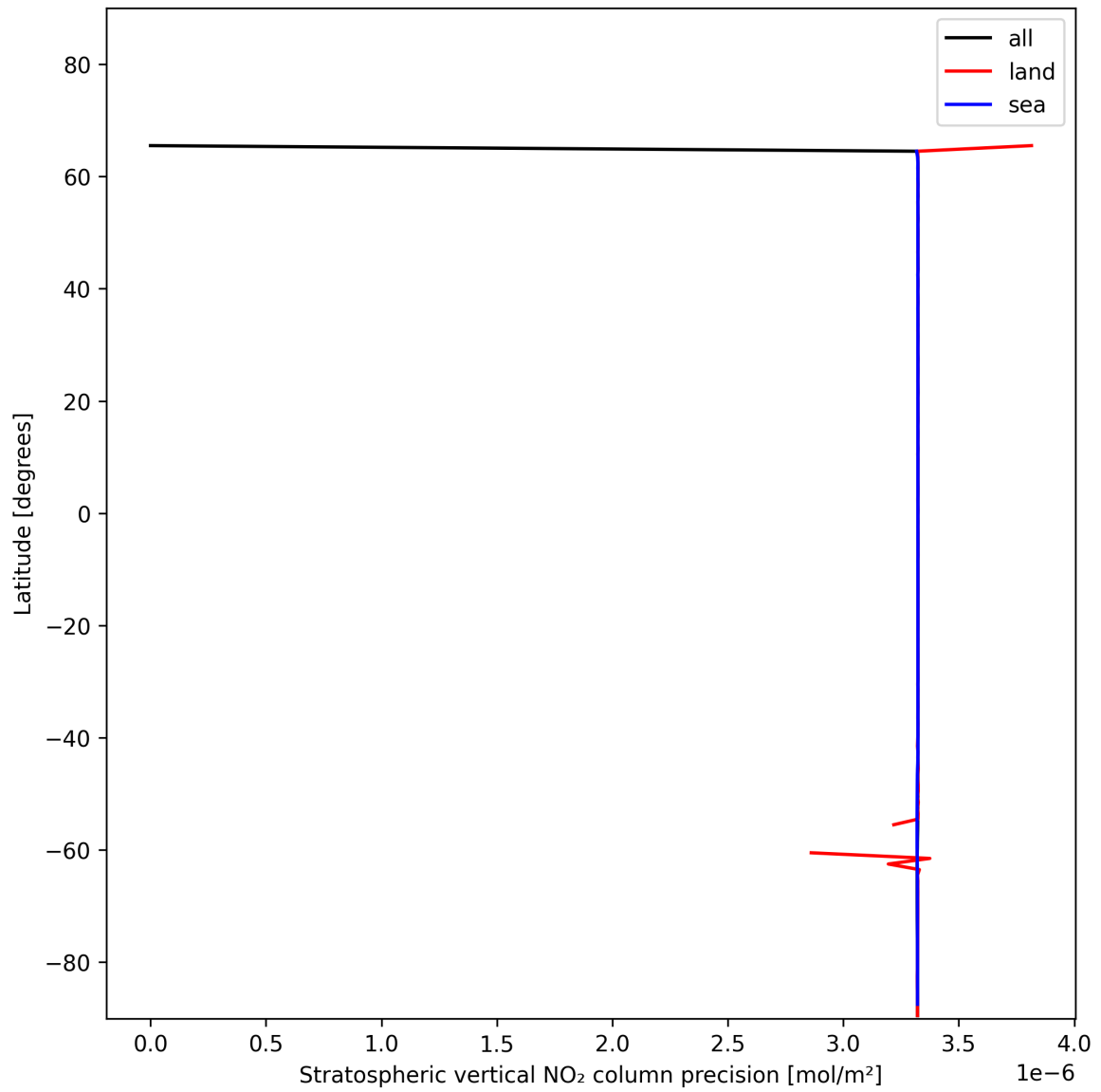
Figure 20: Zonal average of “Stratospheric vertical NO 2 column precision” for 2024-12-30 to 2025-01-01.
