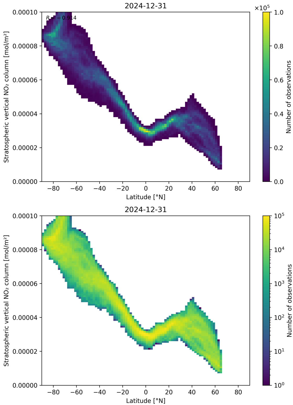
Figure 87: Scatter density plot of “Latitude” against “Stratospheric vertical NO 2 column” for 2024-12-30 to 2025-01-01.
