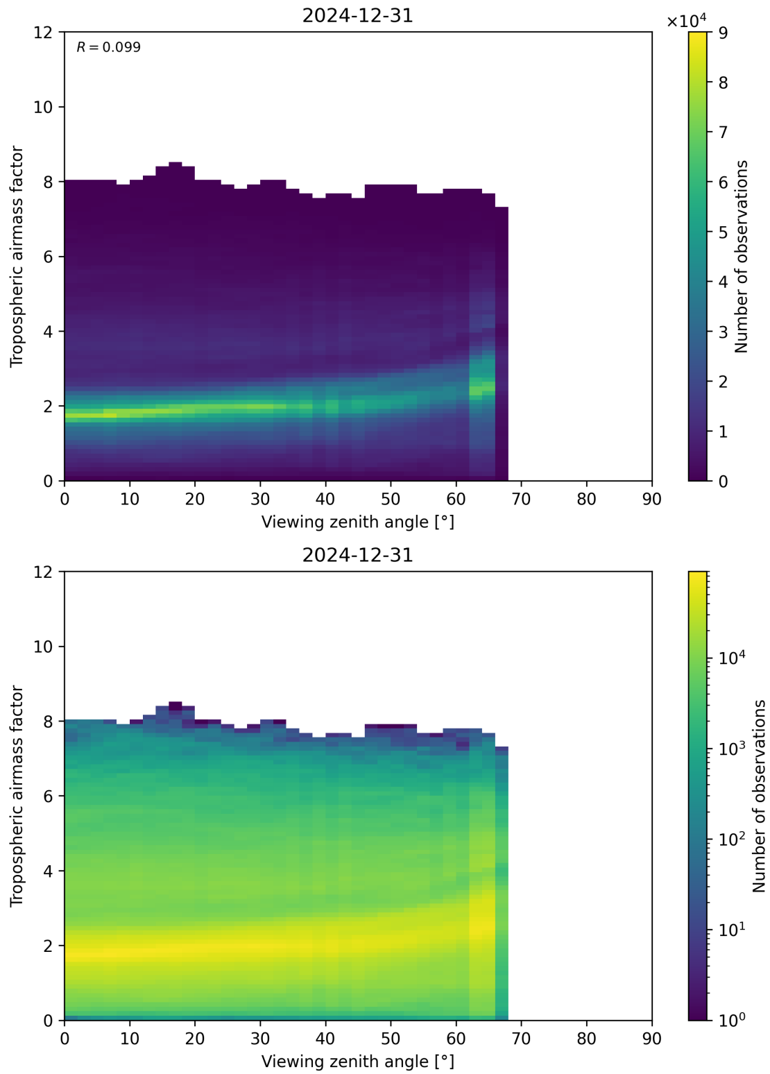
Figure 161: Scatter density plot of “Viewing zenith angle” against “Tropospheric airmass factor” for 2024-12-30 to 2025-01-01.
