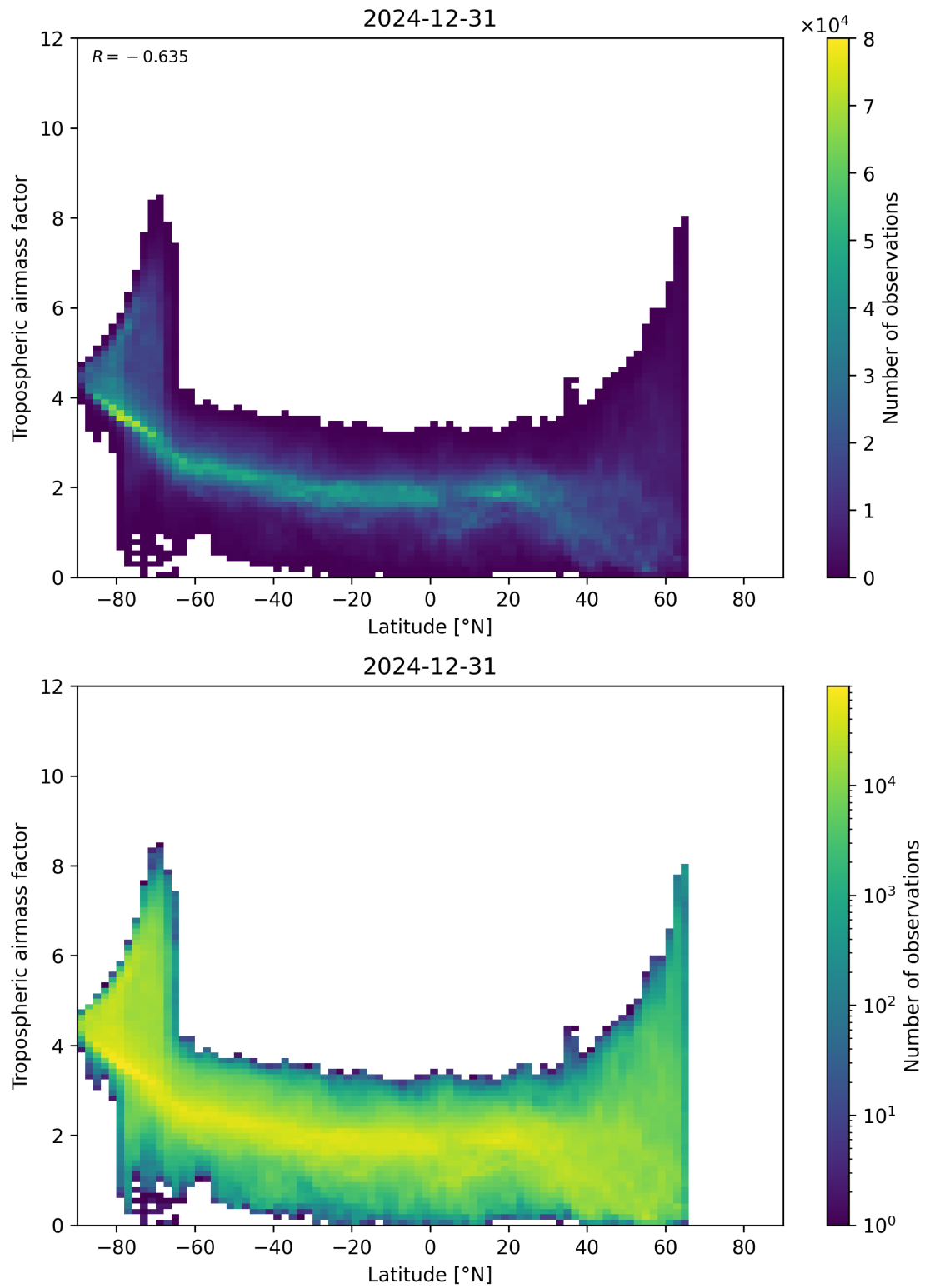
Figure 85: Scatter density plot of “Latitude” against “Tropospheric airmass factor” for 2024-12-30 to 2025-01-01.
