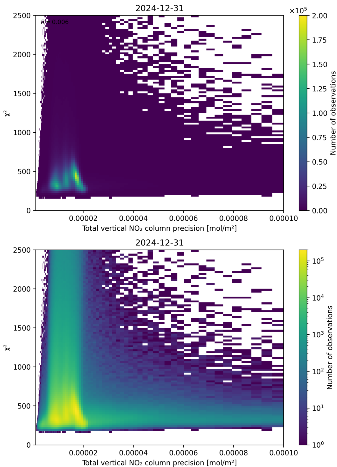
Figure 116: Scatter density plot of “Total vertical NO 2 column precision” against “ \chi^2 ” for 2024-12-30 to 2025-01-01.
