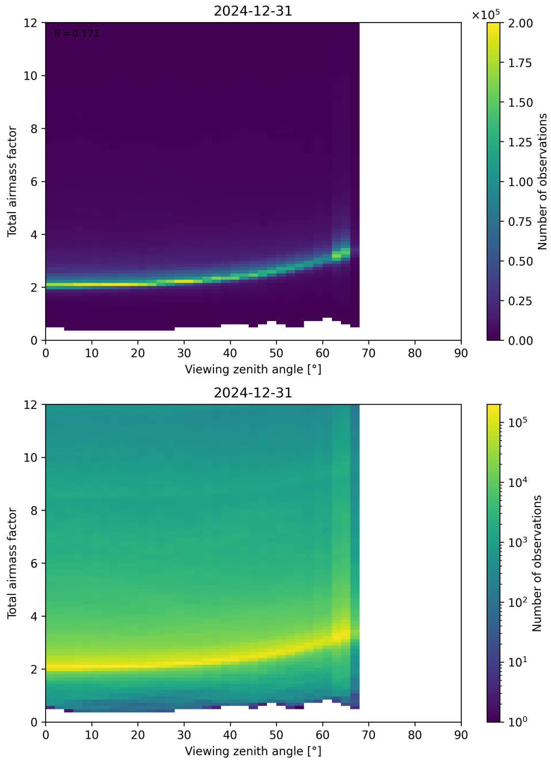
Figure 160: Scatter density plot of “Viewing zenith angle” against “Total airmass factor” for 2024-12-30 to 2025-01-01.
