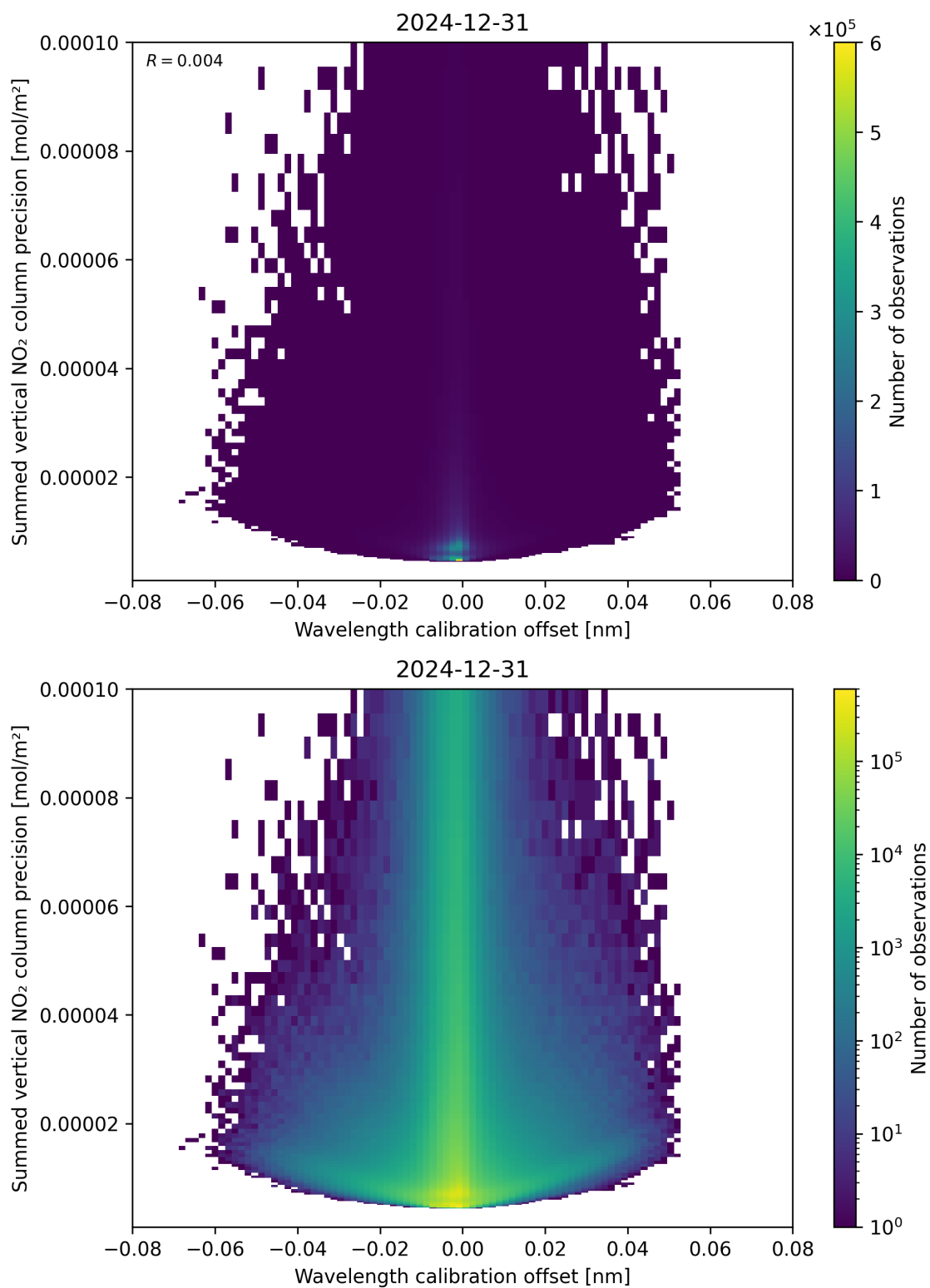
Figure 178: Scatter density plot of “Wavelength calibration offset” against “Summed vertical NO 2 column precision” for 2024-12-30 to 2025-01-01.
