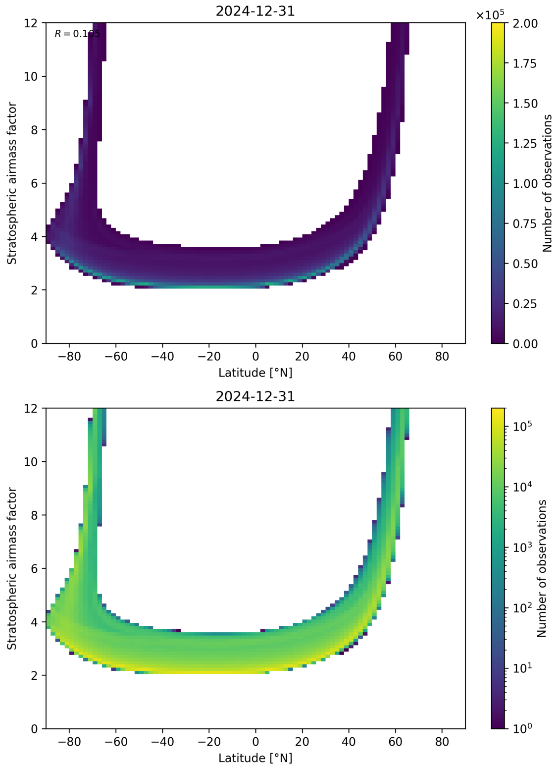
Figure 83: Scatter density plot of “Latitude” against “Stratospheric air mass factor” for 2024-12-30 to 2025-01-01.
