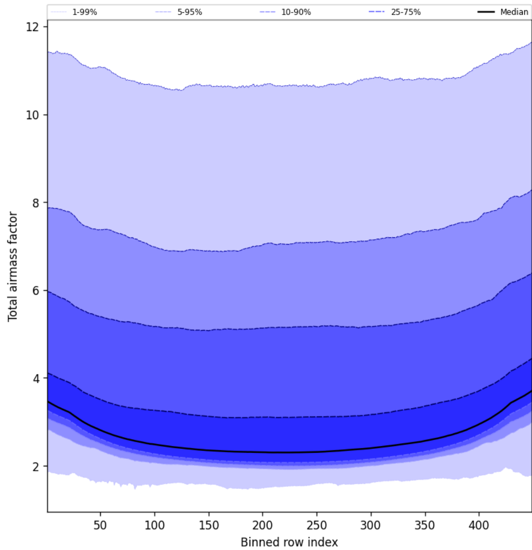
Figure 49: Along track statistics of “Total airmass factor” for 2024-12-30 to 2025-01-01
