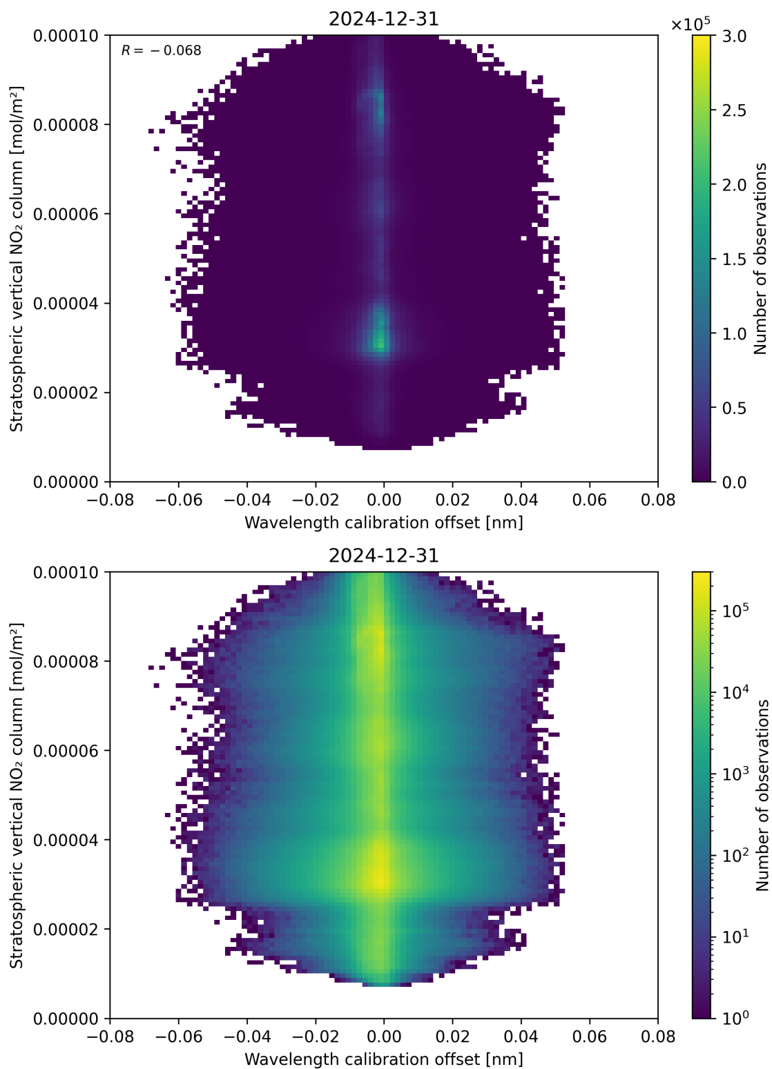
Figure 176: Scatter density plot of “Wavelength calibration offset” against “Stratospheric vertical NO 2 column” for 2024-12-30 to 2025-01-01.
