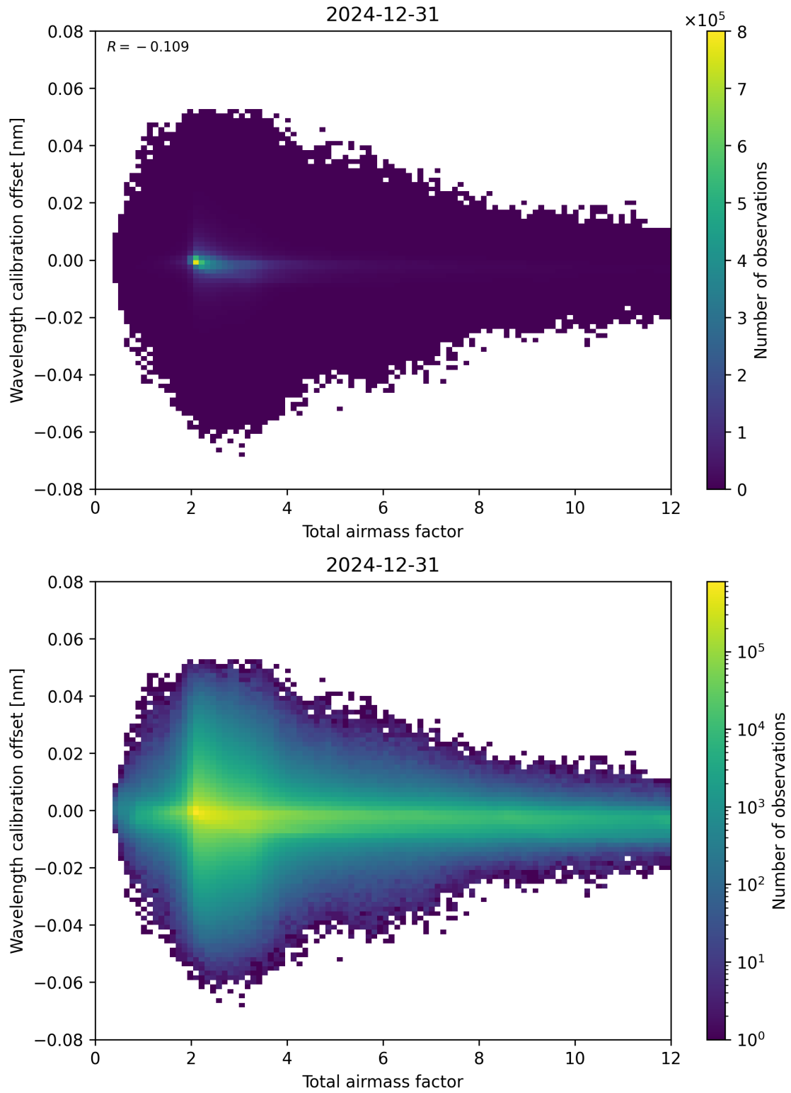
Figure 70: Scatter density plot of “Total airmass factor” against “Wavelength calibration offset” for 2024-12-30 to 2025-01-01.
