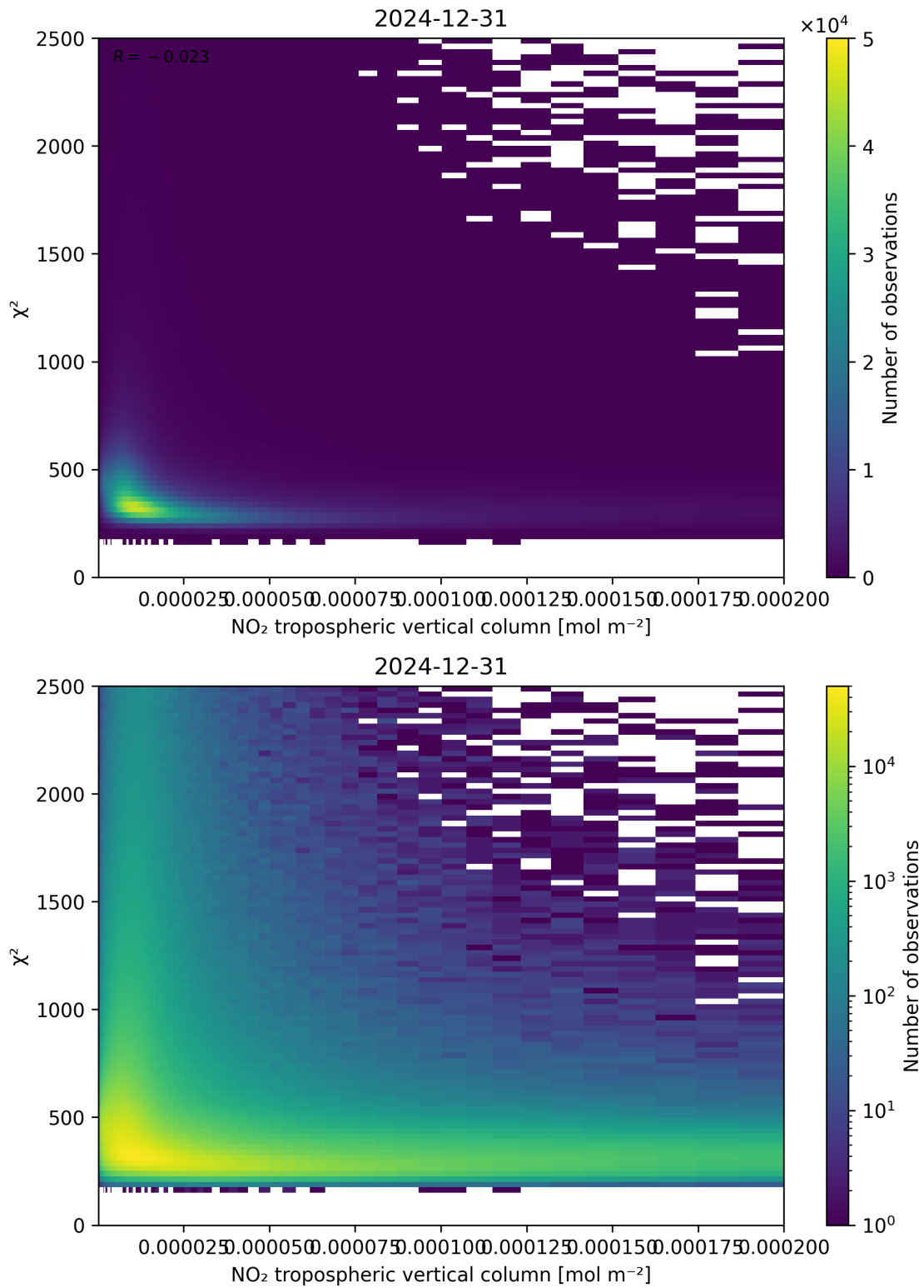
Figure 124: Scatter density plot of “NO 2 tropospheric vertical column” against “ \chi^2 ” for 2024-12-30 to 2025-01-01.
