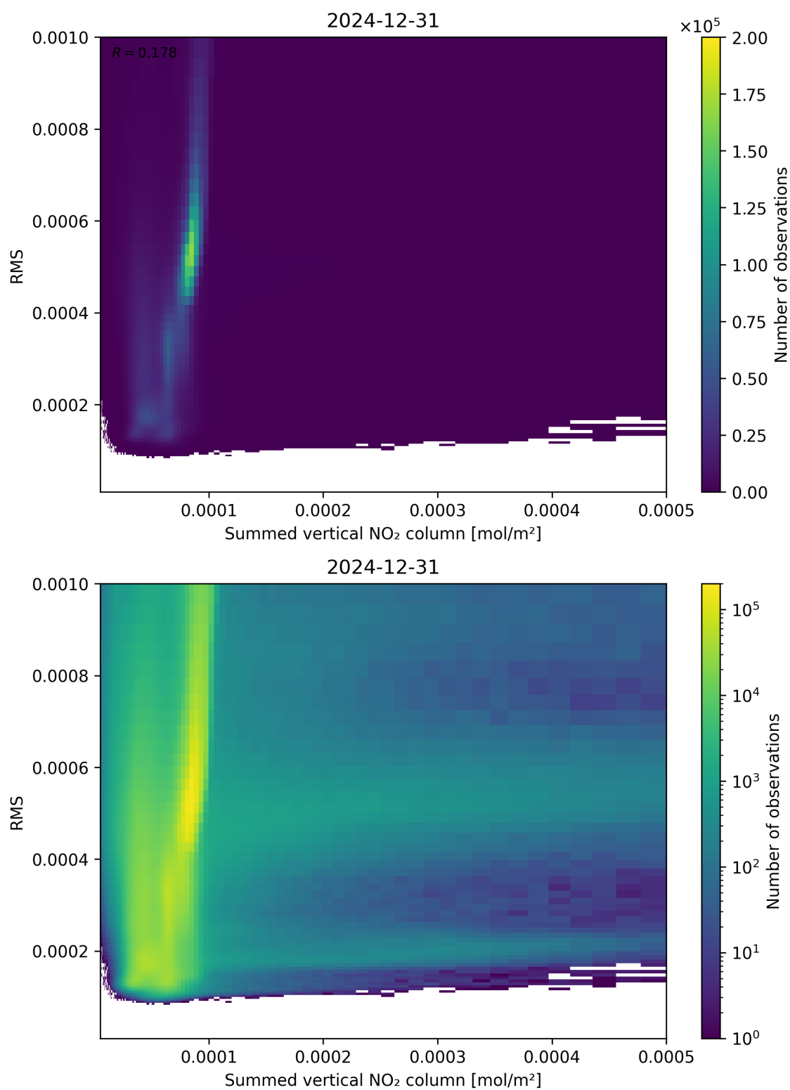
Figure 109: Scatter density plot of “Summed vertical NO 2 column” against “RMS” for 2024-12-30 to 2025-01-01.
