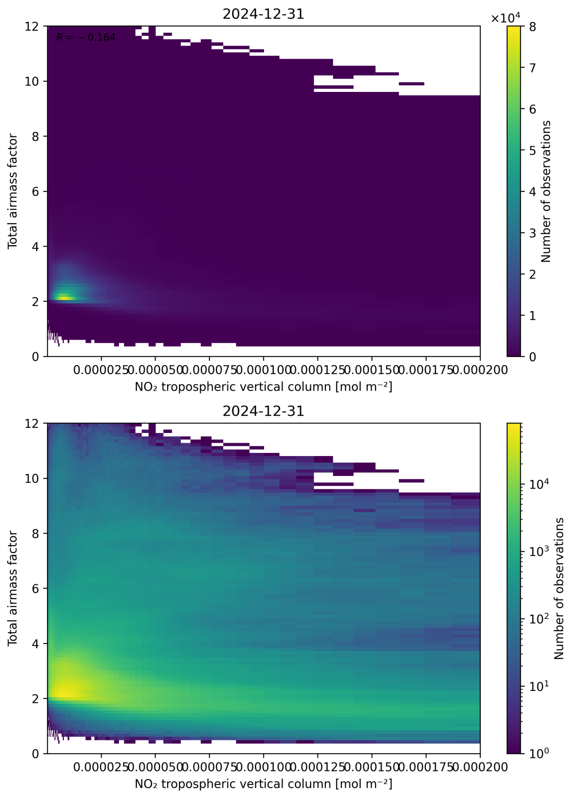
Figure 122: Scatter density plot of “NO 2 tropospheric vertical column” against “Total air mass factor” for 2024-12-30 to 2025-01-01.
