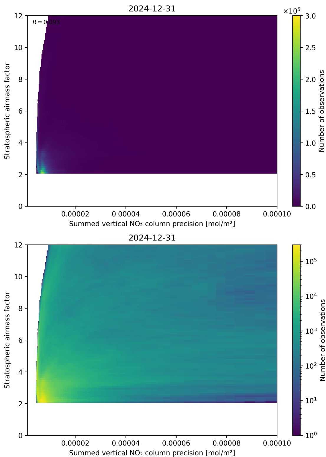
Figure 106: Scatter density plot of “Summed vertical NO 2 column precision” against “Stratospheric airmass factor” for 2024-12-30 to 2025-01-01.
