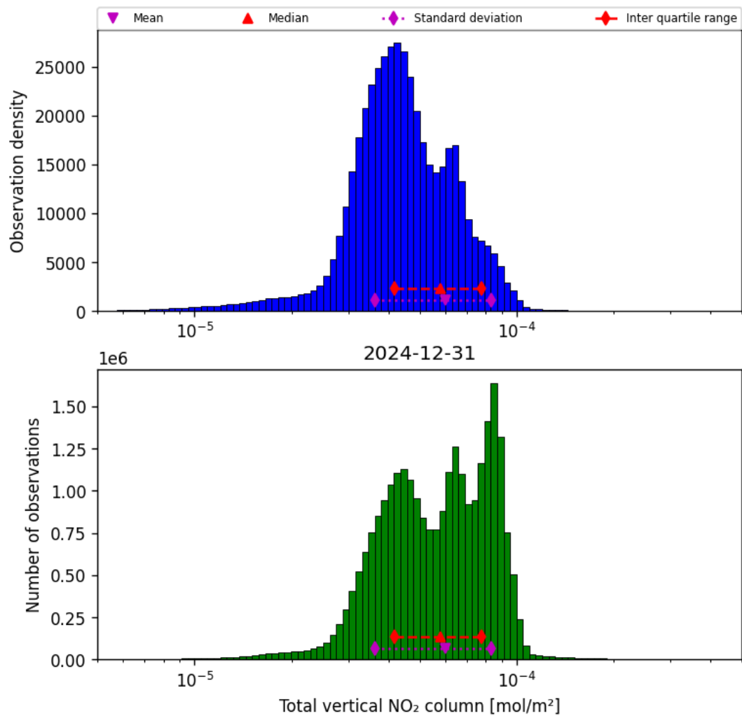
Figure 38: Histogram of “Total vertical NO 2 column” for 2024-12-30 to 2025-01-01
