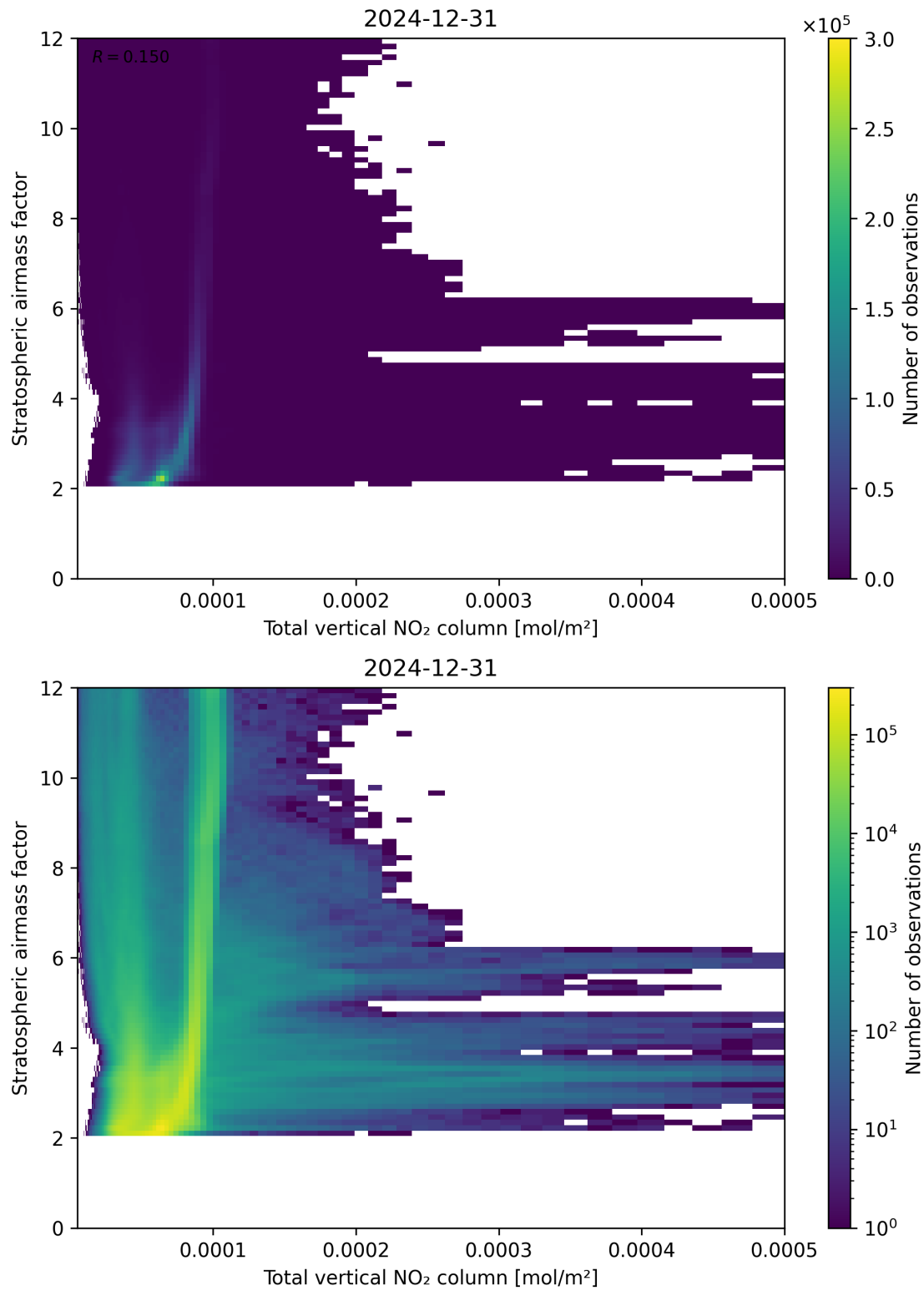
Figure 110: Scatter density plot of “Total vertical NO 2 column” against “Stratospheric airmass factor” for 2024-12-30 to 2025-01-01.
