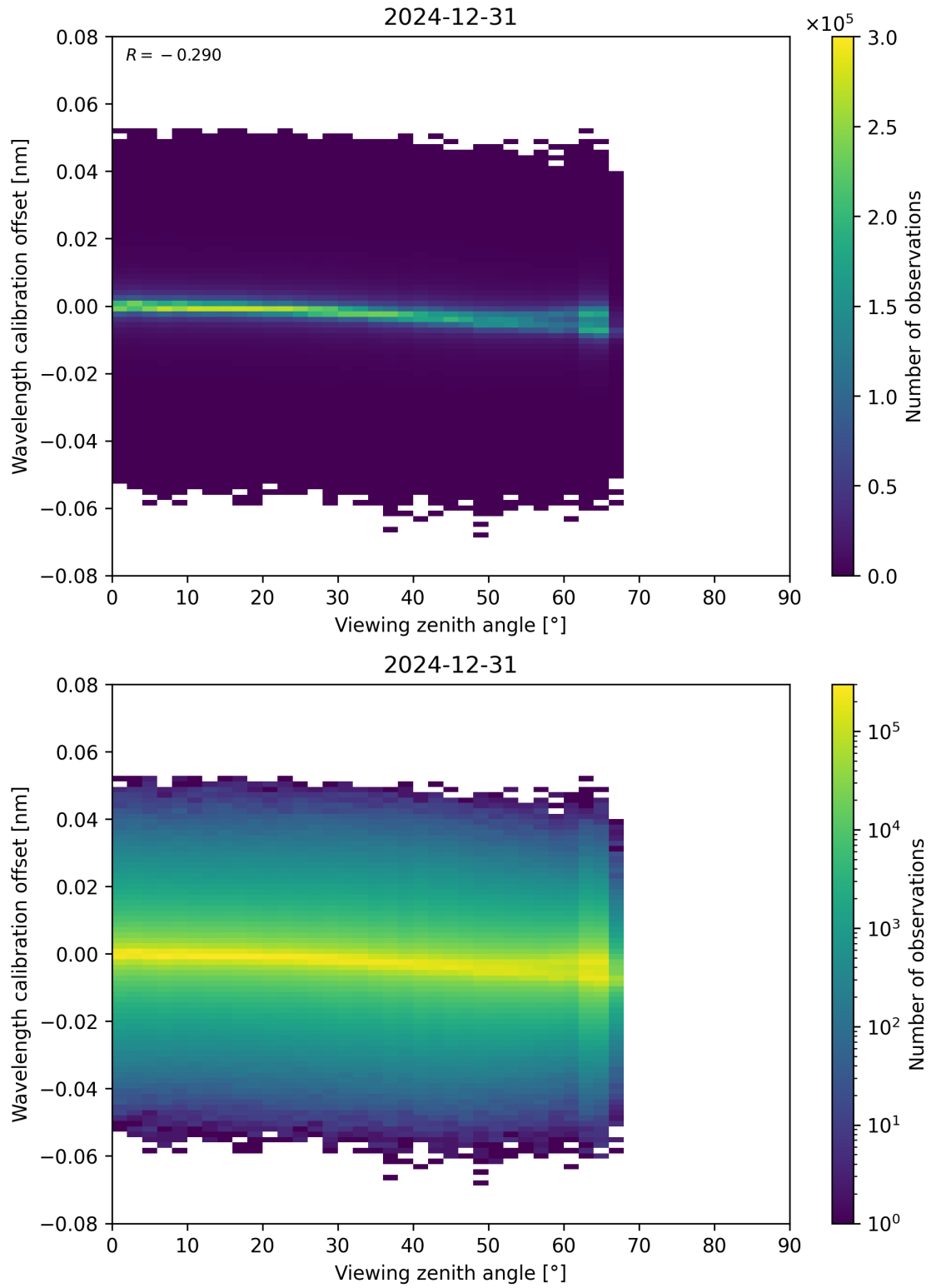
Figure 173: Scatter density plot of “Viewing zenith angle” against “Wavelength calibration offset” for 2024-12-30 to 2025-01-01.
