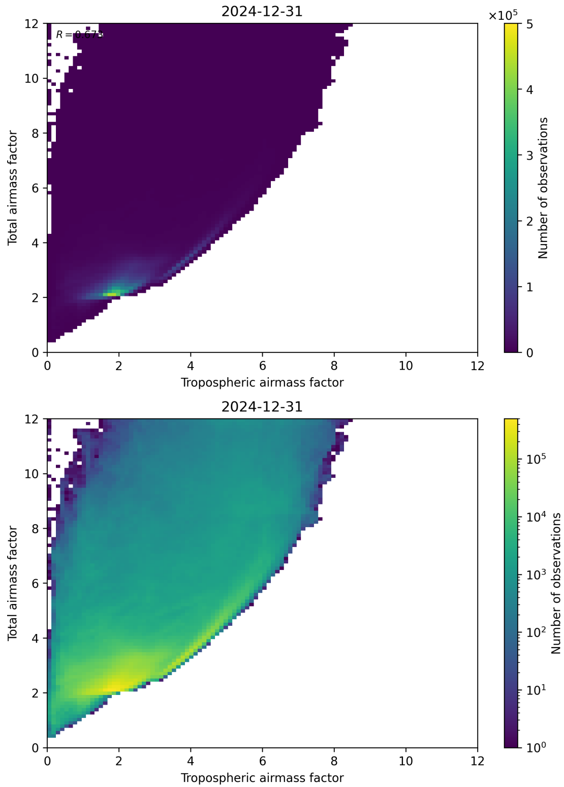
Figure 72: Scatter density plot of “Tropospheric airmass factor” against “Total airmass factor” for 2024-12-30 to 2025-01-01.
