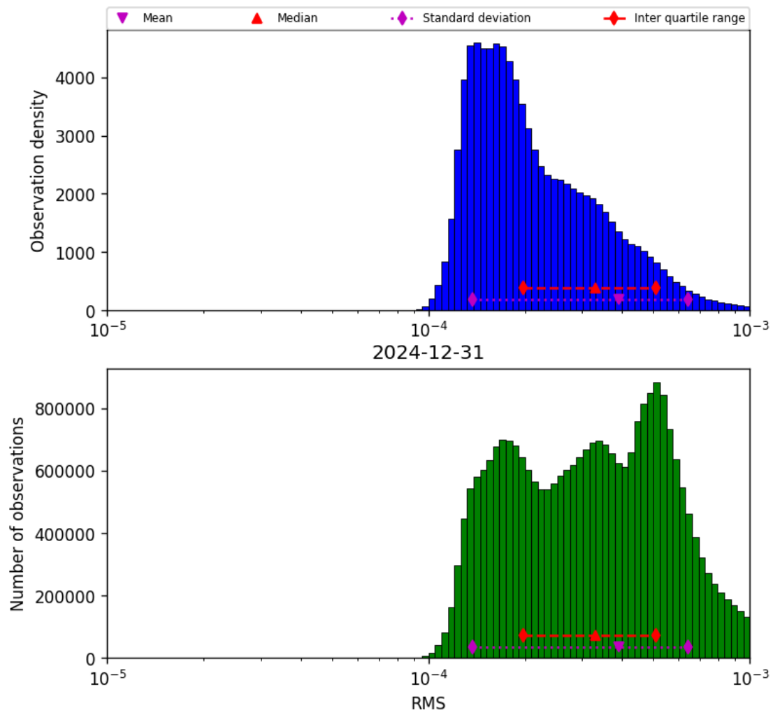
Figure 43: Histogram of “RMS” for 2024-12-30 to 2025-01-01
