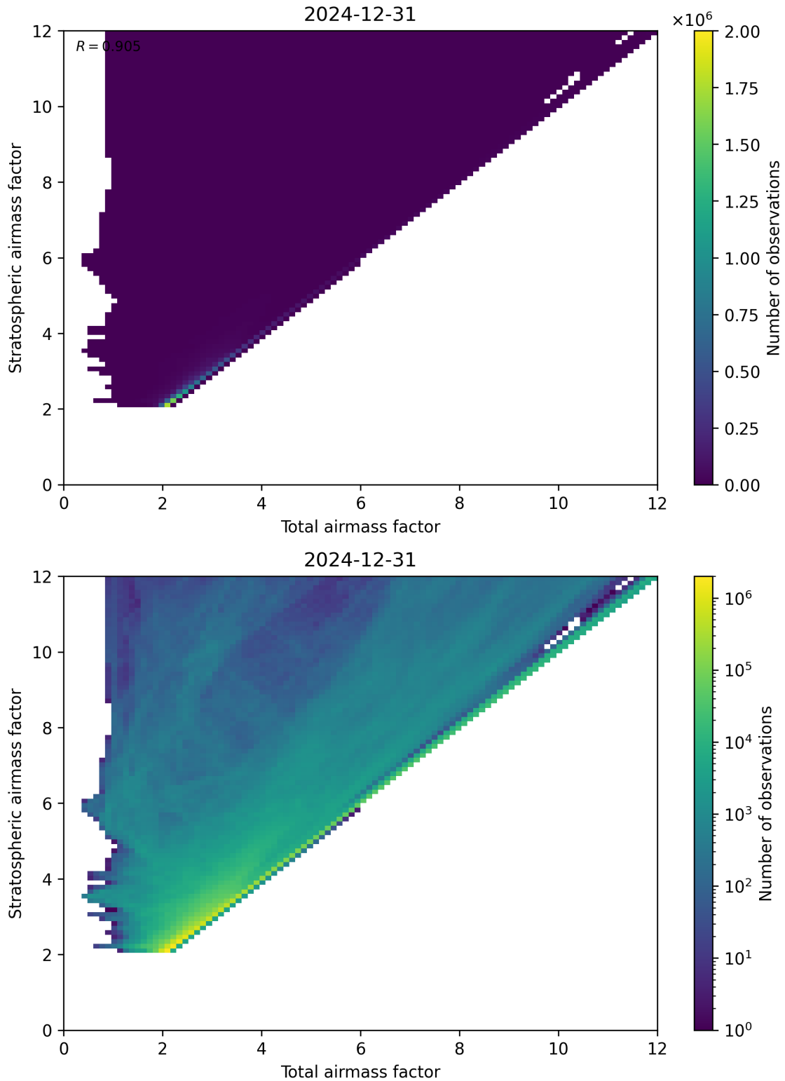
Figure 62: Scatter density plot of “Total airmass factor” against “Stratospheric airmass factor” for 2024-12-30 to 2025-01-01.
