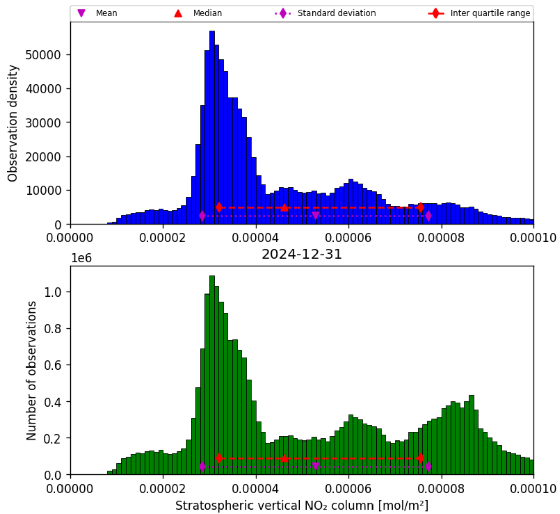
Figure 36: Histogram of “Stratospheric vertical NO 2 column” for 2024-12-30 to 2025-01-01
