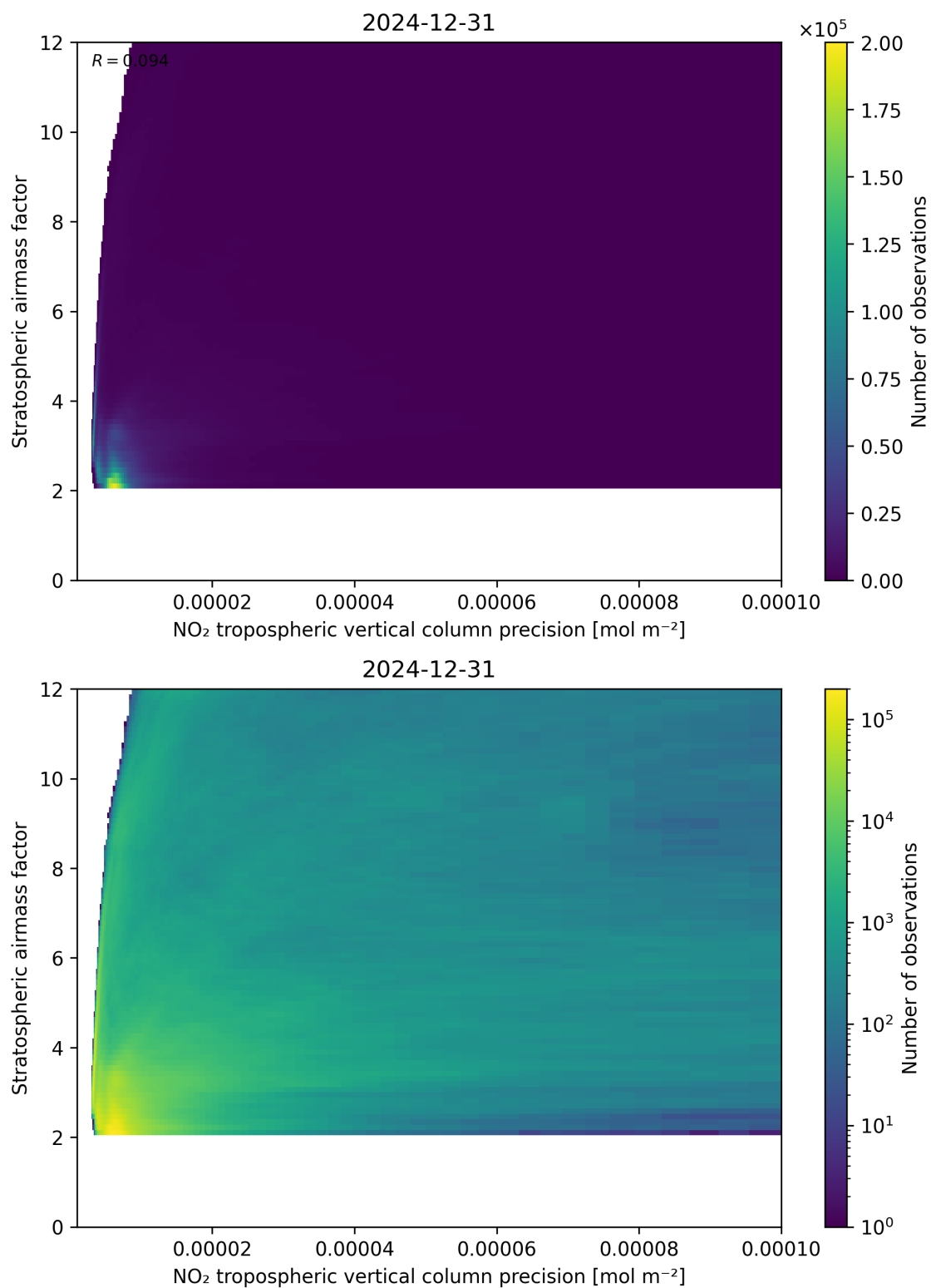
Figure 131: Scatter density plot of “NO 2 tropospheric vertical column precision” against “Stratospheric airmass factor” for 2024-12-30 to 2025-01-01.
