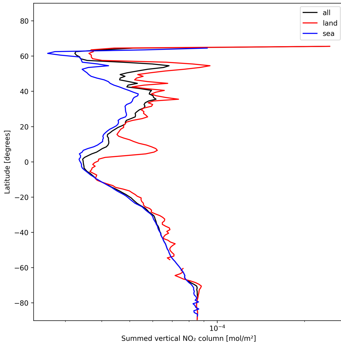
Figure 23: Zonal average of “Summed vertical NO 2 column” for 2024-12-30 to 2025-01-01.
