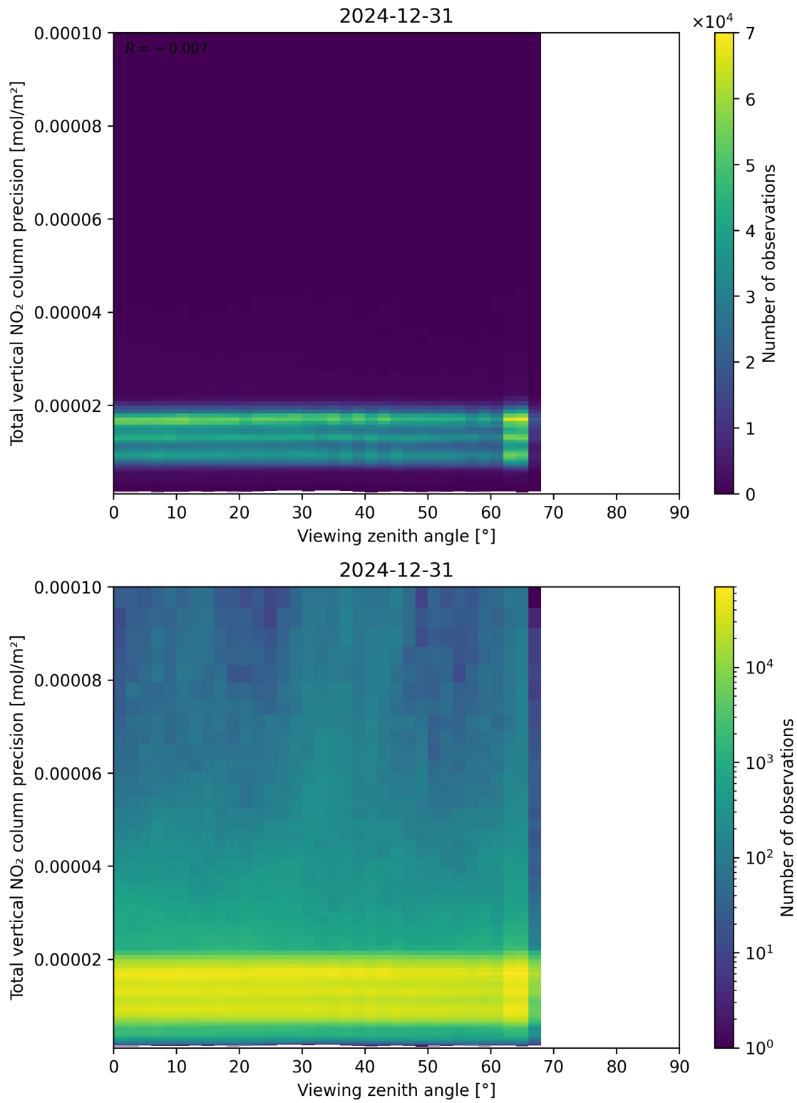
Figure 168: Scatter density plot of “Viewing zenith angle” against “Total vertical NO 2 column precision” for 2024-12-30 to 2025-01-01.
