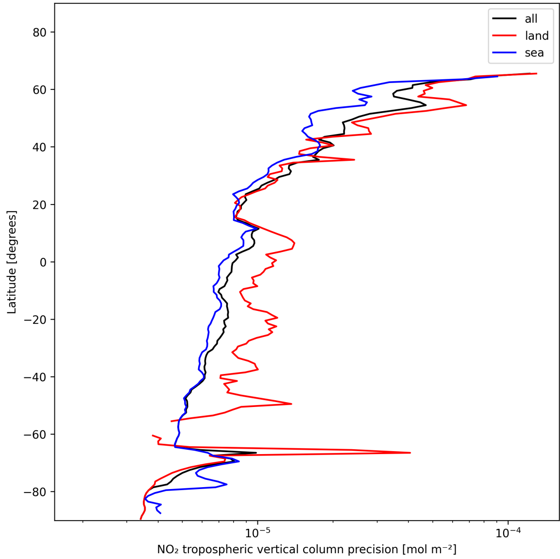
Figure 13: Zonal average of “NO 2 tropospheric vertical column precision” for 2024-12-30 to 2025-01-01.
