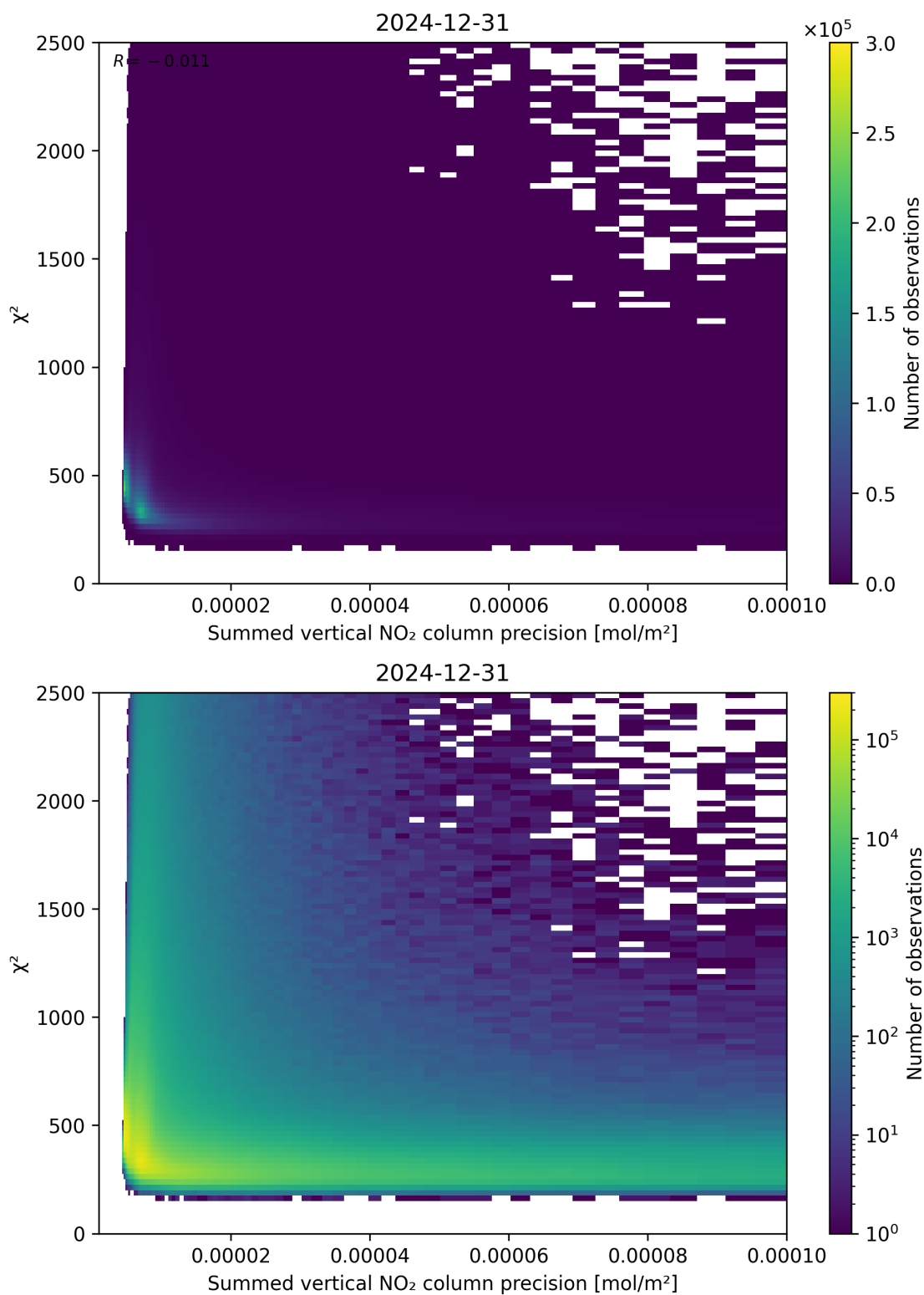
Figure 107: Scatter density plot of “Summed vertical NO 2 column precision” against “ \chi^2 ” for 2024-12-30 to 2025-01-01.
