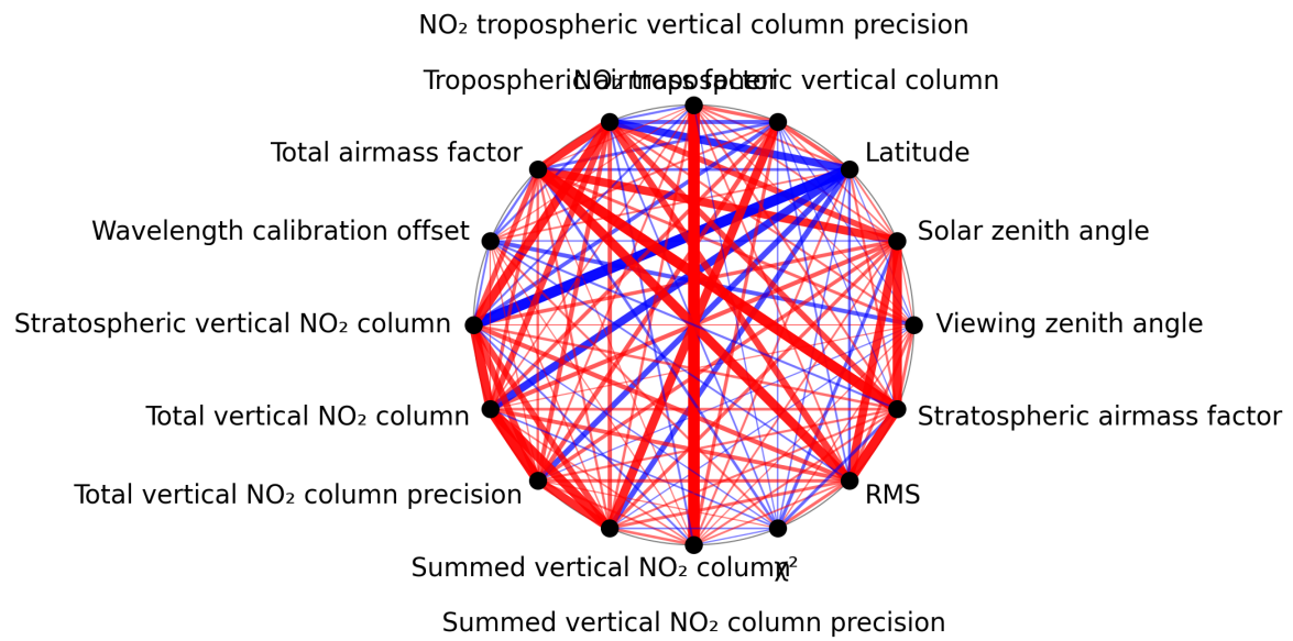
Figure 1: Map of correlation graph for 2024-12-30 to 2025-01-01.
