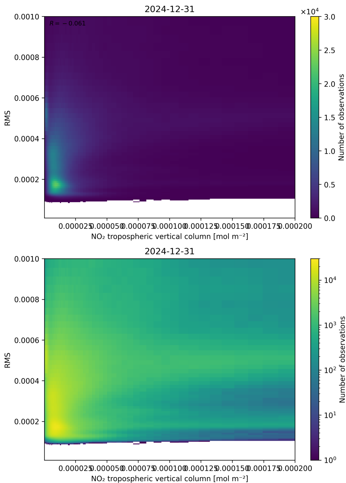
Figure 142: Scatter density plot of “NO 2 tropospheric vertical column” against “RMS” for 2024-12-30 to 2025-01-01.
