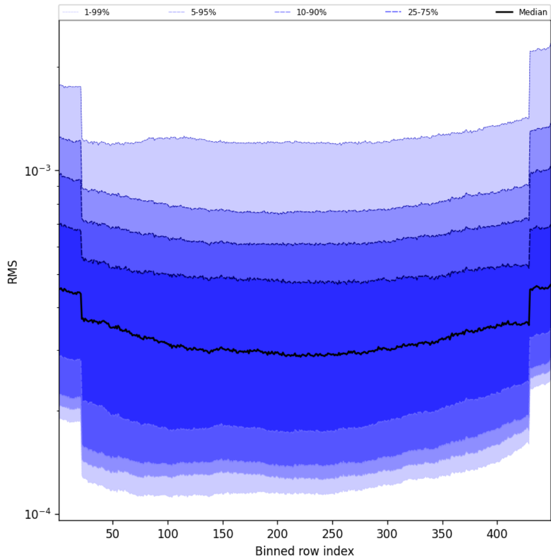
Figure 60: Along track statistics of “RMS” for 2024-12-30 to 2025-01-01
