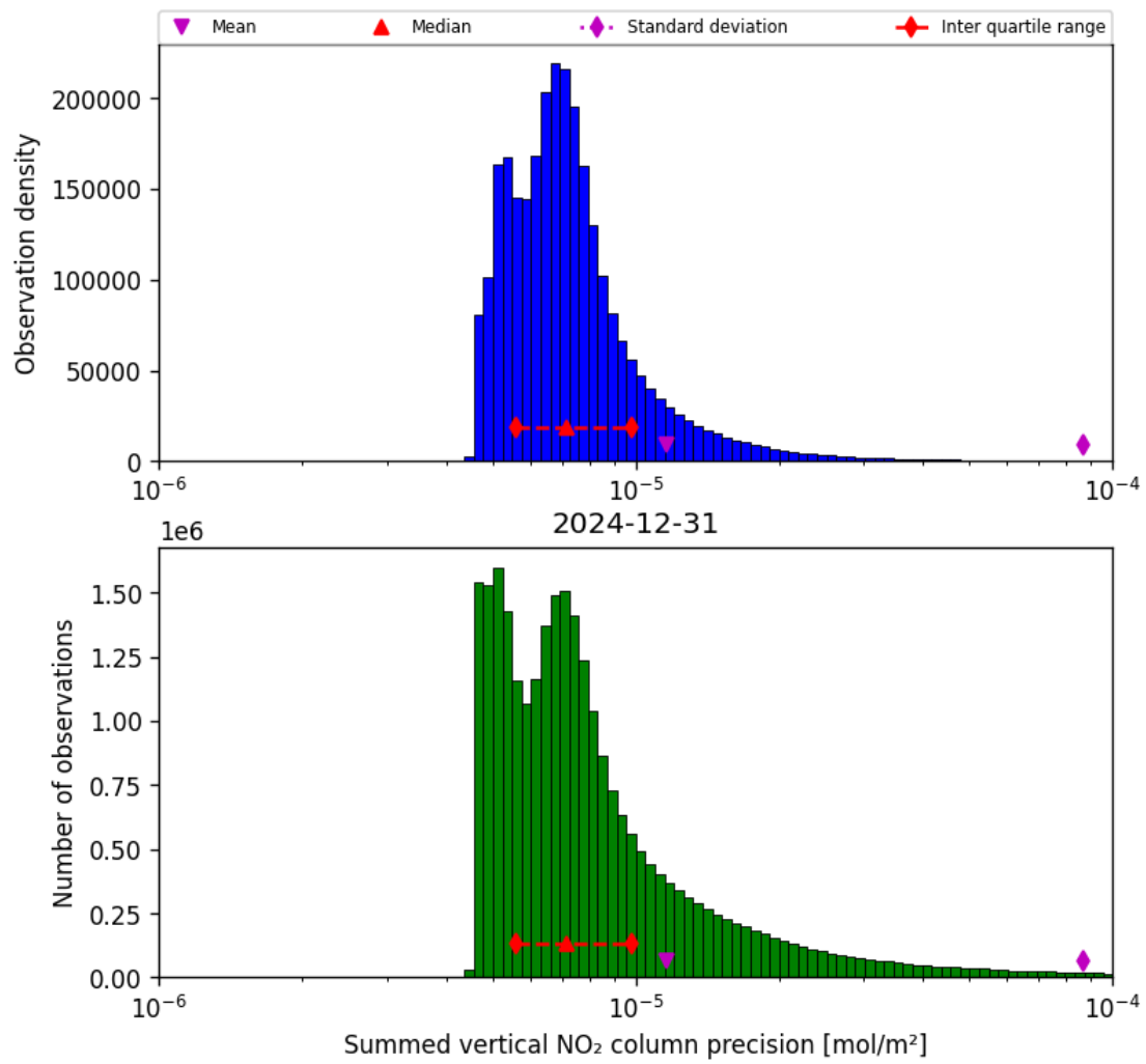
Figure 41: Histogram of “Summed vertical NO 2 column precision” for 2024-12-30 to 2025-01-01
