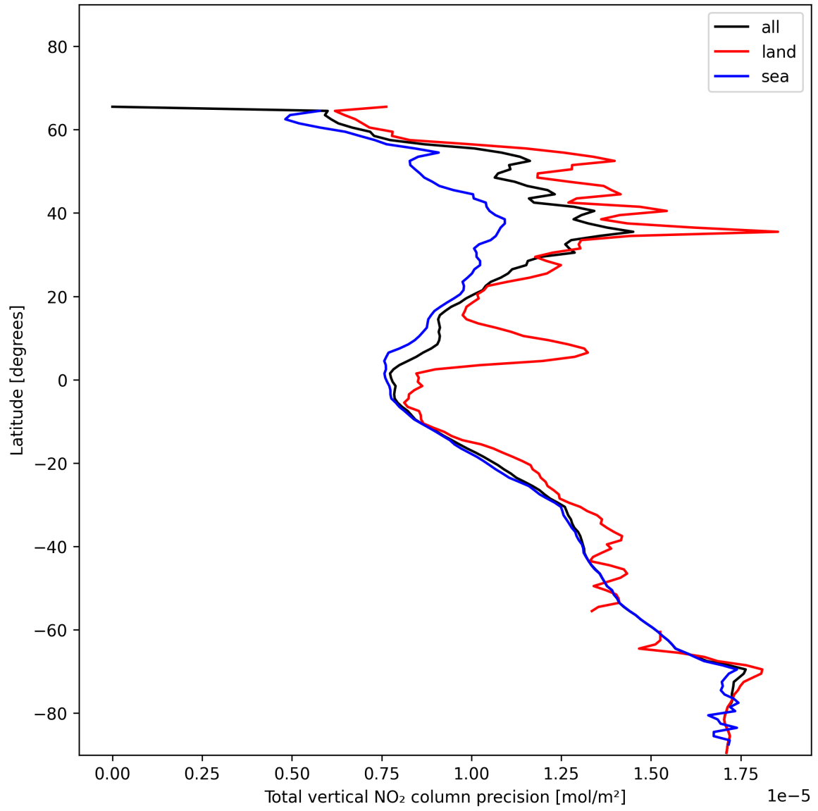
Figure 22: Zonal average of “Total vertical NO 2 column precision” for 2024-12-30 to 2025-01-01.
