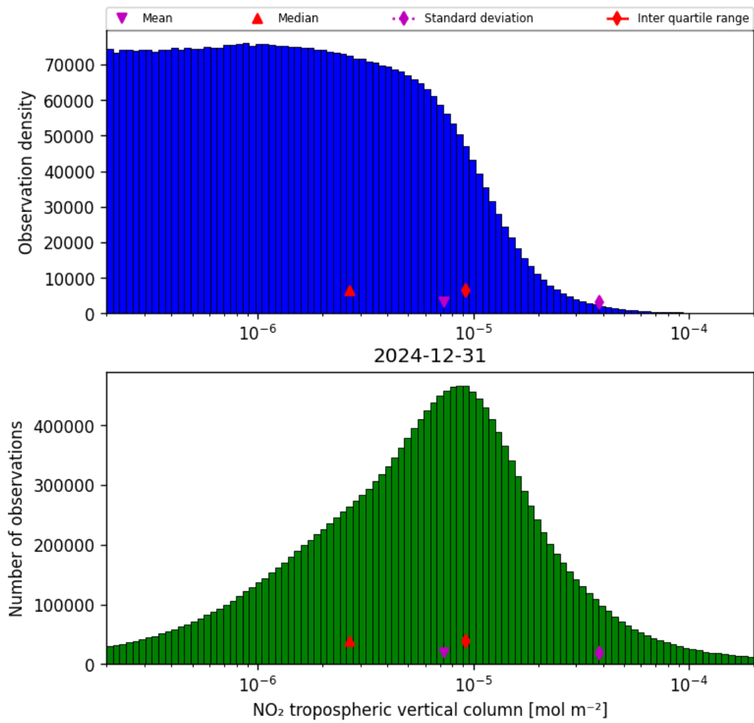
Figure 29: Histogram of “NO 2 tropospheric vertical column” for 2024-12-30 to 2025-01-01
