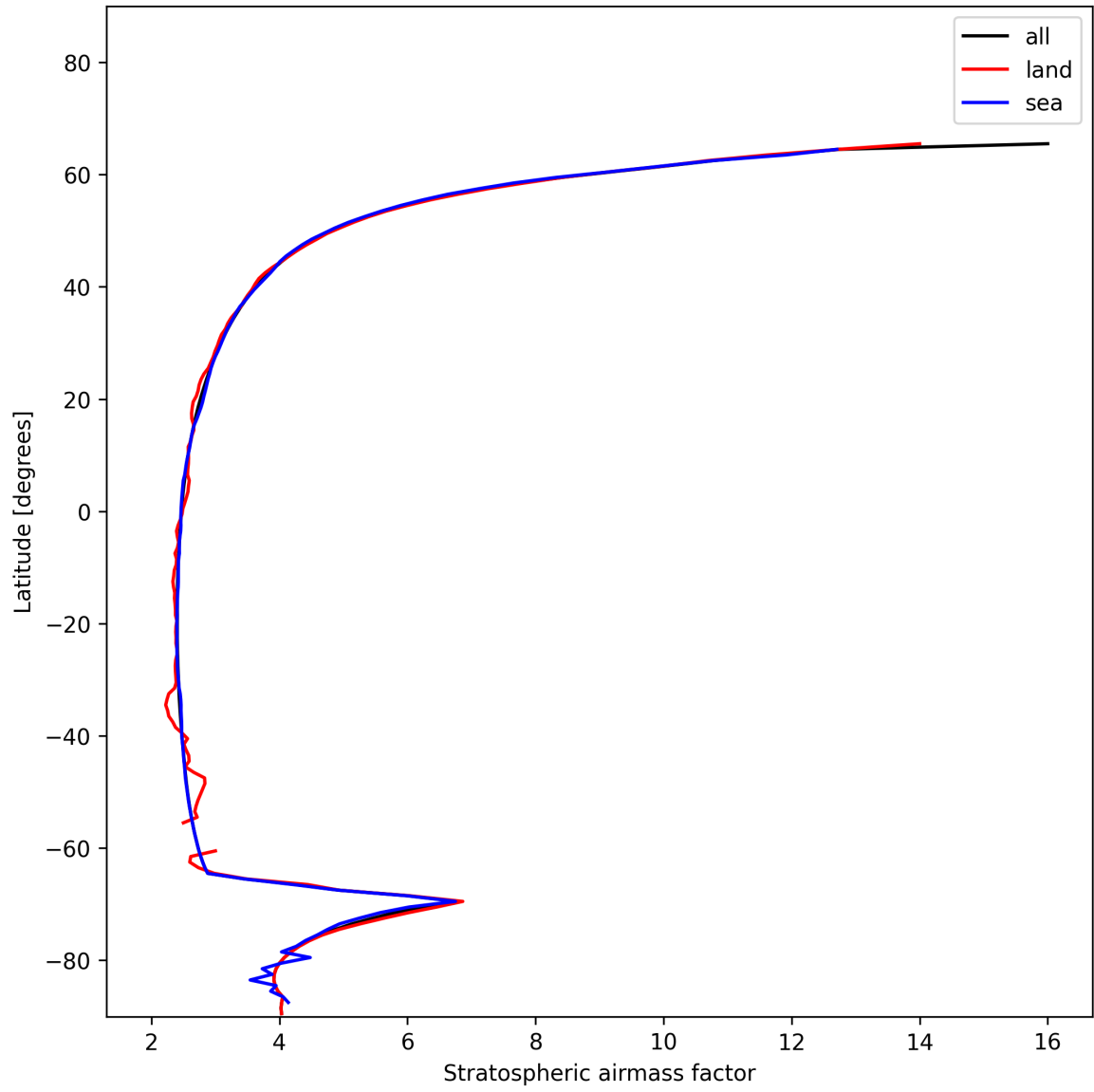
Figure 27: Zonal average of “Stratospheric airmass factor” for 2024-12-30 to 2025-01-01.
