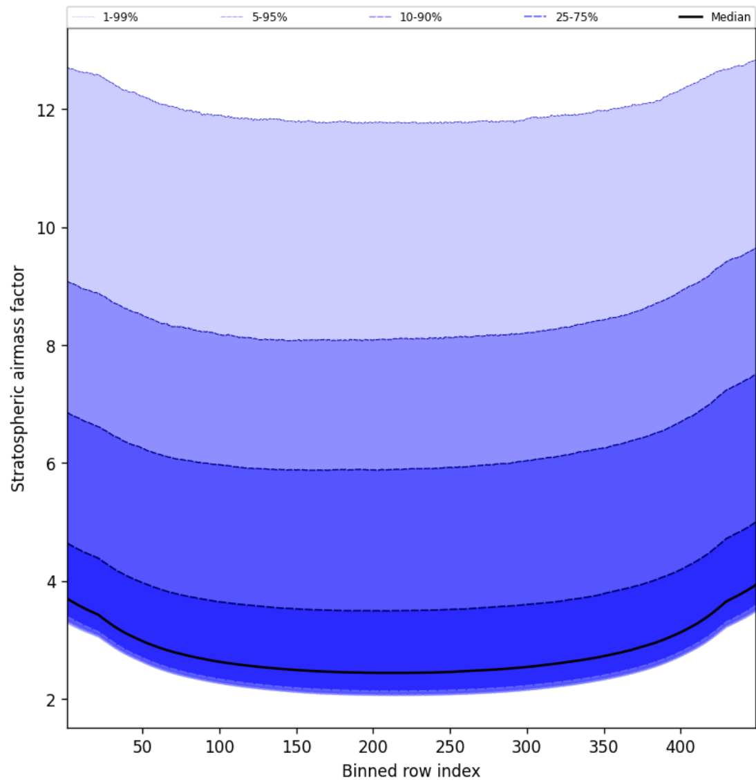
Figure 61: Along track statistics of “Stratospheric airmass factor” for 2024-12-30 to 2025-01-01
