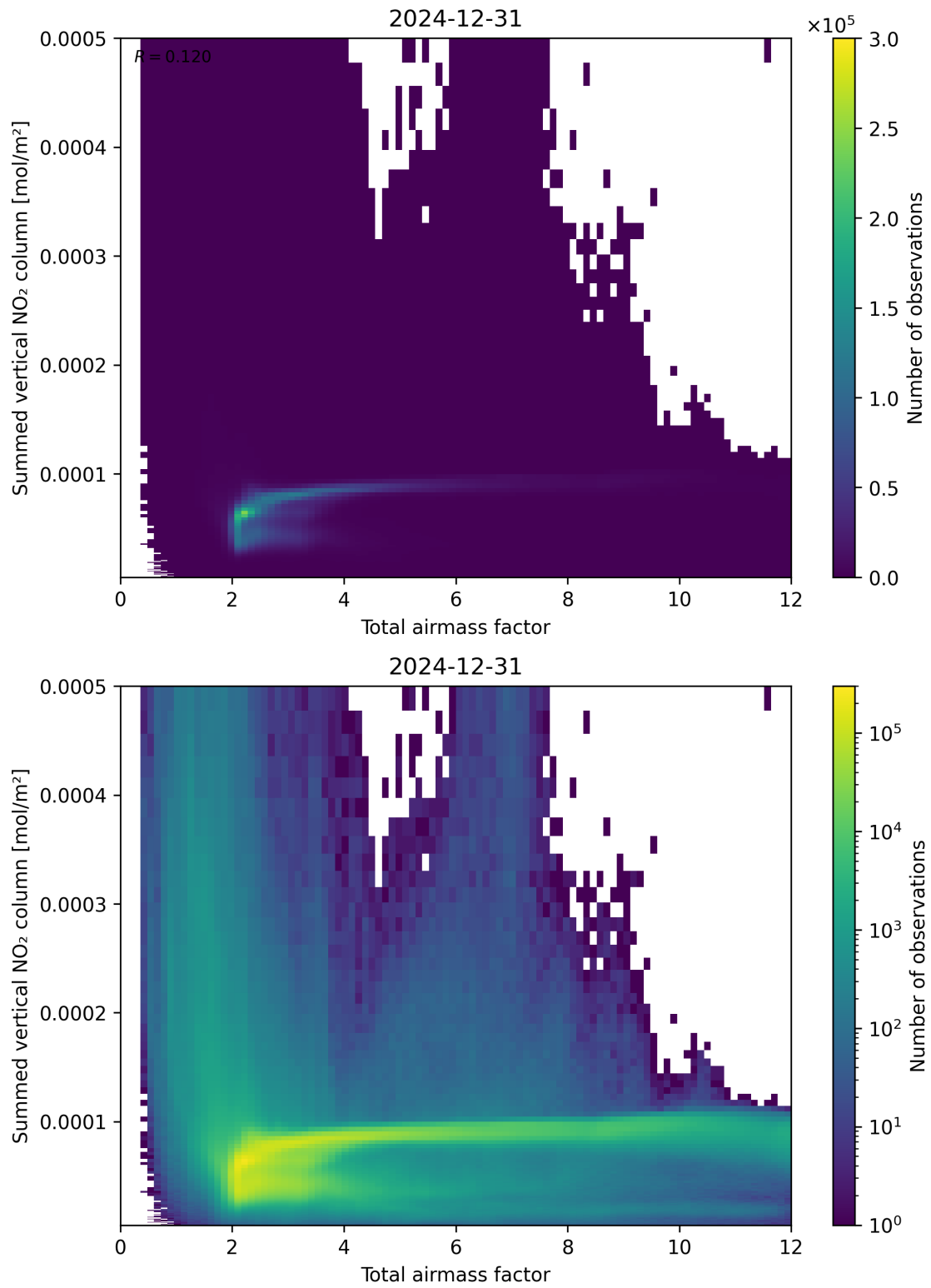
Figure 65: Scatter density plot of “Total airmass factor” against “Summed vertical NO 2 column” for 2024-12-30 to 2025-01-01.
