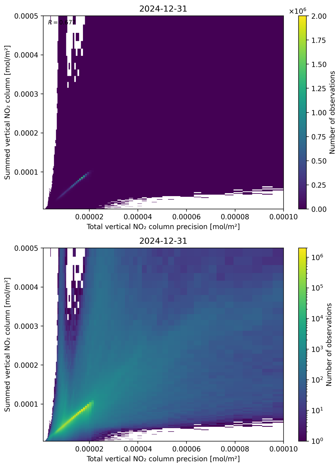
Figure 117: Scatter density plot of “Total vertical NO 2 column precision” against “Summed vertical NO 2 column” for 2024-12-30 to 2025-01-01.
