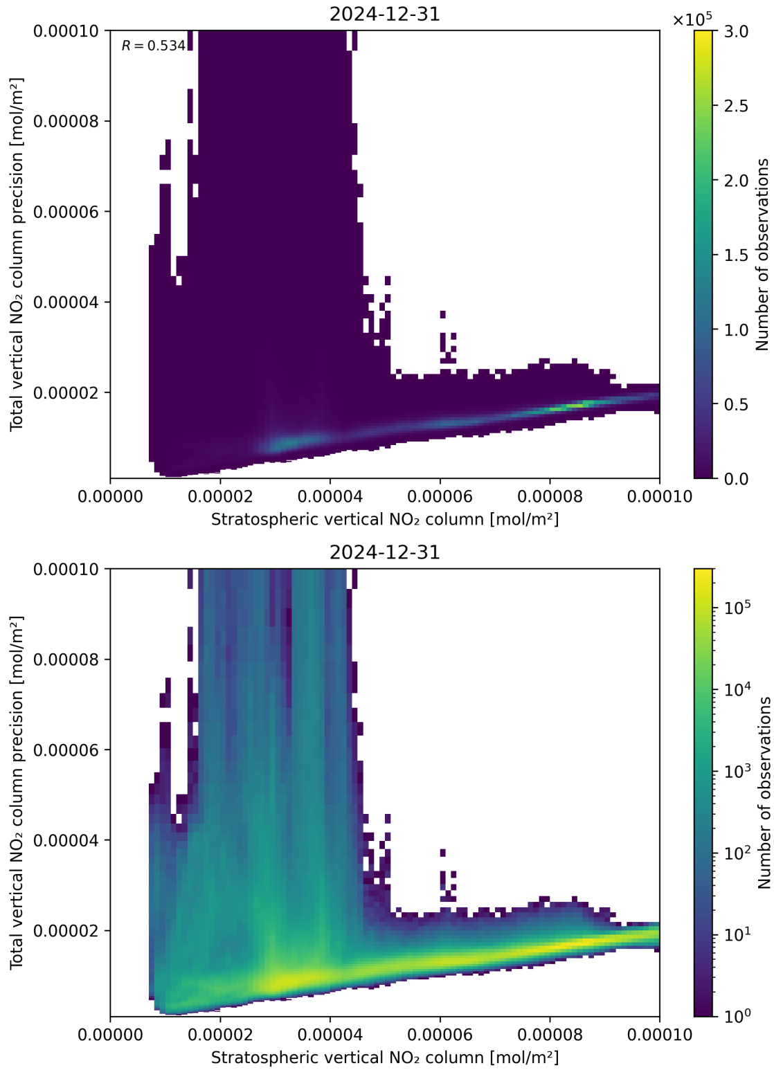
Figure 101: Scatter density plot of “Stratospheric vertical NO 2 column” against “Total vertical NO 2 column precision” for 2024-12-30 to 2025-01-01.
