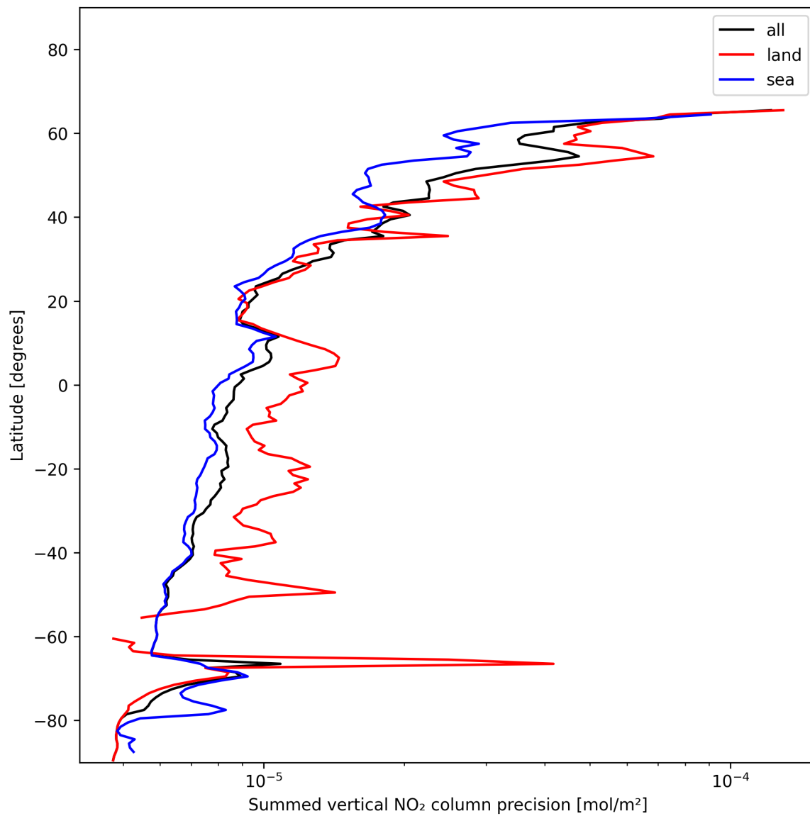
Figure 24: Zonal average of “Summed vertical NO 2 column precision” for 2024-12-30 to 2025-01-01.
