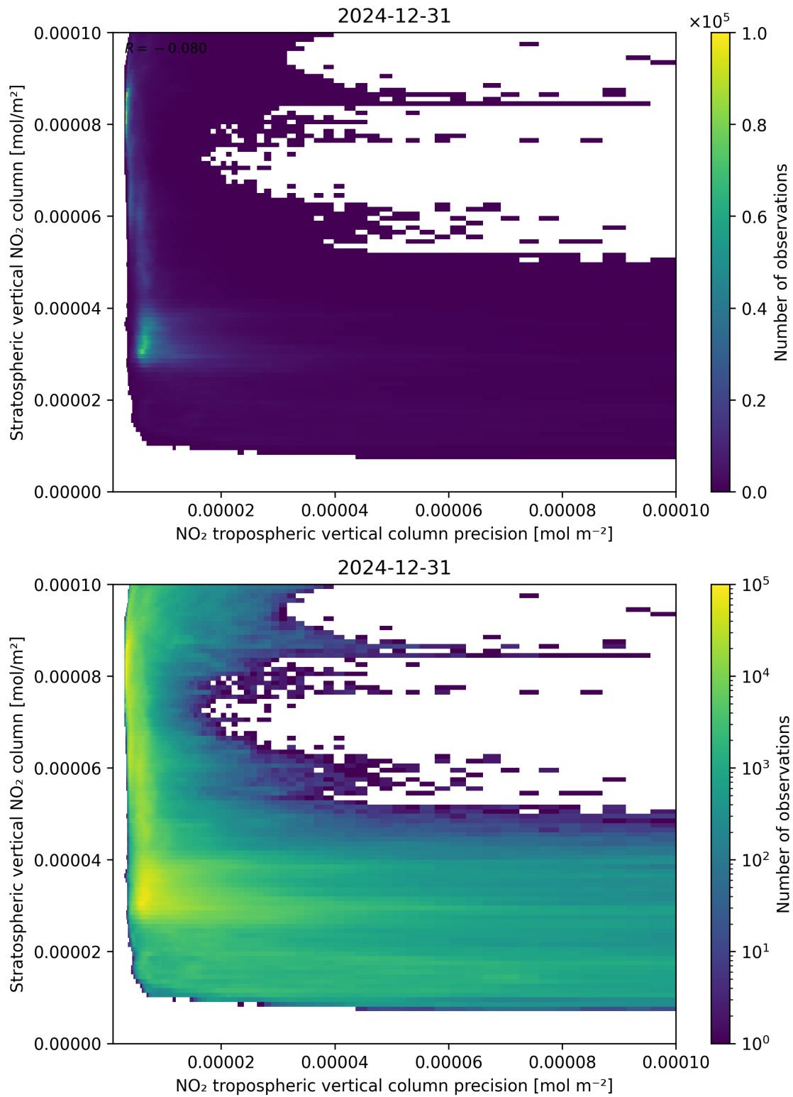
Figure 135: Scatter density plot of “NO 2 tropospheric vertical column precision” against “Stratospheric vertical NO 2 column” for 2024-12-30 to 2025-01-01.
