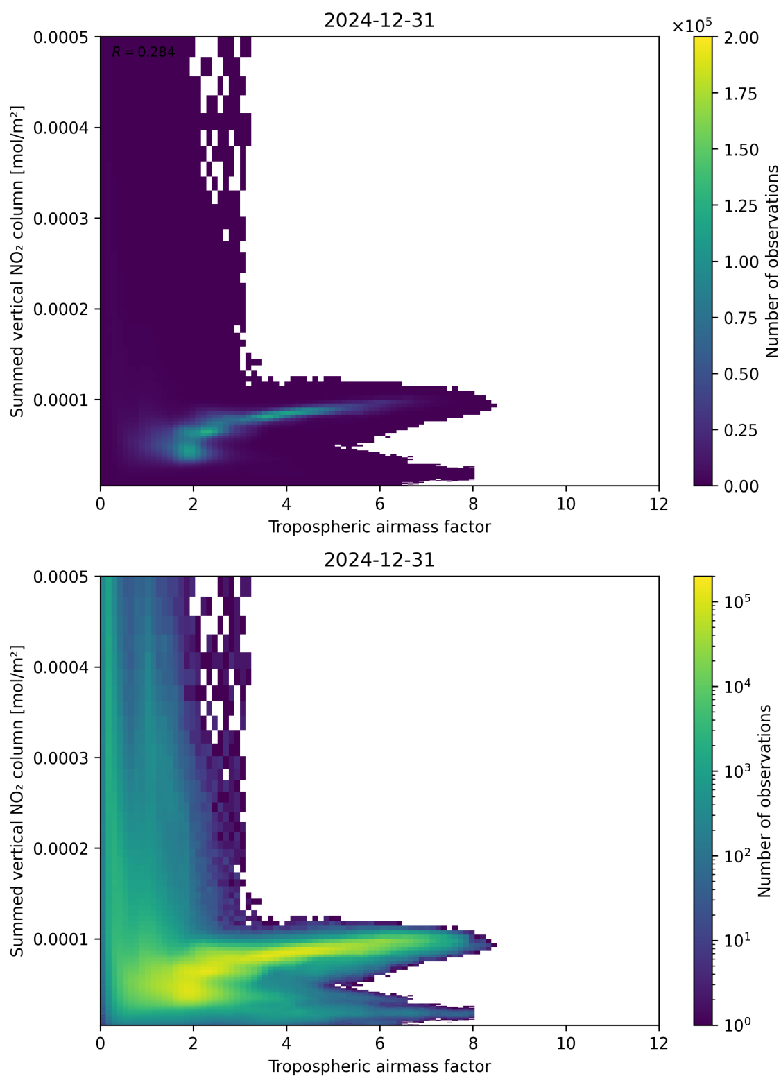
Figure 75: Scatter density plot of “Tropospheric air mass factor” against “Summed vertical NO 2 column” for 2024-12-30 to 2025-01-01.
