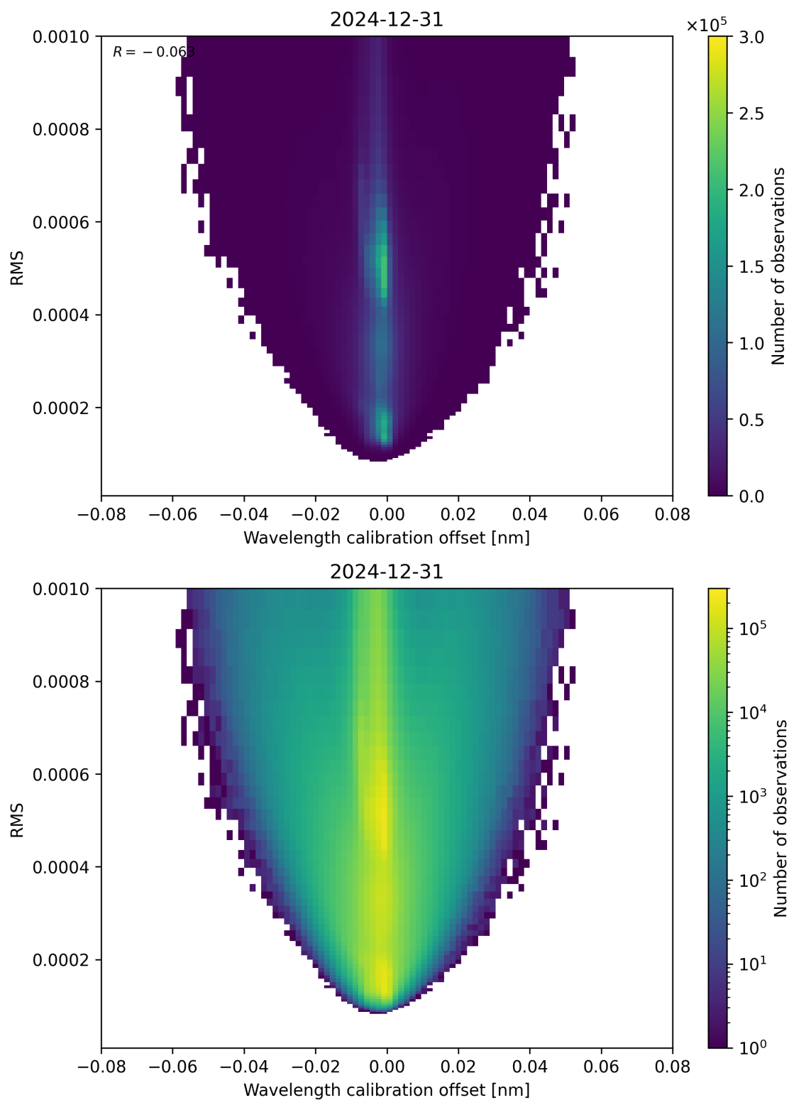
Figure 181: Scatter density plot of “Wavelength calibration offset” against “RMS” for 2024-12-30 to 2025-01-01.
