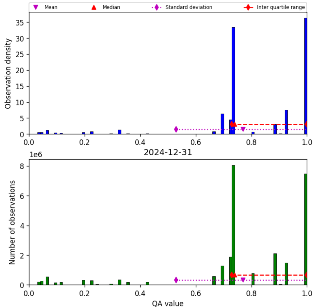
Figure 28: Histogram of “QA value” for 2024-12-30 to 2025-01-01
