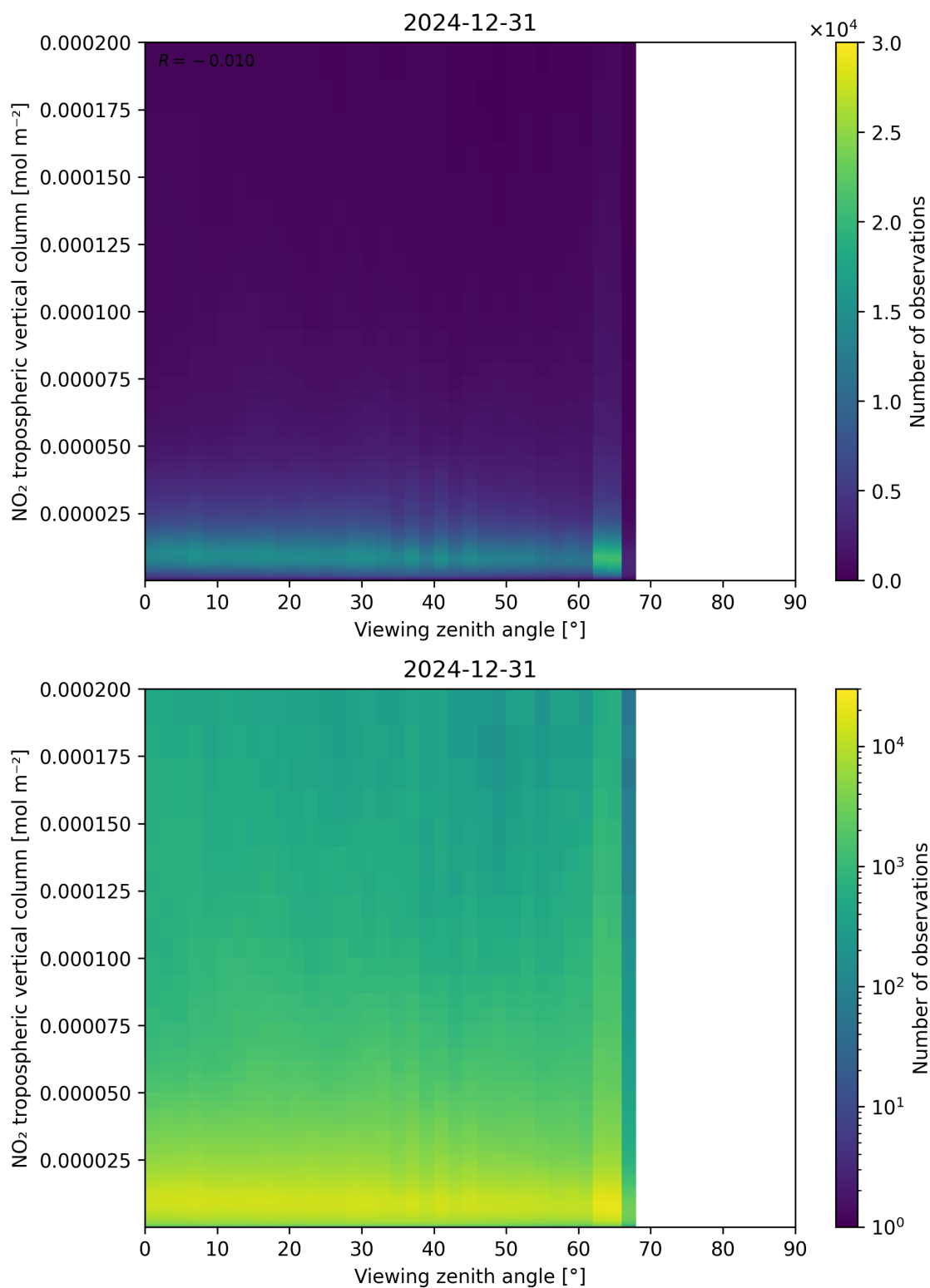
Figure 169: Scatter density plot of “Viewing zenith angle” against “NO 2 tropospheric vertical column” for 2024-12-30 to 2025-01-01.
