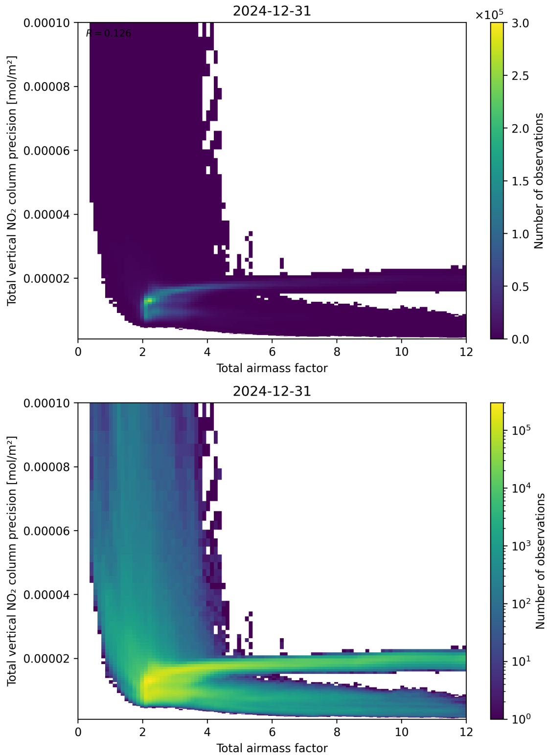
Figure 68: Scatter density plot of “Total airmass factor” against “Total vertical NO 2 column precision” for 2024-12-30 to 2025-01-01.
