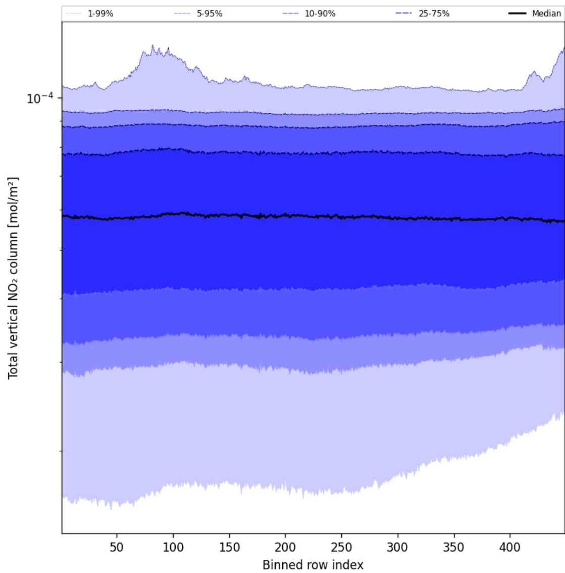
Figure 55: Along track statistics of “Total vertical NO 2 column” for 2024-12-30 to 2025-01-01
