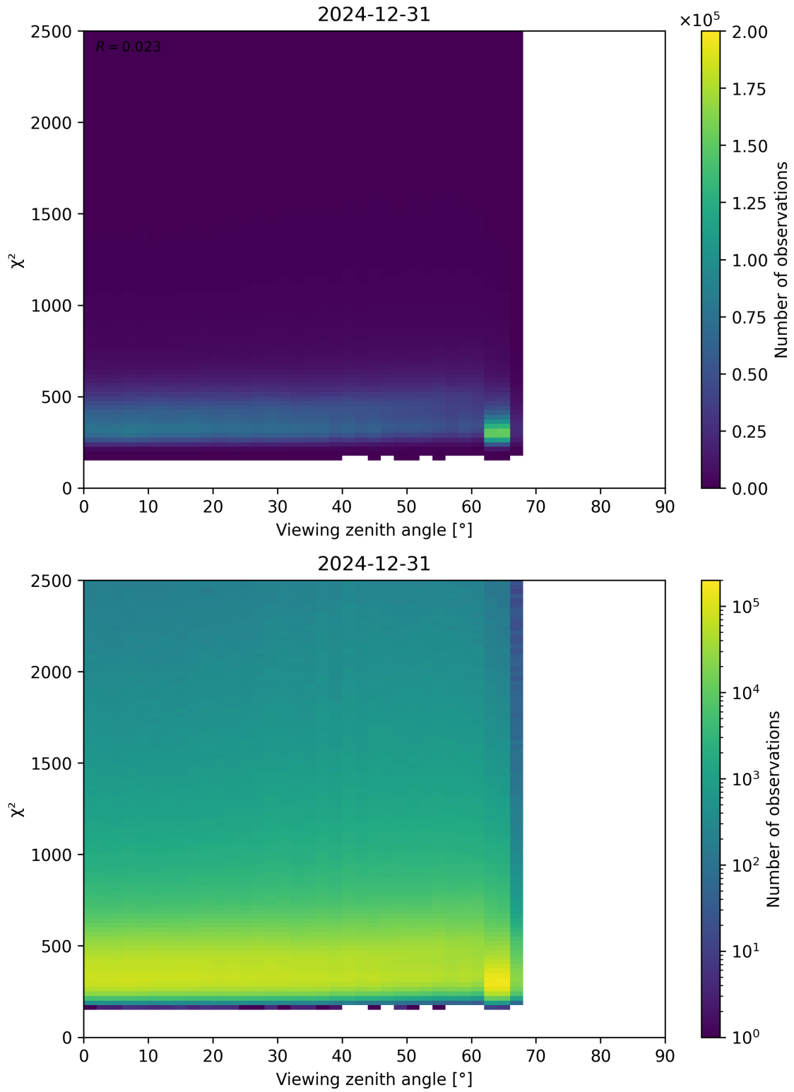
Figure 162: Scatter density plot of “Viewing zenith angle” against “ \chi^2 ” for 2024-12-30 to 2025-01-01.
