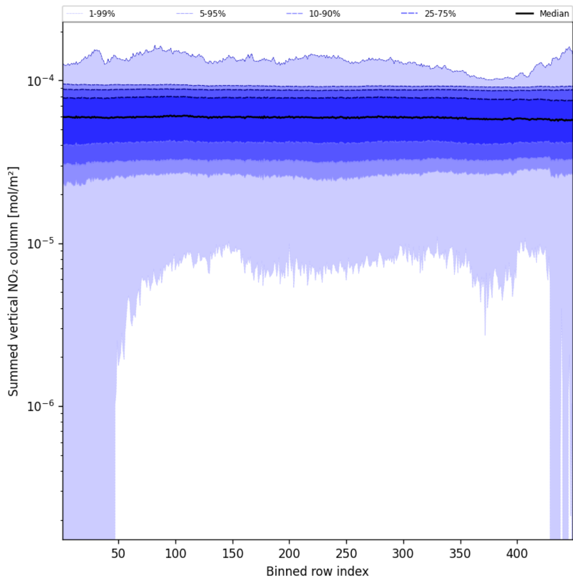
Figure 57: Along track statistics of “Summed vertical NO 2 column” for 2024-12-30 to 2025-01-01
