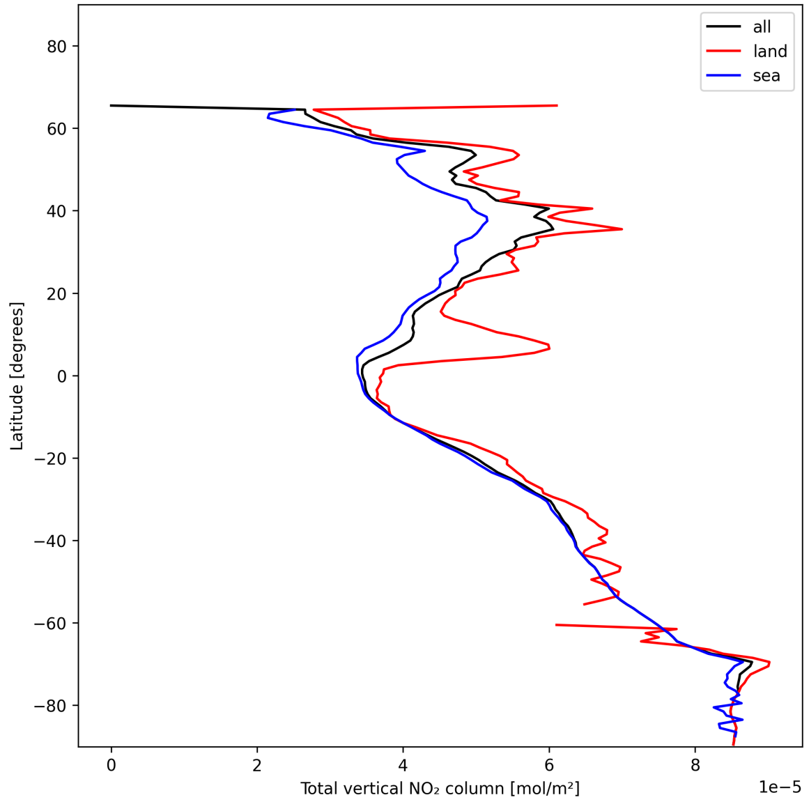
Figure 21: Zonal average of “Total vertical NO 2 column” for 2024-12-30 to 2025-01-01.
