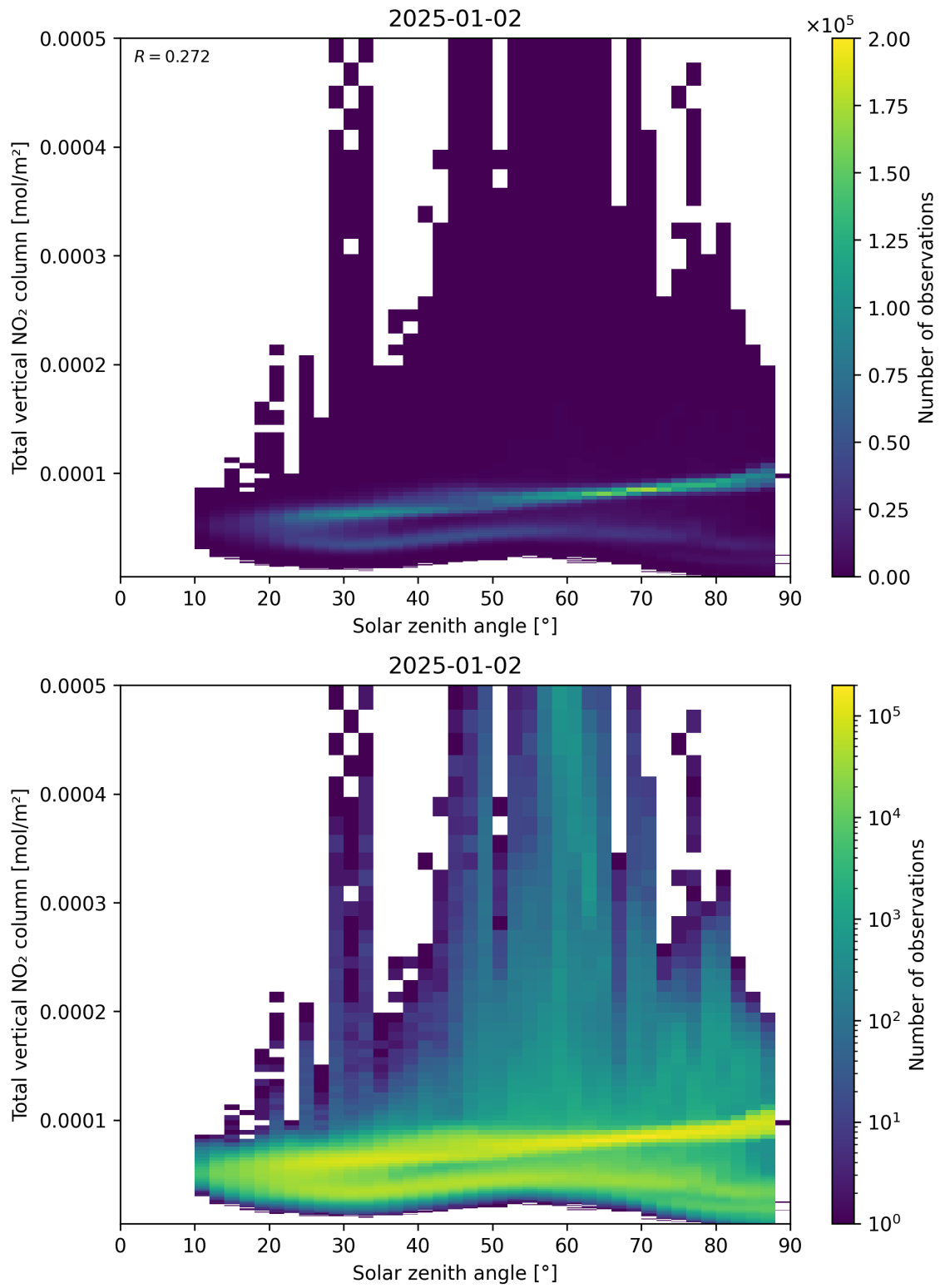
Figure 153: Scatter density plot of “Solar zenith angle” against “Total vertical NO 2 column” for 2025-01-01 to 2025-01-03.
