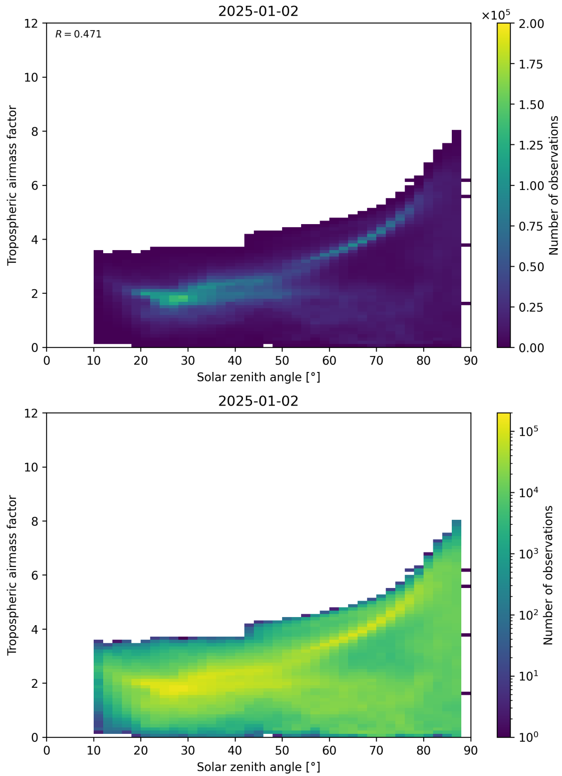
Figure 147: Scatter density plot of “Solar zenith angle” against “Tropospheric airmass factor” for 2025-01-01 to 2025-01-03.
