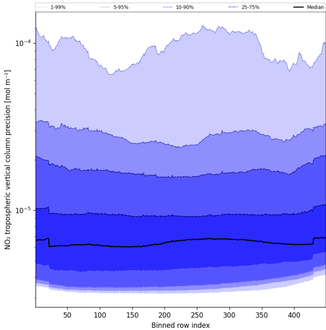
Figure 47: Along track statistics of “NO 2 tropospheric vertical column precision” for 2025-01-01 to 2025-01-03
