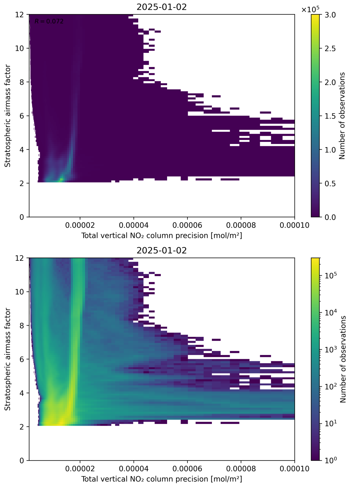
Figure 115: Scatter density plot of “Total vertical NO 2 column precision” against “Stratospheric air mass factor” for 2025-01-01 to 2025-01-03.
