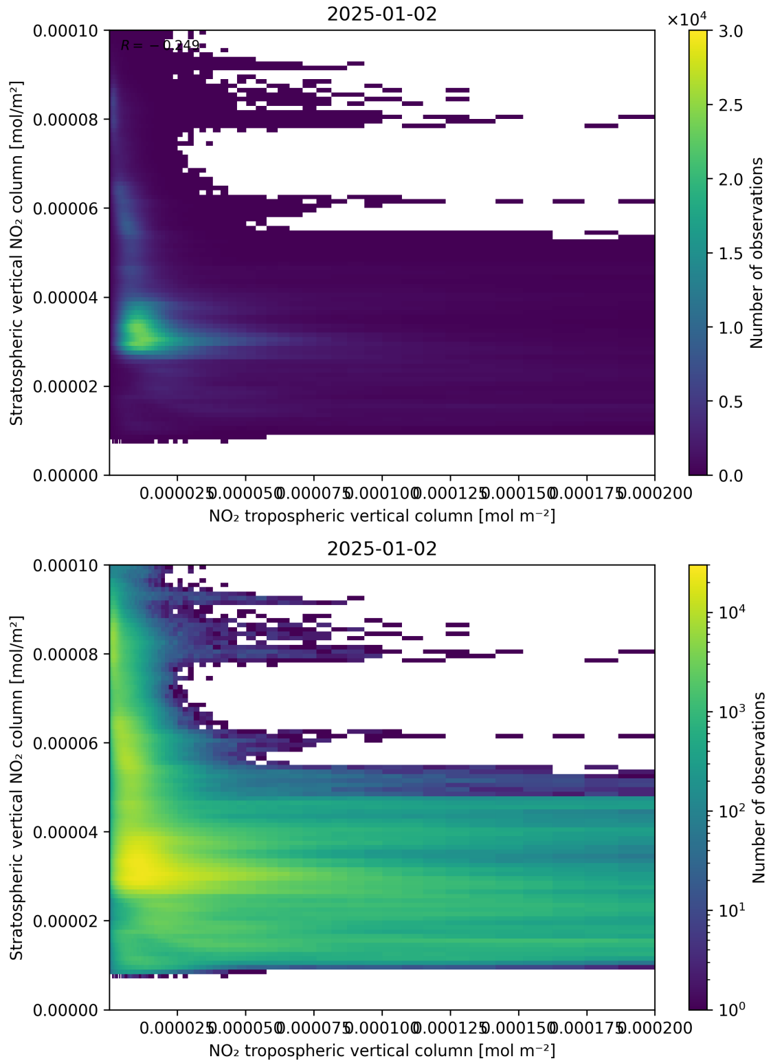
Figure 125: Scatter density plot of “NO 2 tropospheric vertical column” against “Stratospheric vertical NO 2 column” for 2025-01-01 to 2025-01-03.
