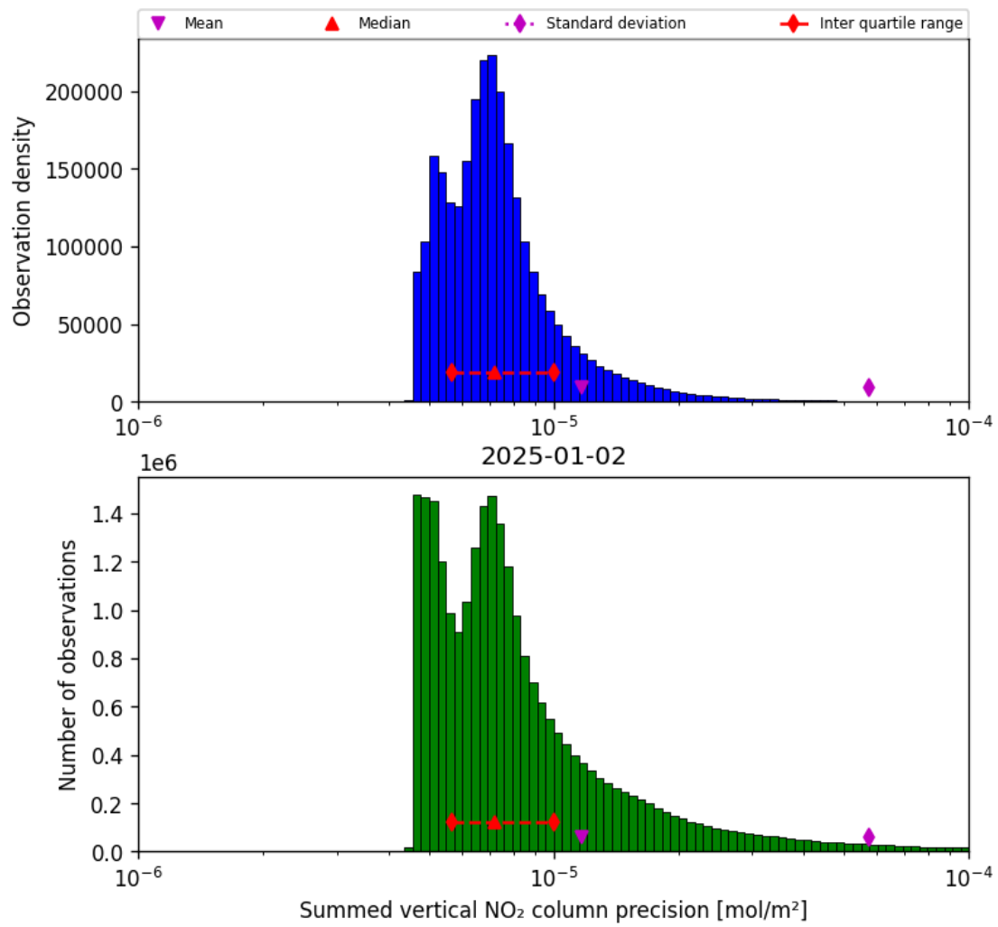
Figure 41: Histogram of "Summed vertical NO 2 column precision" for 2025-01-01 to 2025-01-03
