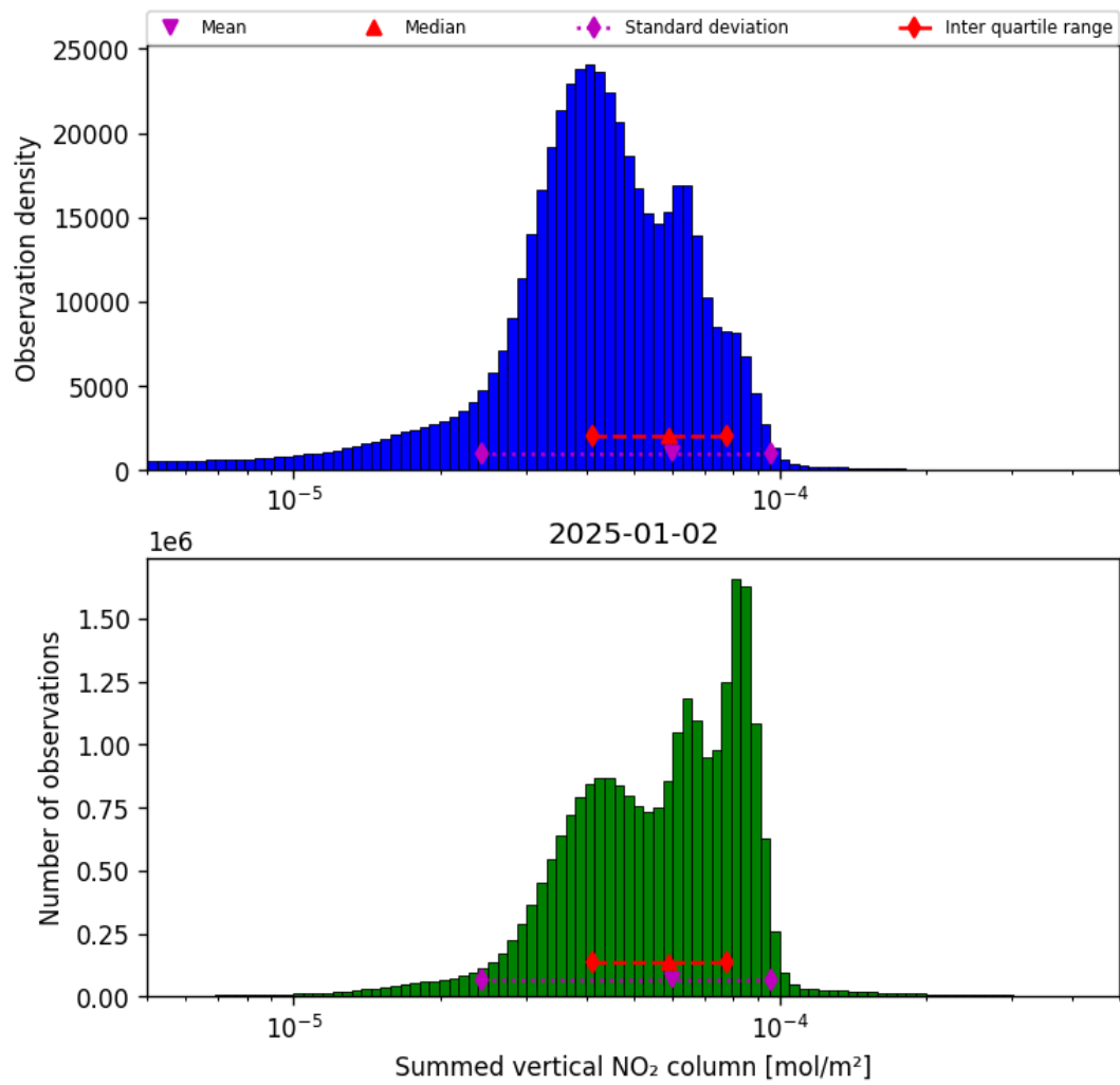
Figure 40: Histogram of “Summed vertical NO 2 column” for 2025-01-01 to 2025-01-03
