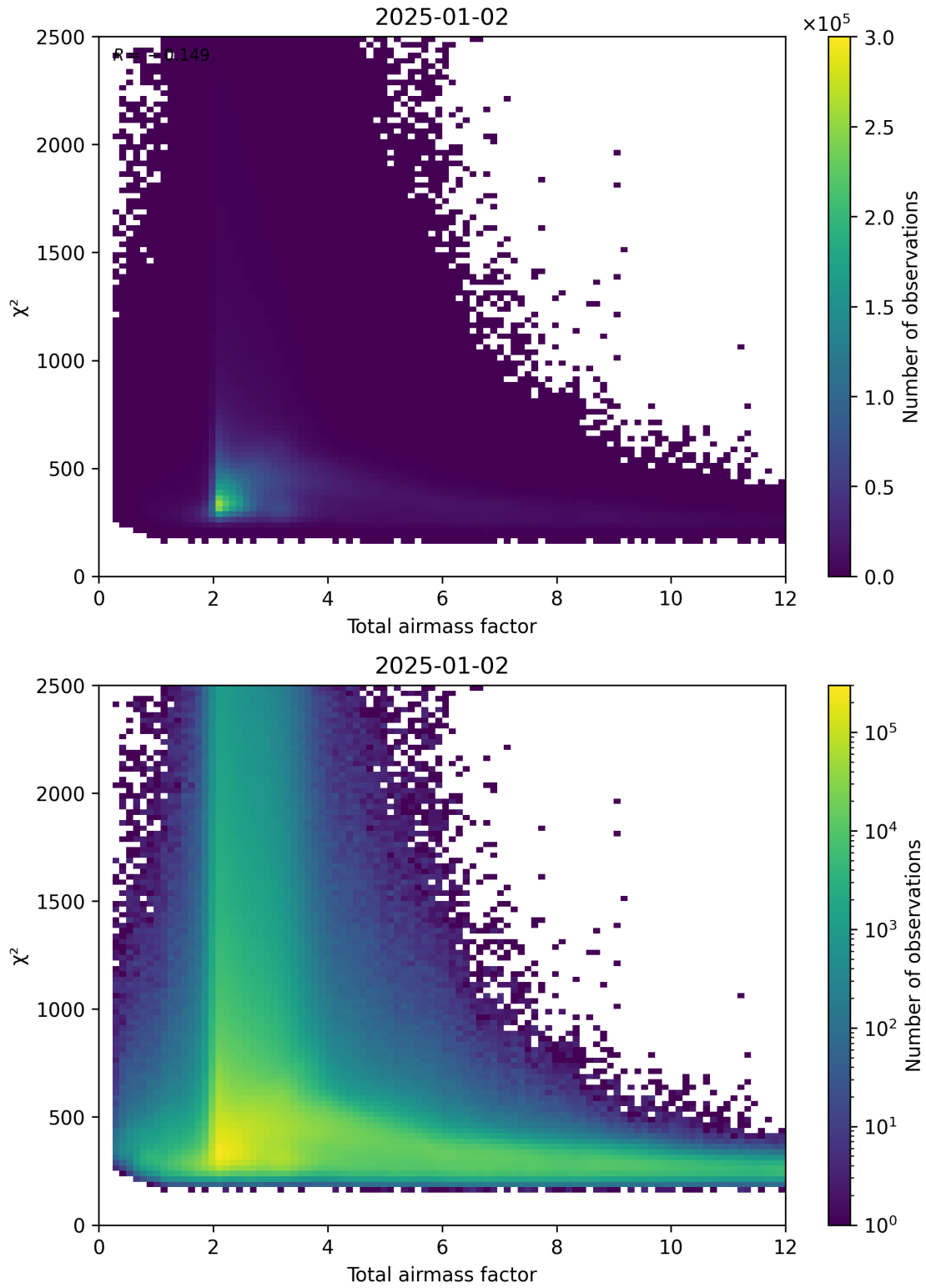
Figure 63: Scatter density plot of “Total airmass factor” against “ \chi^2 ” for 2025-01-01 to 2025-01-03.
