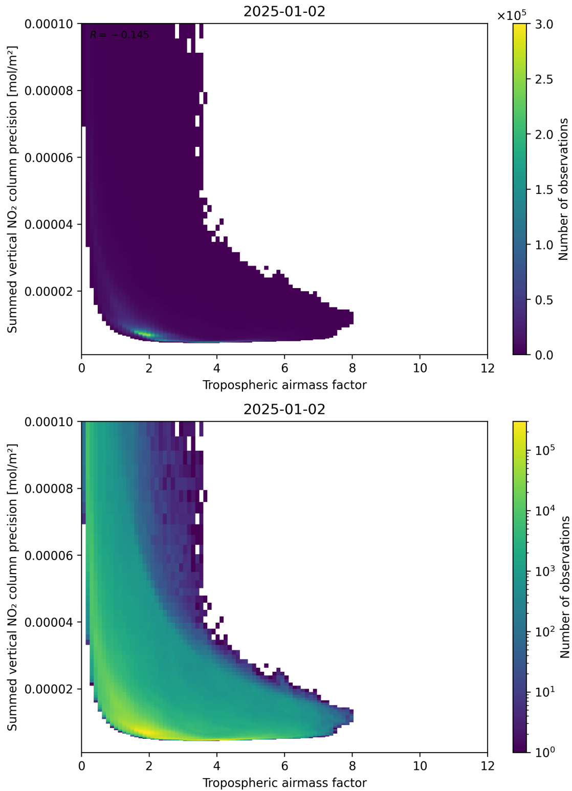
Figure 76: Scatter density plot of “Tropospheric air mass factor” against “Summed vertical NO 2 column precision” for 2025-01-01 to 2025-01-03.
