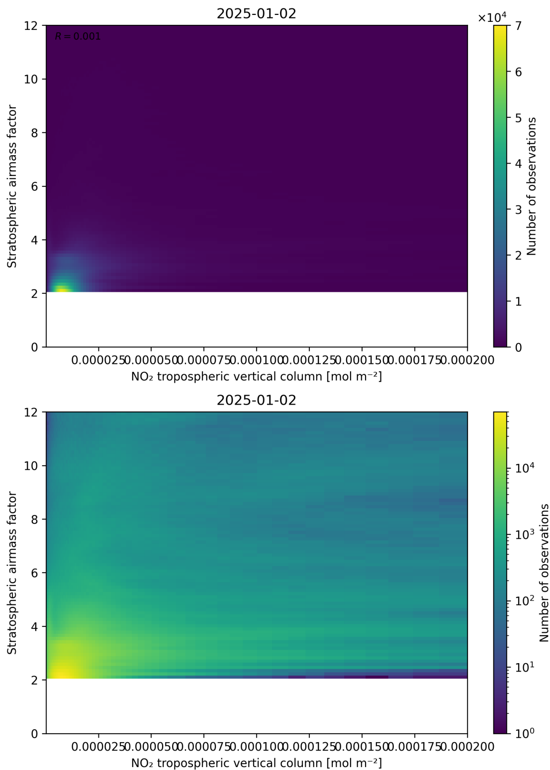
Figure 121: Scatter density plot of “NO 2 tropospheric vertical column” against “Stratospheric airmass factor” for 2025-01-01 to 2025-01-03.
