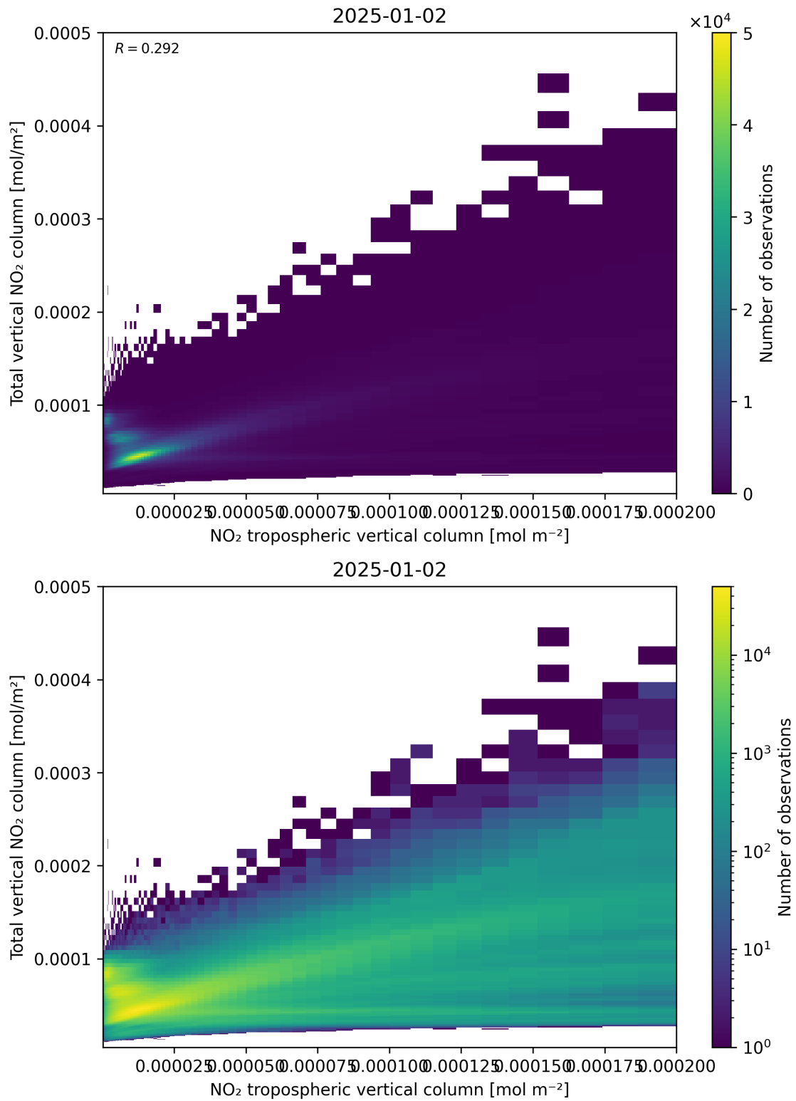
Figure 128: Scatter density plot of “NO 2 tropospheric vertical column” against “Total vertical NO 2 column” for 2025-01-01 to 2025-01-03.
