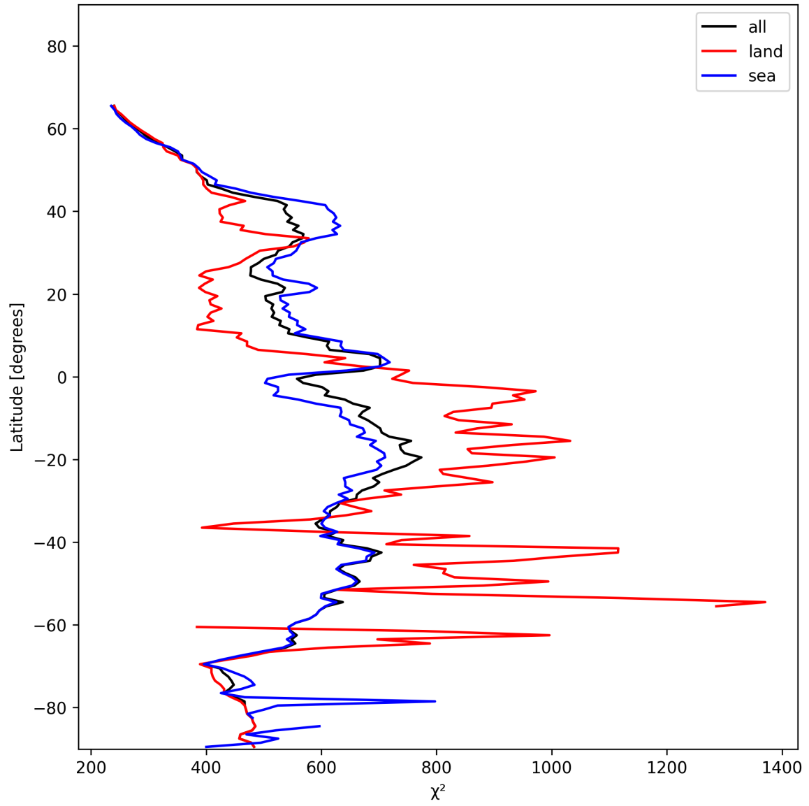
Figure 25: Zonal average of “ \chi^2 ” for 2025-01-01 to 2025-01-03.
