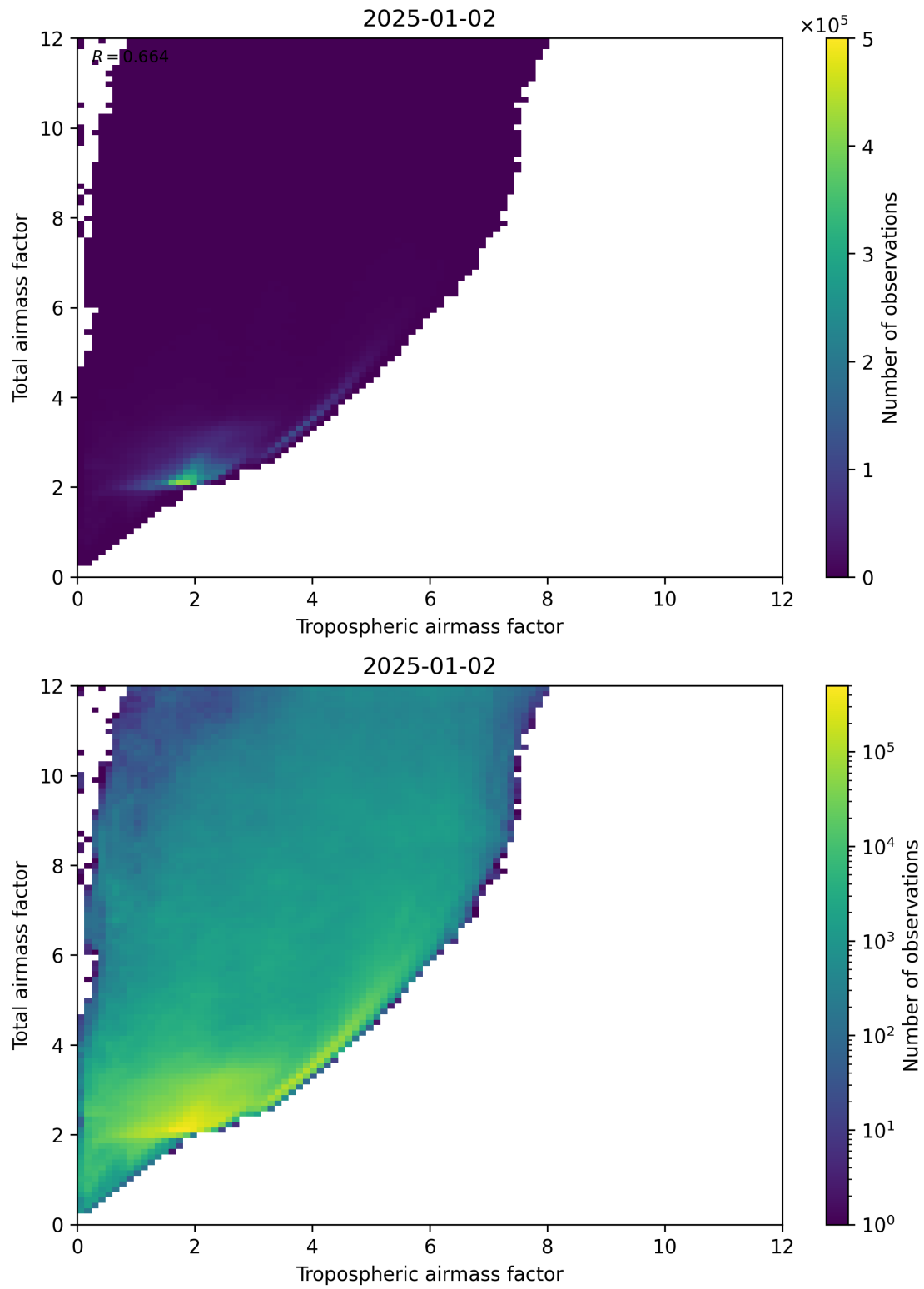
Figure 72: Scatter density plot of “Tropospheric airmass factor” against “Total airmass factor” for 2025-01-01 to 2025-01-03.
