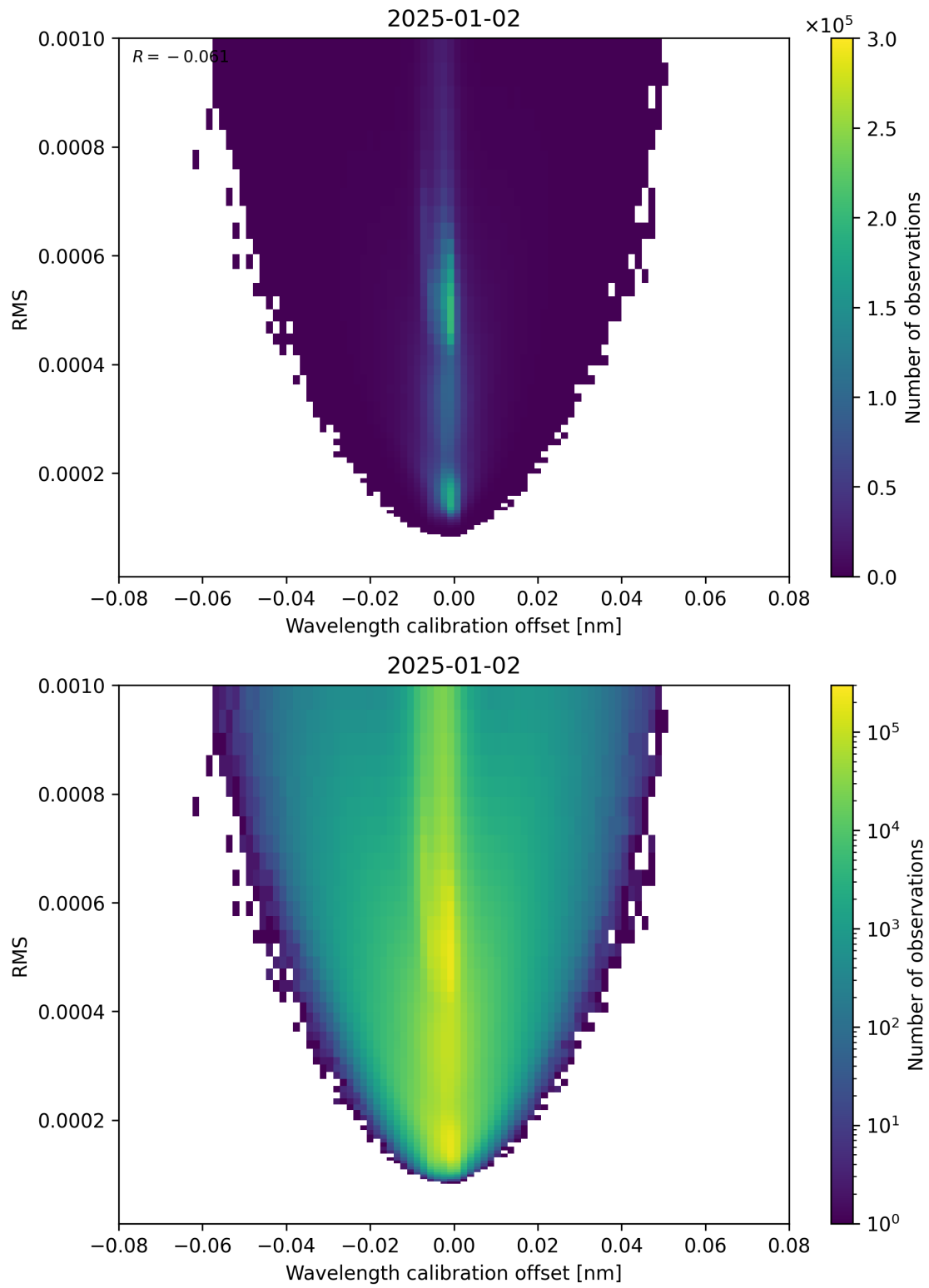
Figure 181: Scatter density plot of “Wavelength calibration offset” against “RMS” for 2025-01-01 to 2025-01-03.
