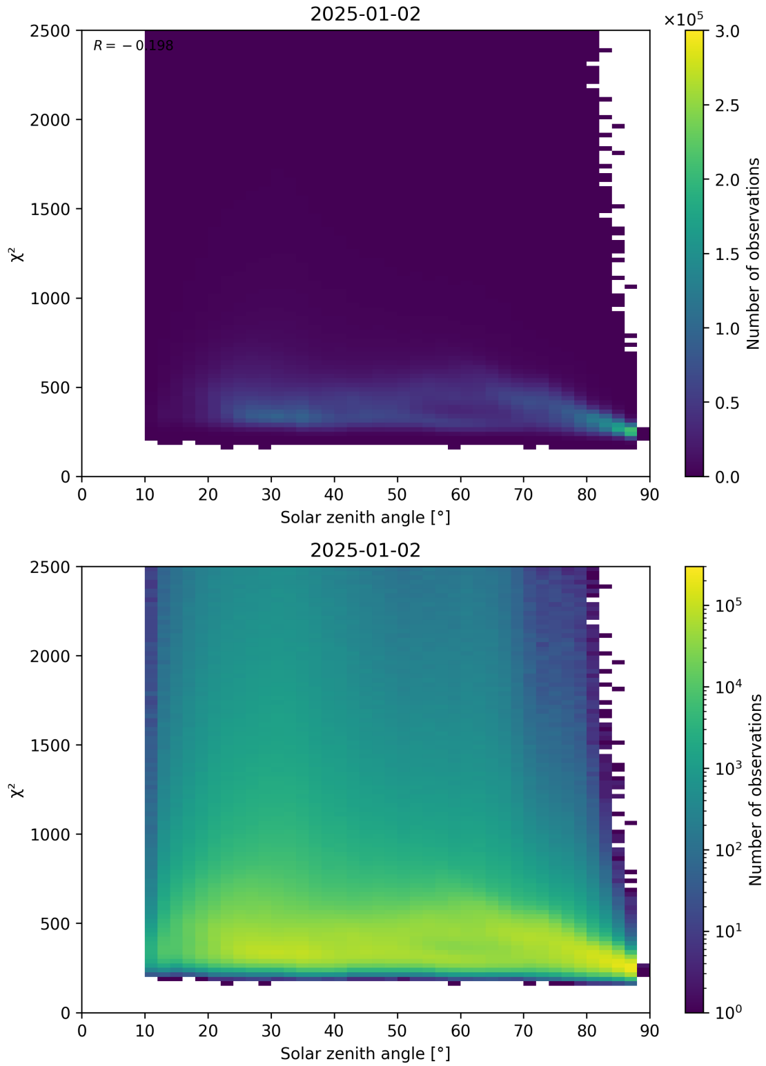
Figure 148: Scatter density plot of “Solar zenith angle” against “ \chi^2 ” for 2025-01-01 to 2025-01-03.
