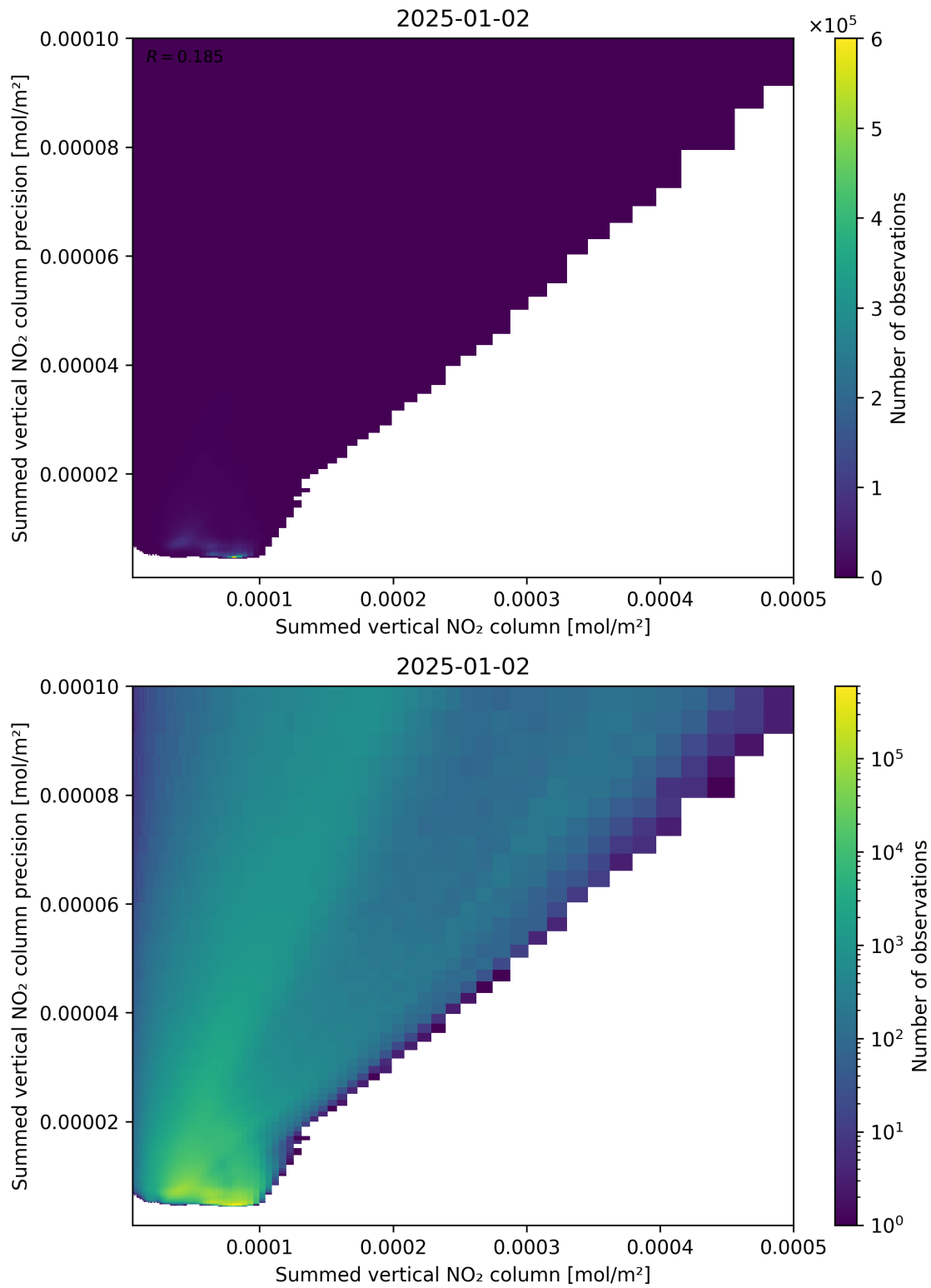
Figure 105: Scatter density plot of “Summed vertical NO 2 column” against “Summed vertical NO 2 column precision” for 2025-01-01 to 2025-01-03.
