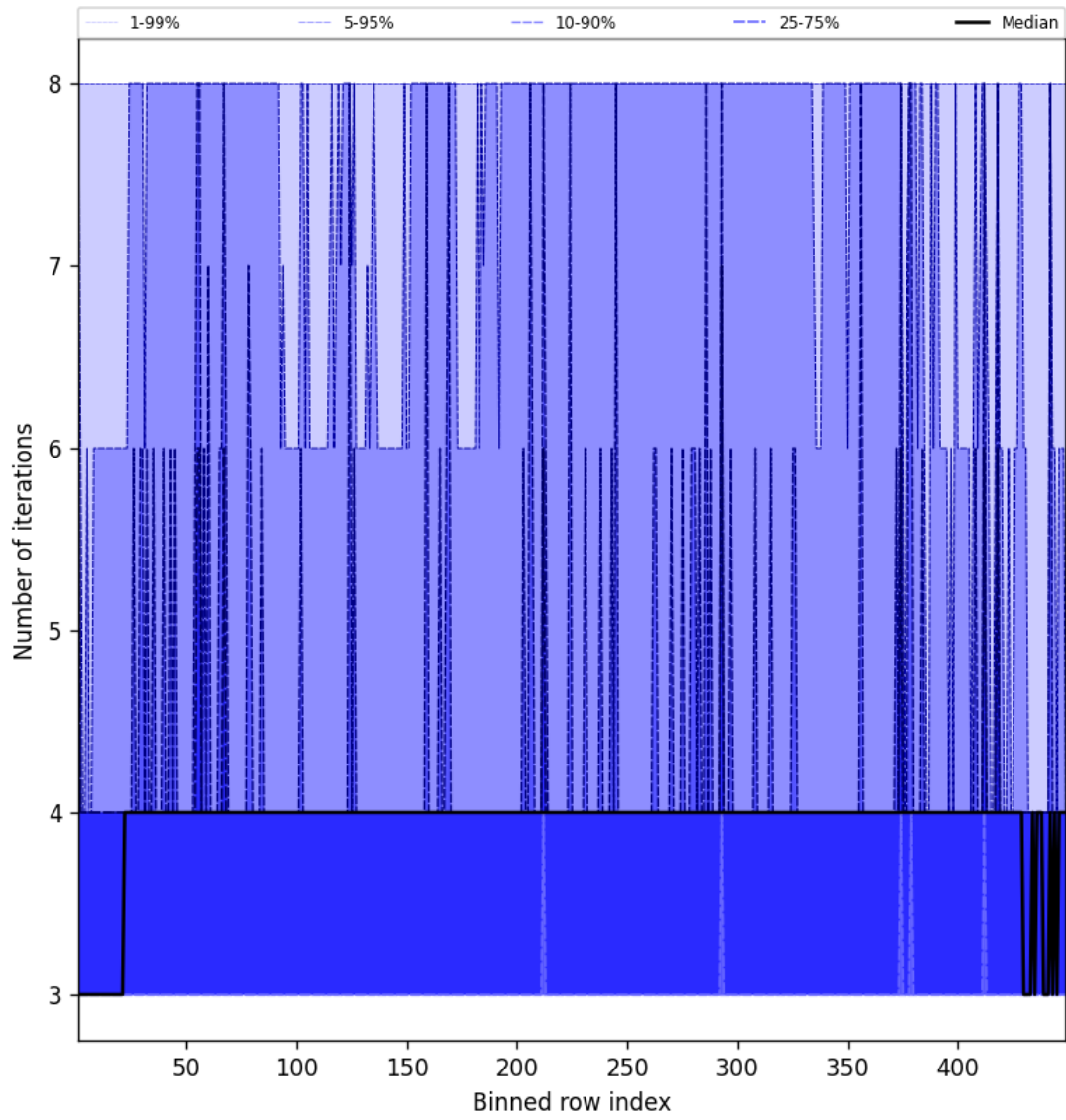
Figure 51: Along track statistics of “Number of iterations” for 2025-01-01 to 2025-01-03
