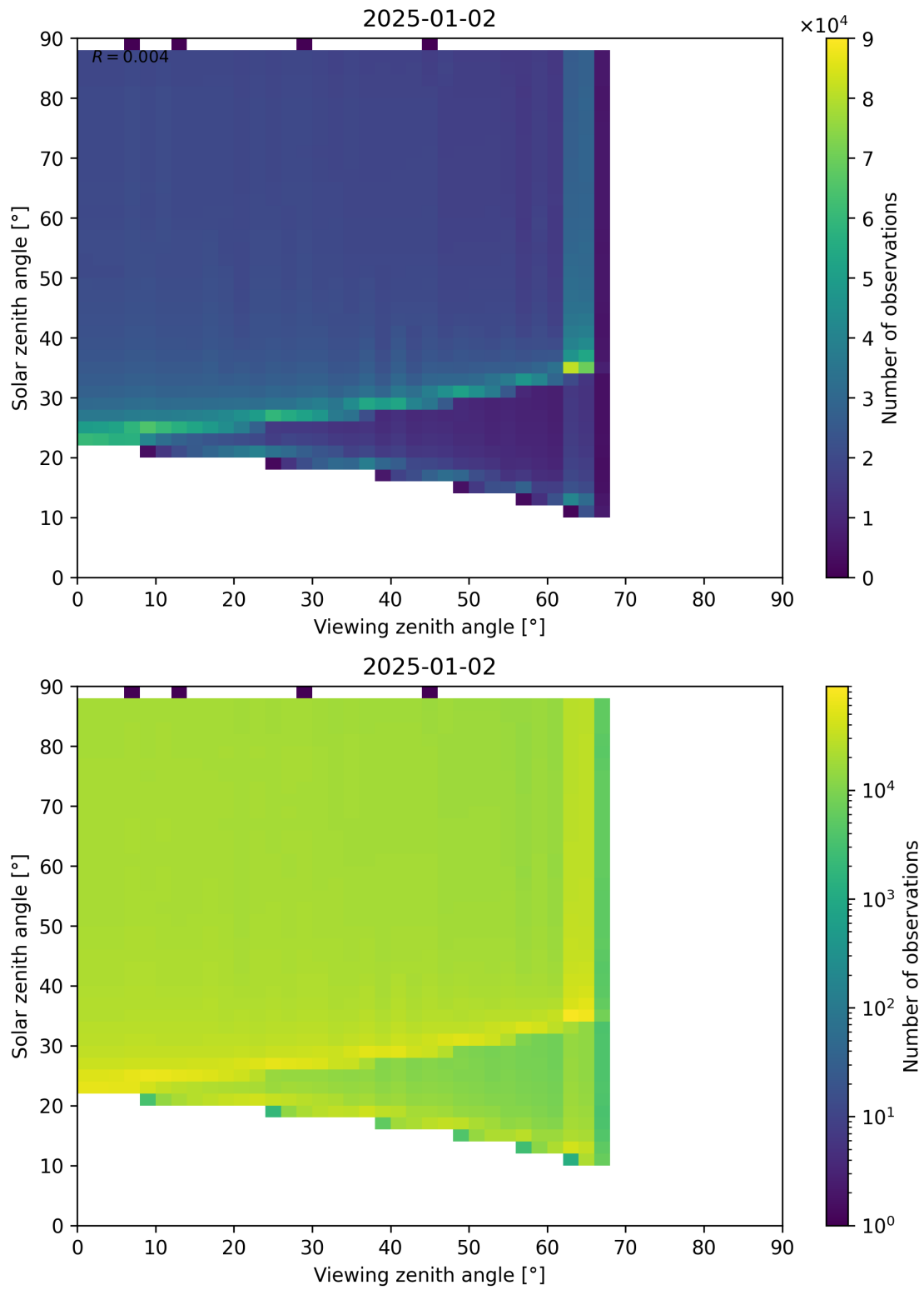
Figure 172: Scatter density plot of “Viewing zenith angle” against “Solar zenith angle” for 2025-01-01 to 2025-01-03.
