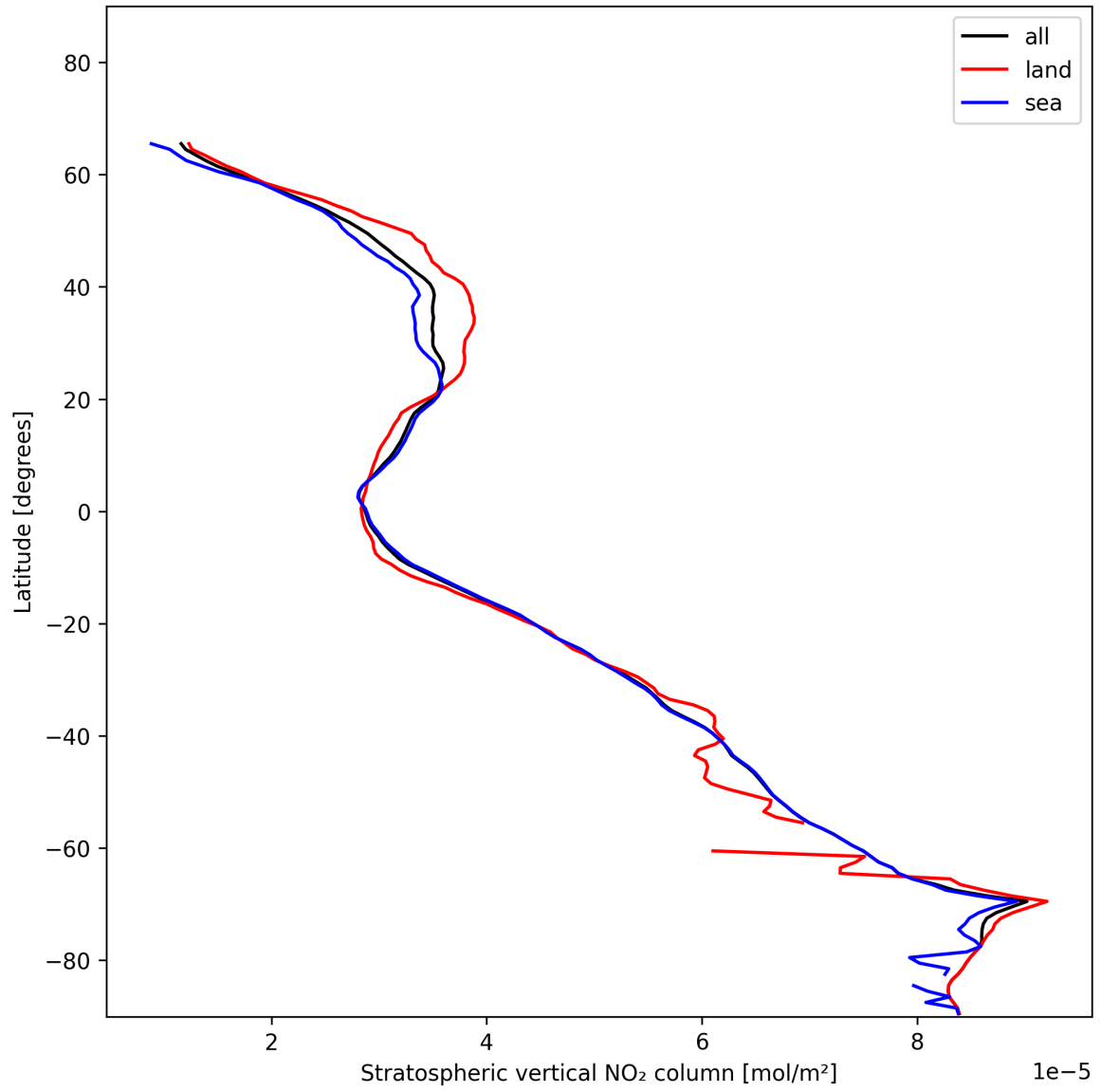
Figure 19: Zonal average of “Stratospheric vertical NO 2 column” for 2025-01-01 to 2025-01-03.
