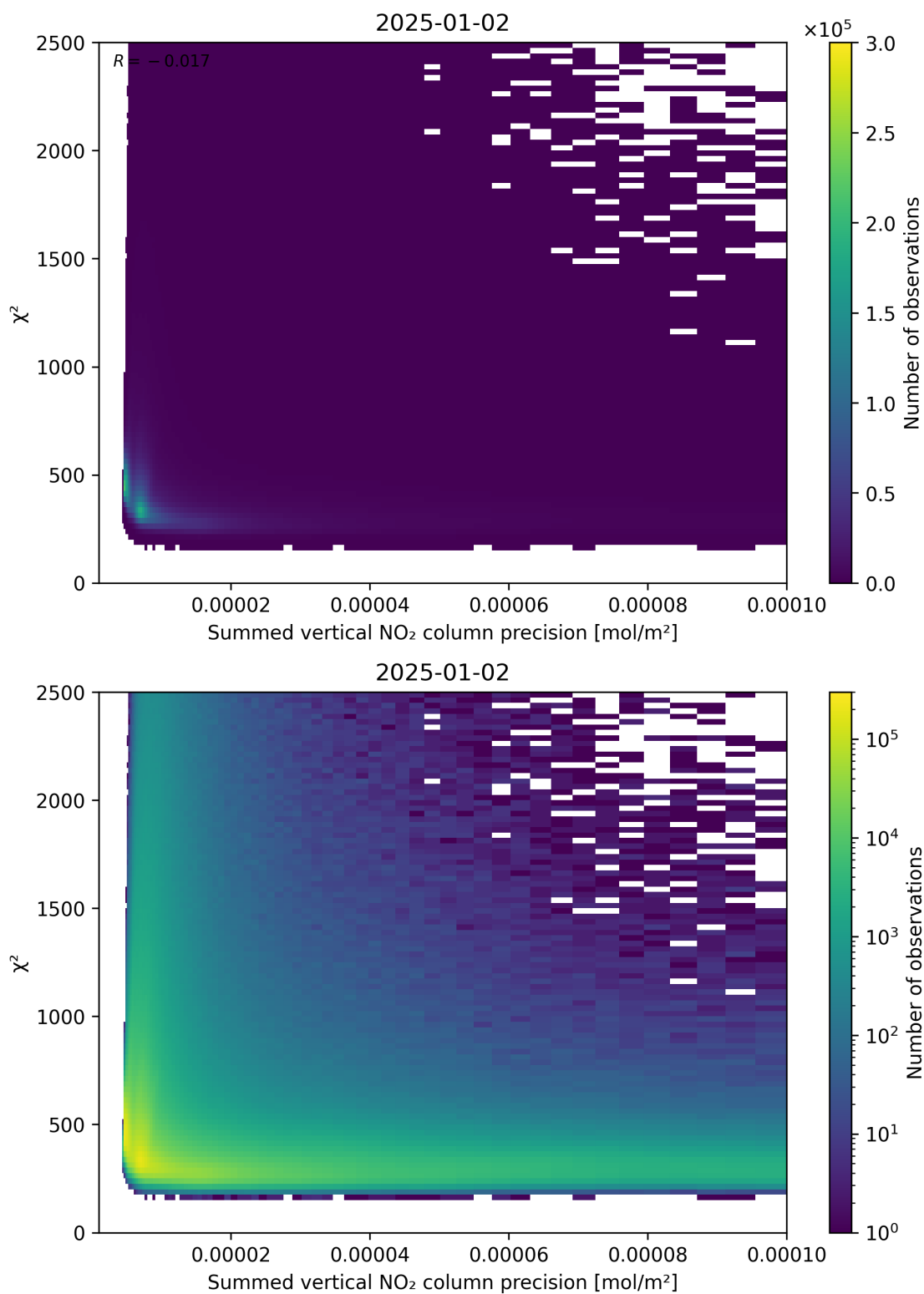
Figure 107: Scatter density plot of “Summed vertical NO 2 column precision” against “ \chi^2 ” for 2025-01-01 to 2025-01-03.
