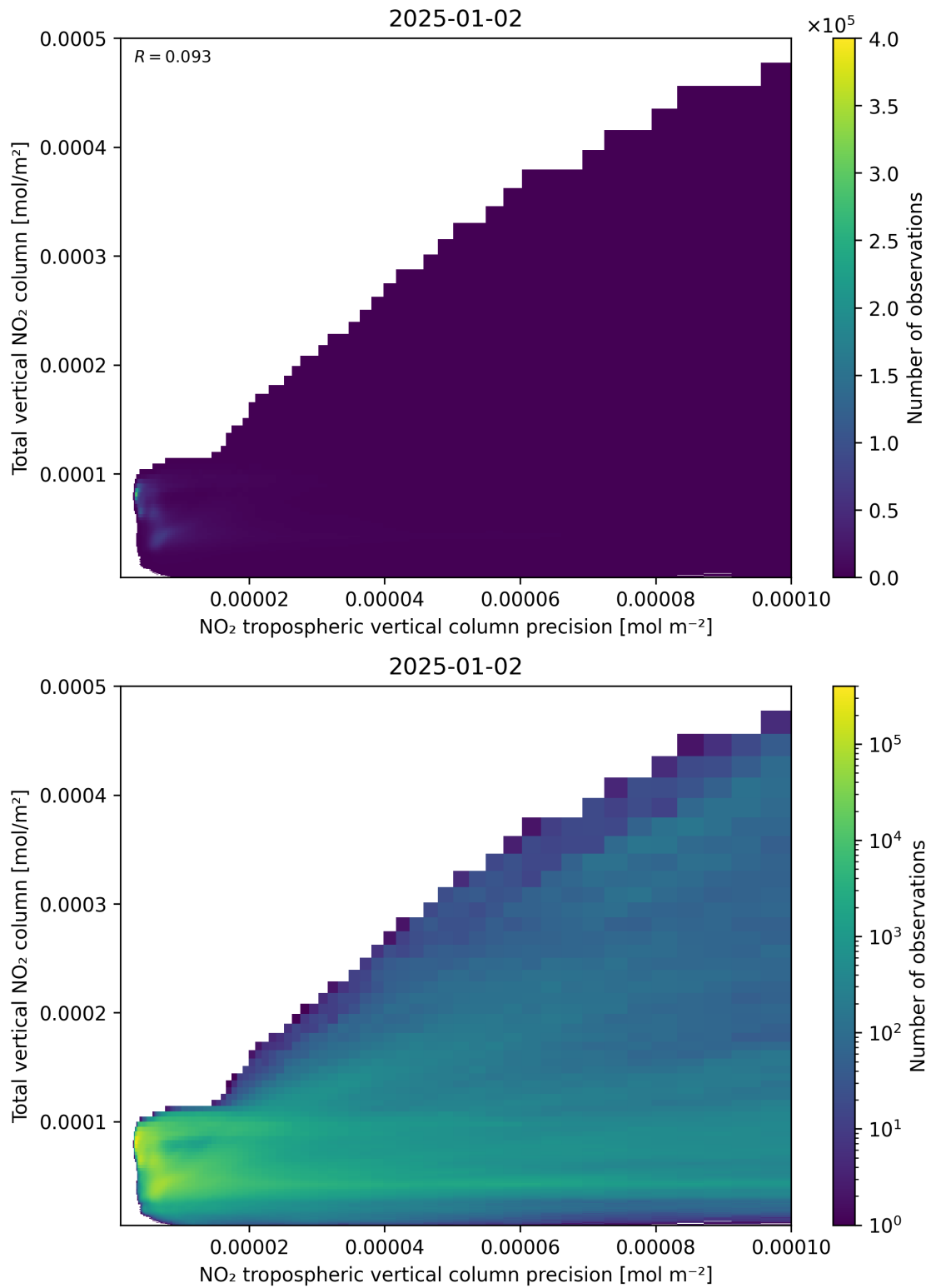
Figure 138: Scatter density plot of “NO 2 tropospheric vertical column precision” against “Total vertical NO 2 column” for 2025-01-01 to 2025-01-03.
