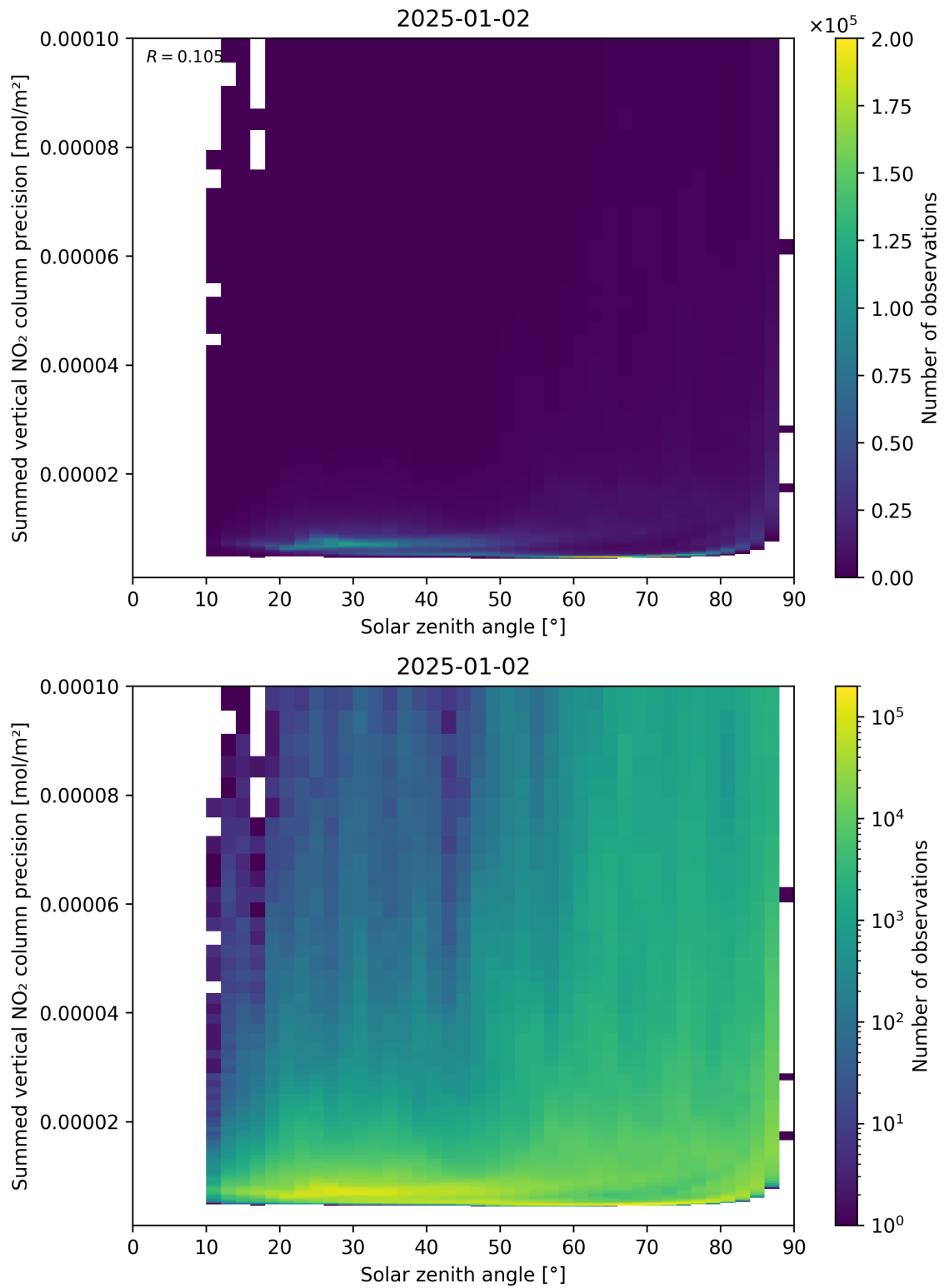
Figure 152: Scatter density plot of “Solar zenith angle” against “Summed vertical NO 2 column precision” for 2025-01-01 to 2025-01-03.
