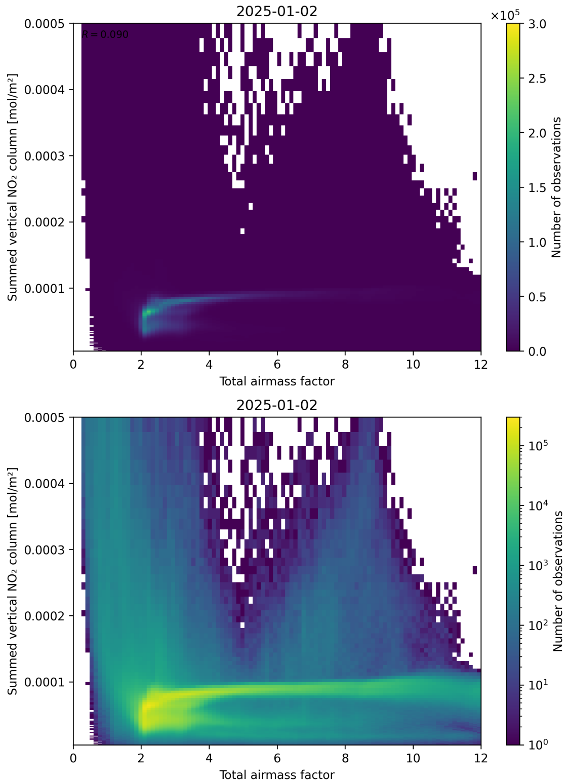
Figure 65: Scatter density plot of “Total airmass factor” against “Summed vertical NO 2 column” for 2025-01-01 to 2025-01-03.
