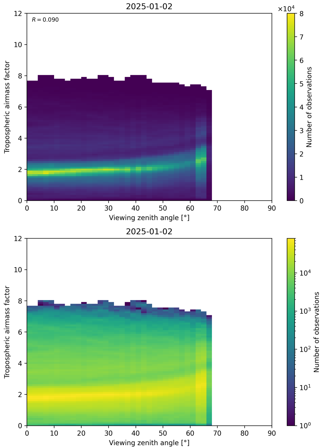
Figure 161: Scatter density plot of “Viewing zenith angle” against “Tropospheric airmass factor” for 2025-01-01 to 2025-01-03.
