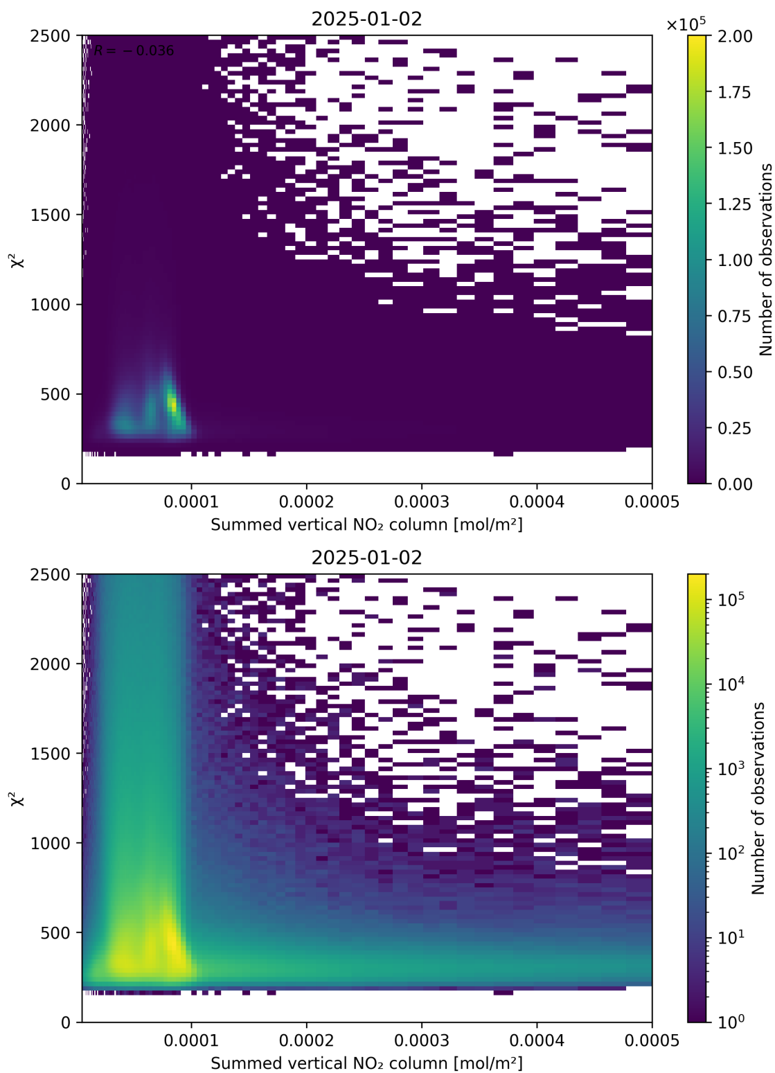
Figure 104: Scatter density plot of “Summed vertical NO 2 column” against “ \chi^2 ” for 2025-01-01 to 2025-01-03.
