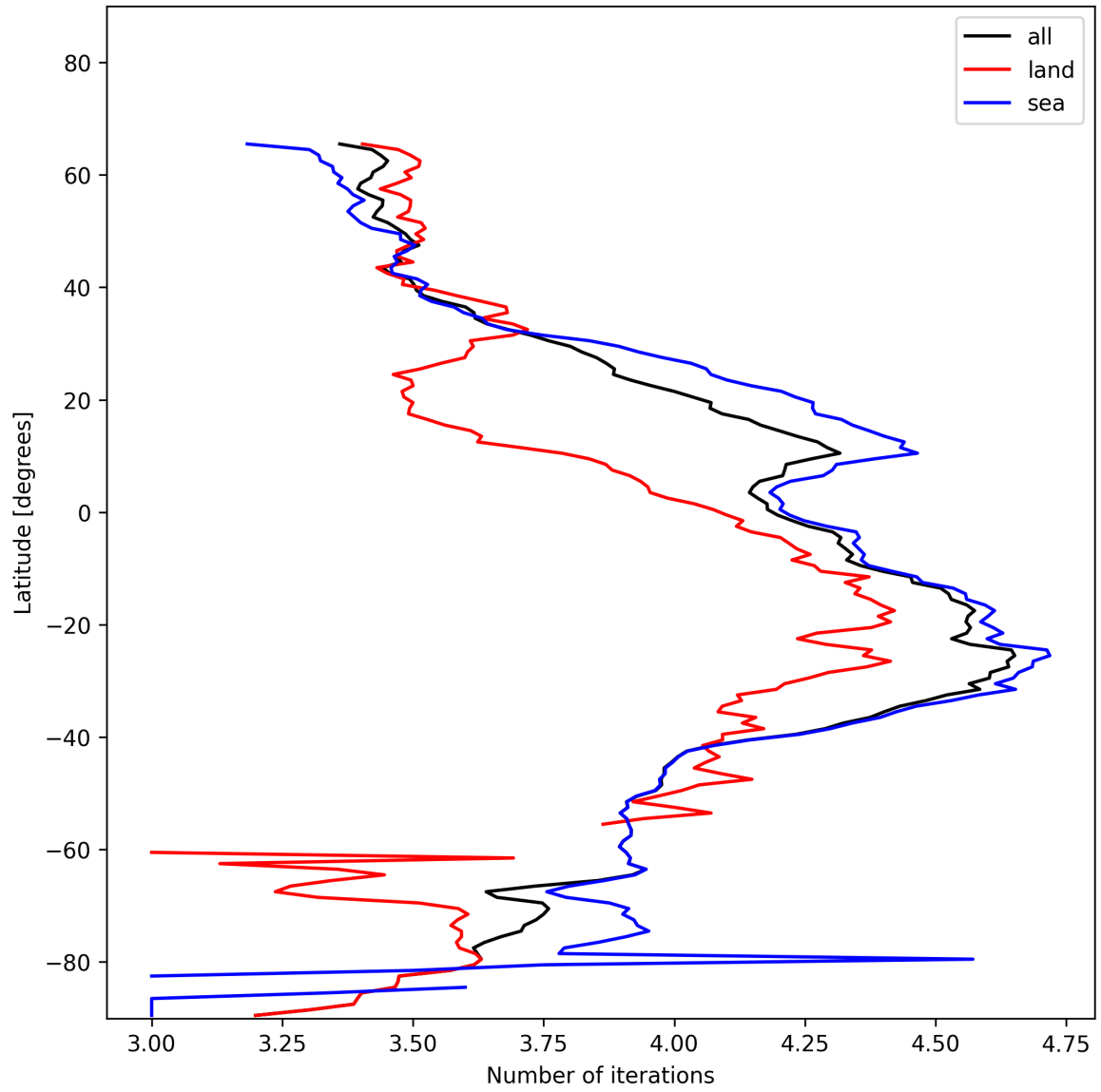
Figure 17: Zonal average of “Number of iterations” for 2025-01-01 to 2025-01-03.
