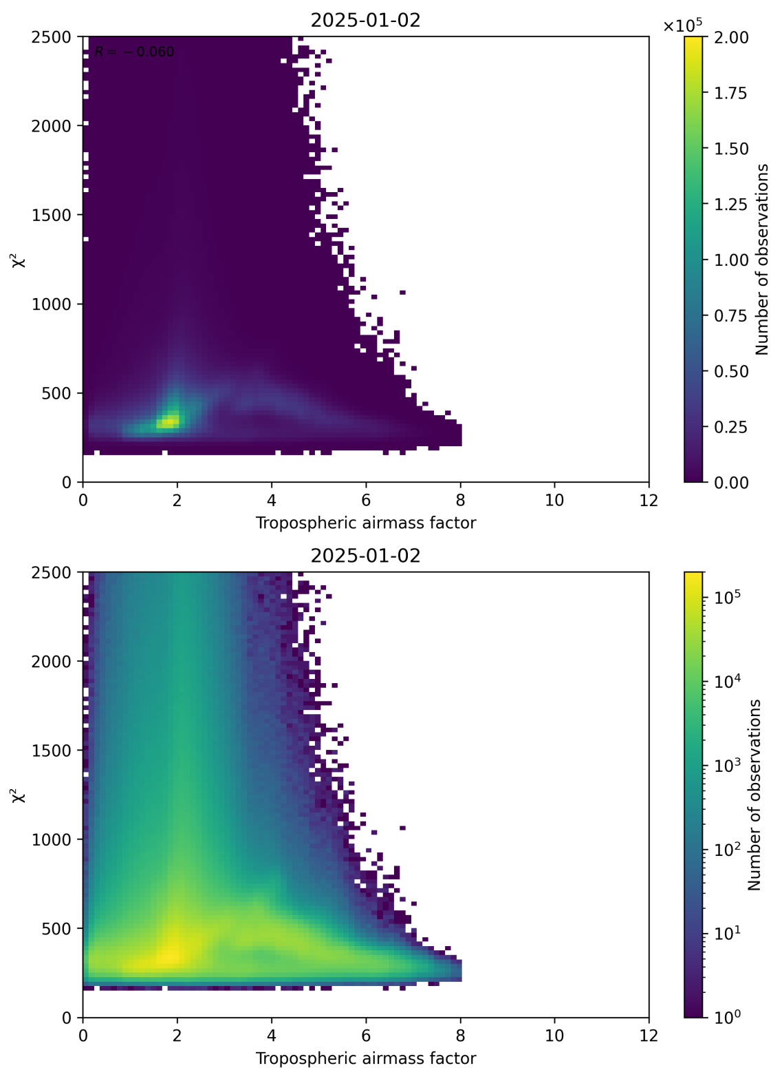
Figure 73: Scatter density plot of “Tropospheric airmass factor” against “ \chi^2 ” for 2025-01-01 to 2025-01-03.
