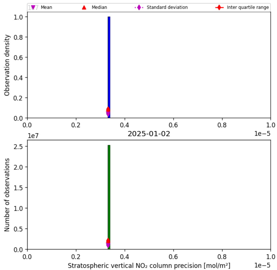
Figure 37: Histogram of “Stratospheric vertical NO 2 column precision” for 2025-01-01 to 2025-01-03
