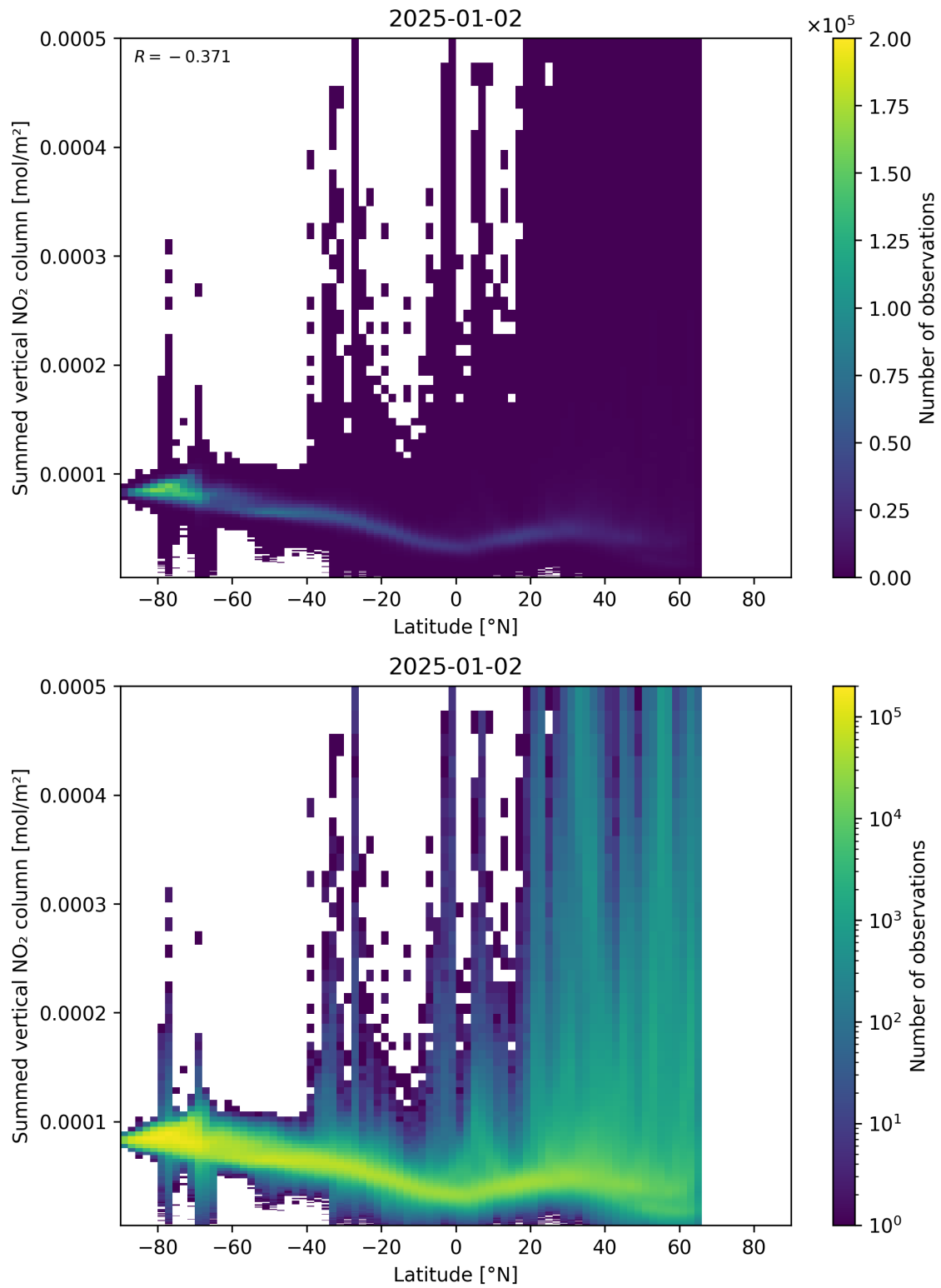
Figure 88: Scatter density plot of “Latitude” against “Summed vertical NO 2 column” for 2025-01-01 to 2025-01-03.
