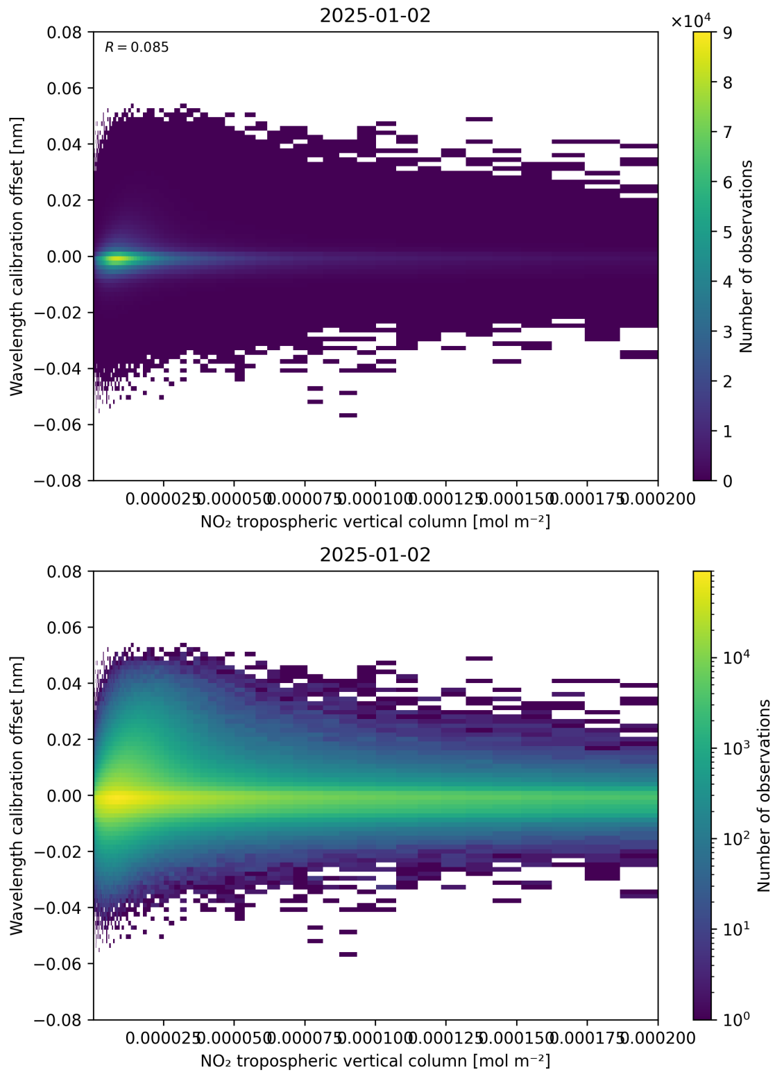
Figure 143: Scatter density plot of “NO 2 tropospheric vertical column” against “Wavelength calibration offset” for 2025-01-01 to 2025-01-03.
