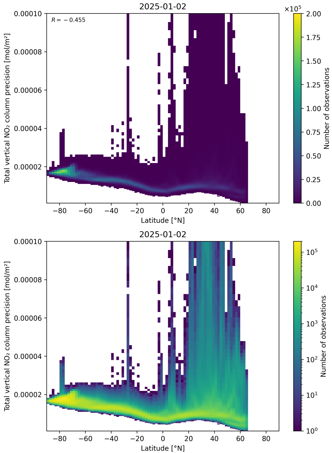
Figure 91: Scatter density plot of “Latitude” against “Total vertical NO 2 column precision” for 2025-01-01 to 2025-01-03.
