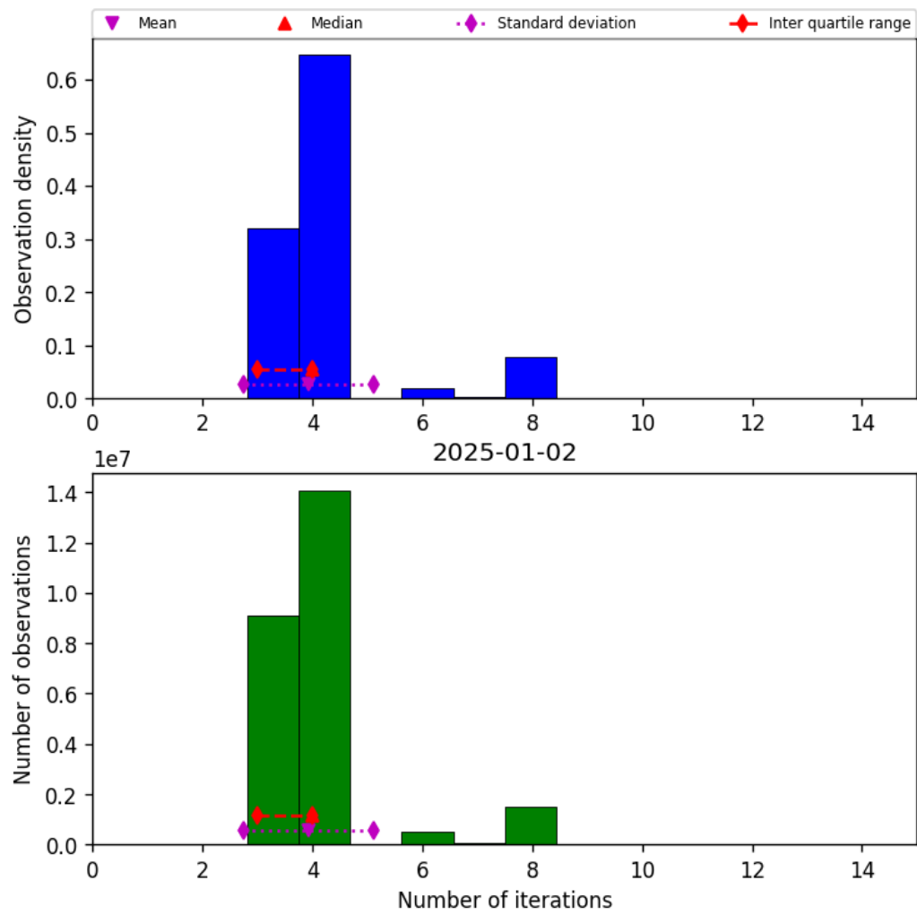
Figure 34: Histogram of “Number of iterations” for 2025-01-01 to 2025-01-03
