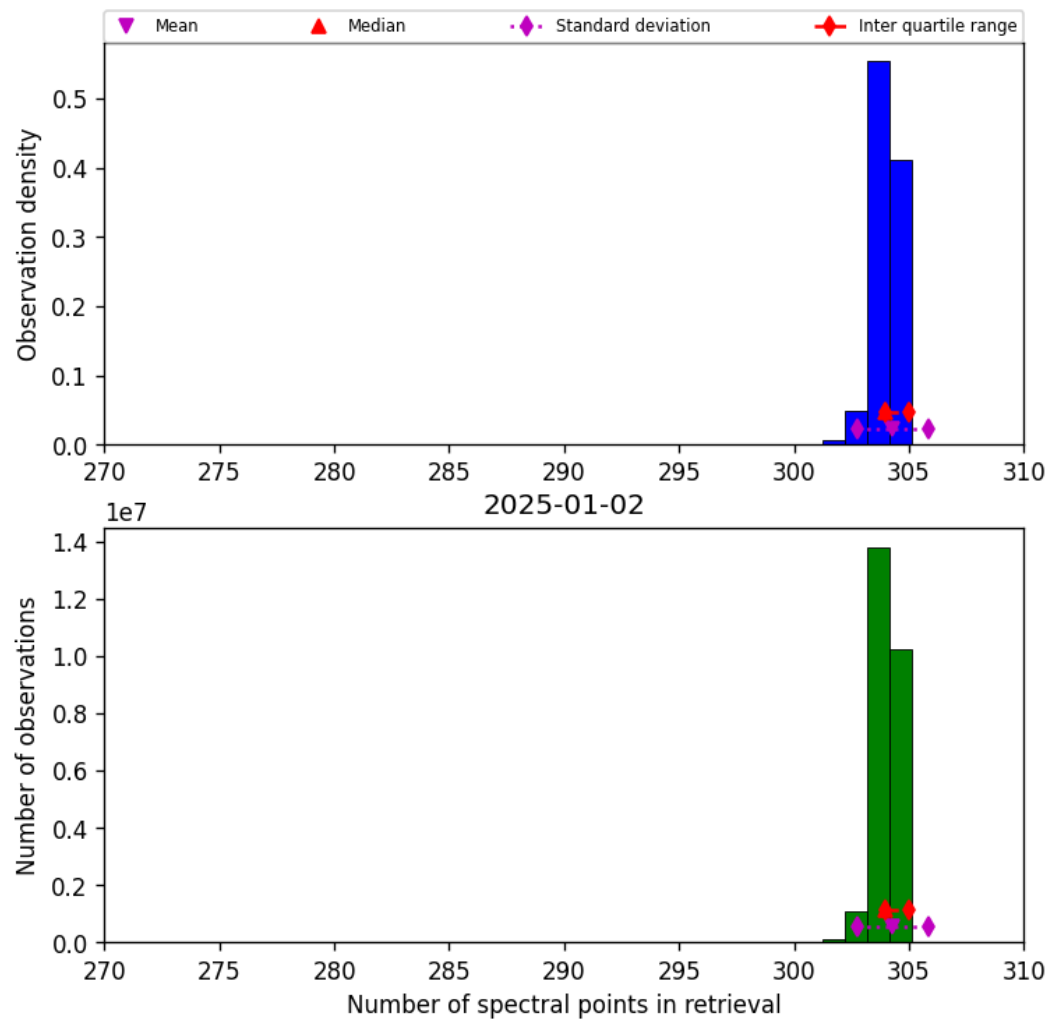
Figure 33: Histogram of “Number of spectral points in retrieval” for 2025-01-01 to 2025-01-03
