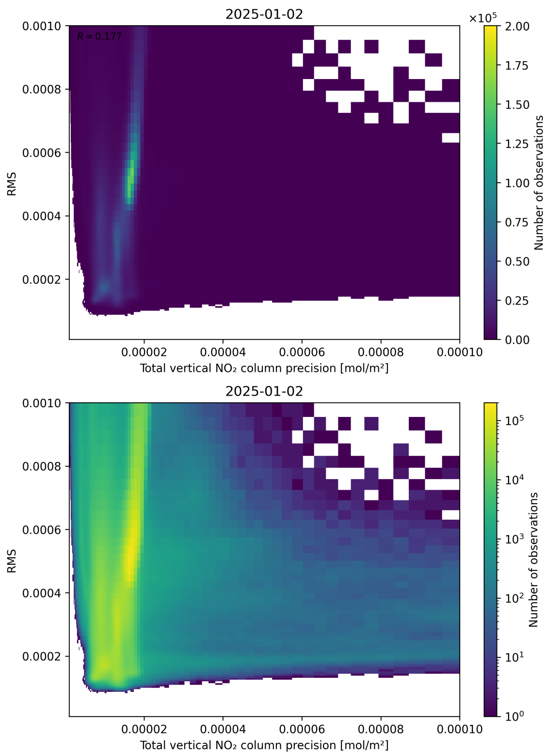
Figure 119: Scatter density plot of “Total vertical NO 2 column precision” against “RMS” for 2025-01-01 to 2025-01-03.
