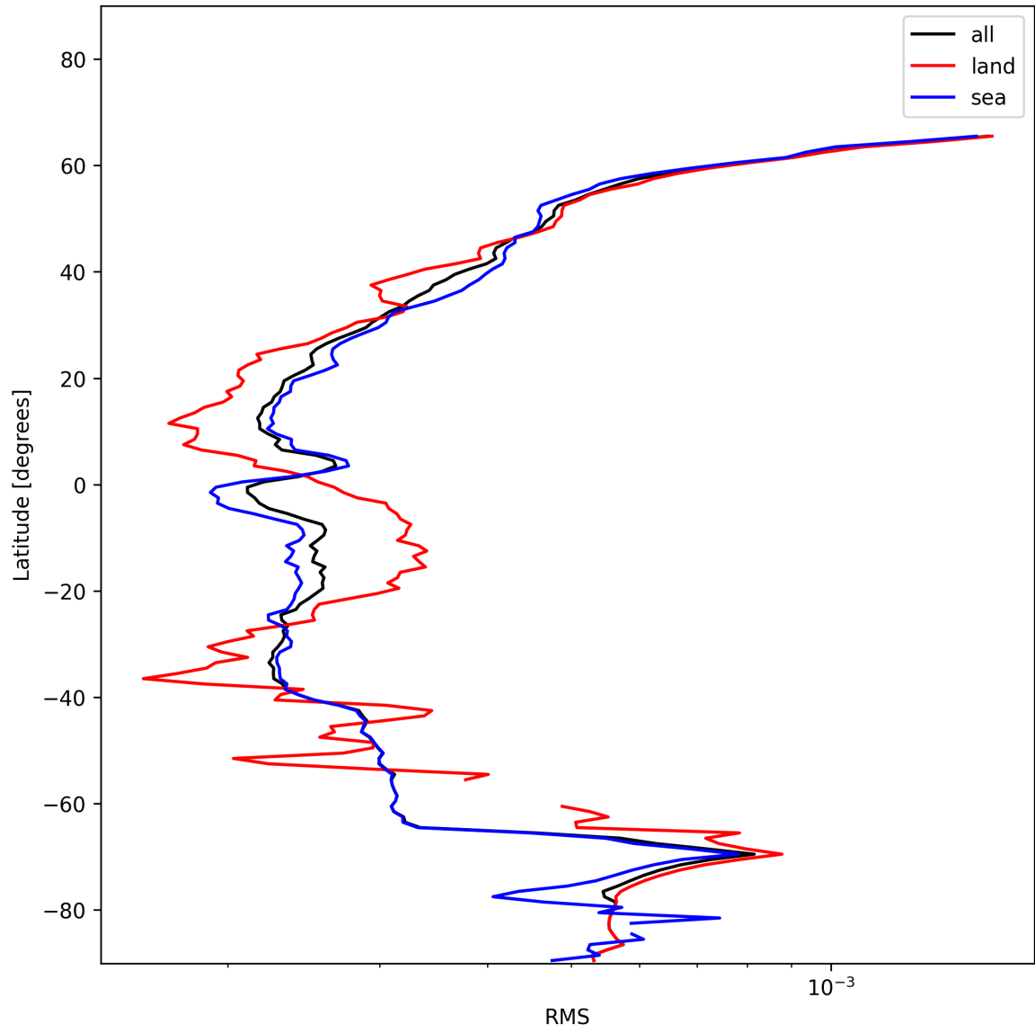
Figure 26: Zonal average of “RMS” for 2025-01-01 to 2025-01-03.
