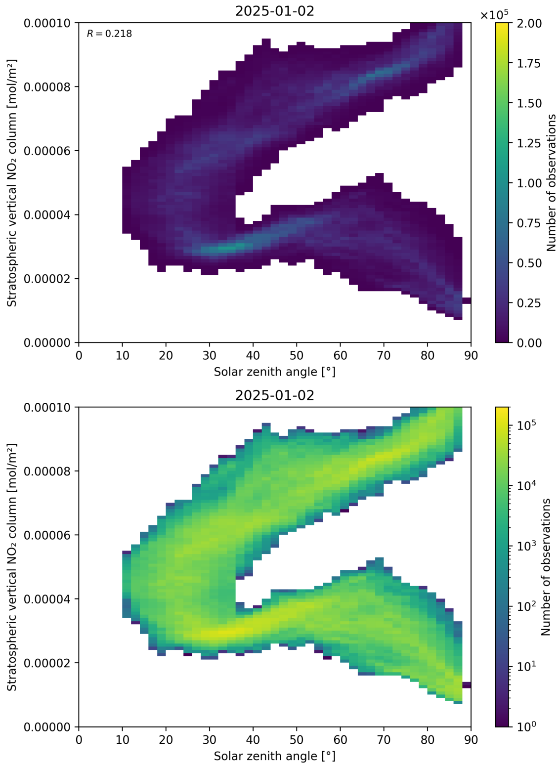
Figure 150: Scatter density plot of “Solar zenith angle” against “Stratospheric vertical NO 2 column” for 2025-01-01 to 2025-01-03.
