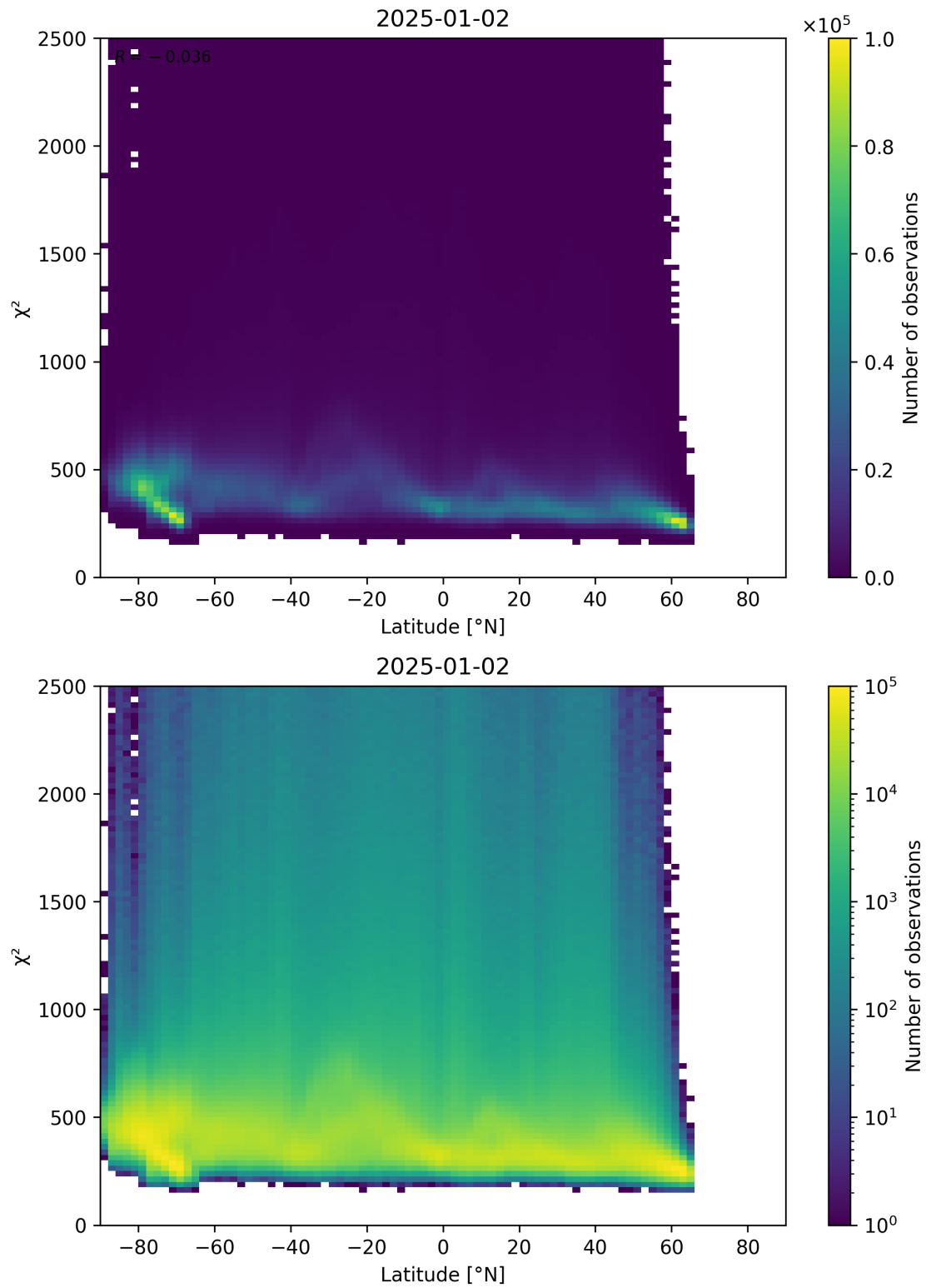
Figure 86: Scatter density plot of “Latitude” against “ \chi^2 ” for 2025-01-01 to 2025-01-03.
