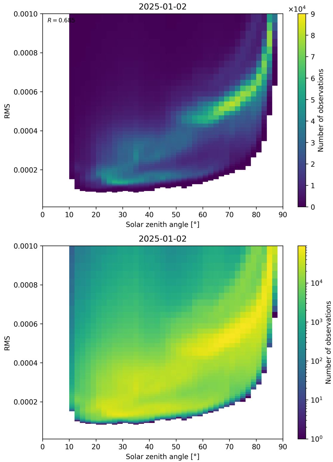
Figure 157: Scatter density plot of “Solar zenith angle” against “RMS” for 2025-01-01 to 2025-01-03.
