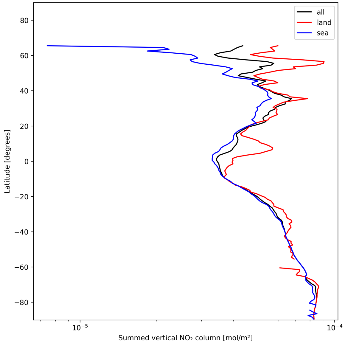
Figure 23: Zonal average of “Summed vertical NO 2 column” for 2025-01-01 to 2025-01-03.
