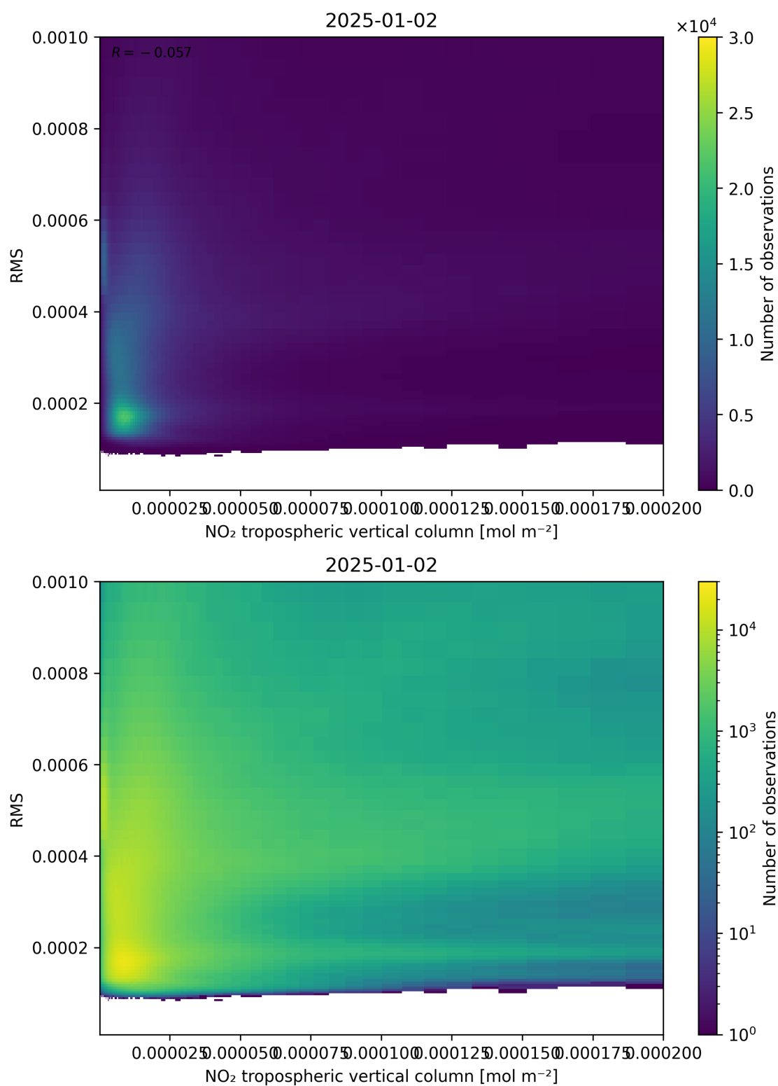
Figure 142: Scatter density plot of “NO 2 tropospheric vertical column” against “RMS” for 2025-01-01 to 2025-01-03.
