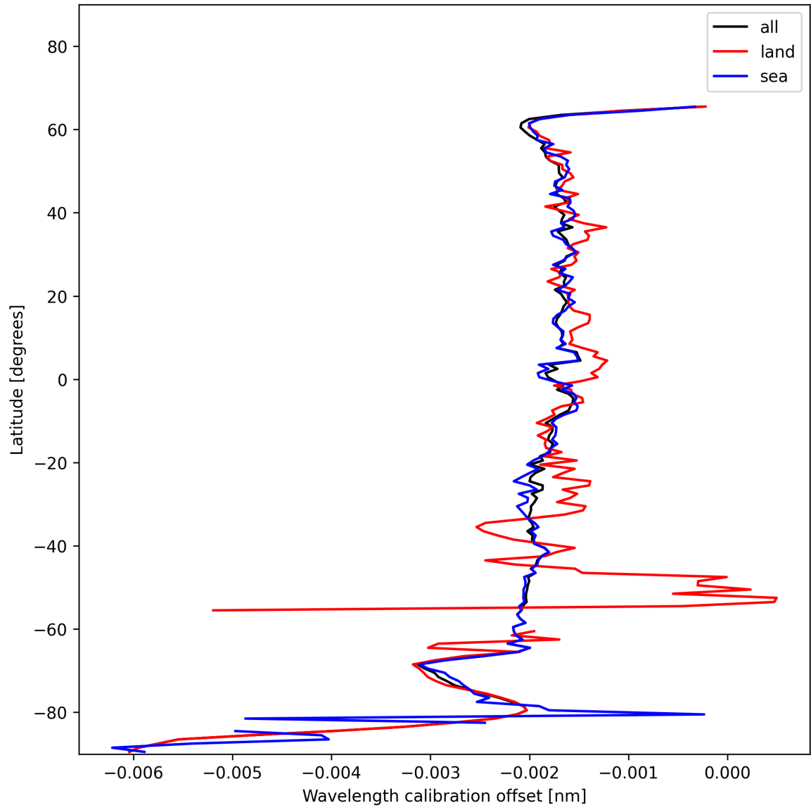
Figure 18: Zonal average of “Wavelength calibration offset” for 2025-01-01 to 2025-01-03.
