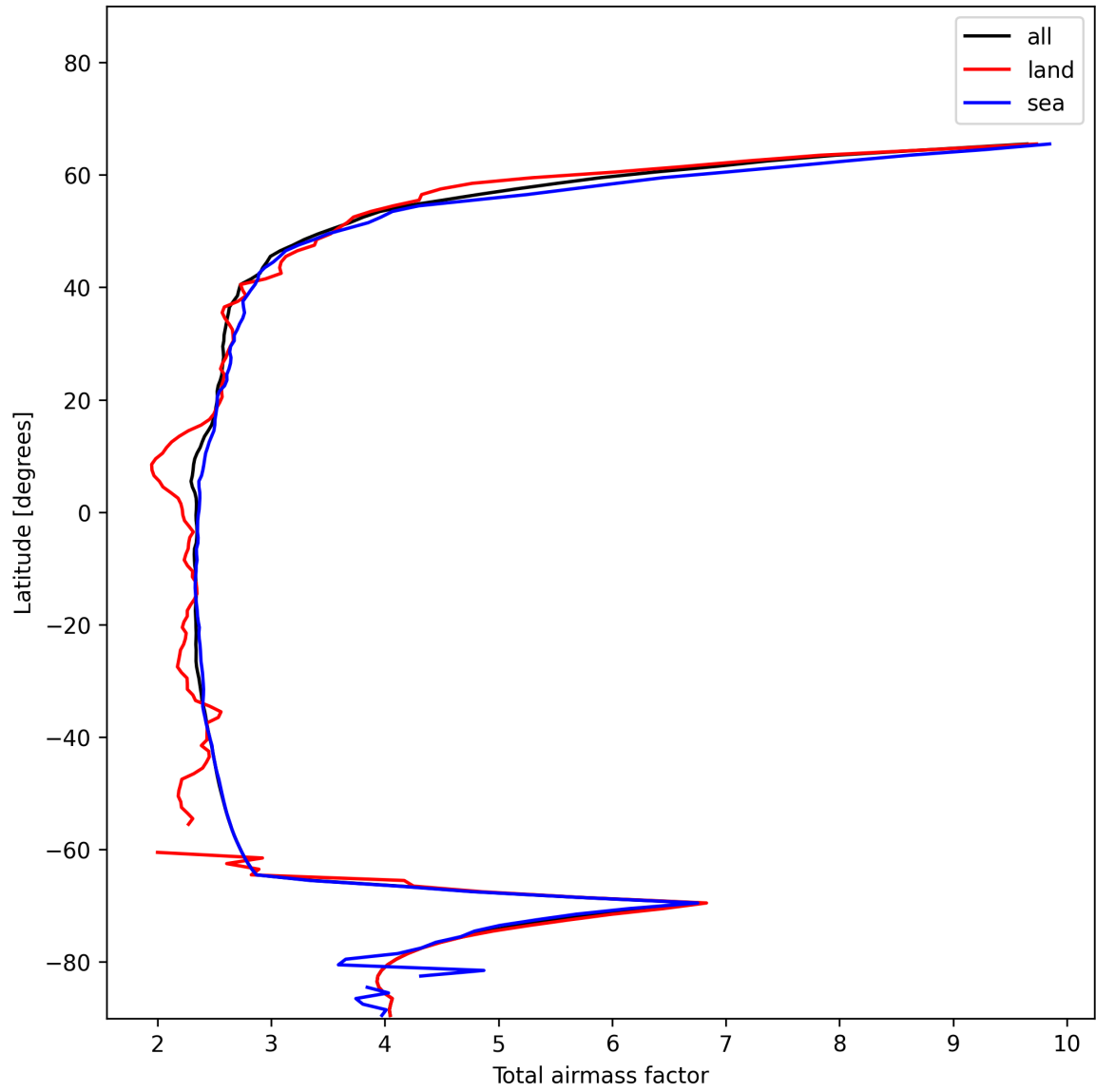
Figure 15: Zonal average of “Total airmass factor” for 2025-01-01 to 2025-01-03.
