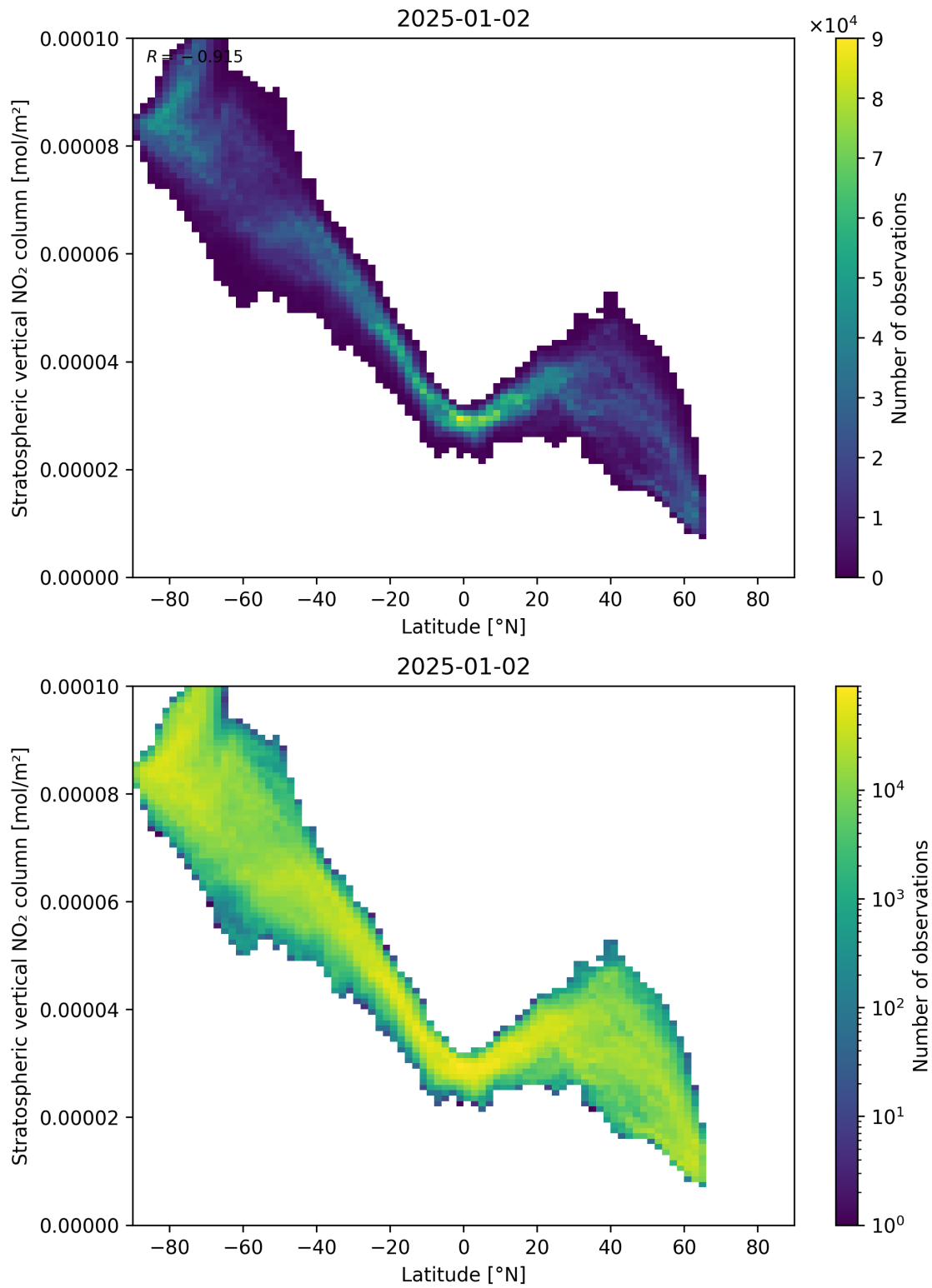
Figure 87: Scatter density plot of “Latitude” against “Stratospheric vertical NO 2 column” for 2025-01-01 to 2025-01-03.
