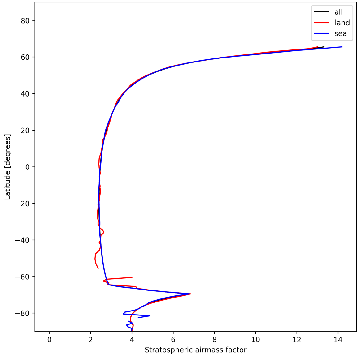
Figure 27: Zonal average of “Stratospheric airmass factor” for 2025-01-01 to 2025-01-03.
