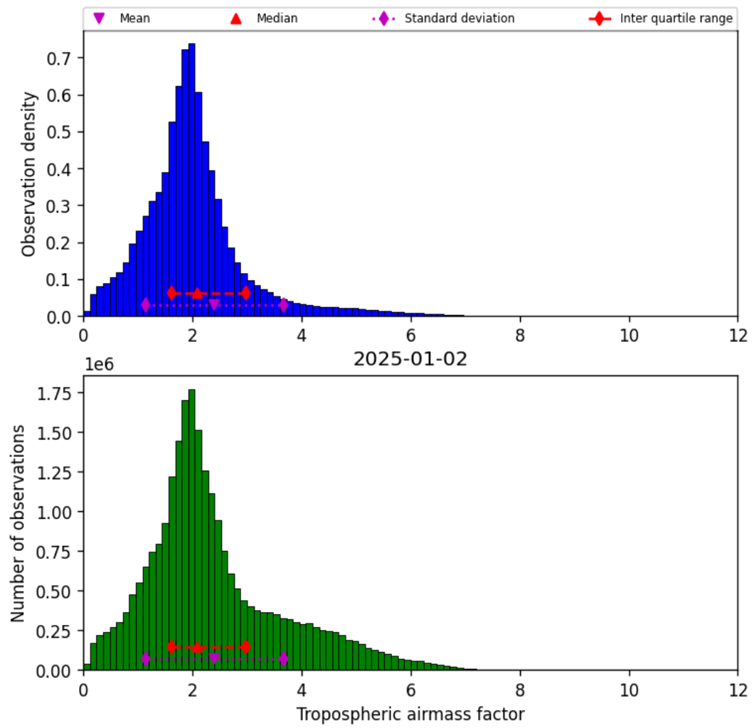
Figure 31: Histogram of “Tropospheric airmass factor” for 2025-01-01 to 2025-01-03
