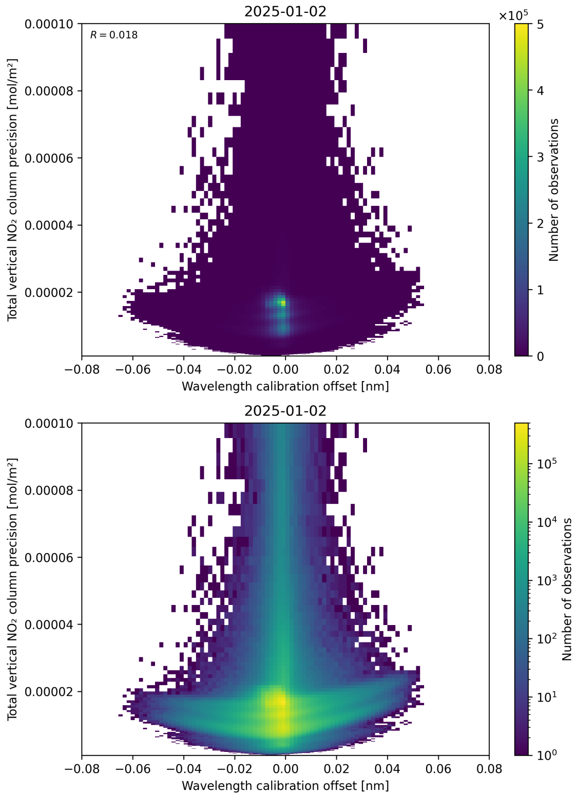
Figure 180: Scatter density plot of “Wavelength calibration offset” against “Total vertical NO 2 column precision” for 2025-01-01 to 2025-01-03.
