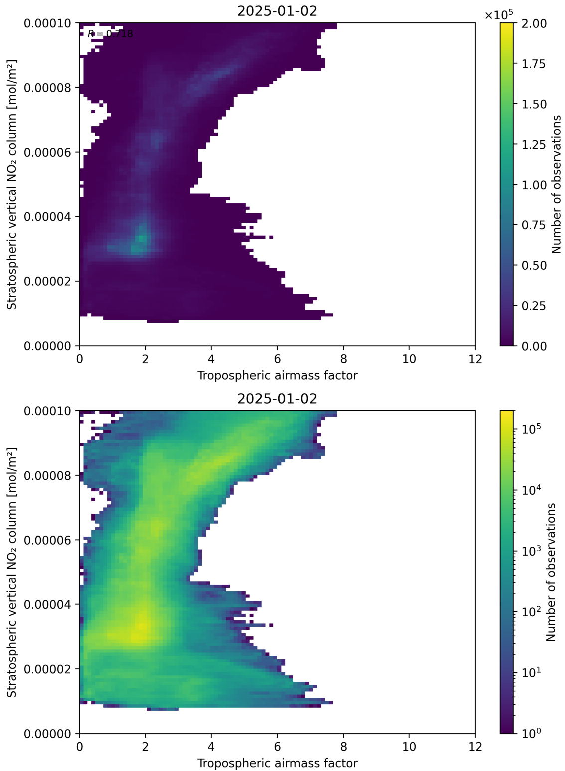
Figure 74: Scatter density plot of “Tropospheric air mass factor” against “Stratospheric vertical NO 2 column” for 2025-01-01 to 2025-01-03.
