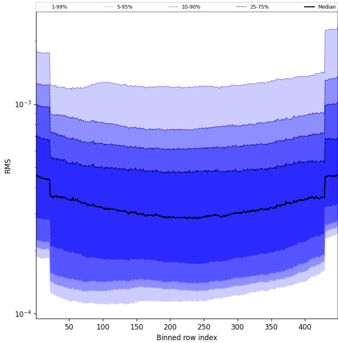
Figure 60: Along track statistics of “RMS” for 2025-01-01 to 2025-01-03
