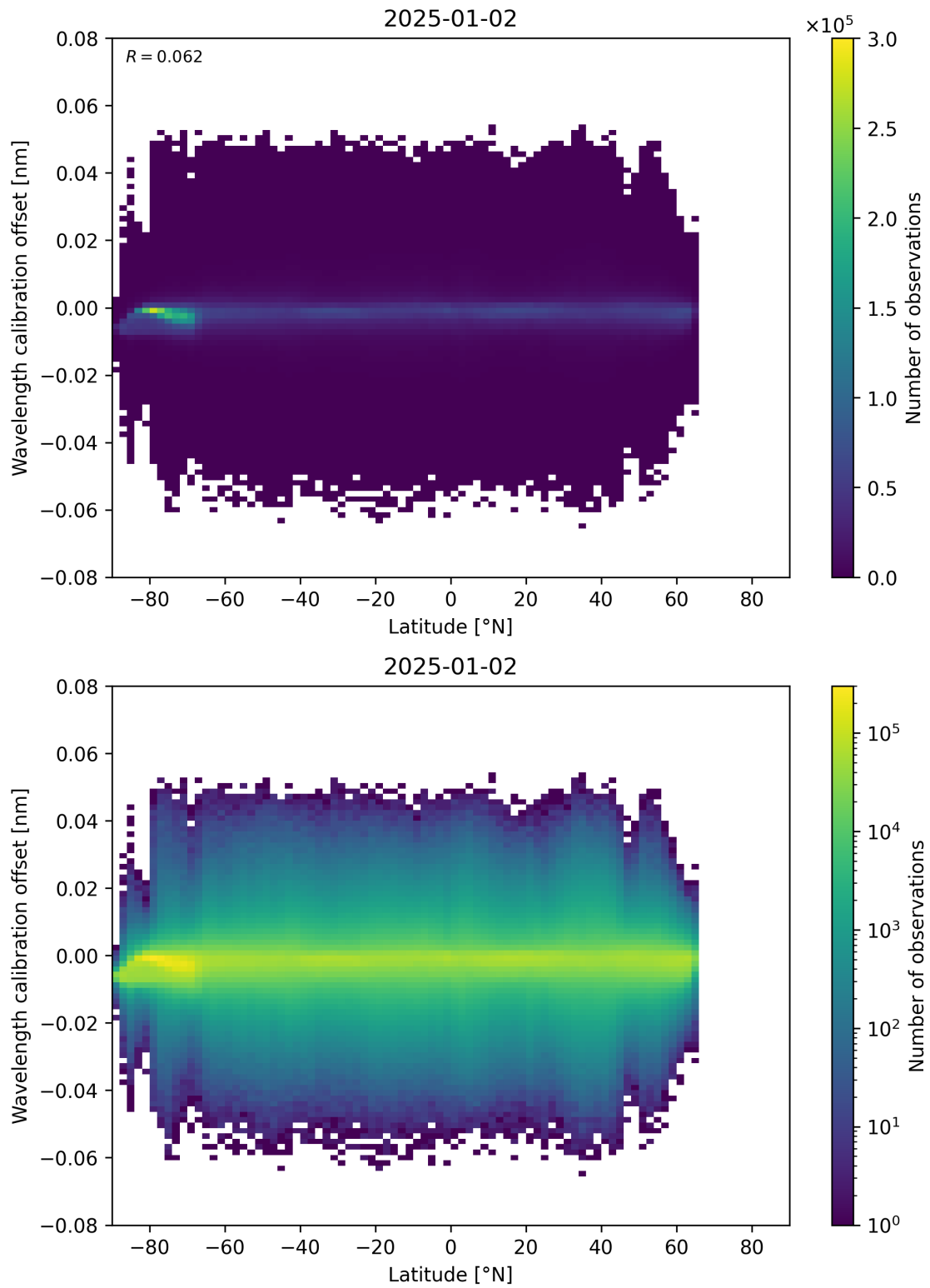
Figure 95: Scatter density plot of “Latitude” against “Wavelength calibration offset” for 2025-01-01 to 2025-01-03.
