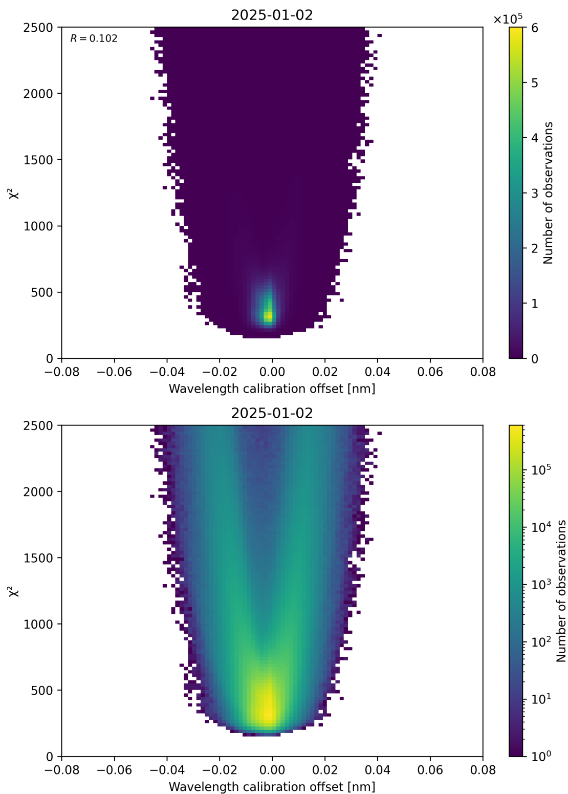
Figure 175: Scatter density plot of “Wavelength calibration offset” against “ \chi^2 ” for 2025-01-01 to 2025-01-03.
