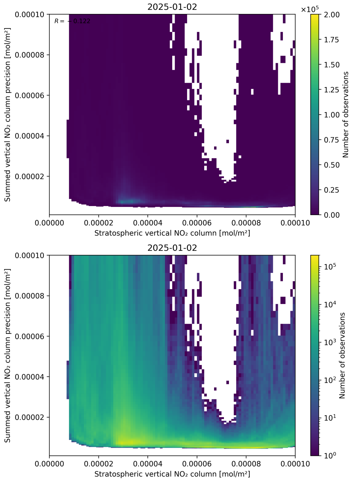
Figure 99: Scatter density plot of “Stratospheric vertical NO 2 column” against “Summed vertical NO 2 column precision” for 2025-01-01 to 2025-01-03.
