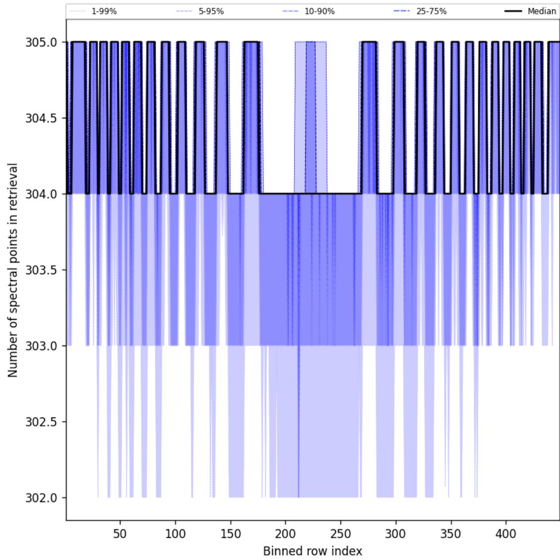
Figure 50: Along track statistics of “Number of spectral points in retrieval” for 2025-01-01 to 2025-01-03
