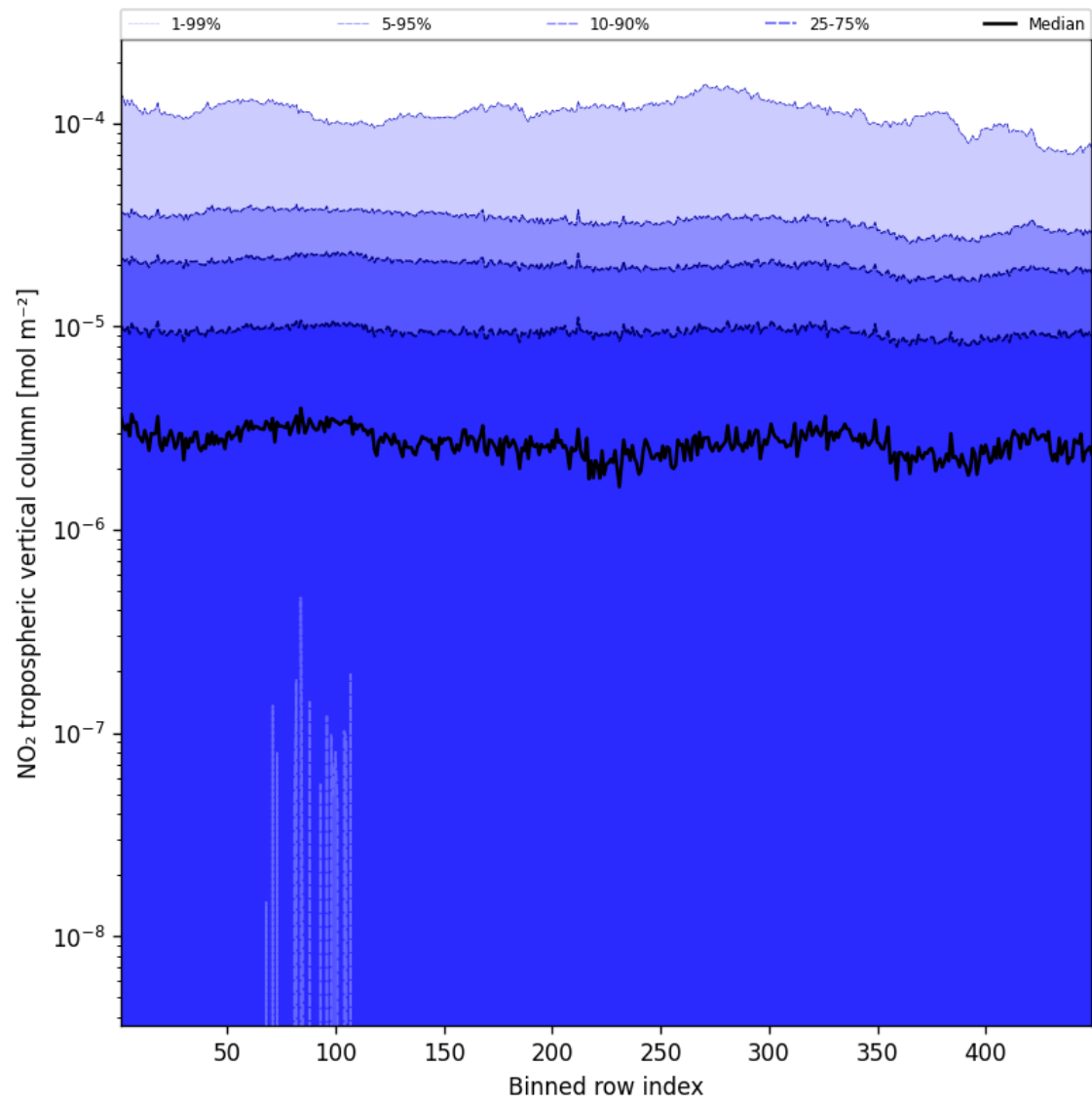
Figure 46: Along track statistics of “NO 2 tropospheric vertical column” for 2025-01-01 to 2025-01-03
