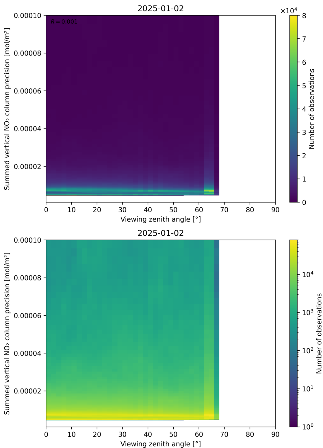
Figure 166: Scatter density plot of “Viewing zenith angle” against “Summed vertical NO 2 column precision” for 2025-01-01 to 2025-01-03.
