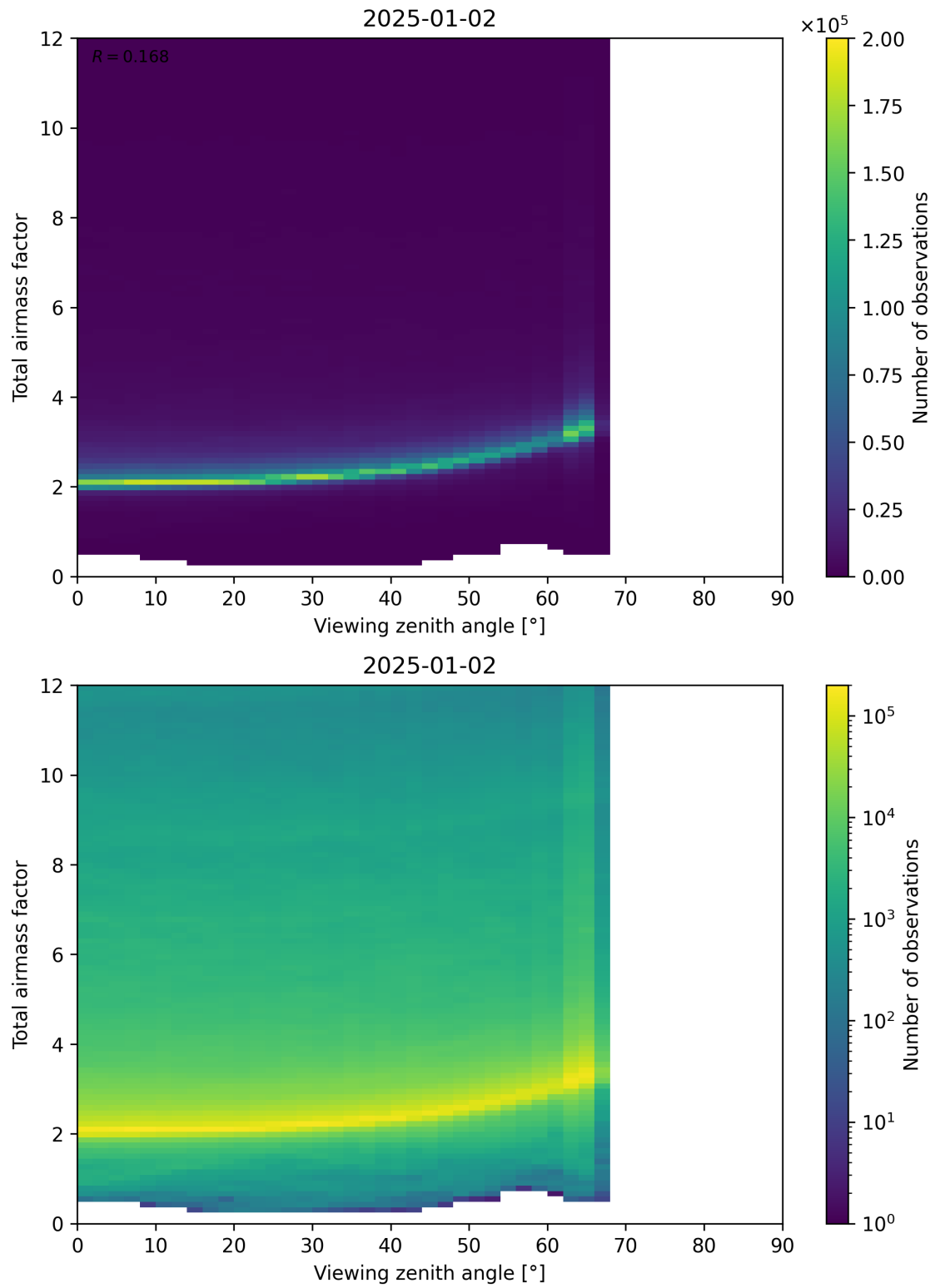
Figure 160: Scatter density plot of “Viewing zenith angle” against “Total airmass factor” for 2025-01-01 to 2025-01-03.
