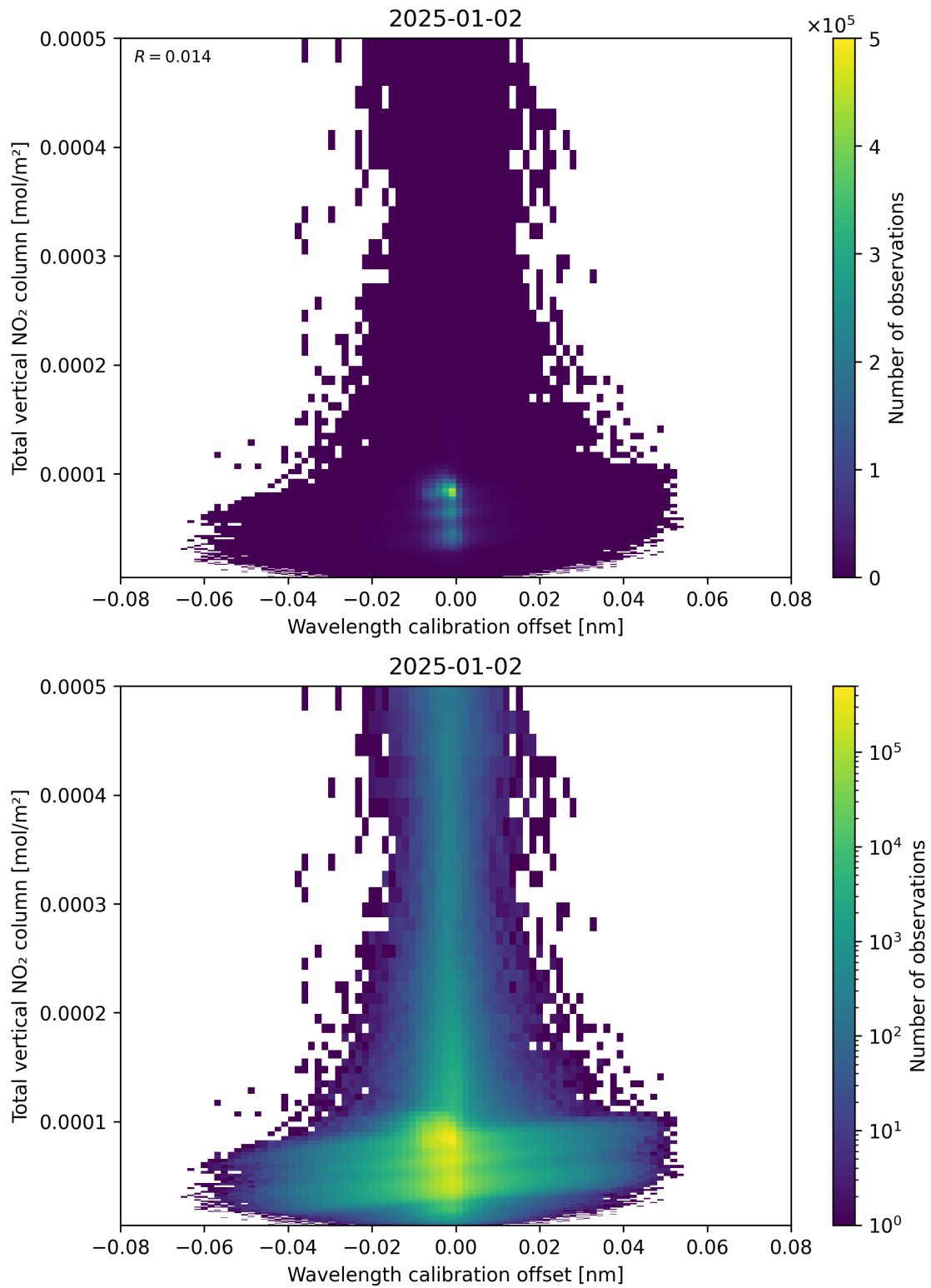
Figure 179: Scatter density plot of “Wavelength calibration offset” against “Total vertical NO 2 column” for 2025-01-01 to 2025-01-03.
