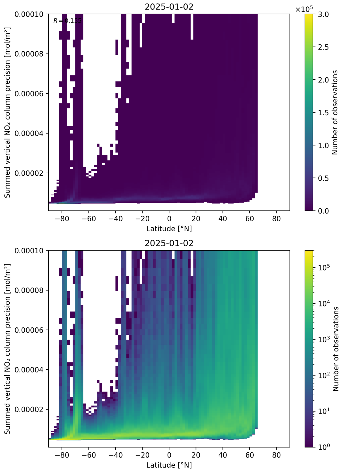
Figure 89: Scatter density plot of “Latitude” against “Summed vertical NO 2 column precision” for 2025-01-01 to 2025-01-03.
