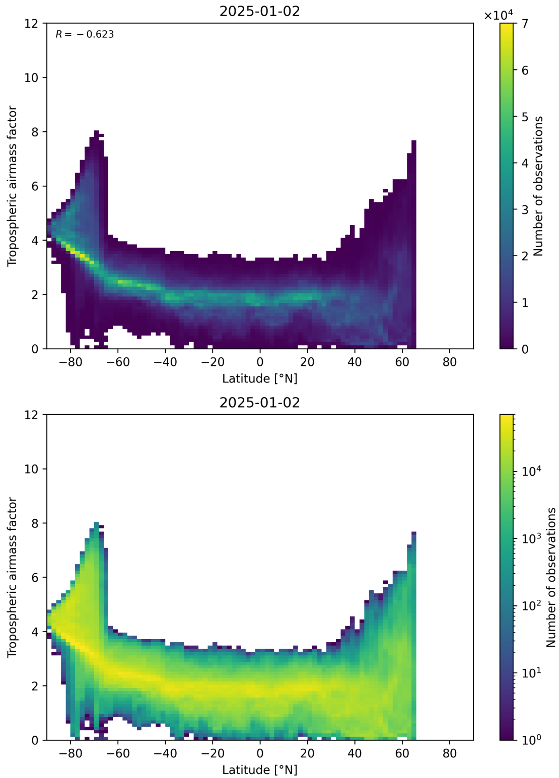
Figure 85: Scatter density plot of “Latitude” against “Tropospheric air mass factor” for 2025-01-01 to 2025-01-03.
