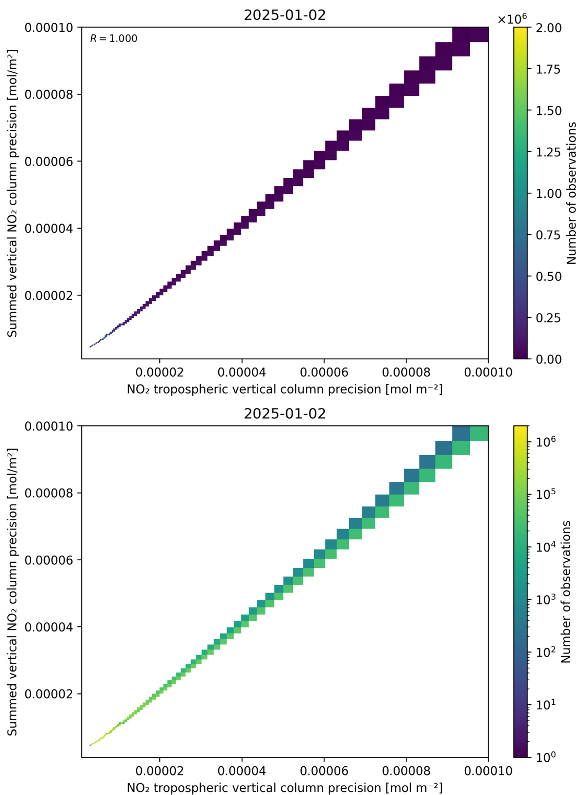
Figure 137: Scatter density plot of “NO 2 tropospheric vertical column precision” against “Summed vertical NO 2 column precision” for 2025-01-01 to 2025-01-03.
