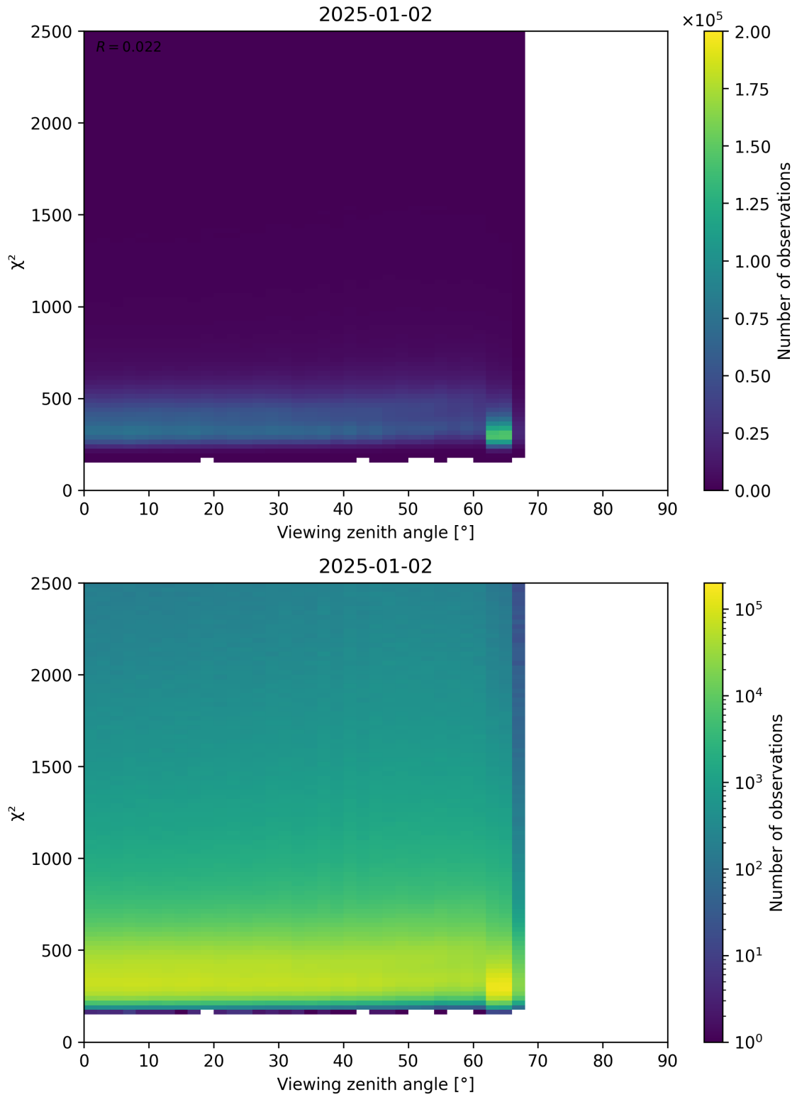
Figure 162: Scatter density plot of “Viewing zenith angle” against “ \chi^2 ” for 2025-01-01 to 2025-01-03.
