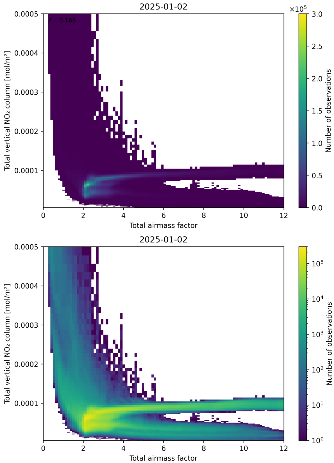
Figure 67: Scatter density plot of “Total airmass factor” against “Total vertical \text{NO}_2 column” for 2025-01-01 to 2025-01-03.
