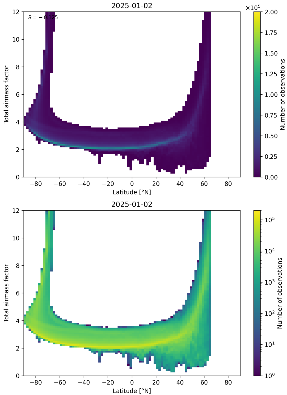
Figure 84: Scatter density plot of “Latitude” against “Total airmass factor” for 2025-01-01 to 2025-01-03.
