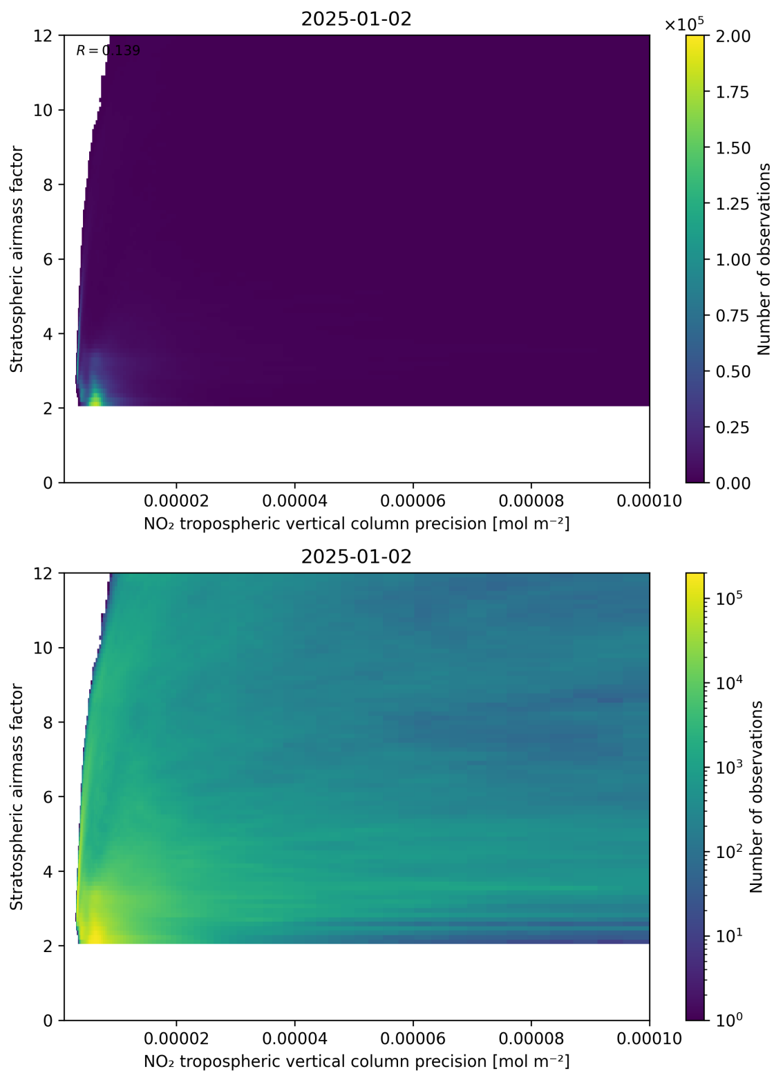
Figure 131: Scatter density plot of “NO 2 tropospheric vertical column precision” against “Stratospheric airmass factor” for 2025-01-01 to 2025-01-03.
