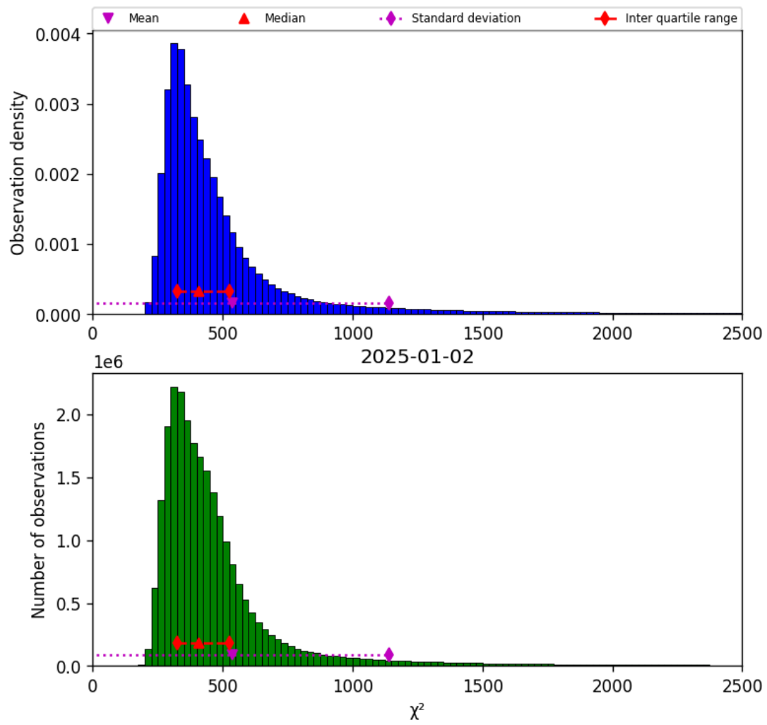
Figure 42: Histogram of " \chi^2 " for 2025-01-01 to 2025-01-03
