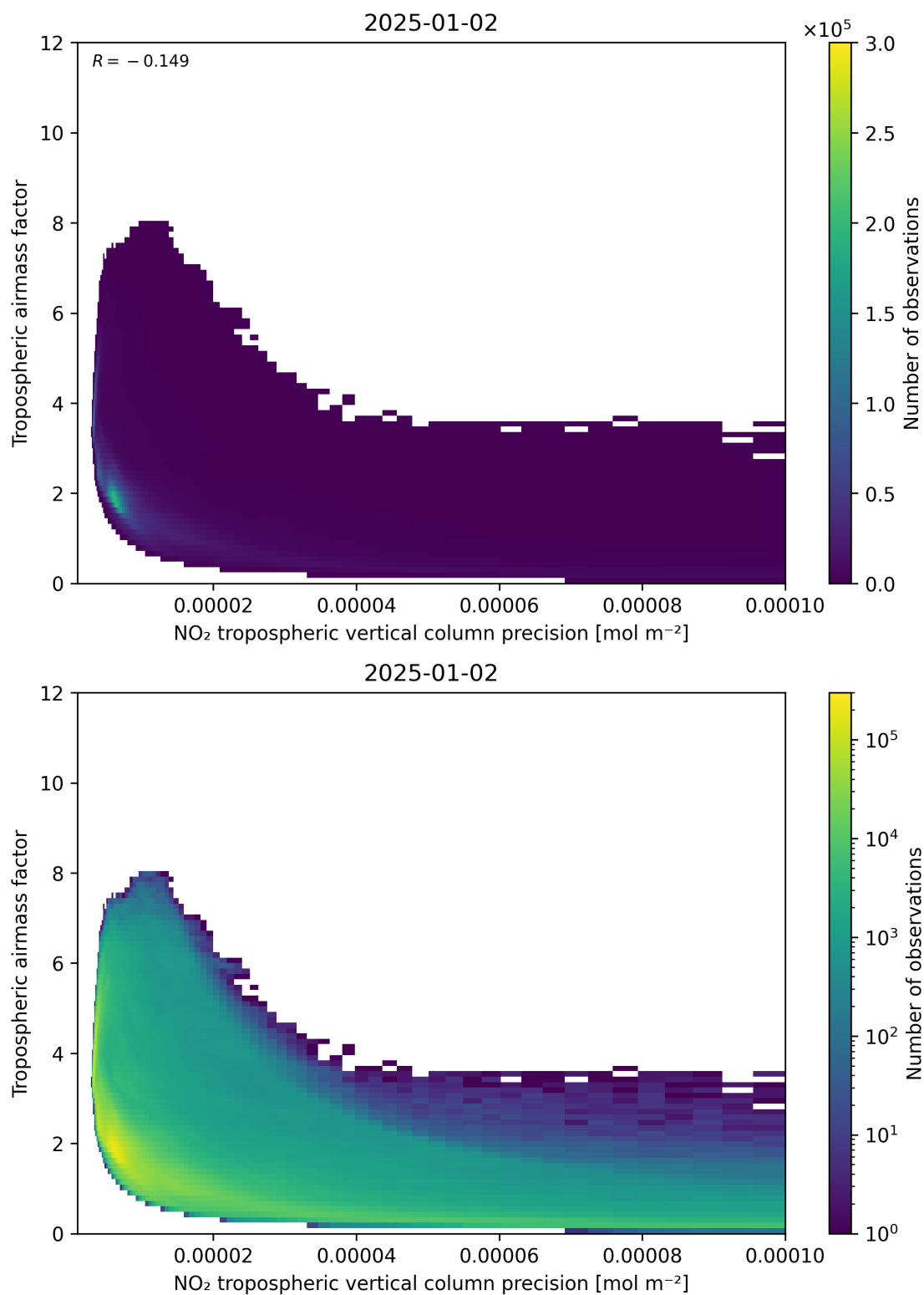
Figure 133: Scatter density plot of “NO 2 tropospheric vertical column precision” against “Tropospheric airmass factor” for 2025-01-01 to 2025-01-03.
