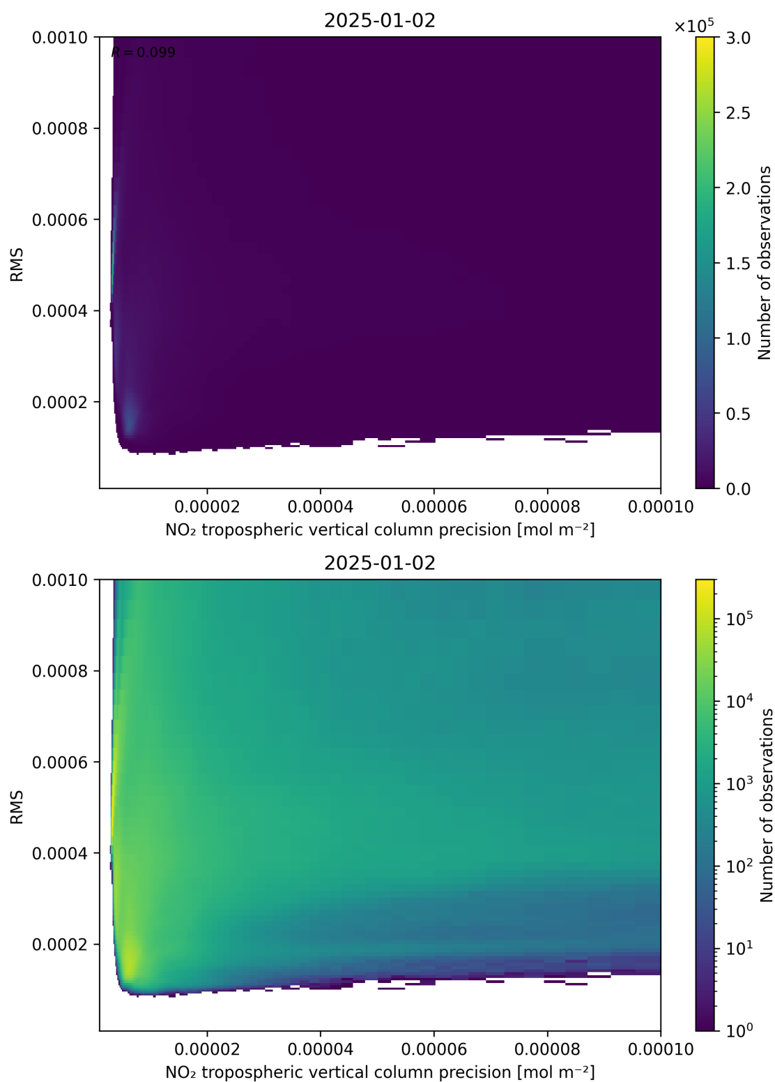
Figure 140: Scatter density plot of “NO 2 tropospheric vertical column precision” against “RMS” for 2025-01-01 to 2025-01-03.
