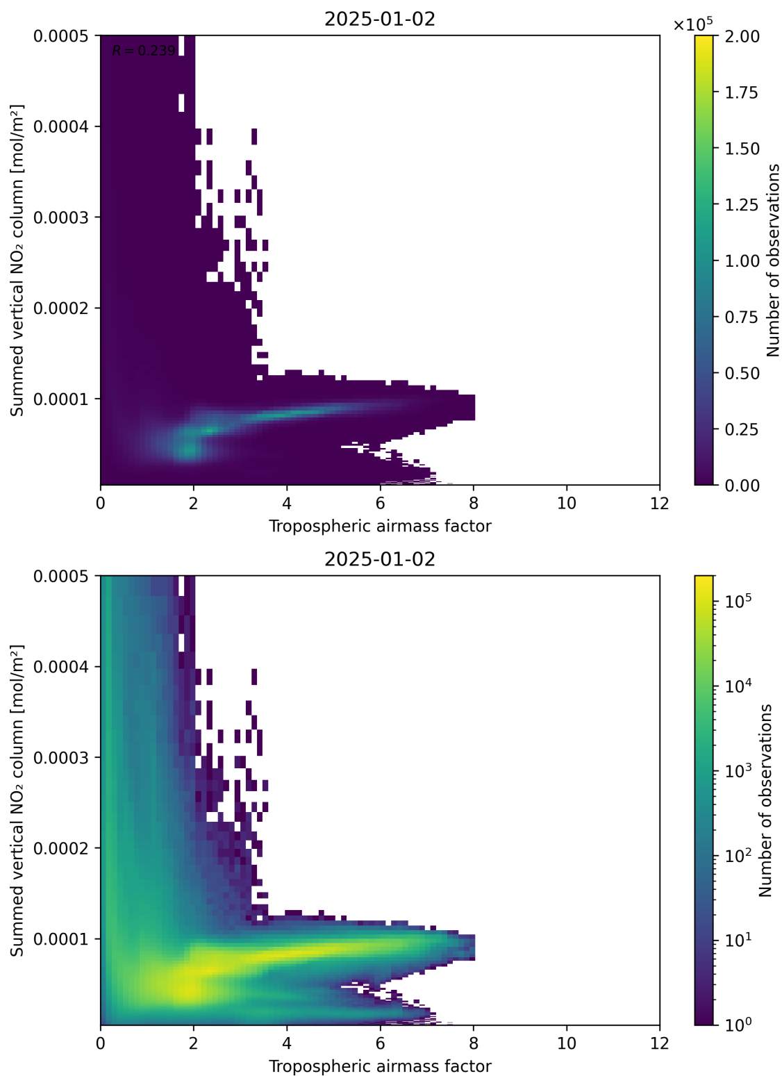
Figure 75: Scatter density plot of “Tropospheric airmass factor” against “Summed vertical NO 2 column” for 2025-01-01 to 2025-01-03.
