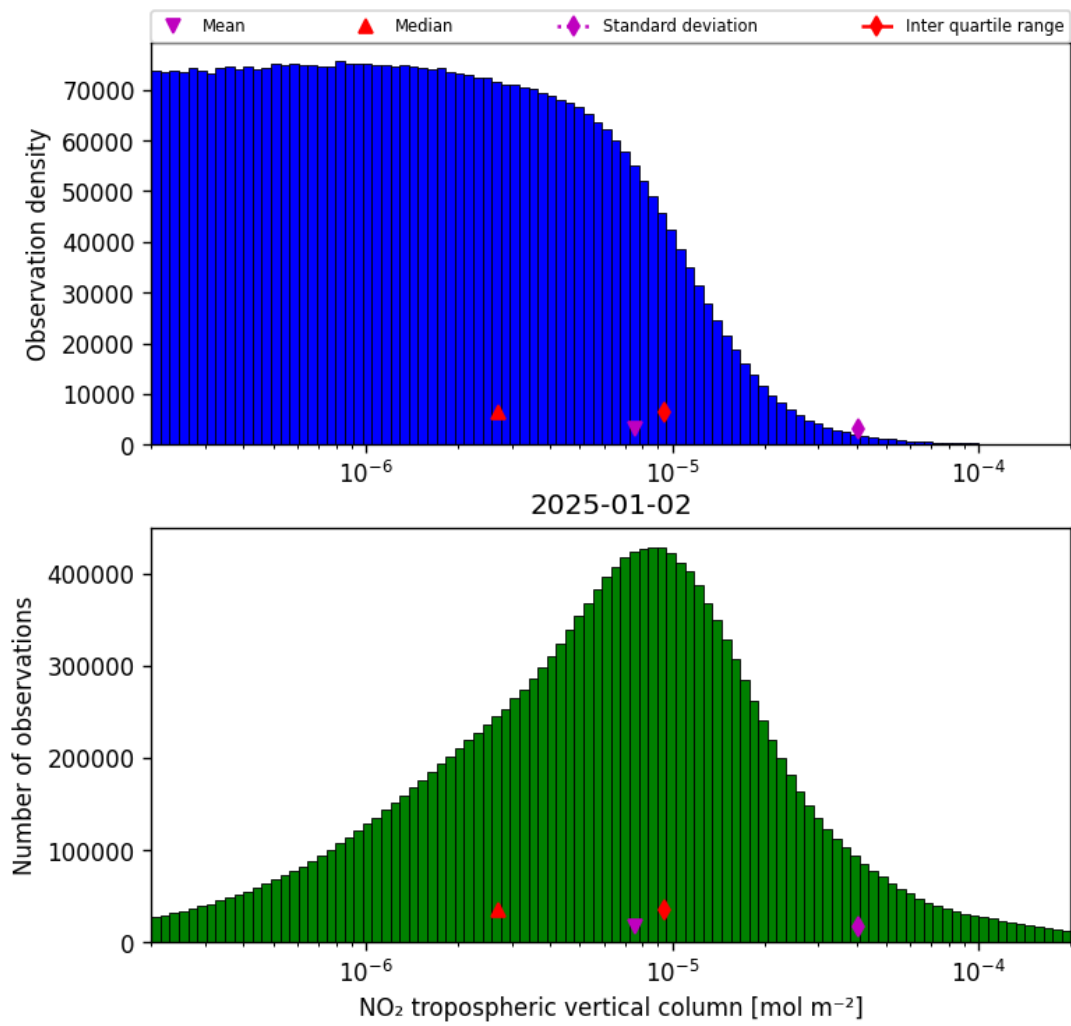
Figure 29: Histogram of “NO 2 tropospheric vertical column” for 2025-01-01 to 2025-01-03
