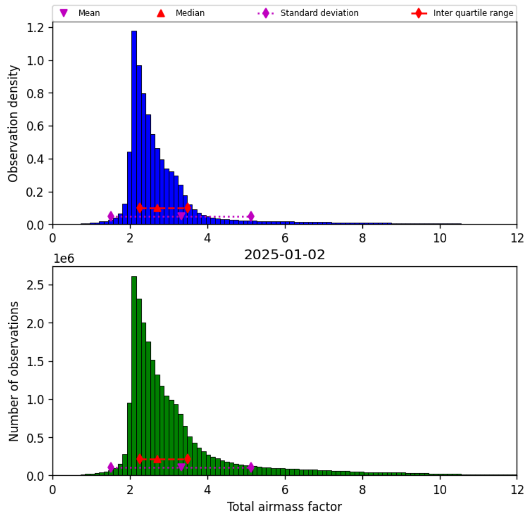
Figure 32: Histogram of “Total airmass factor” for 2025-01-01 to 2025-01-03
