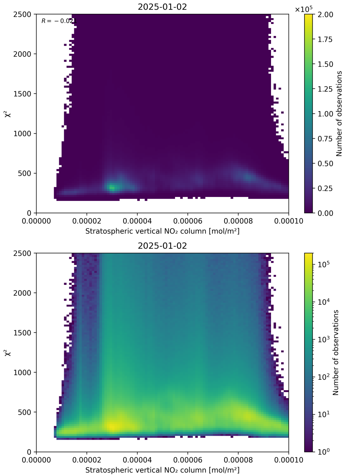
Figure 97: Scatter density plot of “Stratospheric vertical NO 2 column” against “ \chi^2 ” for 2025-01-01 to 2025-01-03.
