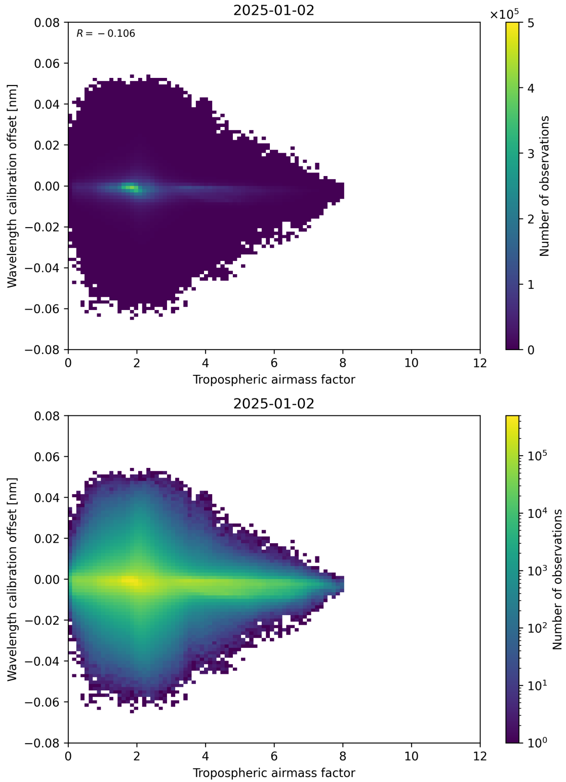
Figure 80: Scatter density plot of “Tropospheric airmass factor” against “Wavelength calibration offset” for 2025-01-01 to 2025-01-03.
