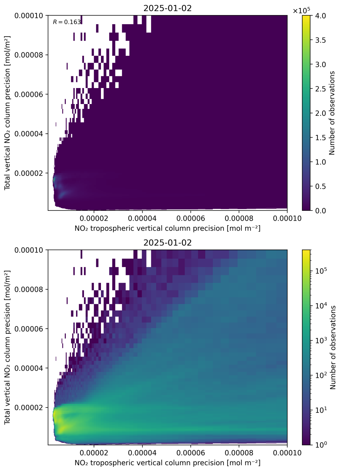
Figure 139: Scatter density plot of “NO 2 tropospheric vertical column precision” against “Total vertical NO 2 column precision” for 2025-01-01 to 2025-01-03.
