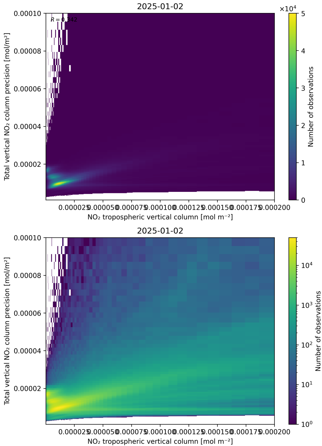
Figure 129: Scatter density plot of “NO 2 tropospheric vertical column” against “Total vertical NO 2 column precision” for 2025-01-01 to 2025-01-03.
