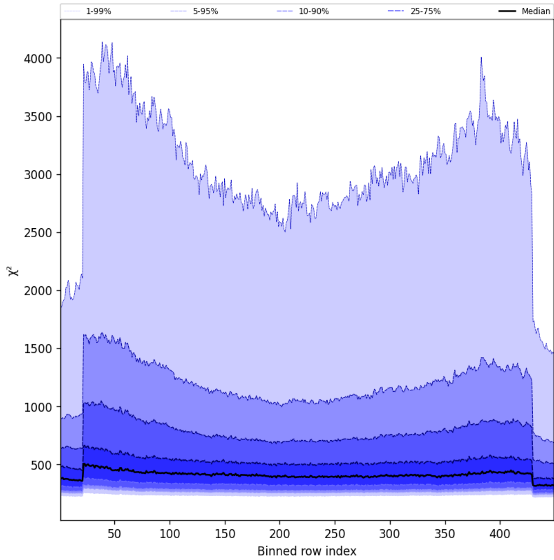
Figure 59: Along track statistics of “ \chi^2 ” for 2025-01-01 to 2025-01-03
