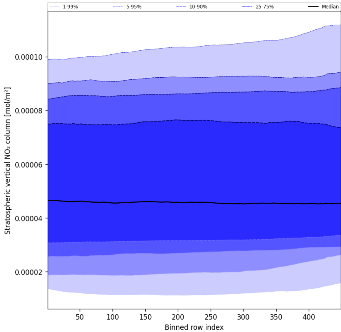
Figure 53: Along track statistics of “Stratospheric vertical NO 2 column” for 2025-01-01 to 2025-01-03
