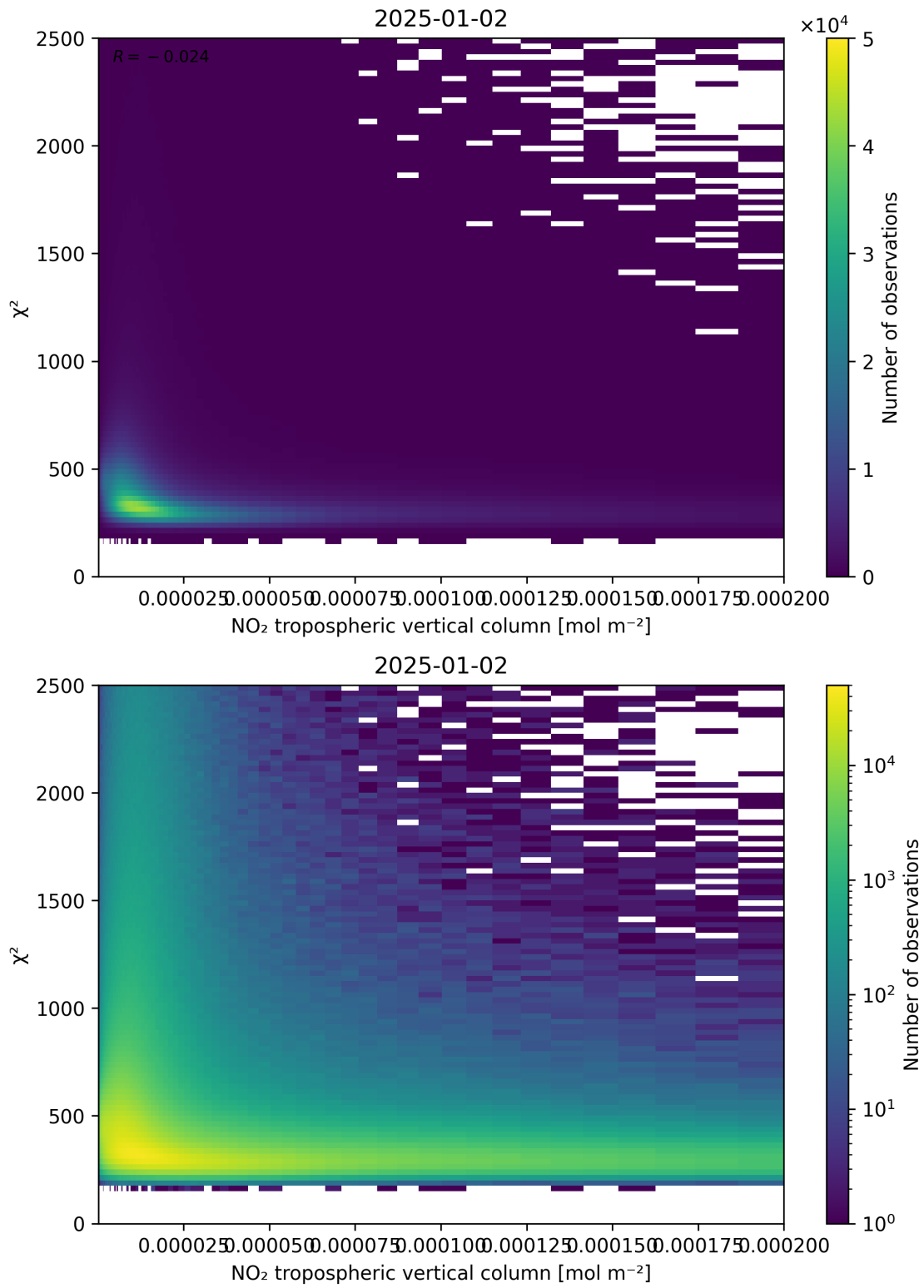
Figure 124: Scatter density plot of “NO 2 tropospheric vertical column” against “ \chi^2 ” for 2025-01-01 to 2025-01-03.
