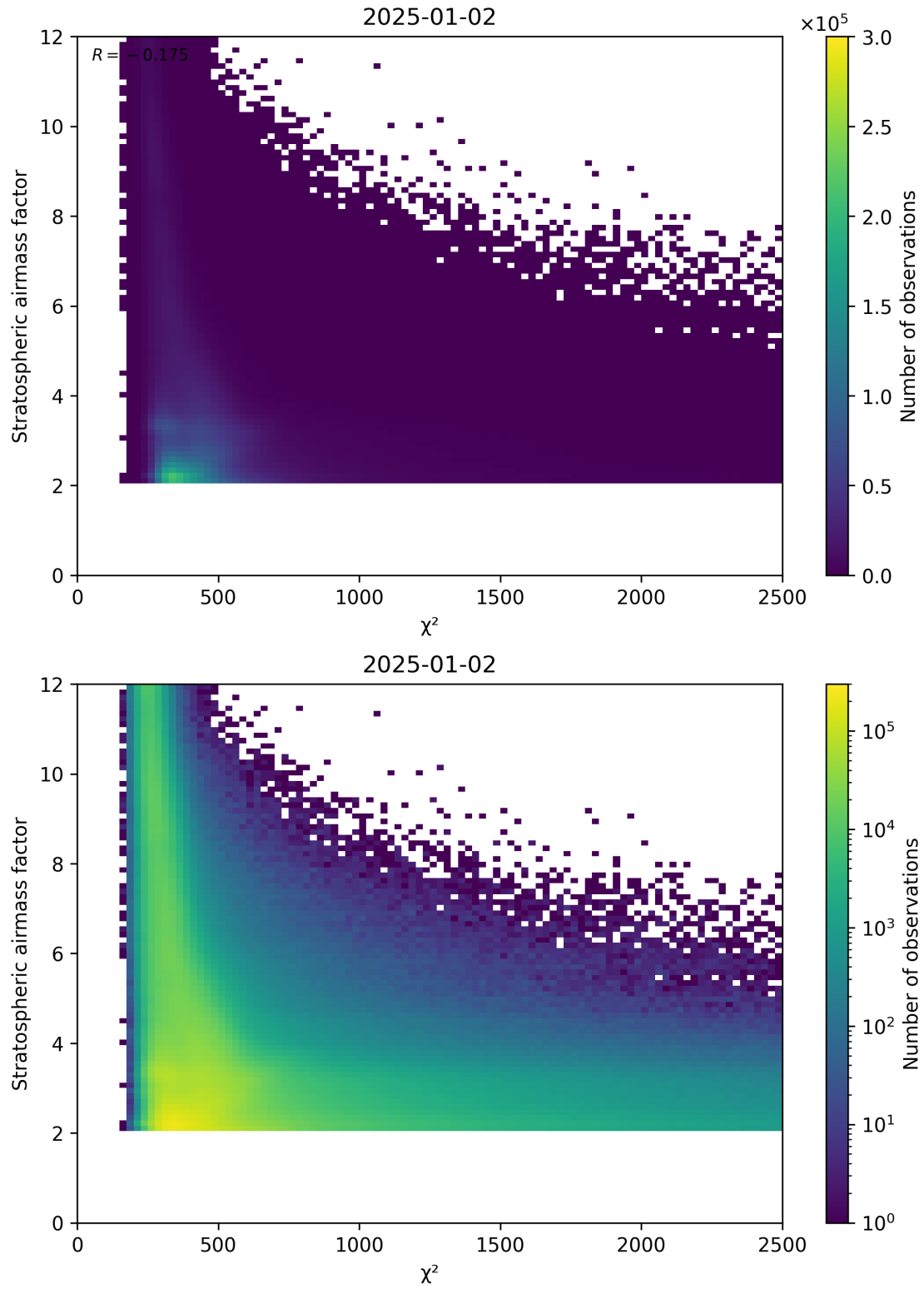
Figure 81: Scatter density plot of “ \chi^2 ” against “Stratospheric airmass factor” for 2025-01-01 to 2025-01-03.
