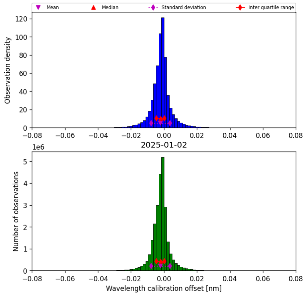
Figure 35: Histogram of “Wavelength calibration offset” for 2025-01-01 to 2025-01-03
