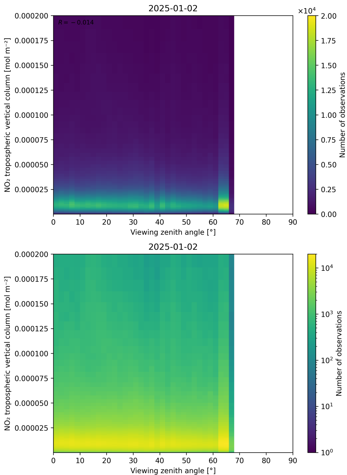
Figure 169: Scatter density plot of “Viewing zenith angle” against “NO 2 tropospheric vertical column” for 2025-01-01 to 2025-01-03.
