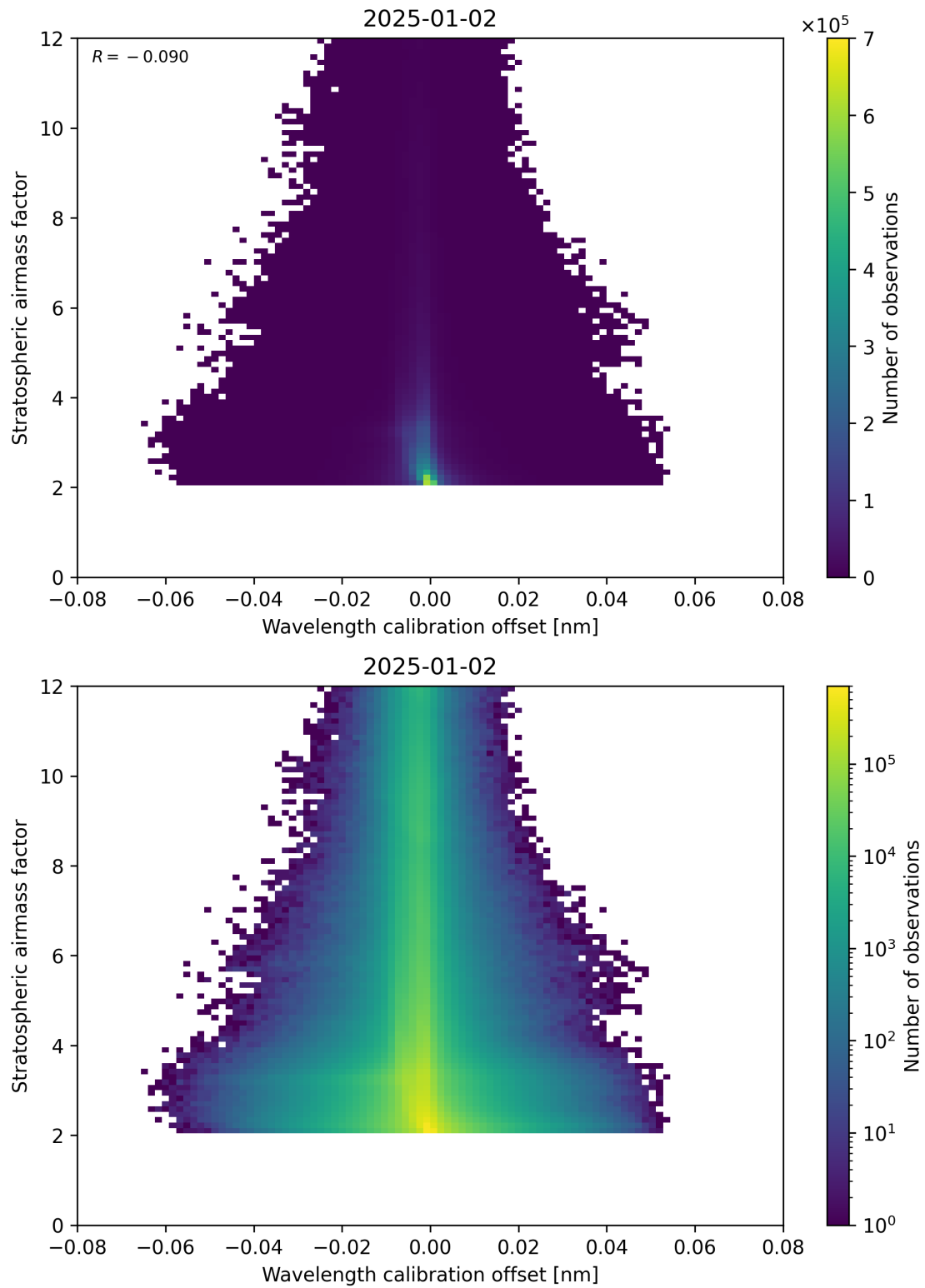
Figure 174: Scatter density plot of “Wavelength calibration offset” against “Stratospheric airmass factor” for 2025-01-01 to 2025-01-03.
