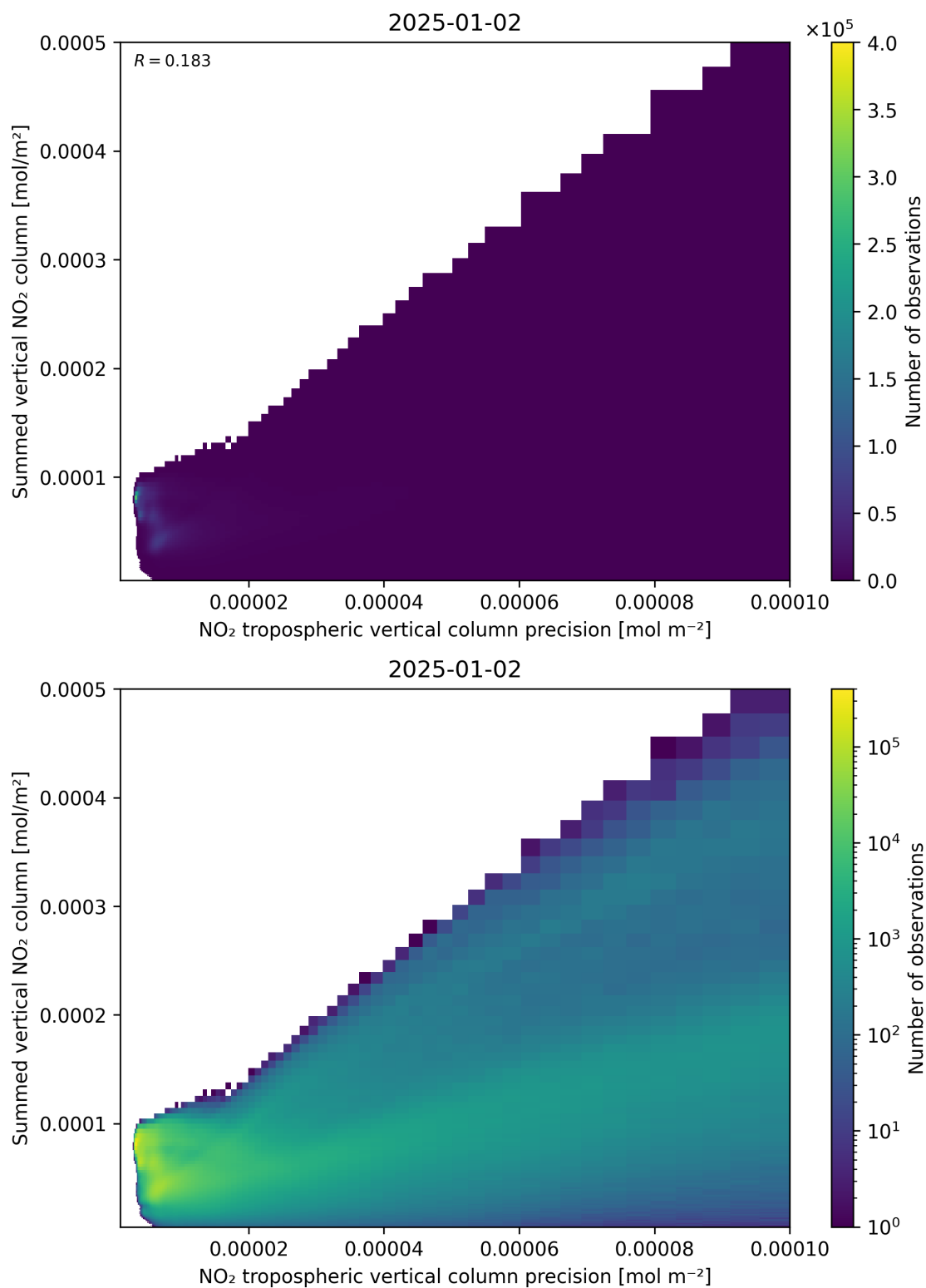
Figure 136: Scatter density plot of “NO 2 tropospheric vertical column precision” against “Summed vertical NO 2 column” for 2025-01-01 to 2025-01-03.
