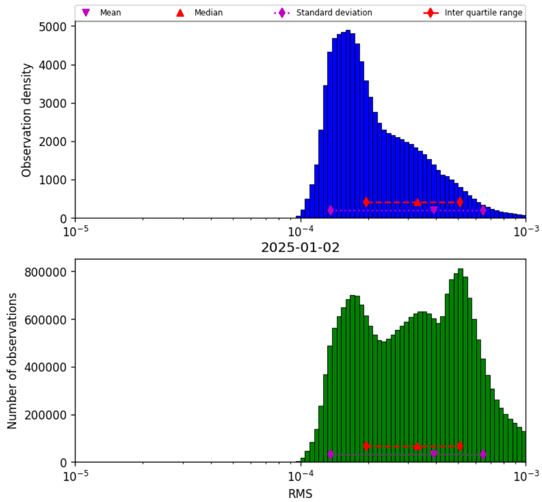
Figure 43: Histogram of “RMS” for 2025-01-01 to 2025-01-03
