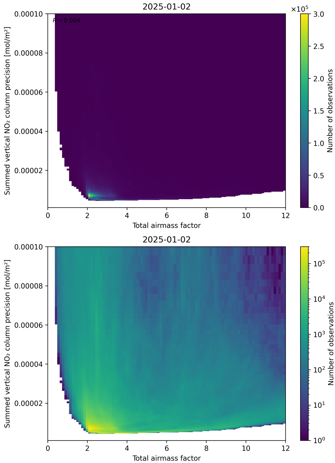
Figure 66: Scatter density plot of “Total airmass factor” against “Summed vertical NO 2 column precision” for 2025-01-01 to 2025-01-03.
