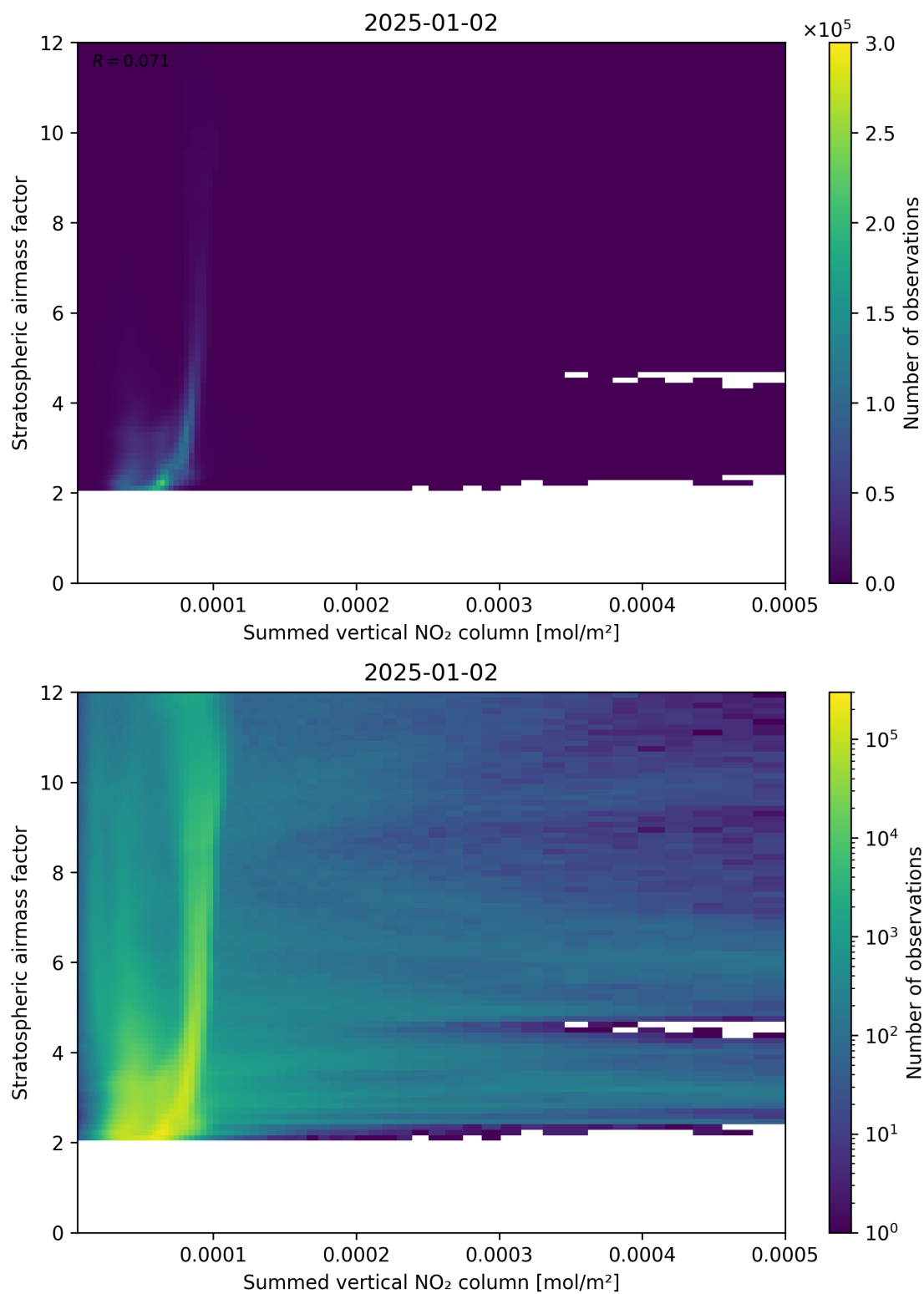
Figure 103: Scatter density plot of “Summed vertical NO 2 column” against “Stratospheric air mass factor” for 2025-01-01 to 2025-01-03.
