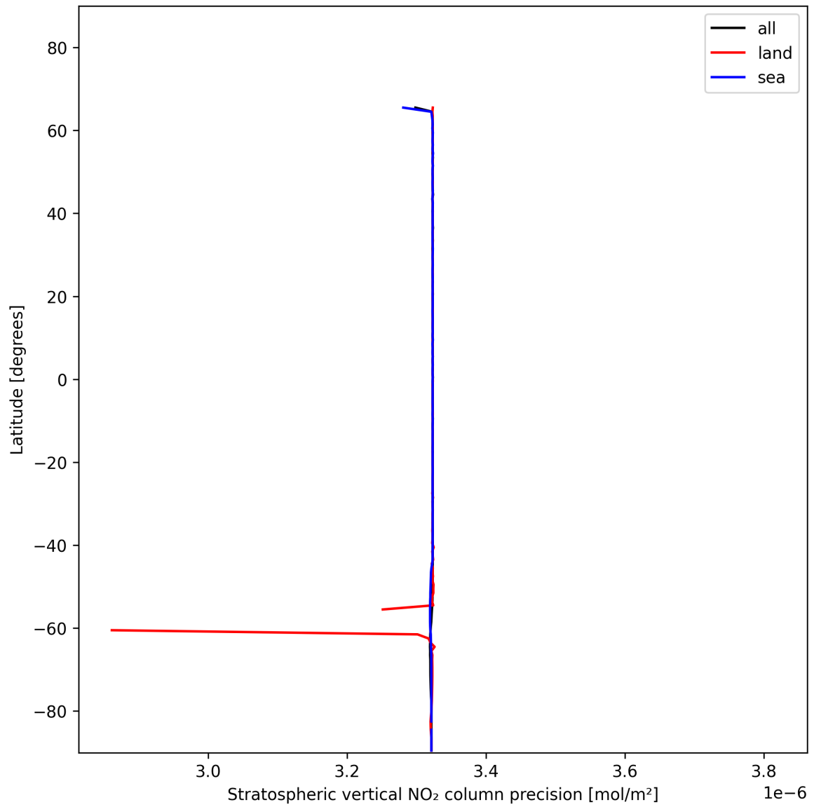
Figure 20: Zonal average of “Stratospheric vertical NO 2 column precision” for 2025-01-01 to 2025-01-03.
