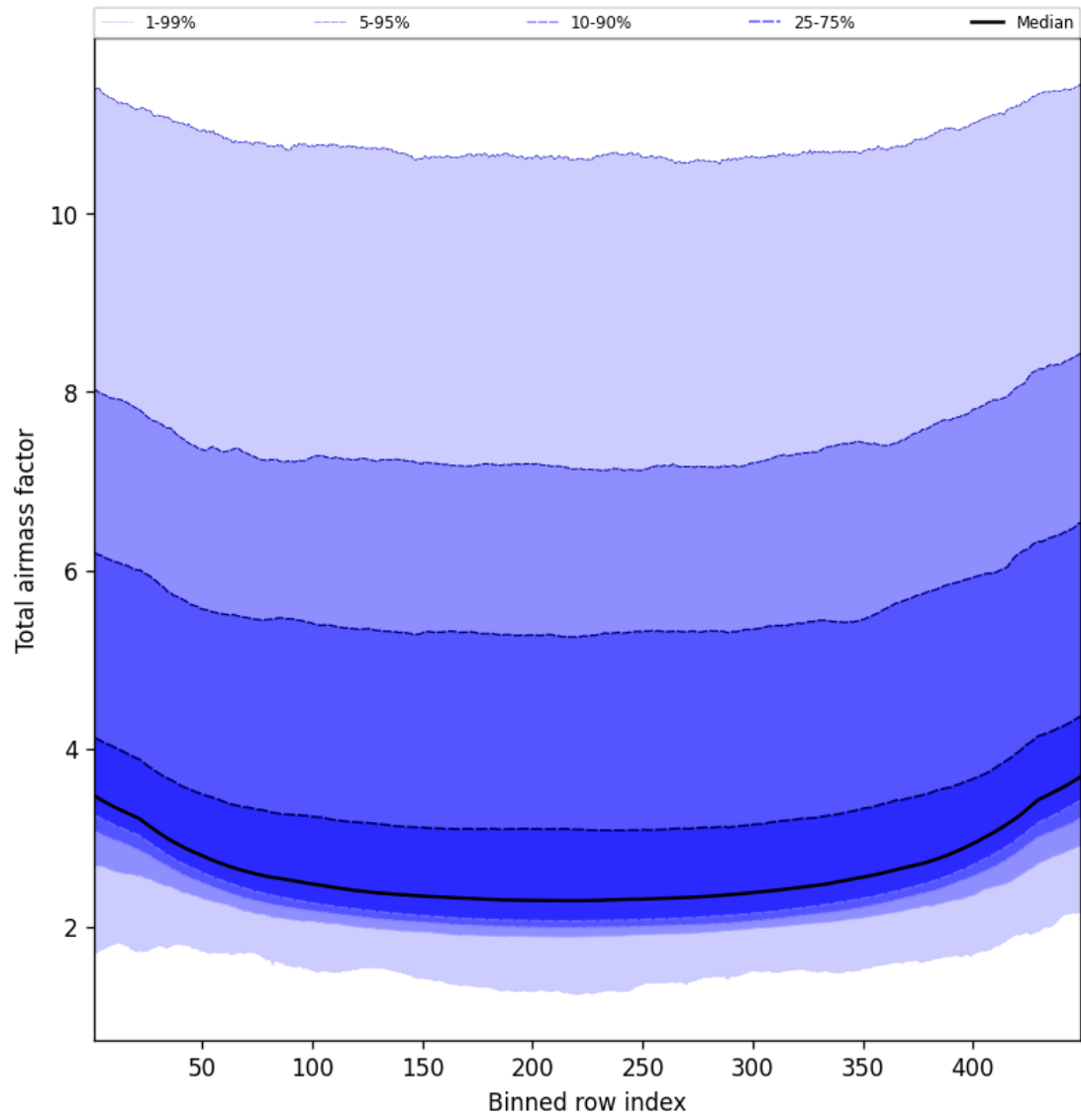
Figure 49: Along track statistics of “Total airmass factor” for 2025-01-01 to 2025-01-03
