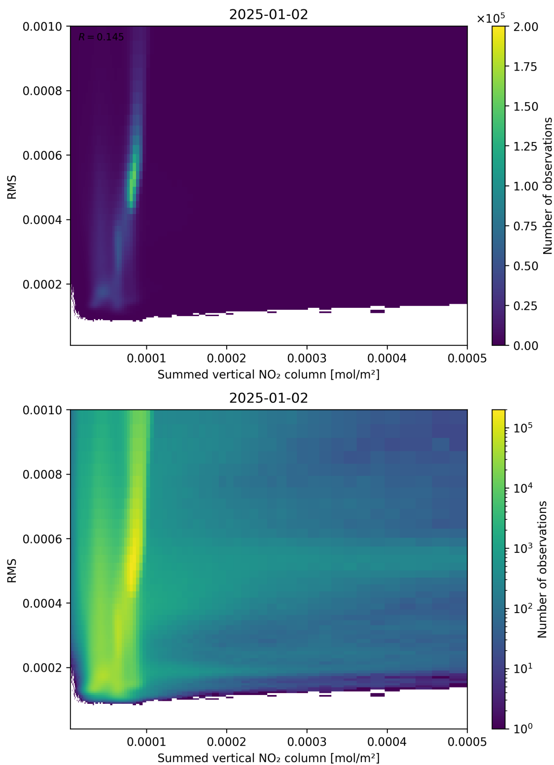
Figure 109: Scatter density plot of “Summed vertical NO 2 column” against “RMS” for 2025-01-01 to 2025-01-03.
