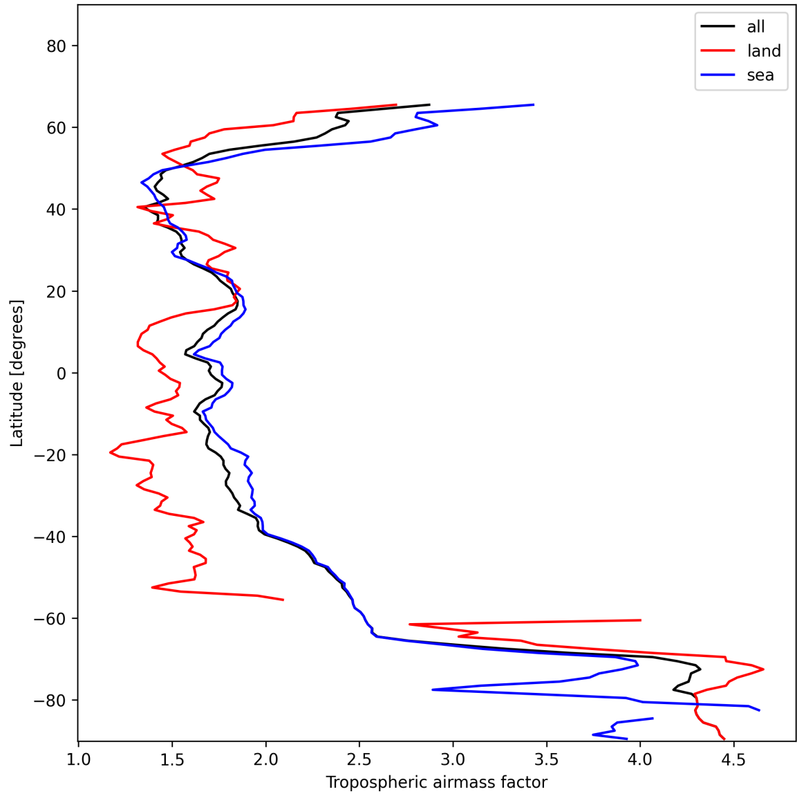
Figure 14: Zonal average of “Tropospheric air mass factor” for 2025-01-01 to 2025-01-03.
