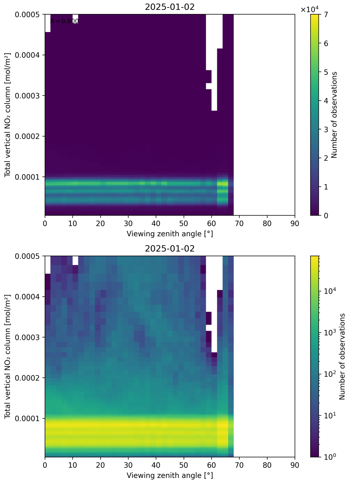
Figure 167: Scatter density plot of “Viewing zenith angle” against “Total vertical NO 2 column” for 2025-01-01 to 2025-01-03.
