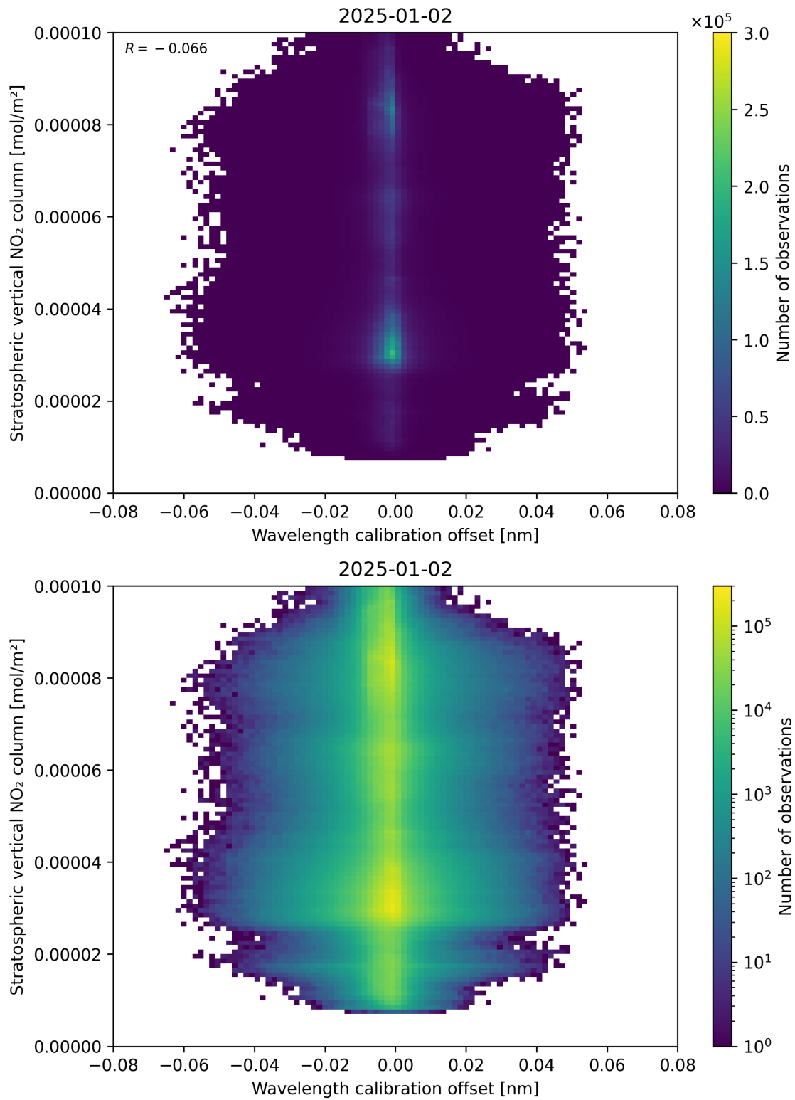
Figure 176: Scatter density plot of “Wavelength calibration offset” against “Stratospheric vertical NO 2 column” for 2025-01-01 to 2025-01-03.
