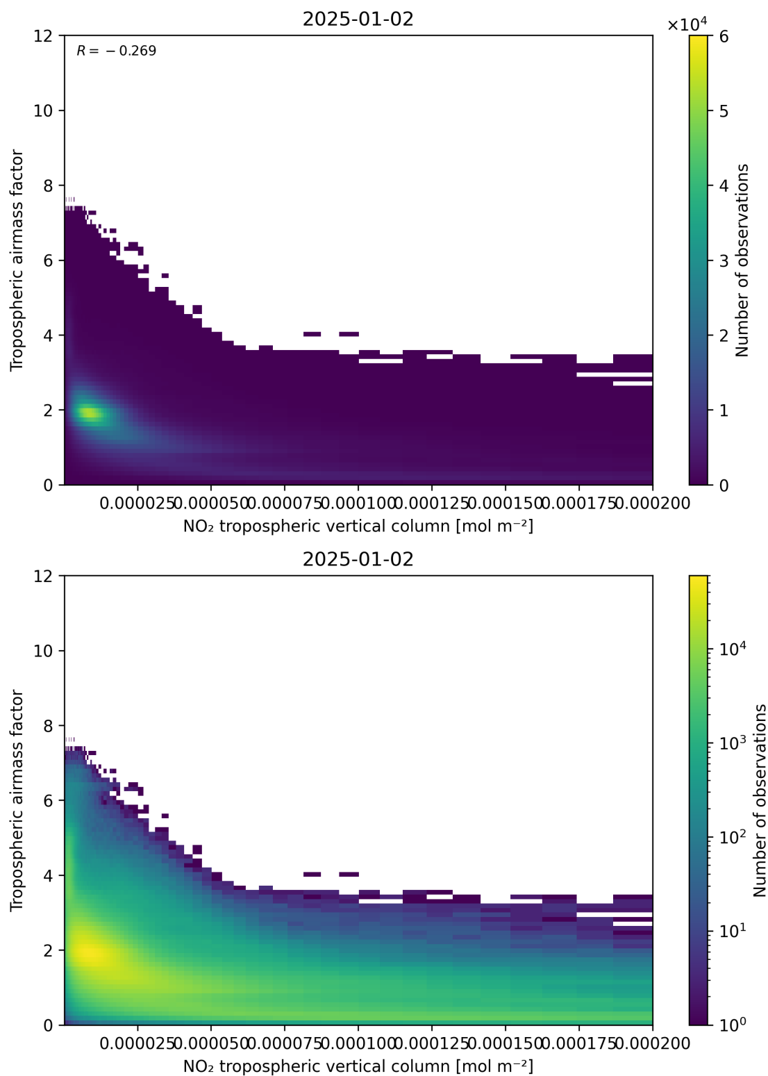
Figure 123: Scatter density plot of “NO 2 tropospheric vertical column” against “Tropospheric air mass factor” for 2025-01-01 to 2025-01-03.
