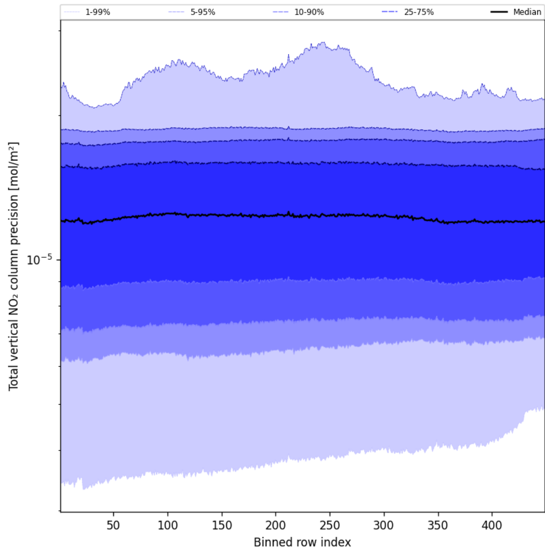
Figure 56: Along track statistics of “Total vertical NO 2 column precision” for 2025-01-01 to 2025-01-03
