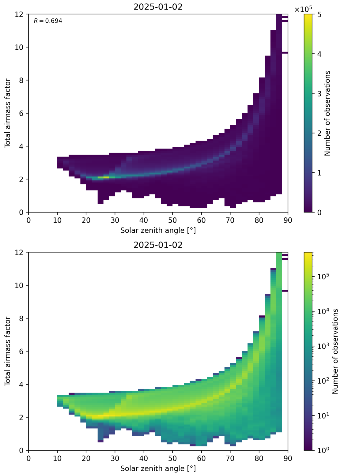
Figure 146: Scatter density plot of “Solar zenith angle” against “Total air mass factor” for 2025-01-01 to 2025-01-03.
