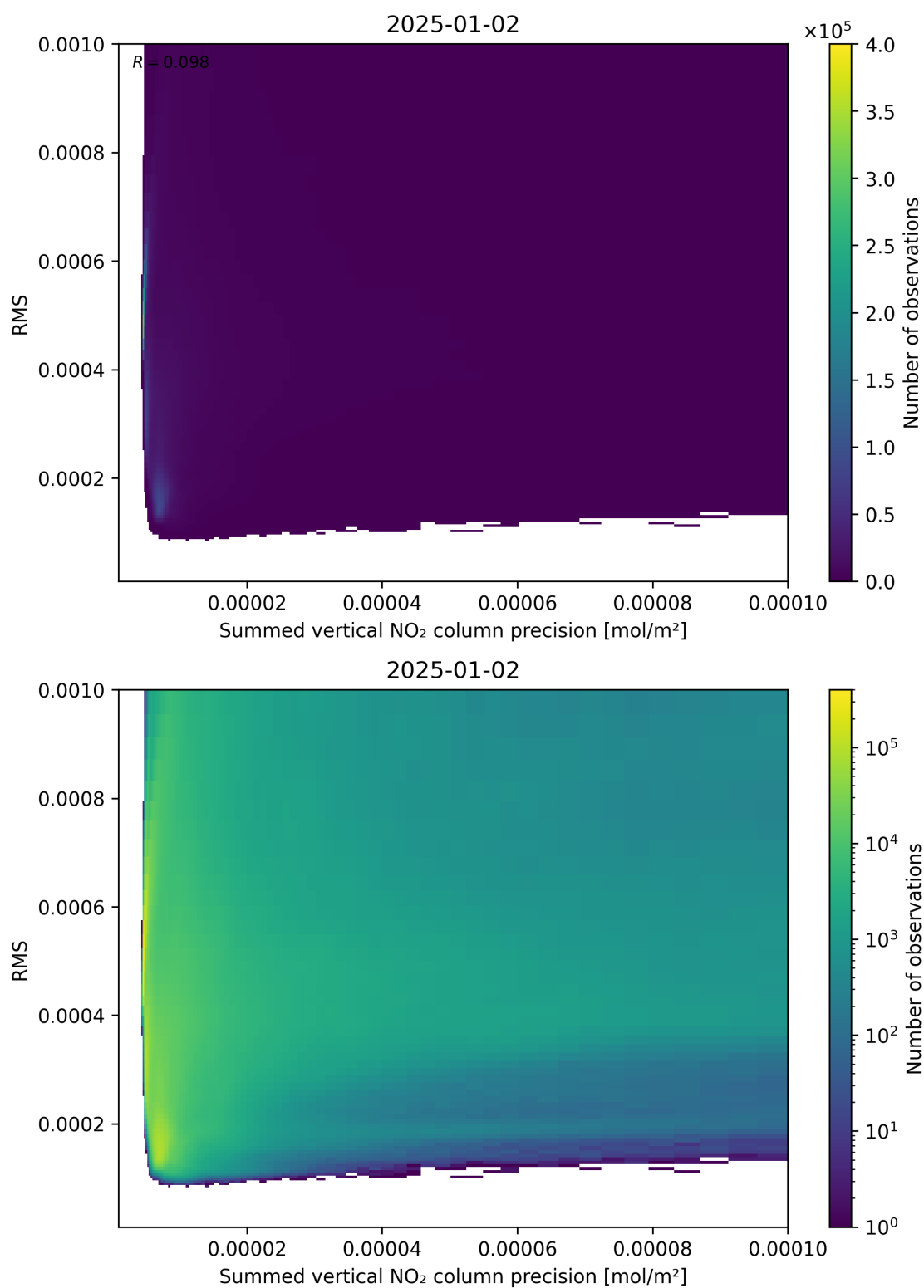
Figure 108: Scatter density plot of “Summed vertical NO 2 column precision” against “RMS” for 2025-01-01 to 2025-01-03.
