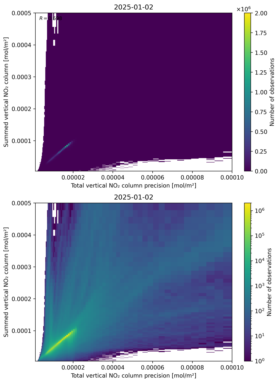
Figure 117: Scatter density plot of “Total vertical NO 2 column precision” against “Summed vertical NO 2 column” for 2025-01-01 to 2025-01-03.
