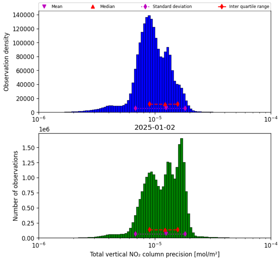
Figure 39: Histogram of “Total vertical NO 2 column precision” for 2025-01-01 to 2025-01-03
