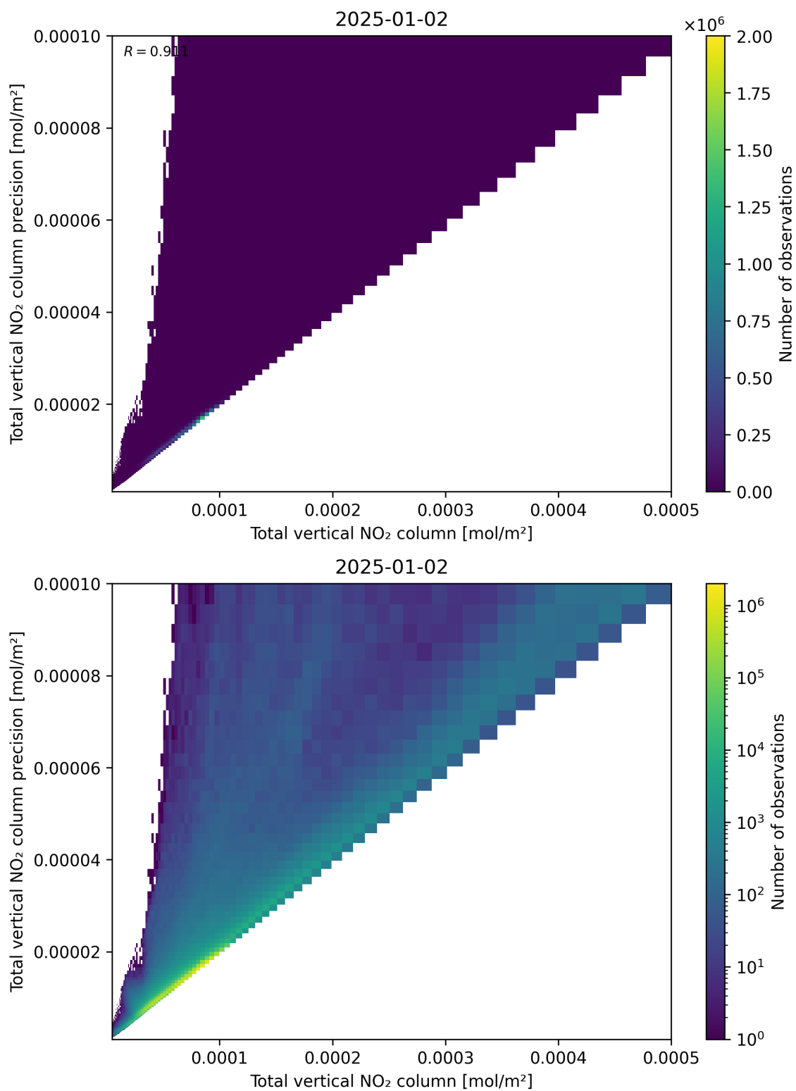
Figure 114: Scatter density plot of “Total vertical NO 2 column” against “Total vertical NO 2 column precision” for 2025-01-01 to 2025-01-03.
