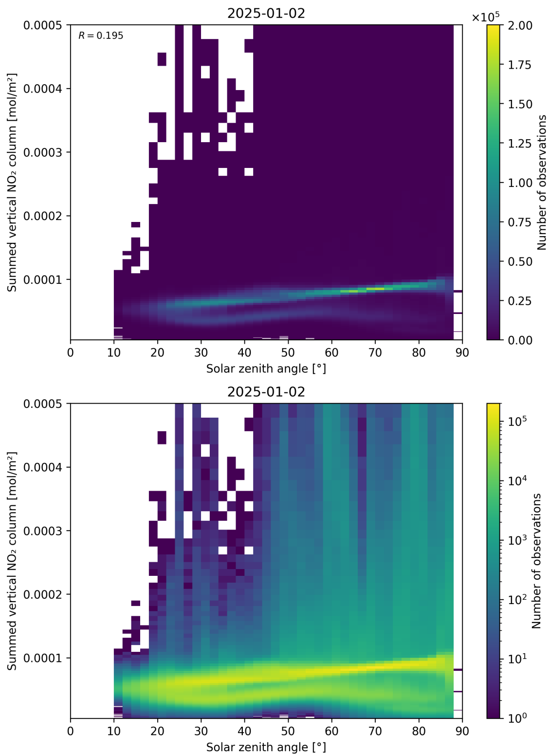
Figure 151: Scatter density plot of “Solar zenith angle” against “Summed vertical NO 2 column” for 2025-01-01 to 2025-01-03.
