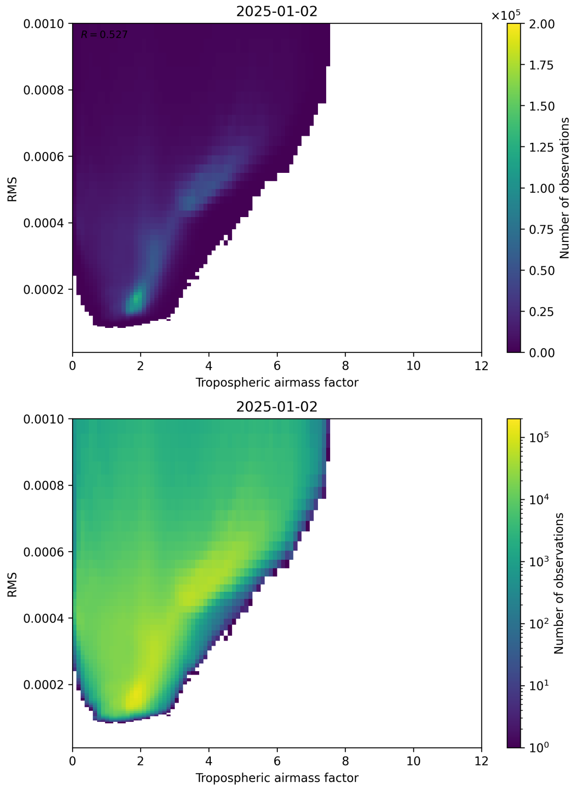
Figure 79: Scatter density plot of “Tropospheric airmass factor” against “RMS” for 2025-01-01 to 2025-01-03.
