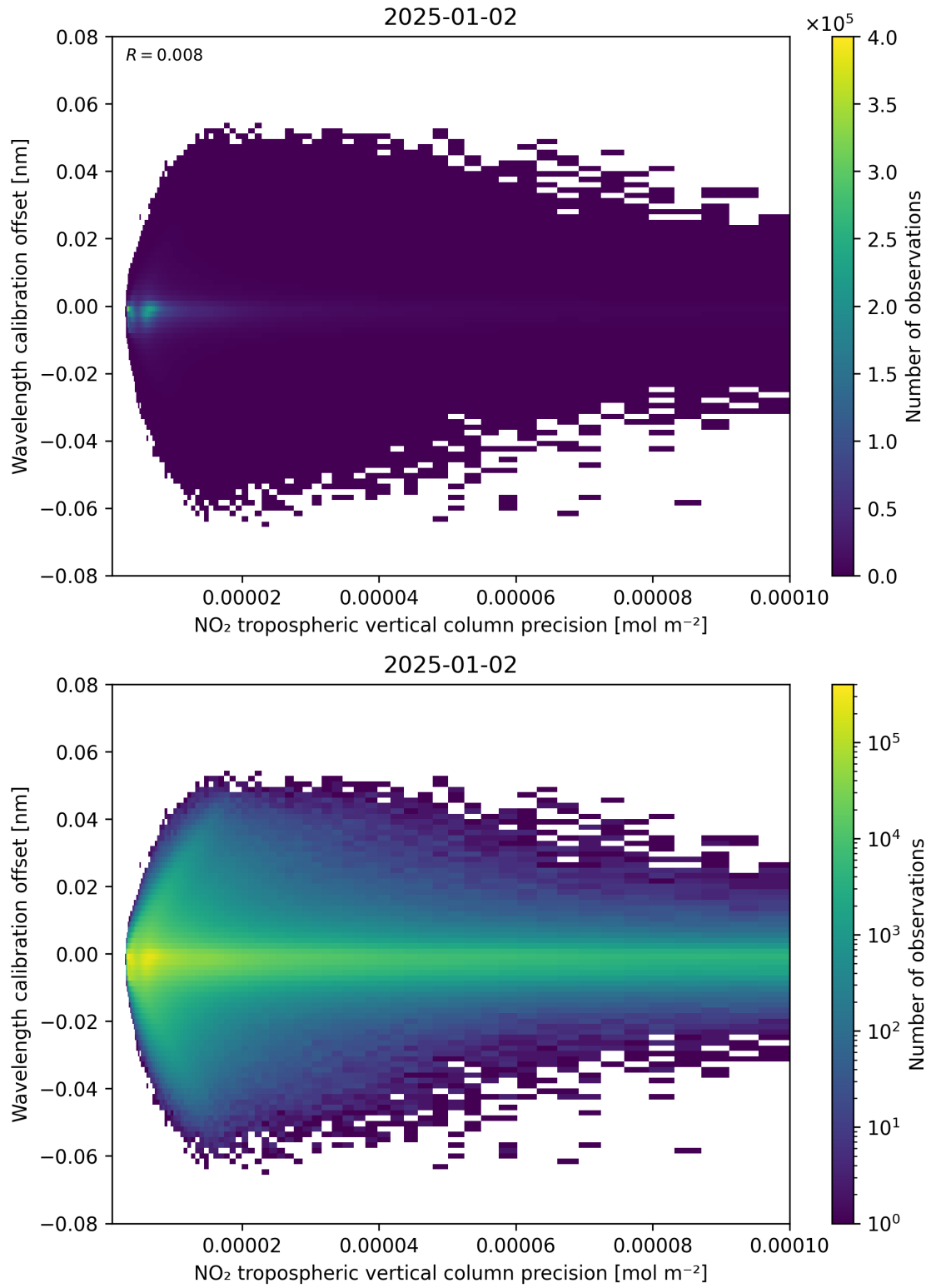
Figure 141: Scatter density plot of “NO 2 tropospheric vertical column precision” against “Wavelength calibration offset” for 2025-01-01 to 2025-01-03.
