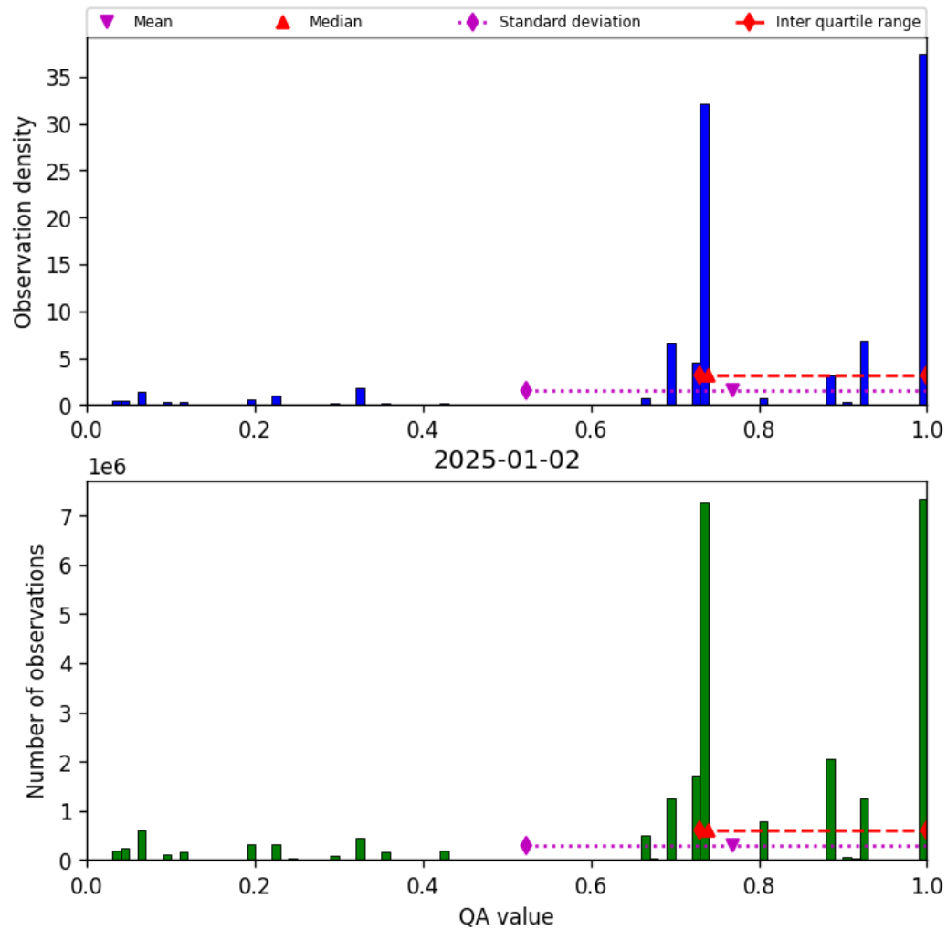
Figure 28: Histogram of “QA value” for 2025-01-01 to 2025-01-03
