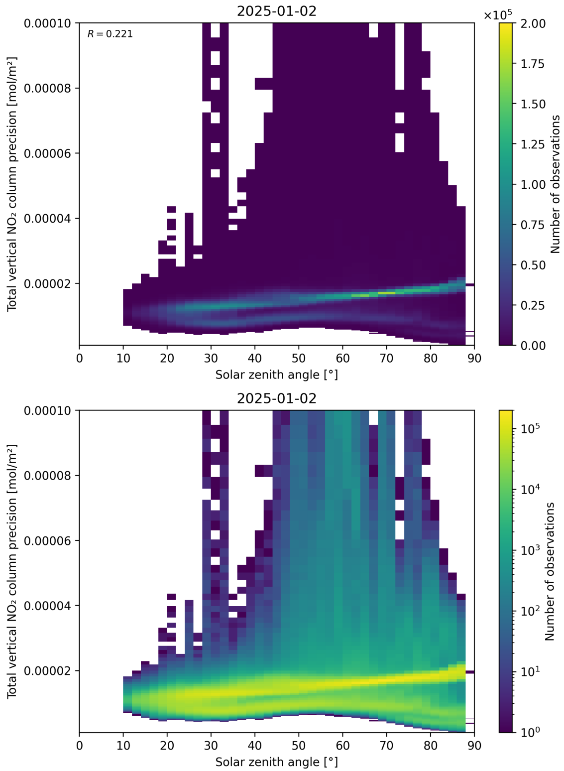
Figure 154: Scatter density plot of “Solar zenith angle” against “Total vertical NO 2 column precision” for 2025-01-01 to 2025-01-03.
