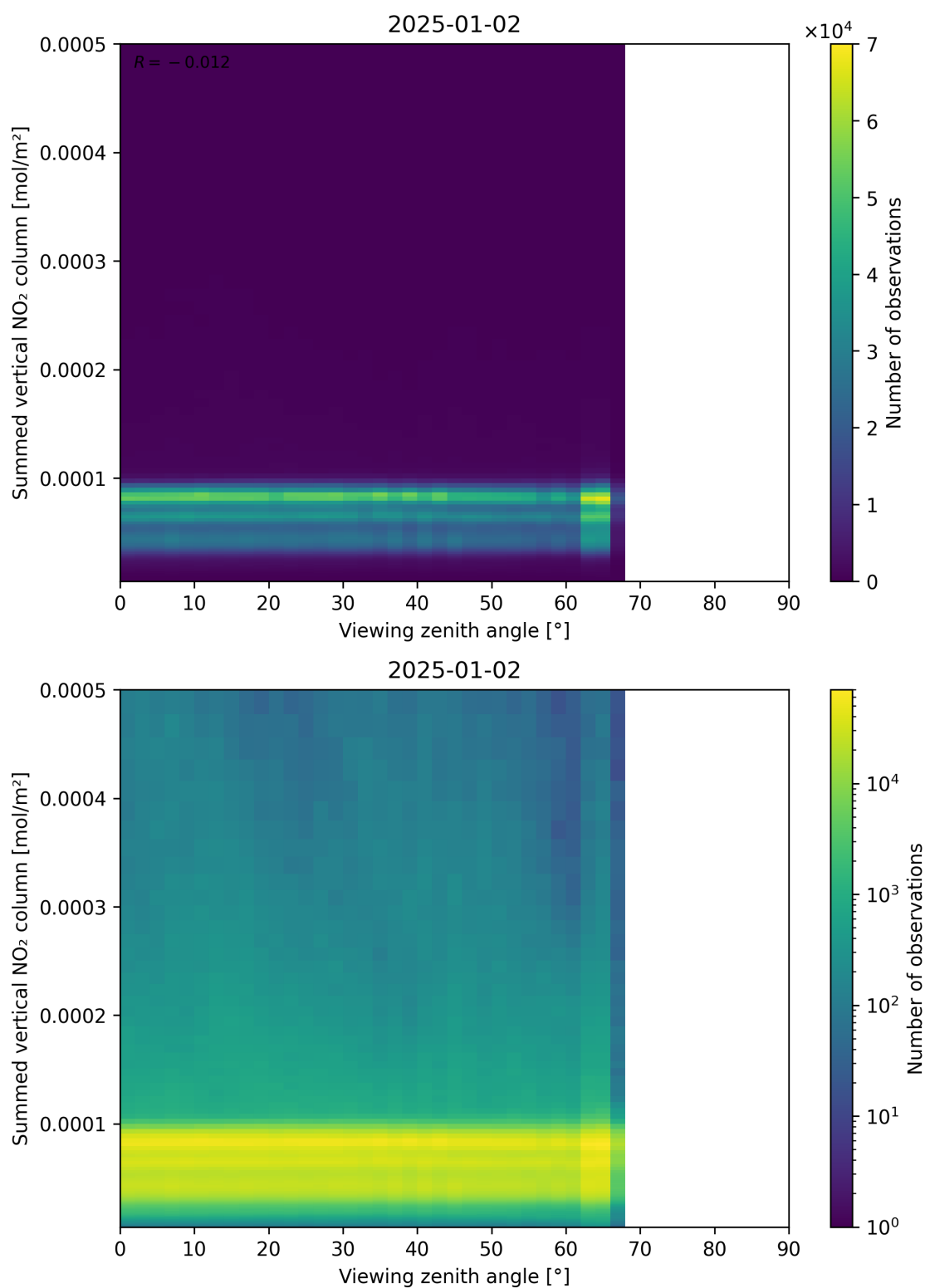
Figure 165: Scatter density plot of “Viewing zenith angle” against “Summed vertical NO 2 column” for 2025-01-01 to 2025-01-03.
