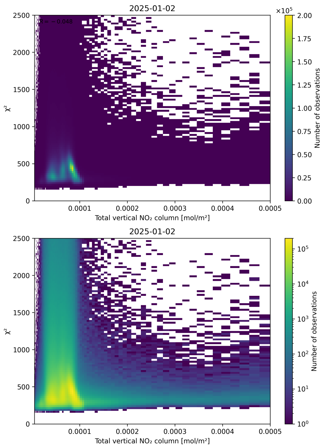
Figure 111: Scatter density plot of “Total vertical NO 2 column” against “ \chi^2 ” for 2025-01-01 to 2025-01-03.
