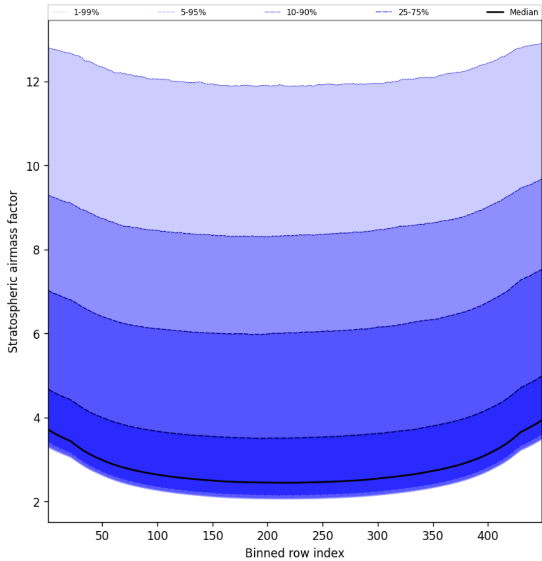
Figure 61: Along track statistics of “Stratospheric airmass factor” for 2025-01-01 to 2025-01-03
