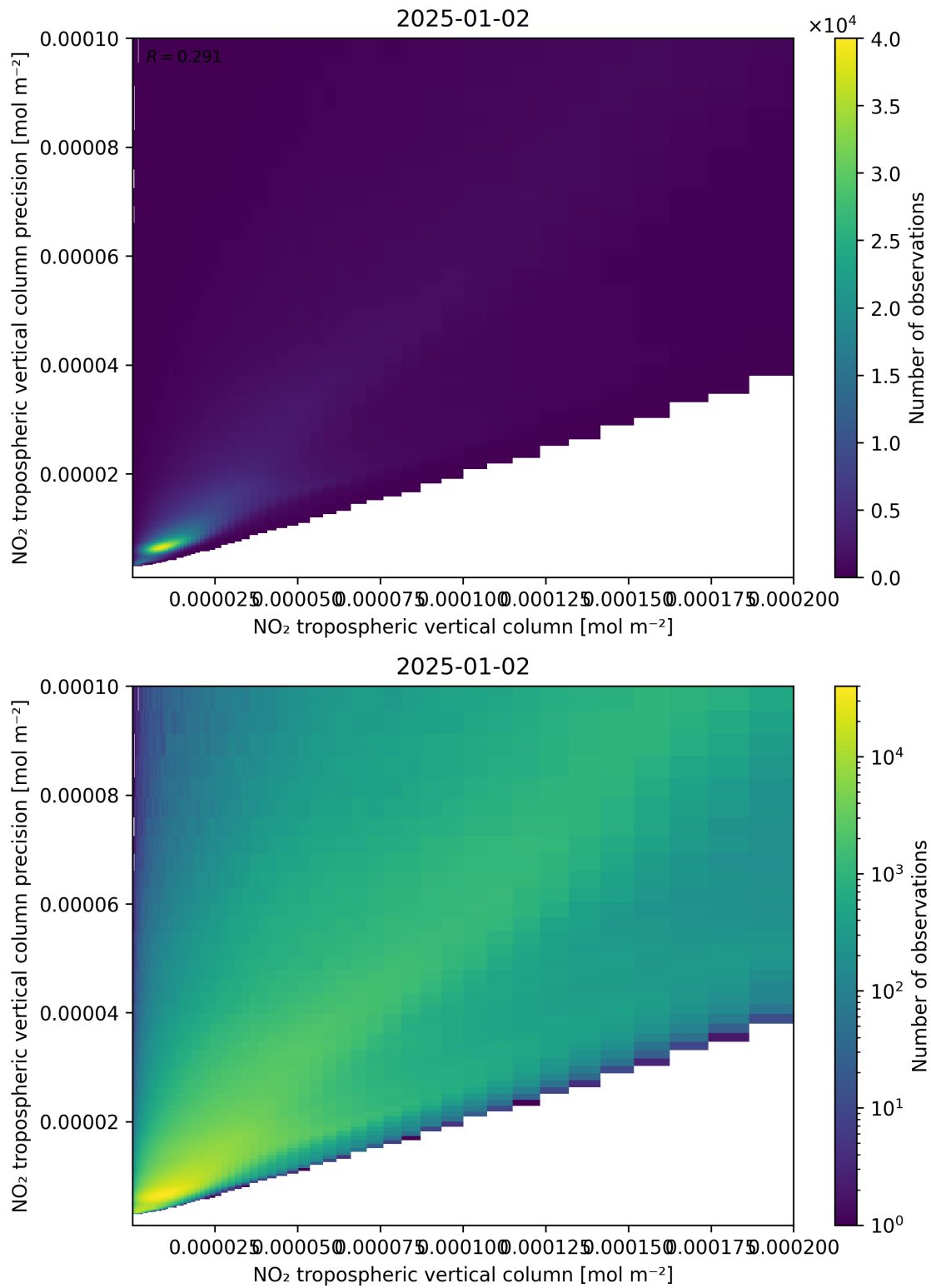
Figure 130: Scatter density plot of “NO 2 tropospheric vertical column” against “NO 2 tropospheric vertical column precision” for 2025-01-01 to 2025-01-03.
