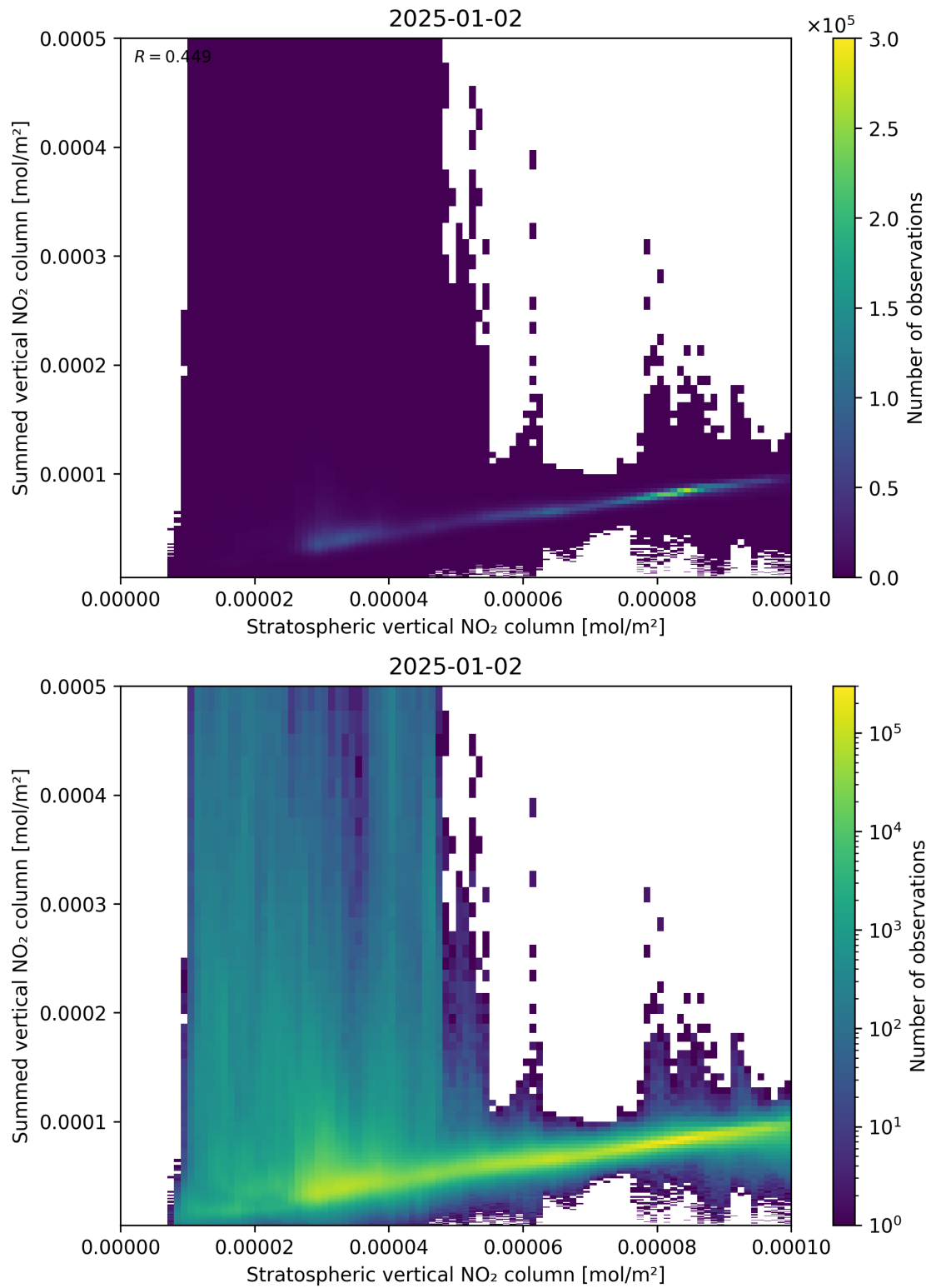
Figure 98: Scatter density plot of “Stratospheric vertical NO 2 column” against “Summed vertical NO 2 column” for 2025-01-01 to 2025-01-03.
