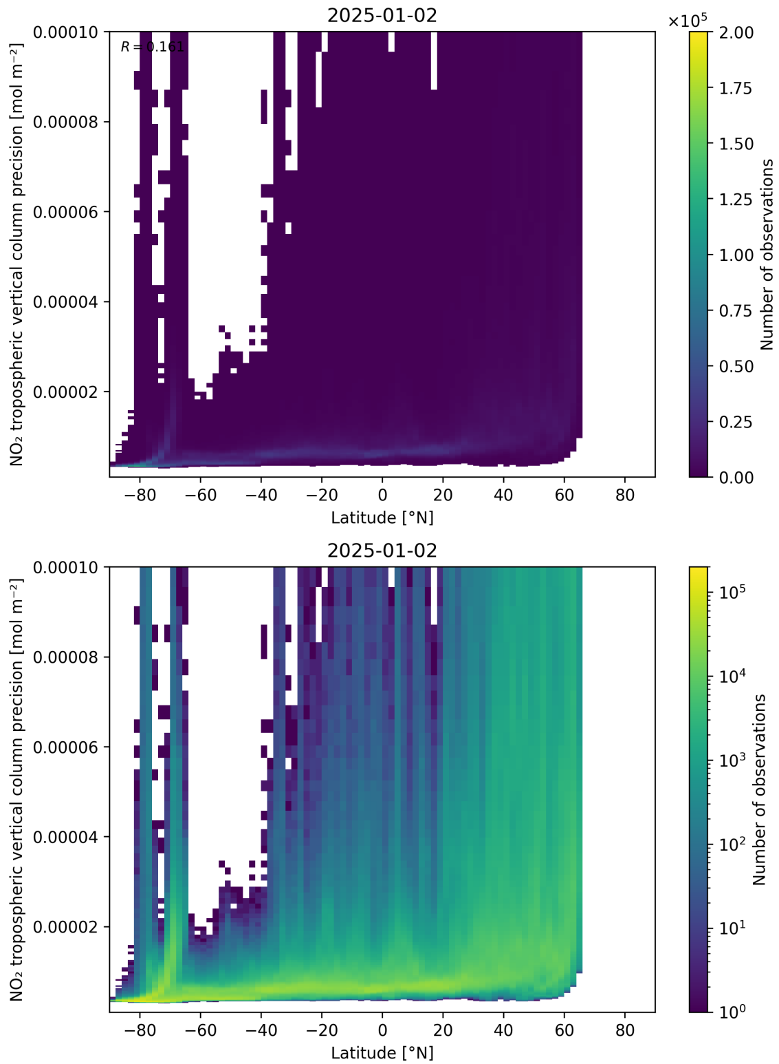
Figure 93: Scatter density plot of “Latitude” against “NO 2 tropospheric vertical column precision” for 2025-01-01 to 2025-01-03.
