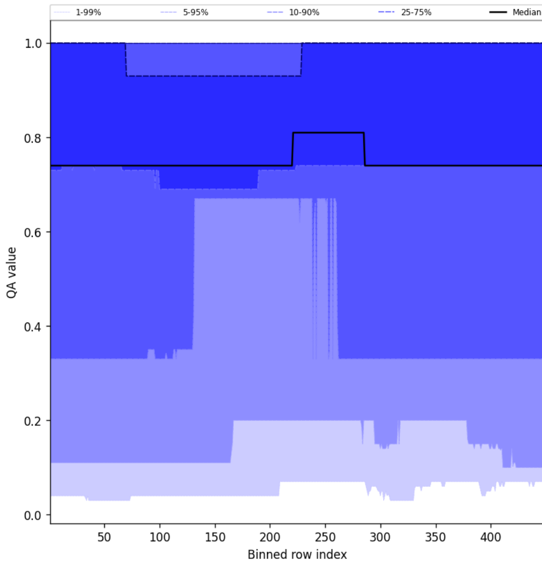
Figure 45: Along track statistics of “QA value” for 2025-01-01 to 2025-01-03
