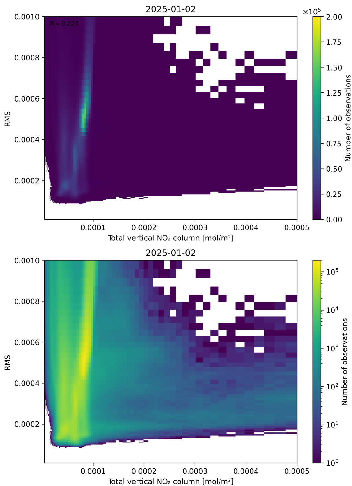
Figure 120: Scatter density plot of “Total vertical NO 2 column” against “RMS” for 2025-01-01 to 2025-01-03.
