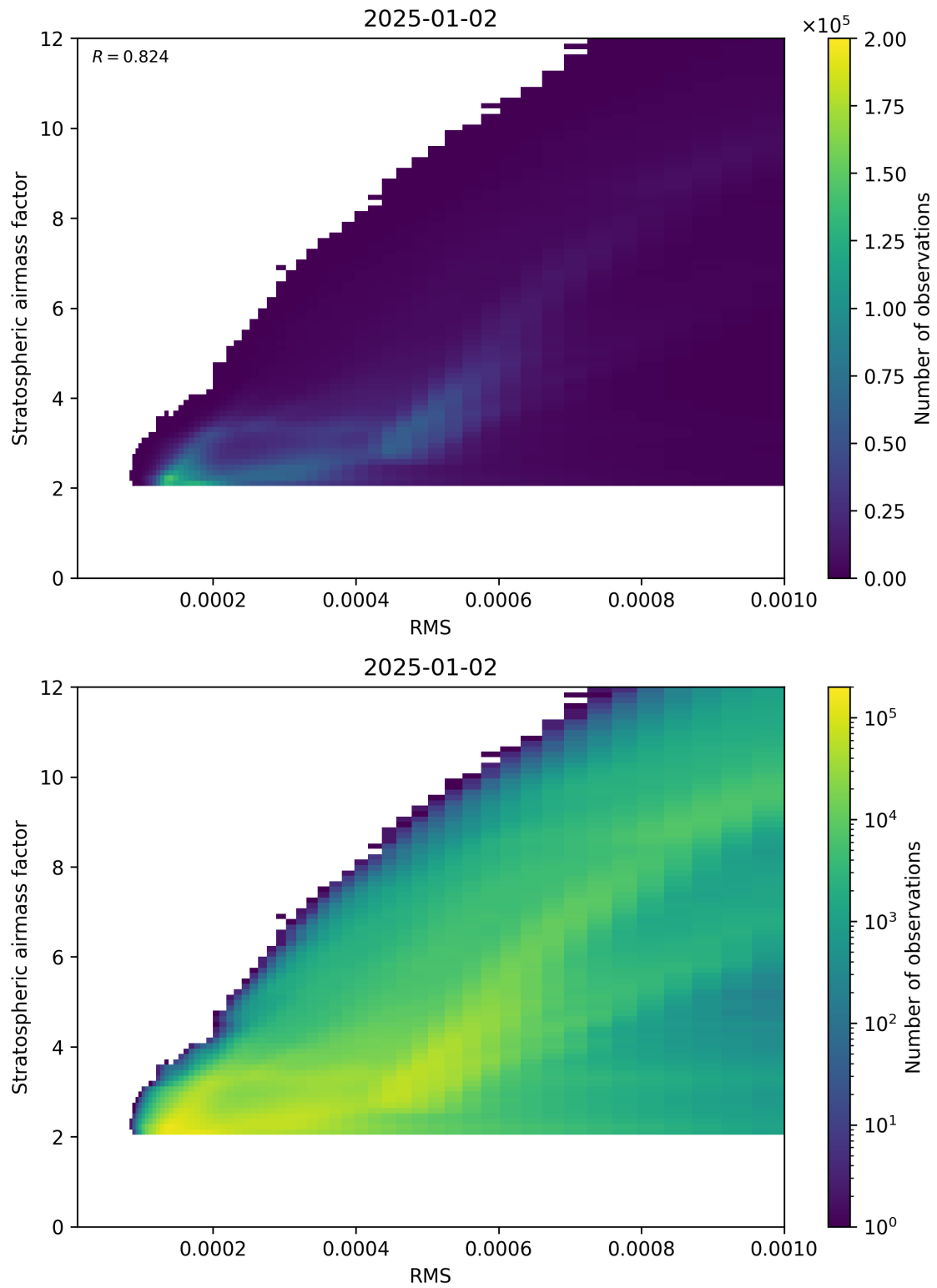
Figure 144: Scatter density plot of “RMS” against “Stratospheric airmass factor” for 2025-01-01 to 2025-01-03.
