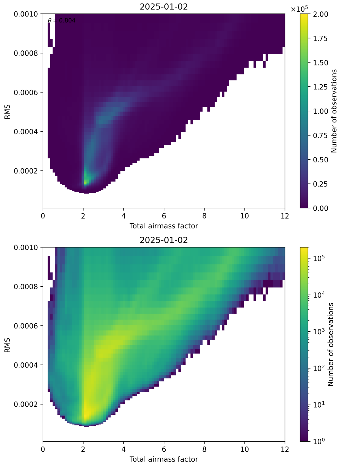
Figure 69: Scatter density plot of “Total airmass factor” against “RMS” for 2025-01-01 to 2025-01-03.
