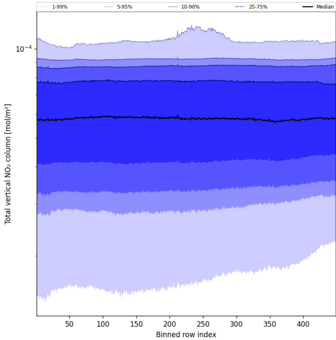
Figure 55: Along track statistics of “Total vertical NO 2 column” for 2025-01-01 to 2025-01-03
