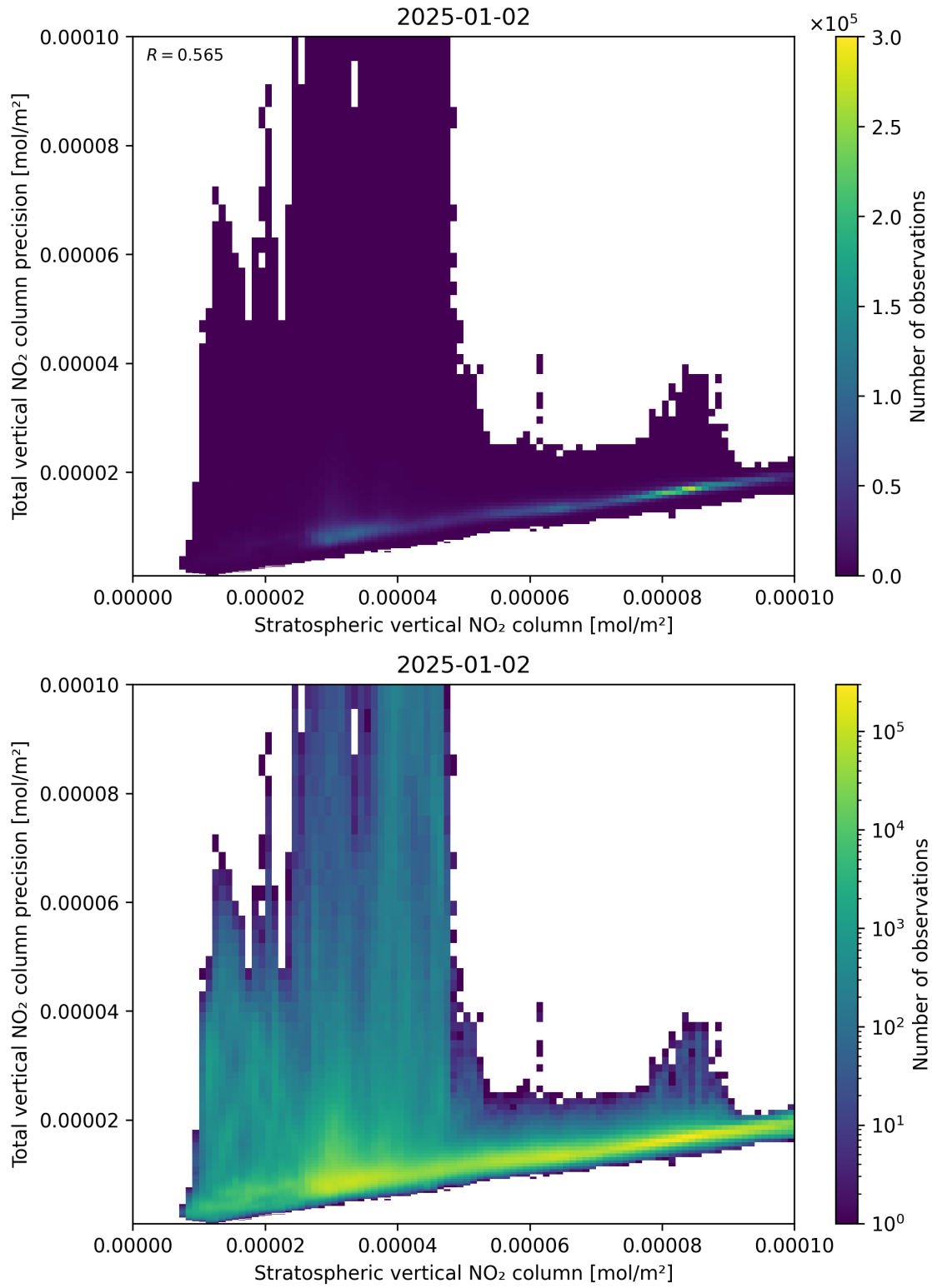
Figure 101: Scatter density plot of “Stratospheric vertical NO 2 column” against “Total vertical NO 2 column precision” for 2025-01-01 to 2025-01-03.
