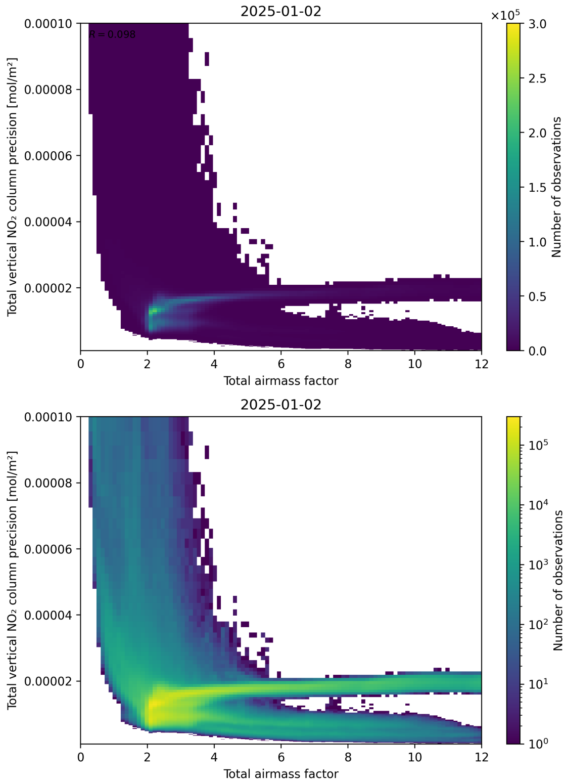
Figure 68: Scatter density plot of “Total airmass factor” against “Total vertical NO 2 column precision” for 2025-01-01 to 2025-01-03.
