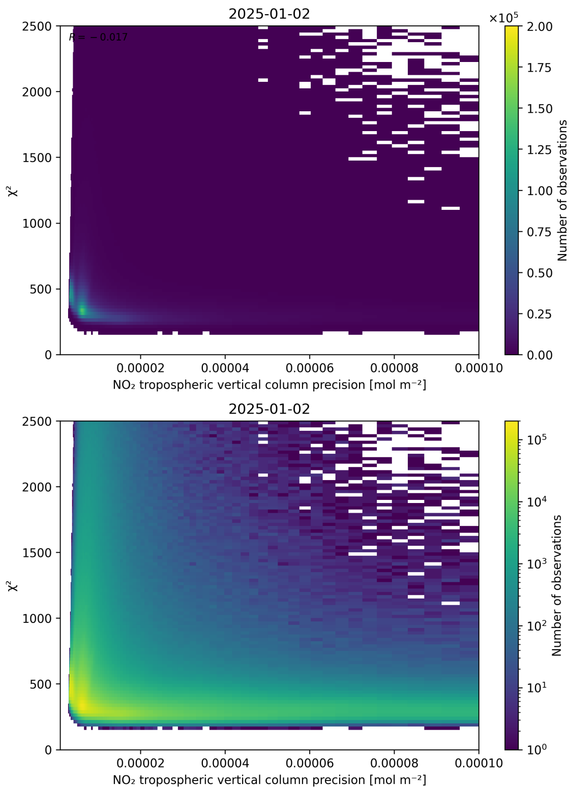
Figure 134: Scatter density plot of “NO 2 tropospheric vertical column precision” against “ \chi^2 ” for 2025-01-01 to 2025-01-03.
