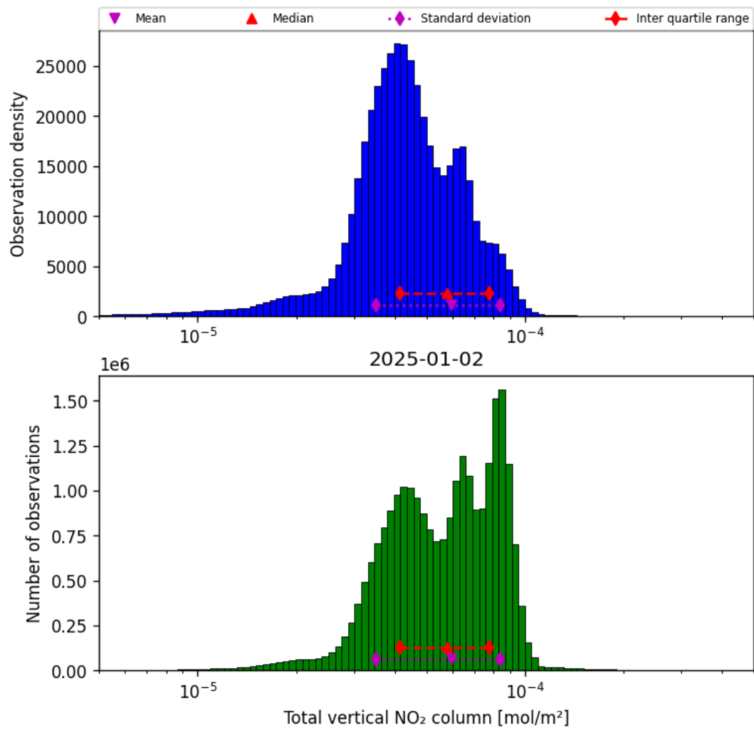
Figure 38: Histogram of “Total vertical NO 2 column” for 2025-01-01 to 2025-01-03
