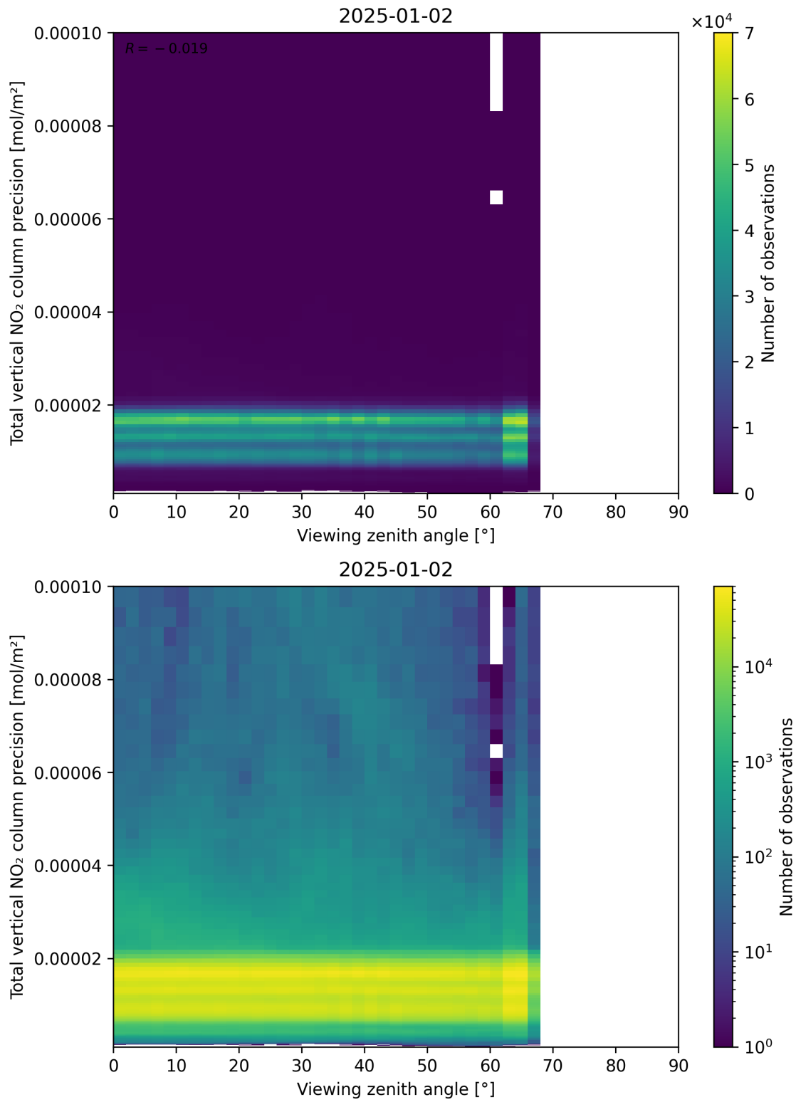
Figure 168: Scatter density plot of “Viewing zenith angle” against “Total vertical NO 2 column precision” for 2025-01-01 to 2025-01-03.
