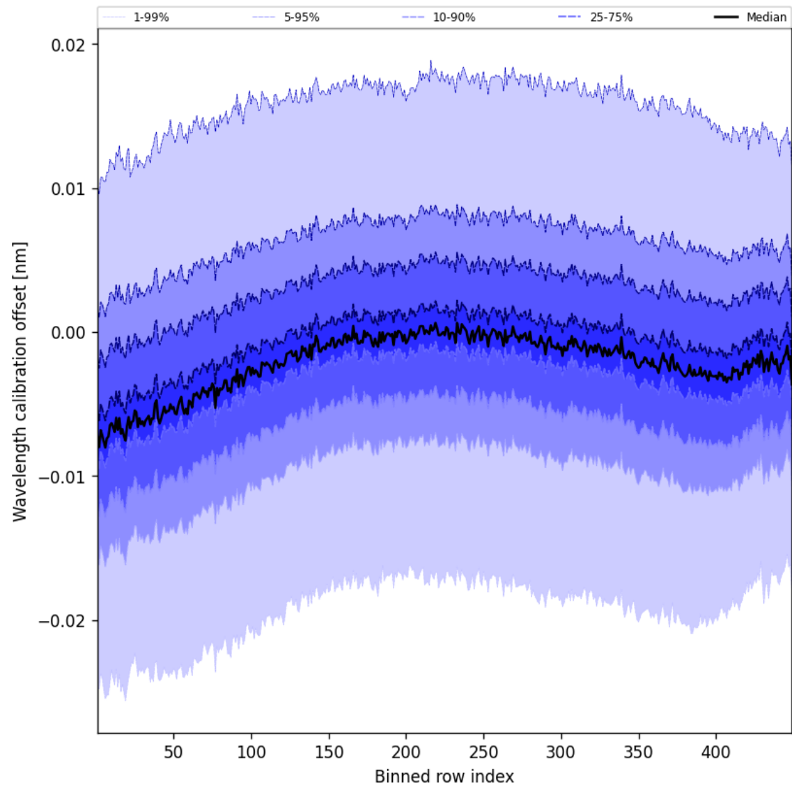
Figure 52: Along track statistics of “Wavelength calibration offset” for 2025-01-01 to 2025-01-03
