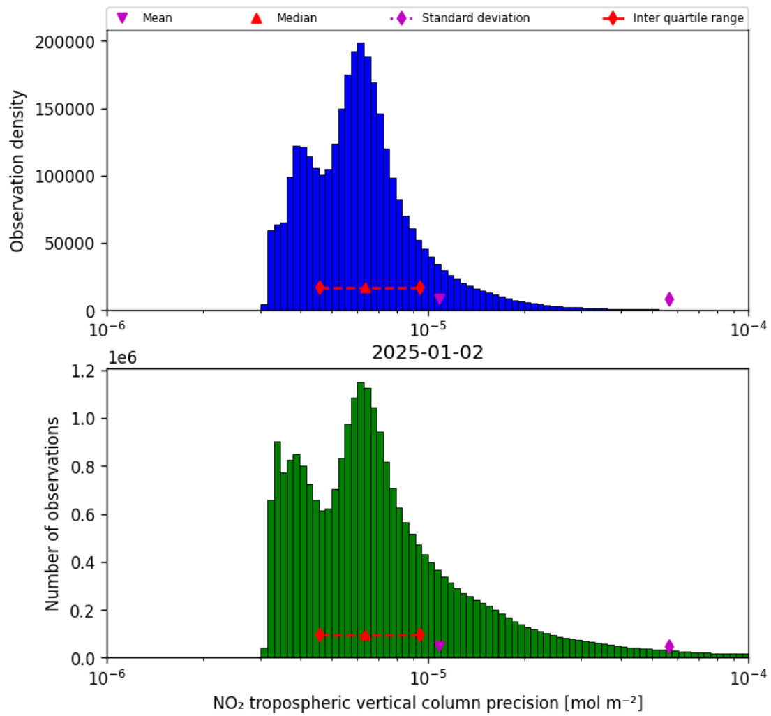
Figure 30: Histogram of “NO 2 tropospheric vertical column precision” for 2025-01-01 to 2025-01-03
