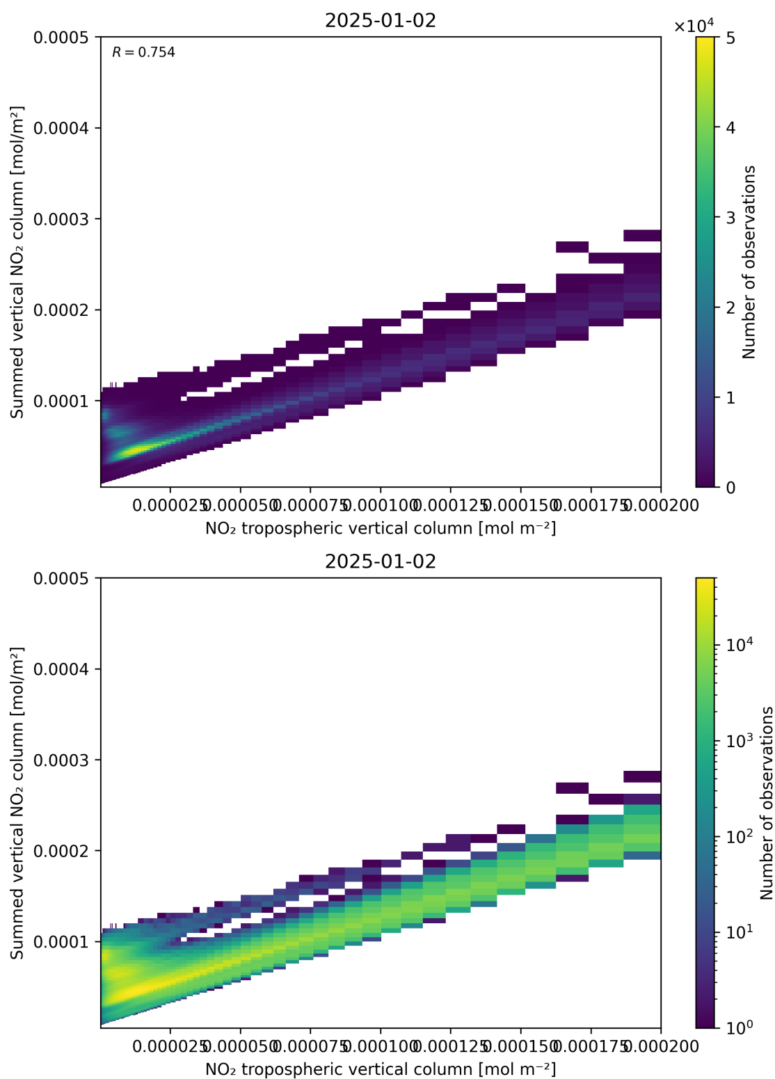
Figure 126: Scatter density plot of “NO 2 tropospheric vertical column” against “Summed vertical NO 2 column” for 2025-01-01 to 2025-01-03.
