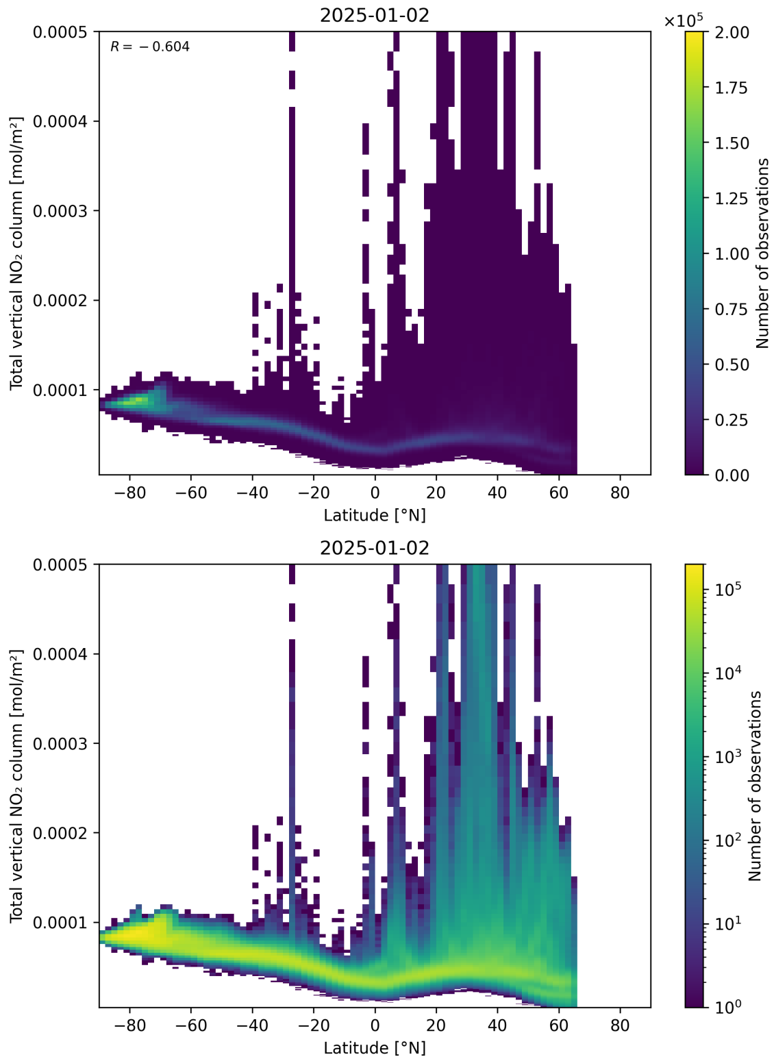
Figure 90: Scatter density plot of “Latitude” against “Total vertical NO 2 column” for 2025-01-01 to 2025-01-03.
