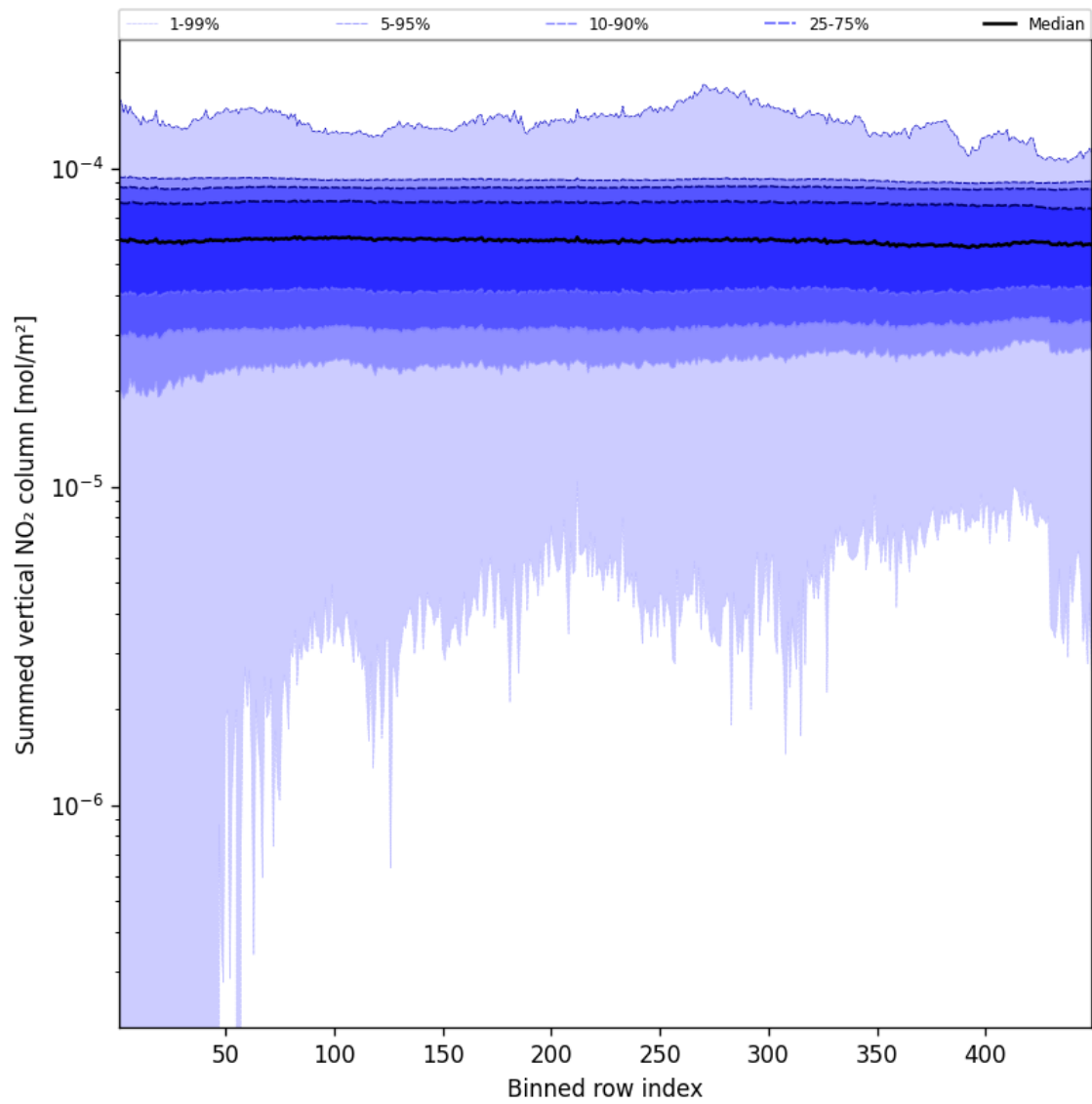
Figure 57: Along track statistics of “Summed vertical NO 2 column” for 2025-01-01 to 2025-01-03
