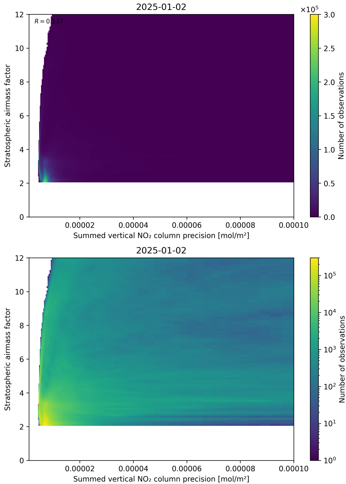
Figure 106: Scatter density plot of “Summed vertical NO 2 column precision” against “Stratospheric airmass factor” for 2025-01-01 to 2025-01-03.
