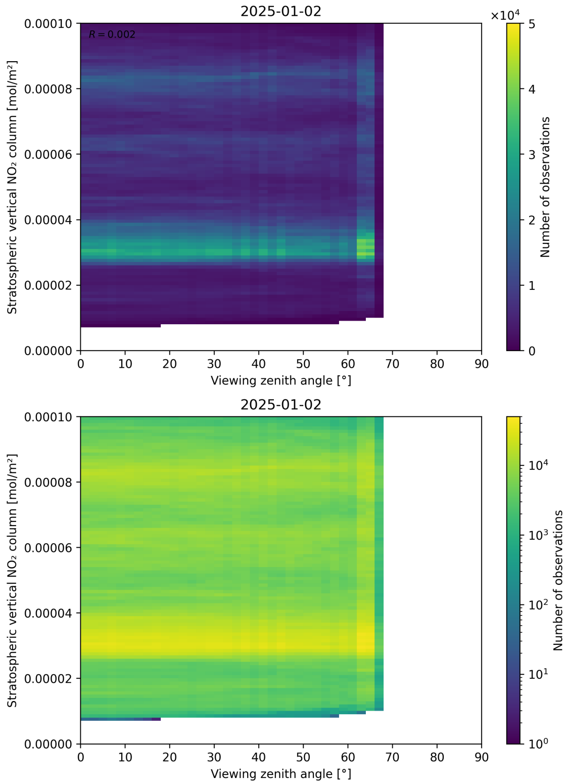
Figure 164: Scatter density plot of “Viewing zenith angle” against “Stratospheric vertical NO 2 column” for 2025-01-01 to 2025-01-03.
