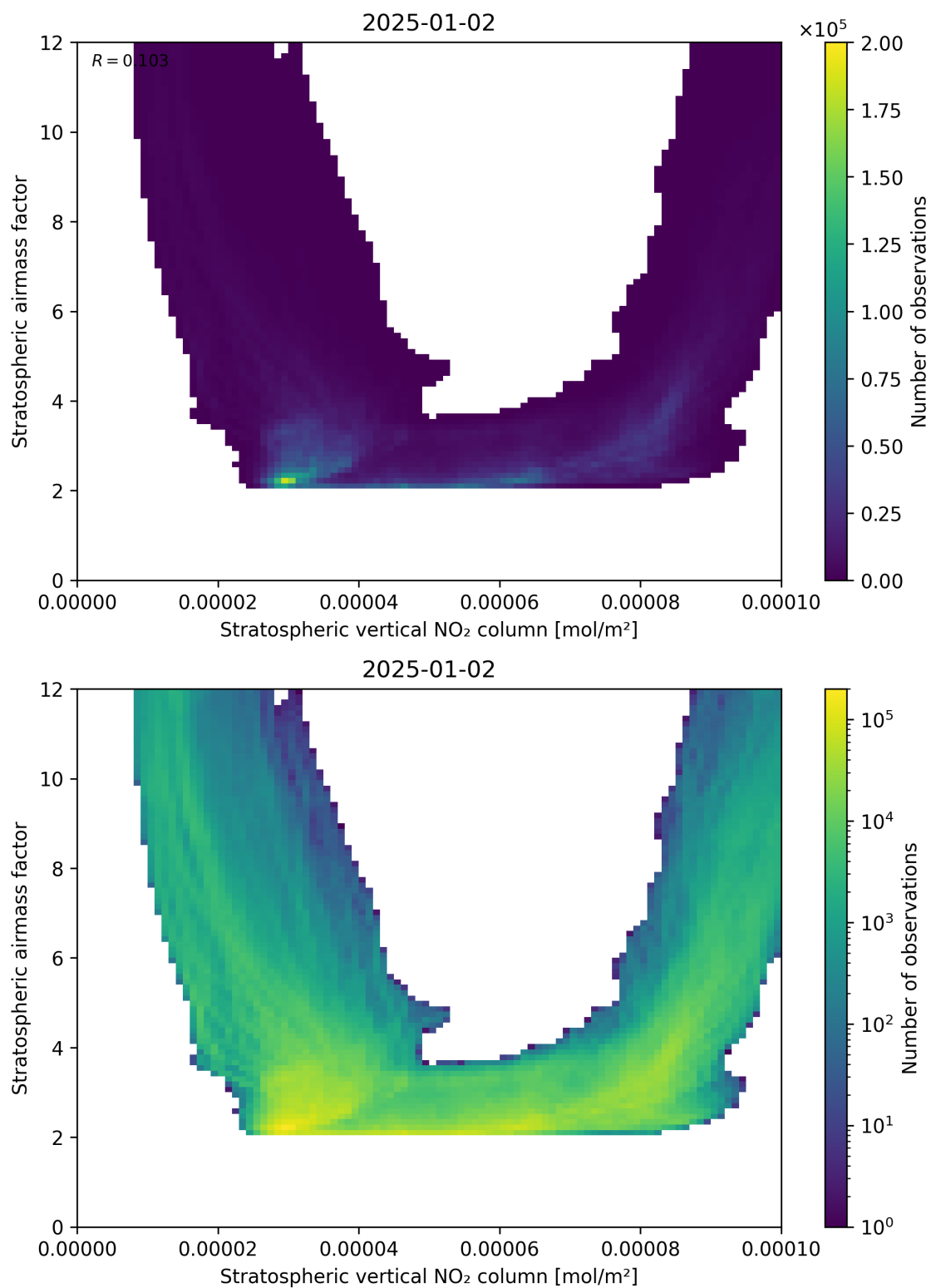
Figure 96: Scatter density plot of “Stratospheric vertical NO 2 column” against “Stratospheric airmass factor” for 2025-01-01 to 2025-01-03.
