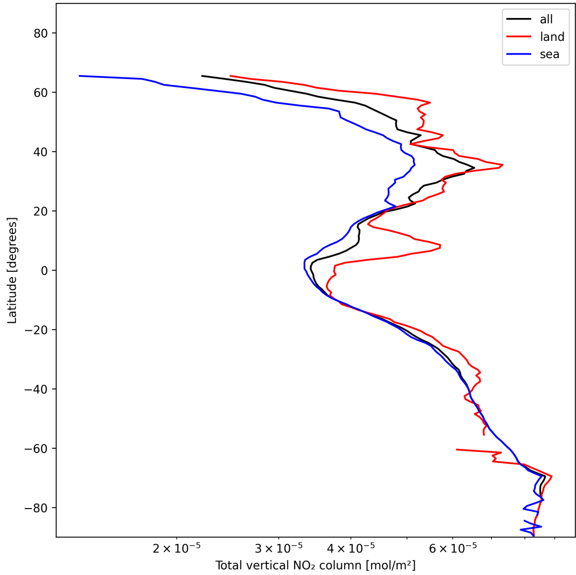
Figure 21: Zonal average of “Total vertical NO 2 column” for 2025-01-01 to 2025-01-03.
