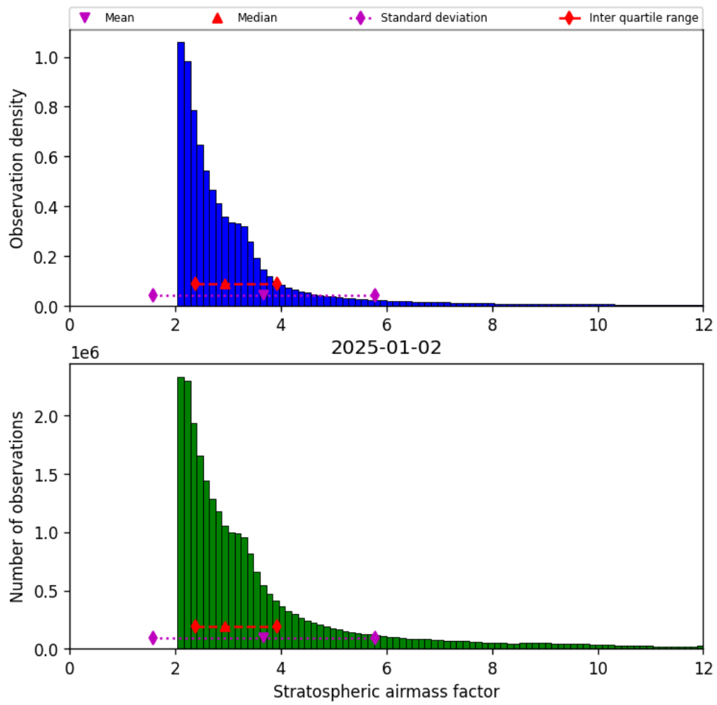
Figure 44: Histogram of “Stratospheric airmass factor” for 2025-01-01 to 2025-01-03
