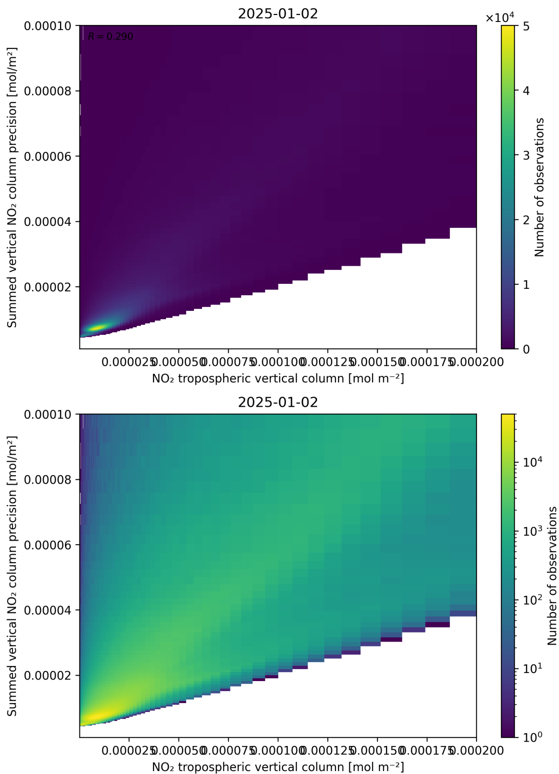
Figure 127: Scatter density plot of “NO 2 tropospheric vertical column” against “Summed vertical NO 2 column precision” for 2025-01-01 to 2025-01-03.
