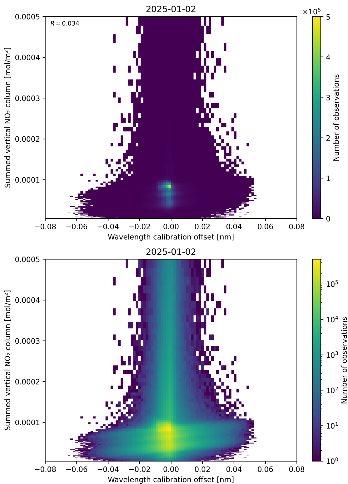
Figure 177: Scatter density plot of “Wavelength calibration offset” against “Summed vertical NO 2 column” for 2025-01-01 to 2025-01-03.
