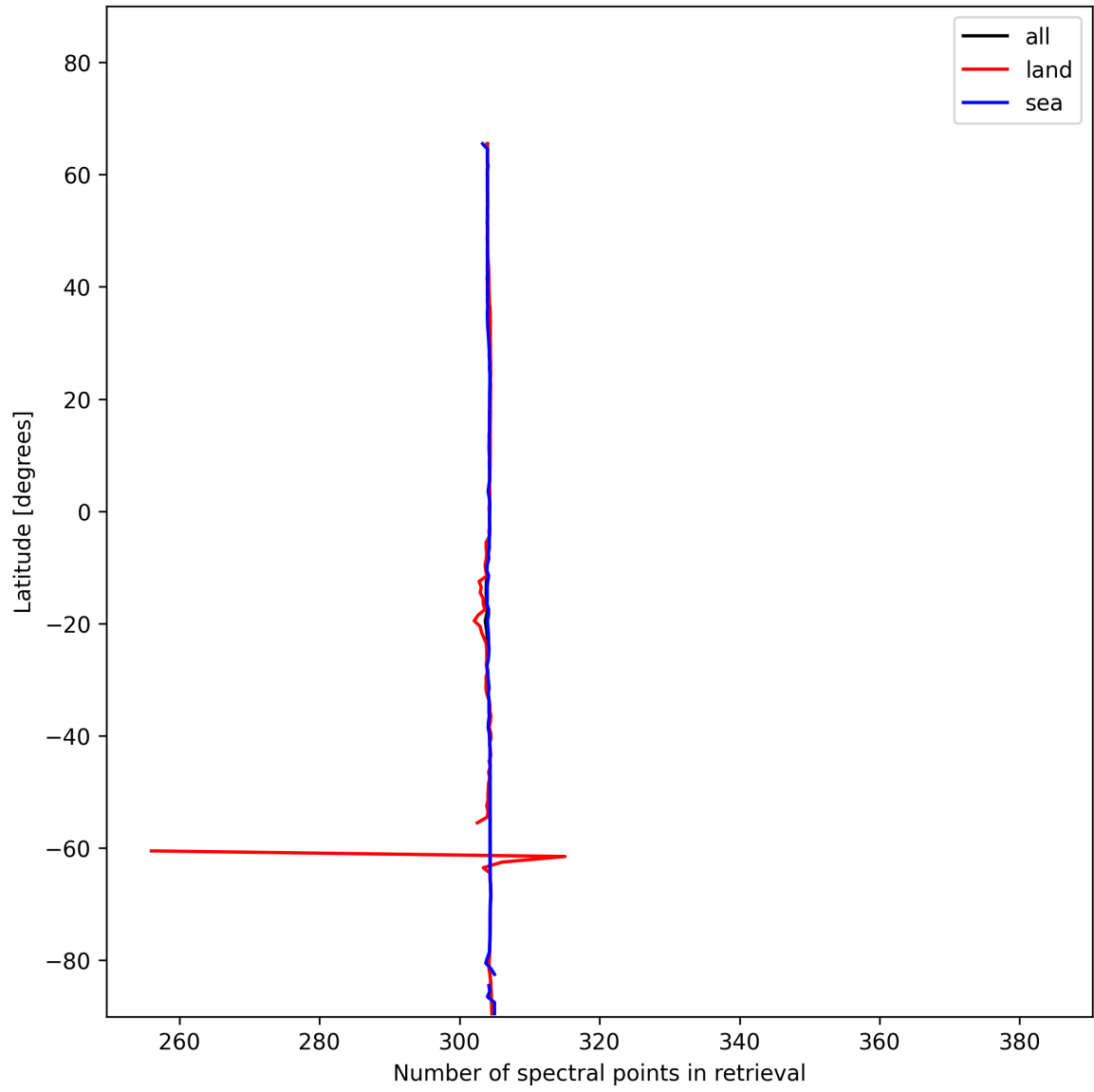
Figure 16: Zonal average of “Number of spectral points in retrieval” for 2025-01-01 to 2025-01-03.
