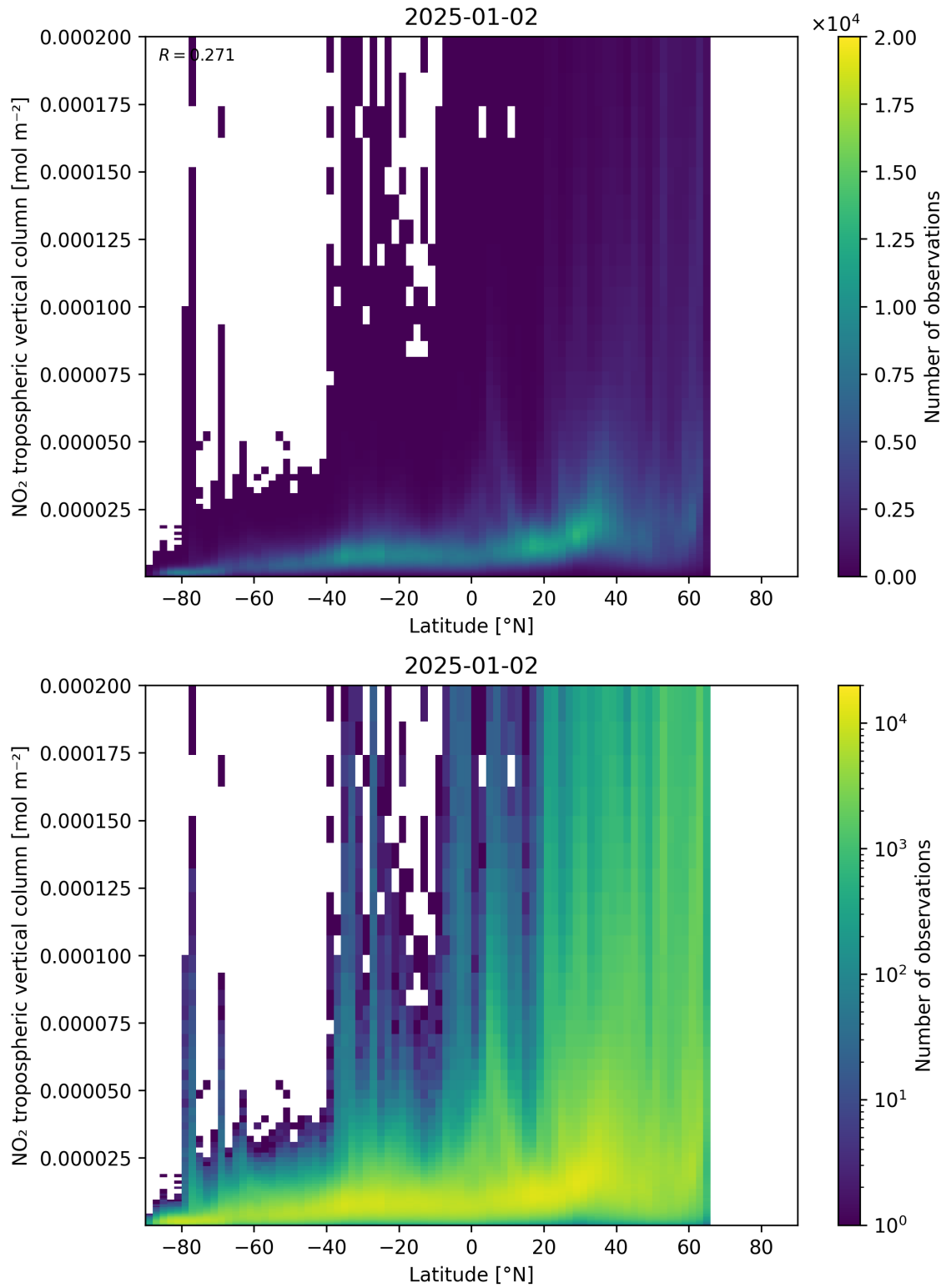
Figure 92: Scatter density plot of “Latitude” against “NO 2 tropospheric vertical column” for 2025-01-01 to 2025-01-03.
