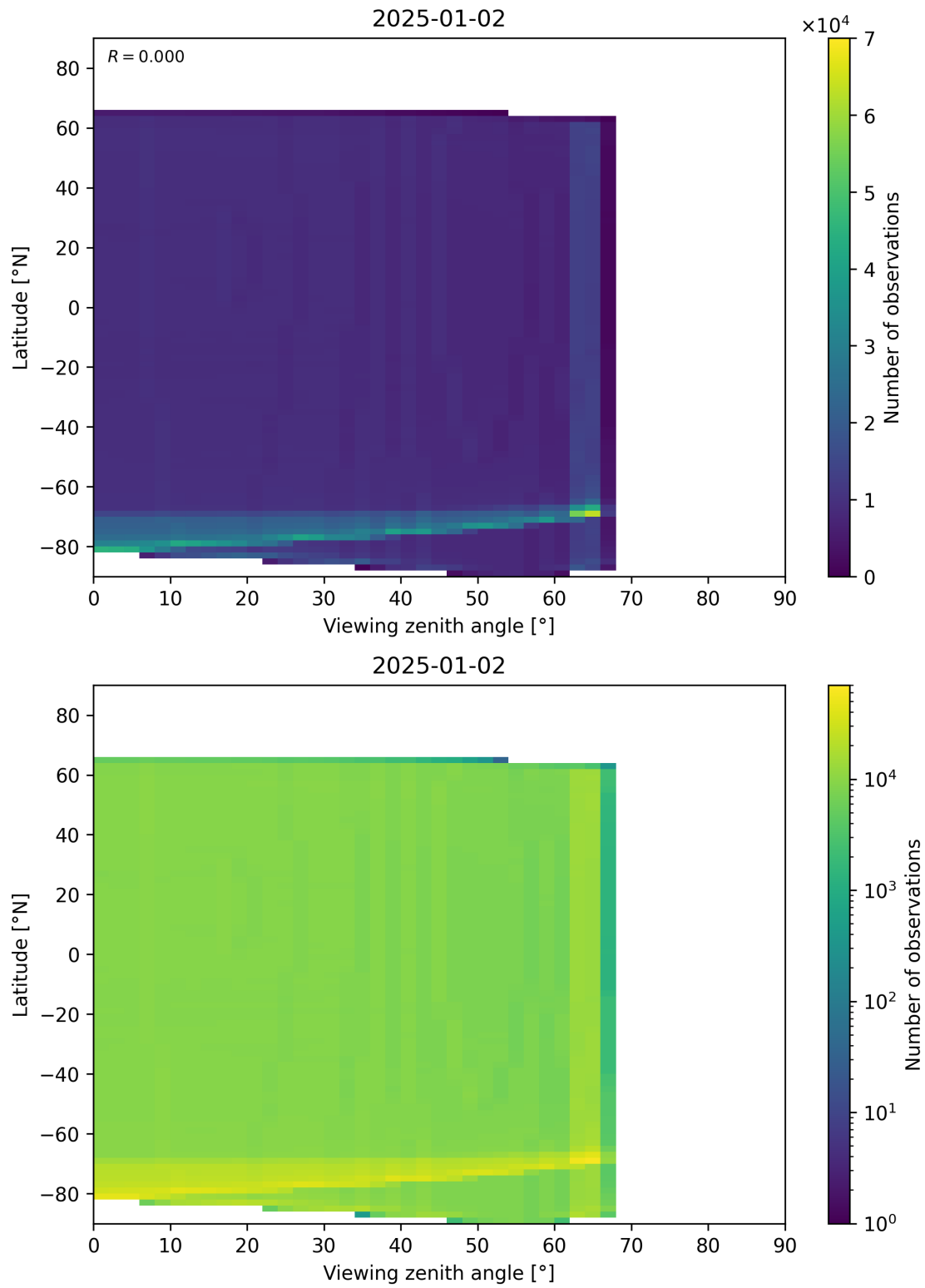
Figure 163: Scatter density plot of “Viewing zenith angle” against “Latitude” for 2025-01-01 to 2025-01-03.
