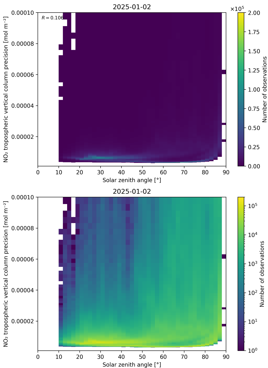
Figure 156: Scatter density plot of “Solar zenith angle” against “NO 2 tropospheric vertical column precision” for 2025-01-01 to 2025-01-03.
