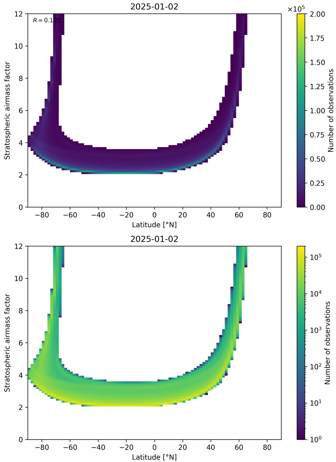
Figure 83: Scatter density plot of “Latitude” against “Stratospheric air mass factor” for 2025-01-01 to 2025-01-03.
