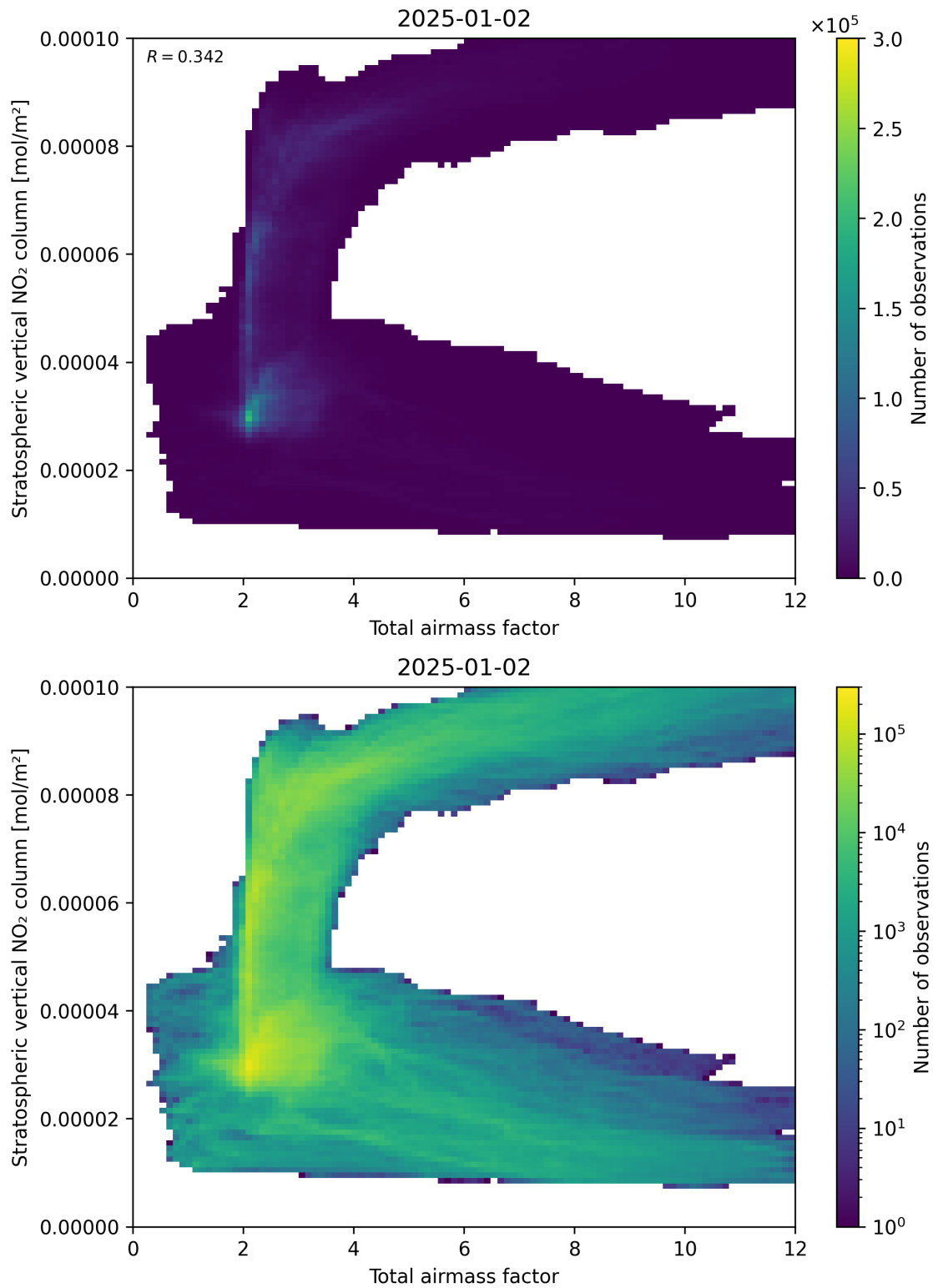
Figure 64: Scatter density plot of “Total airmass factor” against “Stratospheric vertical NO 2 column” for 2025-01-01 to 2025-01-03.
