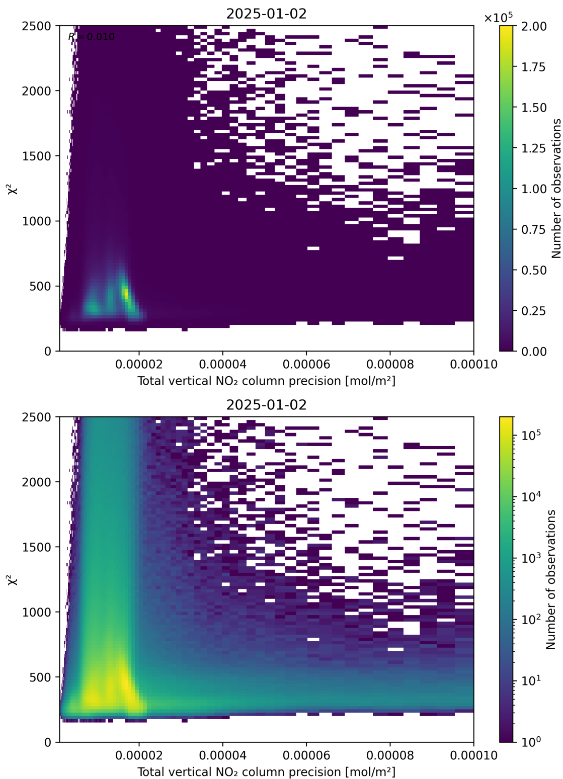
Figure 116: Scatter density plot of “Total vertical NO 2 column precision” against “ \chi^2 ” for 2025-01-01 to 2025-01-03.
