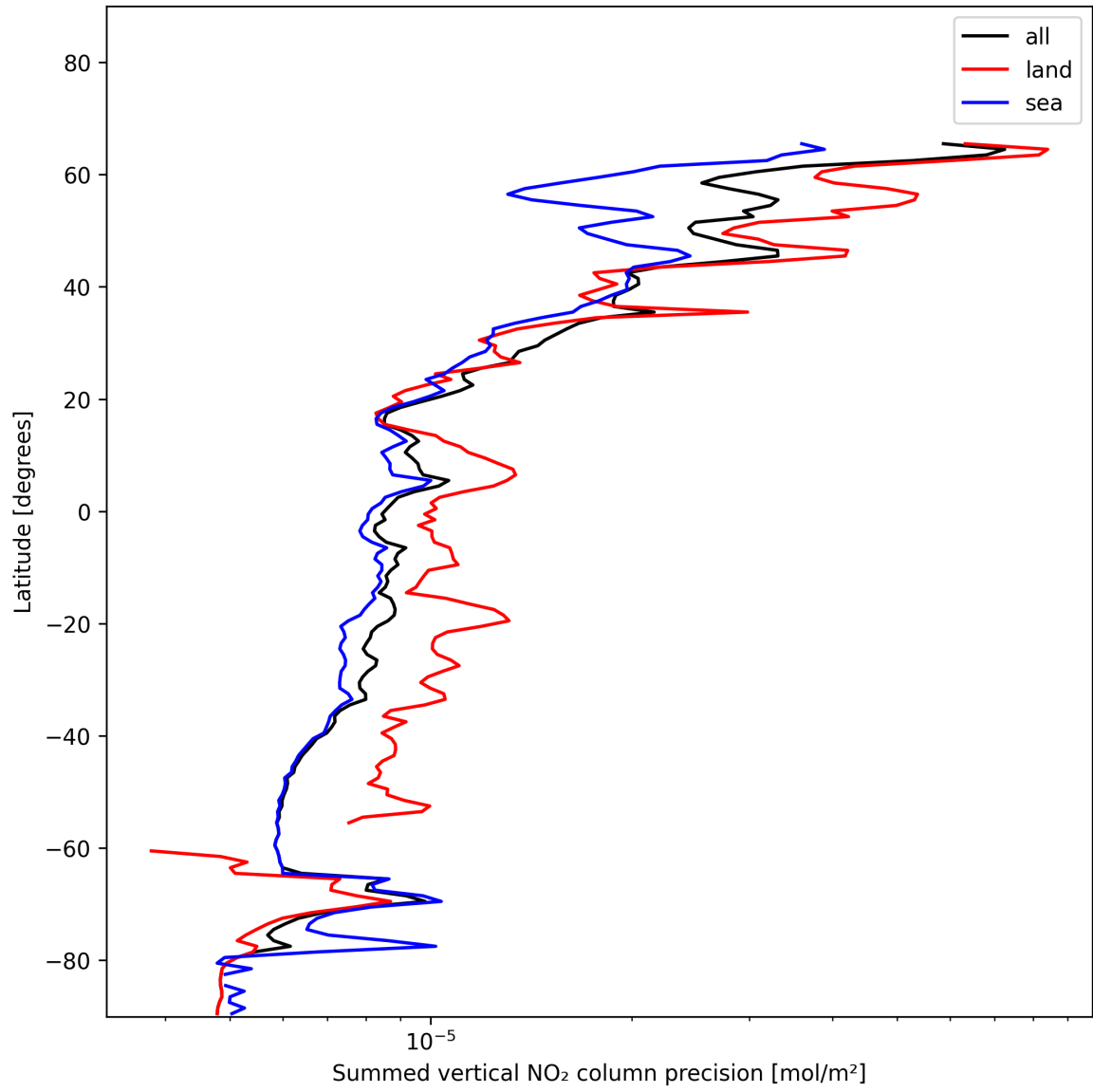
Figure 24: Zonal average of “Summed vertical NO 2 column precision” for 2025-01-01 to 2025-01-03.
