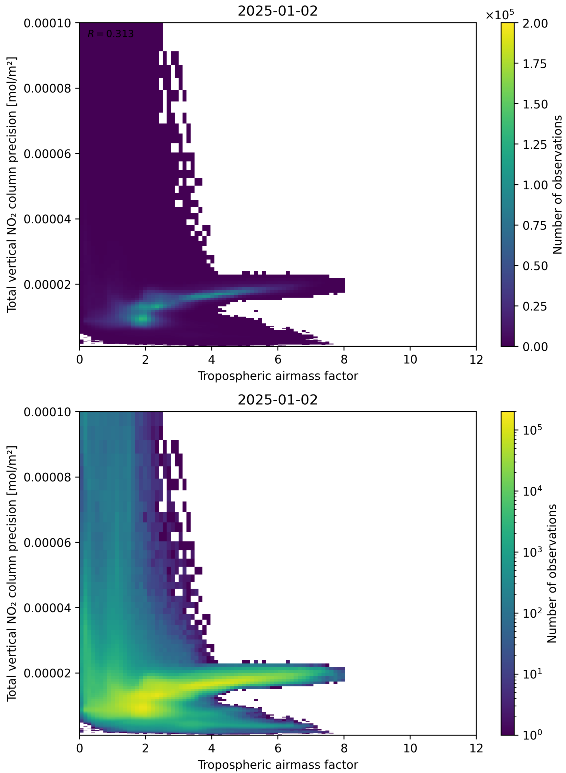
Figure 78: Scatter density plot of “Tropospheric air mass factor” against “Total vertical NO 2 column precision” for 2025-01-01 to 2025-01-03.
