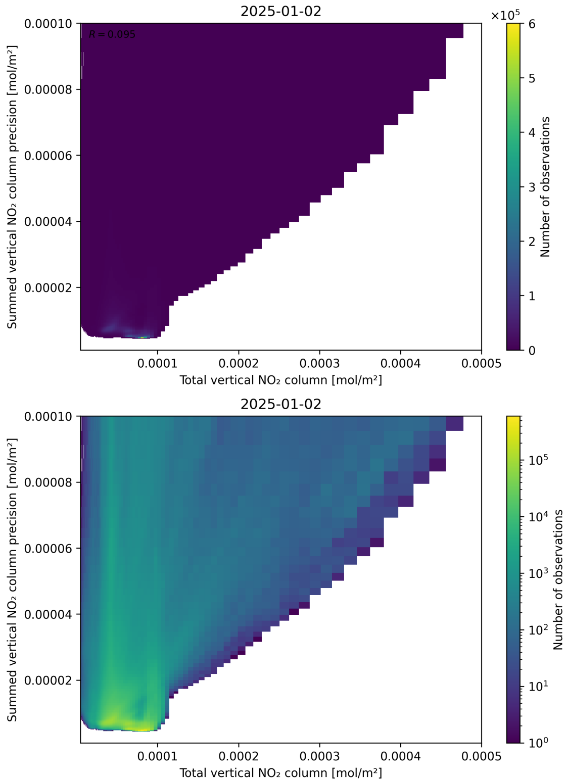
Figure 113: Scatter density plot of “Total vertical NO 2 column” against “Summed vertical NO 2 column precision” for 2025-01-01 to 2025-01-03.
