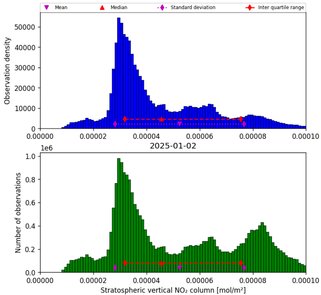
Figure 36: Histogram of “Stratospheric vertical NO 2 column” for 2025-01-01 to 2025-01-03
