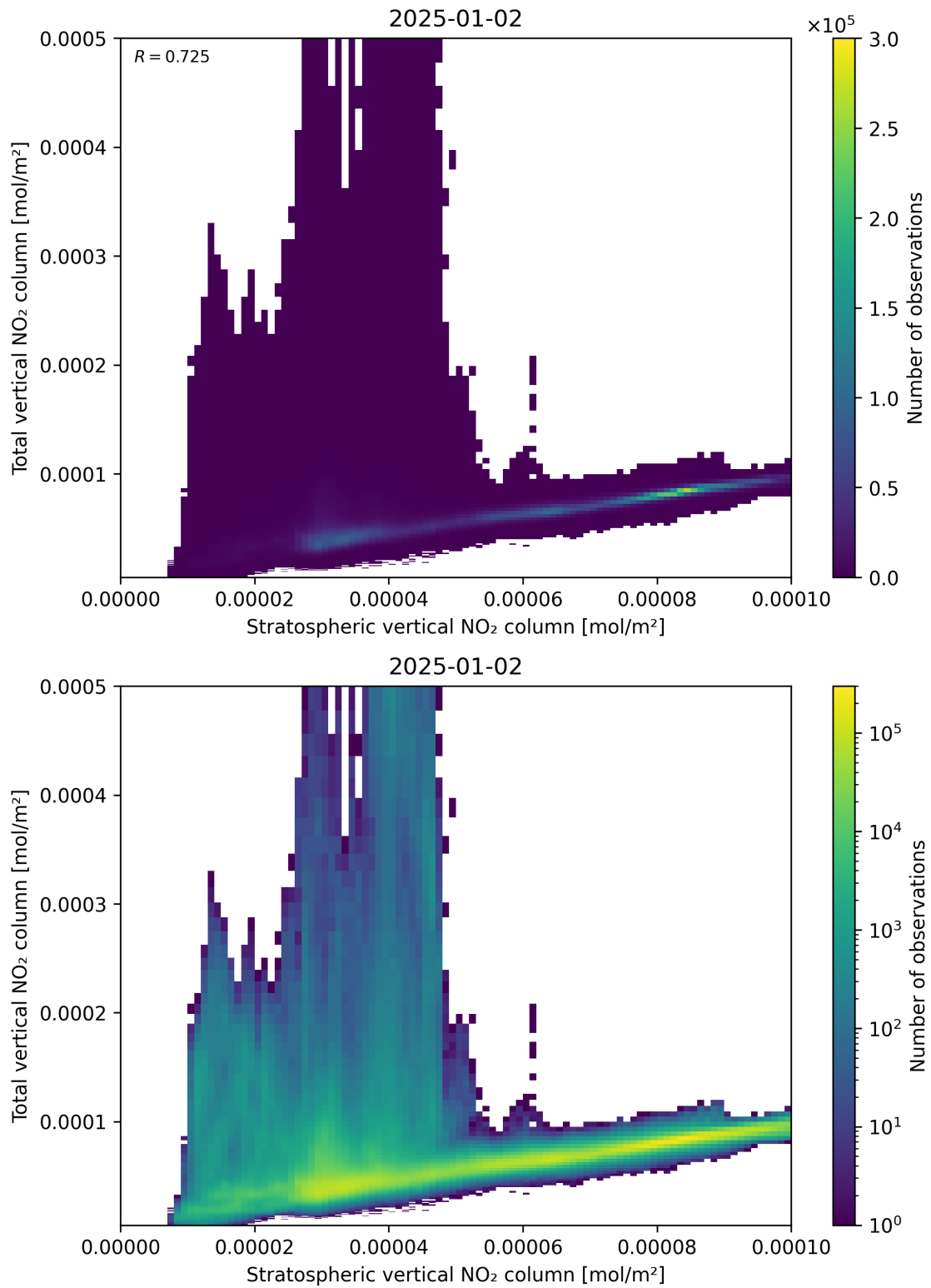
Figure 100: Scatter density plot of “Stratospheric vertical NO 2 column” against “Total vertical NO 2 column” for 2025-01-01 to 2025-01-03.
