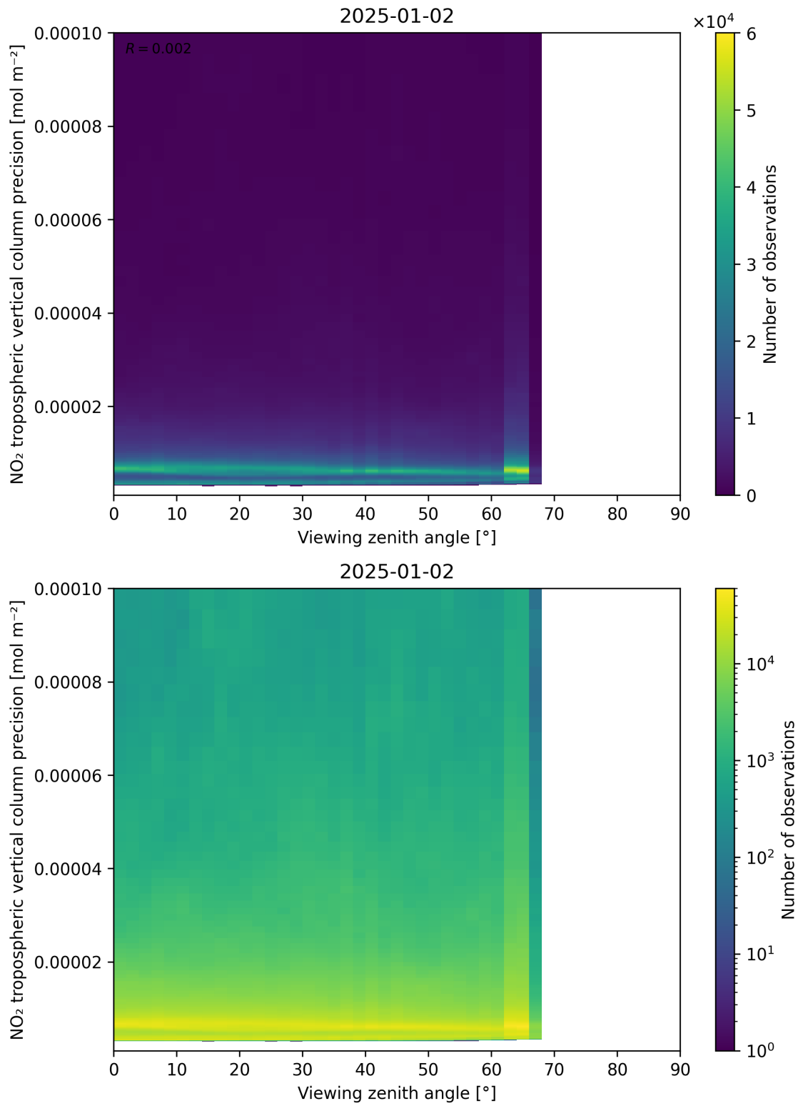
Figure 170: Scatter density plot of “Viewing zenith angle” against “NO 2 tropospheric vertical column precision” for 2025-01-01 to 2025-01-03.
