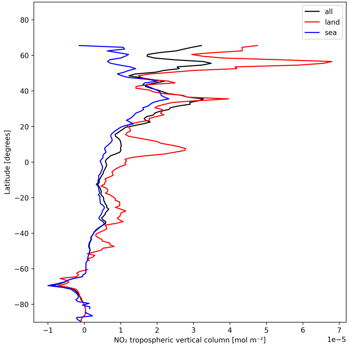
Figure 12: Zonal average of “NO 2 tropospheric vertical column” for 2025-01-01 to 2025-01-03.
