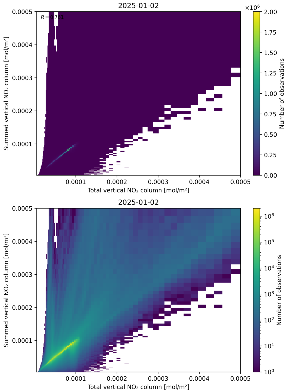
Figure 112: Scatter density plot of “Total vertical NO 2 column” against “Summed vertical NO 2 column” for 2025-01-01 to 2025-01-03.
