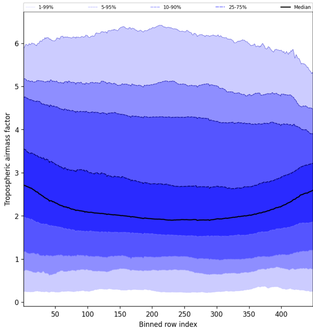
Figure 48: Along track statistics of “Tropospheric airmass factor” for 2025-01-01 to 2025-01-03
