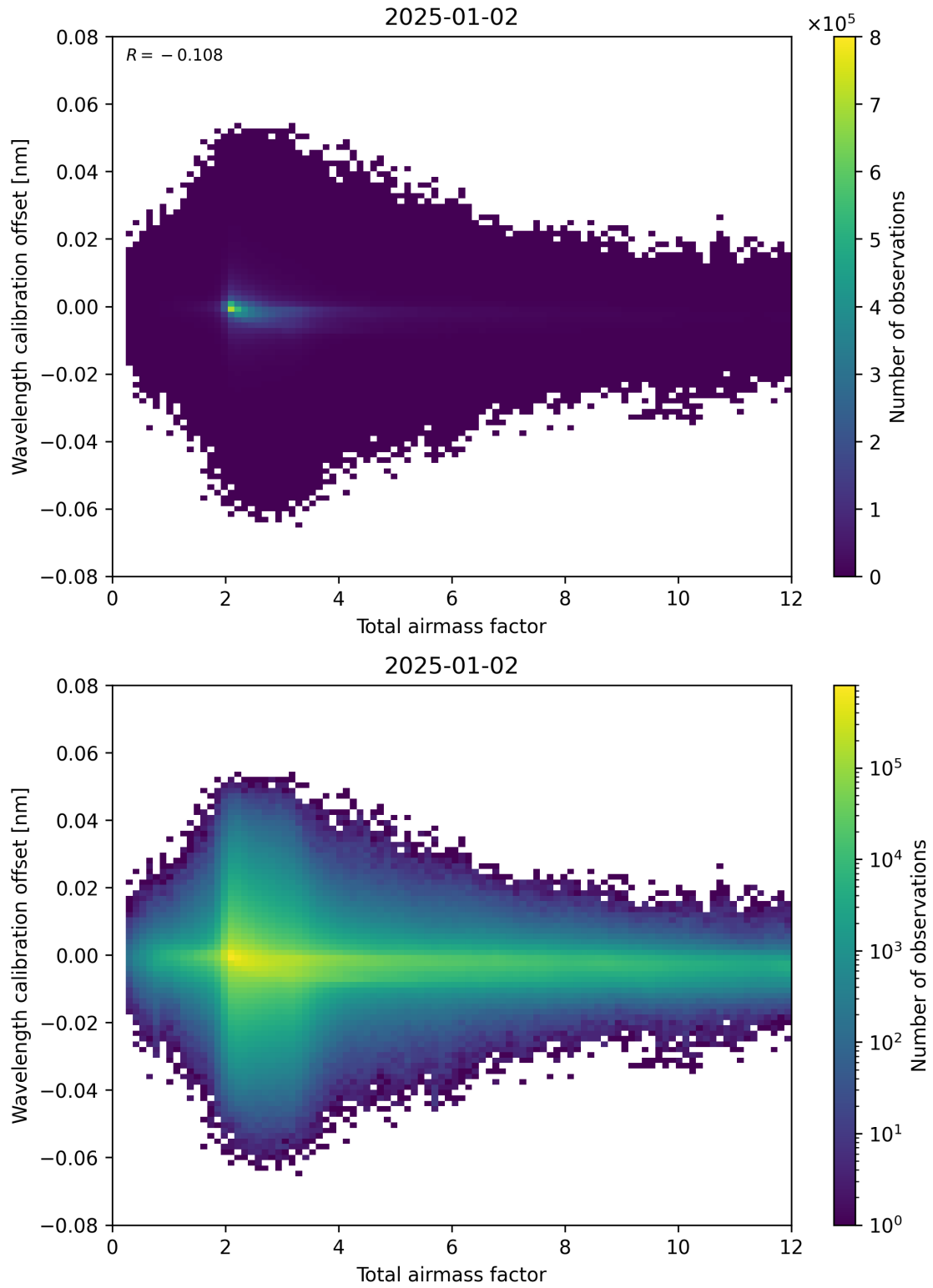
Figure 70: Scatter density plot of “Total airmass factor” against “Wavelength calibration offset” for 2025-01-01 to 2025-01-03.
