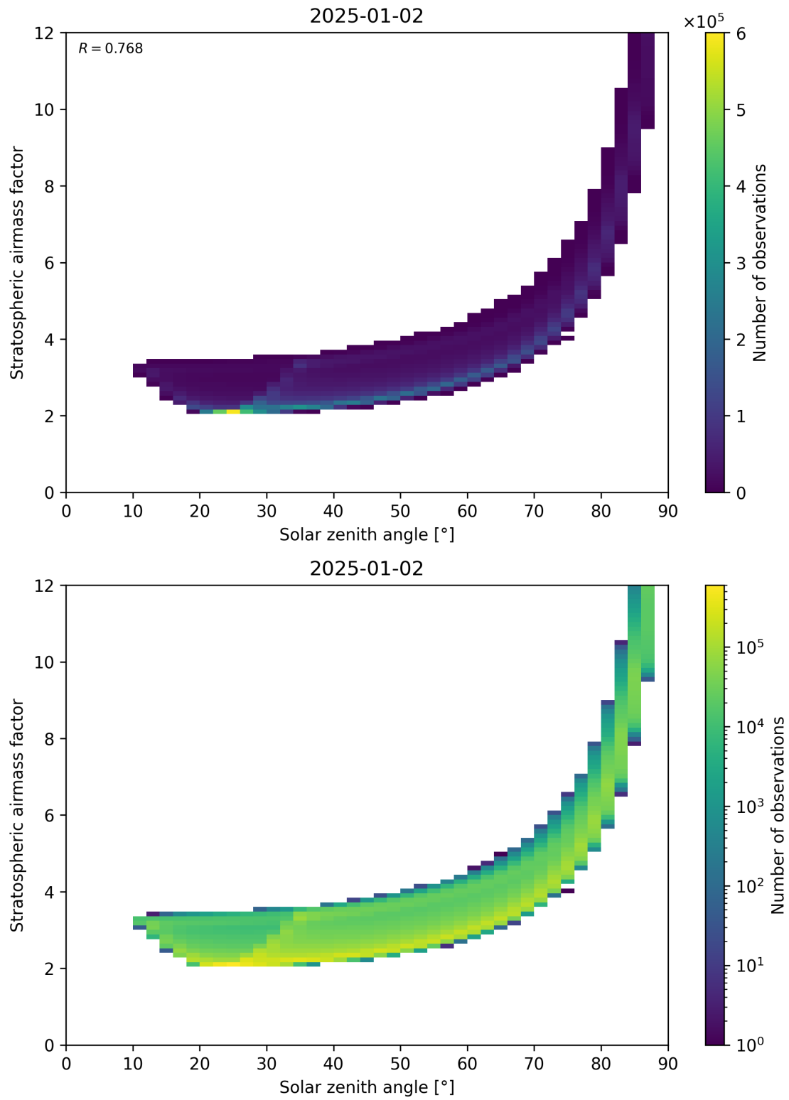
Figure 145: Scatter density plot of “Solar zenith angle” against “Stratospheric airmass factor” for 2025-01-01 to 2025-01-03.
