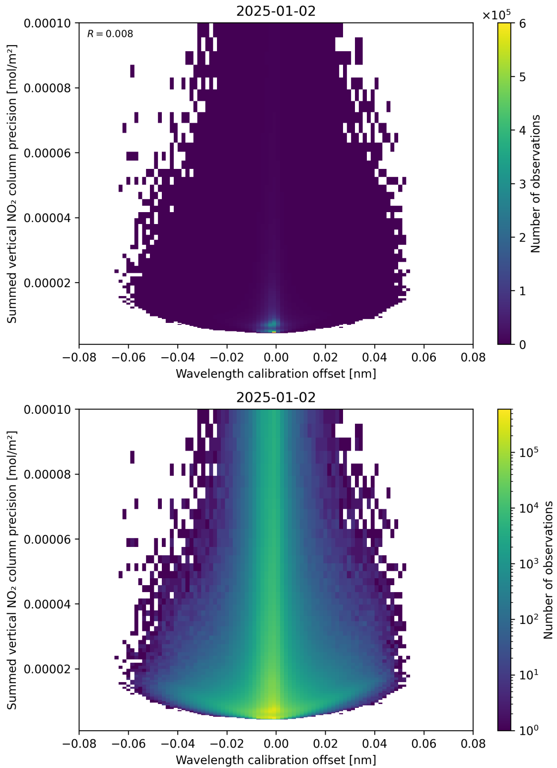
Figure 178: Scatter density plot of “Wavelength calibration offset” against “Summed vertical NO 2 column precision” for 2025-01-01 to 2025-01-03.
