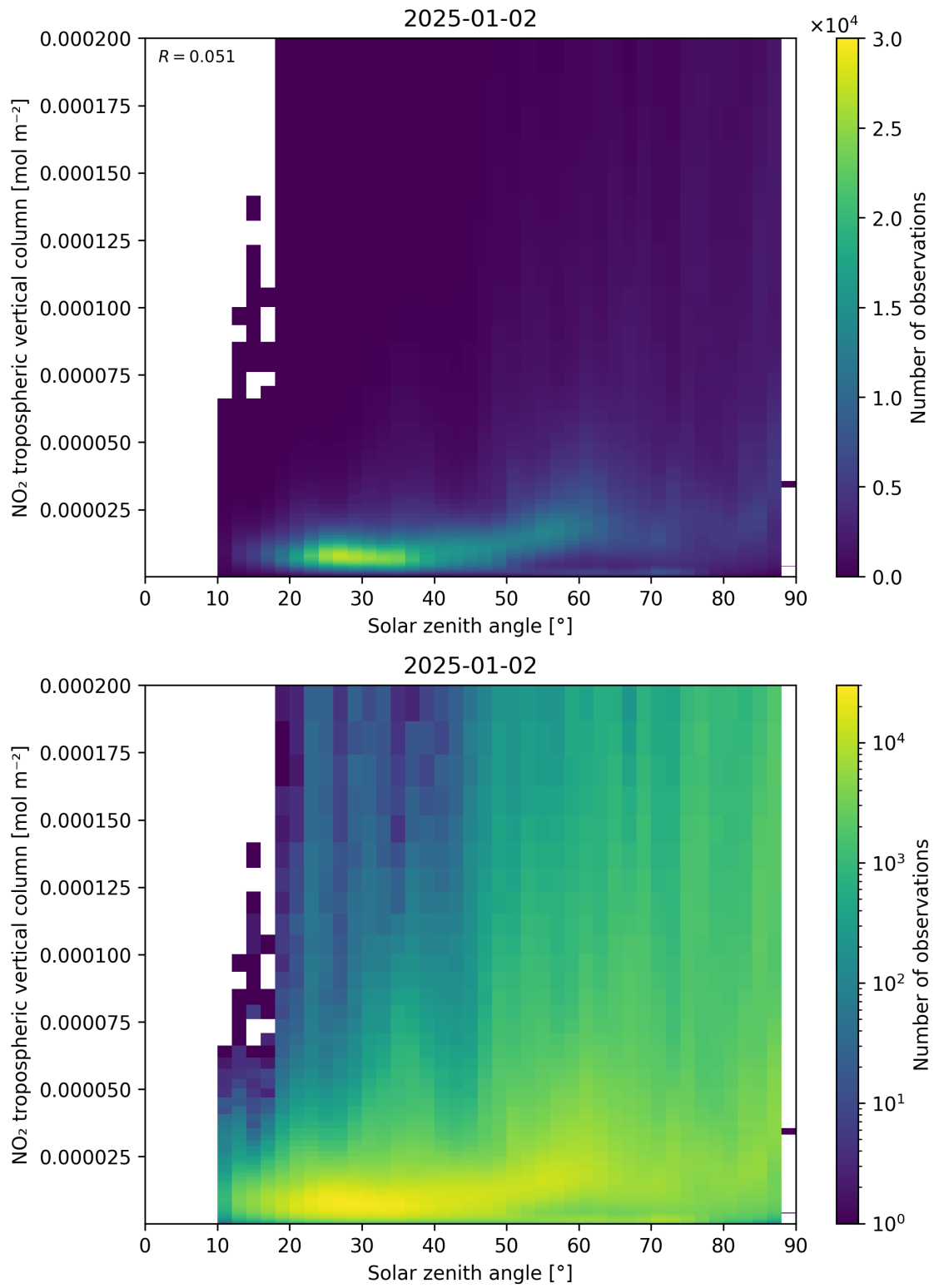
Figure 155: Scatter density plot of “Solar zenith angle” against “NO 2 tropospheric vertical column” for 2025-01-01 to 2025-01-03.
