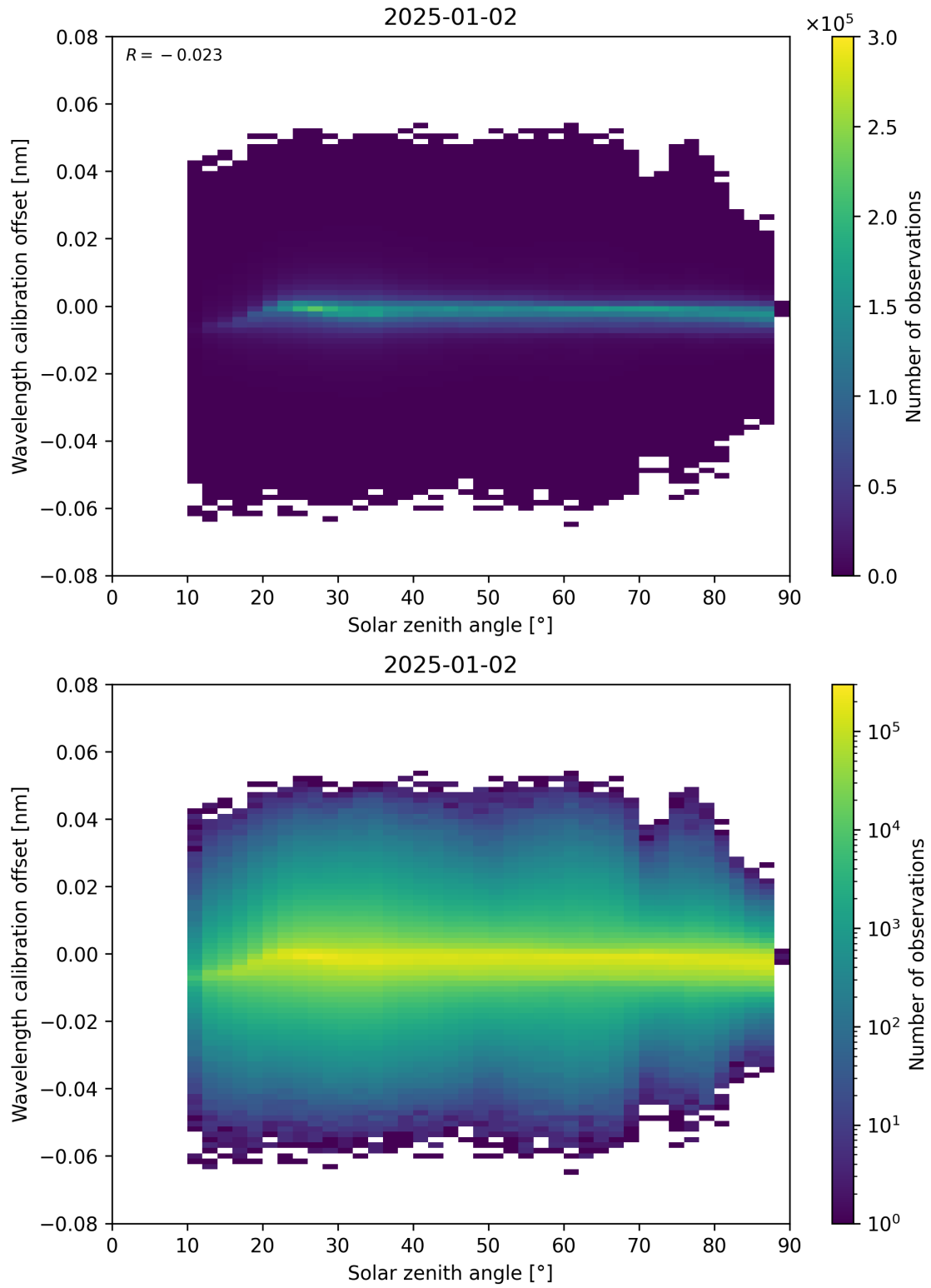
Figure 158: Scatter density plot of “Solar zenith angle” against “Wavelength calibration offset” for 2025-01-01 to 2025-01-03.
