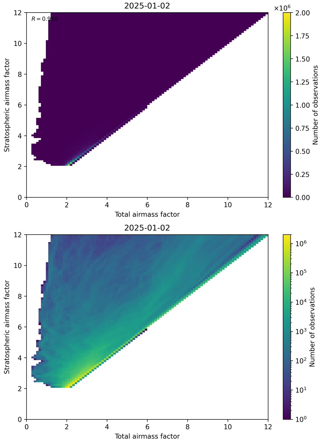
Figure 62: Scatter density plot of “Total airmass factor” against “Stratospheric airmass factor” for 2025-01-01 to 2025-01-03.
