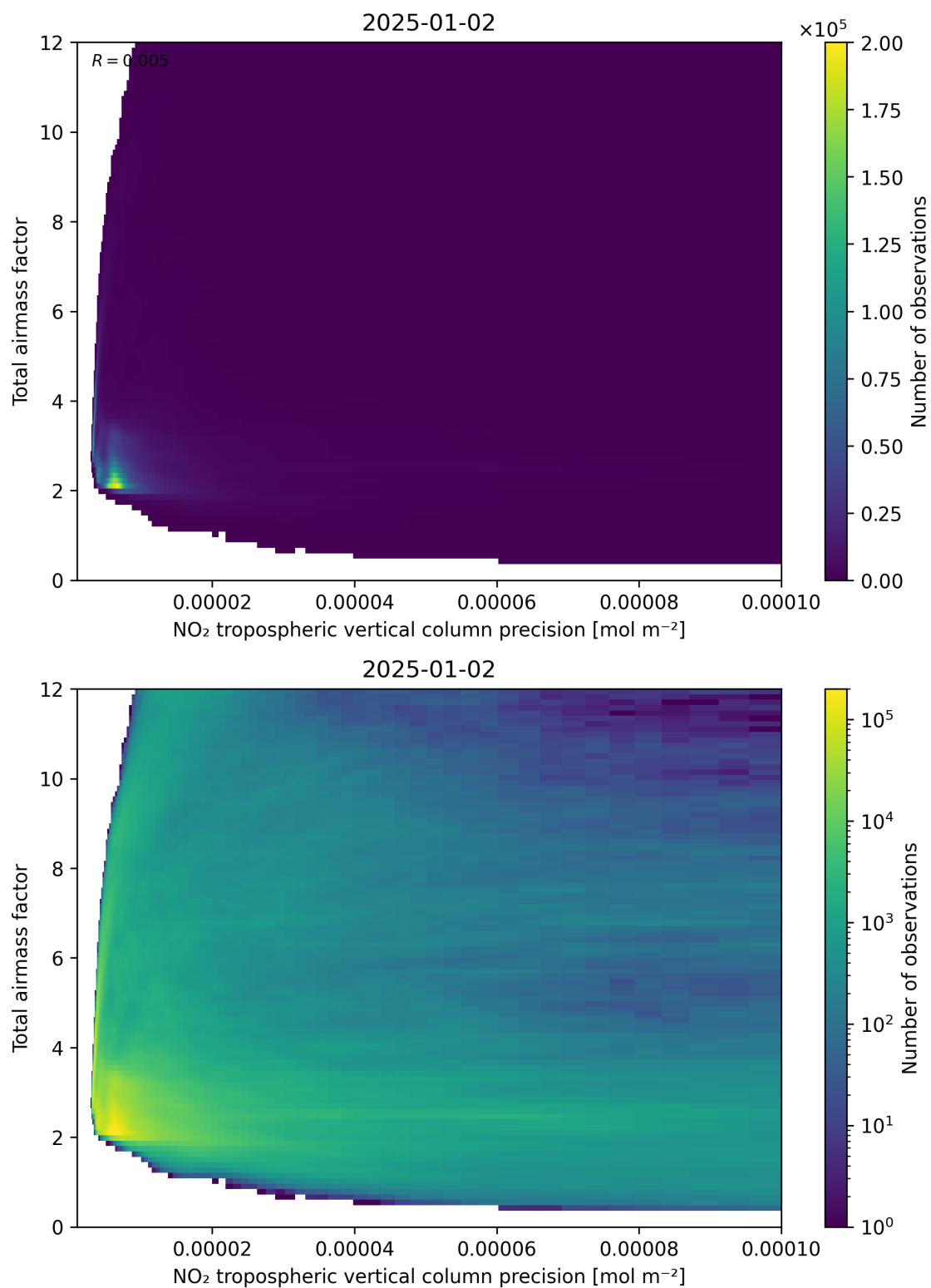
Figure 132: Scatter density plot of “NO 2 tropospheric vertical column precision” against “Total air mass factor” for 2025-01-01 to 2025-01-03.
