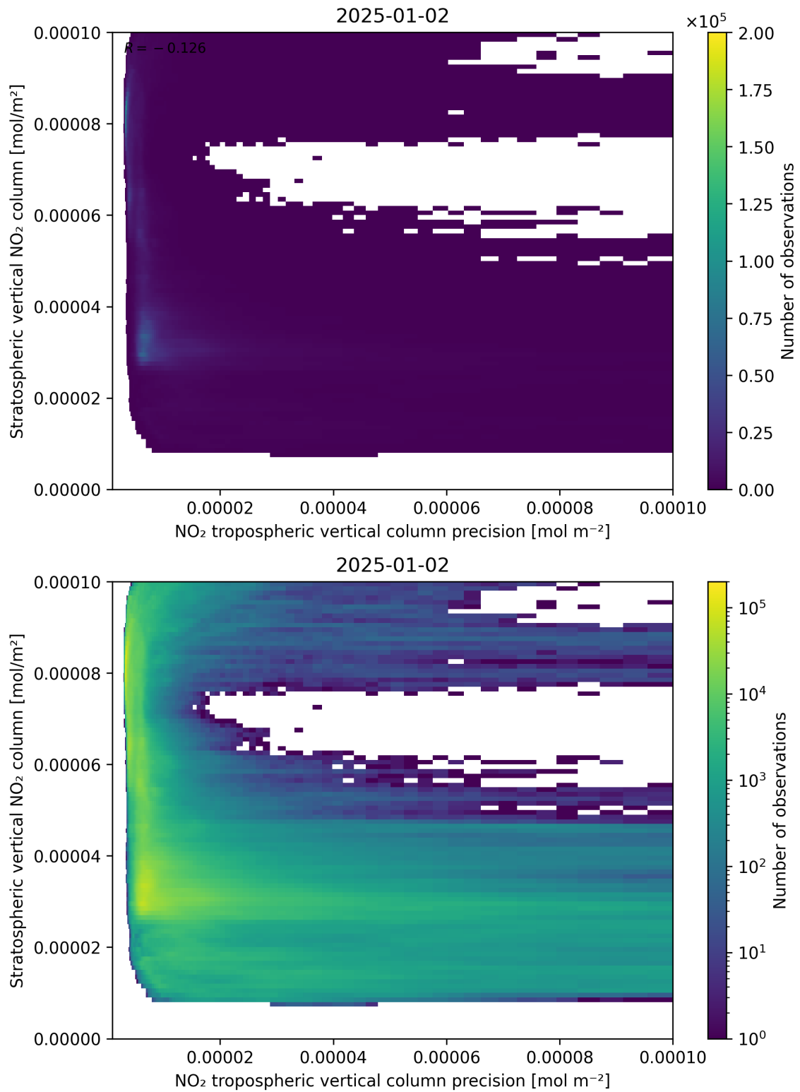
Figure 135: Scatter density plot of “NO 2 tropospheric vertical column precision” against “Stratospheric vertical NO 2 column” for 2025-01-01 to 2025-01-03.
