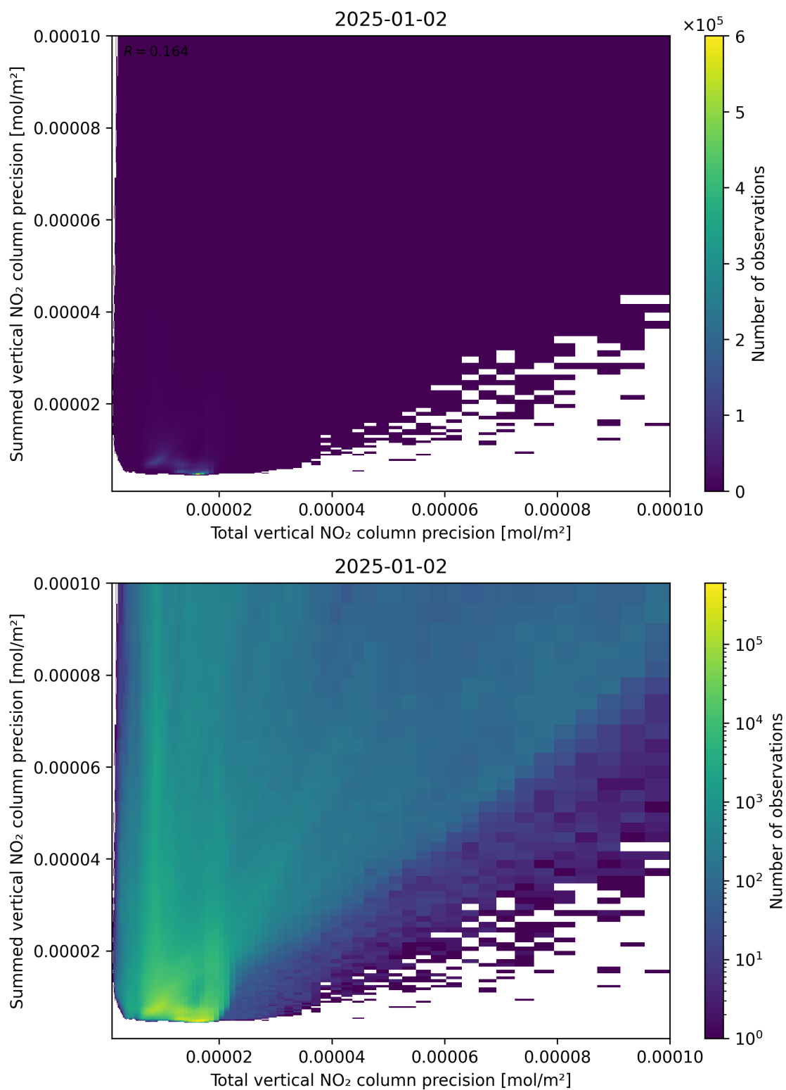
Figure 118: Scatter density plot of “Total vertical NO 2 column precision” against “Summed vertical NO 2 column precision” for 2025-01-01 to 2025-01-03.
