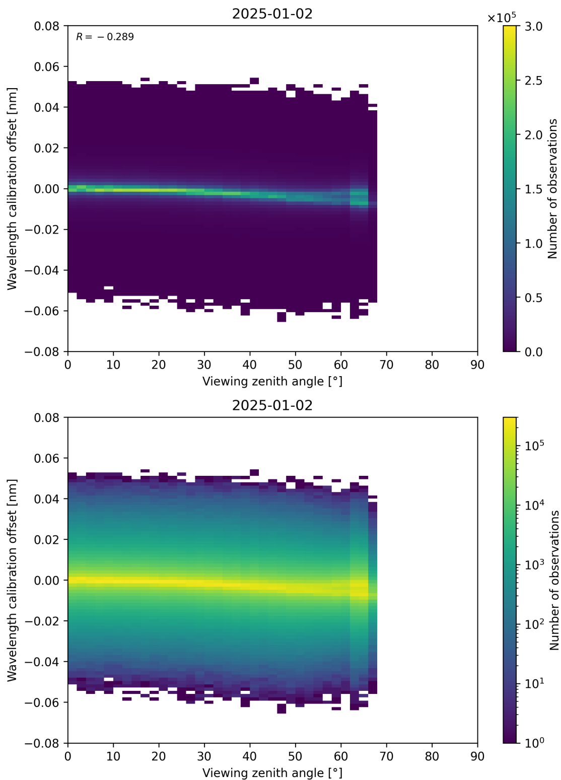
Figure 173: Scatter density plot of “Viewing zenith angle” against “Wavelength calibration offset” for 2025-01-01 to 2025-01-03.
