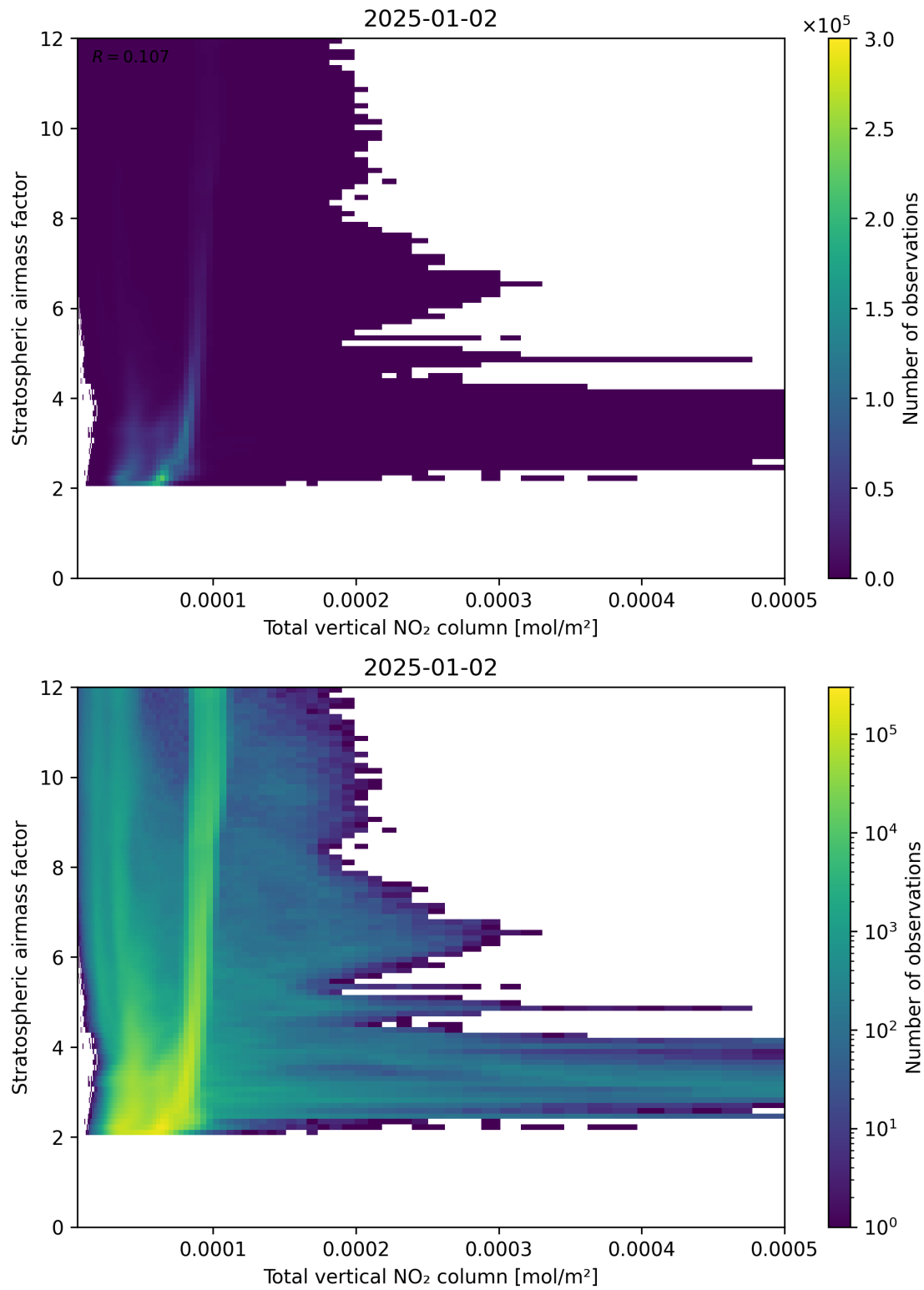
Figure 110: Scatter density plot of “Total vertical NO 2 column” against “Stratospheric airmass factor” for 2025-01-01 to 2025-01-03.
