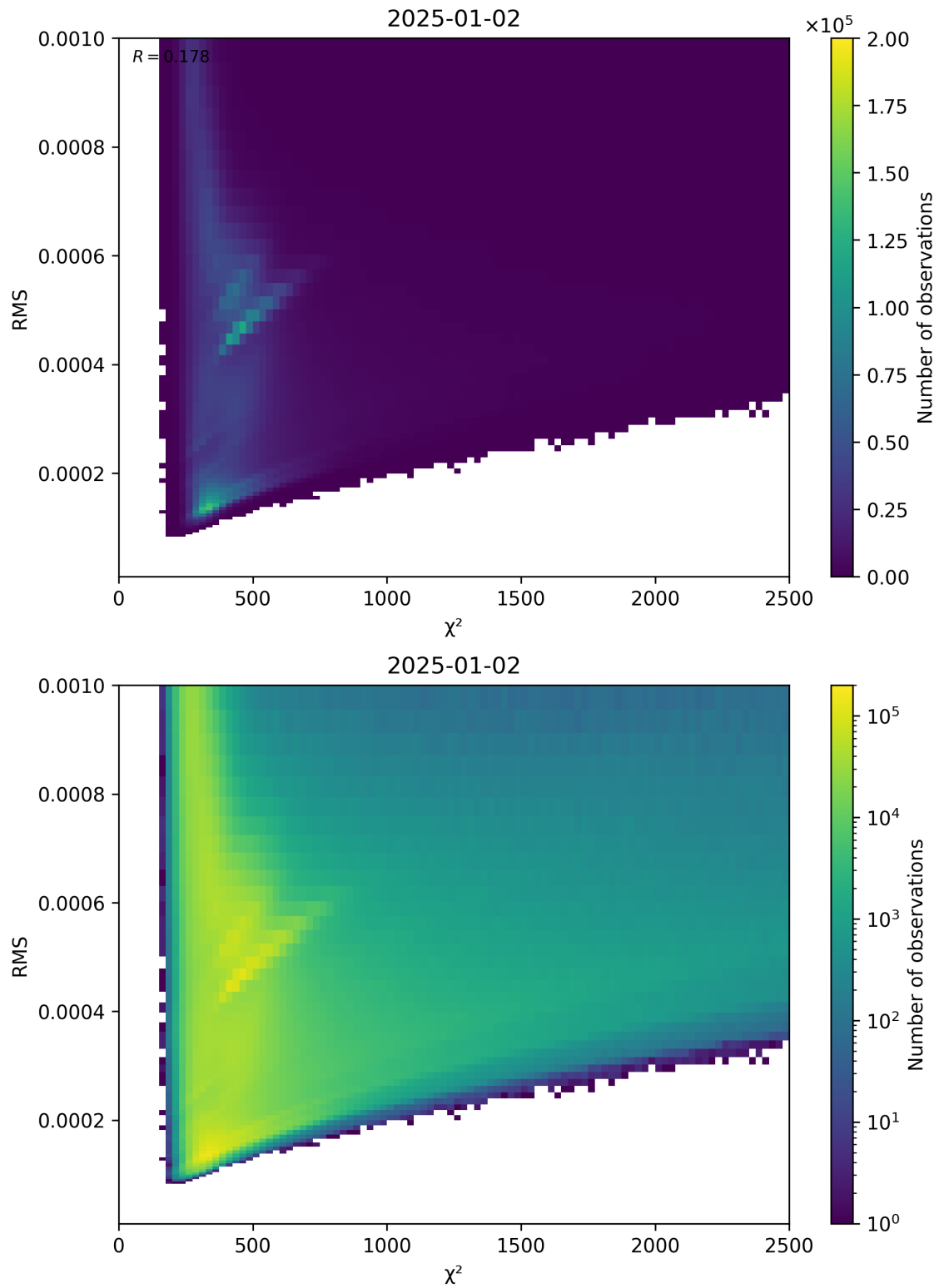
Figure 82: Scatter density plot of “ \chi^2 ” against “RMS” for 2025-01-01 to 2025-01-03.
