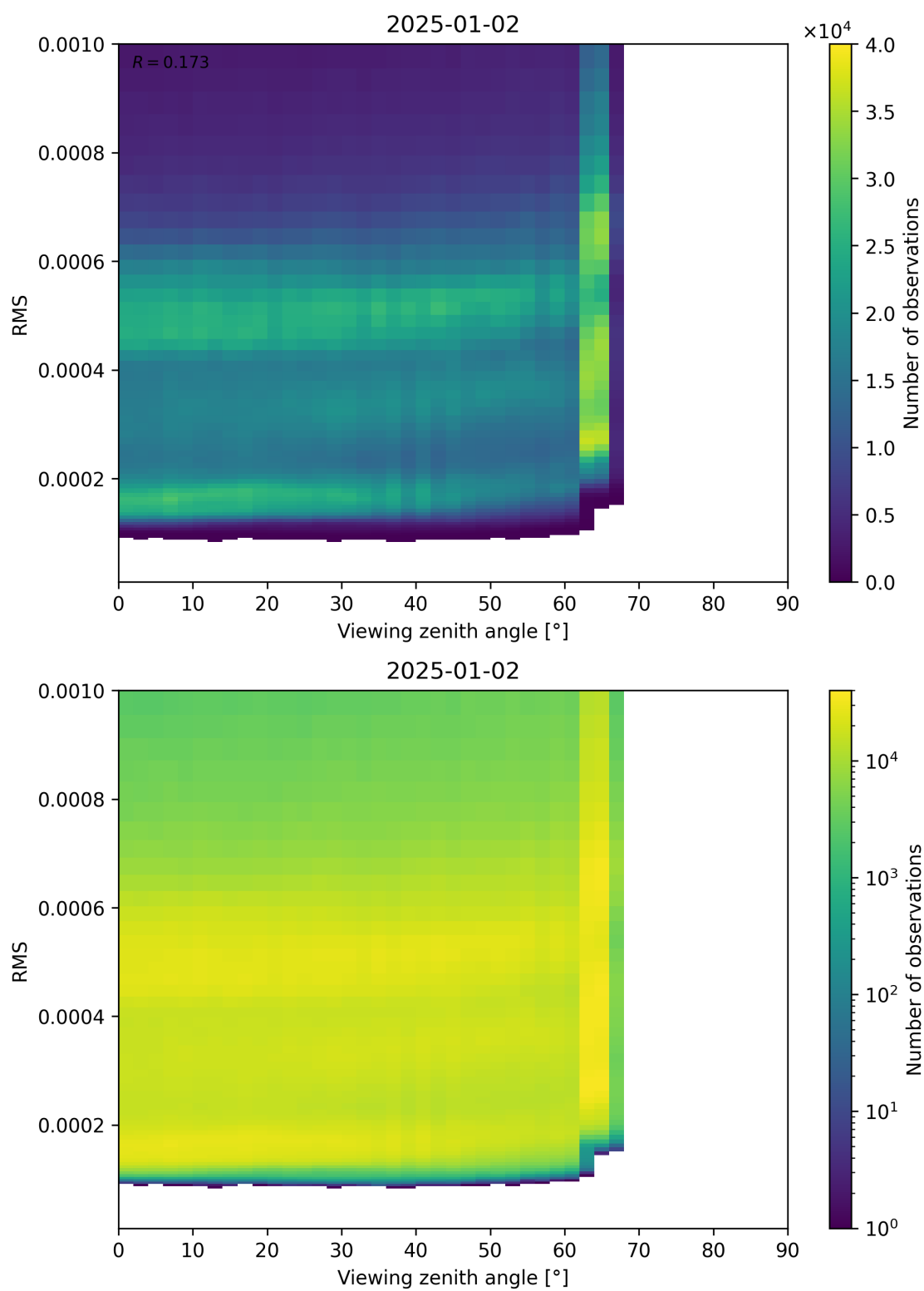
Figure 171: Scatter density plot of “Viewing zenith angle” against “RMS” for 2025-01-01 to 2025-01-03.
