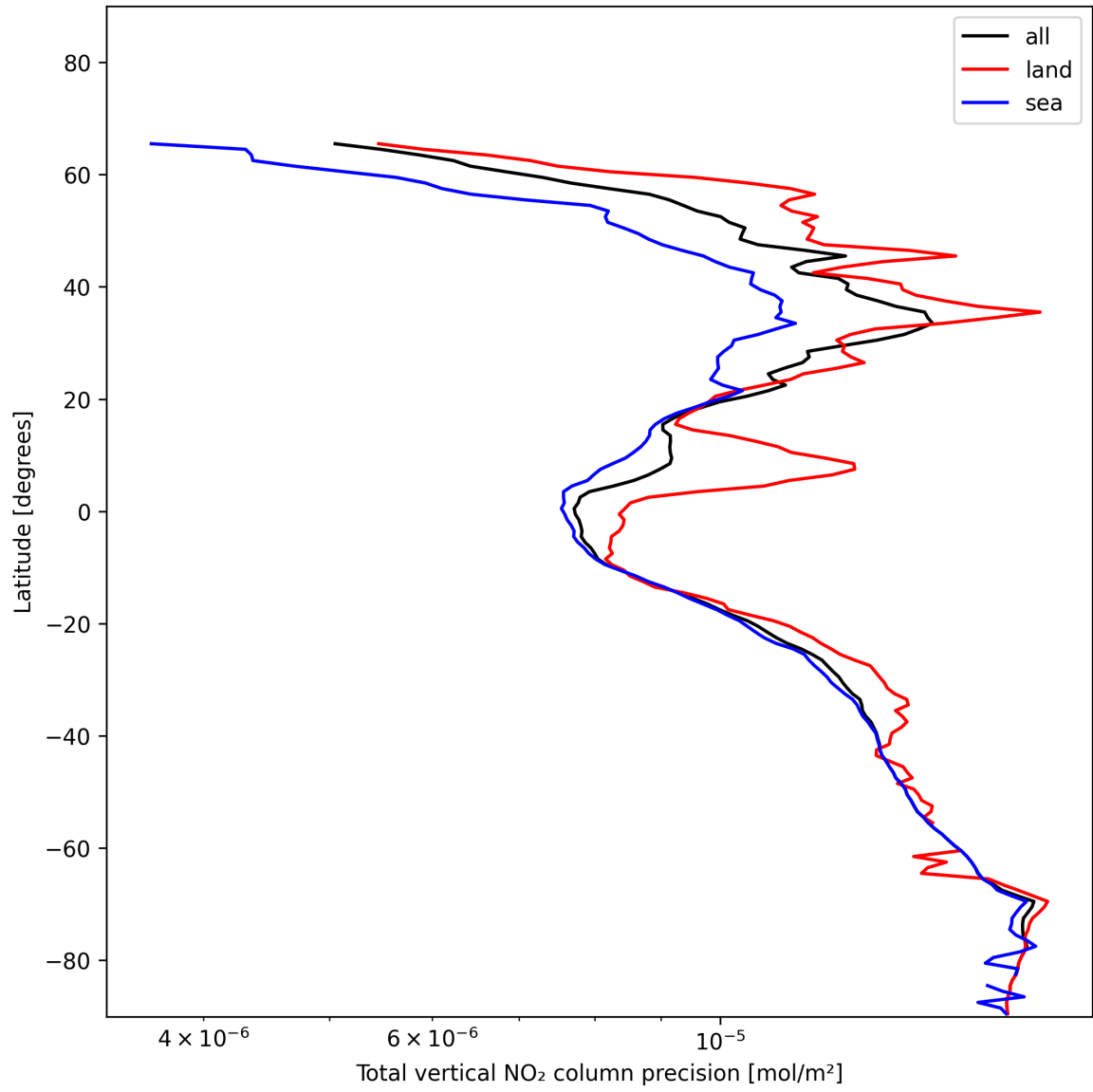
Figure 22: Zonal average of “Total vertical NO 2 column precision” for 2025-01-01 to 2025-01-03.
