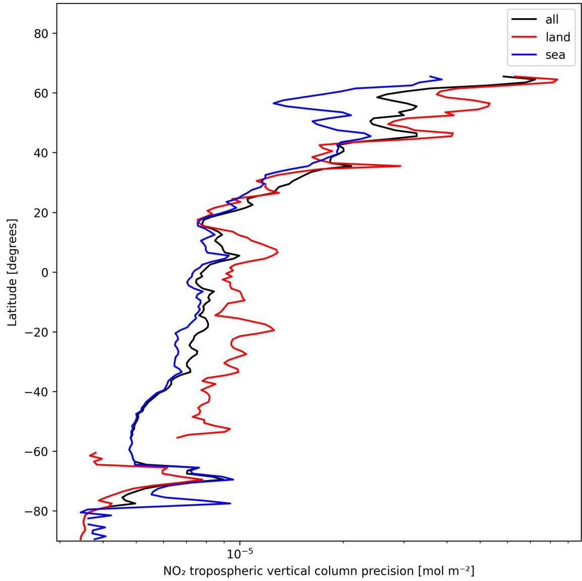
Figure 13: Zonal average of “NO 2 tropospheric vertical column precision” for 2025-01-01 to 2025-01-03.
