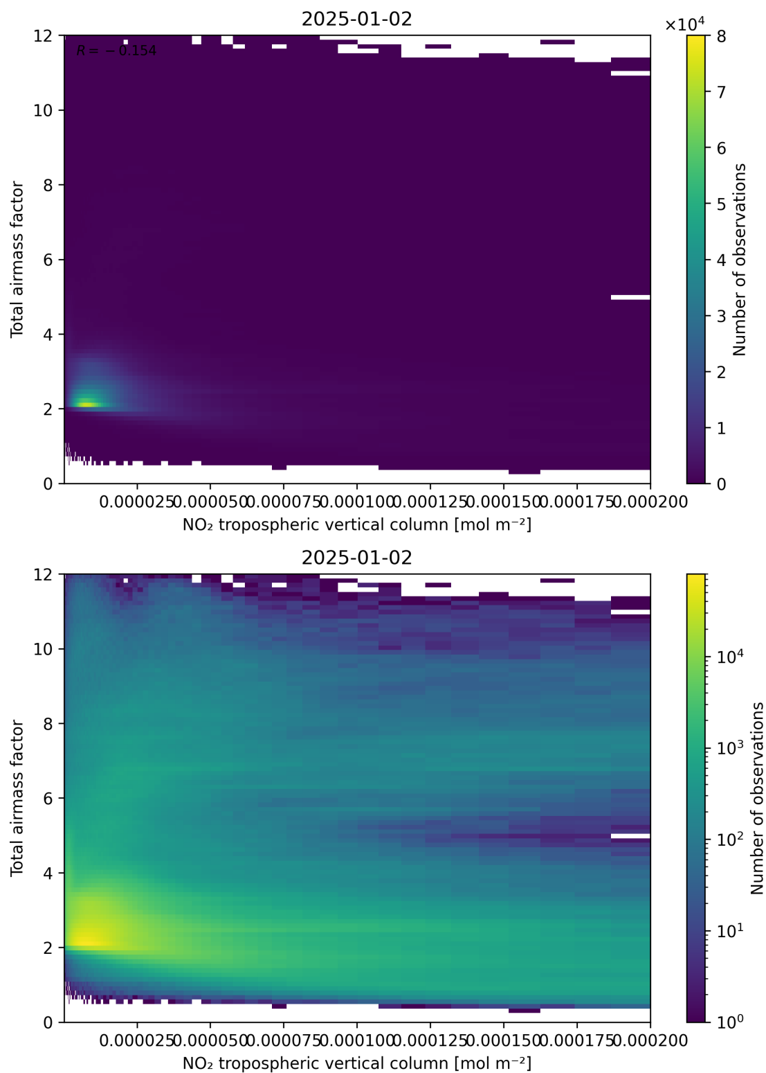
Figure 122: Scatter density plot of “NO 2 tropospheric vertical column” against “Total air mass factor” for 2025-01-01 to 2025-01-03.
