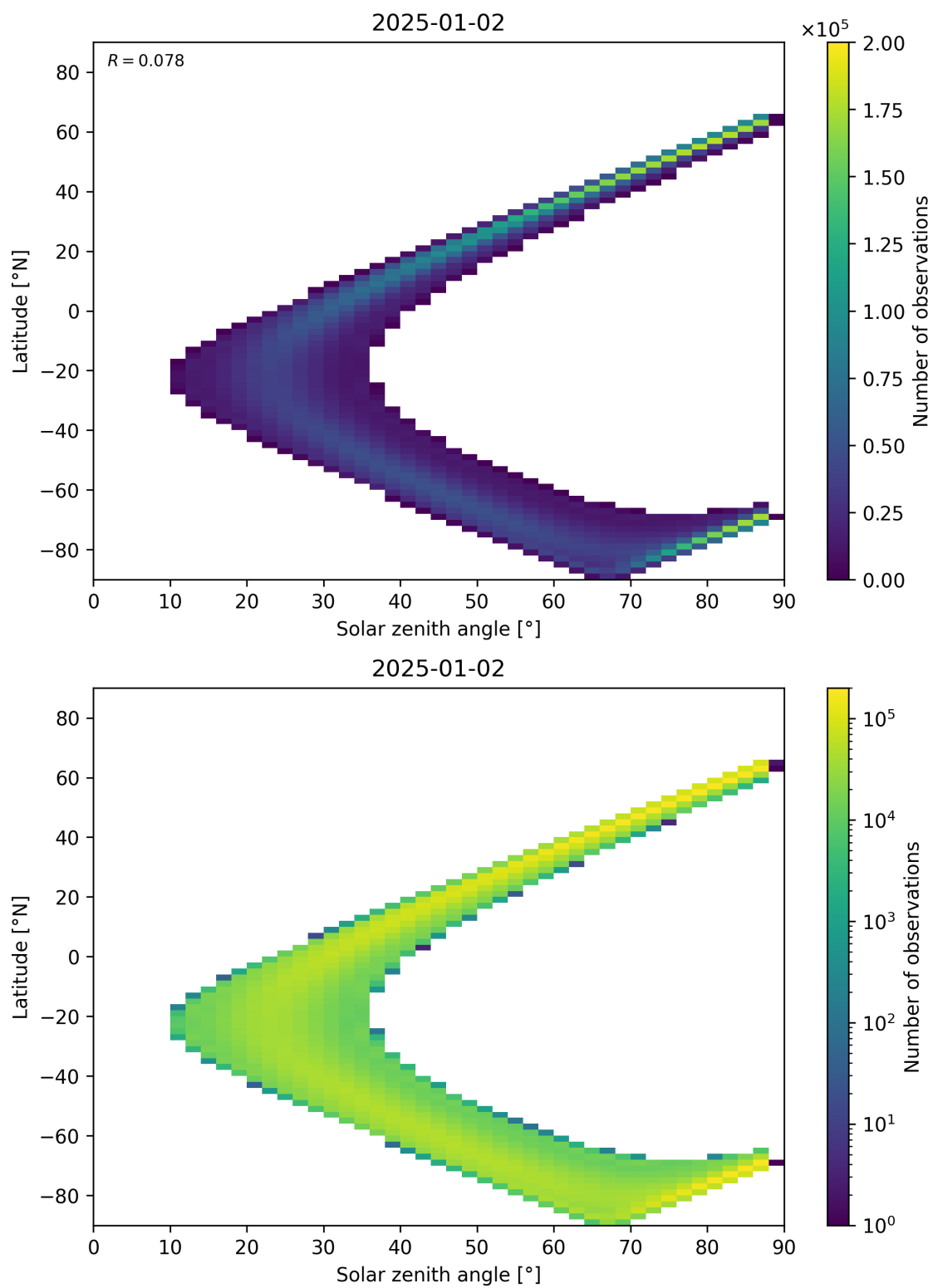
Figure 149: Scatter density plot of “Solar zenith angle” against “Latitude” for 2025-01-01 to 2025-01-03.
