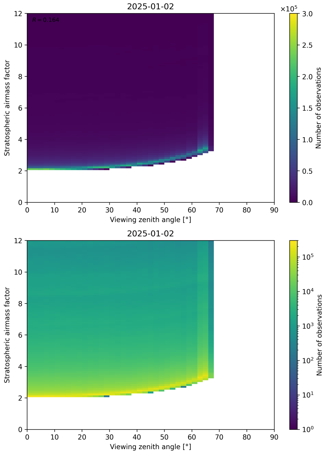
Figure 159: Scatter density plot of “Viewing zenith angle” against “Stratospheric airmass factor” for 2025-01-01 to 2025-01-03.
