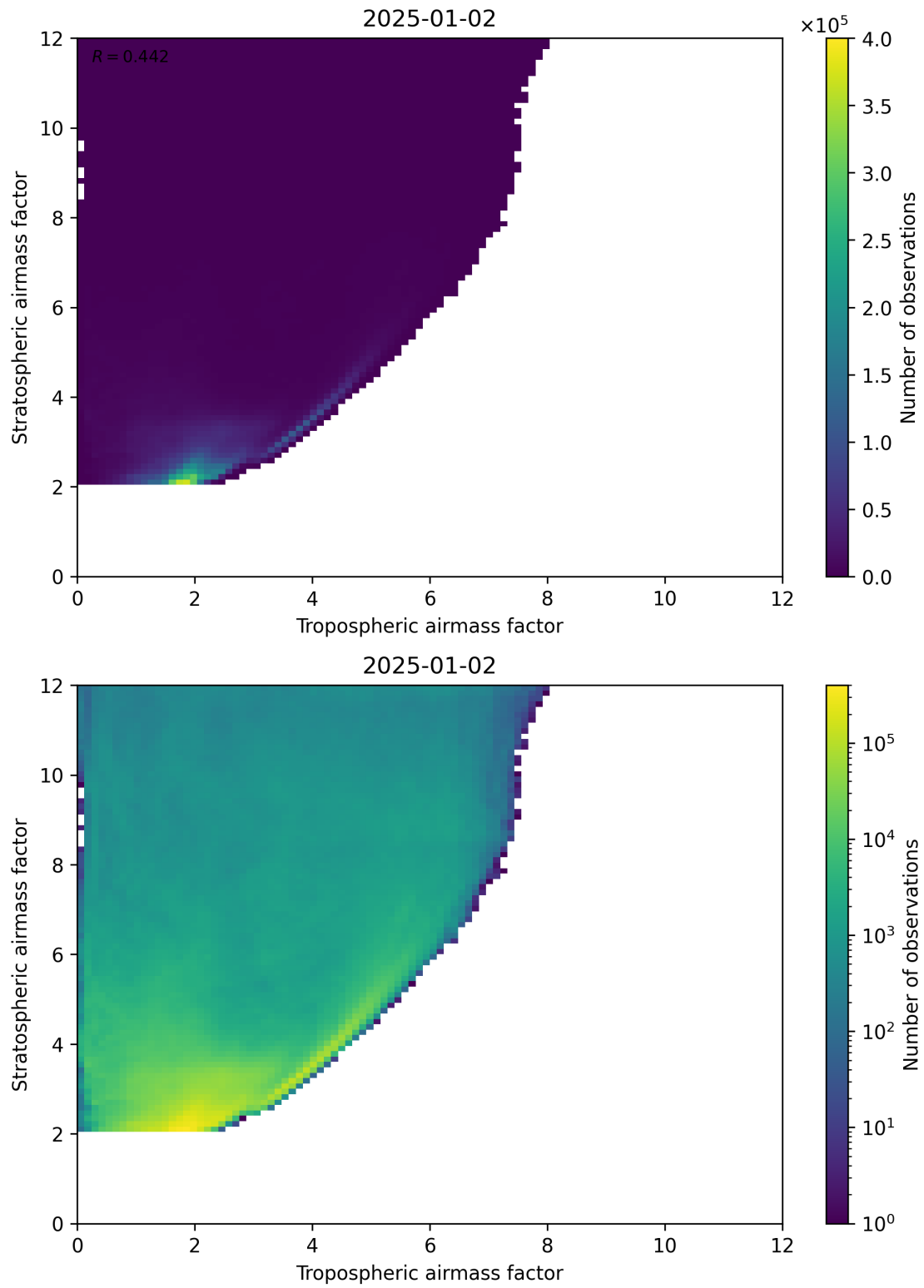
Figure 71: Scatter density plot of “Tropospheric airmass factor” against “Stratospheric airmass factor” for 2025-01-01 to 2025-01-03.
