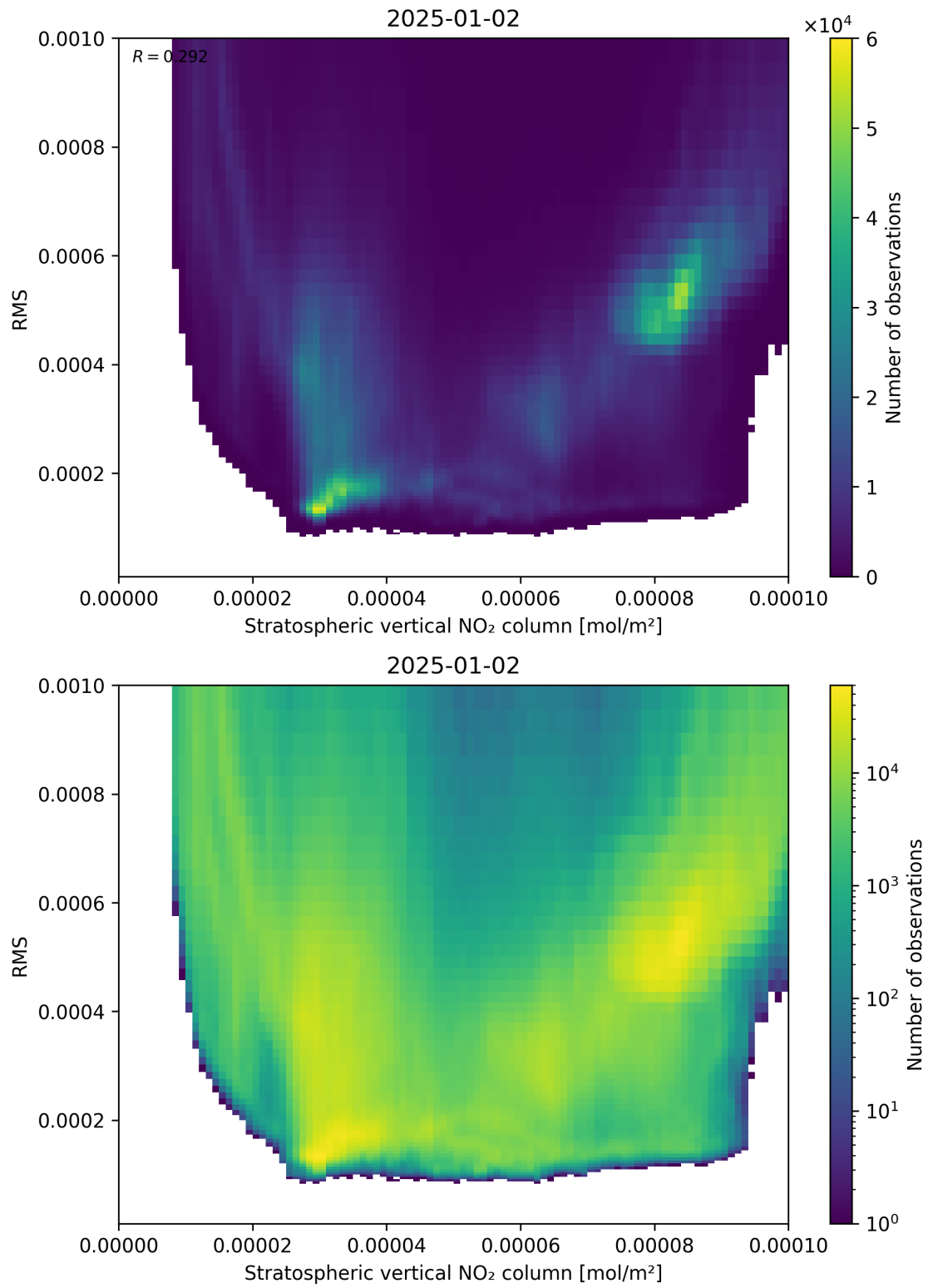
Figure 102: Scatter density plot of “Stratospheric vertical NO 2 column” against “RMS” for 2025-01-01 to 2025-01-03.
