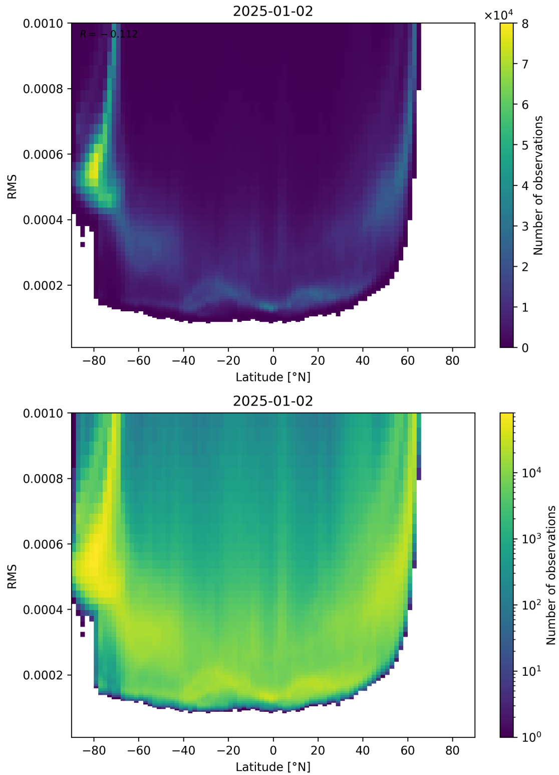
Figure 94: Scatter density plot of “Latitude” against “RMS” for 2025-01-01 to 2025-01-03.
