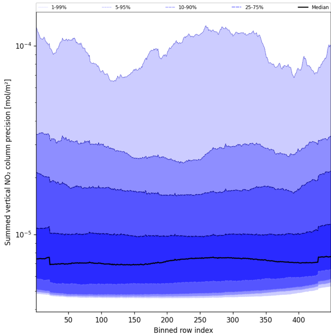
Figure 58: Along track statistics of “Summed vertical NO 2 column precision” for 2025-01-01 to 2025-01-03
