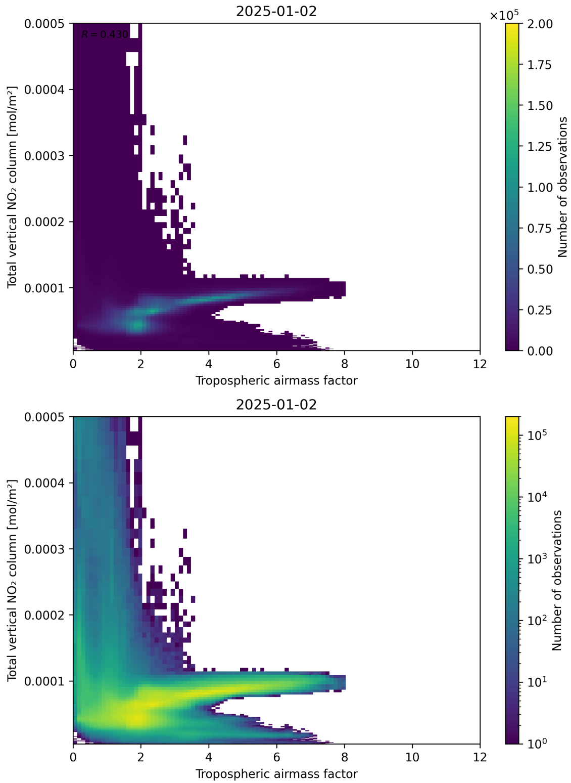
Figure 77: Scatter density plot of “Tropospheric airmass factor” against “Total vertical NO 2 column” for 2025-01-01 to 2025-01-03.
