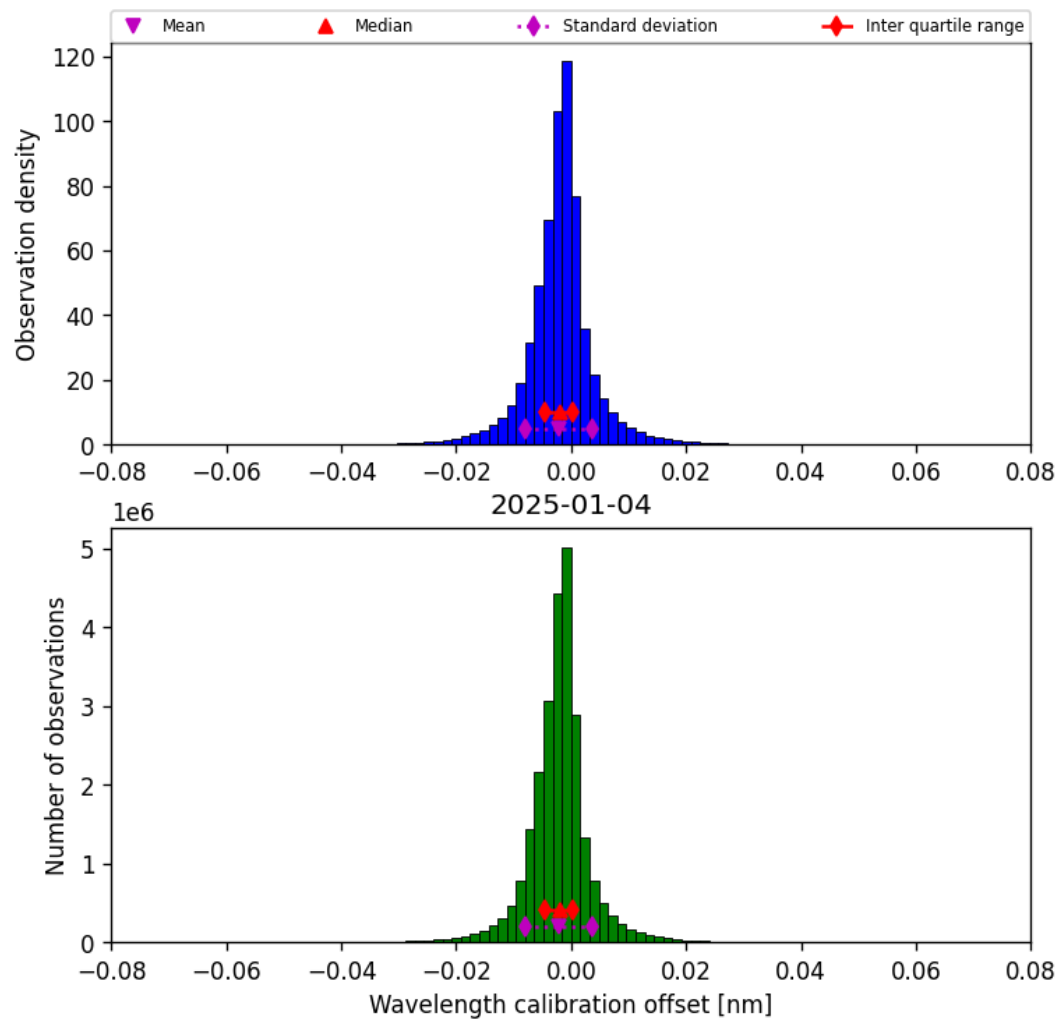
Figure 35: Histogram of “Wavelength calibration offset” for 2025-01-03 to 2025-01-05
