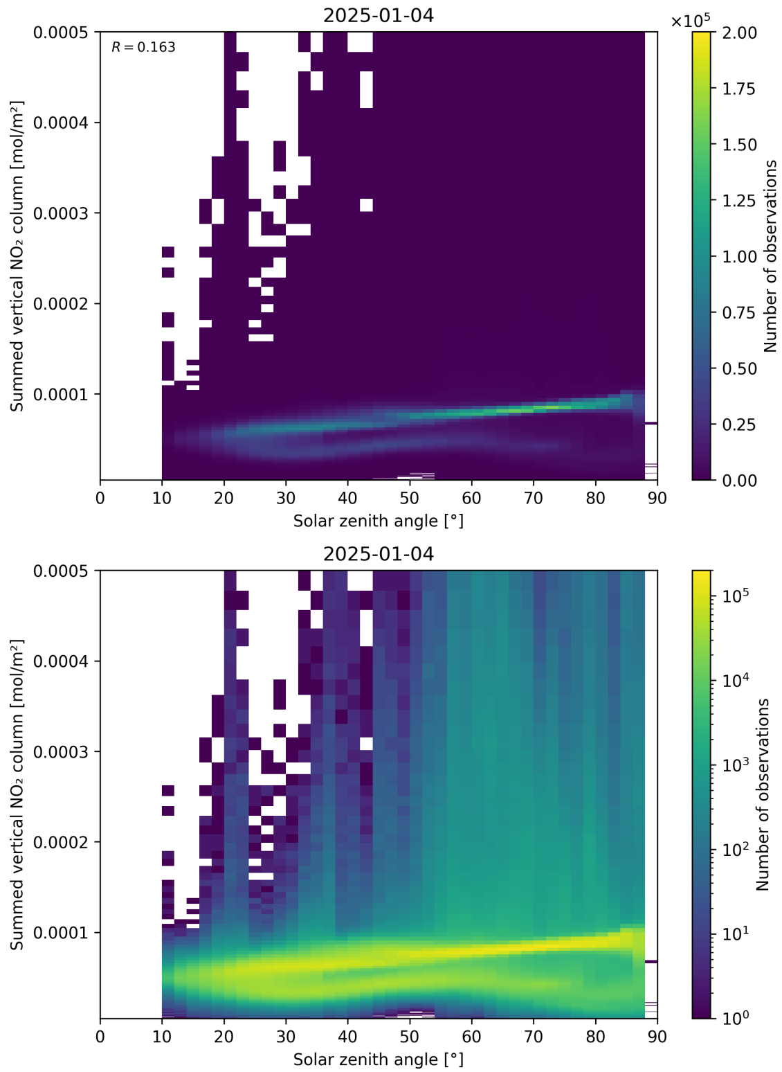
Figure 151: Scatter density plot of “Solar zenith angle” against “Summed vertical NO 2 column” for 2025-01-03 to 2025-01-05.
