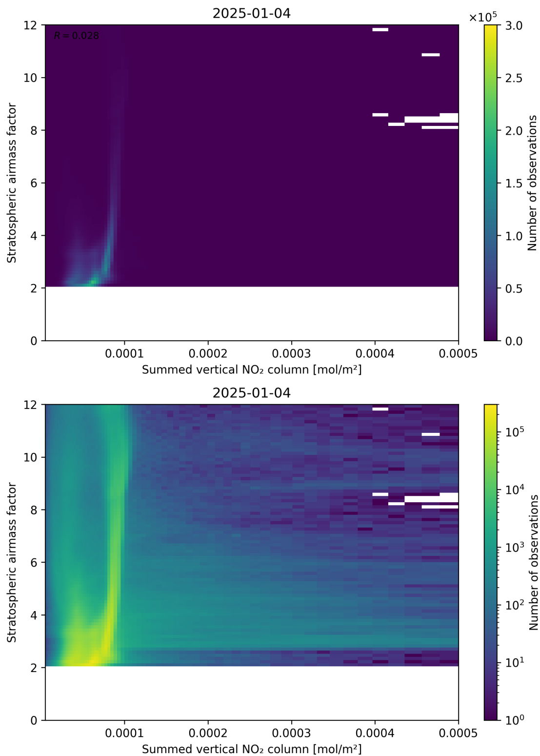
Figure 103: Scatter density plot of “Summed vertical NO 2 column” against “Stratospheric airmass factor” for 2025-01-03 to 2025-01-05.
