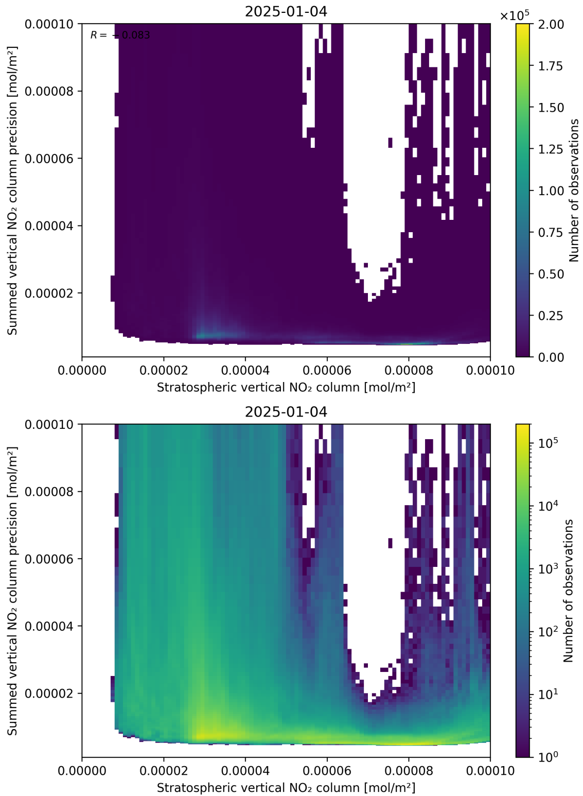
Figure 99: Scatter density plot of “Stratospheric vertical NO 2 column” against “Summed vertical NO 2 column precision” for 2025-01-03 to 2025-01-05.
