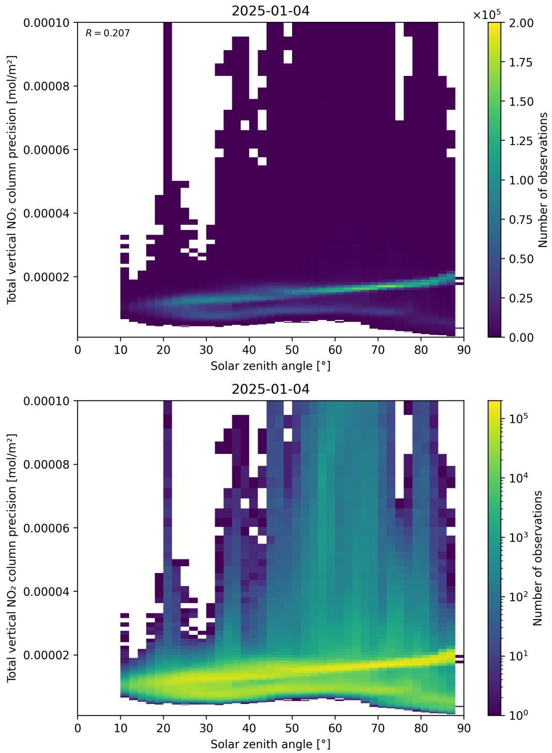
Figure 154: Scatter density plot of “Solar zenith angle” against “Total vertical NO 2 column precision” for 2025-01-03 to 2025-01-05.
