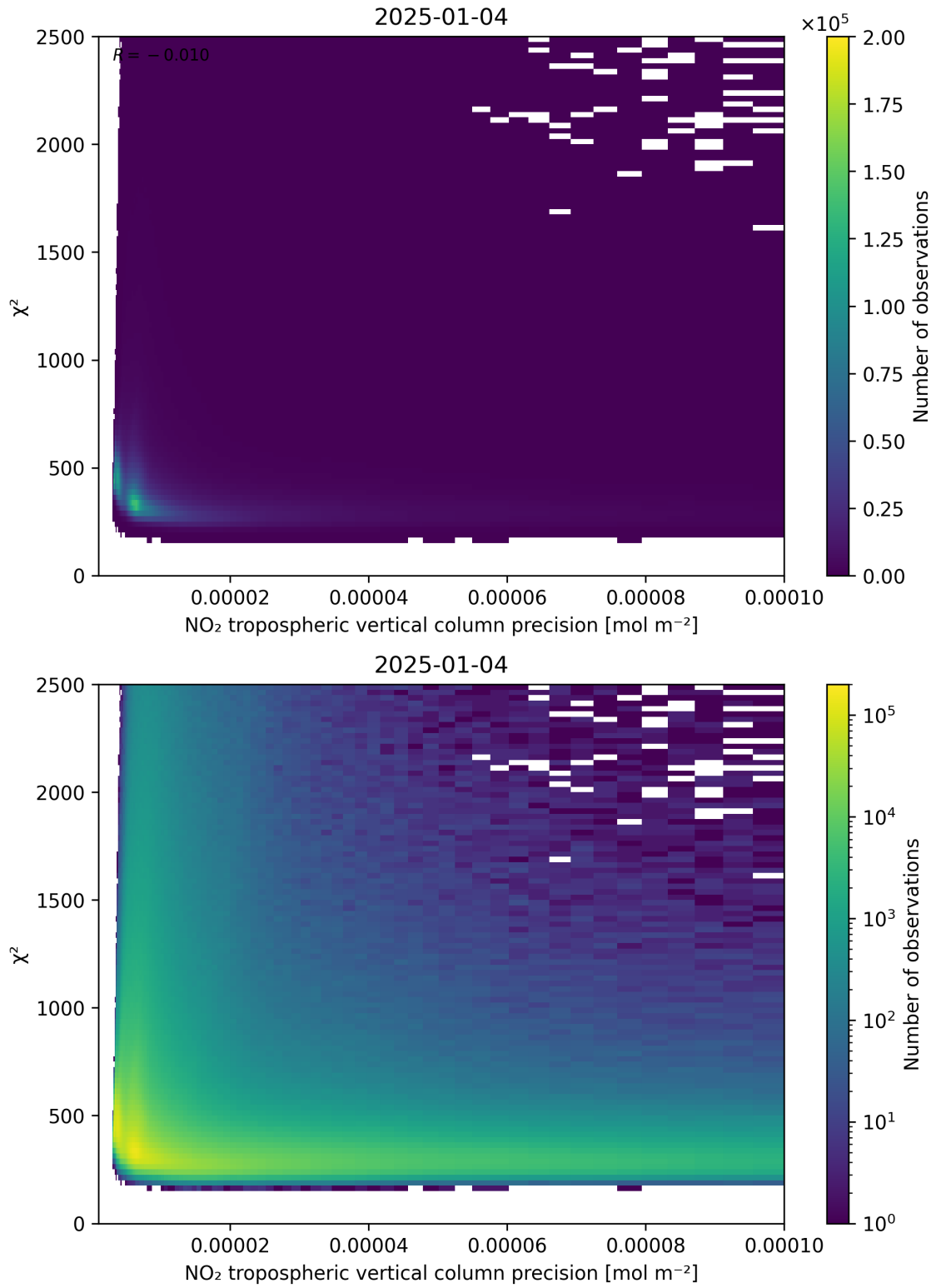
Figure 134: Scatter density plot of “NO 2 tropospheric vertical column precision” against “ \chi^2 ” for 2025-01-03 to 2025-01-05.
