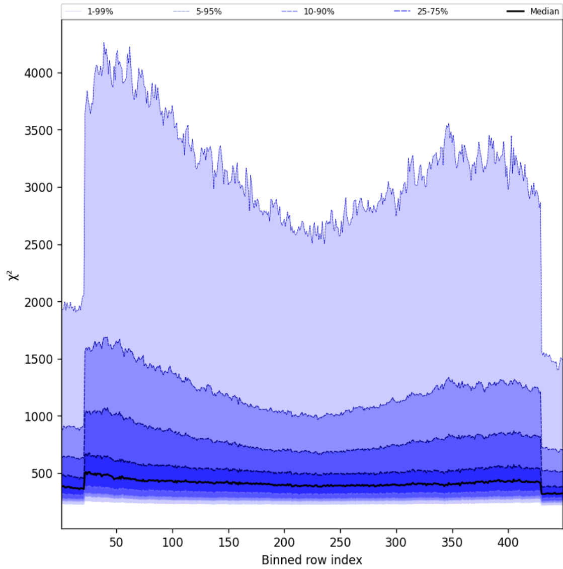
Figure 59: Along track statistics of “ \chi^2 ” for 2025-01-03 to 2025-01-05
