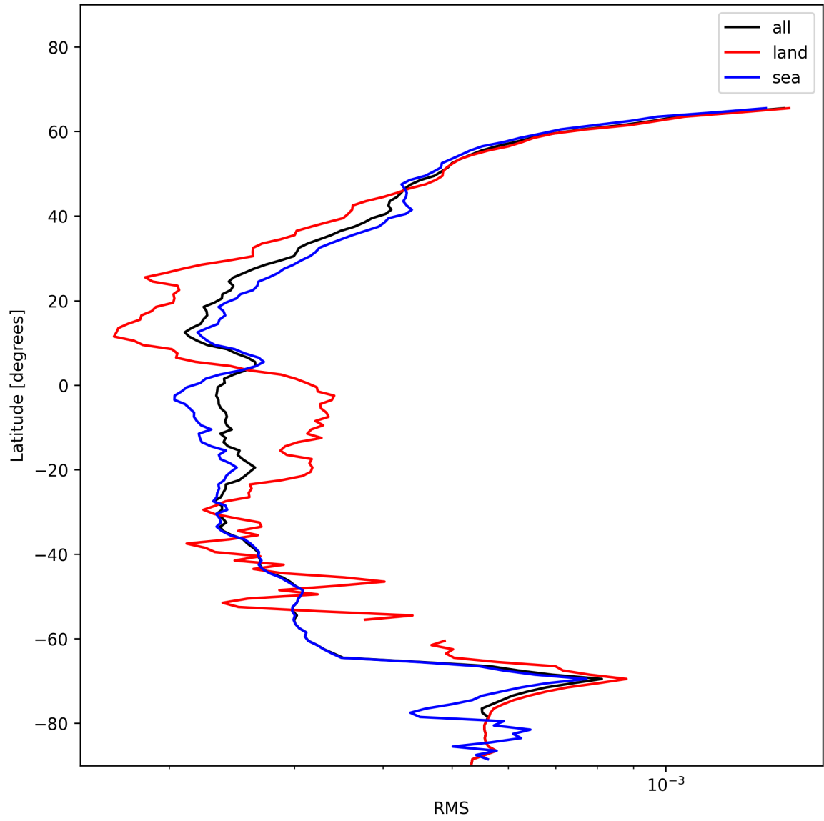
Figure 26: Zonal average of “RMS” for 2025-01-03 to 2025-01-05.
