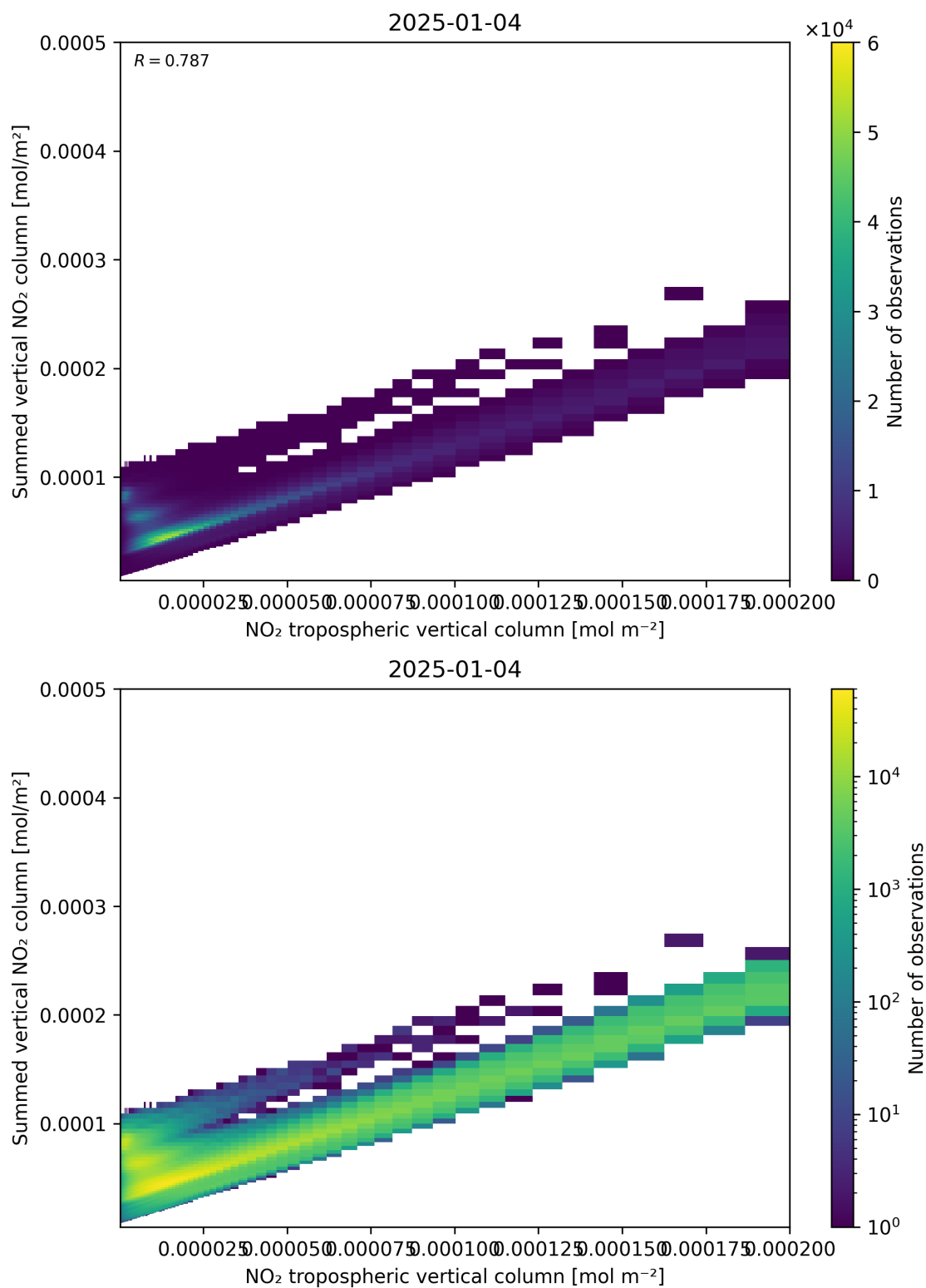
Figure 126: Scatter density plot of “NO 2 tropospheric vertical column” against “Summed vertical NO 2 column” for 2025-01-03 to 2025-01-05.
