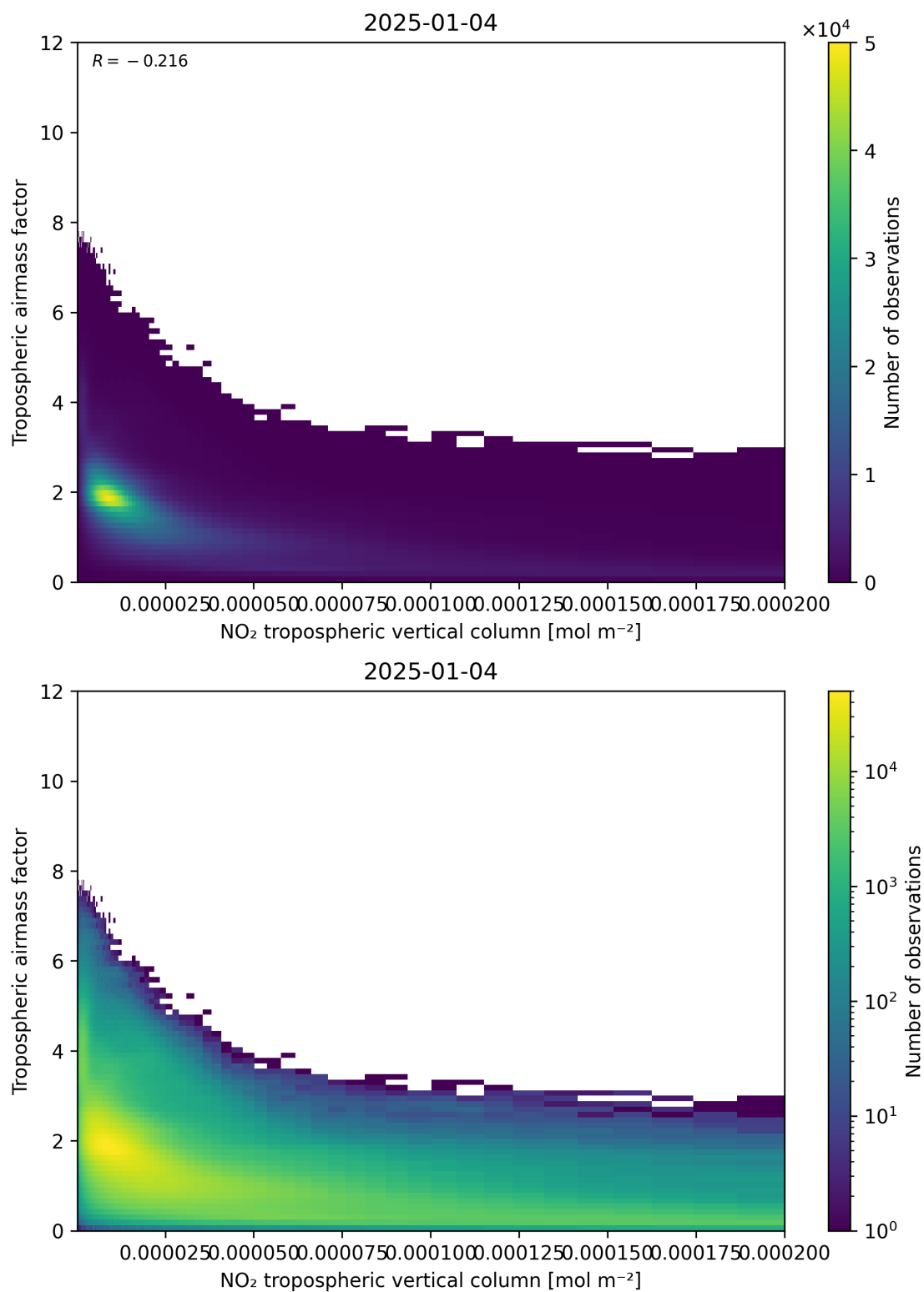
Figure 123: Scatter density plot of “NO 2 tropospheric vertical column” against “Tropospheric air mass factor” for 2025-01-03 to 2025-01-05.
