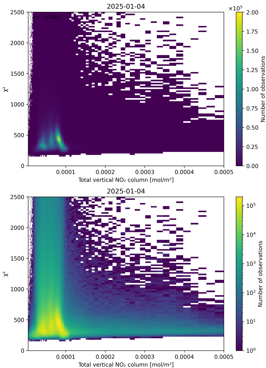
Figure 111: Scatter density plot of “Total vertical NO 2 column” against “ \chi^2 ” for 2025-01-03 to 2025-01-05.
