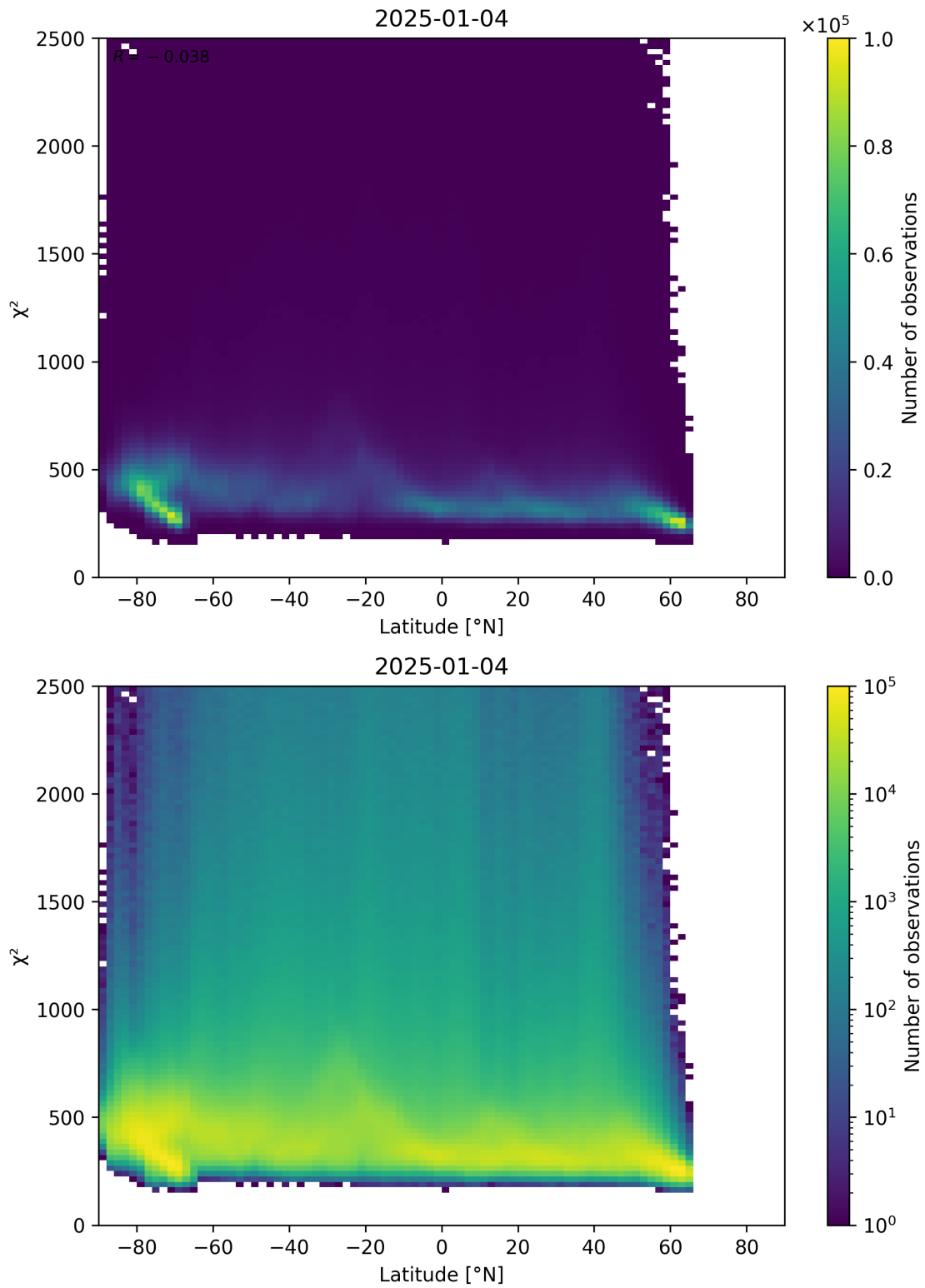
Figure 86: Scatter density plot of “Latitude” against “ \chi^2 ” for 2025-01-03 to 2025-01-05.
