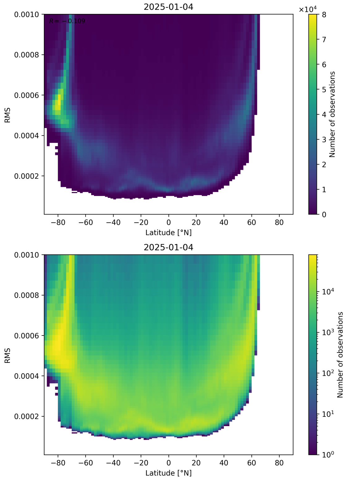
Figure 94: Scatter density plot of “Latitude” against “RMS” for 2025-01-03 to 2025-01-05.
