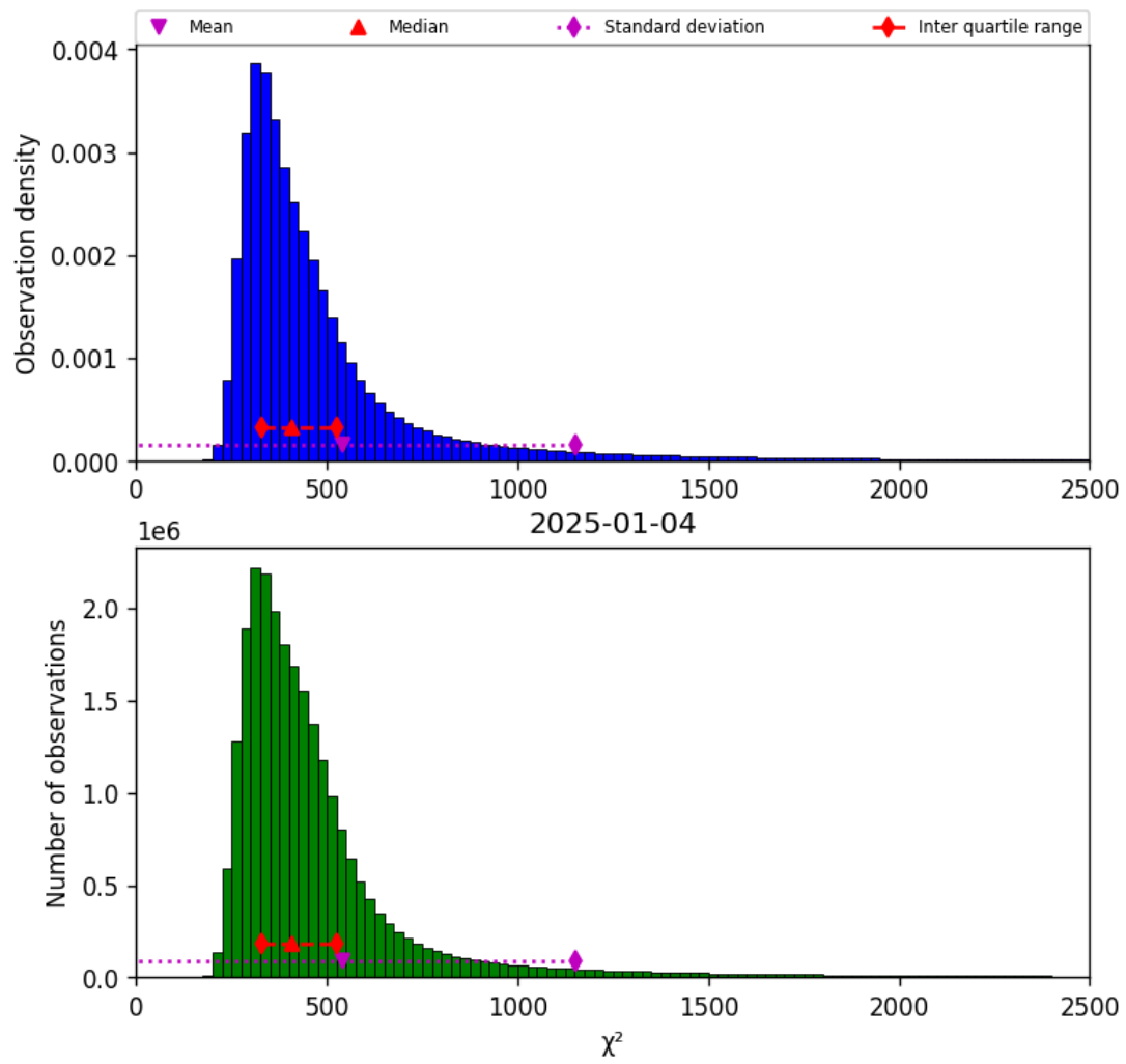
Figure 42: Histogram of “ \chi^2 ” for 2025-01-03 to 2025-01-05
