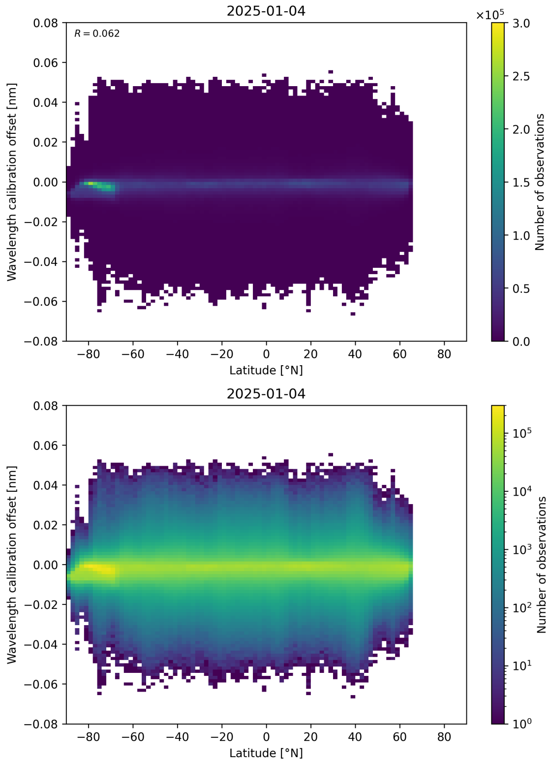
Figure 95: Scatter density plot of “Latitude” against “Wavelength calibration offset” for 2025-01-03 to 2025-01-05.
