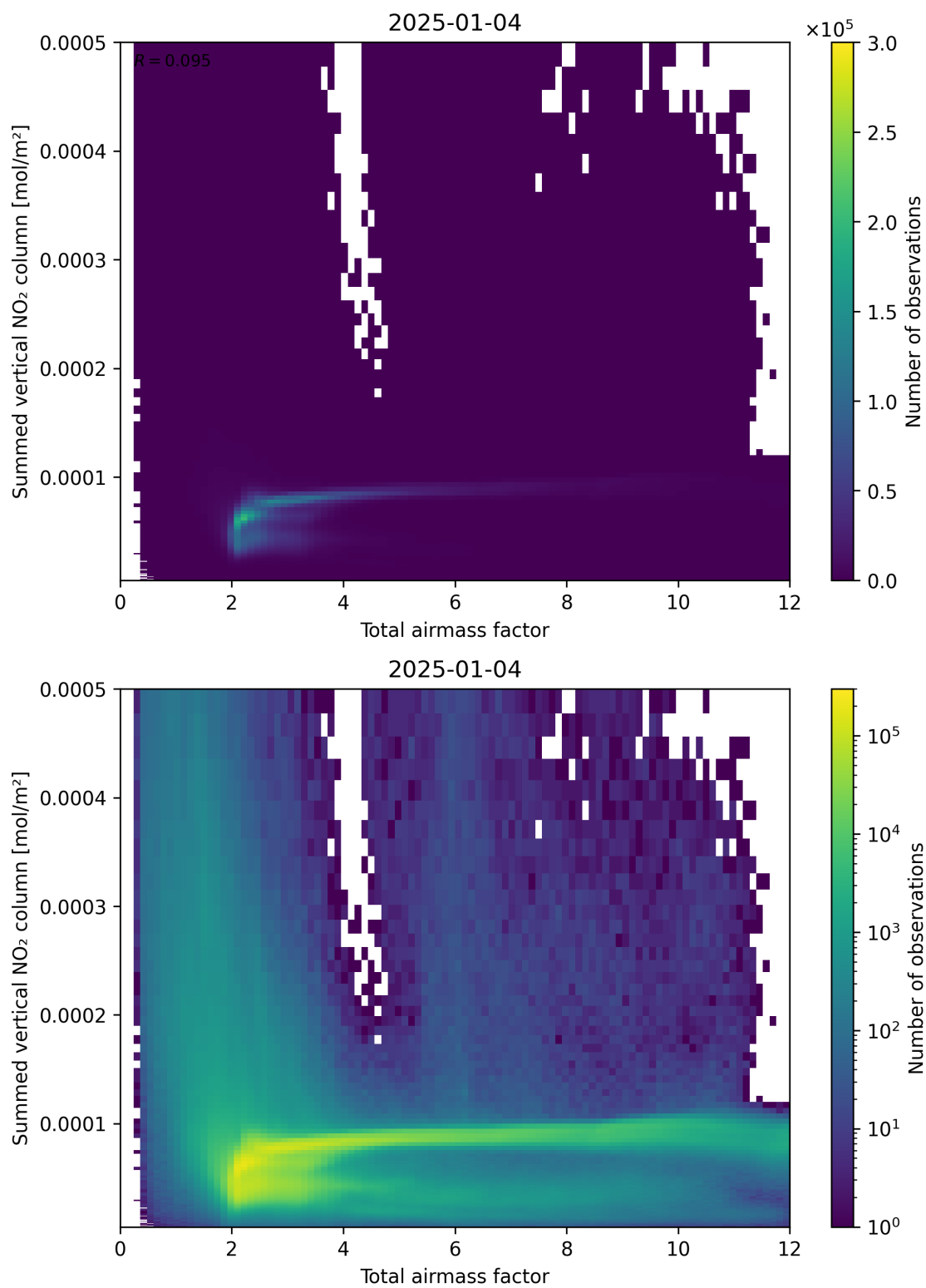
Figure 65: Scatter density plot of “Total airmass factor” against “Summed vertical NO 2 column” for 2025-01-03 to 2025-01-05.
