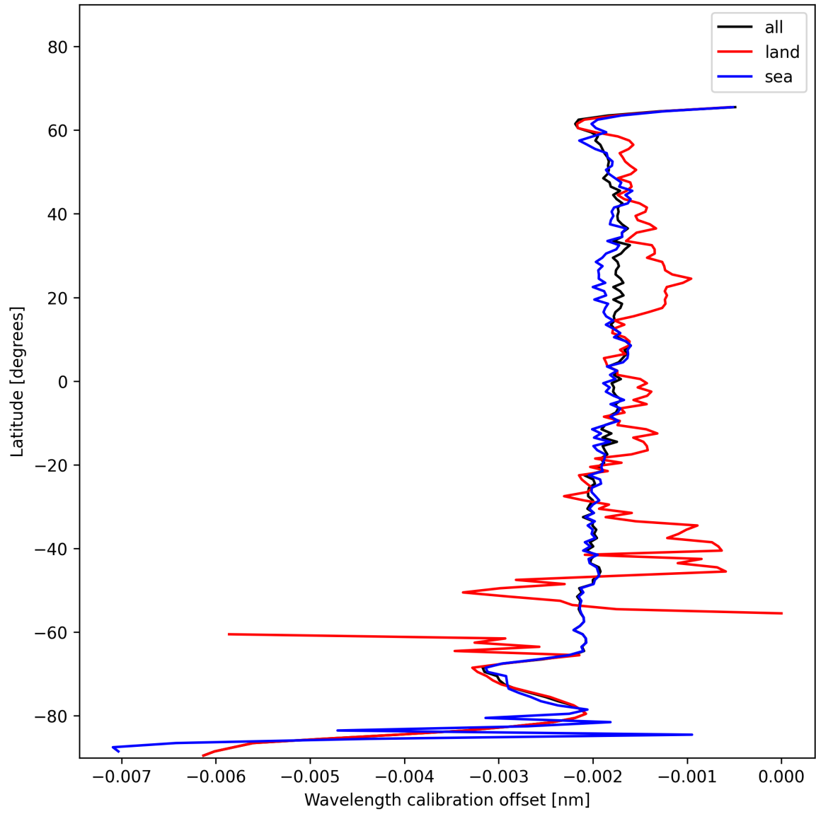
Figure 18: Zonal average of “Wavelength calibration offset” for 2025-01-03 to 2025-01-05.
