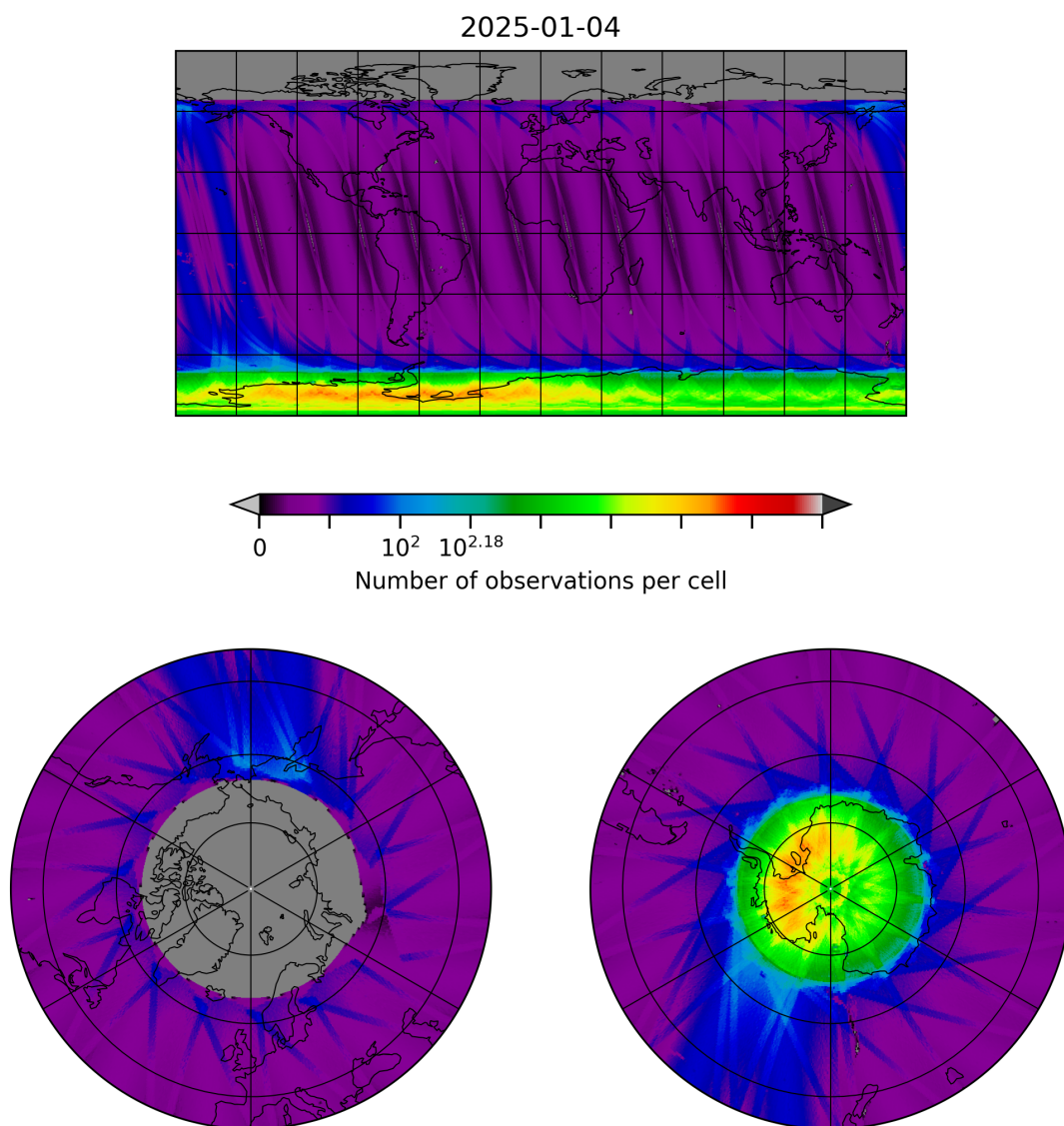
Figure 10: Map of the number of observations for 2025-01-03 to 2025-01-05
