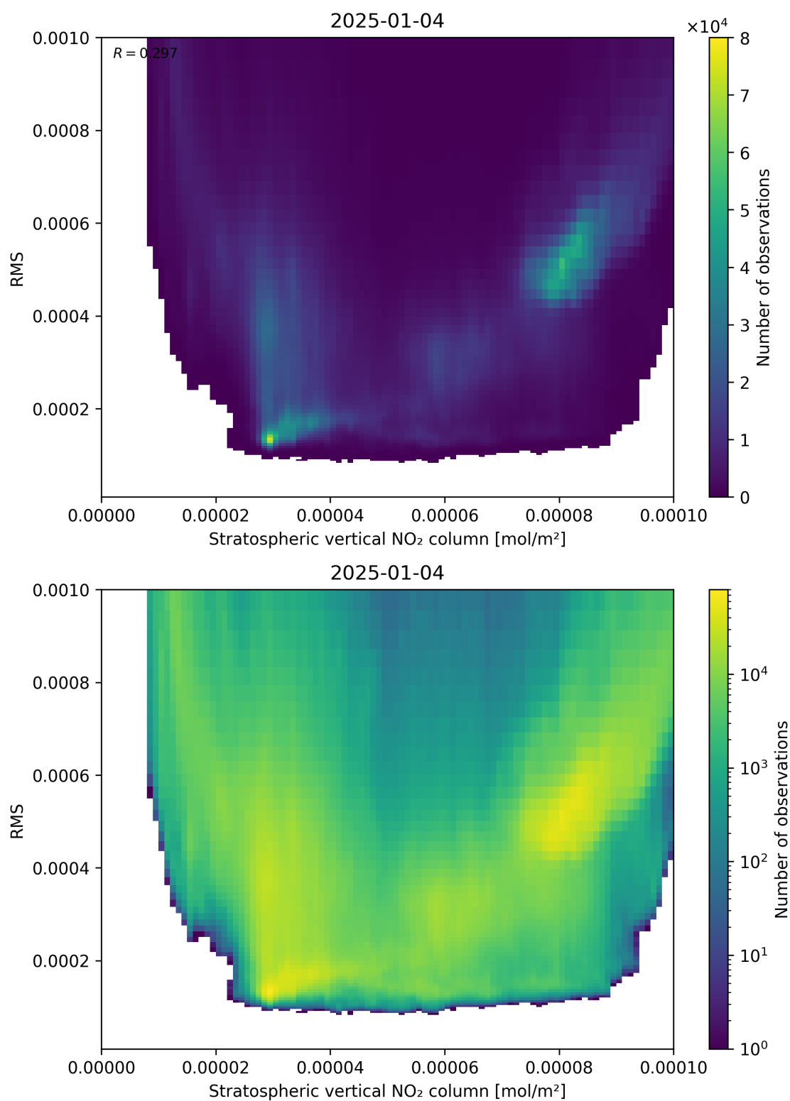
Figure 102: Scatter density plot of “Stratospheric vertical NO 2 column” against “RMS” for 2025-01-03 to 2025-01-05.
