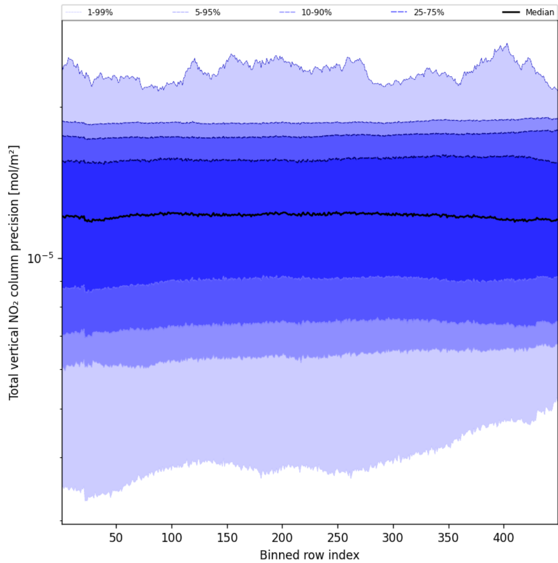
Figure 56: Along track statistics of “Total vertical NO 2 column precision” for 2025-01-03 to 2025-01-05
