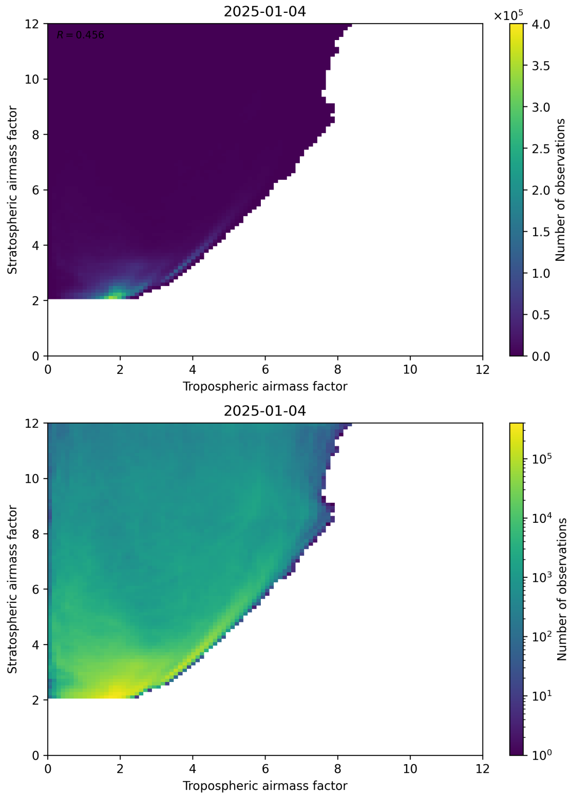
Figure 71: Scatter density plot of “Tropospheric airmass factor” against “Stratospheric airmass factor” for 2025-01-03 to 2025-01-05.
