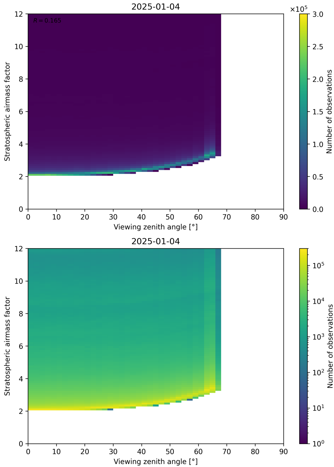
Figure 159: Scatter density plot of “Viewing zenith angle” against “Stratospheric airmass factor” for 2025-01-03 to 2025-01-05.
