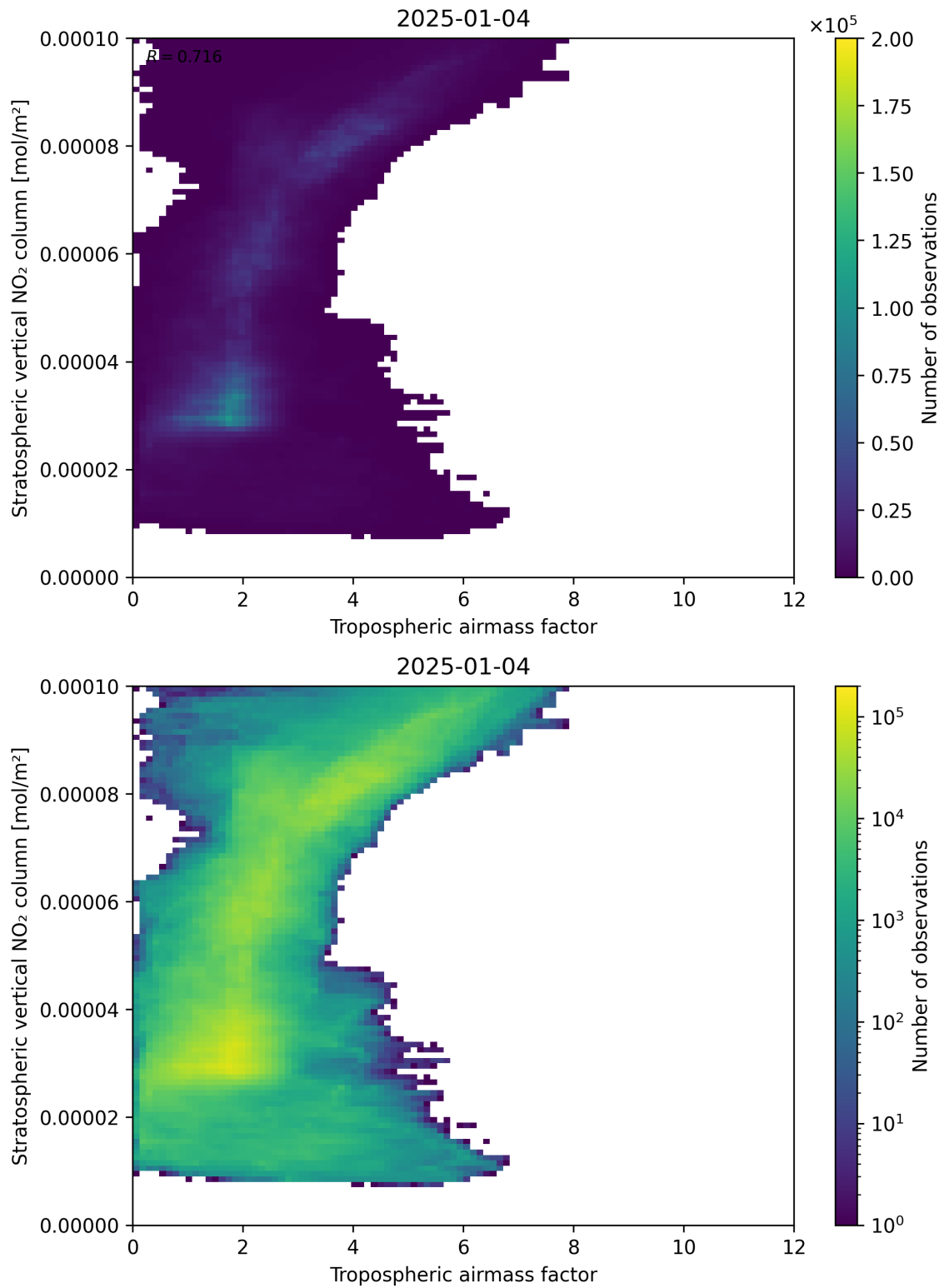
Figure 74: Scatter density plot of “Tropospheric air mass factor” against “Stratospheric vertical NO 2 column” for 2025-01-03 to 2025-01-05.
