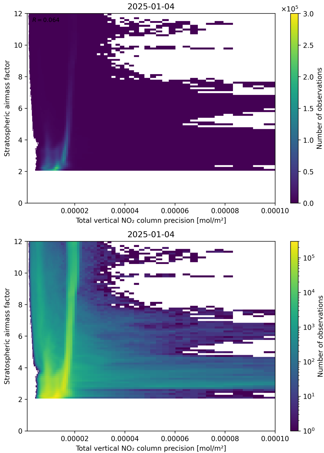
Figure 115: Scatter density plot of “Total vertical NO 2 column precision” against “Stratospheric air mass factor” for 2025-01-03 to 2025-01-05.
