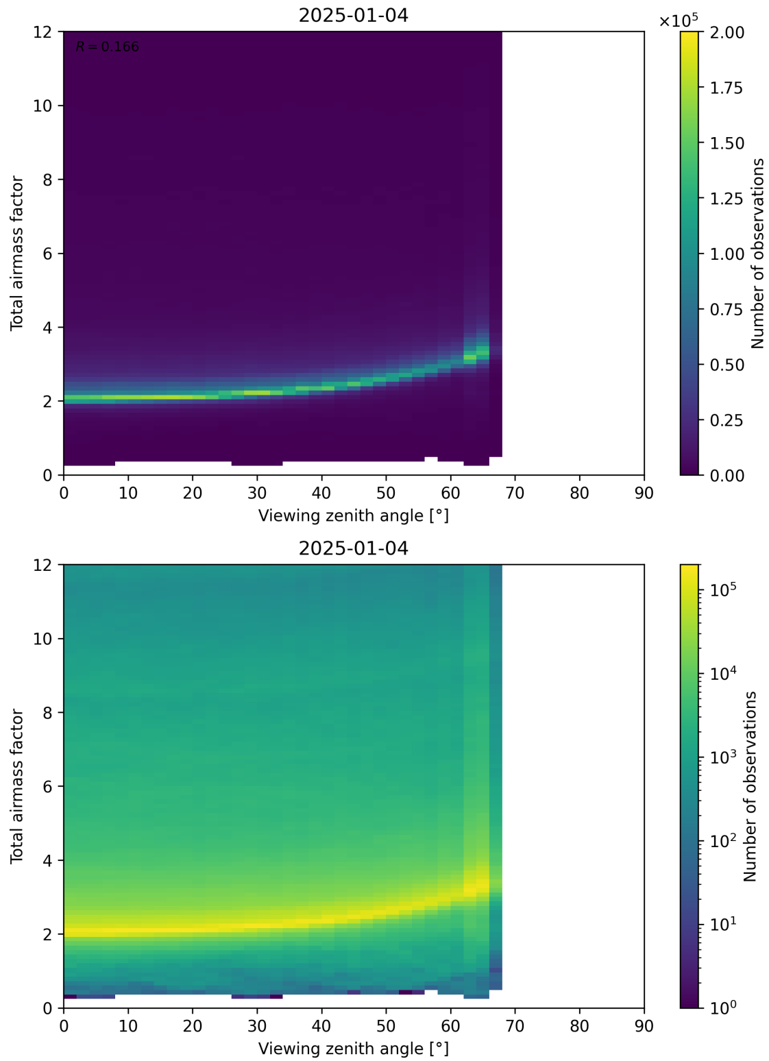
Figure 160: Scatter density plot of “Viewing zenith angle” against “Total airmass factor” for 2025-01-03 to 2025-01-05.
