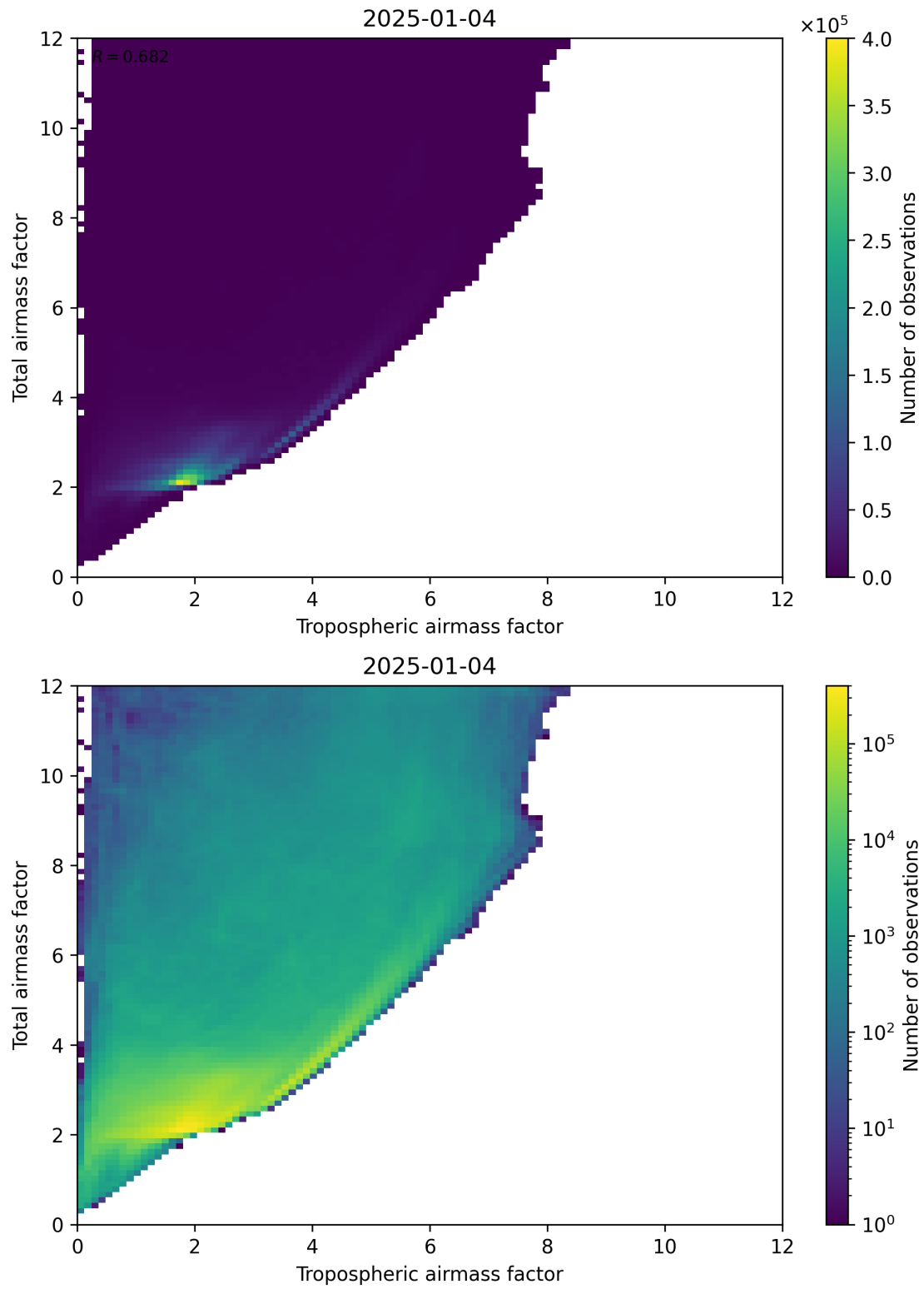
Figure 72: Scatter density plot of “Tropospheric airmass factor” against “Total airmass factor” for 2025-01-03 to 2025-01-05.
