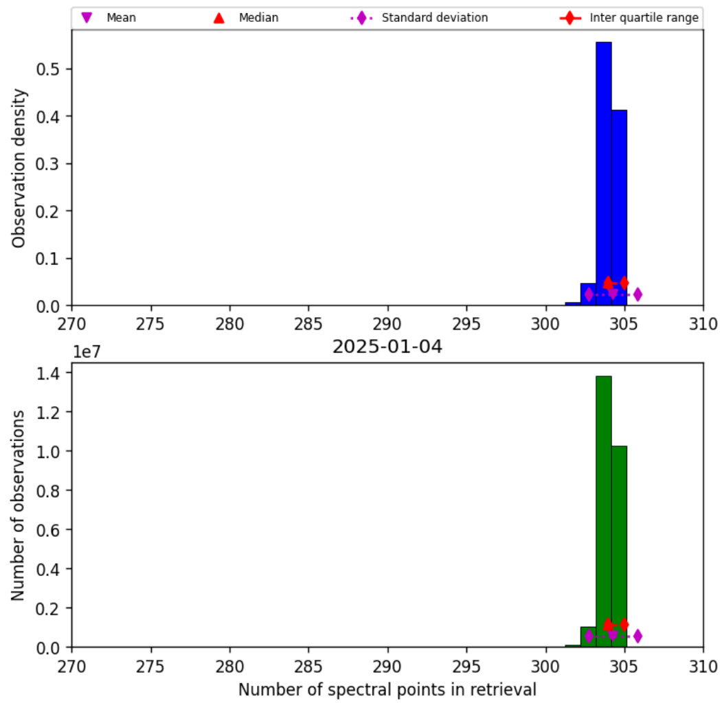
Figure 33: Histogram of “Number of spectral points in retrieval” for 2025-01-03 to 2025-01-05
