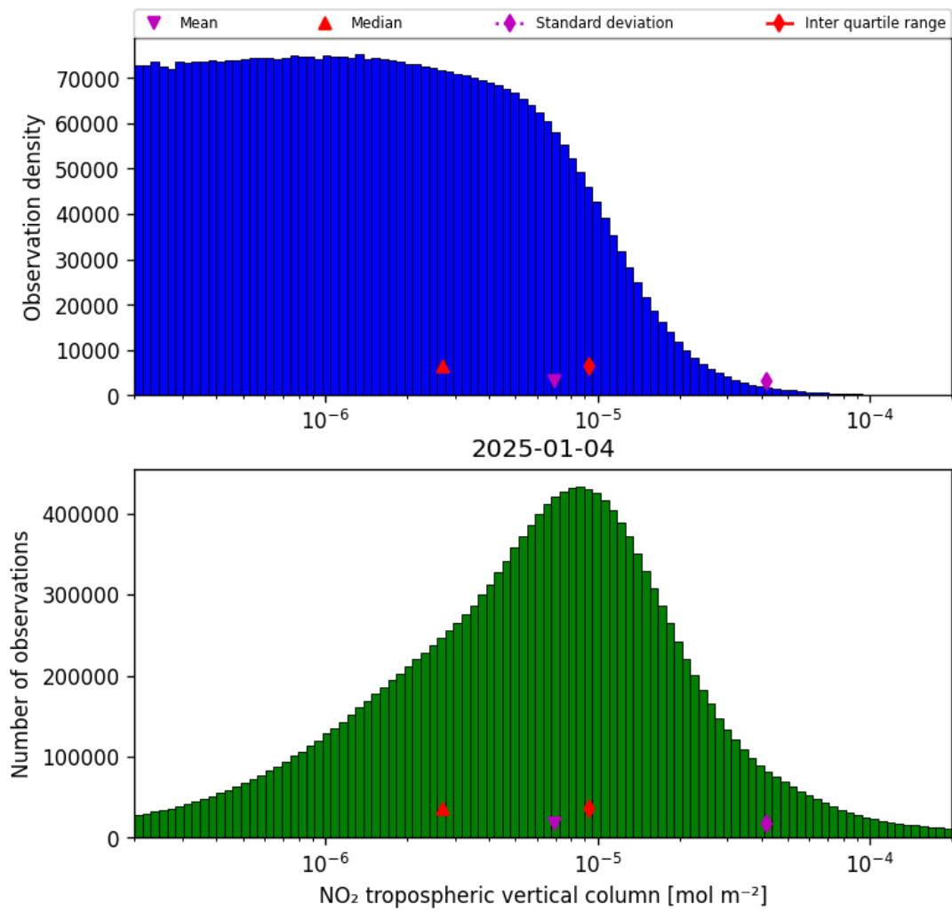
Figure 29: Histogram of “NO 2 tropospheric vertical column” for 2025-01-03 to 2025-01-05
