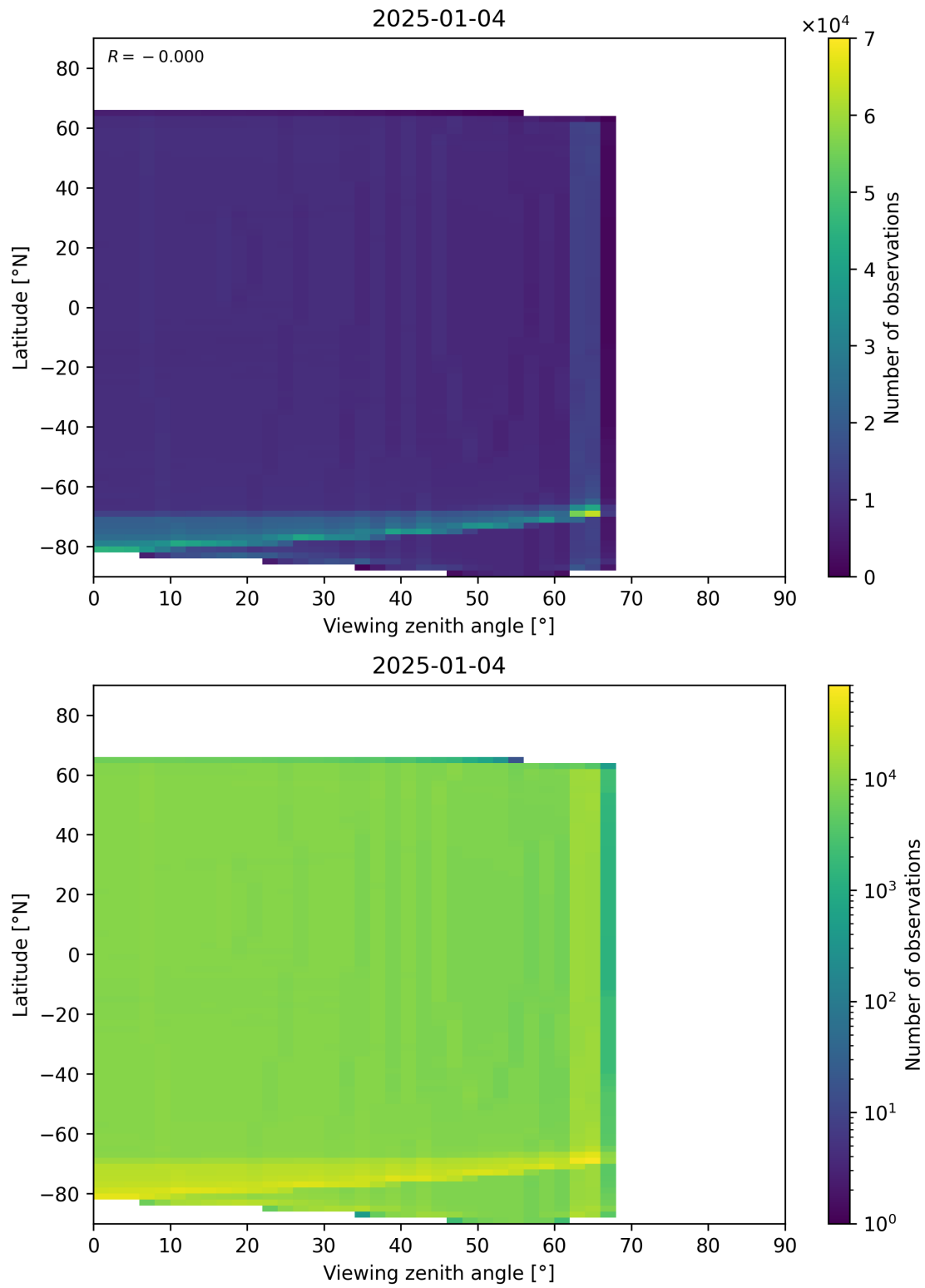
Figure 163: Scatter density plot of “Viewing zenith angle” against “Latitude” for 2025-01-03 to 2025-01-05.
