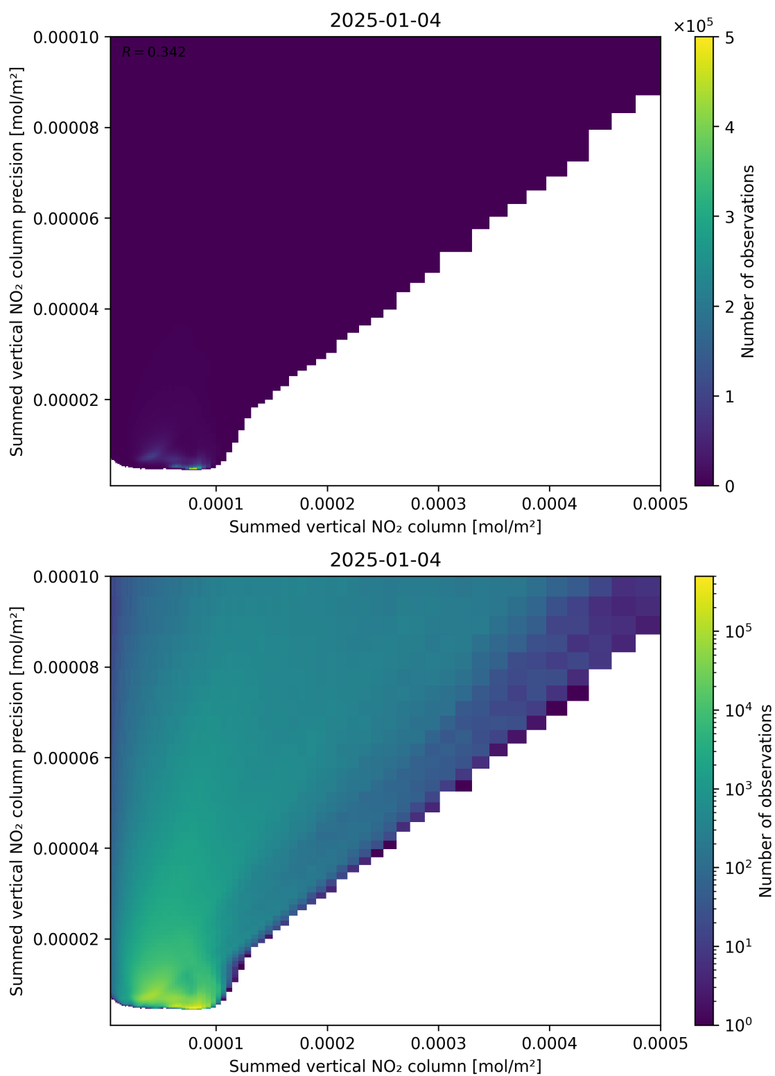
Figure 105: Scatter density plot of “Summed vertical NO 2 column” against “Summed vertical NO 2 column precision” for 2025-01-03 to 2025-01-05.
