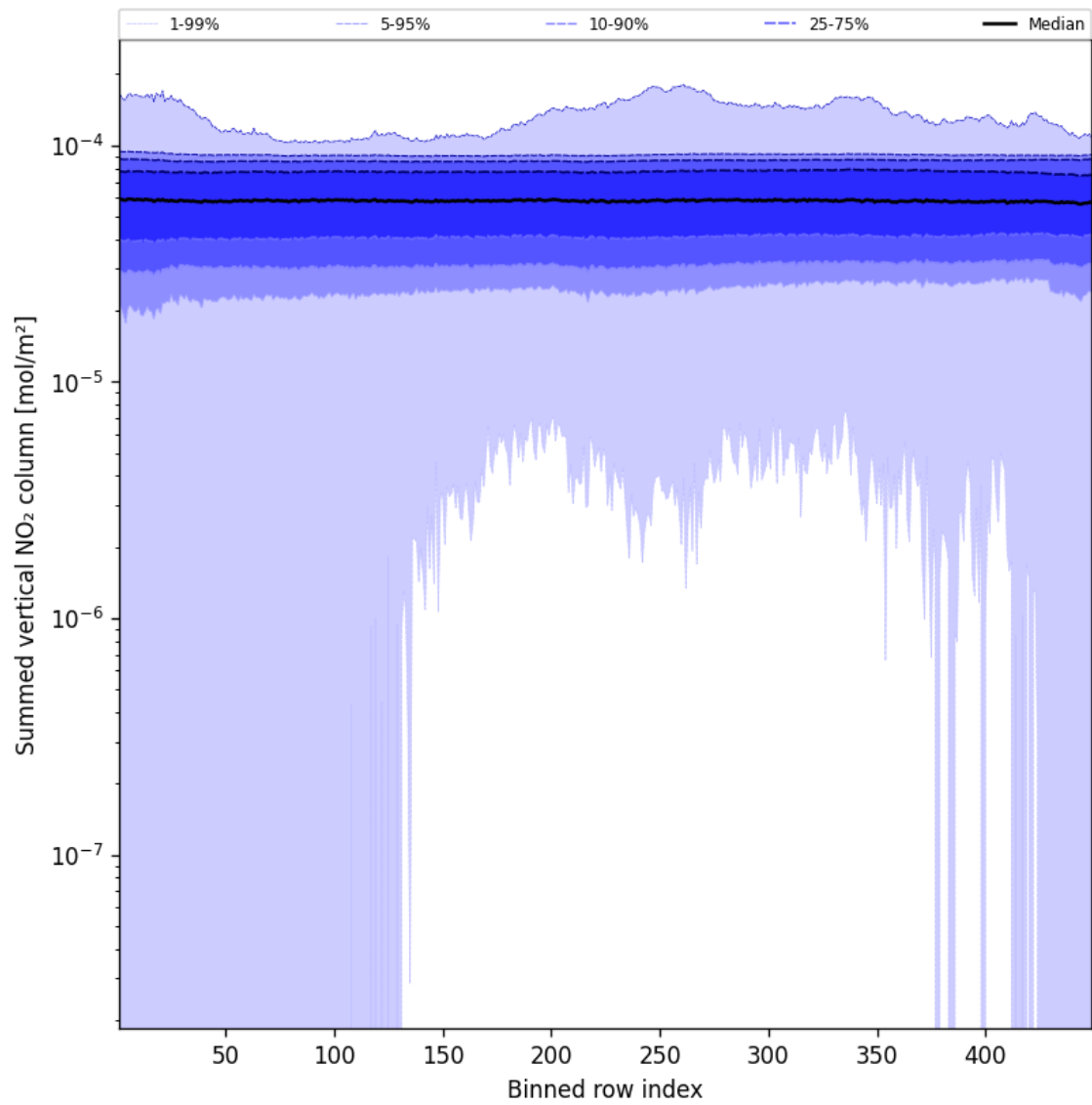
Figure 57: Along track statistics of “Summed vertical NO 2 column” for 2025-01-03 to 2025-01-05
