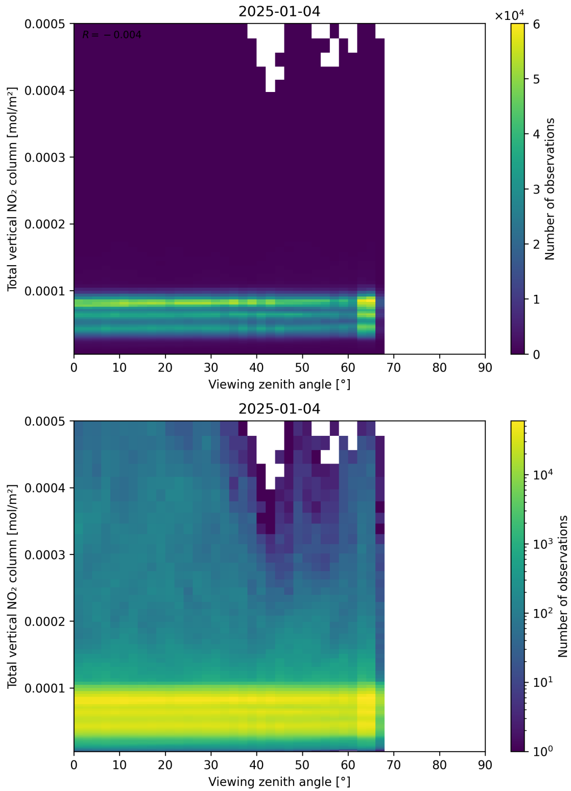
Figure 167: Scatter density plot of “Viewing zenith angle” against “Total vertical NO 2 column” for 2025-01-03 to 2025-01-05.
