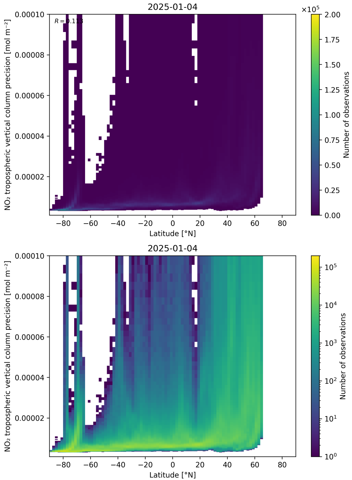
Figure 93: Scatter density plot of “Latitude” against “NO 2 tropospheric vertical column precision” for 2025-01-03 to 2025-01-05.
