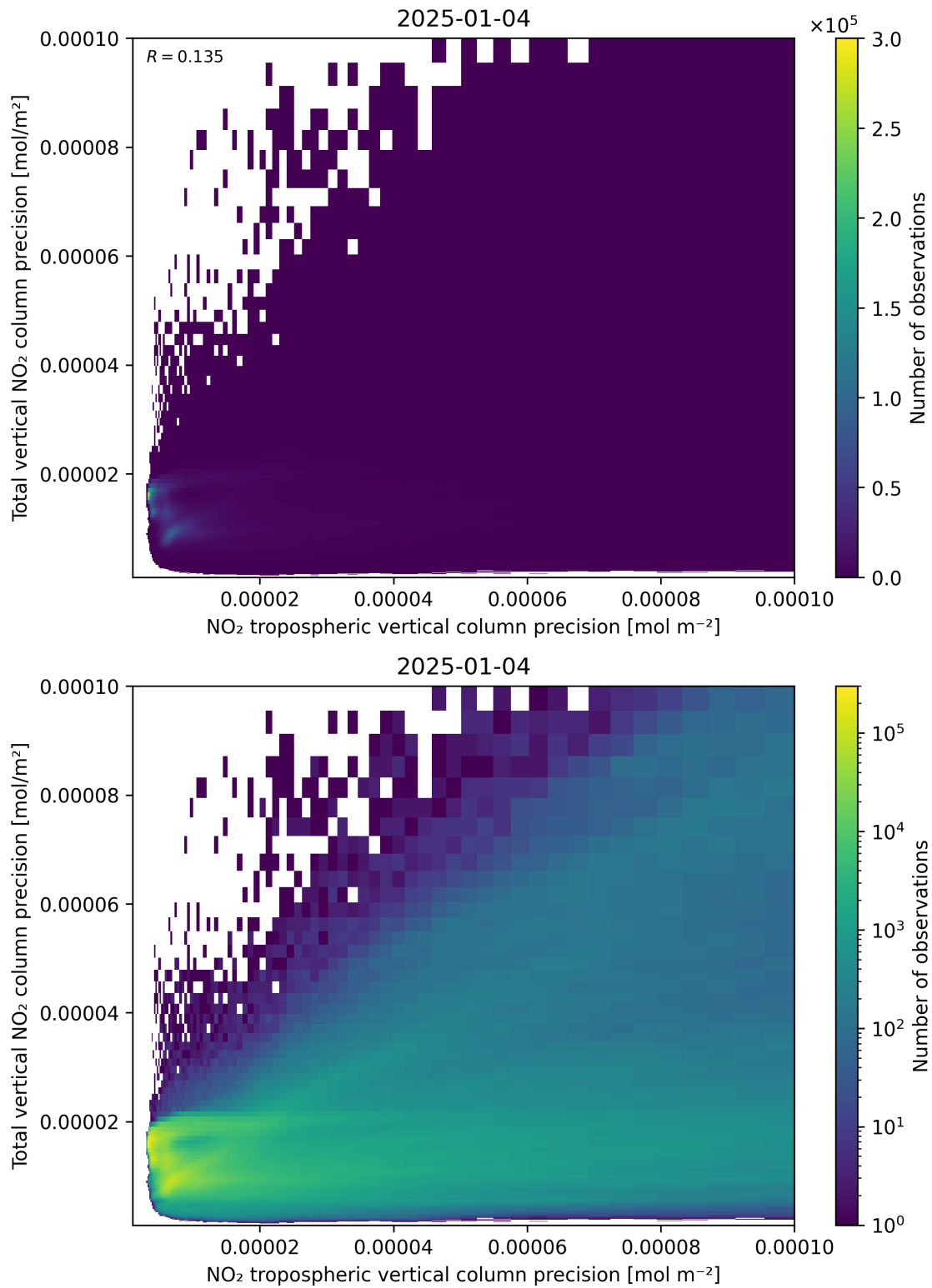
Figure 139: Scatter density plot of “NO 2 tropospheric vertical column precision” against “Total vertical NO 2 column precision” for 2025-01-03 to 2025-01-05.
