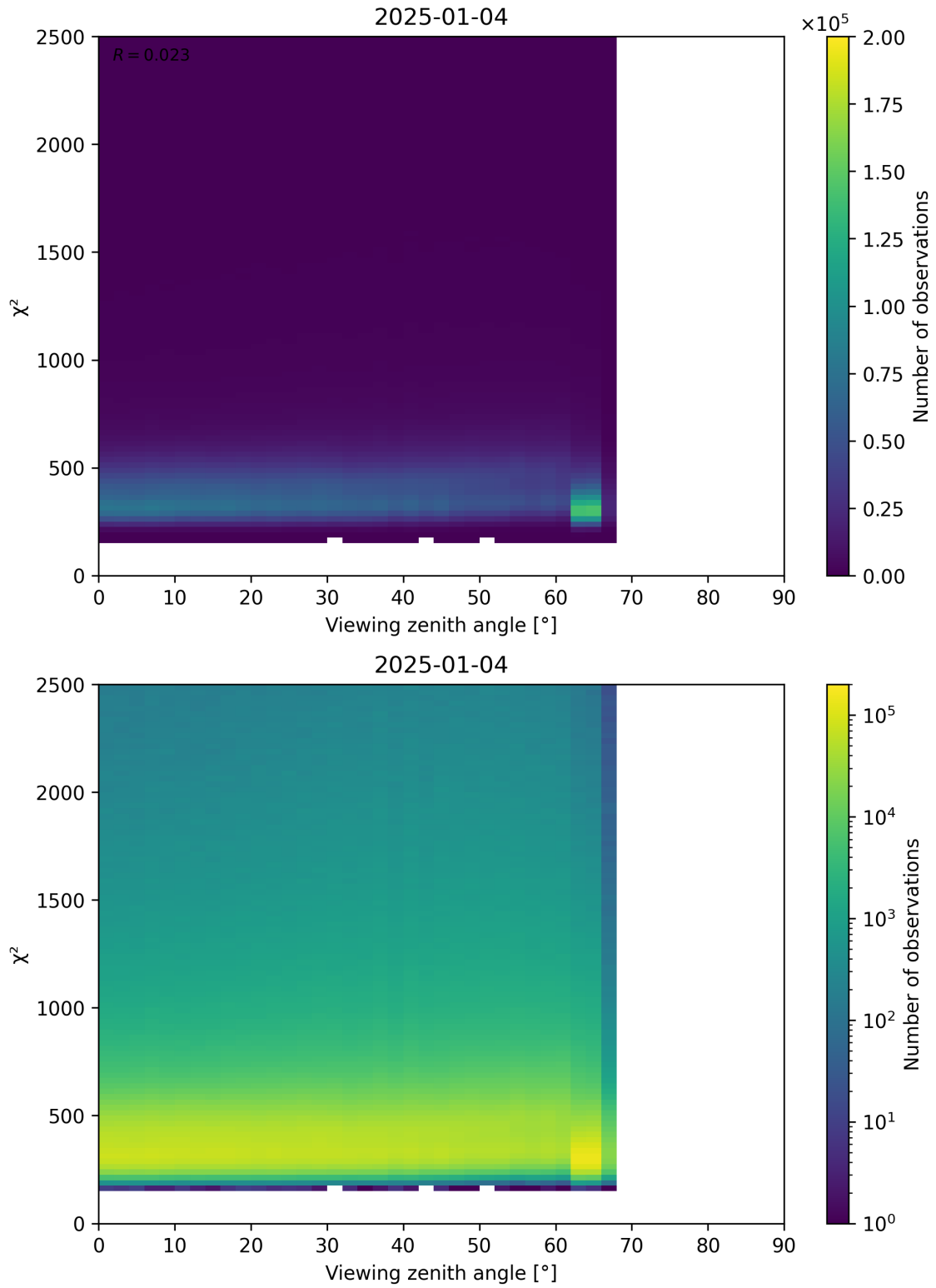
Figure 162: Scatter density plot of “Viewing zenith angle” against “ \chi^2 ” for 2025-01-03 to 2025-01-05.
