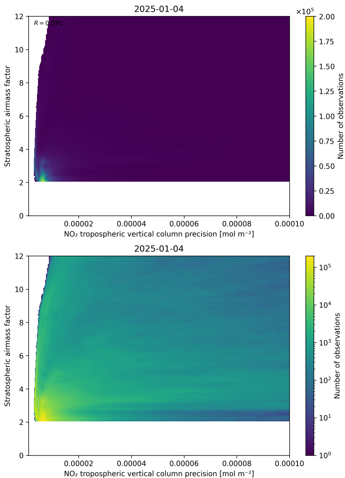
Figure 131: Scatter density plot of “NO 2 tropospheric vertical column precision” against “Stratospheric airmass factor” for 2025-01-03 to 2025-01-05.
