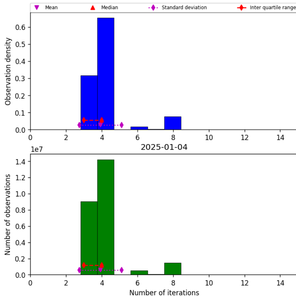
Figure 34: Histogram of “Number of iterations” for 2025-01-03 to 2025-01-05
