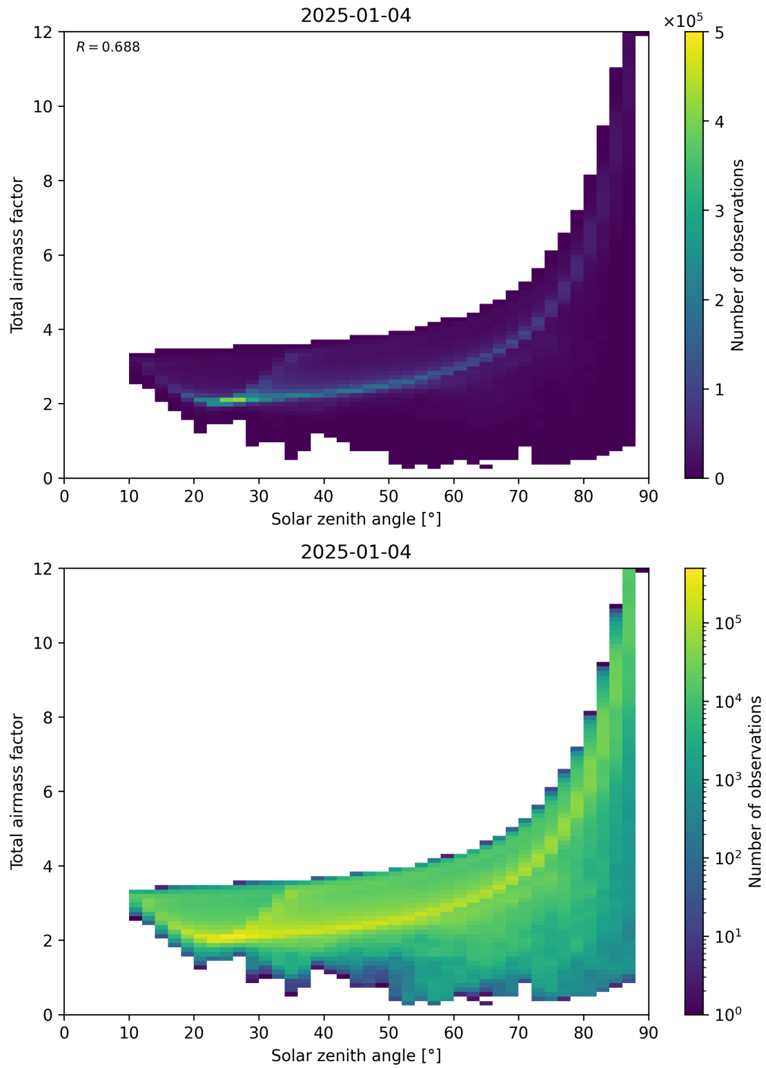
Figure 146: Scatter density plot of “Solar zenith angle” against “Total airmass factor” for 2025-01-03 to 2025-01-05.
