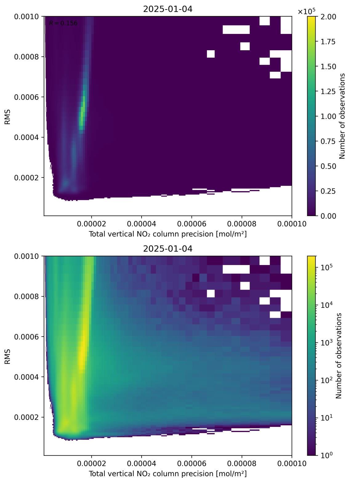
Figure 119: Scatter density plot of “Total vertical NO 2 column precision” against “RMS” for 2025-01-03 to 2025-01-05.
