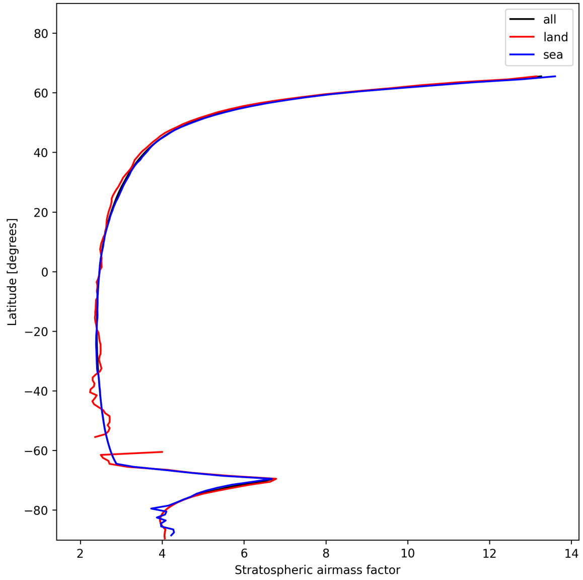
Figure 27: Zonal average of “Stratospheric airmass factor” for 2025-01-03 to 2025-01-05.
