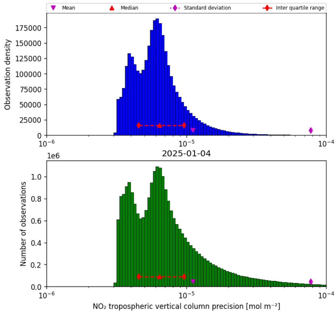
Figure 30: Histogram of “NO 2 tropospheric vertical column precision” for 2025-01-03 to 2025-01-05
