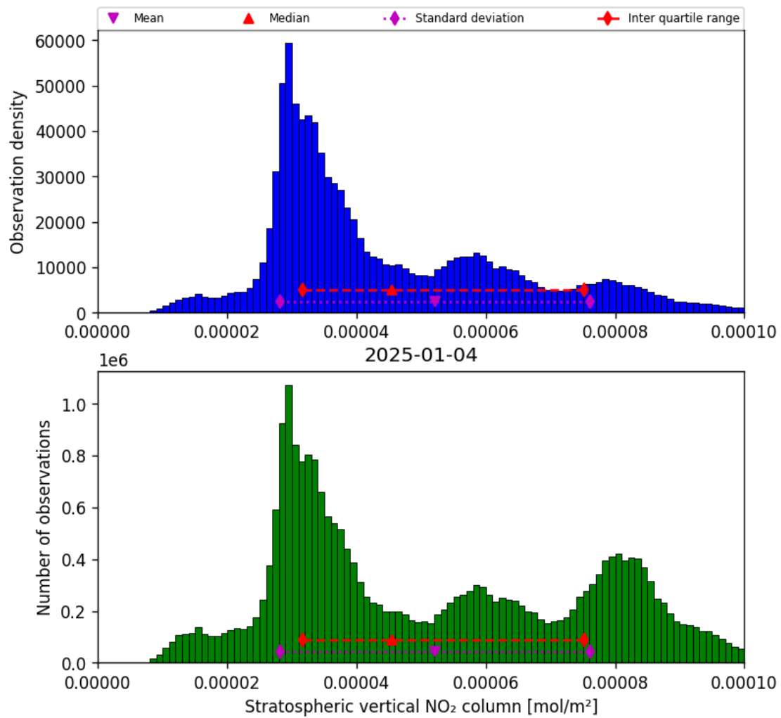
Figure 36: Histogram of “Stratospheric vertical NO 2 column” for 2025-01-03 to 2025-01-05
