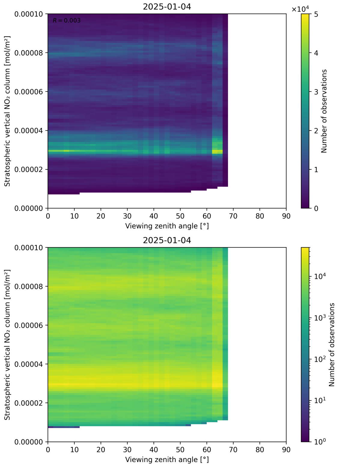
Figure 164: Scatter density plot of “Viewing zenith angle” against “Stratospheric vertical NO 2 column” for 2025-01-03 to 2025-01-05.
