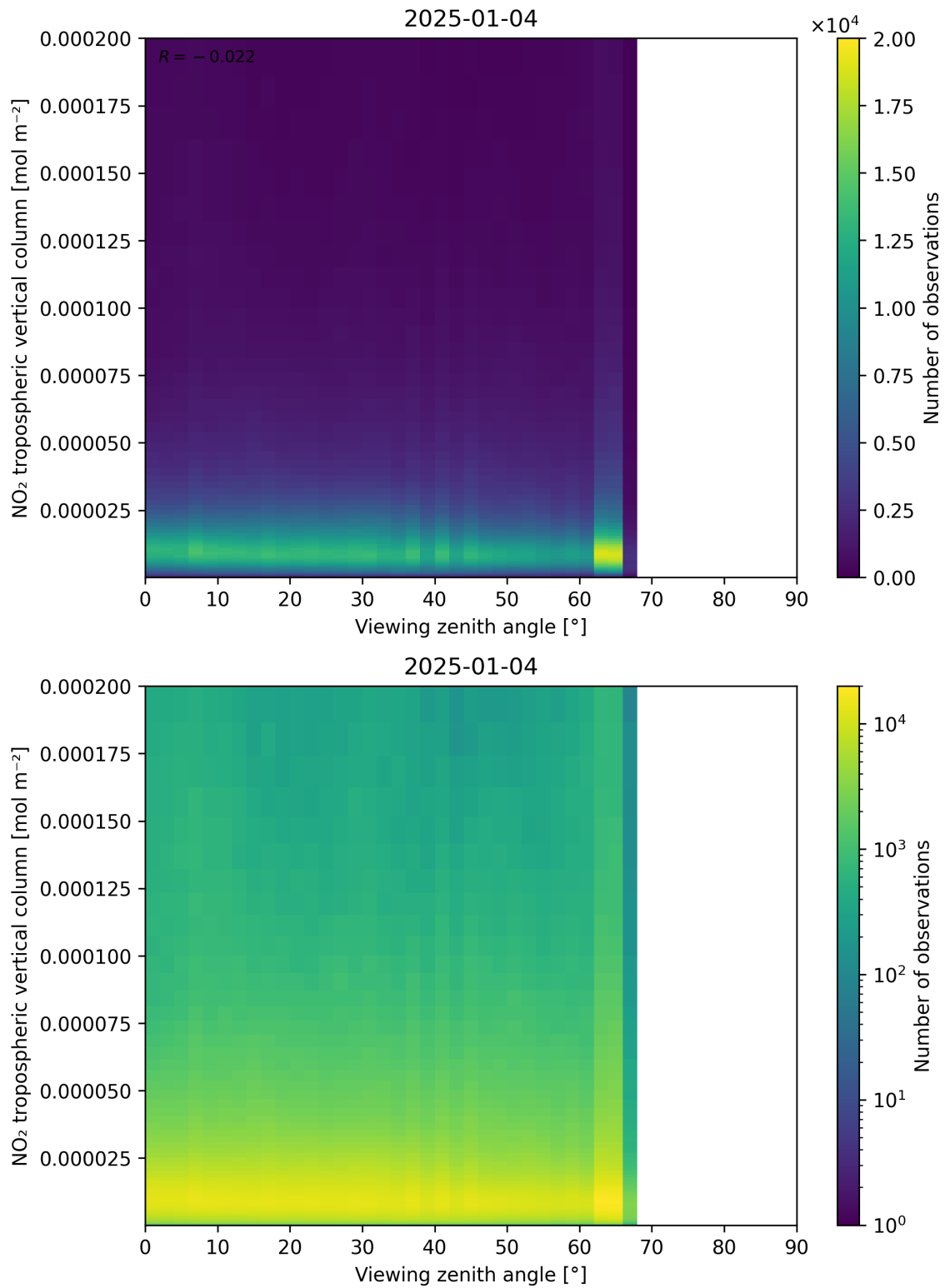
Figure 169: Scatter density plot of “Viewing zenith angle” against “NO 2 tropospheric vertical column” for 2025-01-03 to 2025-01-05.
