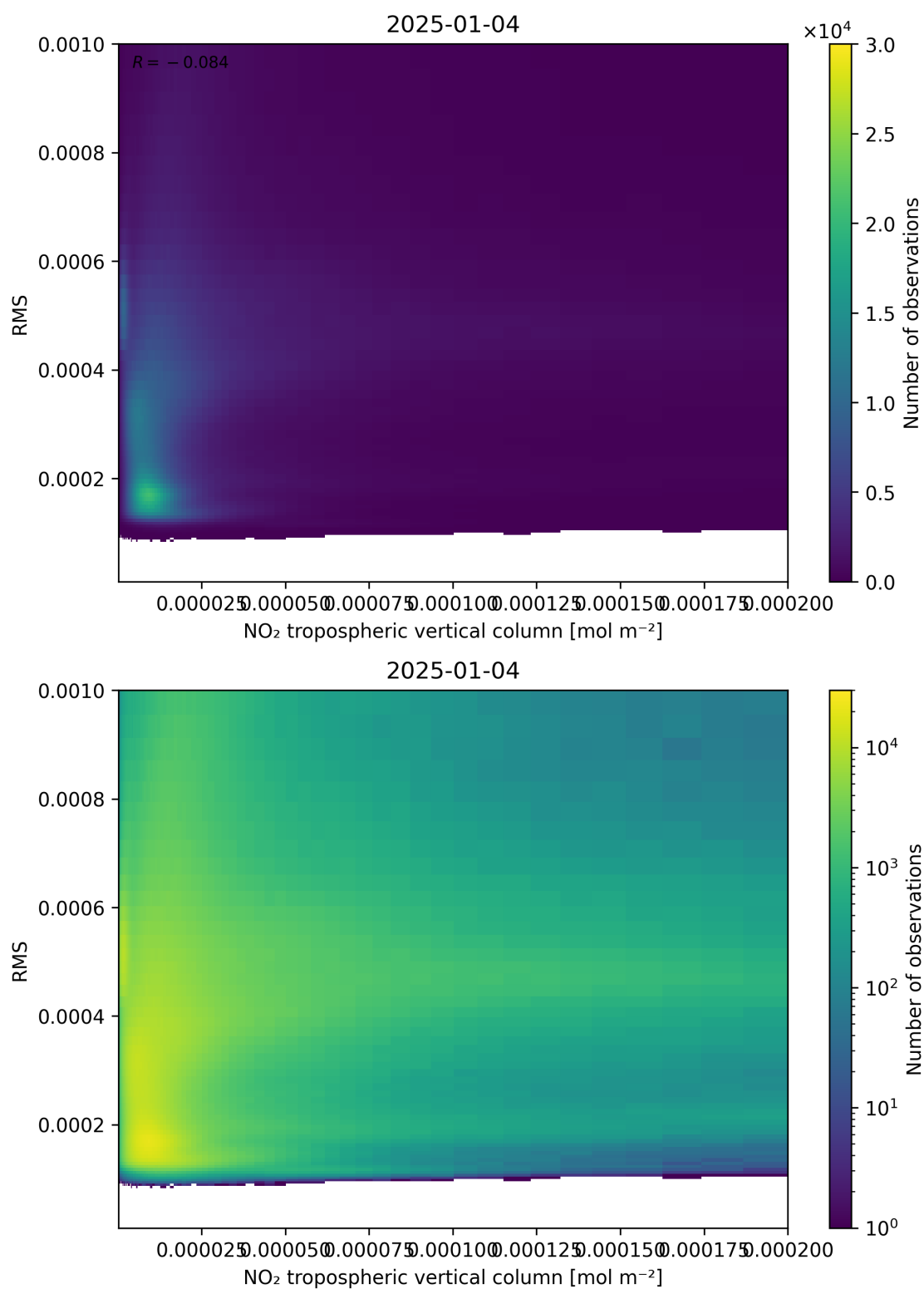
Figure 142: Scatter density plot of “NO 2 tropospheric vertical column” against “RMS” for 2025-01-03 to 2025-01-05.
