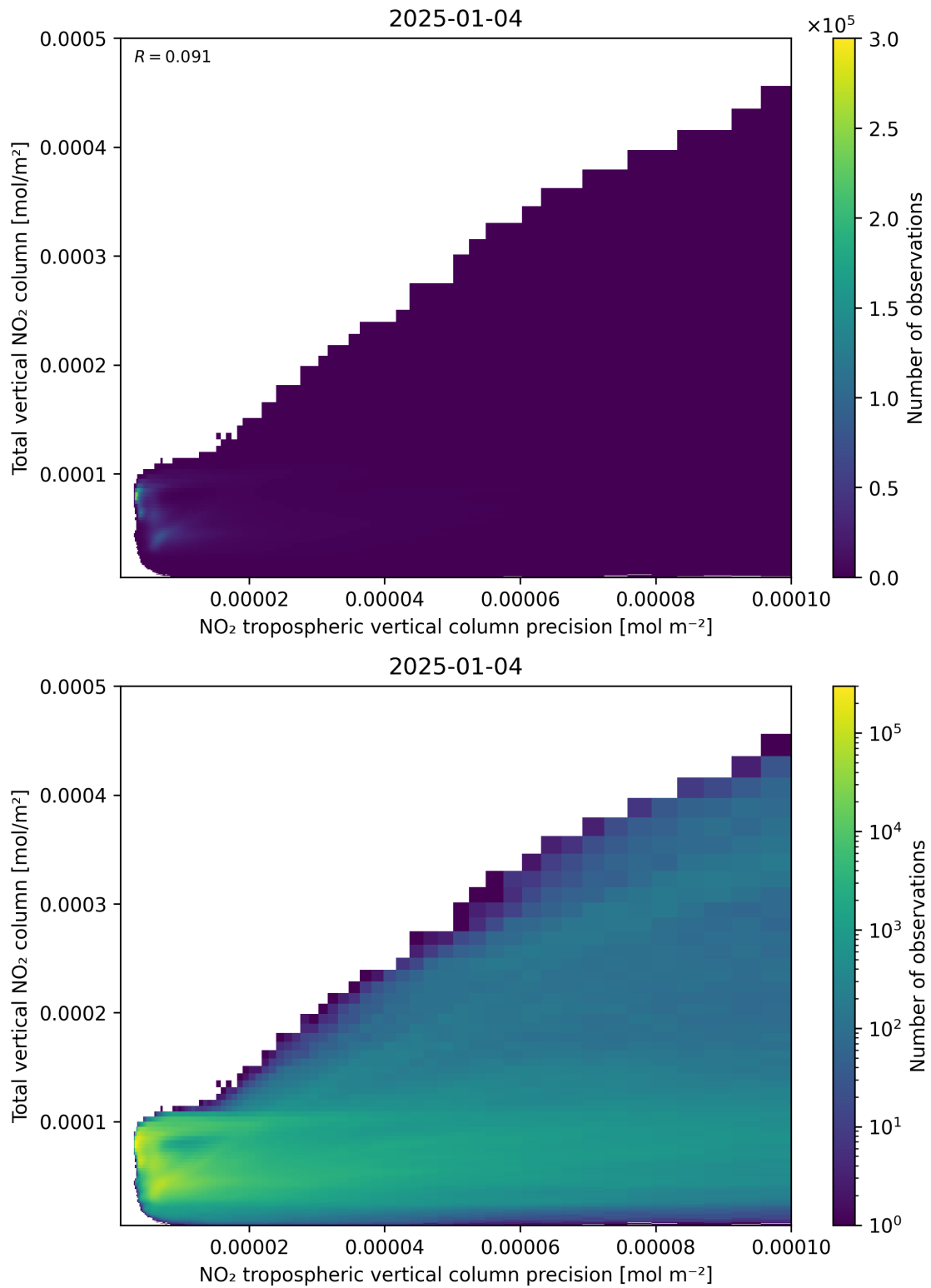
Figure 138: Scatter density plot of “NO 2 tropospheric vertical column precision” against “Total vertical NO 2 column” for 2025-01-03 to 2025-01-05.
