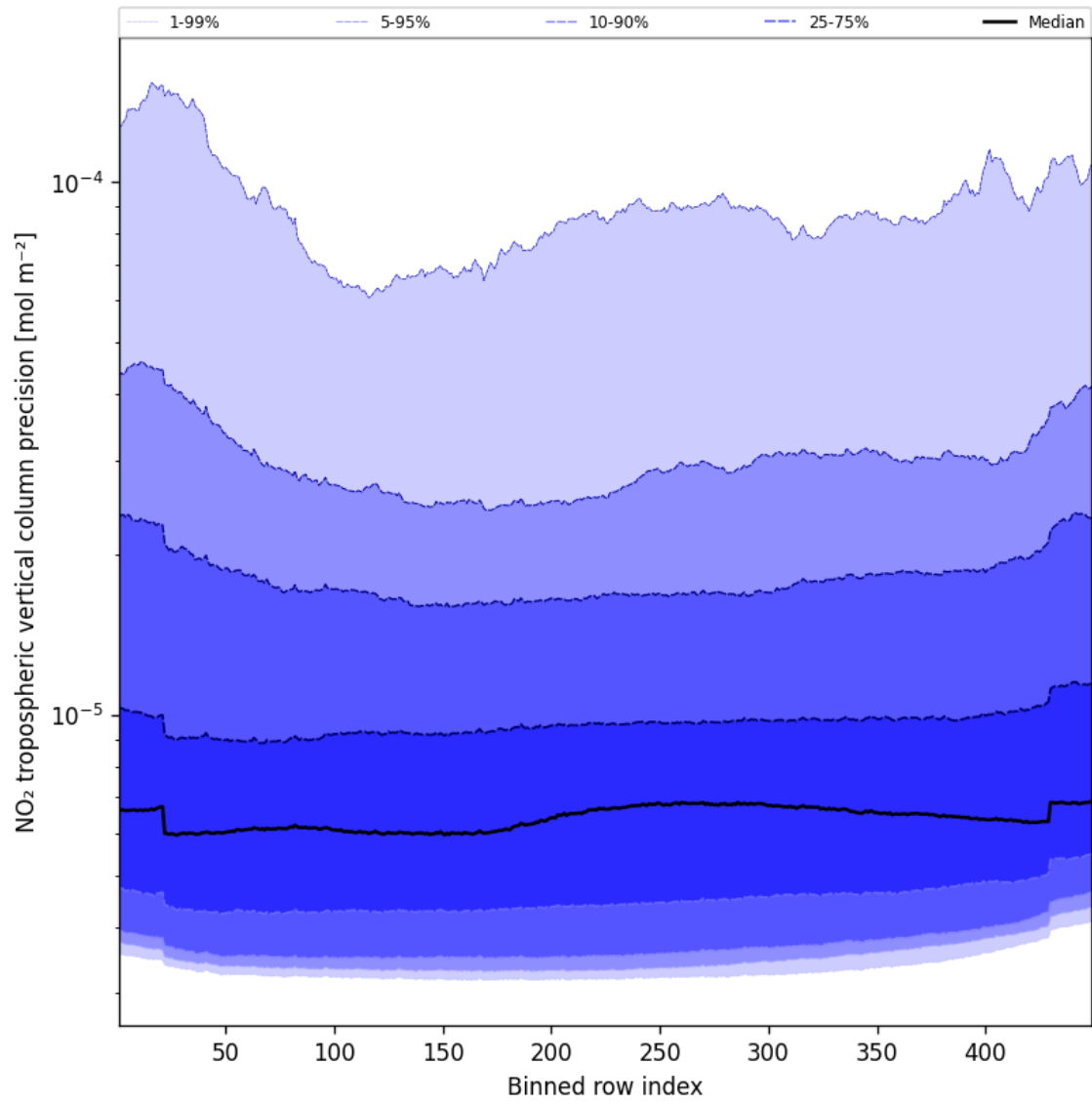
Figure 47: Along track statistics of “NO 2 tropospheric vertical column precision” for 2025-01-03 to 2025-01-05
