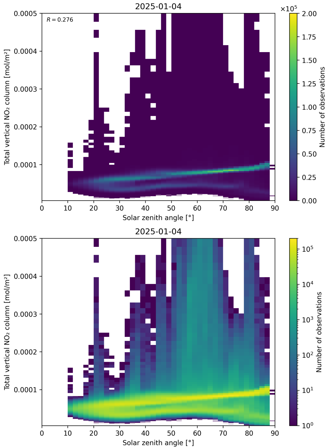
Figure 153: Scatter density plot of “Solar zenith angle” against “Total vertical NO 2 column” for 2025-01-03 to 2025-01-05.
