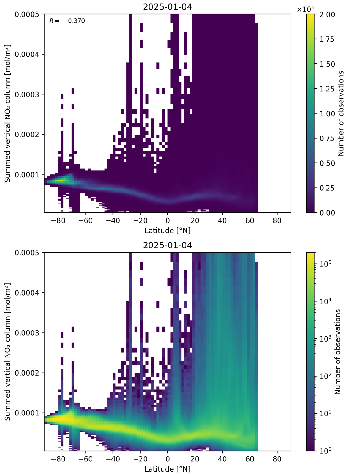
Figure 88: Scatter density plot of “Latitude” against “Summed vertical NO 2 column” for 2025-01-03 to 2025-01-05.
