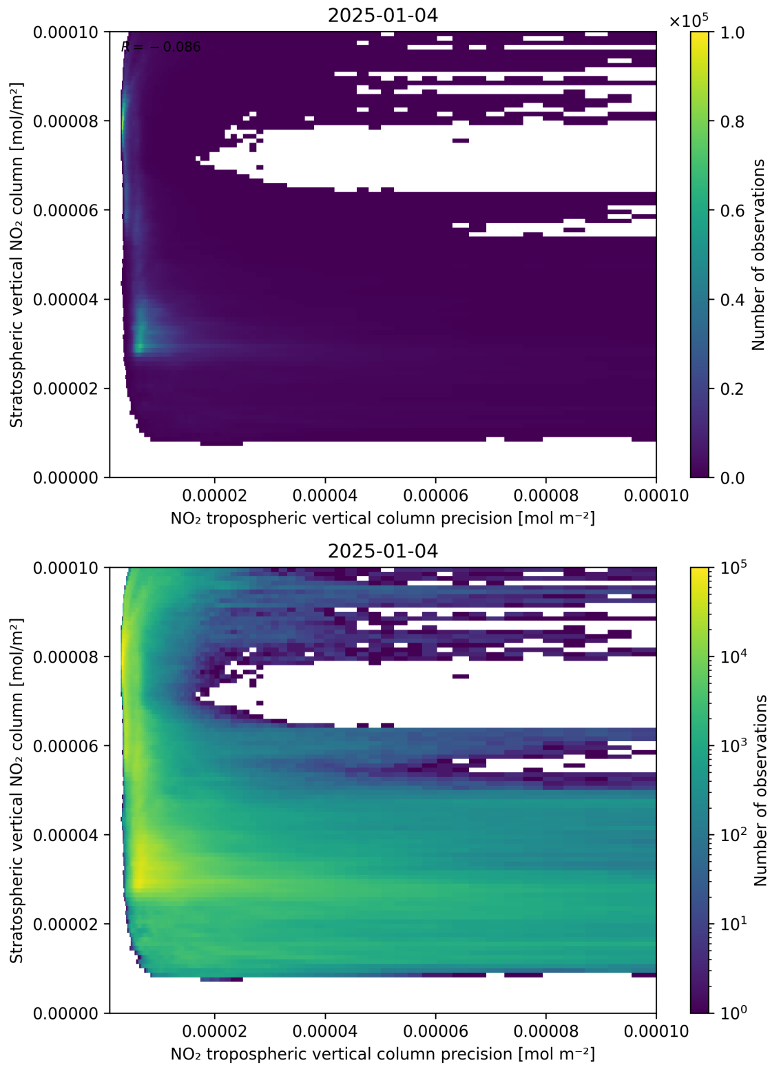
Figure 135: Scatter density plot of “NO 2 tropospheric vertical column precision” against “Stratospheric vertical NO 2 column” for 2025-01-03 to 2025-01-05.
