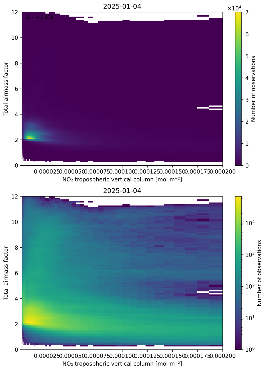
Figure 122: Scatter density plot of “NO 2 tropospheric vertical column” against “Total air mass factor” for 2025-01-03 to 2025-01-05.
