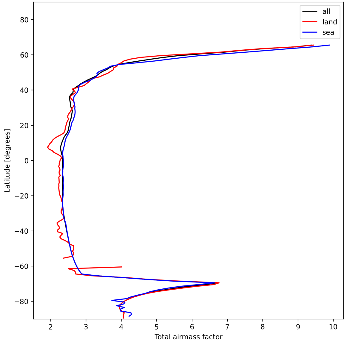
Figure 15: Zonal average of “Total airmass factor” for 2025-01-03 to 2025-01-05.
