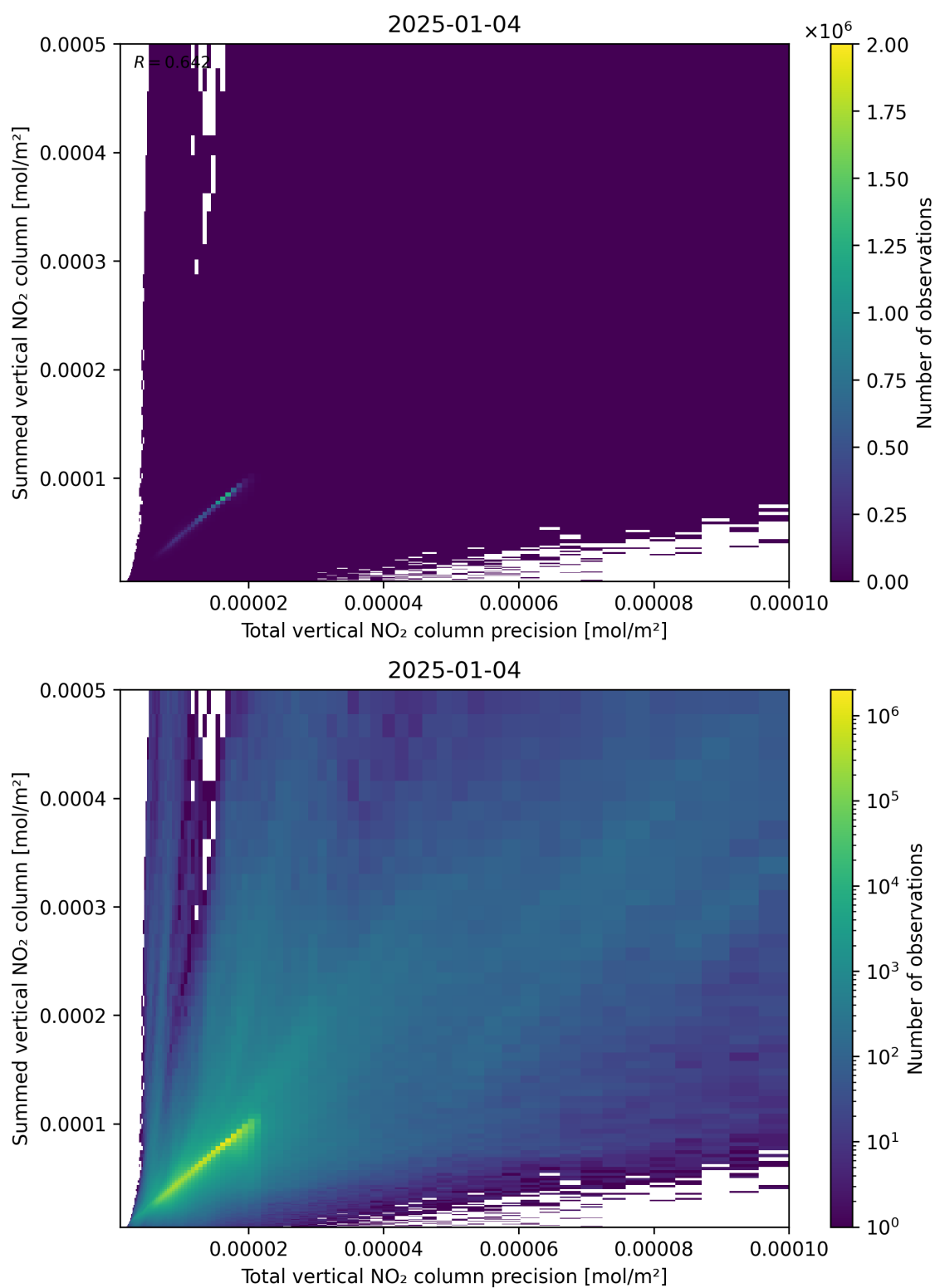
Figure 117: Scatter density plot of “Total vertical NO 2 column precision” against “Summed vertical NO 2 column” for 2025-01-03 to 2025-01-05.
