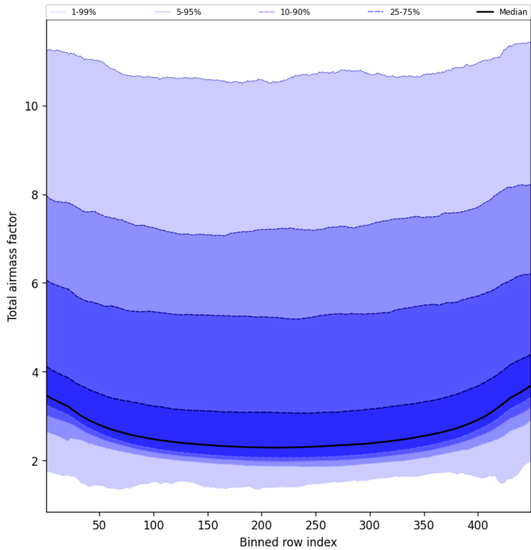
Figure 49: Along track statistics of “Total airmass factor” for 2025-01-03 to 2025-01-05
