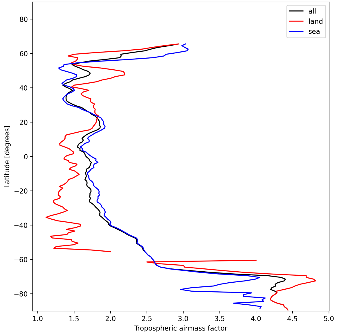
Figure 14: Zonal average of “Tropospheric airmass factor” for 2025-01-03 to 2025-01-05.
