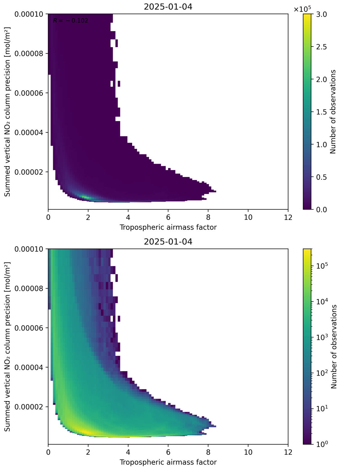
Figure 76: Scatter density plot of “Tropospheric air mass factor” against “Summed vertical NO 2 column precision” for 2025-01-03 to 2025-01-05.
