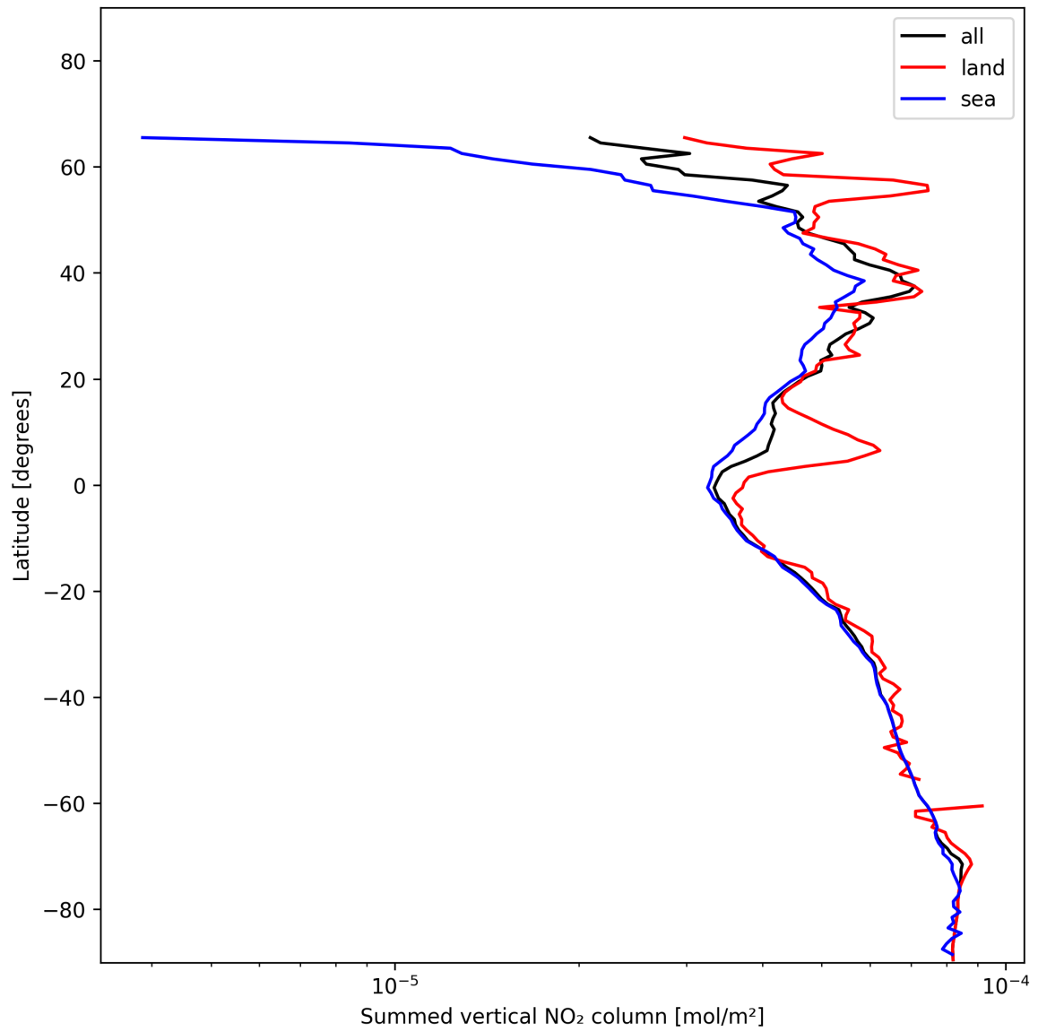
Figure 23: Zonal average of “Summed vertical NO 2 column” for 2025-01-03 to 2025-01-05.
