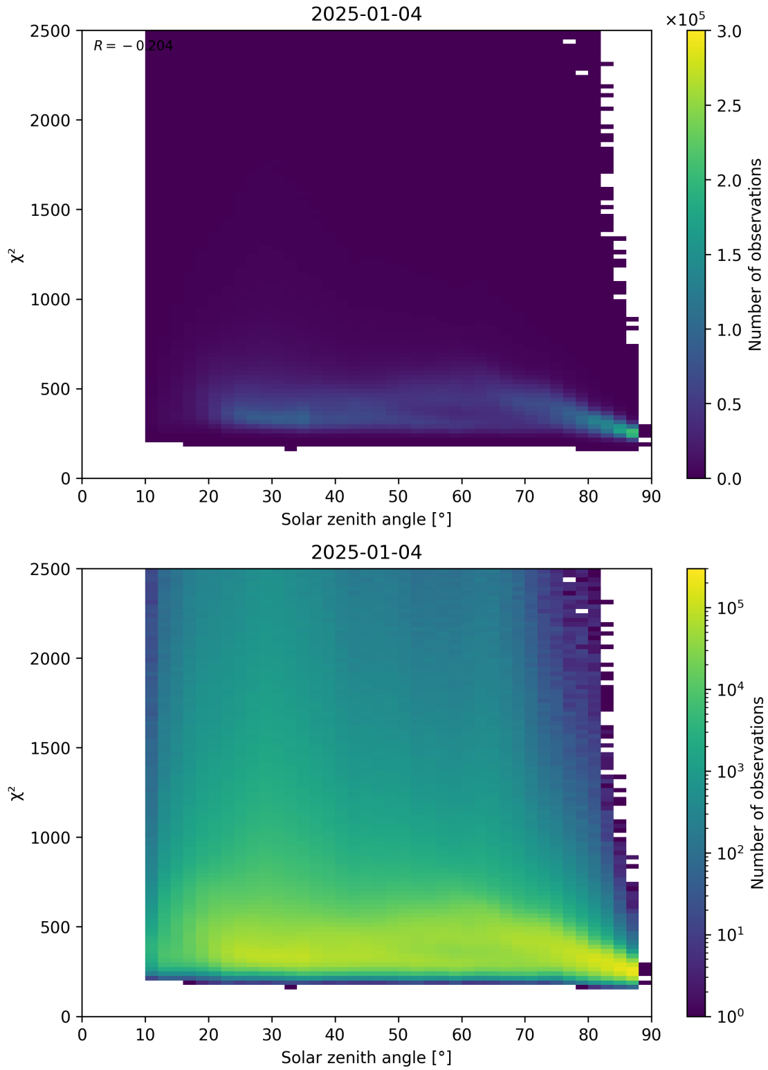
Figure 148: Scatter density plot of “Solar zenith angle” against “ \chi^2 ” for 2025-01-03 to 2025-01-05.
