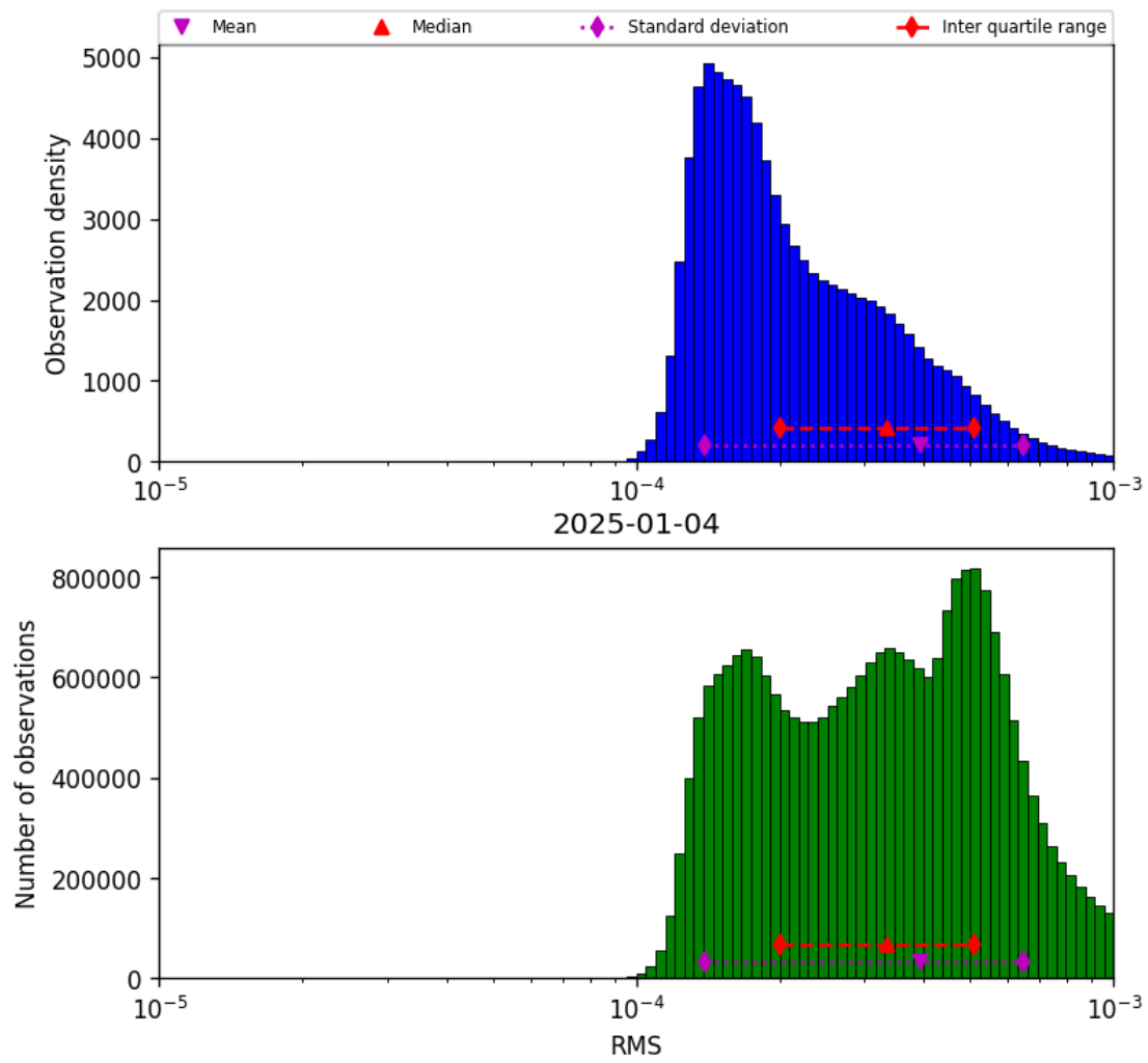
Figure 43: Histogram of “RMS” for 2025-01-03 to 2025-01-05
