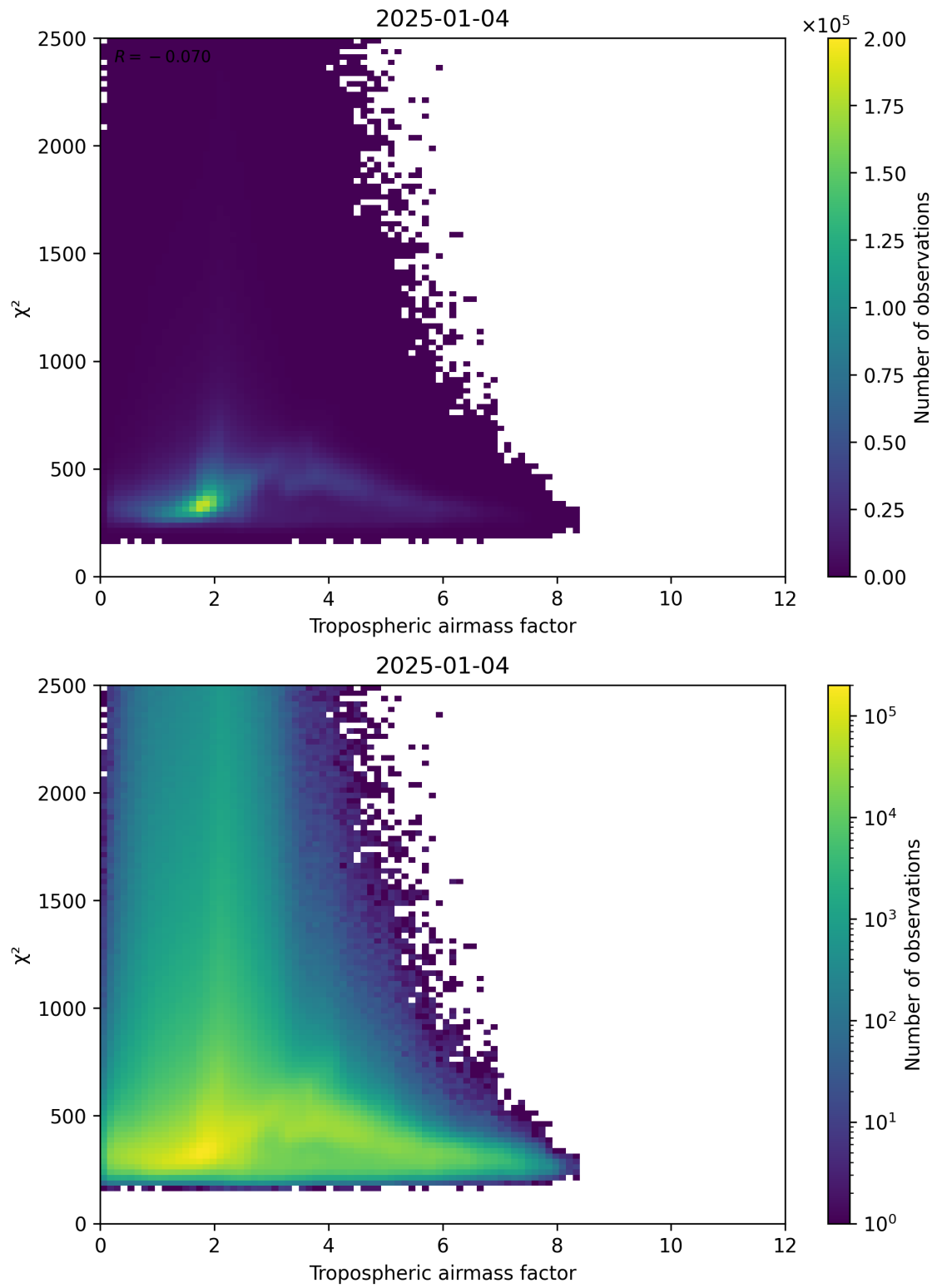
Figure 73: Scatter density plot of “Tropospheric airmass factor” against “ \chi^2 ” for 2025-01-03 to 2025-01-05.
