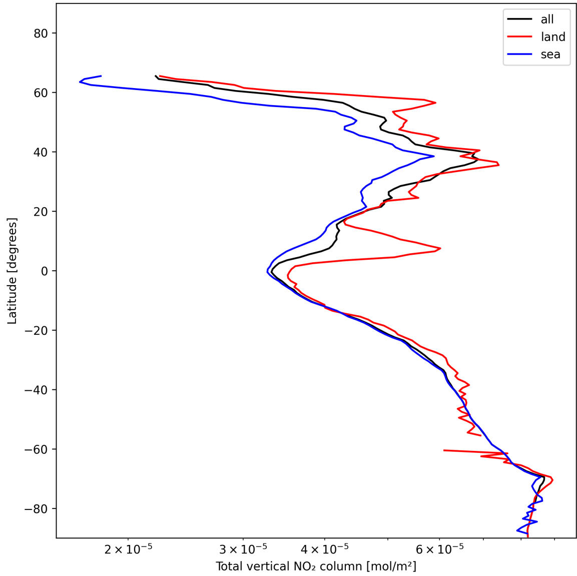
Figure 21: Zonal average of “Total vertical NO 2 column” for 2025-01-03 to 2025-01-05.
