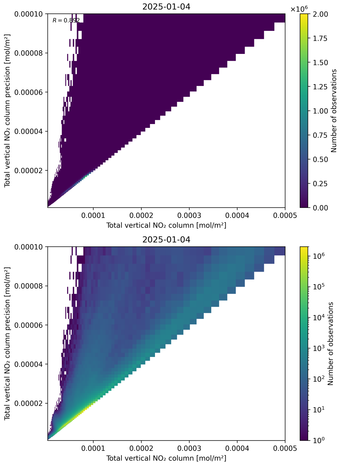
Figure 114: Scatter density plot of “Total vertical NO 2 column” against “Total vertical NO 2 column precision” for 2025-01-03 to 2025-01-05.
