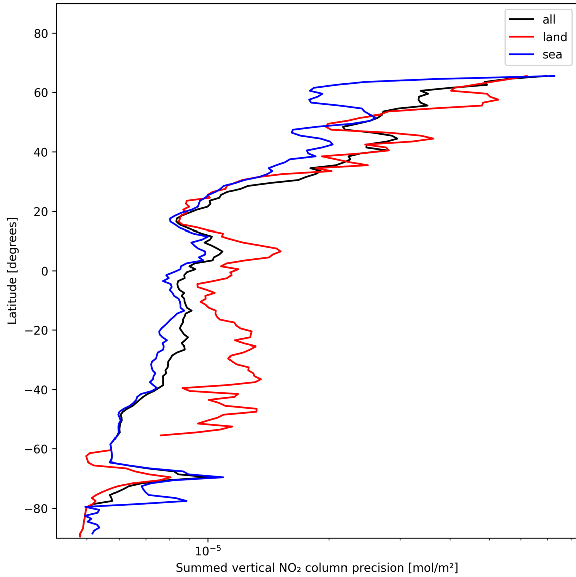
Figure 24: Zonal average of “Summed vertical NO 2 column precision” for 2025-01-03 to 2025-01-05.
