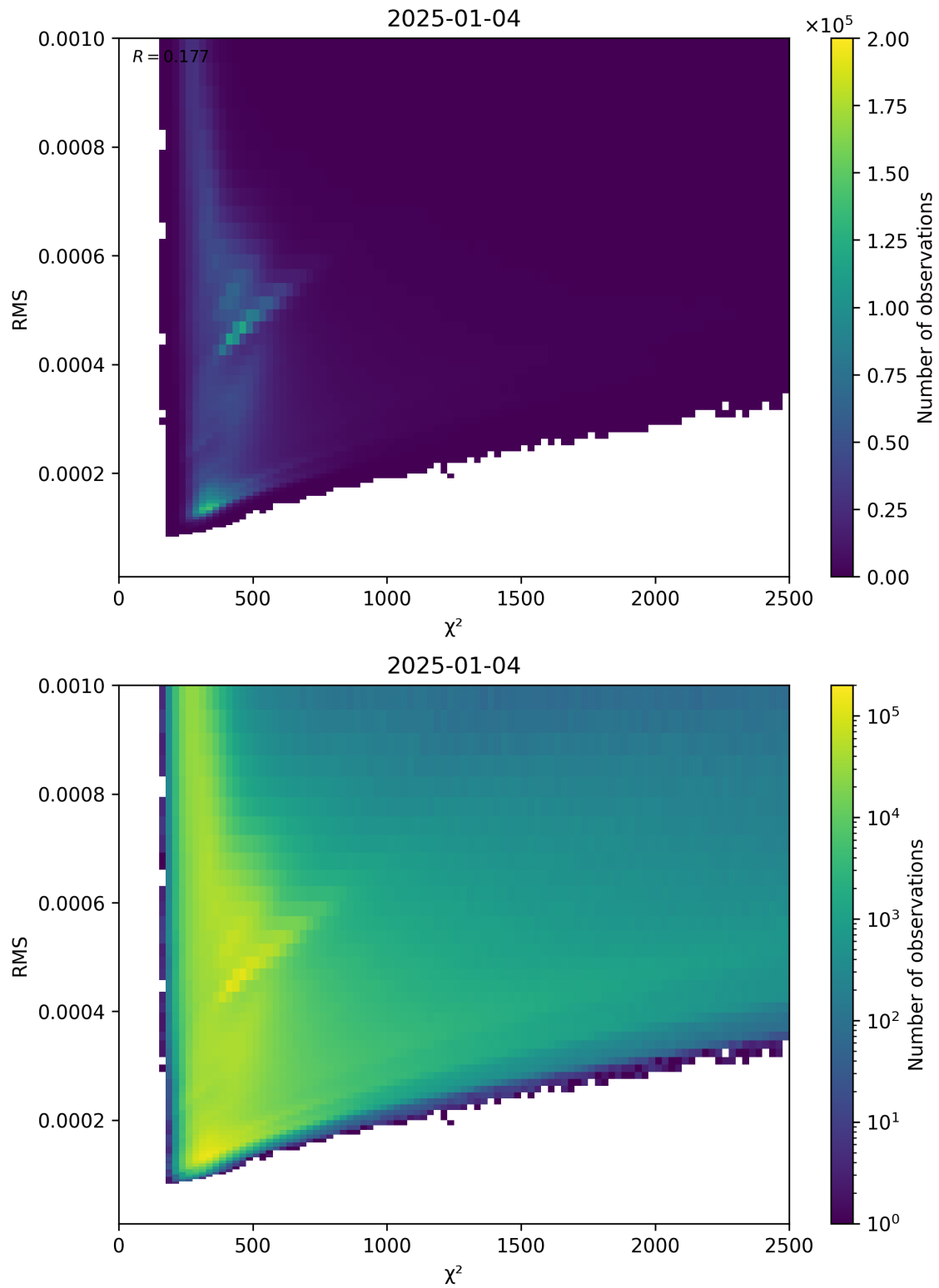
Figure 82: Scatter density plot of “ \chi^2 ” against “RMS” for 2025-01-03 to 2025-01-05.
