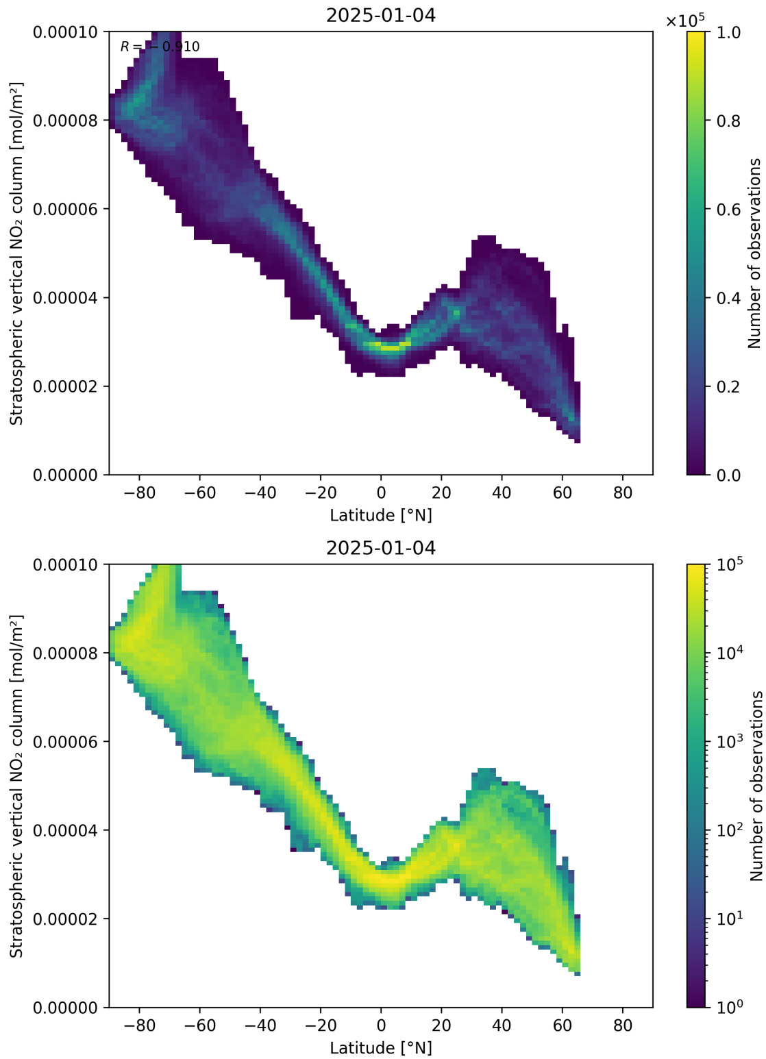
Figure 87: Scatter density plot of “Latitude” against “Stratospheric vertical NO 2 column” for 2025-01-03 to 2025-01-05.
