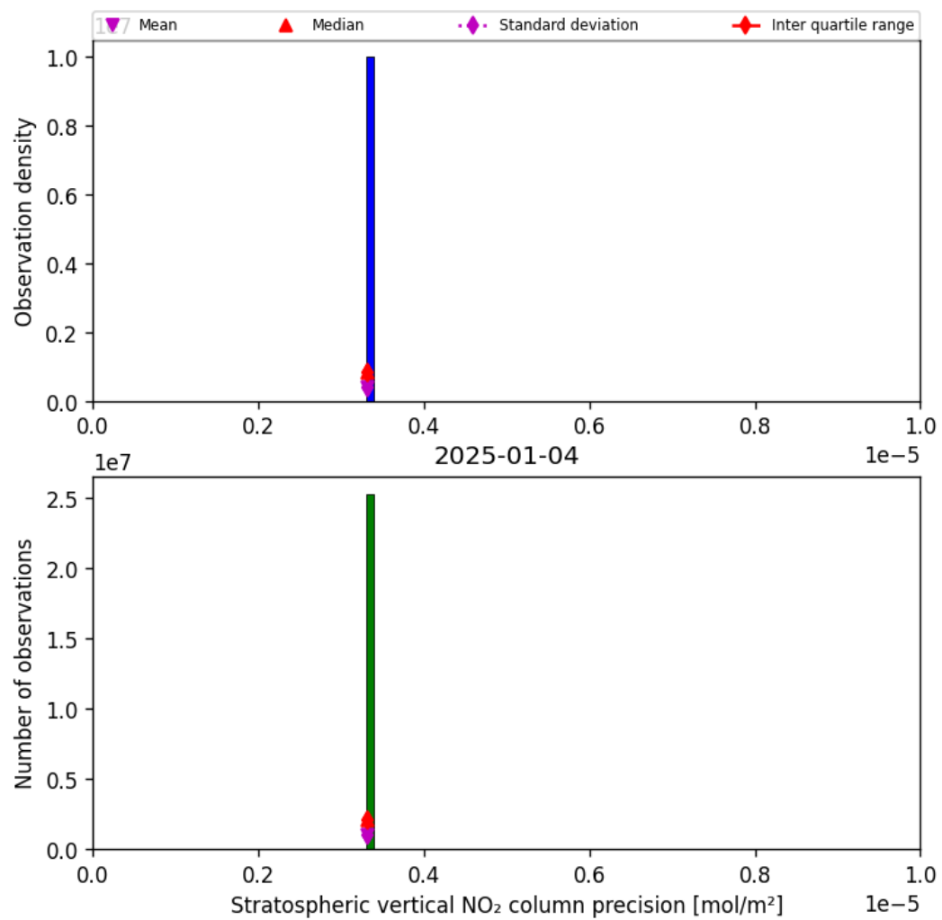
Figure 37: Histogram of “Stratospheric vertical NO 2 column precision” for 2025-01-03 to 2025-01-05
