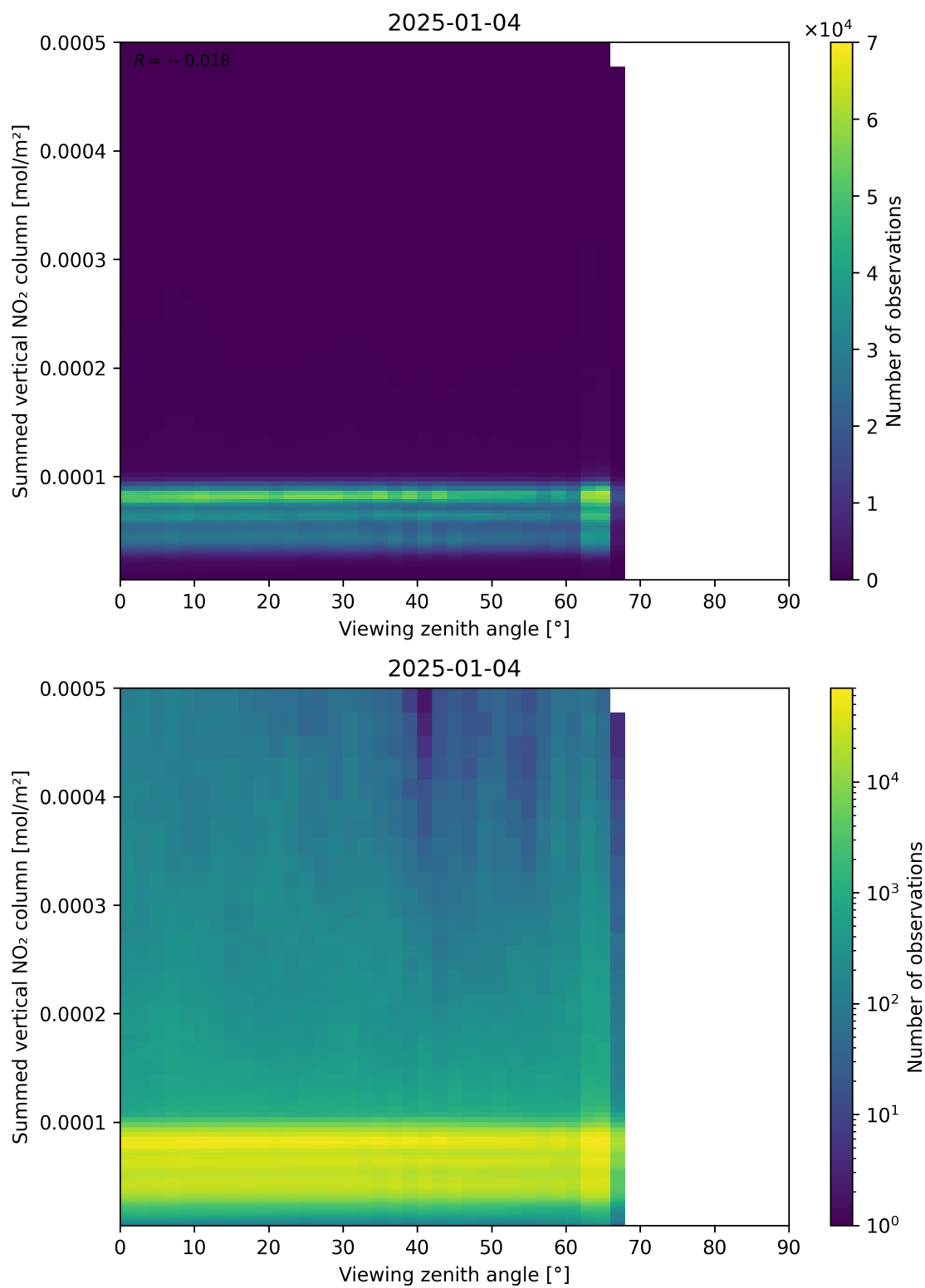
Figure 165: Scatter density plot of “Viewing zenith angle” against “Summed vertical NO 2 column” for 2025-01-03 to 2025-01-05.
