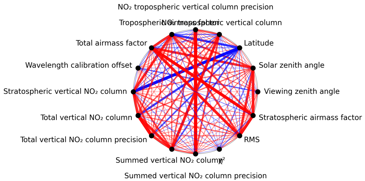
Figure 1: Map of correlation graph for 2025-01-03 to 2025-01-05.
