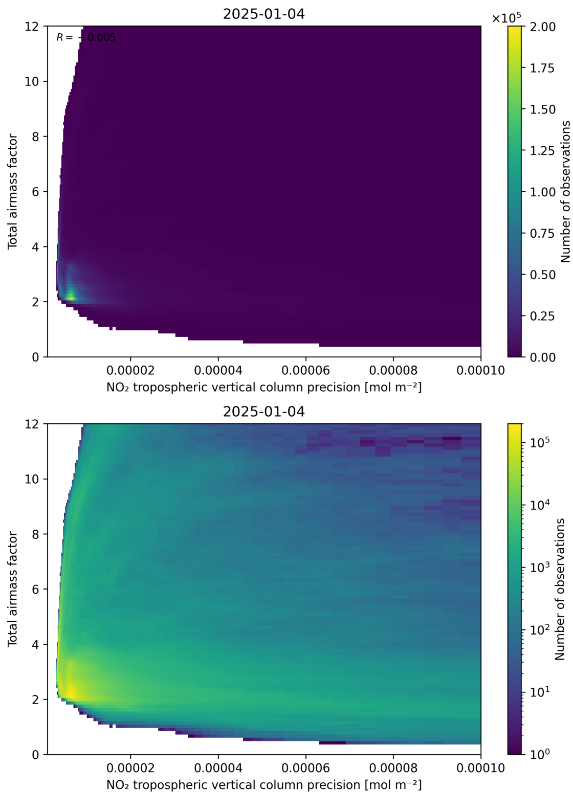
Figure 132: Scatter density plot of “NO 2 tropospheric vertical column precision” against “Total air mass factor” for 2025-01-03 to 2025-01-05.
