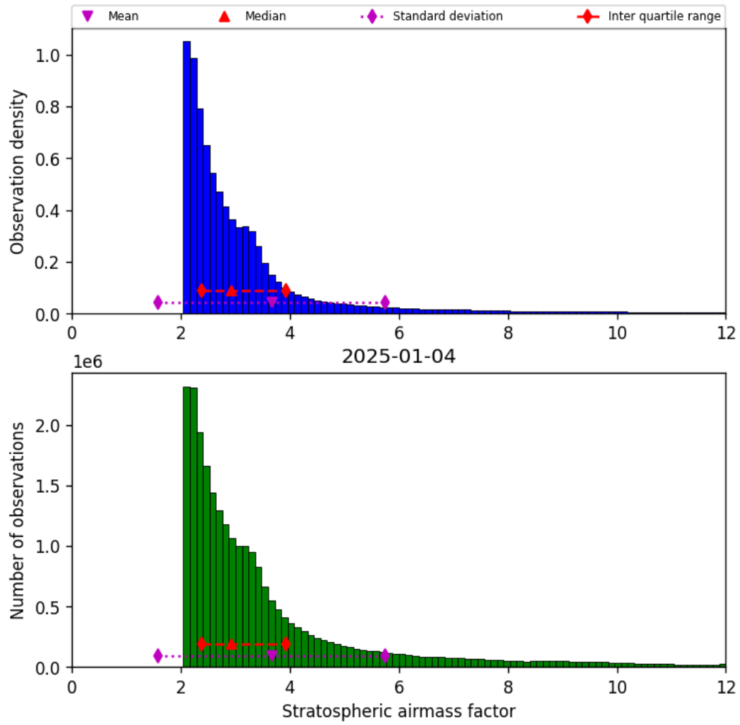
Figure 44: Histogram of “Stratospheric airmass factor” for 2025-01-03 to 2025-01-05
