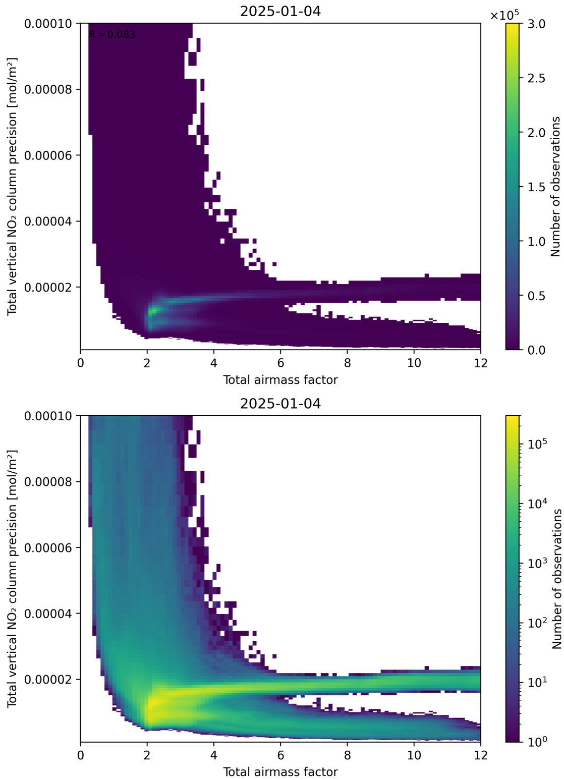
Figure 68: Scatter density plot of “Total airmass factor” against “Total vertical NO 2 column precision” for 2025-01-03 to 2025-01-05.
