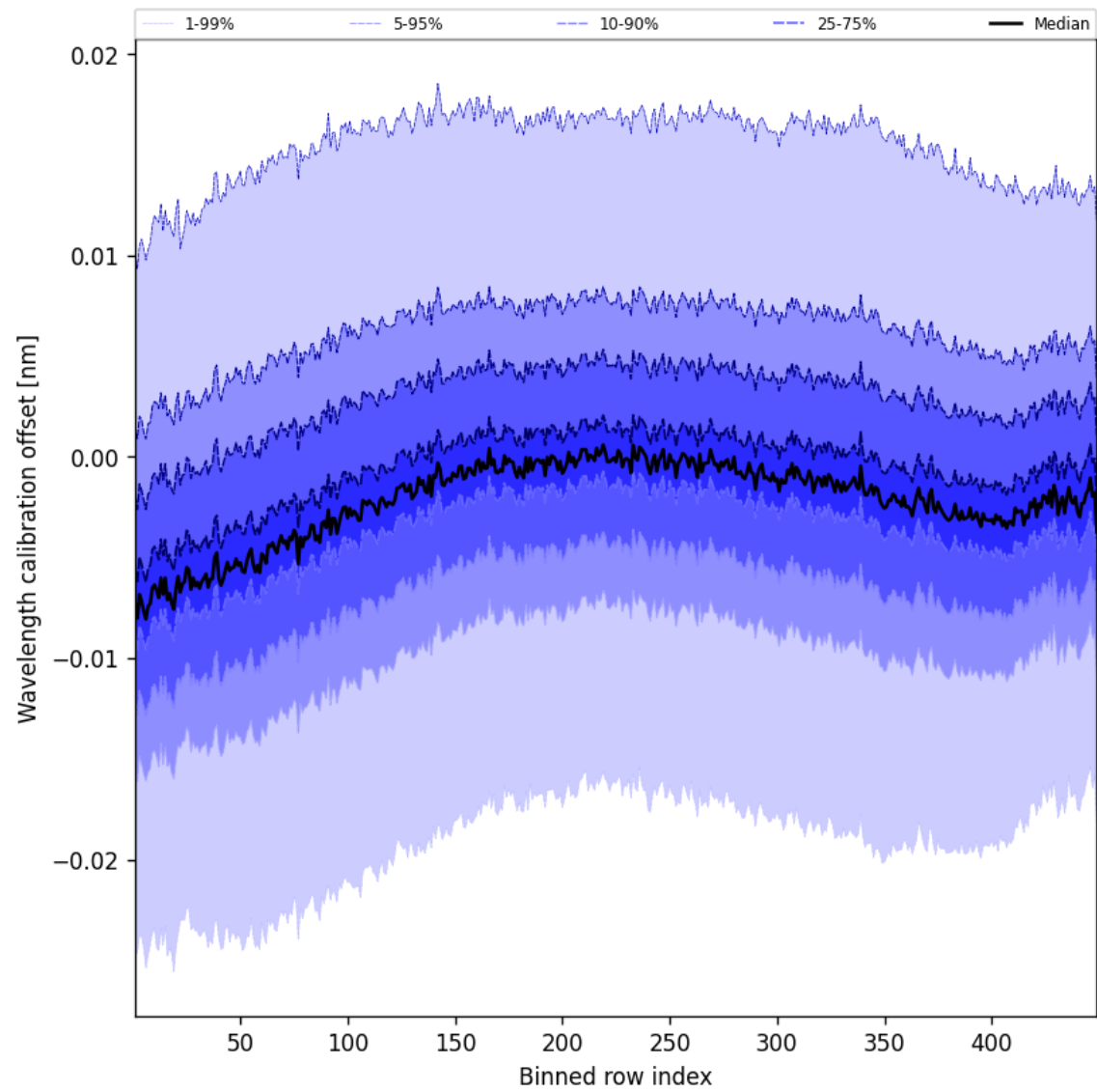
Figure 52: Along track statistics of “Wavelength calibration offset” for 2025-01-03 to 2025-01-05
