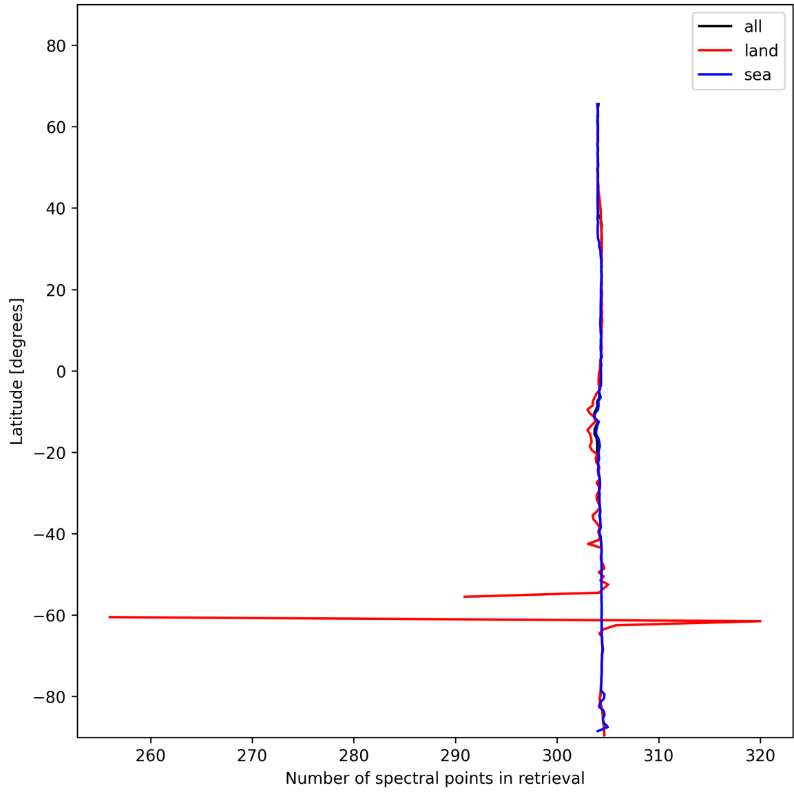
Figure 16: Zonal average of “Number of spectral points in retrieval” for 2025-01-03 to 2025-01-05.
