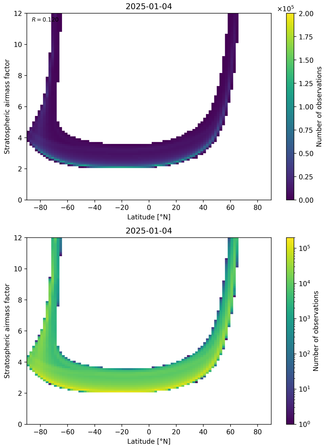
Figure 83: Scatter density plot of “Latitude” against “Stratospheric air mass factor” for 2025-01-03 to 2025-01-05.
