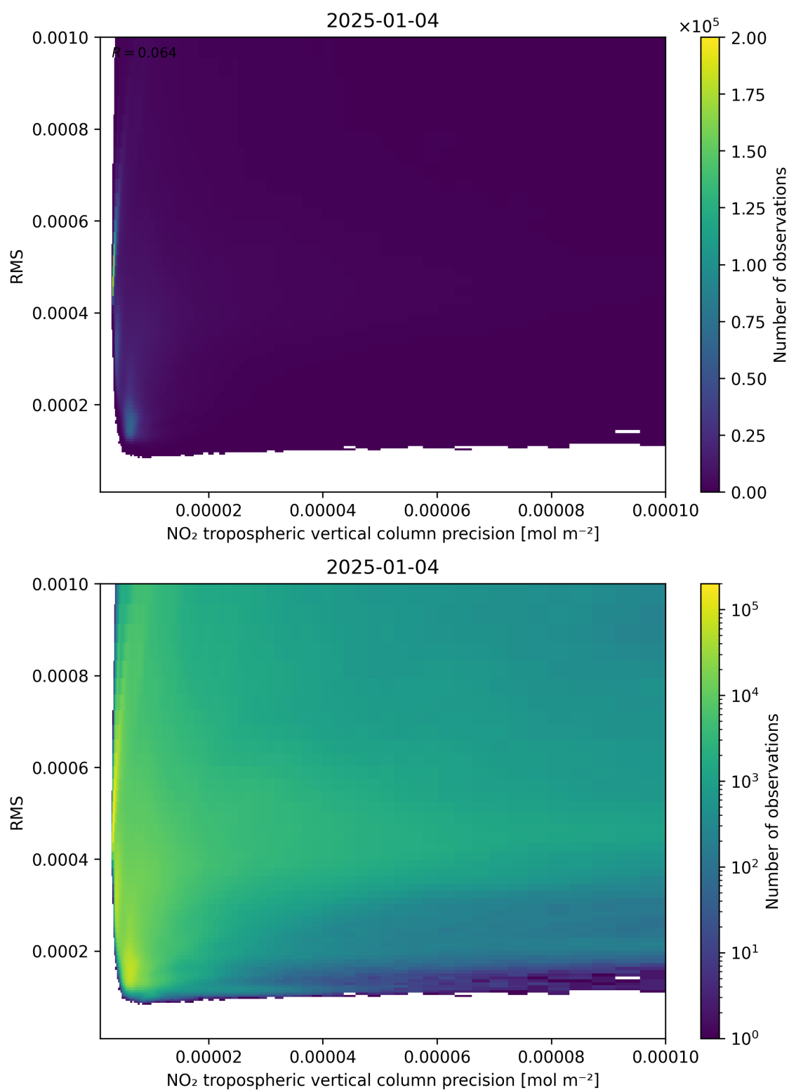
Figure 140: Scatter density plot of “NO 2 tropospheric vertical column precision” against “RMS” for 2025-01-03 to 2025-01-05.
