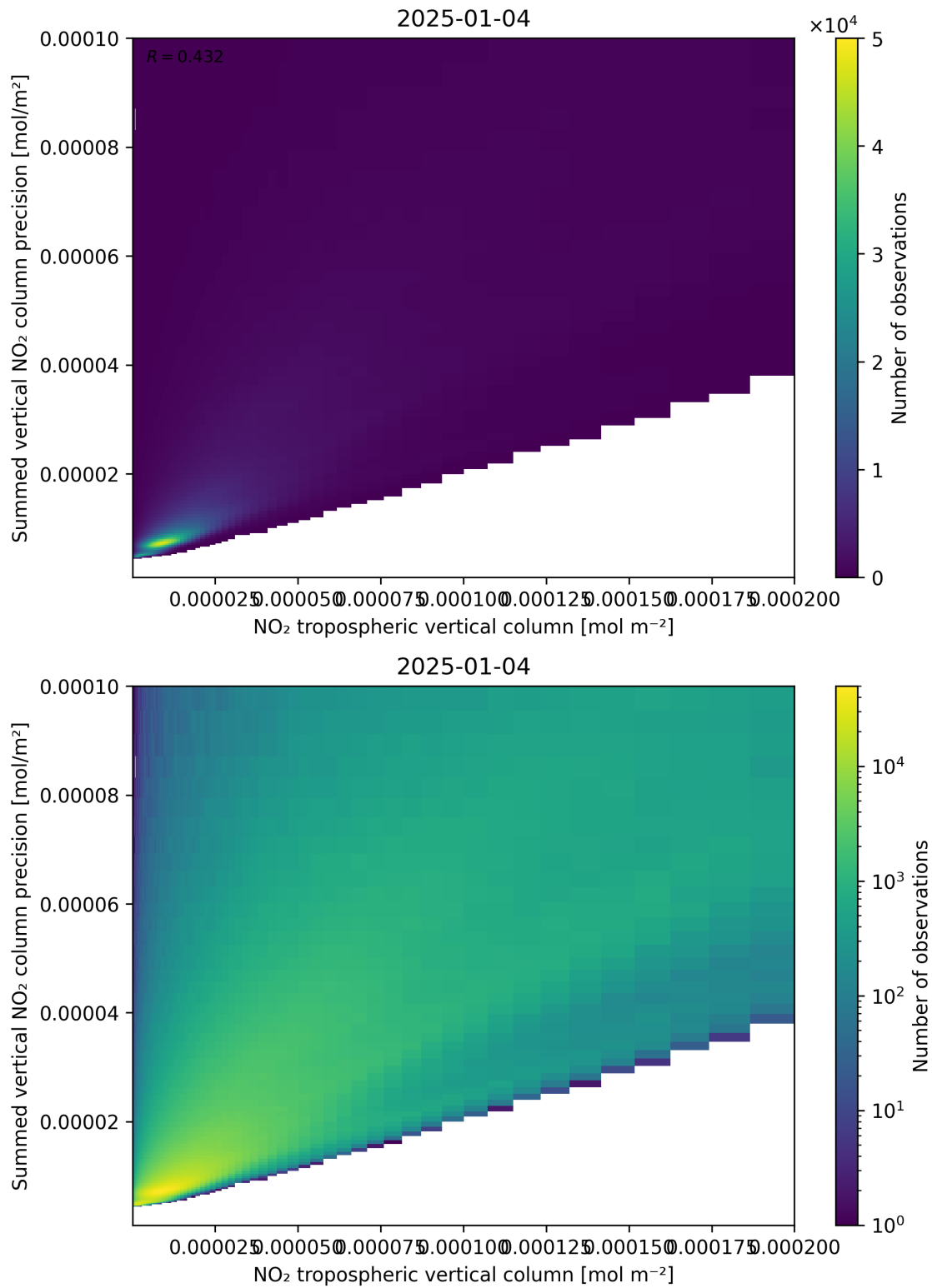
Figure 127: Scatter density plot of “NO 2 tropospheric vertical column” against “Summed vertical NO 2 column precision” for 2025-01-03 to 2025-01-05.
