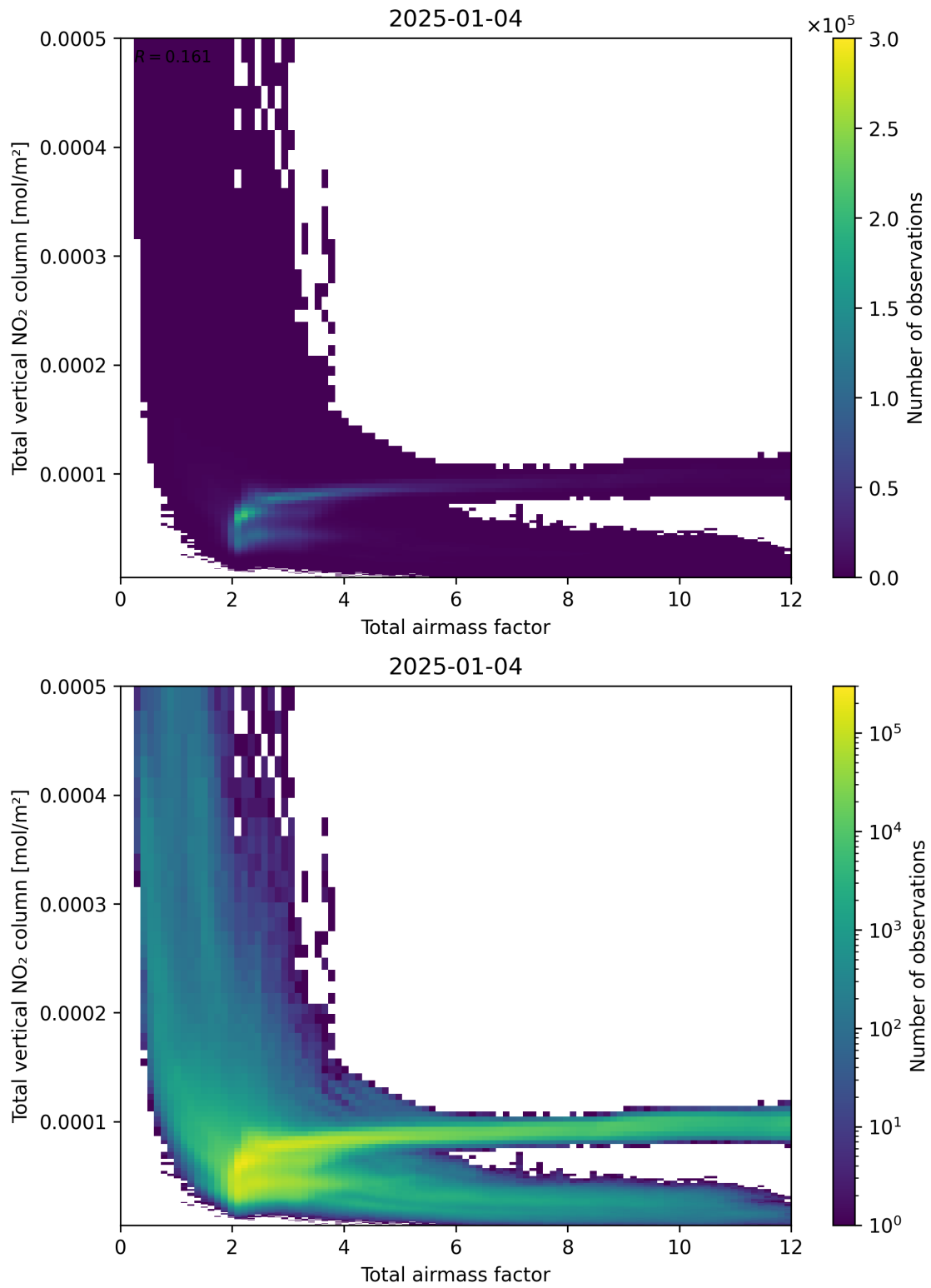
Figure 67: Scatter density plot of “Total airmass factor” against “Total vertical NO 2 column” for 2025-01-03 to 2025-01-05.
