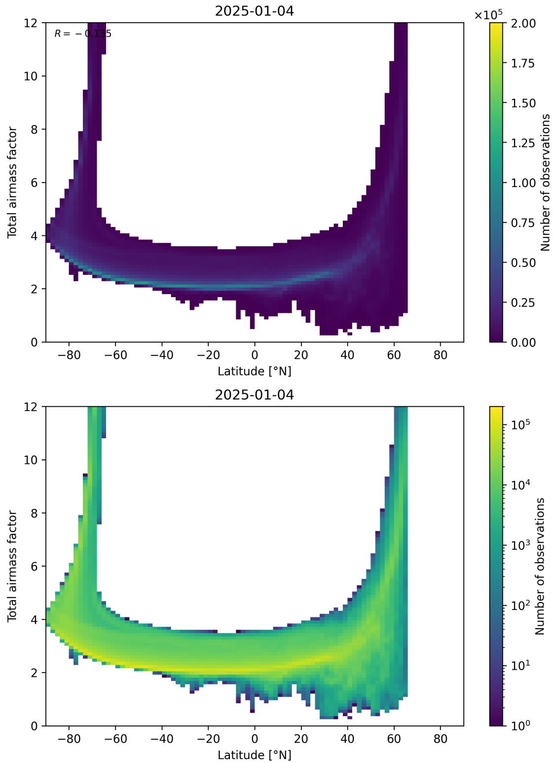
Figure 84: Scatter density plot of “Latitude” against “Total airmass factor” for 2025-01-03 to 2025-01-05.
