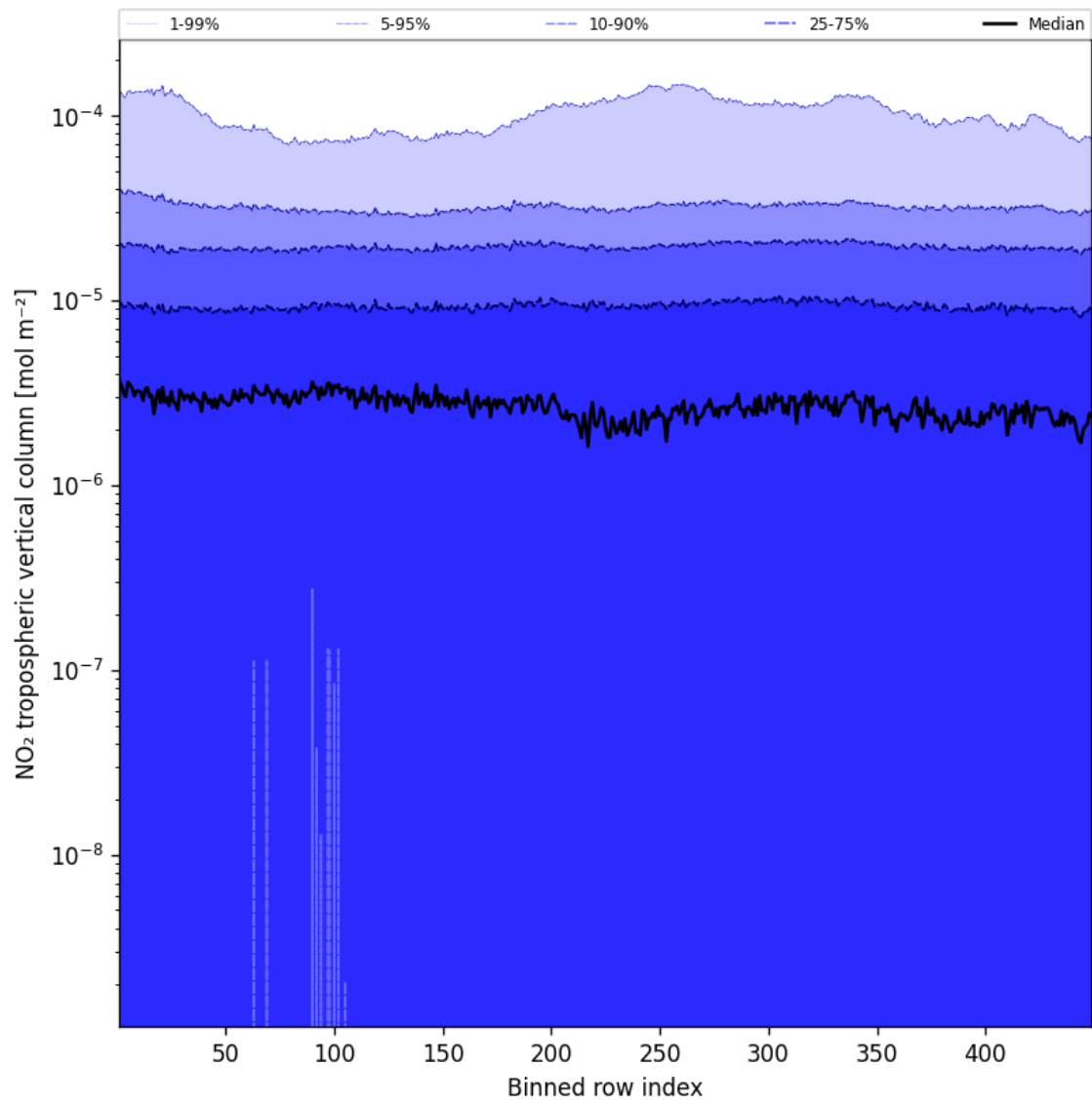
Figure 46: Along track statistics of “ \text{NO}_2 tropospheric vertical column” for 2025-01-03 to 2025-01-05
