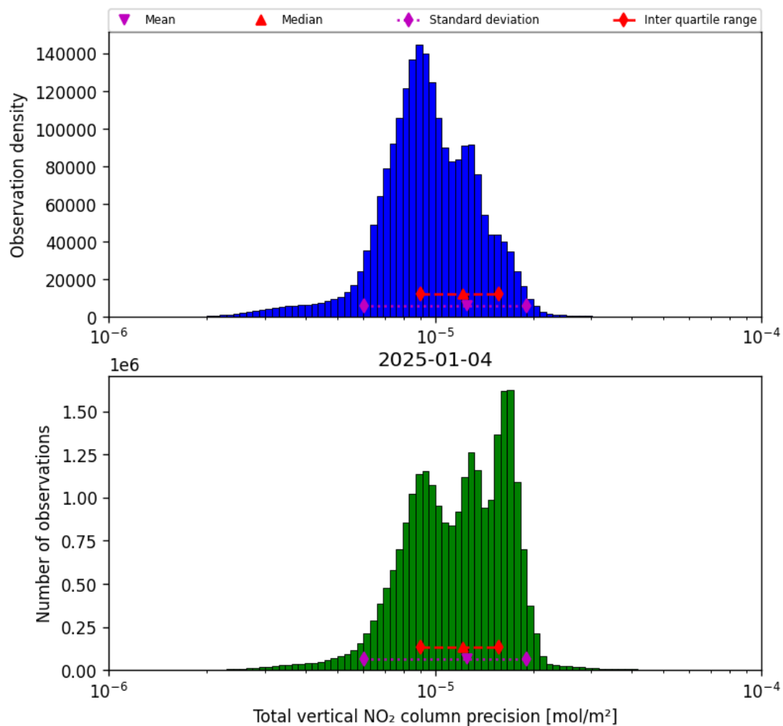
Figure 39: Histogram of “Total vertical NO 2 column precision” for 2025-01-03 to 2025-01-05
