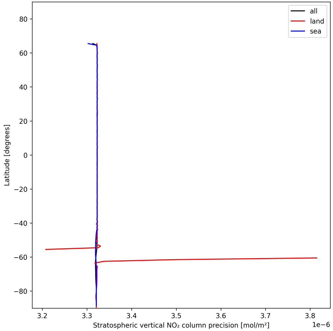
Figure 20: Zonal average of “Stratospheric vertical NO 2 column precision” for 2025-01-03 to 2025-01-05.
