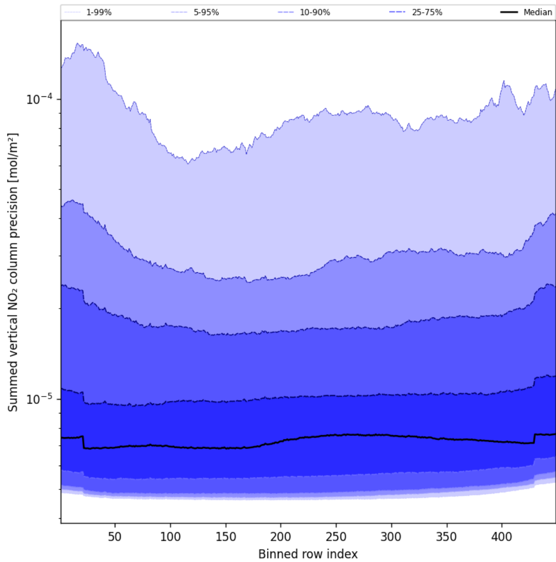
Figure 58: Along track statistics of “Summed vertical NO 2 column precision” for 2025-01-03 to 2025-01-05
