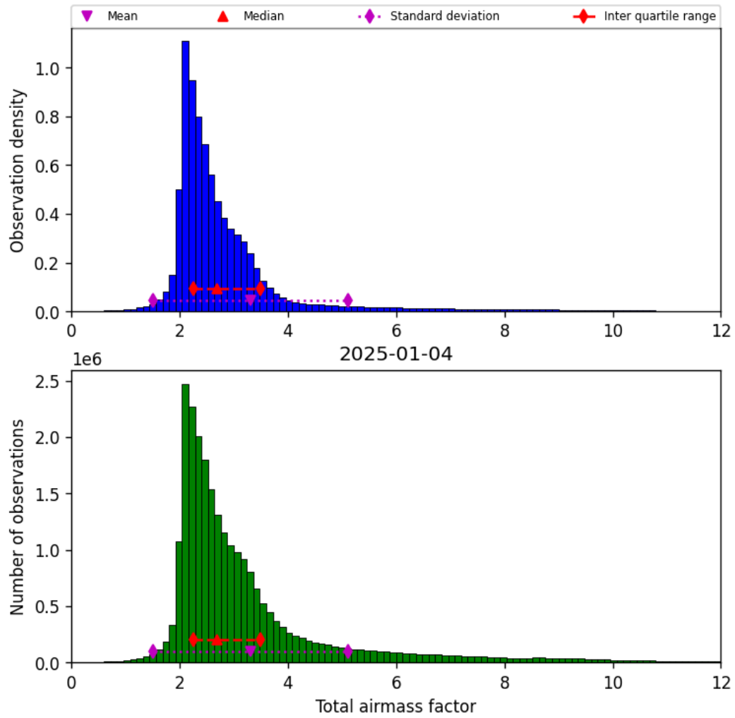
Figure 32: Histogram of “Total airmass factor” for 2025-01-03 to 2025-01-05
