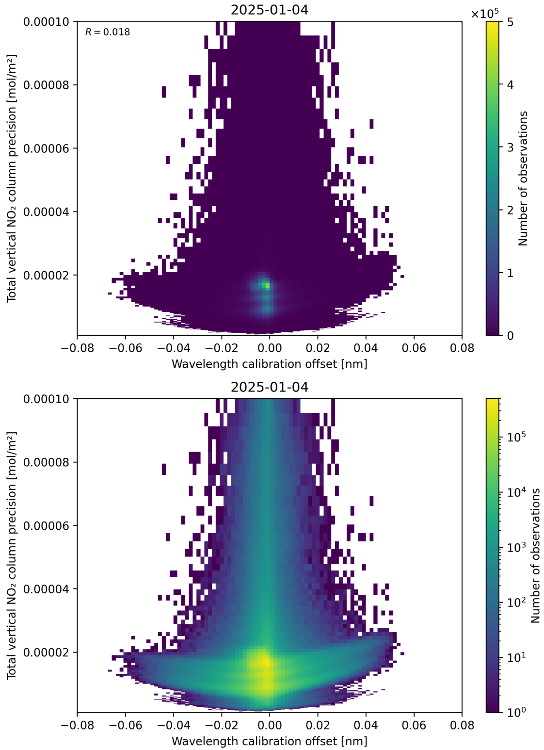
Figure 180: Scatter density plot of “Wavelength calibration offset” against “Total vertical NO 2 column precision” for 2025-01-03 to 2025-01-05.
