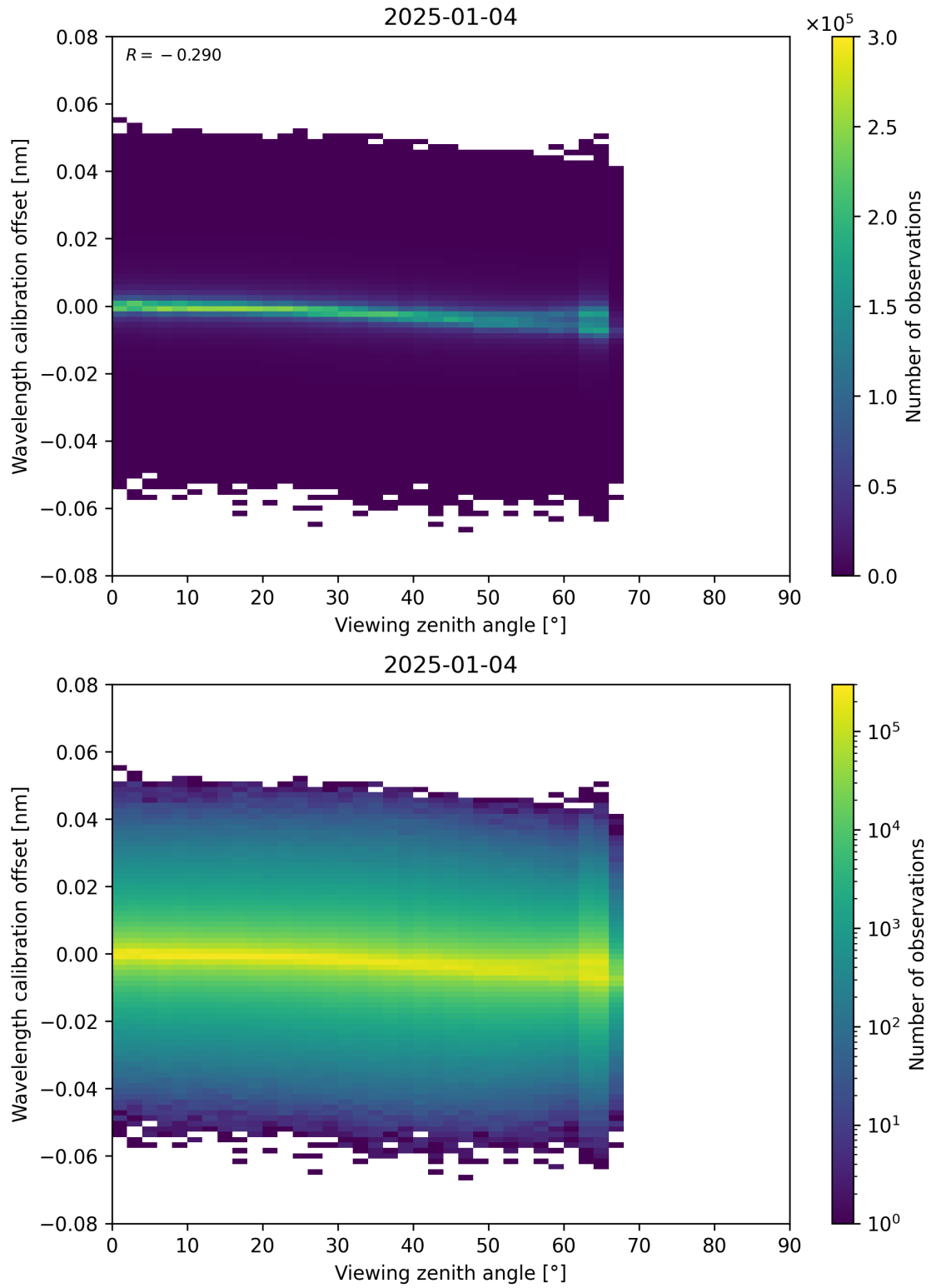
Figure 173: Scatter density plot of “Viewing zenith angle” against “Wavelength calibration offset” for 2025-01-03 to 2025-01-05.
