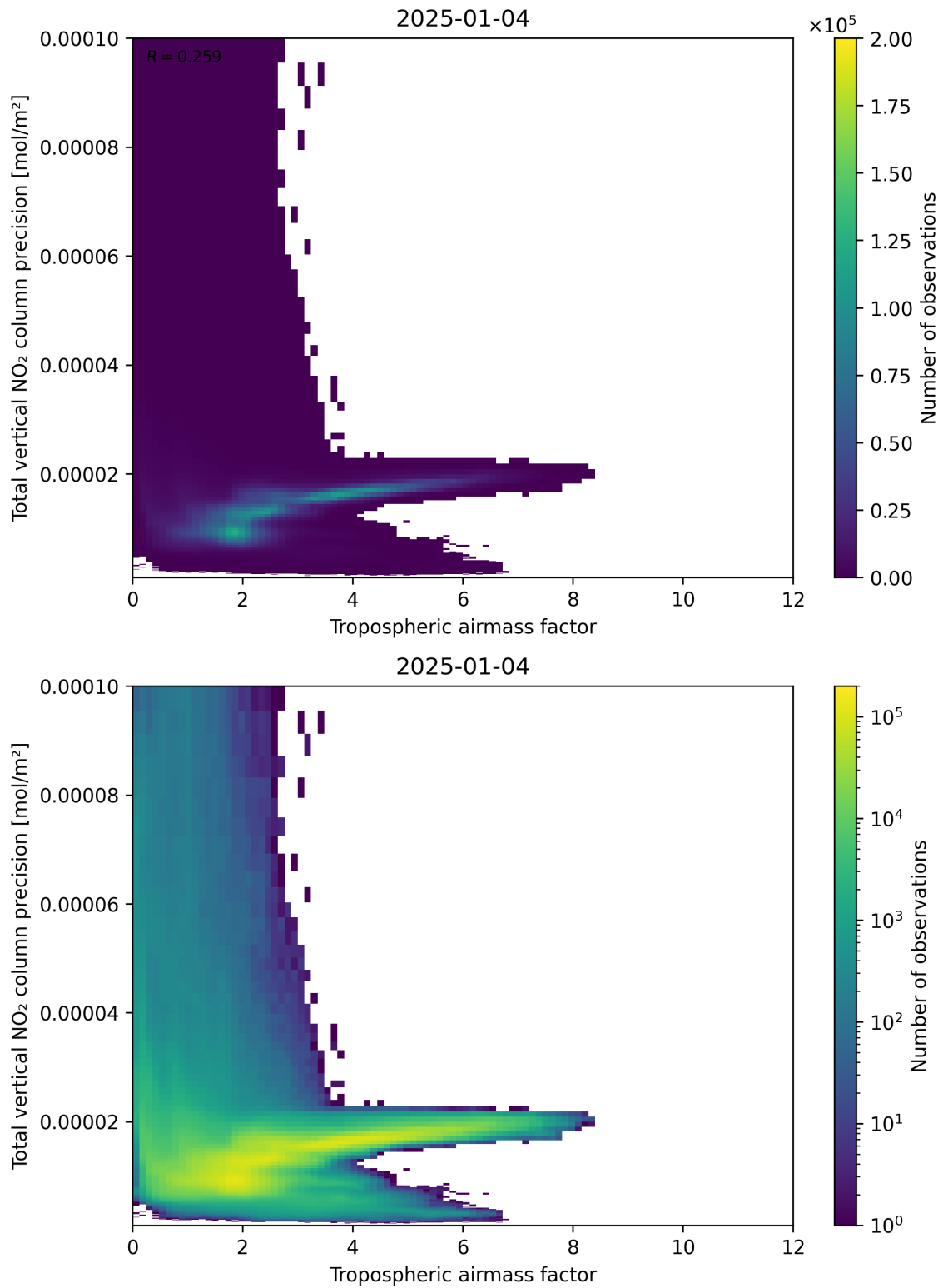
Figure 78: Scatter density plot of “Tropospheric air mass factor” against “Total vertical NO 2 column precision” for 2025-01-03 to 2025-01-05.
