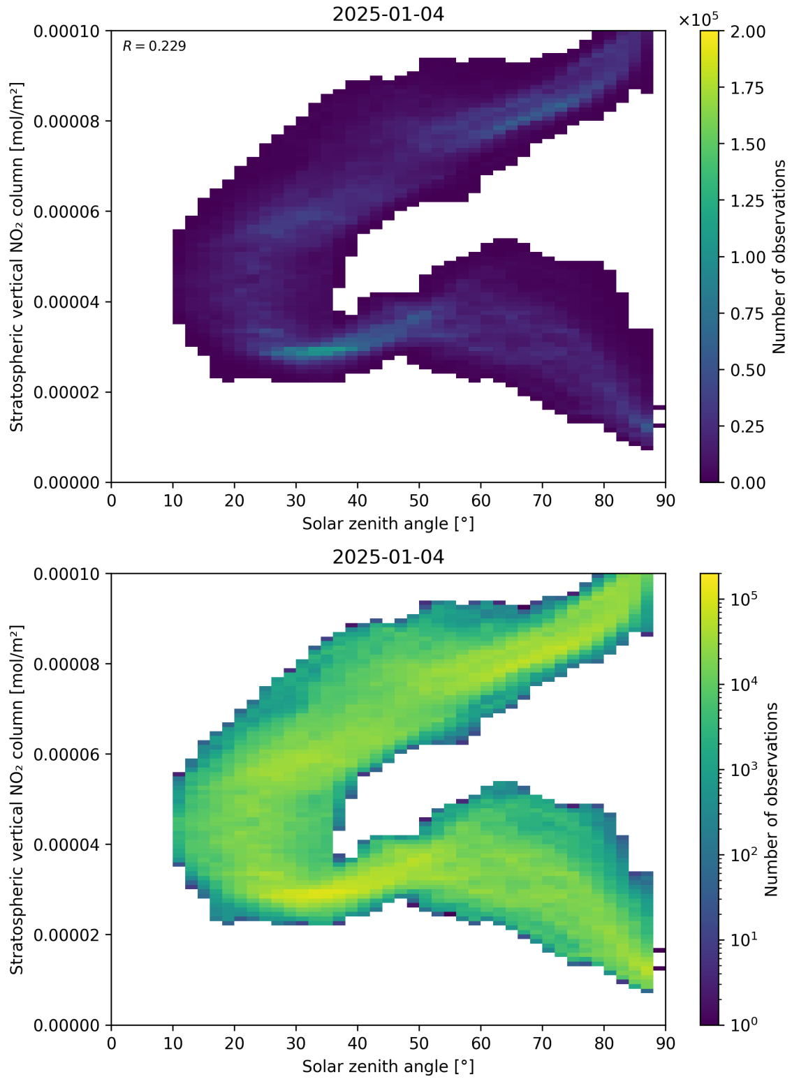
Figure 150: Scatter density plot of “Solar zenith angle” against “Stratospheric vertical NO 2 column” for 2025-01-03 to 2025-01-05.
