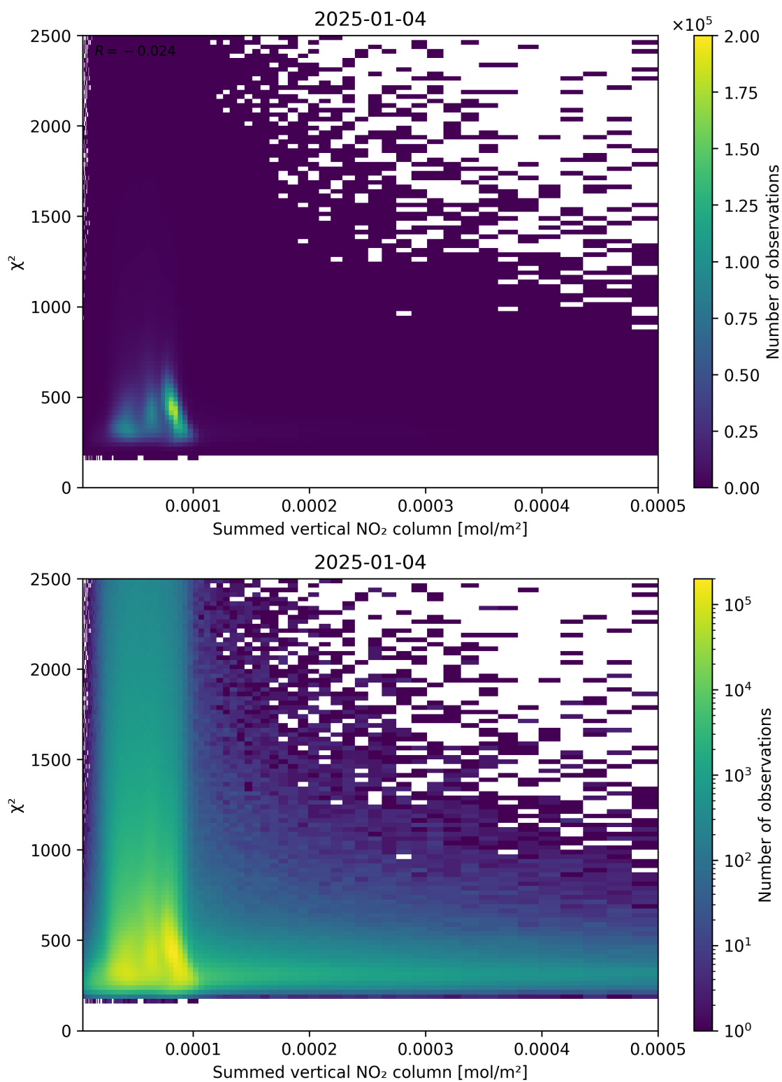
Figure 104: Scatter density plot of “Summed vertical NO 2 column” against “ \chi^2 ” for 2025-01-03 to 2025-01-05.
