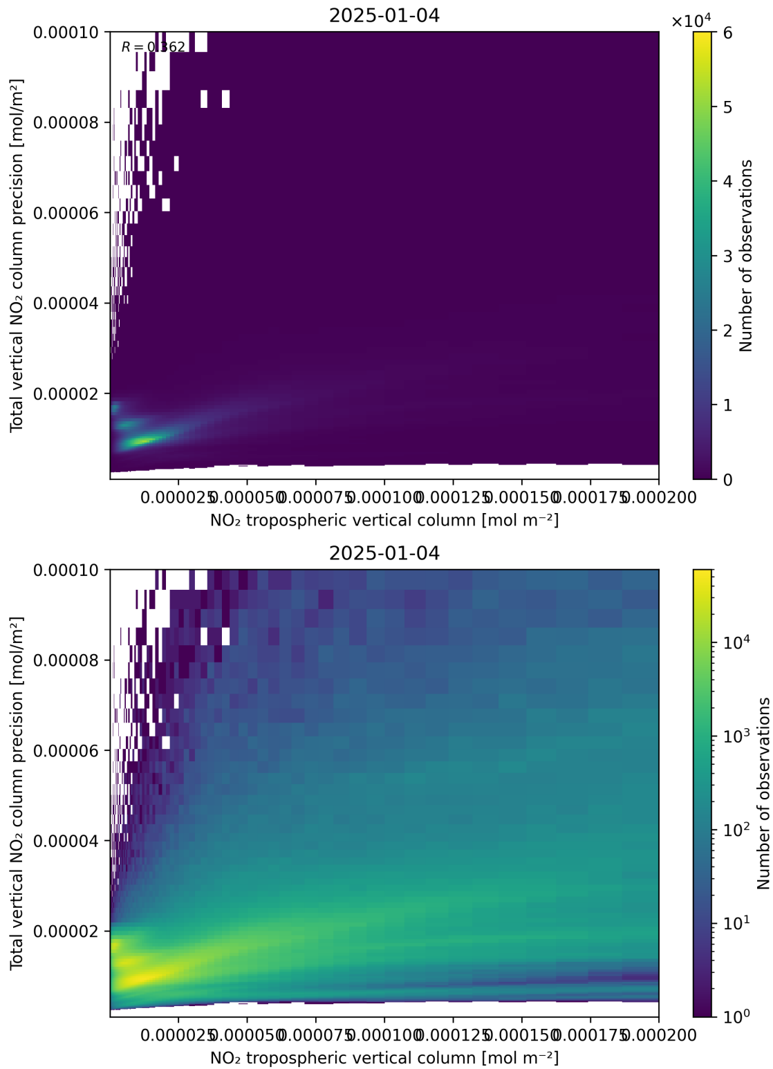
Figure 129: Scatter density plot of “NO 2 tropospheric vertical column” against “Total vertical NO 2 column precision” for 2025-01-03 to 2025-01-05.
