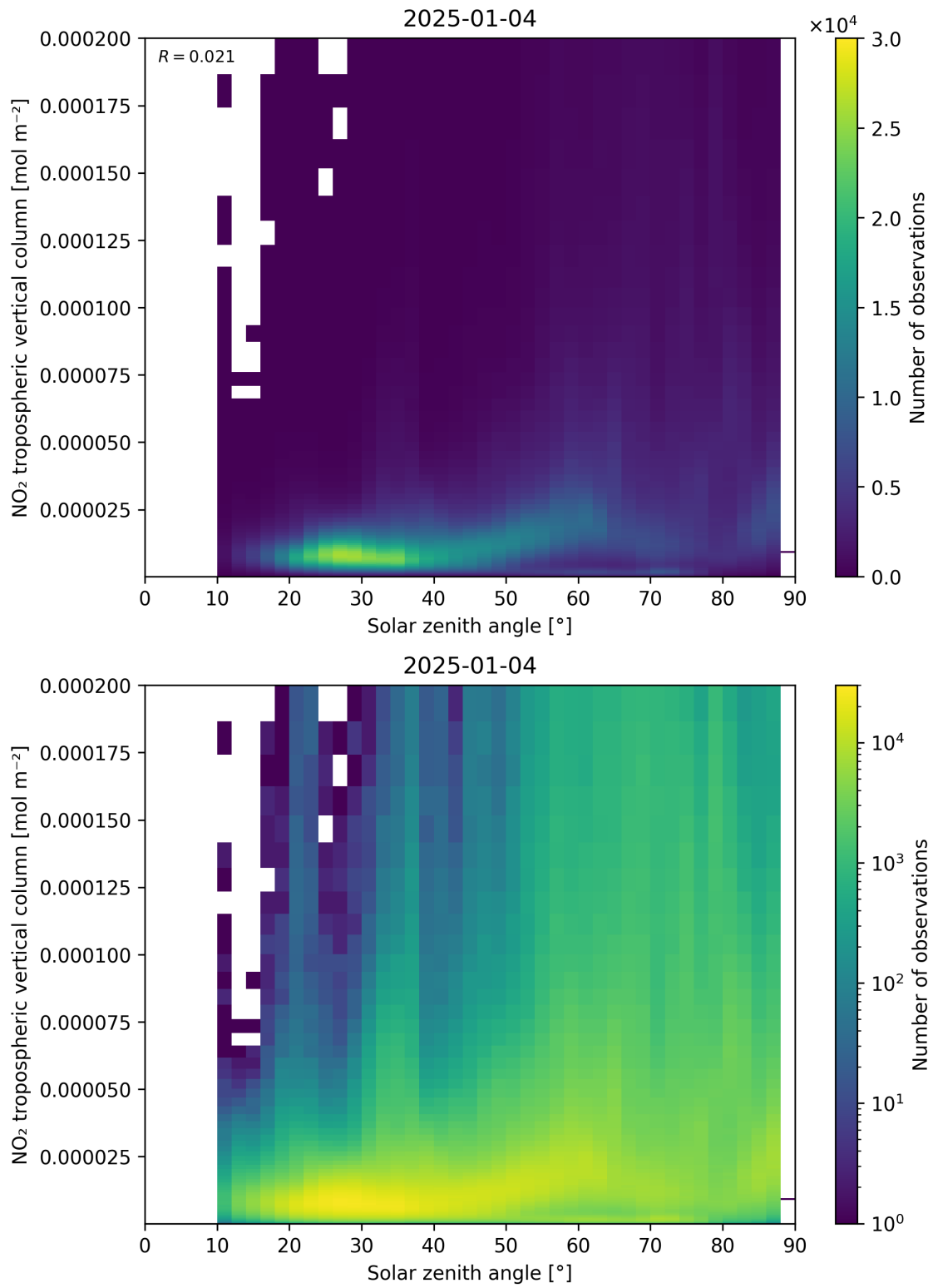
Figure 155: Scatter density plot of “Solar zenith angle” against “NO 2 tropospheric vertical column” for 2025-01-03 to 2025-01-05.
