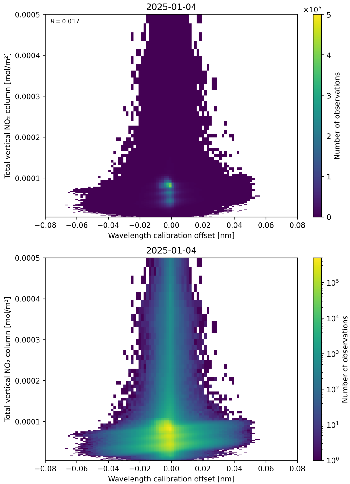
Figure 179: Scatter density plot of “Wavelength calibration offset” against “Total vertical NO 2 column” for 2025-01-03 to 2025-01-05.
