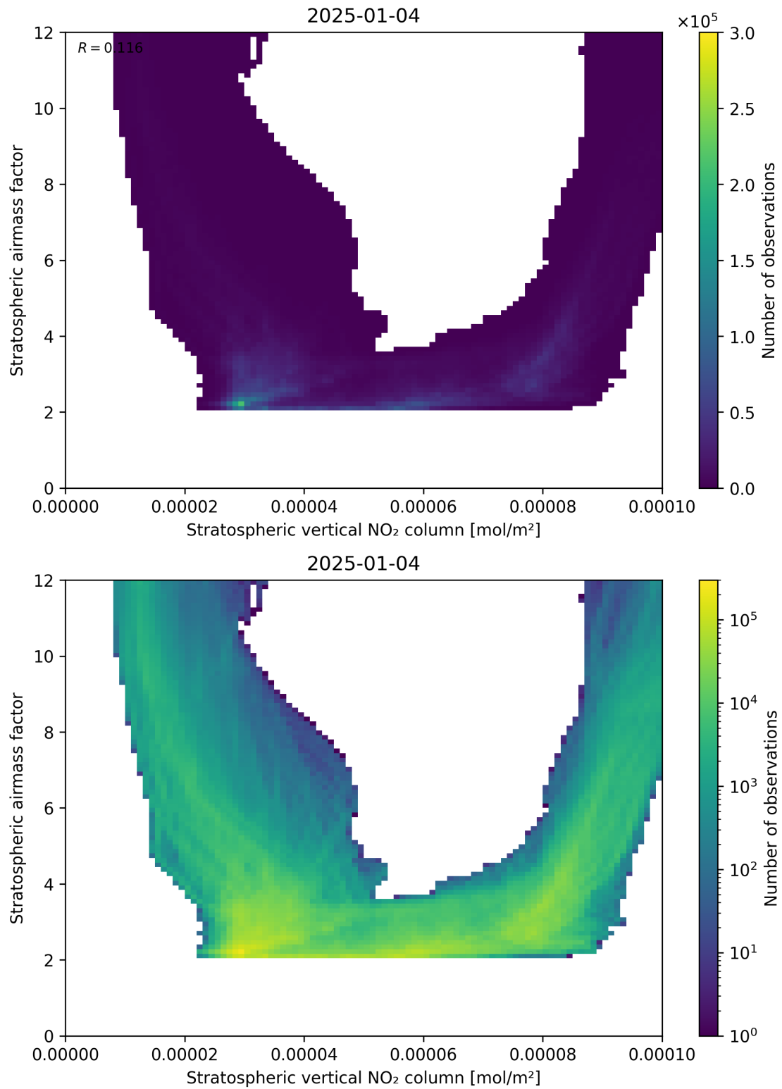
Figure 96: Scatter density plot of “Stratospheric vertical NO 2 column” against “Stratospheric airmass factor” for 2025-01-03 to 2025-01-05.
