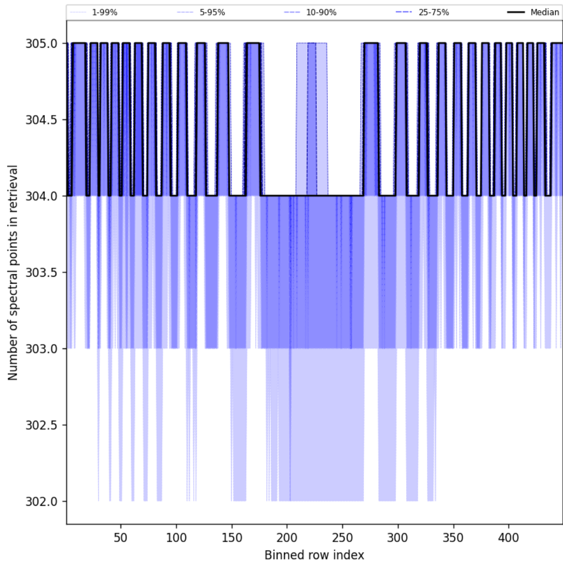
Figure 50: Along track statistics of “Number of spectral points in retrieval” for 2025-01-03 to 2025-01-05
