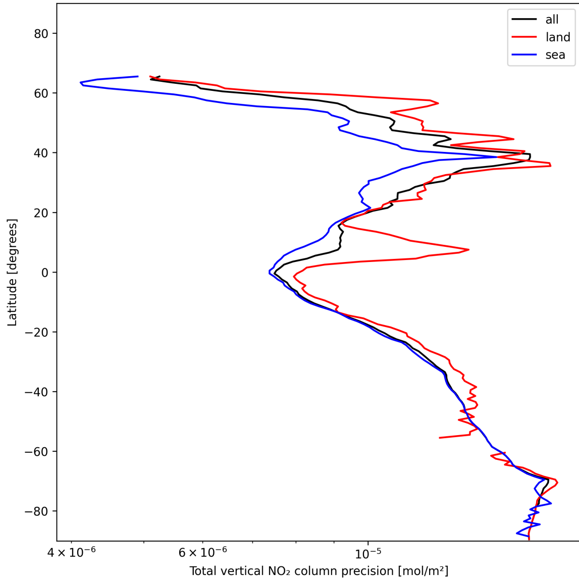
Figure 22: Zonal average of “Total vertical NO 2 column precision” for 2025-01-03 to 2025-01-05.
