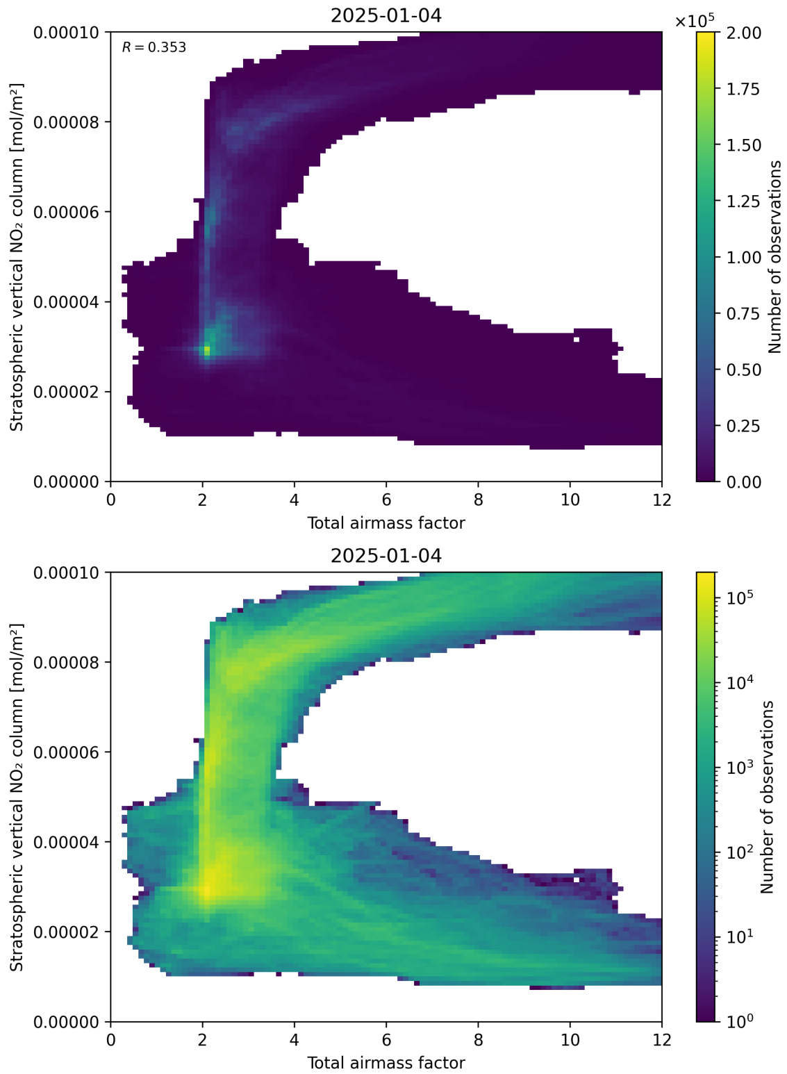
Figure 64: Scatter density plot of “Total airmass factor” against “Stratospheric vertical NO 2 column” for 2025-01-03 to 2025-01-05.
