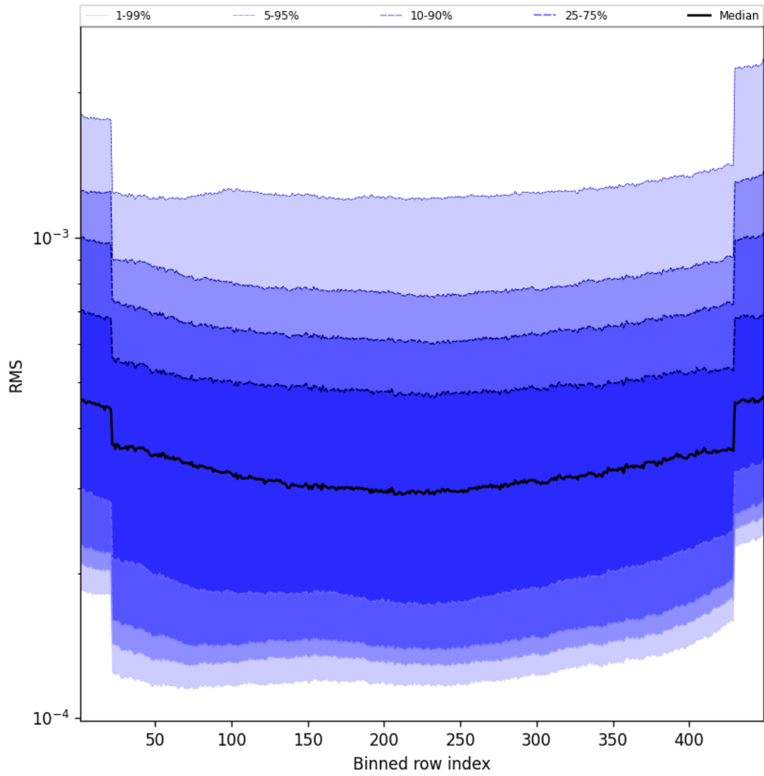
Figure 60: Along track statistics of “RMS” for 2025-01-03 to 2025-01-05
