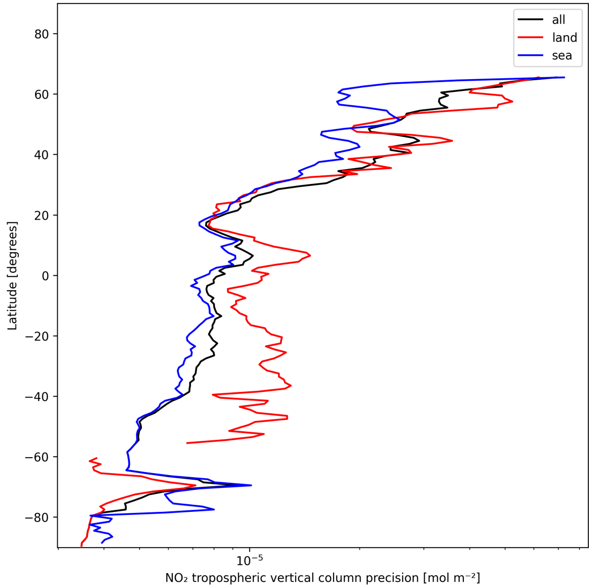
Figure 13: Zonal average of “NO 2 tropospheric vertical column precision” for 2025-01-03 to 2025-01-05.
