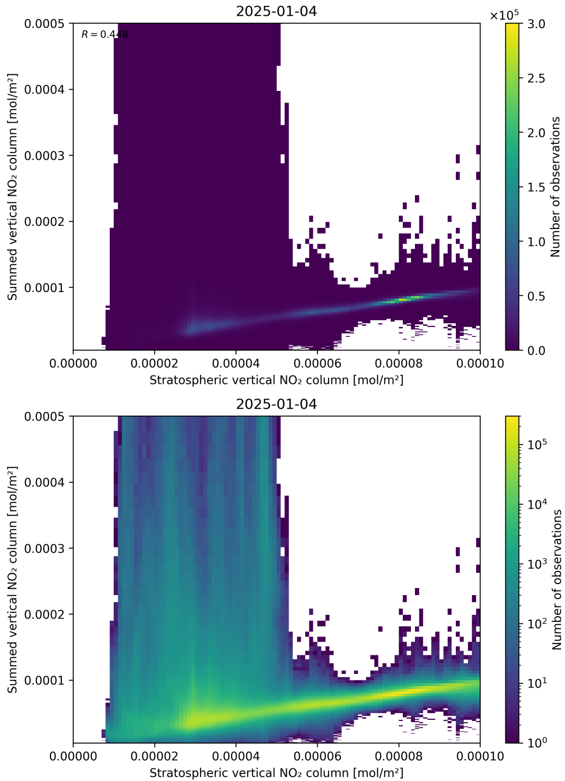
Figure 98: Scatter density plot of “Stratospheric vertical NO 2 column” against “Summed vertical NO 2 column” for 2025-01-03 to 2025-01-05.
