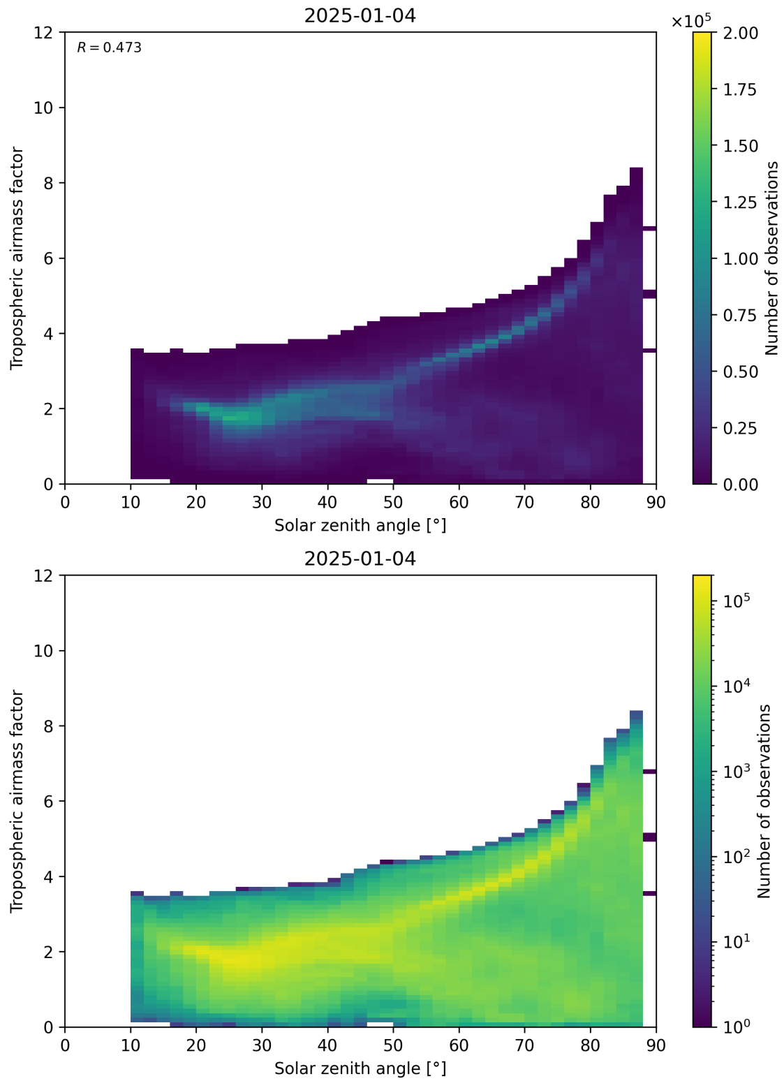
Figure 147: Scatter density plot of “Solar zenith angle” against “Tropospheric airmass factor” for 2025-01-03 to 2025-01-05.
