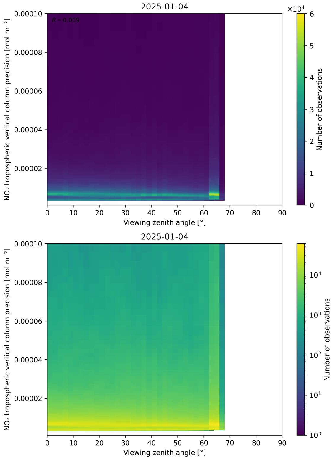
Figure 170: Scatter density plot of “Viewing zenith angle” against “NO 2 tropospheric vertical column precision” for 2025-01-03 to 2025-01-05.
