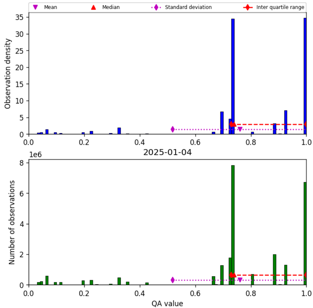
Figure 28: Histogram of “QA value” for 2025-01-03 to 2025-01-05
