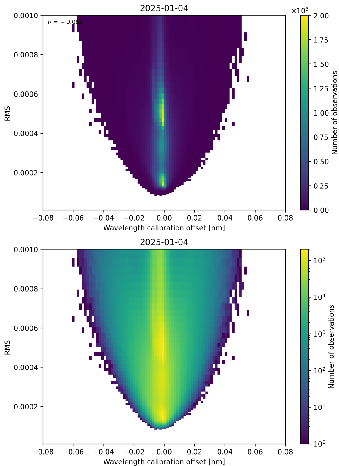
Figure 181: Scatter density plot of “Wavelength calibration offset” against “RMS” for 2025-01-03 to 2025-01-05.
