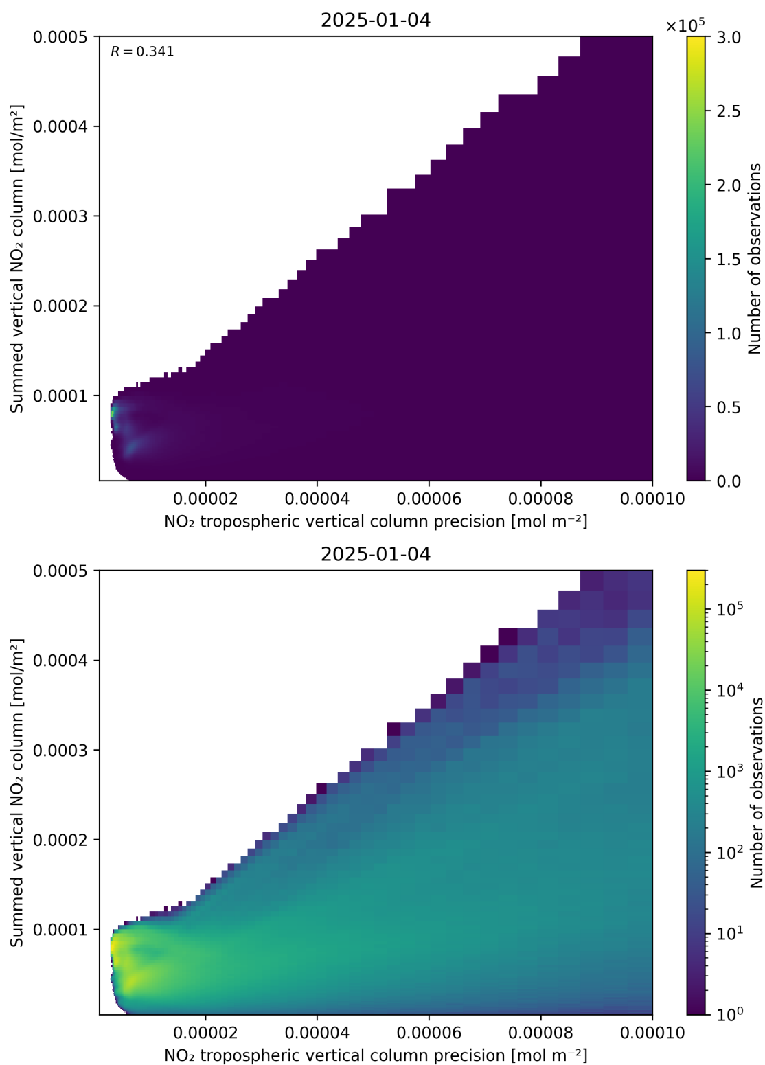
Figure 136: Scatter density plot of “NO 2 tropospheric vertical column precision” against “Summed vertical NO 2 column” for 2025-01-03 to 2025-01-05.
