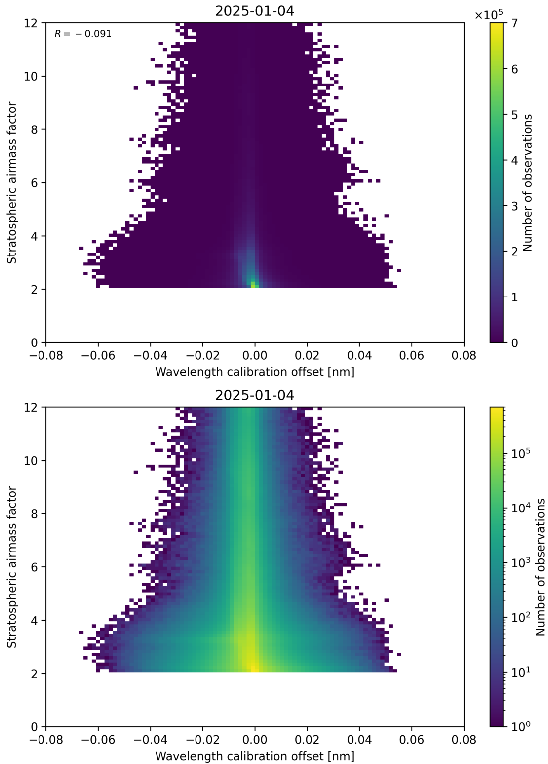
Figure 174: Scatter density plot of “Wavelength calibration offset” against “Stratospheric airmass factor” for 2025-01-03 to 2025-01-05.
