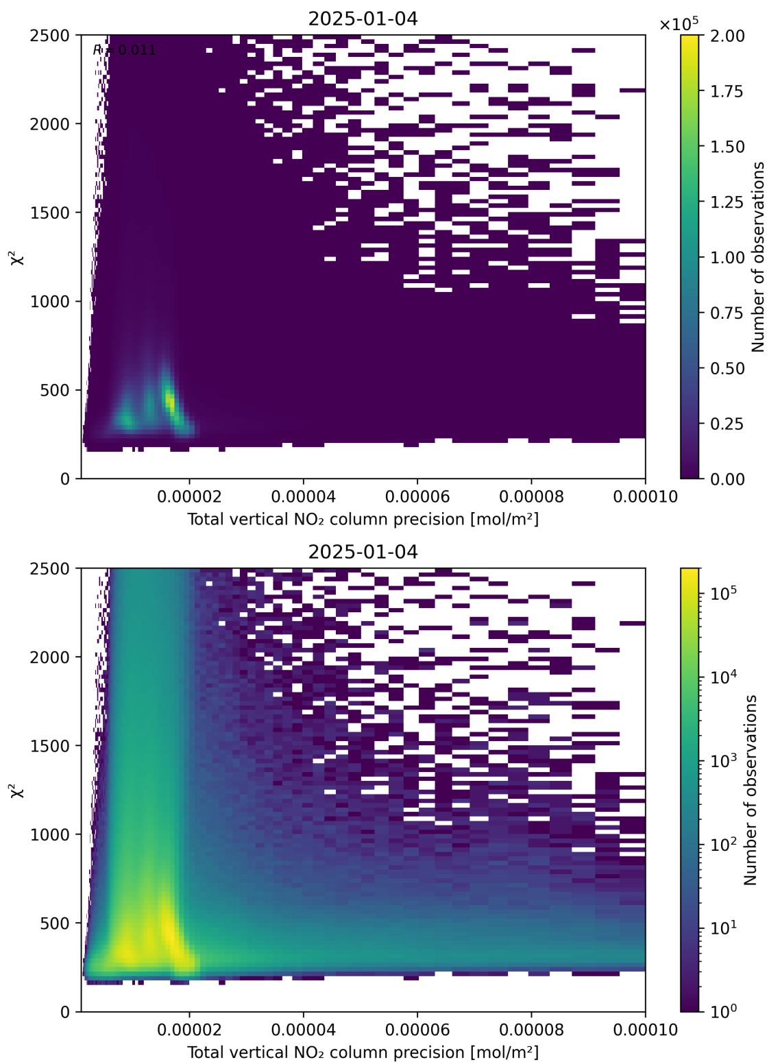
Figure 116: Scatter density plot of “Total vertical NO 2 column precision” against “ \chi^2 ” for 2025-01-03 to 2025-01-05.
