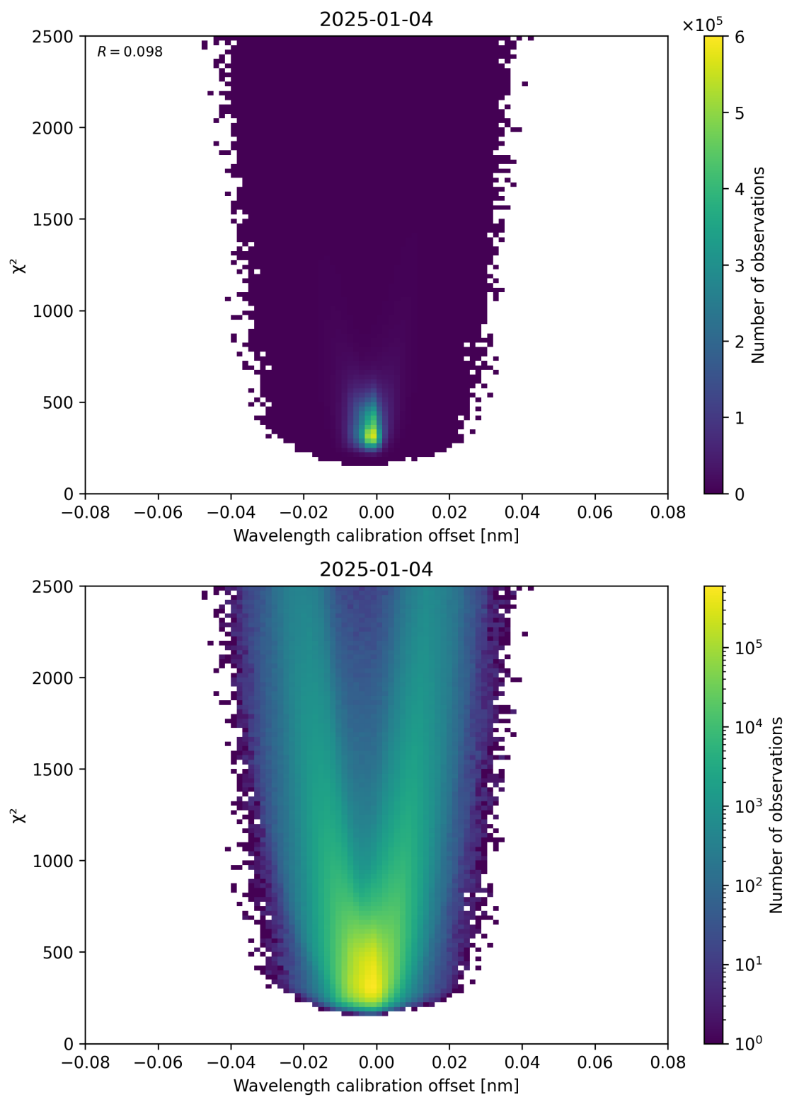
Figure 175: Scatter density plot of “Wavelength calibration offset” against “ \chi^2 ” for 2025-01-03 to 2025-01-05.
