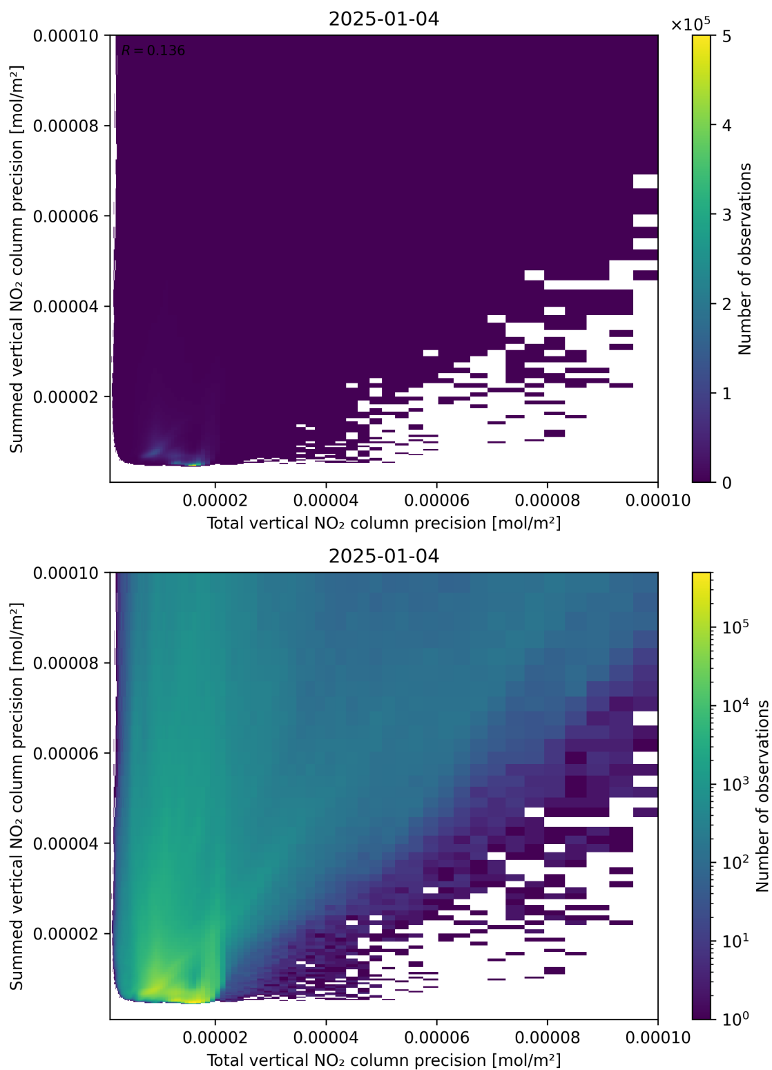
Figure 118: Scatter density plot of “Total vertical NO 2 column precision” against “Summed vertical NO 2 column precision” for 2025-01-03 to 2025-01-05.
