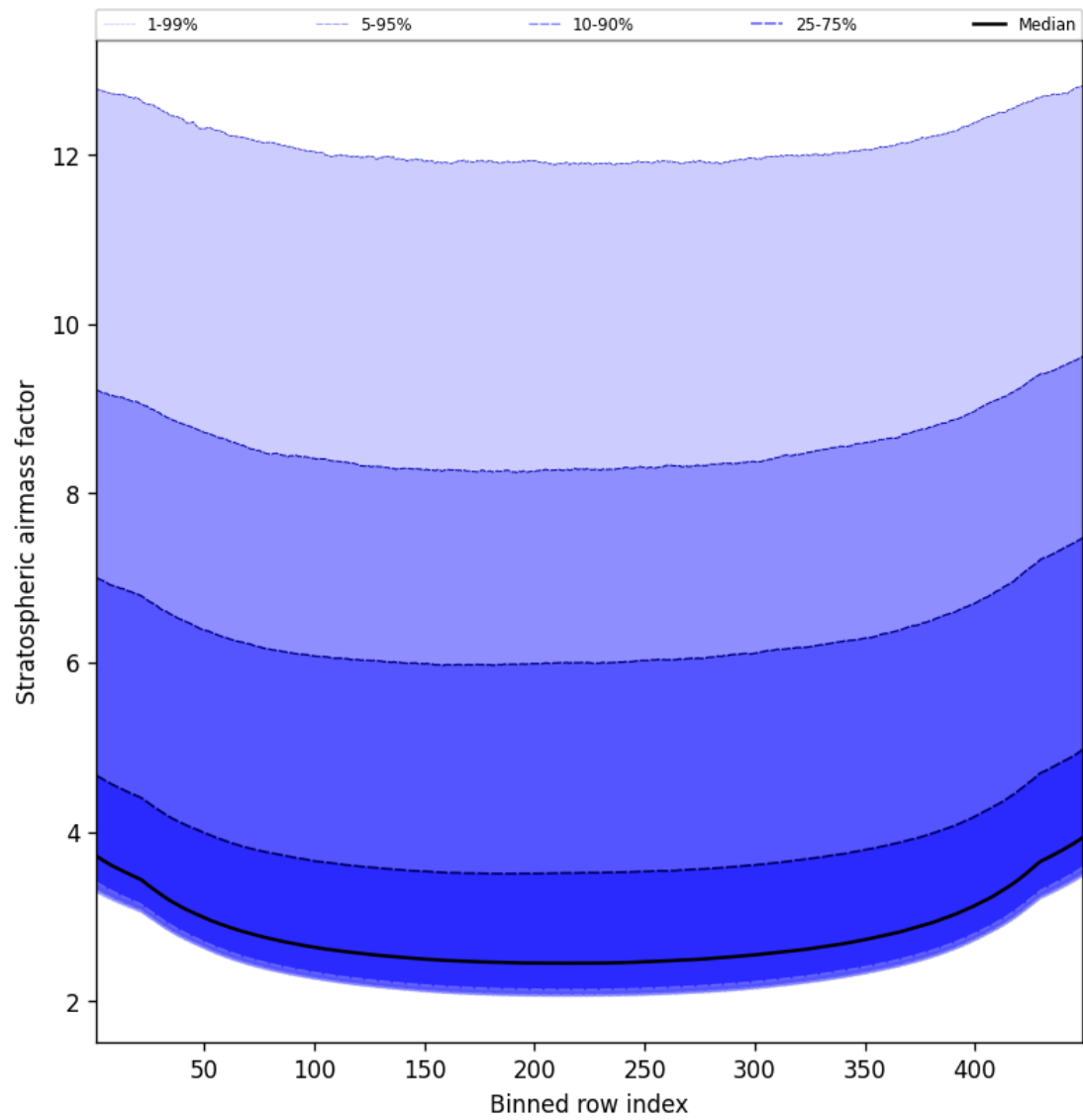
Figure 61: Along track statistics of “Stratospheric airmass factor” for 2025-01-03 to 2025-01-05
