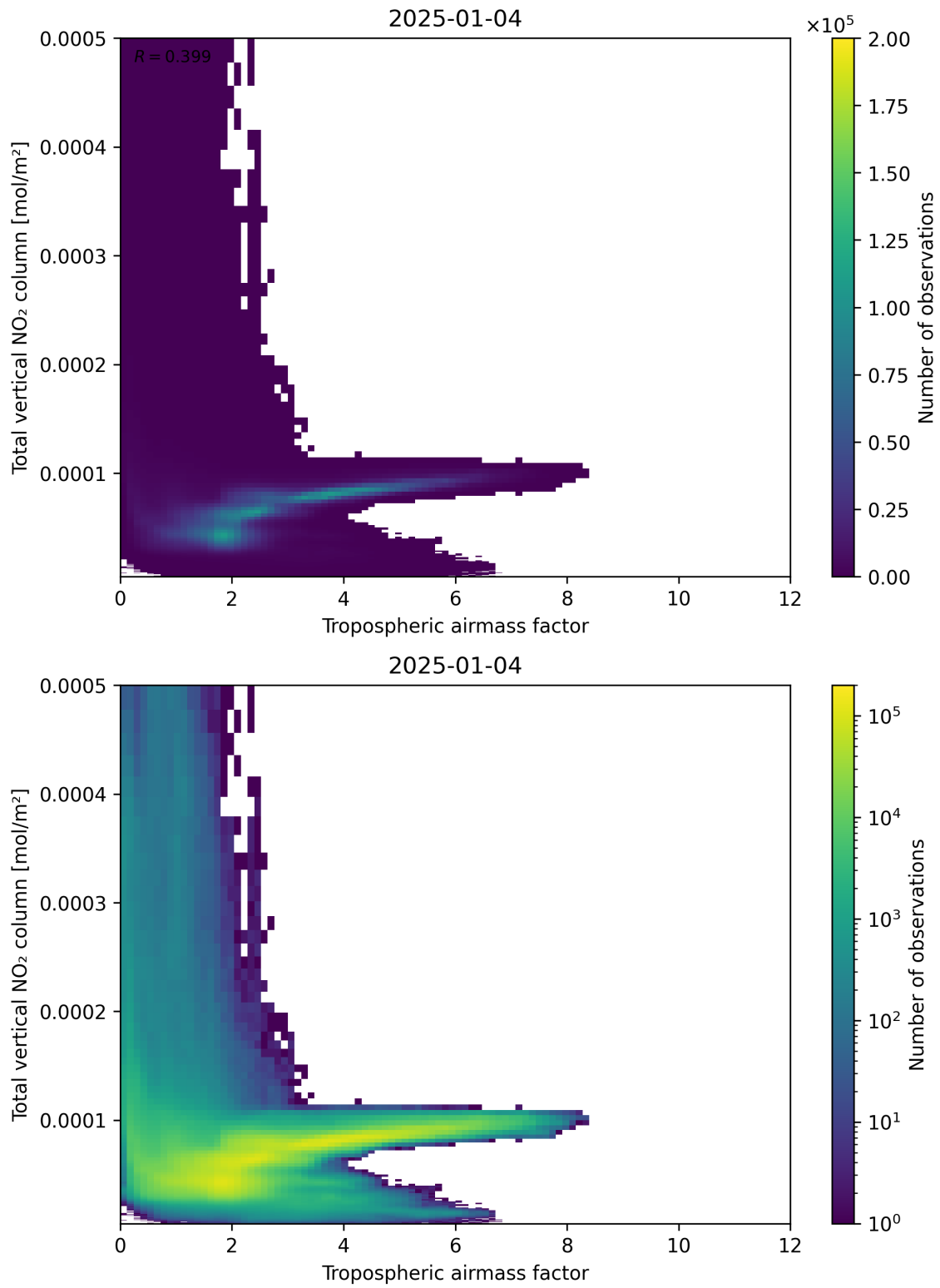
Figure 77: Scatter density plot of “Tropospheric airmass factor” against “Total vertical NO 2 column” for 2025-01-03 to 2025-01-05.
