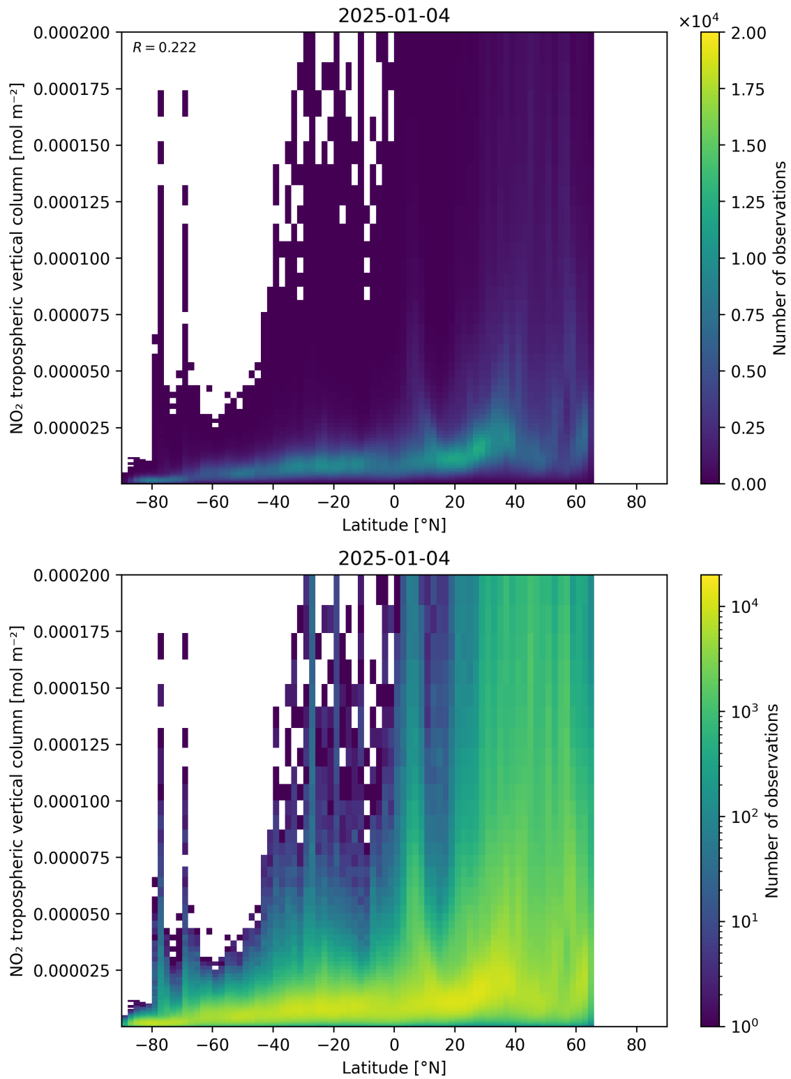
Figure 92: Scatter density plot of “Latitude” against “NO 2 tropospheric vertical column” for 2025-01-03 to 2025-01-05.
