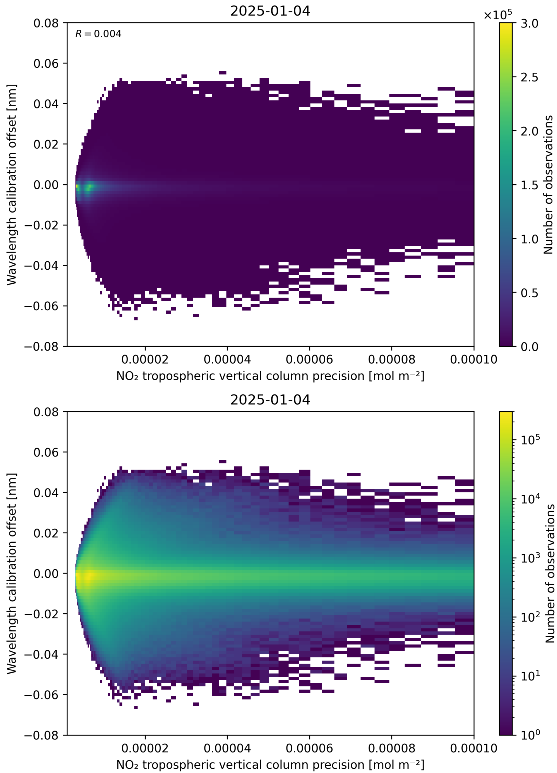
Figure 141: Scatter density plot of “NO 2 tropospheric vertical column precision” against “Wavelength calibration offset” for 2025-01-03 to 2025-01-05.
