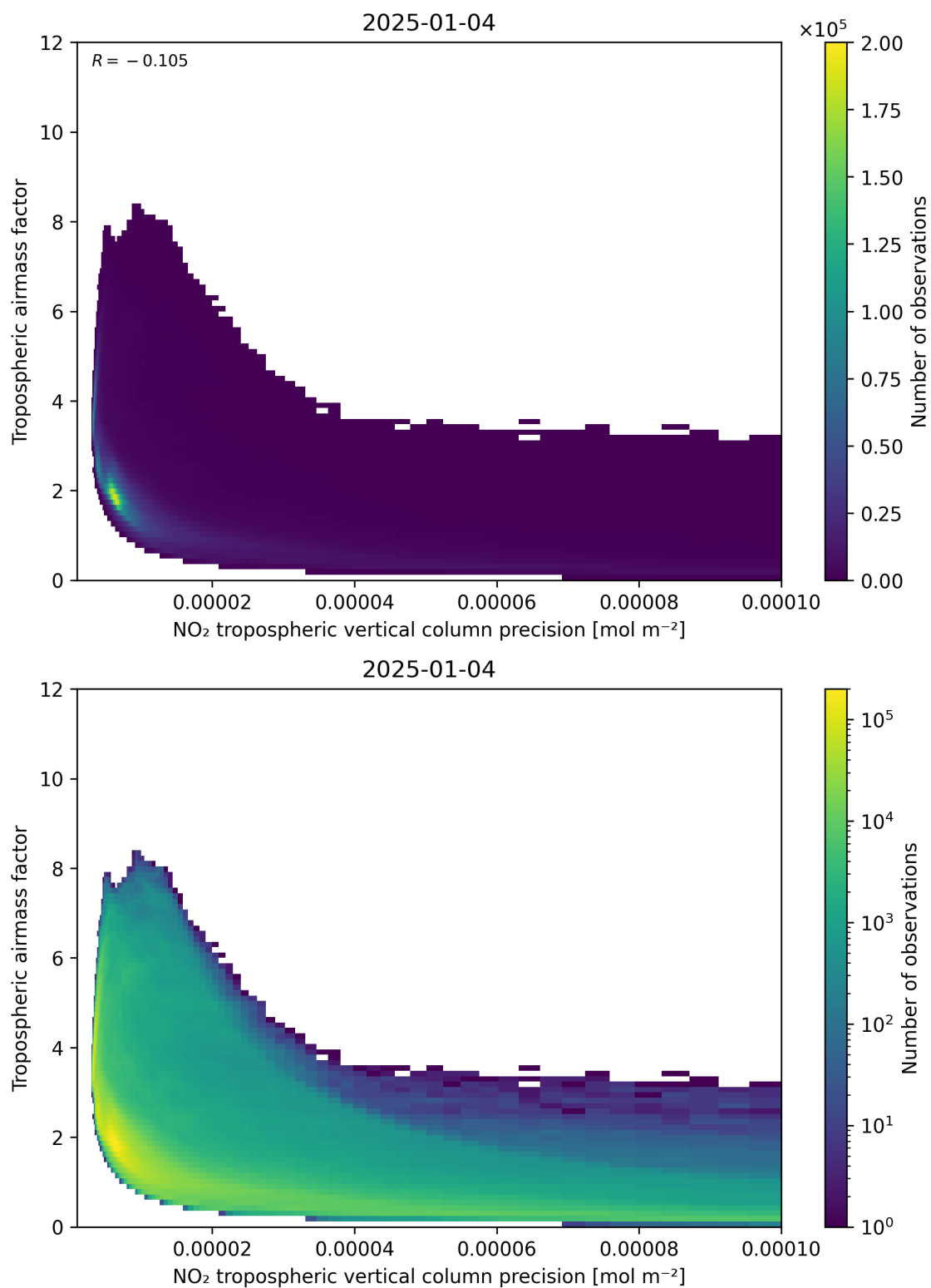
Figure 133: Scatter density plot of “NO 2 tropospheric vertical column precision” against “Tropospheric airmass factor” for 2025-01-03 to 2025-01-05.
