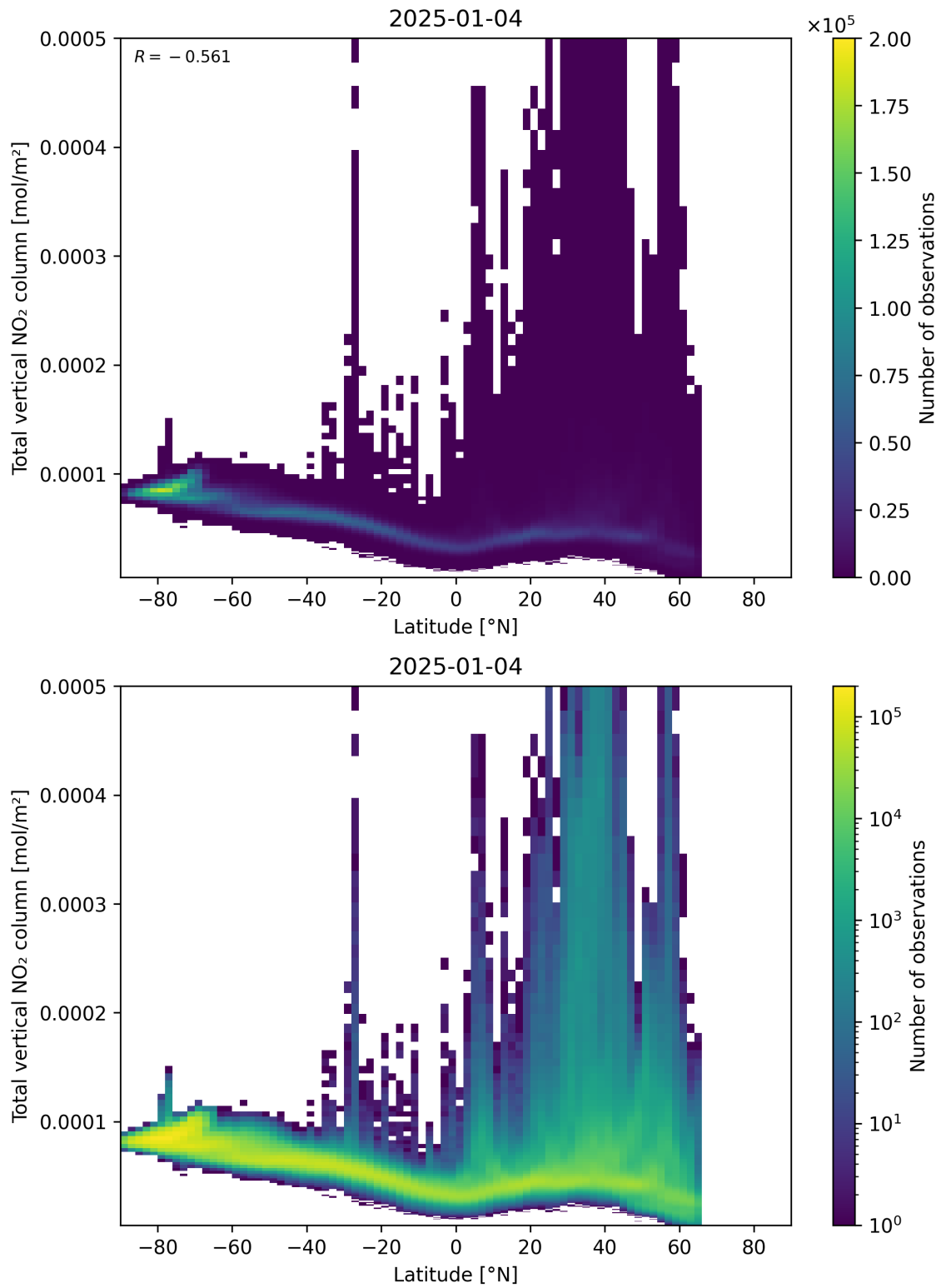
Figure 90: Scatter density plot of “Latitude” against “Total vertical NO 2 column” for 2025-01-03 to 2025-01-05.
