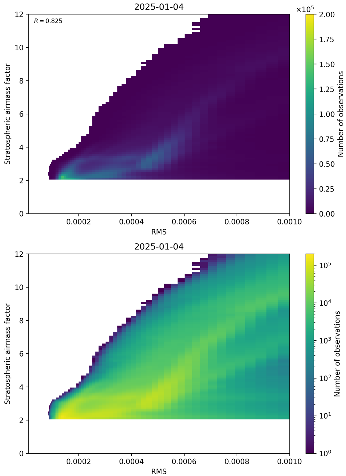
Figure 144: Scatter density plot of “RMS” against “Stratospheric airmass factor” for 2025-01-03 to 2025-01-05.
