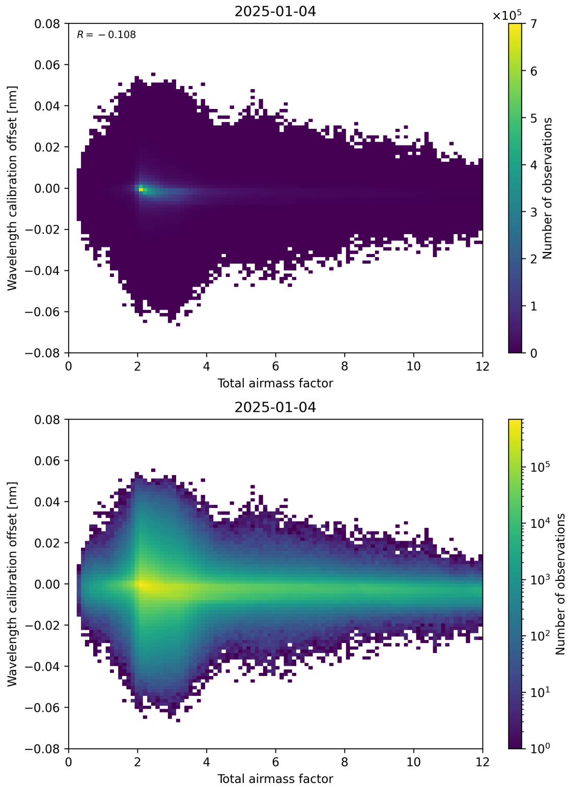
Figure 70: Scatter density plot of “Total airmass factor” against “Wavelength calibration offset” for 2025-01-03 to 2025-01-05.
