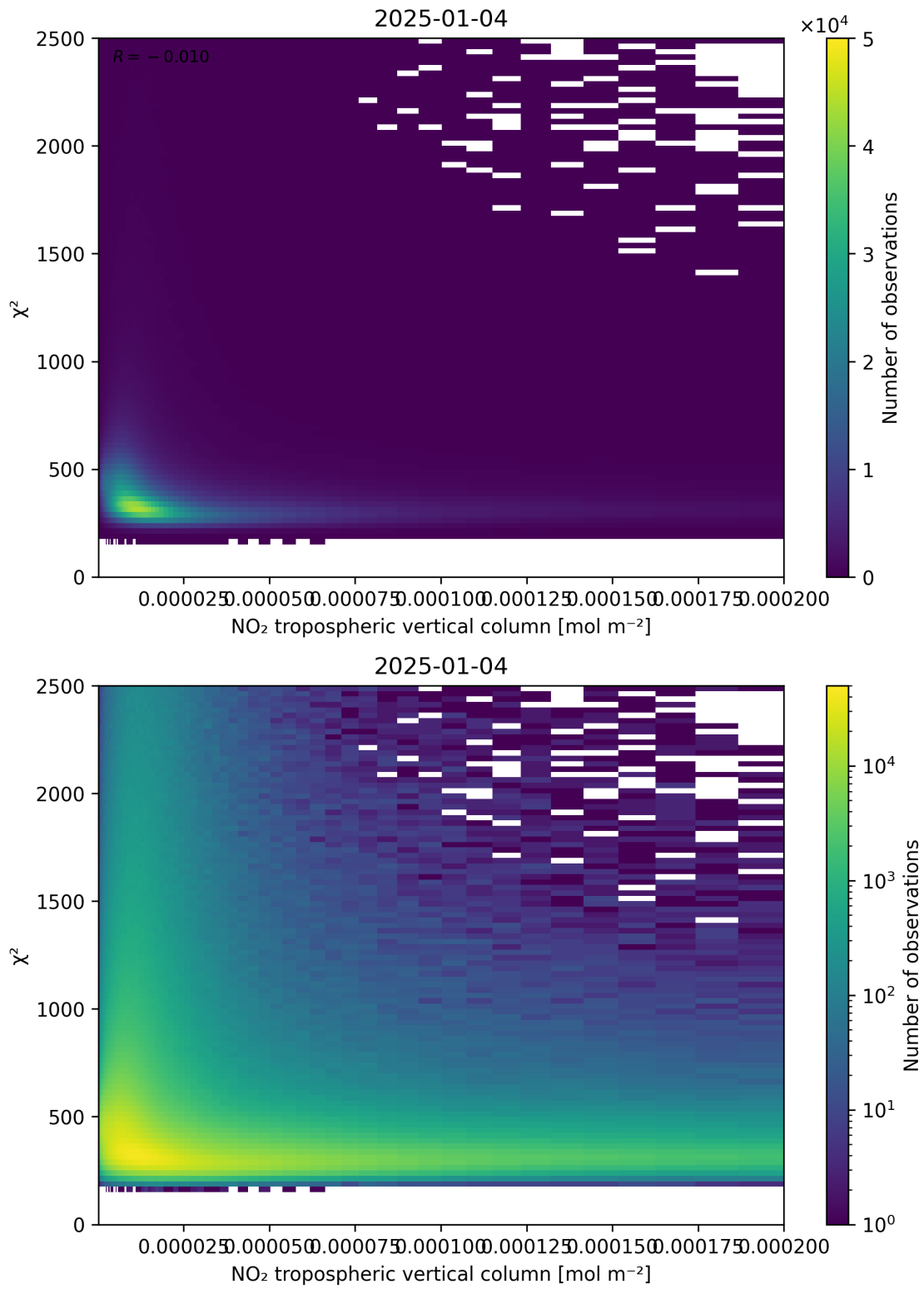
Figure 124: Scatter density plot of “NO 2 tropospheric vertical column” against “ \chi^2 ” for 2025-01-03 to 2025-01-05.
