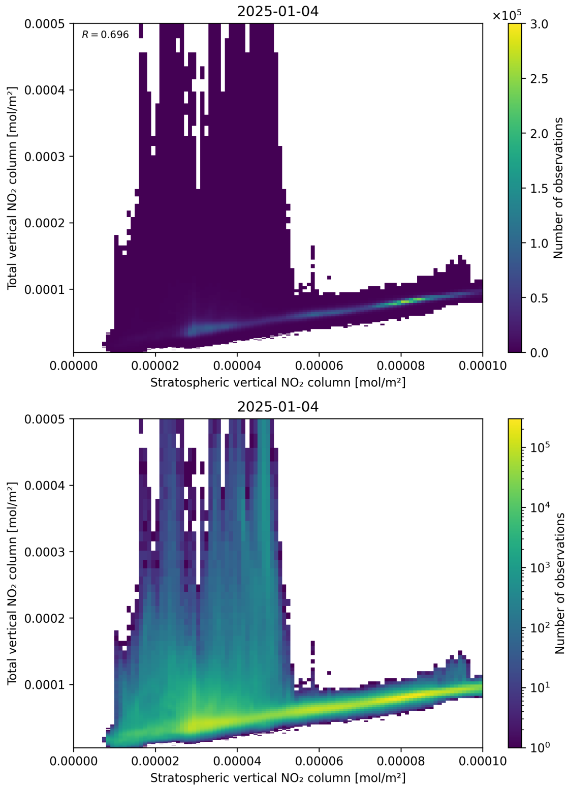
Figure 100: Scatter density plot of “Stratospheric vertical NO 2 column” against “Total vertical NO 2 column” for 2025-01-03 to 2025-01-05.
