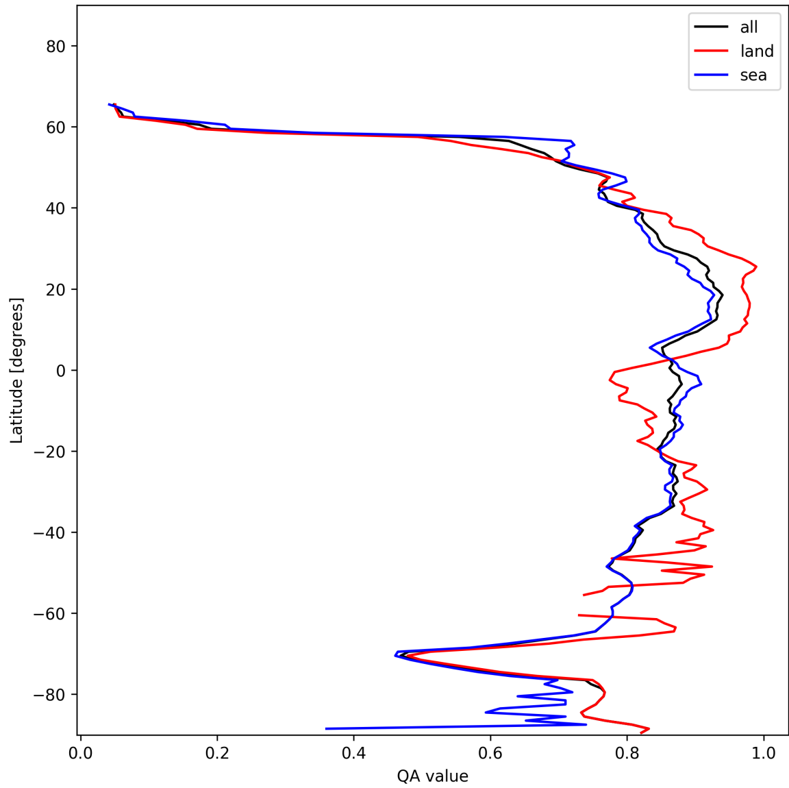
Figure 11: Zonal average of “QA value” for 2025-01-03 to 2025-01-05.
