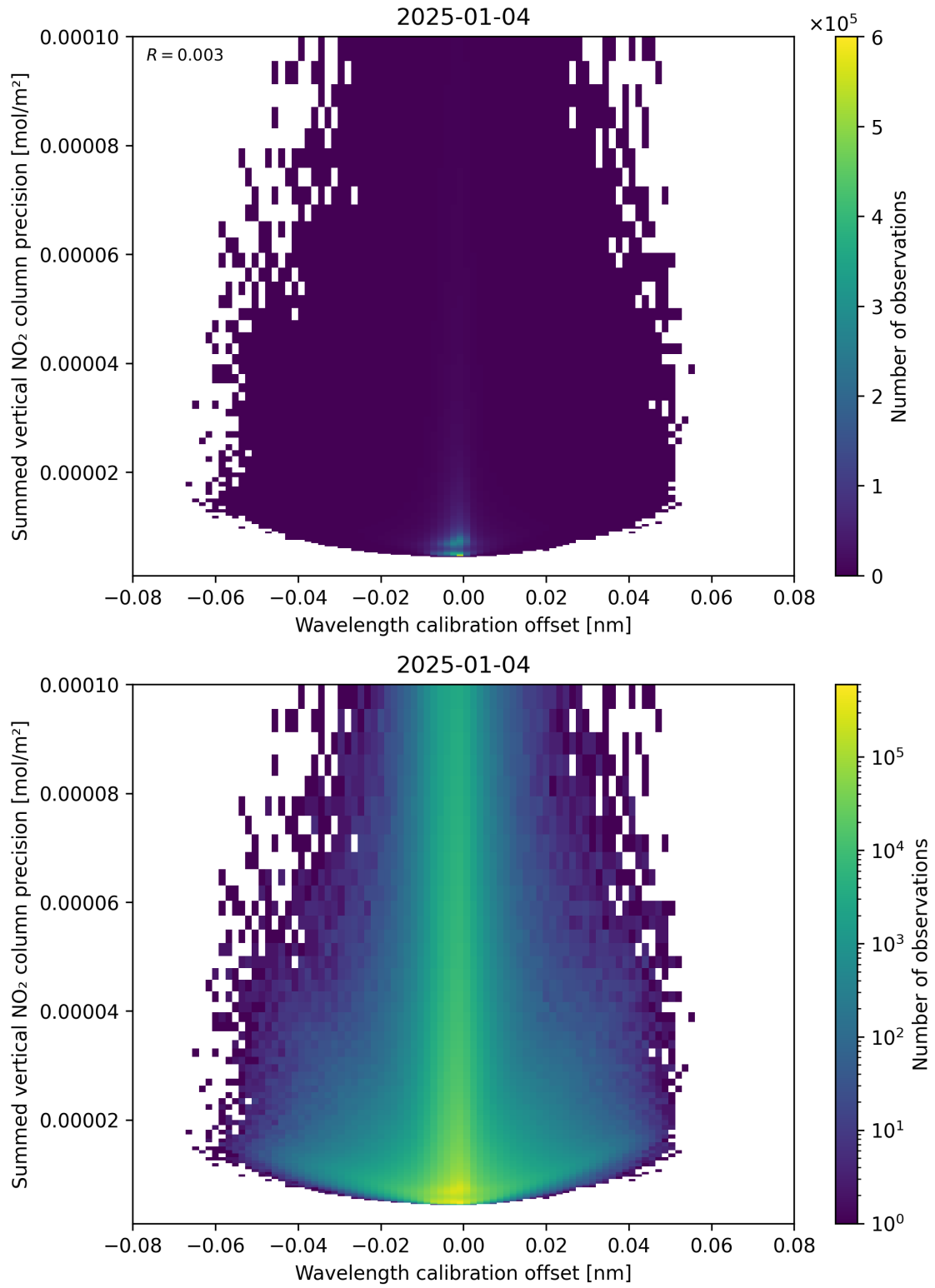
Figure 178: Scatter density plot of “Wavelength calibration offset” against “Summed vertical NO 2 column precision” for 2025-01-03 to 2025-01-05.
