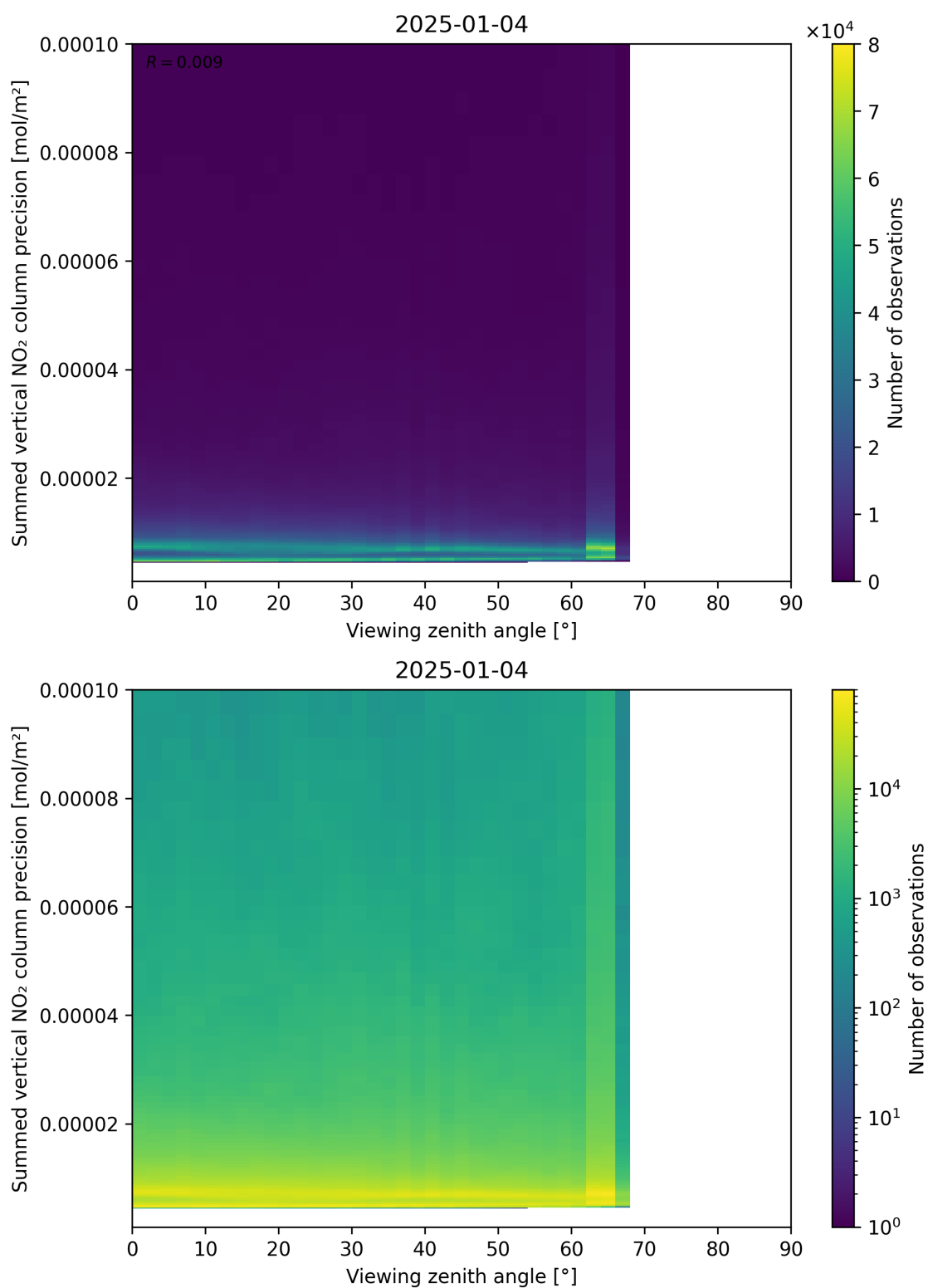
Figure 166: Scatter density plot of “Viewing zenith angle” against “Summed vertical NO 2 column precision” for 2025-01-03 to 2025-01-05.
