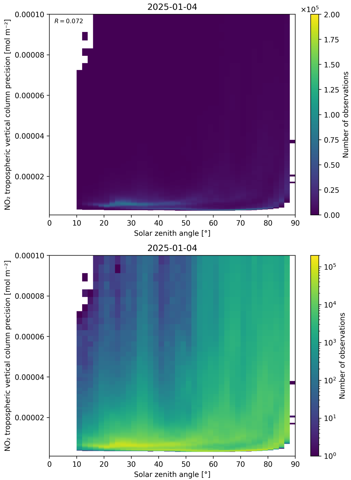
Figure 156: Scatter density plot of “Solar zenith angle” against “NO 2 tropospheric vertical column precision” for 2025-01-03 to 2025-01-05.
