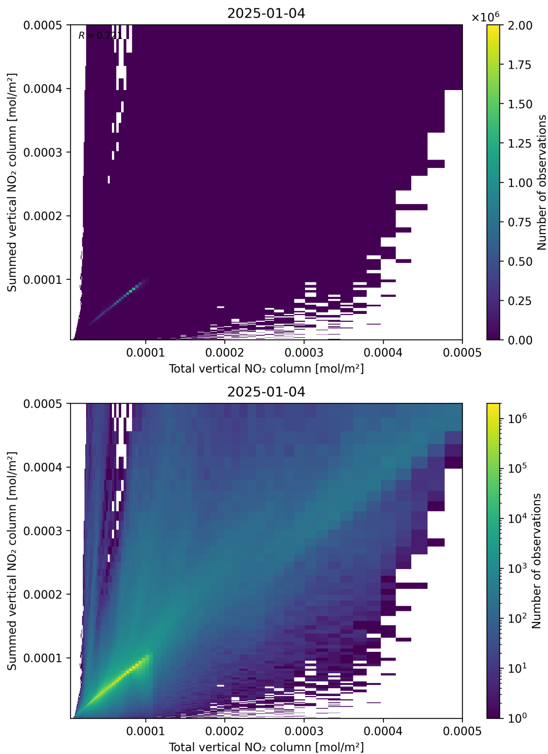
Figure 112: Scatter density plot of “Total vertical NO 2 column” against “Summed vertical NO 2 column” for 2025-01-03 to 2025-01-05.
