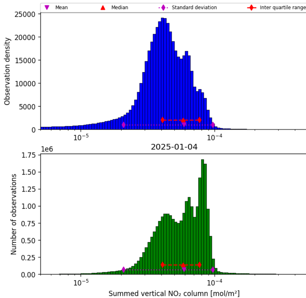
Figure 40: Histogram of “Summed vertical NO 2 column” for 2025-01-03 to 2025-01-05
