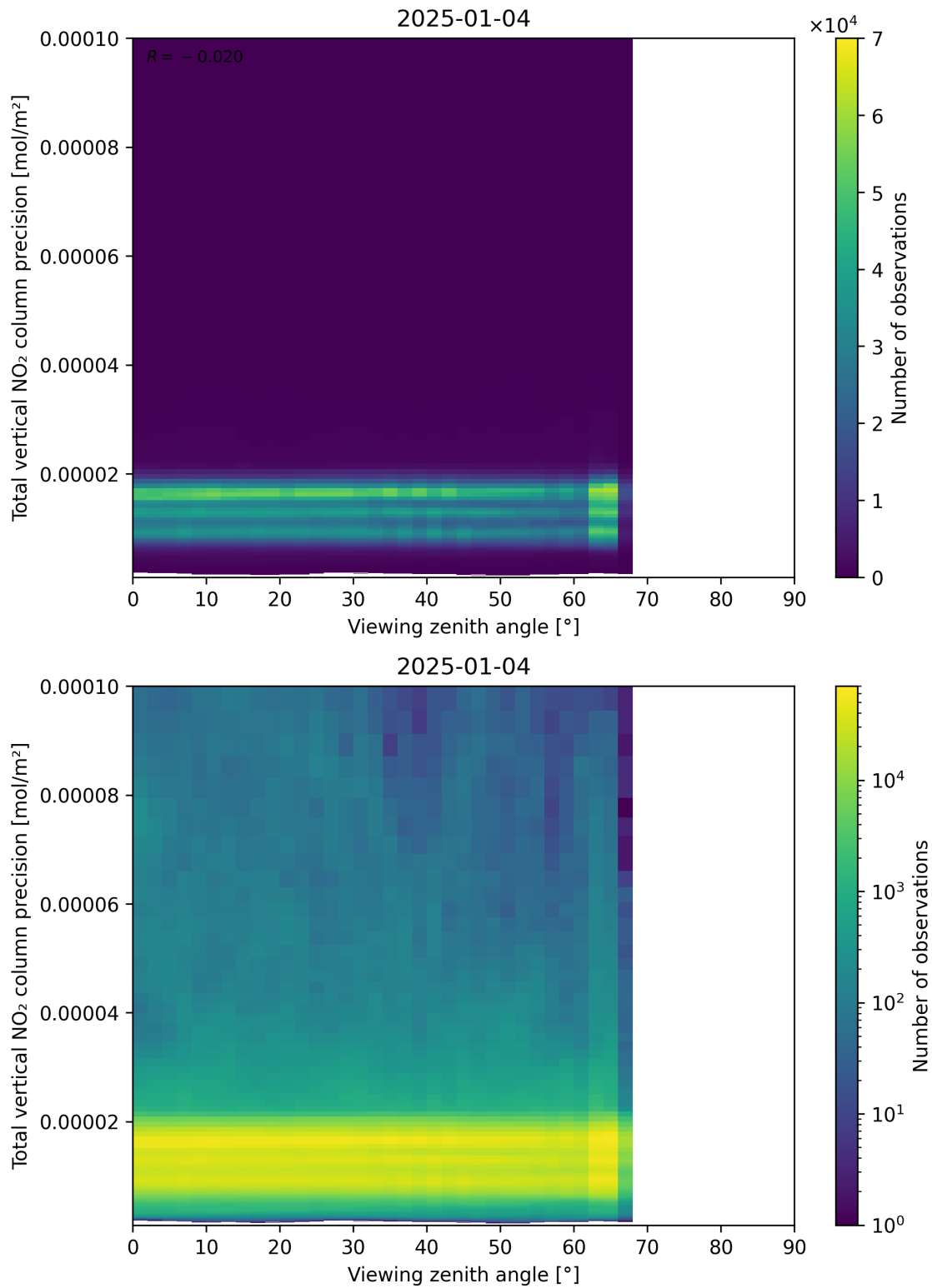
Figure 168: Scatter density plot of “Viewing zenith angle” against “Total vertical NO 2 column precision” for 2025-01-03 to 2025-01-05.
