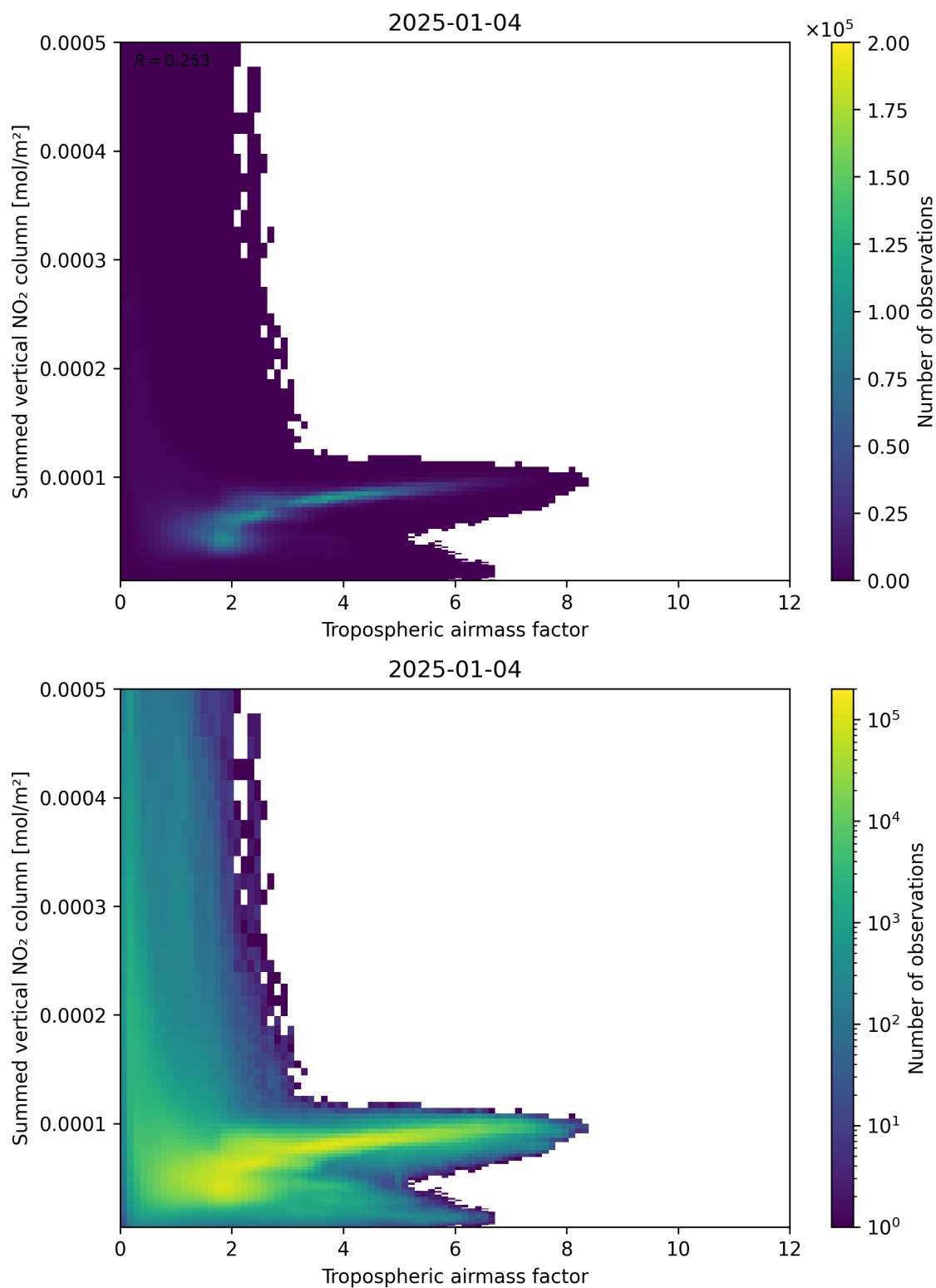
Figure 75: Scatter density plot of “Tropospheric air mass factor” against “Summed vertical NO 2 column” for 2025-01-03 to 2025-01-05.
