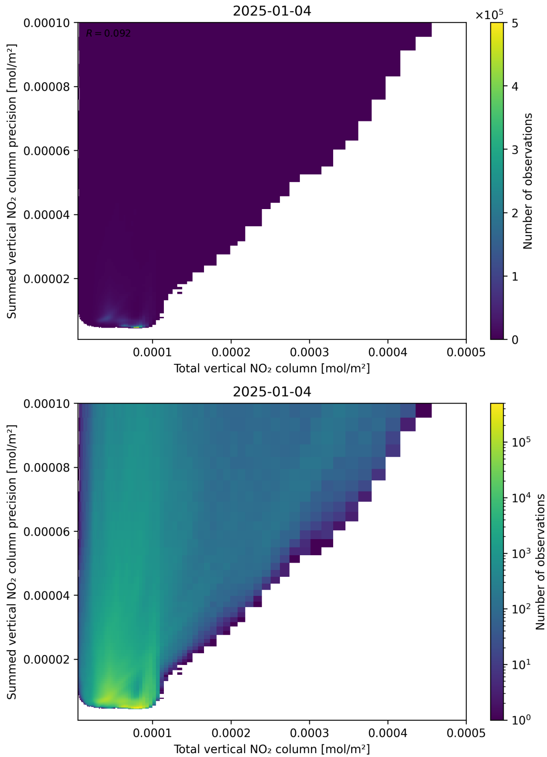
Figure 113: Scatter density plot of “Total vertical NO 2 column” against “Summed vertical NO 2 column precision” for 2025-01-03 to 2025-01-05.
