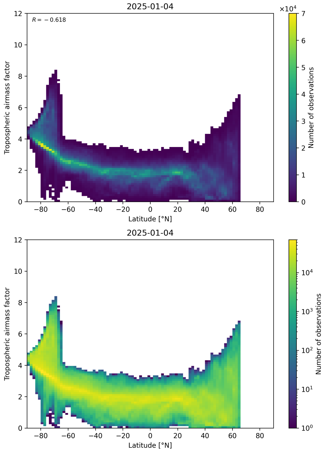
Figure 85: Scatter density plot of “Latitude” against “Tropospheric air mass factor” for 2025-01-03 to 2025-01-05.
