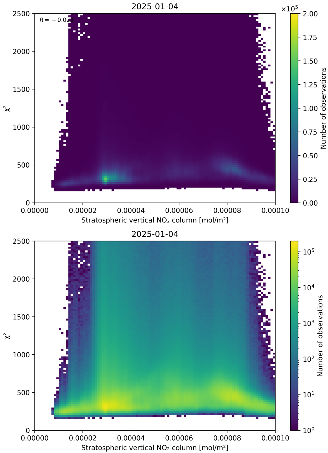
Figure 97: Scatter density plot of “Stratospheric vertical NO 2 column” against “ \chi^2 ” for 2025-01-03 to 2025-01-05.
