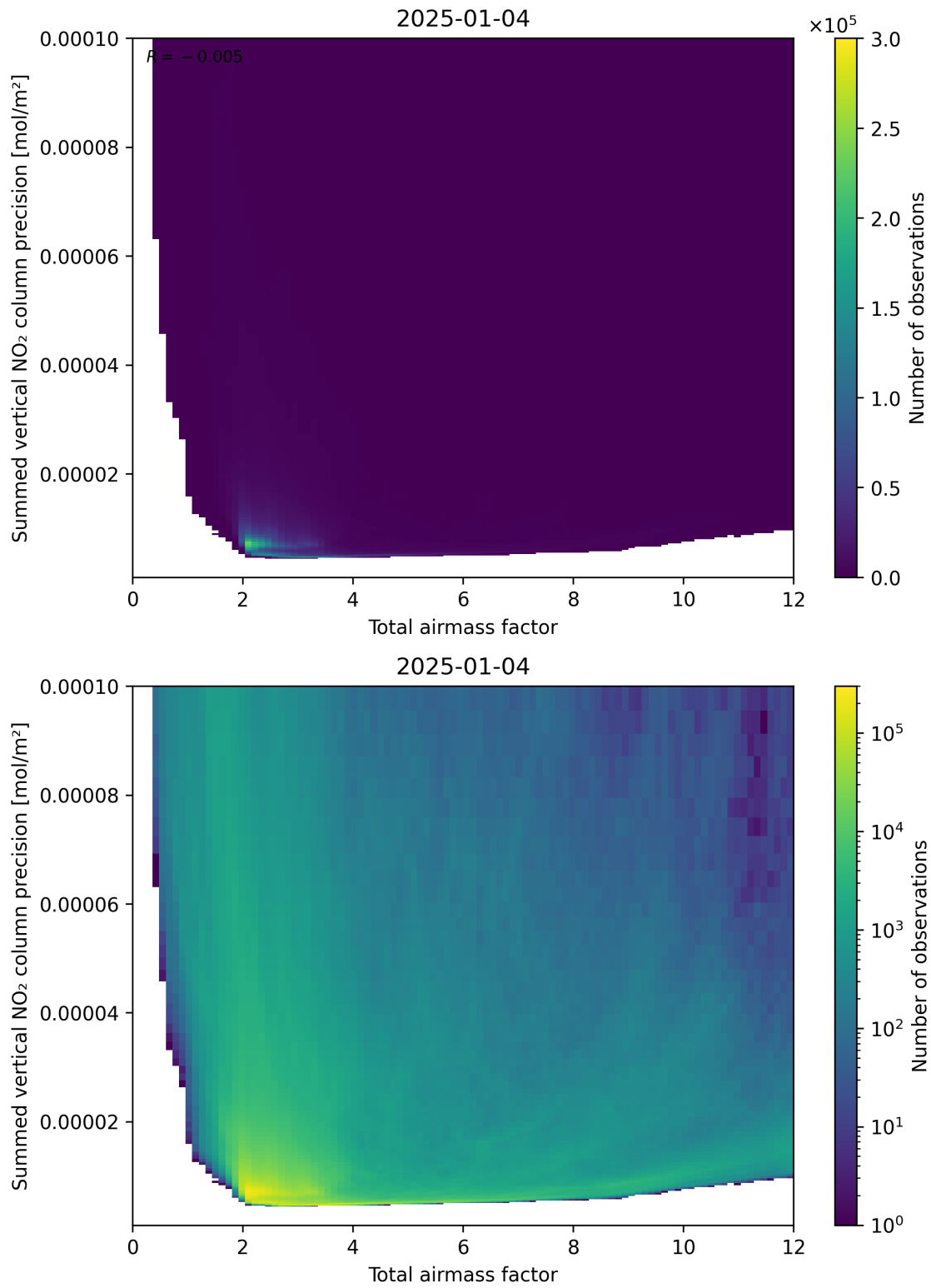
Figure 66: Scatter density plot of “Total airmass factor” against “Summed vertical NO 2 column precision” for 2025-01-03 to 2025-01-05.
