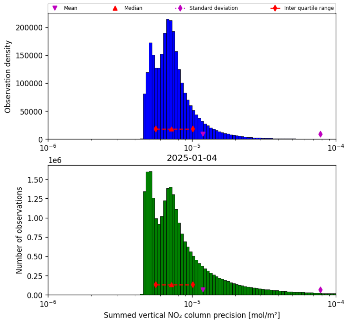
Figure 41: Histogram of “Summed vertical NO 2 column precision” for 2025-01-03 to 2025-01-05
