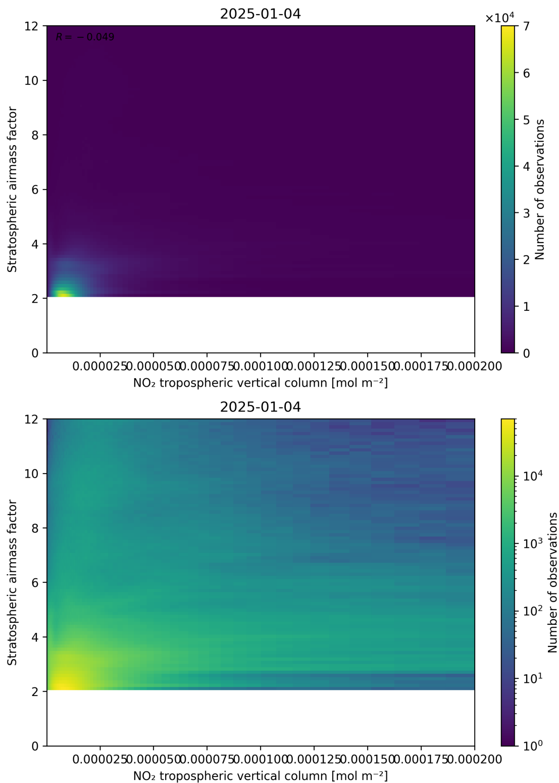
Figure 121: Scatter density plot of “NO 2 tropospheric vertical column” against “Stratospheric airmass factor” for 2025-01-03 to 2025-01-05.
