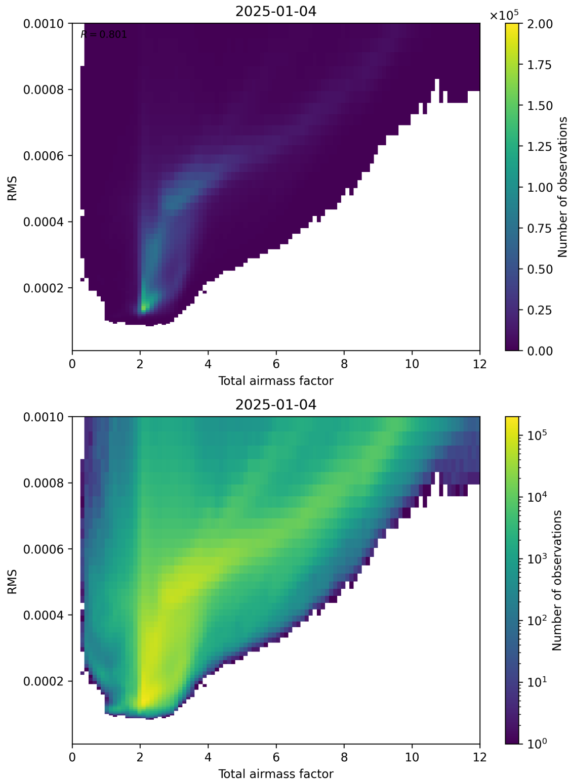
Figure 69: Scatter density plot of “Total airmass factor” against “RMS” for 2025-01-03 to 2025-01-05.
