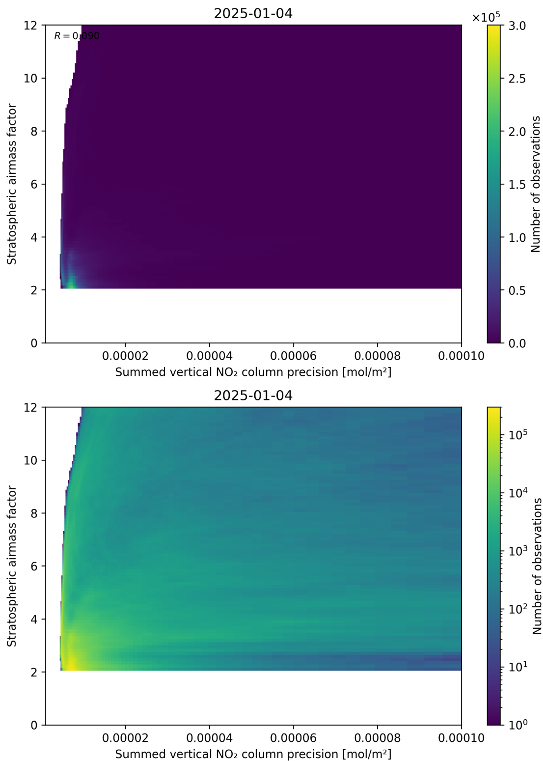
Figure 106: Scatter density plot of “Summed vertical NO 2 column precision” against “Stratospheric airmass factor” for 2025-01-03 to 2025-01-05.
