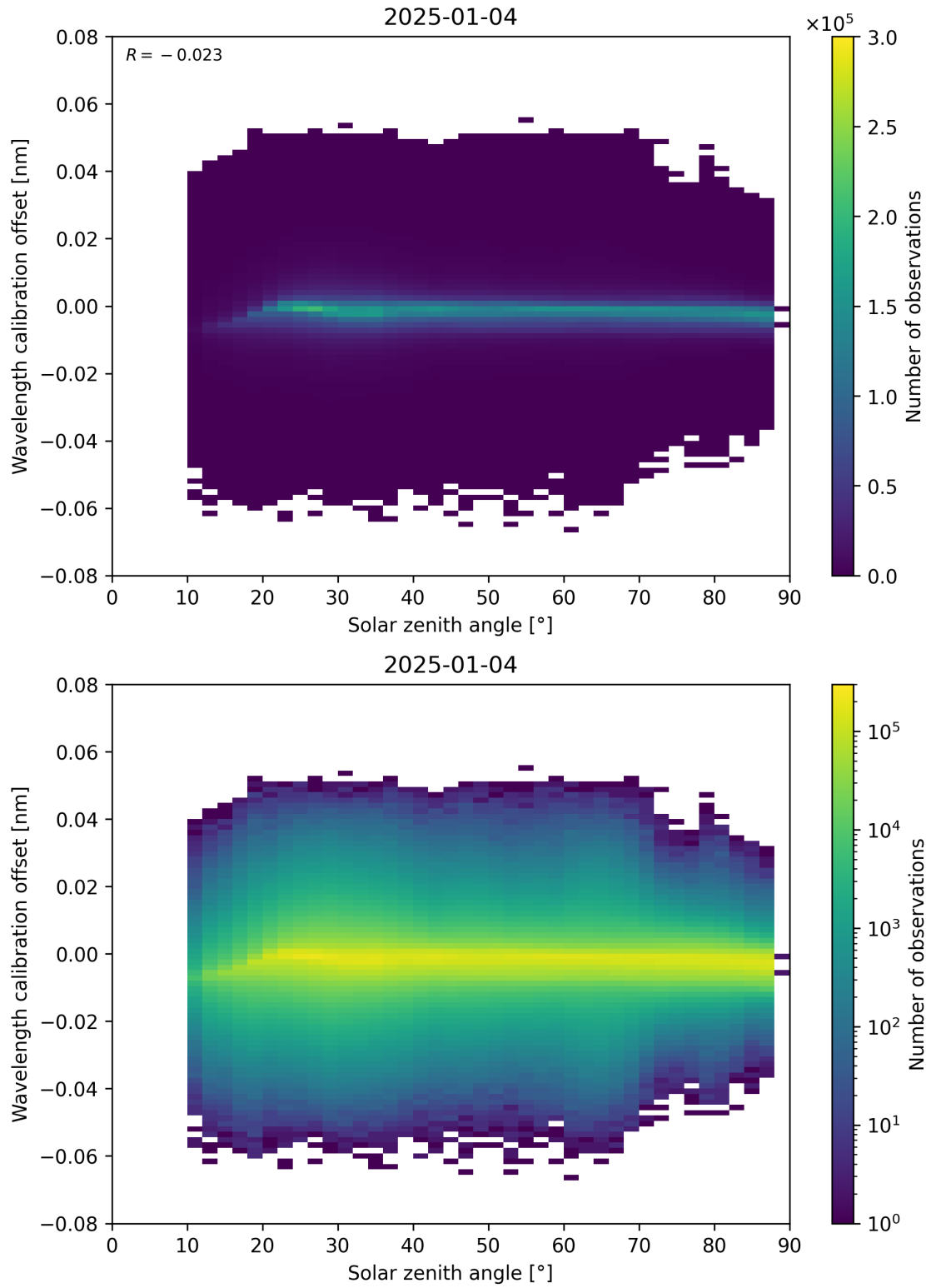
Figure 158: Scatter density plot of “Solar zenith angle” against “Wavelength calibration offset” for 2025-01-03 to 2025-01-05.
