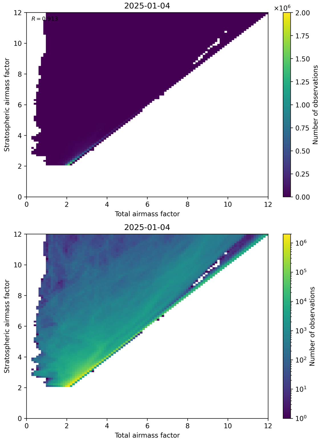
Figure 62: Scatter density plot of “Total airmass factor” against “Stratospheric airmass factor” for 2025-01-03 to 2025-01-05.
