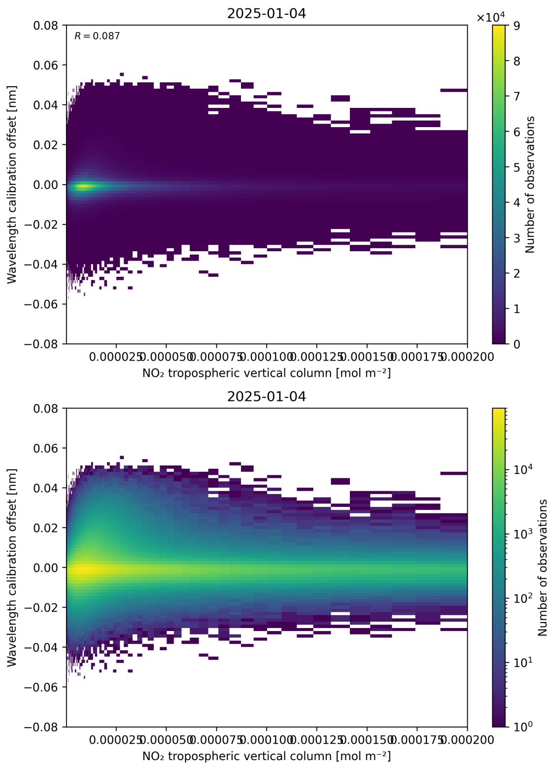
Figure 143: Scatter density plot of “NO 2 tropospheric vertical column” against “Wavelength calibration offset” for 2025-01-03 to 2025-01-05.
