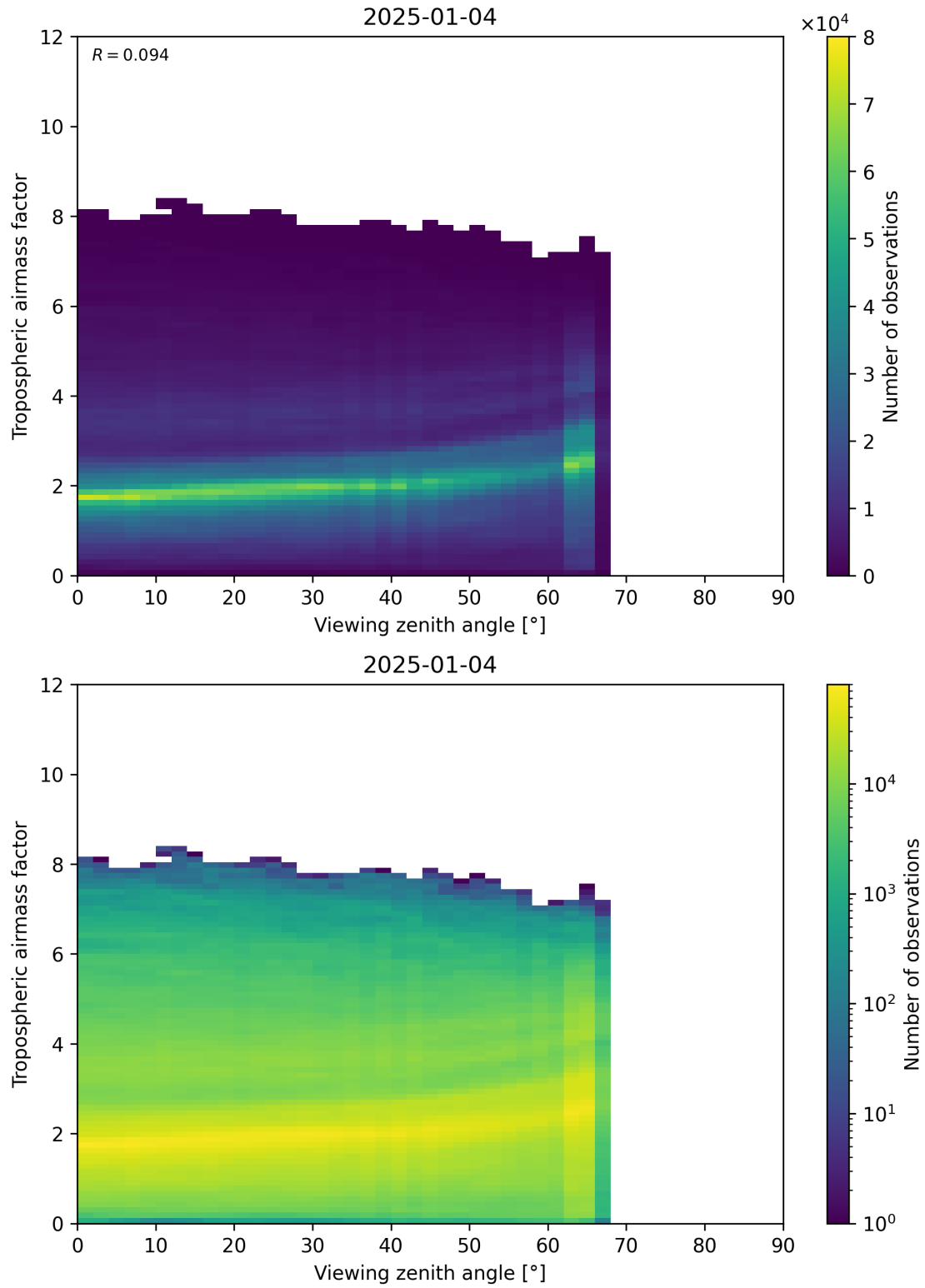
Figure 161: Scatter density plot of “Viewing zenith angle” against “Tropospheric airmass factor” for 2025-01-03 to 2025-01-05.
