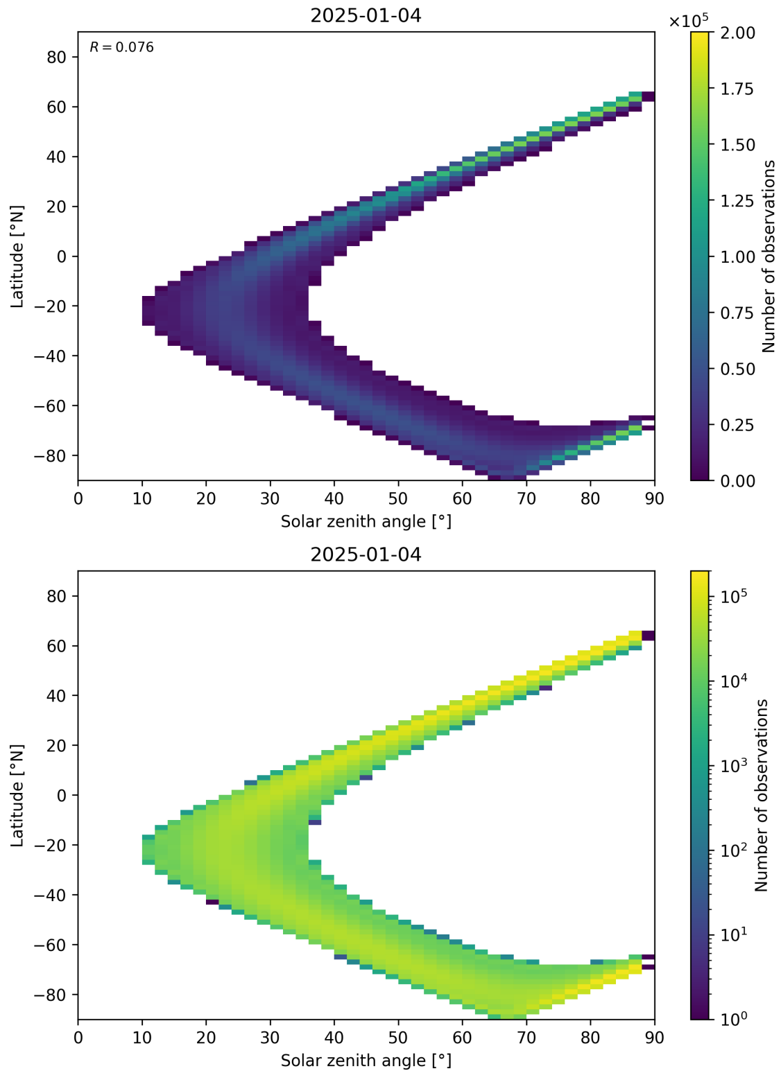
Figure 149: Scatter density plot of “Solar zenith angle” against “Latitude” for 2025-01-03 to 2025-01-05.
