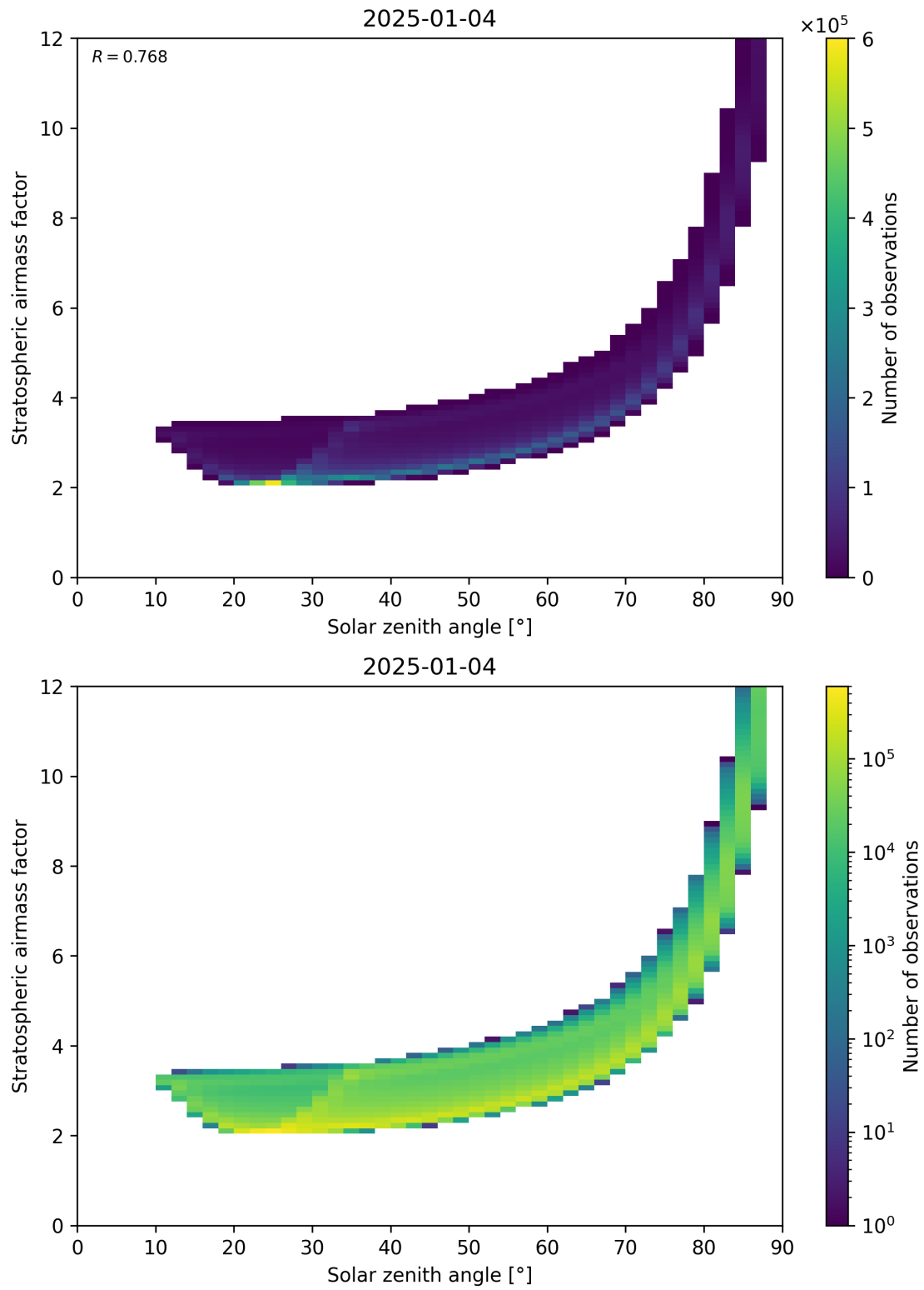
Figure 145: Scatter density plot of “Solar zenith angle” against “Stratospheric airmass factor” for 2025-01-03 to 2025-01-05.
