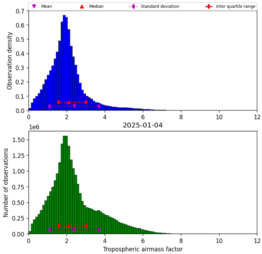
Figure 31: Histogram of “Tropospheric airmass factor” for 2025-01-03 to 2025-01-05
