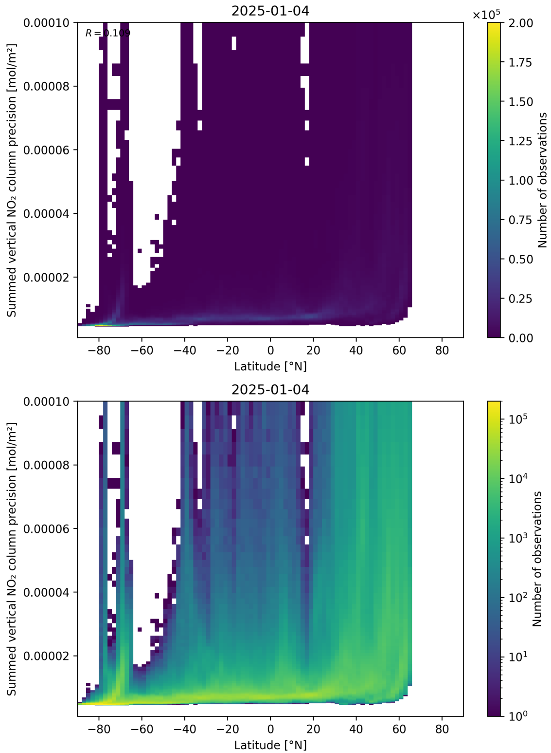
Figure 89: Scatter density plot of “Latitude” against “Summed vertical NO 2 column precision” for 2025-01-03 to 2025-01-05.
