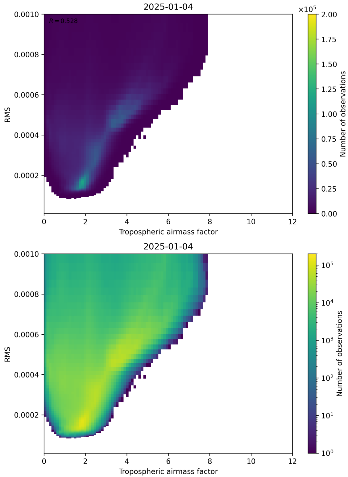
Figure 79: Scatter density plot of “Tropospheric airmass factor” against “RMS” for 2025-01-03 to 2025-01-05.
