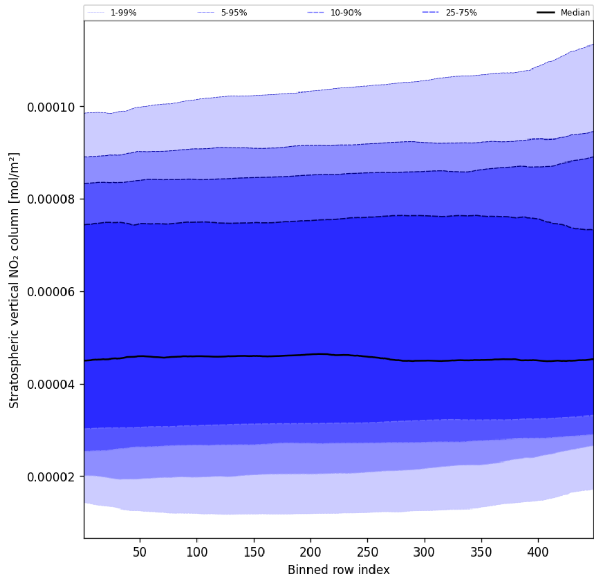
Figure 53: Along track statistics of “Stratospheric vertical NO 2 column” for 2025-01-03 to 2025-01-05
