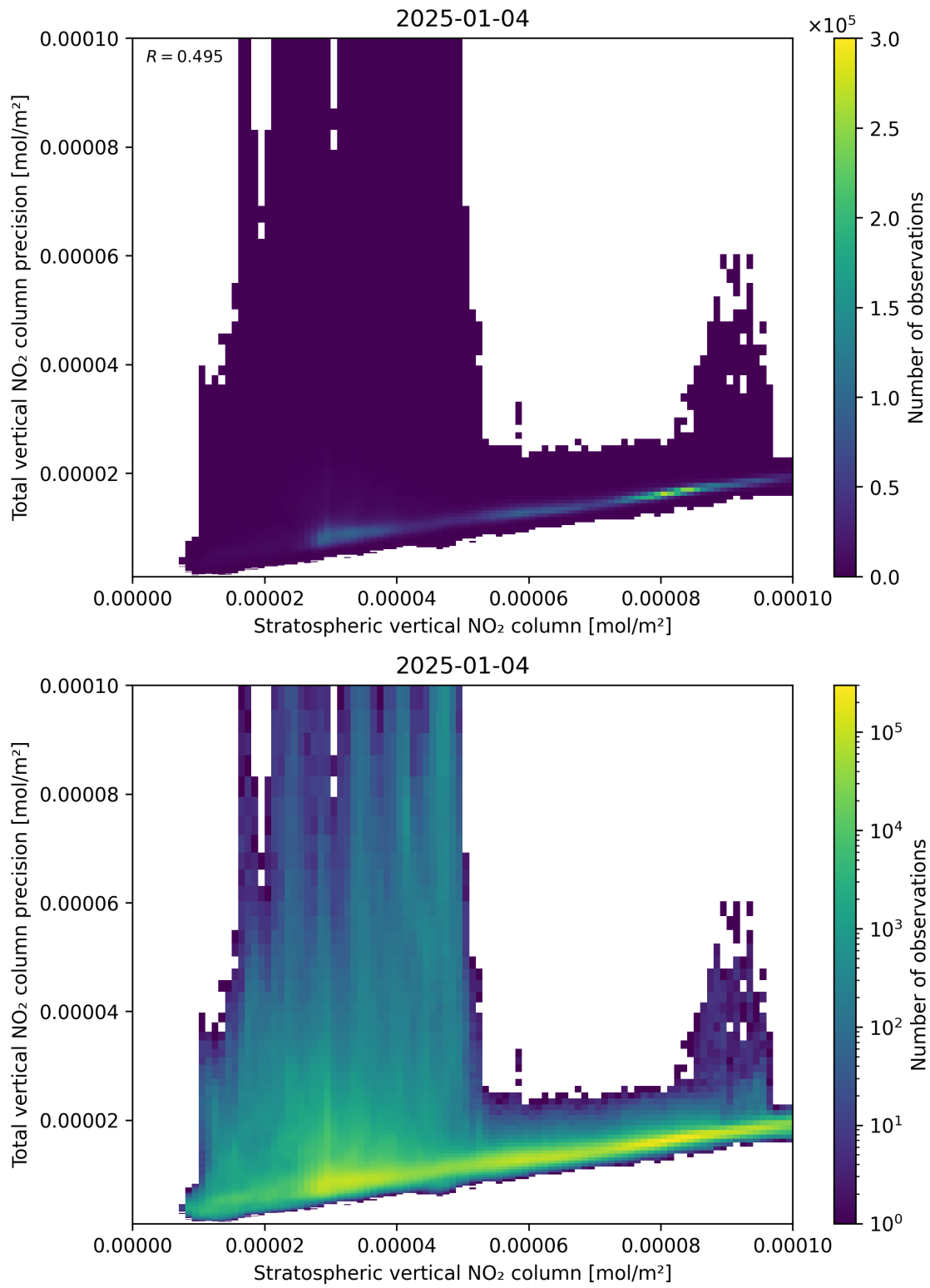
Figure 101: Scatter density plot of “Stratospheric vertical NO 2 column” against “Total vertical NO 2 column precision” for 2025-01-03 to 2025-01-05.
