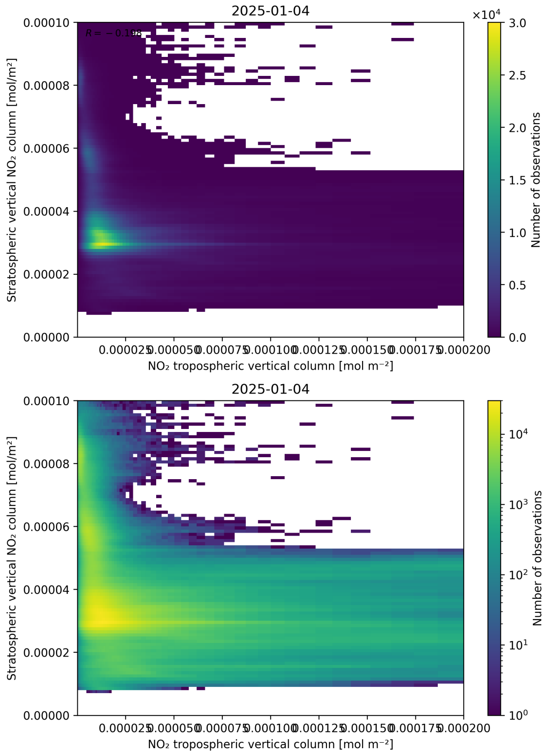
Figure 125: Scatter density plot of “NO 2 tropospheric vertical column” against “Stratospheric vertical NO 2 column” for 2025-01-03 to 2025-01-05.
