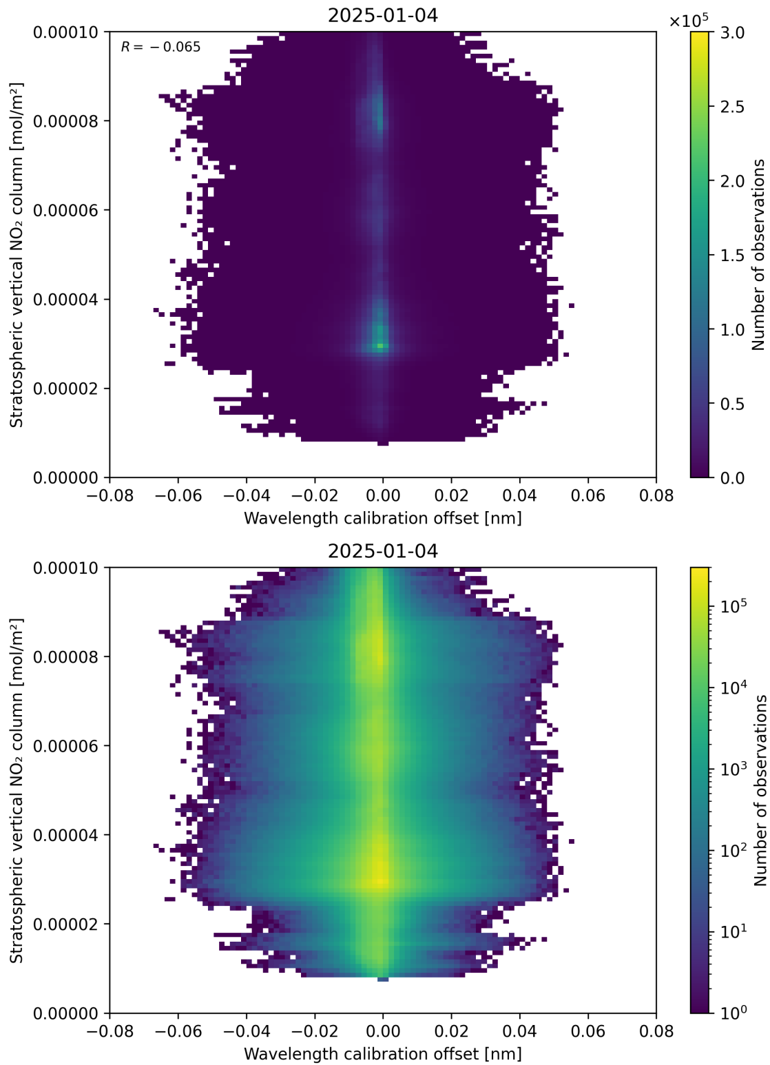
Figure 176: Scatter density plot of “Wavelength calibration offset” against “Stratospheric vertical NO 2 column” for 2025-01-03 to 2025-01-05.
