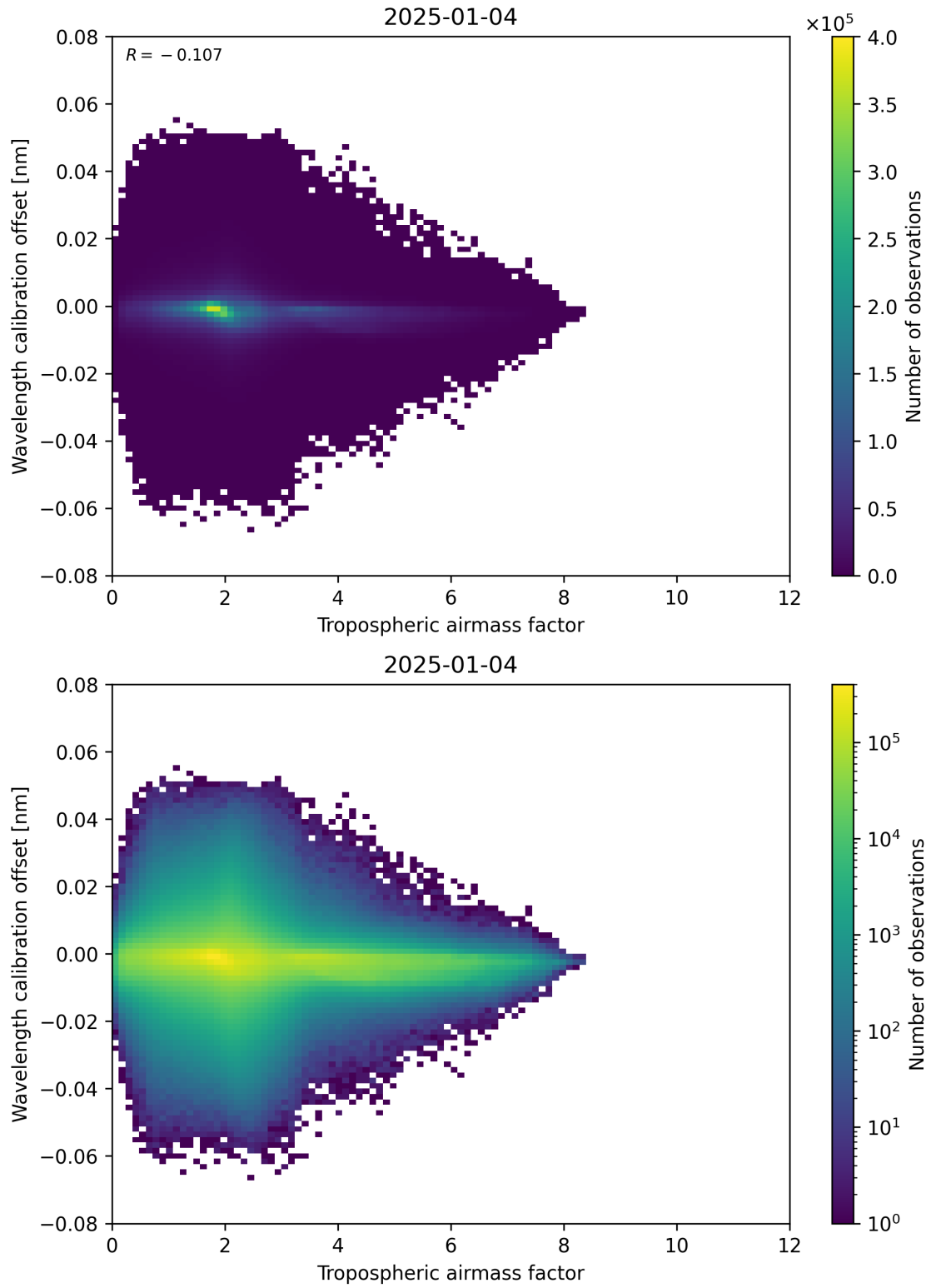
Figure 80: Scatter density plot of “Tropospheric airmass factor” against “Wavelength calibration offset” for 2025-01-03 to 2025-01-05.
