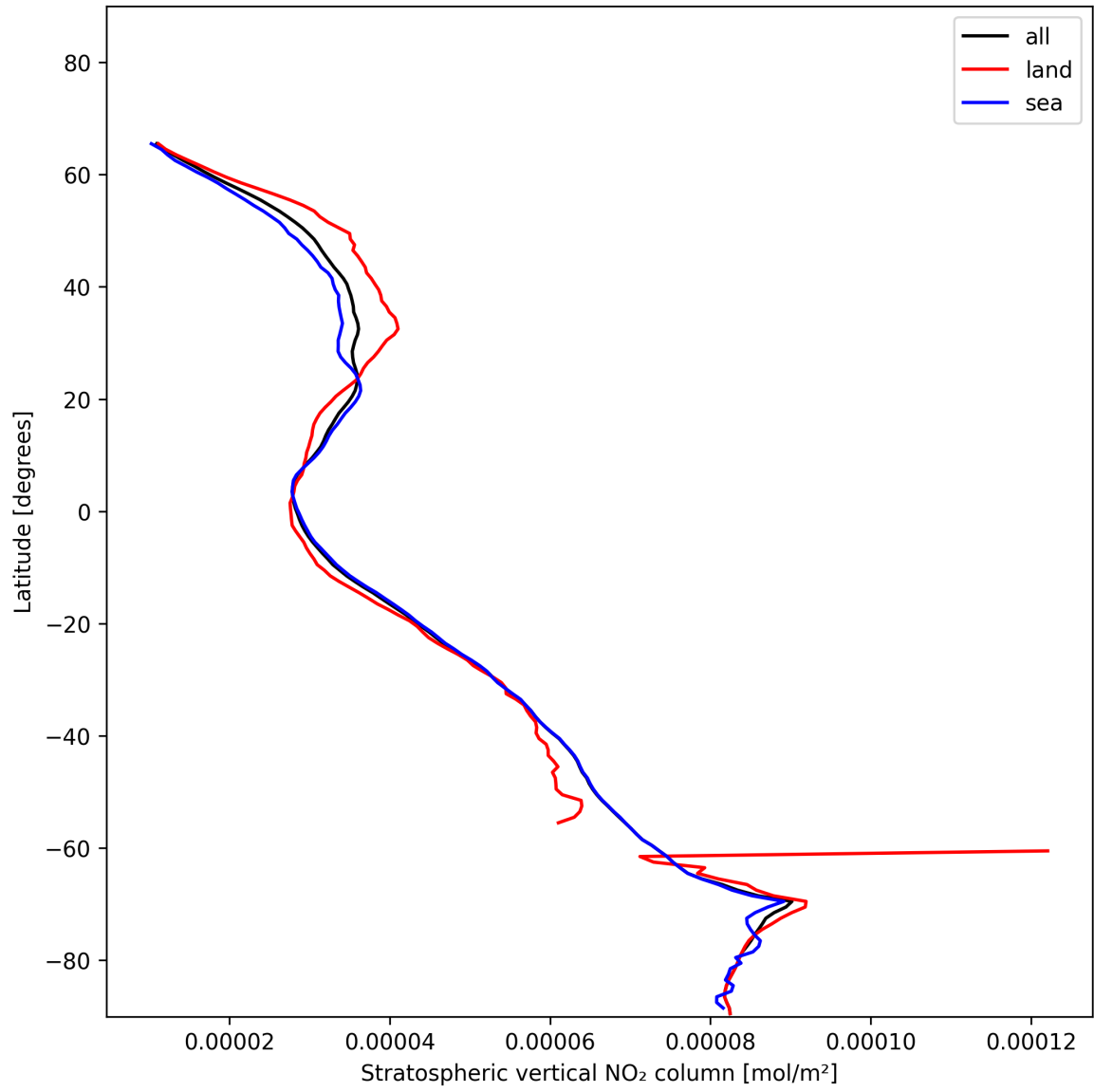
Figure 19: Zonal average of “Stratospheric vertical NO 2 column” for 2025-01-03 to 2025-01-05.
