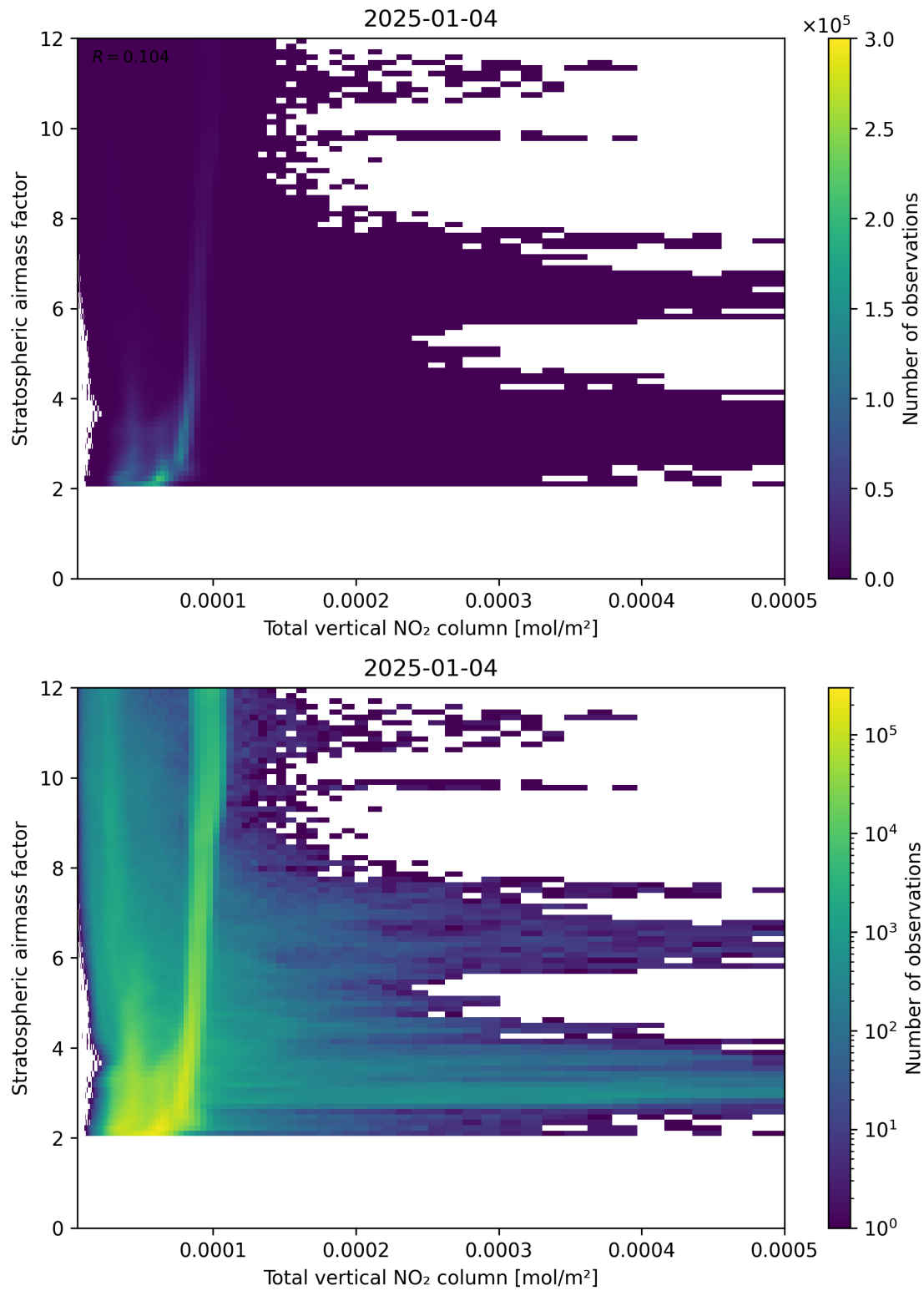
Figure 110: Scatter density plot of “Total vertical NO 2 column” against “Stratospheric air mass factor” for 2025-01-03 to 2025-01-05.
