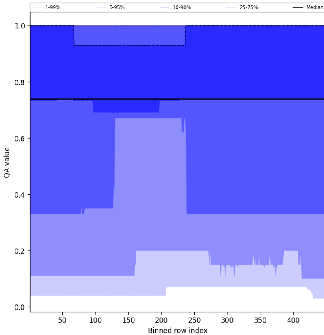
Figure 45: Along track statistics of “QA value” for 2025-01-03 to 2025-01-05
