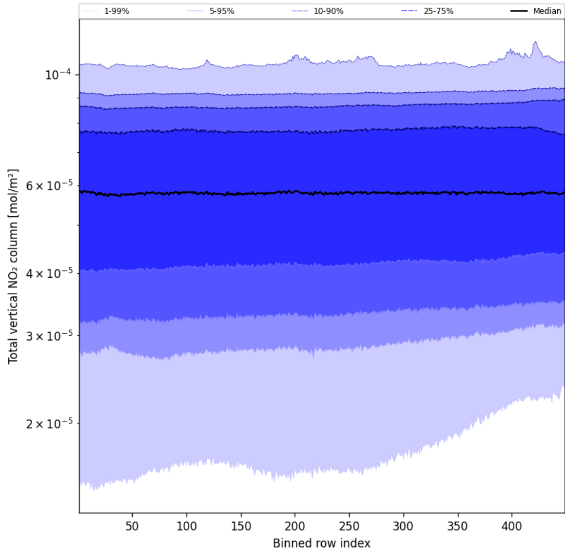
Figure 55: Along track statistics of “Total vertical NO 2 column” for 2025-01-03 to 2025-01-05
