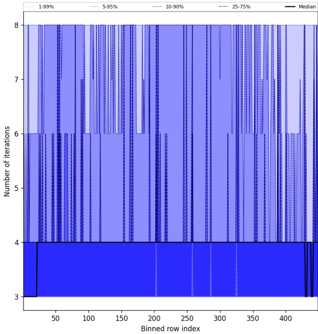
Figure 51: Along track statistics of “Number of iterations” for 2025-01-03 to 2025-01-05
