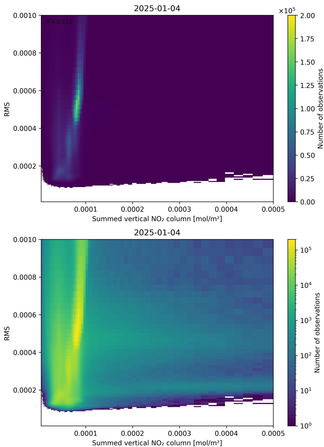
Figure 109: Scatter density plot of “Summed vertical NO 2 column” against “RMS” for 2025-01-03 to 2025-01-05.
