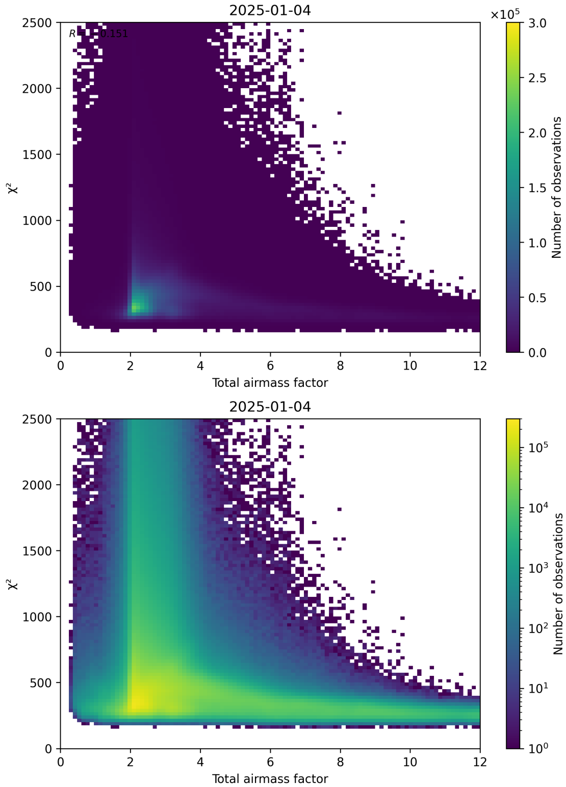
Figure 63: Scatter density plot of “Total airmass factor” against “ \chi^2 ” for 2025-01-03 to 2025-01-05.
