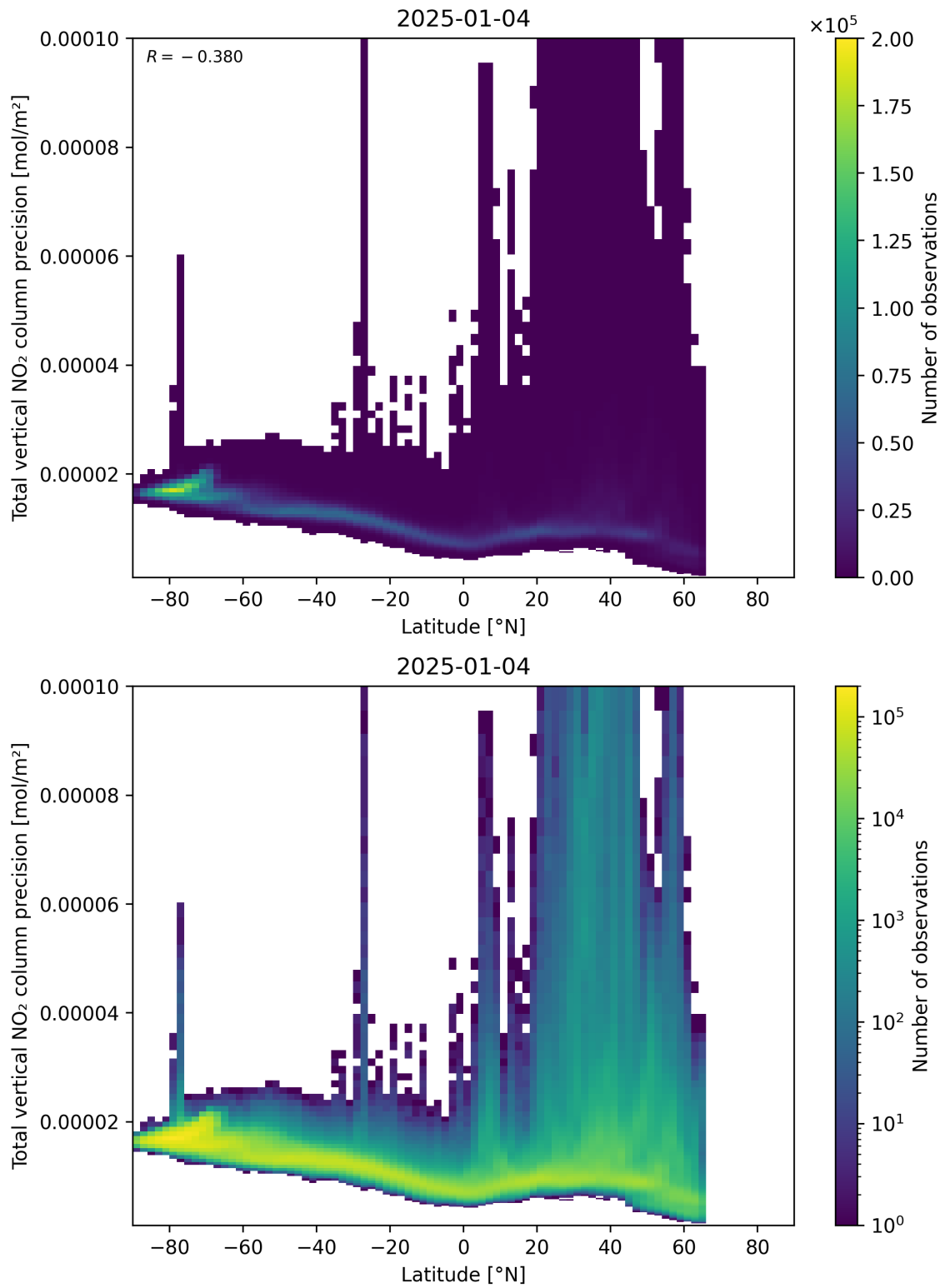
Figure 91: Scatter density plot of “Latitude” against “Total vertical NO 2 column precision” for 2025-01-03 to 2025-01-05.
