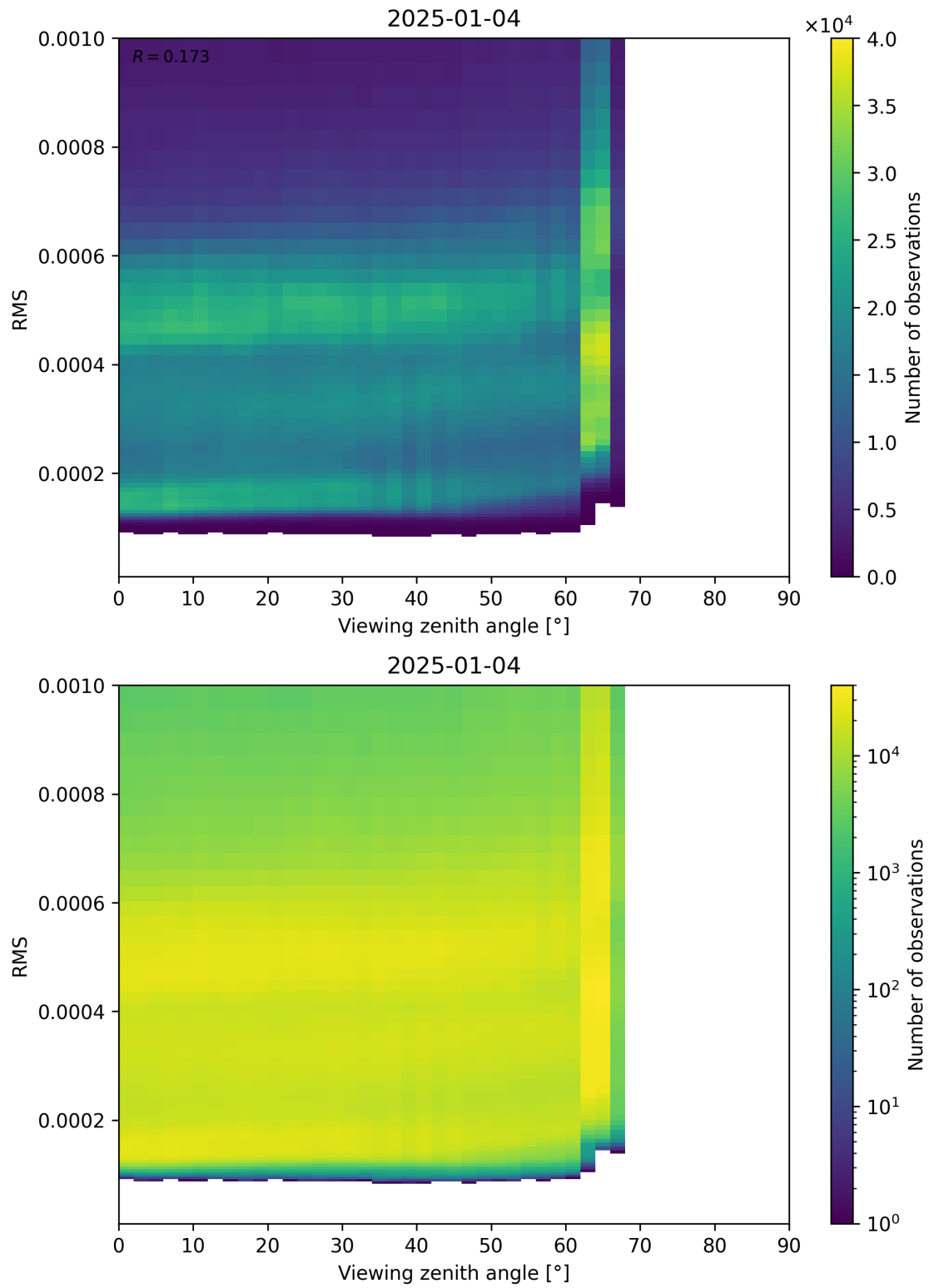
Figure 171: Scatter density plot of “Viewing zenith angle” against “RMS” for 2025-01-03 to 2025-01-05.
