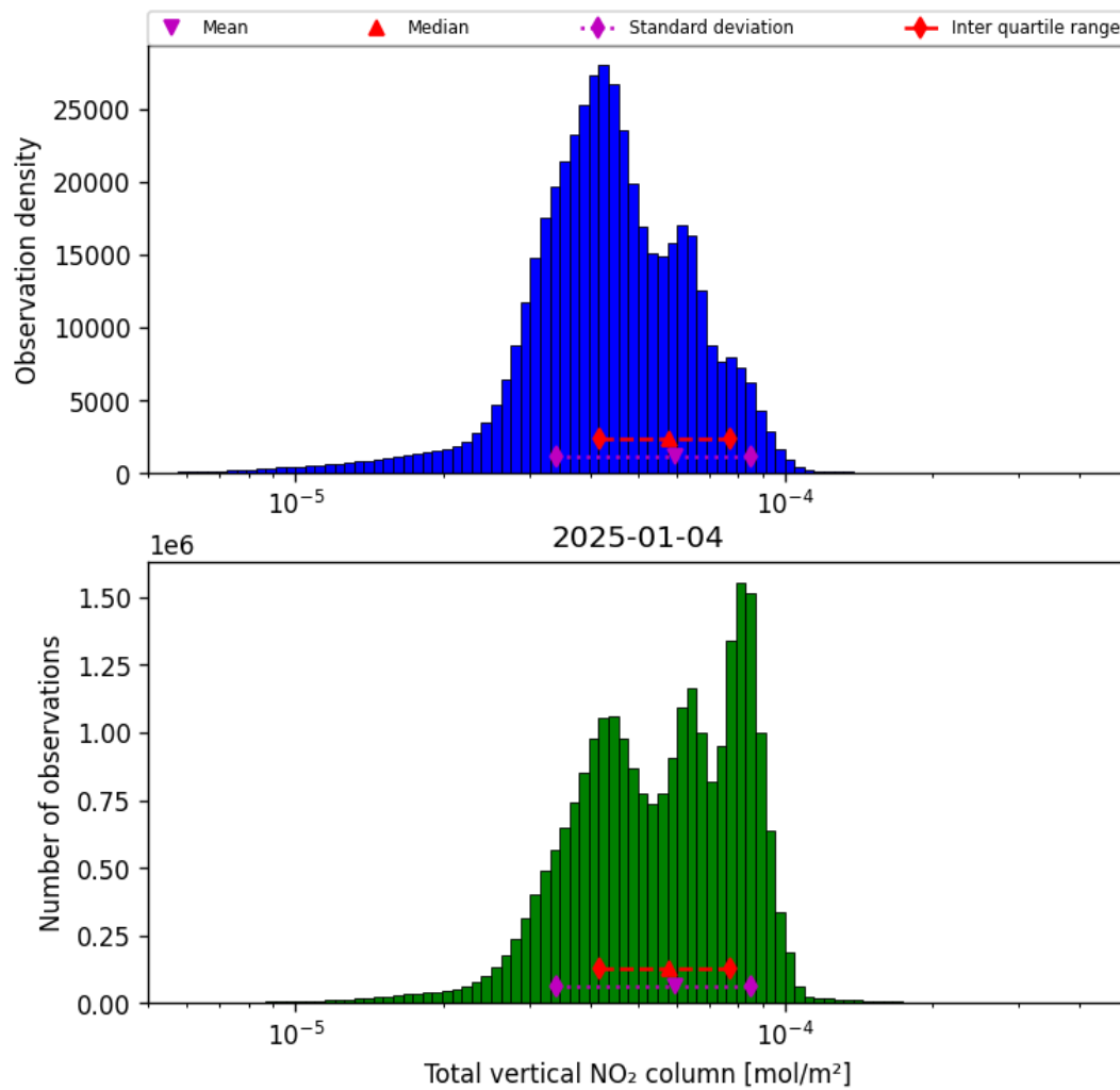
Figure 38: Histogram of “Total vertical NO 2 column” for 2025-01-03 to 2025-01-05
