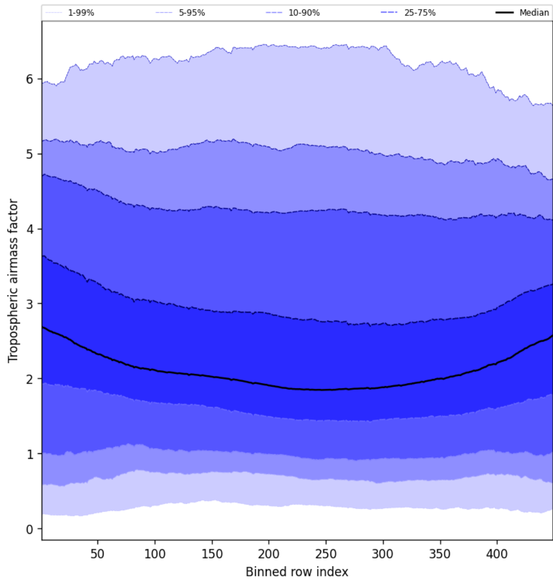
Figure 48: Along track statistics of “Tropospheric air mass factor” for 2025-01-03 to 2025-01-05
