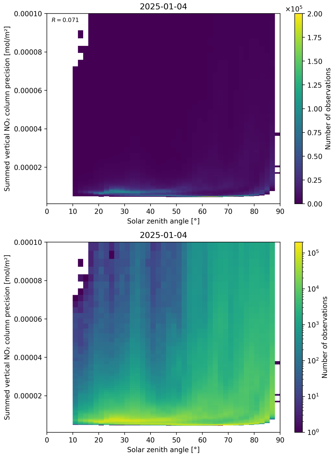
Figure 152: Scatter density plot of “Solar zenith angle” against “Summed vertical NO 2 column precision” for 2025-01-03 to 2025-01-05.
