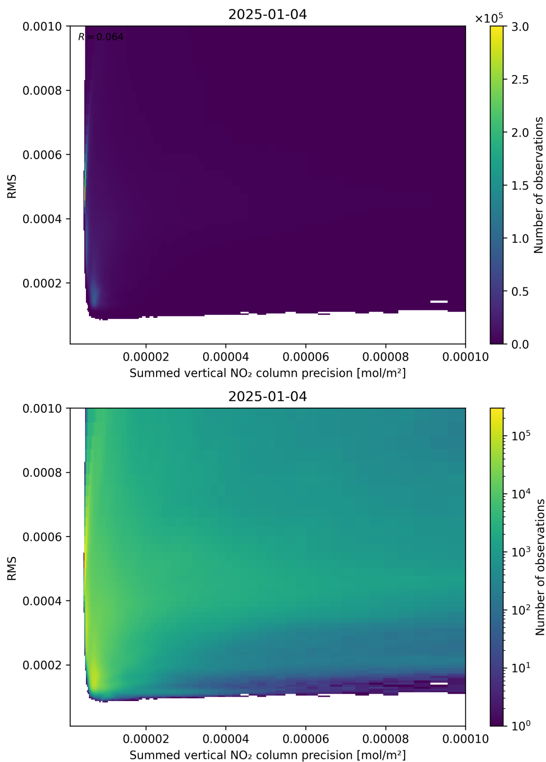
Figure 108: Scatter density plot of “Summed vertical NO 2 column precision” against “RMS” for 2025-01-03 to 2025-01-05.
