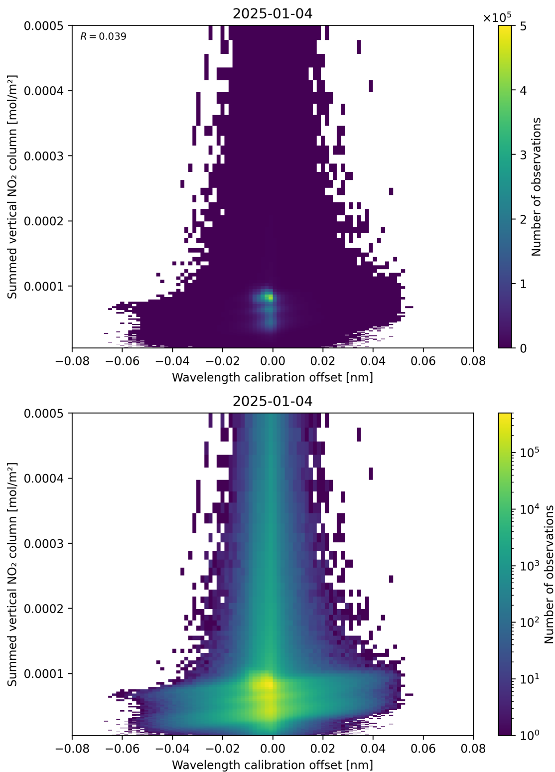
Figure 177: Scatter density plot of “Wavelength calibration offset” against “Summed vertical NO 2 column” for 2025-01-03 to 2025-01-05.
