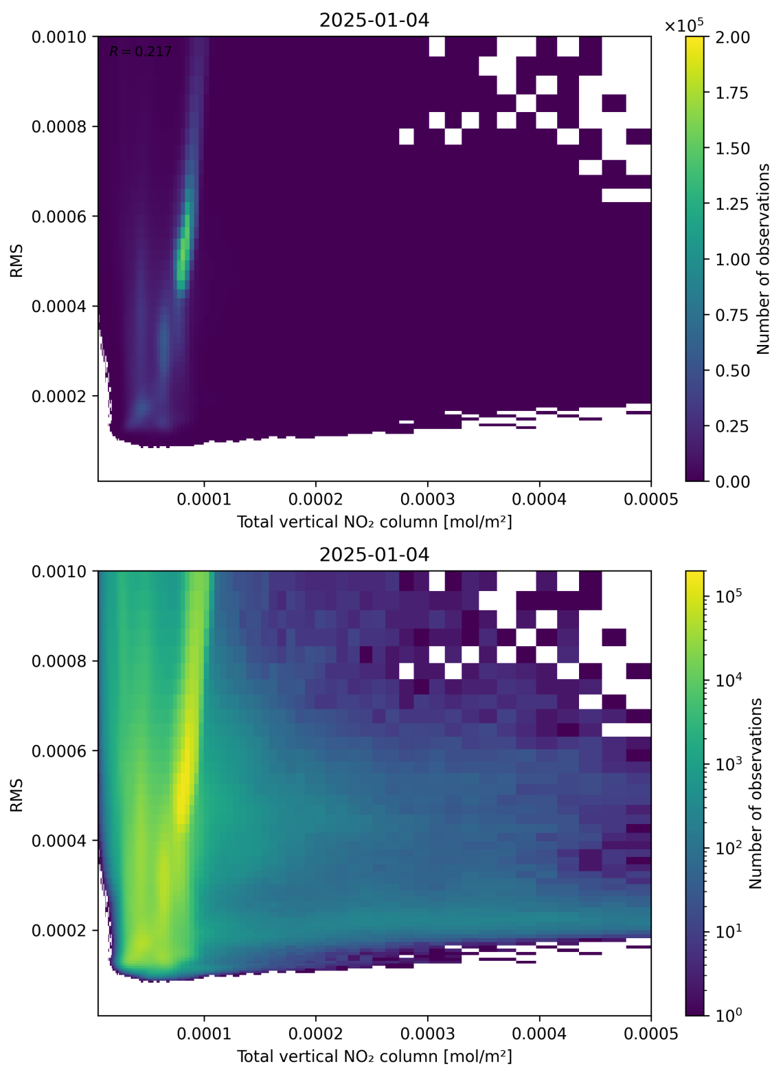
Figure 120: Scatter density plot of “Total vertical NO 2 column” against “RMS” for 2025-01-03 to 2025-01-05.
