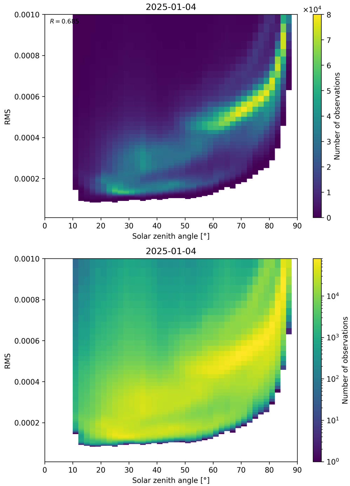
Figure 157: Scatter density plot of “Solar zenith angle” against “RMS” for 2025-01-03 to 2025-01-05.
