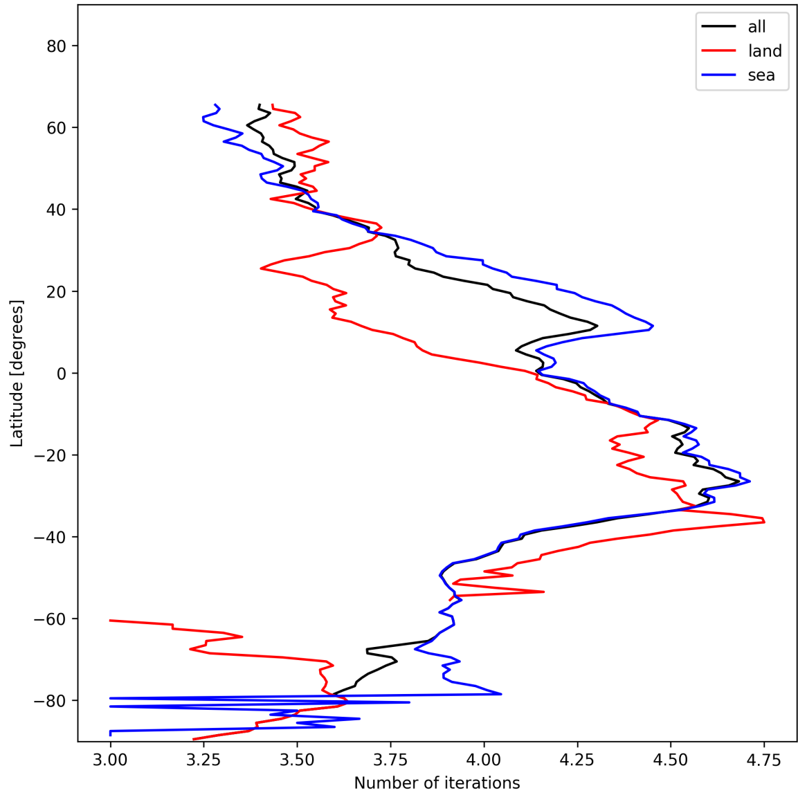
Figure 17: Zonal average of “Number of iterations” for 2025-01-03 to 2025-01-05.
