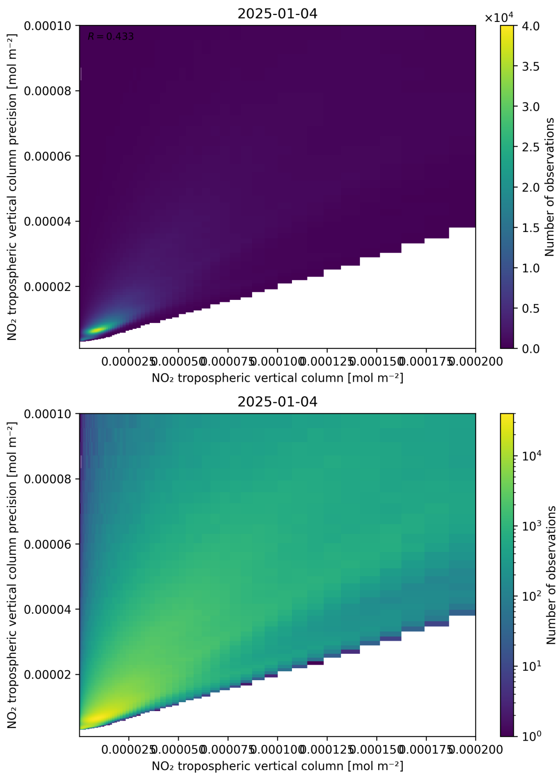
Figure 130: Scatter density plot of “NO 2 tropospheric vertical column” against “NO 2 tropospheric vertical column precision” for 2025-01-03 to 2025-01-05.
