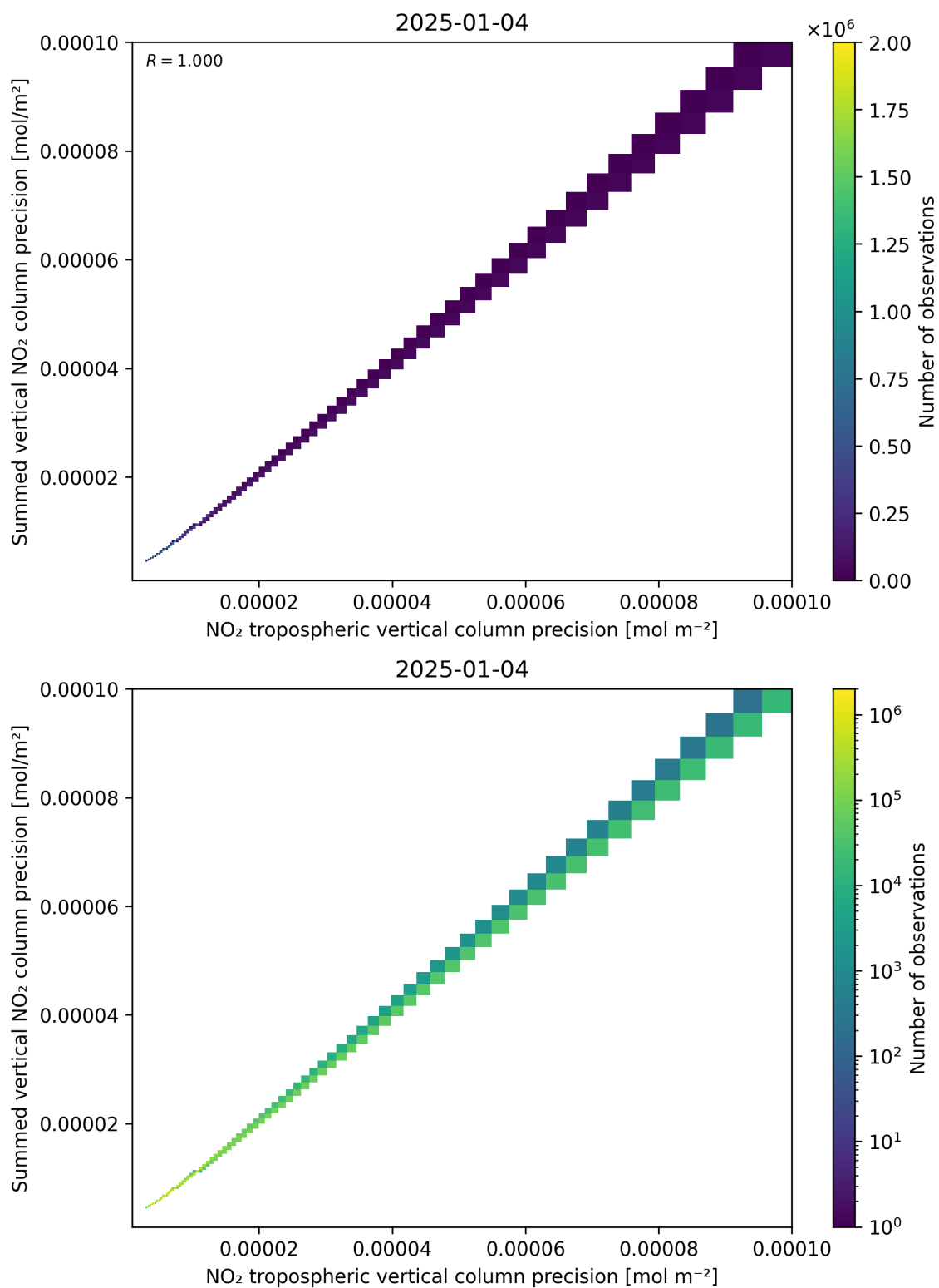
Figure 137: Scatter density plot of “NO 2 tropospheric vertical column precision” against “Summed vertical NO 2 column precision” for 2025-01-03 to 2025-01-05.
