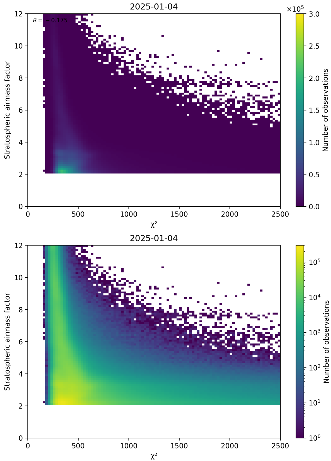
Figure 81: Scatter density plot of “ \chi^2 ” against “Stratospheric airmass factor” for 2025-01-03 to 2025-01-05.
