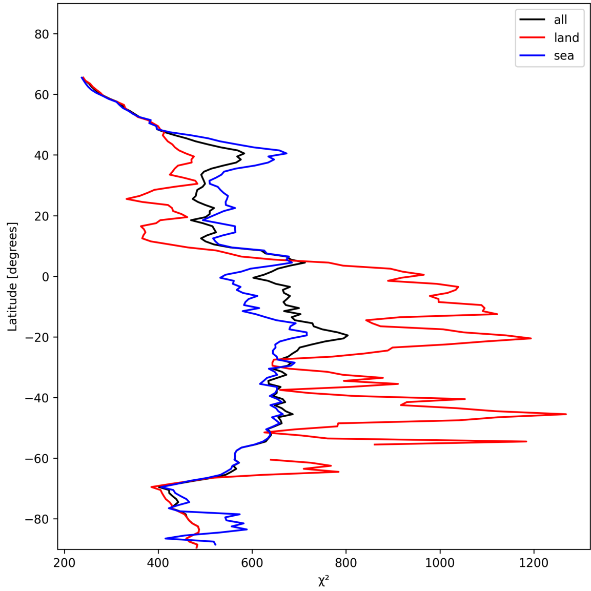
Figure 25: Zonal average of “ \chi^2 ” for 2025-01-03 to 2025-01-05.
