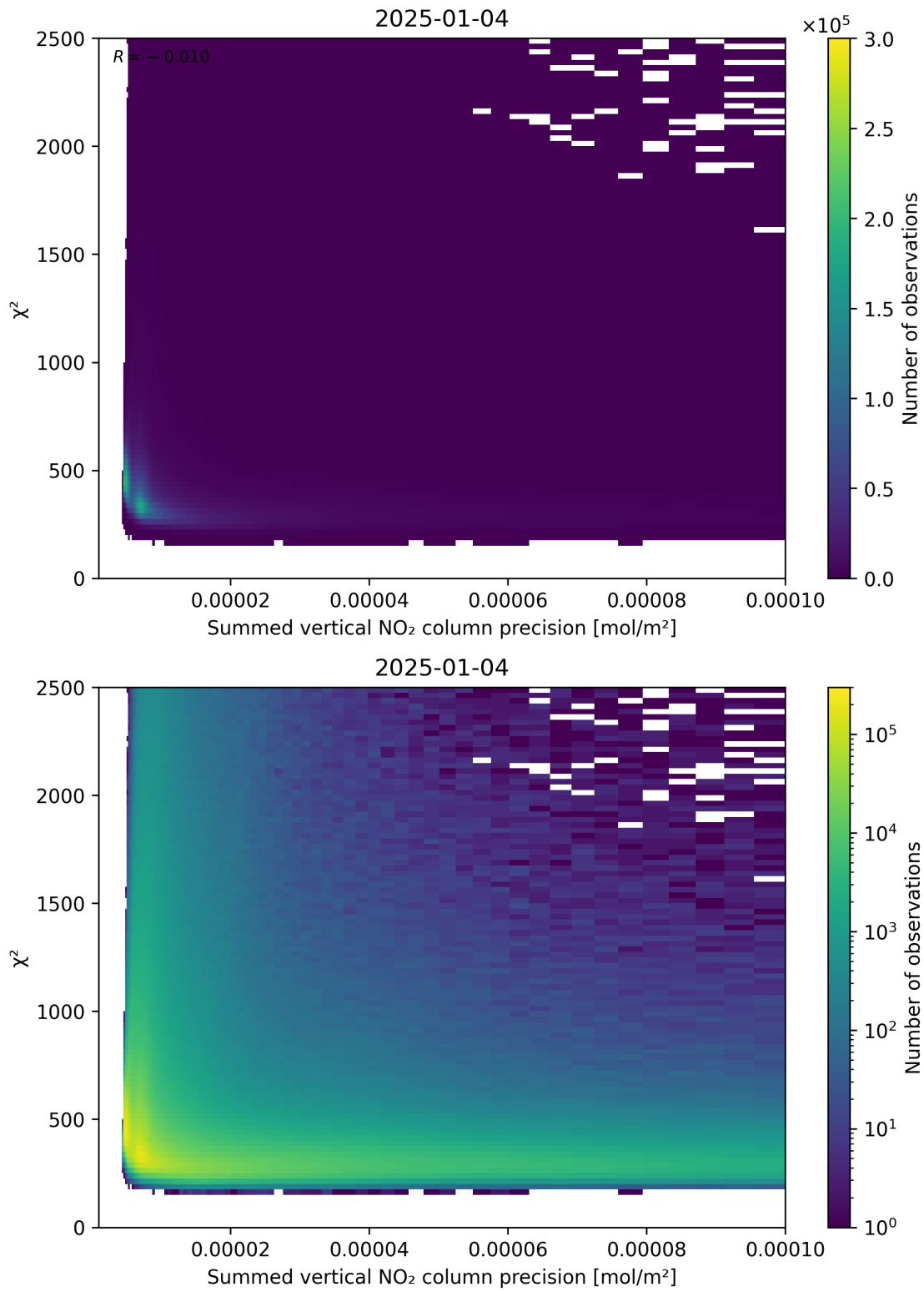
Figure 107: Scatter density plot of “Summed vertical NO 2 column precision” against “ \chi^2 ” for 2025-01-03 to 2025-01-05.
