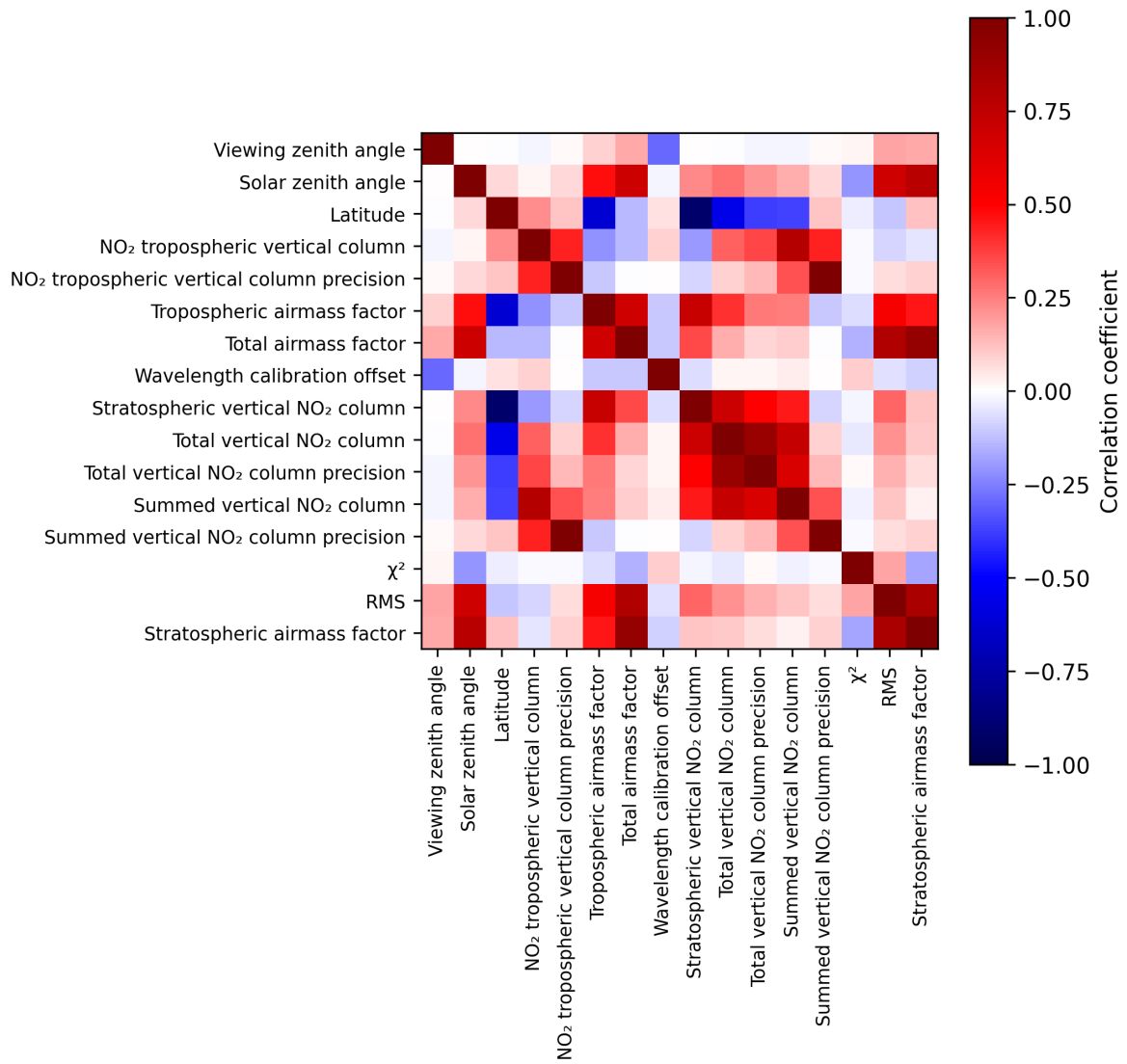
Figure 2: Map of correlation matrix for 2025-01-03 to 2025-01-05.
