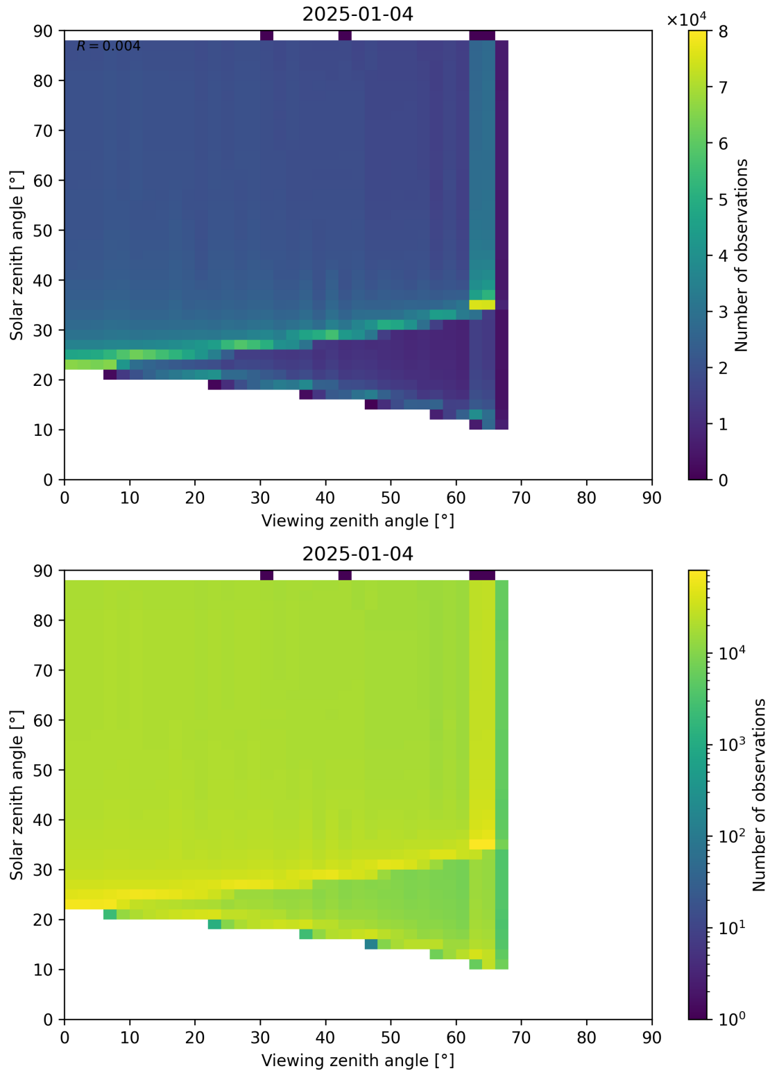
Figure 172: Scatter density plot of “Viewing zenith angle” against “Solar zenith angle” for 2025-01-03 to 2025-01-05.
