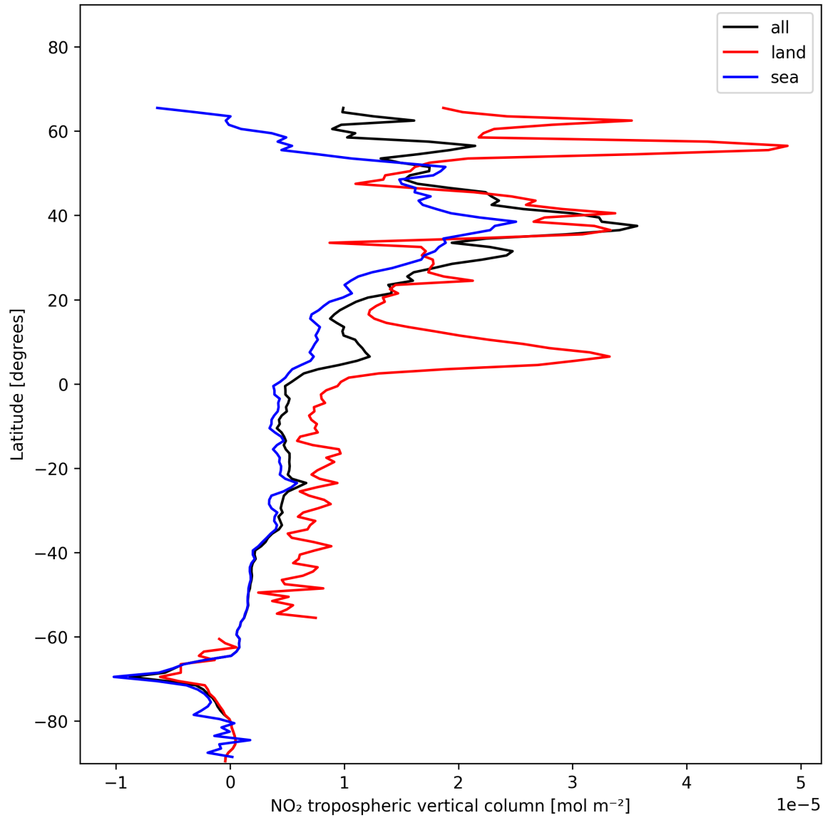
Figure 12: Zonal average of “NO 2 tropospheric vertical column” for 2025-01-03 to 2025-01-05.
