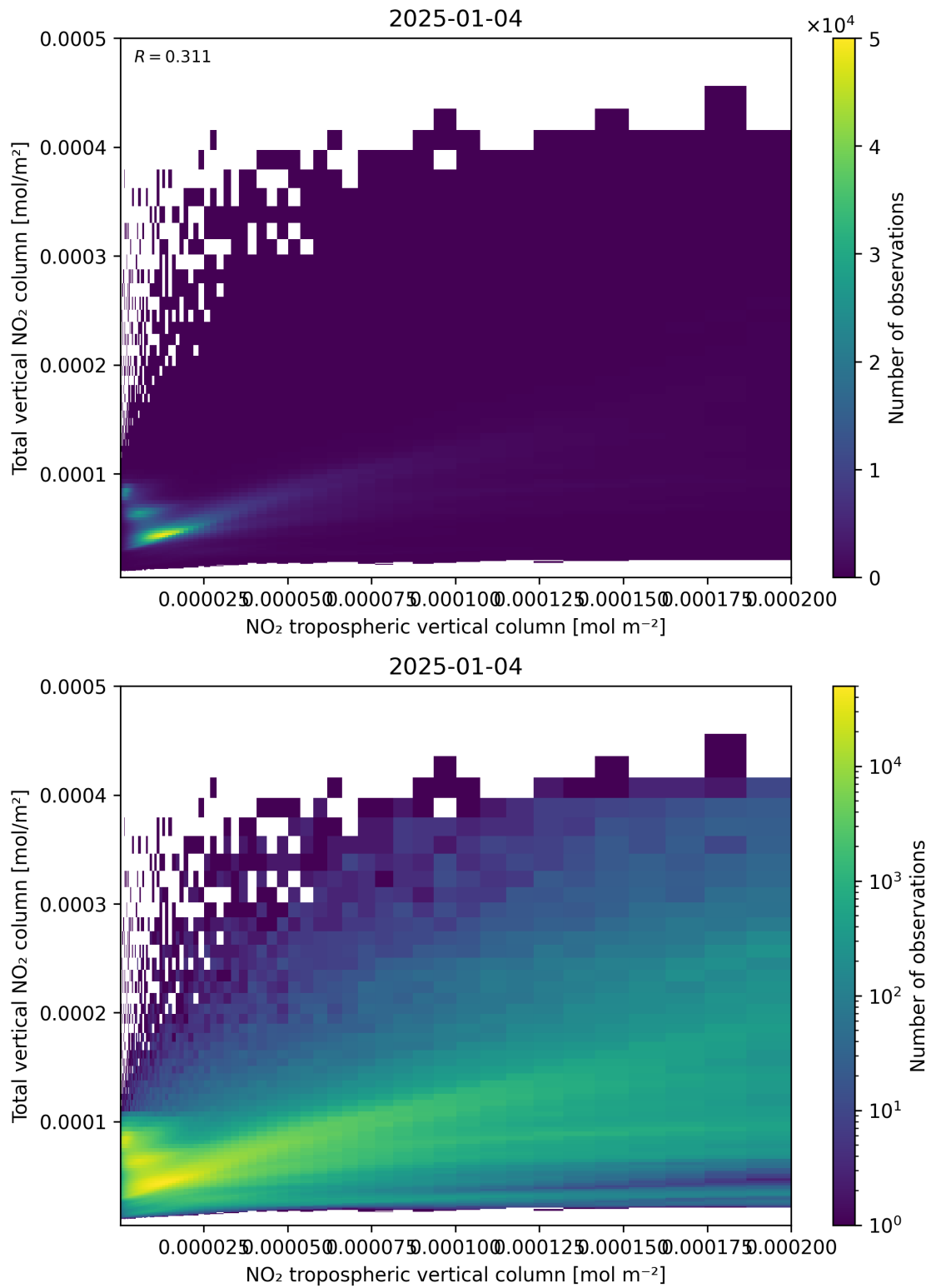
Figure 128: Scatter density plot of “NO 2 tropospheric vertical column” against “Total vertical NO 2 column” for 2025-01-03 to 2025-01-05.
