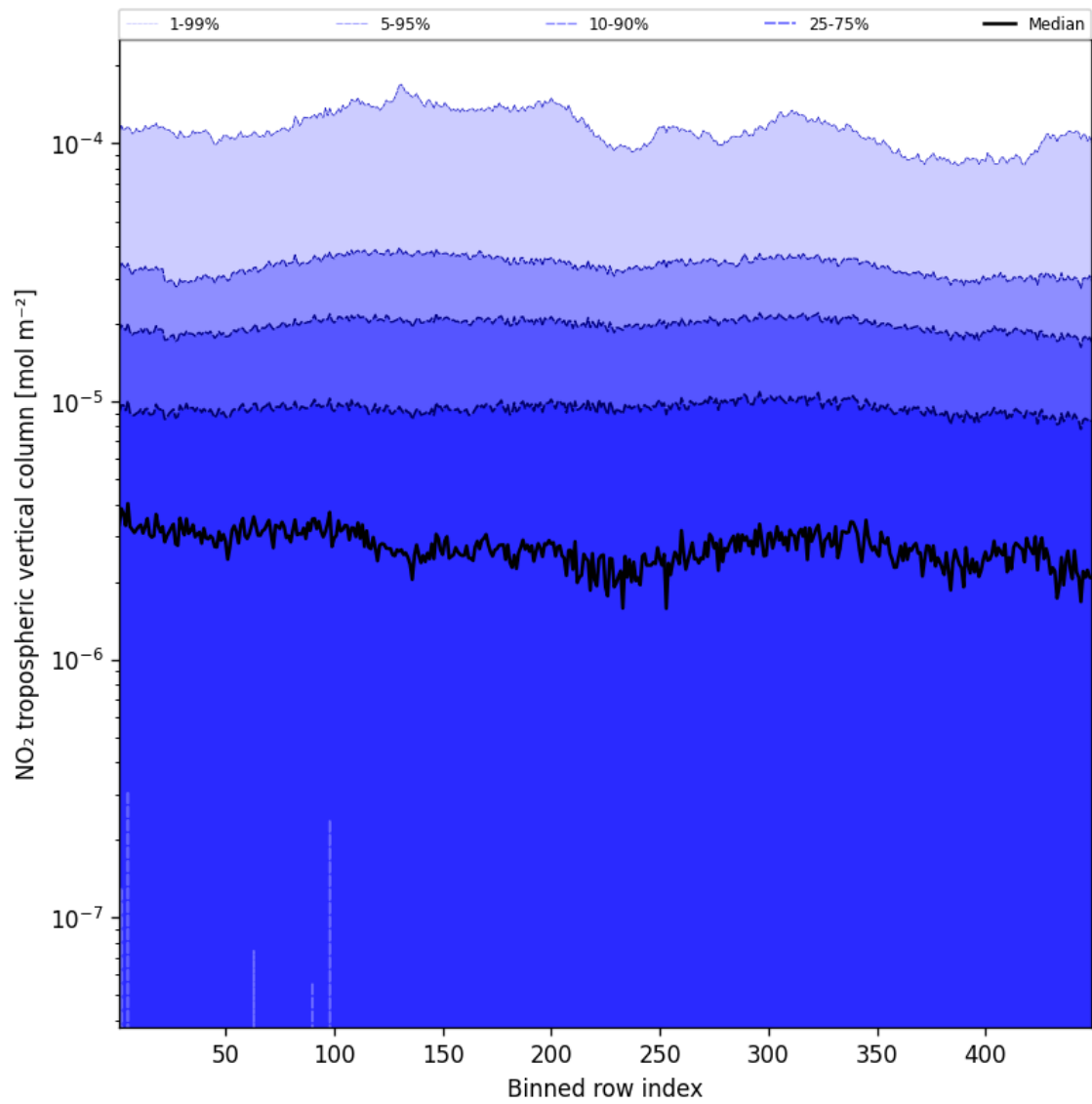
Figure 46: Along track statistics of “NO 2 tropospheric vertical column” for 2025-01-04 to 2025-01-06
