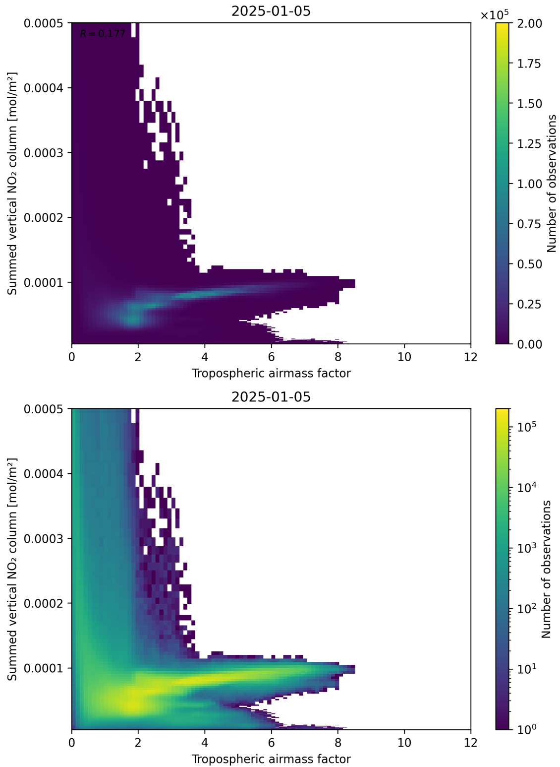
Figure 75: Scatter density plot of “Tropospheric air mass factor” against “Summed vertical NO 2 column” for 2025-01-04 to 2025-01-06.
