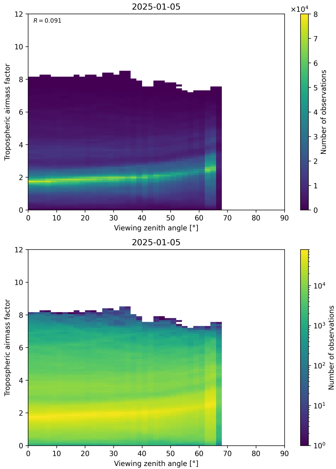
Figure 161: Scatter density plot of “Viewing zenith angle” against “Tropospheric airmass factor” for 2025-01-04 to 2025-01-06.
