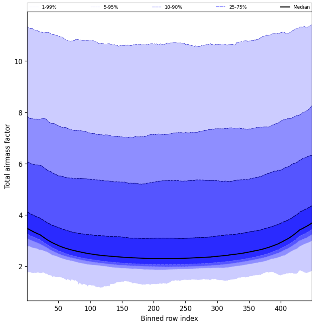
Figure 49: Along track statistics of “Total airmass factor” for 2025-01-04 to 2025-01-06
