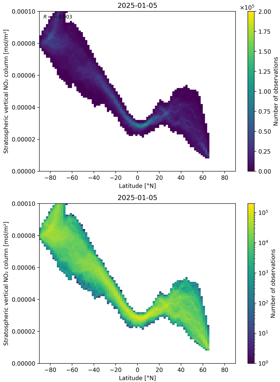
Figure 87: Scatter density plot of “Latitude” against “Stratospheric vertical NO 2 column” for 2025-01-04 to 2025-01-06.
