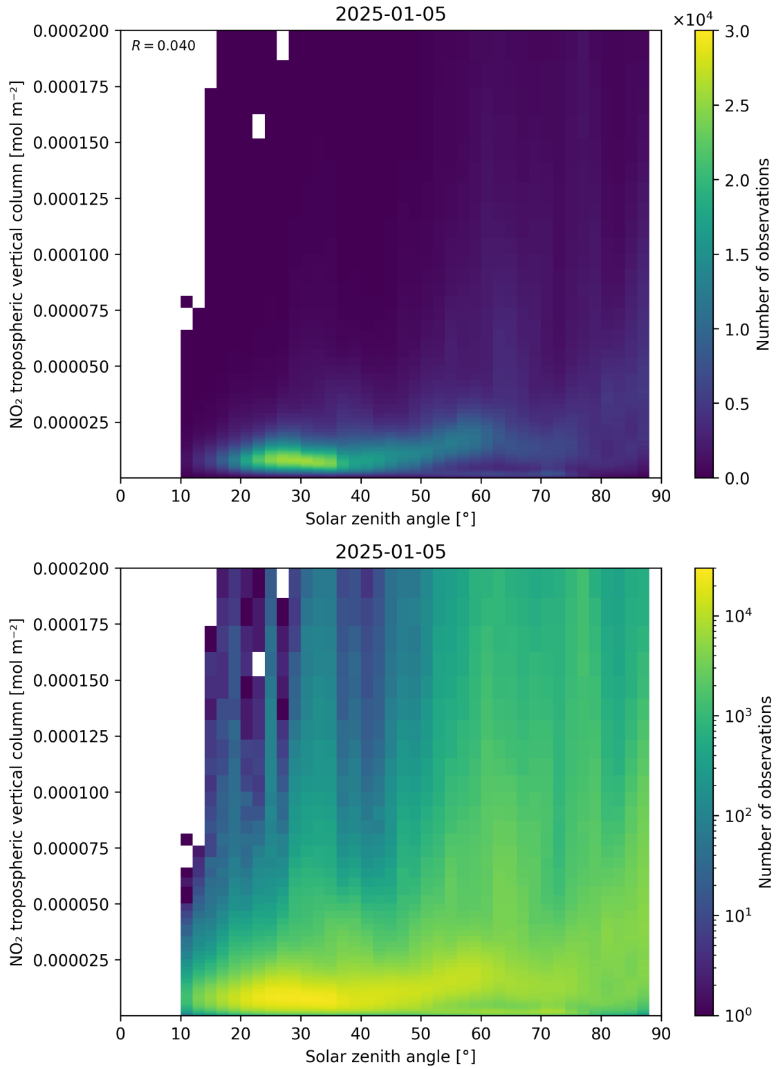
Figure 155: Scatter density plot of “Solar zenith angle” against “NO 2 tropospheric vertical column” for 2025-01-04 to 2025-01-06.
