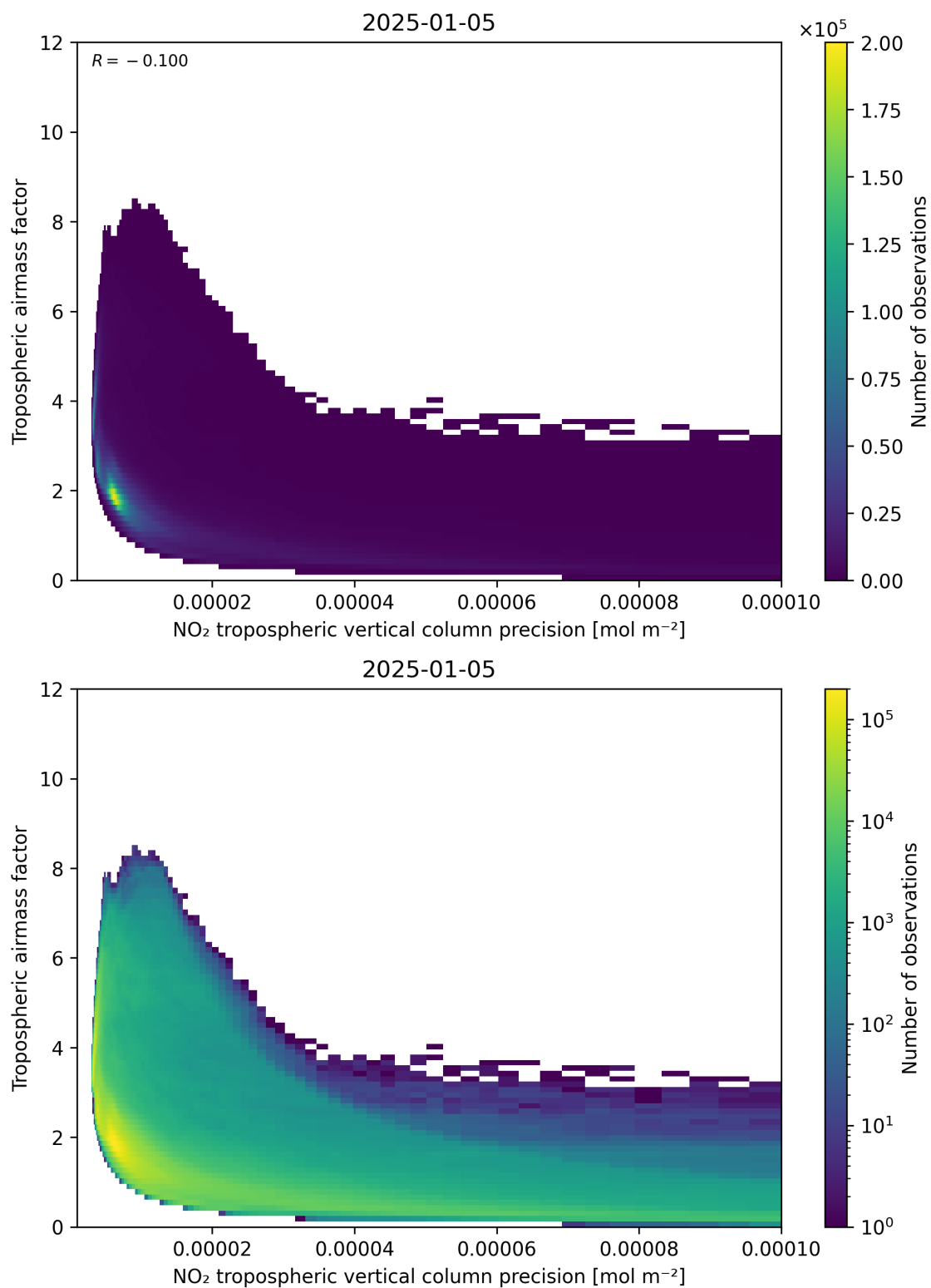
Figure 133: Scatter density plot of “NO 2 tropospheric vertical column precision” against “Tropospheric airmass factor” for 2025-01-04 to 2025-01-06.
