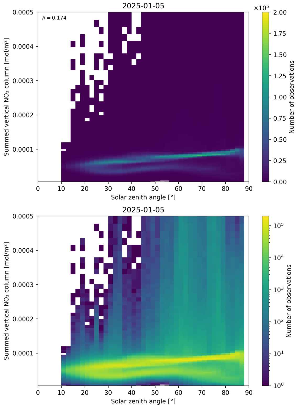
Figure 151: Scatter density plot of “Solar zenith angle” against “Summed vertical NO 2 column” for 2025-01-04 to 2025-01-06.
