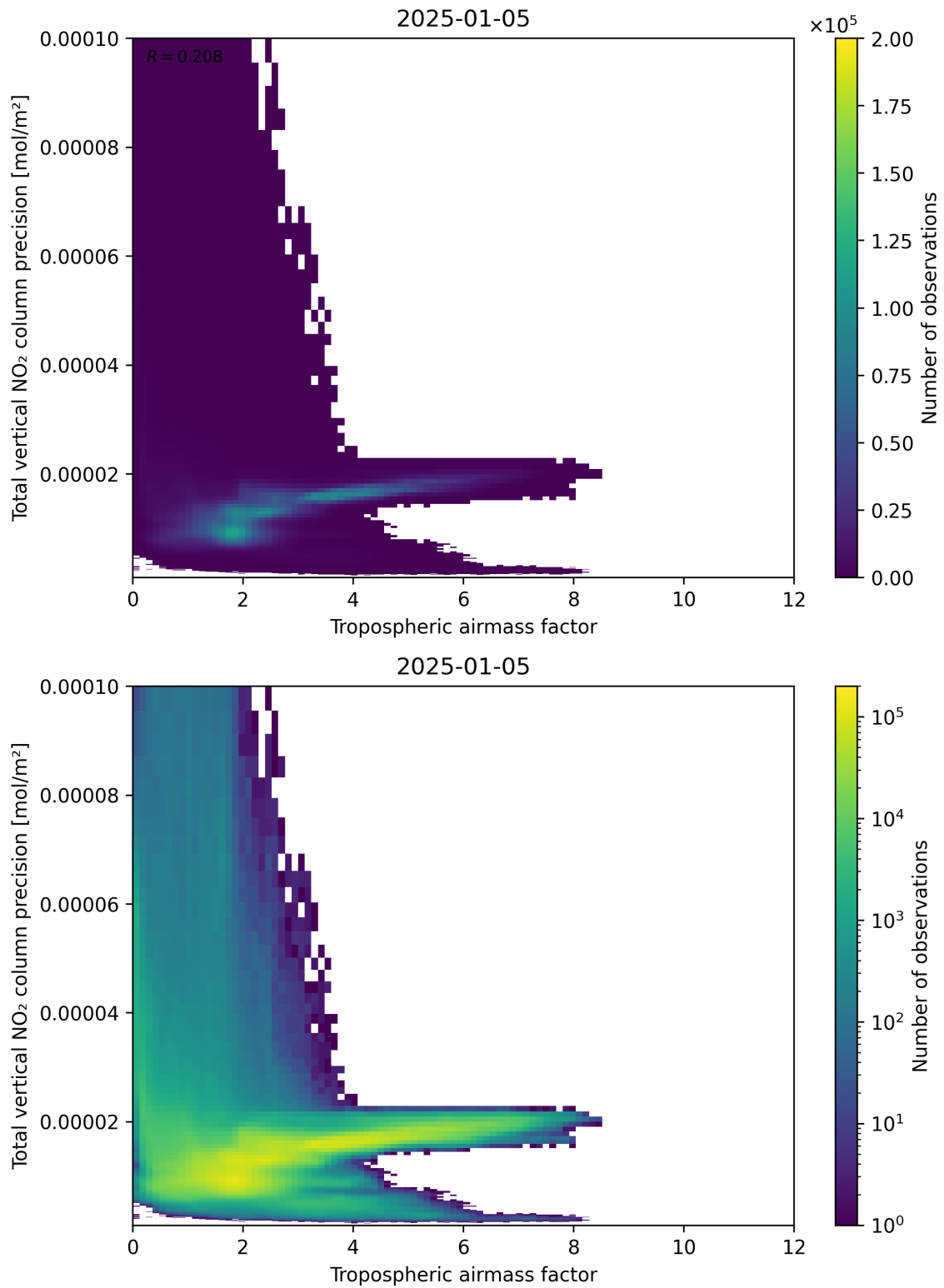
Figure 78: Scatter density plot of “Tropospheric air mass factor” against “Total vertical NO 2 column precision” for 2025-01-04 to 2025-01-06.
