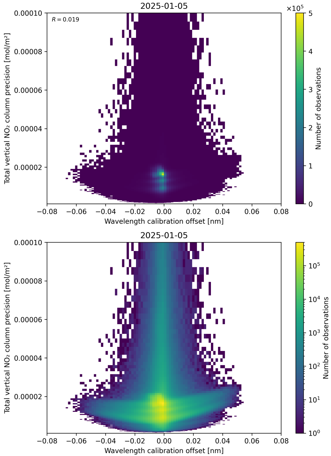
Figure 180: Scatter density plot of “Wavelength calibration offset” against “Total vertical NO 2 column precision” for 2025-01-04 to 2025-01-06.
