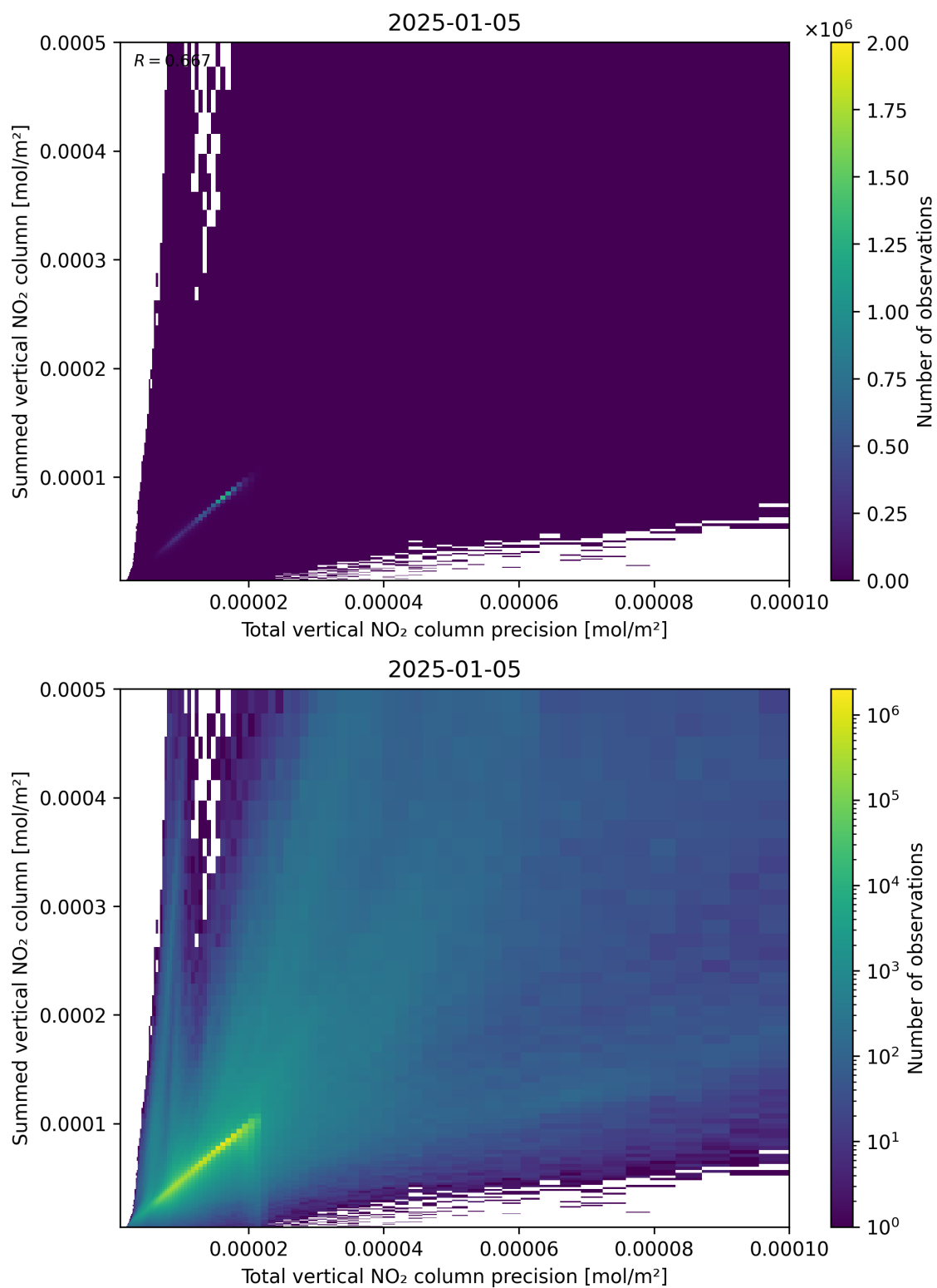
Figure 117: Scatter density plot of “Total vertical NO 2 column precision” against “Summed vertical NO 2 column” for 2025-01-04 to 2025-01-06.
