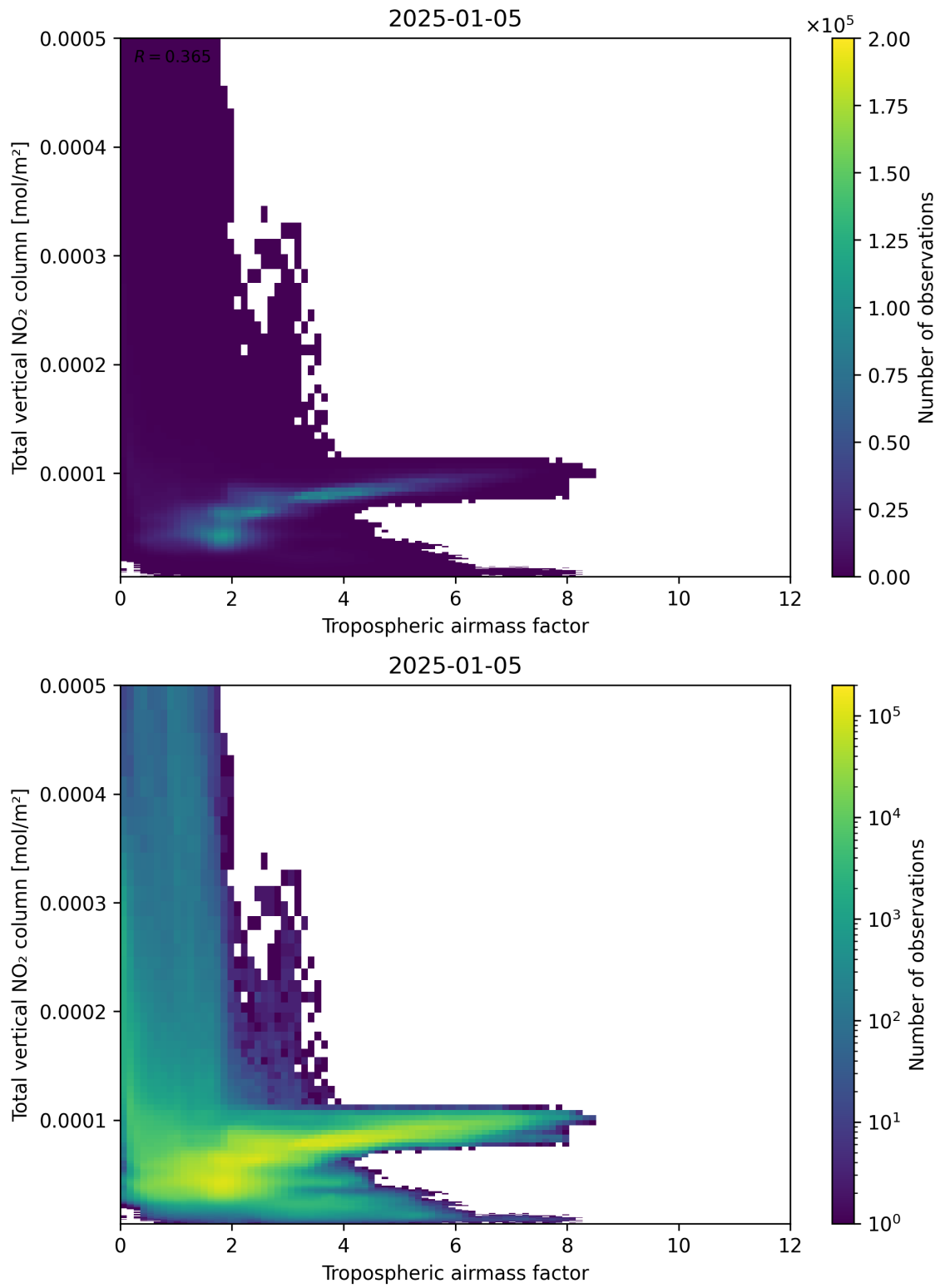
Figure 77: Scatter density plot of “Tropospheric airmass factor” against “Total vertical NO 2 column” for 2025-01-04 to 2025-01-06.
