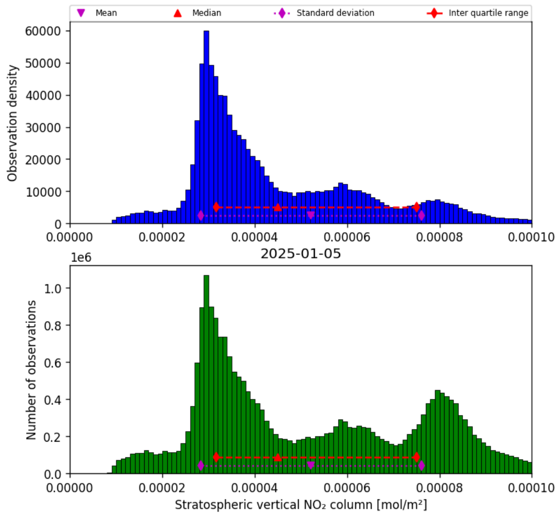
Figure 36: Histogram of “Stratospheric vertical NO 2 column” for 2025-01-04 to 2025-01-06
