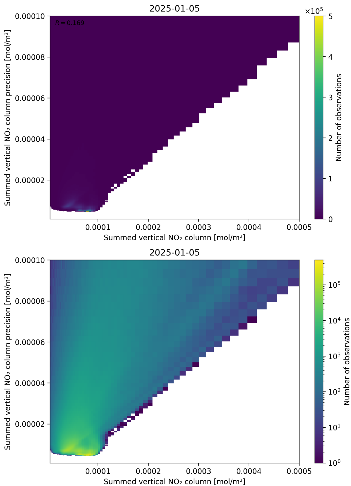
Figure 105: Scatter density plot of “Summed vertical NO 2 column” against “Summed vertical NO 2 column precision” for 2025-01-04 to 2025-01-06.
