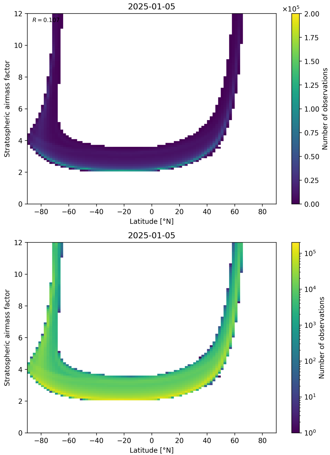
Figure 83: Scatter density plot of “Latitude” against “Stratospheric air mass factor” for 2025-01-04 to 2025-01-06.
