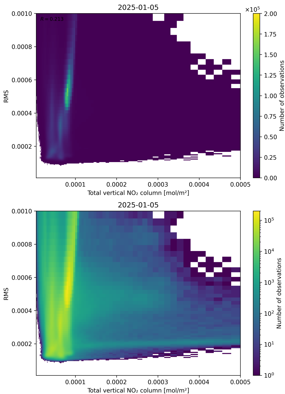
Figure 120: Scatter density plot of “Total vertical NO 2 column” against “RMS” for 2025-01-04 to 2025-01-06.
