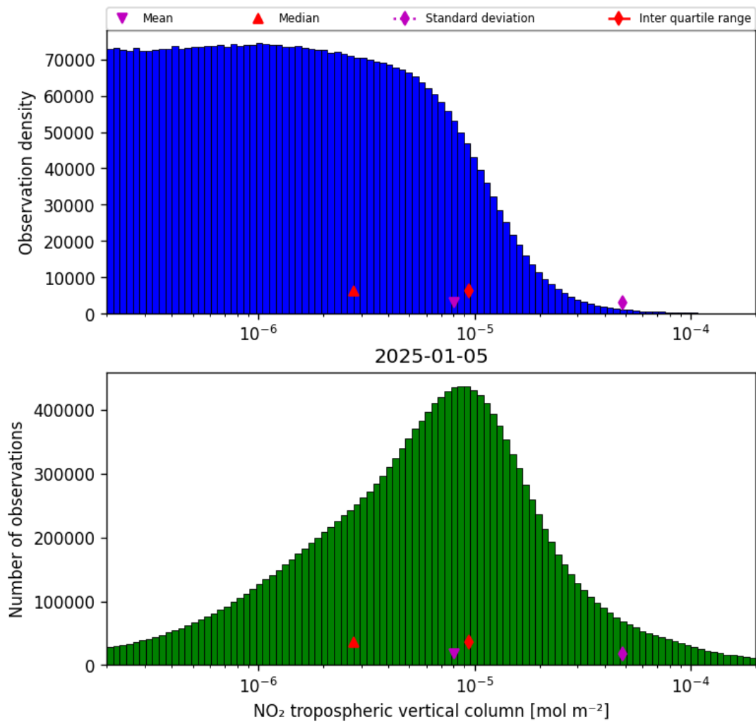
Figure 29: Histogram of “NO 2 tropospheric vertical column” for 2025-01-04 to 2025-01-06
