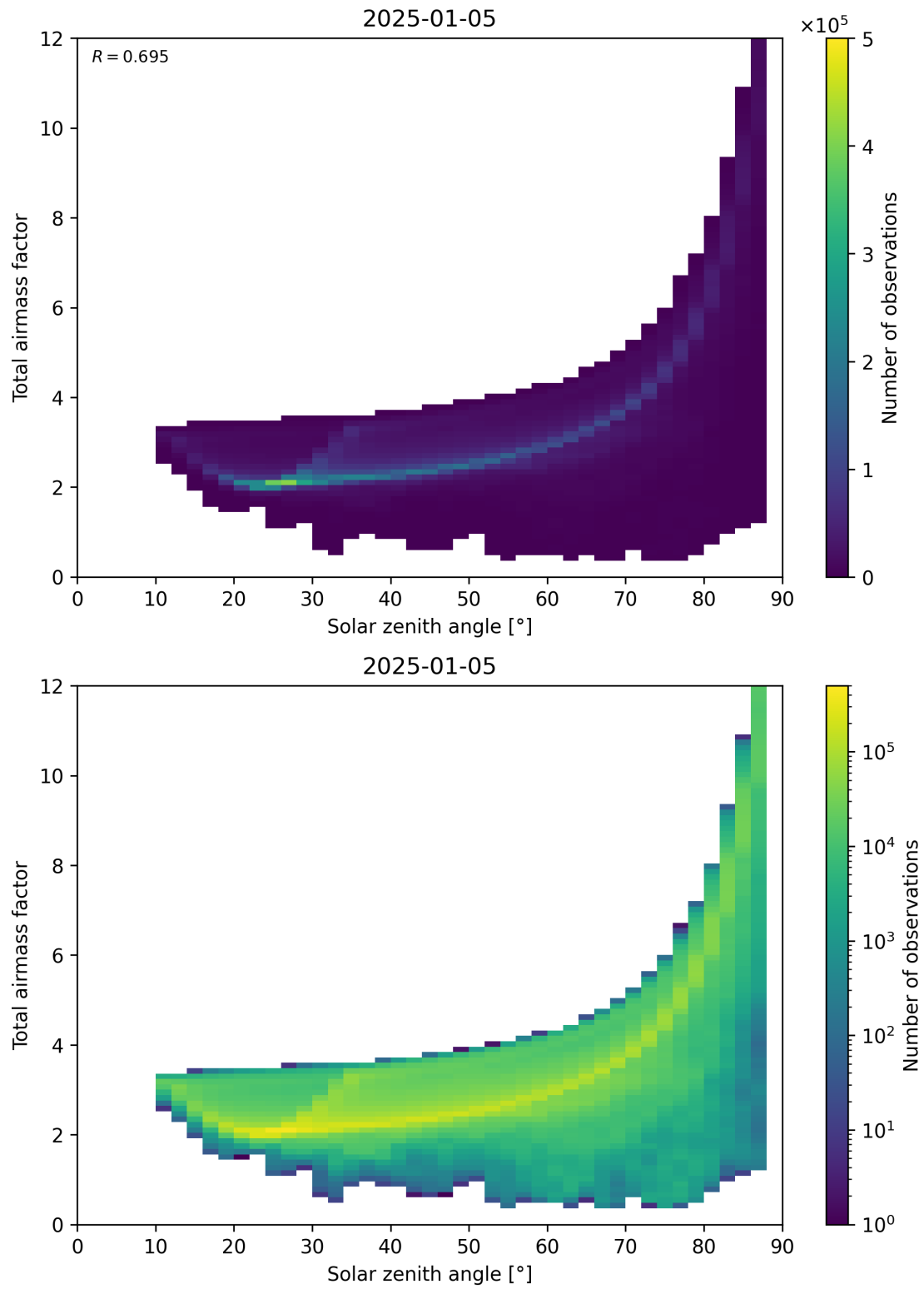
Figure 146: Scatter density plot of “Solar zenith angle” against “Total airmass factor” for 2025-01-04 to 2025-01-06.
