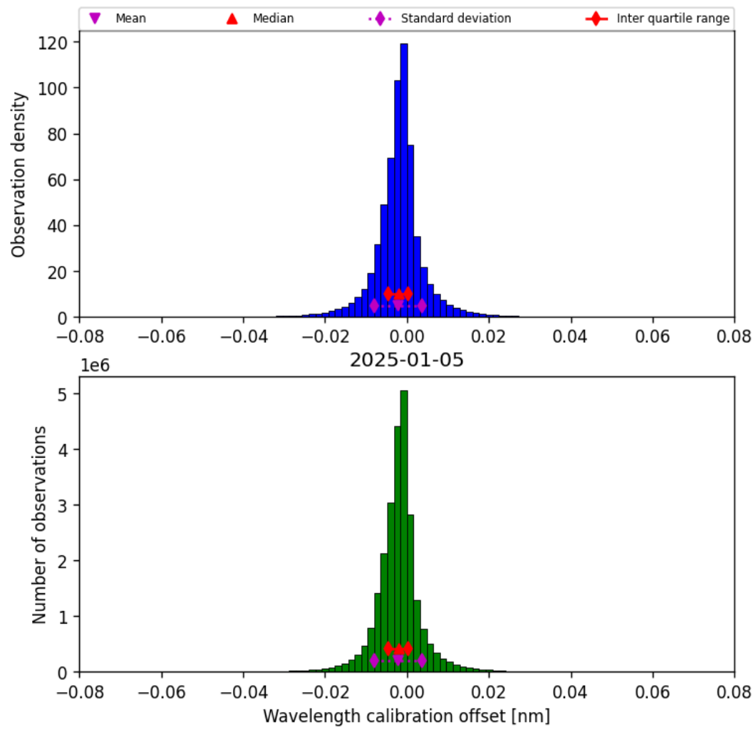
Figure 35: Histogram of “Wavelength calibration offset” for 2025-01-04 to 2025-01-06
