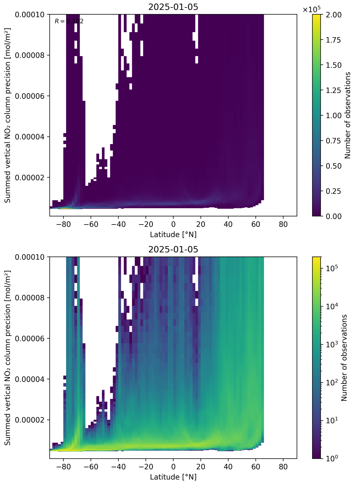
Figure 89: Scatter density plot of “Latitude” against “Summed vertical NO 2 column precision” for 2025-01-04 to 2025-01-06.
