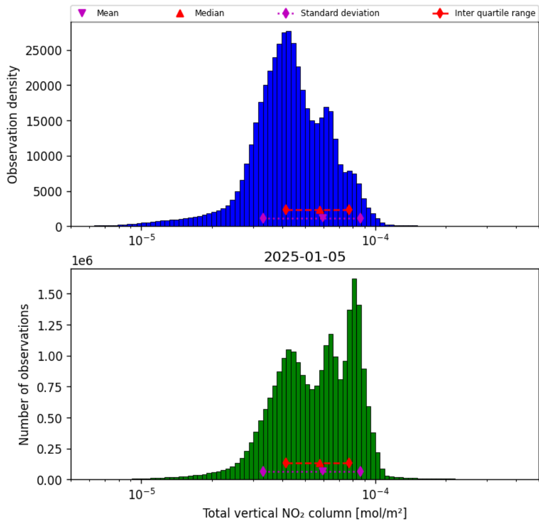
Figure 38: Histogram of “Total vertical NO 2 column” for 2025-01-04 to 2025-01-06
