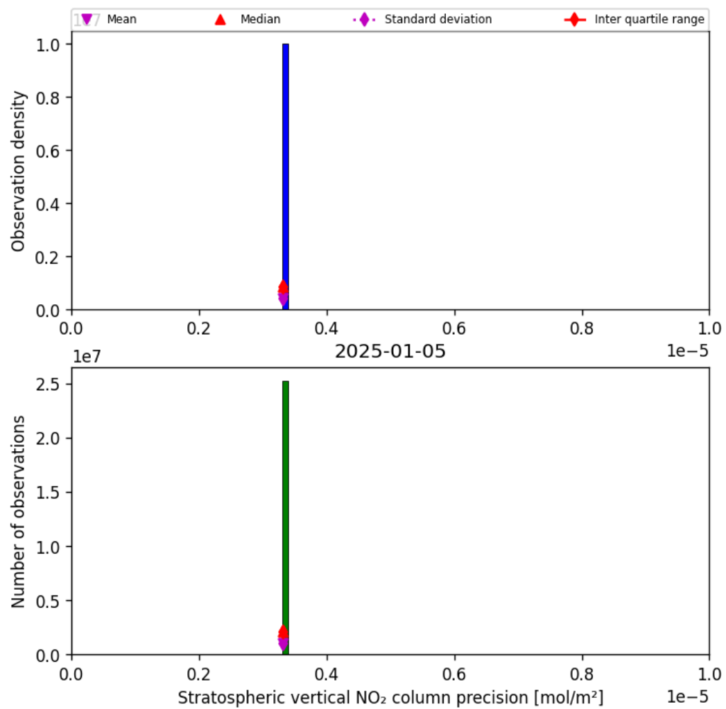
Figure 37: Histogram of “Stratospheric vertical NO 2 column precision” for 2025-01-04 to 2025-01-06
