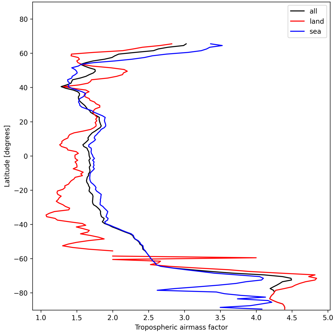
Figure 14: Zonal average of “Tropospheric airmass factor” for 2025-01-04 to 2025-01-06.
