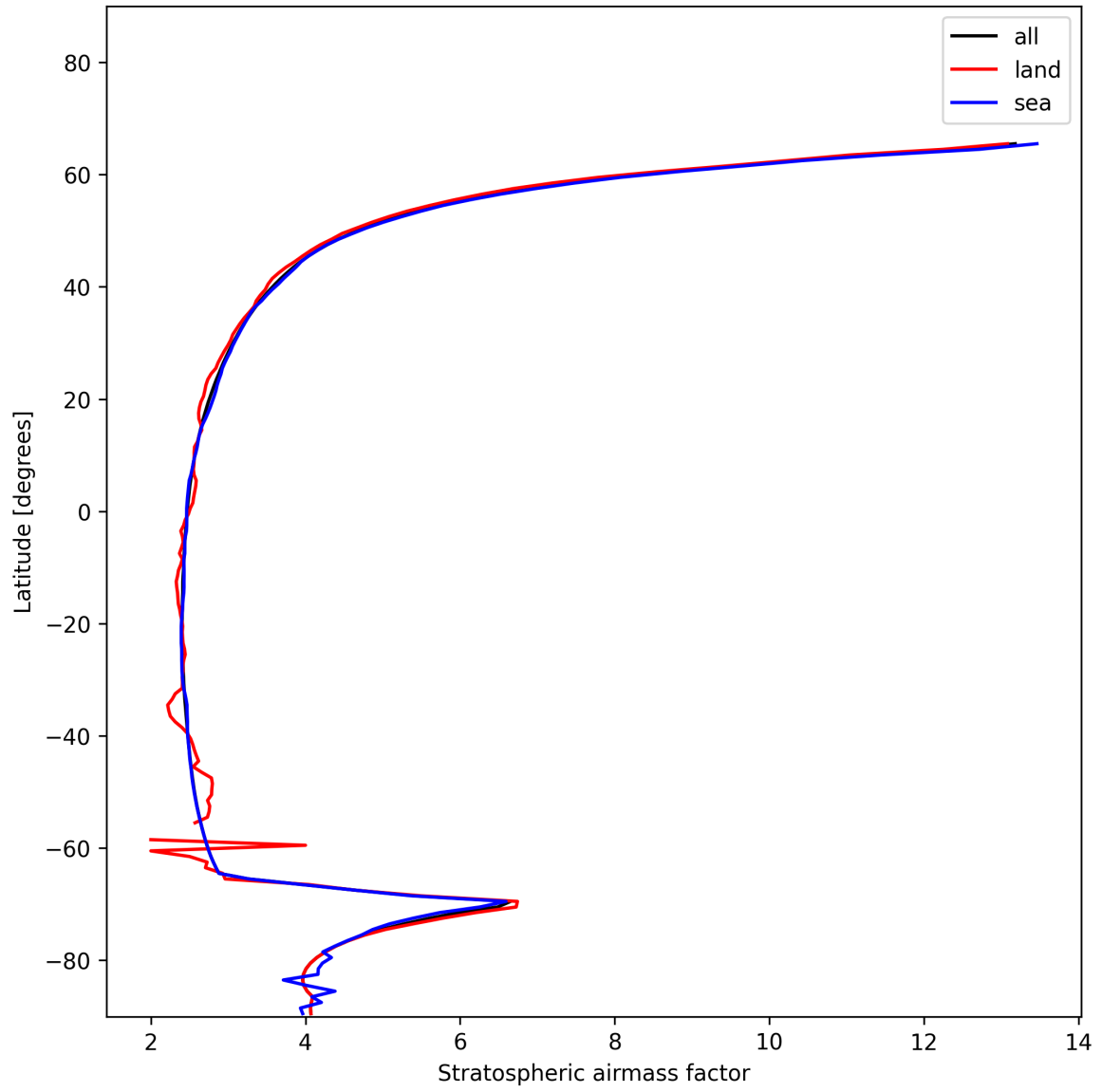
Figure 27: Zonal average of “Stratospheric airmass factor” for 2025-01-04 to 2025-01-06.
