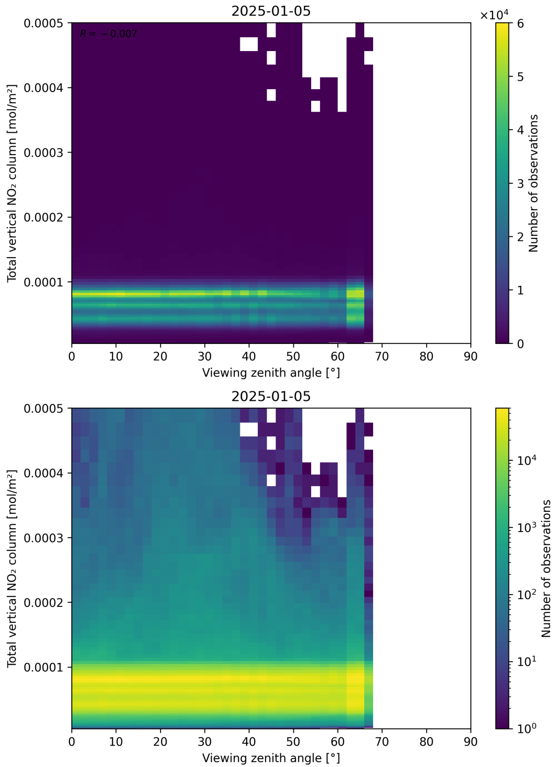
Figure 167: Scatter density plot of “Viewing zenith angle” against “Total vertical NO 2 column” for 2025-01-04 to 2025-01-06.
