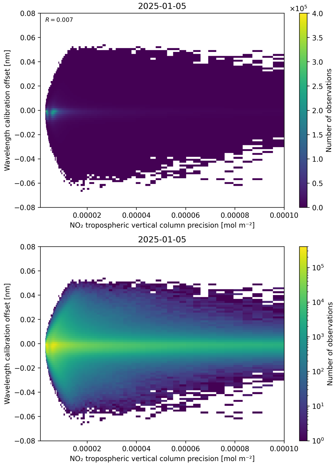
Figure 141: Scatter density plot of “NO 2 tropospheric vertical column precision” against “Wavelength calibration offset” for 2025-01-04 to 2025-01-06.
