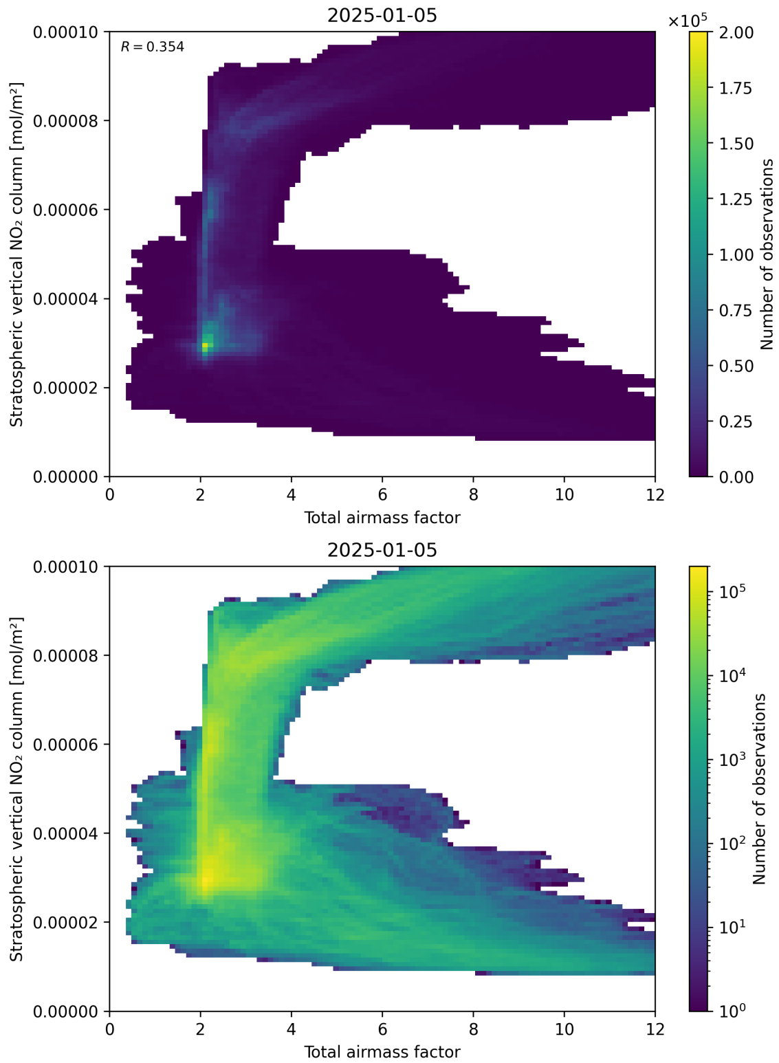
Figure 64: Scatter density plot of “Total airmass factor” against “Stratospheric vertical NO 2 column” for 2025-01-04 to 2025-01-06.
