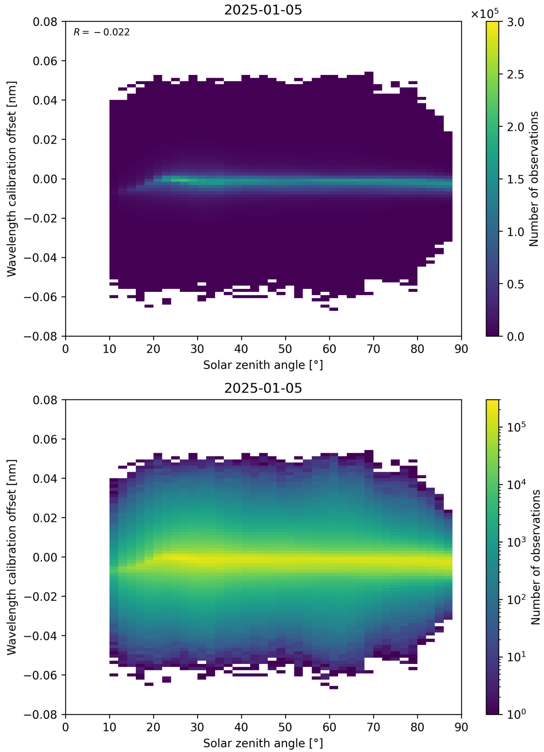
Figure 158: Scatter density plot of “Solar zenith angle” against “Wavelength calibration offset” for 2025-01-04 to 2025-01-06.
