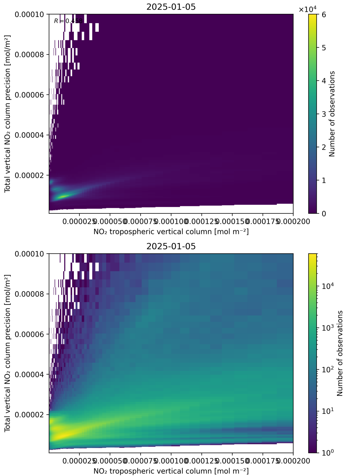
Figure 129: Scatter density plot of “NO 2 tropospheric vertical column” against “Total vertical NO 2 column precision” for 2025-01-04 to 2025-01-06.
