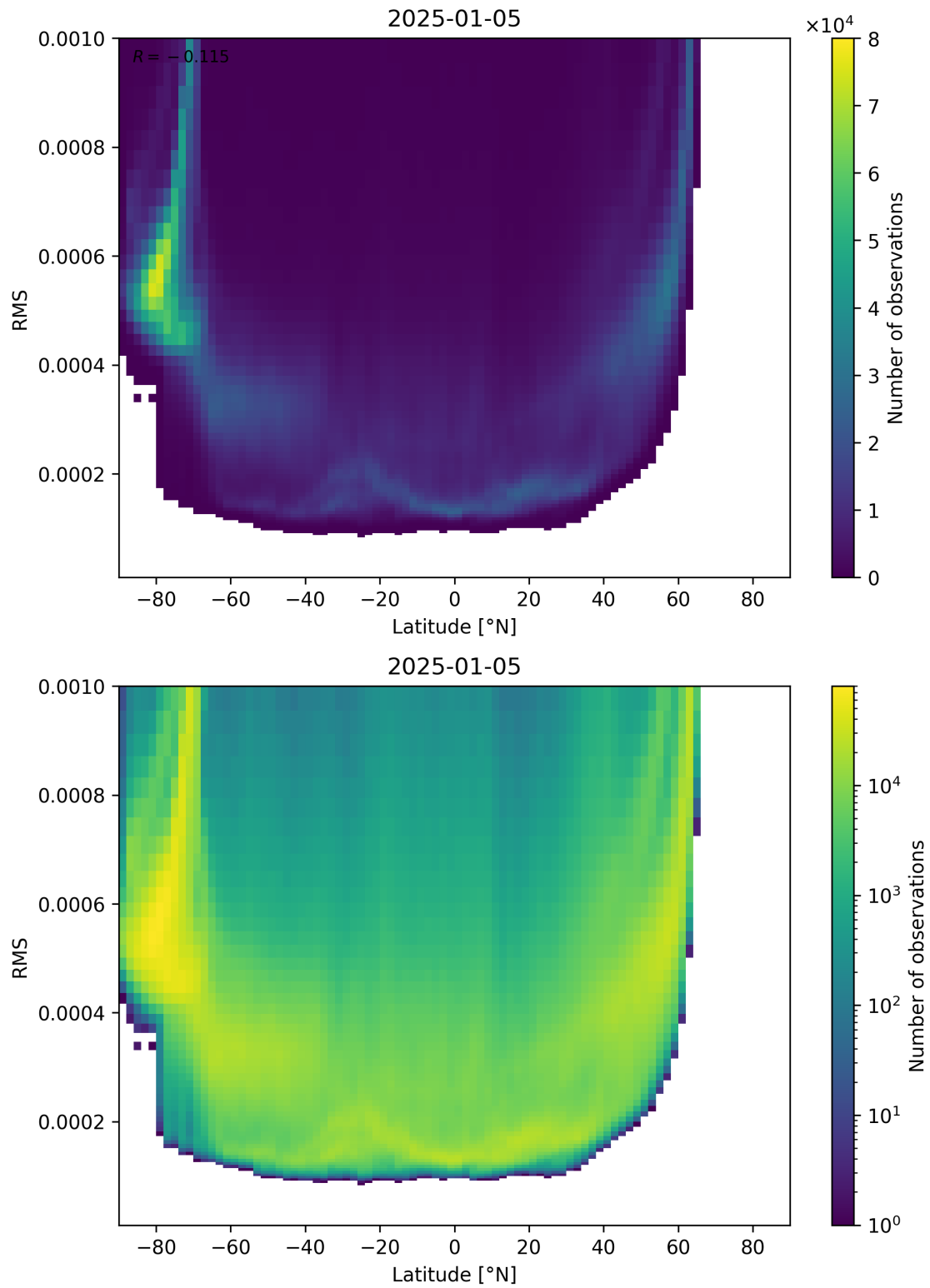
Figure 94: Scatter density plot of “Latitude” against “RMS” for 2025-01-04 to 2025-01-06.
