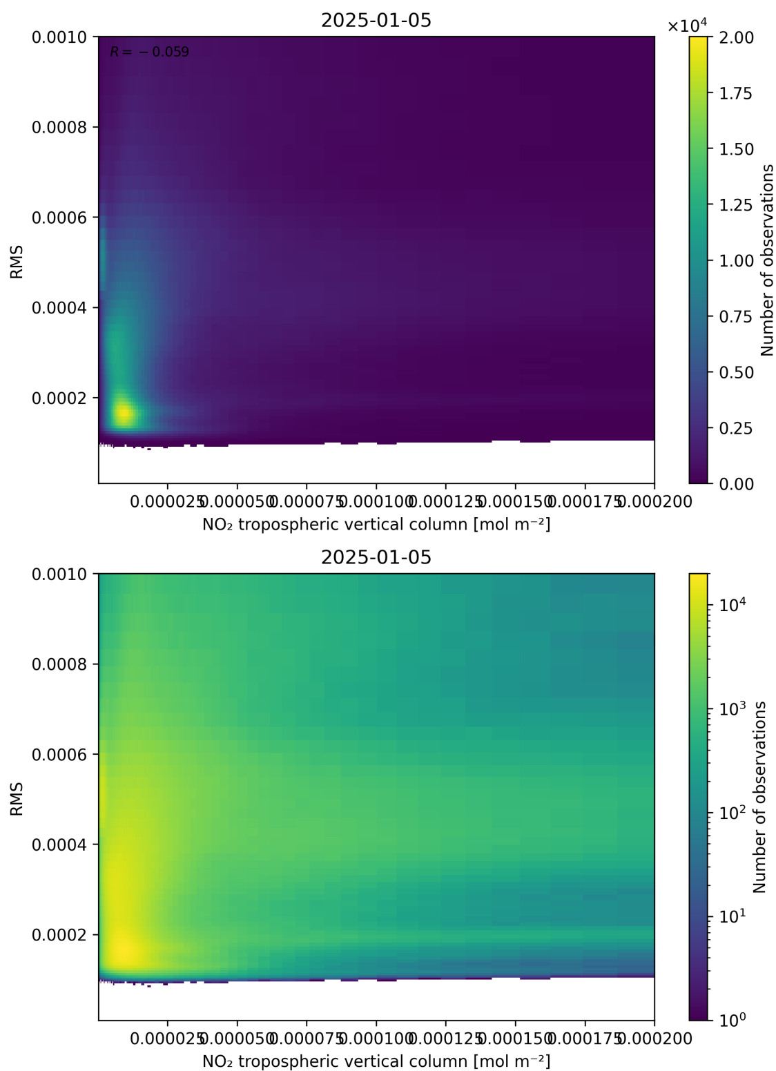
Figure 142: Scatter density plot of “NO 2 tropospheric vertical column” against “RMS” for 2025-01-04 to 2025-01-06.
