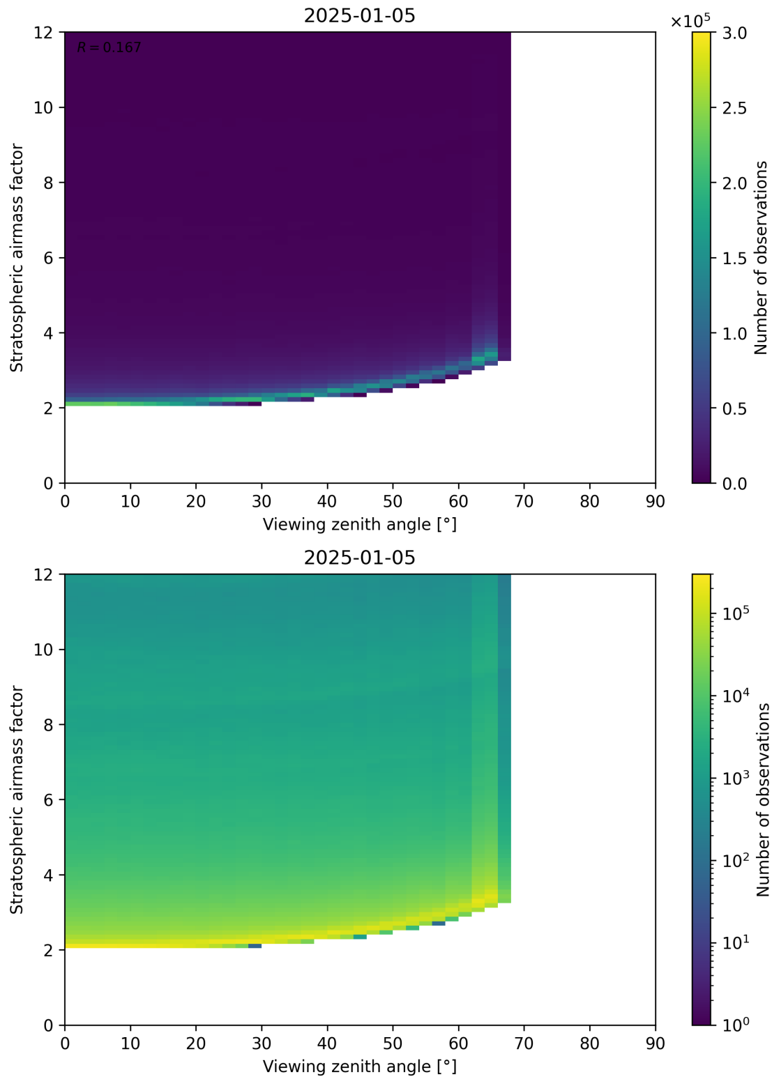
Figure 159: Scatter density plot of “Viewing zenith angle” against “Stratospheric airmass factor” for 2025-01-04 to 2025-01-06.
