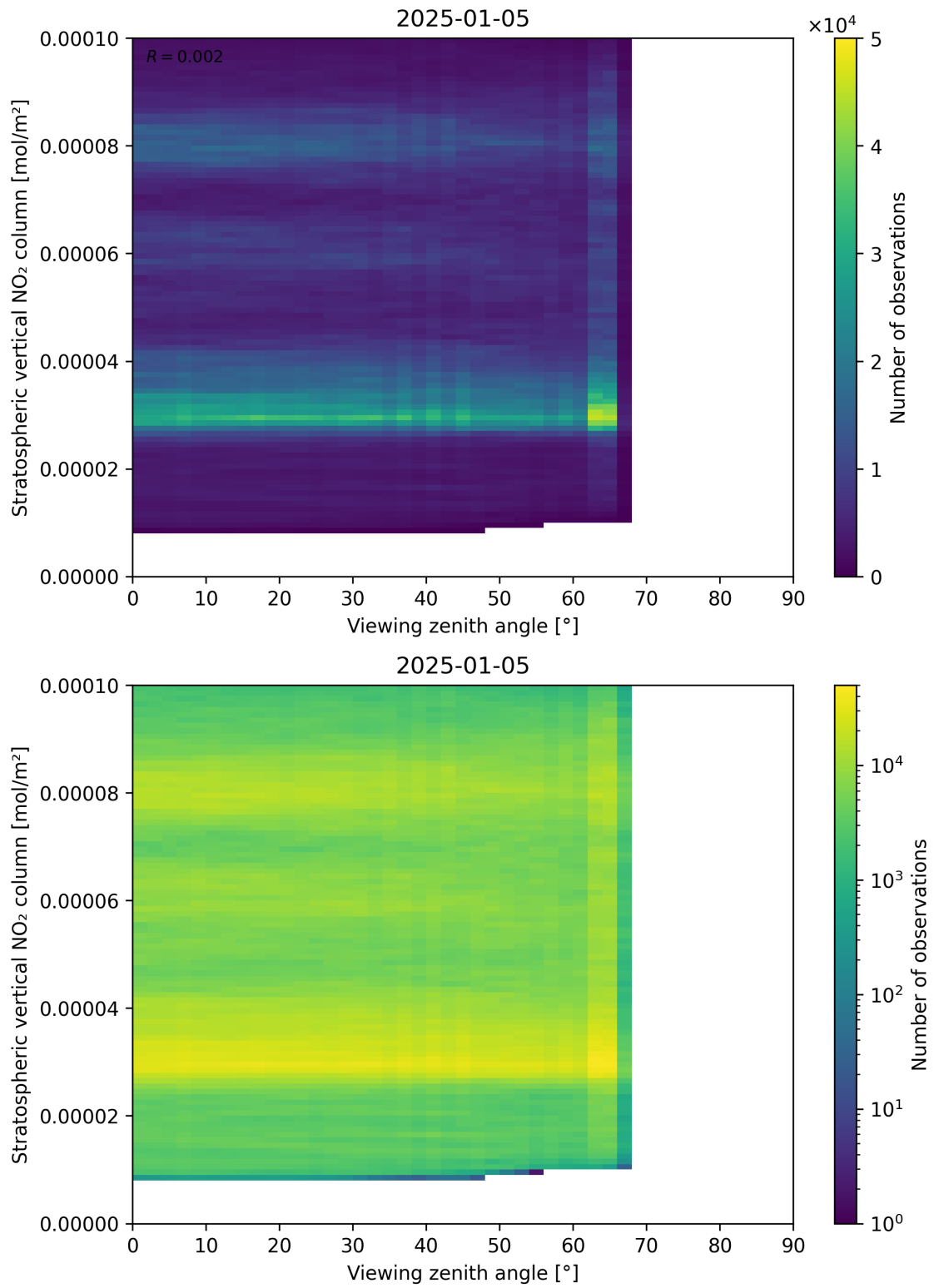
Figure 164: Scatter density plot of “Viewing zenith angle” against “Stratospheric vertical NO 2 column” for 2025-01-04 to 2025-01-06.
