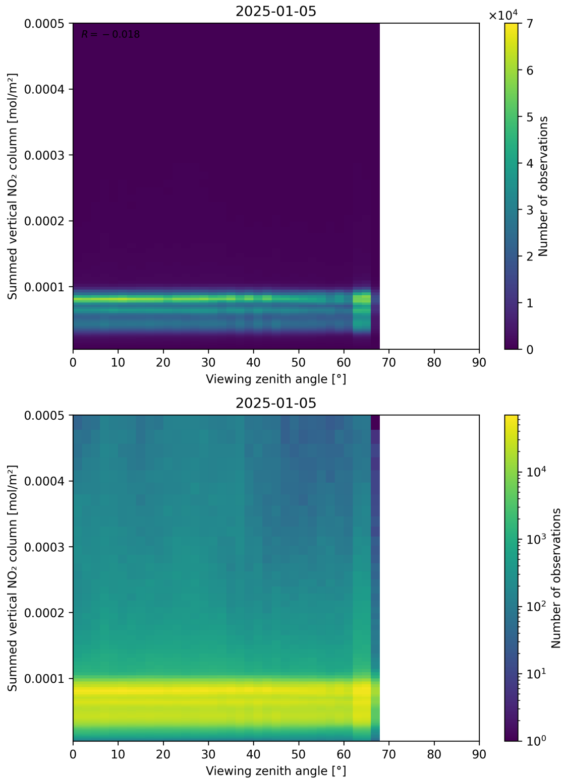
Figure 165: Scatter density plot of “Viewing zenith angle” against “Summed vertical NO 2 column” for 2025-01-04 to 2025-01-06.
