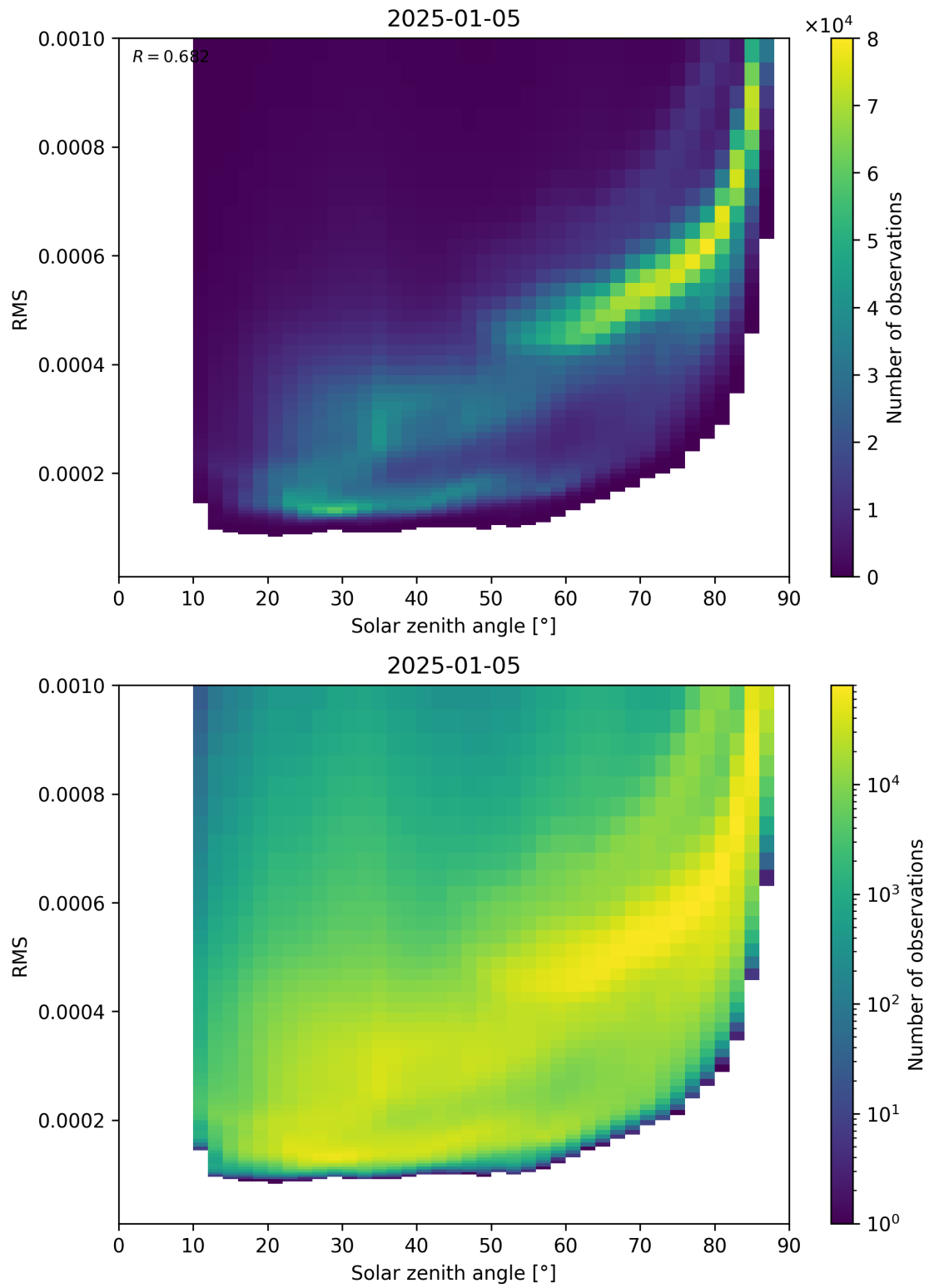
Figure 157: Scatter density plot of “Solar zenith angle” against “RMS” for 2025-01-04 to 2025-01-06.
