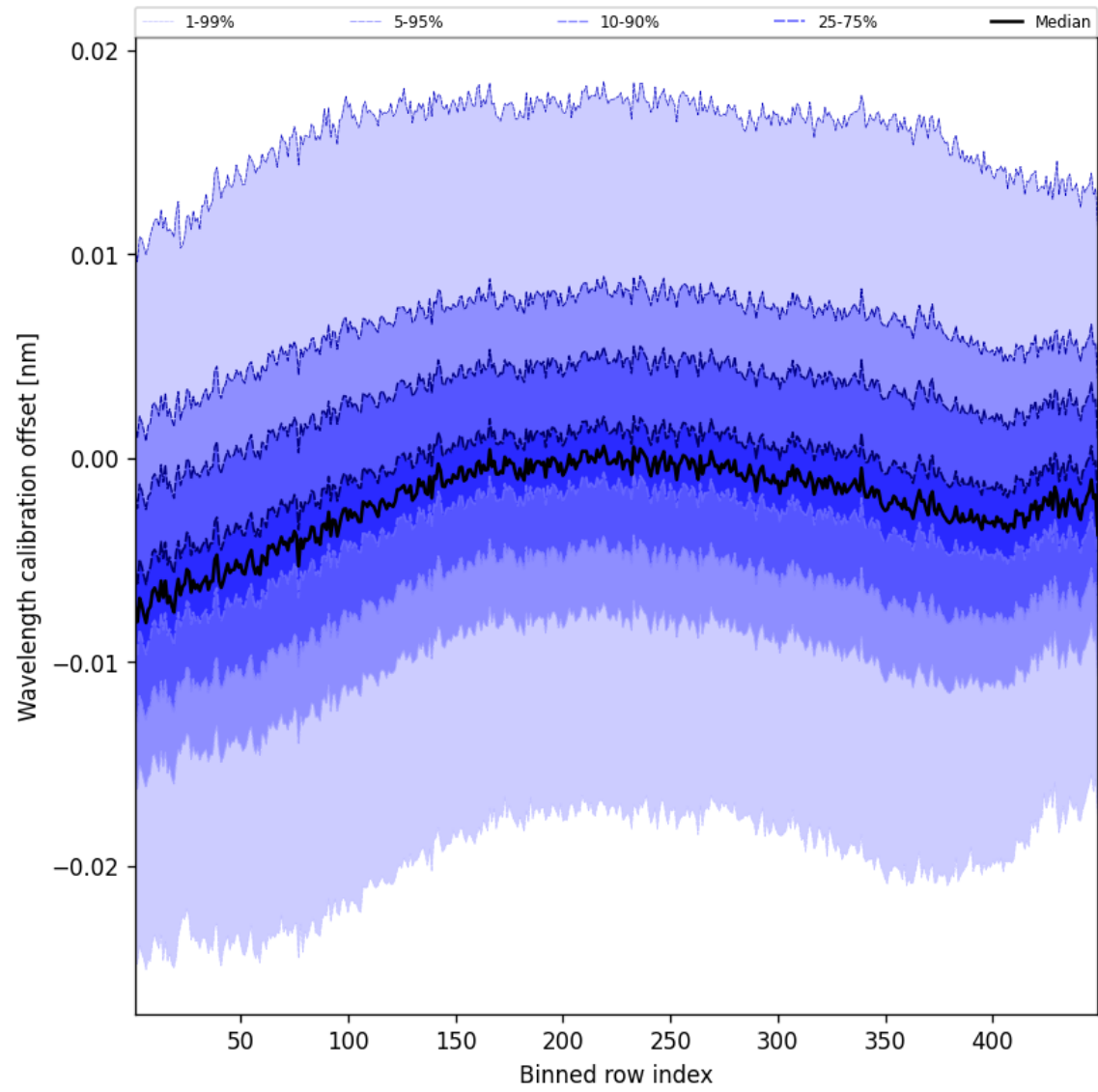
Figure 52: Along track statistics of “Wavelength calibration offset” for 2025-01-04 to 2025-01-06
