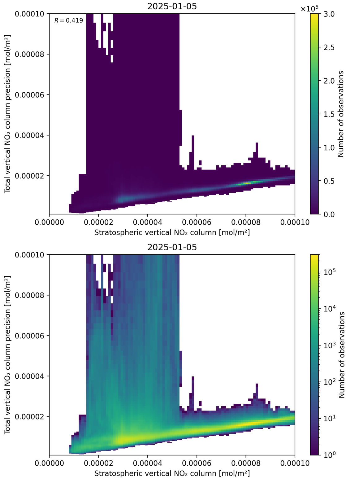
Figure 101: Scatter density plot of “Stratospheric vertical NO 2 column” against “Total vertical NO 2 column precision” for 2025-01-04 to 2025-01-06.
