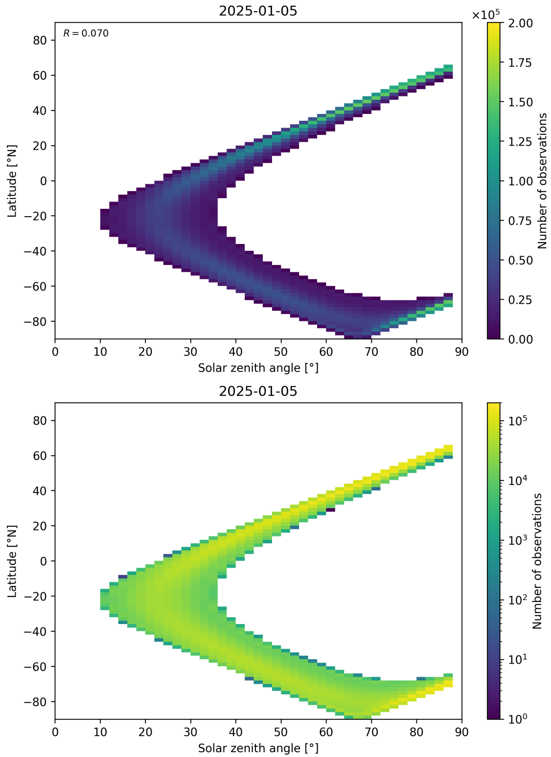
Figure 149: Scatter density plot of “Solar zenith angle” against “Latitude” for 2025-01-04 to 2025-01-06.
