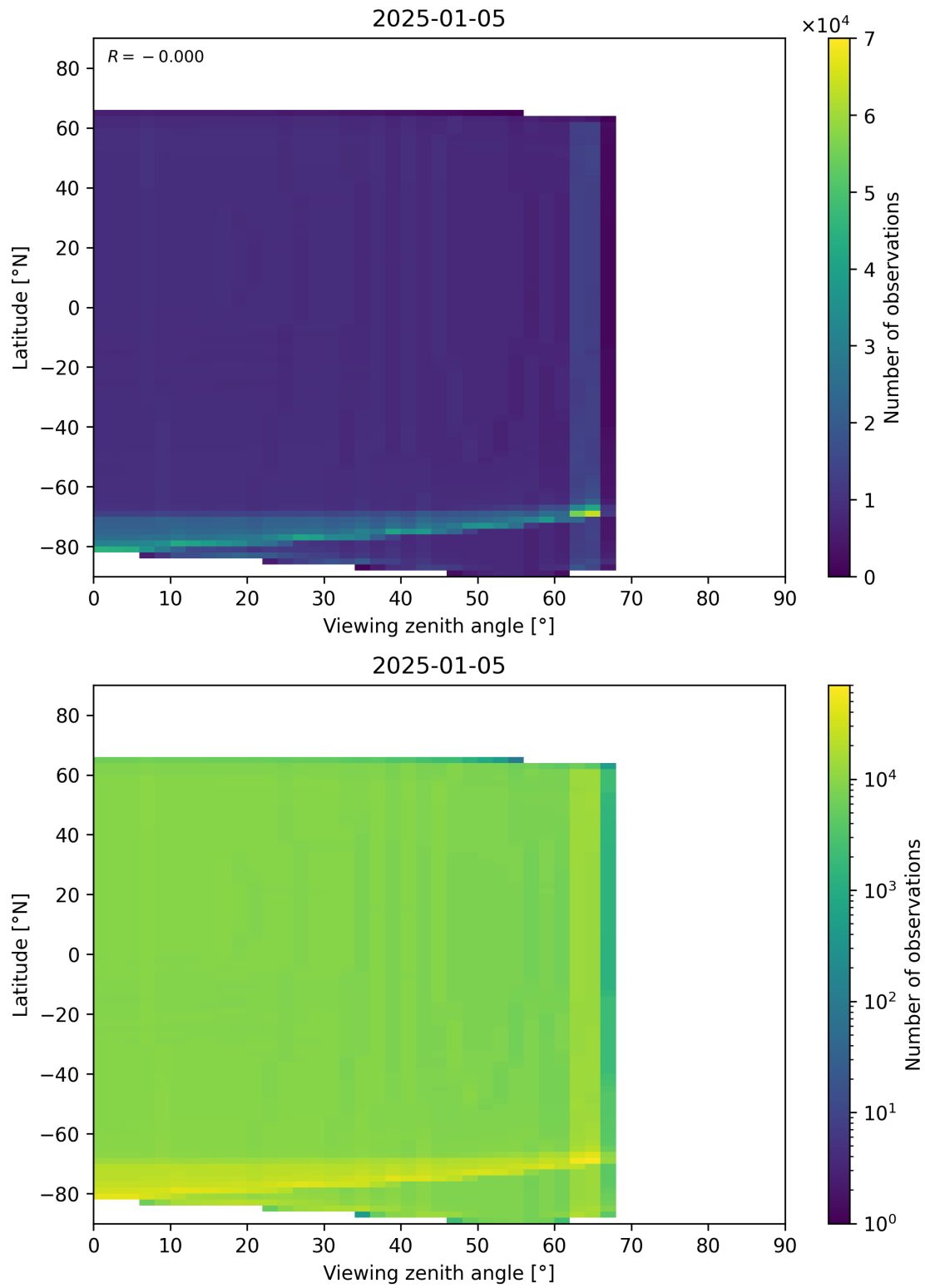
Figure 163: Scatter density plot of “Viewing zenith angle” against “Latitude” for 2025-01-04 to 2025-01-06.
