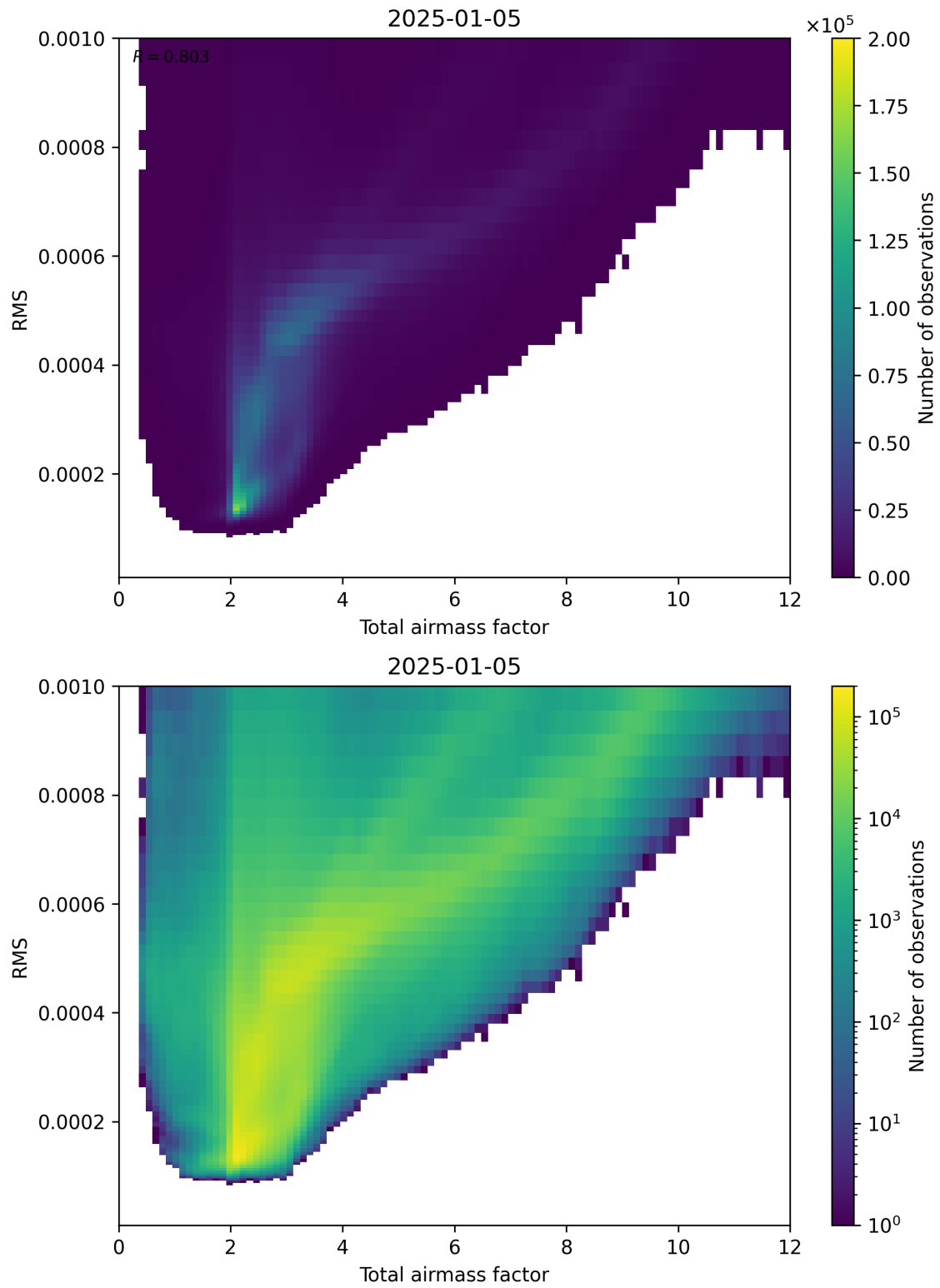
Figure 69: Scatter density plot of “Total airmass factor” against “RMS” for 2025-01-04 to 2025-01-06.
