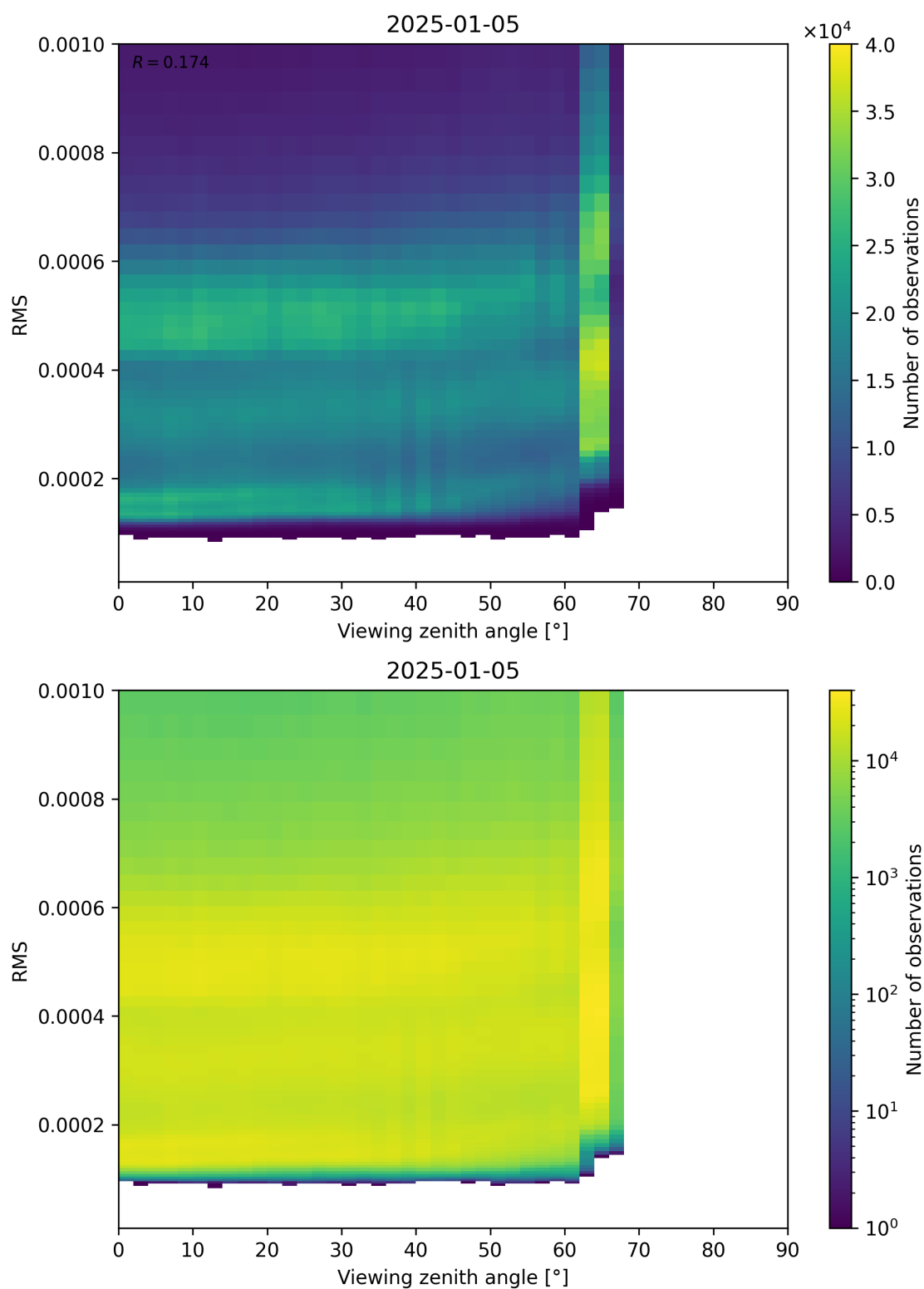
Figure 171: Scatter density plot of “Viewing zenith angle” against “RMS” for 2025-01-04 to 2025-01-06.
