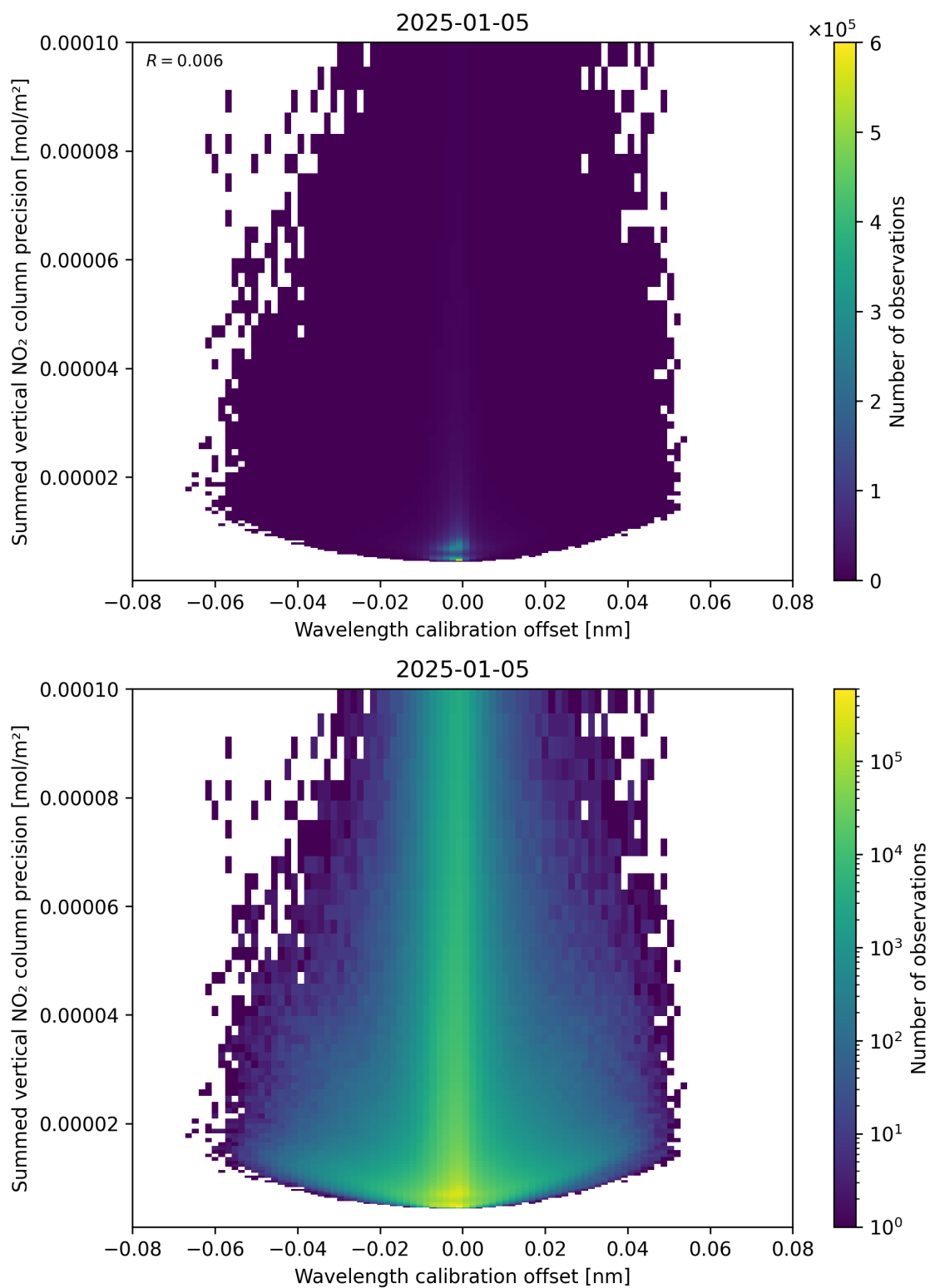
Figure 178: Scatter density plot of “Wavelength calibration offset” against “Summed vertical NO 2 column precision” for 2025-01-04 to 2025-01-06.
