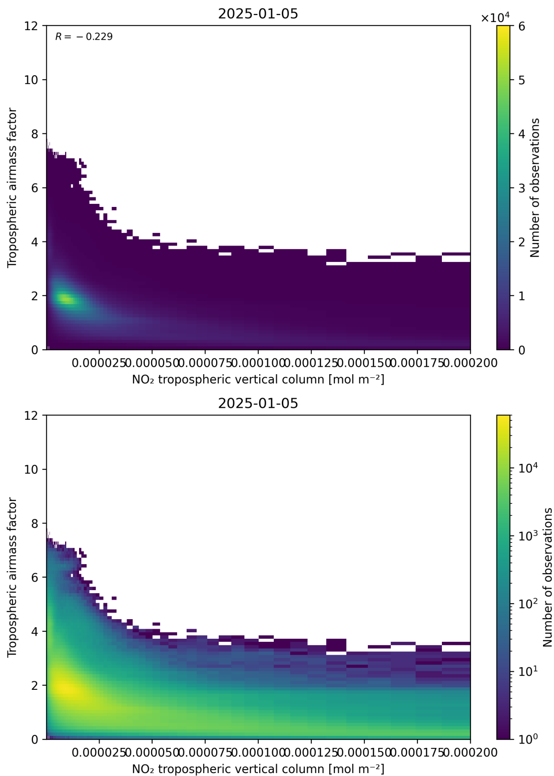
Figure 123: Scatter density plot of “NO 2 tropospheric vertical column” against “Tropospheric air mass factor” for 2025-01-04 to 2025-01-06.
