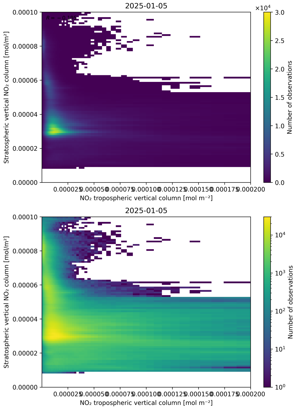
Figure 125: Scatter density plot of “NO 2 tropospheric vertical column” against “Stratospheric vertical NO 2 column” for 2025-01-04 to 2025-01-06.
