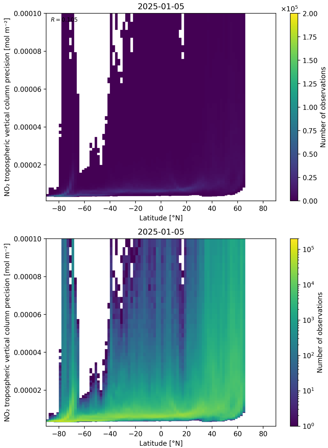
Figure 93: Scatter density plot of “Latitude” against “NO 2 tropospheric vertical column precision” for 2025-01-04 to 2025-01-06.
