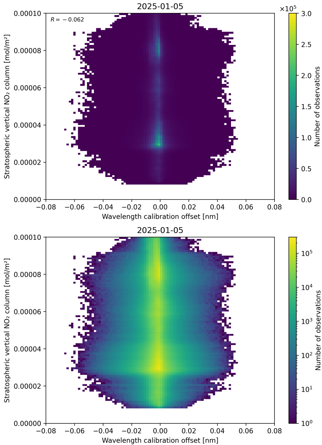
Figure 176: Scatter density plot of “Wavelength calibration offset” against “Stratospheric vertical NO 2 column” for 2025-01-04 to 2025-01-06.
