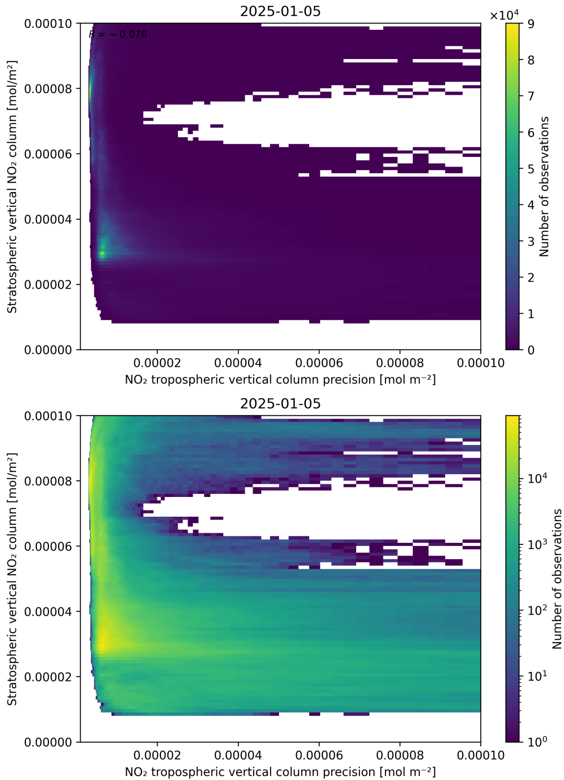
Figure 135: Scatter density plot of “NO 2 tropospheric vertical column precision” against “Stratospheric vertical NO 2 column” for 2025-01-04 to 2025-01-06.
