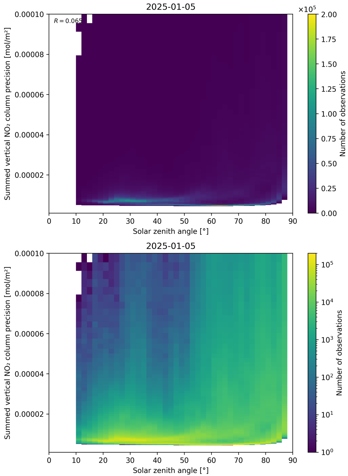
Figure 152: Scatter density plot of “Solar zenith angle” against “Summed vertical NO 2 column precision” for 2025-01-04 to 2025-01-06.
