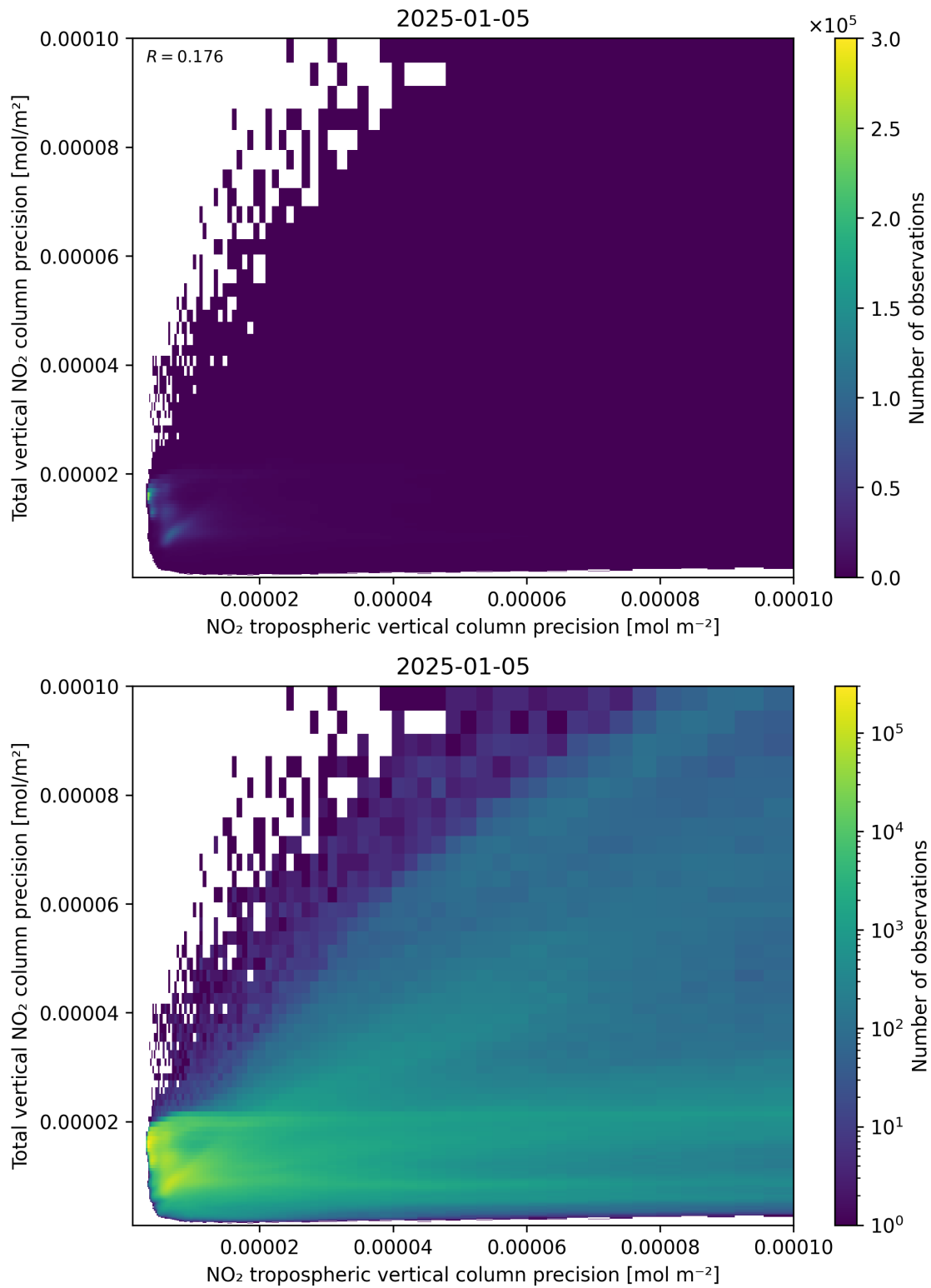
Figure 139: Scatter density plot of “NO 2 tropospheric vertical column precision” against “Total vertical NO 2 column precision” for 2025-01-04 to 2025-01-06.
