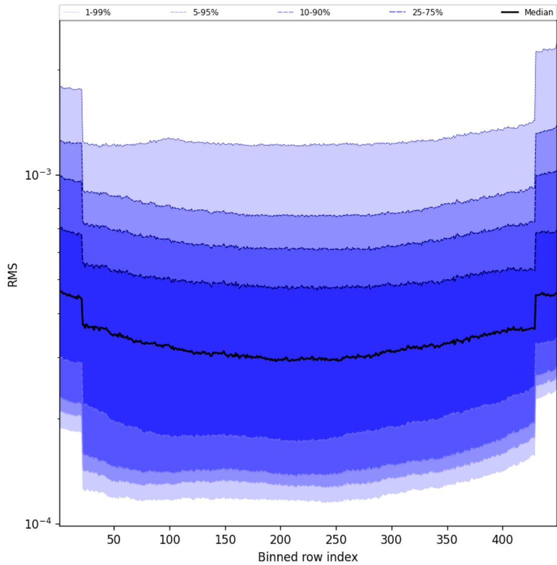
Figure 60: Along track statistics of “RMS” for 2025-01-04 to 2025-01-06
