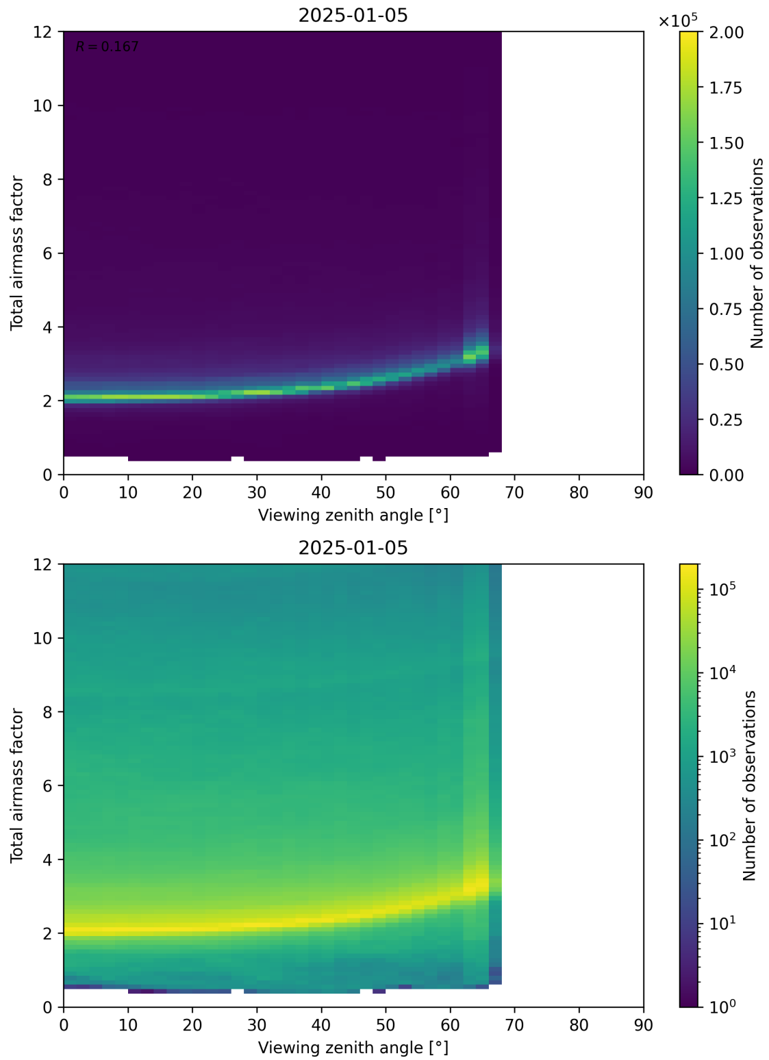
Figure 160: Scatter density plot of “Viewing zenith angle” against “Total airmass factor” for 2025-01-04 to 2025-01-06.
