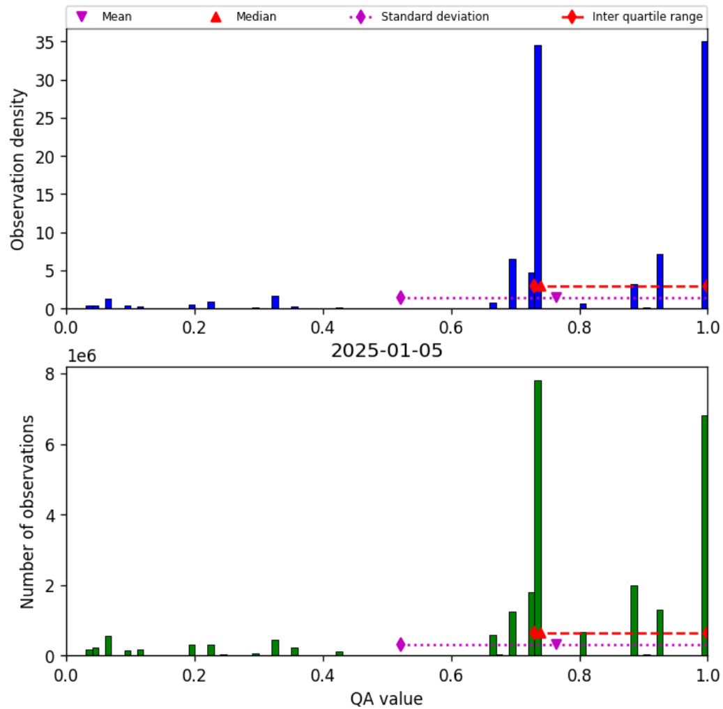
Figure 28: Histogram of “QA value” for 2025-01-04 to 2025-01-06
