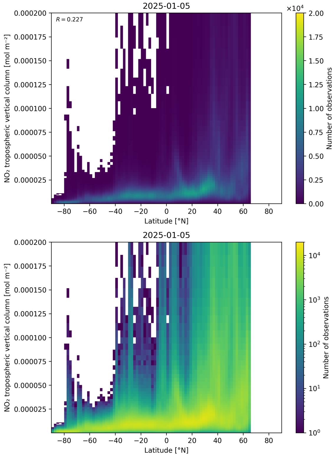
Figure 92: Scatter density plot of “Latitude” against “NO 2 tropospheric vertical column” for 2025-01-04 to 2025-01-06.
