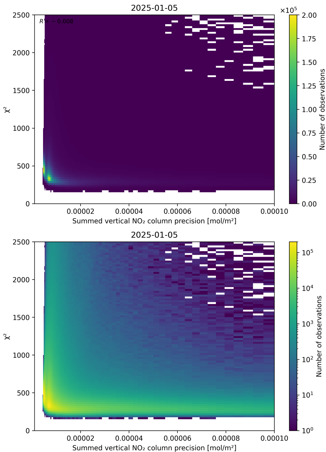
Figure 107: Scatter density plot of “Summed vertical NO 2 column precision” against “ \chi^2 ” for 2025-01-04 to 2025-01-06.
