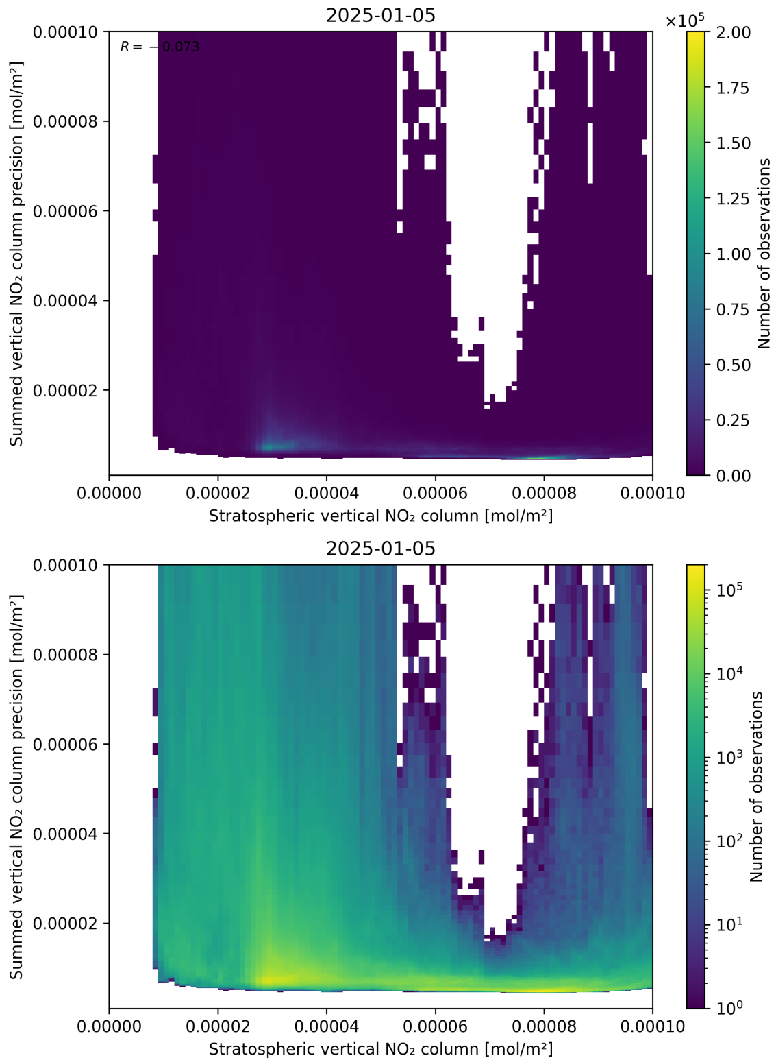
Figure 99: Scatter density plot of “Stratospheric vertical NO 2 column” against “Summed vertical NO 2 column precision” for 2025-01-04 to 2025-01-06.
