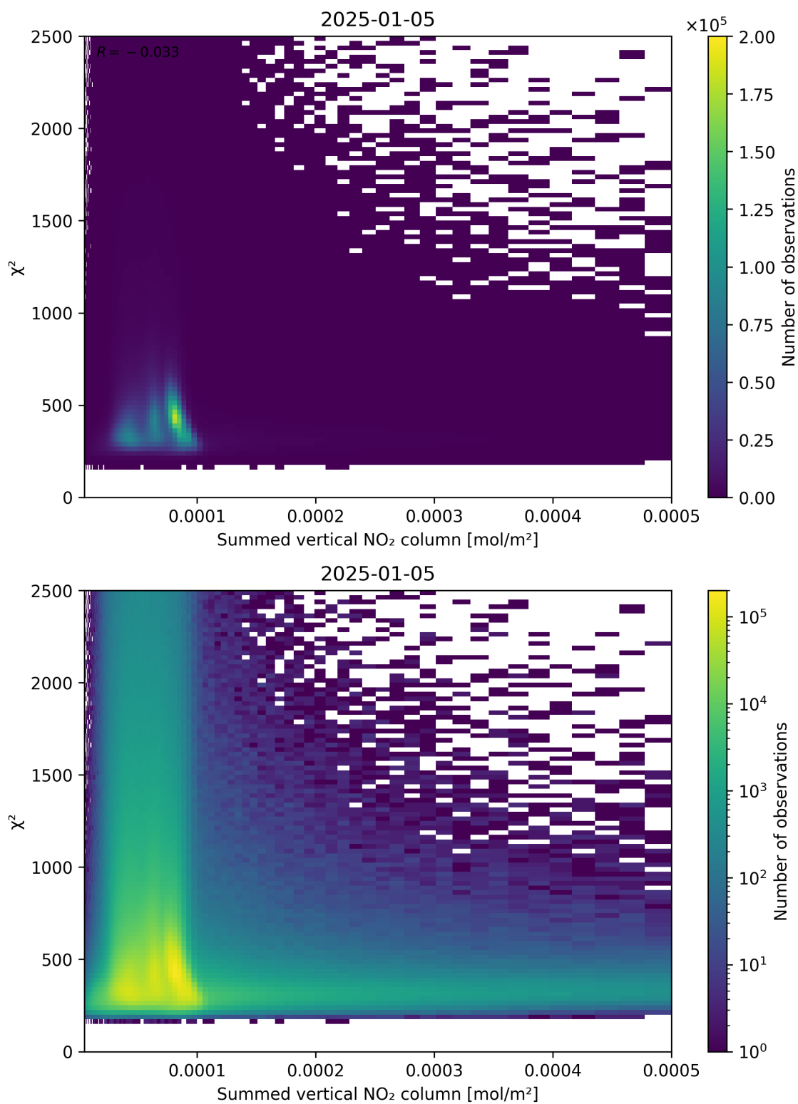
Figure 104: Scatter density plot of “Summed vertical NO 2 column” against “ \chi^2 ” for 2025-01-04 to 2025-01-06.
