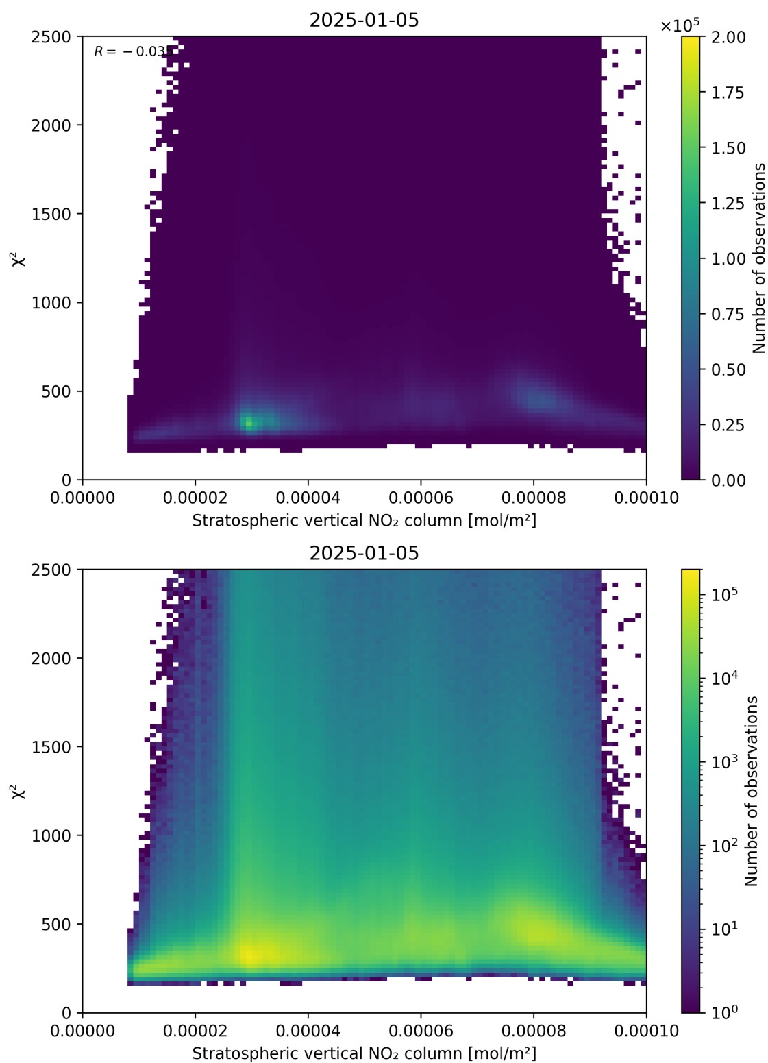
Figure 97: Scatter density plot of “Stratospheric vertical NO 2 column” against “ \chi^2 ” for 2025-01-04 to 2025-01-06.
