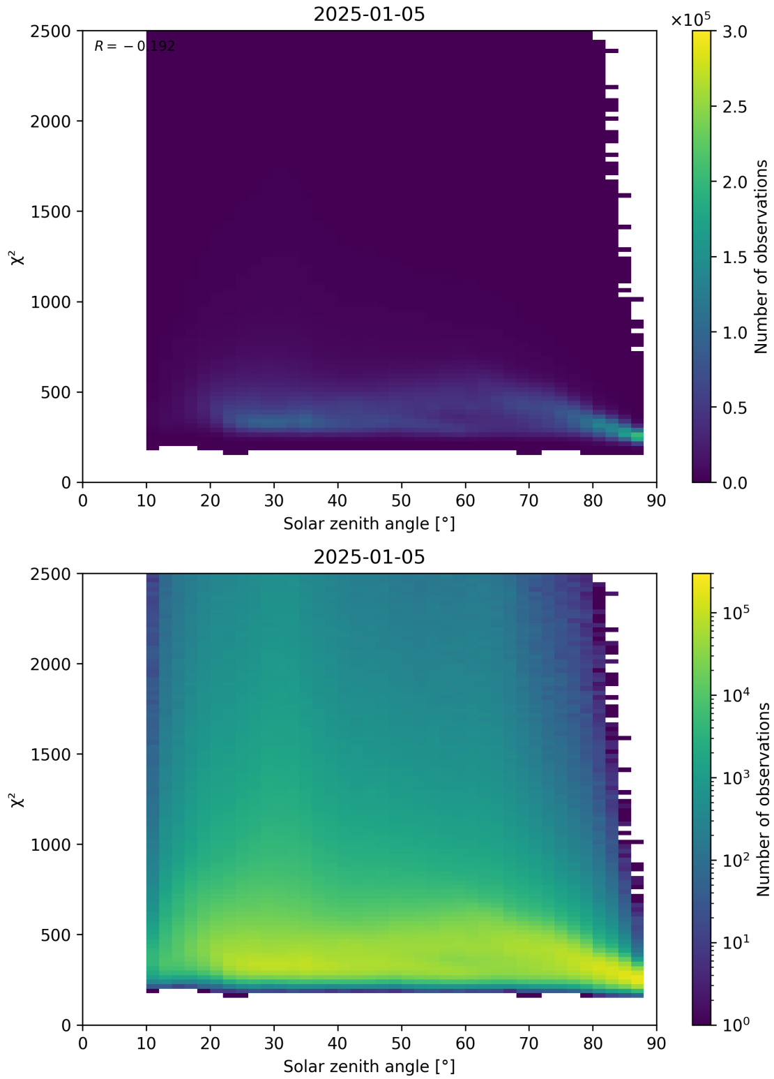
Figure 148: Scatter density plot of “Solar zenith angle” against “ \chi^2 ” for 2025-01-04 to 2025-01-06.
