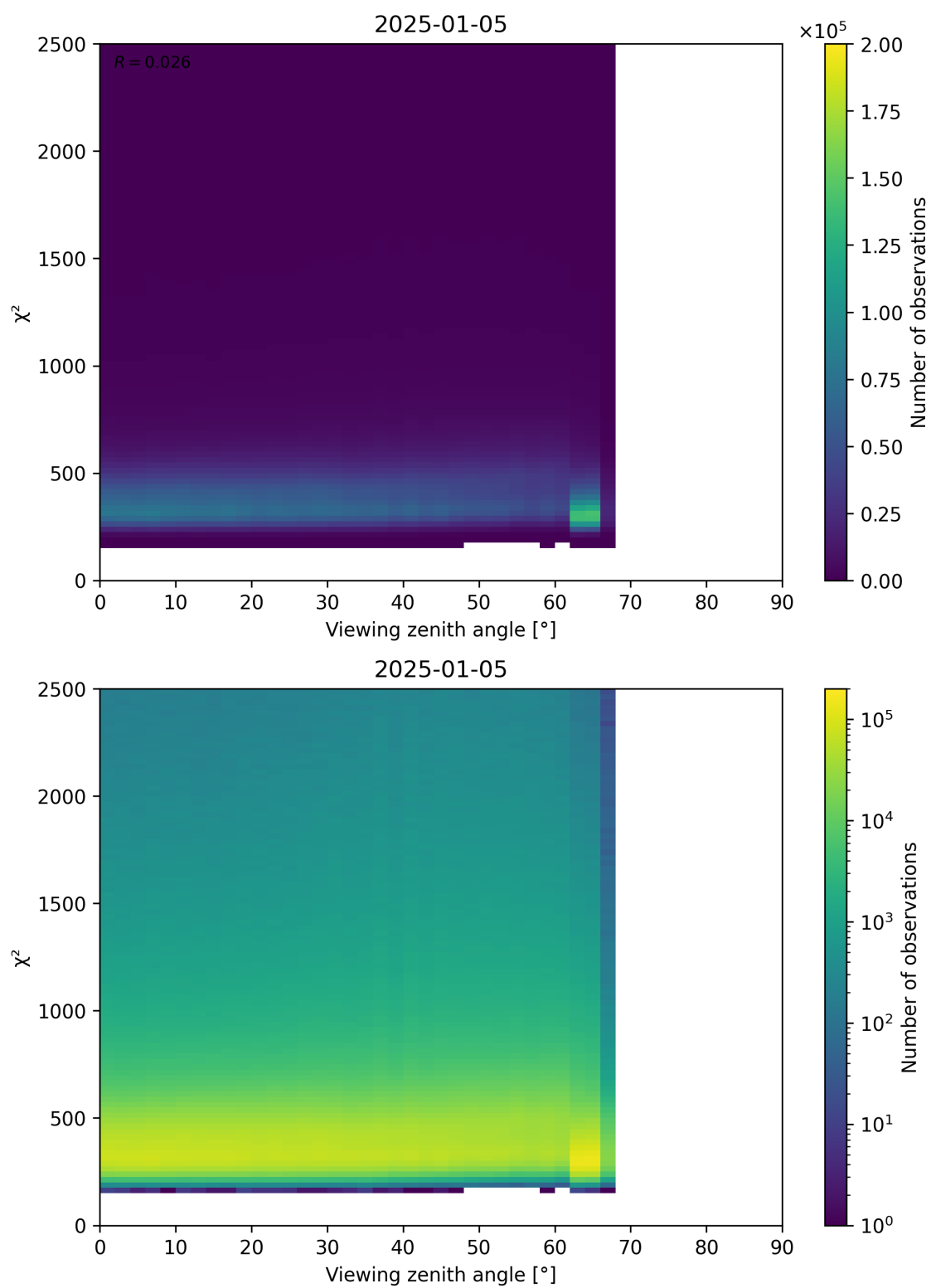
Figure 162: Scatter density plot of “Viewing zenith angle” against “ \chi^2 ” for 2025-01-04 to 2025-01-06.
