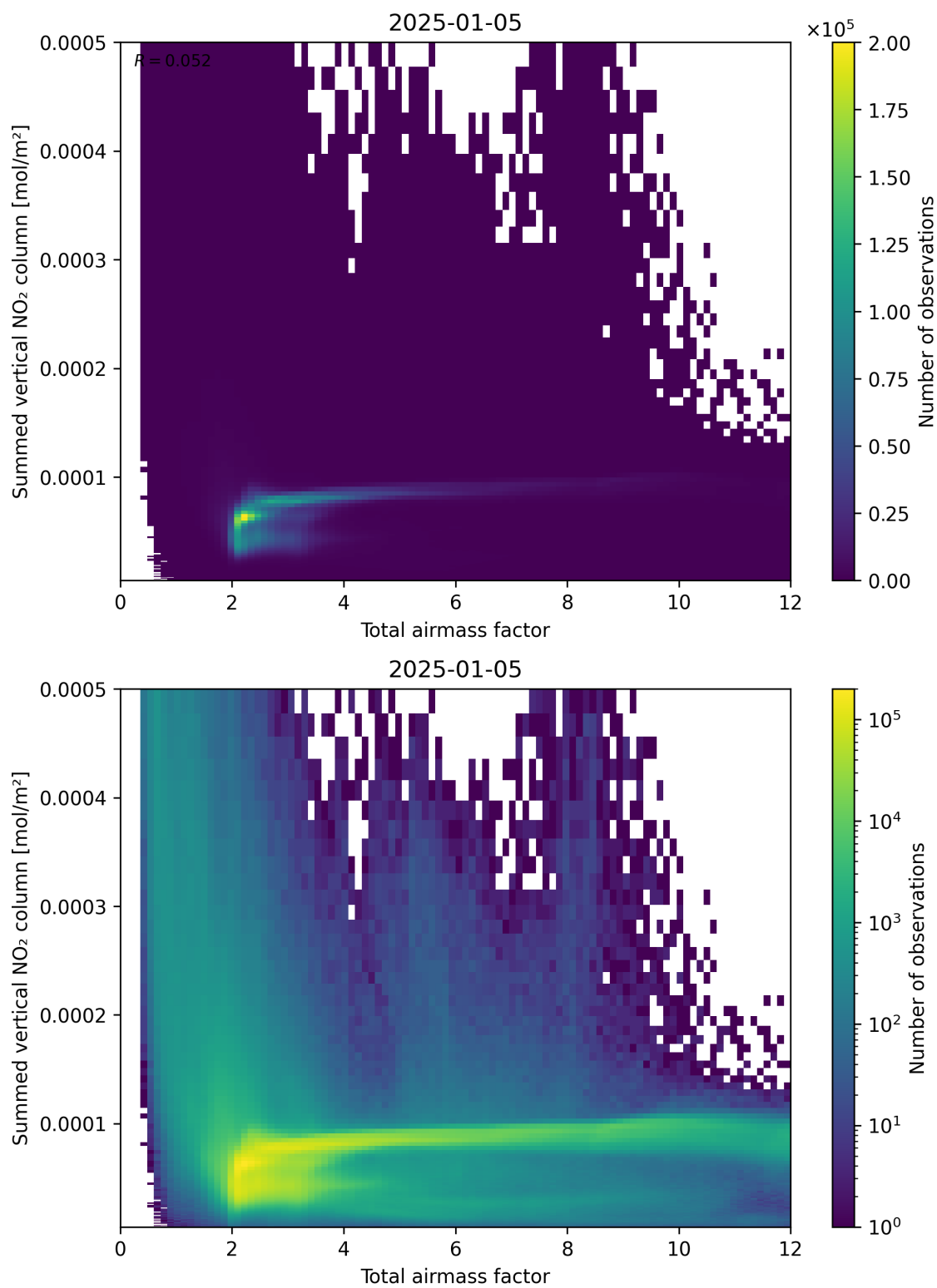
Figure 65: Scatter density plot of “Total airmass factor” against “Summed vertical NO 2 column” for 2025-01-04 to 2025-01-06.
