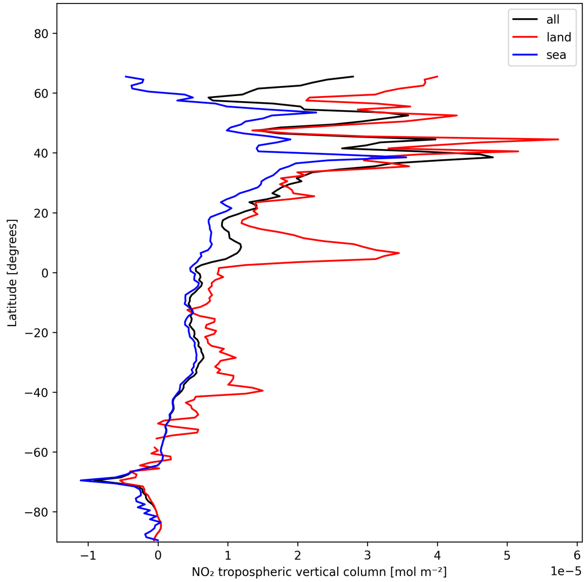
Figure 12: Zonal average of “NO 2 tropospheric vertical column” for 2025-01-04 to 2025-01-06.
