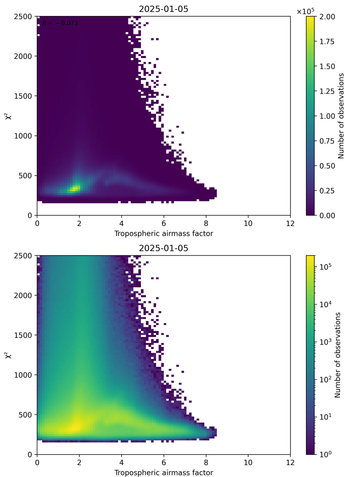
Figure 73: Scatter density plot of “Tropospheric airmass factor” against “ \chi^2 ” for 2025-01-04 to 2025-01-06.
