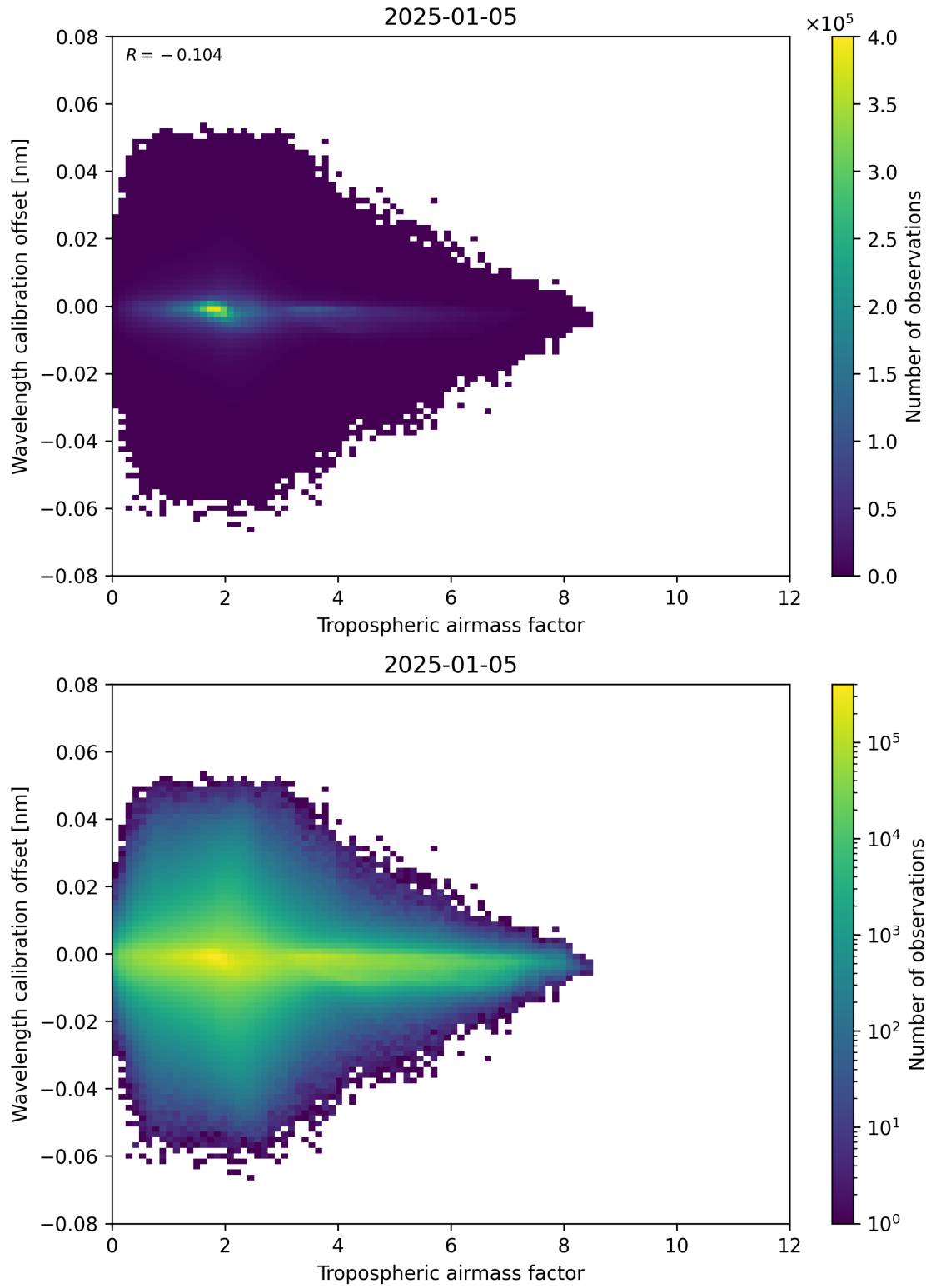
Figure 80: Scatter density plot of “Tropospheric airmass factor” against “Wavelength calibration offset” for 2025-01-04 to 2025-01-06.
