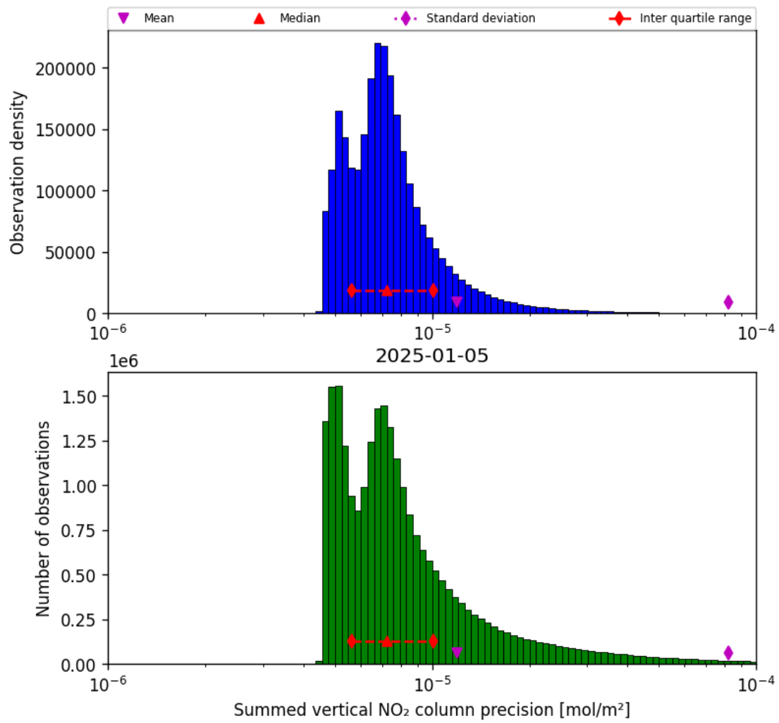
Figure 41: Histogram of “Summed vertical NO 2 column precision” for 2025-01-04 to 2025-01-06
