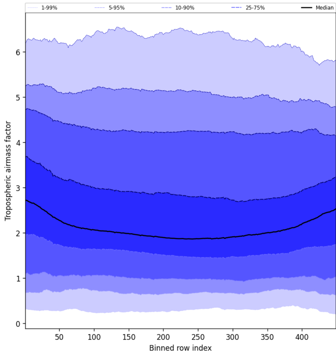
Figure 48: Along track statistics of “Tropospheric air mass factor” for 2025-01-04 to 2025-01-06
