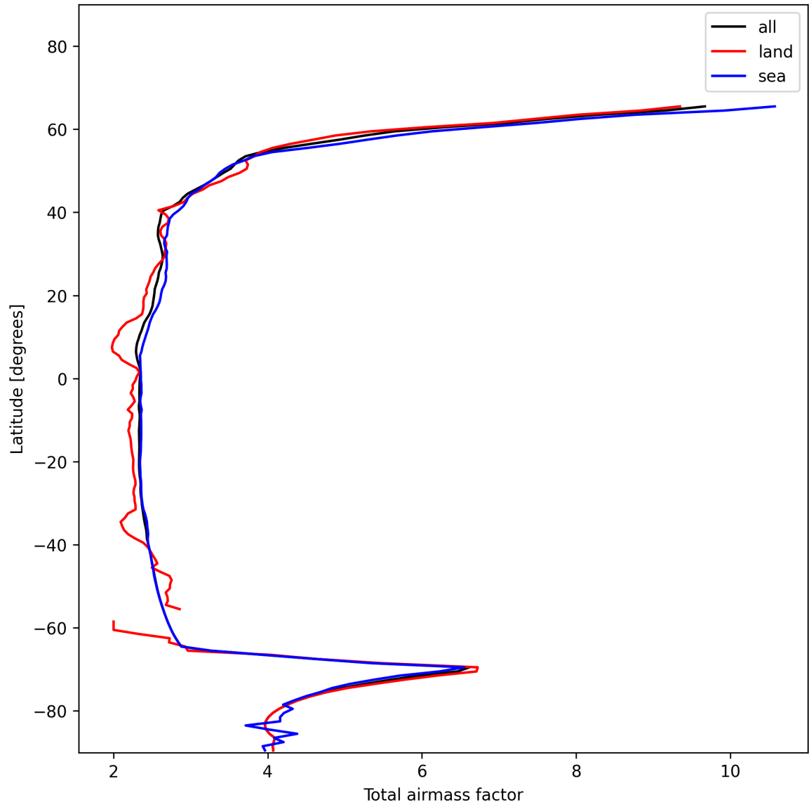
Figure 15: Zonal average of “Total airmass factor” for 2025-01-04 to 2025-01-06.
