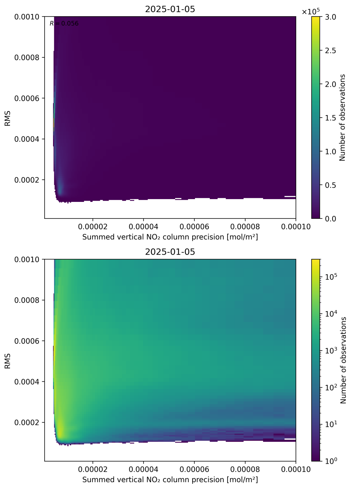
Figure 108: Scatter density plot of “Summed vertical NO 2 column precision” against “RMS” for 2025-01-04 to 2025-01-06.
