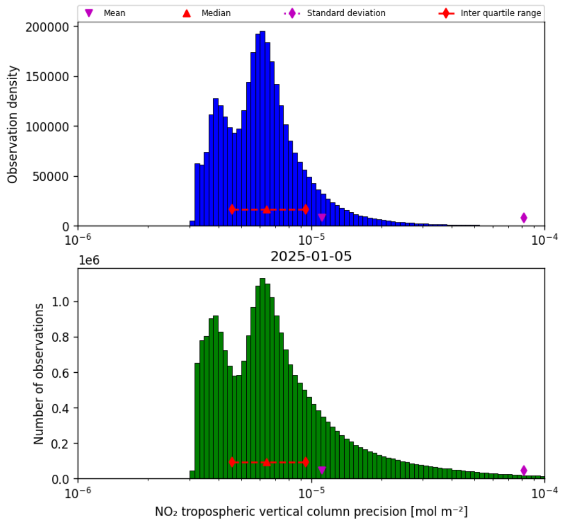
Figure 30: Histogram of “NO 2 tropospheric vertical column precision” for 2025-01-04 to 2025-01-06
