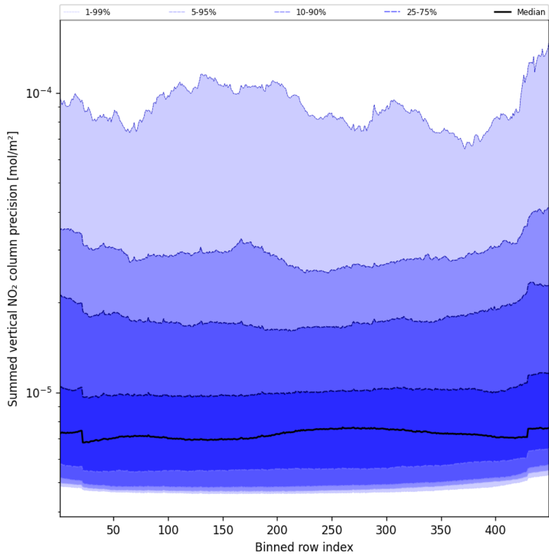
Figure 58: Along track statistics of “Summed vertical NO 2 column precision” for 2025-01-04 to 2025-01-06
