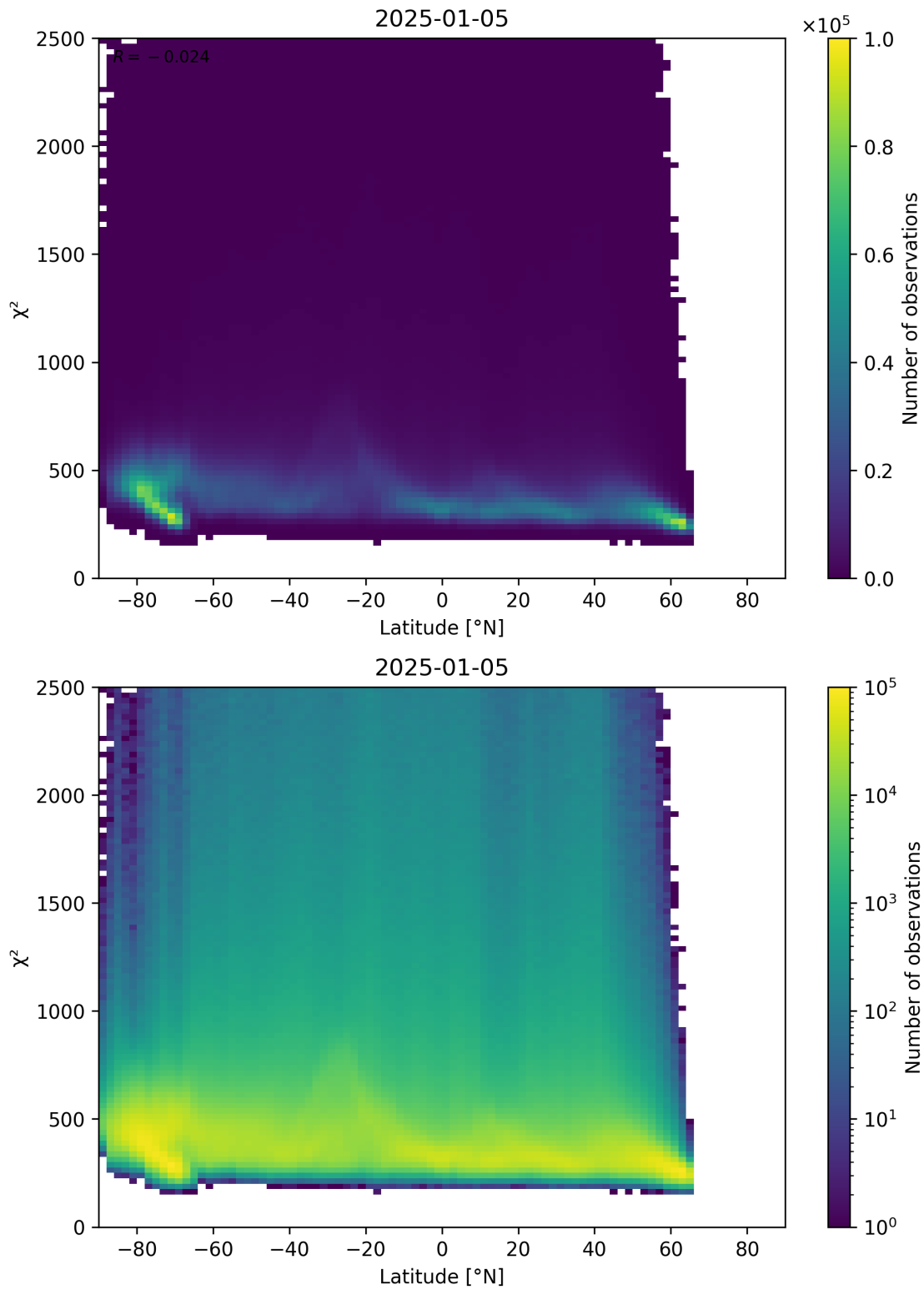
Figure 86: Scatter density plot of “Latitude” against “ \chi^2 ” for 2025-01-04 to 2025-01-06.
