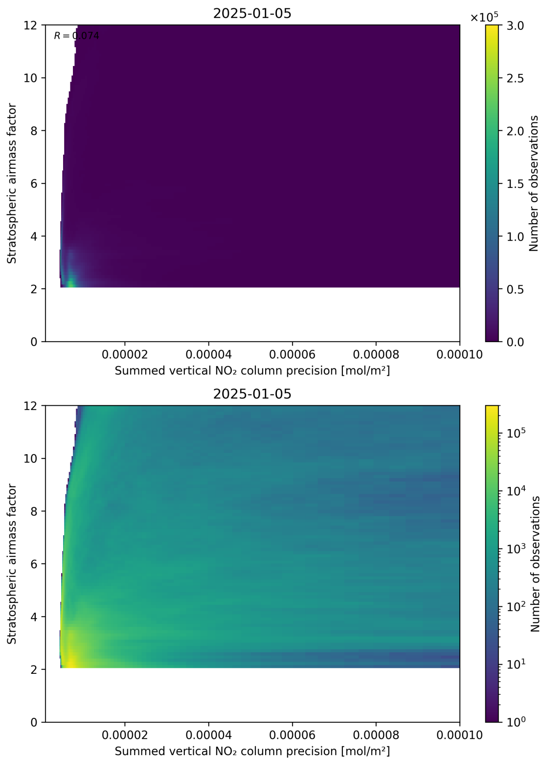
Figure 106: Scatter density plot of “Summed vertical NO 2 column precision” against “Stratospheric airmass factor” for 2025-01-04 to 2025-01-06.
