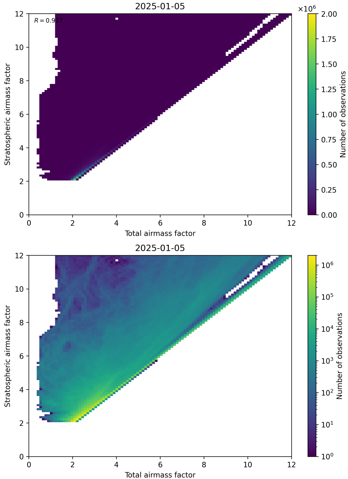
Figure 62: Scatter density plot of “Total airmass factor” against “Stratospheric airmass factor” for 2025-01-04 to 2025-01-06.
