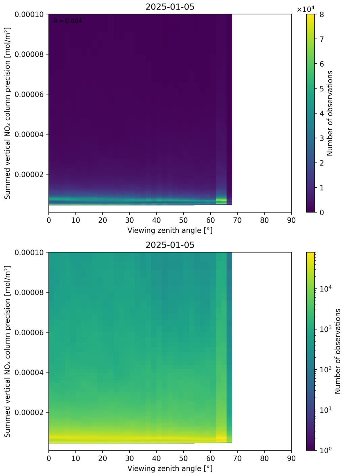
Figure 166: Scatter density plot of “Viewing zenith angle” against “Summed vertical NO 2 column precision” for 2025-01-04 to 2025-01-06.
