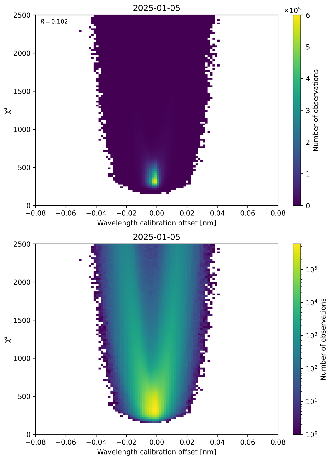
Figure 175: Scatter density plot of “Wavelength calibration offset” against “ \chi^2 ” for 2025-01-04 to 2025-01-06.
