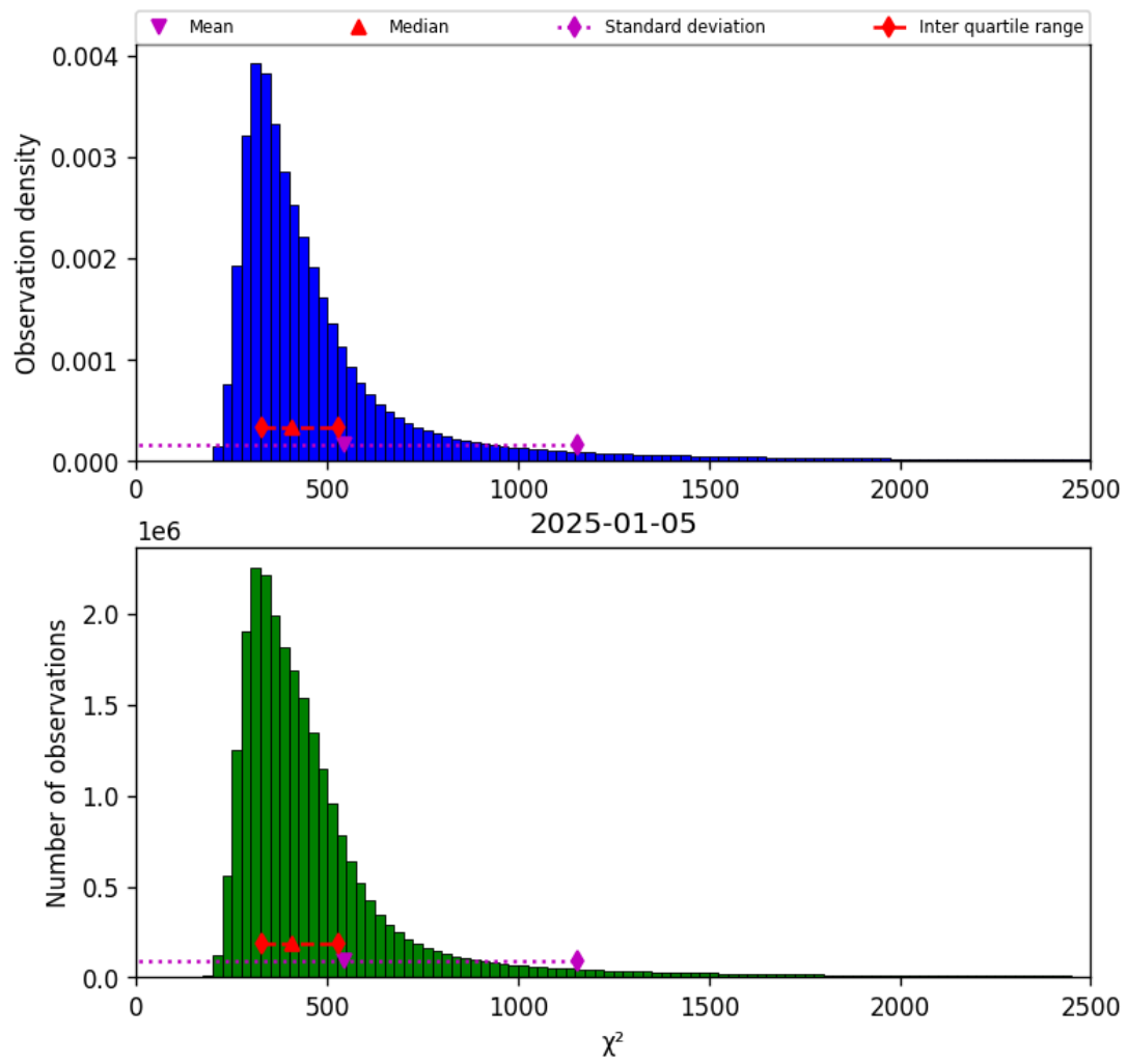
Figure 42: Histogram of “ \chi^2 ” for 2025-01-04 to 2025-01-06
