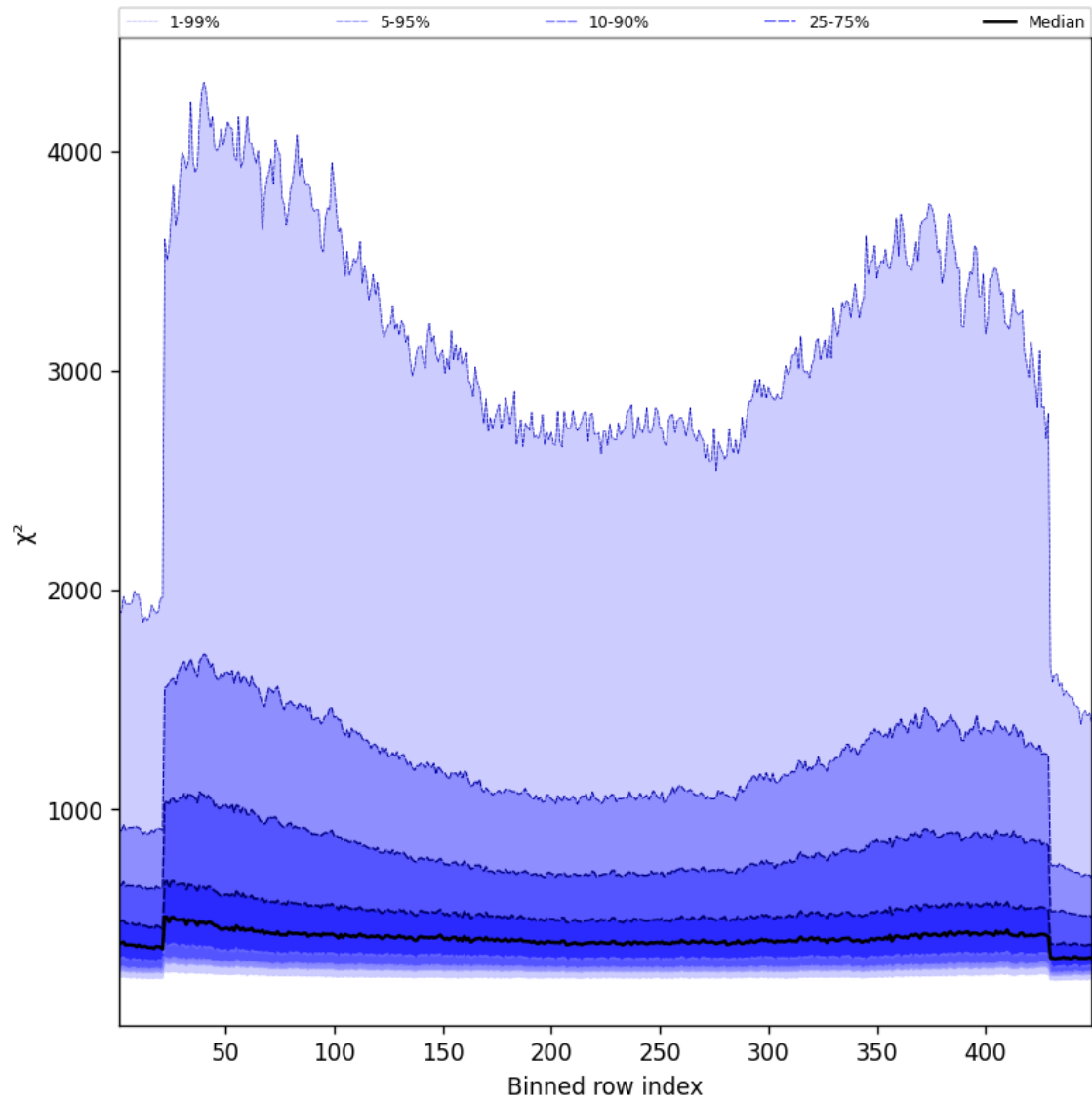
Figure 59: Along track statistics of “ \chi^2 ” for 2025-01-04 to 2025-01-06
