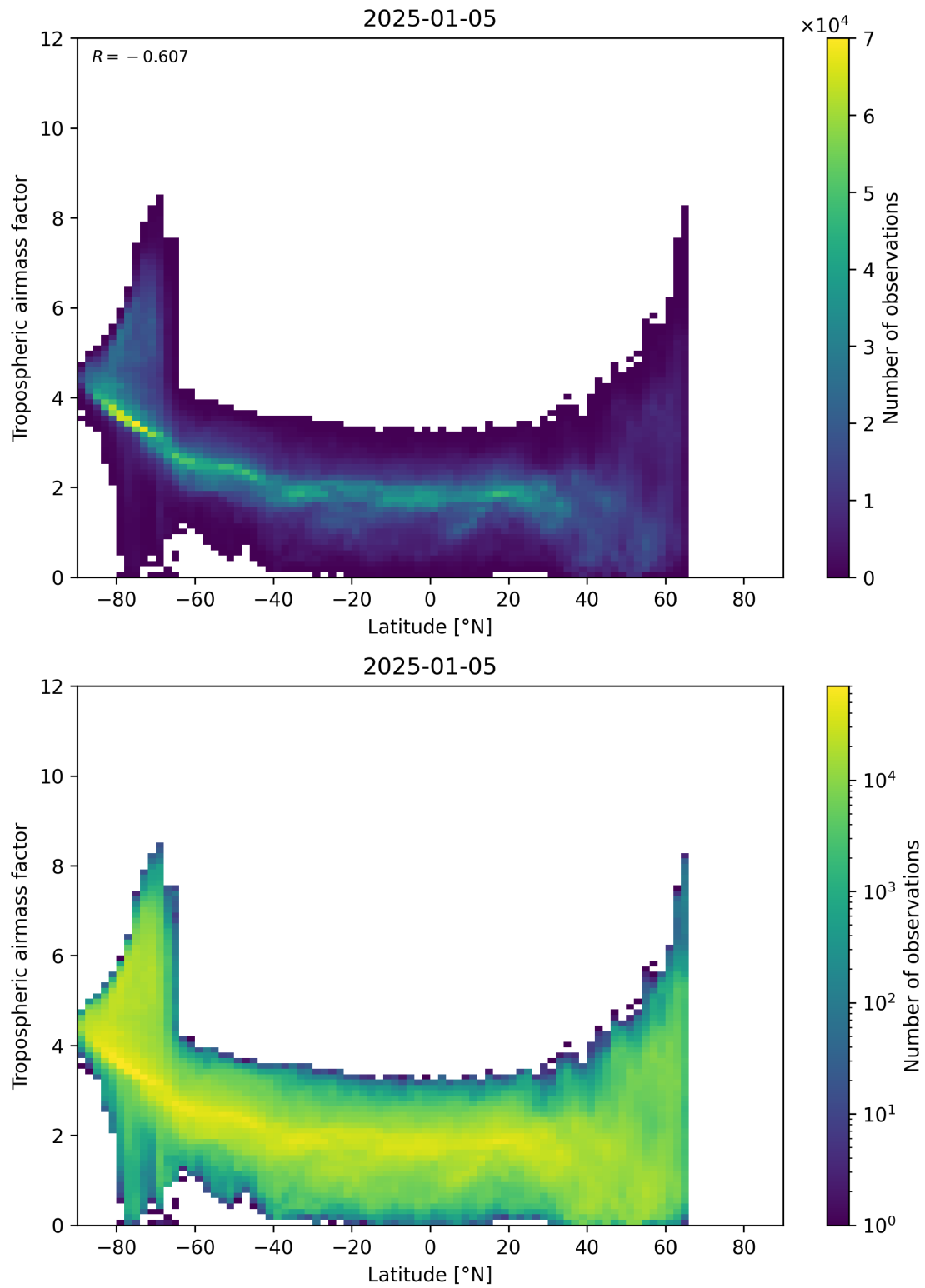
Figure 85: Scatter density plot of “Latitude” against “Tropospheric air mass factor” for 2025-01-04 to 2025-01-06.
