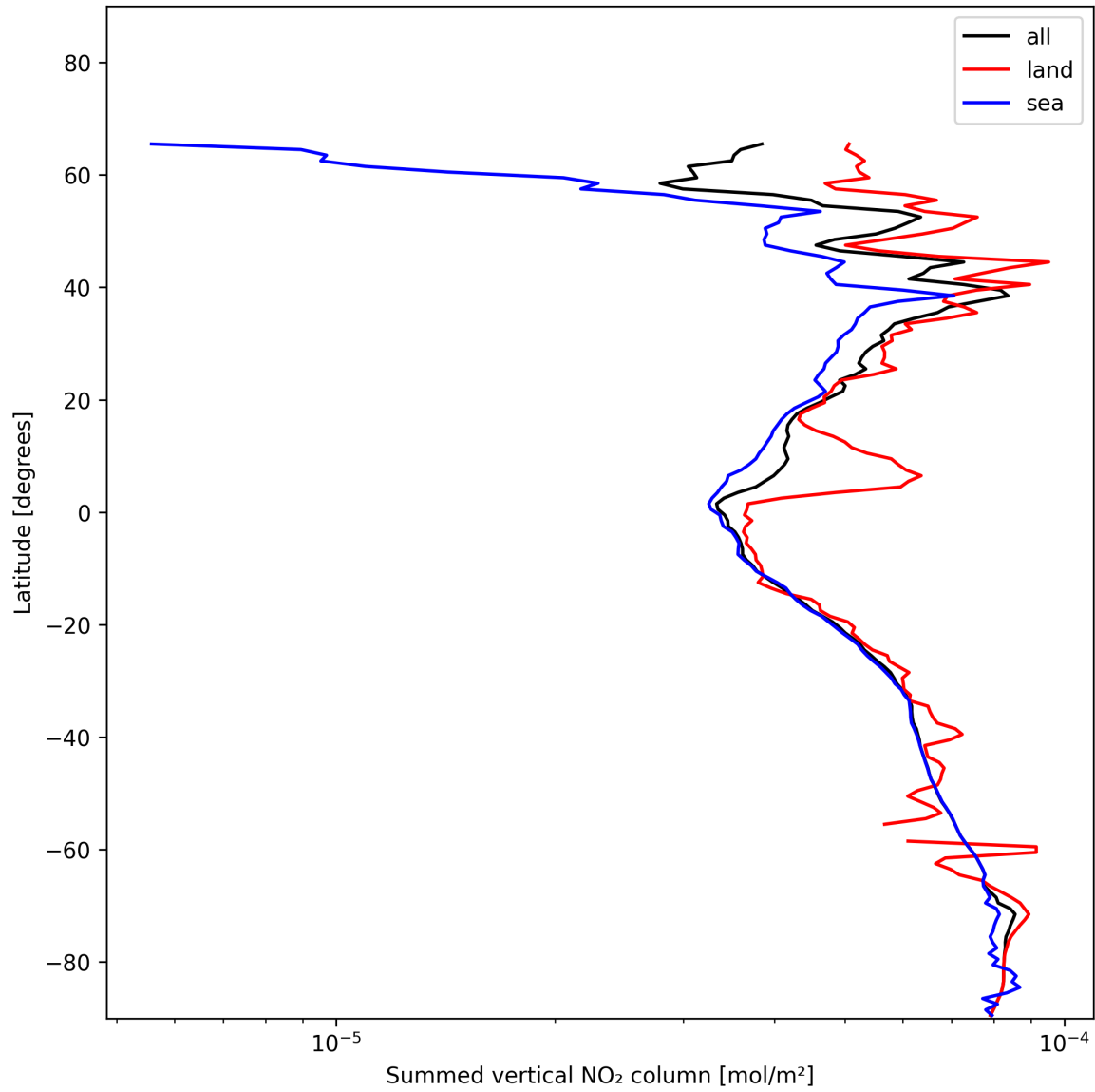
Figure 23: Zonal average of “Summed vertical NO 2 column” for 2025-01-04 to 2025-01-06.
