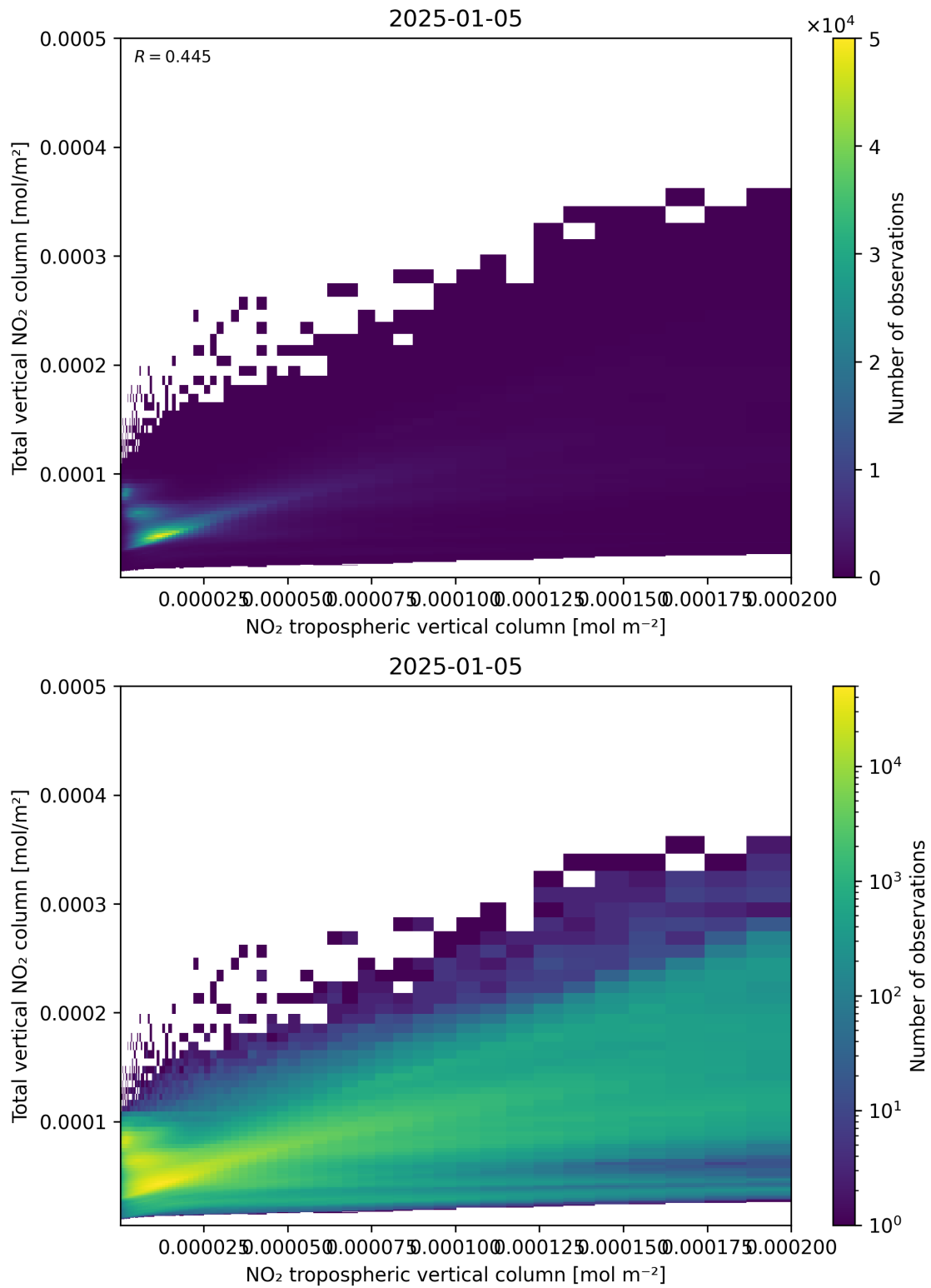
Figure 128: Scatter density plot of “NO 2 tropospheric vertical column” against “Total vertical NO 2 column” for 2025-01-04 to 2025-01-06.
