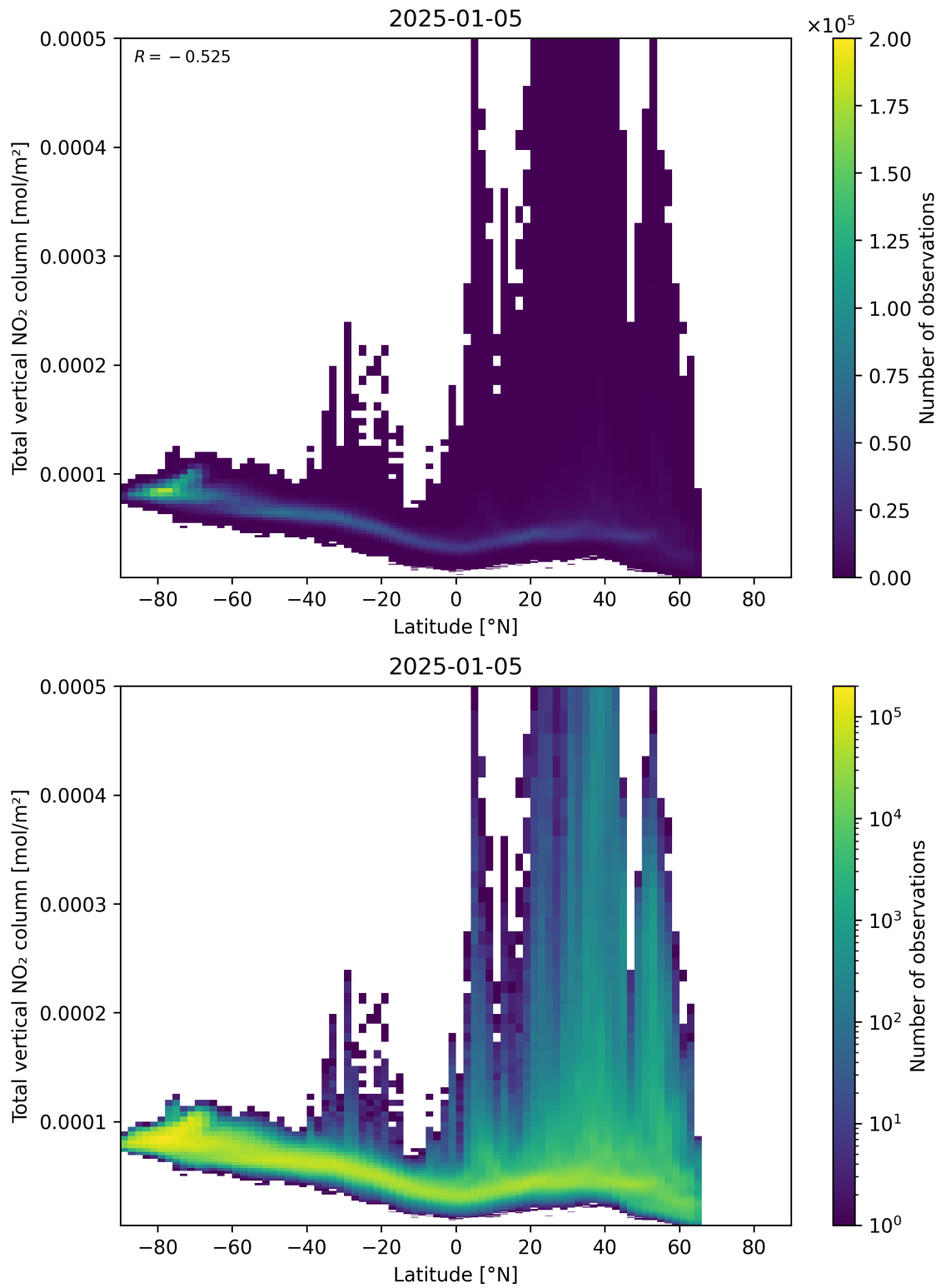
Figure 90: Scatter density plot of “Latitude” against “Total vertical NO 2 column” for 2025-01-04 to 2025-01-06.
