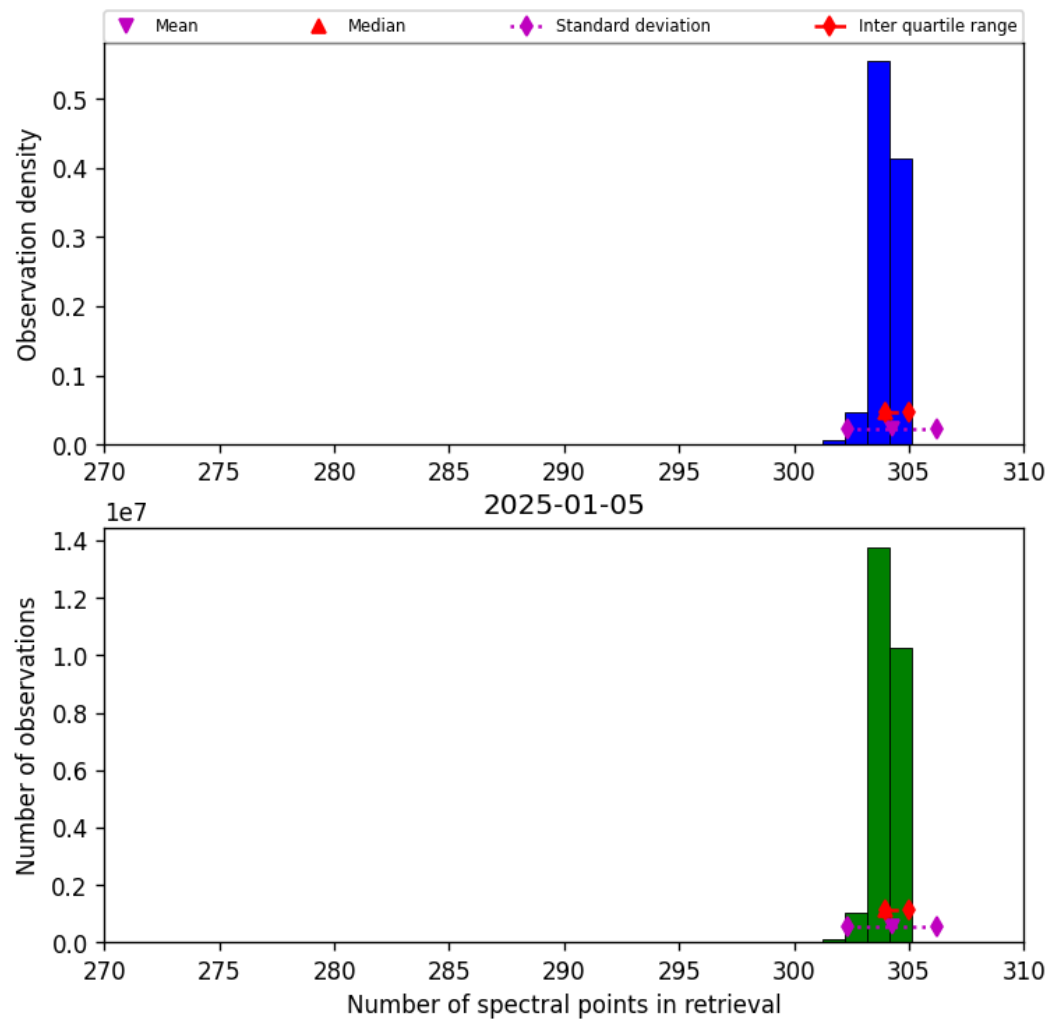
Figure 33: Histogram of “Number of spectral points in retrieval” for 2025-01-04 to 2025-01-06
