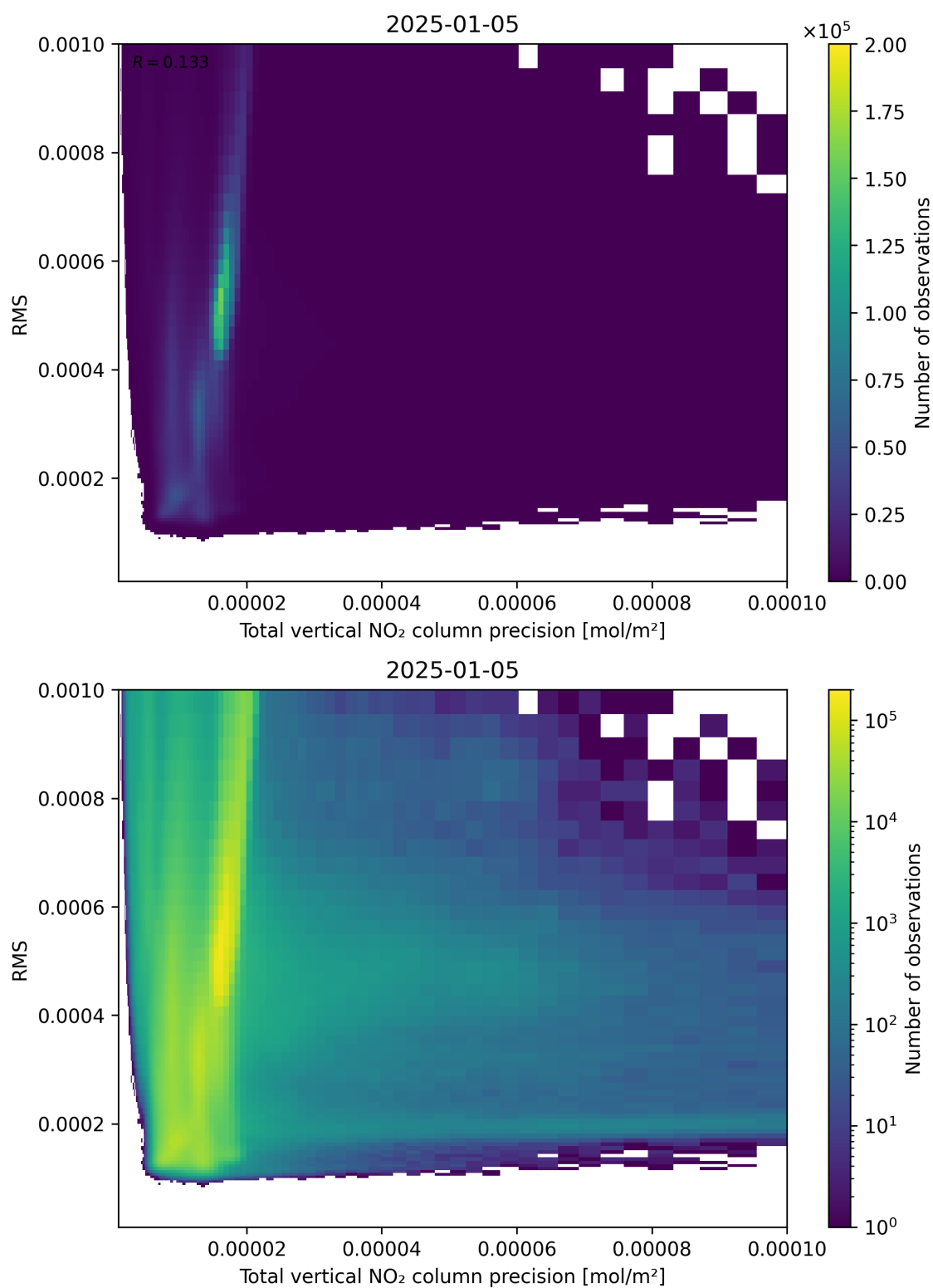
Figure 119: Scatter density plot of “Total vertical NO 2 column precision” against “RMS” for 2025-01-04 to 2025-01-06.
