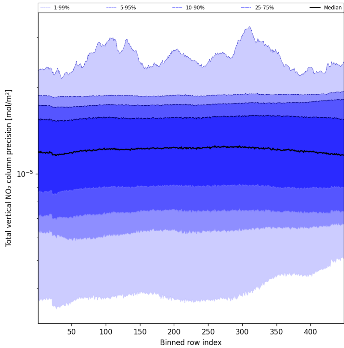
Figure 56: Along track statistics of “Total vertical NO 2 column precision” for 2025-01-04 to 2025-01-06
