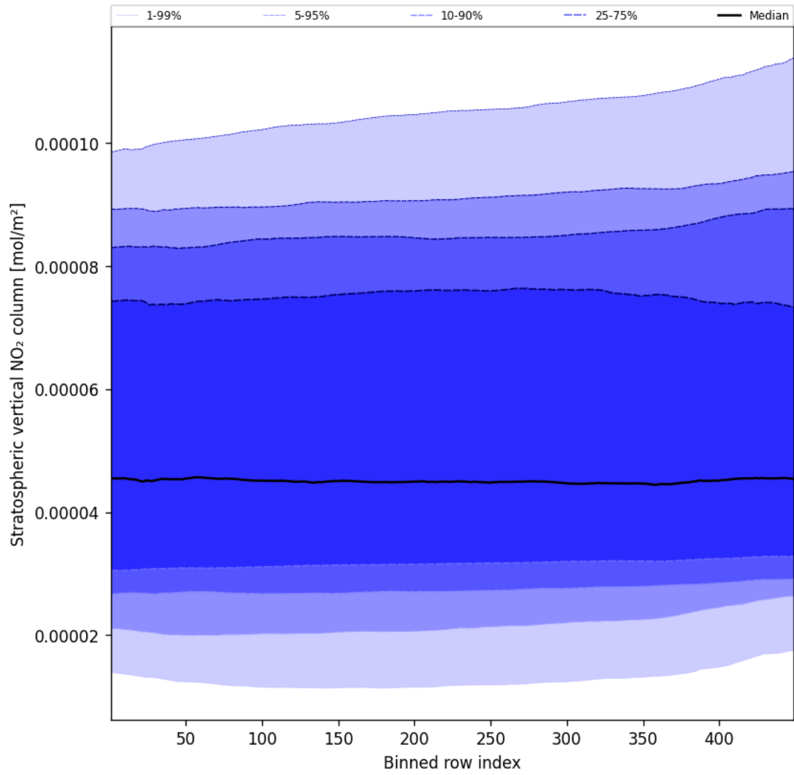
Figure 53: Along track statistics of “Stratospheric vertical NO 2 column” for 2025-01-04 to 2025-01-06
