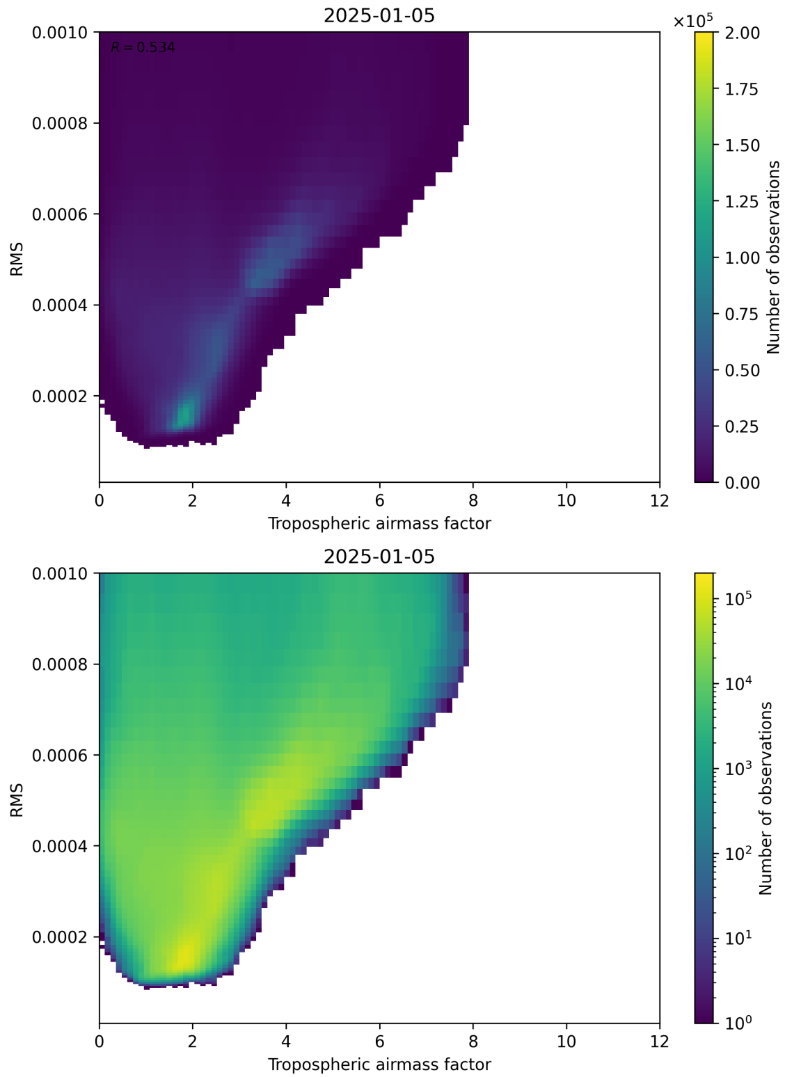
Figure 79: Scatter density plot of “Tropospheric airmass factor” against “RMS” for 2025-01-04 to 2025-01-06.
