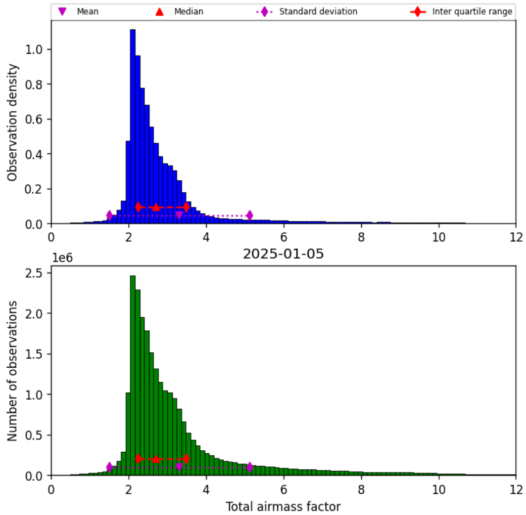
Figure 32: Histogram of “Total airmass factor” for 2025-01-04 to 2025-01-06
