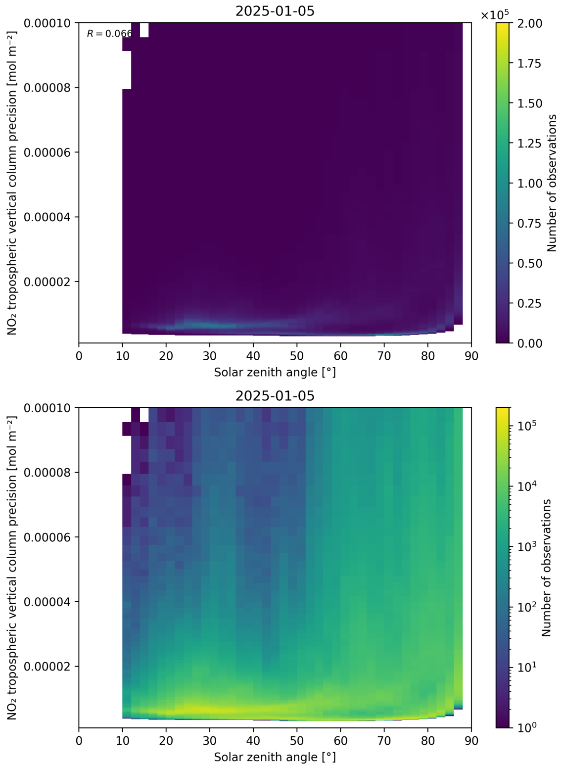
Figure 156: Scatter density plot of “Solar zenith angle” against “NO 2 tropospheric vertical column precision” for 2025-01-04 to 2025-01-06.
