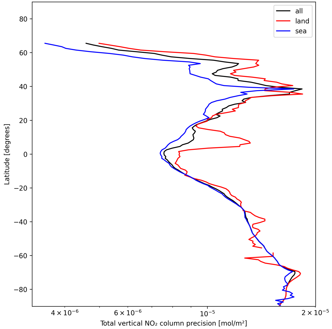
Figure 22: Zonal average of “Total vertical NO 2 column precision” for 2025-01-04 to 2025-01-06.
