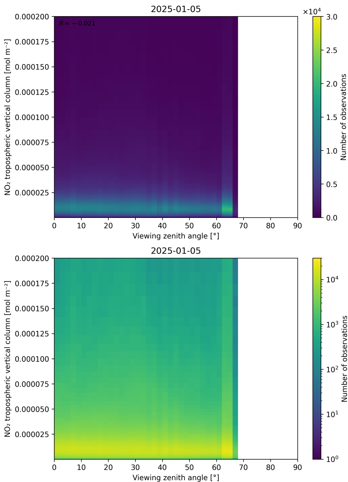
Figure 169: Scatter density plot of “Viewing zenith angle” against “NO 2 tropospheric vertical column” for 2025-01-04 to 2025-01-06.
