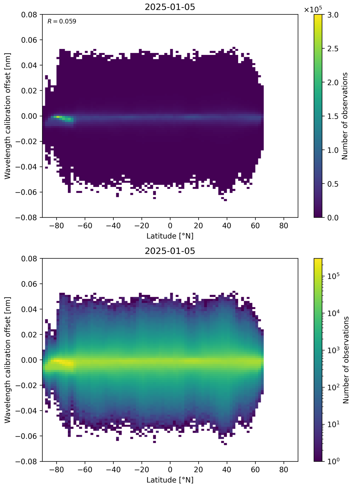
Figure 95: Scatter density plot of “Latitude” against “Wavelength calibration offset” for 2025-01-04 to 2025-01-06.
