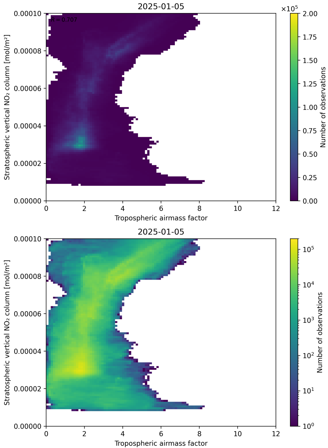
Figure 74: Scatter density plot of “Tropospheric air mass factor” against “Stratospheric vertical NO 2 column” for 2025-01-04 to 2025-01-06.
