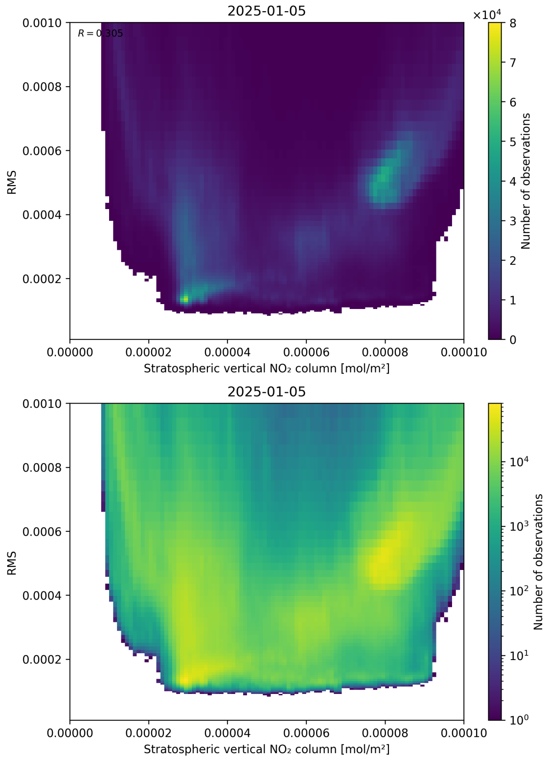
Figure 102: Scatter density plot of “Stratospheric vertical NO 2 column” against “RMS” for 2025-01-04 to 2025-01-06.
