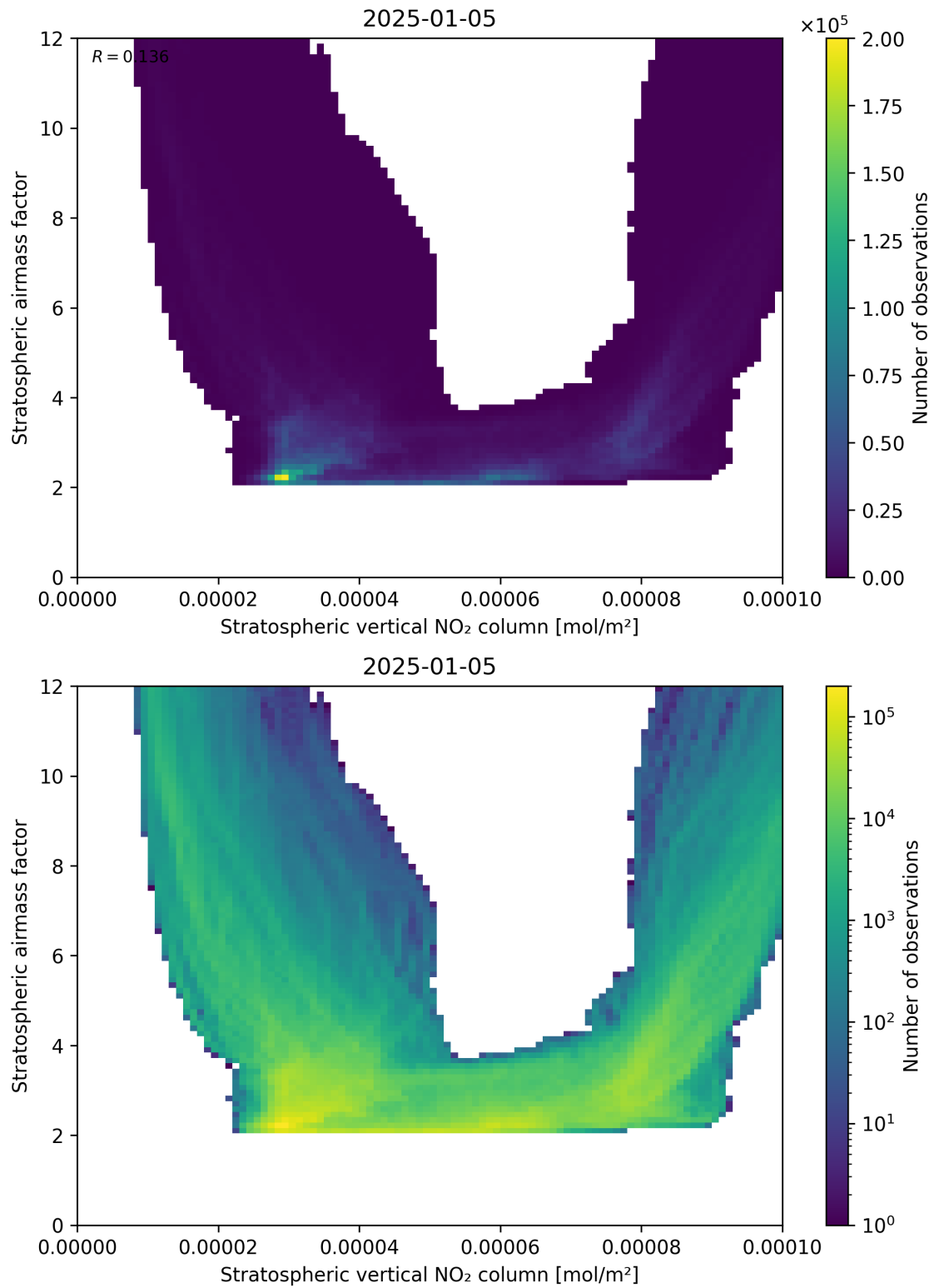
Figure 96: Scatter density plot of “Stratospheric vertical NO 2 column” against “Stratospheric airmass factor” for 2025-01-04 to 2025-01-06.
