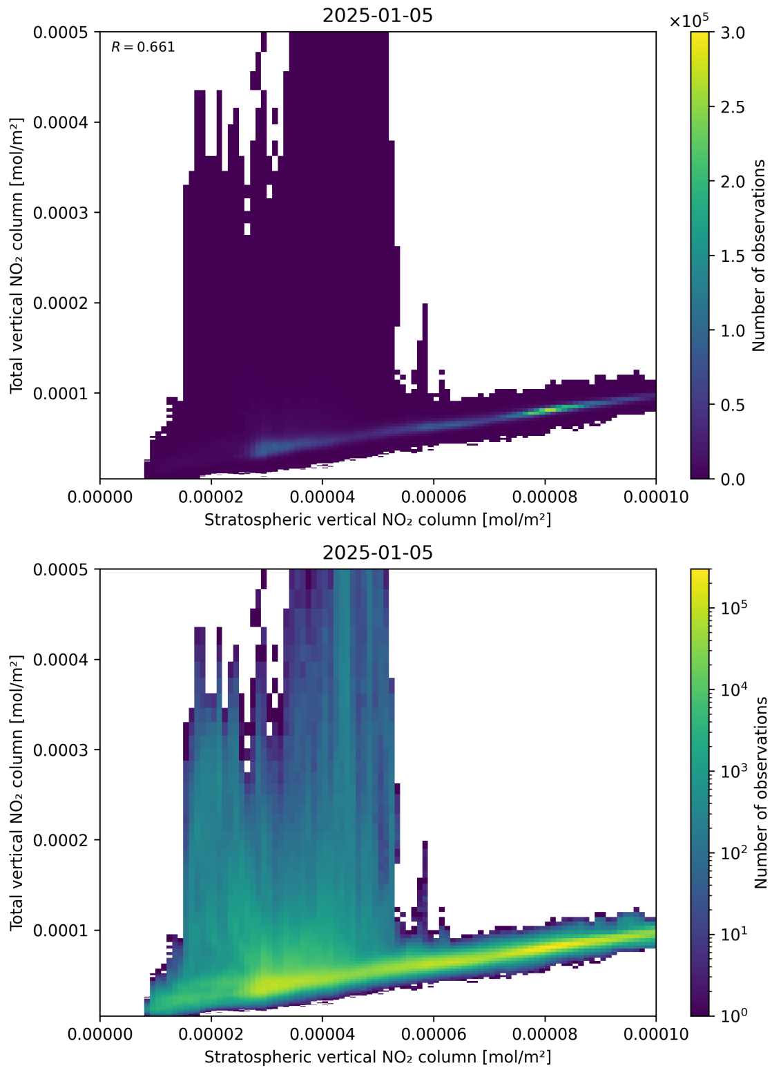
Figure 100: Scatter density plot of “Stratospheric vertical NO 2 column” against “Total vertical NO 2 column” for 2025-01-04 to 2025-01-06.
