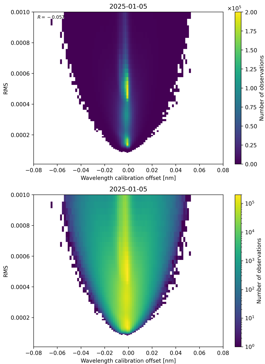
Figure 181: Scatter density plot of “Wavelength calibration offset” against “RMS” for 2025-01-04 to 2025-01-06.
