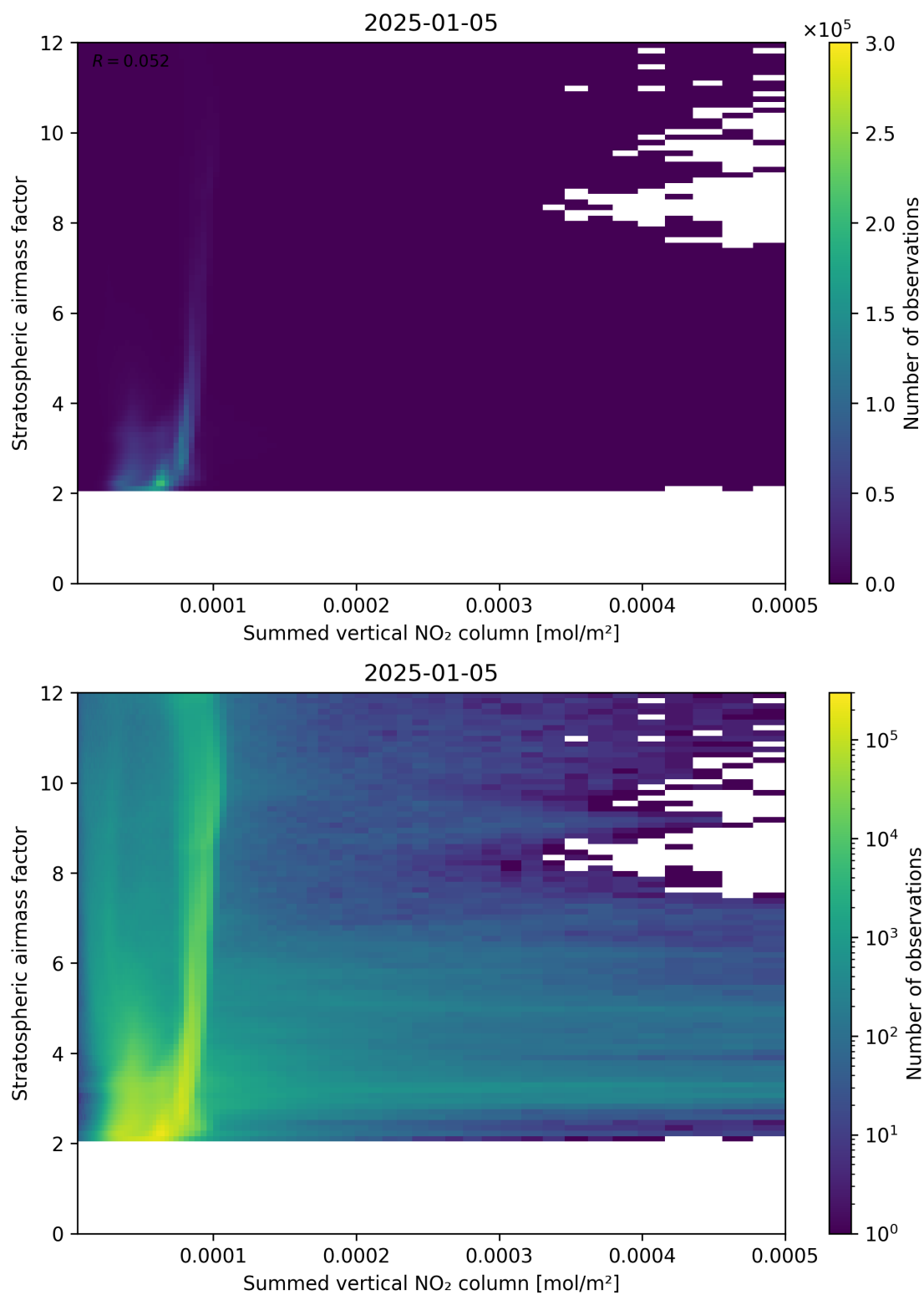
Figure 103: Scatter density plot of “Summed vertical NO 2 column” against “Stratospheric airmass factor” for 2025-01-04 to 2025-01-06.
