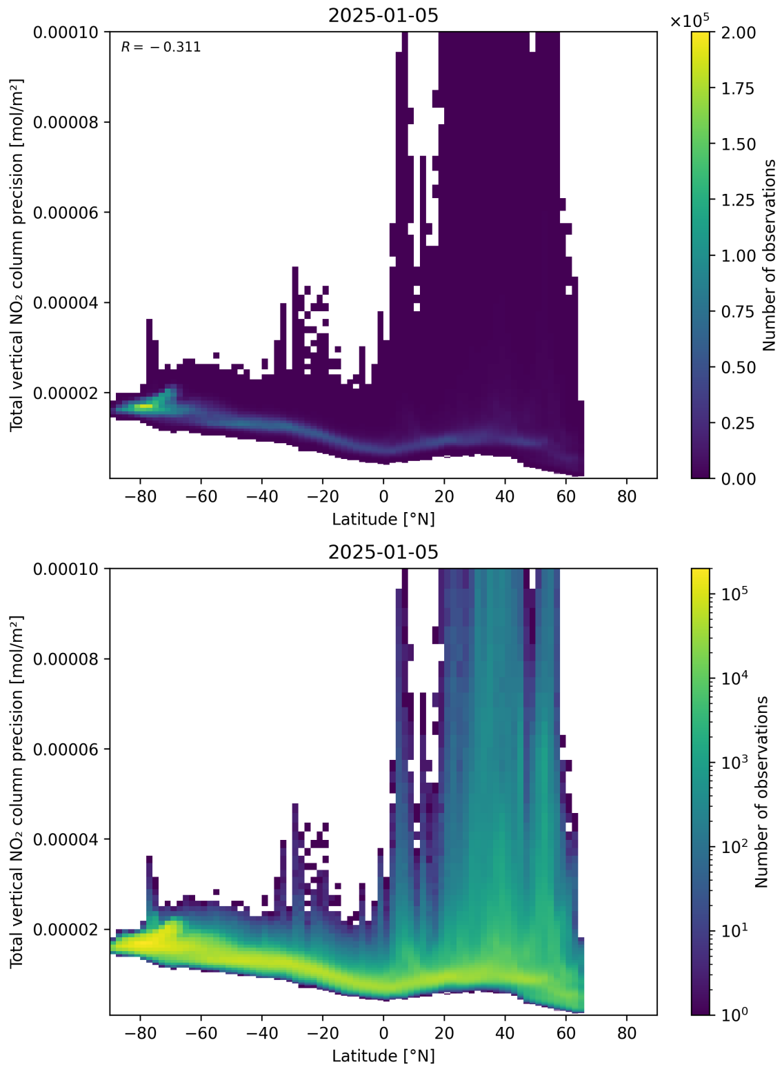
Figure 91: Scatter density plot of “Latitude” against “Total vertical NO 2 column precision” for 2025-01-04 to 2025-01-06.
