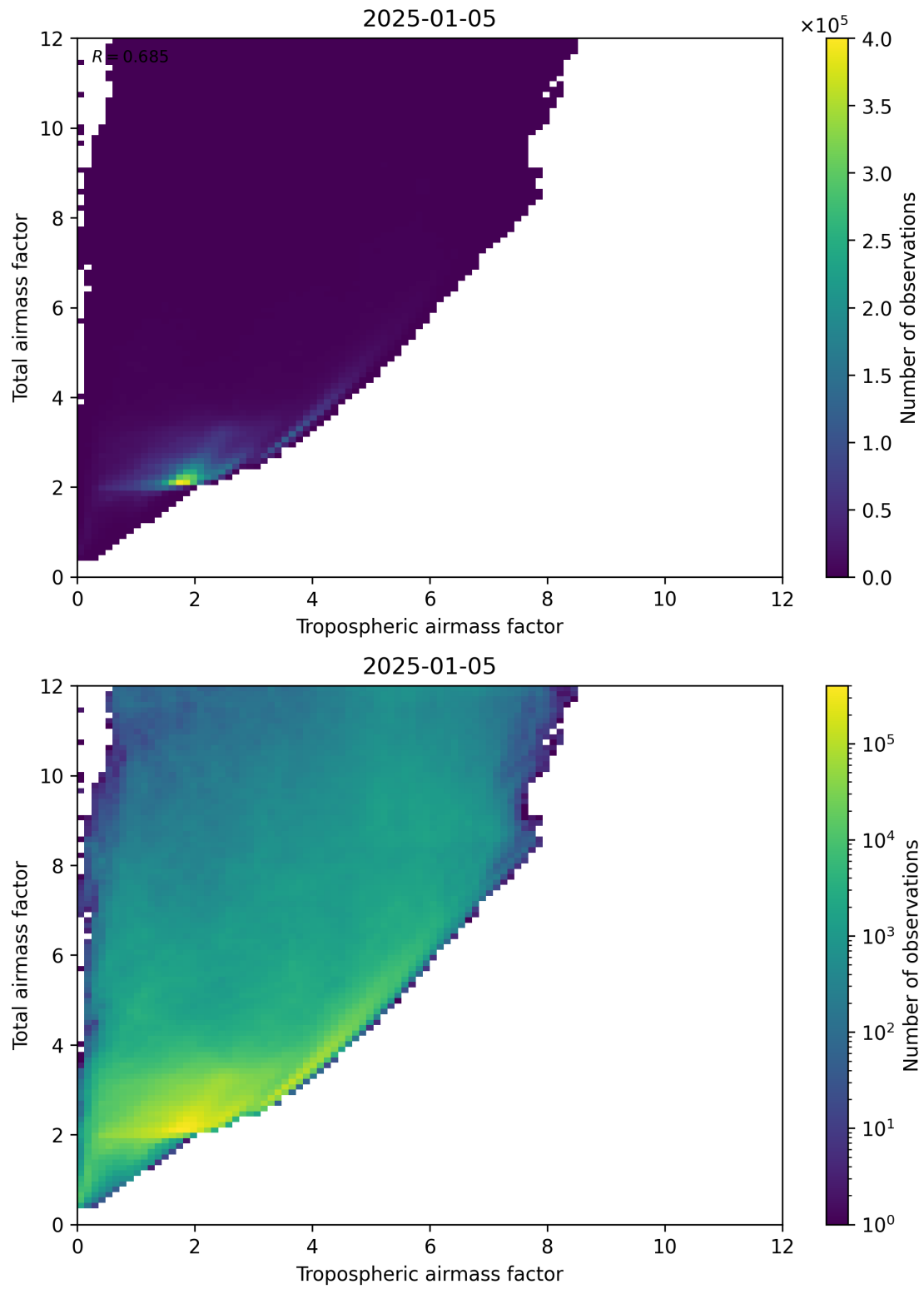
Figure 72: Scatter density plot of “Tropospheric airmass factor” against “Total airmass factor” for 2025-01-04 to 2025-01-06.
