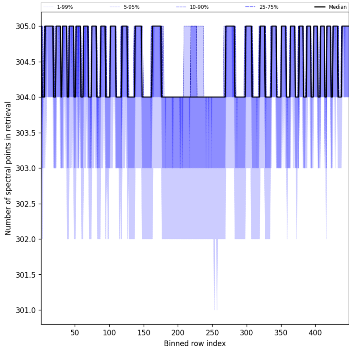
Figure 50: Along track statistics of “Number of spectral points in retrieval” for 2025-01-04 to 2025-01-06
