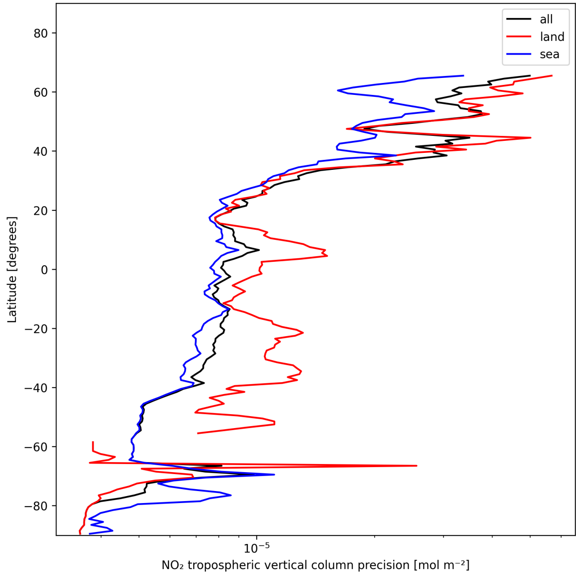
Figure 13: Zonal average of “NO 2 tropospheric vertical column precision” for 2025-01-04 to 2025-01-06.
