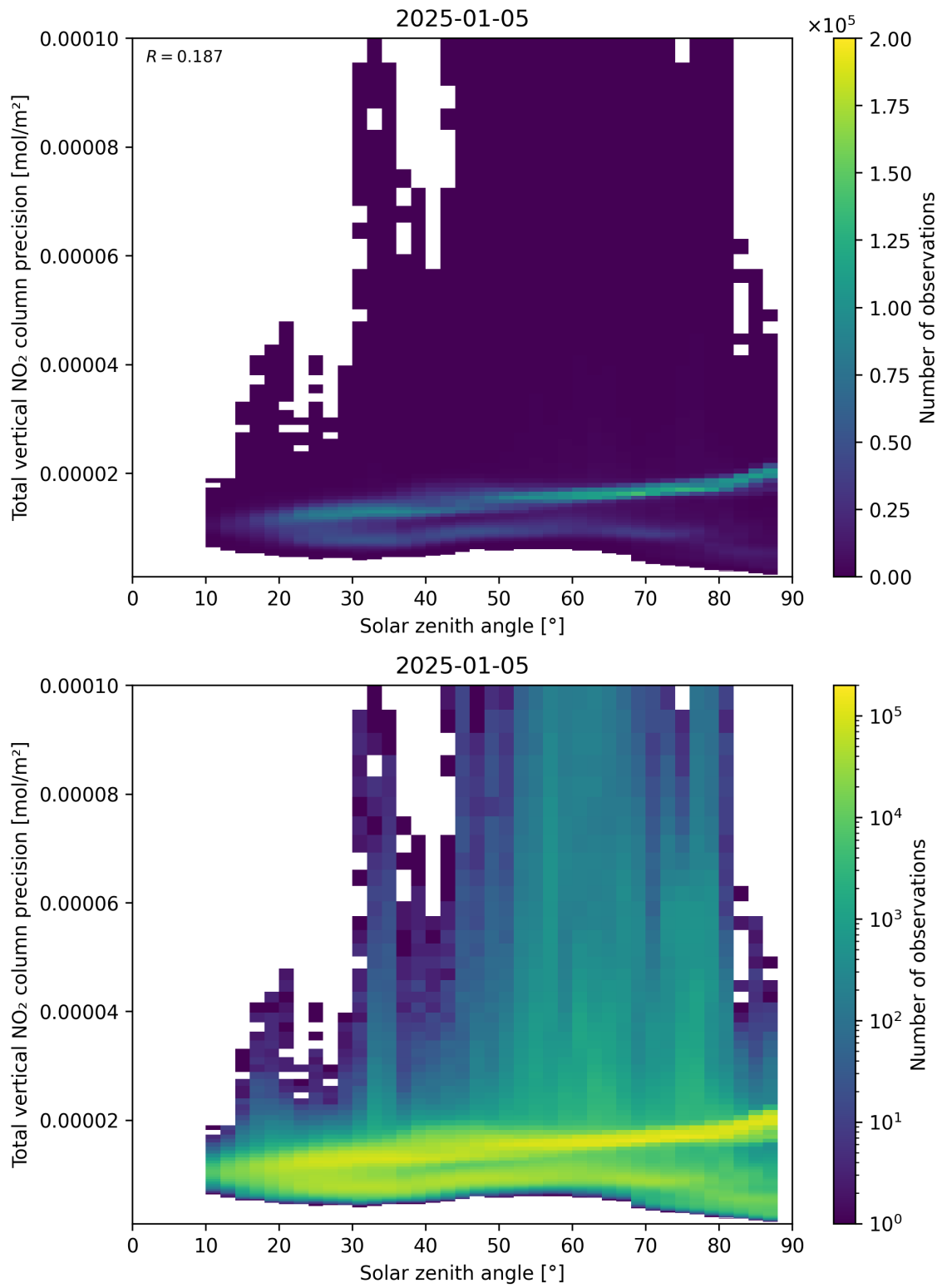
Figure 154: Scatter density plot of “Solar zenith angle” against “Total vertical NO 2 column precision” for 2025-01-04 to 2025-01-06.
