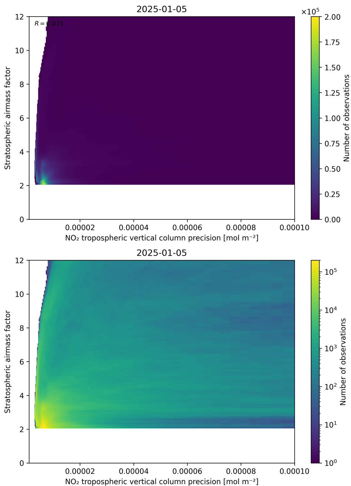
Figure 131: Scatter density plot of “NO 2 tropospheric vertical column precision” against “Stratospheric airmass factor” for 2025-01-04 to 2025-01-06.
