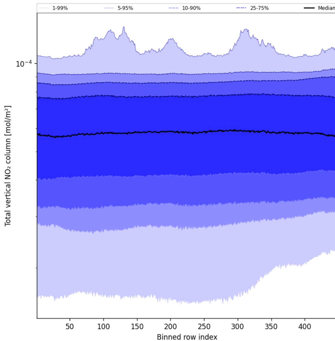
Figure 55: Along track statistics of “Total vertical NO 2 column” for 2025-01-04 to 2025-01-06
