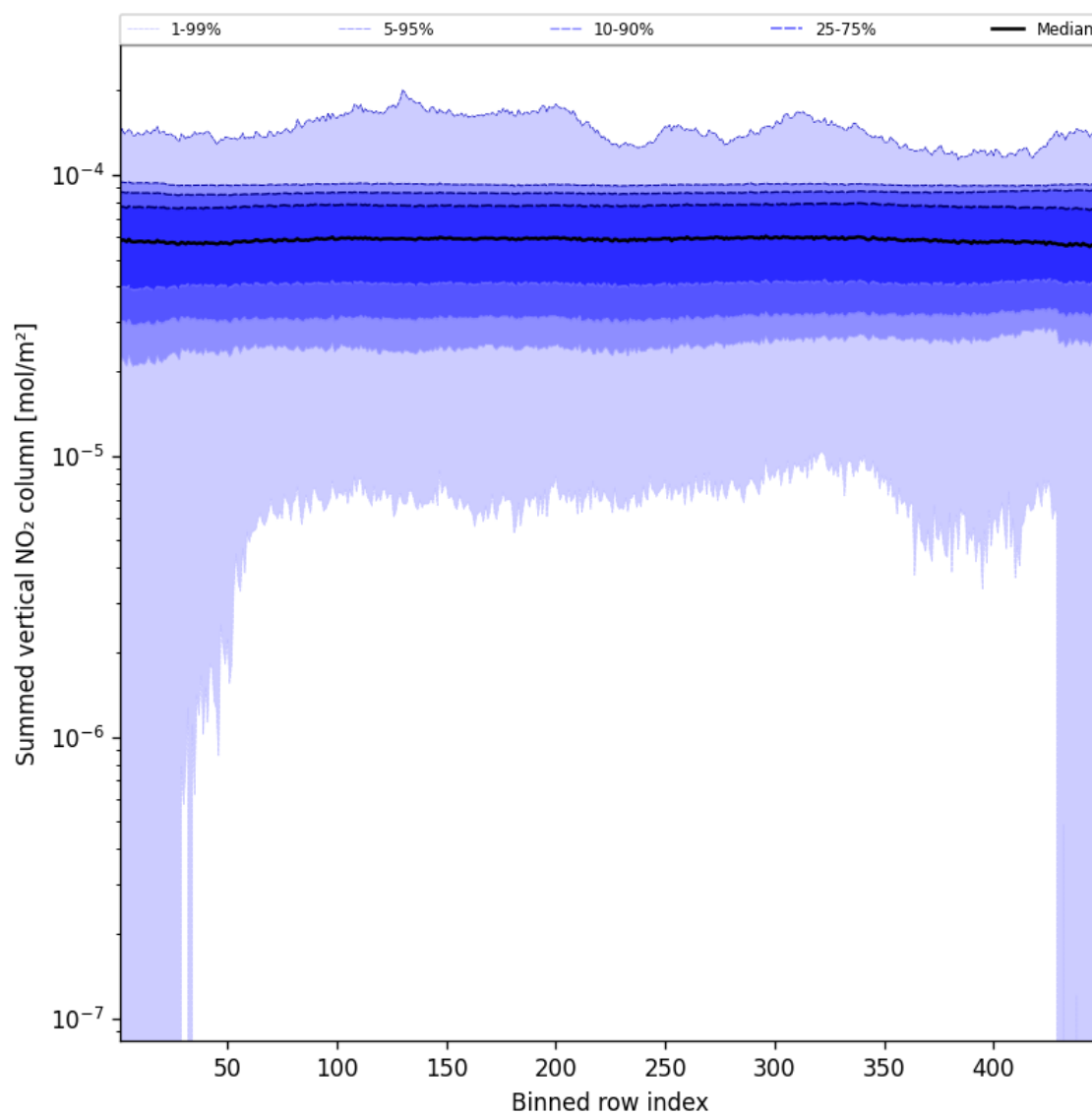
Figure 57: Along track statistics of “Summed vertical NO 2 column” for 2025-01-04 to 2025-01-06
