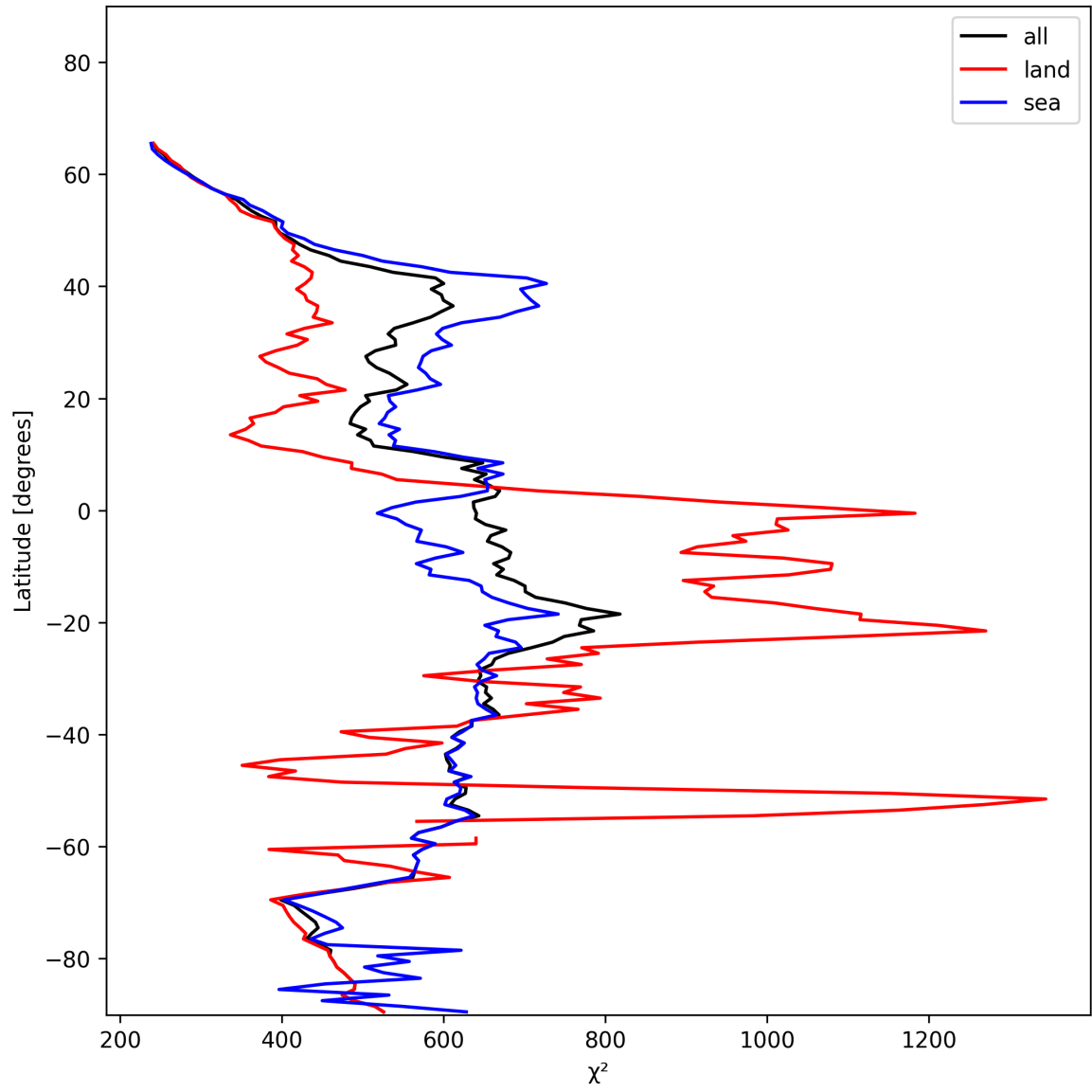
Figure 25: Zonal average of “ \chi^2 ” for 2025-01-04 to 2025-01-06.
