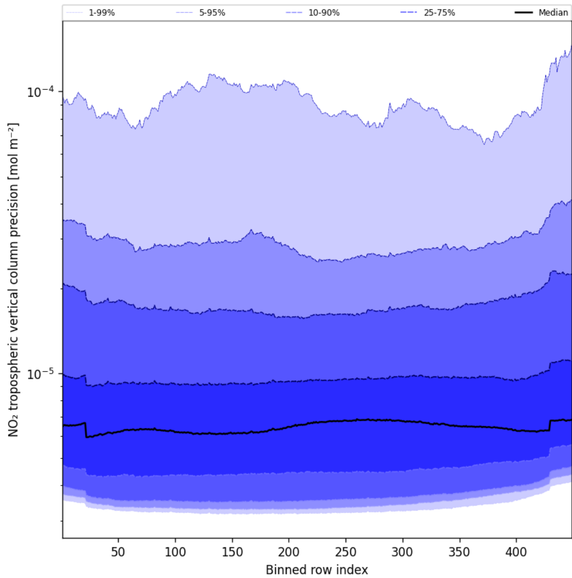
Figure 47: Along track statistics of “NO 2 tropospheric vertical column precision” for 2025-01-04 to 2025-01-06
