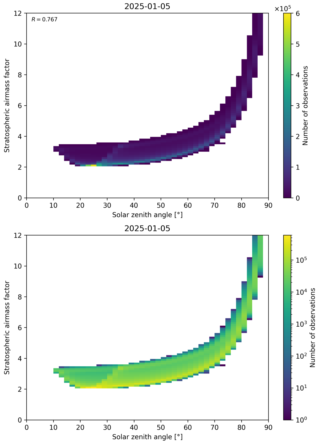
Figure 145: Scatter density plot of “Solar zenith angle” against “Stratospheric airmass factor” for 2025-01-04 to 2025-01-06.
