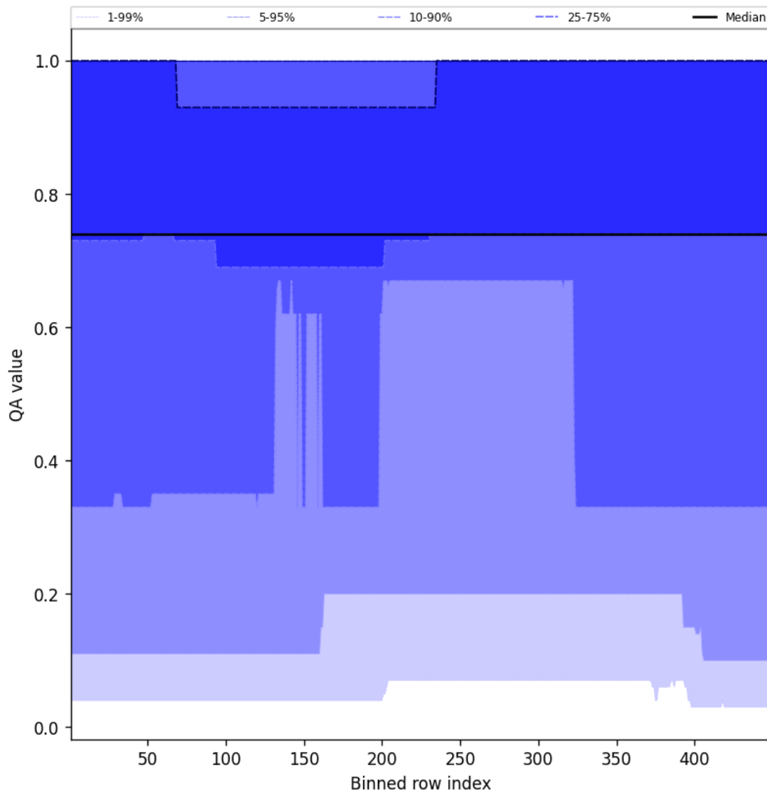
Figure 45: Along track statistics of "QA value" for 2025-01-04 to 2025-01-06
