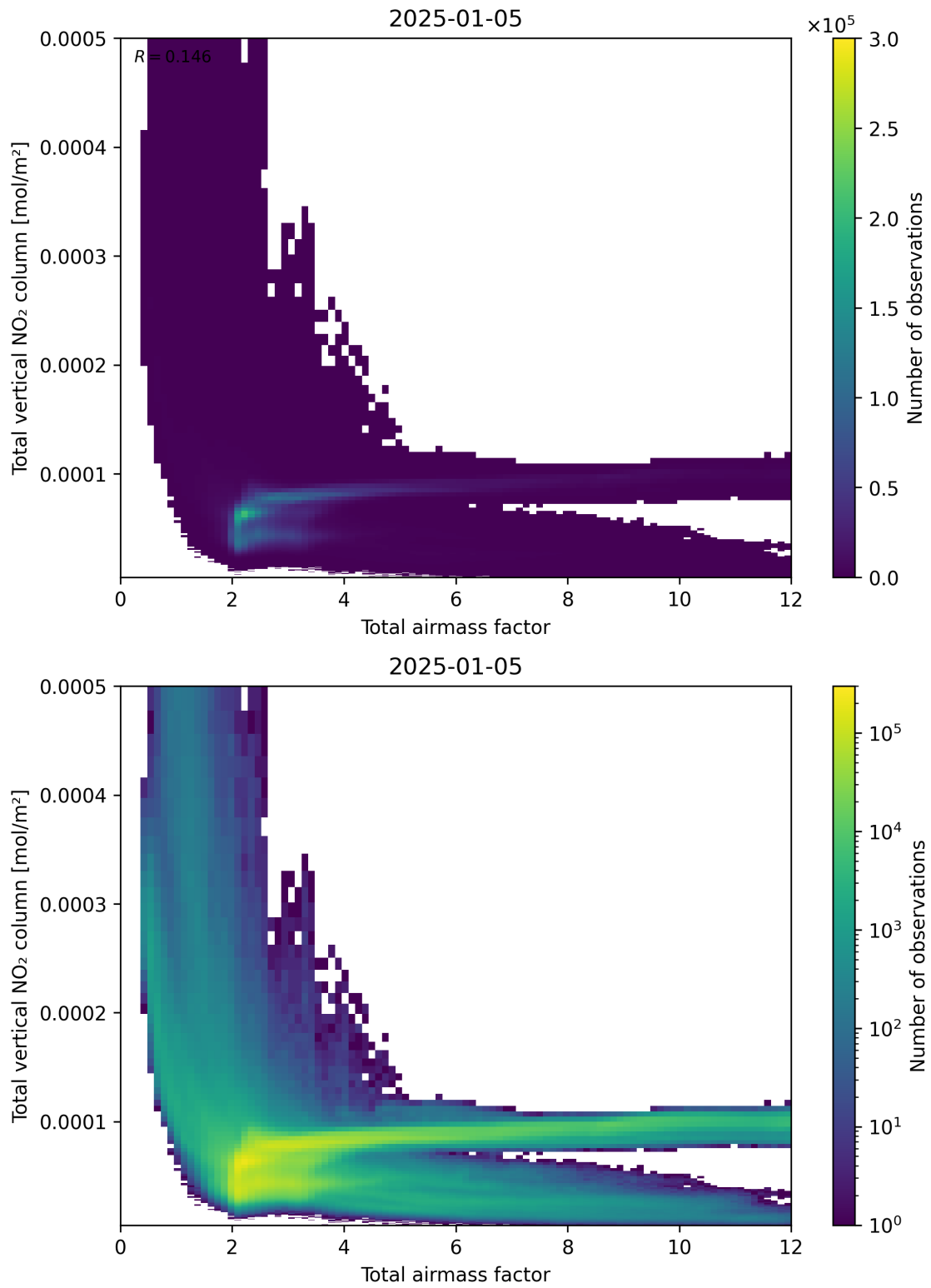
Figure 67: Scatter density plot of “Total airmass factor” against “Total vertical NO 2 column” for 2025-01-04 to 2025-01-06.
