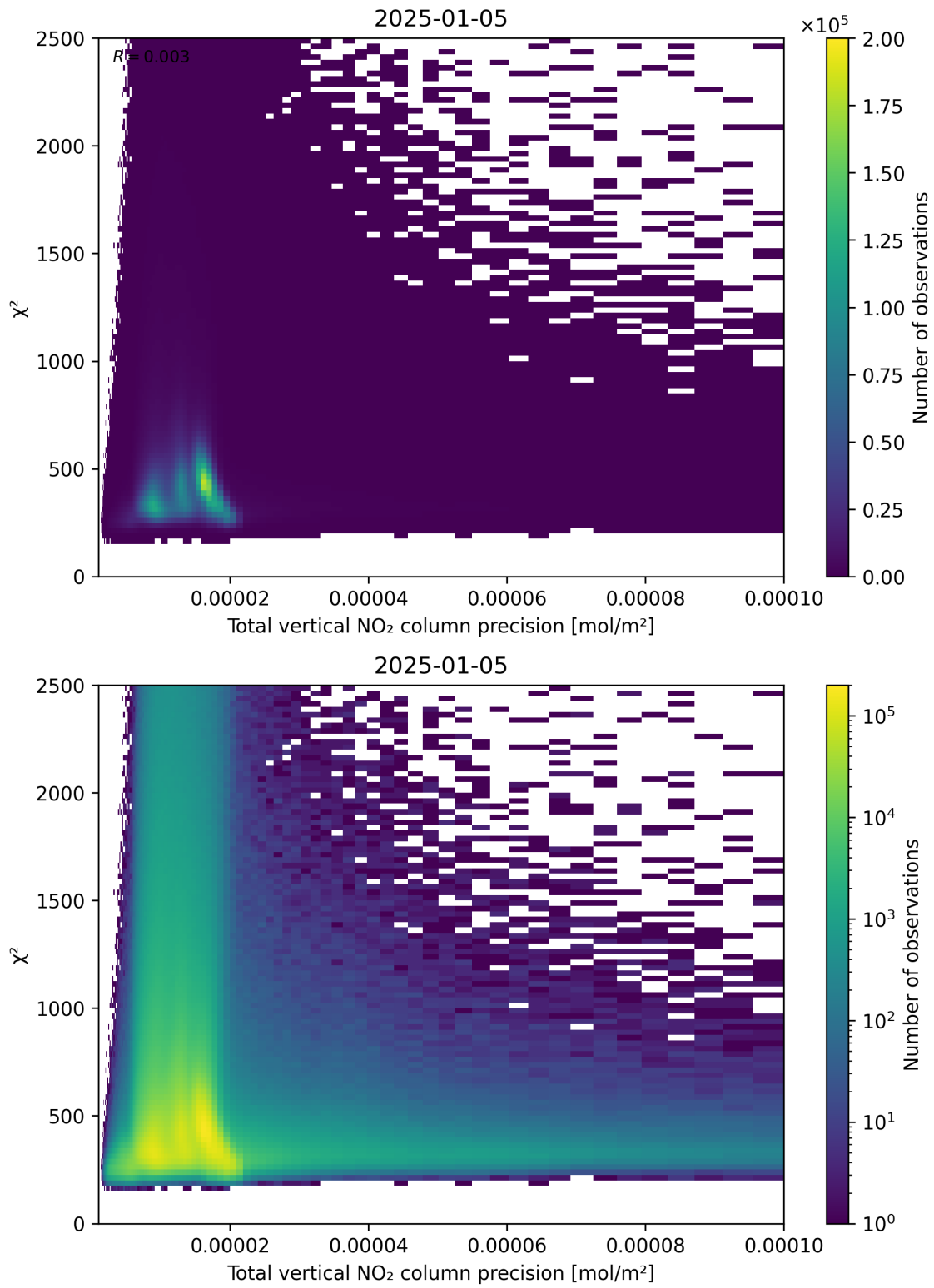
Figure 116: Scatter density plot of “Total vertical NO 2 column precision” against “ \chi^2 ” for 2025-01-04 to 2025-01-06.
