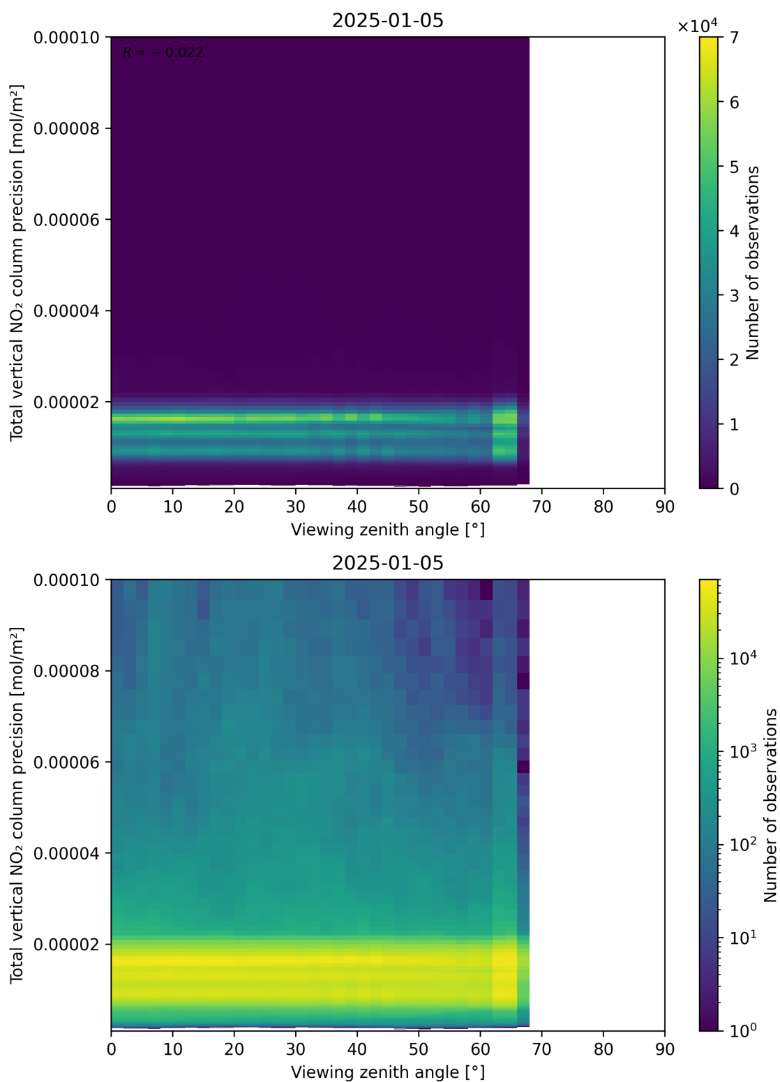
Figure 168: Scatter density plot of “Viewing zenith angle” against “Total vertical NO 2 column precision” for 2025-01-04 to 2025-01-06.
