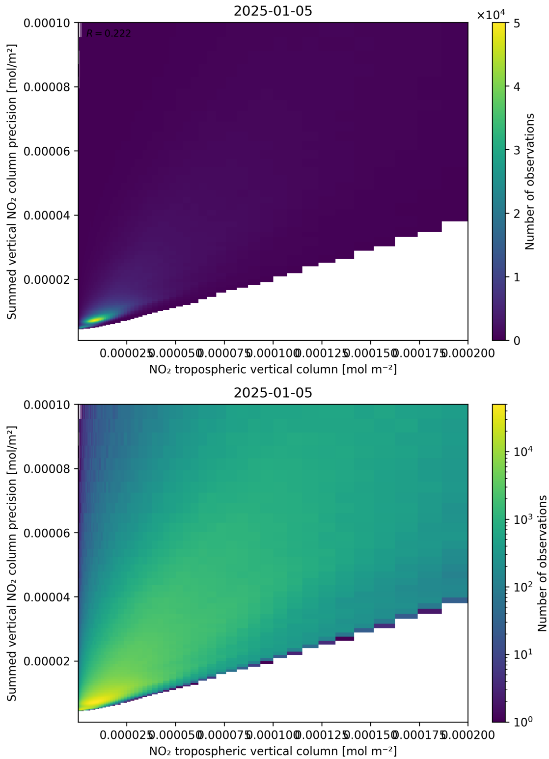
Figure 127: Scatter density plot of “NO 2 tropospheric vertical column” against “Summed vertical NO 2 column precision” for 2025-01-04 to 2025-01-06.
