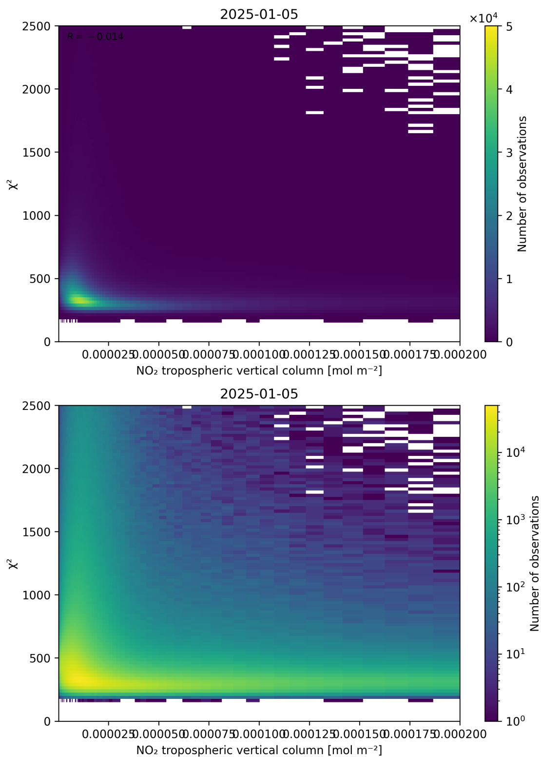
Figure 124: Scatter density plot of “NO 2 tropospheric vertical column” against “ \chi^2 ” for 2025-01-04 to 2025-01-06.
