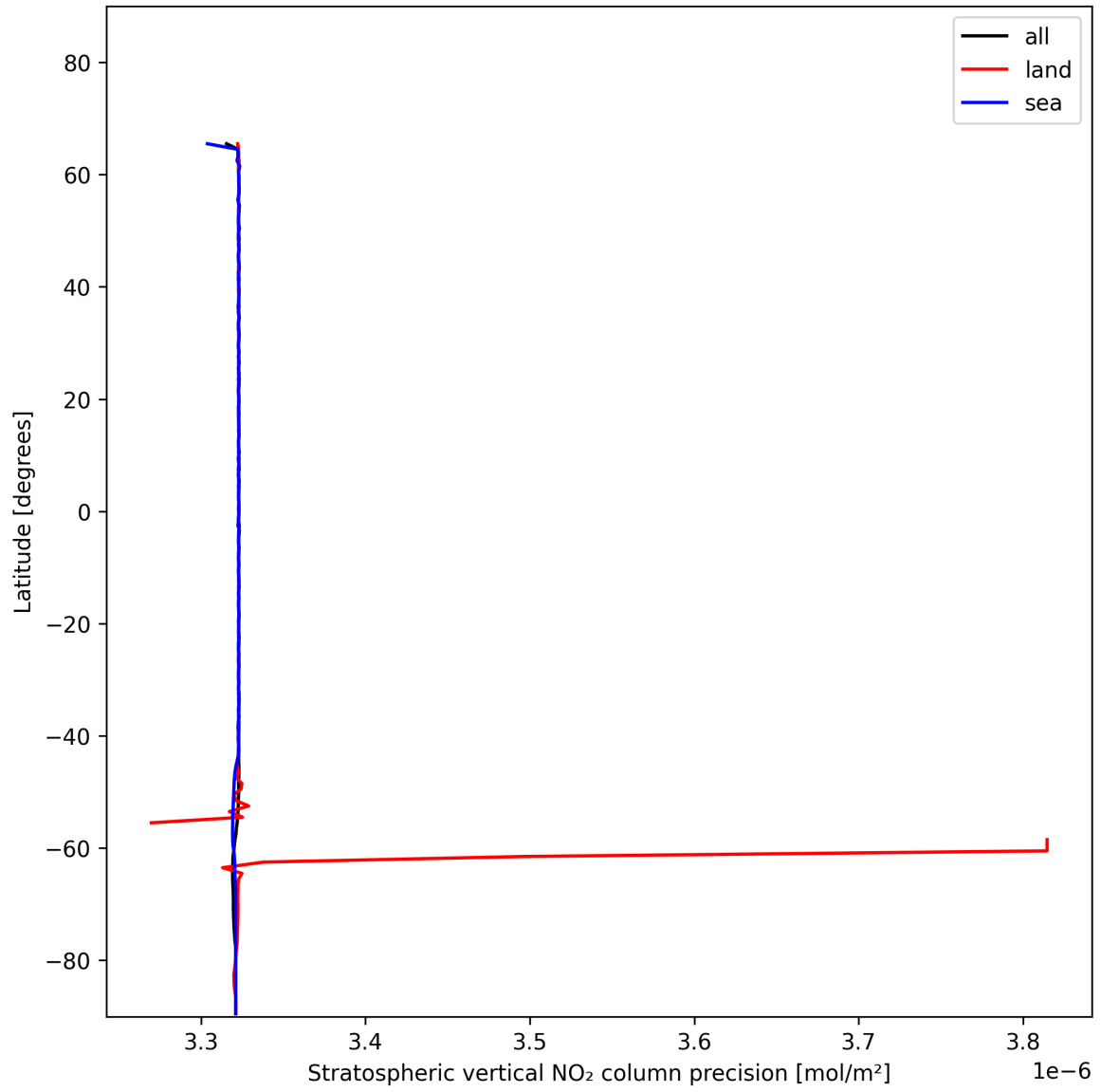
Figure 20: Zonal average of “Stratospheric vertical NO 2 column precision” for 2025-01-04 to 2025-01-06.
