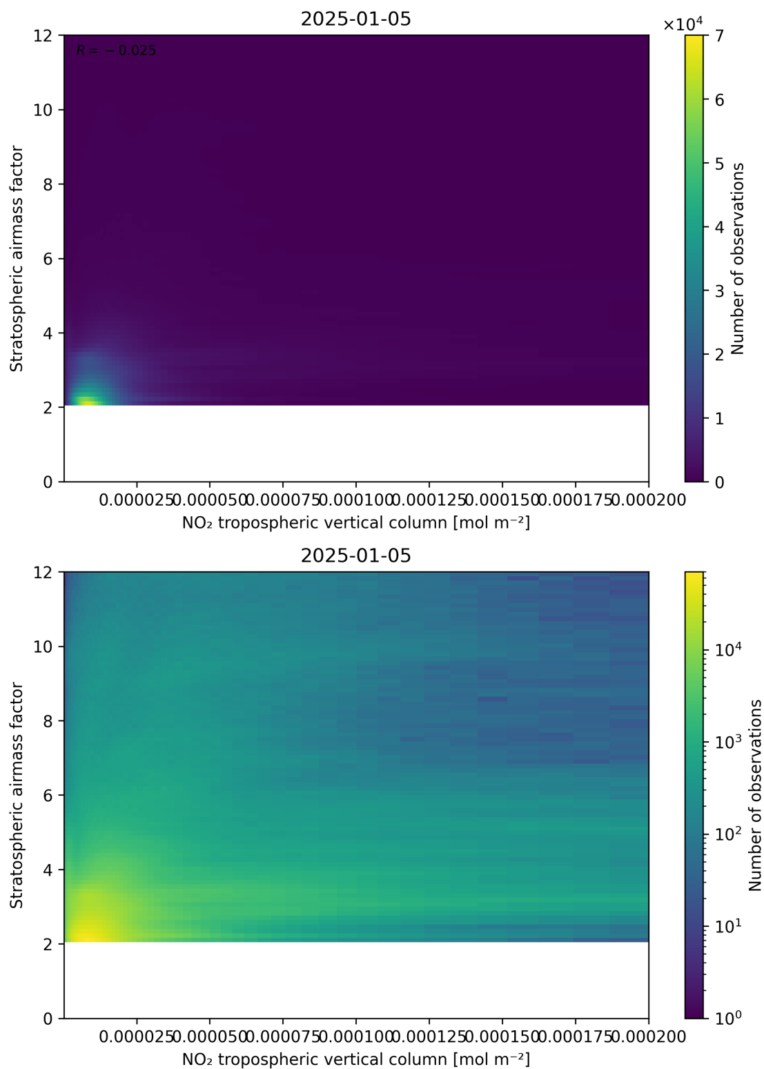
Figure 121: Scatter density plot of “NO 2 tropospheric vertical column” against “Stratospheric airmass factor” for 2025-01-04 to 2025-01-06.
