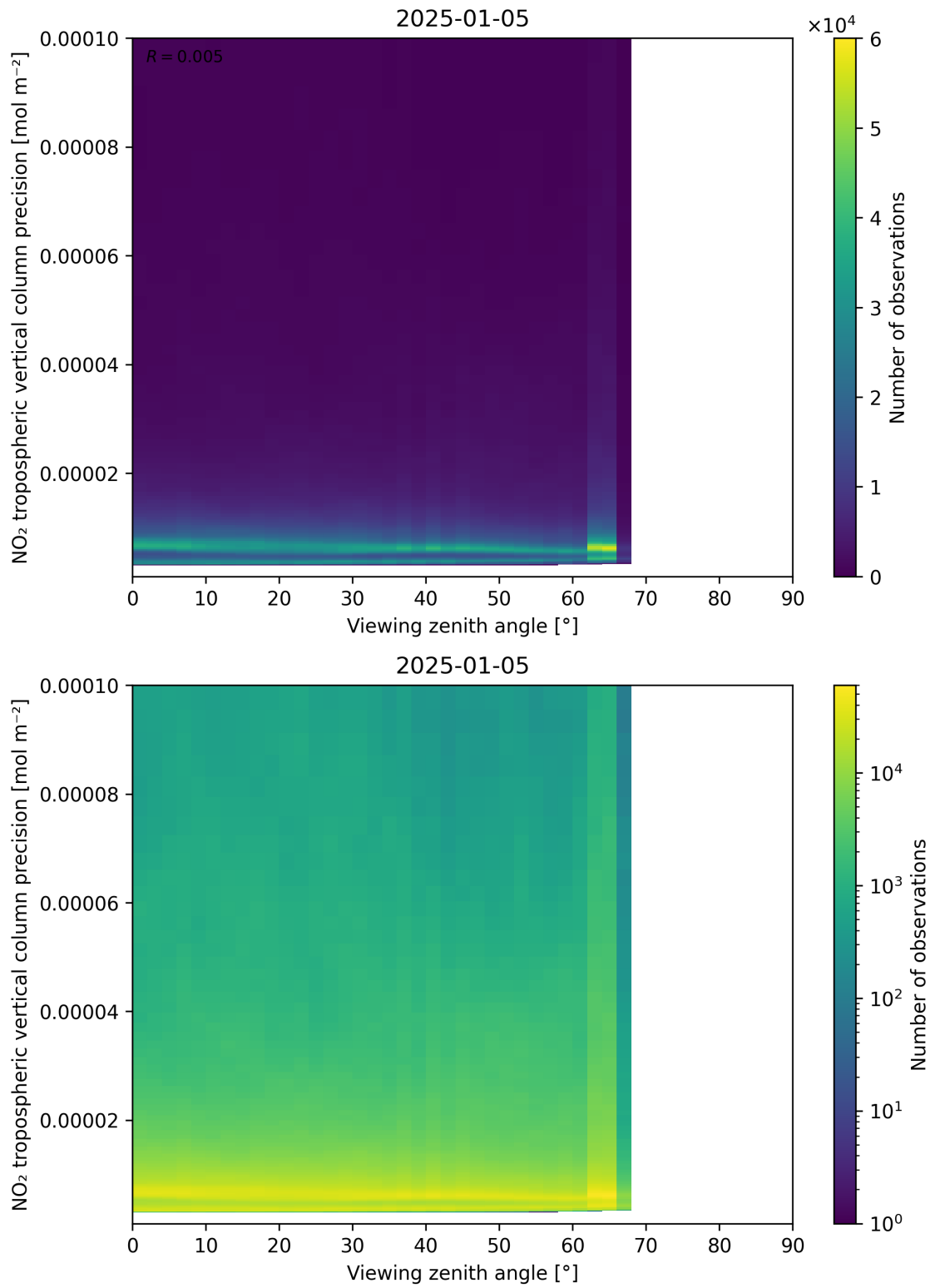
Figure 170: Scatter density plot of “Viewing zenith angle” against “NO 2 tropospheric vertical column precision” for 2025-01-04 to 2025-01-06.
