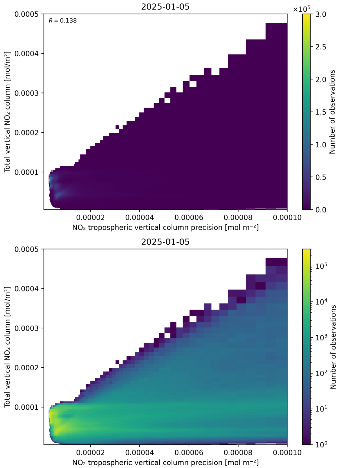
Figure 138: Scatter density plot of “NO 2 tropospheric vertical column precision” against “Total vertical NO 2 column” for 2025-01-04 to 2025-01-06.
