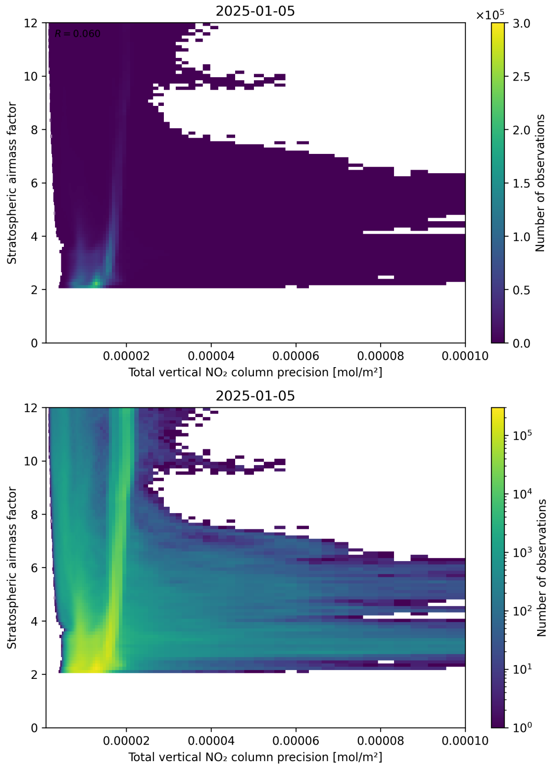
Figure 115: Scatter density plot of “Total vertical NO 2 column precision” against “Stratospheric airmass factor” for 2025-01-04 to 2025-01-06.
