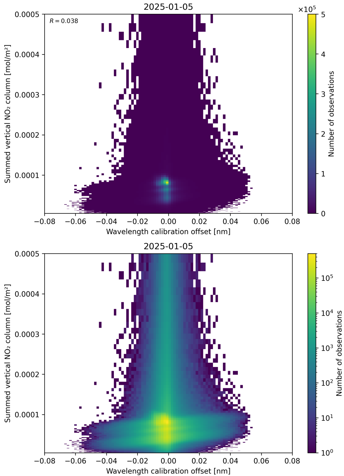
Figure 177: Scatter density plot of “Wavelength calibration offset” against “Summed vertical NO 2 column” for 2025-01-04 to 2025-01-06.
