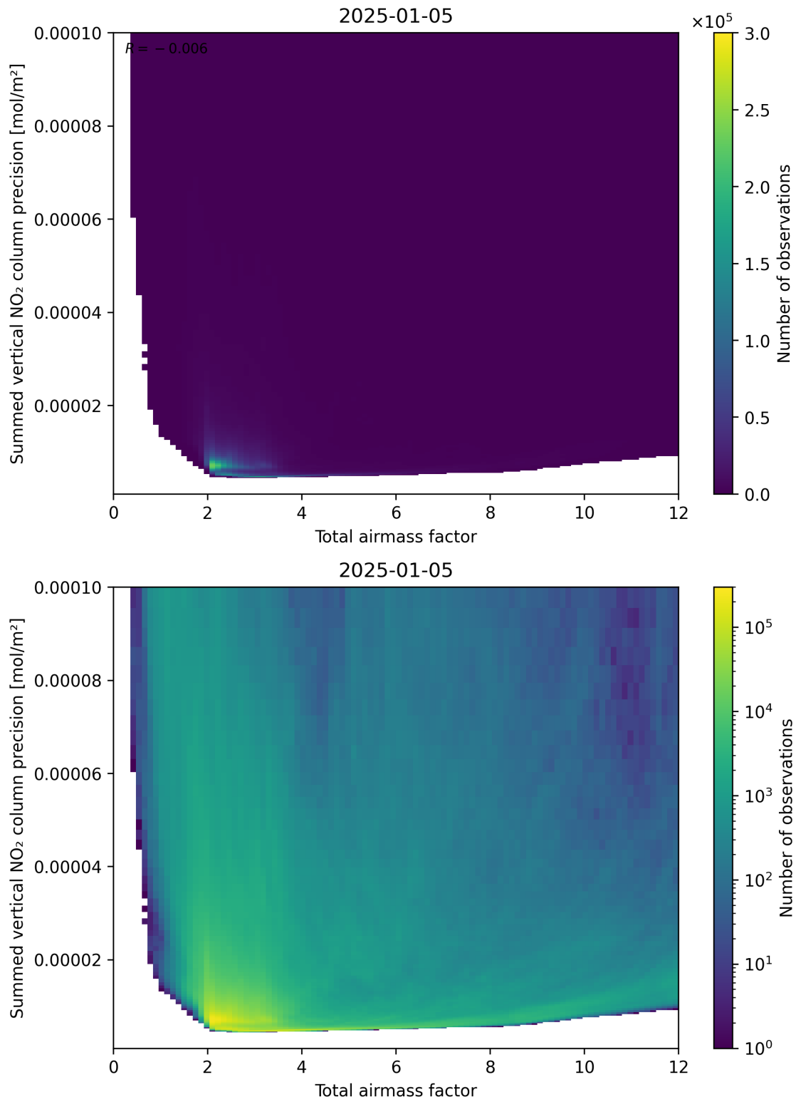
Figure 66: Scatter density plot of “Total airmass factor” against “Summed vertical NO 2 column precision” for 2025-01-04 to 2025-01-06.
