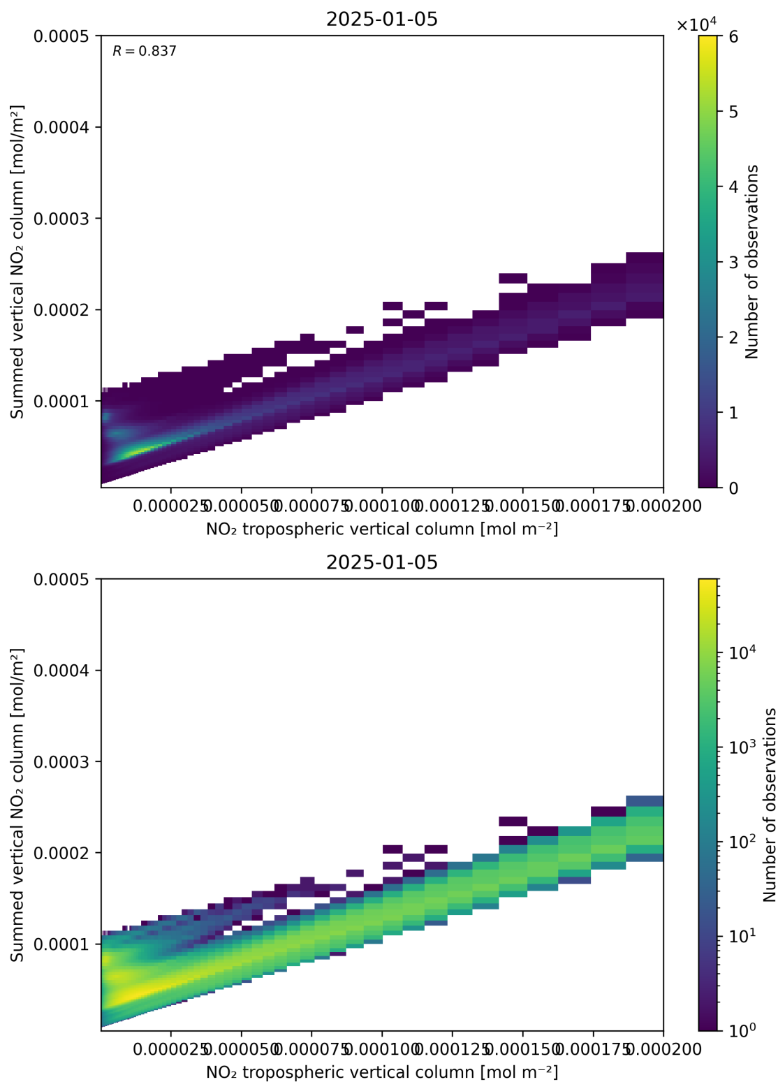
Figure 126: Scatter density plot of “NO 2 tropospheric vertical column” against “Summed vertical NO 2 column” for 2025-01-04 to 2025-01-06.
