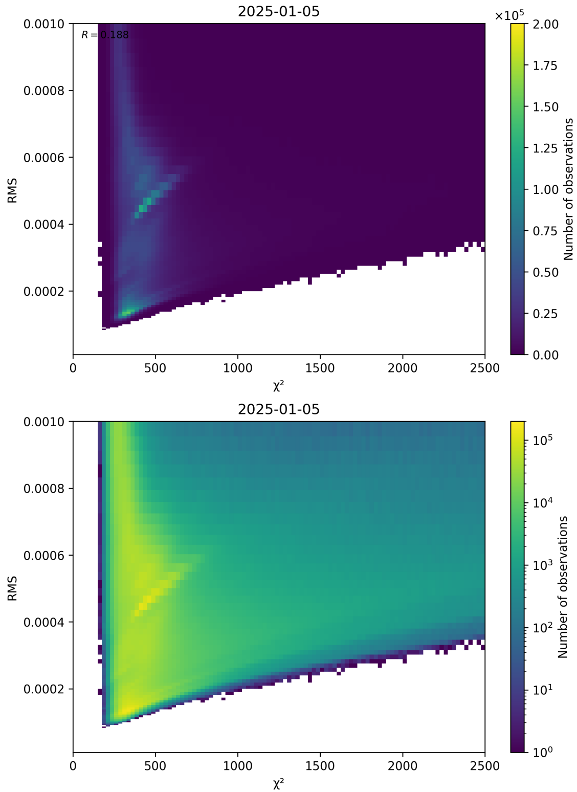
Figure 82: Scatter density plot of “ \chi^2 ” against “RMS” for 2025-01-04 to 2025-01-06.
