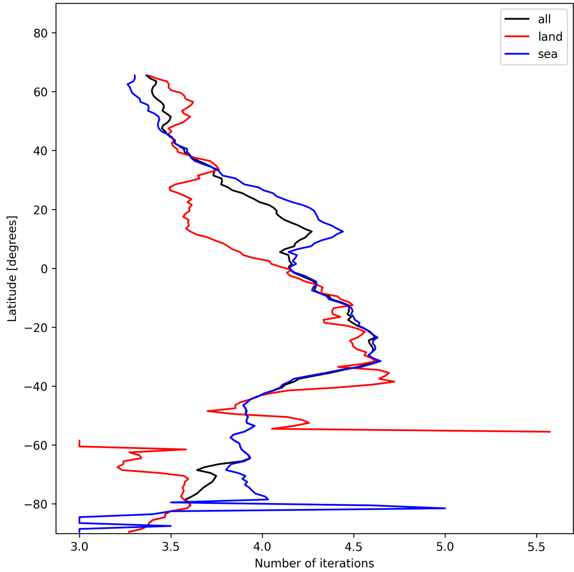
Figure 17: Zonal average of “Number of iterations” for 2025-01-04 to 2025-01-06.
