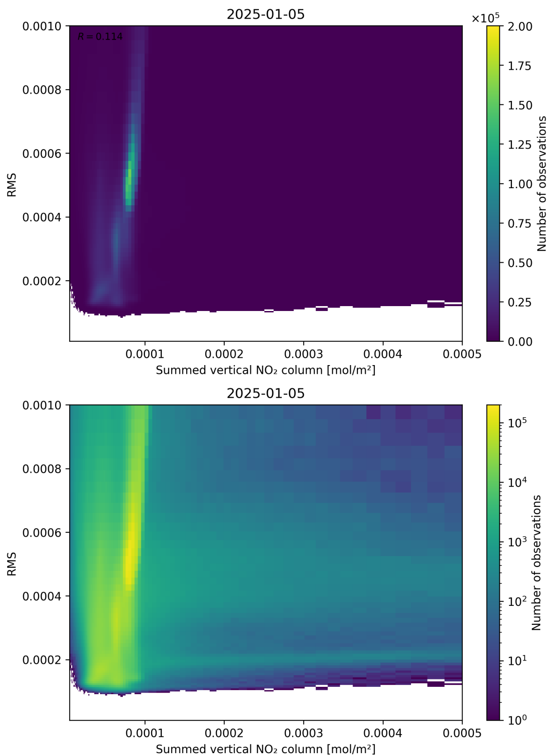
Figure 109: Scatter density plot of “Summed vertical NO 2 column” against “RMS” for 2025-01-04 to 2025-01-06.
