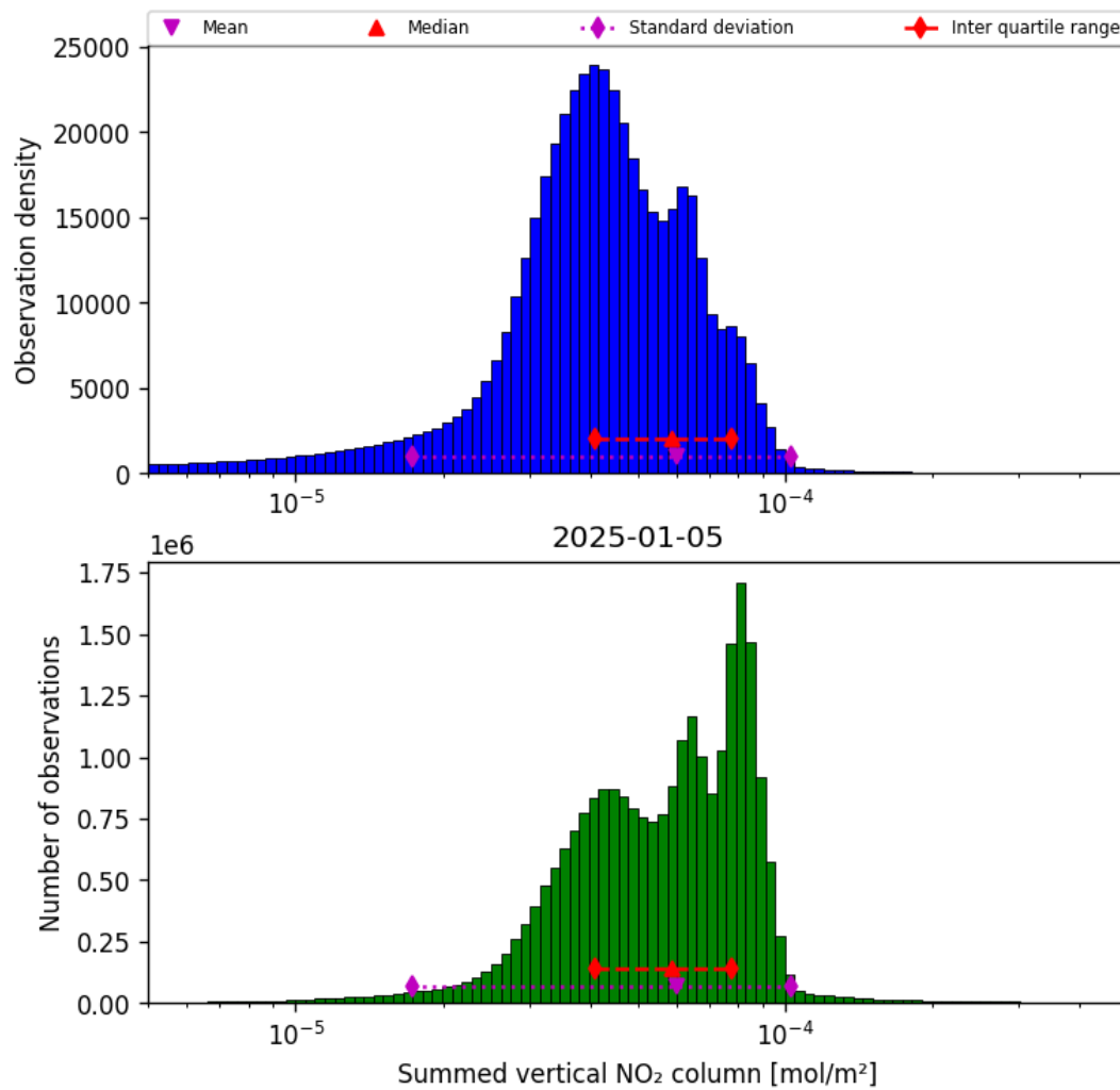
Figure 40: Histogram of “Summed vertical NO 2 column” for 2025-01-04 to 2025-01-06
