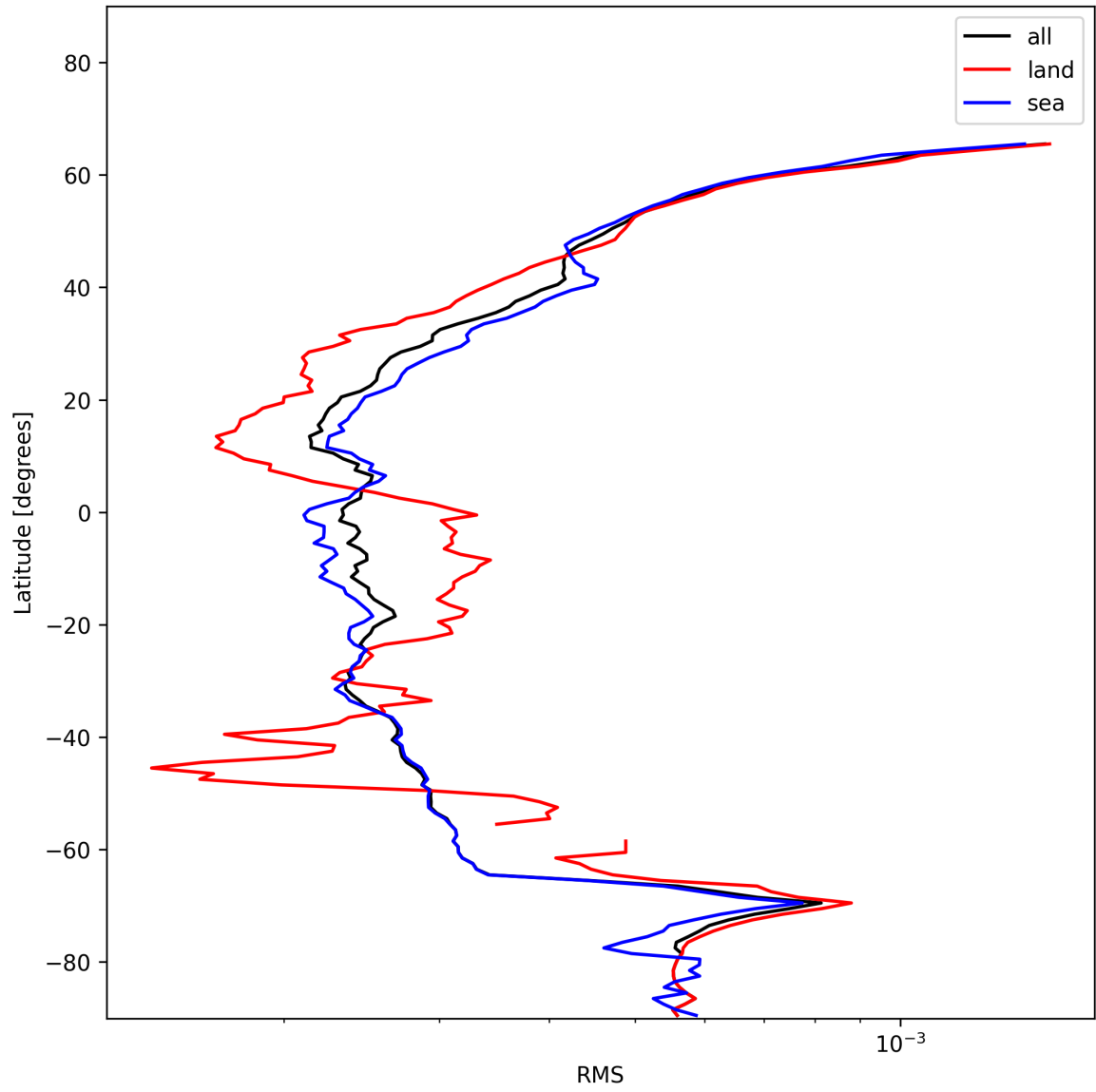
Figure 26: Zonal average of “RMS” for 2025-01-04 to 2025-01-06.
