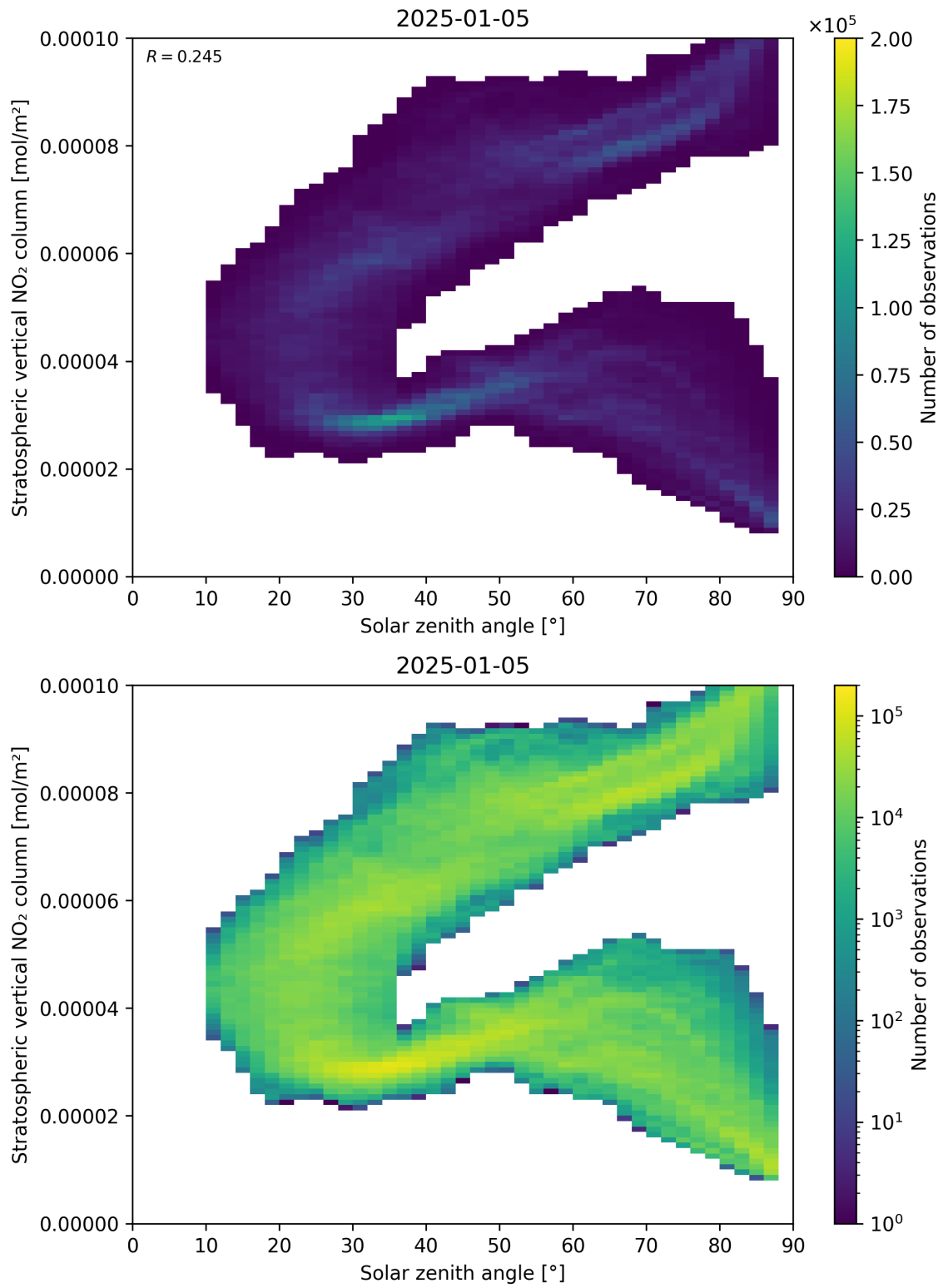
Figure 150: Scatter density plot of “Solar zenith angle” against “Stratospheric vertical NO 2 column” for 2025-01-04 to 2025-01-06.
