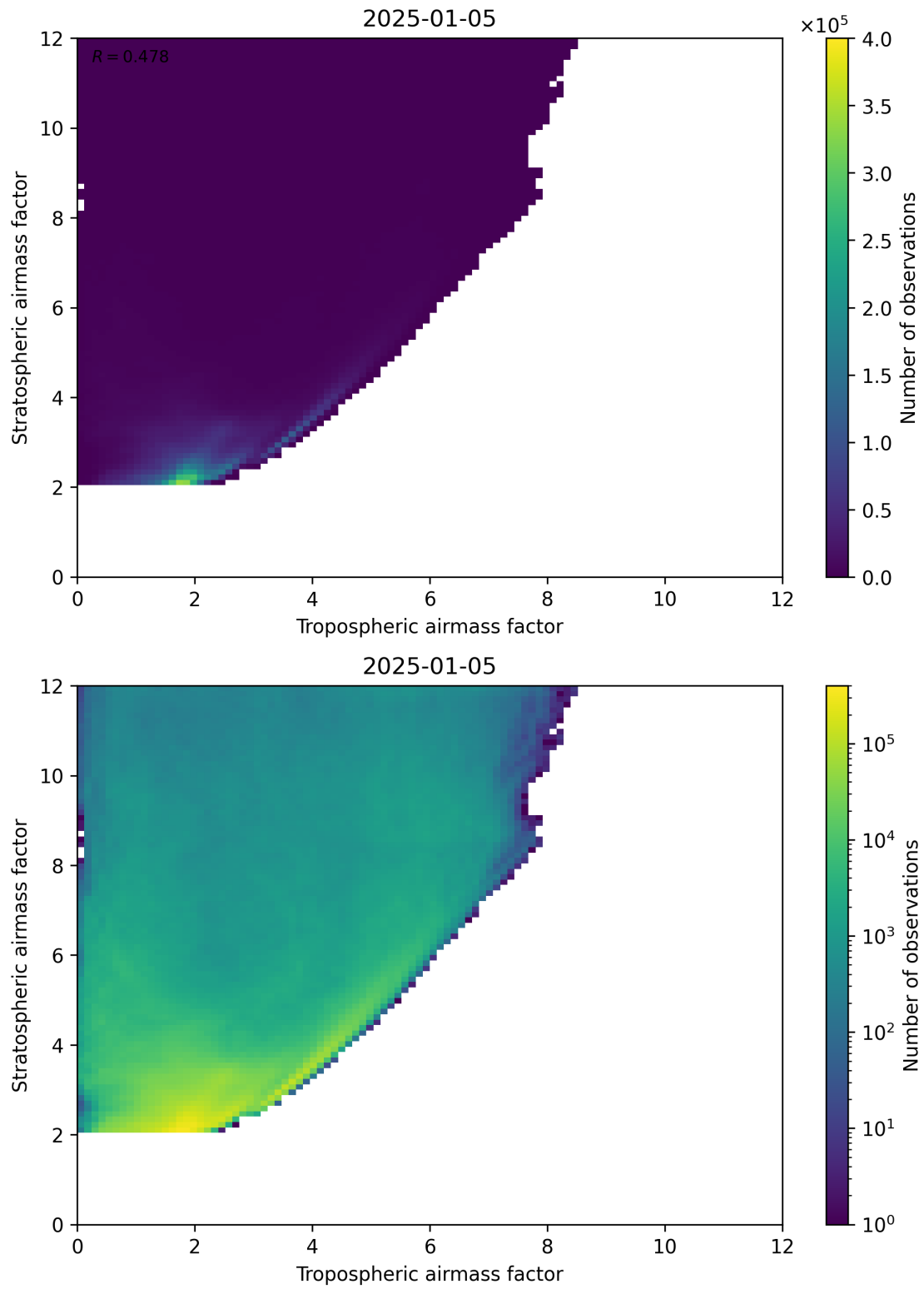
Figure 71: Scatter density plot of “Tropospheric airmass factor” against “Stratospheric airmass factor” for 2025-01-04 to 2025-01-06.
