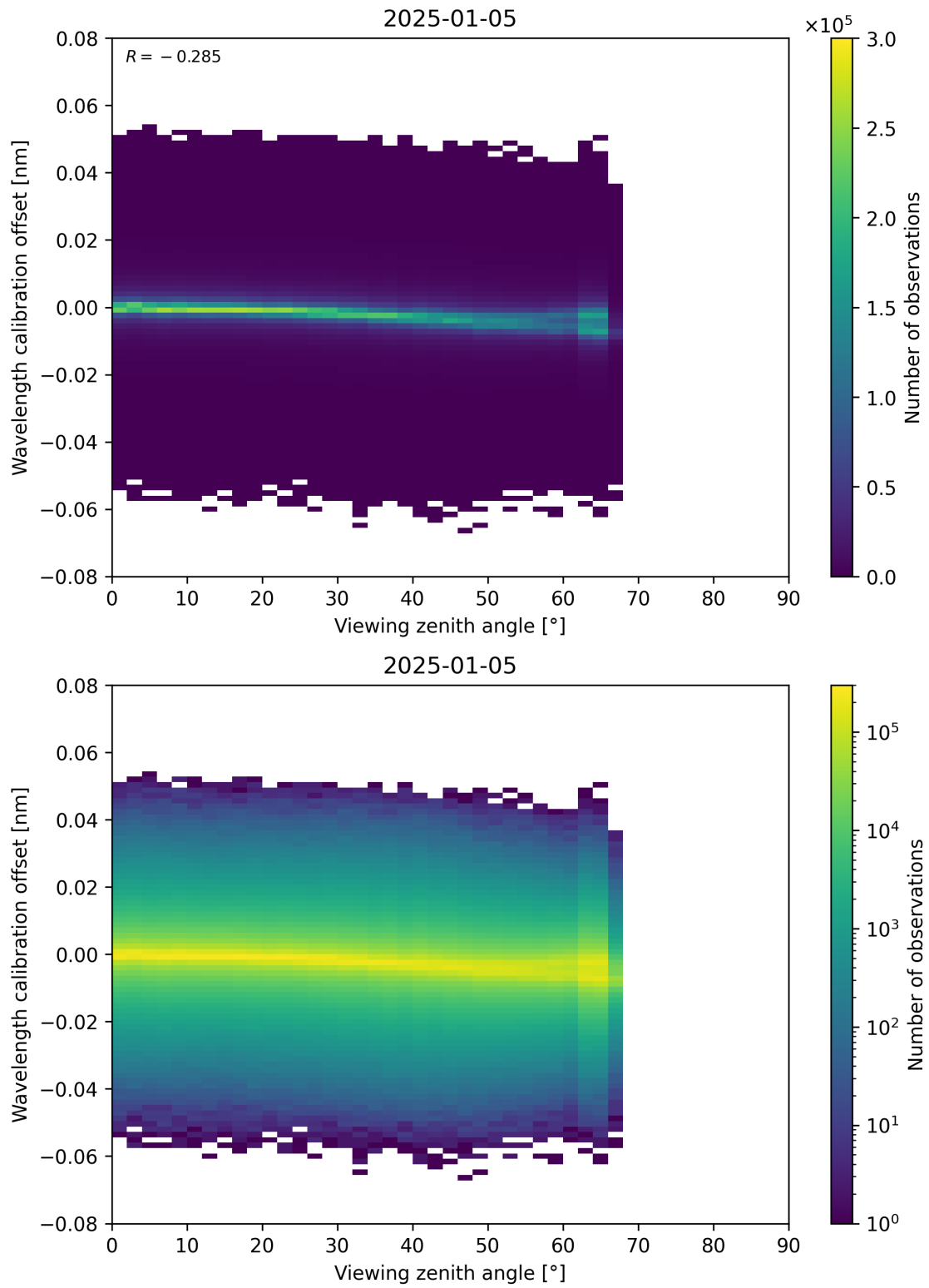
Figure 173: Scatter density plot of “Viewing zenith angle” against “Wavelength calibration offset” for 2025-01-04 to 2025-01-06.
