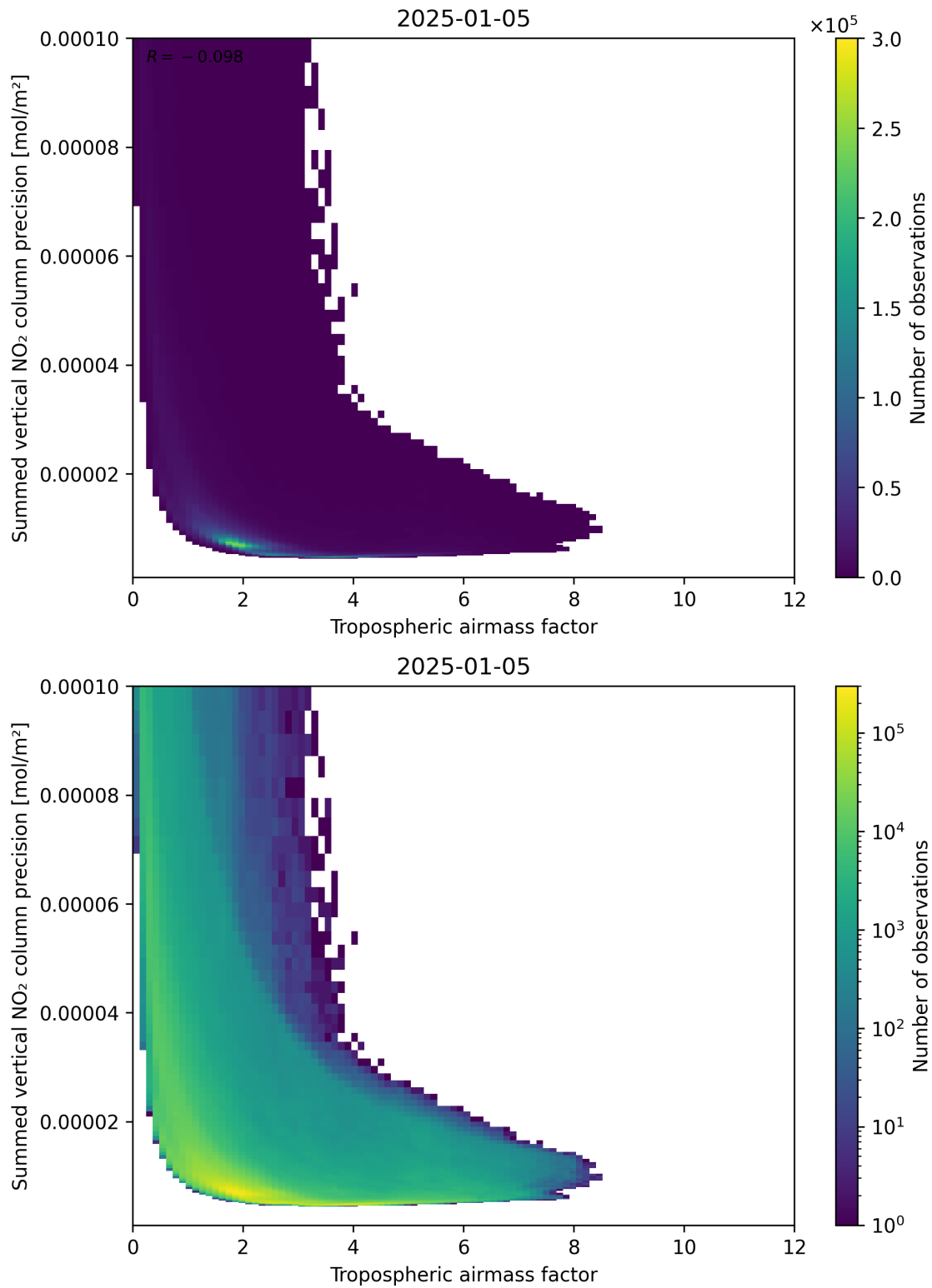
Figure 76: Scatter density plot of “Tropospheric air mass factor” against “Summed vertical NO 2 column precision” for 2025-01-04 to 2025-01-06.
