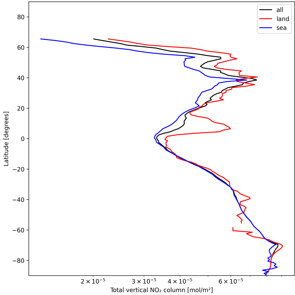
Figure 21: Zonal average of “Total vertical NO 2 column” for 2025-01-04 to 2025-01-06.
