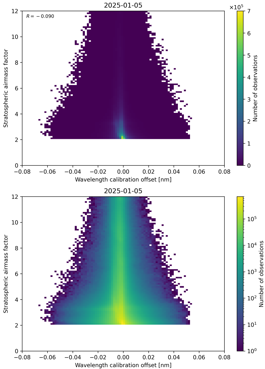
Figure 174: Scatter density plot of “Wavelength calibration offset” against “Stratospheric airmass factor” for 2025-01-04 to 2025-01-06.
