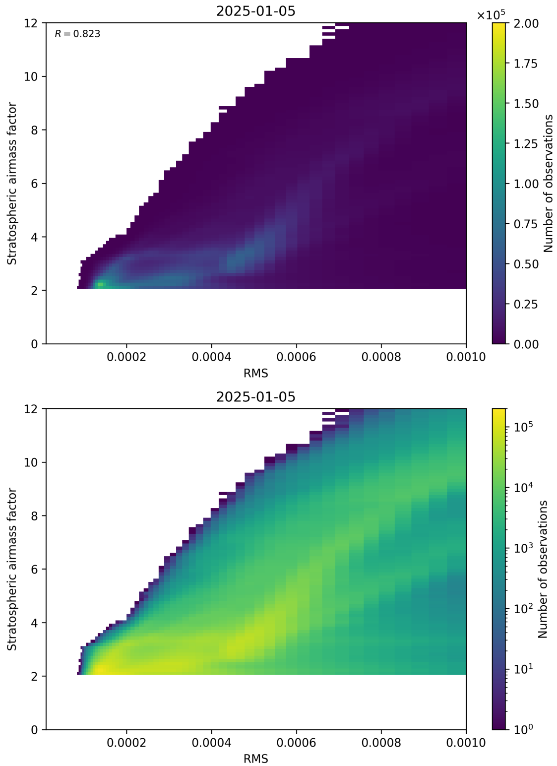
Figure 144: Scatter density plot of “RMS” against “Stratospheric airmass factor” for 2025-01-04 to 2025-01-06.
