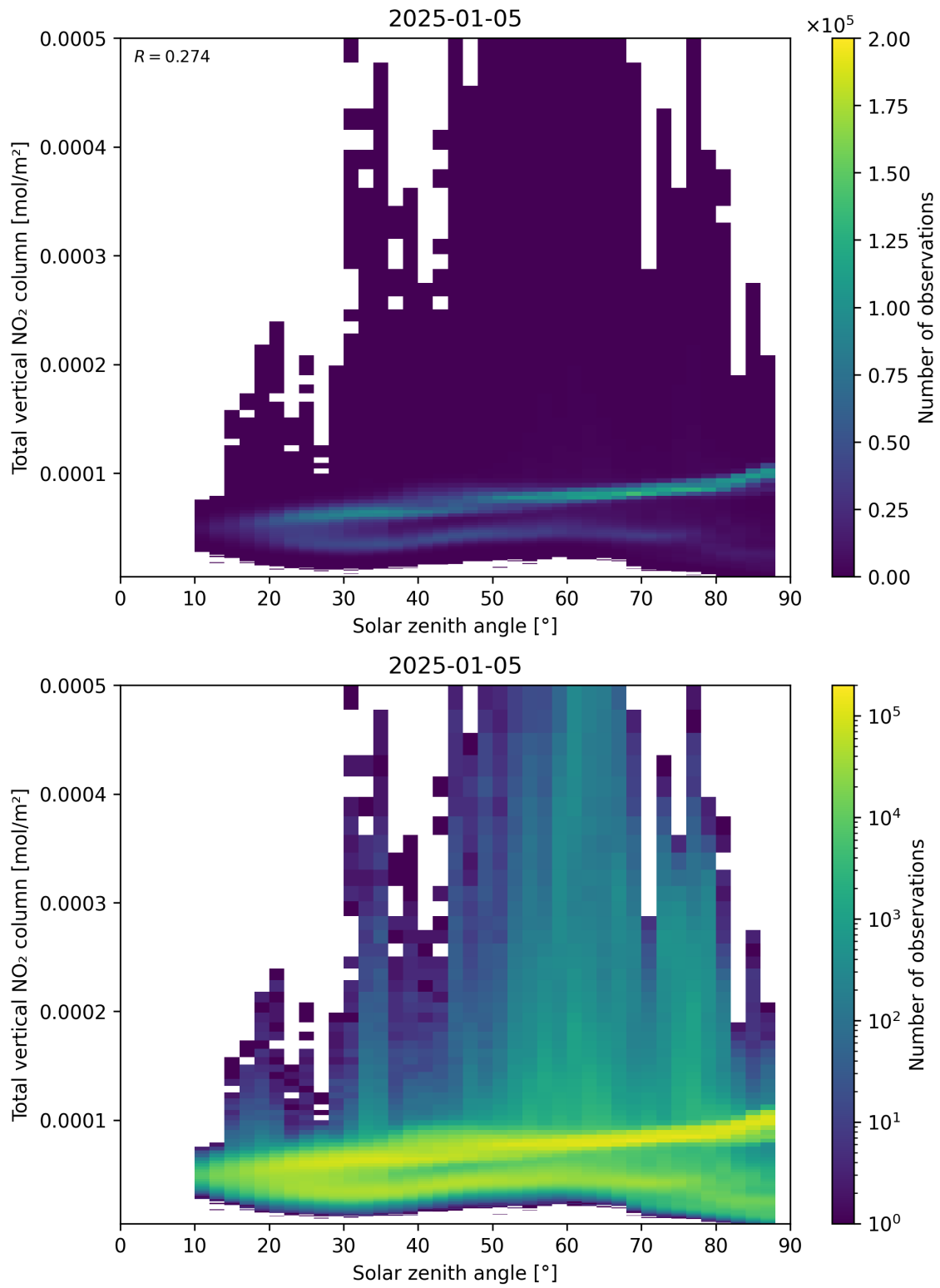
Figure 153: Scatter density plot of “Solar zenith angle” against “Total vertical NO 2 column” for 2025-01-04 to 2025-01-06.
