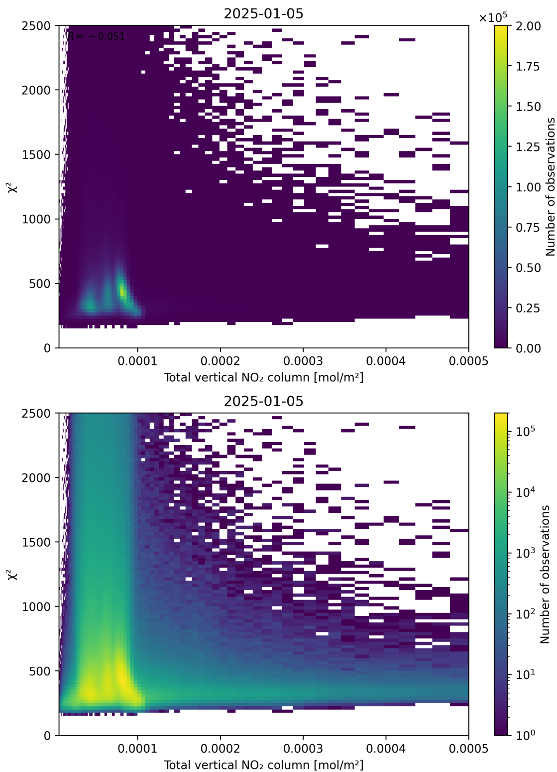
Figure 111: Scatter density plot of “Total vertical NO 2 column” against “ \chi^2 ” for 2025-01-04 to 2025-01-06.
