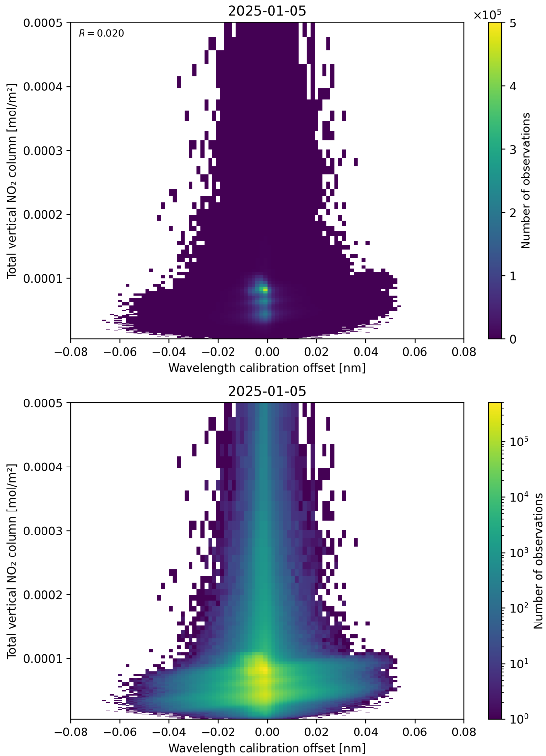
Figure 179: Scatter density plot of “Wavelength calibration offset” against “Total vertical NO 2 column” for 2025-01-04 to 2025-01-06.
