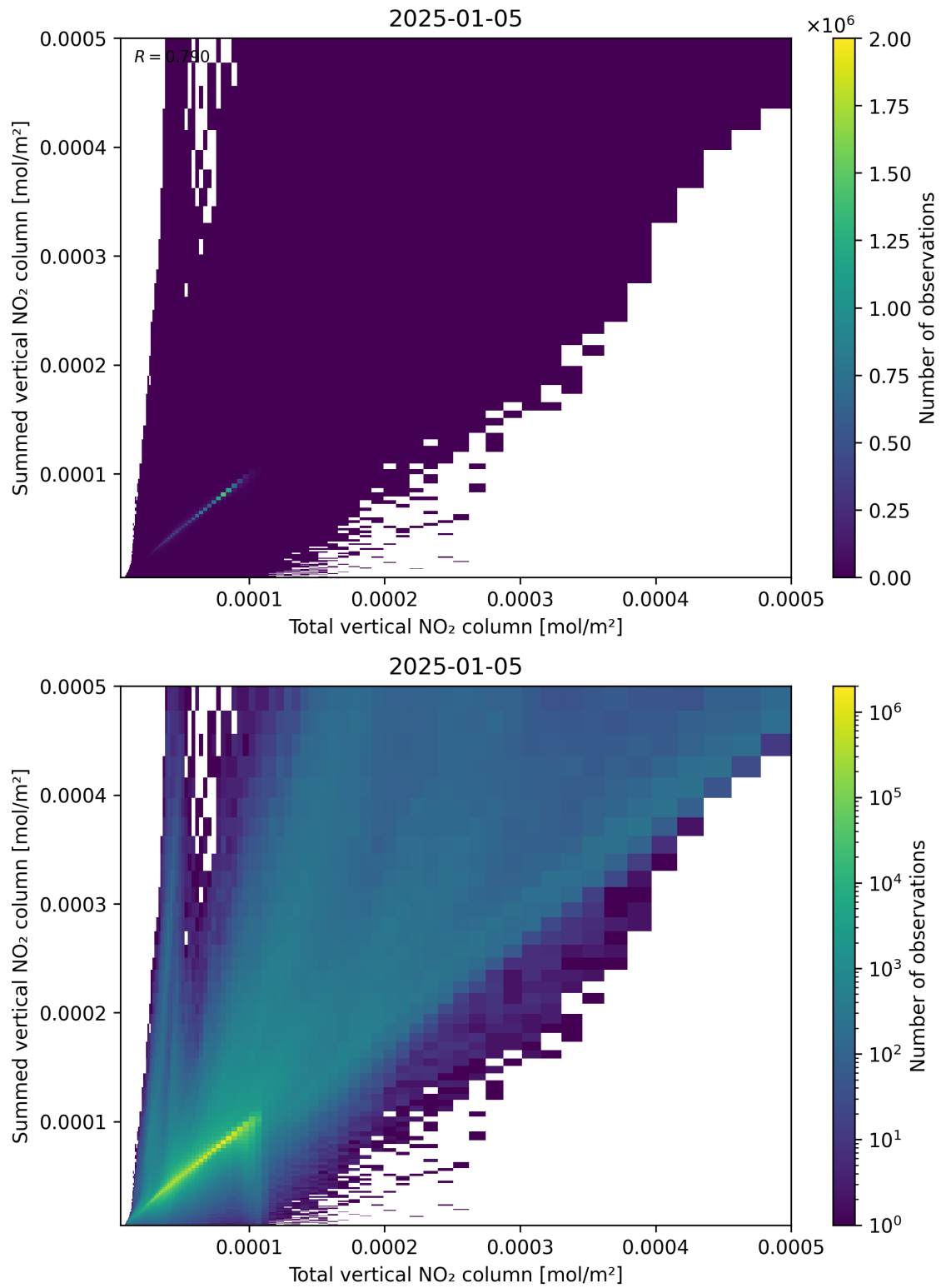
Figure 112: Scatter density plot of “Total vertical NO 2 column” against “Summed vertical NO 2 column” for 2025-01-04 to 2025-01-06.
