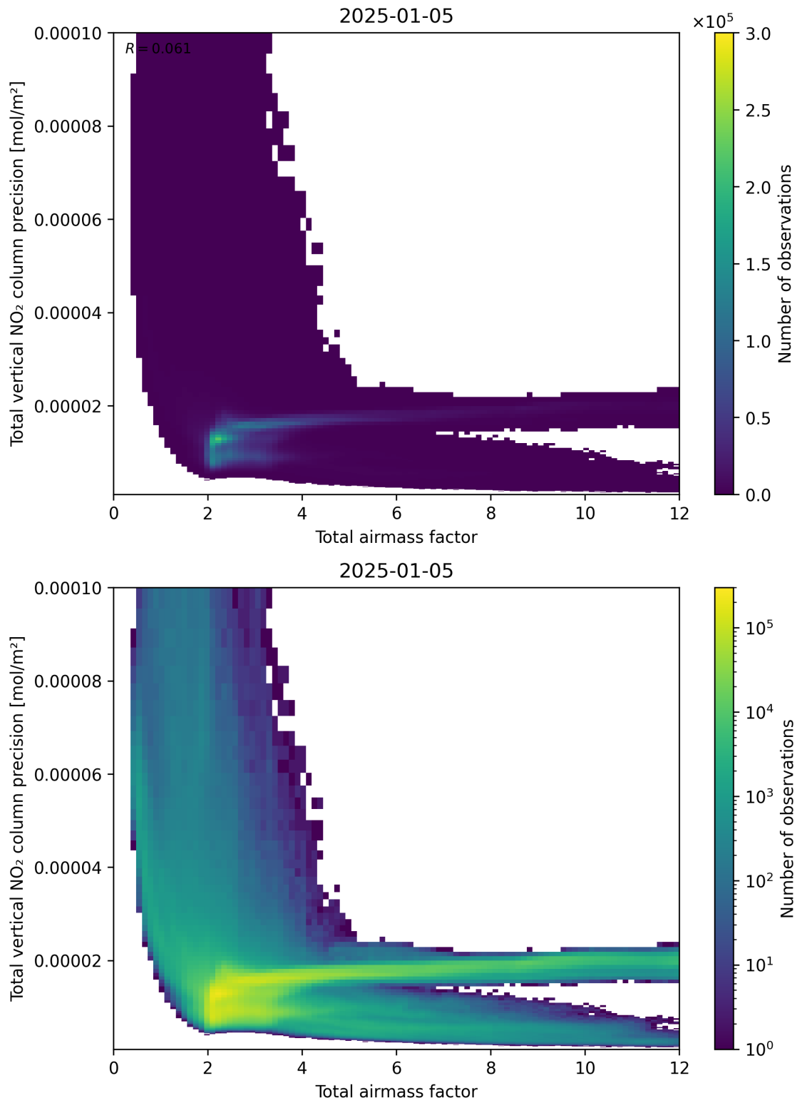
Figure 68: Scatter density plot of “Total airmass factor” against “Total vertical NO 2 column precision” for 2025-01-04 to 2025-01-06.
