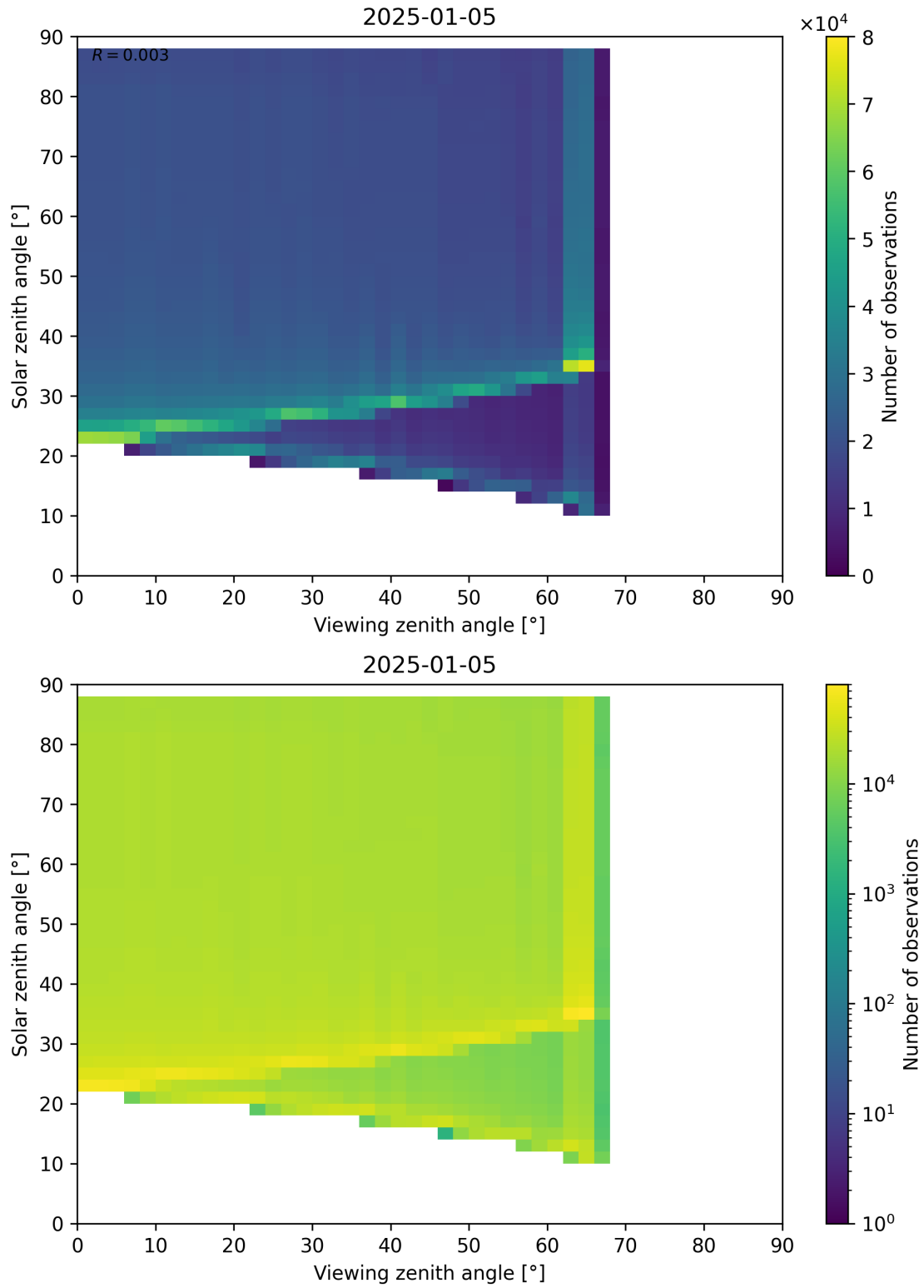
Figure 172: Scatter density plot of “Viewing zenith angle” against “Solar zenith angle” for 2025-01-04 to 2025-01-06.
