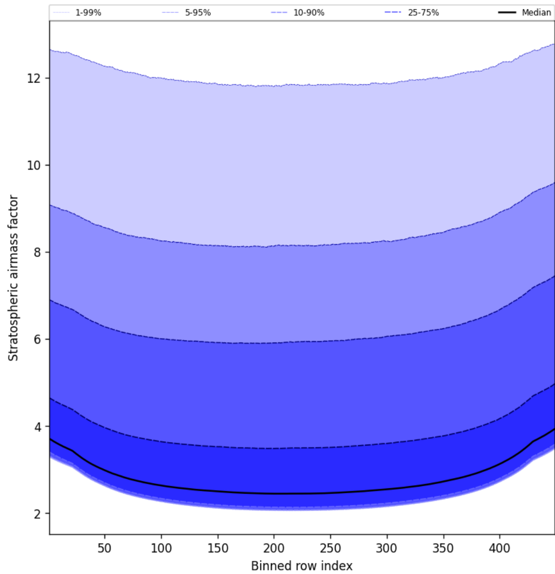
Figure 61: Along track statistics of “Stratospheric airmass factor” for 2025-01-04 to 2025-01-06
