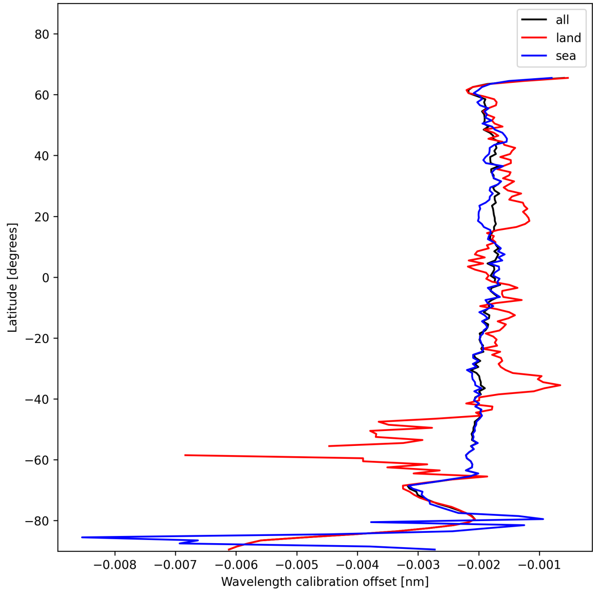
Figure 18: Zonal average of “Wavelength calibration offset” for 2025-01-04 to 2025-01-06.
