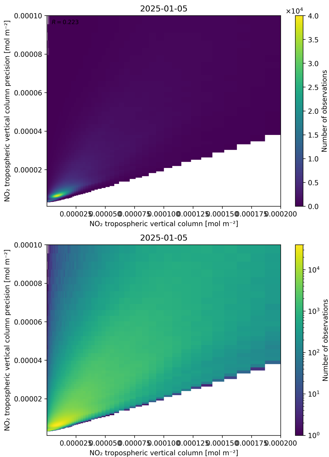
Figure 130: Scatter density plot of “NO 2 tropospheric vertical column” against “NO 2 tropospheric vertical column precision” for 2025-01-04 to 2025-01-06.
