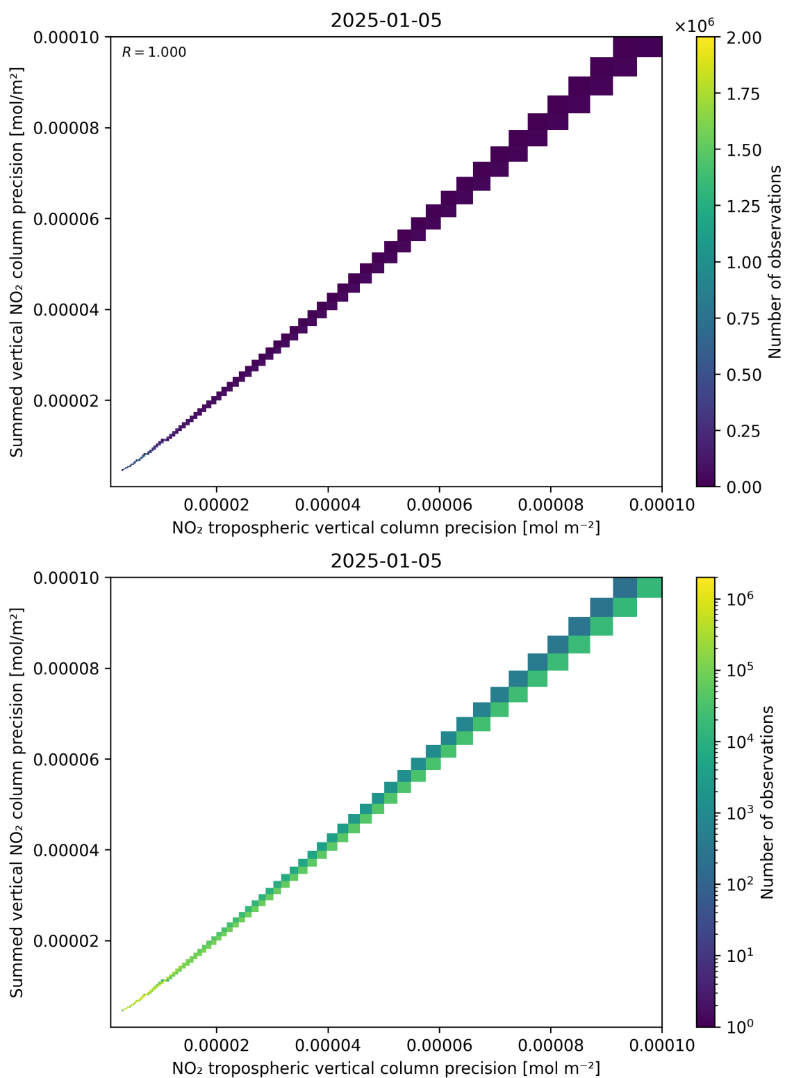
Figure 137: Scatter density plot of “NO 2 tropospheric vertical column precision” against “Summed vertical NO 2 column precision” for 2025-01-04 to 2025-01-06.
