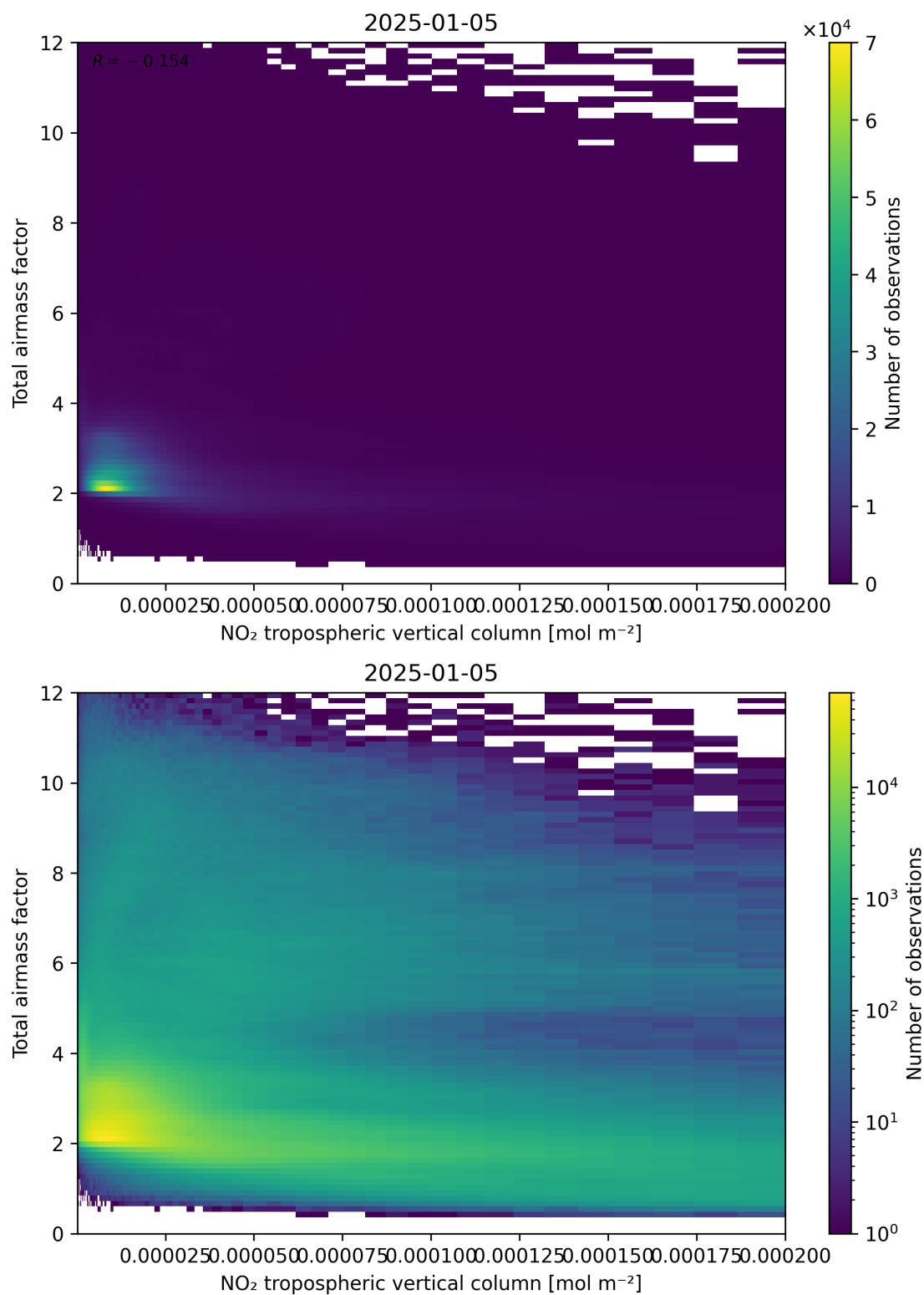
Figure 122: Scatter density plot of “NO 2 tropospheric vertical column” against “Total air mass factor” for 2025-01-04 to 2025-01-06.
