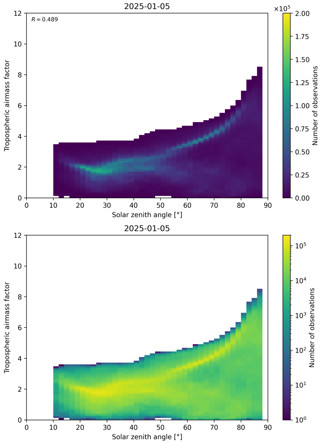
Figure 147: Scatter density plot of “Solar zenith angle” against “Tropospheric airmass factor” for 2025-01-04 to 2025-01-06.
