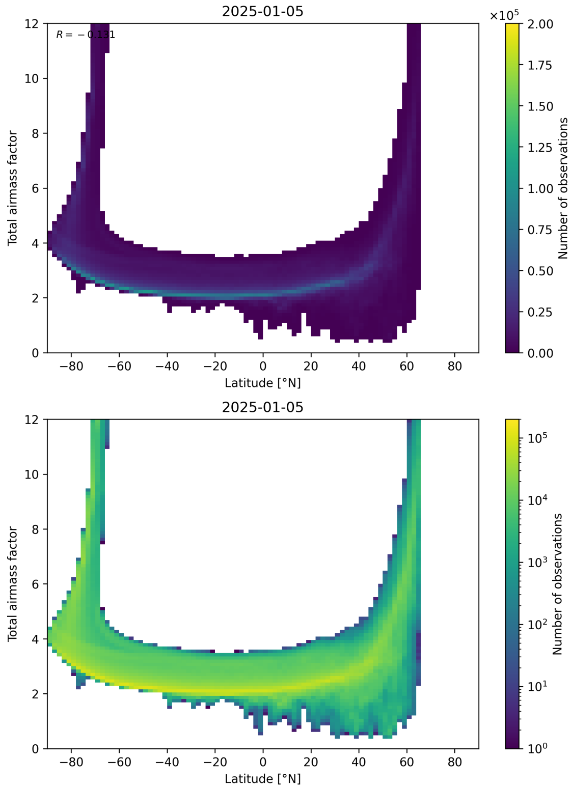
Figure 84: Scatter density plot of “Latitude” against “Total airmass factor” for 2025-01-04 to 2025-01-06.
