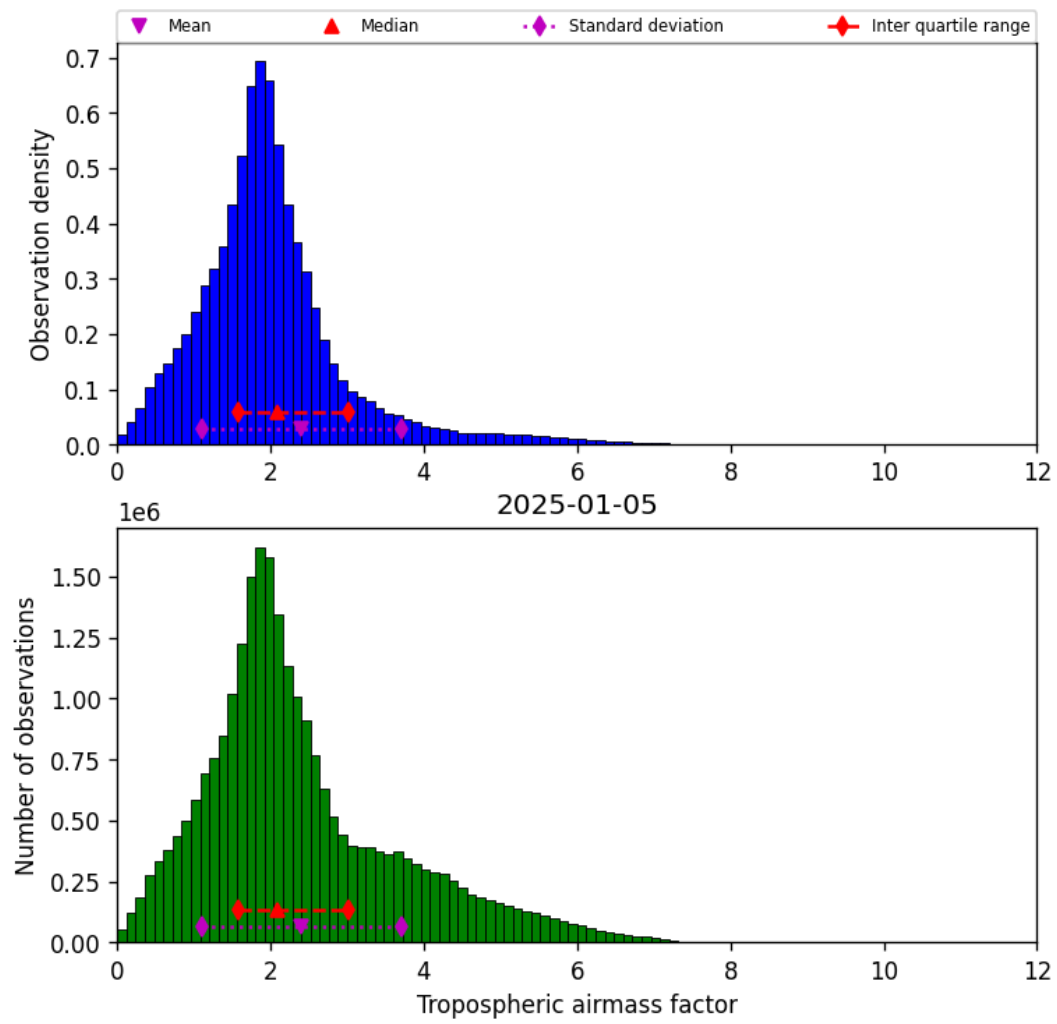
Figure 31: Histogram of “Tropospheric airmass factor” for 2025-01-04 to 2025-01-06
