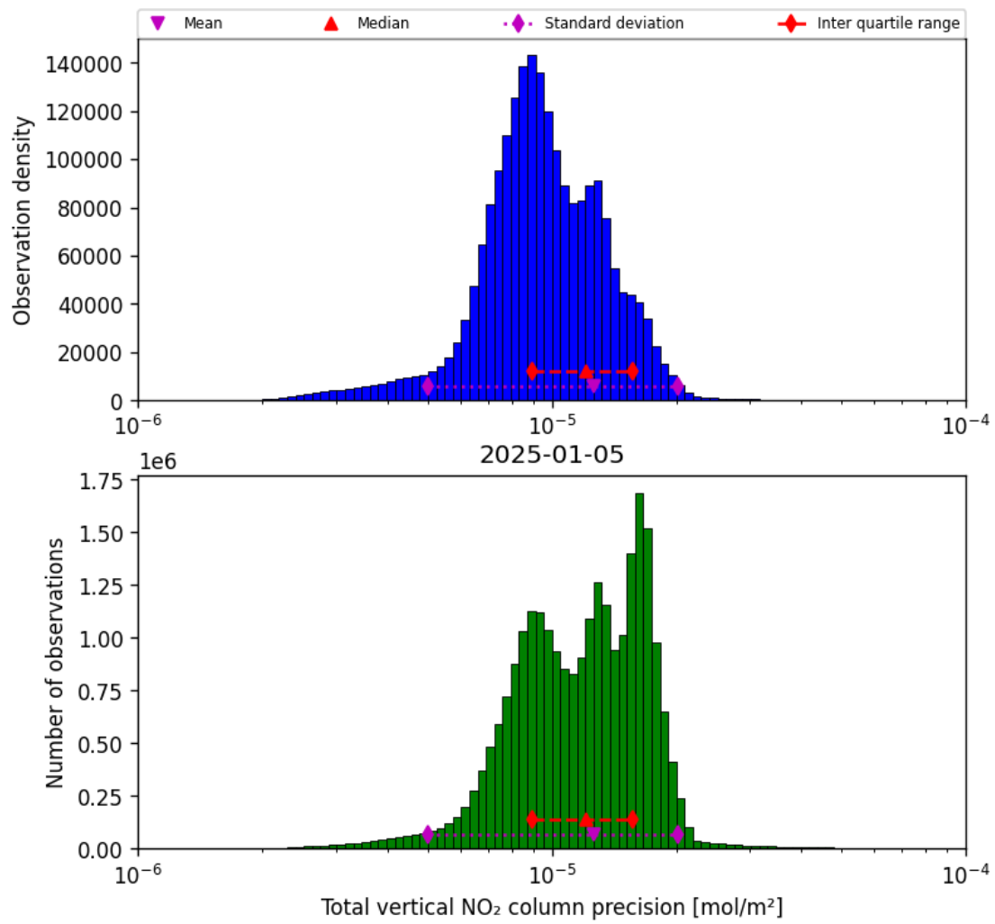
Figure 39: Histogram of “Total vertical NO 2 column precision” for 2025-01-04 to 2025-01-06
