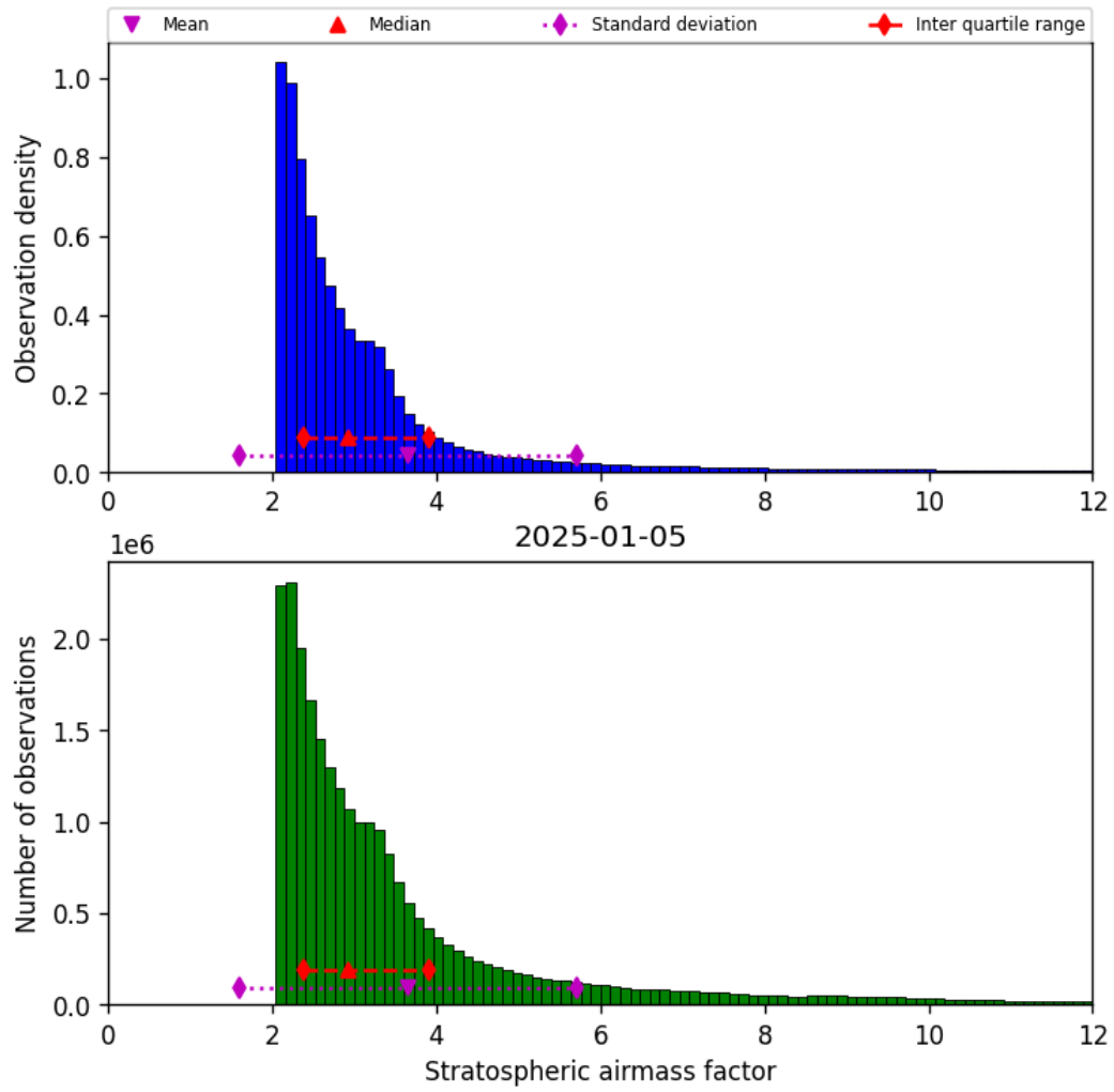
Figure 44: Histogram of “Stratospheric airmass factor” for 2025-01-04 to 2025-01-06
