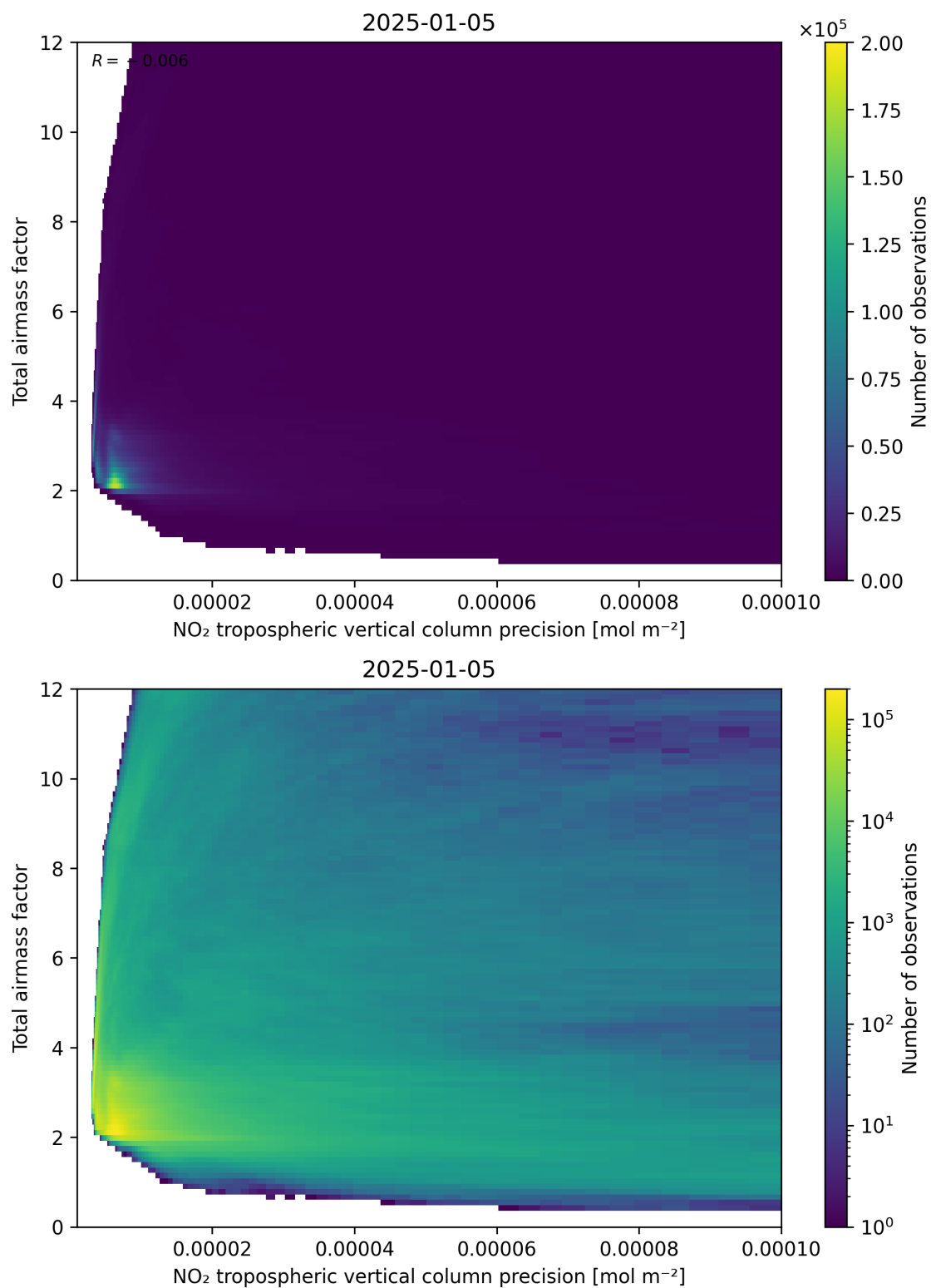
Figure 132: Scatter density plot of “NO 2 tropospheric vertical column precision” against “Total air mass factor” for 2025-01-04 to 2025-01-06.
