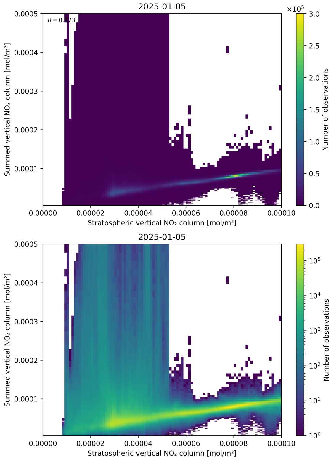
Figure 98: Scatter density plot of “Stratospheric vertical NO 2 column” against “Summed vertical NO 2 column” for 2025-01-04 to 2025-01-06.
