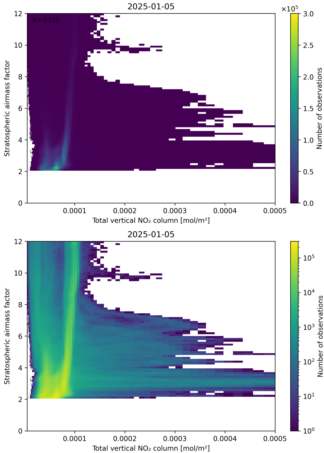
Figure 110: Scatter density plot of “Total vertical NO 2 column” against “Stratospheric airmass factor” for 2025-01-04 to 2025-01-06.
