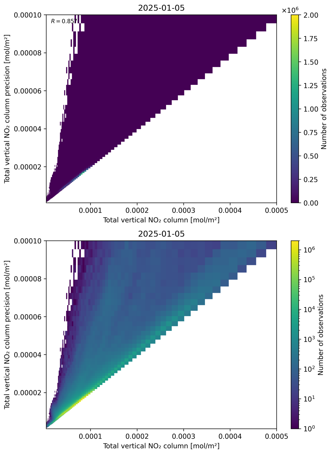
Figure 114: Scatter density plot of “Total vertical NO 2 column” against “Total vertical NO 2 column precision” for 2025-01-04 to 2025-01-06.
