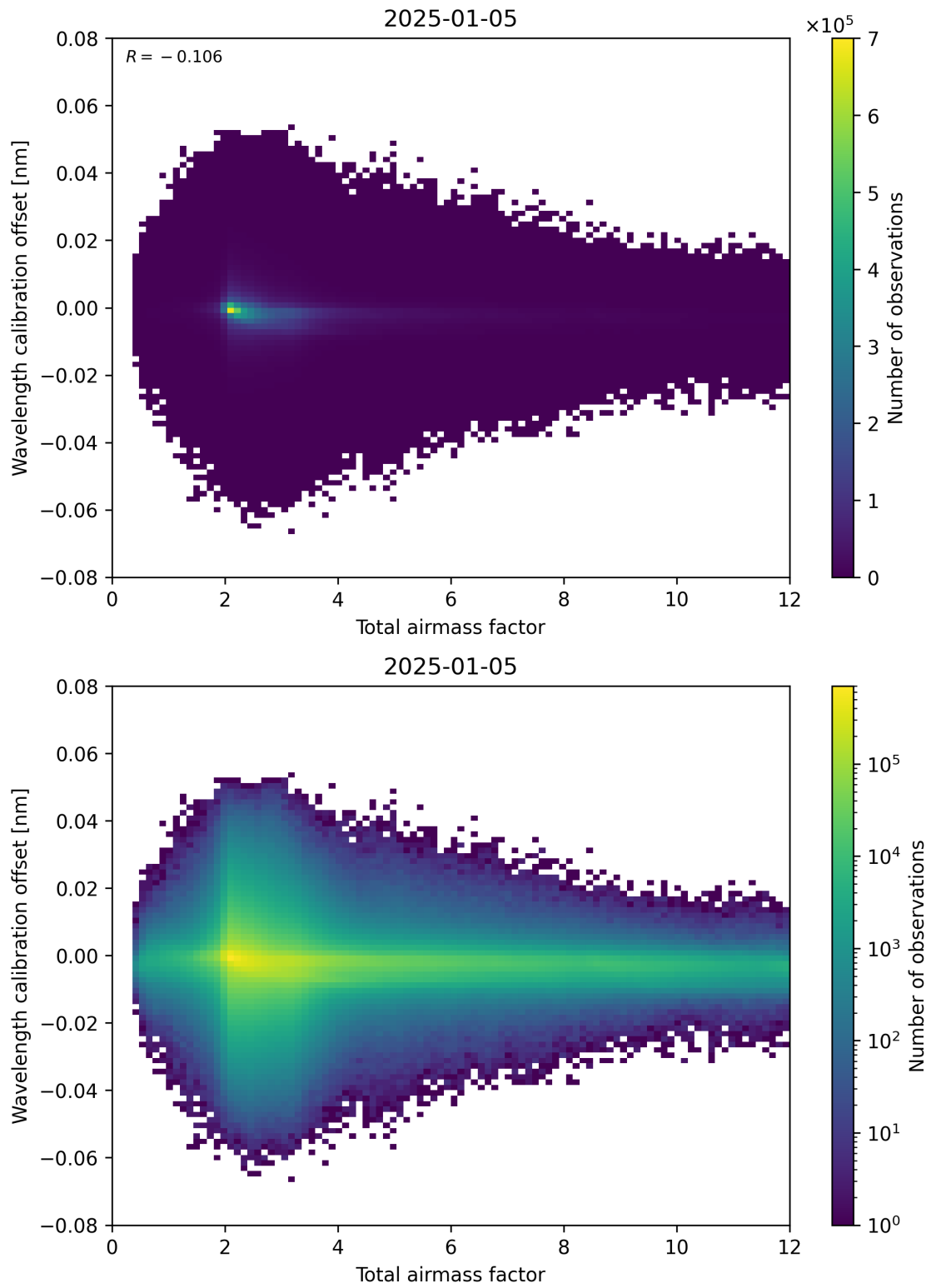
Figure 70: Scatter density plot of “Total airmass factor” against “Wavelength calibration offset” for 2025-01-04 to 2025-01-06.
