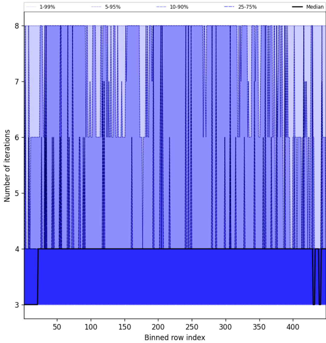
Figure 51: Along track statistics of “Number of iterations” for 2025-01-04 to 2025-01-06
