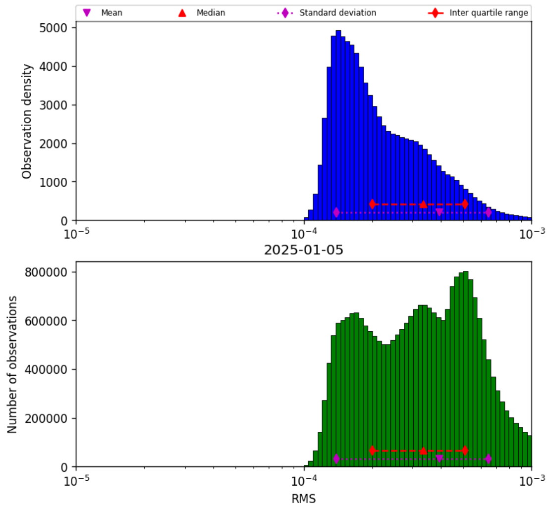
Figure 43: Histogram of “RMS” for 2025-01-04 to 2025-01-06
