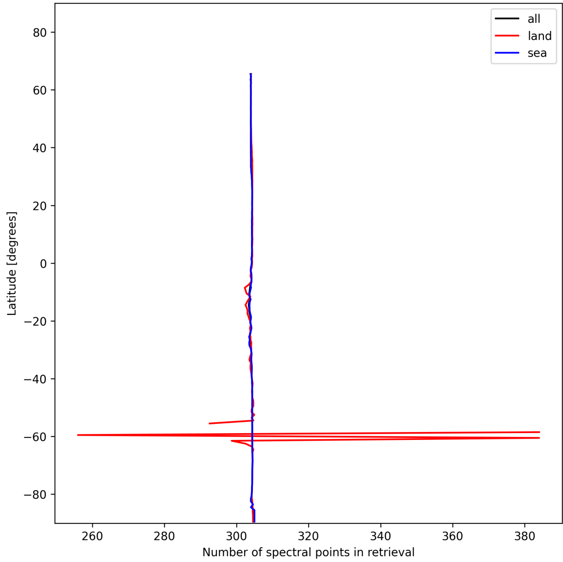
Figure 16: Zonal average of “Number of spectral points in retrieval” for 2025-01-04 to 2025-01-06.
