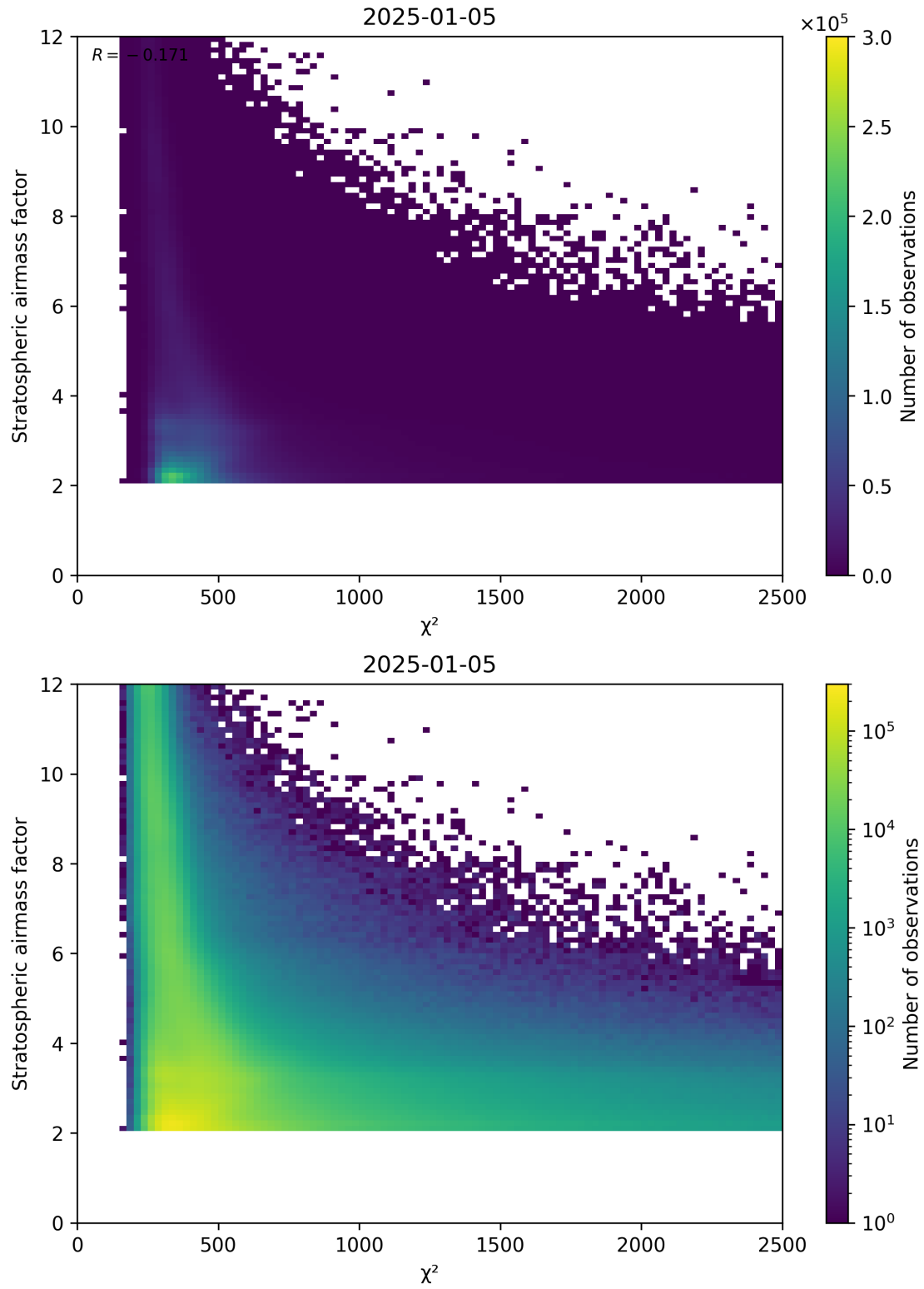
Figure 81: Scatter density plot of “ \chi^2 ” against “Stratospheric airmass factor” for 2025-01-04 to 2025-01-06.
