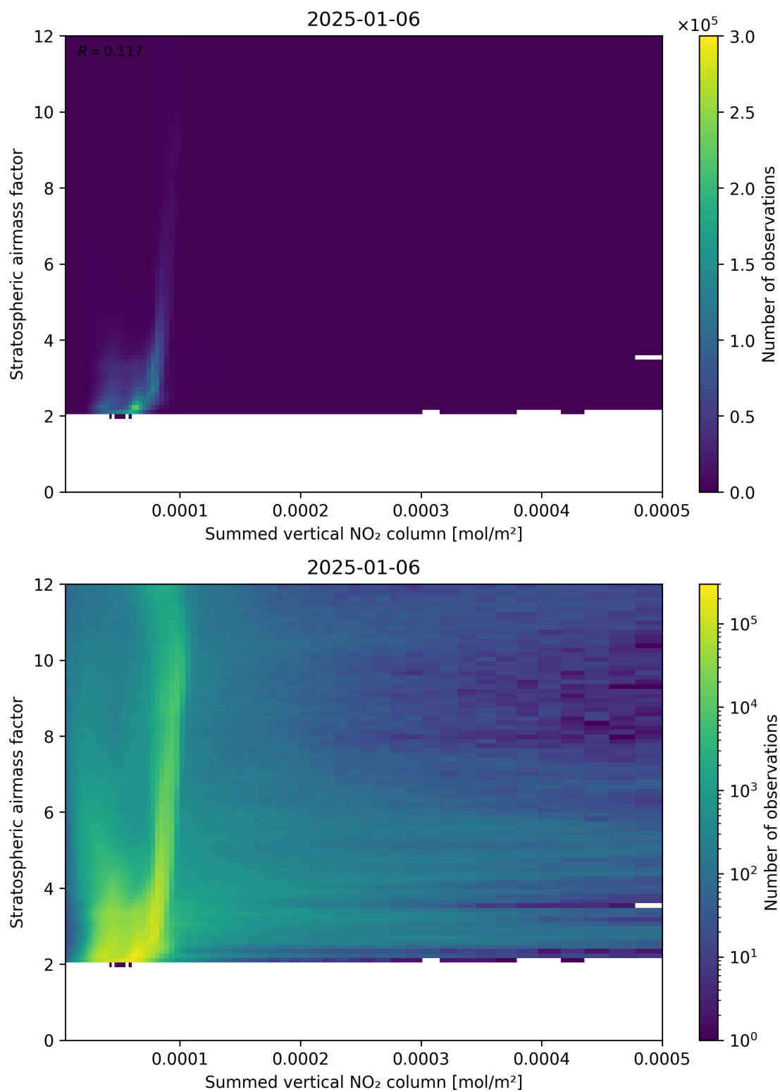
Figure 103: Scatter density plot of “Summed vertical NO 2 column” against “Stratospheric airmass factor” for 2025-01-05 to 2025-01-07.
