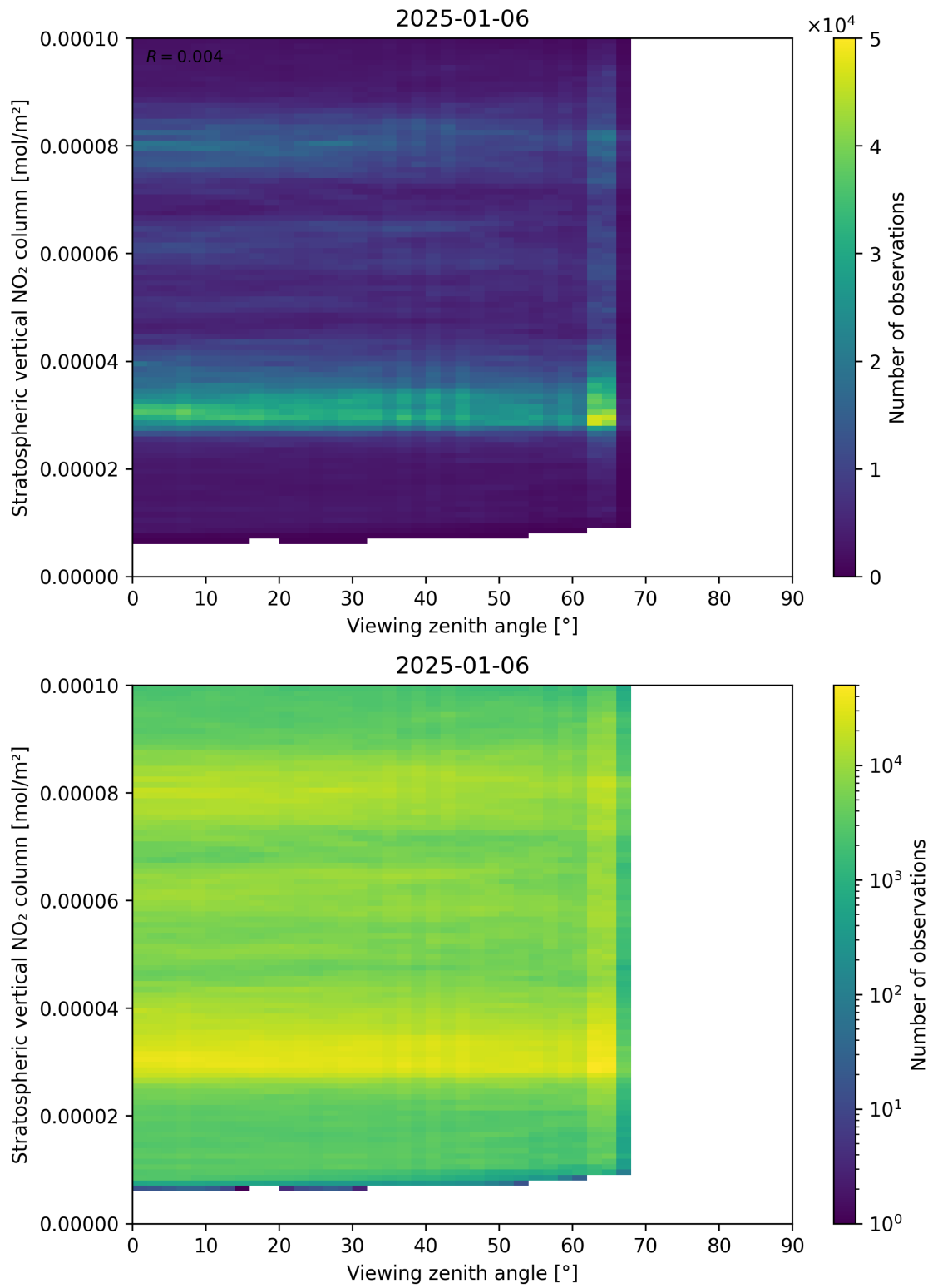
Figure 164: Scatter density plot of “Viewing zenith angle” against “Stratospheric vertical NO 2 column” for 2025-01-05 to 2025-01-07.
