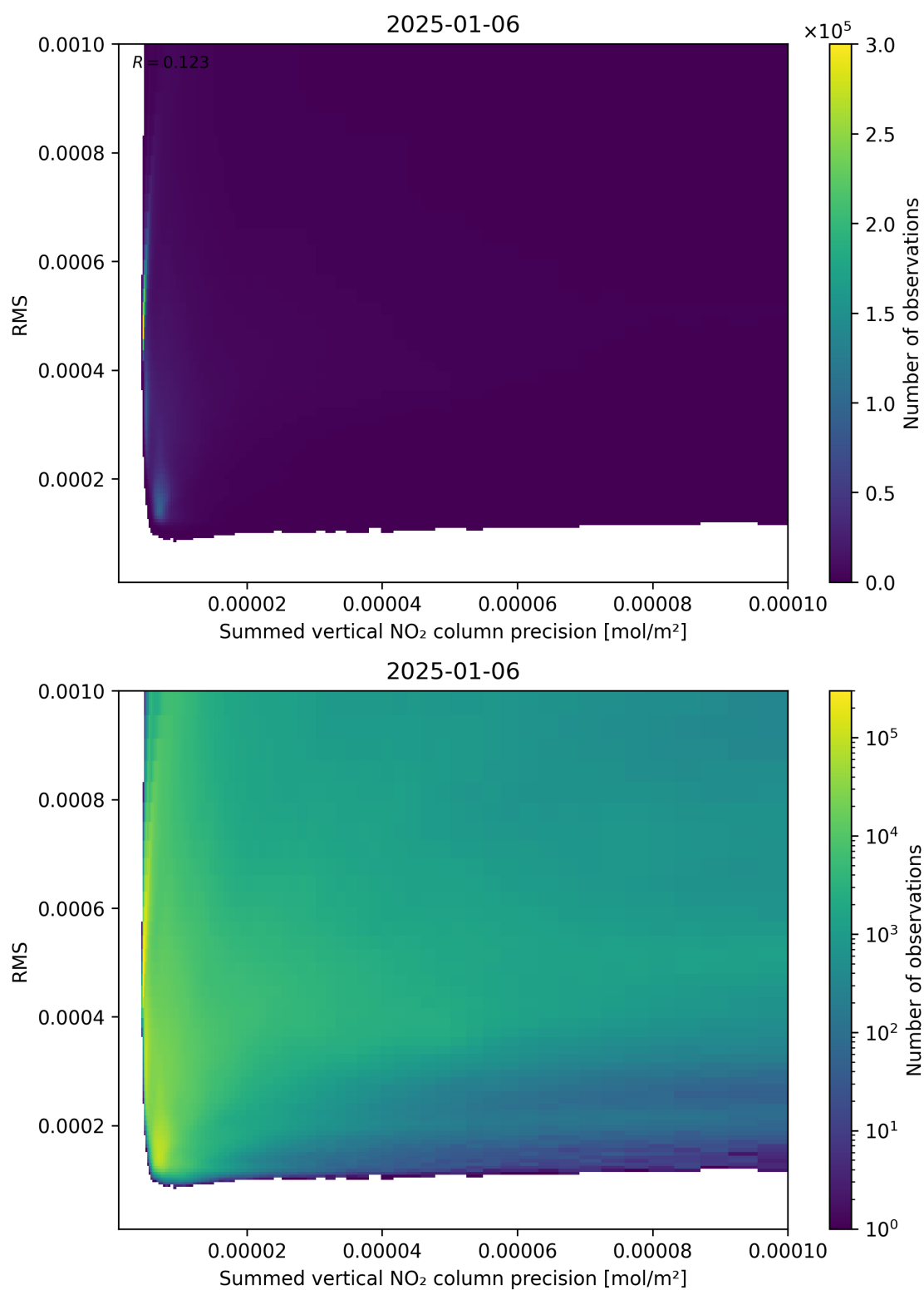
Figure 108: Scatter density plot of “Summed vertical NO 2 column precision” against “RMS” for 2025-01-05 to 2025-01-07.
