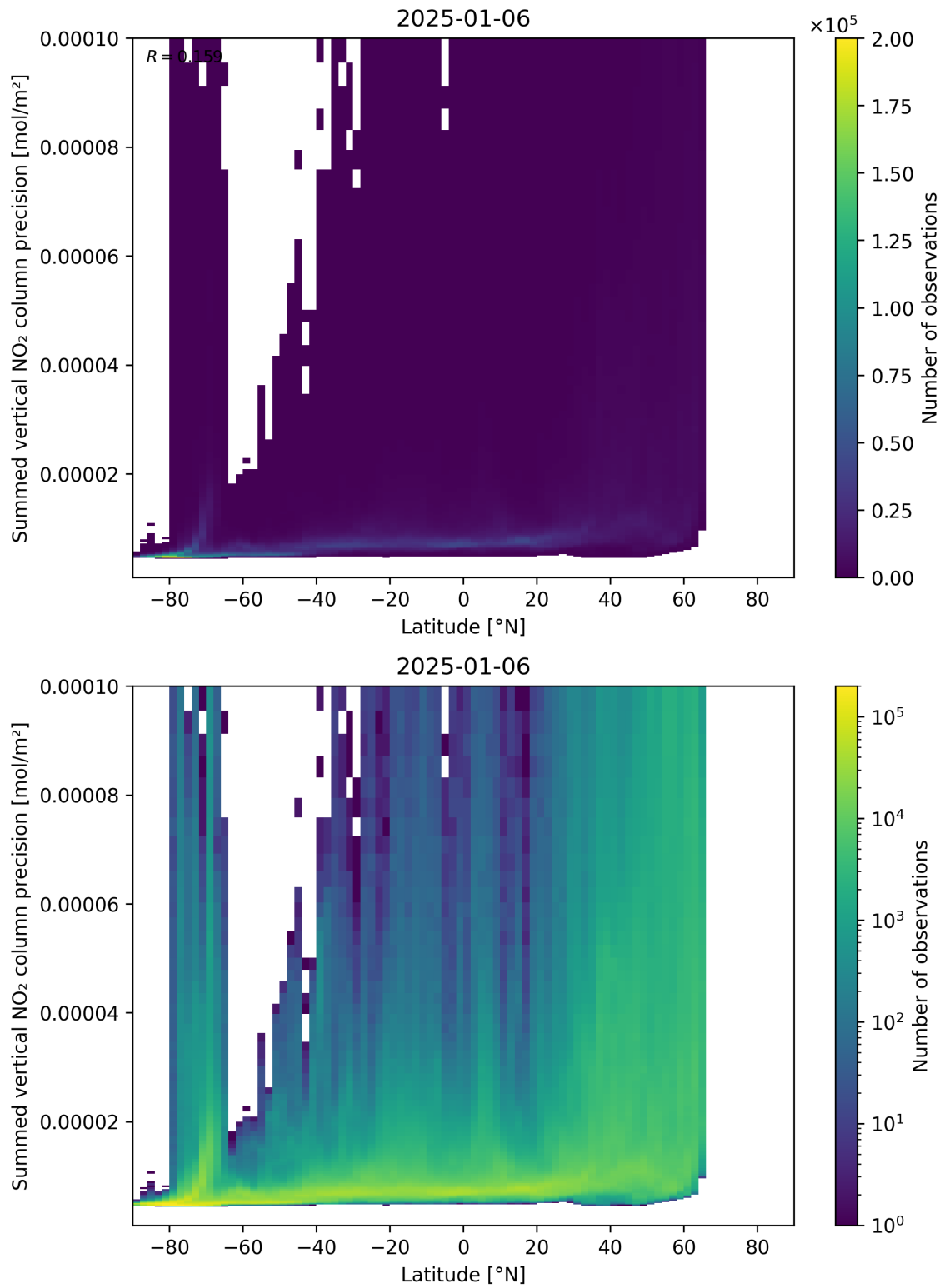
Figure 89: Scatter density plot of “Latitude” against “Summed vertical NO 2 column precision” for 2025-01-05 to 2025-01-07.
