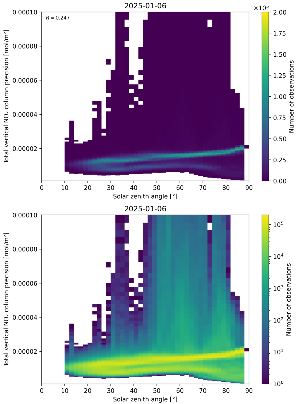
Figure 154: Scatter density plot of “Solar zenith angle” against “Total vertical NO 2 column precision” for 2025-01-05 to 2025-01-07.
