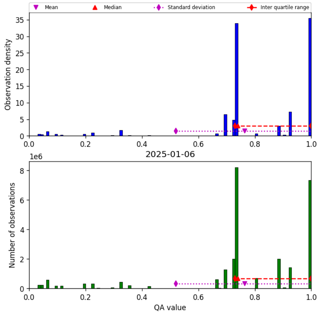
Figure 28: Histogram of “QA value” for 2025-01-05 to 2025-01-07
