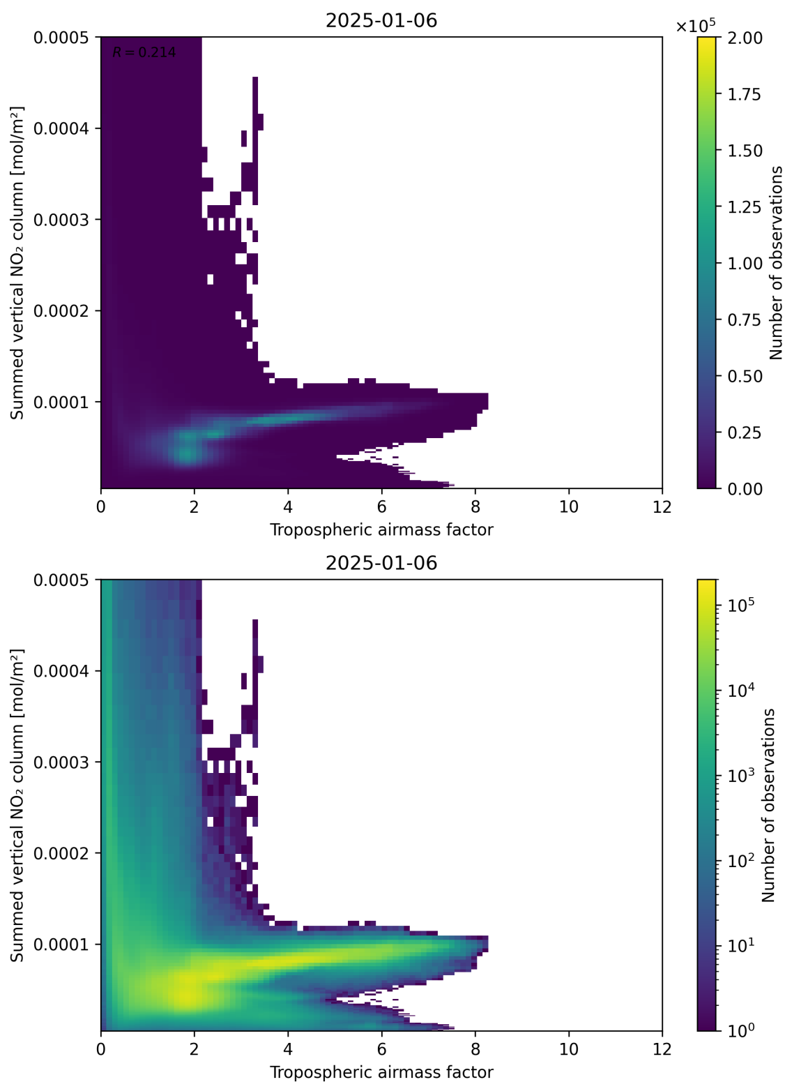
Figure 75: Scatter density plot of “Tropospheric air mass factor” against “Summed vertical NO 2 column” for 2025-01-05 to 2025-01-07.
