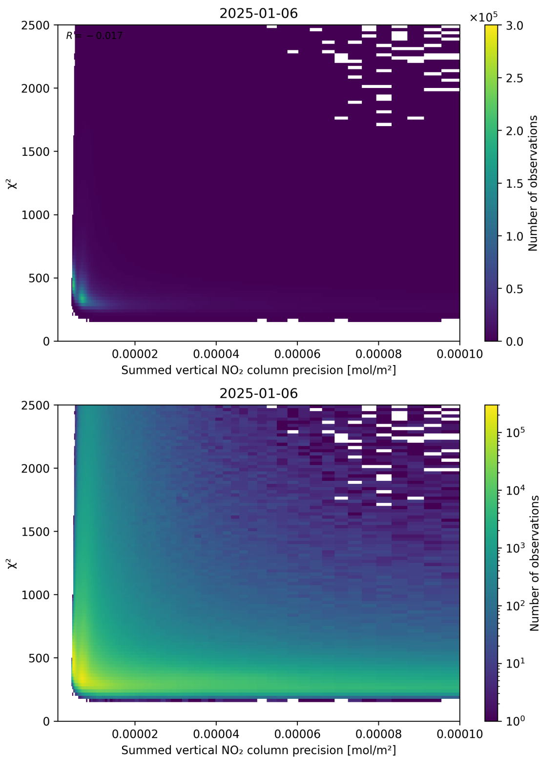
Figure 107: Scatter density plot of “Summed vertical NO 2 column precision” against “ \chi^2 ” for 2025-01-05 to 2025-01-07.
