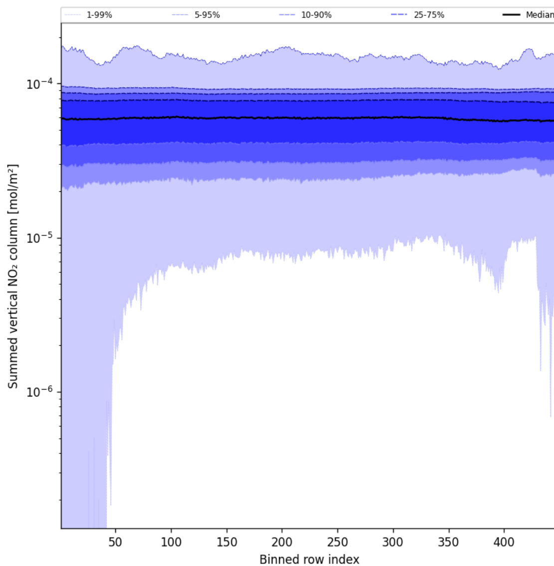
Figure 57: Along track statistics of “Summed vertical NO 2 column” for 2025-01-05 to 2025-01-07
