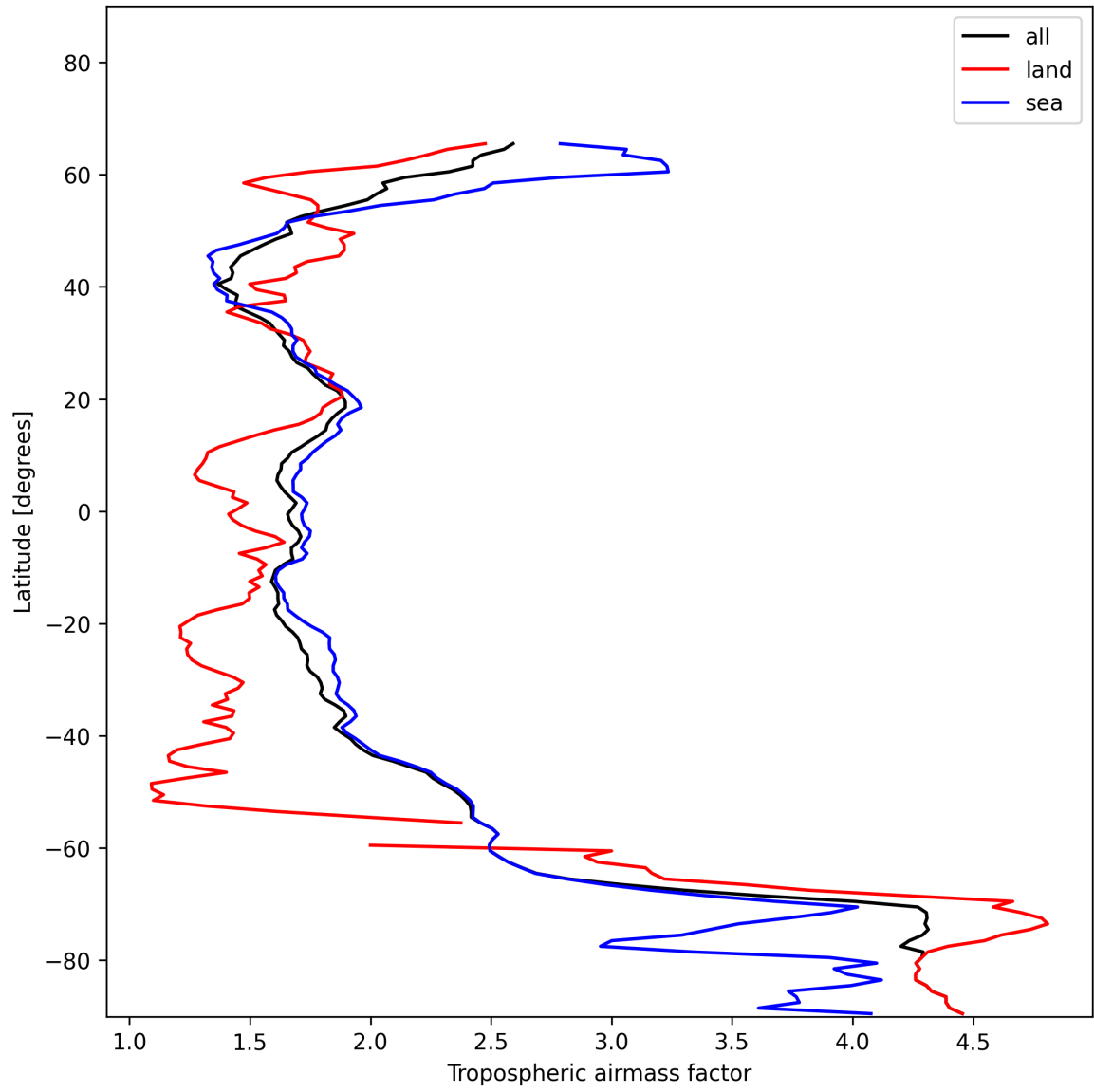
Figure 14: Zonal average of “Tropospheric airmass factor” for 2025-01-05 to 2025-01-07.
