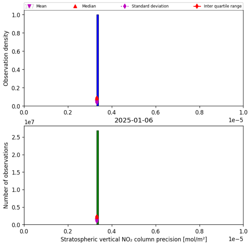
Figure 37: Histogram of “Stratospheric vertical NO 2 column precision” for 2025-01-05 to 2025-01-07
