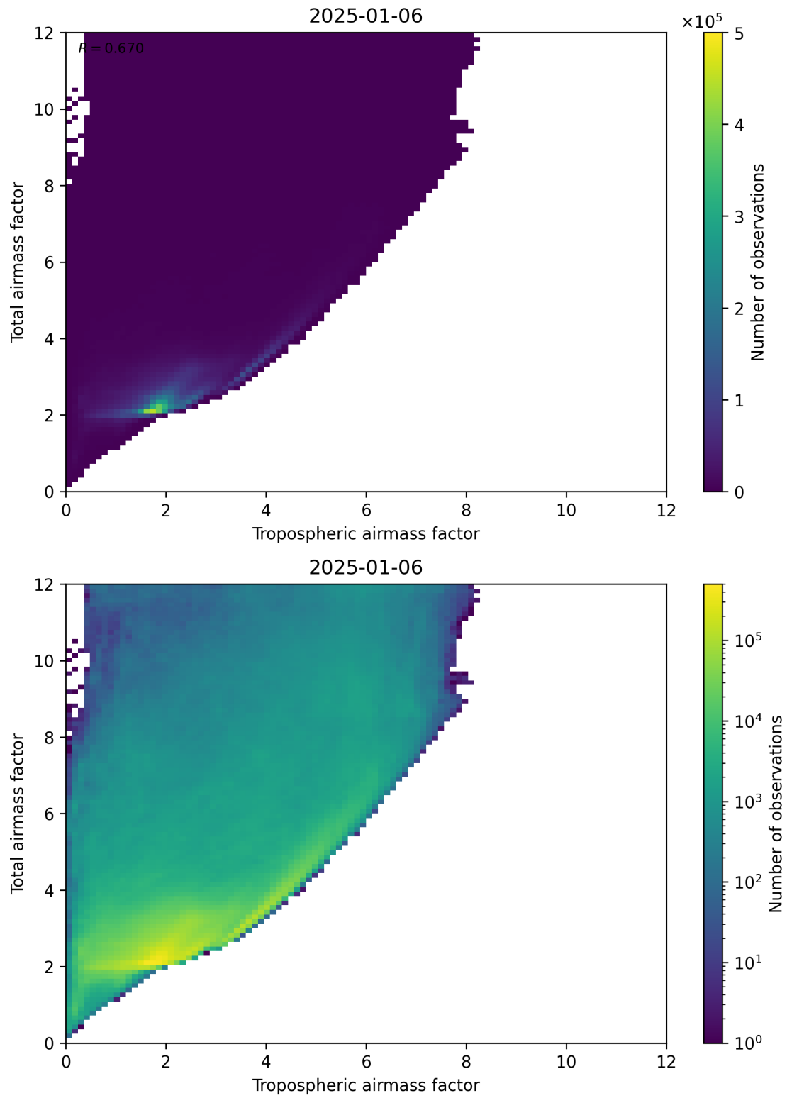
Figure 72: Scatter density plot of “Tropospheric airmass factor” against “Total airmass factor” for 2025-01-05 to 2025-01-07.
