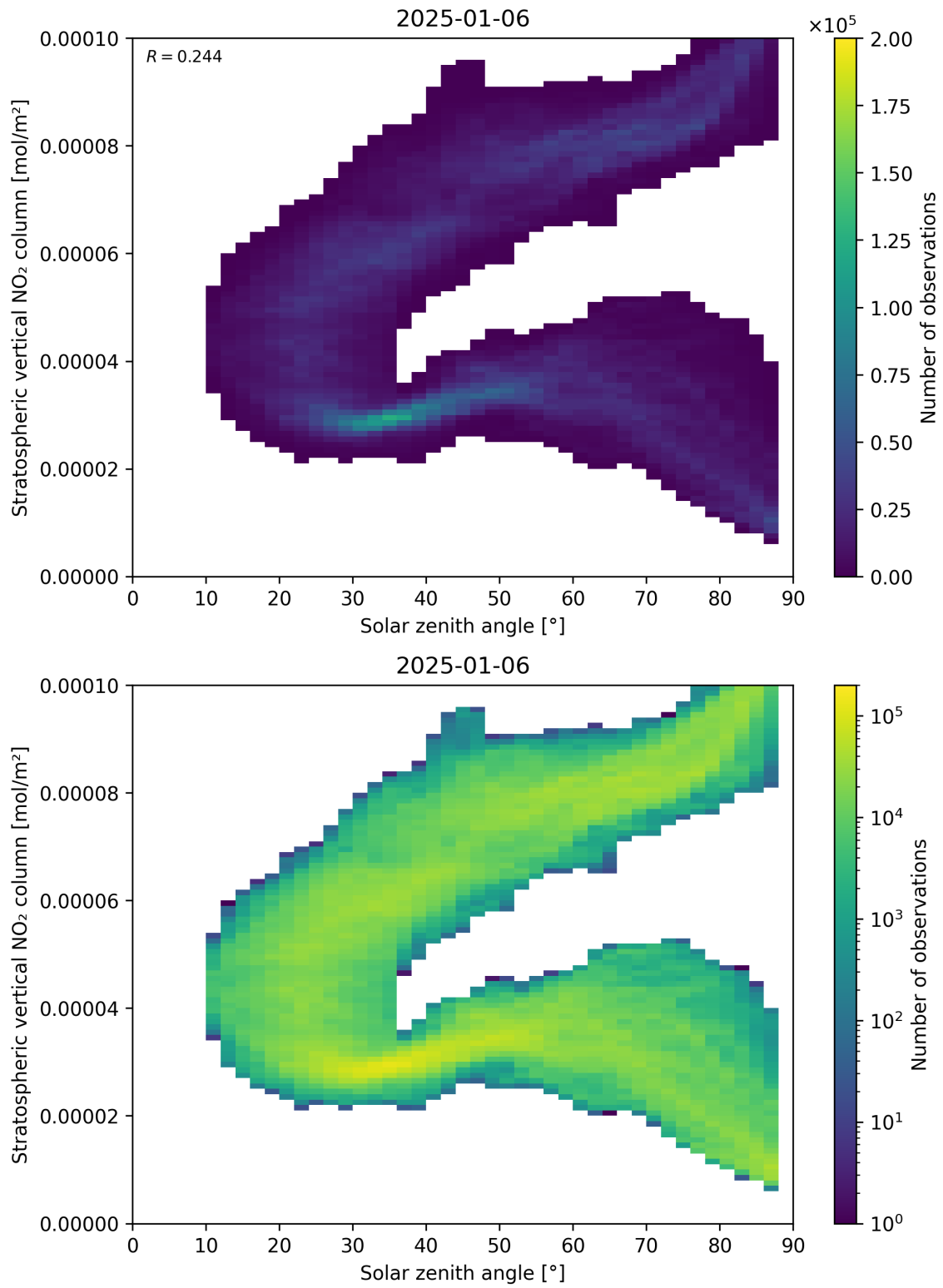
Figure 150: Scatter density plot of “Solar zenith angle” against “Stratospheric vertical NO 2 column” for 2025-01-05 to 2025-01-07.
