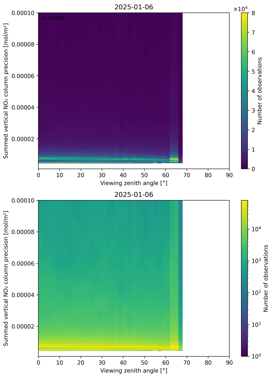
Figure 166: Scatter density plot of “Viewing zenith angle” against “Summed vertical NO 2 column precision” for 2025-01-05 to 2025-01-07.
