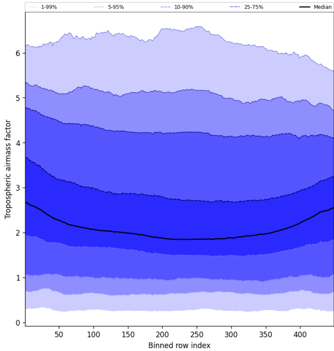
Figure 48: Along track statistics of “Tropospheric air mass factor” for 2025-01-05 to 2025-01-07
