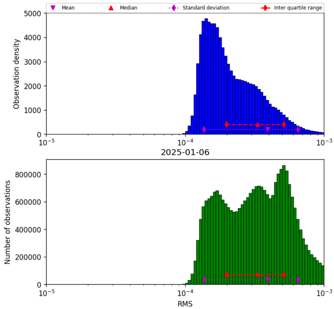
Figure 43: Histogram of “RMS” for 2025-01-05 to 2025-01-07
