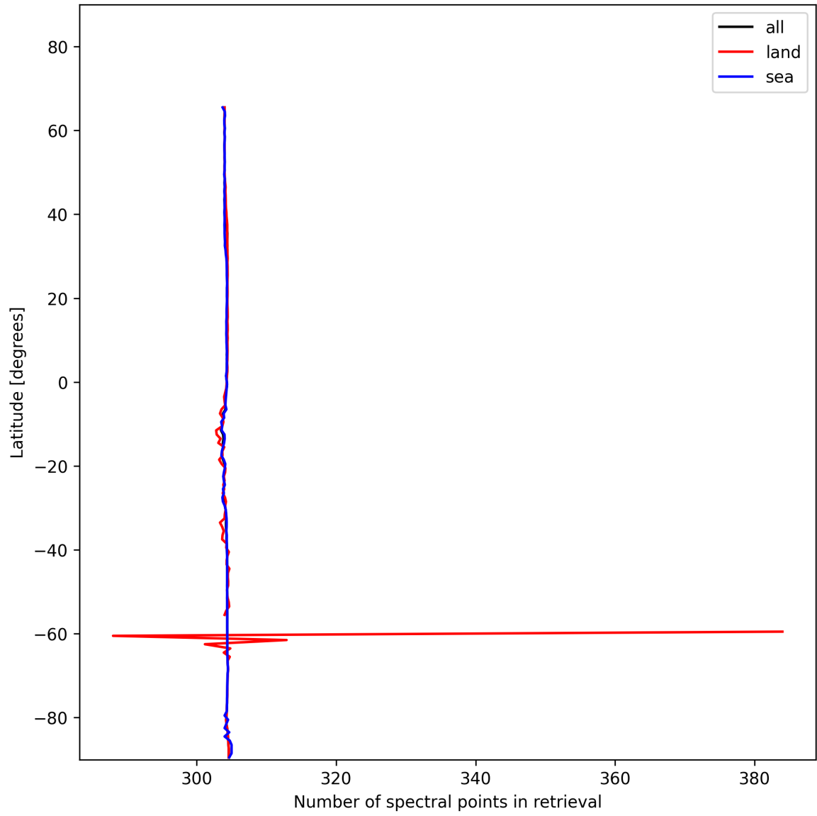
Figure 16: Zonal average of “Number of spectral points in retrieval” for 2025-01-05 to 2025-01-07.
