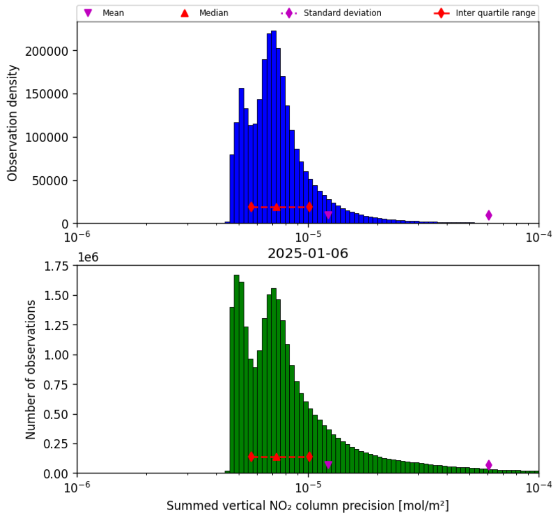
Figure 41: Histogram of “Summed vertical NO 2 column precision” for 2025-01-05 to 2025-01-07
