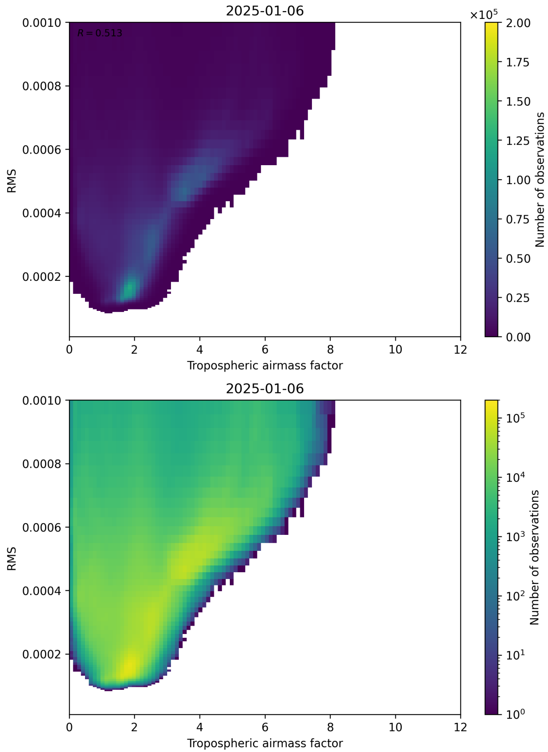
Figure 79: Scatter density plot of “Tropospheric airmass factor” against “RMS” for 2025-01-05 to 2025-01-07.
