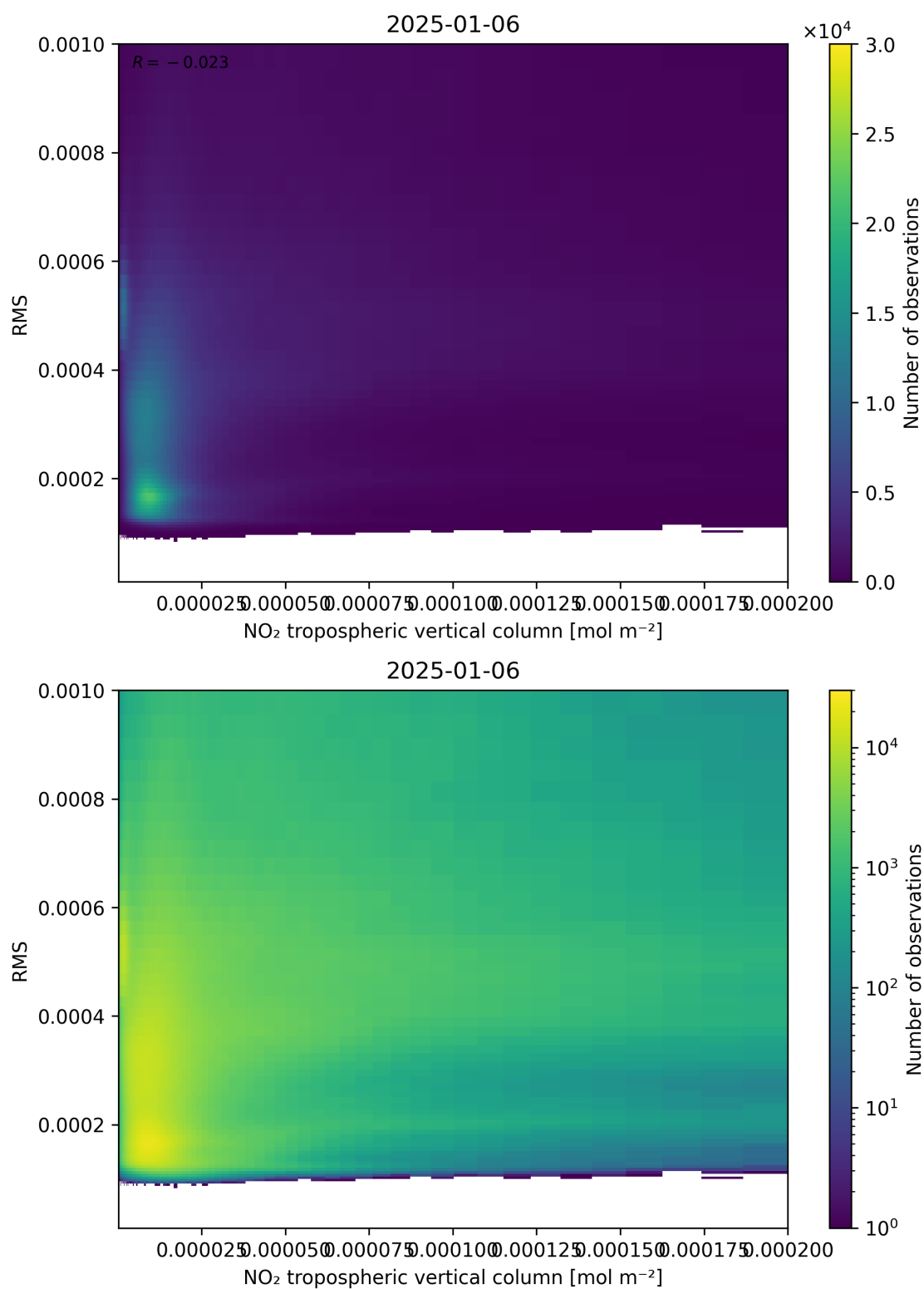
Figure 142: Scatter density plot of “NO 2 tropospheric vertical column” against “RMS” for 2025-01-05 to 2025-01-07.
