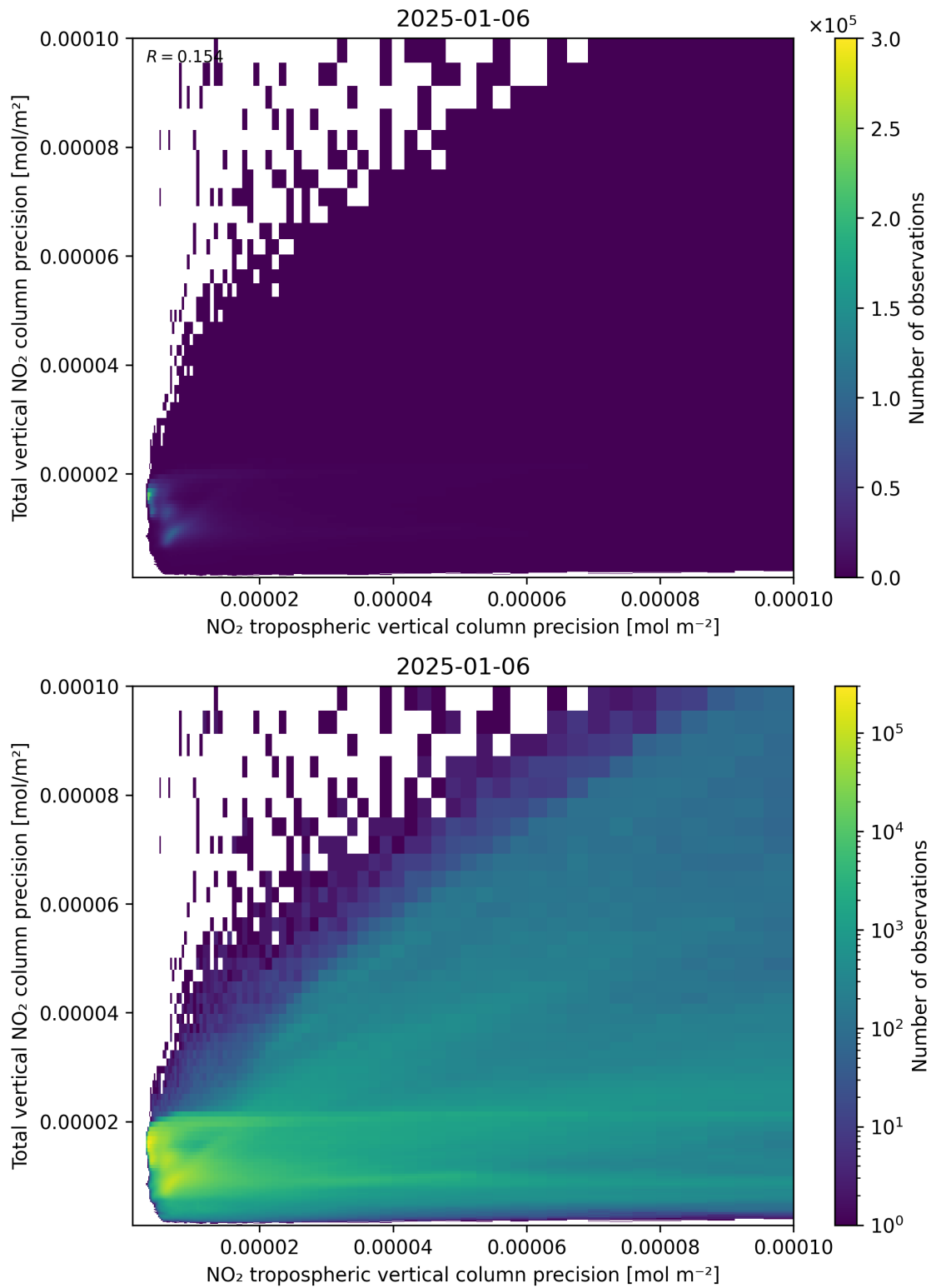
Figure 139: Scatter density plot of “NO 2 tropospheric vertical column precision” against “Total vertical NO 2 column precision” for 2025-01-05 to 2025-01-07.
