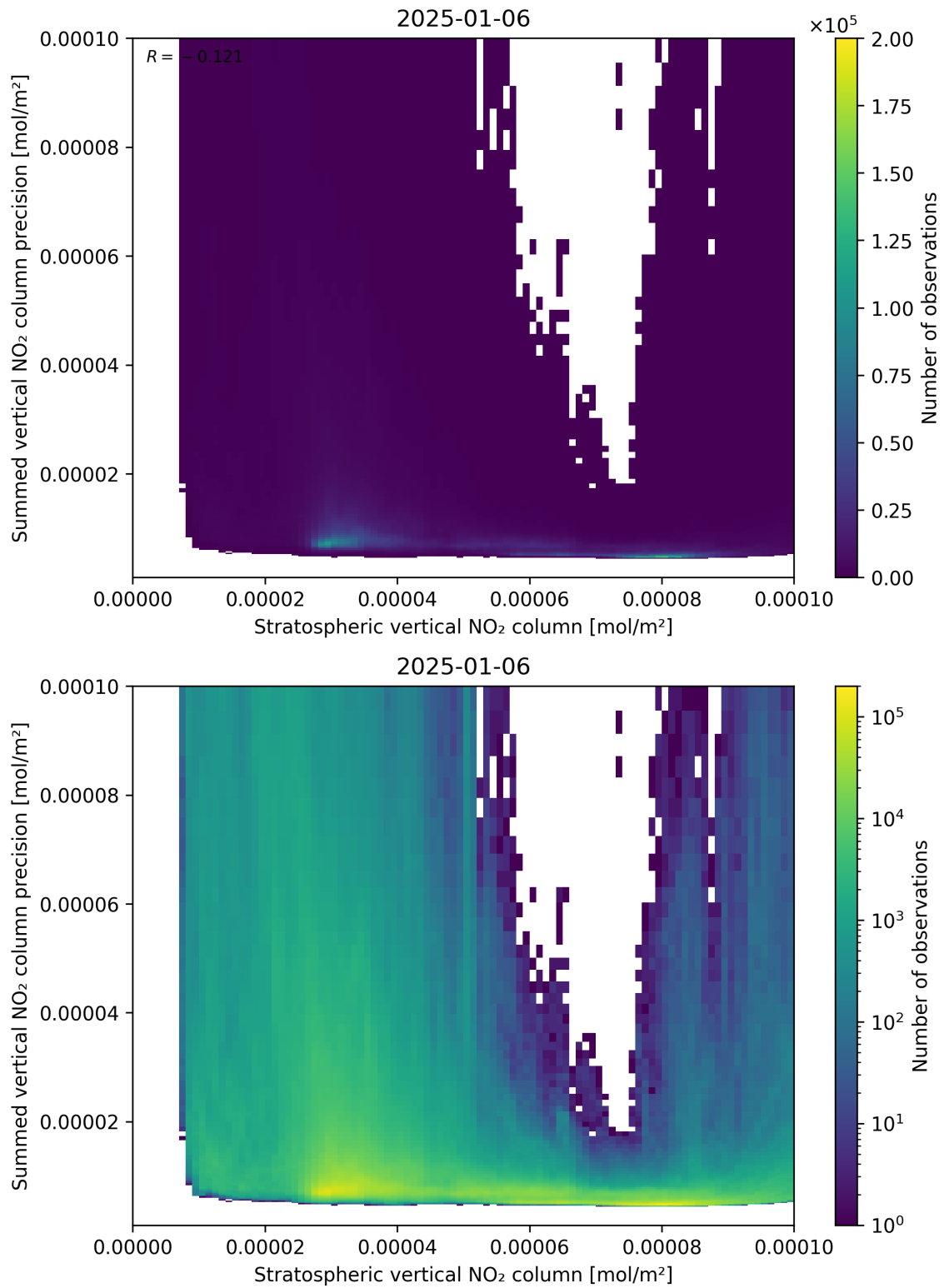
Figure 99: Scatter density plot of “Stratospheric vertical NO 2 column” against “Summed vertical NO 2 column precision” for 2025-01-05 to 2025-01-07.
