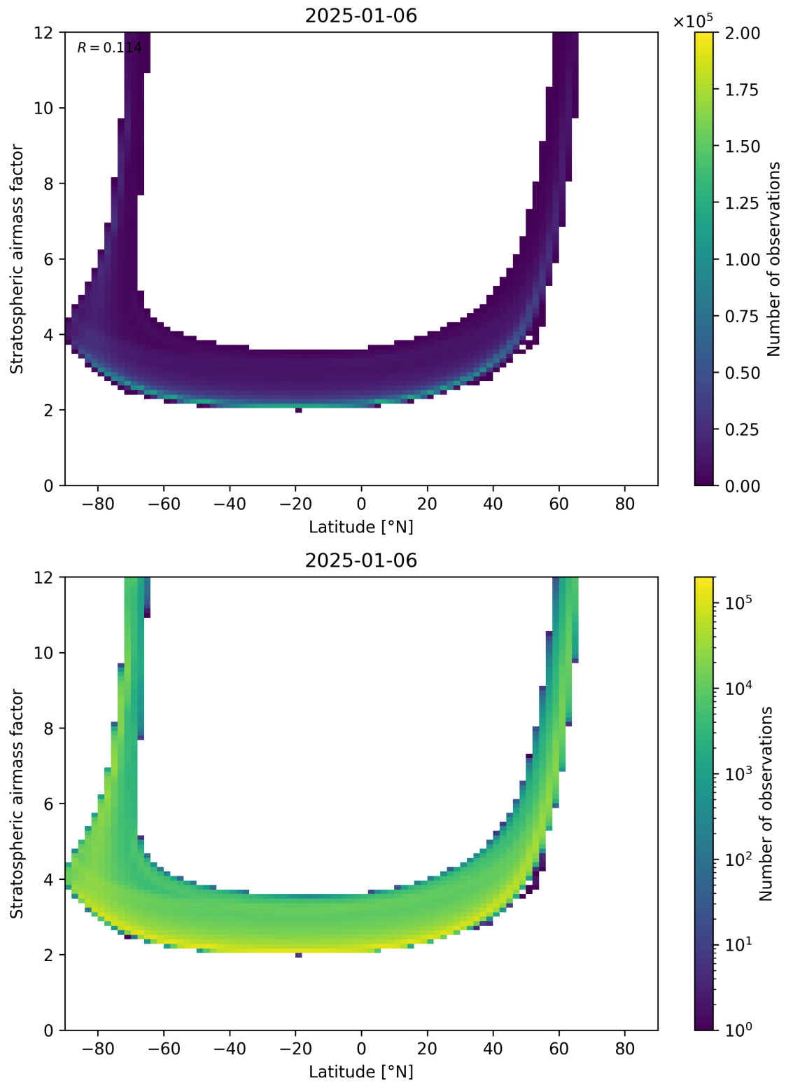
Figure 83: Scatter density plot of “Latitude” against “Stratospheric airmass factor” for 2025-01-05 to 2025-01-07.
