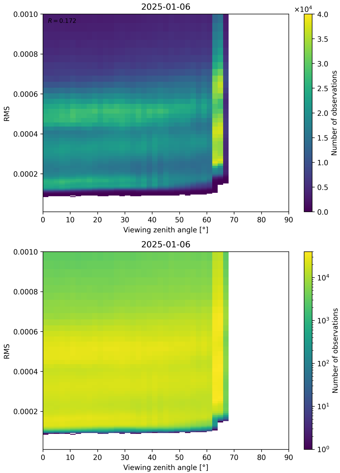
Figure 171: Scatter density plot of “Viewing zenith angle” against “RMS” for 2025-01-05 to 2025-01-07.
