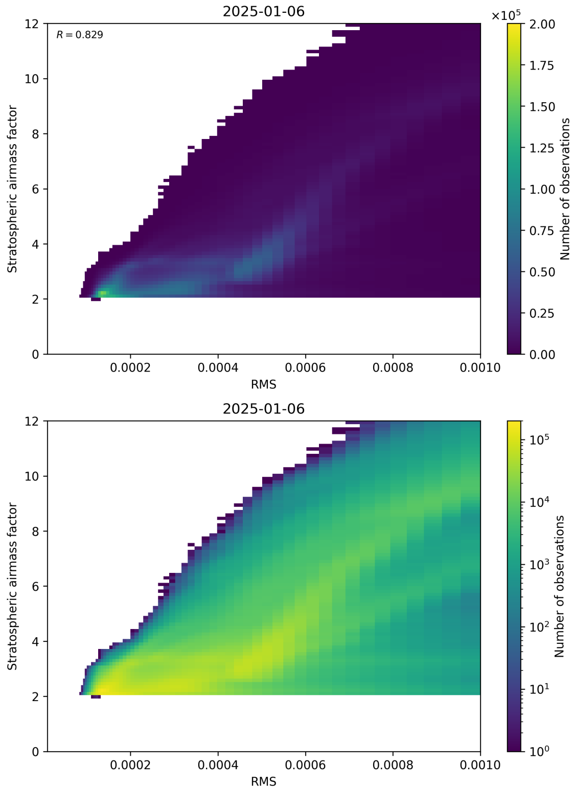
Figure 144: Scatter density plot of “RMS” against “Stratospheric airmass factor” for 2025-01-05 to 2025-01-07.
