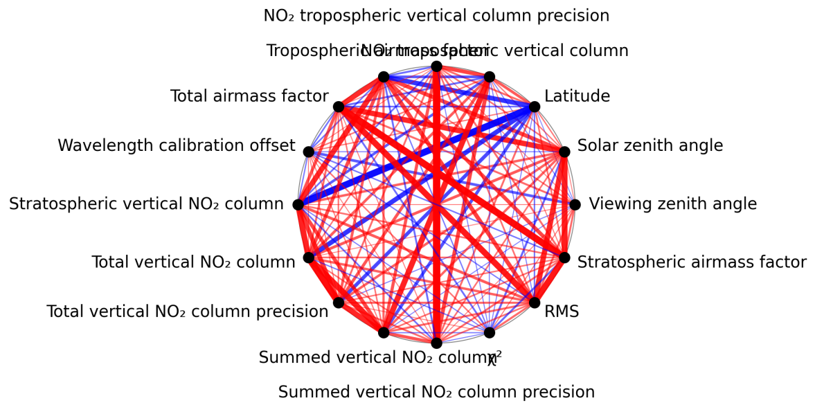
Figure 1: Map of correlation graph for 2025-01-05 to 2025-01-07.
