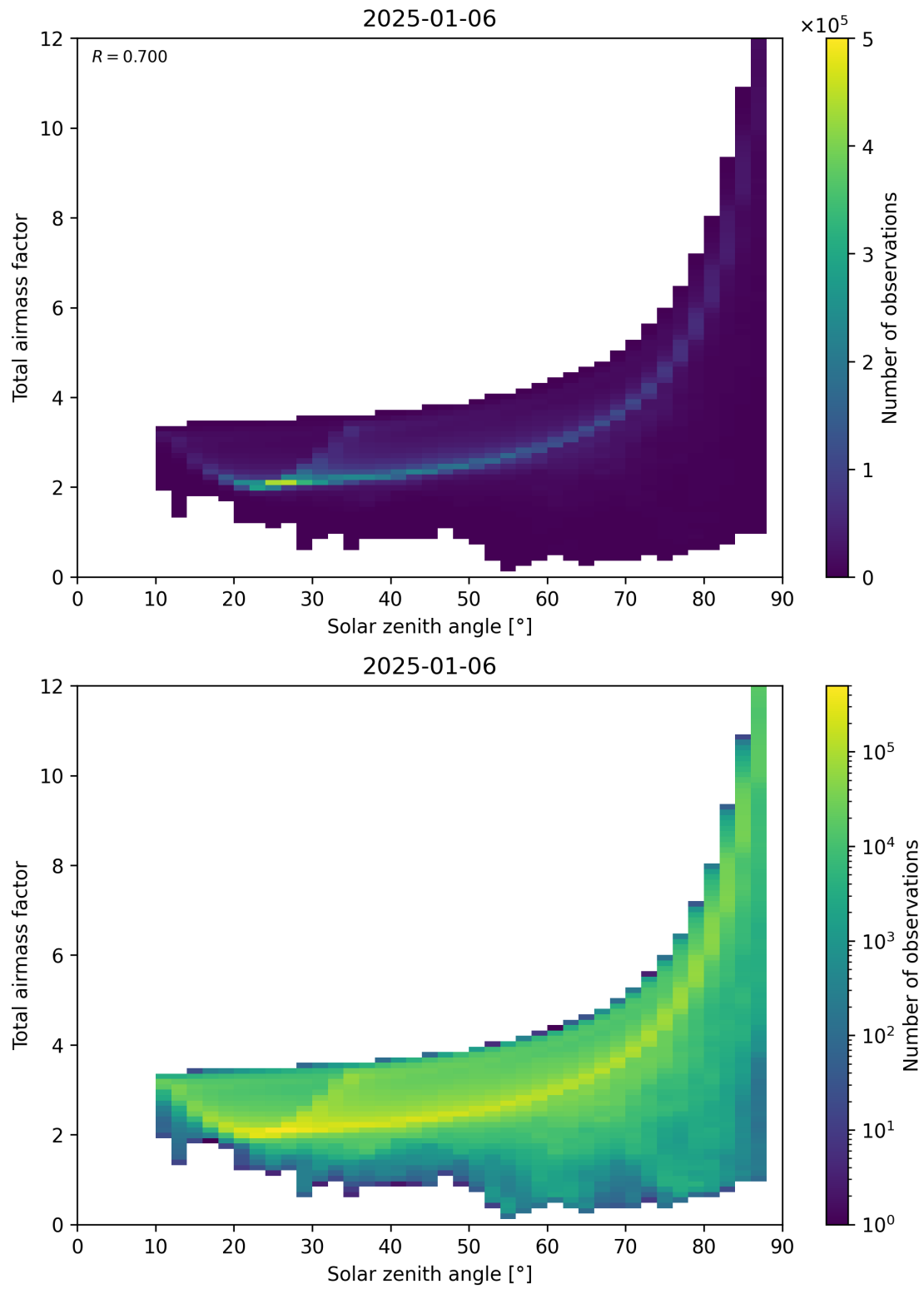
Figure 146: Scatter density plot of “Solar zenith angle” against “Total air mass factor” for 2025-01-05 to 2025-01-07.
