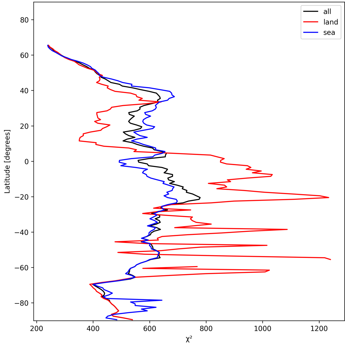
Figure 25: Zonal average of “ \chi^2 ” for 2025-01-05 to 2025-01-07.
