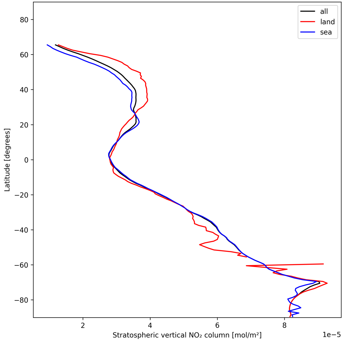
Figure 19: Zonal average of “Stratospheric vertical NO 2 column” for 2025-01-05 to 2025-01-07.
