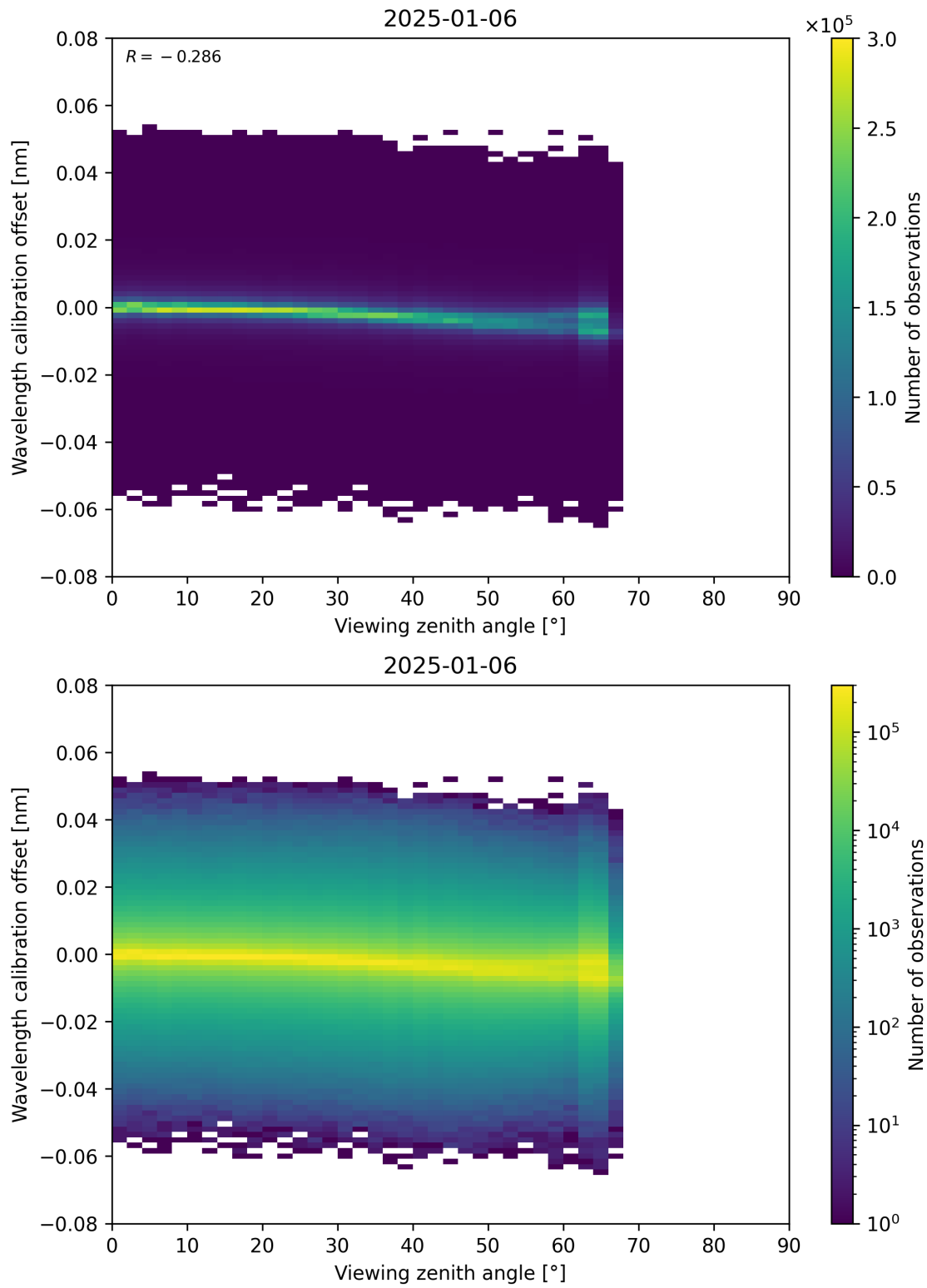
Figure 173: Scatter density plot of “Viewing zenith angle” against “Wavelength calibration offset” for 2025-01-05 to 2025-01-07.
