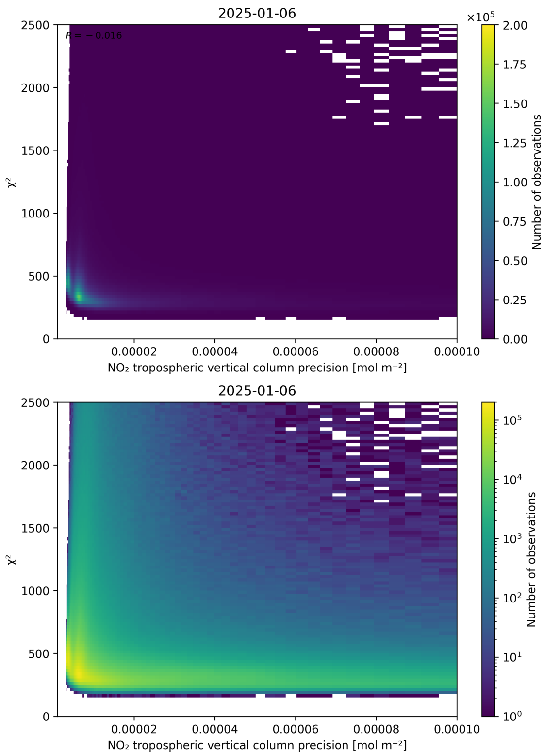
Figure 134: Scatter density plot of “NO 2 tropospheric vertical column precision” against “ \chi^2 ” for 2025-01-05 to 2025-01-07.
