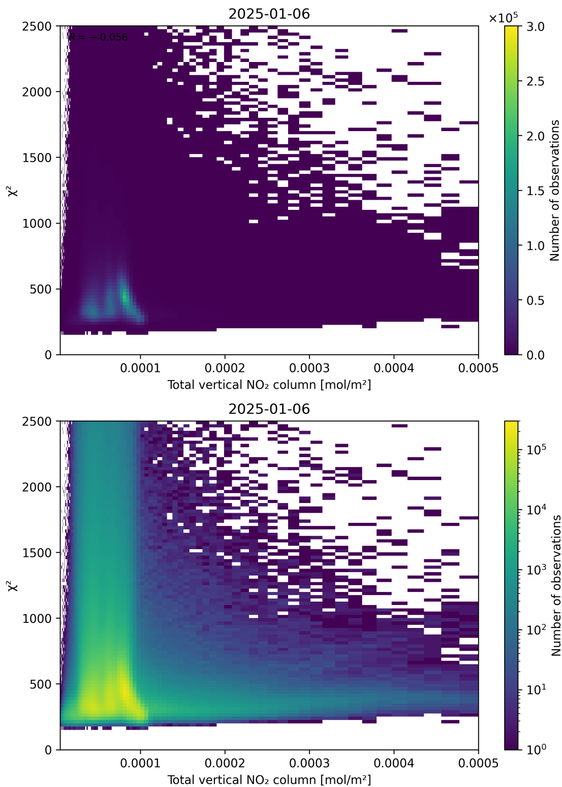
Figure 111: Scatter density plot of “Total vertical NO 2 column” against “ \chi^2 ” for 2025-01-05 to 2025-01-07.
