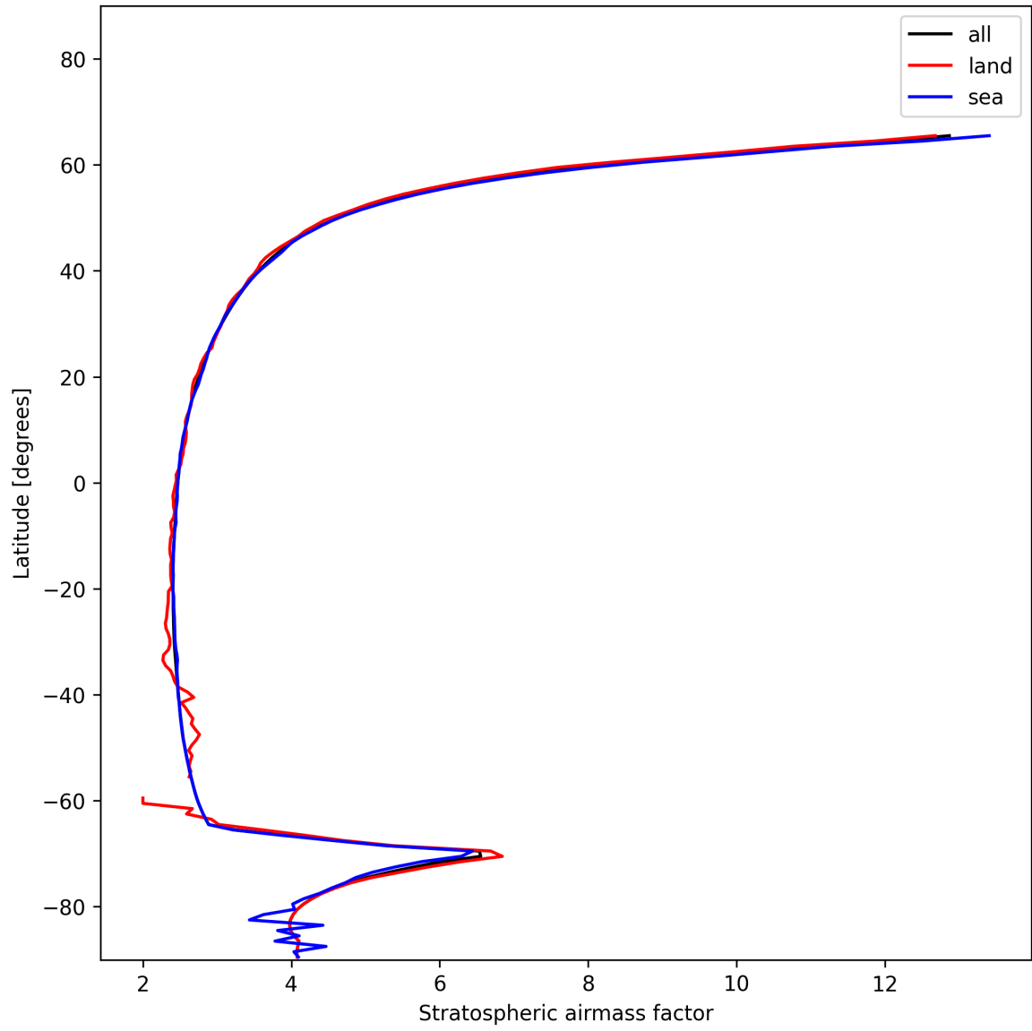
Figure 27: Zonal average of “Stratospheric air mass factor” for 2025-01-05 to 2025-01-07.
