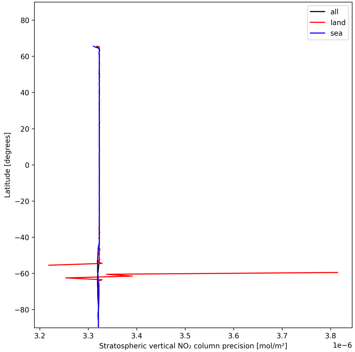
Figure 20: Zonal average of “Stratospheric vertical NO 2 column precision” for 2025-01-05 to 2025-01-07.
