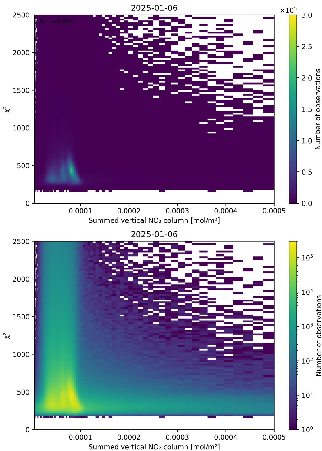
Figure 104: Scatter density plot of “Summed vertical NO 2 column” against “ \chi^2 ” for 2025-01-05 to 2025-01-07.
