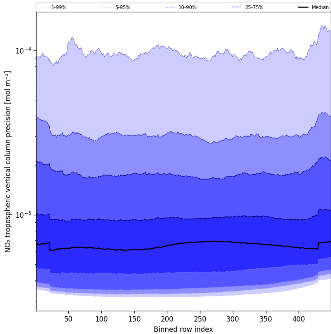
Figure 47: Along track statistics of “NO 2 tropospheric vertical column precision” for 2025-01-05 to 2025-01-07
