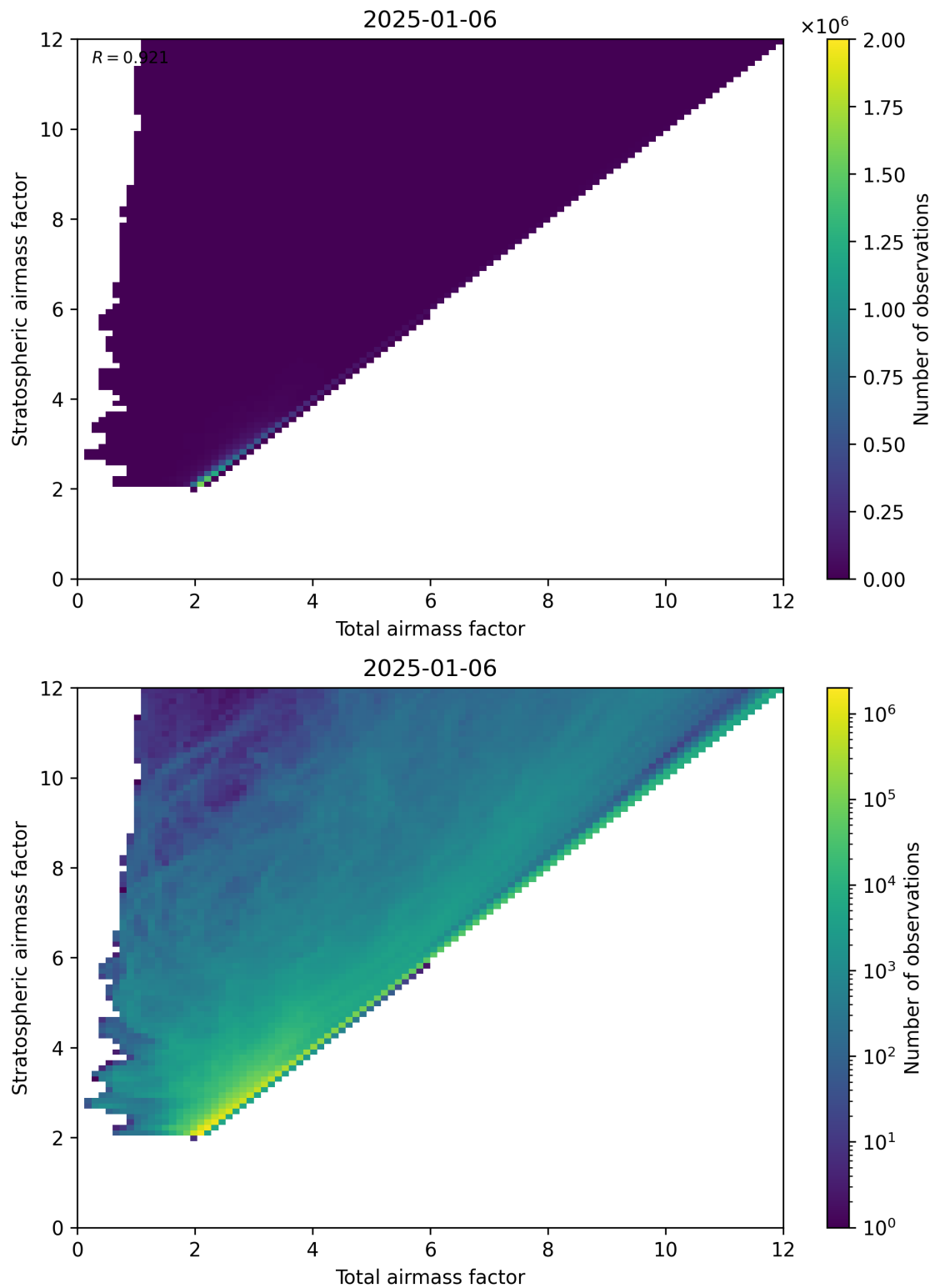
Figure 62: Scatter density plot of “Total airmass factor” against “Stratospheric airmass factor” for 2025-01-05 to 2025-01-07.
