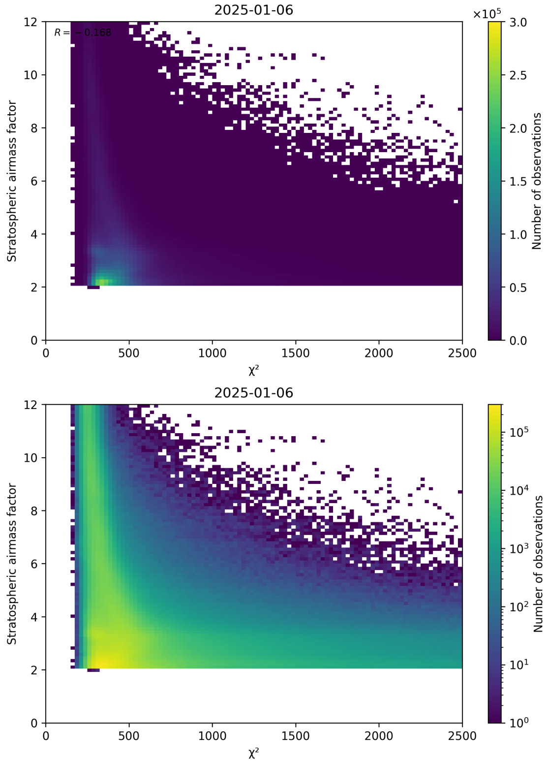
Figure 81: Scatter density plot of “ \chi^2 ” against “Stratospheric airmass factor” for 2025-01-05 to 2025-01-07.
