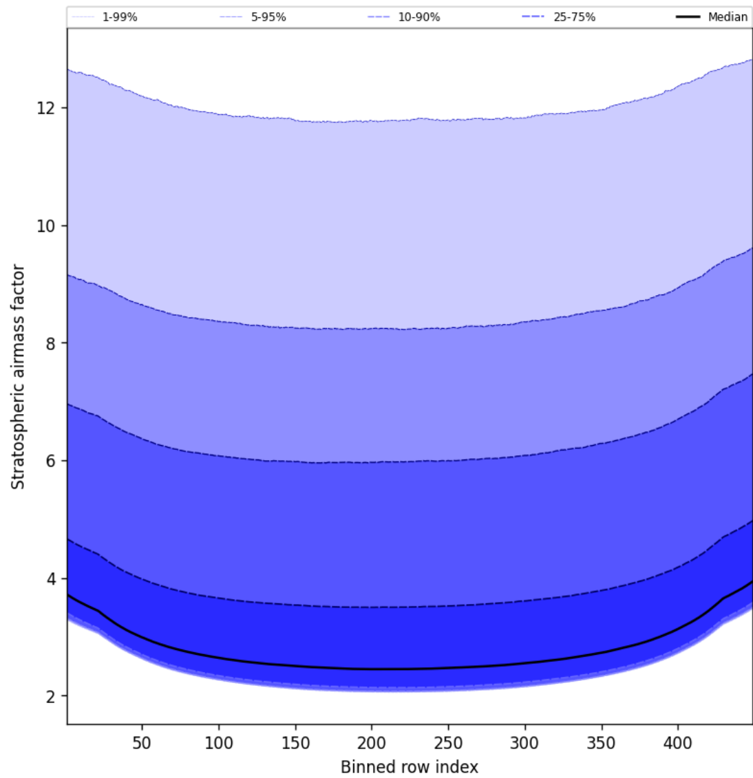
Figure 61: Along track statistics of “Stratospheric air mass factor” for 2025-01-05 to 2025-01-07
