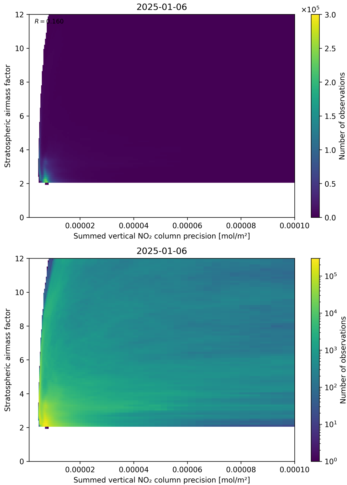
Figure 106: Scatter density plot of “Summed vertical NO 2 column precision” against “Stratospheric airmass factor” for 2025-01-05 to 2025-01-07.
