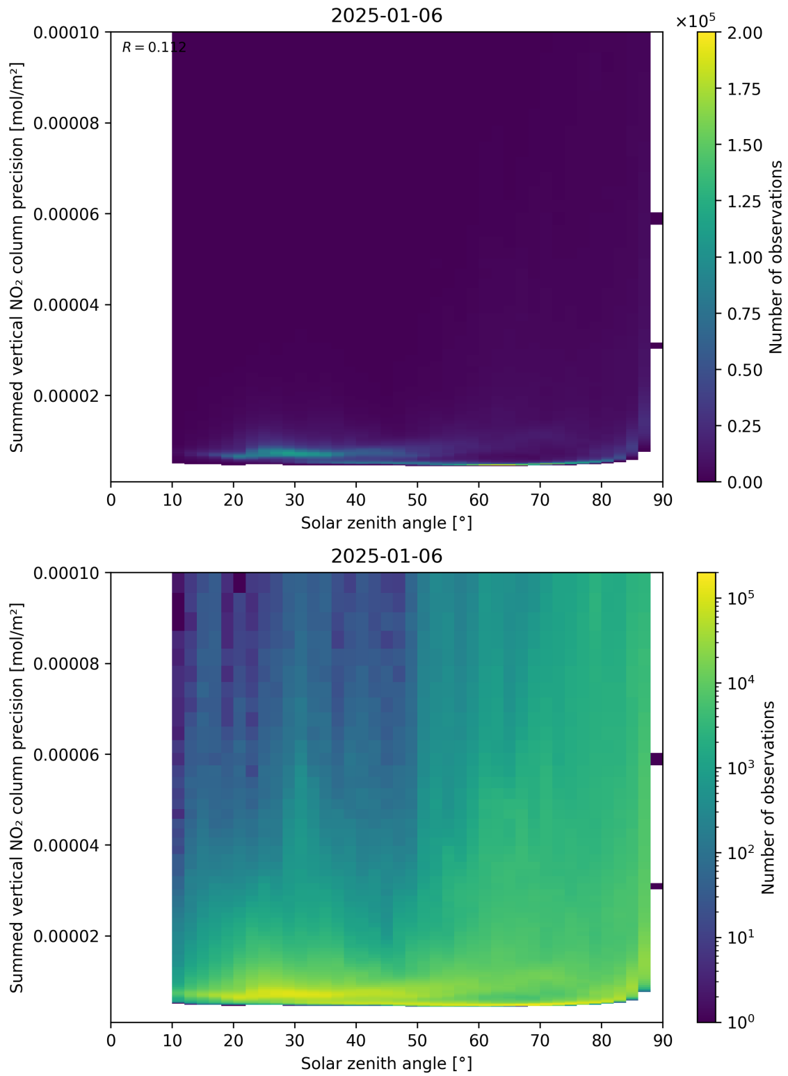
Figure 152: Scatter density plot of “Solar zenith angle” against “Summed vertical NO 2 column precision” for 2025-01-05 to 2025-01-07.
