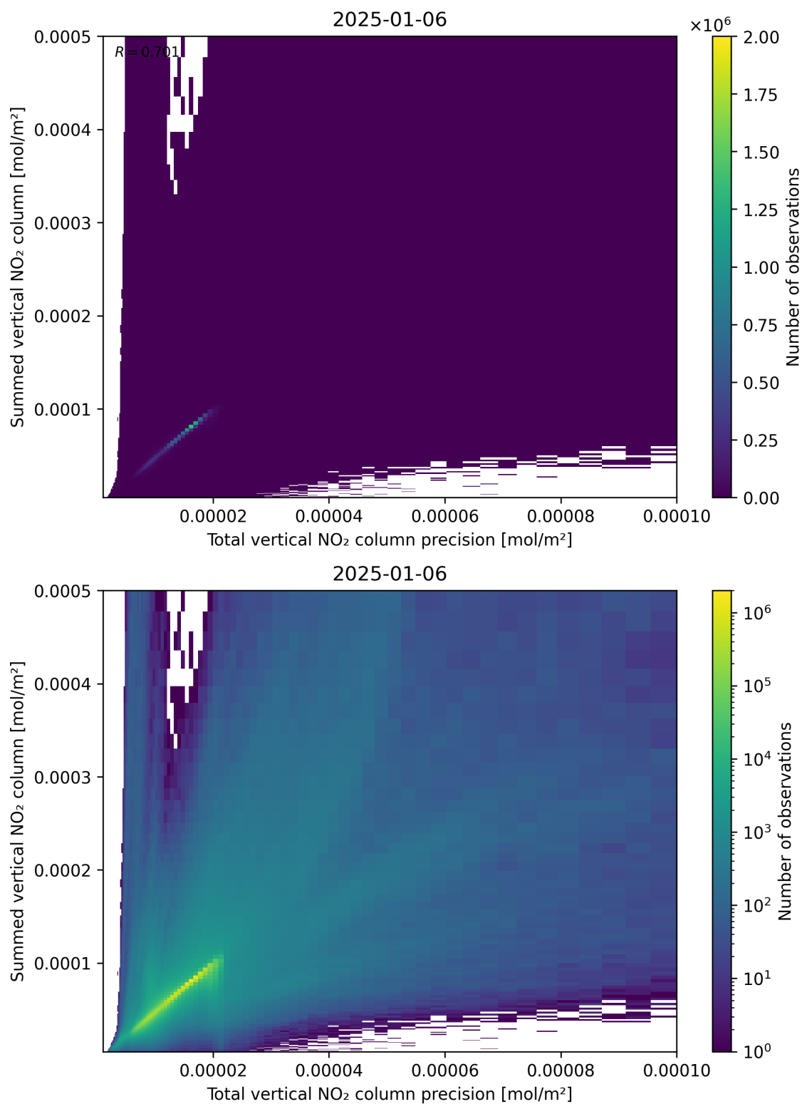
Figure 117: Scatter density plot of “Total vertical NO 2 column precision” against “Summed vertical NO 2 column” for 2025-01-05 to 2025-01-07.
