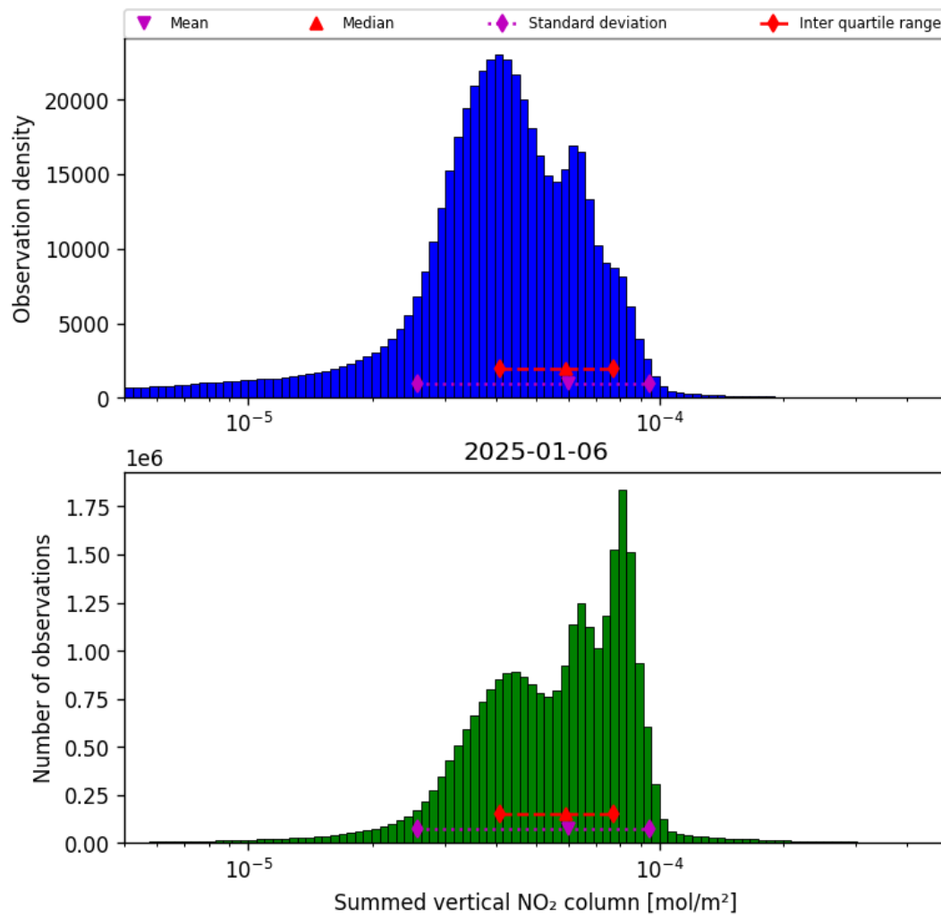
Figure 40: Histogram of “Summed vertical NO 2 column” for 2025-01-05 to 2025-01-07
