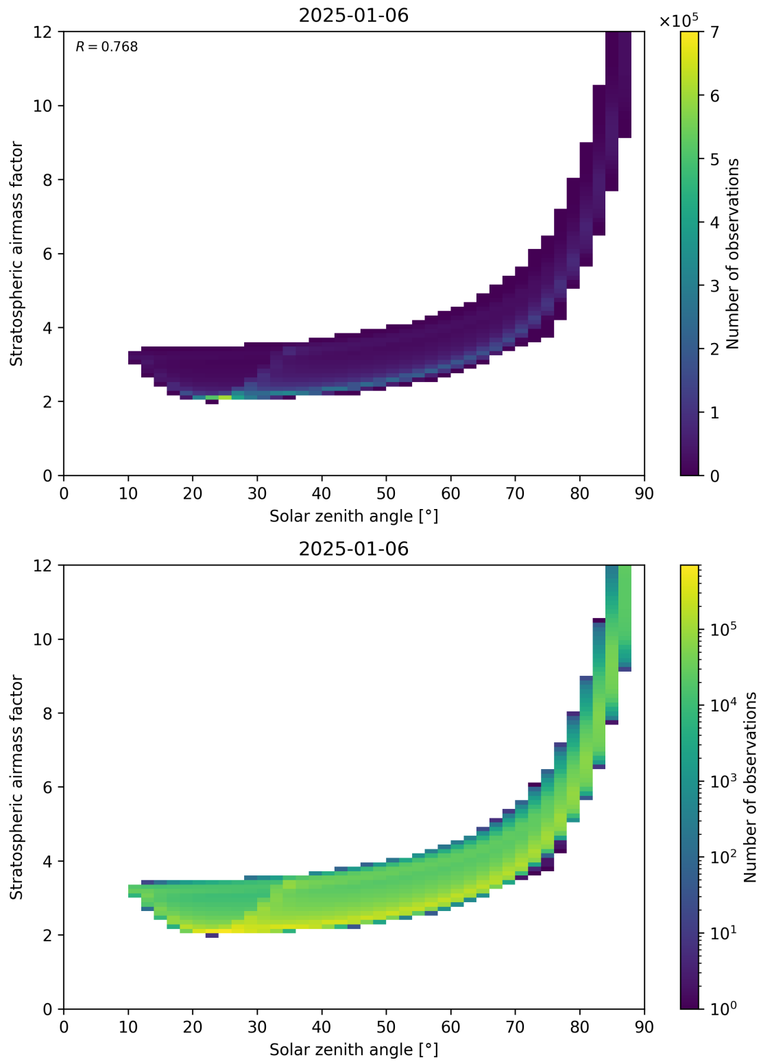
Figure 145: Scatter density plot of “Solar zenith angle” against “Stratospheric airmass factor” for 2025-01-05 to 2025-01-07.
