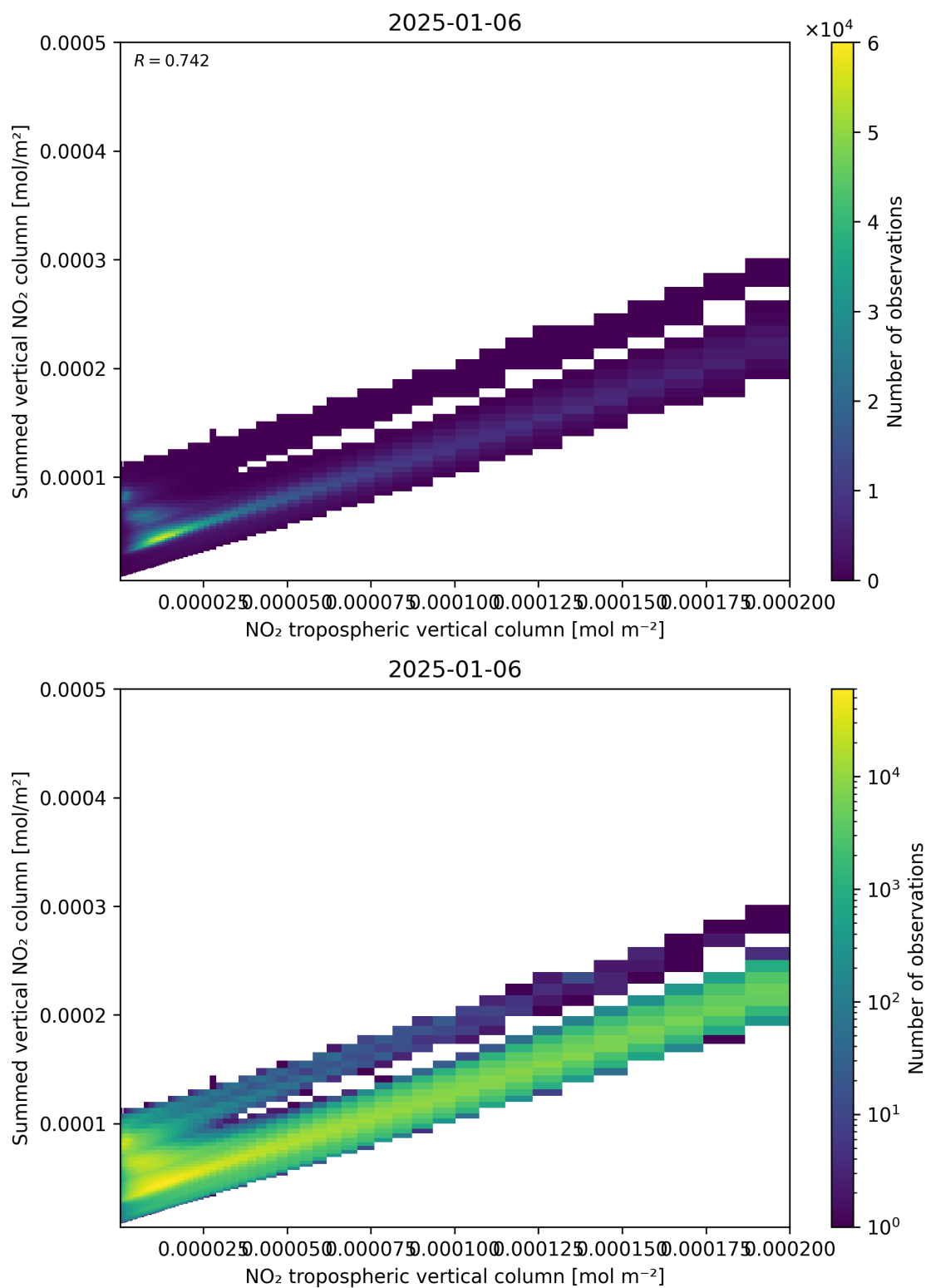
Figure 126: Scatter density plot of “NO 2 tropospheric vertical column” against “Summed vertical NO 2 column” for 2025-01-05 to 2025-01-07.
