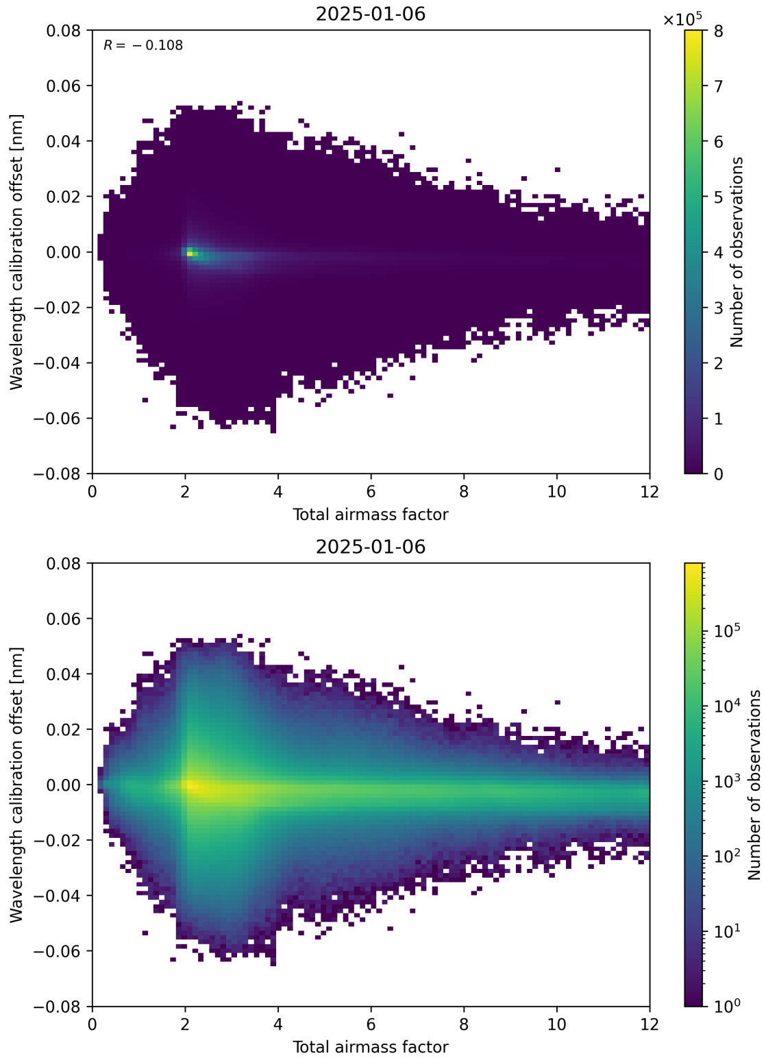
Figure 70: Scatter density plot of “Total airmass factor” against “Wavelength calibration offset” for 2025-01-05 to 2025-01-07.
