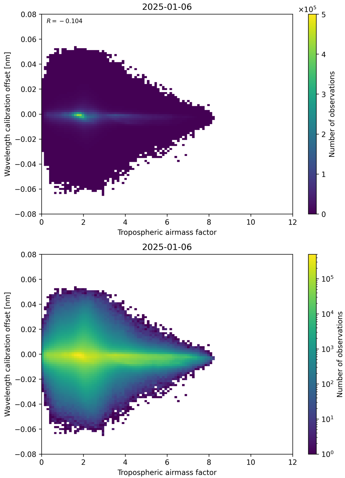
Figure 80: Scatter density plot of “Tropospheric airmass factor” against “Wavelength calibration offset” for 2025-01-05 to 2025-01-07.
