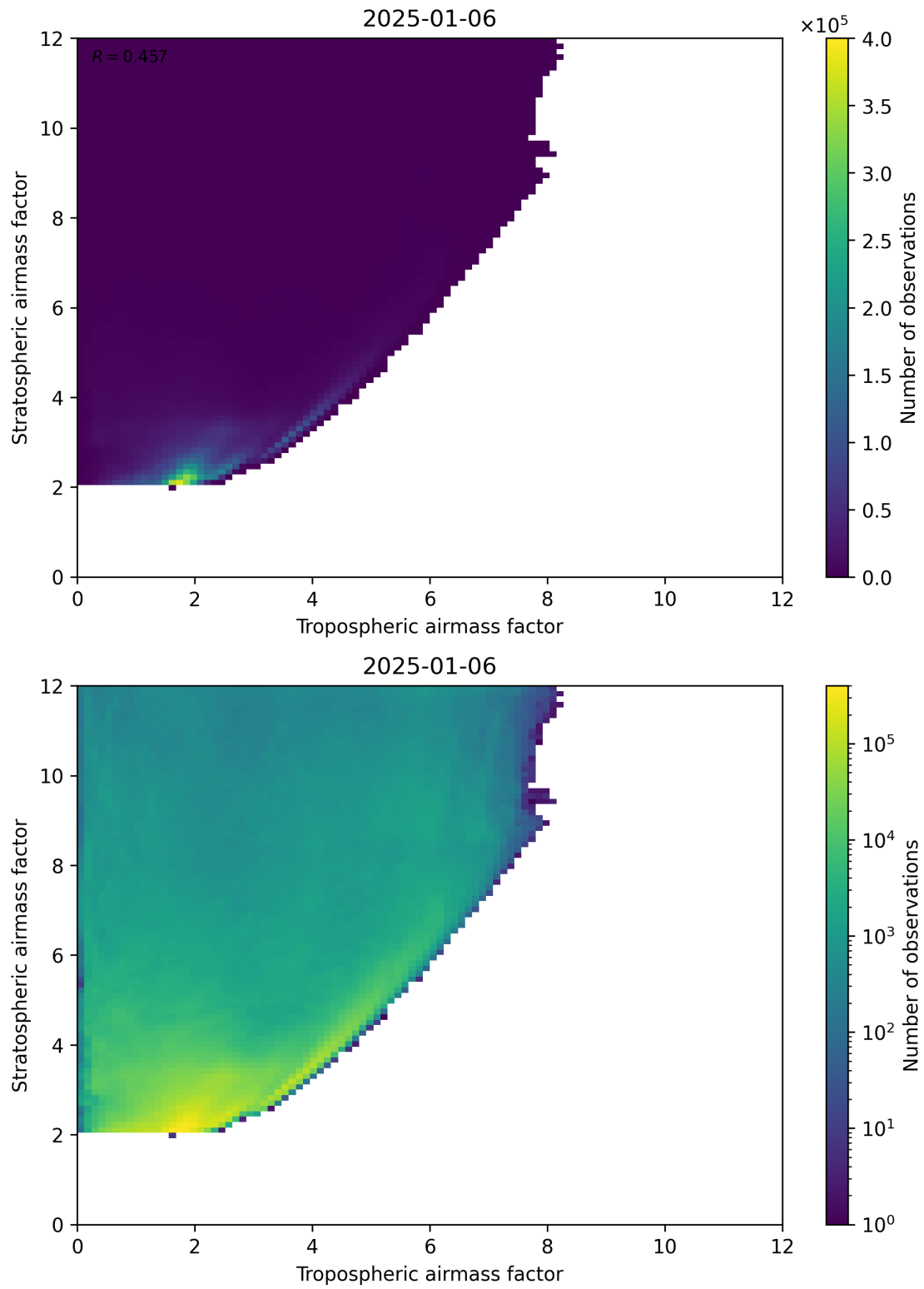
Figure 71: Scatter density plot of “Tropospheric airmass factor” against “Stratospheric airmass factor” for 2025-01-05 to 2025-01-07.
