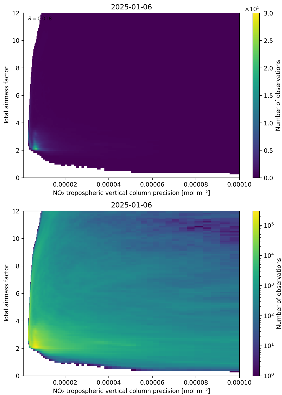
Figure 132: Scatter density plot of “NO 2 tropospheric vertical column precision” against “Total air mass factor” for 2025-01-05 to 2025-01-07.
