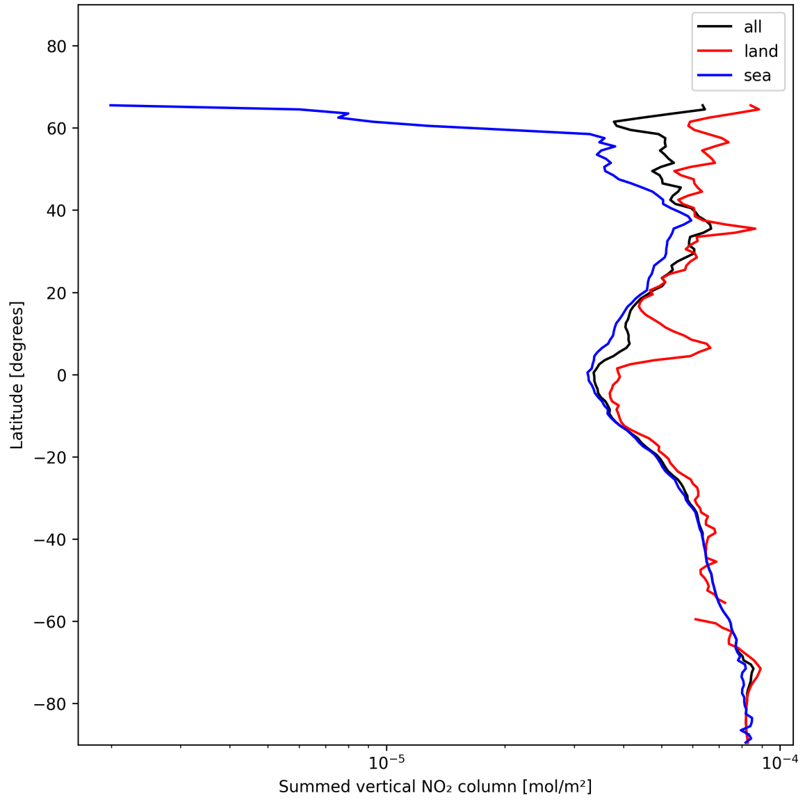
Figure 23: Zonal average of “Summed vertical NO 2 column” for 2025-01-05 to 2025-01-07.
