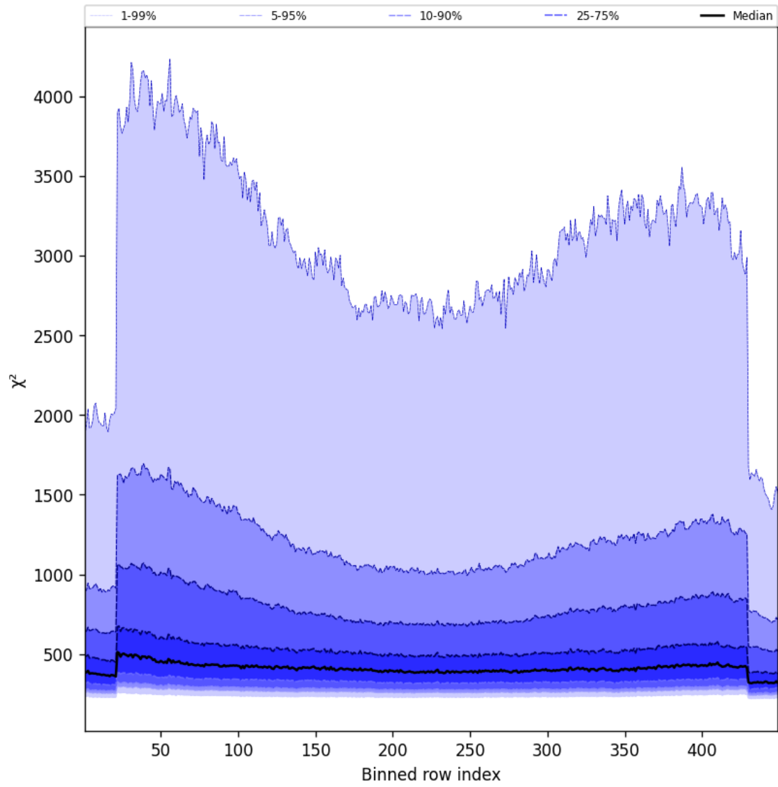
Figure 59: Along track statistics of “ \chi^2 ” for 2025-01-05 to 2025-01-07
