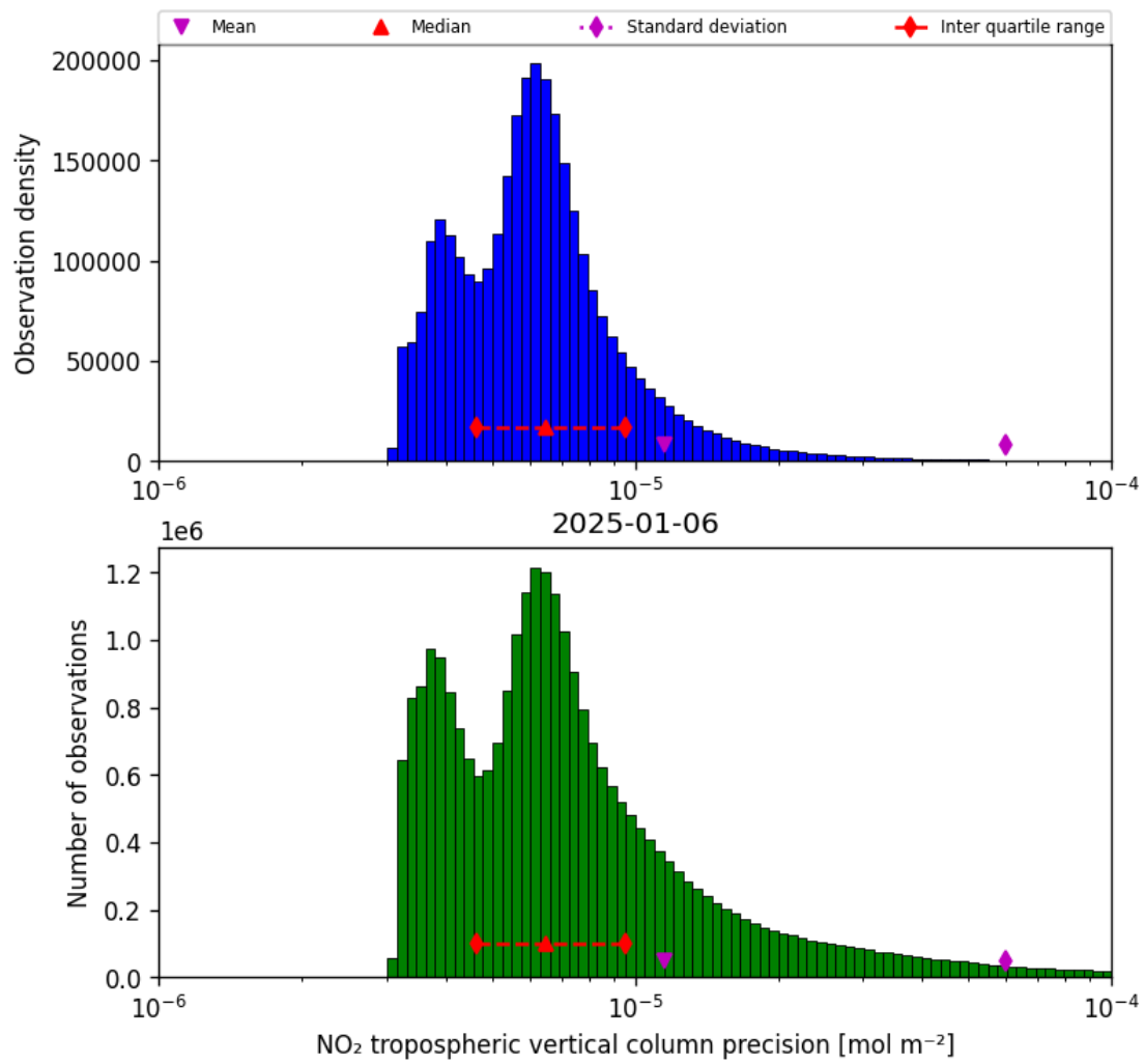
Figure 30: Histogram of “NO 2 tropospheric vertical column precision” for 2025-01-05 to 2025-01-07
