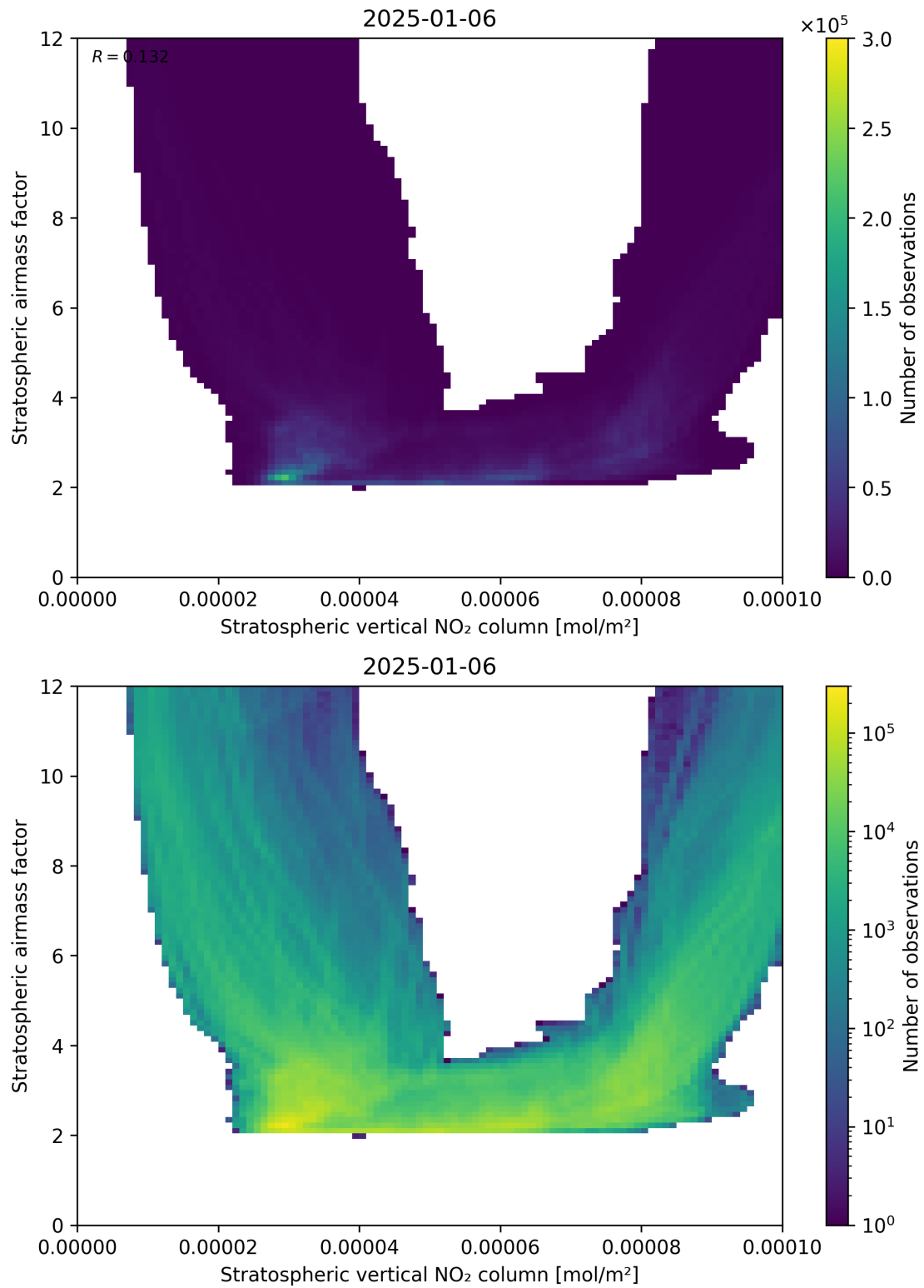
Figure 96: Scatter density plot of “Stratospheric vertical NO 2 column” against “Stratospheric airmass factor” for 2025-01-05 to 2025-01-07.
