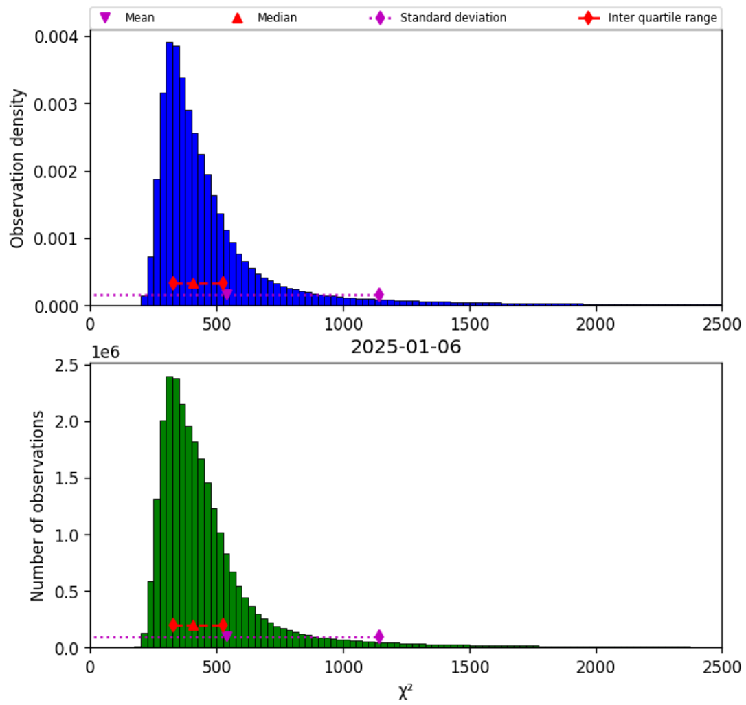
Figure 42: Histogram of “ \chi^2 ” for 2025-01-05 to 2025-01-07
