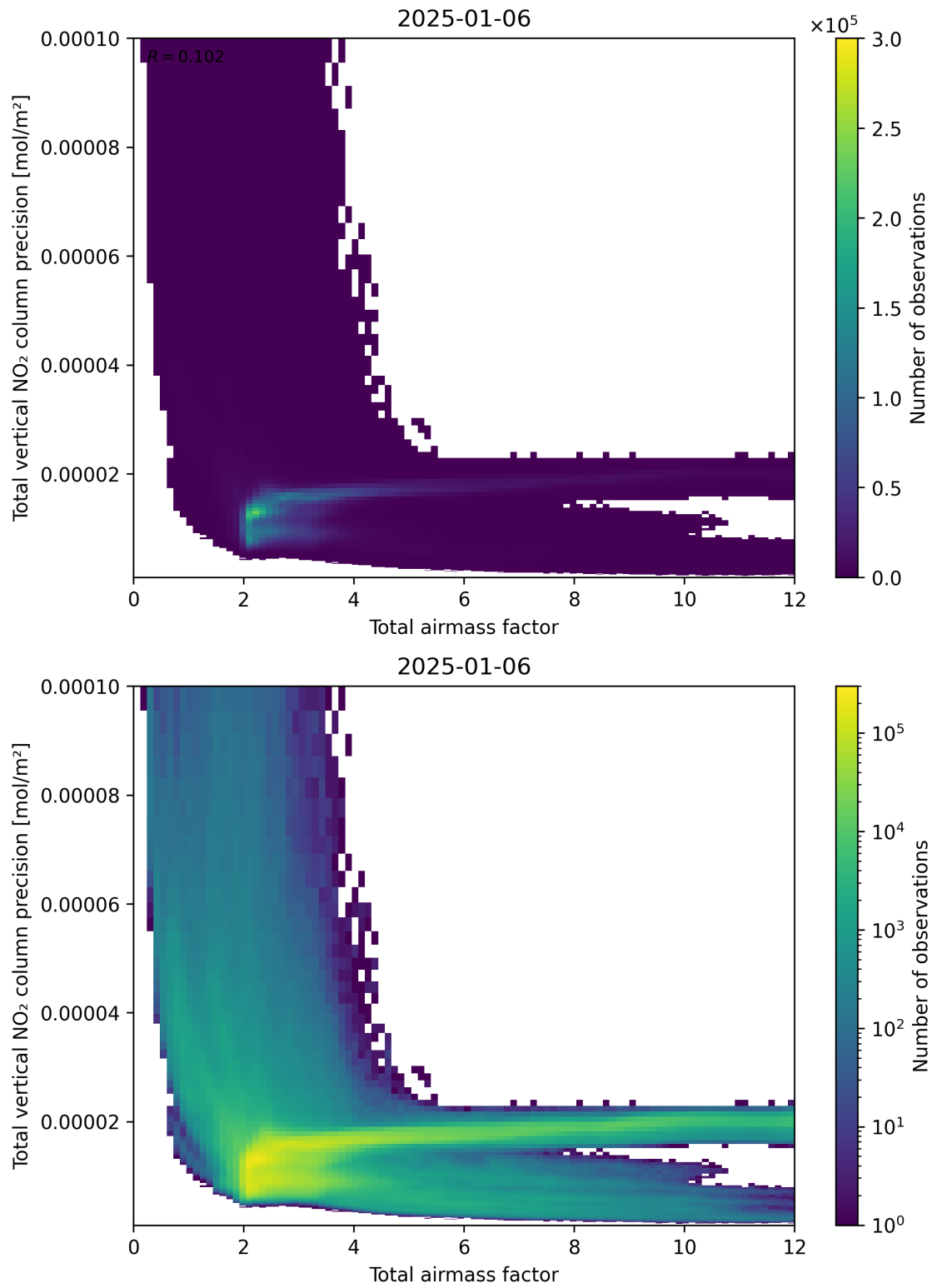
Figure 68: Scatter density plot of “Total airmass factor” against “Total vertical NO 2 column precision” for 2025-01-05 to 2025-01-07.
