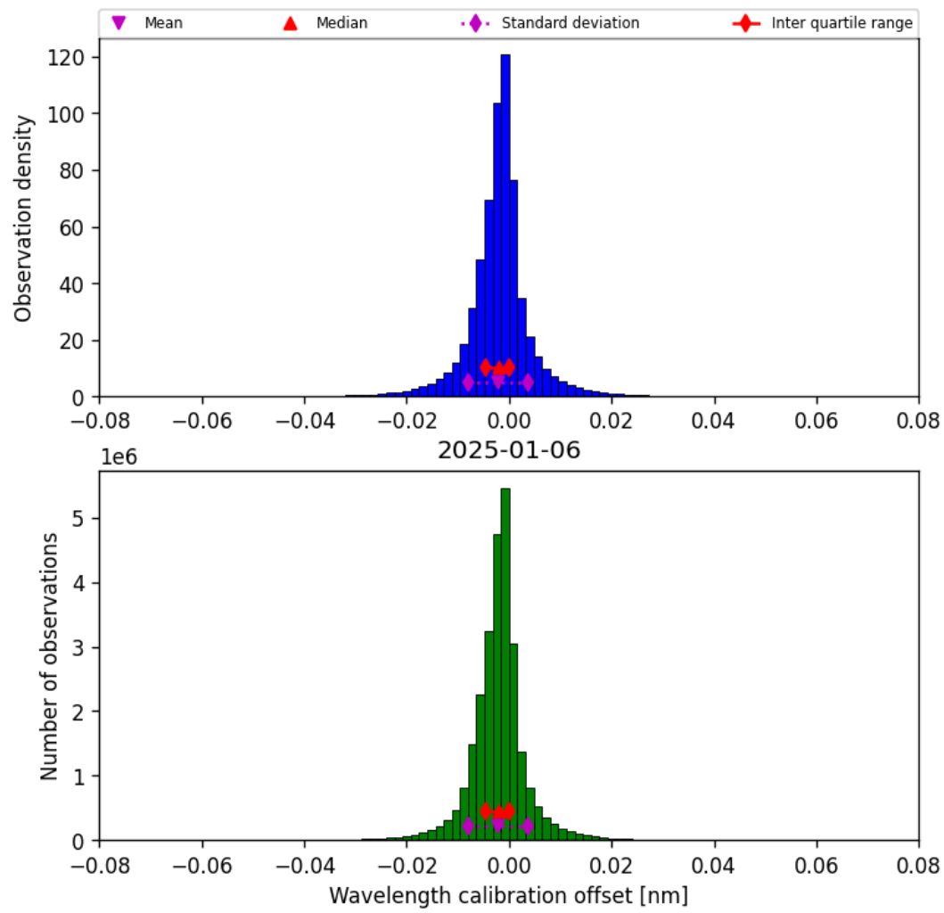
Figure 35: Histogram of “Wavelength calibration offset” for 2025-01-05 to 2025-01-07
