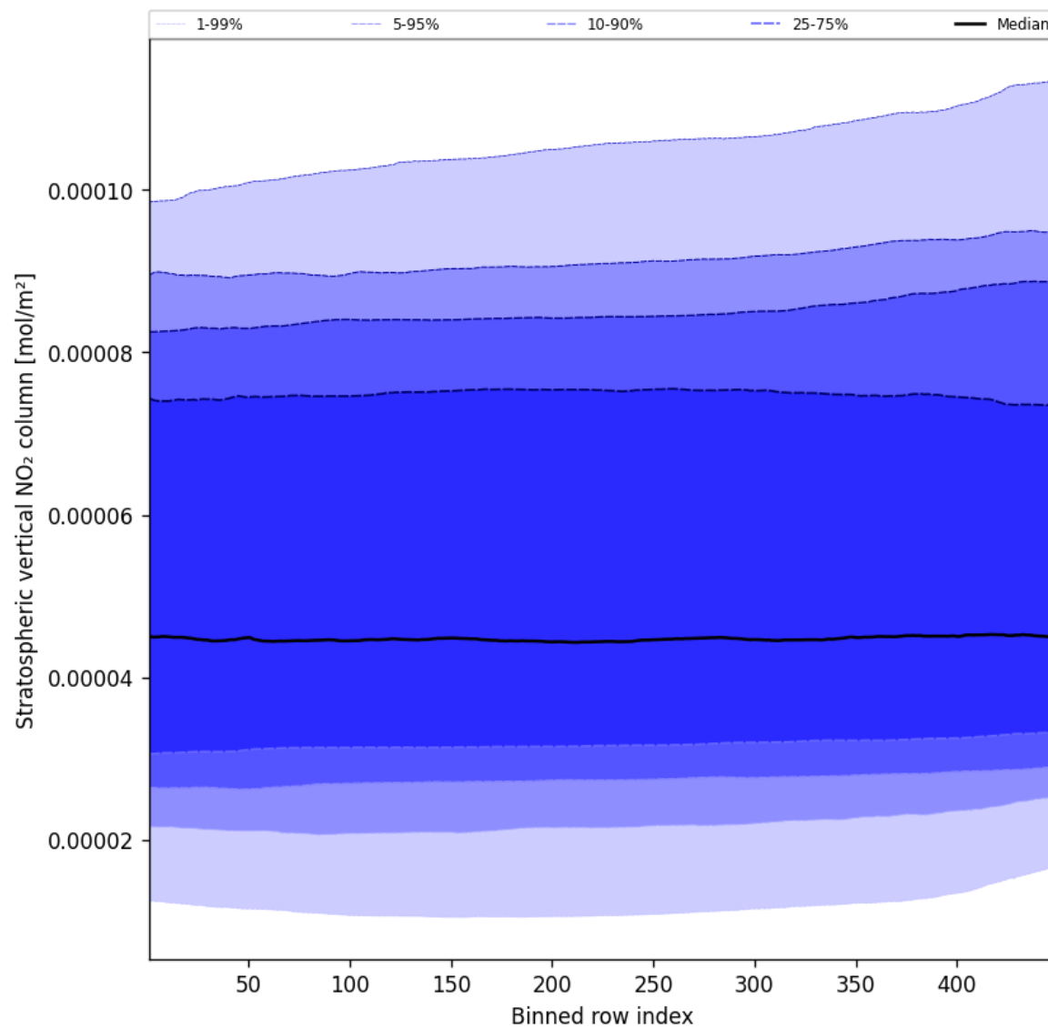
Figure 53: Along track statistics of “Stratospheric vertical NO 2 column” for 2025-01-05 to 2025-01-07
