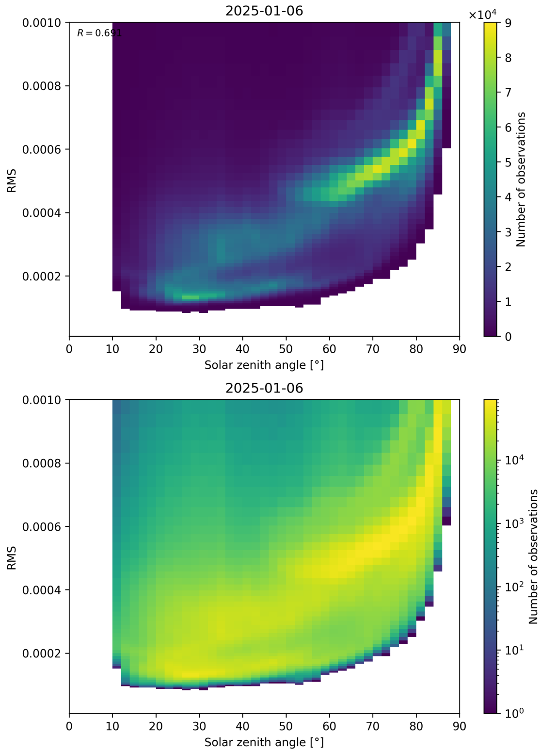
Figure 157: Scatter density plot of “Solar zenith angle” against “RMS” for 2025-01-05 to 2025-01-07.
