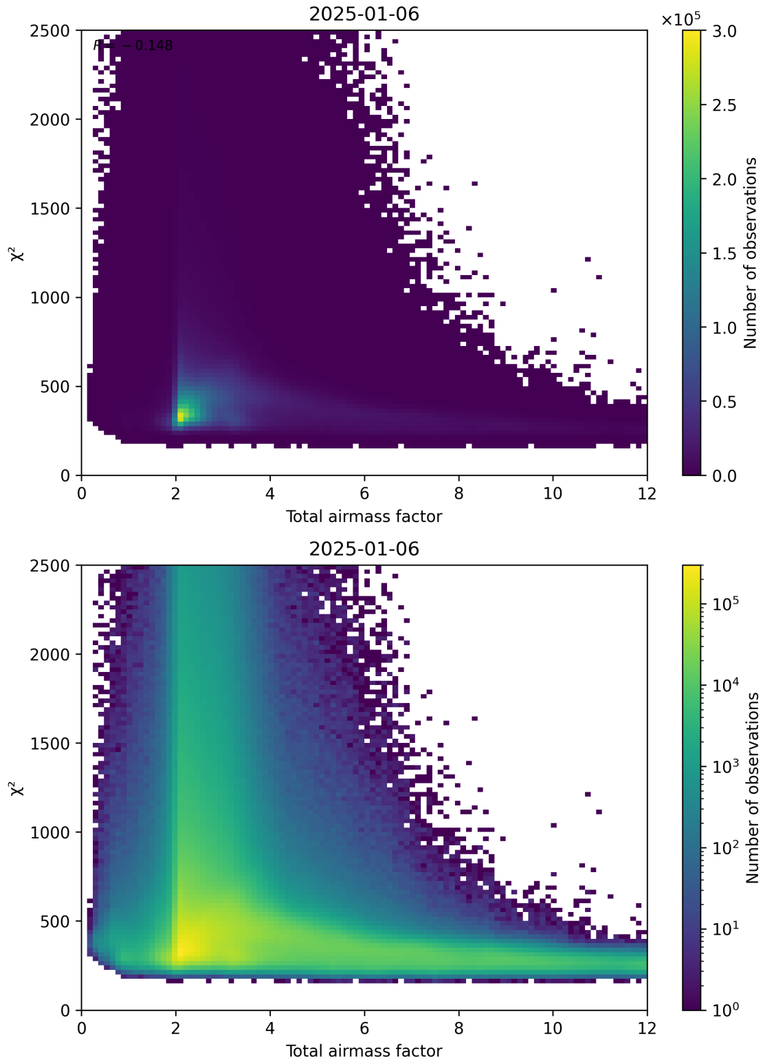
Figure 63: Scatter density plot of “Total airmass factor” against “ \chi^2 ” for 2025-01-05 to 2025-01-07.
