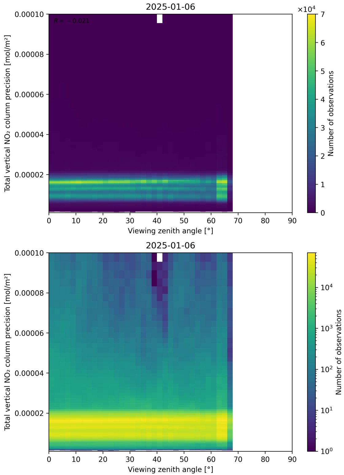
Figure 168: Scatter density plot of “Viewing zenith angle” against “Total vertical NO 2 column precision” for 2025-01-05 to 2025-01-07.
