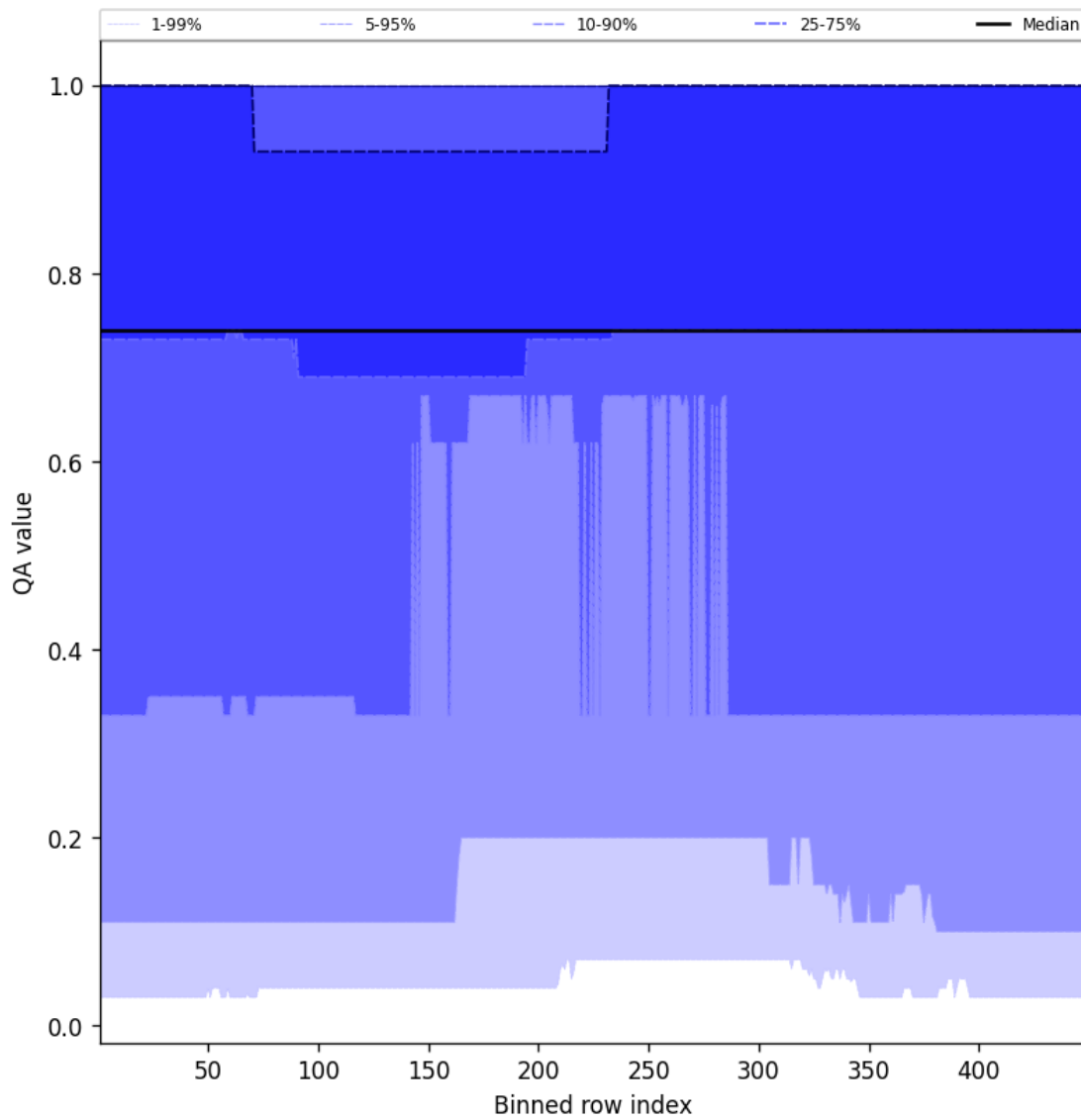
Figure 45: Along track statistics of “QA value” for 2025-01-05 to 2025-01-07
