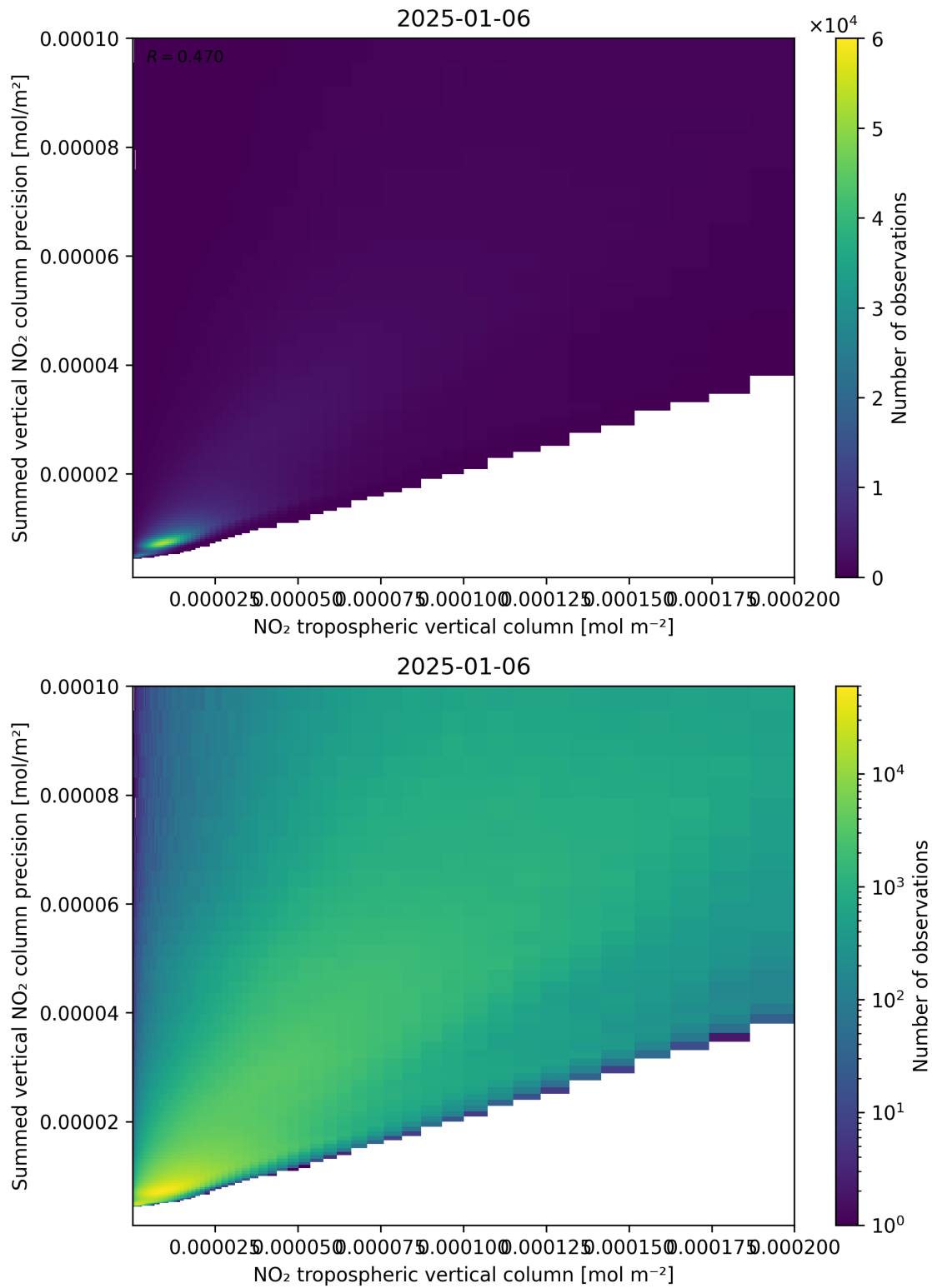
Figure 127: Scatter density plot of “NO 2 tropospheric vertical column” against “Summed vertical NO 2 column precision” for 2025-01-05 to 2025-01-07.
