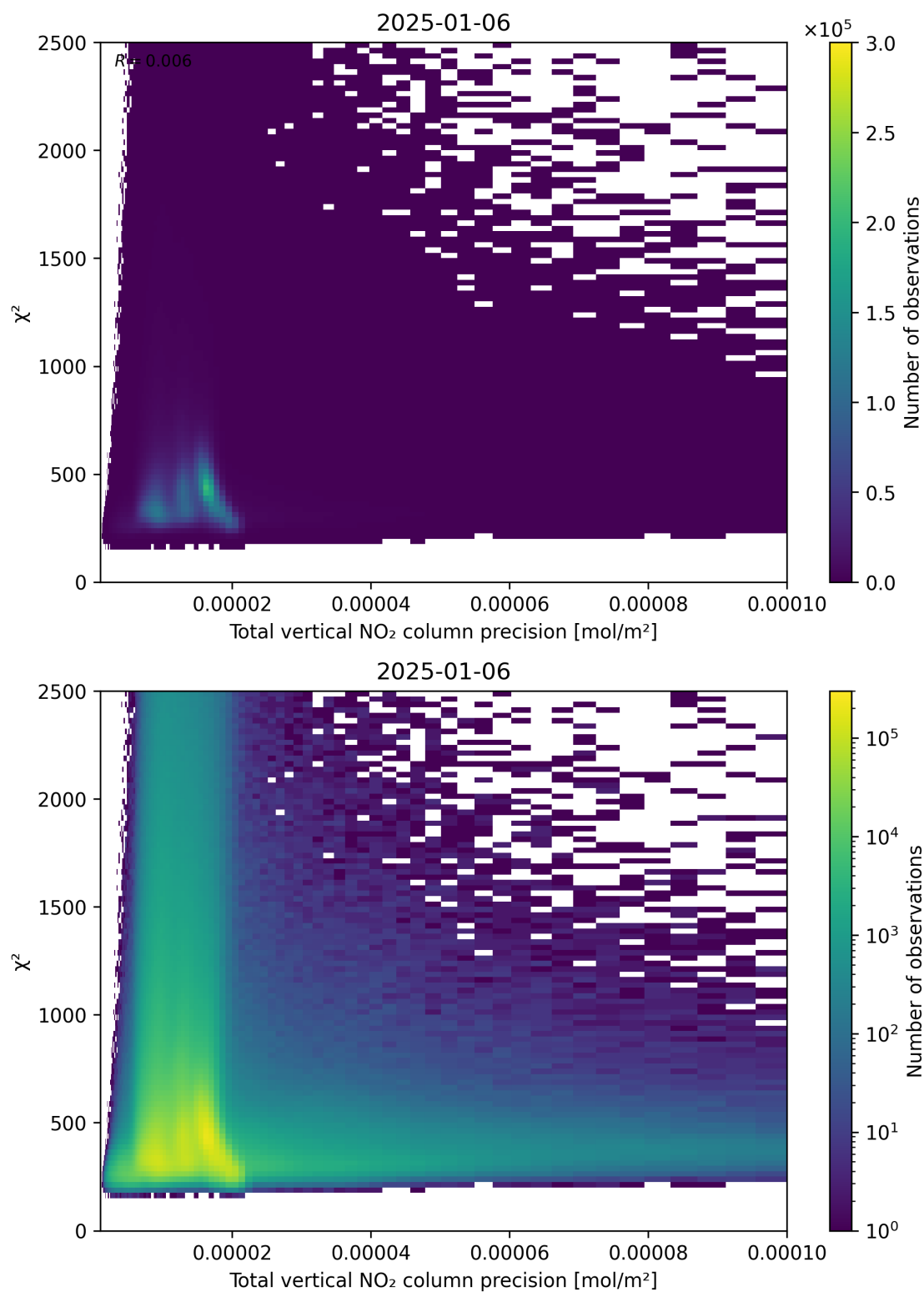
Figure 116: Scatter density plot of “Total vertical NO 2 column precision” against “ \chi^2 ” for 2025-01-05 to 2025-01-07.
