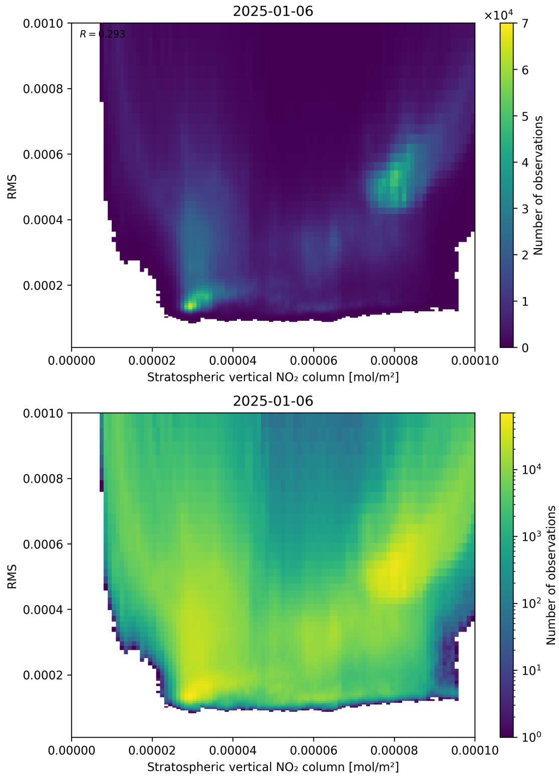
Figure 102: Scatter density plot of “Stratospheric vertical NO 2 column” against “RMS” for 2025-01-05 to 2025-01-07.
