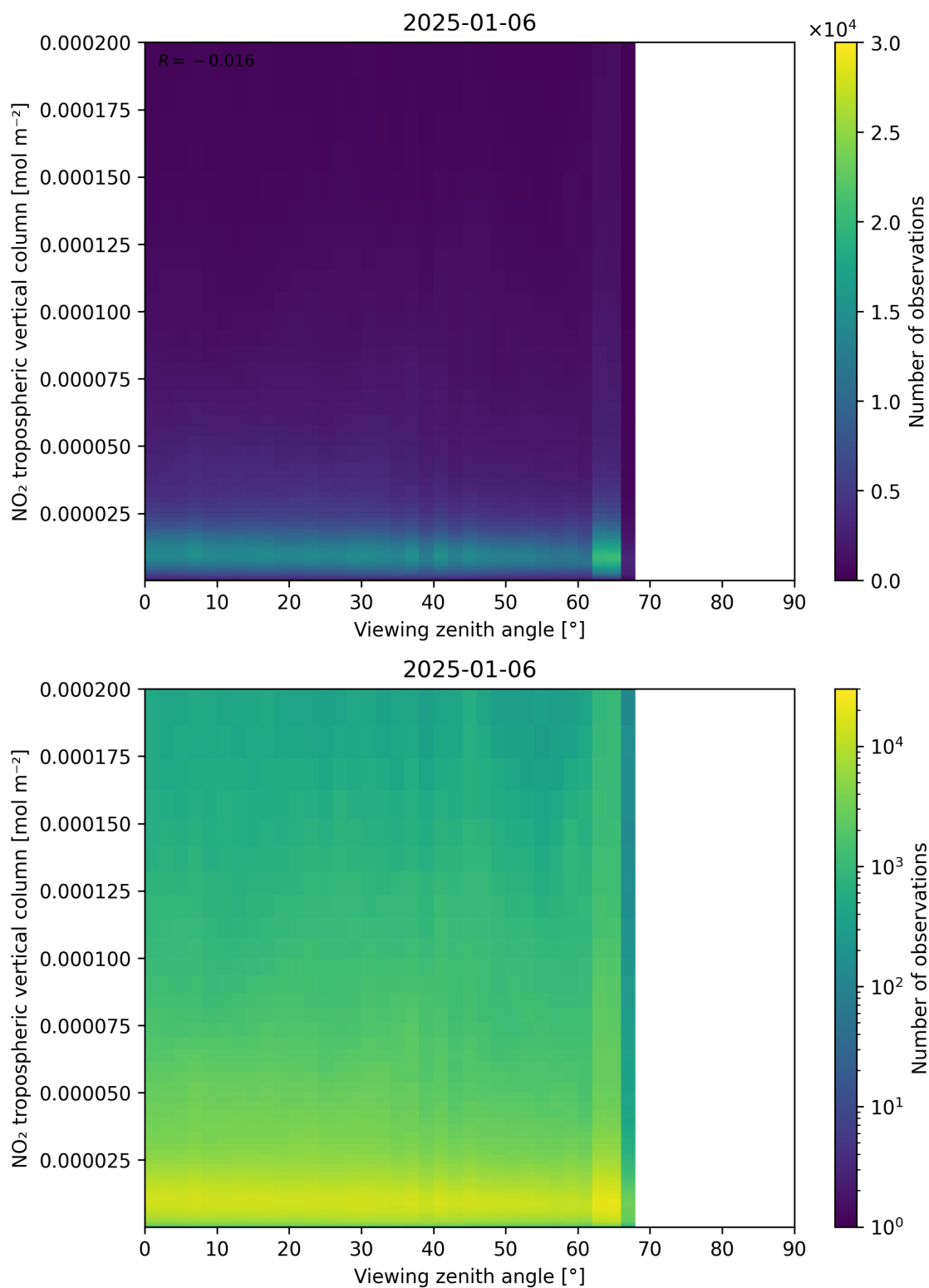
Figure 169: Scatter density plot of “Viewing zenith angle” against “NO 2 tropospheric vertical column” for 2025-01-05 to 2025-01-07.
