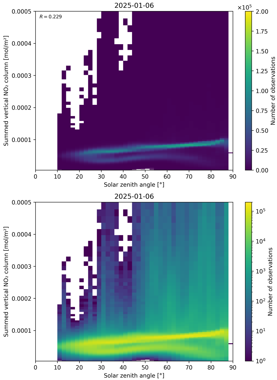
Figure 151: Scatter density plot of “Solar zenith angle” against “Summed vertical NO 2 column” for 2025-01-05 to 2025-01-07.
