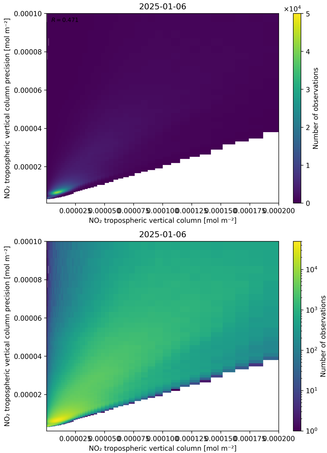
Figure 130: Scatter density plot of “NO 2 tropospheric vertical column” against “NO 2 tropospheric vertical column precision” for 2025-01-05 to 2025-01-07.
