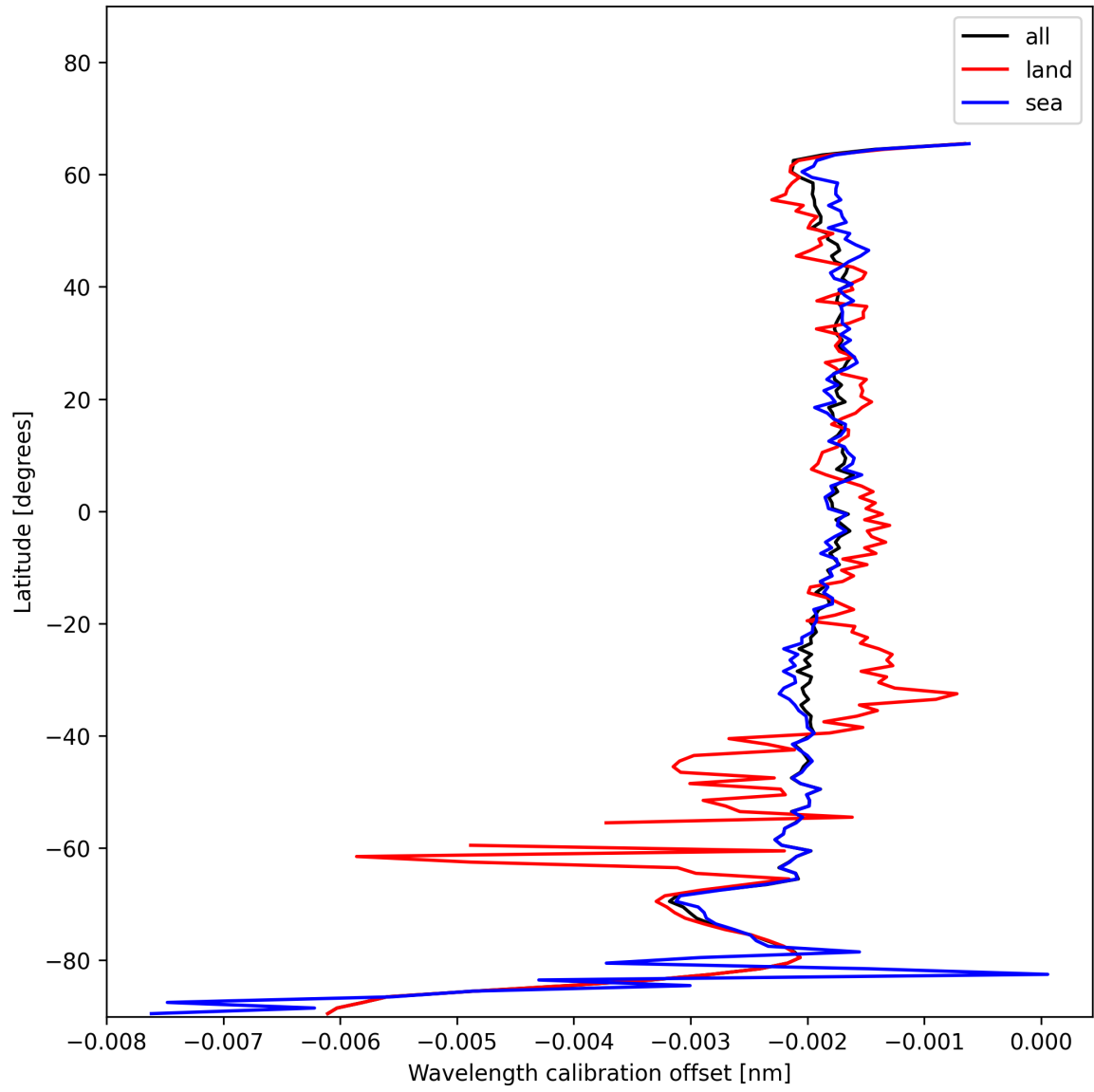
Figure 18: Zonal average of “Wavelength calibration offset” for 2025-01-05 to 2025-01-07.
