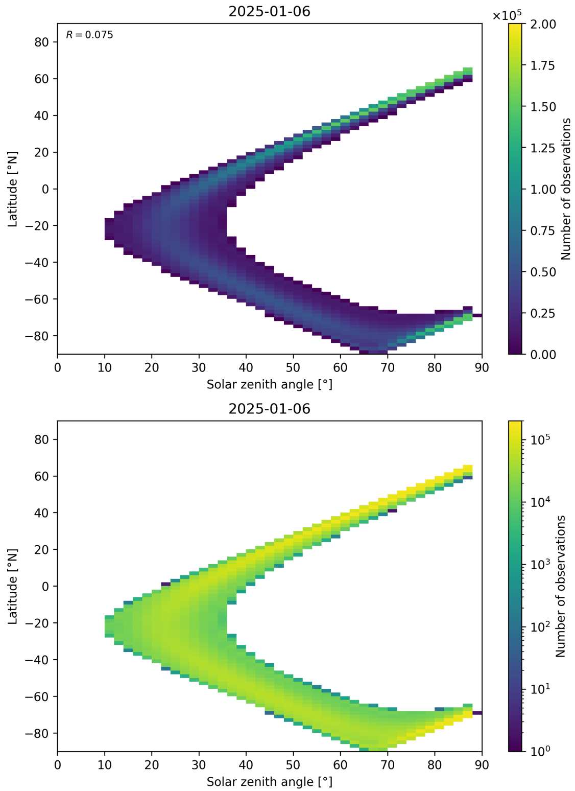
Figure 149: Scatter density plot of “Solar zenith angle” against “Latitude” for 2025-01-05 to 2025-01-07.
