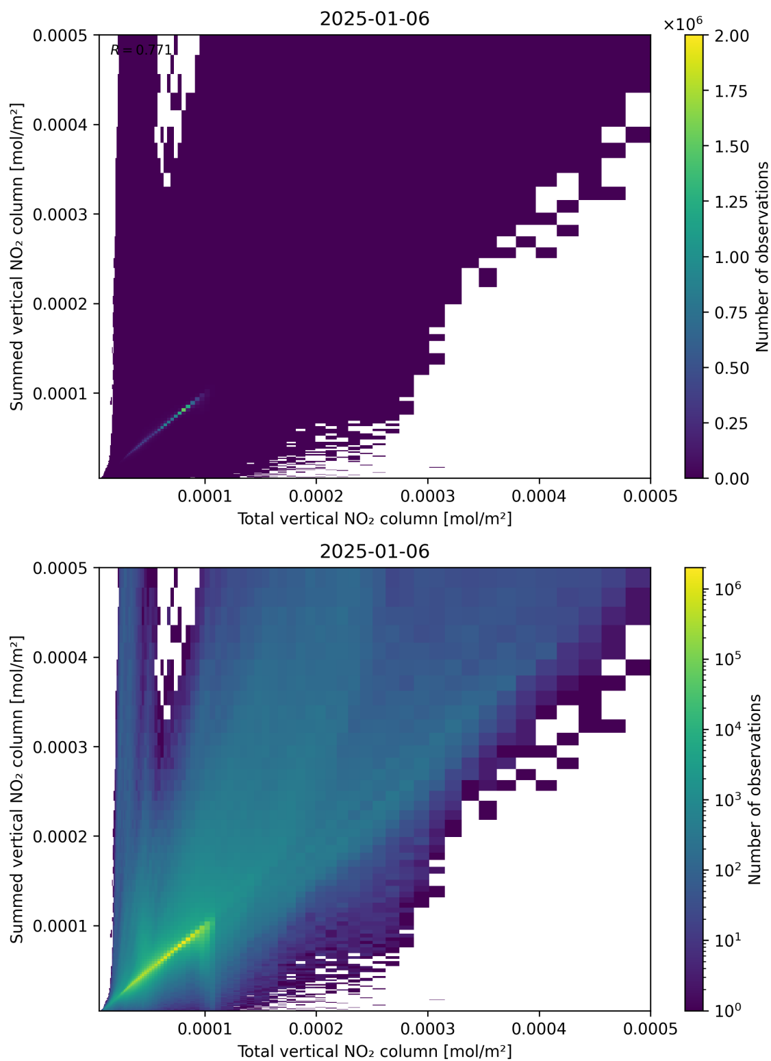
Figure 112: Scatter density plot of “Total vertical NO 2 column” against “Summed vertical NO 2 column” for 2025-01-05 to 2025-01-07.
