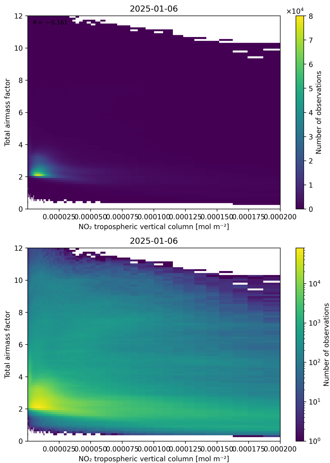
Figure 122: Scatter density plot of “NO 2 tropospheric vertical column” against “Total air mass factor” for 2025-01-05 to 2025-01-07.
