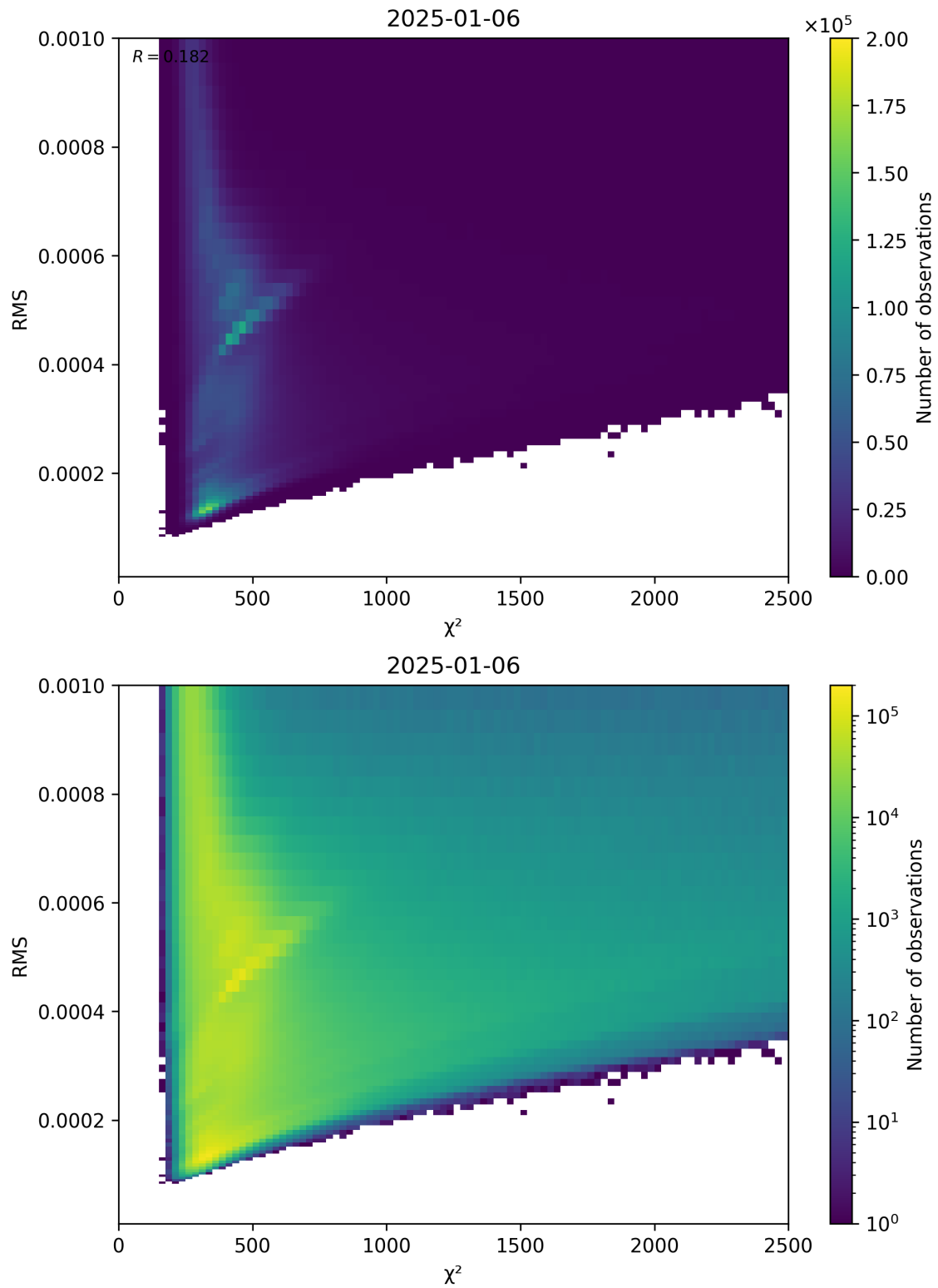
Figure 82: Scatter density plot of “ \chi^2 ” against “RMS” for 2025-01-05 to 2025-01-07.
