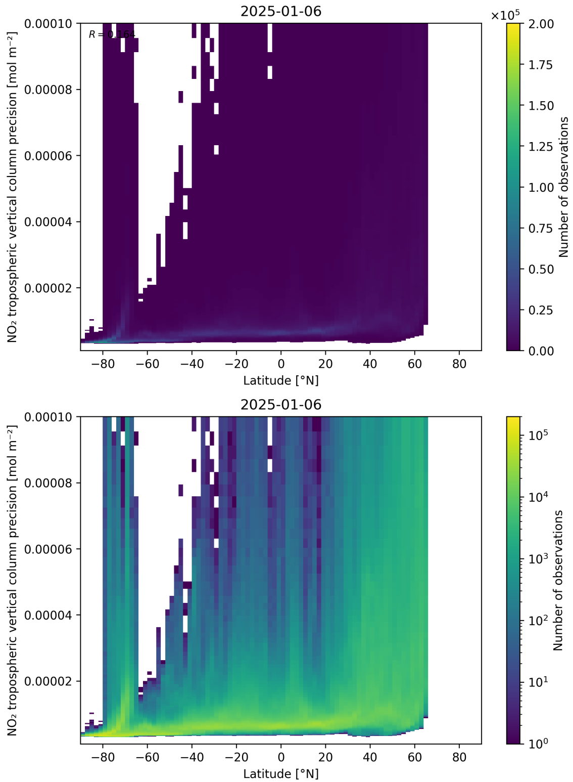
Figure 93: Scatter density plot of “Latitude” against “NO 2 tropospheric vertical column precision” for 2025-01-05 to 2025-01-07.
