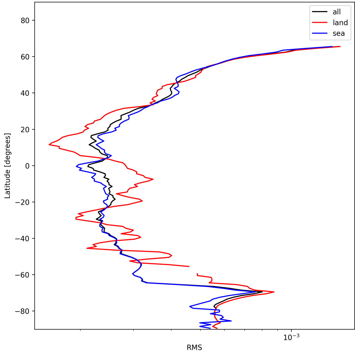
Figure 26: Zonal average of “RMS” for 2025-01-05 to 2025-01-07.
