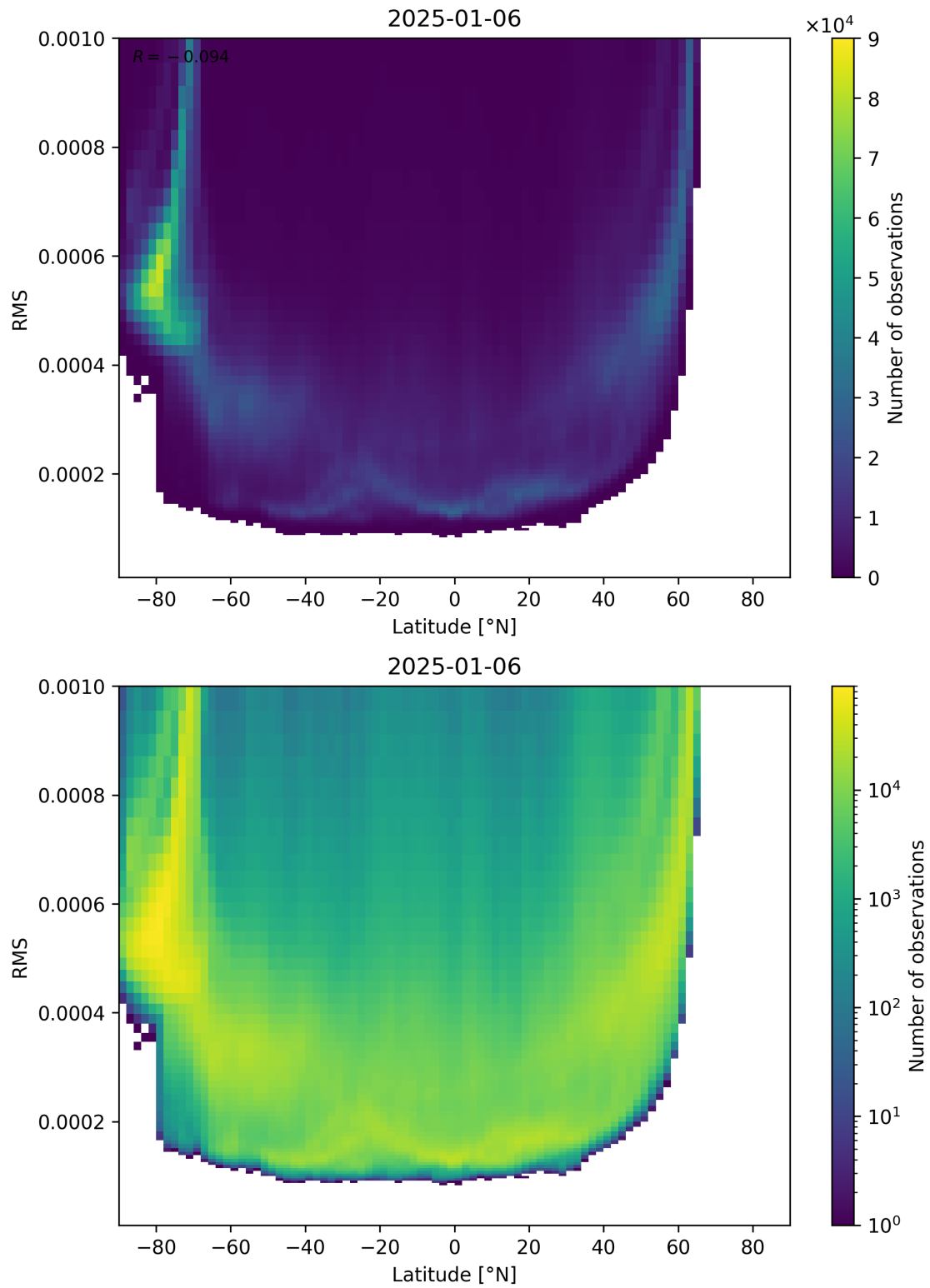
Figure 94: Scatter density plot of “Latitude” against “RMS” for 2025-01-05 to 2025-01-07.
