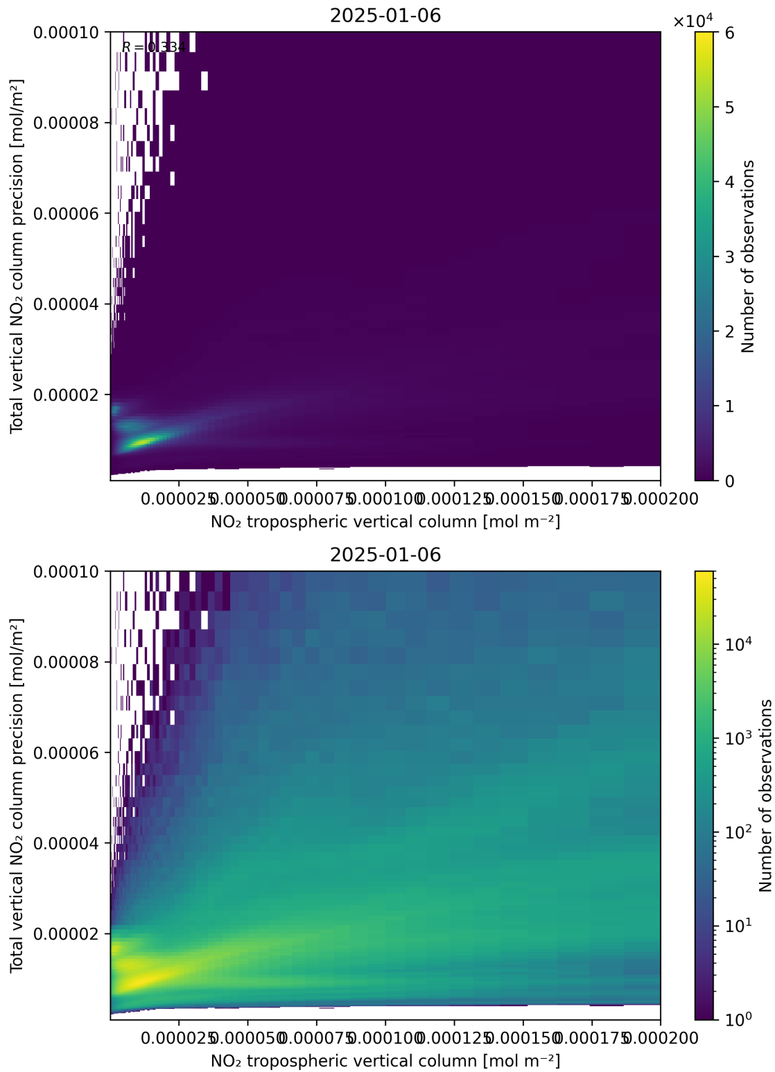
Figure 129: Scatter density plot of “NO 2 tropospheric vertical column” against “Total vertical NO 2 column precision” for 2025-01-05 to 2025-01-07.
