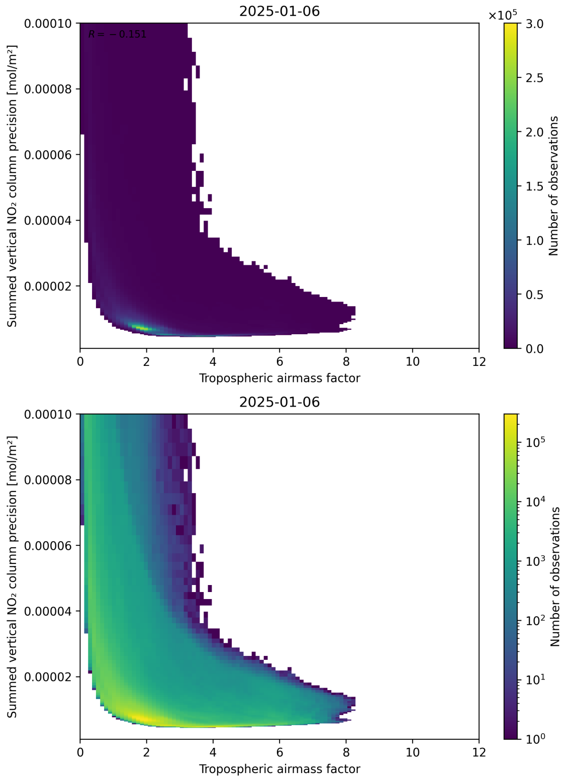
Figure 76: Scatter density plot of “Tropospheric air mass factor” against “Summed vertical NO 2 column precision” for 2025-01-05 to 2025-01-07.
