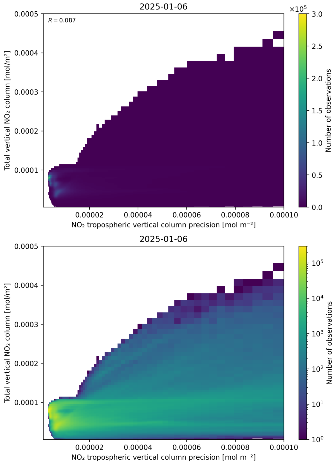
Figure 138: Scatter density plot of “NO 2 tropospheric vertical column precision” against “Total vertical NO 2 column” for 2025-01-05 to 2025-01-07.
