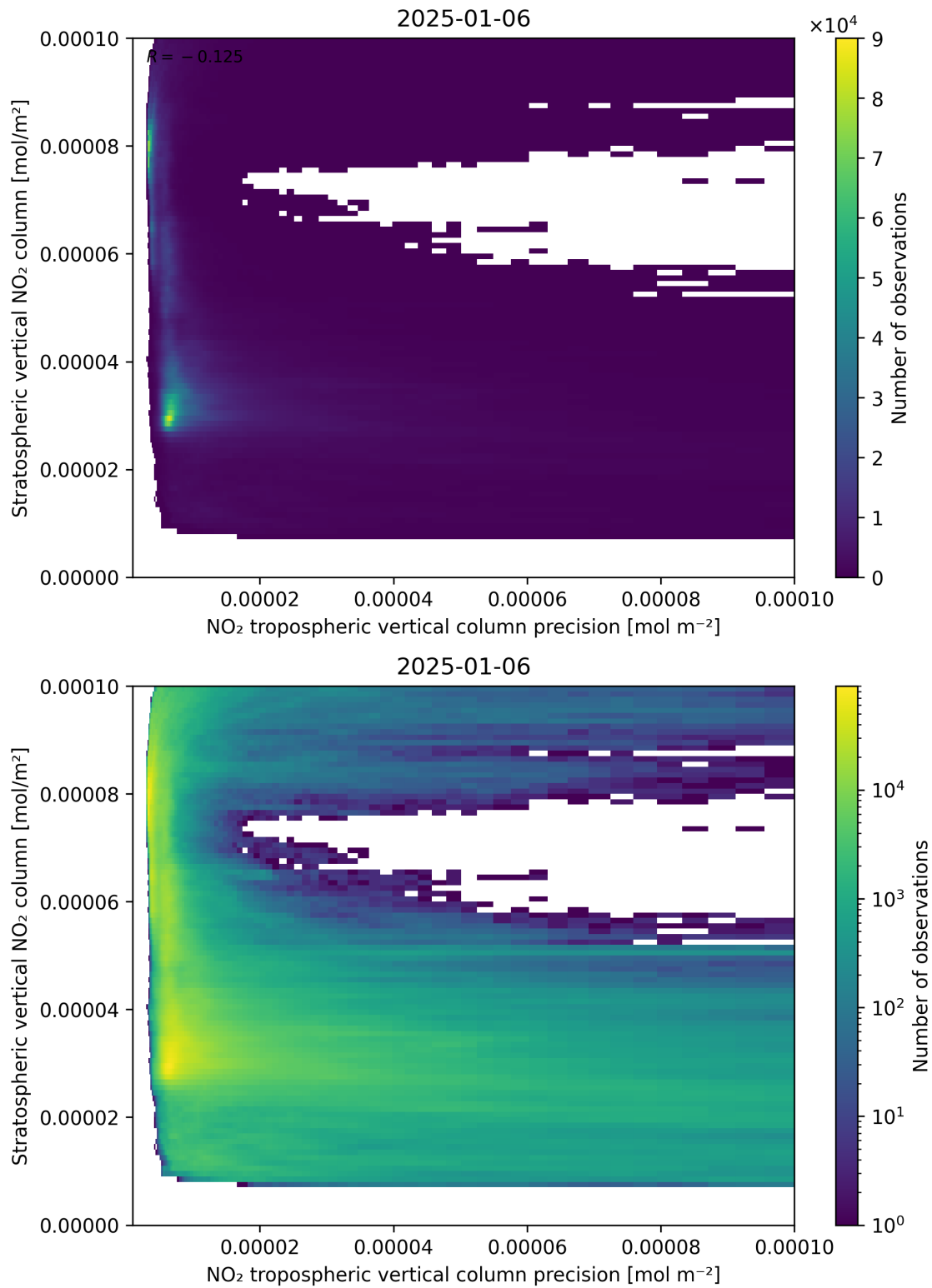
Figure 135: Scatter density plot of “NO 2 tropospheric vertical column precision” against “Stratospheric vertical NO 2 column” for 2025-01-05 to 2025-01-07.
