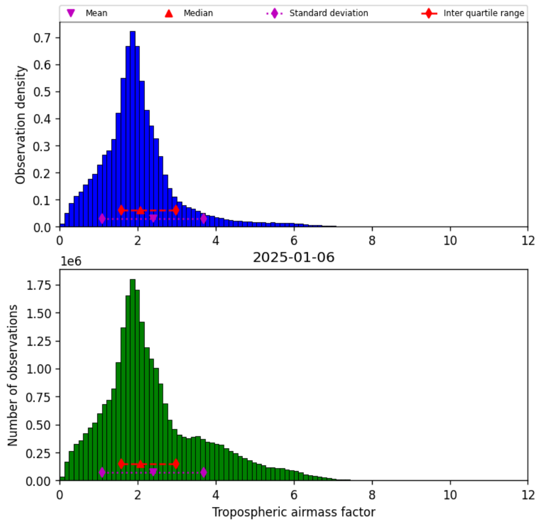
Figure 31: Histogram of “Tropospheric airmass factor” for 2025-01-05 to 2025-01-07
