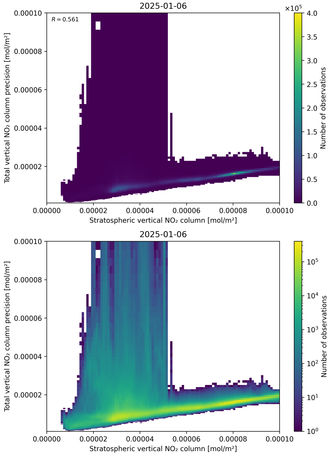
Figure 101: Scatter density plot of “Stratospheric vertical NO 2 column” against “Total vertical NO 2 column precision” for 2025-01-05 to 2025-01-07.
