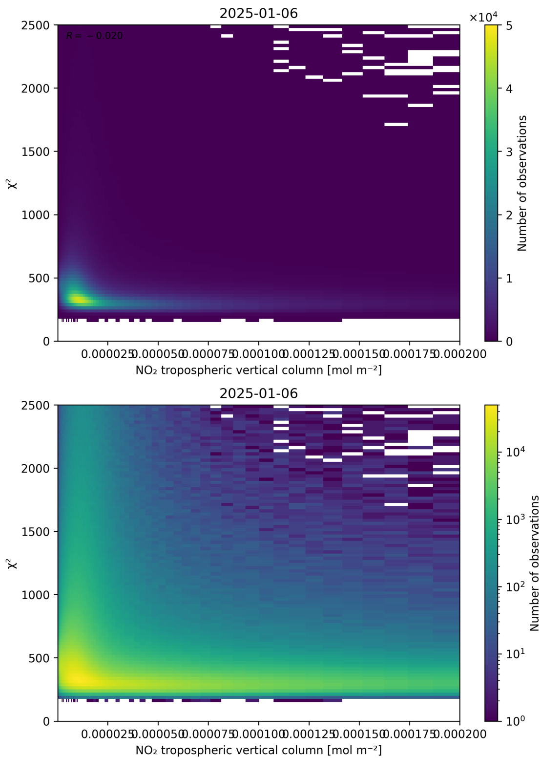
Figure 124: Scatter density plot of “NO 2 tropospheric vertical column” against “ \chi^2 ” for 2025-01-05 to 2025-01-07.
