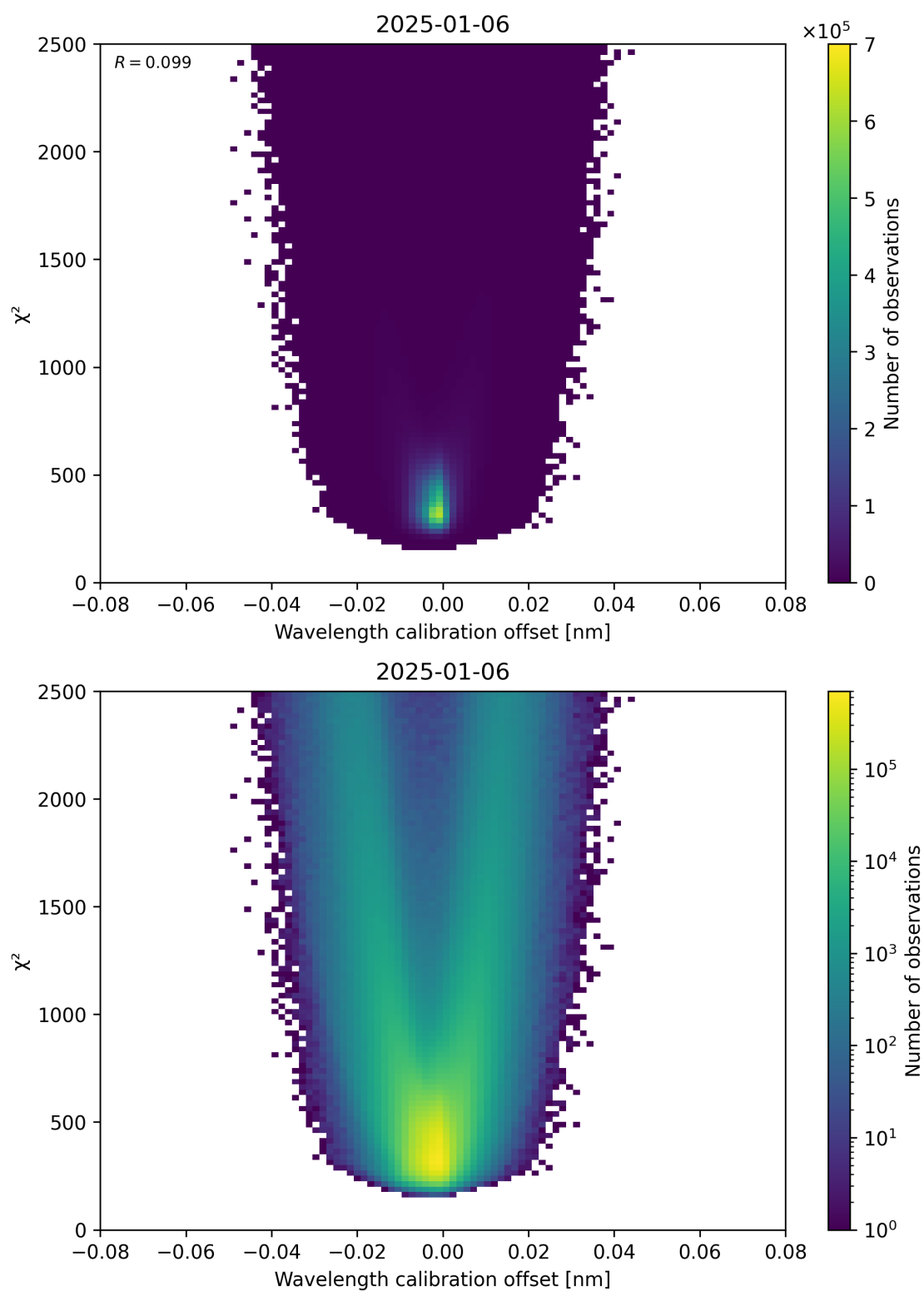
Figure 175: Scatter density plot of “Wavelength calibration offset” against “ \chi^2 ” for 2025-01-05 to 2025-01-07.
