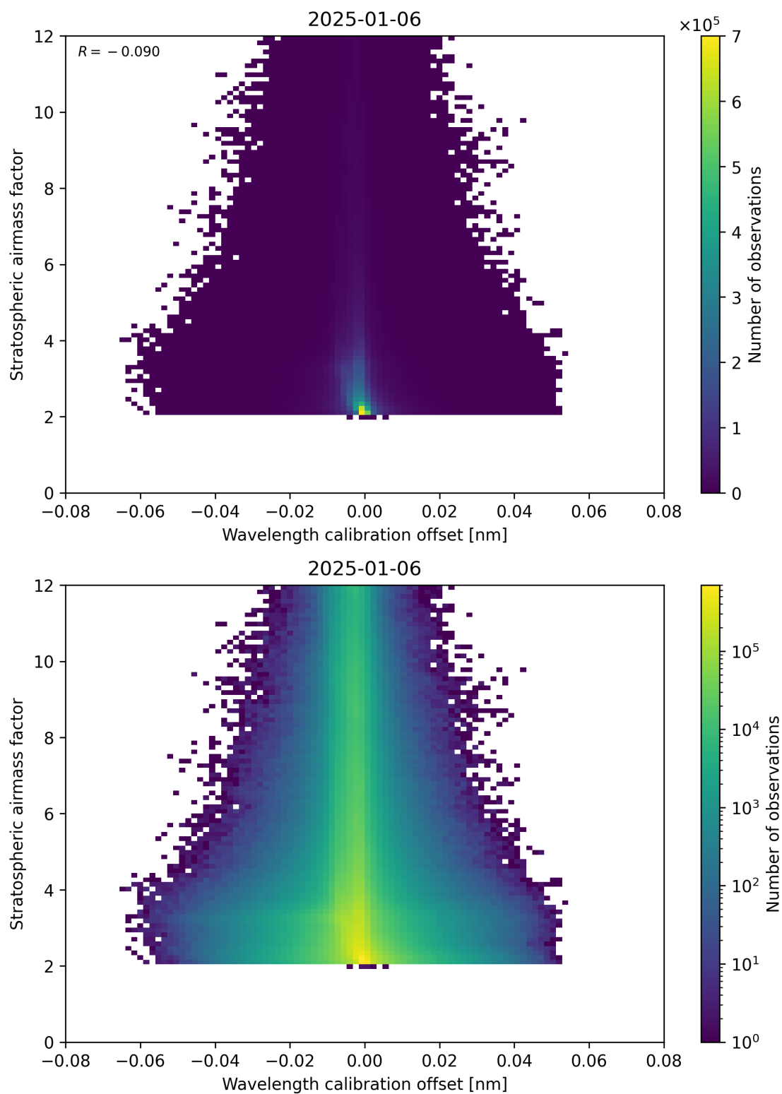
Figure 174: Scatter density plot of “Wavelength calibration offset” against “Stratospheric airmass factor” for 2025-01-05 to 2025-01-07.
