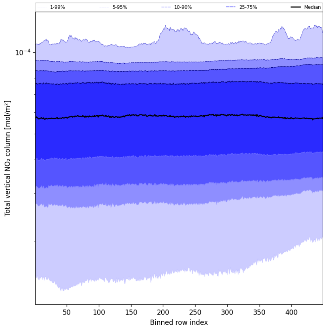
Figure 55: Along track statistics of “Total vertical NO 2 column” for 2025-01-05 to 2025-01-07
