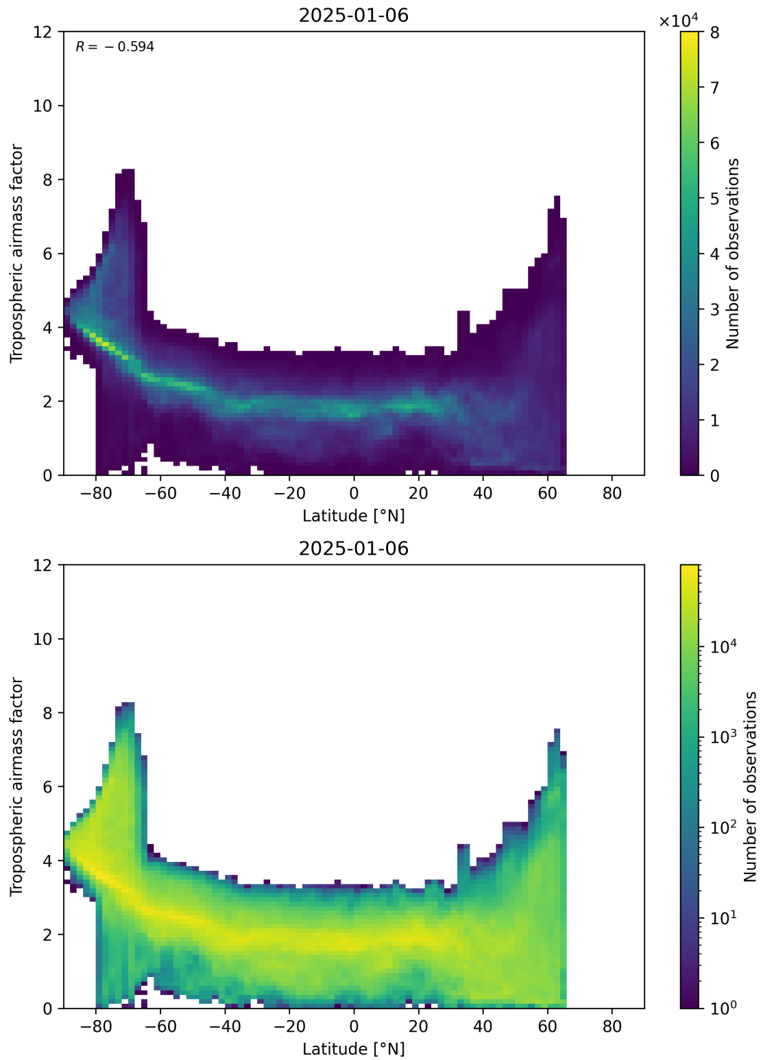
Figure 85: Scatter density plot of “Latitude” against “Tropospheric airmass factor” for 2025-01-05 to 2025-01-07.
