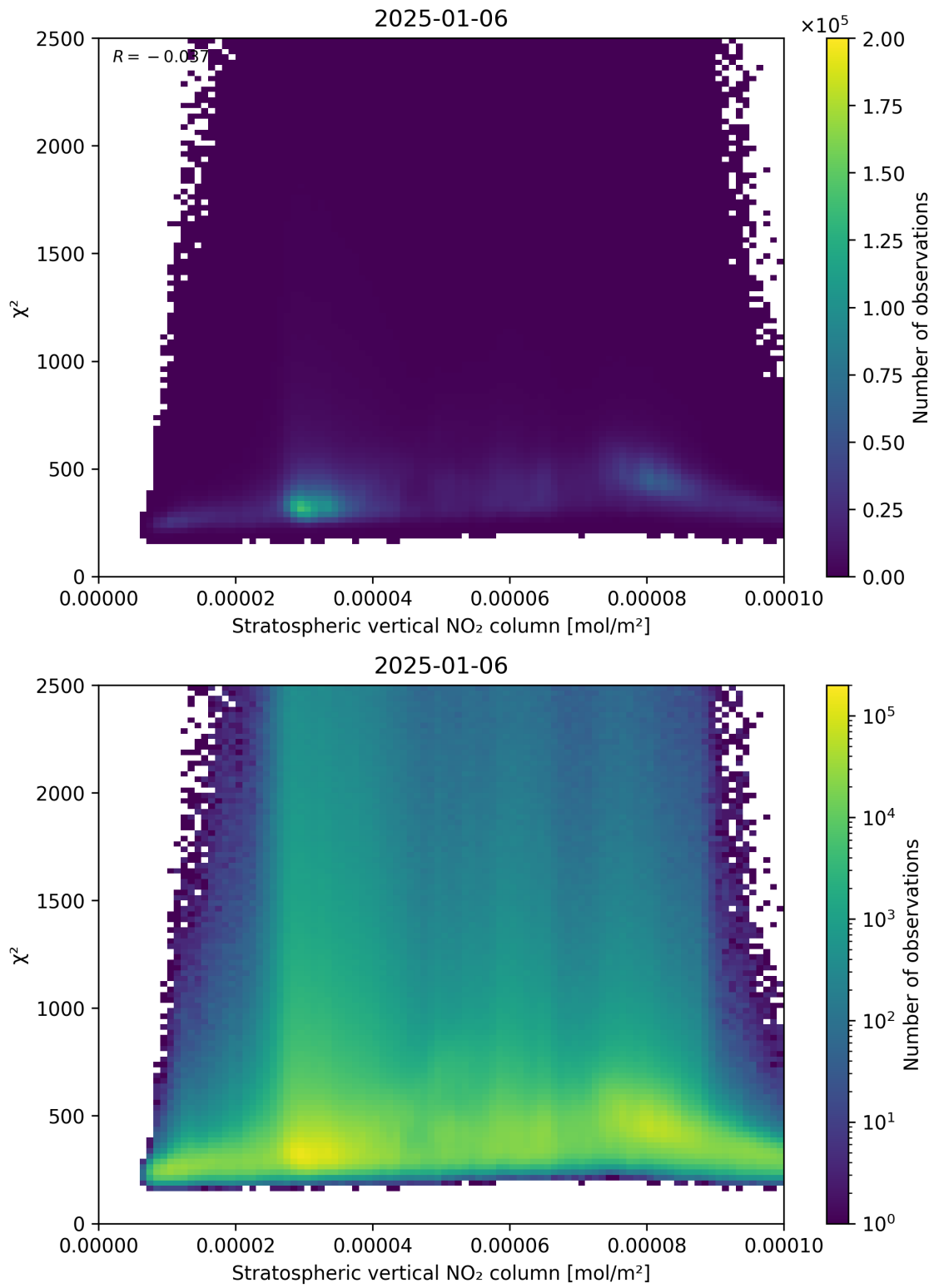
Figure 97: Scatter density plot of “Stratospheric vertical NO 2 column” against “ \chi^2 ” for 2025-01-05 to 2025-01-07.
