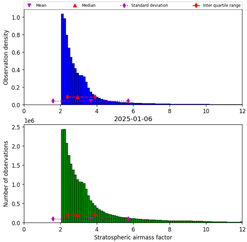
Figure 44: Histogram of “Stratospheric airmass factor” for 2025-01-05 to 2025-01-07
