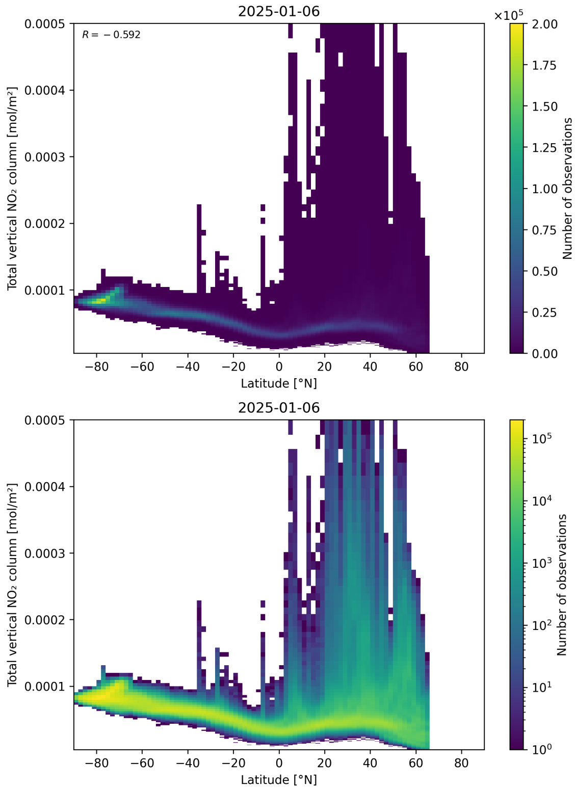
Figure 90: Scatter density plot of “Latitude” against “Total vertical NO 2 column” for 2025-01-05 to 2025-01-07.
