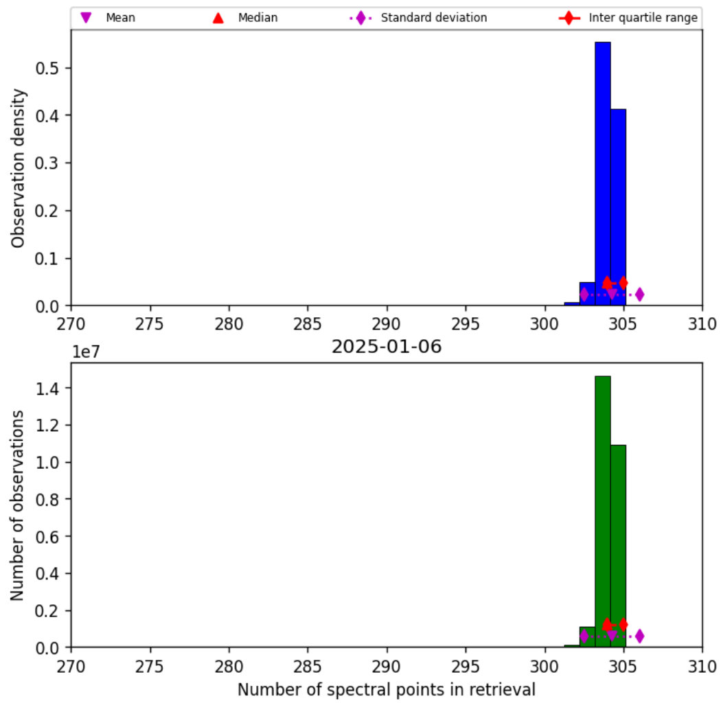
Figure 33: Histogram of “Number of spectral points in retrieval” for 2025-01-05 to 2025-01-07
