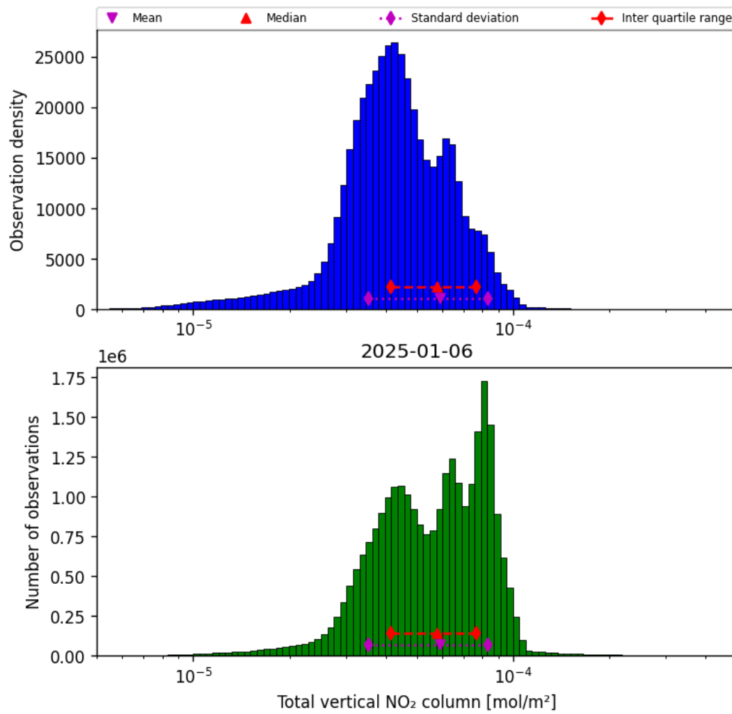
Figure 38: Histogram of “Total vertical NO 2 column” for 2025-01-05 to 2025-01-07
