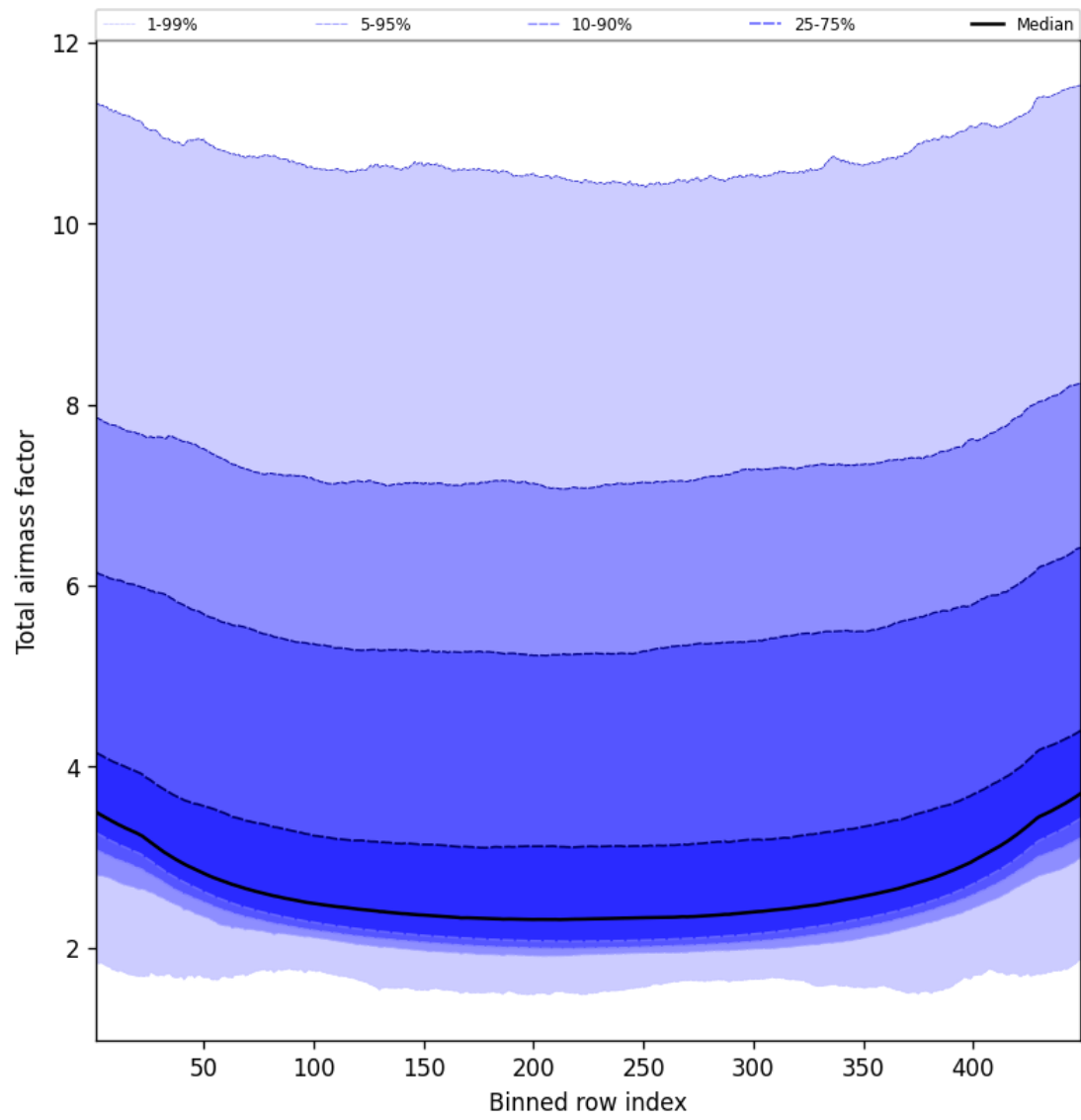
Figure 49: Along track statistics of “Total airmass factor” for 2025-01-05 to 2025-01-07
