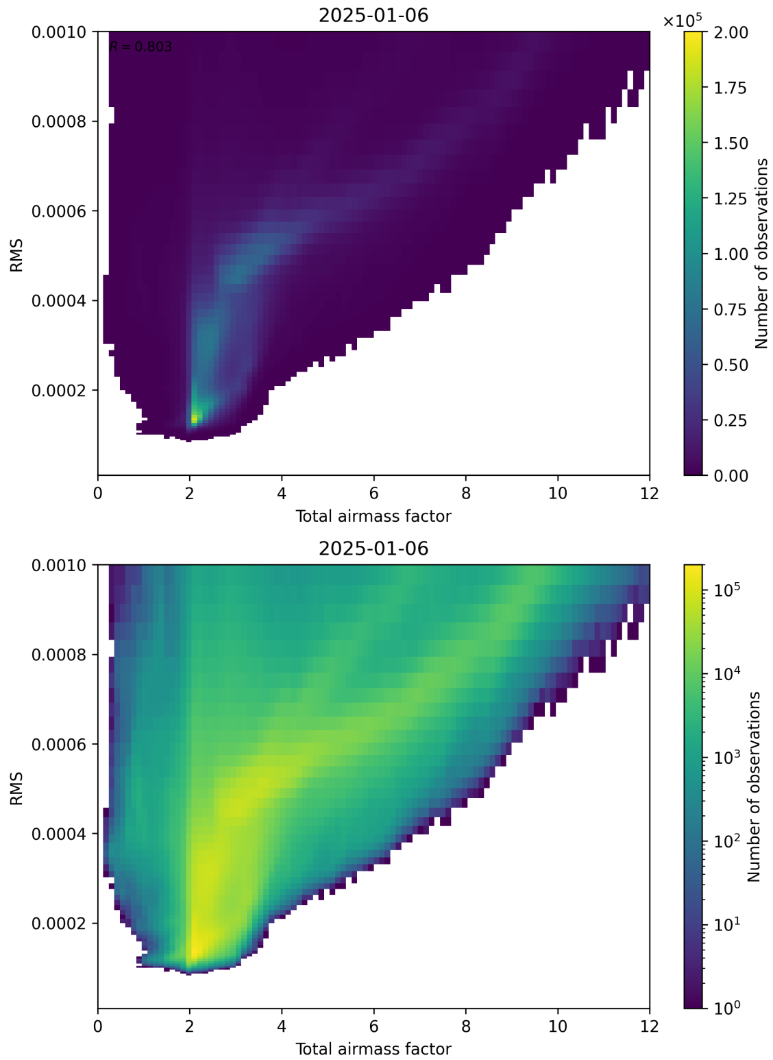
Figure 69: Scatter density plot of “Total airmass factor” against “RMS” for 2025-01-05 to 2025-01-07.
