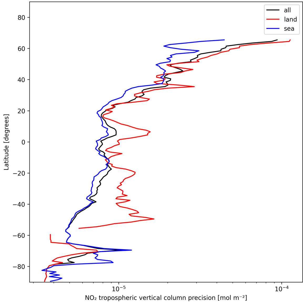
Figure 13: Zonal average of “NO 2 tropospheric vertical column precision” for 2025-01-05 to 2025-01-07.
