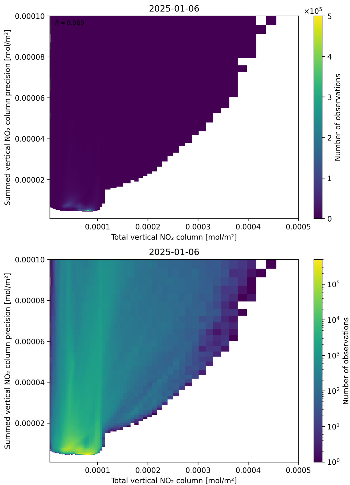
Figure 113: Scatter density plot of “Total vertical NO 2 column” against “Summed vertical NO 2 column precision” for 2025-01-05 to 2025-01-07.
