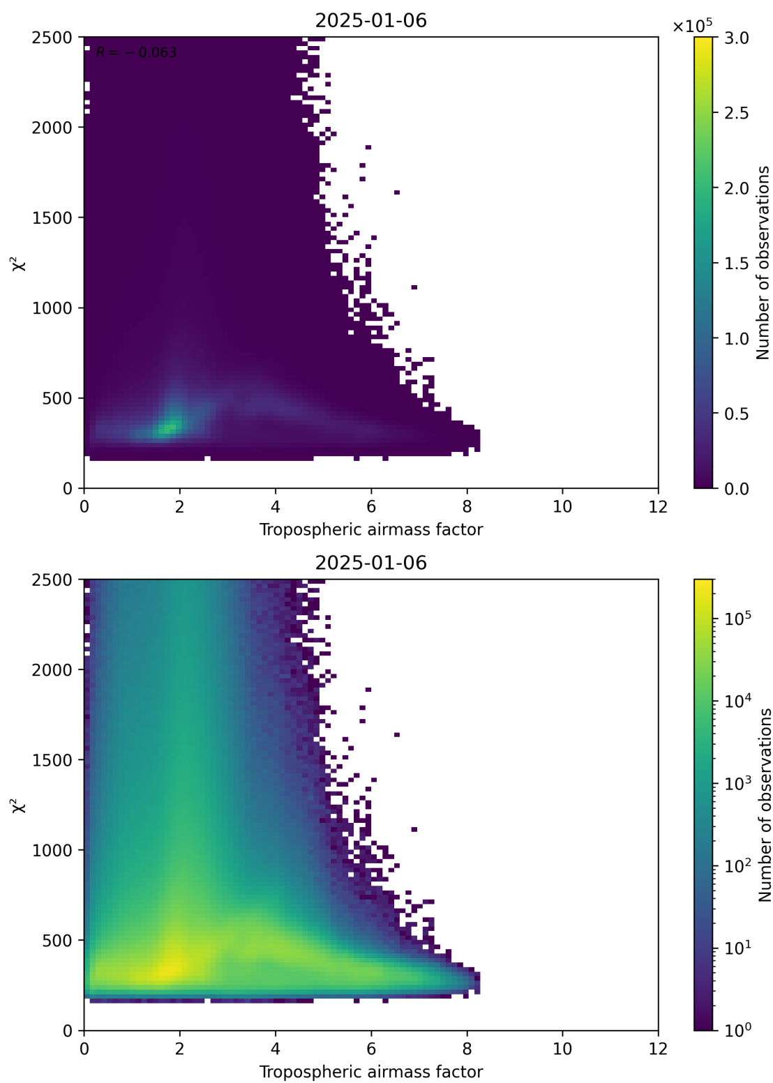
Figure 73: Scatter density plot of “Tropospheric airmass factor” against “ \chi^2 ” for 2025-01-05 to 2025-01-07.
