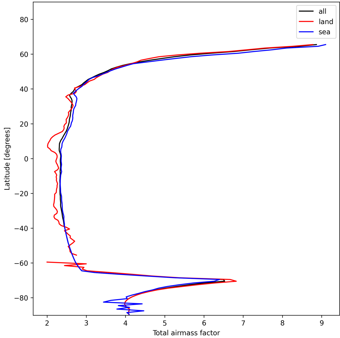
Figure 15: Zonal average of “Total airmass factor” for 2025-01-05 to 2025-01-07.
