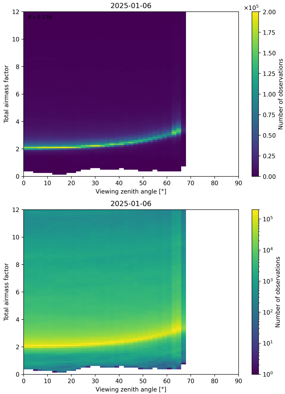
Figure 160: Scatter density plot of “Viewing zenith angle” against “Total airmass factor” for 2025-01-05 to 2025-01-07.
