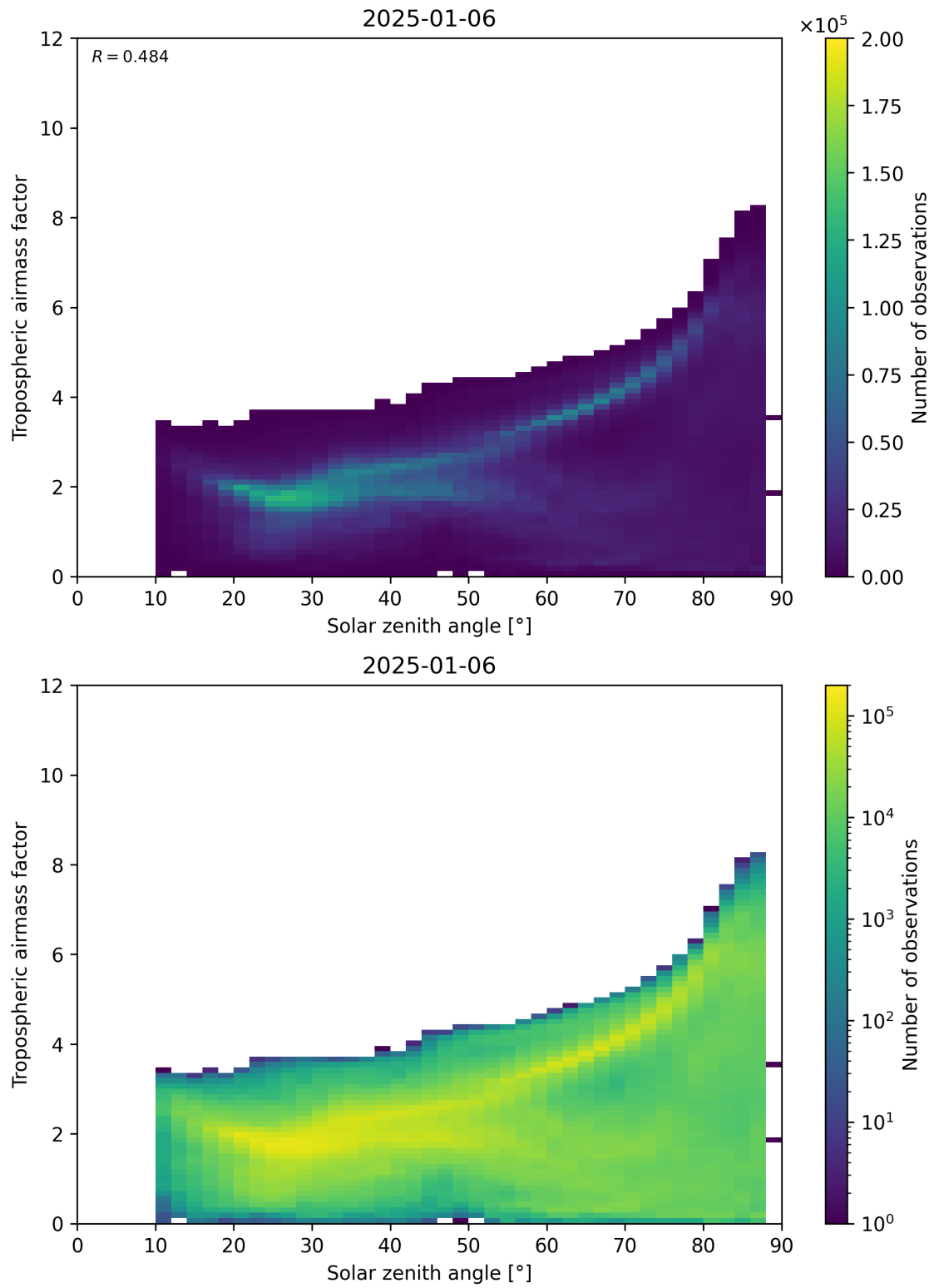
Figure 147: Scatter density plot of “Solar zenith angle” against “Tropospheric airmass factor” for 2025-01-05 to 2025-01-07.
