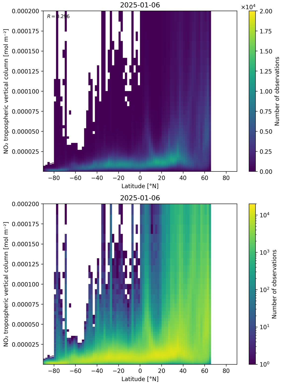
Figure 92: Scatter density plot of “Latitude” against “NO 2 tropospheric vertical column” for 2025-01-05 to 2025-01-07.
