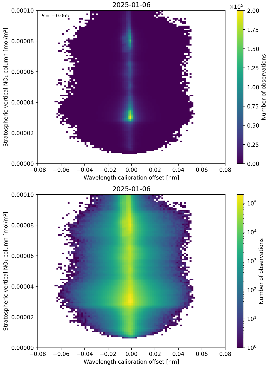
Figure 176: Scatter density plot of “Wavelength calibration offset” against “Stratospheric vertical NO 2 column” for 2025-01-05 to 2025-01-07.
