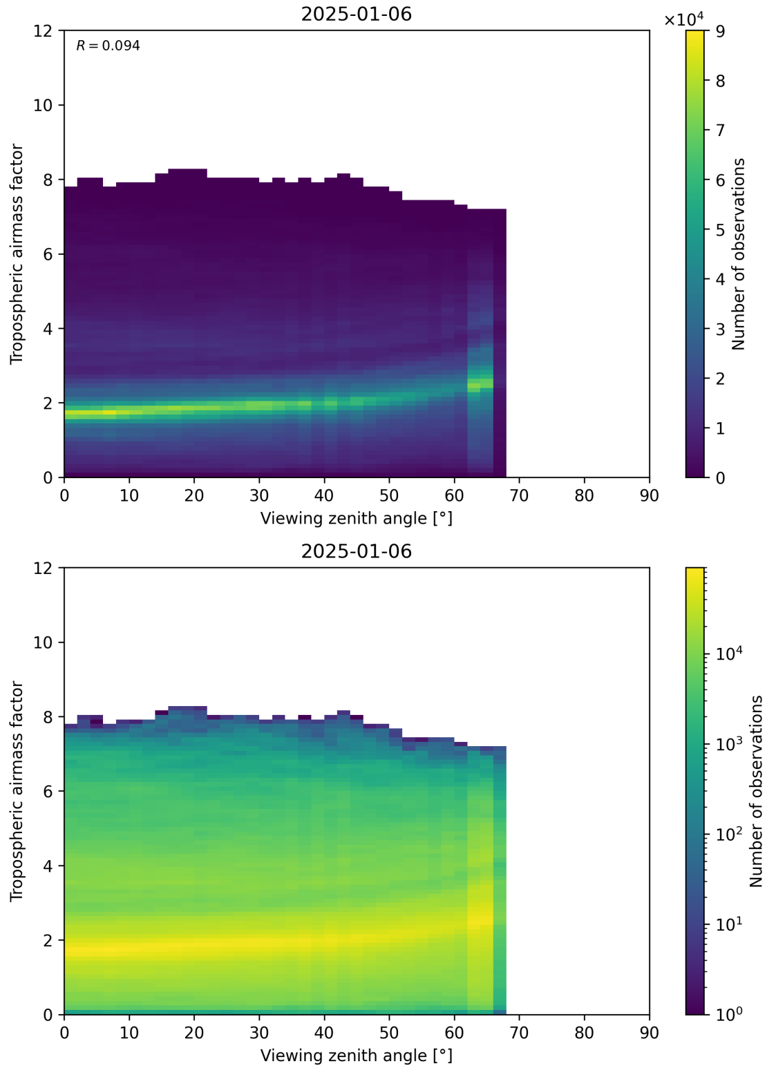
Figure 161: Scatter density plot of “Viewing zenith angle” against “Tropospheric airmass factor” for 2025-01-05 to 2025-01-07.
