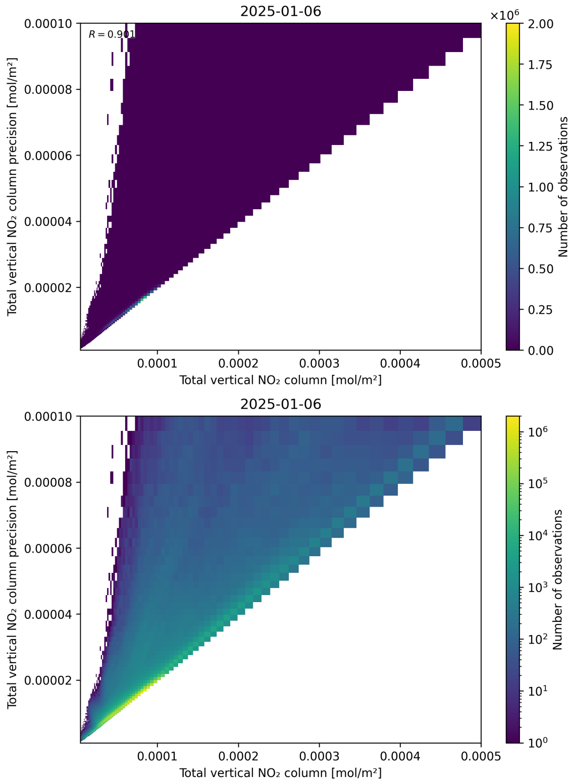
Figure 114: Scatter density plot of “Total vertical NO 2 column” against “Total vertical NO 2 column precision” for 2025-01-05 to 2025-01-07.
