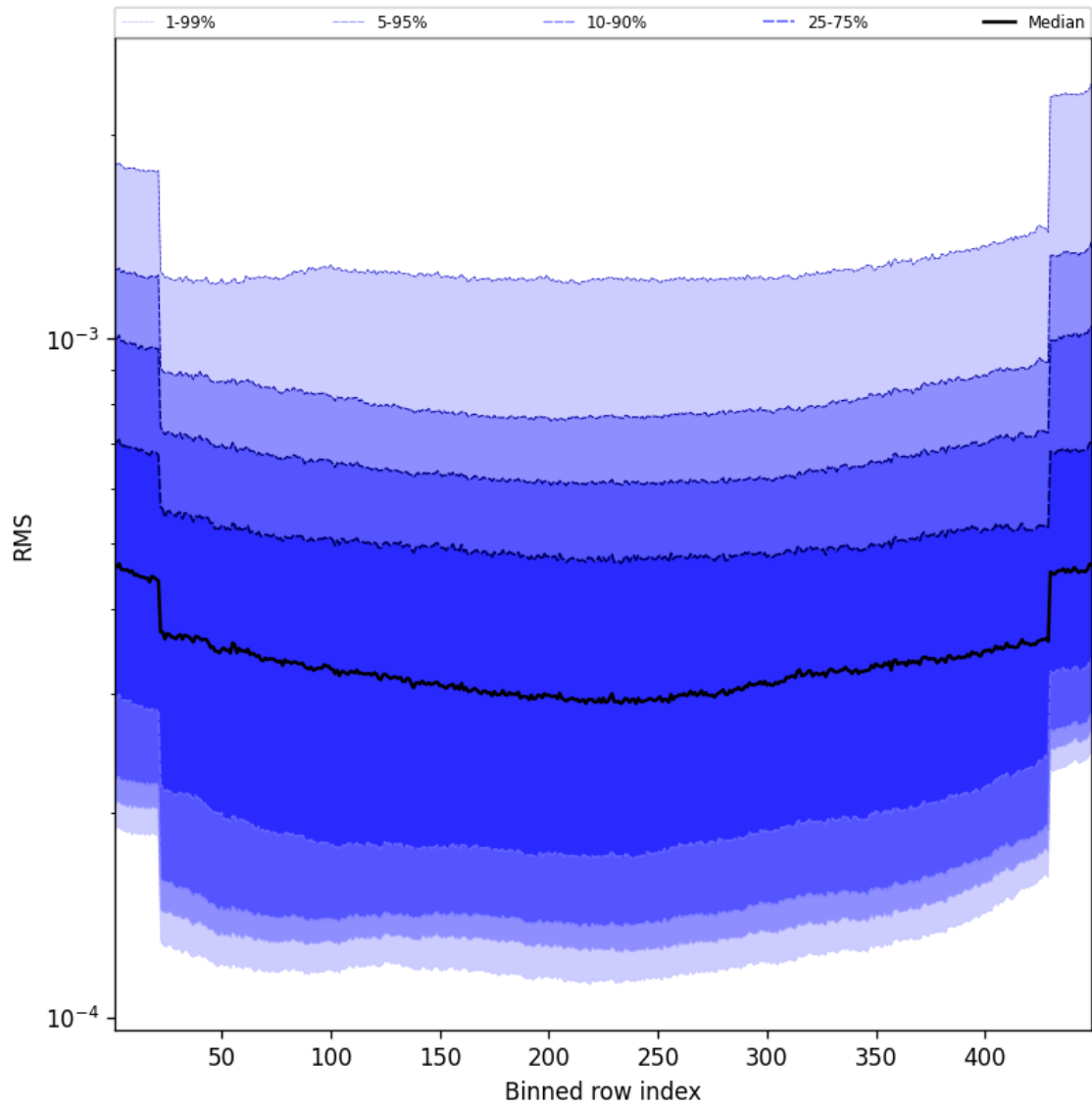
Figure 60: Along track statistics of “RMS” for 2025-01-05 to 2025-01-07
