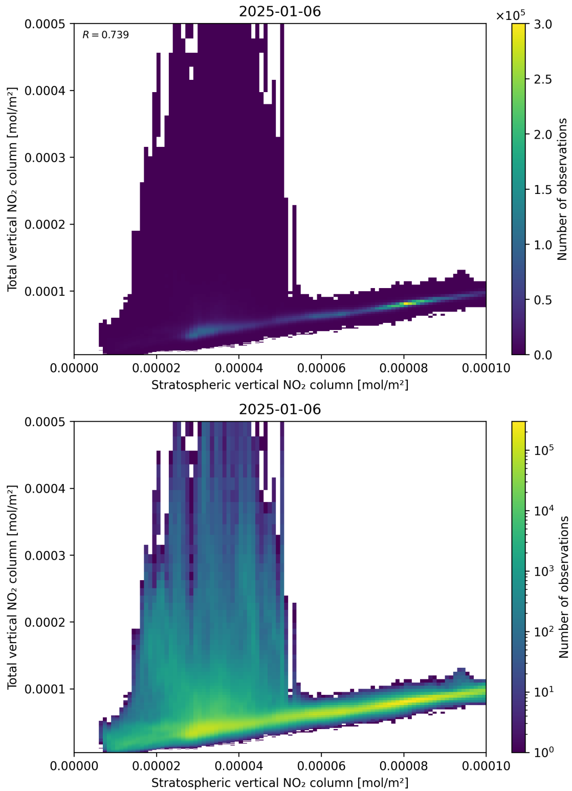
Figure 100: Scatter density plot of “Stratospheric vertical NO 2 column” against “Total vertical NO 2 column” for 2025-01-05 to 2025-01-07.
