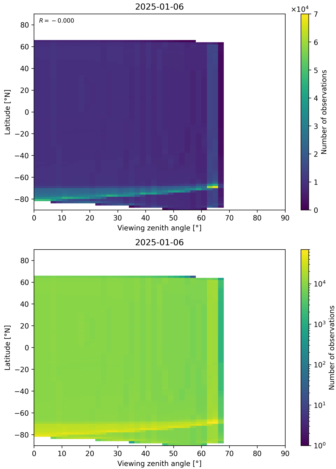
Figure 163: Scatter density plot of “Viewing zenith angle” against “Latitude” for 2025-01-05 to 2025-01-07.
