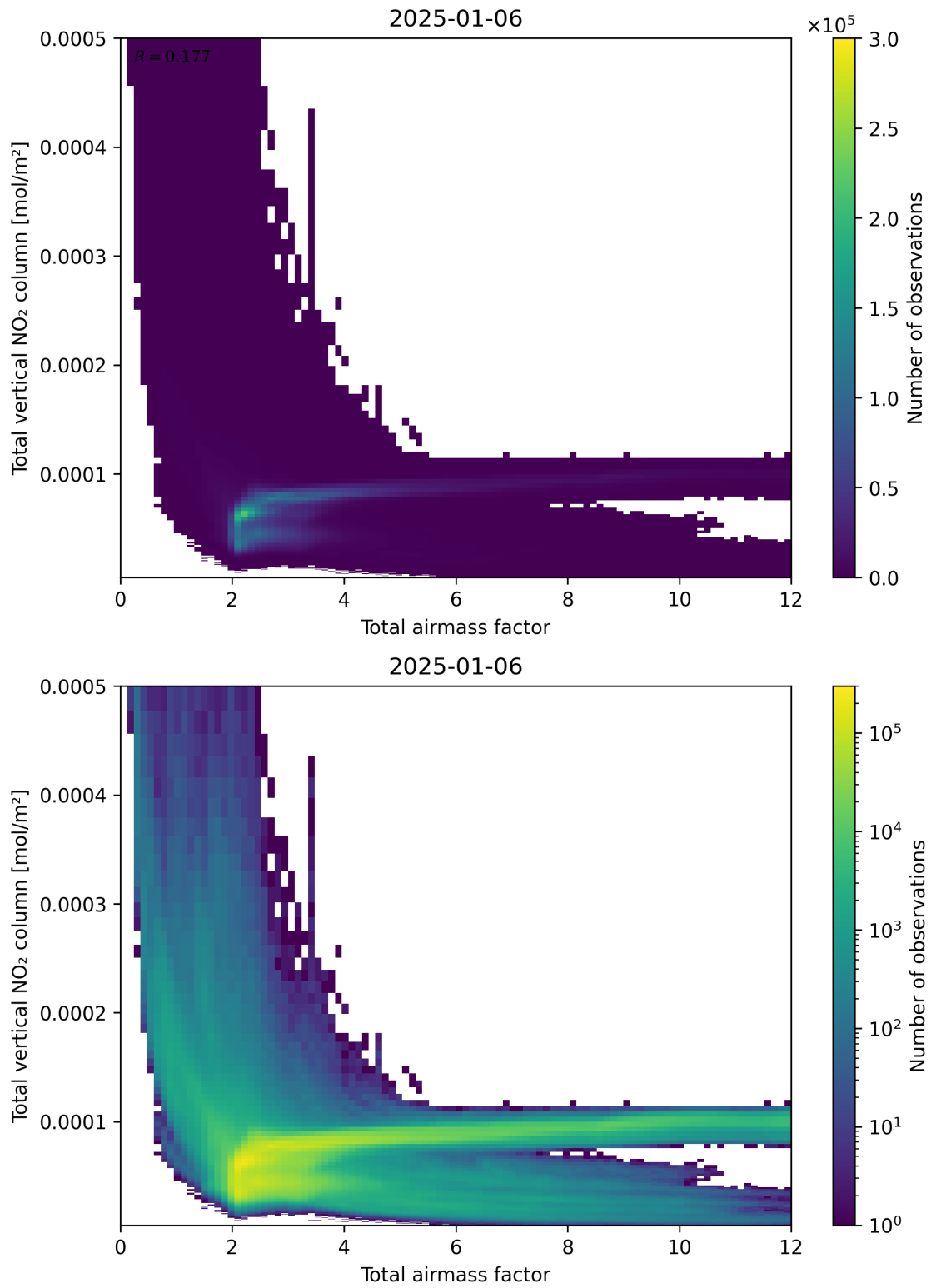
Figure 67: Scatter density plot of “Total airmass factor” against “Total vertical NO 2 column” for 2025-01-05 to 2025-01-07.
