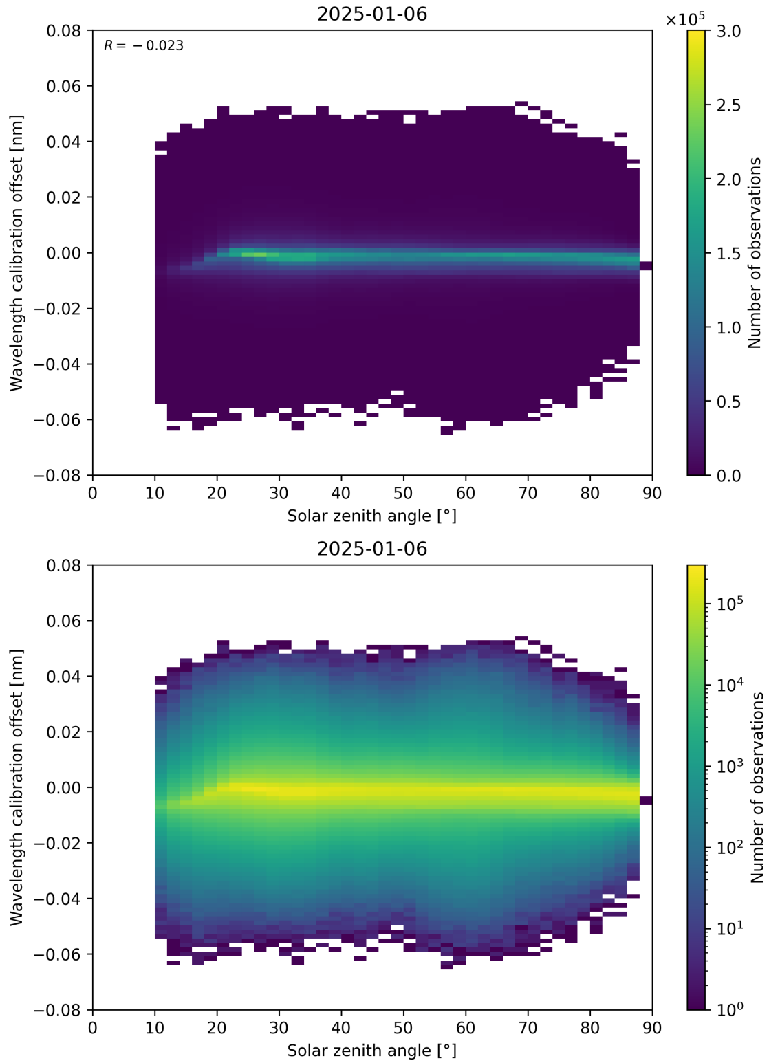
Figure 158: Scatter density plot of “Solar zenith angle” against “Wavelength calibration offset” for 2025-01-05 to 2025-01-07.
