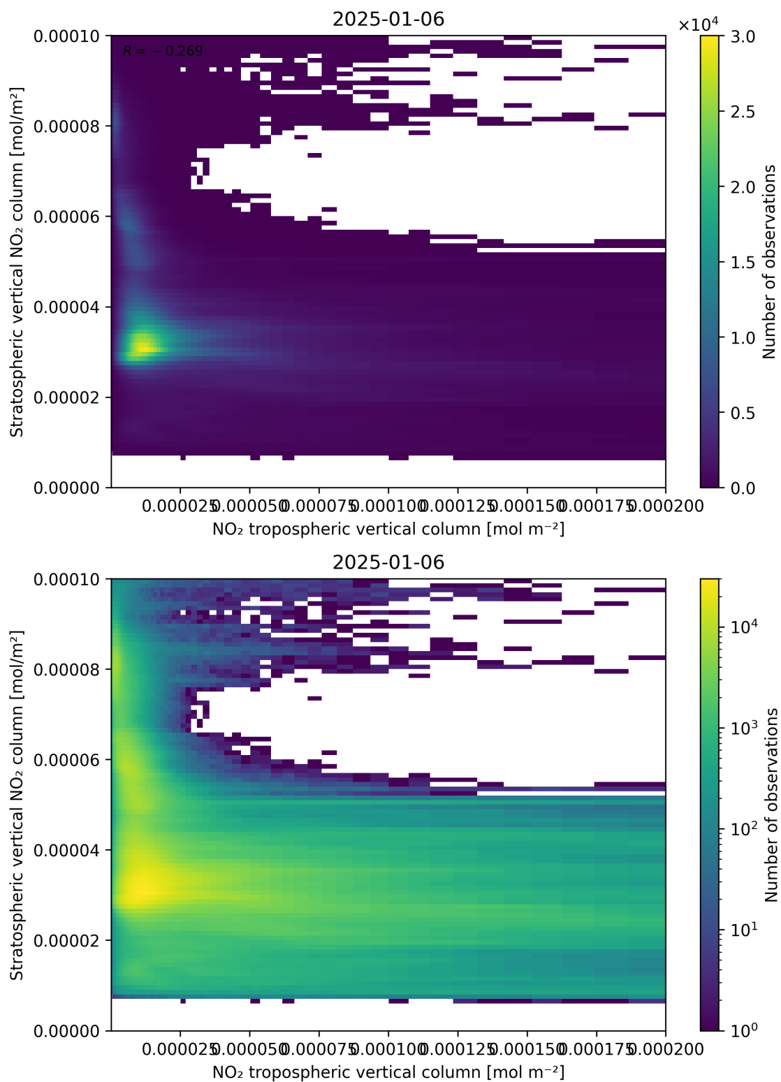
Figure 125: Scatter density plot of “NO 2 tropospheric vertical column” against “Stratospheric vertical NO 2 column” for 2025-01-05 to 2025-01-07.
