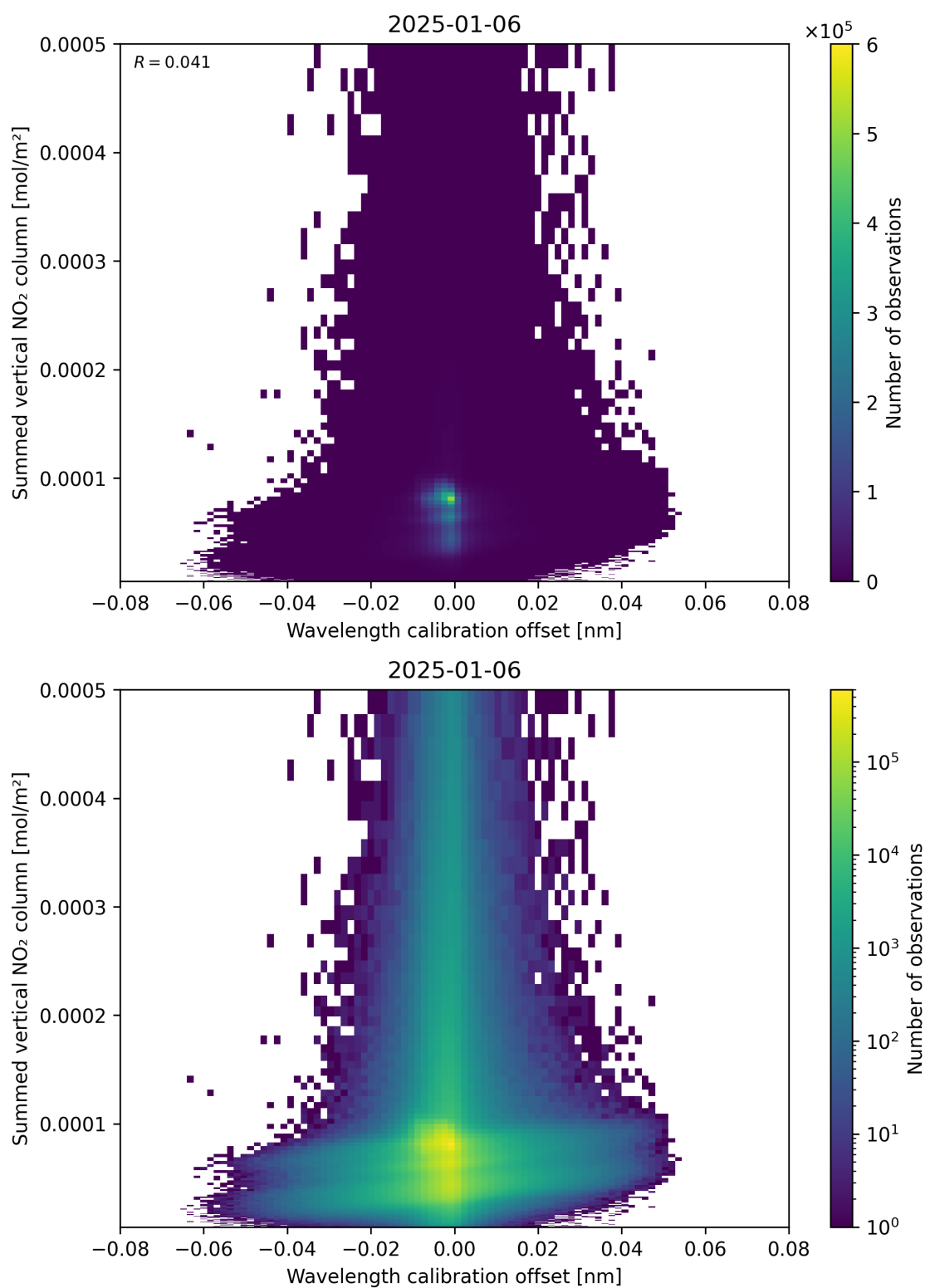
Figure 177: Scatter density plot of “Wavelength calibration offset” against “Summed vertical NO 2 column” for 2025-01-05 to 2025-01-07.
