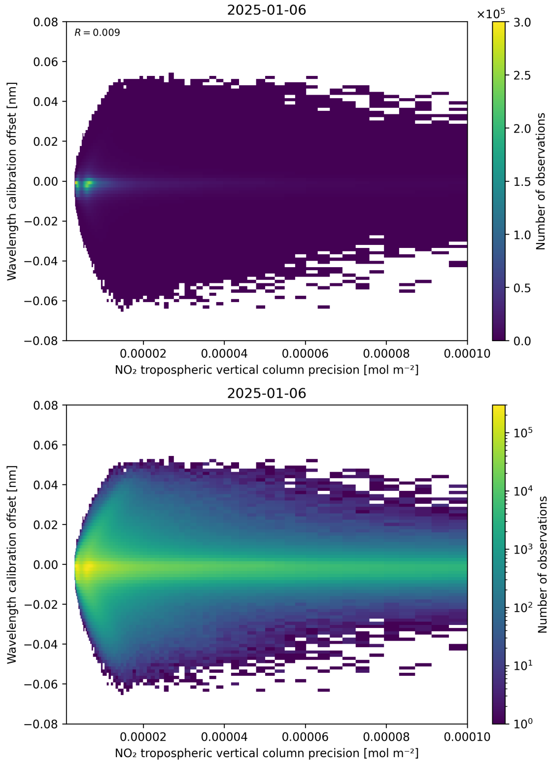
Figure 141: Scatter density plot of “NO 2 tropospheric vertical column precision” against “Wavelength calibration offset” for 2025-01-05 to 2025-01-07.
