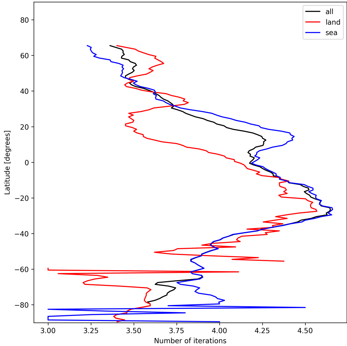
Figure 17: Zonal average of “Number of iterations” for 2025-01-05 to 2025-01-07.
