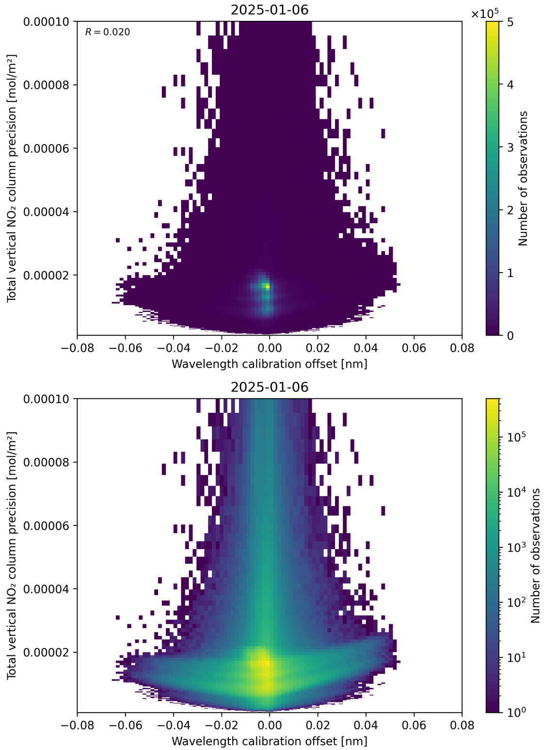
Figure 180: Scatter density plot of “Wavelength calibration offset” against “Total vertical NO 2 column precision” for 2025-01-05 to 2025-01-07.
