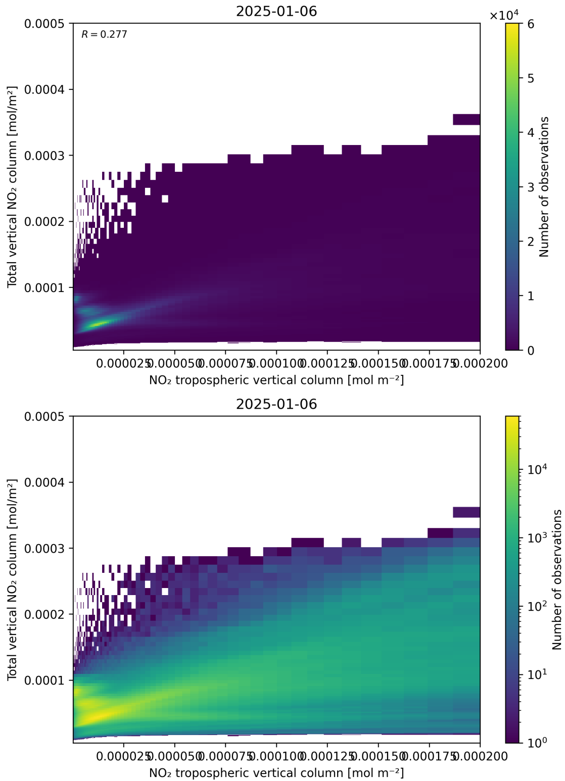
Figure 128: Scatter density plot of “NO 2 tropospheric vertical column” against “Total vertical NO 2 column” for 2025-01-05 to 2025-01-07.
