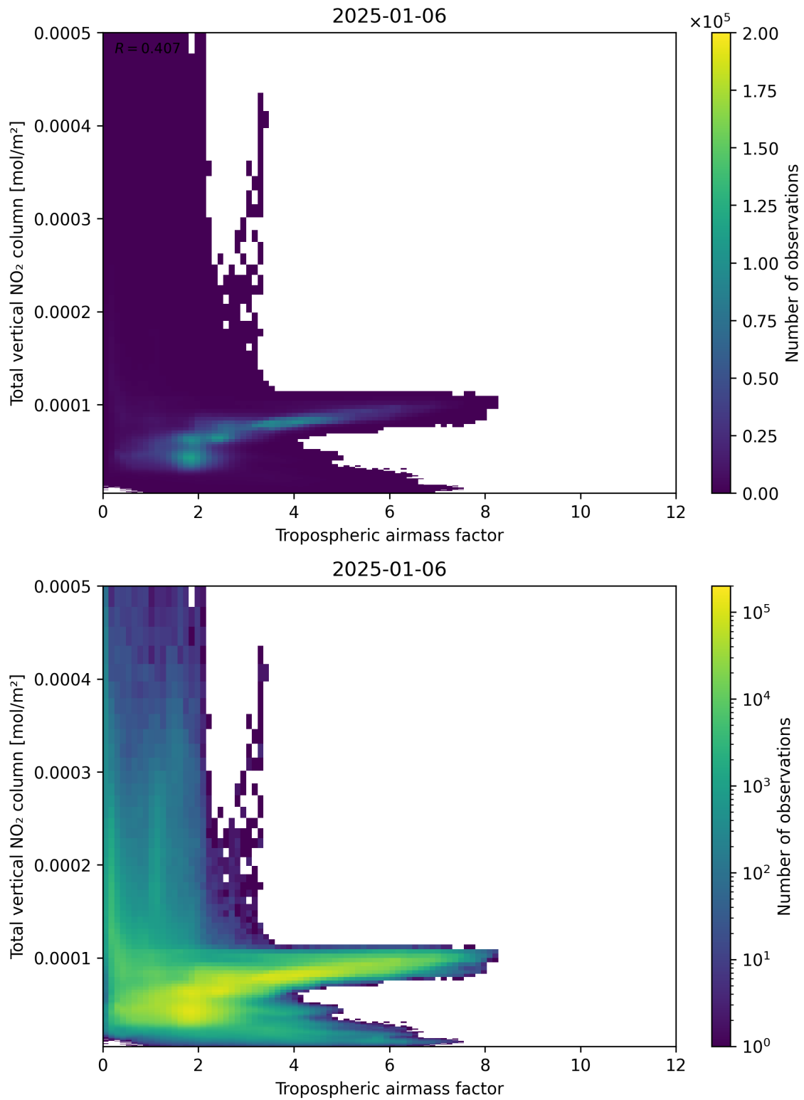
Figure 77: Scatter density plot of “Tropospheric airmass factor” against “Total vertical NO 2 column” for 2025-01-05 to 2025-01-07.
