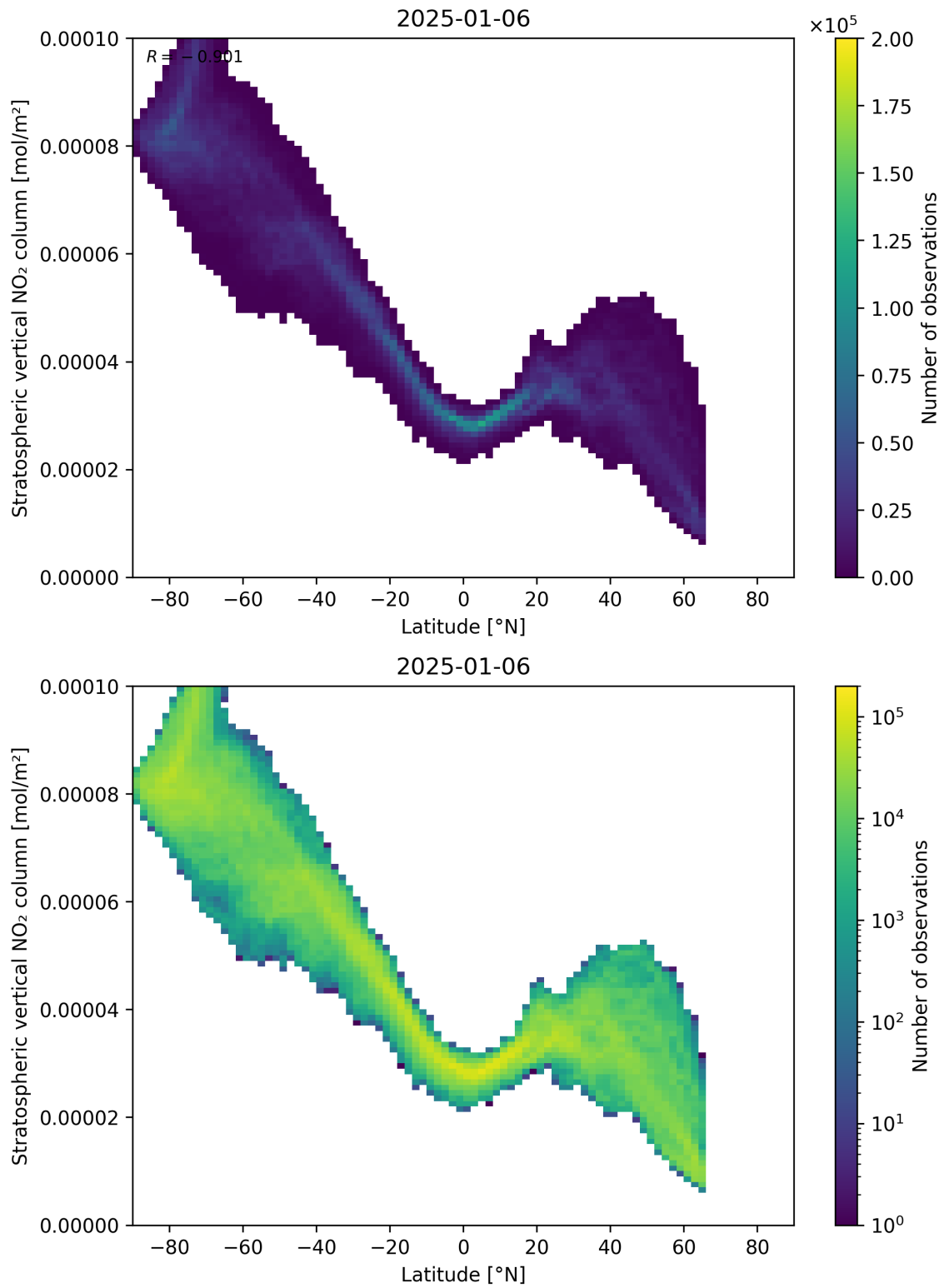
Figure 87: Scatter density plot of “Latitude” against “Stratospheric vertical NO 2 column” for 2025-01-05 to 2025-01-07.
