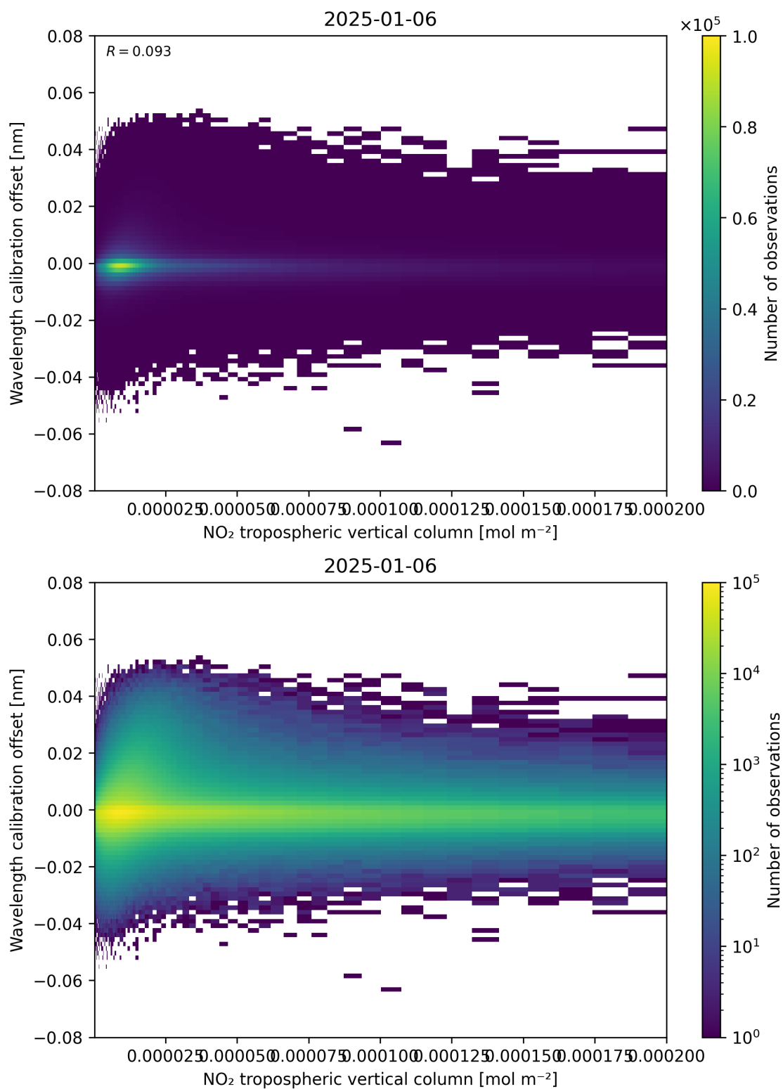
Figure 143: Scatter density plot of “NO 2 tropospheric vertical column” against “Wavelength calibration offset” for 2025-01-05 to 2025-01-07.
