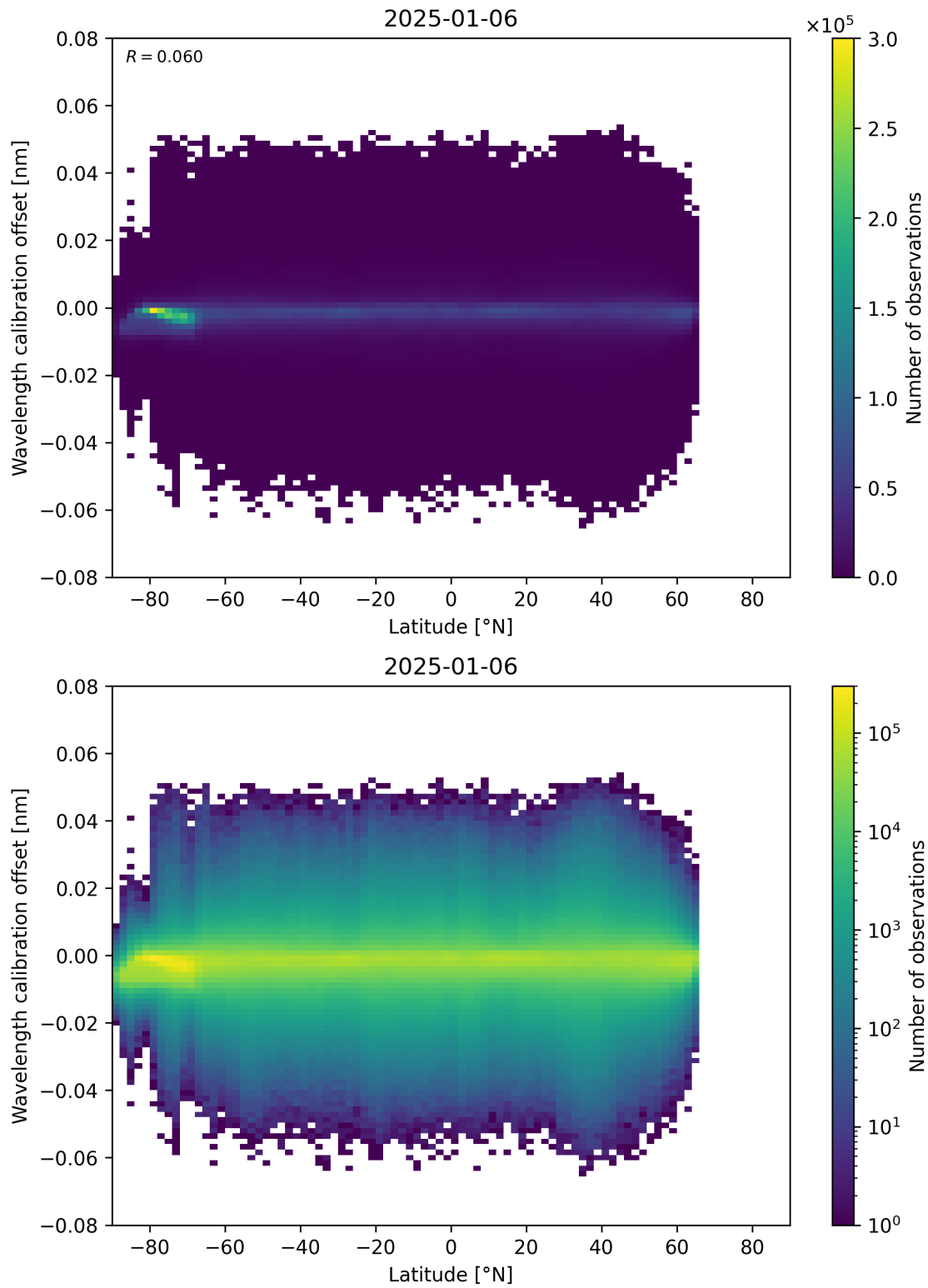
Figure 95: Scatter density plot of “Latitude” against “Wavelength calibration offset” for 2025-01-05 to 2025-01-07.
