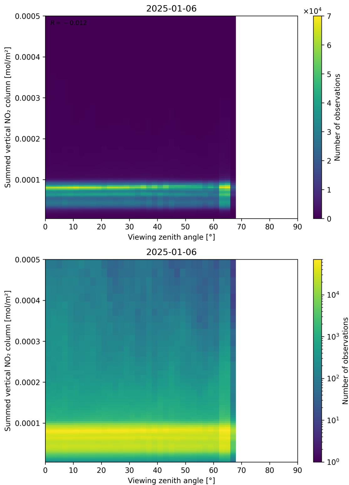
Figure 165: Scatter density plot of “Viewing zenith angle” against “Summed vertical NO 2 column” for 2025-01-05 to 2025-01-07.
