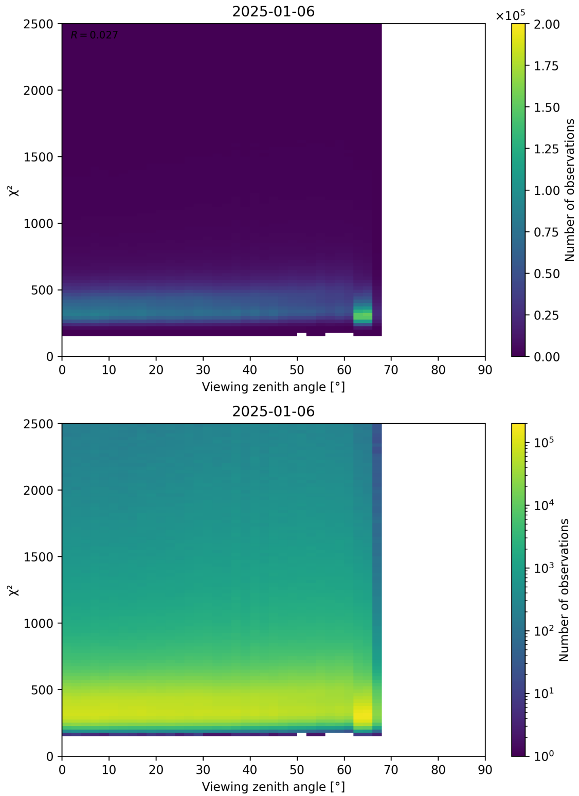
Figure 162: Scatter density plot of “Viewing zenith angle” against “ \chi^2 ” for 2025-01-05 to 2025-01-07.
