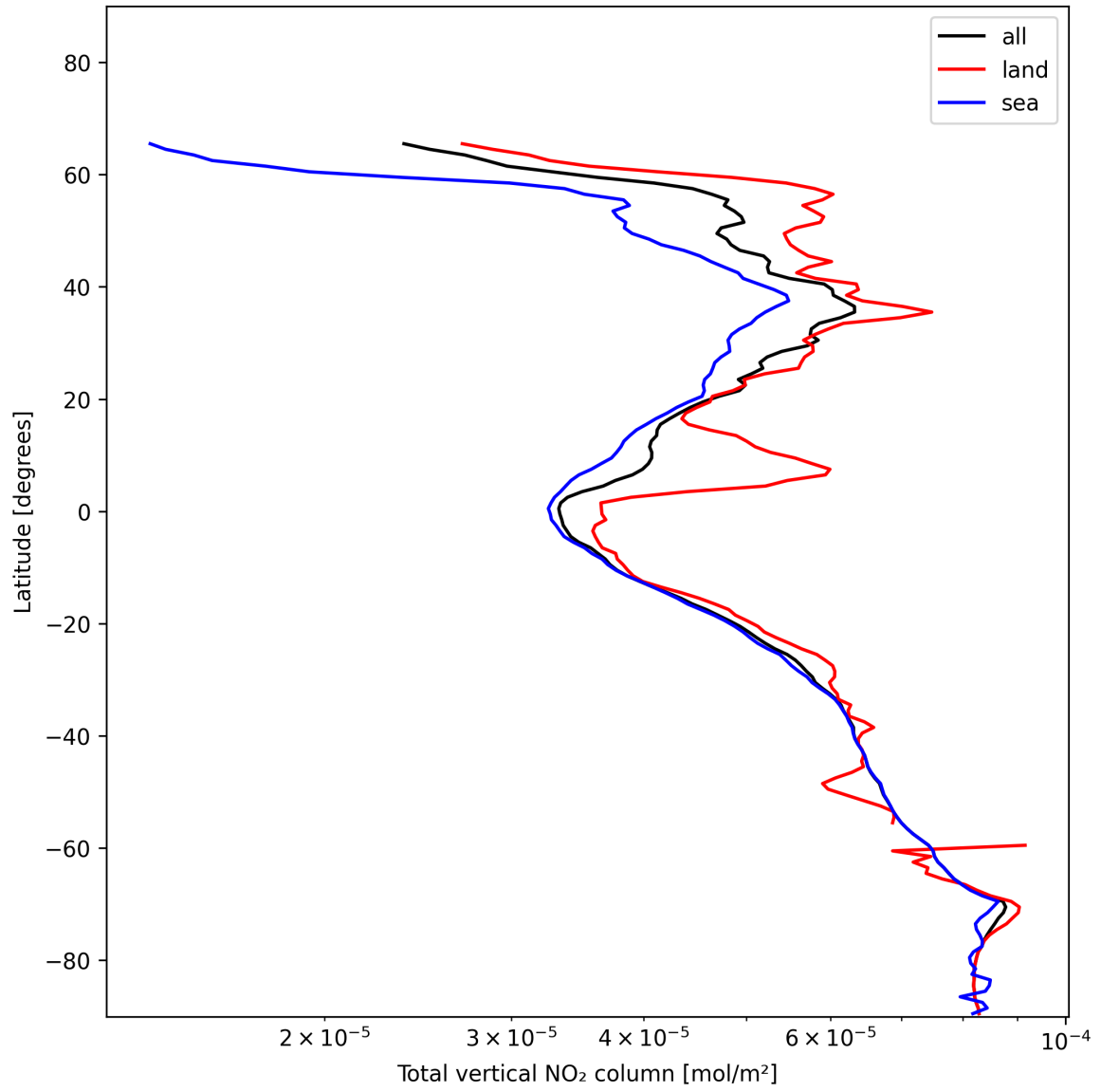
Figure 21: Zonal average of “Total vertical NO 2 column” for 2025-01-05 to 2025-01-07.
