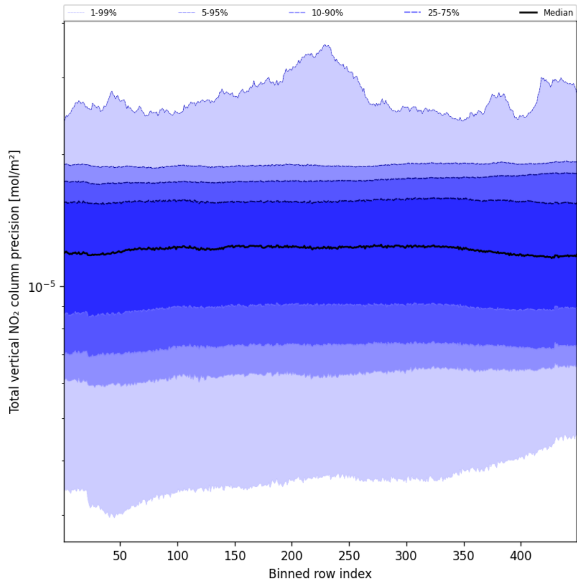
Figure 56: Along track statistics of “Total vertical NO 2 column precision” for 2025-01-05 to 2025-01-07
