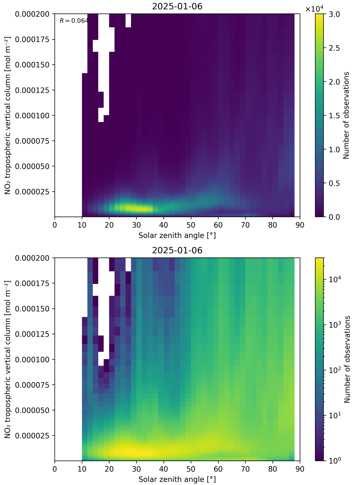
Figure 155: Scatter density plot of “Solar zenith angle” against “NO 2 tropospheric vertical column” for 2025-01-05 to 2025-01-07.
