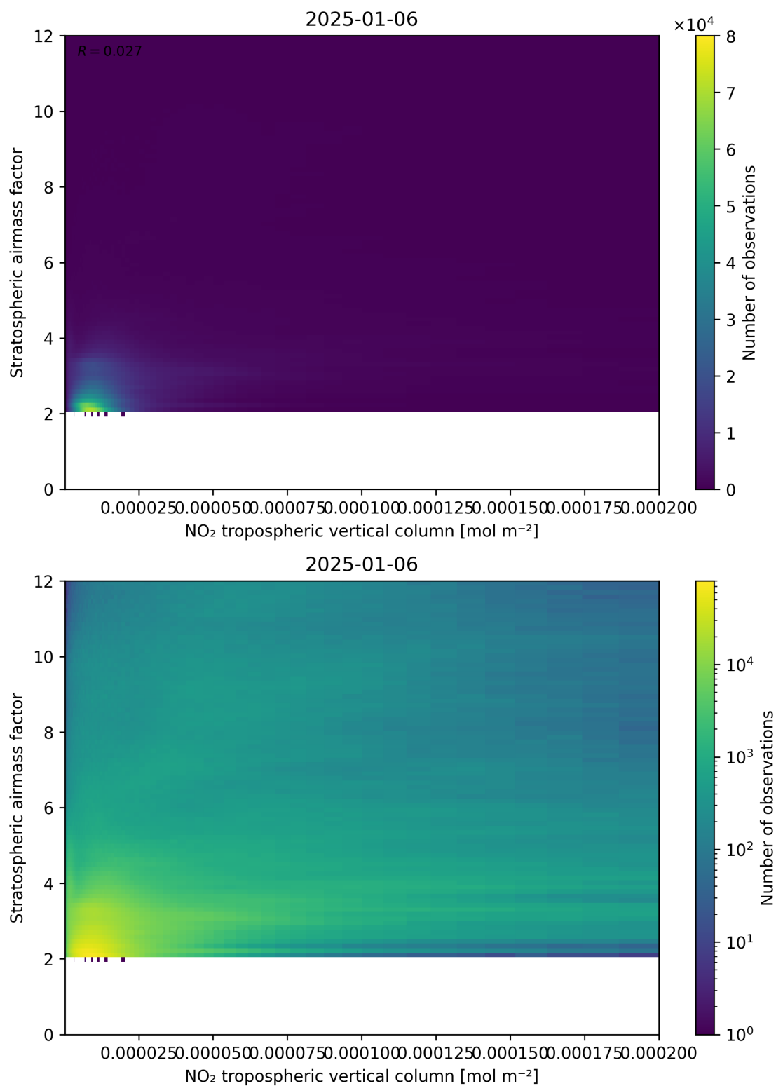
Figure 121: Scatter density plot of “NO 2 tropospheric vertical column” against “Stratospheric airmass factor” for 2025-01-05 to 2025-01-07.
