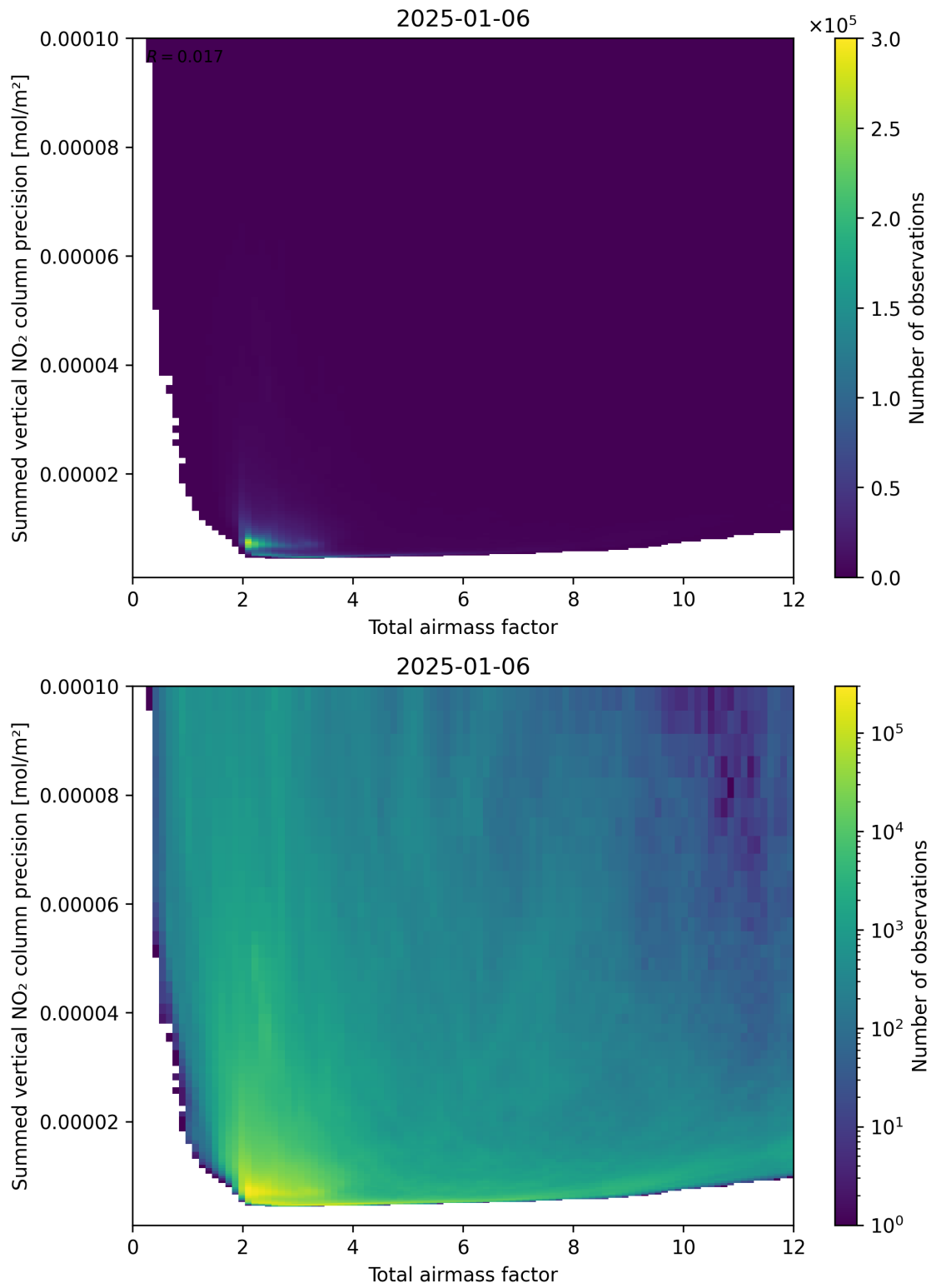
Figure 66: Scatter density plot of “Total airmass factor” against “Summed vertical NO 2 column precision” for 2025-01-05 to 2025-01-07.
