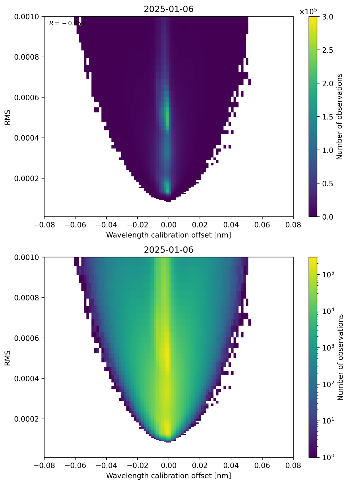
Figure 181: Scatter density plot of “Wavelength calibration offset” against “RMS” for 2025-01-05 to 2025-01-07.
