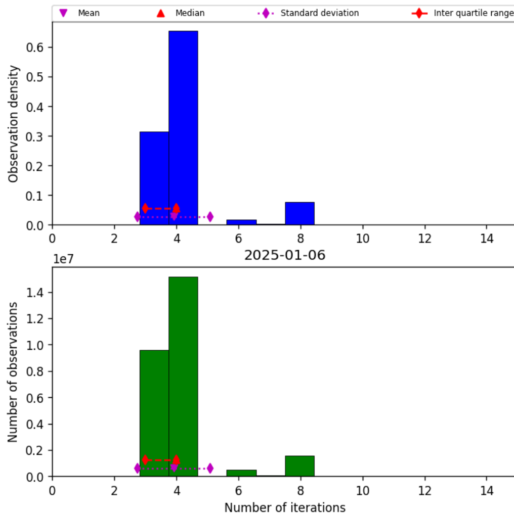
Figure 34: Histogram of “Number of iterations” for 2025-01-05 to 2025-01-07
