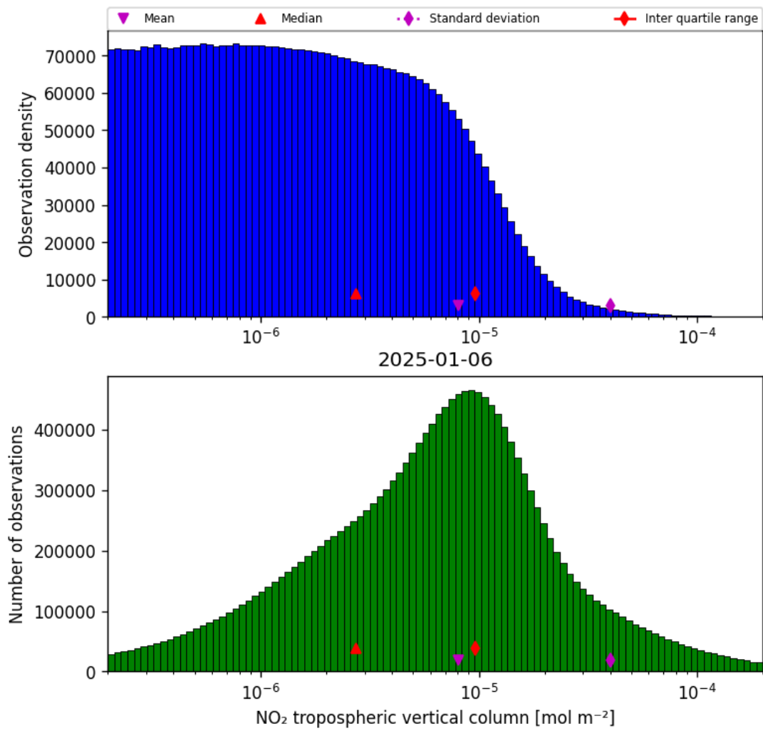
Figure 29: Histogram of “NO 2 tropospheric vertical column” for 2025-01-05 to 2025-01-07
