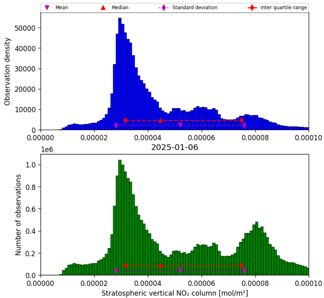
Figure 36: Histogram of “Stratospheric vertical NO 2 column” for 2025-01-05 to 2025-01-07
