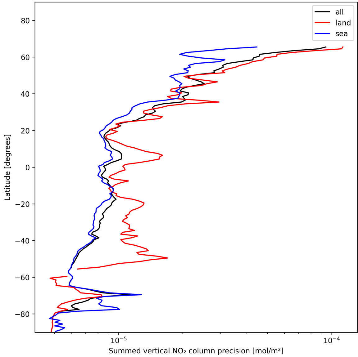
Figure 24: Zonal average of “Summed vertical NO 2 column precision” for 2025-01-05 to 2025-01-07.
