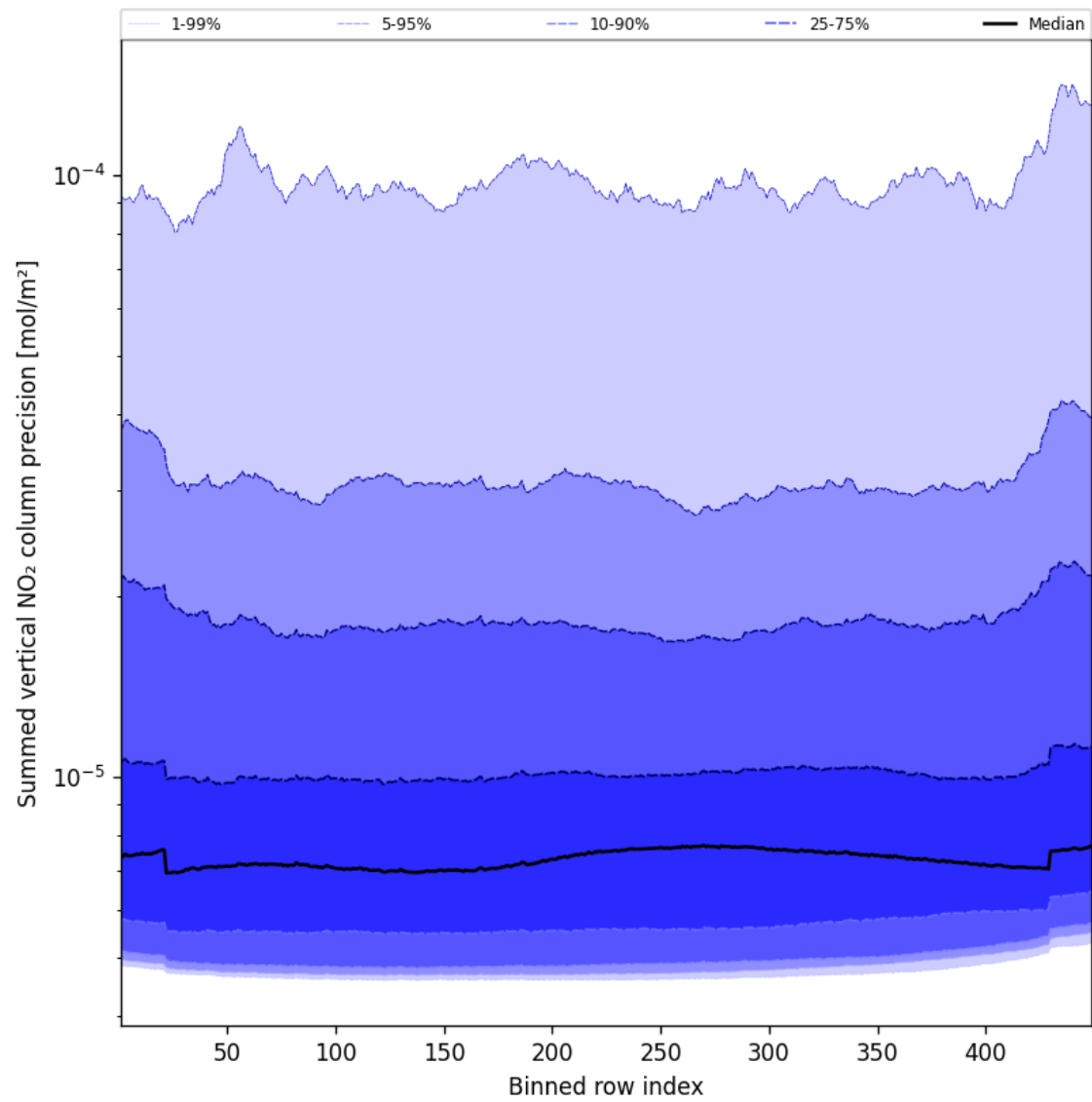
Figure 58: Along track statistics of “Summed vertical NO 2 column precision” for 2025-01-05 to 2025-01-07
