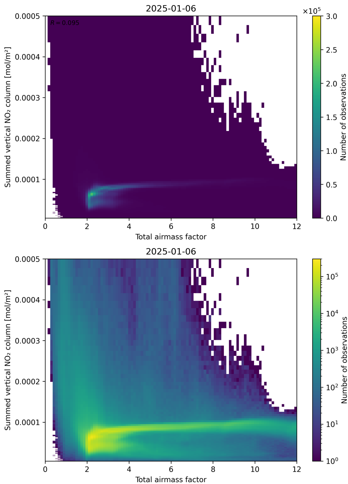
Figure 65: Scatter density plot of “Total airmass factor” against “Summed vertical NO 2 column” for 2025-01-05 to 2025-01-07.
