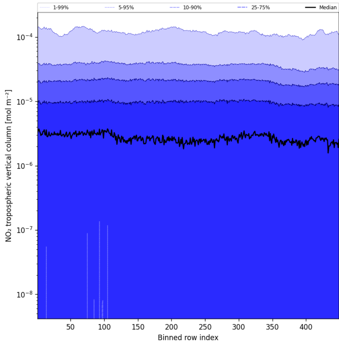
Figure 46: Along track statistics of “NO 2 tropospheric vertical column” for 2025-01-05 to 2025-01-07
