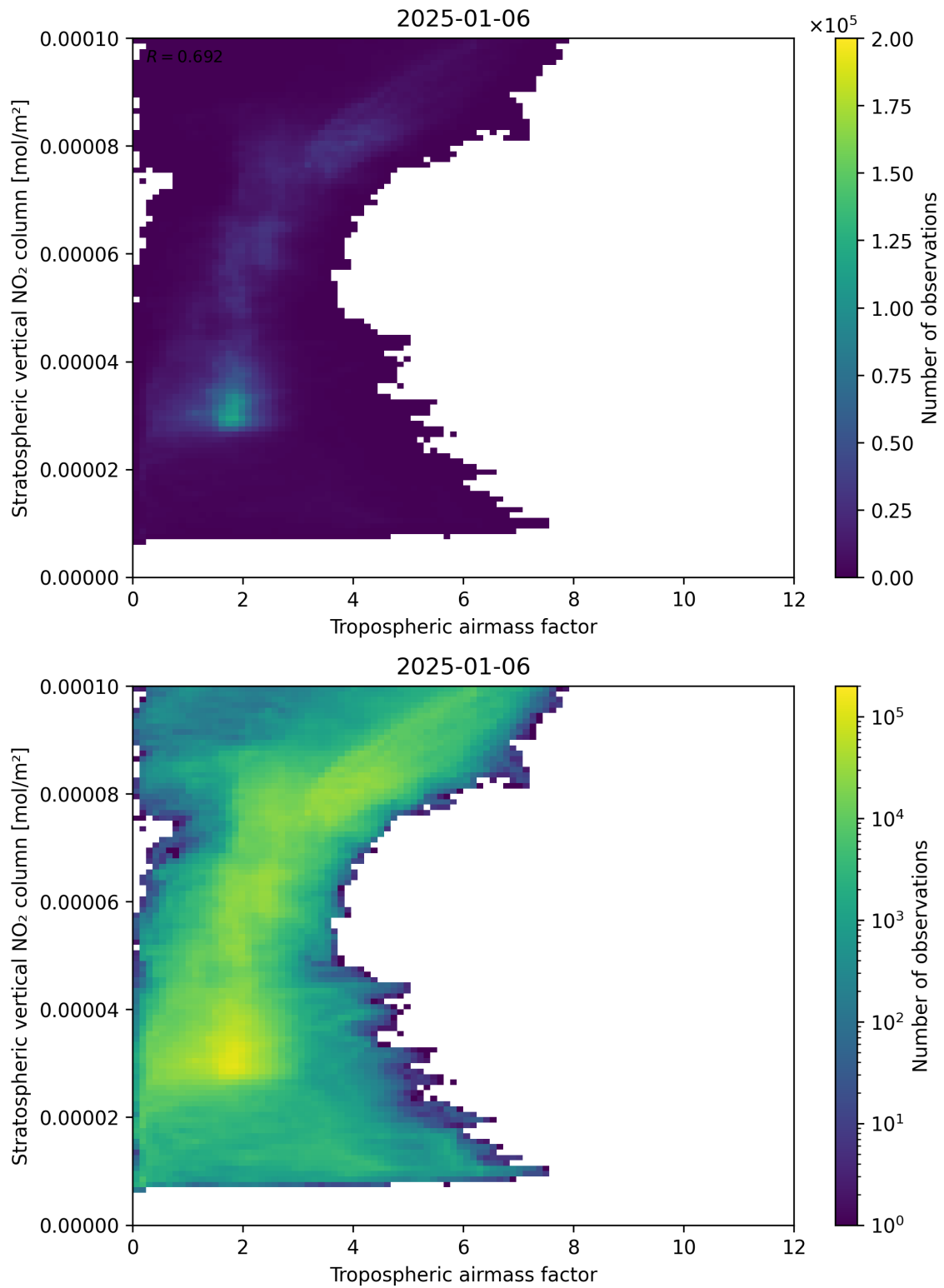
Figure 74: Scatter density plot of “Tropospheric air mass factor” against “Stratospheric vertical NO 2 column” for 2025-01-05 to 2025-01-07.
