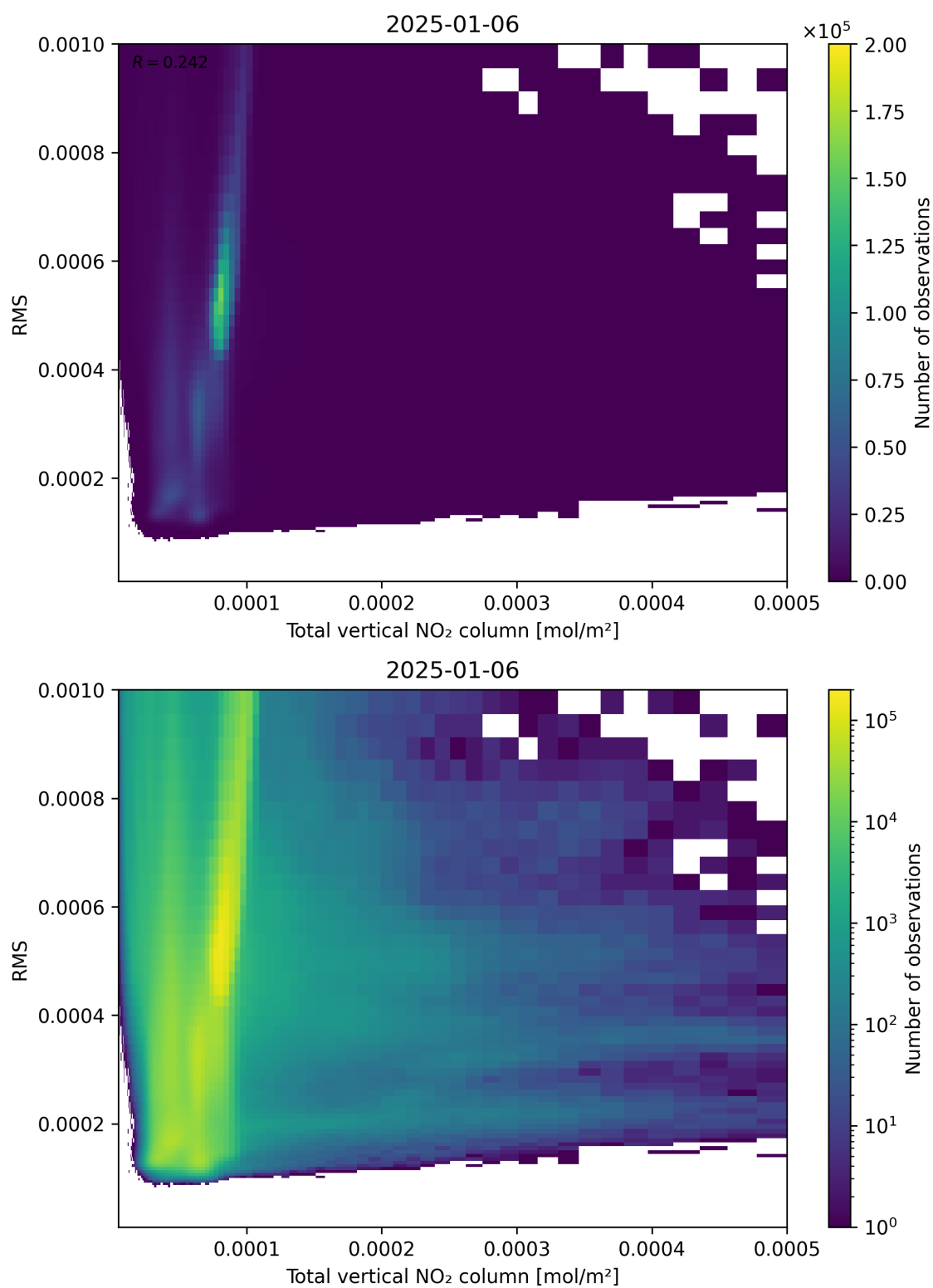
Figure 120: Scatter density plot of “Total vertical NO 2 column” against “RMS” for 2025-01-05 to 2025-01-07.
