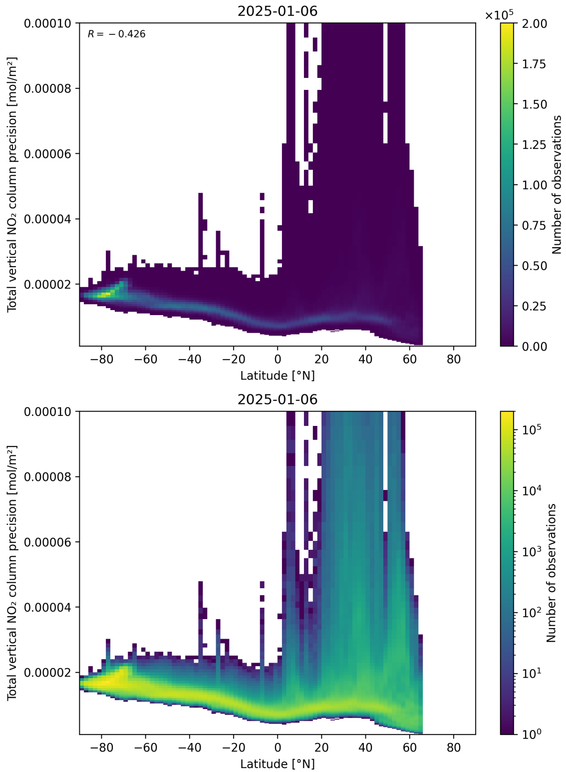
Figure 91: Scatter density plot of “Latitude” against “Total vertical NO 2 column precision” for 2025-01-05 to 2025-01-07.
