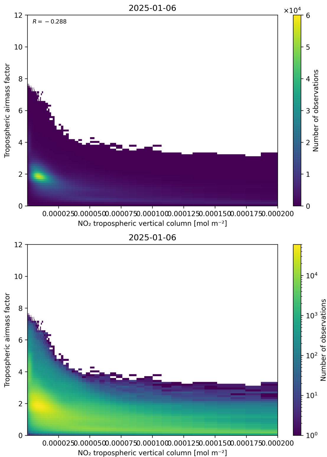
Figure 123: Scatter density plot of “NO 2 tropospheric vertical column” against “Tropospheric air mass factor” for 2025-01-05 to 2025-01-07.
