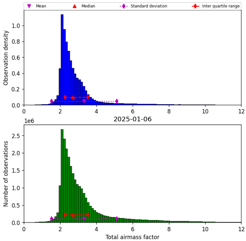
Figure 32: Histogram of “Total airmass factor” for 2025-01-05 to 2025-01-07
