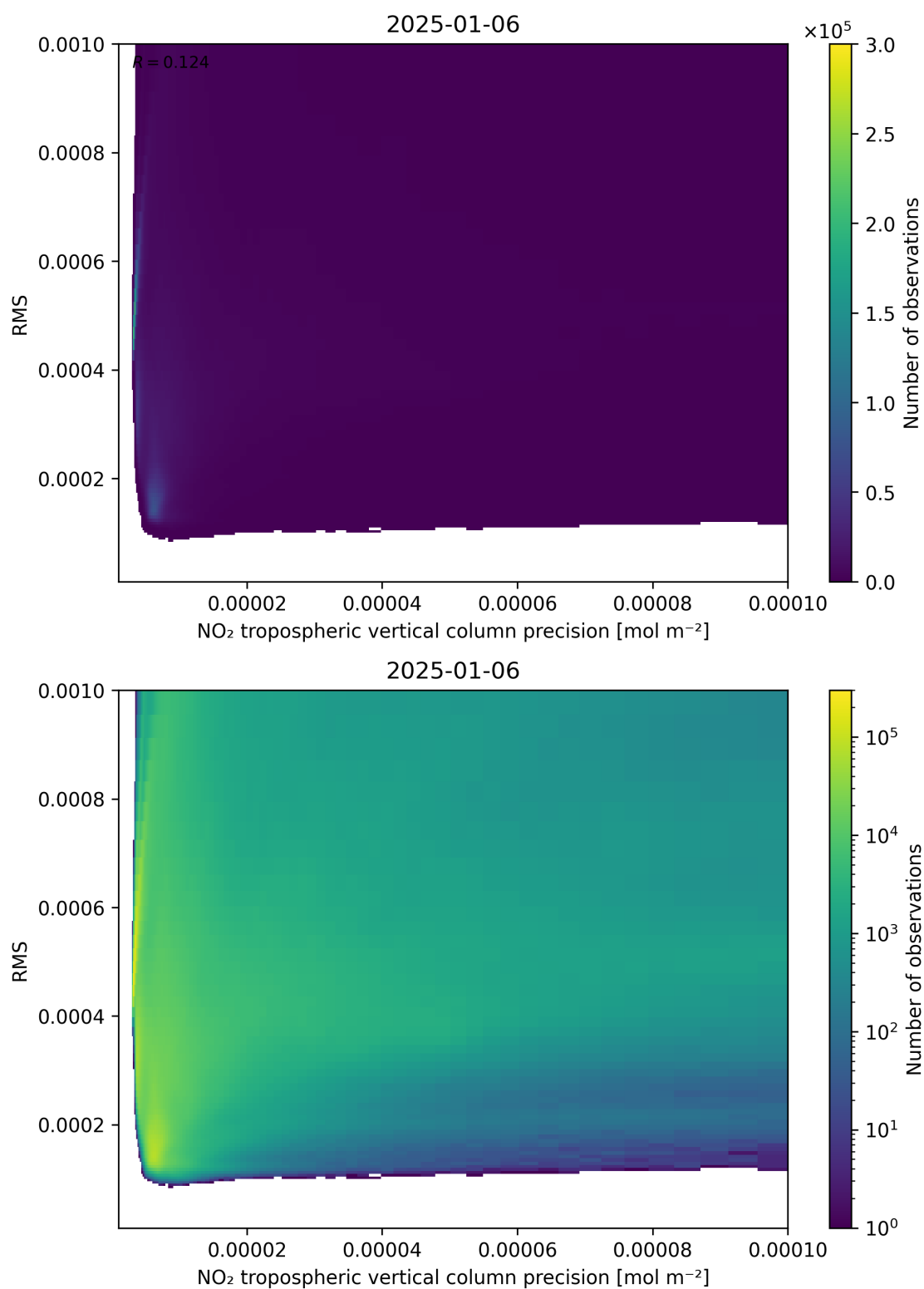
Figure 140: Scatter density plot of “NO 2 tropospheric vertical column precision” against “RMS” for 2025-01-05 to 2025-01-07.
