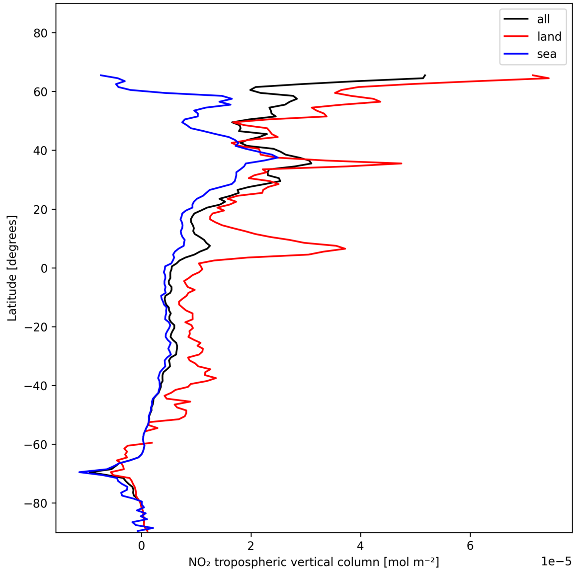
Figure 12: Zonal average of “NO 2 tropospheric vertical column” for 2025-01-05 to 2025-01-07.
