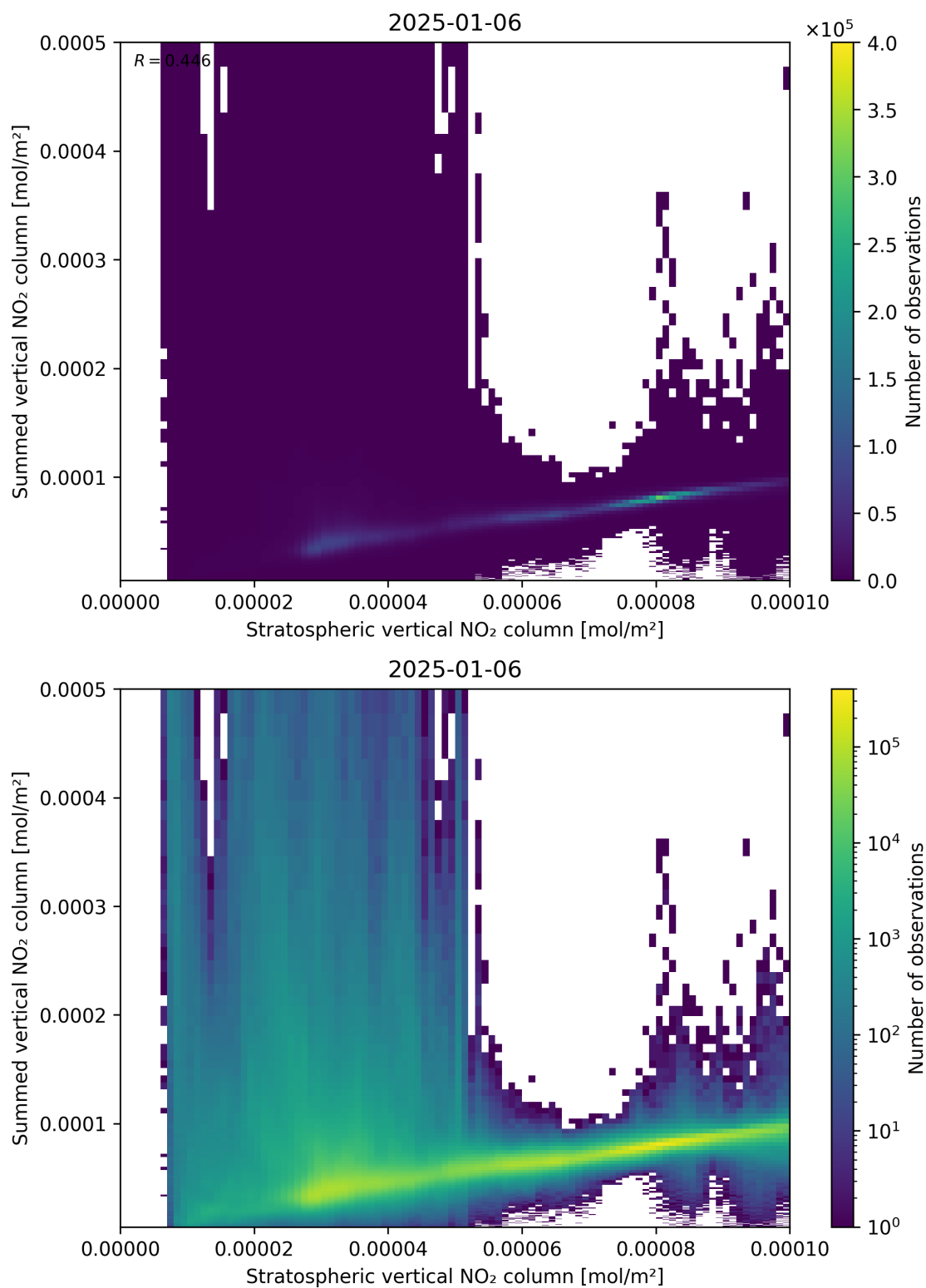
Figure 98: Scatter density plot of “Stratospheric vertical NO 2 column” against “Summed vertical NO 2 column” for 2025-01-05 to 2025-01-07.
