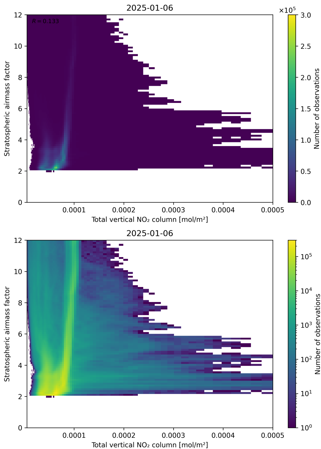
Figure 110: Scatter density plot of “Total vertical NO 2 column” against “Stratospheric airmass factor” for 2025-01-05 to 2025-01-07.
