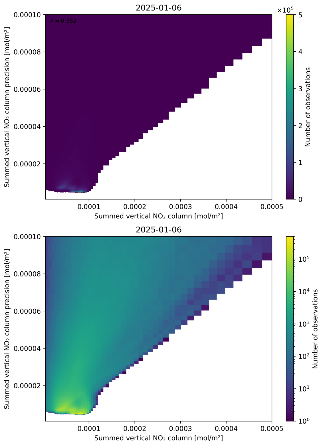
Figure 105: Scatter density plot of “Summed vertical NO 2 column” against “Summed vertical NO 2 column precision” for 2025-01-05 to 2025-01-07.
