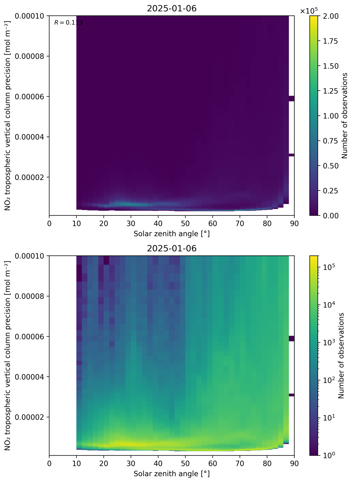
Figure 156: Scatter density plot of “Solar zenith angle” against “NO 2 tropospheric vertical column precision” for 2025-01-05 to 2025-01-07.
