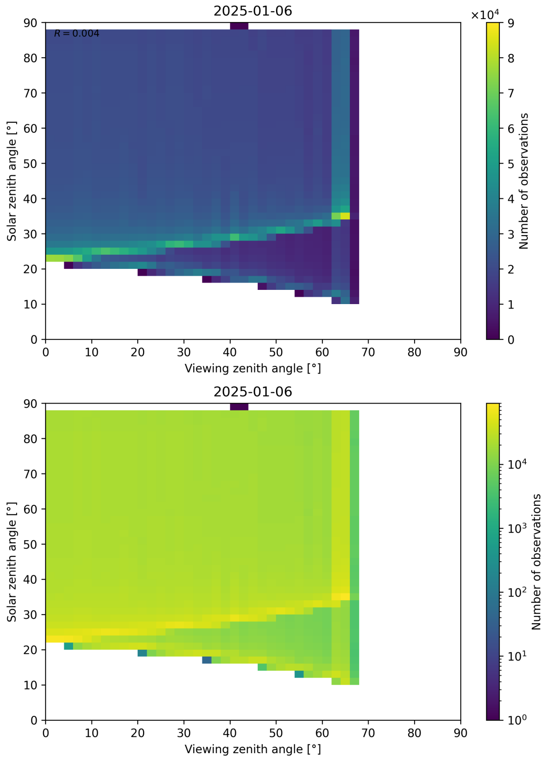
Figure 172: Scatter density plot of “Viewing zenith angle” against “Solar zenith angle” for 2025-01-05 to 2025-01-07.
