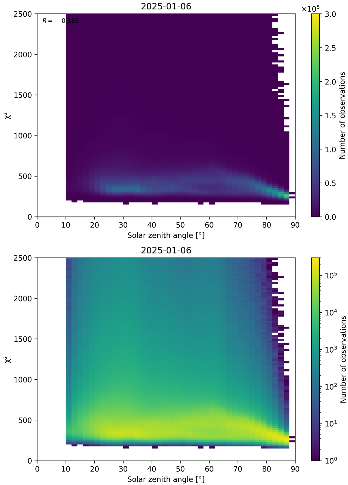
Figure 148: Scatter density plot of “Solar zenith angle” against “ \chi^2 ” for 2025-01-05 to 2025-01-07.
