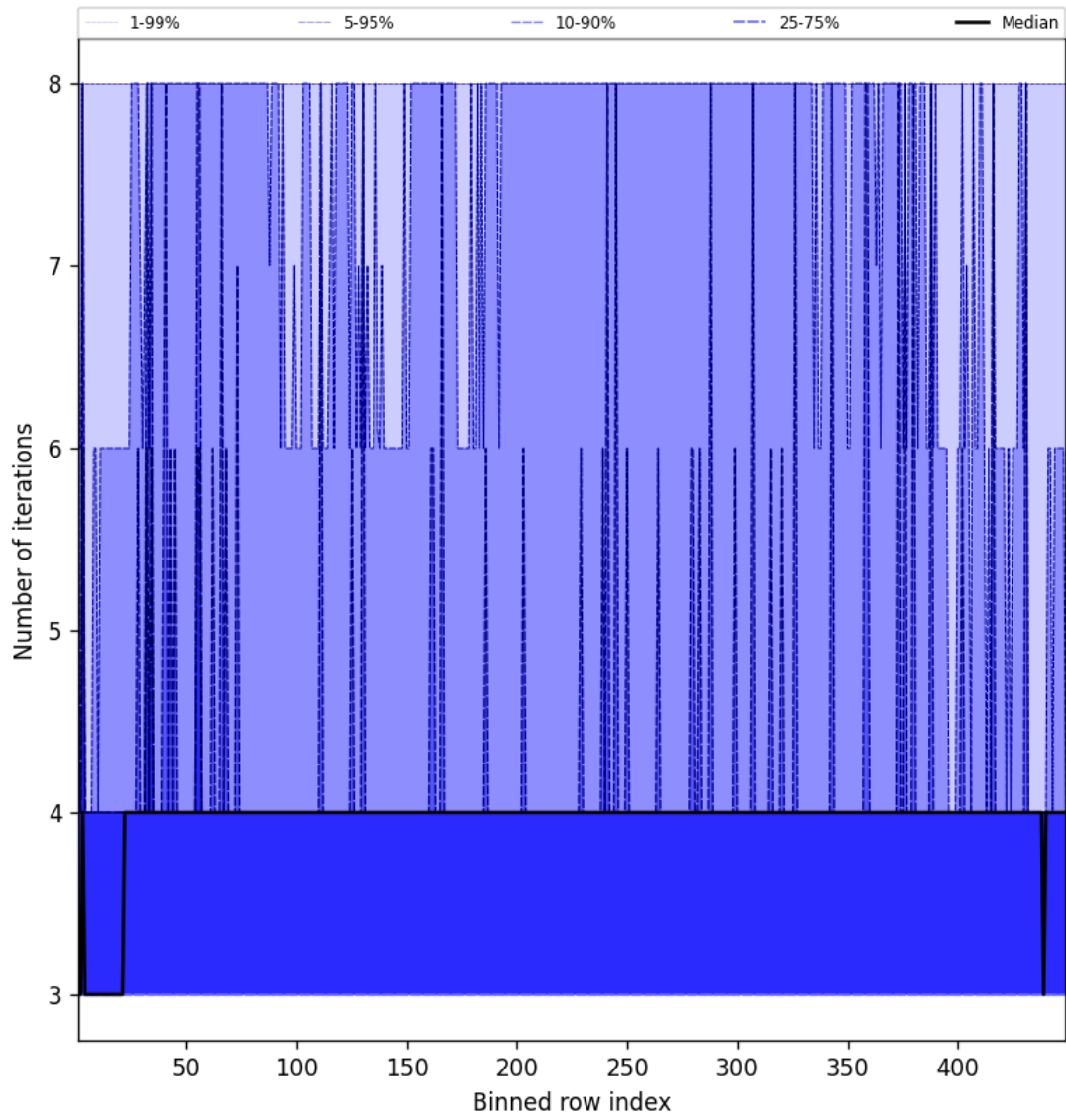
Figure 51: Along track statistics of “Number of iterations” for 2025-01-05 to 2025-01-07
