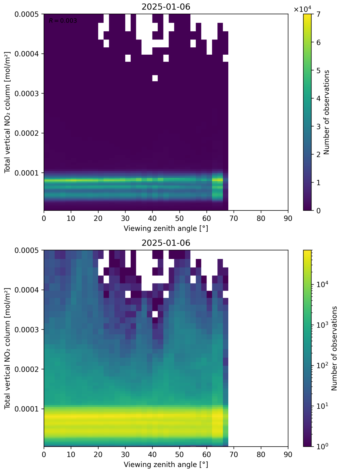
Figure 167: Scatter density plot of “Viewing zenith angle” against “Total vertical NO 2 column” for 2025-01-05 to 2025-01-07.
