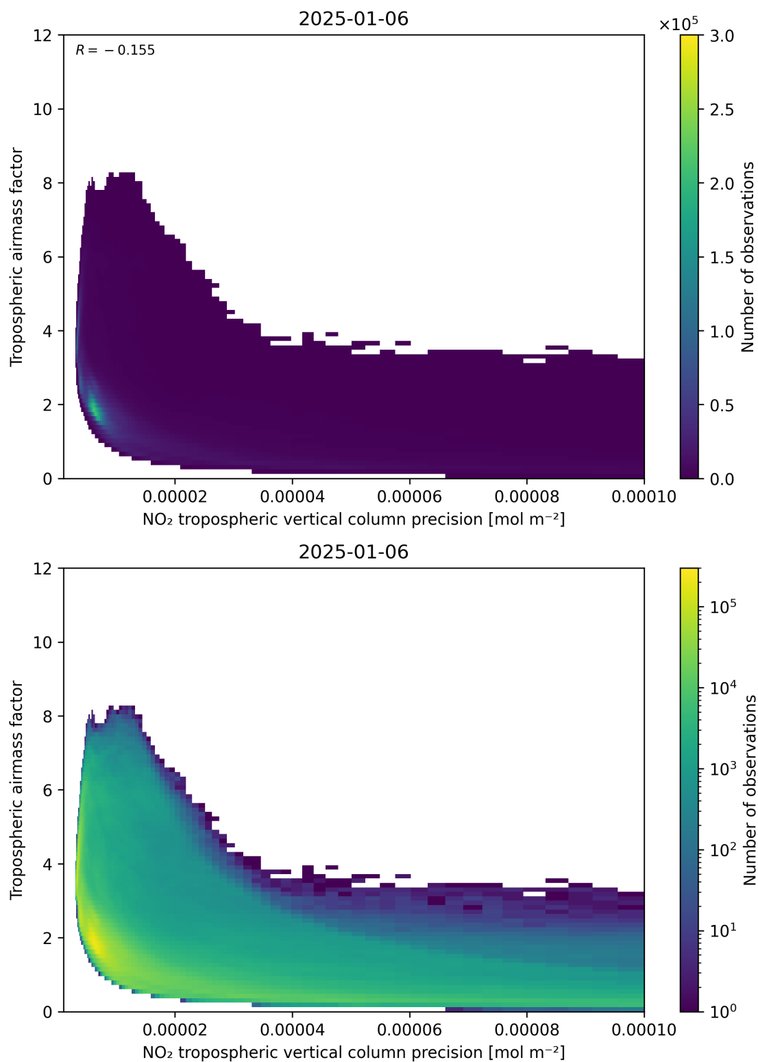
Figure 133: Scatter density plot of “NO 2 tropospheric vertical column precision” against “Tropospheric air mass factor” for 2025-01-05 to 2025-01-07.
