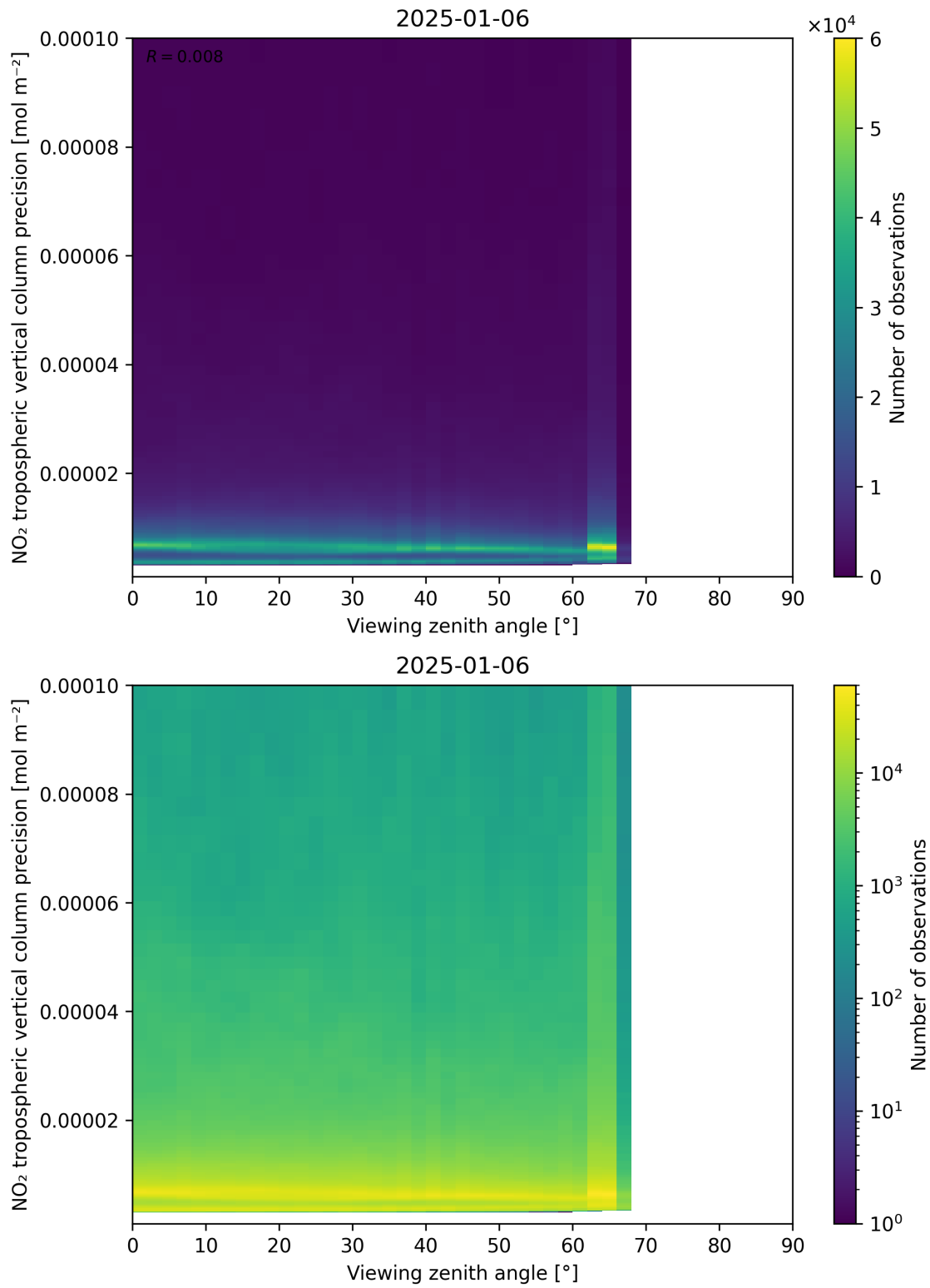
Figure 170: Scatter density plot of “Viewing zenith angle” against “NO 2 tropospheric vertical column precision” for 2025-01-05 to 2025-01-07.
