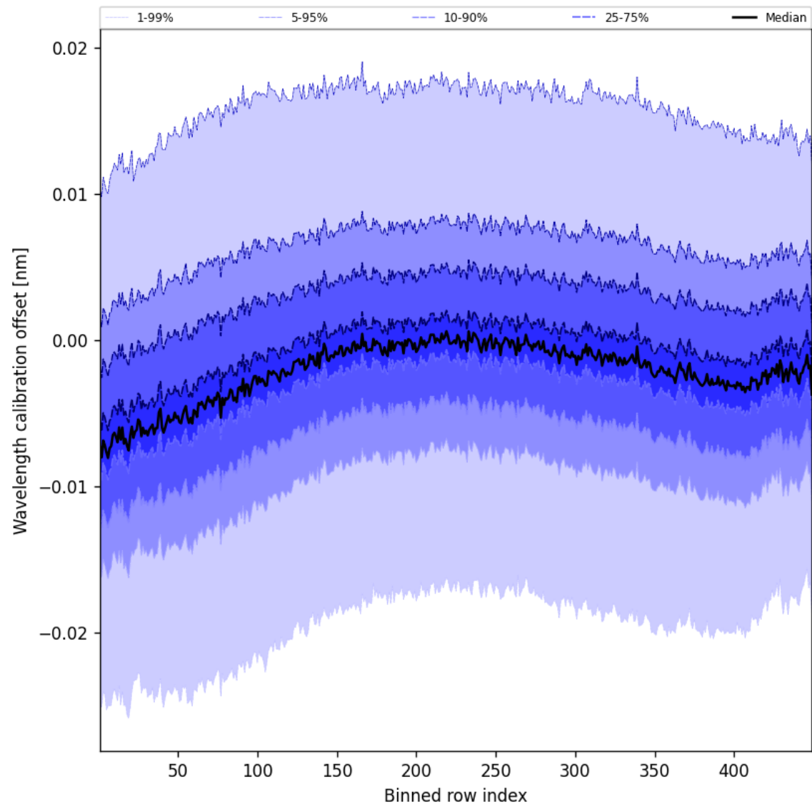
Figure 52: Along track statistics of “Wavelength calibration offset” for 2025-01-05 to 2025-01-07
