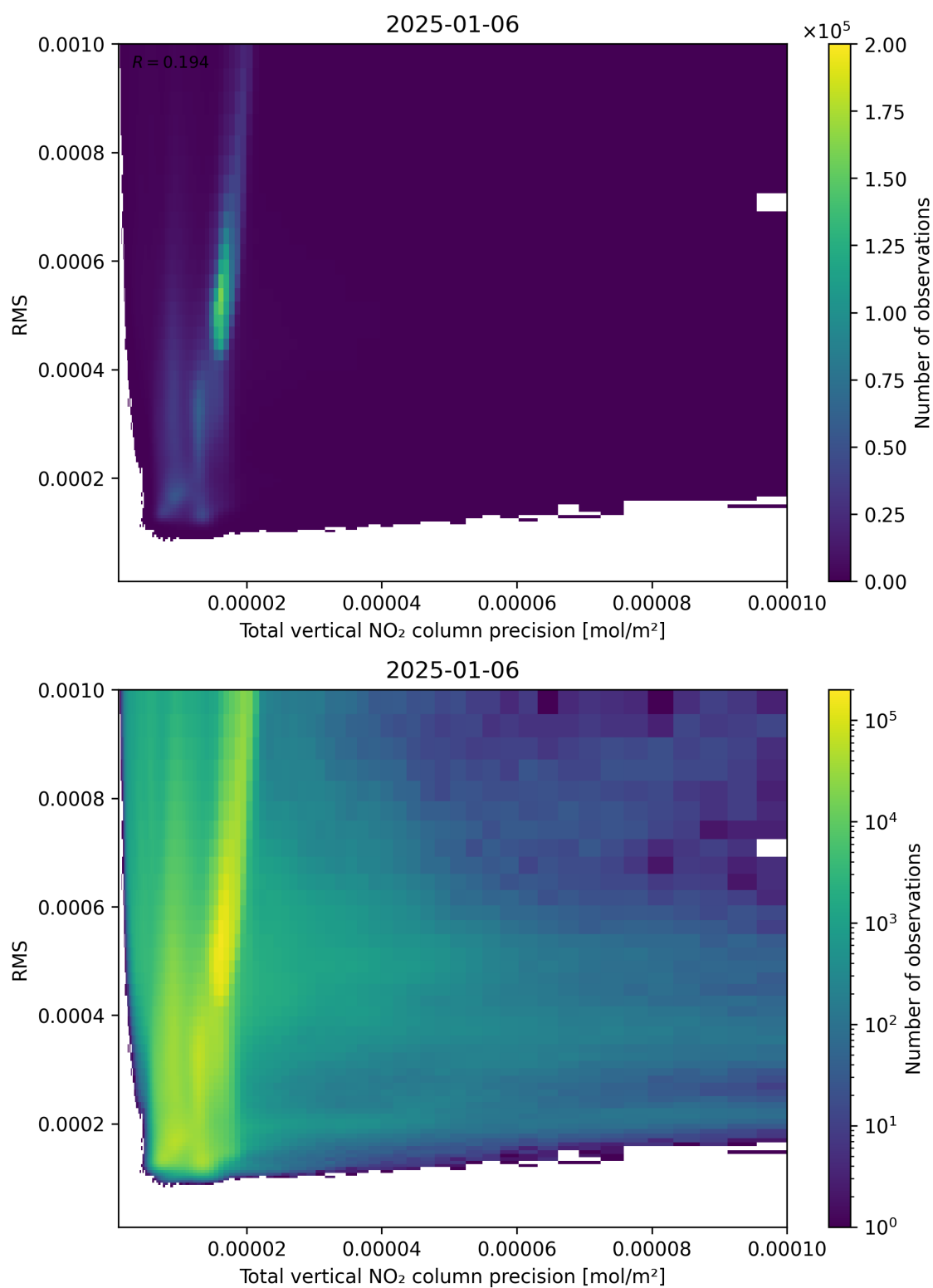
Figure 119: Scatter density plot of “Total vertical NO 2 column precision” against “RMS” for 2025-01-05 to 2025-01-07.
