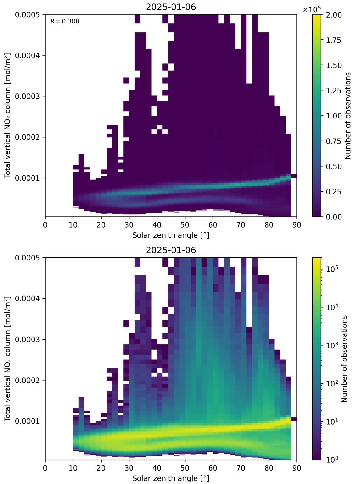
Figure 153: Scatter density plot of “Solar zenith angle” against “Total vertical NO 2 column” for 2025-01-05 to 2025-01-07.
