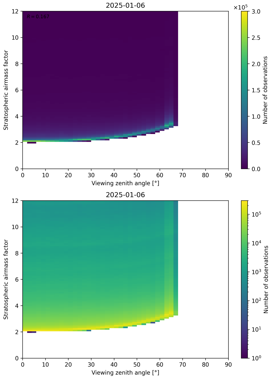
Figure 159: Scatter density plot of “Viewing zenith angle” against “Stratospheric airmass factor” for 2025-01-05 to 2025-01-07.
