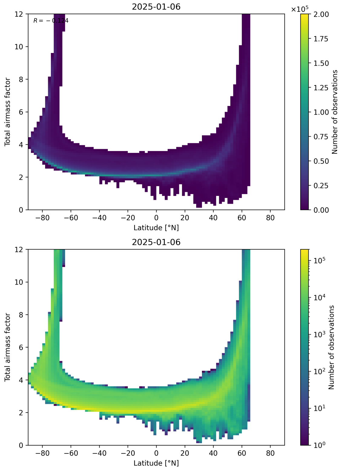
Figure 84: Scatter density plot of “Latitude” against “Total airmass factor” for 2025-01-05 to 2025-01-07.
