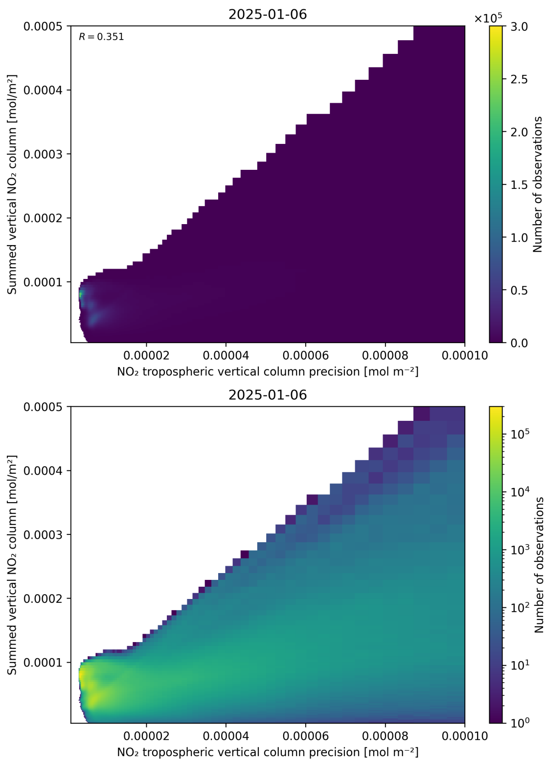
Figure 136: Scatter density plot of “NO 2 tropospheric vertical column precision” against “Summed vertical NO 2 column” for 2025-01-05 to 2025-01-07.
