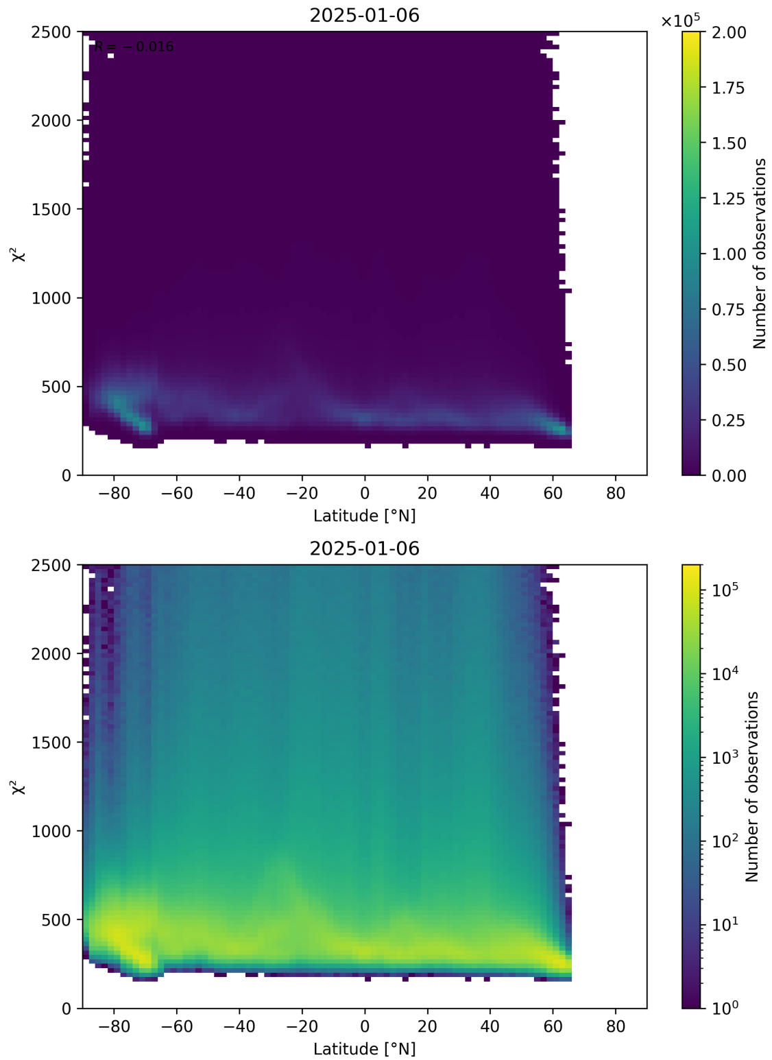
Figure 86: Scatter density plot of “Latitude” against “ \chi^2 ” for 2025-01-05 to 2025-01-07.
