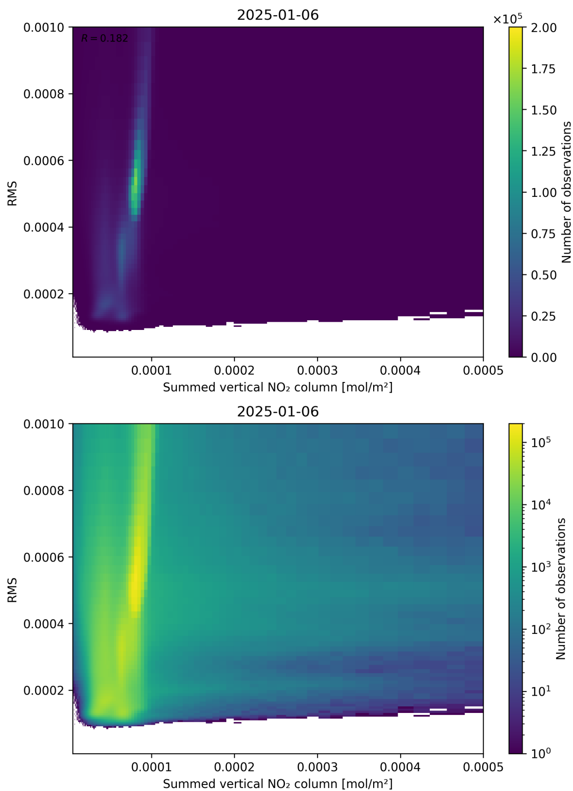
Figure 109: Scatter density plot of “Summed vertical NO 2 column” against “RMS” for 2025-01-05 to 2025-01-07.
