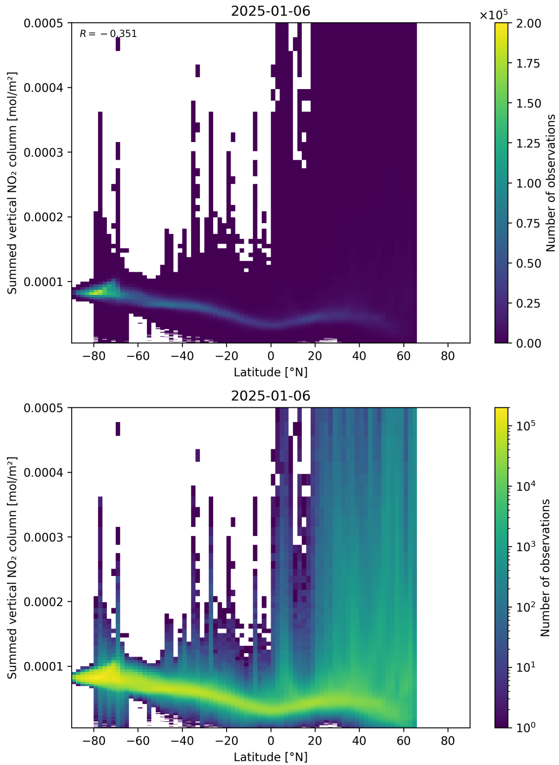
Figure 88: Scatter density plot of “Latitude” against “Summed vertical NO 2 column” for 2025-01-05 to 2025-01-07.
