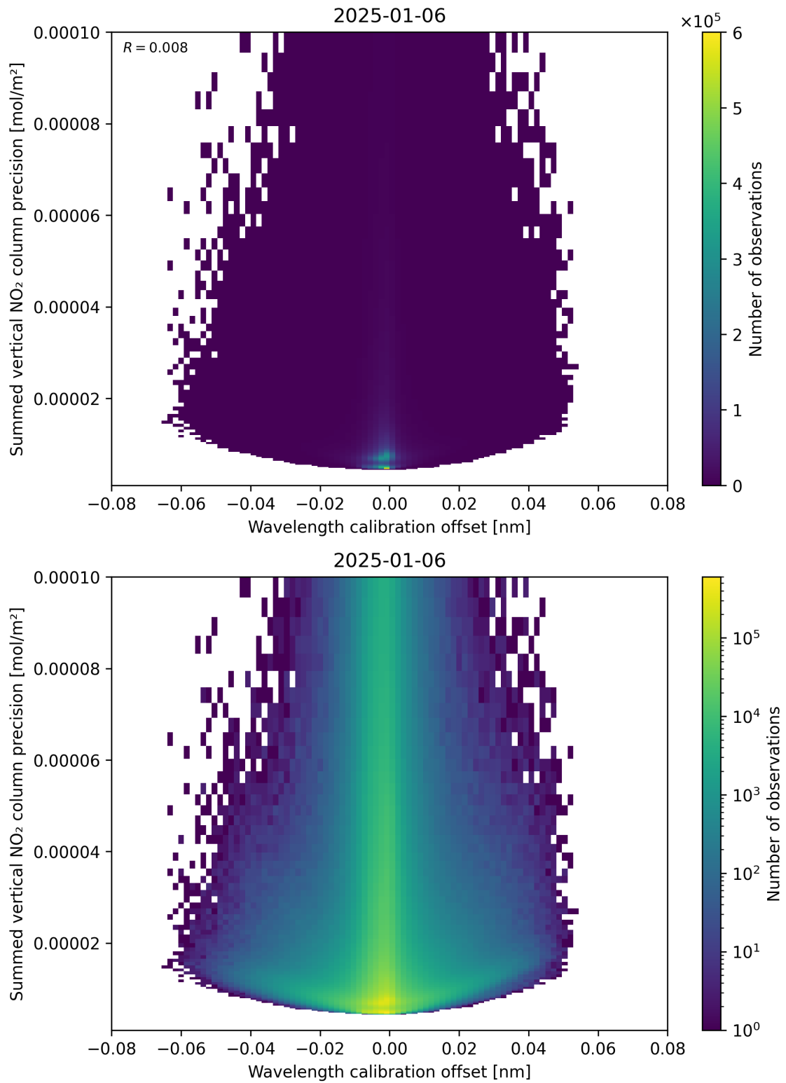
Figure 178: Scatter density plot of “Wavelength calibration offset” against “Summed vertical NO 2 column precision” for 2025-01-05 to 2025-01-07.
