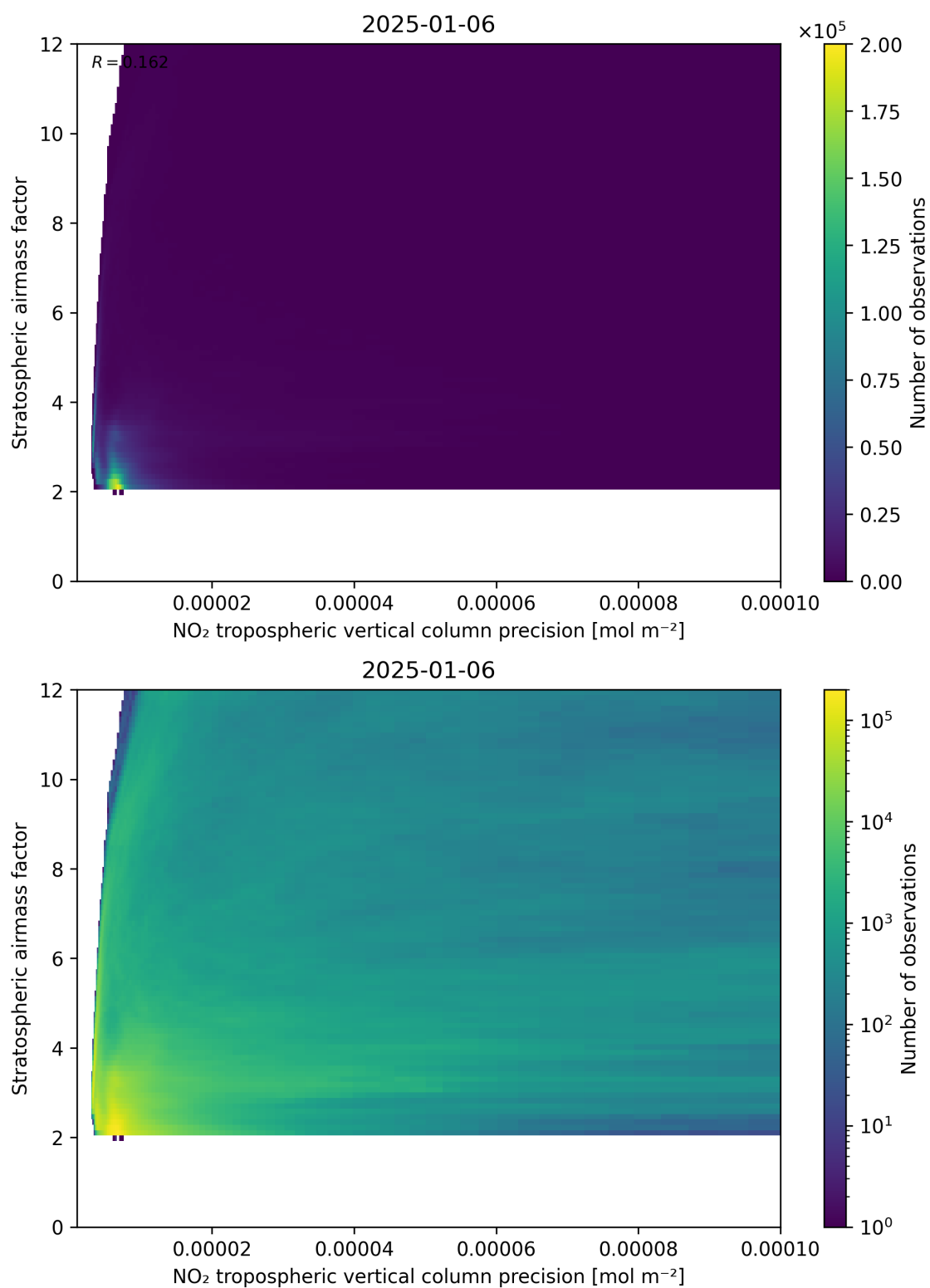
Figure 131: Scatter density plot of “NO 2 tropospheric vertical column precision” against “Stratospheric airmass factor” for 2025-01-05 to 2025-01-07.
