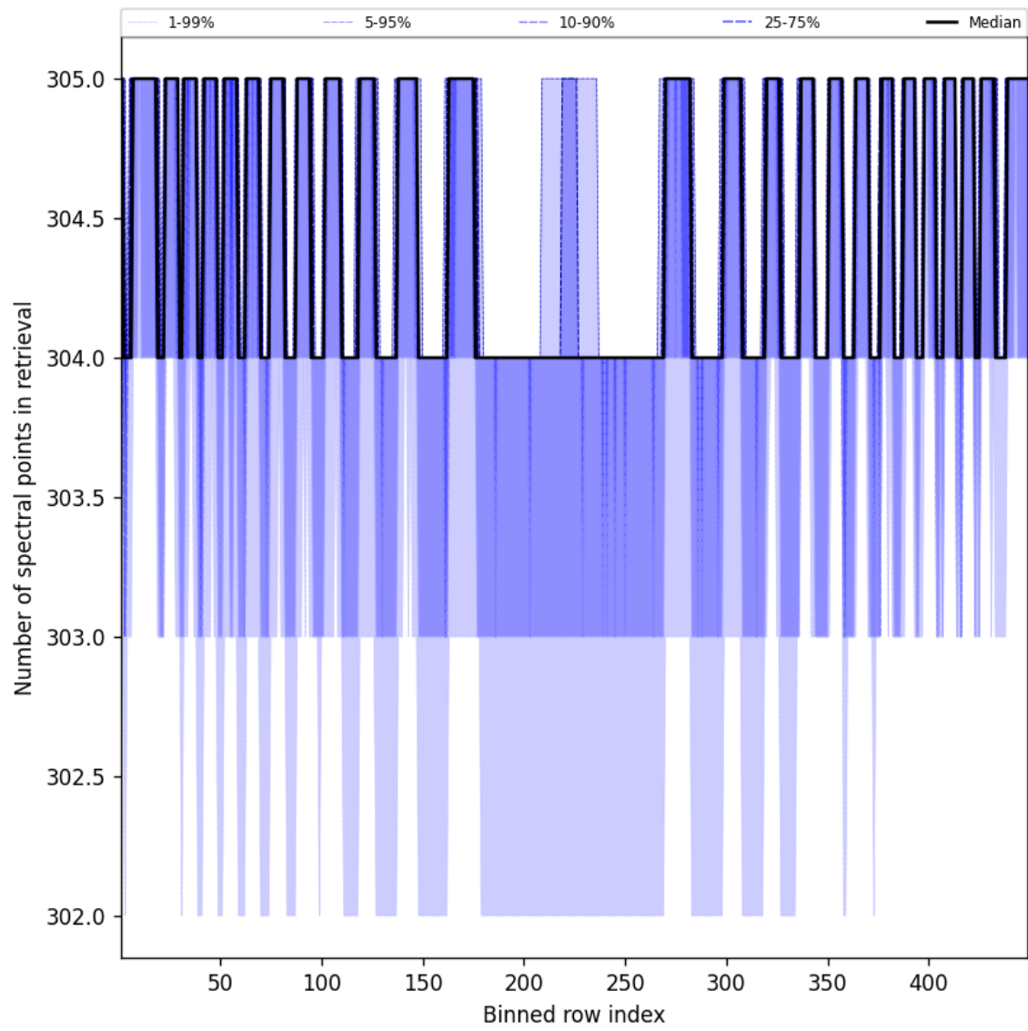
Figure 50: Along track statistics of “Number of spectral points in retrieval” for 2025-01-05 to 2025-01-07
