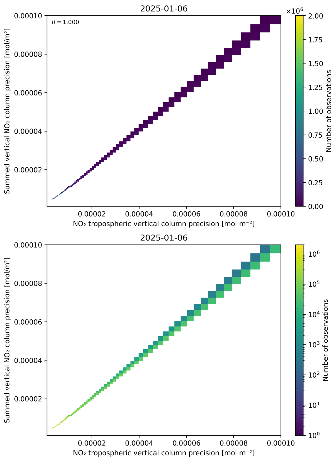
Figure 137: Scatter density plot of “NO 2 tropospheric vertical column precision” against “Summed vertical NO 2 column precision” for 2025-01-05 to 2025-01-07.
