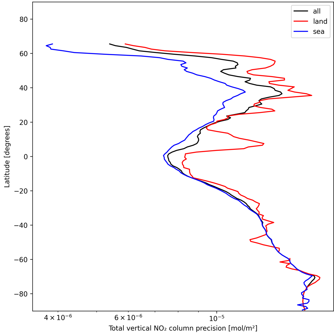
Figure 22: Zonal average of "Total vertical NO 2 column precision" for 2025-01-05 to 2025-01-07.
