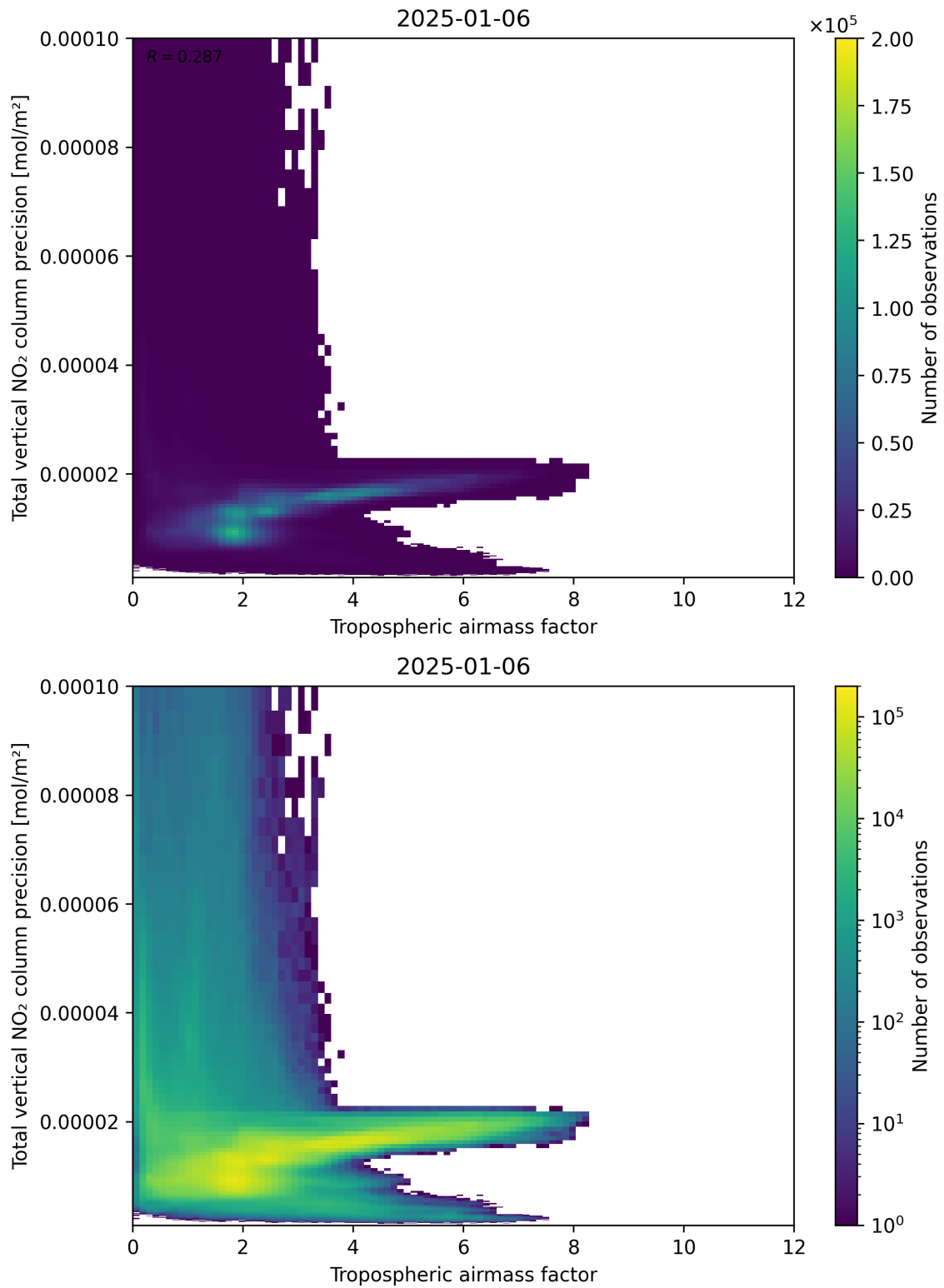
Figure 78: Scatter density plot of “Tropospheric airmass factor” against “Total vertical NO 2 column precision” for 2025-01-05 to 2025-01-07.
