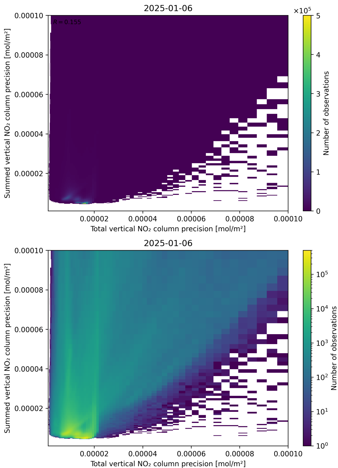
Figure 118: Scatter density plot of “Total vertical NO 2 column precision” against “Summed vertical NO 2 column precision” for 2025-01-05 to 2025-01-07.
