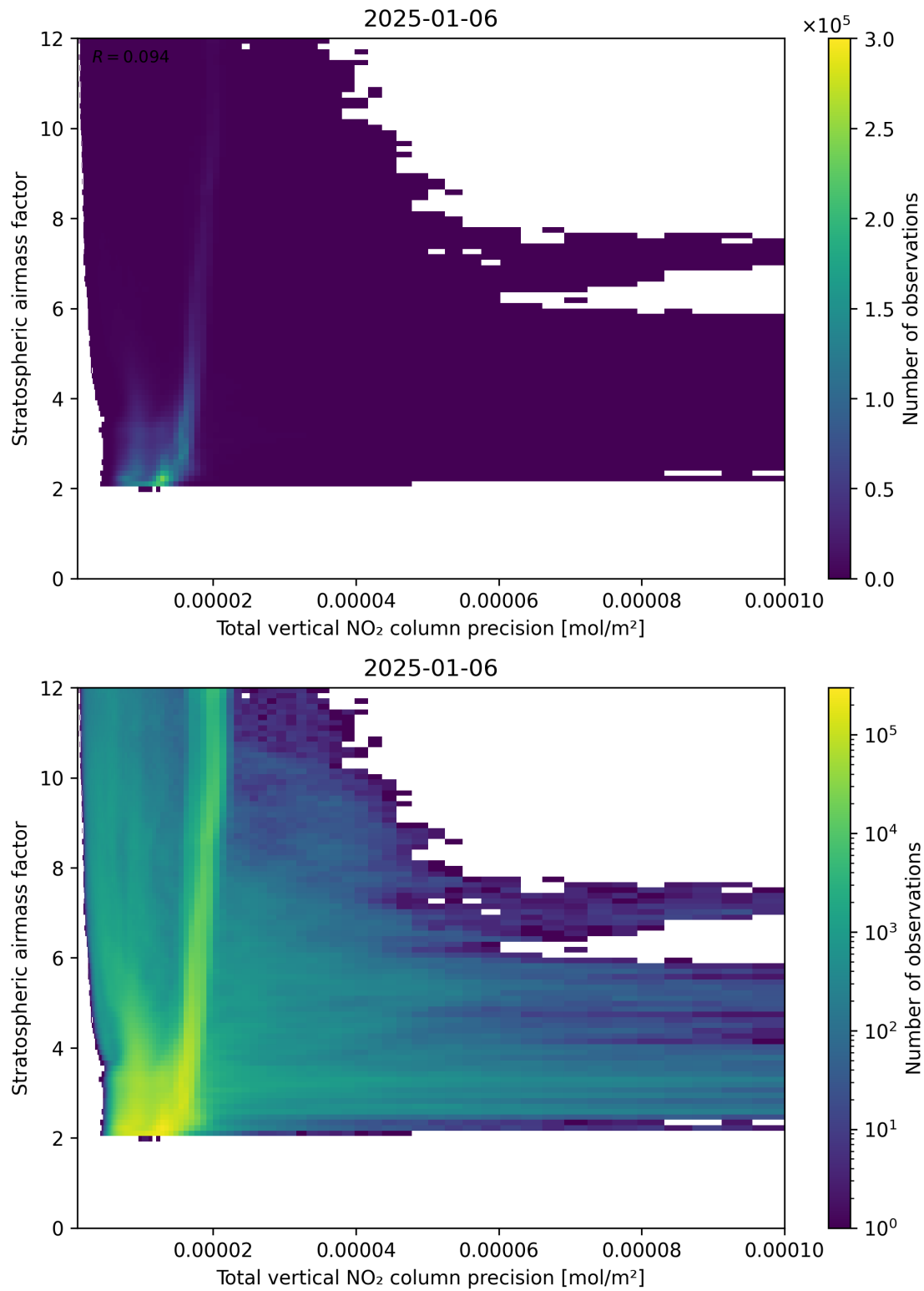
Figure 115: Scatter density plot of “Total vertical NO 2 column precision” against “Stratospheric air mass factor” for 2025-01-05 to 2025-01-07.
