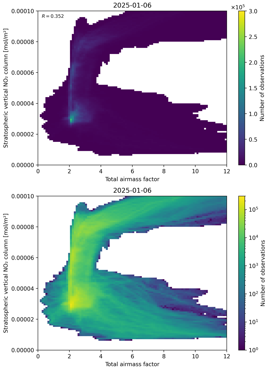
Figure 64: Scatter density plot of “Total airmass factor” against “Stratospheric vertical NO 2 column” for 2025-01-05 to 2025-01-07.
