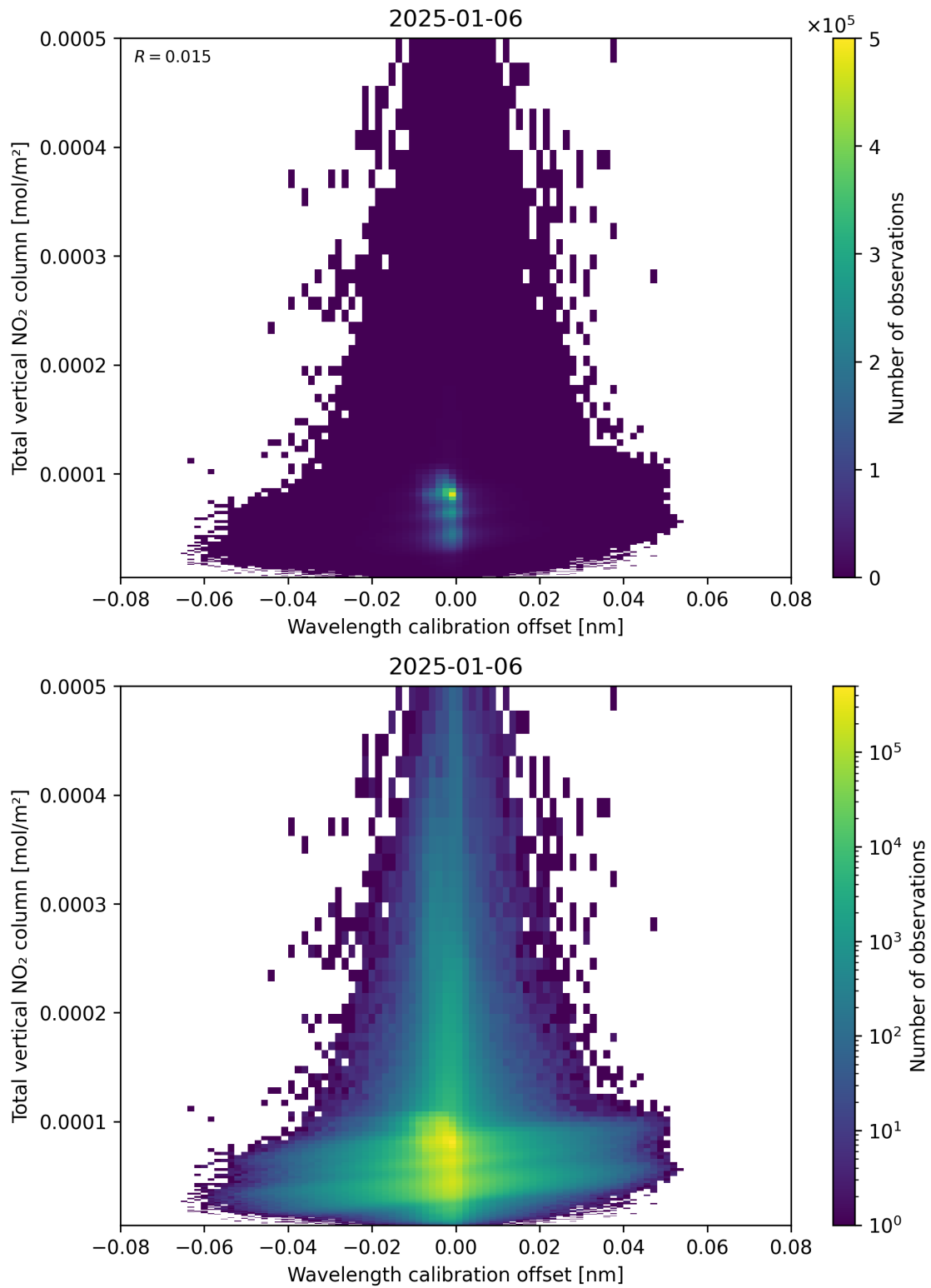
Figure 179: Scatter density plot of “Wavelength calibration offset” against “Total vertical NO 2 column” for 2025-01-05 to 2025-01-07.
