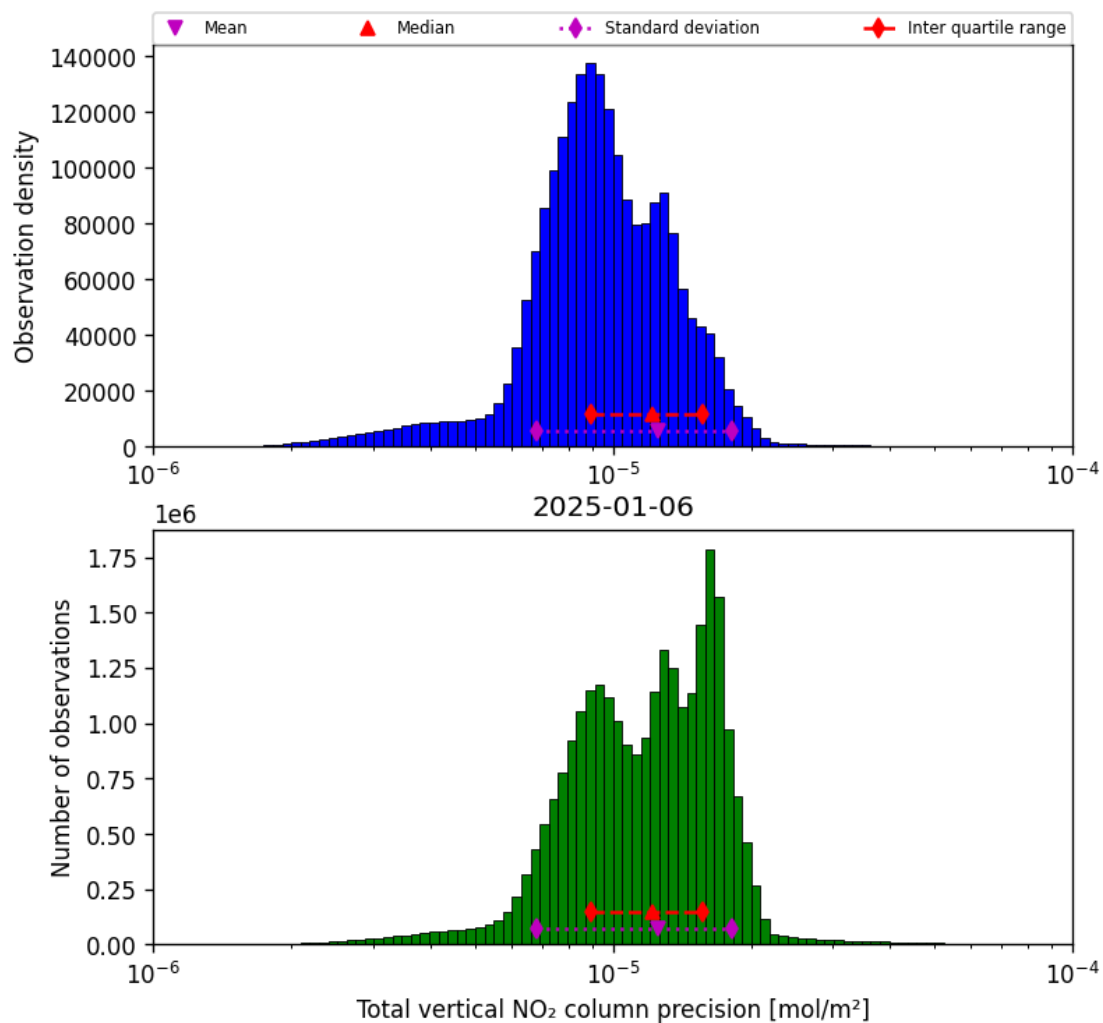
Figure 39: Histogram of “Total vertical NO 2 column precision” for 2025-01-05 to 2025-01-07
