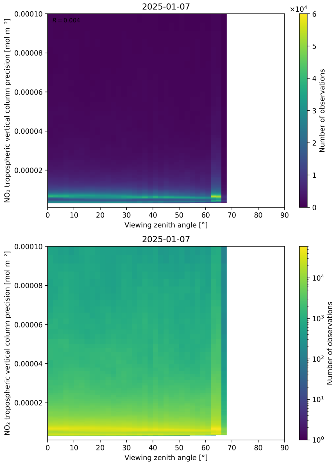
Figure 170: Scatter density plot of “Viewing zenith angle” against “NO 2 tropospheric vertical column precision” for 2025-01-07 to 2025-01-08.
