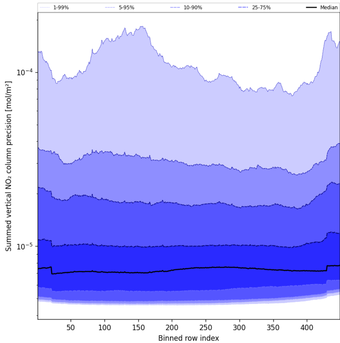
Figure 58: Along track statistics of “Summed vertical NO 2 column precision” for 2025-01-07 to 2025-01-08
