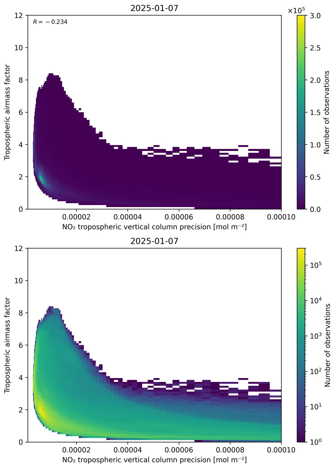
Figure 133: Scatter density plot of “NO 2 tropospheric vertical column precision” against “Tropospheric air mass factor” for 2025-01-07 to 2025-01-08.
