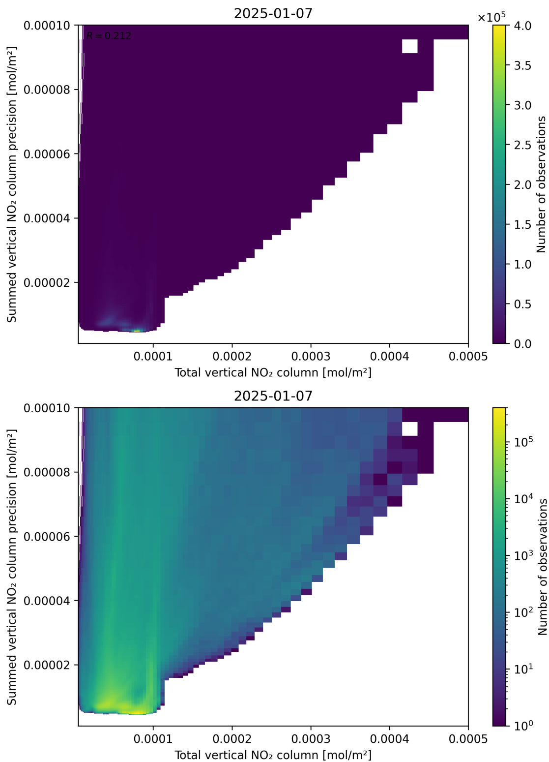
Figure 113: Scatter density plot of “Total vertical NO 2 column” against “Summed vertical NO 2 column precision” for 2025-01-07 to 2025-01-08.
