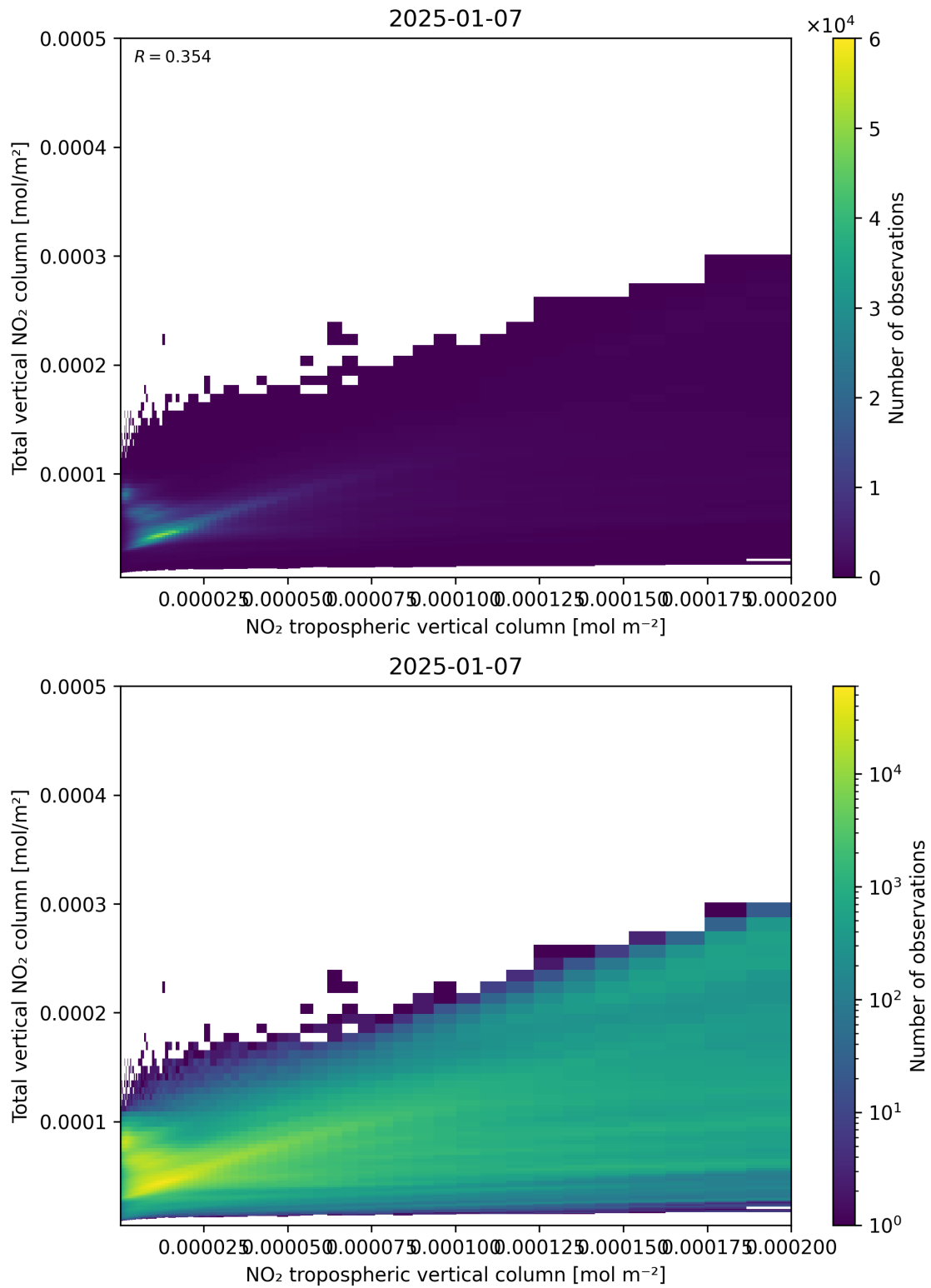
Figure 128: Scatter density plot of “NO 2 tropospheric vertical column” against “Total vertical NO 2 column” for 2025-01-07 to 2025-01-08.
