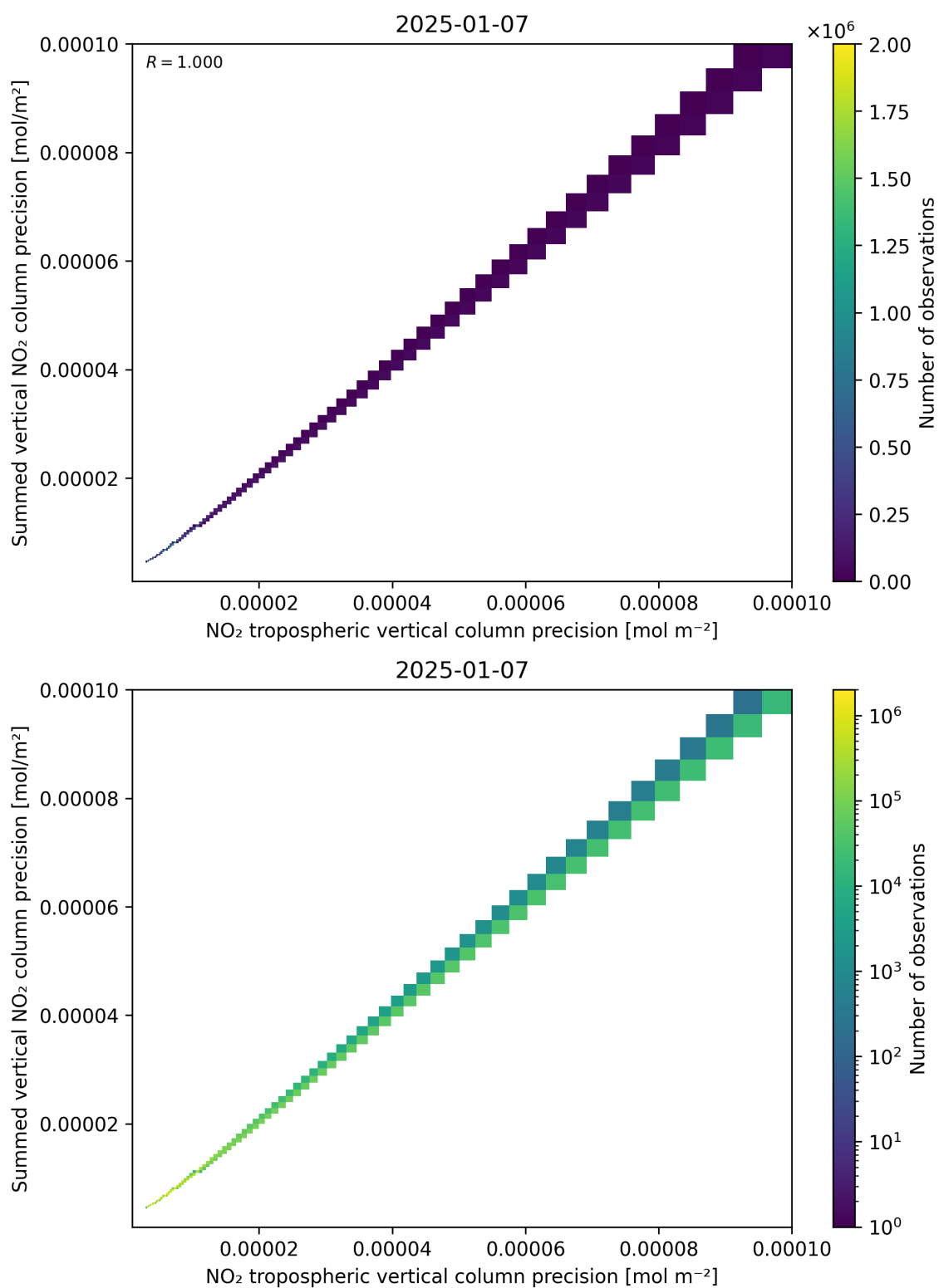
Figure 137: Scatter density plot of “NO 2 tropospheric vertical column precision” against “Summed vertical NO 2 column precision” for 2025-01-07 to 2025-01-08.
