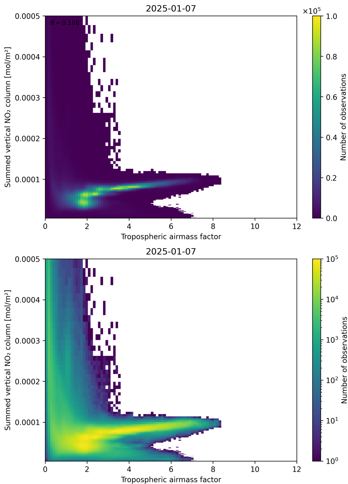
Figure 75: Scatter density plot of “Tropospheric air mass factor” against “Summed vertical NO 2 column” for 2025-01-07 to 2025-01-08.
