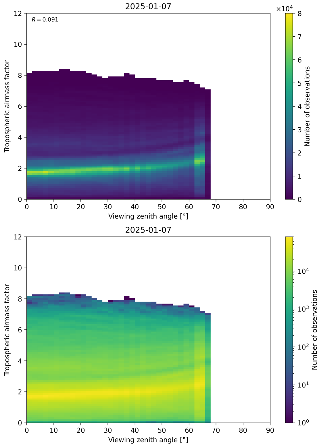
Figure 161: Scatter density plot of “Viewing zenith angle” against “Tropospheric airmass factor” for 2025-01-07 to 2025-01-08.
