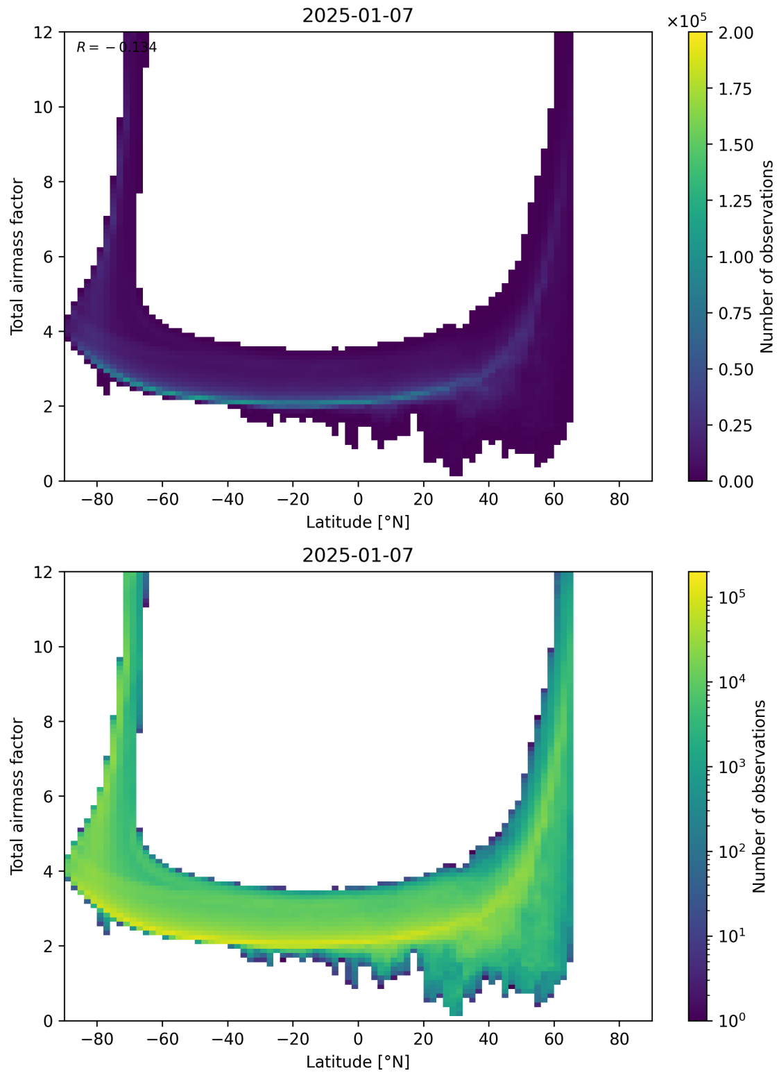
Figure 84: Scatter density plot of “Latitude” against “Total airmass factor” for 2025-01-07 to 2025-01-08.
