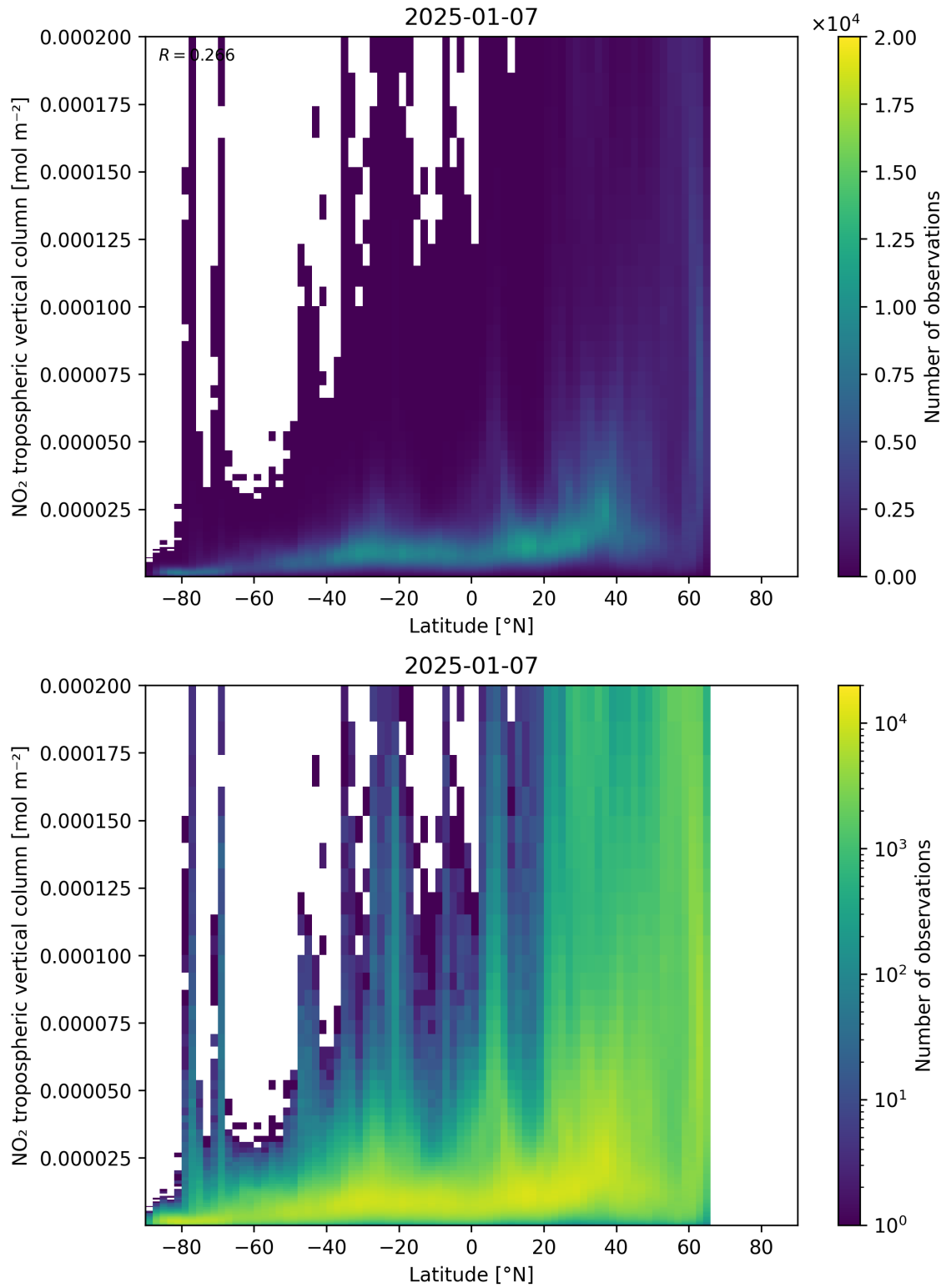
Figure 92: Scatter density plot of “Latitude” against “NO 2 tropospheric vertical column” for 2025-01-07 to 2025-01-08.
