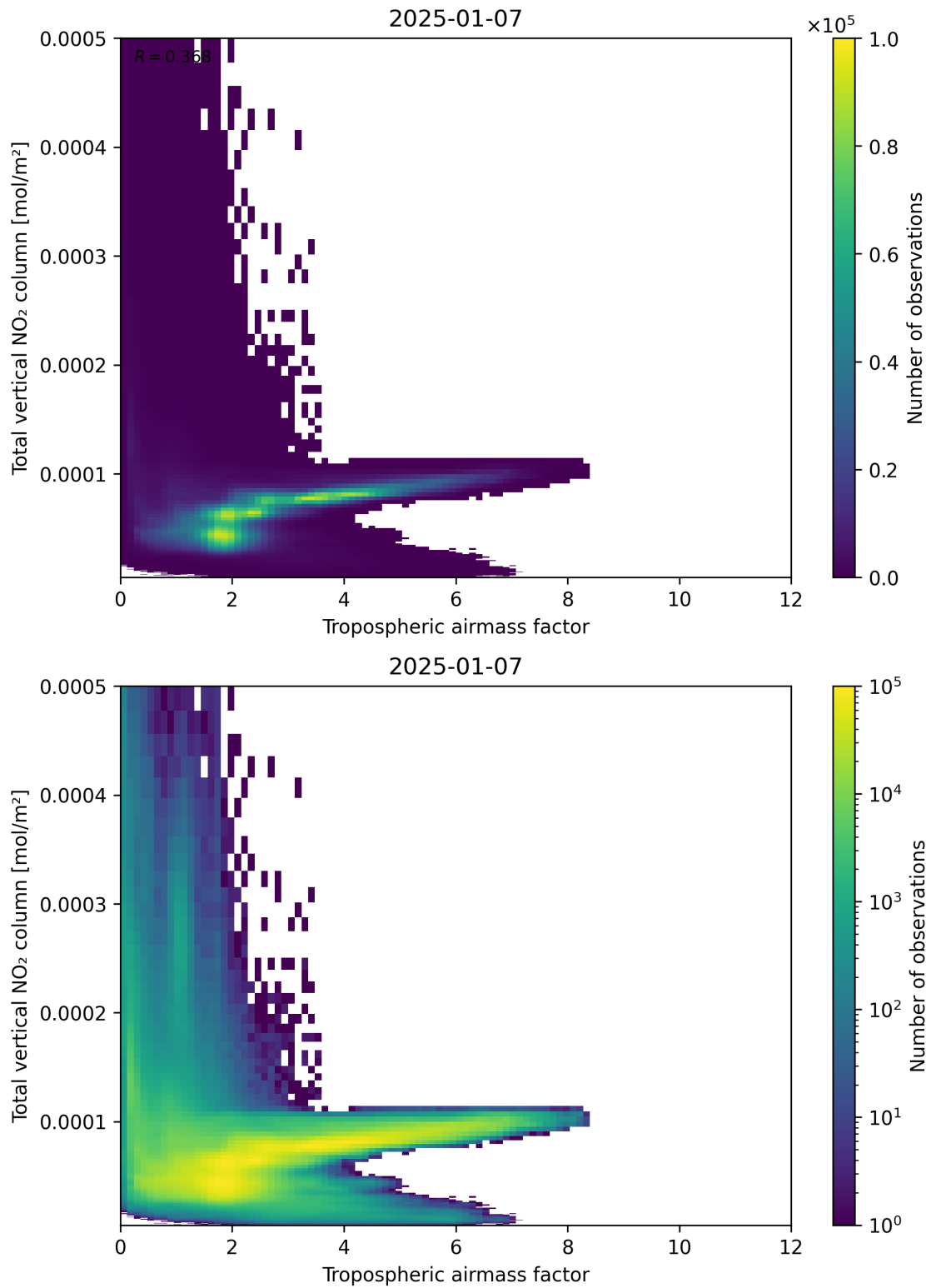
Figure 77: Scatter density plot of “Tropospheric airmass factor” against “Total vertical NO 2 column” for 2025-01-07 to 2025-01-08.
