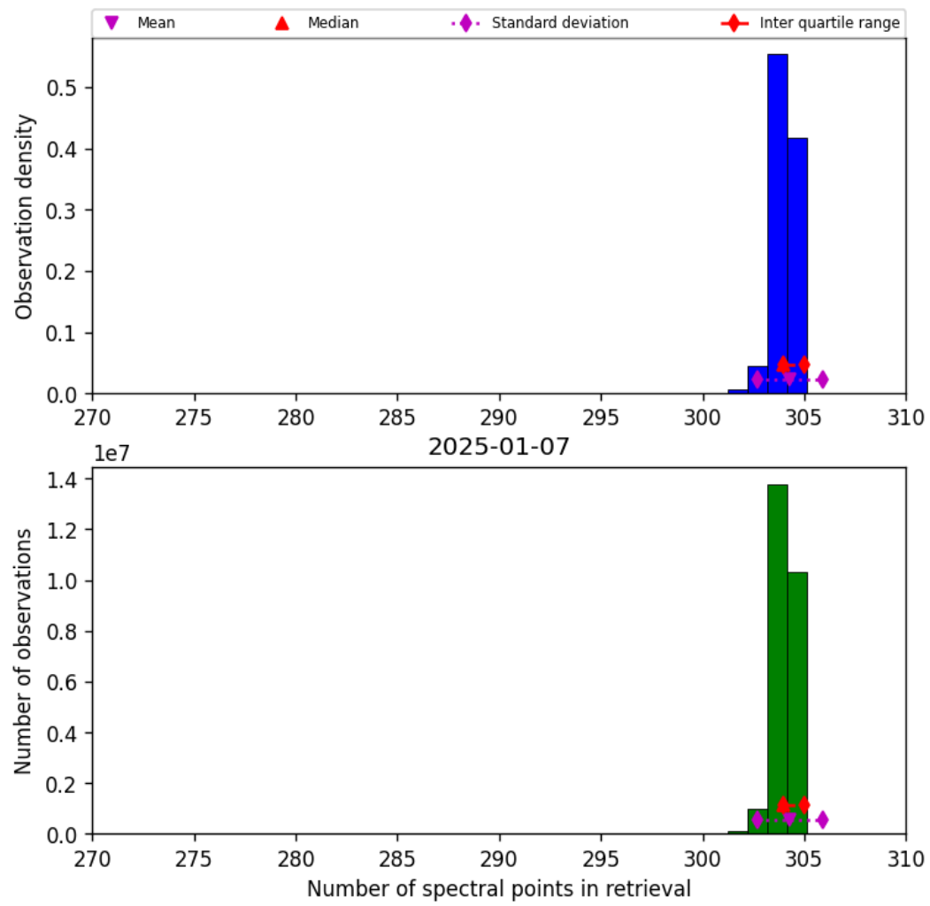
Figure 33: Histogram of “Number of spectral points in retrieval” for 2025-01-07 to 2025-01-08
