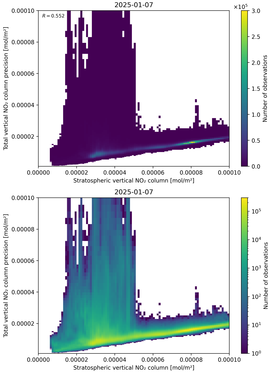
Figure 101: Scatter density plot of “Stratospheric vertical NO 2 column” against “Total vertical NO 2 column precision” for 2025-01-07 to 2025-01-08.
