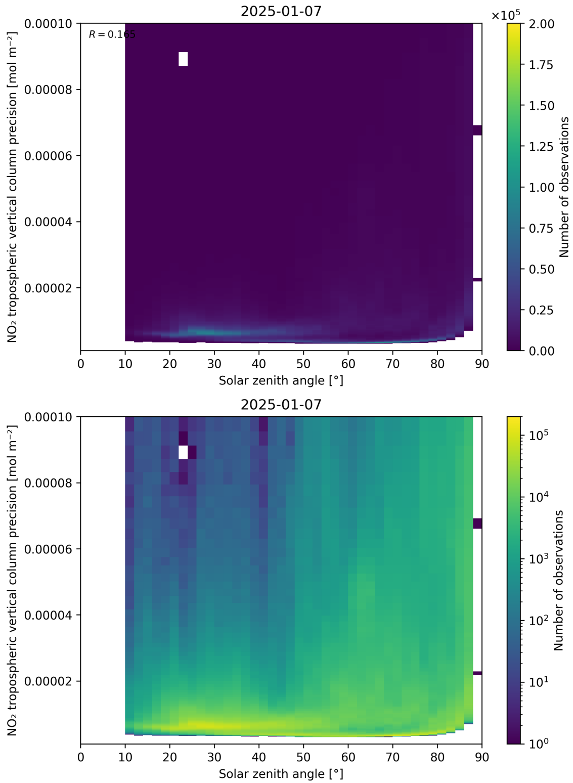
Figure 156: Scatter density plot of “Solar zenith angle” against “NO 2 tropospheric vertical column precision” for 2025-01-07 to 2025-01-08.
