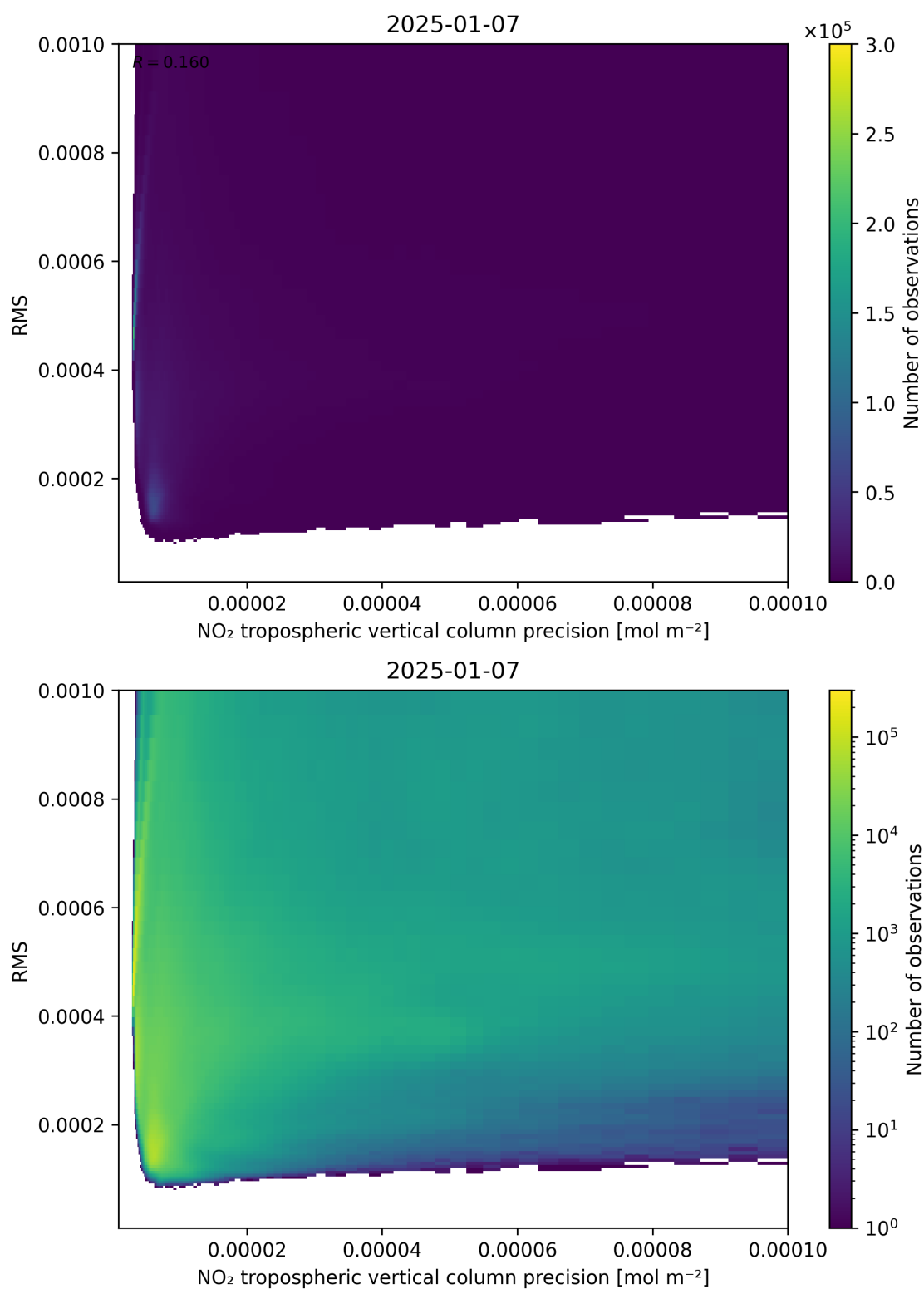
Figure 140: Scatter density plot of “NO 2 tropospheric vertical column precision” against “RMS” for 2025-01-07 to 2025-01-08.
