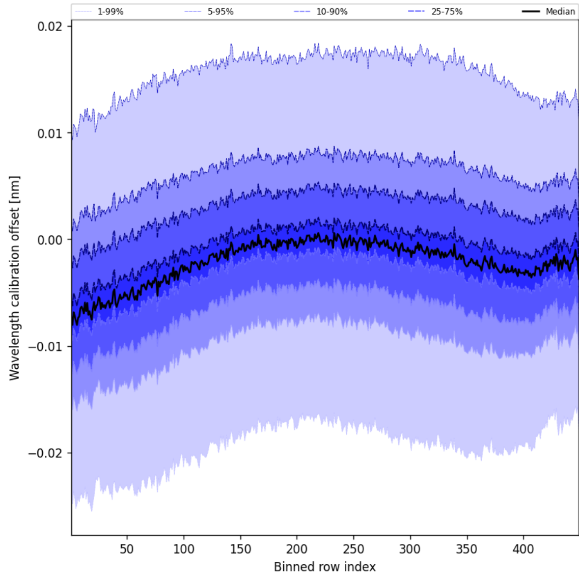
Figure 52: Along track statistics of “Wavelength calibration offset” for 2025-01-07 to 2025-01-08
