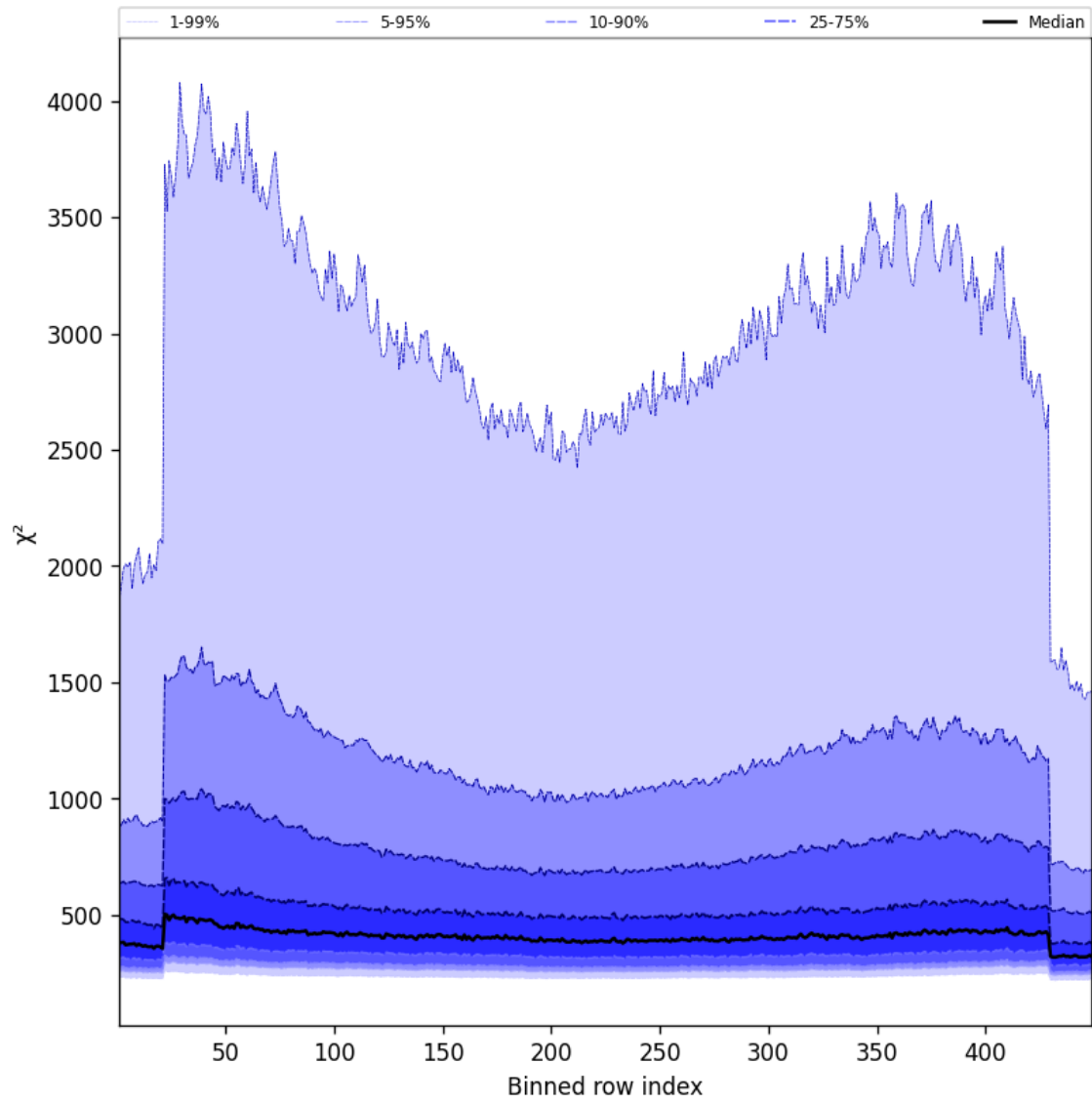
Figure 59: Along track statistics of “ \chi^2 ” for 2025-01-07 to 2025-01-08
