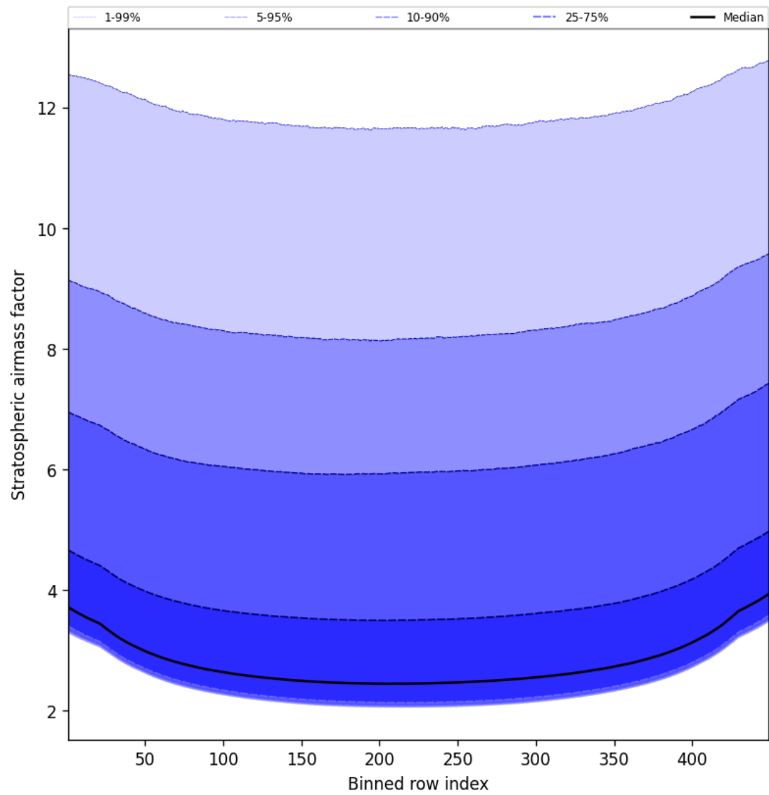
Figure 61: Along track statistics of “Stratospheric air mass factor” for 2025-01-07 to 2025-01-08
