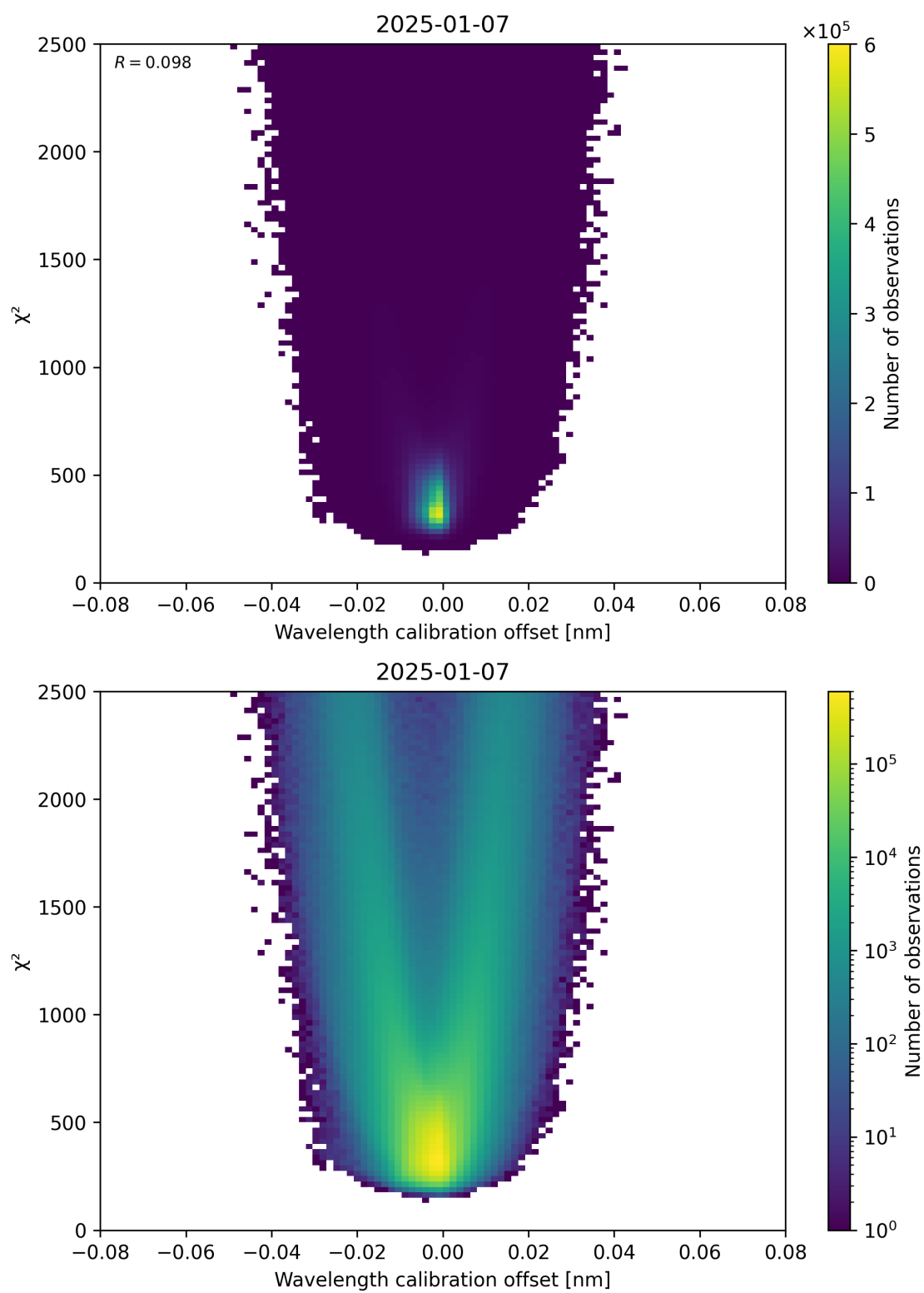
Figure 175: Scatter density plot of “Wavelength calibration offset” against “ \chi^2 ” for 2025-01-07 to 2025-01-08.
