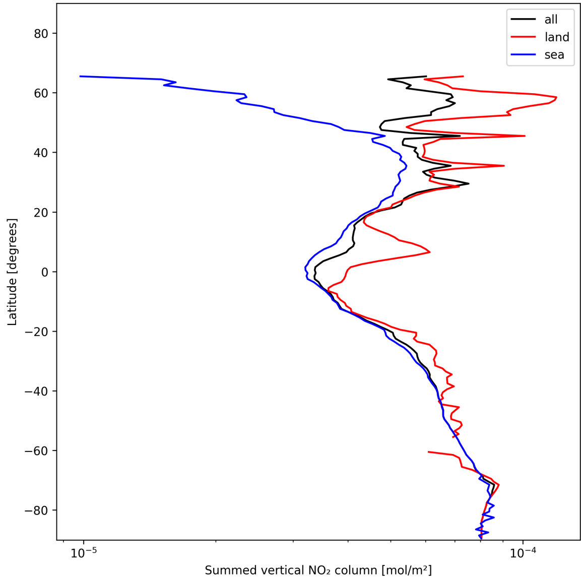
Figure 23: Zonal average of “Summed vertical NO 2 column” for 2025-01-07 to 2025-01-08.
