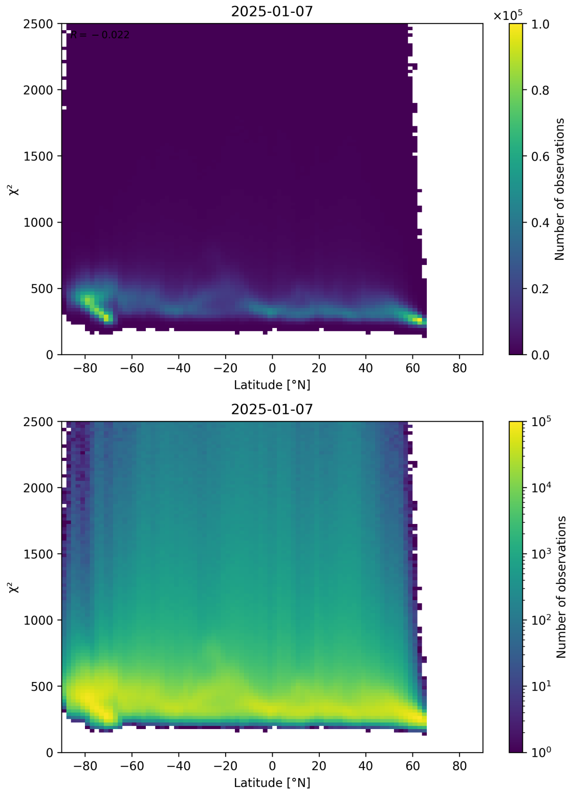
Figure 86: Scatter density plot of “Latitude” against “ \chi^2 ” for 2025-01-07 to 2025-01-08.
