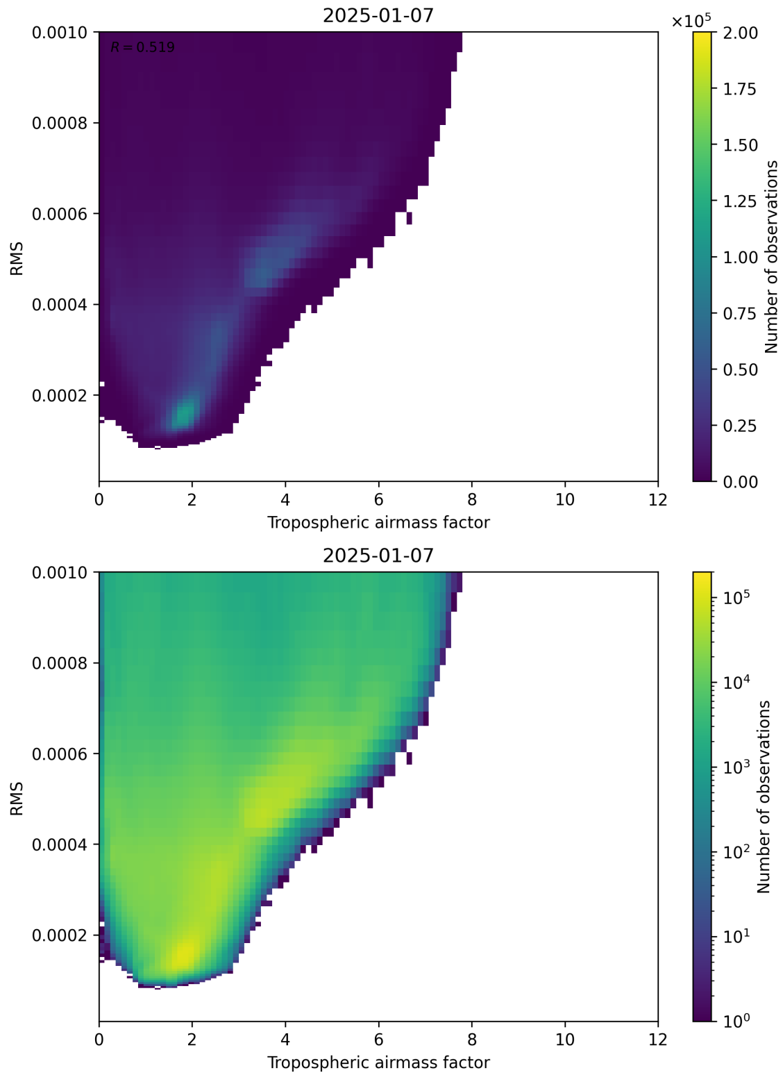
Figure 79: Scatter density plot of “Tropospheric airmass factor” against “RMS” for 2025-01-07 to 2025-01-08.
