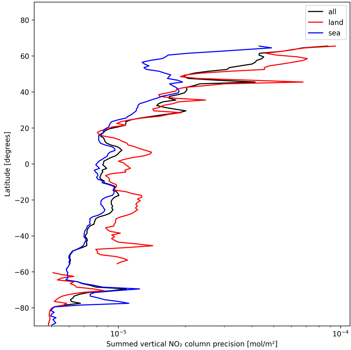
Figure 24: Zonal average of “Summed vertical NO 2 column precision” for 2025-01-07 to 2025-01-08.
