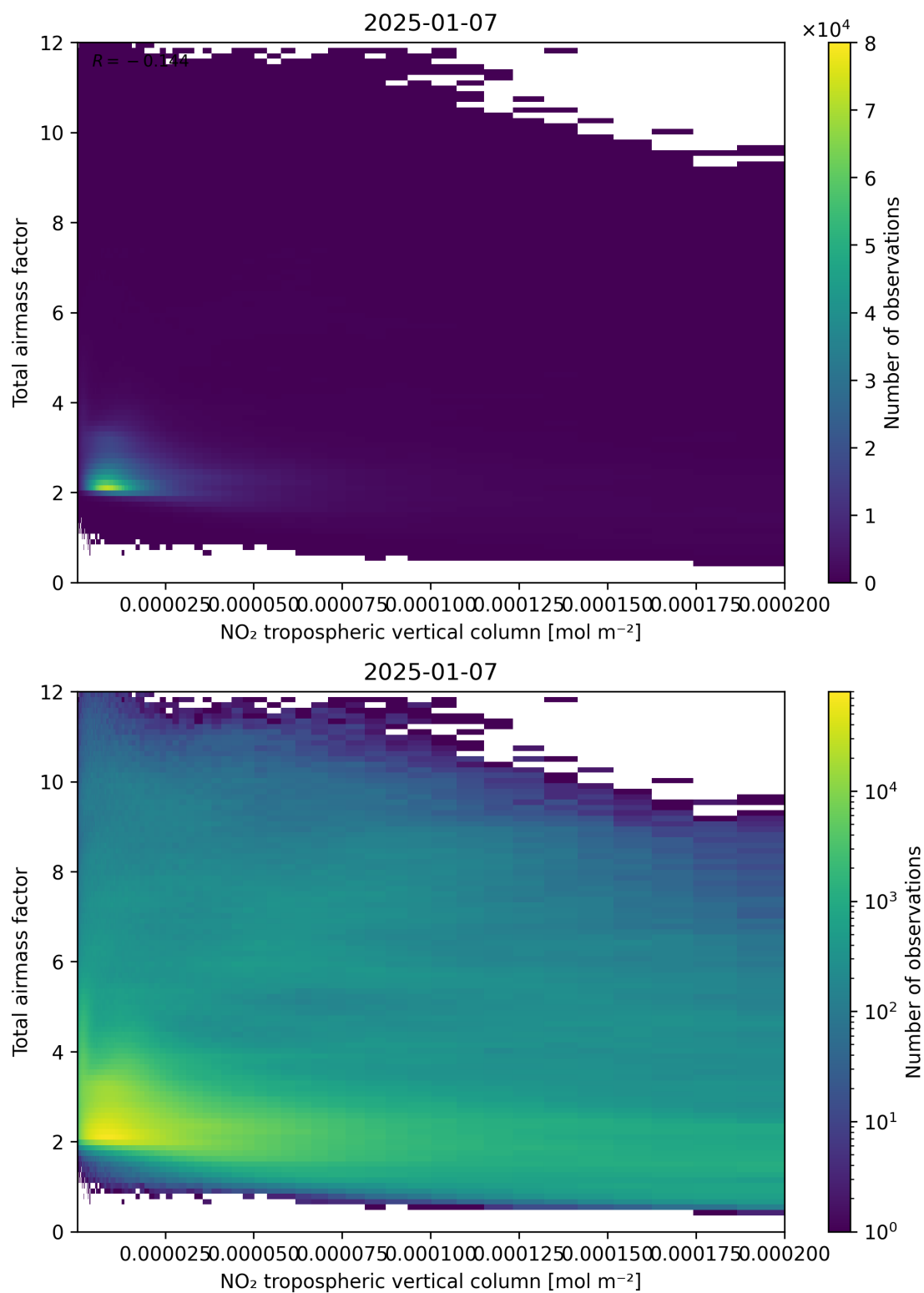
Figure 122: Scatter density plot of “NO 2 tropospheric vertical column” against “Total air mass factor” for 2025-01-07 to 2025-01-08.
