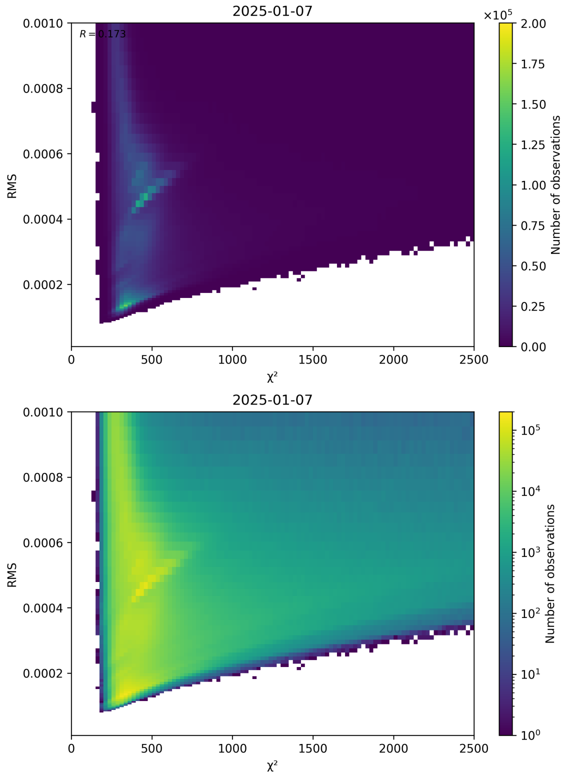
Figure 82: Scatter density plot of “ \chi^2 ” against “RMS” for 2025-01-07 to 2025-01-08.
