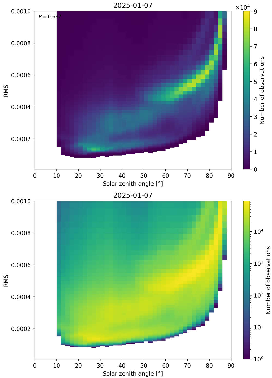
Figure 157: Scatter density plot of “Solar zenith angle” against “RMS” for 2025-01-07 to 2025-01-08.
