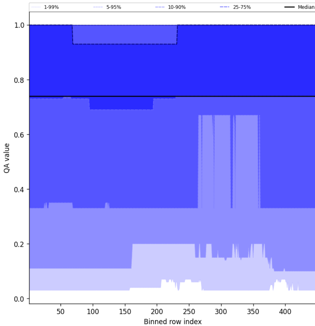
Figure 45: Along track statistics of “QA value” for 2025-01-07 to 2025-01-08
