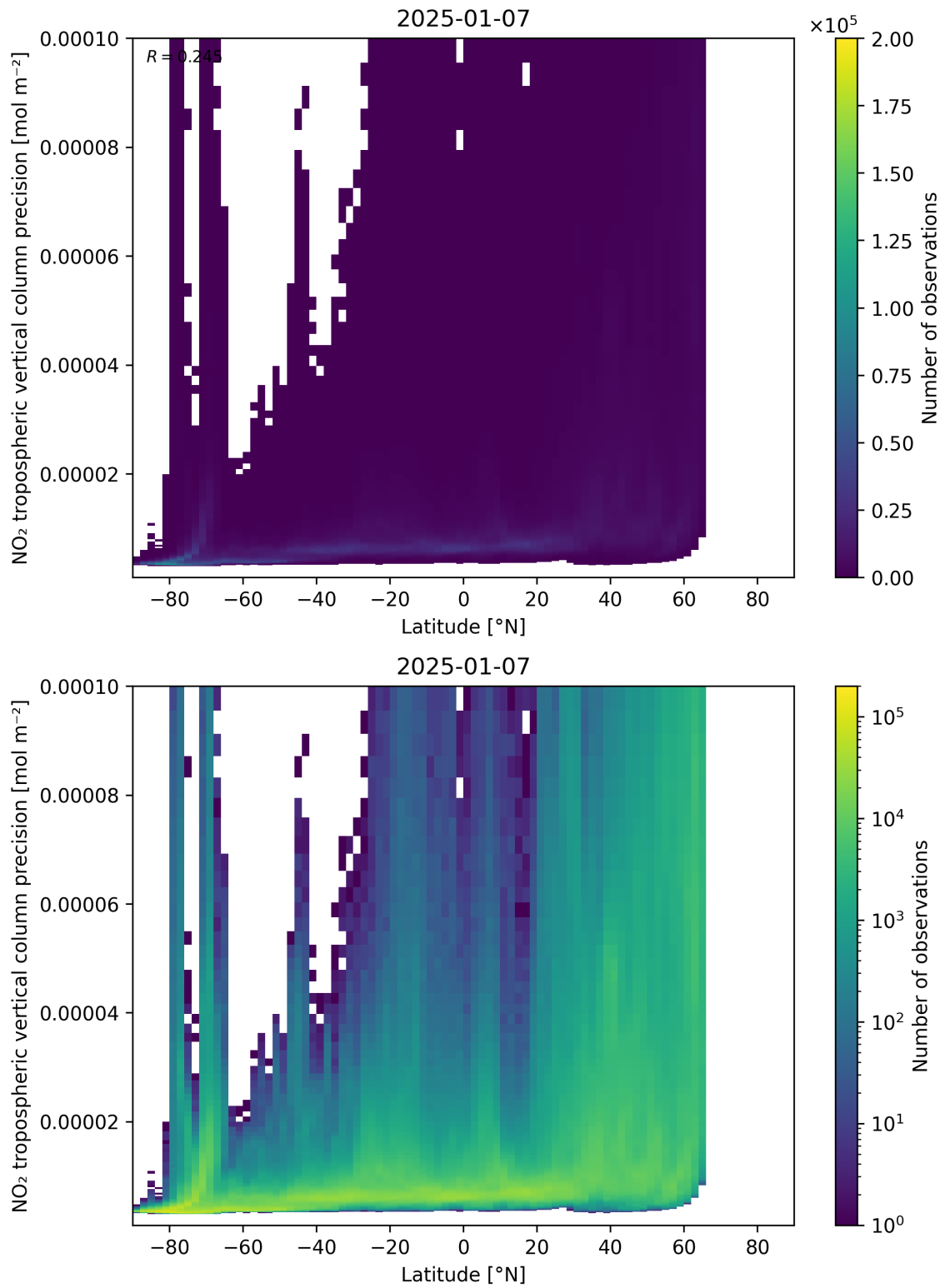
Figure 93: Scatter density plot of “Latitude” against “NO 2 tropospheric vertical column precision” for 2025-01-07 to 2025-01-08.
