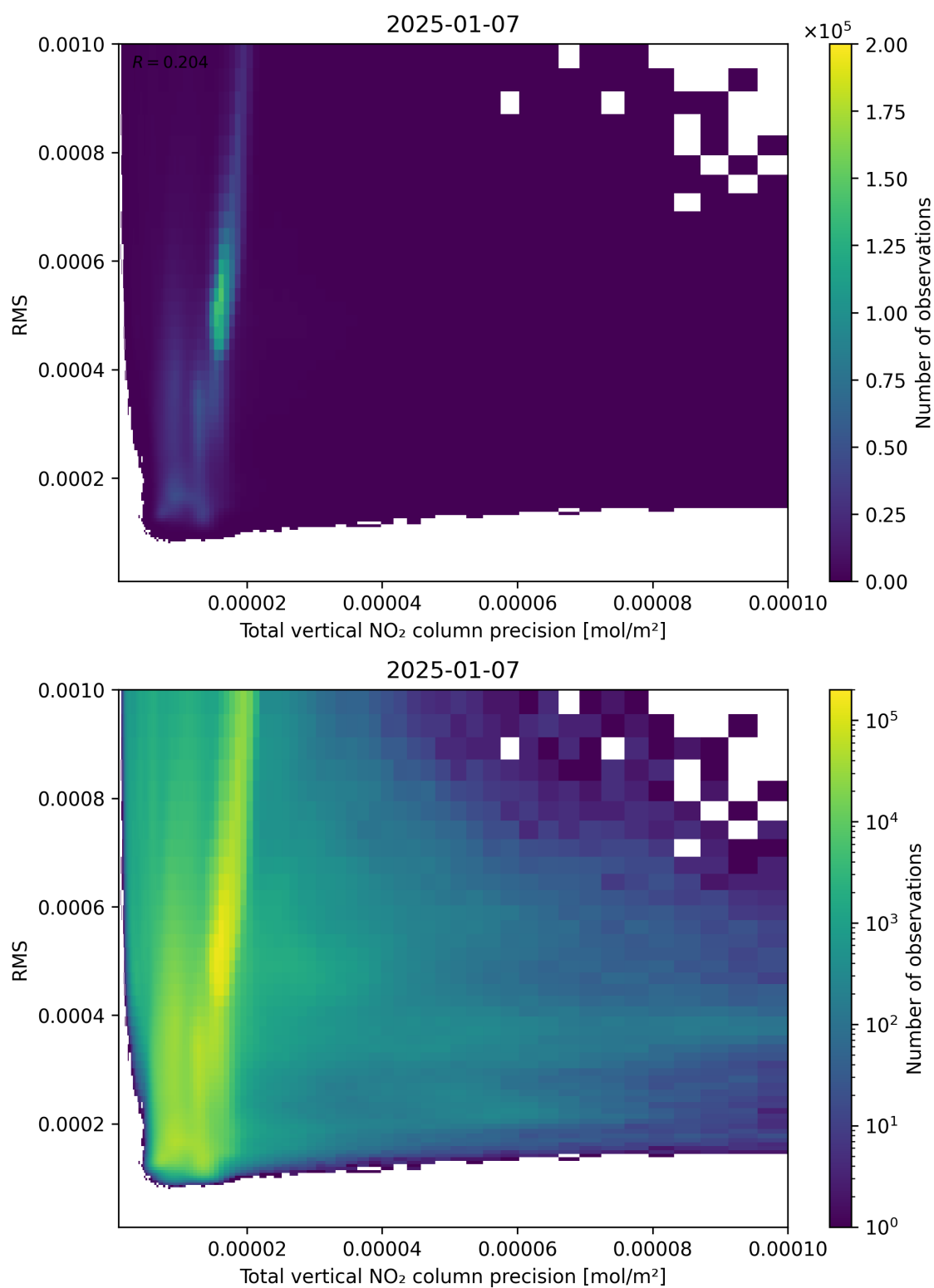
Figure 119: Scatter density plot of “Total vertical NO 2 column precision” against “RMS” for 2025-01-07 to 2025-01-08.
