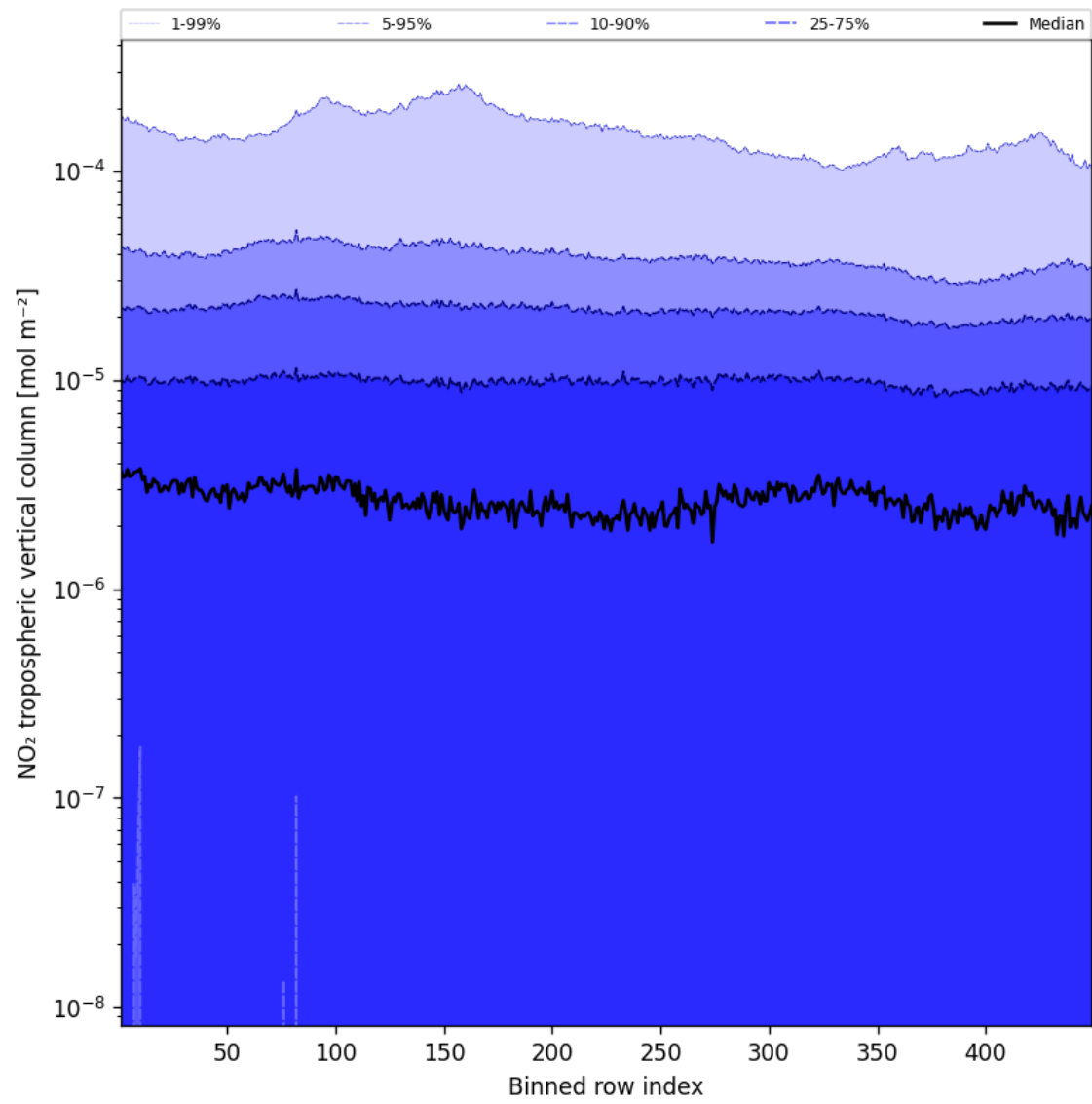
Figure 46: Along track statistics of “NO 2 tropospheric vertical column” for 2025-01-07 to 2025-01-08
