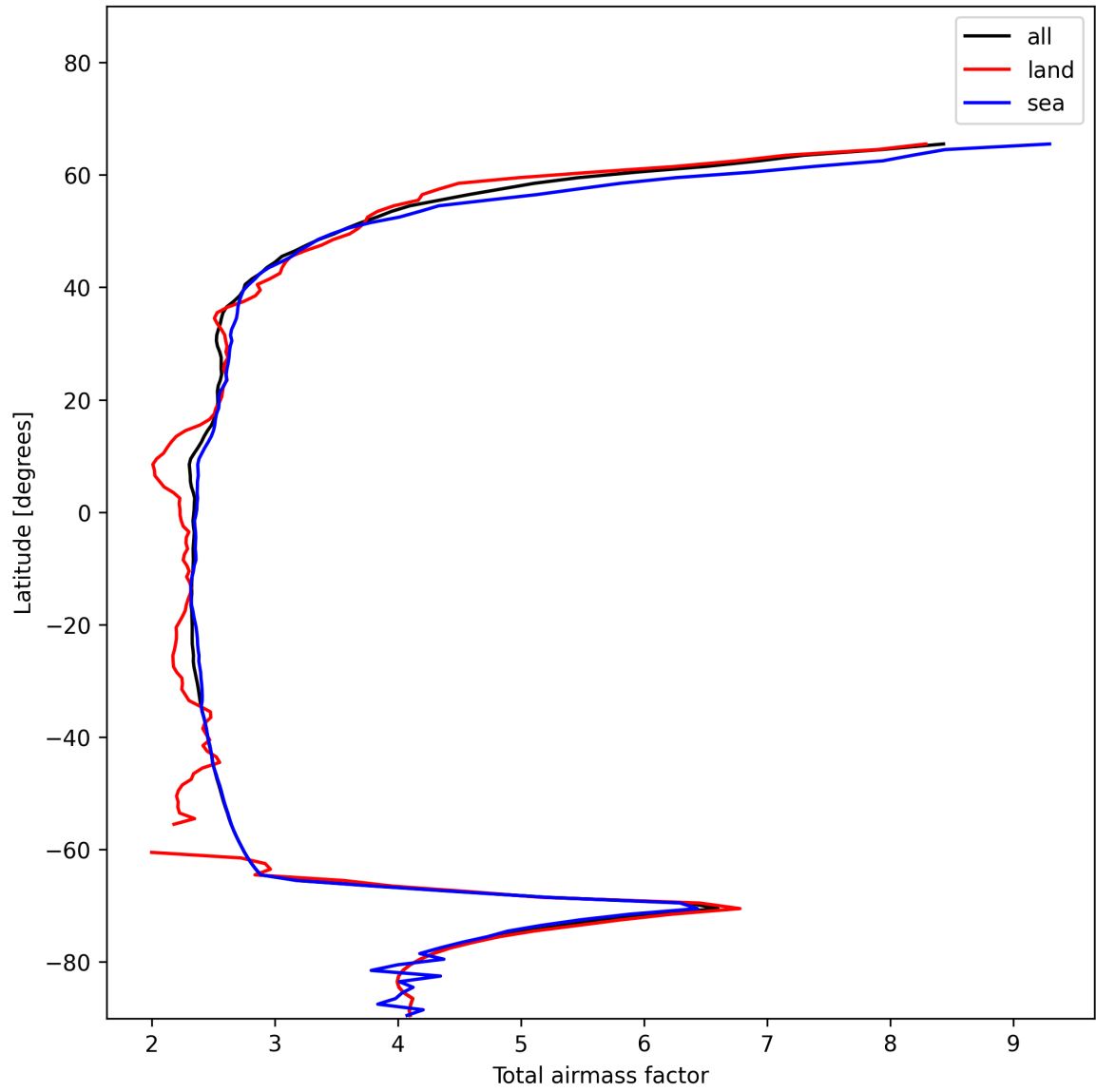
Figure 15: Zonal average of “Total airmass factor” for 2025-01-07 to 2025-01-08.
