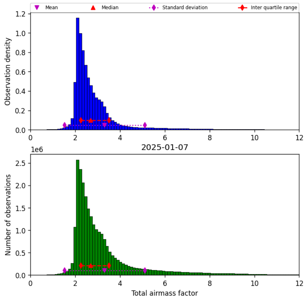
Figure 32: Histogram of “Total airmass factor” for 2025-01-07 to 2025-01-08
