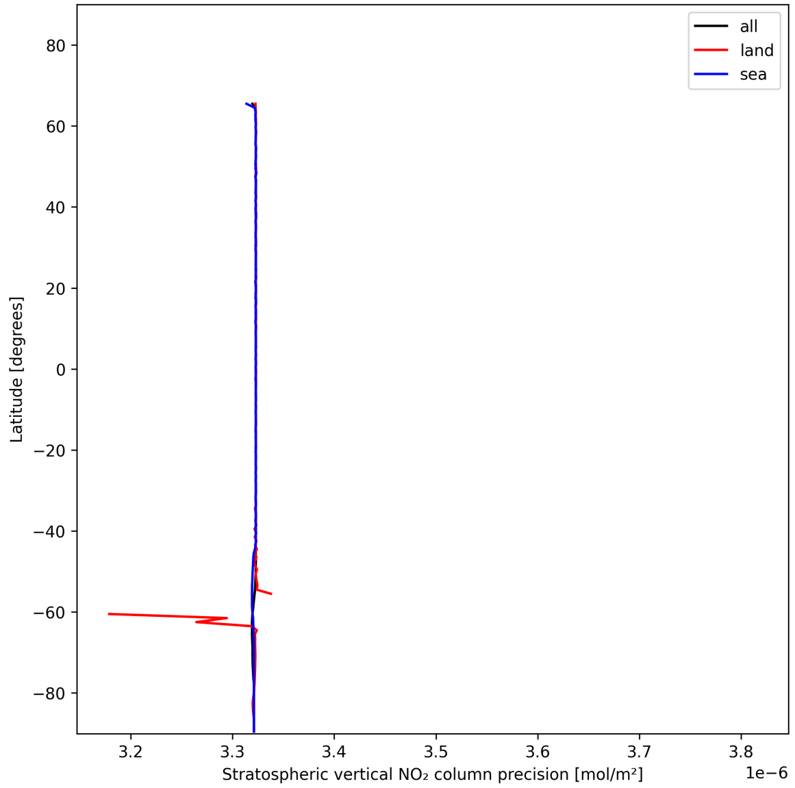
Figure 20: Zonal average of “Stratospheric vertical NO 2 column precision” for 2025-01-07 to 2025-01-08.
