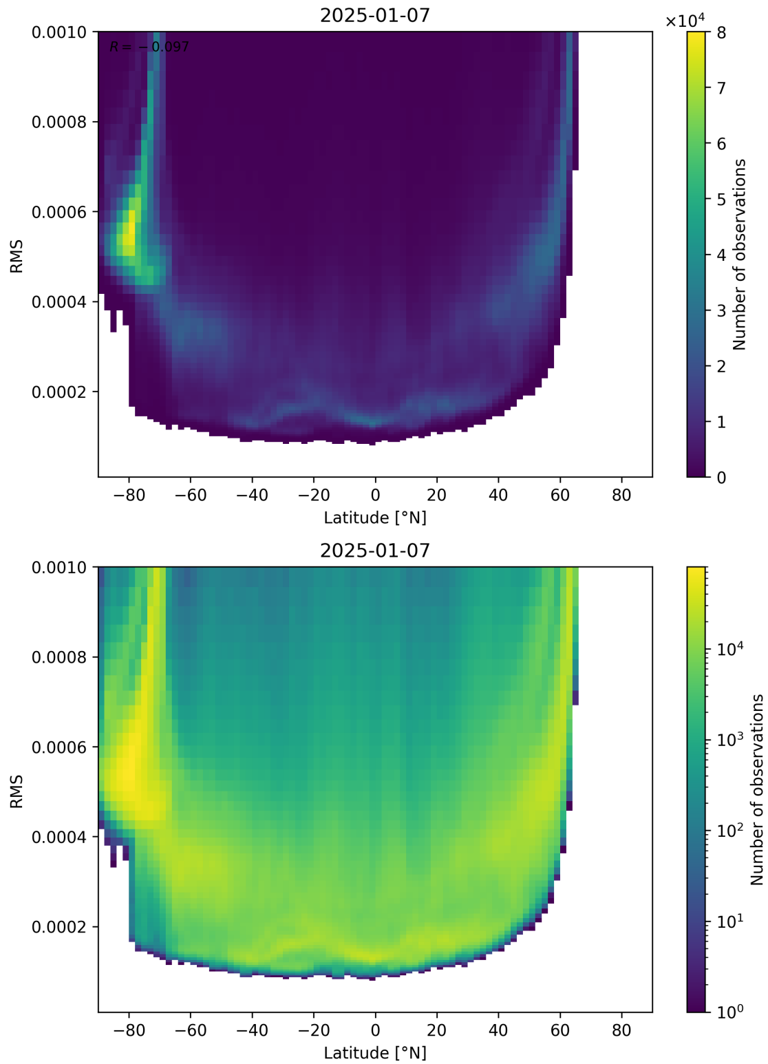
Figure 94: Scatter density plot of “Latitude” against “RMS” for 2025-01-07 to 2025-01-08.
