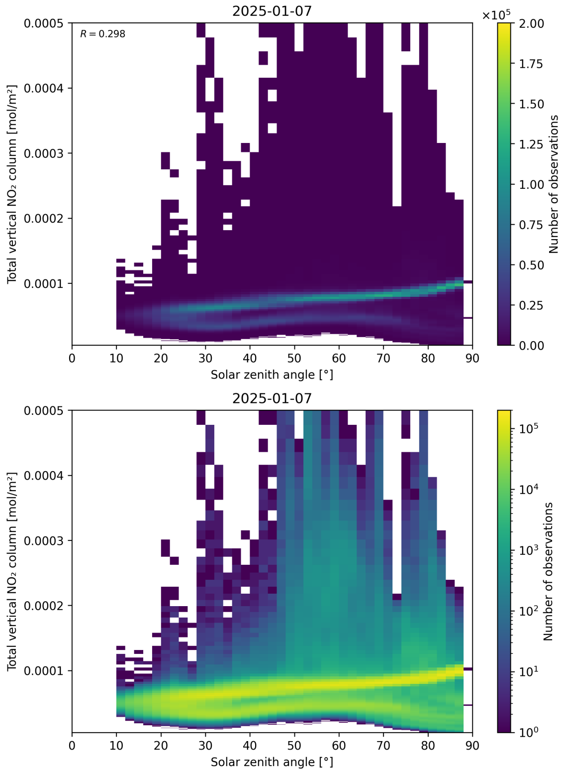
Figure 153: Scatter density plot of “Solar zenith angle” against “Total vertical NO 2 column” for 2025-01-07 to 2025-01-08.
