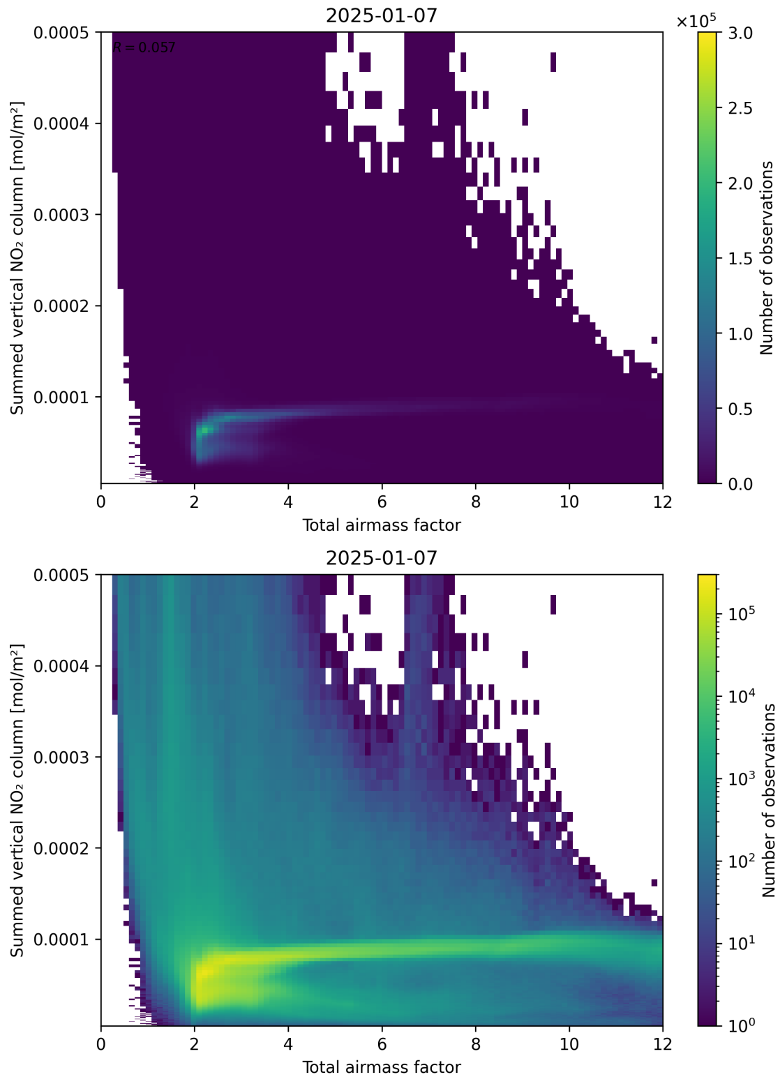
Figure 65: Scatter density plot of “Total airmass factor” against “Summed vertical NO 2 column” for 2025-01-07 to 2025-01-08.
