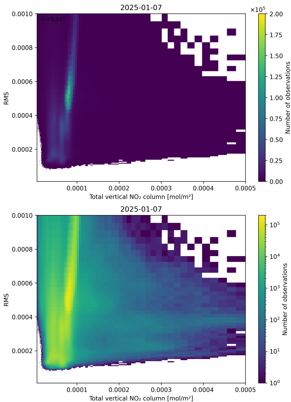
Figure 120: Scatter density plot of “Total vertical NO 2 column” against “RMS” for 2025-01-07 to 2025-01-08.
