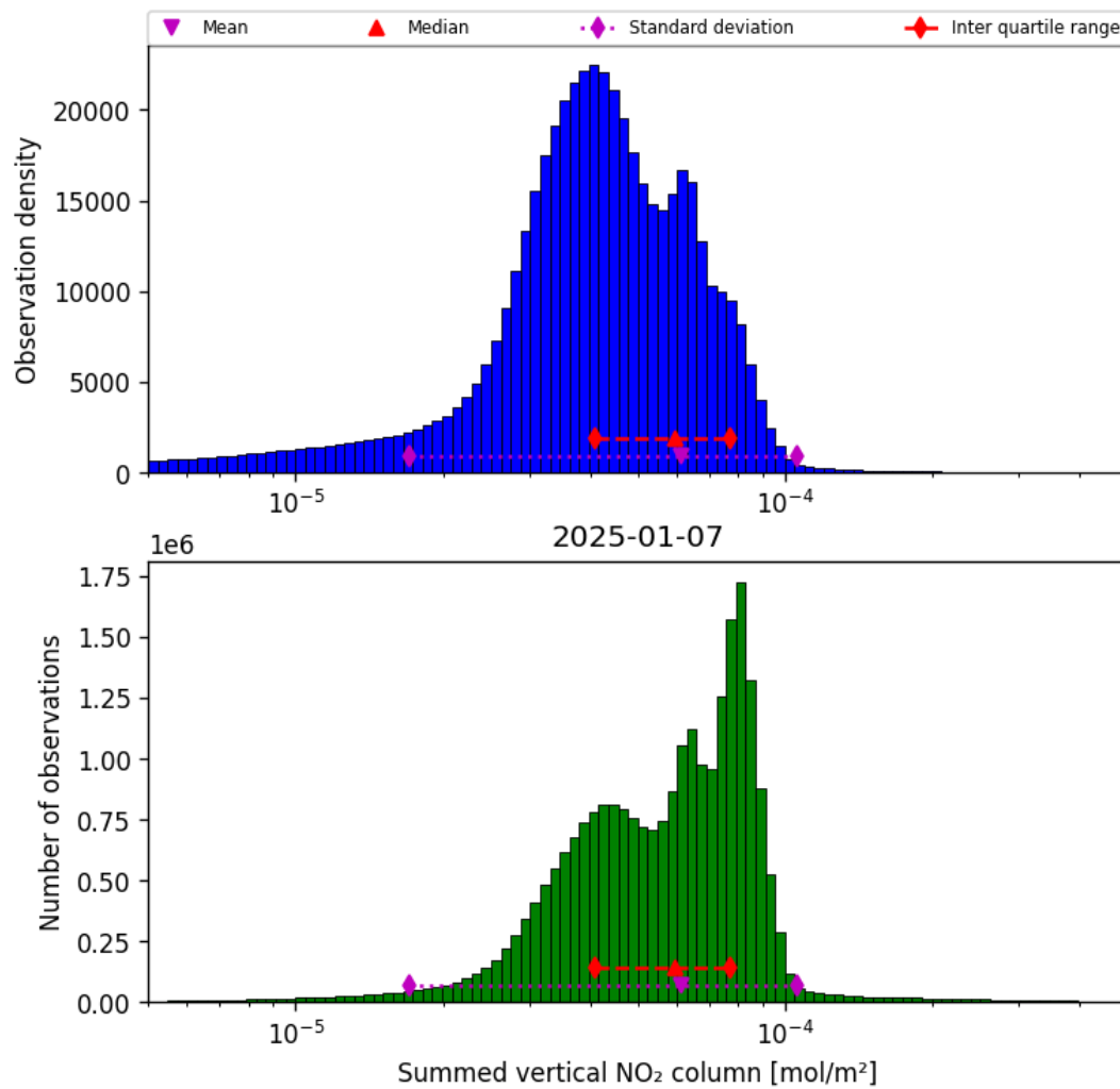
Figure 40: Histogram of “Summed vertical NO 2 column” for 2025-01-07 to 2025-01-08
