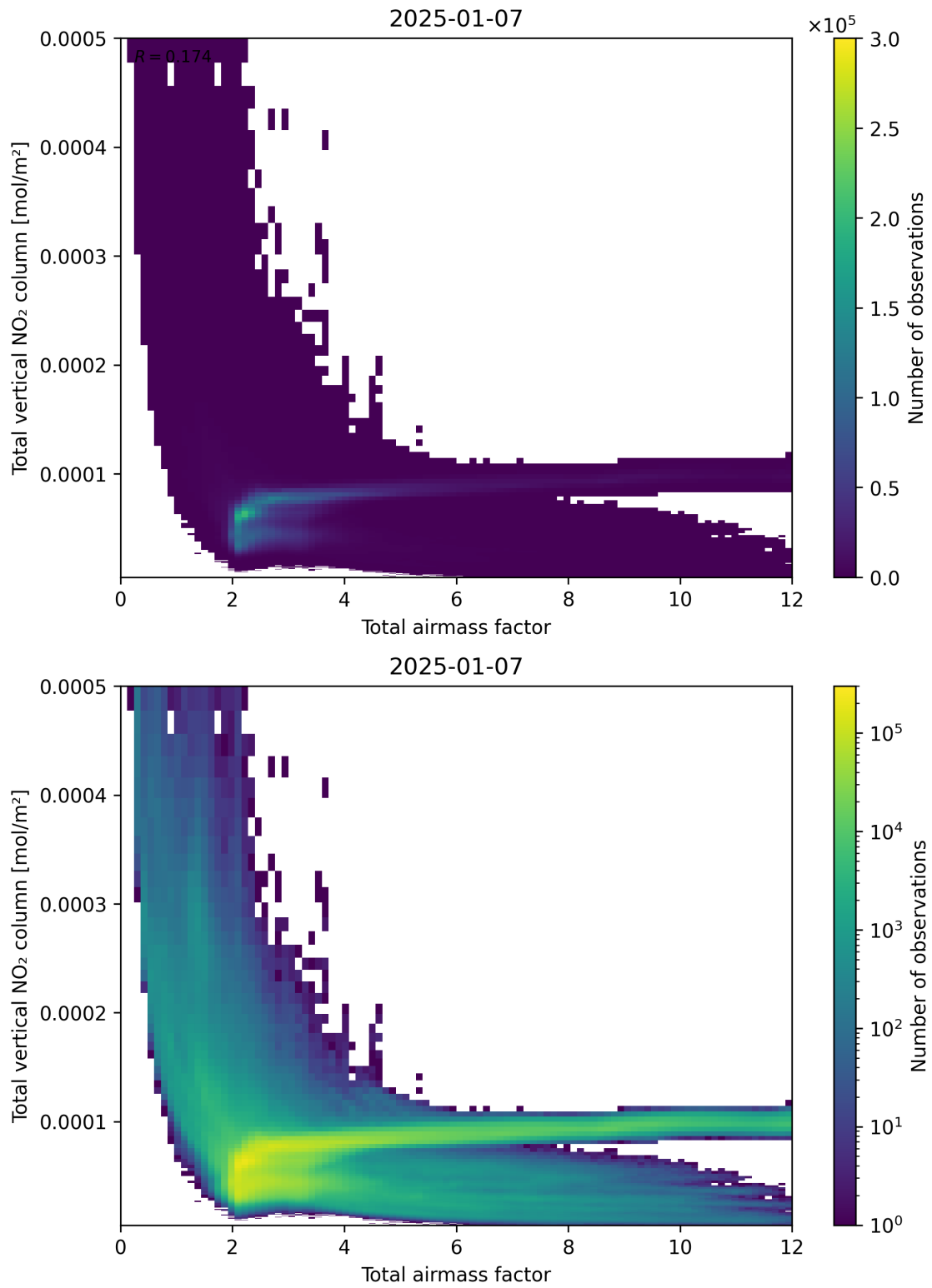
Figure 67: Scatter density plot of “Total airmass factor” against “Total vertical NO 2 column” for 2025-01-07 to 2025-01-08.
