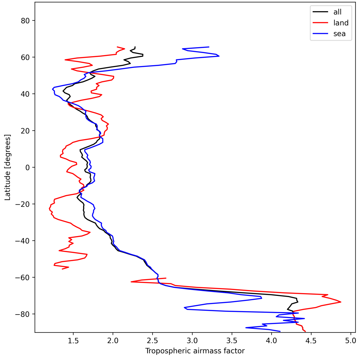
Figure 14: Zonal average of “Tropospheric airmass factor” for 2025-01-07 to 2025-01-08.
