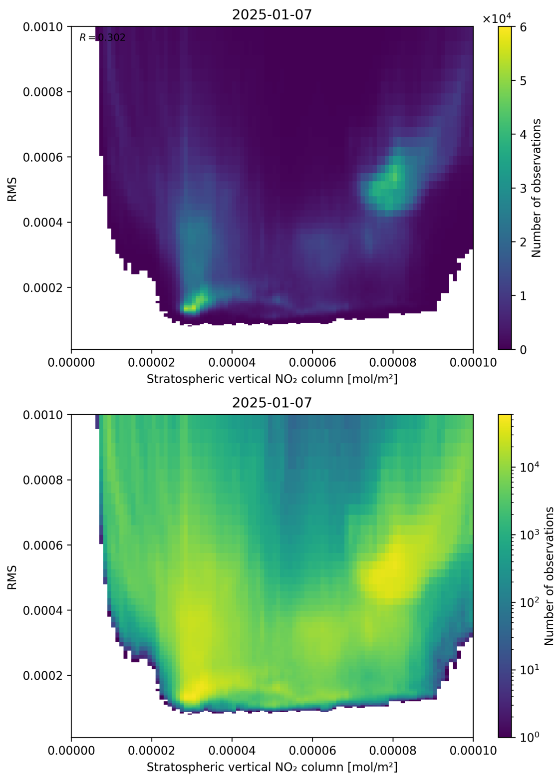
Figure 102: Scatter density plot of “Stratospheric vertical NO 2 column” against “RMS” for 2025-01-07 to 2025-01-08.
