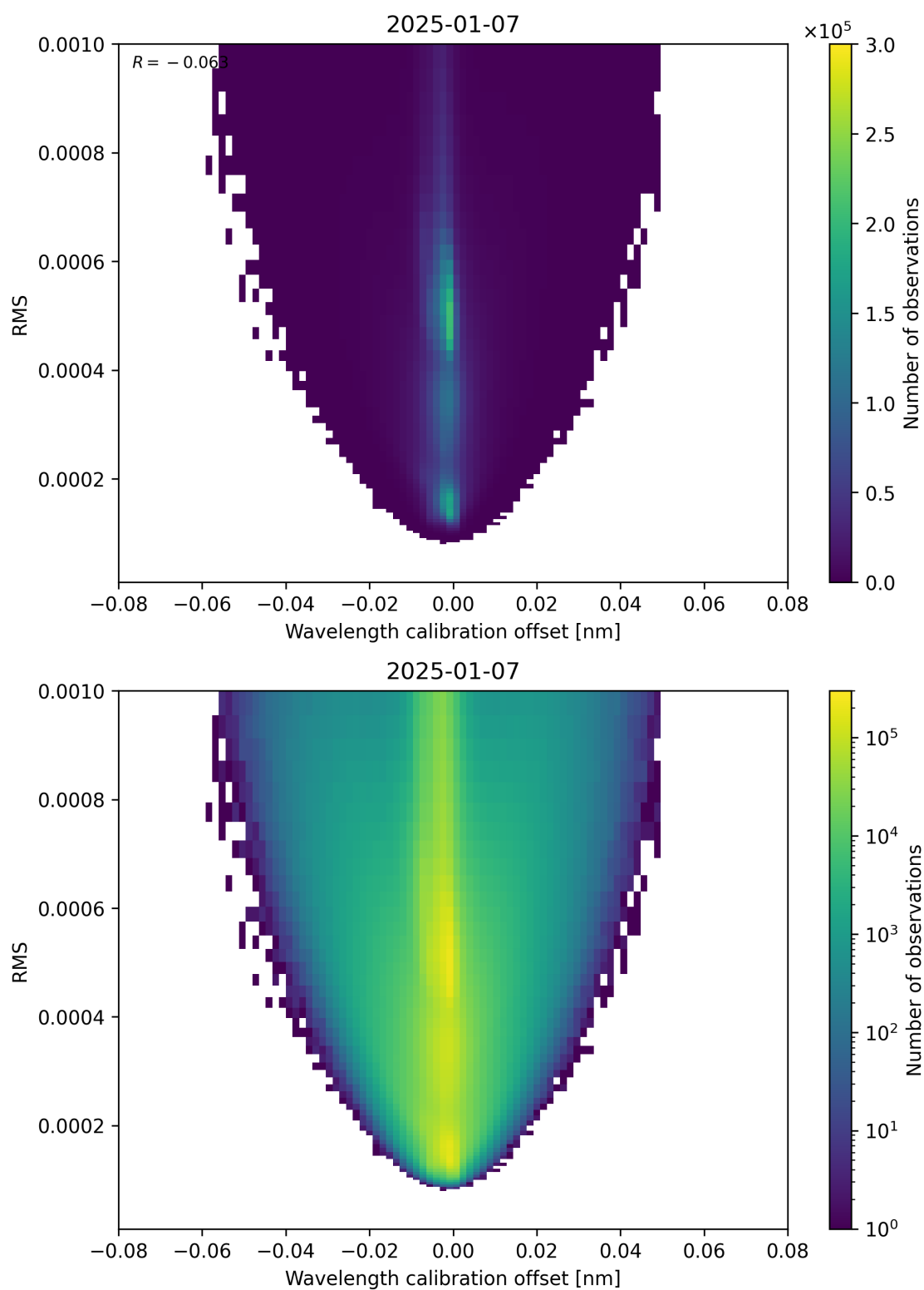
Figure 181: Scatter density plot of “Wavelength calibration offset” against “RMS” for 2025-01-07 to 2025-01-08.
