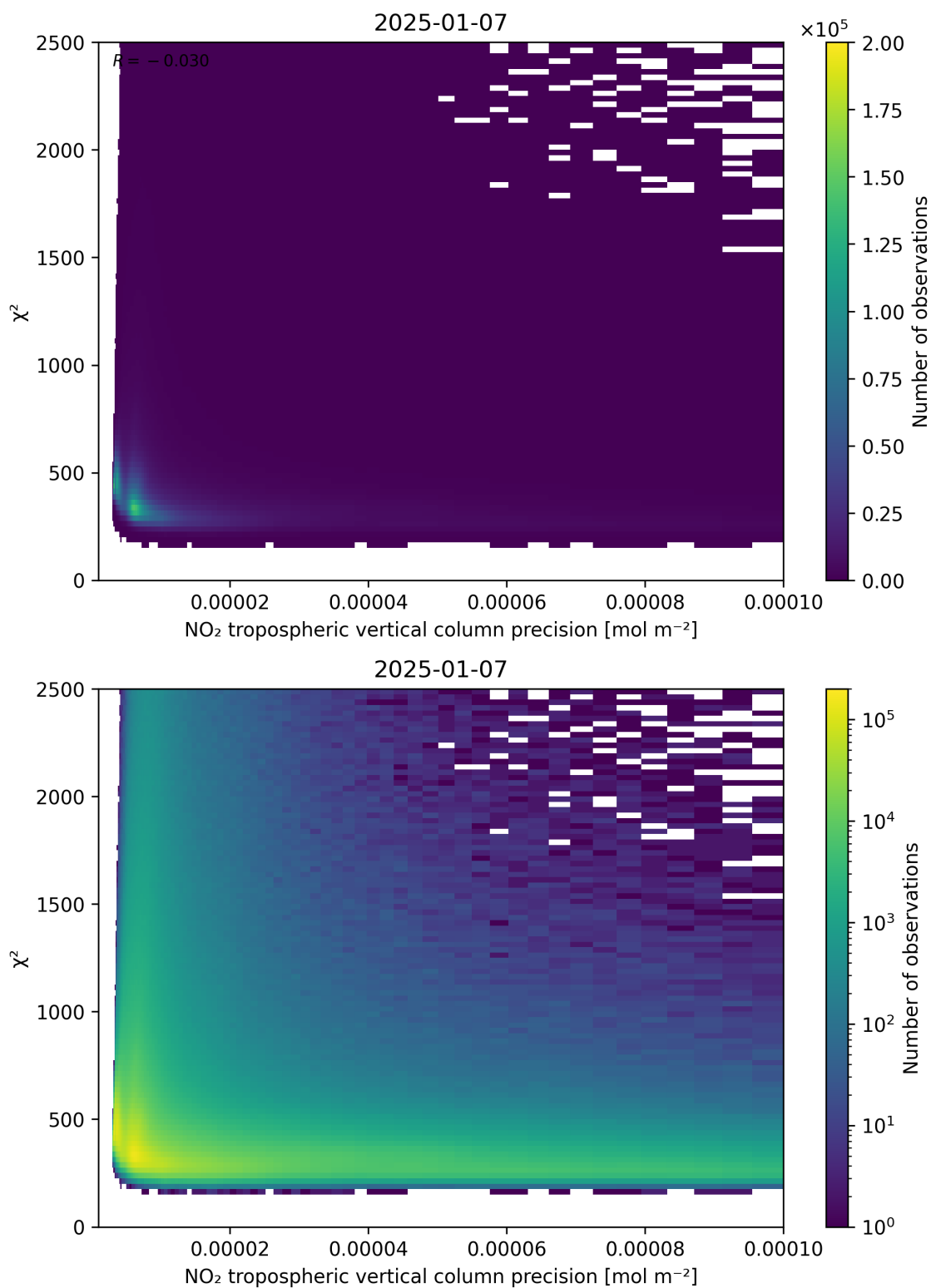
Figure 134: Scatter density plot of “NO 2 tropospheric vertical column precision” against “ \chi^2 ” for 2025-01-07 to 2025-01-08.
