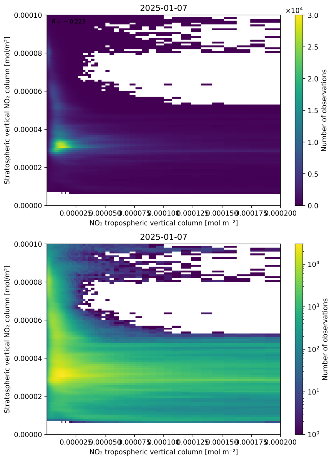
Figure 125: Scatter density plot of “NO 2 tropospheric vertical column” against “Stratospheric vertical NO 2 column” for 2025-01-07 to 2025-01-08.
