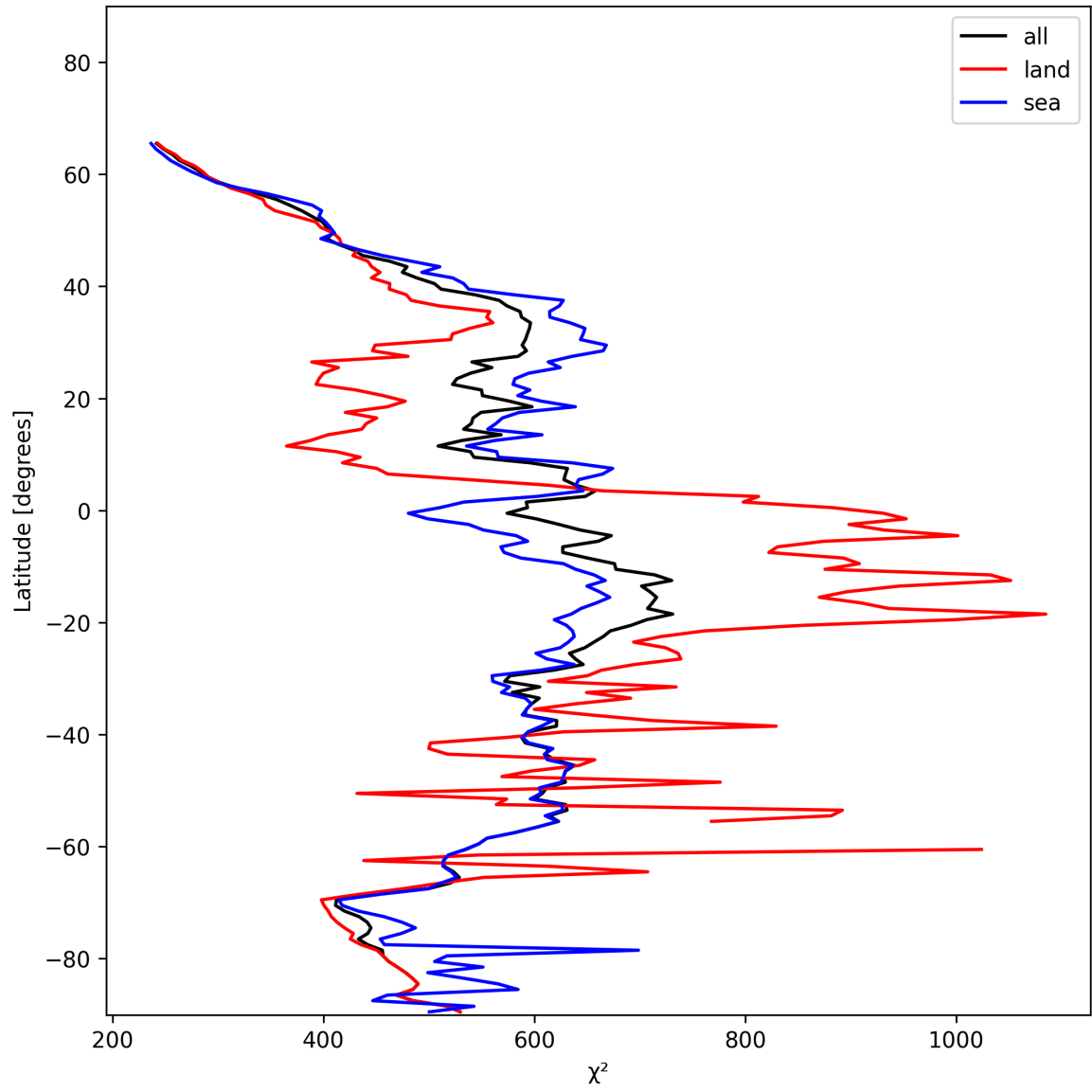
Figure 25: Zonal average of “ \chi^2 ” for 2025-01-07 to 2025-01-08.
