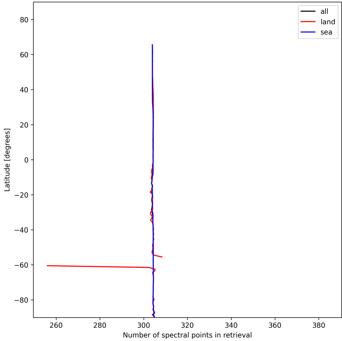
Figure 16: Zonal average of “Number of spectral points in retrieval” for 2025-01-07 to 2025-01-08.
