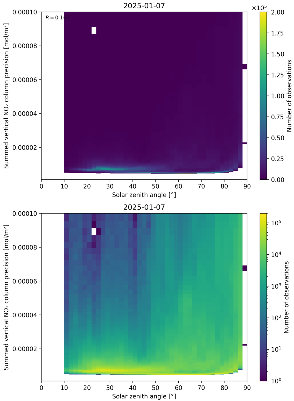
Figure 152: Scatter density plot of “Solar zenith angle” against “Summed vertical NO 2 column precision” for 2025-01-07 to 2025-01-08.
