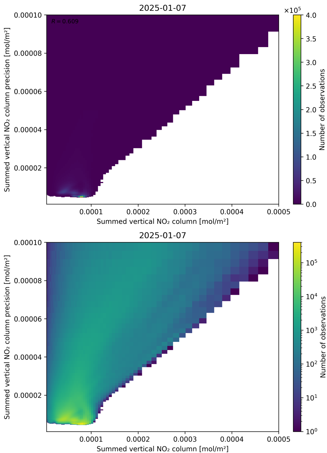
Figure 105: Scatter density plot of “Summed vertical NO 2 column” against “Summed vertical NO 2 column precision” for 2025-01-07 to 2025-01-08.
