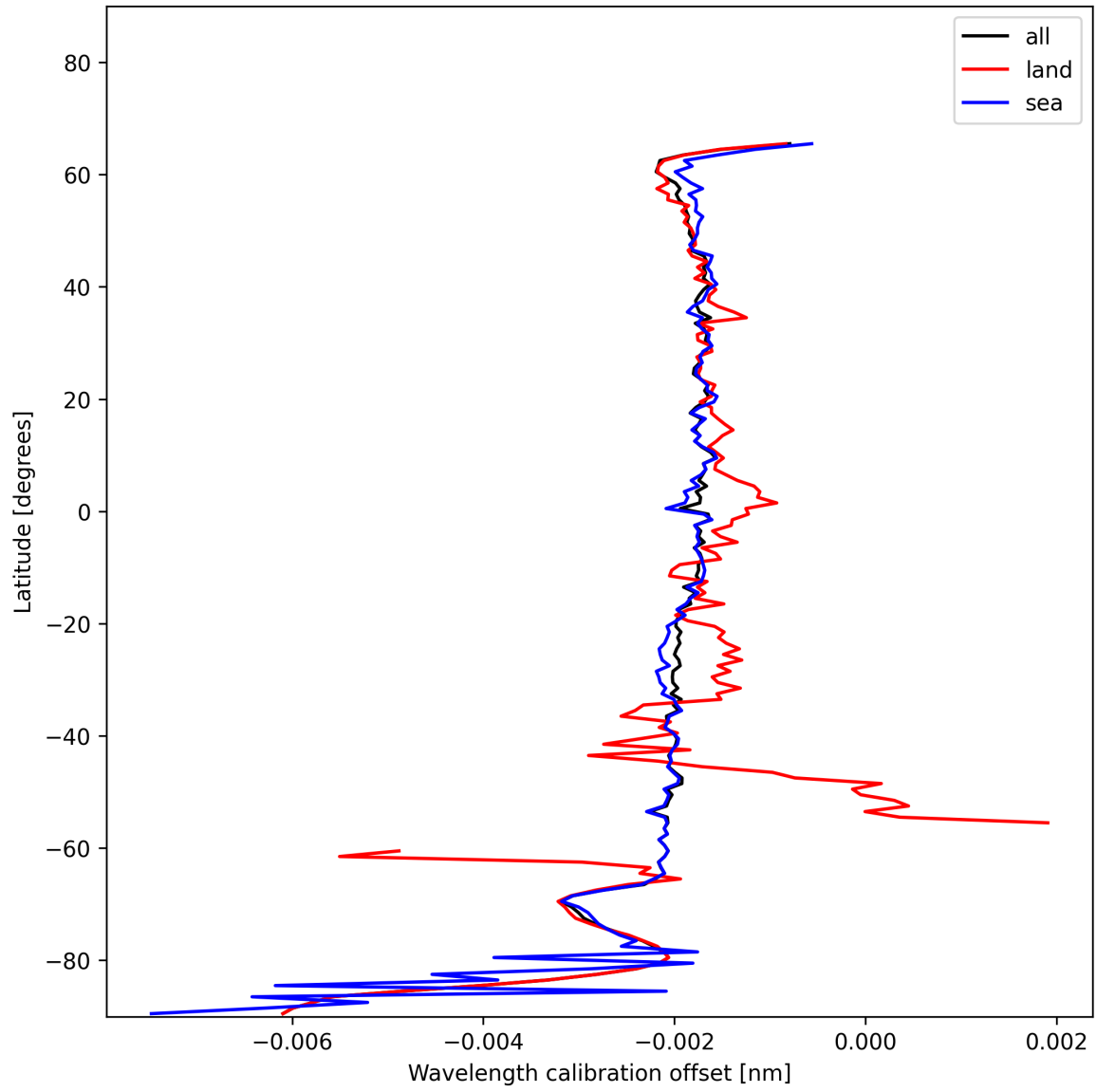
Figure 18: Zonal average of “Wavelength calibration offset” for 2025-01-07 to 2025-01-08.
