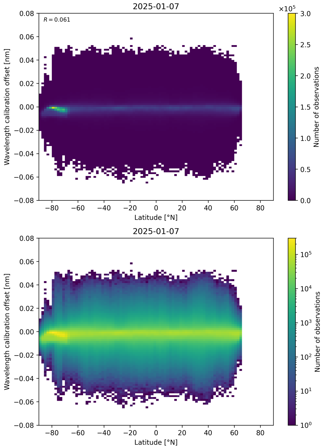
Figure 95: Scatter density plot of “Latitude” against “Wavelength calibration offset” for 2025-01-07 to 2025-01-08.
