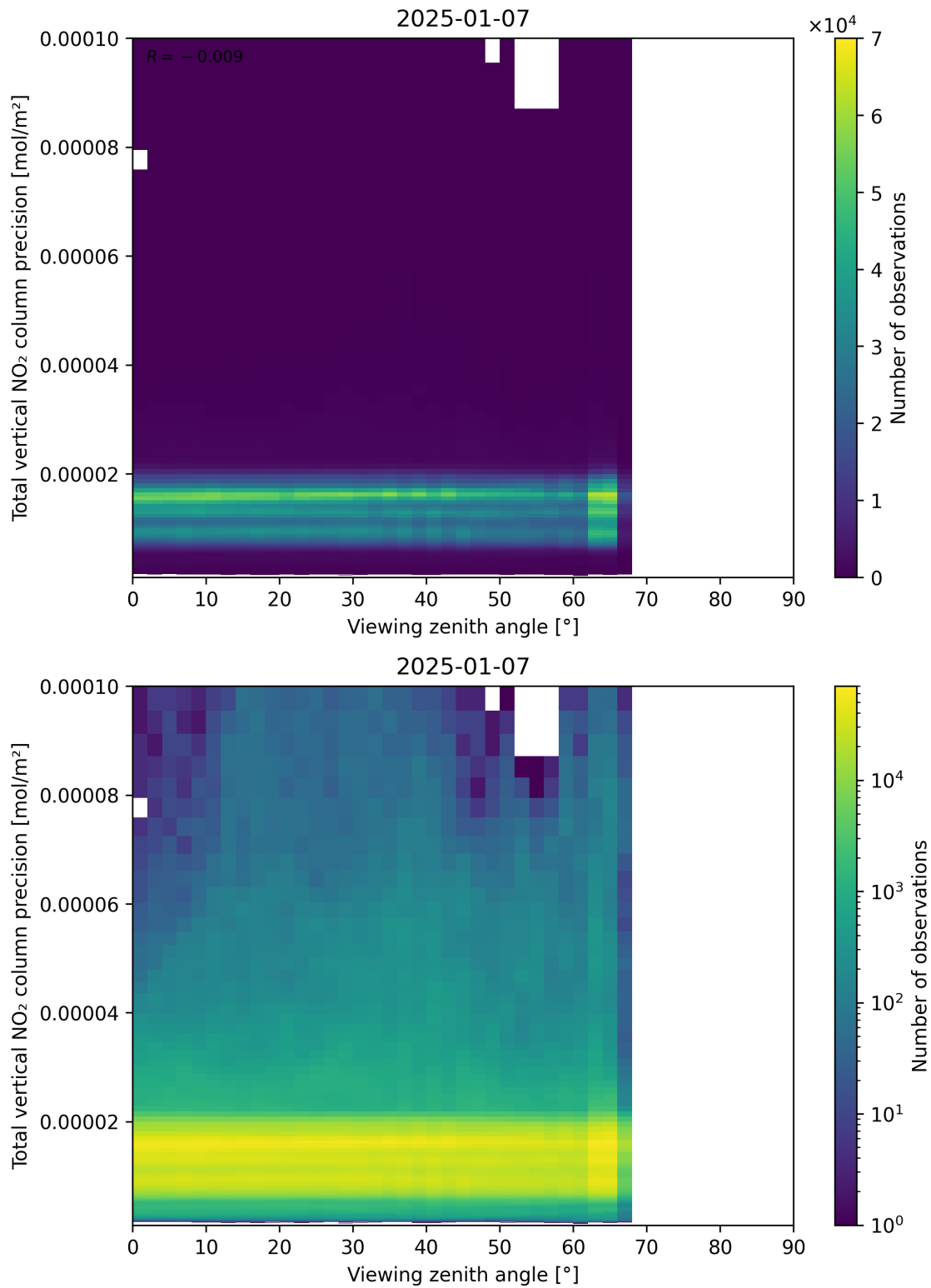
Figure 168: Scatter density plot of “Viewing zenith angle” against “Total vertical NO 2 column precision” for 2025-01-07 to 2025-01-08.
