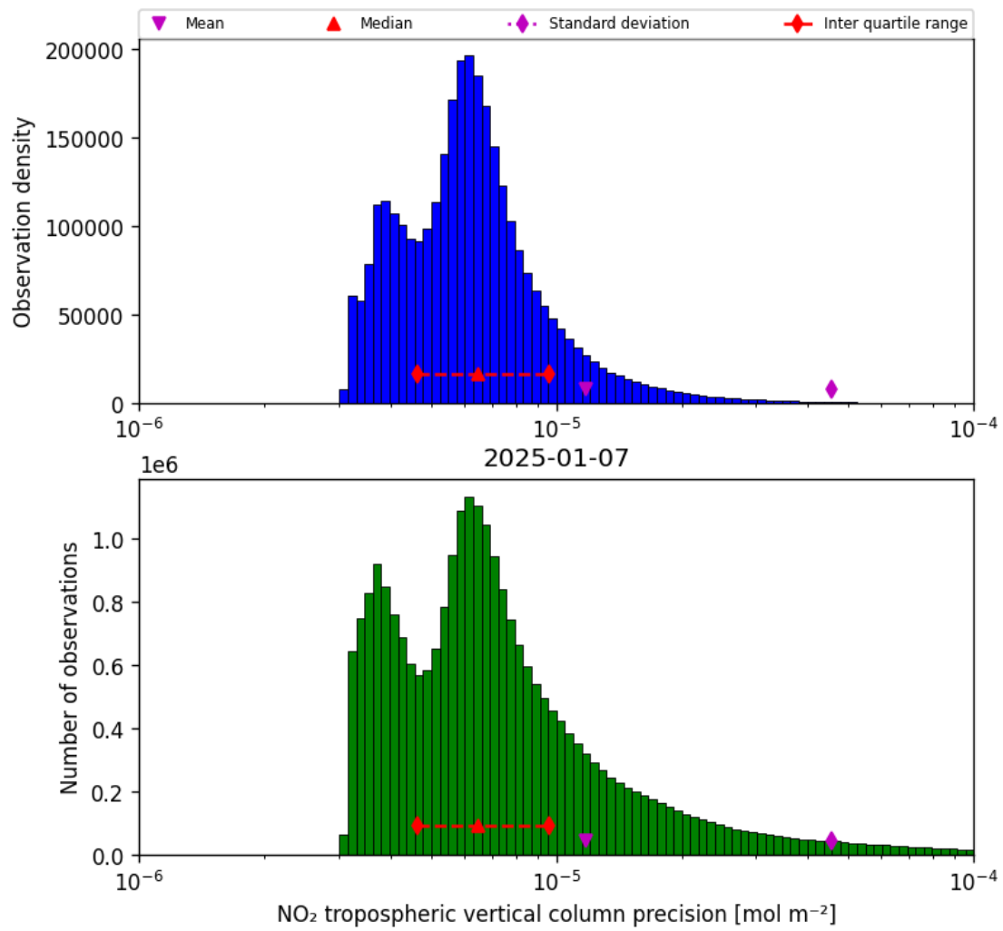
Figure 30: Histogram of “NO 2 tropospheric vertical column precision” for 2025-01-07 to 2025-01-08
