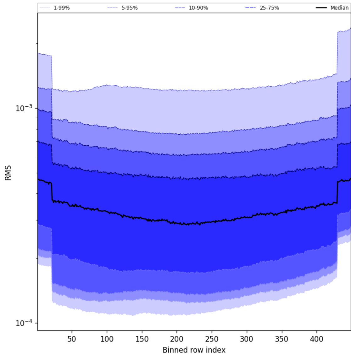
Figure 60: Along track statistics of “RMS” for 2025-01-07 to 2025-01-08
