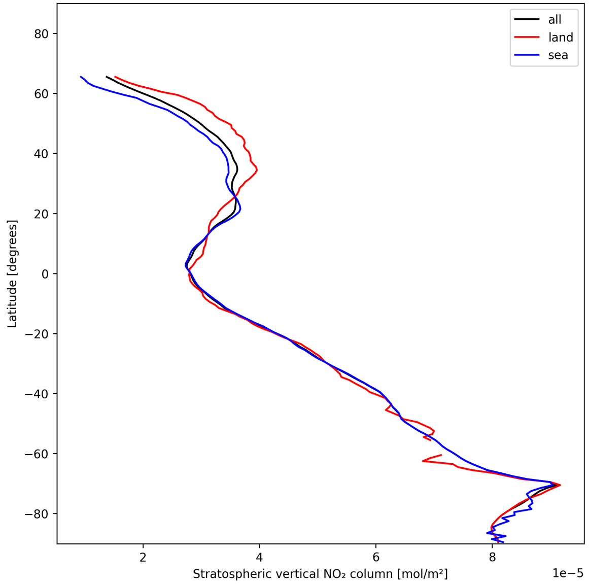
Figure 19: Zonal average of “Stratospheric vertical NO 2 column” for 2025-01-07 to 2025-01-08.
