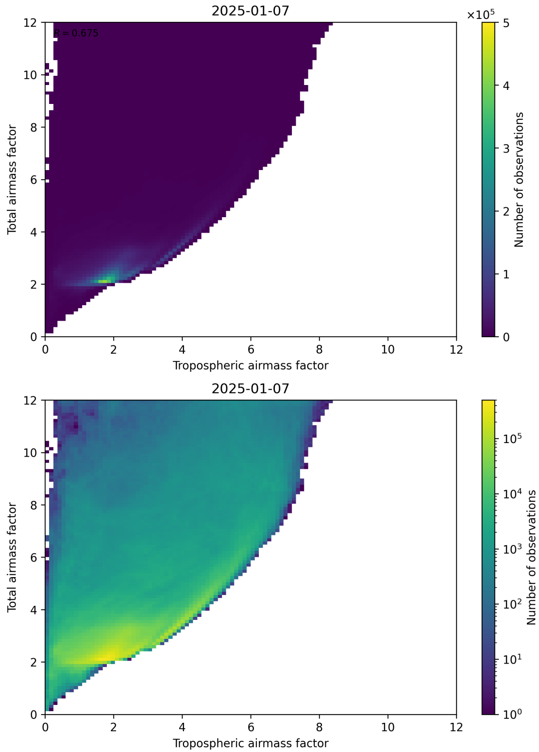
Figure 72: Scatter density plot of “Tropospheric airmass factor” against “Total airmass factor” for 2025-01-07 to 2025-01-08.
