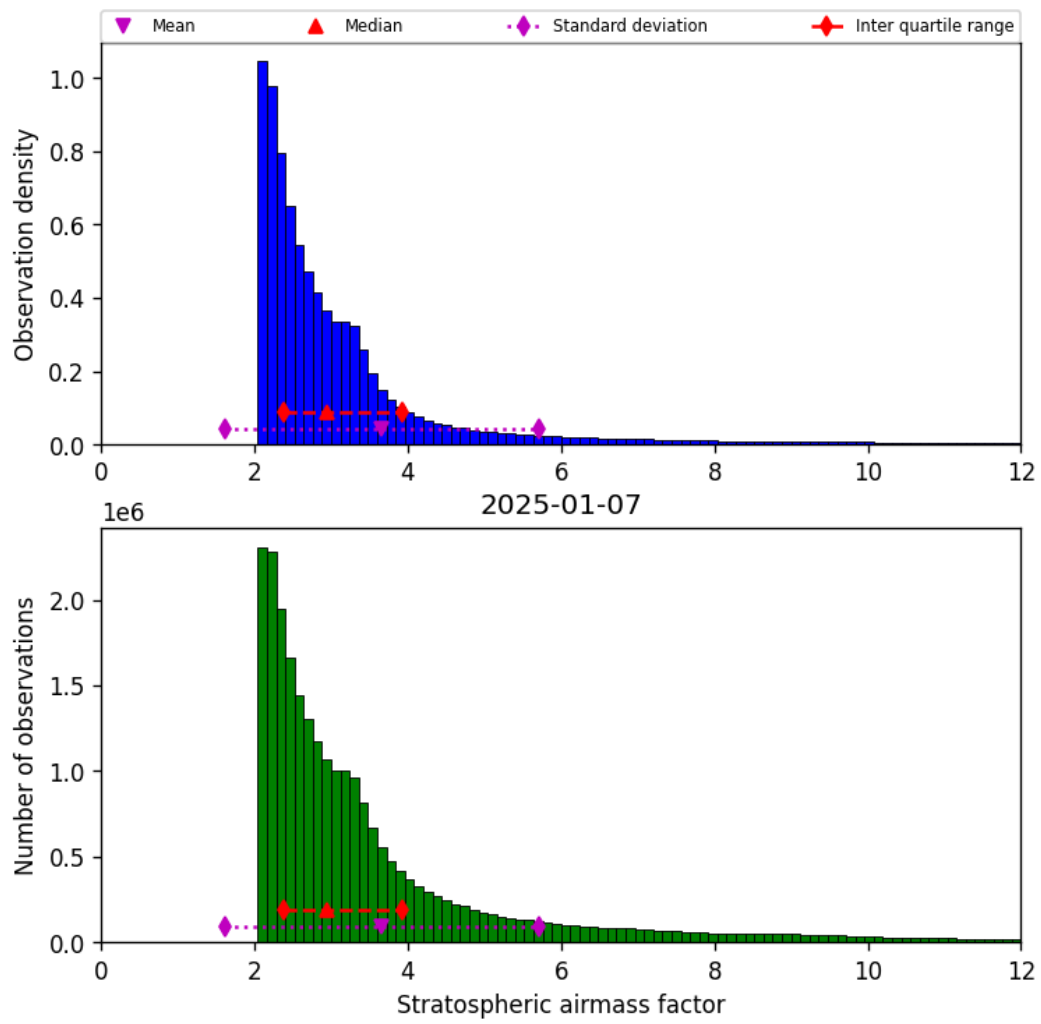
Figure 44: Histogram of “Stratospheric airmass factor” for 2025-01-07 to 2025-01-08
