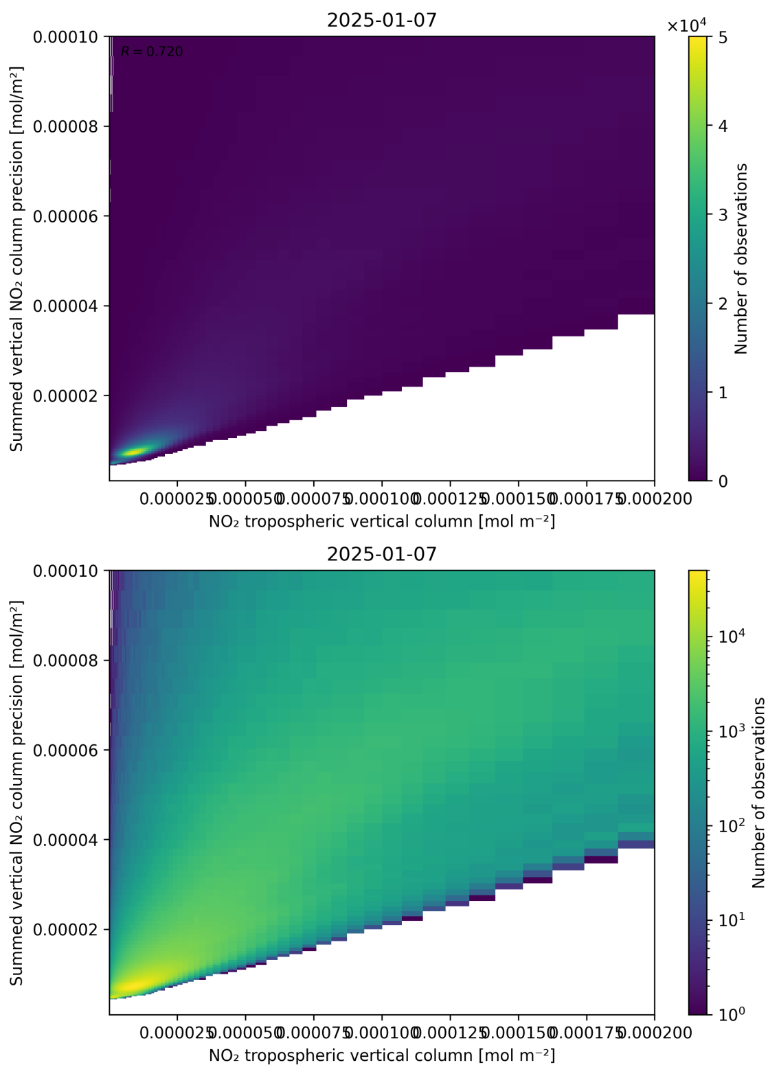
Figure 127: Scatter density plot of “NO 2 tropospheric vertical column” against “Summed vertical NO 2 column precision” for 2025-01-07 to 2025-01-08.
