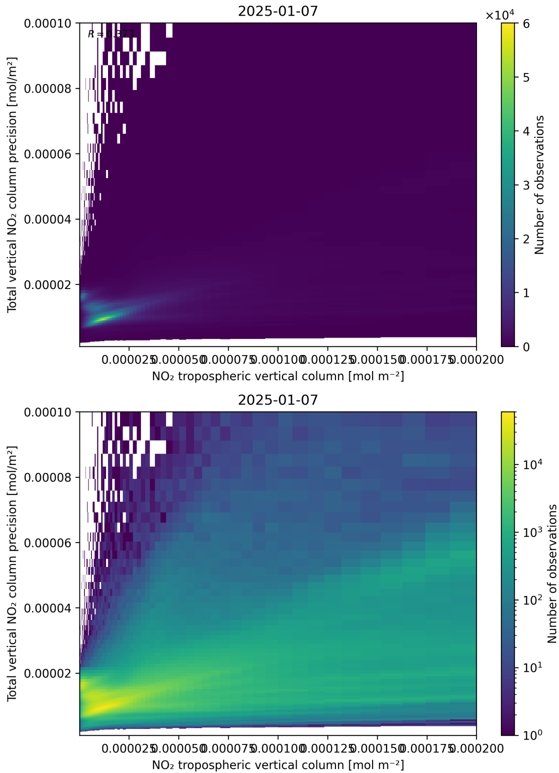
Figure 129: Scatter density plot of “NO 2 tropospheric vertical column” against “Total vertical NO 2 column precision” for 2025-01-07 to 2025-01-08.
