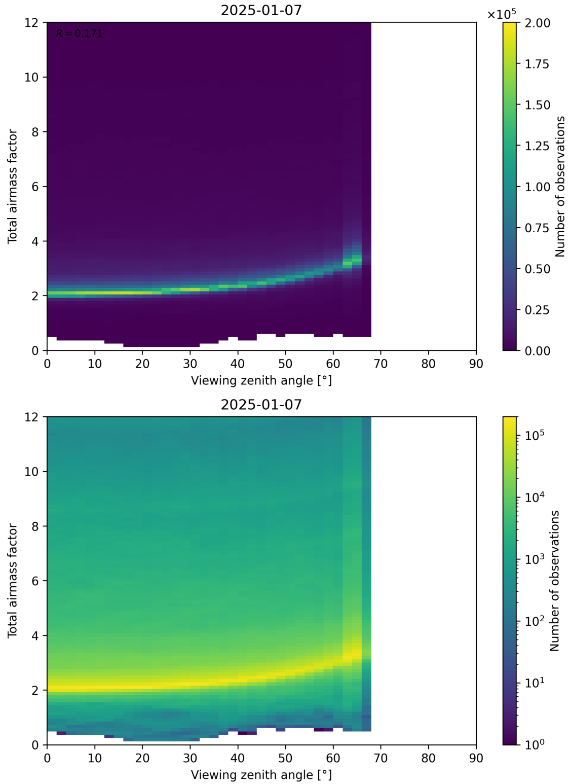
Figure 160: Scatter density plot of “Viewing zenith angle” against “Total airmass factor” for 2025-01-07 to 2025-01-08.
