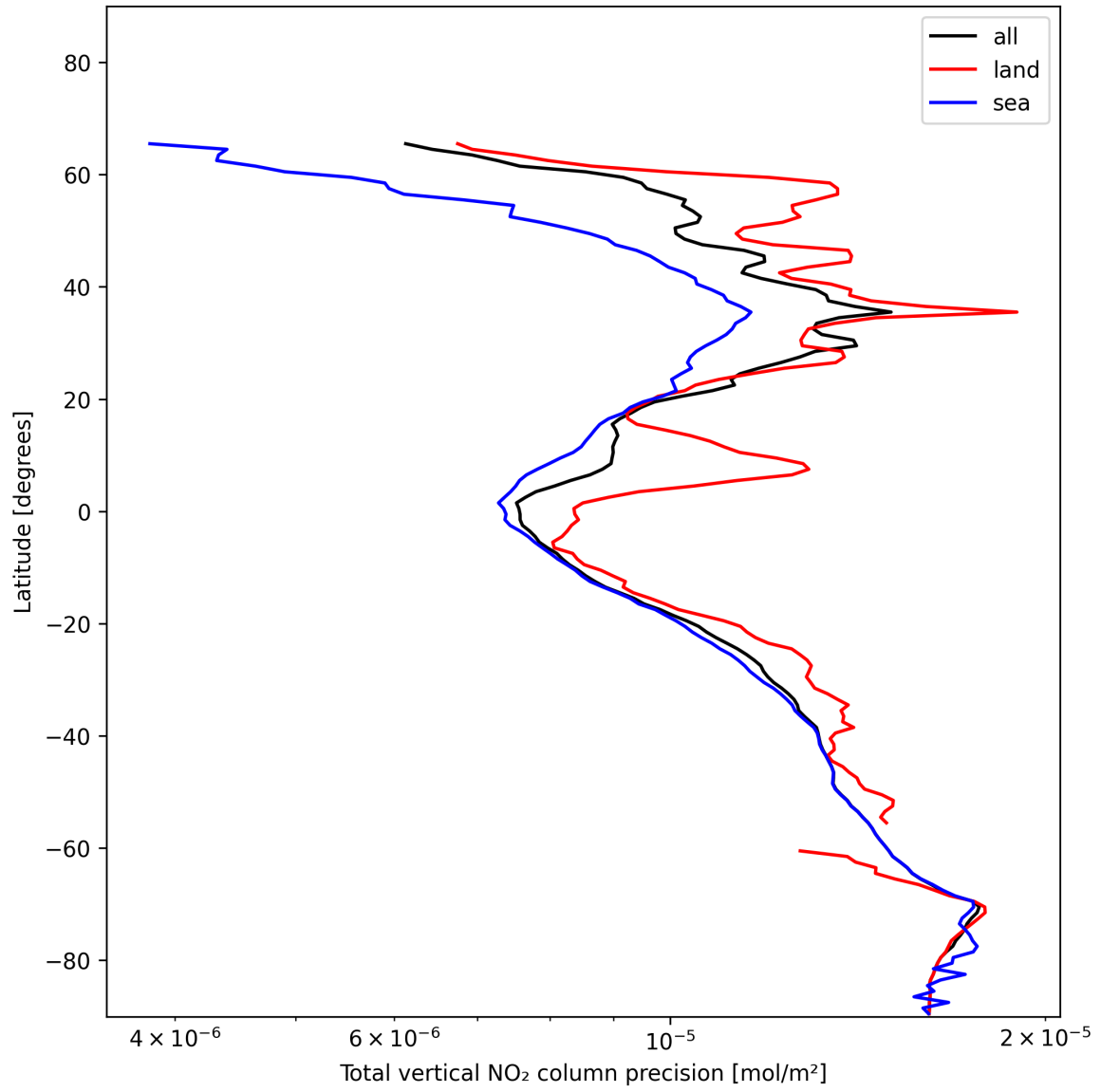
Figure 22: Zonal average of “Total vertical NO 2 column precision” for 2025-01-07 to 2025-01-08.
