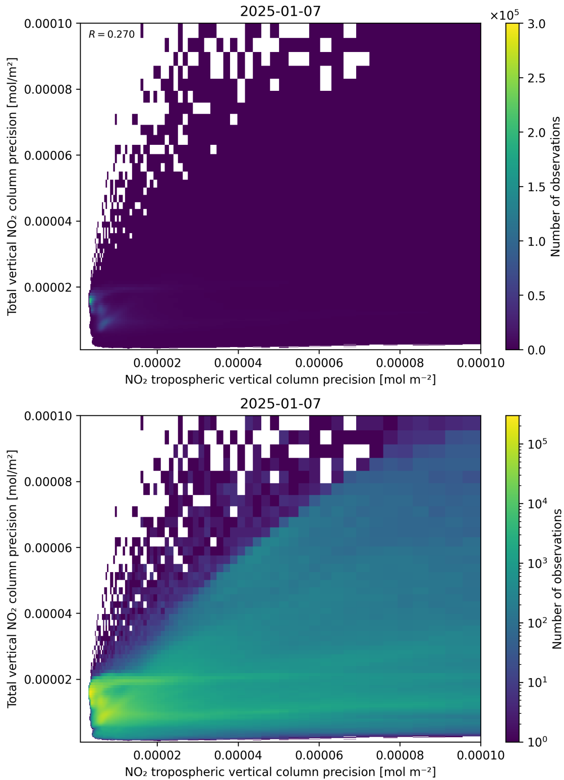
Figure 139: Scatter density plot of “NO 2 tropospheric vertical column precision” against “Total vertical NO 2 column precision” for 2025-01-07 to 2025-01-08.
