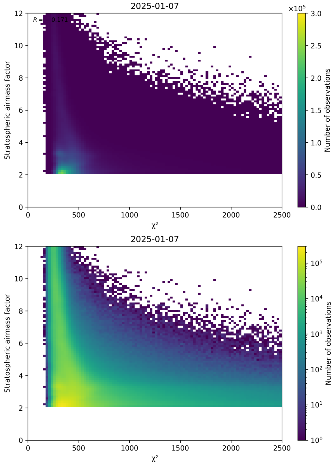
Figure 81: Scatter density plot of “ \chi^2 ” against “Stratospheric airmass factor” for 2025-01-07 to 2025-01-08.
