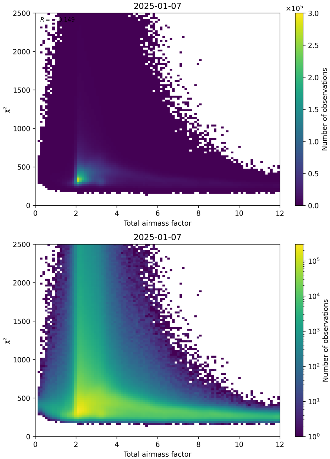
Figure 63: Scatter density plot of “Total airmass factor” against “ \chi^2 ” for 2025-01-07 to 2025-01-08.
