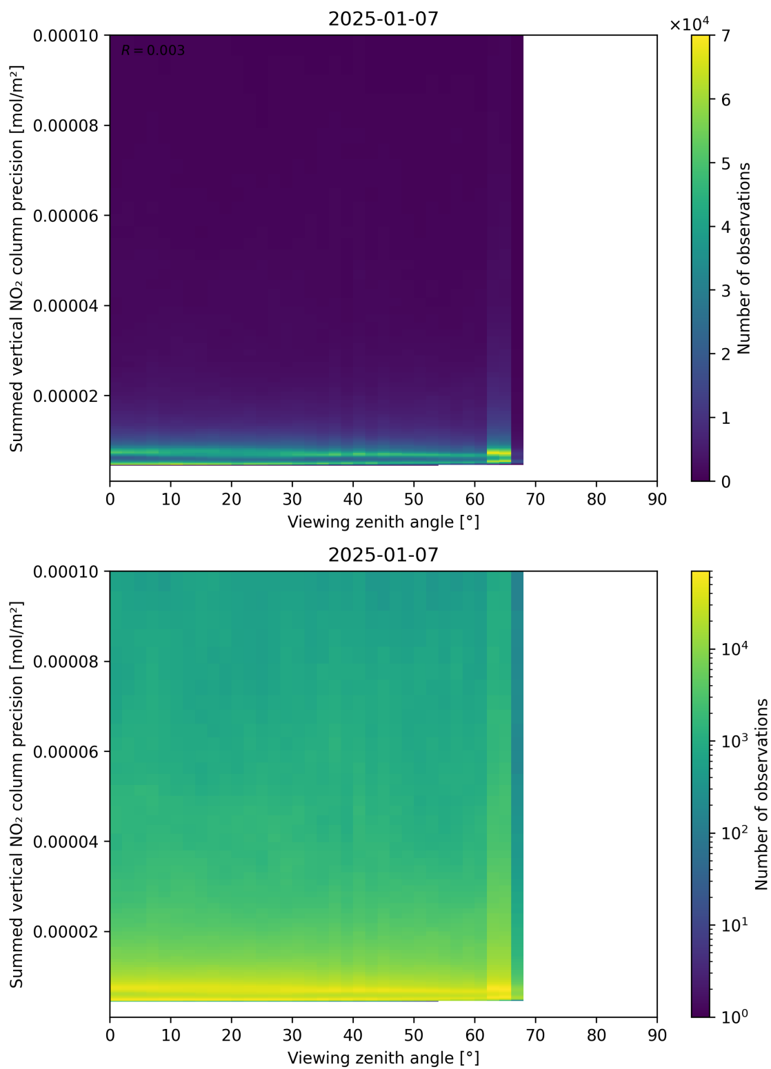
Figure 166: Scatter density plot of “Viewing zenith angle” against “Summed vertical NO 2 column precision” for 2025-01-07 to 2025-01-08.
