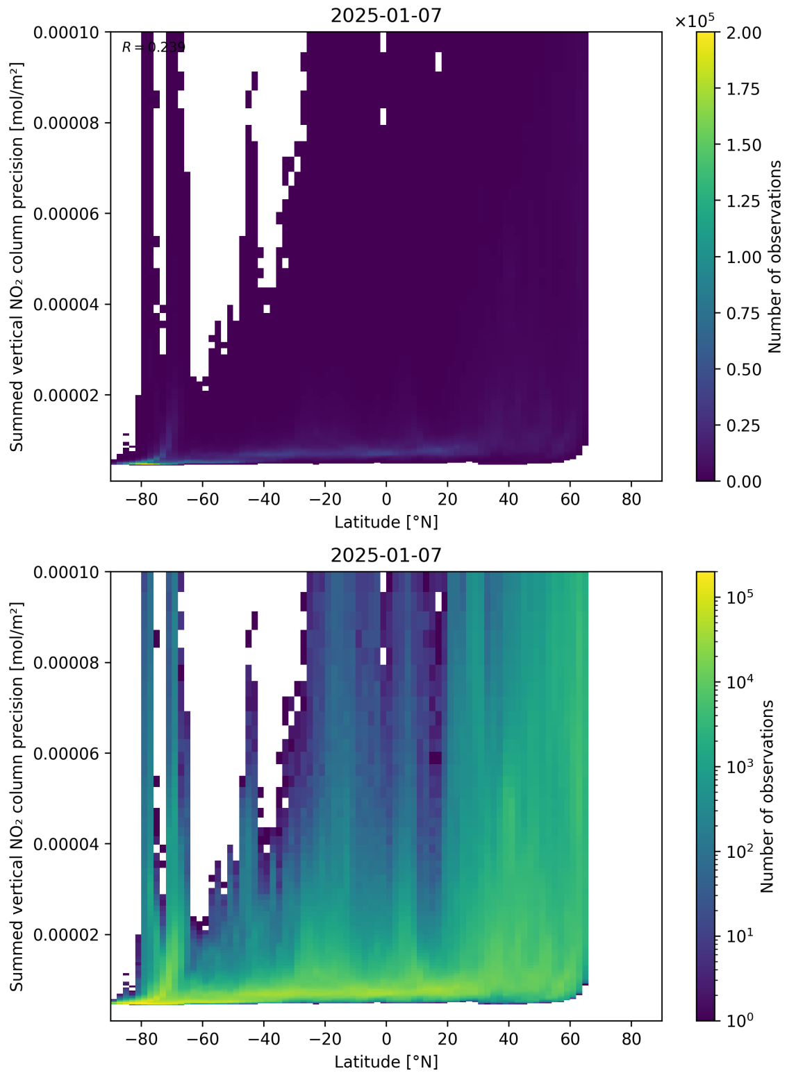
Figure 89: Scatter density plot of “Latitude” against “Summed vertical NO 2 column precision” for 2025-01-07 to 2025-01-08.
