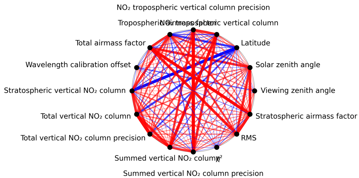
Figure 1: Map of correlation graph for 2025-01-07 to 2025-01-08.
