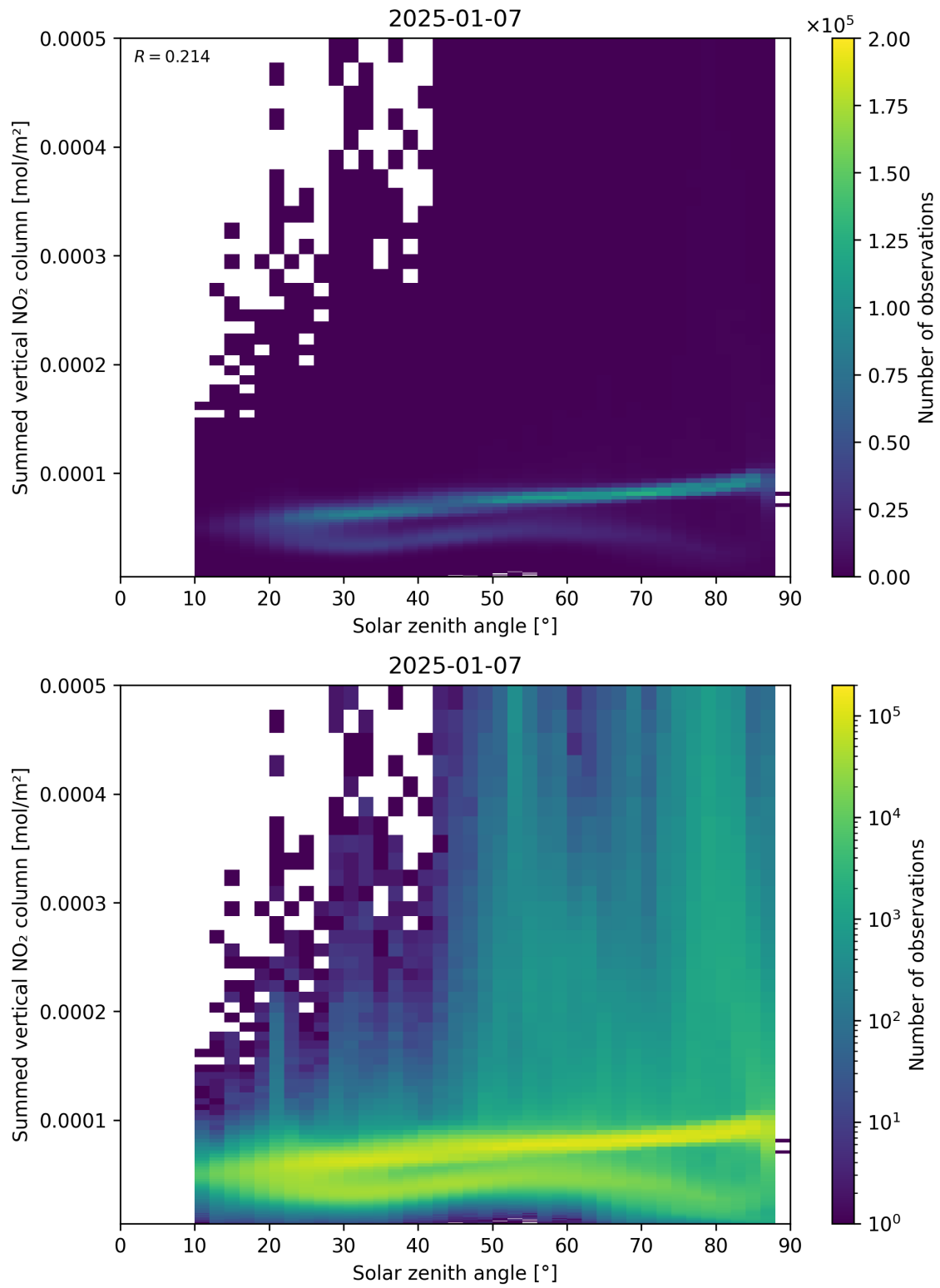
Figure 151: Scatter density plot of “Solar zenith angle” against “Summed vertical NO 2 column” for 2025-01-07 to 2025-01-08.
