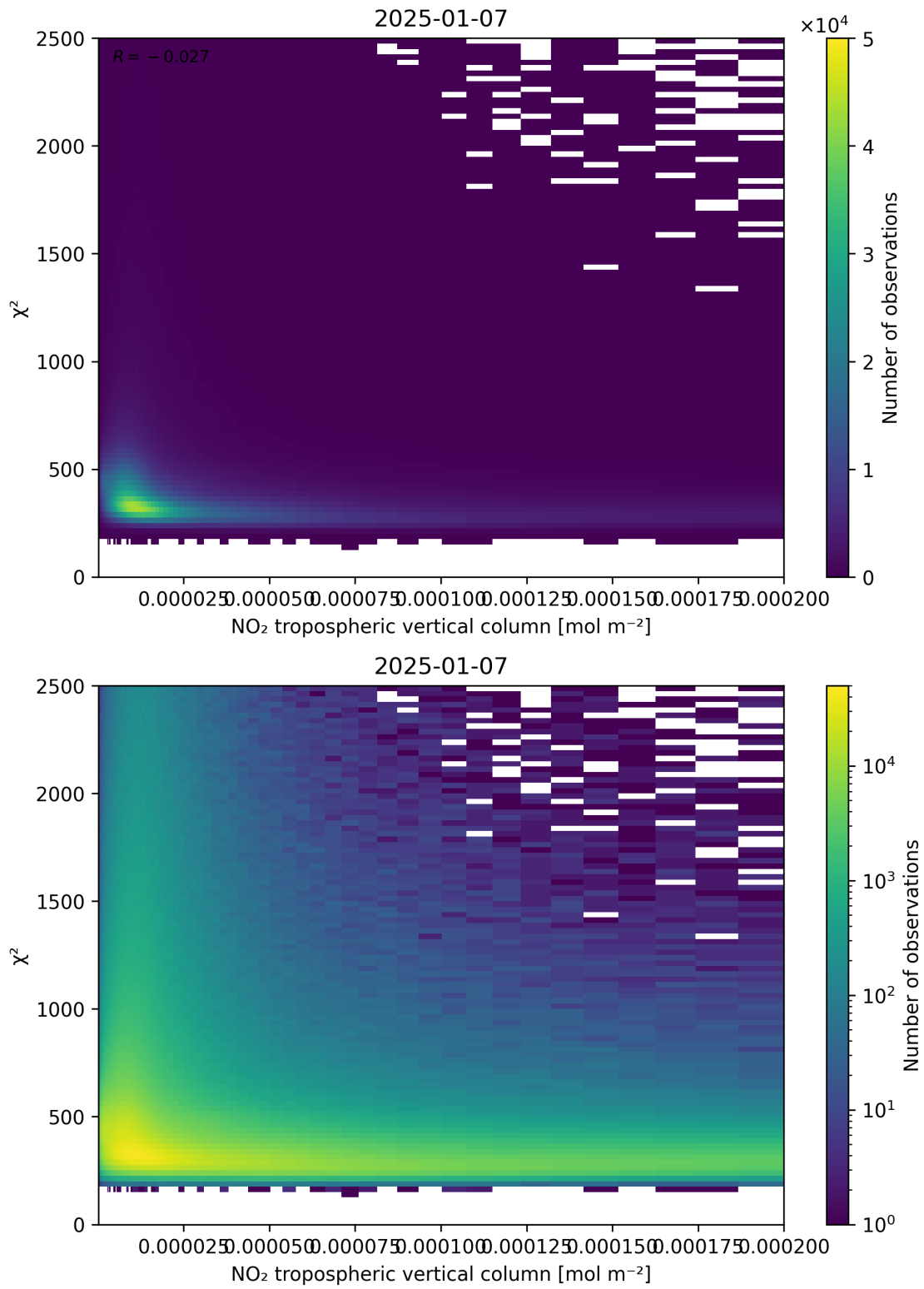
Figure 124: Scatter density plot of “NO 2 tropospheric vertical column” against “ \chi^2 ” for 2025-01-07 to 2025-01-08.
