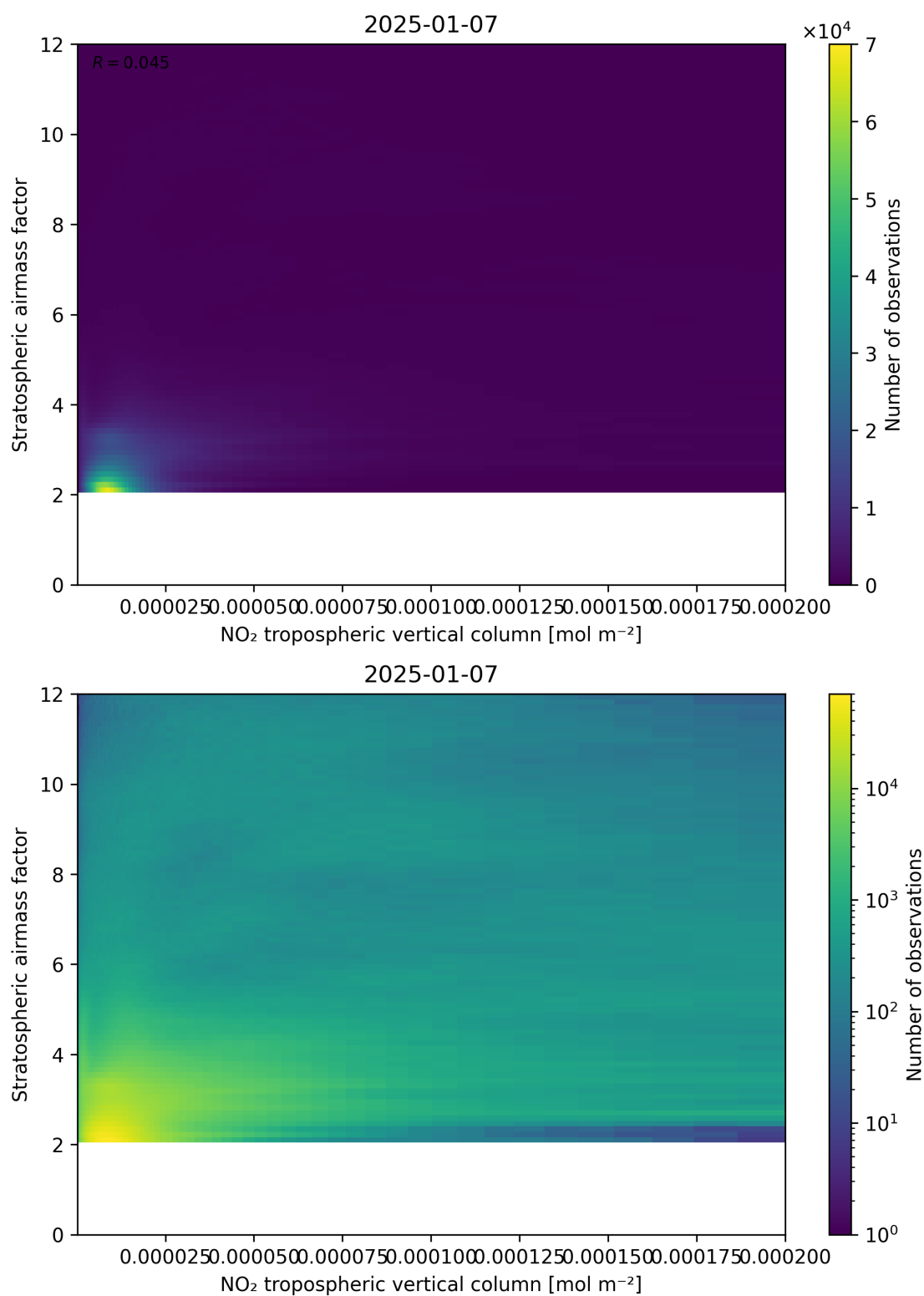
Figure 121: Scatter density plot of “NO 2 tropospheric vertical column” against “Stratospheric airmass factor” for 2025-01-07 to 2025-01-08.
