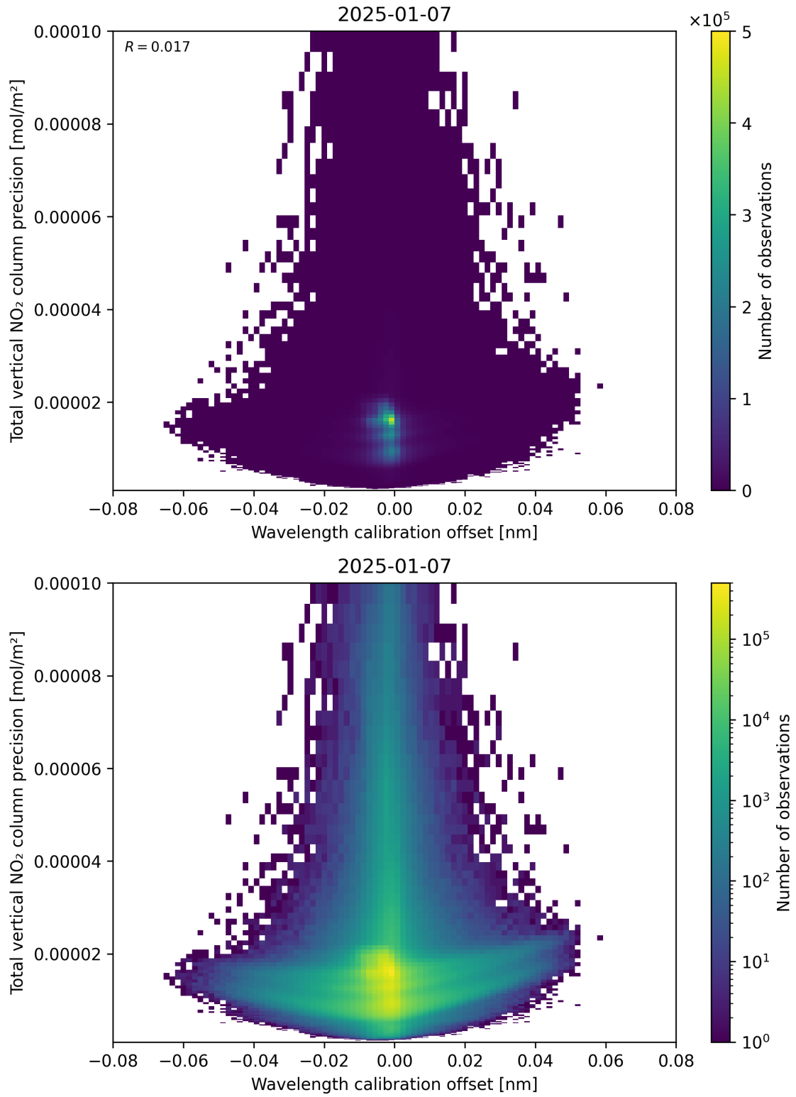
Figure 180: Scatter density plot of “Wavelength calibration offset” against “Total vertical NO 2 column precision” for 2025-01-07 to 2025-01-08.
