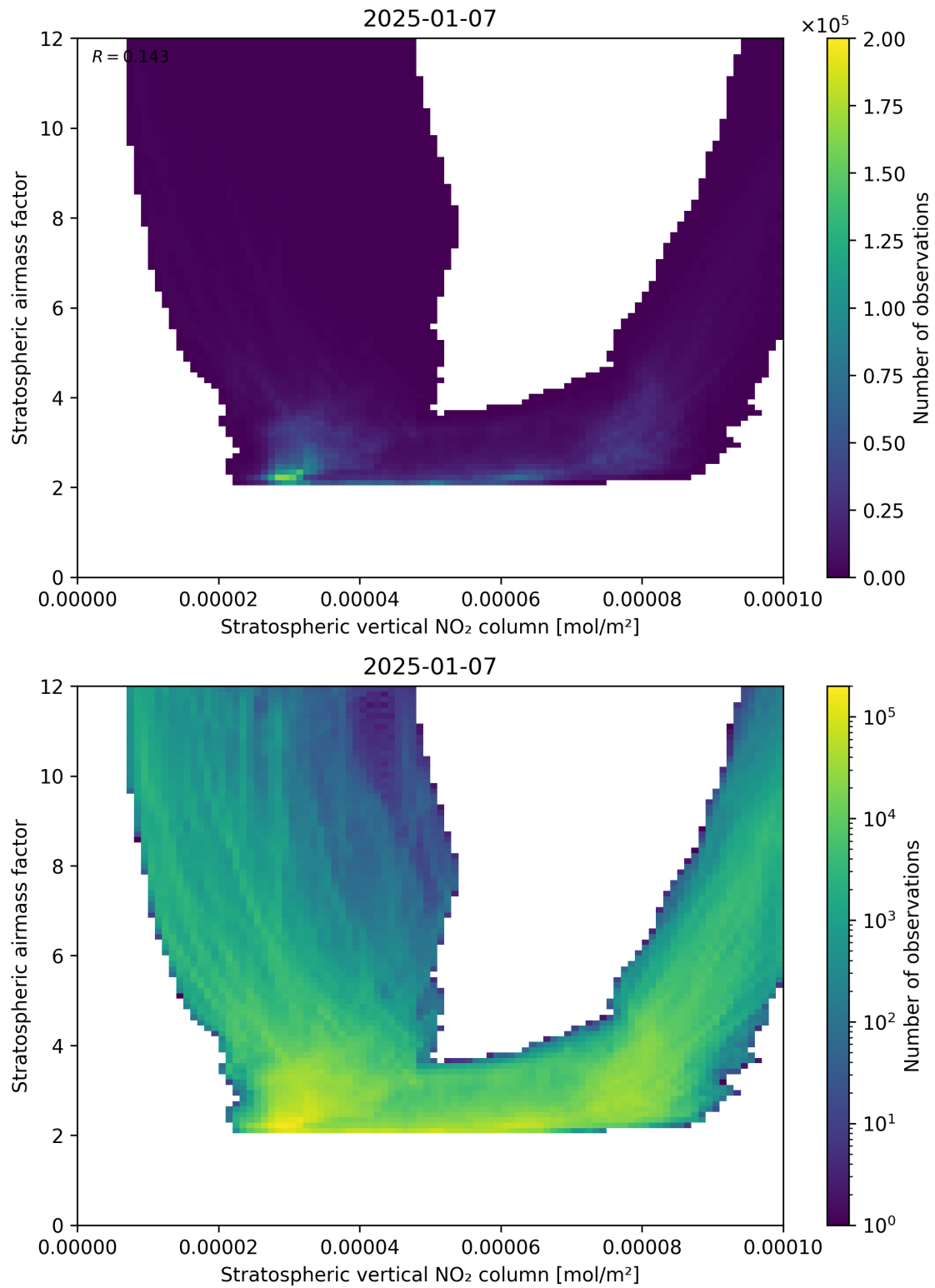
Figure 96: Scatter density plot of “Stratospheric vertical NO 2 column” against “Stratospheric airmass factor” for 2025-01-07 to 2025-01-08.
