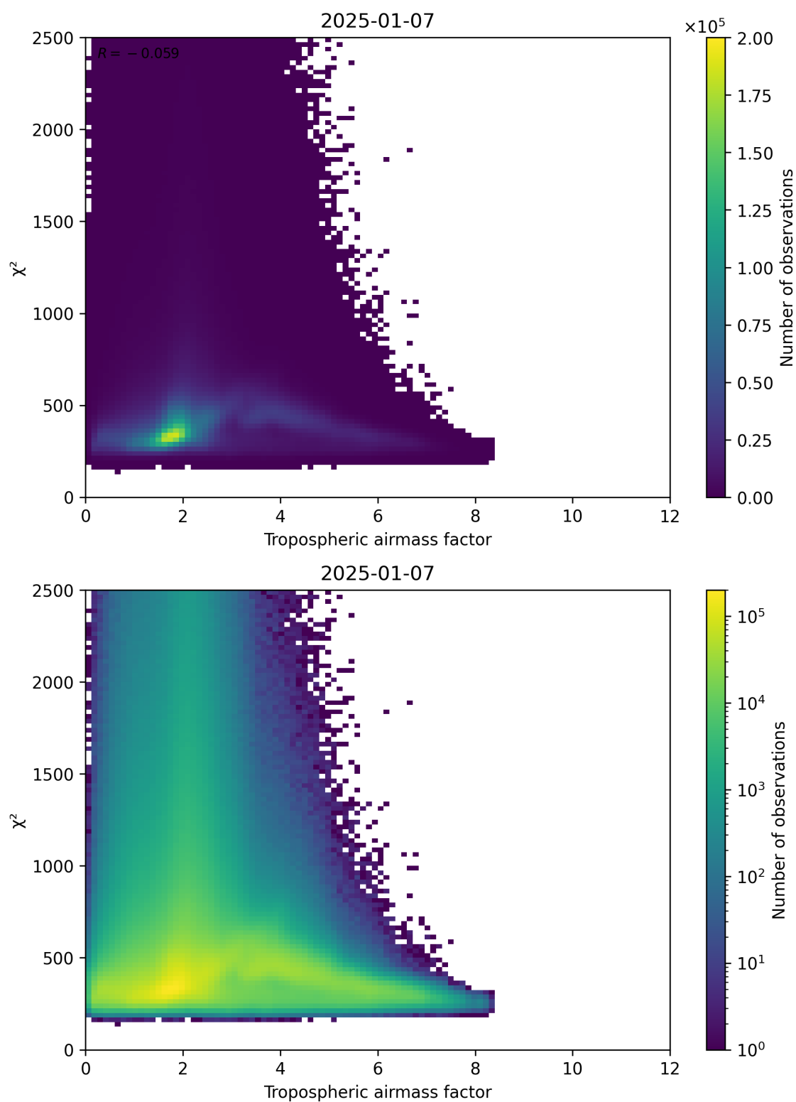
Figure 73: Scatter density plot of “Tropospheric airmass factor” against “ \chi^2 ” for 2025-01-07 to 2025-01-08.
