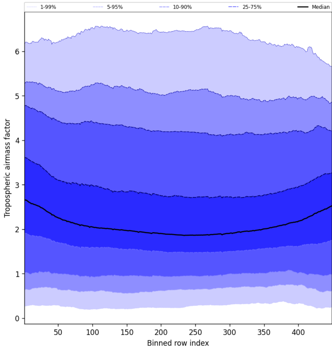
Figure 48: Along track statistics of “Tropospheric airmass factor” for 2025-01-07 to 2025-01-08
