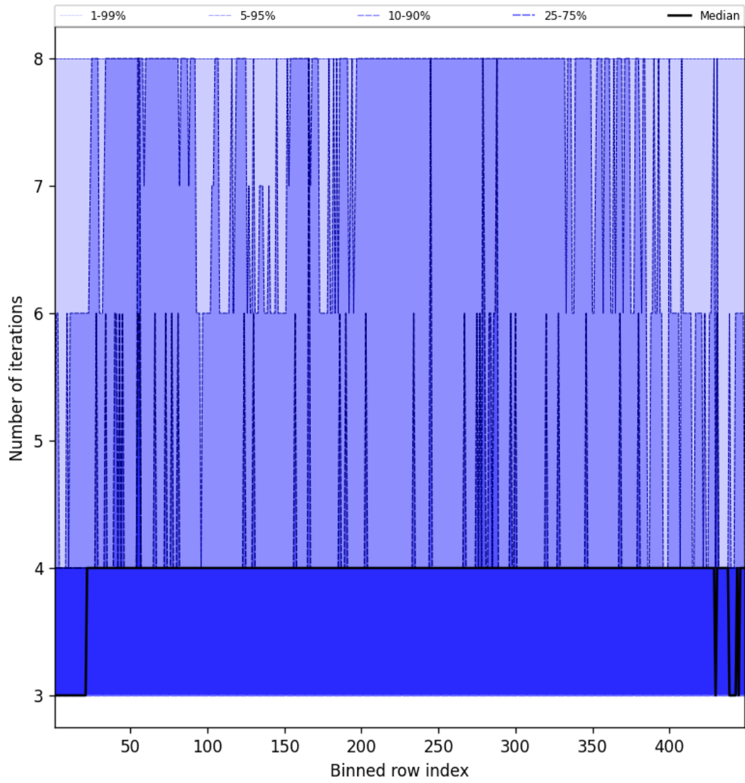
Figure 51: Along track statistics of “Number of iterations” for 2025-01-07 to 2025-01-08
