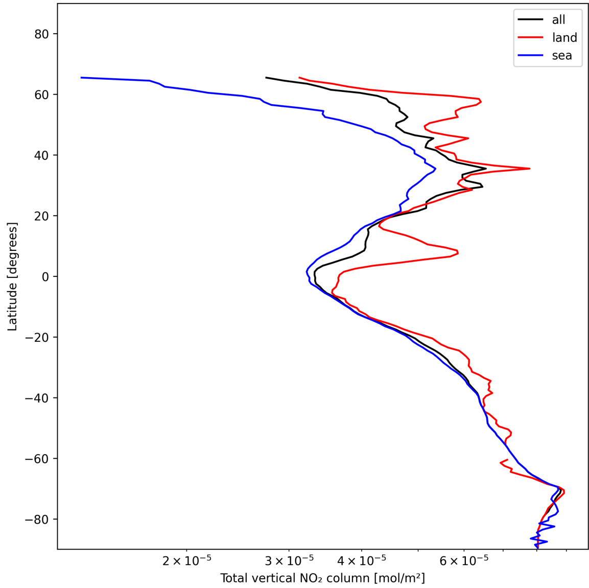
Figure 21: Zonal average of “Total vertical NO 2 column” for 2025-01-07 to 2025-01-08.
