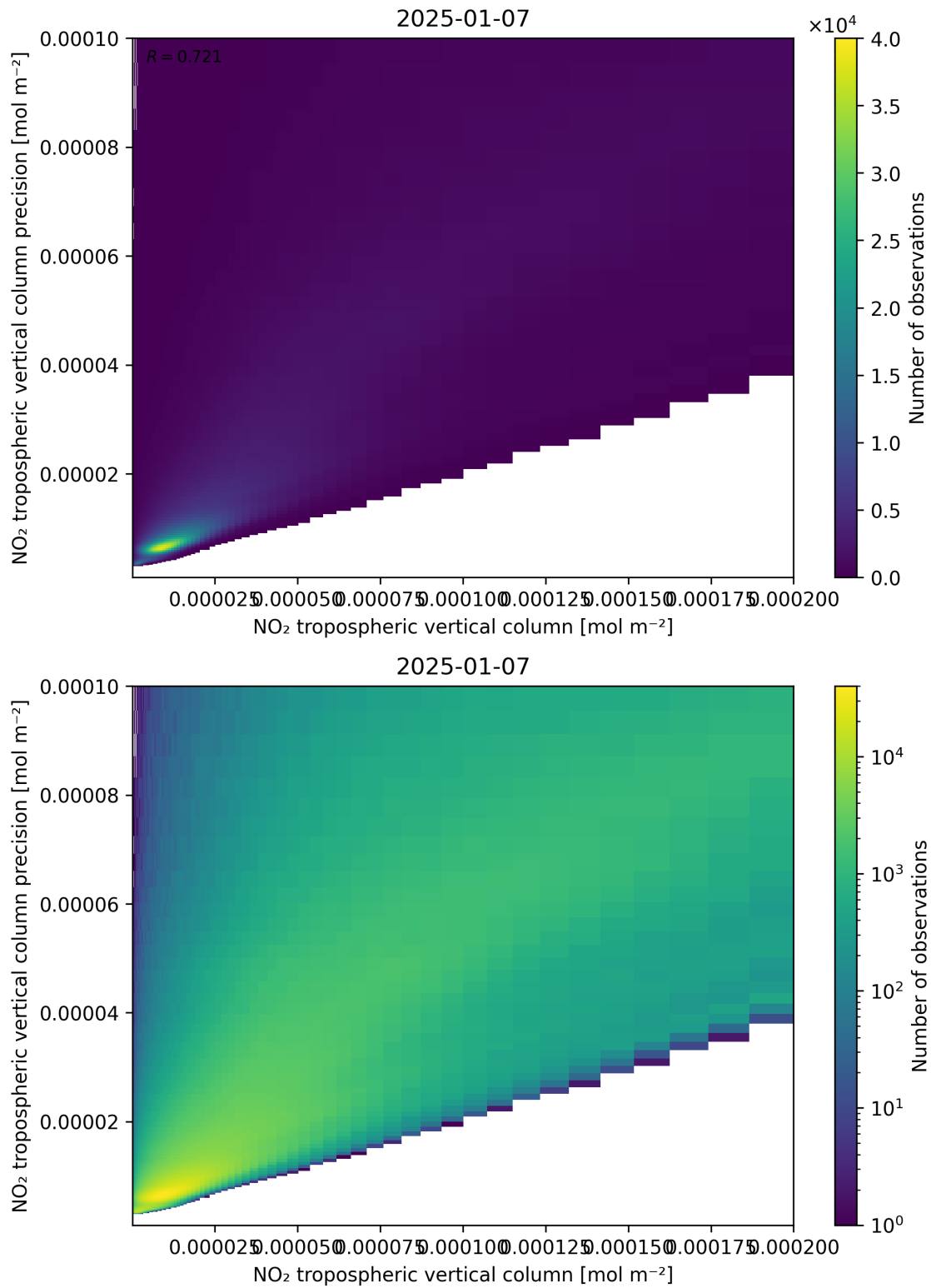
Figure 130: Scatter density plot of “NO 2 tropospheric vertical column” against “NO 2 tropospheric vertical column precision” for 2025-01-07 to 2025-01-08.
