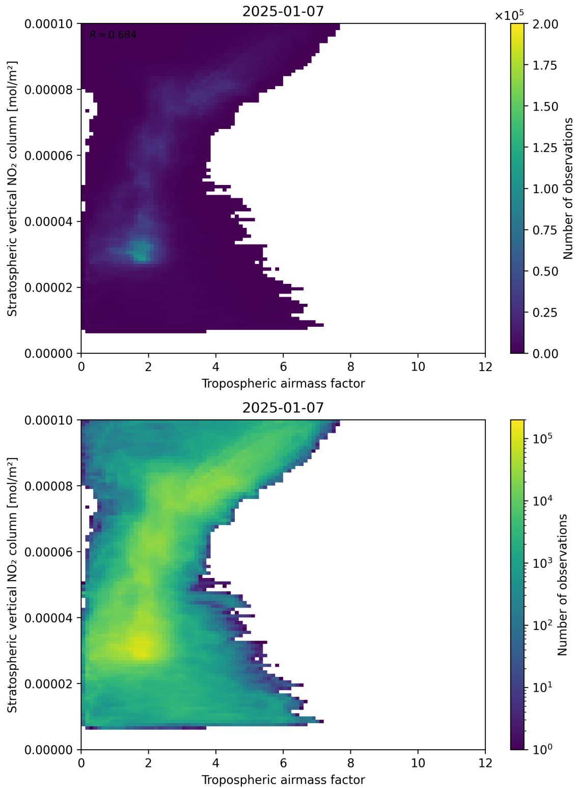
Figure 74: Scatter density plot of “Tropospheric airmass factor” against “Stratospheric vertical NO 2 column” for 2025-01-07 to 2025-01-08.
