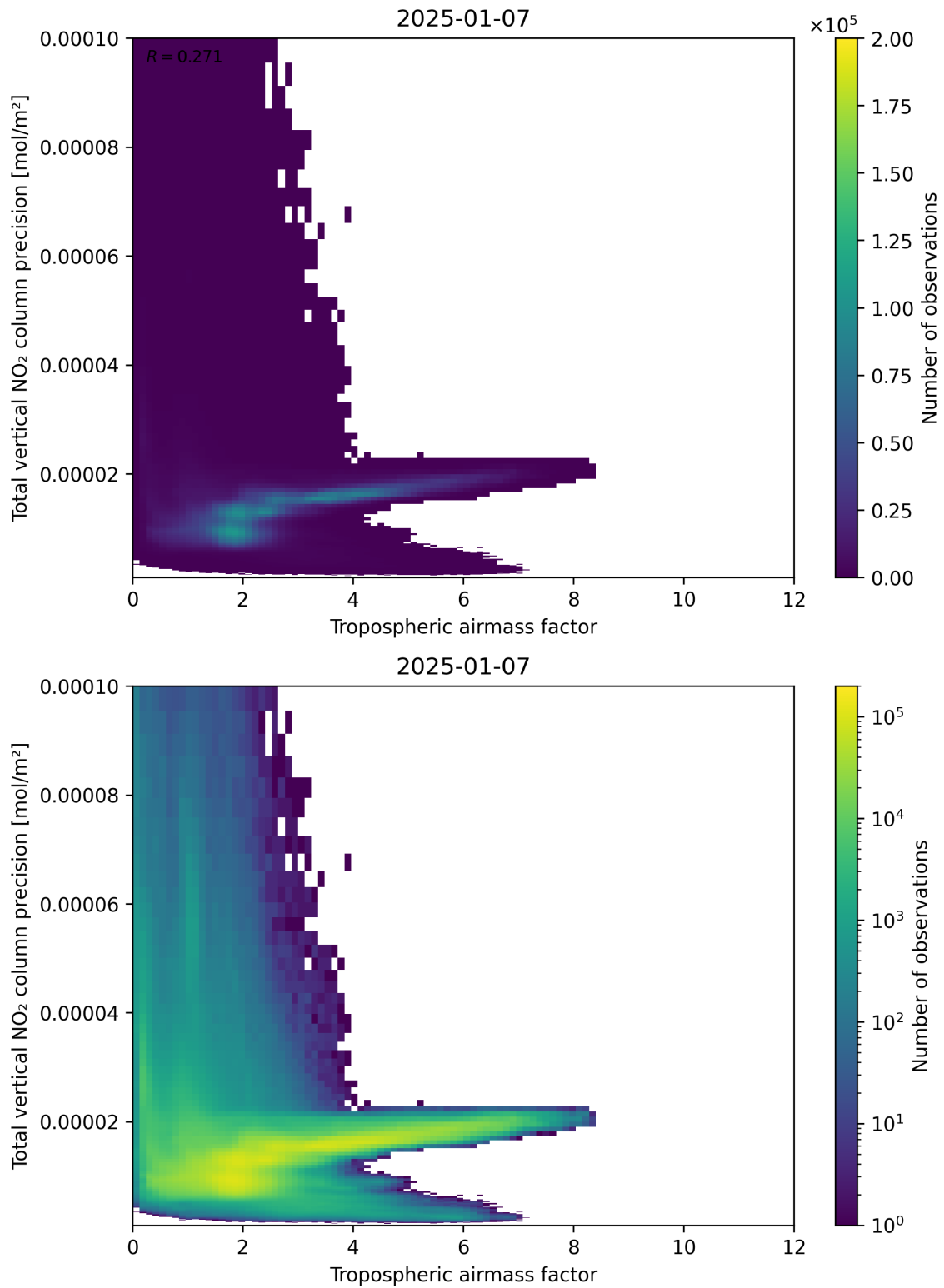
Figure 78: Scatter density plot of “Tropospheric air mass factor” against “Total vertical NO 2 column precision” for 2025-01-07 to 2025-01-08.
