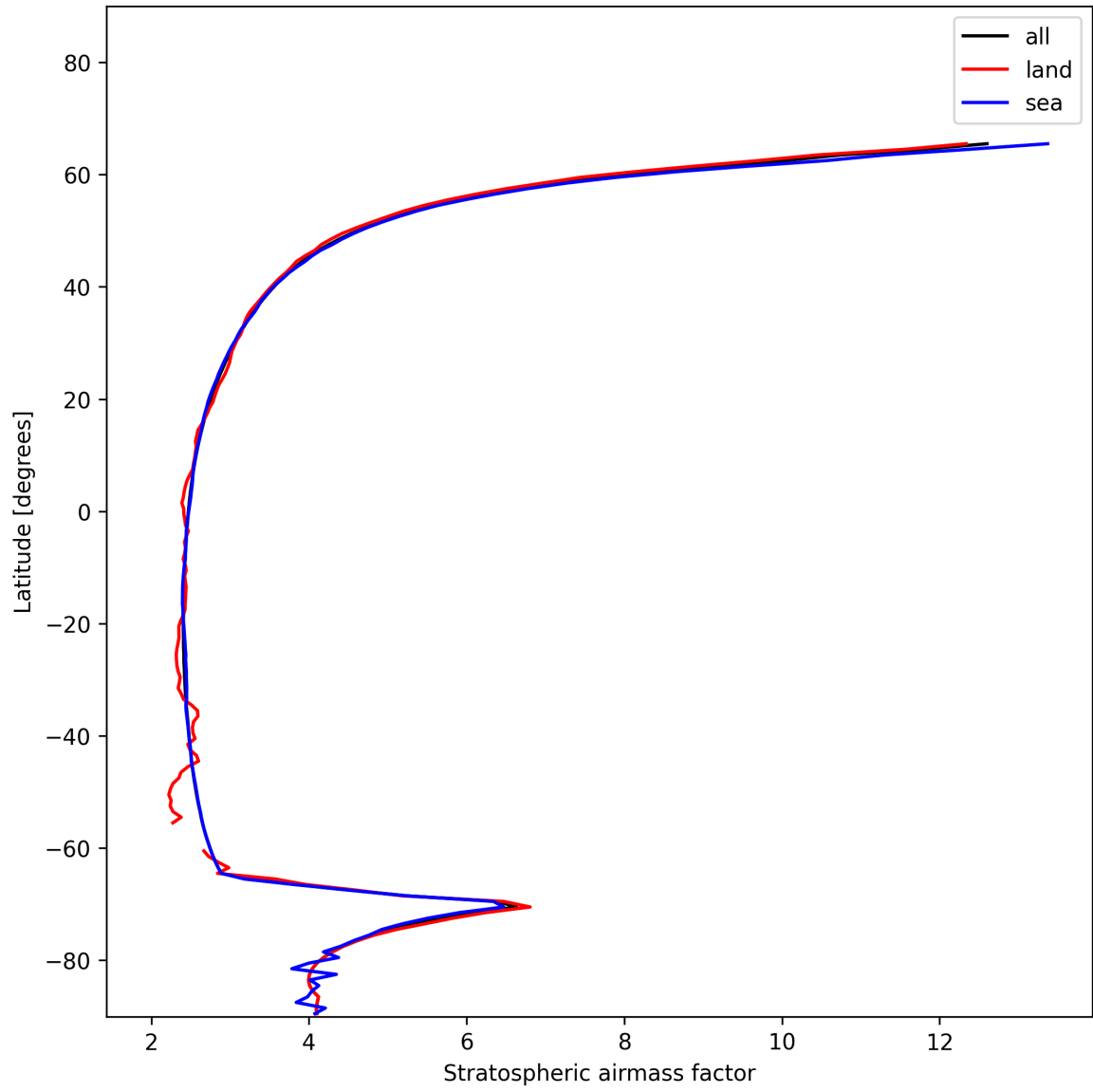
Figure 27: Zonal average of “Stratospheric air mass factor” for 2025-01-07 to 2025-01-08.
