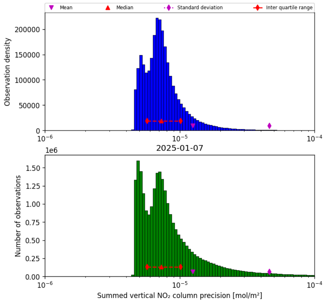
Figure 41: Histogram of “Summed vertical NO 2 column precision” for 2025-01-07 to 2025-01-08
