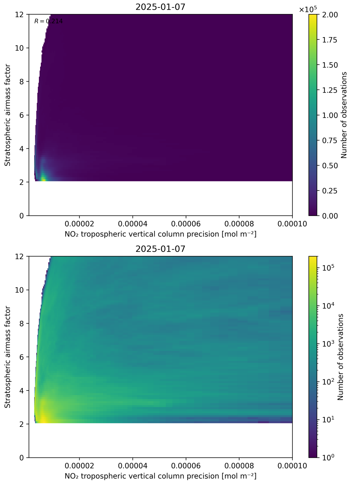
Figure 131: Scatter density plot of “NO 2 tropospheric vertical column precision” against “Stratospheric airmass factor” for 2025-01-07 to 2025-01-08.
