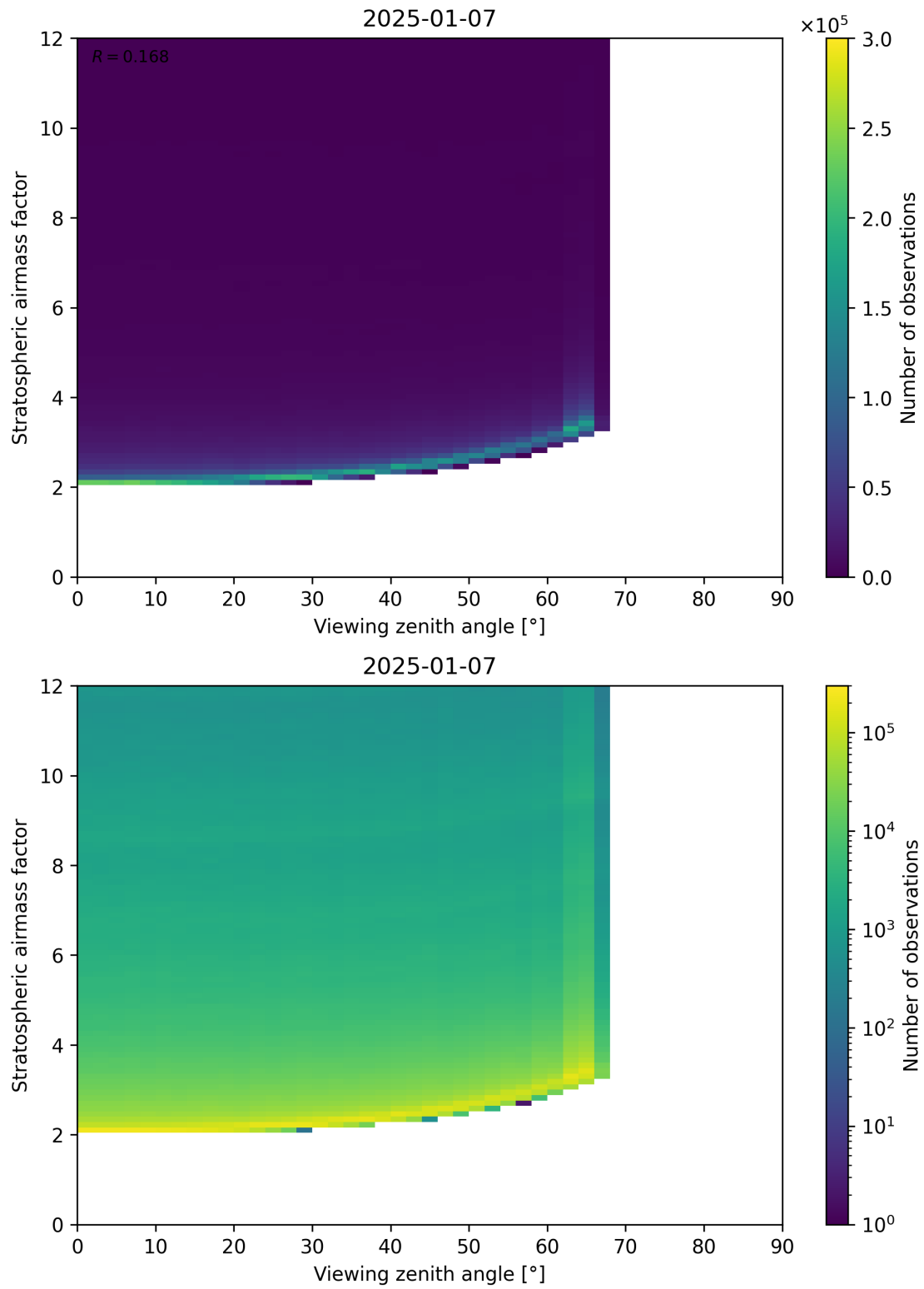
Figure 159: Scatter density plot of “Viewing zenith angle” against “Stratospheric airmass factor” for 2025-01-07 to 2025-01-08.
