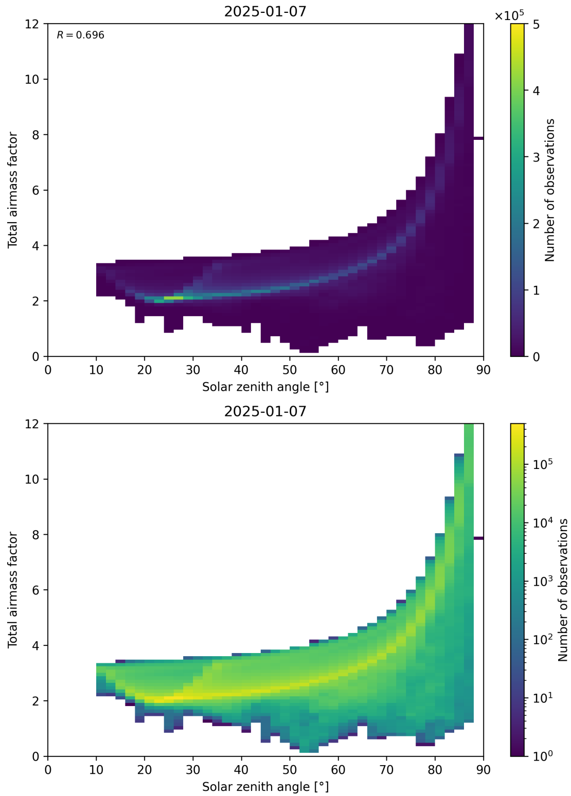
Figure 146: Scatter density plot of “Solar zenith angle” against “Total air mass factor” for 2025-01-07 to 2025-01-08.
