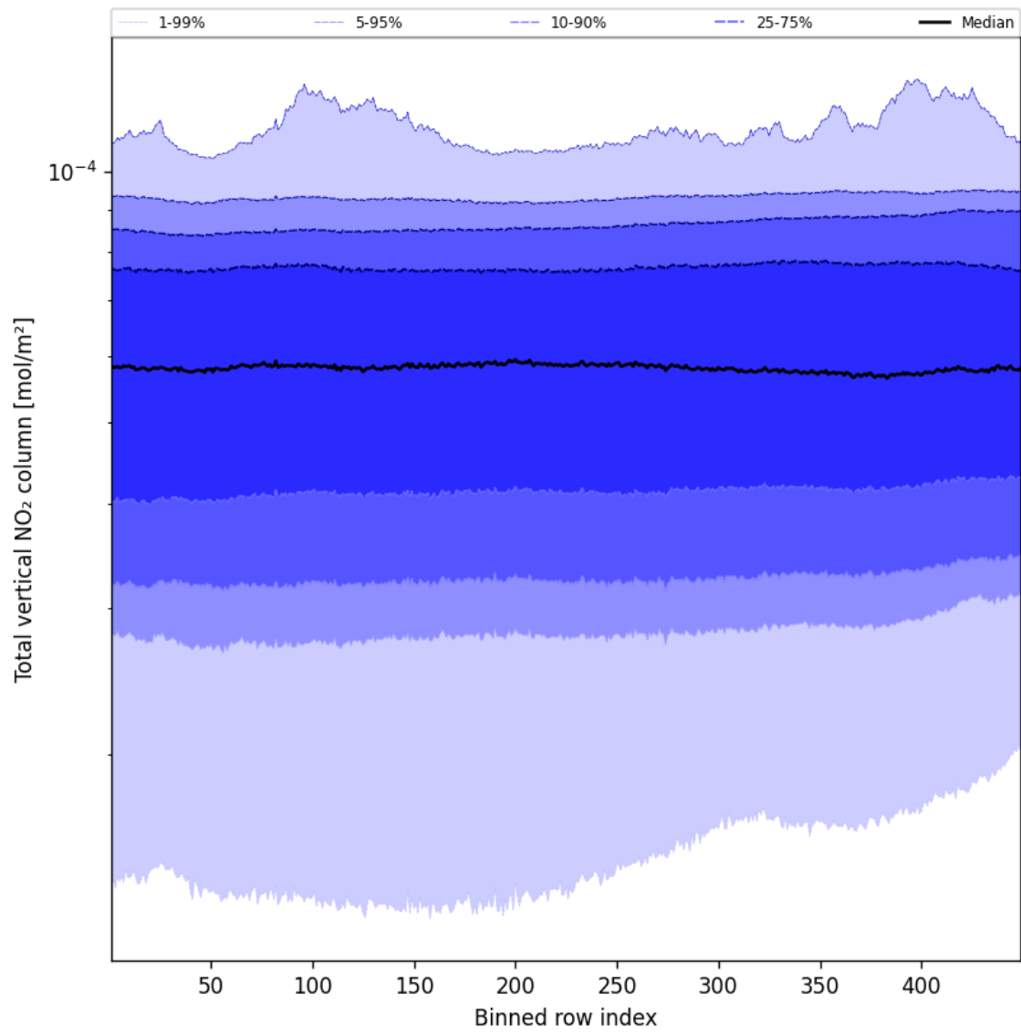
Figure 55: Along track statistics of “Total vertical NO 2 column” for 2025-01-07 to 2025-01-08
