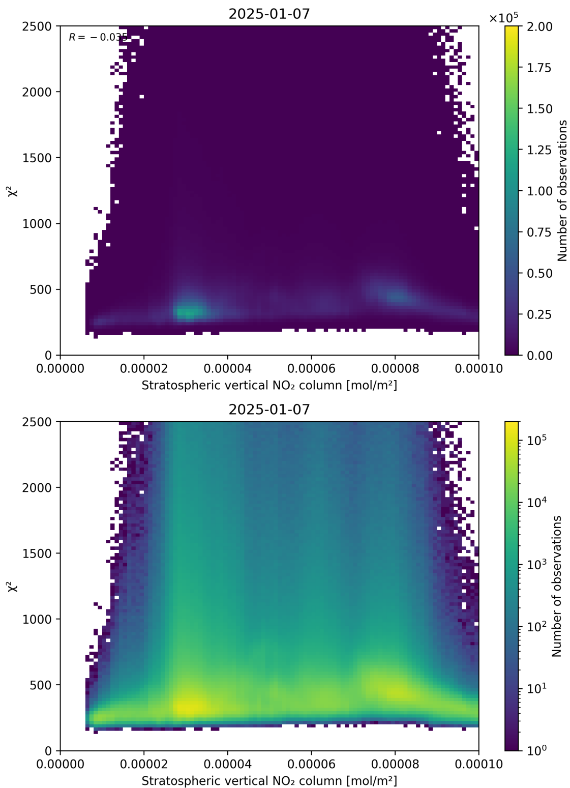
Figure 97: Scatter density plot of “Stratospheric vertical NO 2 column” against “ \chi^2 ” for 2025-01-07 to 2025-01-08.
