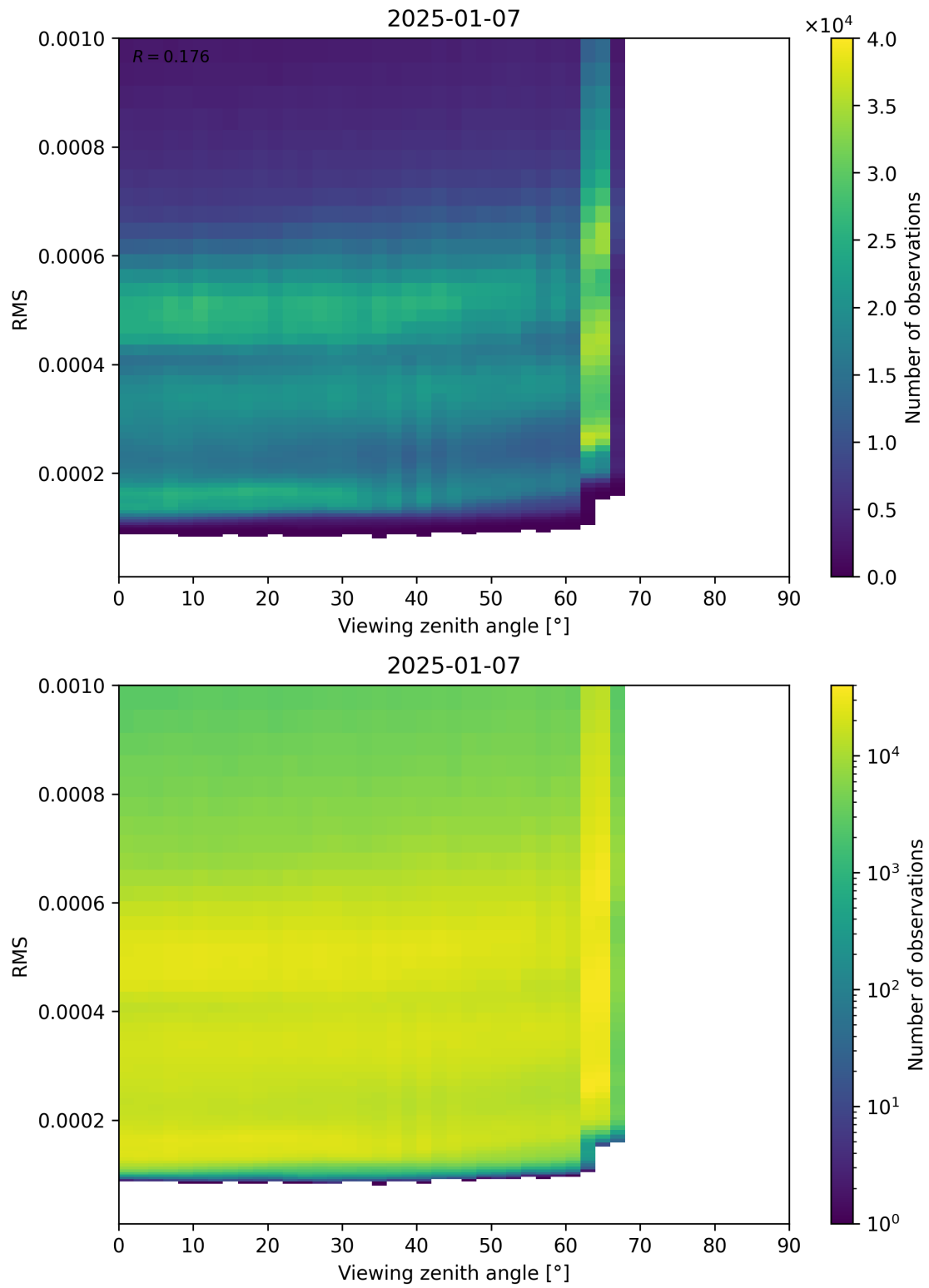
Figure 171: Scatter density plot of “Viewing zenith angle” against “RMS” for 2025-01-07 to 2025-01-08.
