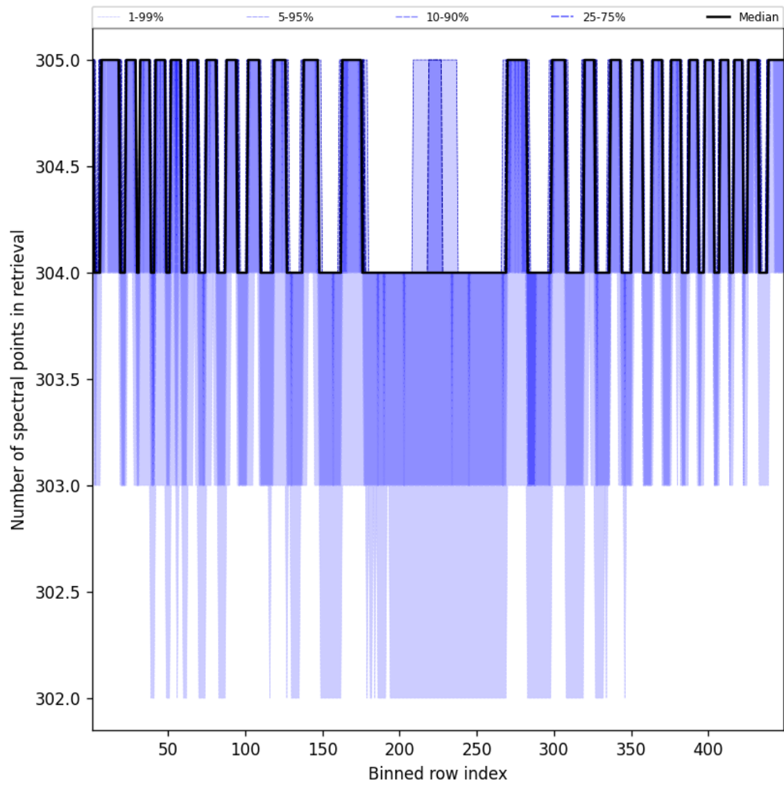
Figure 50: Along track statistics of “Number of spectral points in retrieval” for 2025-01-07 to 2025-01-08
