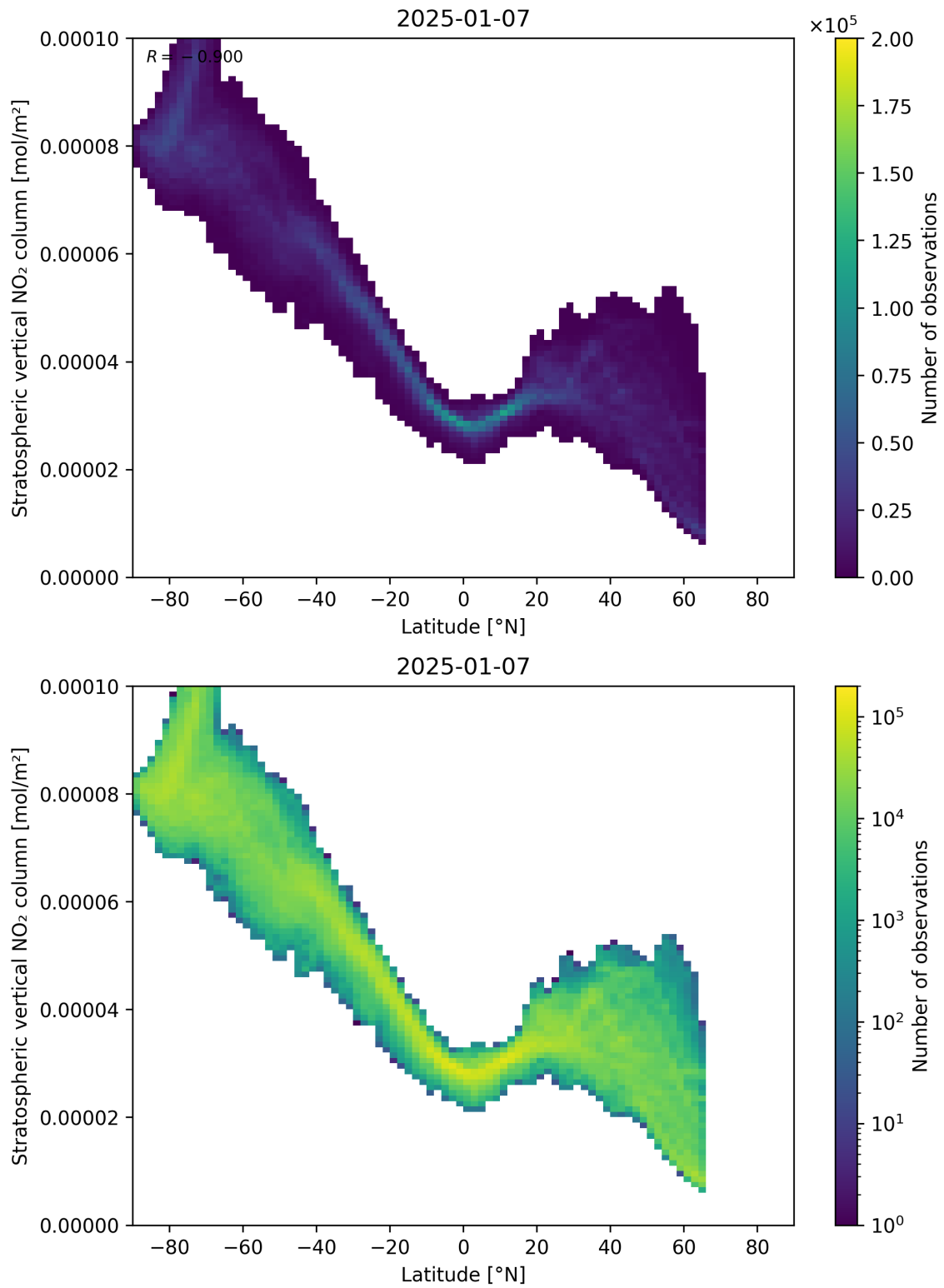
Figure 87: Scatter density plot of “Latitude” against “Stratospheric vertical NO 2 column” for 2025-01-07 to 2025-01-08.
