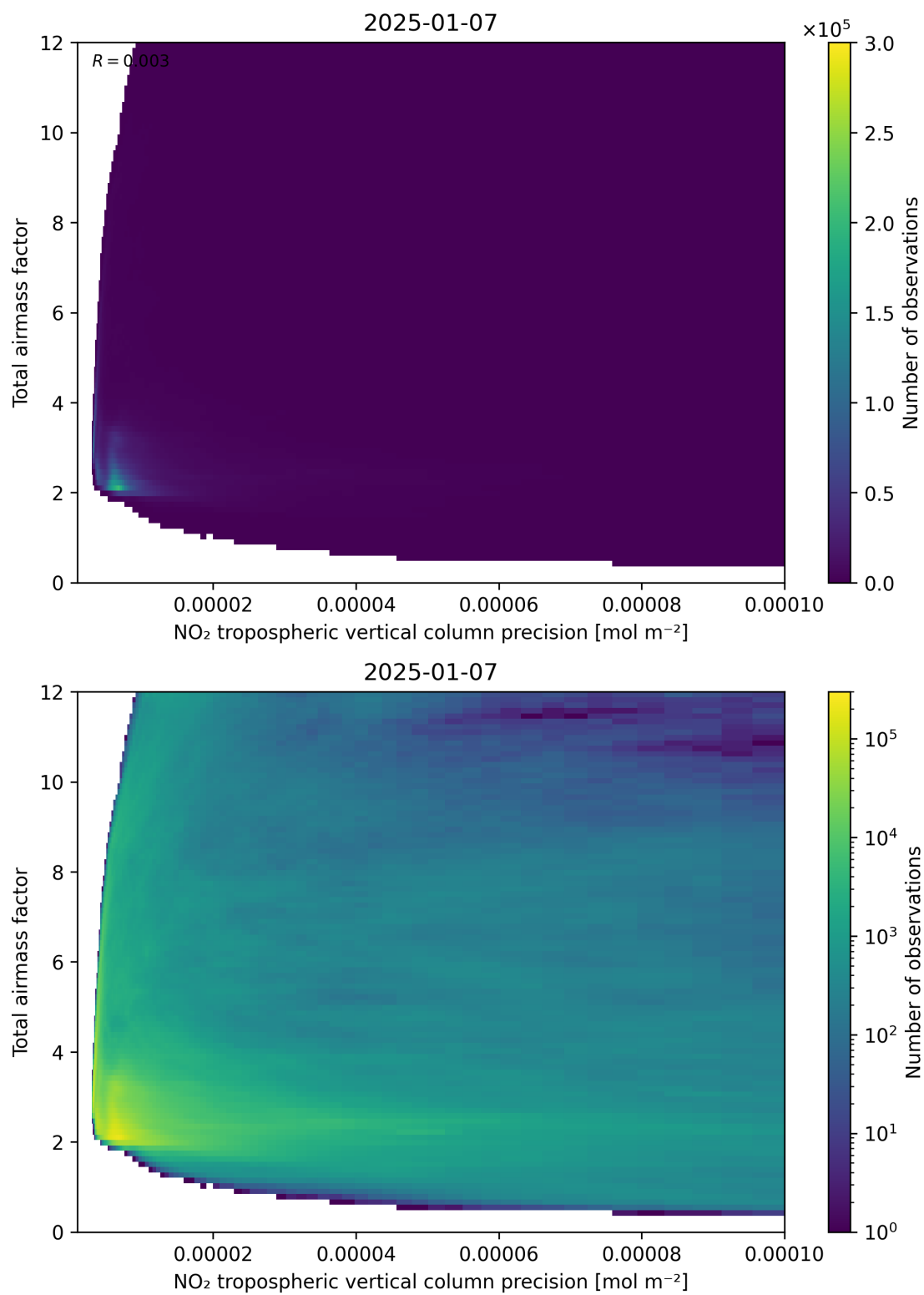
Figure 132: Scatter density plot of “NO 2 tropospheric vertical column precision” against “Total air mass factor” for 2025-01-07 to 2025-01-08.
