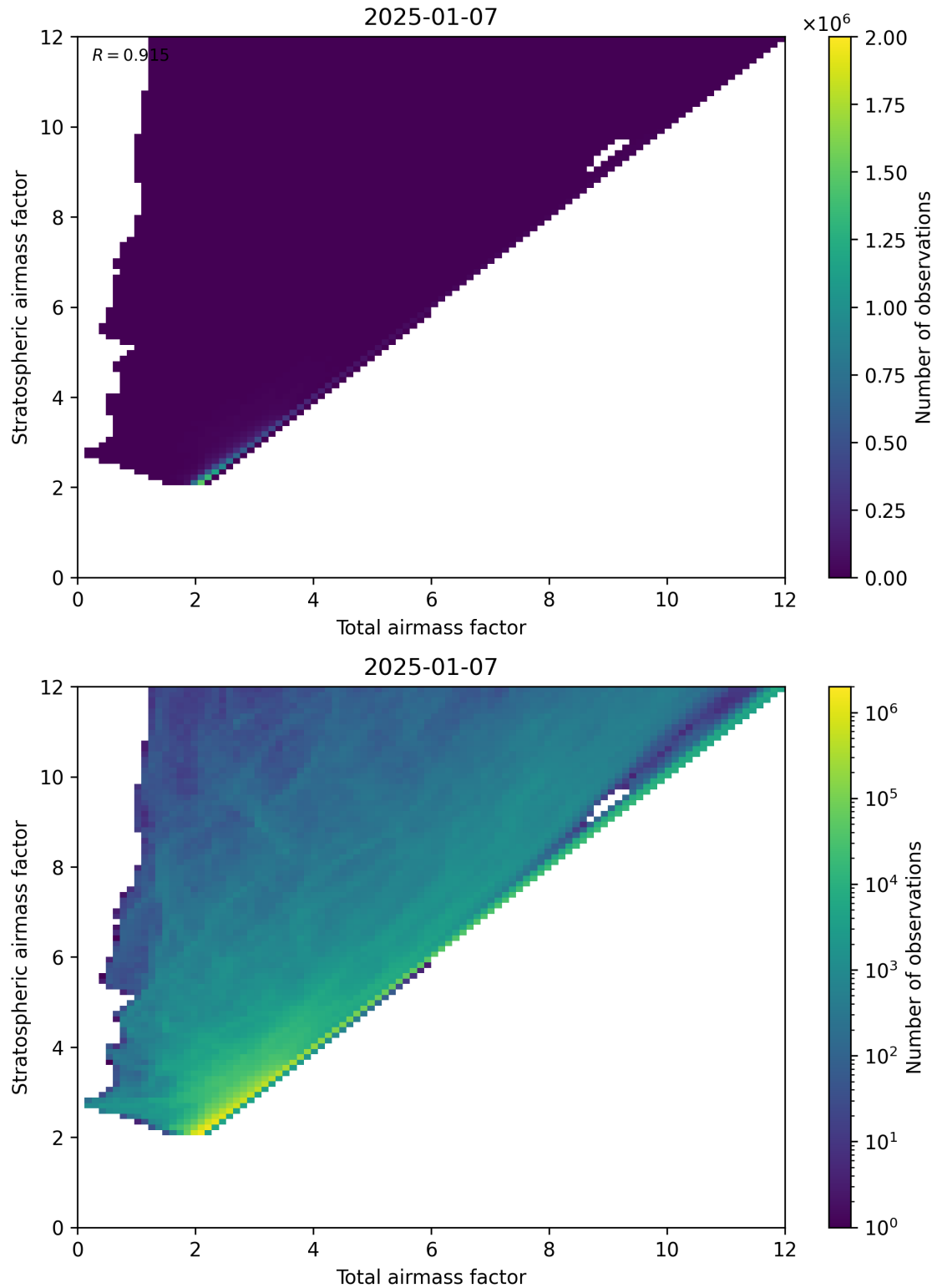
Figure 62: Scatter density plot of “Total airmass factor” against “Stratospheric airmass factor” for 2025-01-07 to 2025-01-08.
