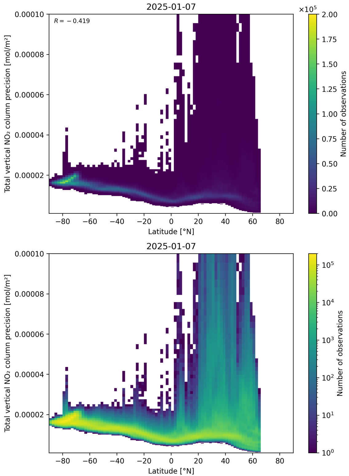
Figure 91: Scatter density plot of “Latitude” against “Total vertical NO 2 column precision” for 2025-01-07 to 2025-01-08.
