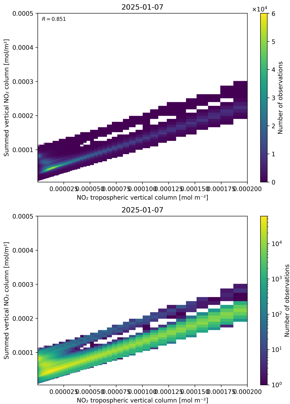
Figure 126: Scatter density plot of “NO 2 tropospheric vertical column” against “Summed vertical NO 2 column” for 2025-01-07 to 2025-01-08.
