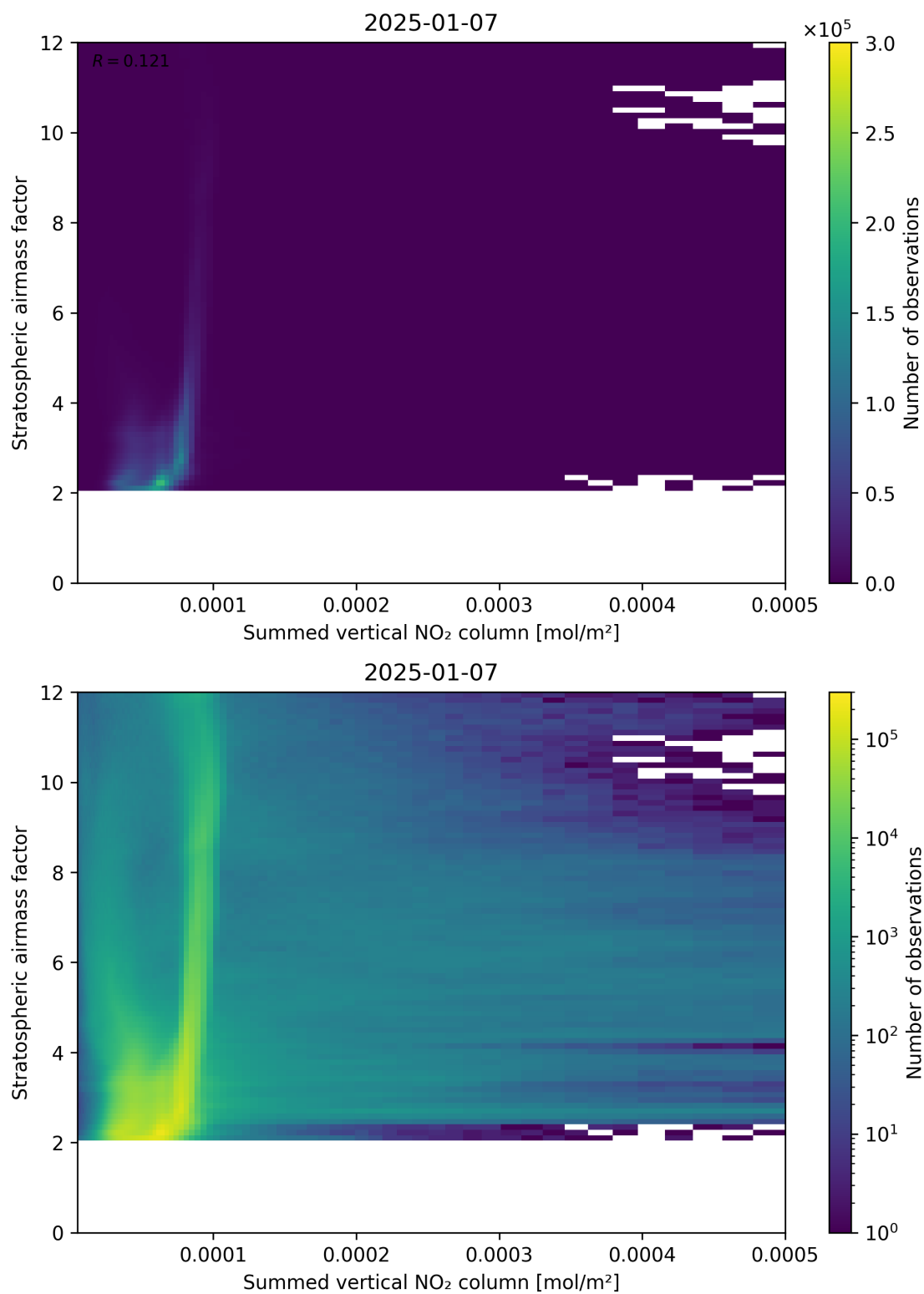
Figure 103: Scatter density plot of “Summed vertical NO 2 column” against “Stratospheric airmass factor” for 2025-01-07 to 2025-01-08.
