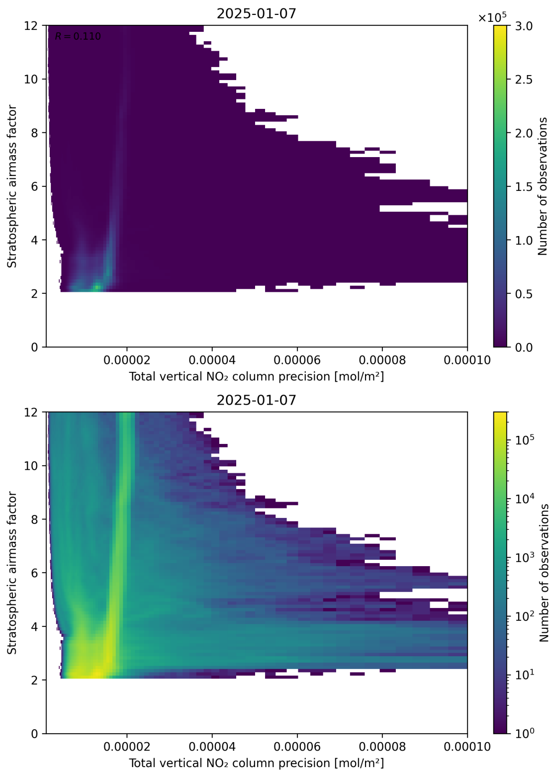
Figure 115: Scatter density plot of “Total vertical NO 2 column precision” against “Stratospheric airmass factor” for 2025-01-07 to 2025-01-08.
