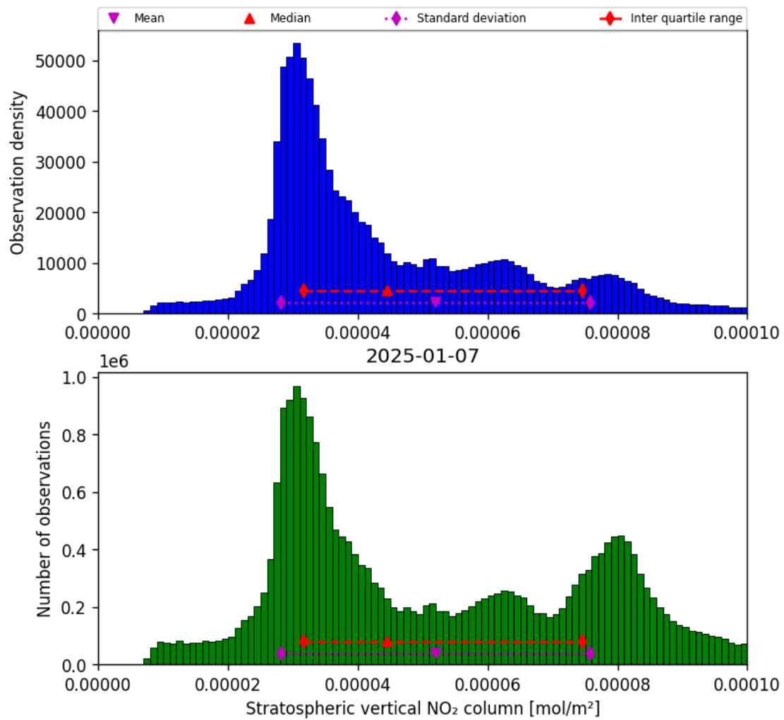
Figure 36: Histogram of “Stratospheric vertical NO 2 column” for 2025-01-07 to 2025-01-08
