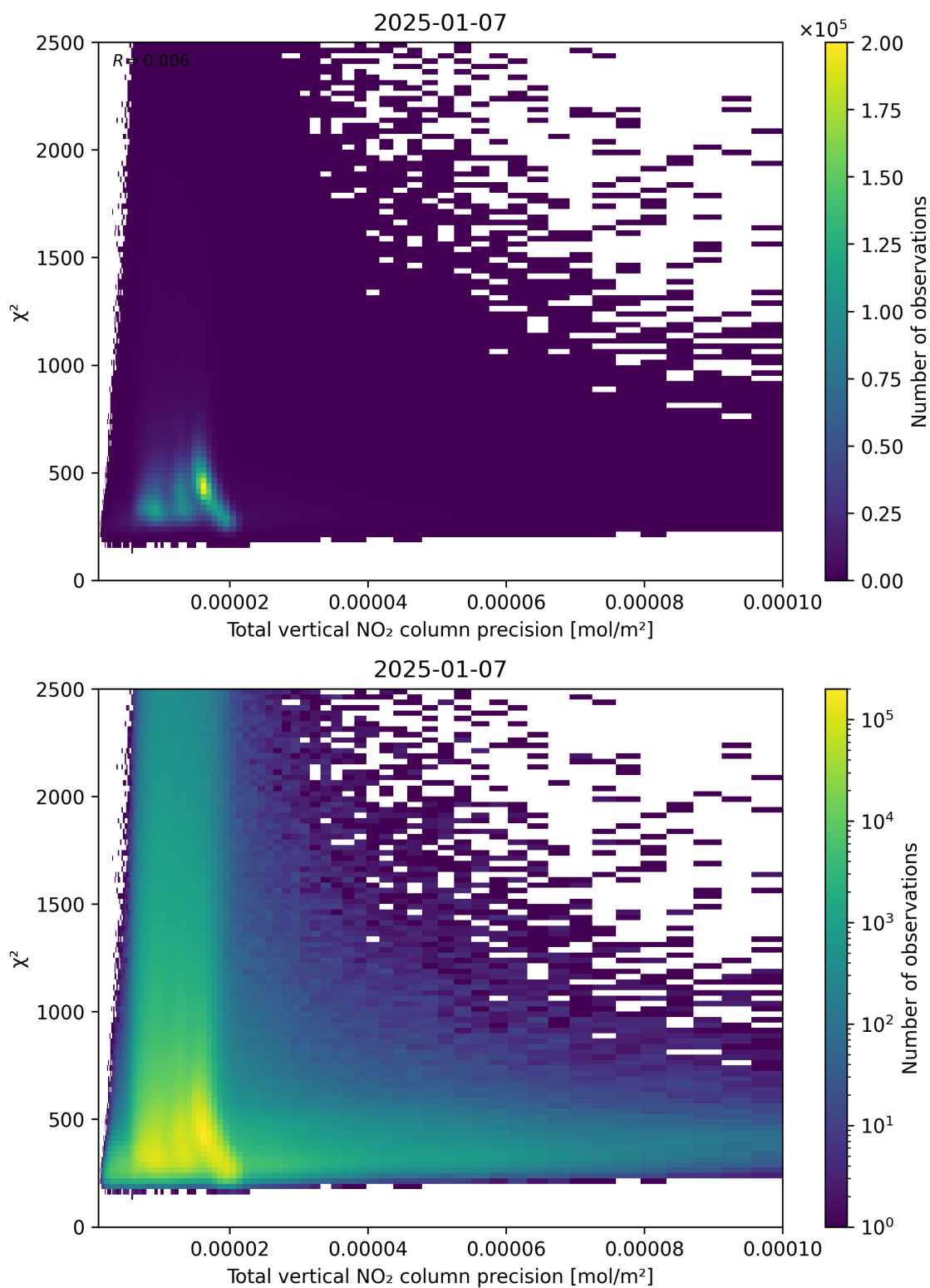
Figure 116: Scatter density plot of “Total vertical NO 2 column precision” against “ \chi^2 ” for 2025-01-07 to 2025-01-08.
