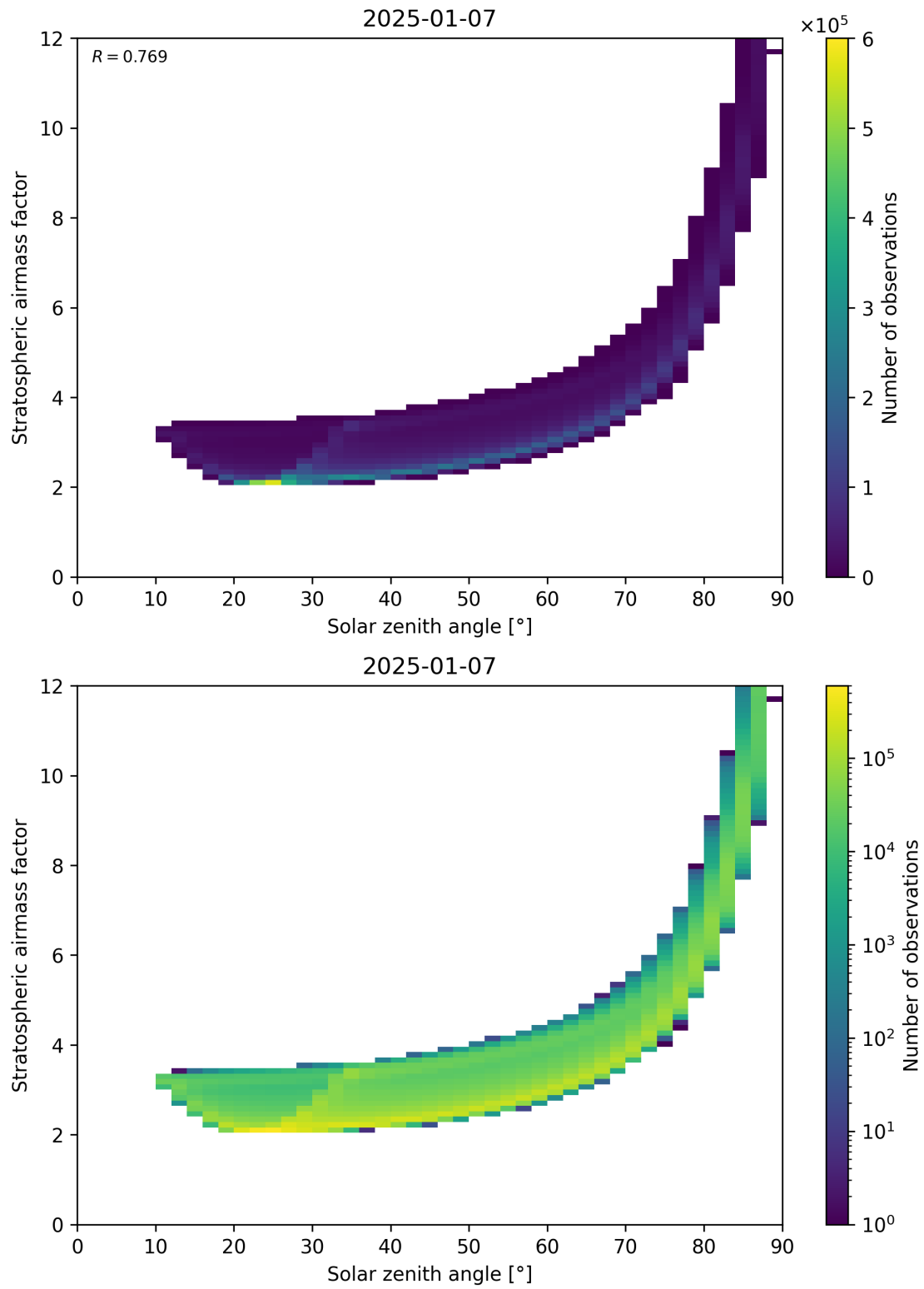
Figure 145: Scatter density plot of “Solar zenith angle” against “Stratospheric airmass factor” for 2025-01-07 to 2025-01-08.
