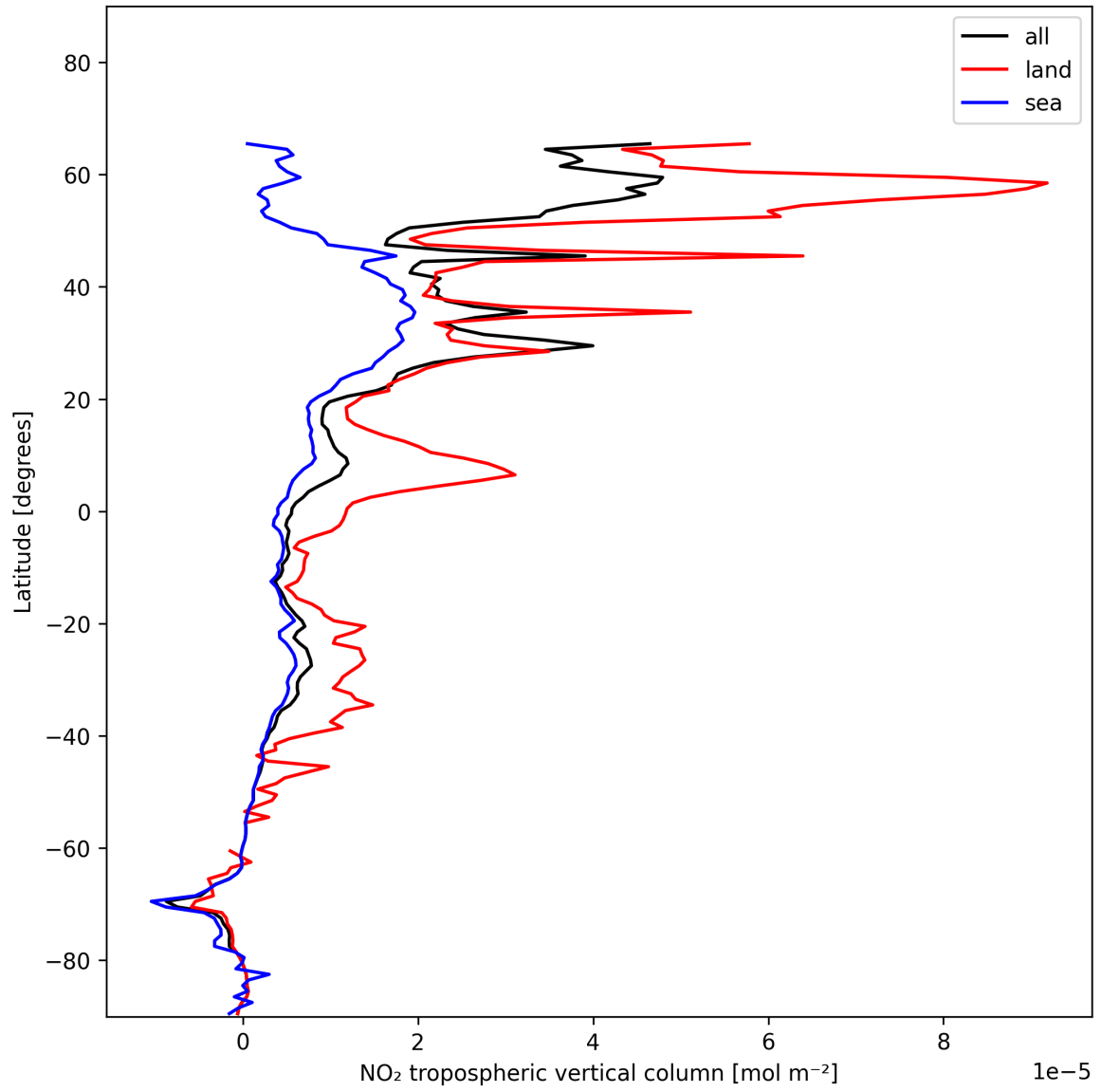
Figure 12: Zonal average of “NO 2 tropospheric vertical column” for 2025-01-07 to 2025-01-08.
