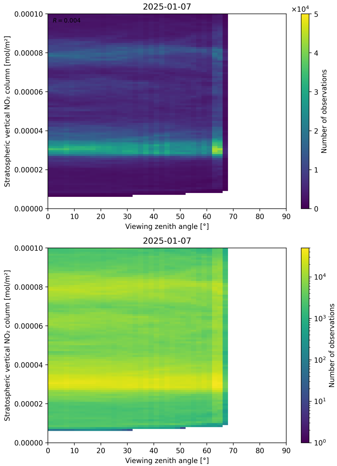
Figure 164: Scatter density plot of “Viewing zenith angle” against “Stratospheric vertical NO 2 column” for 2025-01-07 to 2025-01-08.
