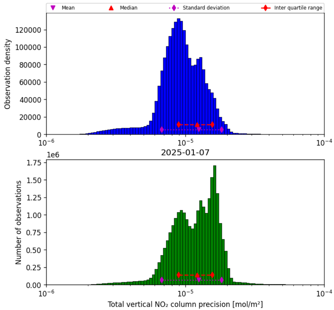
Figure 39: Histogram of “Total vertical NO 2 column precision” for 2025-01-07 to 2025-01-08
