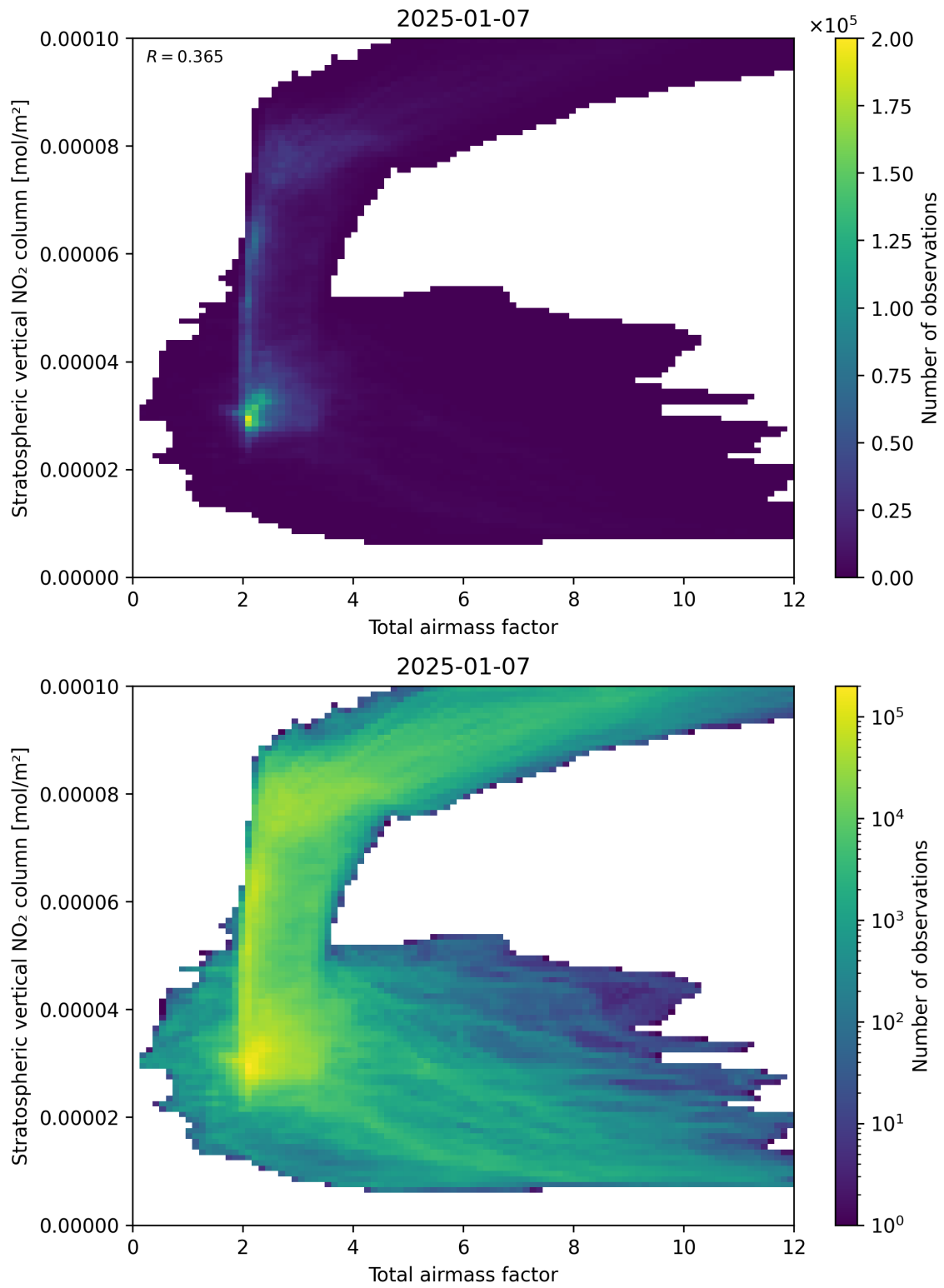
Figure 64: Scatter density plot of “Total airmass factor” against “Stratospheric vertical NO 2 column” for 2025-01-07 to 2025-01-08.
