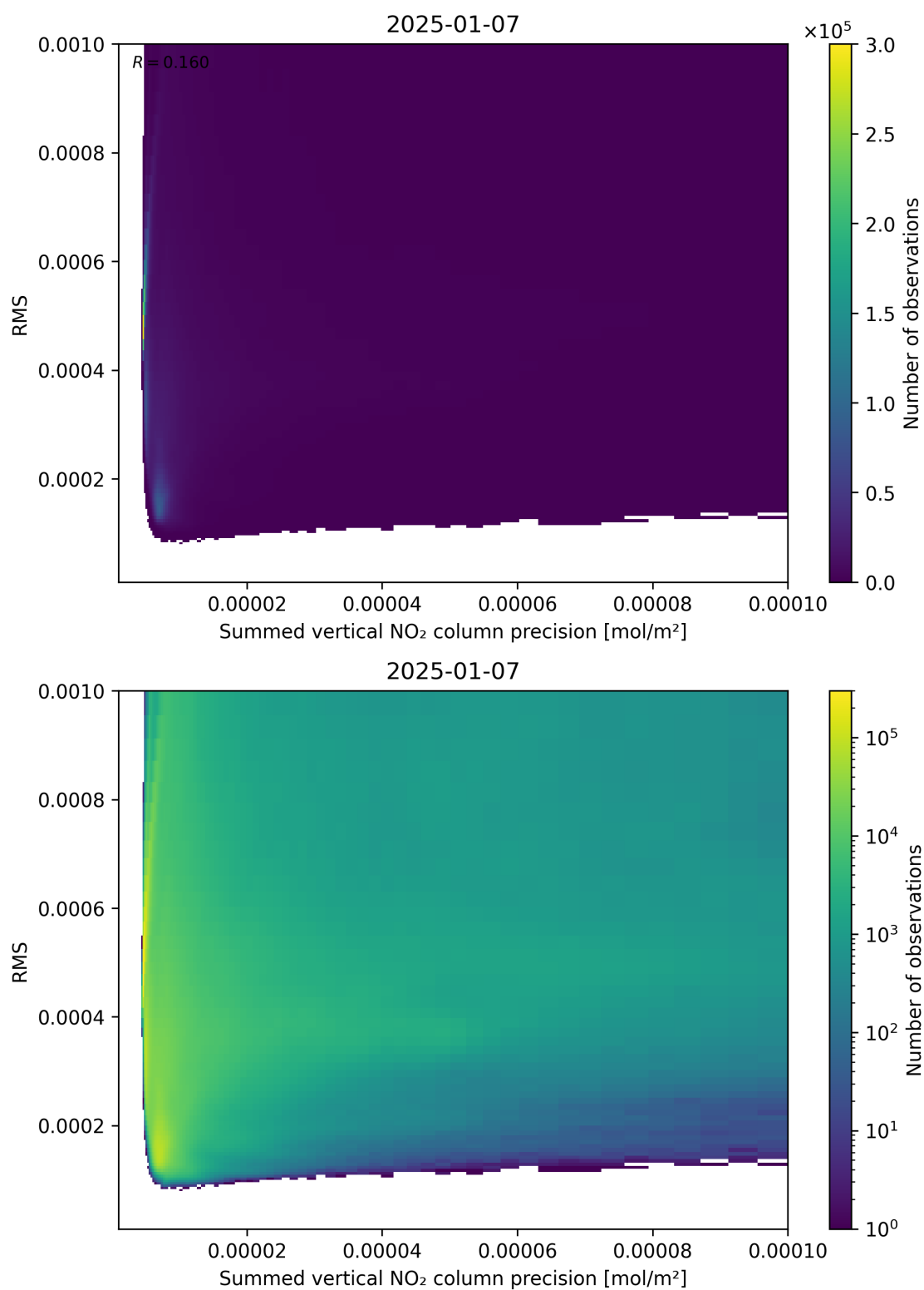
Figure 108: Scatter density plot of “Summed vertical NO 2 column precision” against “RMS” for 2025-01-07 to 2025-01-08.
