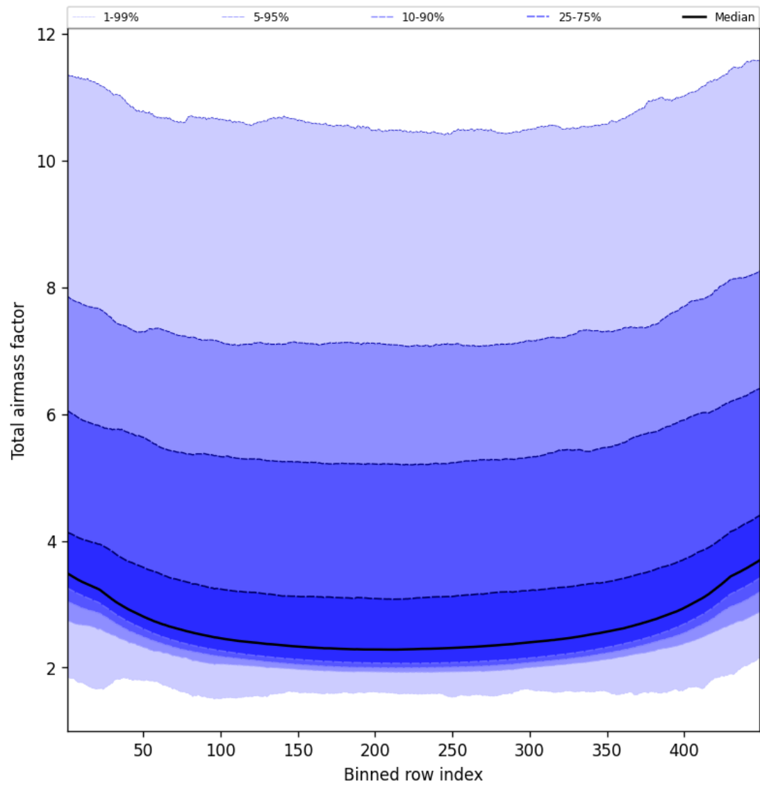
Figure 49: Along track statistics of “Total airmass factor” for 2025-01-07 to 2025-01-08
