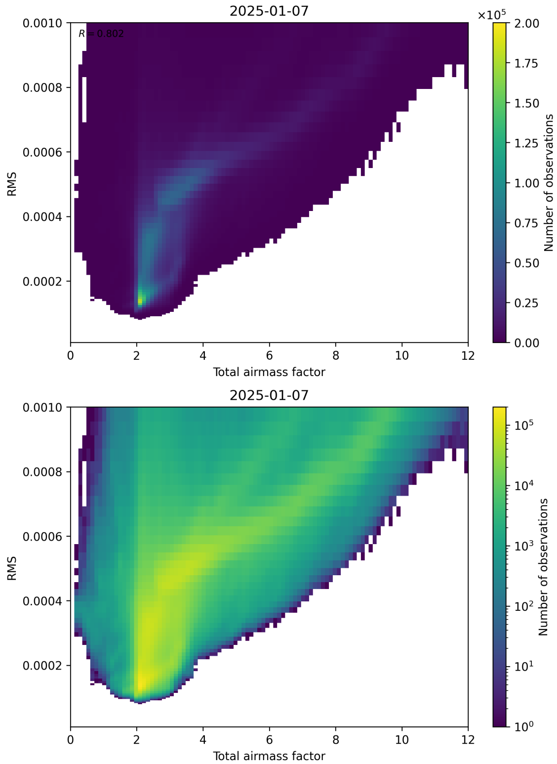
Figure 69: Scatter density plot of “Total airmass factor” against “RMS” for 2025-01-07 to 2025-01-08.
