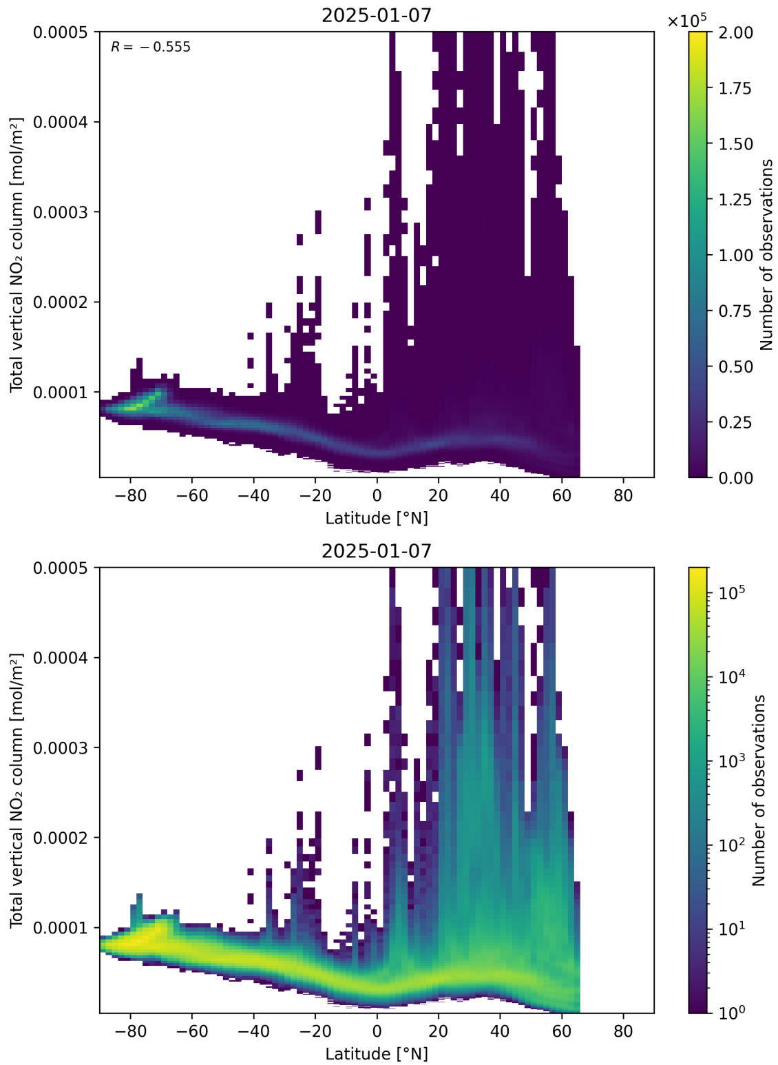
Figure 90: Scatter density plot of “Latitude” against “Total vertical NO 2 column” for 2025-01-07 to 2025-01-08.
