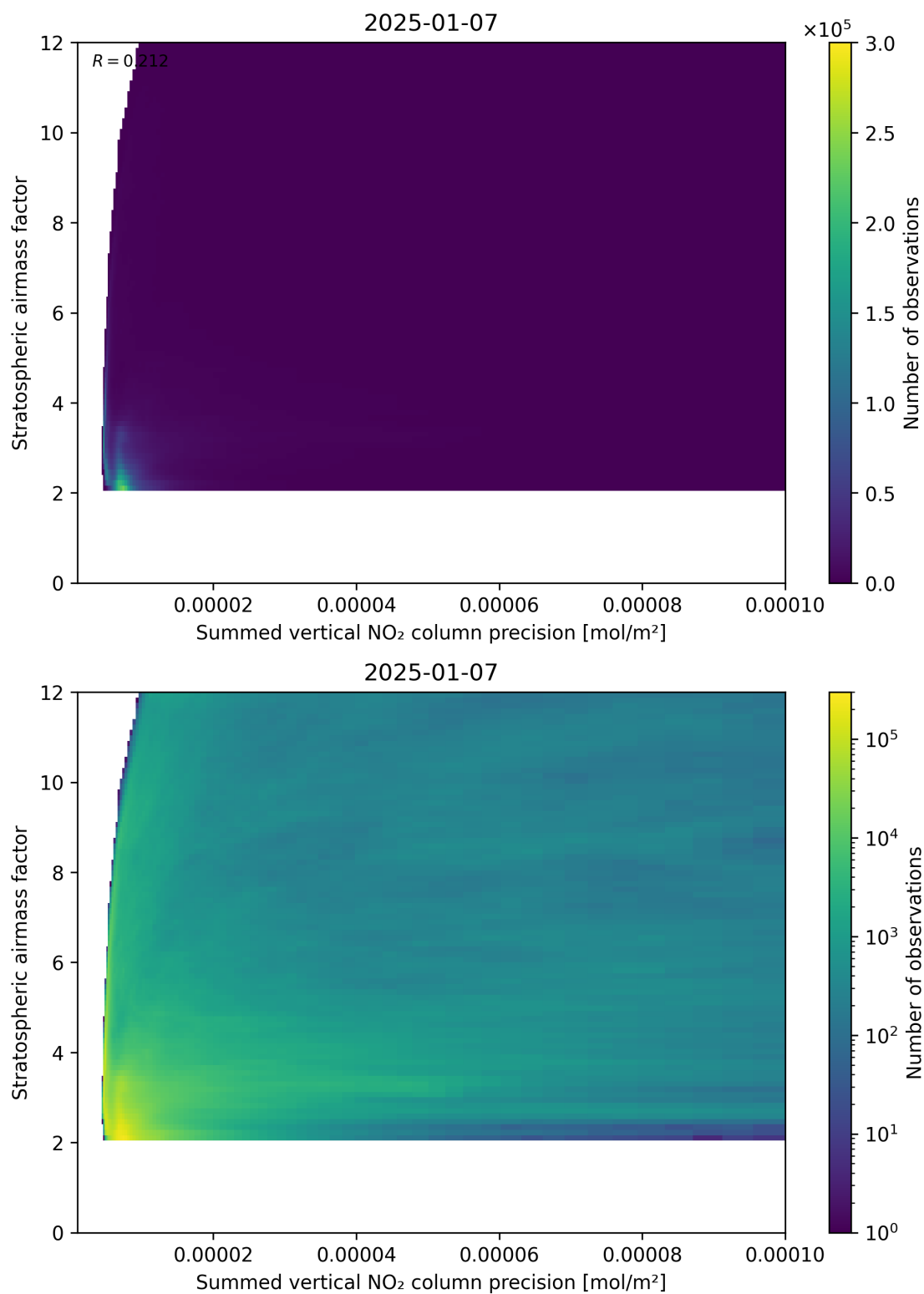
Figure 106: Scatter density plot of “Summed vertical NO 2 column precision” against “Stratospheric airmass factor” for 2025-01-07 to 2025-01-08.
