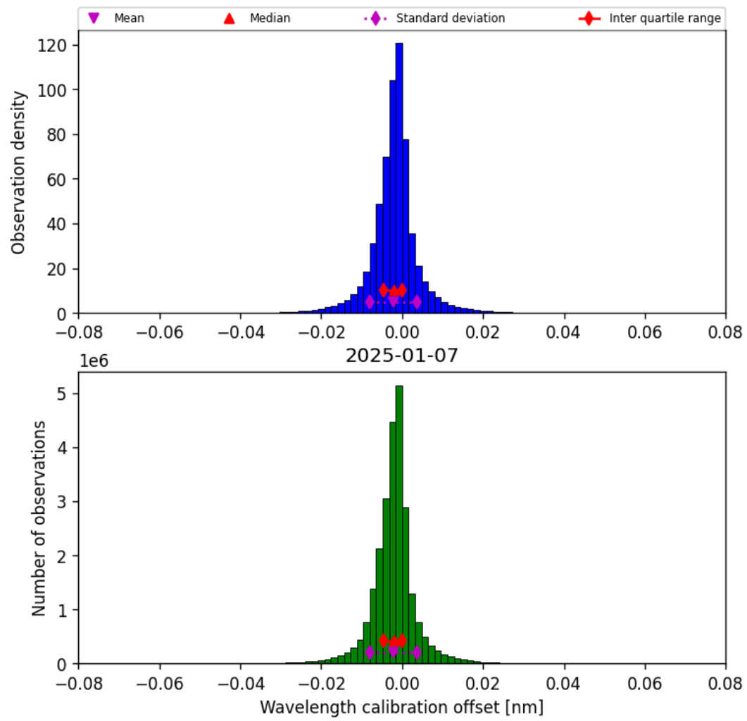
Figure 35: Histogram of “Wavelength calibration offset” for 2025-01-07 to 2025-01-08
