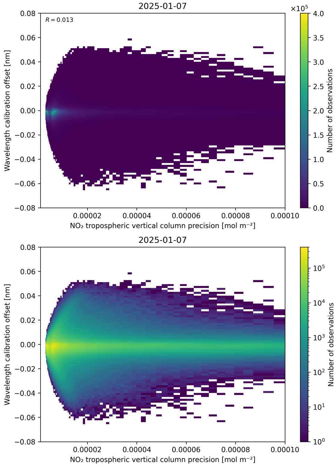
Figure 141: Scatter density plot of “NO 2 tropospheric vertical column precision” against “Wavelength calibration offset” for 2025-01-07 to 2025-01-08.
