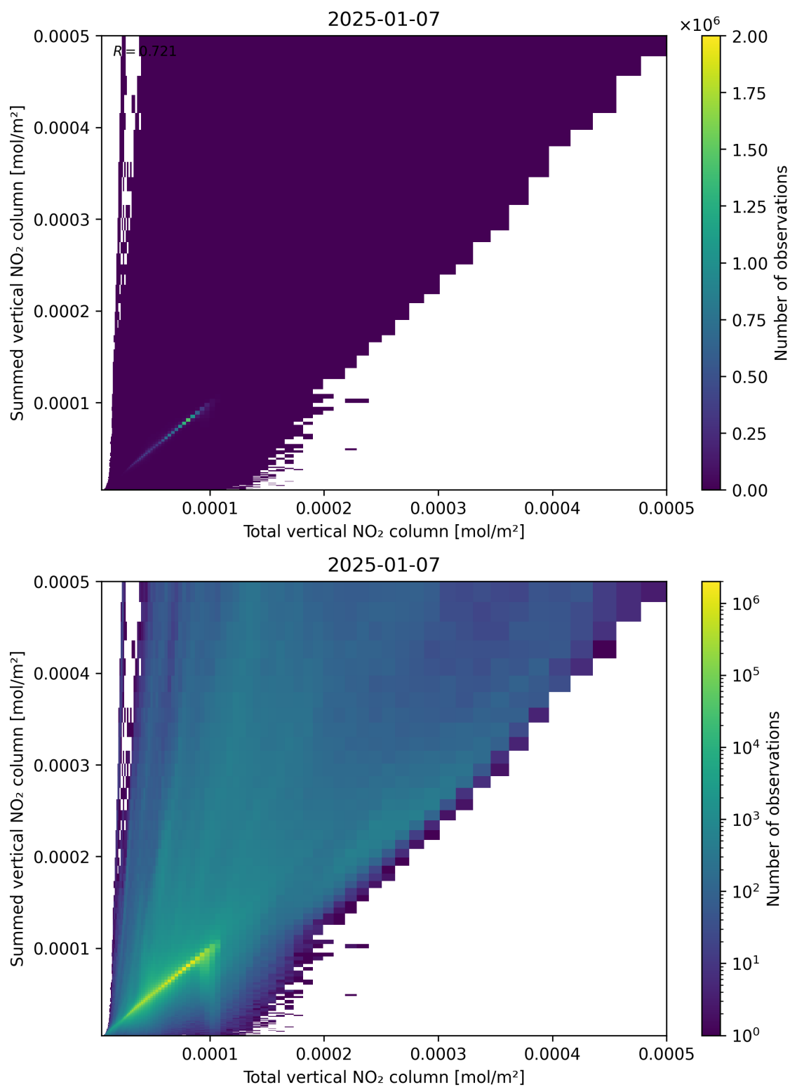
Figure 112: Scatter density plot of “Total vertical NO 2 column” against “Summed vertical NO 2 column” for 2025-01-07 to 2025-01-08.
