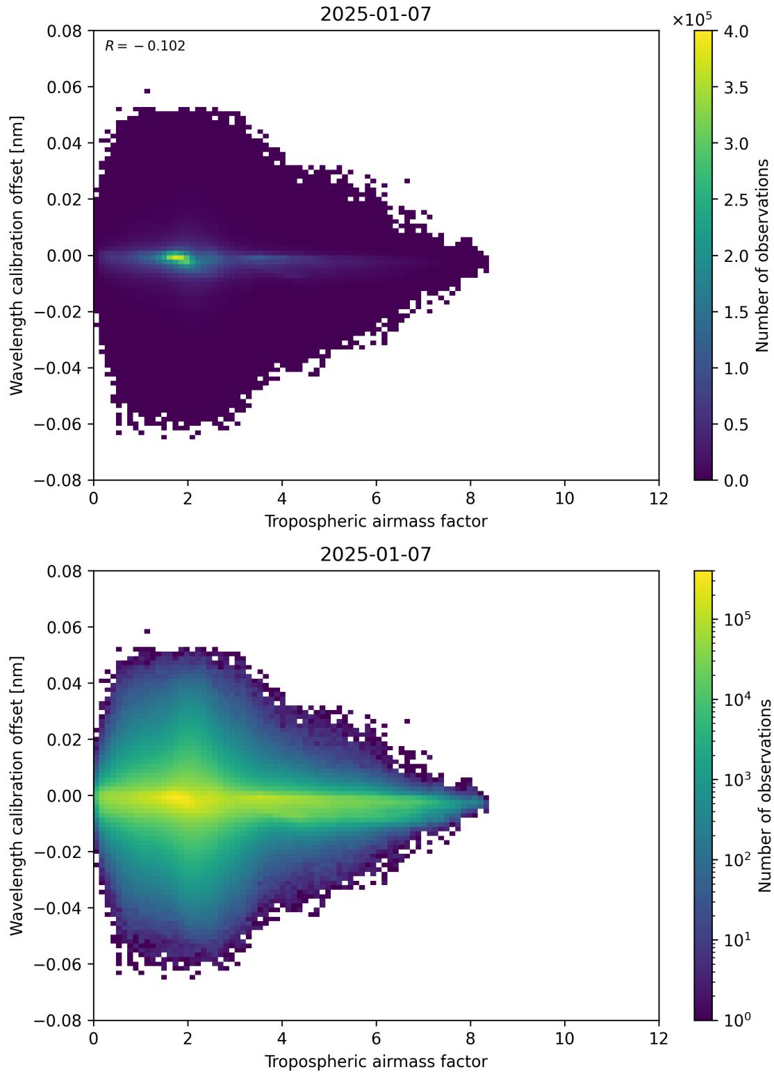
Figure 80: Scatter density plot of “Tropospheric airmass factor” against “Wavelength calibration offset” for 2025-01-07 to 2025-01-08.
