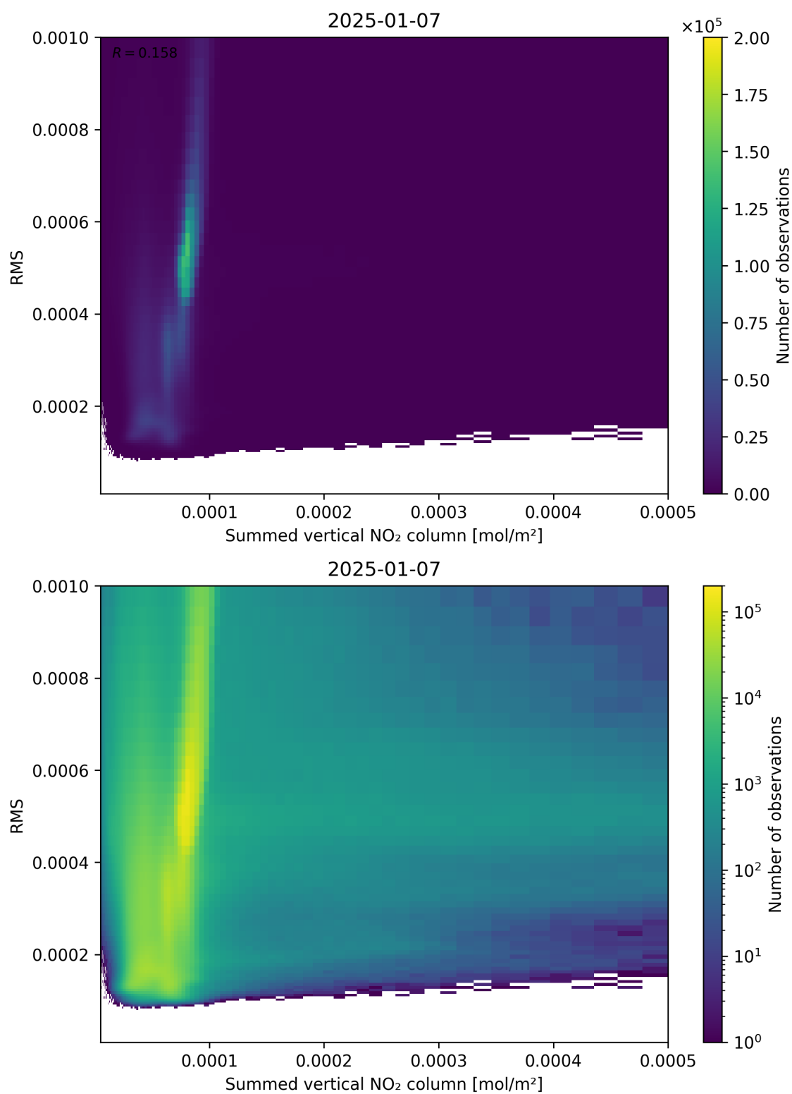
Figure 109: Scatter density plot of “Summed vertical NO 2 column” against “RMS” for 2025-01-07 to 2025-01-08.
