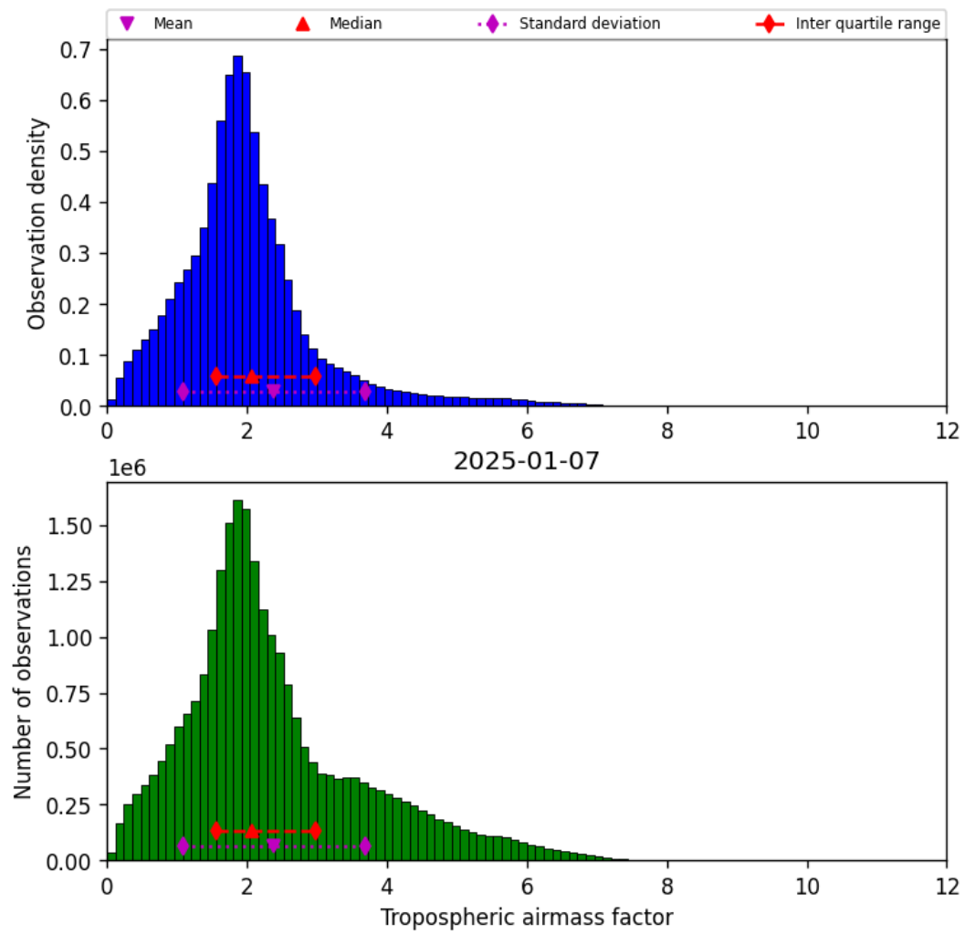
Figure 31: Histogram of “Tropospheric airmass factor” for 2025-01-07 to 2025-01-08
