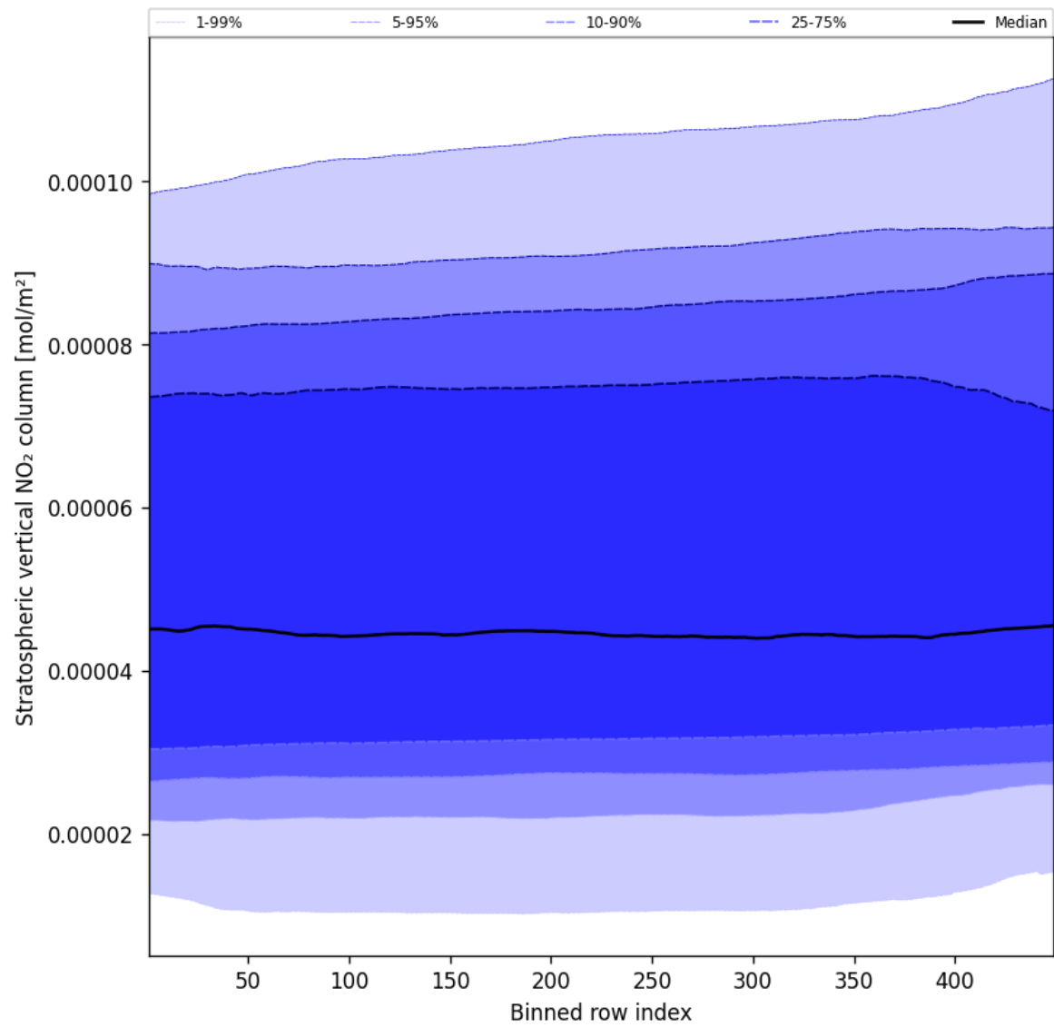
Figure 53: Along track statistics of “Stratospheric vertical NO 2 column” for 2025-01-07 to 2025-01-08
