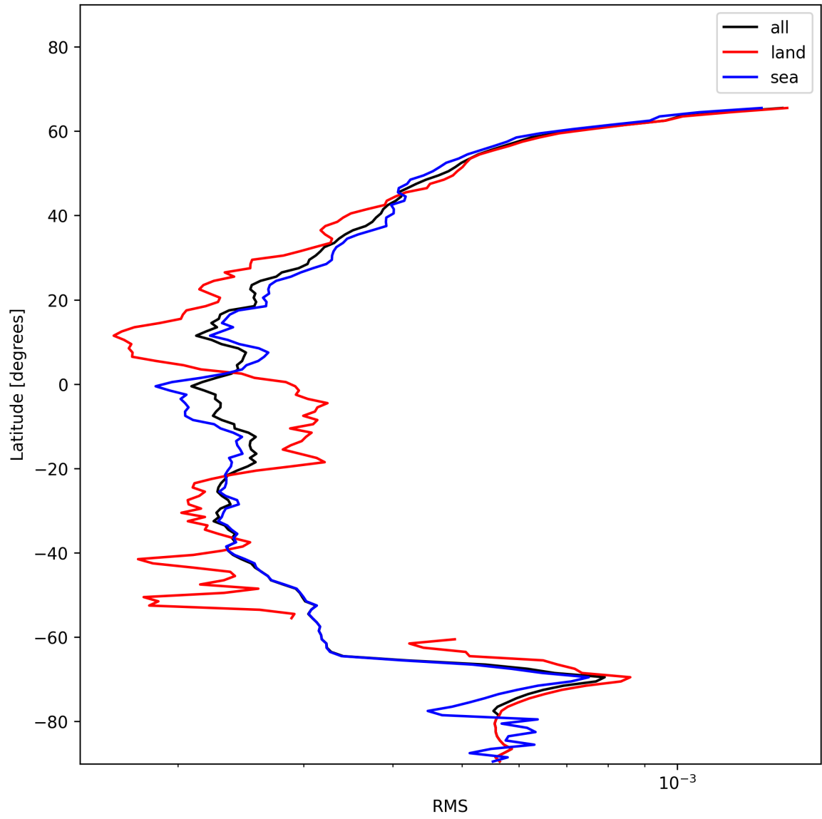
Figure 26: Zonal average of “RMS” for 2025-01-07 to 2025-01-08.
