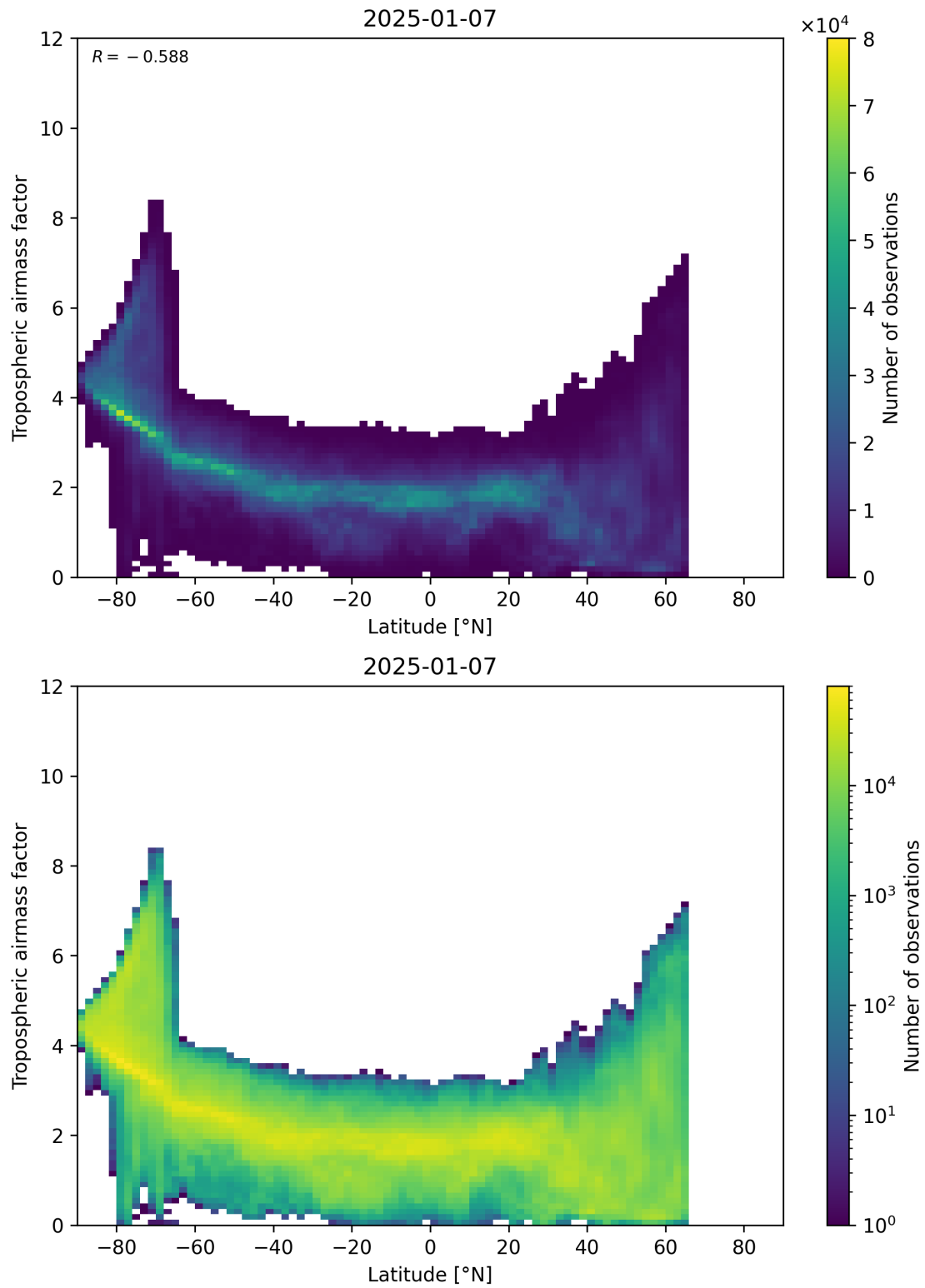
Figure 85: Scatter density plot of “Latitude” against “Tropospheric airmass factor” for 2025-01-07 to 2025-01-08.
