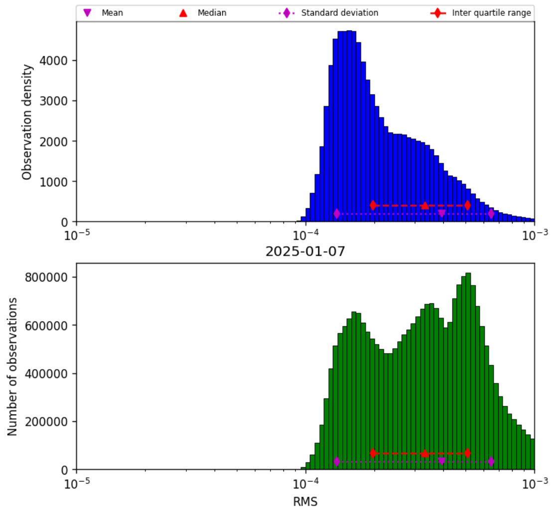
Figure 43: Histogram of “RMS” for 2025-01-07 to 2025-01-08
