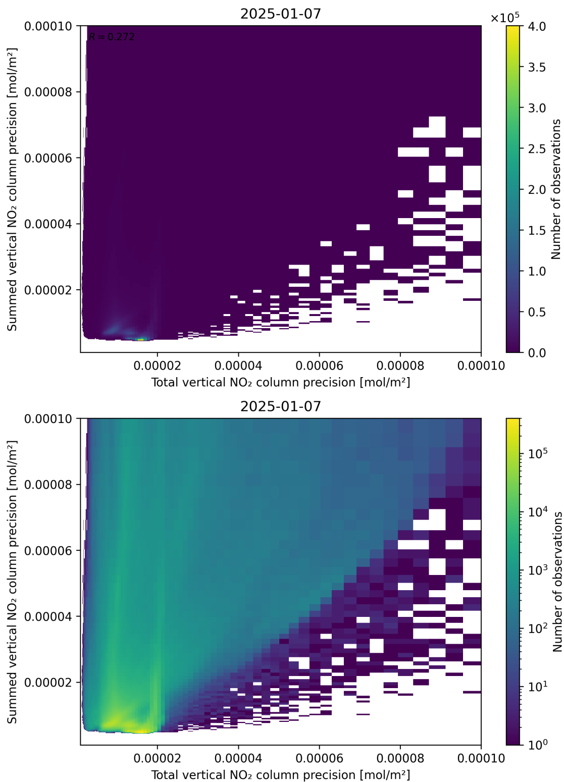
Figure 118: Scatter density plot of “Total vertical NO 2 column precision” against “Summed vertical NO 2 column precision” for 2025-01-07 to 2025-01-08.
