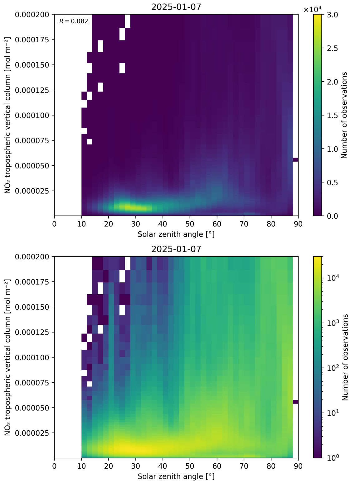
Figure 155: Scatter density plot of “Solar zenith angle” against “NO 2 tropospheric vertical column” for 2025-01-07 to 2025-01-08.
