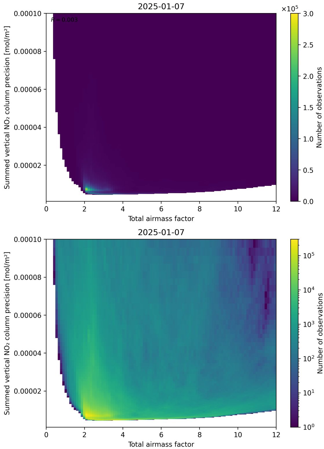
Figure 66: Scatter density plot of “Total airmass factor” against “Summed vertical NO 2 column precision” for 2025-01-07 to 2025-01-08.
