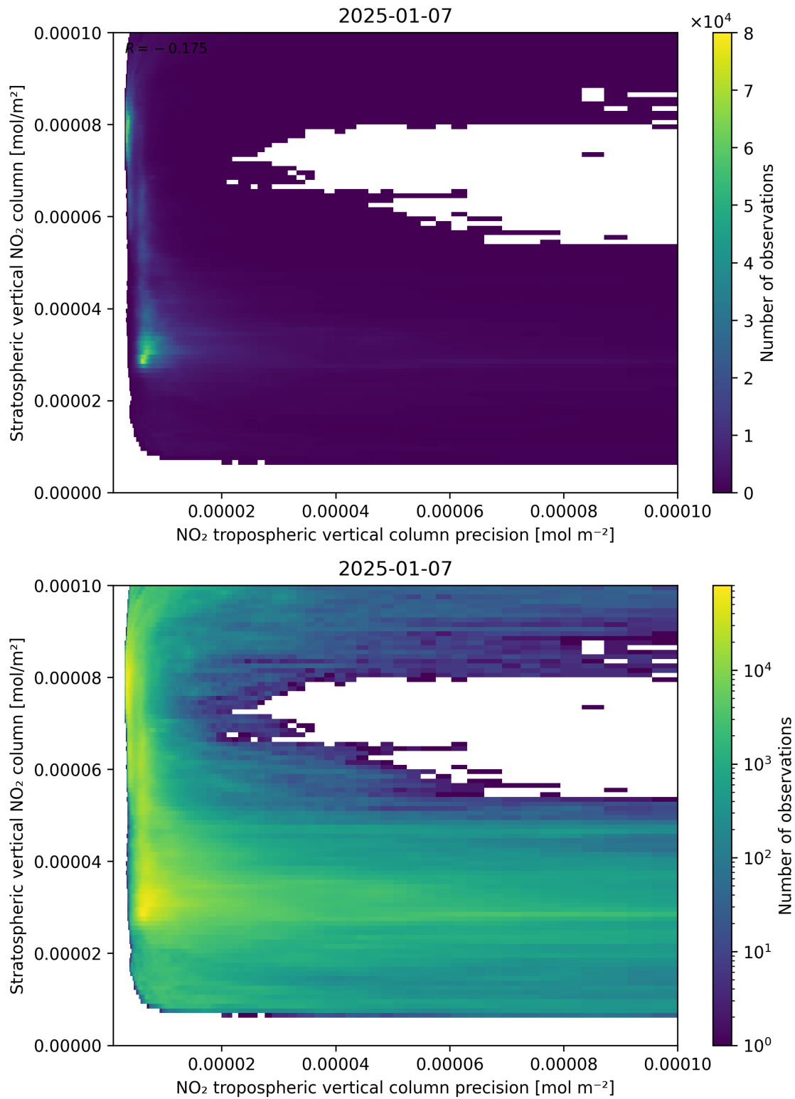
Figure 135: Scatter density plot of “NO 2 tropospheric vertical column precision” against “Stratospheric vertical NO 2 column” for 2025-01-07 to 2025-01-08.
