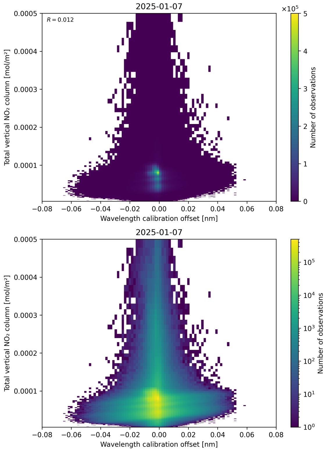
Figure 179: Scatter density plot of “Wavelength calibration offset” against “Total vertical NO 2 column” for 2025-01-07 to 2025-01-08.
