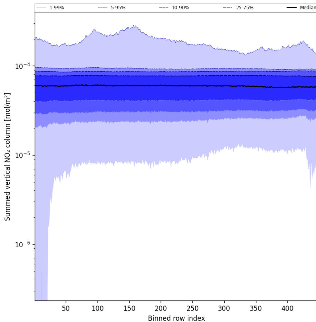
Figure 57: Along track statistics of “Summed vertical NO 2 column” for 2025-01-07 to 2025-01-08
