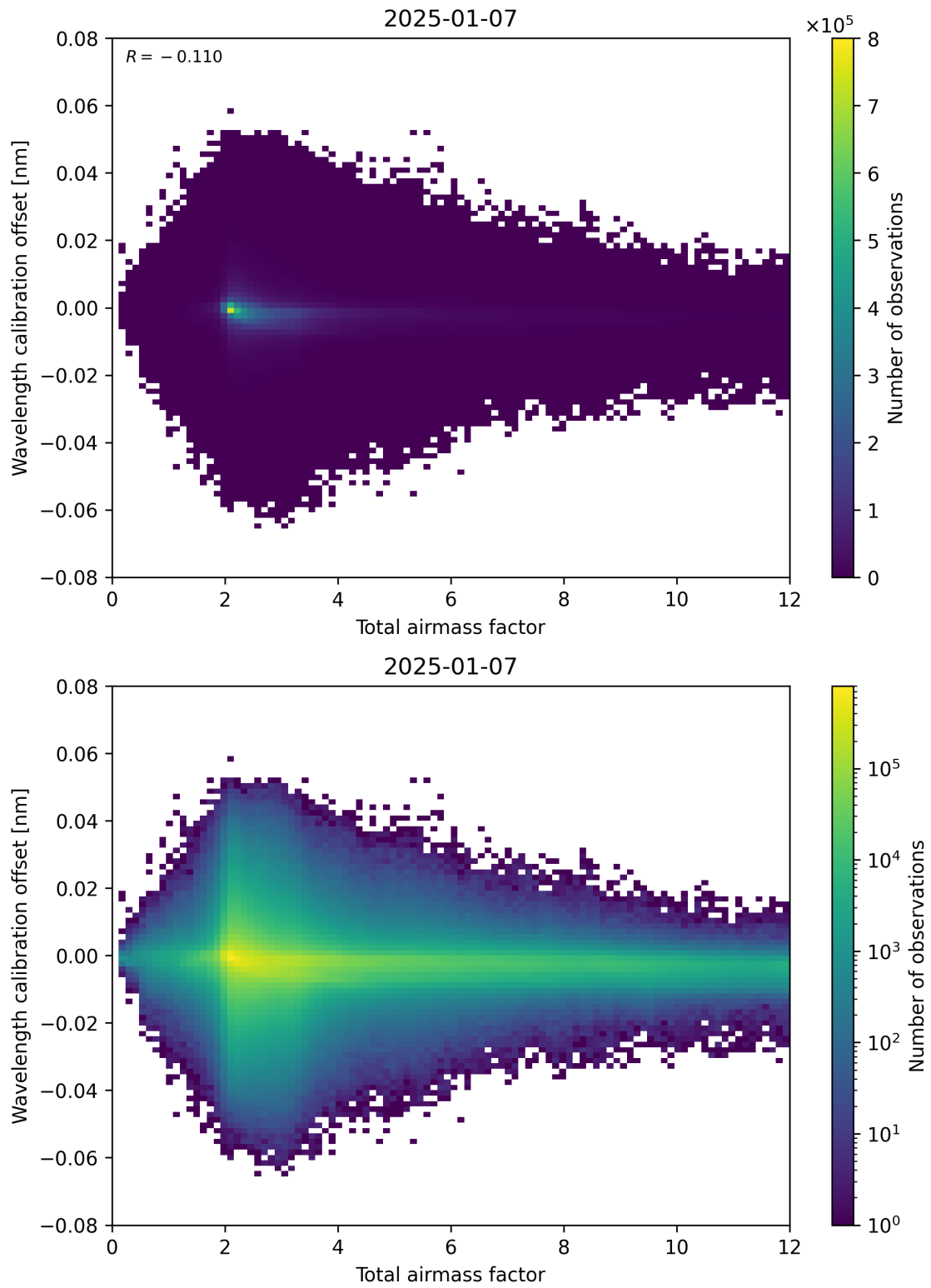
Figure 70: Scatter density plot of “Total airmass factor” against “Wavelength calibration offset” for 2025-01-07 to 2025-01-08.
