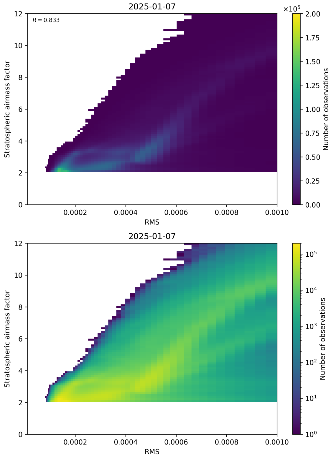
Figure 144: Scatter density plot of “RMS” against “Stratospheric airmass factor” for 2025-01-07 to 2025-01-08.
