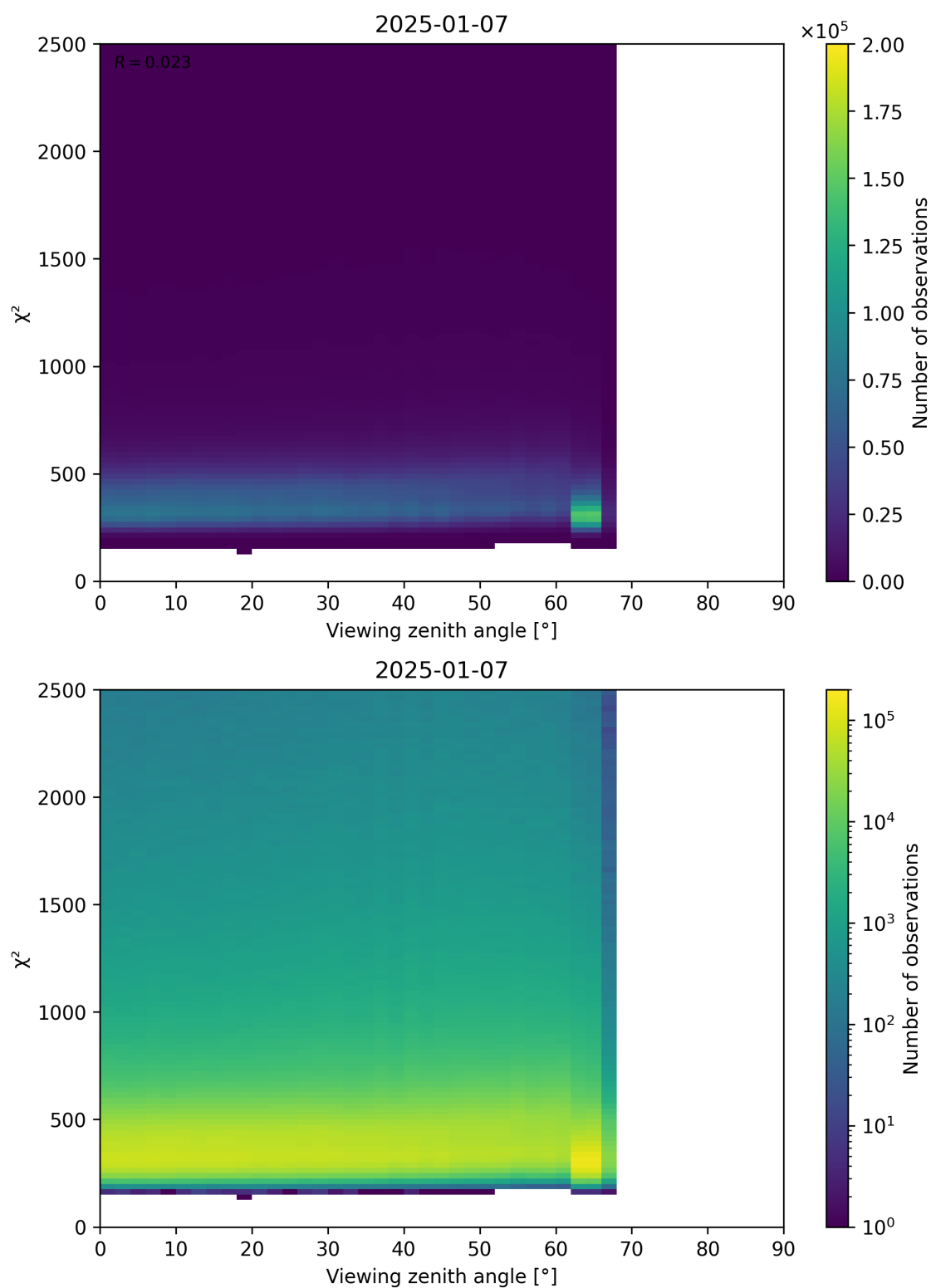
Figure 162: Scatter density plot of “Viewing zenith angle” against “ \chi^2 ” for 2025-01-07 to 2025-01-08.
