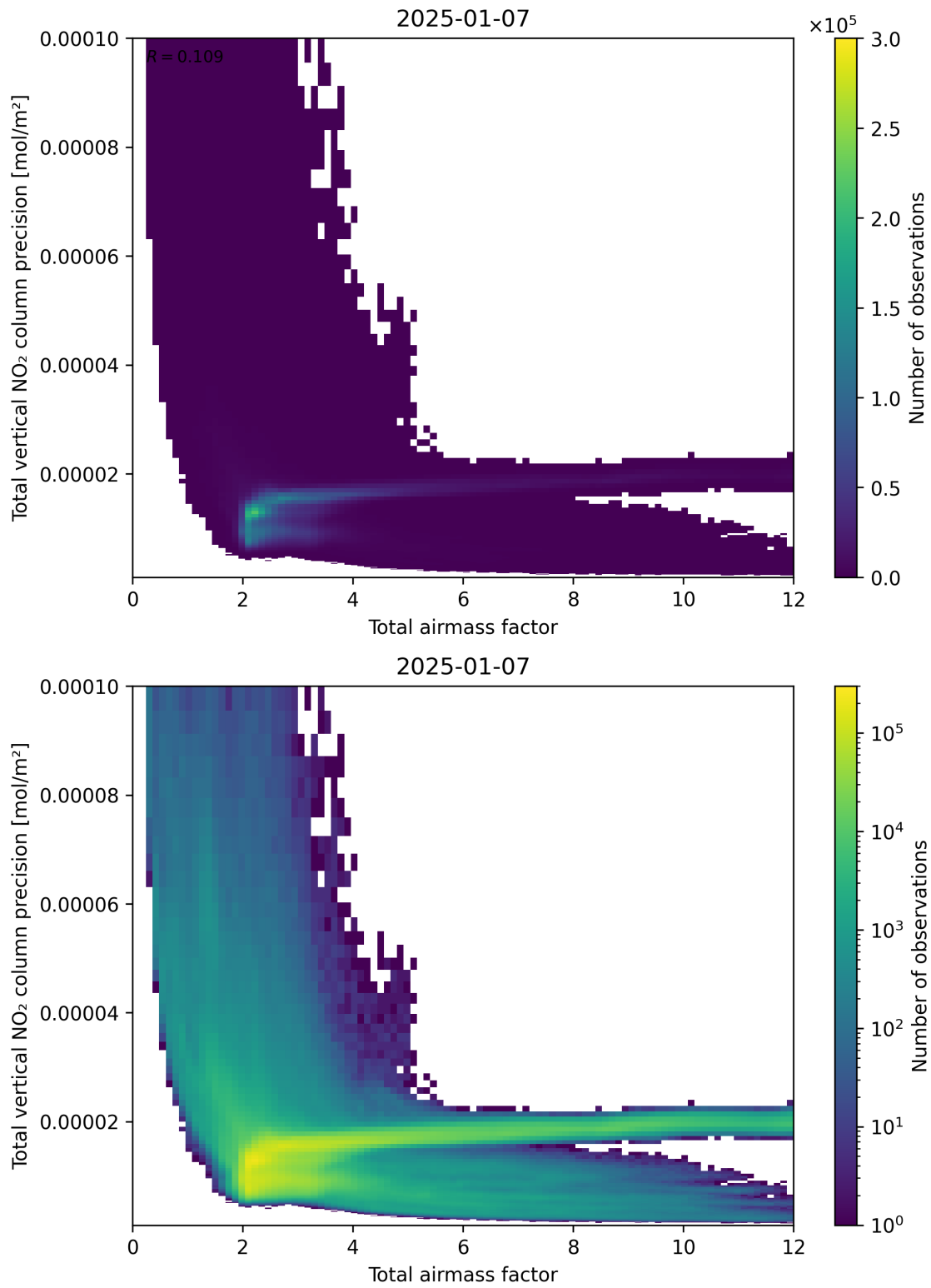
Figure 68: Scatter density plot of “Total airmass factor” against “Total vertical NO 2 column precision” for 2025-01-07 to 2025-01-08.
