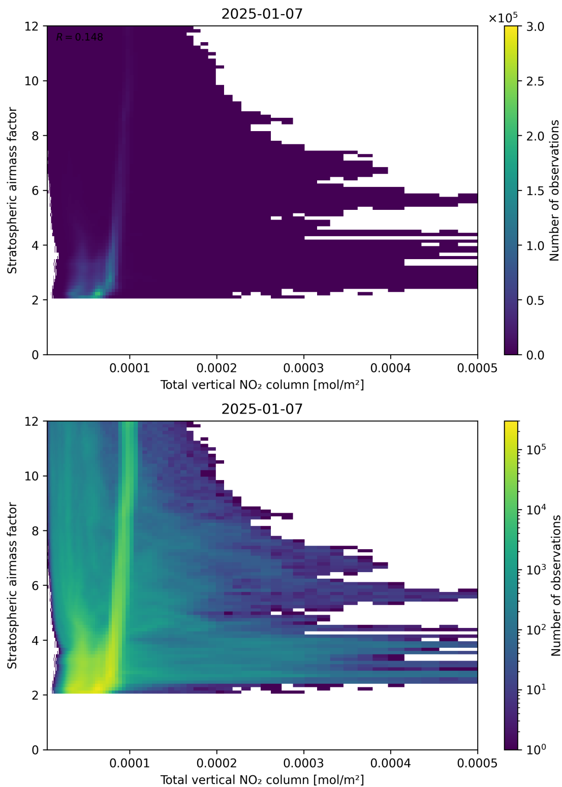
Figure 110: Scatter density plot of “Total vertical NO 2 column” against “Stratospheric airmass factor” for 2025-01-07 to 2025-01-08.
