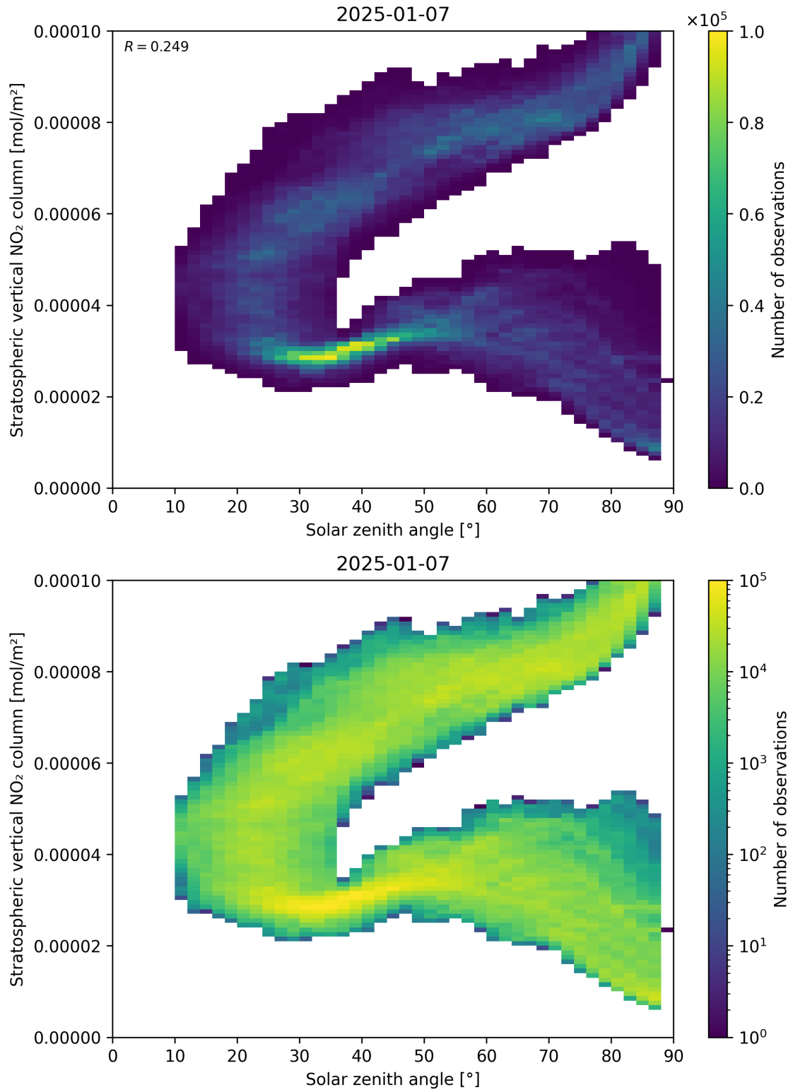
Figure 150: Scatter density plot of “Solar zenith angle” against “Stratospheric vertical NO 2 column” for 2025-01-07 to 2025-01-08.
