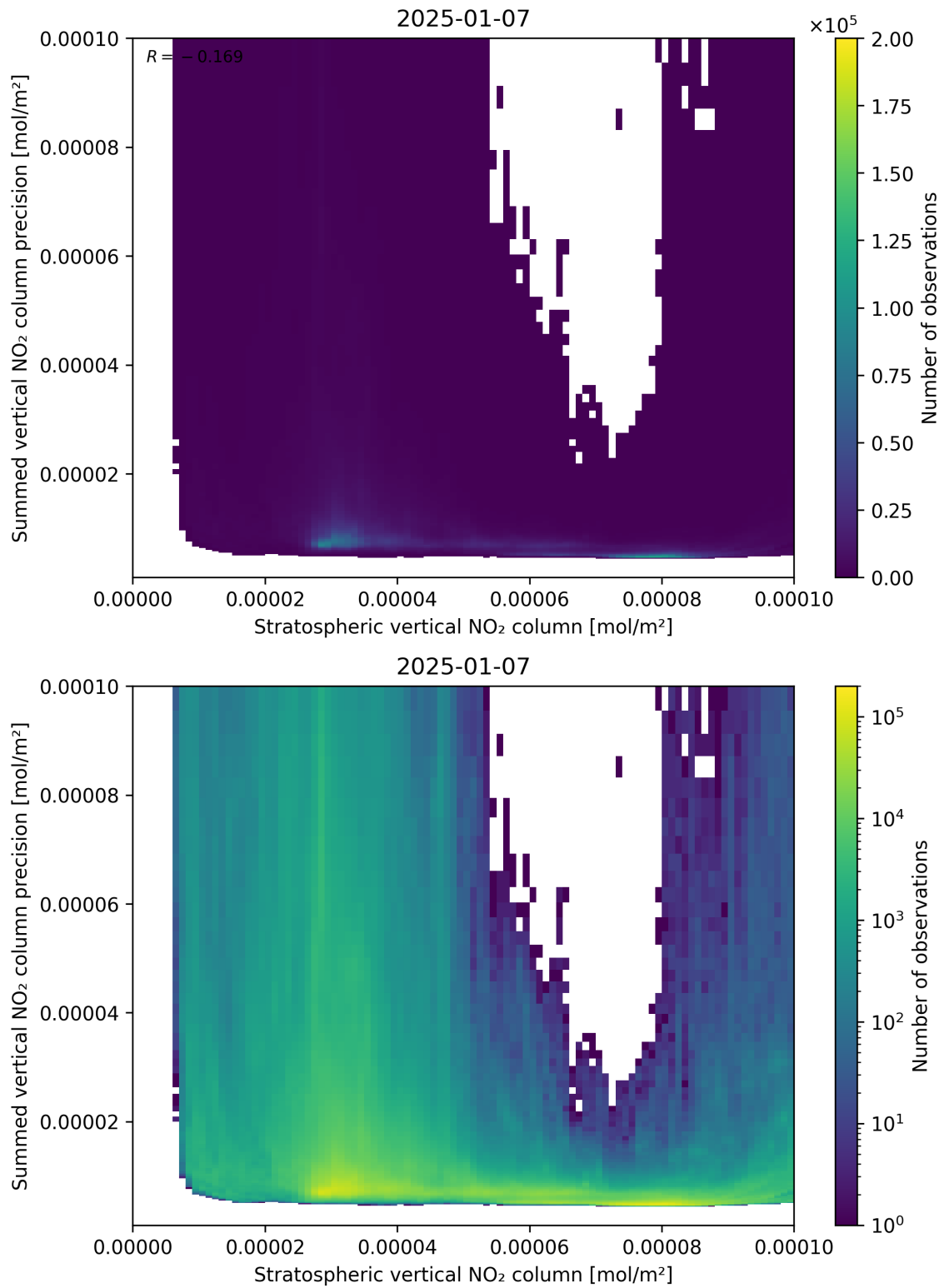
Figure 99: Scatter density plot of “Stratospheric vertical NO 2 column” against “Summed vertical NO 2 column precision” for 2025-01-07 to 2025-01-08.
