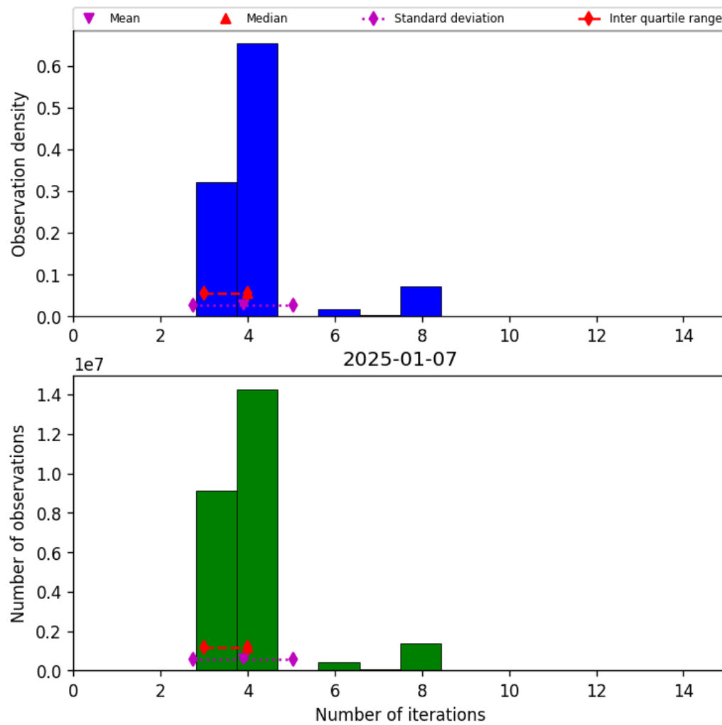
Figure 34: Histogram of “Number of iterations” for 2025-01-07 to 2025-01-08
