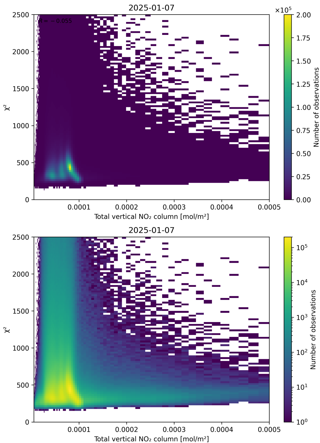
Figure 111: Scatter density plot of “Total vertical NO 2 column” against “ \chi^2 ” for 2025-01-07 to 2025-01-08.
