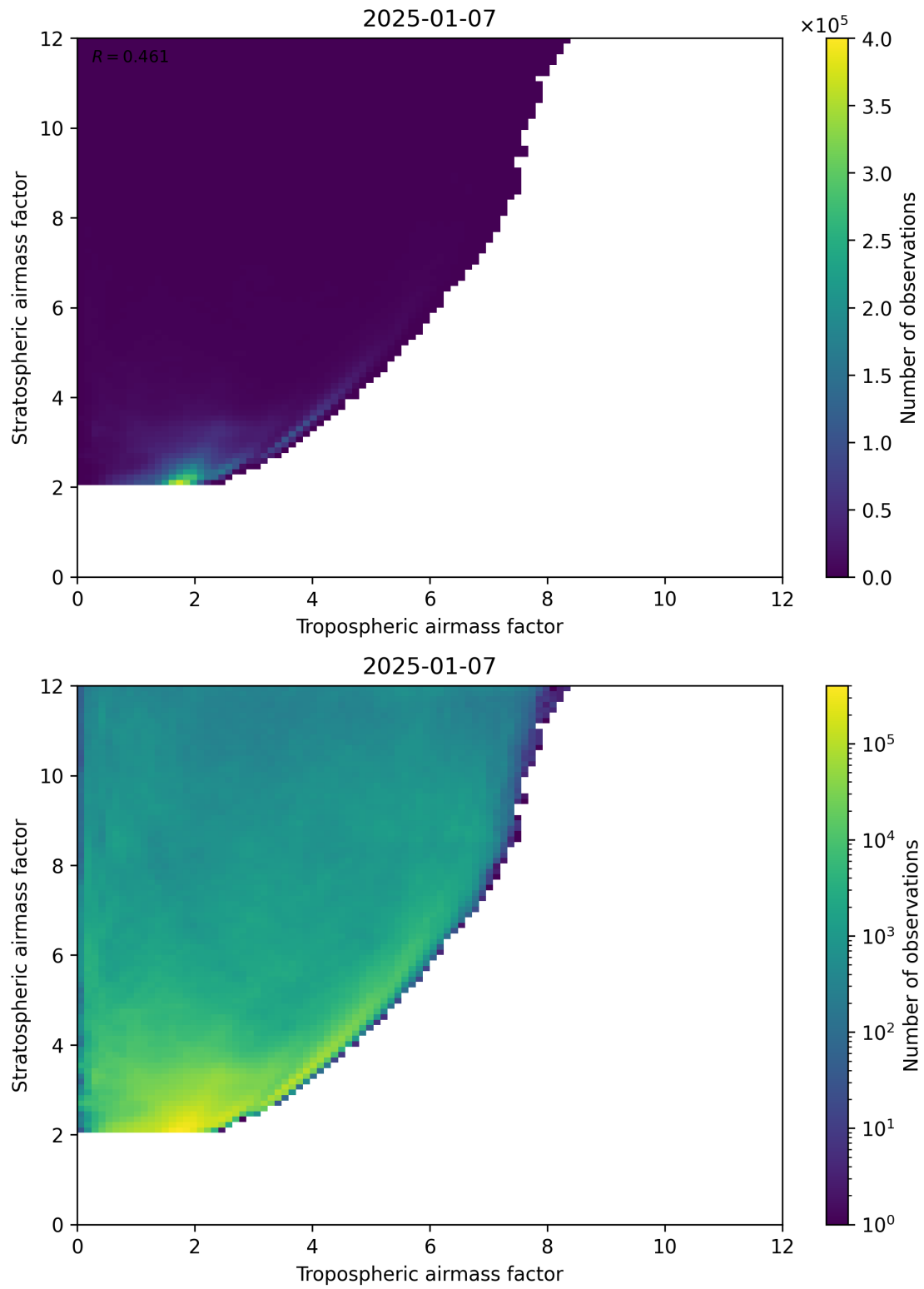
Figure 71: Scatter density plot of “Tropospheric airmass factor” against “Stratospheric airmass factor” for 2025-01-07 to 2025-01-08.
