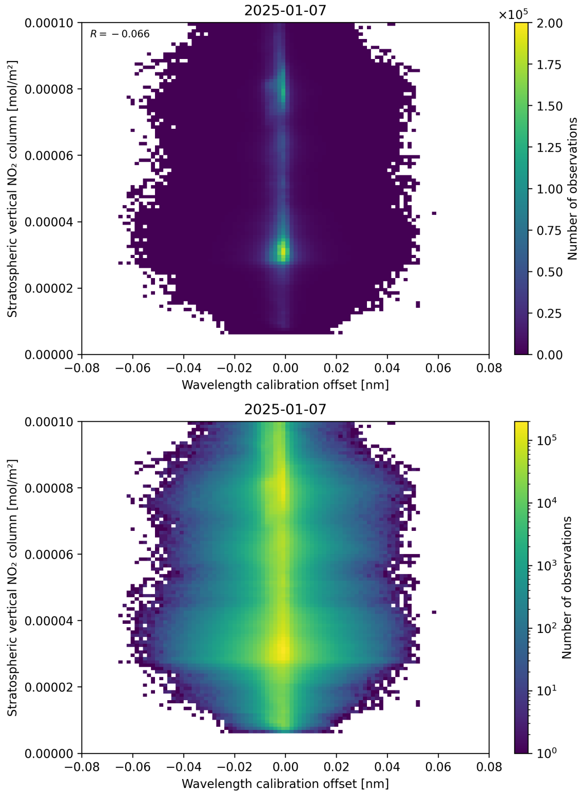
Figure 176: Scatter density plot of “Wavelength calibration offset” against “Stratospheric vertical NO 2 column” for 2025-01-07 to 2025-01-08.
