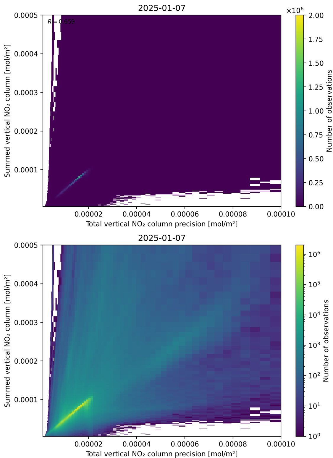
Figure 117: Scatter density plot of “Total vertical NO 2 column precision” against “Summed vertical NO 2 column” for 2025-01-07 to 2025-01-08.
