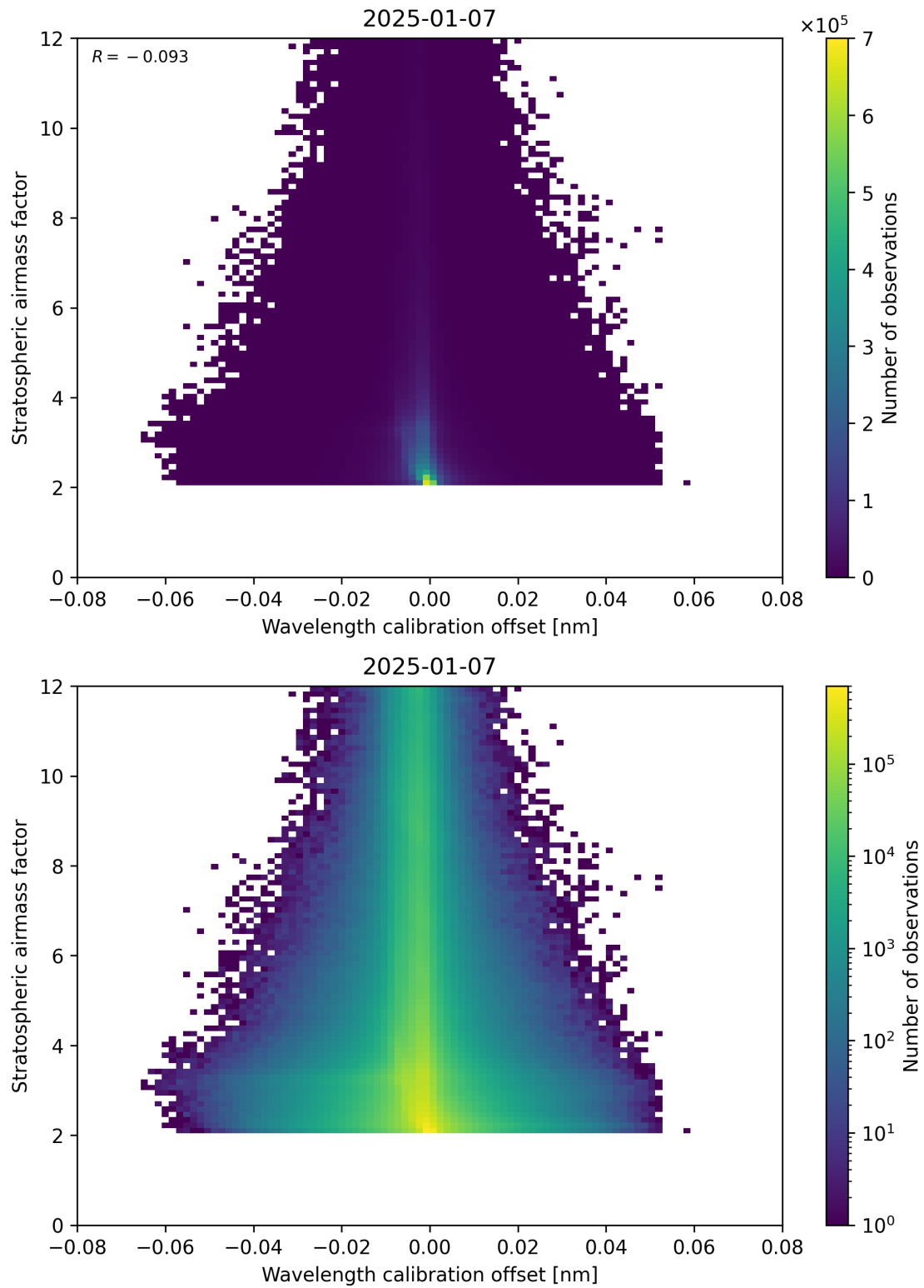
Figure 174: Scatter density plot of “Wavelength calibration offset” against “Stratospheric airmass factor” for 2025-01-07 to 2025-01-08.
