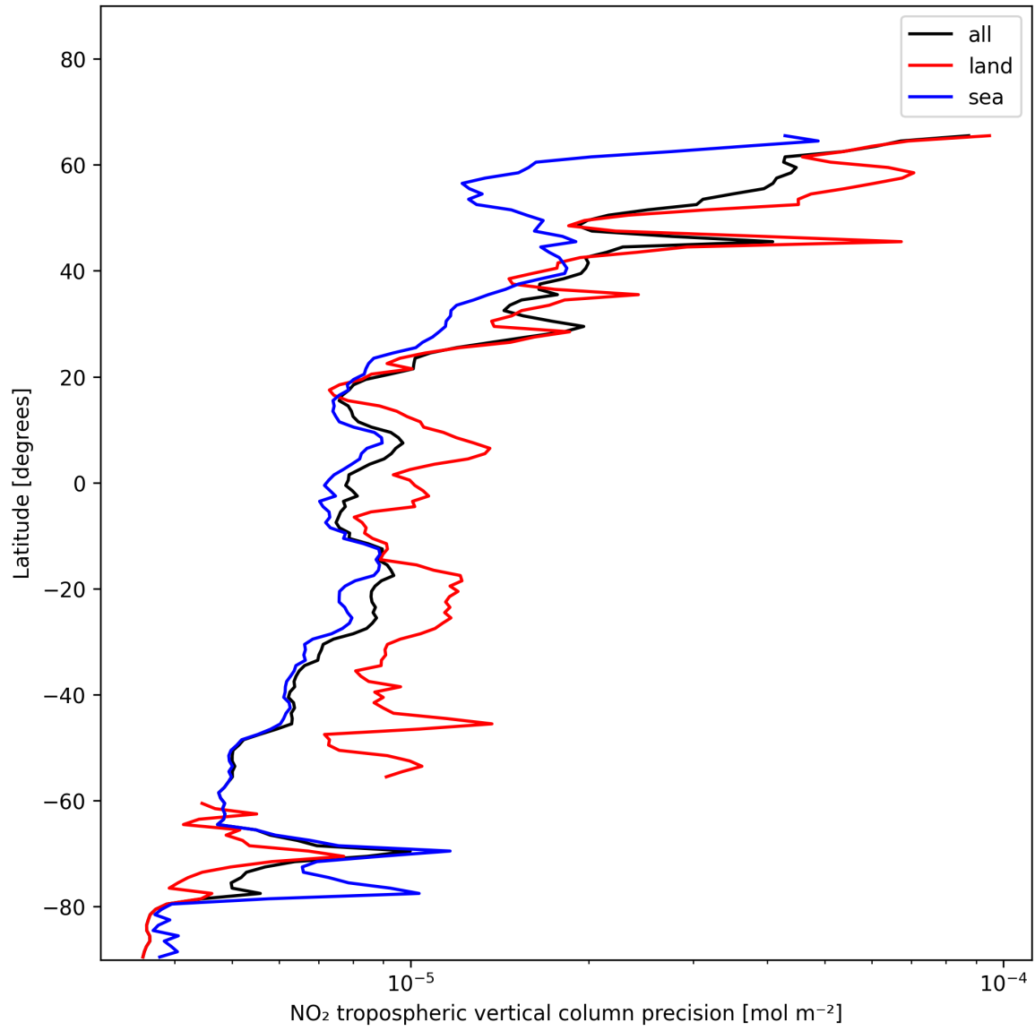
Figure 13: Zonal average of “NO 2 tropospheric vertical column precision” for 2025-01-07 to 2025-01-08.
