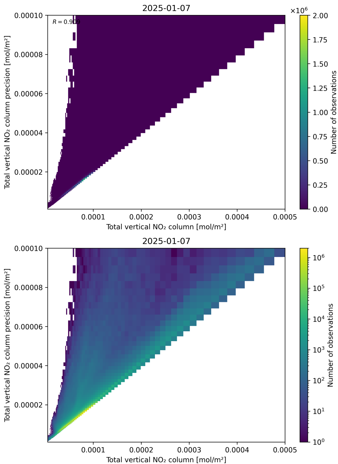
Figure 114: Scatter density plot of “Total vertical NO 2 column” against “Total vertical NO 2 column precision” for 2025-01-07 to 2025-01-08.
