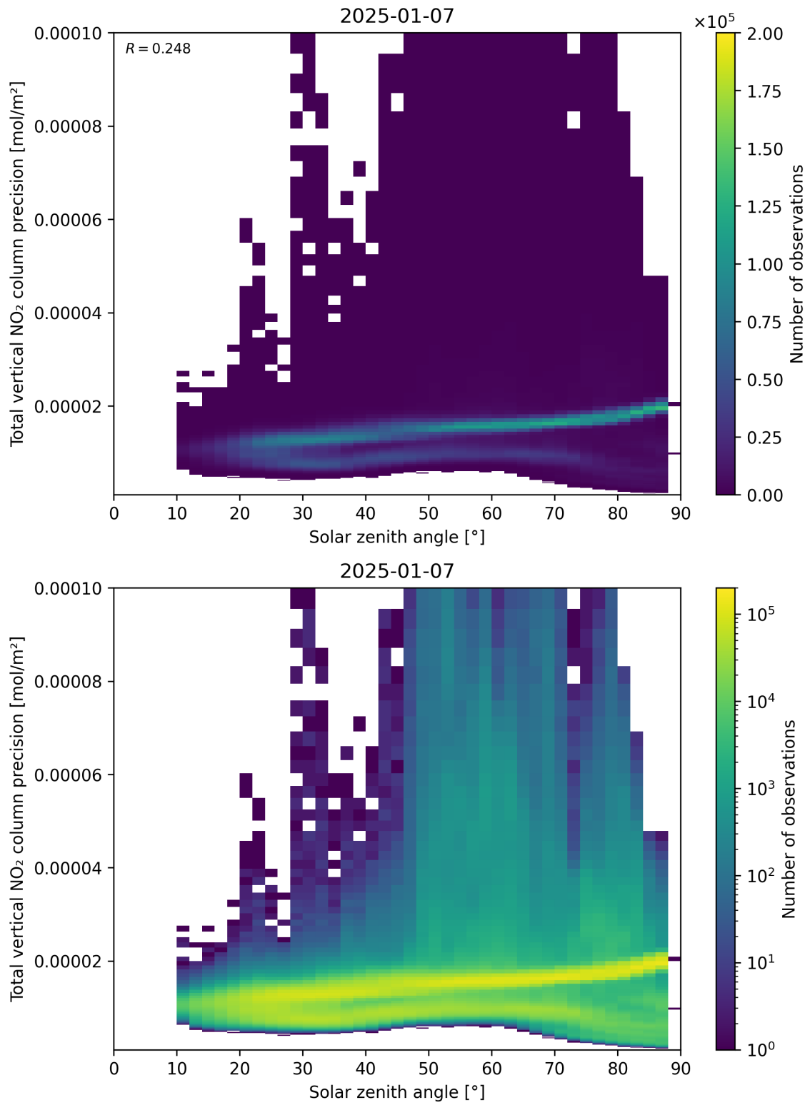
Figure 154: Scatter density plot of “Solar zenith angle” against “Total vertical NO 2 column precision” for 2025-01-07 to 2025-01-08.
