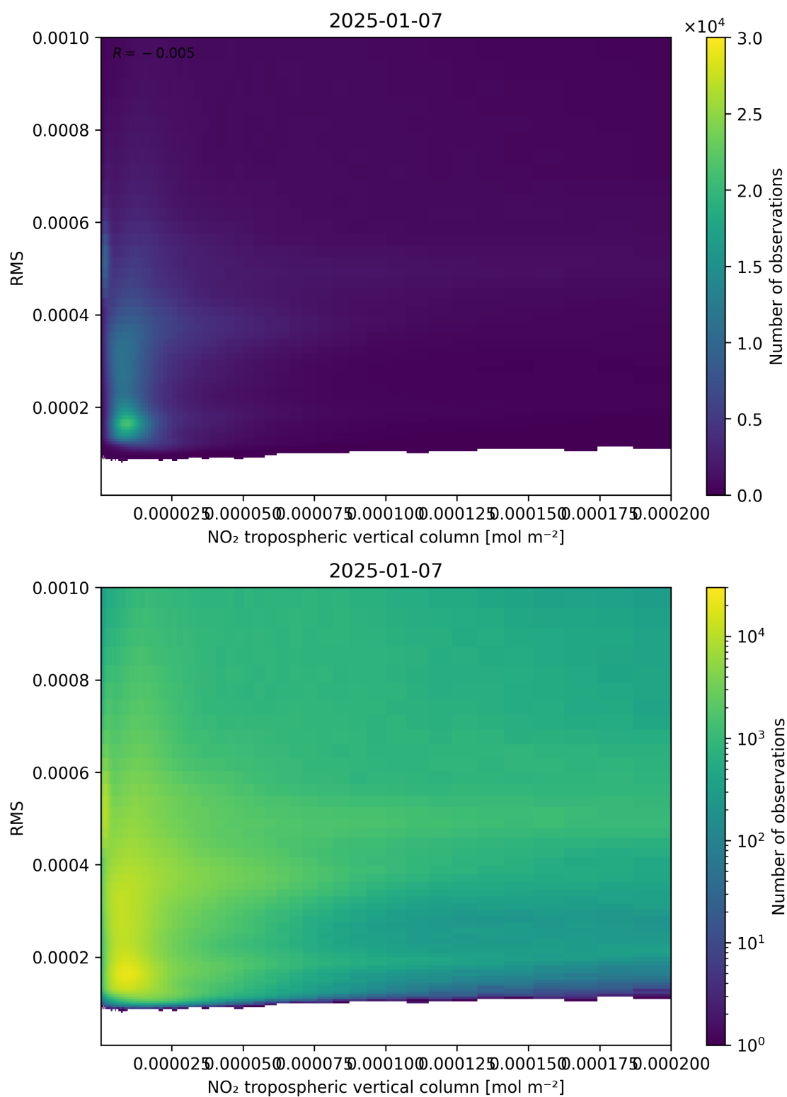
Figure 142: Scatter density plot of “NO 2 tropospheric vertical column” against “RMS” for 2025-01-07 to 2025-01-08.
