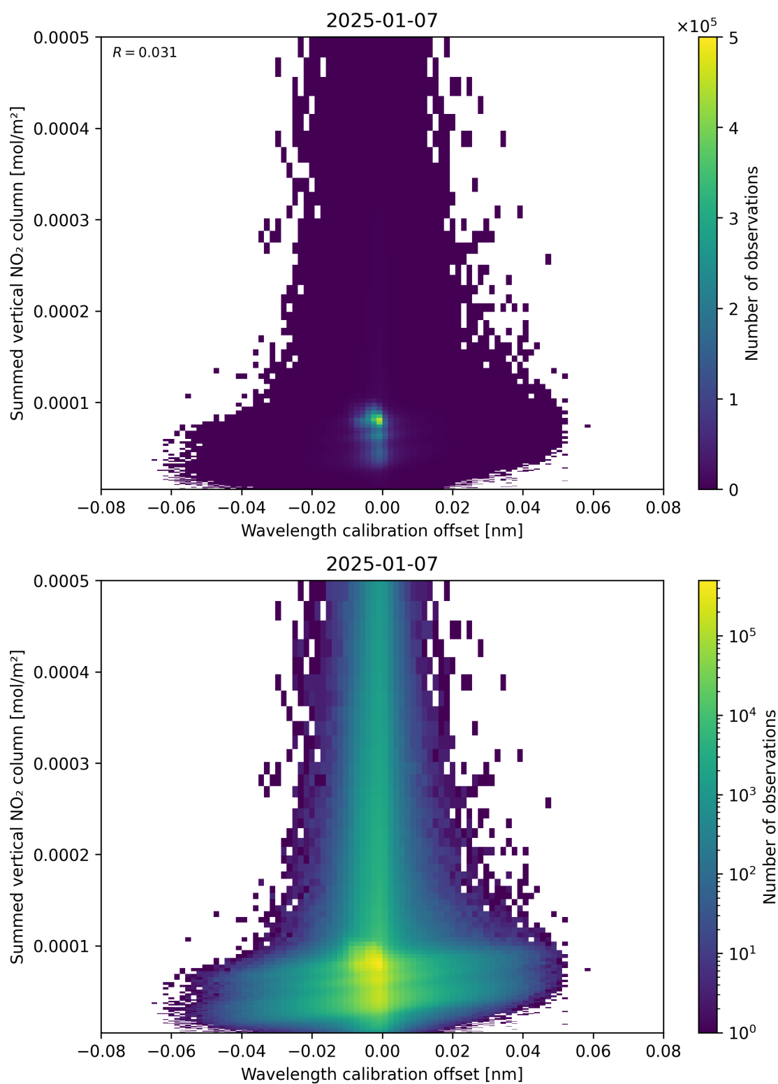
Figure 177: Scatter density plot of “Wavelength calibration offset” against “Summed vertical NO 2 column” for 2025-01-07 to 2025-01-08.
