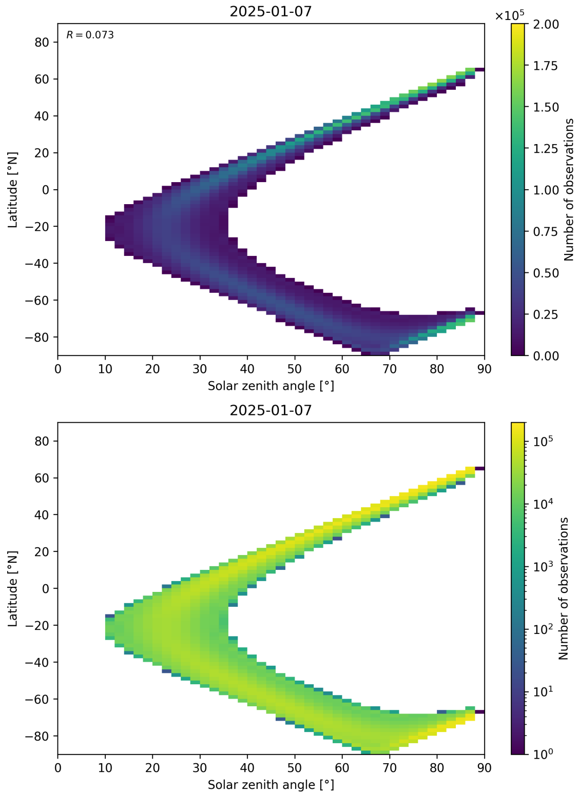
Figure 149: Scatter density plot of “Solar zenith angle” against “Latitude” for 2025-01-07 to 2025-01-08.
