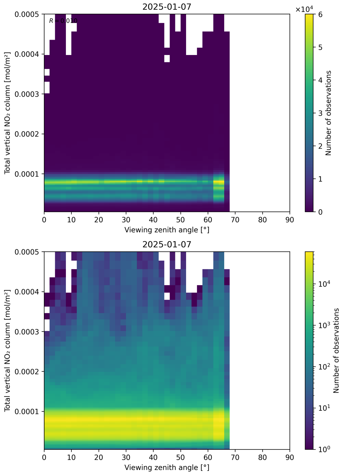
Figure 167: Scatter density plot of “Viewing zenith angle” against “Total vertical NO 2 column” for 2025-01-07 to 2025-01-08.
