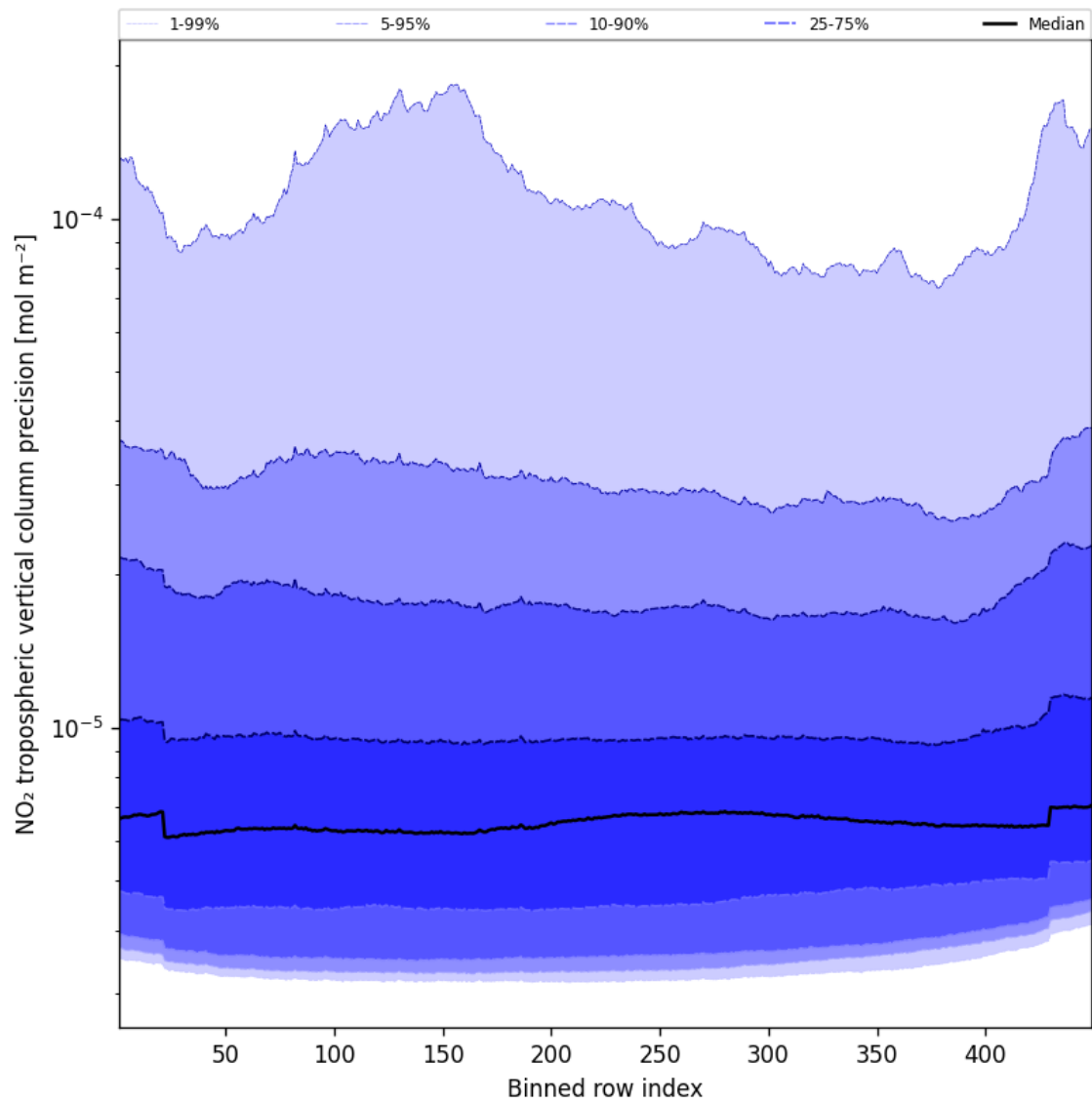
Figure 47: Along track statistics of “NO 2 tropospheric vertical column precision” for 2025-01-07 to 2025-01-08
