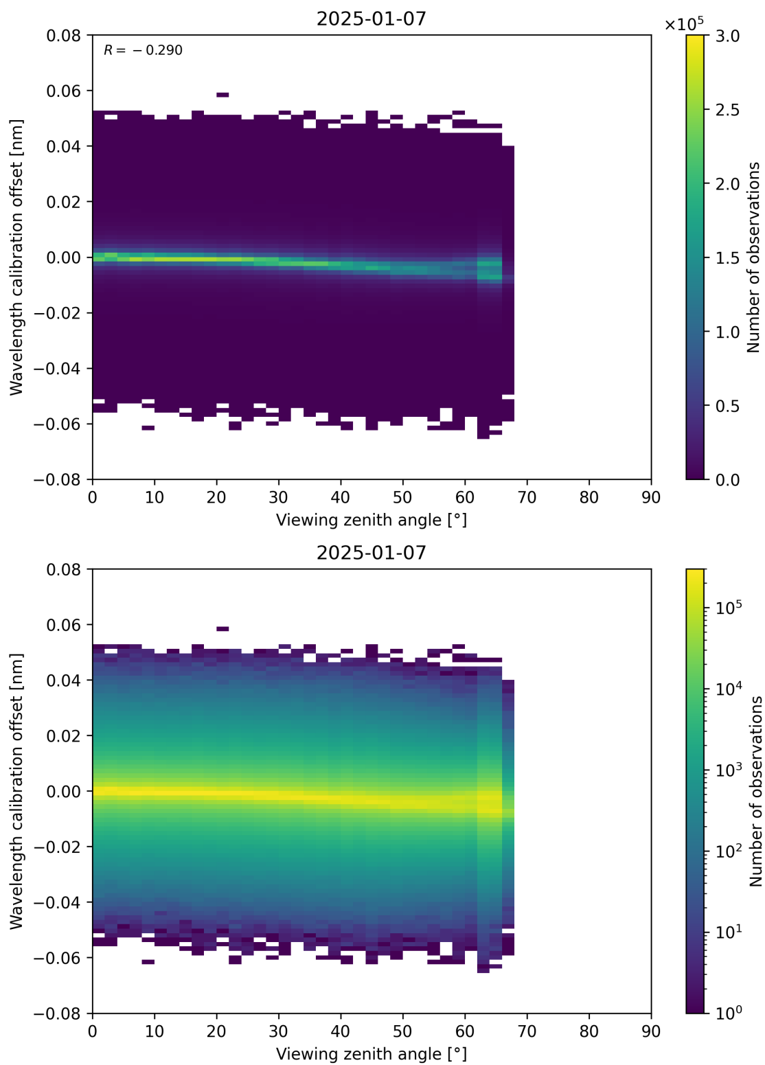
Figure 173: Scatter density plot of “Viewing zenith angle” against “Wavelength calibration offset” for 2025-01-07 to 2025-01-08.
