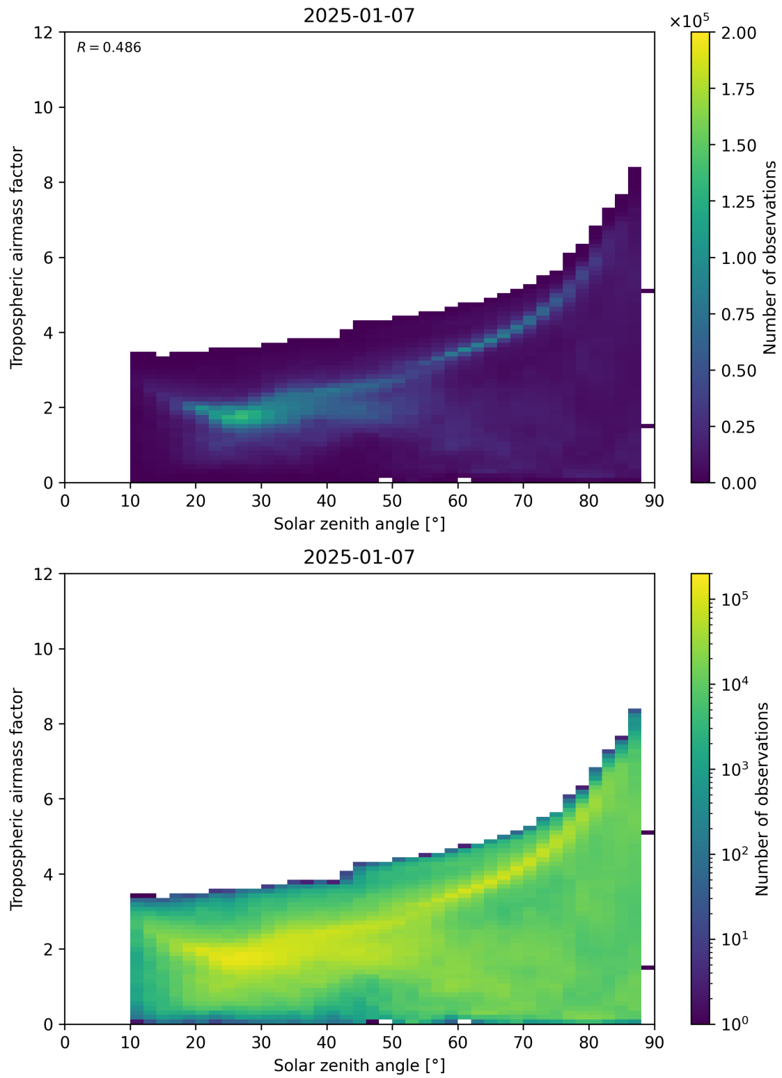
Figure 147: Scatter density plot of “Solar zenith angle” against “Tropospheric airmass factor” for 2025-01-07 to 2025-01-08.
