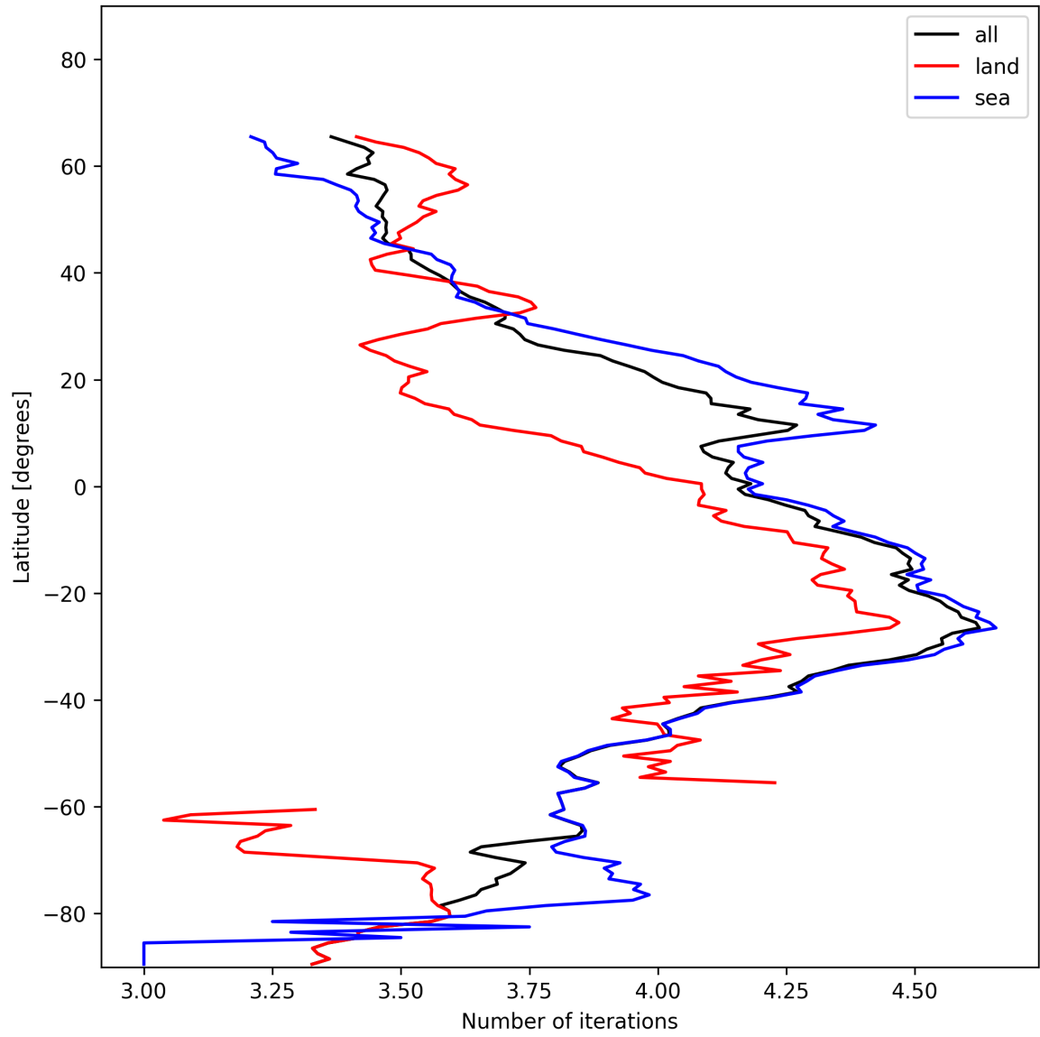
Figure 17: Zonal average of “Number of iterations” for 2025-01-07 to 2025-01-08.
