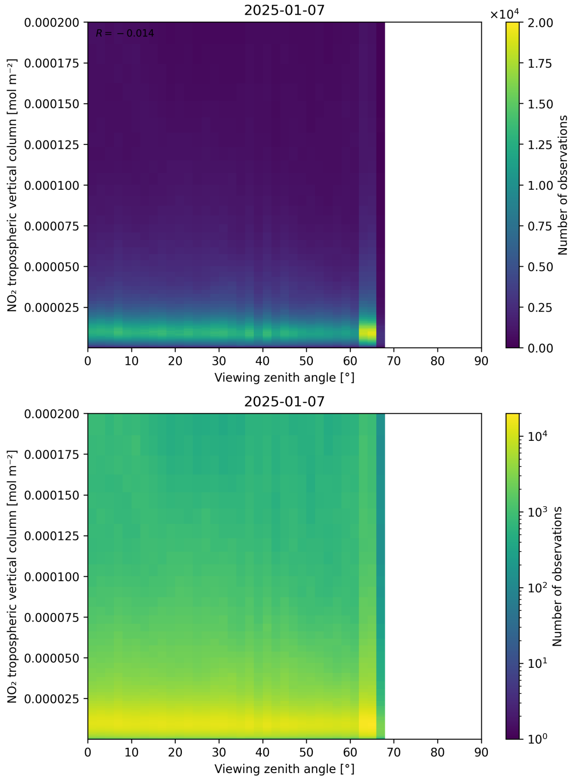
Figure 169: Scatter density plot of “Viewing zenith angle” against “NO 2 tropospheric vertical column” for 2025-01-07 to 2025-01-08.
