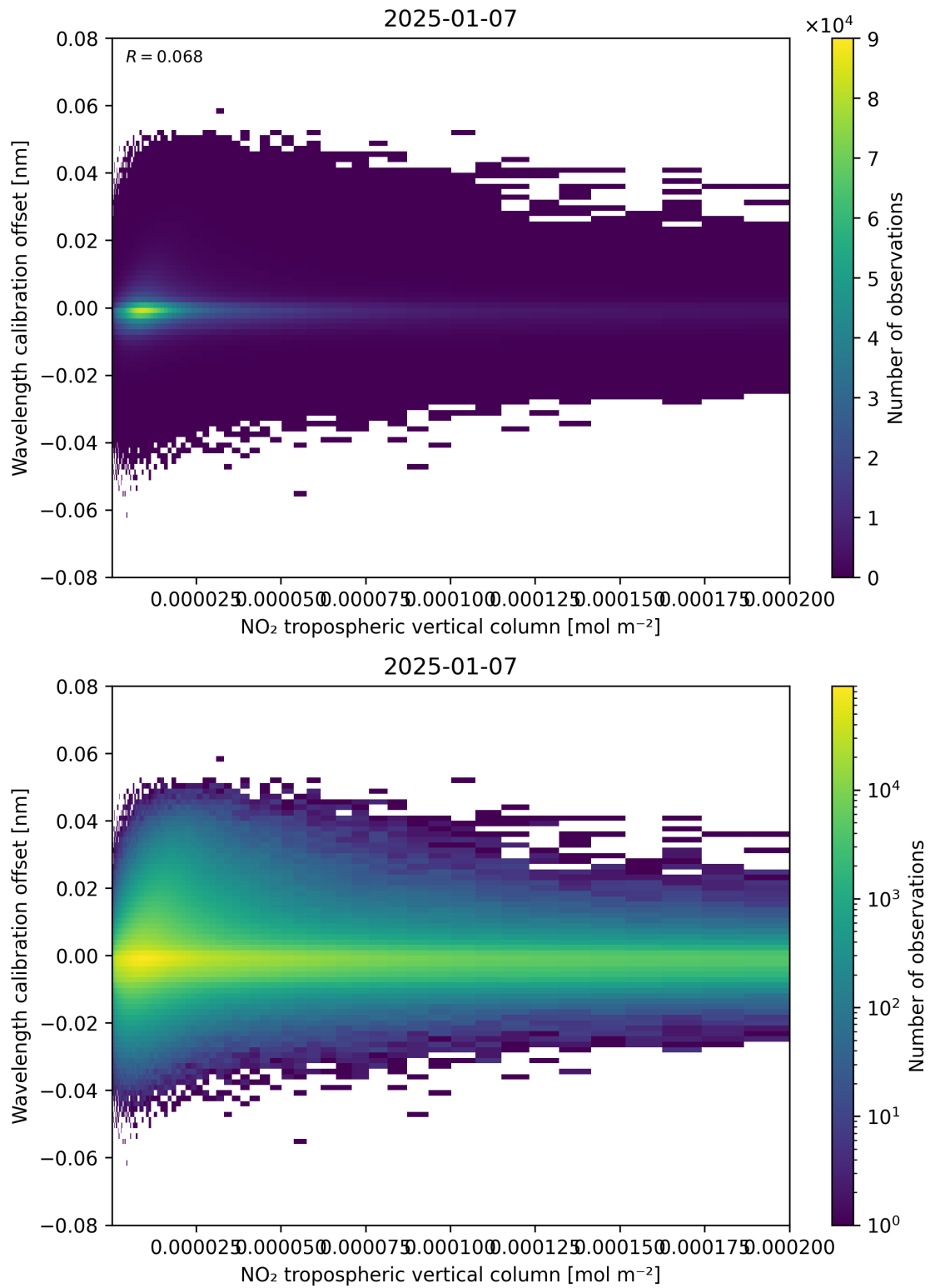
Figure 143: Scatter density plot of “NO 2 tropospheric vertical column” against “Wavelength calibration offset” for 2025-01-07 to 2025-01-08.
