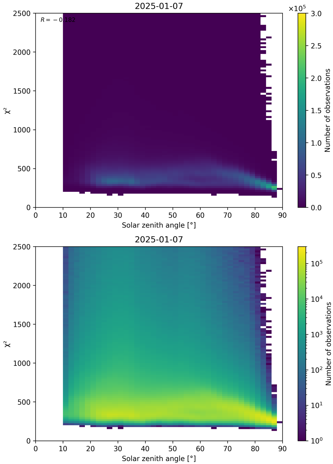
Figure 148: Scatter density plot of “Solar zenith angle” against “ \chi^2 ” for 2025-01-07 to 2025-01-08.
