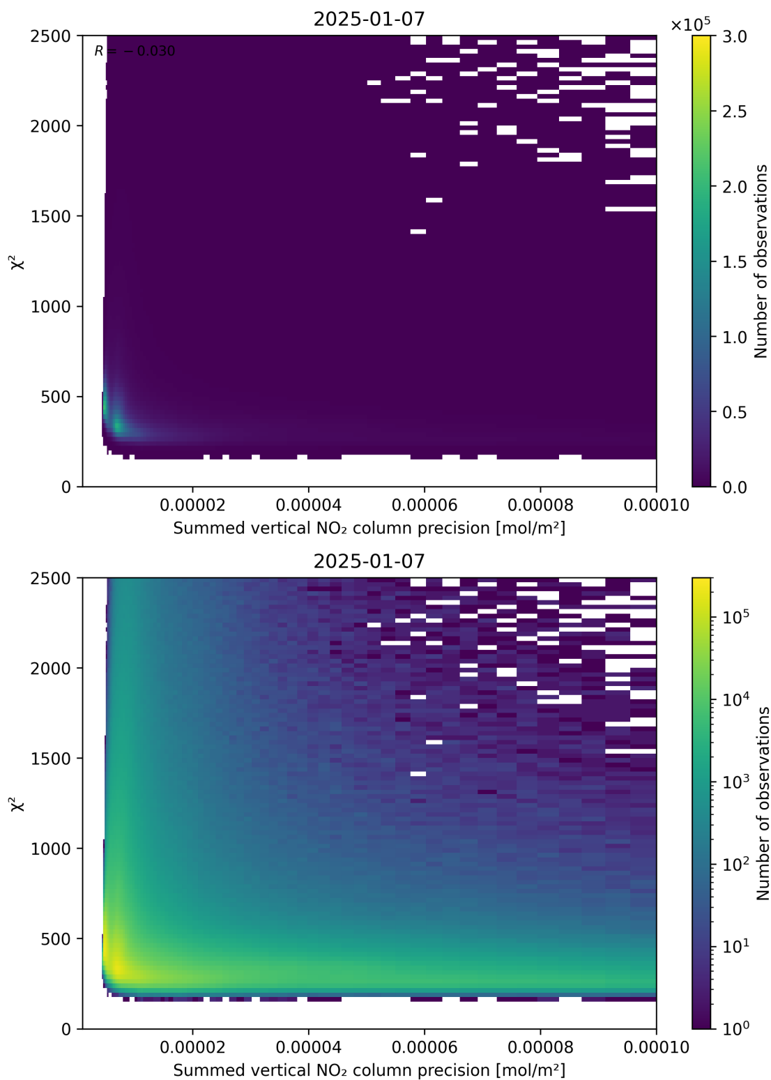
Figure 107: Scatter density plot of “Summed vertical NO 2 column precision” against “ \chi^2 ” for 2025-01-07 to 2025-01-08.
