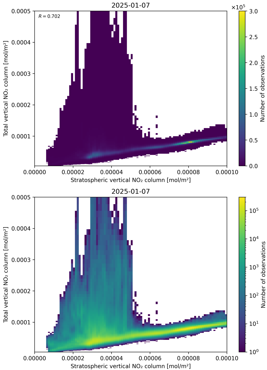
Figure 100: Scatter density plot of “Stratospheric vertical NO 2 column” against “Total vertical NO 2 column” for 2025-01-07 to 2025-01-08.
