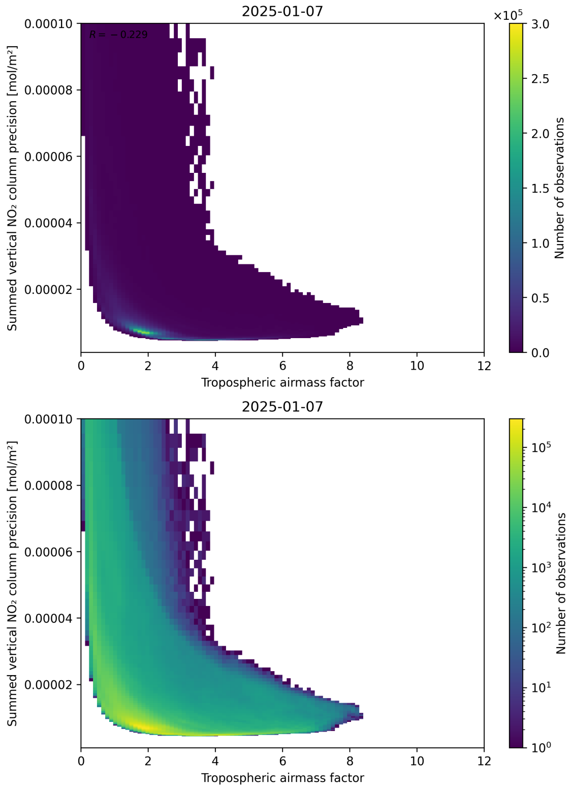
Figure 76: Scatter density plot of “Tropospheric air mass factor” against “Summed vertical NO 2 column precision” for 2025-01-07 to 2025-01-08.
