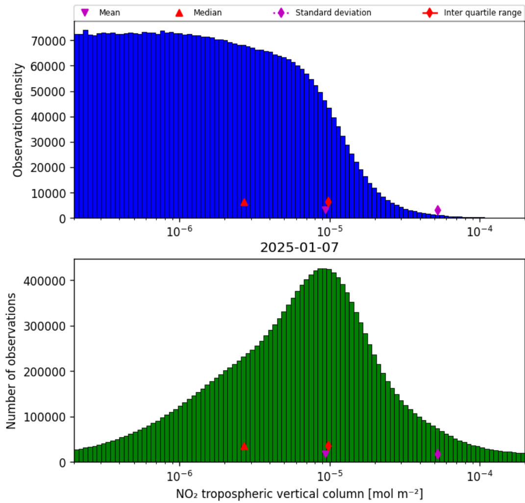
Figure 29: Histogram of “NO 2 tropospheric vertical column” for 2025-01-07 to 2025-01-08
