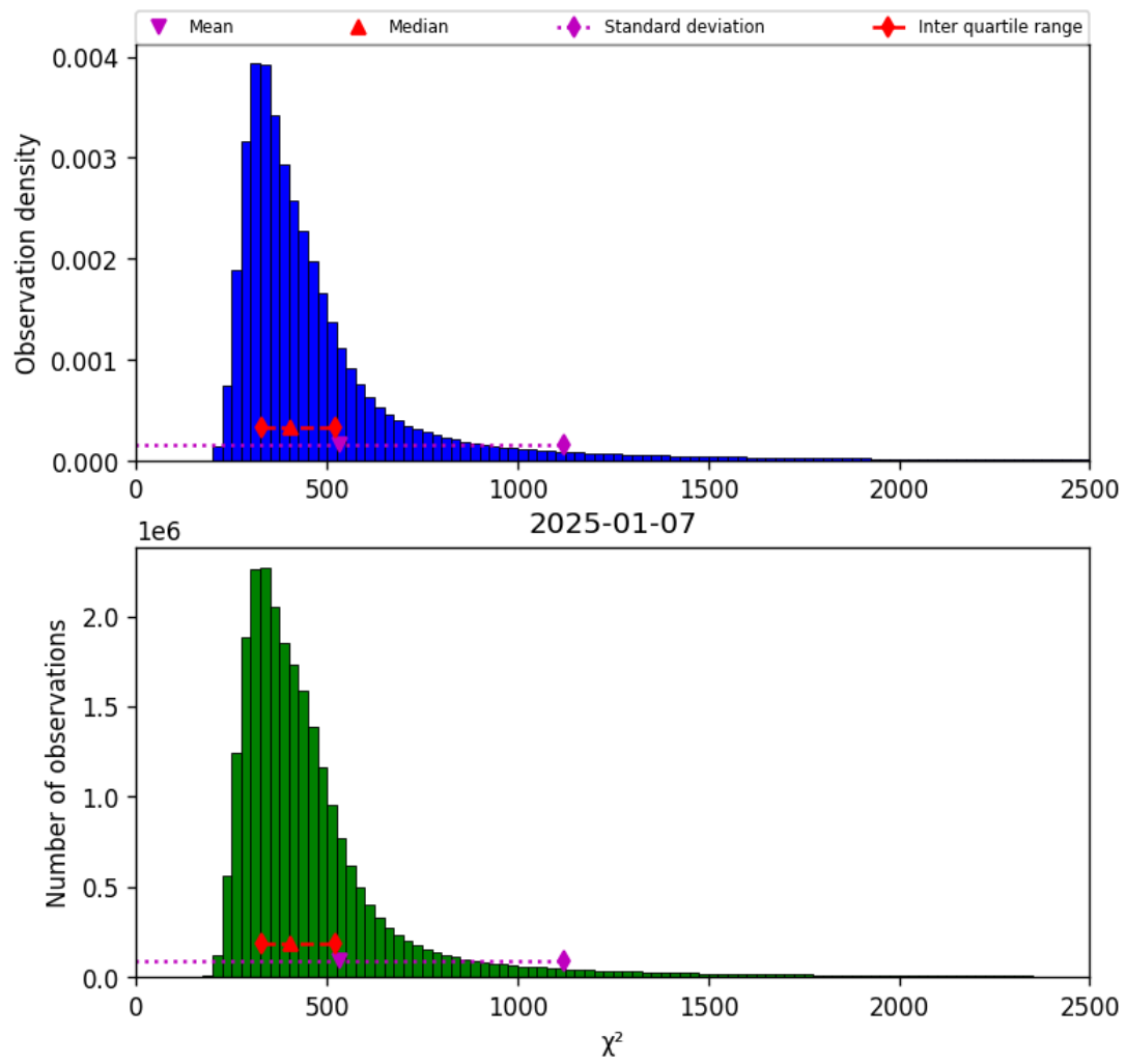
Figure 42: Histogram of " \chi^2 " for 2025-01-07 to 2025-01-08
