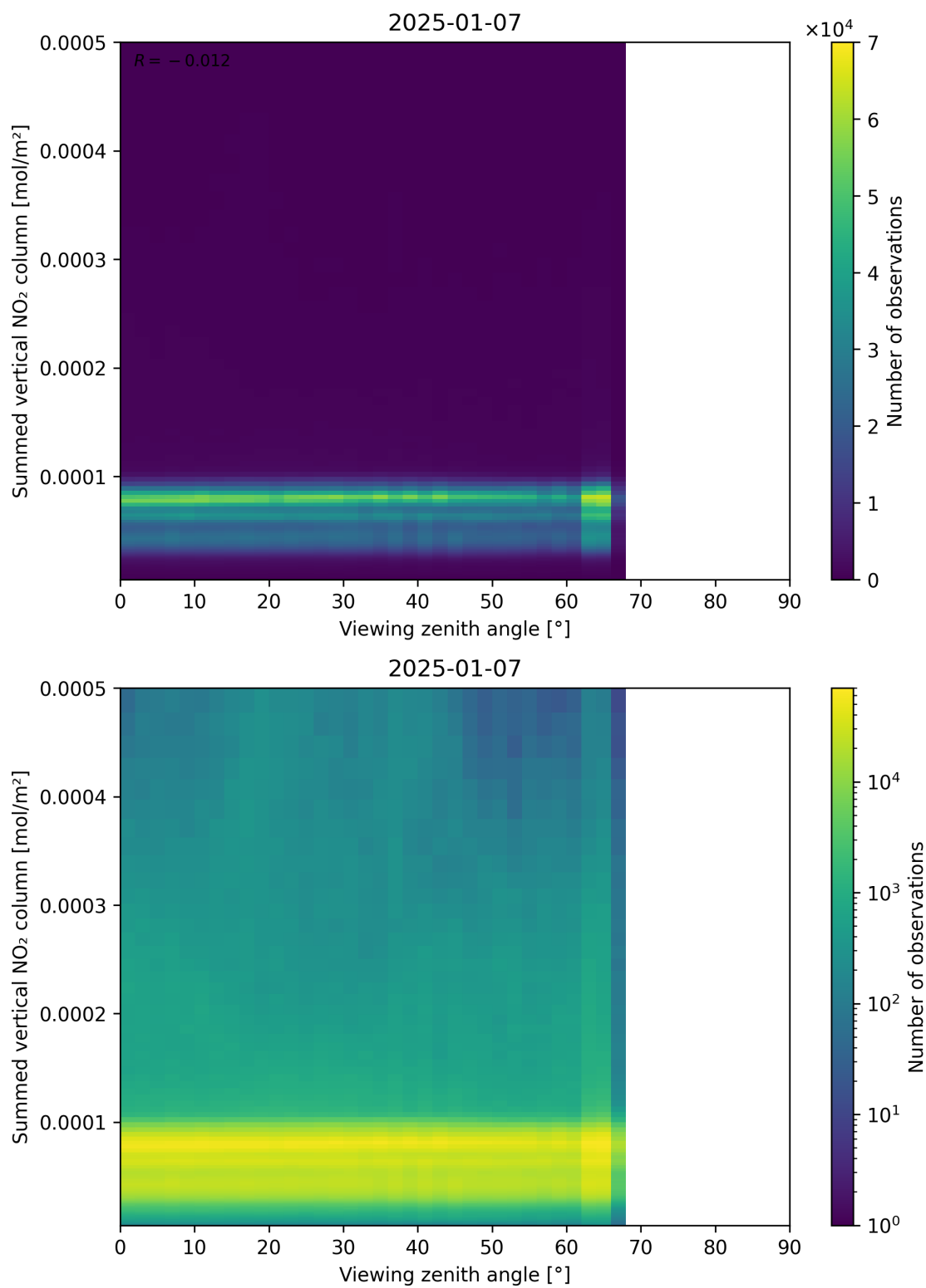
Figure 165: Scatter density plot of “Viewing zenith angle” against “Summed vertical NO 2 column” for 2025-01-07 to 2025-01-08.
