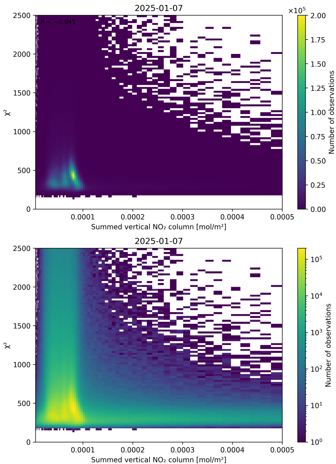
Figure 104: Scatter density plot of “Summed vertical NO 2 column” against “ \chi^2 ” for 2025-01-07 to 2025-01-08.
