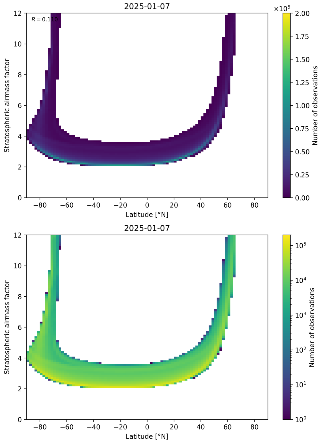
Figure 83: Scatter density plot of “Latitude” against “Stratospheric air mass factor” for 2025-01-07 to 2025-01-08.
