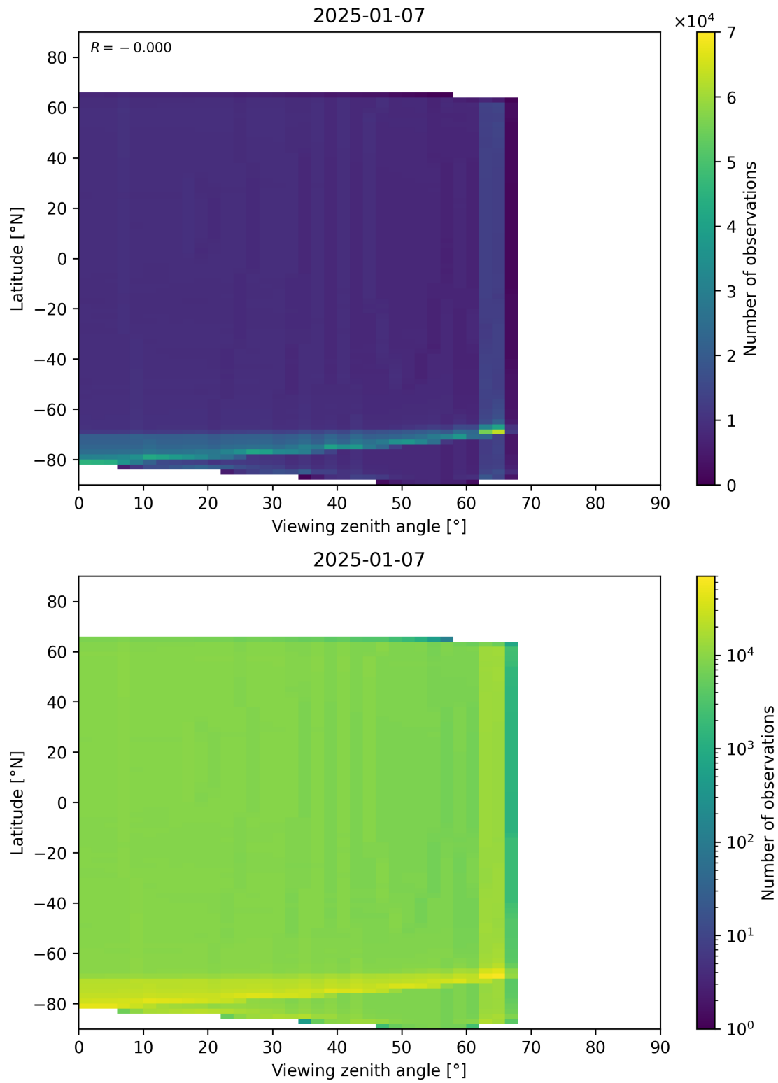
Figure 163: Scatter density plot of “Viewing zenith angle” against “Latitude” for 2025-01-07 to 2025-01-08.
