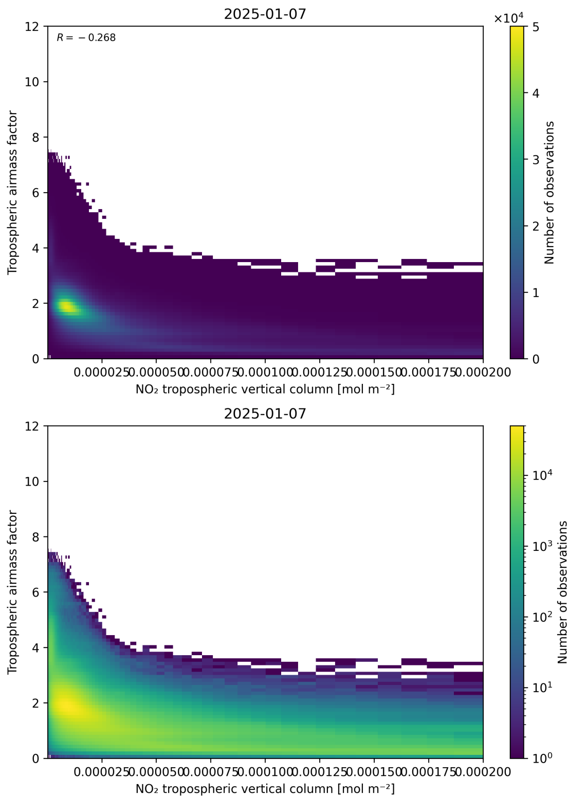
Figure 123: Scatter density plot of “NO 2 tropospheric vertical column” against “Tropospheric air mass factor” for 2025-01-07 to 2025-01-08.
