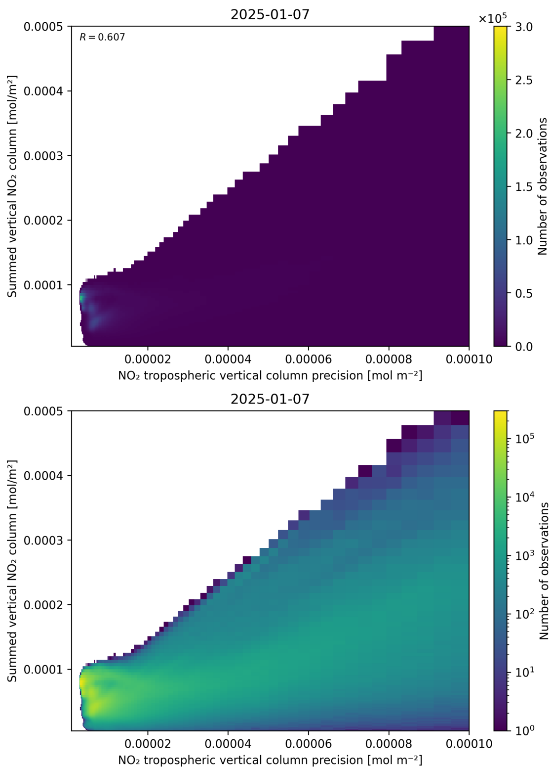
Figure 136: Scatter density plot of “NO 2 tropospheric vertical column precision” against “Summed vertical NO 2 column” for 2025-01-07 to 2025-01-08.
