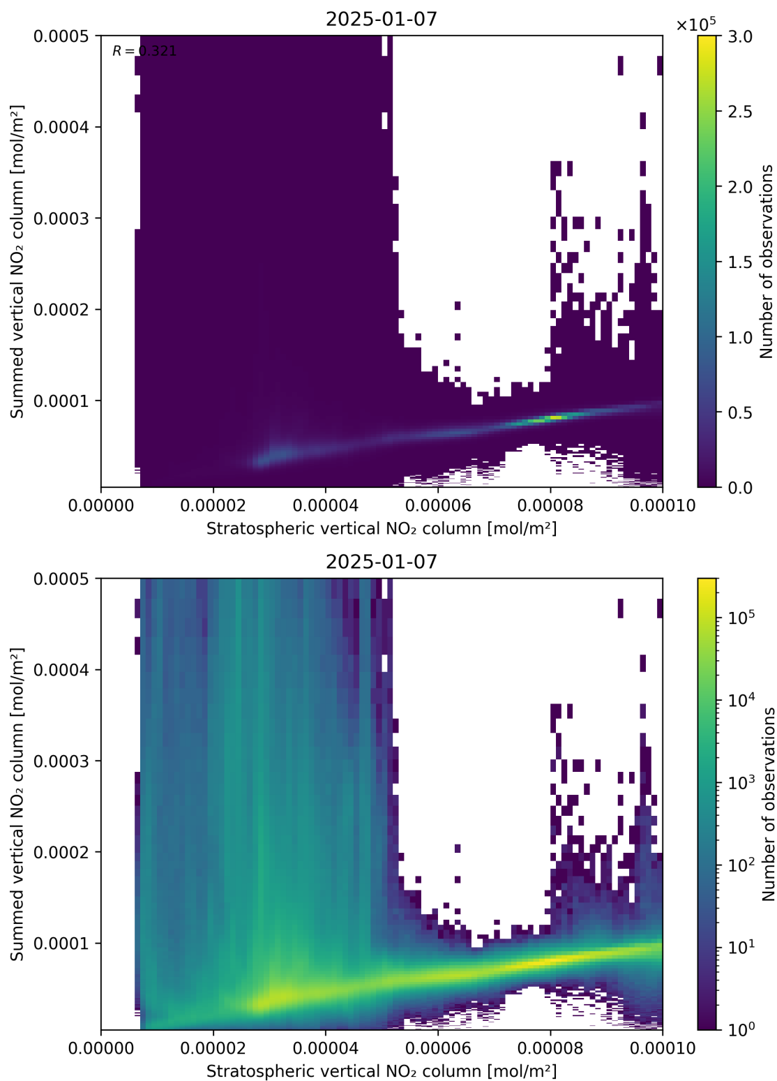
Figure 98: Scatter density plot of “Stratospheric vertical NO 2 column” against “Summed vertical NO 2 column” for 2025-01-07 to 2025-01-08.
