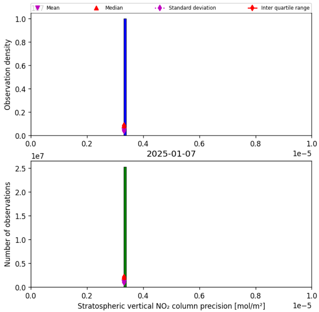
Figure 37: Histogram of “Stratospheric vertical NO 2 column precision” for 2025-01-07 to 2025-01-08
