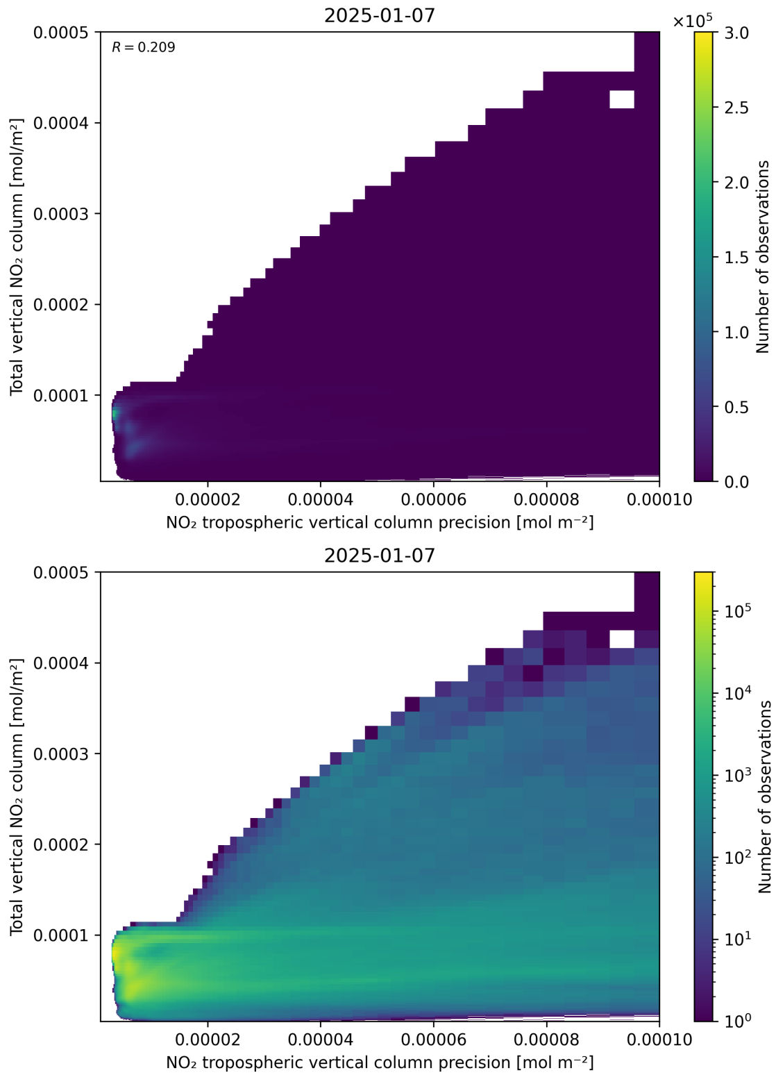
Figure 138: Scatter density plot of “NO 2 tropospheric vertical column precision” against “Total vertical NO 2 column” for 2025-01-07 to 2025-01-08.
