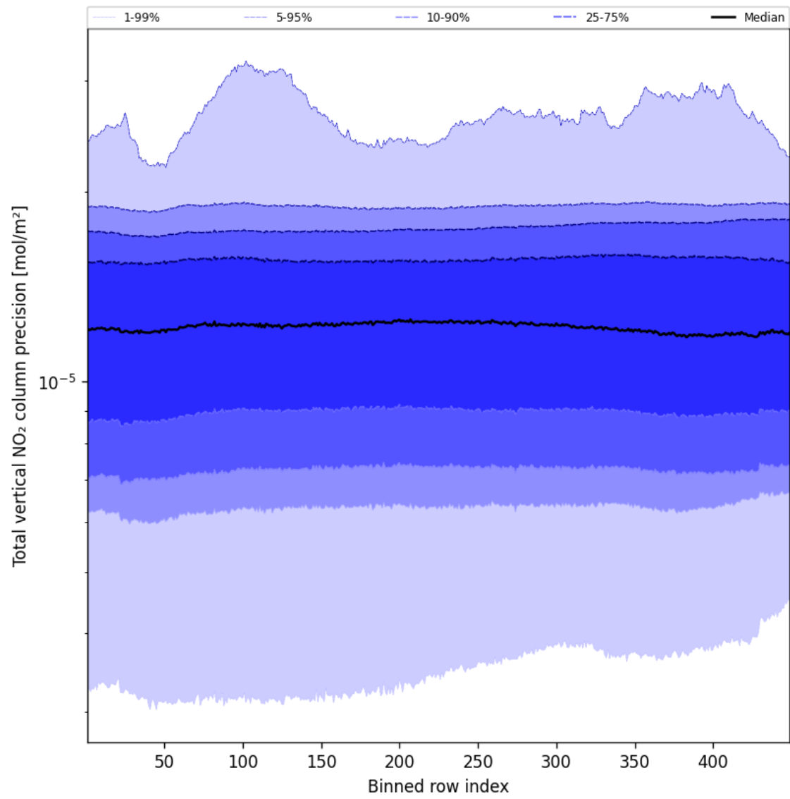
Figure 56: Along track statistics of “Total vertical NO 2 column precision” for 2025-01-07 to 2025-01-08
