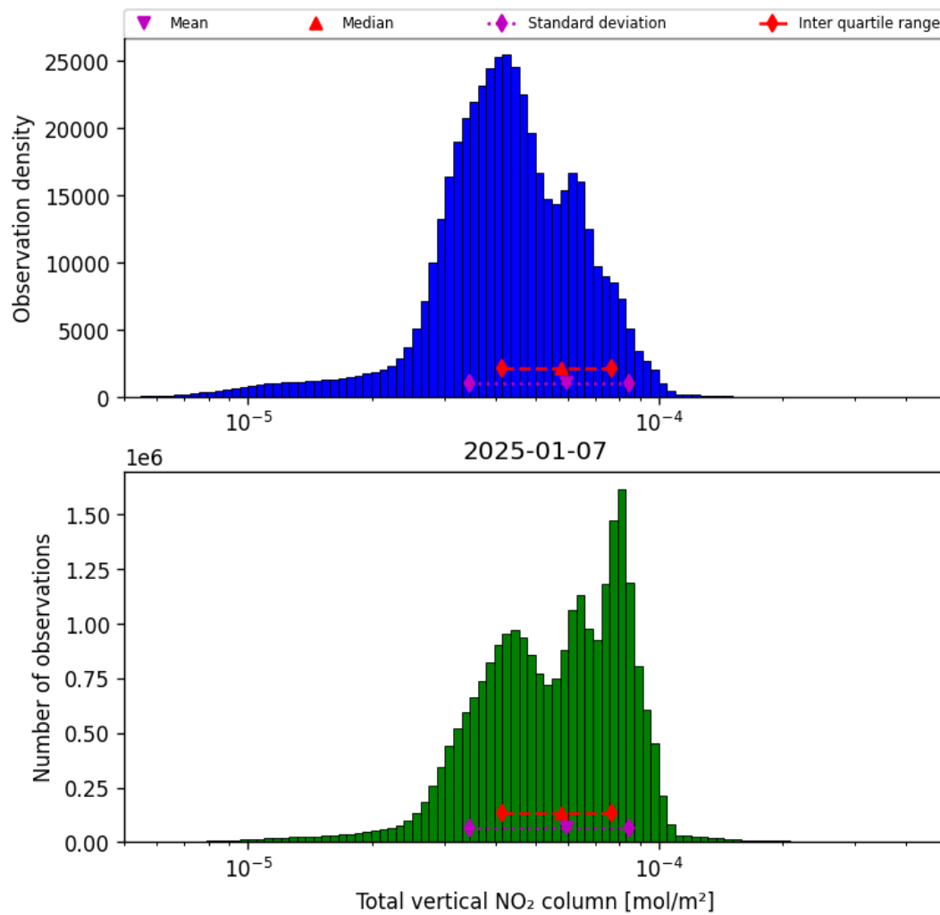
Figure 38: Histogram of “Total vertical NO 2 column” for 2025-01-07 to 2025-01-08
