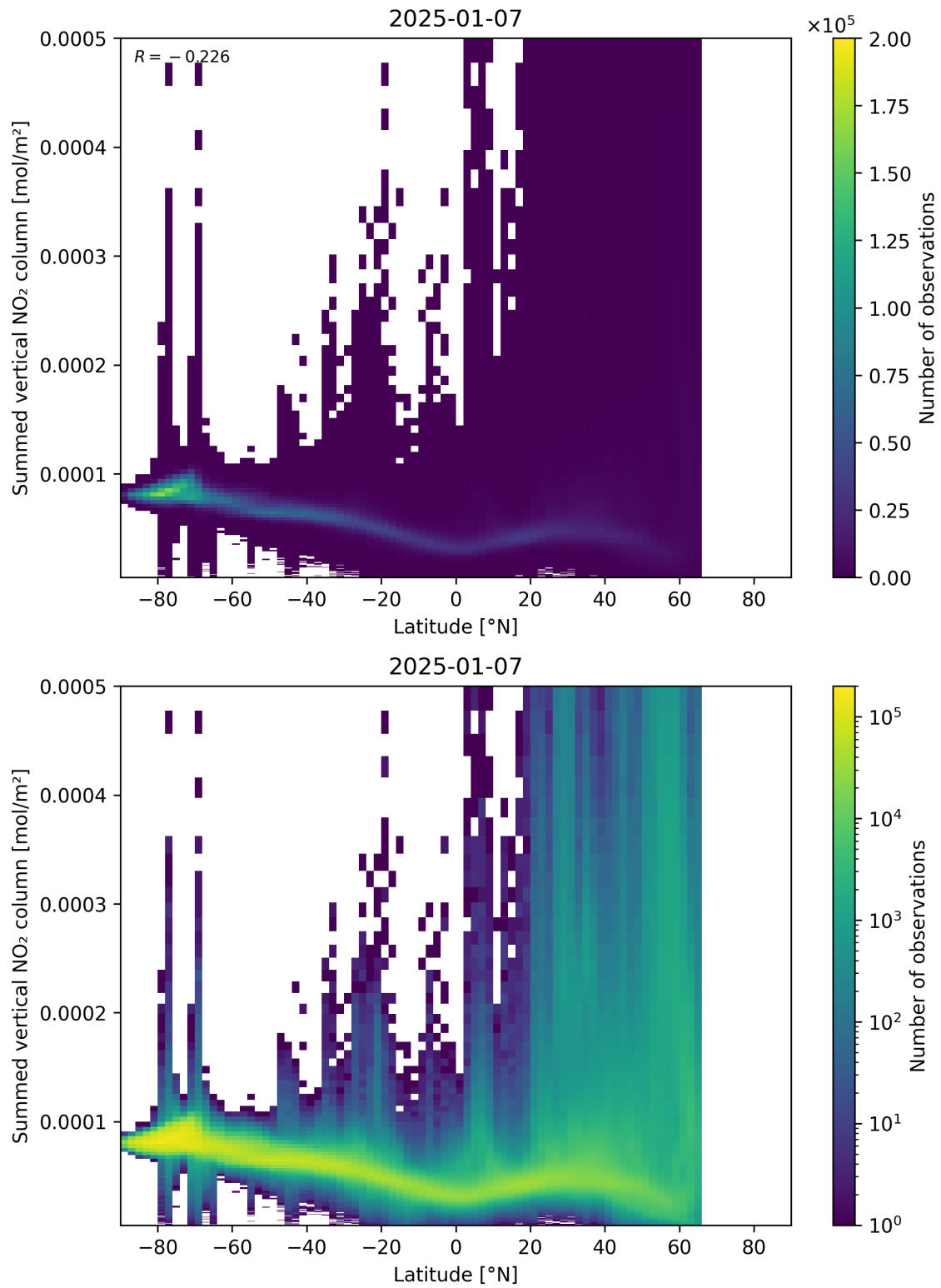
Figure 88: Scatter density plot of “Latitude” against “Summed vertical NO 2 column” for 2025-01-07 to 2025-01-08.
