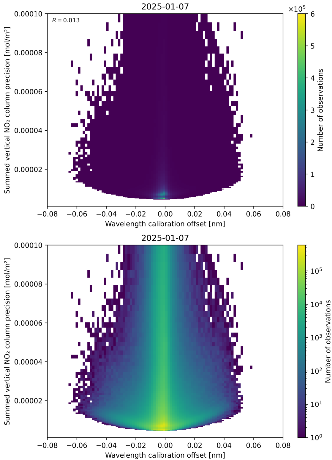
Figure 178: Scatter density plot of “Wavelength calibration offset” against “Summed vertical NO 2 column precision” for 2025-01-07 to 2025-01-08.
