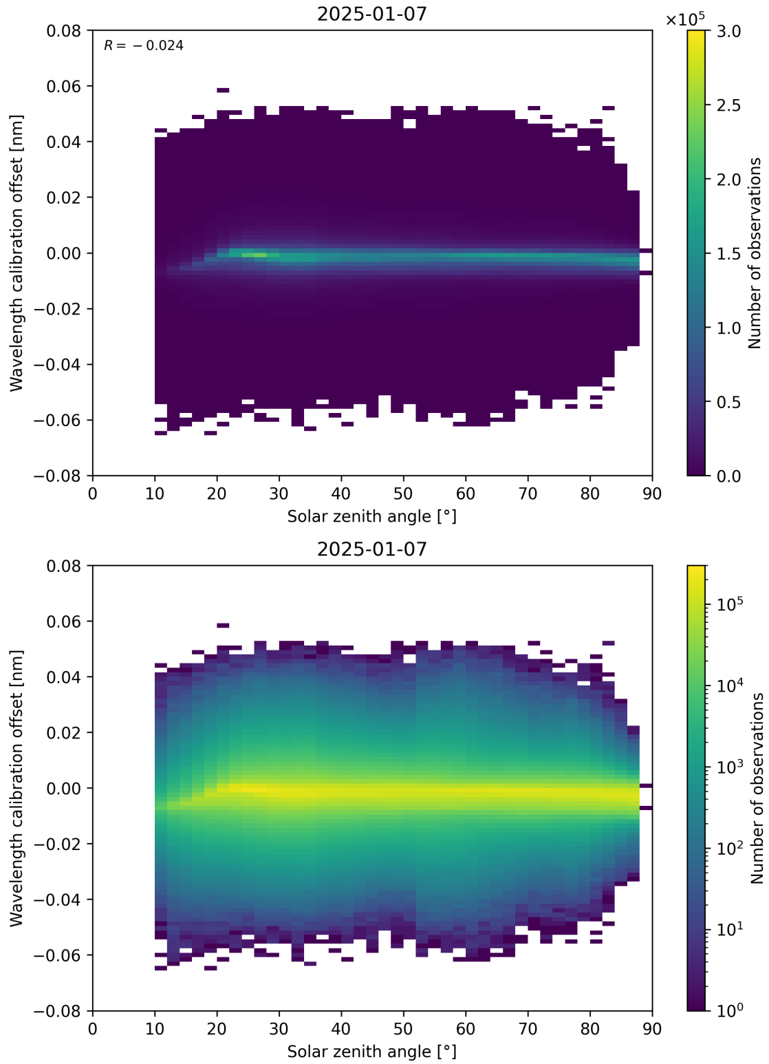
Figure 158: Scatter density plot of “Solar zenith angle” against “Wavelength calibration offset” for 2025-01-07 to 2025-01-08.
