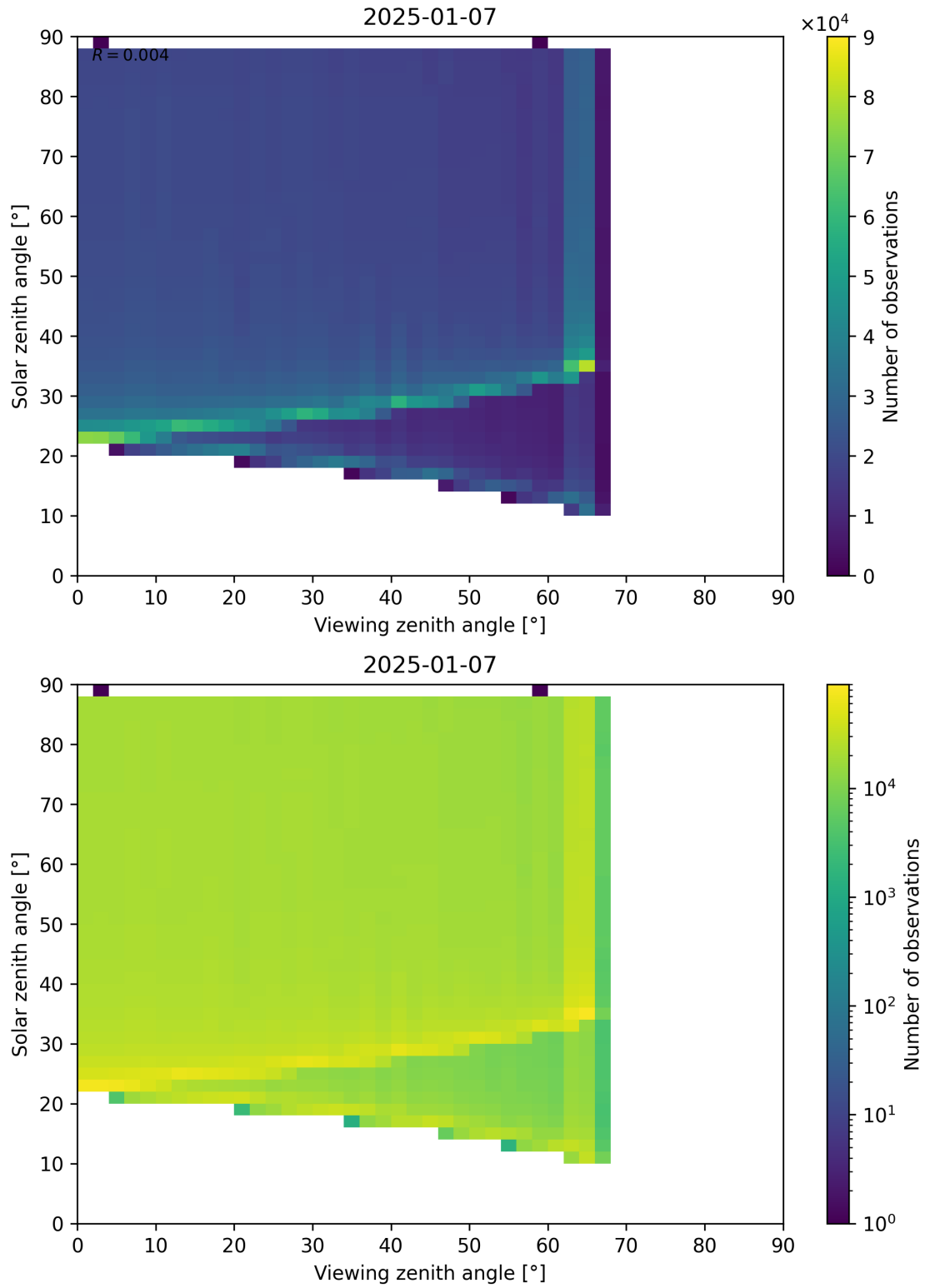
Figure 172: Scatter density plot of “Viewing zenith angle” against “Solar zenith angle” for 2025-01-07 to 2025-01-08.
