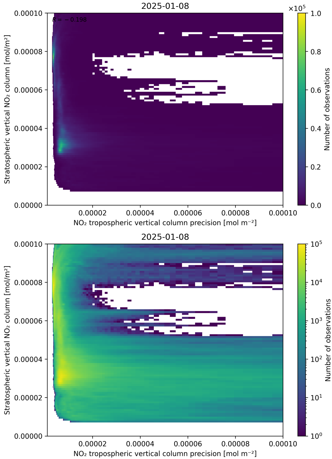
Figure 135: Scatter density plot of “NO 2 tropospheric vertical column precision” against “Stratospheric vertical NO 2 column” for 2025-01-07 to 2025-01-09.
