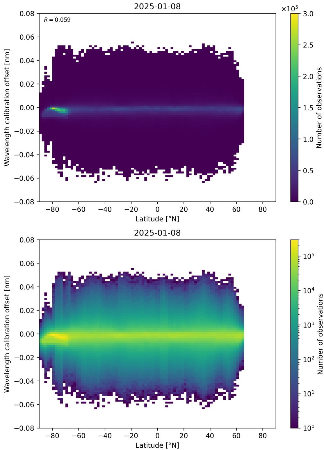
Figure 95: Scatter density plot of “Latitude” against “Wavelength calibration offset” for 2025-01-07 to 2025-01-09.
