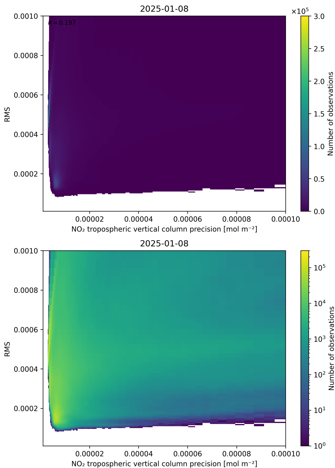
Figure 140: Scatter density plot of “NO 2 tropospheric vertical column precision” against “RMS” for 2025-01-07 to 2025-01-09.
