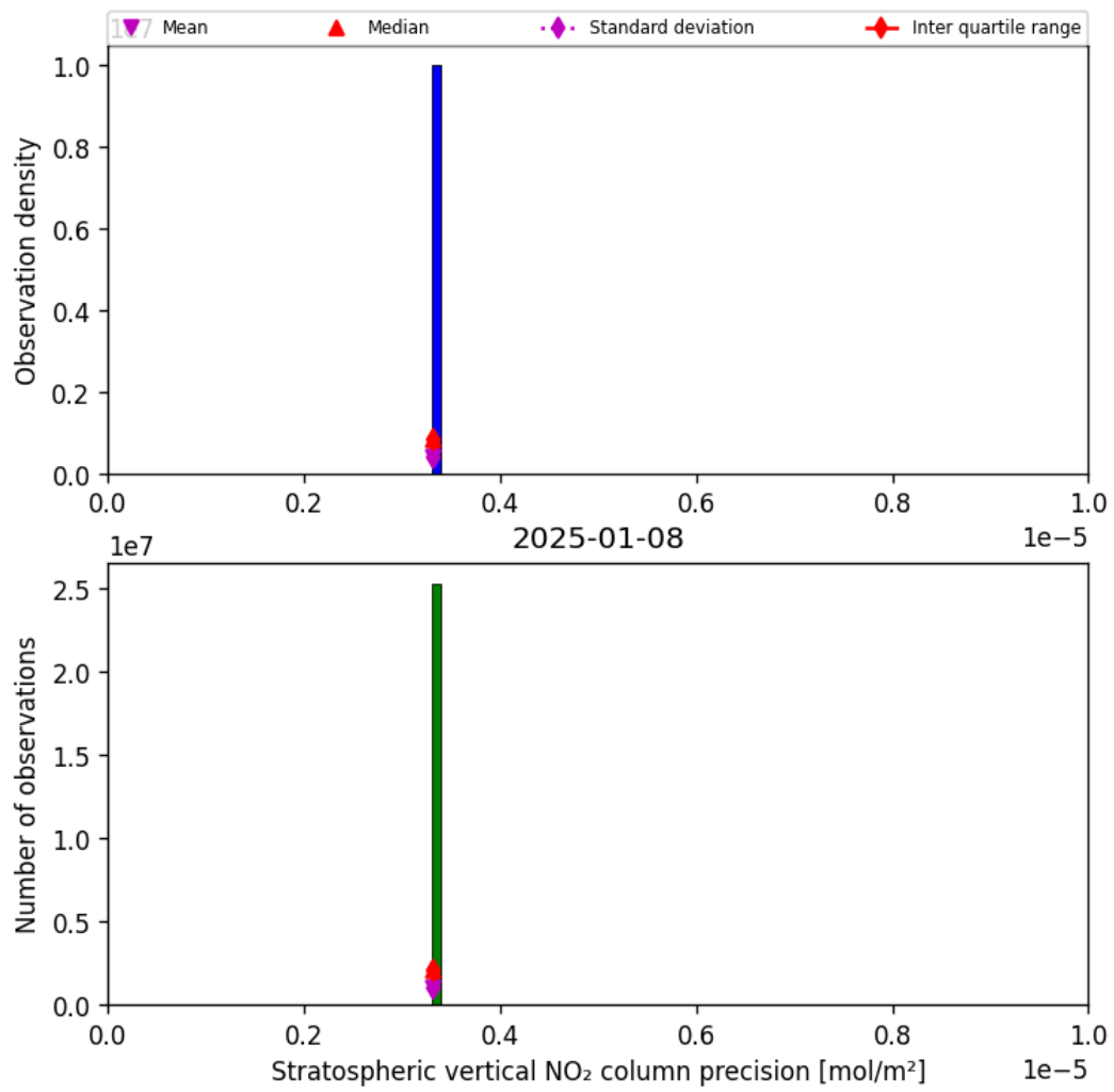
Figure 37: Histogram of “Stratospheric vertical NO 2 column precision” for 2025-01-07 to 2025-01-09
