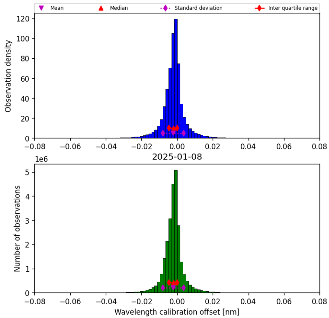
Figure 35: Histogram of “Wavelength calibration offset” for 2025-01-07 to 2025-01-09
