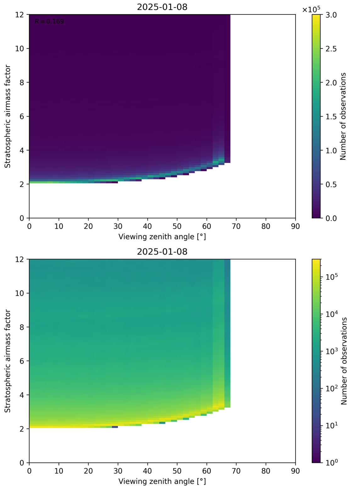
Figure 159: Scatter density plot of “Viewing zenith angle” against “Stratospheric airmass factor” for 2025-01-07 to 2025-01-09.
