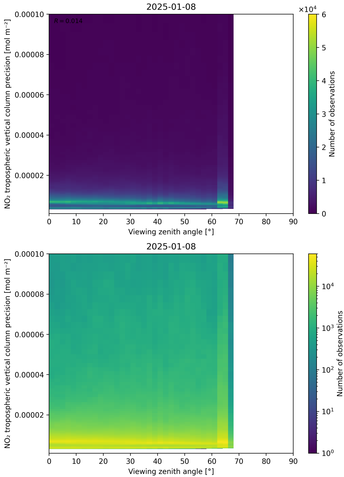
Figure 170: Scatter density plot of “Viewing zenith angle” against “NO 2 tropospheric vertical column precision” for 2025-01-07 to 2025-01-09.
