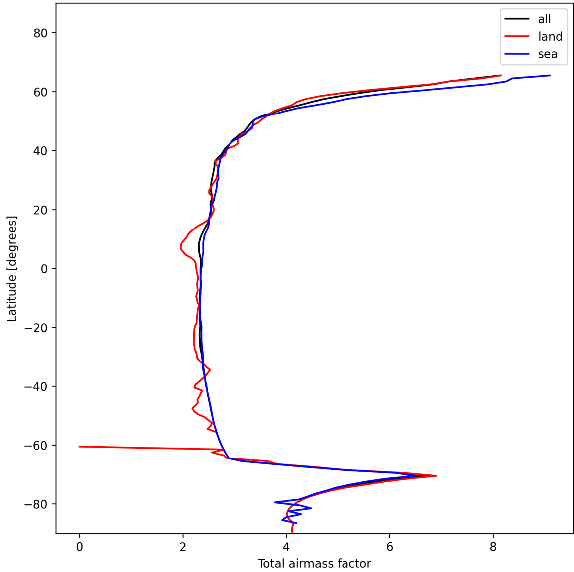
Figure 15: Zonal average of “Total airmass factor” for 2025-01-07 to 2025-01-09.
