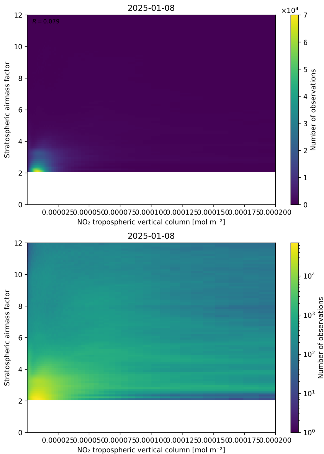
Figure 121: Scatter density plot of “NO 2 tropospheric vertical column” against “Stratospheric airmass factor” for 2025-01-07 to 2025-01-09.
