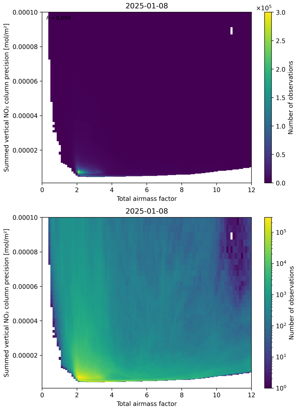
Figure 66: Scatter density plot of “Total airmass factor” against “Summed vertical NO 2 column precision” for 2025-01-07 to 2025-01-09.
