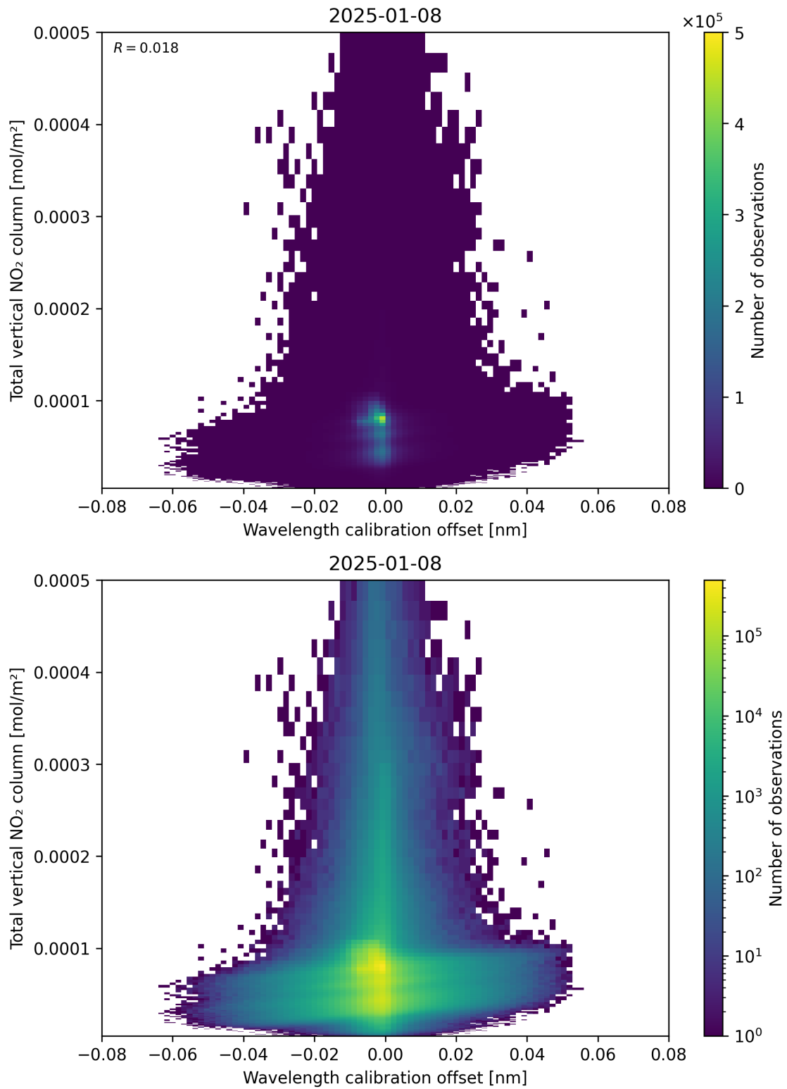
Figure 179: Scatter density plot of “Wavelength calibration offset” against “Total vertical NO 2 column” for 2025-01-07 to 2025-01-09.
