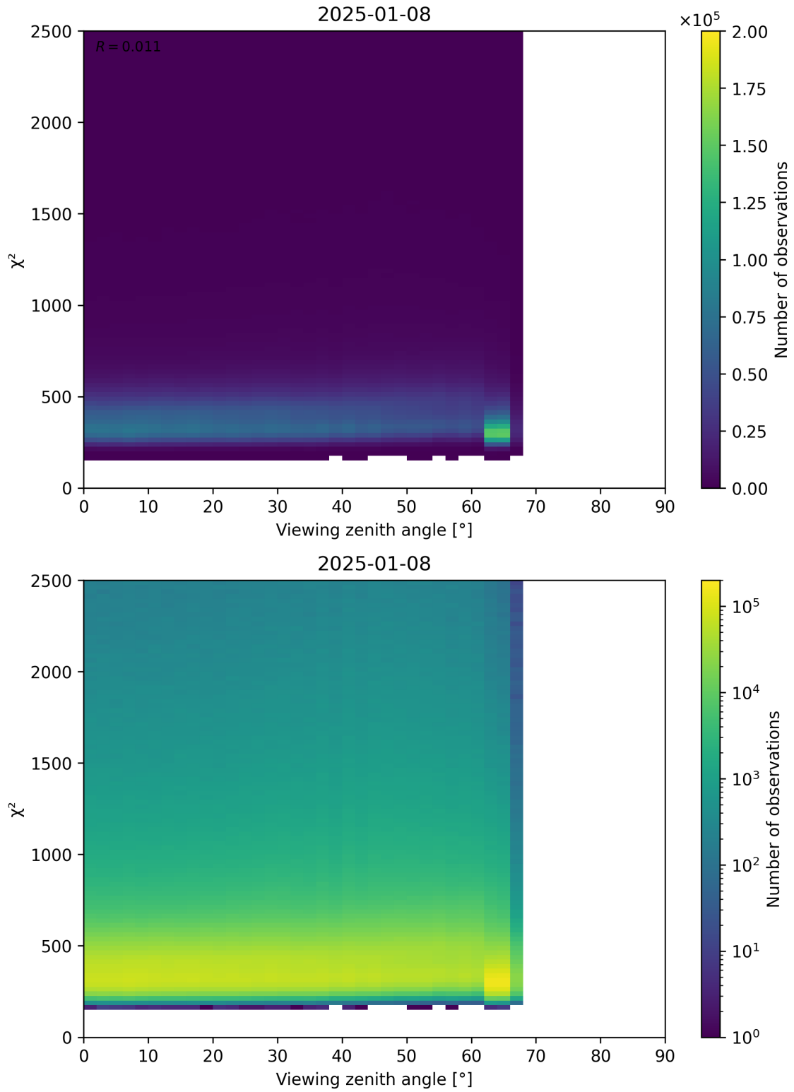
Figure 162: Scatter density plot of “Viewing zenith angle” against “ \chi^2 ” for 2025-01-07 to 2025-01-09.
