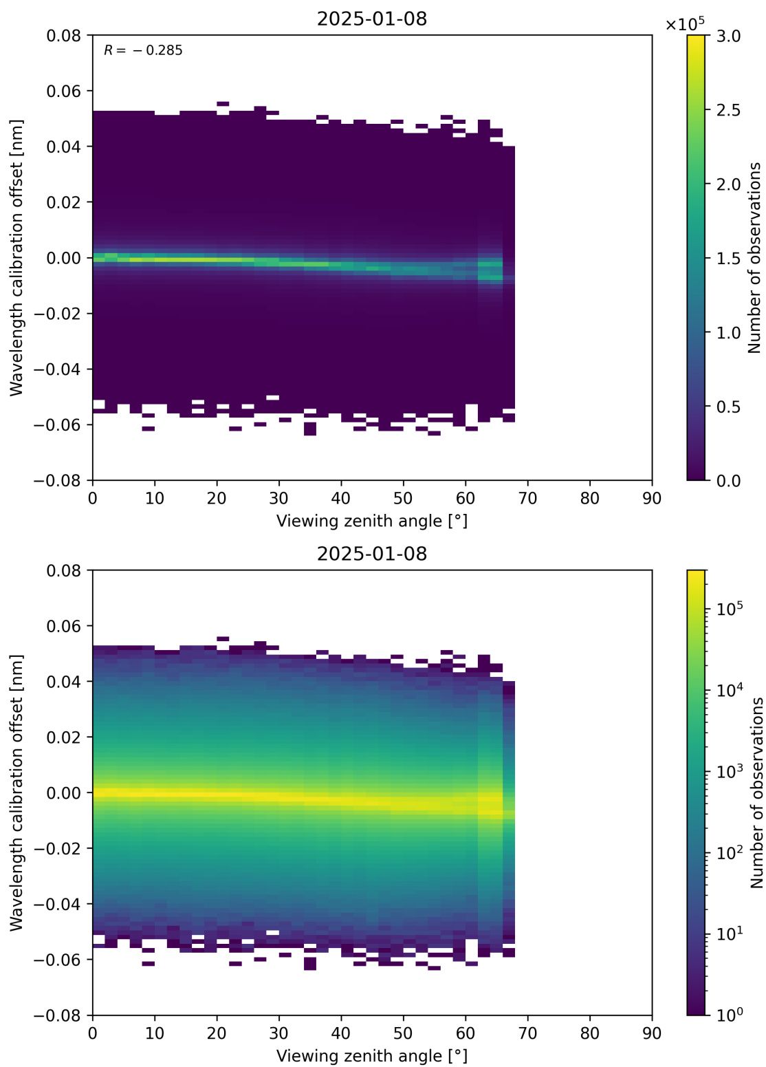
Figure 173: Scatter density plot of “Viewing zenith angle” against “Wavelength calibration offset” for 2025-01-07 to 2025-01-09.
