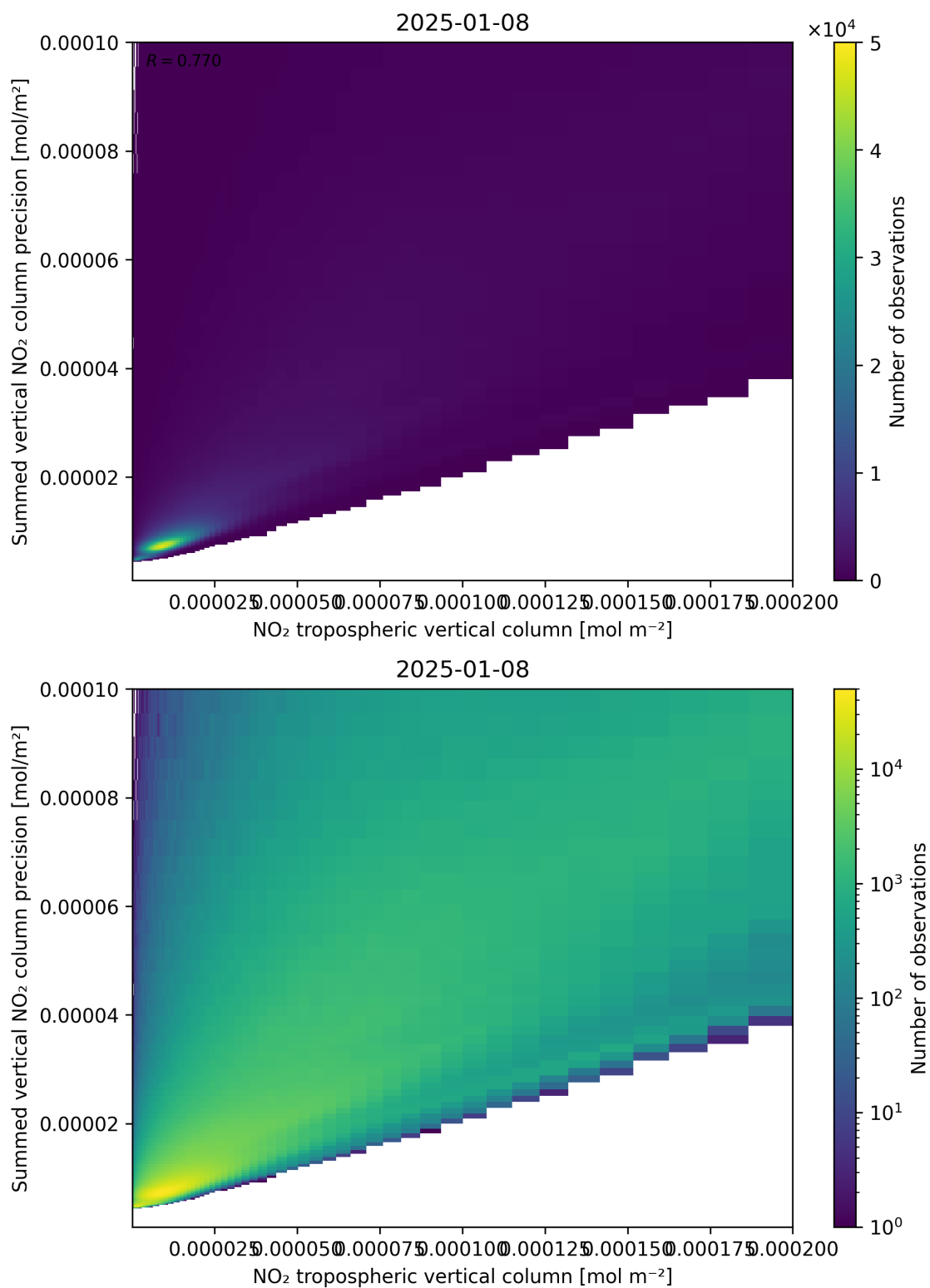
Figure 127: Scatter density plot of “NO 2 tropospheric vertical column” against “Summed vertical NO 2 column precision” for 2025-01-07 to 2025-01-09.
