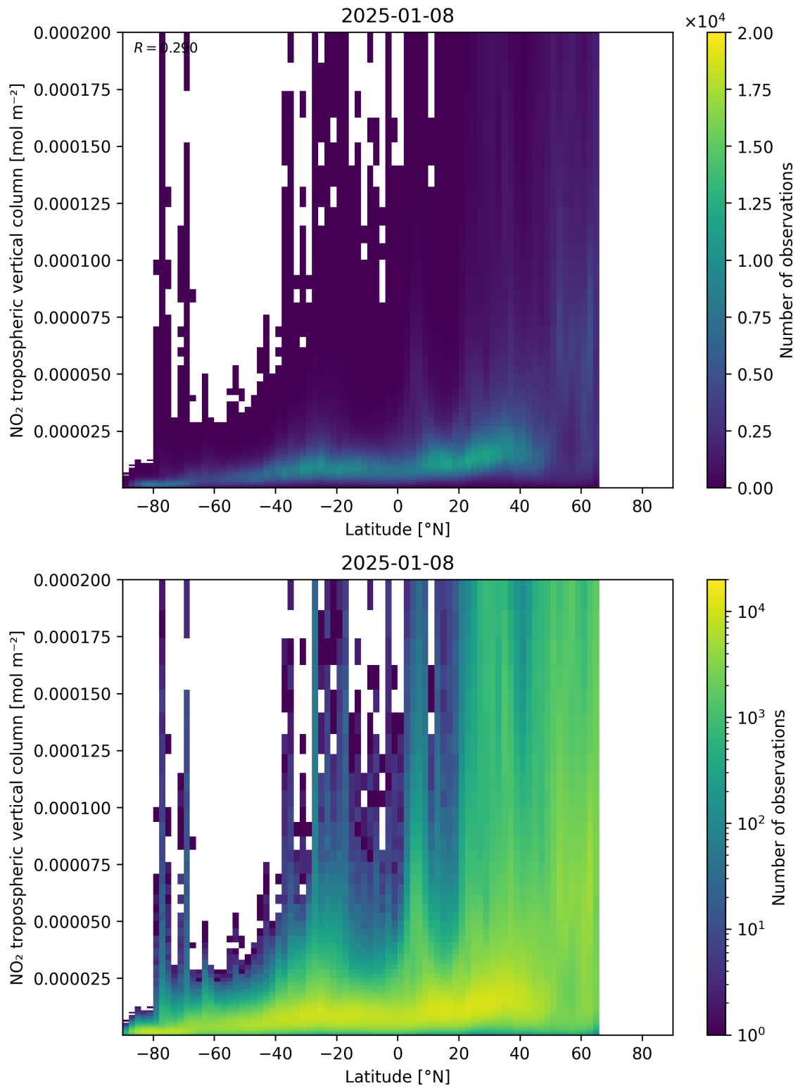
Figure 92: Scatter density plot of “Latitude” against “NO 2 tropospheric vertical column” for 2025-01-07 to 2025-01-09.
