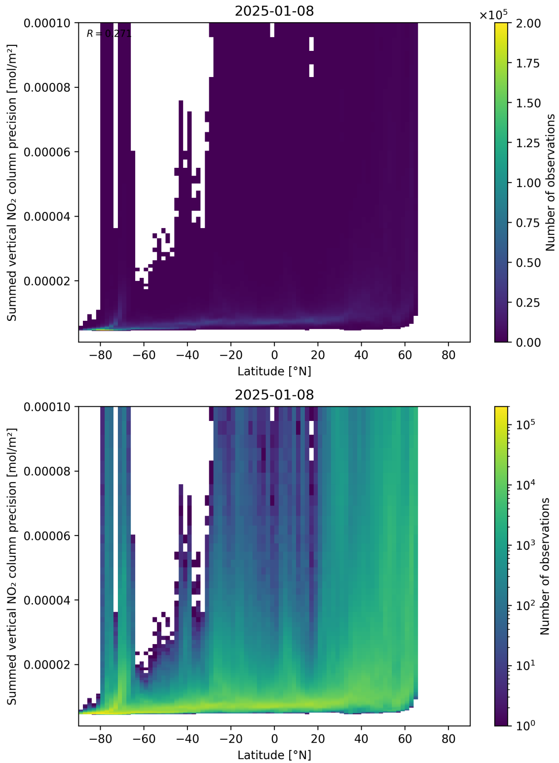
Figure 89: Scatter density plot of “Latitude” against “Summed vertical NO 2 column precision” for 2025-01-07 to 2025-01-09.
