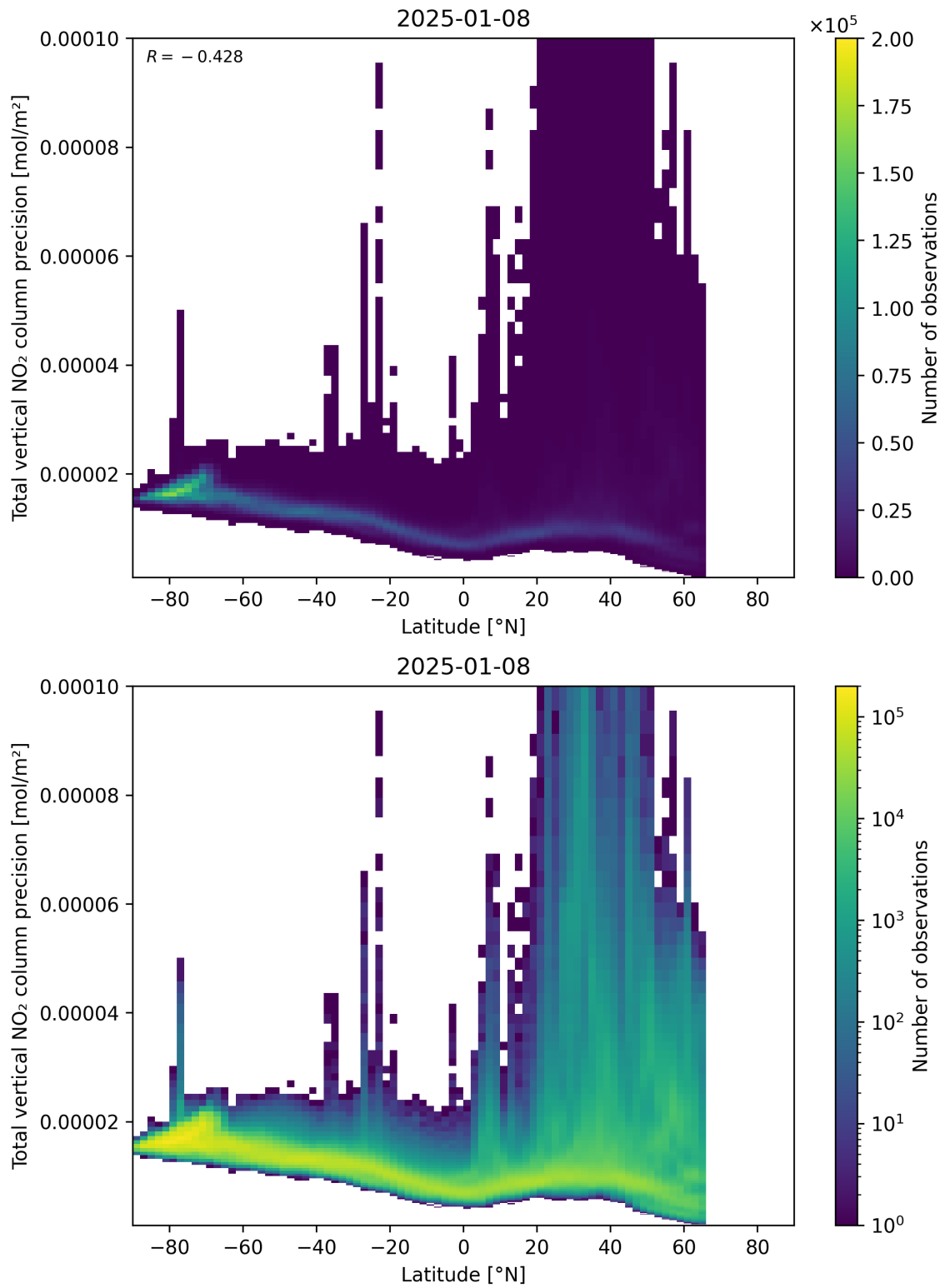
Figure 91: Scatter density plot of “Latitude” against “Total vertical NO 2 column precision” for 2025-01-07 to 2025-01-09.
