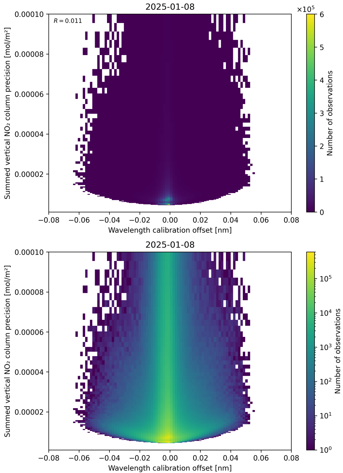
Figure 178: Scatter density plot of “Wavelength calibration offset” against “Summed vertical NO 2 column precision” for 2025-01-07 to 2025-01-09.
