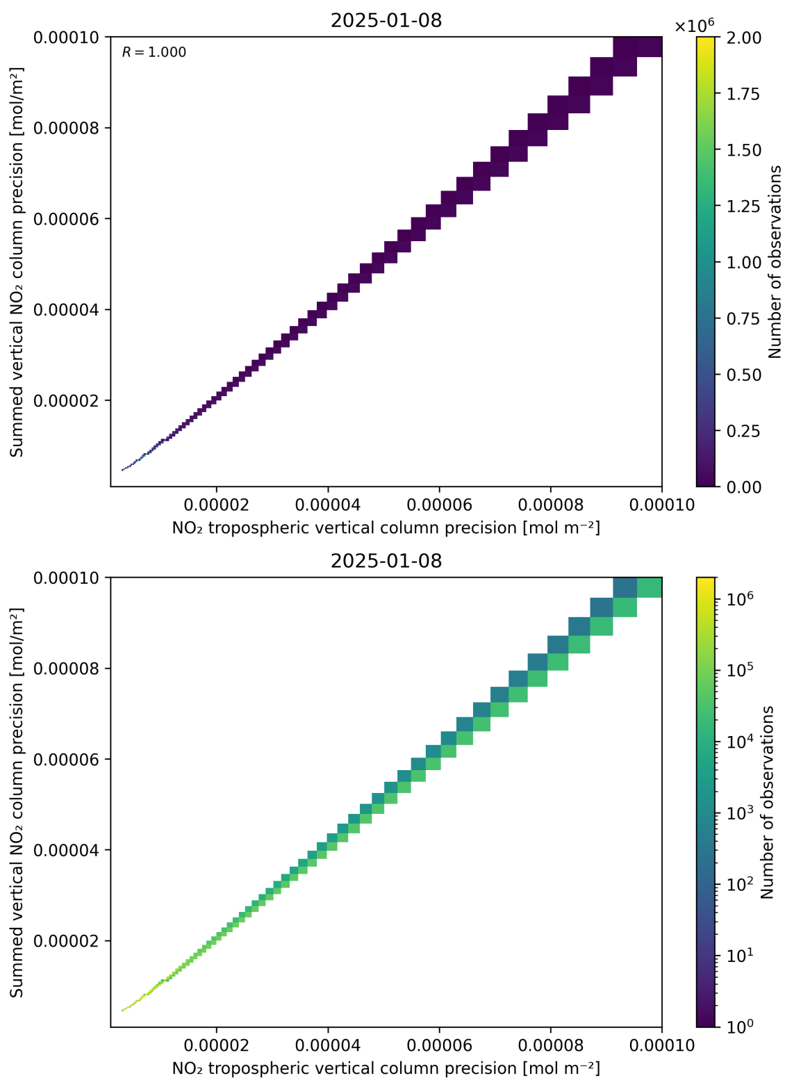
Figure 137: Scatter density plot of “NO 2 tropospheric vertical column precision” against “Summed vertical NO 2 column precision” for 2025-01-07 to 2025-01-09.
