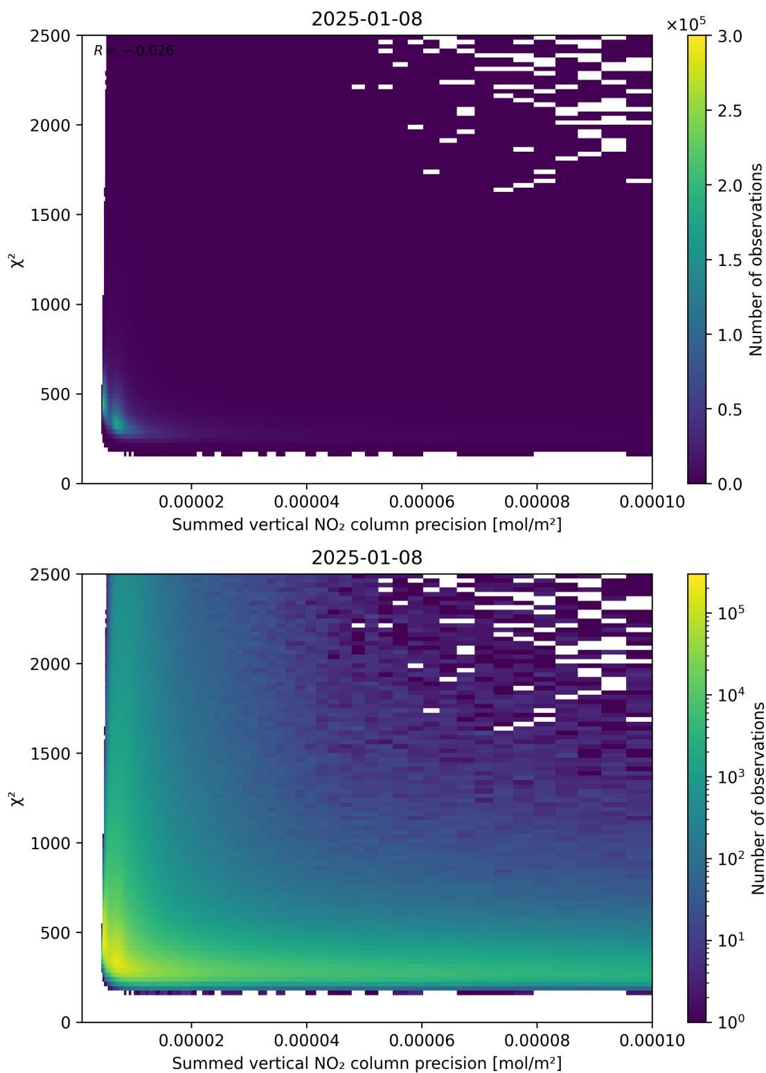
Figure 107: Scatter density plot of “Summed vertical NO 2 column precision” against “ \chi^2 ” for 2025-01-07 to 2025-01-09.
