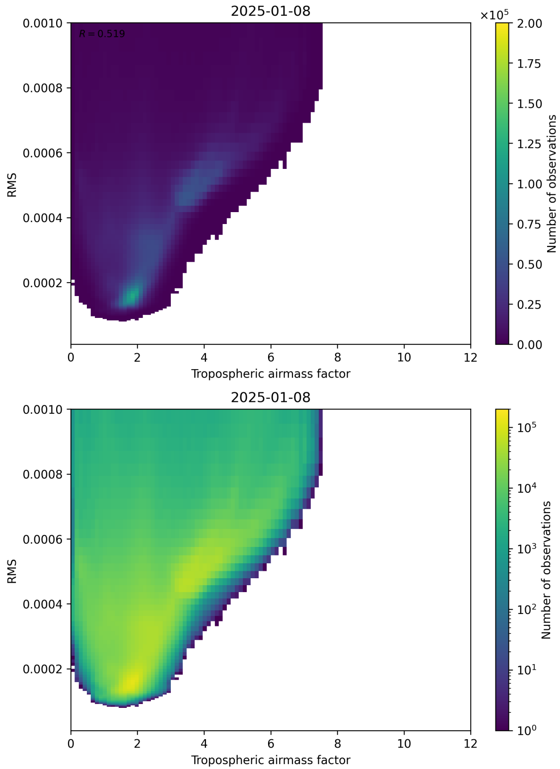
Figure 79: Scatter density plot of “Tropospheric airmass factor” against “RMS” for 2025-01-07 to 2025-01-09.
