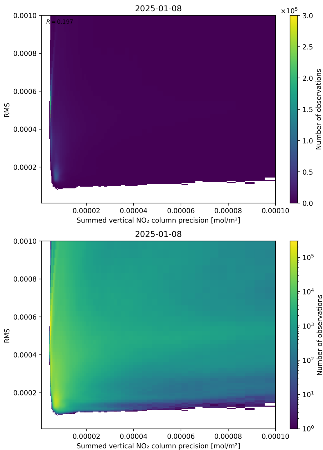
Figure 108: Scatter density plot of “Summed vertical NO 2 column precision” against “RMS” for 2025-01-07 to 2025-01-09.
