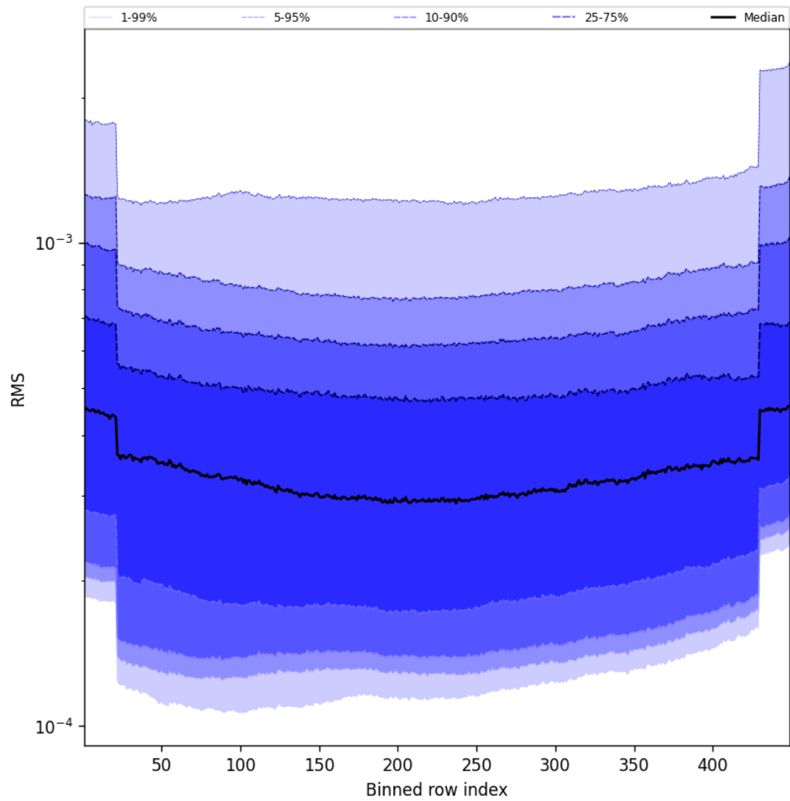
Figure 60: Along track statistics of “RMS” for 2025-01-07 to 2025-01-09
