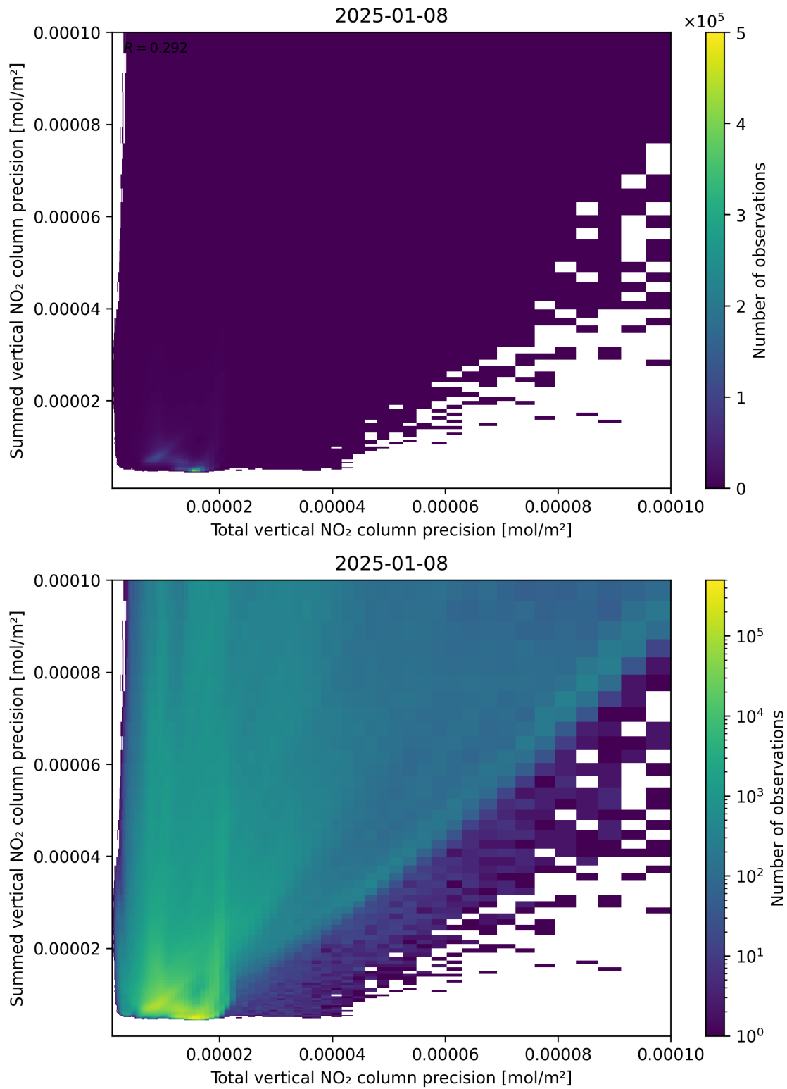
Figure 118: Scatter density plot of “Total vertical NO 2 column precision” against “Summed vertical NO 2 column precision” for 2025-01-07 to 2025-01-09.
