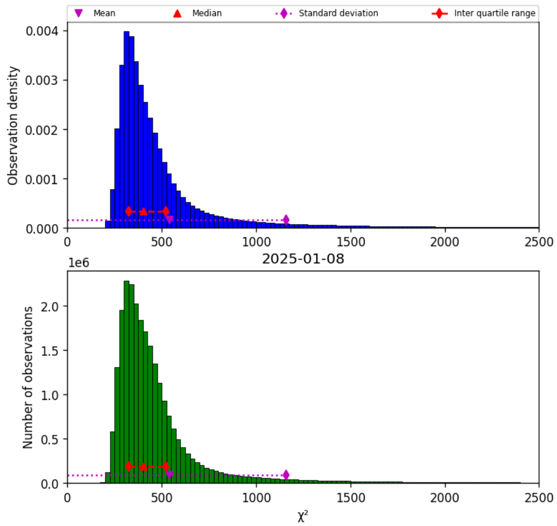
Figure 42: Histogram of “ \chi^2 ” for 2025-01-07 to 2025-01-09
