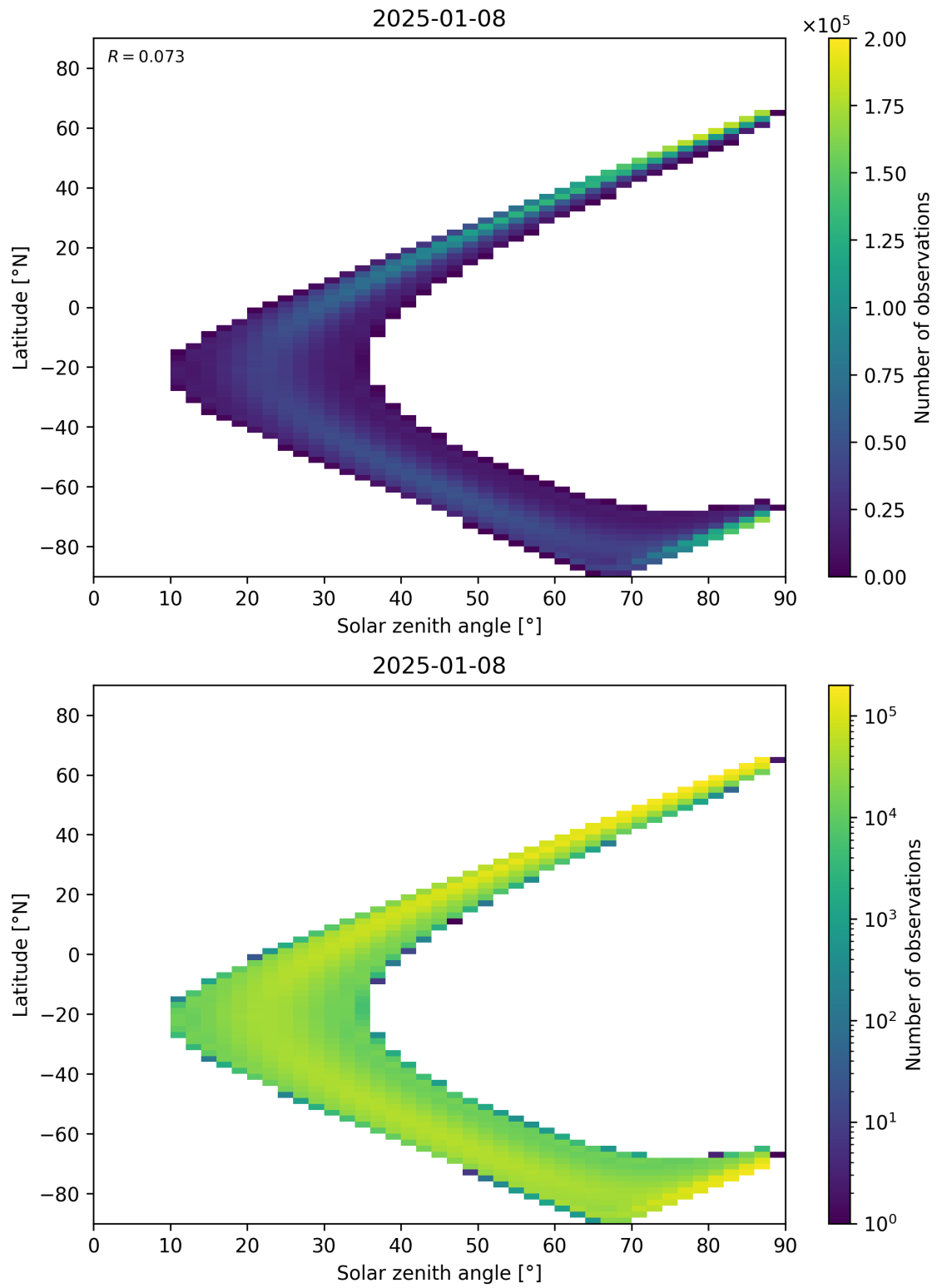
Figure 149: Scatter density plot of “Solar zenith angle” against “Latitude” for 2025-01-07 to 2025-01-09.
