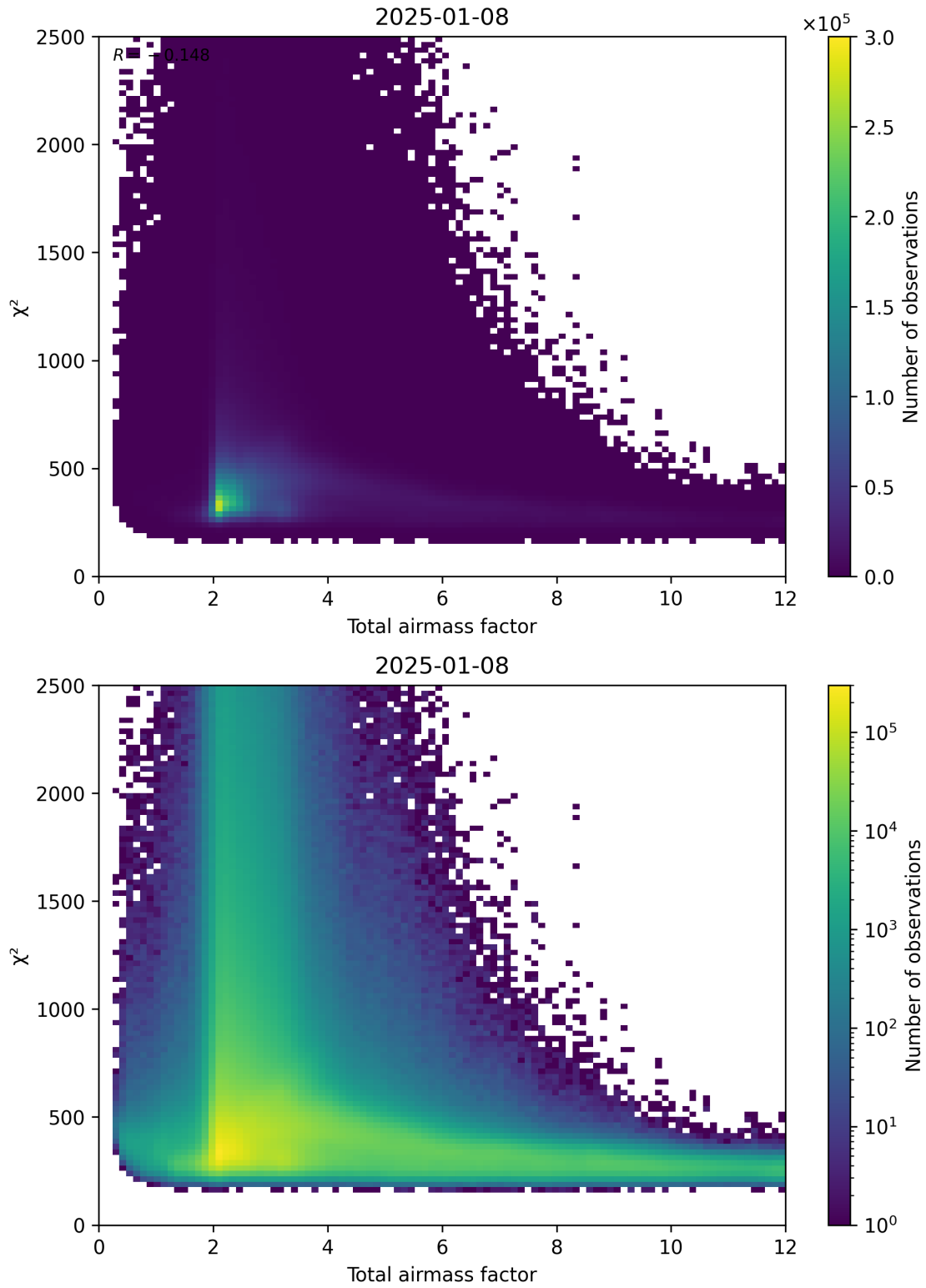
Figure 63: Scatter density plot of “Total airmass factor” against “ \chi^2 ” for 2025-01-07 to 2025-01-09.
