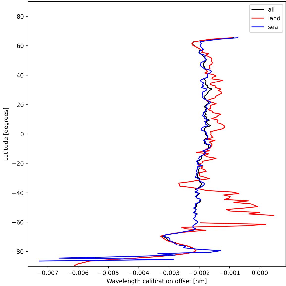
Figure 18: Zonal average of “Wavelength calibration offset” for 2025-01-07 to 2025-01-09.
