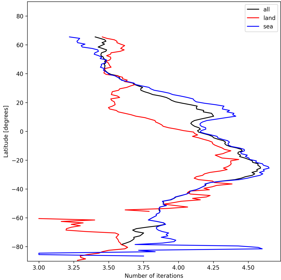
Figure 17: Zonal average of “Number of iterations” for 2025-01-07 to 2025-01-09.
