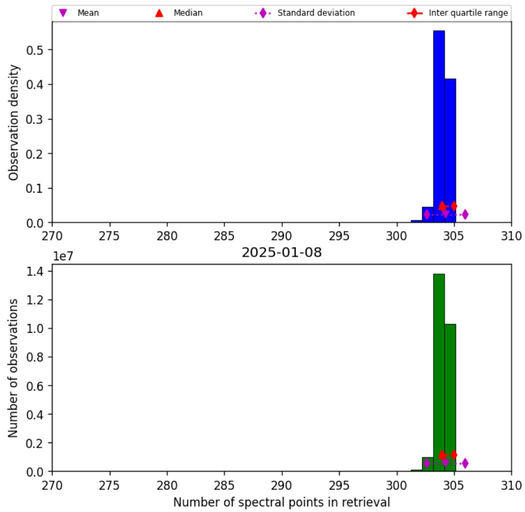
Figure 33: Histogram of “Number of spectral points in retrieval” for 2025-01-07 to 2025-01-09
