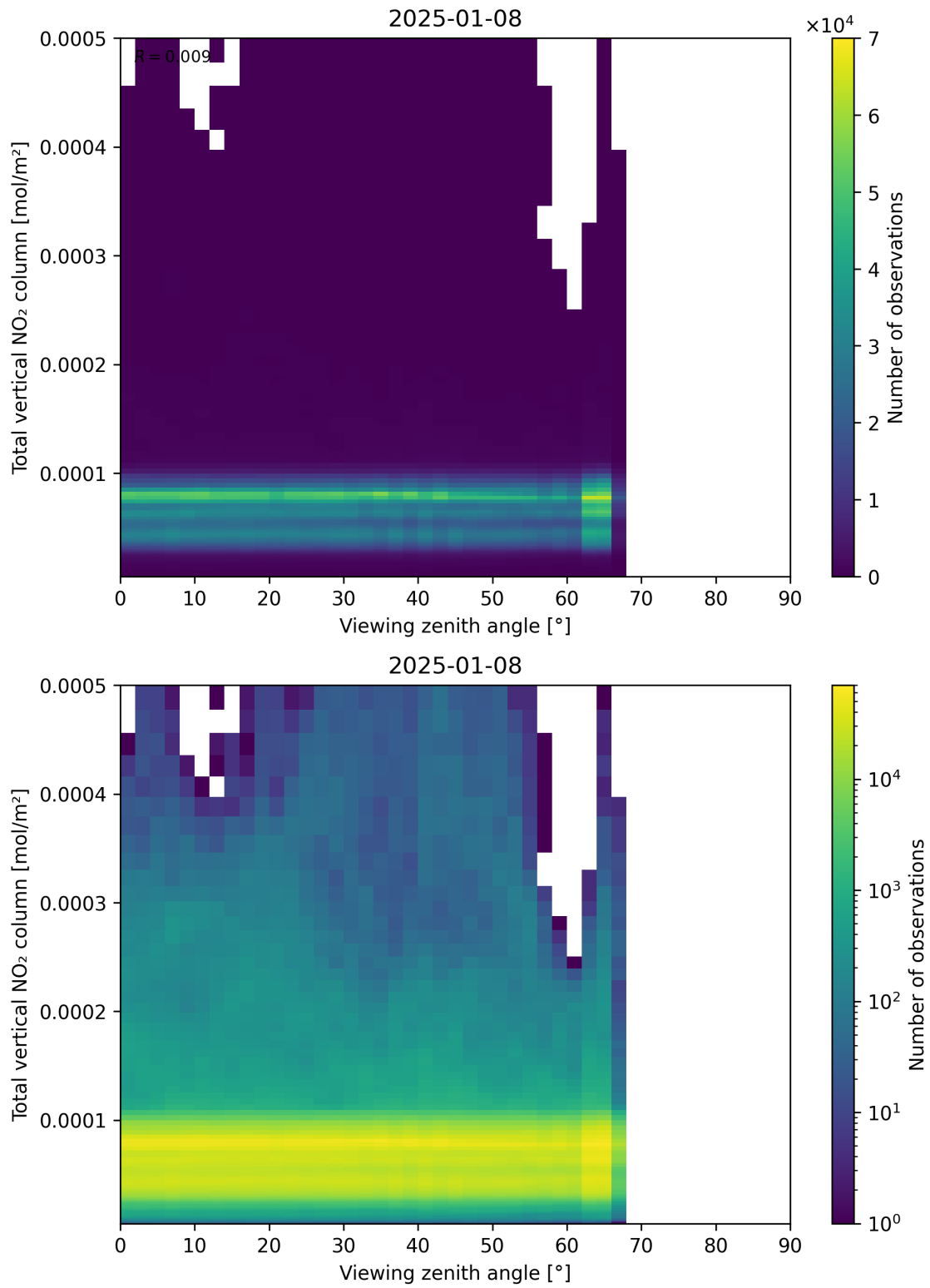
Figure 167: Scatter density plot of “Viewing zenith angle” against “Total vertical NO 2 column” for 2025-01-07 to 2025-01-09.
