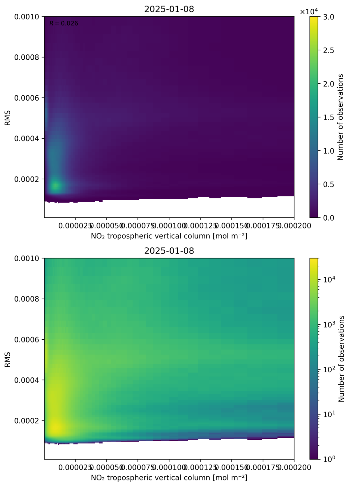
Figure 142: Scatter density plot of “NO 2 tropospheric vertical column” against “RMS” for 2025-01-07 to 2025-01-09.
