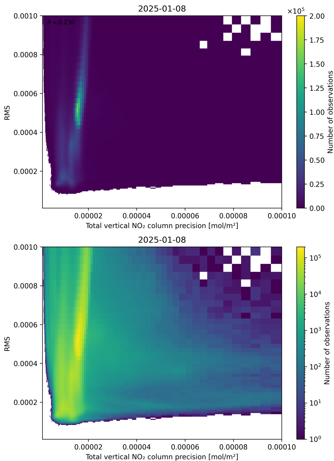
Figure 119: Scatter density plot of “Total vertical NO 2 column precision” against “RMS” for 2025-01-07 to 2025-01-09.
