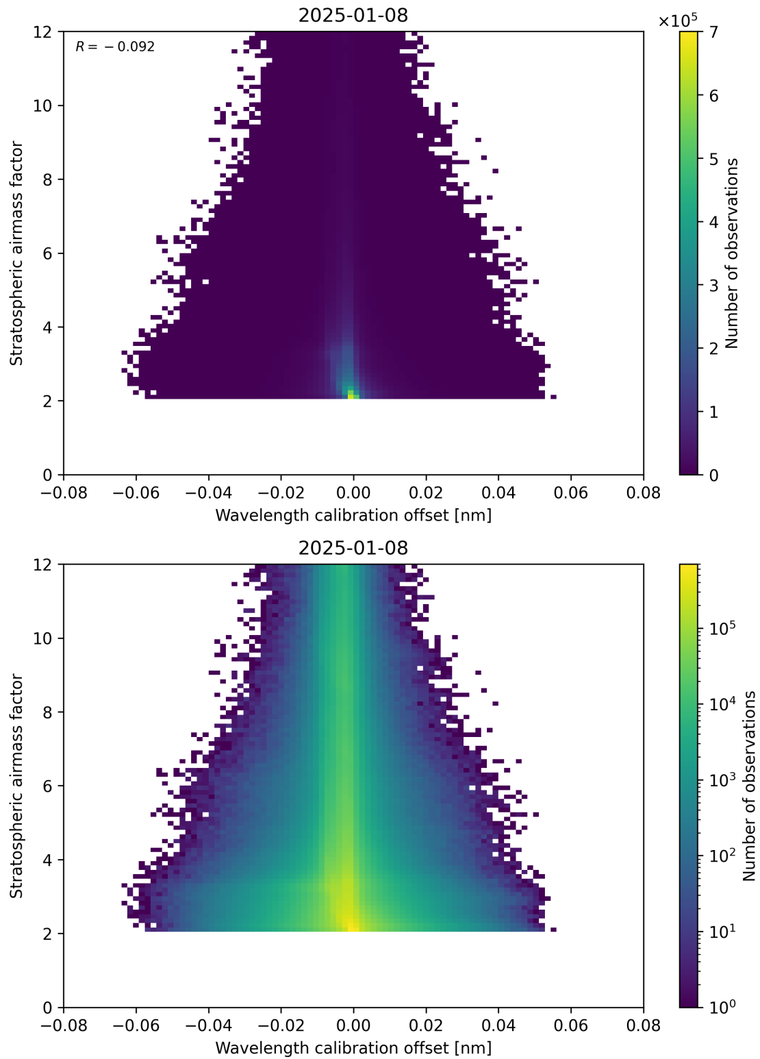
Figure 174: Scatter density plot of “Wavelength calibration offset” against “Stratospheric airmass factor” for 2025-01-07 to 2025-01-09.
