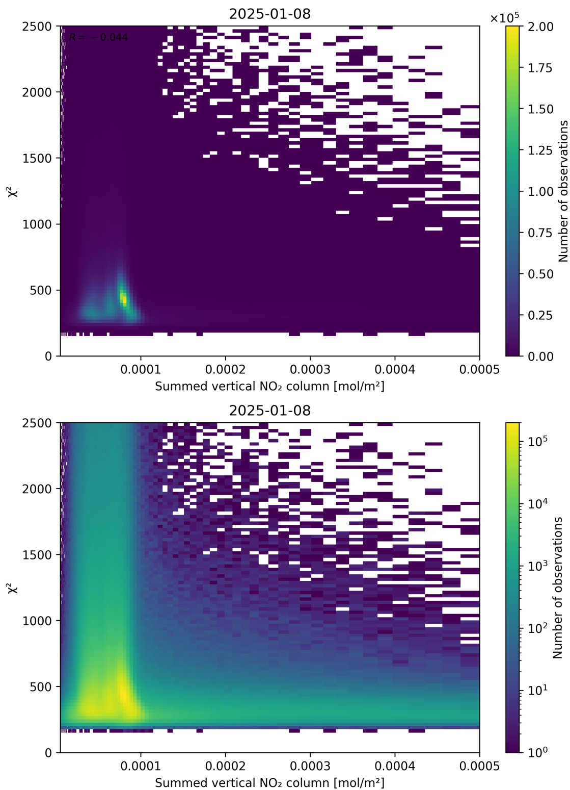
Figure 104: Scatter density plot of “Summed vertical NO 2 column” against “ \chi^2 ” for 2025-01-07 to 2025-01-09.
