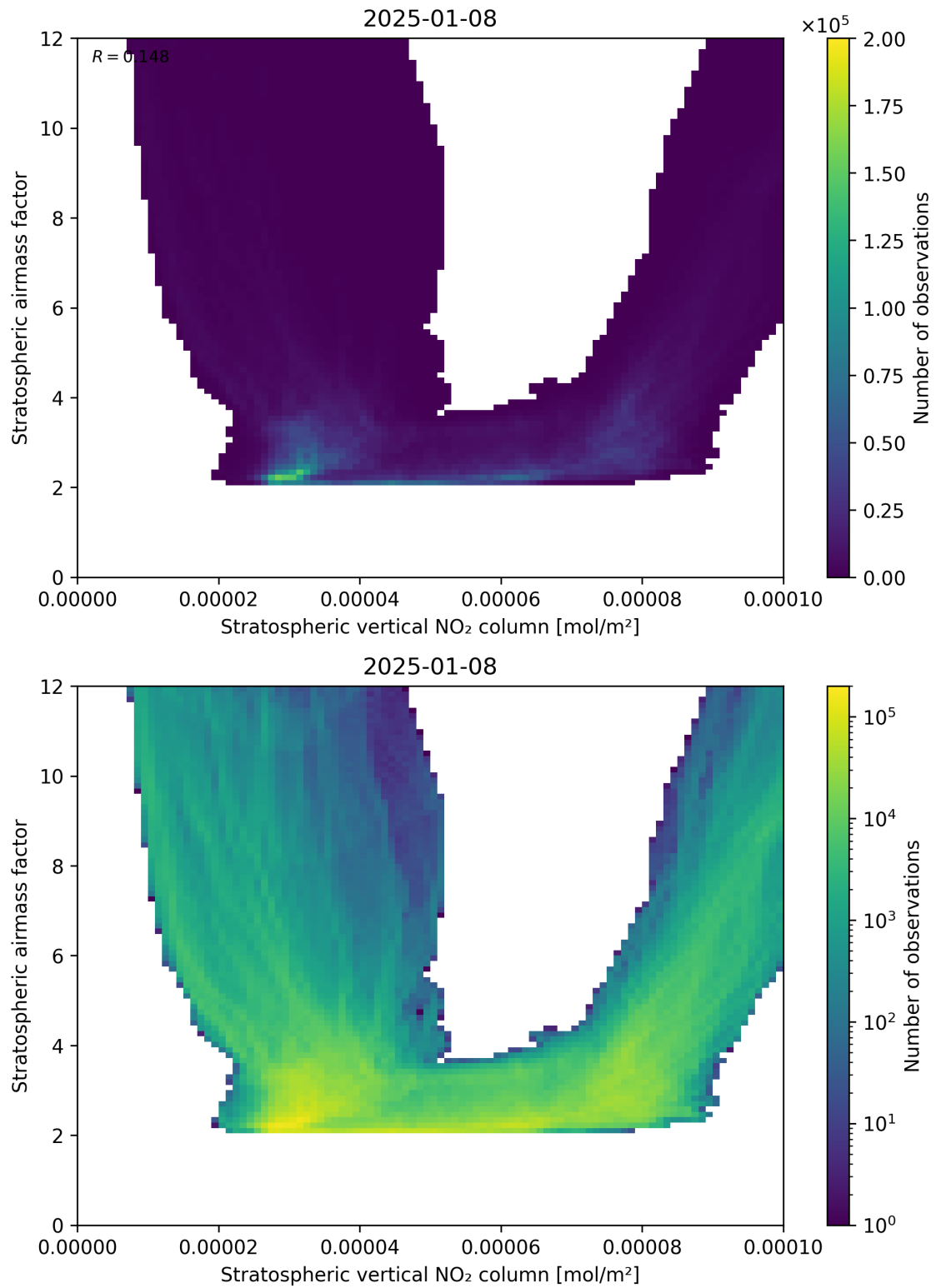
Figure 96: Scatter density plot of “Stratospheric vertical NO 2 column” against “Stratospheric airmass factor” for 2025-01-07 to 2025-01-09.
