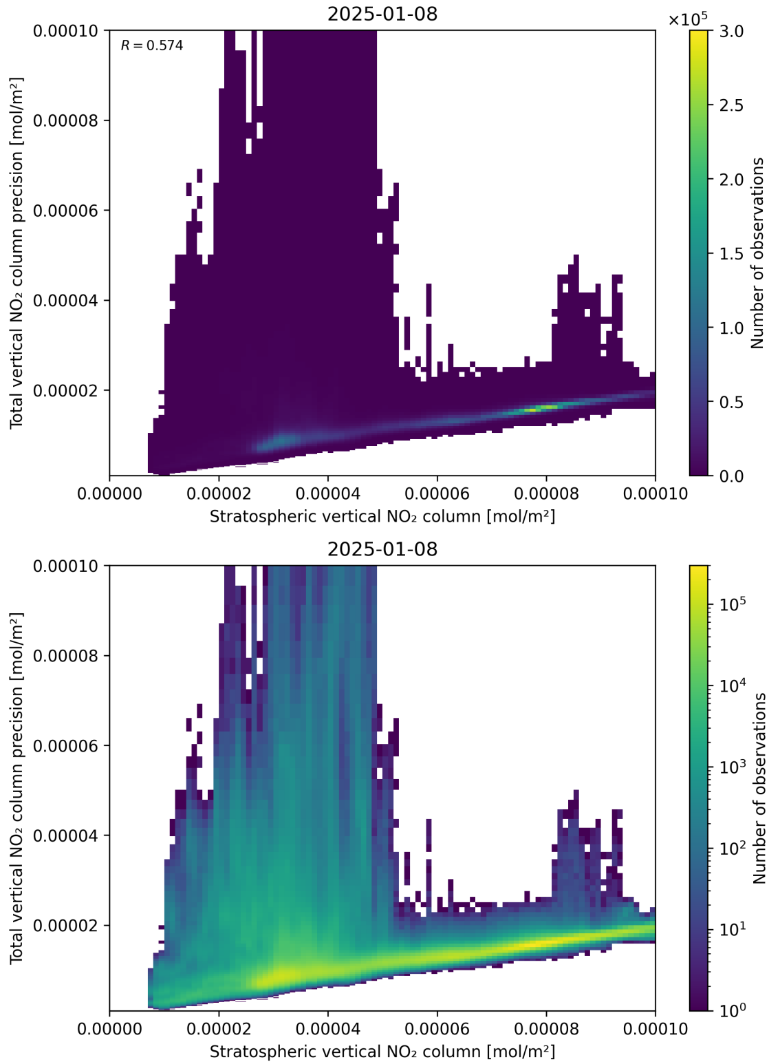
Figure 101: Scatter density plot of “Stratospheric vertical NO 2 column” against “Total vertical NO 2 column precision” for 2025-01-07 to 2025-01-09.
