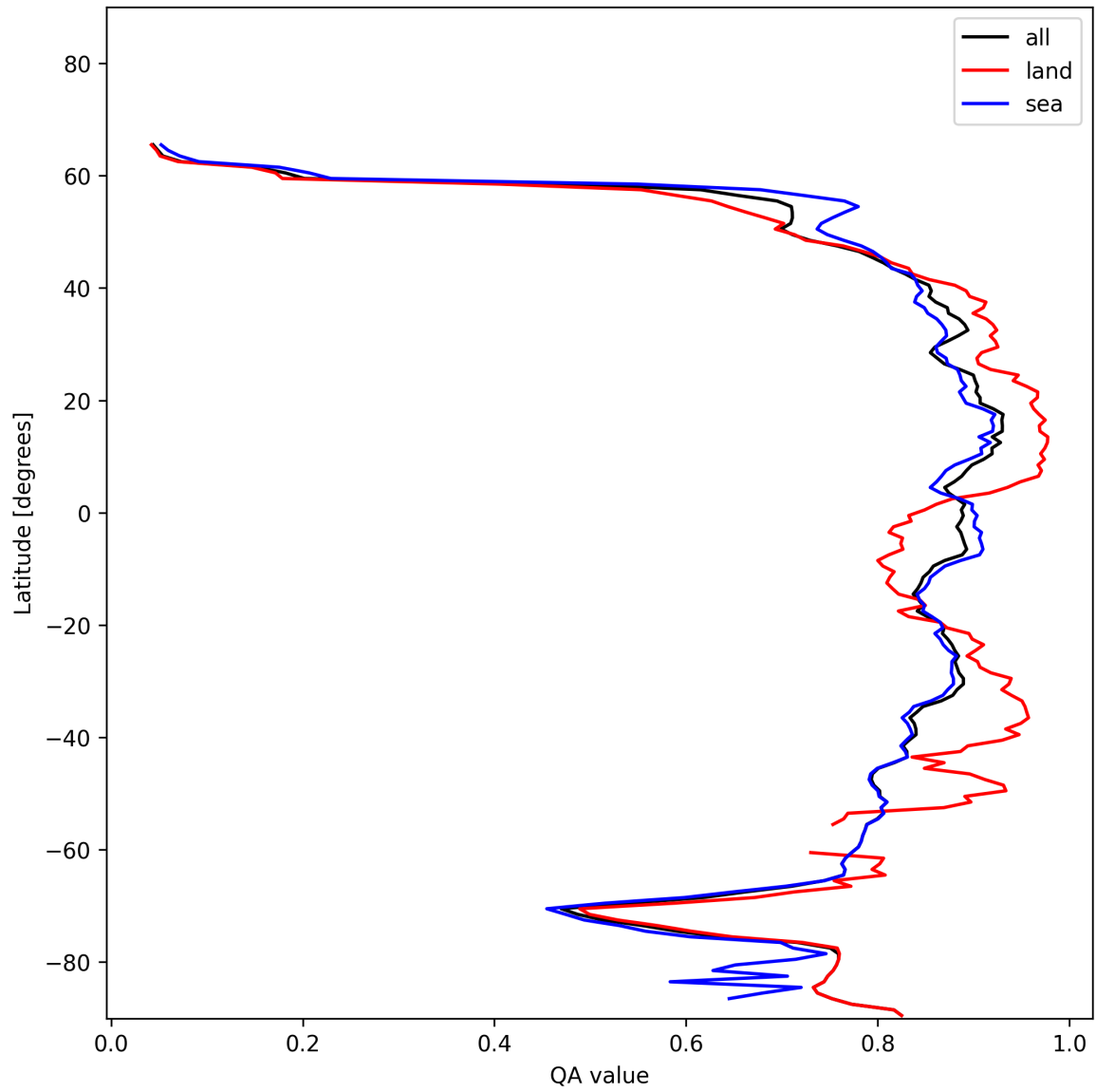
Figure 11: Zonal average of “QA value” for 2025-01-07 to 2025-01-09.
