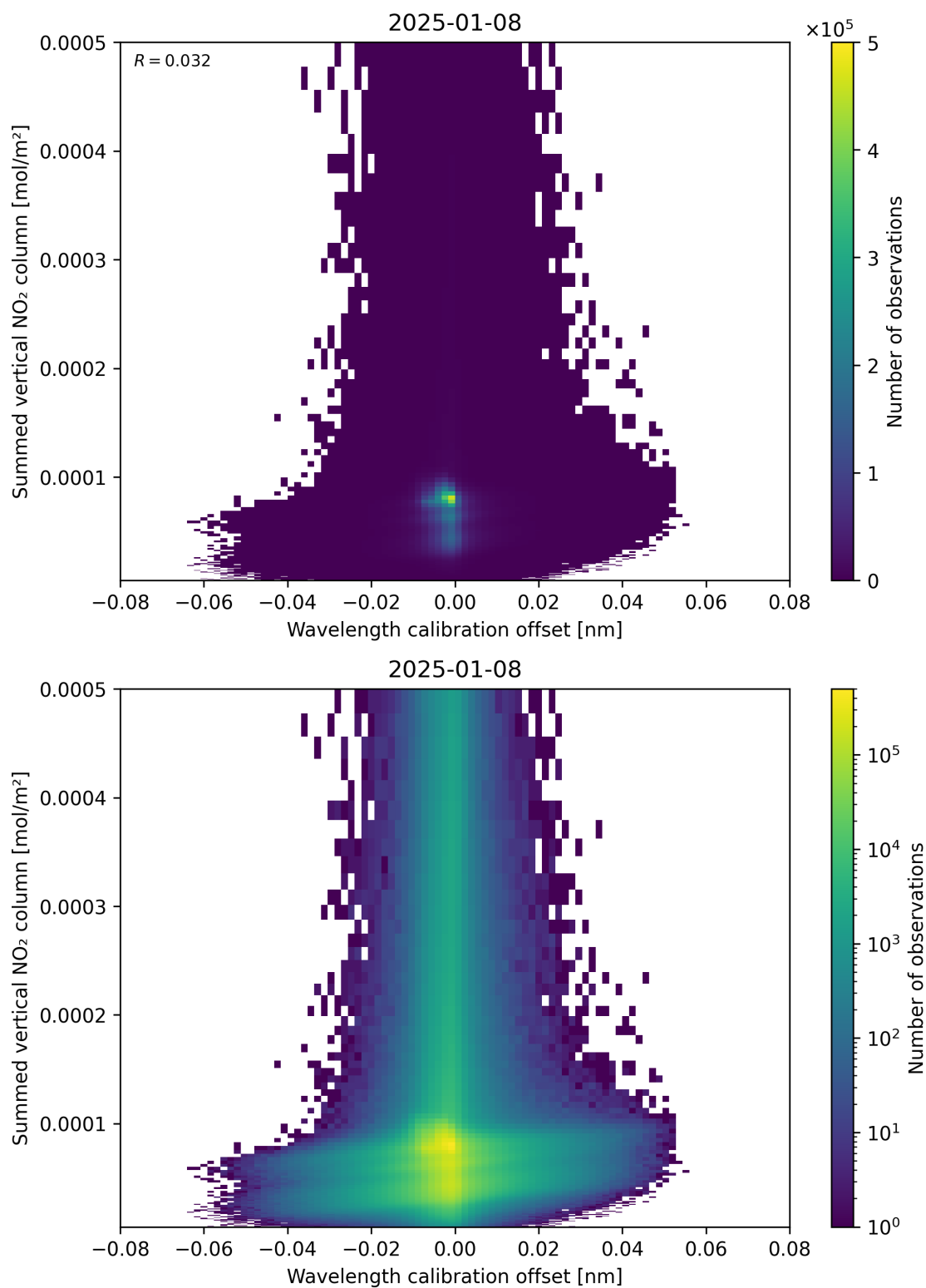
Figure 177: Scatter density plot of “Wavelength calibration offset” against “Summed vertical NO 2 column” for 2025-01-07 to 2025-01-09.
