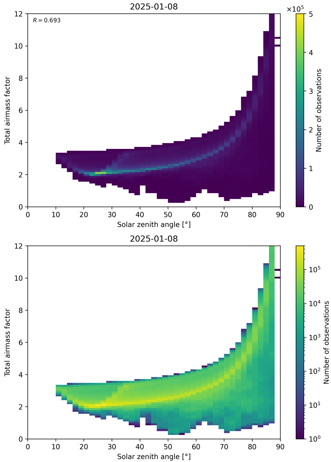
Figure 146: Scatter density plot of “Solar zenith angle” against “Total air mass factor” for 2025-01-07 to 2025-01-09.
