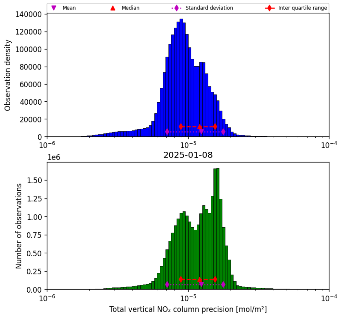
Figure 39: Histogram of “Total vertical NO 2 column precision” for 2025-01-07 to 2025-01-09
