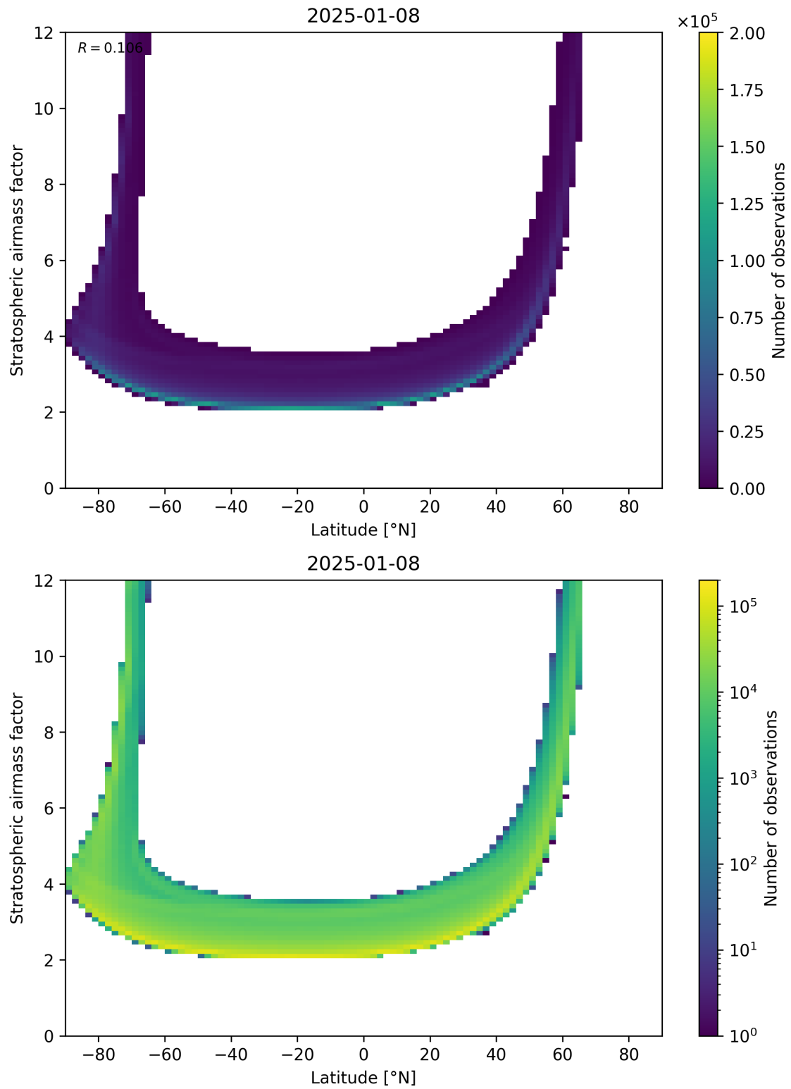
Figure 83: Scatter density plot of “Latitude” against “Stratospheric airmass factor” for 2025-01-07 to 2025-01-09.
