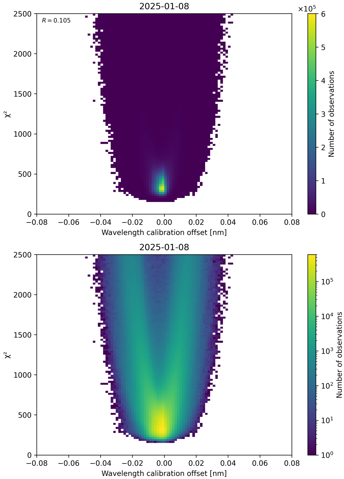
Figure 175: Scatter density plot of “Wavelength calibration offset” against “ \chi^2 ” for 2025-01-07 to 2025-01-09.
