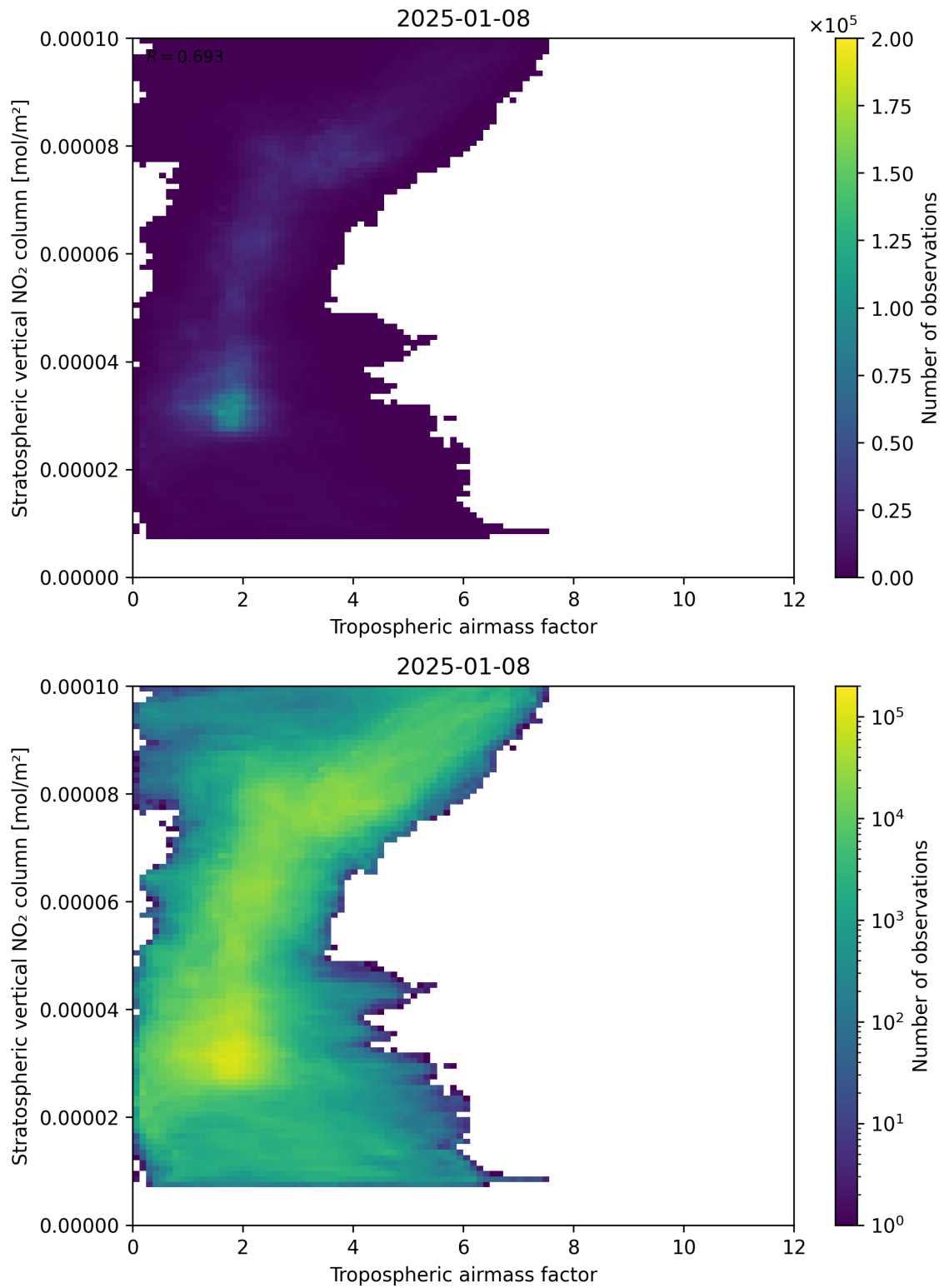
Figure 74: Scatter density plot of “Tropospheric air mass factor” against “Stratospheric vertical NO 2 column” for 2025-01-07 to 2025-01-09.
