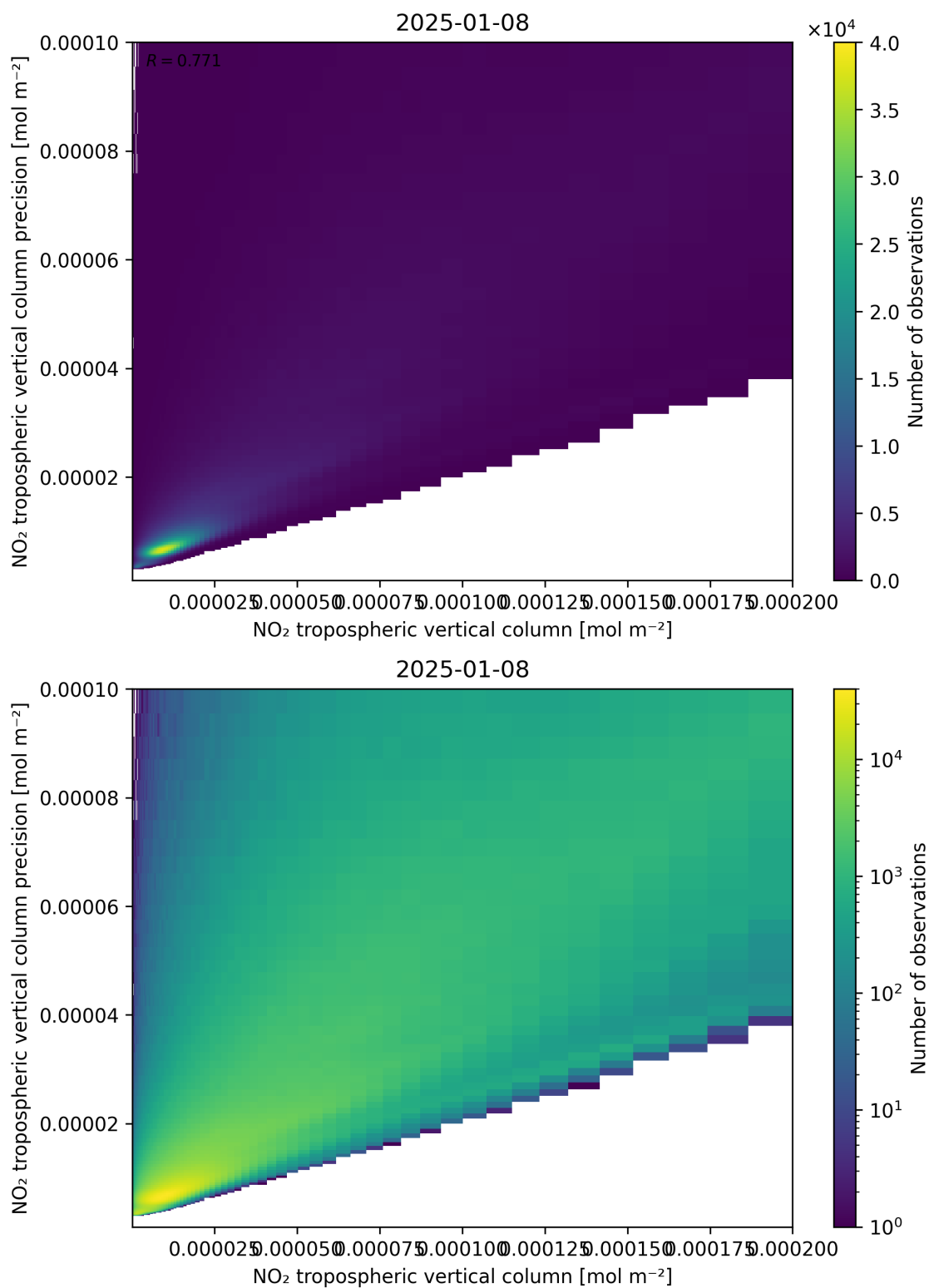
Figure 130: Scatter density plot of “NO 2 tropospheric vertical column” against “NO 2 tropospheric vertical column precision” for 2025-01-07 to 2025-01-09.
