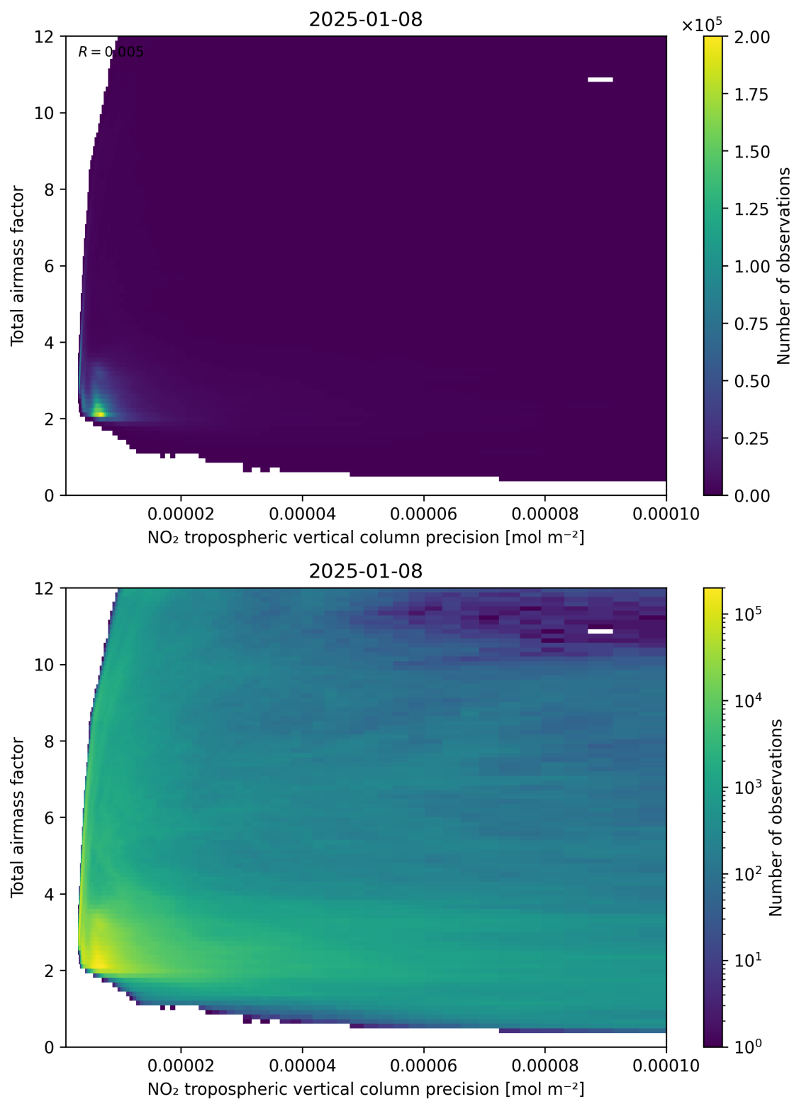
Figure 132: Scatter density plot of “NO 2 tropospheric vertical column precision” against “Total air mass factor” for 2025-01-07 to 2025-01-09.
