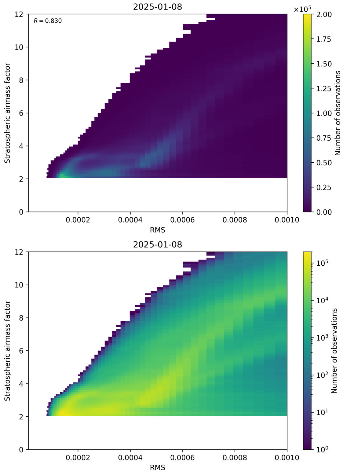
Figure 144: Scatter density plot of “RMS” against “Stratospheric airmass factor” for 2025-01-07 to 2025-01-09.
