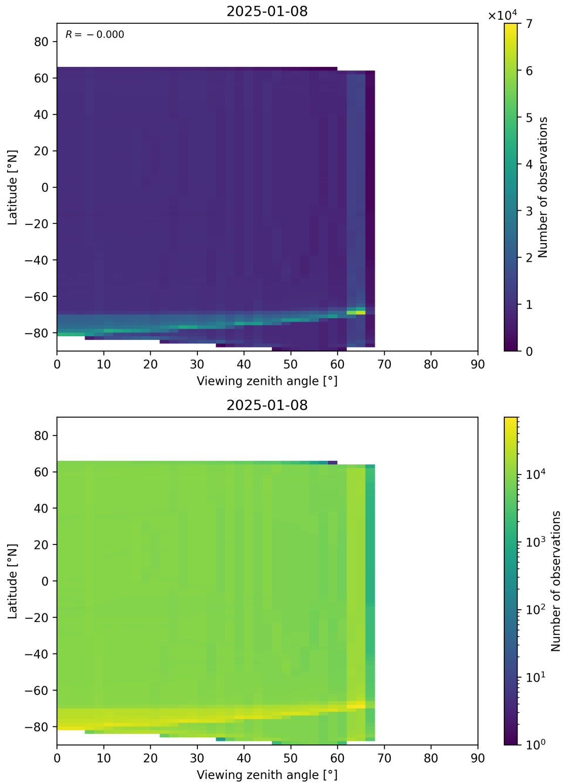
Figure 163: Scatter density plot of “Viewing zenith angle” against “Latitude” for 2025-01-07 to 2025-01-09.
