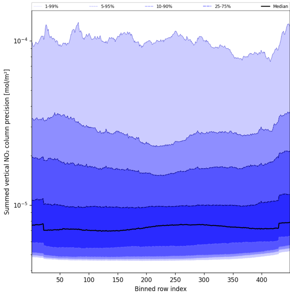
Figure 58: Along track statistics of “Summed vertical NO 2 column precision” for 2025-01-07 to 2025-01-09
