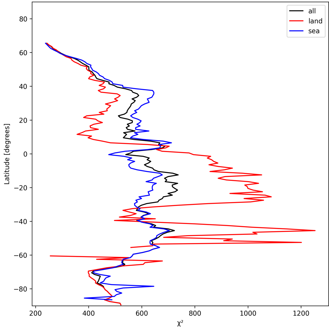
Figure 25: Zonal average of “ \chi^2 ” for 2025-01-07 to 2025-01-09.
