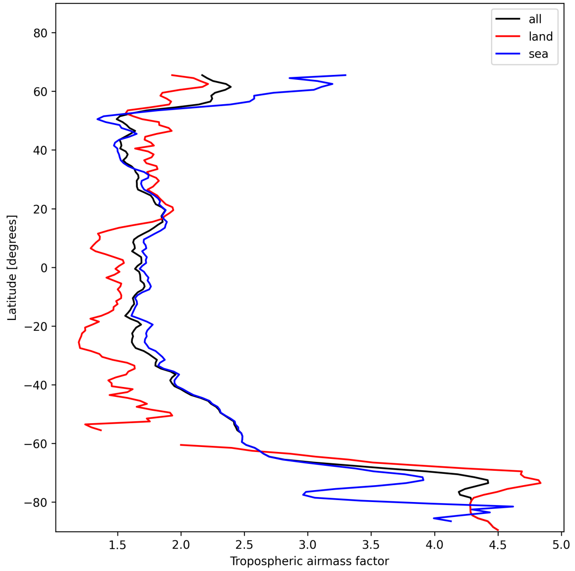
Figure 14: Zonal average of “Tropospheric airmass factor” for 2025-01-07 to 2025-01-09.
