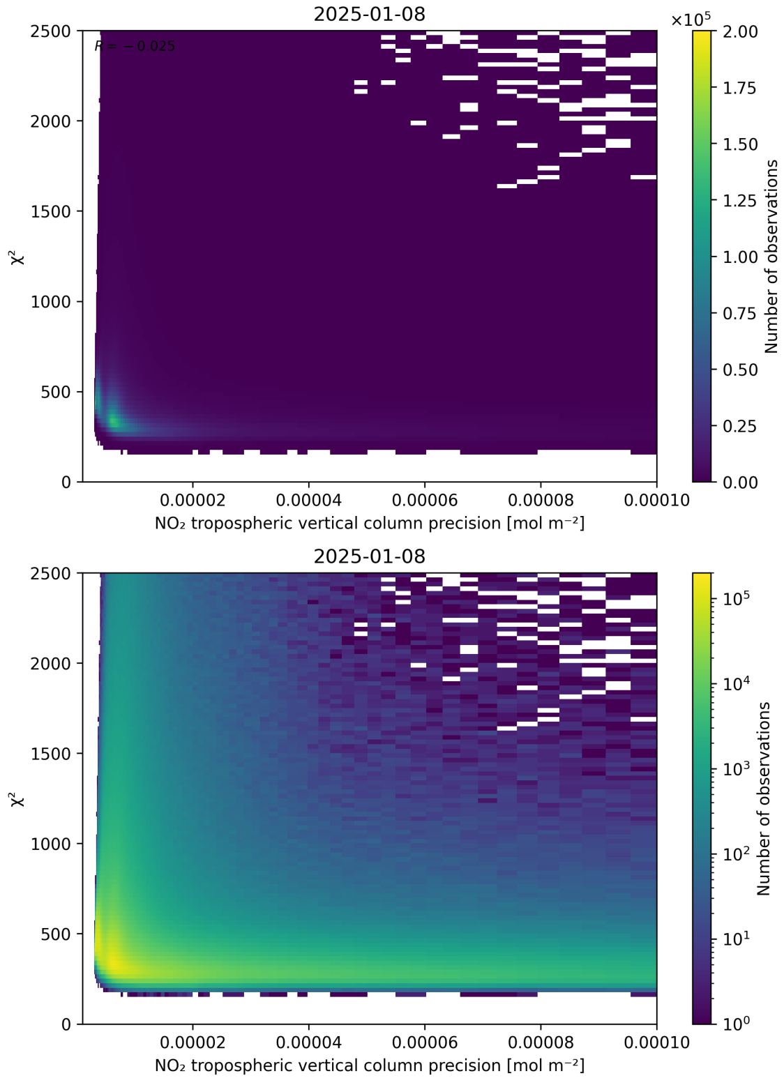
Figure 134: Scatter density plot of “NO 2 tropospheric vertical column precision” against “ \chi^2 ” for 2025-01-07 to 2025-01-09.
