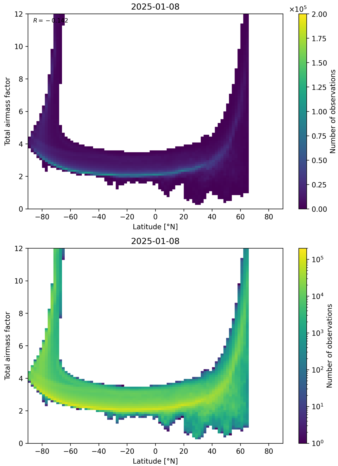
Figure 84: Scatter density plot of “Latitude” against “Total airmass factor” for 2025-01-07 to 2025-01-09.
