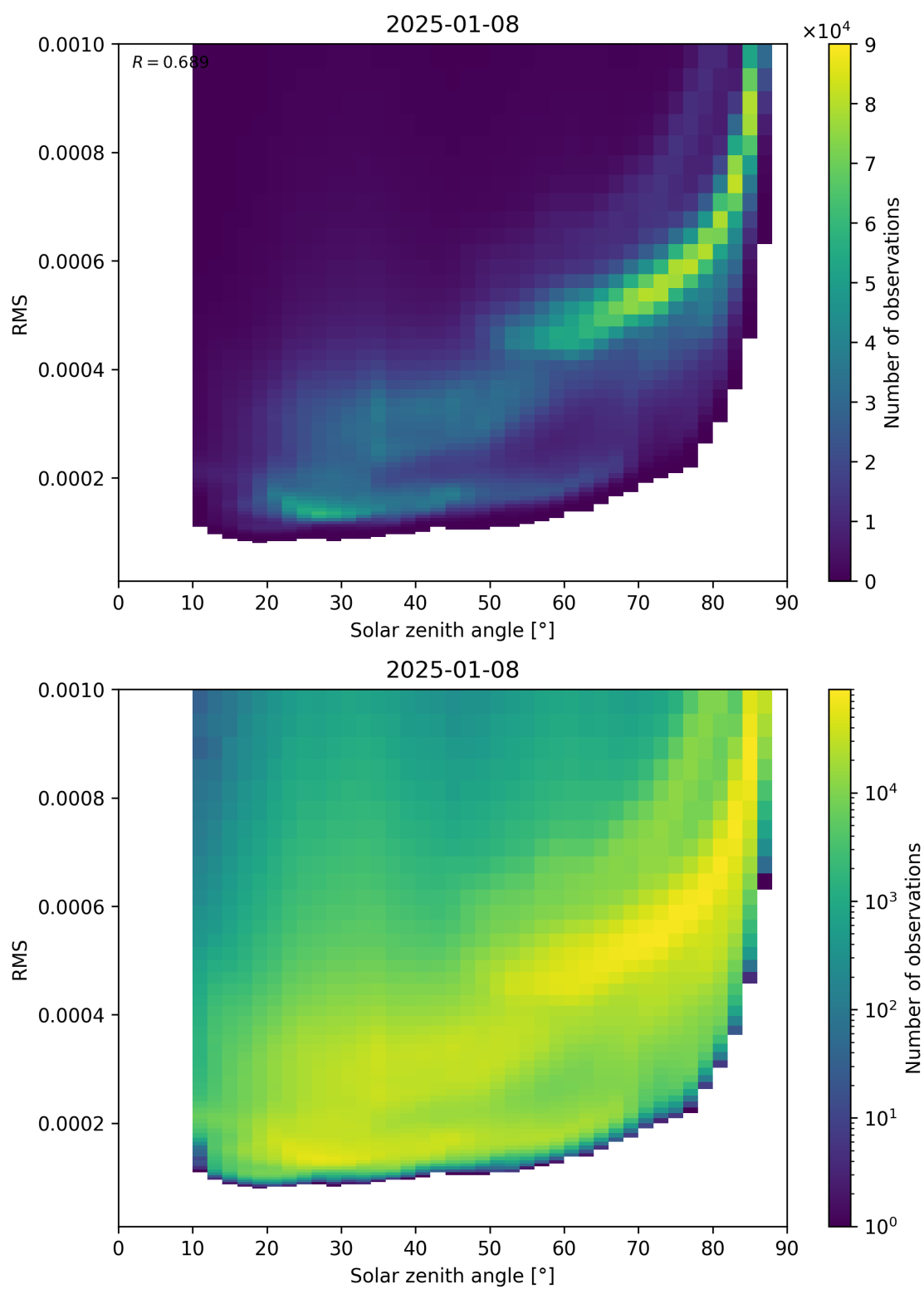
Figure 157: Scatter density plot of “Solar zenith angle” against “RMS” for 2025-01-07 to 2025-01-09.
