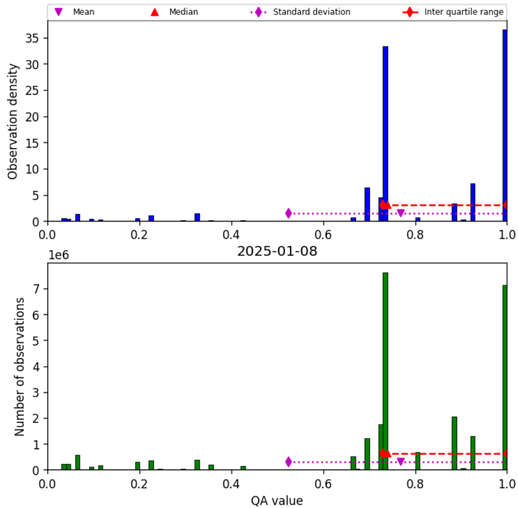
Figure 28: Histogram of “QA value” for 2025-01-07 to 2025-01-09
