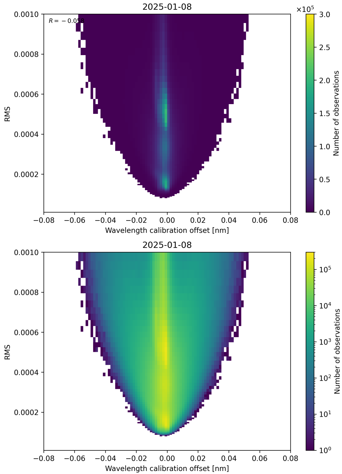
Figure 181: Scatter density plot of “Wavelength calibration offset” against “RMS” for 2025-01-07 to 2025-01-09.
