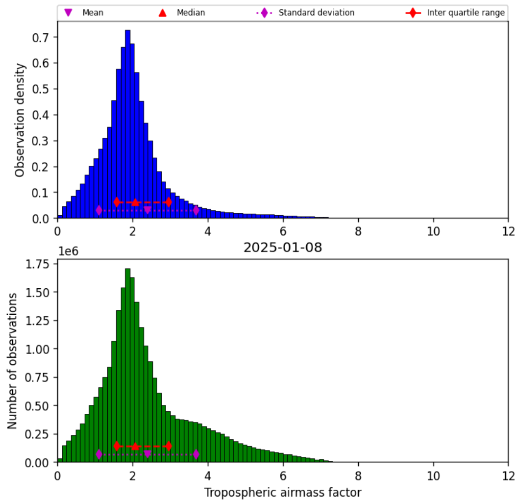
Figure 31: Histogram of “Tropospheric airmass factor” for 2025-01-07 to 2025-01-09
