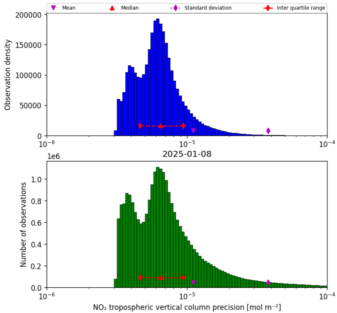
Figure 30: Histogram of “NO 2 tropospheric vertical column precision” for 2025-01-07 to 2025-01-09
