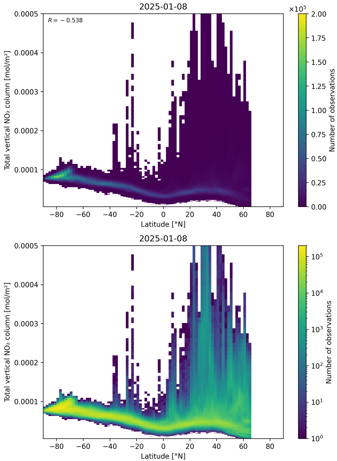
Figure 90: Scatter density plot of “Latitude” against “Total vertical NO 2 column” for 2025-01-07 to 2025-01-09.
