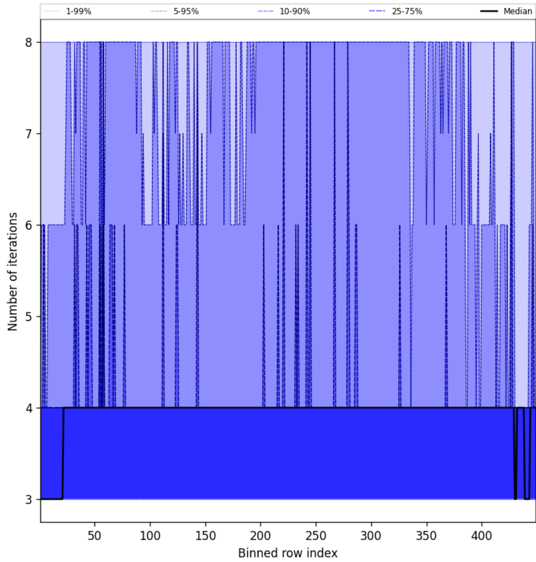
Figure 51: Along track statistics of “Number of iterations” for 2025-01-07 to 2025-01-09
