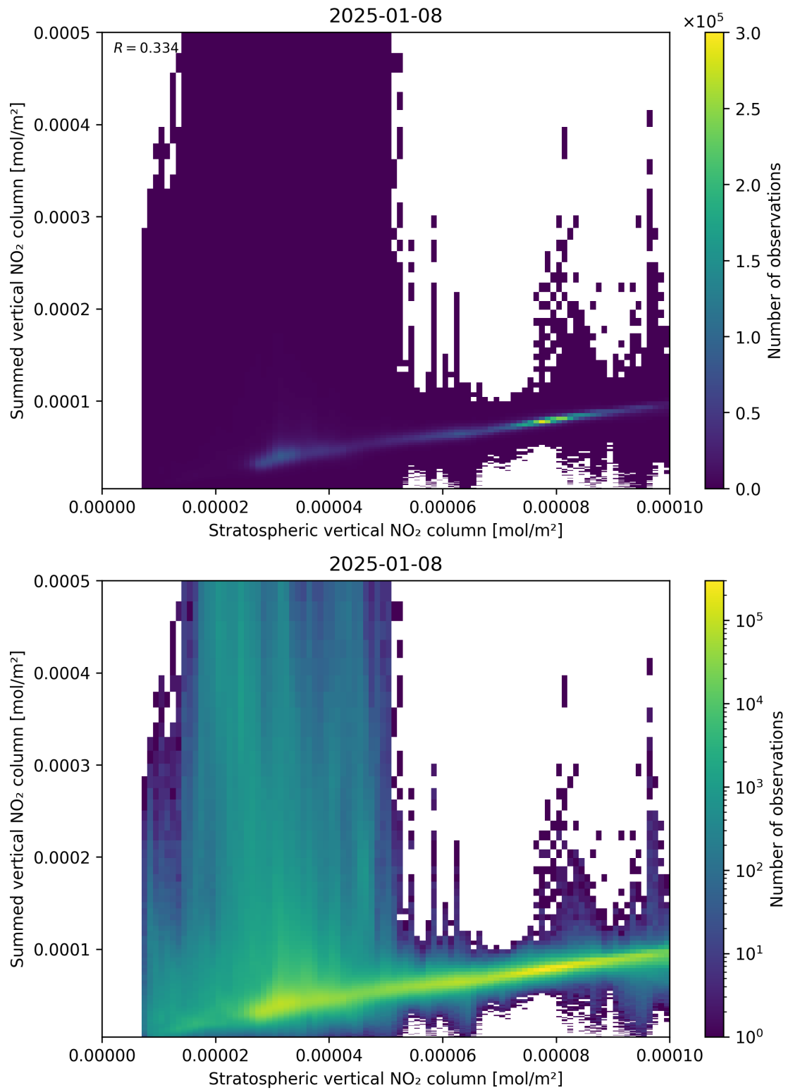
Figure 98: Scatter density plot of “Stratospheric vertical NO 2 column” against “Summed vertical NO 2 column” for 2025-01-07 to 2025-01-09.
