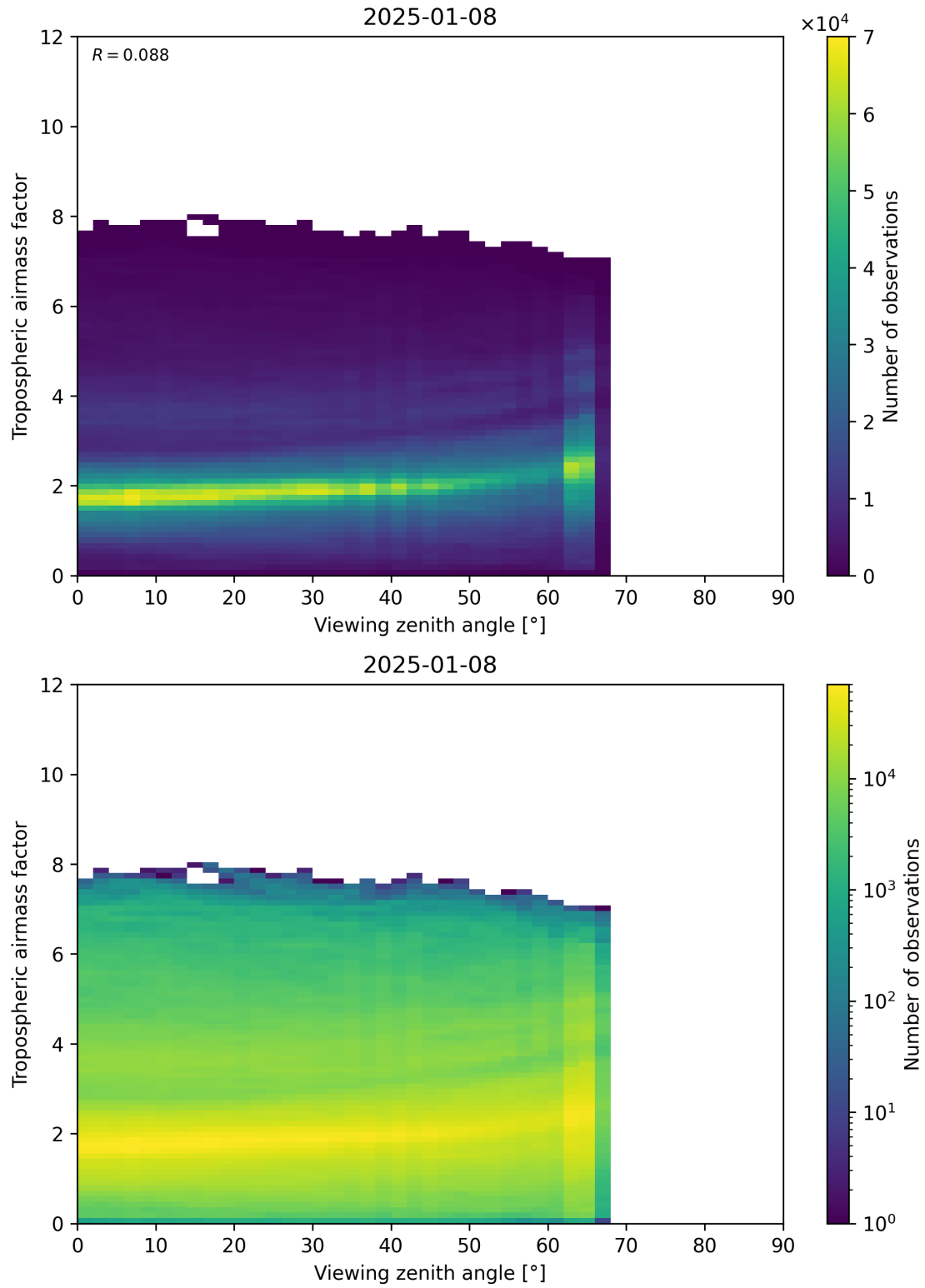
Figure 161: Scatter density plot of “Viewing zenith angle” against “Tropospheric airmass factor” for 2025-01-07 to 2025-01-09.
