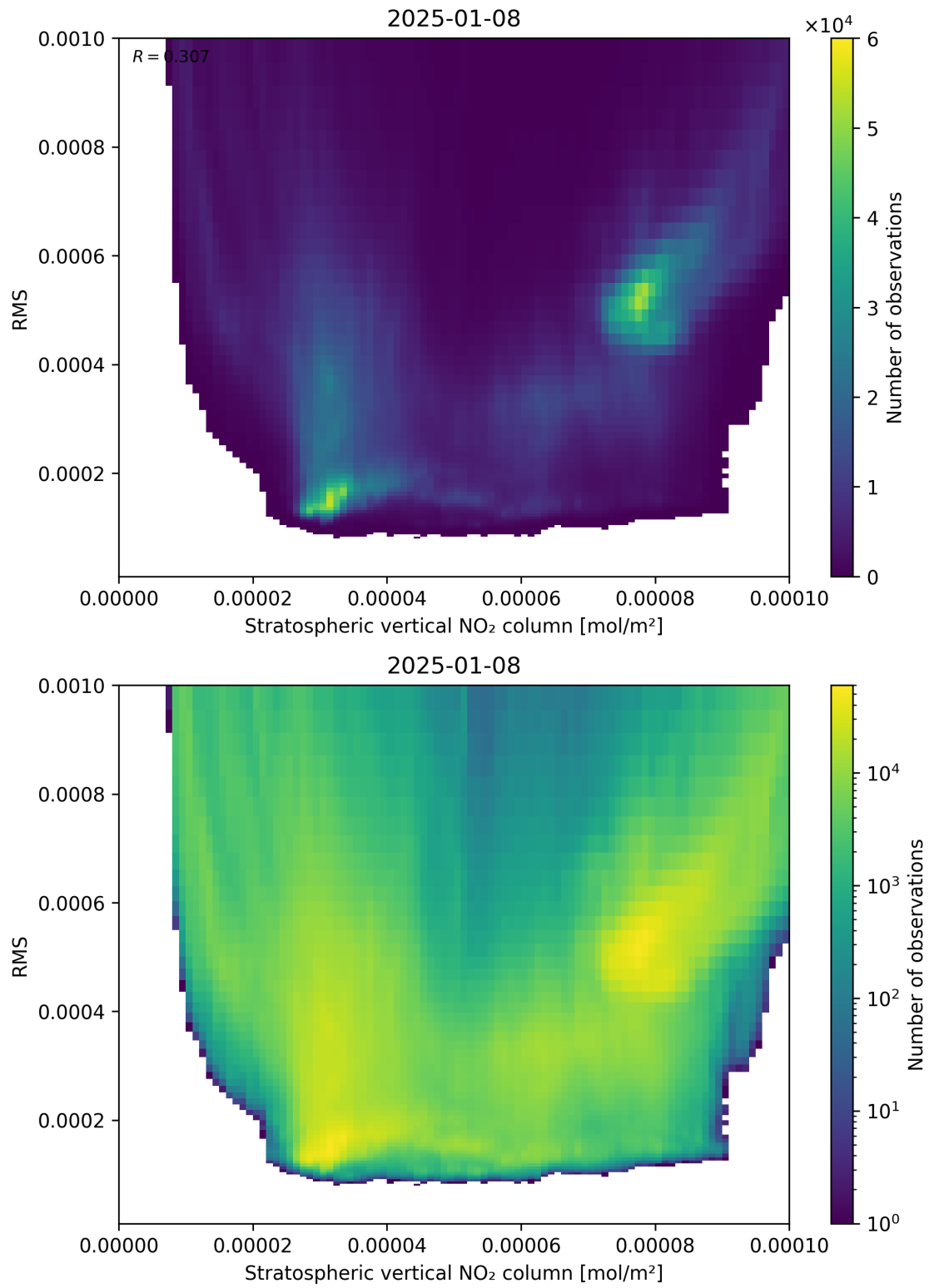
Figure 102: Scatter density plot of “Stratospheric vertical NO 2 column” against “RMS” for 2025-01-07 to 2025-01-09.
