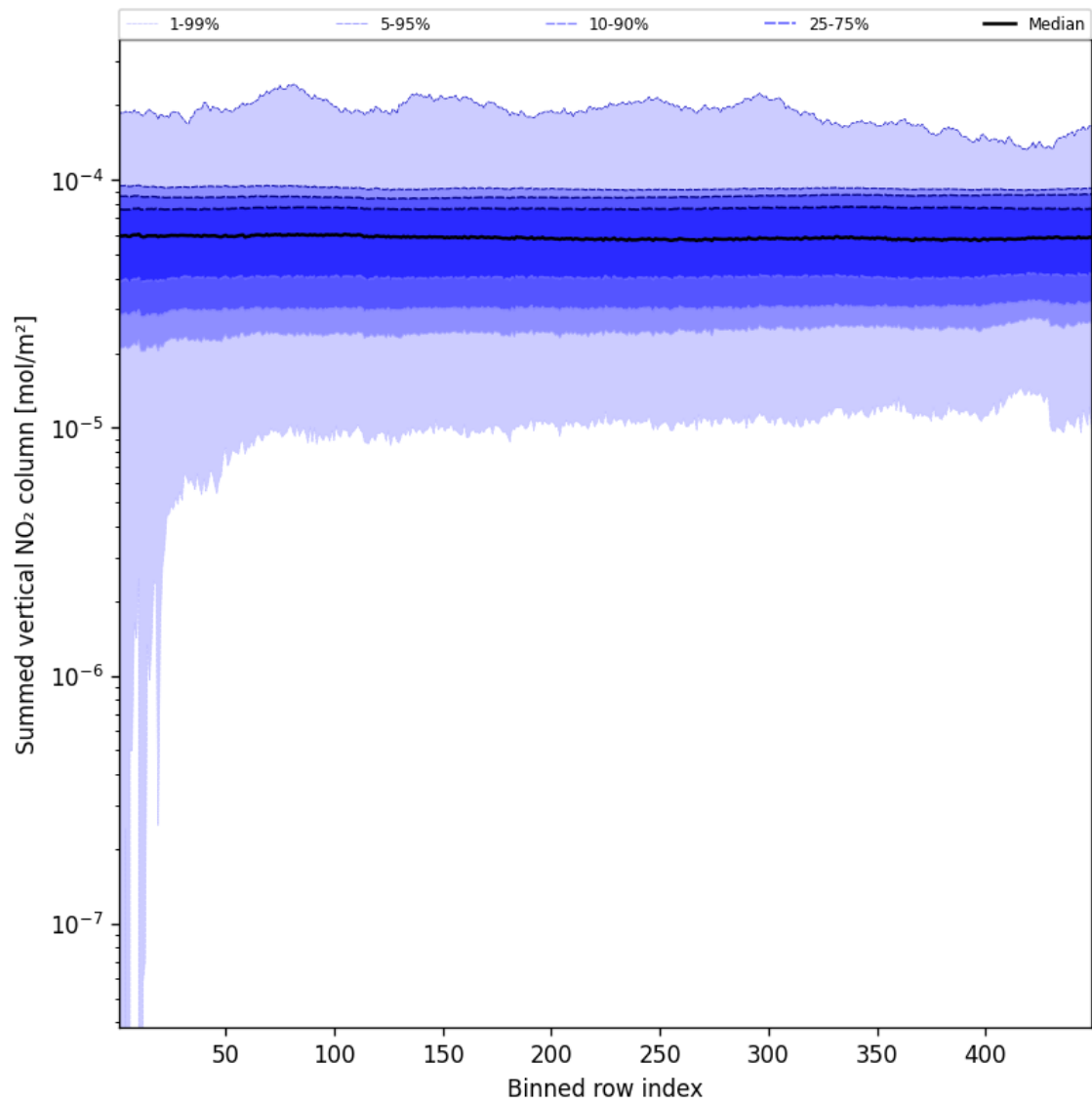
Figure 57: Along track statistics of “Summed vertical NO 2 column” for 2025-01-07 to 2025-01-09
