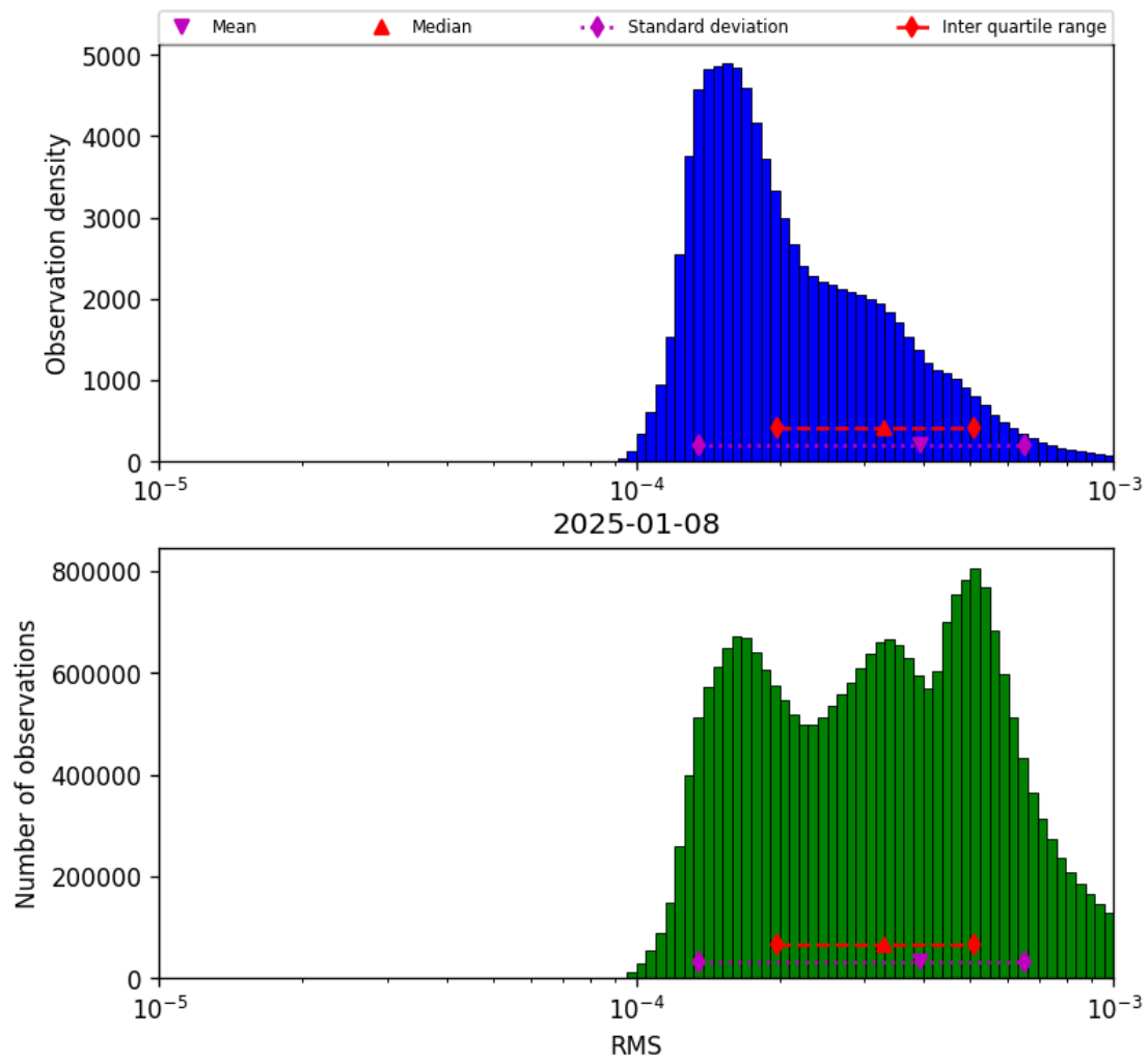
Figure 43: Histogram of “RMS” for 2025-01-07 to 2025-01-09
