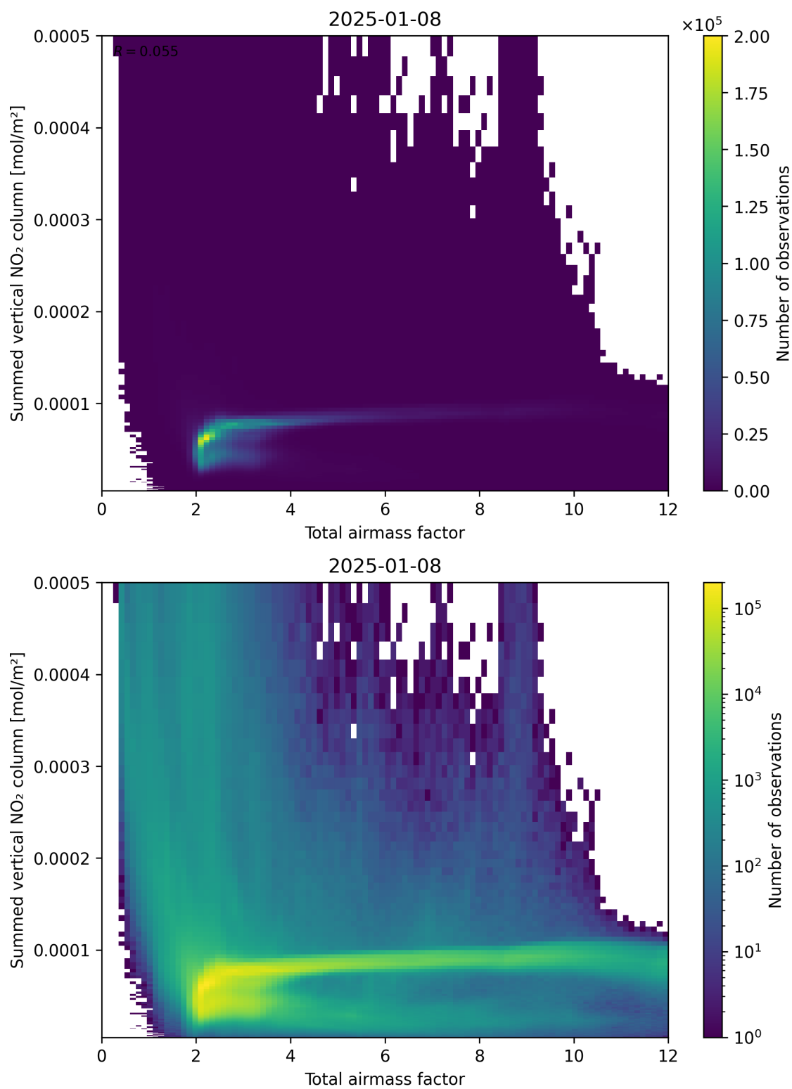
Figure 65: Scatter density plot of “Total airmass factor” against “Summed vertical NO 2 column” for 2025-01-07 to 2025-01-09.
