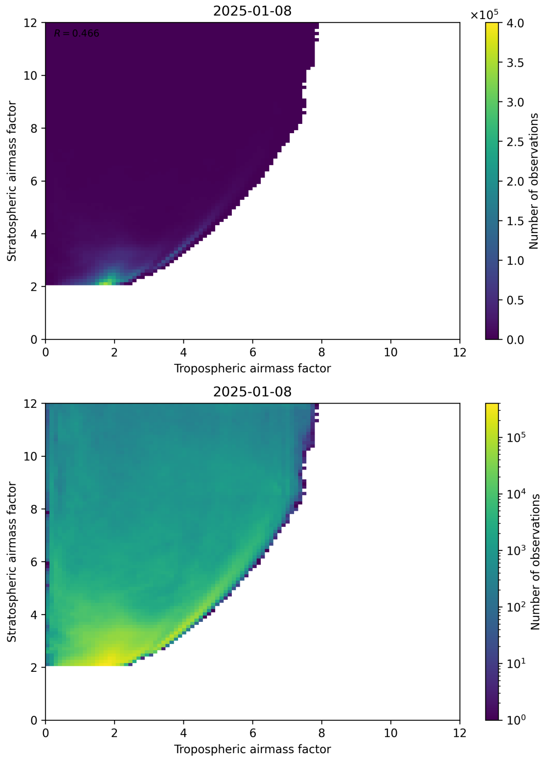
Figure 71: Scatter density plot of “Tropospheric airmass factor” against “Stratospheric airmass factor” for 2025-01-07 to 2025-01-09.
