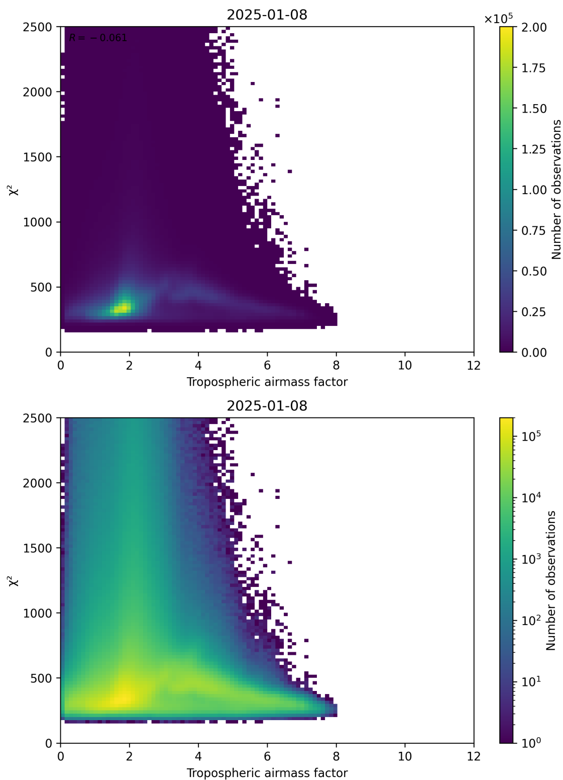
Figure 73: Scatter density plot of “Tropospheric airmass factor” against “ \chi^2 ” for 2025-01-07 to 2025-01-09.
