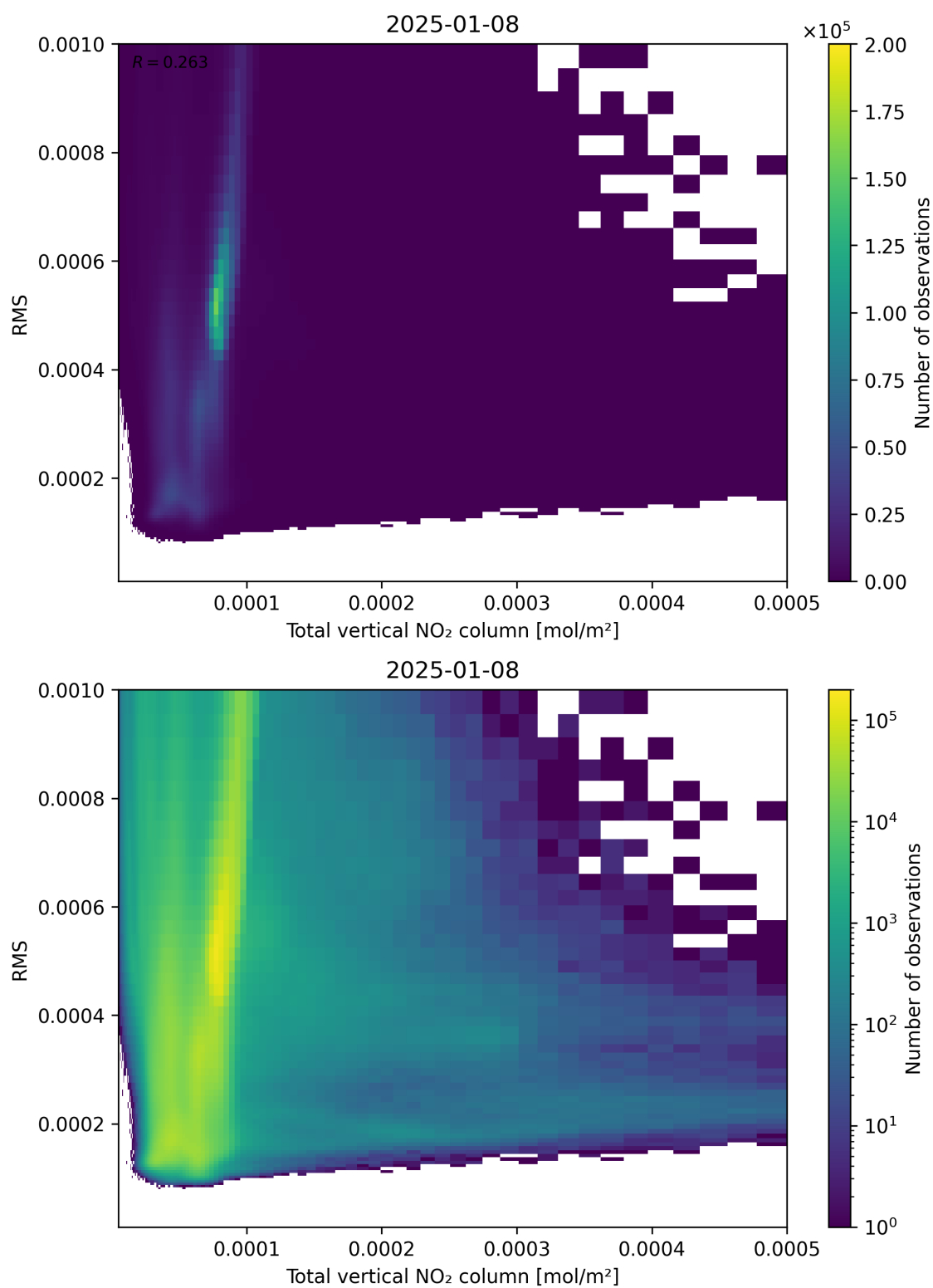
Figure 120: Scatter density plot of “Total vertical NO 2 column” against “RMS” for 2025-01-07 to 2025-01-09.
