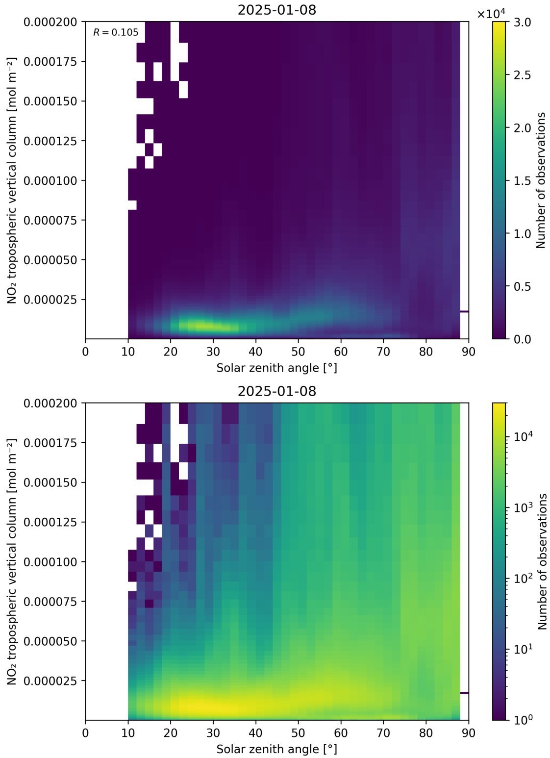
Figure 155: Scatter density plot of “Solar zenith angle” against “NO 2 tropospheric vertical column” for 2025-01-07 to 2025-01-09.
