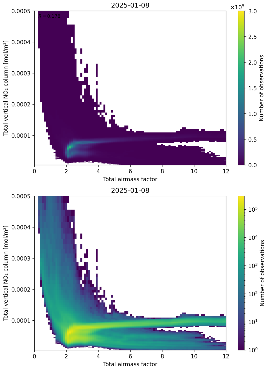
Figure 67: Scatter density plot of “Total airmass factor” against “Total vertical NO 2 column” for 2025-01-07 to 2025-01-09.
