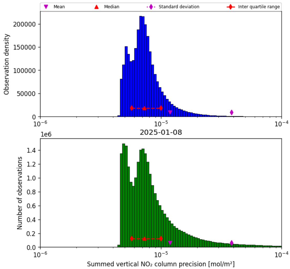
Figure 41: Histogram of “Summed vertical NO 2 column precision” for 2025-01-07 to 2025-01-09
