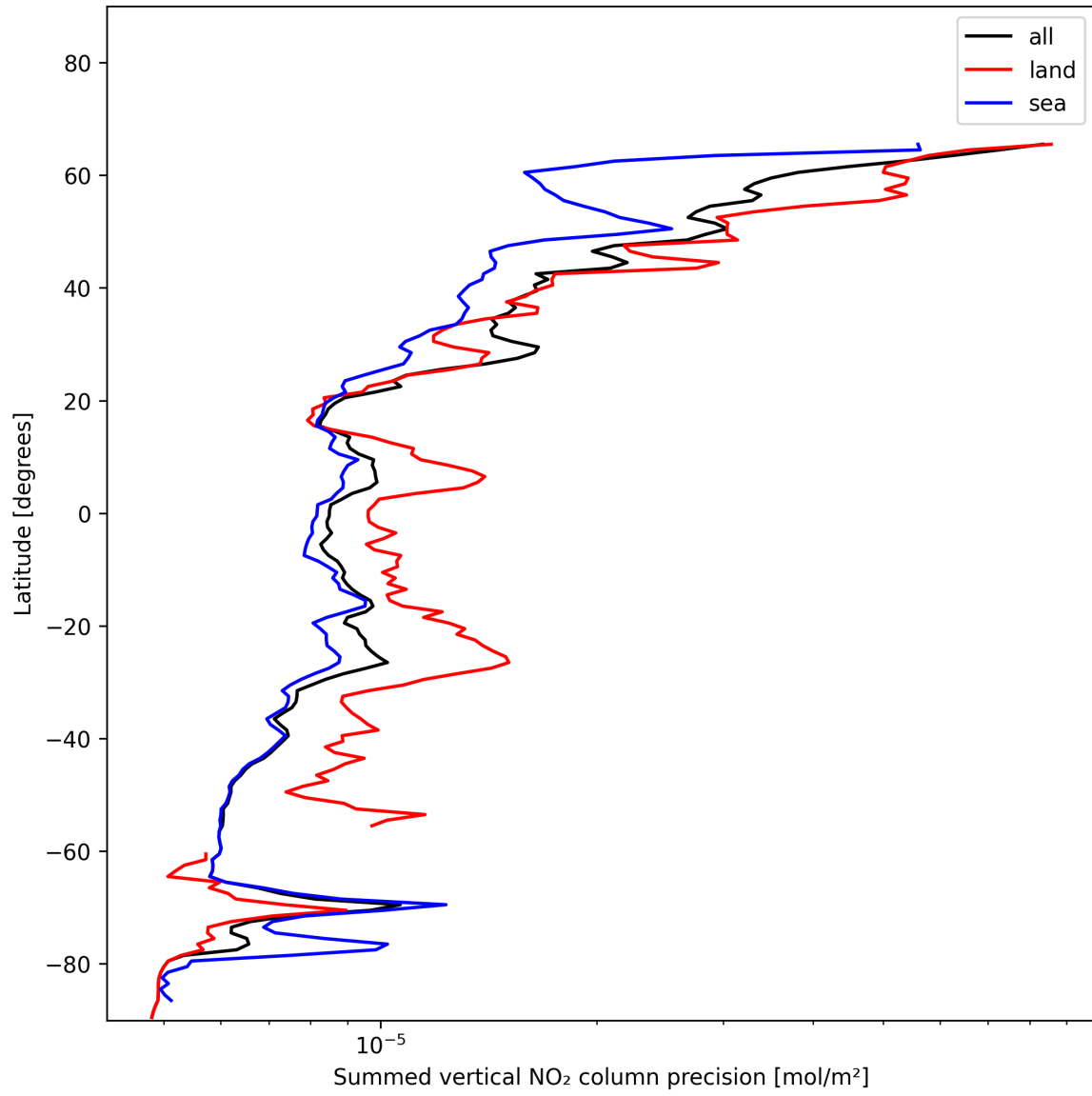
Figure 24: Zonal average of “Summed vertical NO 2 column precision” for 2025-01-07 to 2025-01-09.
