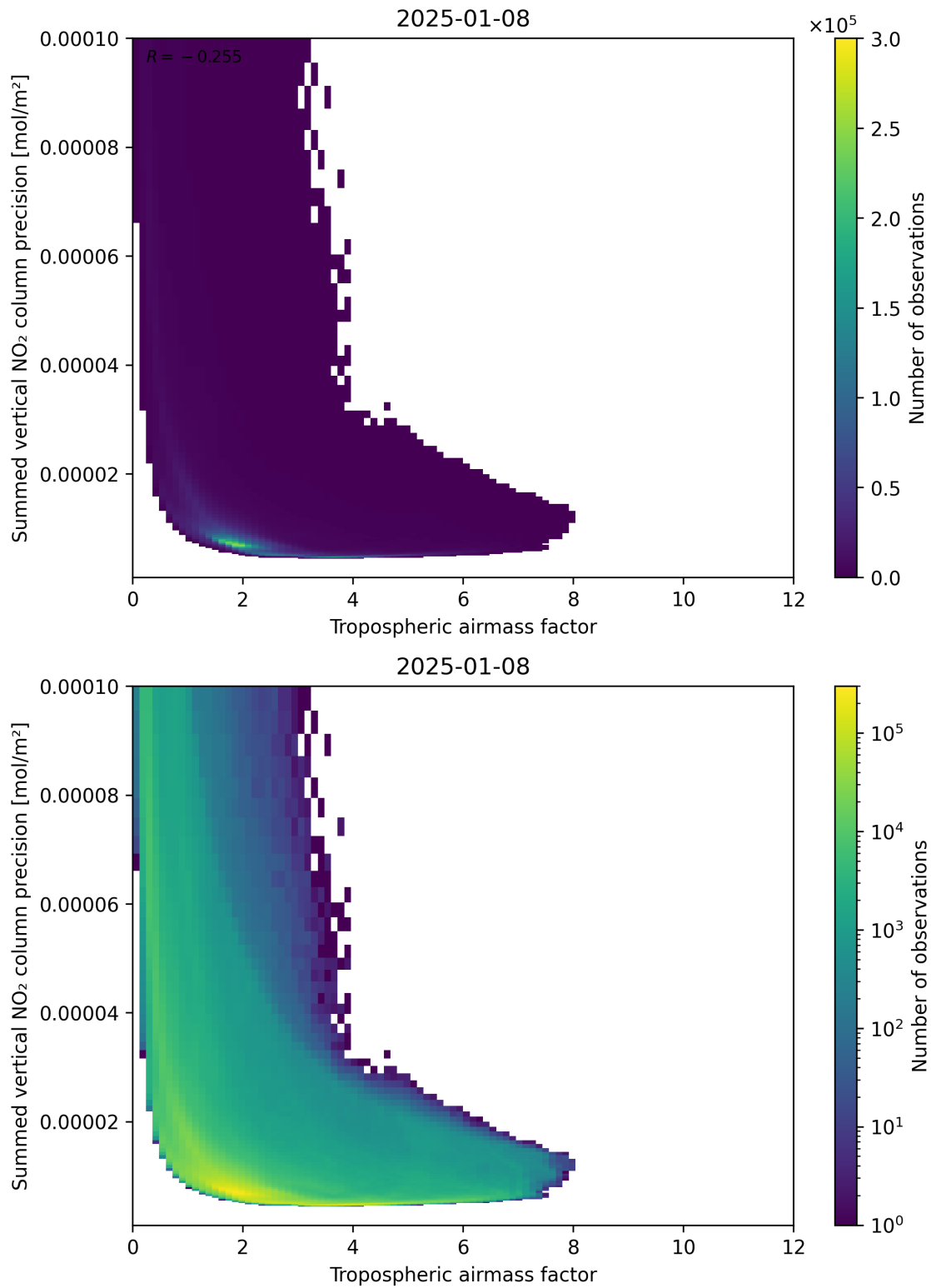
Figure 76: Scatter density plot of “Tropospheric air mass factor” against “Summed vertical NO 2 column precision” for 2025-01-07 to 2025-01-09.
