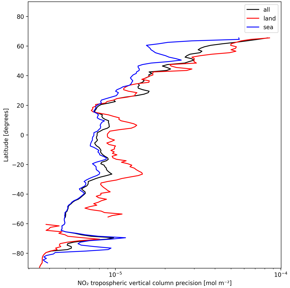
Figure 13: Zonal average of “NO 2 tropospheric vertical column precision” for 2025-01-07 to 2025-01-09.
