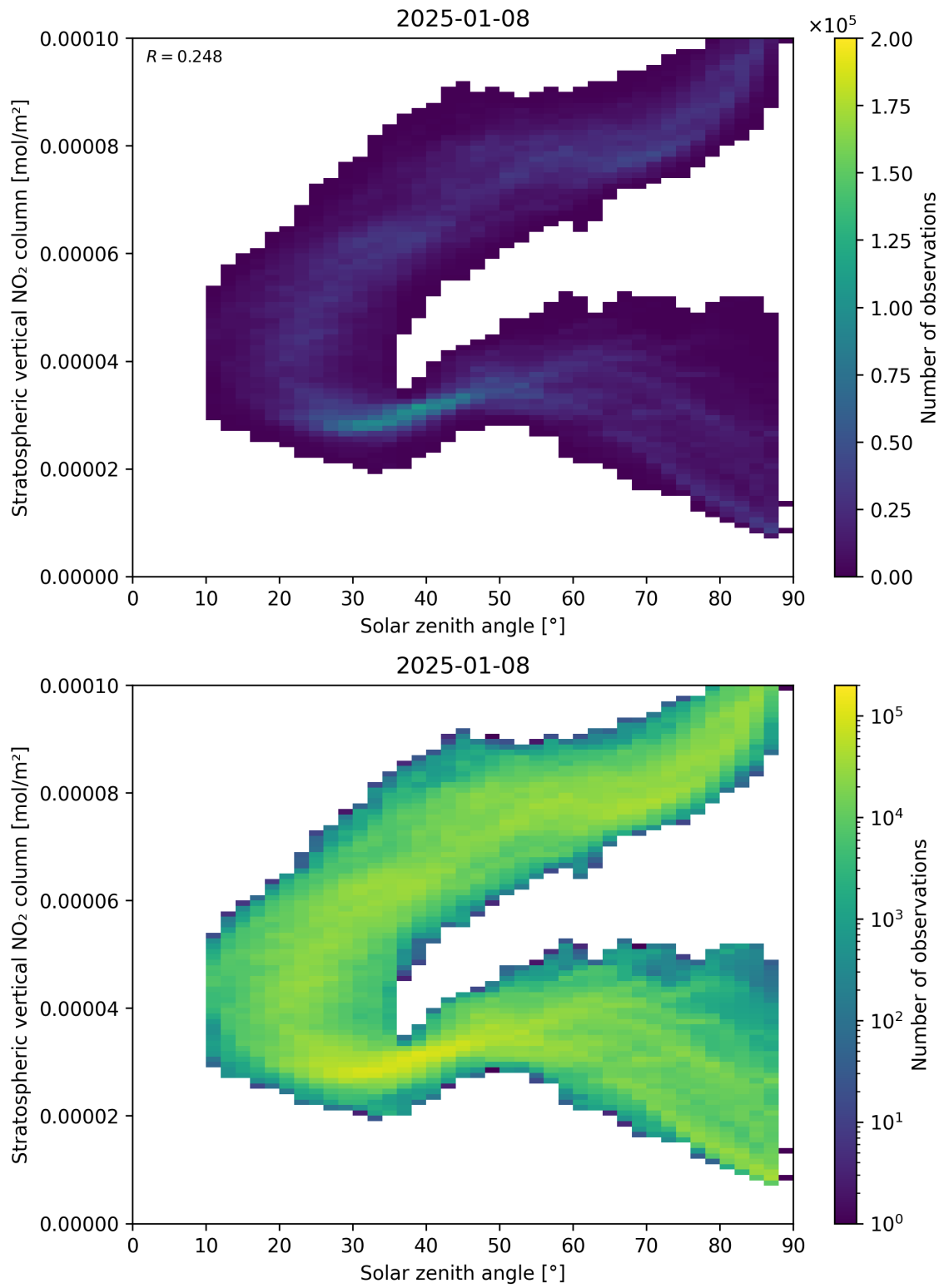
Figure 150: Scatter density plot of “Solar zenith angle” against “Stratospheric vertical NO 2 column” for 2025-01-07 to 2025-01-09.
