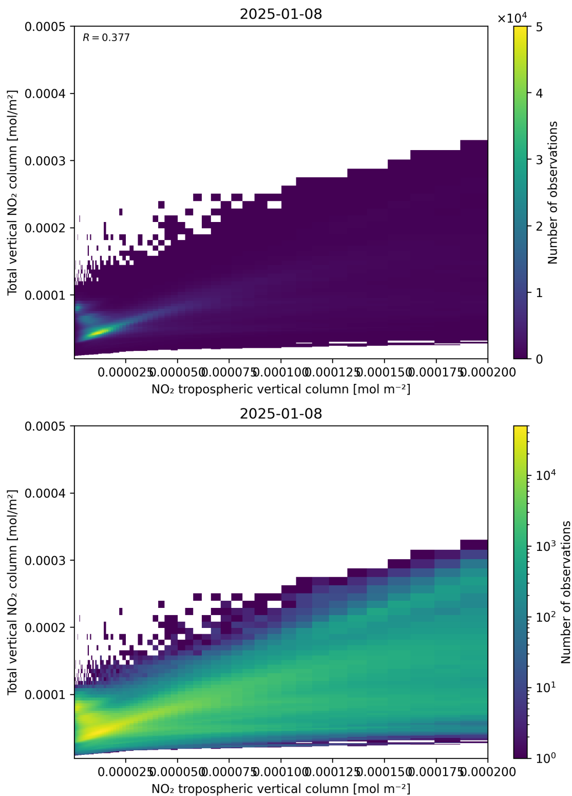
Figure 128: Scatter density plot of “NO 2 tropospheric vertical column” against “Total vertical NO 2 column” for 2025-01-07 to 2025-01-09.
