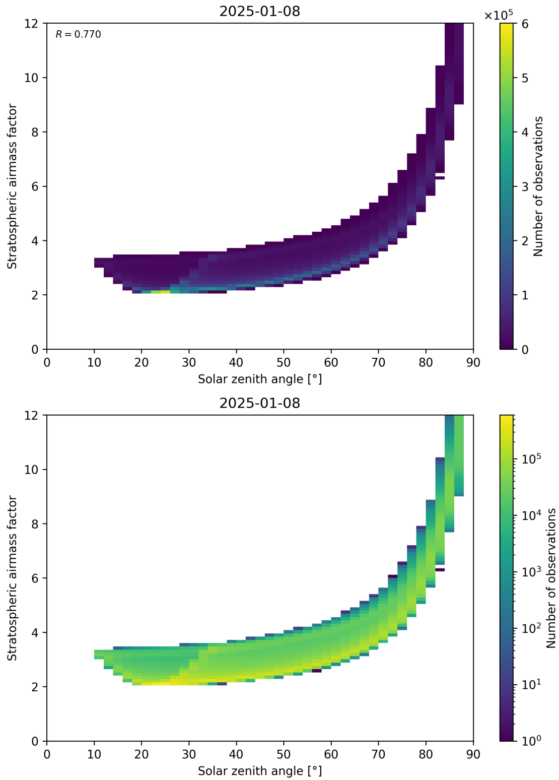
Figure 145: Scatter density plot of “Solar zenith angle” against “Stratospheric airmass factor” for 2025-01-07 to 2025-01-09.
