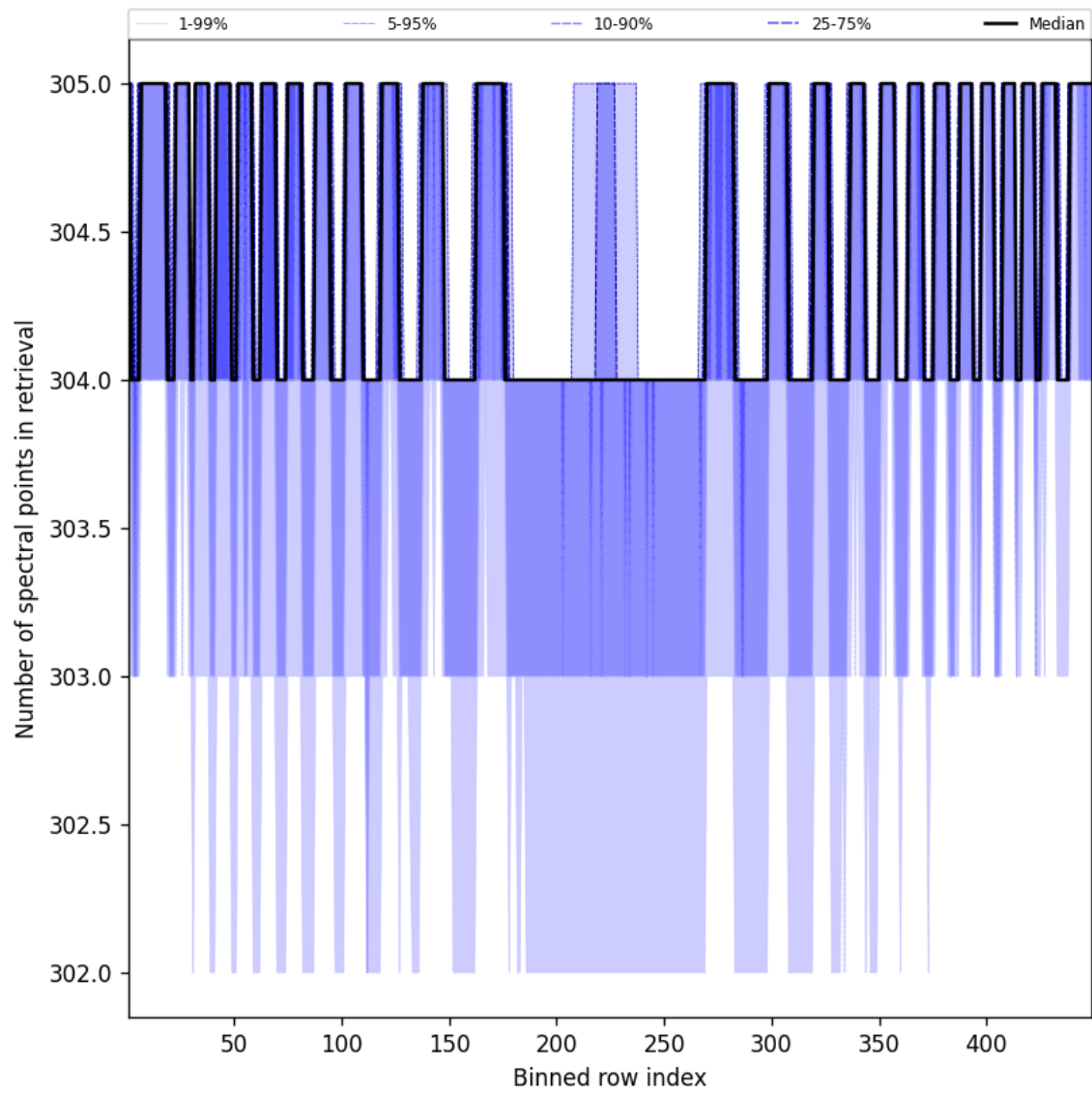
Figure 50: Along track statistics of “Number of spectral points in retrieval” for 2025-01-07 to 2025-01-09
