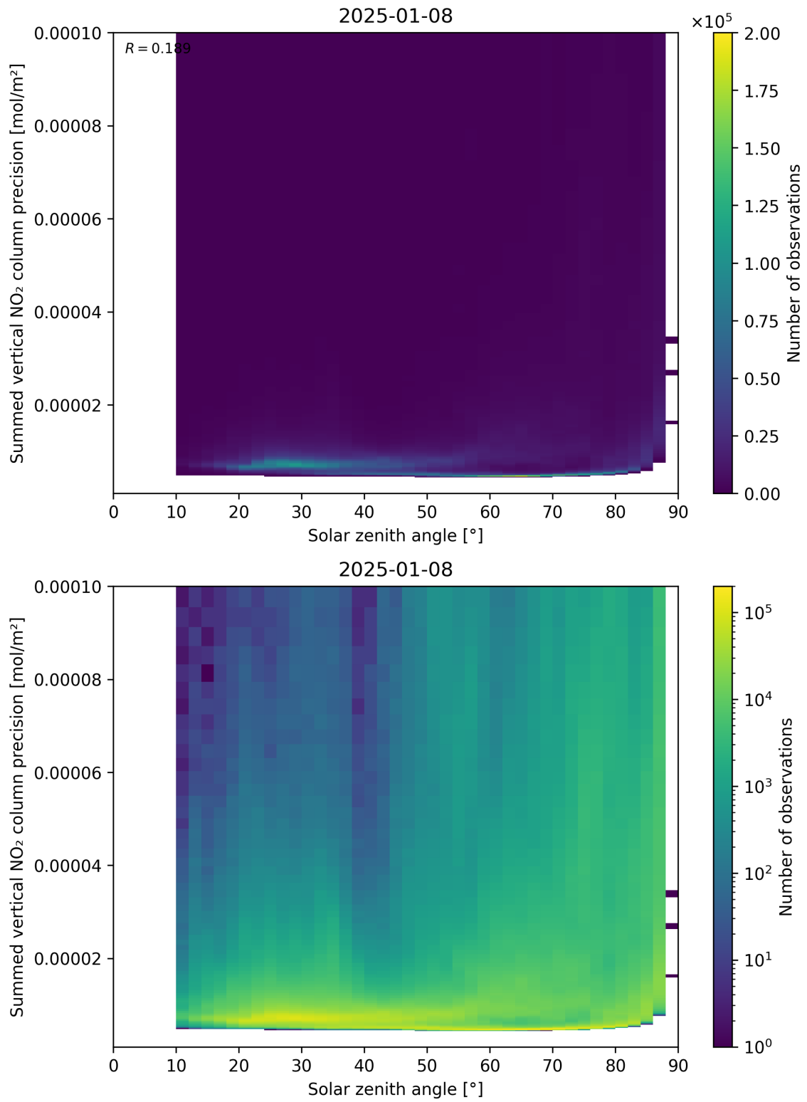
Figure 152: Scatter density plot of “Solar zenith angle” against “Summed vertical NO 2 column precision” for 2025-01-07 to 2025-01-09.
