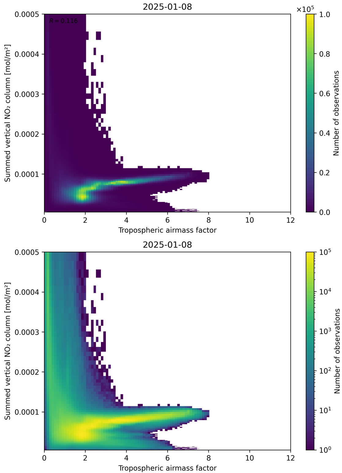
Figure 75: Scatter density plot of “Tropospheric airmass factor” against “Summed vertical NO 2 column” for 2025-01-07 to 2025-01-09.
