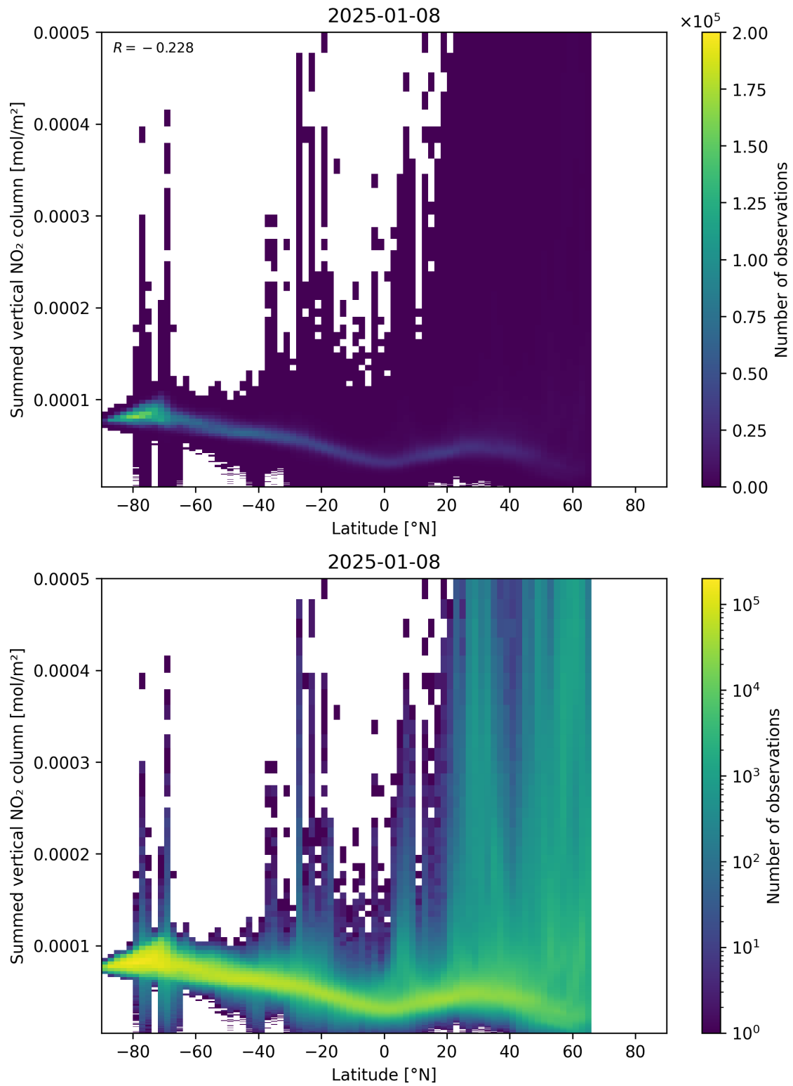
Figure 88: Scatter density plot of “Latitude” against “Summed vertical NO 2 column” for 2025-01-07 to 2025-01-09.
