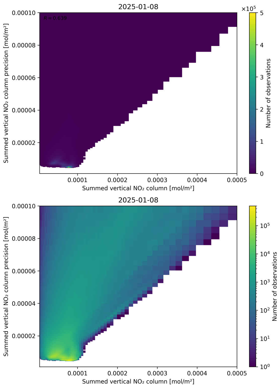
Figure 105: Scatter density plot of “Summed vertical NO 2 column” against “Summed vertical NO 2 column precision” for 2025-01-07 to 2025-01-09.
