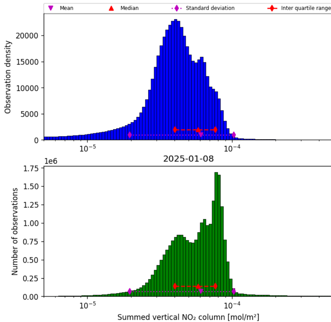
Figure 40: Histogram of “Summed vertical NO 2 column” for 2025-01-07 to 2025-01-09
