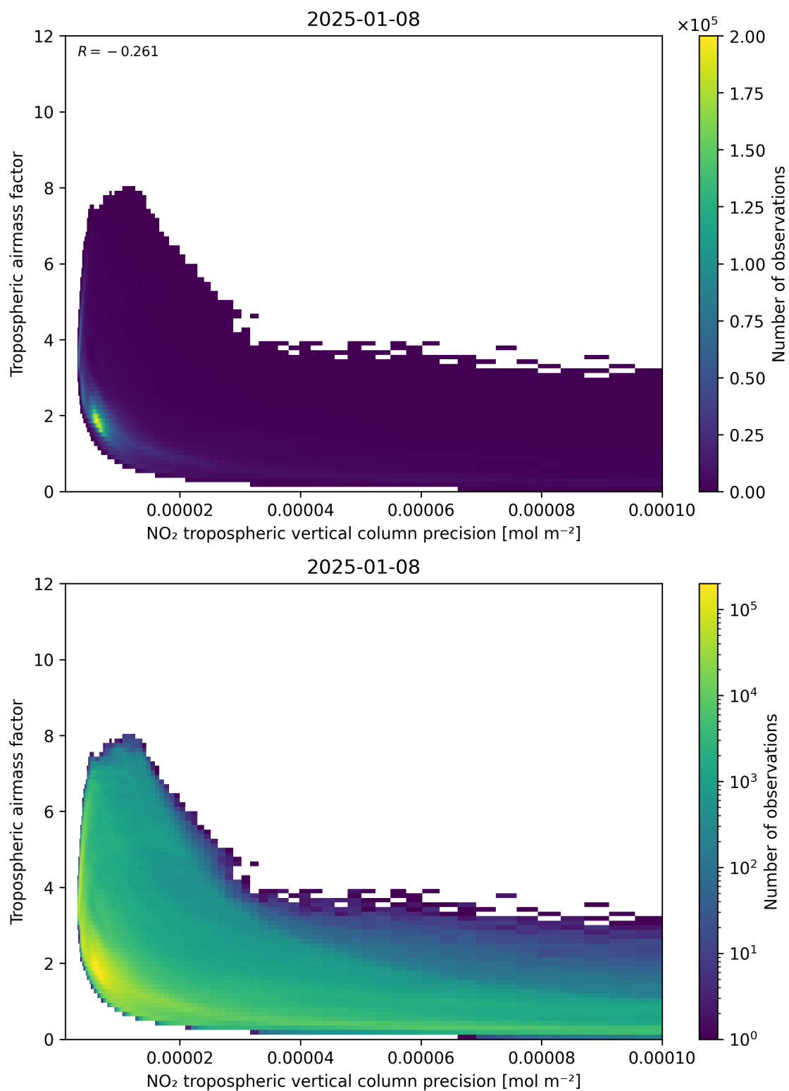
Figure 133: Scatter density plot of “NO 2 tropospheric vertical column precision” against “Tropospheric air mass factor” for 2025-01-07 to 2025-01-09.
