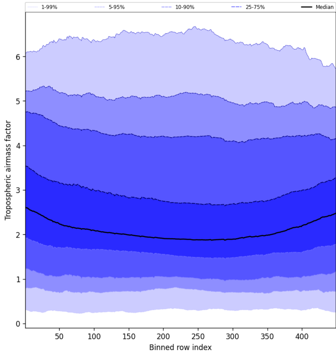
Figure 48: Along track statistics of “Tropospheric airmass factor” for 2025-01-07 to 2025-01-09
