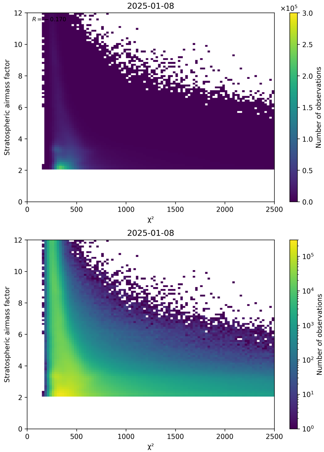
Figure 81: Scatter density plot of “ \chi^2 ” against “Stratospheric airmass factor” for 2025-01-07 to 2025-01-09.
