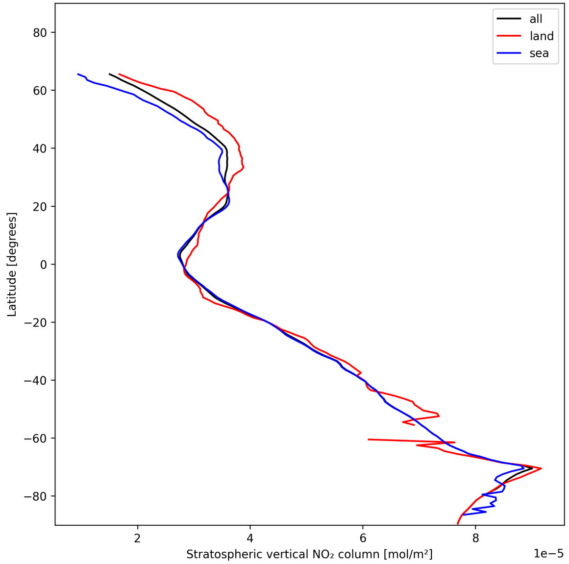
Figure 19: Zonal average of “Stratospheric vertical NO 2 column” for 2025-01-07 to 2025-01-09.
