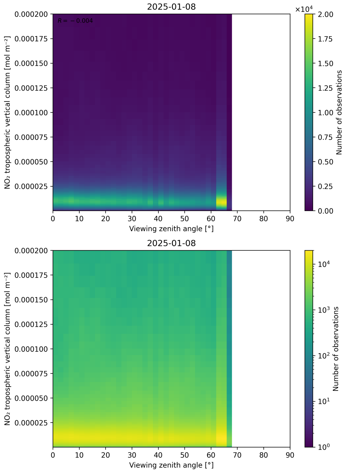
Figure 169: Scatter density plot of “Viewing zenith angle” against “NO 2 tropospheric vertical column” for 2025-01-07 to 2025-01-09.
