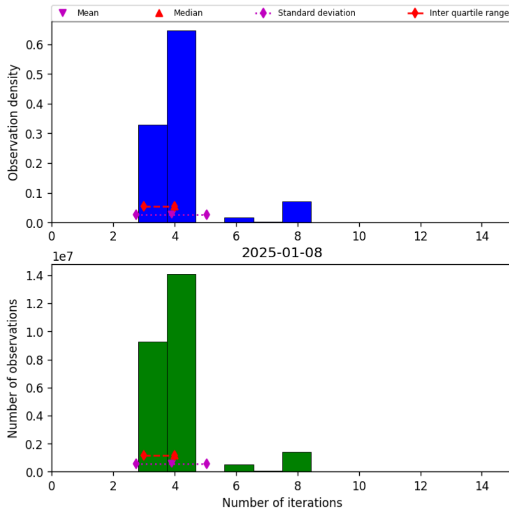
Figure 34: Histogram of “Number of iterations” for 2025-01-07 to 2025-01-09
