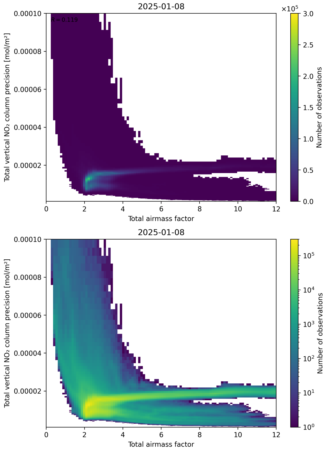
Figure 68: Scatter density plot of “Total airmass factor” against “Total vertical NO 2 column precision” for 2025-01-07 to 2025-01-09.
