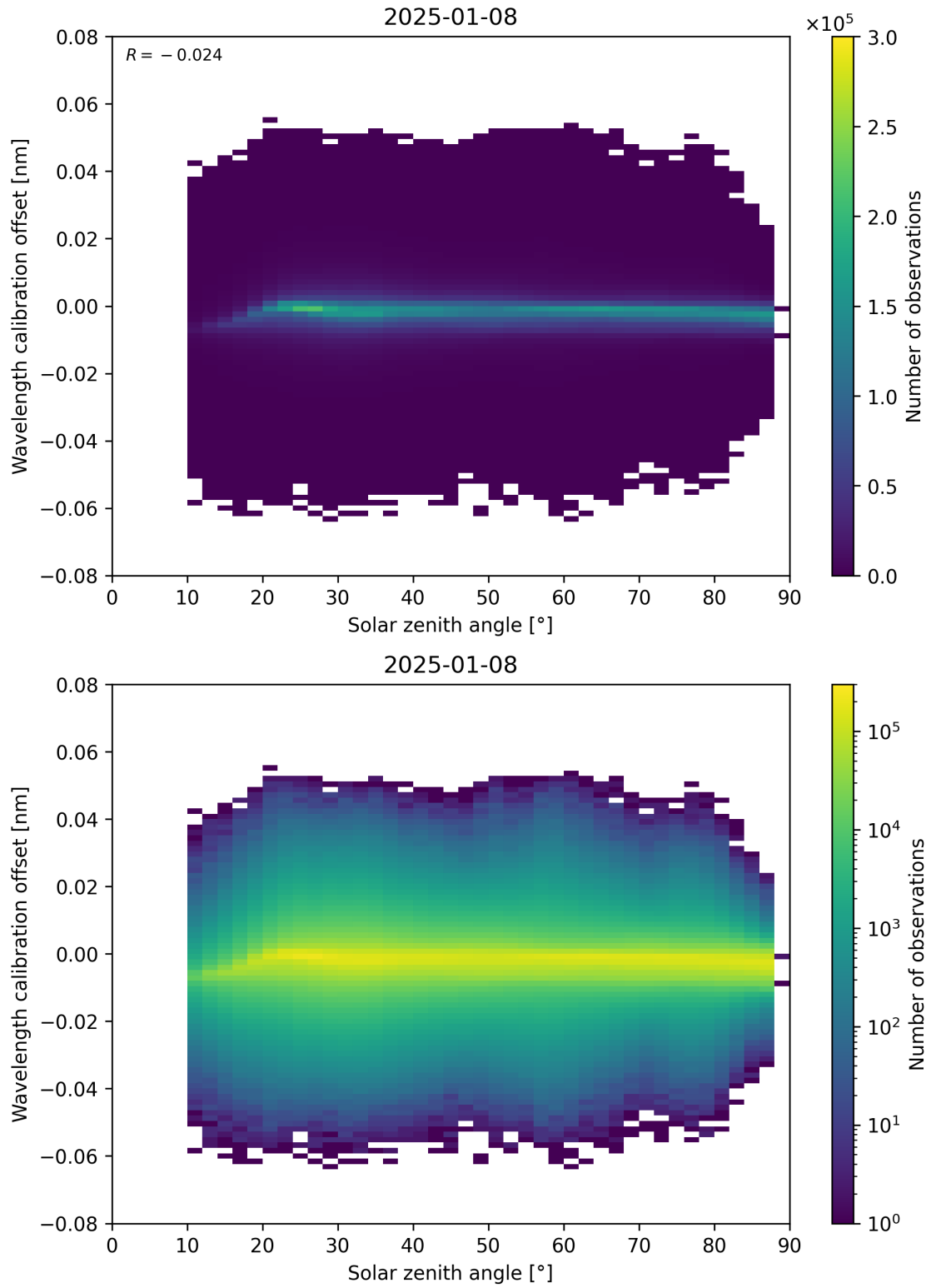
Figure 158: Scatter density plot of “Solar zenith angle” against “Wavelength calibration offset” for 2025-01-07 to 2025-01-09.
