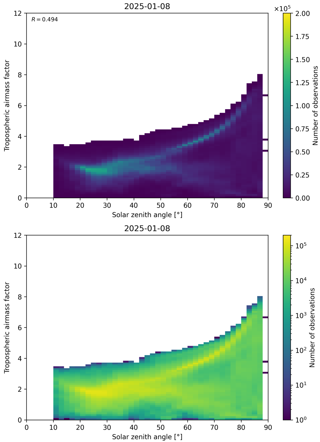
Figure 147: Scatter density plot of “Solar zenith angle” against “Tropospheric airmass factor” for 2025-01-07 to 2025-01-09.
