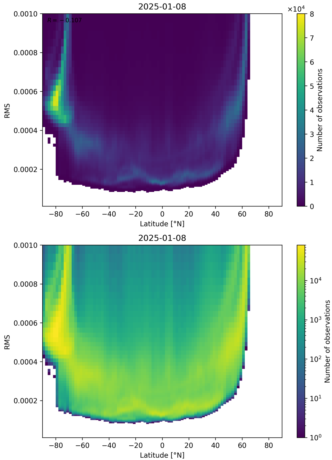
Figure 94: Scatter density plot of “Latitude” against “RMS” for 2025-01-07 to 2025-01-09.
