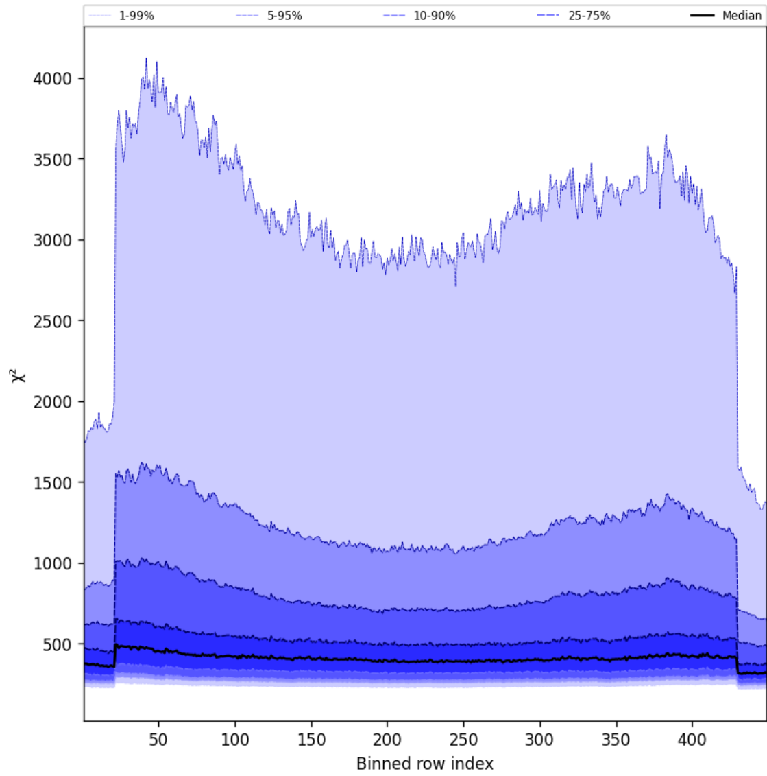
Figure 59: Along track statistics of “ \chi^2 ” for 2025-01-07 to 2025-01-09
