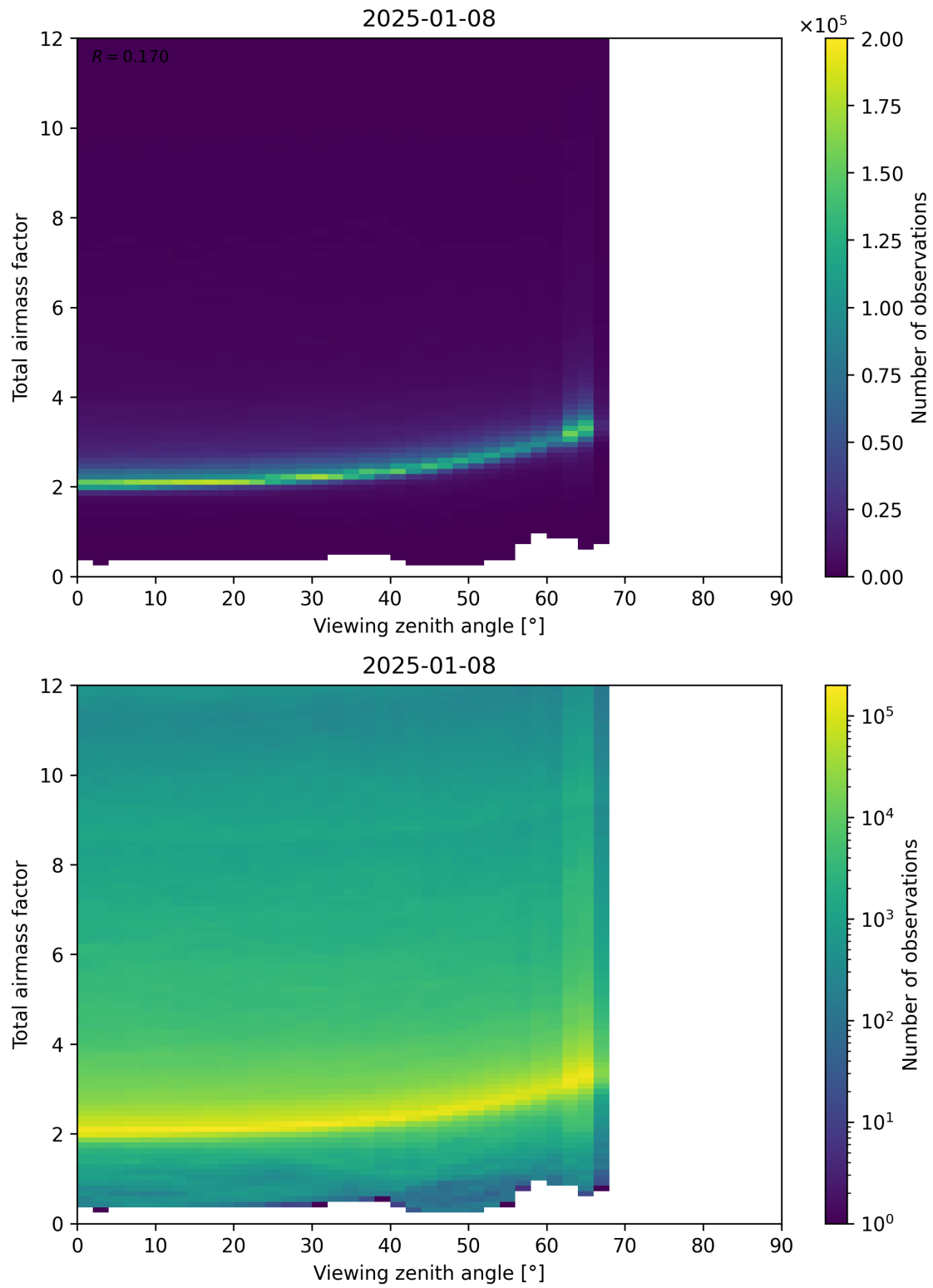
Figure 160: Scatter density plot of “Viewing zenith angle” against “Total airmass factor” for 2025-01-07 to 2025-01-09.
