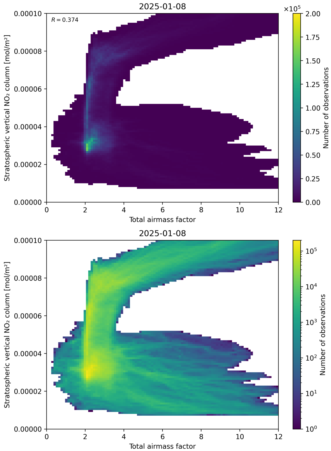
Figure 64: Scatter density plot of “Total airmass factor” against “Stratospheric vertical \text{NO}_2 column” for 2025-01-07 to 2025-01-09.
