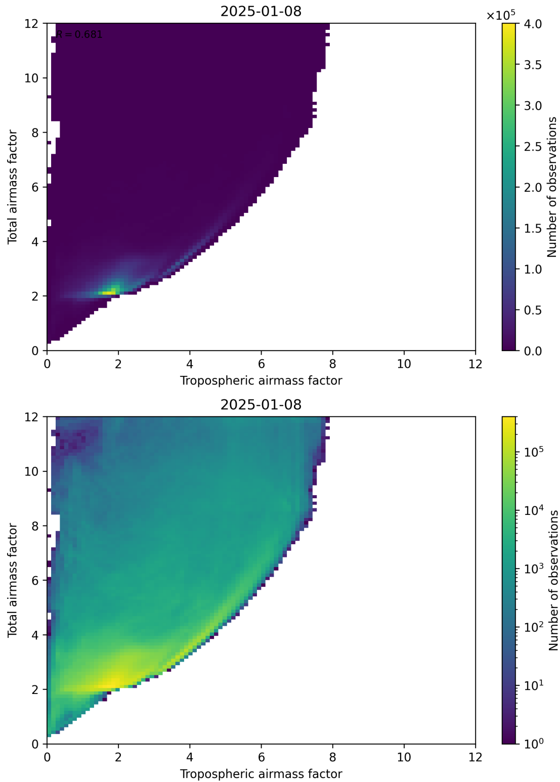
Figure 72: Scatter density plot of “Tropospheric airmass factor” against “Total airmass factor” for 2025-01-07 to 2025-01-09.
