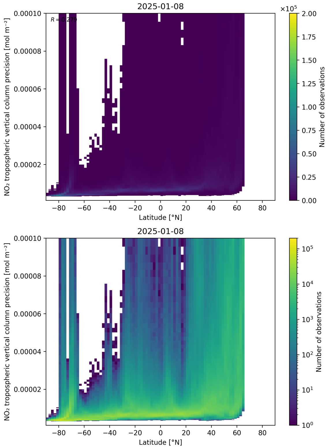
Figure 93: Scatter density plot of “Latitude” against “NO 2 tropospheric vertical column precision” for 2025-01-07 to 2025-01-09.
