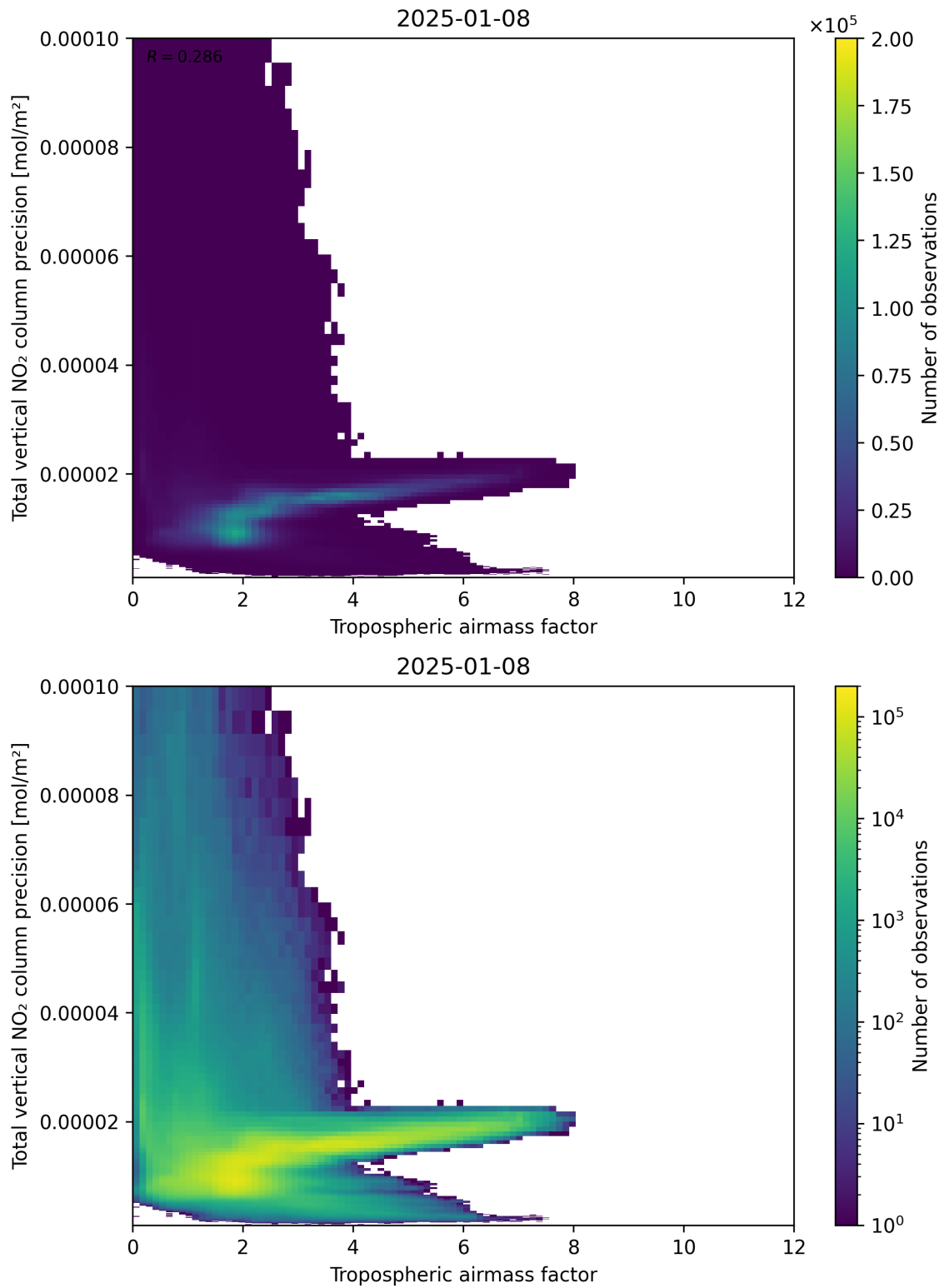
Figure 78: Scatter density plot of “Tropospheric air mass factor” against “Total vertical NO 2 column precision” for 2025-01-07 to 2025-01-09.
