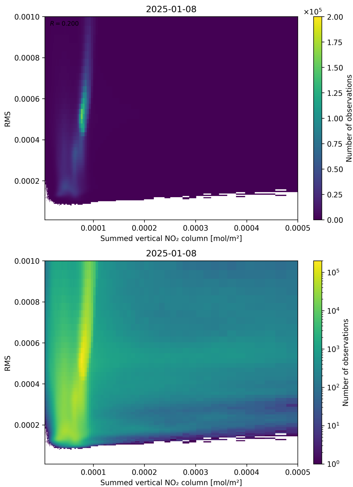
Figure 109: Scatter density plot of “Summed vertical NO 2 column” against “RMS” for 2025-01-07 to 2025-01-09.
