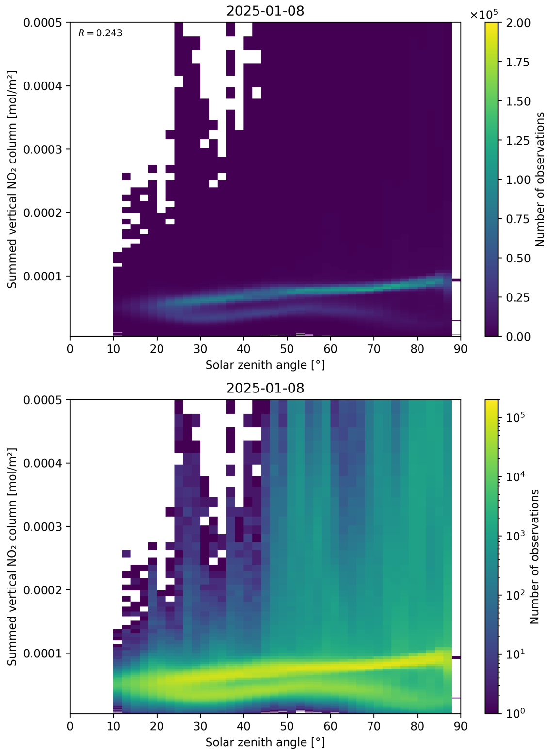
Figure 151: Scatter density plot of “Solar zenith angle” against “Summed vertical NO 2 column” for 2025-01-07 to 2025-01-09.
