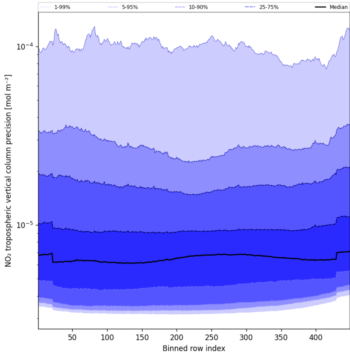
Figure 47: Along track statistics of “NO 2 tropospheric vertical column precision” for 2025-01-07 to 2025-01-09
