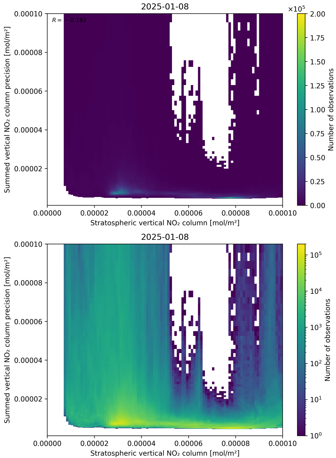
Figure 99: Scatter density plot of “Stratospheric vertical NO 2 column” against “Summed vertical NO 2 column precision” for 2025-01-07 to 2025-01-09.
