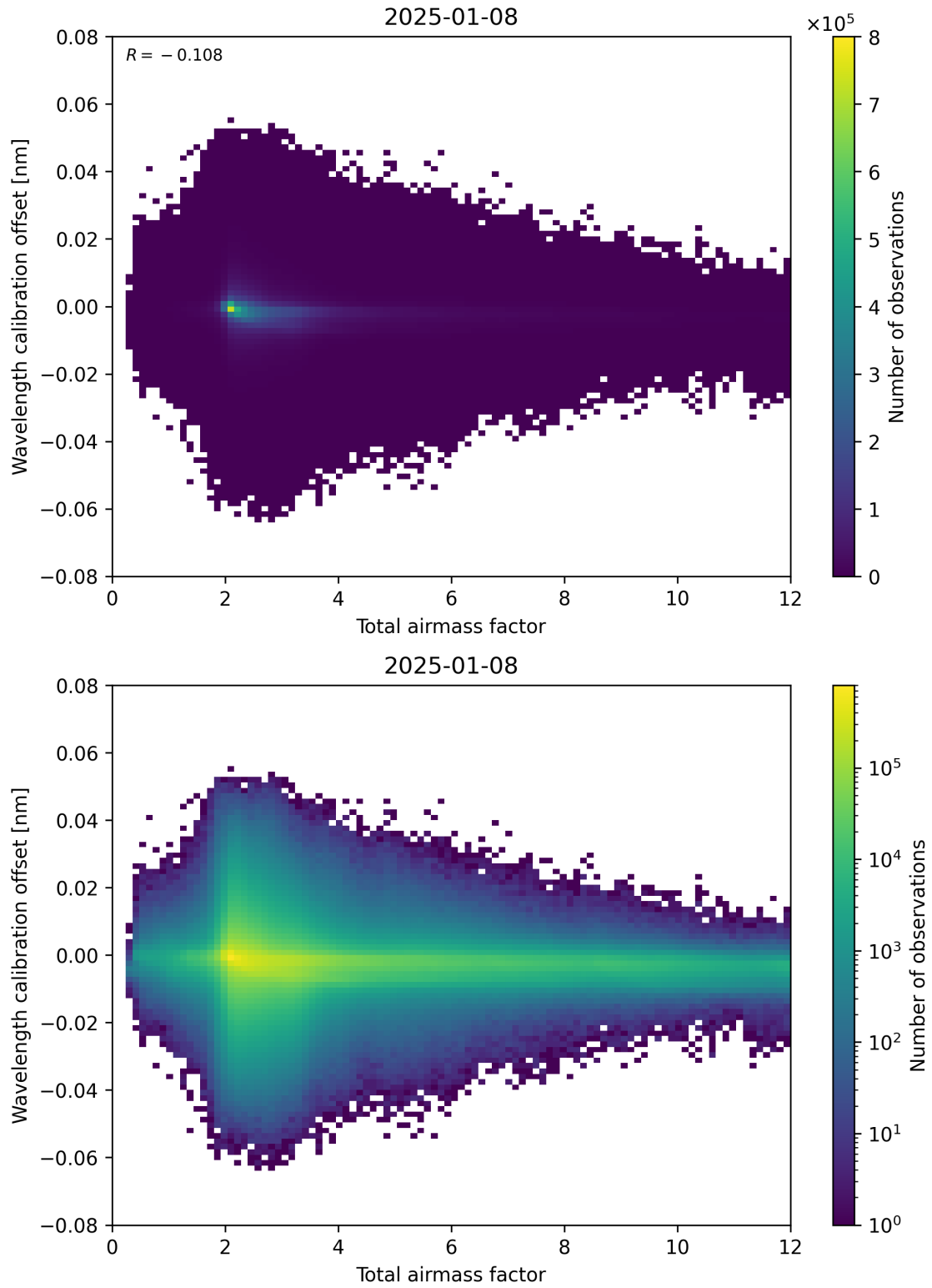
Figure 70: Scatter density plot of “Total airmass factor” against “Wavelength calibration offset” for 2025-01-07 to 2025-01-09.
