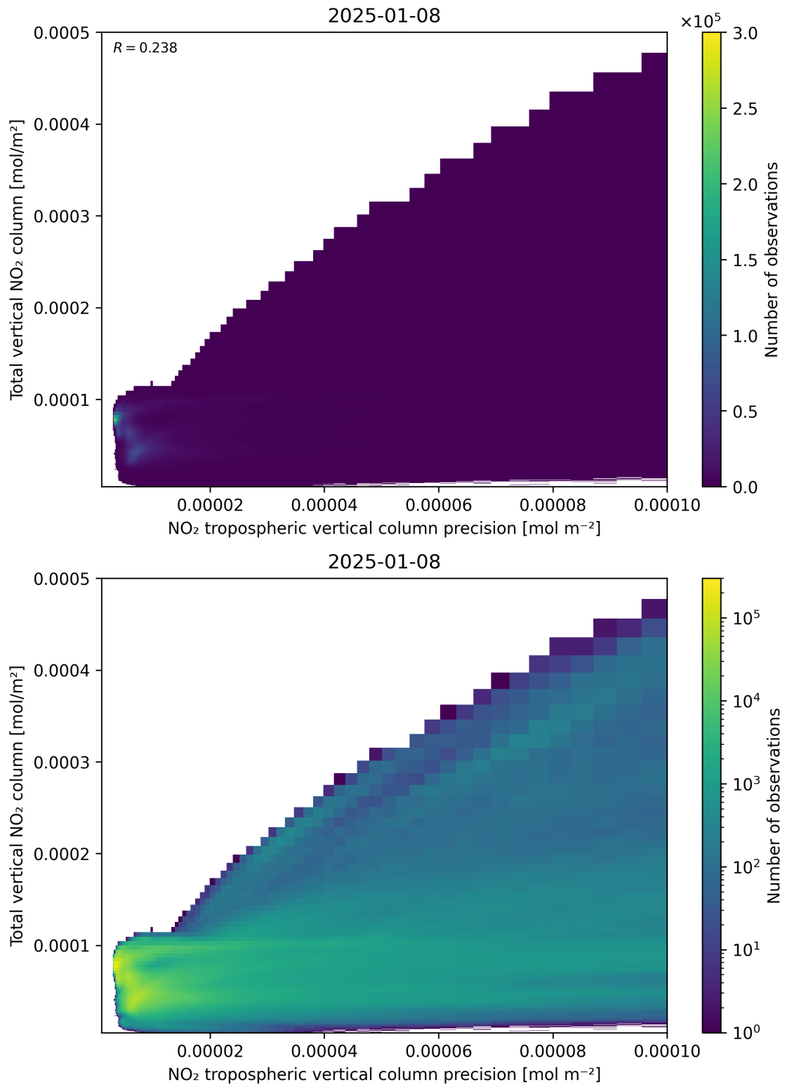
Figure 138: Scatter density plot of “NO 2 tropospheric vertical column precision” against “Total vertical NO 2 column” for 2025-01-07 to 2025-01-09.
