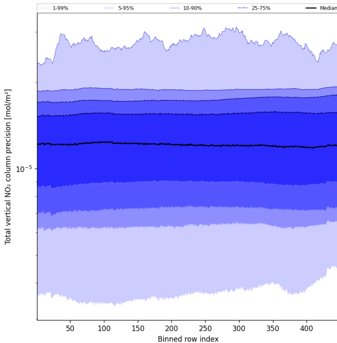
Figure 56: Along track statistics of “Total vertical NO 2 column precision” for 2025-01-07 to 2025-01-09
