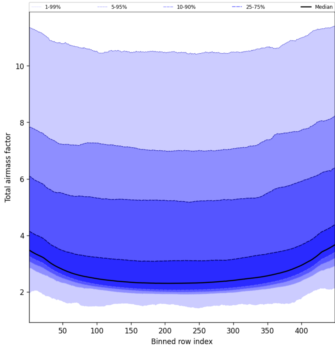
Figure 49: Along track statistics of “Total airmass factor” for 2025-01-07 to 2025-01-09
