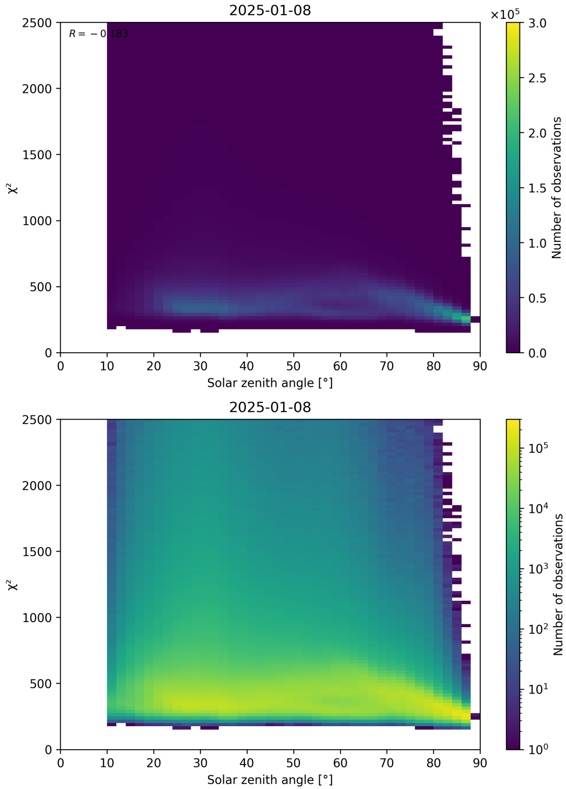
Figure 148: Scatter density plot of “Solar zenith angle” against “ \chi^2 ” for 2025-01-07 to 2025-01-09.
