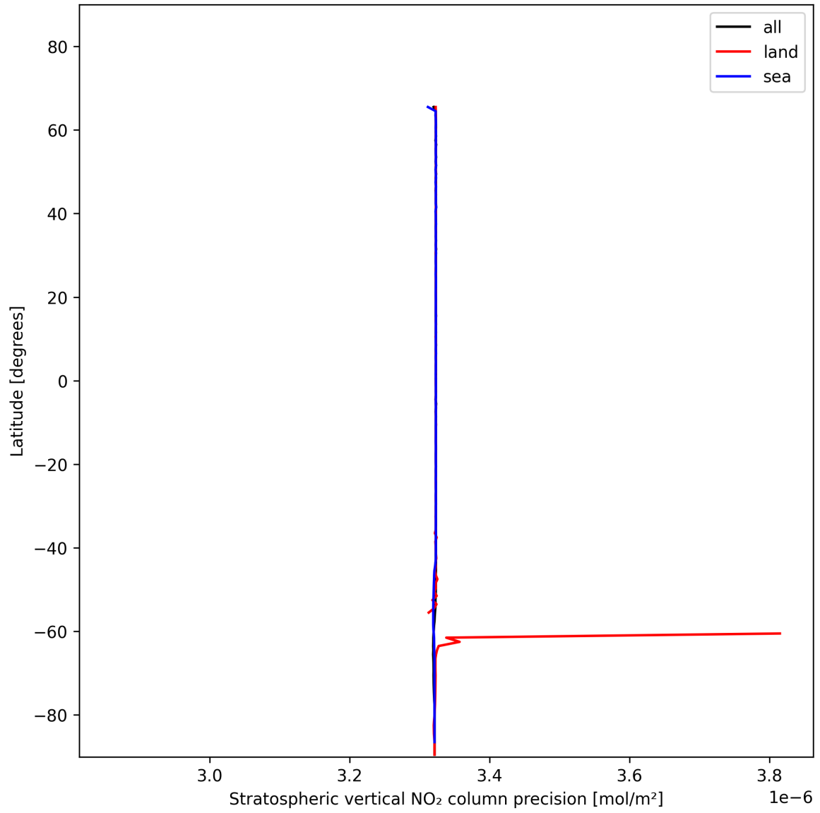
Figure 20: Zonal average of “Stratospheric vertical NO 2 column precision” for 2025-01-07 to 2025-01-09.
