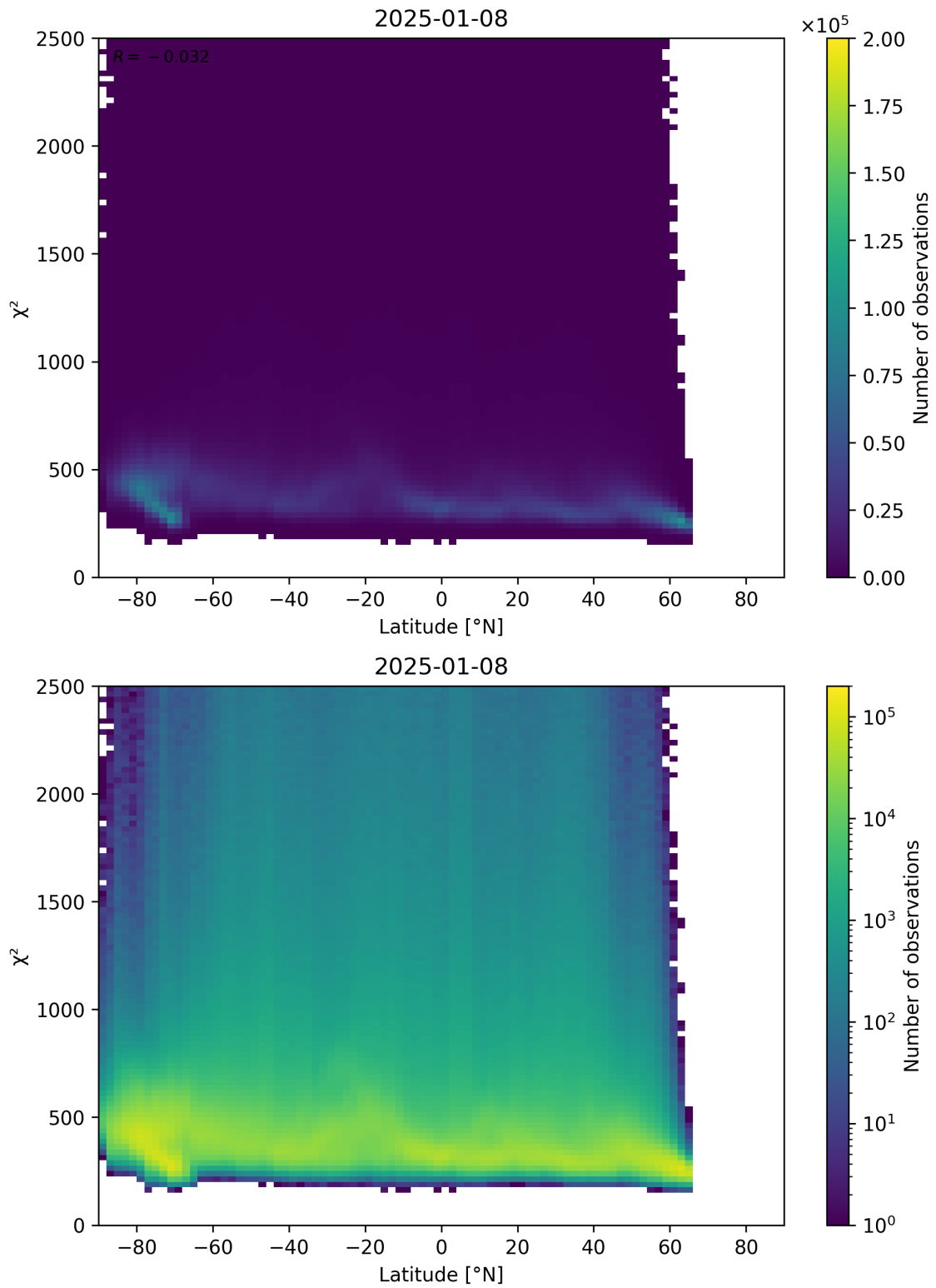
Figure 86: Scatter density plot of “Latitude” against “ \chi^2 ” for 2025-01-07 to 2025-01-09.
