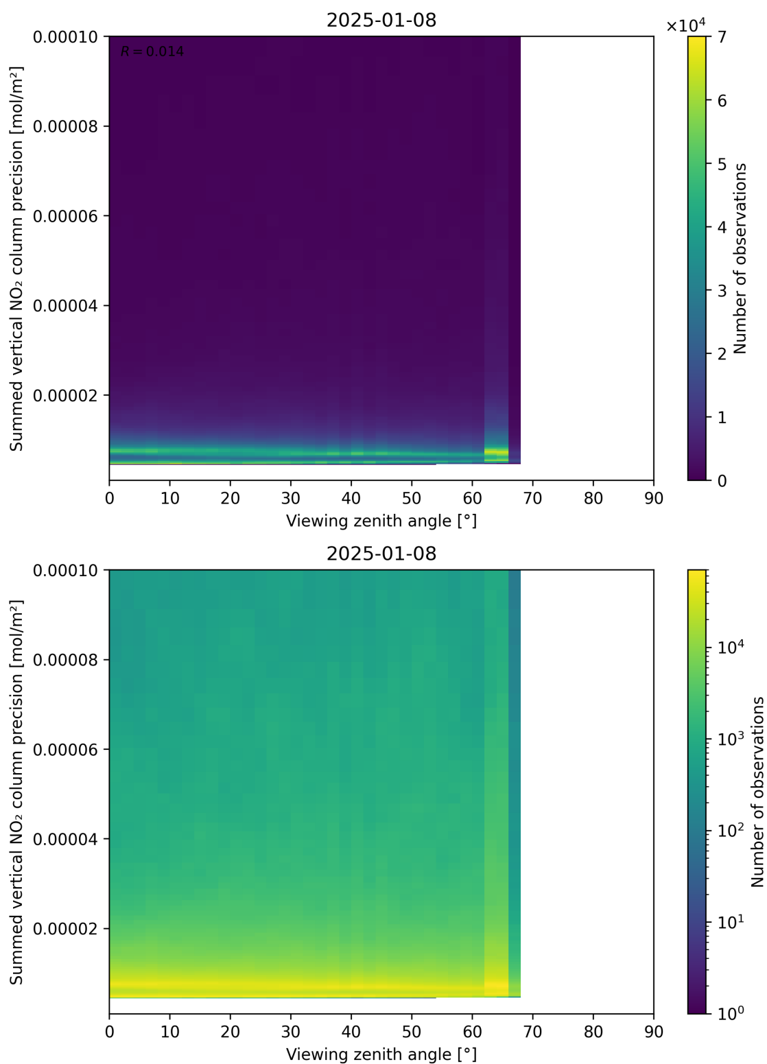
Figure 166: Scatter density plot of “Viewing zenith angle” against “Summed vertical NO 2 column precision” for 2025-01-07 to 2025-01-09.
