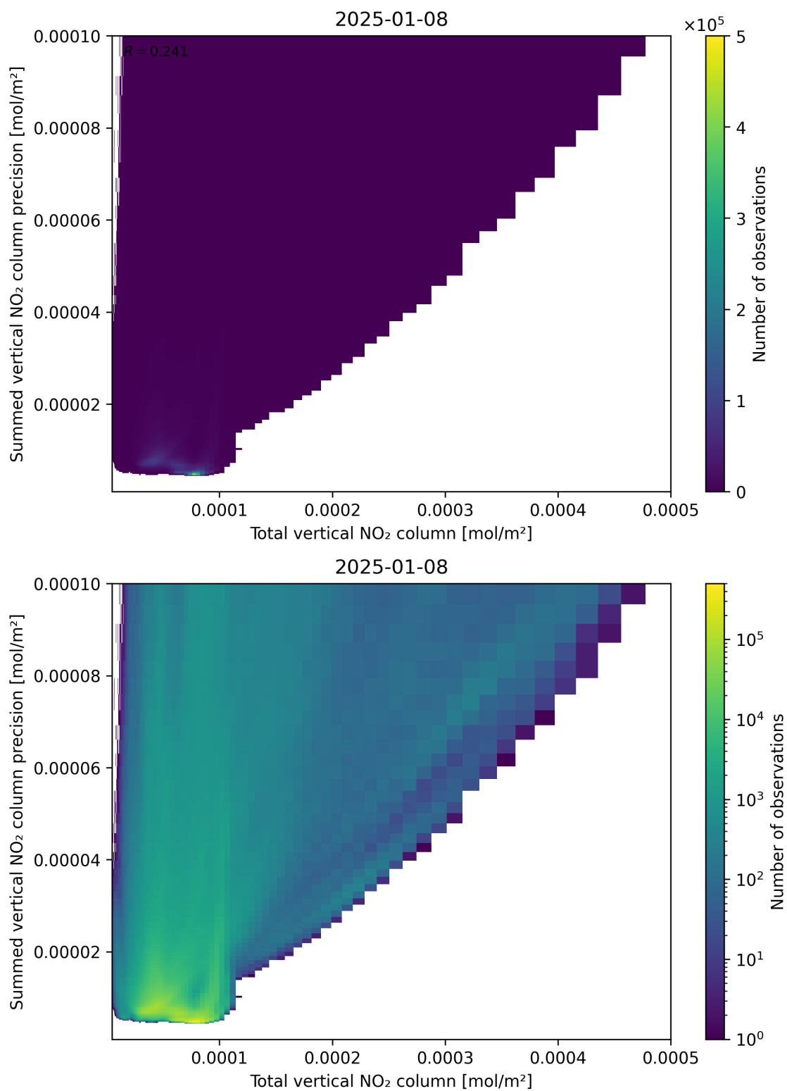
Figure 113: Scatter density plot of “Total vertical NO 2 column” against “Summed vertical NO 2 column precision” for 2025-01-07 to 2025-01-09.
