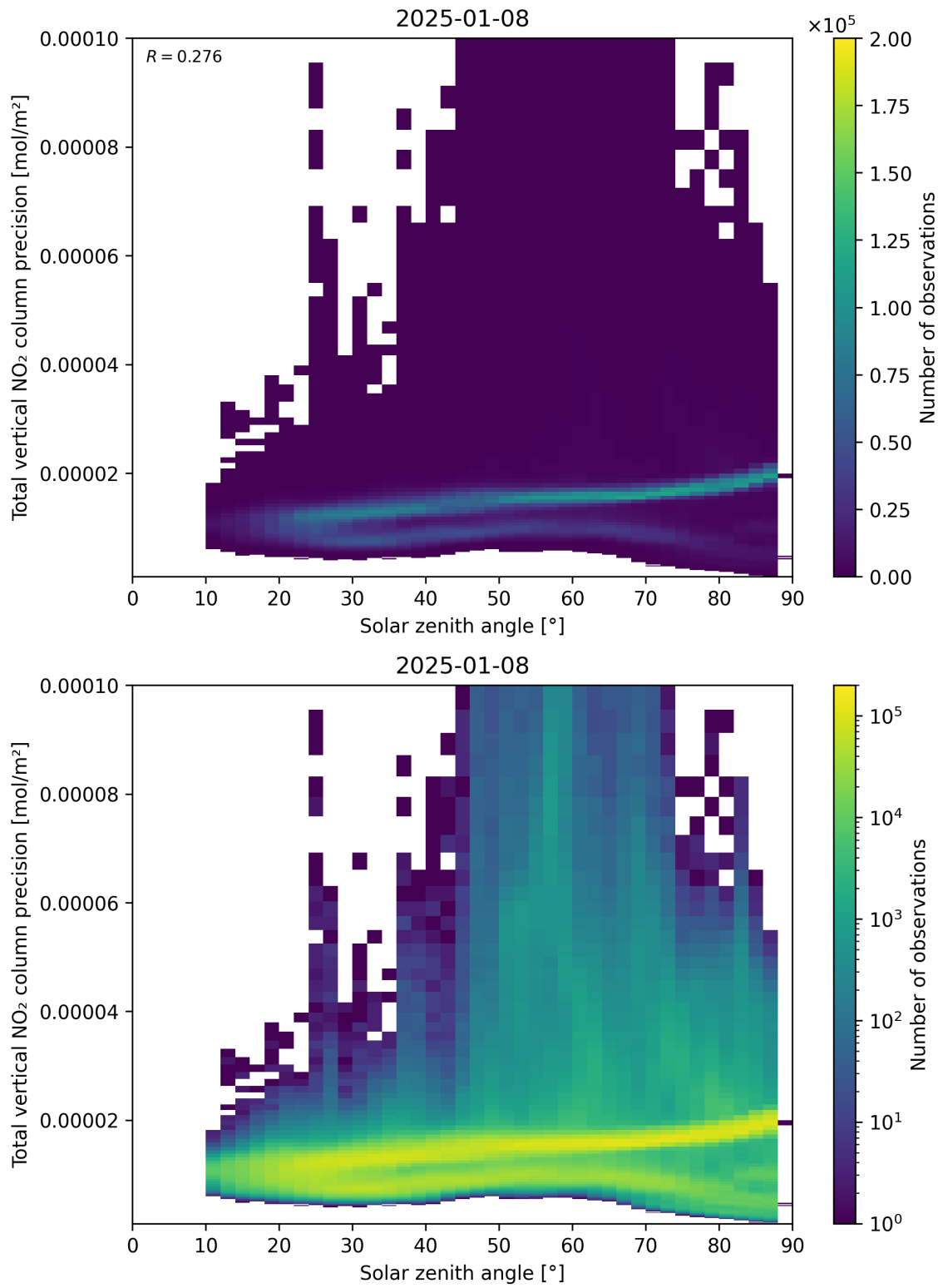
Figure 154: Scatter density plot of “Solar zenith angle” against “Total vertical NO 2 column precision” for 2025-01-07 to 2025-01-09.
