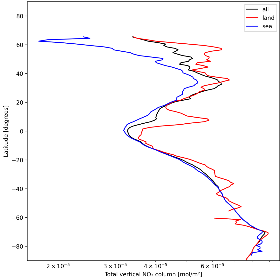
Figure 21: Zonal average of “Total vertical NO 2 column” for 2025-01-07 to 2025-01-09.
