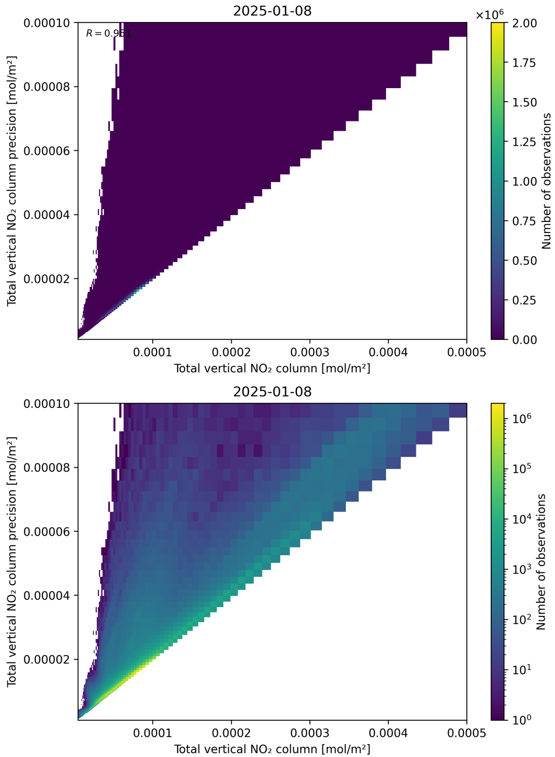
Figure 114: Scatter density plot of “Total vertical NO 2 column” against “Total vertical NO 2 column precision” for 2025-01-07 to 2025-01-09.
