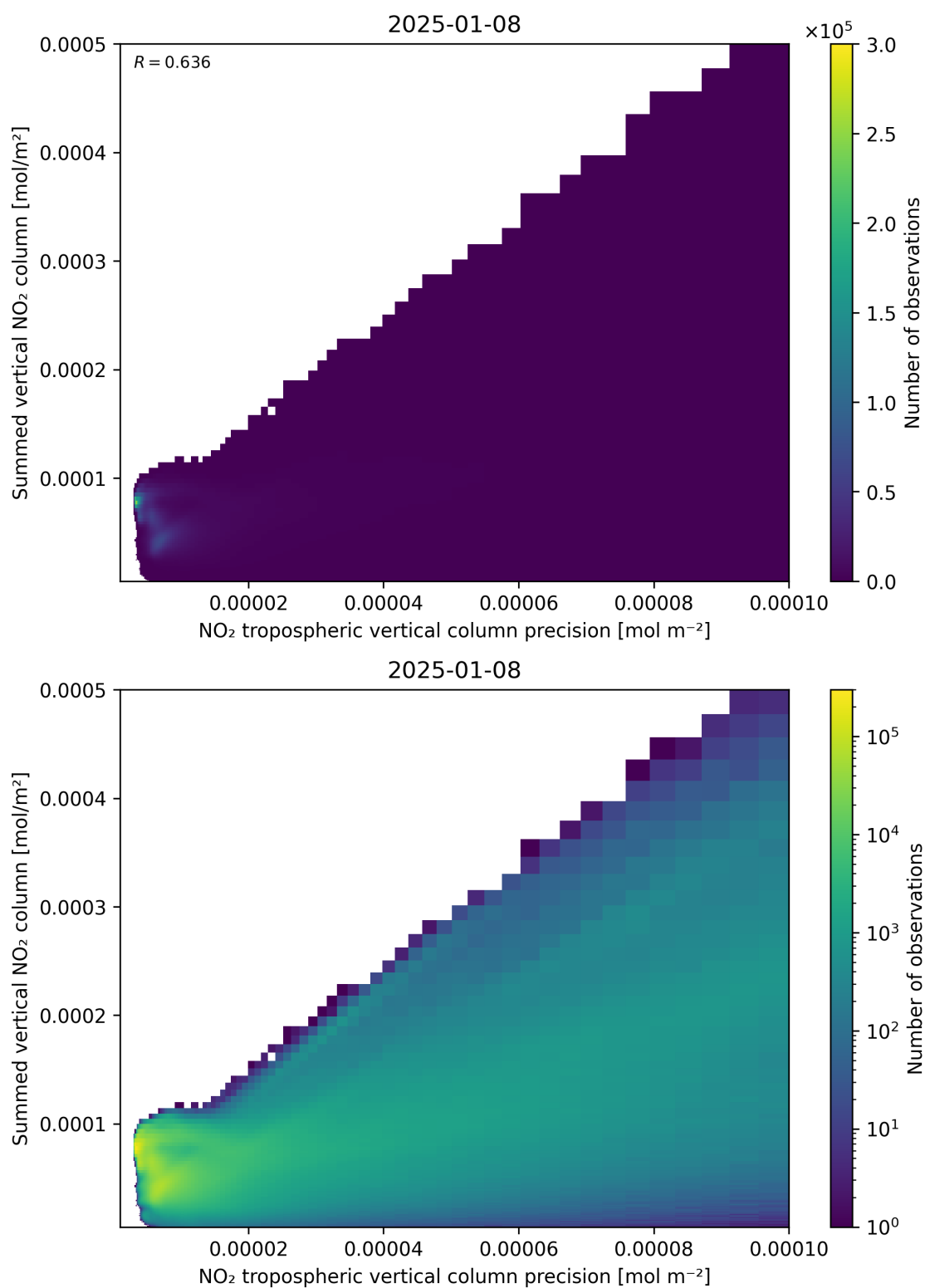
Figure 136: Scatter density plot of “NO 2 tropospheric vertical column precision” against “Summed vertical NO 2 column” for 2025-01-07 to 2025-01-09.
