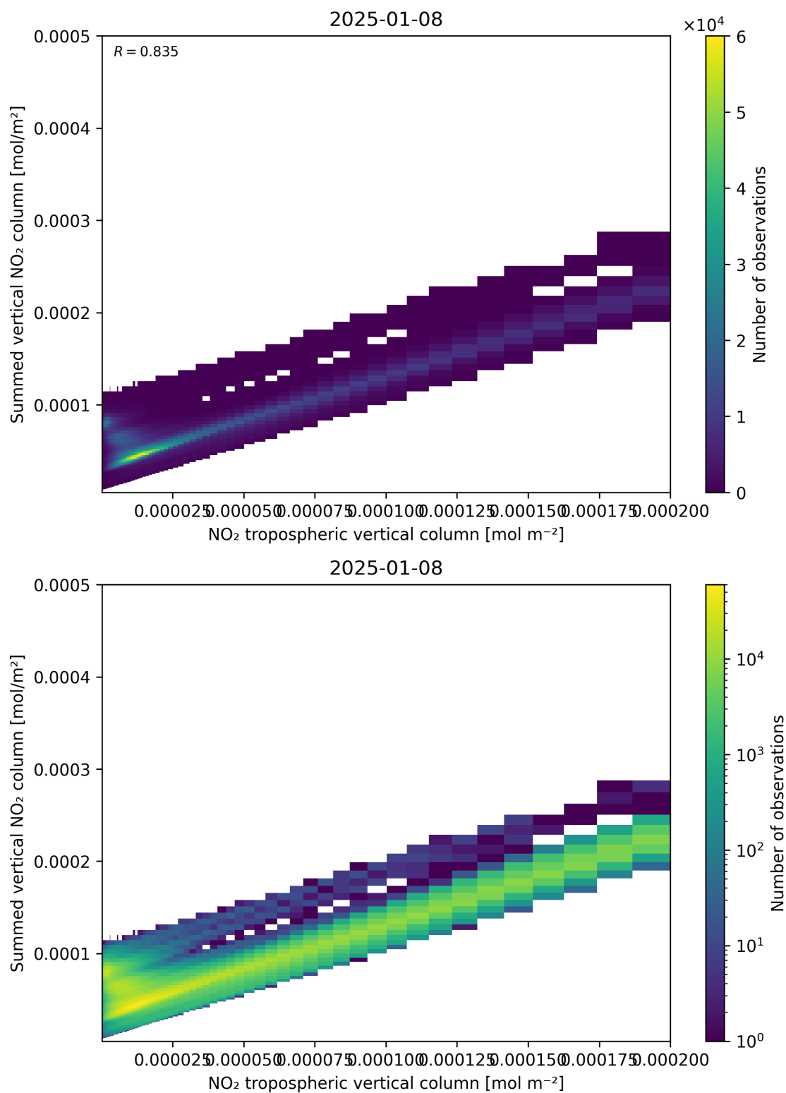
Figure 126: Scatter density plot of “NO 2 tropospheric vertical column” against “Summed vertical NO 2 column” for 2025-01-07 to 2025-01-09.
