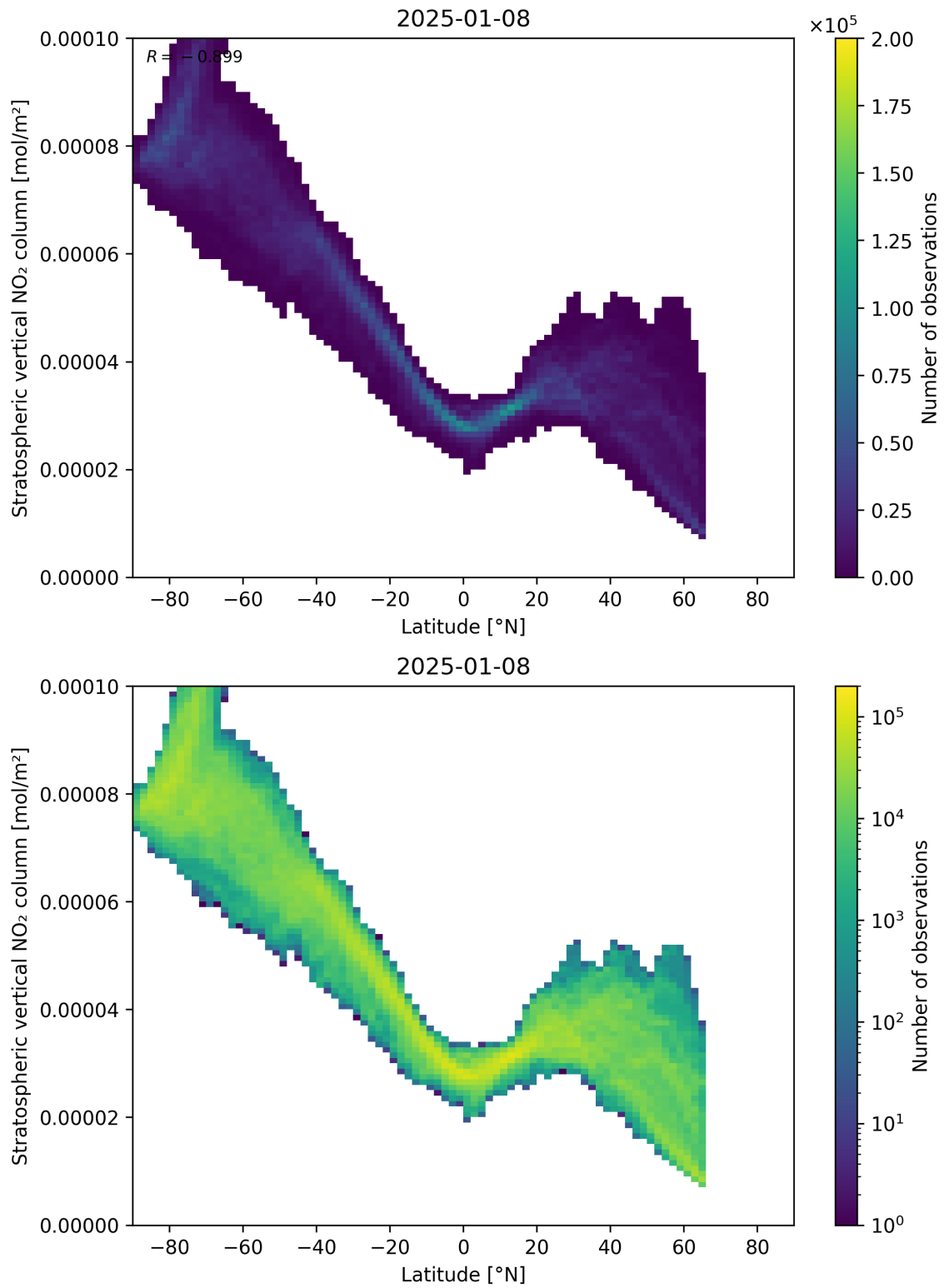
Figure 87: Scatter density plot of “Latitude” against “Stratospheric vertical NO 2 column” for 2025-01-07 to 2025-01-09.
