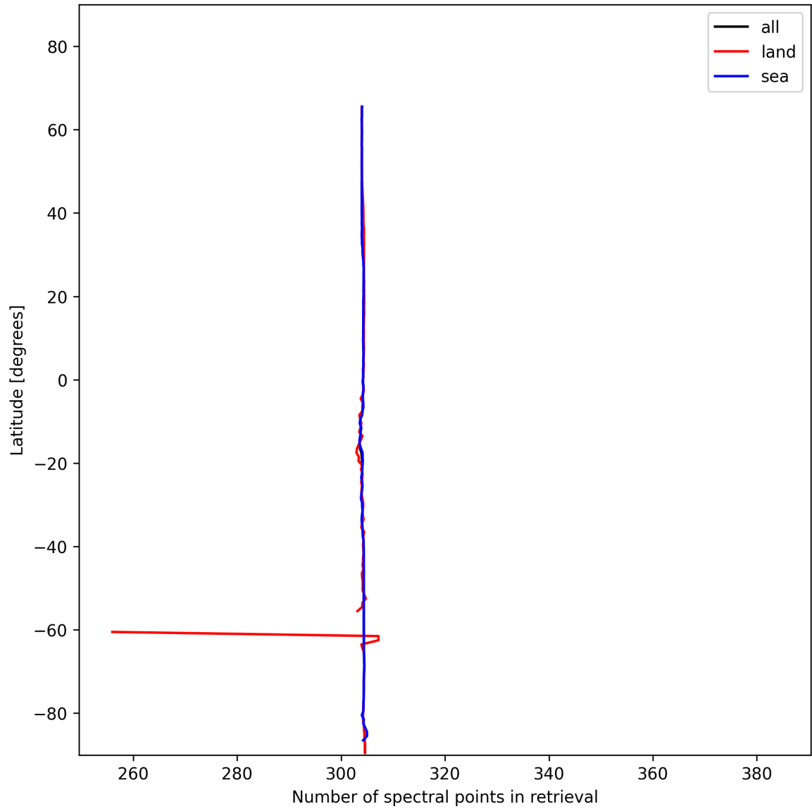
Figure 16: Zonal average of “Number of spectral points in retrieval” for 2025-01-07 to 2025-01-09.
