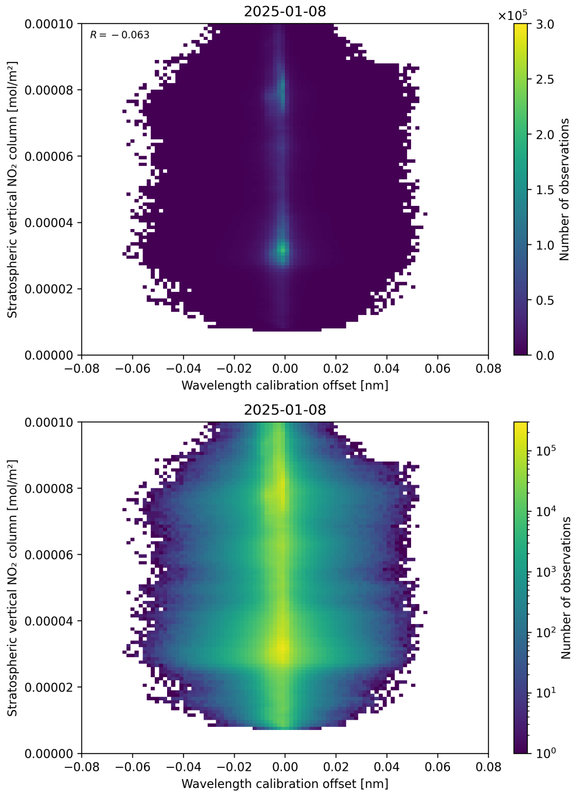
Figure 176: Scatter density plot of “Wavelength calibration offset” against “Stratospheric vertical NO 2 column” for 2025-01-07 to 2025-01-09.
