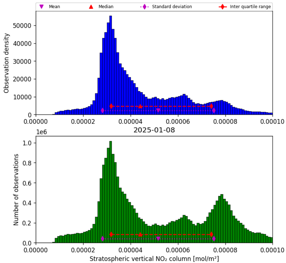
Figure 36: Histogram of “Stratospheric vertical NO 2 column” for 2025-01-07 to 2025-01-09
