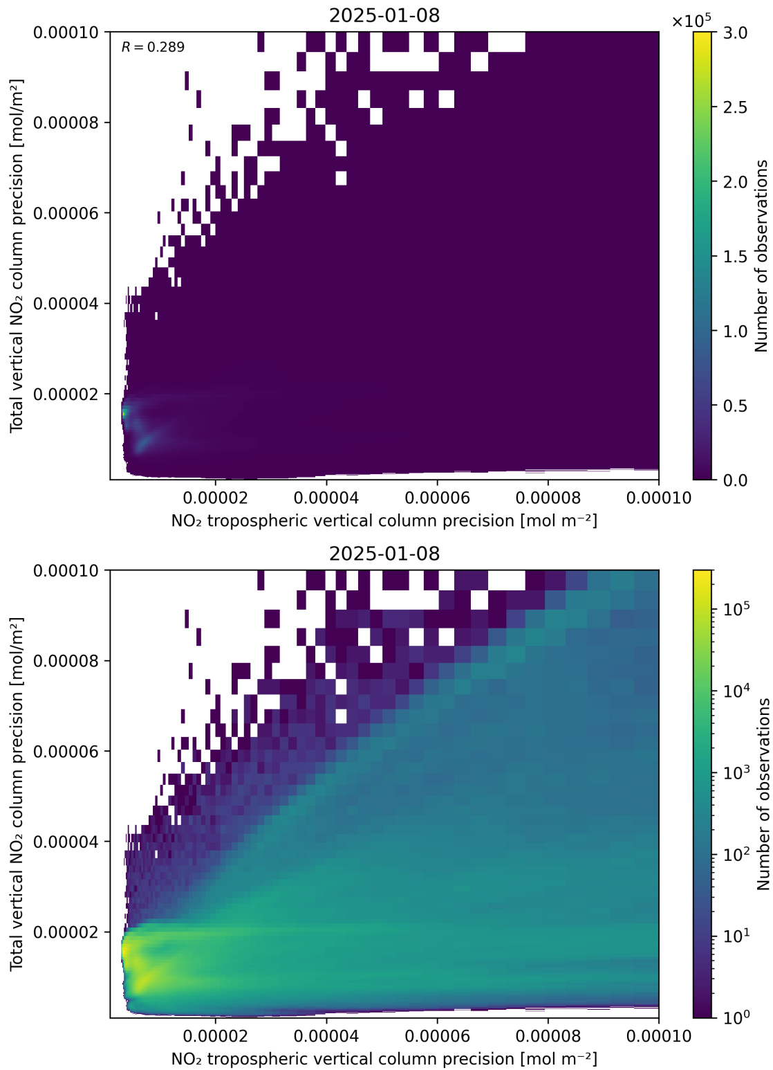
Figure 139: Scatter density plot of “NO 2 tropospheric vertical column precision” against “Total vertical NO 2 column precision” for 2025-01-07 to 2025-01-09.
