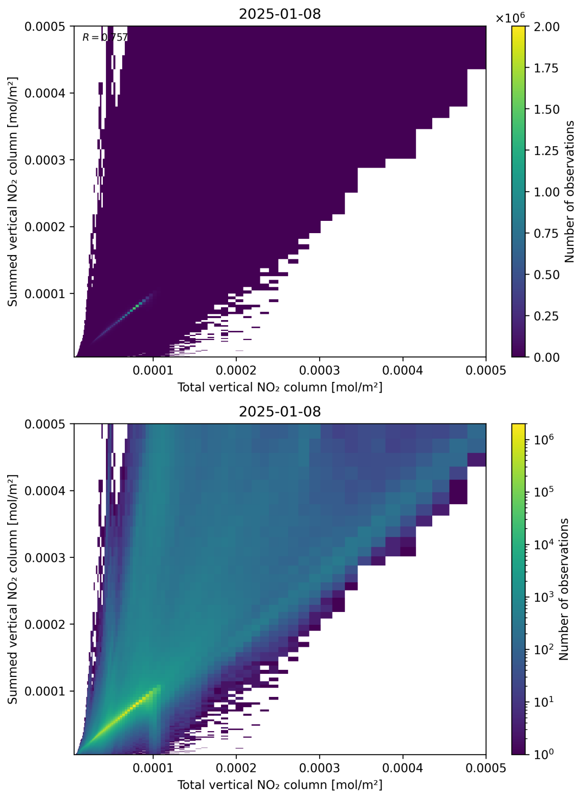
Figure 112: Scatter density plot of “Total vertical NO 2 column” against “Summed vertical NO 2 column” for 2025-01-07 to 2025-01-09.
