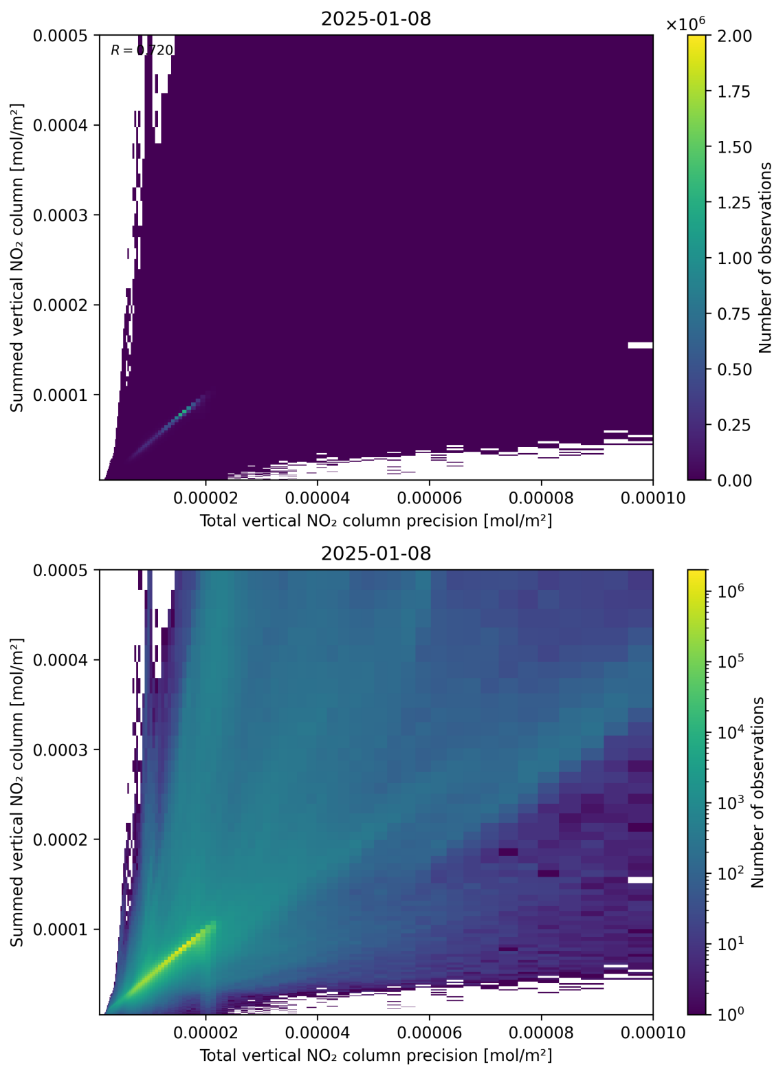
Figure 117: Scatter density plot of “Total vertical NO 2 column precision” against “Summed vertical NO 2 column” for 2025-01-07 to 2025-01-09.
