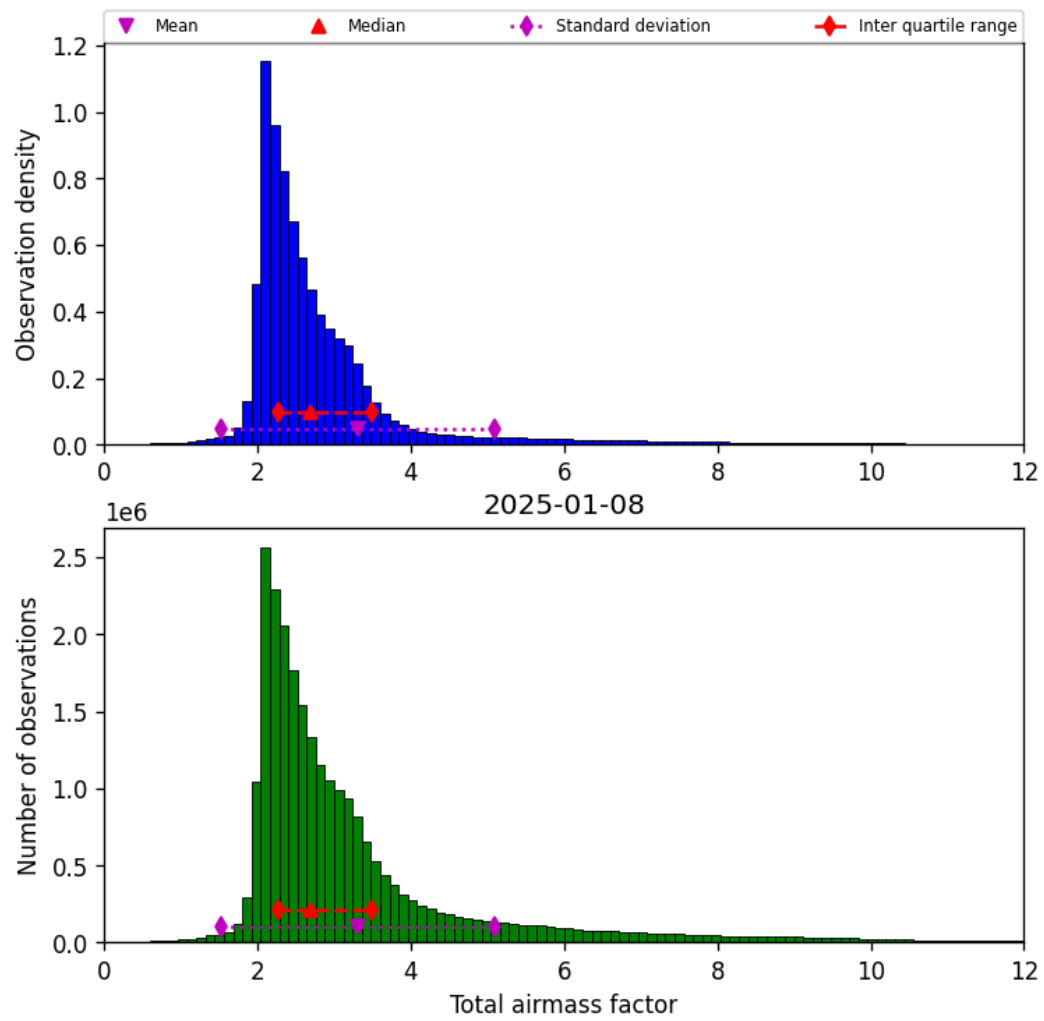
Figure 32: Histogram of “Total airmass factor” for 2025-01-07 to 2025-01-09
