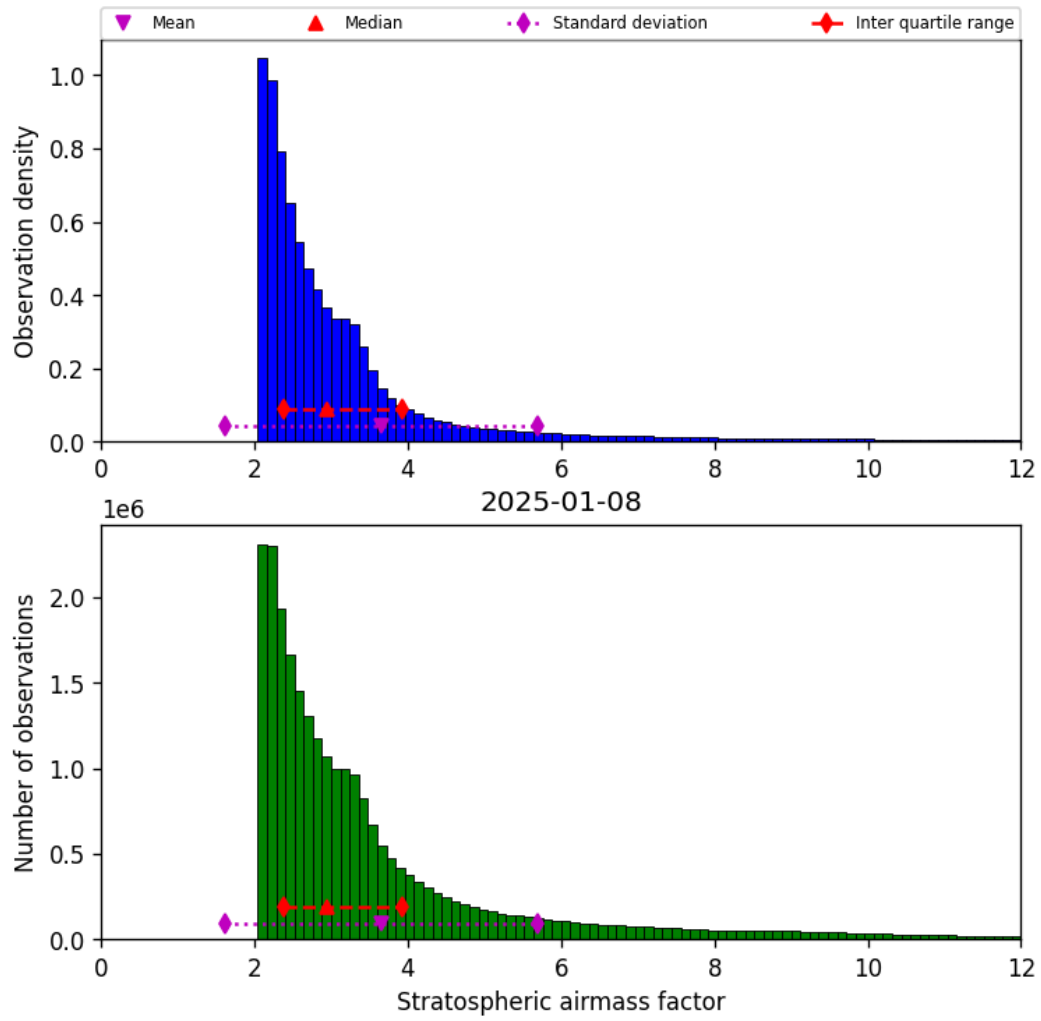
Figure 44: Histogram of “Stratospheric airmass factor” for 2025-01-07 to 2025-01-09
