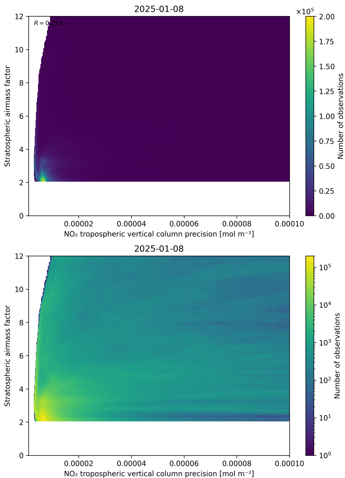
Figure 131: Scatter density plot of “NO 2 tropospheric vertical column precision” against “Stratospheric airmass factor” for 2025-01-07 to 2025-01-09.
