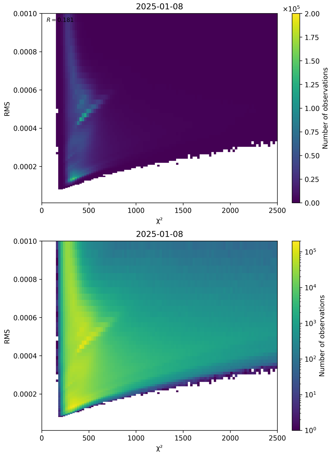
Figure 82: Scatter density plot of “ \chi^2 ” against “RMS” for 2025-01-07 to 2025-01-09.
