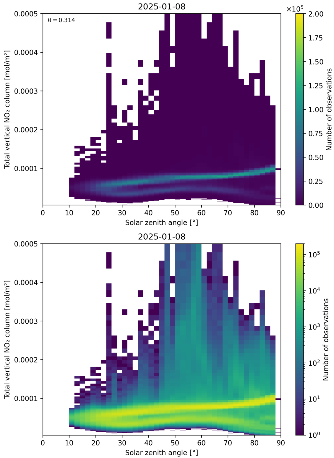
Figure 153: Scatter density plot of “Solar zenith angle” against “Total vertical NO 2 column” for 2025-01-07 to 2025-01-09.
