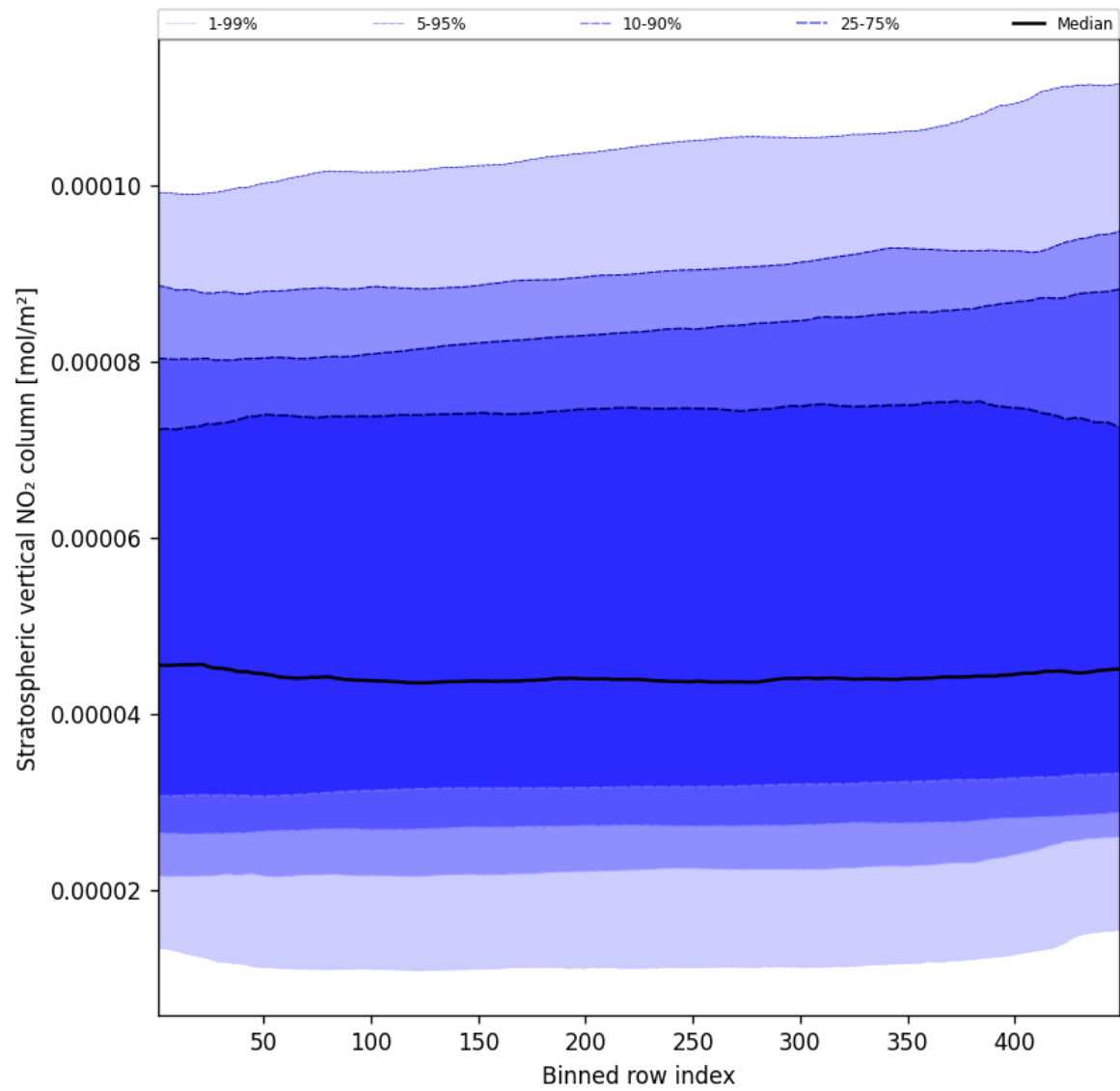
Figure 53: Along track statistics of “Stratospheric vertical NO 2 column” for 2025-01-07 to 2025-01-09
