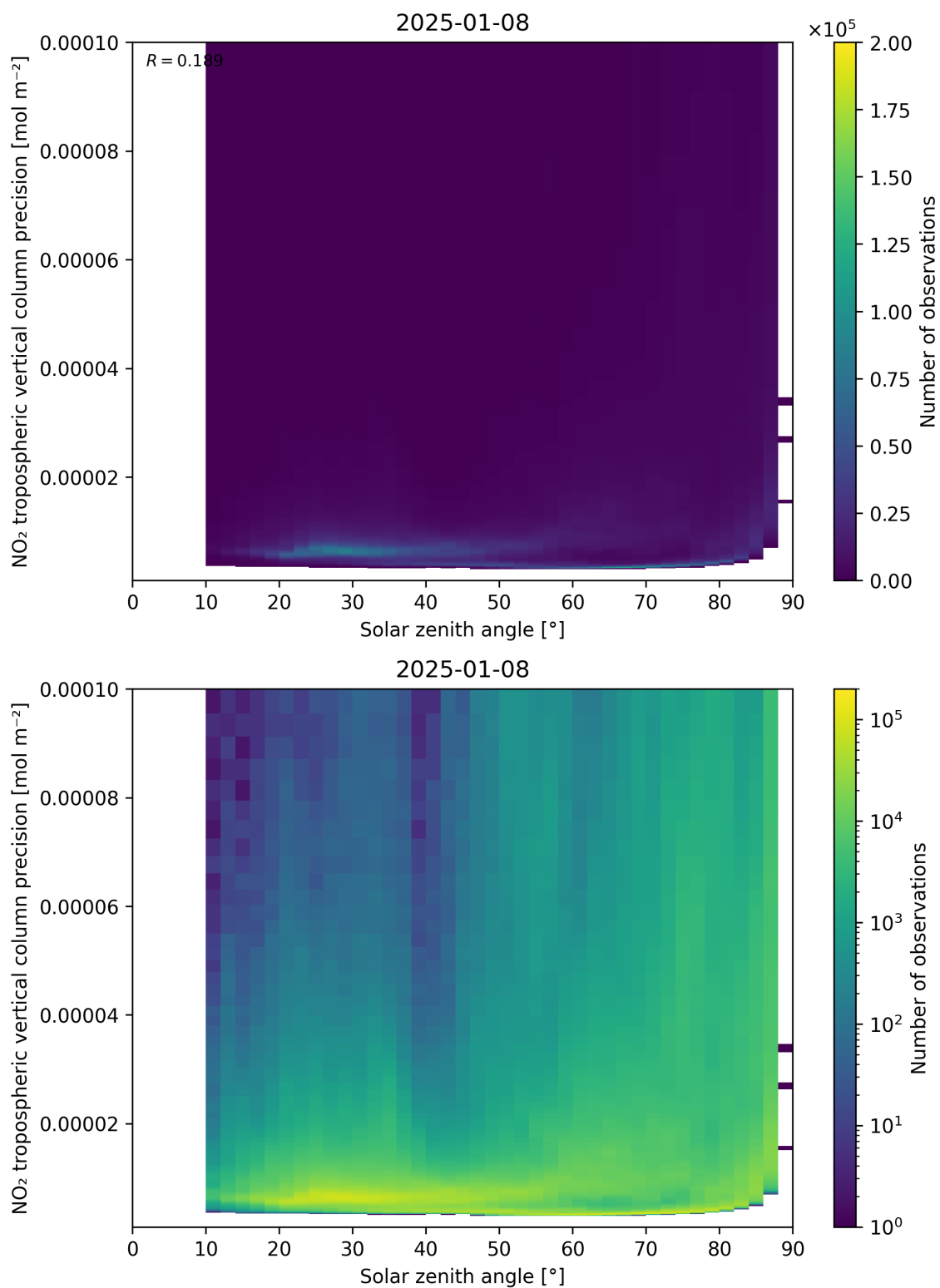
Figure 156: Scatter density plot of “Solar zenith angle” against “NO 2 tropospheric vertical column precision” for 2025-01-07 to 2025-01-09.
