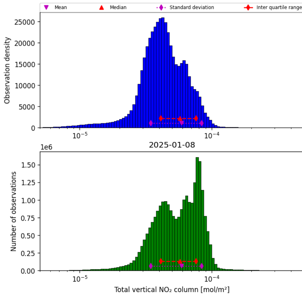
Figure 38: Histogram of “Total vertical NO 2 column” for 2025-01-07 to 2025-01-09
