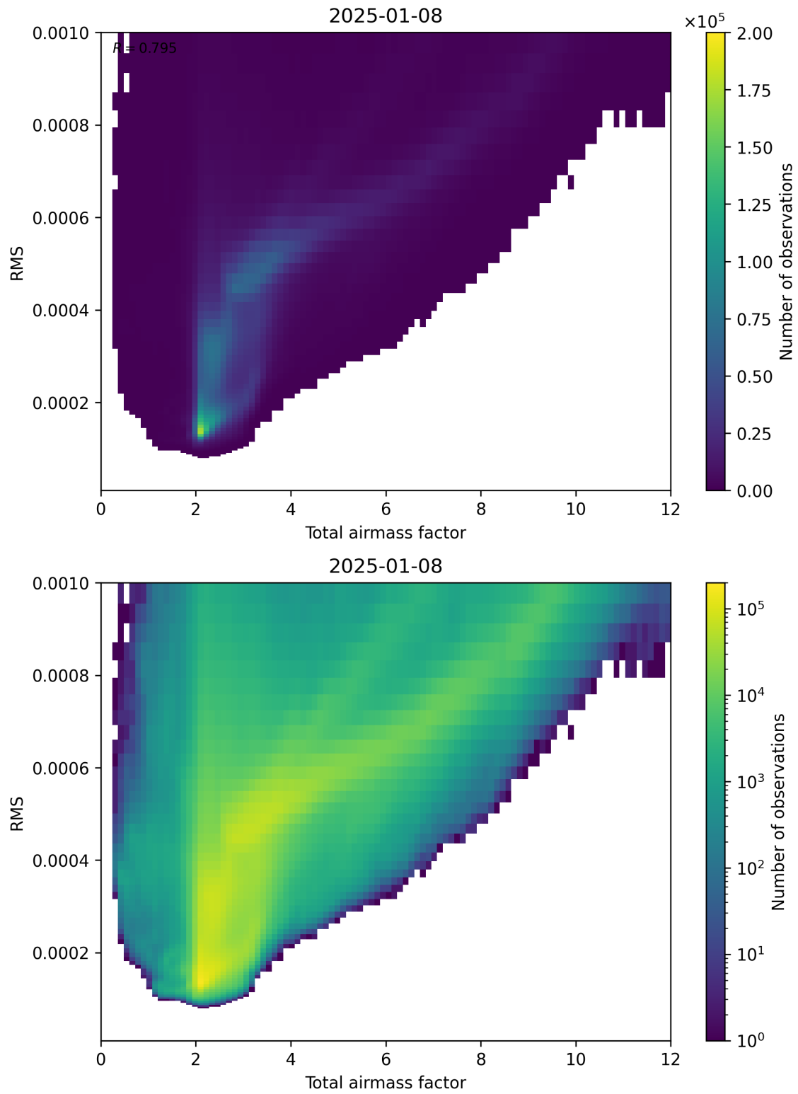
Figure 69: Scatter density plot of “Total airmass factor” against “RMS” for 2025-01-07 to 2025-01-09.
