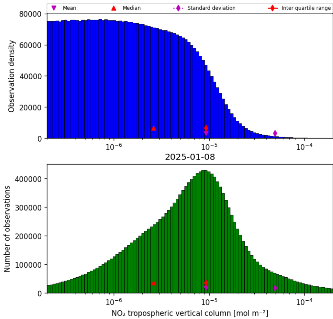
Figure 29: Histogram of “NO 2 tropospheric vertical column” for 2025-01-07 to 2025-01-09
