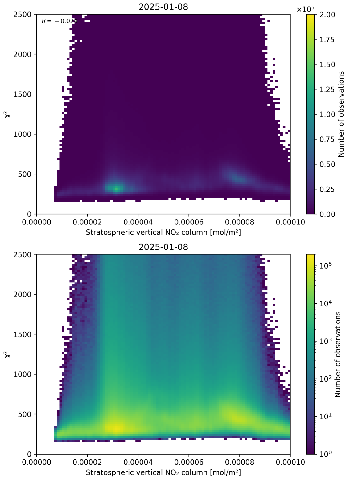
Figure 97: Scatter density plot of “Stratospheric vertical NO 2 column” against “ \chi^2 ” for 2025-01-07 to 2025-01-09.
