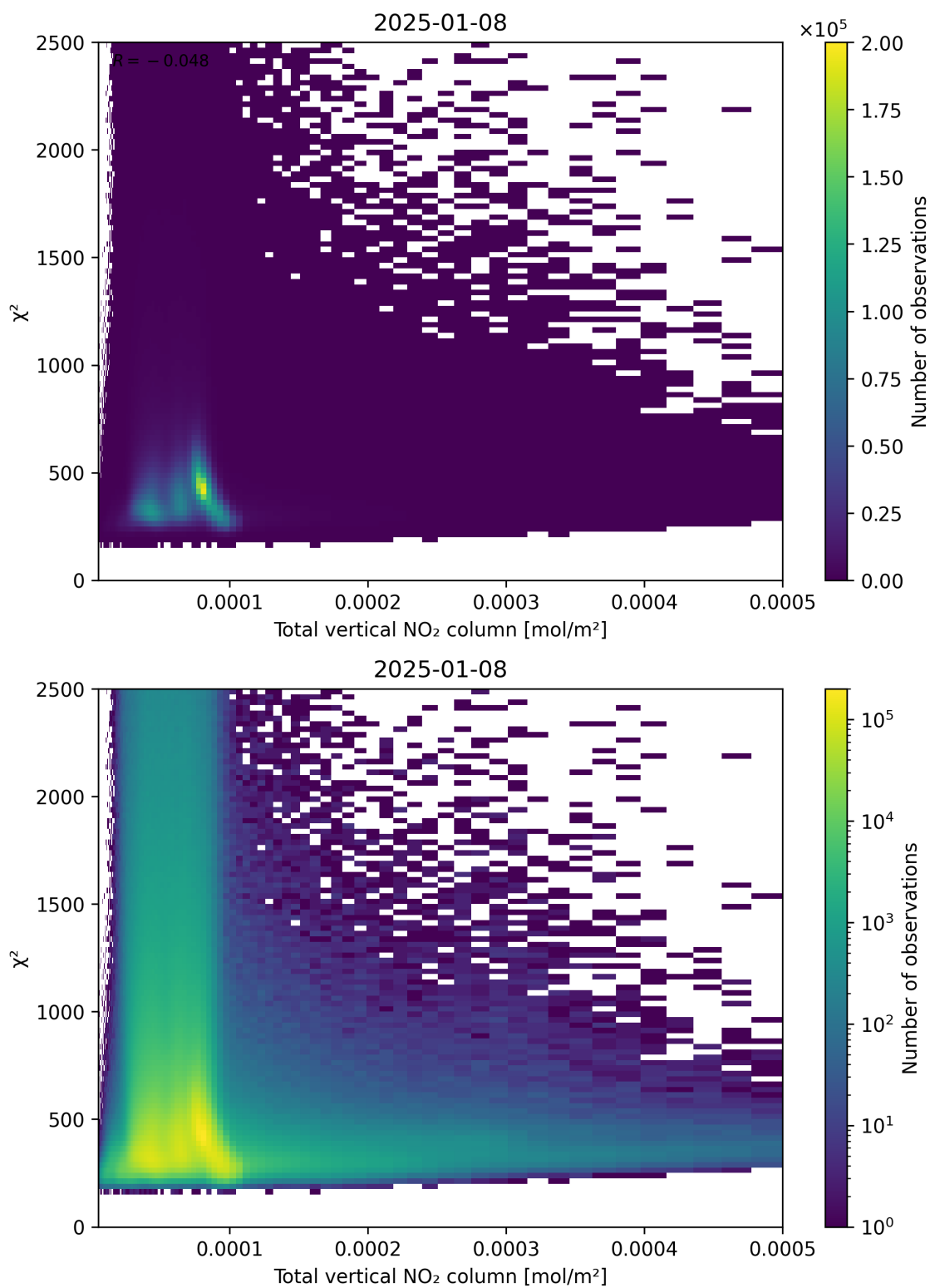
Figure 111: Scatter density plot of “Total vertical NO 2 column” against “ \chi^2 ” for 2025-01-07 to 2025-01-09.
