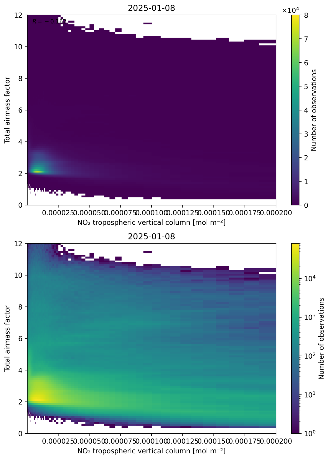
Figure 122: Scatter density plot of “NO 2 tropospheric vertical column” against “Total air mass factor” for 2025-01-07 to 2025-01-09.
