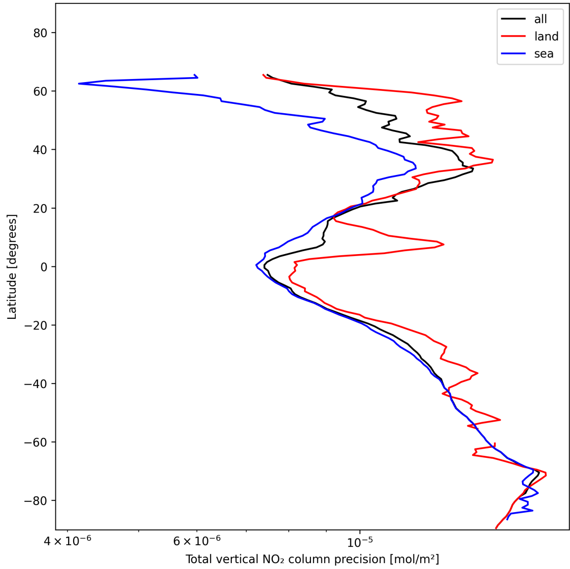
Figure 22: Zonal average of “Total vertical NO 2 column precision” for 2025-01-07 to 2025-01-09.
