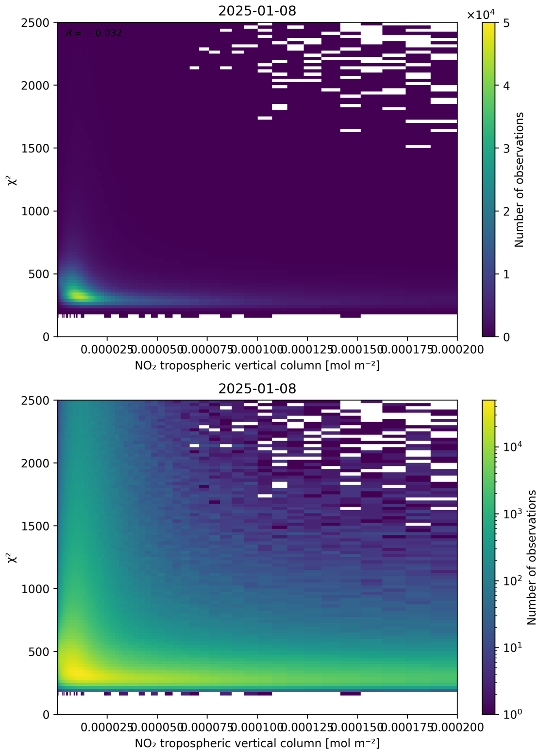
Figure 124: Scatter density plot of “NO 2 tropospheric vertical column” against “ \chi^2 ” for 2025-01-07 to 2025-01-09.
