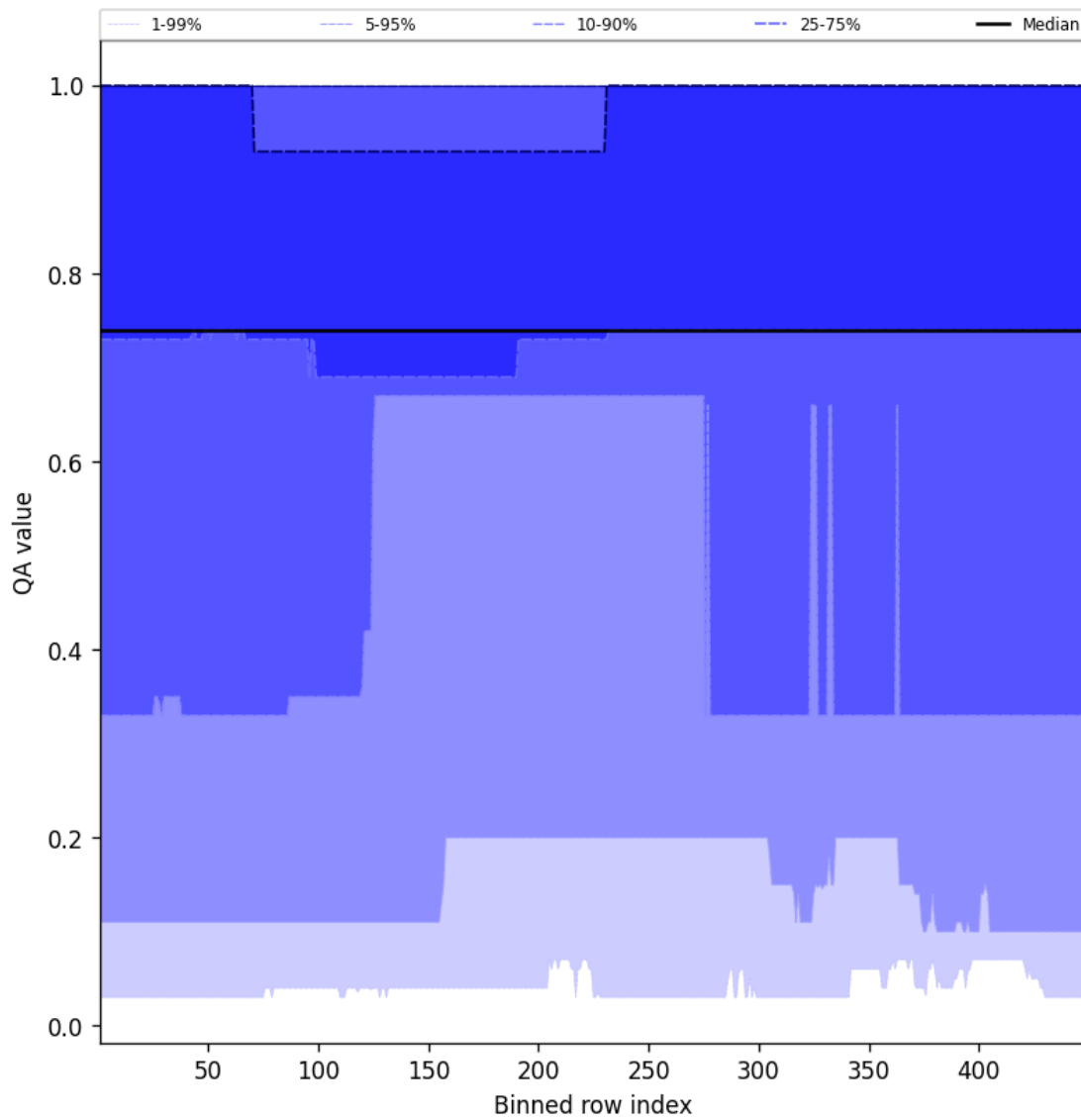
Figure 45: Along track statistics of “QA value” for 2025-01-07 to 2025-01-09
