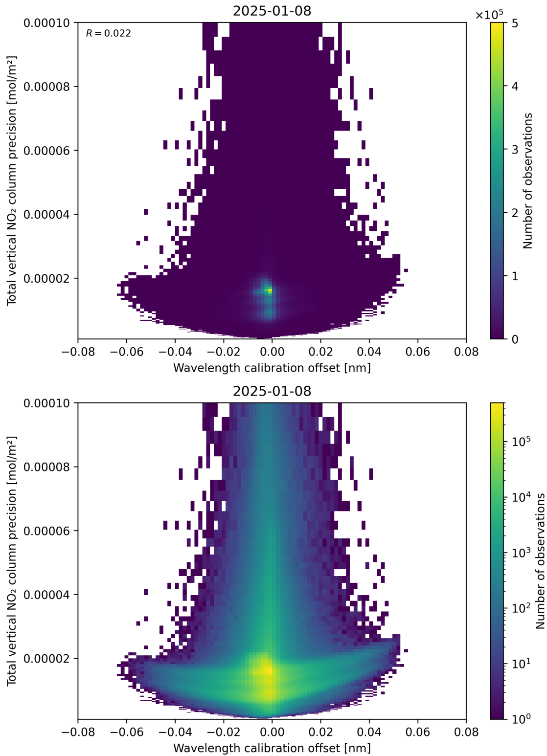
Figure 180: Scatter density plot of “Wavelength calibration offset” against “Total vertical NO 2 column precision” for 2025-01-07 to 2025-01-09.
