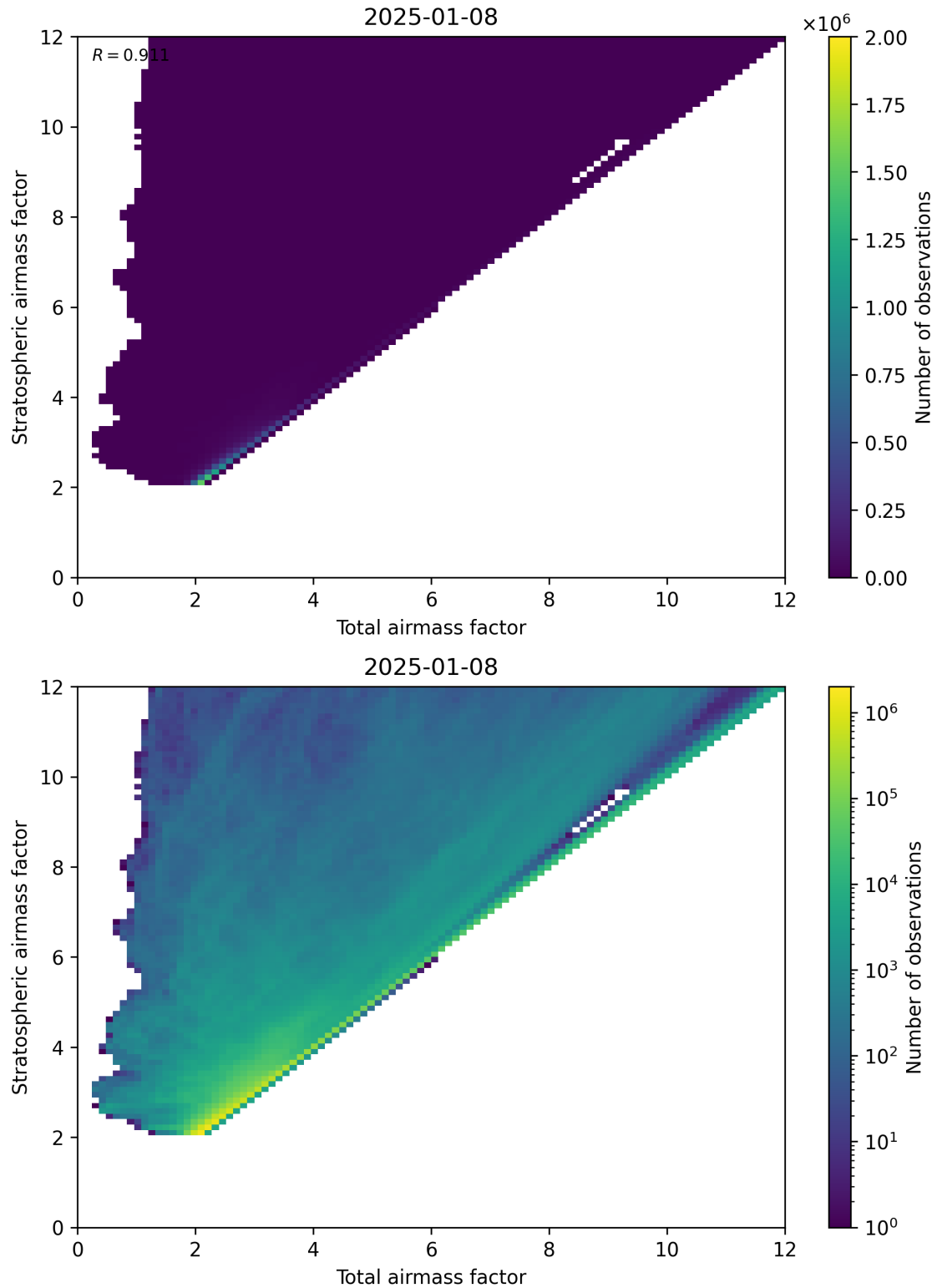
Figure 62: Scatter density plot of “Total airmass factor” against “Stratospheric airmass factor” for 2025-01-07 to 2025-01-09.
