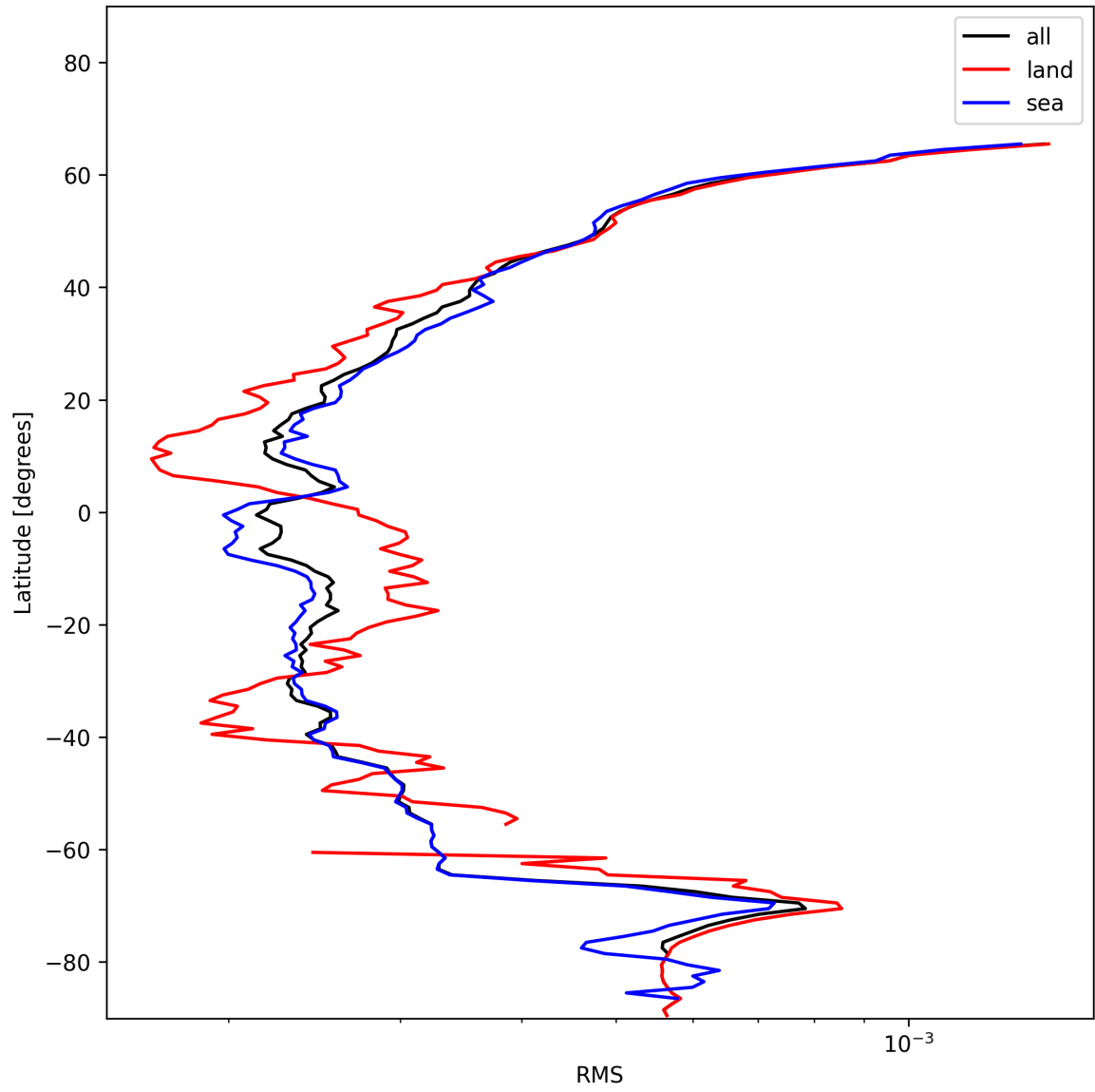
Figure 26: Zonal average of “RMS” for 2025-01-07 to 2025-01-09.
