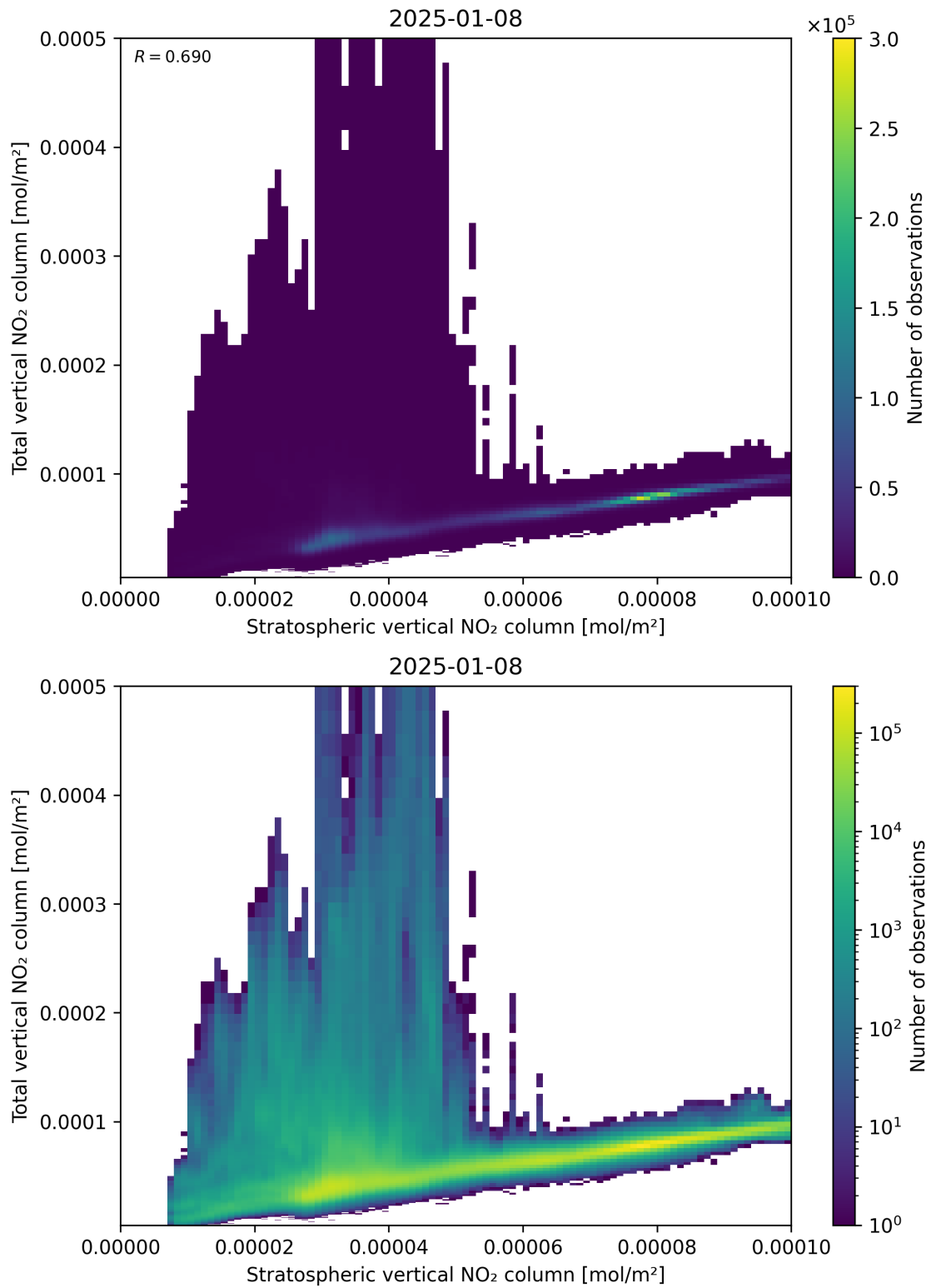
Figure 100: Scatter density plot of “Stratospheric vertical NO 2 column” against “Total vertical NO 2 column” for 2025-01-07 to 2025-01-09.
