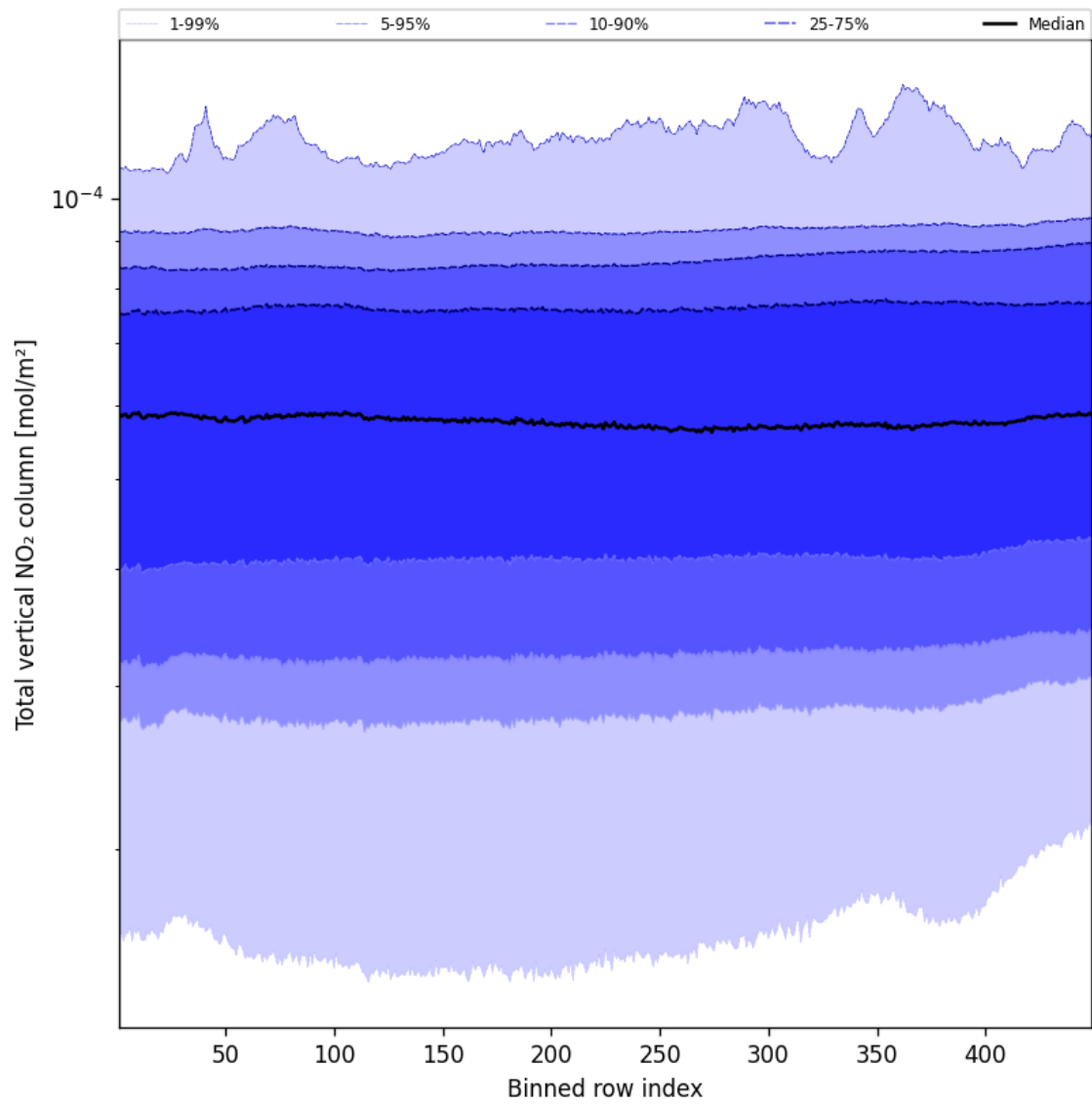
Figure 55: Along track statistics of “Total vertical NO 2 column” for 2025-01-07 to 2025-01-09
