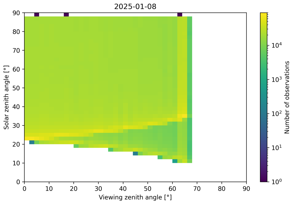
Figure 172: Scatter density plot of “Viewing zenith angle” against “Solar zenith angle” for 2025-01-07 to 2025-01-09.
