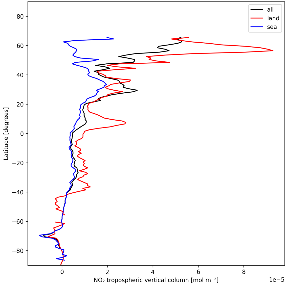
Figure 12: Zonal average of “NO 2 tropospheric vertical column” for 2025-01-07 to 2025-01-09.
