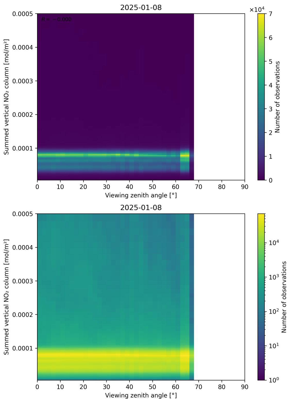
Figure 165: Scatter density plot of “Viewing zenith angle” against “Summed vertical NO 2 column” for 2025-01-07 to 2025-01-09.
