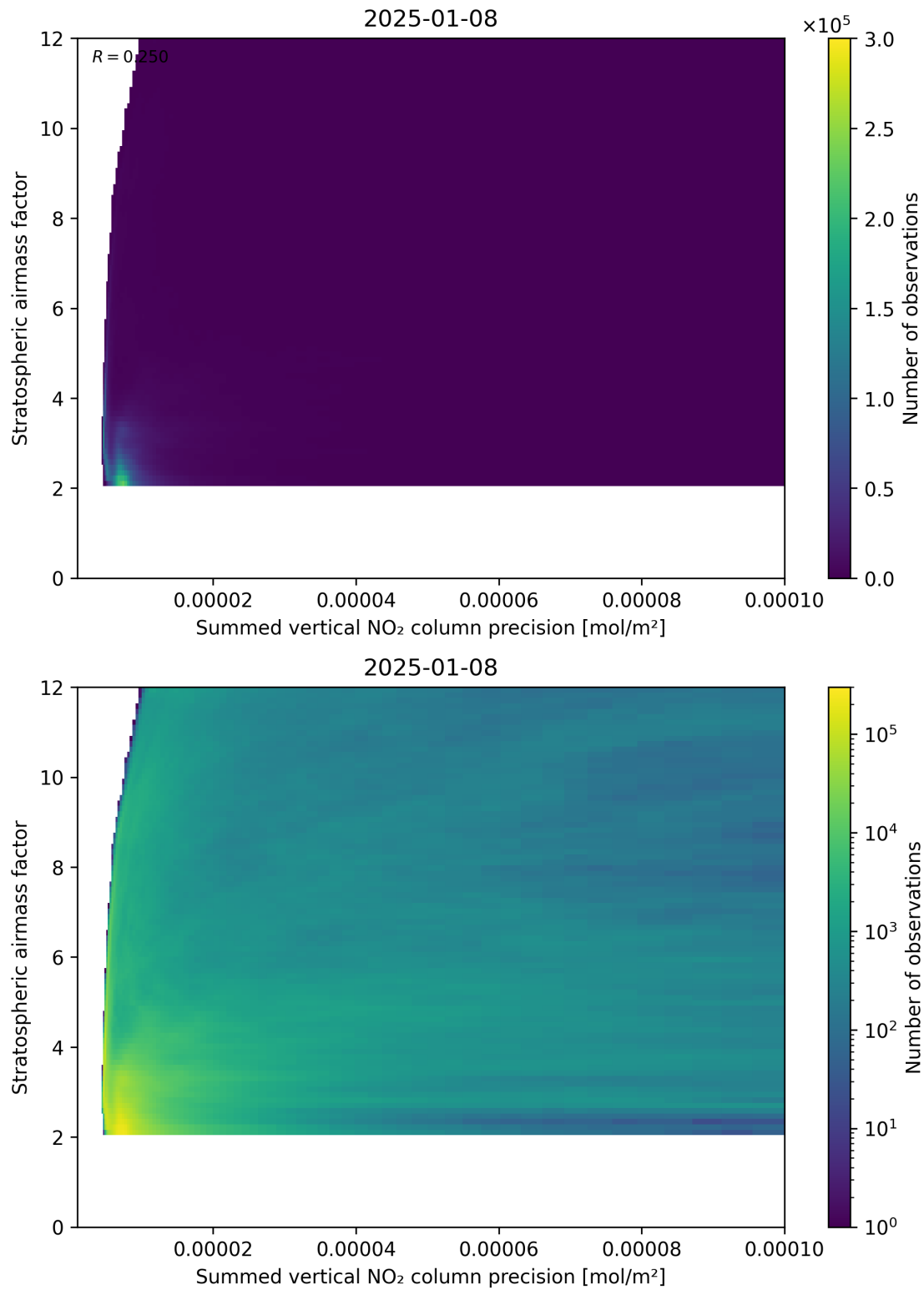
Figure 106: Scatter density plot of “Summed vertical NO 2 column precision” against “Stratospheric airmass factor” for 2025-01-07 to 2025-01-09.
