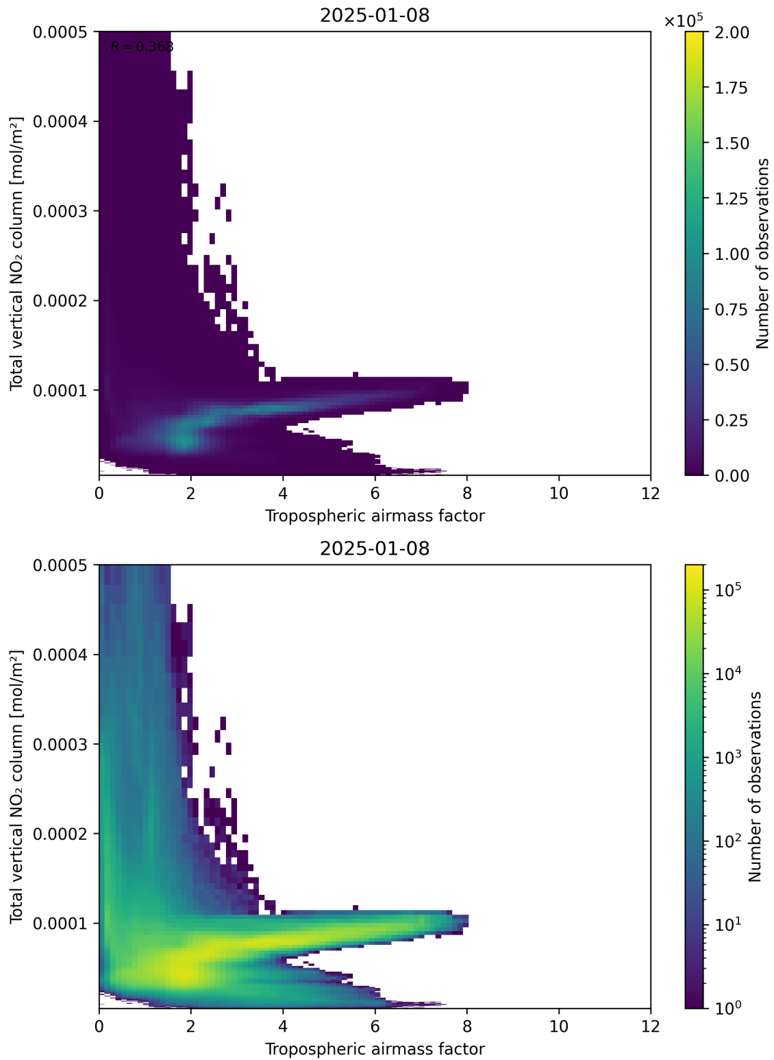
Figure 77: Scatter density plot of “Tropospheric airmass factor” against “Total vertical NO 2 column” for 2025-01-07 to 2025-01-09.
