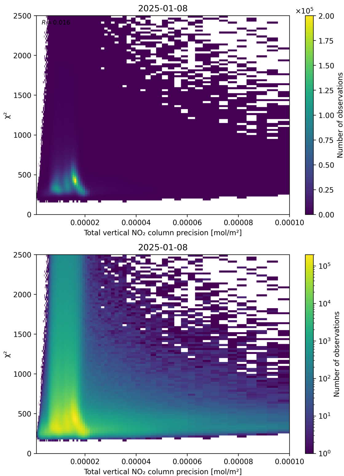
Figure 116: Scatter density plot of “Total vertical NO 2 column precision” against “ \chi^2 ” for 2025-01-07 to 2025-01-09.
