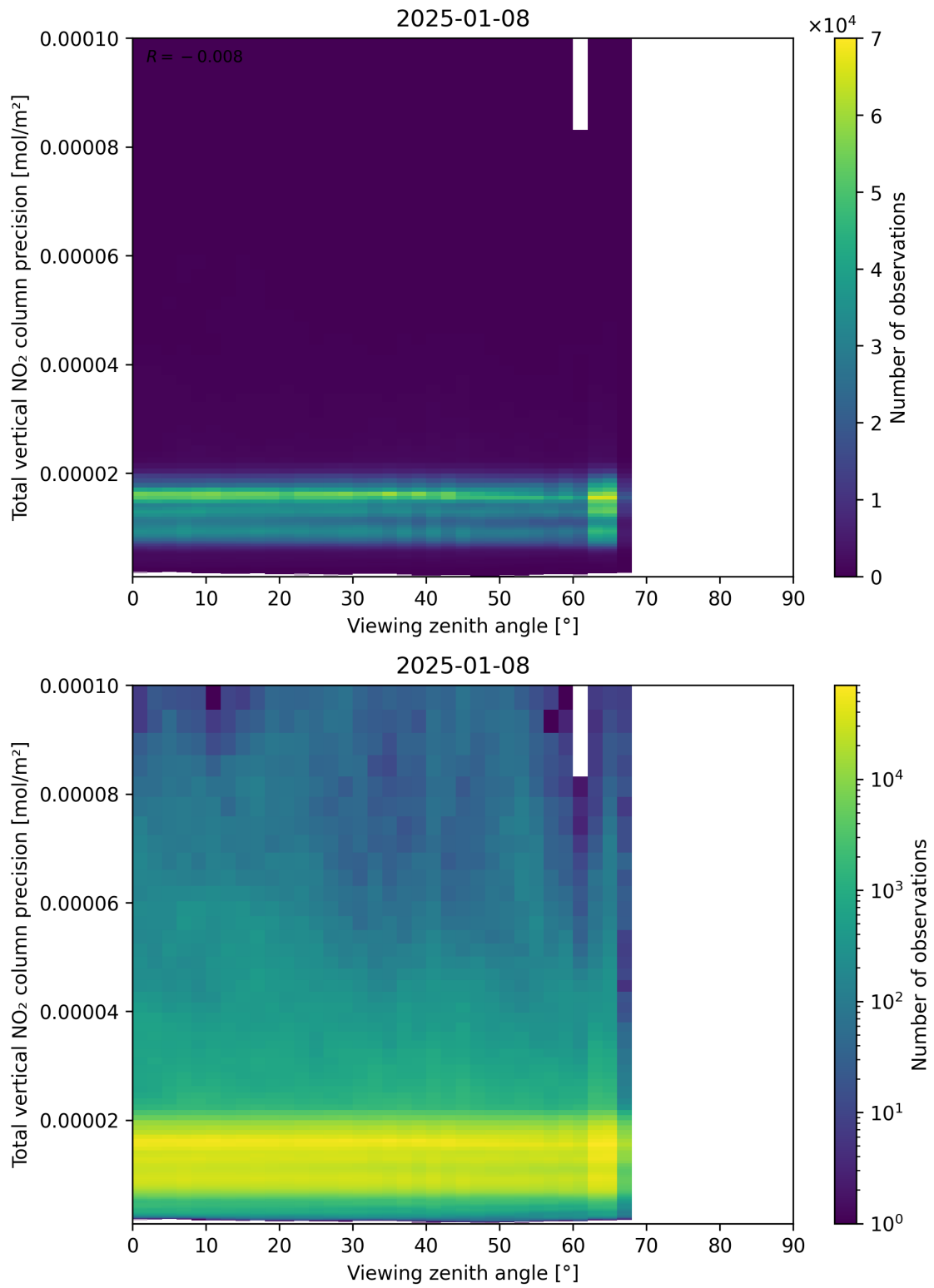
Figure 168: Scatter density plot of “Viewing zenith angle” against “Total vertical NO 2 column precision” for 2025-01-07 to 2025-01-09.
