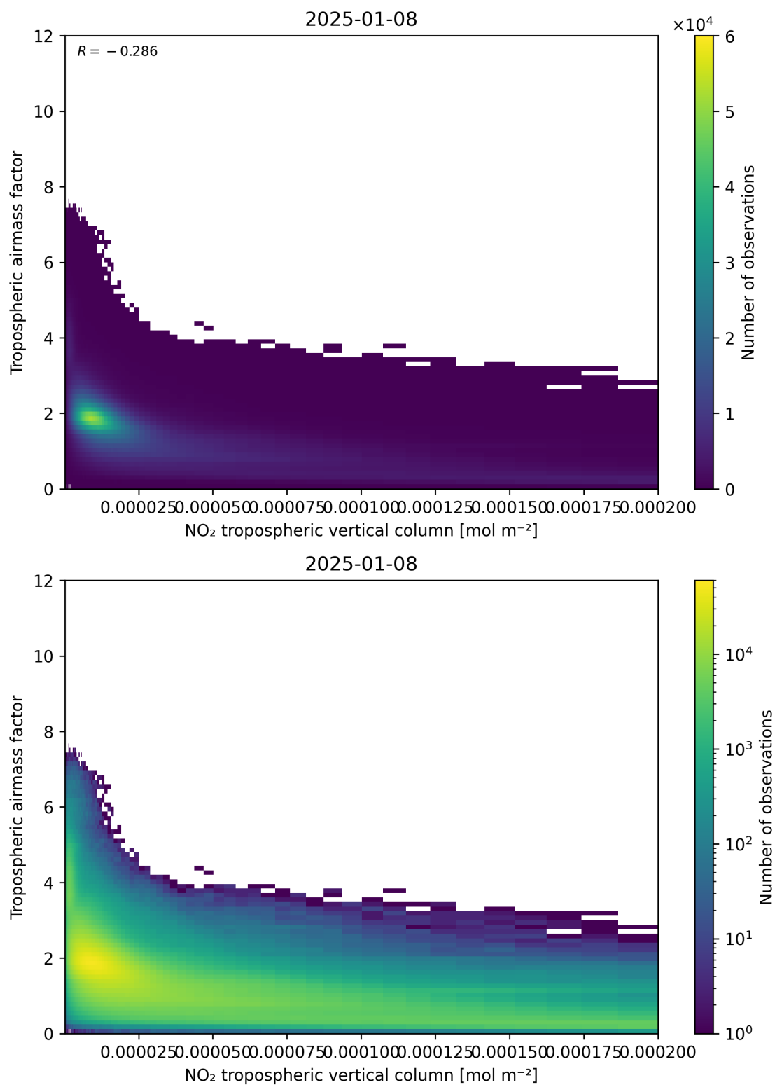
Figure 123: Scatter density plot of “NO 2 tropospheric vertical column” against “Tropospheric air mass factor” for 2025-01-07 to 2025-01-09.
