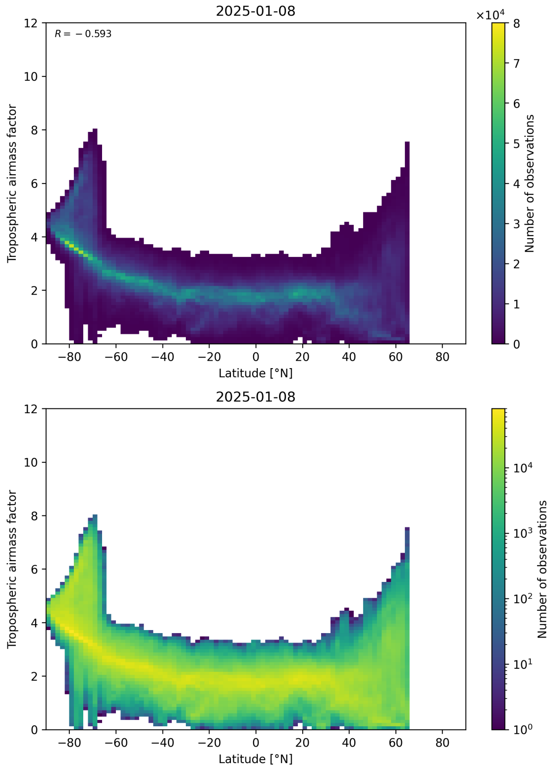
Figure 85: Scatter density plot of “Latitude” against “Tropospheric airmass factor” for 2025-01-07 to 2025-01-09.
