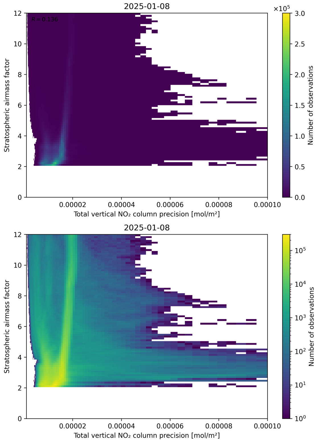
Figure 115: Scatter density plot of “Total vertical NO 2 column precision” against “Stratospheric air mass factor” for 2025-01-07 to 2025-01-09.
