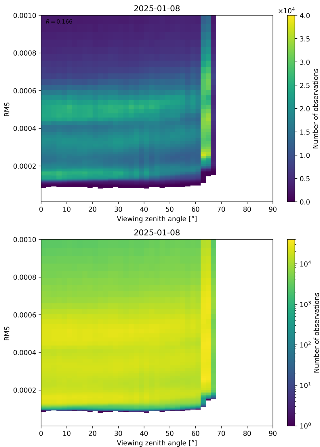
Figure 171: Scatter density plot of “Viewing zenith angle” against “RMS” for 2025-01-07 to 2025-01-09.
