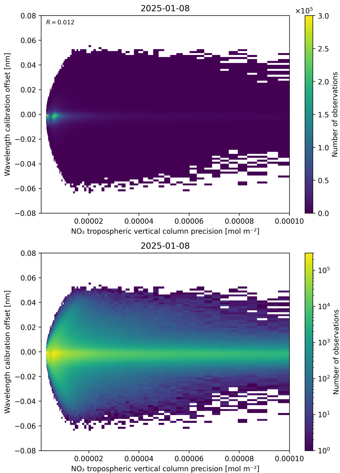
Figure 141: Scatter density plot of “NO 2 tropospheric vertical column precision” against “Wavelength calibration offset” for 2025-01-07 to 2025-01-09.
