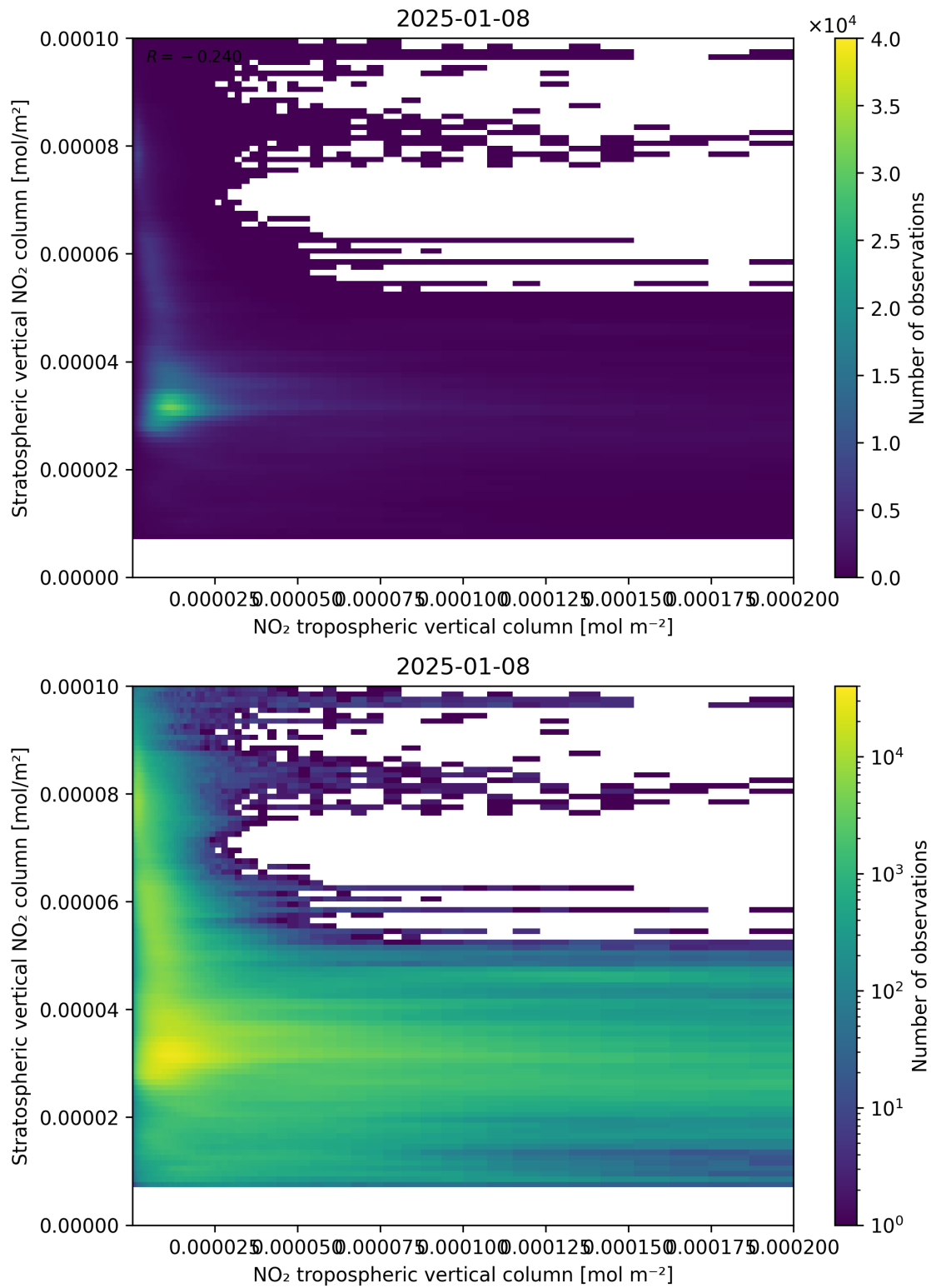
Figure 125: Scatter density plot of “NO 2 tropospheric vertical column” against “Stratospheric vertical NO 2 column” for 2025-01-07 to 2025-01-09.
