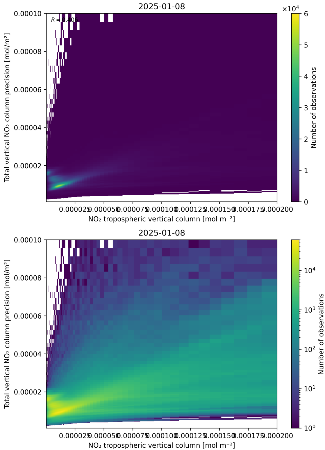
Figure 129: Scatter density plot of “NO 2 tropospheric vertical column” against “Total vertical NO 2 column precision” for 2025-01-07 to 2025-01-09.
