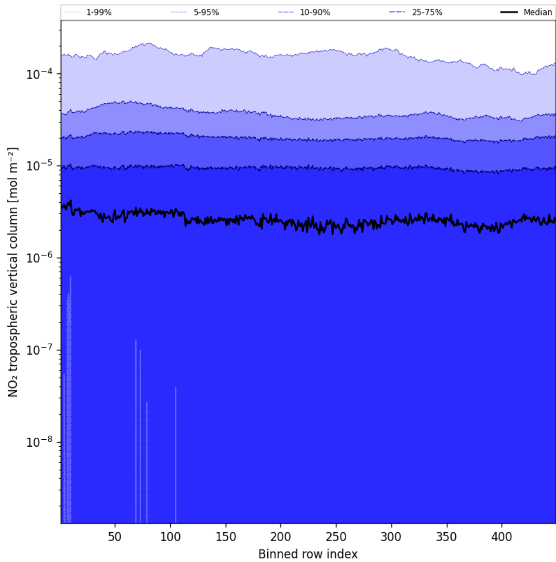
Figure 46: Along track statistics of “NO 2 tropospheric vertical column” for 2025-01-07 to 2025-01-09
