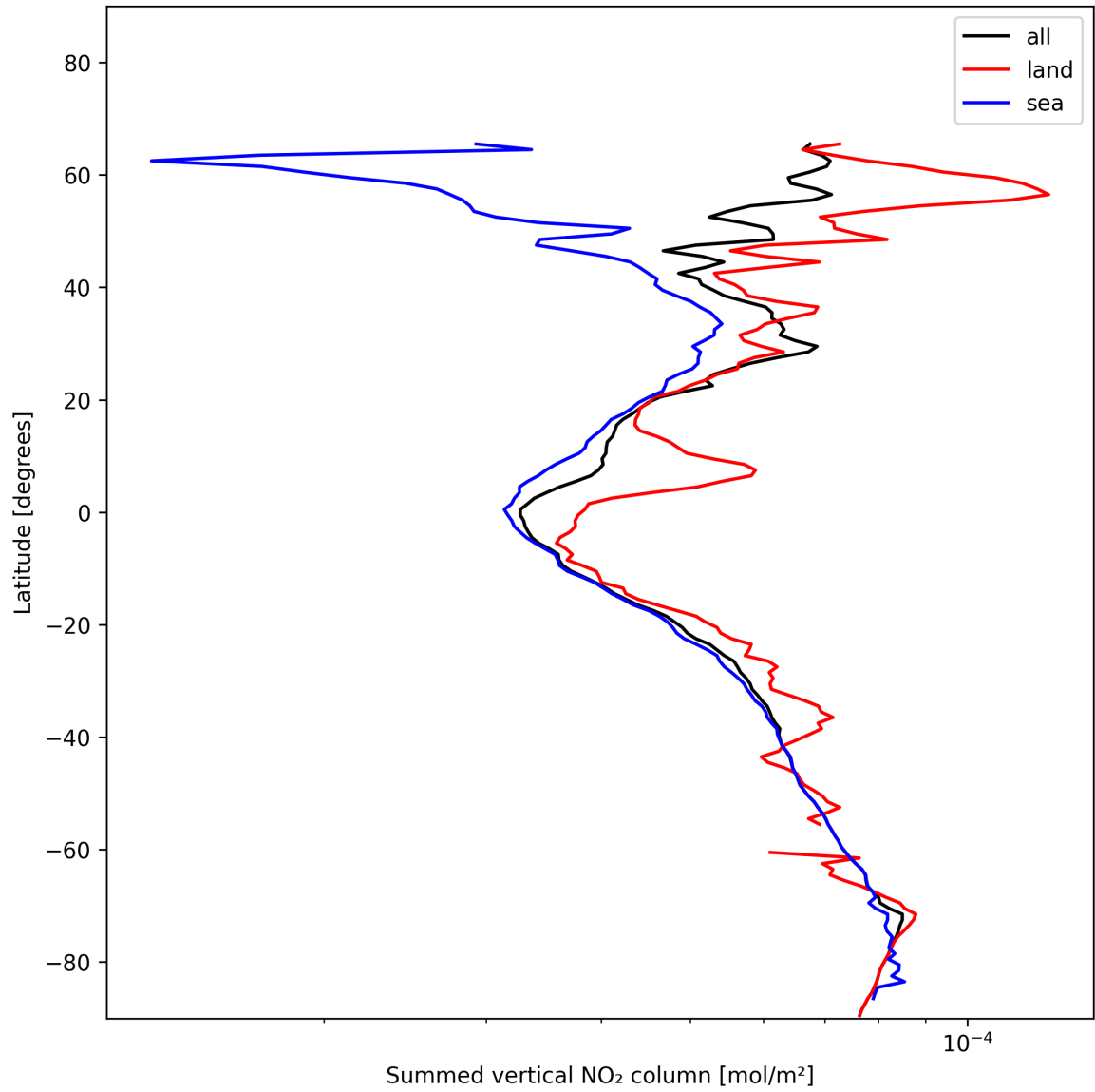
Figure 23: Zonal average of “Summed vertical NO 2 column” for 2025-01-07 to 2025-01-09.
