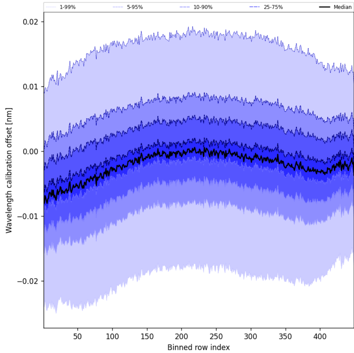
Figure 52: Along track statistics of “Wavelength calibration offset” for 2025-01-07 to 2025-01-09
