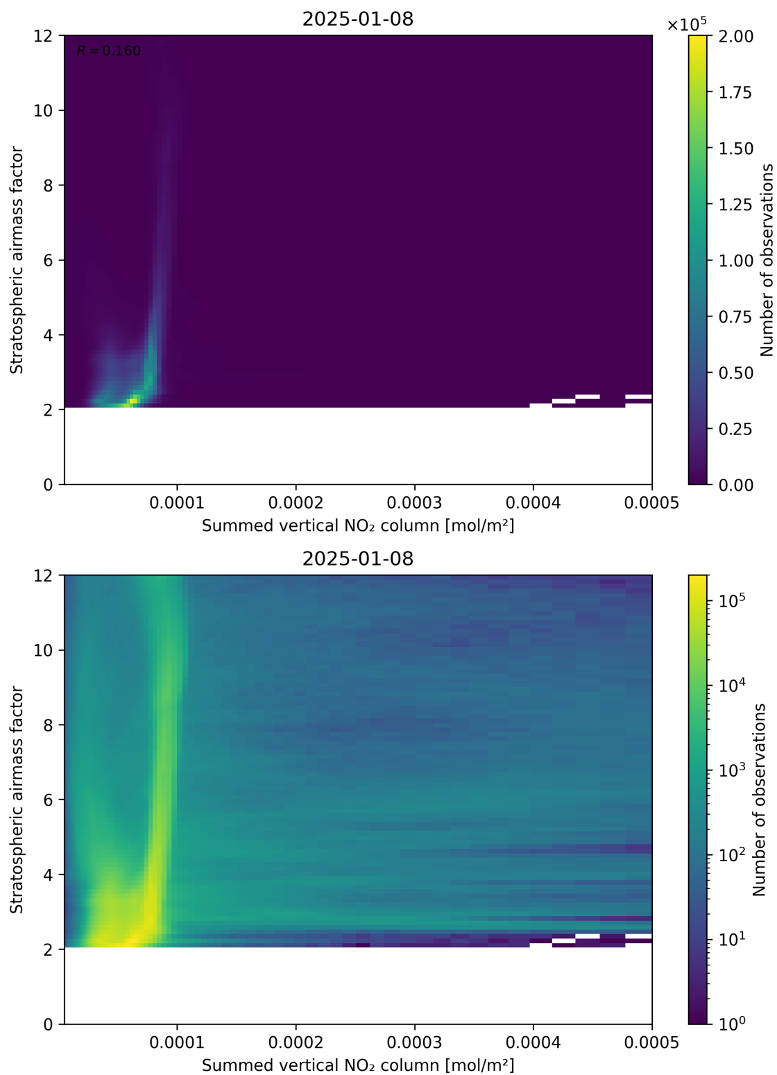
Figure 103: Scatter density plot of “Summed vertical NO 2 column” against “Stratospheric airmass factor” for 2025-01-07 to 2025-01-09.
