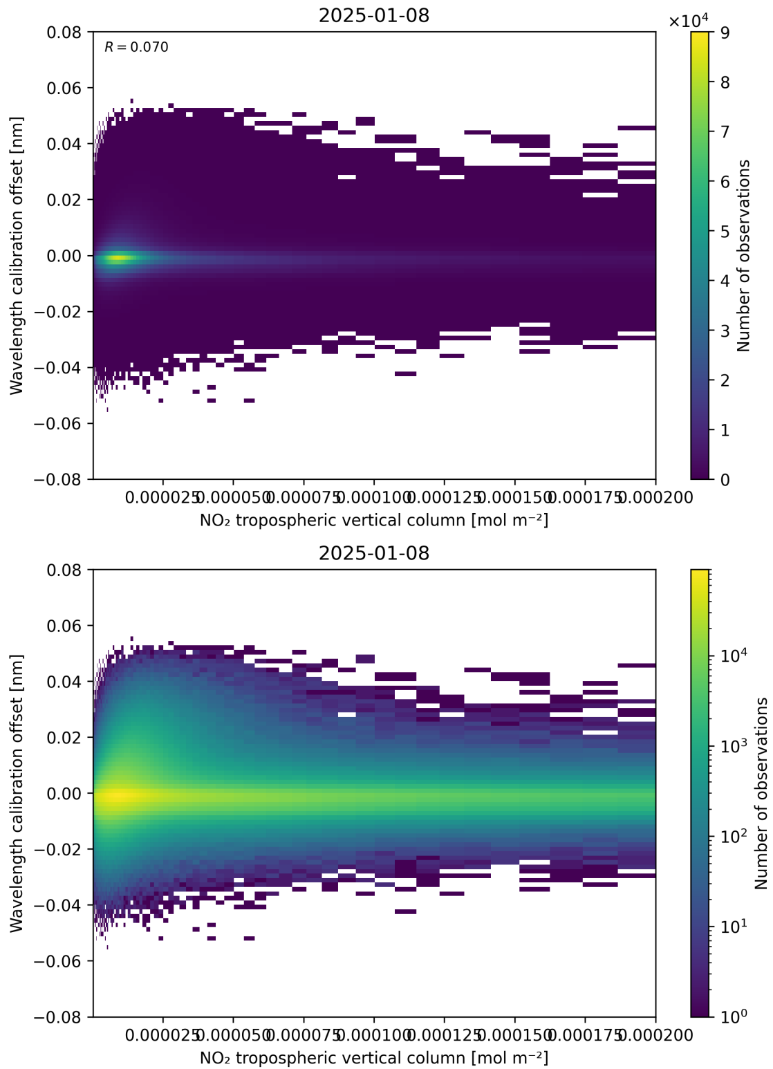
Figure 143: Scatter density plot of “NO 2 tropospheric vertical column” against “Wavelength calibration offset” for 2025-01-07 to 2025-01-09.
