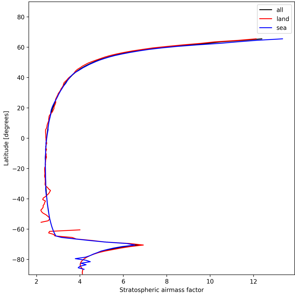
Figure 27: Zonal average of “Stratospheric air mass factor” for 2025-01-07 to 2025-01-09.
