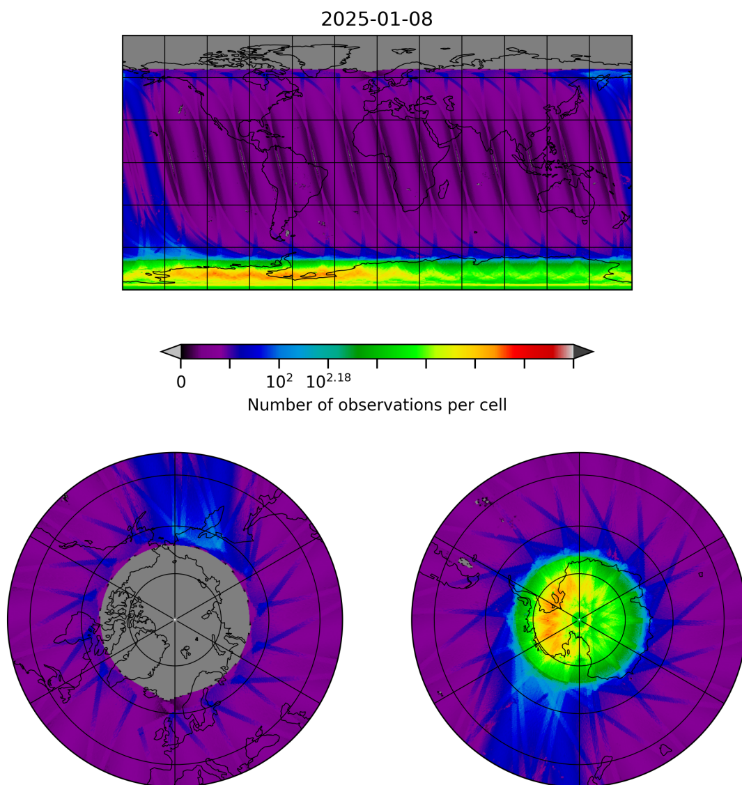
Figure 10: Map of the number of observations for 2025-01-07 to 2025-01-09
