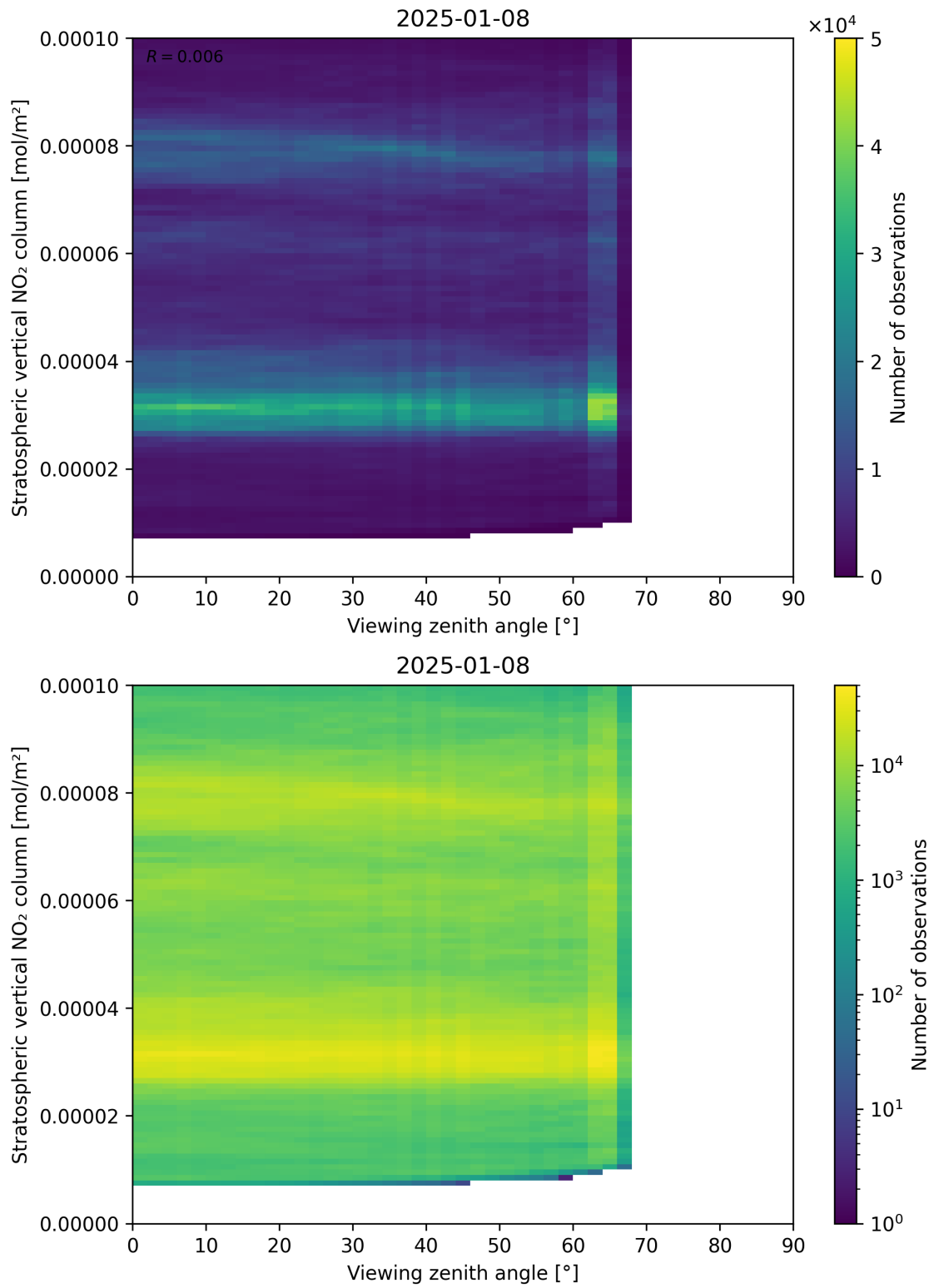
Figure 164: Scatter density plot of “Viewing zenith angle” against “Stratospheric vertical NO 2 column” for 2025-01-07 to 2025-01-09.
