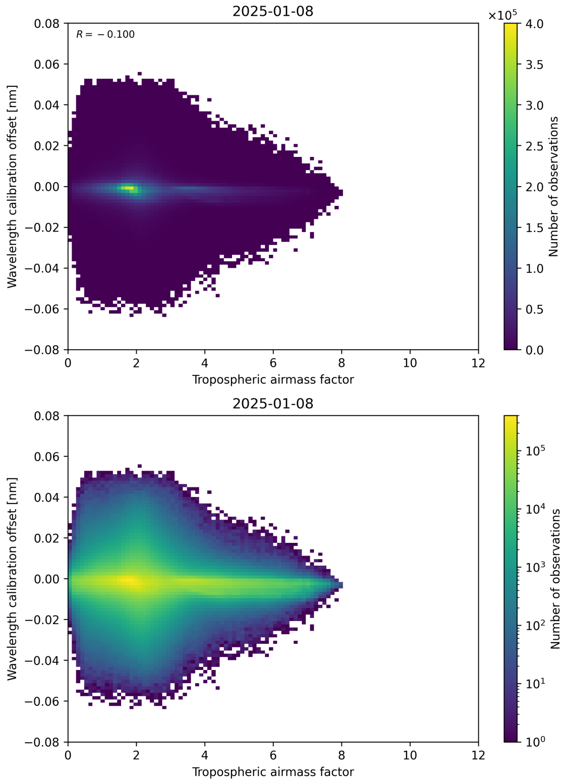
Figure 80: Scatter density plot of “Tropospheric airmass factor” against “Wavelength calibration offset” for 2025-01-07 to 2025-01-09.
