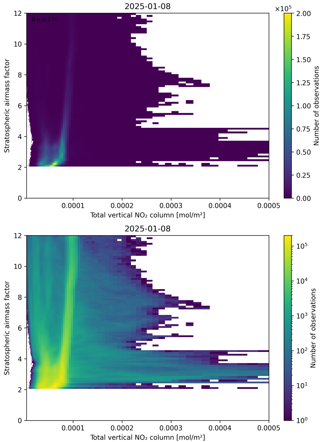
Figure 110: Scatter density plot of “Total vertical NO 2 column” against “Stratospheric air mass factor” for 2025-01-07 to 2025-01-09.
