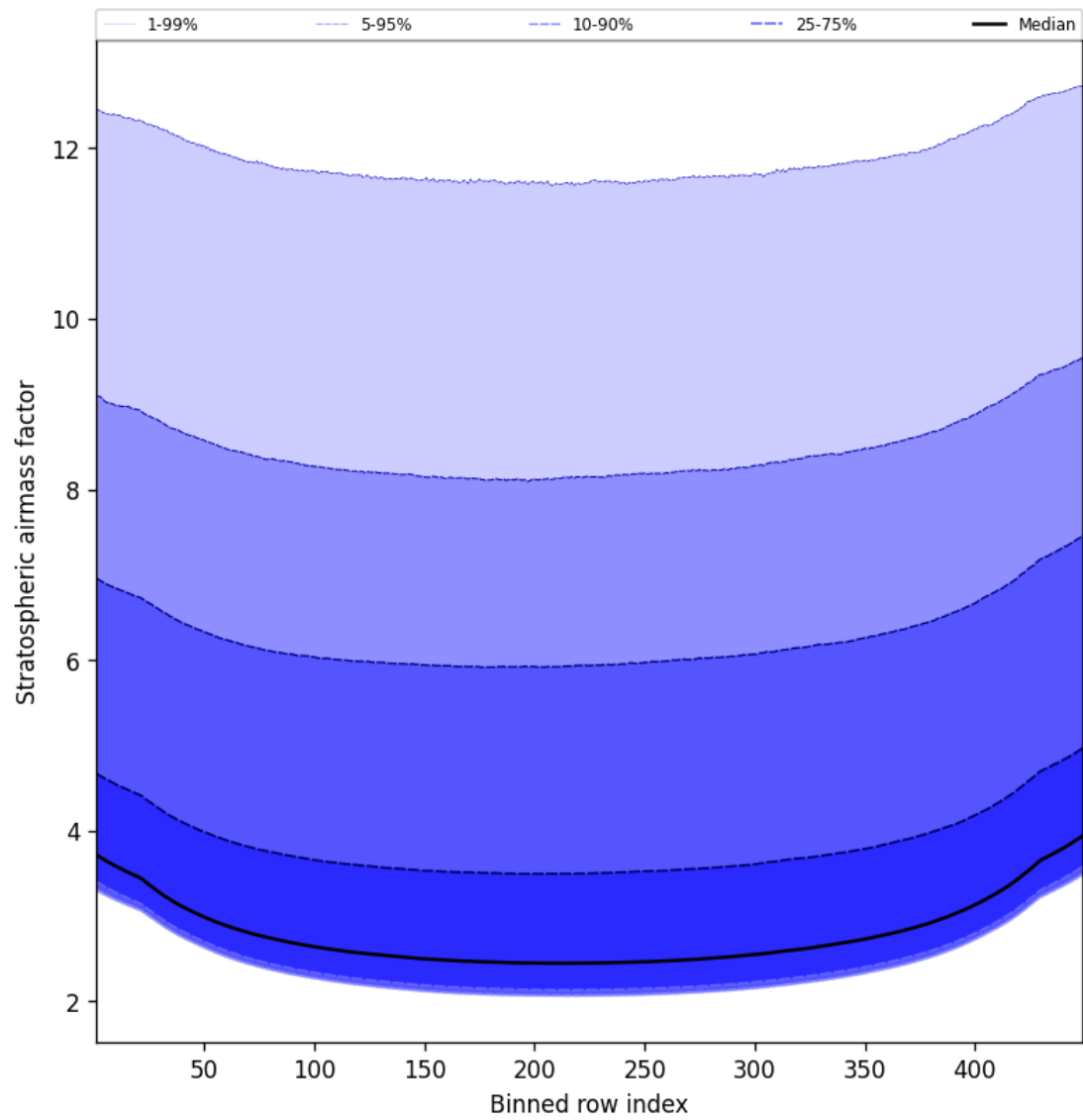
Figure 61: Along track statistics of “Stratospheric airmass factor” for 2025-01-07 to 2025-01-09
