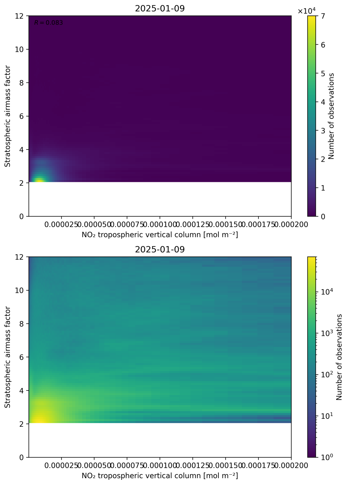
Figure 121: Scatter density plot of “NO 2 tropospheric vertical column” against “Stratospheric airmass factor” for 2025-01-08 to 2025-01-10.
