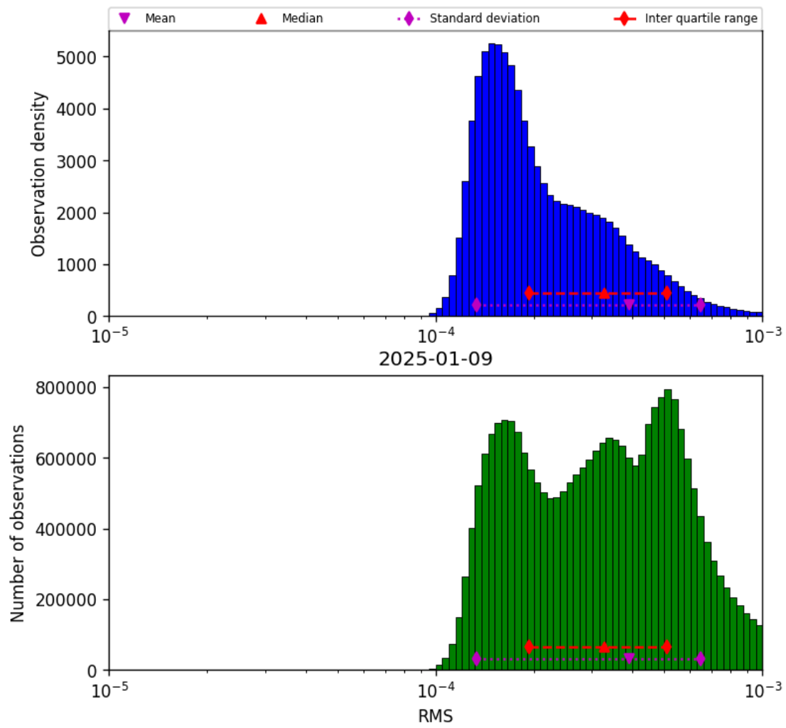
Figure 43: Histogram of “RMS” for 2025-01-08 to 2025-01-10
