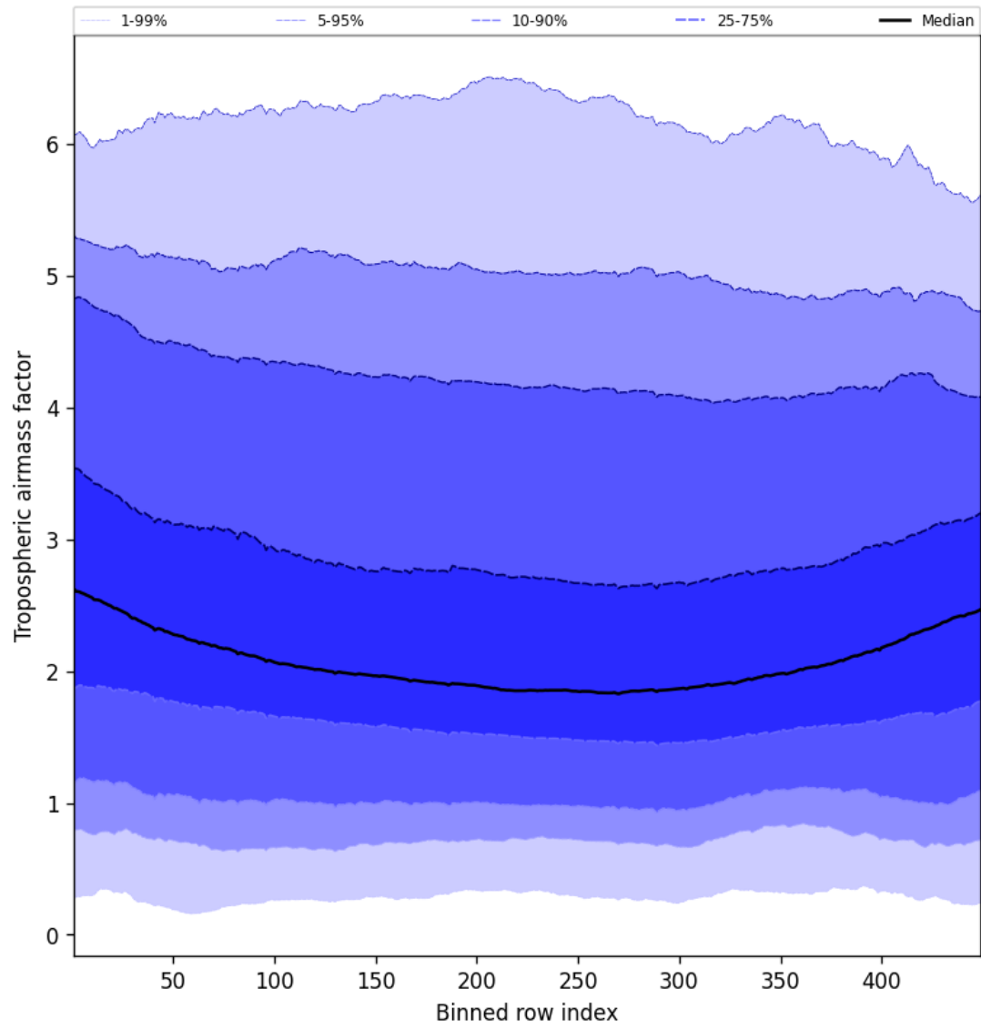
Figure 48: Along track statistics of “Tropospheric airmass factor” for 2025-01-08 to 2025-01-10
