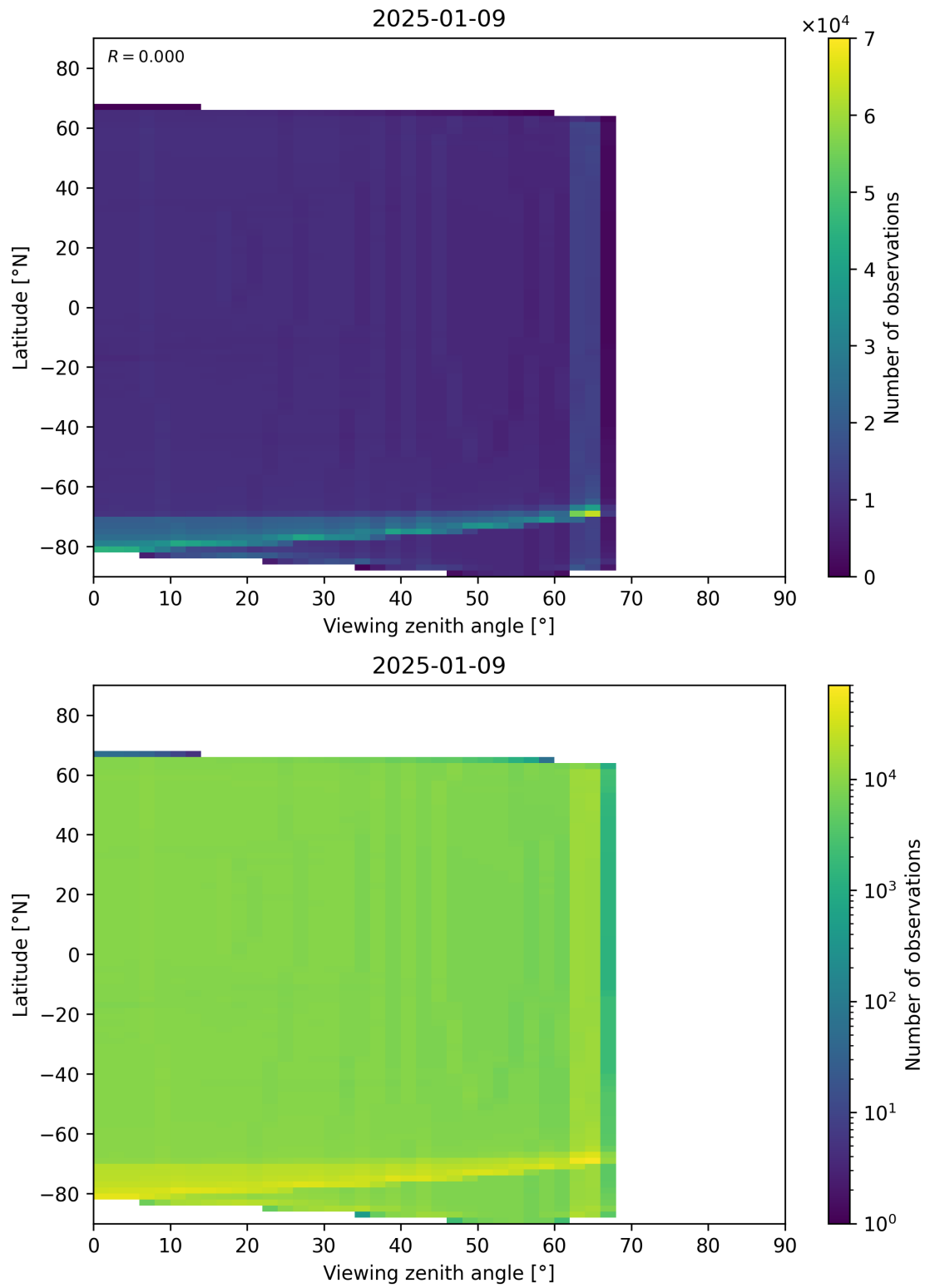
Figure 163: Scatter density plot of “Viewing zenith angle” against “Latitude” for 2025-01-08 to 2025-01-10.
