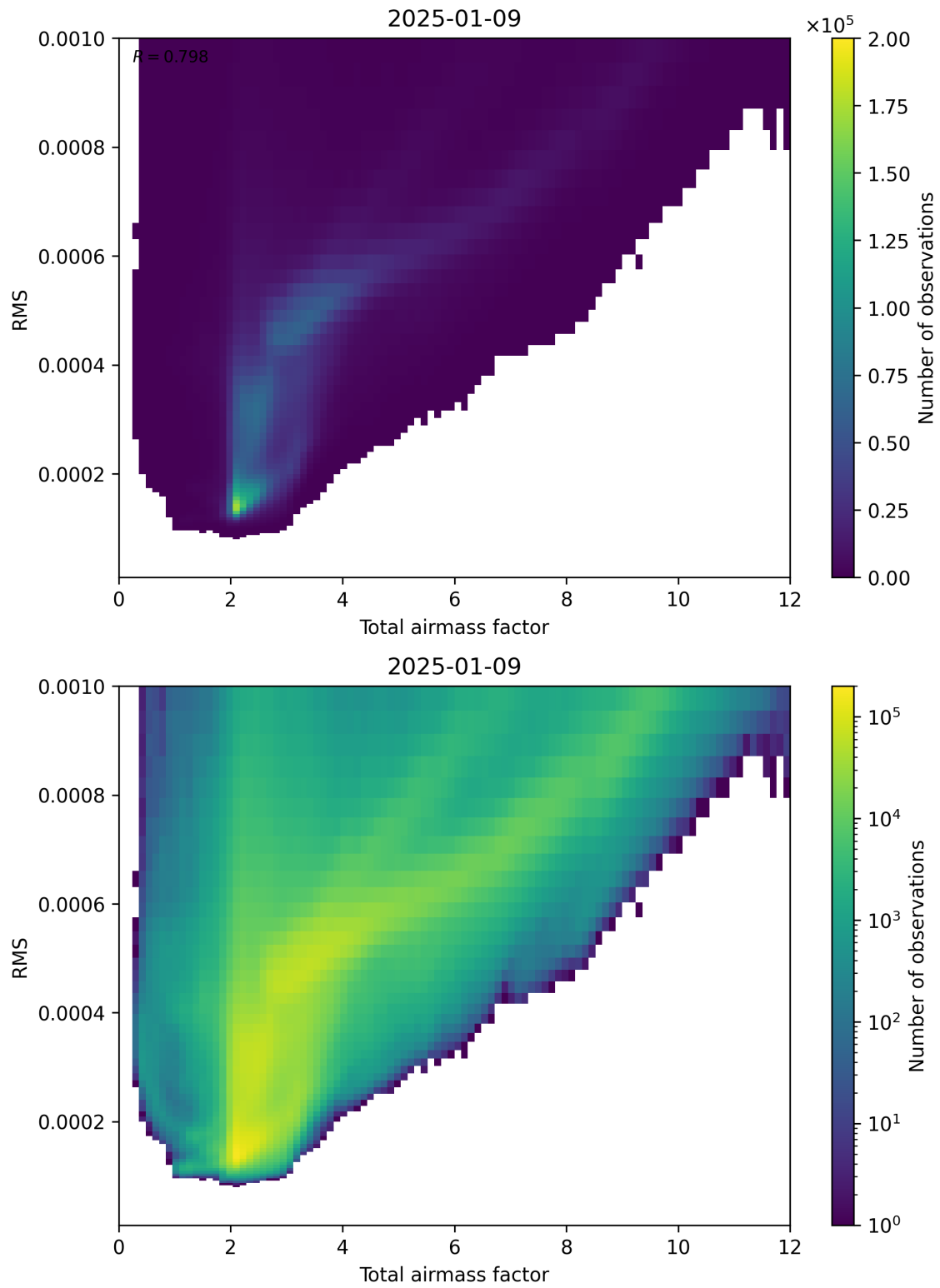
Figure 69: Scatter density plot of “Total airmass factor” against “RMS” for 2025-01-08 to 2025-01-10.
