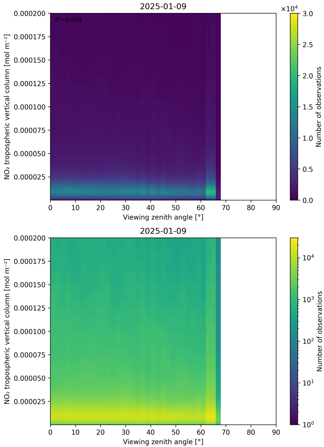
Figure 169: Scatter density plot of “Viewing zenith angle” against “NO 2 tropospheric vertical column” for 2025-01-08 to 2025-01-10.
