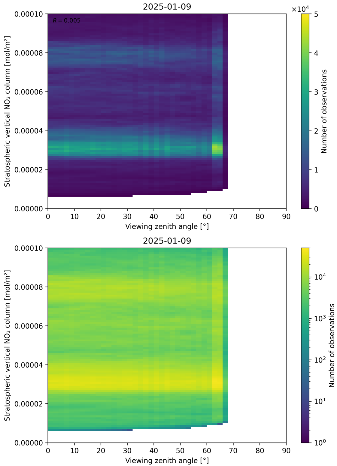
Figure 164: Scatter density plot of “Viewing zenith angle” against “Stratospheric vertical NO 2 column” for 2025-01-08 to 2025-01-10.
