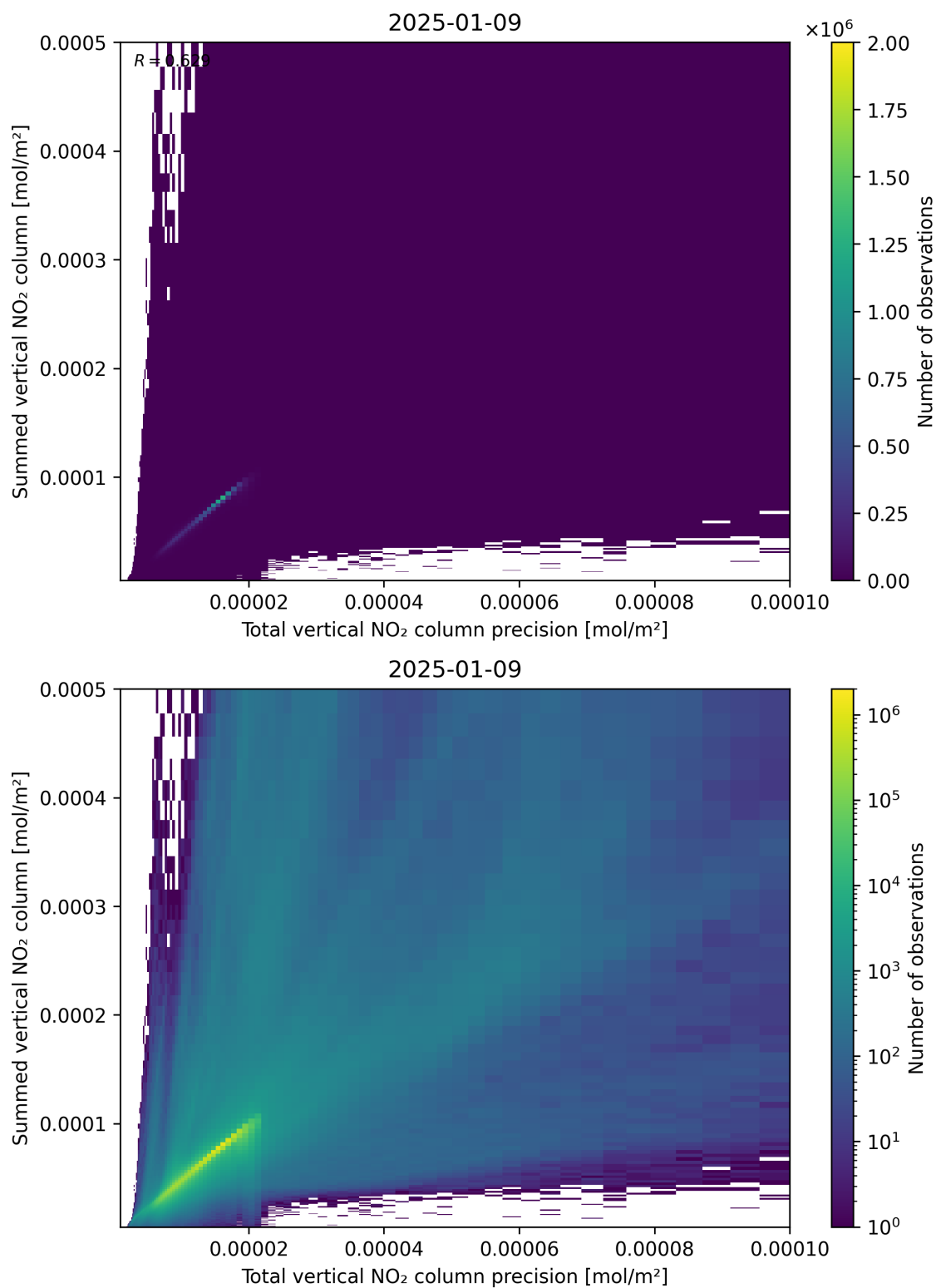
Figure 117: Scatter density plot of “Total vertical NO 2 column precision” against “Summed vertical NO 2 column” for 2025-01-08 to 2025-01-10.
