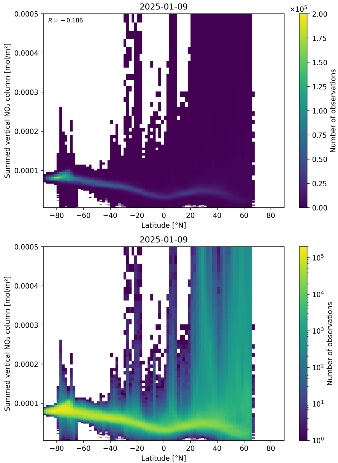
Figure 88: Scatter density plot of “Latitude” against “Summed vertical NO 2 column” for 2025-01-08 to 2025-01-10.
