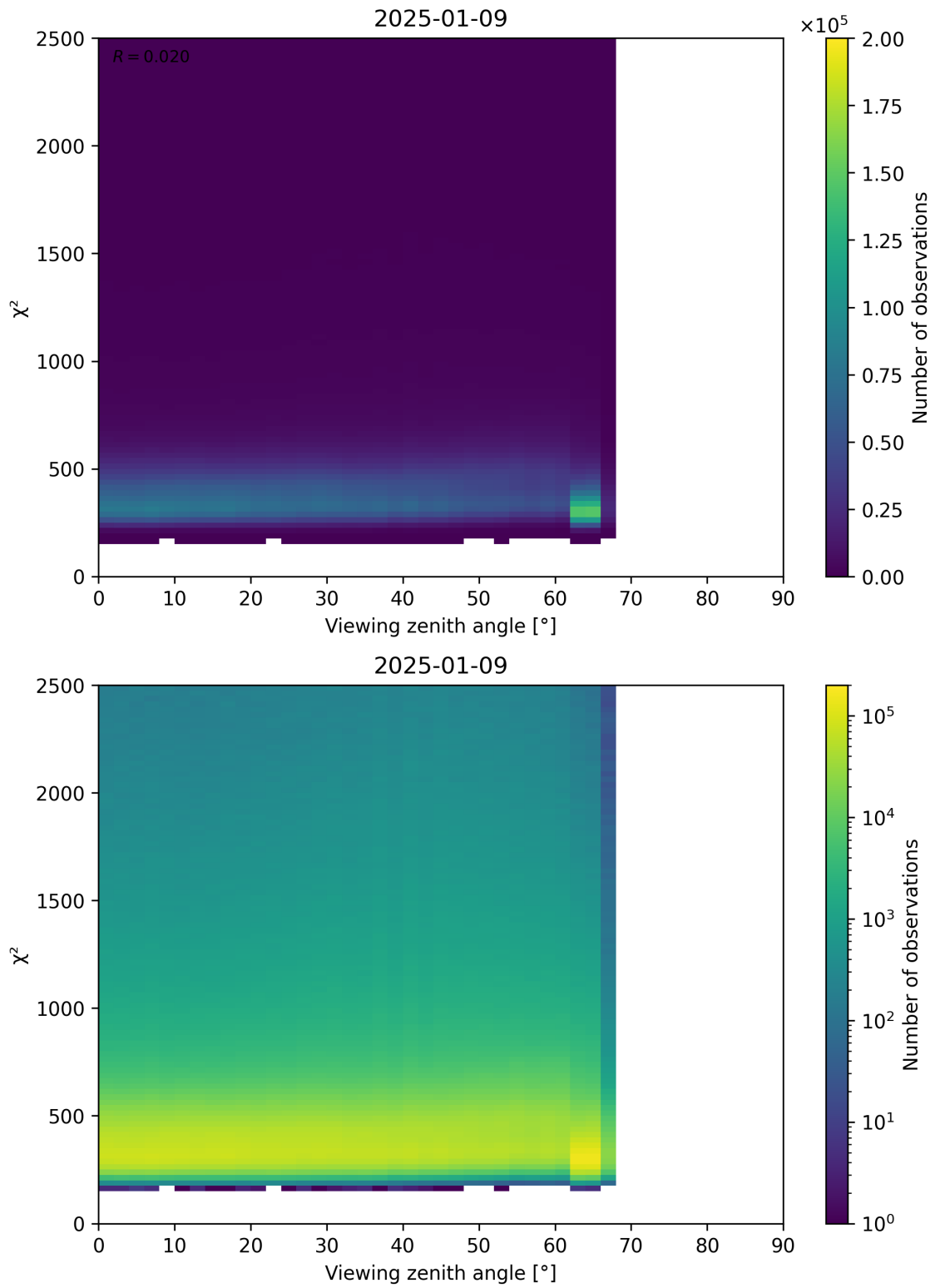
Figure 162: Scatter density plot of “Viewing zenith angle” against “ \chi^2 ” for 2025-01-08 to 2025-01-10.
