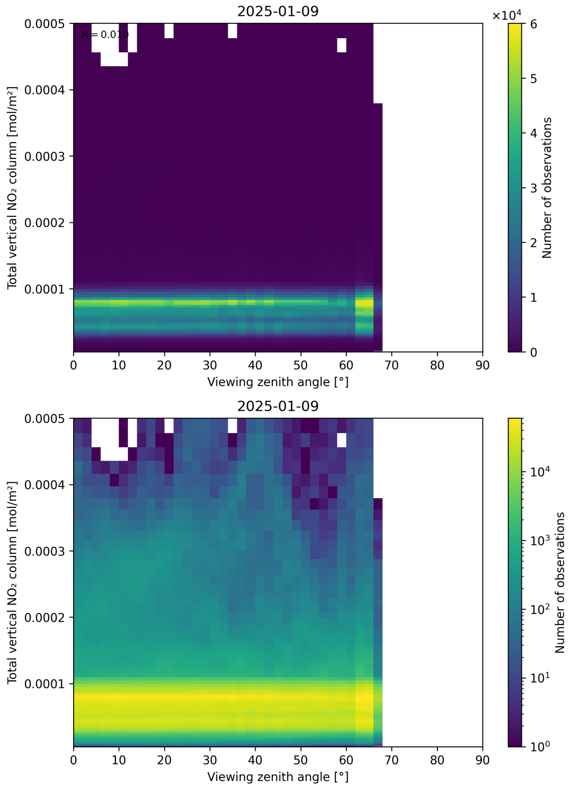
Figure 167: Scatter density plot of “Viewing zenith angle” against “Total vertical NO 2 column” for 2025-01-08 to 2025-01-10.
