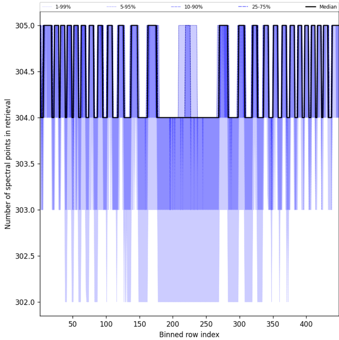
Figure 50: Along track statistics of “Number of spectral points in retrieval” for 2025-01-08 to 2025-01-10
