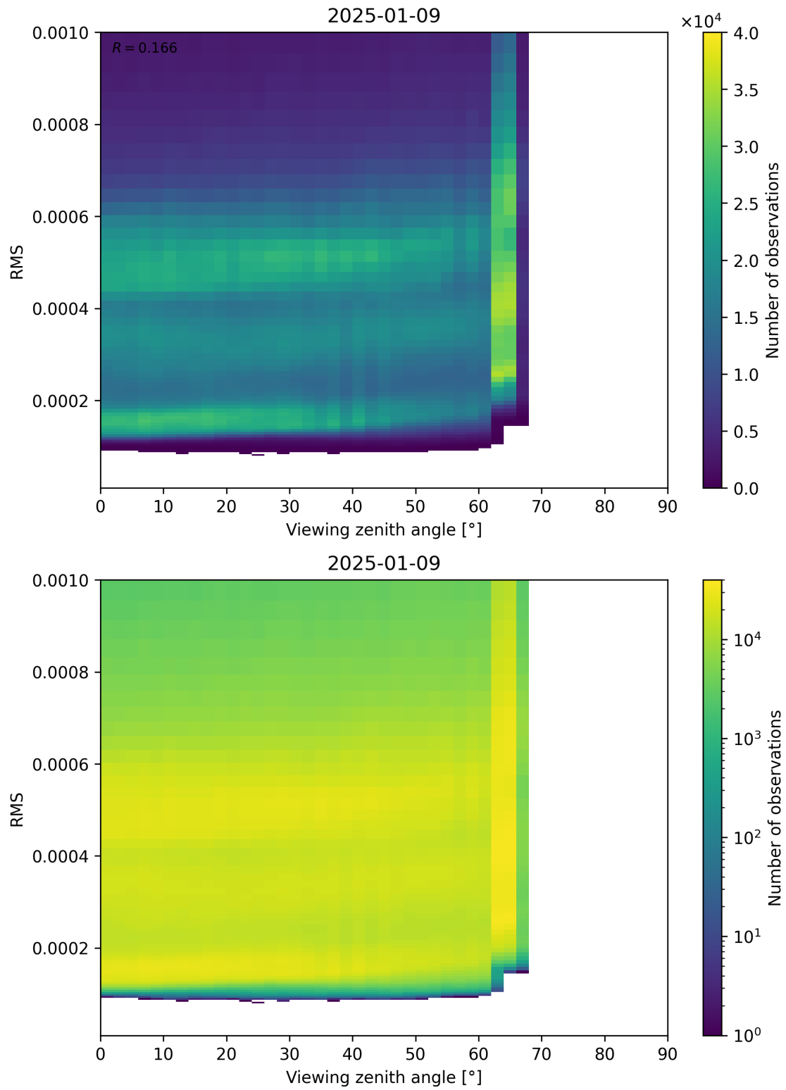
Figure 171: Scatter density plot of “Viewing zenith angle” against “RMS” for 2025-01-08 to 2025-01-10.
