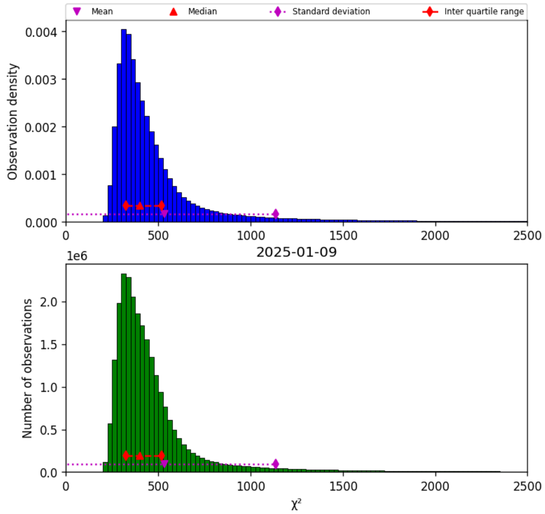
Figure 42: Histogram of “ \chi^2 ” for 2025-01-08 to 2025-01-10
