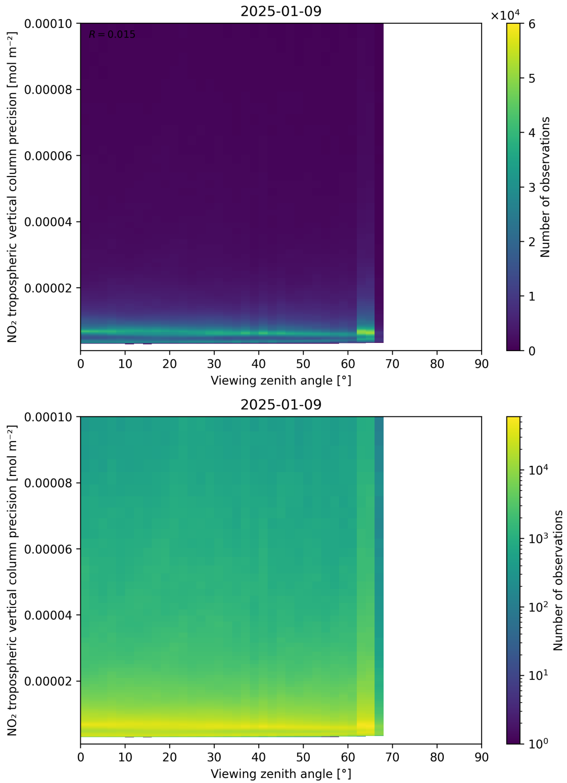
Figure 170: Scatter density plot of “Viewing zenith angle” against “NO 2 tropospheric vertical column precision” for 2025-01-08 to 2025-01-10.
