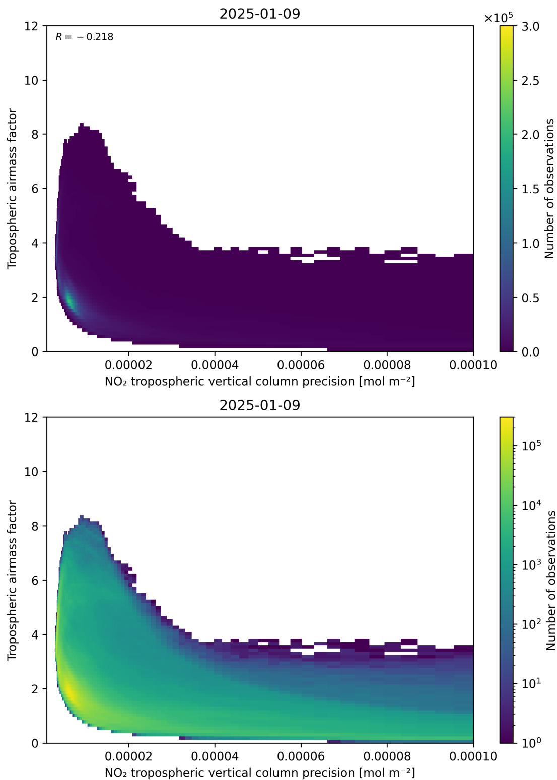
Figure 133: Scatter density plot of “NO 2 tropospheric vertical column precision” against “Tropospheric airmass factor” for 2025-01-08 to 2025-01-10.
