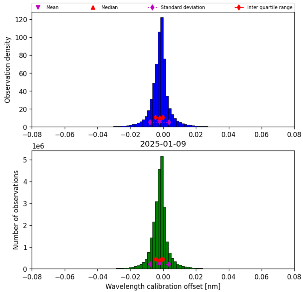
Figure 35: Histogram of “Wavelength calibration offset” for 2025-01-08 to 2025-01-10
