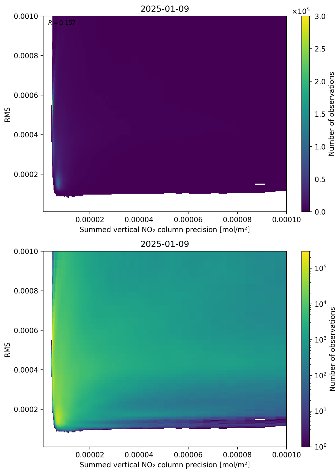
Figure 108: Scatter density plot of “Summed vertical NO 2 column precision” against “RMS” for 2025-01-08 to 2025-01-10.
