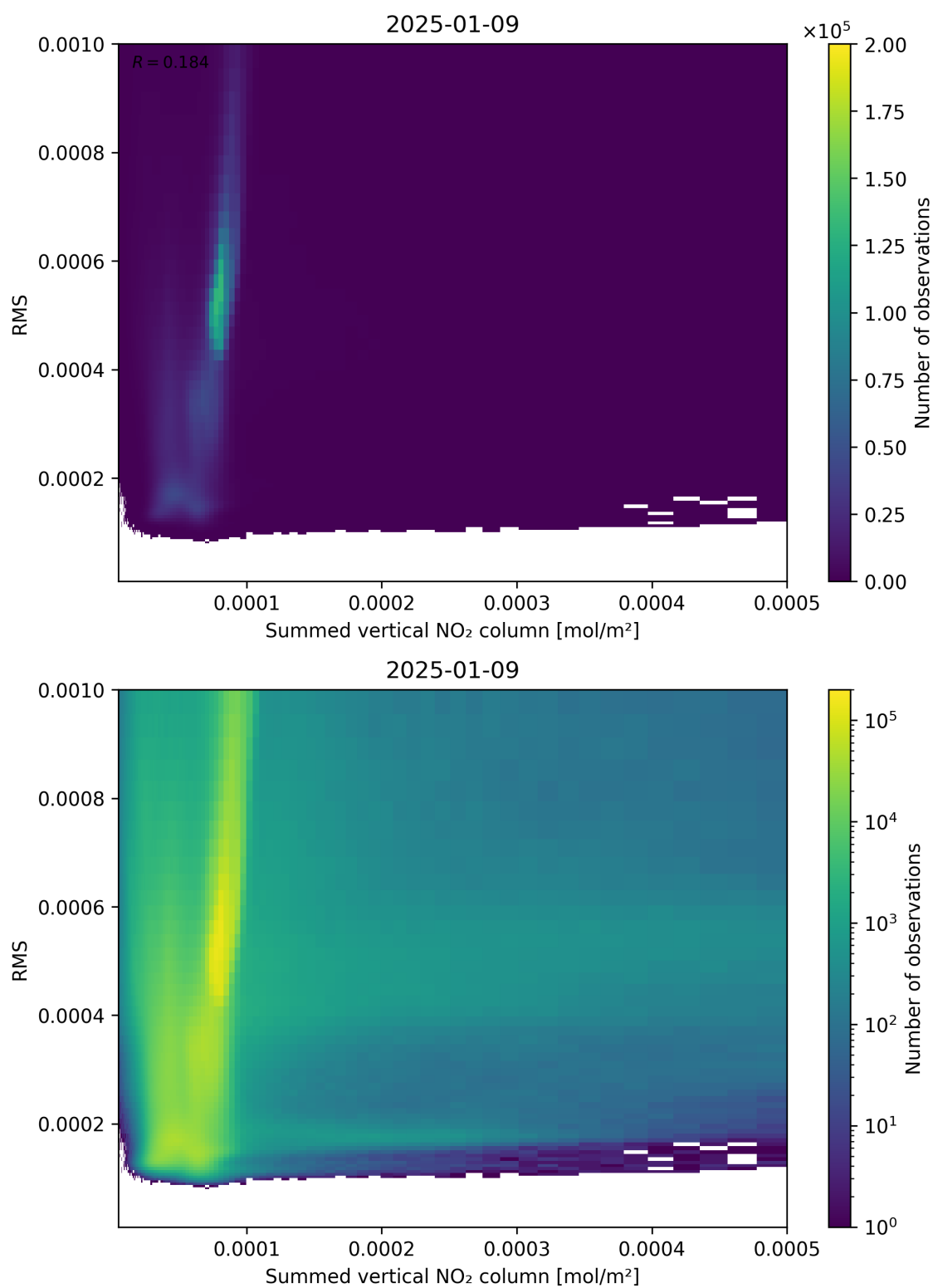
Figure 109: Scatter density plot of “Summed vertical NO 2 column” against “RMS” for 2025-01-08 to 2025-01-10.
