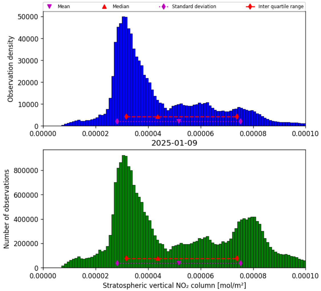
Figure 36: Histogram of “Stratospheric vertical NO 2 column” for 2025-01-08 to 2025-01-10
