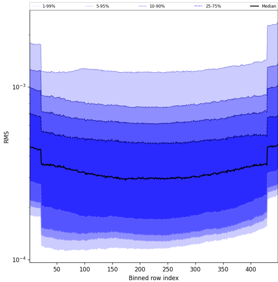
Figure 60: Along track statistics of “RMS” for 2025-01-08 to 2025-01-10
