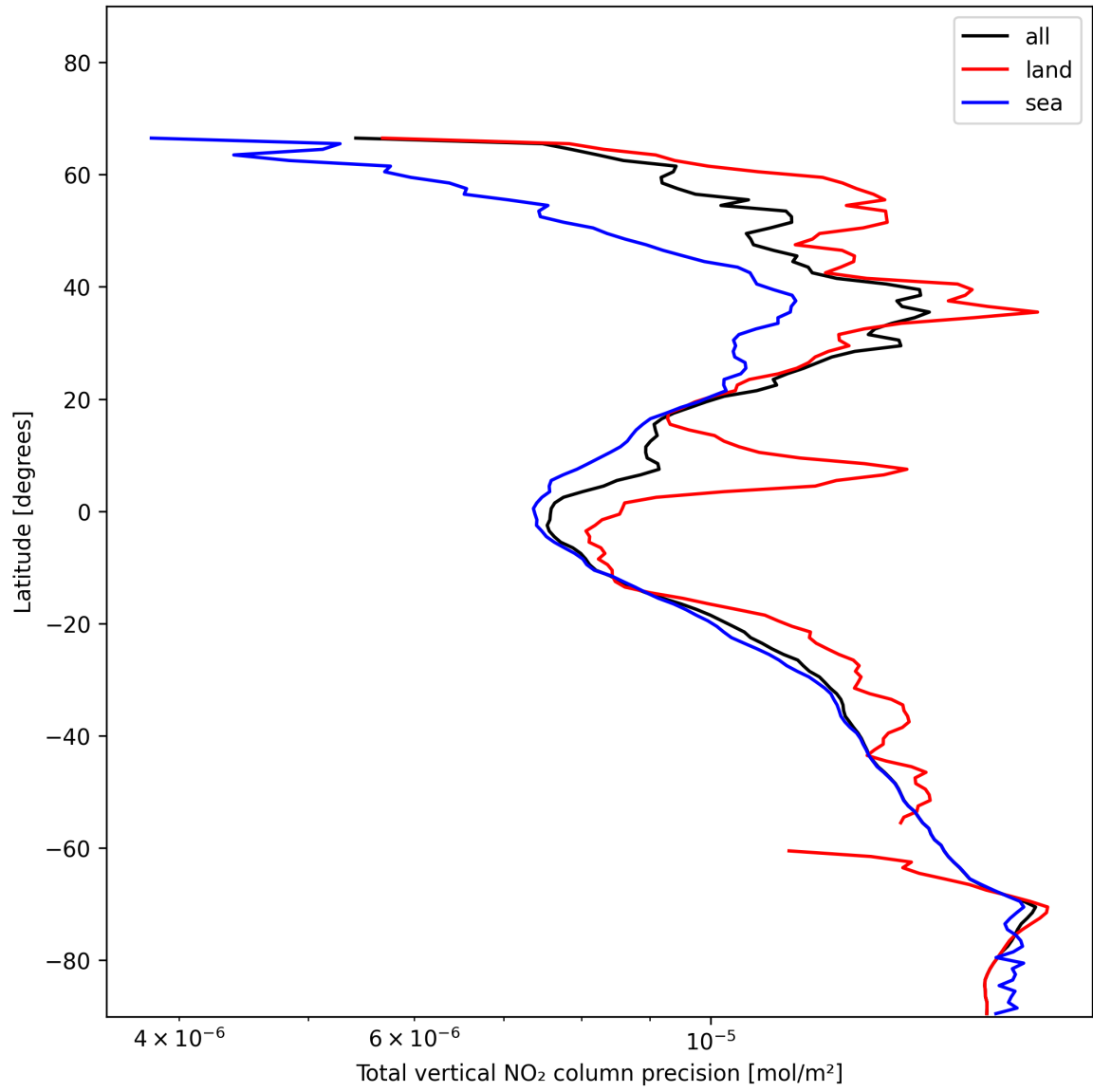
Figure 22: Zonal average of “Total vertical NO 2 column precision” for 2025-01-08 to 2025-01-10.
