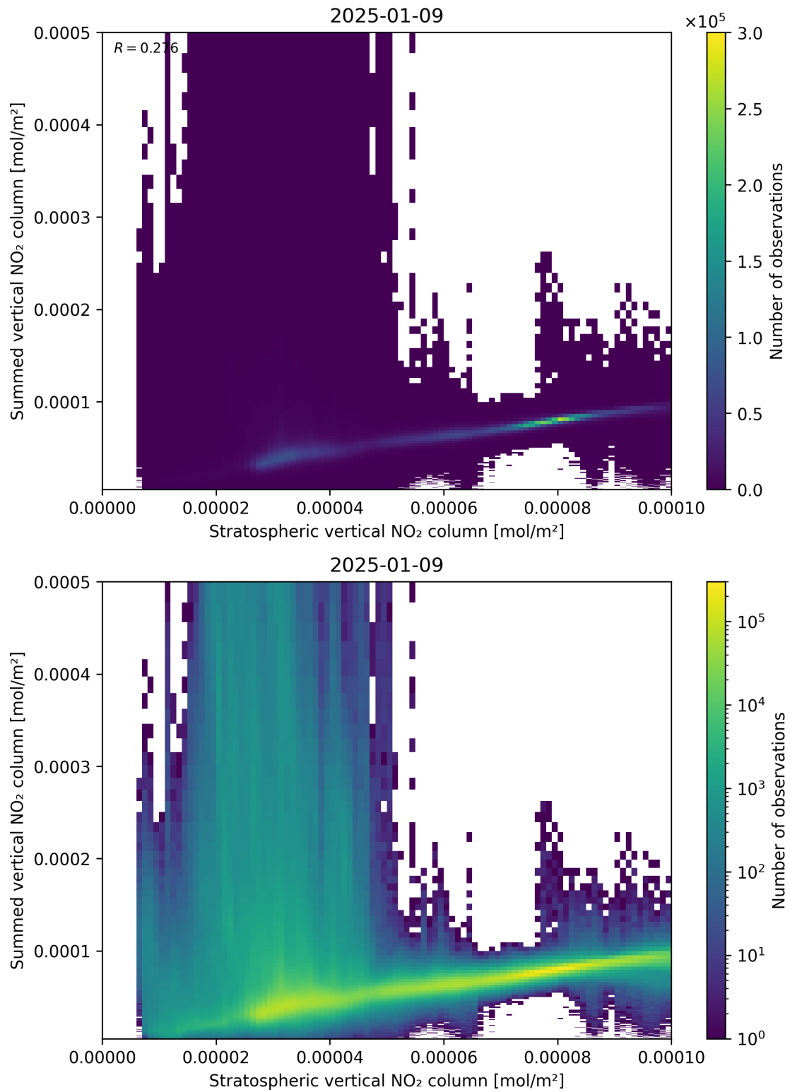
Figure 98: Scatter density plot of “Stratospheric vertical NO 2 column” against “Summed vertical NO 2 column” for 2025-01-08 to 2025-01-10.
