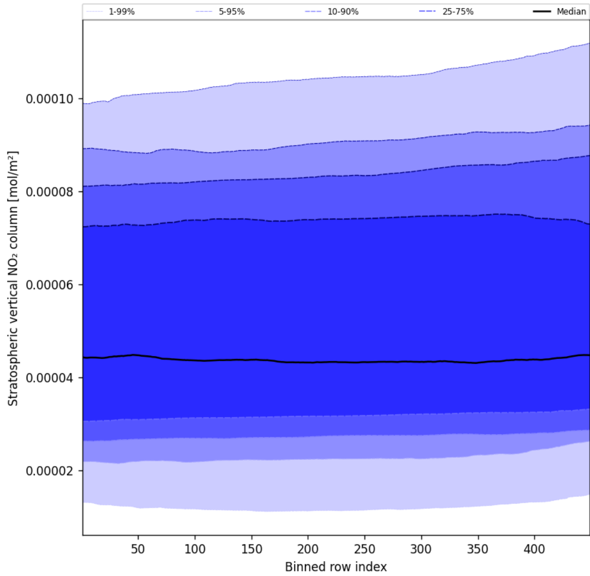
Figure 53: Along track statistics of “Stratospheric vertical NO 2 column” for 2025-01-08 to 2025-01-10
