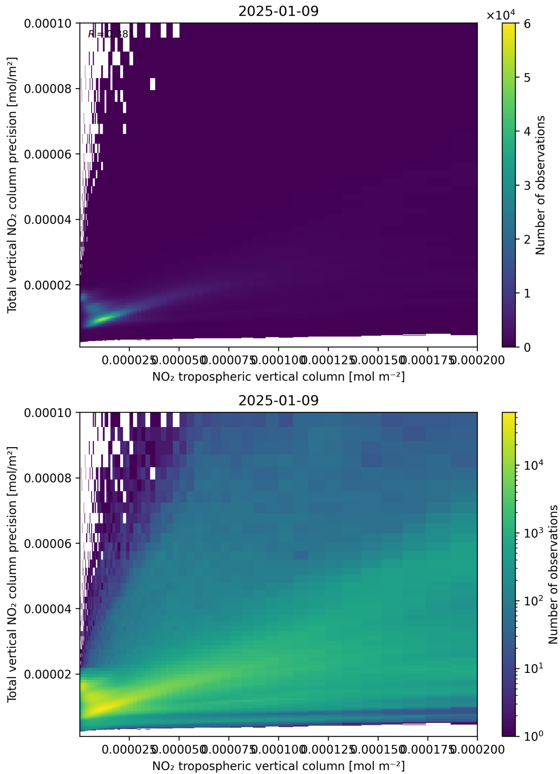
Figure 129: Scatter density plot of “NO 2 tropospheric vertical column” against “Total vertical NO 2 column precision” for 2025-01-08 to 2025-01-10.
