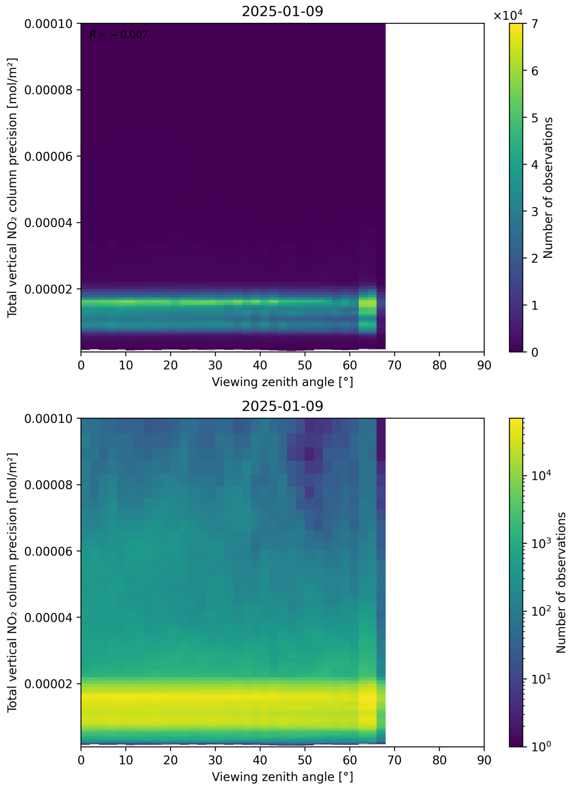
Figure 168: Scatter density plot of “Viewing zenith angle” against “Total vertical NO 2 column precision” for 2025-01-08 to 2025-01-10.
