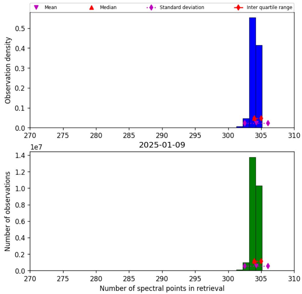
Figure 33: Histogram of “Number of spectral points in retrieval” for 2025-01-08 to 2025-01-10
