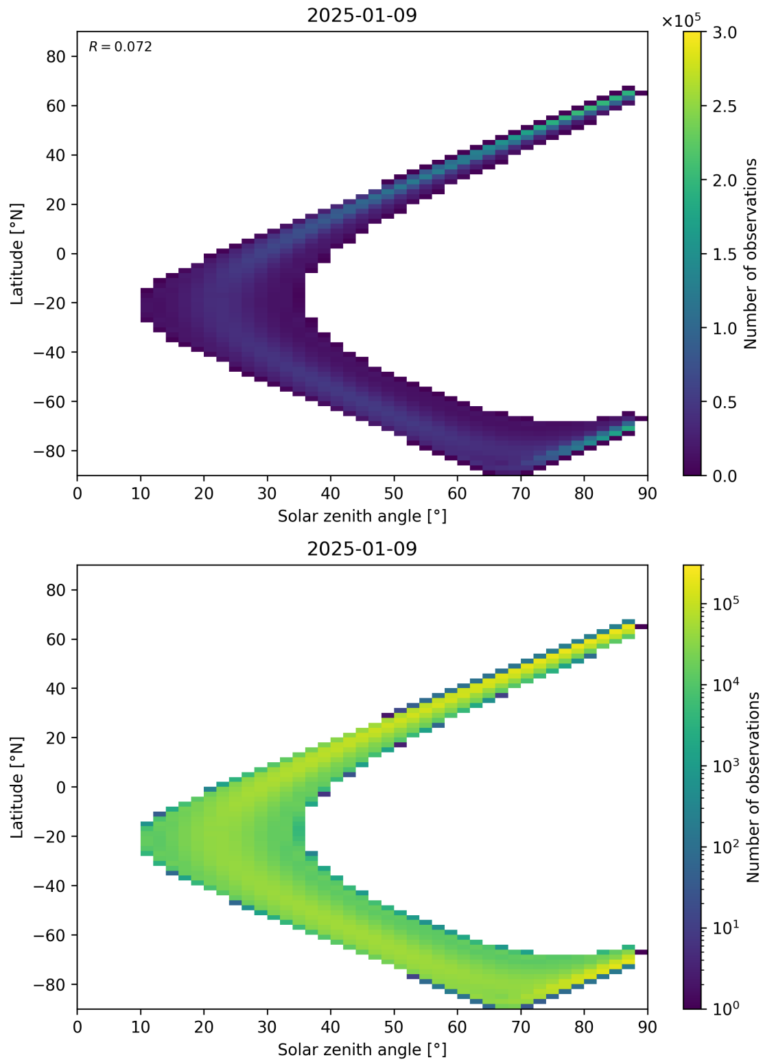
Figure 149: Scatter density plot of “Solar zenith angle” against “Latitude” for 2025-01-08 to 2025-01-10.
