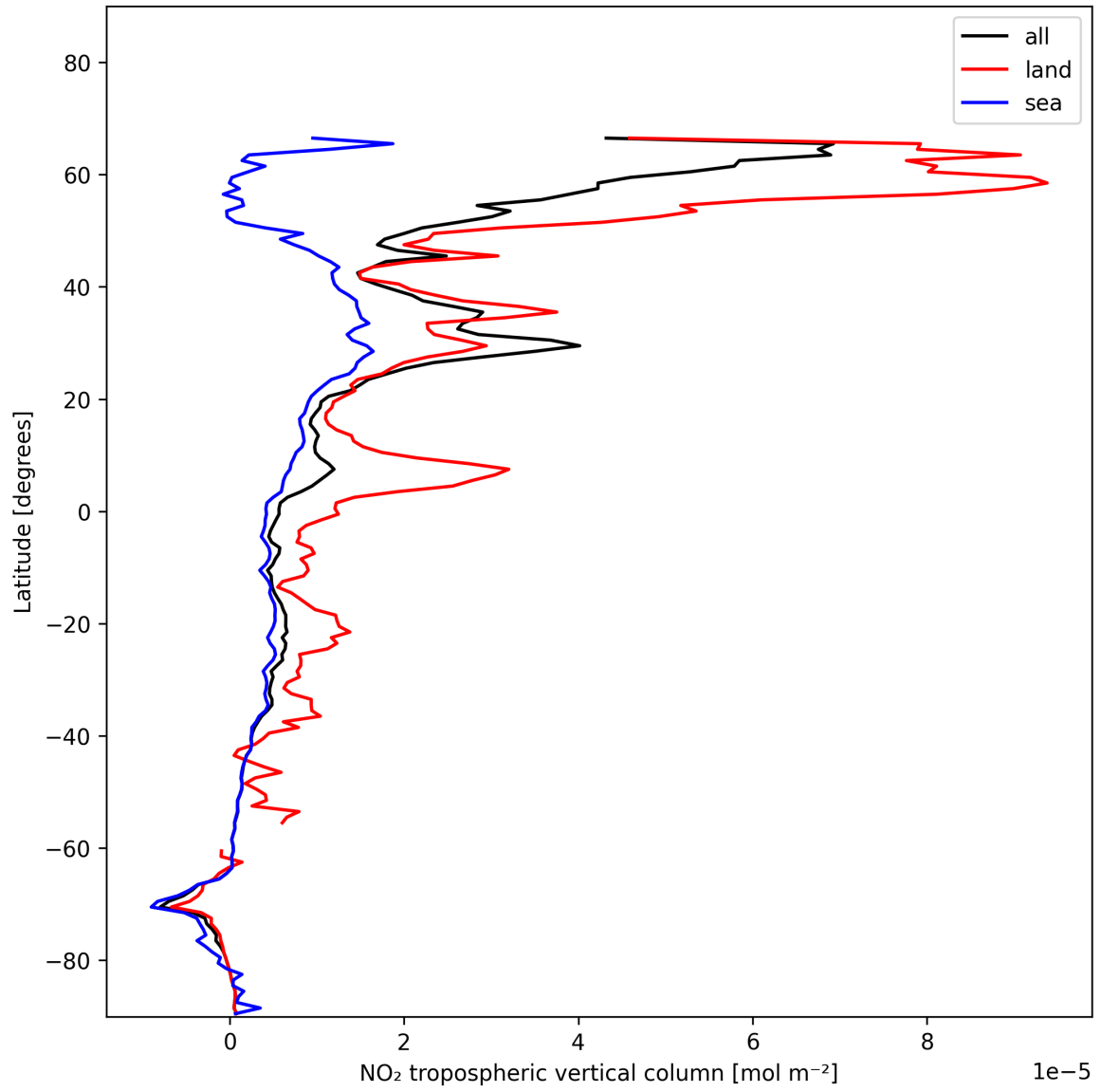
Figure 12: Zonal average of “NO 2 tropospheric vertical column” for 2025-01-08 to 2025-01-10.
