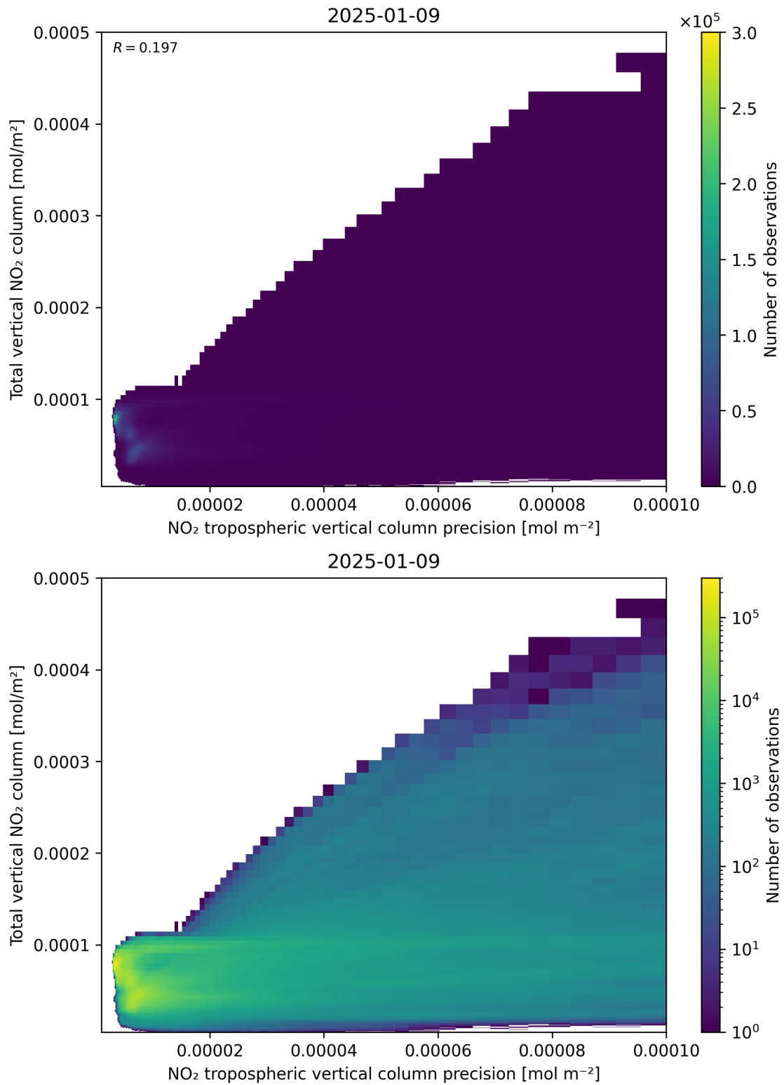
Figure 138: Scatter density plot of “NO 2 tropospheric vertical column precision” against “Total vertical NO 2 column” for 2025-01-08 to 2025-01-10.
