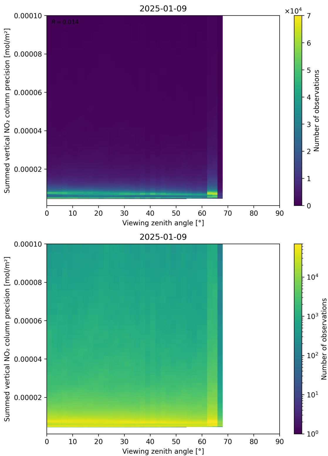
Figure 166: Scatter density plot of “Viewing zenith angle” against “Summed vertical NO 2 column precision” for 2025-01-08 to 2025-01-10.
