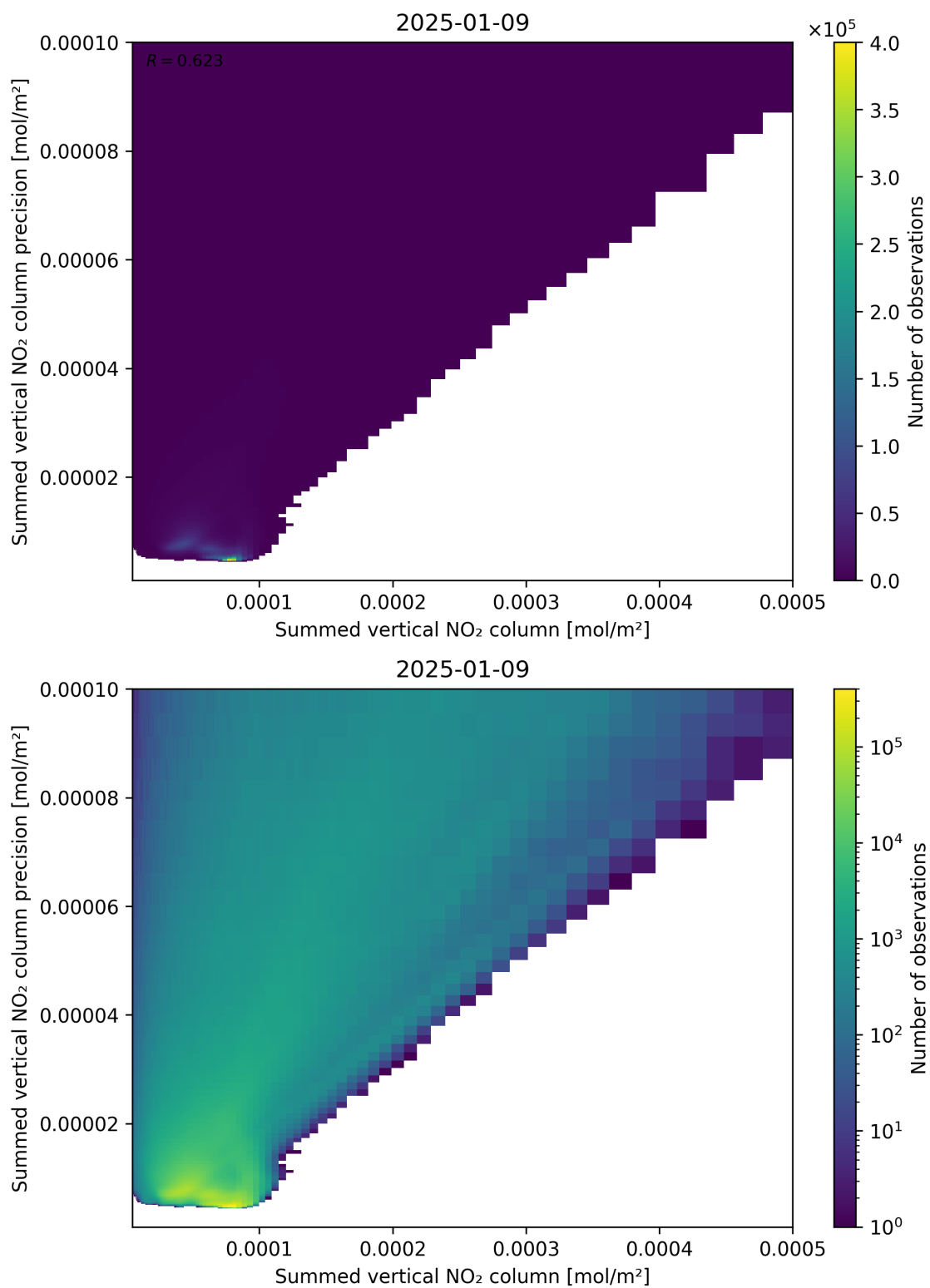
Figure 105: Scatter density plot of “Summed vertical NO 2 column” against “Summed vertical NO 2 column precision” for 2025-01-08 to 2025-01-10.
