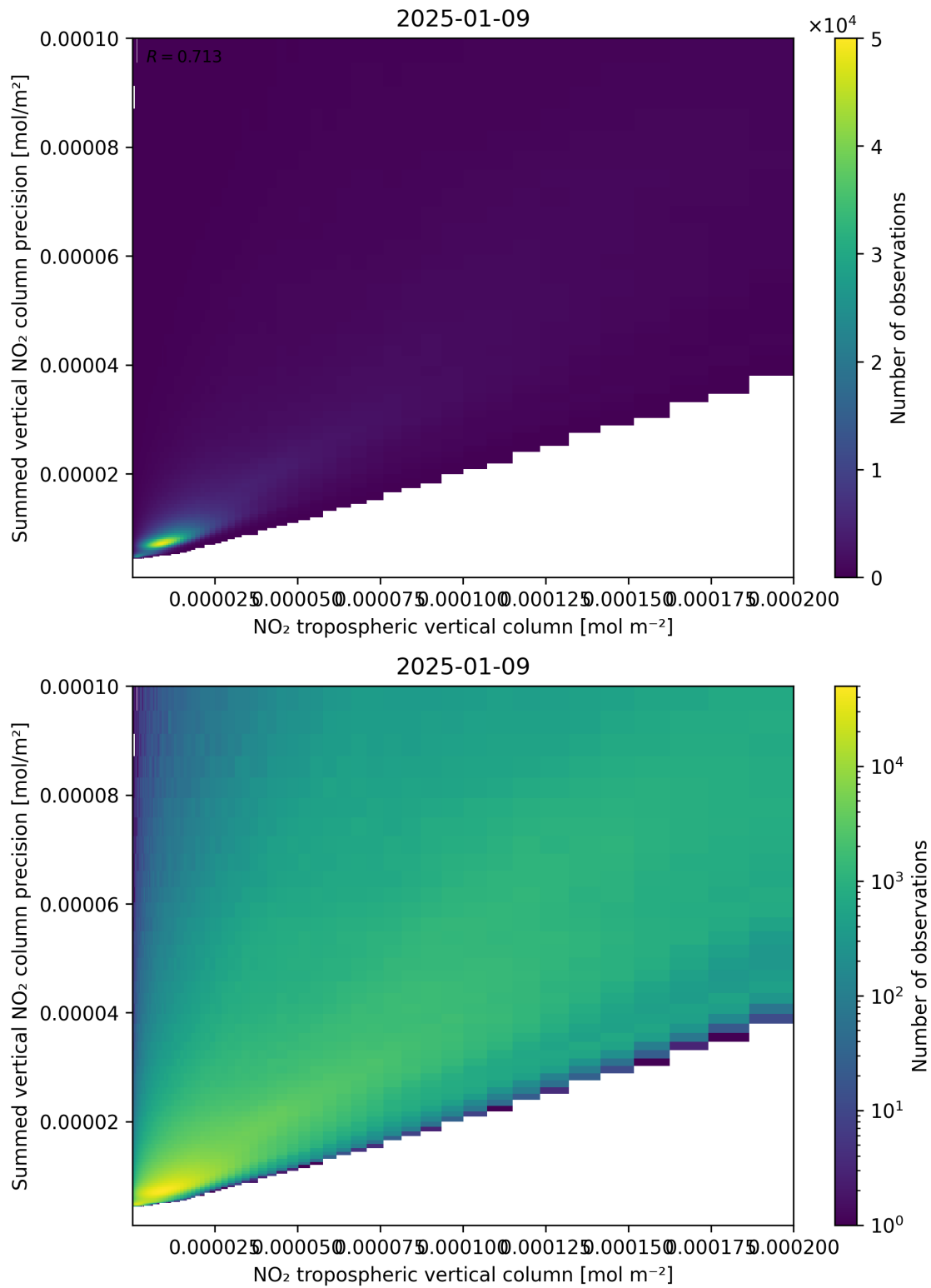
Figure 127: Scatter density plot of “NO 2 tropospheric vertical column” against “Summed vertical NO 2 column precision” for 2025-01-08 to 2025-01-10.
