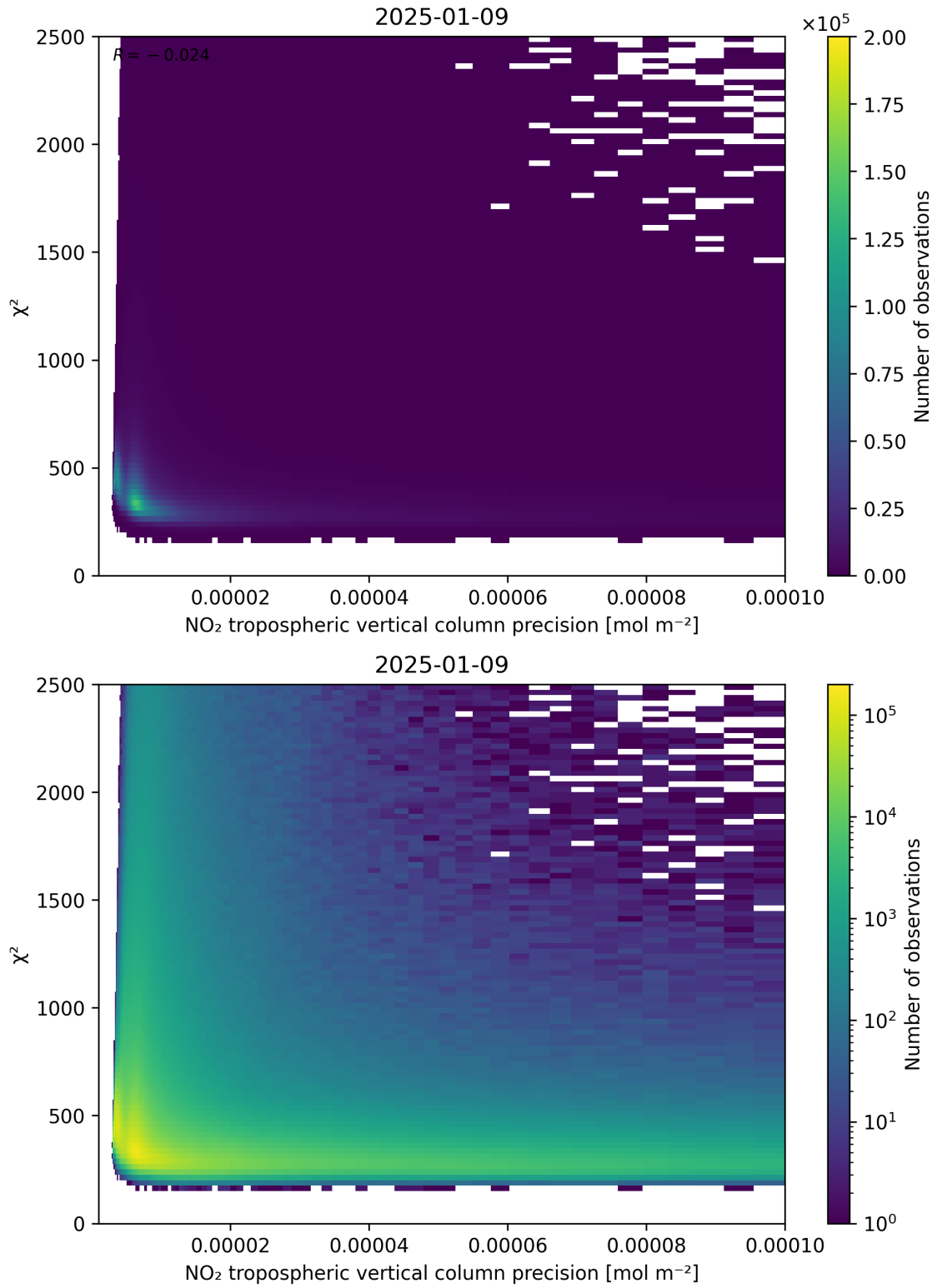
Figure 134: Scatter density plot of “NO 2 tropospheric vertical column precision” against “ \chi^2 ” for 2025-01-08 to 2025-01-10.
