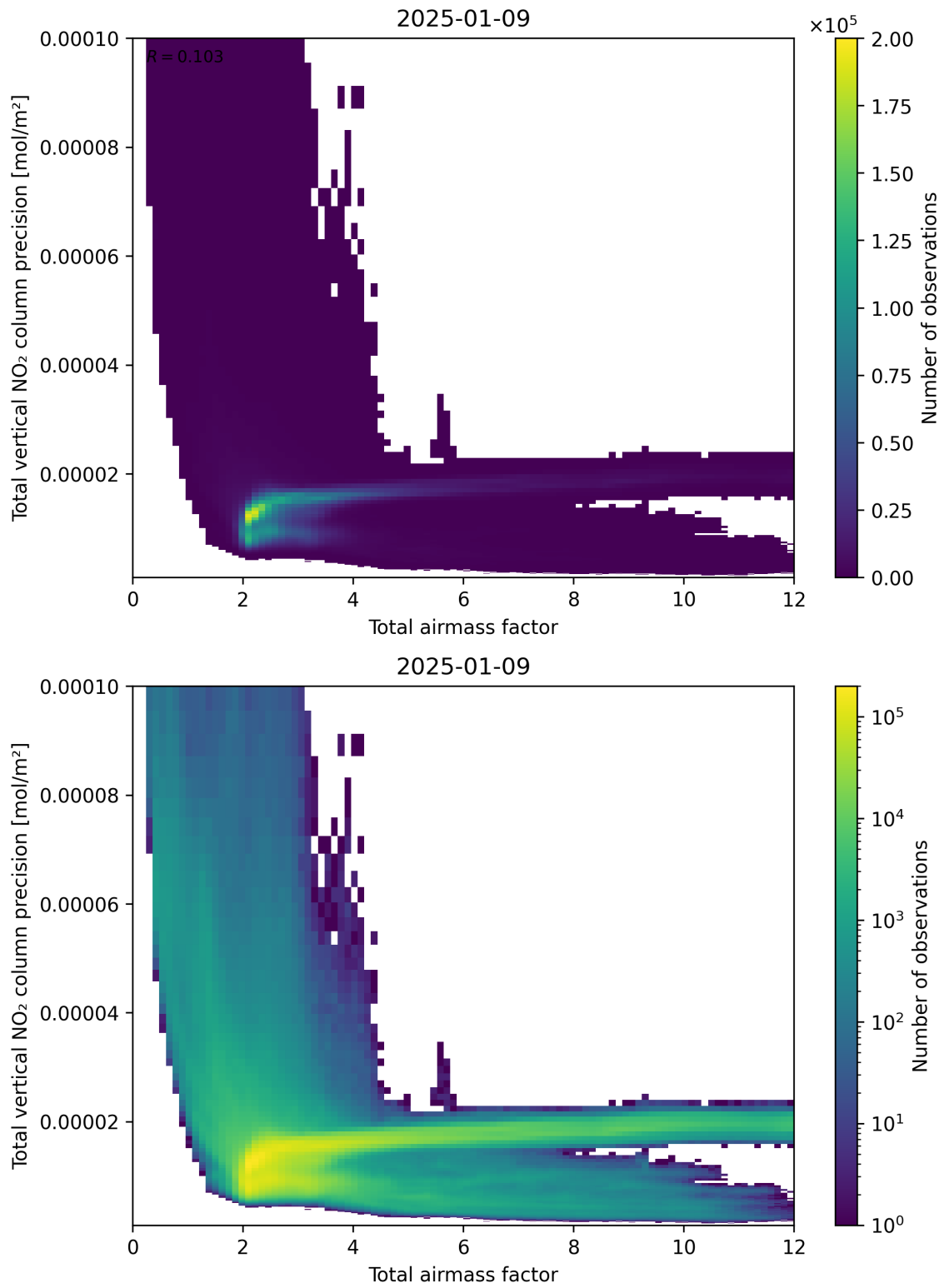
Figure 68: Scatter density plot of “Total airmass factor” against “Total vertical NO 2 column precision” for 2025-01-08 to 2025-01-10.
