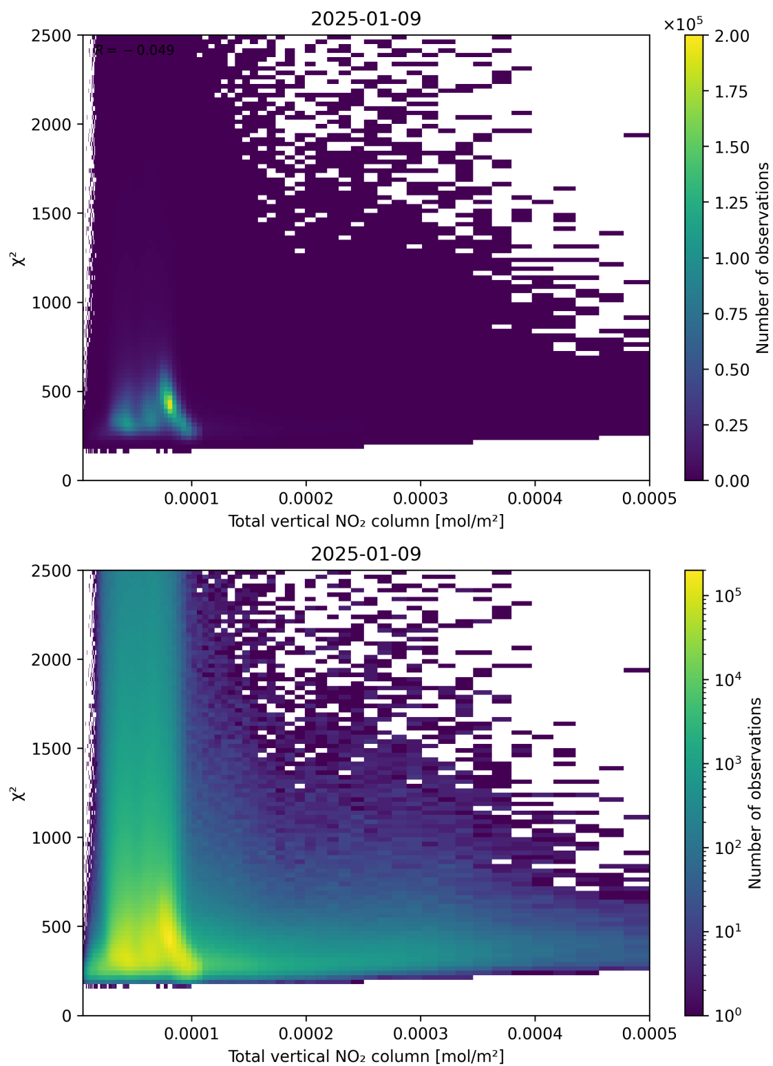
Figure 111: Scatter density plot of “Total vertical NO 2 column” against “ \chi^2 ” for 2025-01-08 to 2025-01-10.
