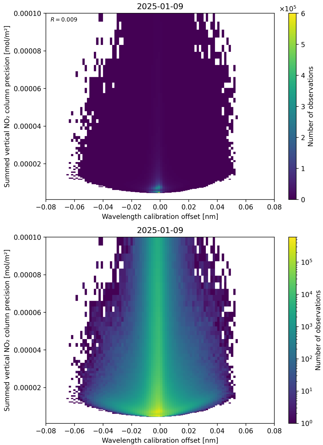
Figure 178: Scatter density plot of “Wavelength calibration offset” against “Summed vertical NO 2 column precision” for 2025-01-08 to 2025-01-10.
