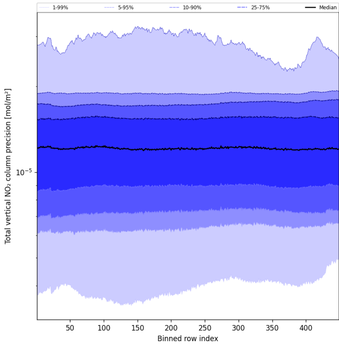
Figure 56: Along track statistics of “Total vertical NO 2 column precision” for 2025-01-08 to 2025-01-10
