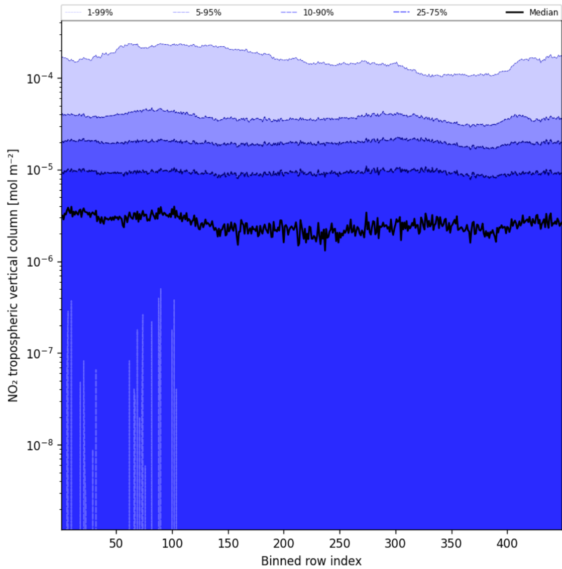
Figure 46: Along track statistics of “NO 2 tropospheric vertical column” for 2025-01-08 to 2025-01-10
