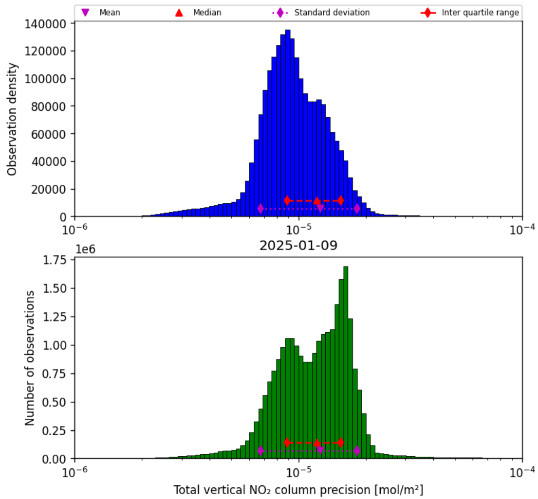
Figure 39: Histogram of “Total vertical NO 2 column precision” for 2025-01-08 to 2025-01-10
