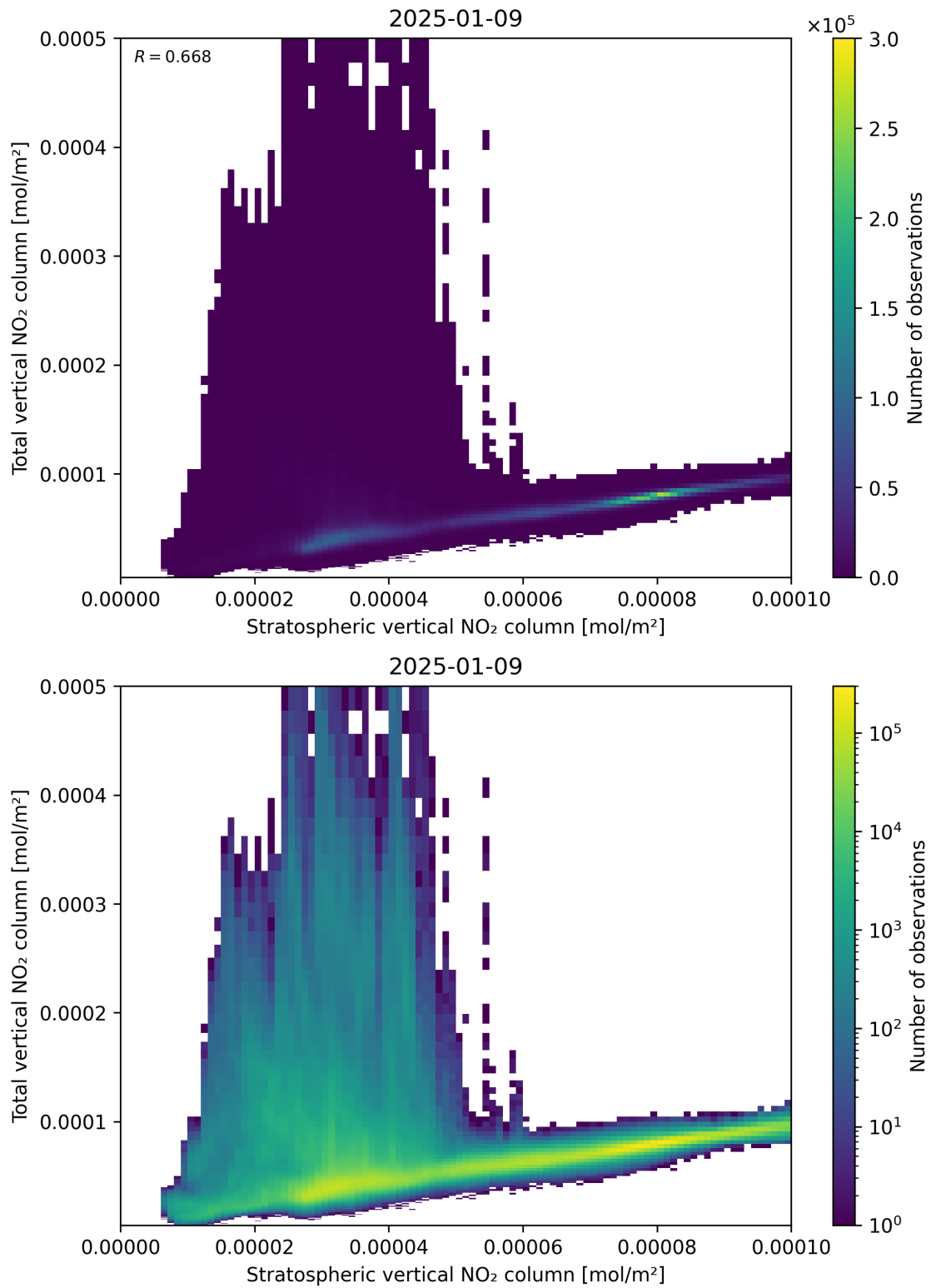
Figure 100: Scatter density plot of “Stratospheric vertical NO 2 column” against “Total vertical NO 2 column” for 2025-01-08 to 2025-01-10.
