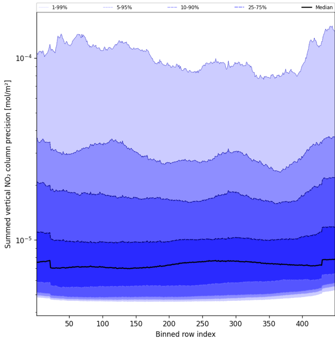
Figure 58: Along track statistics of “Summed vertical NO 2 column precision” for 2025-01-08 to 2025-01-10
