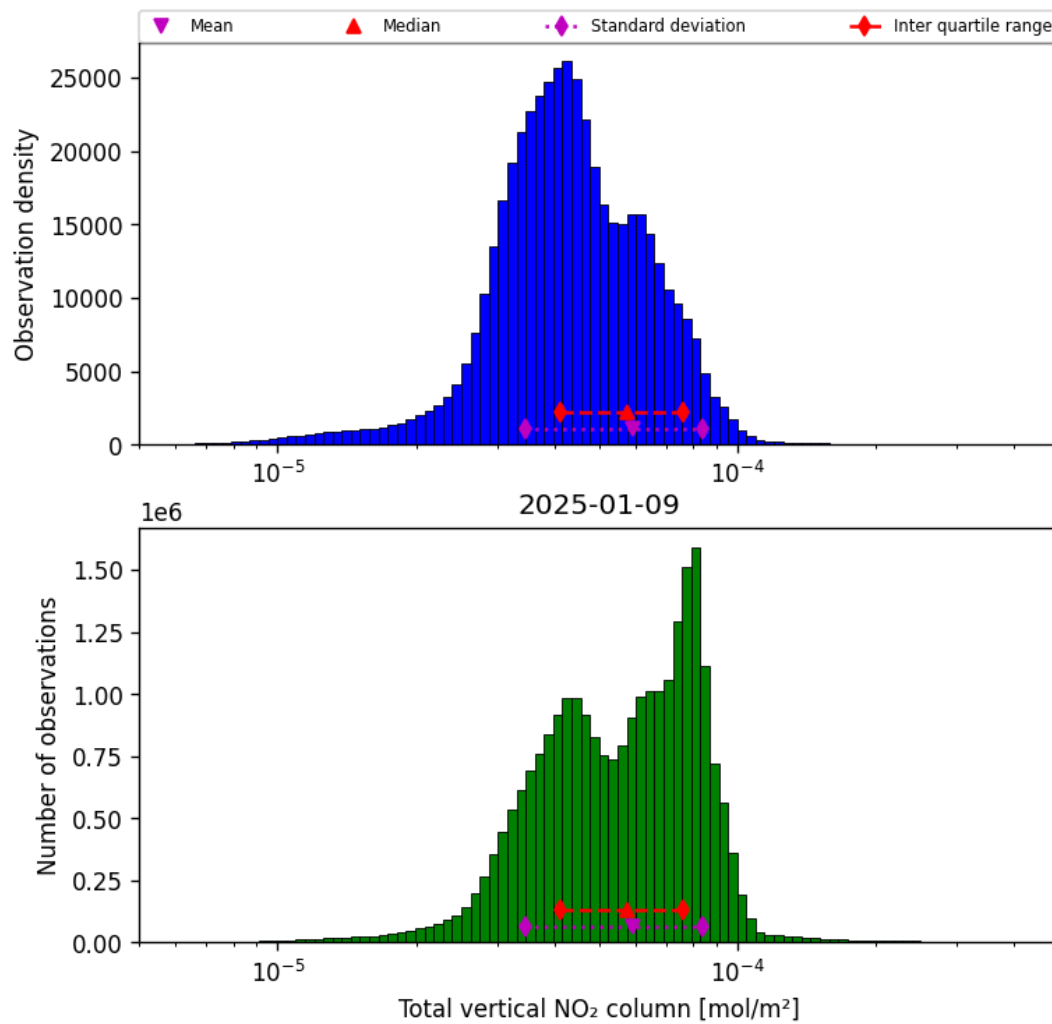
Figure 38: Histogram of “Total vertical NO 2 column” for 2025-01-08 to 2025-01-10
