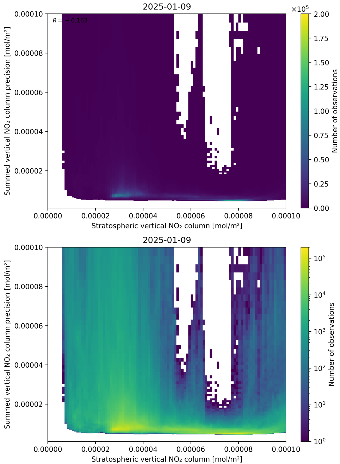
Figure 99: Scatter density plot of “Stratospheric vertical NO 2 column” against “Summed vertical NO 2 column precision” for 2025-01-08 to 2025-01-10.
