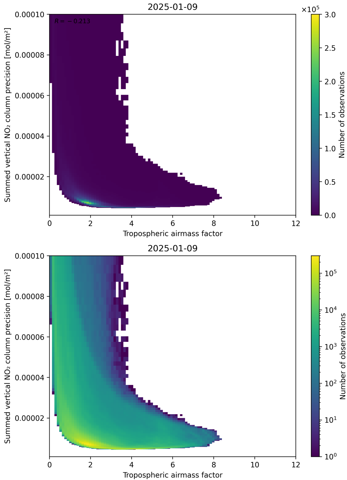
Figure 76: Scatter density plot of “Tropospheric air mass factor” against “Summed vertical NO 2 column precision” for 2025-01-08 to 2025-01-10.
