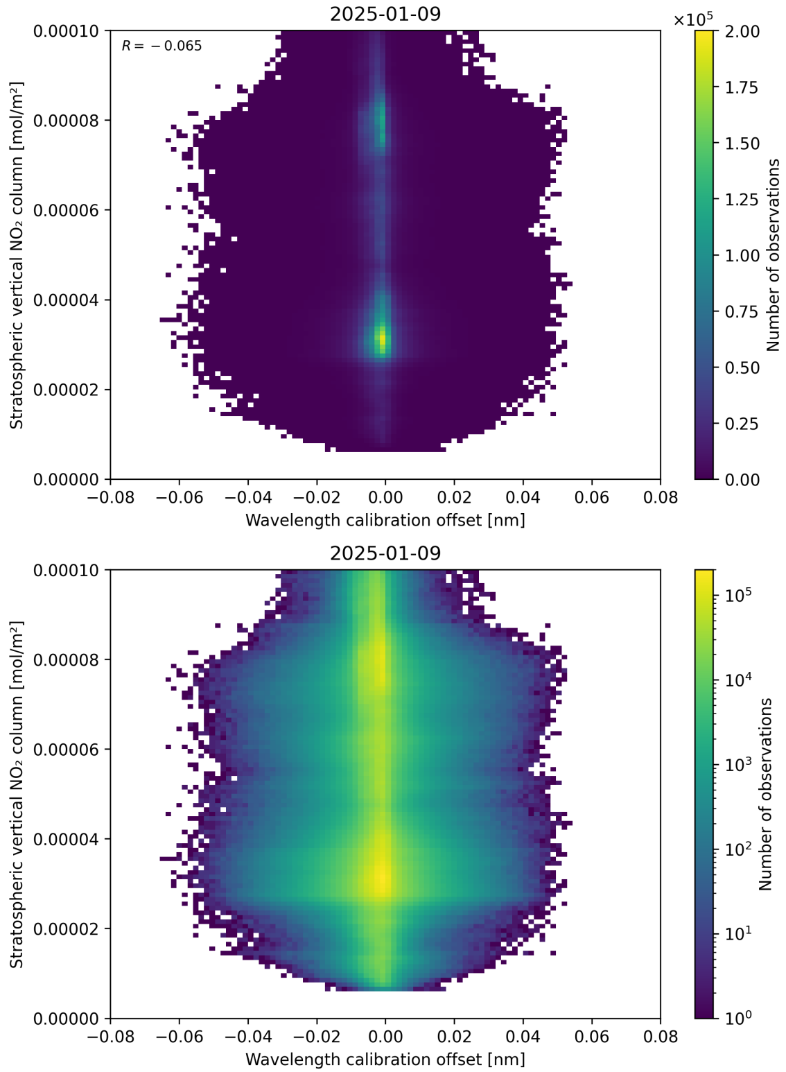
Figure 176: Scatter density plot of “Wavelength calibration offset” against “Stratospheric vertical NO 2 column” for 2025-01-08 to 2025-01-10.
