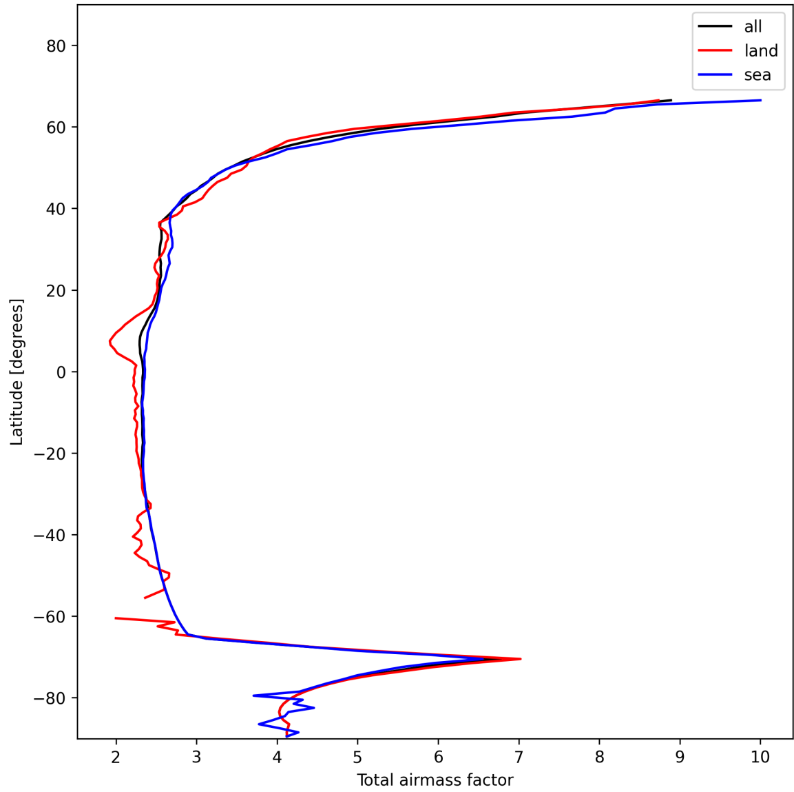
Figure 15: Zonal average of “Total airmass factor” for 2025-01-08 to 2025-01-10.
