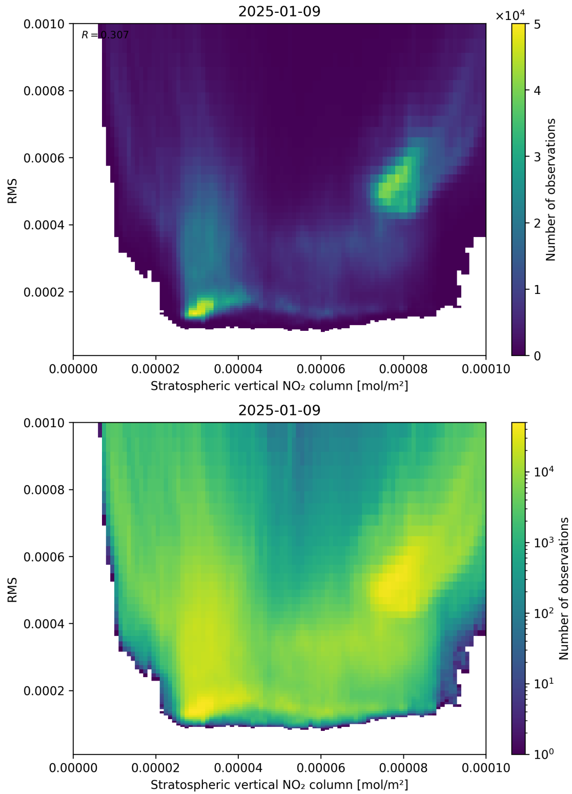
Figure 102: Scatter density plot of “Stratospheric vertical NO 2 column” against “RMS” for 2025-01-08 to 2025-01-10.
