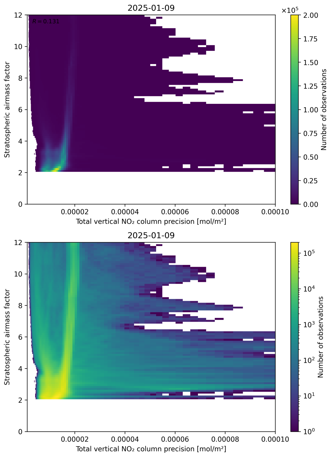
Figure 115: Scatter density plot of “Total vertical NO 2 column precision” against “Stratospheric air mass factor” for 2025-01-08 to 2025-01-10.
