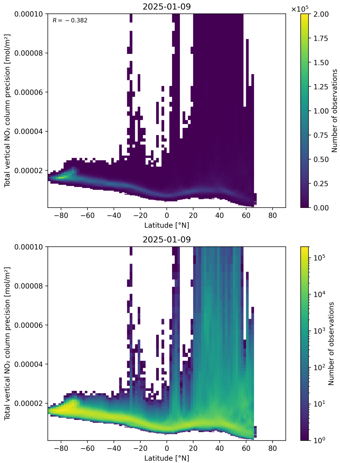
Figure 91: Scatter density plot of “Latitude” against “Total vertical NO 2 column precision” for 2025-01-08 to 2025-01-10.
