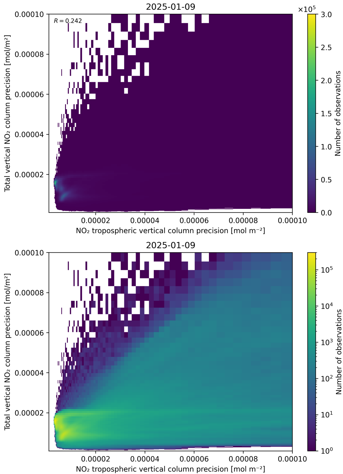
Figure 139: Scatter density plot of “NO 2 tropospheric vertical column precision” against “Total vertical NO 2 column precision” for 2025-01-08 to 2025-01-10.
