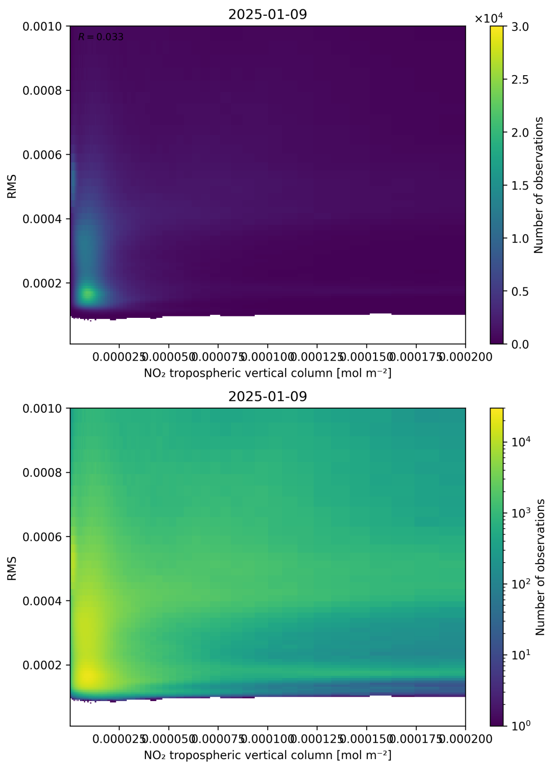
Figure 142: Scatter density plot of “NO 2 tropospheric vertical column” against “RMS” for 2025-01-08 to 2025-01-10.
