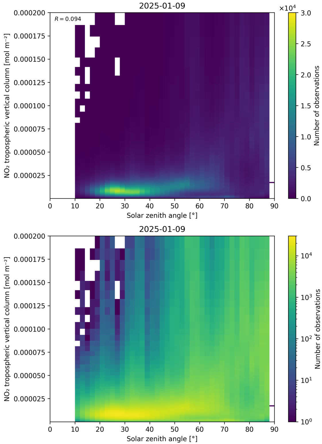
Figure 155: Scatter density plot of “Solar zenith angle” against “NO 2 tropospheric vertical column” for 2025-01-08 to 2025-01-10.
