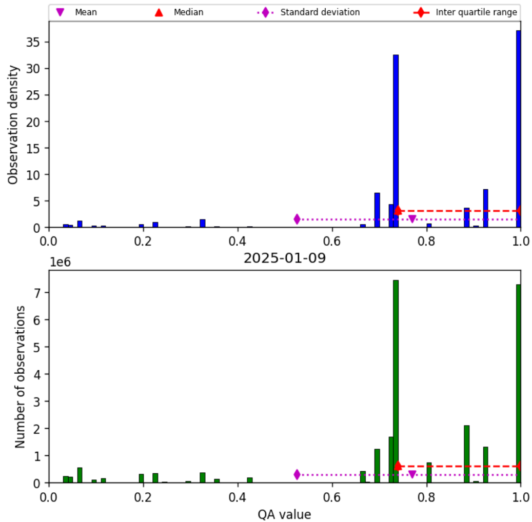
Figure 28: Histogram of “QA value” for 2025-01-08 to 2025-01-10
