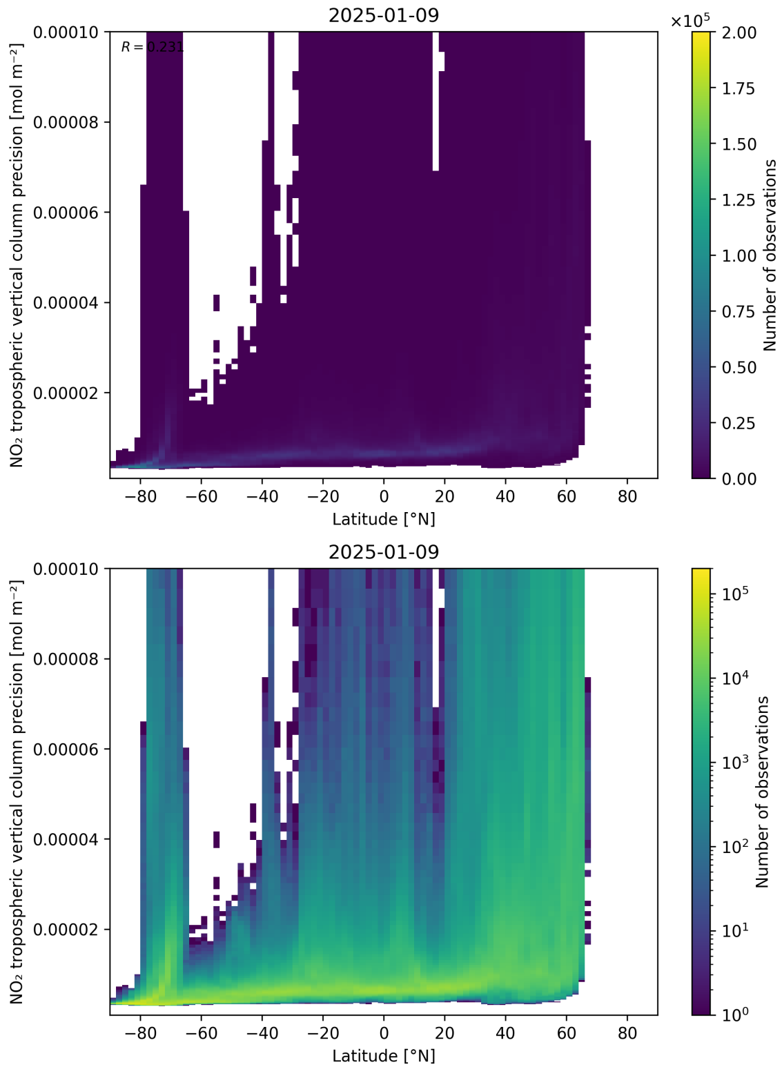
Figure 93: Scatter density plot of “Latitude” against “NO 2 tropospheric vertical column precision” for 2025-01-08 to 2025-01-10.
