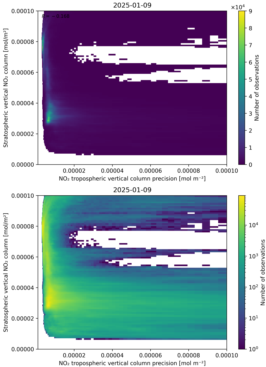
Figure 135: Scatter density plot of “NO 2 tropospheric vertical column precision” against “Stratospheric vertical NO 2 column” for 2025-01-08 to 2025-01-10.
