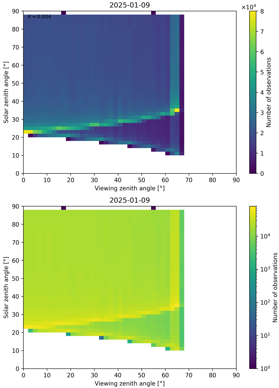
Figure 172: Scatter density plot of “Viewing zenith angle” against “Solar zenith angle” for 2025-01-08 to 2025-01-10.
