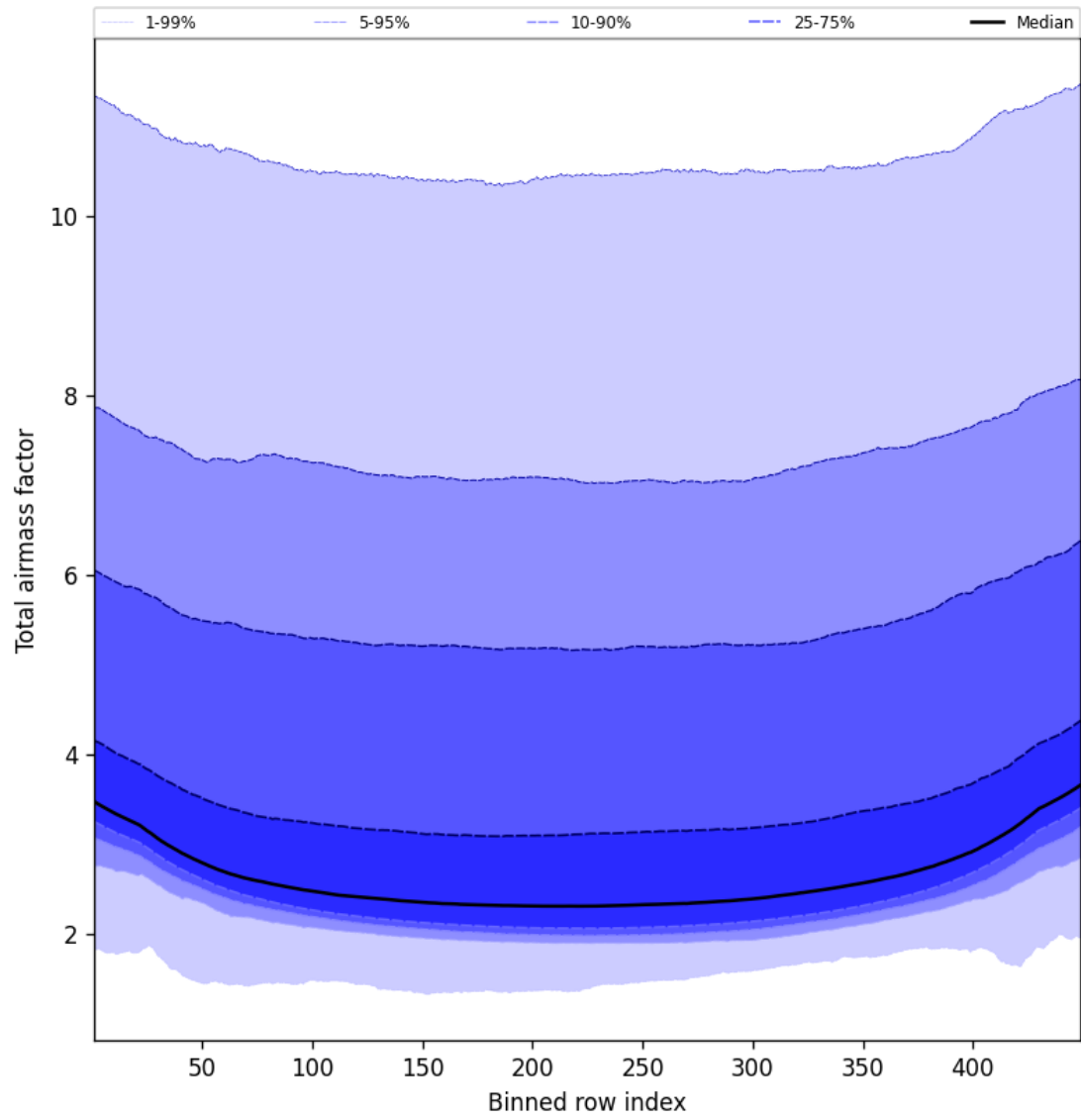
Figure 49: Along track statistics of “Total airmass factor” for 2025-01-08 to 2025-01-10
