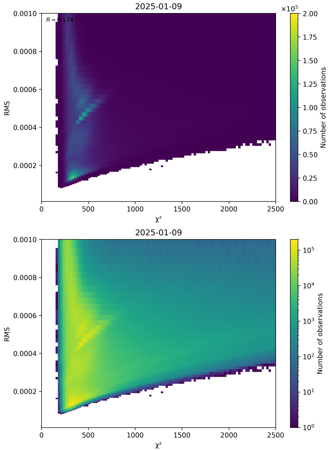
Figure 82: Scatter density plot of “ \chi^2 ” against “RMS” for 2025-01-08 to 2025-01-10.
