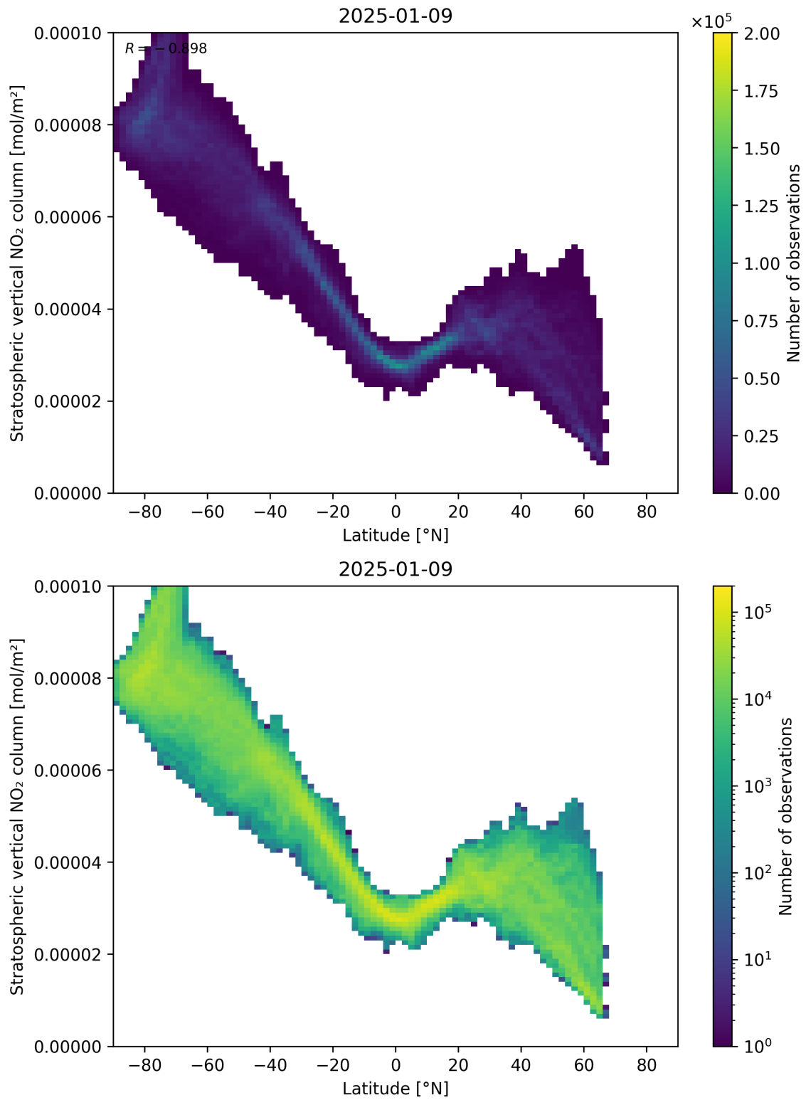
Figure 87: Scatter density plot of “Latitude” against “Stratospheric vertical NO 2 column” for 2025-01-08 to 2025-01-10.
