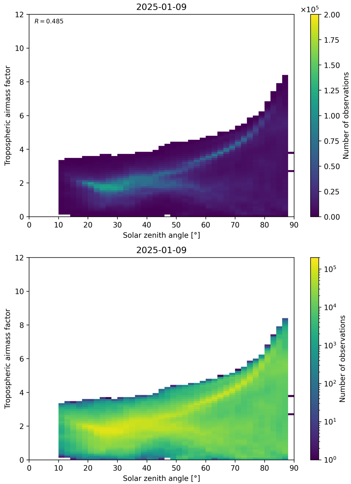
Figure 147: Scatter density plot of “Solar zenith angle” against “Tropospheric airmass factor” for 2025-01-08 to 2025-01-10.
