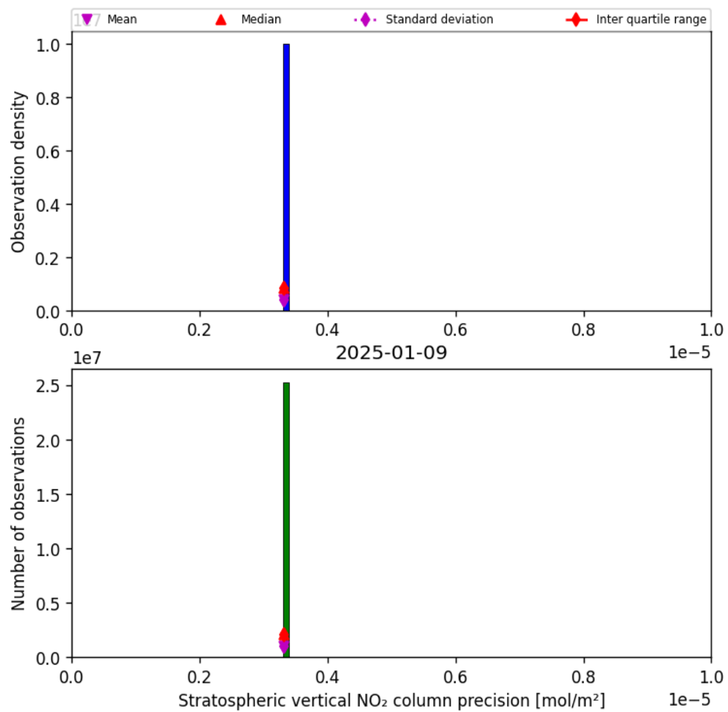
Figure 37: Histogram of “Stratospheric vertical NO 2 column precision” for 2025-01-08 to 2025-01-10
