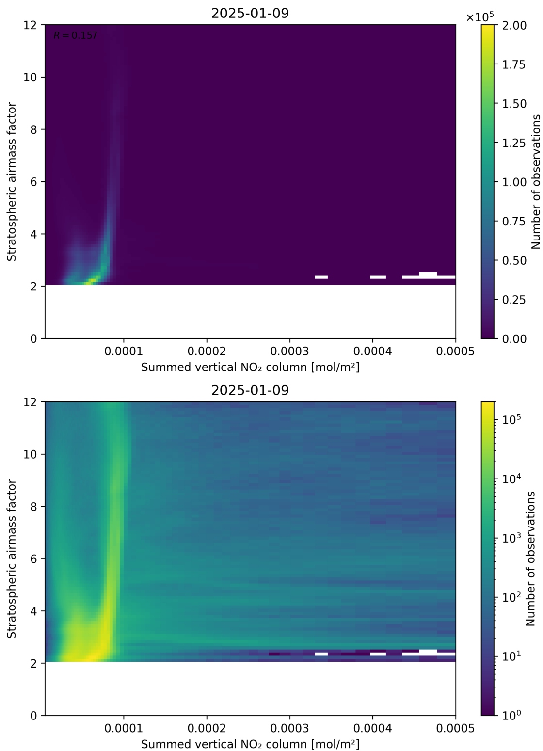
Figure 103: Scatter density plot of “Summed vertical NO 2 column” against “Stratospheric airmass factor” for 2025-01-08 to 2025-01-10.
