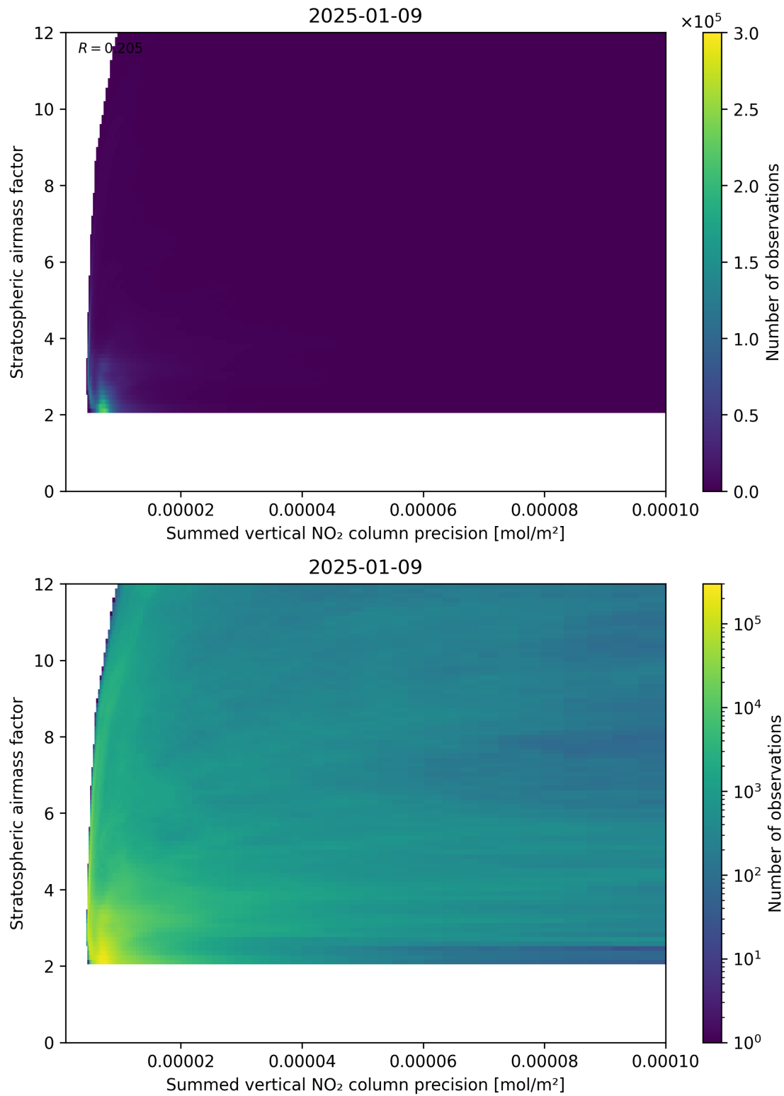
Figure 106: Scatter density plot of “Summed vertical NO 2 column precision” against “Stratospheric airmass factor” for 2025-01-08 to 2025-01-10.
