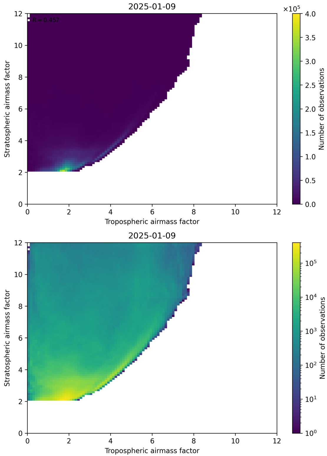
Figure 71: Scatter density plot of “Tropospheric airmass factor” against “Stratospheric airmass factor” for 2025-01-08 to 2025-01-10.
