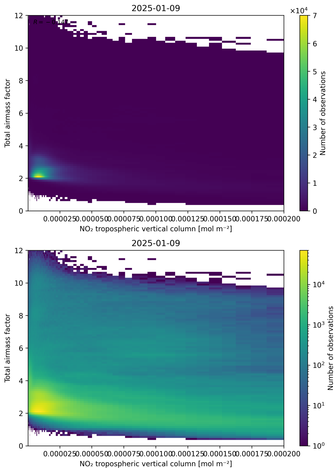
Figure 122: Scatter density plot of “NO 2 tropospheric vertical column” against “Total air mass factor” for 2025-01-08 to 2025-01-10.
