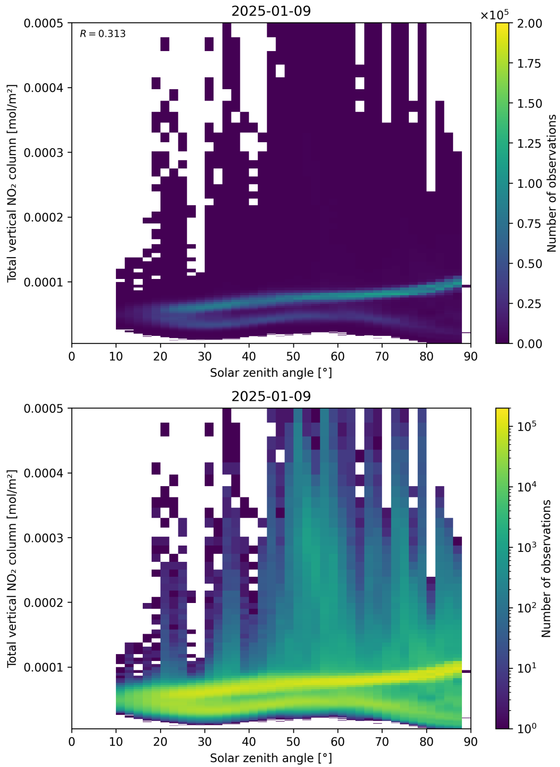
Figure 153: Scatter density plot of “Solar zenith angle” against “Total vertical NO 2 column” for 2025-01-08 to 2025-01-10.
