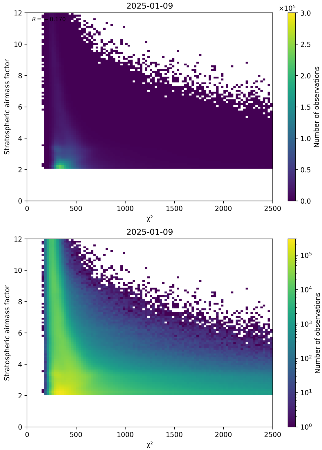
Figure 81: Scatter density plot of “ \chi^2 ” against “Stratospheric airmass factor” for 2025-01-08 to 2025-01-10.
