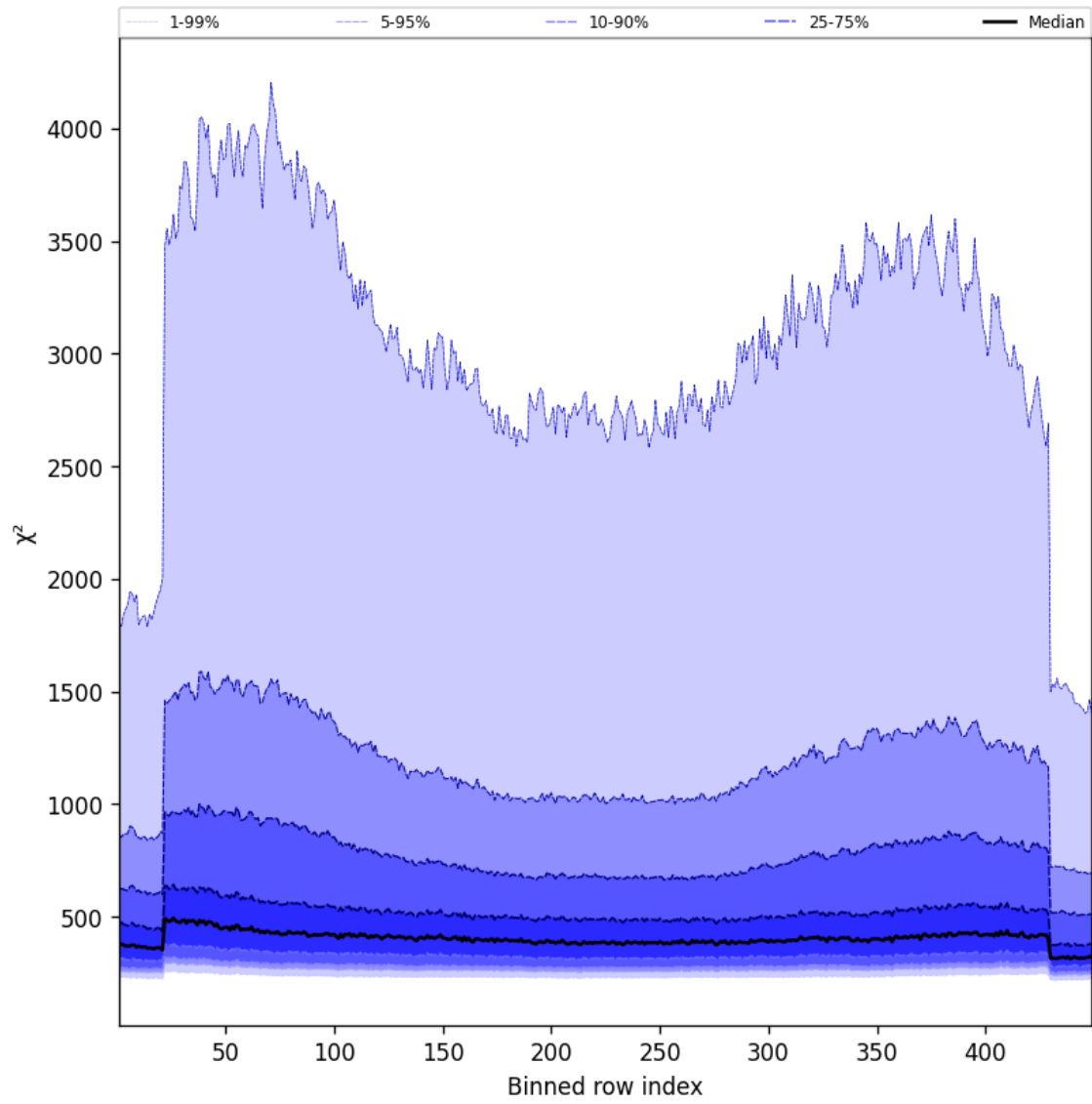
Figure 59: Along track statistics of “ \chi^2 ” for 2025-01-08 to 2025-01-10
