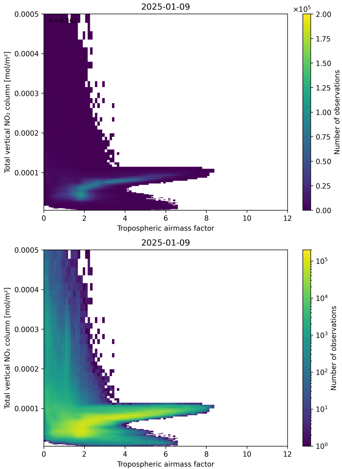
Figure 77: Scatter density plot of “Tropospheric airmass factor” against “Total vertical NO 2 column” for 2025-01-08 to 2025-01-10.
