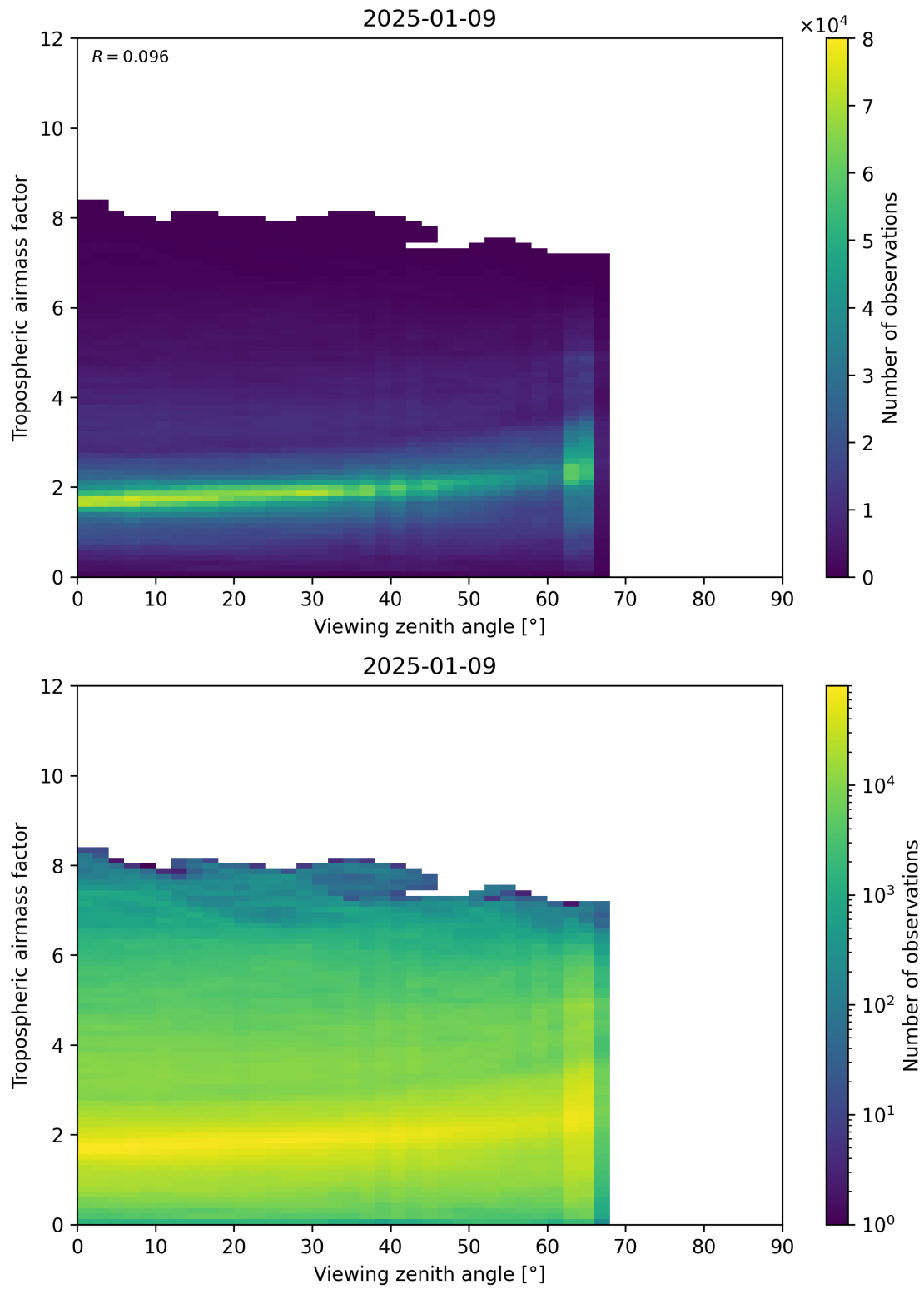
Figure 161: Scatter density plot of “Viewing zenith angle” against “Tropospheric airmass factor” for 2025-01-08 to 2025-01-10.
