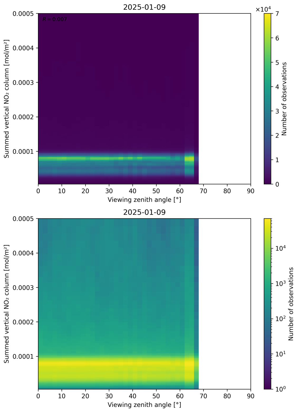
Figure 165: Scatter density plot of “Viewing zenith angle” against “Summed vertical NO 2 column” for 2025-01-08 to 2025-01-10.
