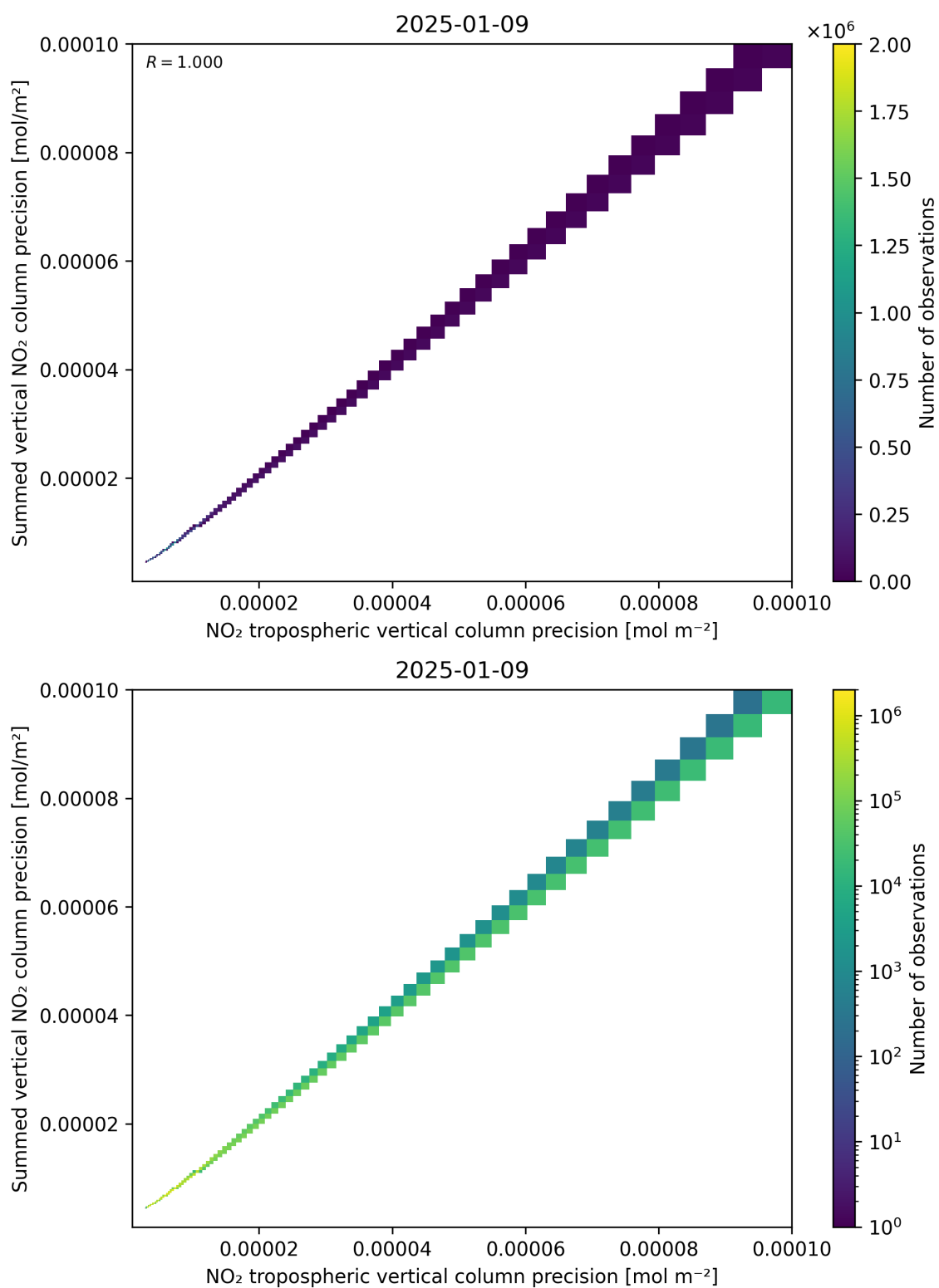
Figure 137: Scatter density plot of “NO 2 tropospheric vertical column precision” against “Summed vertical NO 2 column precision” for 2025-01-08 to 2025-01-10.
