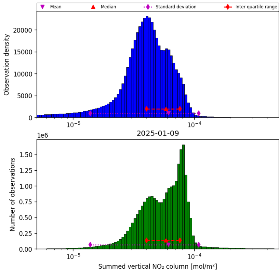
Figure 40: Histogram of “Summed vertical NO 2 column” for 2025-01-08 to 2025-01-10
