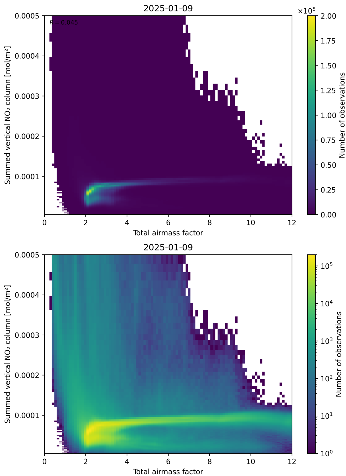
Figure 65: Scatter density plot of “Total airmass factor” against “Summed vertical NO 2 column” for 2025-01-08 to 2025-01-10.
