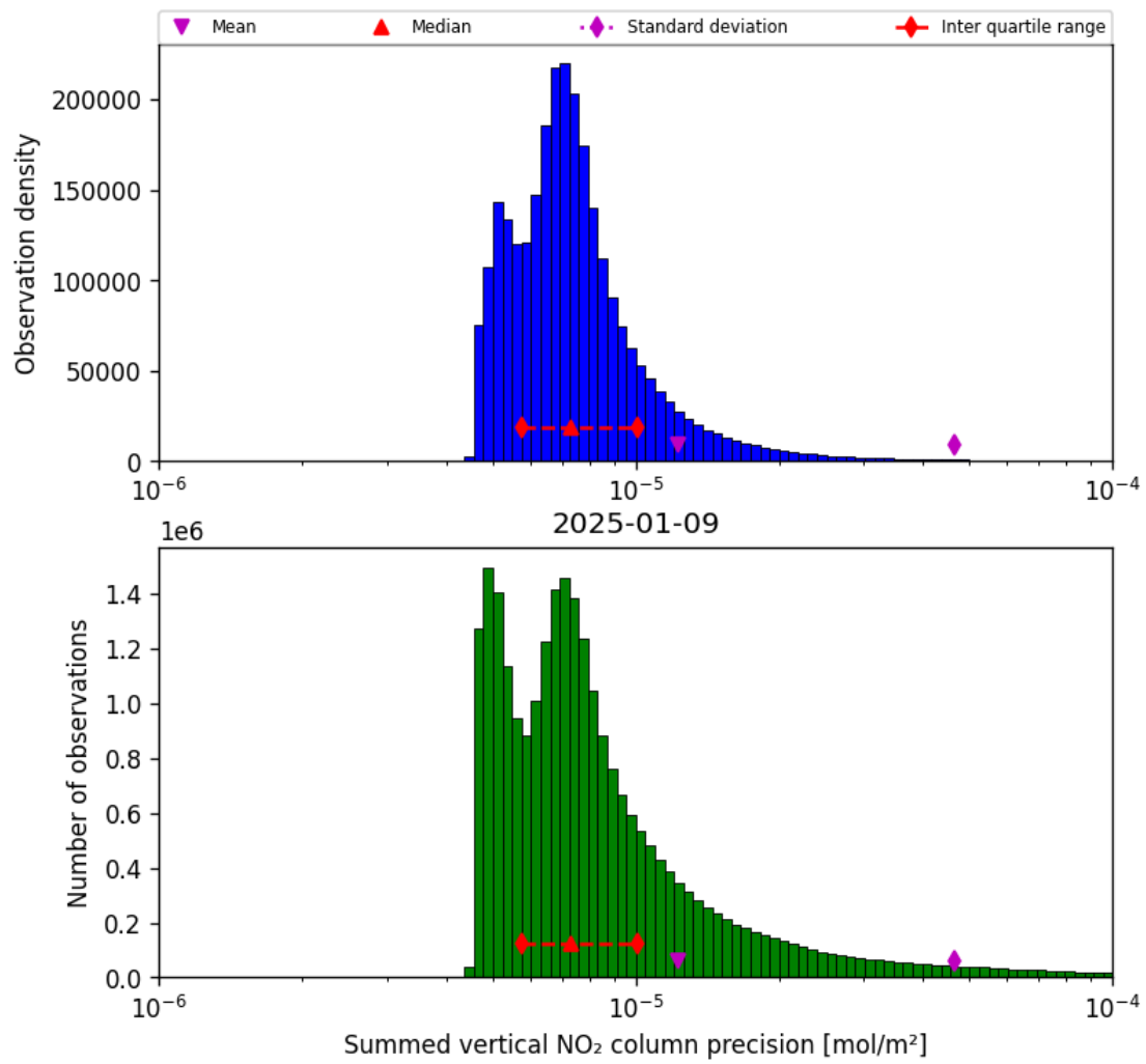
Figure 41: Histogram of “Summed vertical NO 2 column precision” for 2025-01-08 to 2025-01-10
