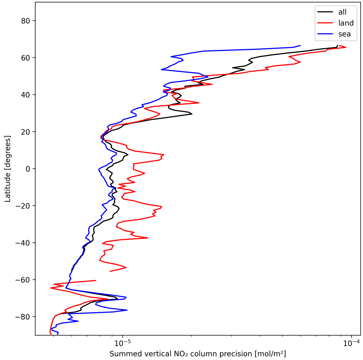
Figure 24: Zonal average of “Summed vertical NO 2 column precision” for 2025-01-08 to 2025-01-10.
