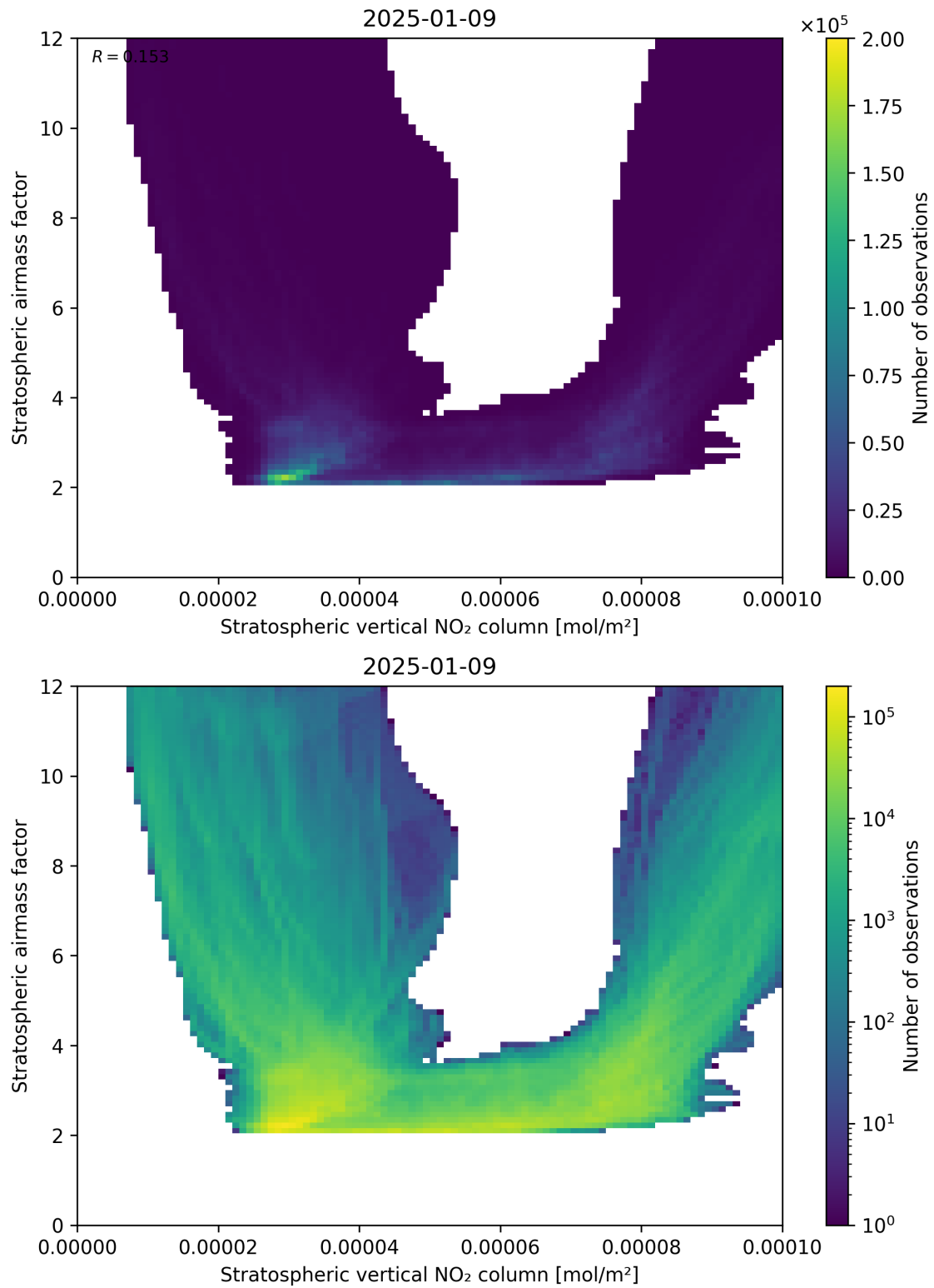
Figure 96: Scatter density plot of “Stratospheric vertical NO 2 column” against “Stratospheric airmass factor” for 2025-01-08 to 2025-01-10.
