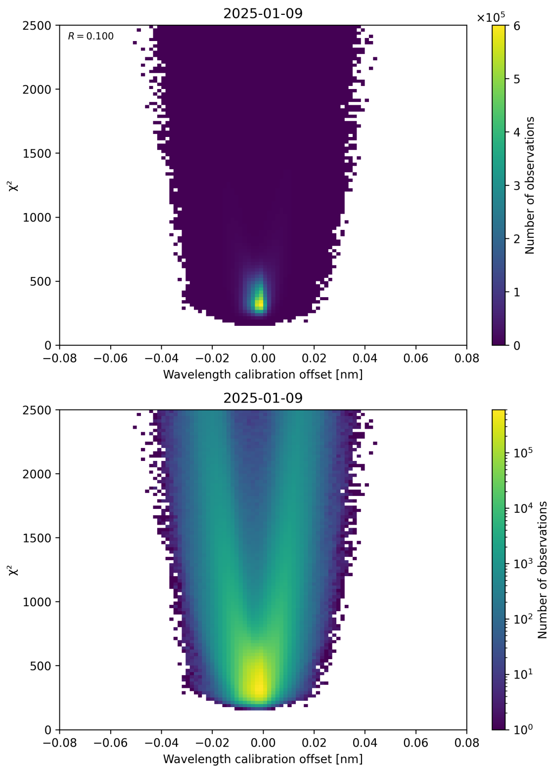
Figure 175: Scatter density plot of “Wavelength calibration offset” against “ \chi^2 ” for 2025-01-08 to 2025-01-10.
