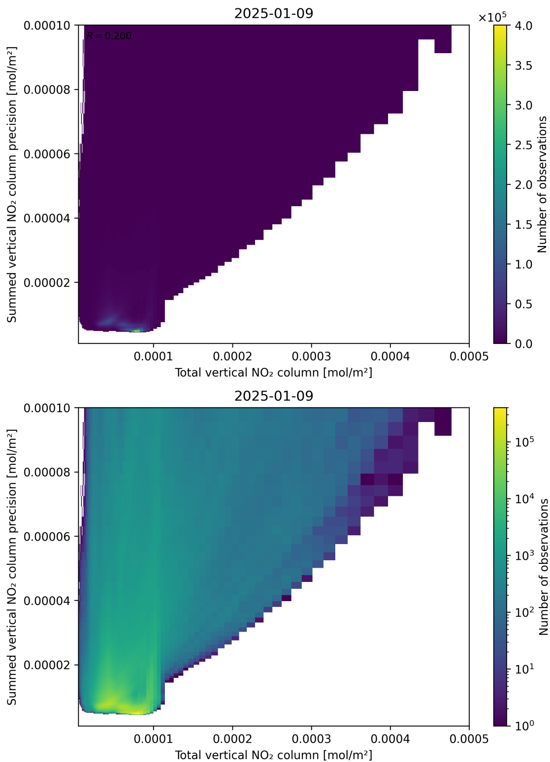
Figure 113: Scatter density plot of “Total vertical NO 2 column” against “Summed vertical NO 2 column precision” for 2025-01-08 to 2025-01-10.
