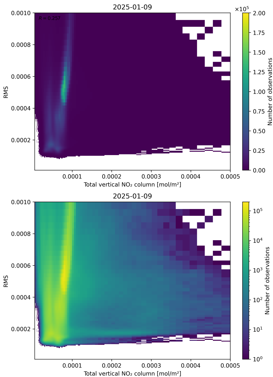
Figure 120: Scatter density plot of “Total vertical NO 2 column” against “RMS” for 2025-01-08 to 2025-01-10.
