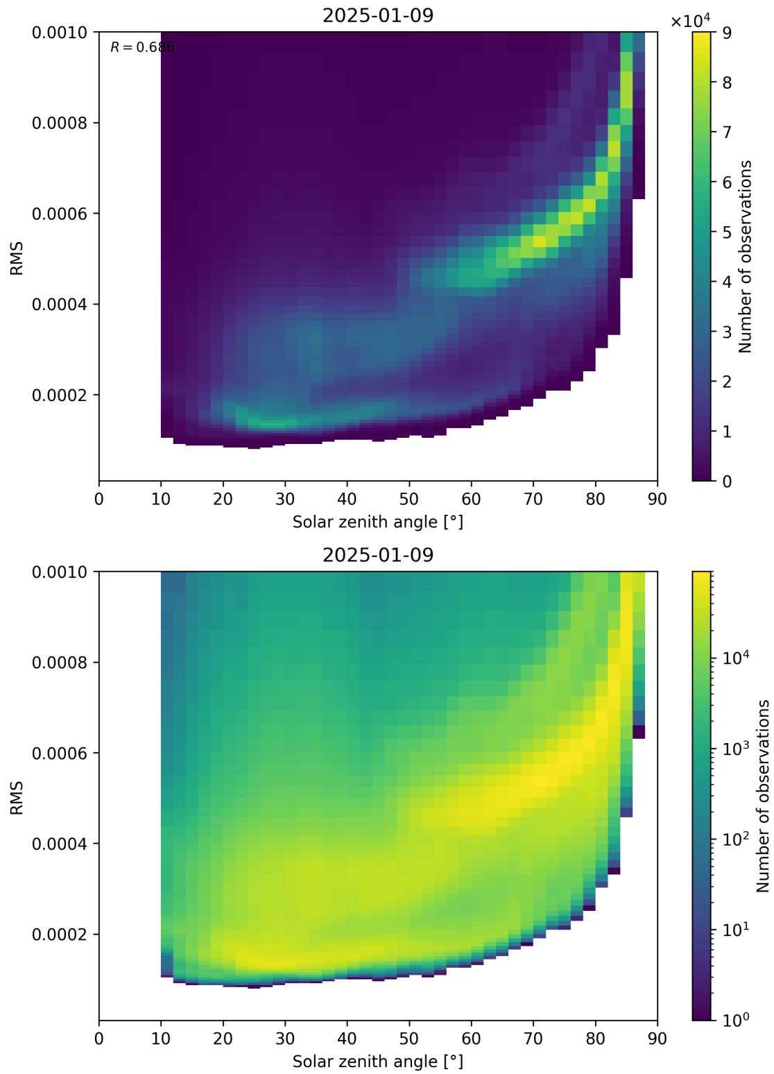
Figure 157: Scatter density plot of “Solar zenith angle” against “RMS” for 2025-01-08 to 2025-01-10.
