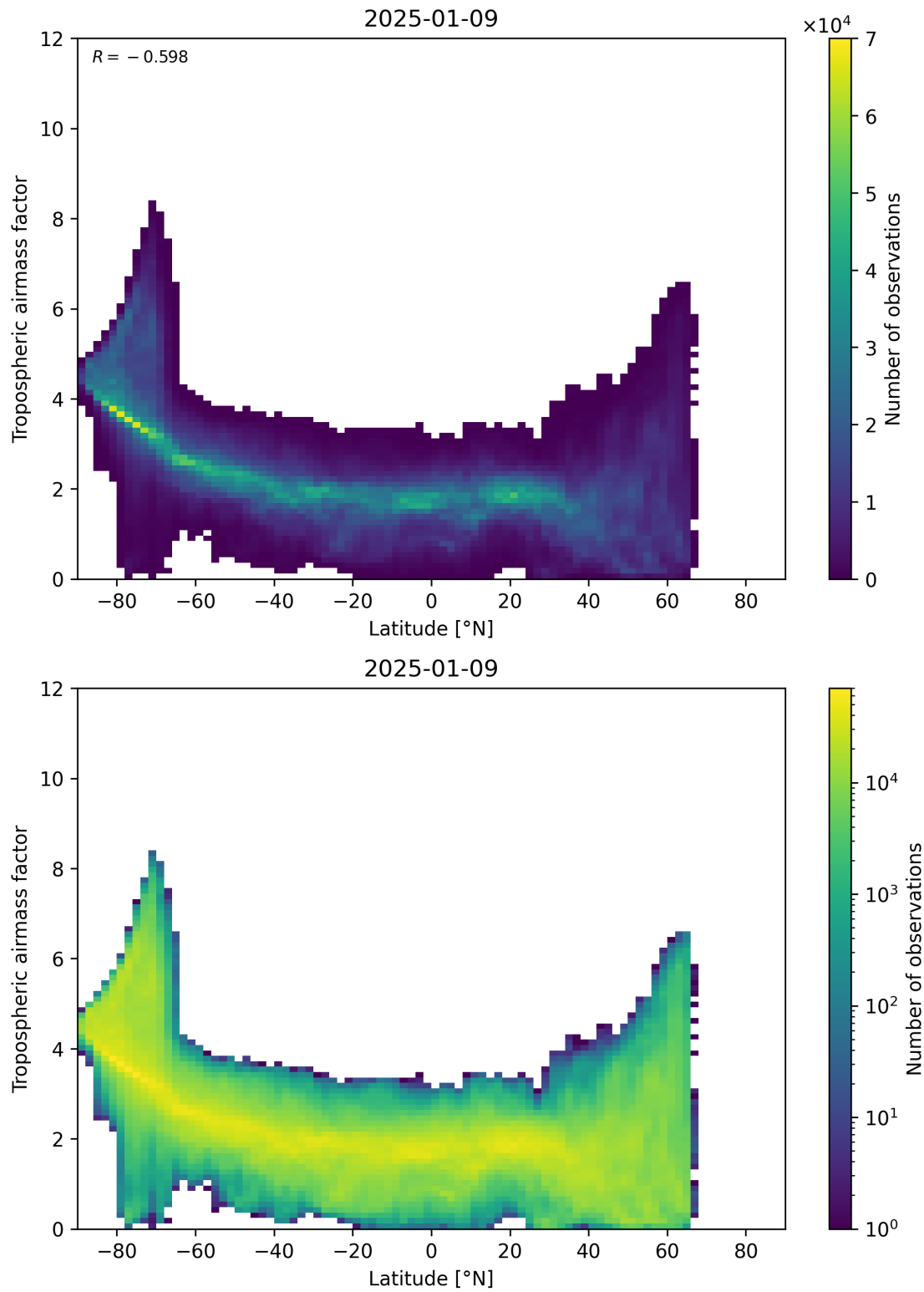
Figure 85: Scatter density plot of “Latitude” against “Tropospheric airmass factor” for 2025-01-08 to 2025-01-10.
