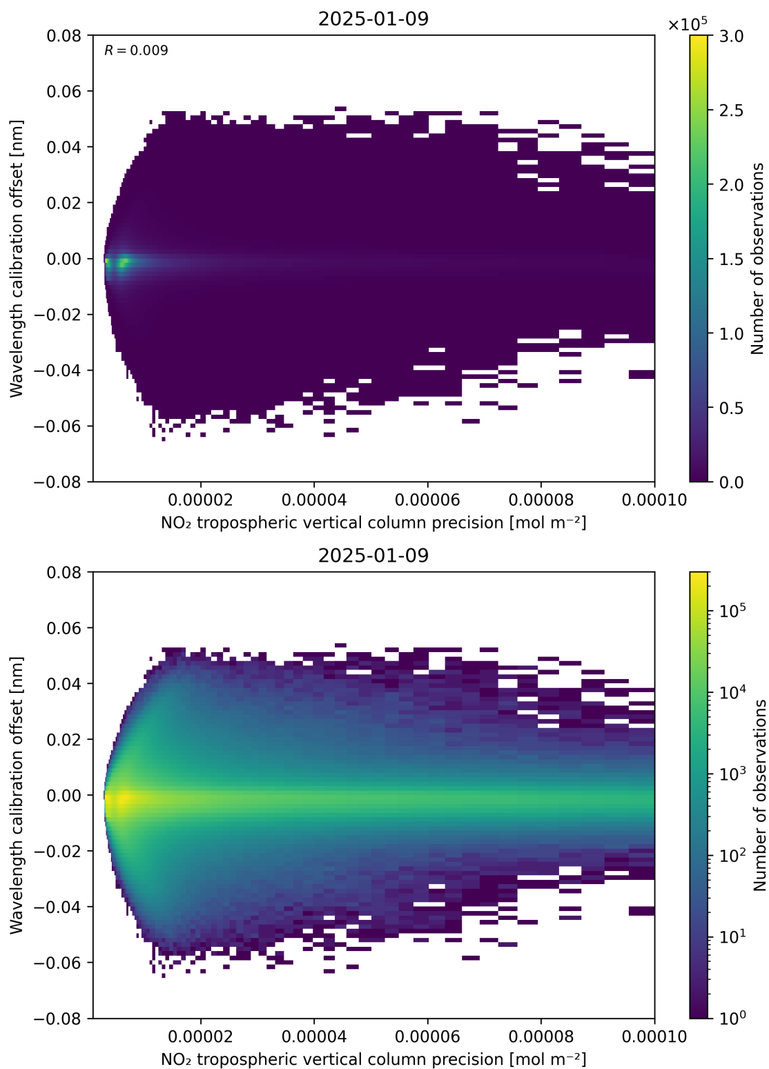
Figure 141: Scatter density plot of “NO 2 tropospheric vertical column precision” against “Wavelength calibration offset” for 2025-01-08 to 2025-01-10.
