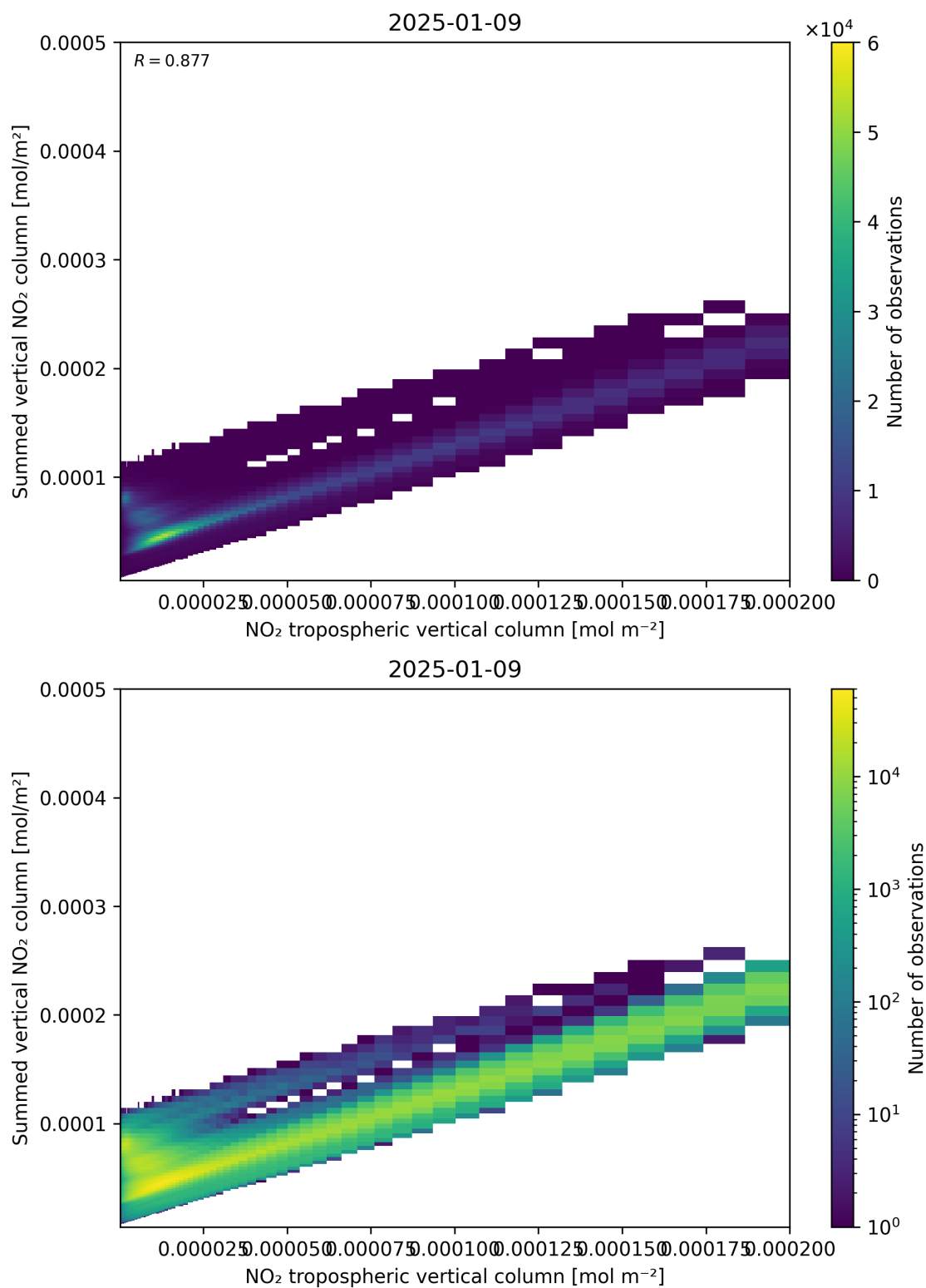
Figure 126: Scatter density plot of “NO 2 tropospheric vertical column” against “Summed vertical NO 2 column” for 2025-01-08 to 2025-01-10.
