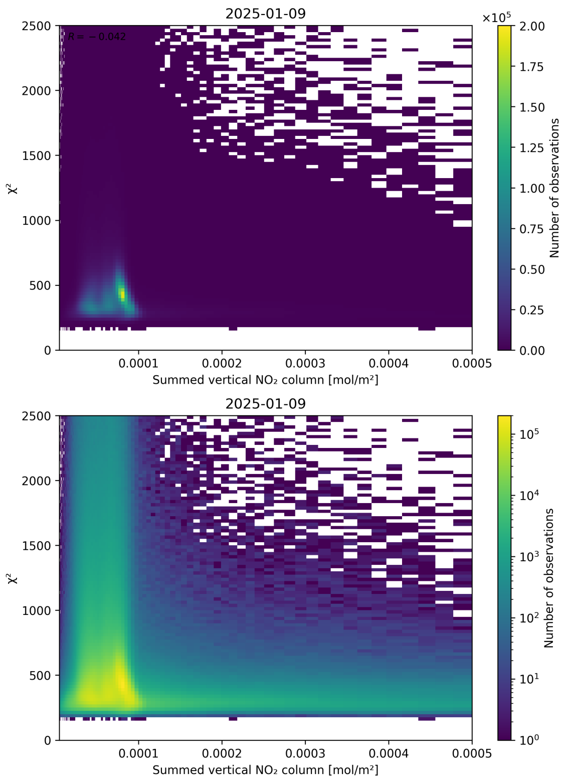
Figure 104: Scatter density plot of “Summed vertical NO 2 column” against “ \chi^2 ” for 2025-01-08 to 2025-01-10.
