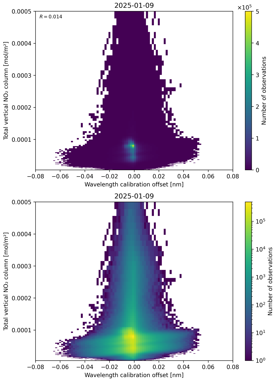
Figure 179: Scatter density plot of “Wavelength calibration offset” against “Total vertical NO 2 column” for 2025-01-08 to 2025-01-10.
