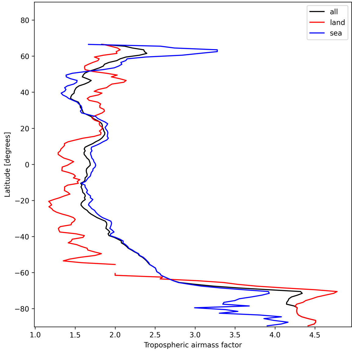
Figure 14: Zonal average of “Tropospheric air mass factor” for 2025-01-08 to 2025-01-10.
