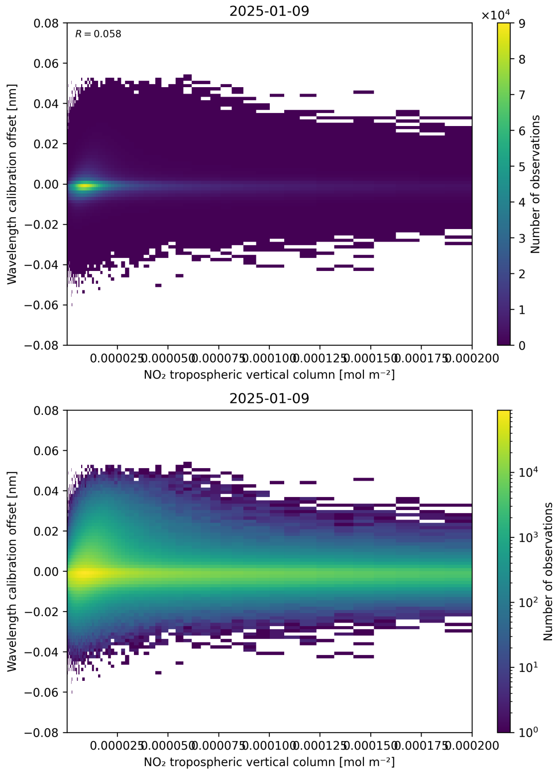
Figure 143: Scatter density plot of “NO 2 tropospheric vertical column” against “Wavelength calibration offset” for 2025-01-08 to 2025-01-10.
