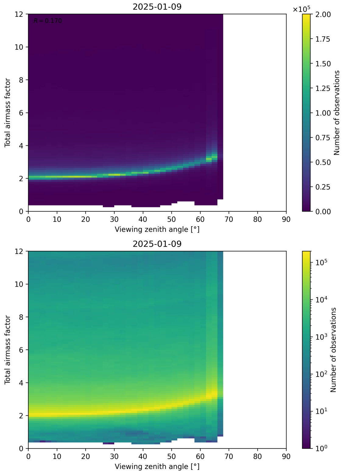
Figure 160: Scatter density plot of “Viewing zenith angle” against “Total airmass factor” for 2025-01-08 to 2025-01-10.
