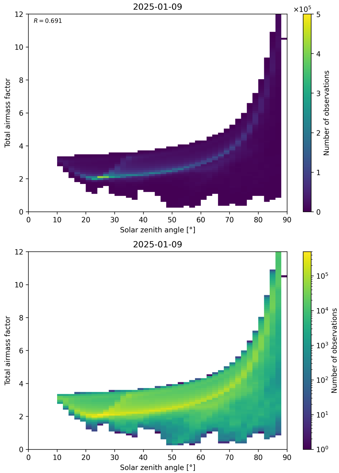
Figure 146: Scatter density plot of “Solar zenith angle” against “Total air mass factor” for 2025-01-08 to 2025-01-10.
