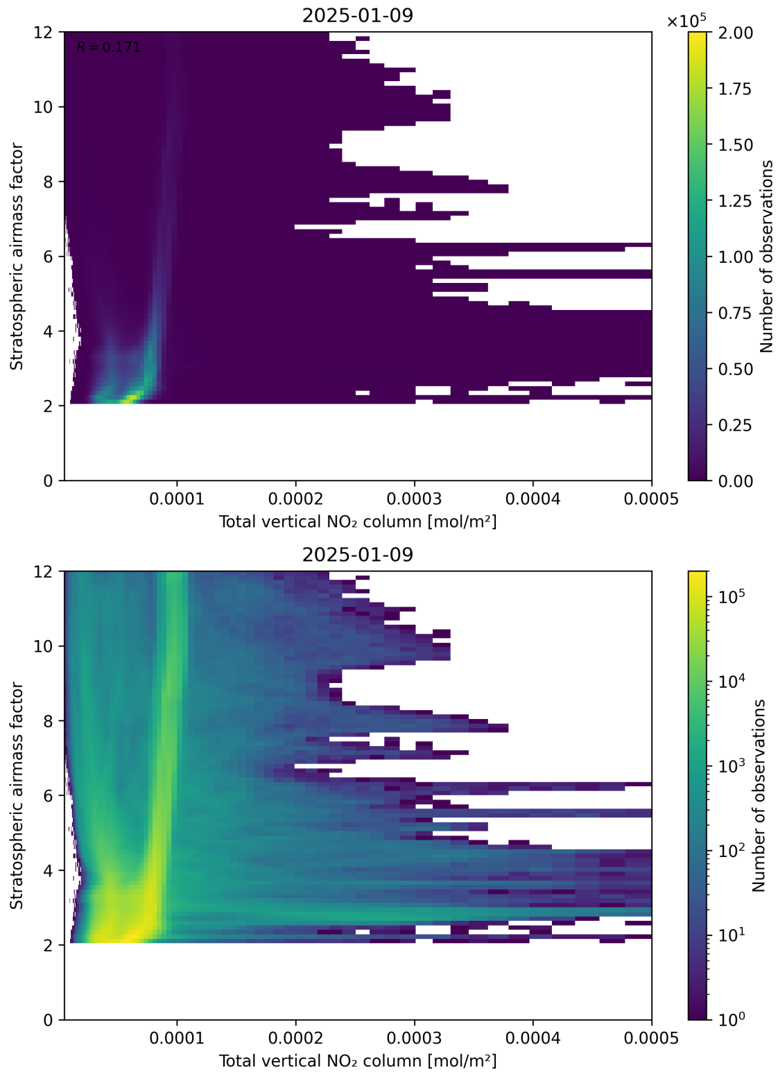
Figure 110: Scatter density plot of “Total vertical NO 2 column” against “Stratospheric airmass factor” for 2025-01-08 to 2025-01-10.
