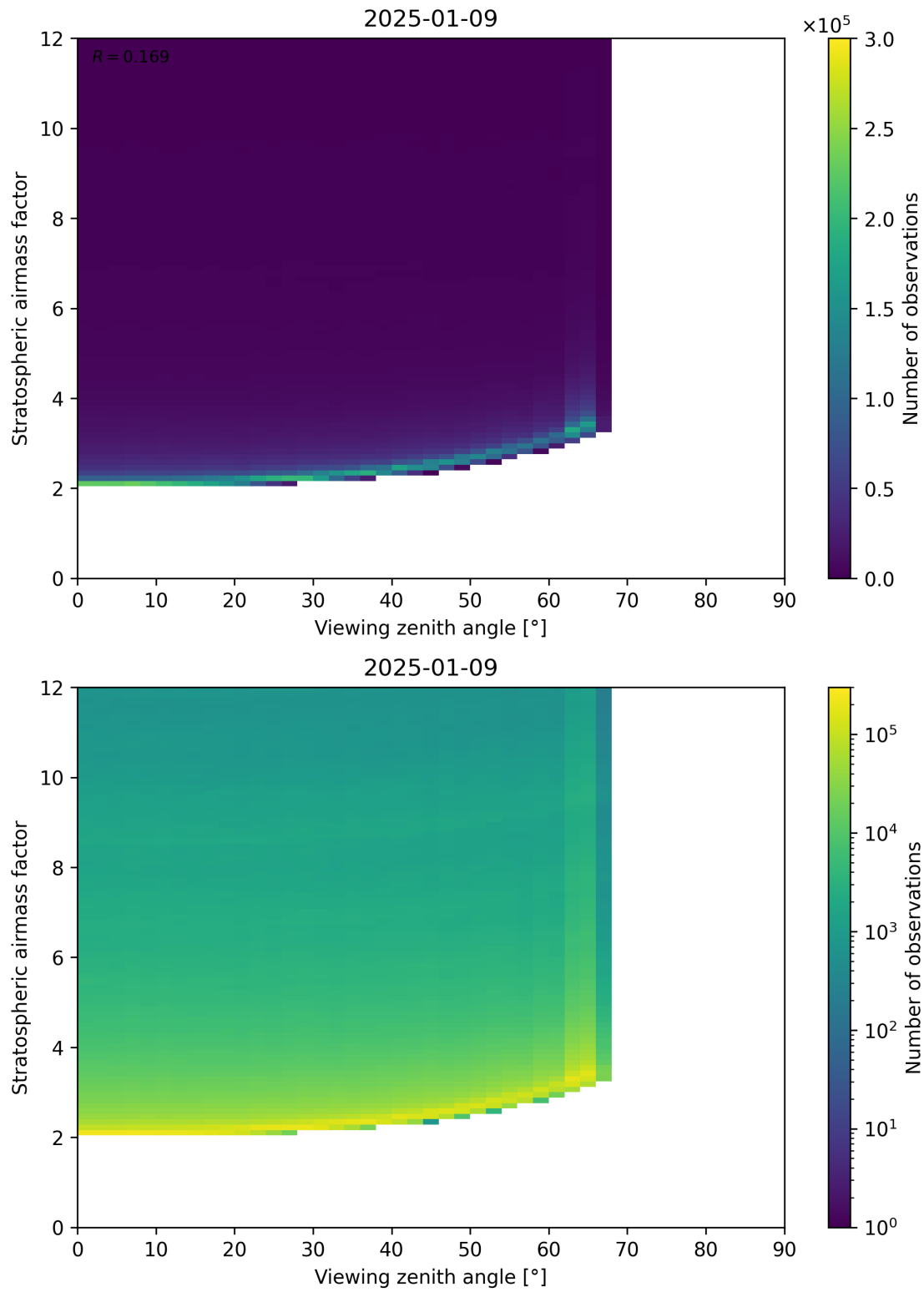
Figure 159: Scatter density plot of “Viewing zenith angle” against “Stratospheric airmass factor” for 2025-01-08 to 2025-01-10.
