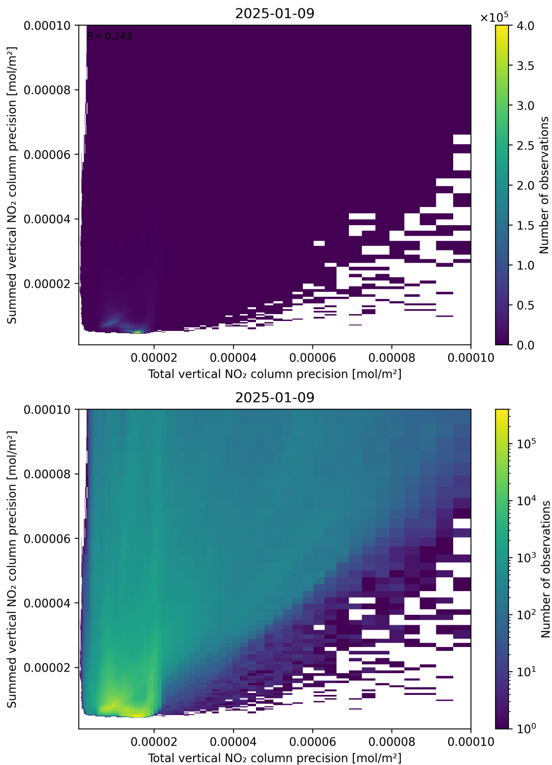
Figure 118: Scatter density plot of “Total vertical NO 2 column precision” against “Summed vertical NO 2 column precision” for 2025-01-08 to 2025-01-10.
