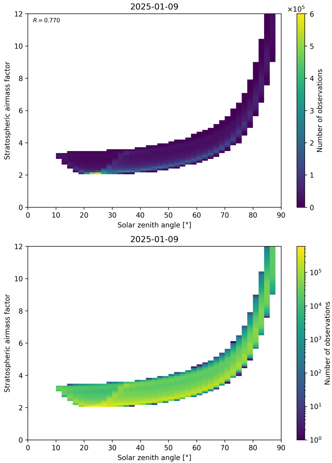
Figure 145: Scatter density plot of “Solar zenith angle” against “Stratospheric airmass factor” for 2025-01-08 to 2025-01-10.
