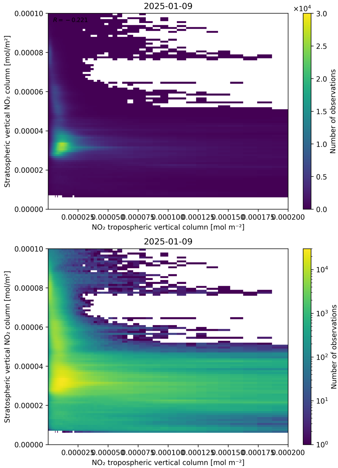
Figure 125: Scatter density plot of “NO 2 tropospheric vertical column” against “Stratospheric vertical NO 2 column” for 2025-01-08 to 2025-01-10.
