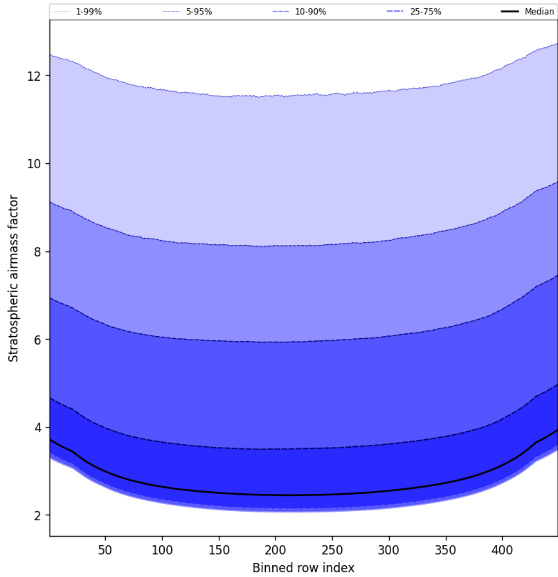
Figure 61: Along track statistics of “Stratospheric air mass factor” for 2025-01-08 to 2025-01-10
