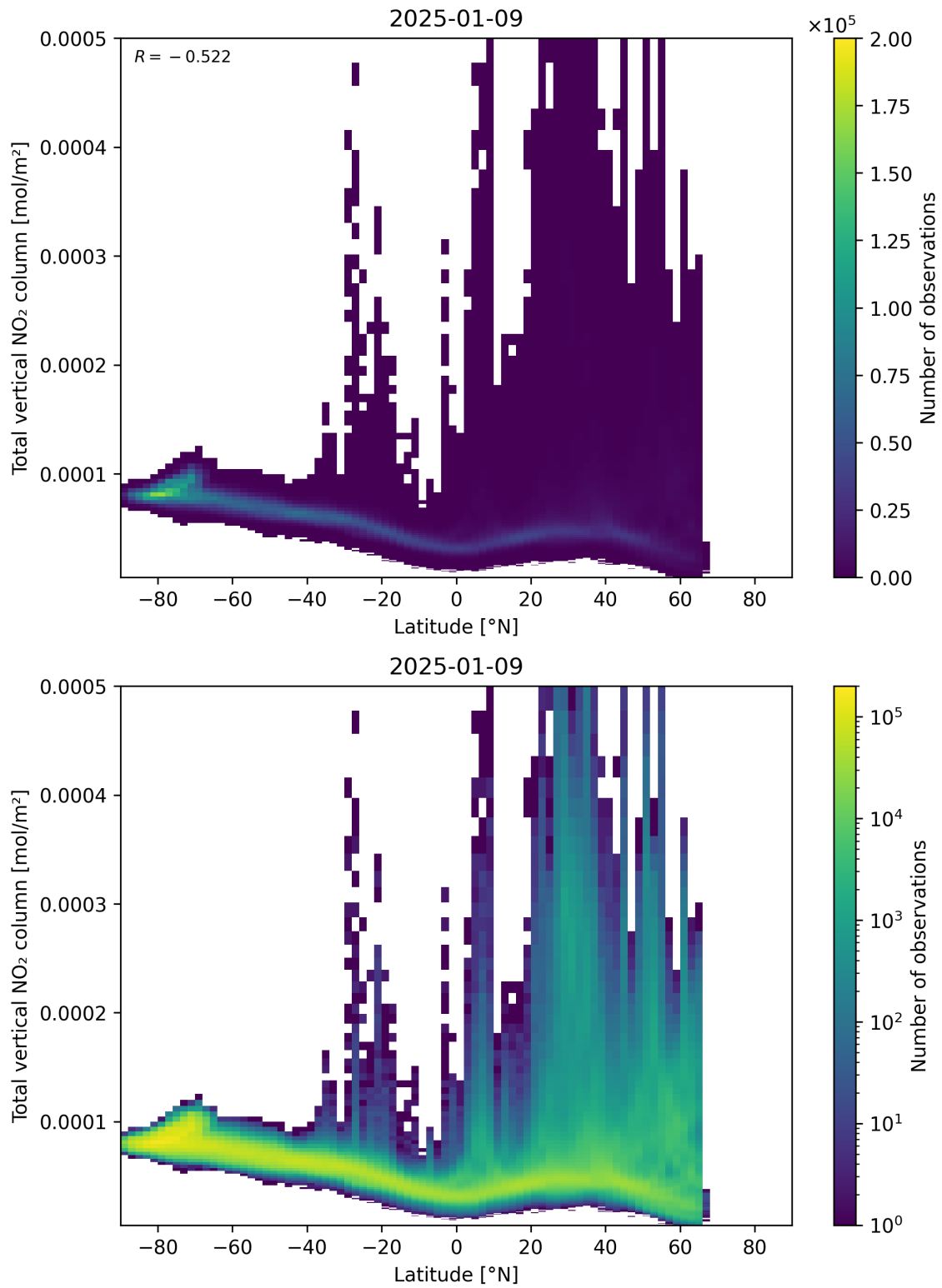
Figure 90: Scatter density plot of “Latitude” against “Total vertical NO 2 column” for 2025-01-08 to 2025-01-10.
