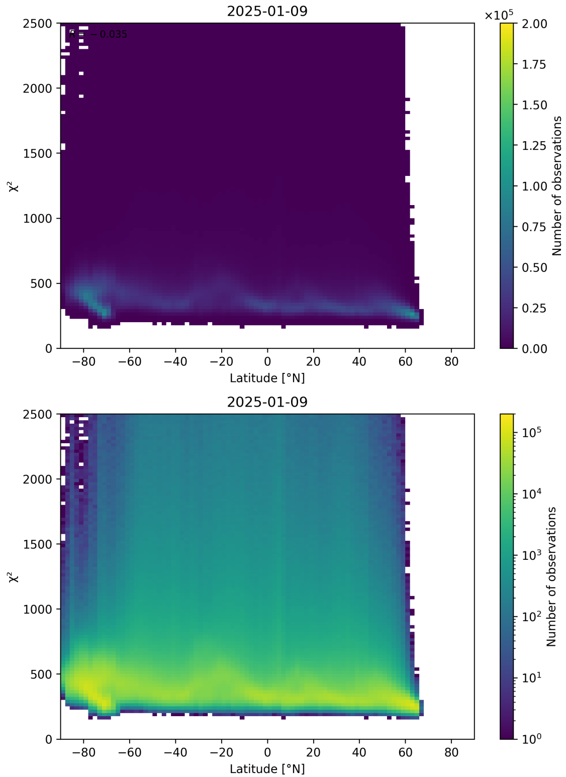
Figure 86: Scatter density plot of “Latitude” against “ \chi^2 ” for 2025-01-08 to 2025-01-10.
