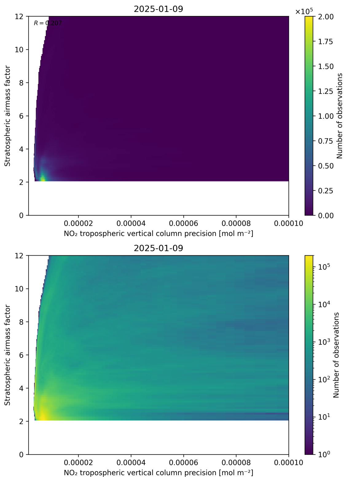
Figure 131: Scatter density plot of “NO 2 tropospheric vertical column precision” against “Stratospheric airmass factor” for 2025-01-08 to 2025-01-10.
