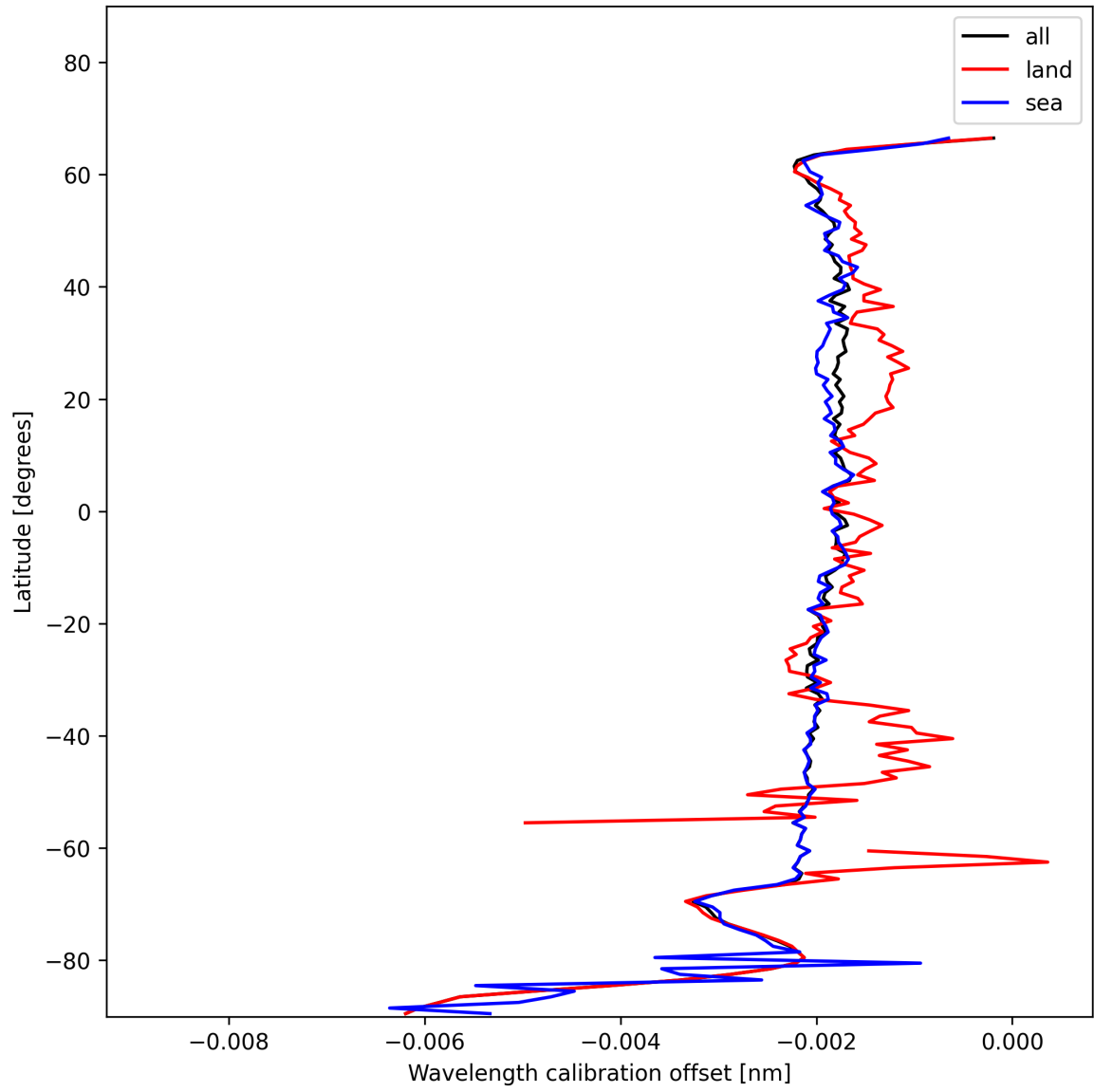
Figure 18: Zonal average of “Wavelength calibration offset” for 2025-01-08 to 2025-01-10.
