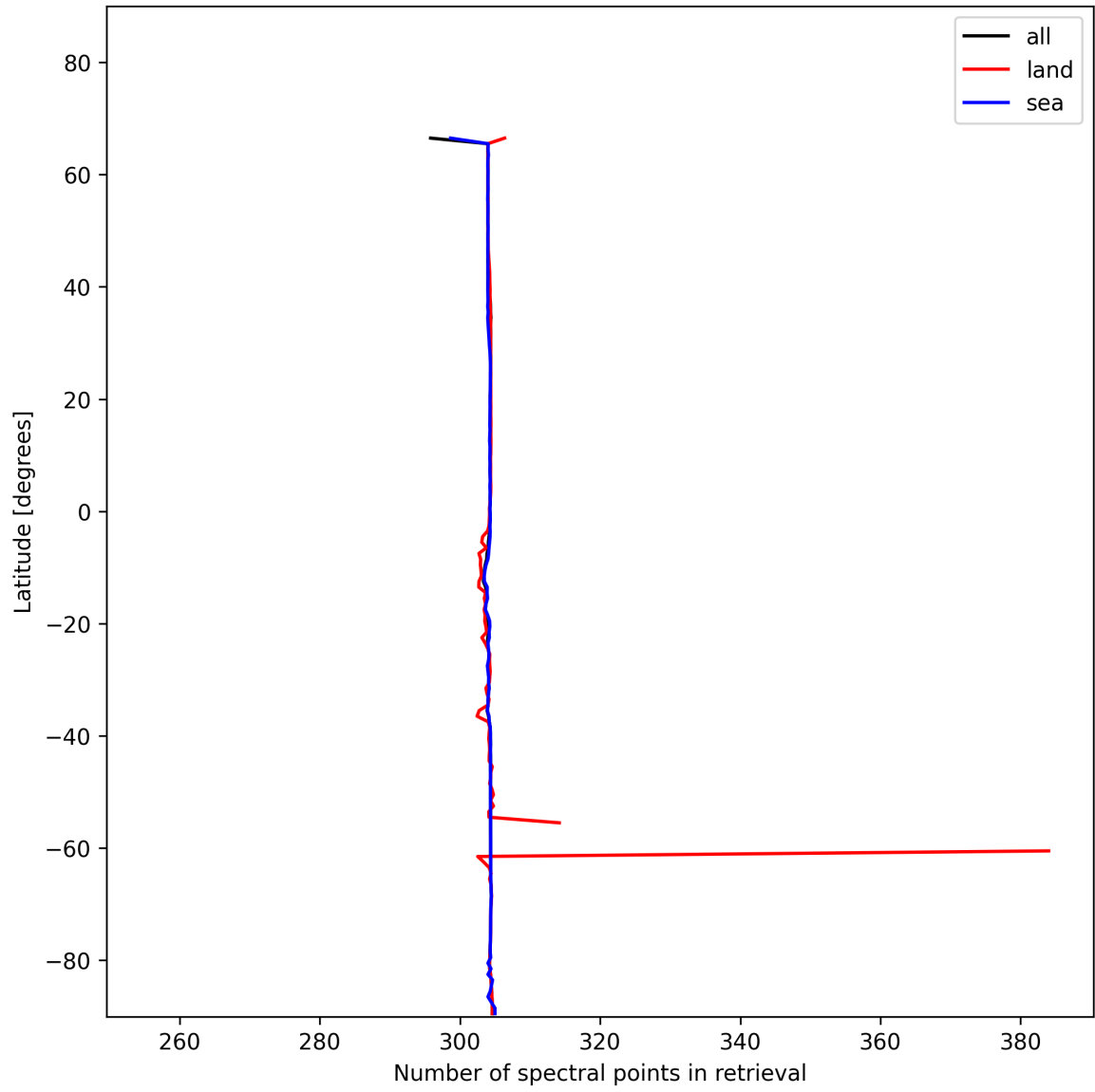
Figure 16: Zonal average of “Number of spectral points in retrieval” for 2025-01-08 to 2025-01-10.
