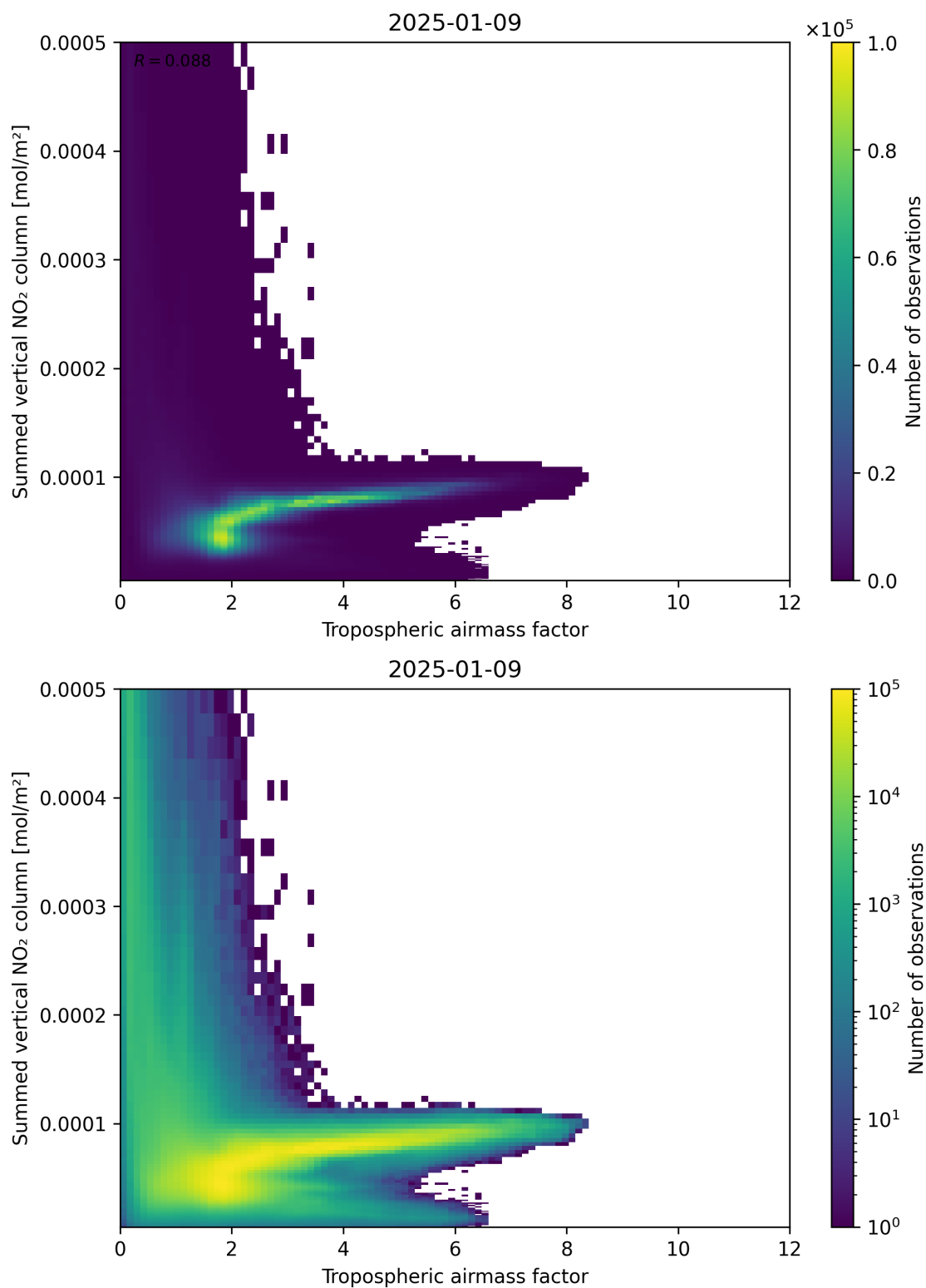
Figure 75: Scatter density plot of “Tropospheric air mass factor” against “Summed vertical NO 2 column” for 2025-01-08 to 2025-01-10.
