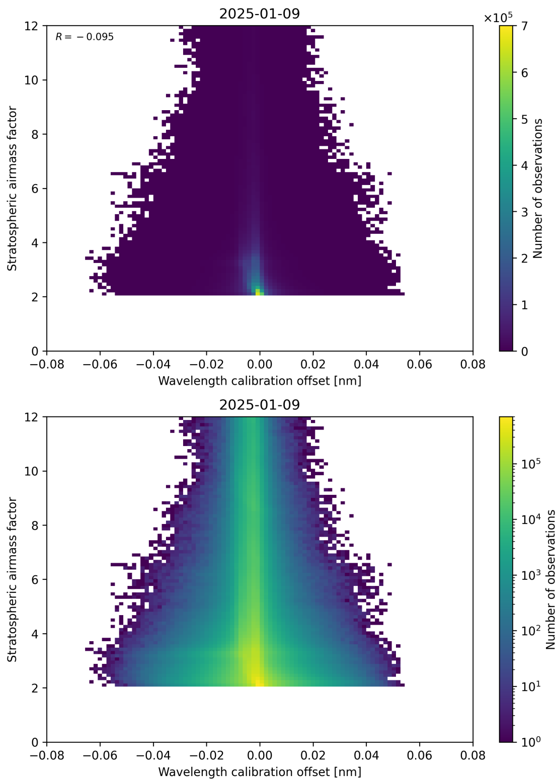
Figure 174: Scatter density plot of “Wavelength calibration offset” against “Stratospheric airmass factor” for 2025-01-08 to 2025-01-10.
