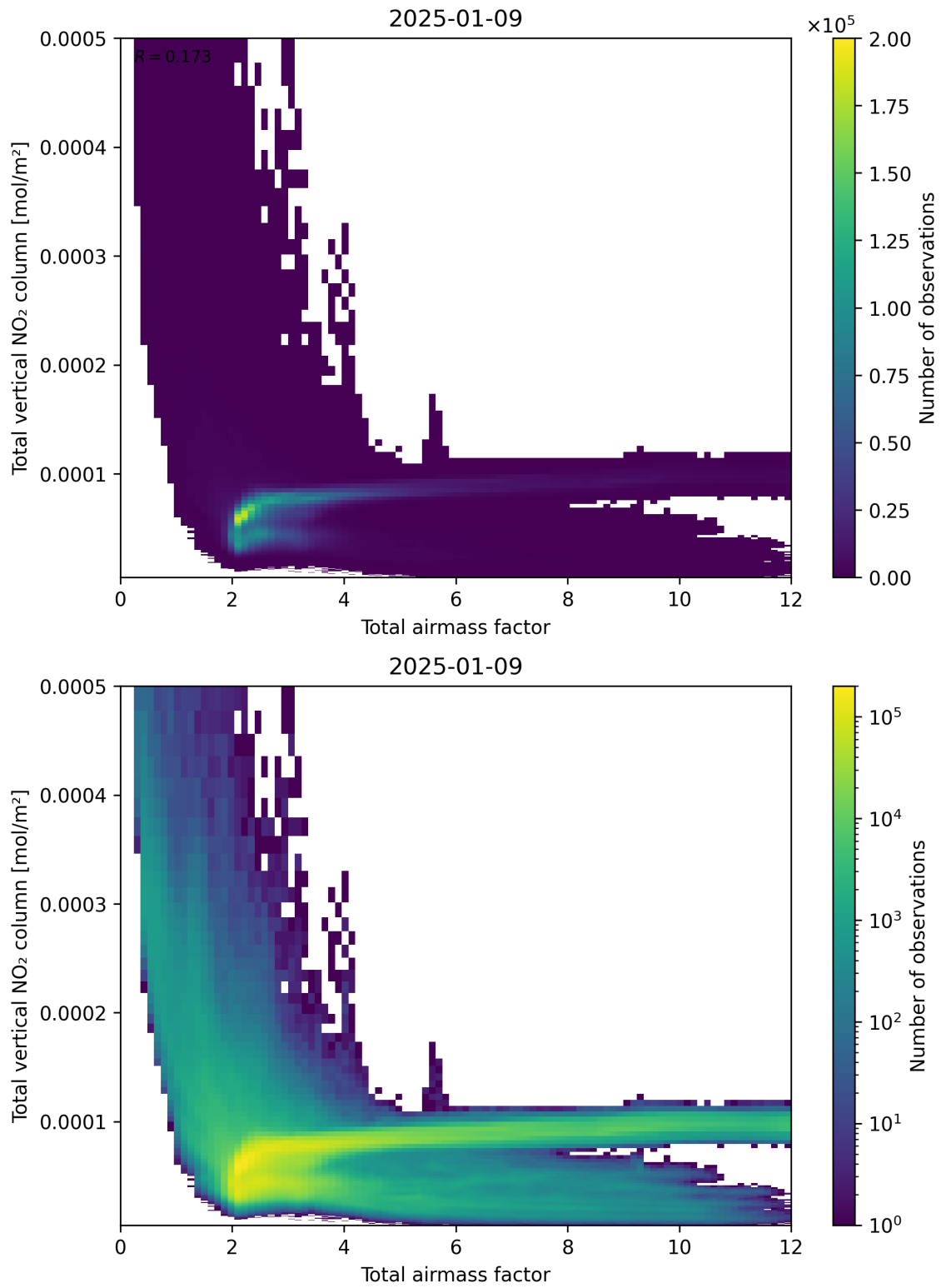
Figure 67: Scatter density plot of “Total airmass factor” against “Total vertical NO 2 column” for 2025-01-08 to 2025-01-10.
