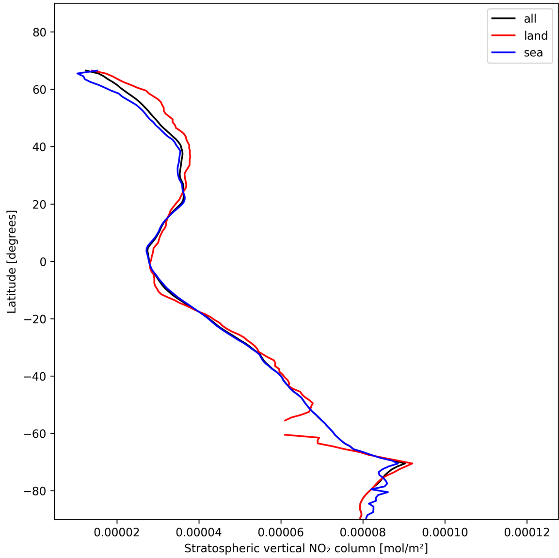
Figure 19: Zonal average of “Stratospheric vertical NO 2 column” for 2025-01-08 to 2025-01-10.
