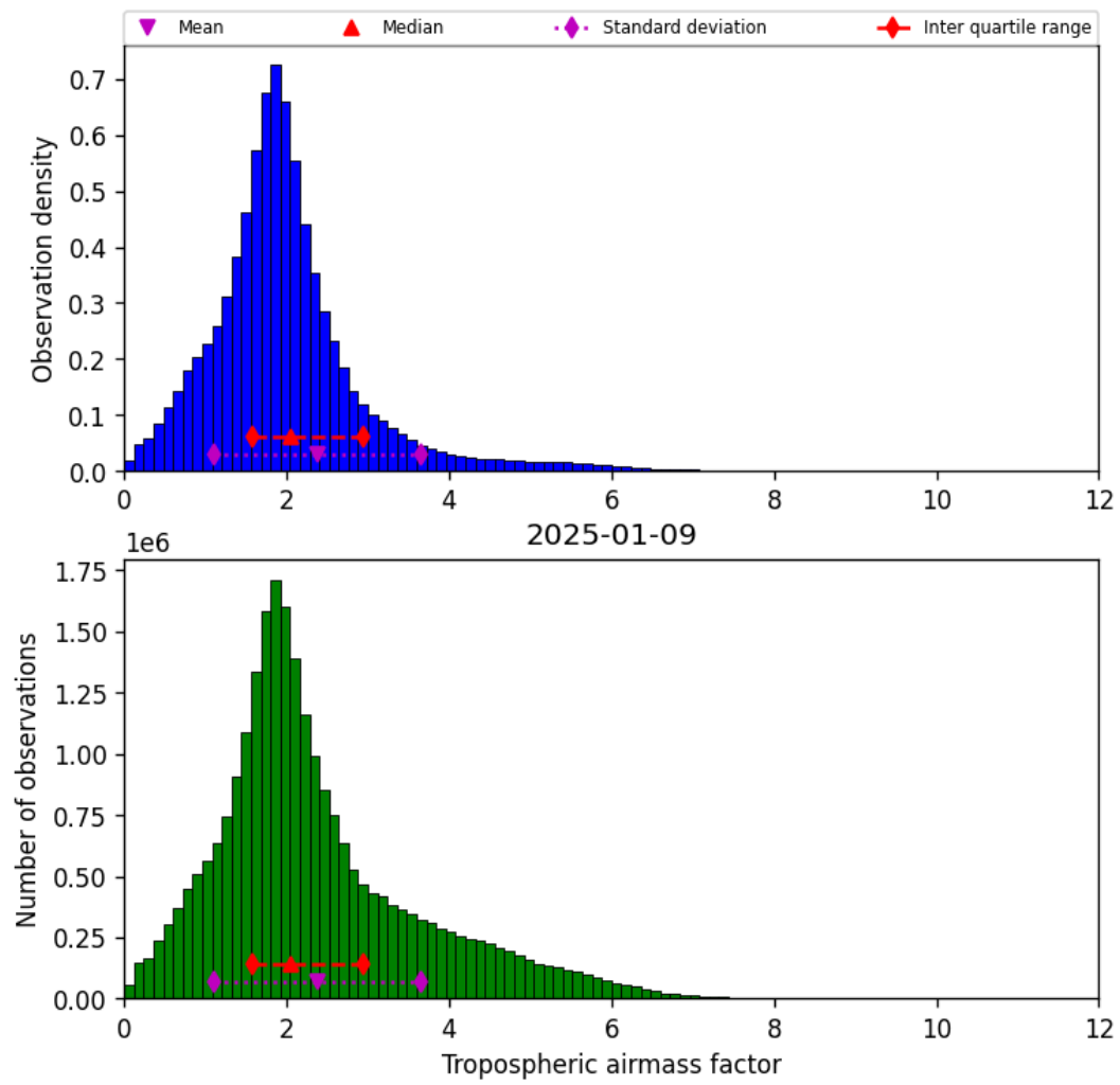
Figure 31: Histogram of “Tropospheric airmass factor” for 2025-01-08 to 2025-01-10
