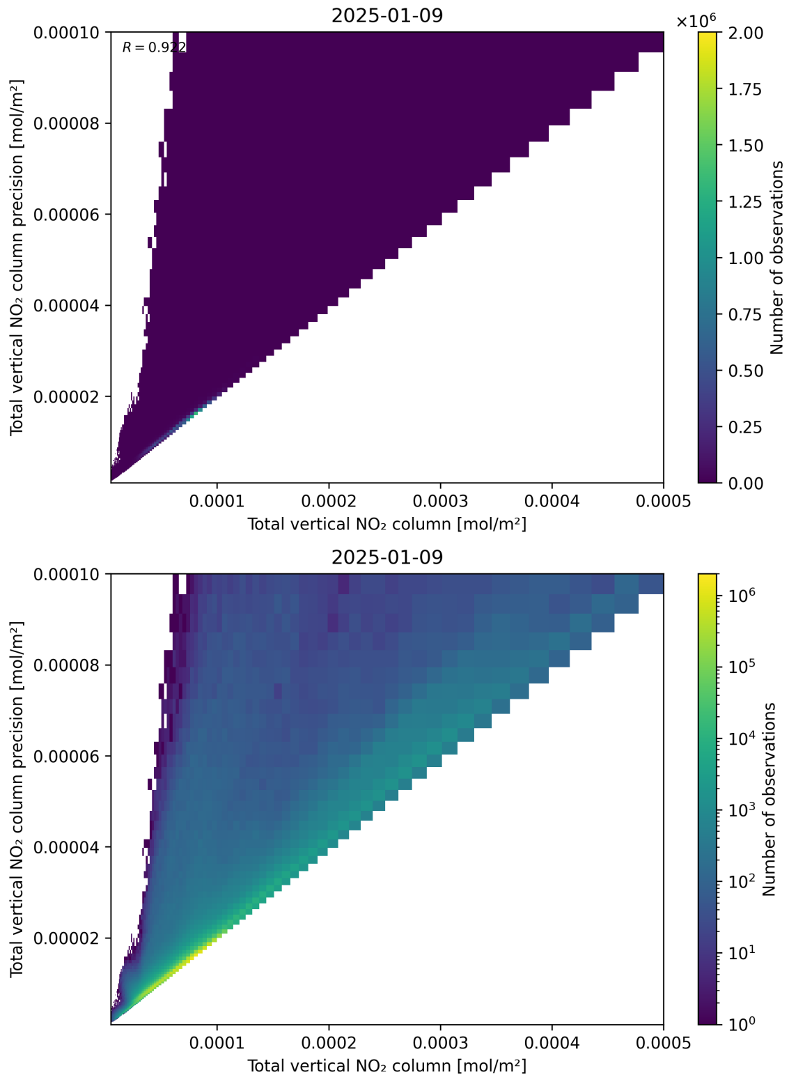
Figure 114: Scatter density plot of “Total vertical NO 2 column” against “Total vertical NO 2 column precision” for 2025-01-08 to 2025-01-10.
