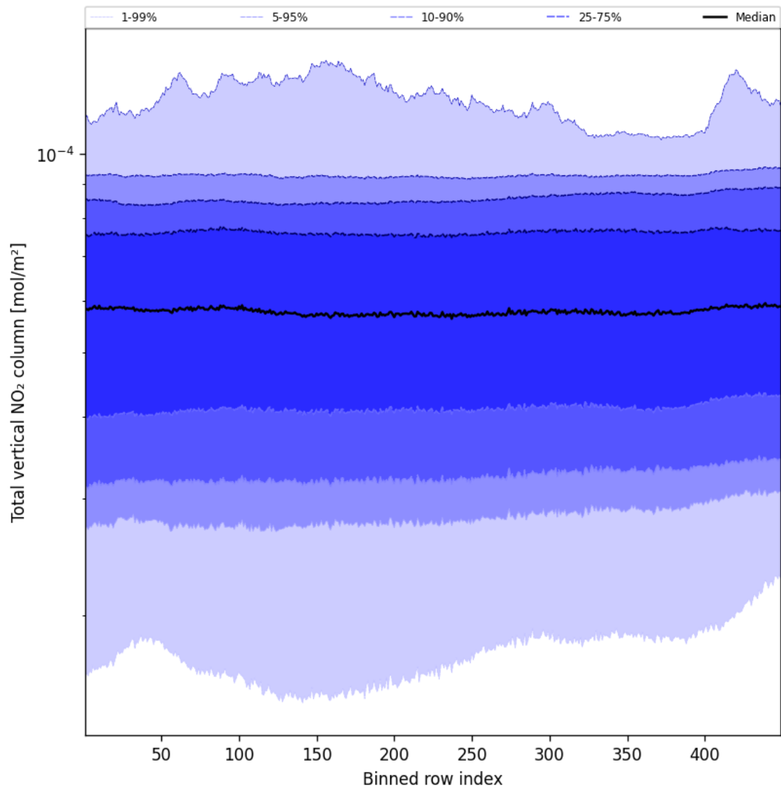
Figure 55: Along track statistics of “Total vertical NO 2 column” for 2025-01-08 to 2025-01-10
