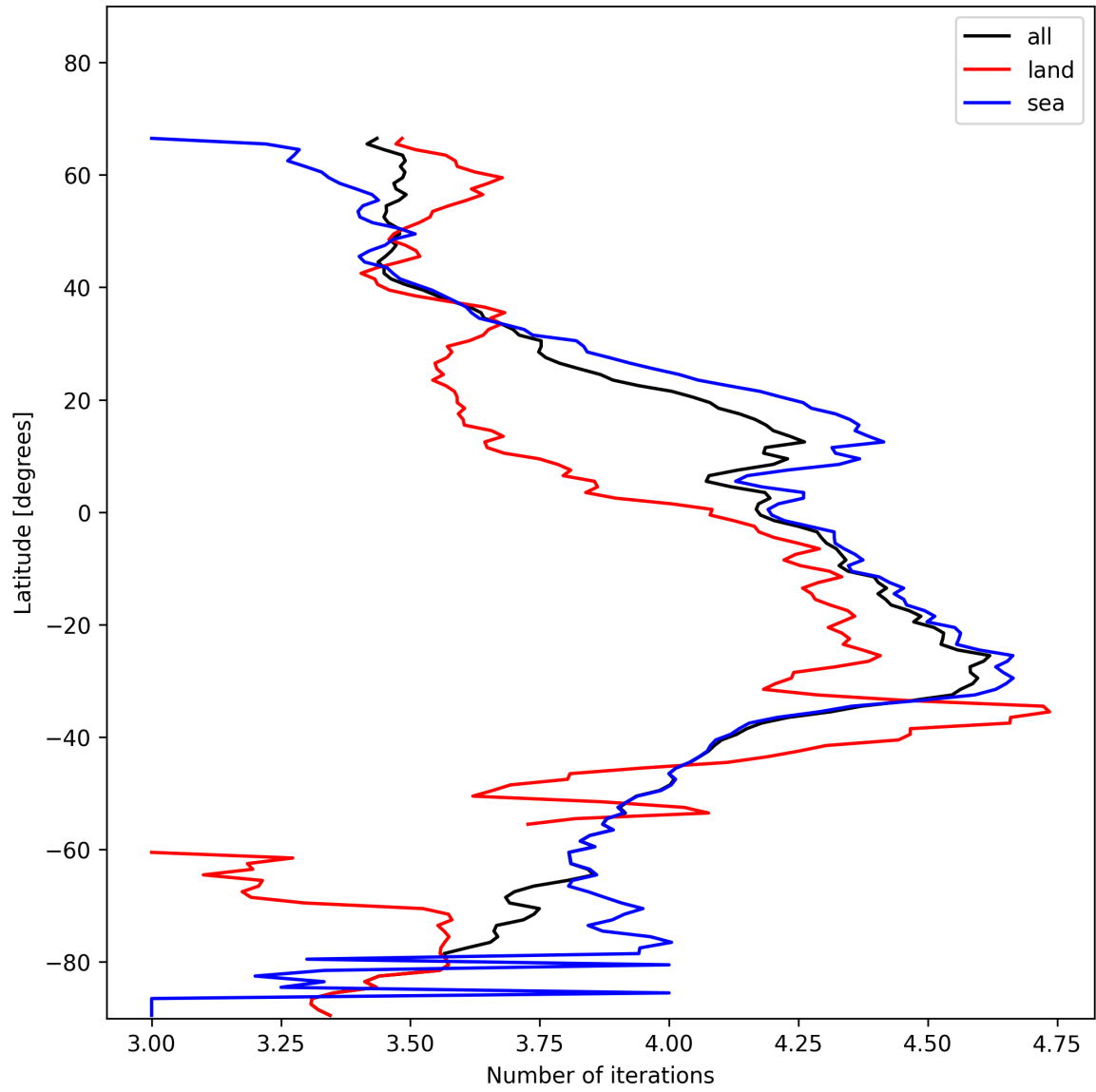
Figure 17: Zonal average of “Number of iterations” for 2025-01-08 to 2025-01-10.
