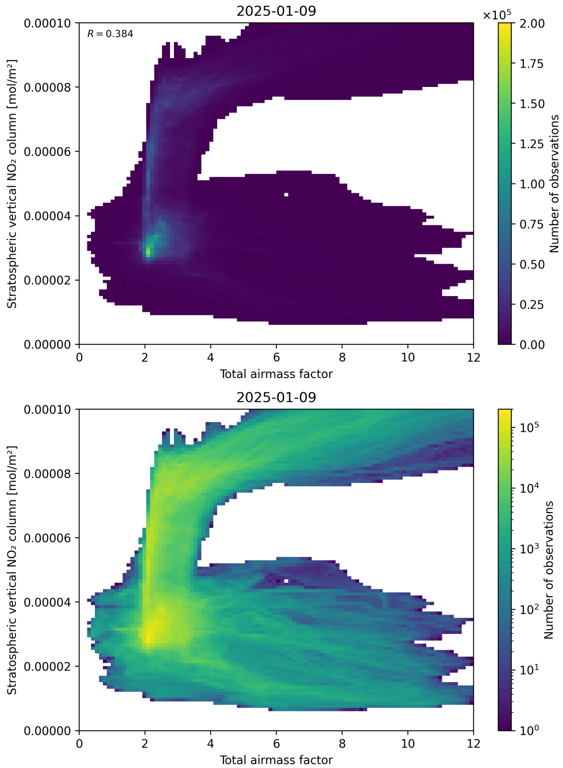
Figure 64: Scatter density plot of “Total airmass factor” against “Stratospheric vertical NO 2 column” for 2025-01-08 to 2025-01-10.
