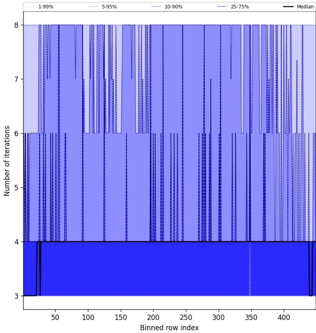
Figure 51: Along track statistics of “Number of iterations” for 2025-01-08 to 2025-01-10
