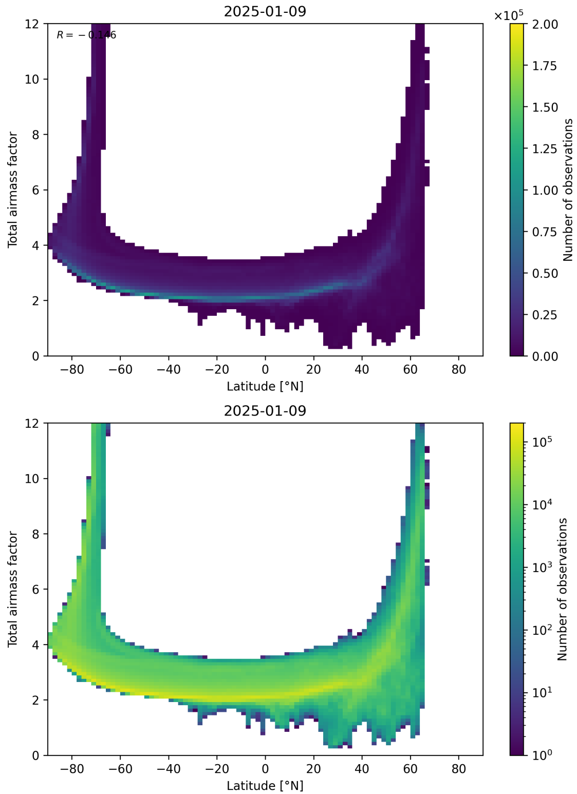
Figure 84: Scatter density plot of “Latitude” against “Total airmass factor” for 2025-01-08 to 2025-01-10.
