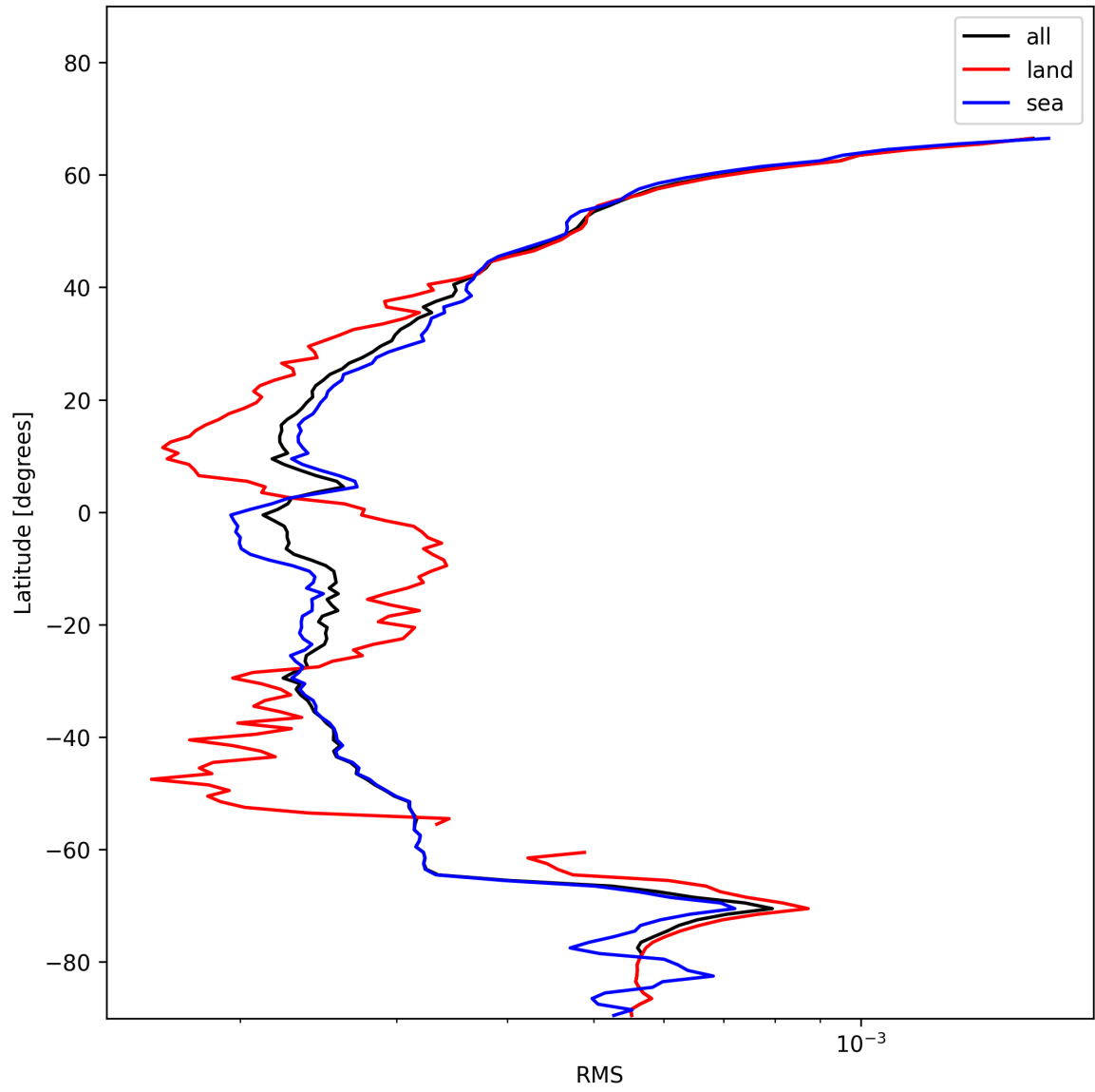
Figure 26: Zonal average of “RMS” for 2025-01-08 to 2025-01-10.
