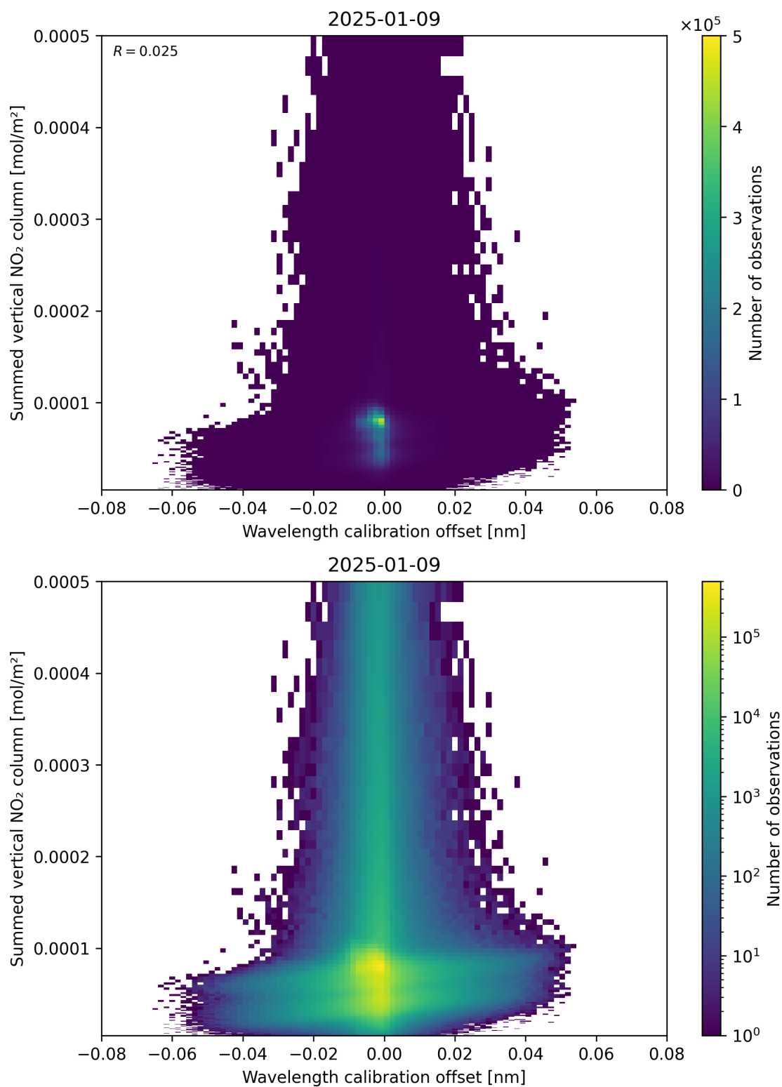
Figure 177: Scatter density plot of “Wavelength calibration offset” against “Summed vertical NO 2 column” for 2025-01-08 to 2025-01-10.
