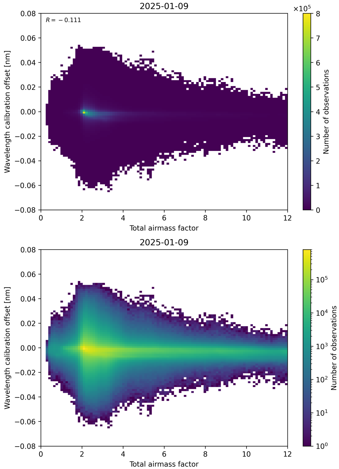
Figure 70: Scatter density plot of “Total airmass factor” against “Wavelength calibration offset” for 2025-01-08 to 2025-01-10.
