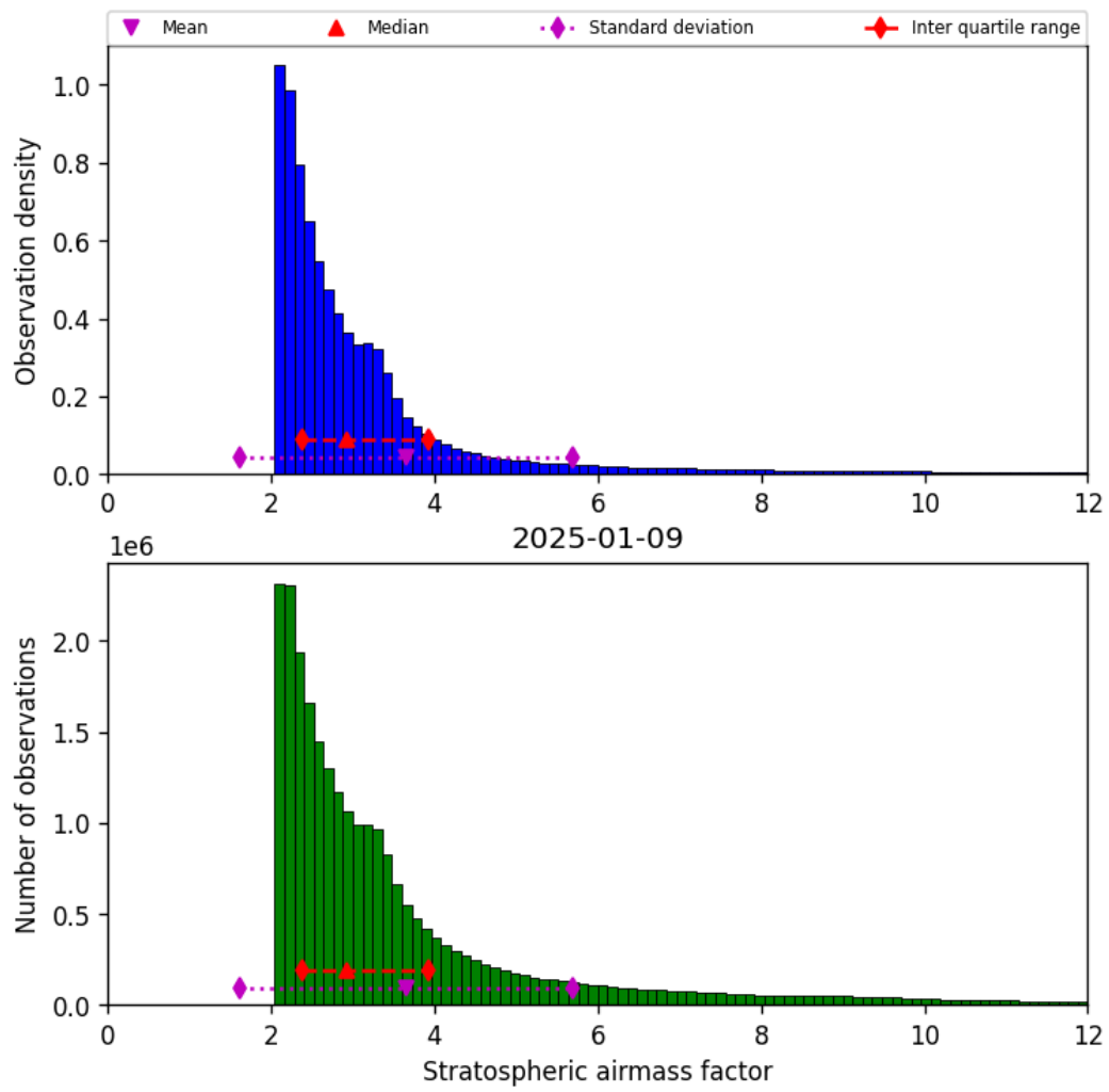
Figure 44: Histogram of “Stratospheric airmass factor” for 2025-01-08 to 2025-01-10
