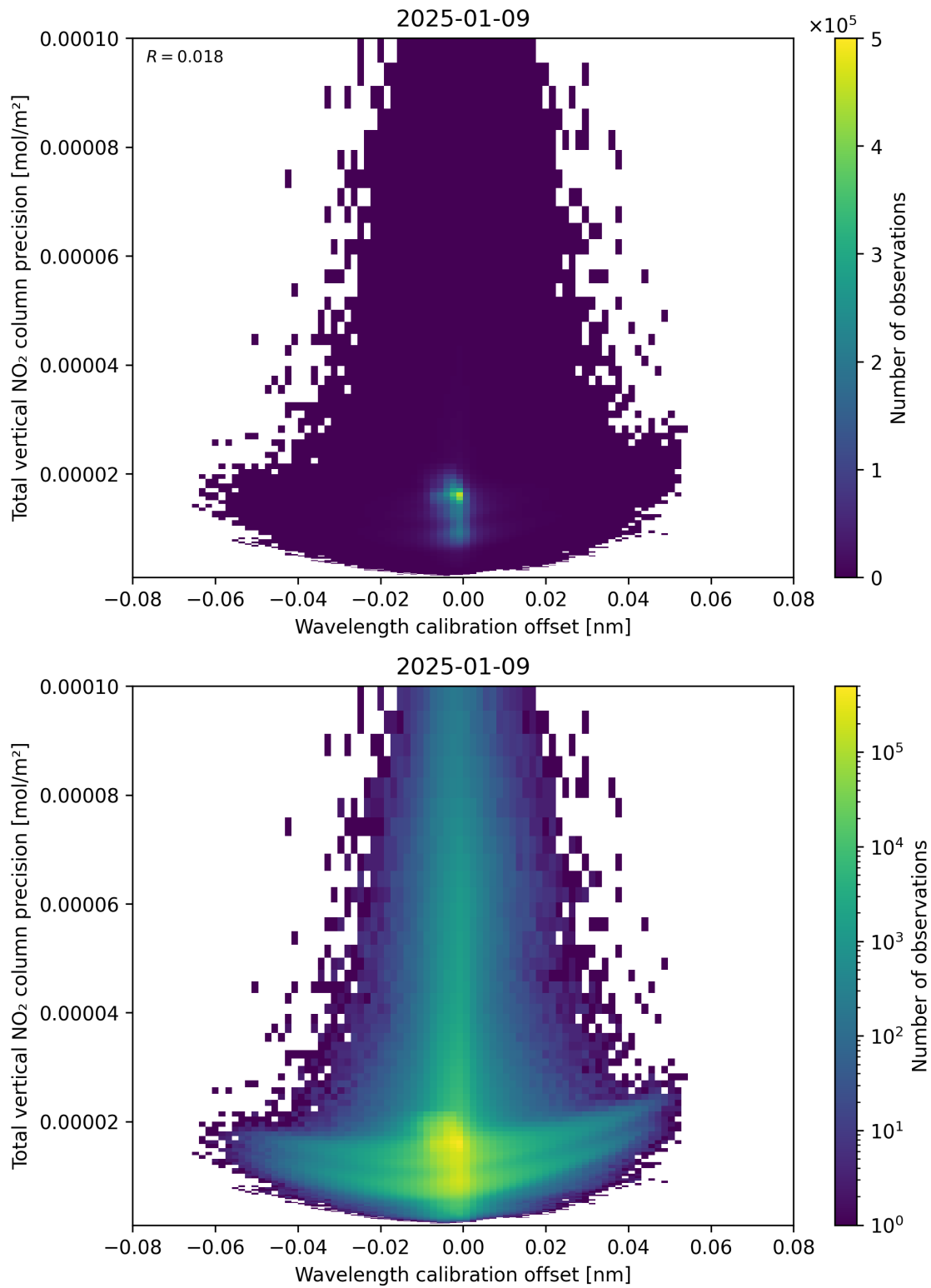
Figure 180: Scatter density plot of “Wavelength calibration offset” against “Total vertical NO 2 column precision” for 2025-01-08 to 2025-01-10.
