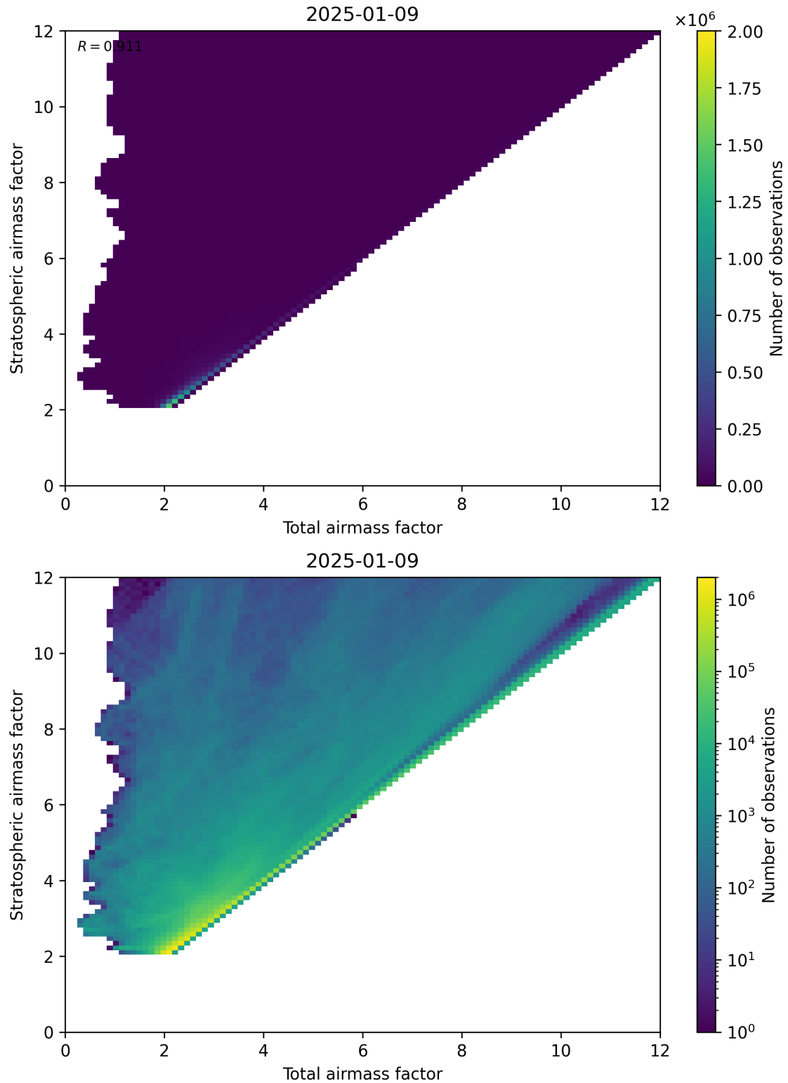
Figure 62: Scatter density plot of “Total airmass factor” against “Stratospheric airmass factor” for 2025-01-08 to 2025-01-10.
