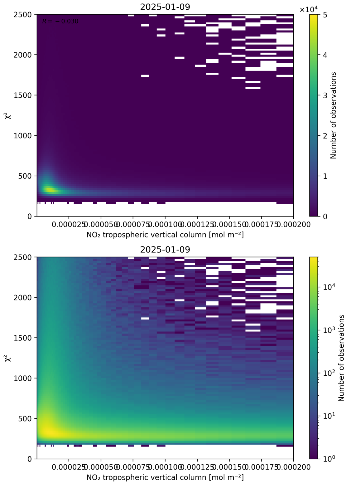
Figure 124: Scatter density plot of “NO 2 tropospheric vertical column” against “ \chi^2 ” for 2025-01-08 to 2025-01-10.
