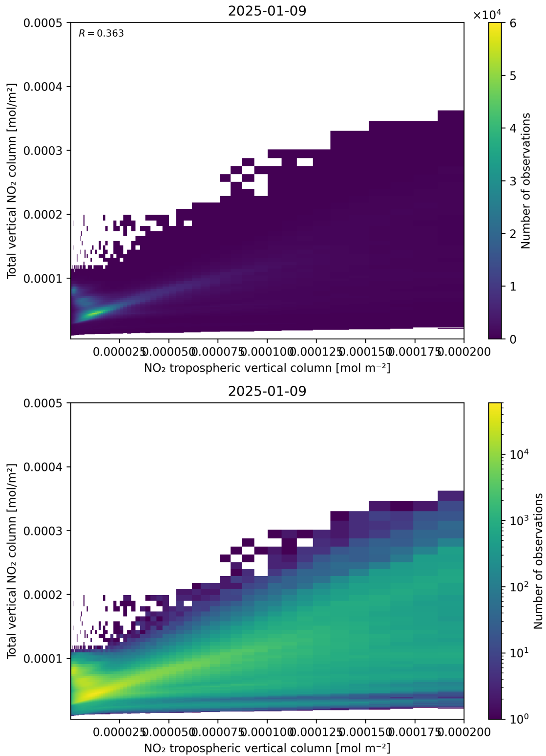
Figure 128: Scatter density plot of “NO 2 tropospheric vertical column” against “Total vertical NO 2 column” for 2025-01-08 to 2025-01-10.
