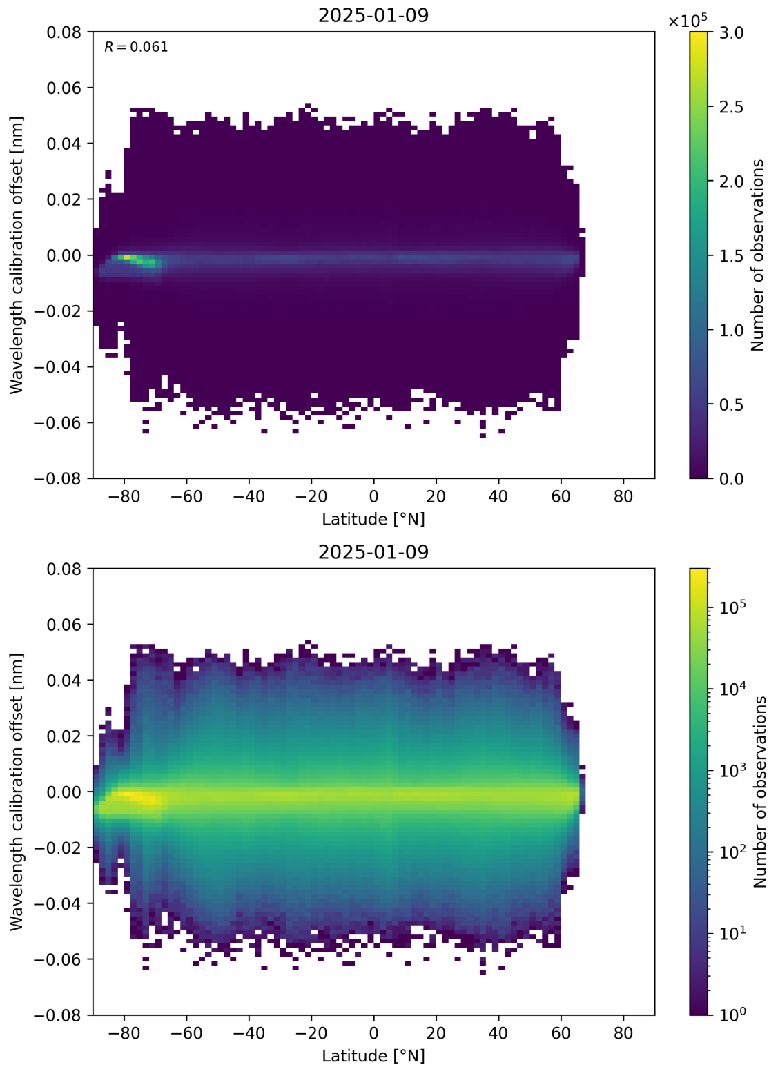
Figure 95: Scatter density plot of “Latitude” against “Wavelength calibration offset” for 2025-01-08 to 2025-01-10.
