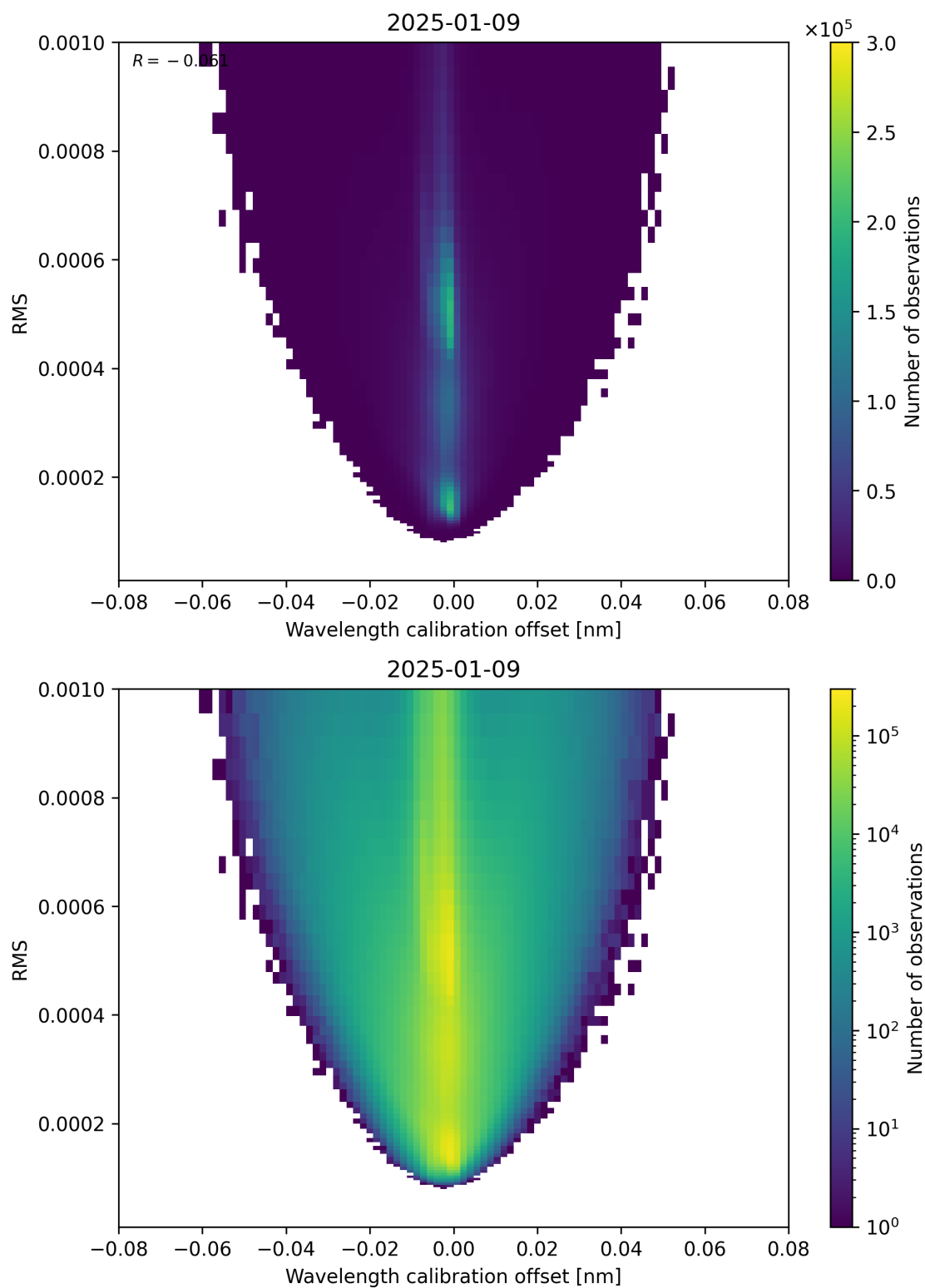
Figure 181: Scatter density plot of “Wavelength calibration offset” against “RMS” for 2025-01-08 to 2025-01-10.
