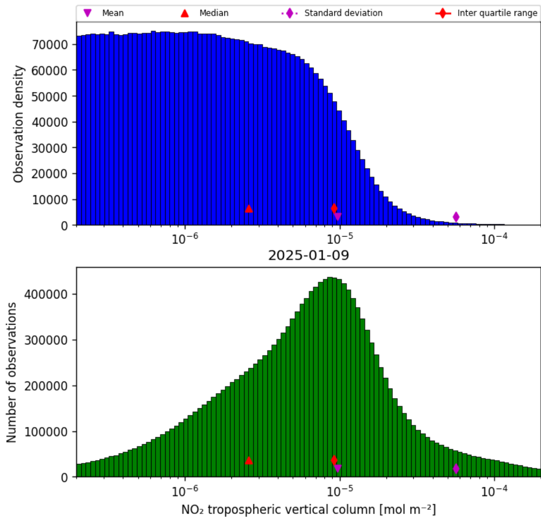
Figure 29: Histogram of “NO 2 tropospheric vertical column” for 2025-01-08 to 2025-01-10
