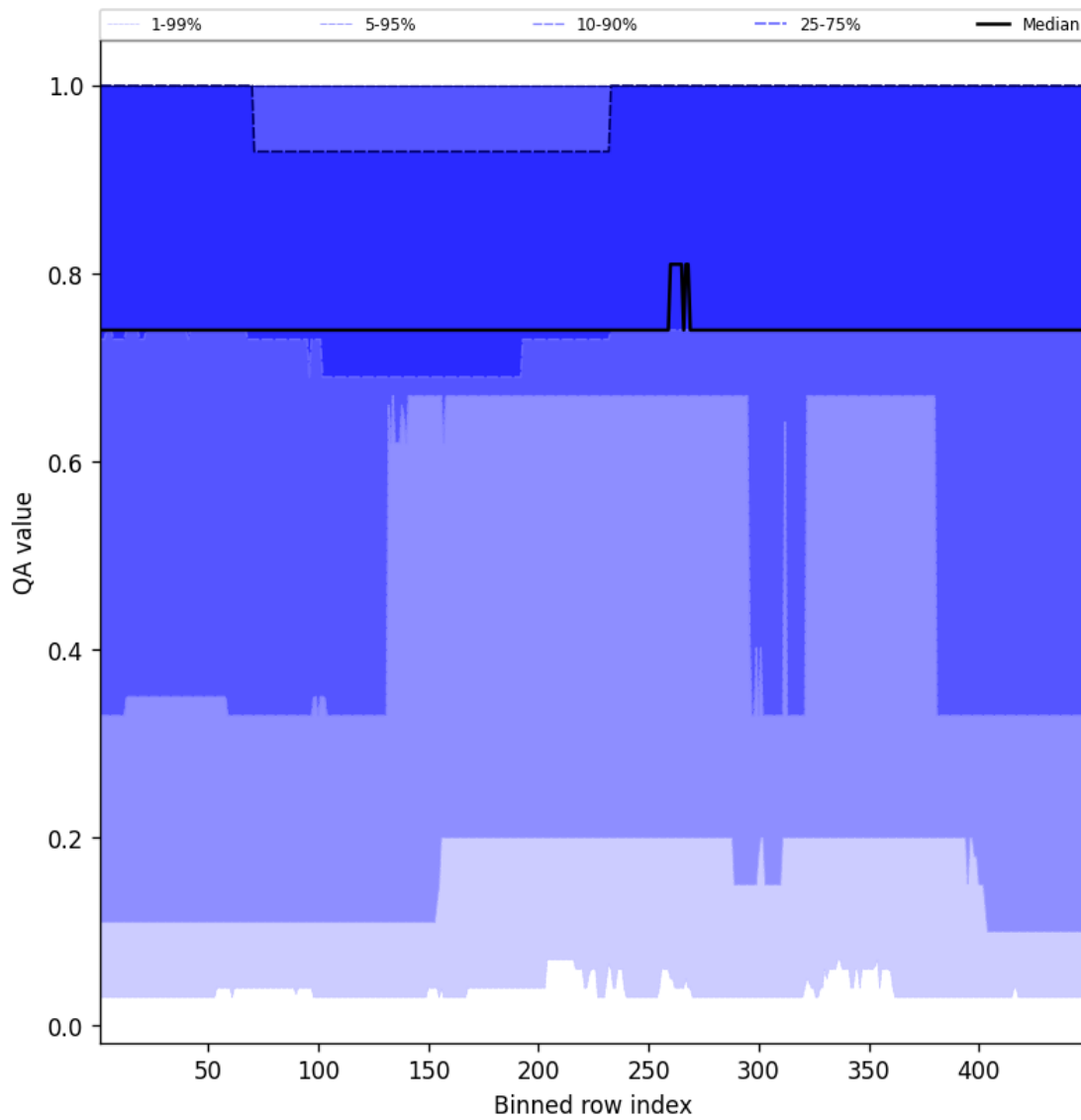
Figure 45: Along track statistics of “QA value” for 2025-01-08 to 2025-01-10
