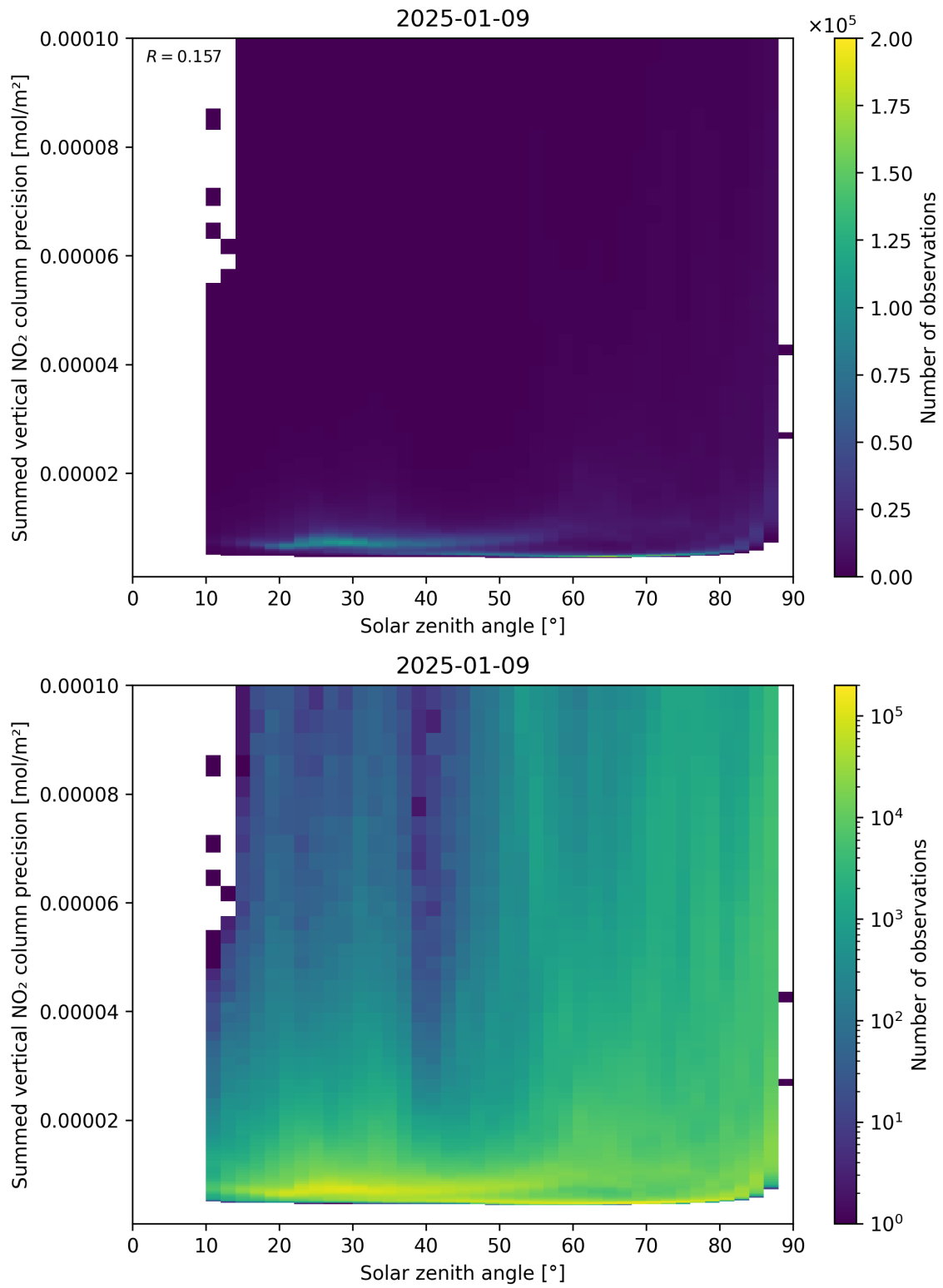
Figure 152: Scatter density plot of “Solar zenith angle” against “Summed vertical NO 2 column precision” for 2025-01-08 to 2025-01-10.
