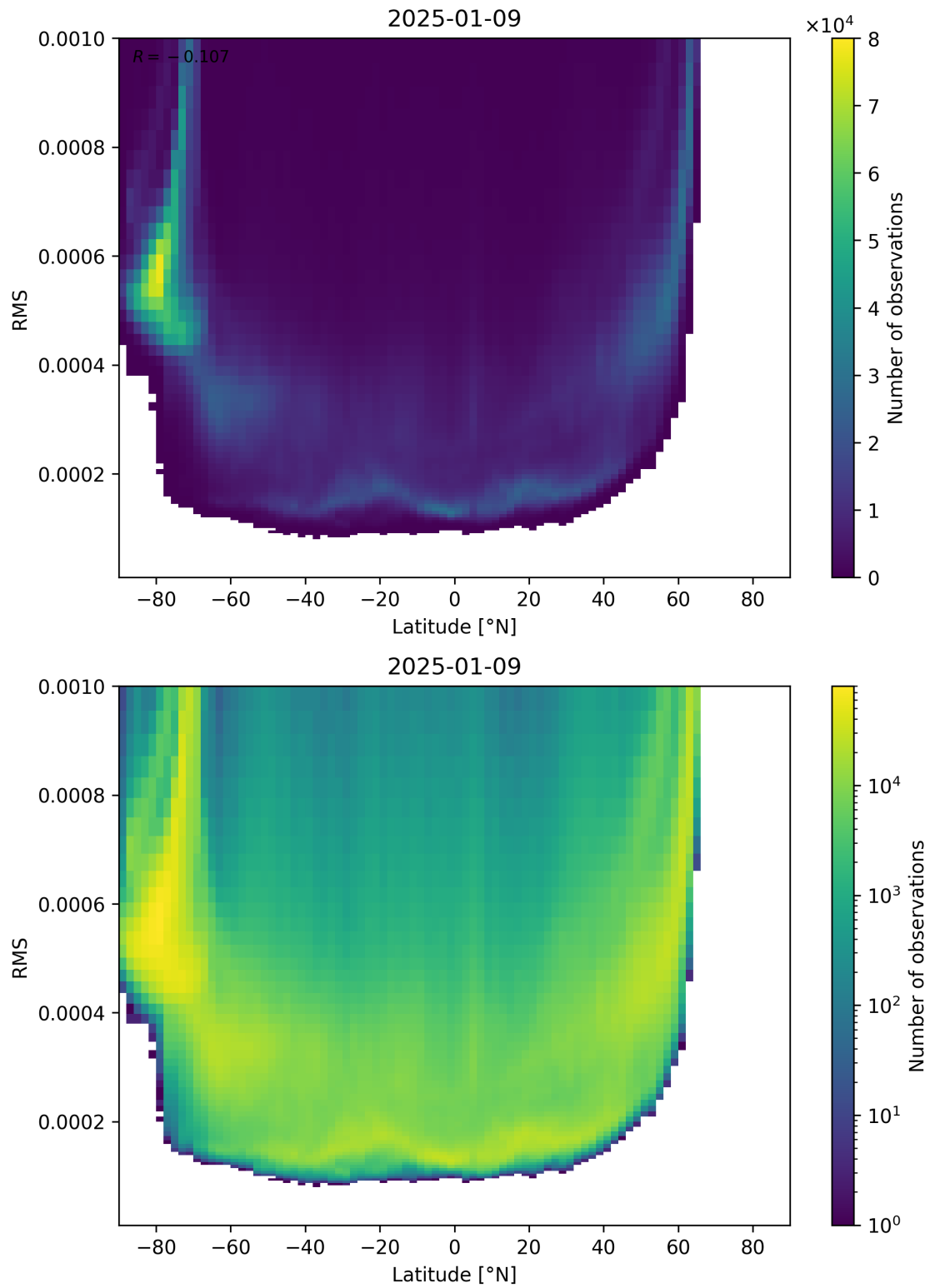
Figure 94: Scatter density plot of “Latitude” against “RMS” for 2025-01-08 to 2025-01-10.
