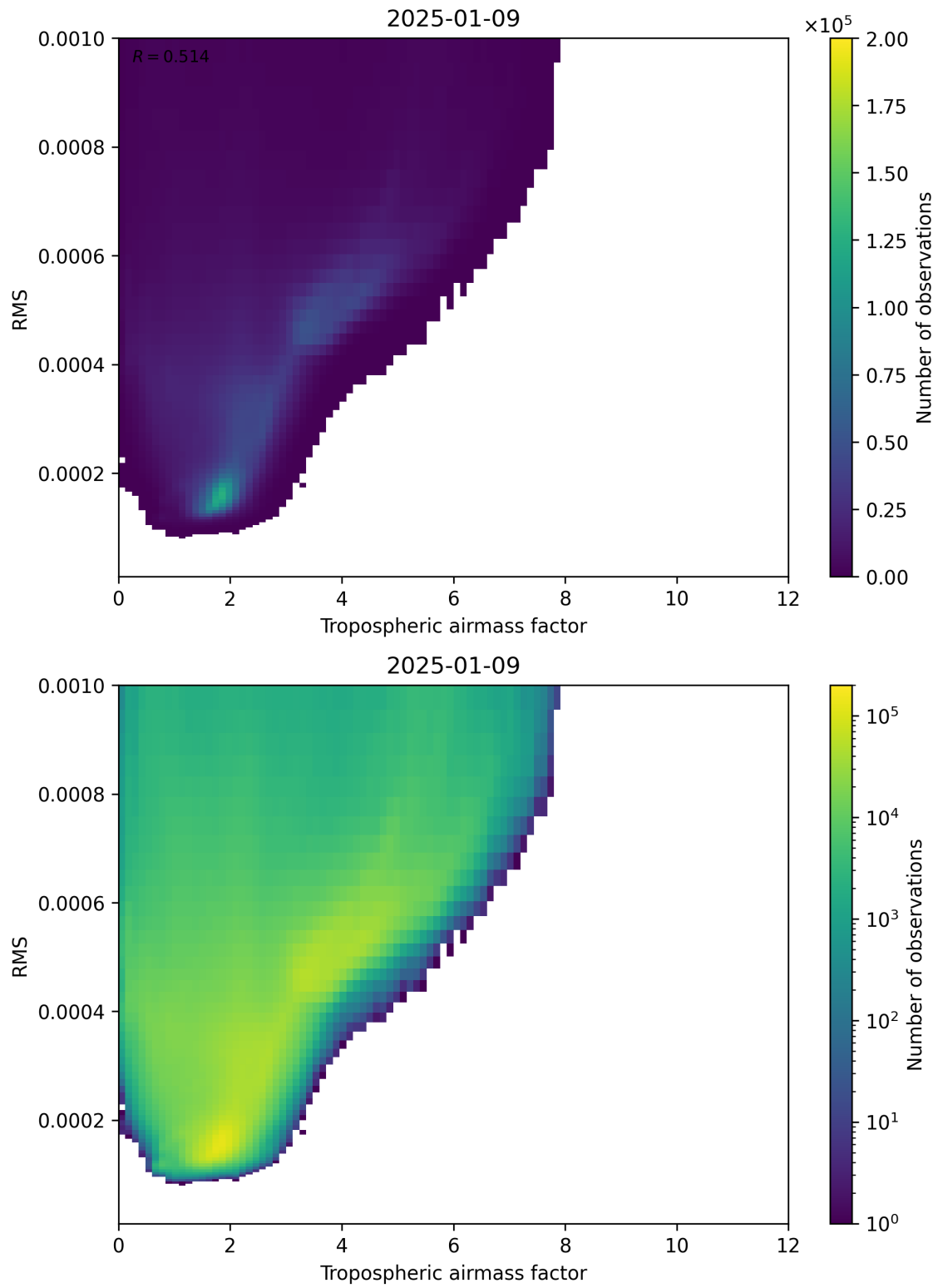
Figure 79: Scatter density plot of “Tropospheric airmass factor” against “RMS” for 2025-01-08 to 2025-01-10.
