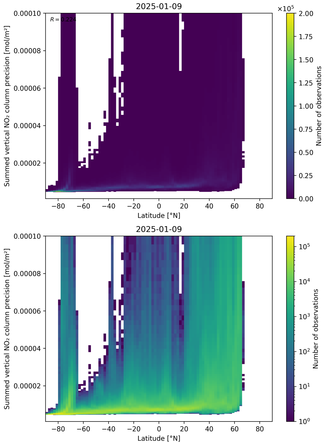
Figure 89: Scatter density plot of “Latitude” against “Summed vertical NO 2 column precision” for 2025-01-08 to 2025-01-10.
