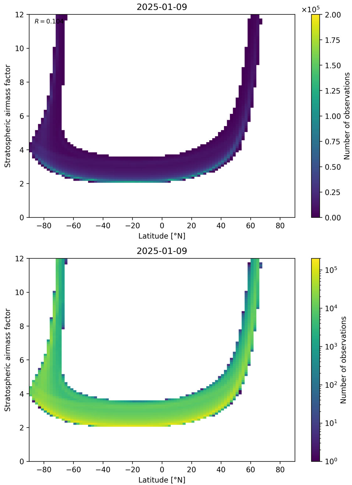
Figure 83: Scatter density plot of “Latitude” against “Stratospheric airmass factor” for 2025-01-08 to 2025-01-10.
