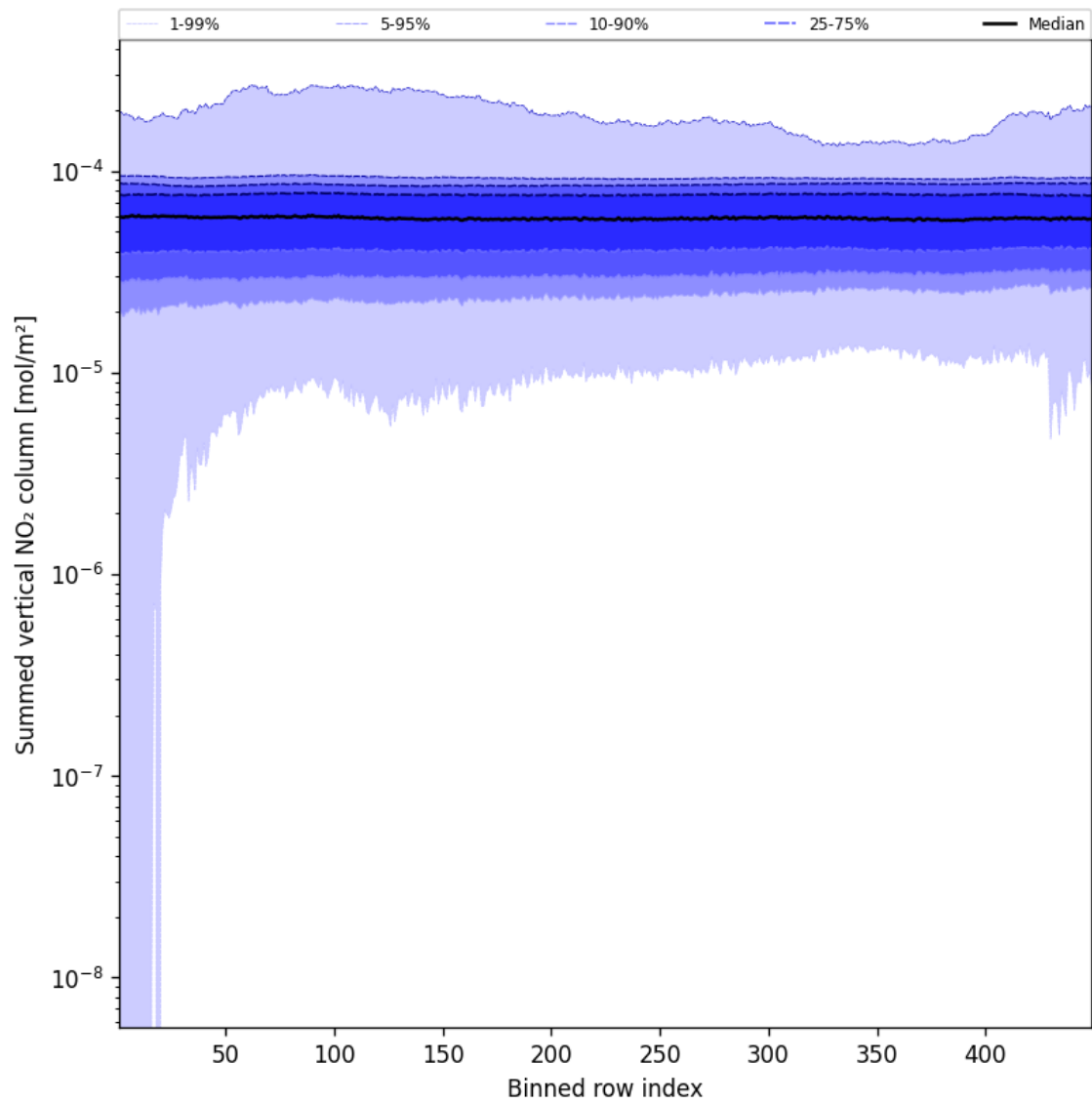
Figure 57: Along track statistics of “Summed vertical NO 2 column” for 2025-01-08 to 2025-01-10
