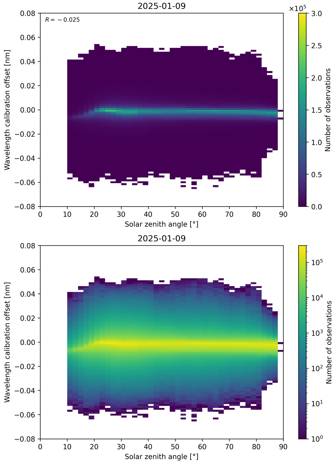
Figure 158: Scatter density plot of “Solar zenith angle” against “Wavelength calibration offset” for 2025-01-08 to 2025-01-10.
