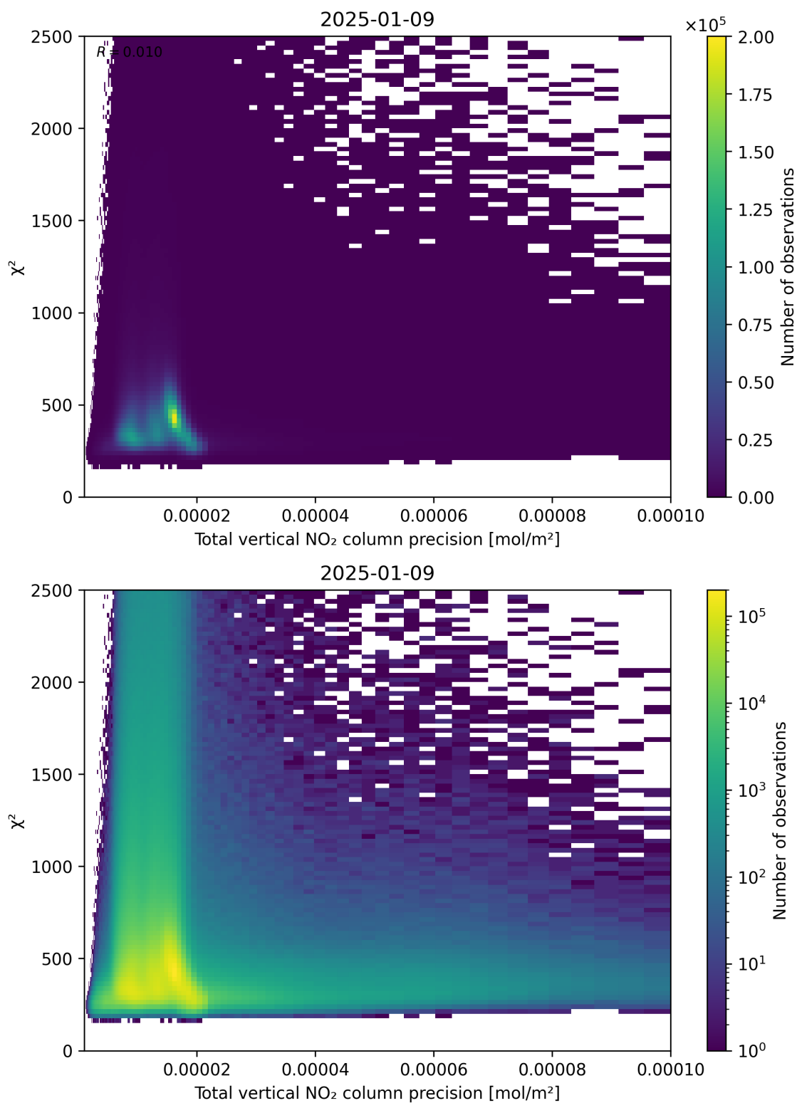
Figure 116: Scatter density plot of “Total vertical NO 2 column precision” against “ \chi^2 ” for 2025-01-08 to 2025-01-10.
