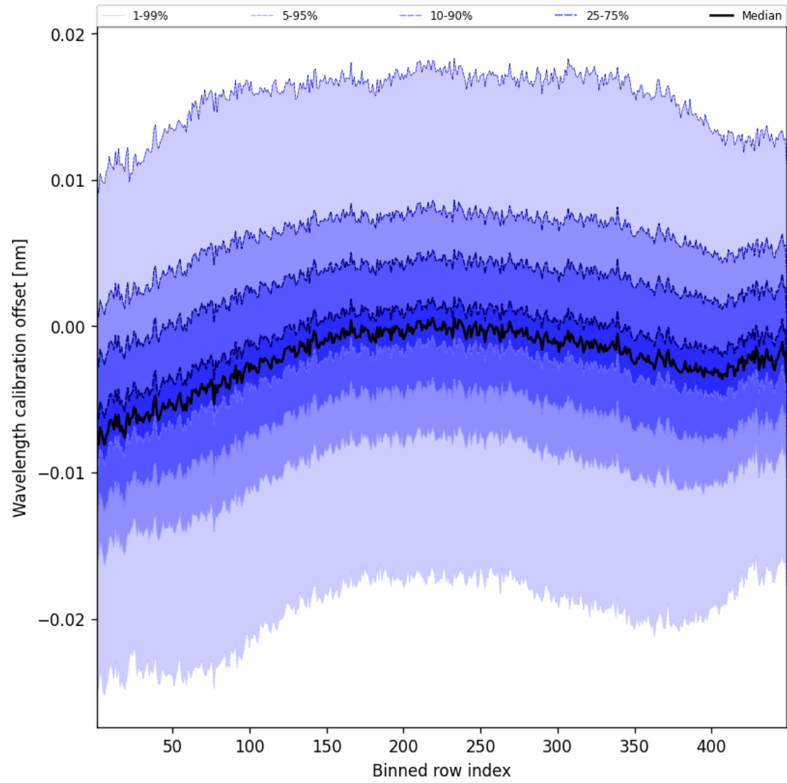
Figure 52: Along track statistics of “Wavelength calibration offset” for 2025-01-08 to 2025-01-10
