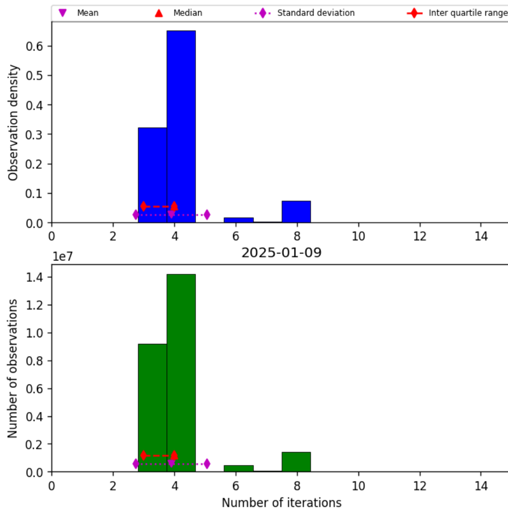
Figure 34: Histogram of “Number of iterations” for 2025-01-08 to 2025-01-10
