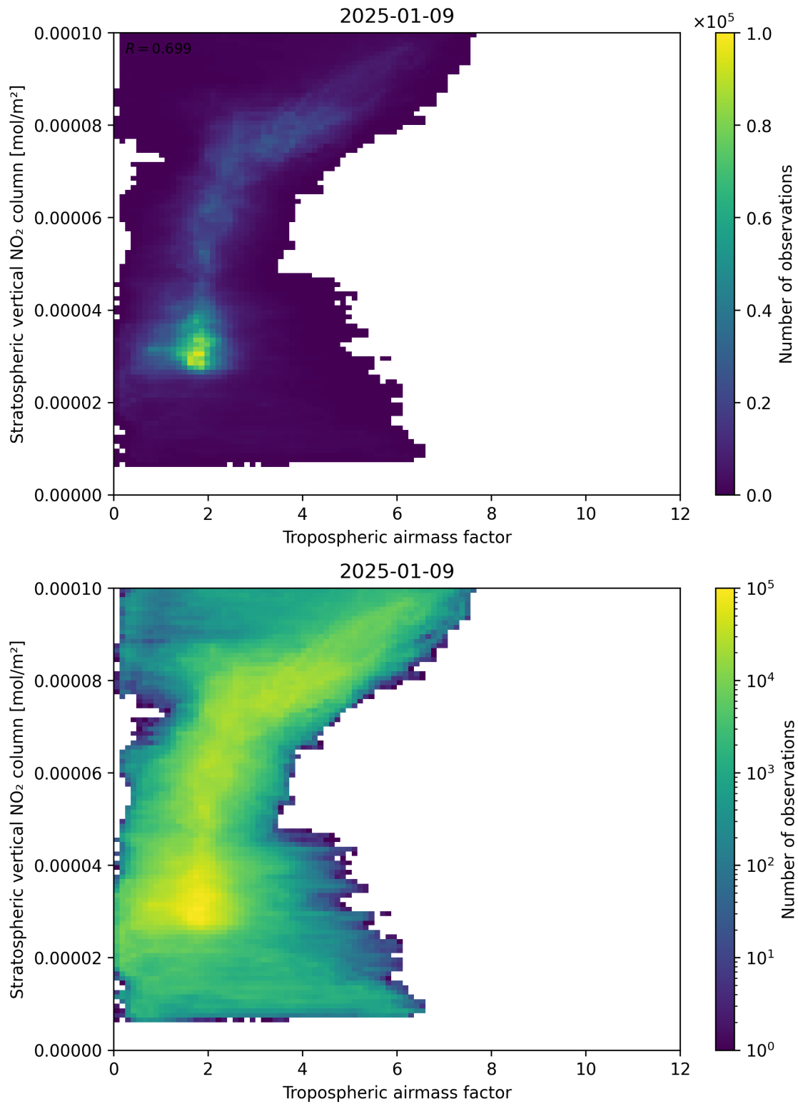
Figure 74: Scatter density plot of “Tropospheric air mass factor” against “Stratospheric vertical NO 2 column” for 2025-01-08 to 2025-01-10.
