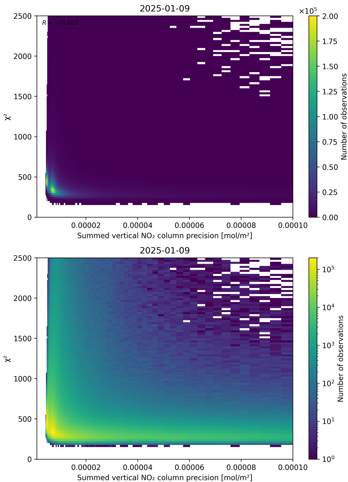
Figure 107: Scatter density plot of “Summed vertical NO 2 column precision” against “ \chi^2 ” for 2025-01-08 to 2025-01-10.
