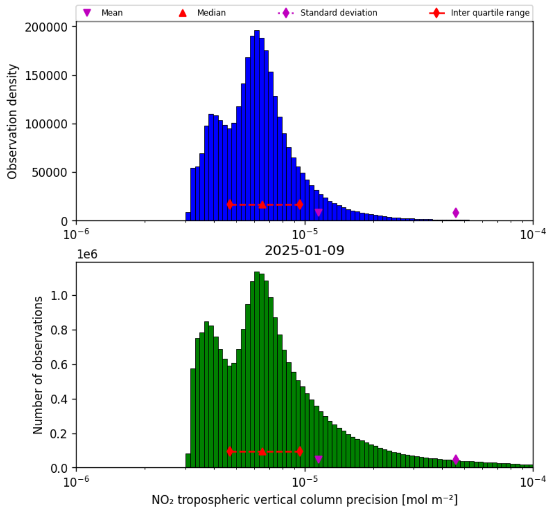
Figure 30: Histogram of “NO 2 tropospheric vertical column precision” for 2025-01-08 to 2025-01-10
