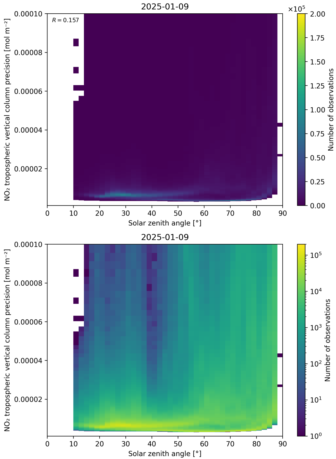
Figure 156: Scatter density plot of “Solar zenith angle” against “NO 2 tropospheric vertical column precision” for 2025-01-08 to 2025-01-10.
