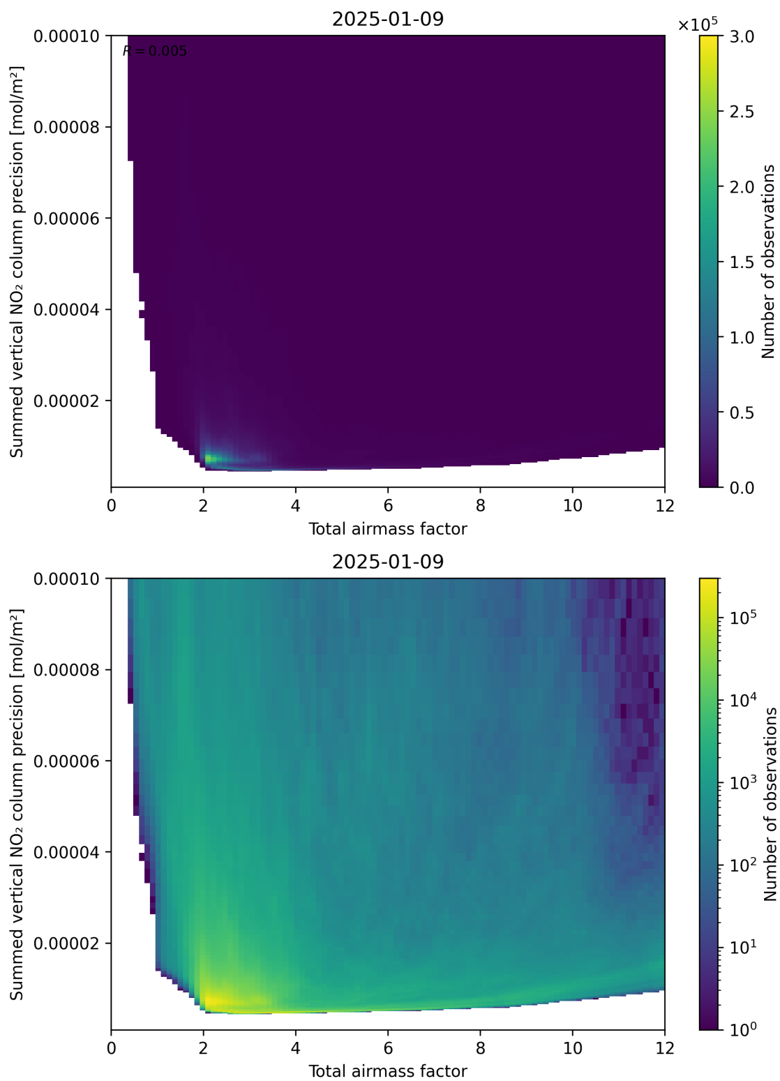
Figure 66: Scatter density plot of “Total airmass factor” against “Summed vertical NO 2 column precision” for 2025-01-08 to 2025-01-10.
