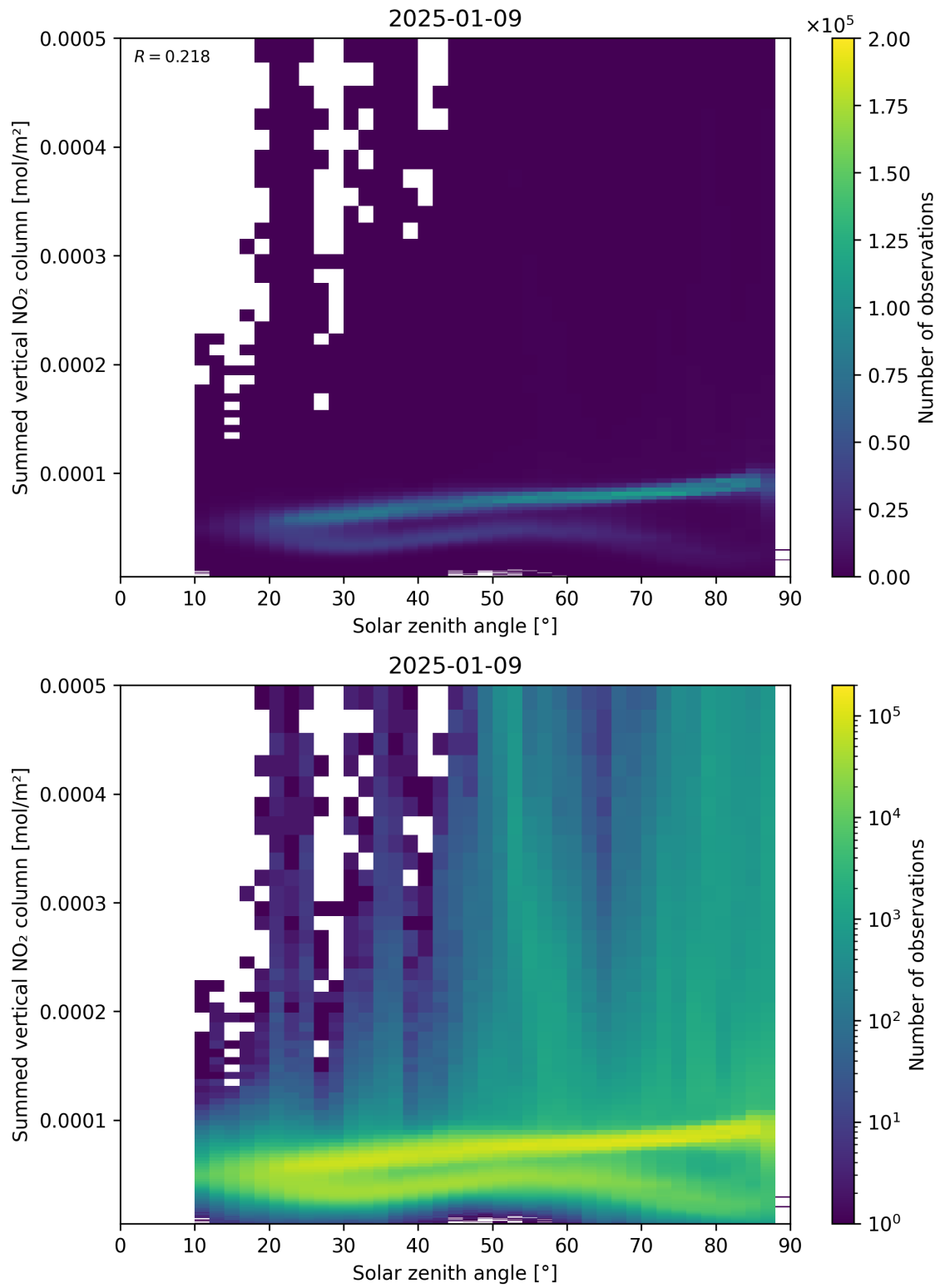
Figure 151: Scatter density plot of “Solar zenith angle” against “Summed vertical NO 2 column” for 2025-01-08 to 2025-01-10.
