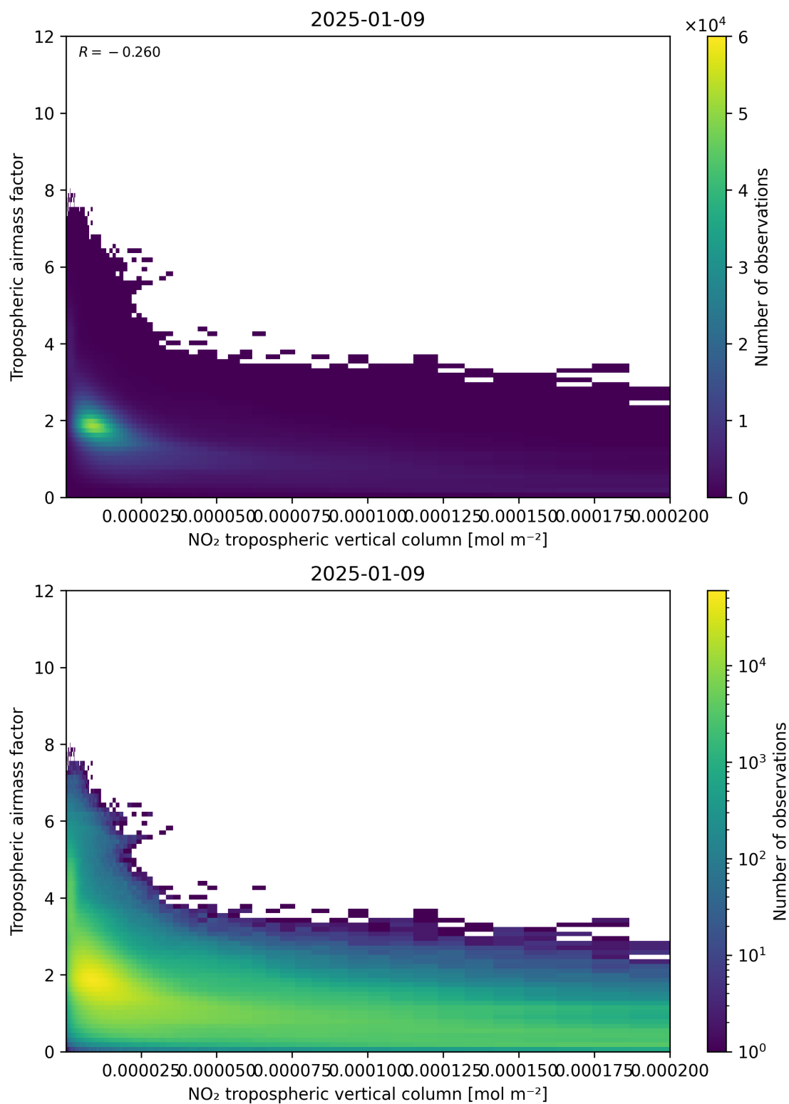
Figure 123: Scatter density plot of “NO 2 tropospheric vertical column” against “Tropospheric air mass factor” for 2025-01-08 to 2025-01-10.
