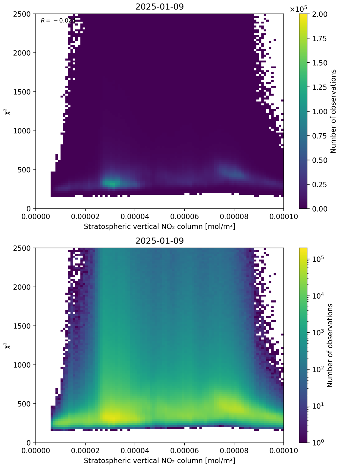
Figure 97: Scatter density plot of “Stratospheric vertical NO 2 column” against “ \chi^2 ” for 2025-01-08 to 2025-01-10.
