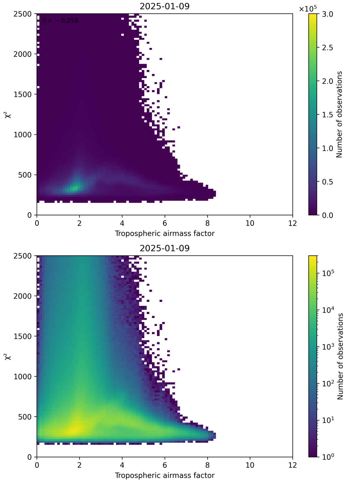
Figure 73: Scatter density plot of “Tropospheric airmass factor” against “ \chi^2 ” for 2025-01-08 to 2025-01-10.
