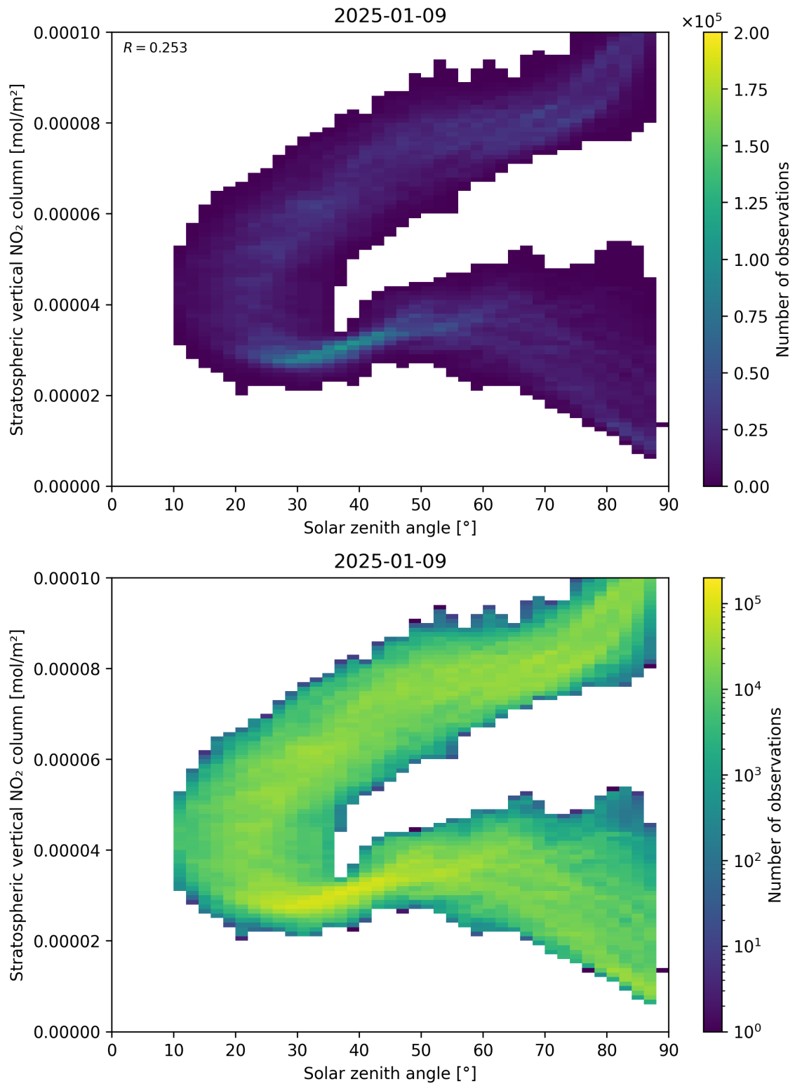
Figure 150: Scatter density plot of “Solar zenith angle” against “Stratospheric vertical NO 2 column” for 2025-01-08 to 2025-01-10.
