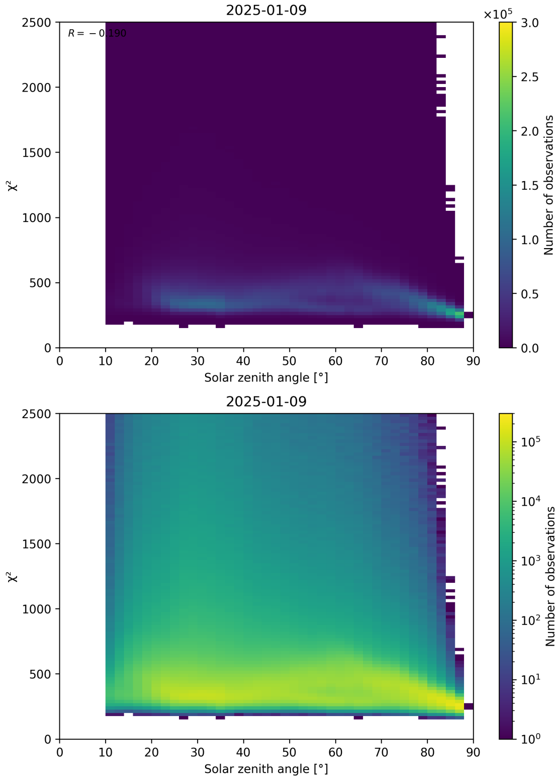
Figure 148: Scatter density plot of “Solar zenith angle” against “ \chi^2 ” for 2025-01-08 to 2025-01-10.
