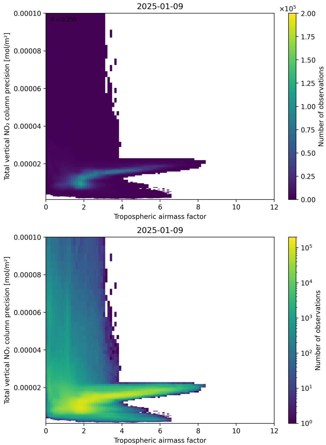
Figure 78: Scatter density plot of “Tropospheric air mass factor” against “Total vertical NO 2 column precision” for 2025-01-08 to 2025-01-10.
