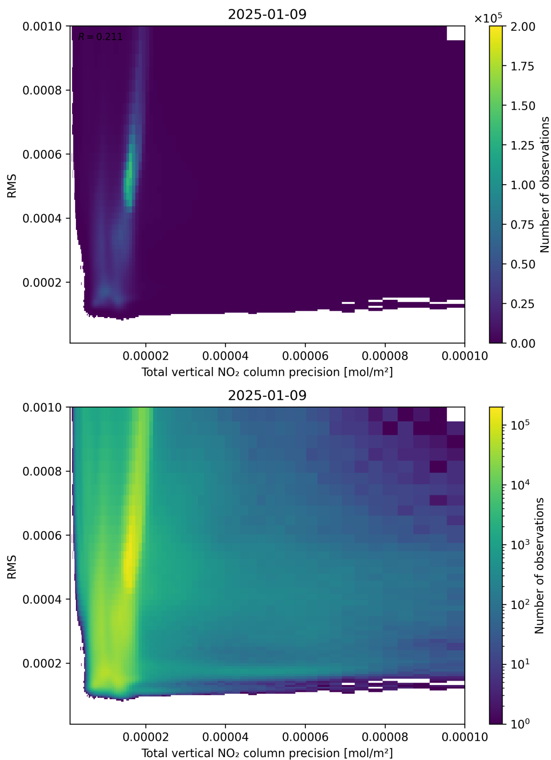
Figure 119: Scatter density plot of “Total vertical NO 2 column precision” against “RMS” for 2025-01-08 to 2025-01-10.
