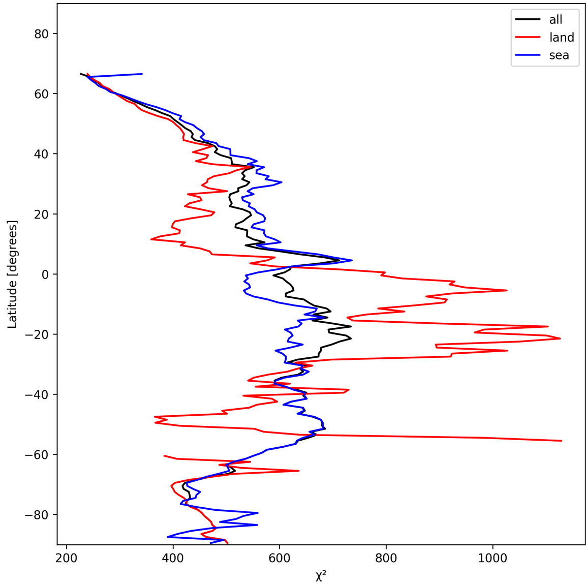
Figure 25: Zonal average of “ \chi^2 ” for 2025-01-08 to 2025-01-10.
