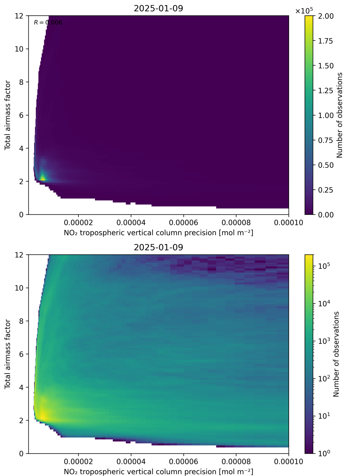
Figure 132: Scatter density plot of “NO 2 tropospheric vertical column precision” against “Total air mass factor” for 2025-01-08 to 2025-01-10.
