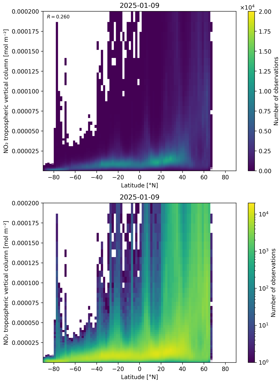
Figure 92: Scatter density plot of “Latitude” against “NO 2 tropospheric vertical column” for 2025-01-08 to 2025-01-10.
