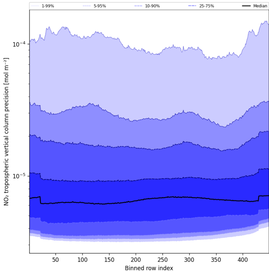
Figure 47: Along track statistics of “NO 2 tropospheric vertical column precision” for 2025-01-08 to 2025-01-10
