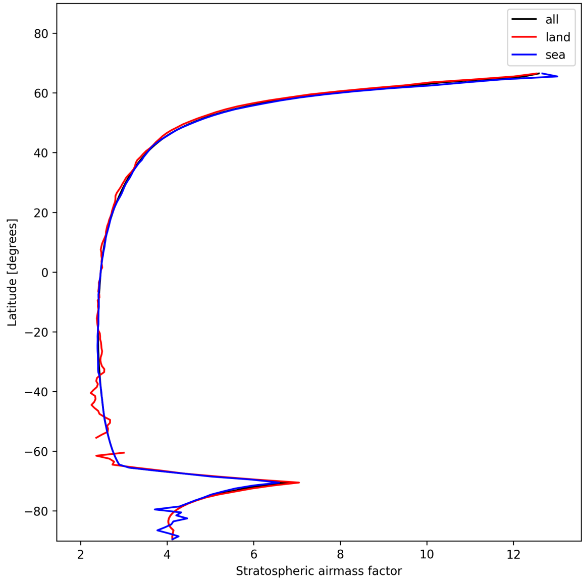
Figure 27: Zonal average of “Stratospheric air mass factor” for 2025-01-08 to 2025-01-10.
