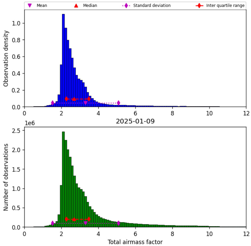
Figure 32: Histogram of “Total airmass factor” for 2025-01-08 to 2025-01-10
