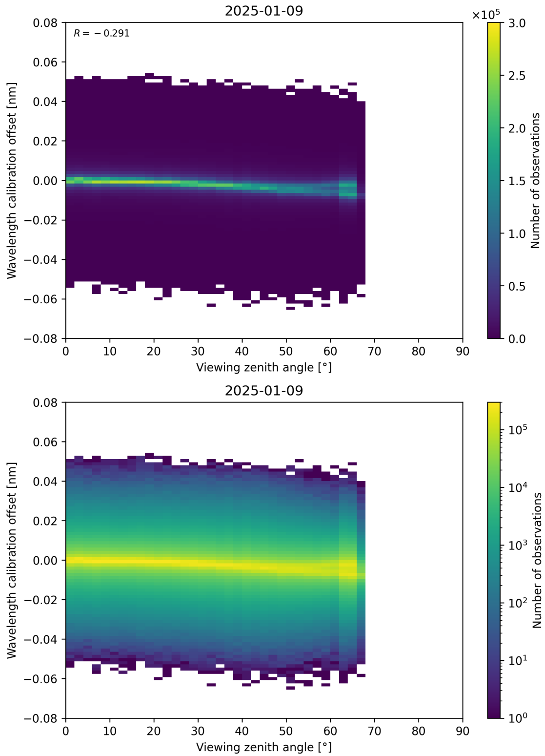
Figure 173: Scatter density plot of “Viewing zenith angle” against “Wavelength calibration offset” for 2025-01-08 to 2025-01-10.
