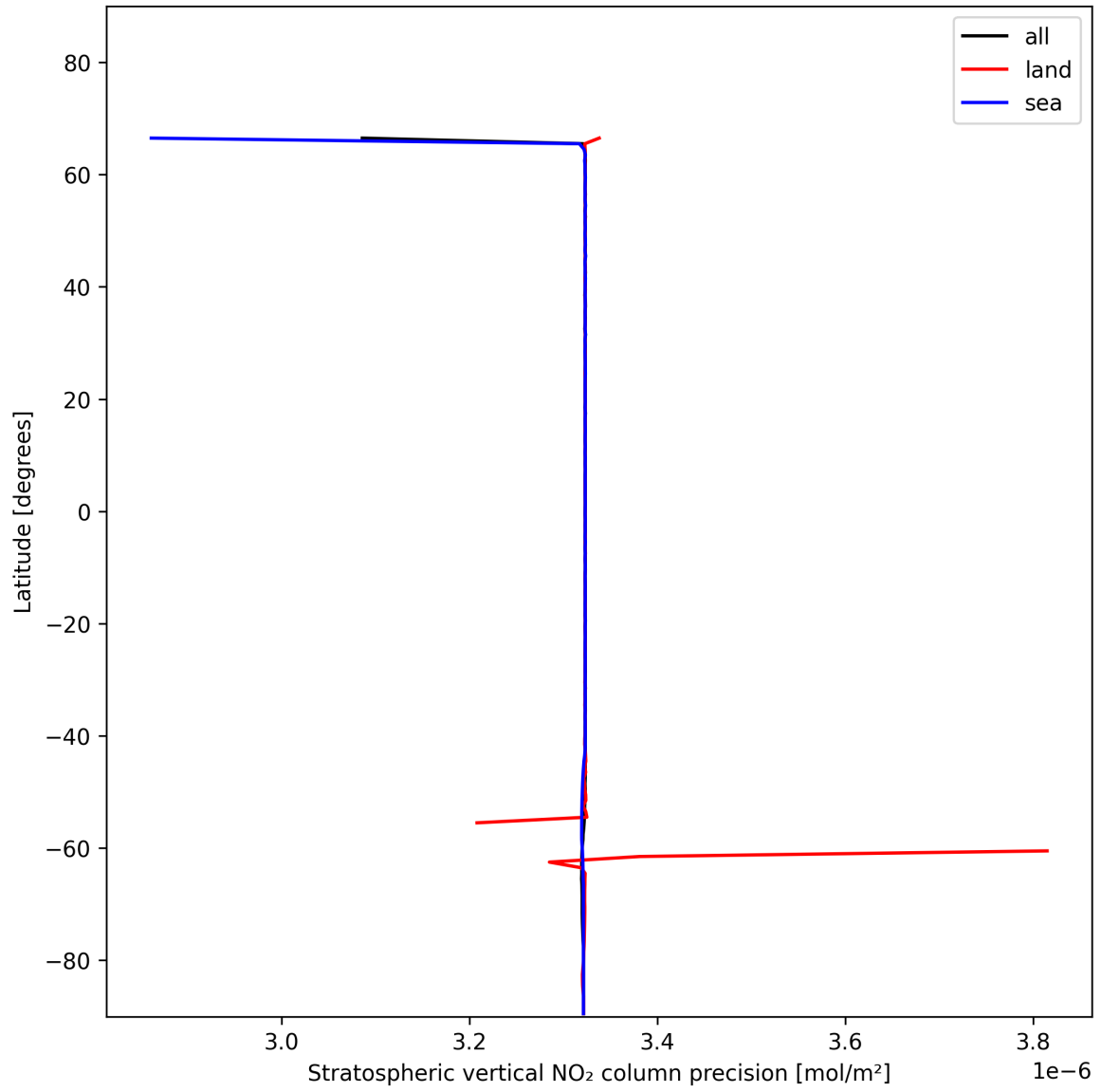
Figure 20: Zonal average of “Stratospheric vertical NO 2 column precision” for 2025-01-08 to 2025-01-10.
