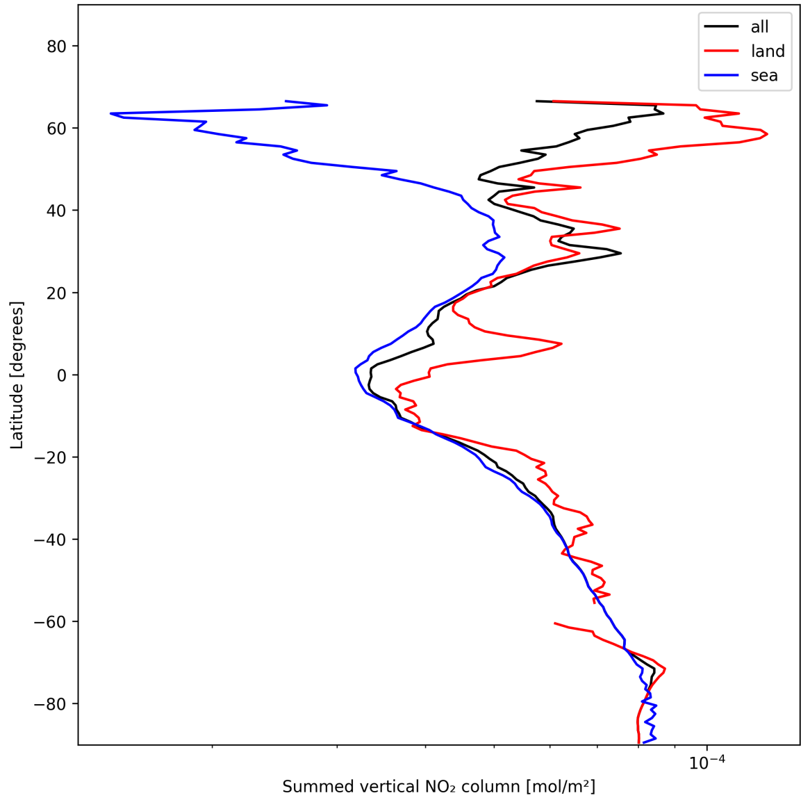
Figure 23: Zonal average of “Summed vertical NO 2 column” for 2025-01-08 to 2025-01-10.
