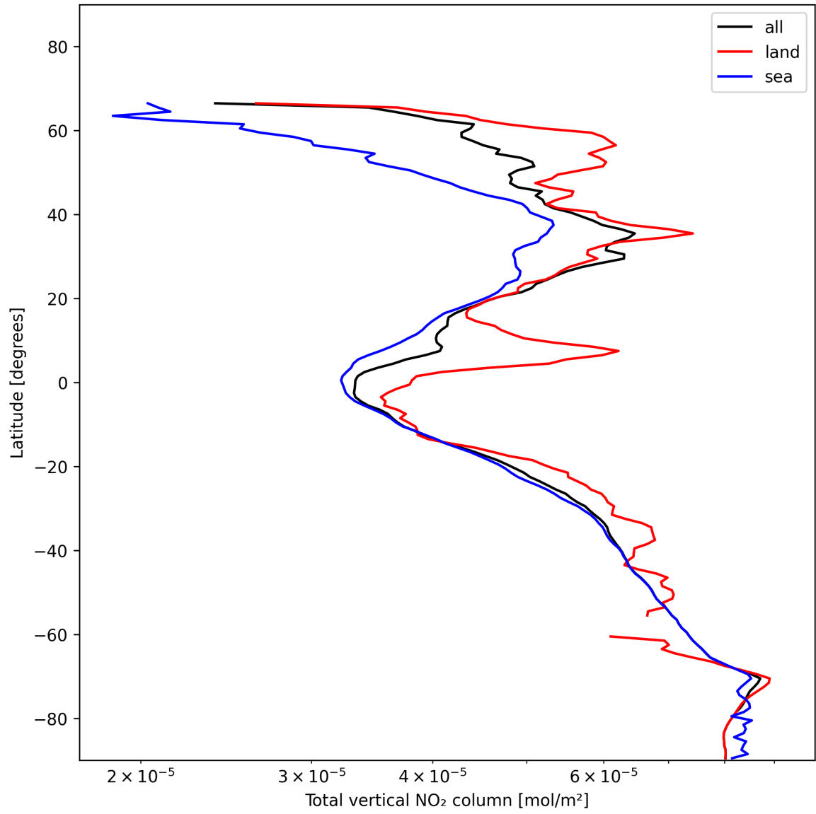
Figure 21: Zonal average of “Total vertical NO 2 column” for 2025-01-08 to 2025-01-10.
