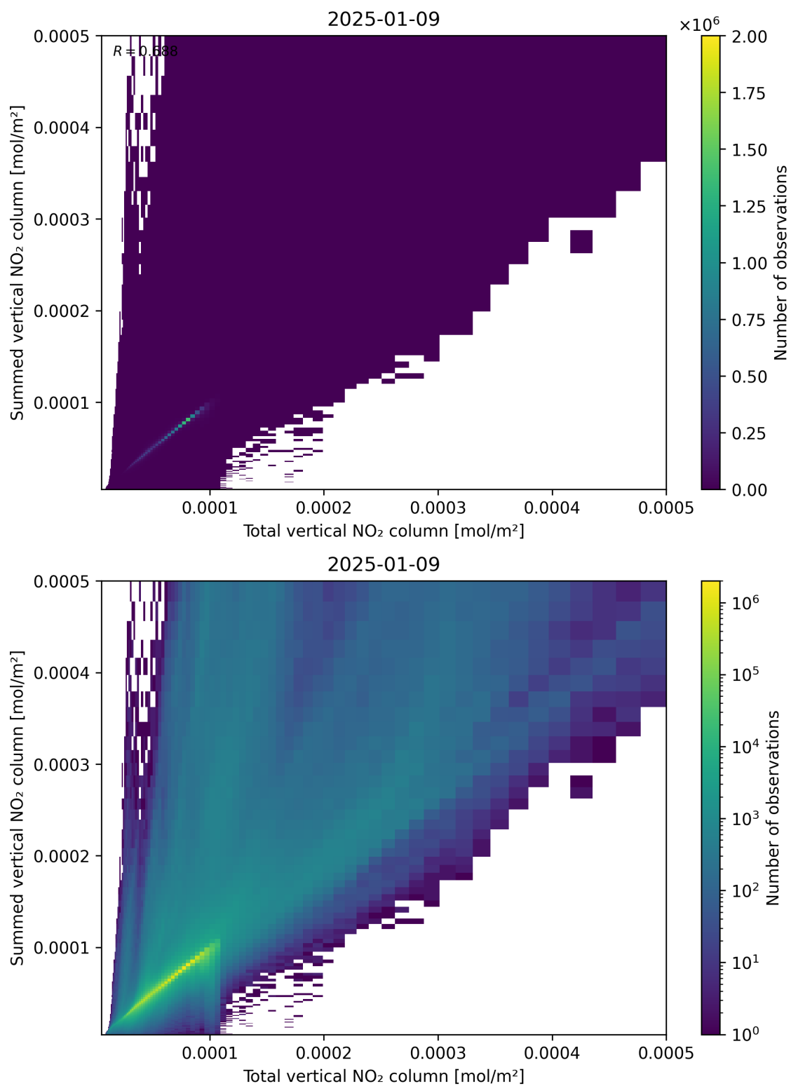
Figure 112: Scatter density plot of “Total vertical NO 2 column” against “Summed vertical NO 2 column” for 2025-01-08 to 2025-01-10.
