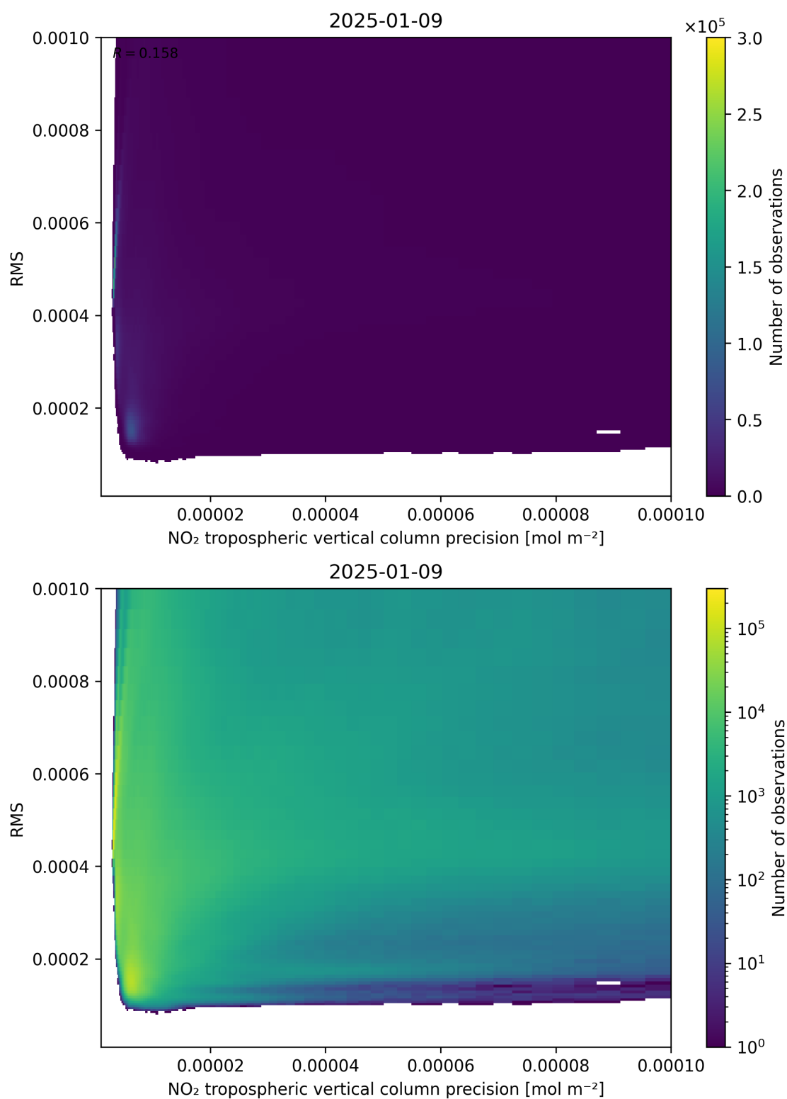
Figure 140: Scatter density plot of “NO 2 tropospheric vertical column precision” against “RMS” for 2025-01-08 to 2025-01-10.
