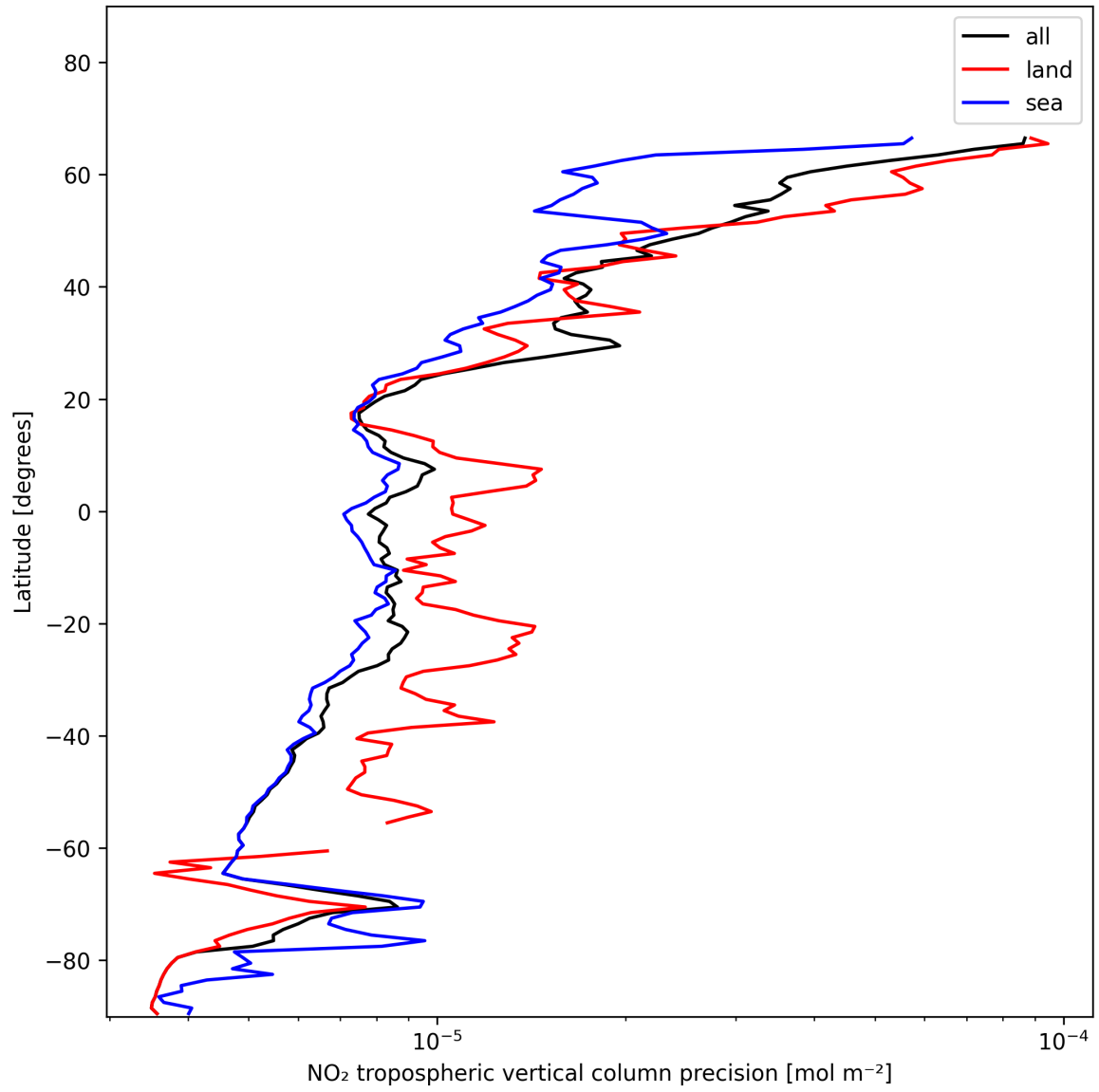
Figure 13: Zonal average of “NO 2 tropospheric vertical column precision” for 2025-01-08 to 2025-01-10.
