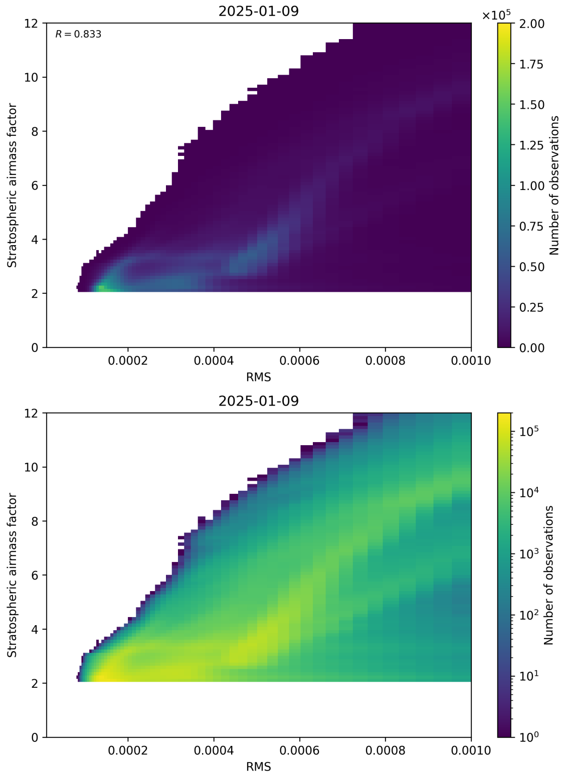
Figure 144: Scatter density plot of “RMS” against “Stratospheric airmass factor” for 2025-01-08 to 2025-01-10.
