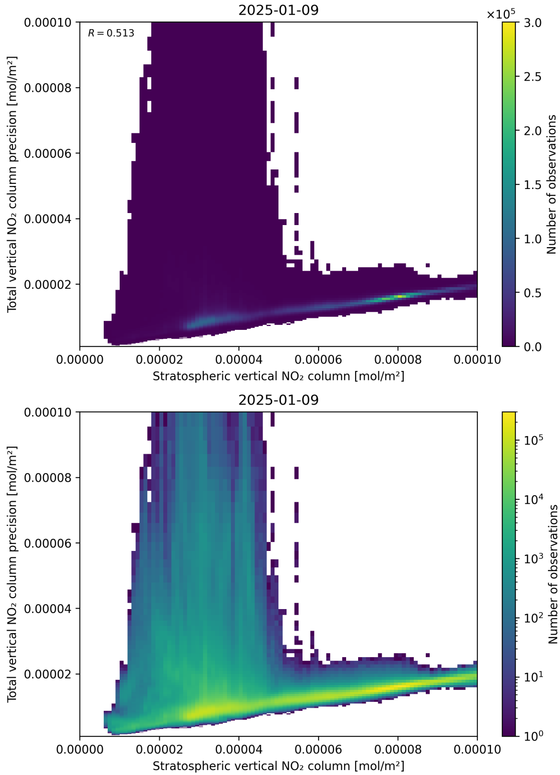
Figure 101: Scatter density plot of “Stratospheric vertical NO 2 column” against “Total vertical NO 2 column precision” for 2025-01-08 to 2025-01-10.
