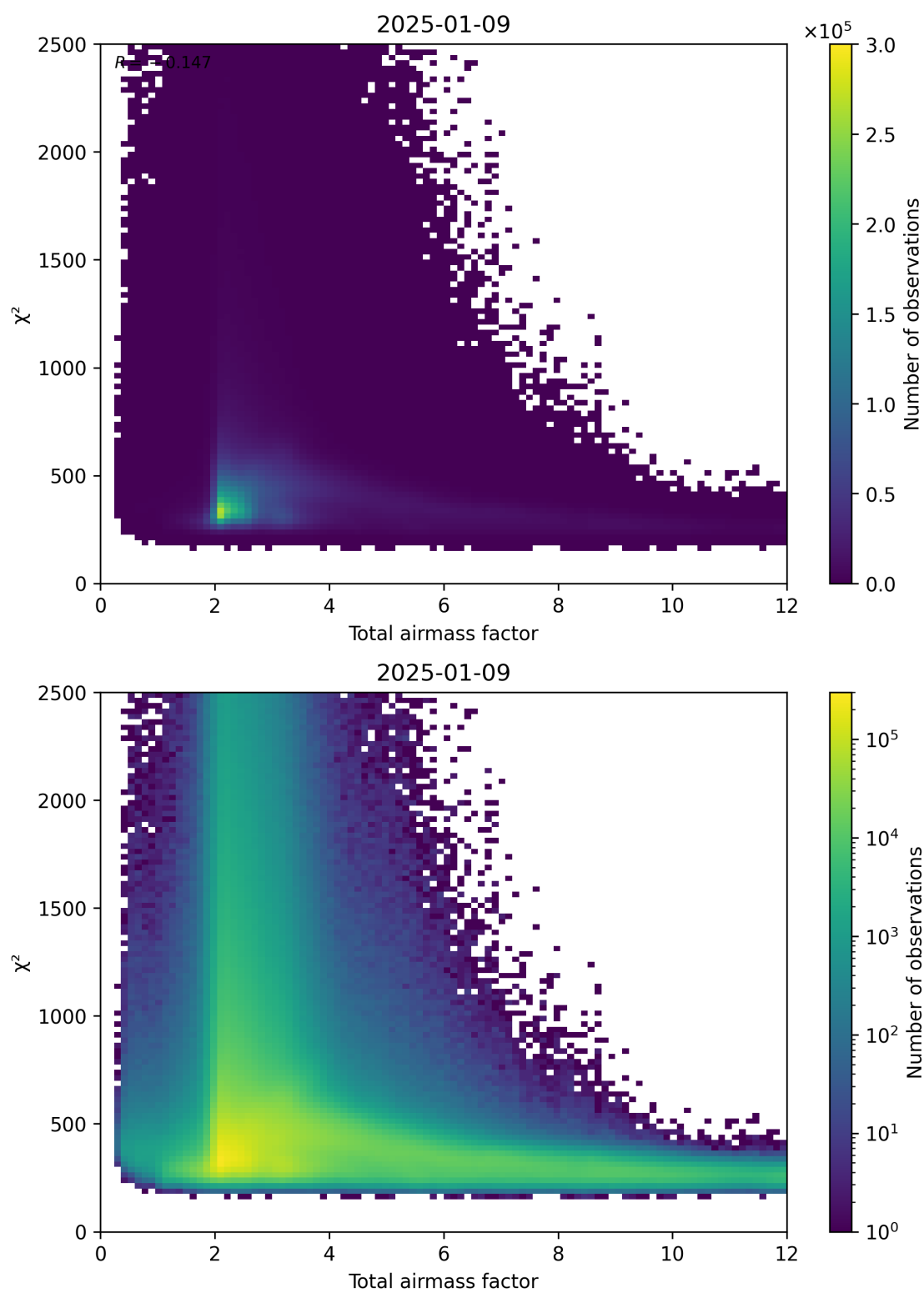
Figure 63: Scatter density plot of “Total airmass factor” against “ \chi^2 ” for 2025-01-08 to 2025-01-10.
