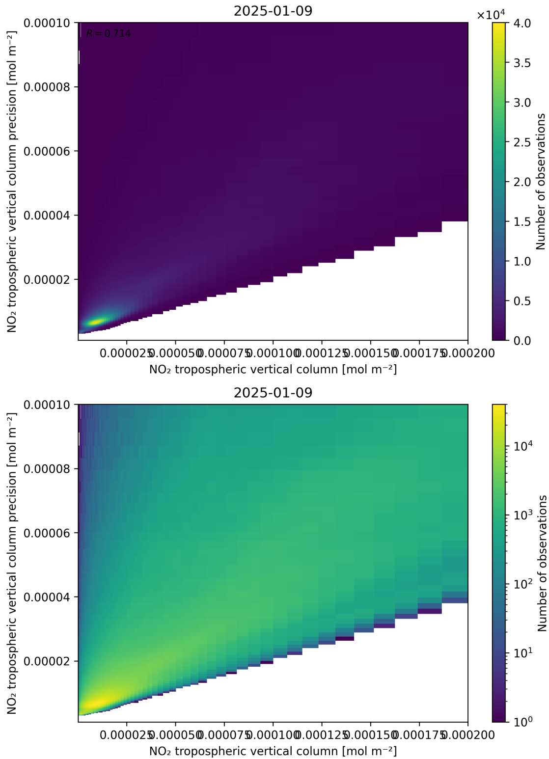
Figure 130: Scatter density plot of “NO 2 tropospheric vertical column” against “NO 2 tropospheric vertical column precision” for 2025-01-08 to 2025-01-10.
