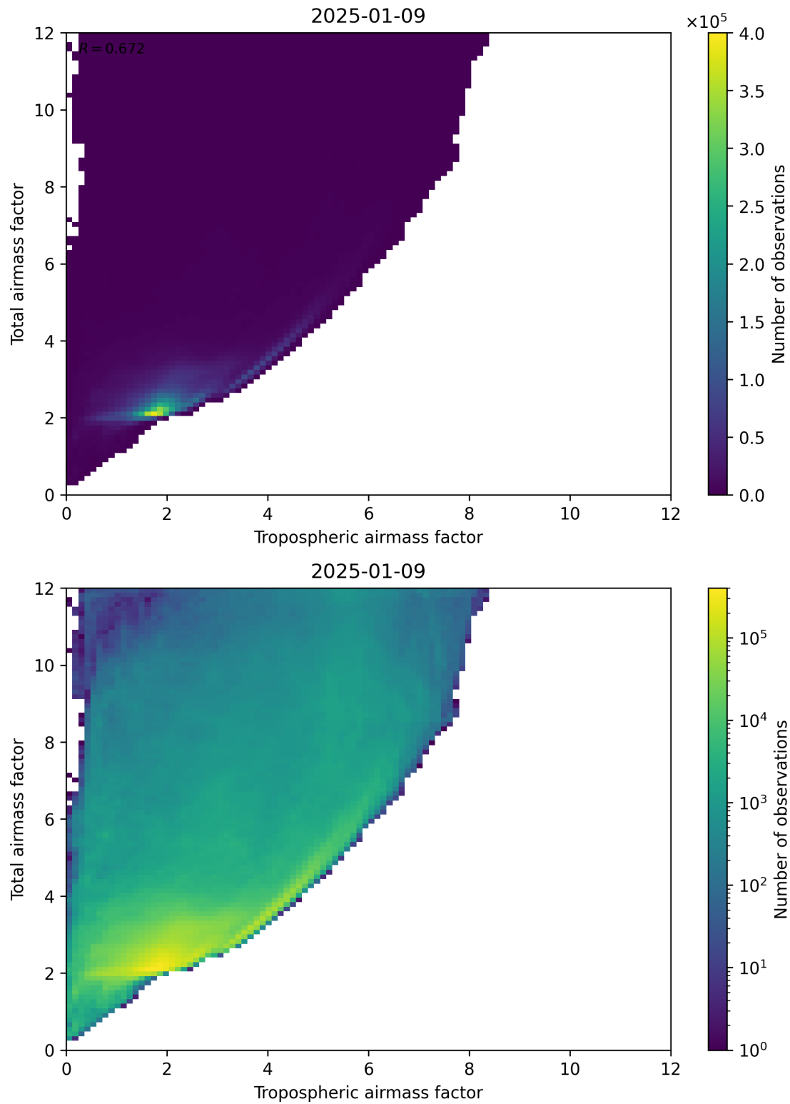
Figure 72: Scatter density plot of “Tropospheric airmass factor” against “Total airmass factor” for 2025-01-08 to 2025-01-10.
