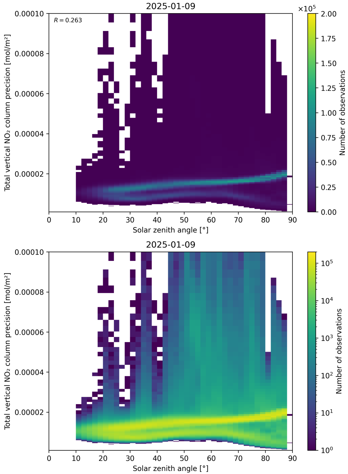
Figure 154: Scatter density plot of “Solar zenith angle” against “Total vertical NO 2 column precision” for 2025-01-08 to 2025-01-10.
