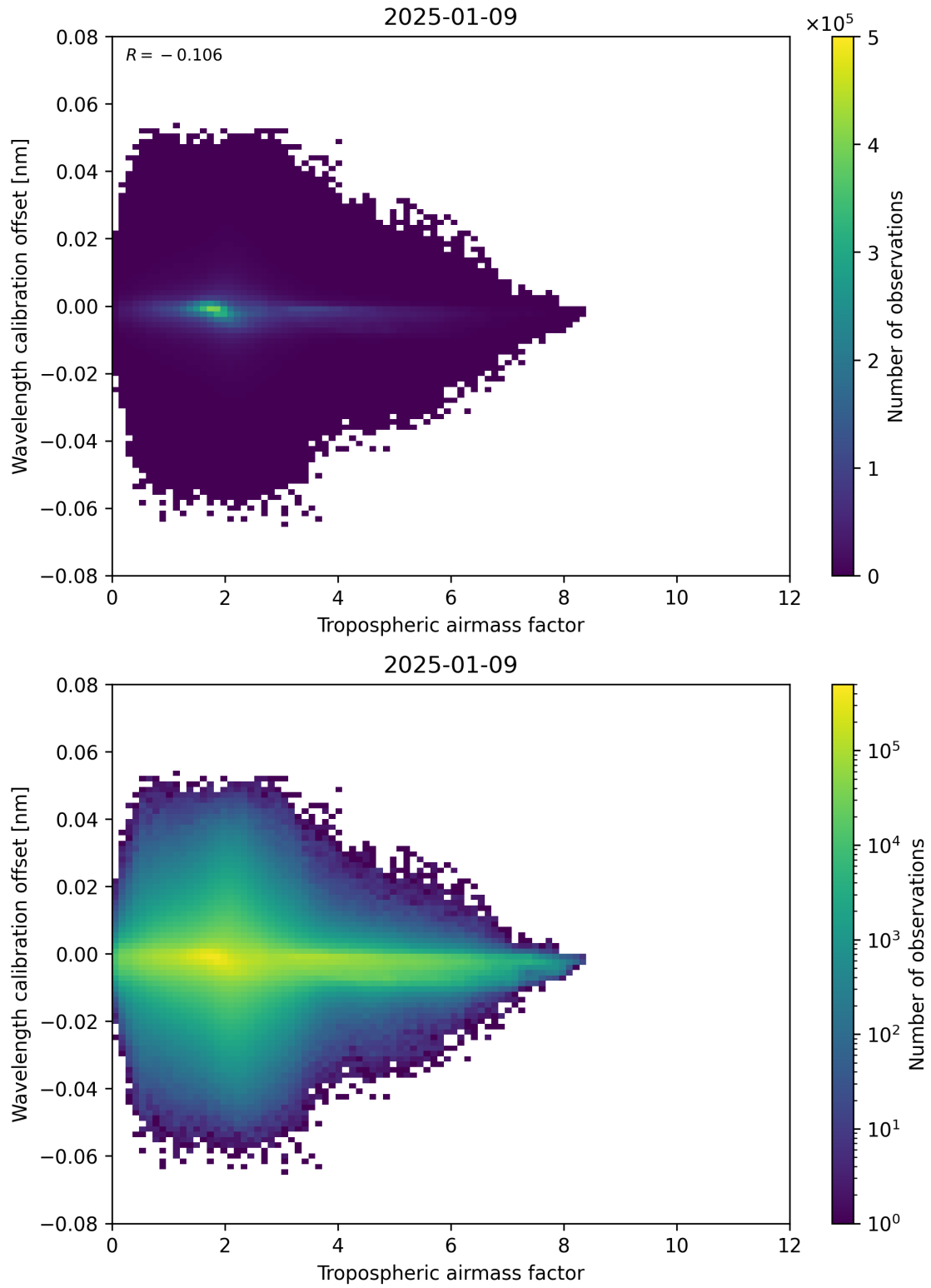
Figure 80: Scatter density plot of “Tropospheric airmass factor” against “Wavelength calibration offset” for 2025-01-08 to 2025-01-10.
