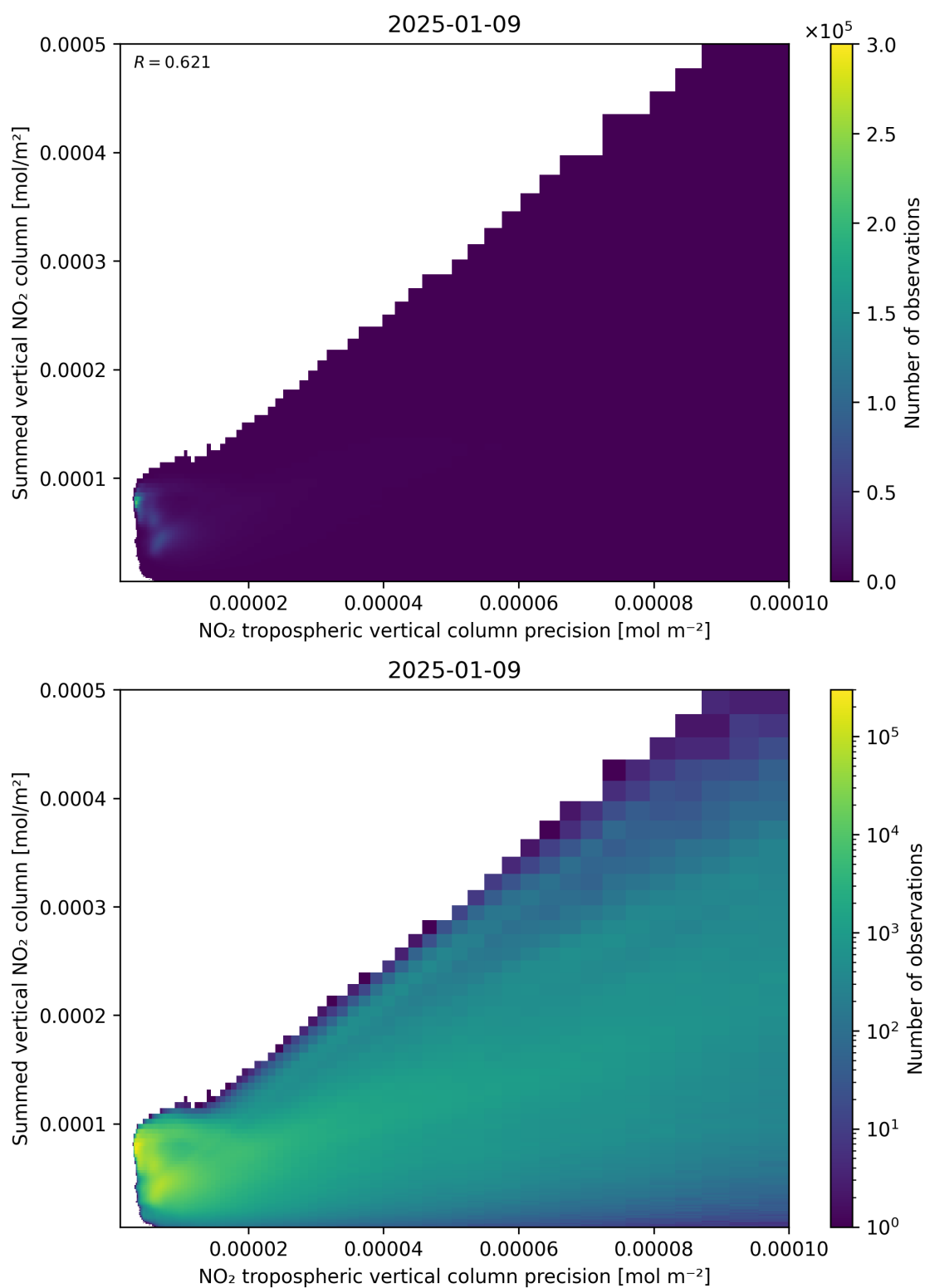
Figure 136: Scatter density plot of “NO 2 tropospheric vertical column precision” against “Summed vertical NO 2 column” for 2025-01-08 to 2025-01-10.
