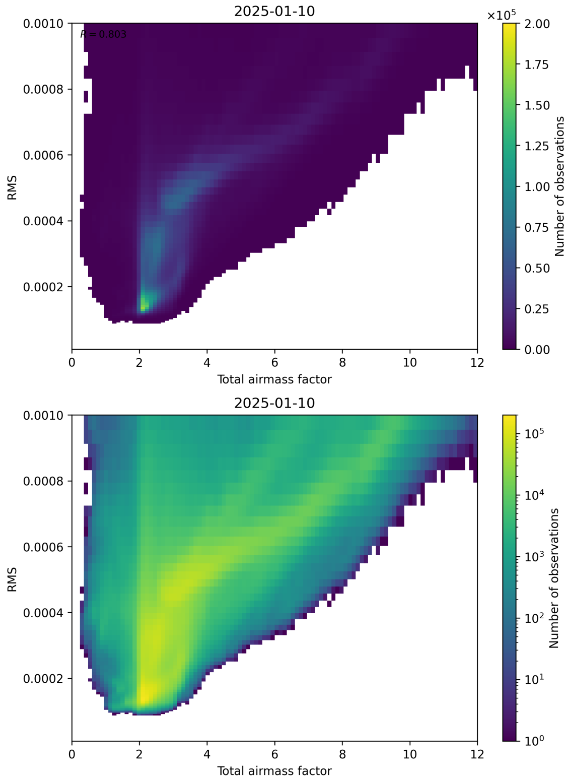
Figure 69: Scatter density plot of “Total airmass factor” against “RMS” for 2025-01-09 to 2025-01-11.
