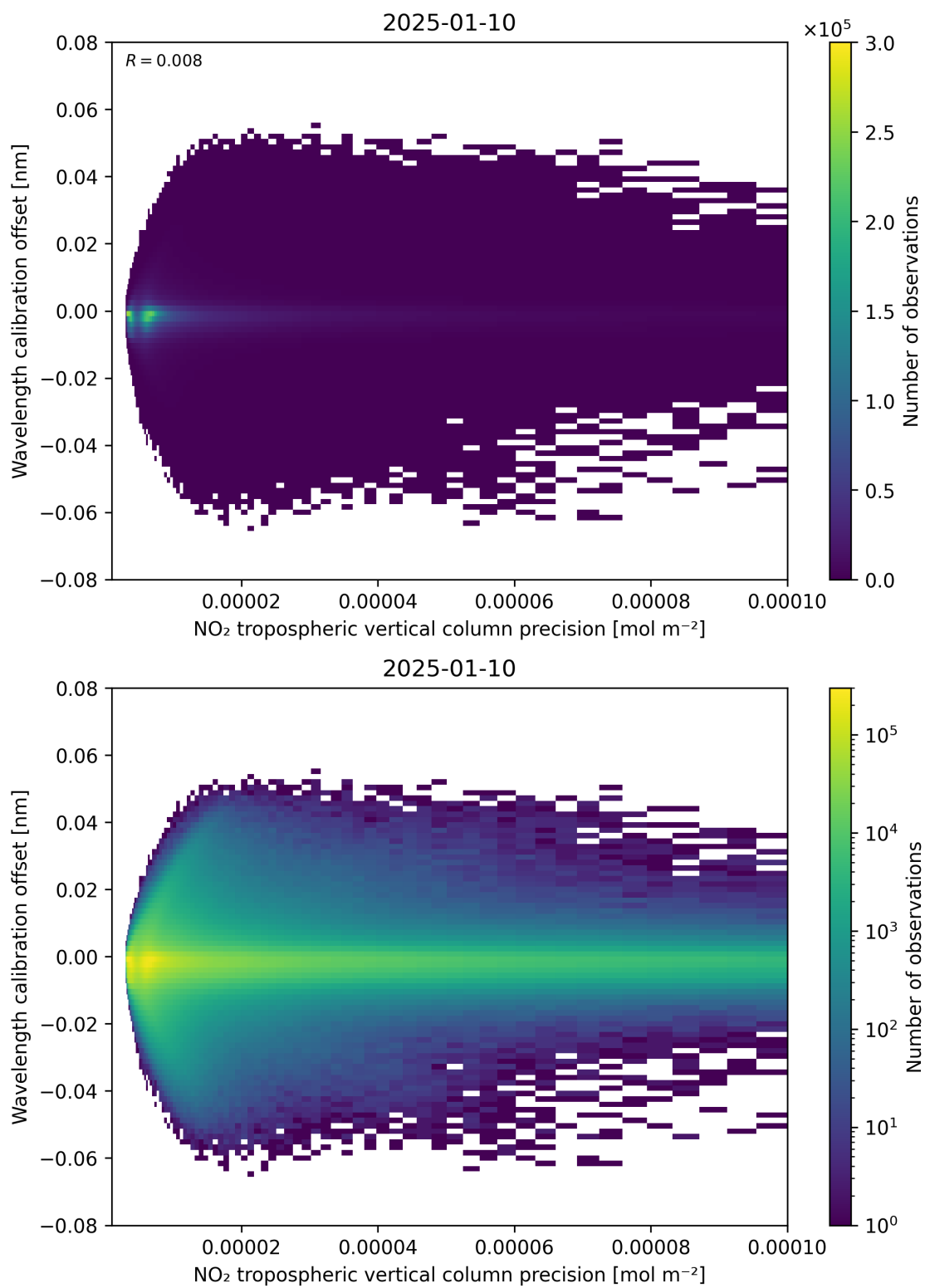
Figure 141: Scatter density plot of “NO 2 tropospheric vertical column precision” against “Wavelength calibration offset” for 2025-01-09 to 2025-01-11.
