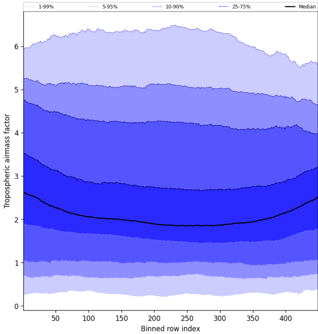
Figure 48: Along track statistics of “Tropospheric air mass factor” for 2025-01-09 to 2025-01-11
