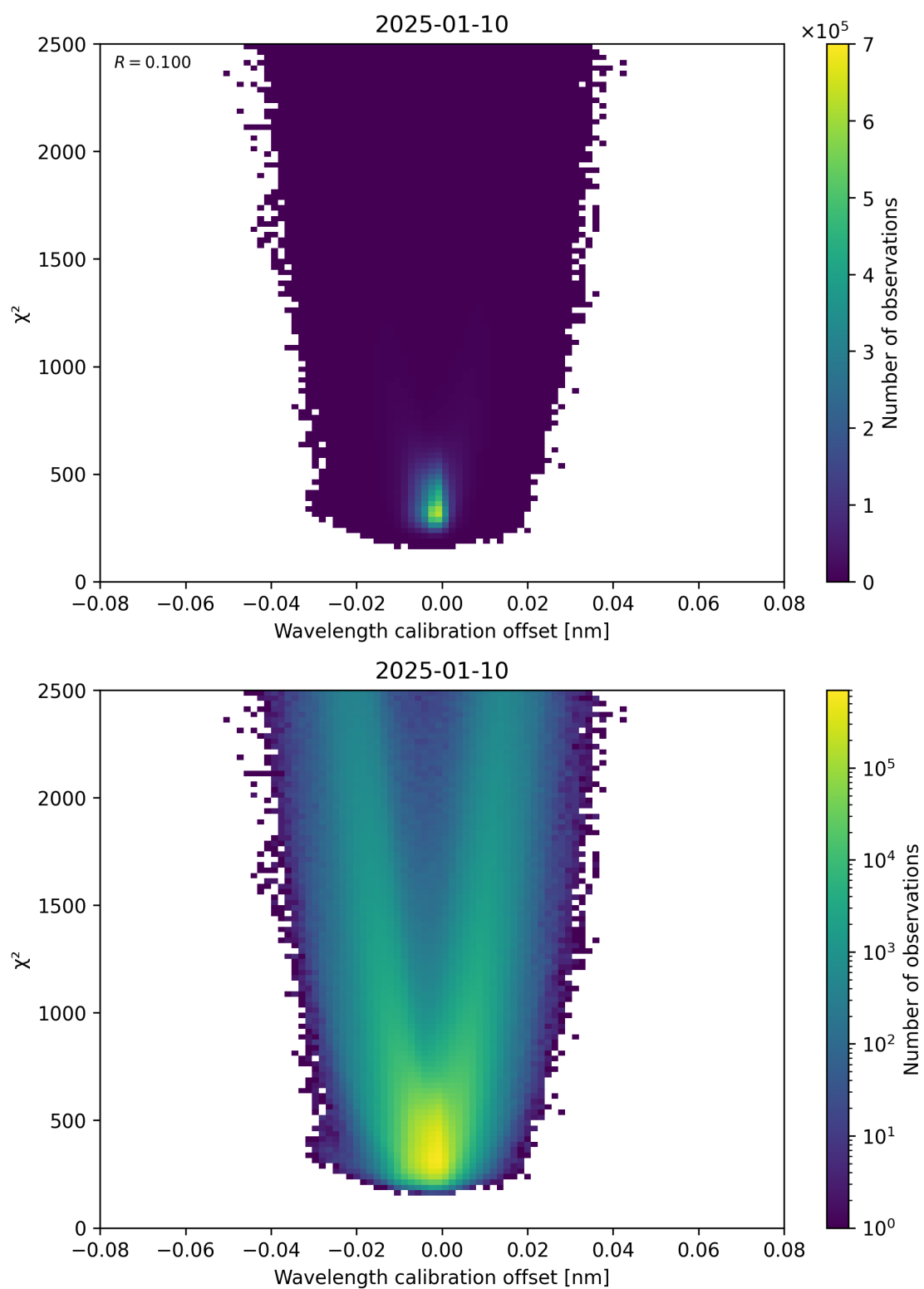
Figure 175: Scatter density plot of “Wavelength calibration offset” against “ \chi^2 ” for 2025-01-09 to 2025-01-11.
