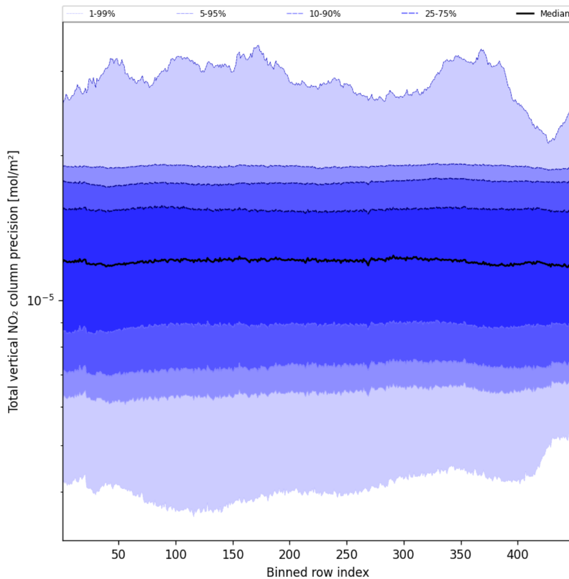
Figure 56: Along track statistics of “Total vertical NO 2 column precision” for 2025-01-09 to 2025-01-11
