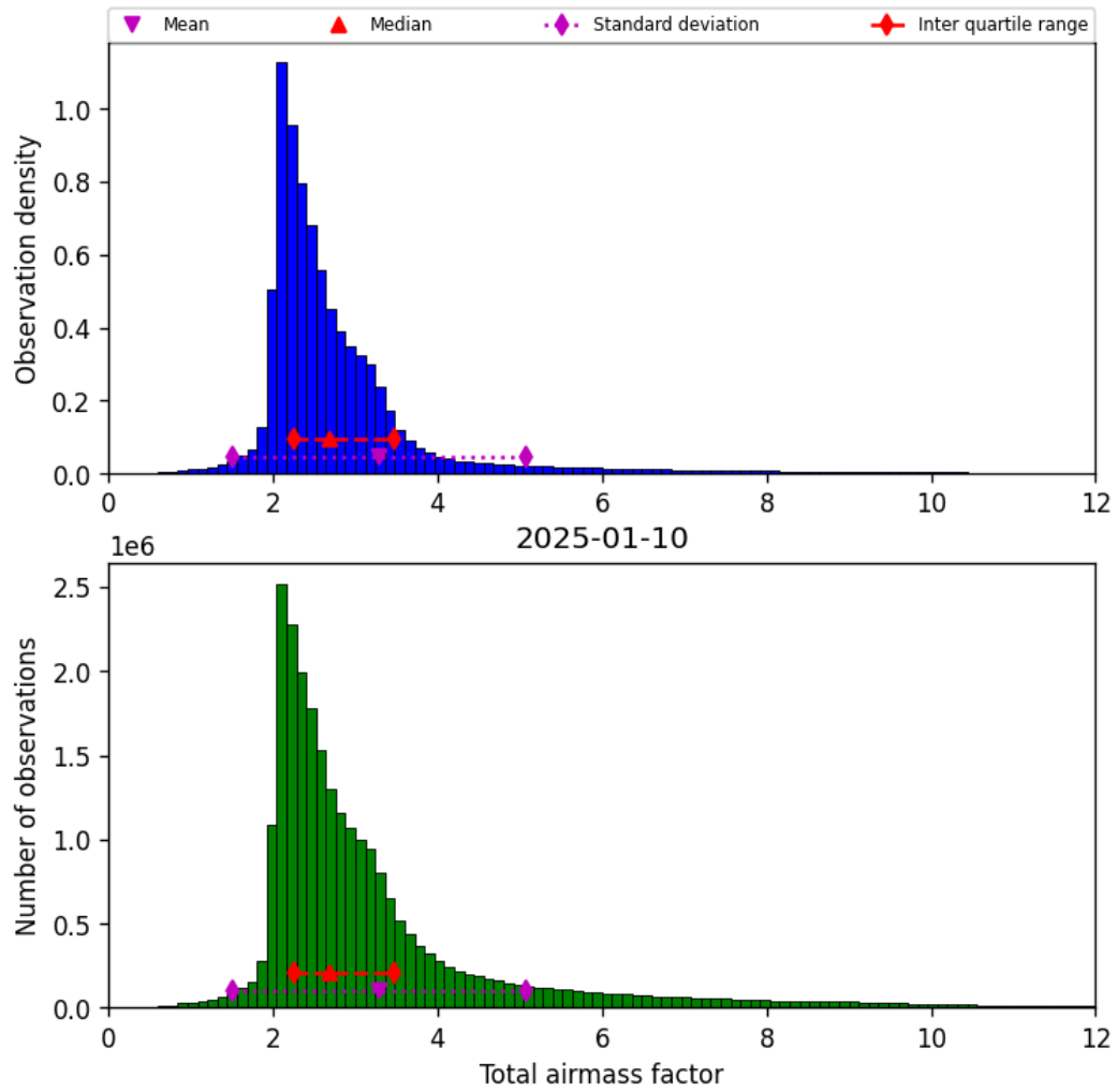
Figure 32: Histogram of “Total airmass factor” for 2025-01-09 to 2025-01-11
