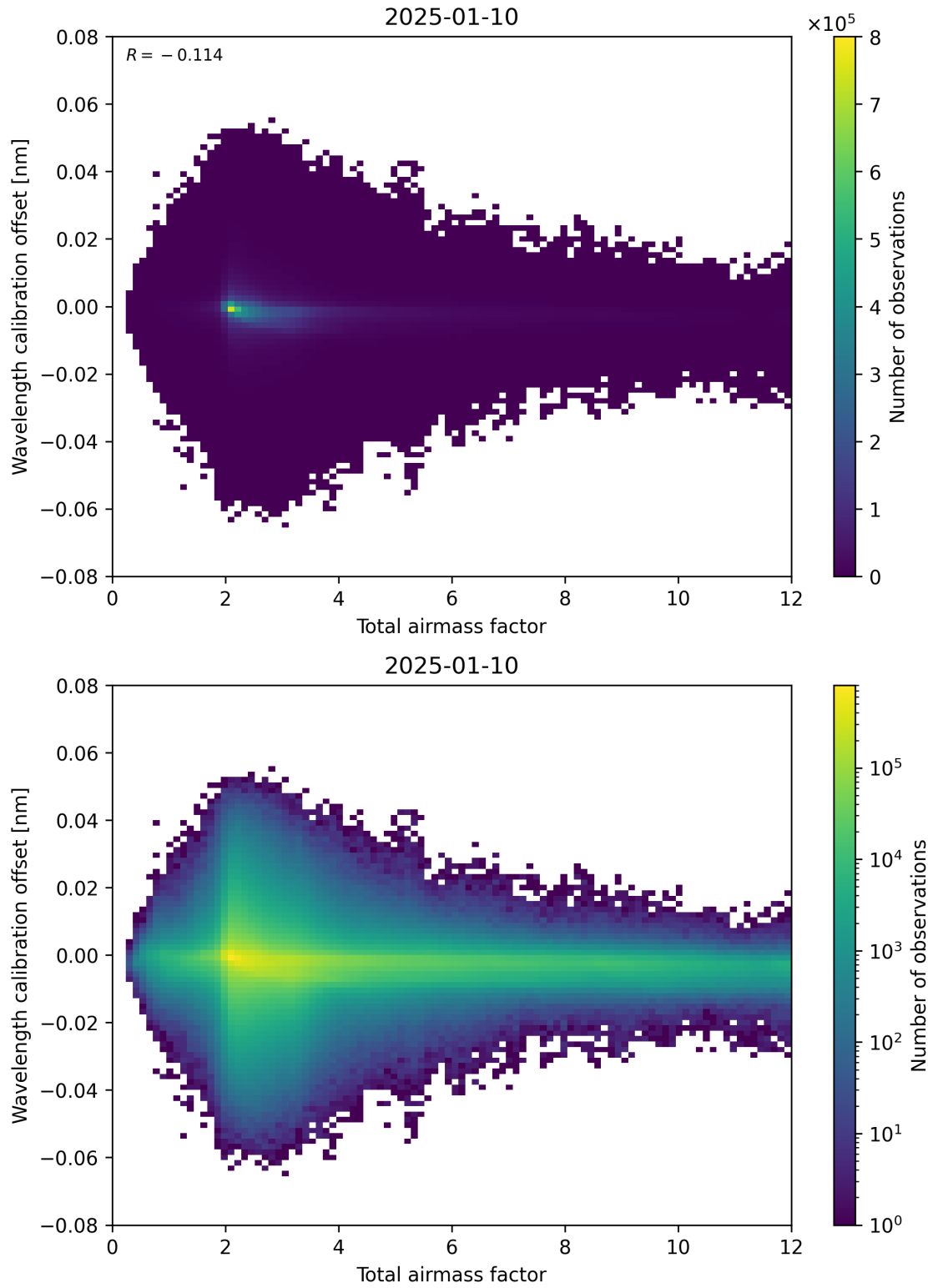
Figure 70: Scatter density plot of “Total airmass factor” against “Wavelength calibration offset” for 2025-01-09 to 2025-01-11.
