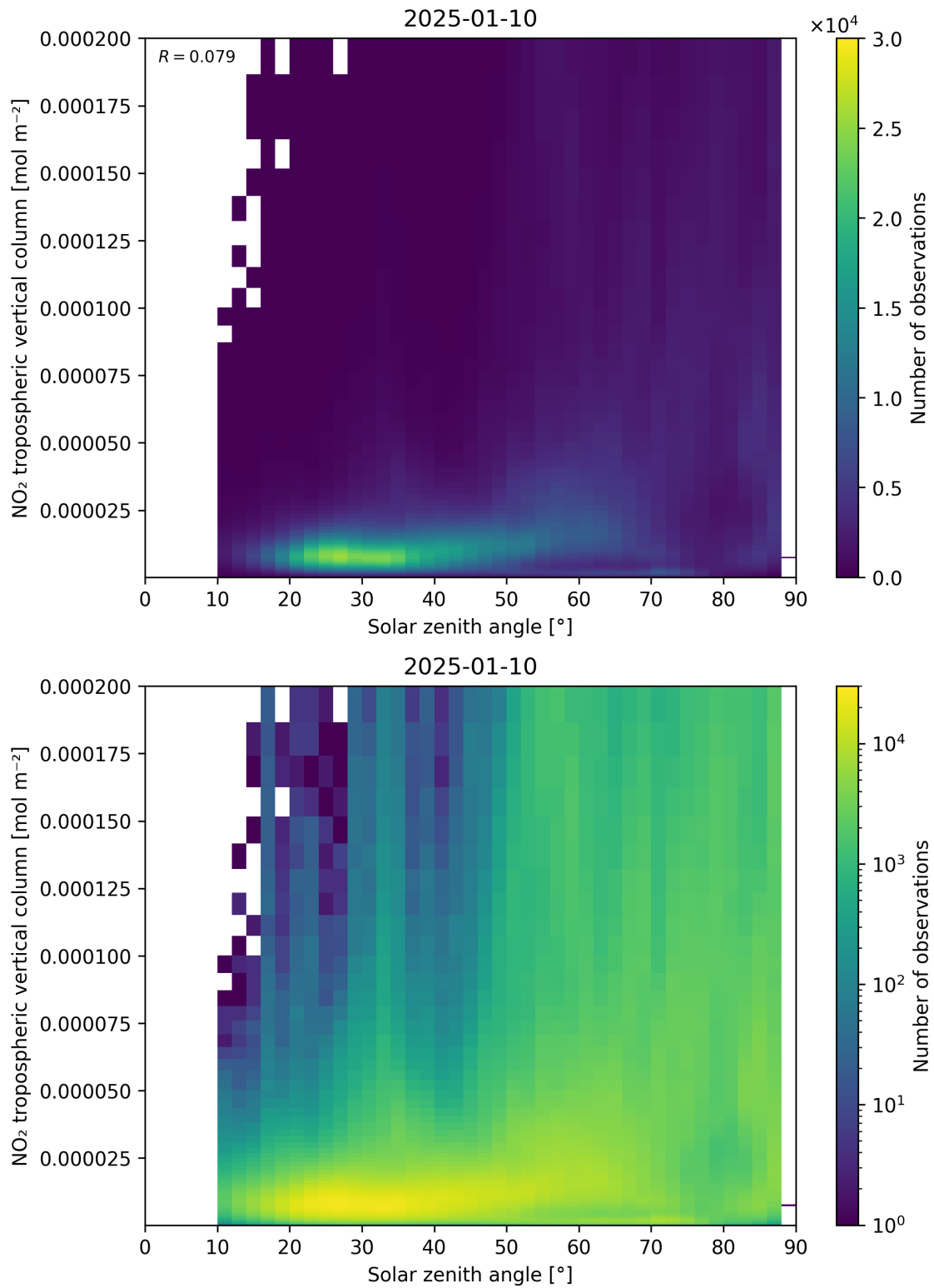
Figure 155: Scatter density plot of “Solar zenith angle” against “NO 2 tropospheric vertical column” for 2025-01-09 to 2025-01-11.
