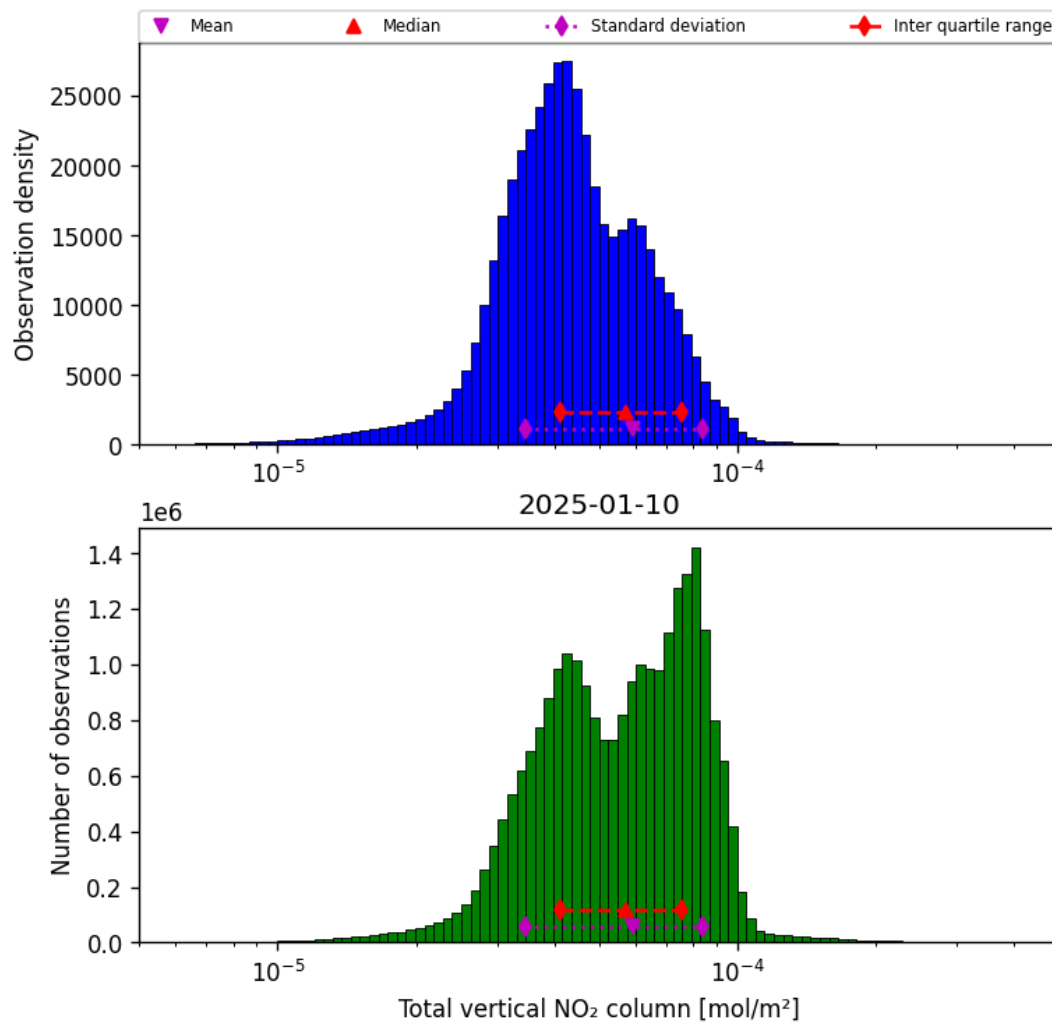
Figure 38: Histogram of “Total vertical NO 2 column” for 2025-01-09 to 2025-01-11
