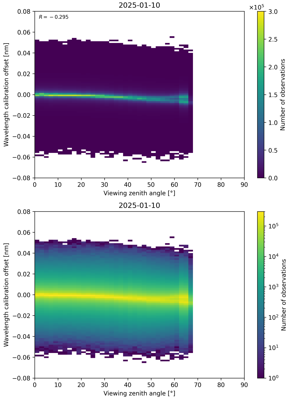
Figure 173: Scatter density plot of “Viewing zenith angle” against “Wavelength calibration offset” for 2025-01-09 to 2025-01-11.
