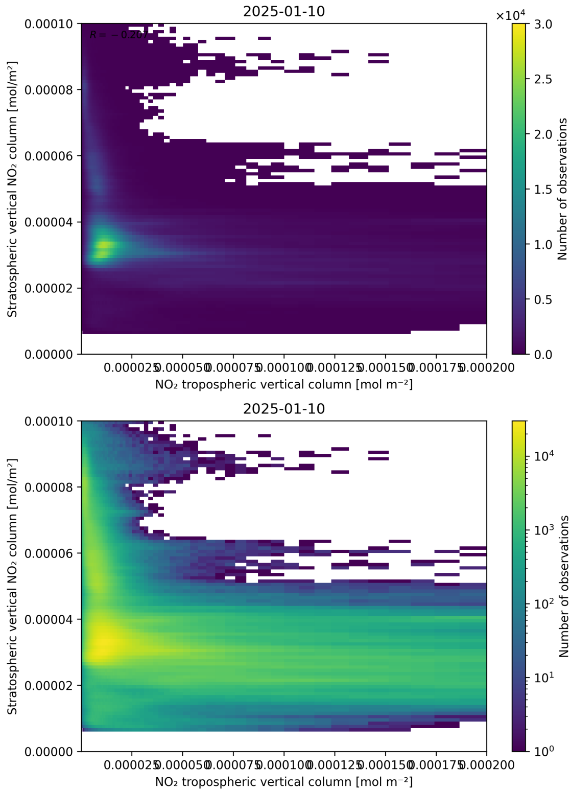
Figure 125: Scatter density plot of “NO 2 tropospheric vertical column” against “Stratospheric vertical NO 2 column” for 2025-01-09 to 2025-01-11.
