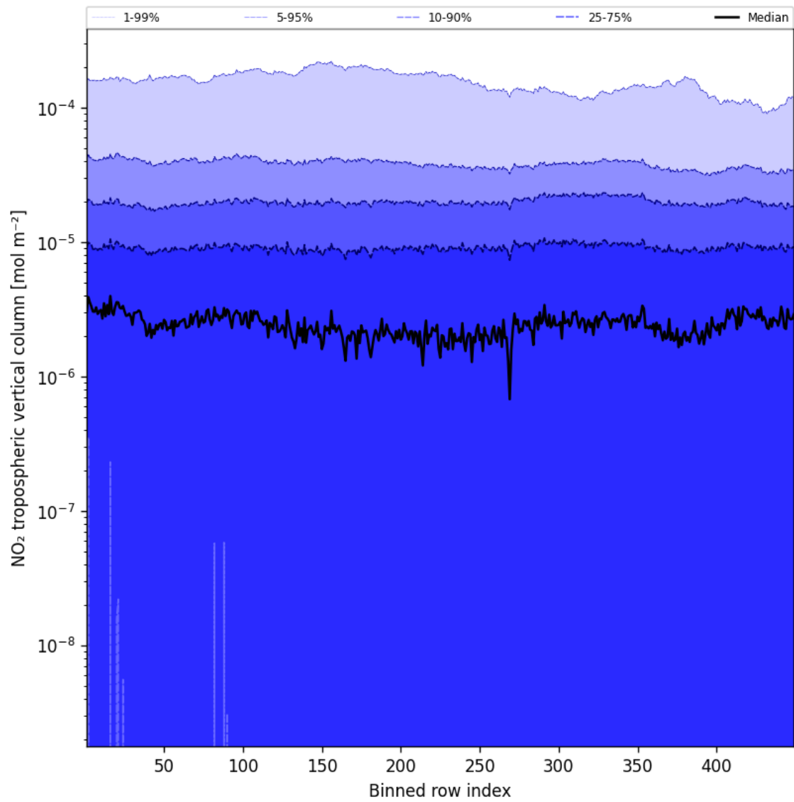
Figure 46: Along track statistics of “NO 2 tropospheric vertical column” for 2025-01-09 to 2025-01-11
