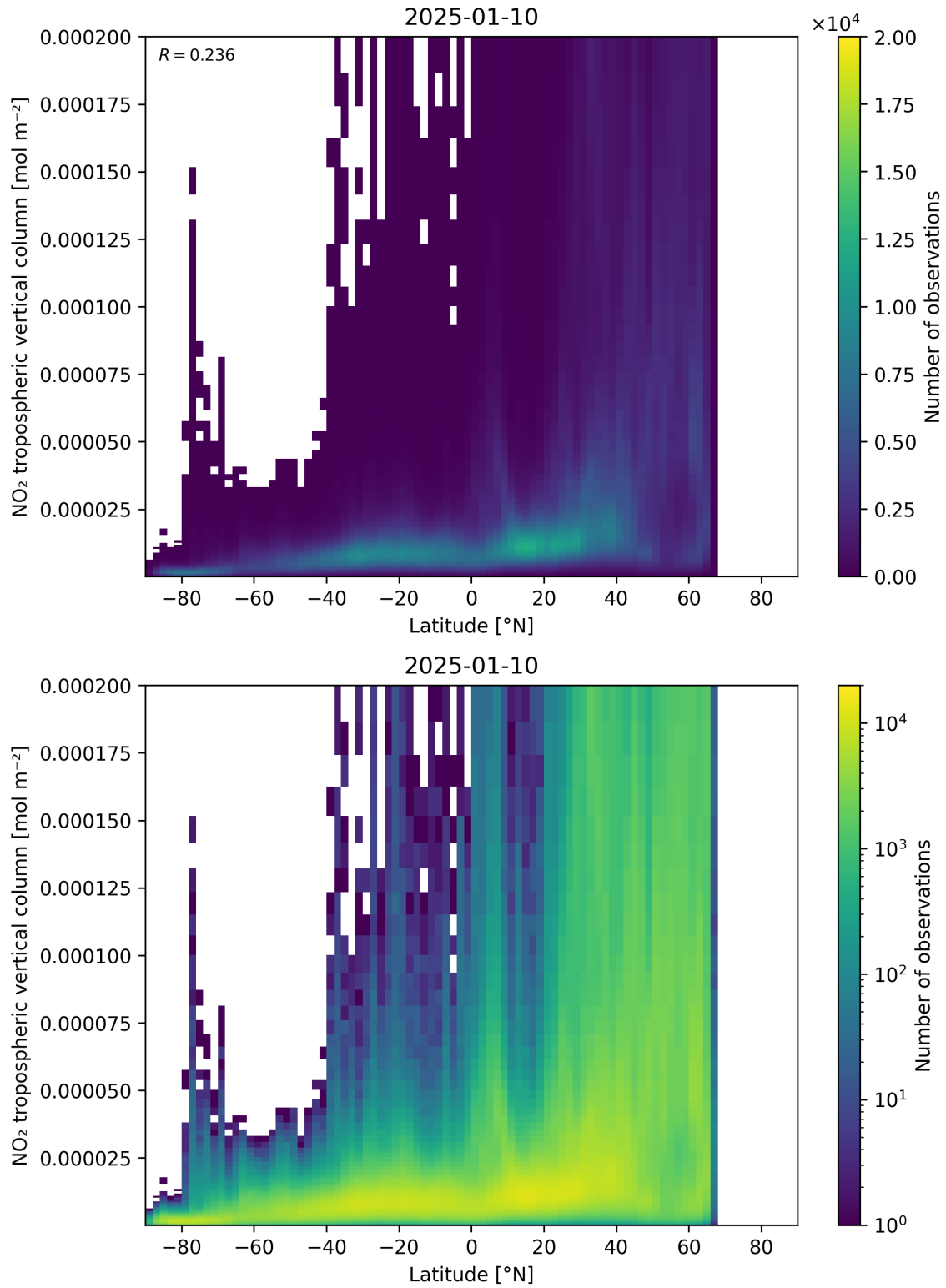
Figure 92: Scatter density plot of “Latitude” against “NO 2 tropospheric vertical column” for 2025-01-09 to 2025-01-11.
