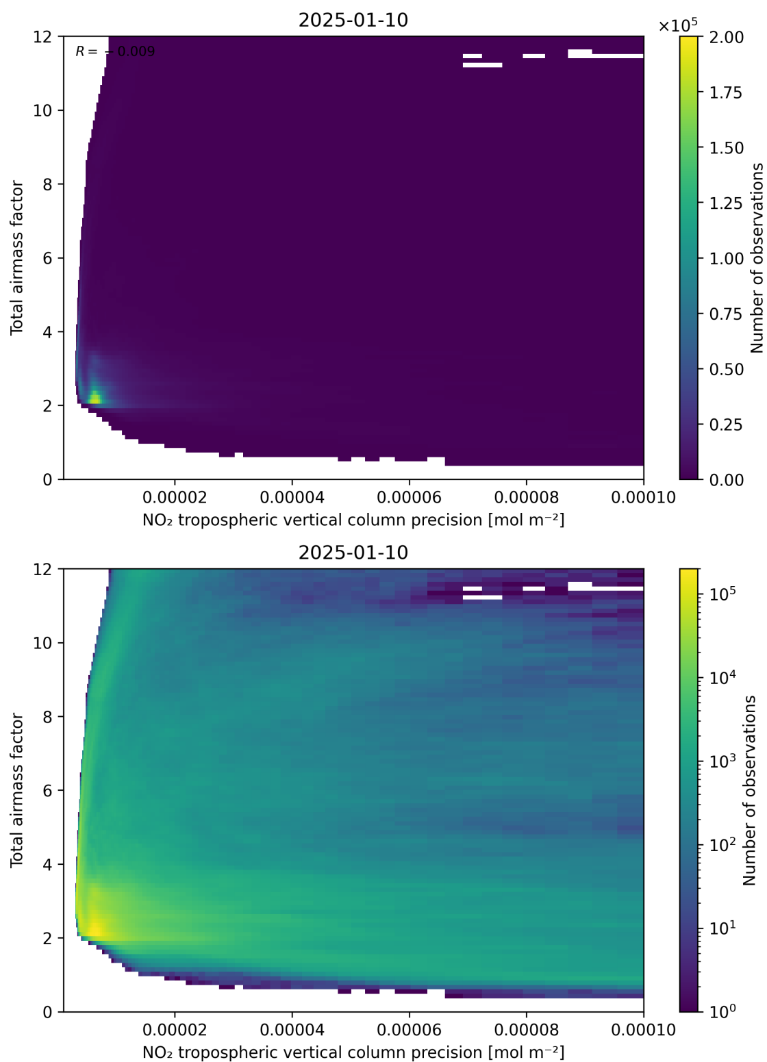
Figure 132: Scatter density plot of “NO 2 tropospheric vertical column precision” against “Total air mass factor” for 2025-01-09 to 2025-01-11.
