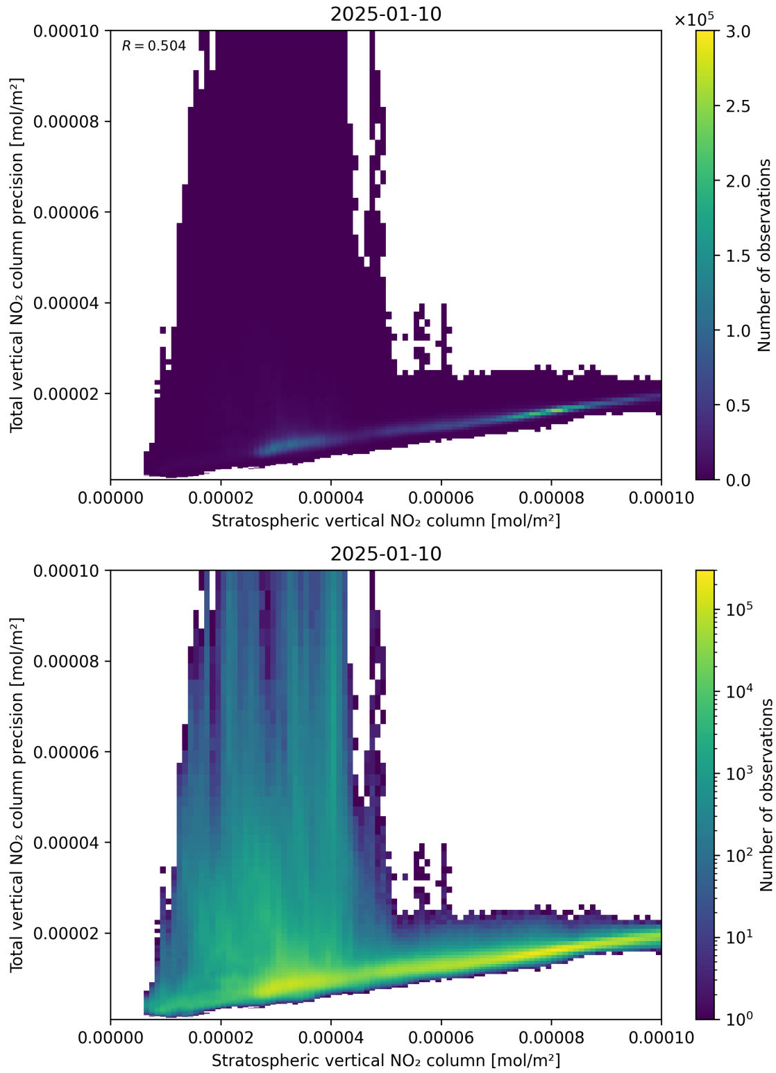
Figure 101: Scatter density plot of “Stratospheric vertical NO 2 column” against “Total vertical NO 2 column precision” for 2025-01-09 to 2025-01-11.
