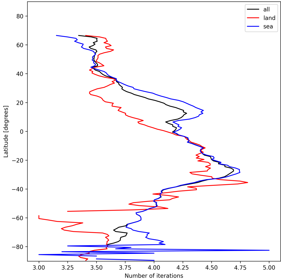
Figure 17: Zonal average of “Number of iterations” for 2025-01-09 to 2025-01-11.
