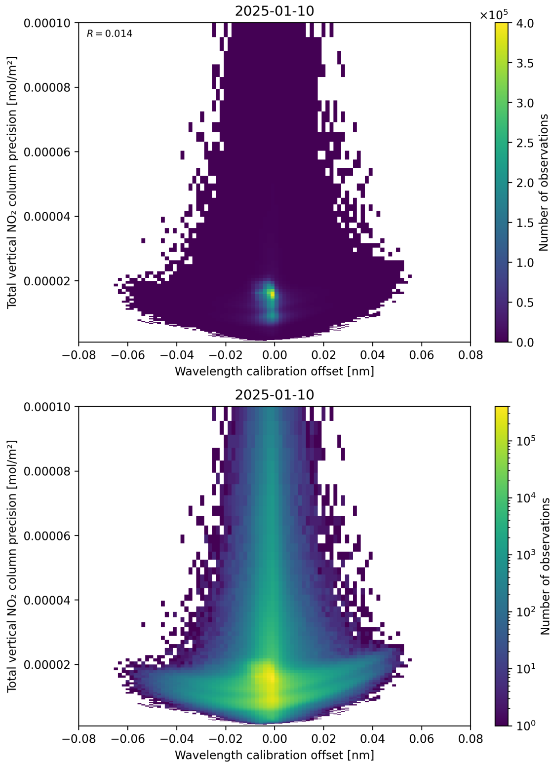
Figure 180: Scatter density plot of “Wavelength calibration offset” against “Total vertical NO 2 column precision” for 2025-01-09 to 2025-01-11.
