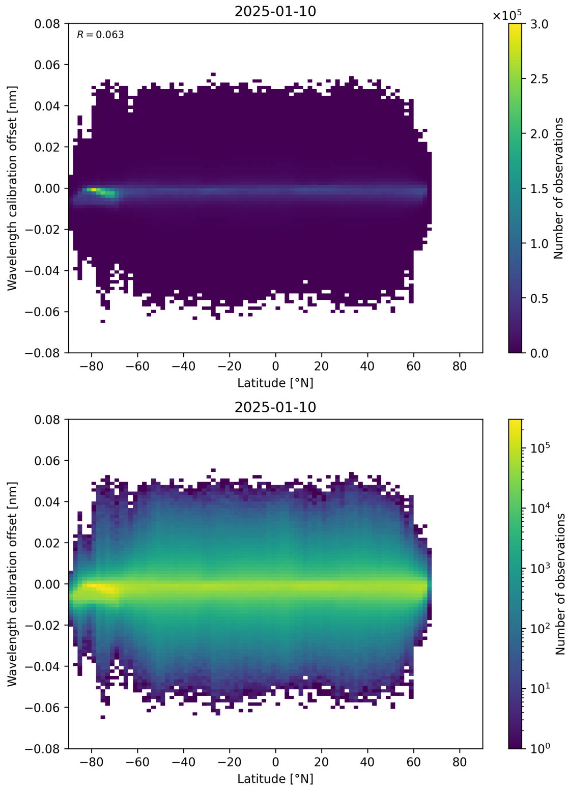
Figure 95: Scatter density plot of “Latitude” against “Wavelength calibration offset” for 2025-01-09 to 2025-01-11.
