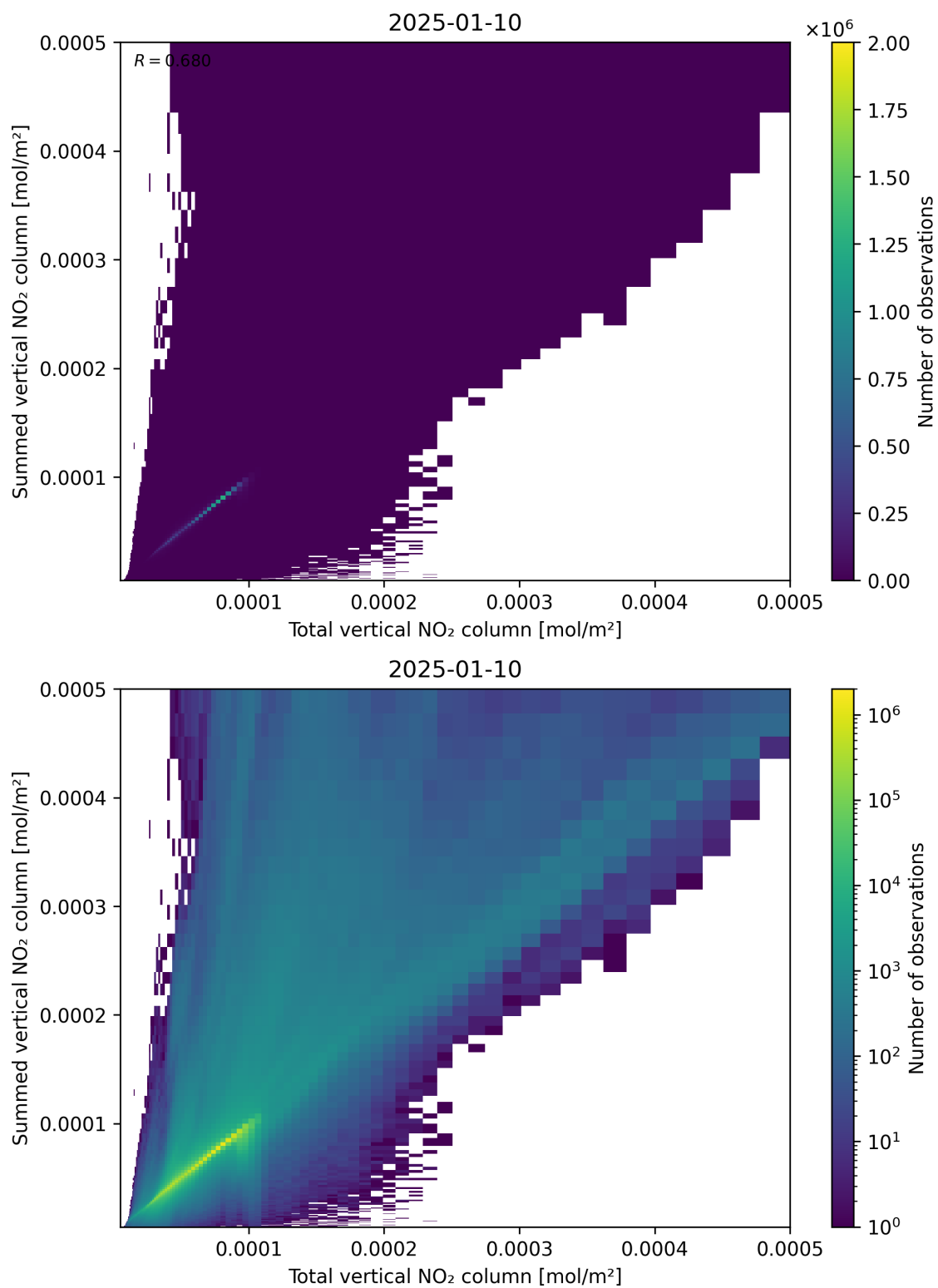
Figure 112: Scatter density plot of “Total vertical NO 2 column” against “Summed vertical NO 2 column” for 2025-01-09 to 2025-01-11.
