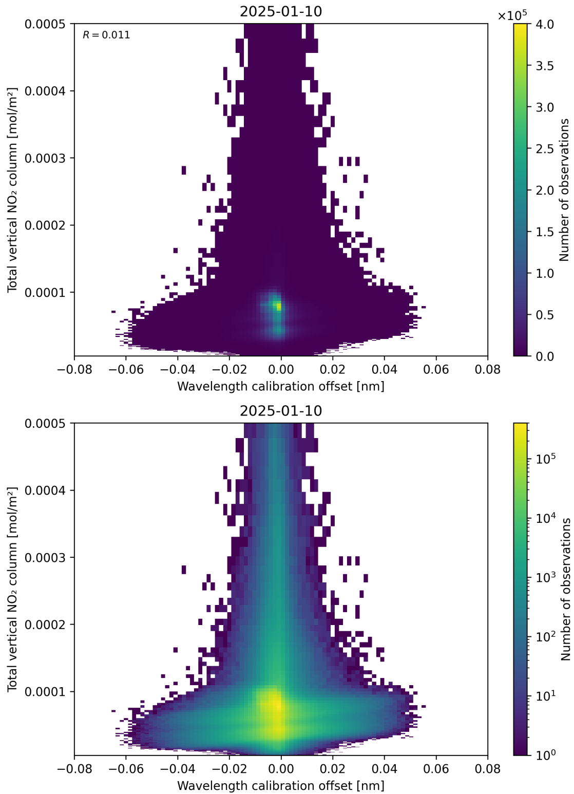
Figure 179: Scatter density plot of “Wavelength calibration offset” against “Total vertical NO 2 column” for 2025-01-09 to 2025-01-11.
