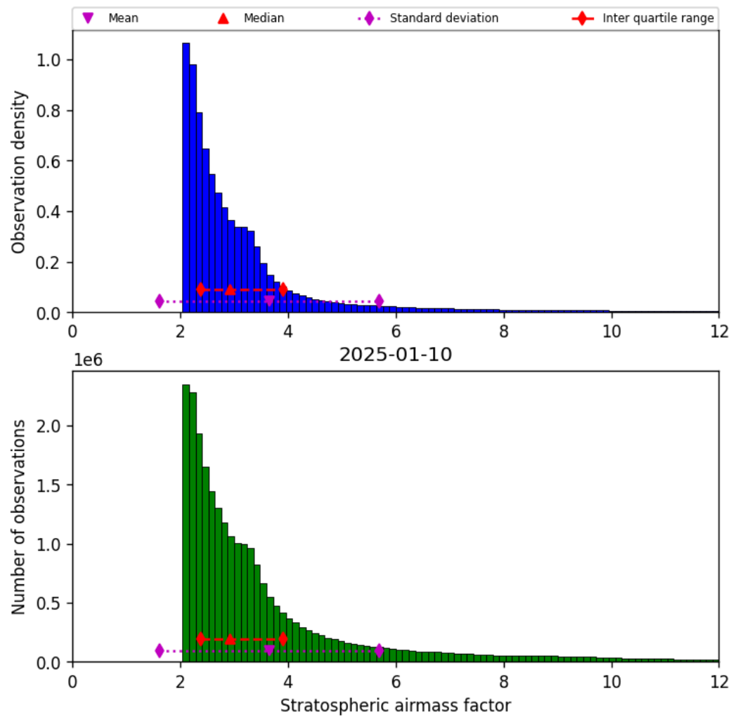
Figure 44: Histogram of “Stratospheric airmass factor” for 2025-01-09 to 2025-01-11
