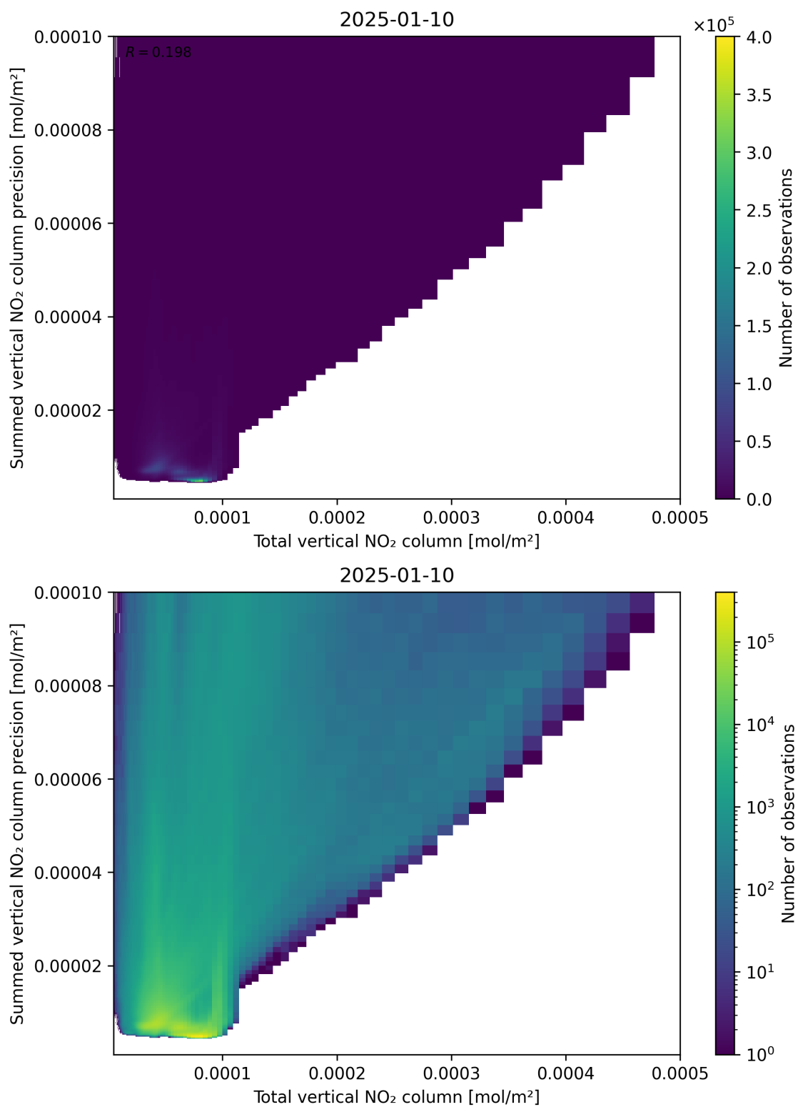
Figure 113: Scatter density plot of “Total vertical NO 2 column” against “Summed vertical NO 2 column precision” for 2025-01-09 to 2025-01-11.
