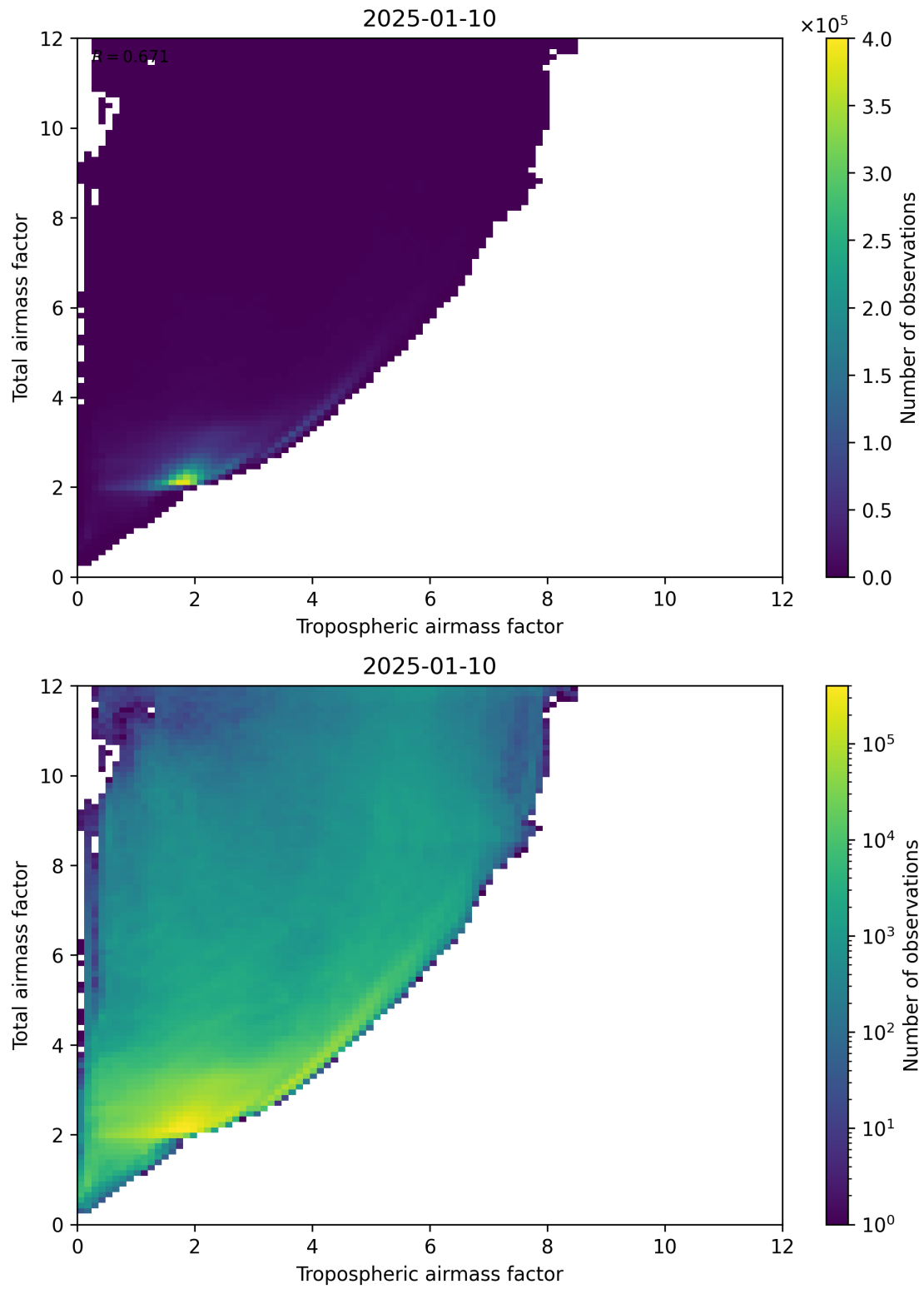
Figure 72: Scatter density plot of “Tropospheric airmass factor” against “Total airmass factor” for 2025-01-09 to 2025-01-11.
