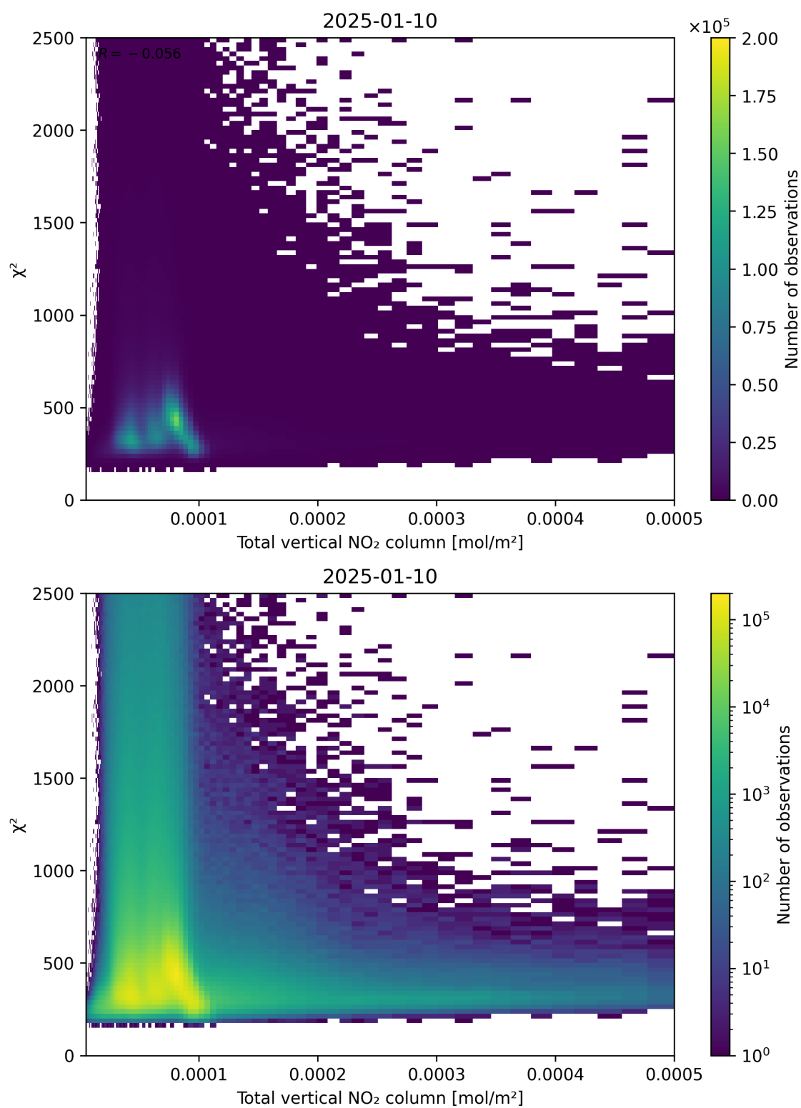
Figure 111: Scatter density plot of “Total vertical NO 2 column” against “ \chi^2 ” for 2025-01-09 to 2025-01-11.
