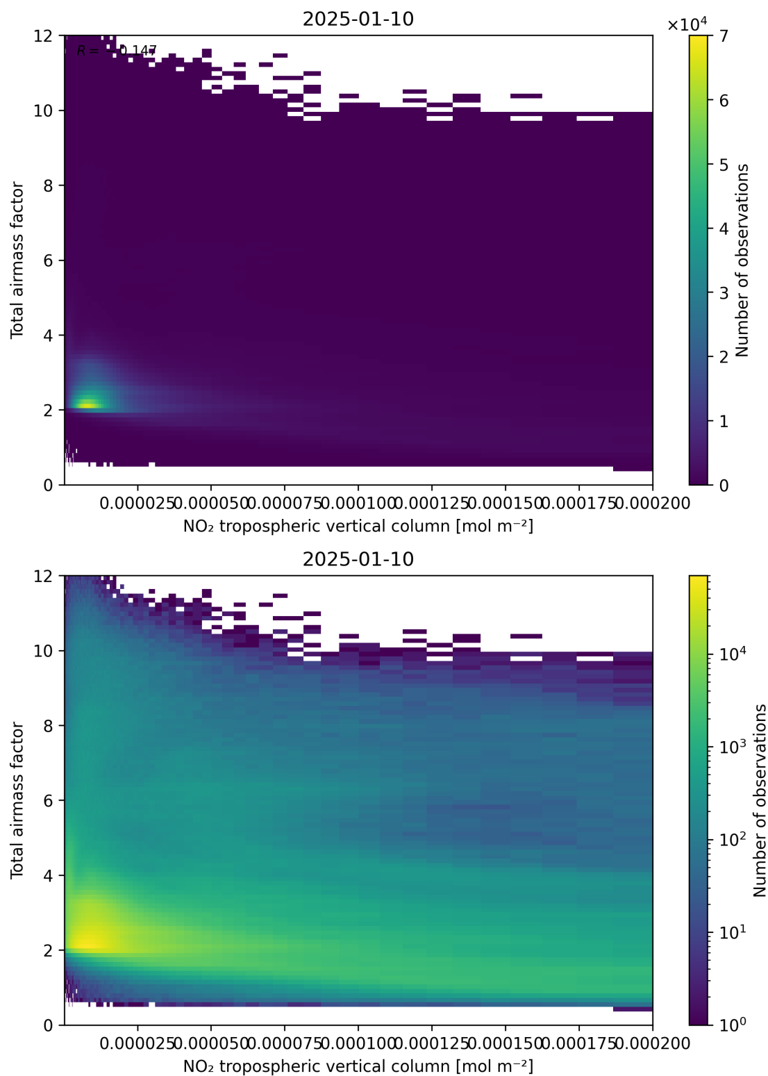
Figure 122: Scatter density plot of “NO 2 tropospheric vertical column” against “Total air mass factor” for 2025-01-09 to 2025-01-11.
