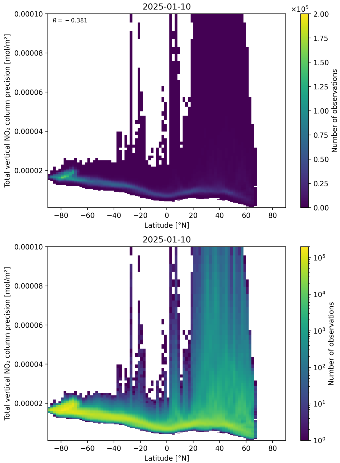
Figure 91: Scatter density plot of “Latitude” against “Total vertical NO 2 column precision” for 2025-01-09 to 2025-01-11.
