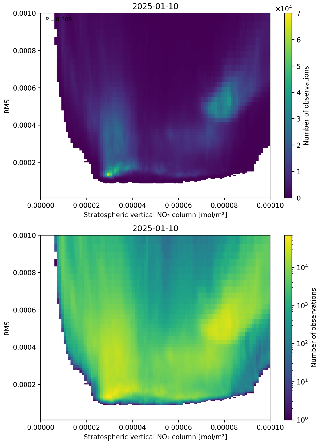
Figure 102: Scatter density plot of “Stratospheric vertical NO 2 column” against “RMS” for 2025-01-09 to 2025-01-11.
