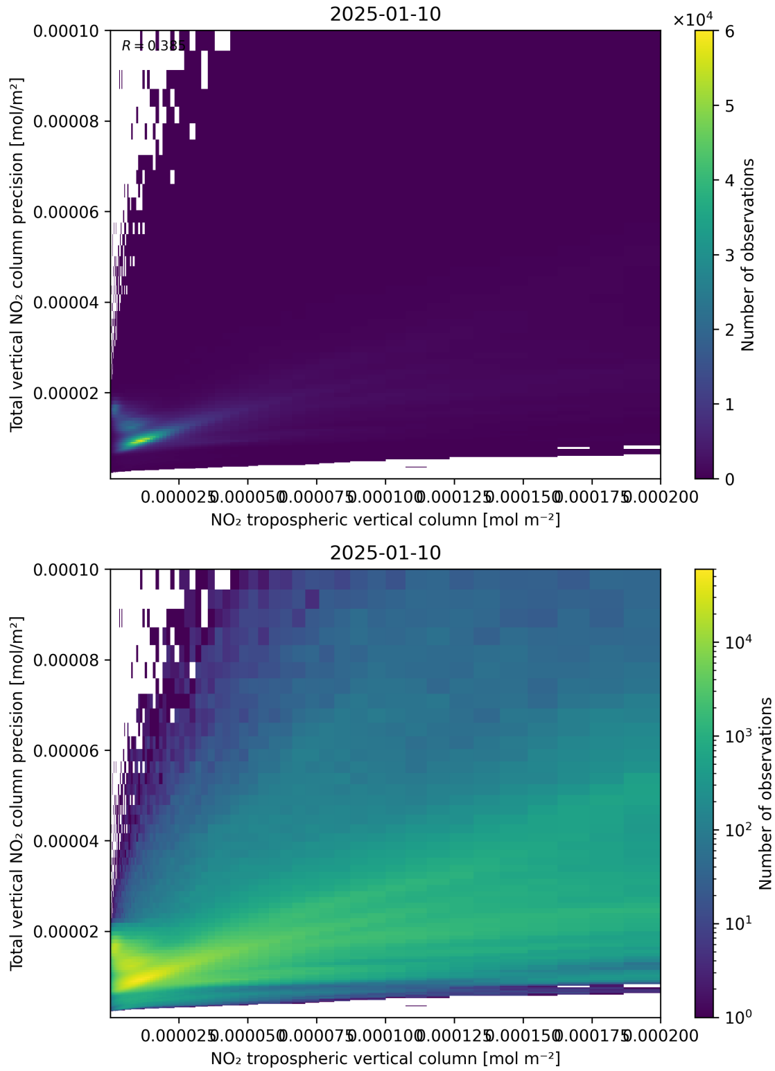
Figure 129: Scatter density plot of “NO 2 tropospheric vertical column” against “Total vertical NO 2 column precision” for 2025-01-09 to 2025-01-11.
