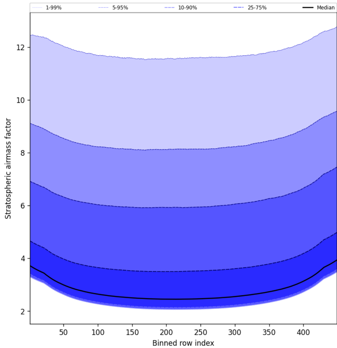
Figure 61: Along track statistics of “Stratospheric airmass factor” for 2025-01-09 to 2025-01-11
