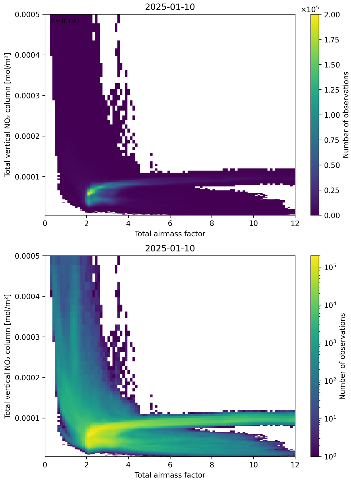
Figure 67: Scatter density plot of “Total airmass factor” against “Total vertical NO 2 column” for 2025-01-09 to 2025-01-11.
