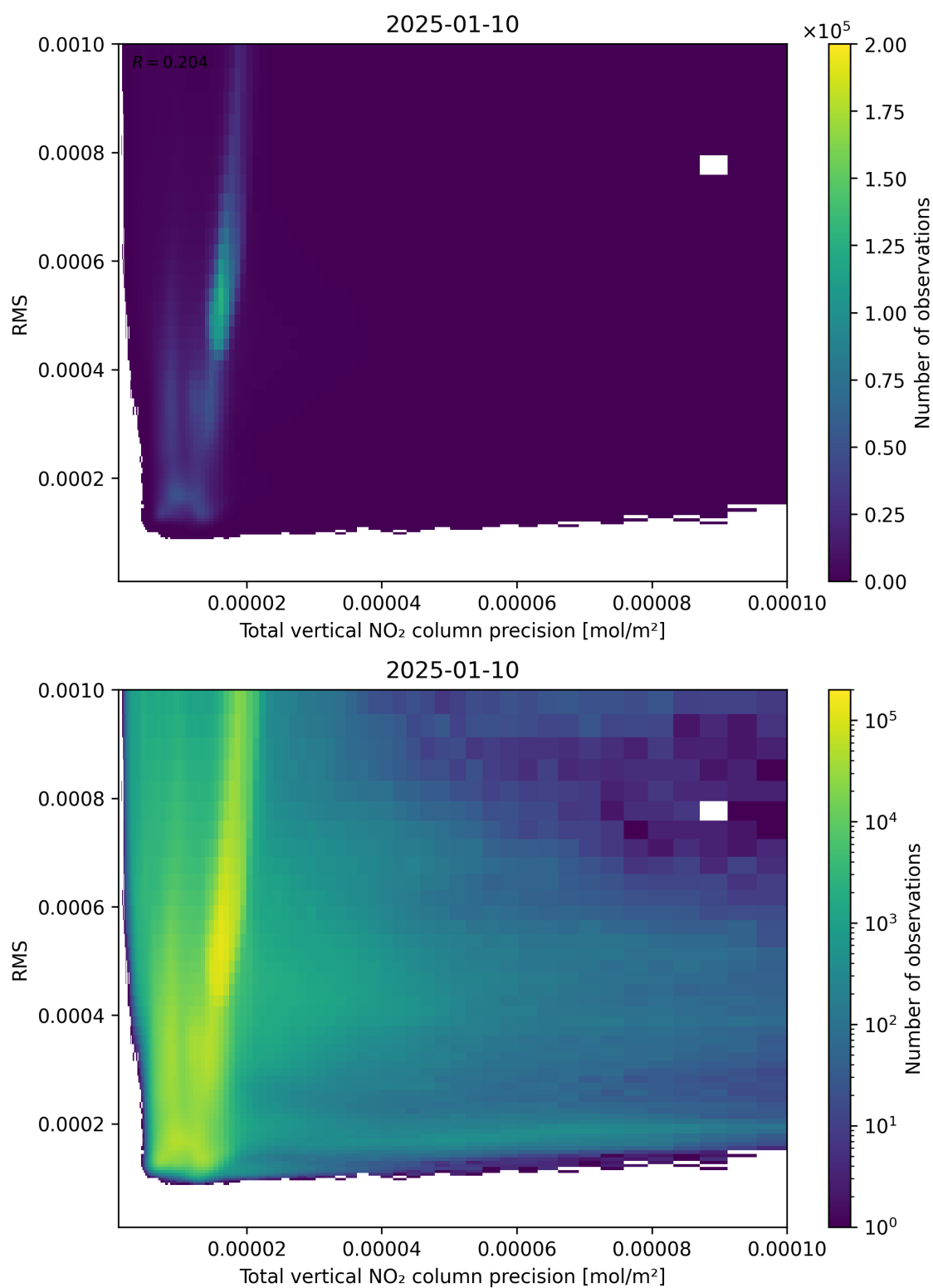
Figure 119: Scatter density plot of “Total vertical NO 2 column precision” against “RMS” for 2025-01-09 to 2025-01-11.
