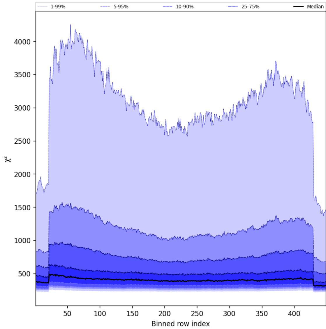
Figure 59: Along track statistics of “ \chi^2 ” for 2025-01-09 to 2025-01-11
