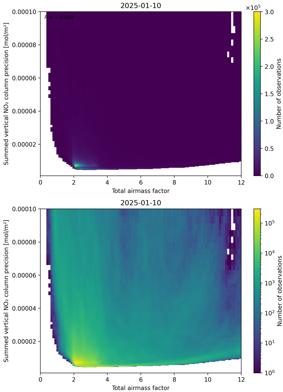
Figure 66: Scatter density plot of “Total airmass factor” against “Summed vertical NO 2 column precision” for 2025-01-09 to 2025-01-11.
