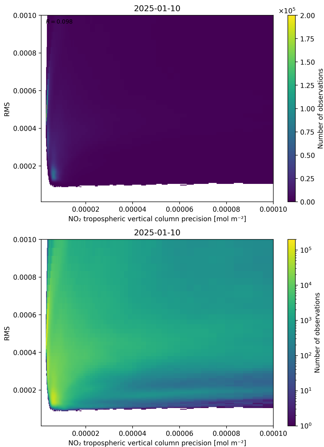
Figure 140: Scatter density plot of “NO 2 tropospheric vertical column precision” against “RMS” for 2025-01-09 to 2025-01-11.
