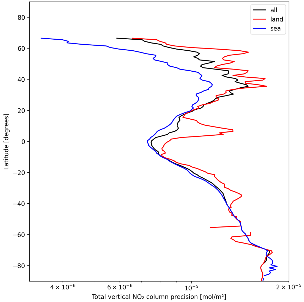
Figure 22: Zonal average of “Total vertical NO 2 column precision” for 2025-01-09 to 2025-01-11.
