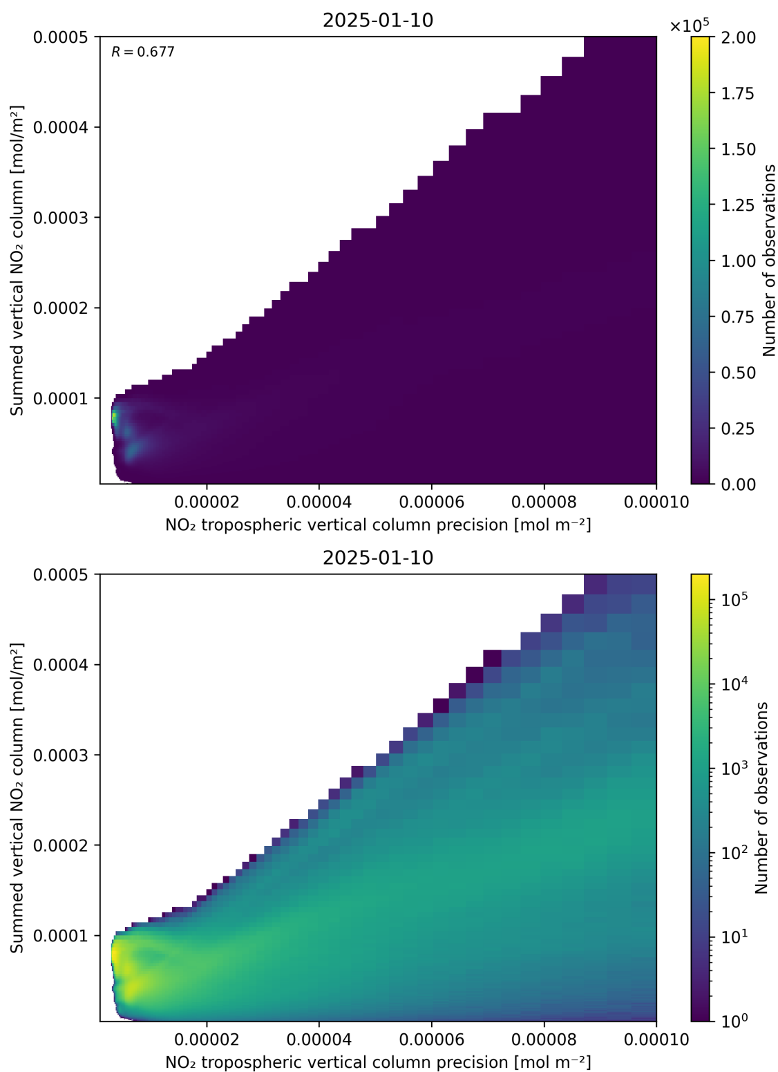
Figure 136: Scatter density plot of “NO 2 tropospheric vertical column precision” against “Summed vertical NO 2 column” for 2025-01-09 to 2025-01-11.
