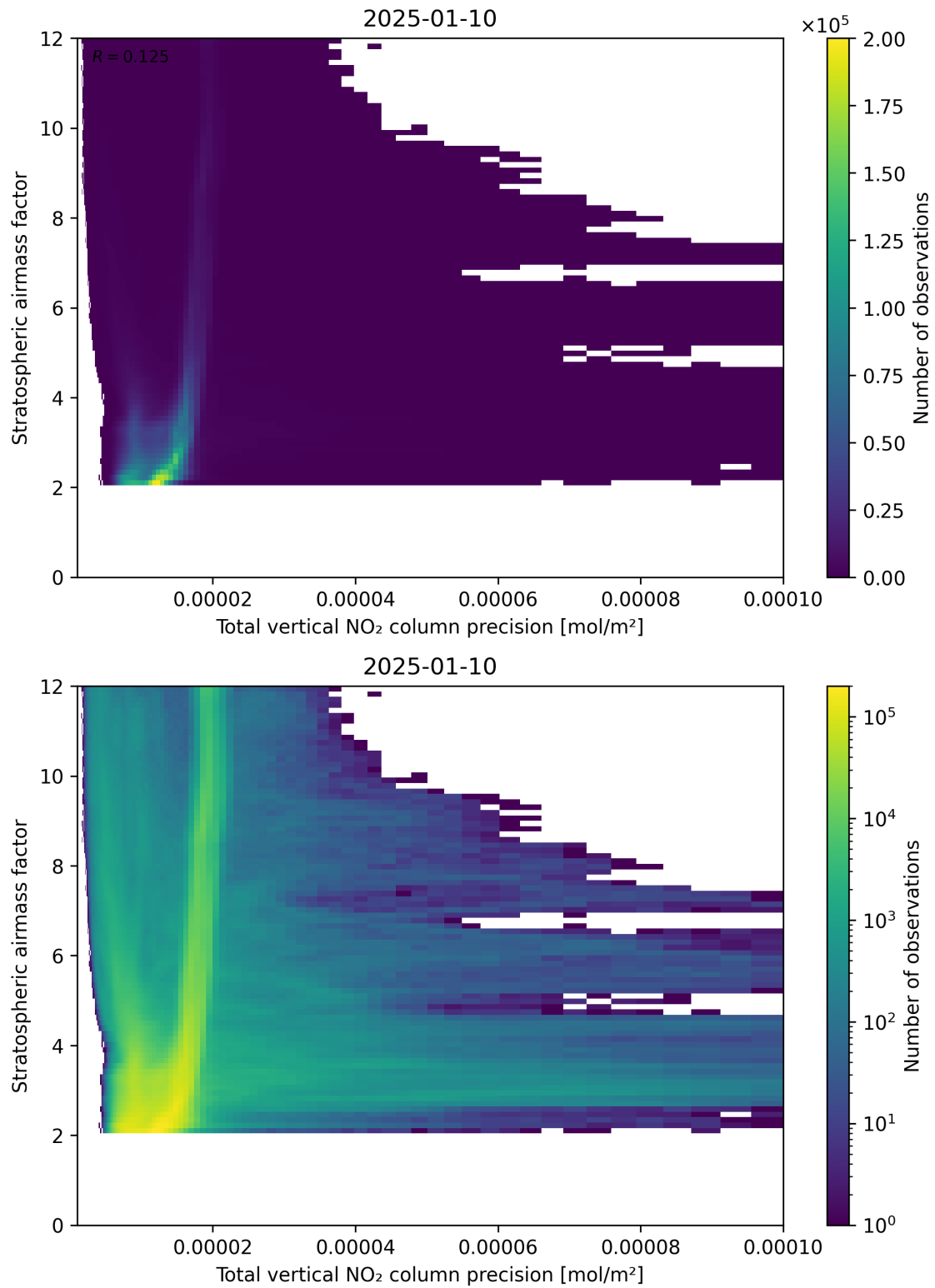
Figure 115: Scatter density plot of “Total vertical NO 2 column precision” against “Stratospheric air mass factor” for 2025-01-09 to 2025-01-11.
