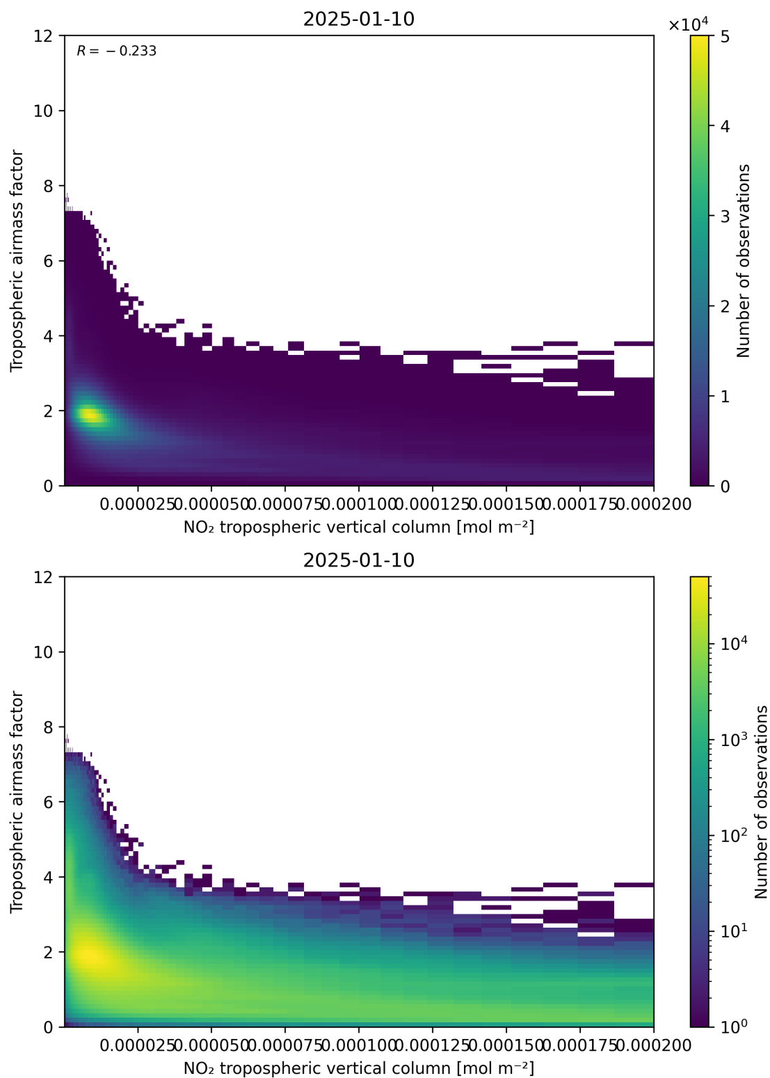
Figure 123: Scatter density plot of “NO 2 tropospheric vertical column” against “Tropospheric air mass factor” for 2025-01-09 to 2025-01-11.
