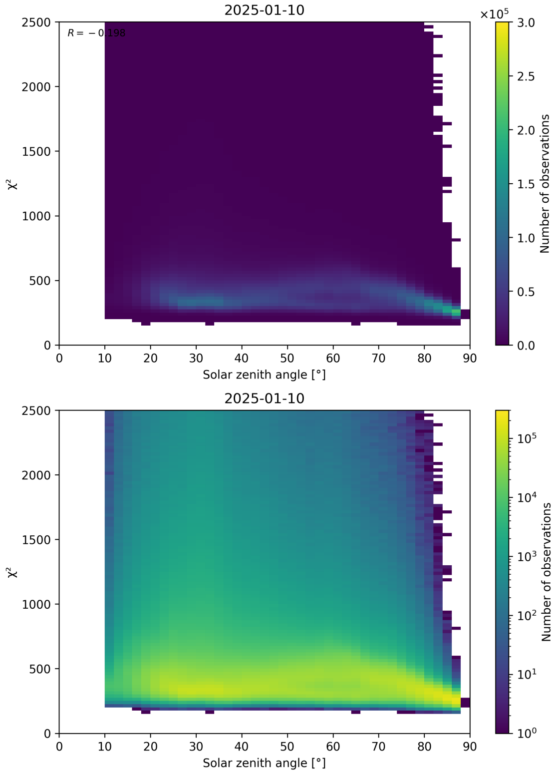
Figure 148: Scatter density plot of “Solar zenith angle” against “ \chi^2 ” for 2025-01-09 to 2025-01-11.
