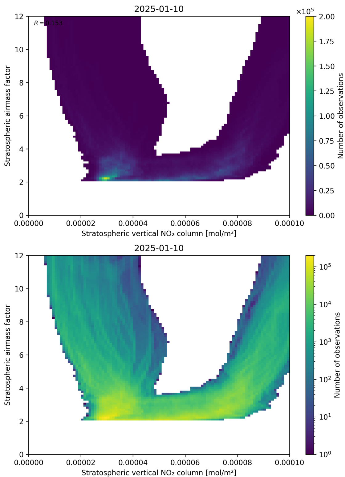
Figure 96: Scatter density plot of “Stratospheric vertical NO 2 column” against “Stratospheric airmass factor” for 2025-01-09 to 2025-01-11.
