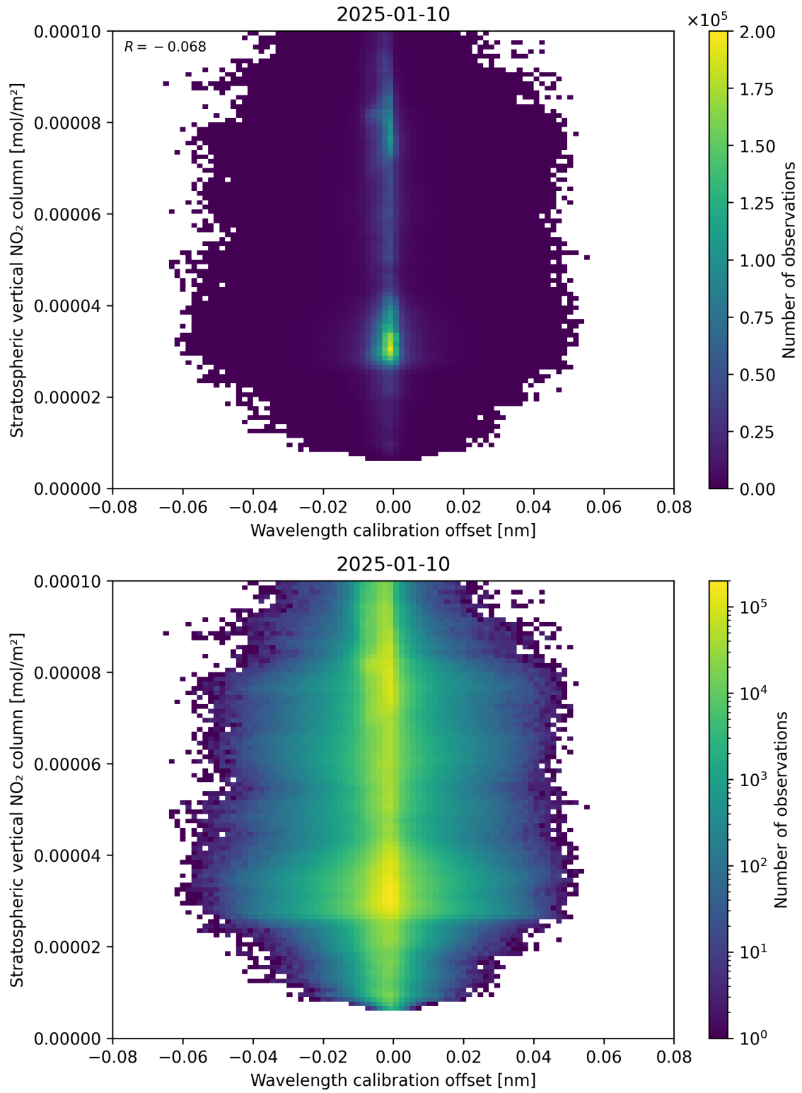
Figure 176: Scatter density plot of “Wavelength calibration offset” against “Stratospheric vertical NO 2 column” for 2025-01-09 to 2025-01-11.
