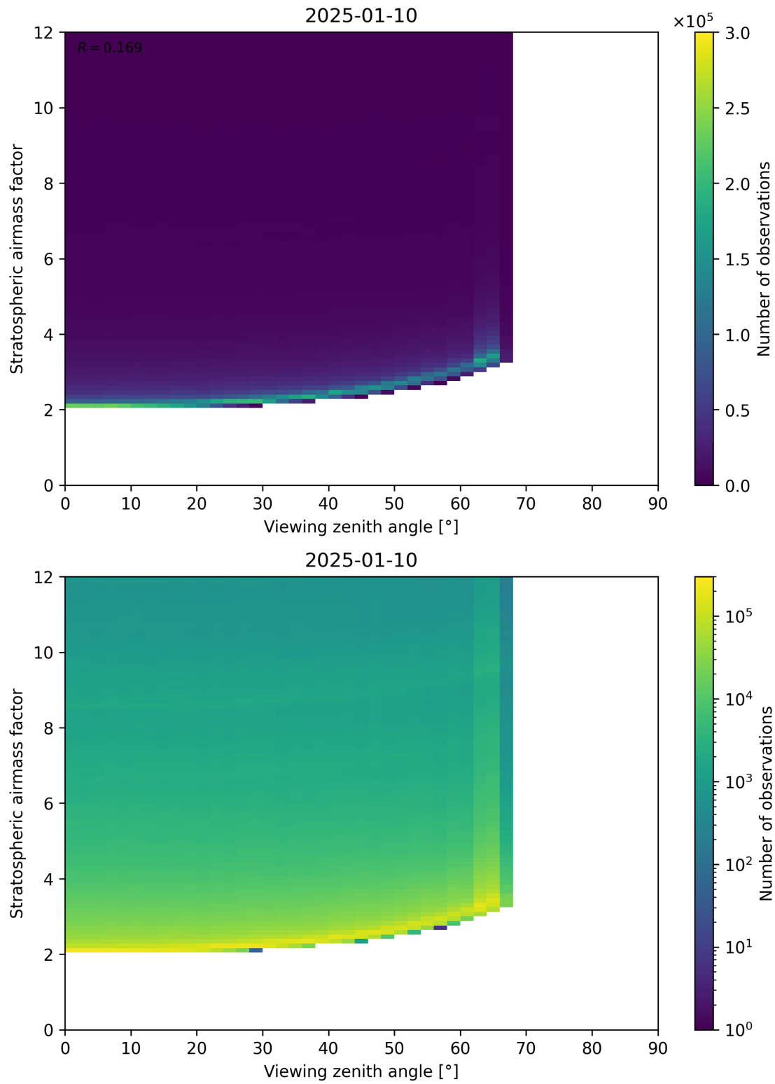
Figure 159: Scatter density plot of “Viewing zenith angle” against “Stratospheric airmass factor” for 2025-01-09 to 2025-01-11.
