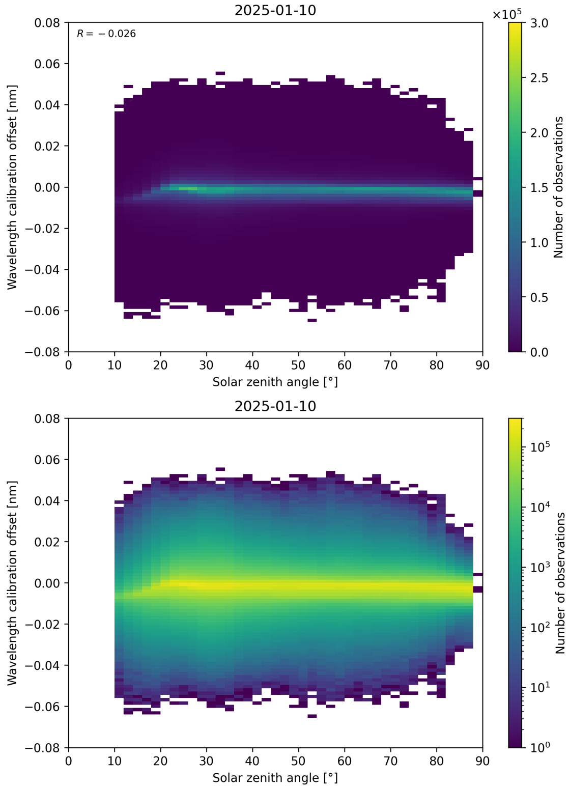
Figure 158: Scatter density plot of “Solar zenith angle” against “Wavelength calibration offset” for 2025-01-09 to 2025-01-11.
