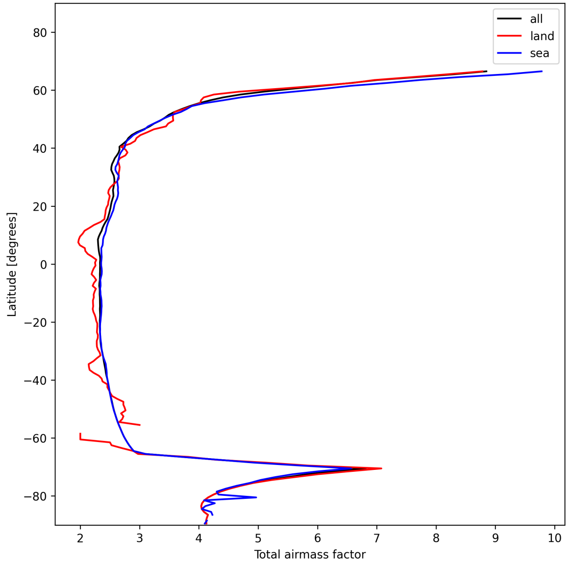
Figure 15: Zonal average of “Total airmass factor” for 2025-01-09 to 2025-01-11.
