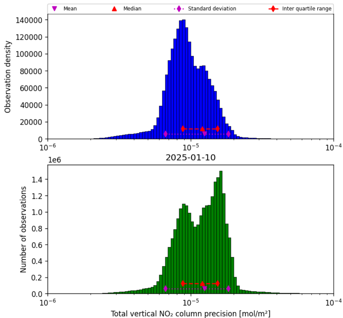
Figure 39: Histogram of “Total vertical NO 2 column precision” for 2025-01-09 to 2025-01-11
