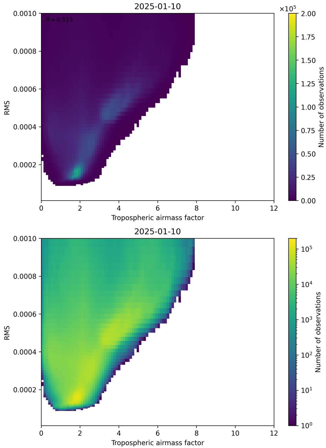
Figure 79: Scatter density plot of “Tropospheric airmass factor” against “RMS” for 2025-01-09 to 2025-01-11.
