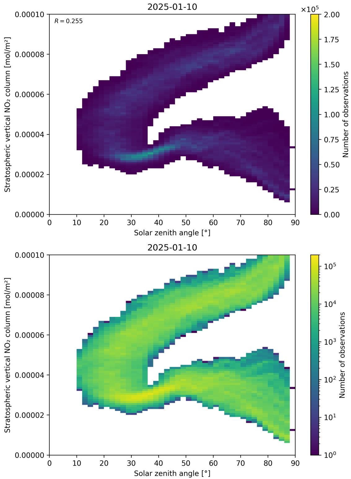
Figure 150: Scatter density plot of “Solar zenith angle” against “Stratospheric vertical NO 2 column” for 2025-01-09 to 2025-01-11.
