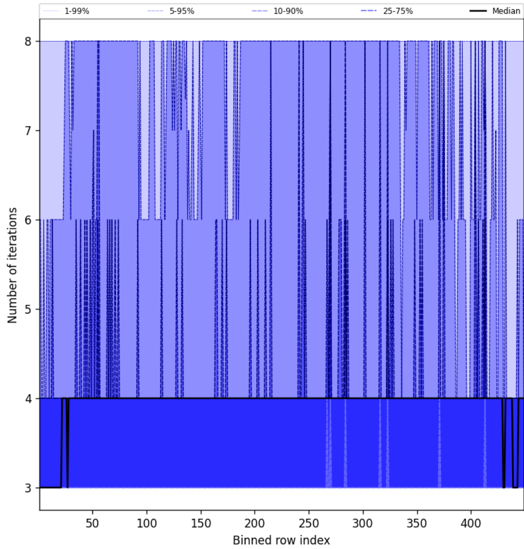
Figure 51: Along track statistics of “Number of iterations” for 2025-01-09 to 2025-01-11
