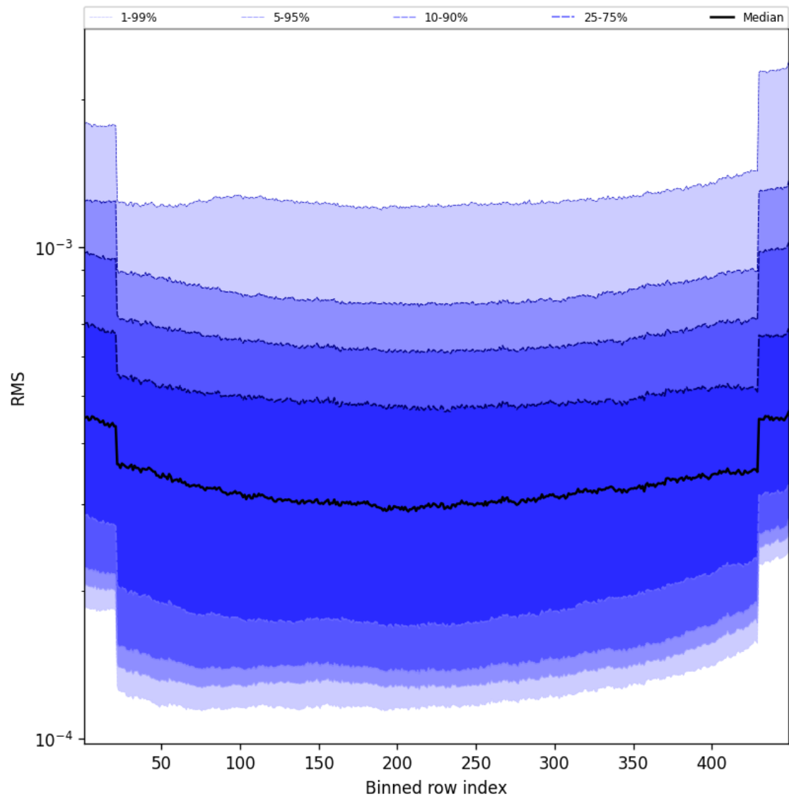
Figure 60: Along track statistics of “RMS” for 2025-01-09 to 2025-01-11
