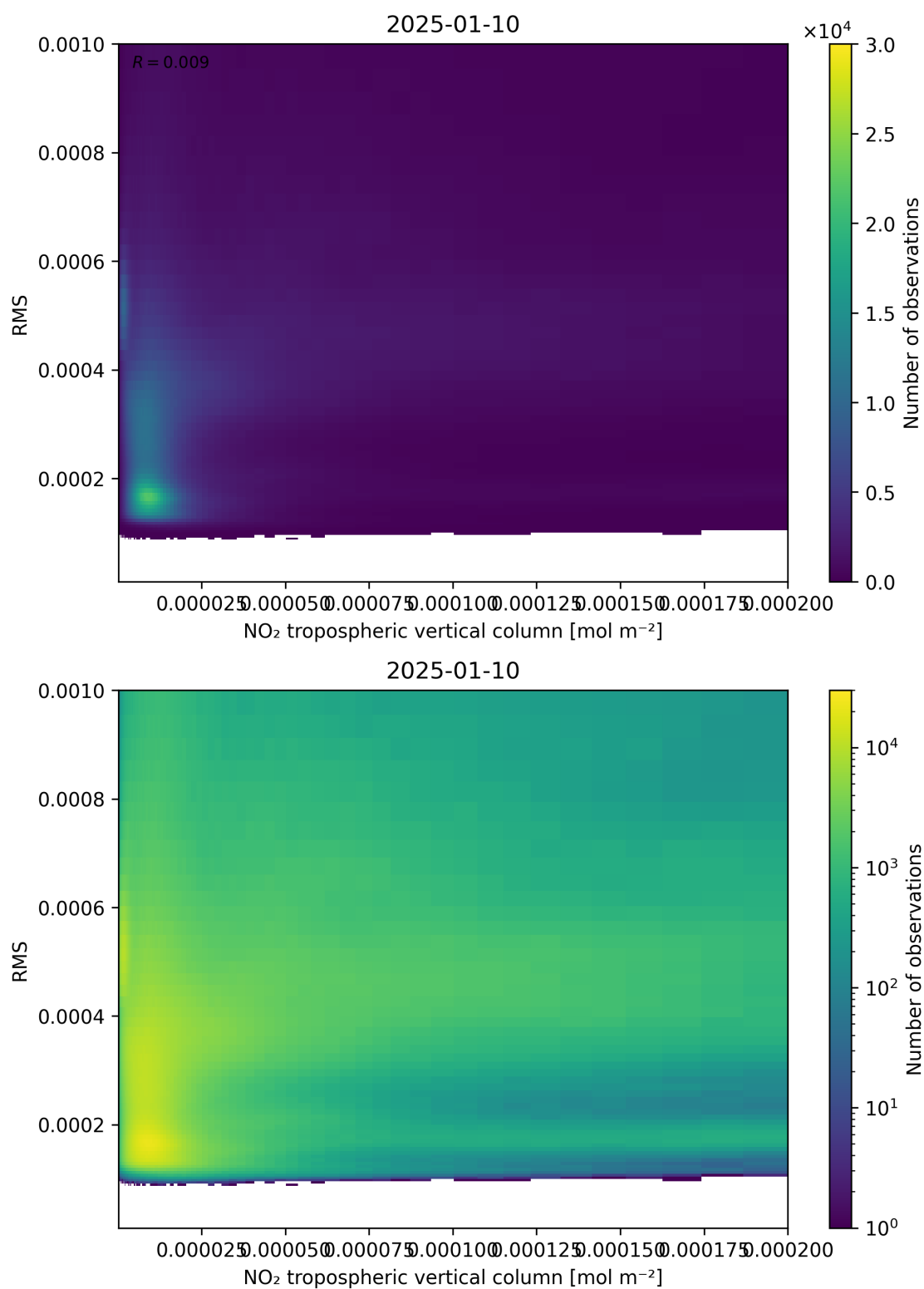
Figure 142: Scatter density plot of “NO 2 tropospheric vertical column” against “RMS” for 2025-01-09 to 2025-01-11.
