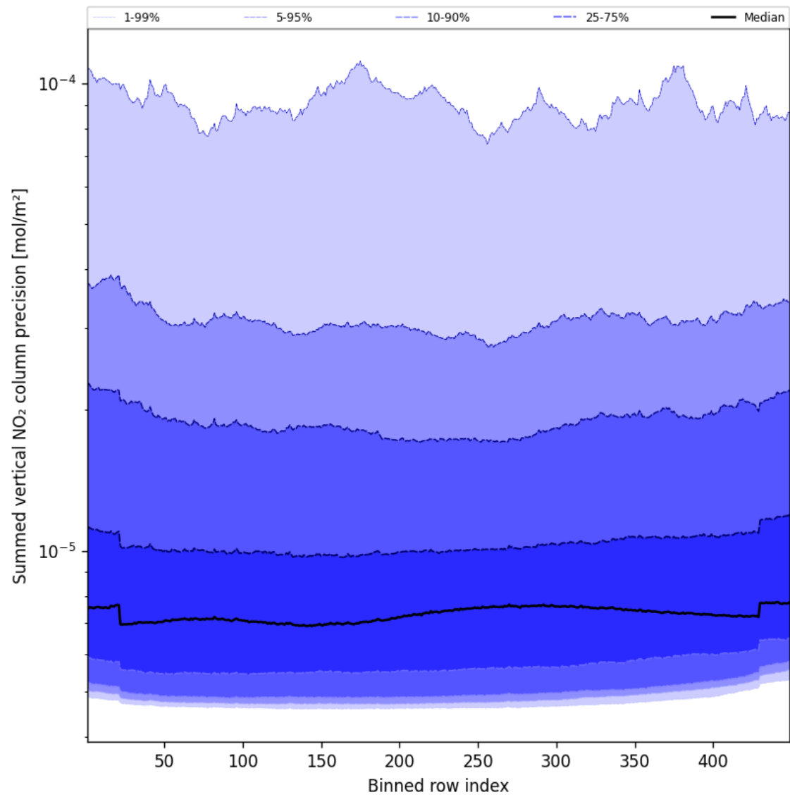
Figure 58: Along track statistics of “Summed vertical NO 2 column precision” for 2025-01-09 to 2025-01-11
