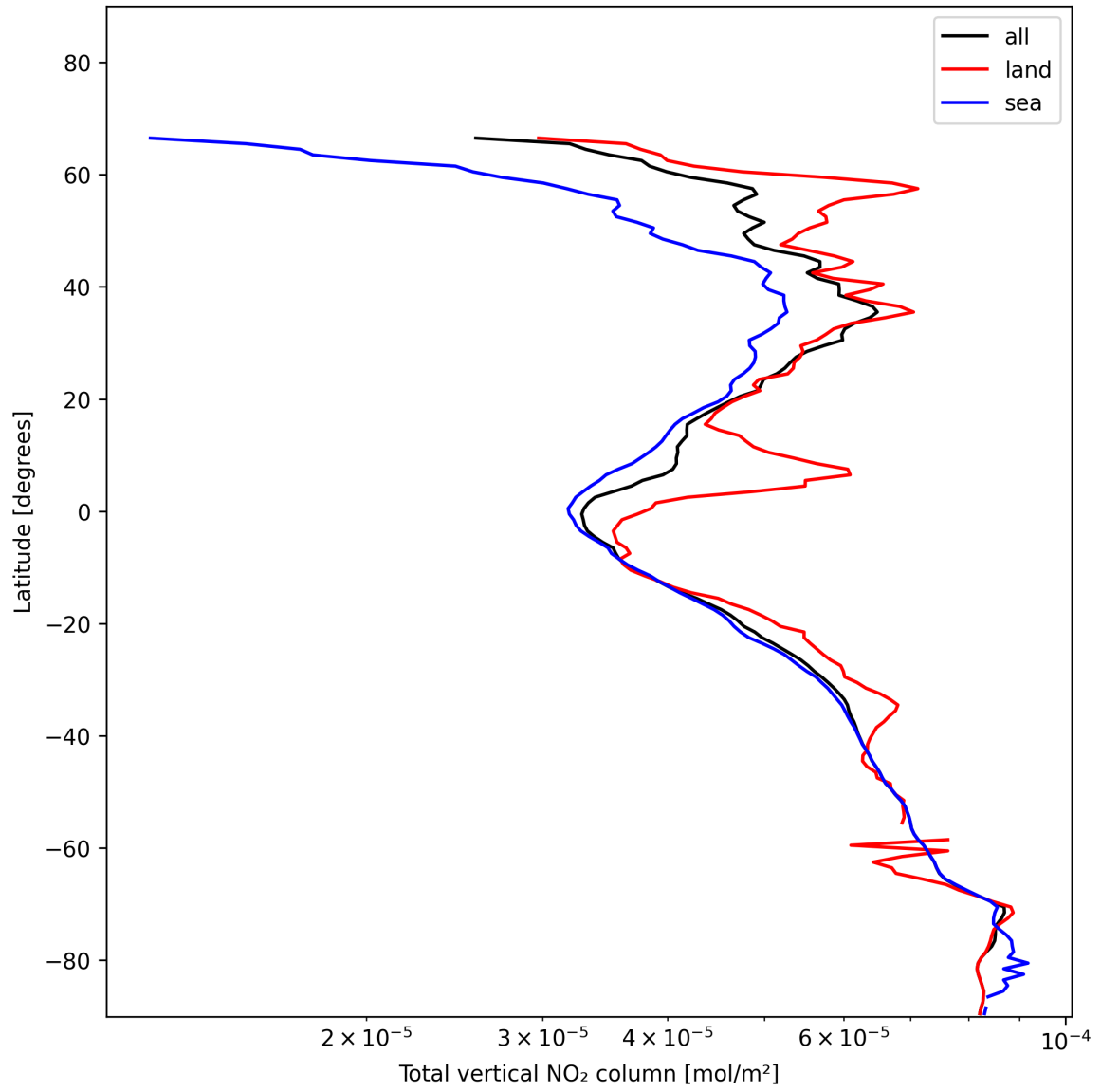
Figure 21: Zonal average of “Total vertical NO 2 column” for 2025-01-09 to 2025-01-11.
