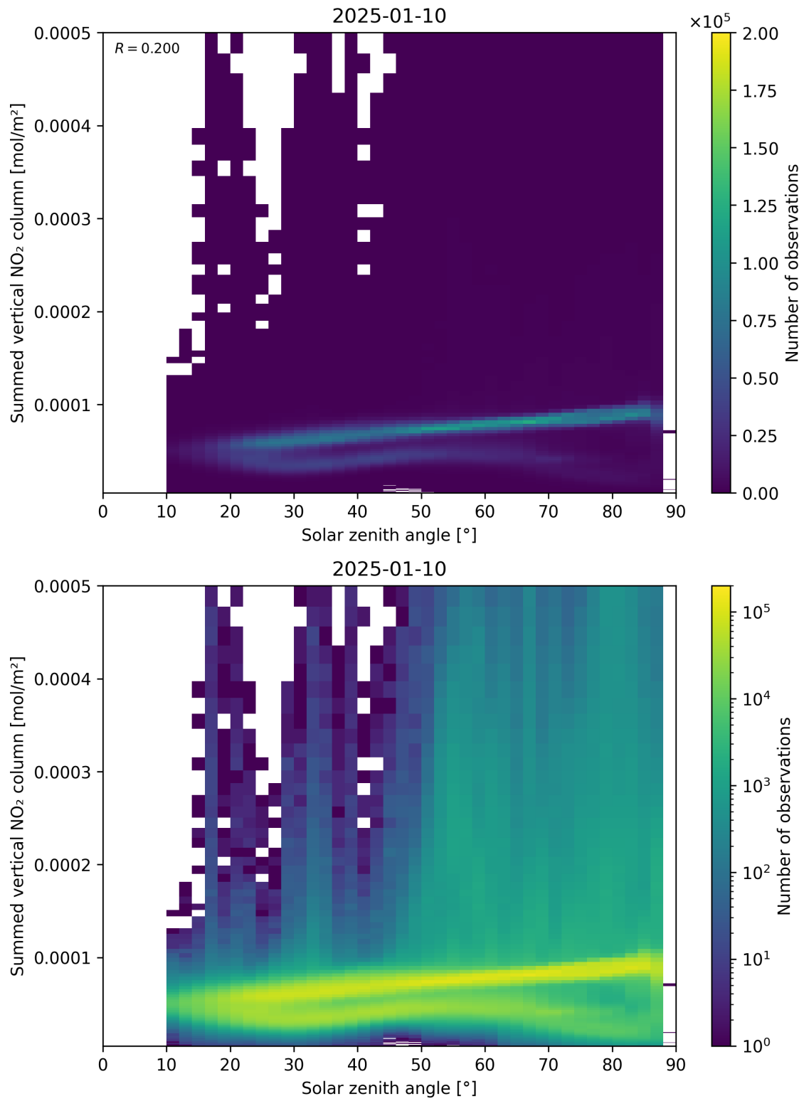
Figure 151: Scatter density plot of “Solar zenith angle” against “Summed vertical NO 2 column” for 2025-01-09 to 2025-01-11.
