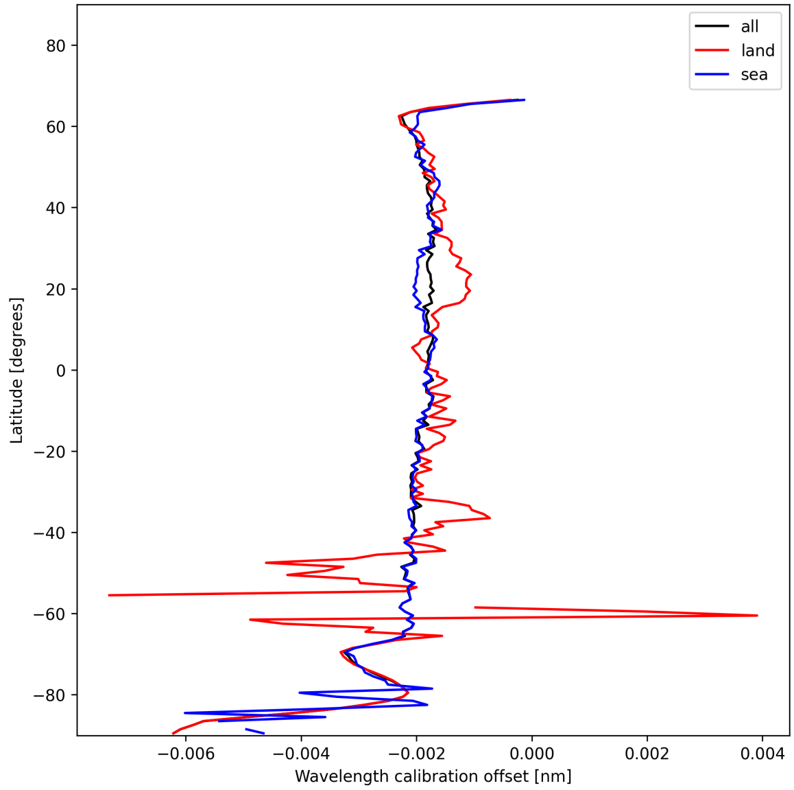
Figure 18: Zonal average of “Wavelength calibration offset” for 2025-01-09 to 2025-01-11.
