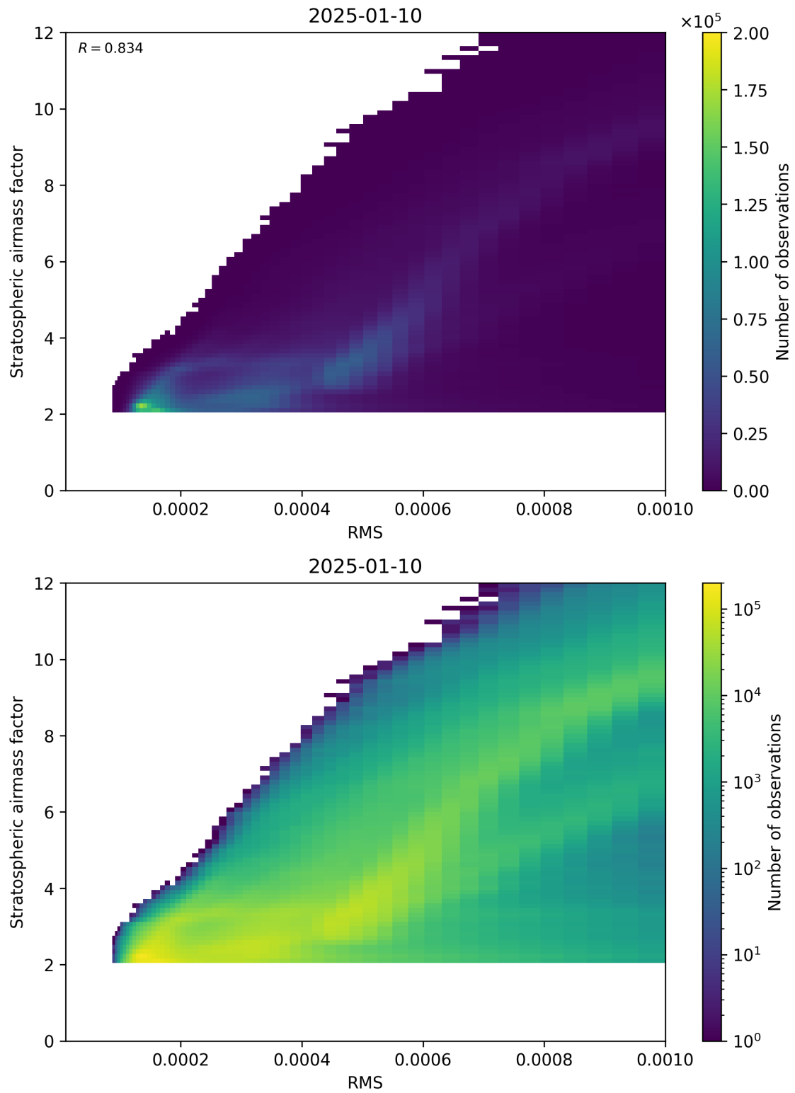
Figure 144: Scatter density plot of “RMS” against “Stratospheric airmass factor” for 2025-01-09 to 2025-01-11.
