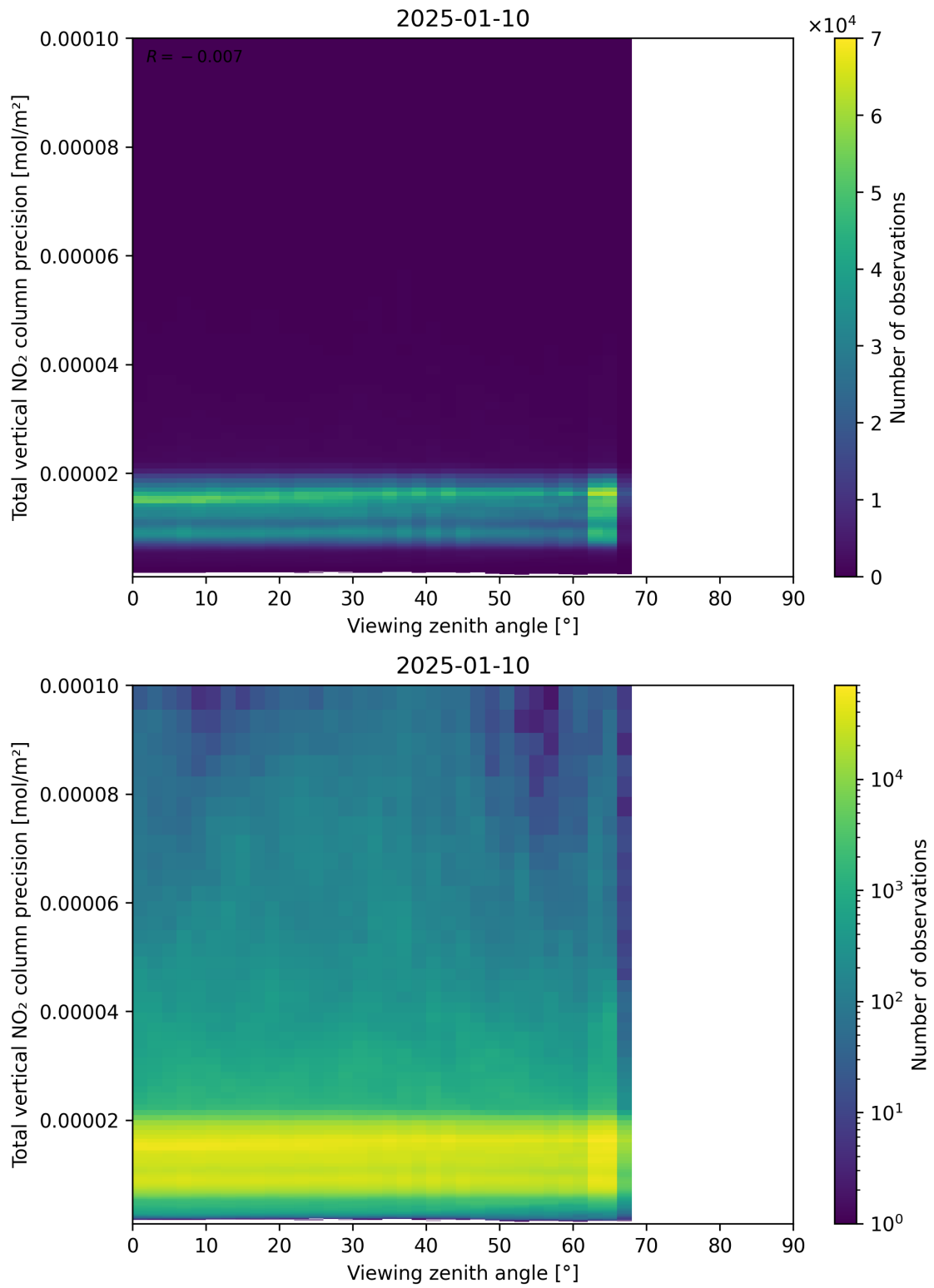
Figure 168: Scatter density plot of “Viewing zenith angle” against “Total vertical NO 2 column precision” for 2025-01-09 to 2025-01-11.
