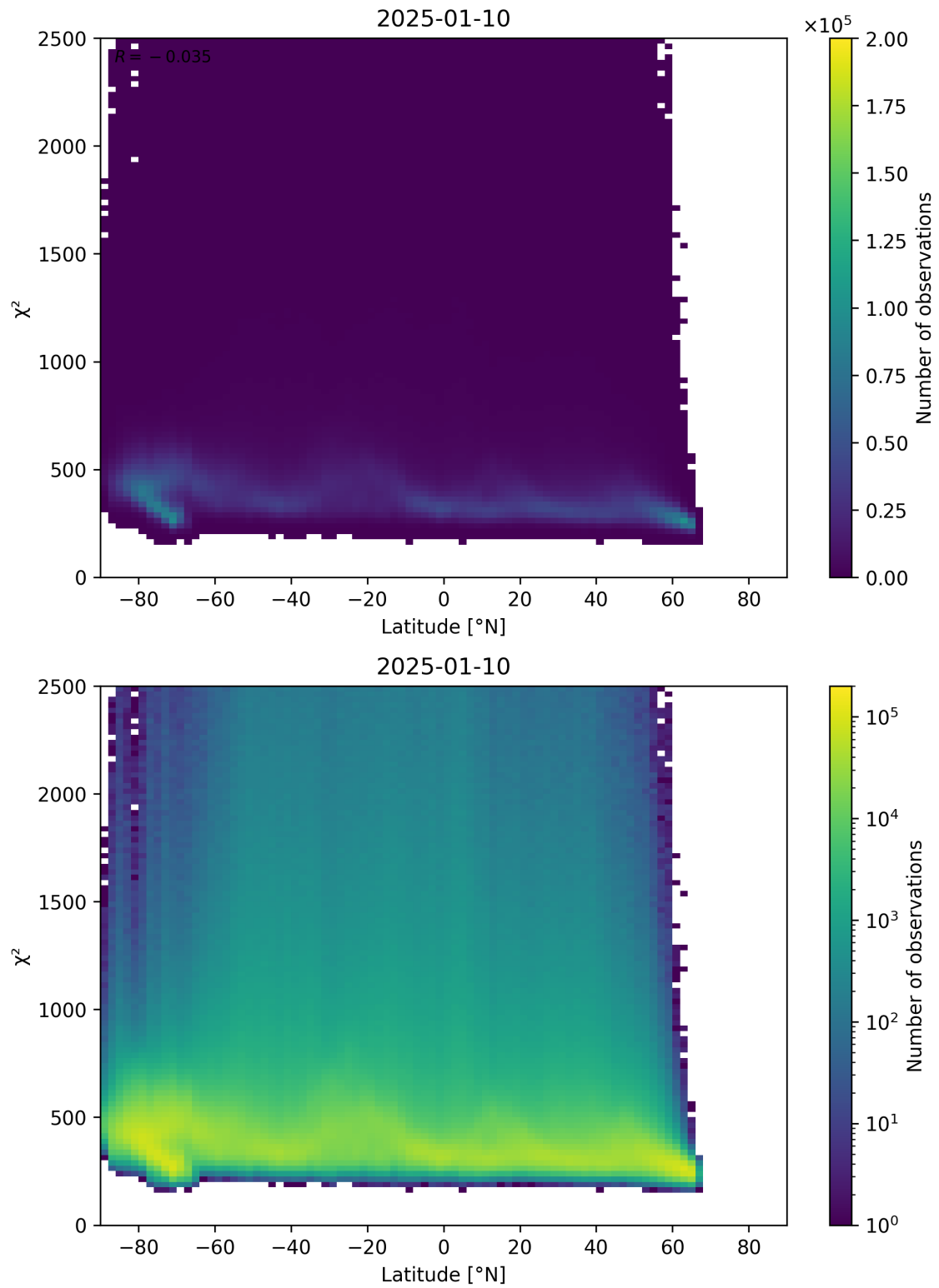
Figure 86: Scatter density plot of “Latitude” against “ \chi^2 ” for 2025-01-09 to 2025-01-11.
