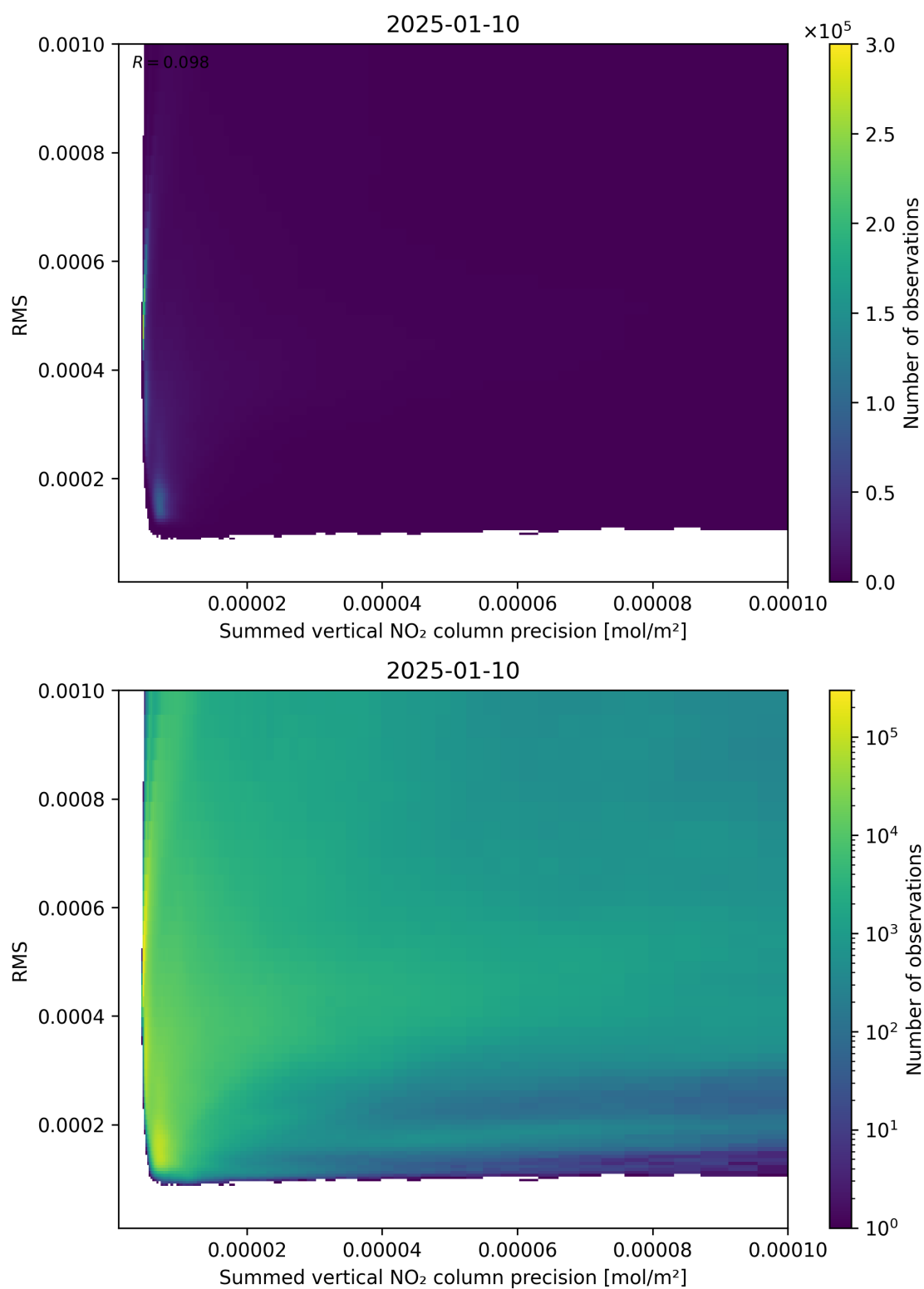
Figure 108: Scatter density plot of “Summed vertical NO 2 column precision” against “RMS” for 2025-01-09 to 2025-01-11.
