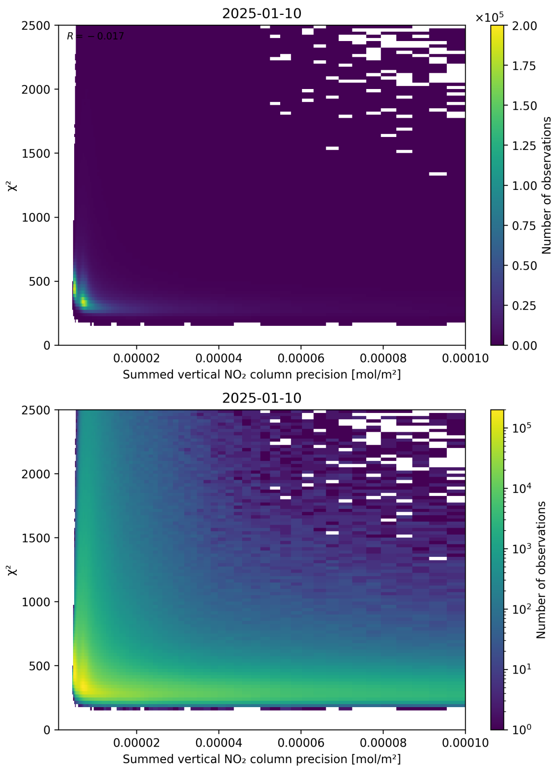
Figure 107: Scatter density plot of “Summed vertical NO 2 column precision” against “ \chi^2 ” for 2025-01-09 to 2025-01-11.
