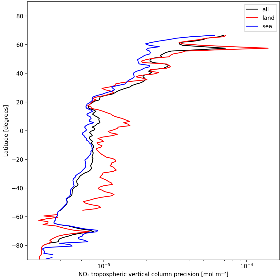
Figure 13: Zonal average of “NO 2 tropospheric vertical column precision” for 2025-01-09 to 2025-01-11.
