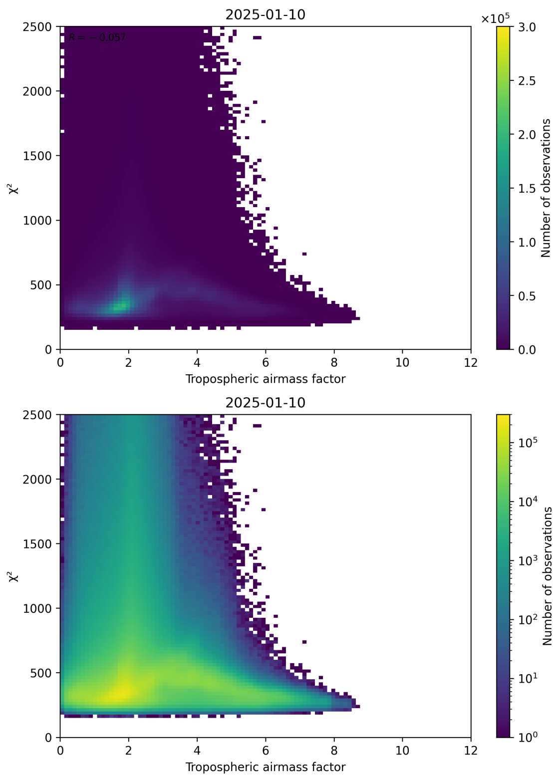
Figure 73: Scatter density plot of “Tropospheric airmass factor” against “ \chi^2 ” for 2025-01-09 to 2025-01-11.
