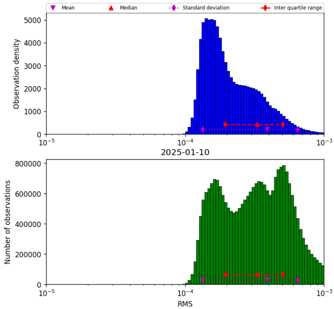
Figure 43: Histogram of “RMS” for 2025-01-09 to 2025-01-11
