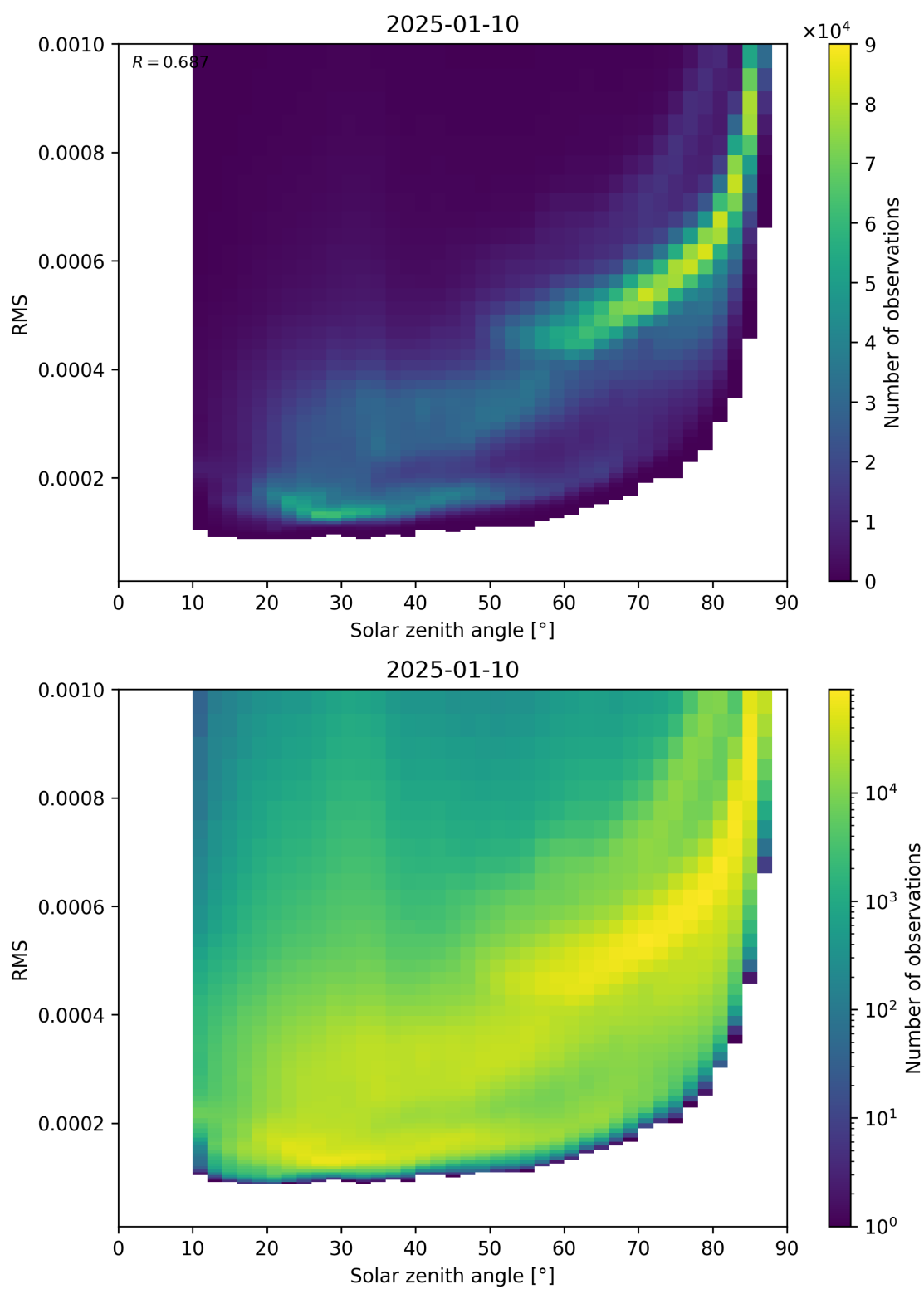
Figure 157: Scatter density plot of “Solar zenith angle” against “RMS” for 2025-01-09 to 2025-01-11.
