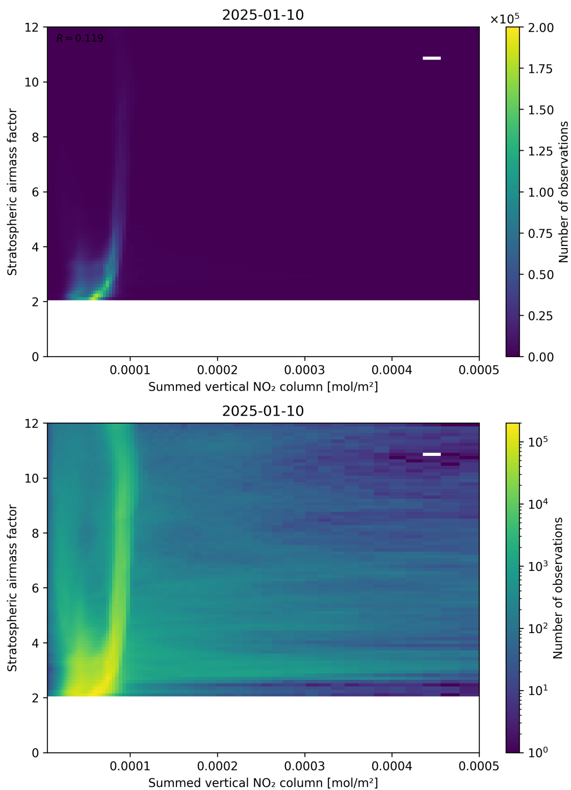
Figure 103: Scatter density plot of “Summed vertical NO 2 column” against “Stratospheric airmass factor” for 2025-01-09 to 2025-01-11.
