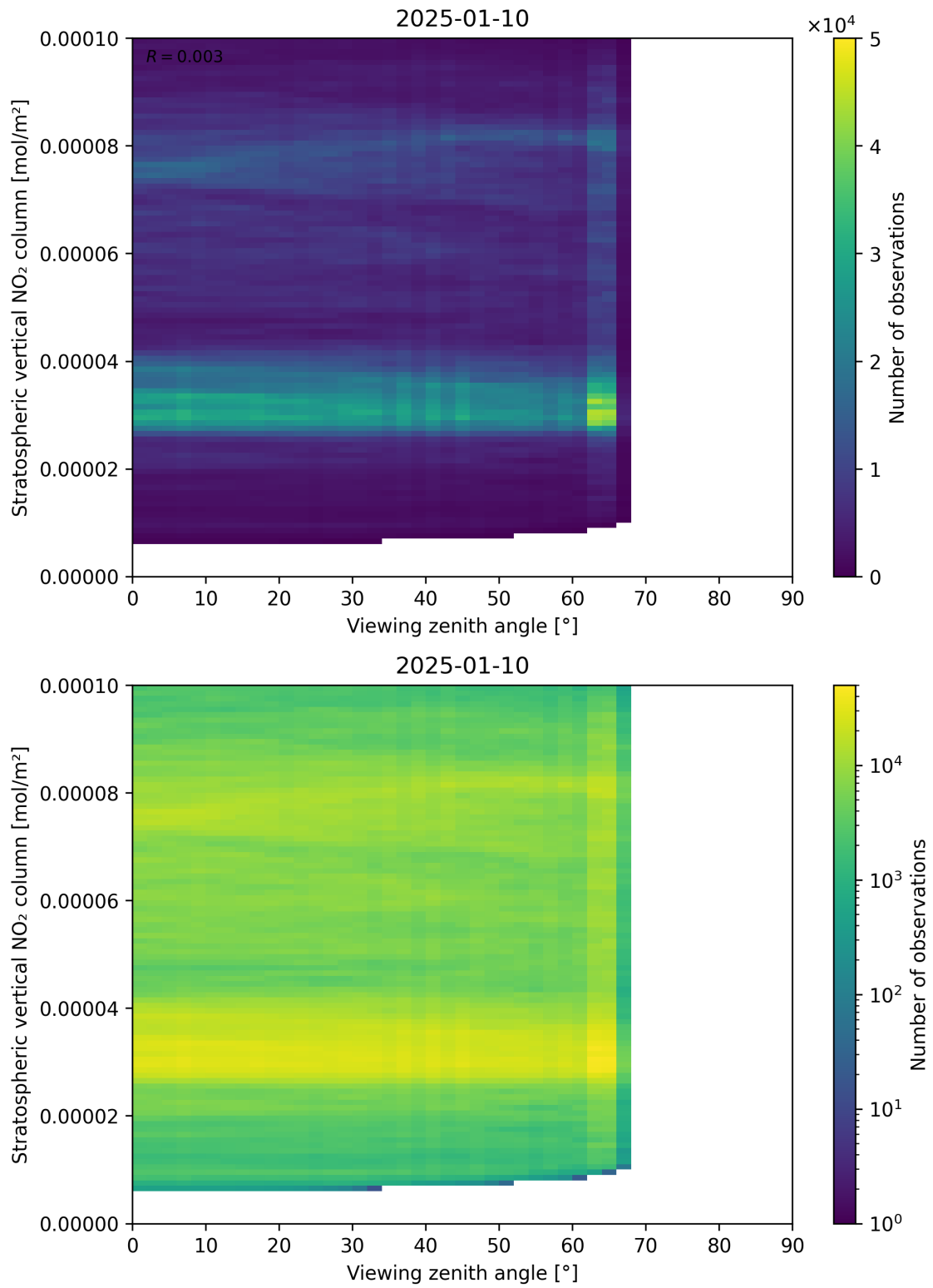
Figure 164: Scatter density plot of “Viewing zenith angle” against “Stratospheric vertical NO 2 column” for 2025-01-09 to 2025-01-11.
