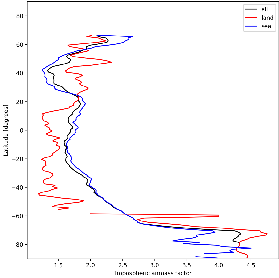
Figure 14: Zonal average of “Tropospheric airmass factor” for 2025-01-09 to 2025-01-11.
