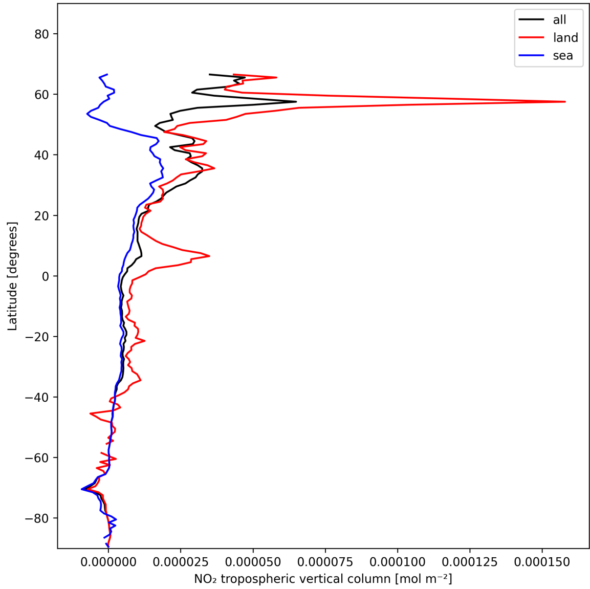
Figure 12: Zonal average of “NO 2 tropospheric vertical column” for 2025-01-09 to 2025-01-11.
