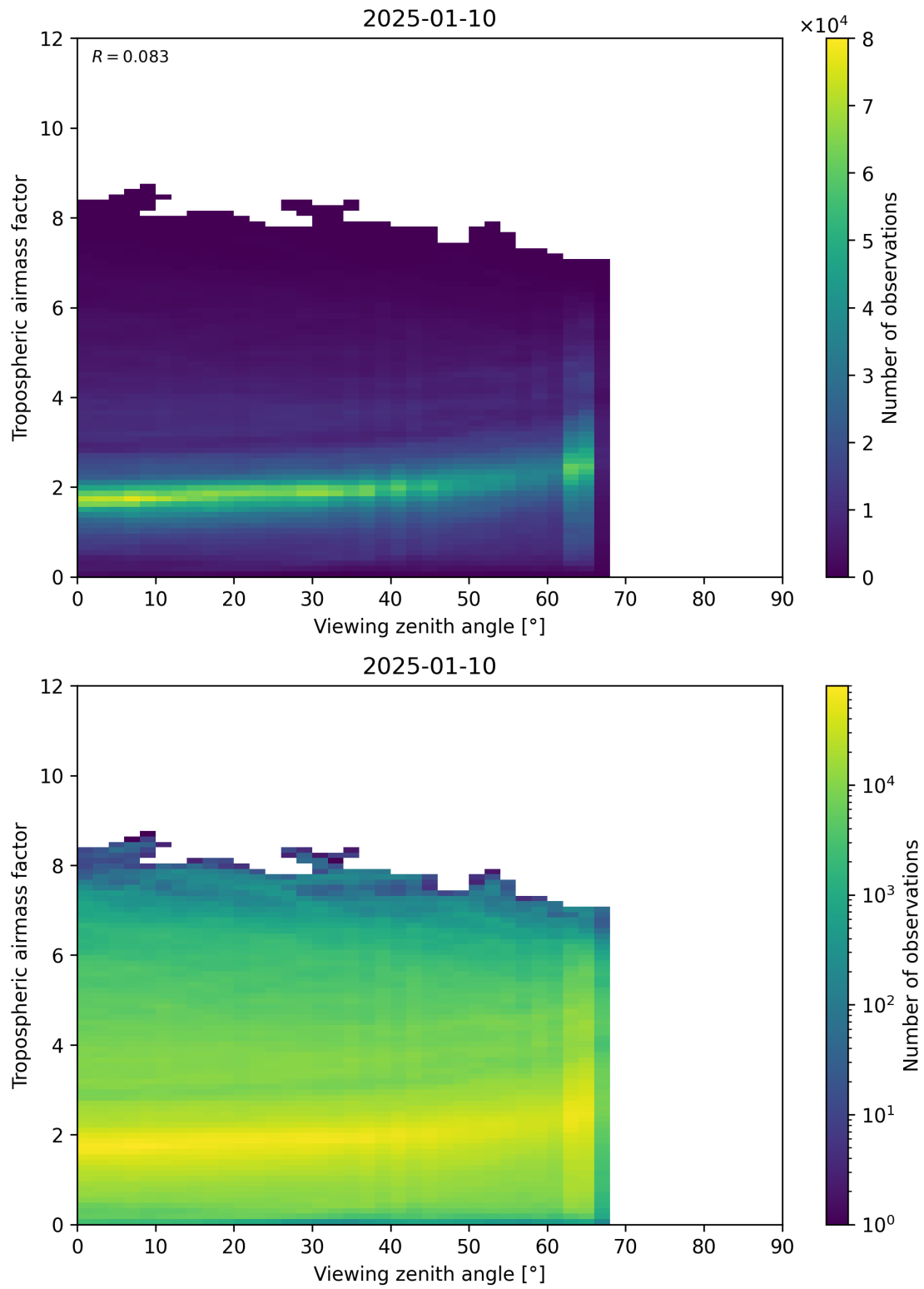
Figure 161: Scatter density plot of “Viewing zenith angle” against “Tropospheric airmass factor” for 2025-01-09 to 2025-01-11.
