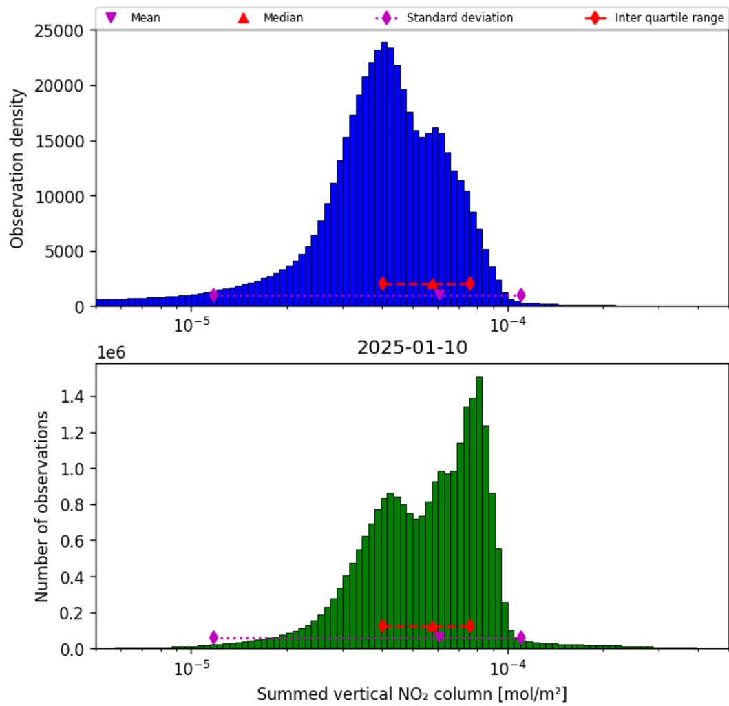
Figure 40: Histogram of “Summed vertical NO 2 column” for 2025-01-09 to 2025-01-11
