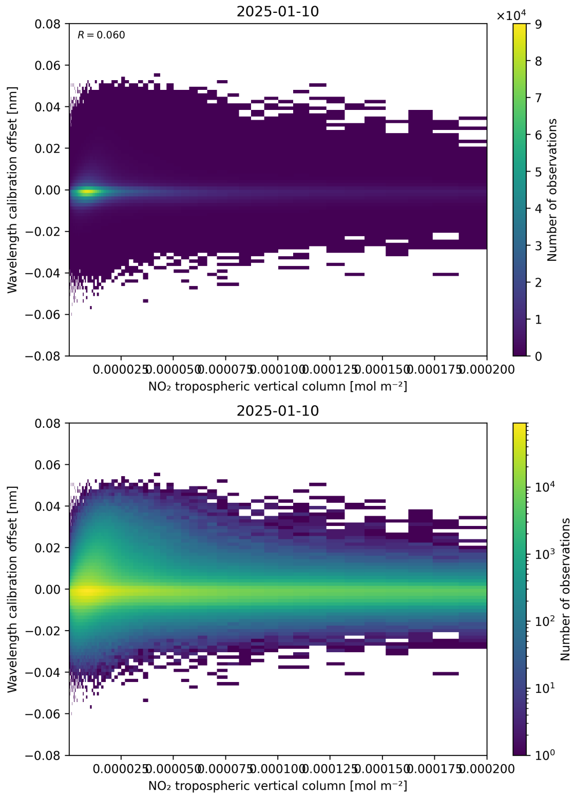
Figure 143: Scatter density plot of “NO 2 tropospheric vertical column” against “Wavelength calibration offset” for 2025-01-09 to 2025-01-11.
