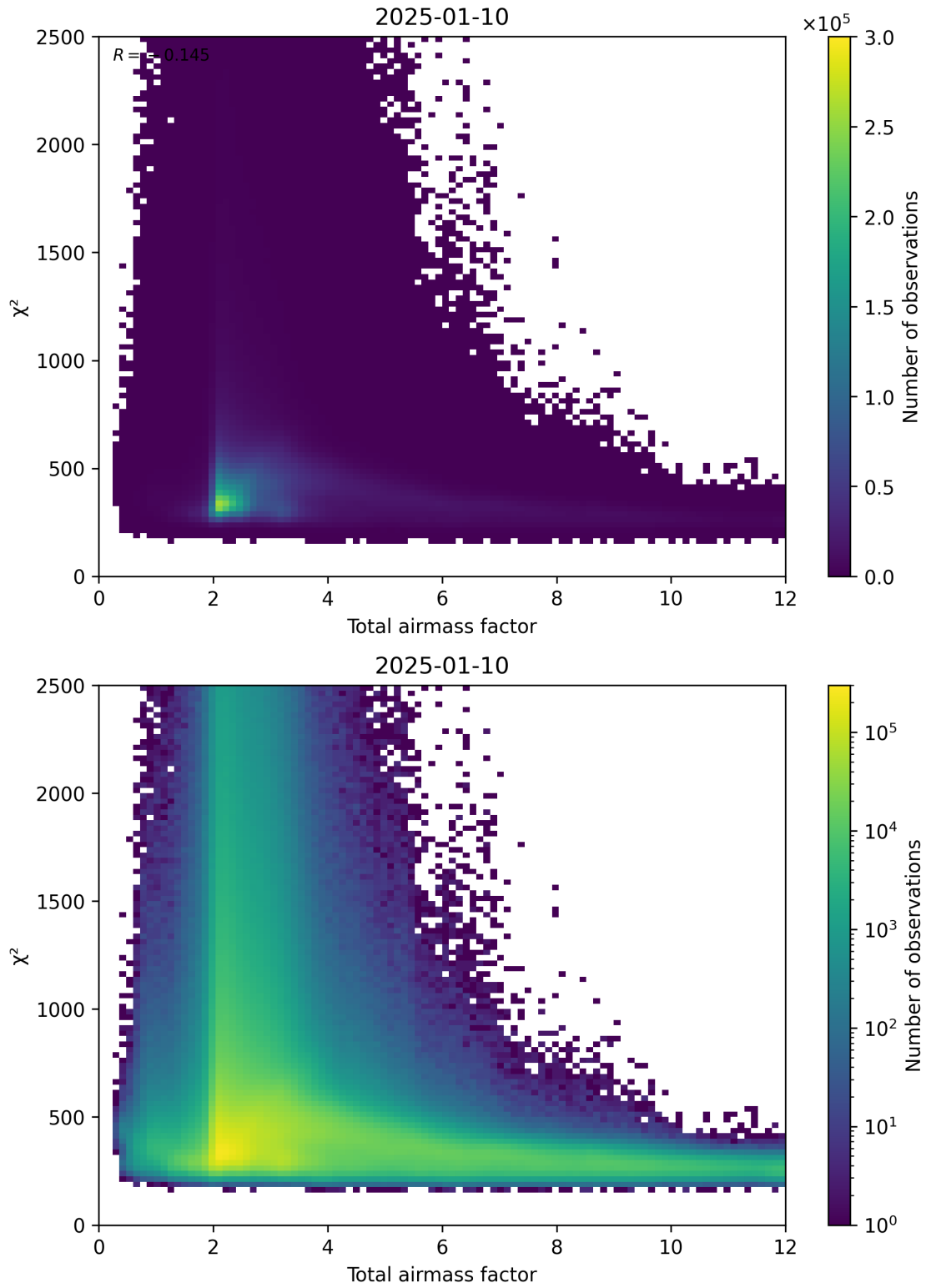
Figure 63: Scatter density plot of “Total airmass factor” against “ \chi^2 ” for 2025-01-09 to 2025-01-11.
