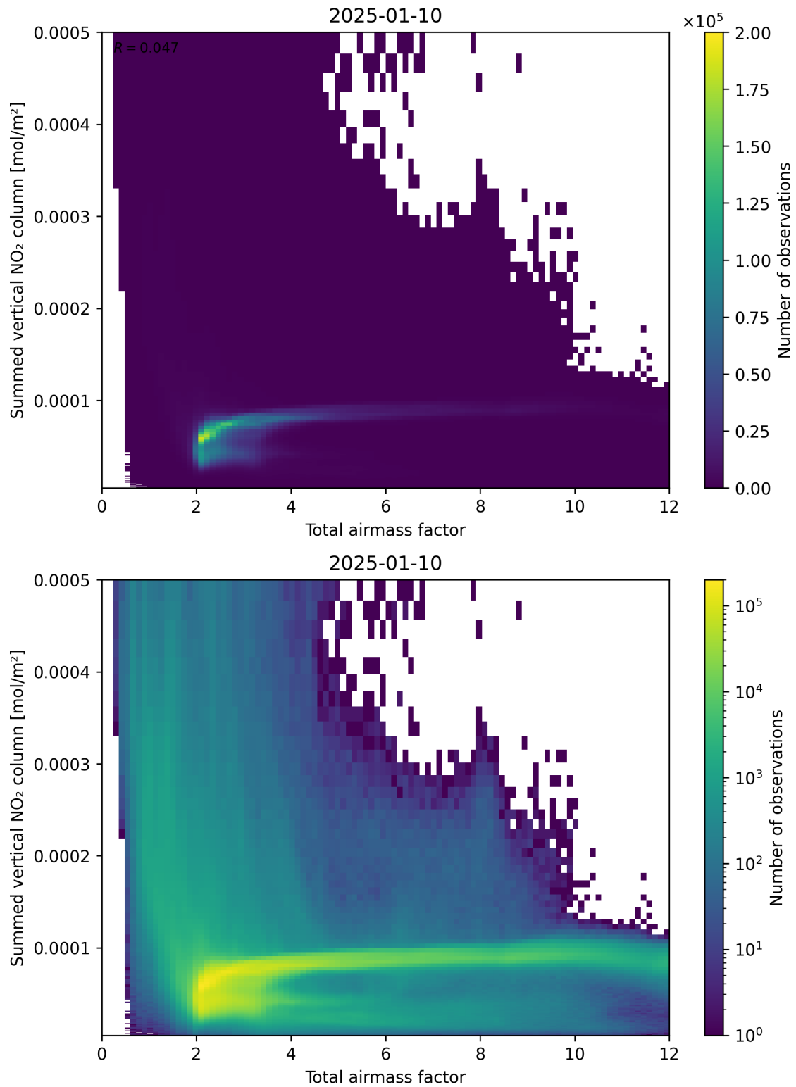
Figure 65: Scatter density plot of “Total airmass factor” against “Summed vertical NO 2 column” for 2025-01-09 to 2025-01-11.
