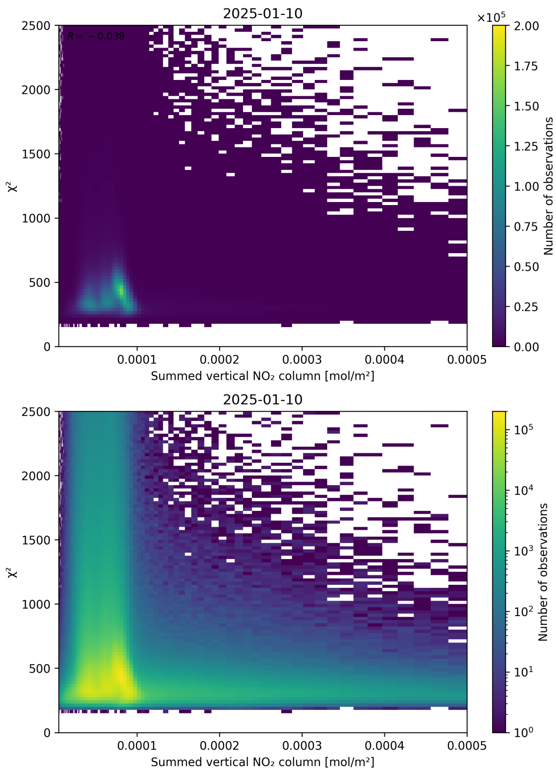
Figure 104: Scatter density plot of “Summed vertical NO 2 column” against “ \chi^2 ” for 2025-01-09 to 2025-01-11.
