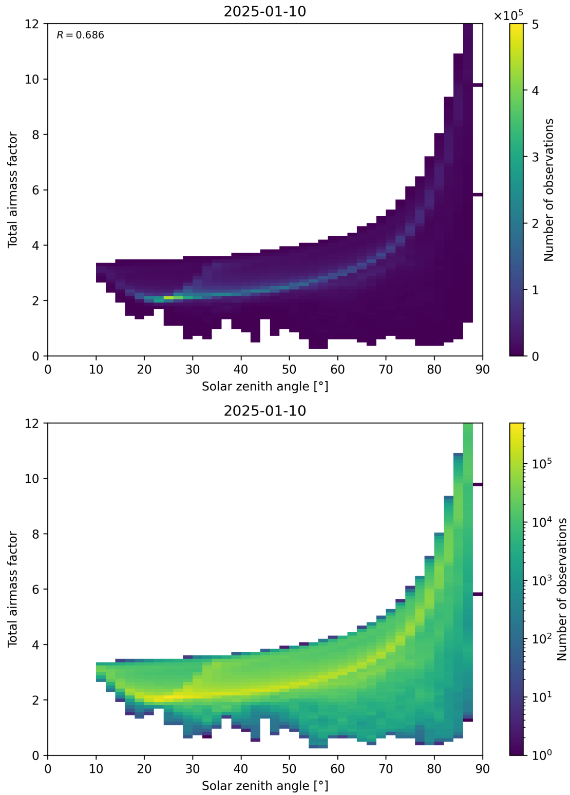
Figure 146: Scatter density plot of “Solar zenith angle” against “Total airmass factor” for 2025-01-09 to 2025-01-11.
