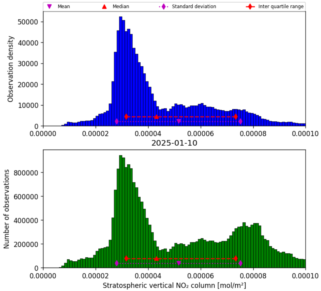
Figure 36: Histogram of “Stratospheric vertical NO 2 column” for 2025-01-09 to 2025-01-11
