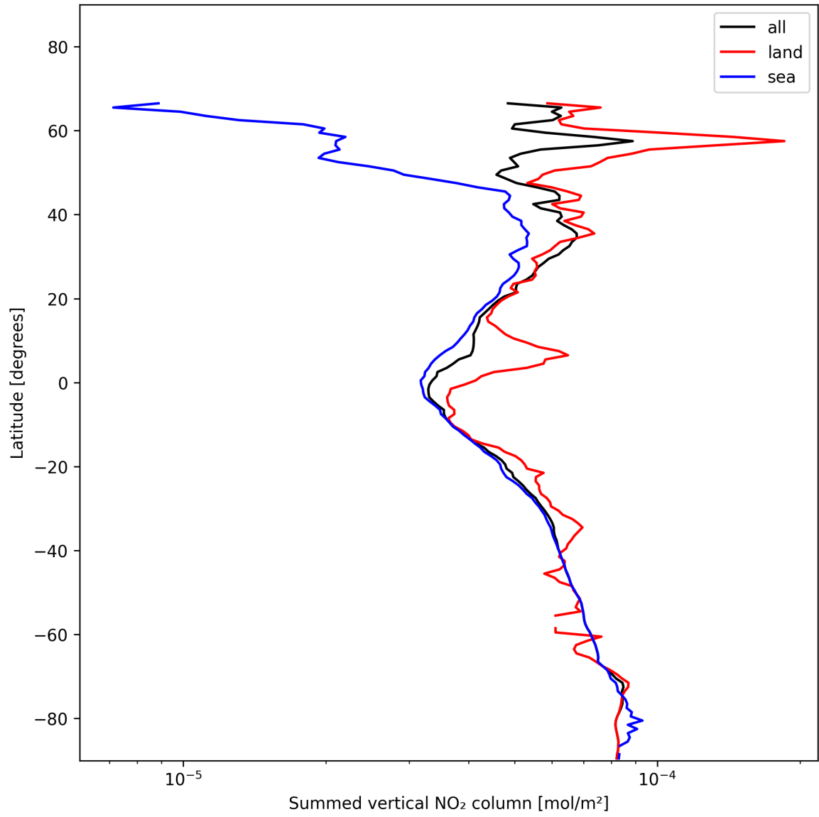
Figure 23: Zonal average of “Summed vertical NO 2 column” for 2025-01-09 to 2025-01-11.
