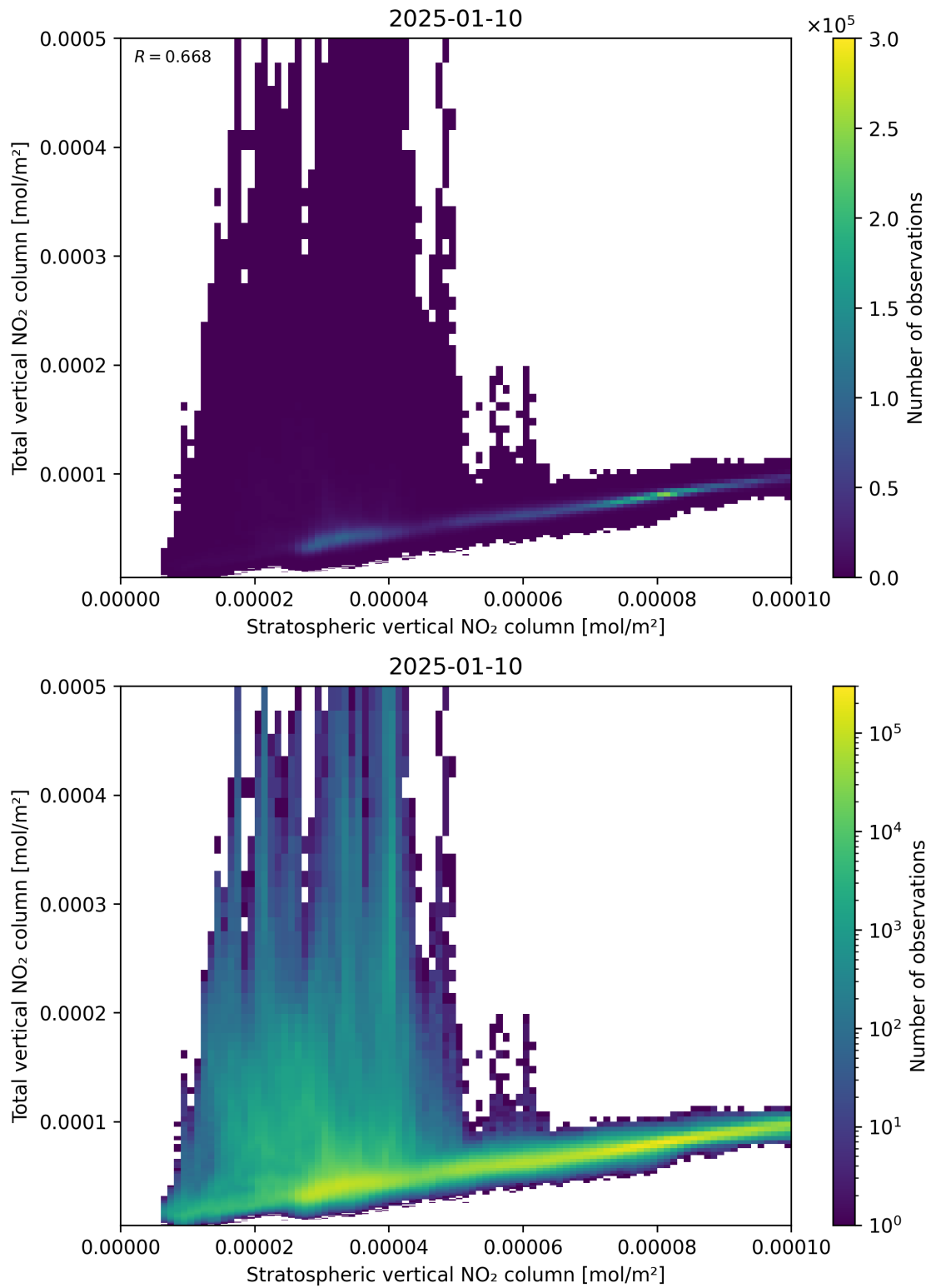
Figure 100: Scatter density plot of “Stratospheric vertical NO 2 column” against “Total vertical NO 2 column” for 2025-01-09 to 2025-01-11.
