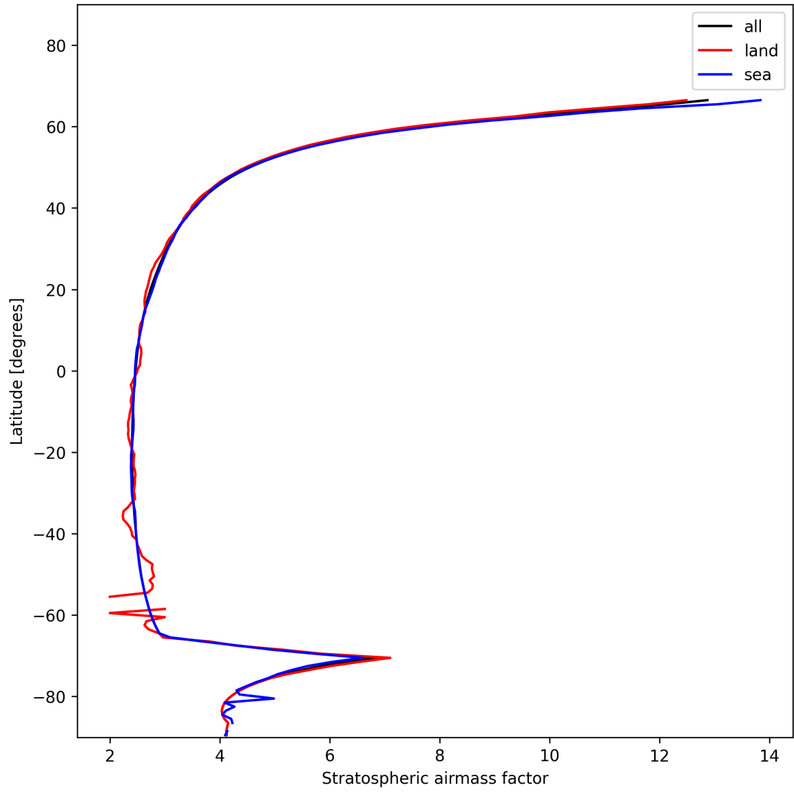
Figure 27: Zonal average of “Stratospheric air mass factor” for 2025-01-09 to 2025-01-11.
