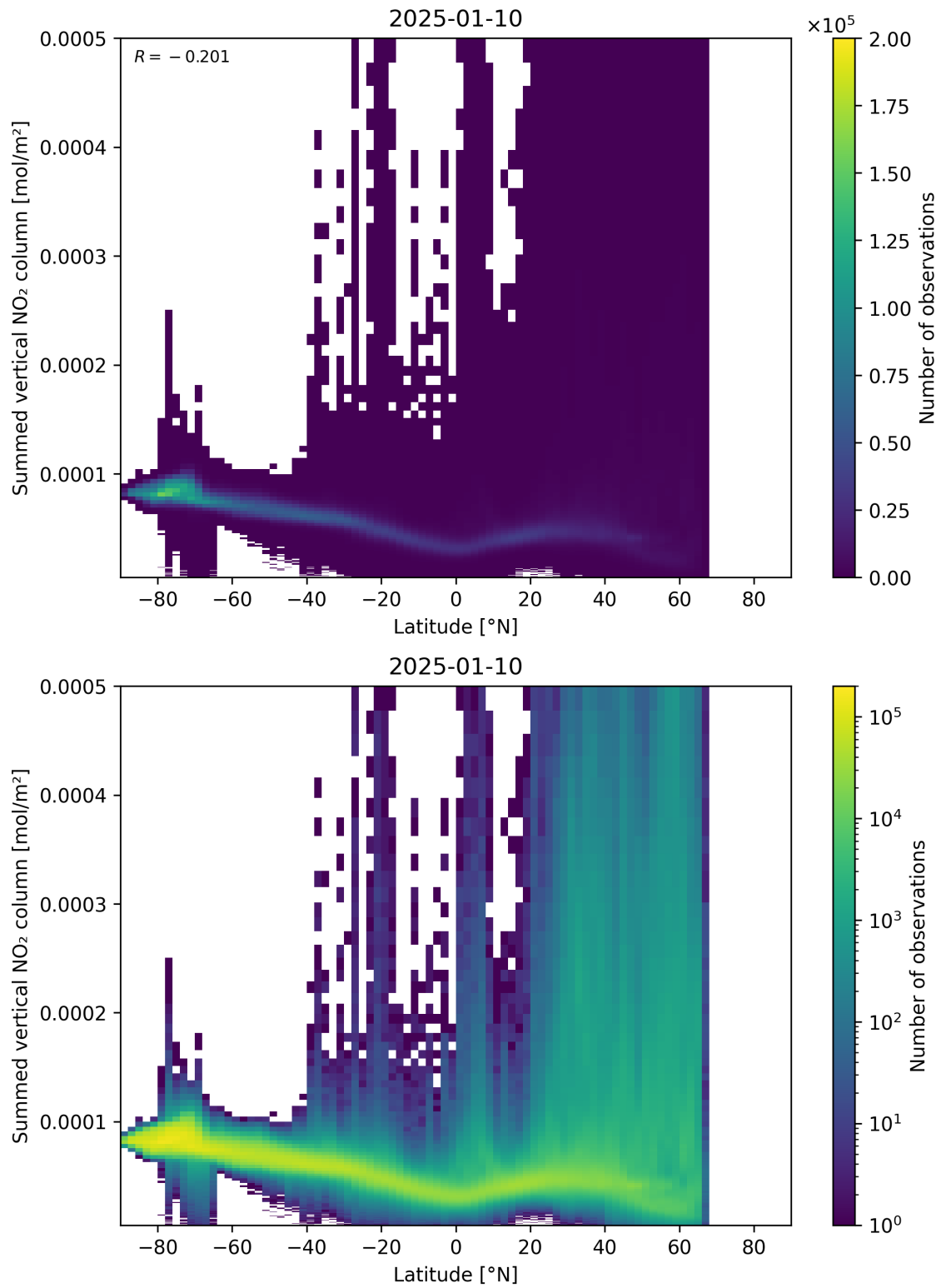
Figure 88: Scatter density plot of “Latitude” against “Summed vertical NO 2 column” for 2025-01-09 to 2025-01-11.
