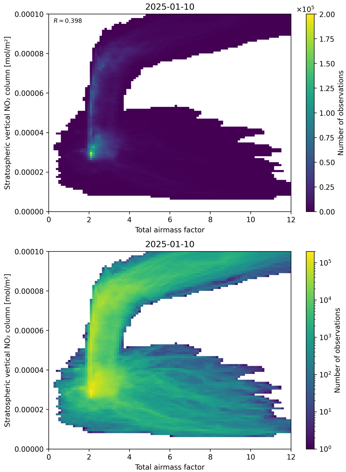
Figure 64: Scatter density plot of “Total airmass factor” against “Stratospheric vertical NO 2 column” for 2025-01-09 to 2025-01-11.
