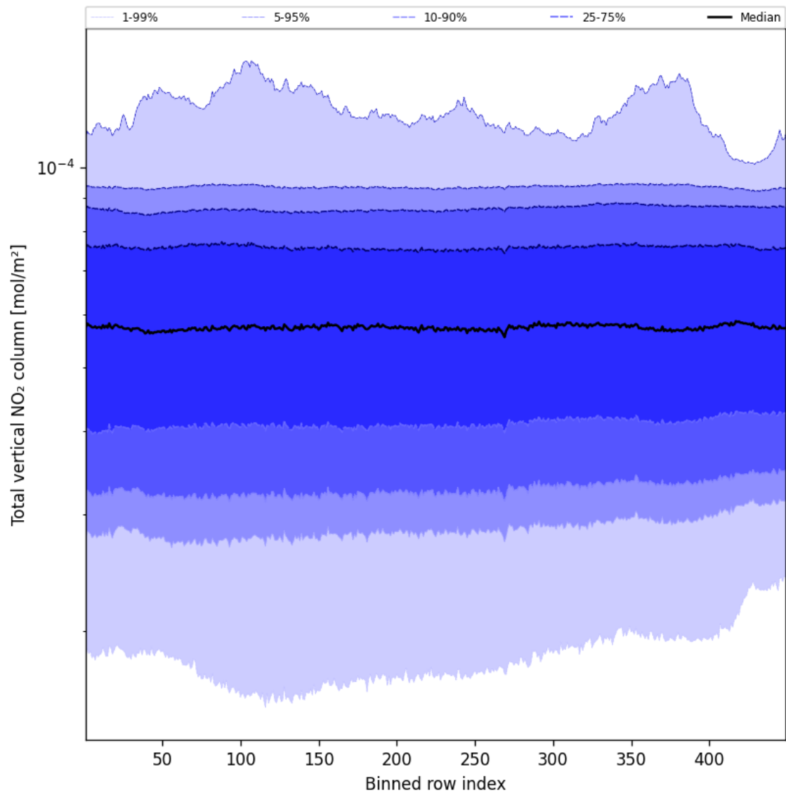
Figure 55: Along track statistics of “Total vertical NO 2 column” for 2025-01-09 to 2025-01-11
