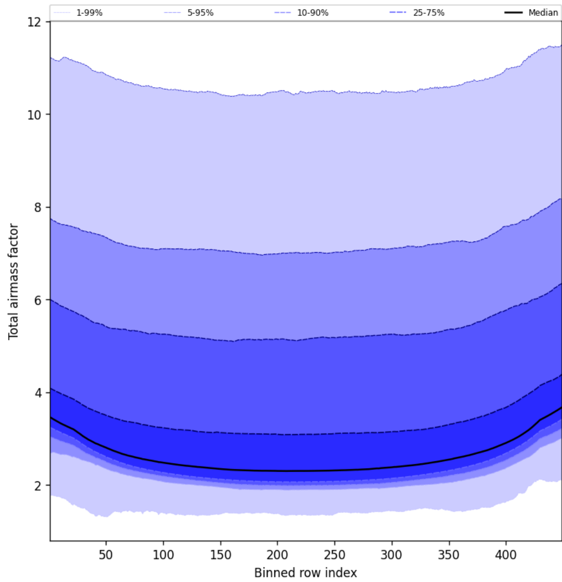
Figure 49: Along track statistics of “Total airmass factor” for 2025-01-09 to 2025-01-11
