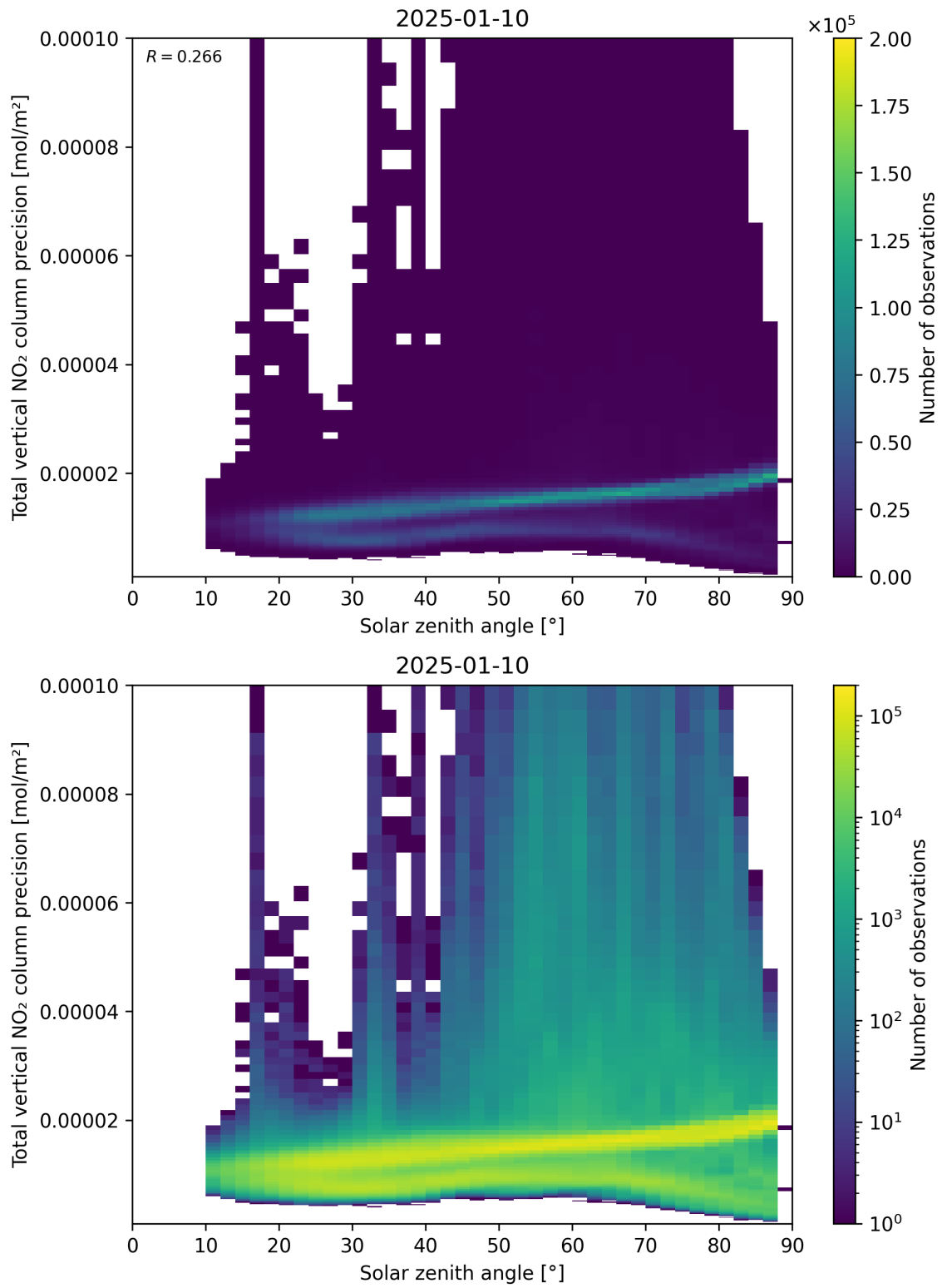
Figure 154: Scatter density plot of “Solar zenith angle” against “Total vertical NO 2 column precision” for 2025-01-09 to 2025-01-11.
