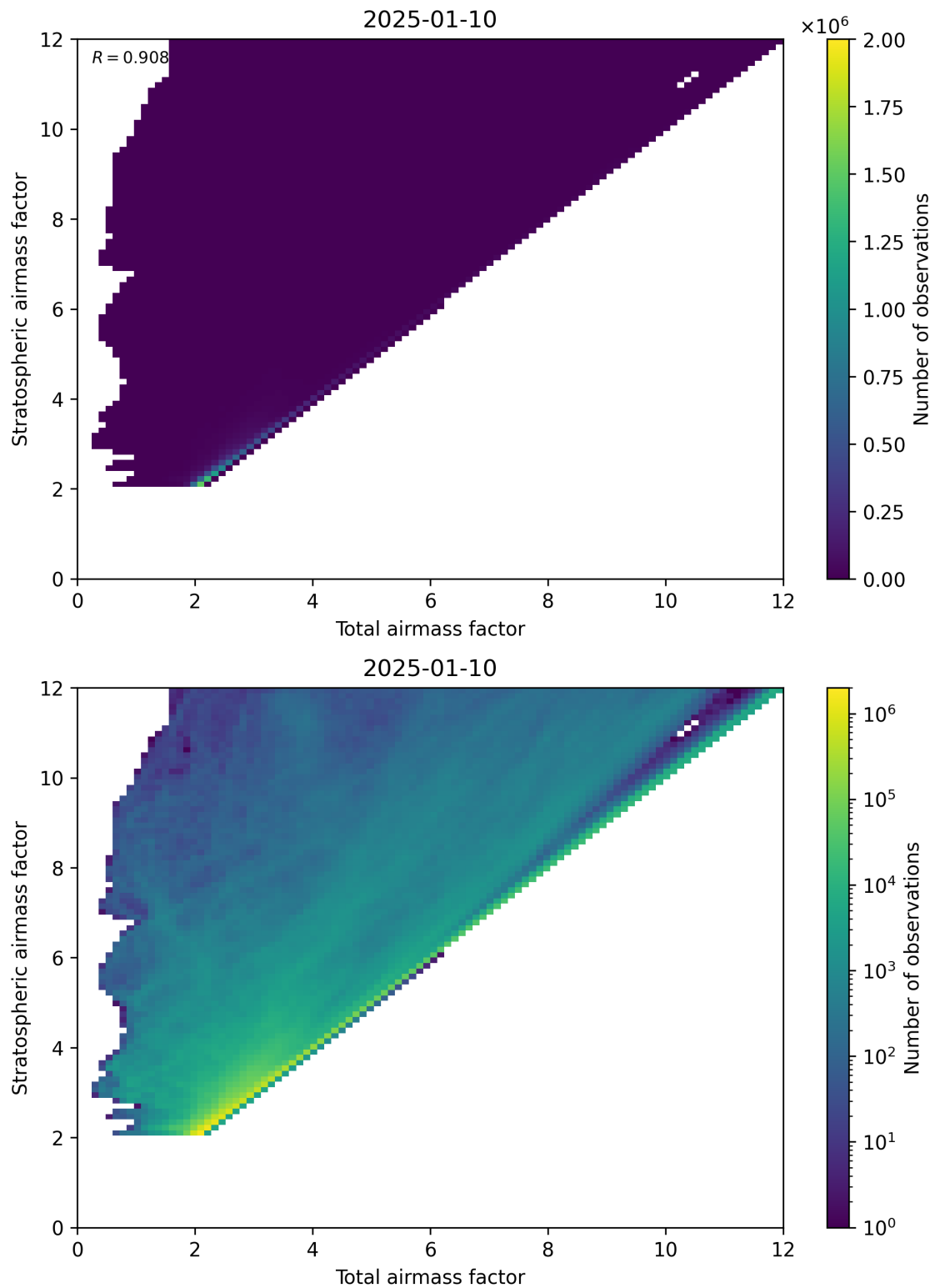
Figure 62: Scatter density plot of “Total airmass factor” against “Stratospheric airmass factor” for 2025-01-09 to 2025-01-11.
