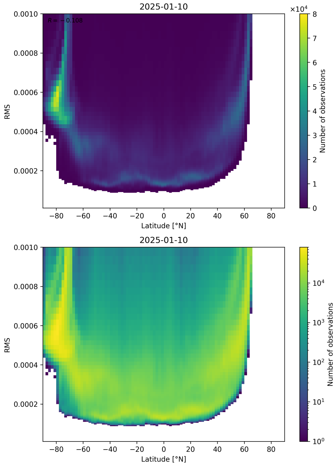
Figure 94: Scatter density plot of “Latitude” against “RMS” for 2025-01-09 to 2025-01-11.
