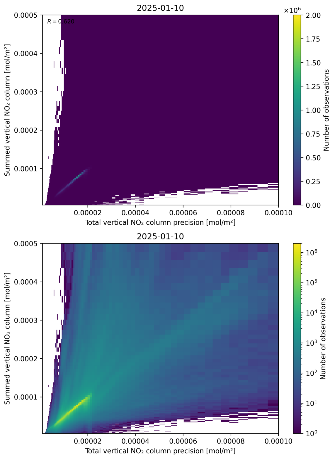
Figure 117: Scatter density plot of “Total vertical NO 2 column precision” against “Summed vertical NO 2 column” for 2025-01-09 to 2025-01-11.
