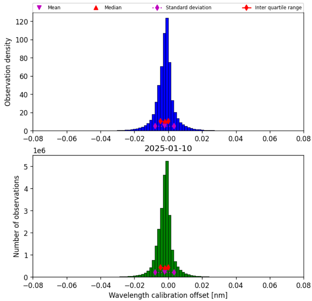
Figure 35: Histogram of “Wavelength calibration offset” for 2025-01-09 to 2025-01-11
