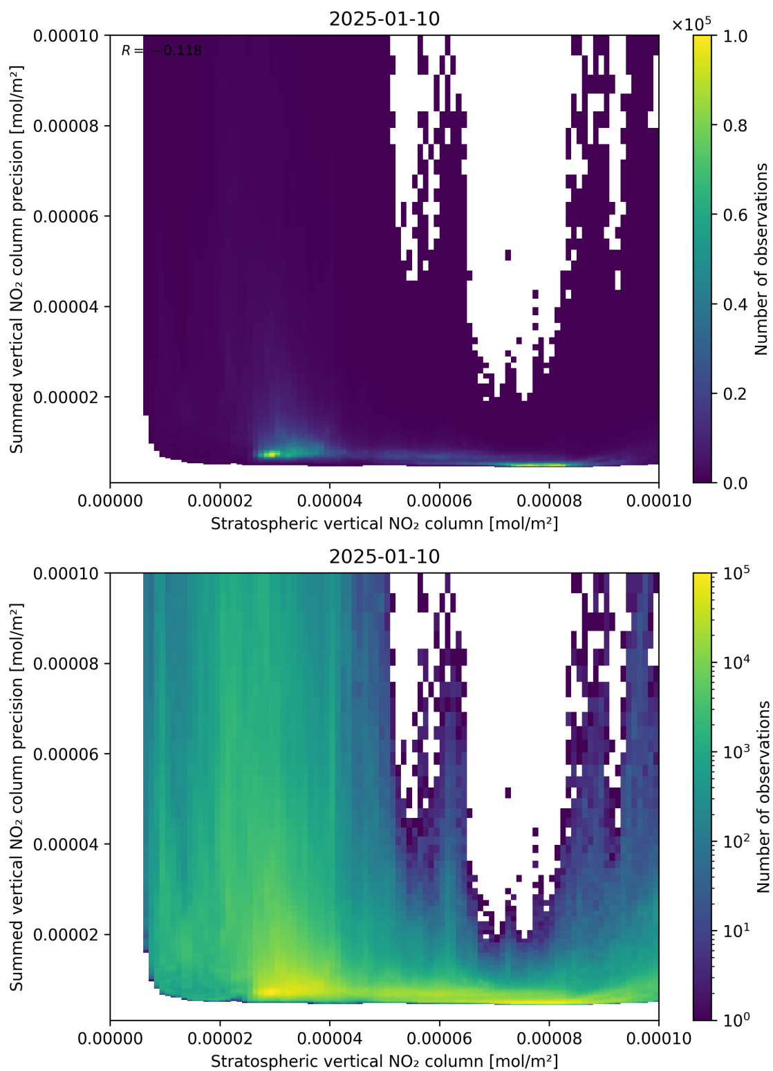
Figure 99: Scatter density plot of “Stratospheric vertical NO 2 column” against “Summed vertical NO 2 column precision” for 2025-01-09 to 2025-01-11.
