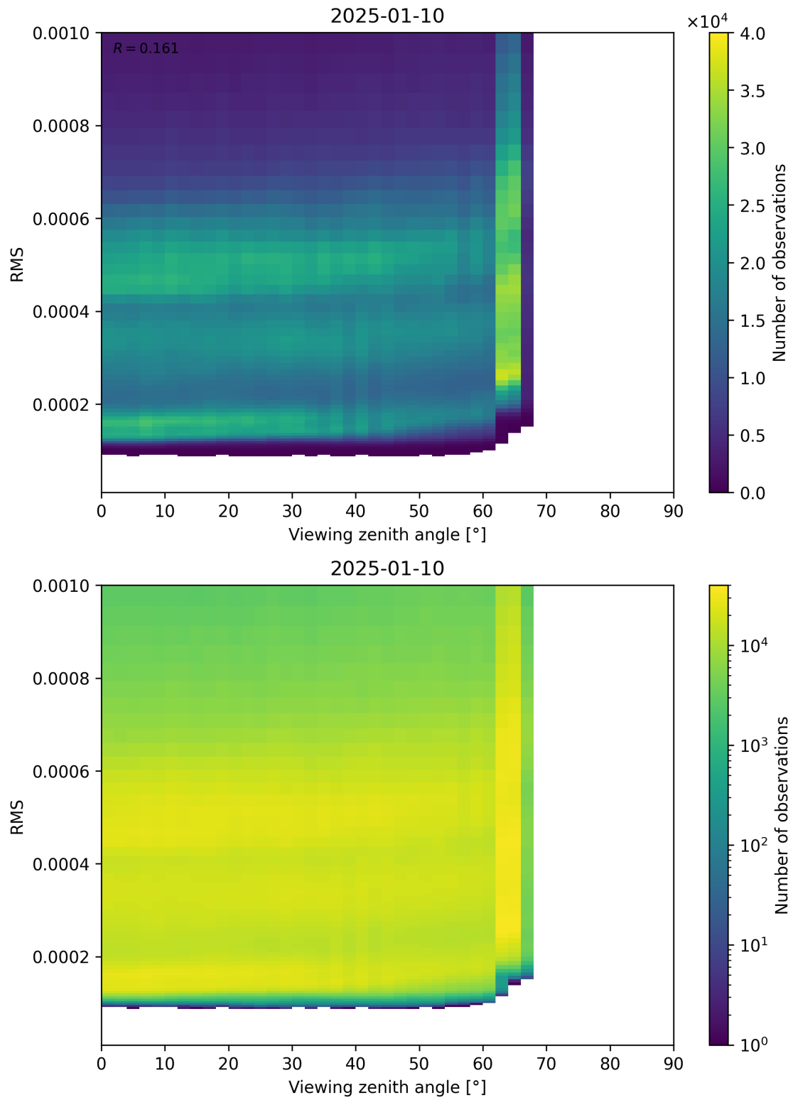
Figure 171: Scatter density plot of “Viewing zenith angle” against “RMS” for 2025-01-09 to 2025-01-11.
