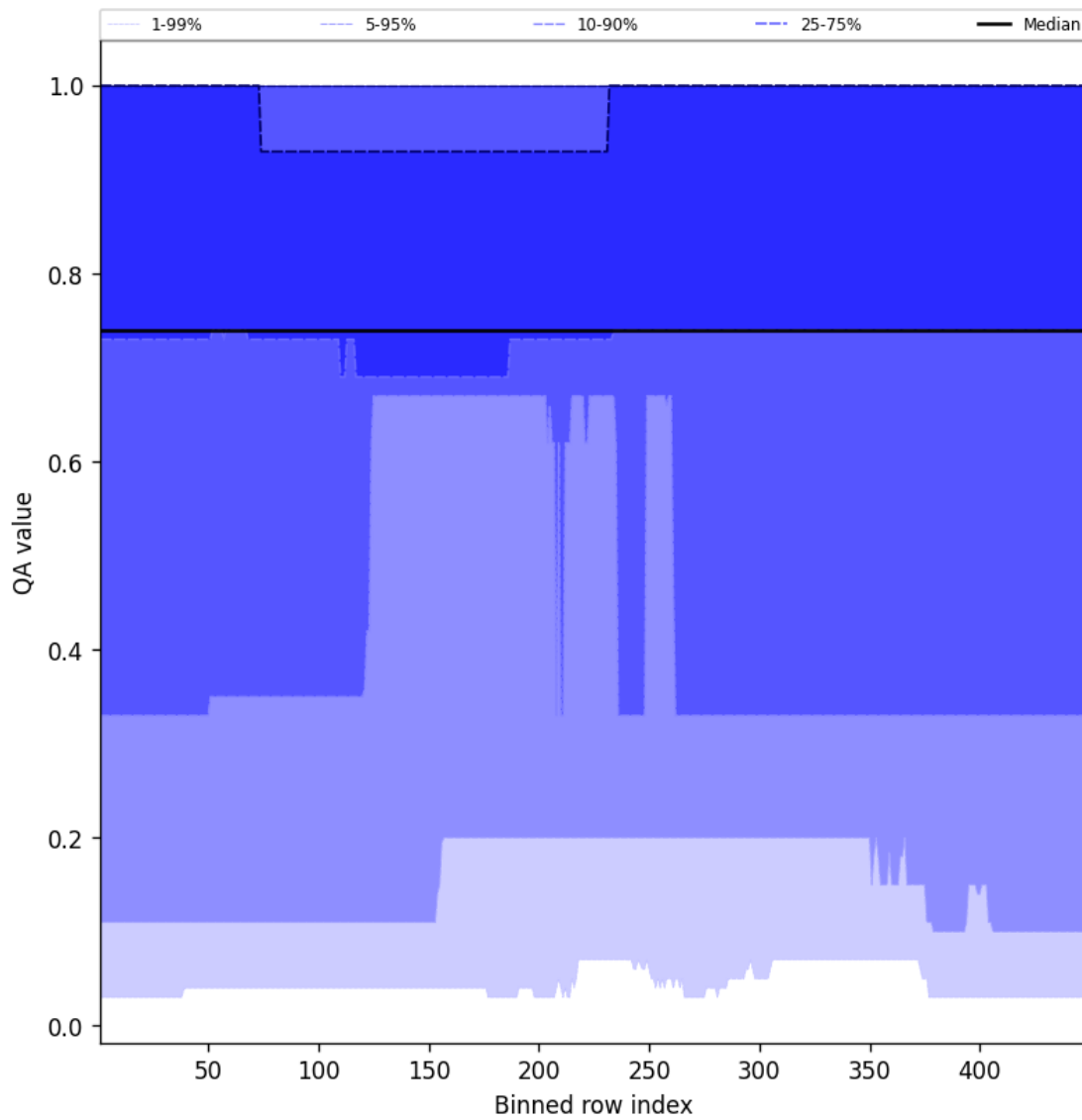
Figure 45: Along track statistics of “QA value” for 2025-01-09 to 2025-01-11
