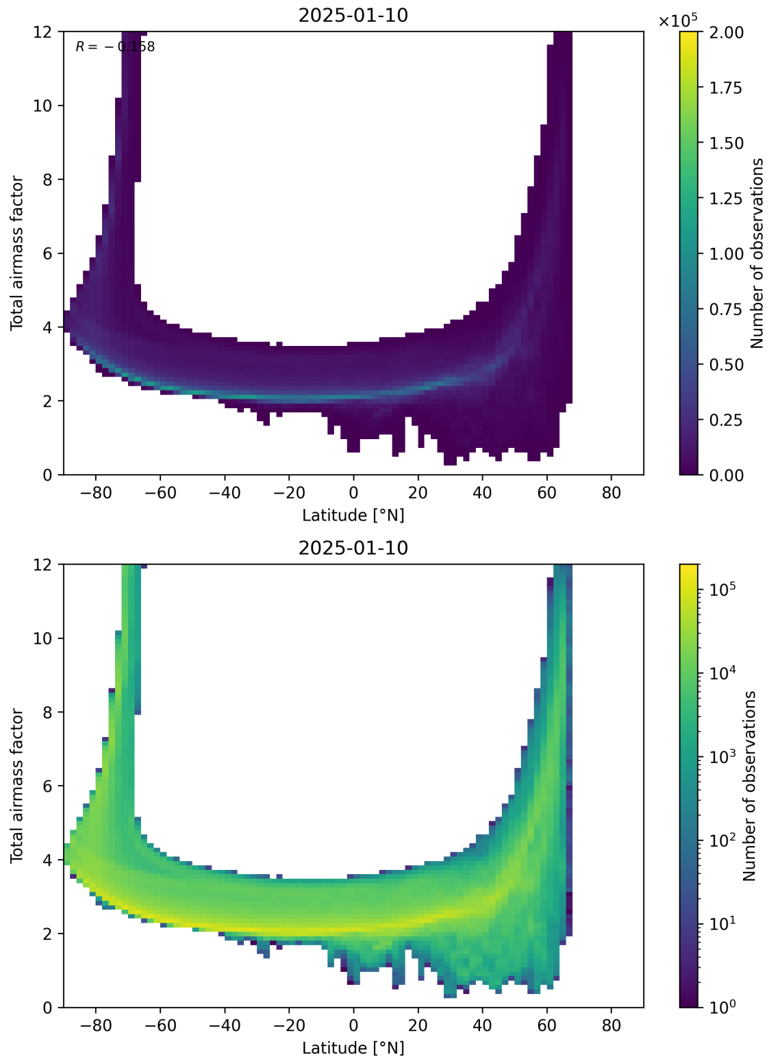
Figure 84: Scatter density plot of “Latitude” against “Total airmass factor” for 2025-01-09 to 2025-01-11.
