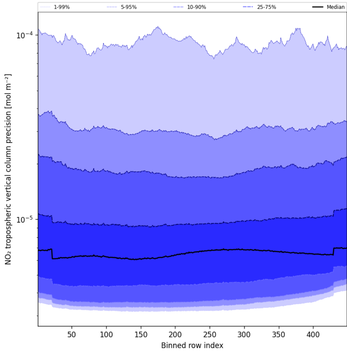
Figure 47: Along track statistics of “NO 2 tropospheric vertical column precision” for 2025-01-09 to 2025-01-11
