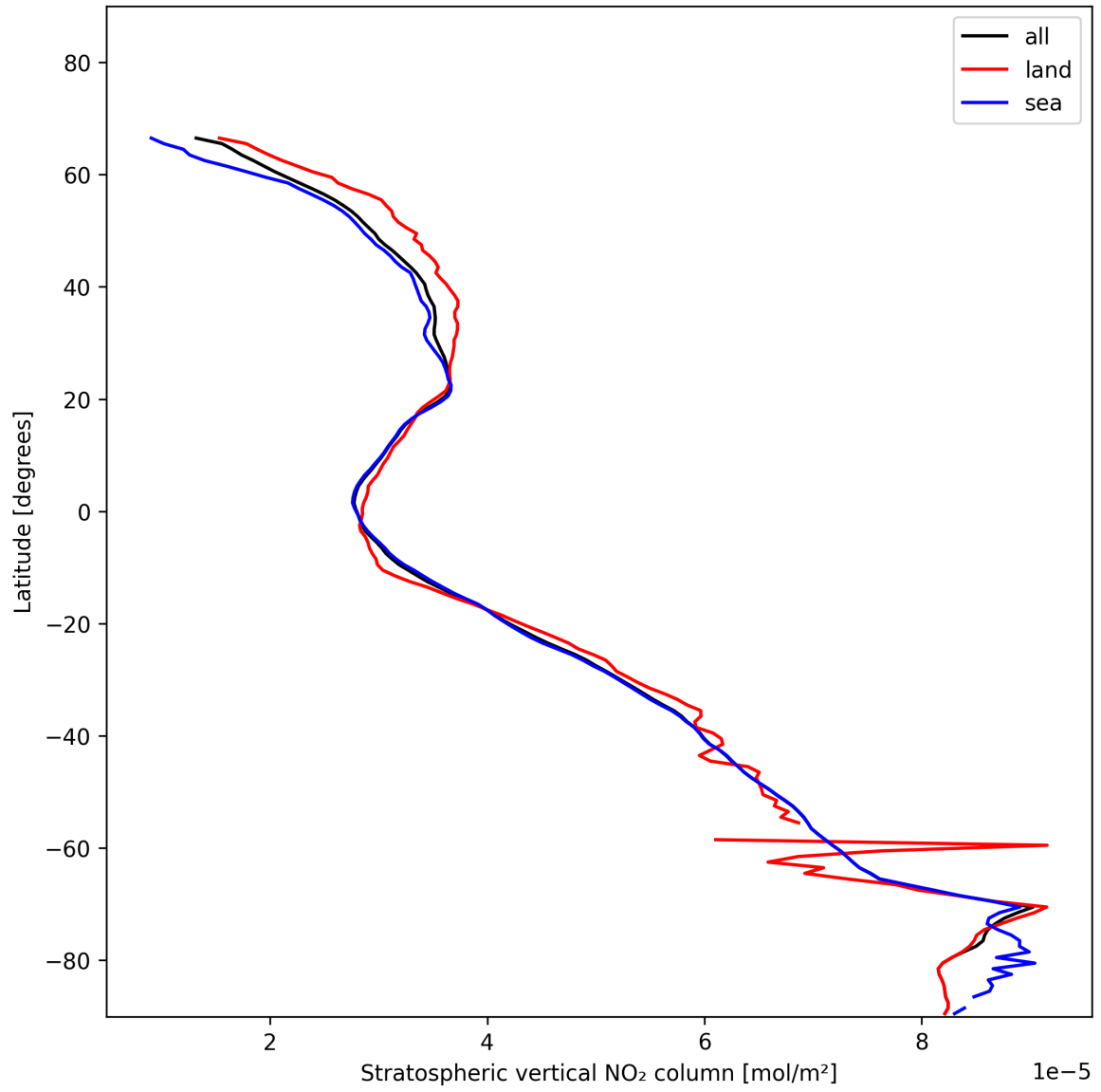
Figure 19: Zonal average of “Stratospheric vertical NO 2 column” for 2025-01-09 to 2025-01-11.
