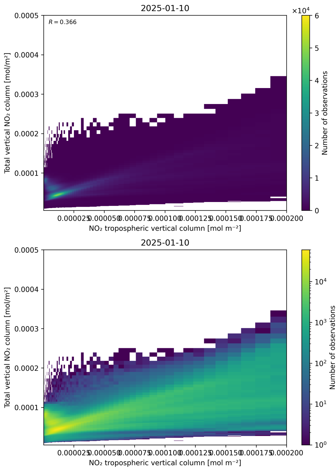
Figure 128: Scatter density plot of “NO 2 tropospheric vertical column” against “Total vertical NO 2 column” for 2025-01-09 to 2025-01-11.
