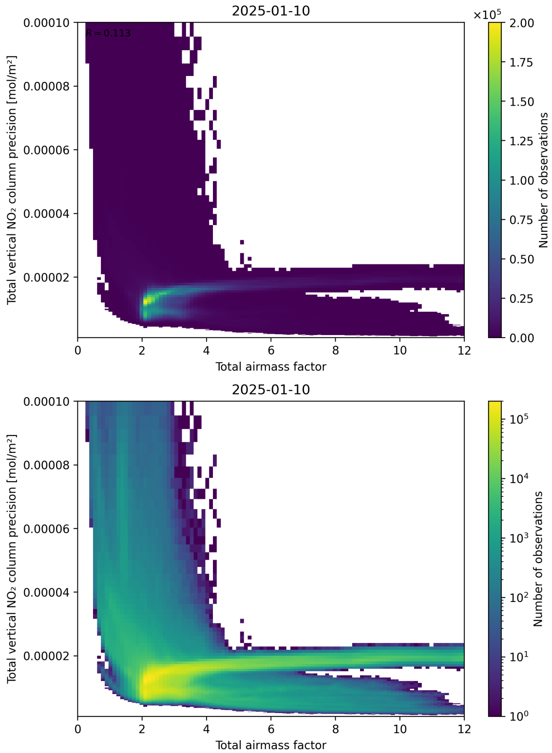
Figure 68: Scatter density plot of “Total airmass factor” against “Total vertical NO 2 column precision” for 2025-01-09 to 2025-01-11.
