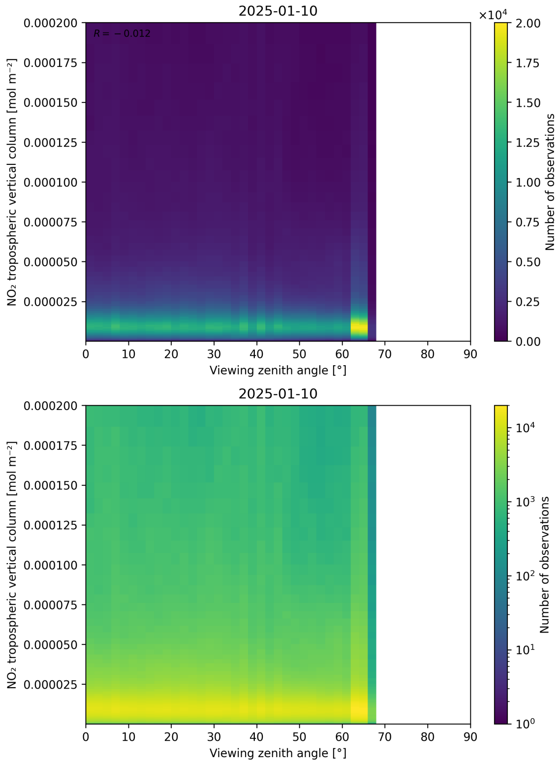
Figure 169: Scatter density plot of “Viewing zenith angle” against “NO 2 tropospheric vertical column” for 2025-01-09 to 2025-01-11.
