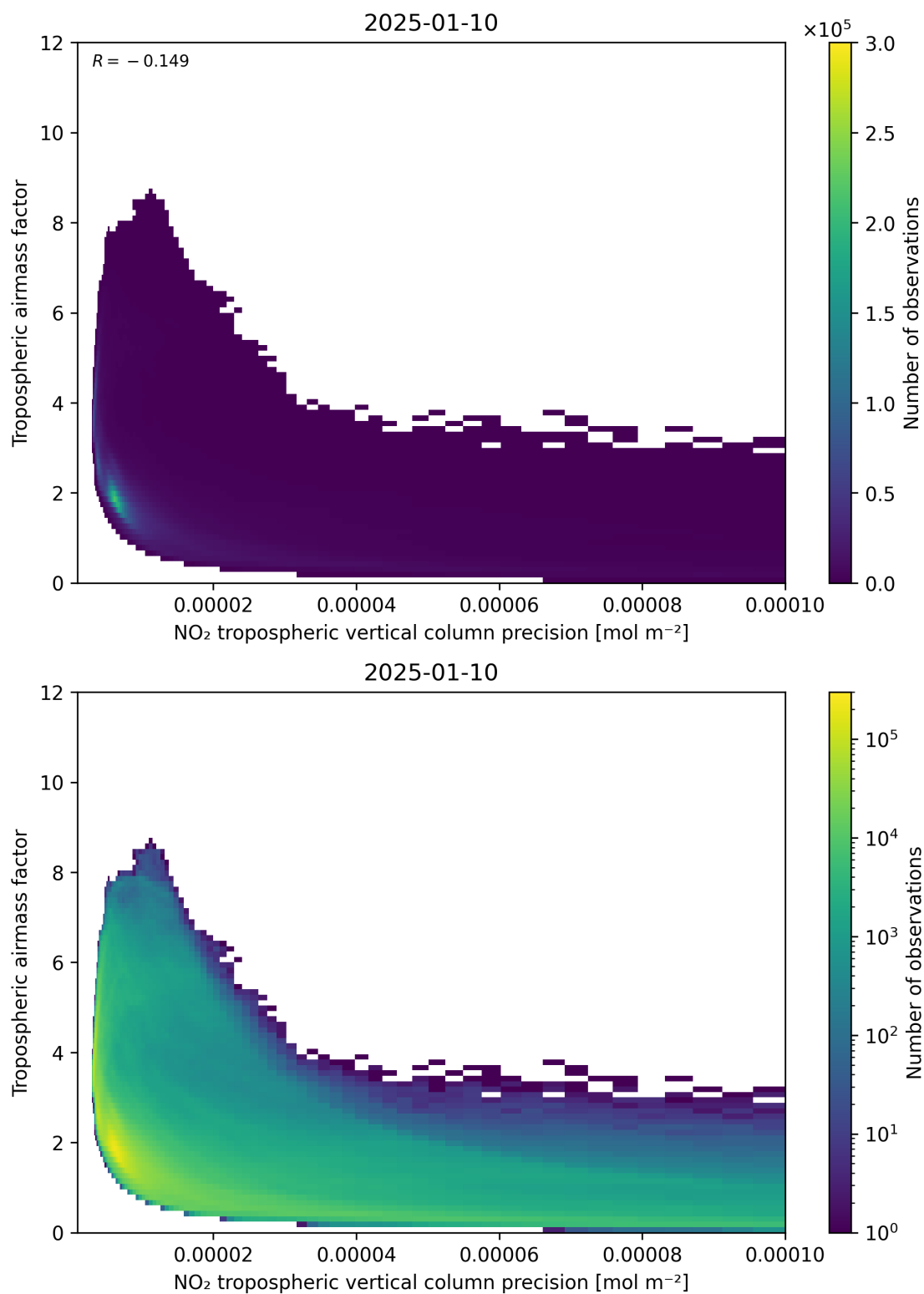
Figure 133: Scatter density plot of “NO 2 tropospheric vertical column precision” against “Tropospheric airmass factor” for 2025-01-09 to 2025-01-11.
