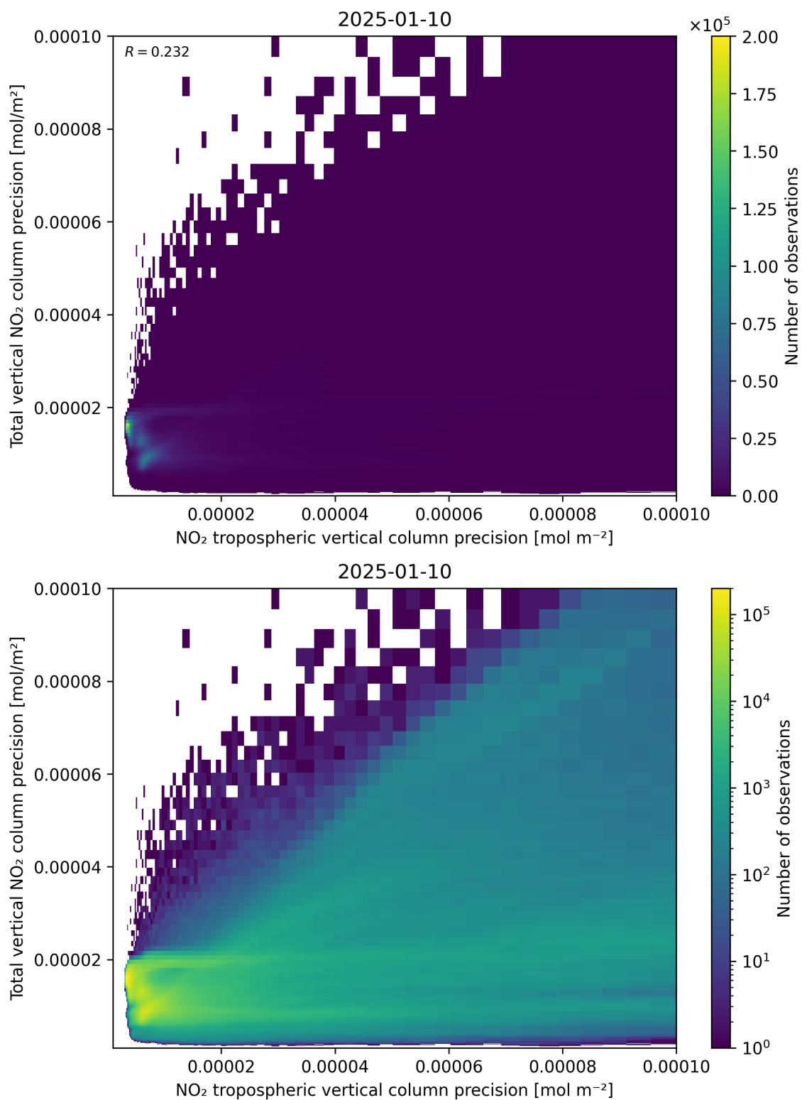
Figure 139: Scatter density plot of “NO 2 tropospheric vertical column precision” against “Total vertical NO 2 column precision” for 2025-01-09 to 2025-01-11.
