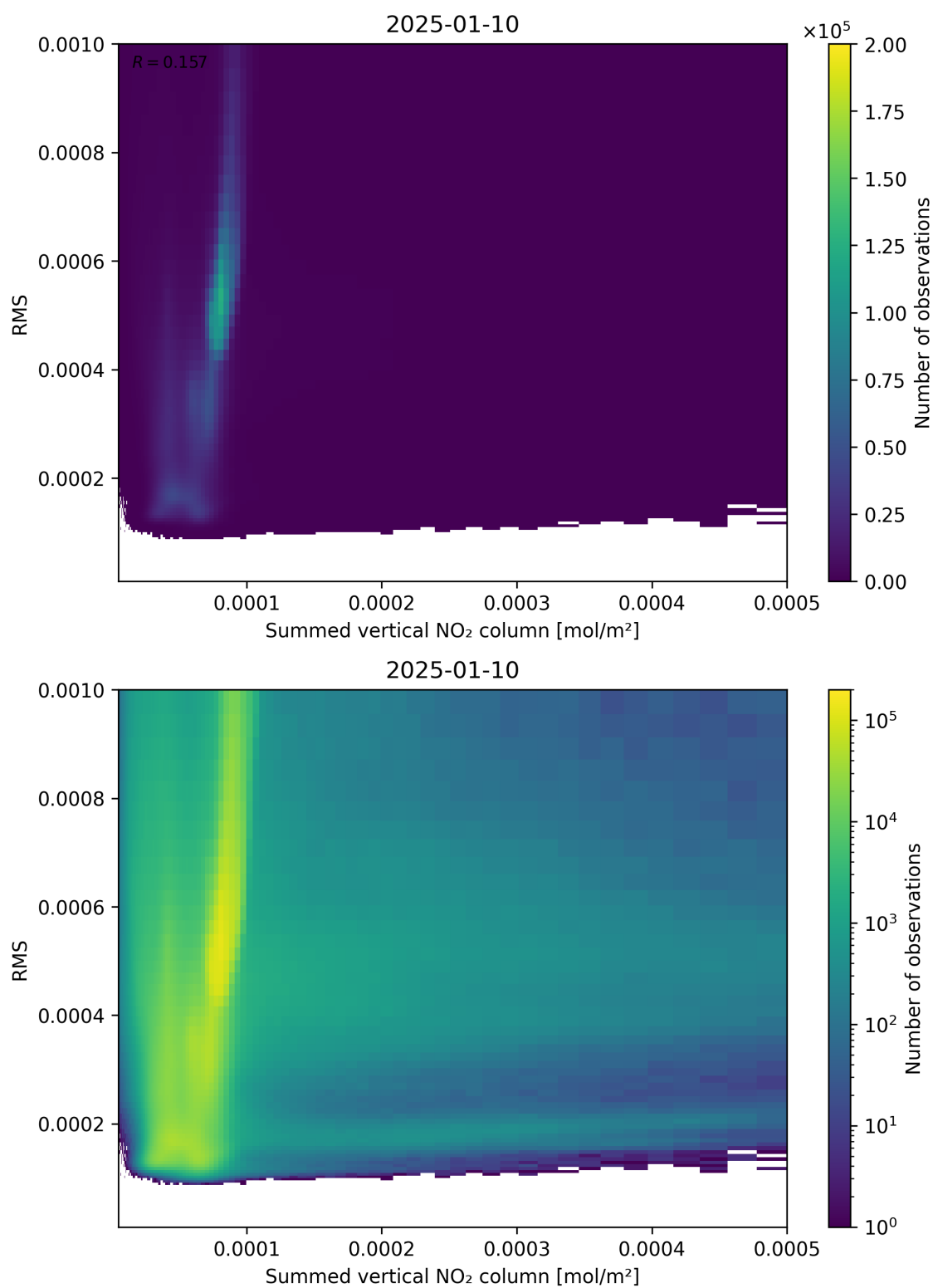
Figure 109: Scatter density plot of “Summed vertical NO 2 column” against “RMS” for 2025-01-09 to 2025-01-11.
