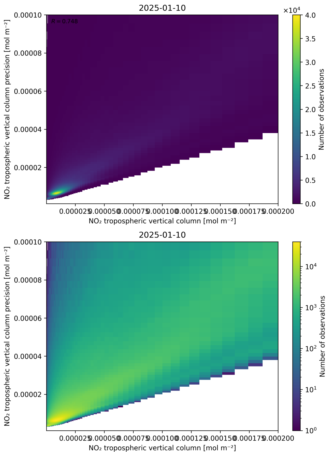
Figure 130: Scatter density plot of “NO 2 tropospheric vertical column” against “NO 2 tropospheric vertical column precision” for 2025-01-09 to 2025-01-11.
