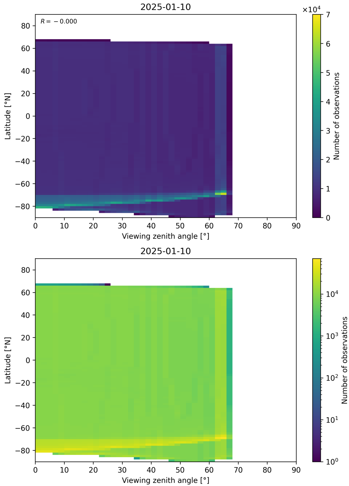
Figure 163: Scatter density plot of “Viewing zenith angle” against “Latitude” for 2025-01-09 to 2025-01-11.
