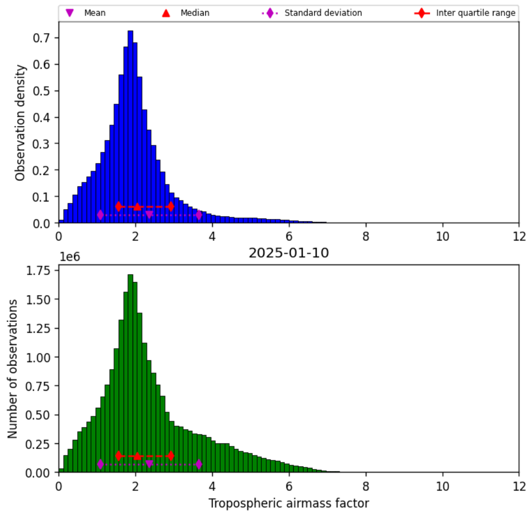
Figure 31: Histogram of “Tropospheric airmass factor” for 2025-01-09 to 2025-01-11
