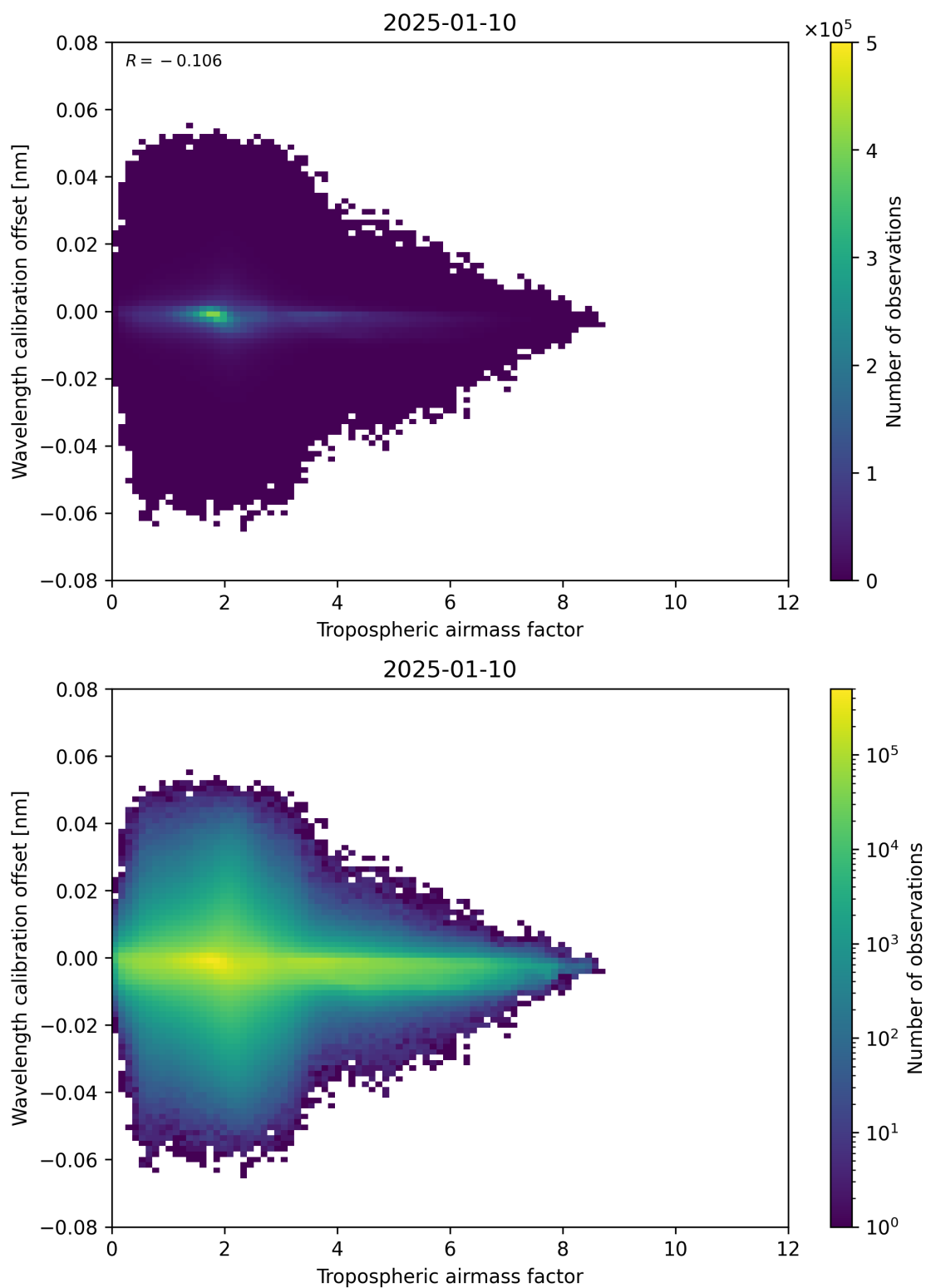
Figure 80: Scatter density plot of “Tropospheric airmass factor” against “Wavelength calibration offset” for 2025-01-09 to 2025-01-11.
