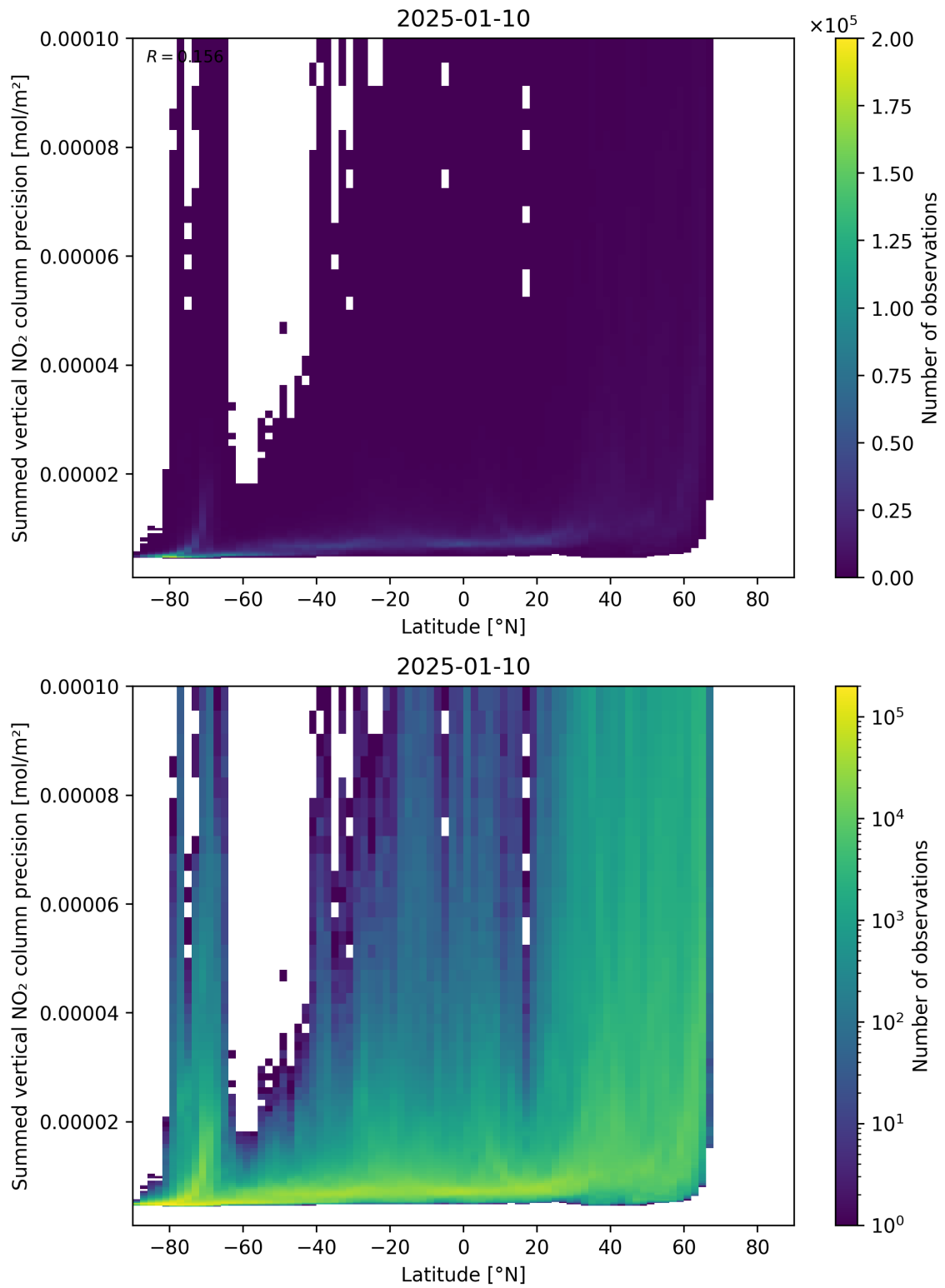
Figure 89: Scatter density plot of “Latitude” against “Summed vertical NO 2 column precision” for 2025-01-09 to 2025-01-11.
