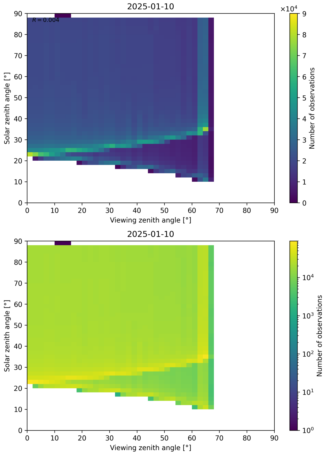
Figure 172: Scatter density plot of “Viewing zenith angle” against “Solar zenith angle” for 2025-01-09 to 2025-01-11.
