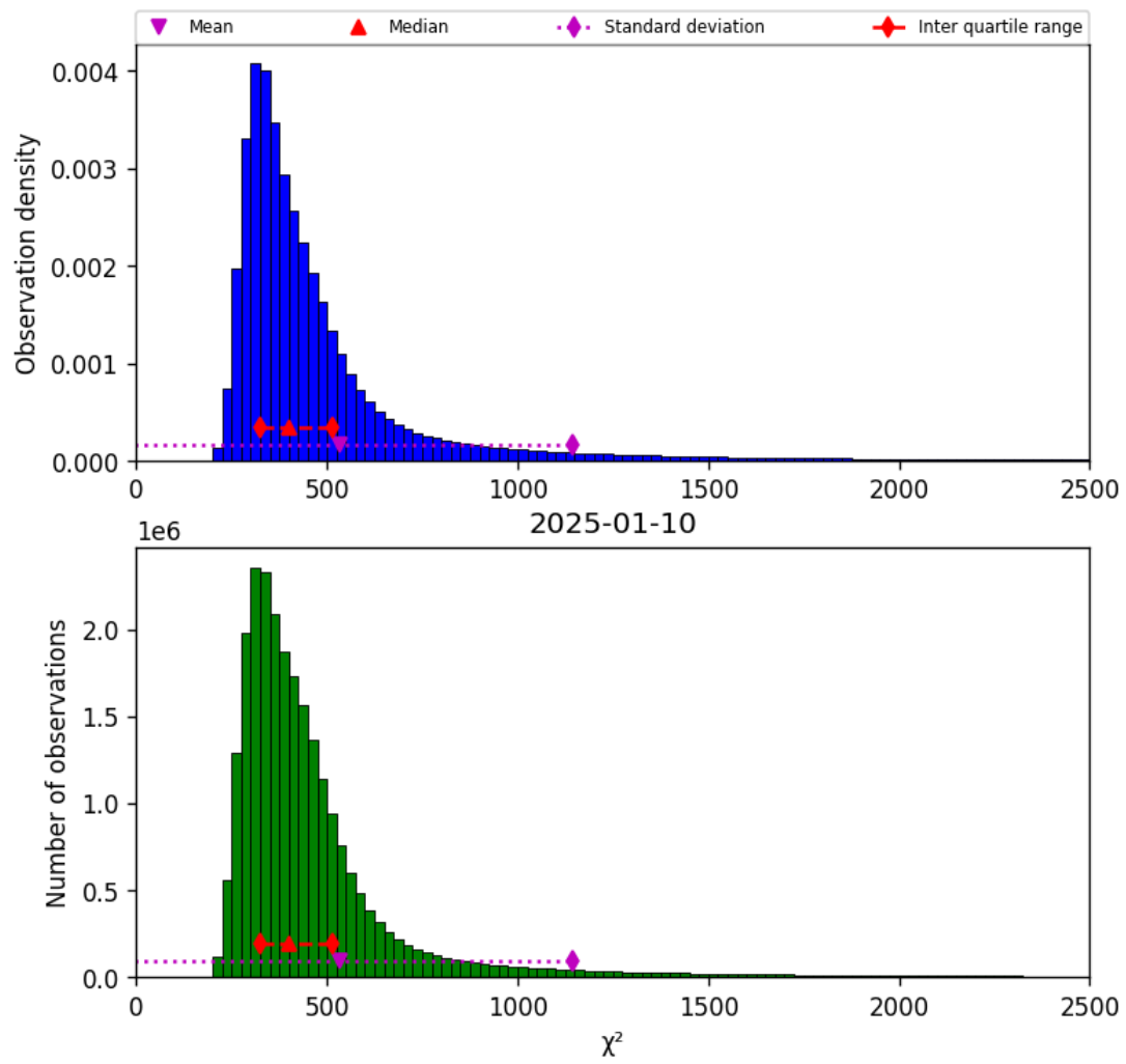
Figure 42: Histogram of “ \chi^2 ” for 2025-01-09 to 2025-01-11
