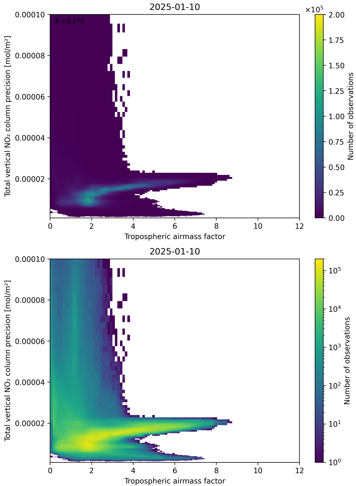
Figure 78: Scatter density plot of “Tropospheric air mass factor” against “Total vertical NO 2 column precision” for 2025-01-09 to 2025-01-11.
