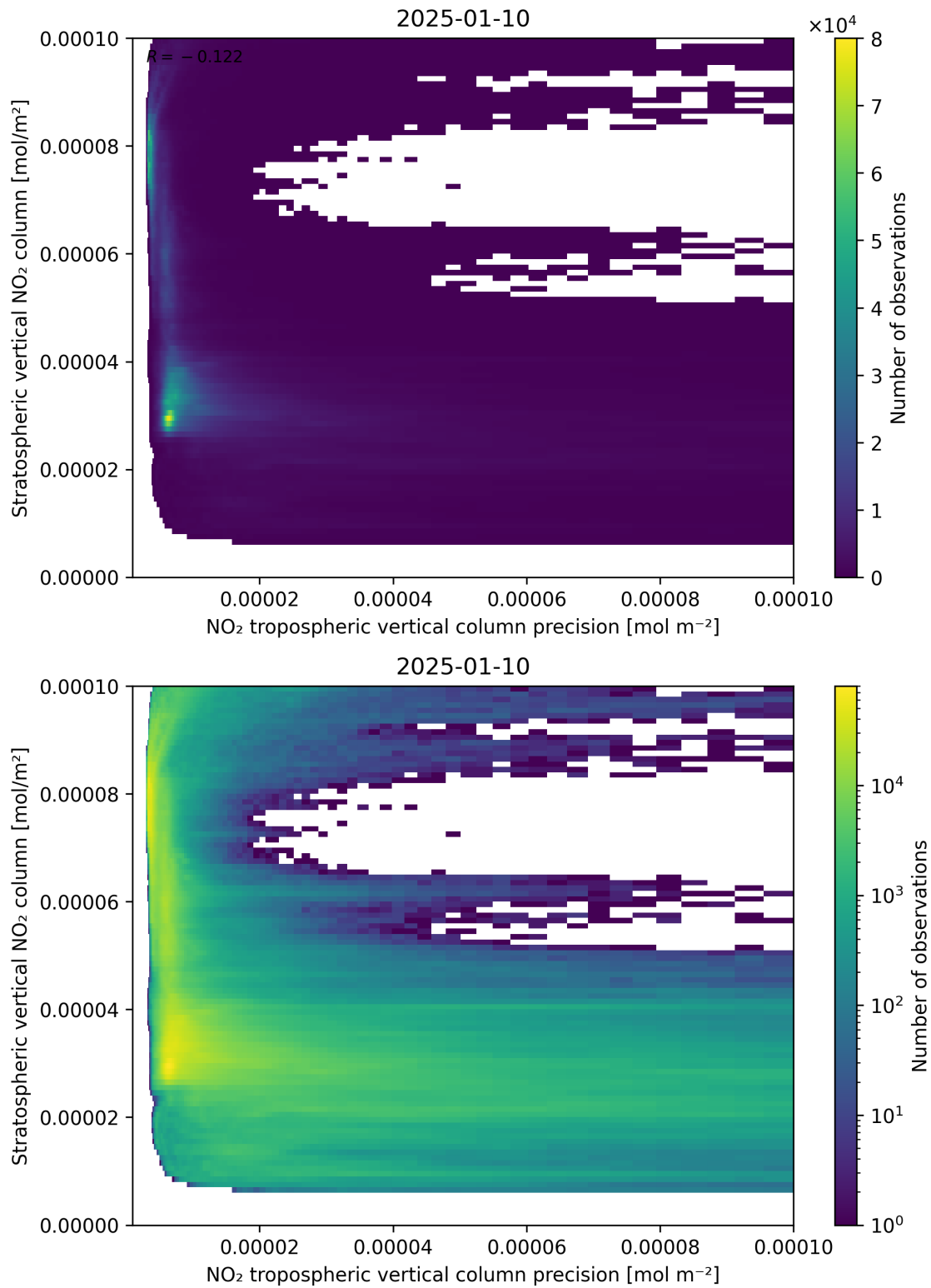
Figure 135: Scatter density plot of “NO 2 tropospheric vertical column precision” against “Stratospheric vertical NO 2 column” for 2025-01-09 to 2025-01-11.
