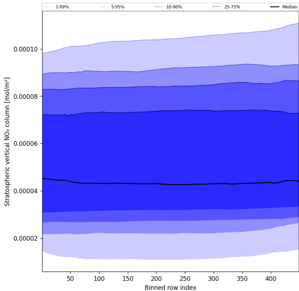
Figure 53: Along track statistics of “Stratospheric vertical NO 2 column” for 2025-01-09 to 2025-01-11
