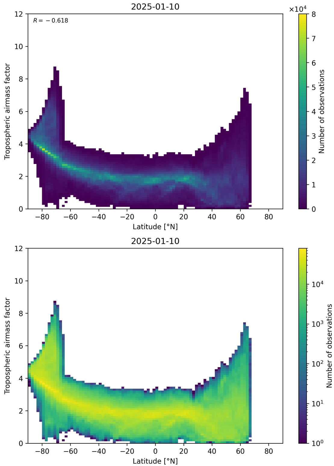
Figure 85: Scatter density plot of “Latitude” against “Tropospheric airmass factor” for 2025-01-09 to 2025-01-11.
