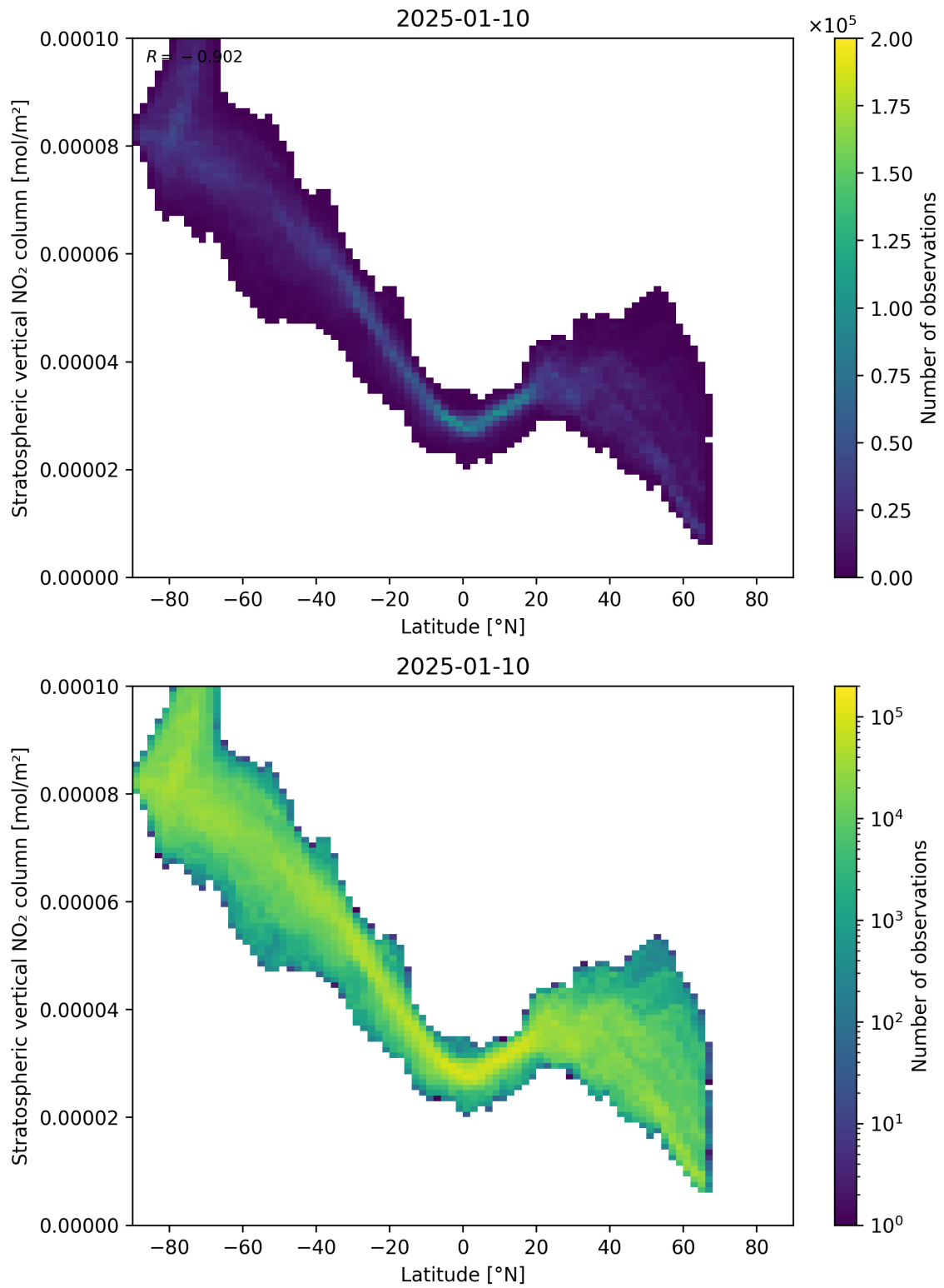
Figure 87: Scatter density plot of “Latitude” against “Stratospheric vertical NO 2 column” for 2025-01-09 to 2025-01-11.
