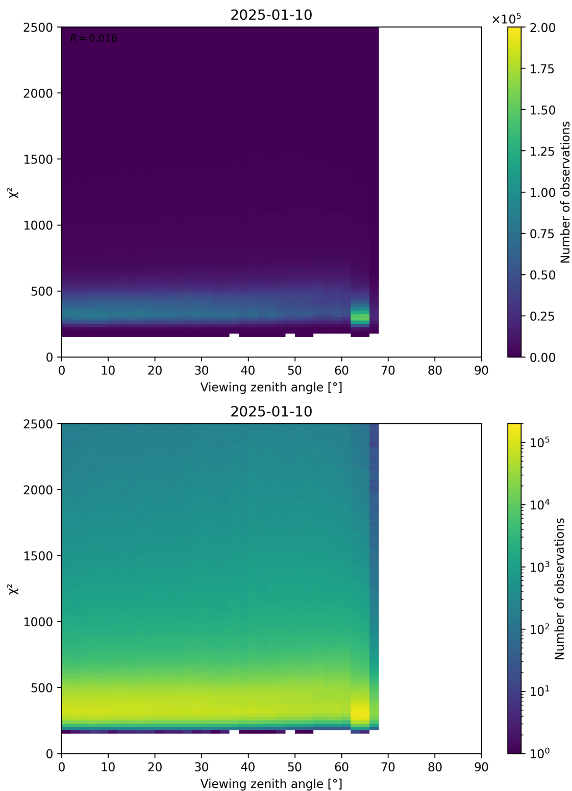
Figure 162: Scatter density plot of “Viewing zenith angle” against “ \chi^2 ” for 2025-01-09 to 2025-01-11.
