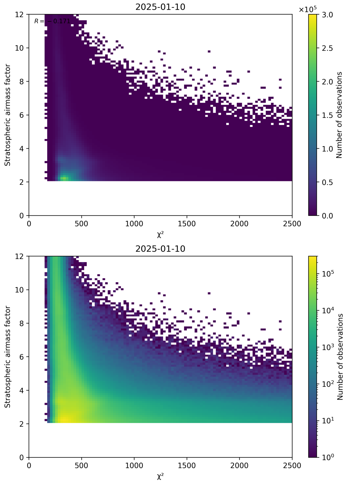
Figure 81: Scatter density plot of “ \chi^2 ” against “Stratospheric airmass factor” for 2025-01-09 to 2025-01-11.
