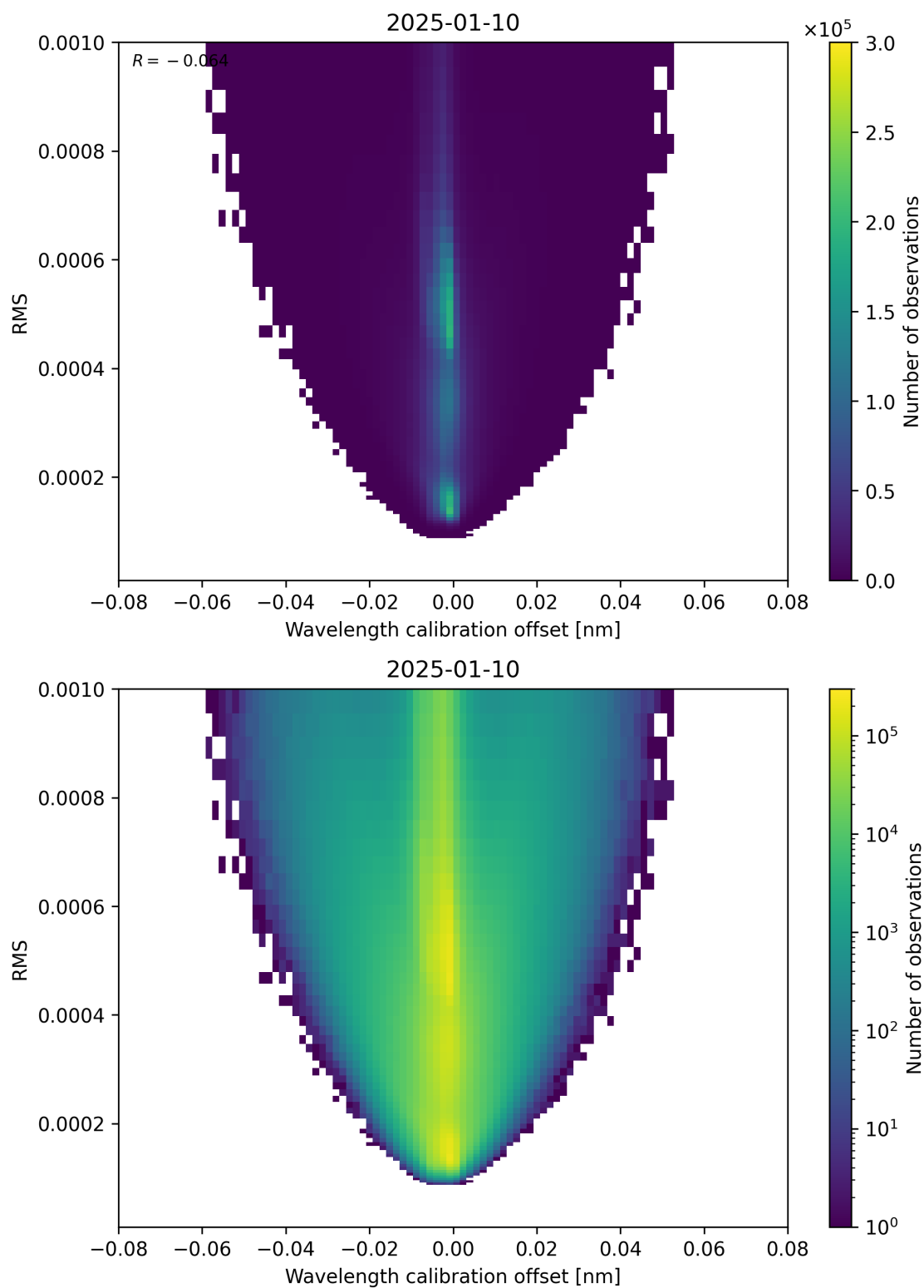
Figure 181: Scatter density plot of “Wavelength calibration offset” against “RMS” for 2025-01-09 to 2025-01-11.
