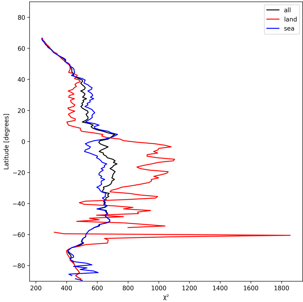
Figure 25: Zonal average of “ \chi^2 ” for 2025-01-09 to 2025-01-11.
