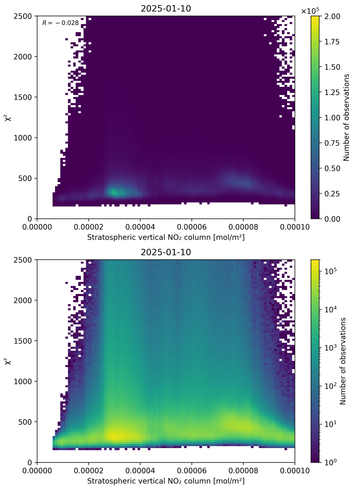
Figure 97: Scatter density plot of “Stratospheric vertical NO 2 column” against “ \chi^2 ” for 2025-01-09 to 2025-01-11.
