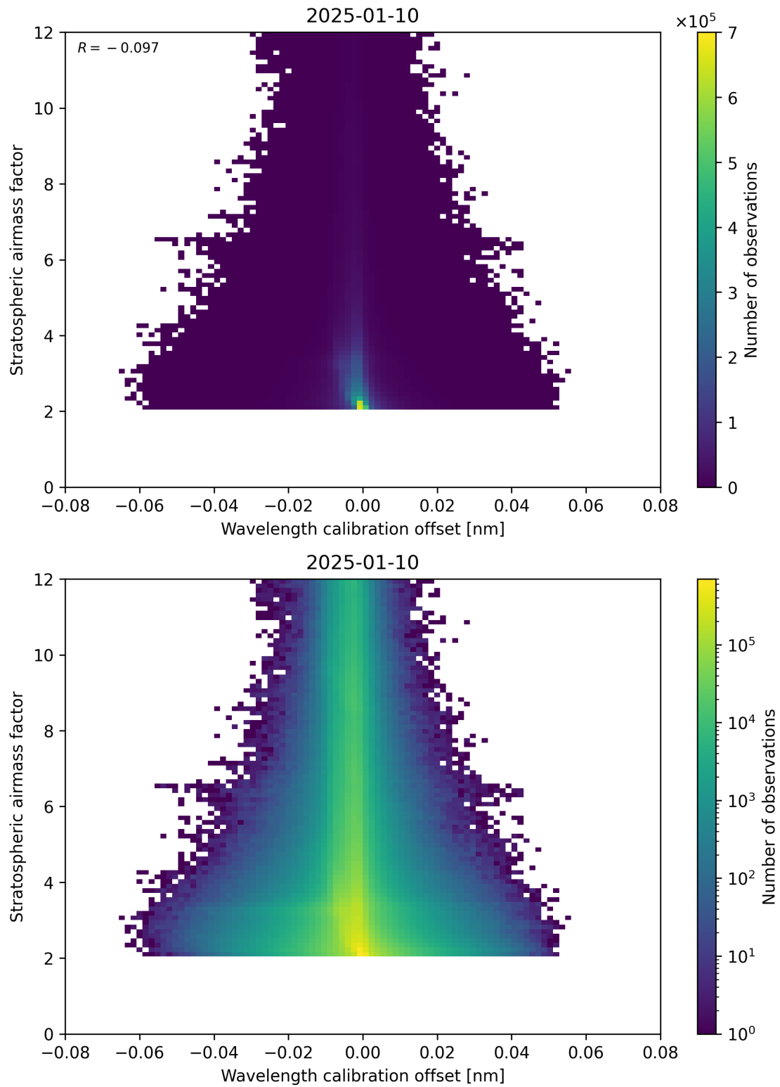
Figure 174: Scatter density plot of “Wavelength calibration offset” against “Stratospheric airmass factor” for 2025-01-09 to 2025-01-11.
