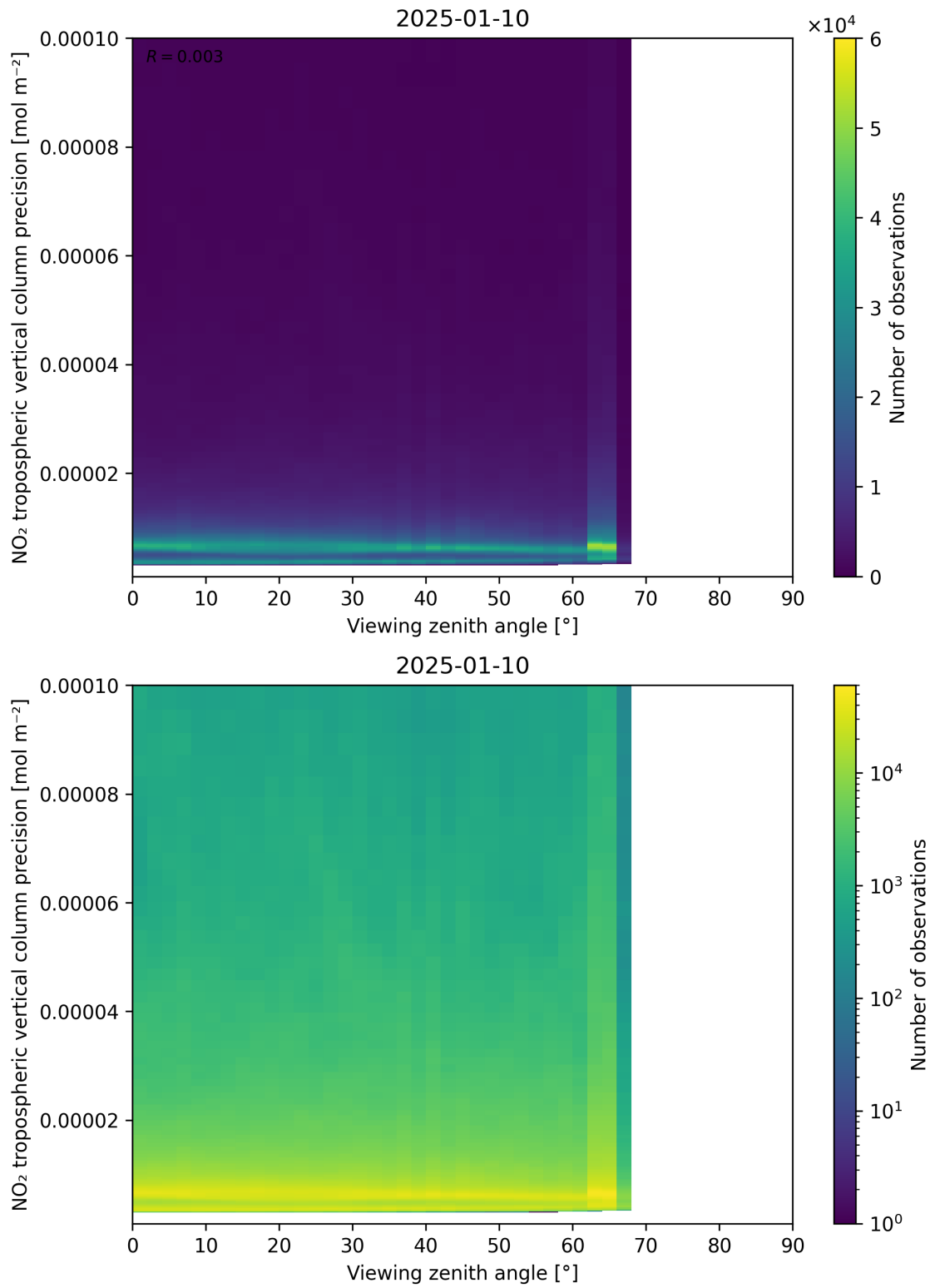
Figure 170: Scatter density plot of “Viewing zenith angle” against “NO 2 tropospheric vertical column precision” for 2025-01-09 to 2025-01-11.
