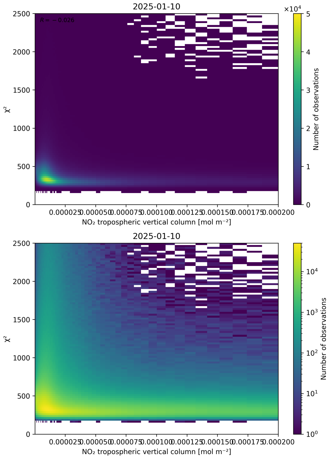
Figure 124: Scatter density plot of “NO 2 tropospheric vertical column” against “ \chi^2 ” for 2025-01-09 to 2025-01-11.
