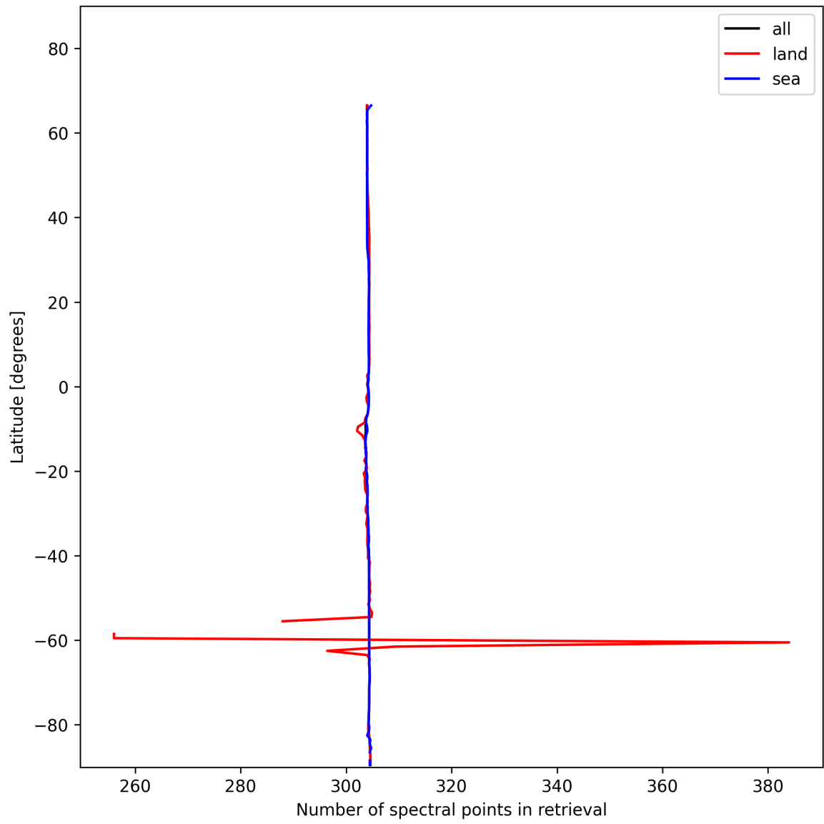
Figure 16: Zonal average of “Number of spectral points in retrieval” for 2025-01-09 to 2025-01-11.
