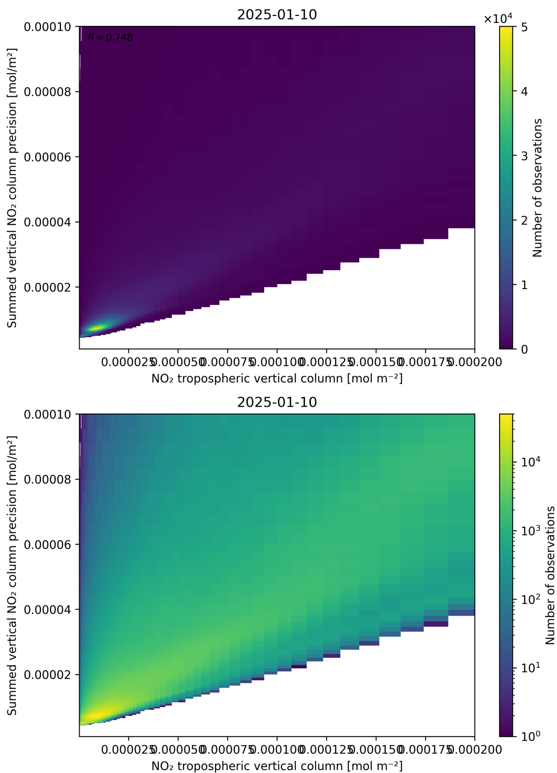
Figure 127: Scatter density plot of “NO 2 tropospheric vertical column” against “Summed vertical NO 2 column precision” for 2025-01-09 to 2025-01-11.
