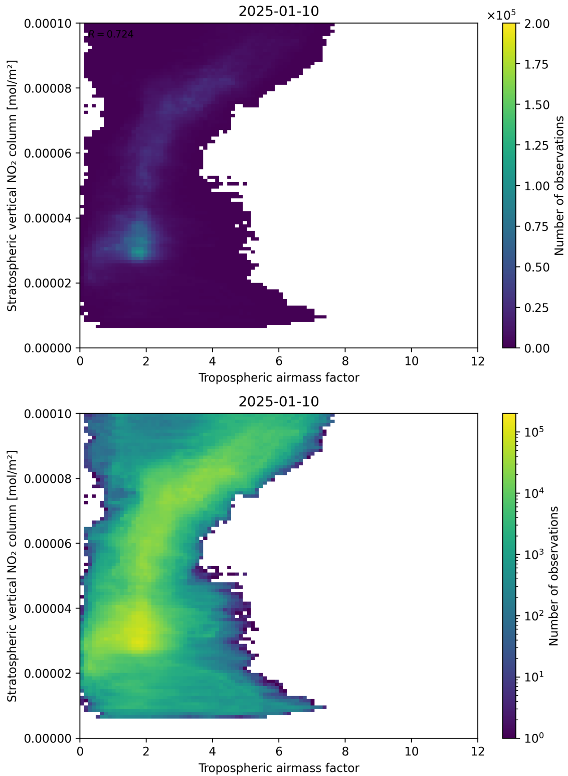
Figure 74: Scatter density plot of “Tropospheric air mass factor” against “Stratospheric vertical NO 2 column” for 2025-01-09 to 2025-01-11.
