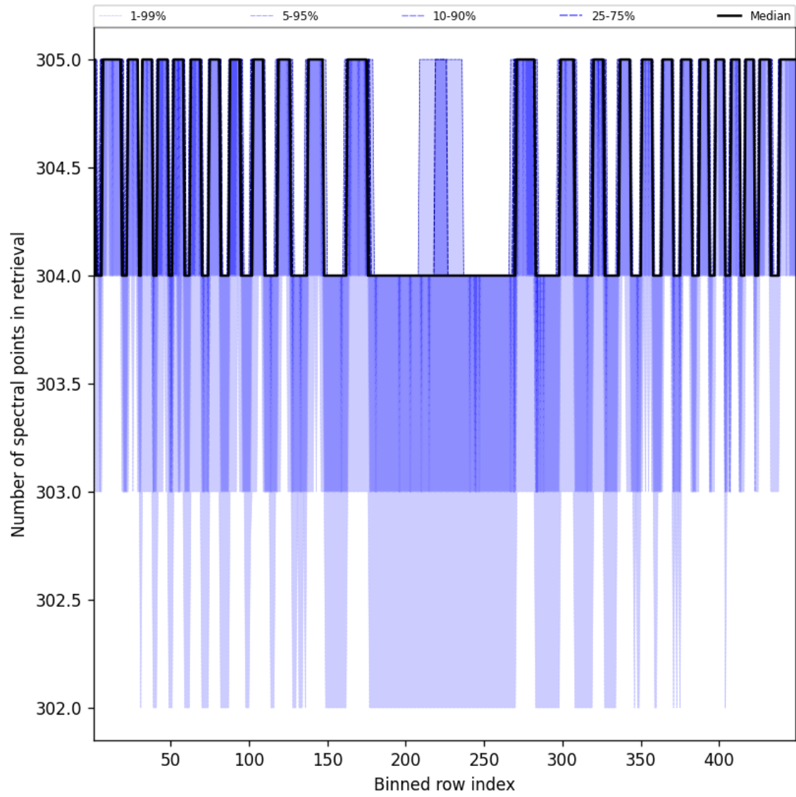
Figure 50: Along track statistics of “Number of spectral points in retrieval” for 2025-01-09 to 2025-01-11
