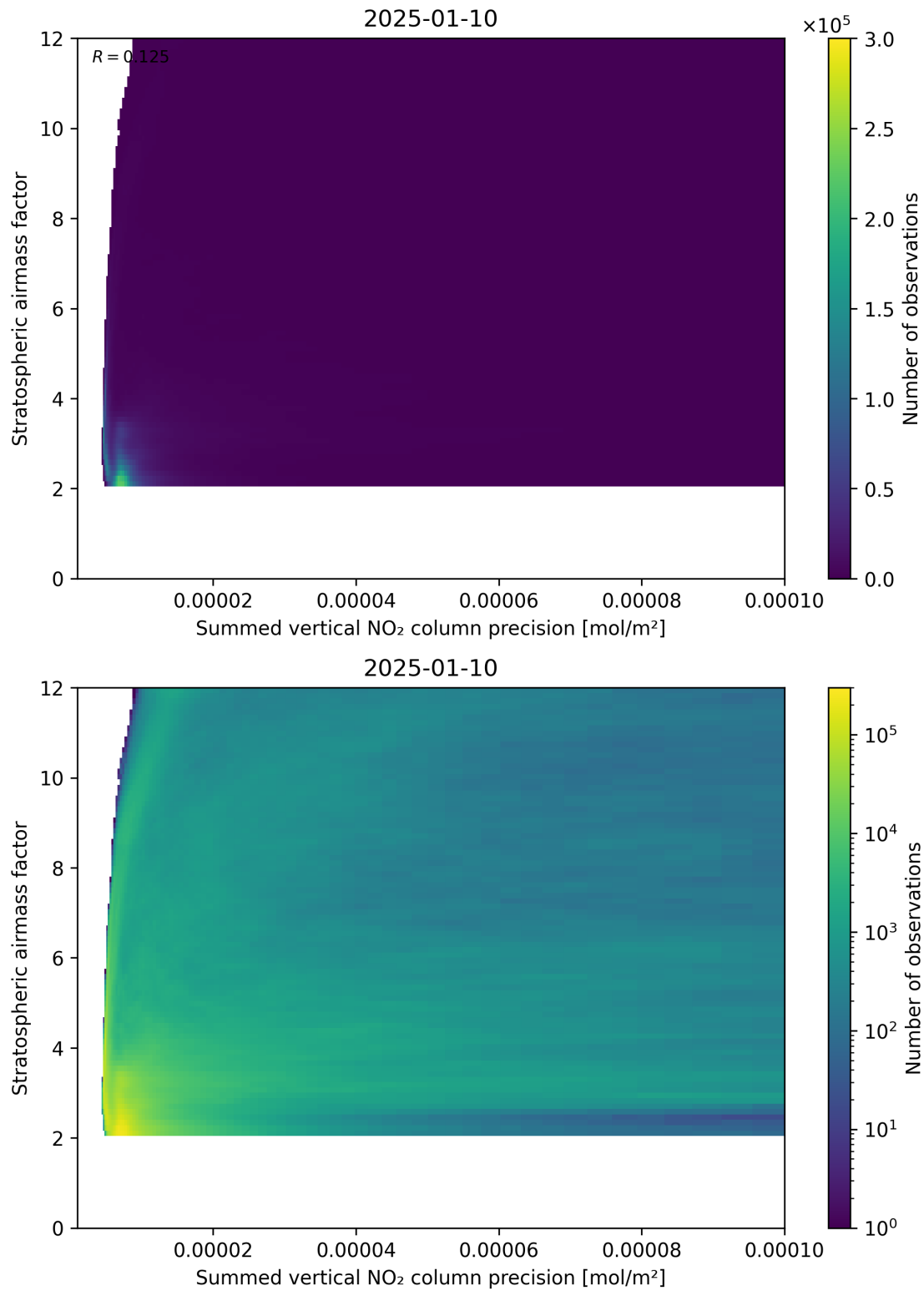
Figure 106: Scatter density plot of “Summed vertical NO 2 column precision” against “Stratospheric airmass factor” for 2025-01-09 to 2025-01-11.
