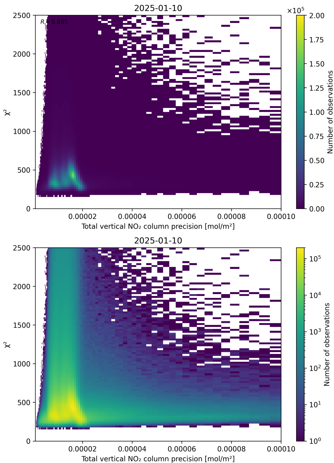
Figure 116: Scatter density plot of “Total vertical NO 2 column precision” against “ \chi^2 ” for 2025-01-09 to 2025-01-11.
