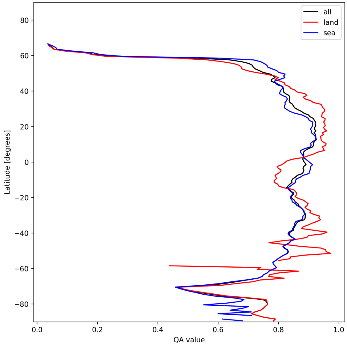
Figure 11: Zonal average of “QA value” for 2025-01-09 to 2025-01-11.
