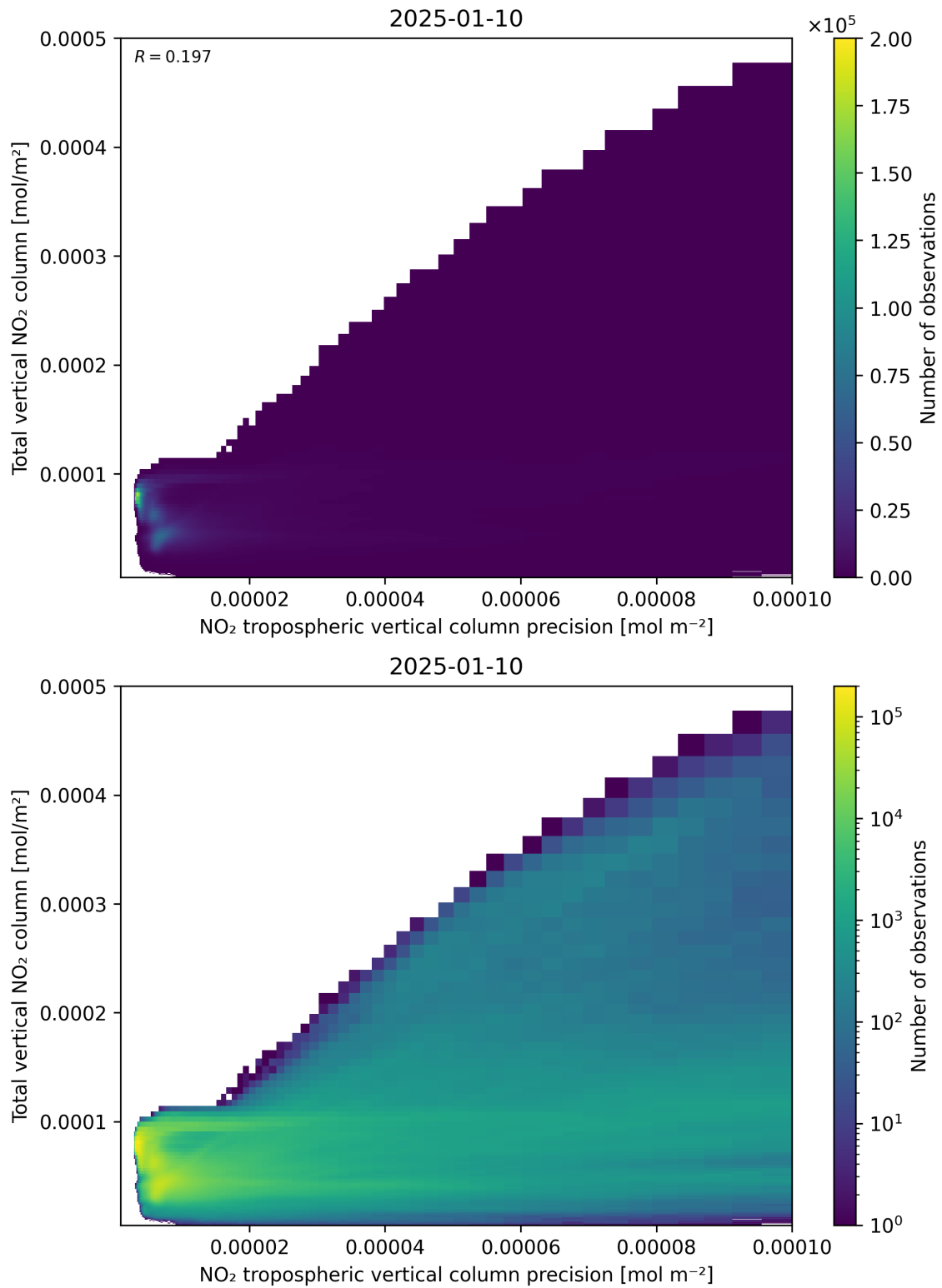
Figure 138: Scatter density plot of “NO 2 tropospheric vertical column precision” against “Total vertical NO 2 column” for 2025-01-09 to 2025-01-11.
