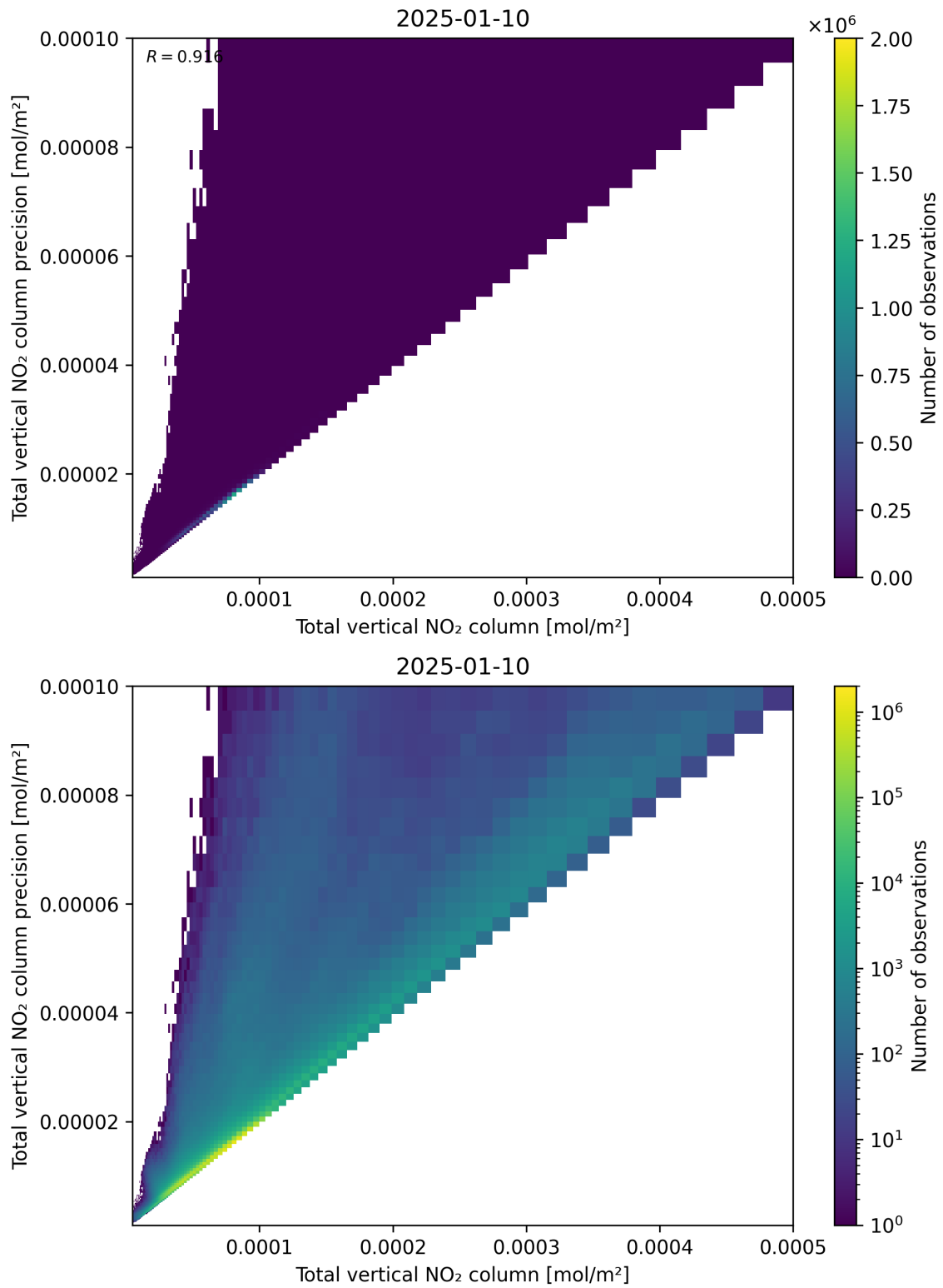
Figure 114: Scatter density plot of “Total vertical NO 2 column” against “Total vertical NO 2 column precision” for 2025-01-09 to 2025-01-11.
