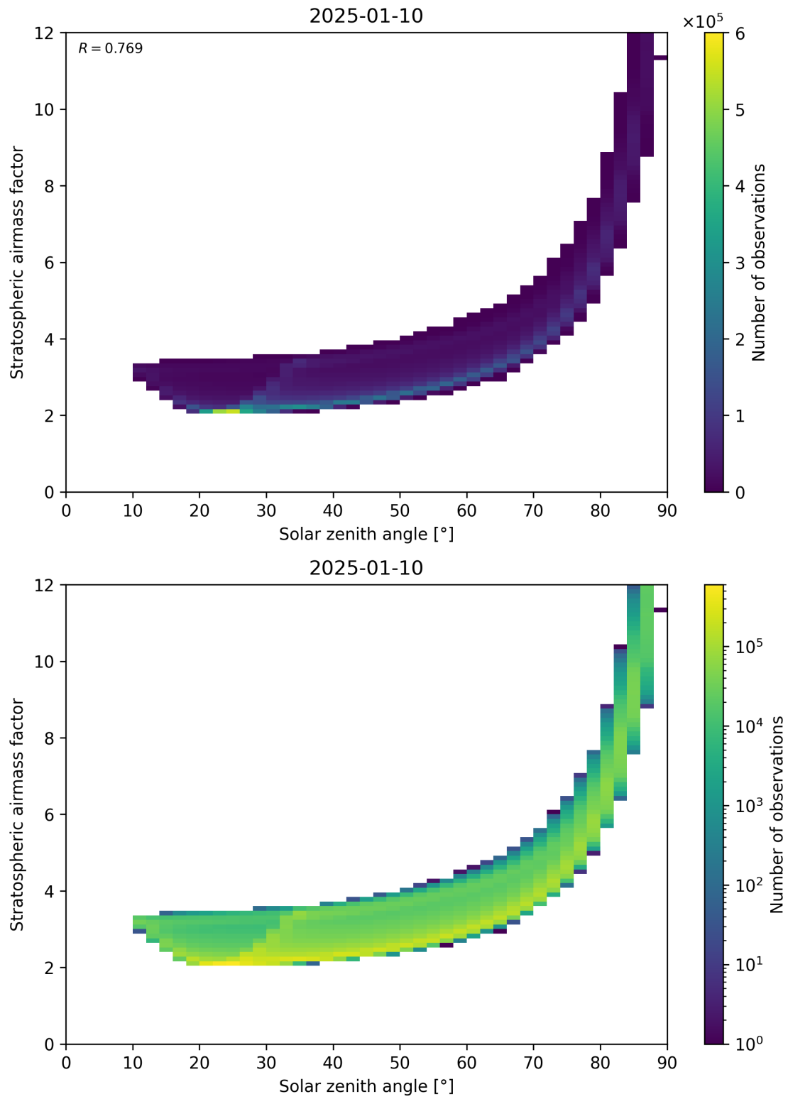
Figure 145: Scatter density plot of “Solar zenith angle” against “Stratospheric airmass factor” for 2025-01-09 to 2025-01-11.
