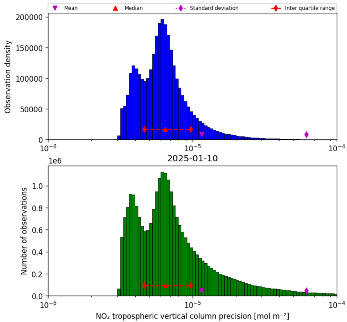
Figure 30: Histogram of “NO 2 tropospheric vertical column precision” for 2025-01-09 to 2025-01-11
