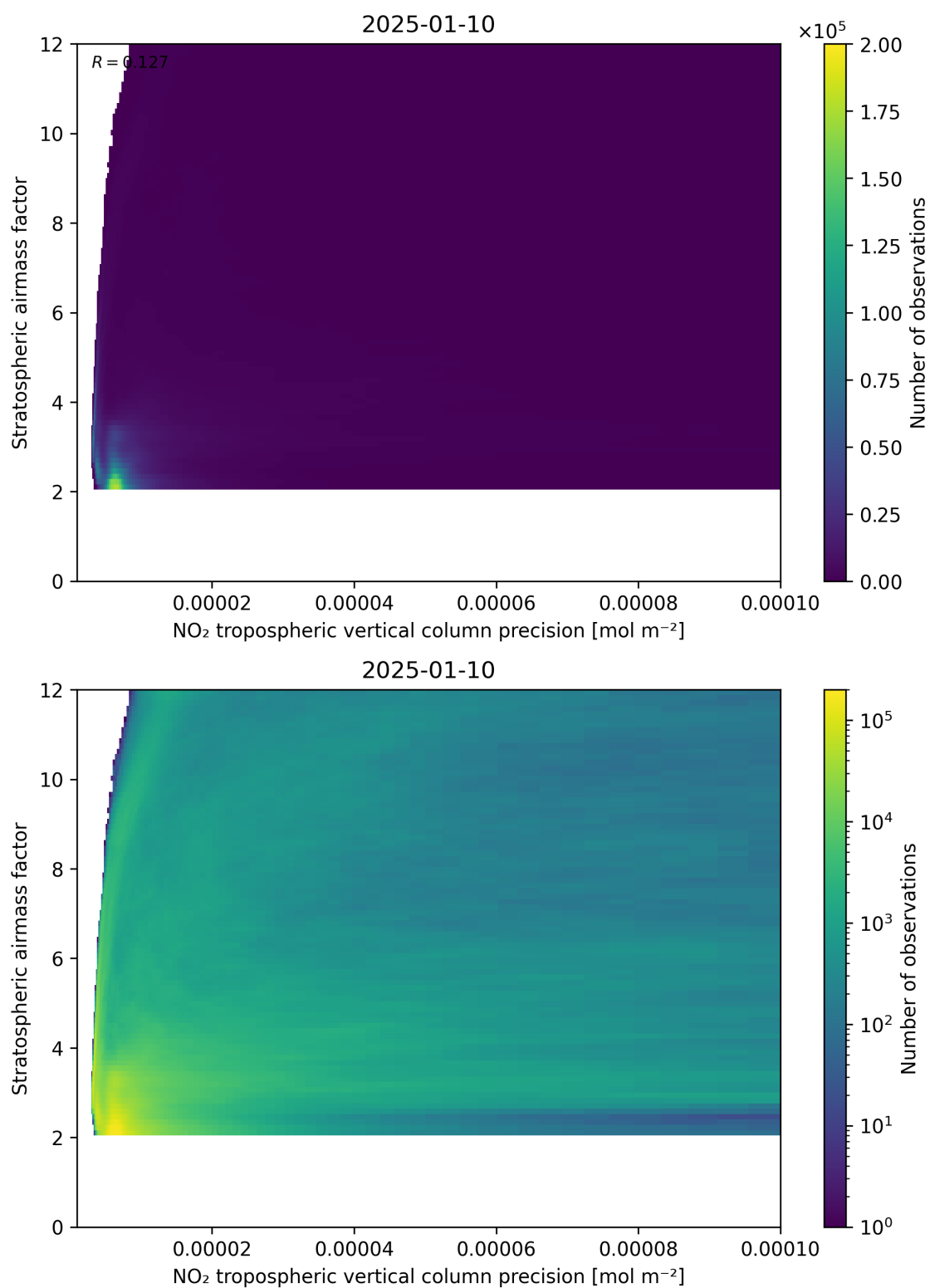
Figure 131: Scatter density plot of “NO 2 tropospheric vertical column precision” against “Stratospheric airmass factor” for 2025-01-09 to 2025-01-11.
