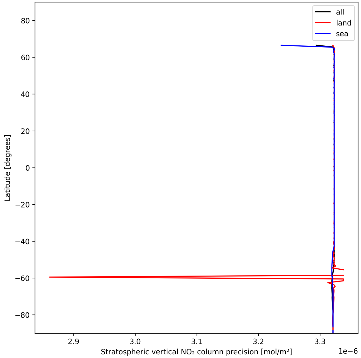
Figure 20: Zonal average of “Stratospheric vertical NO 2 column precision” for 2025-01-09 to 2025-01-11.
