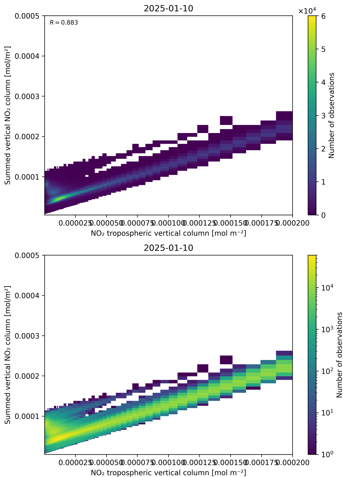
Figure 126: Scatter density plot of “NO 2 tropospheric vertical column” against “Summed vertical NO 2 column” for 2025-01-09 to 2025-01-11.
