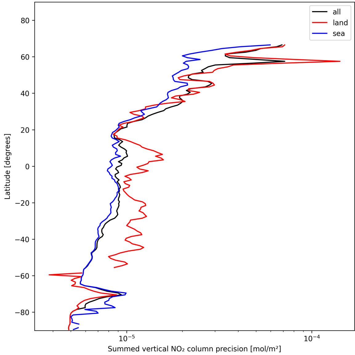
Figure 24: Zonal average of “Summed vertical NO 2 column precision” for 2025-01-09 to 2025-01-11.
