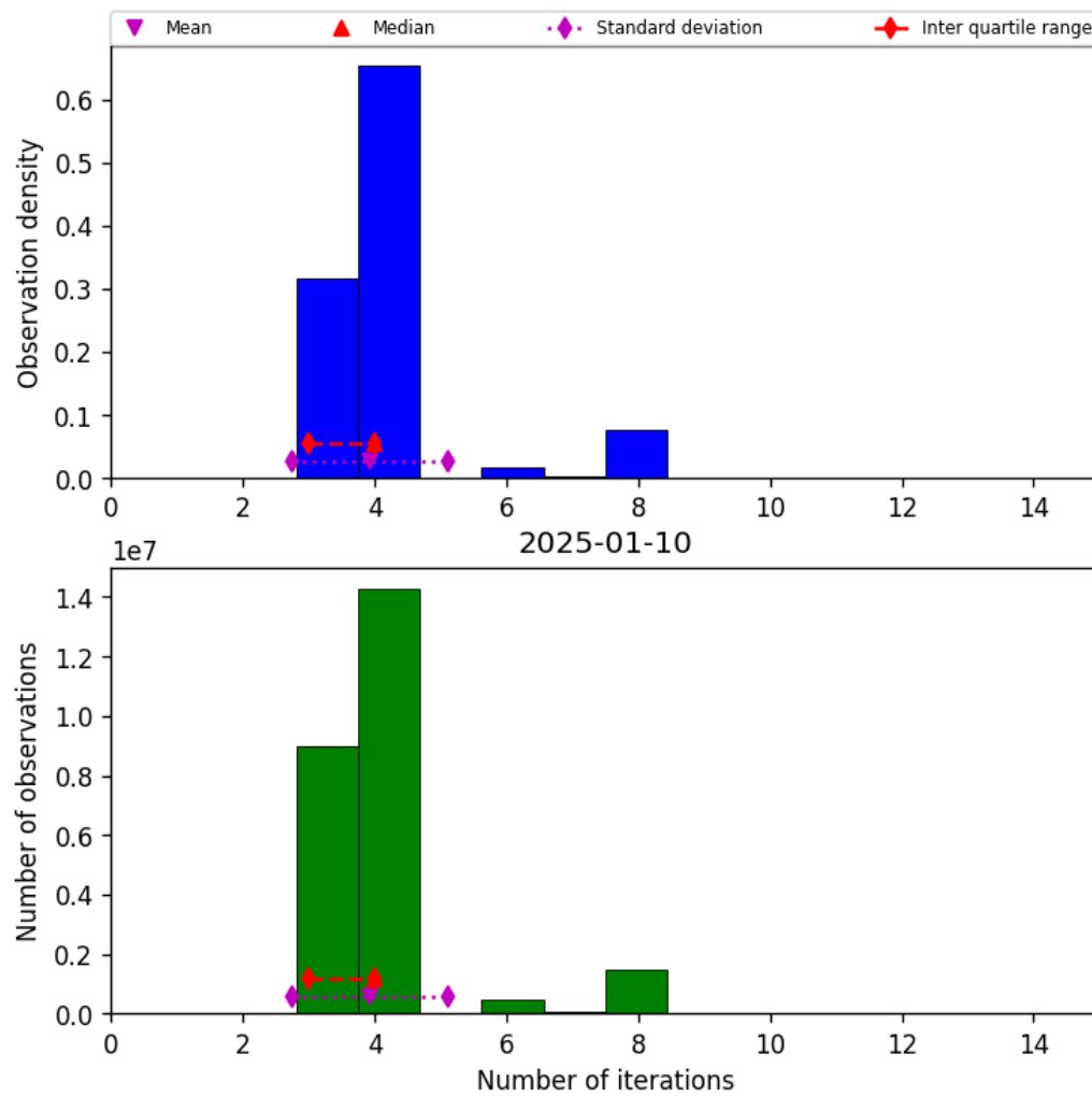
Figure 34: Histogram of “Number of iterations” for 2025-01-09 to 2025-01-11
