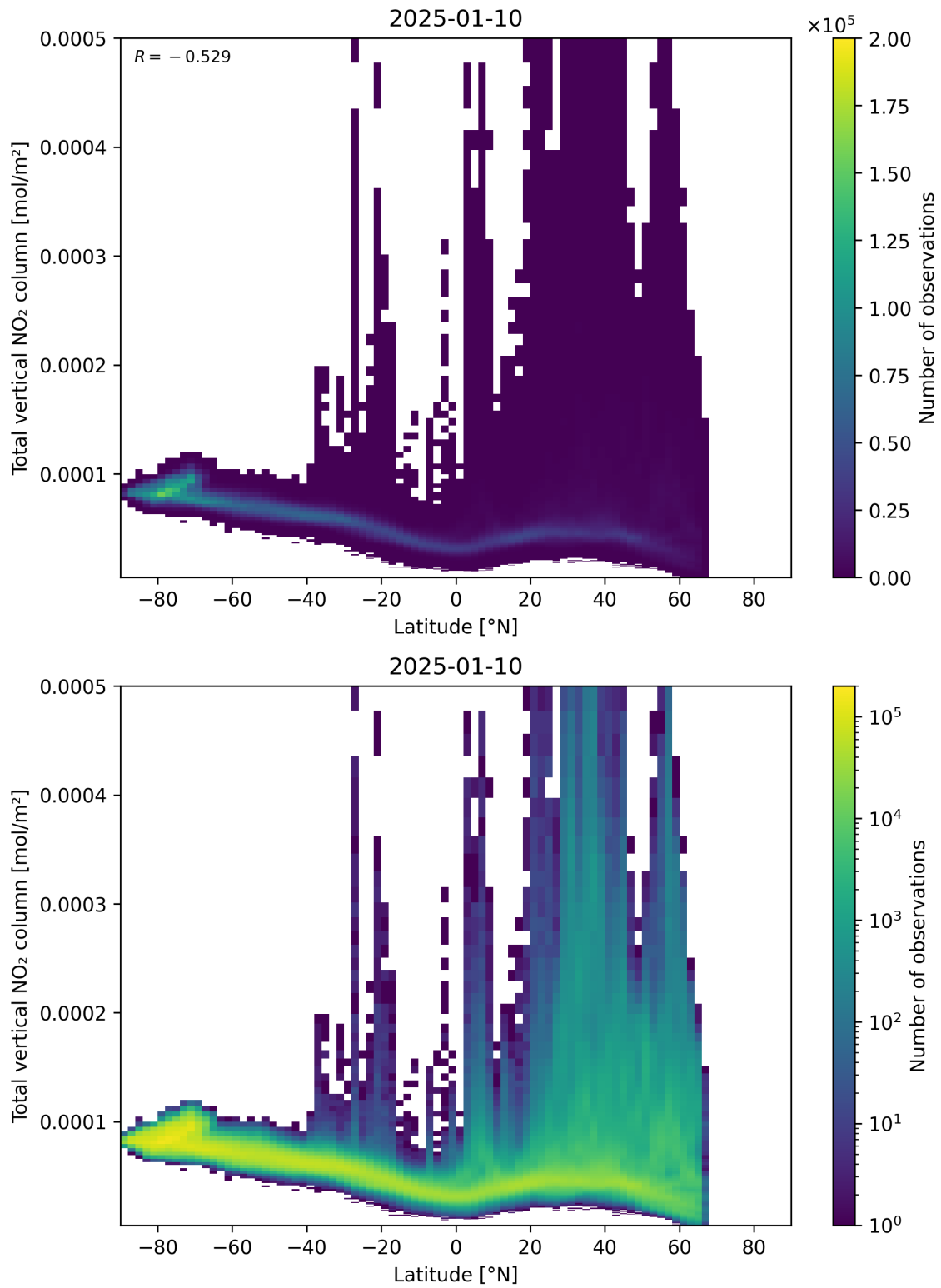
Figure 90: Scatter density plot of “Latitude” against “Total vertical NO 2 column” for 2025-01-09 to 2025-01-11.
