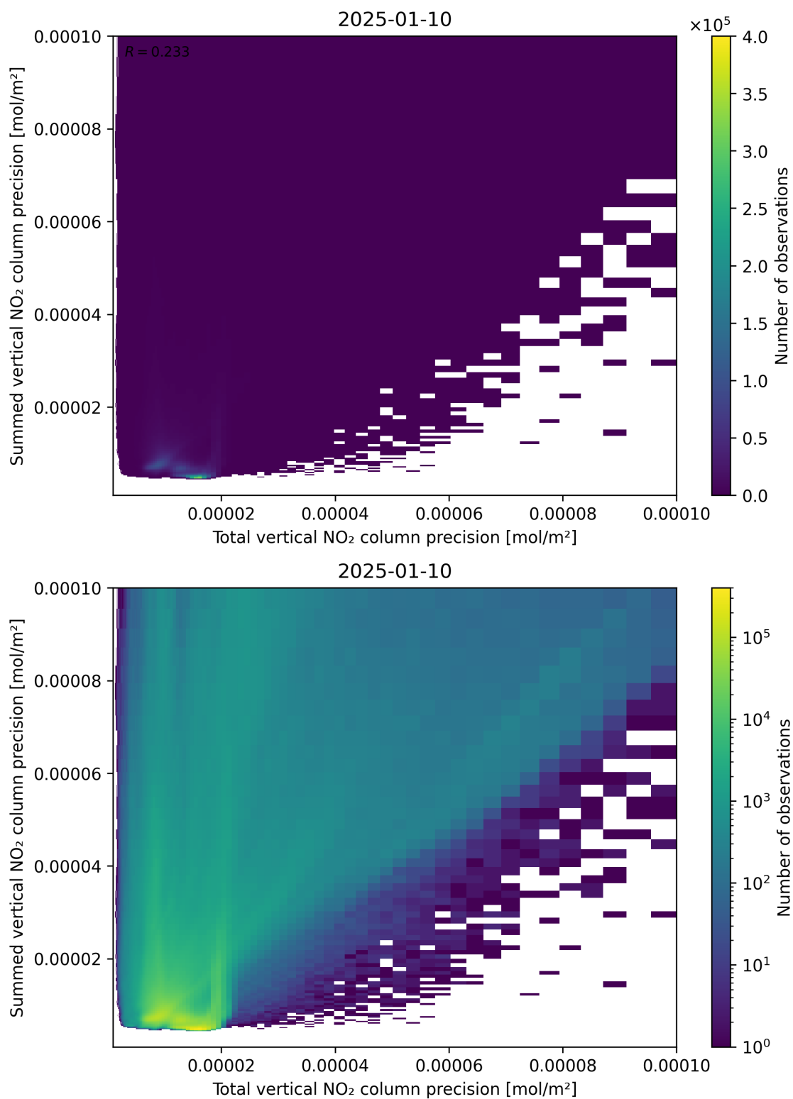
Figure 118: Scatter density plot of “Total vertical NO 2 column precision” against “Summed vertical NO 2 column precision” for 2025-01-09 to 2025-01-11.
