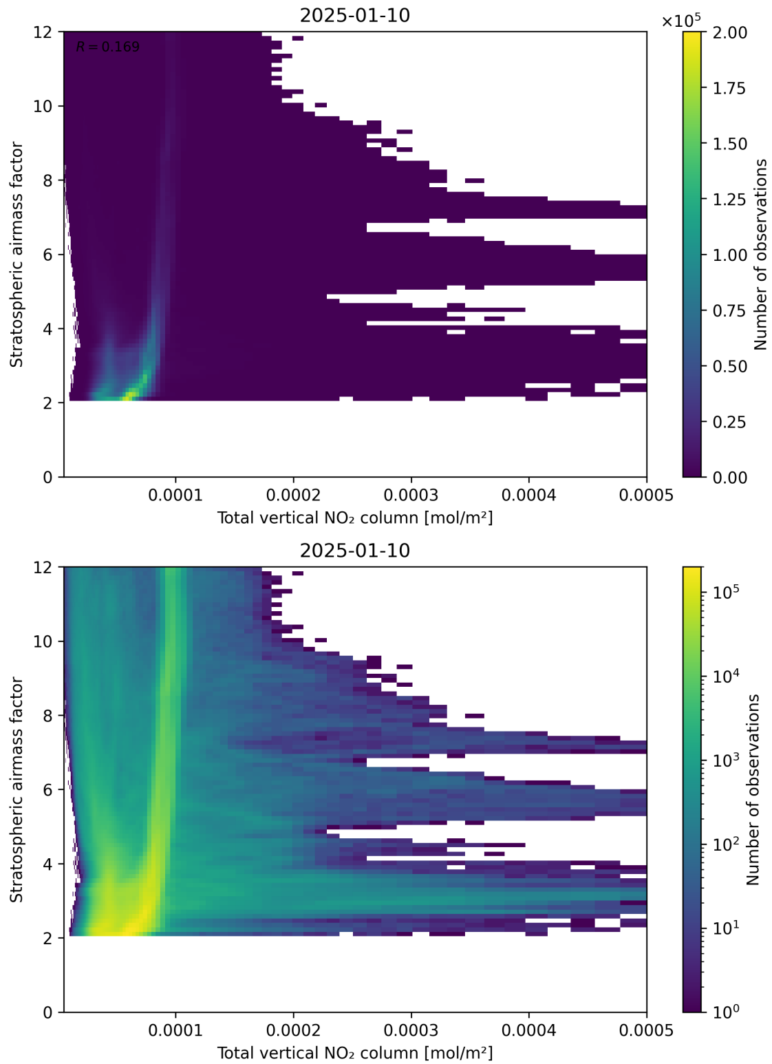
Figure 110: Scatter density plot of “Total vertical NO 2 column” against “Stratospheric airmass factor” for 2025-01-09 to 2025-01-11.
