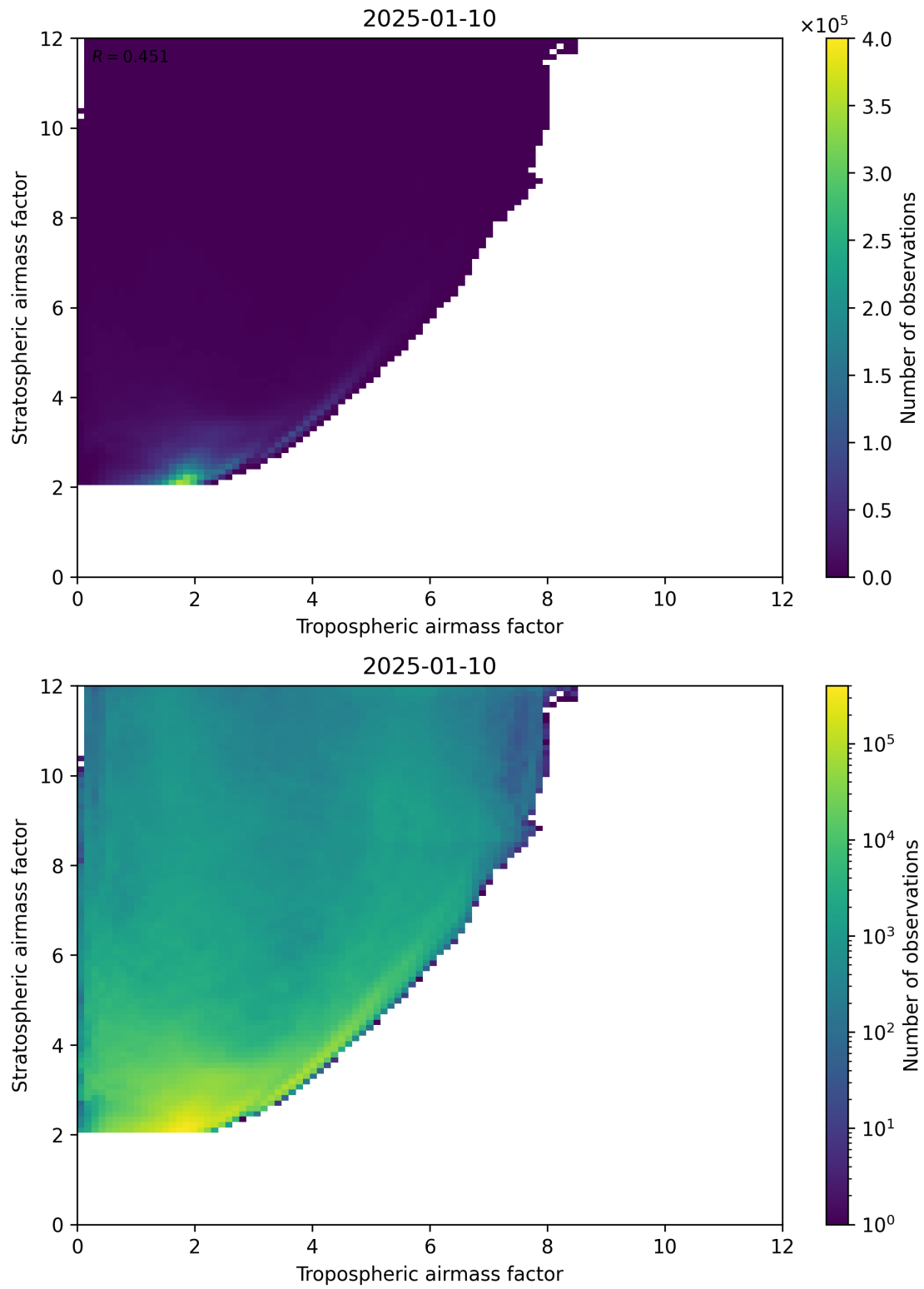
Figure 71: Scatter density plot of “Tropospheric airmass factor” against “Stratospheric airmass factor” for 2025-01-09 to 2025-01-11.
