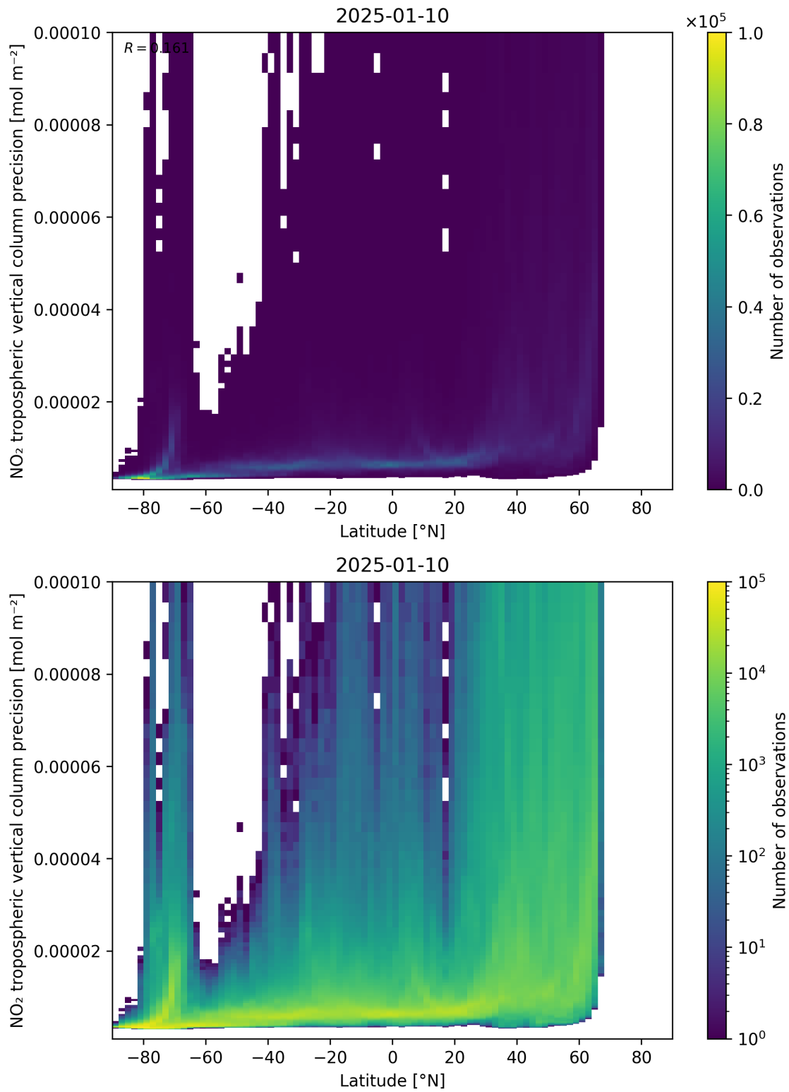
Figure 93: Scatter density plot of “Latitude” against “NO 2 tropospheric vertical column precision” for 2025-01-09 to 2025-01-11.
