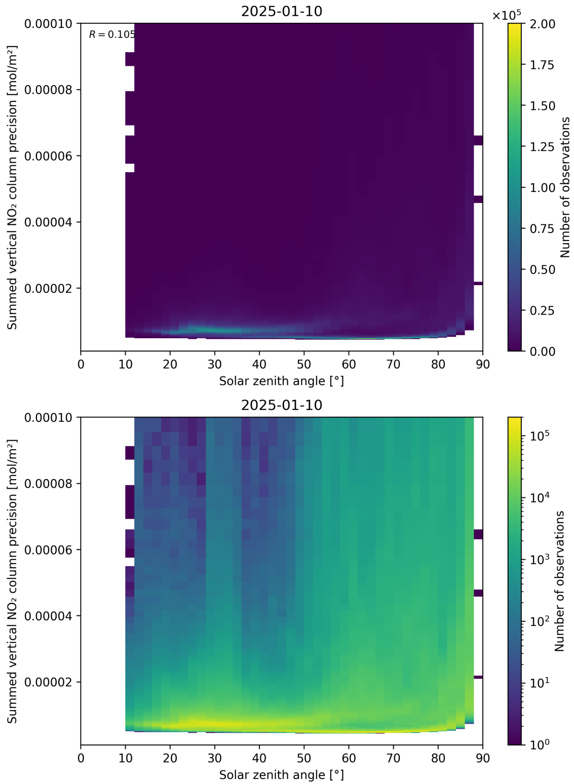
Figure 152: Scatter density plot of “Solar zenith angle” against “Summed vertical NO 2 column precision” for 2025-01-09 to 2025-01-11.
