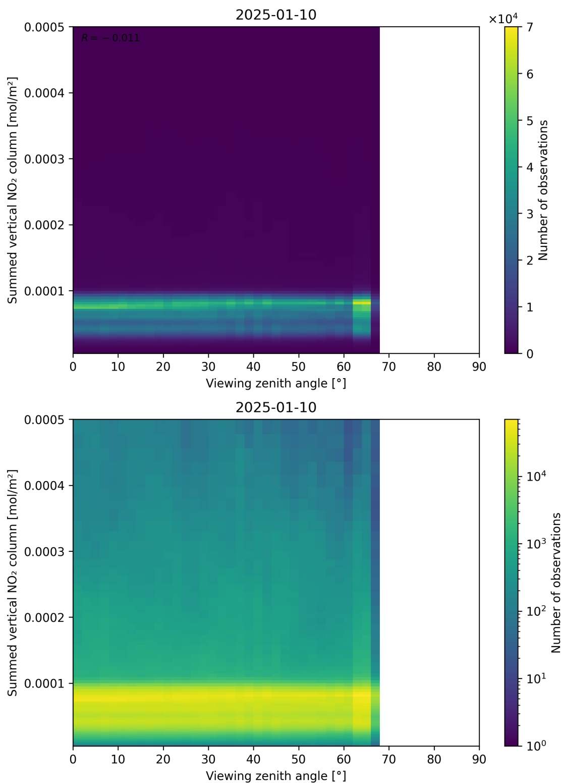
Figure 165: Scatter density plot of “Viewing zenith angle” against “Summed vertical NO 2 column” for 2025-01-09 to 2025-01-11.
