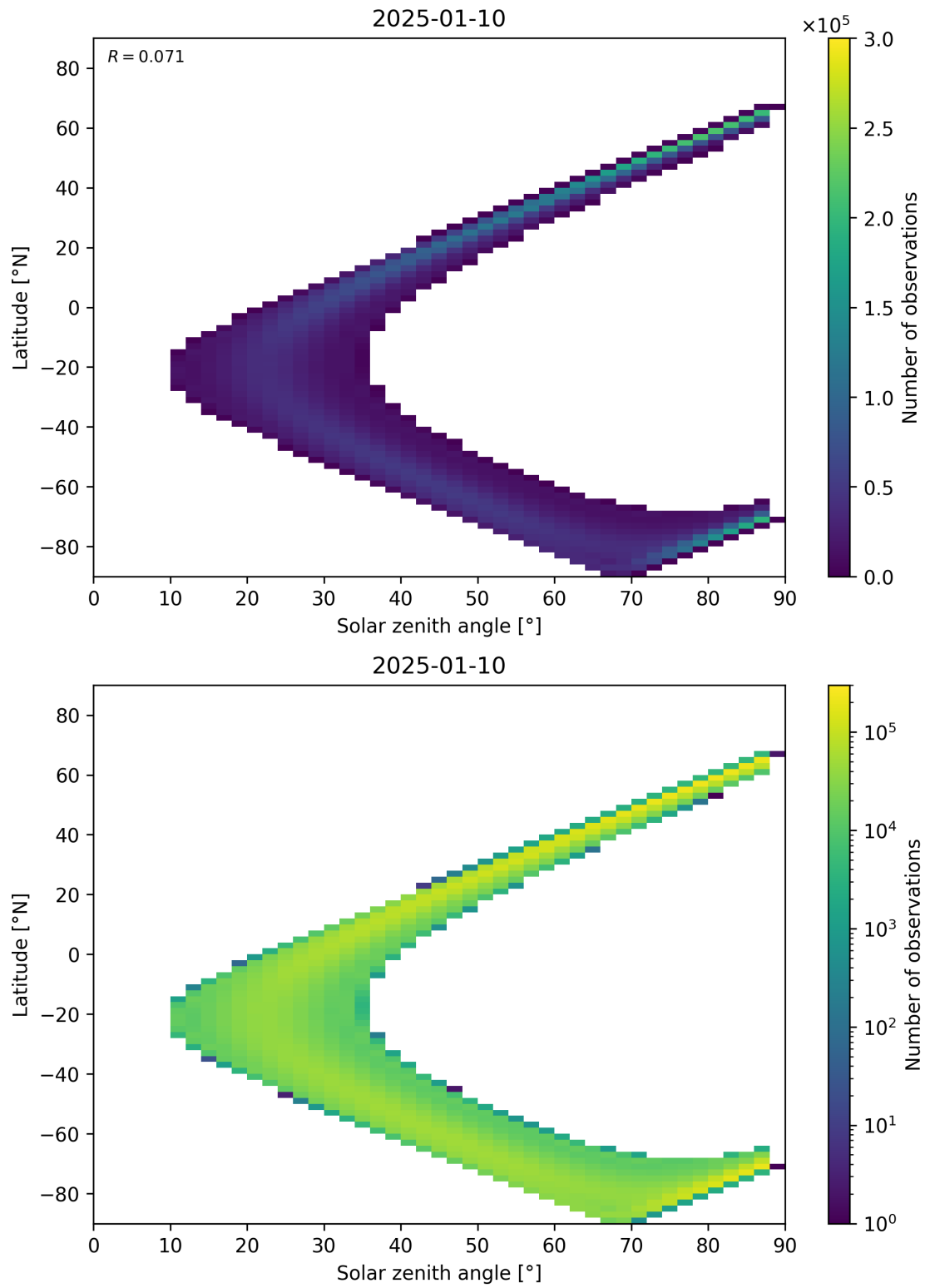
Figure 149: Scatter density plot of “Solar zenith angle” against “Latitude” for 2025-01-09 to 2025-01-11.
