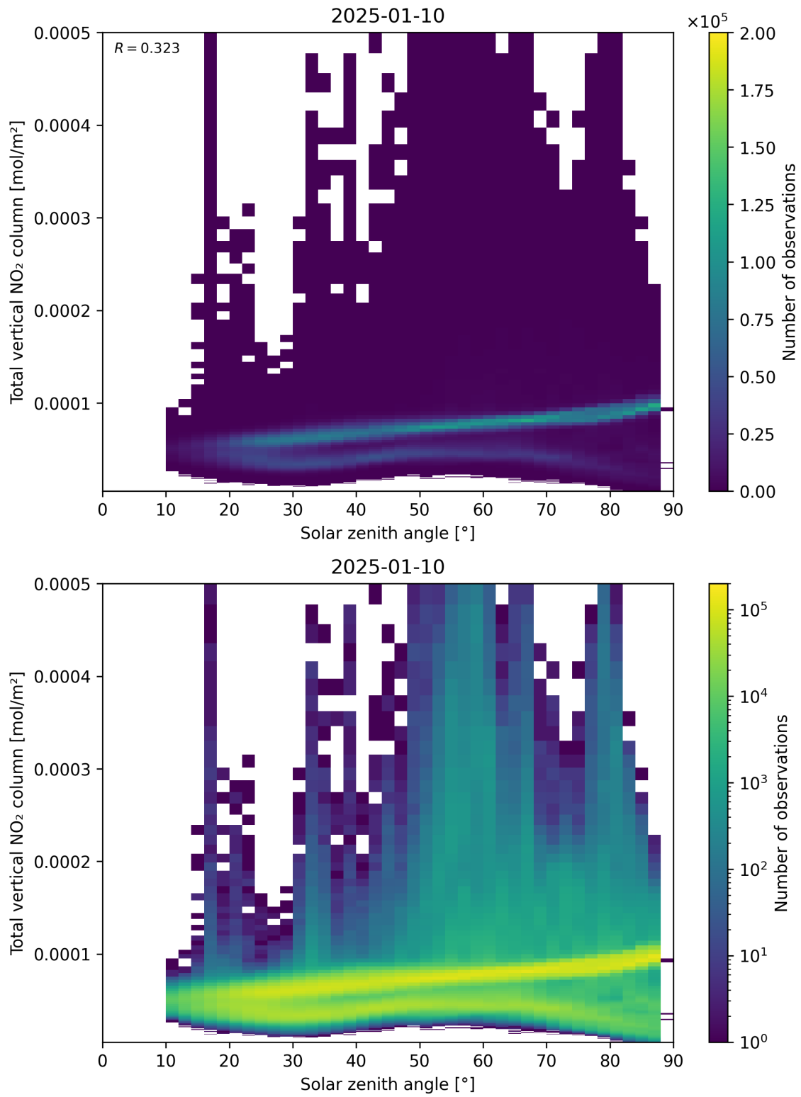
Figure 153: Scatter density plot of “Solar zenith angle” against “Total vertical NO 2 column” for 2025-01-09 to 2025-01-11.
