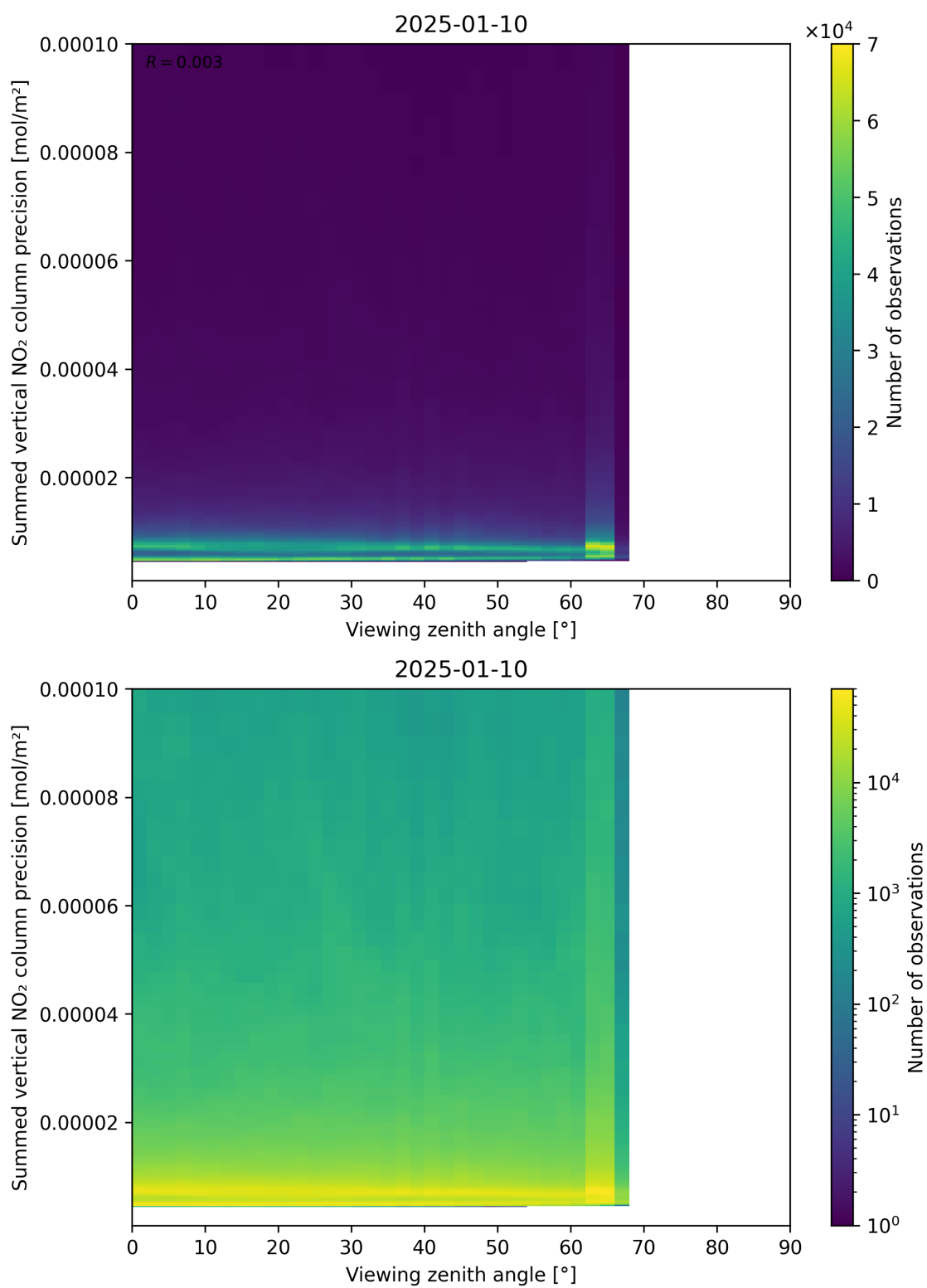
Figure 166: Scatter density plot of “Viewing zenith angle” against “Summed vertical NO 2 column precision” for 2025-01-09 to 2025-01-11.
