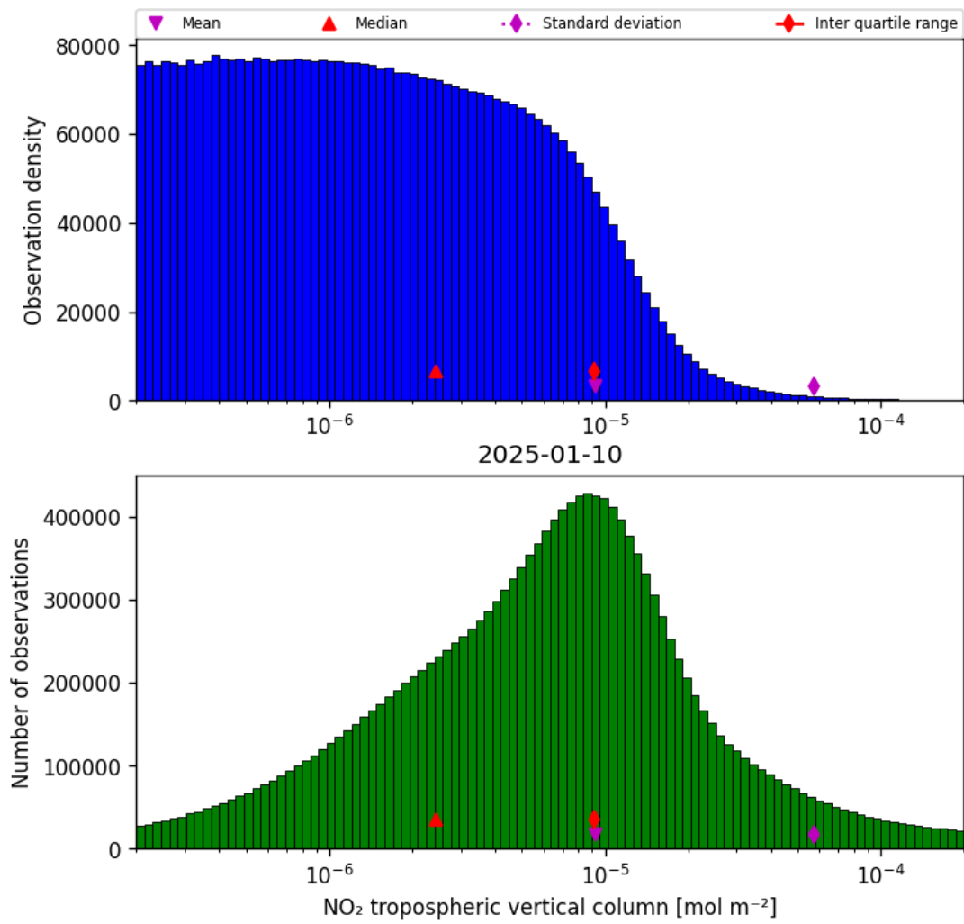
Figure 29: Histogram of “NO 2 tropospheric vertical column” for 2025-01-09 to 2025-01-11
