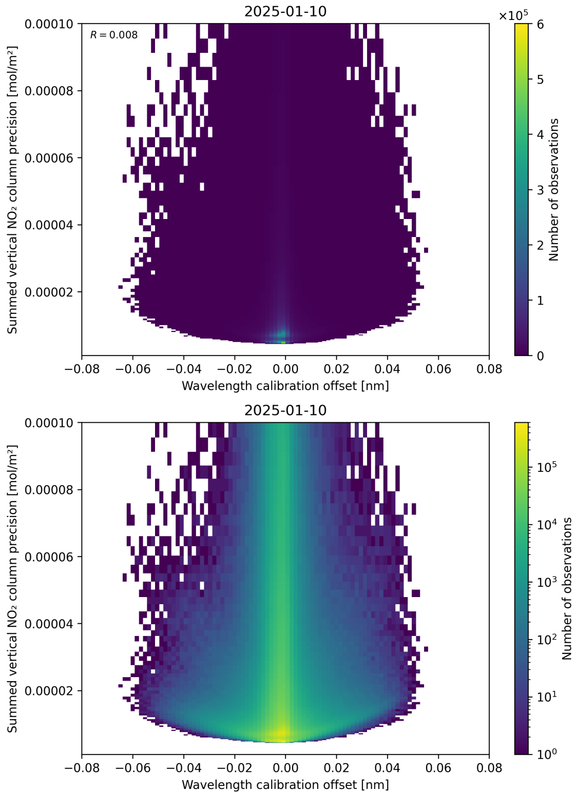
Figure 178: Scatter density plot of “Wavelength calibration offset” against “Summed vertical NO 2 column precision” for 2025-01-09 to 2025-01-11.
