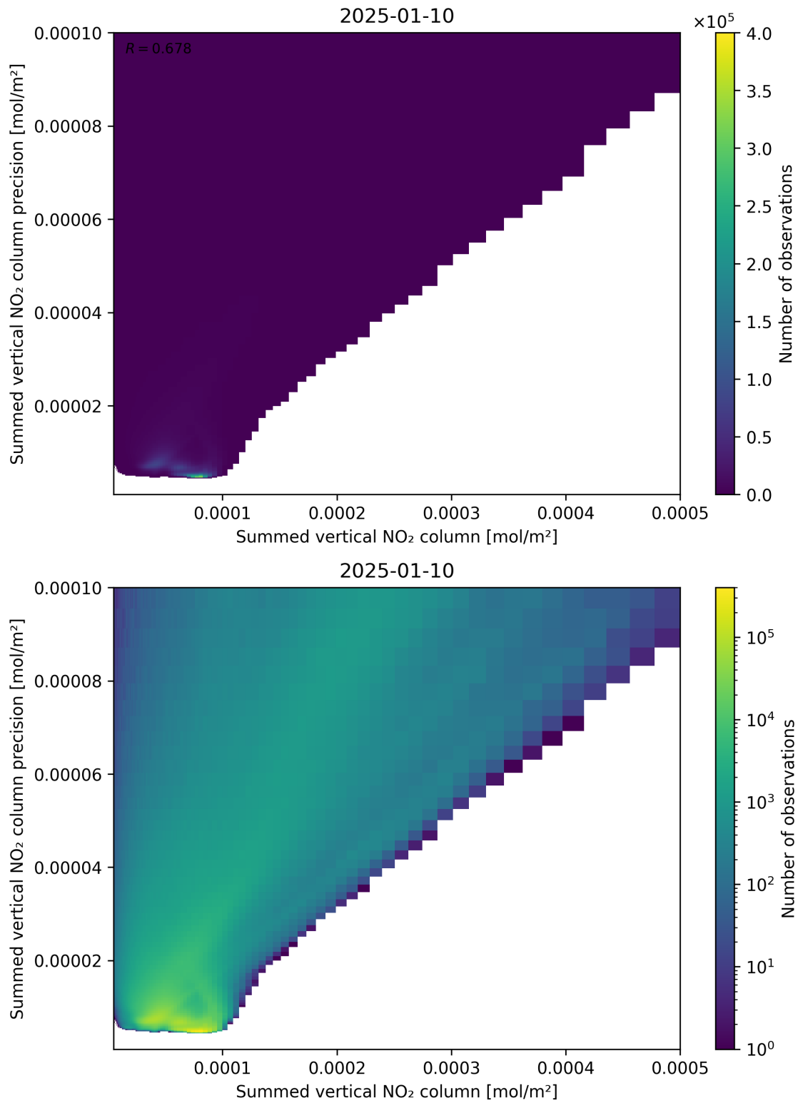
Figure 105: Scatter density plot of “Summed vertical NO 2 column” against “Summed vertical NO 2 column precision” for 2025-01-09 to 2025-01-11.
