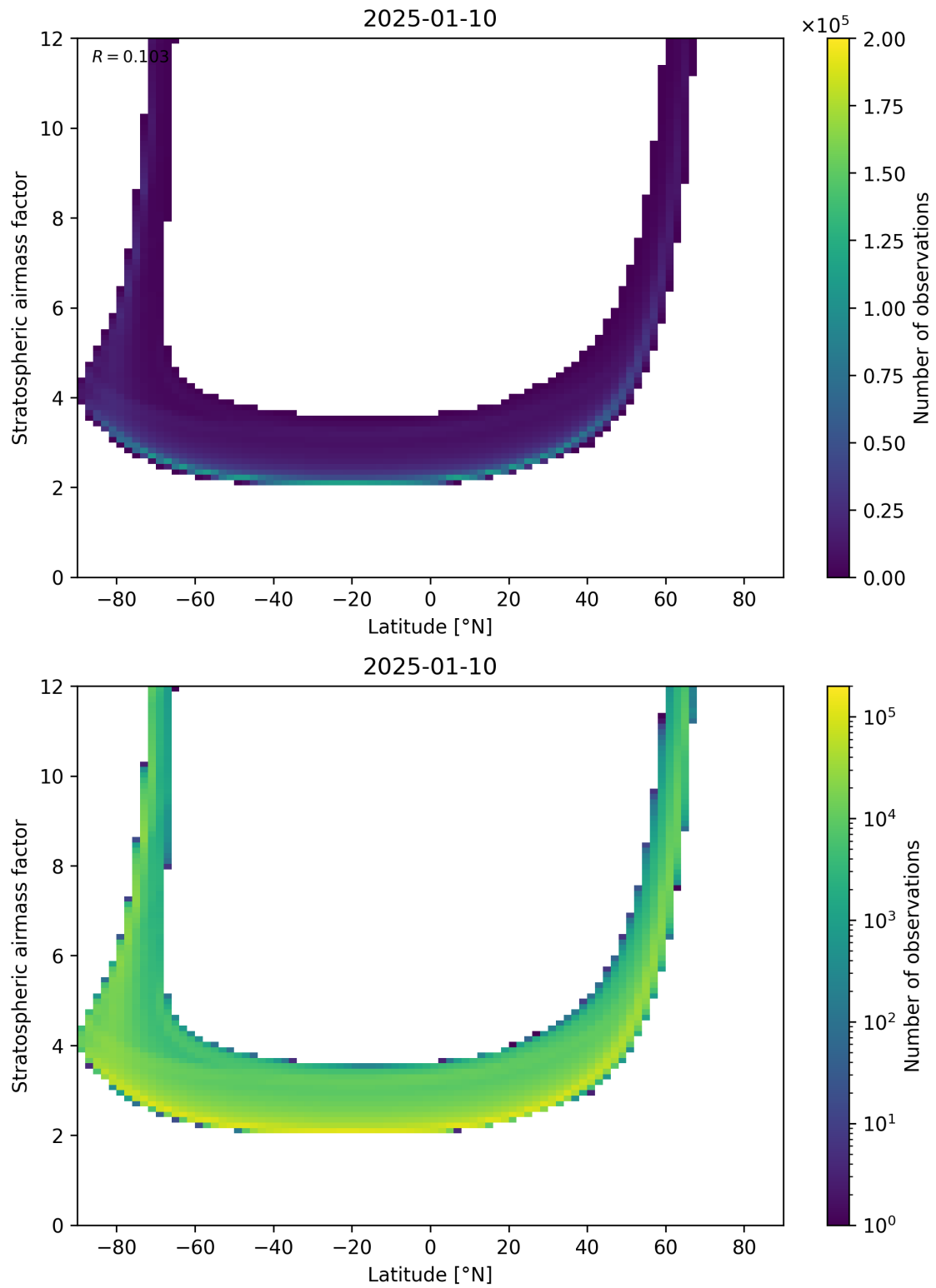
Figure 83: Scatter density plot of “Latitude” against “Stratospheric air mass factor” for 2025-01-09 to 2025-01-11.
