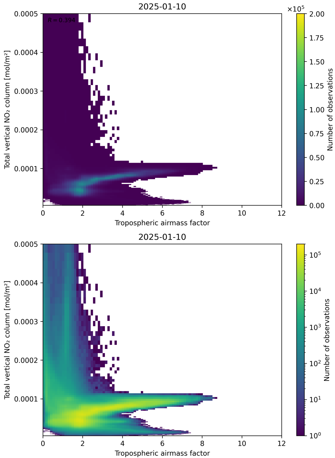
Figure 77: Scatter density plot of “Tropospheric airmass factor” against “Total vertical NO 2 column” for 2025-01-09 to 2025-01-11.
