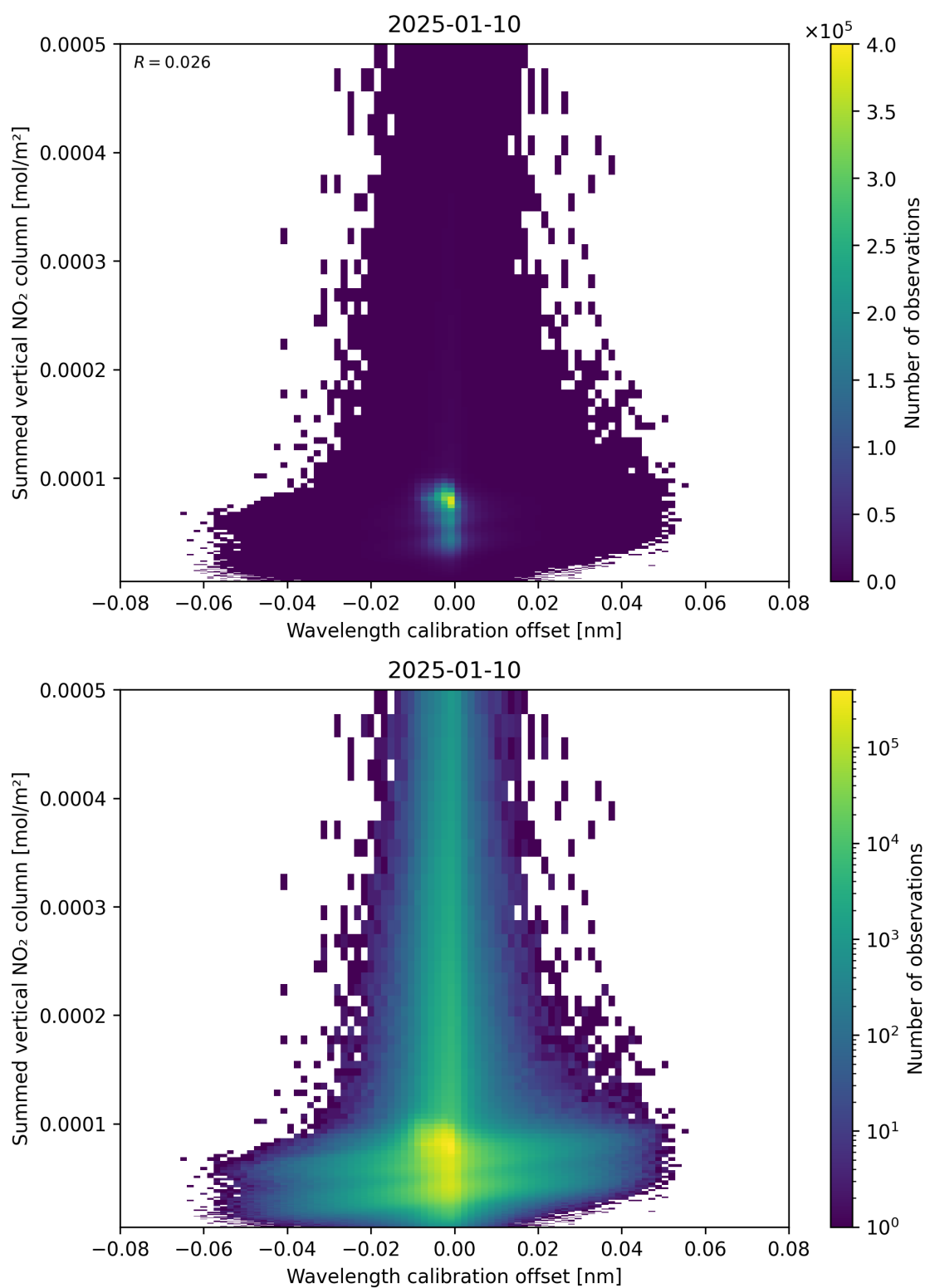
Figure 177: Scatter density plot of “Wavelength calibration offset” against “Summed vertical NO 2 column” for 2025-01-09 to 2025-01-11.
