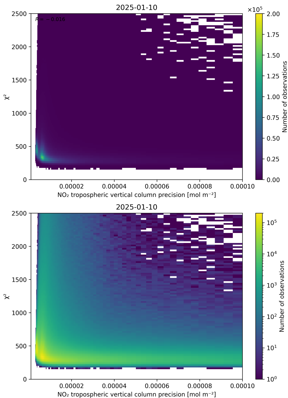
Figure 134: Scatter density plot of “NO 2 tropospheric vertical column precision” against “ \chi^2 ” for 2025-01-09 to 2025-01-11.
