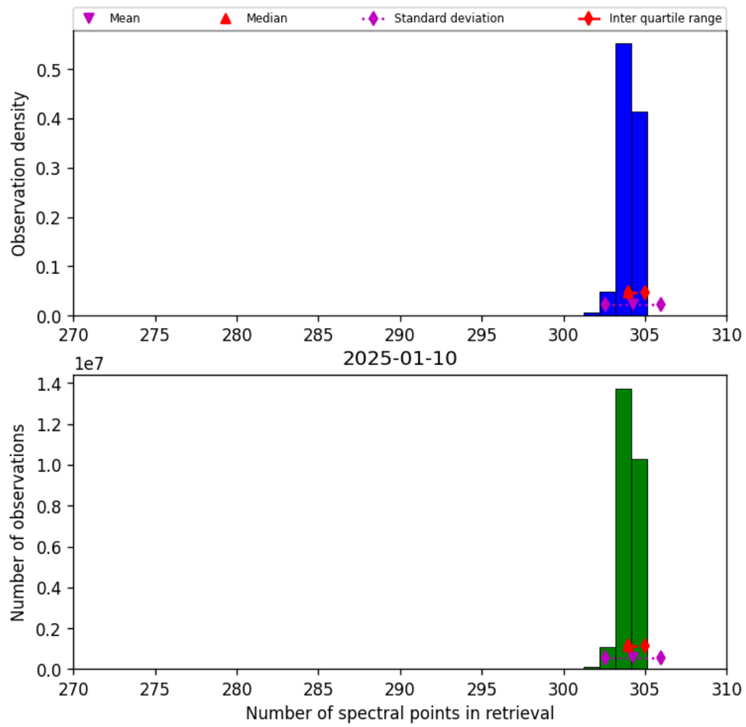
Figure 33: Histogram of “Number of spectral points in retrieval” for 2025-01-09 to 2025-01-11
