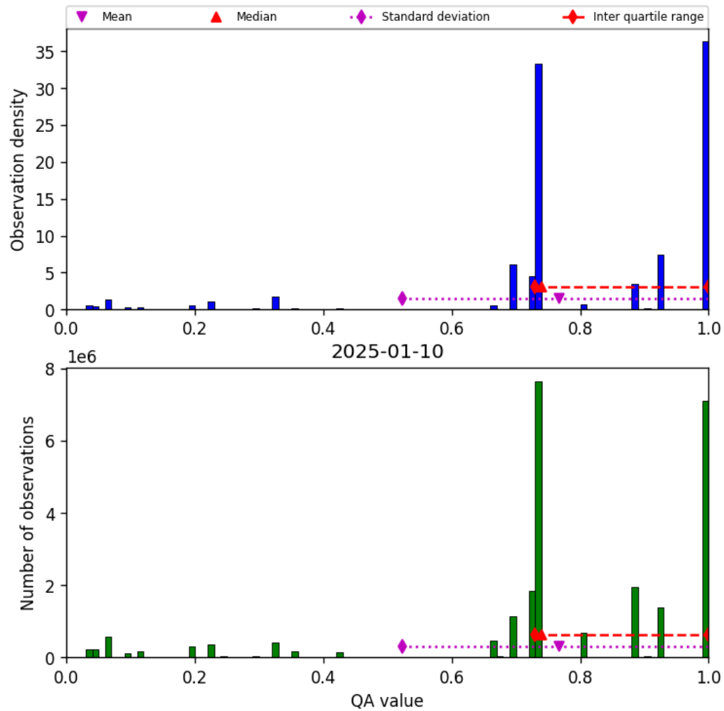
Figure 28: Histogram of “QA value” for 2025-01-09 to 2025-01-11
