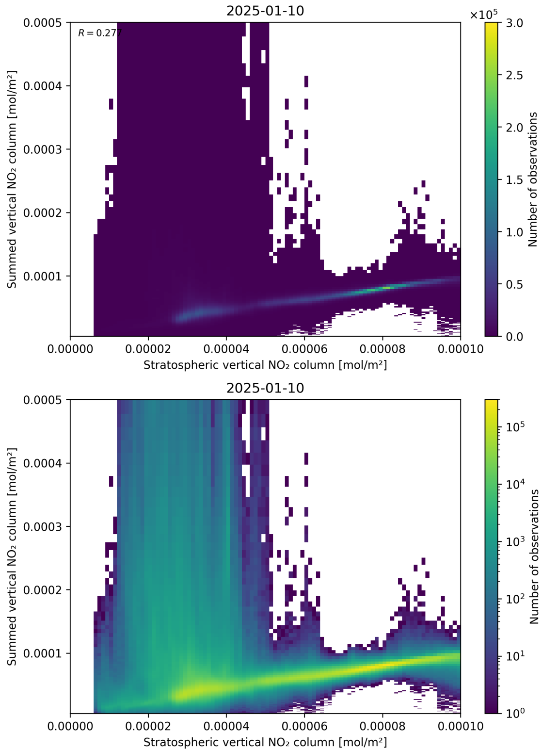
Figure 98: Scatter density plot of “Stratospheric vertical NO 2 column” against “Summed vertical NO 2 column” for 2025-01-09 to 2025-01-11.
