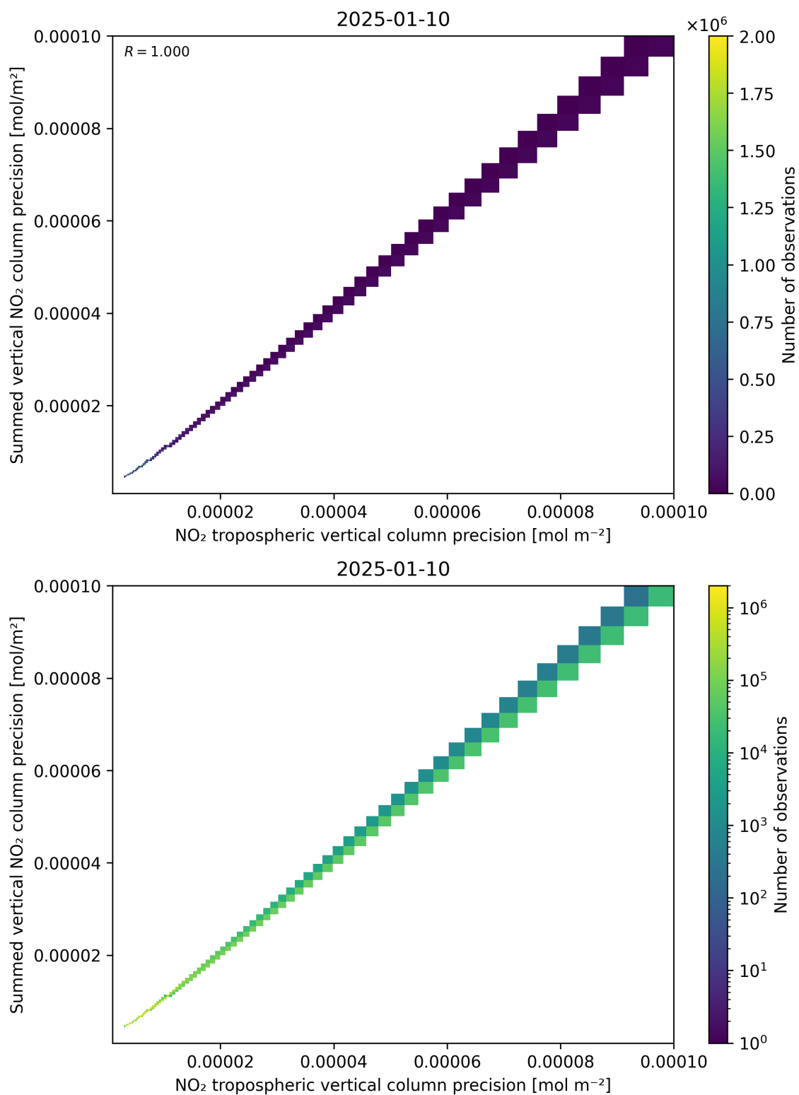
Figure 137: Scatter density plot of “NO 2 tropospheric vertical column precision” against “Summed vertical NO 2 column precision” for 2025-01-09 to 2025-01-11.
