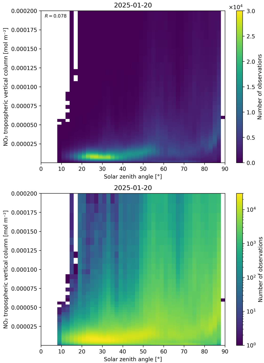
Figure 155: Scatter density plot of “Solar zenith angle” against “NO 2 tropospheric vertical column” for 2025-01-19 to 2025-01-21.
