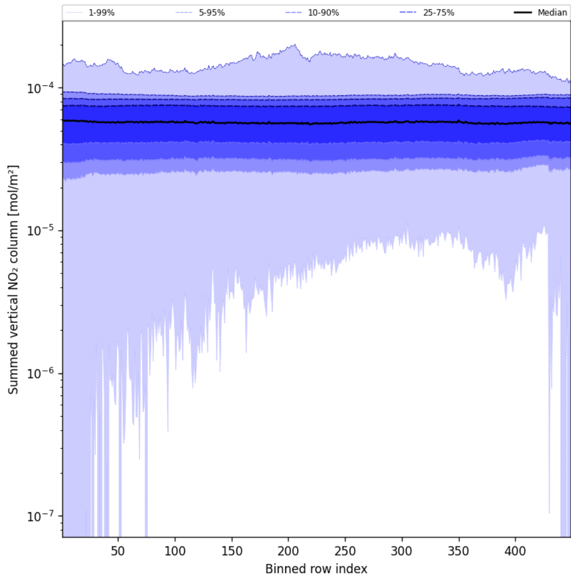
Figure 57: Along track statistics of “Summed vertical NO 2 column” for 2025-01-19 to 2025-01-21
