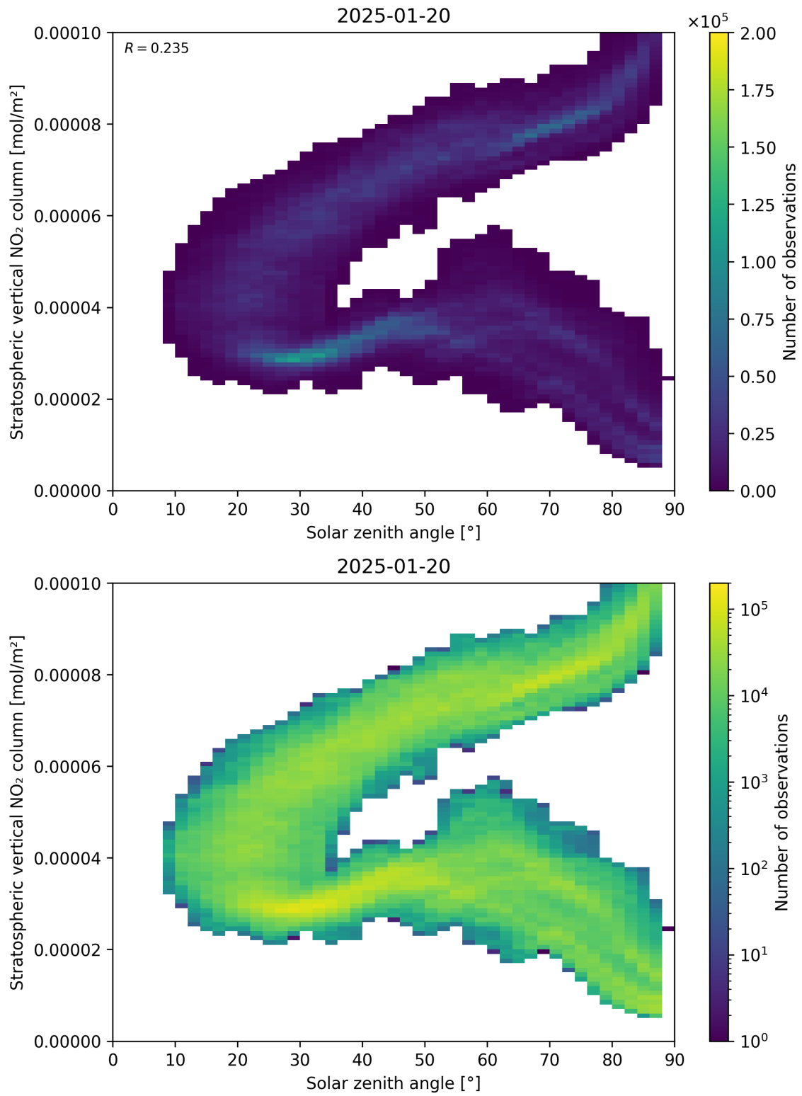
Figure 150: Scatter density plot of “Solar zenith angle” against “Stratospheric vertical NO 2 column” for 2025-01-19 to 2025-01-21.
