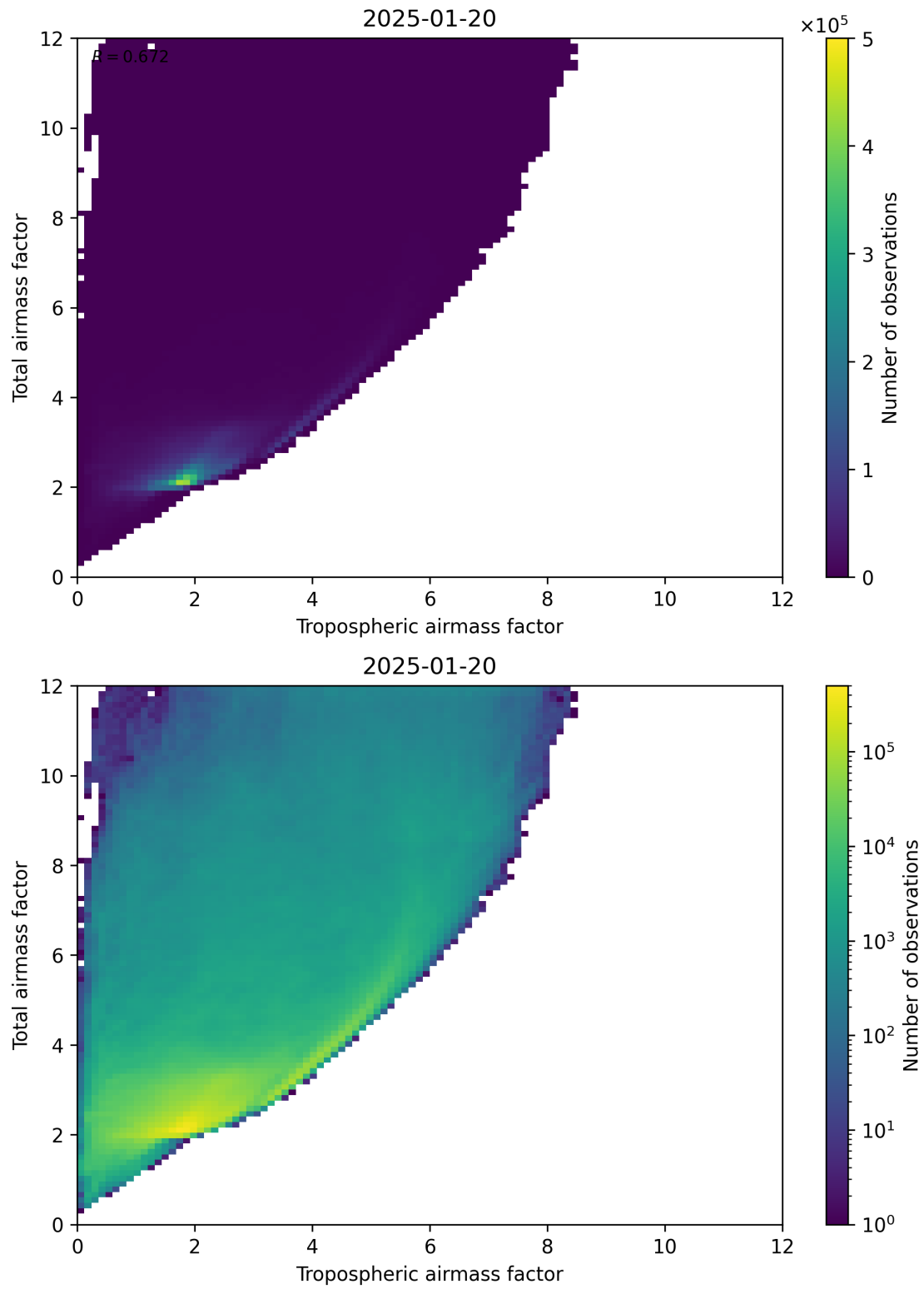
Figure 72: Scatter density plot of “Tropospheric airmass factor” against “Total airmass factor” for 2025-01-19 to 2025-01-21.
