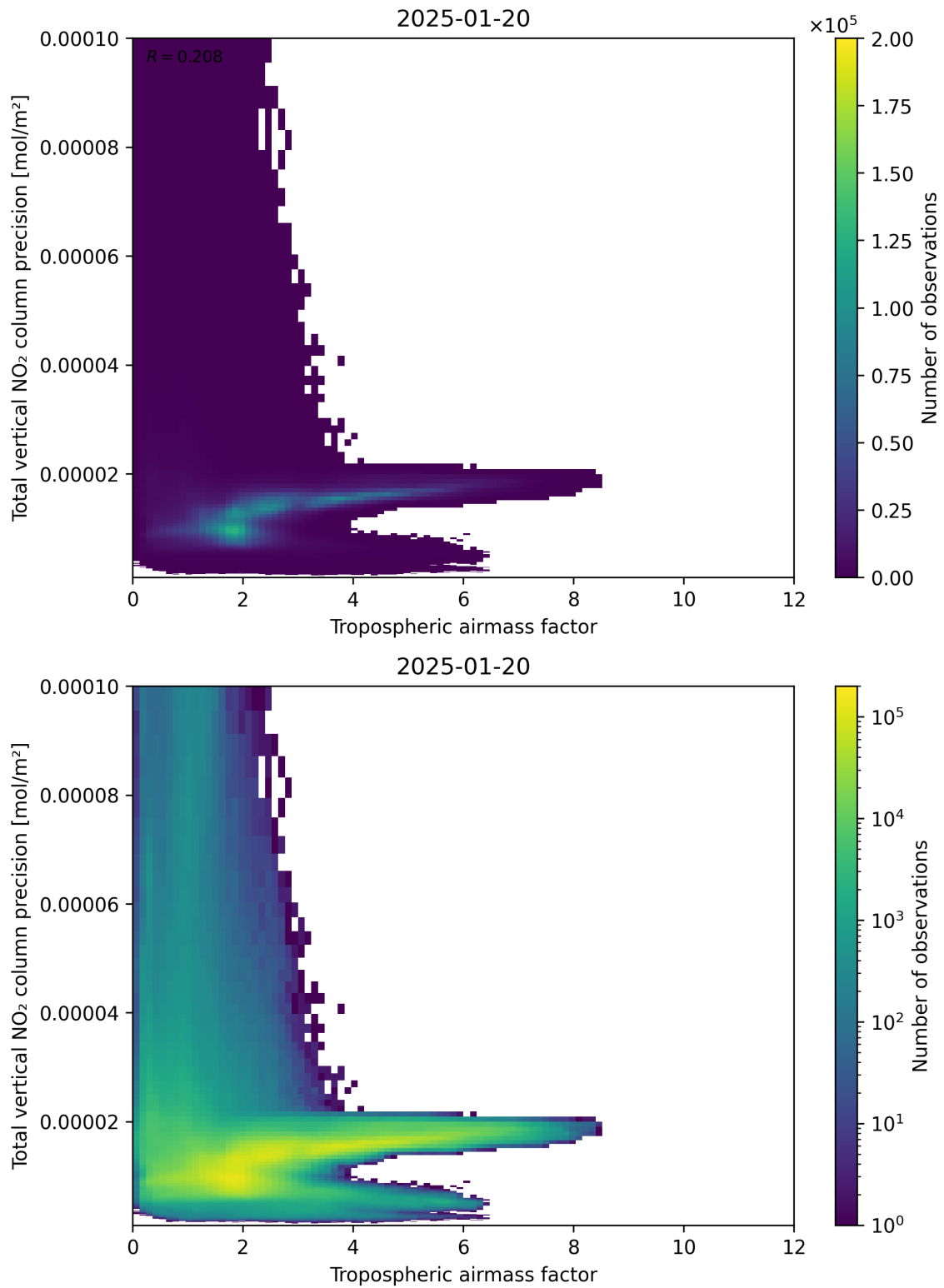
Figure 78: Scatter density plot of “Tropospheric air mass factor” against “Total vertical NO 2 column precision” for 2025-01-19 to 2025-01-21.
