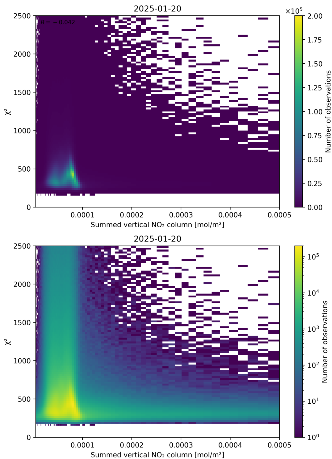
Figure 104: Scatter density plot of “Summed vertical NO 2 column” against “ \chi^2 ” for 2025-01-19 to 2025-01-21.
