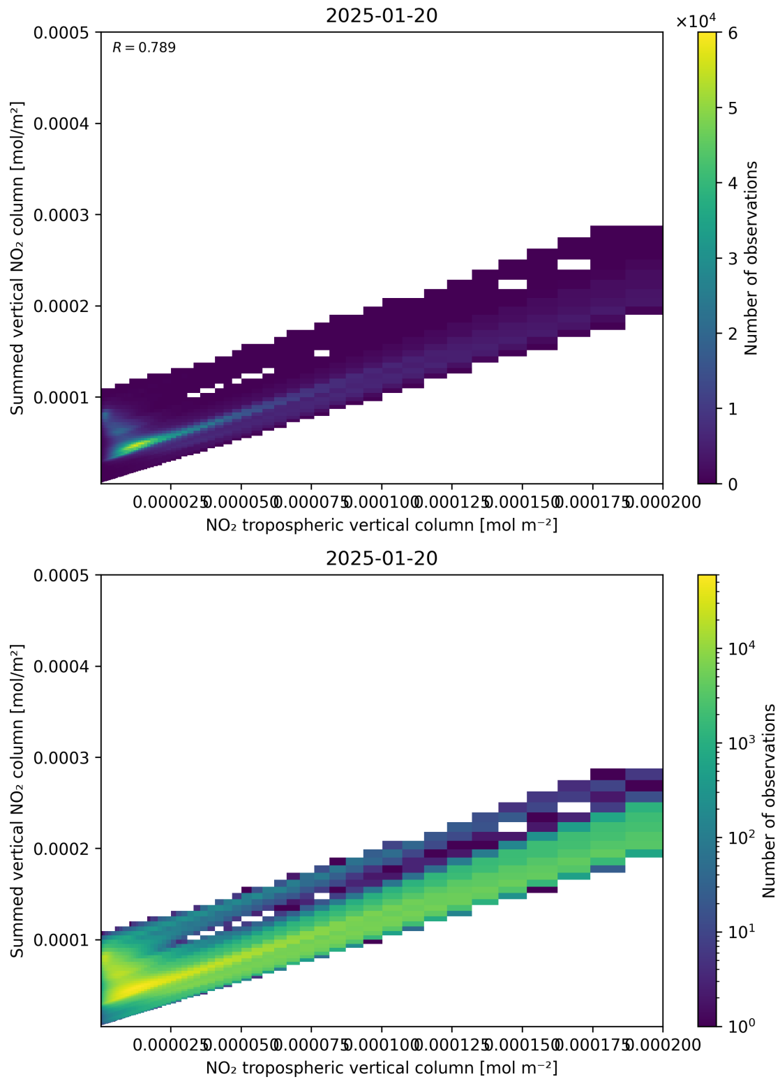
Figure 126: Scatter density plot of “NO 2 tropospheric vertical column” against “Summed vertical NO 2 column” for 2025-01-19 to 2025-01-21.
