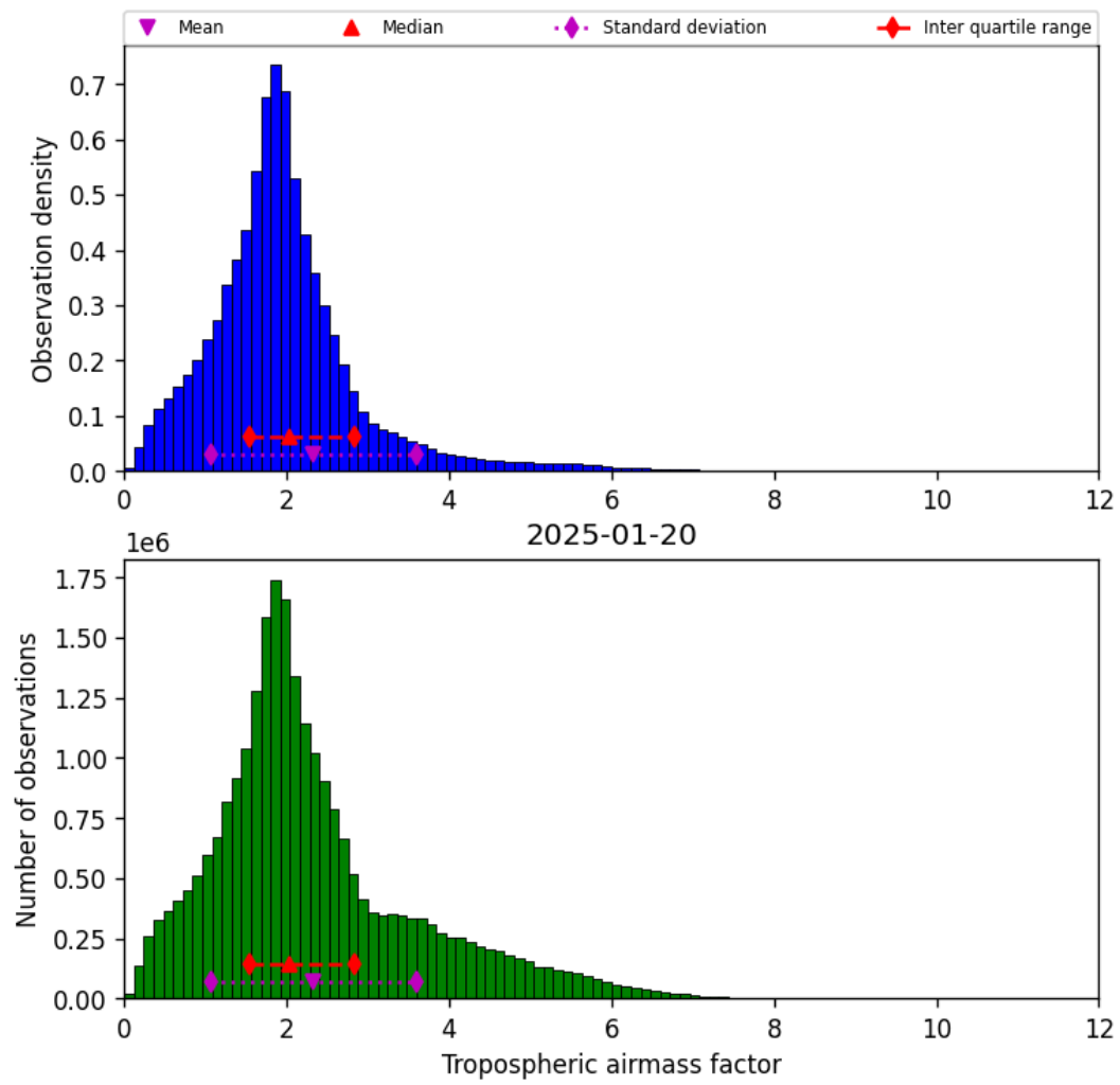
Figure 31: Histogram of “Tropospheric airmass factor” for 2025-01-19 to 2025-01-21
