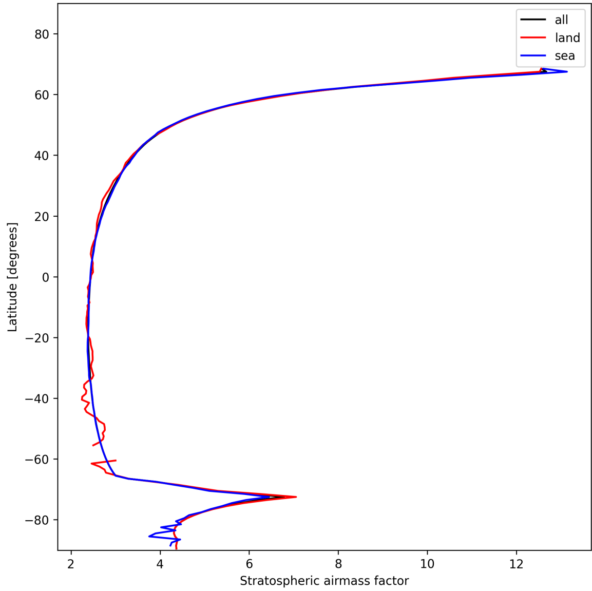
Figure 27: Zonal average of “Stratospheric airmass factor” for 2025-01-19 to 2025-01-21.
