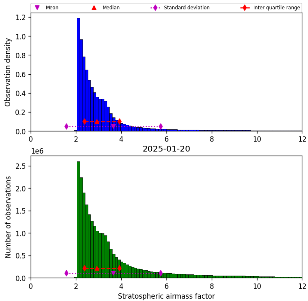
Figure 44: Histogram of “Stratospheric airmass factor” for 2025-01-19 to 2025-01-21
