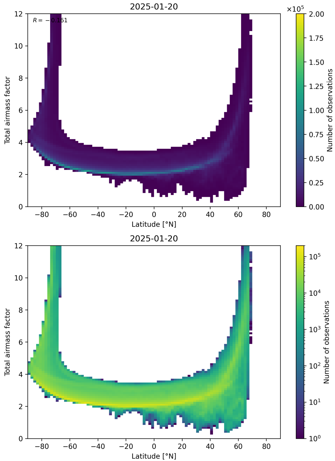
Figure 84: Scatter density plot of “Latitude” against “Total airmass factor” for 2025-01-19 to 2025-01-21.
