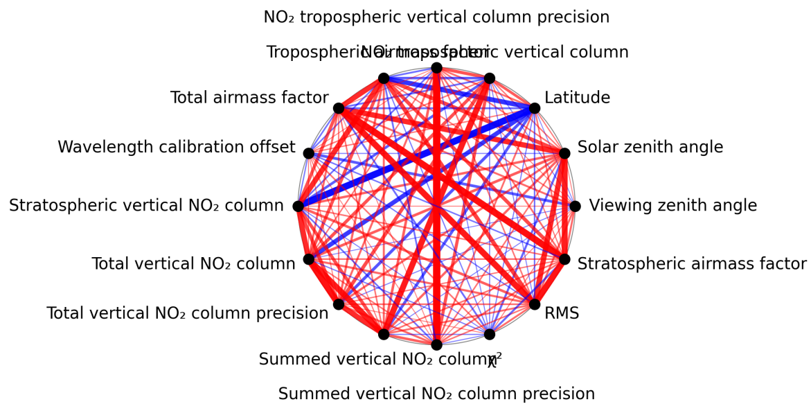
Figure 1: Map of correlation graph for 2025-01-19 to 2025-01-21.
