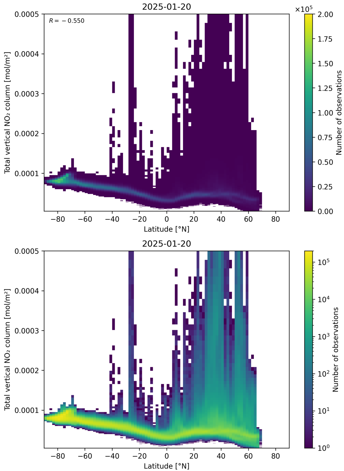
Figure 90: Scatter density plot of “Latitude” against “Total vertical NO 2 column” for 2025-01-19 to 2025-01-21.
