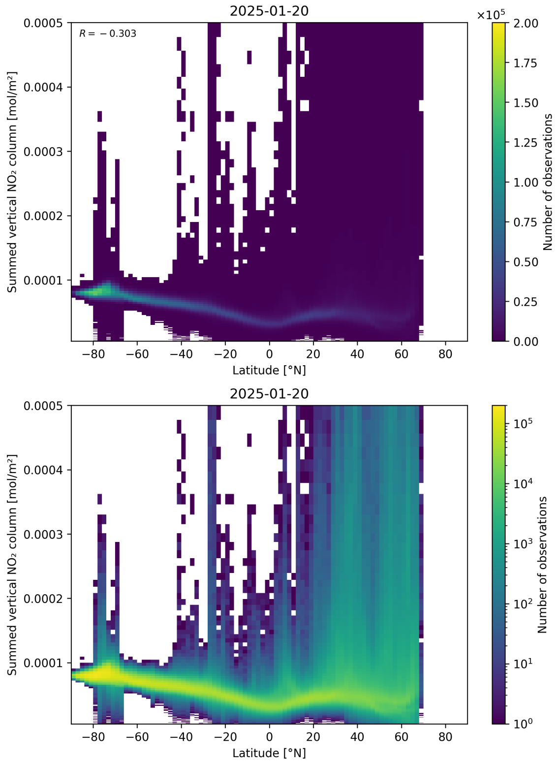
Figure 88: Scatter density plot of “Latitude” against “Summed vertical NO 2 column” for 2025-01-19 to 2025-01-21.
