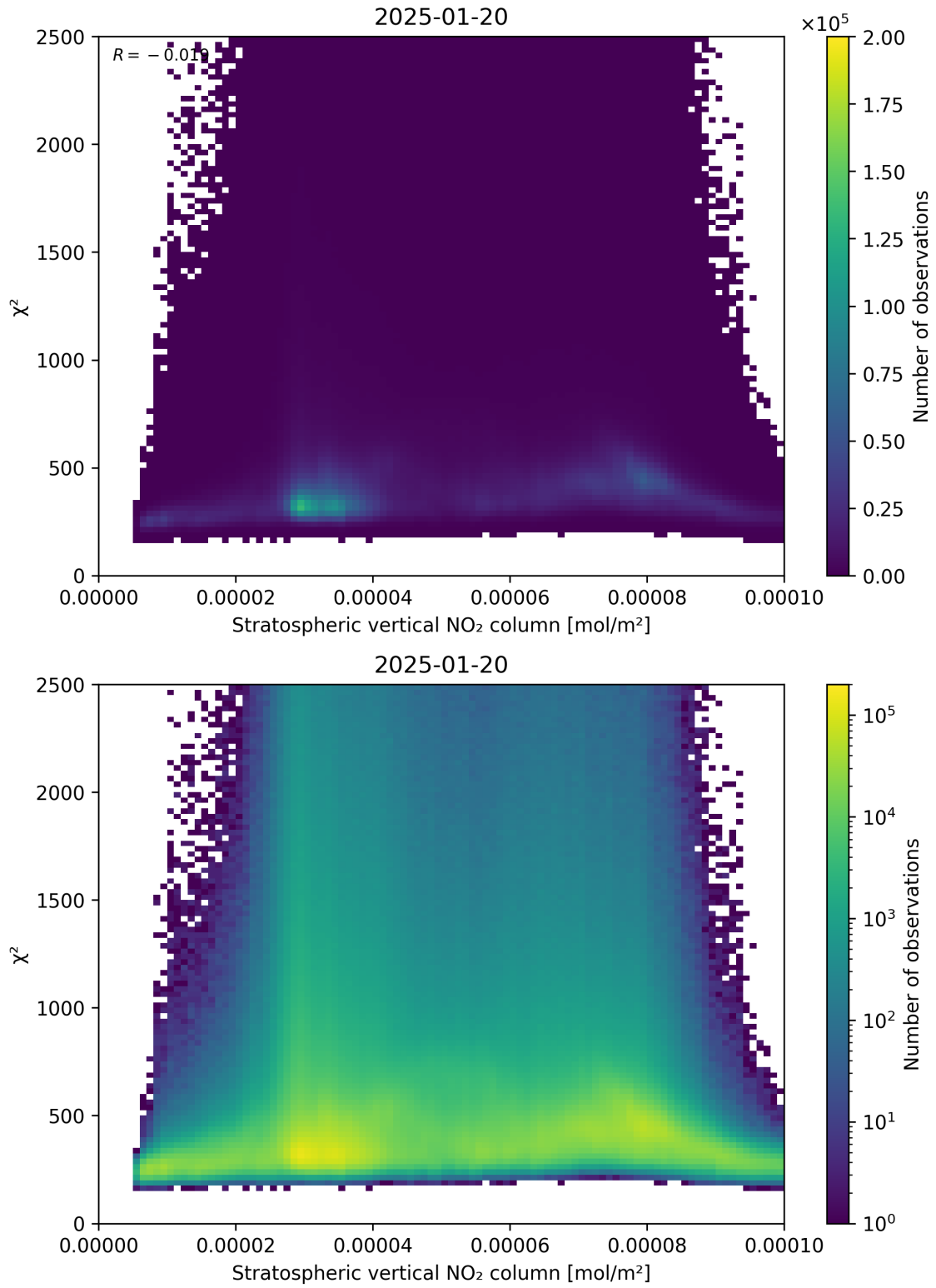
Figure 97: Scatter density plot of “Stratospheric vertical NO 2 column” against “ \chi^2 ” for 2025-01-19 to 2025-01-21.
