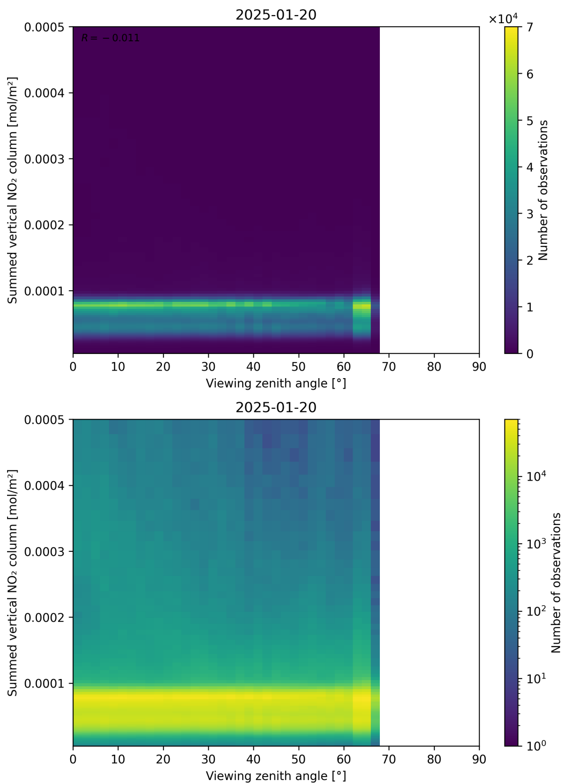
Figure 165: Scatter density plot of “Viewing zenith angle” against “Summed vertical NO 2 column” for 2025-01-19 to 2025-01-21.
