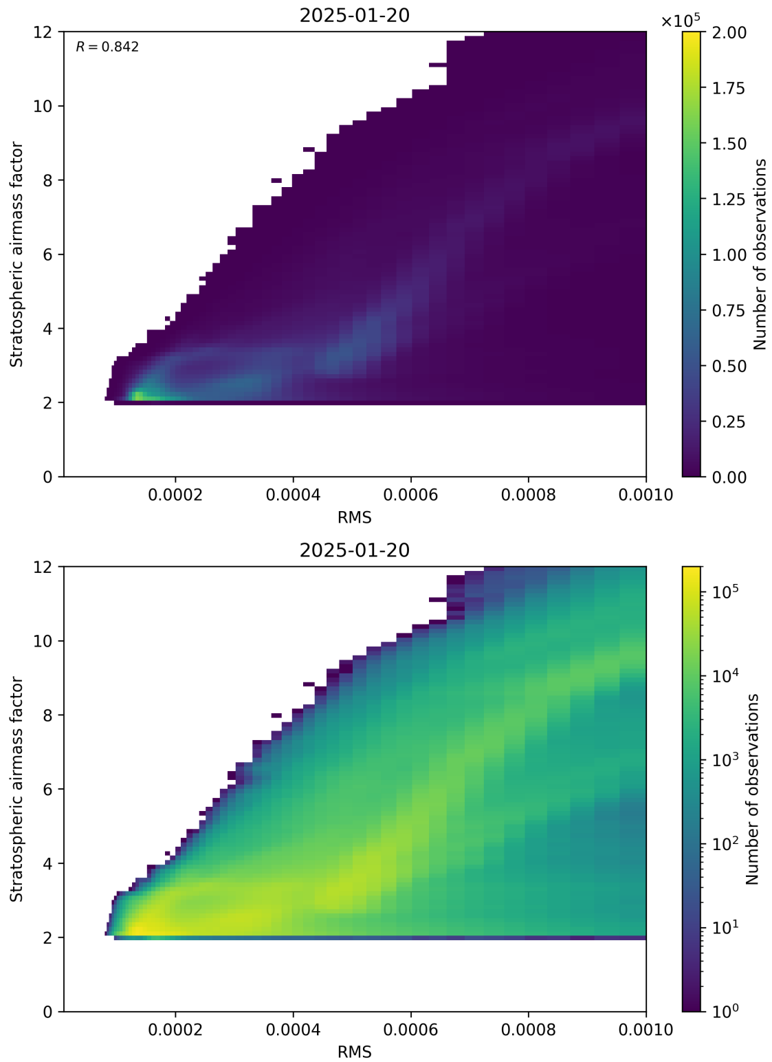
Figure 144: Scatter density plot of “RMS” against “Stratospheric airmass factor” for 2025-01-19 to 2025-01-21.
