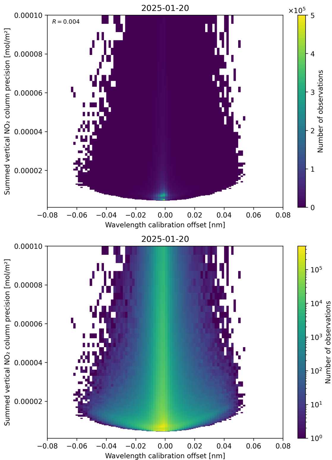
Figure 178: Scatter density plot of “Wavelength calibration offset” against “Summed vertical NO 2 column precision” for 2025-01-19 to 2025-01-21.
