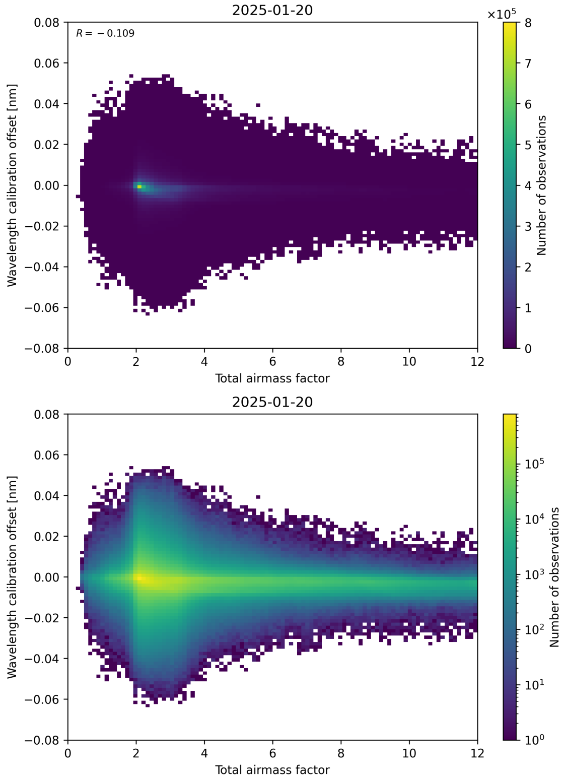
Figure 70: Scatter density plot of “Total airmass factor” against “Wavelength calibration offset” for 2025-01-19 to 2025-01-21.
