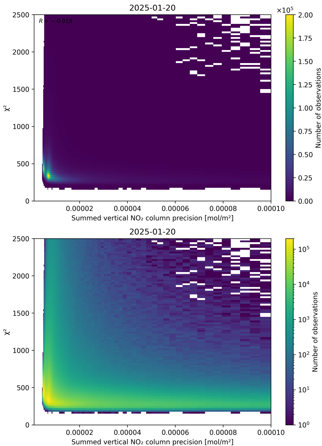
Figure 107: Scatter density plot of “Summed vertical NO 2 column precision” against “ \chi^2 ” for 2025-01-19 to 2025-01-21.
