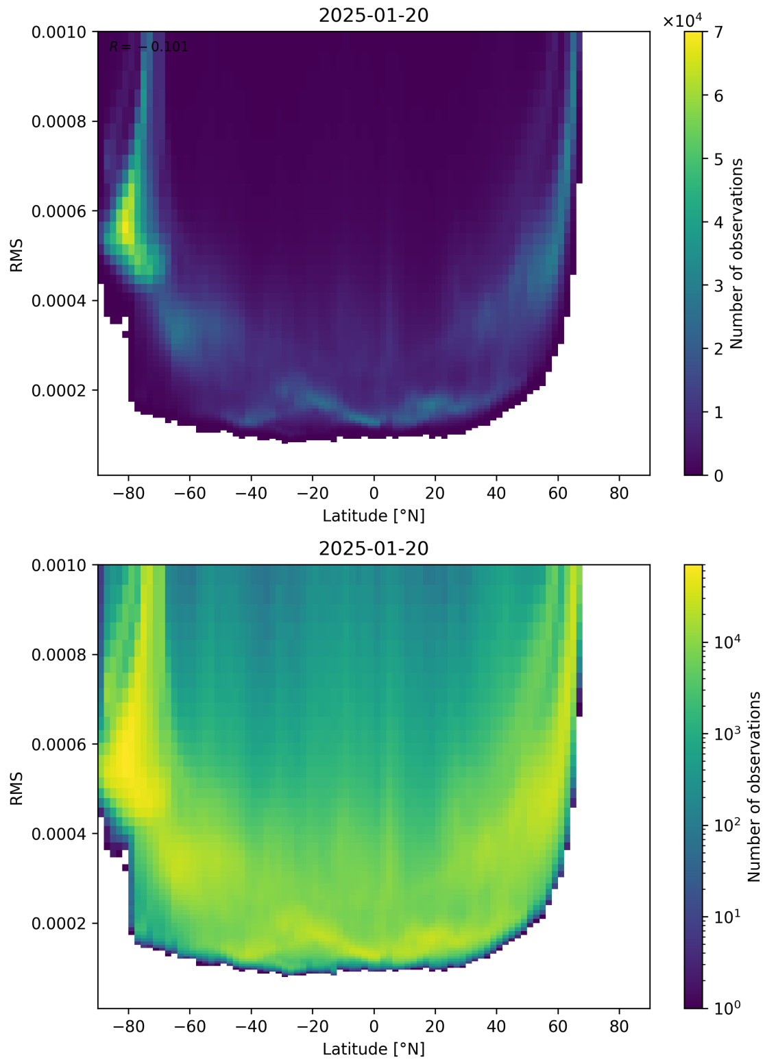
Figure 94: Scatter density plot of “Latitude” against “RMS” for 2025-01-19 to 2025-01-21.
