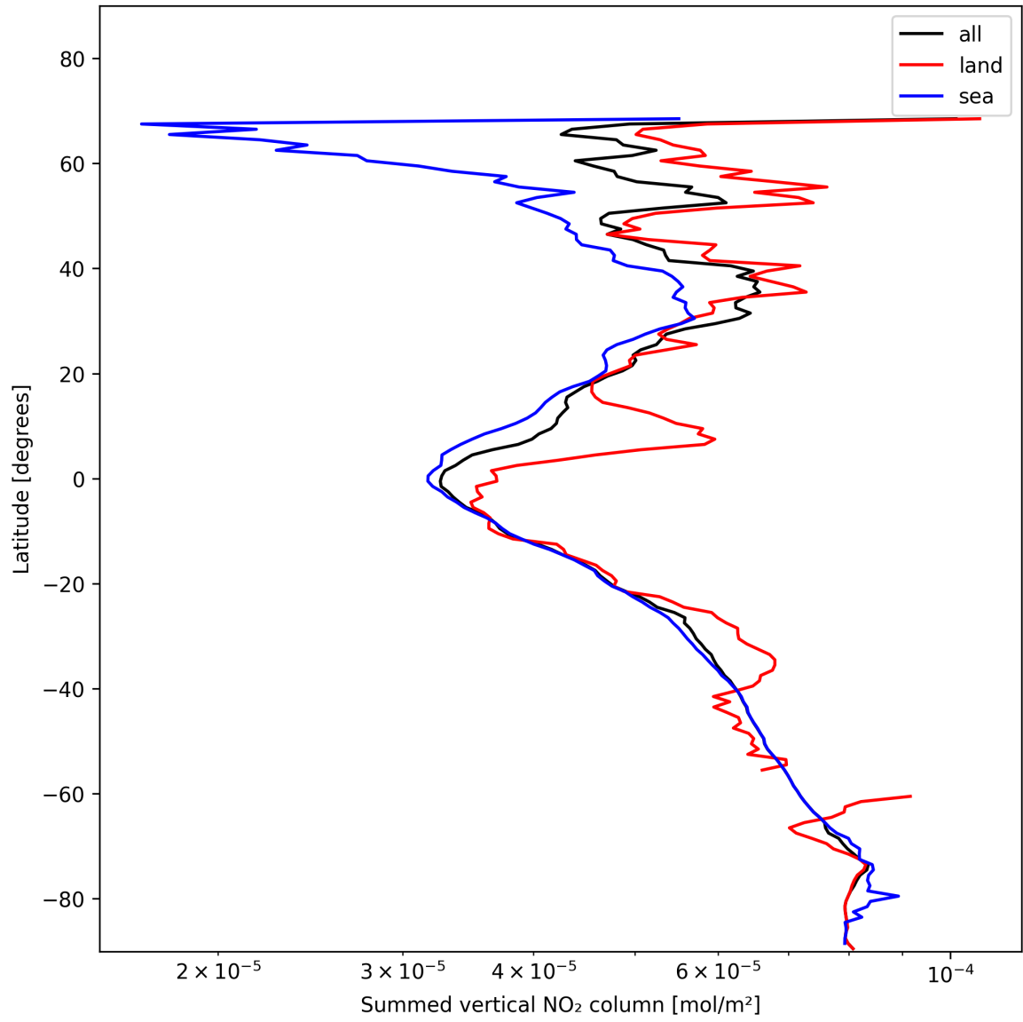
Figure 23: Zonal average of “Summed vertical NO 2 column” for 2025-01-19 to 2025-01-21.
