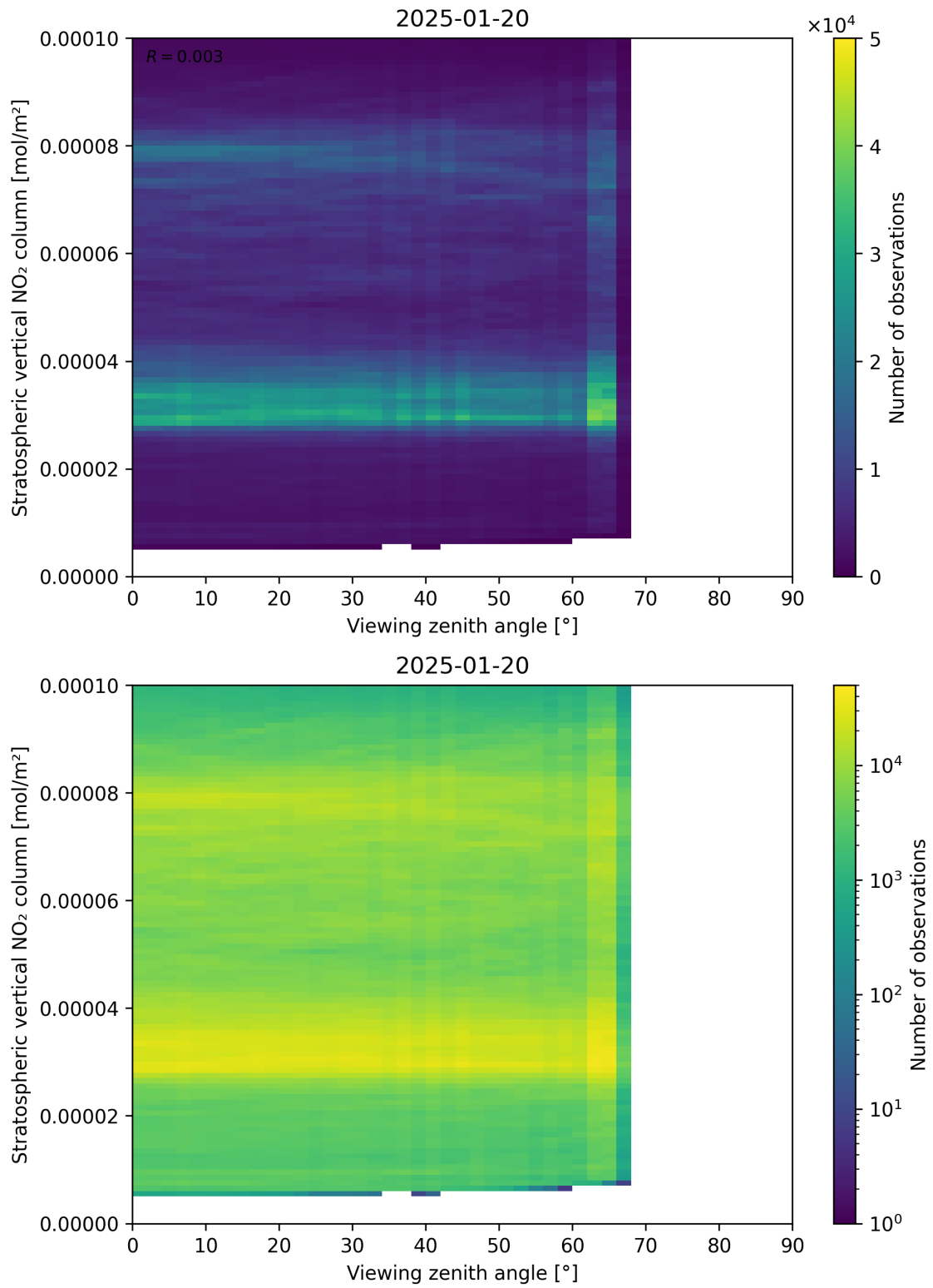
Figure 164: Scatter density plot of “Viewing zenith angle” against “Stratospheric vertical NO 2 column” for 2025-01-19 to 2025-01-21.
