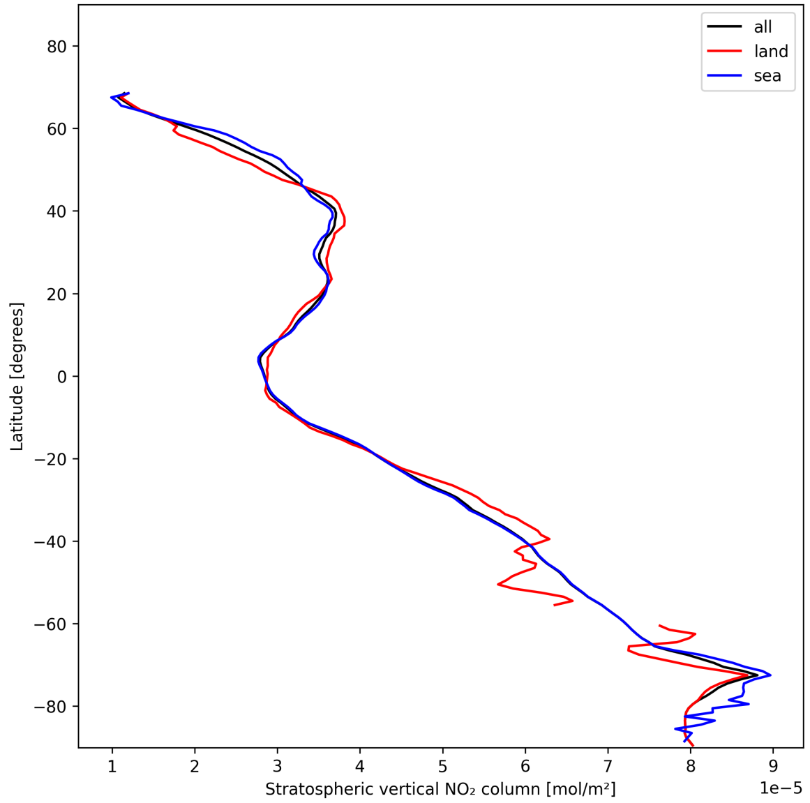
Figure 19: Zonal average of “Stratospheric vertical NO 2 column” for 2025-01-19 to 2025-01-21.
