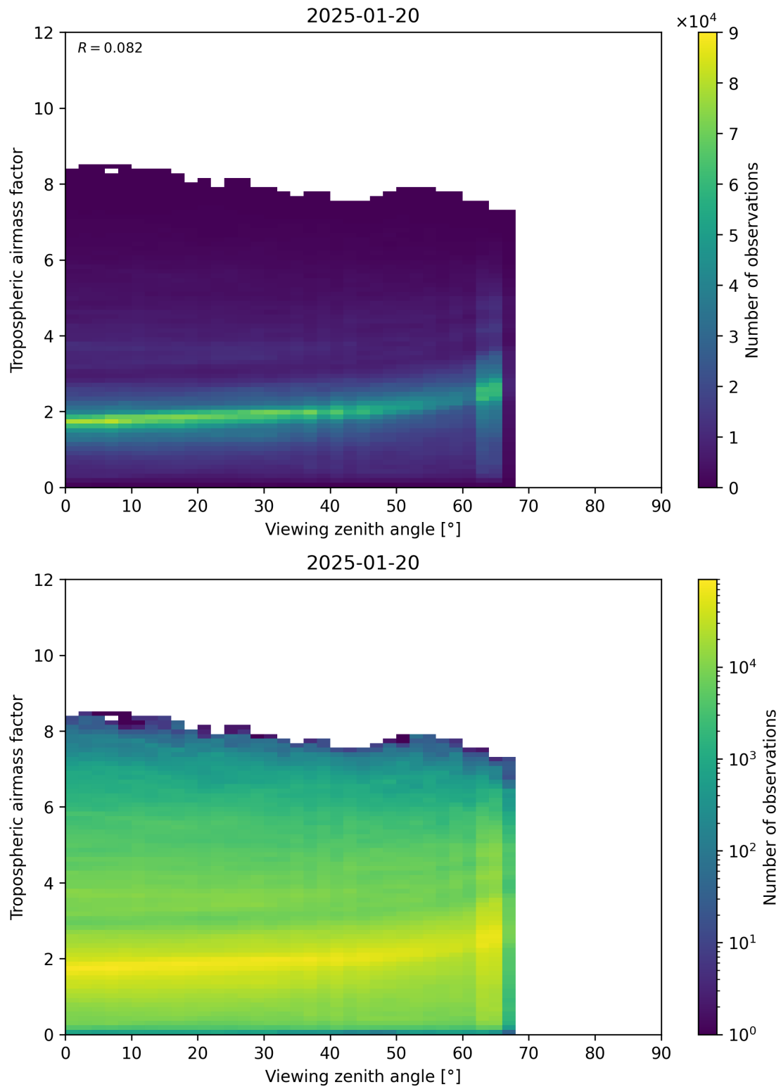
Figure 161: Scatter density plot of “Viewing zenith angle” against “Tropospheric airmass factor” for 2025-01-19 to 2025-01-21.
