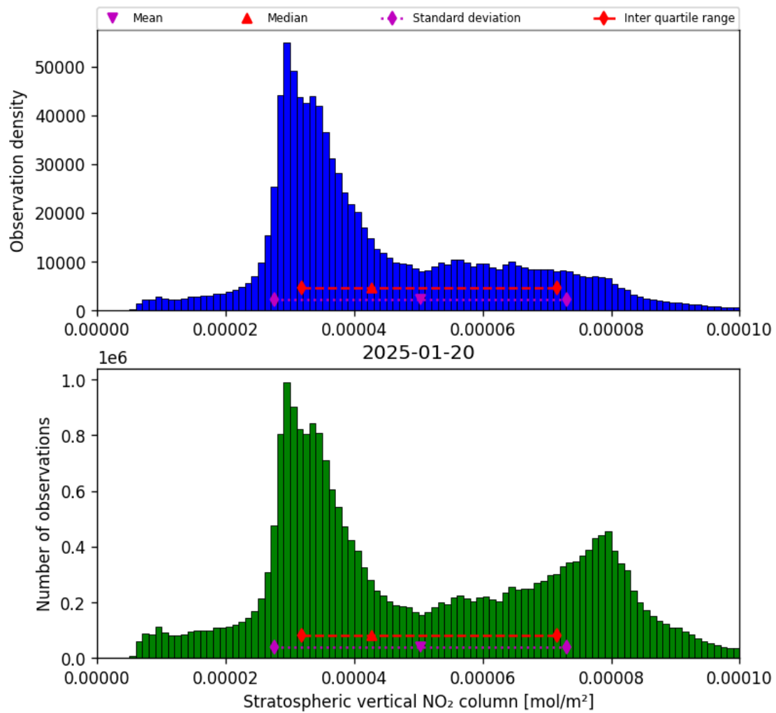
Figure 36: Histogram of “Stratospheric vertical NO 2 column” for 2025-01-19 to 2025-01-21
