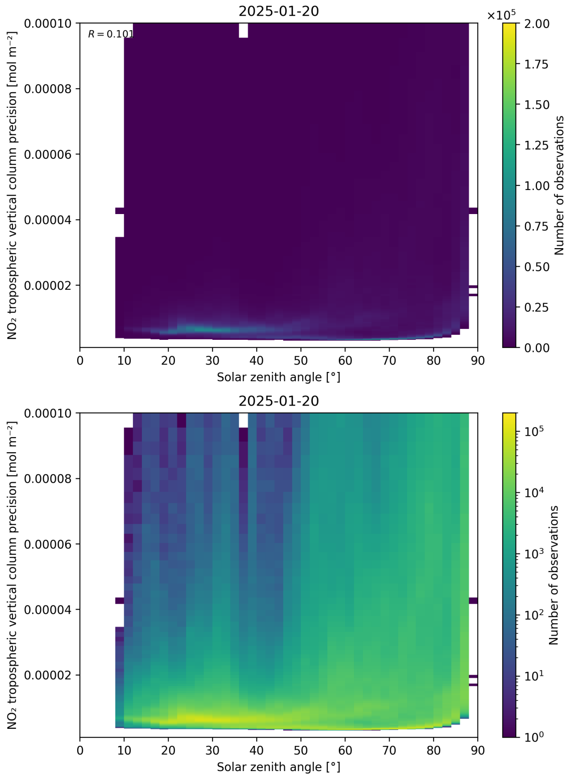
Figure 156: Scatter density plot of “Solar zenith angle” against “NO 2 tropospheric vertical column precision” for 2025-01-19 to 2025-01-21.
