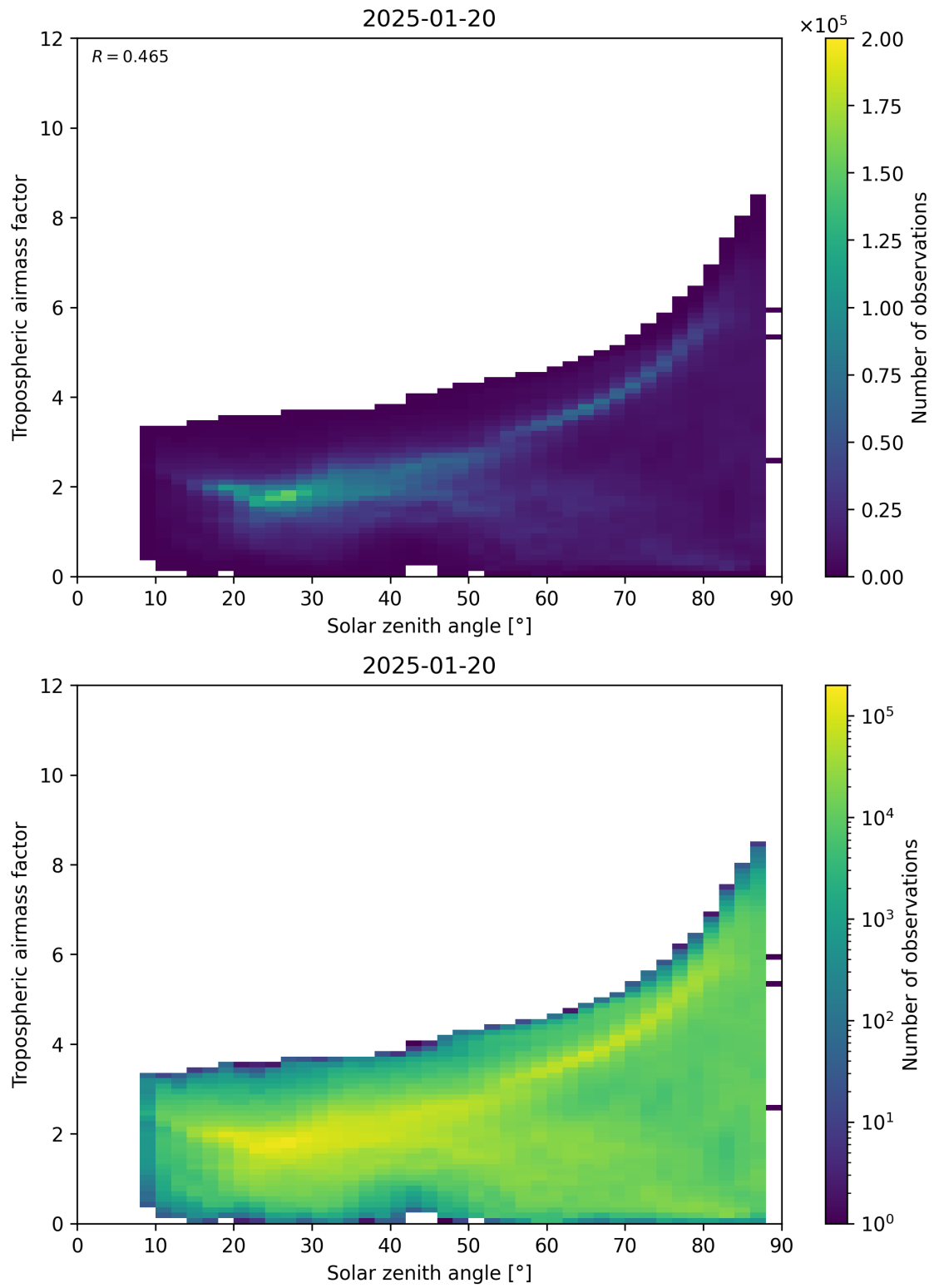
Figure 147: Scatter density plot of “Solar zenith angle” against “Tropospheric airmass factor” for 2025-01-19 to 2025-01-21.
