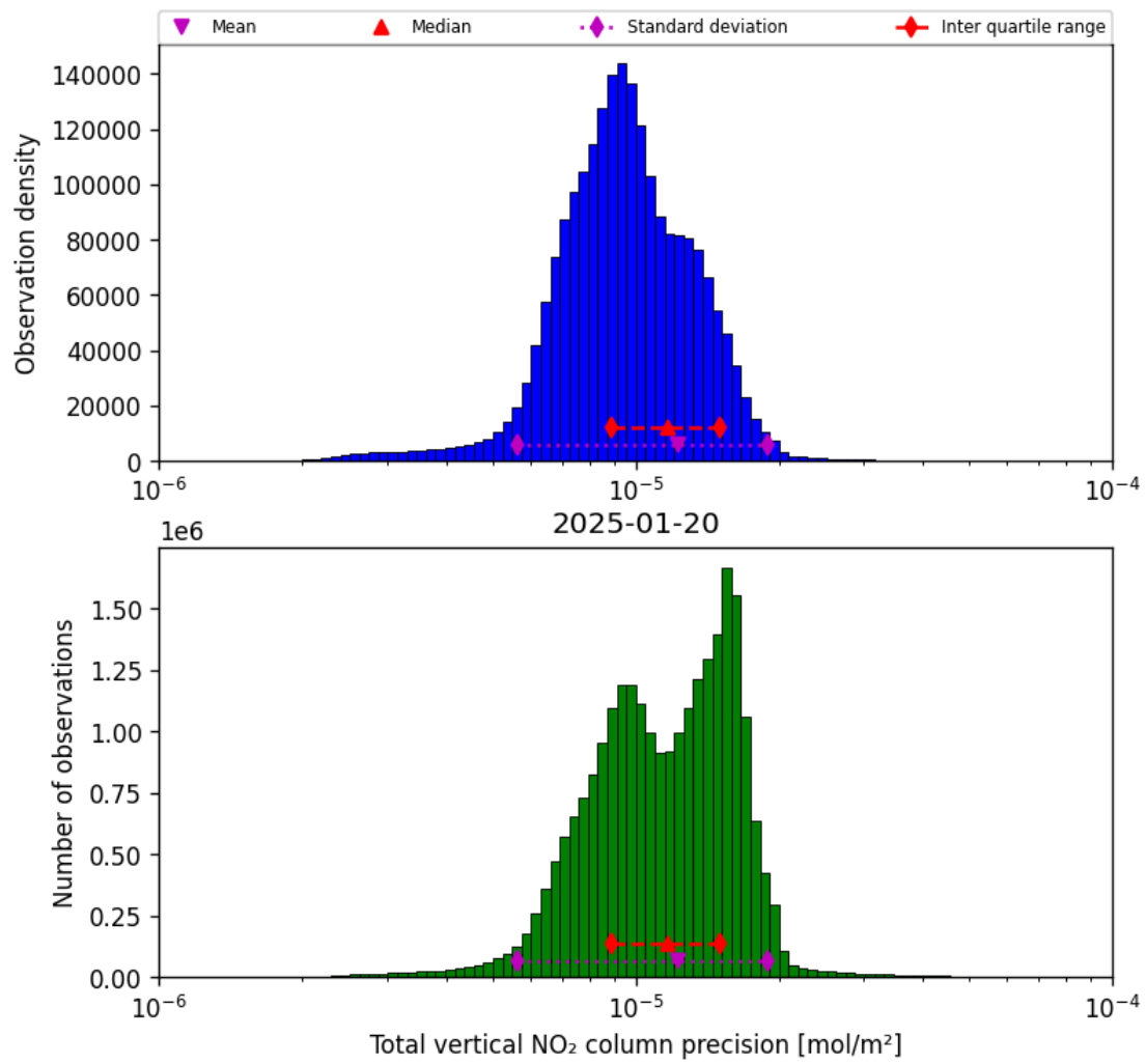
Figure 39: Histogram of “Total vertical NO 2 column precision” for 2025-01-19 to 2025-01-21
