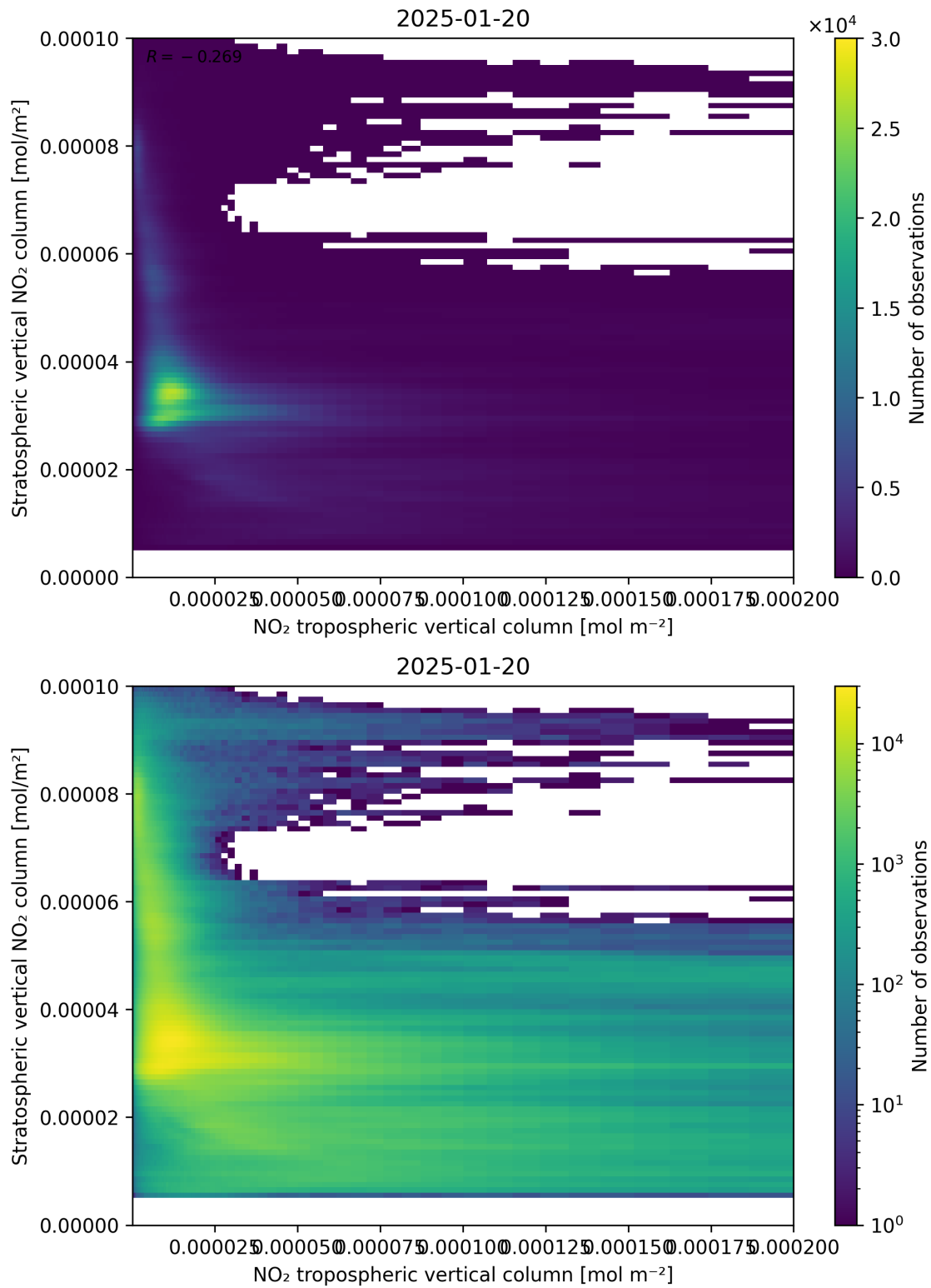
Figure 125: Scatter density plot of “NO 2 tropospheric vertical column” against “Stratospheric vertical NO 2 column” for 2025-01-19 to 2025-01-21.
