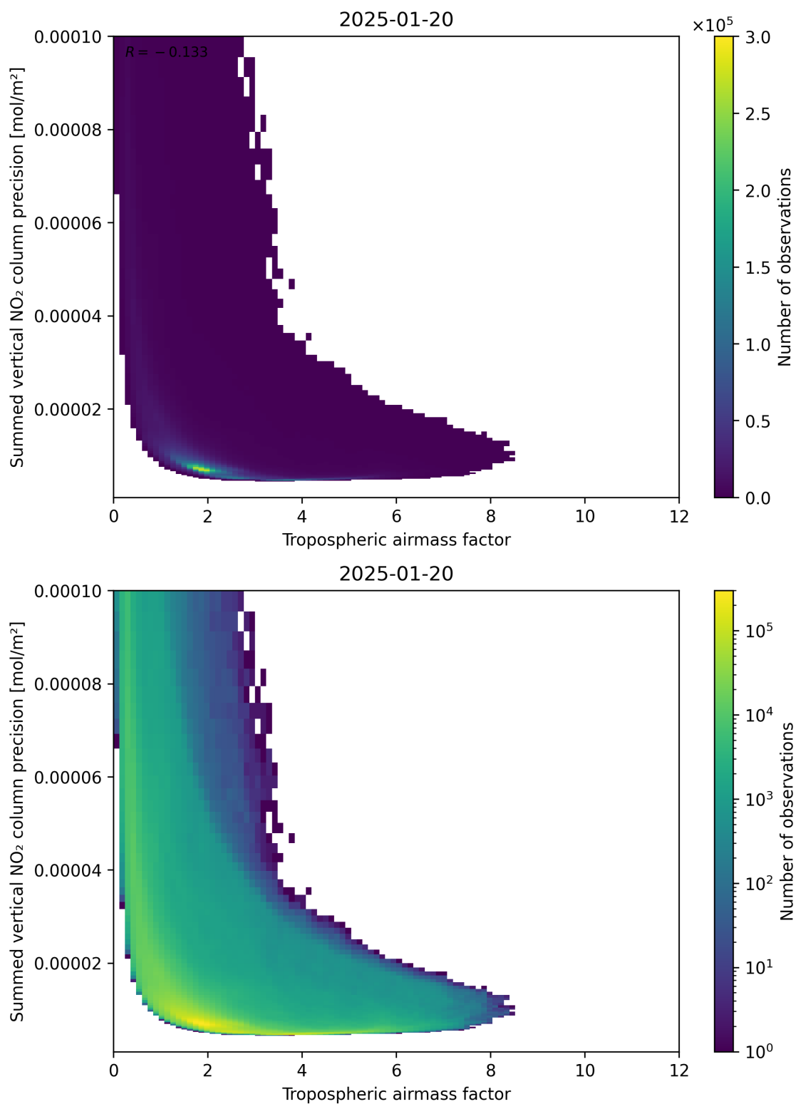
Figure 76: Scatter density plot of “Tropospheric air mass factor” against “Summed vertical NO 2 column precision” for 2025-01-19 to 2025-01-21.
