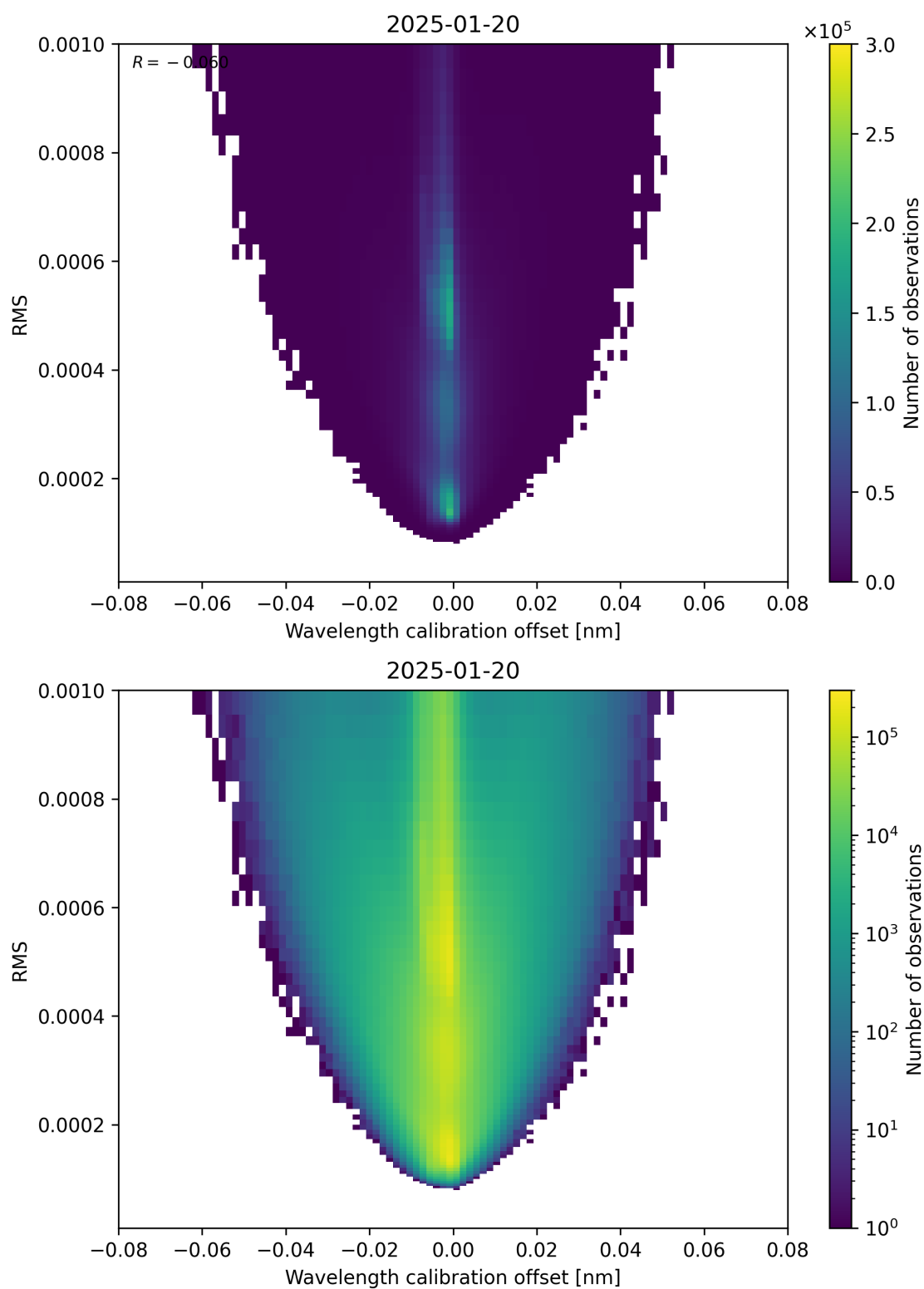
Figure 181: Scatter density plot of “Wavelength calibration offset” against “RMS” for 2025-01-19 to 2025-01-21.
