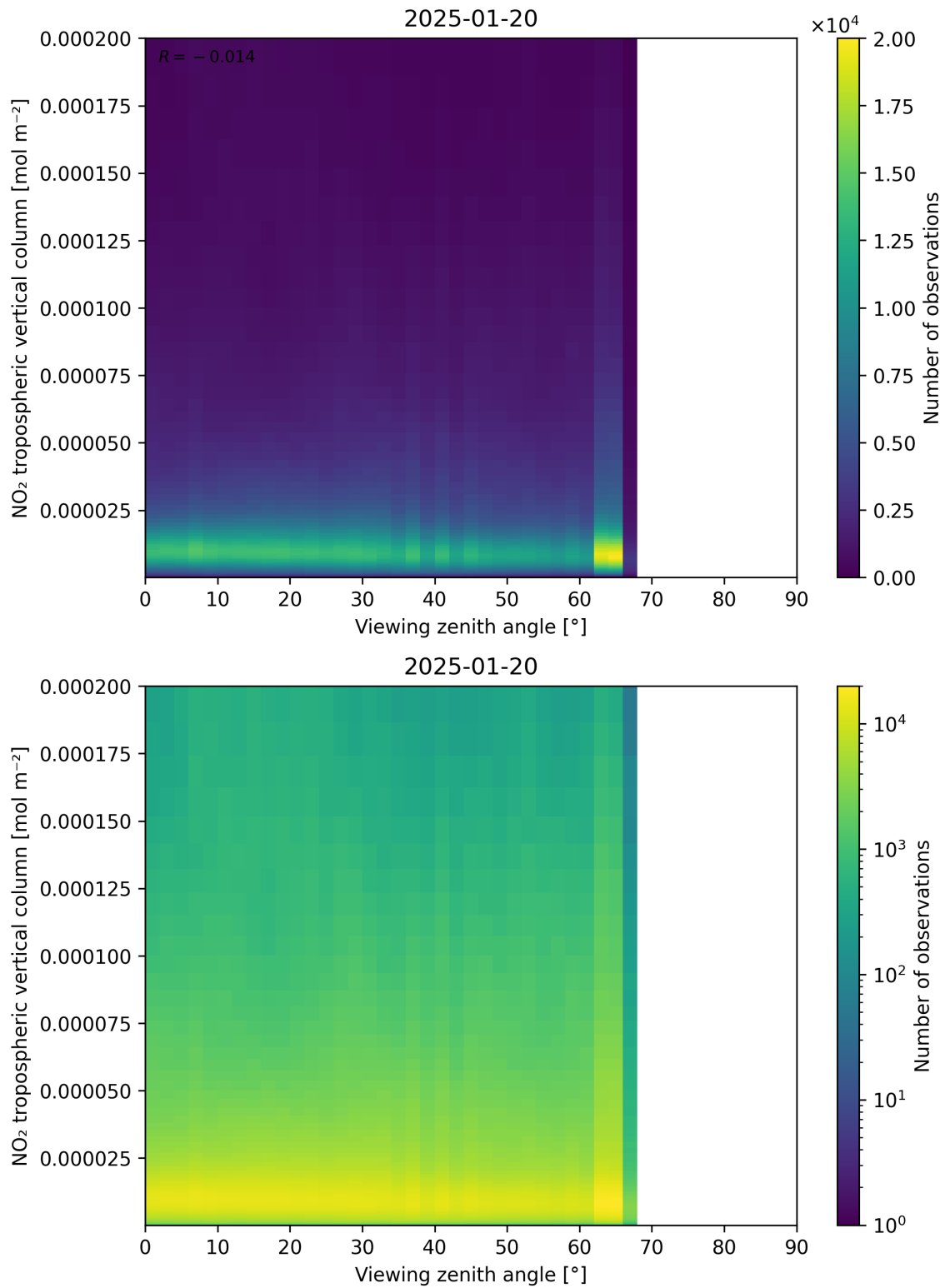
Figure 169: Scatter density plot of “Viewing zenith angle” against “NO 2 tropospheric vertical column” for 2025-01-19 to 2025-01-21.
