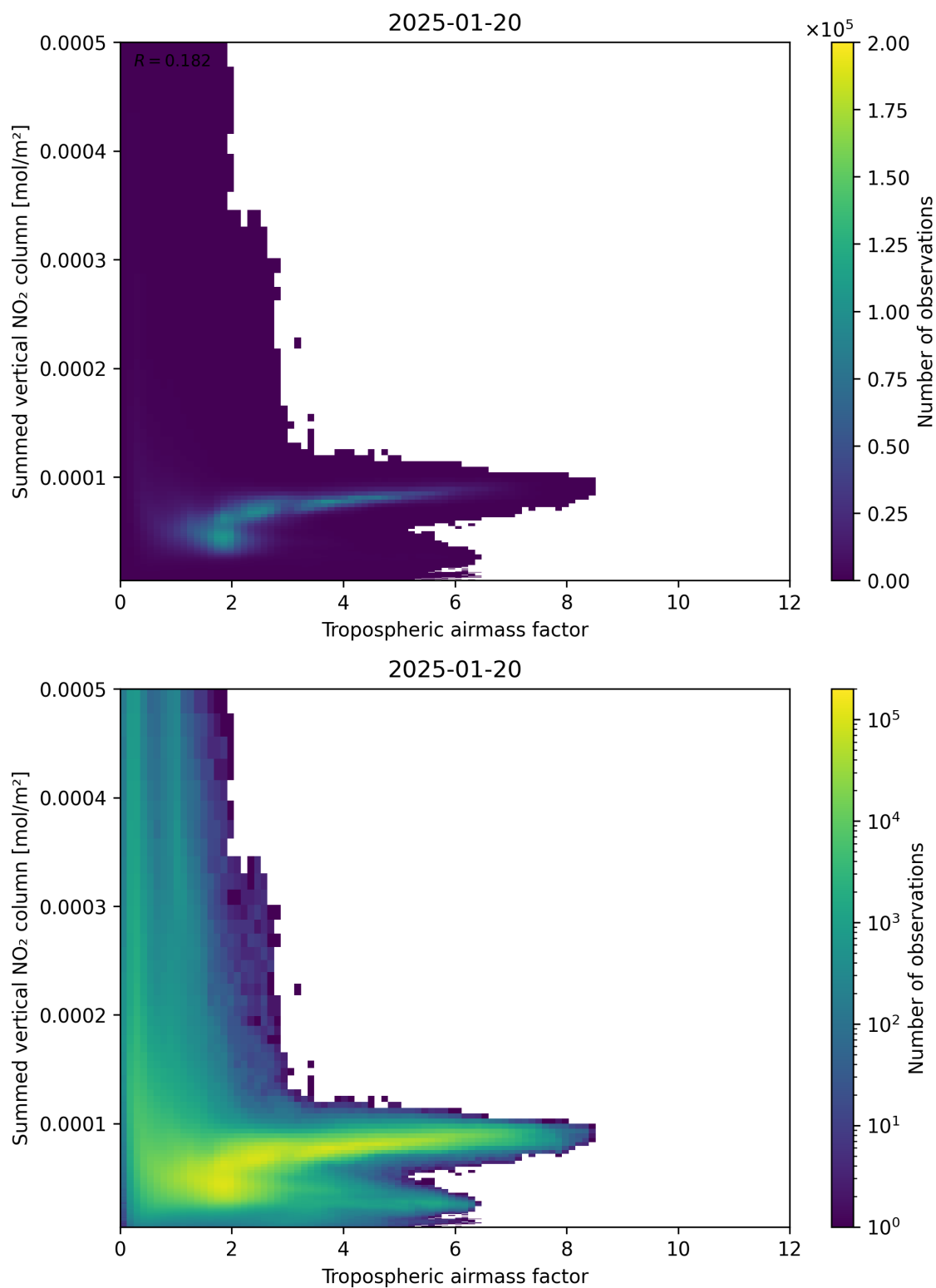
Figure 75: Scatter density plot of “Tropospheric air mass factor” against “Summed vertical NO 2 column” for 2025-01-19 to 2025-01-21.
