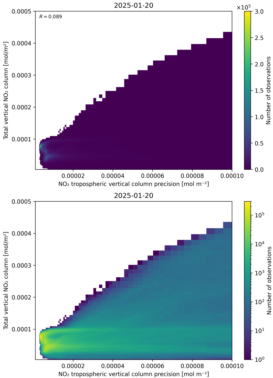
Figure 138: Scatter density plot of “NO 2 tropospheric vertical column precision” against “Total vertical NO 2 column” for 2025-01-19 to 2025-01-21.
