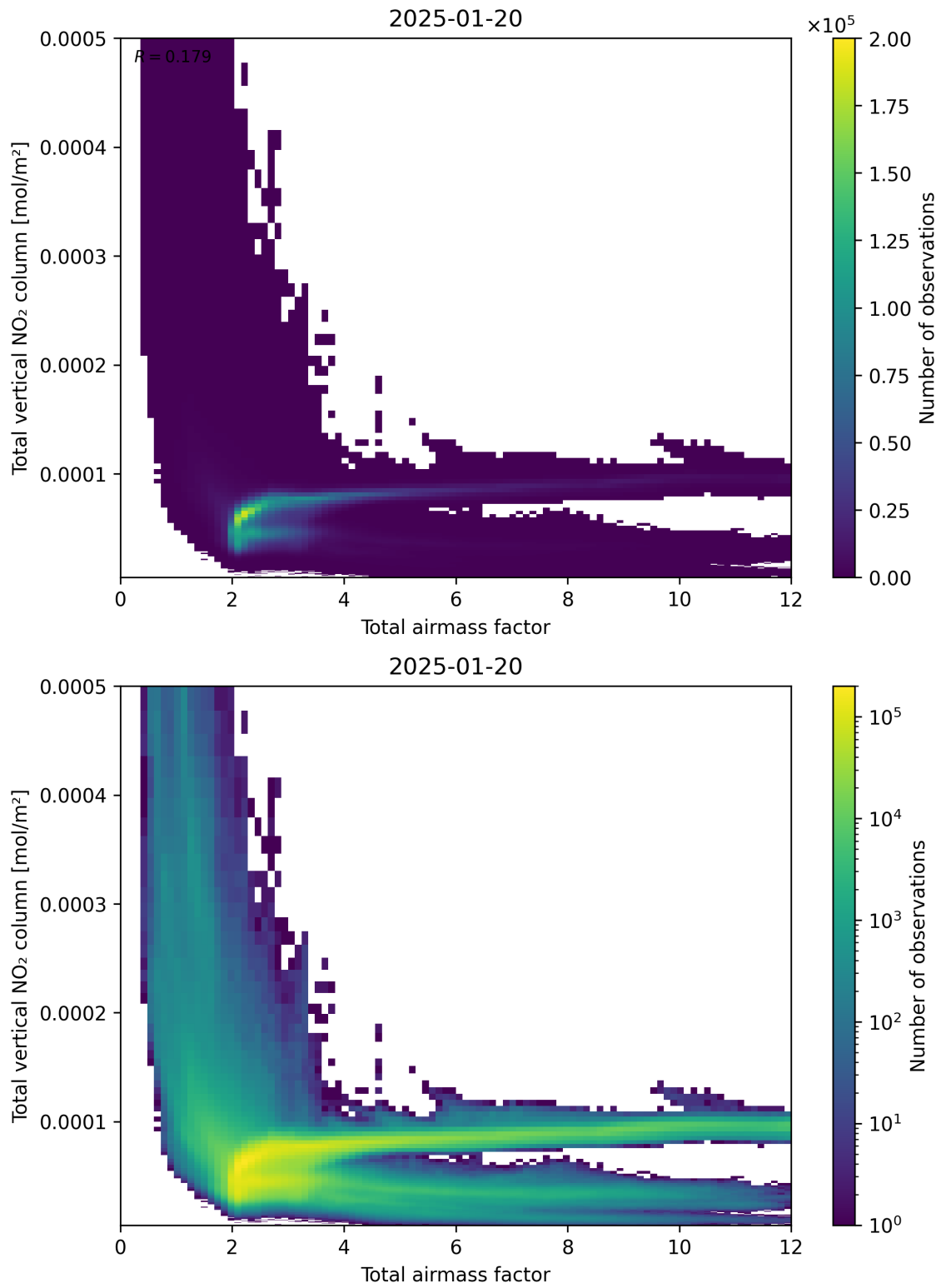
Figure 67: Scatter density plot of “Total airmass factor” against “Total vertical NO 2 column” for 2025-01-19 to 2025-01-21.
