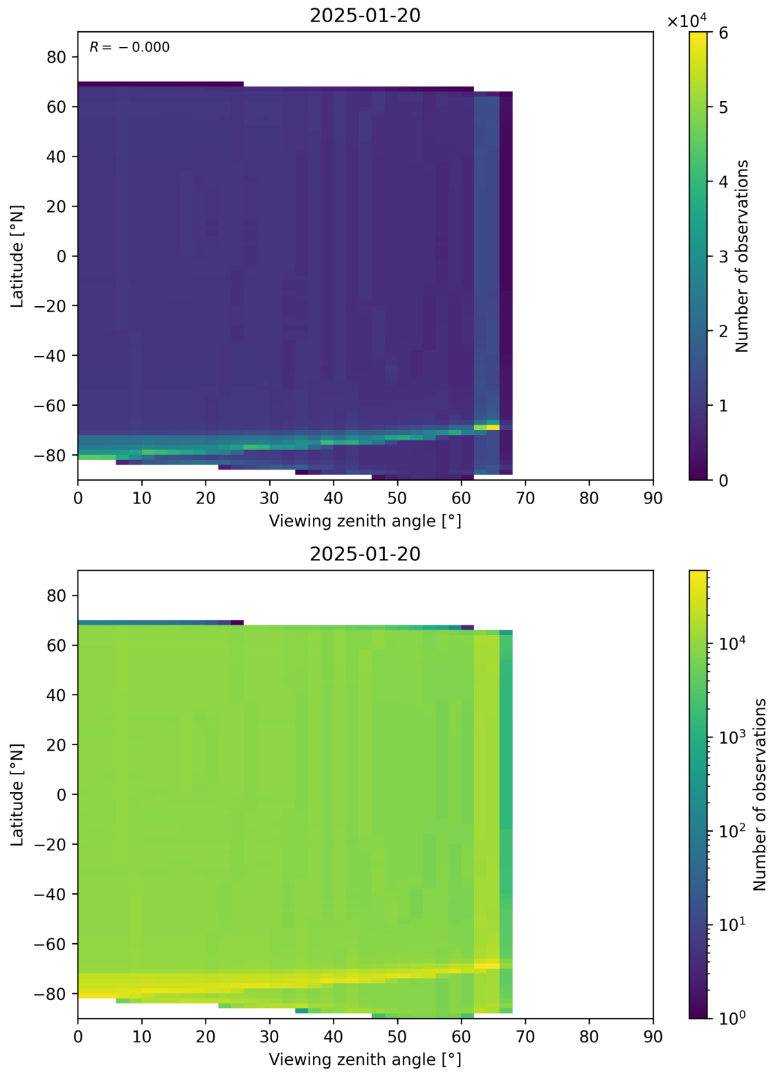
Figure 163: Scatter density plot of “Viewing zenith angle” against “Latitude” for 2025-01-19 to 2025-01-21.
