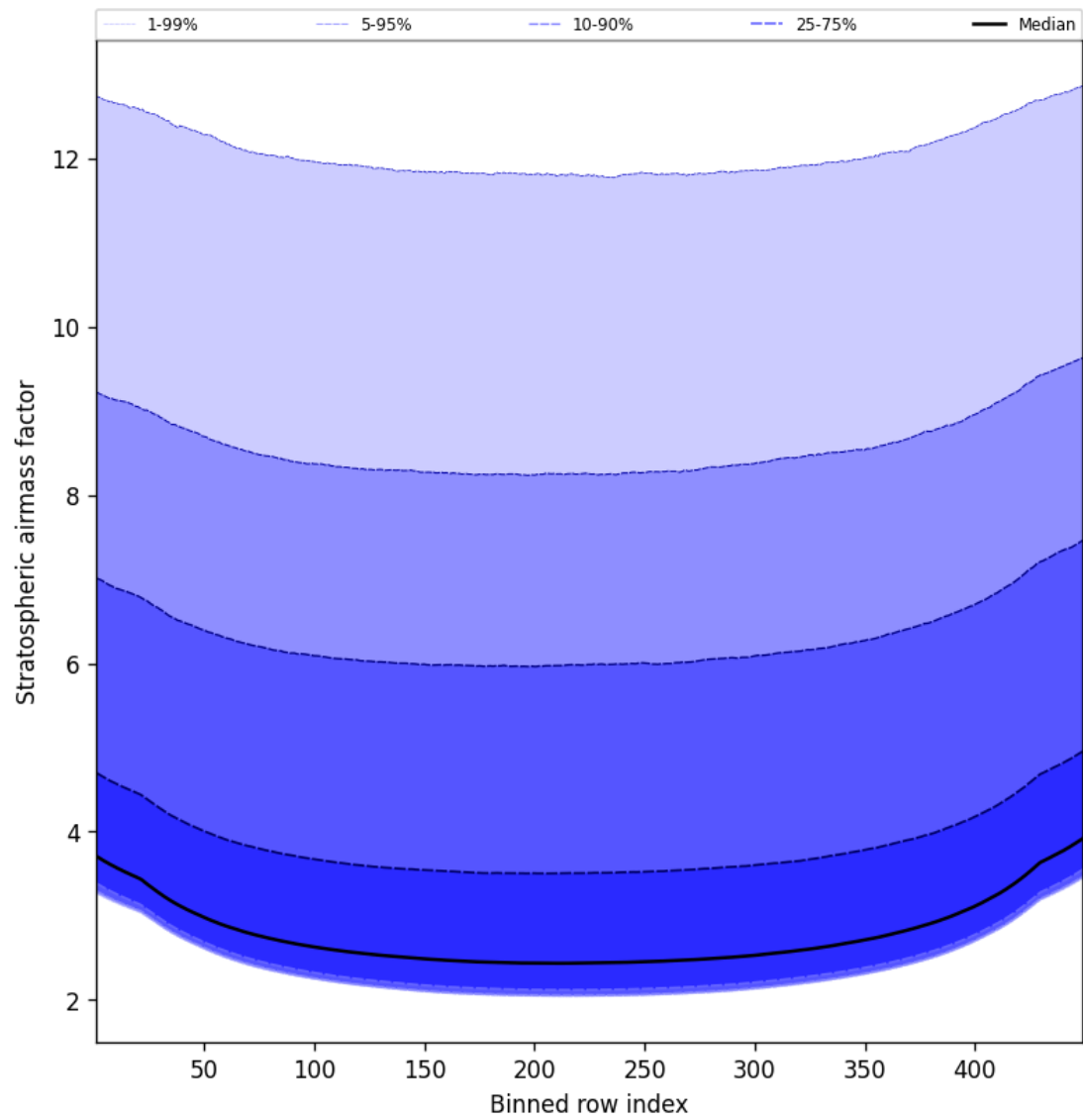
Figure 61: Along track statistics of “Stratospheric airmass factor” for 2025-01-19 to 2025-01-21
