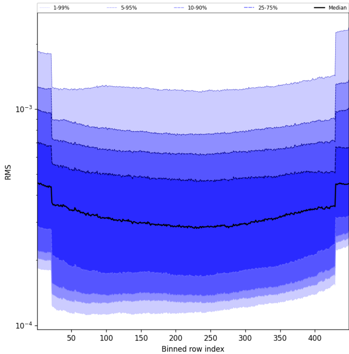
Figure 60: Along track statistics of “RMS” for 2025-01-19 to 2025-01-21
