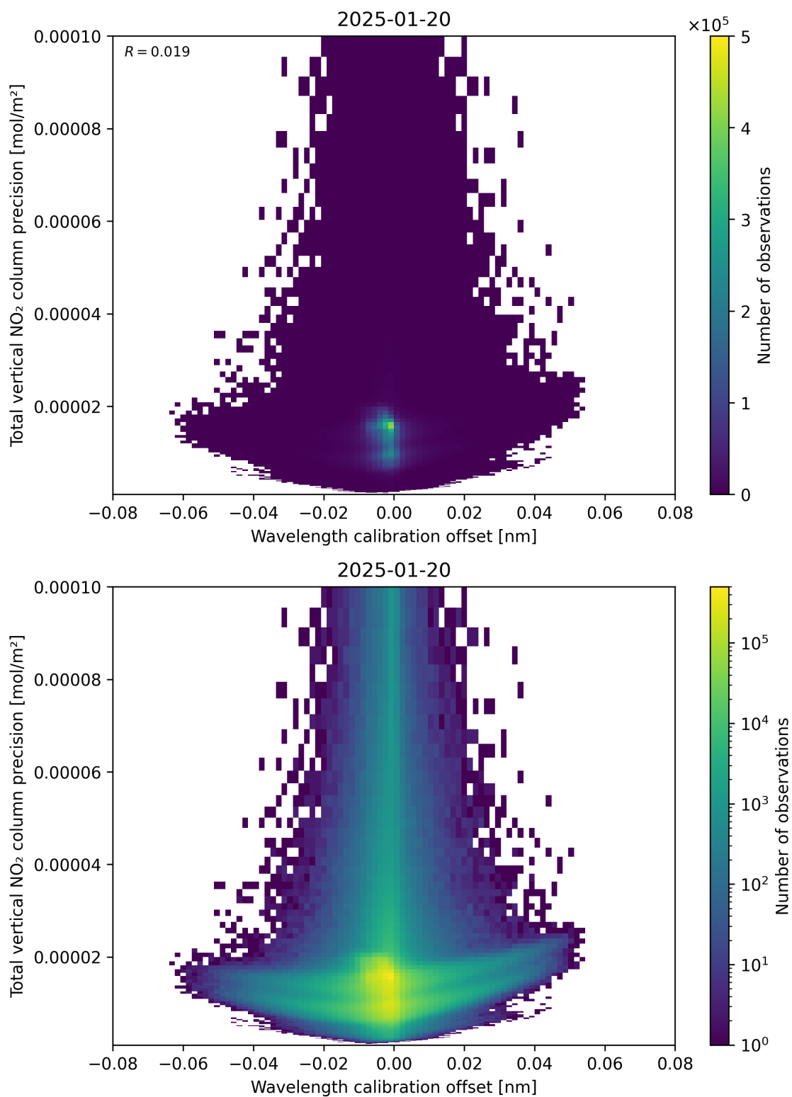
Figure 180: Scatter density plot of “Wavelength calibration offset” against “Total vertical NO 2 column precision” for 2025-01-19 to 2025-01-21.
