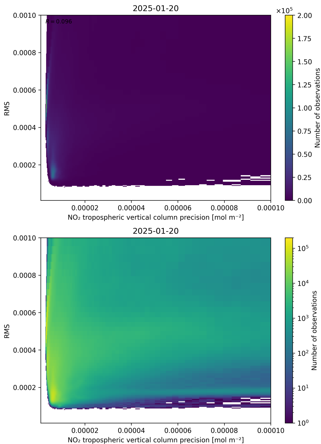
Figure 140: Scatter density plot of “NO 2 tropospheric vertical column precision” against “RMS” for 2025-01-19 to 2025-01-21.
