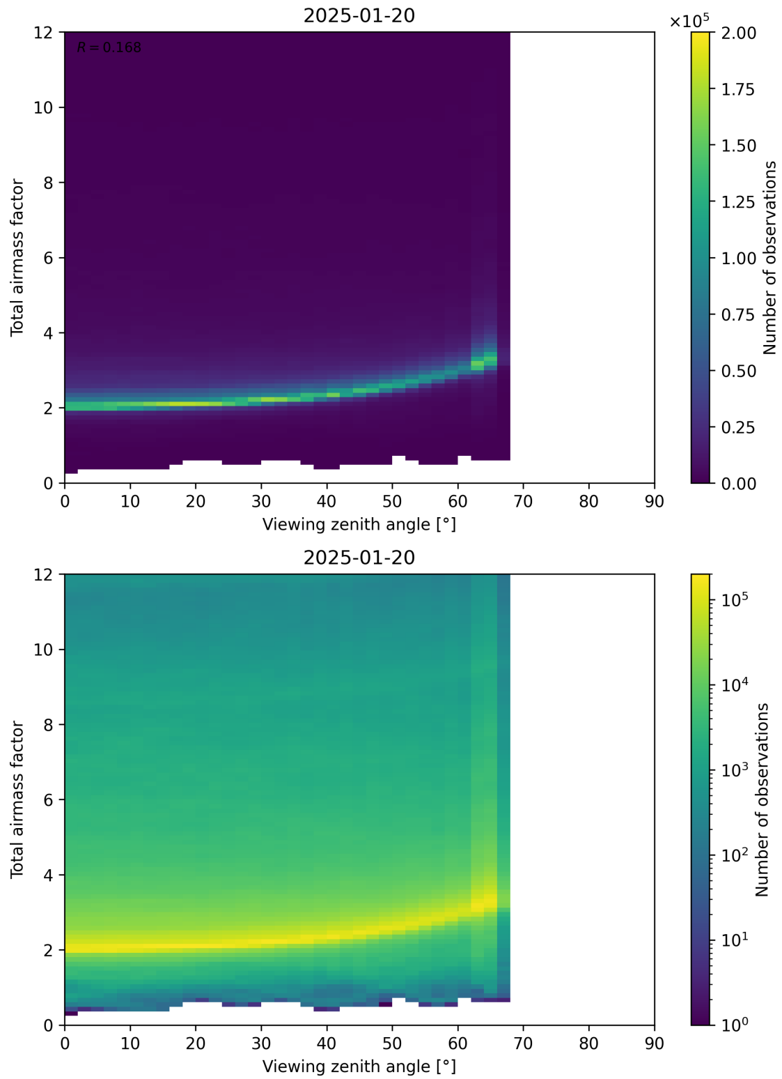
Figure 160: Scatter density plot of “Viewing zenith angle” against “Total airmass factor” for 2025-01-19 to 2025-01-21.
