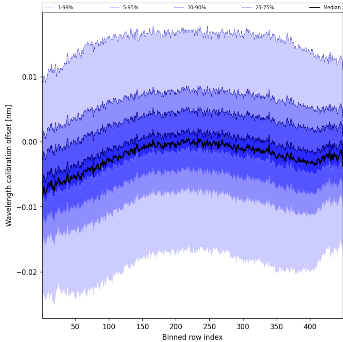
Figure 52: Along track statistics of “Wavelength calibration offset” for 2025-01-19 to 2025-01-21
