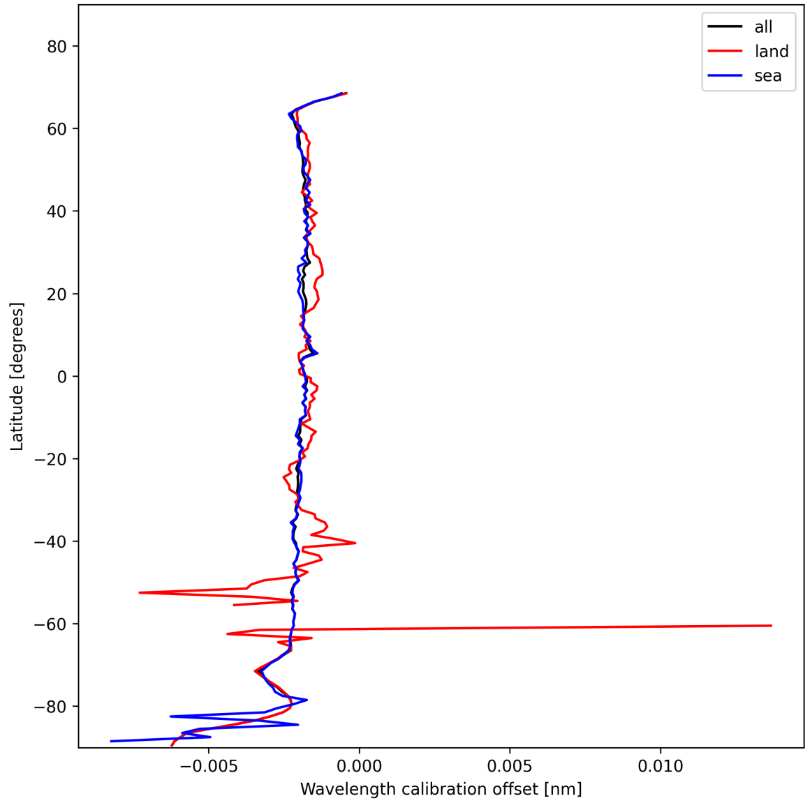
Figure 18: Zonal average of “Wavelength calibration offset” for 2025-01-19 to 2025-01-21.
