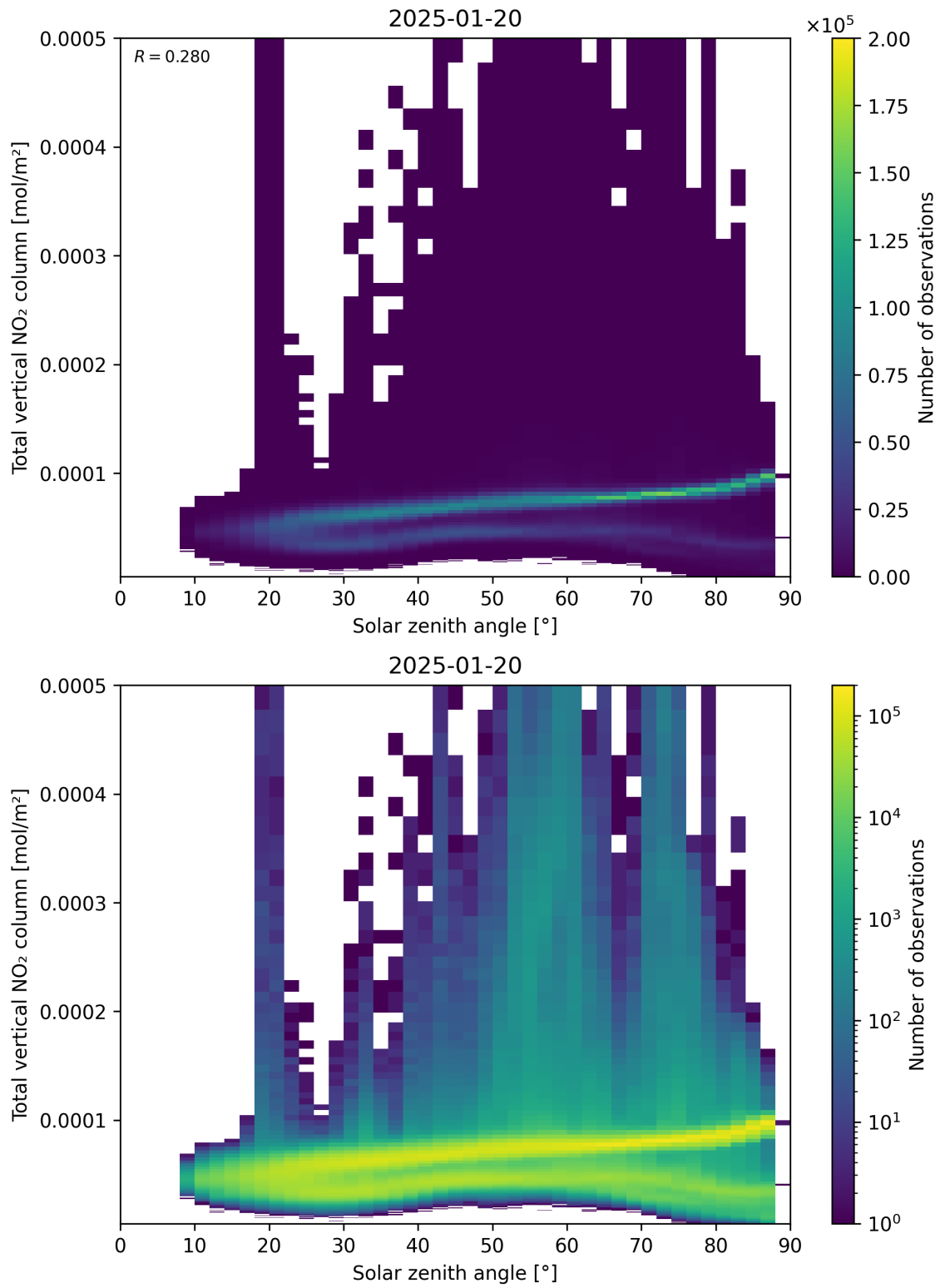
Figure 153: Scatter density plot of “Solar zenith angle” against “Total vertical NO 2 column” for 2025-01-19 to 2025-01-21.
