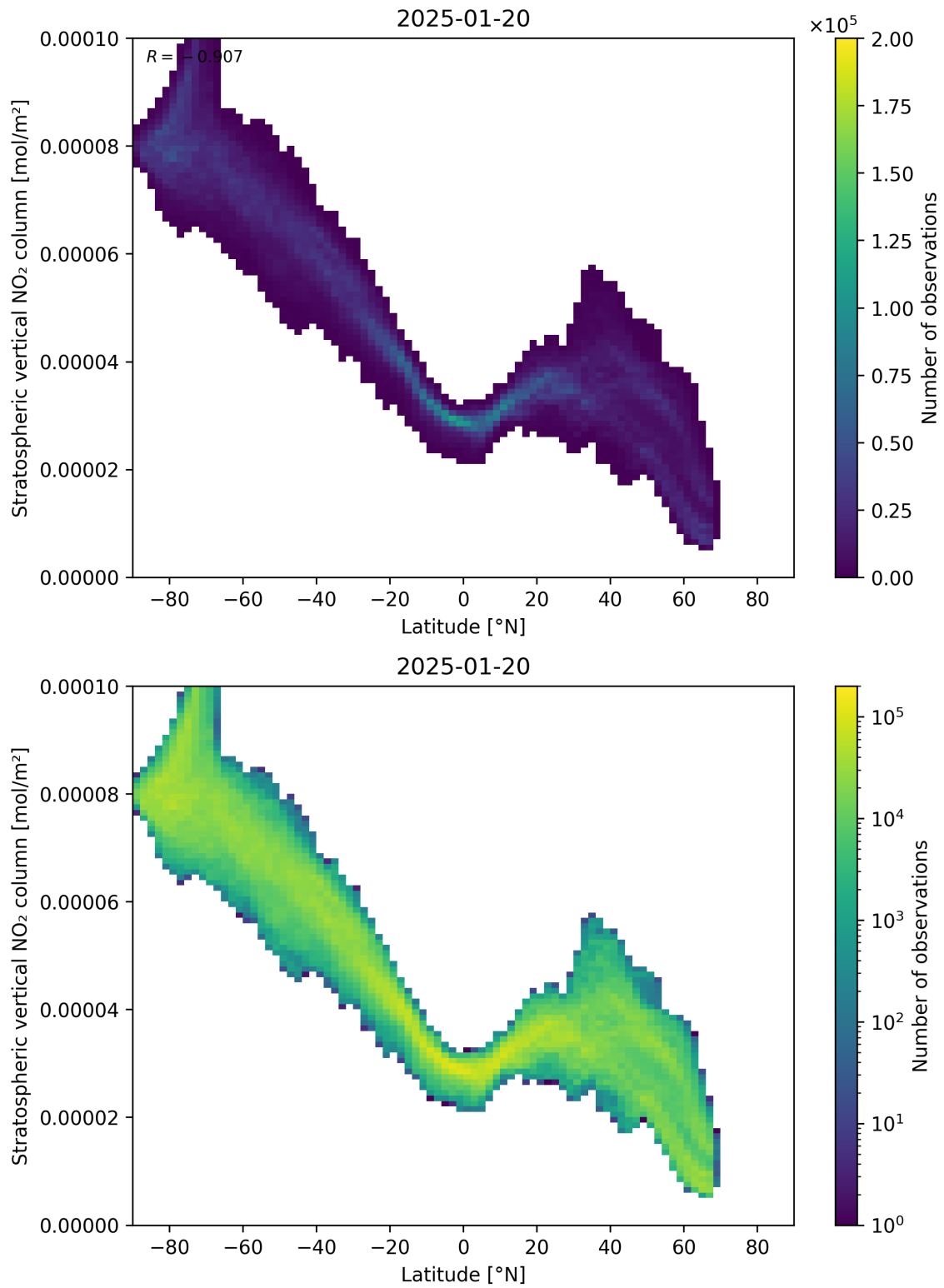
Figure 87: Scatter density plot of “Latitude” against “Stratospheric vertical NO 2 column” for 2025-01-19 to 2025-01-21.
