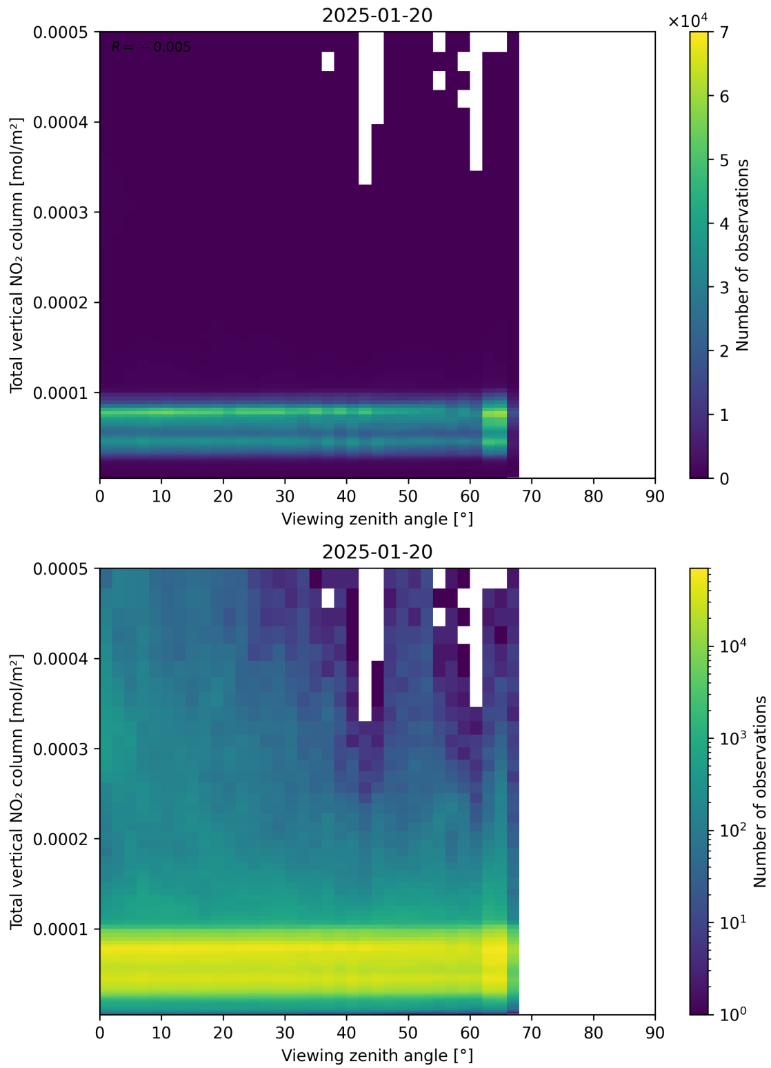
Figure 167: Scatter density plot of “Viewing zenith angle” against “Total vertical NO 2 column” for 2025-01-19 to 2025-01-21.
