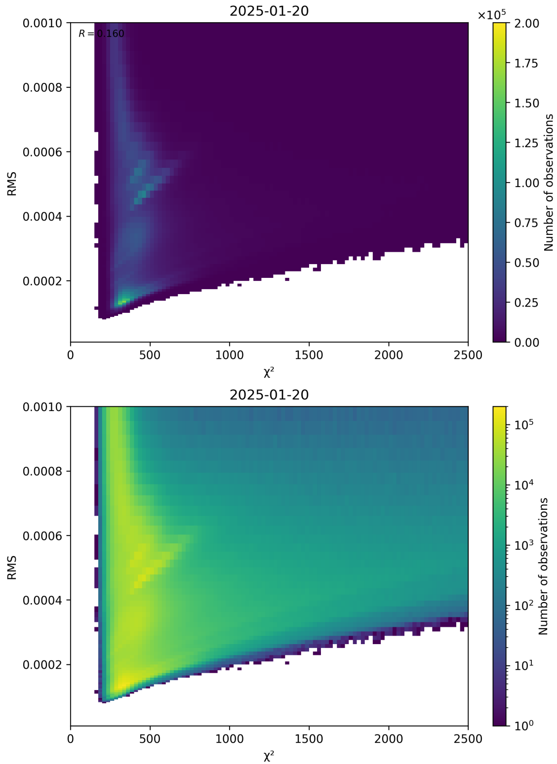
Figure 82: Scatter density plot of “ \chi^2 ” against “RMS” for 2025-01-19 to 2025-01-21.
