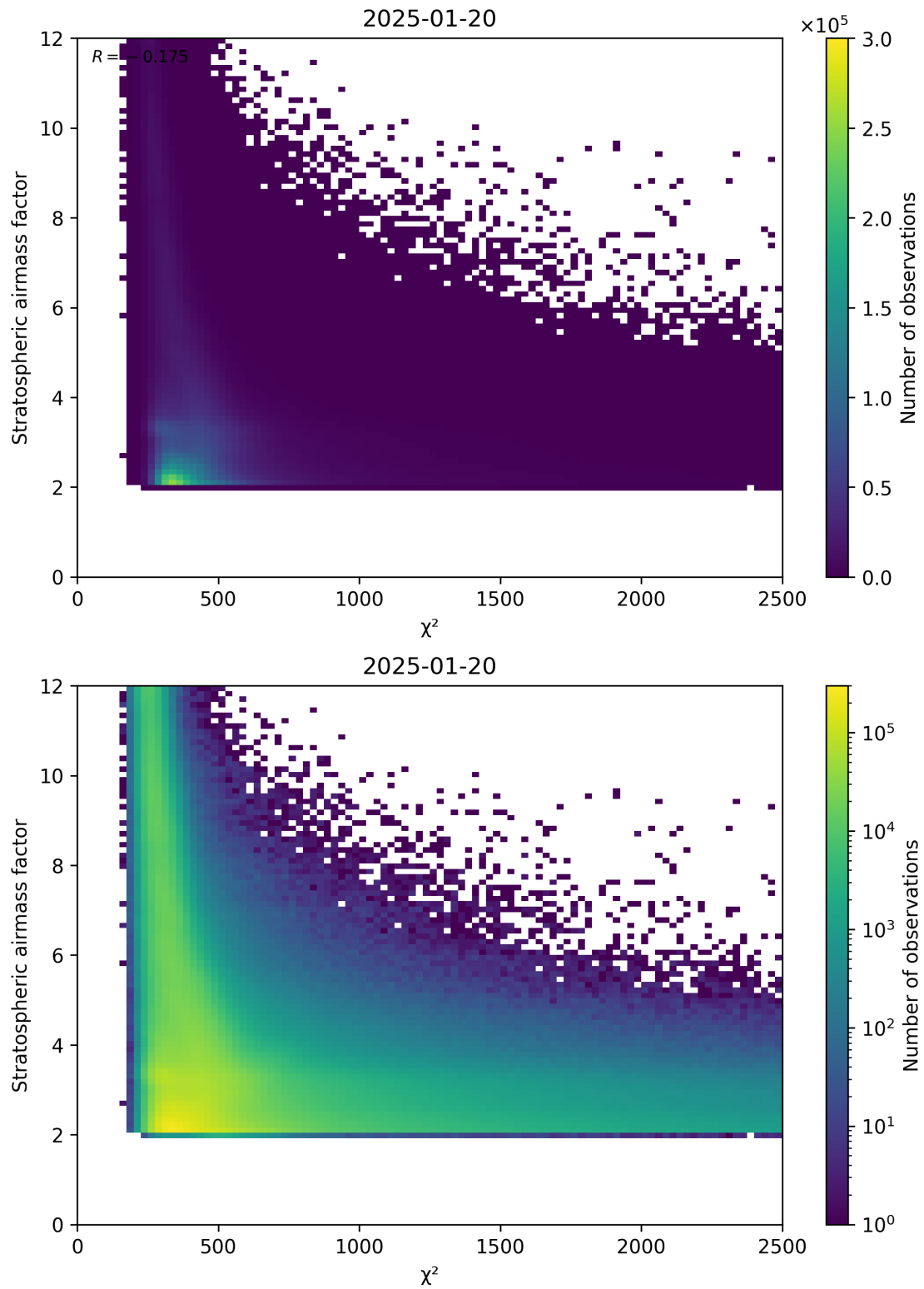
Figure 81: Scatter density plot of “ \chi^2 ” against “Stratospheric airmass factor” for 2025-01-19 to 2025-01-21.
