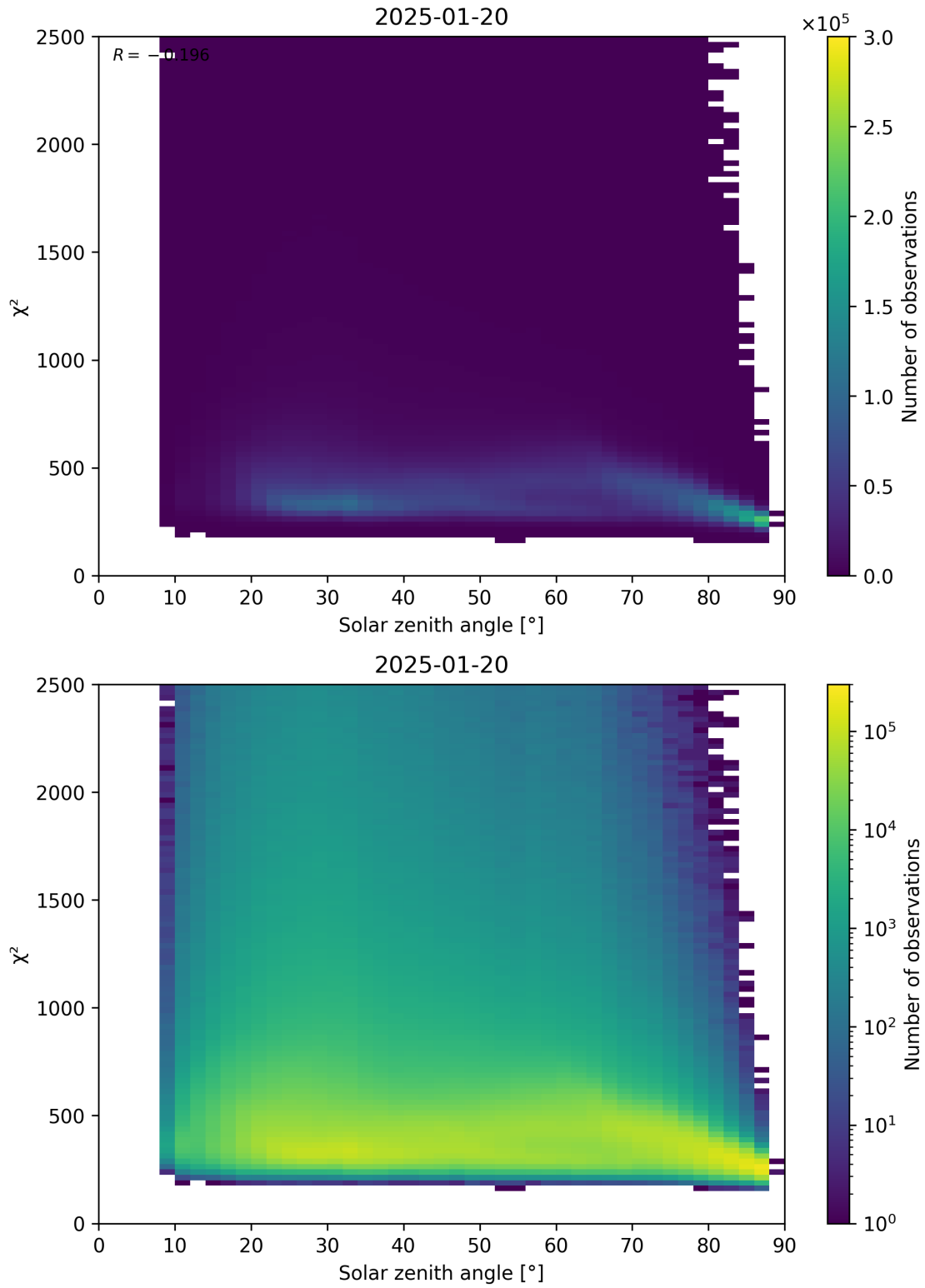
Figure 148: Scatter density plot of “Solar zenith angle” against “ \chi^2 ” for 2025-01-19 to 2025-01-21.
