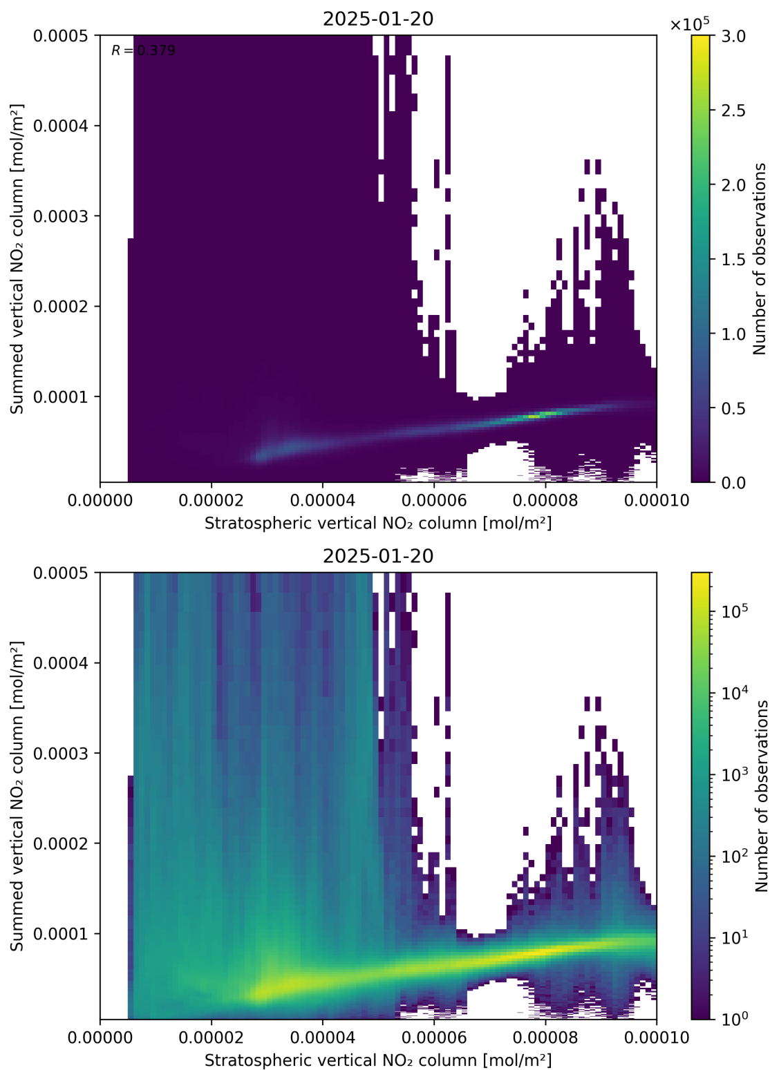
Figure 98: Scatter density plot of “Stratospheric vertical NO 2 column” against “Summed vertical NO 2 column” for 2025-01-19 to 2025-01-21.
