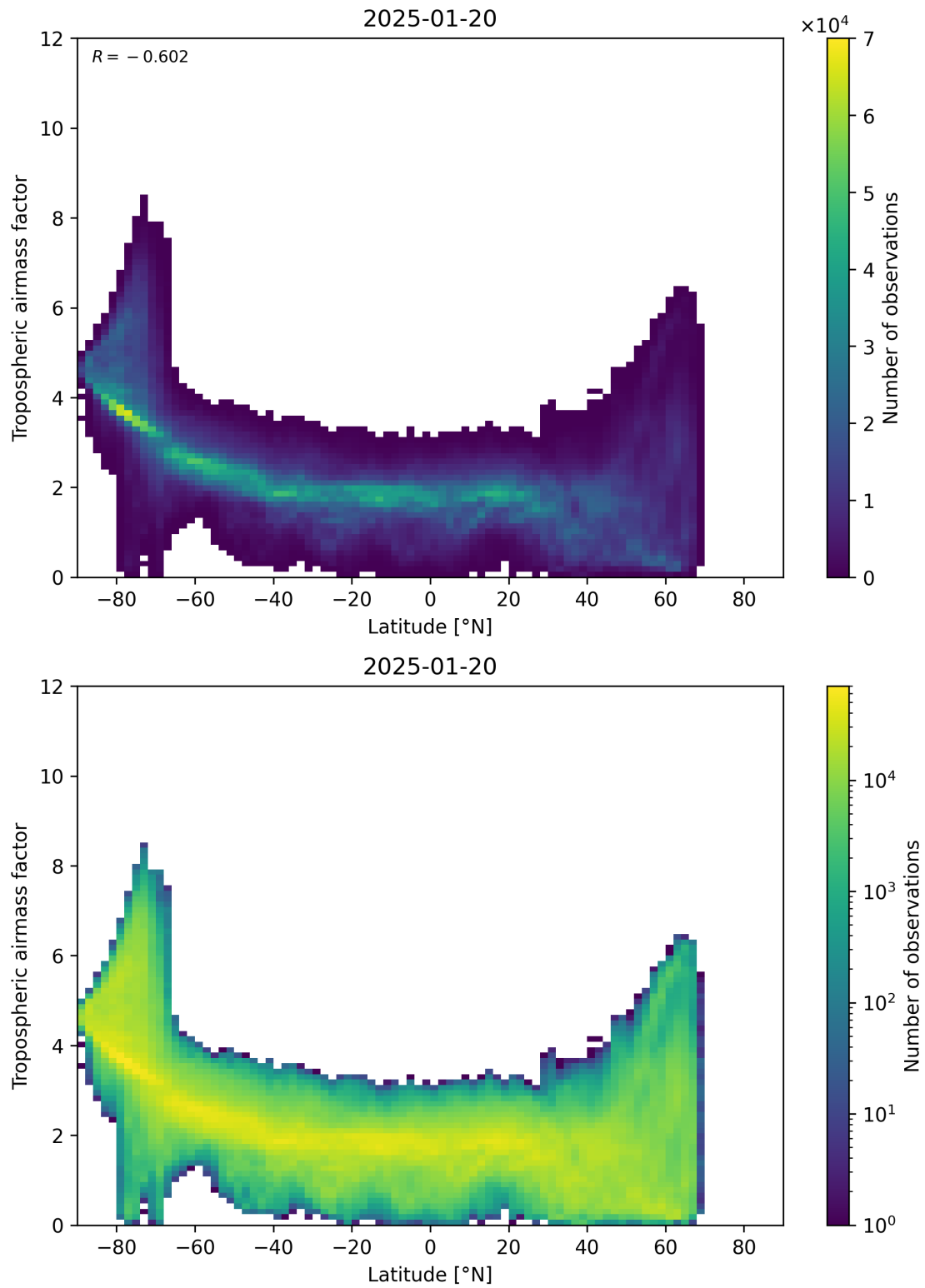
Figure 85: Scatter density plot of “Latitude” against “Tropospheric air mass factor” for 2025-01-19 to 2025-01-21.
