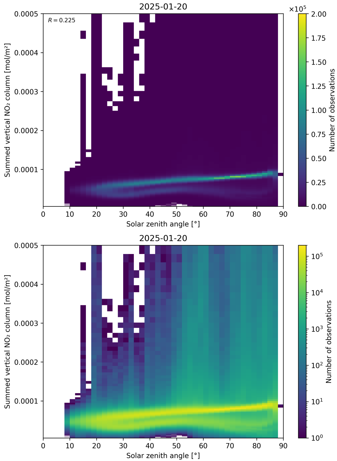
Figure 151: Scatter density plot of “Solar zenith angle” against “Summed vertical NO 2 column” for 2025-01-19 to 2025-01-21.
