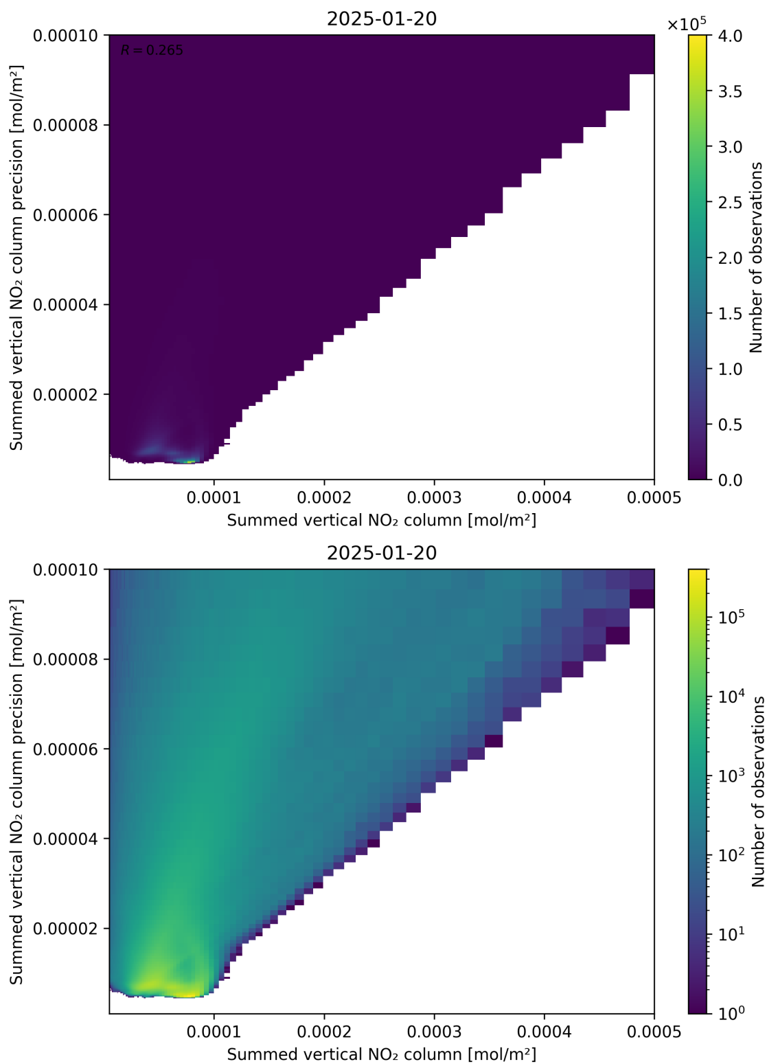
Figure 105: Scatter density plot of “Summed vertical NO 2 column” against “Summed vertical NO 2 column precision” for 2025-01-19 to 2025-01-21.
