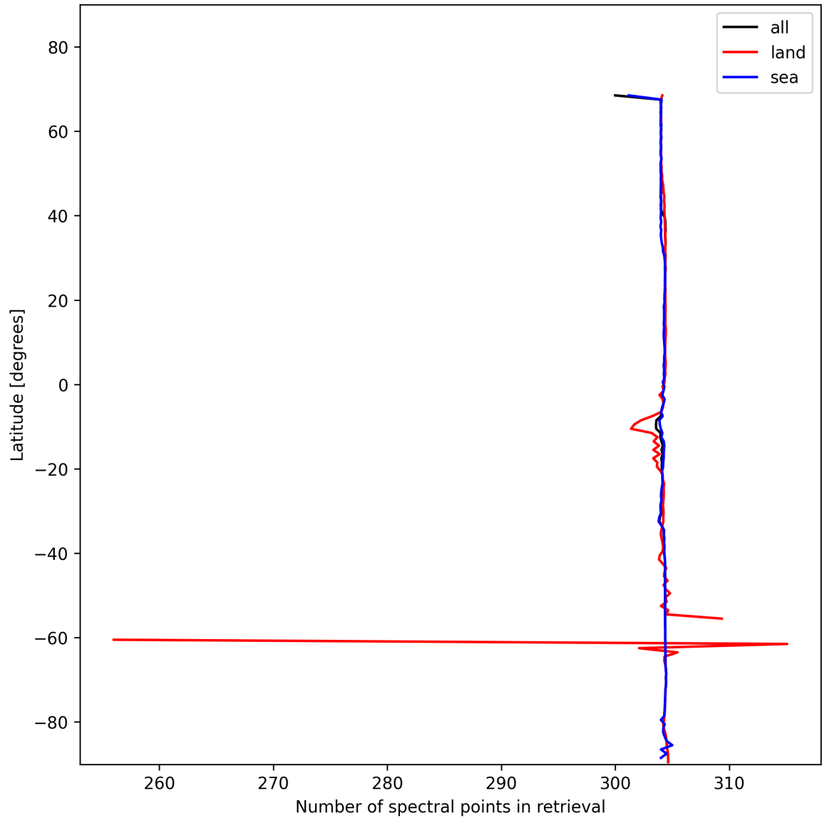
Figure 16: Zonal average of “Number of spectral points in retrieval” for 2025-01-19 to 2025-01-21.
