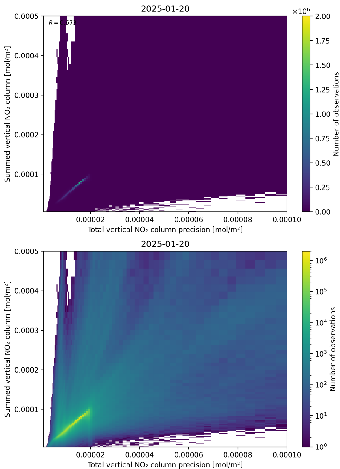
Figure 117: Scatter density plot of “Total vertical NO 2 column precision” against “Summed vertical NO 2 column” for 2025-01-19 to 2025-01-21.
