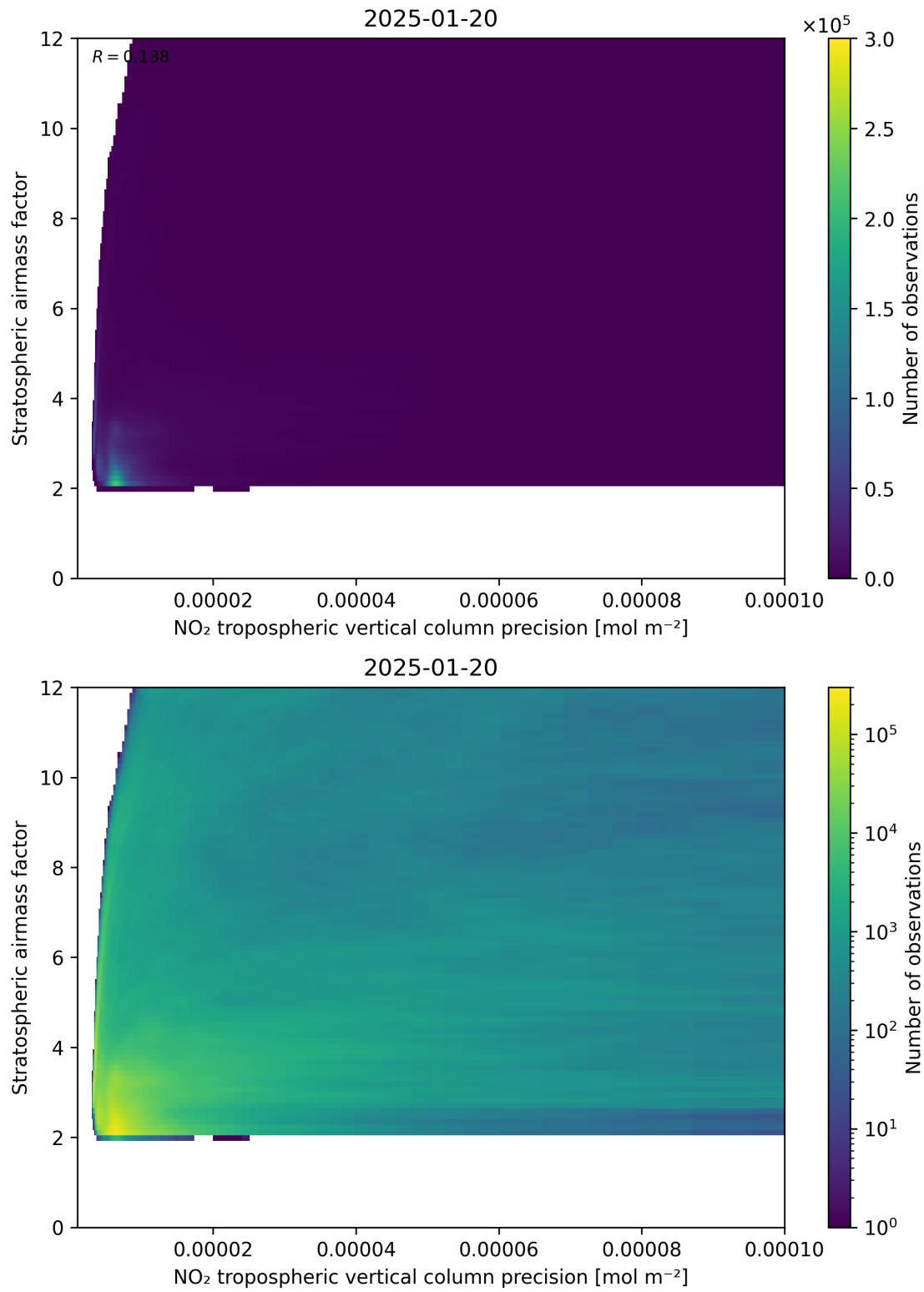
Figure 131: Scatter density plot of “NO 2 tropospheric vertical column precision” against “Stratospheric airmass factor” for 2025-01-19 to 2025-01-21.
