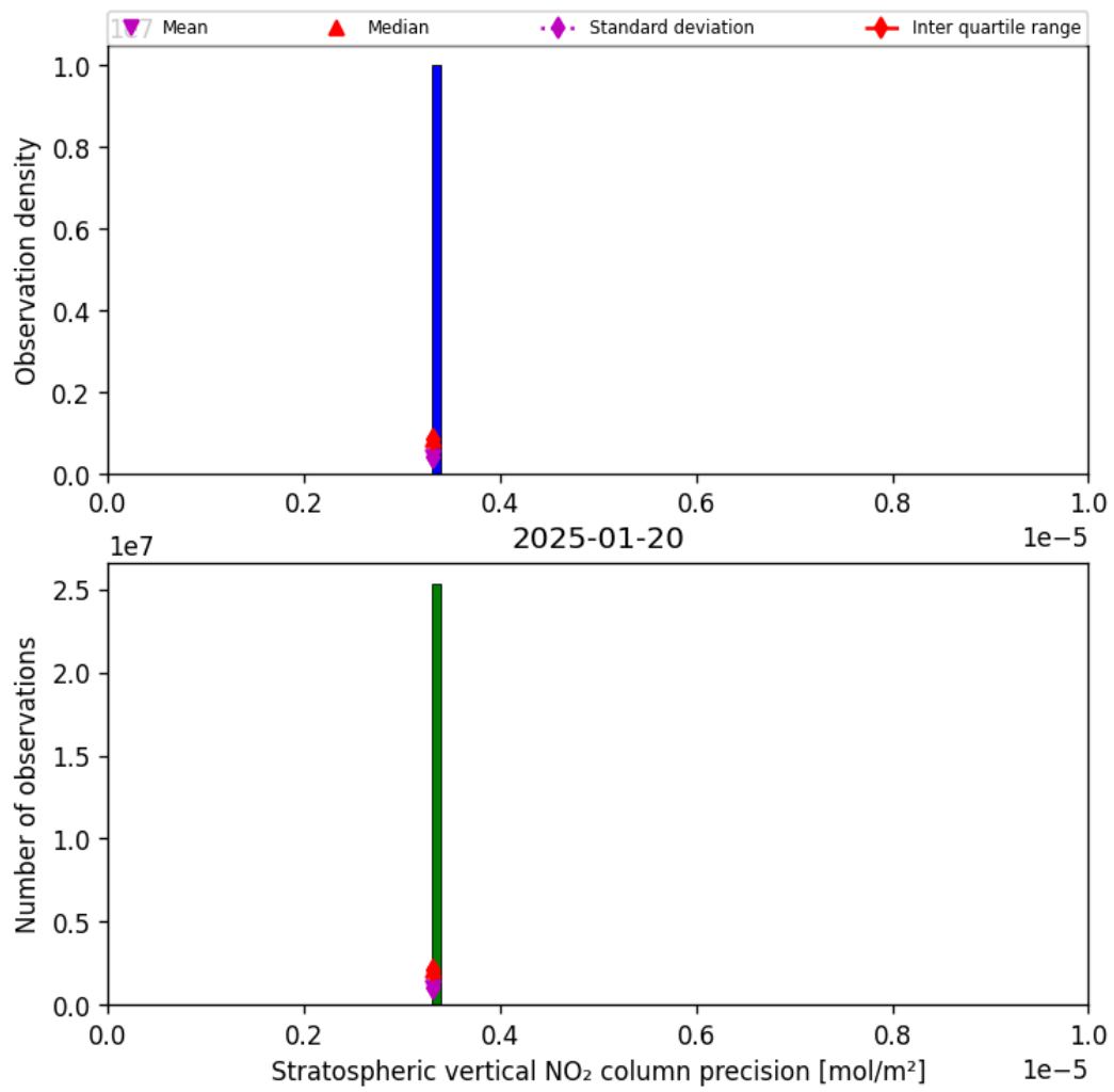
Figure 37: Histogram of “Stratospheric vertical NO 2 column precision” for 2025-01-19 to 2025-01-21
