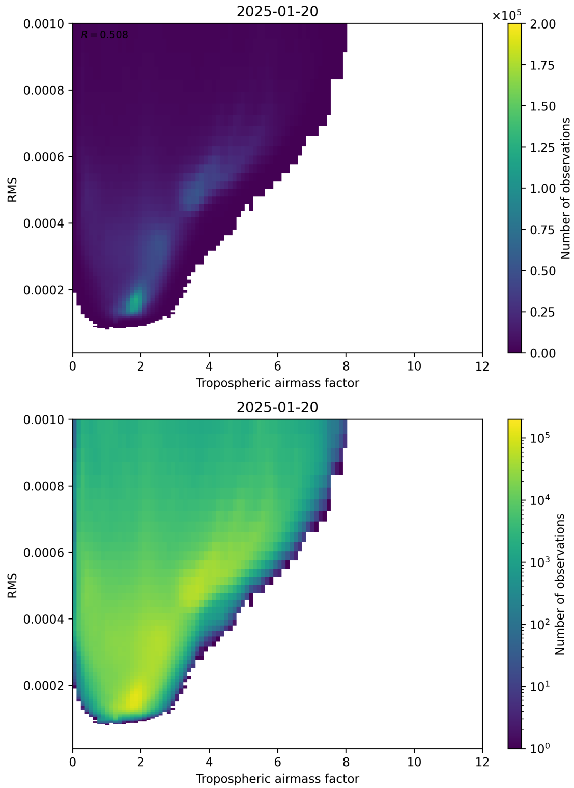
Figure 79: Scatter density plot of “Tropospheric airmass factor” against “RMS” for 2025-01-19 to 2025-01-21.
