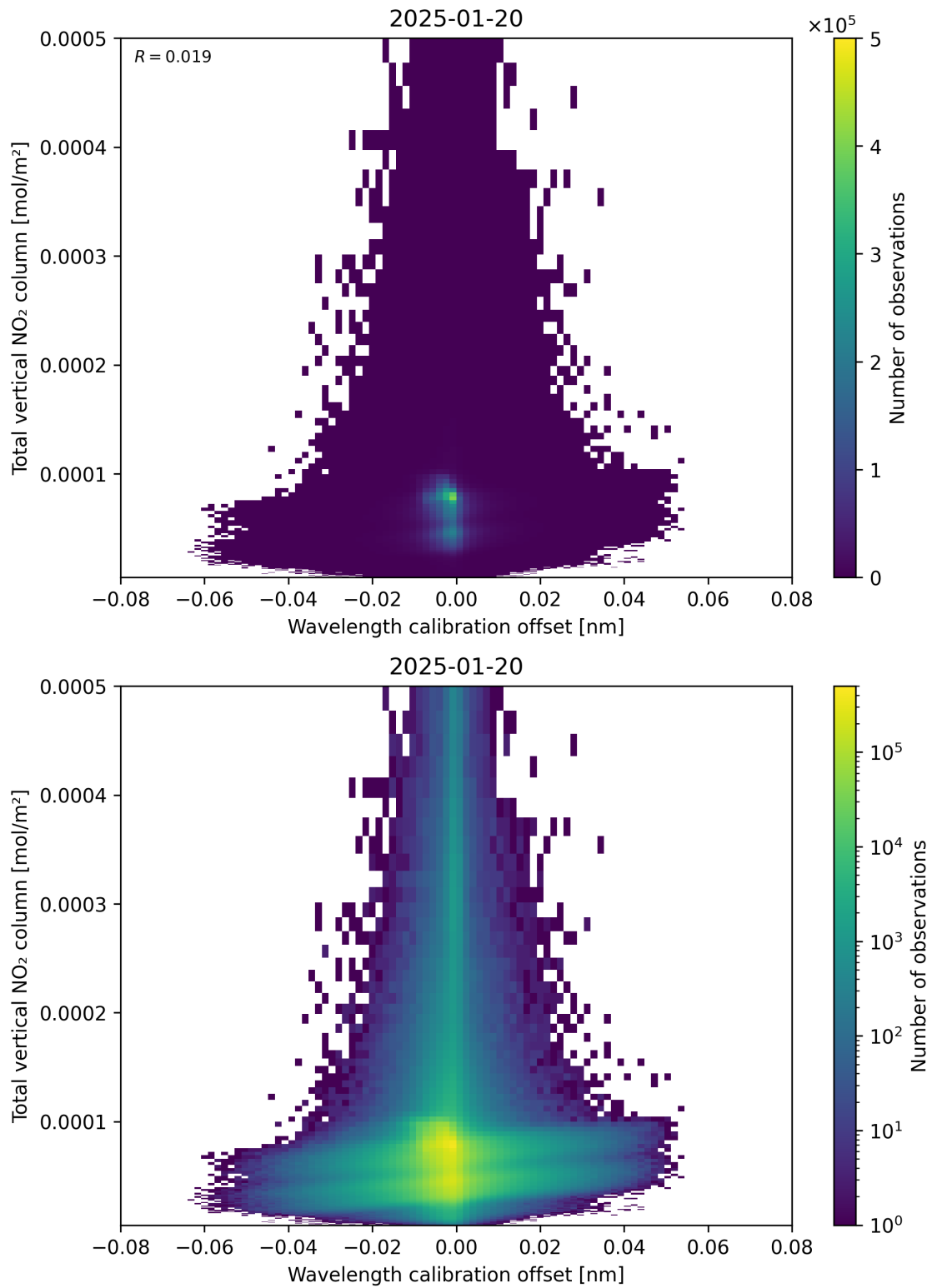
Figure 179: Scatter density plot of “Wavelength calibration offset” against “Total vertical NO 2 column” for 2025-01-19 to 2025-01-21.
