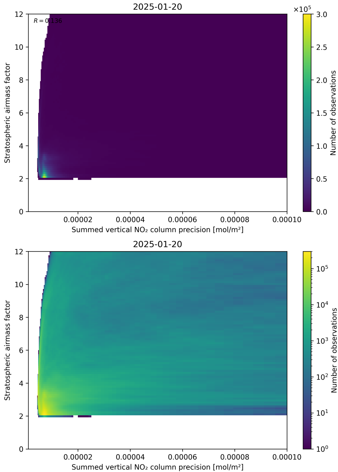
Figure 106: Scatter density plot of “Summed vertical NO 2 column precision” against “Stratospheric airmass factor” for 2025-01-19 to 2025-01-21.
