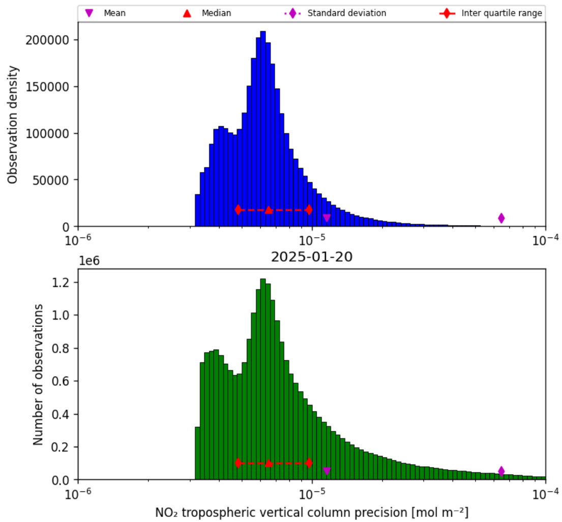
Figure 30: Histogram of “NO 2 tropospheric vertical column precision” for 2025-01-19 to 2025-01-21
