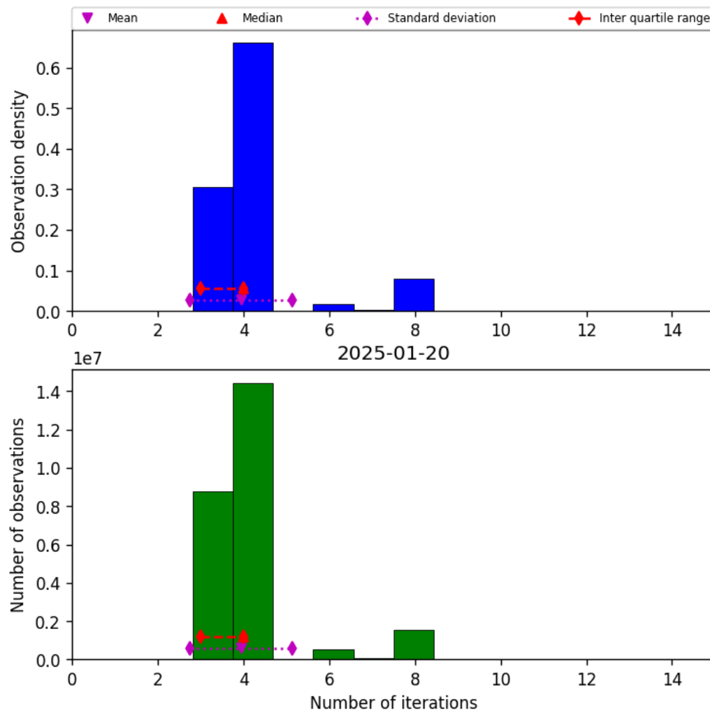
Figure 34: Histogram of “Number of iterations” for 2025-01-19 to 2025-01-21
