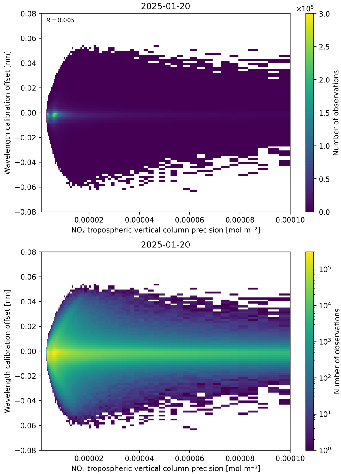
Figure 141: Scatter density plot of “NO 2 tropospheric vertical column precision” against “Wavelength calibration offset” for 2025-01-19 to 2025-01-21.
