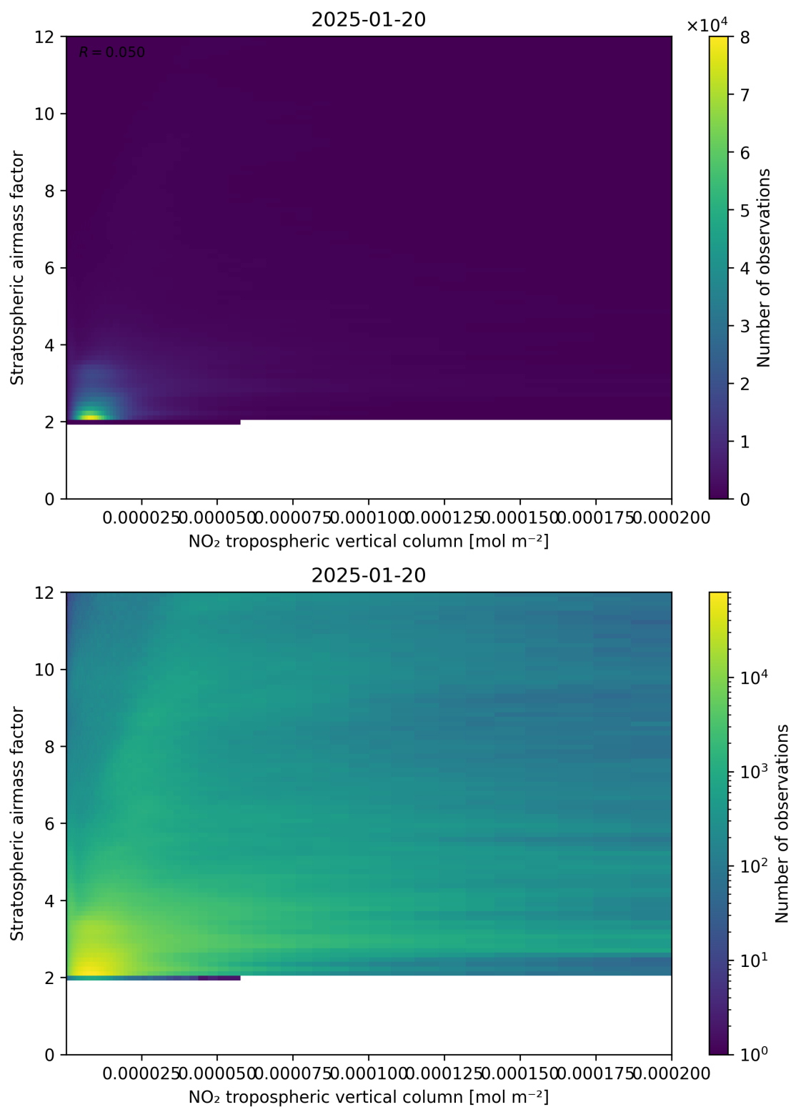
Figure 121: Scatter density plot of “NO 2 tropospheric vertical column” against “Stratospheric airmass factor” for 2025-01-19 to 2025-01-21.
