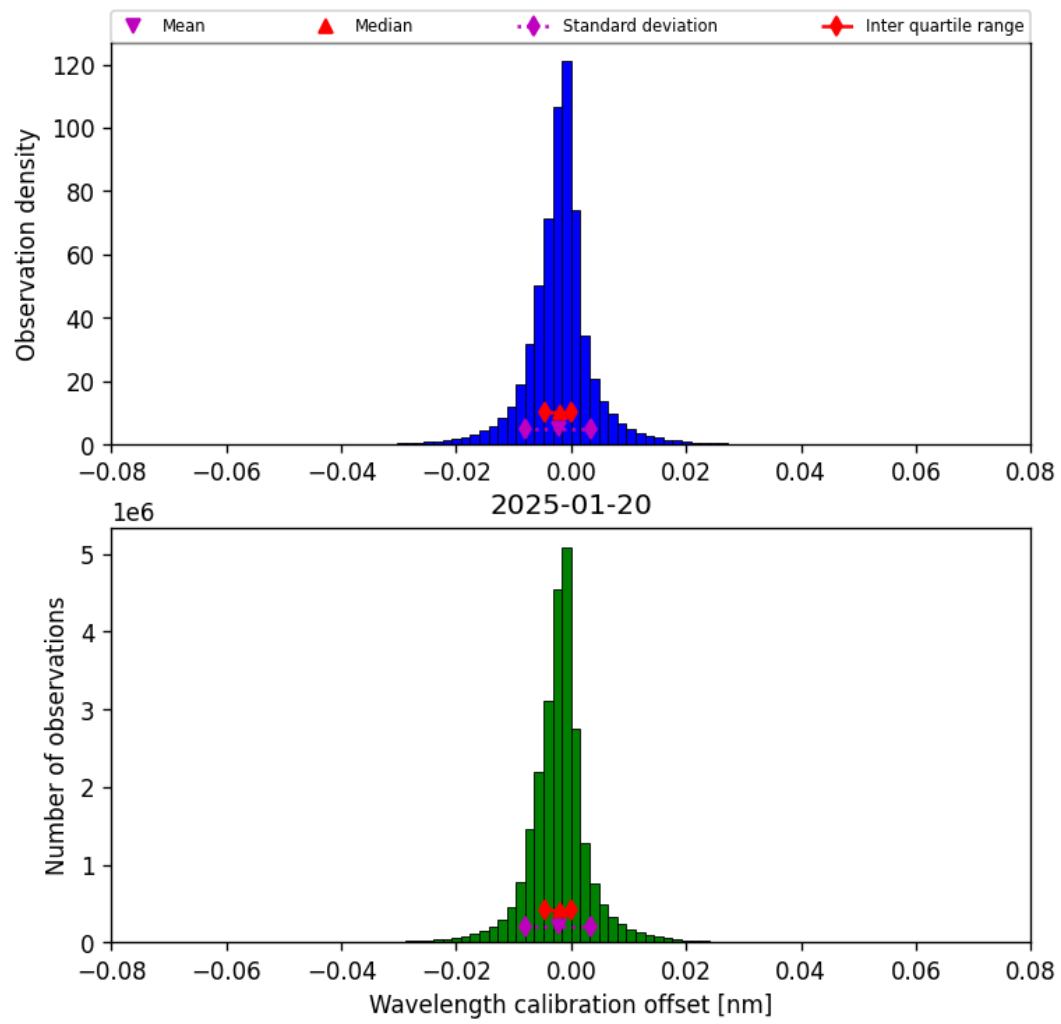
Figure 35: Histogram of “Wavelength calibration offset” for 2025-01-19 to 2025-01-21
