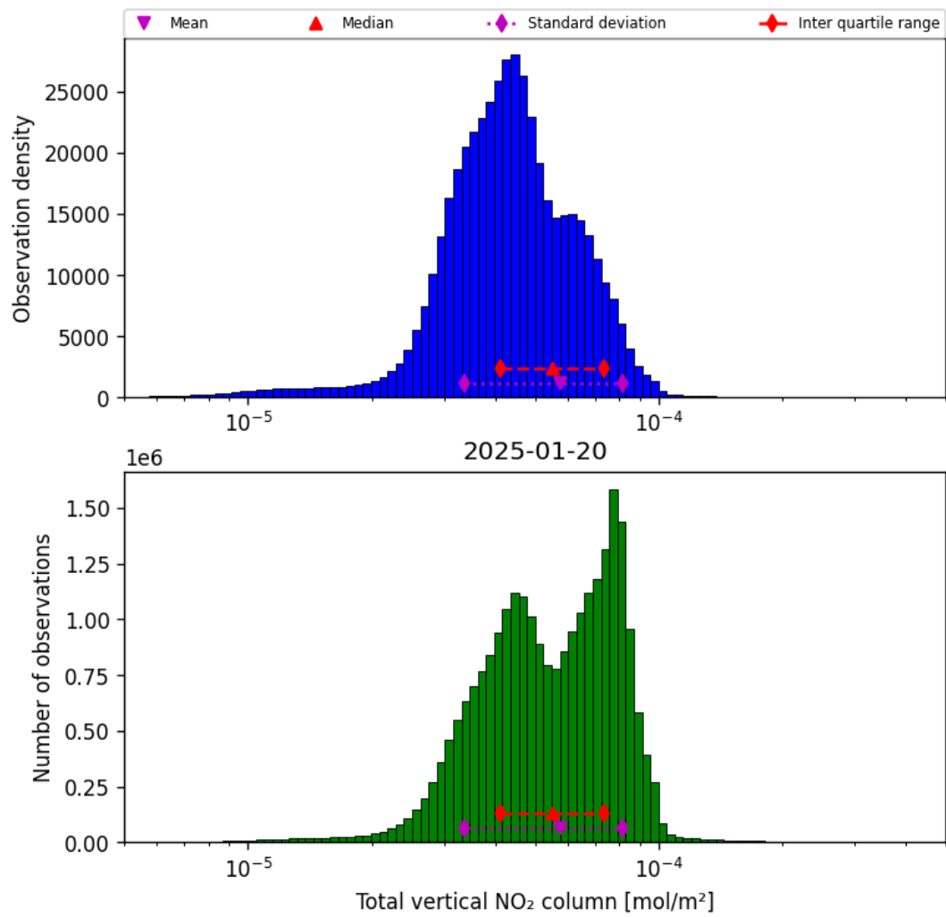
Figure 38: Histogram of “Total vertical NO 2 column” for 2025-01-19 to 2025-01-21
