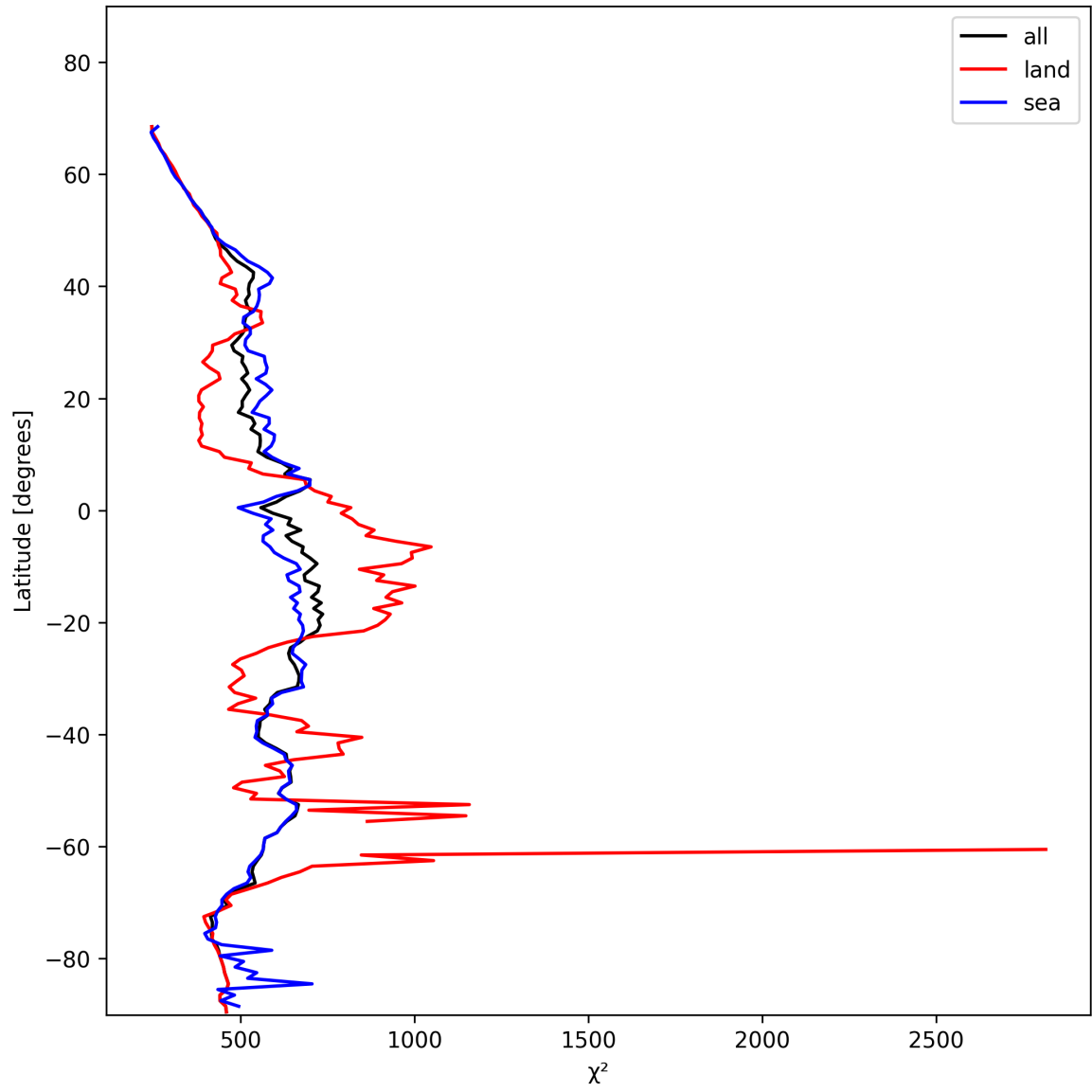
Figure 25: Zonal average of “ \chi^2 ” for 2025-01-19 to 2025-01-21.
