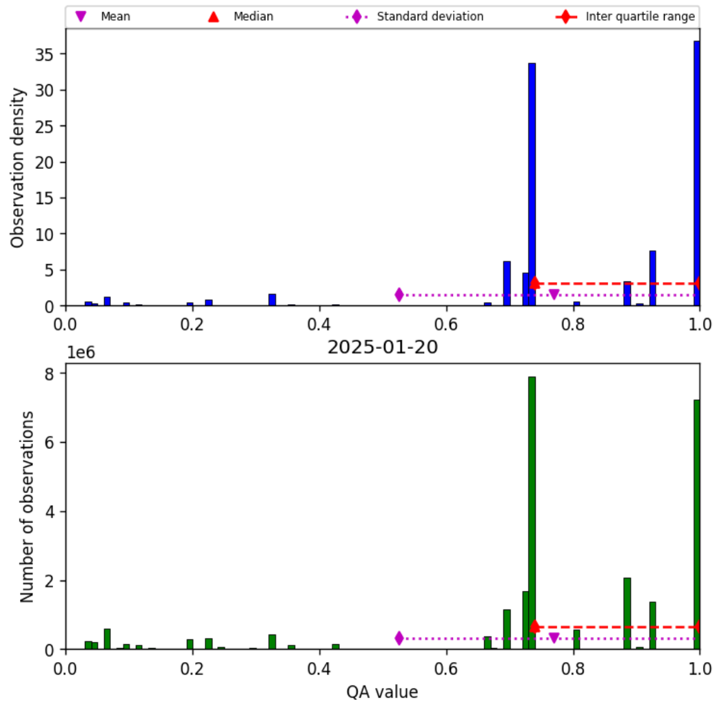
Figure 28: Histogram of “QA value” for 2025-01-19 to 2025-01-21
