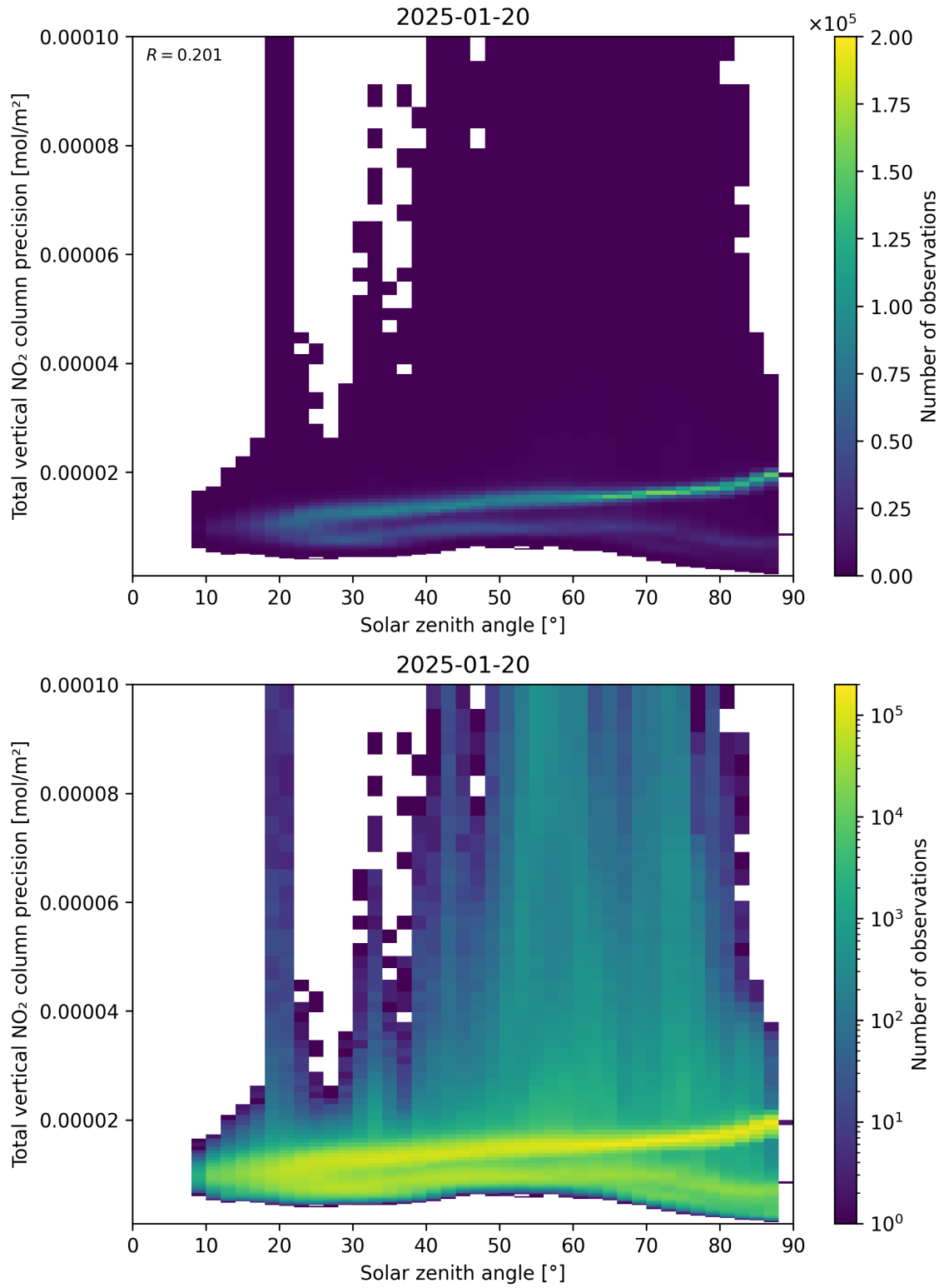
Figure 154: Scatter density plot of “Solar zenith angle” against “Total vertical NO 2 column precision” for 2025-01-19 to 2025-01-21.
