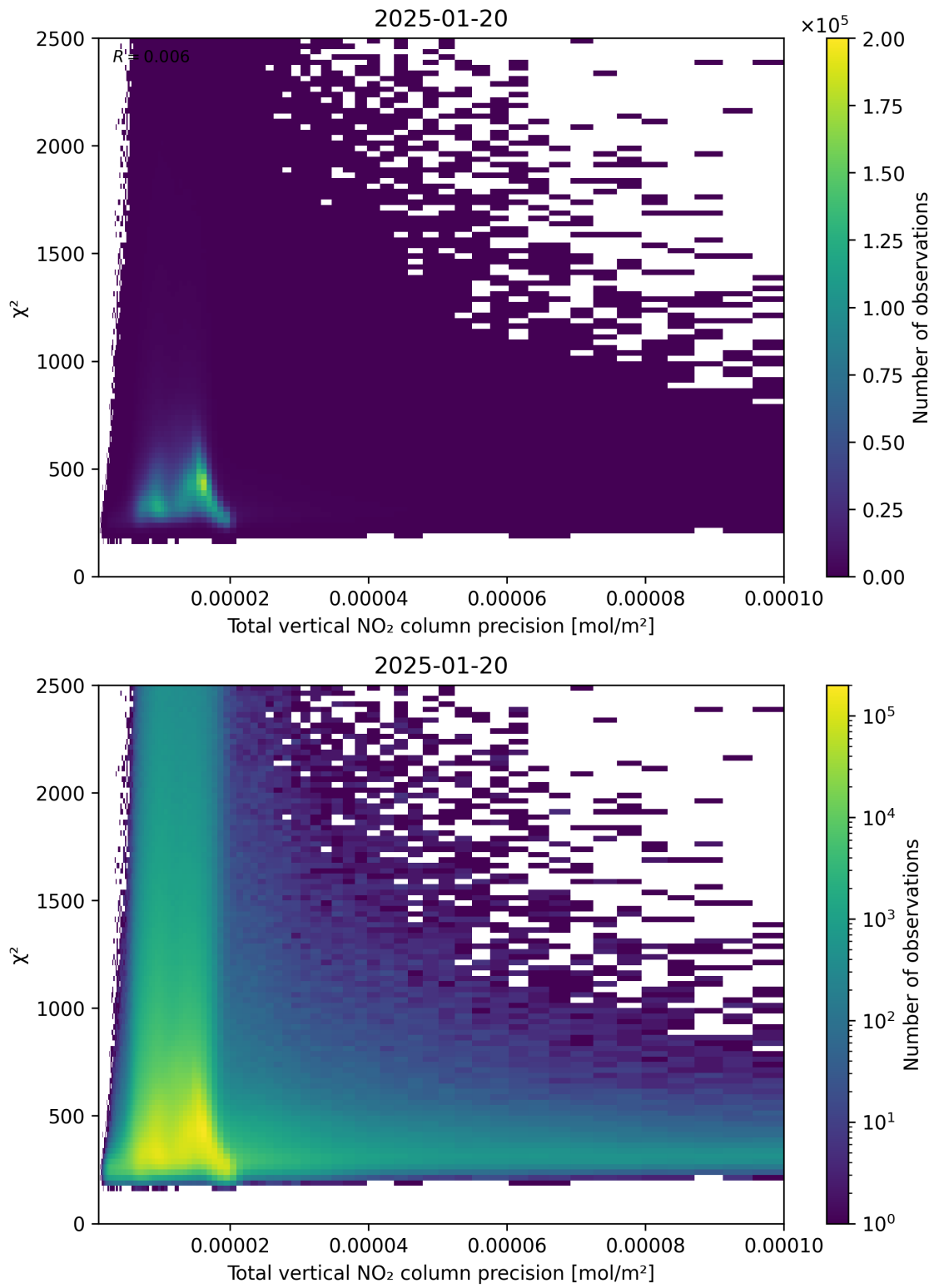
Figure 116: Scatter density plot of “Total vertical NO 2 column precision” against “ \chi^2 ” for 2025-01-19 to 2025-01-21.
