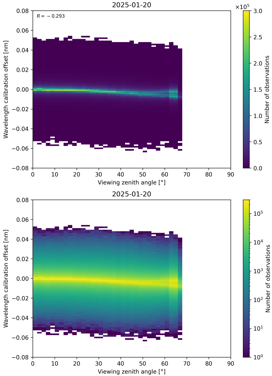
Figure 173: Scatter density plot of “Viewing zenith angle” against “Wavelength calibration offset” for 2025-01-19 to 2025-01-21.
