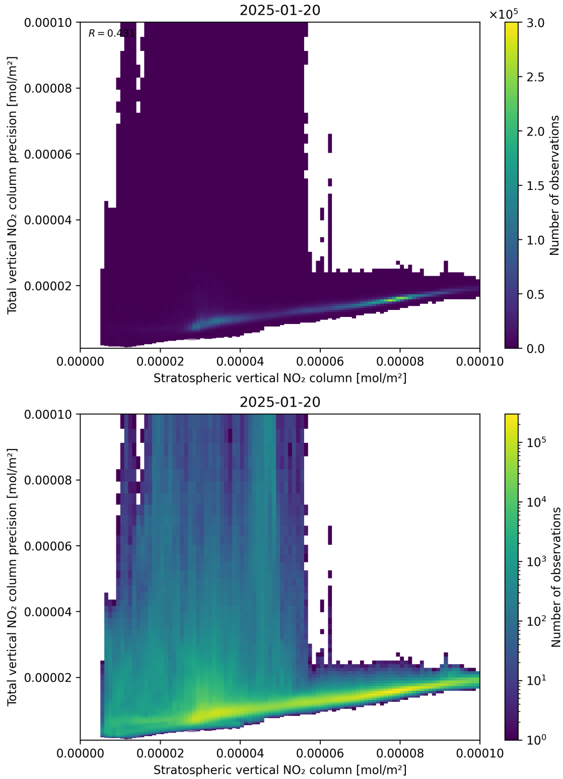
Figure 101: Scatter density plot of “Stratospheric vertical NO 2 column” against “Total vertical NO 2 column precision” for 2025-01-19 to 2025-01-21.
