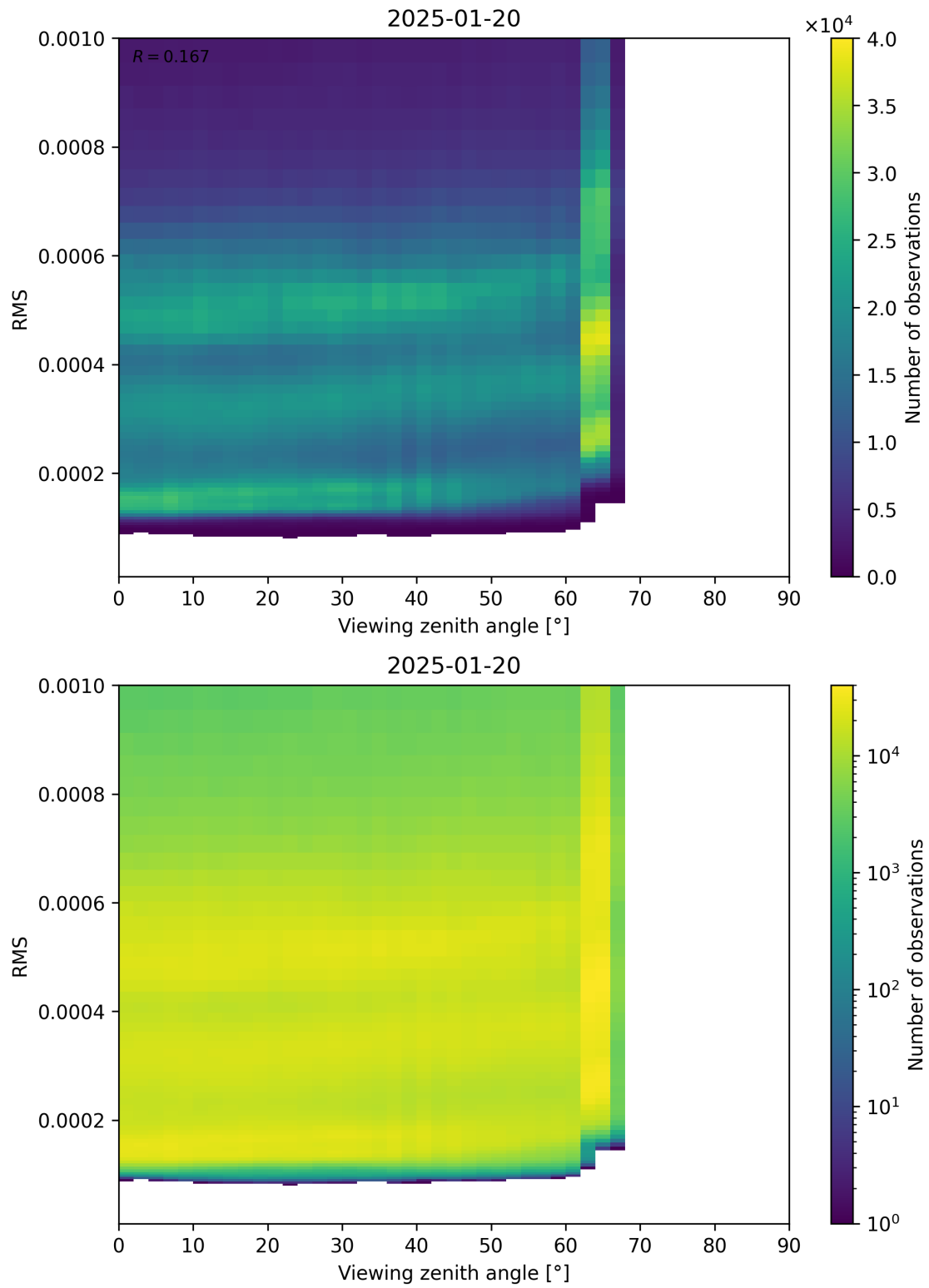
Figure 171: Scatter density plot of “Viewing zenith angle” against “RMS” for 2025-01-19 to 2025-01-21.
