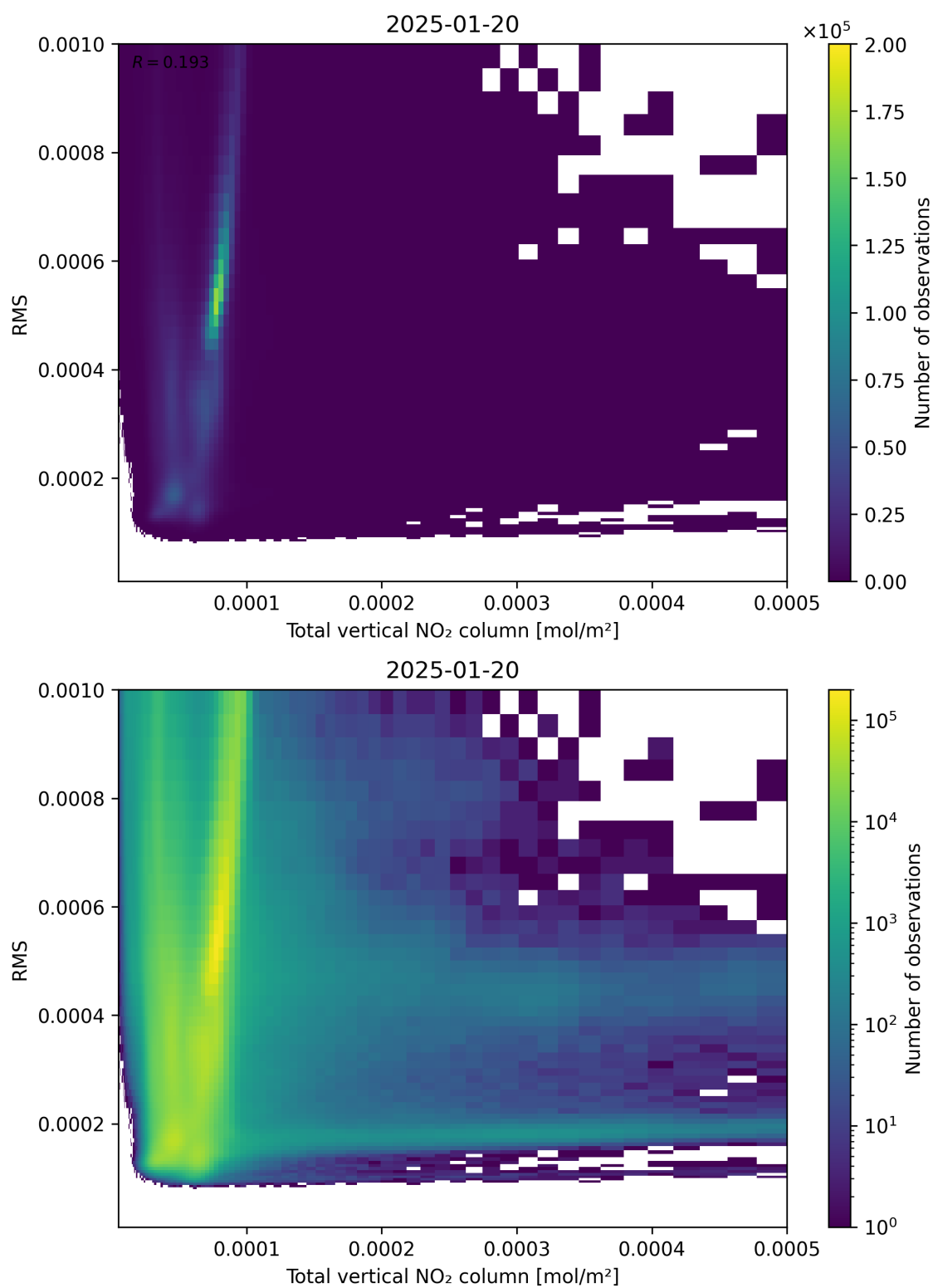
Figure 120: Scatter density plot of “Total vertical NO 2 column” against “RMS” for 2025-01-19 to 2025-01-21.
