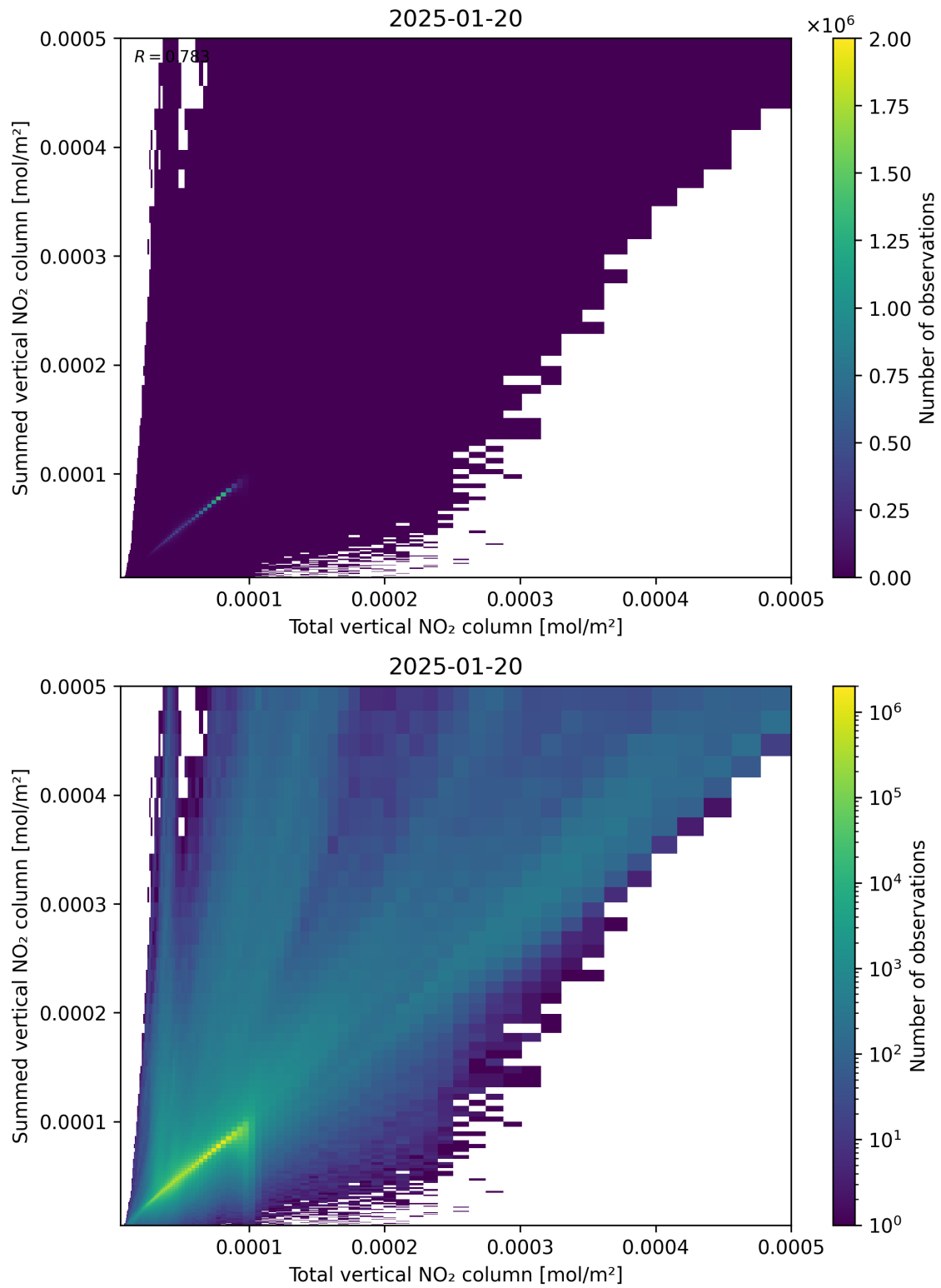
Figure 112: Scatter density plot of “Total vertical NO 2 column” against “Summed vertical NO 2 column” for 2025-01-19 to 2025-01-21.
