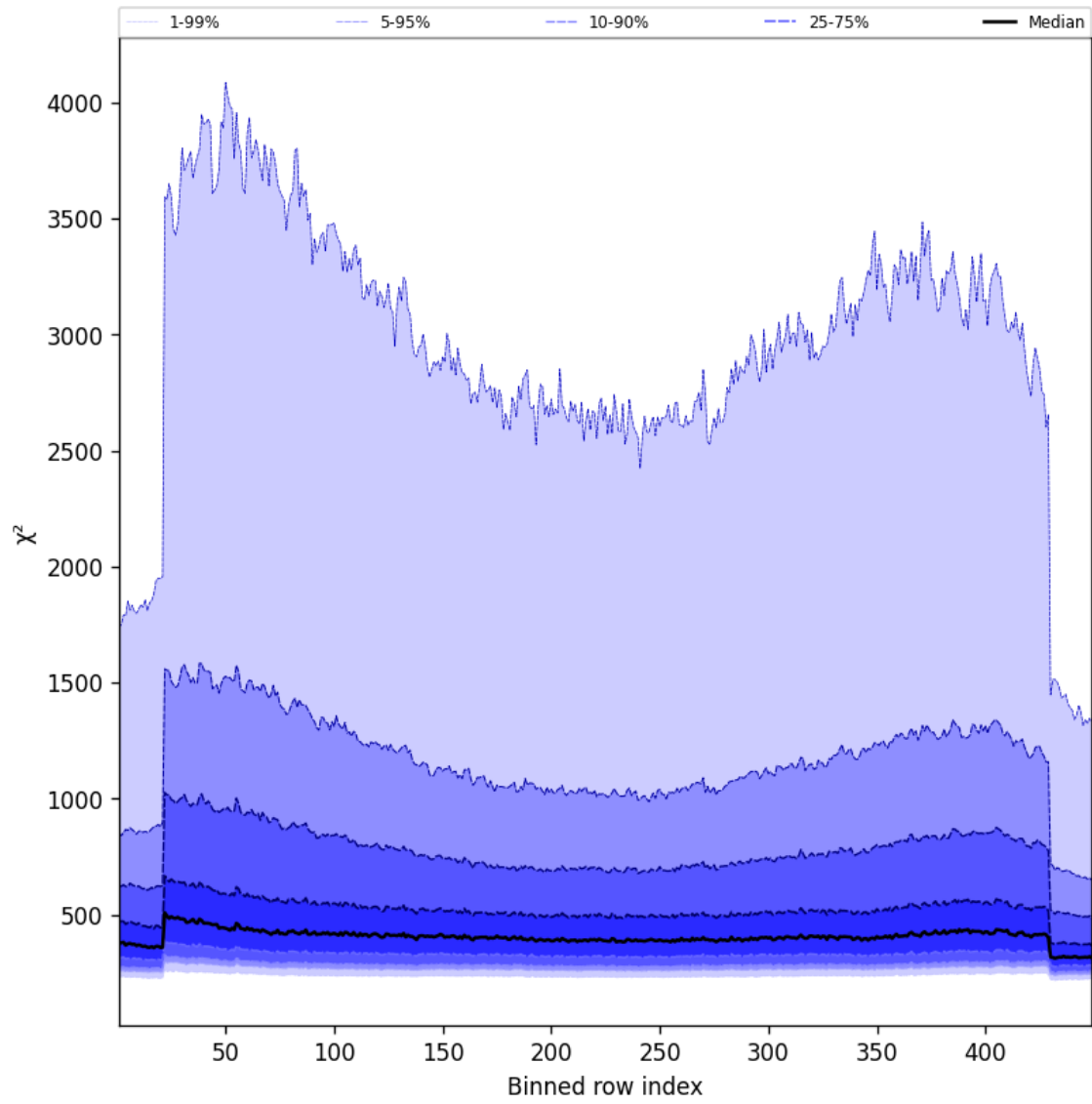
Figure 59: Along track statistics of “ \chi^2 ” for 2025-01-19 to 2025-01-21
