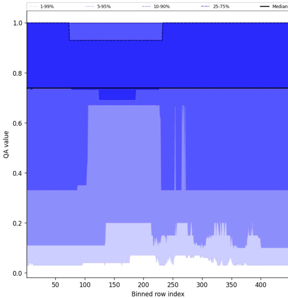
Figure 45: Along track statistics of “QA value” for 2025-01-19 to 2025-01-21
