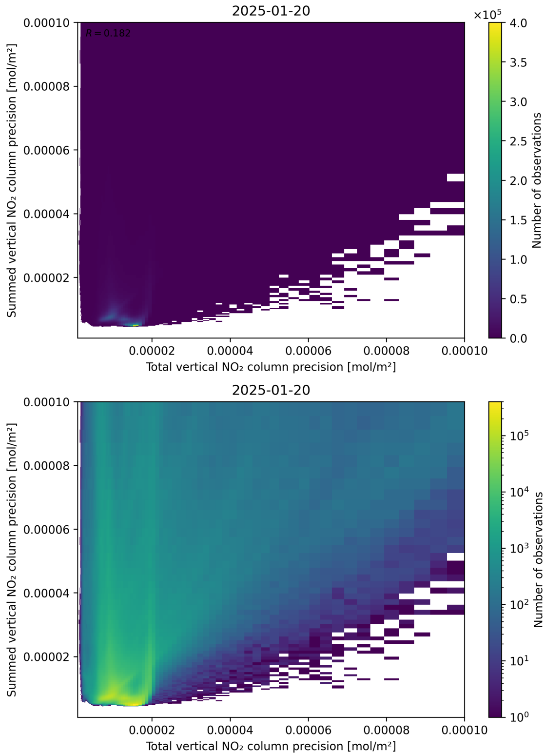
Figure 118: Scatter density plot of “Total vertical NO 2 column precision” against “Summed vertical NO 2 column precision” for 2025-01-19 to 2025-01-21.
