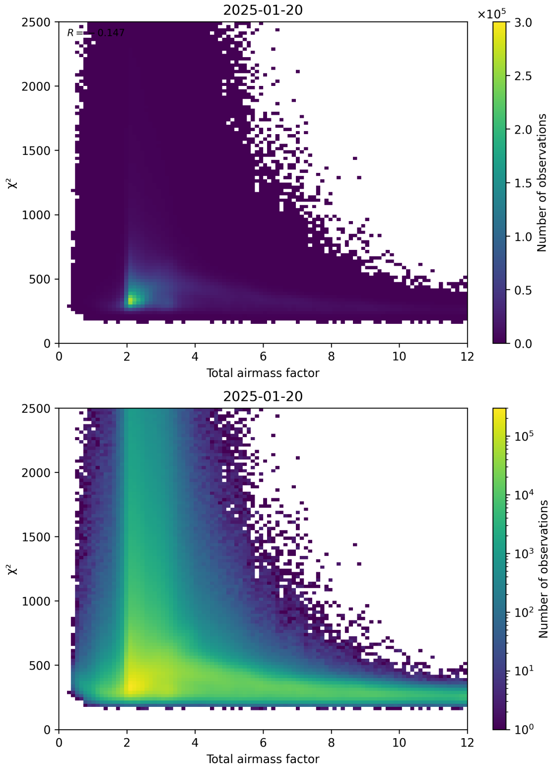
Figure 63: Scatter density plot of “Total airmass factor” against “ \chi^2 ” for 2025-01-19 to 2025-01-21.
