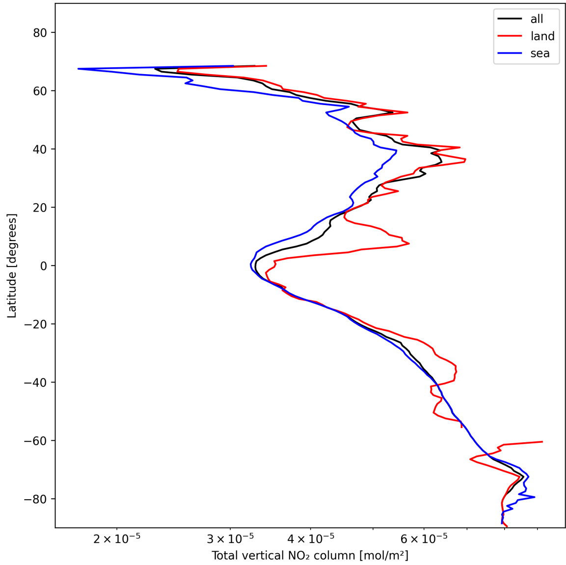
Figure 21: Zonal average of “Total vertical NO 2 column” for 2025-01-19 to 2025-01-21.
