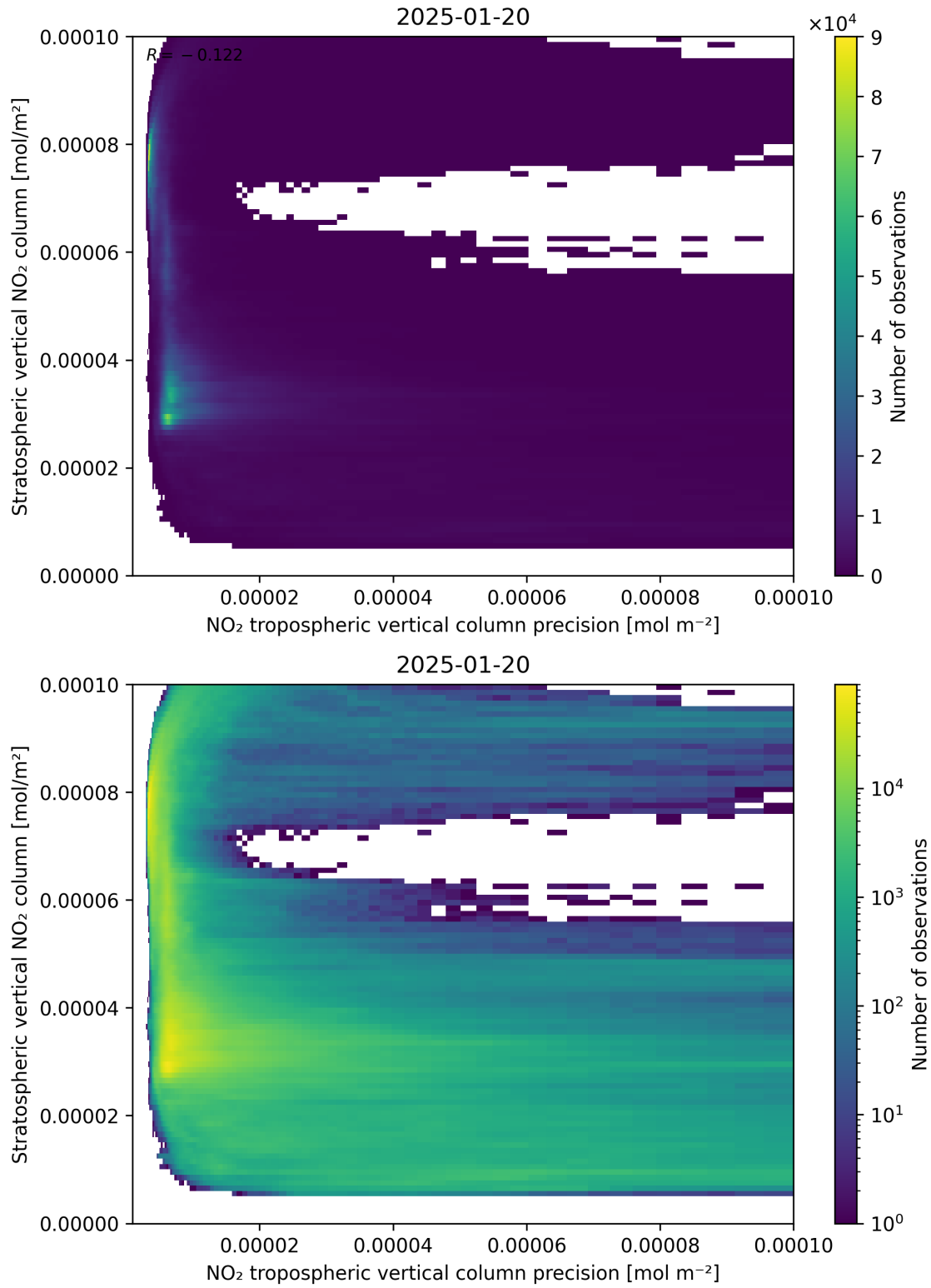
Figure 135: Scatter density plot of “NO 2 tropospheric vertical column precision” against “Stratospheric vertical NO 2 column” for 2025-01-19 to 2025-01-21.
