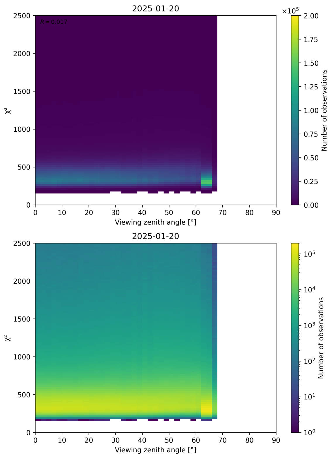
Figure 162: Scatter density plot of “Viewing zenith angle” against “ \chi^2 ” for 2025-01-19 to 2025-01-21.
