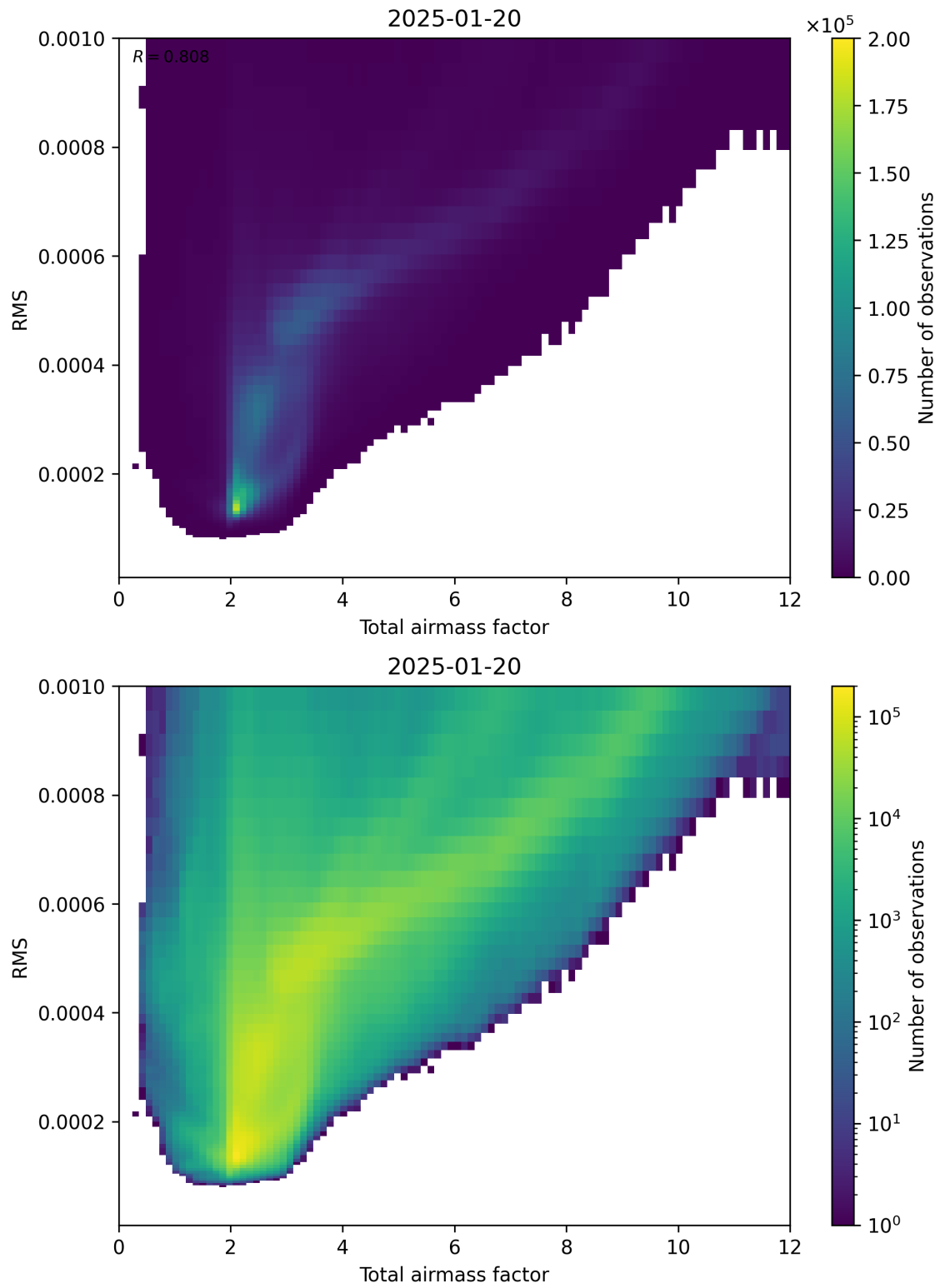
Figure 69: Scatter density plot of “Total airmass factor” against “RMS” for 2025-01-19 to 2025-01-21.
