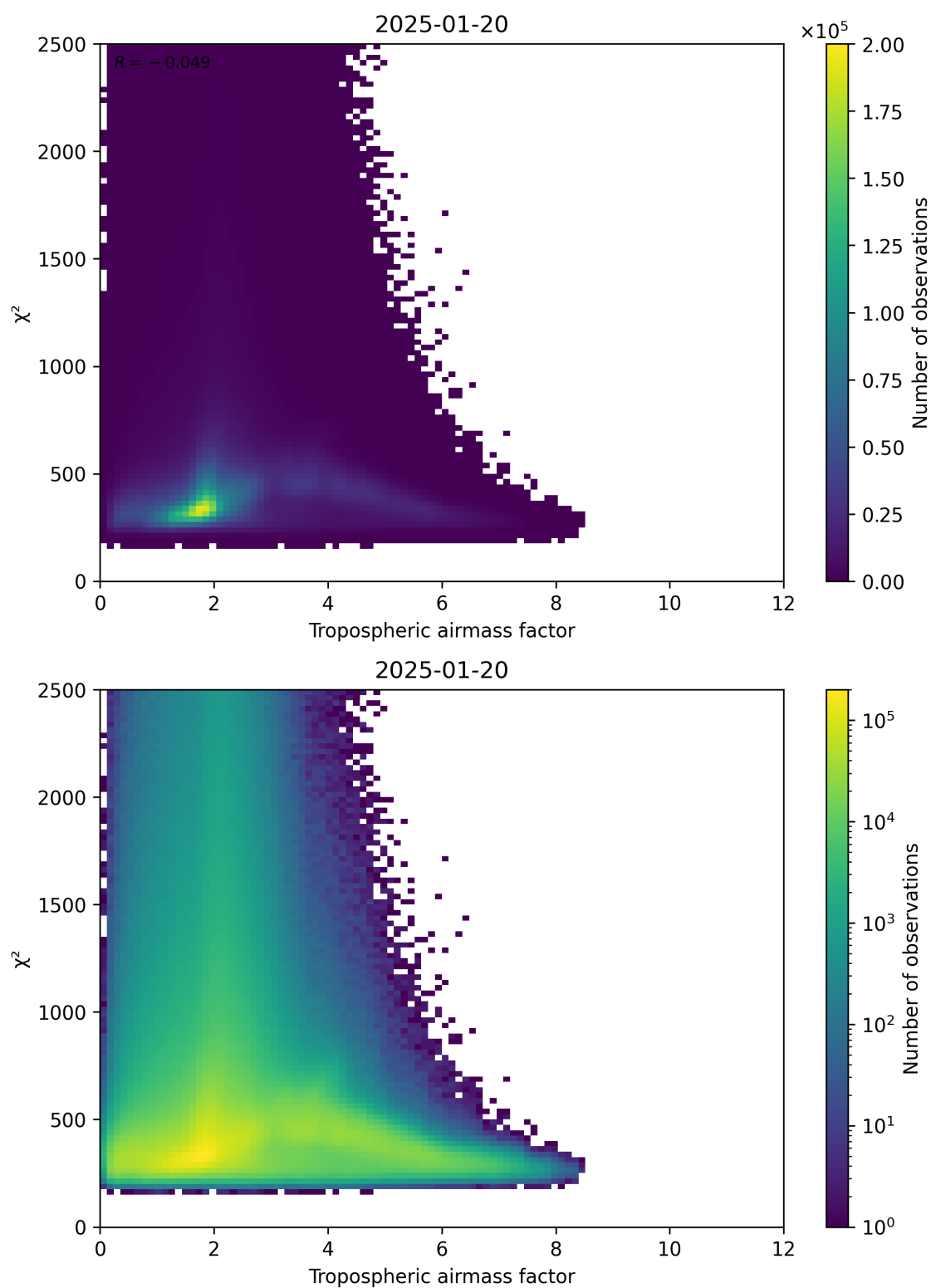
Figure 73: Scatter density plot of “Tropospheric airmass factor” against “ \chi^2 ” for 2025-01-19 to 2025-01-21.
