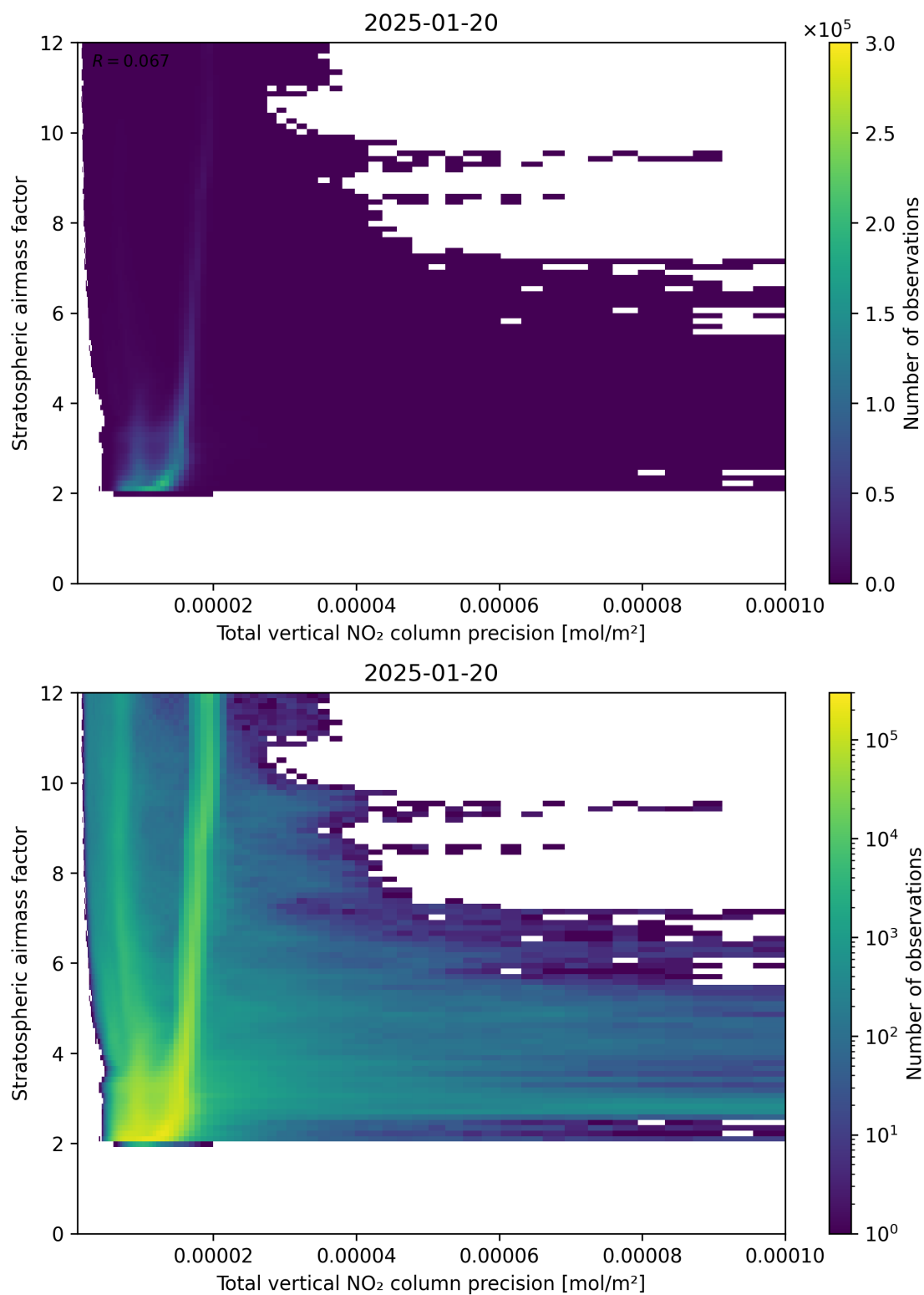
Figure 115: Scatter density plot of “Total vertical NO 2 column precision” against “Stratospheric air mass factor” for 2025-01-19 to 2025-01-21.
