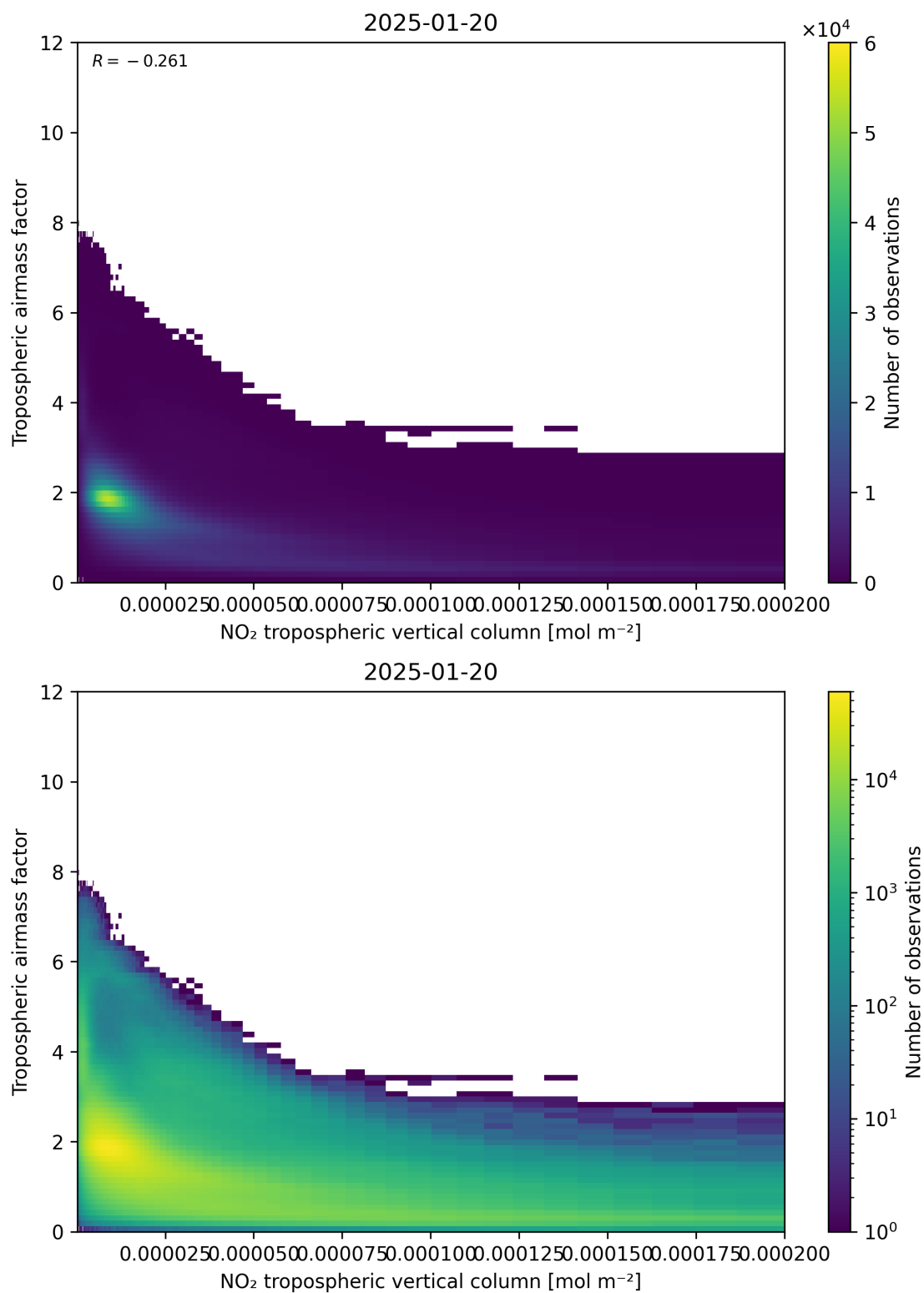
Figure 123: Scatter density plot of “NO 2 tropospheric vertical column” against “Tropospheric air mass factor” for 2025-01-19 to 2025-01-21.
