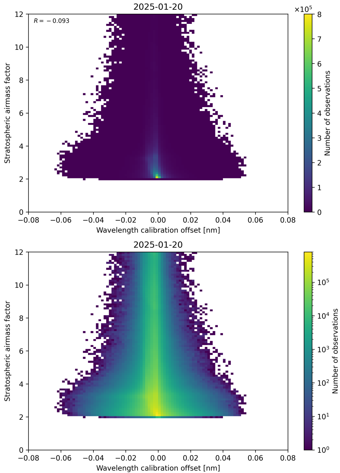
Figure 174: Scatter density plot of “Wavelength calibration offset” against “Stratospheric airmass factor” for 2025-01-19 to 2025-01-21.
