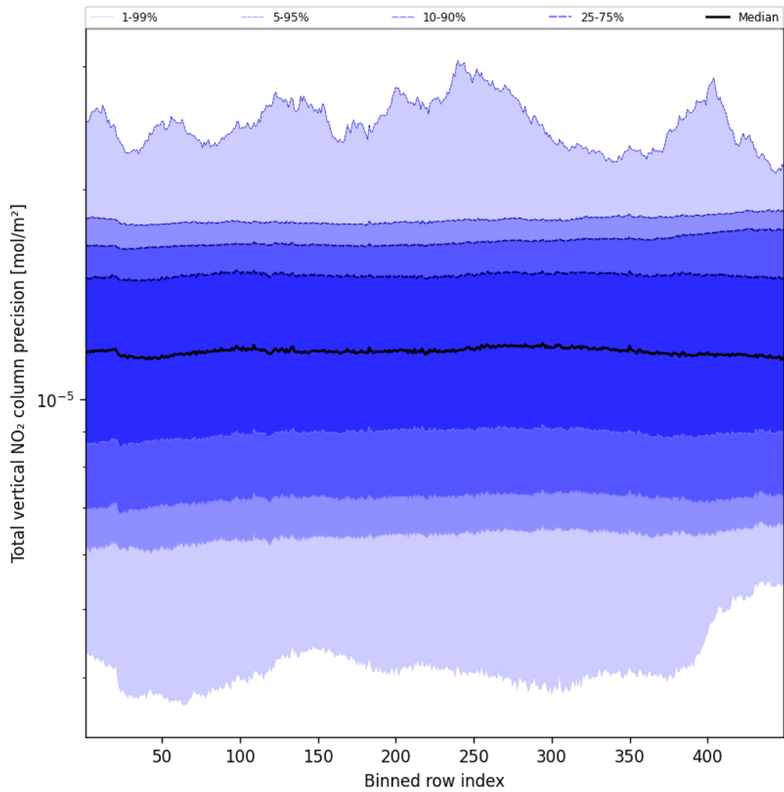
Figure 56: Along track statistics of “Total vertical NO 2 column precision” for 2025-01-19 to 2025-01-21
