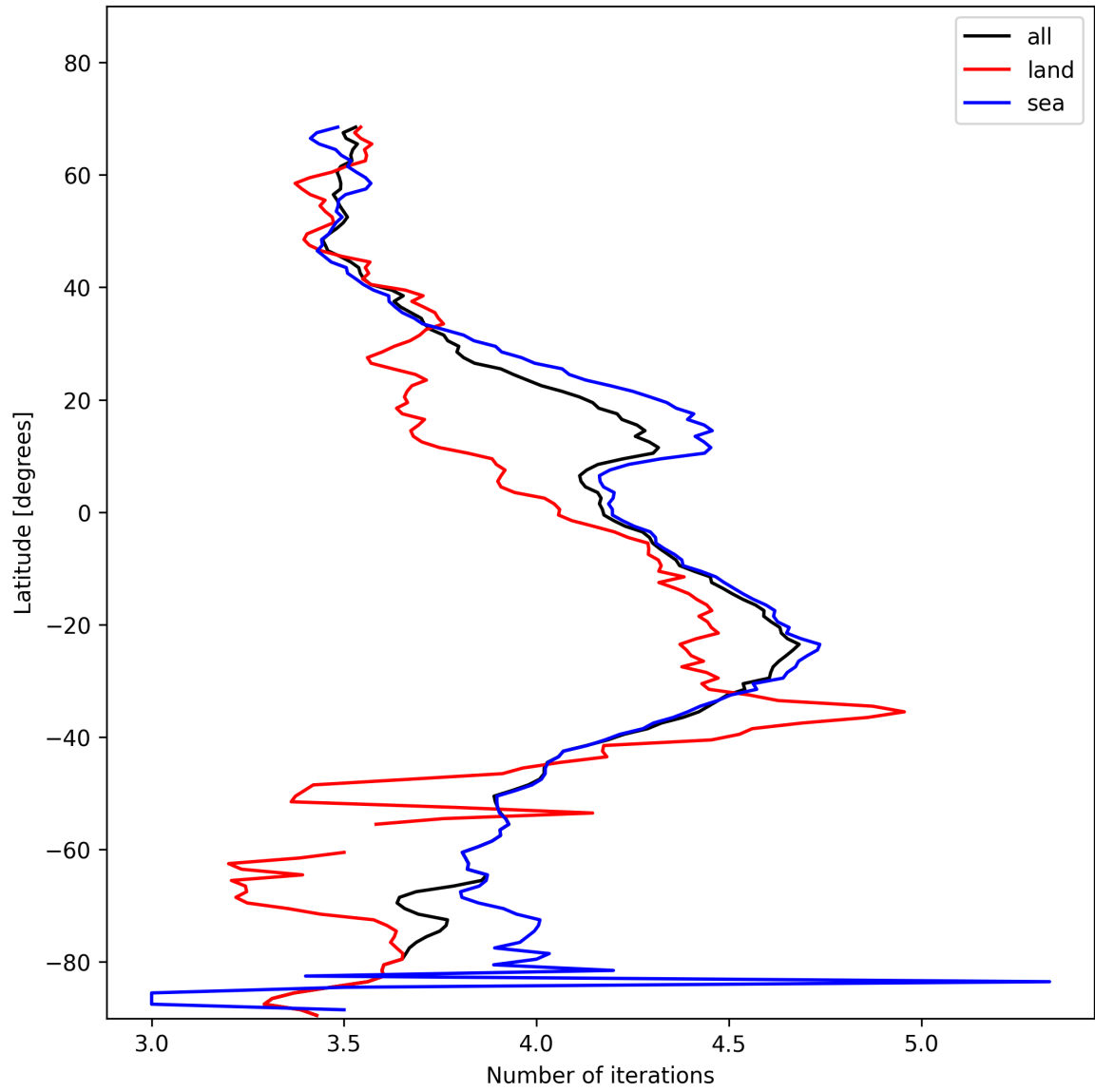
Figure 17: Zonal average of “Number of iterations” for 2025-01-19 to 2025-01-21.
