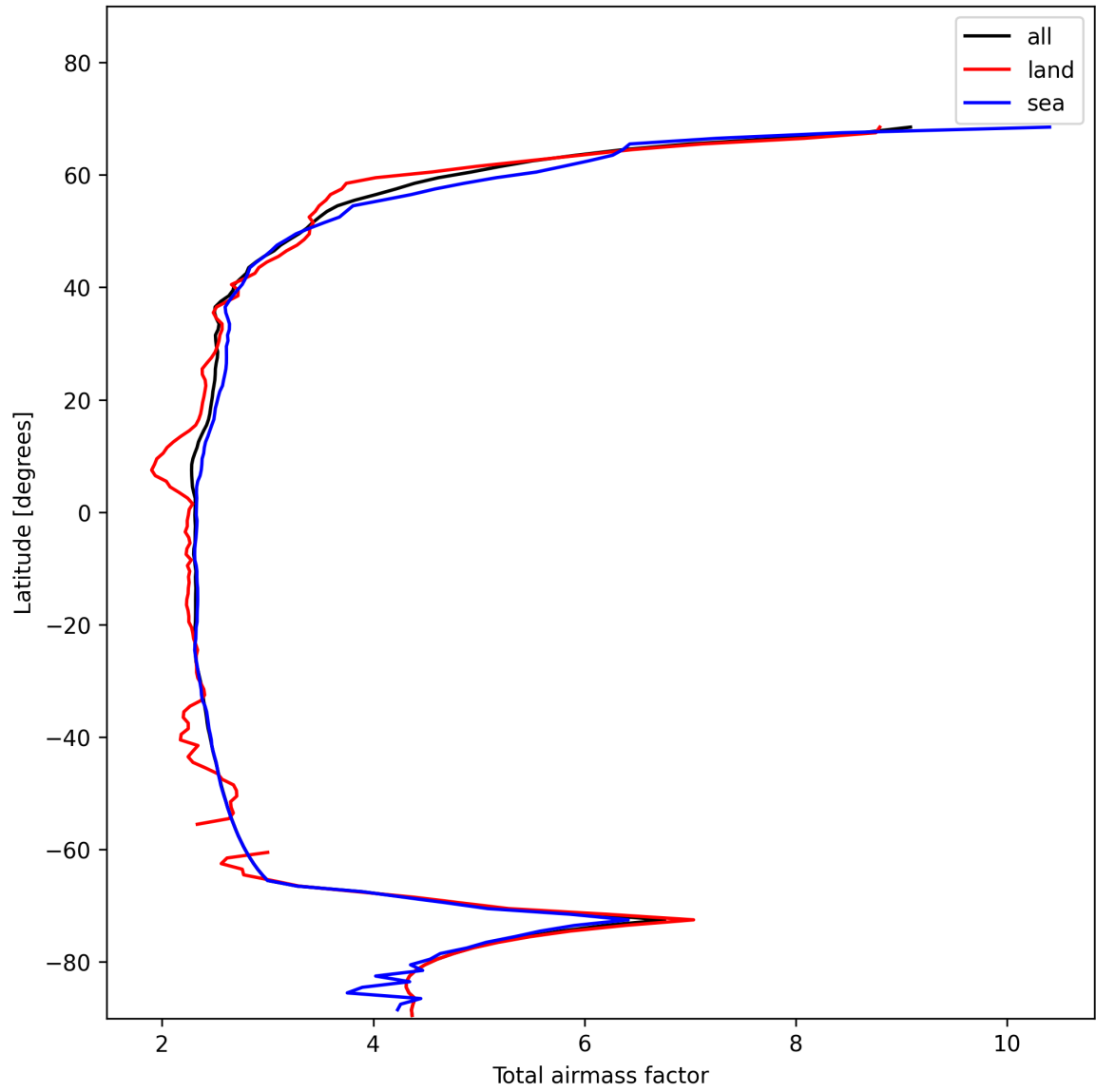
Figure 15: Zonal average of “Total airmass factor” for 2025-01-19 to 2025-01-21.
