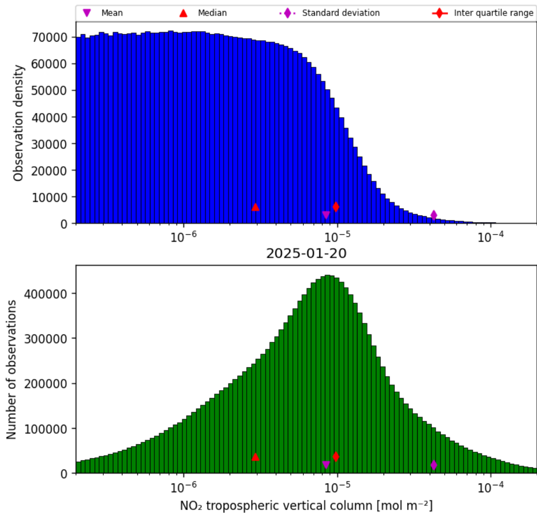
Figure 29: Histogram of “NO 2 tropospheric vertical column” for 2025-01-19 to 2025-01-21
