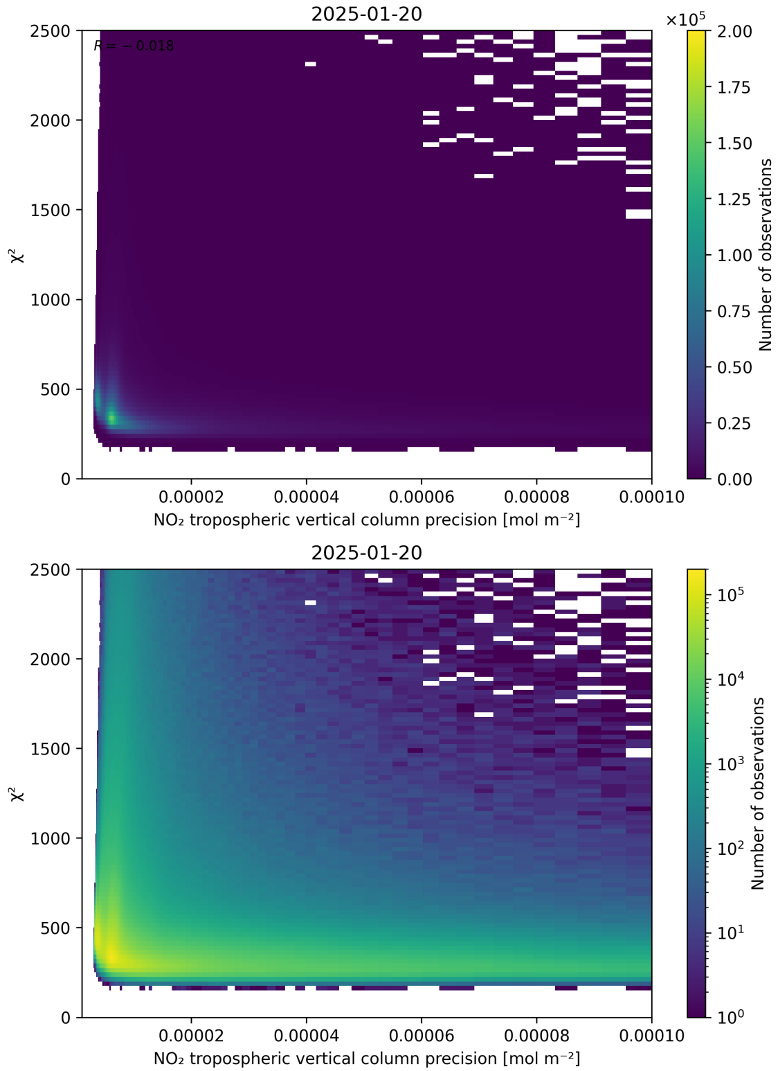
Figure 134: Scatter density plot of “NO 2 tropospheric vertical column precision” against “ \chi^2 ” for 2025-01-19 to 2025-01-21.
