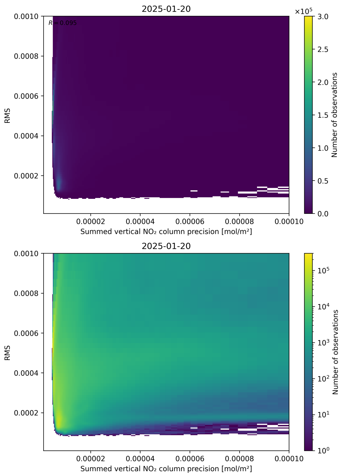
Figure 108: Scatter density plot of “Summed vertical NO 2 column precision” against “RMS” for 2025-01-19 to 2025-01-21.
