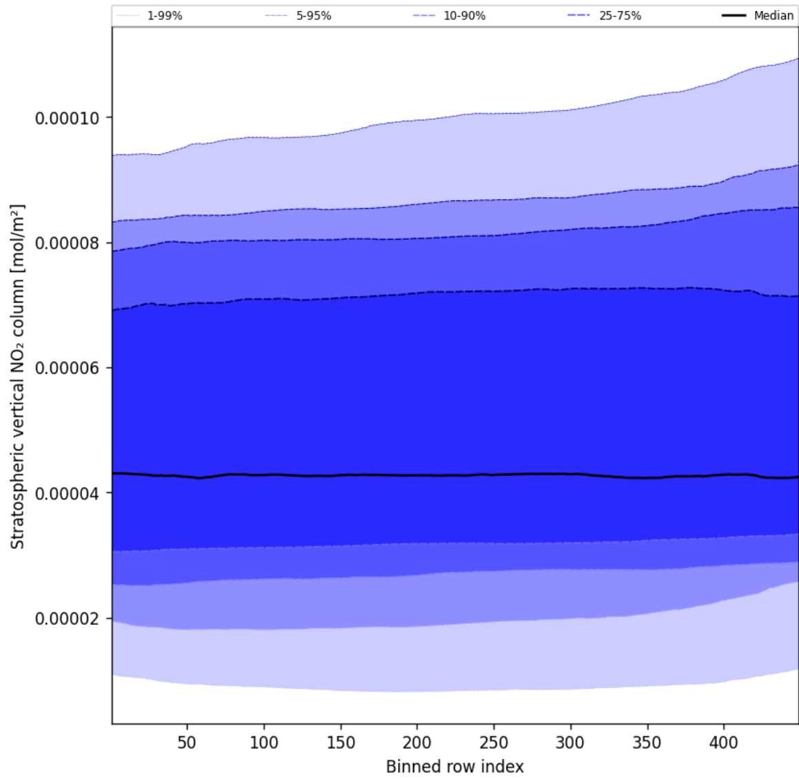
Figure 53: Along track statistics of “Stratospheric vertical NO 2 column” for 2025-01-19 to 2025-01-21
