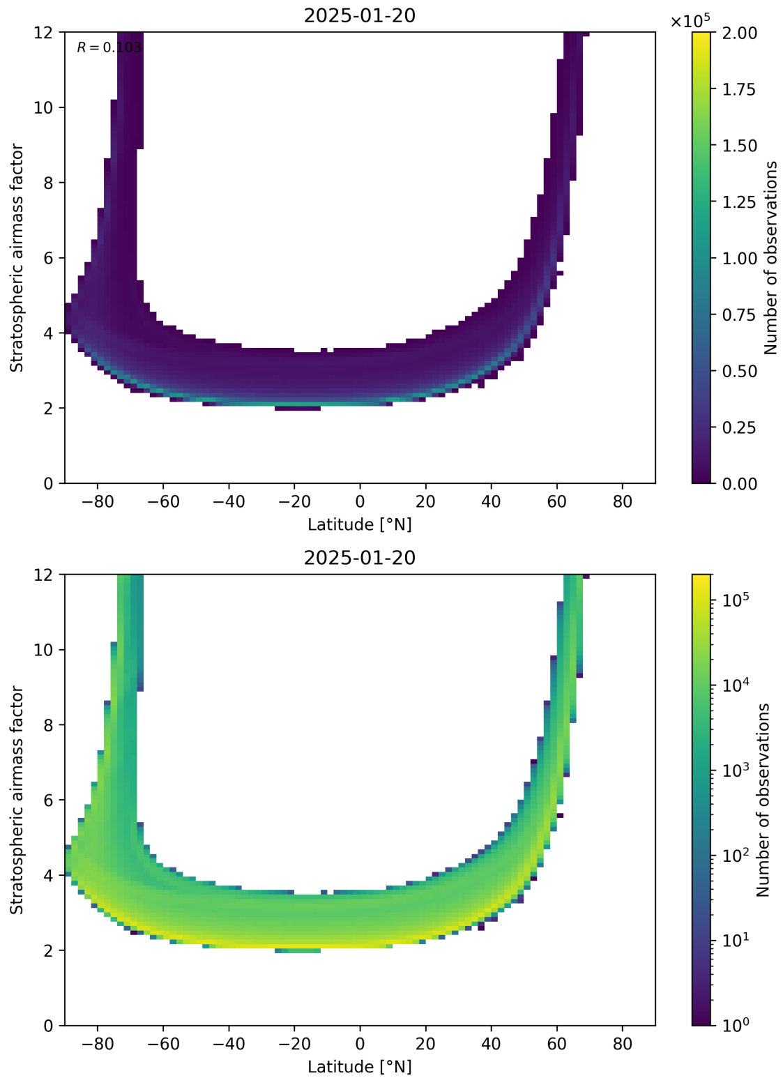
Figure 83: Scatter density plot of “Latitude” against “Stratospheric airmass factor” for 2025-01-19 to 2025-01-21.
