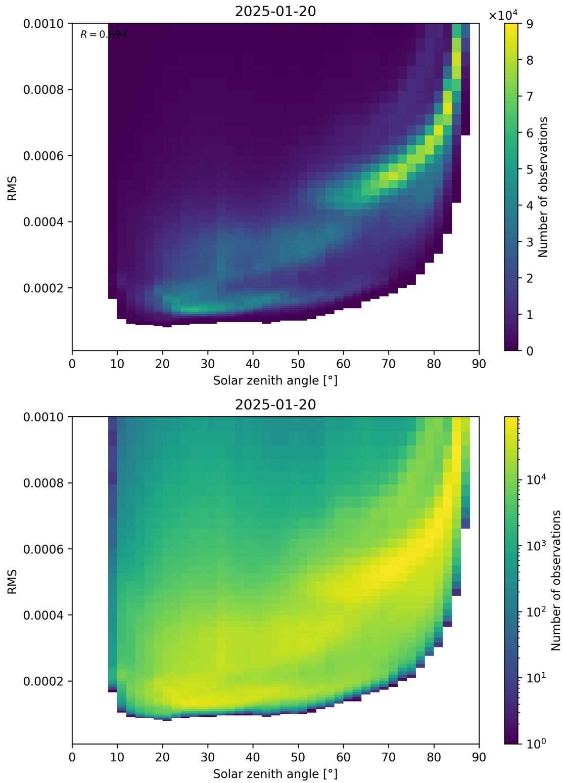
Figure 157: Scatter density plot of “Solar zenith angle” against “RMS” for 2025-01-19 to 2025-01-21.
