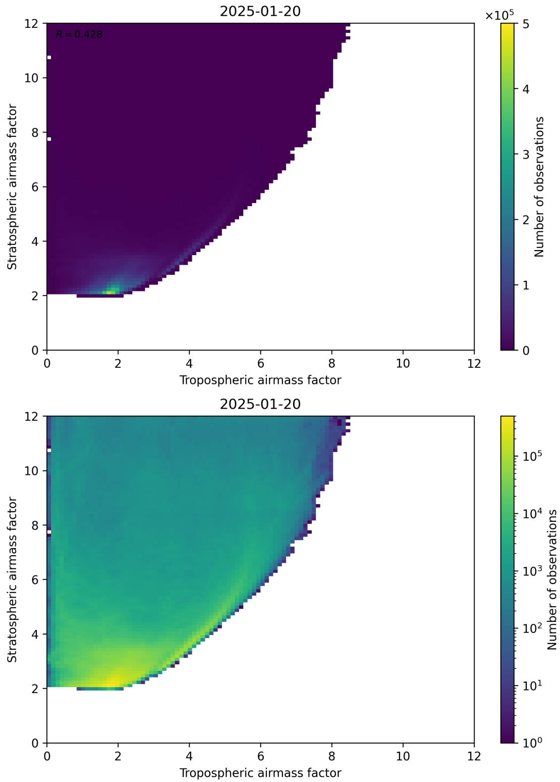
Figure 71: Scatter density plot of “Tropospheric airmass factor” against “Stratospheric airmass factor” for 2025-01-19 to 2025-01-21.
