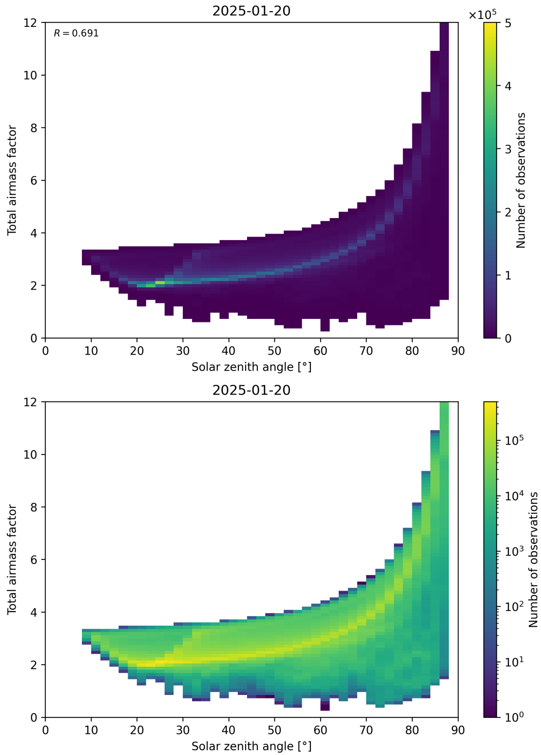
Figure 146: Scatter density plot of “Solar zenith angle” against “Total airmass factor” for 2025-01-19 to 2025-01-21.
