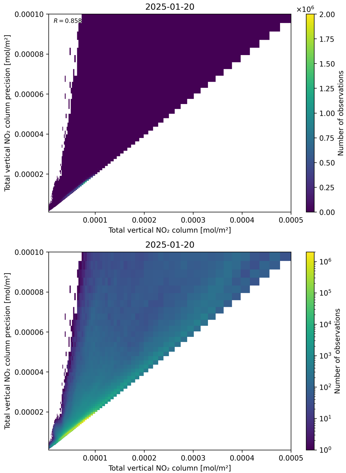
Figure 114: Scatter density plot of “Total vertical NO 2 column” against “Total vertical NO 2 column precision” for 2025-01-19 to 2025-01-21.
