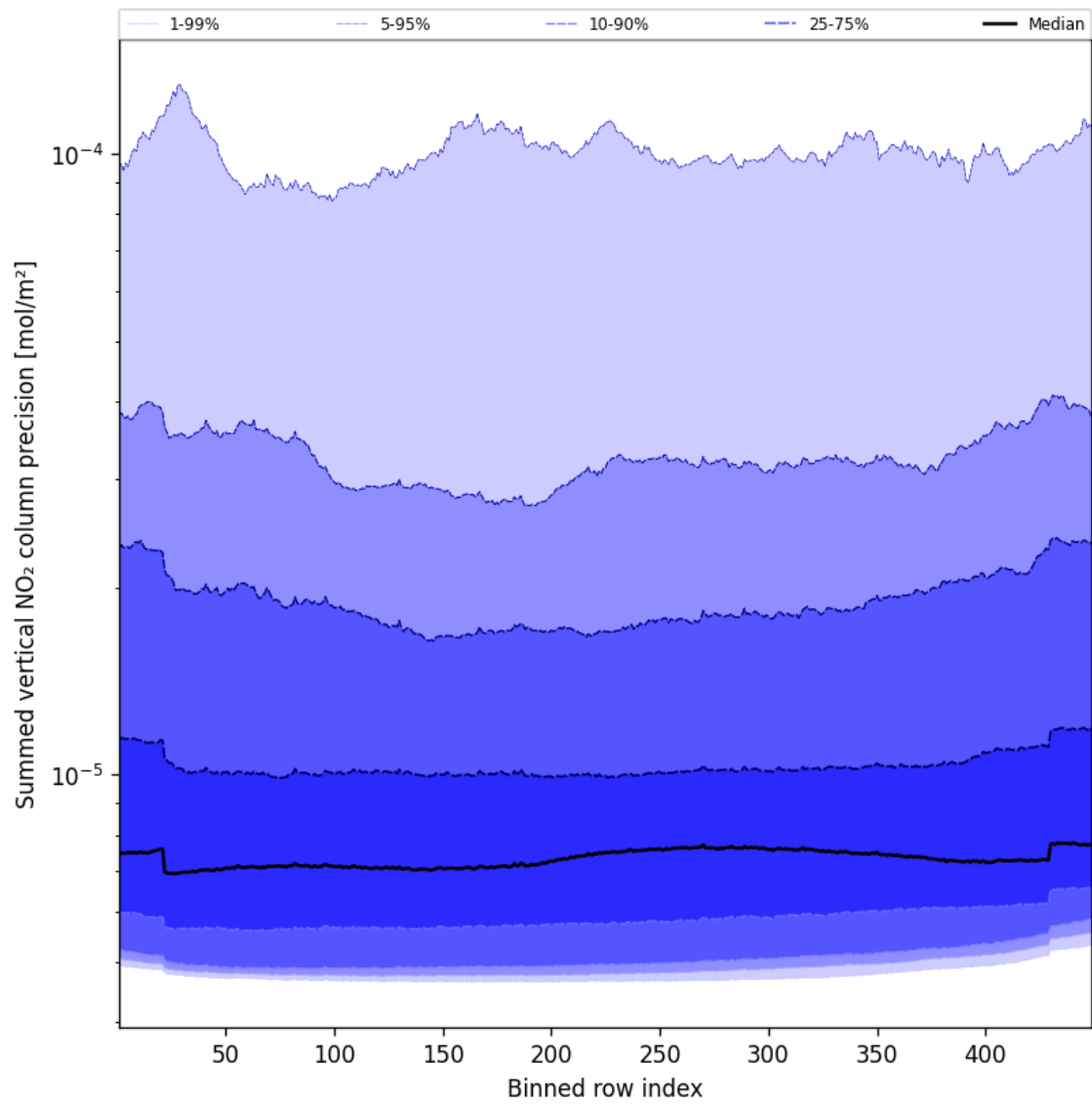
Figure 58: Along track statistics of “Summed vertical NO 2 column precision” for 2025-01-19 to 2025-01-21
