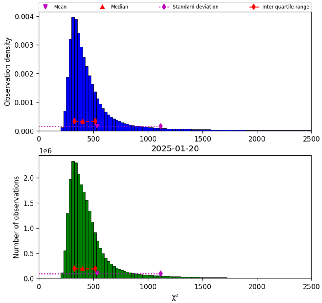
Figure 42: Histogram of “ \chi^2 ” for 2025-01-19 to 2025-01-21
