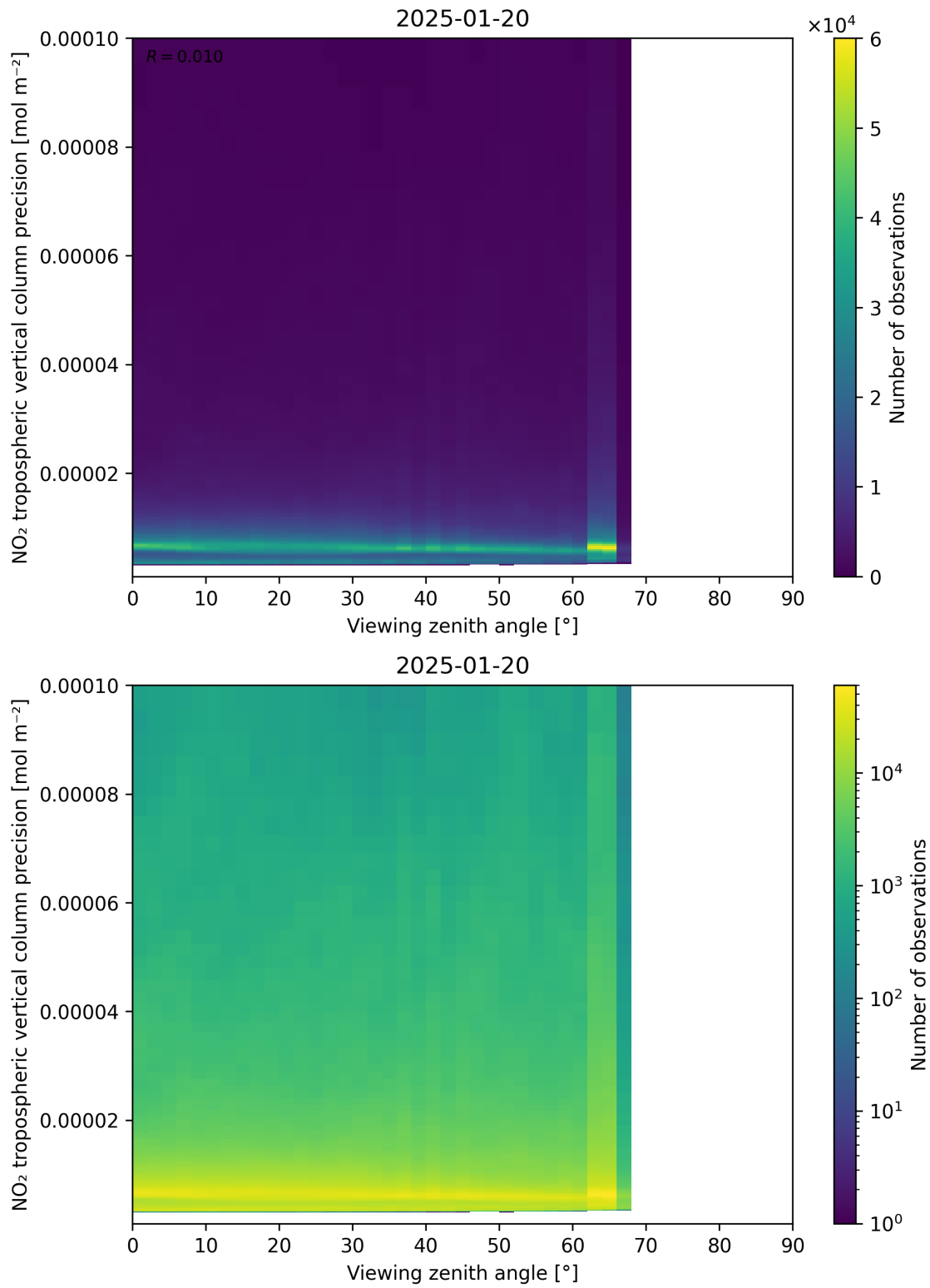
Figure 170: Scatter density plot of “Viewing zenith angle” against “NO 2 tropospheric vertical column precision” for 2025-01-19 to 2025-01-21.
