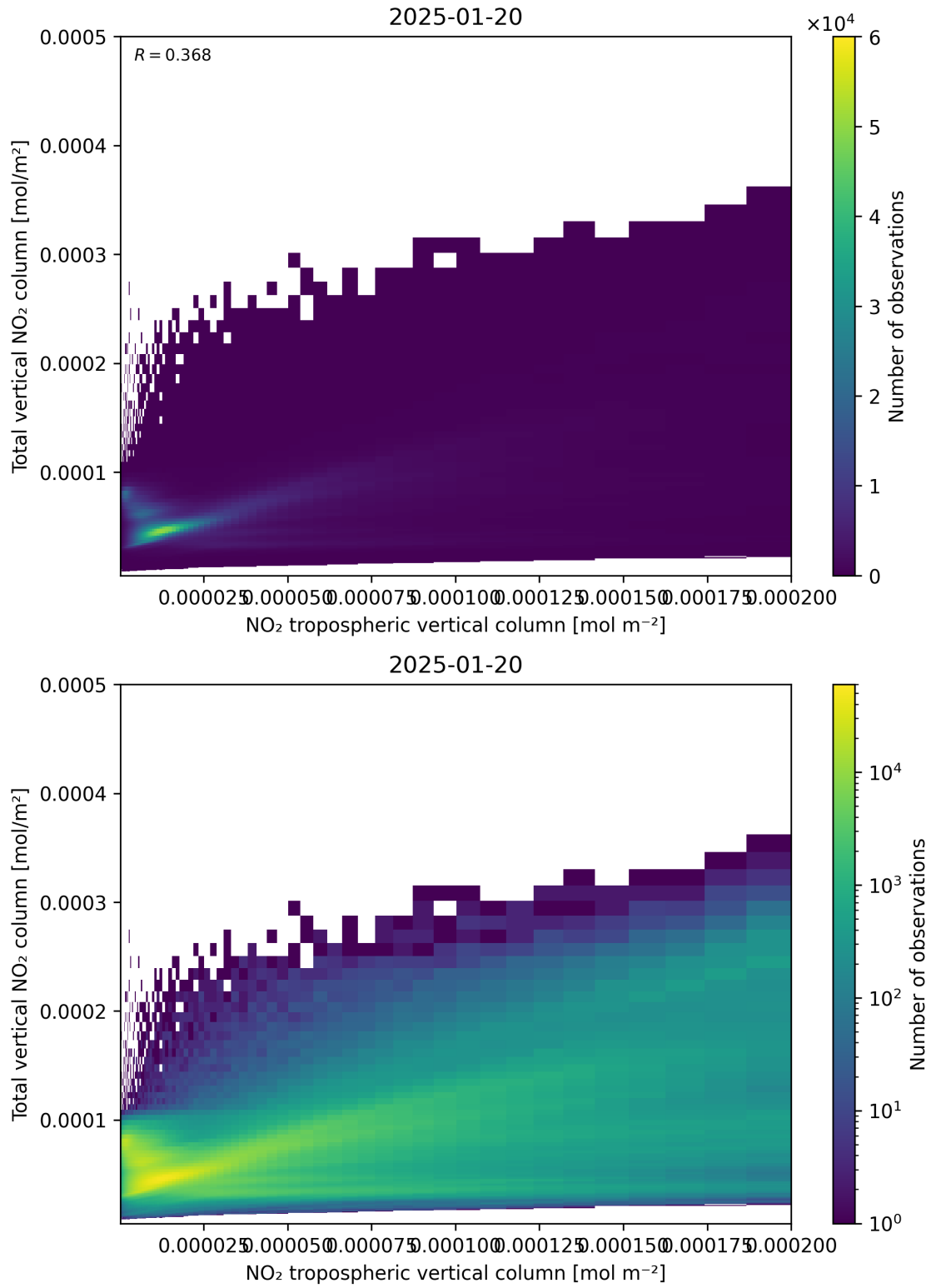
Figure 128: Scatter density plot of “NO 2 tropospheric vertical column” against “Total vertical NO 2 column” for 2025-01-19 to 2025-01-21.
