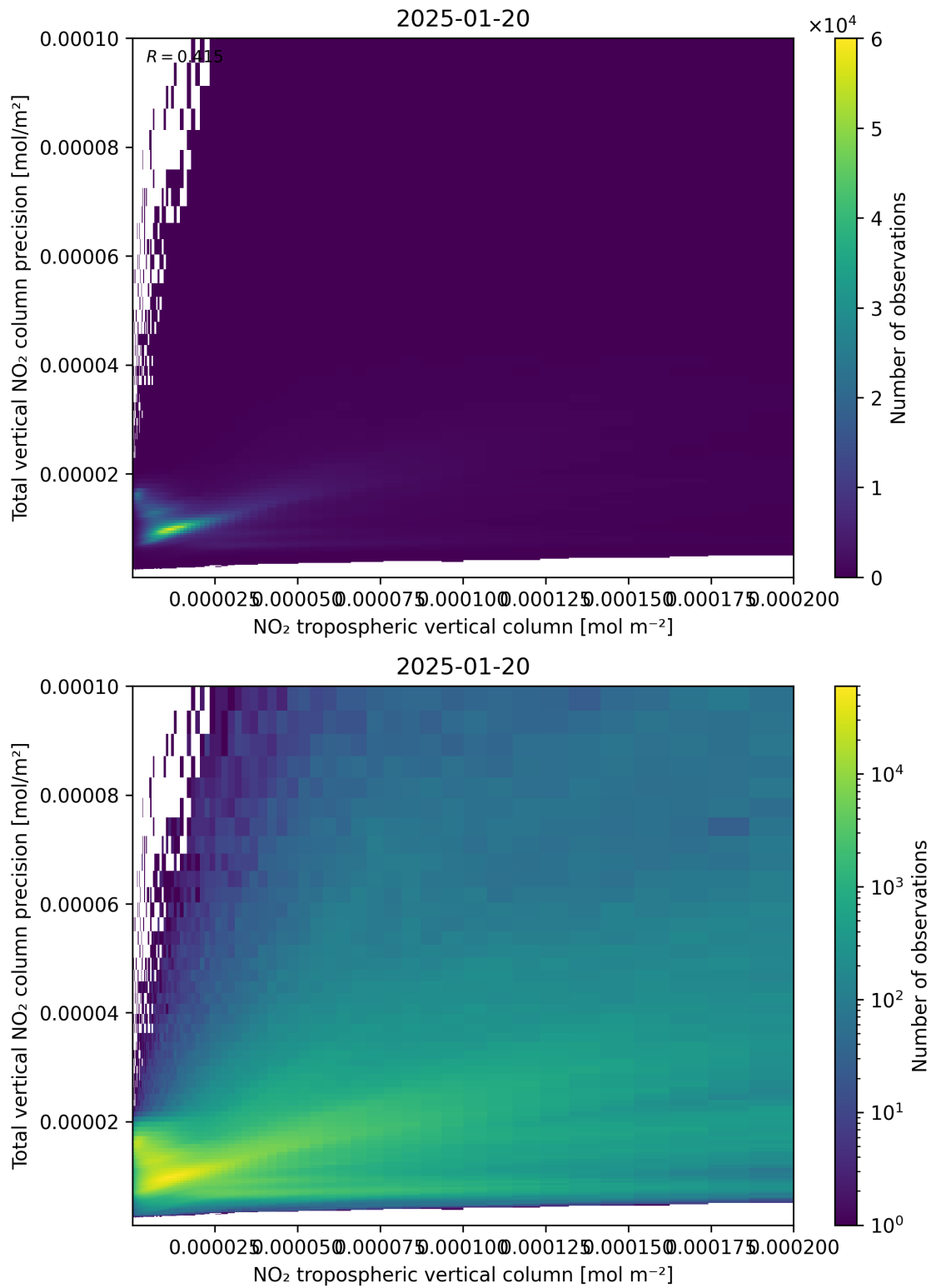
Figure 129: Scatter density plot of “NO 2 tropospheric vertical column” against “Total vertical NO 2 column precision” for 2025-01-19 to 2025-01-21.
