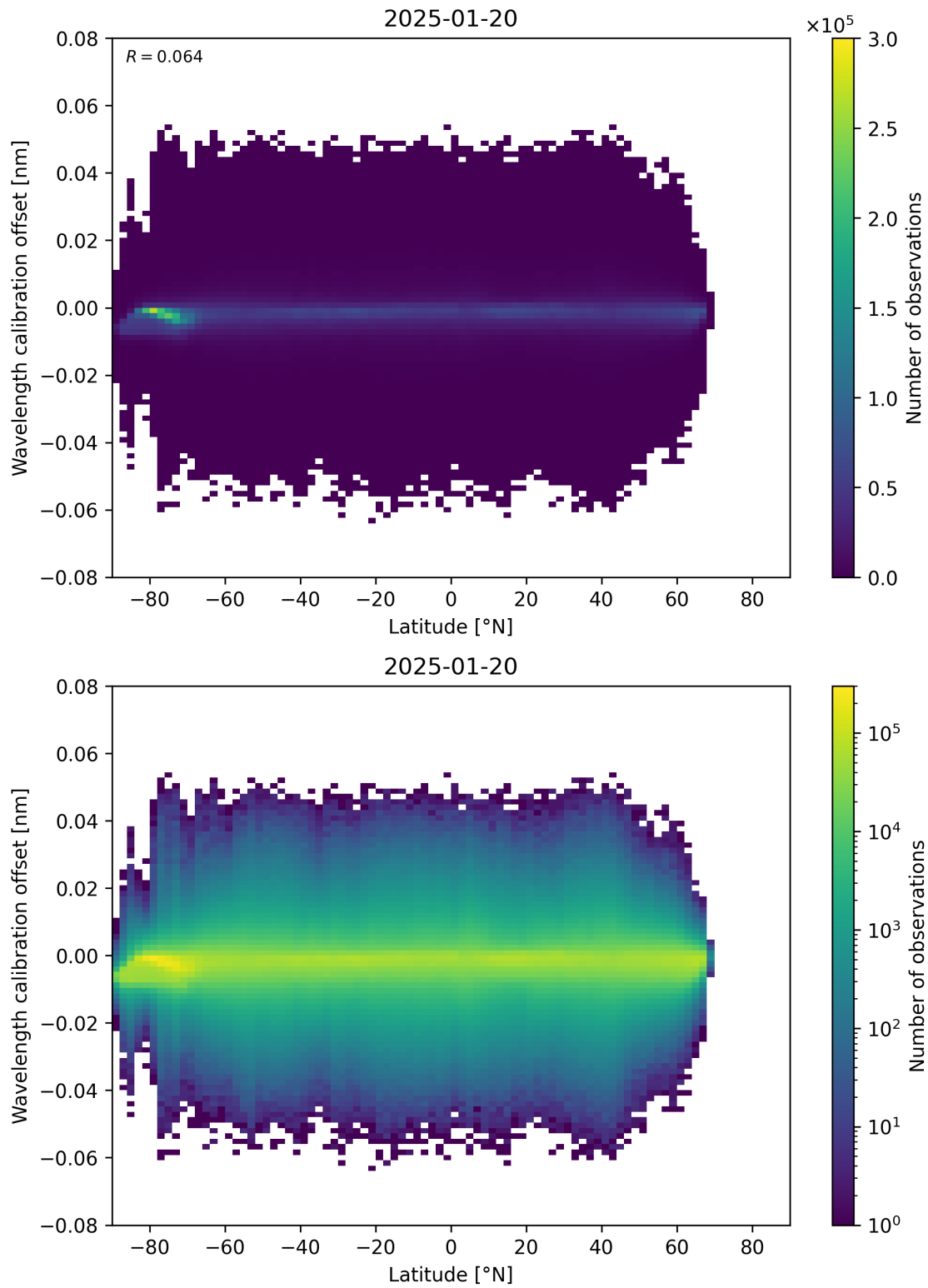
Figure 95: Scatter density plot of “Latitude” against “Wavelength calibration offset” for 2025-01-19 to 2025-01-21.
