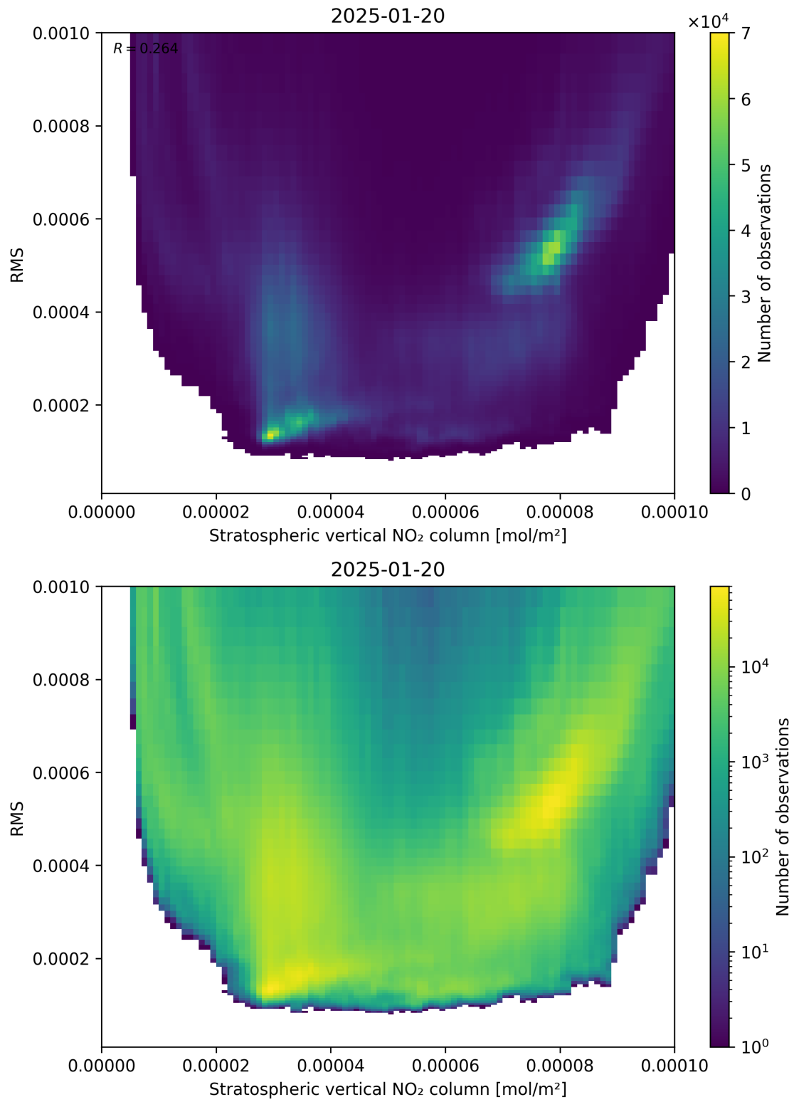
Figure 102: Scatter density plot of “Stratospheric vertical NO 2 column” against “RMS” for 2025-01-19 to 2025-01-21.
