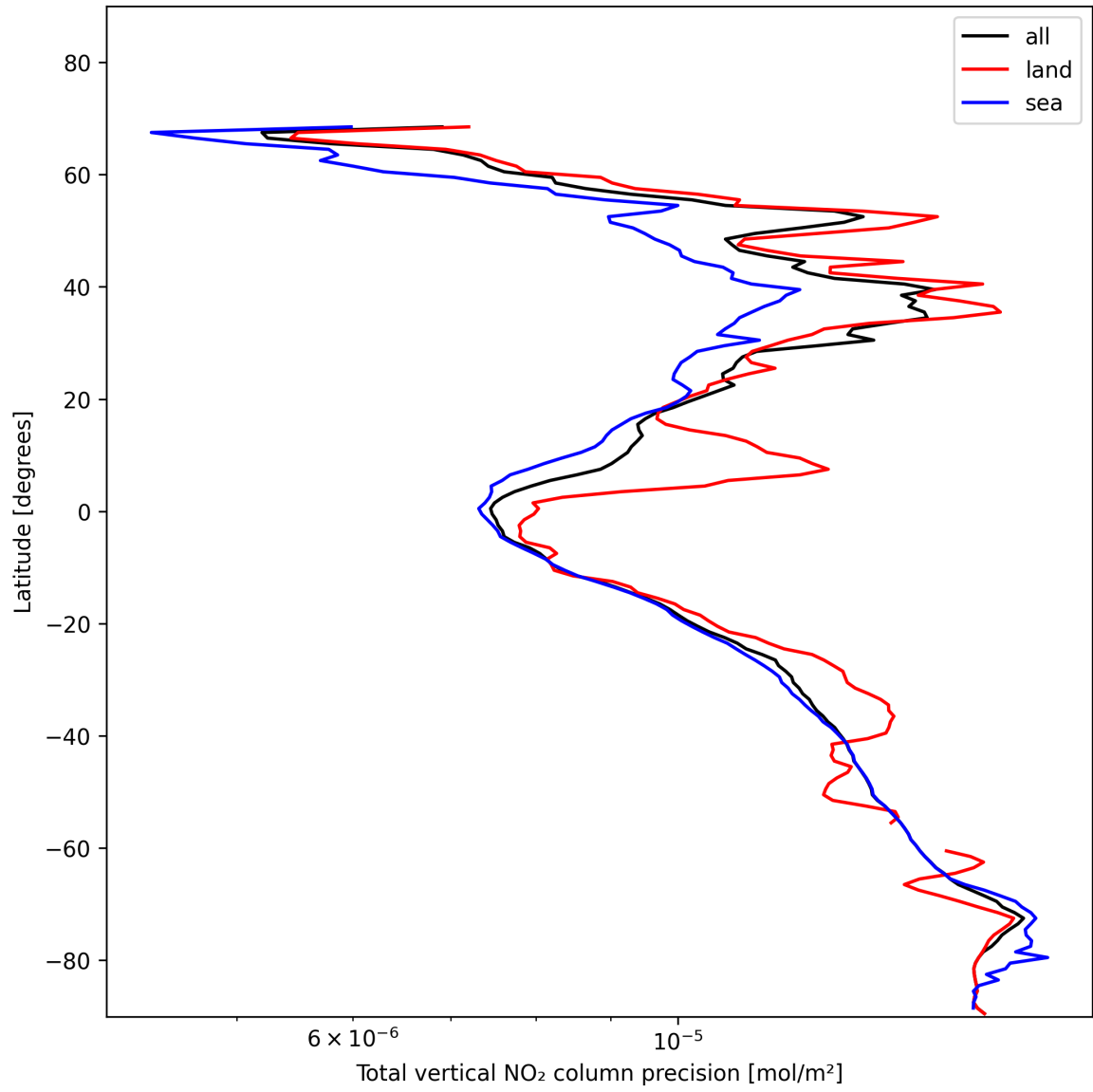
Figure 22: Zonal average of "Total vertical NO 2 column precision" for 2025-01-19 to 2025-01-21.
