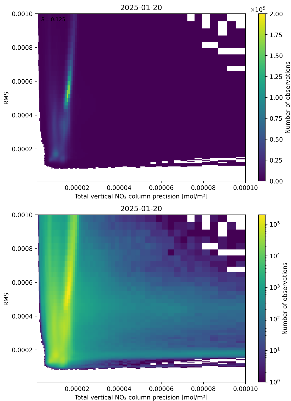
Figure 119: Scatter density plot of “Total vertical NO 2 column precision” against “RMS” for 2025-01-19 to 2025-01-21.
