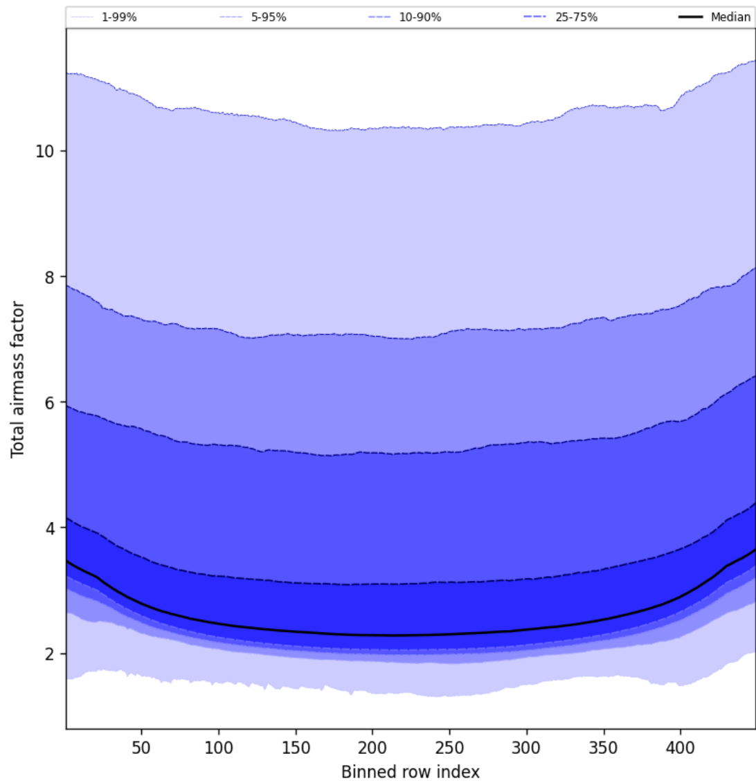
Figure 49: Along track statistics of “Total airmass factor” for 2025-01-19 to 2025-01-21
