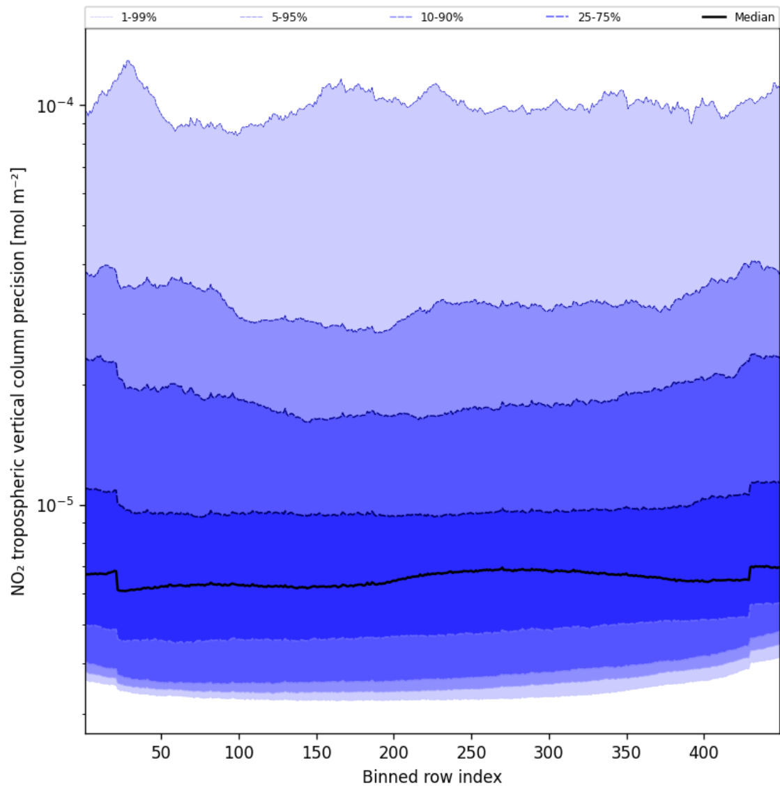
Figure 47: Along track statistics of “NO 2 tropospheric vertical column precision” for 2025-01-19 to 2025-01-21
