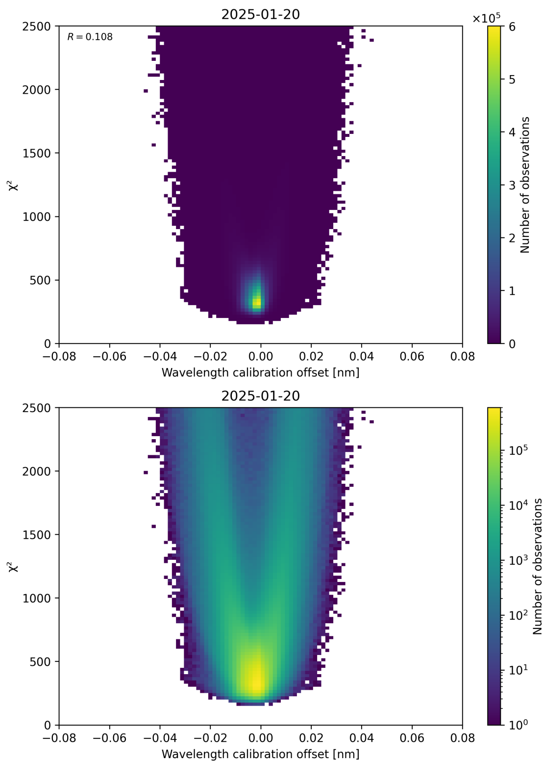
Figure 175: Scatter density plot of “Wavelength calibration offset” against “ \chi^2 ” for 2025-01-19 to 2025-01-21.
