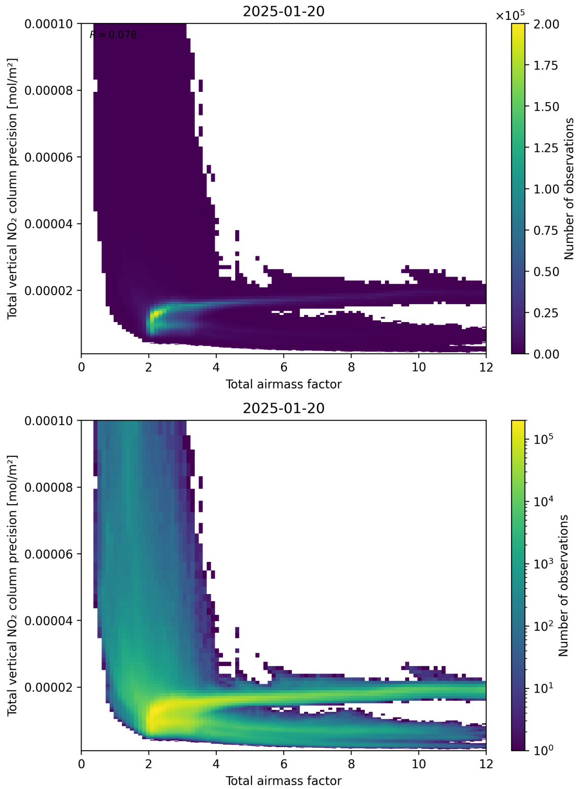
Figure 68: Scatter density plot of “Total airmass factor” against “Total vertical NO 2 column precision” for 2025-01-19 to 2025-01-21.
