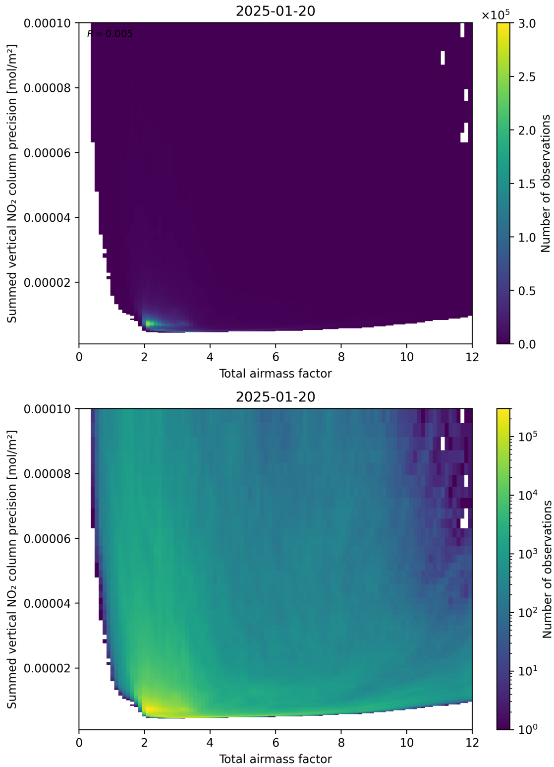
Figure 66: Scatter density plot of “Total airmass factor” against “Summed vertical NO 2 column precision” for 2025-01-19 to 2025-01-21.
