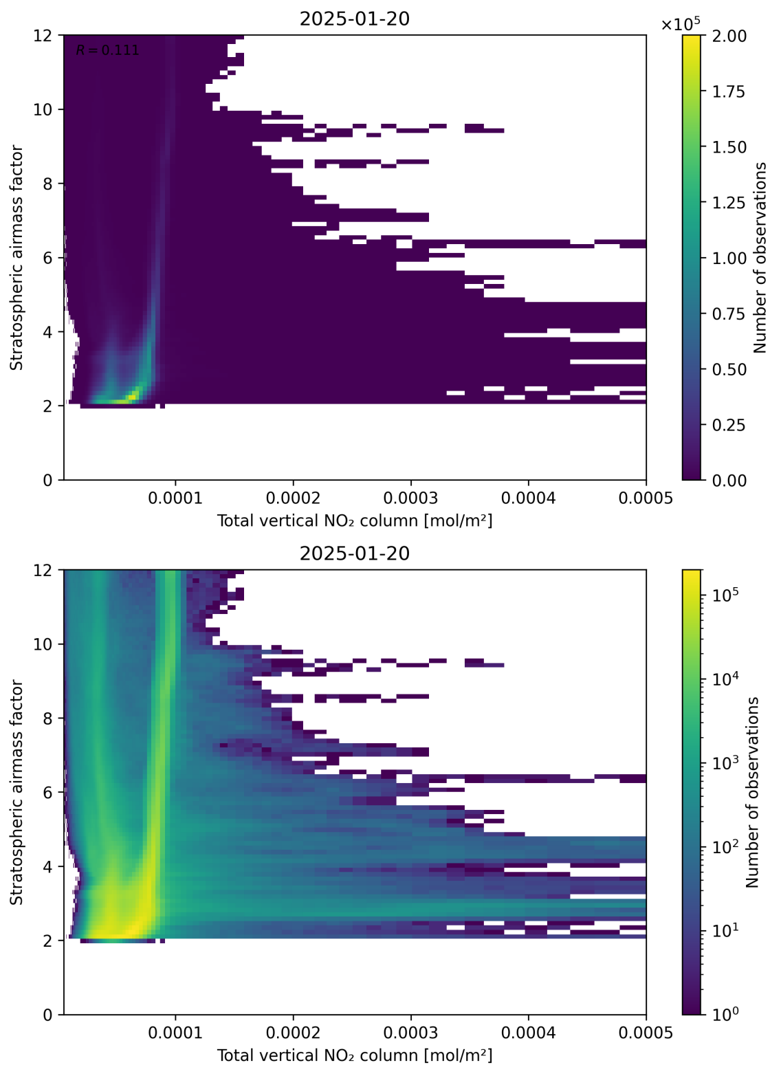
Figure 110: Scatter density plot of “Total vertical NO 2 column” against “Stratospheric airmass factor” for 2025-01-19 to 2025-01-21.
