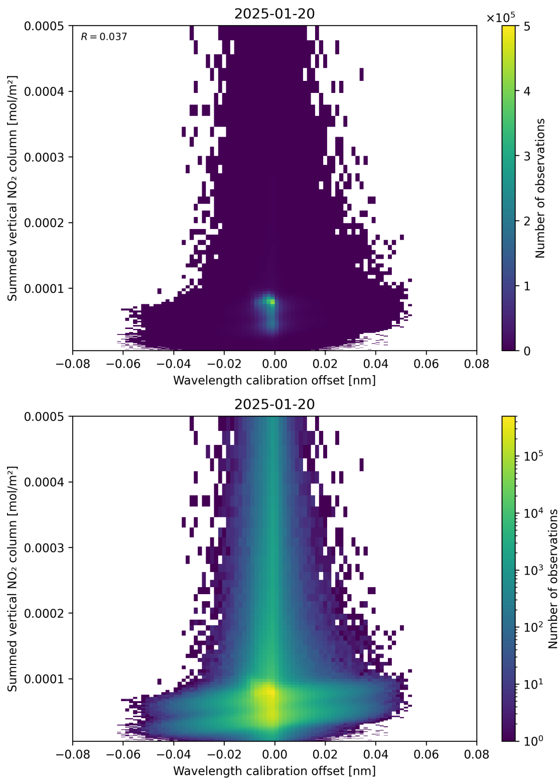
Figure 177: Scatter density plot of “Wavelength calibration offset” against “Summed vertical NO 2 column” for 2025-01-19 to 2025-01-21.
