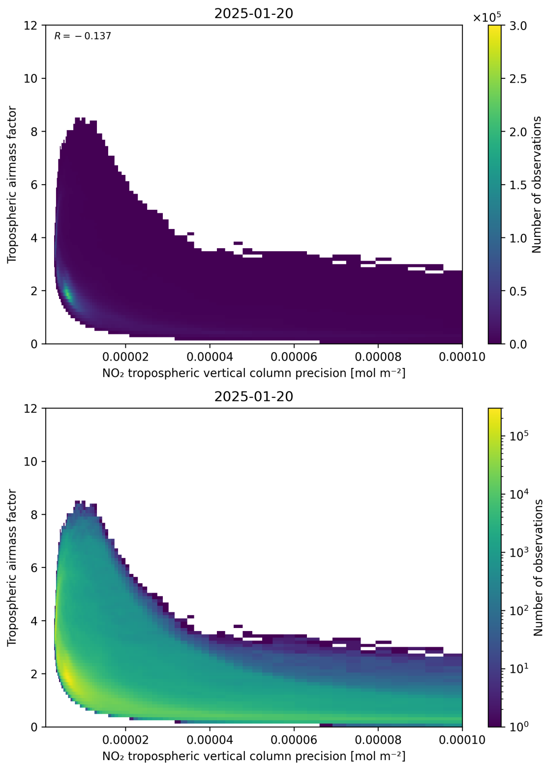
Figure 133: Scatter density plot of “NO 2 tropospheric vertical column precision” against “Tropospheric air mass factor” for 2025-01-19 to 2025-01-21.
