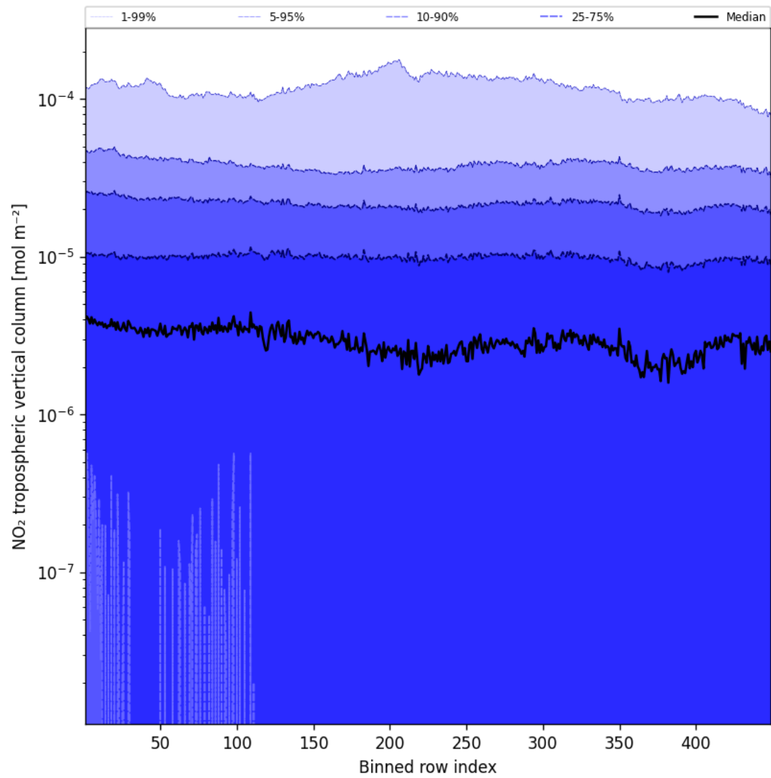
Figure 46: Along track statistics of "NO 2 tropospheric vertical column" for 2025-01-19 to 2025-01-21
