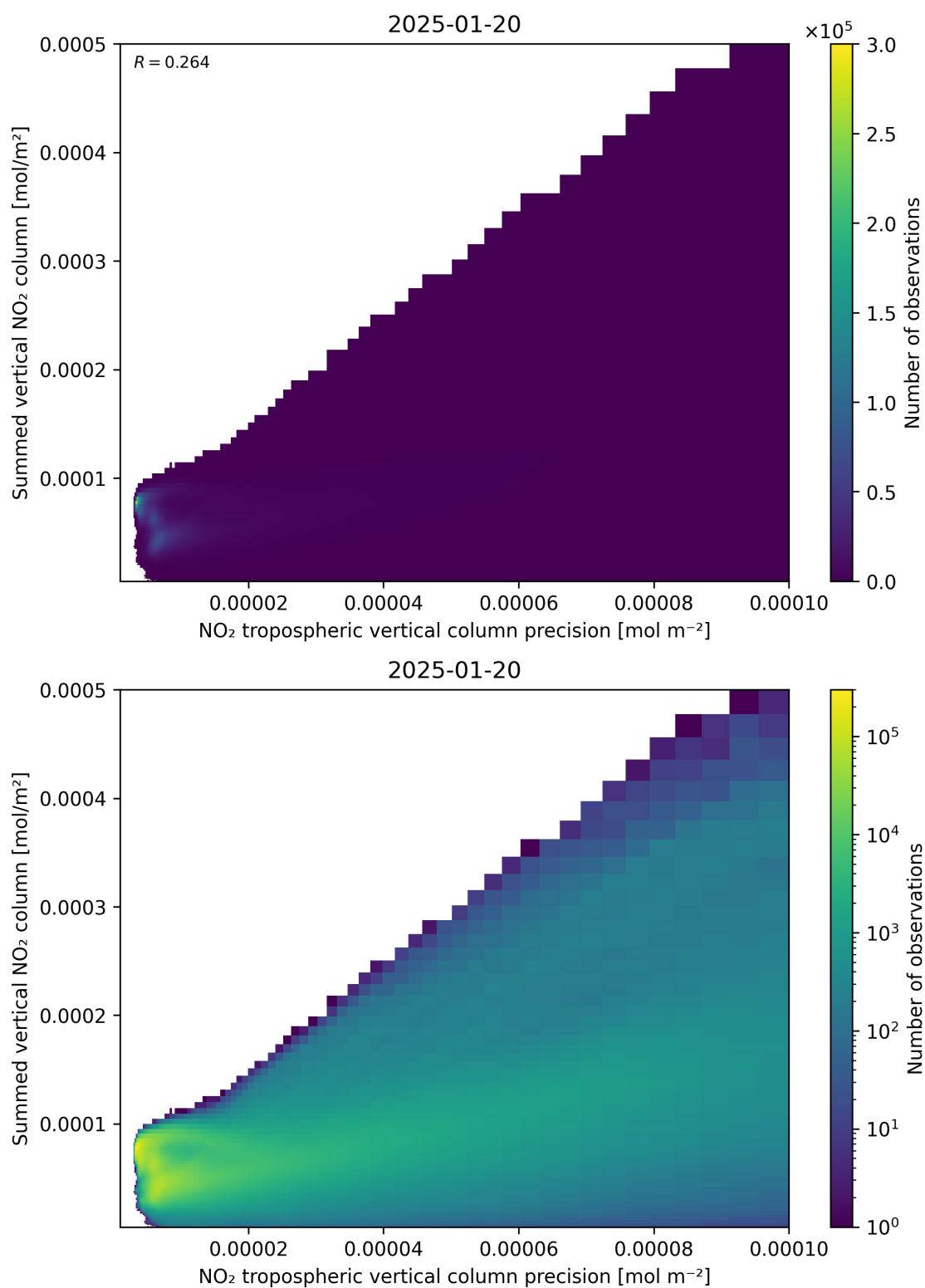
Figure 136: Scatter density plot of “NO 2 tropospheric vertical column precision” against “Summed vertical NO 2 column” for 2025-01-19 to 2025-01-21.
