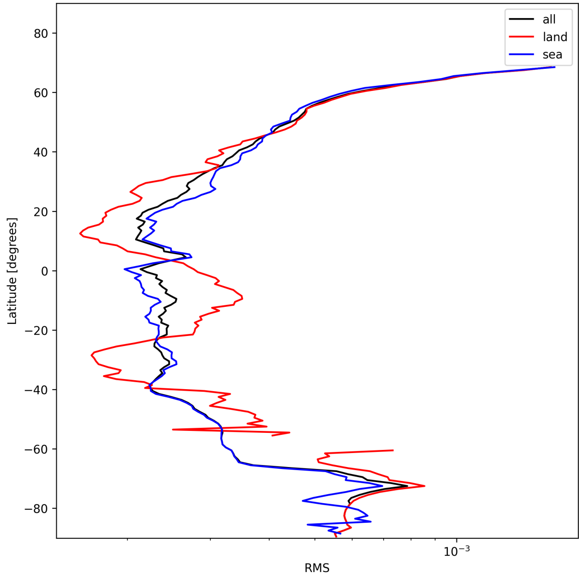
Figure 26: Zonal average of “RMS” for 2025-01-19 to 2025-01-21.
