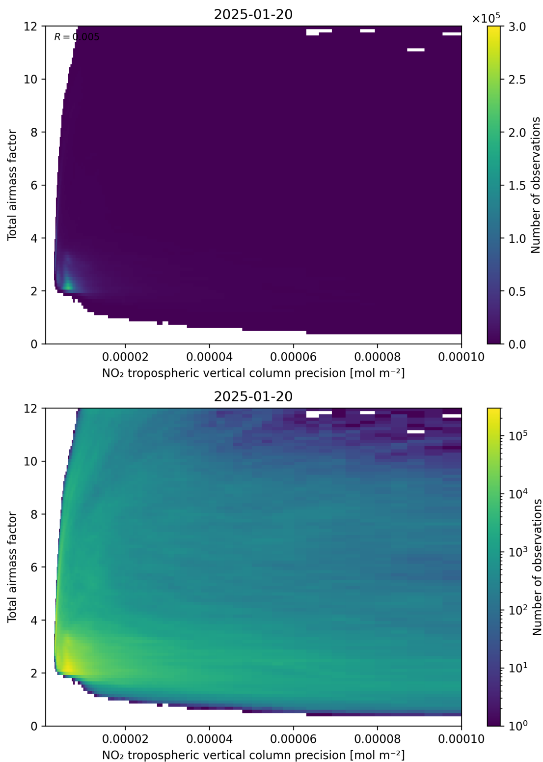
Figure 132: Scatter density plot of “NO 2 tropospheric vertical column precision” against “Total airmass factor” for 2025-01-19 to 2025-01-21.
