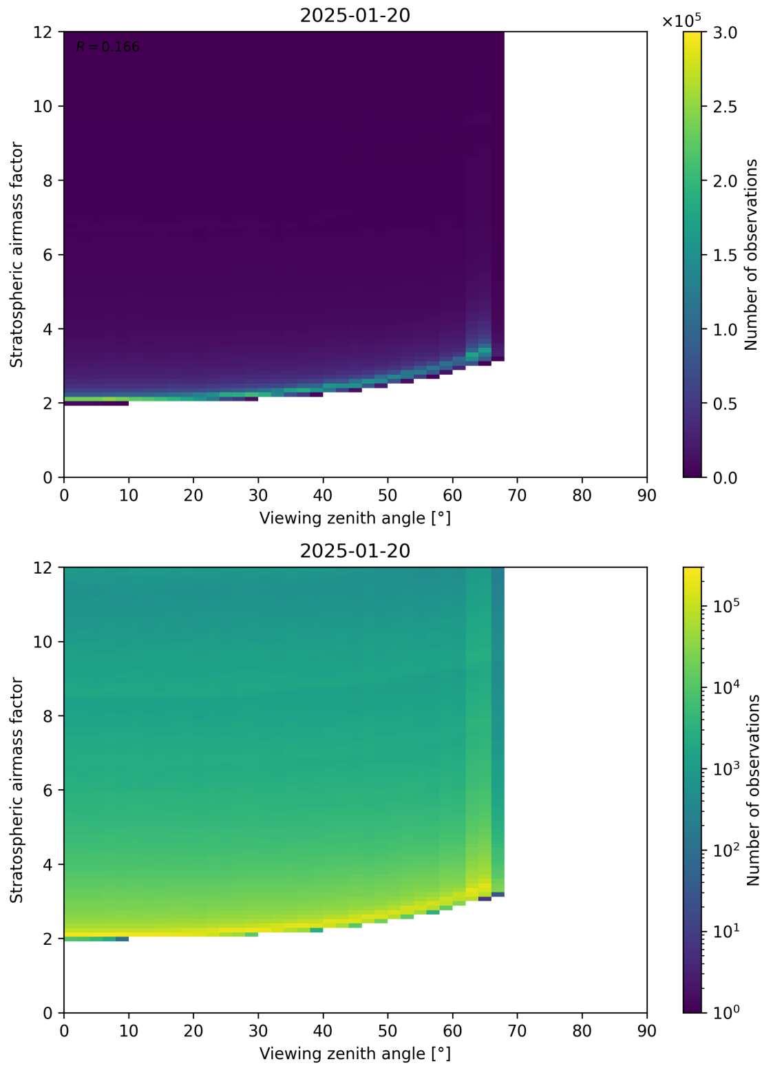
Figure 159: Scatter density plot of “Viewing zenith angle” against “Stratospheric airmass factor” for 2025-01-19 to 2025-01-21.
