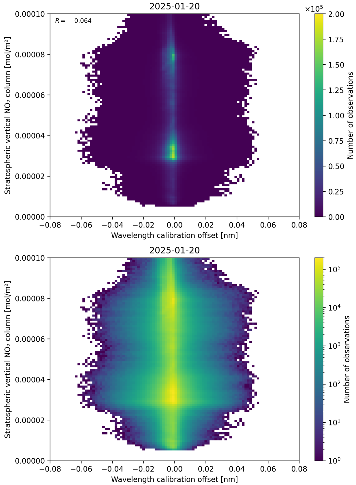
Figure 176: Scatter density plot of “Wavelength calibration offset” against “Stratospheric vertical NO 2 column” for 2025-01-19 to 2025-01-21.
