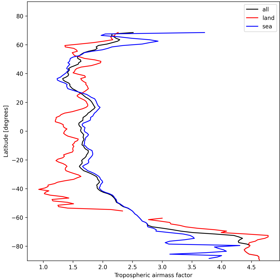
Figure 14: Zonal average of “Tropospheric airmass factor” for 2025-01-19 to 2025-01-21.
