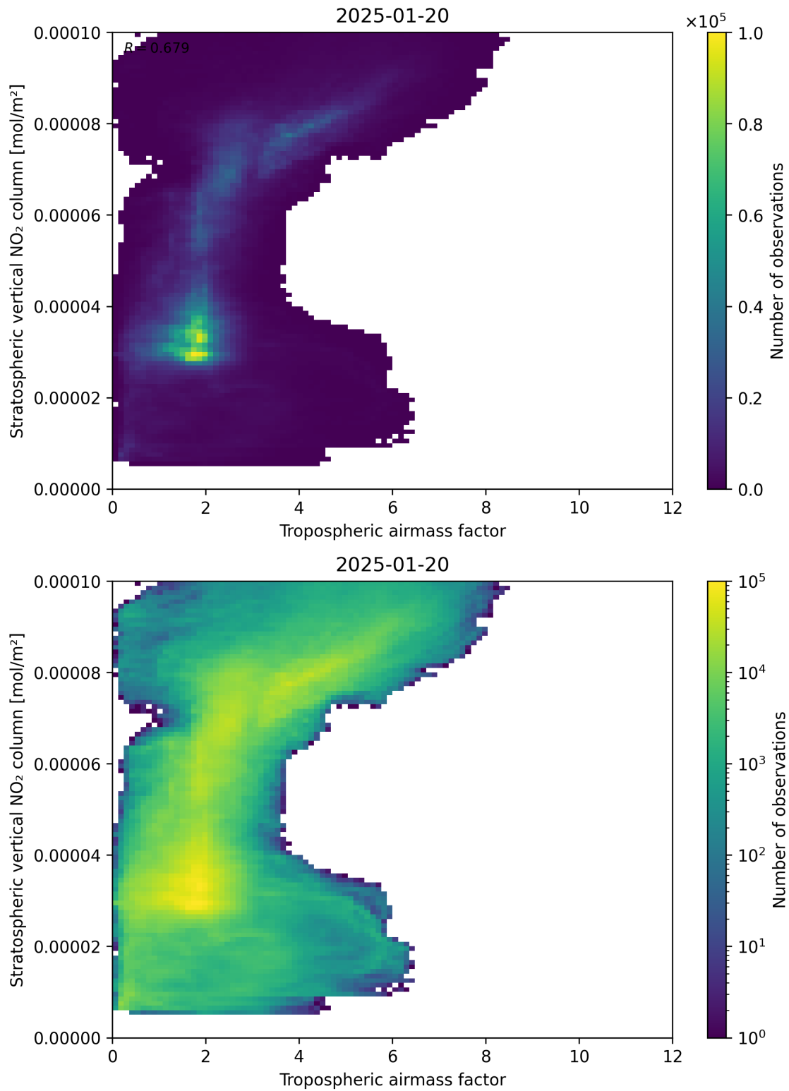
Figure 74: Scatter density plot of “Tropospheric air mass factor” against “Stratospheric vertical NO 2 column” for 2025-01-19 to 2025-01-21.
