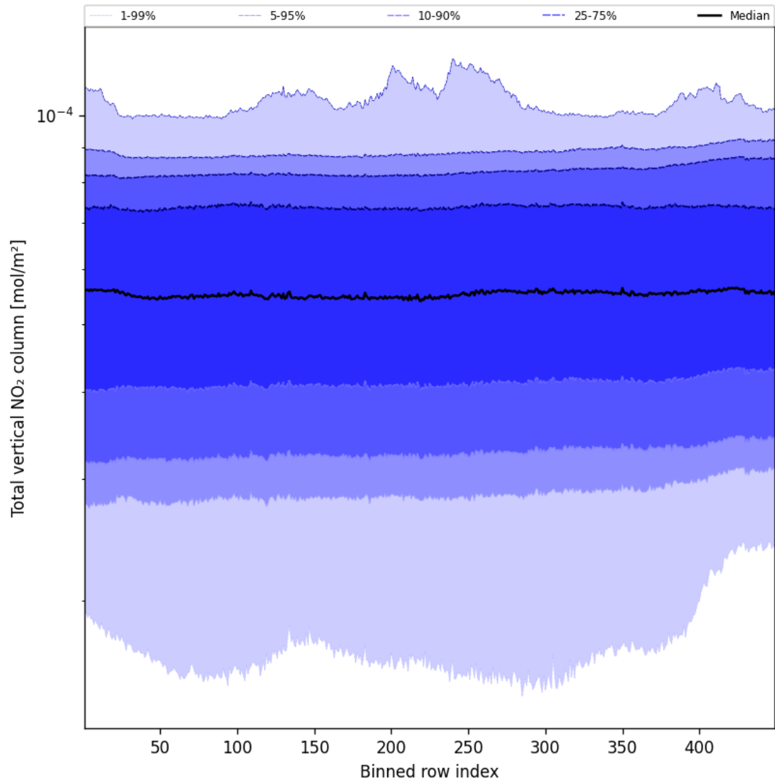
Figure 55: Along track statistics of “Total vertical NO 2 column” for 2025-01-19 to 2025-01-21
