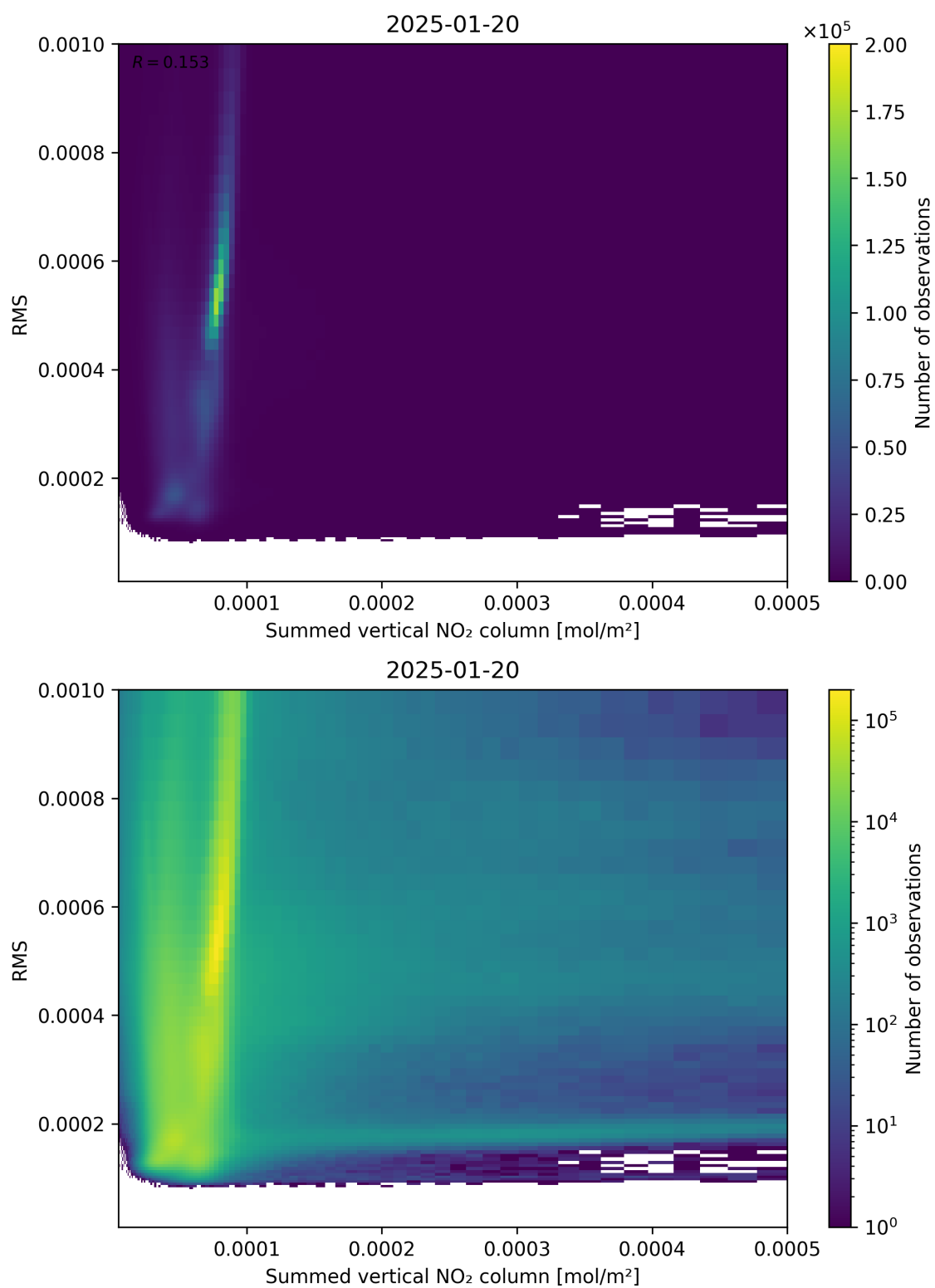
Figure 109: Scatter density plot of “Summed vertical NO 2 column” against “RMS” for 2025-01-19 to 2025-01-21.
