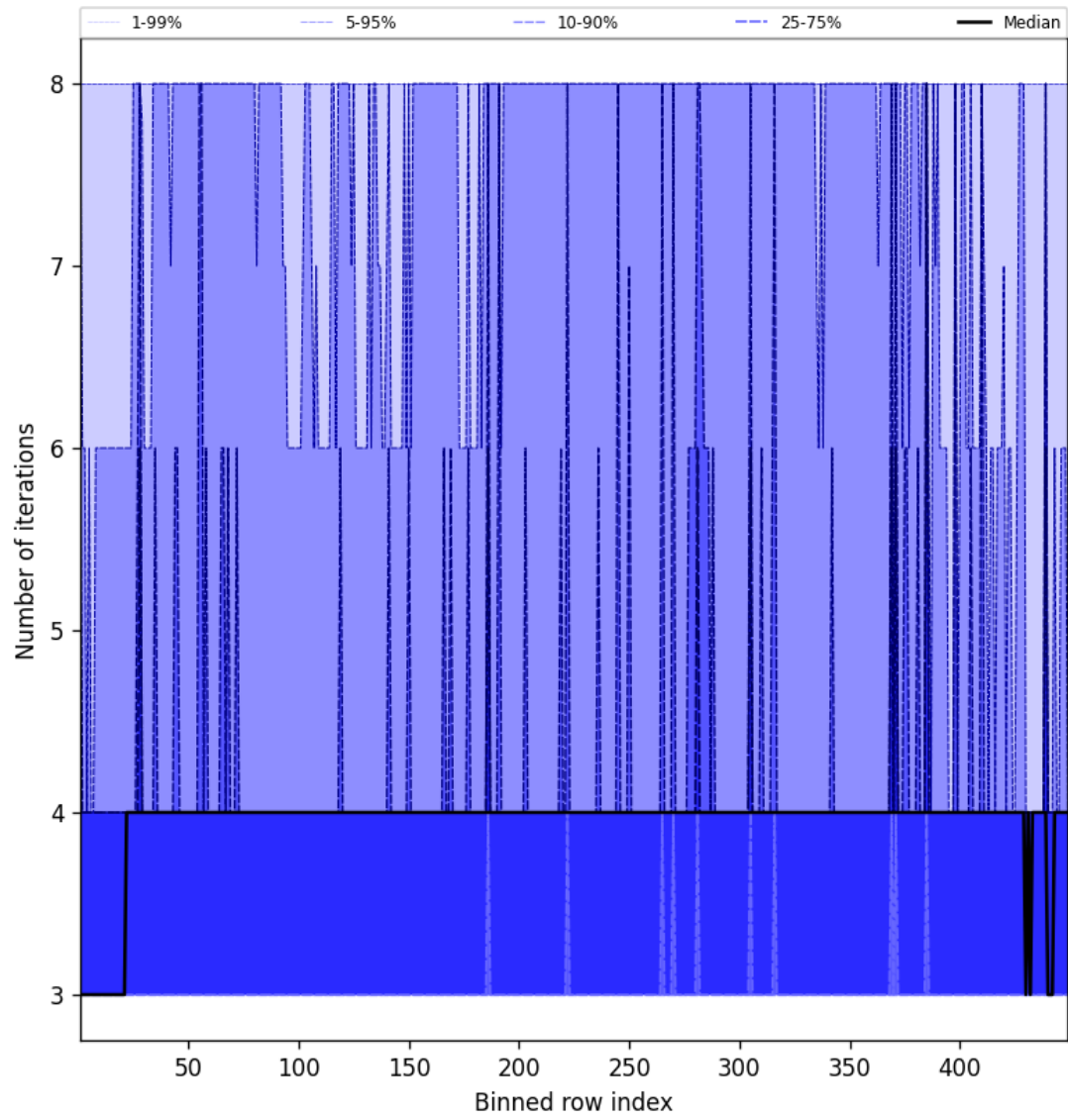
Figure 51: Along track statistics of “Number of iterations” for 2025-01-19 to 2025-01-21
