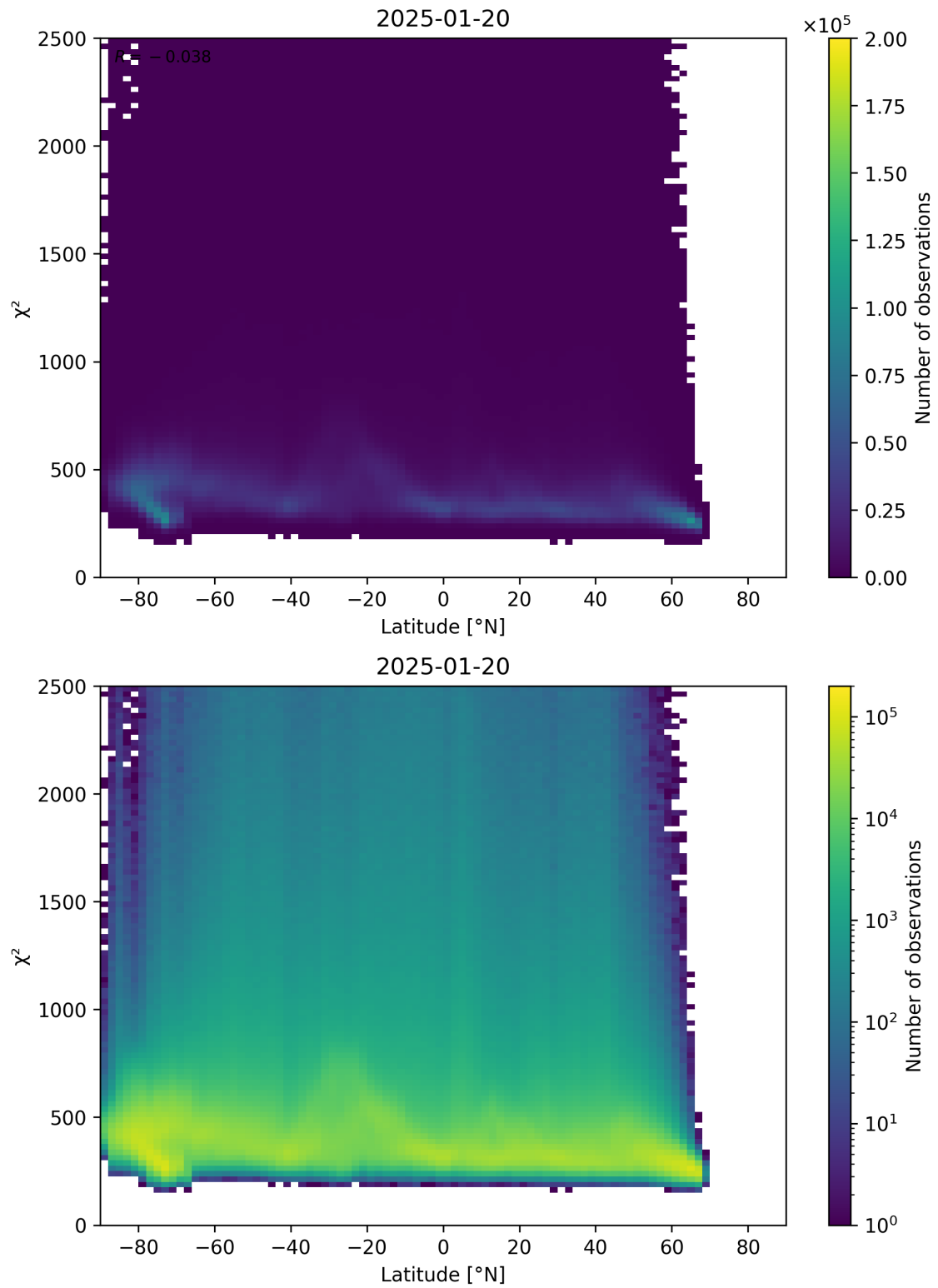
Figure 86: Scatter density plot of “Latitude” against “ \chi^2 ” for 2025-01-19 to 2025-01-21.
