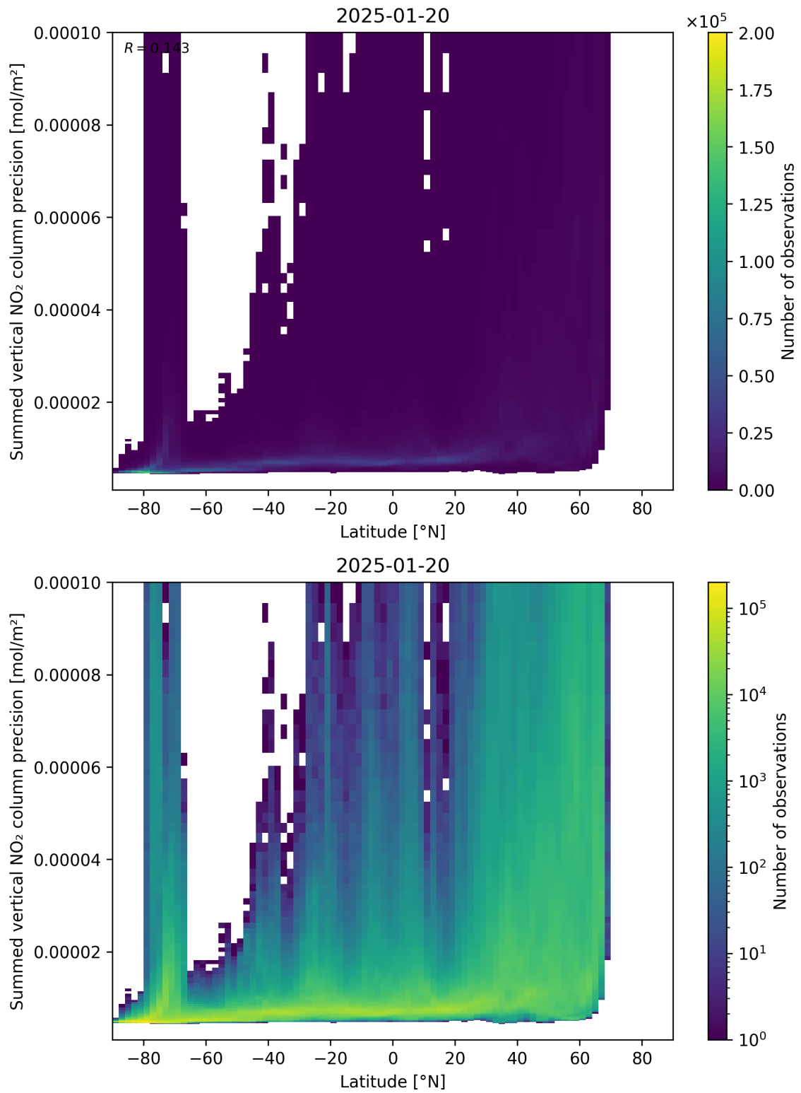
Figure 89: Scatter density plot of “Latitude” against “Summed vertical NO 2 column precision” for 2025-01-19 to 2025-01-21.
