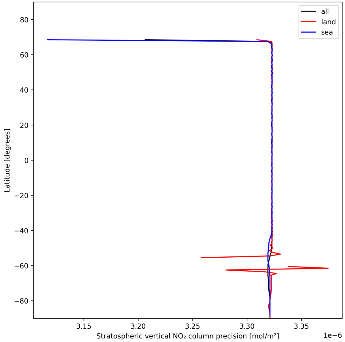
Figure 20: Zonal average of “Stratospheric vertical NO 2 column precision” for 2025-01-19 to 2025-01-21.
