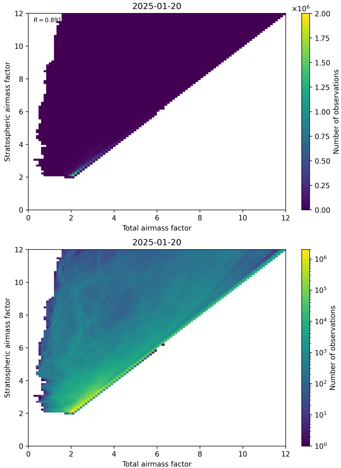
Figure 62: Scatter density plot of “Total airmass factor” against “Stratospheric airmass factor” for 2025-01-19 to 2025-01-21.
