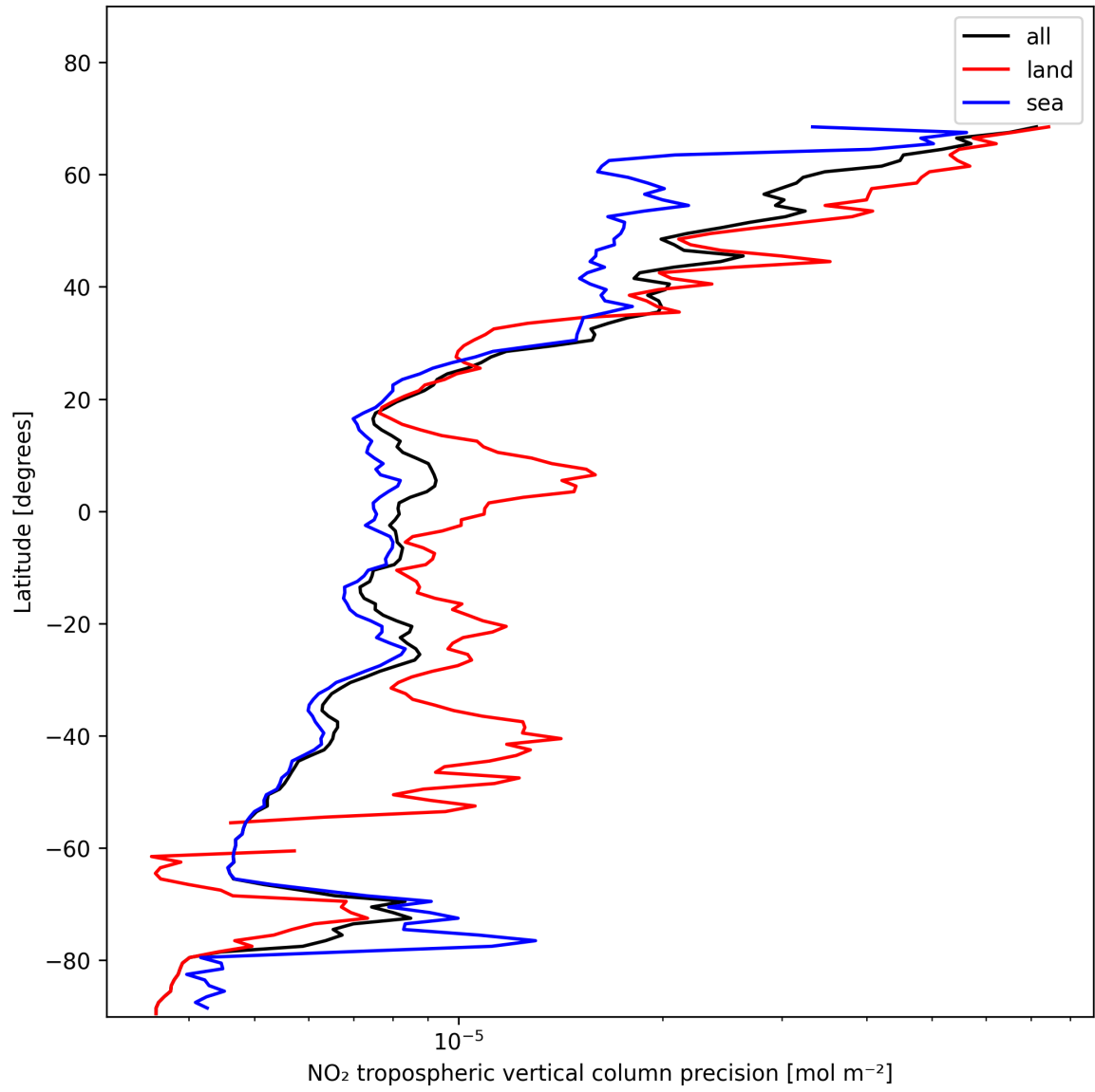
Figure 13: Zonal average of “NO 2 tropospheric vertical column precision” for 2025-01-19 to 2025-01-21.
