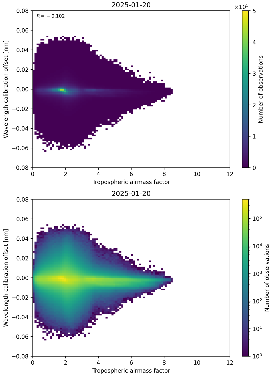
Figure 80: Scatter density plot of “Tropospheric airmass factor” against “Wavelength calibration offset” for 2025-01-19 to 2025-01-21.
