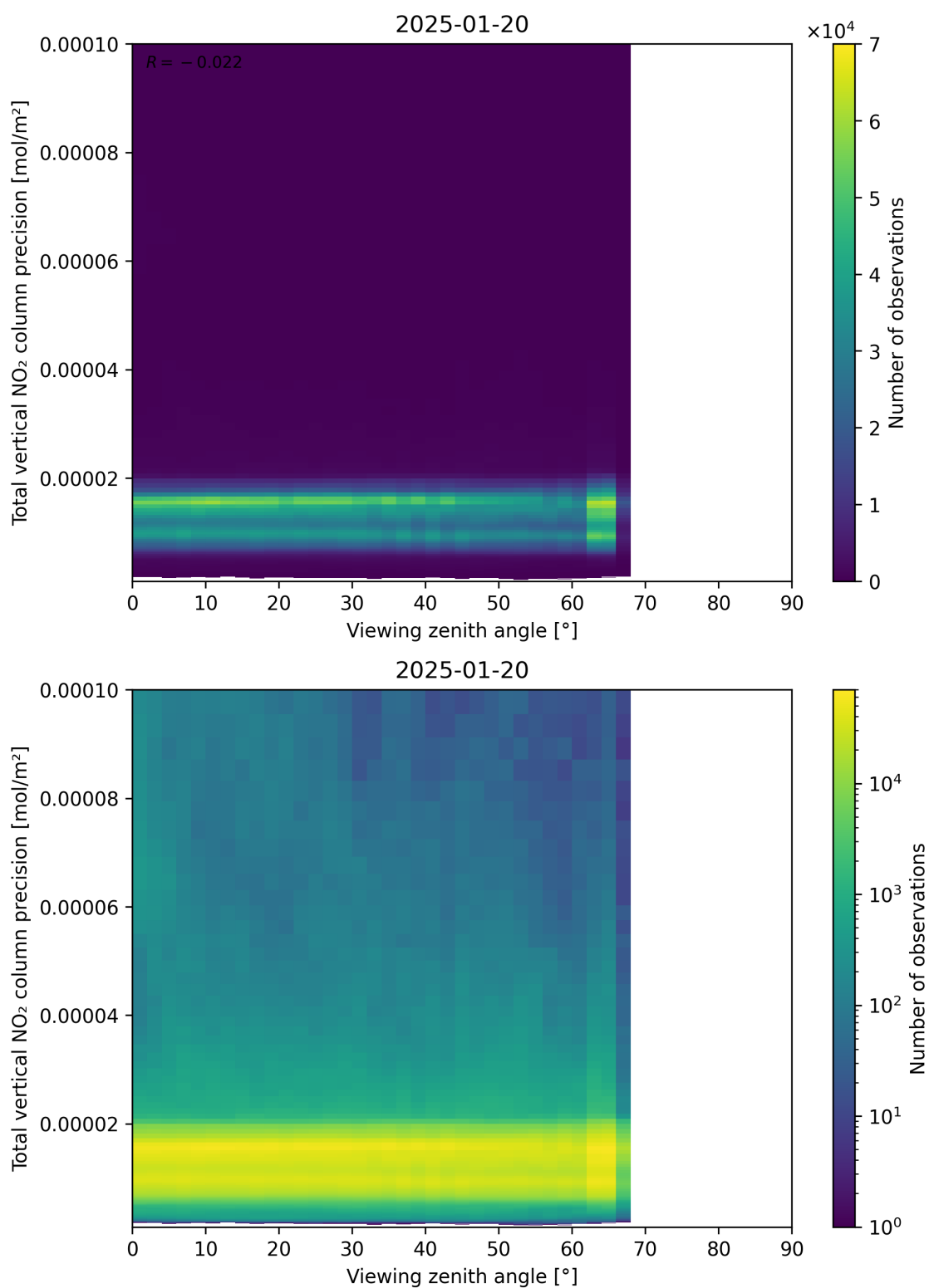
Figure 168: Scatter density plot of “Viewing zenith angle” against “Total vertical NO 2 column precision” for 2025-01-19 to 2025-01-21.
