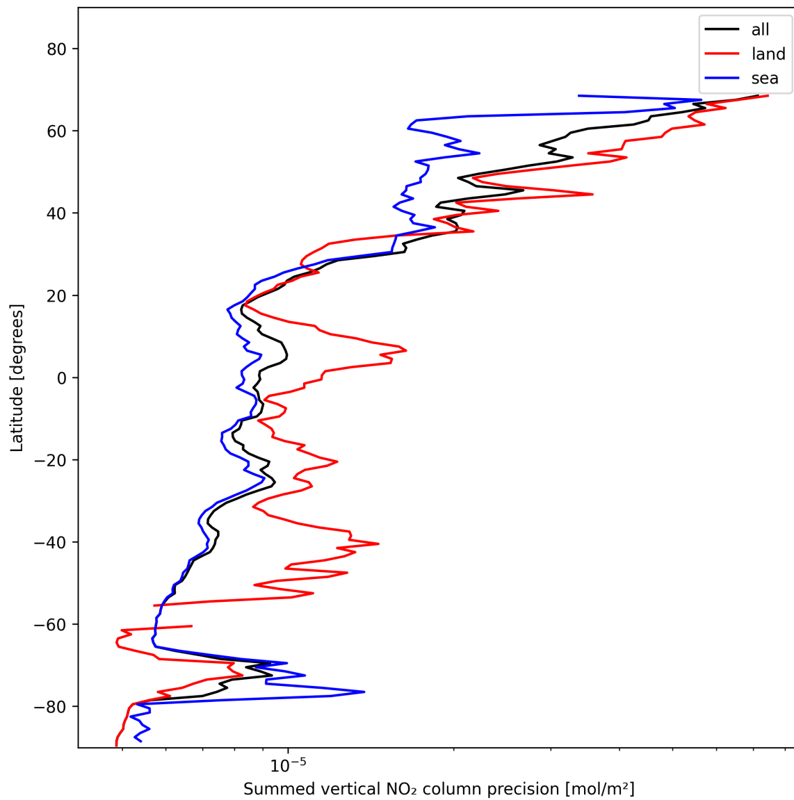
Figure 24: Zonal average of “Summed vertical NO 2 column precision” for 2025-01-19 to 2025-01-21.
