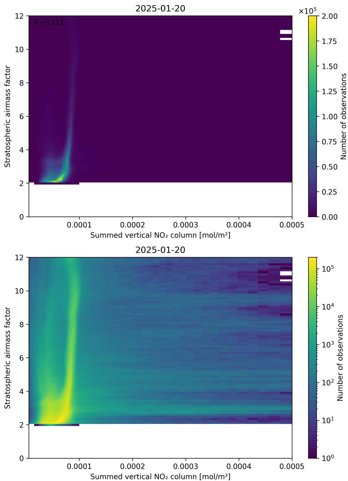
Figure 103: Scatter density plot of “Summed vertical NO 2 column” against “Stratospheric airmass factor” for 2025-01-19 to 2025-01-21.
