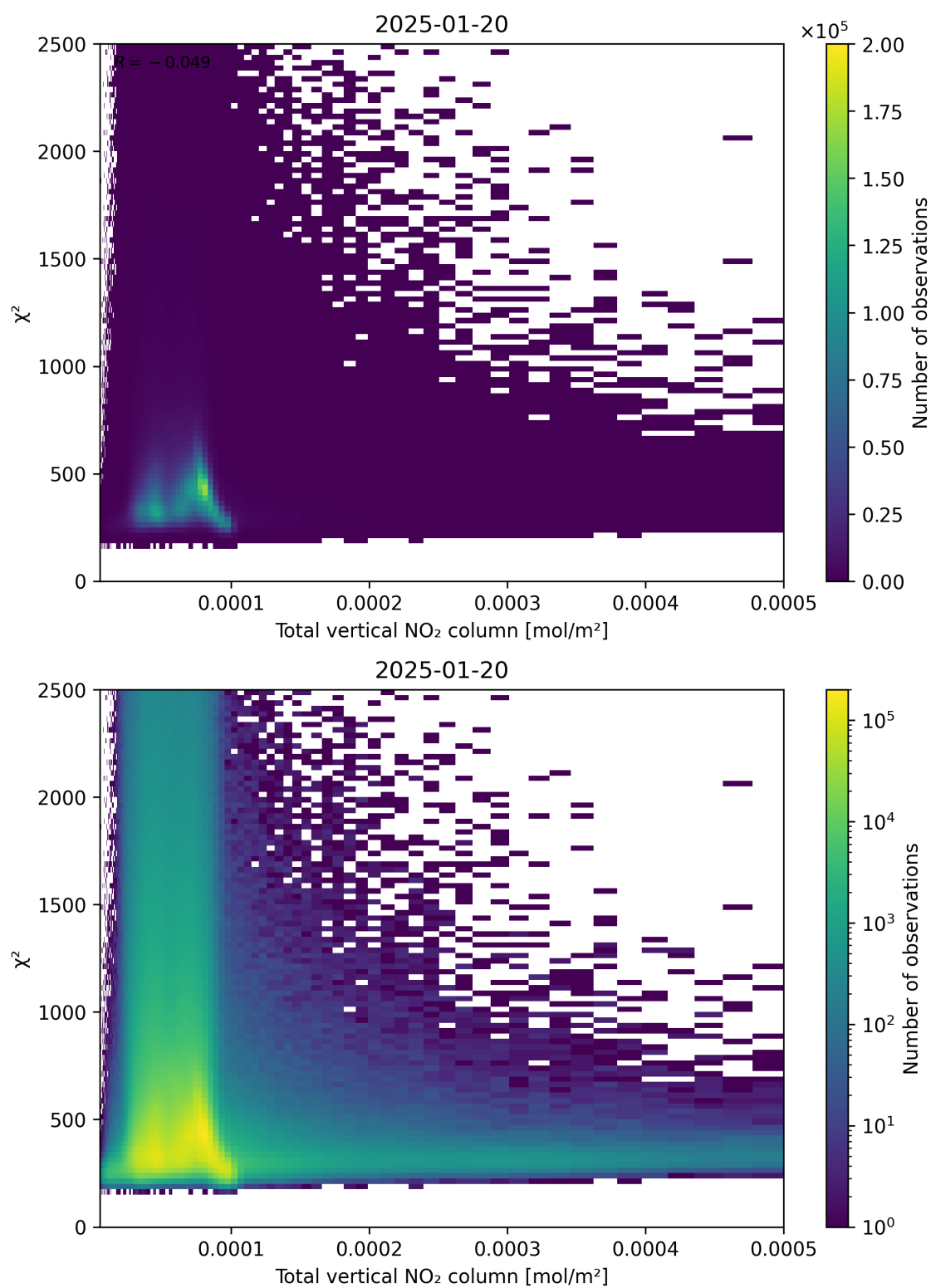
Figure 111: Scatter density plot of “Total vertical NO 2 column” against “ \chi^2 ” for 2025-01-19 to 2025-01-21.
