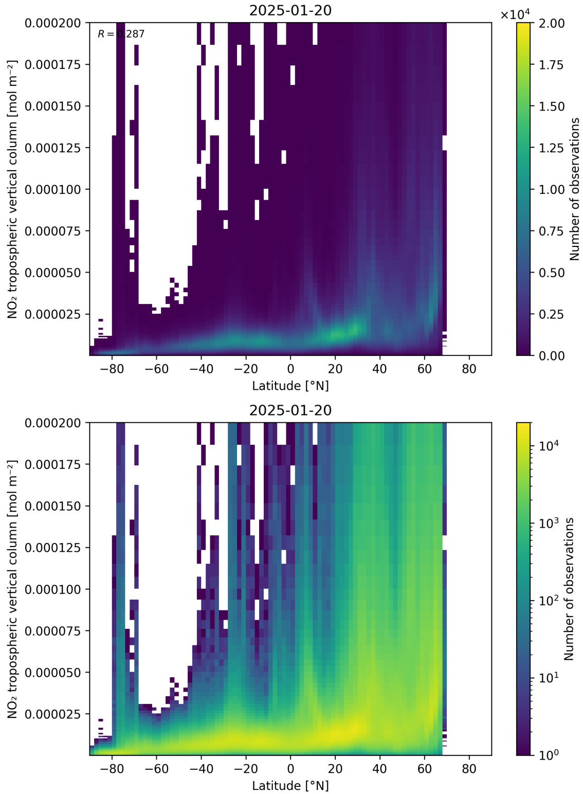
Figure 92: Scatter density plot of “Latitude” against “NO 2 tropospheric vertical column” for 2025-01-19 to 2025-01-21.
