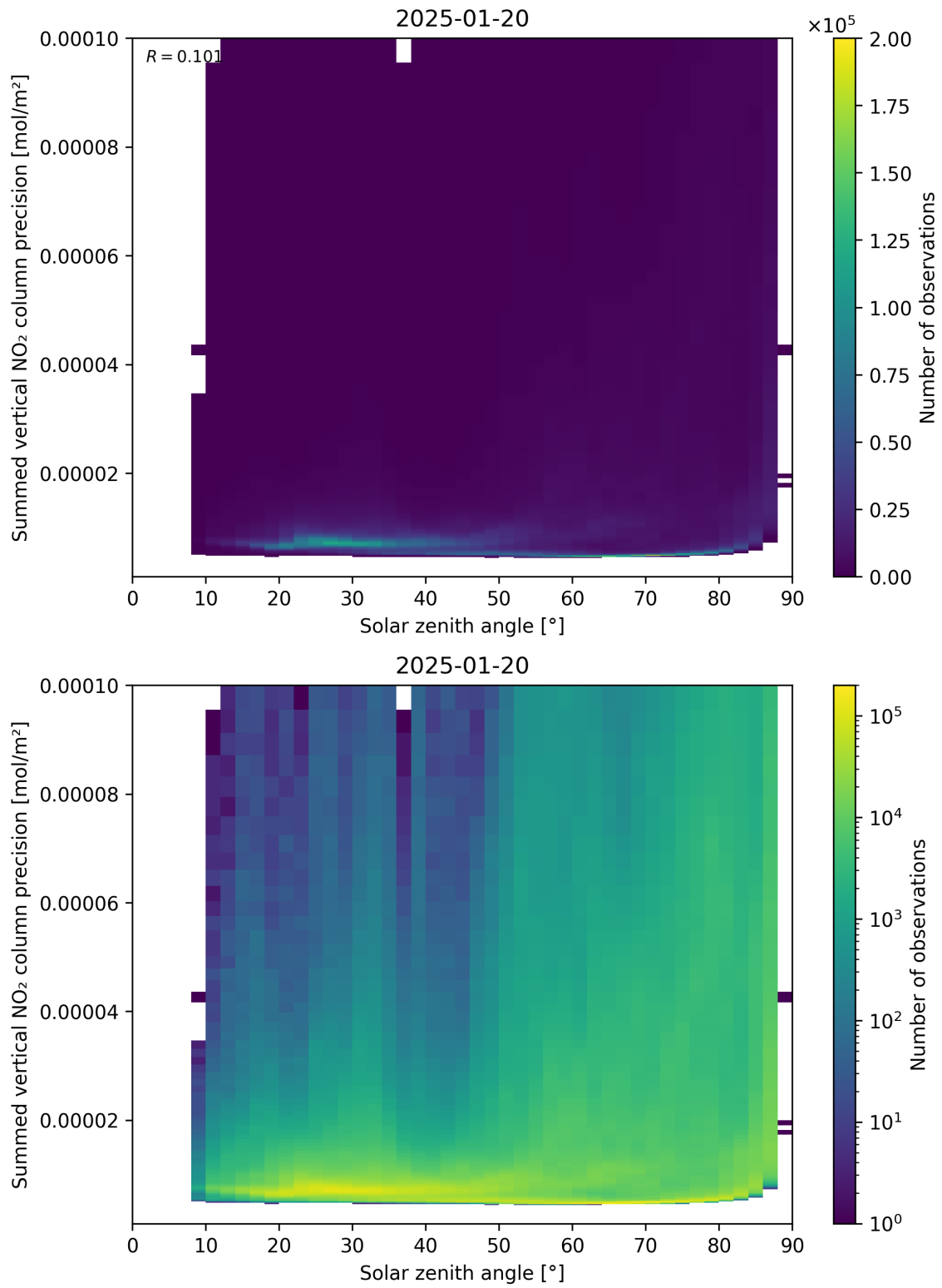
Figure 152: Scatter density plot of “Solar zenith angle” against “Summed vertical NO 2 column precision” for 2025-01-19 to 2025-01-21.
