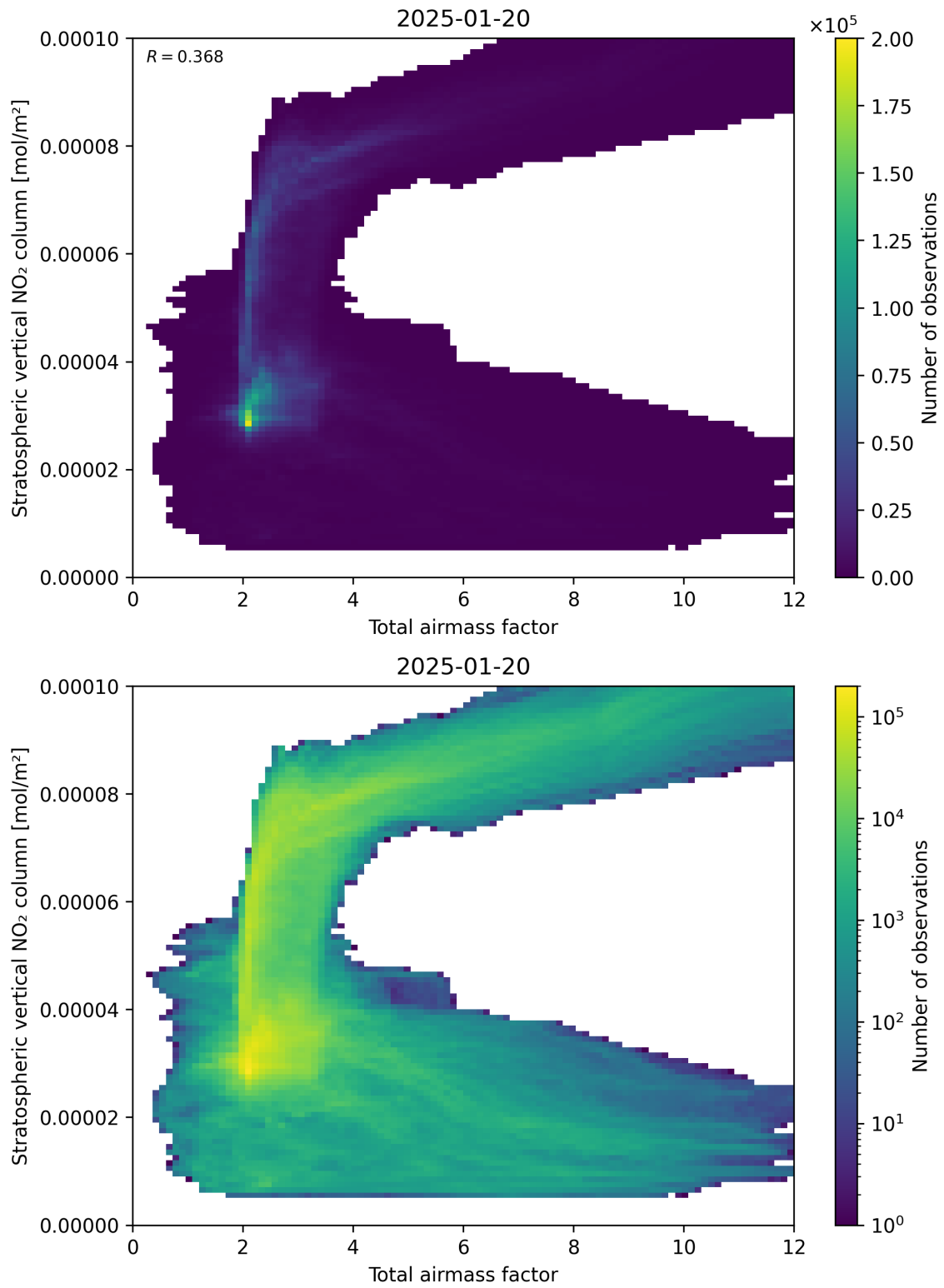
Figure 64: Scatter density plot of “Total airmass factor” against “Stratospheric vertical NO 2 column” for 2025-01-19 to 2025-01-21.
