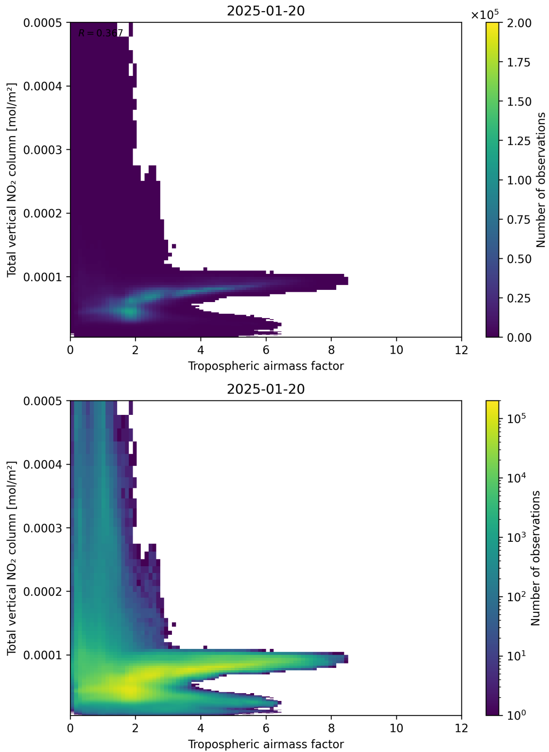
Figure 77: Scatter density plot of “Tropospheric airmass factor” against “Total vertical NO 2 column” for 2025-01-19 to 2025-01-21.
