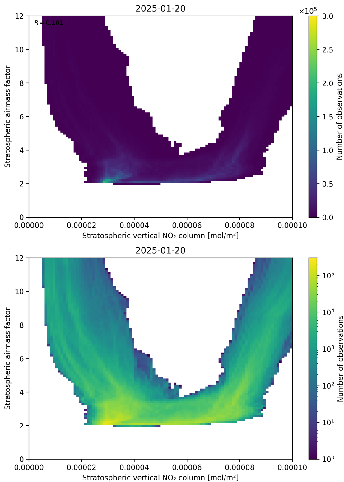
Figure 96: Scatter density plot of “Stratospheric vertical NO 2 column” against “Stratospheric airmass factor” for 2025-01-19 to 2025-01-21.
