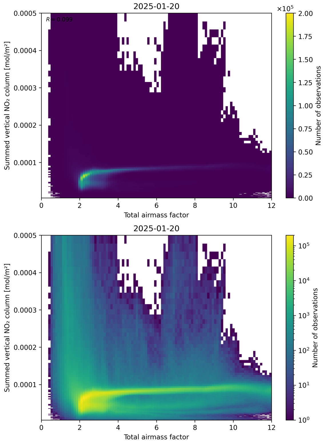
Figure 65: Scatter density plot of “Total airmass factor” against “Summed vertical NO 2 column” for 2025-01-19 to 2025-01-21.
