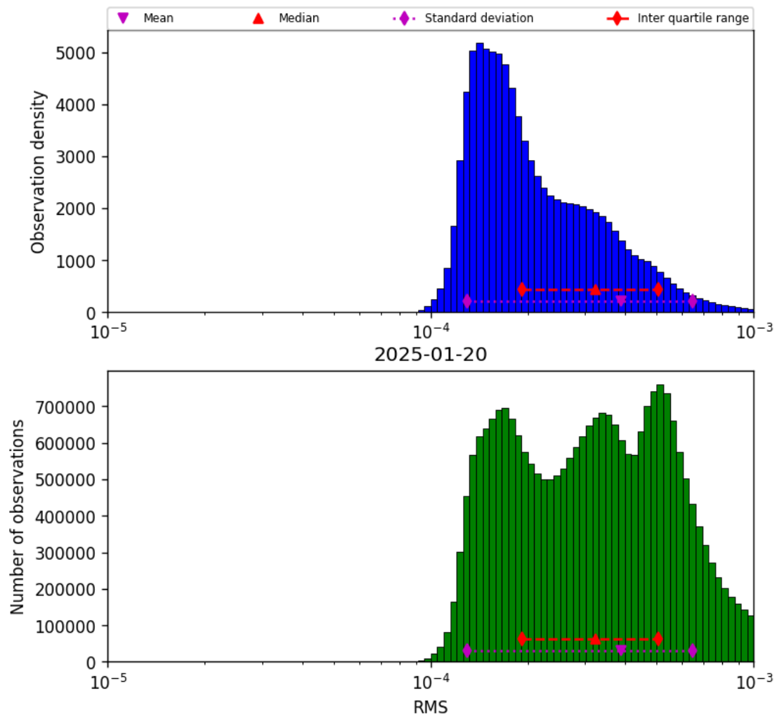
Figure 43: Histogram of “RMS” for 2025-01-19 to 2025-01-21
