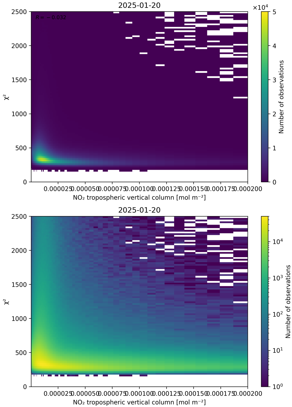
Figure 124: Scatter density plot of “NO 2 tropospheric vertical column” against “ \chi^2 ” for 2025-01-19 to 2025-01-21.
