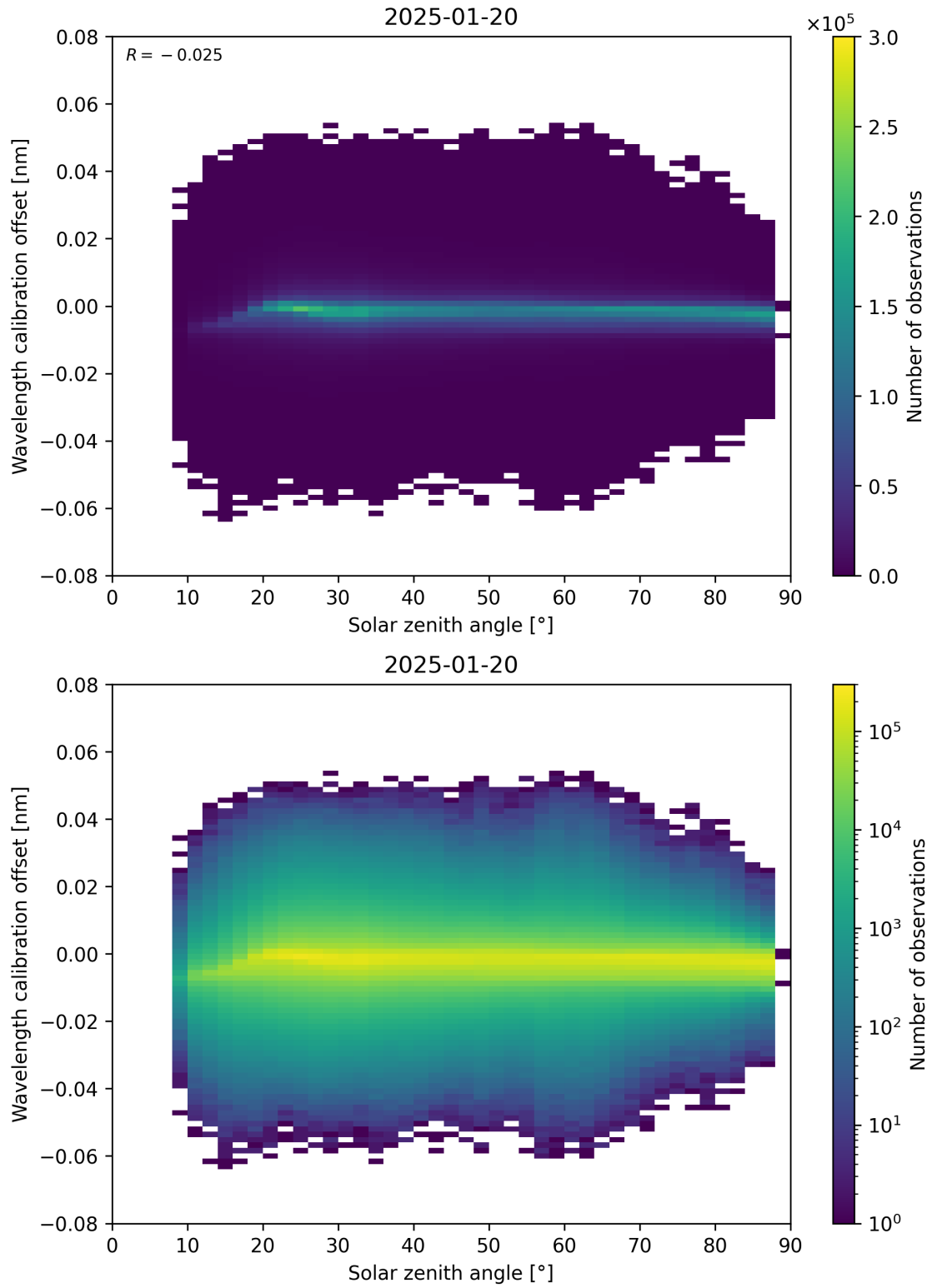
Figure 158: Scatter density plot of “Solar zenith angle” against “Wavelength calibration offset” for 2025-01-19 to 2025-01-21.
