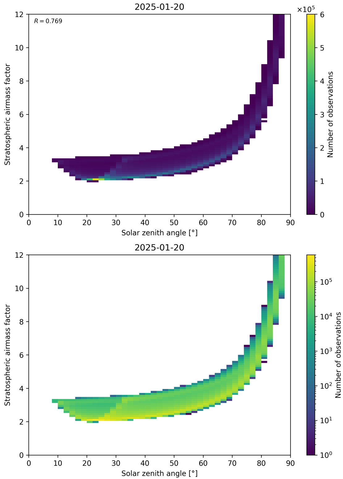
Figure 145: Scatter density plot of “Solar zenith angle” against “Stratospheric airmass factor” for 2025-01-19 to 2025-01-21.
