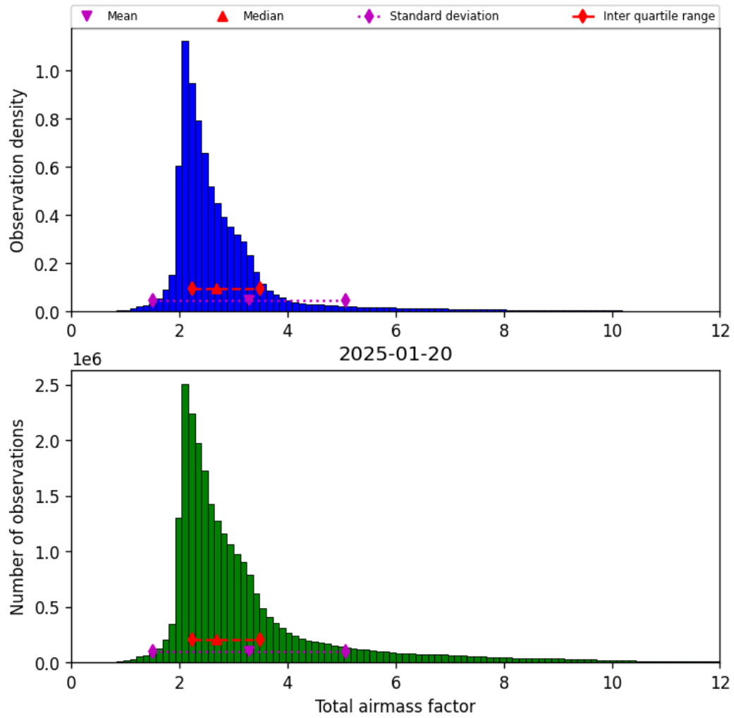
Figure 32: Histogram of “Total airmass factor” for 2025-01-19 to 2025-01-21
