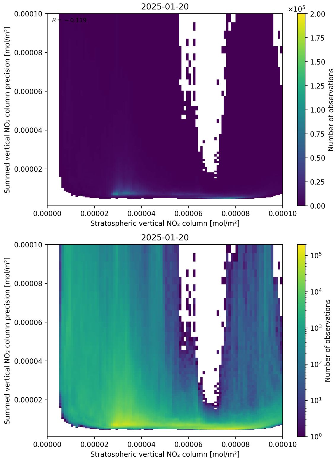
Figure 99: Scatter density plot of “Stratospheric vertical NO 2 column” against “Summed vertical NO 2 column precision” for 2025-01-19 to 2025-01-21.
