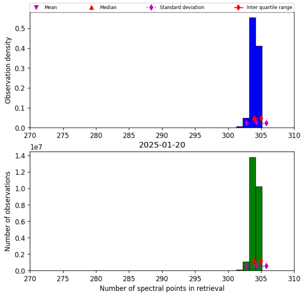
Figure 33: Histogram of “Number of spectral points in retrieval” for 2025-01-19 to 2025-01-21
