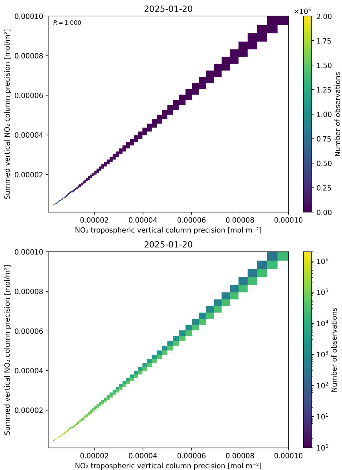
Figure 137: Scatter density plot of “NO 2 tropospheric vertical column precision” against “Summed vertical NO 2 column precision” for 2025-01-19 to 2025-01-21.
