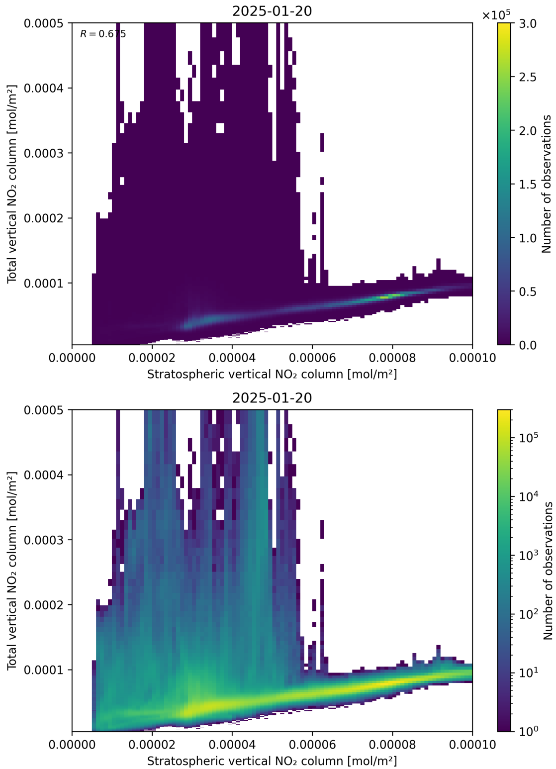
Figure 100: Scatter density plot of “Stratospheric vertical NO 2 column” against “Total vertical NO 2 column” for 2025-01-19 to 2025-01-21.
