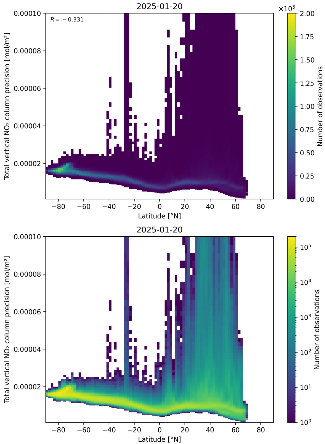
Figure 91: Scatter density plot of “Latitude” against “Total vertical NO 2 column precision” for 2025-01-19 to 2025-01-21.
