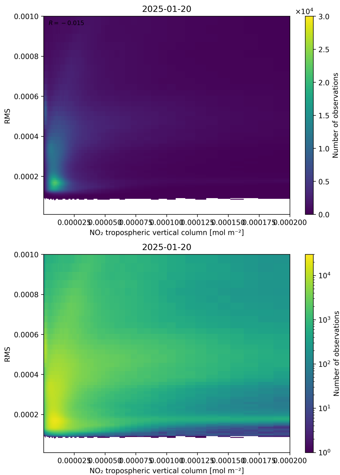
Figure 142: Scatter density plot of “NO 2 tropospheric vertical column” against “RMS” for 2025-01-19 to 2025-01-21.
