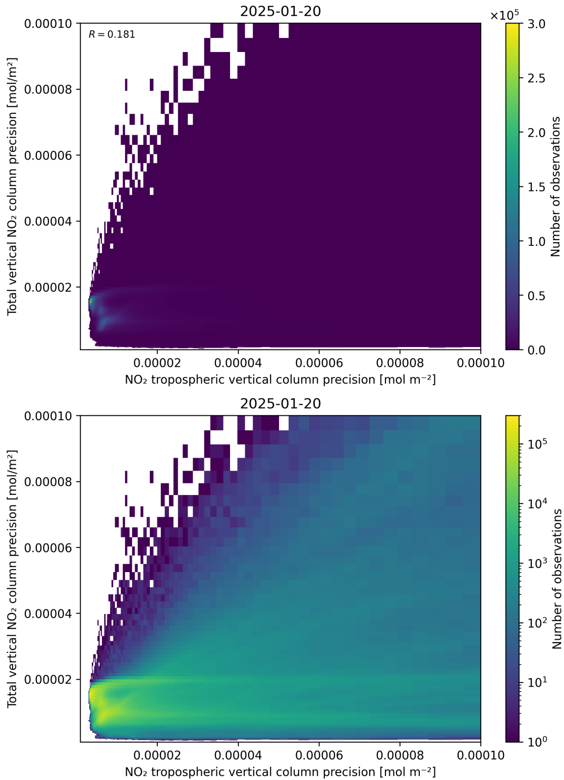
Figure 139: Scatter density plot of “NO 2 tropospheric vertical column precision” against “Total vertical NO 2 column precision” for 2025-01-19 to 2025-01-21.
