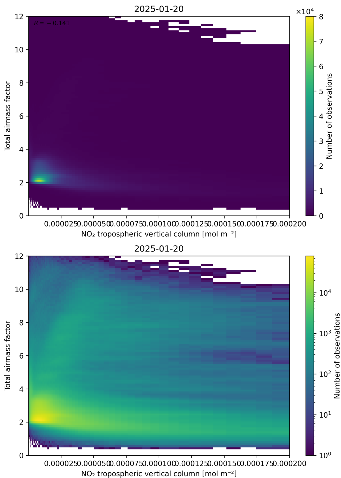
Figure 122: Scatter density plot of “NO 2 tropospheric vertical column” against “Total air mass factor” for 2025-01-19 to 2025-01-21.
