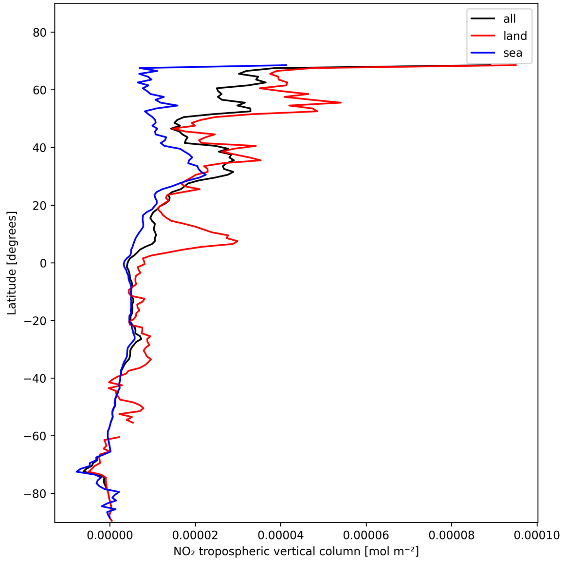
Figure 12: Zonal average of “NO 2 tropospheric vertical column” for 2025-01-19 to 2025-01-21.
