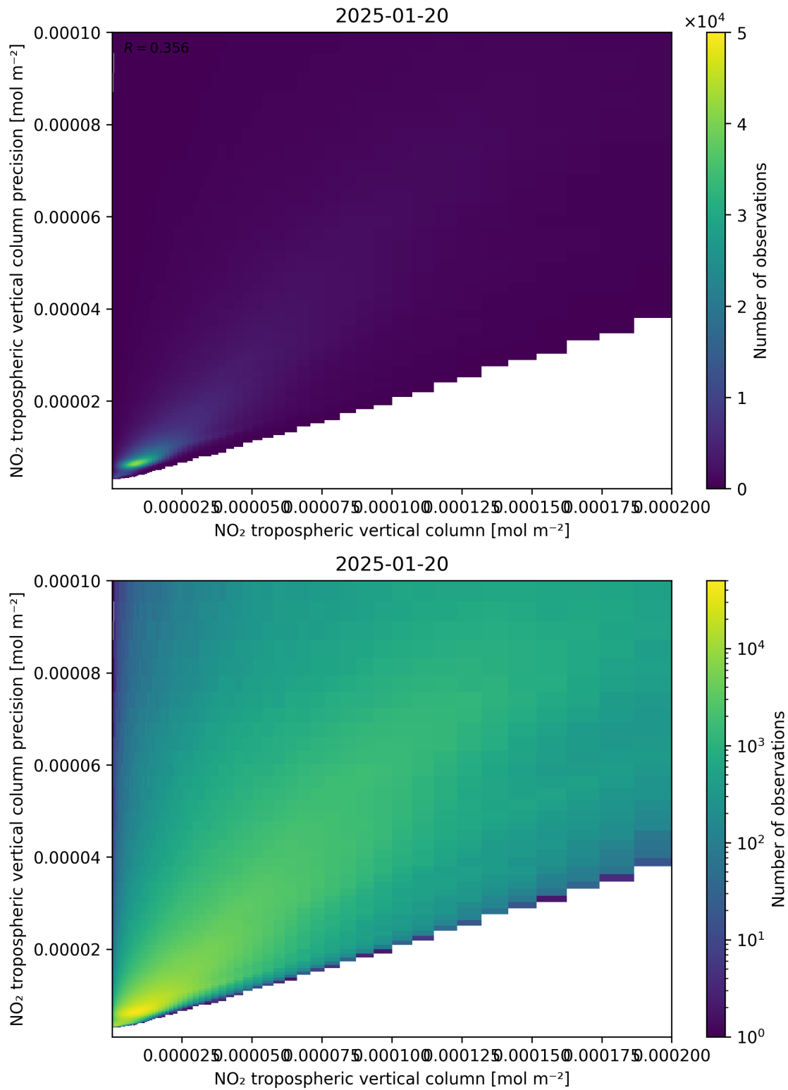
Figure 130: Scatter density plot of “NO 2 tropospheric vertical column” against “NO 2 tropospheric vertical column precision” for 2025-01-19 to 2025-01-21.
