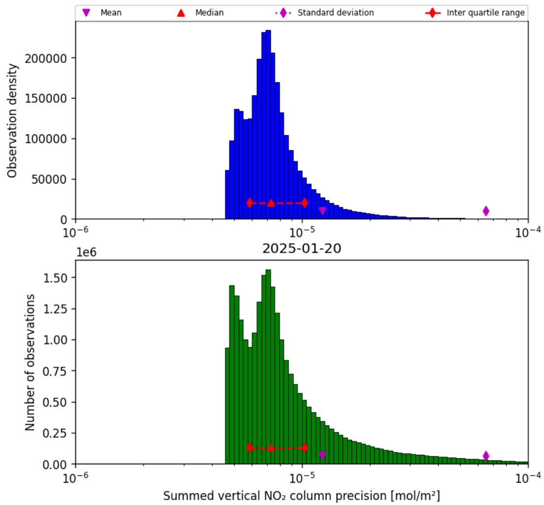
Figure 41: Histogram of “Summed vertical NO 2 column precision” for 2025-01-19 to 2025-01-21
