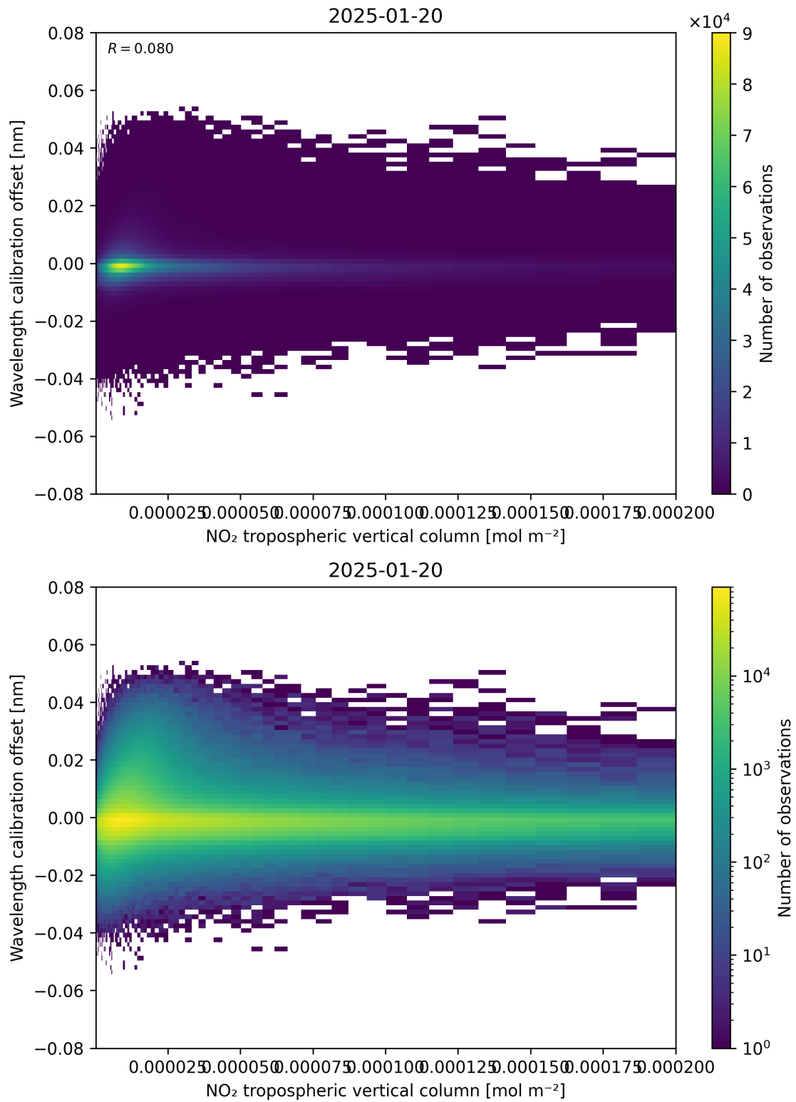
Figure 143: Scatter density plot of “NO 2 tropospheric vertical column” against “Wavelength calibration offset” for 2025-01-19 to 2025-01-21.
