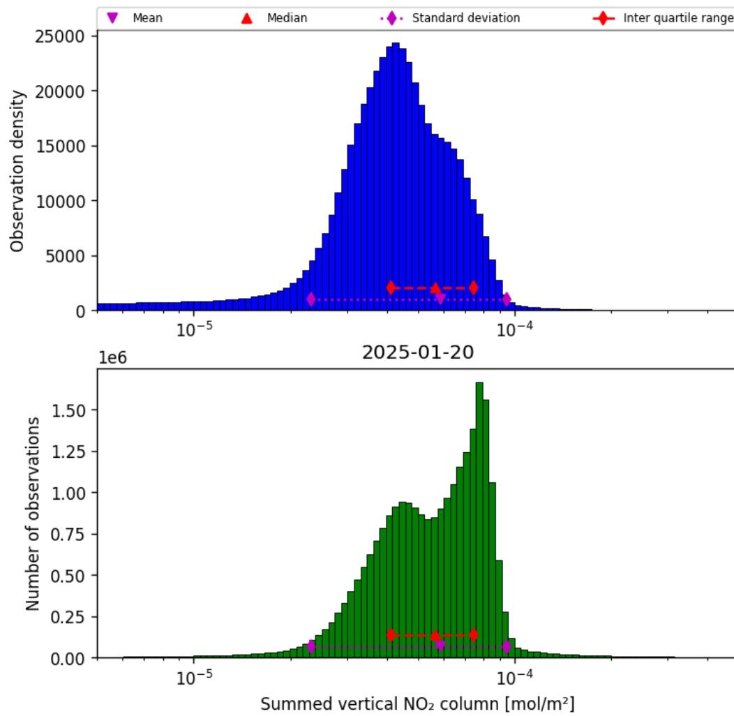
Figure 40: Histogram of “Summed vertical NO 2 column” for 2025-01-19 to 2025-01-21
