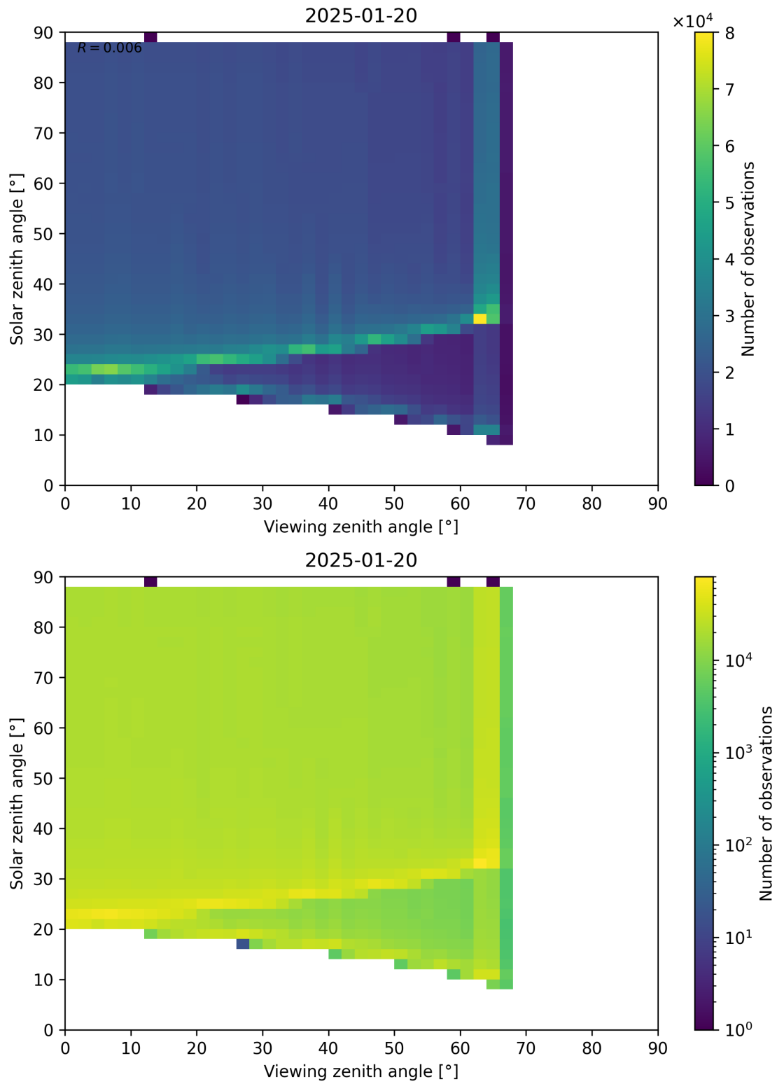
Figure 172: Scatter density plot of “Viewing zenith angle” against “Solar zenith angle” for 2025-01-19 to 2025-01-21.
