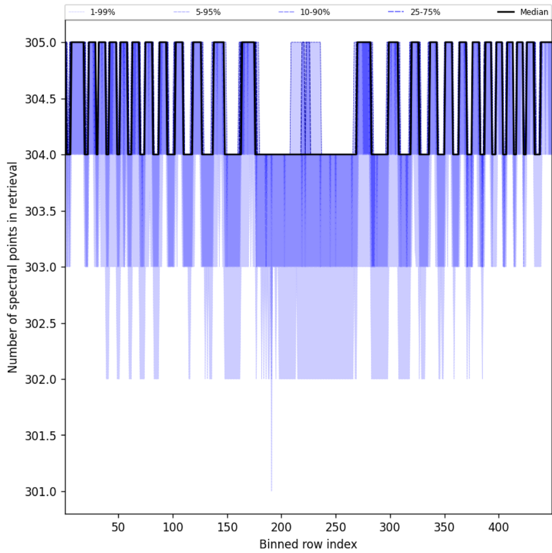
Figure 50: Along track statistics of “Number of spectral points in retrieval” for 2025-01-19 to 2025-01-21
