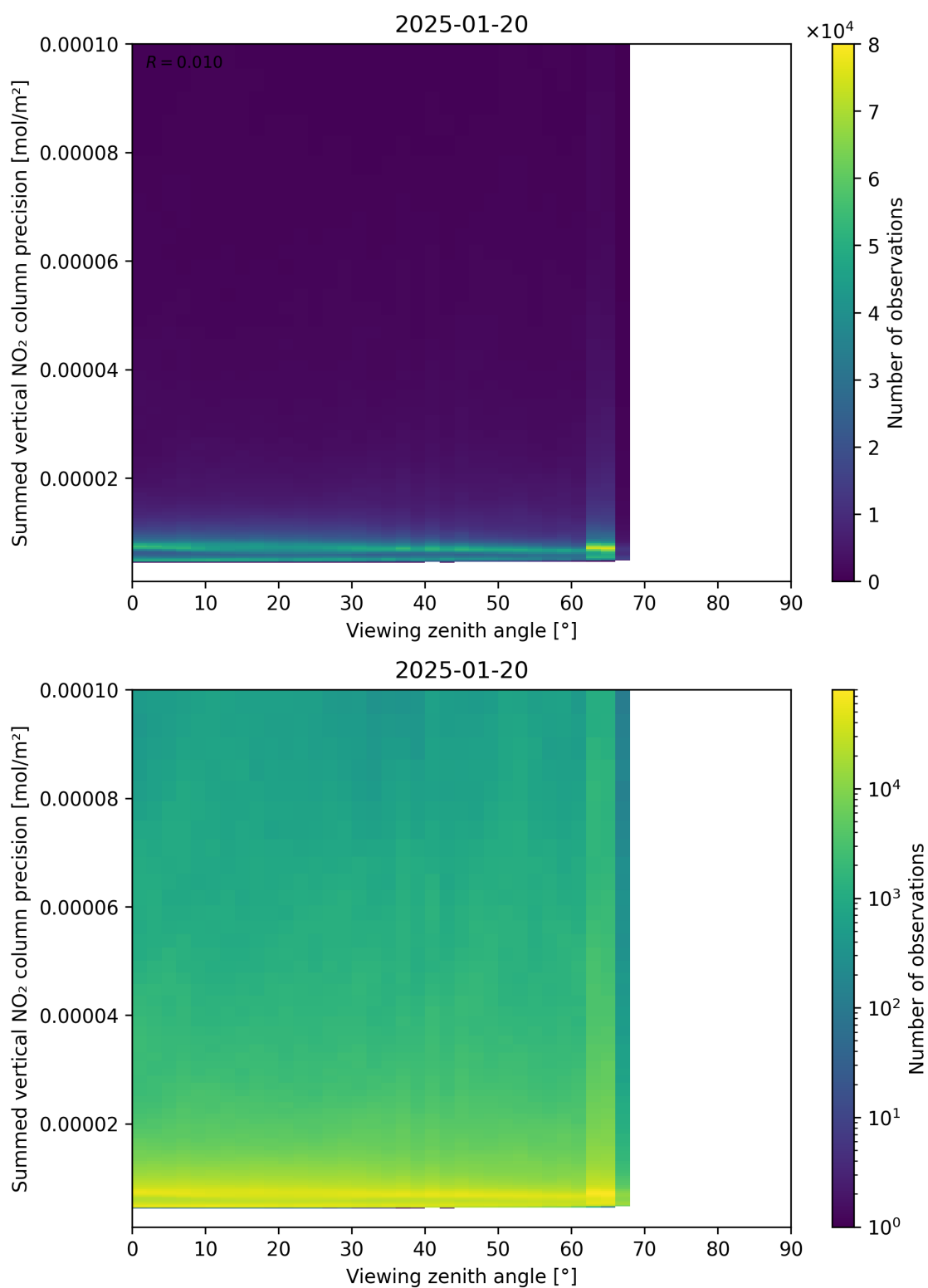
Figure 166: Scatter density plot of “Viewing zenith angle” against “Summed vertical NO 2 column precision” for 2025-01-19 to 2025-01-21.
