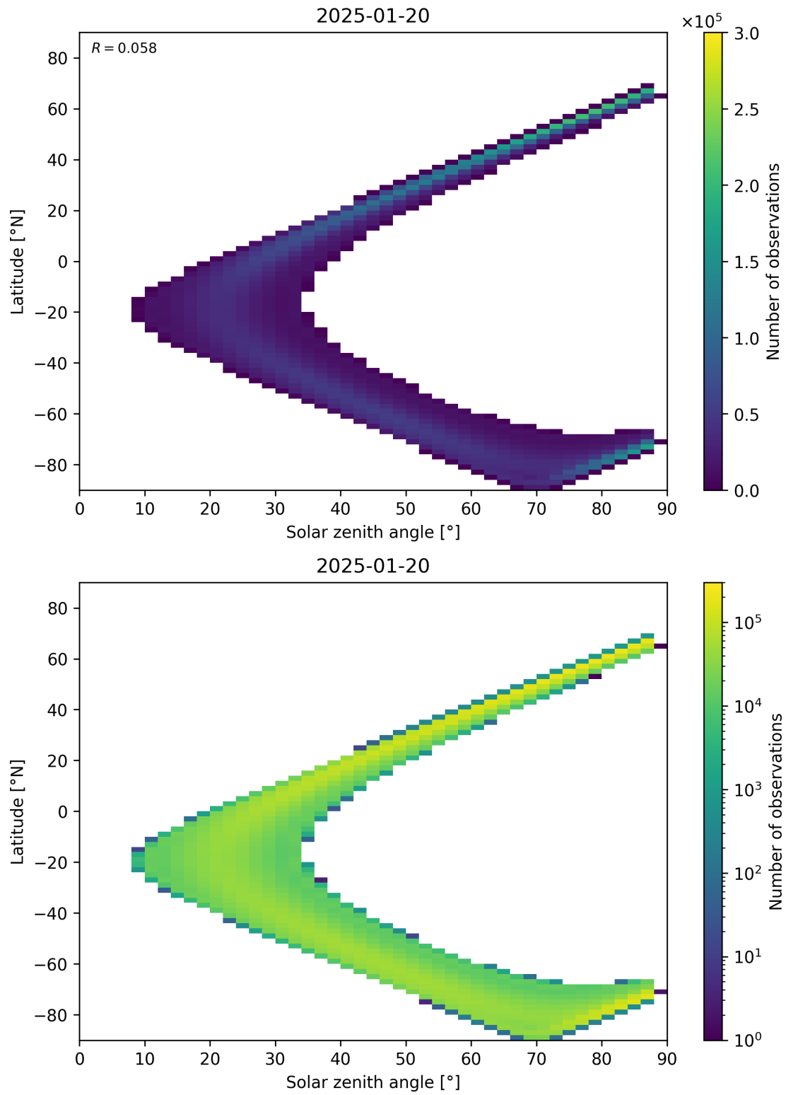
Figure 149: Scatter density plot of “Solar zenith angle” against “Latitude” for 2025-01-19 to 2025-01-21.
