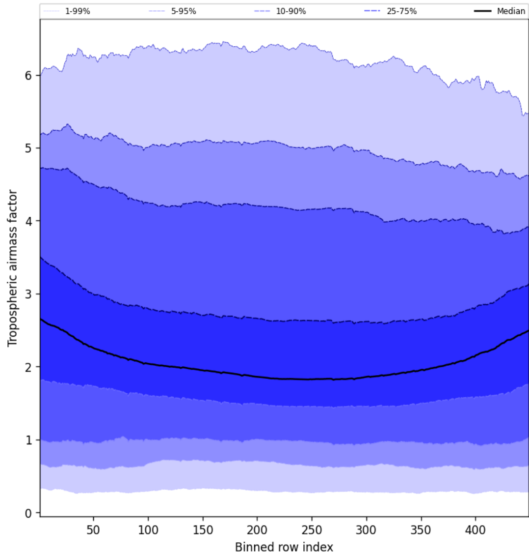
Figure 48: Along track statistics of “Tropospheric airmass factor” for 2025-01-19 to 2025-01-21
