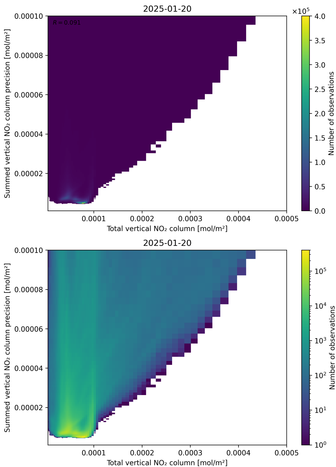
Figure 113: Scatter density plot of “Total vertical NO 2 column” against “Summed vertical NO 2 column precision” for 2025-01-19 to 2025-01-21.
