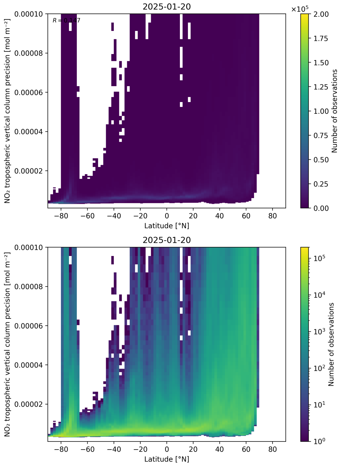
Figure 93: Scatter density plot of “Latitude” against “NO 2 tropospheric vertical column precision” for 2025-01-19 to 2025-01-21.
