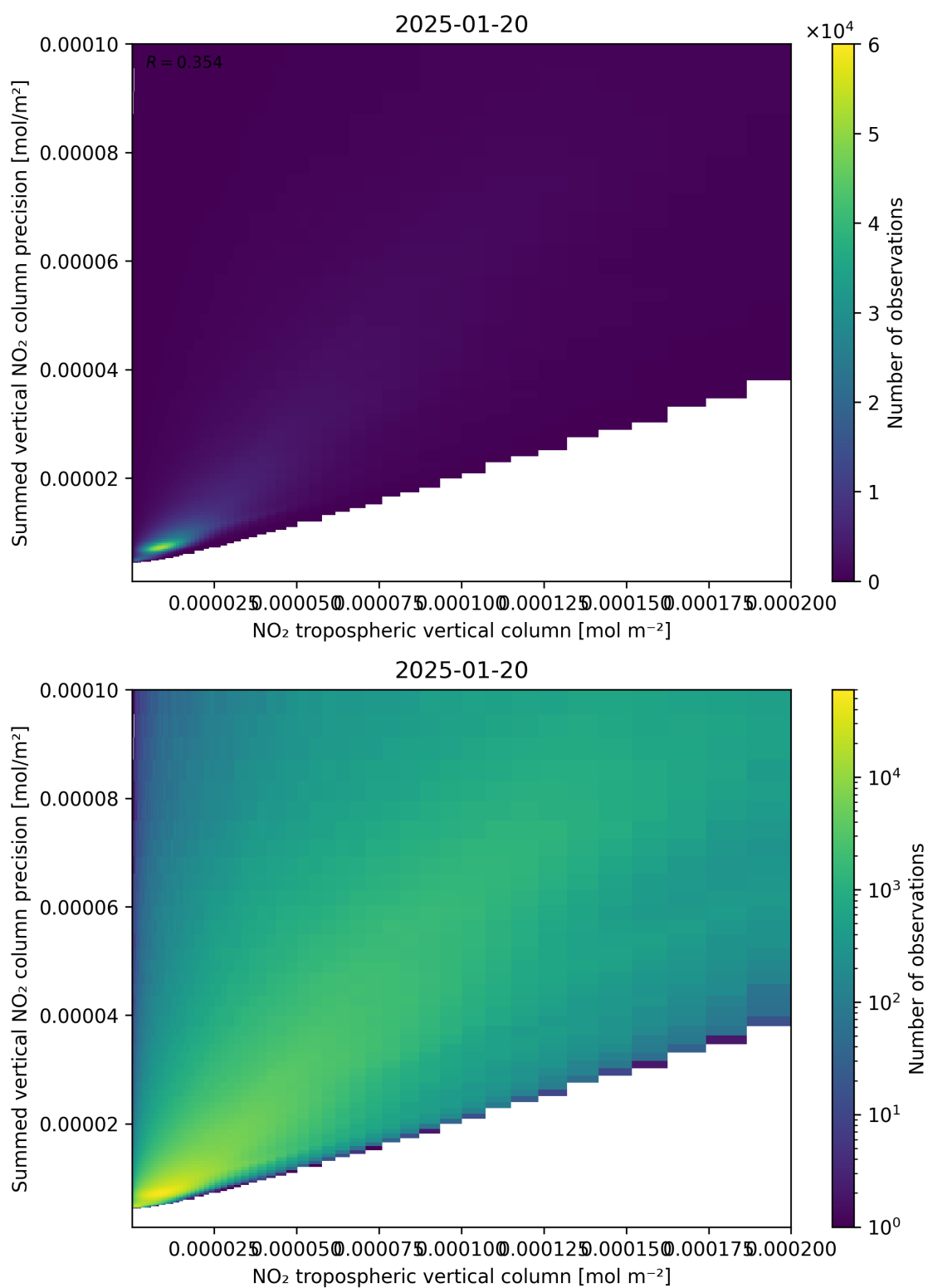
Figure 127: Scatter density plot of “NO 2 tropospheric vertical column” against “Summed vertical NO 2 column precision” for 2025-01-19 to 2025-01-21.
