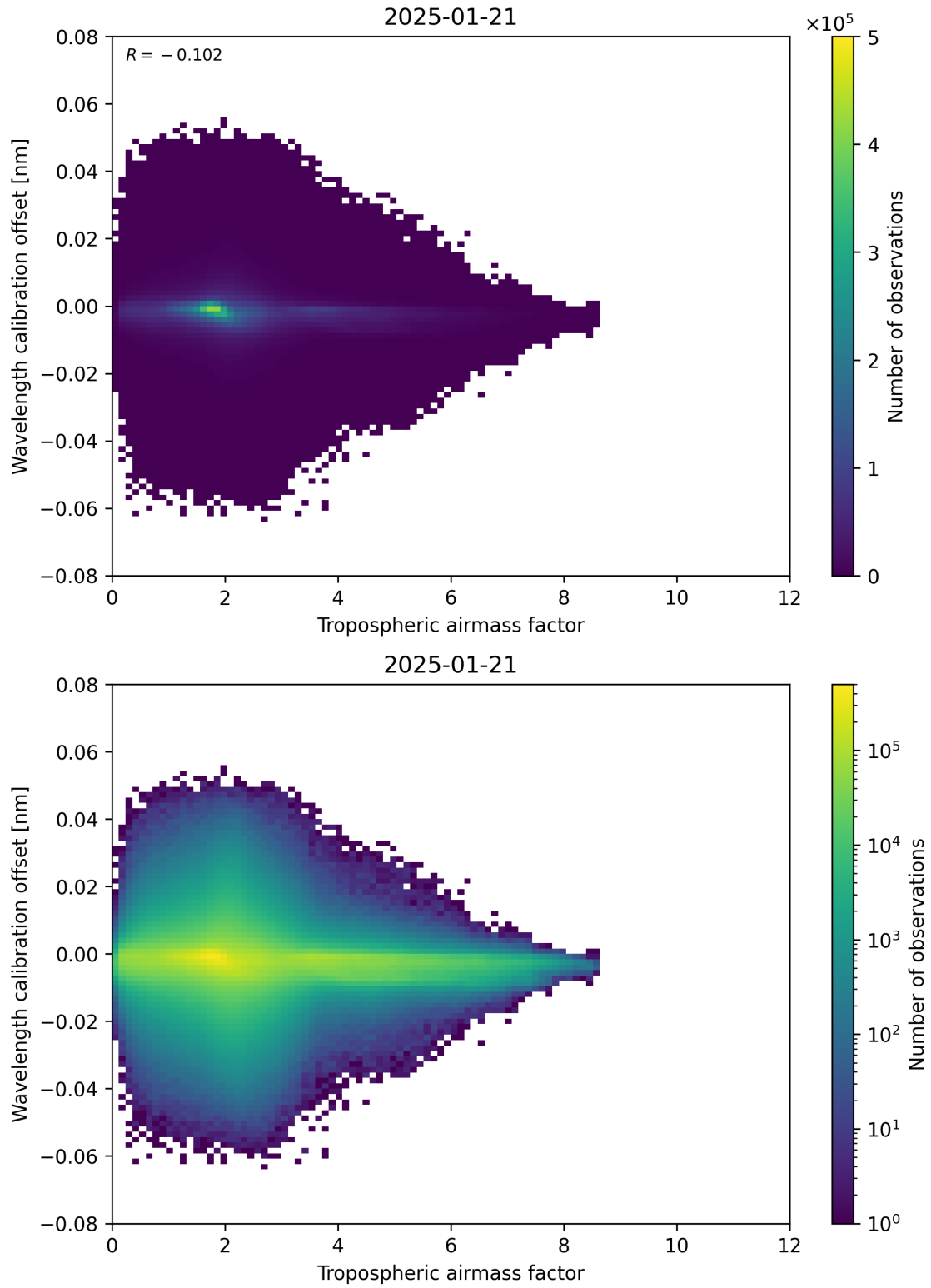
Figure 80: Scatter density plot of “Tropospheric airmass factor” against “Wavelength calibration offset” for 2025-01-20 to 2025-01-22.
