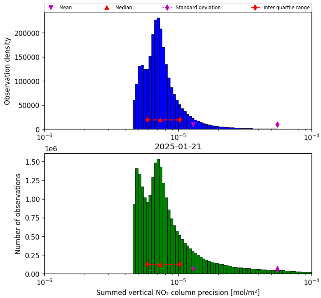
Figure 41: Histogram of “Summed vertical NO 2 column precision” for 2025-01-20 to 2025-01-22
