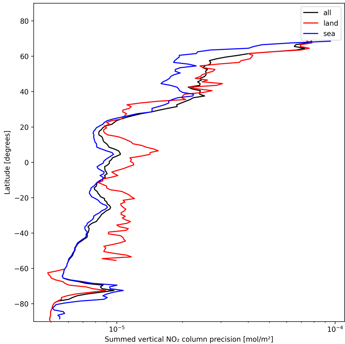
Figure 24: Zonal average of “Summed vertical NO 2 column precision” for 2025-01-20 to 2025-01-22.
