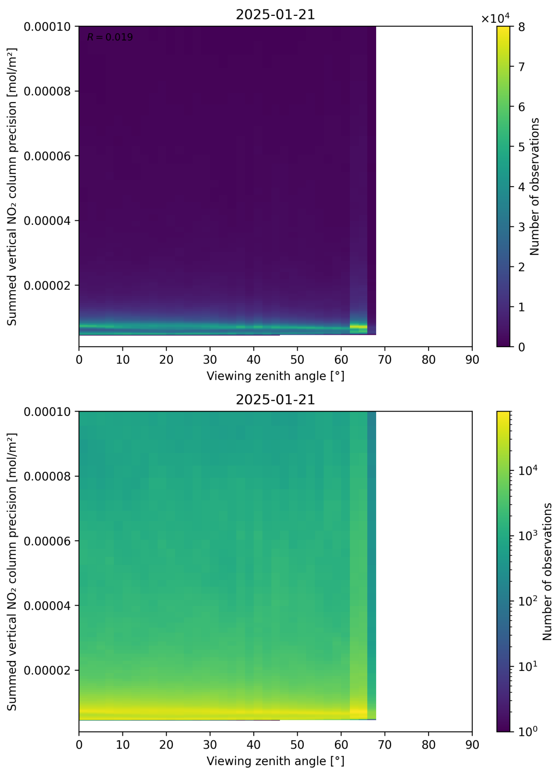
Figure 166: Scatter density plot of “Viewing zenith angle” against “Summed vertical NO 2 column precision” for 2025-01-20 to 2025-01-22.
