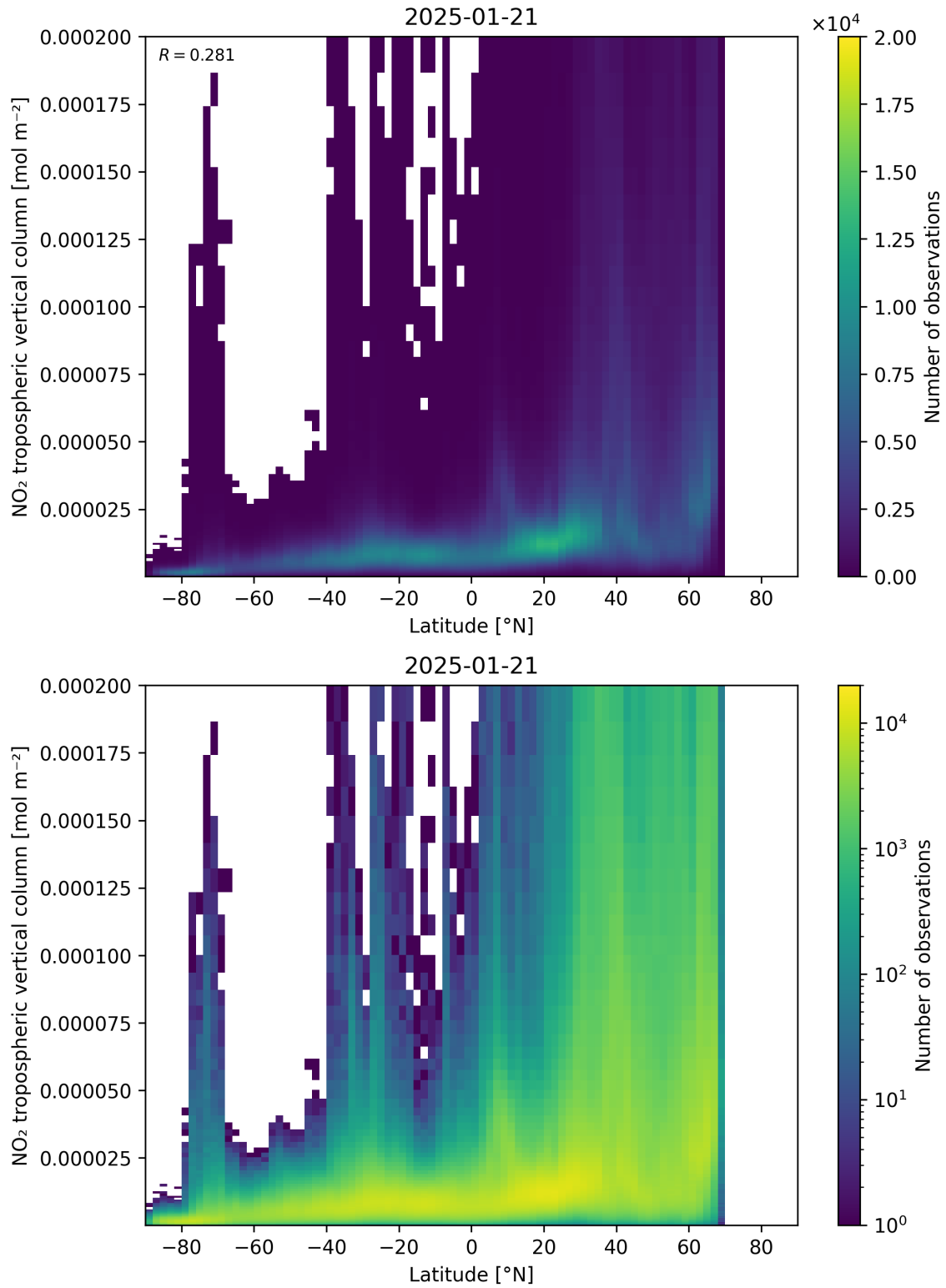
Figure 92: Scatter density plot of “Latitude” against “NO 2 tropospheric vertical column” for 2025-01-20 to 2025-01-22.
