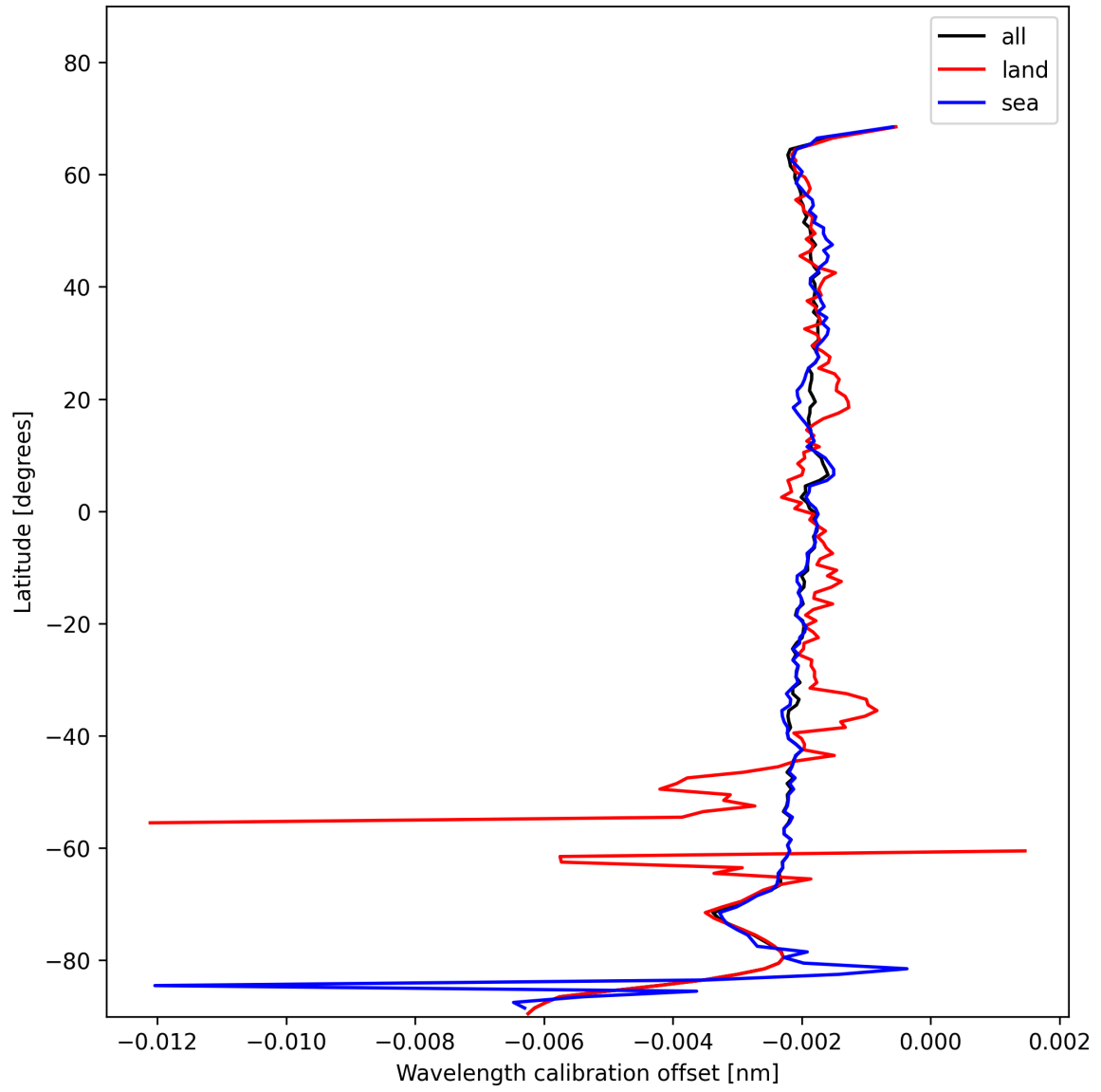
Figure 18: Zonal average of “Wavelength calibration offset” for 2025-01-20 to 2025-01-22.
