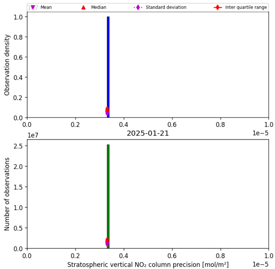
Figure 37: Histogram of “Stratospheric vertical NO 2 column precision” for 2025-01-20 to 2025-01-22
