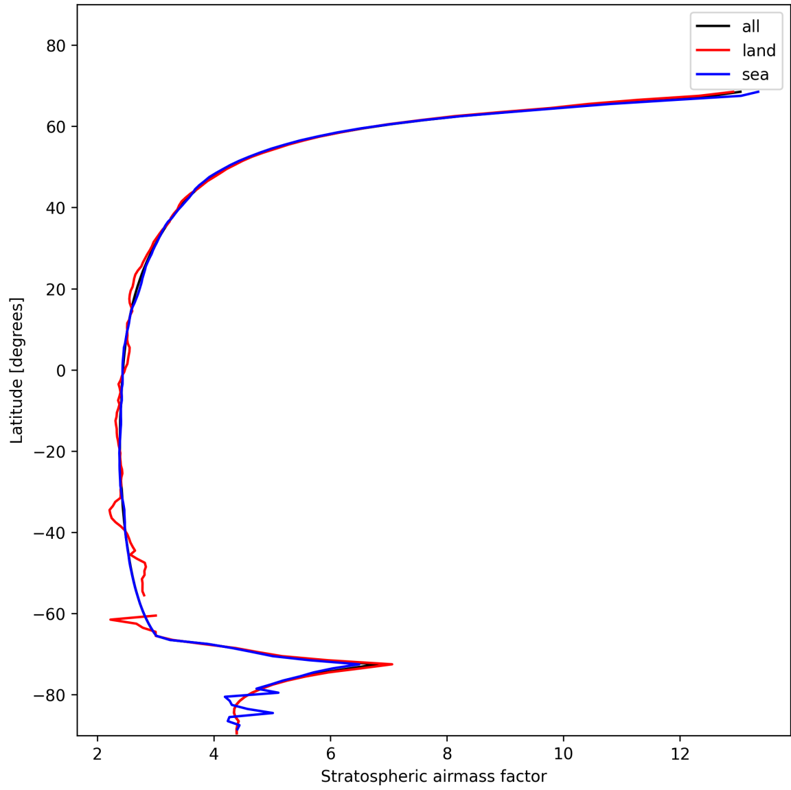
Figure 27: Zonal average of “Stratospheric airmass factor” for 2025-01-20 to 2025-01-22.
