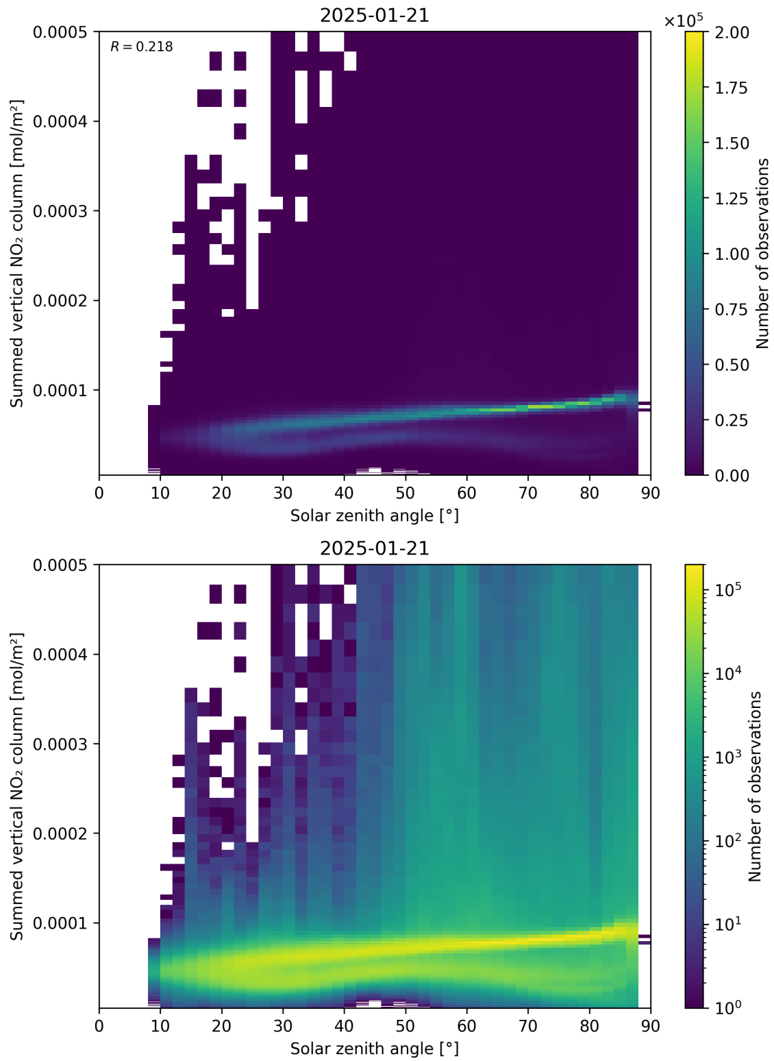
Figure 151: Scatter density plot of “Solar zenith angle” against “Summed vertical NO 2 column” for 2025-01-20 to 2025-01-22.
