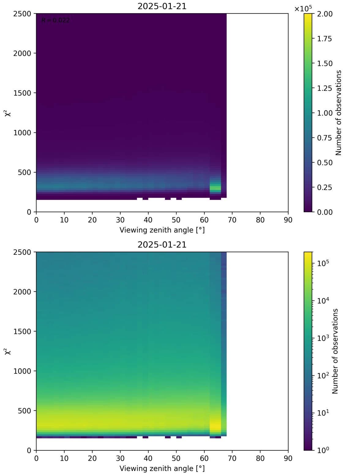
Figure 162: Scatter density plot of “Viewing zenith angle” against “ \chi^2 ” for 2025-01-20 to 2025-01-22.
