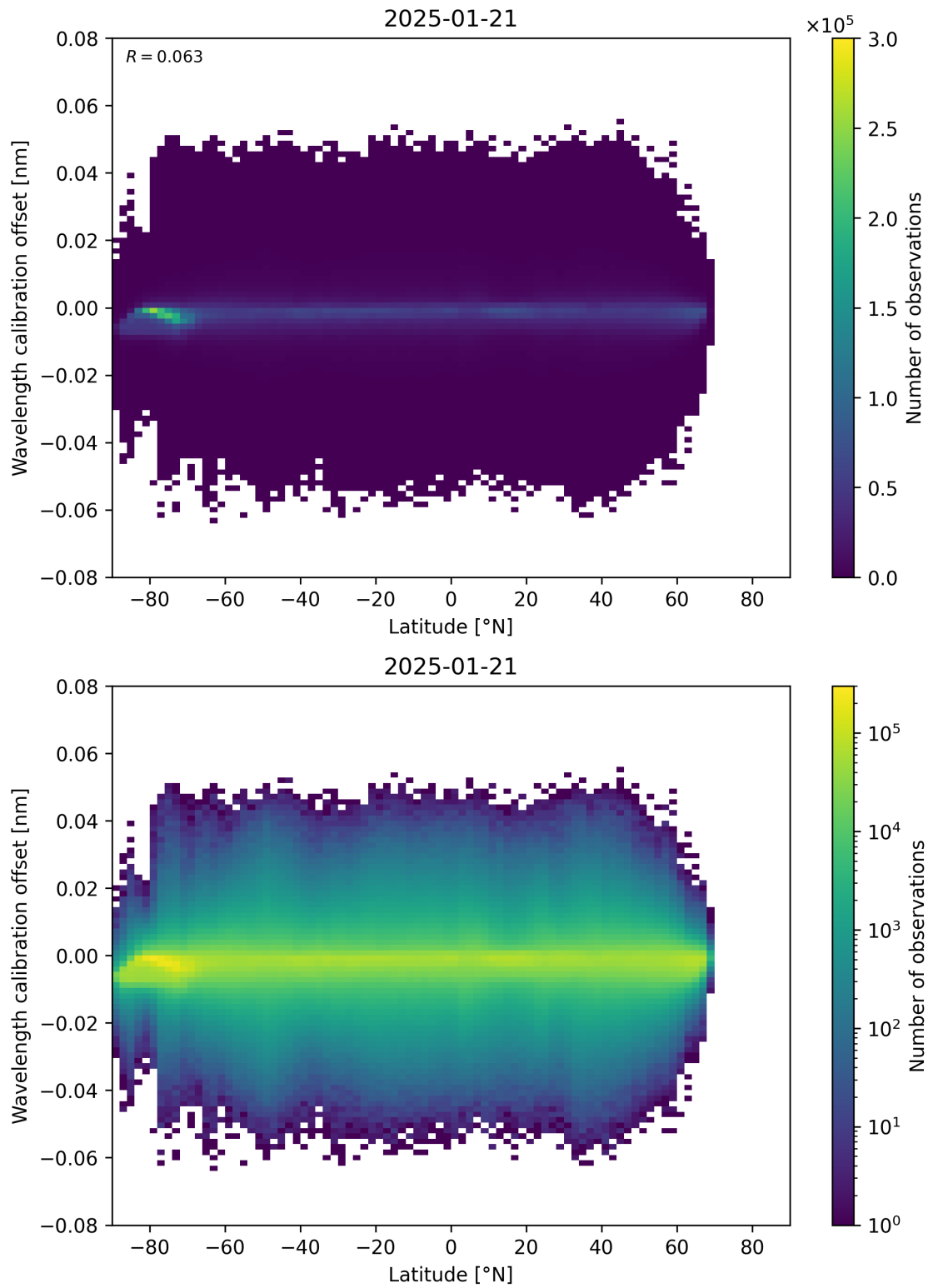
Figure 95: Scatter density plot of “Latitude” against “Wavelength calibration offset” for 2025-01-20 to 2025-01-22.
