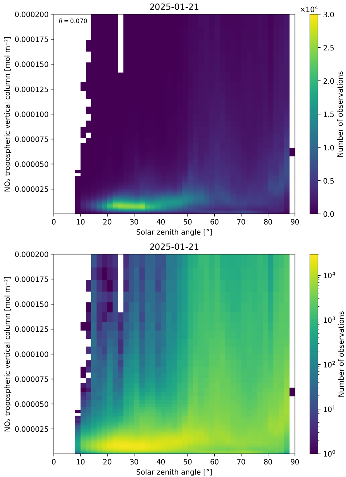
Figure 155: Scatter density plot of “Solar zenith angle” against “NO 2 tropospheric vertical column” for 2025-01-20 to 2025-01-22.
