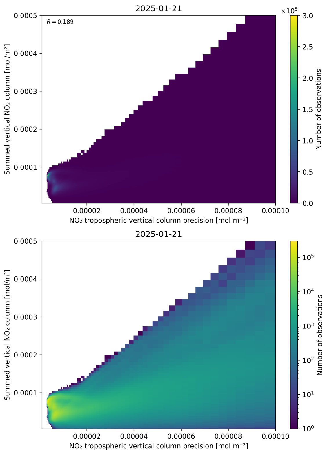
Figure 136: Scatter density plot of “NO 2 tropospheric vertical column precision” against “Summed vertical NO 2 column” for 2025-01-20 to 2025-01-22.
