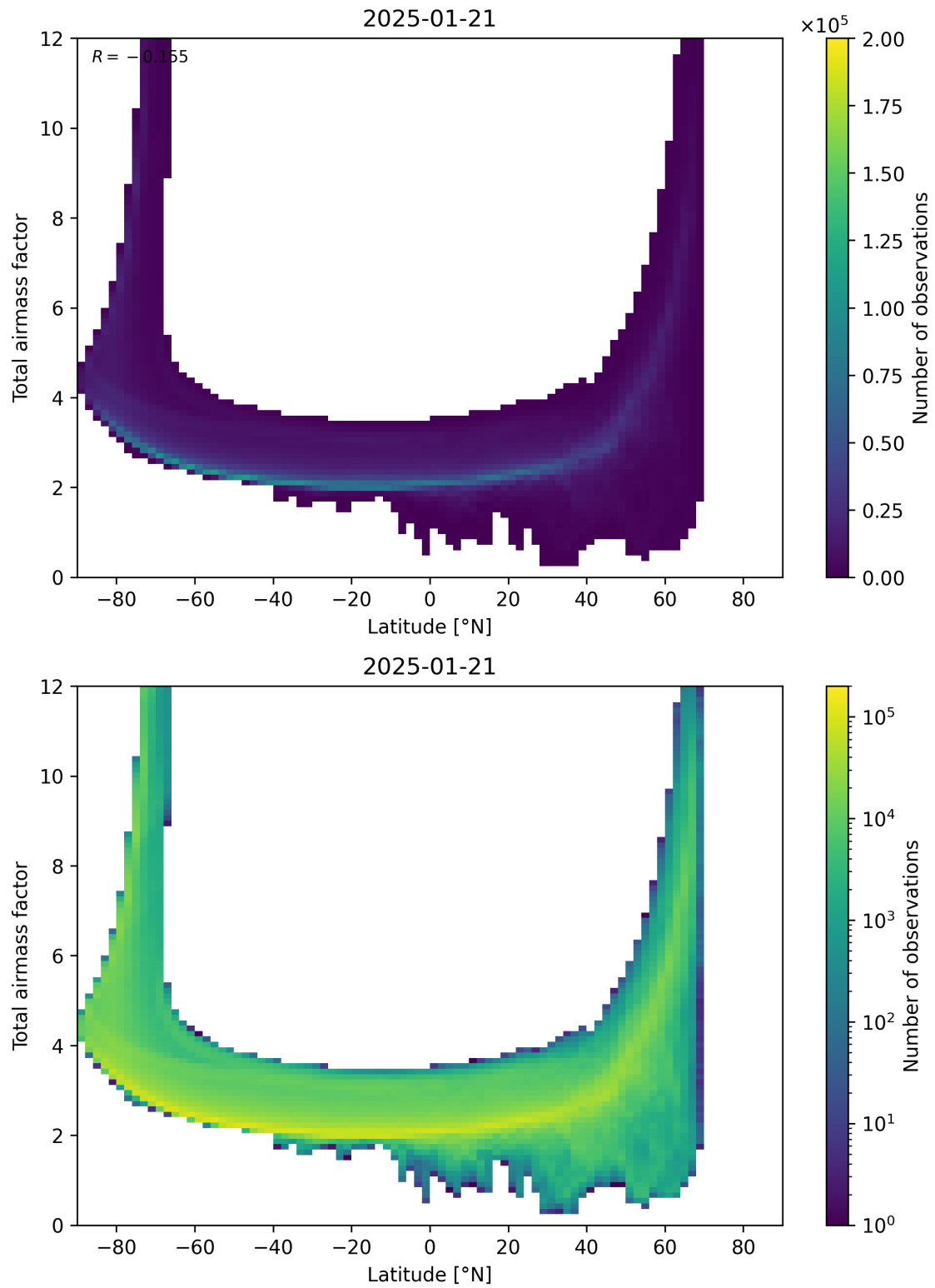
Figure 84: Scatter density plot of “Latitude” against “Total airmass factor” for 2025-01-20 to 2025-01-22.
