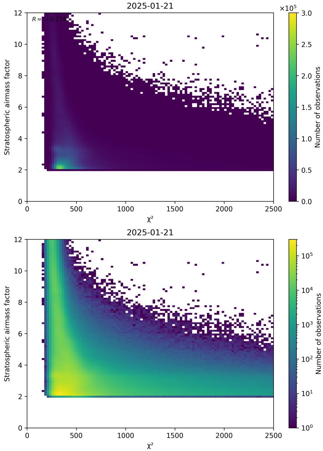
Figure 81: Scatter density plot of “ \chi^2 ” against “Stratospheric airmass factor” for 2025-01-20 to 2025-01-22.
