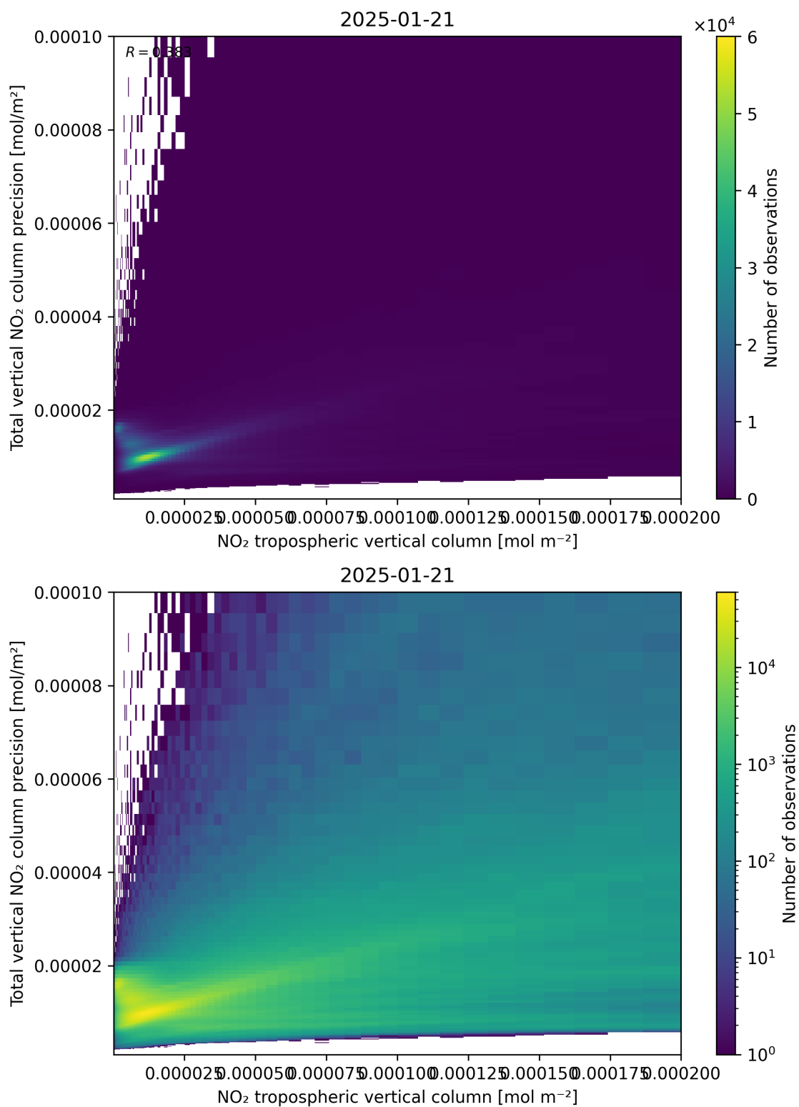
Figure 129: Scatter density plot of “NO 2 tropospheric vertical column” against “Total vertical NO 2 column precision” for 2025-01-20 to 2025-01-22.
