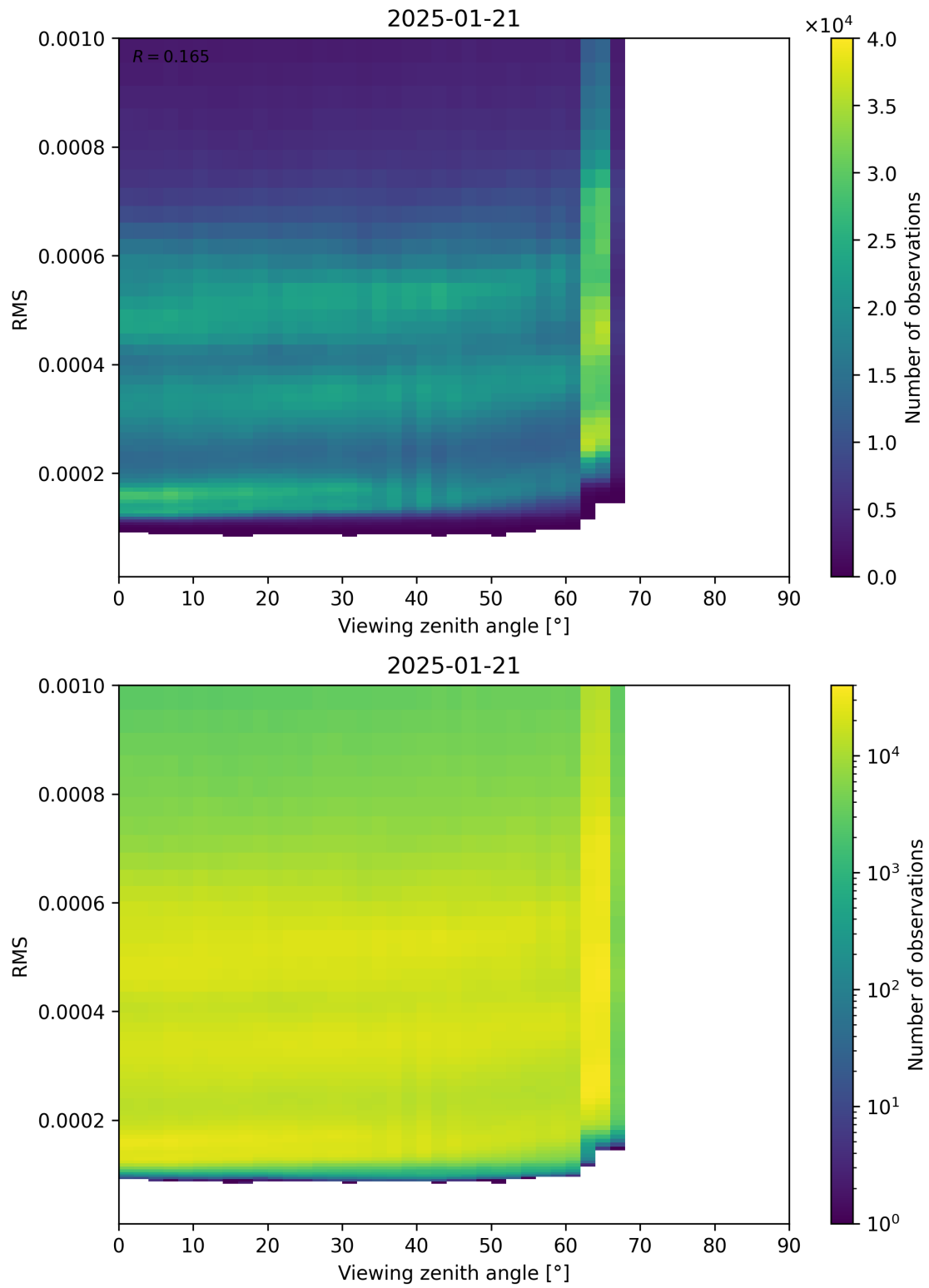
Figure 171: Scatter density plot of “Viewing zenith angle” against “RMS” for 2025-01-20 to 2025-01-22.
