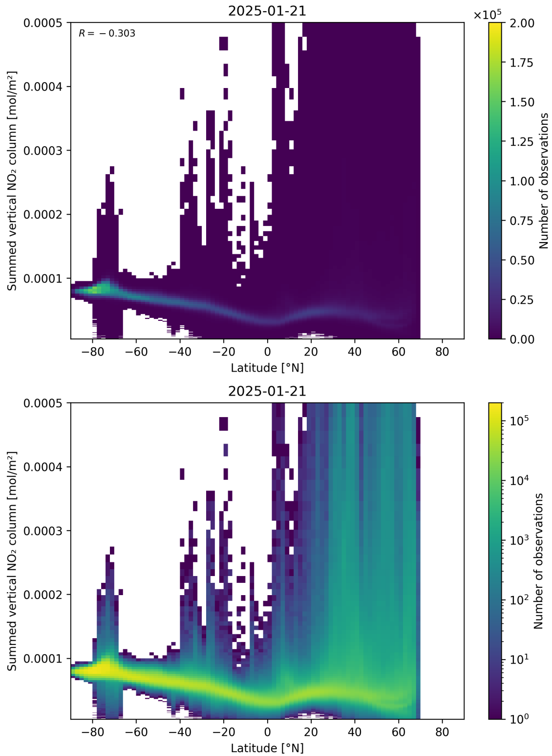
Figure 88: Scatter density plot of “Latitude” against “Summed vertical NO 2 column” for 2025-01-20 to 2025-01-22.
