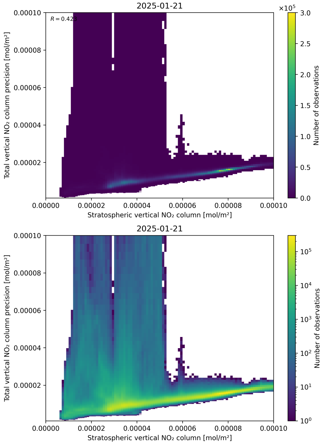
Figure 101: Scatter density plot of “Stratospheric vertical NO 2 column” against “Total vertical NO 2 column precision” for 2025-01-20 to 2025-01-22.
