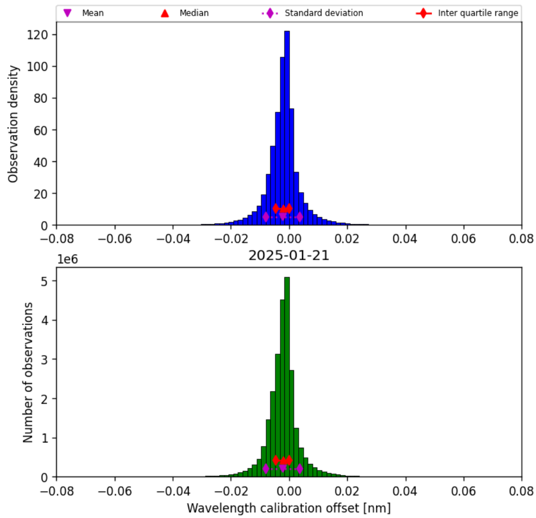
Figure 35: Histogram of “Wavelength calibration offset” for 2025-01-20 to 2025-01-22
