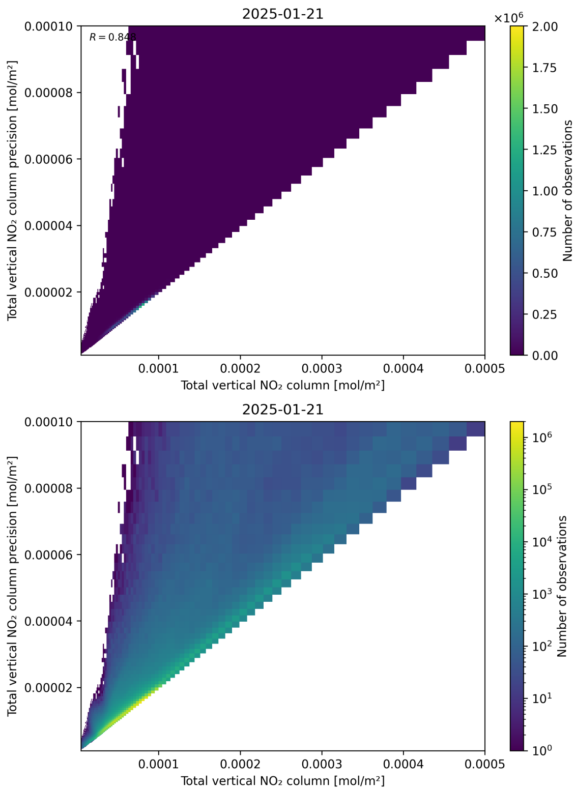
Figure 114: Scatter density plot of “Total vertical NO 2 column” against “Total vertical NO 2 column precision” for 2025-01-20 to 2025-01-22.
