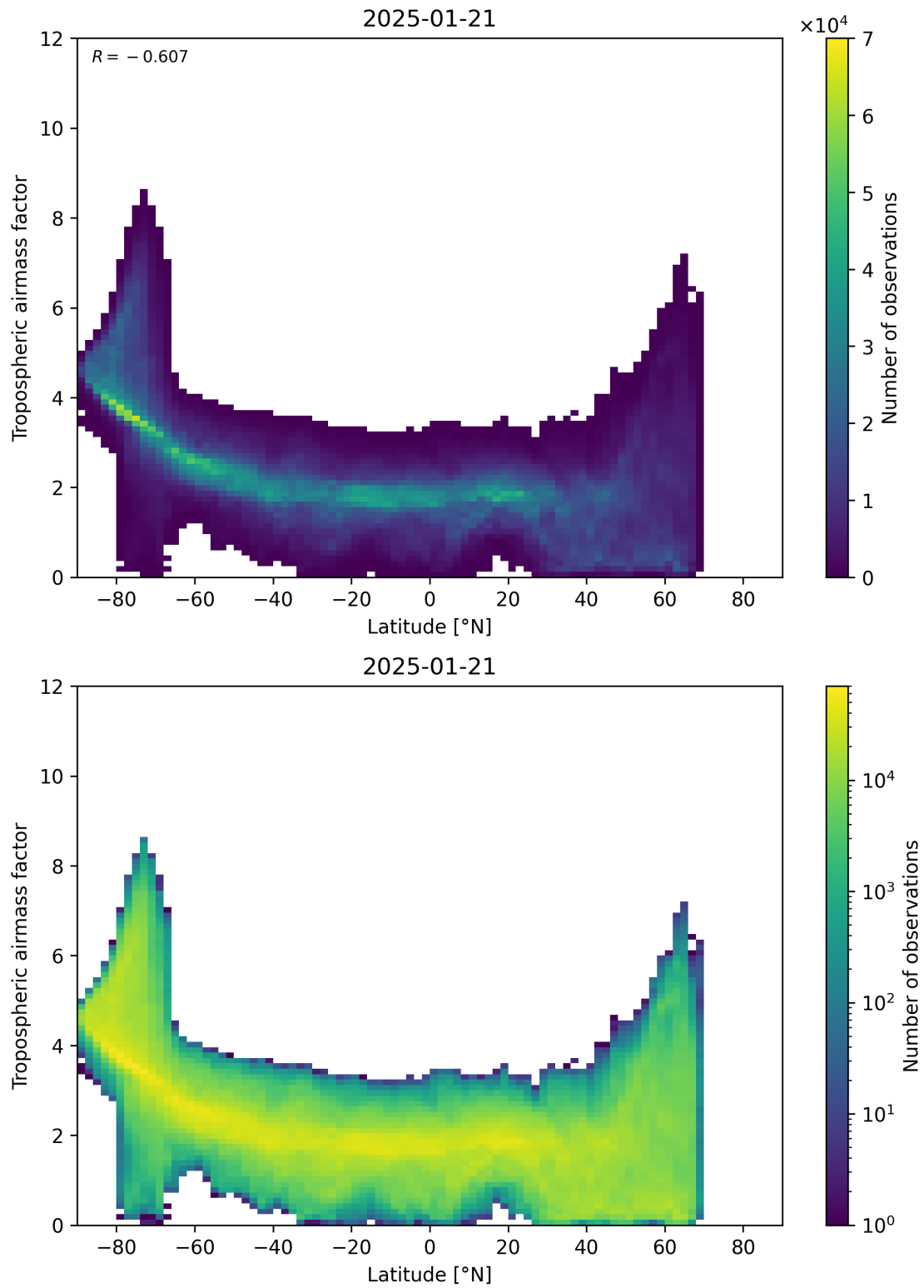
Figure 85: Scatter density plot of “Latitude” against “Tropospheric air mass factor” for 2025-01-20 to 2025-01-22.
