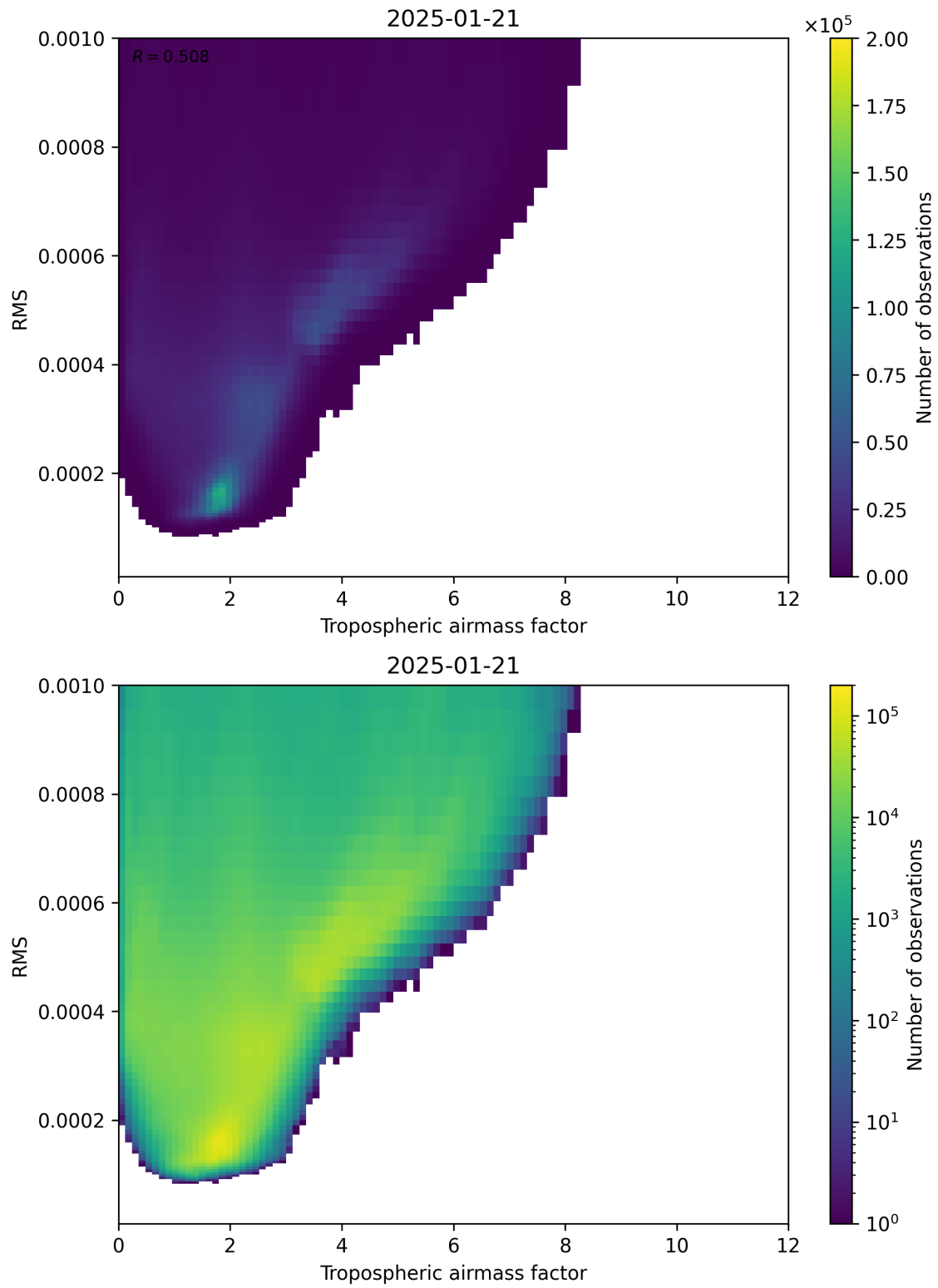
Figure 79: Scatter density plot of “Tropospheric airmass factor” against “RMS” for 2025-01-20 to 2025-01-22.
