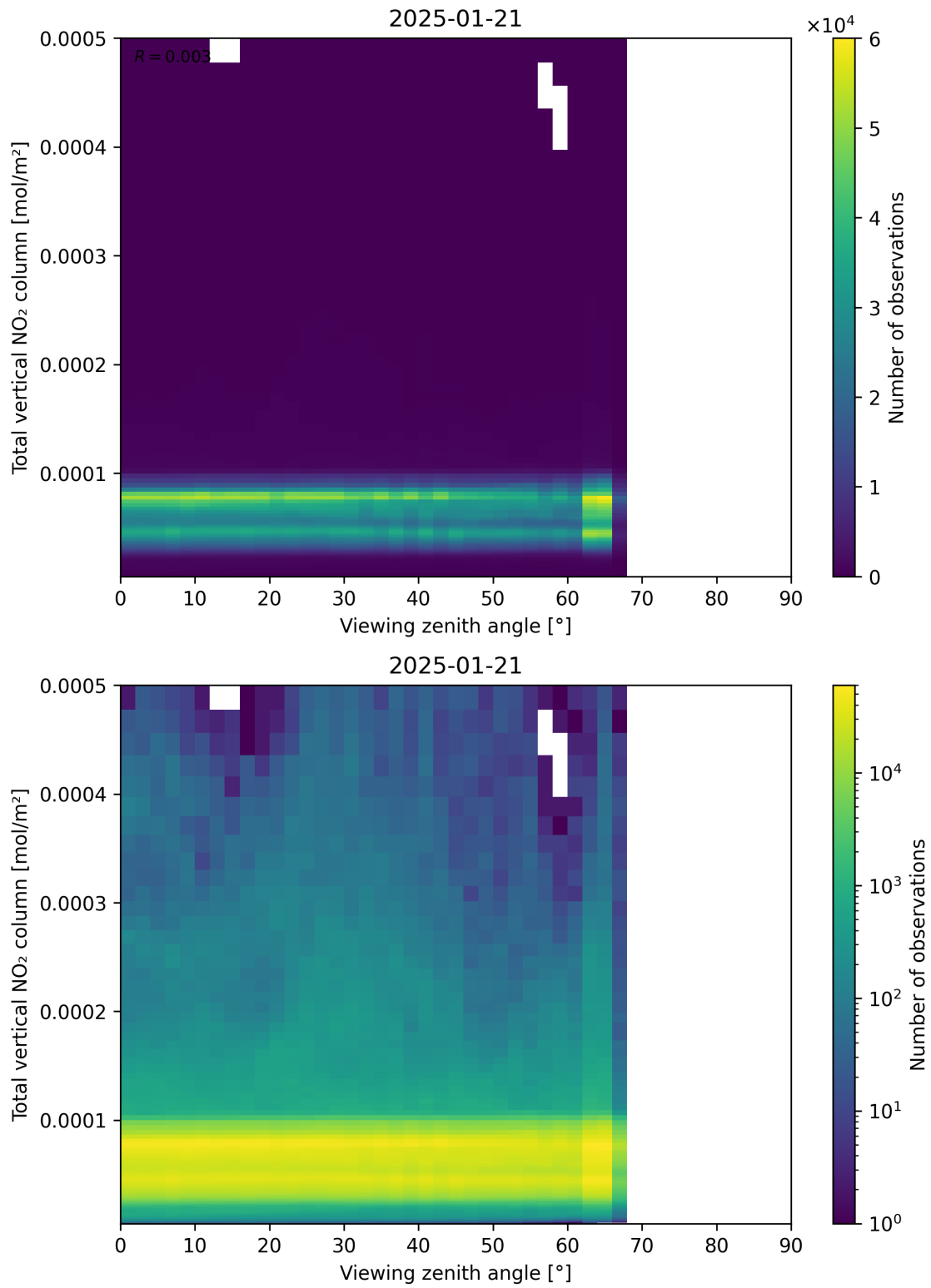
Figure 167: Scatter density plot of “Viewing zenith angle” against “Total vertical NO 2 column” for 2025-01-20 to 2025-01-22.
