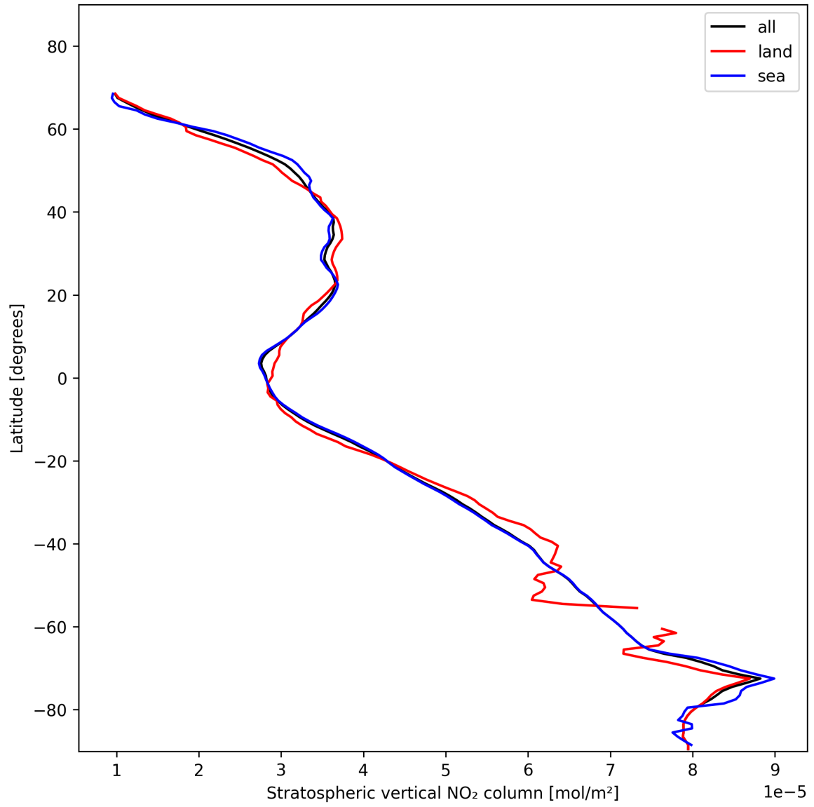
Figure 19: Zonal average of “Stratospheric vertical NO 2 column” for 2025-01-20 to 2025-01-22.
