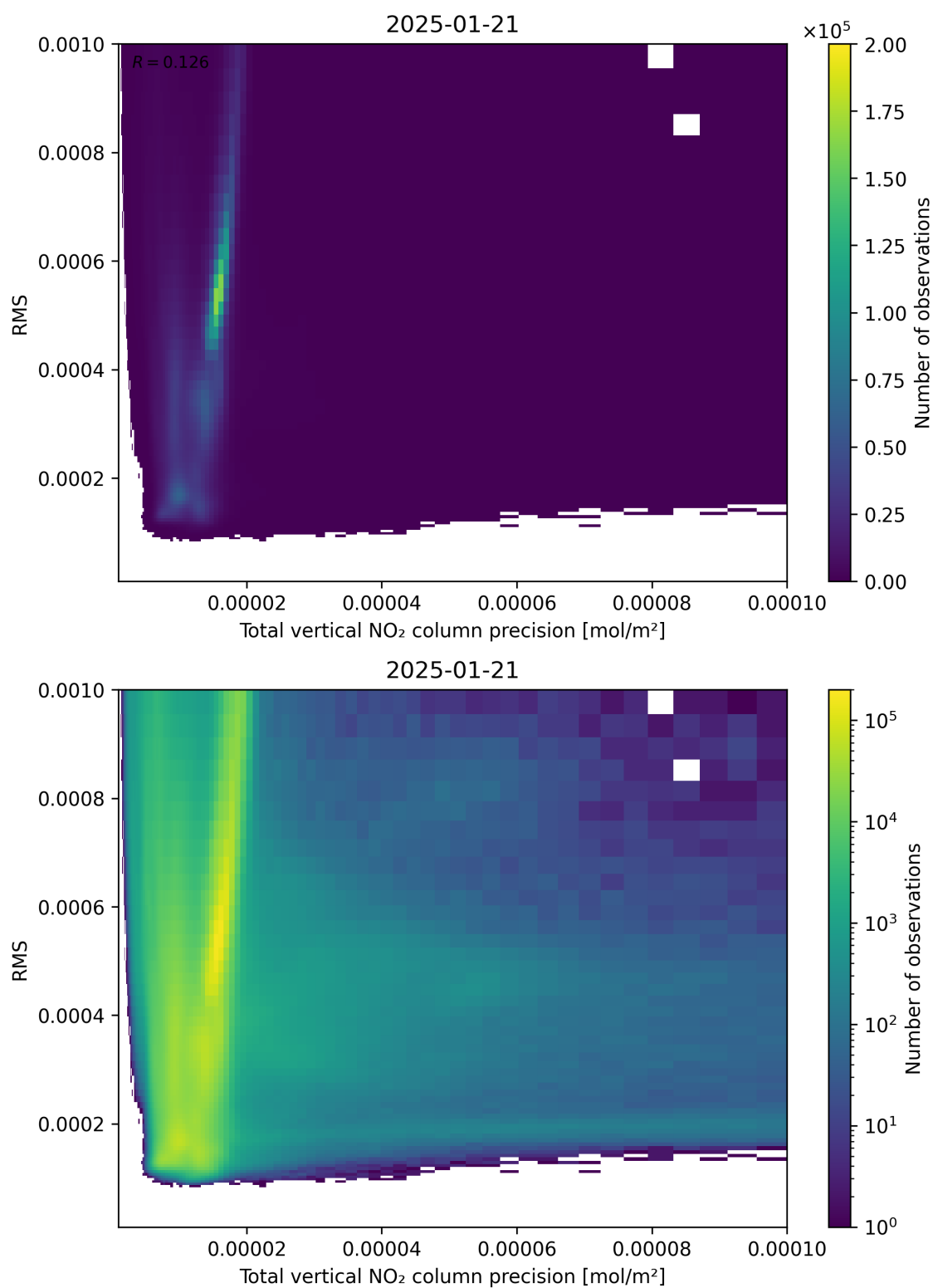
Figure 119: Scatter density plot of “Total vertical NO 2 column precision” against “RMS” for 2025-01-20 to 2025-01-22.
