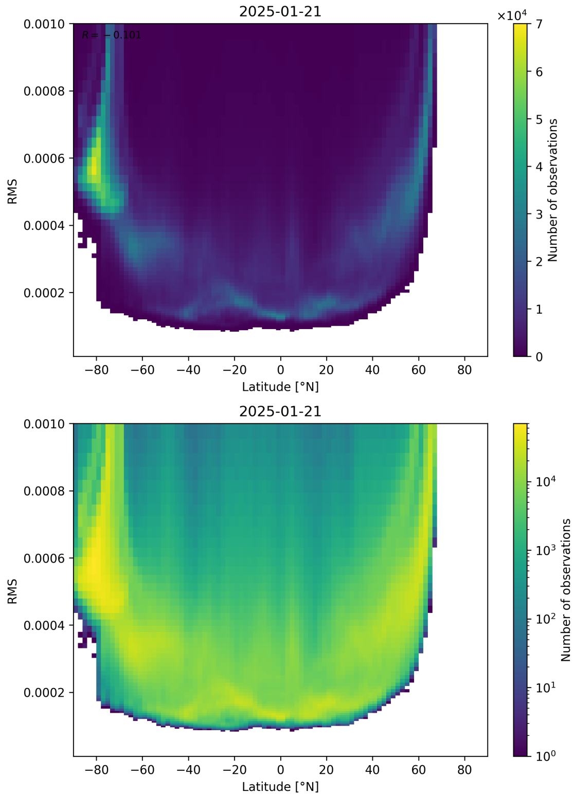
Figure 94: Scatter density plot of “Latitude” against “RMS” for 2025-01-20 to 2025-01-22.
