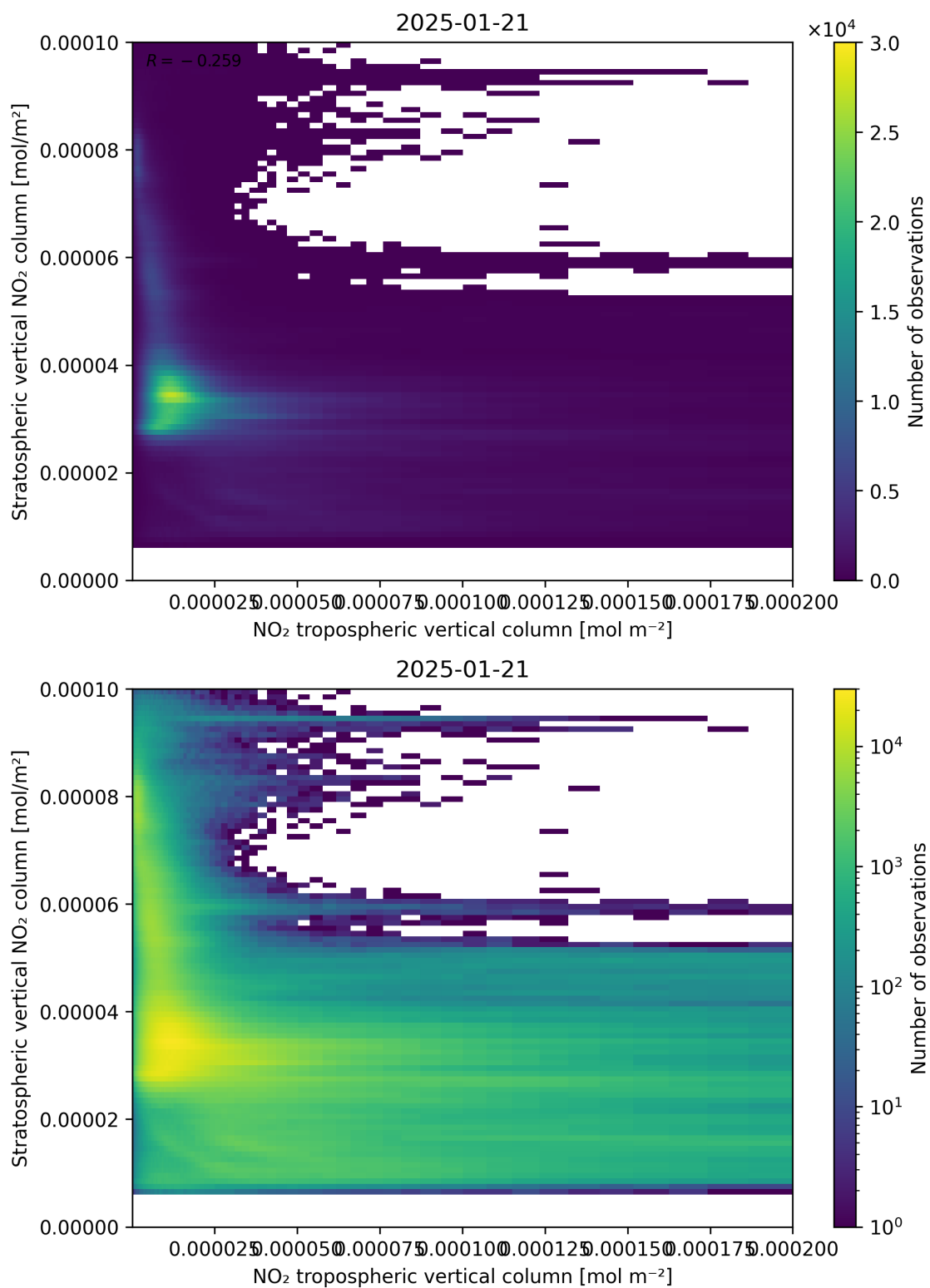
Figure 125: Scatter density plot of “NO 2 tropospheric vertical column” against “Stratospheric vertical NO 2 column” for 2025-01-20 to 2025-01-22.
