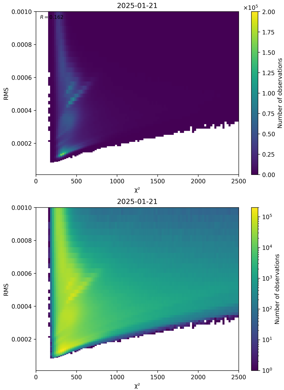
Figure 82: Scatter density plot of “ \chi^2 ” against “RMS” for 2025-01-20 to 2025-01-22.
