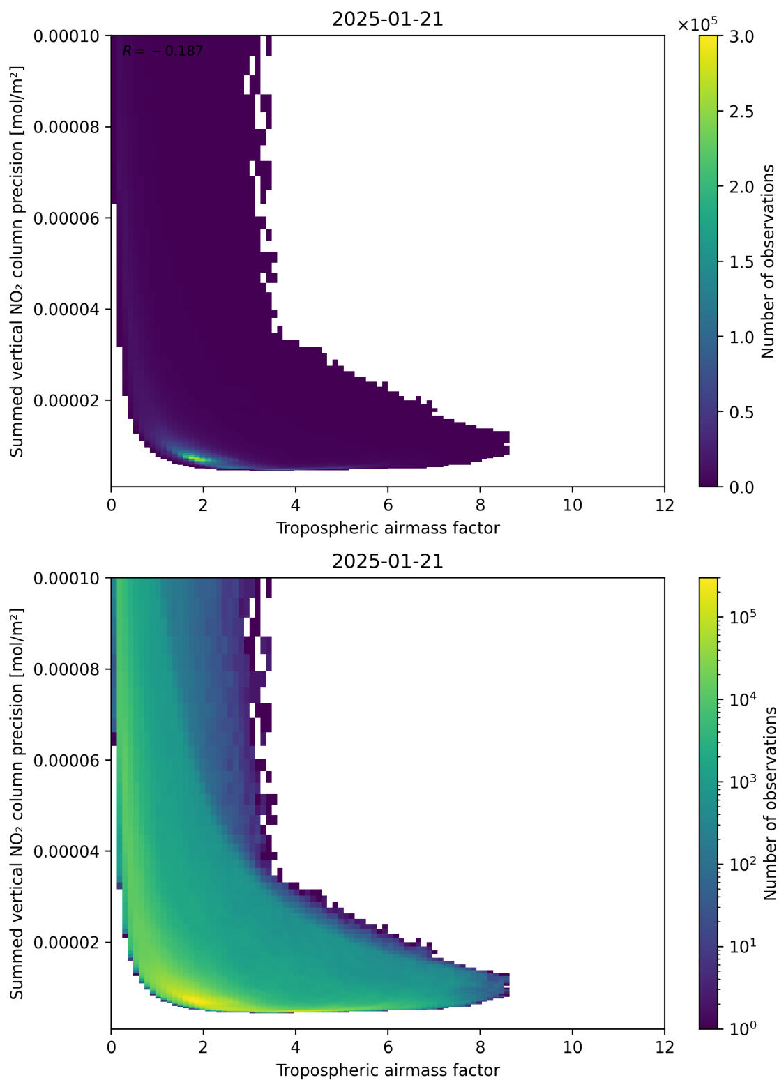
Figure 76: Scatter density plot of “Tropospheric air mass factor” against “Summed vertical NO 2 column precision” for 2025-01-20 to 2025-01-22.
