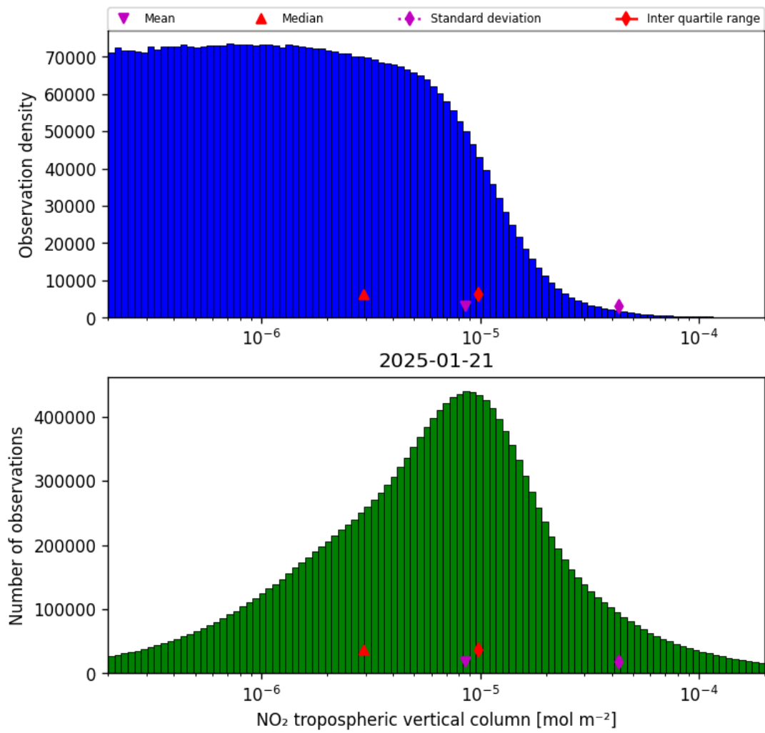
Figure 29: Histogram of “NO 2 tropospheric vertical column” for 2025-01-20 to 2025-01-22
