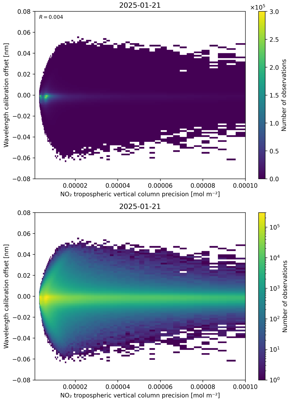
Figure 141: Scatter density plot of “NO 2 tropospheric vertical column precision” against “Wavelength calibration offset” for 2025-01-20 to 2025-01-22.
