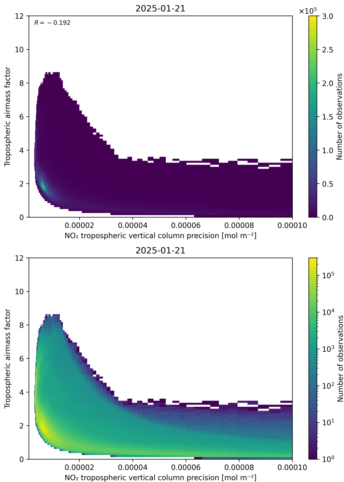
Figure 133: Scatter density plot of “NO 2 tropospheric vertical column precision” against “Tropospheric airmass factor” for 2025-01-20 to 2025-01-22.
