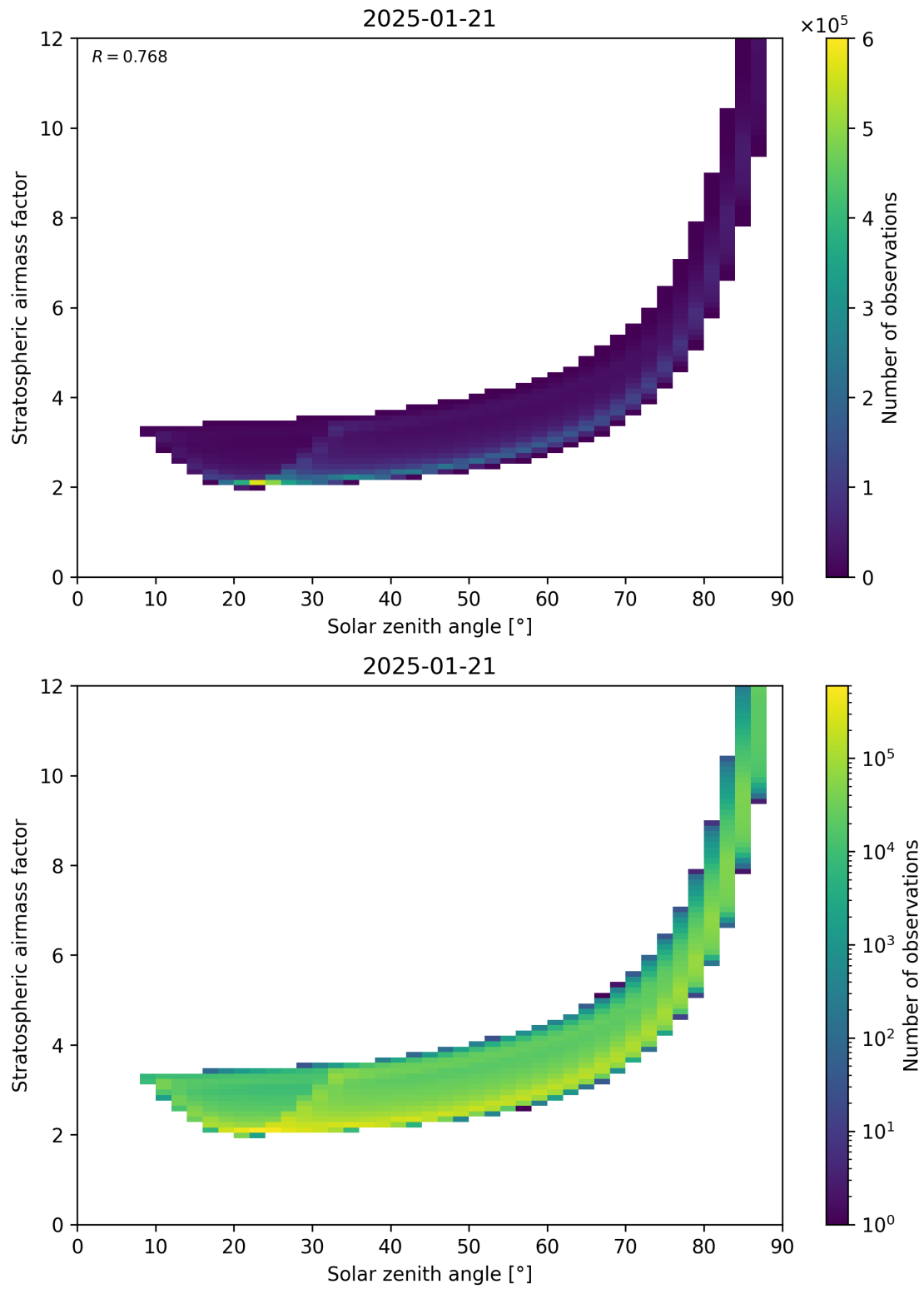
Figure 145: Scatter density plot of “Solar zenith angle” against “Stratospheric airmass factor” for 2025-01-20 to 2025-01-22.
