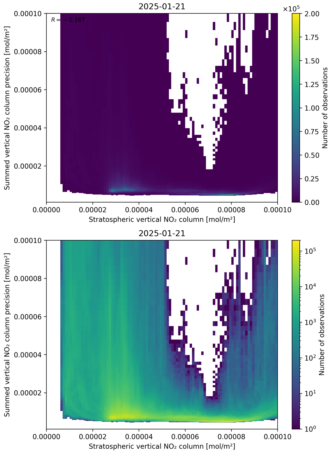
Figure 99: Scatter density plot of “Stratospheric vertical NO 2 column” against “Summed vertical NO 2 column precision” for 2025-01-20 to 2025-01-22.
