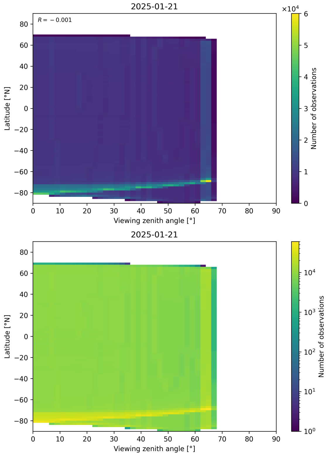
Figure 163: Scatter density plot of “Viewing zenith angle” against “Latitude” for 2025-01-20 to 2025-01-22.
