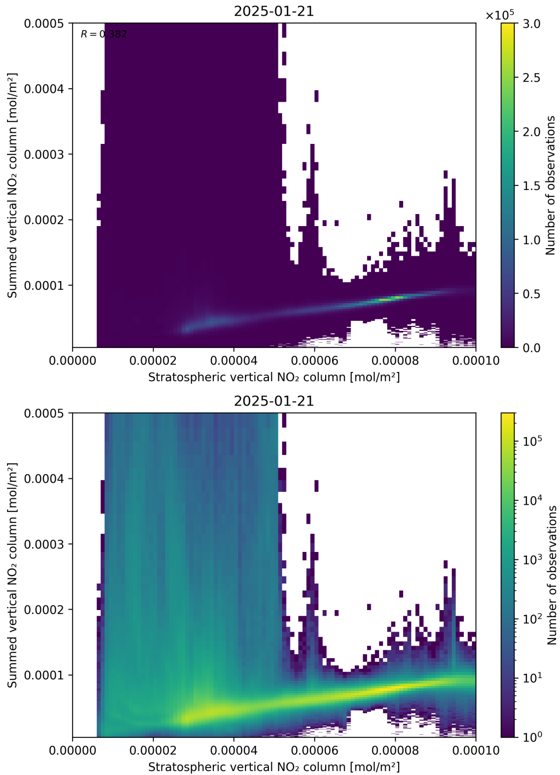
Figure 98: Scatter density plot of “Stratospheric vertical NO 2 column” against “Summed vertical NO 2 column” for 2025-01-20 to 2025-01-22.
