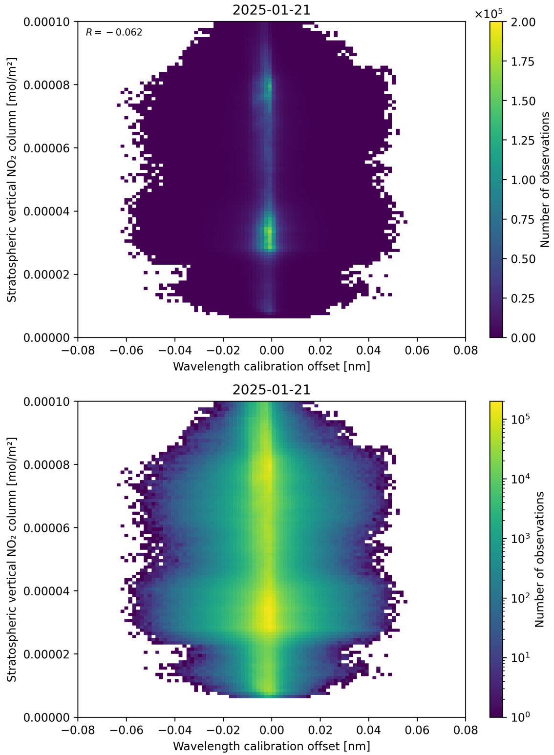
Figure 176: Scatter density plot of “Wavelength calibration offset” against “Stratospheric vertical NO 2 column” for 2025-01-20 to 2025-01-22.
