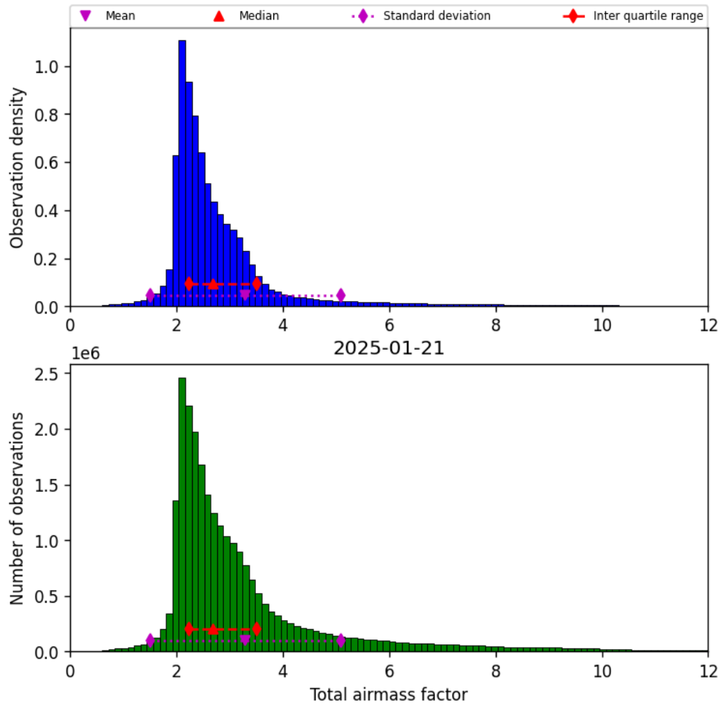
Figure 32: Histogram of “Total airmass factor” for 2025-01-20 to 2025-01-22
