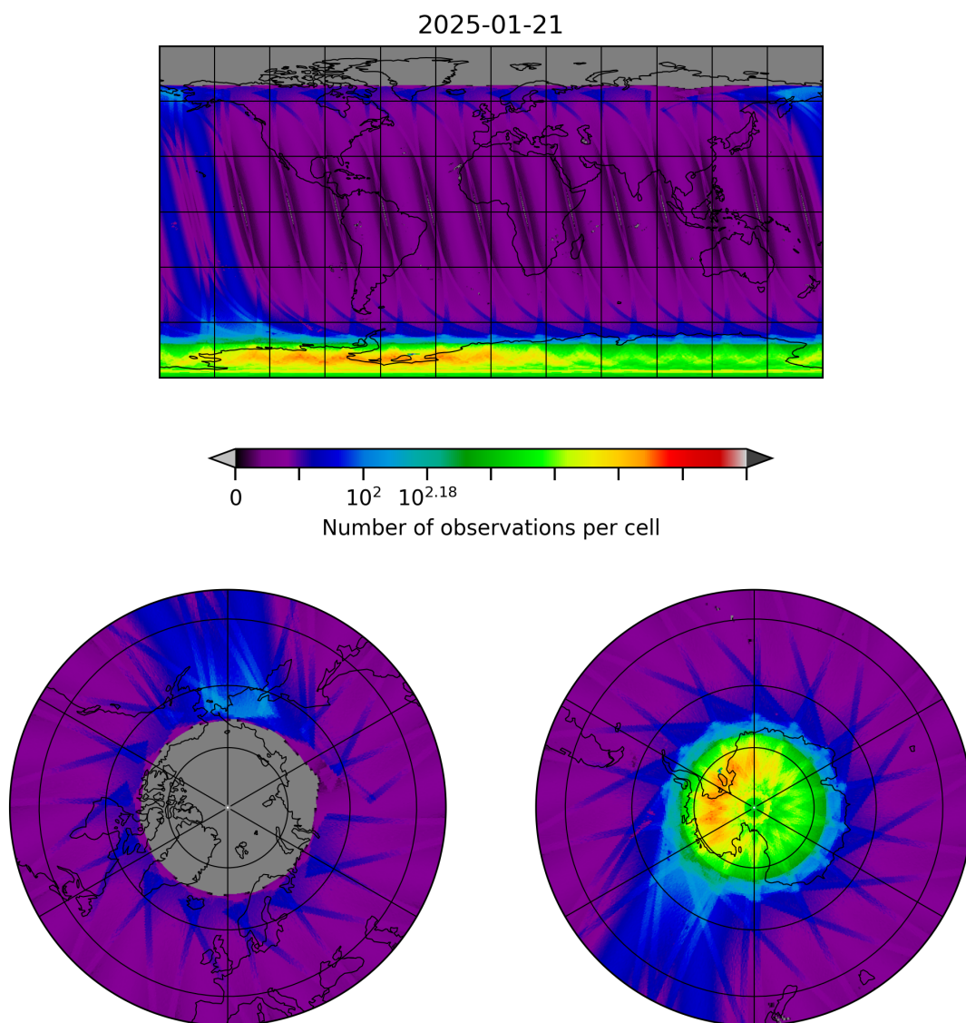
Figure 10: Map of the number of observations for 2025-01-20 to 2025-01-22
