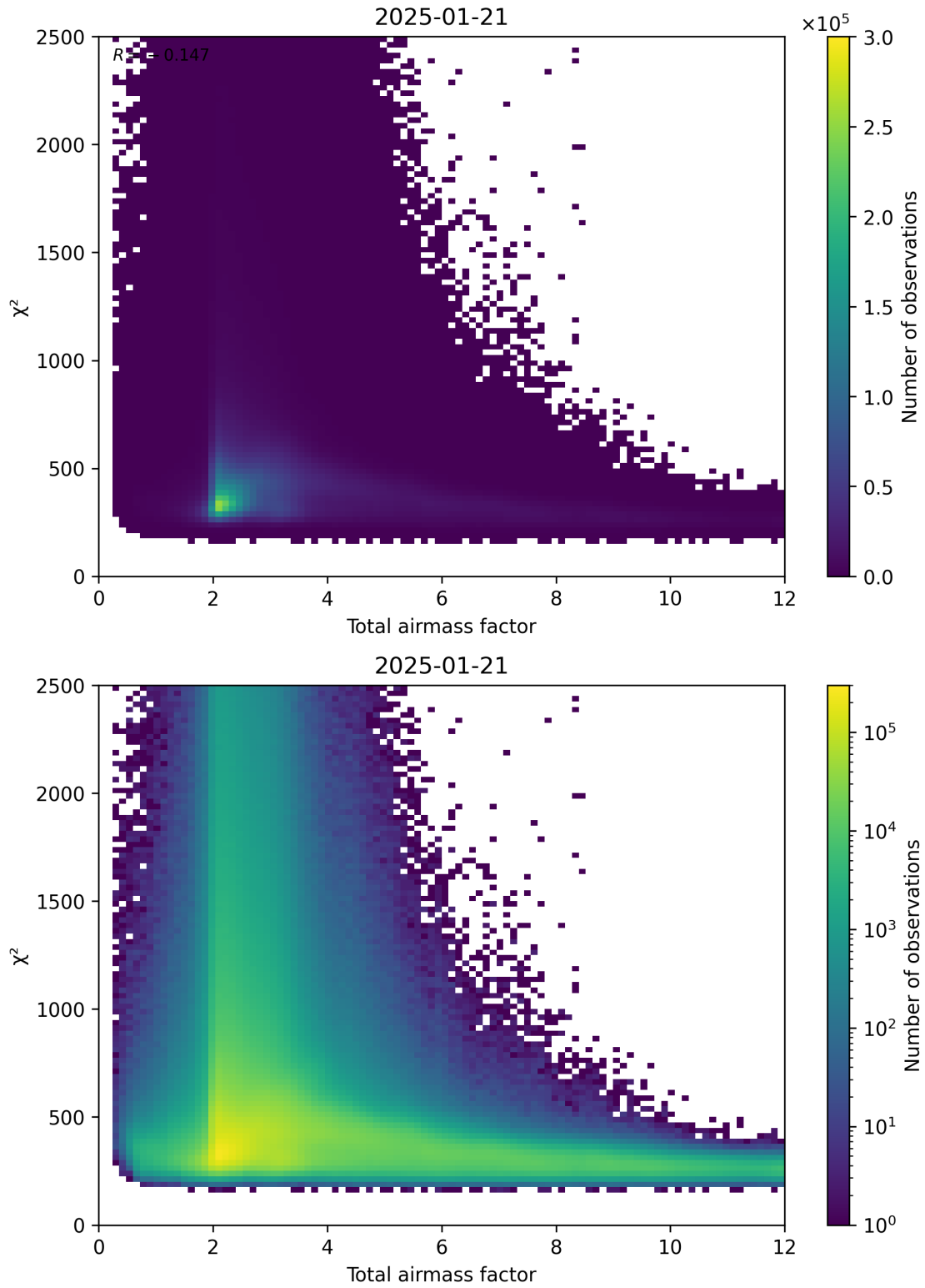
Figure 63: Scatter density plot of “Total airmass factor” against “ \chi^2 ” for 2025-01-20 to 2025-01-22.
