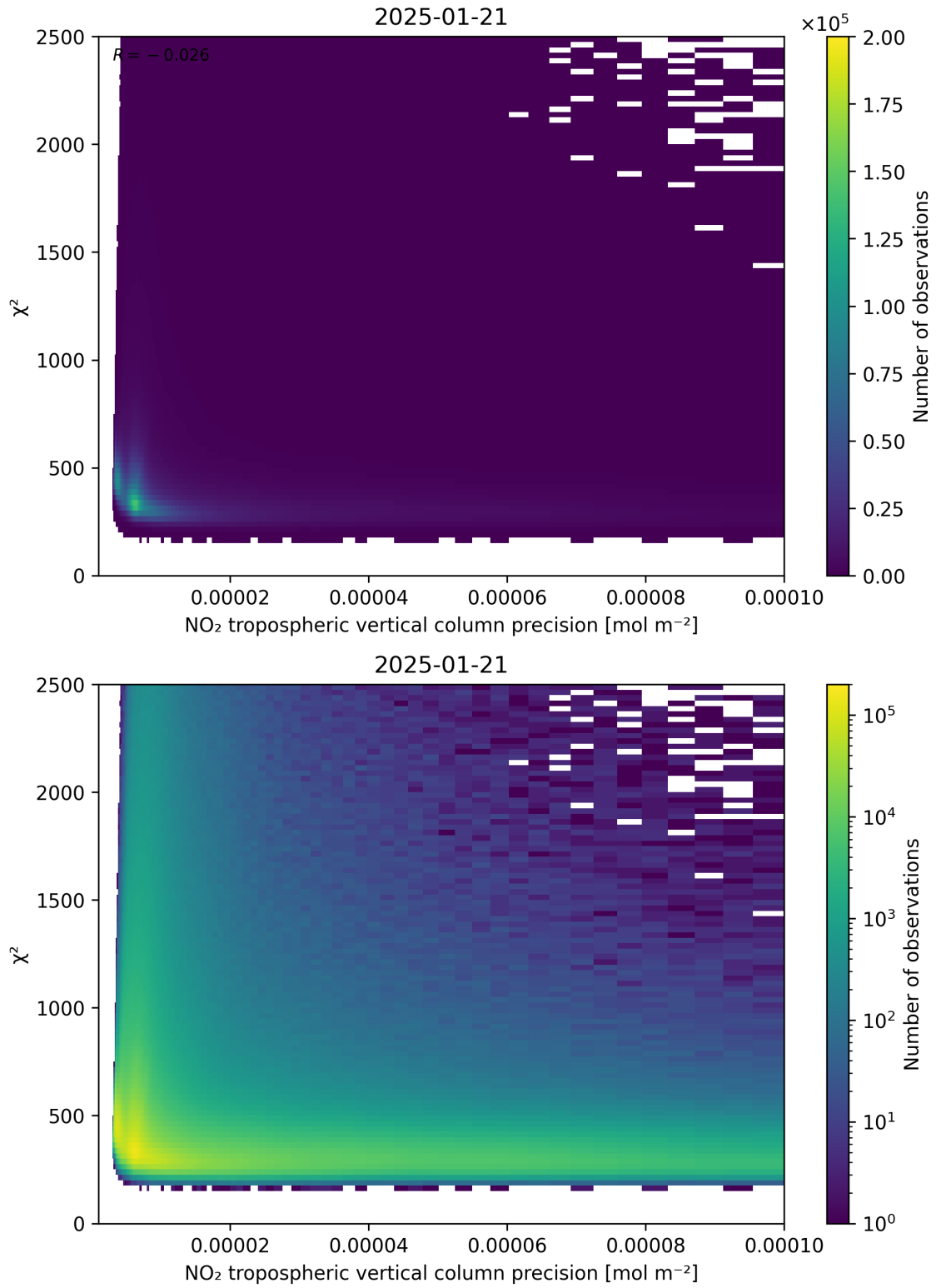
Figure 134: Scatter density plot of “NO 2 tropospheric vertical column precision” against “ \chi^2 ” for 2025-01-20 to 2025-01-22.
