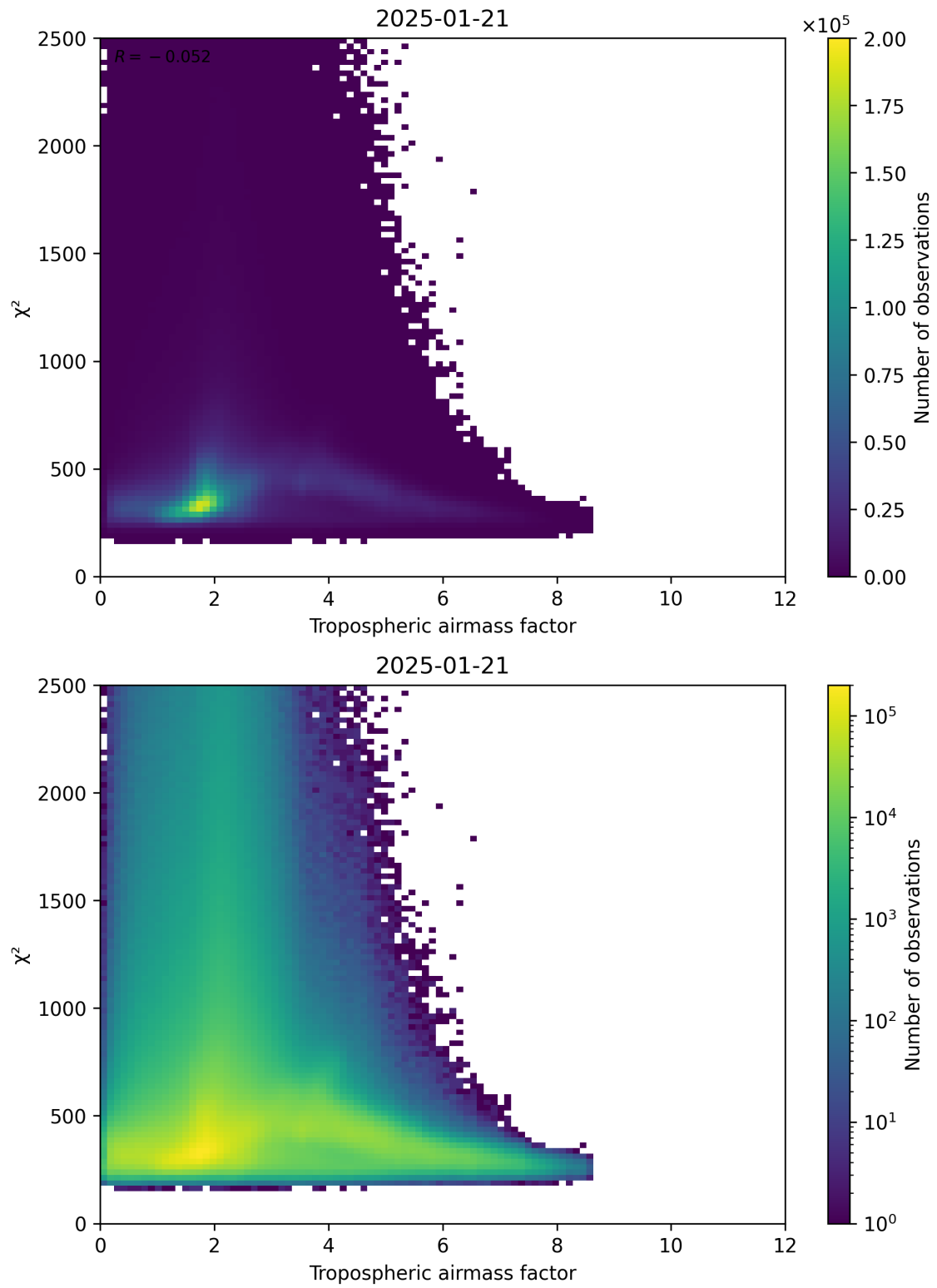
Figure 73: Scatter density plot of “Tropospheric airmass factor” against “ \chi^2 ” for 2025-01-20 to 2025-01-22.
