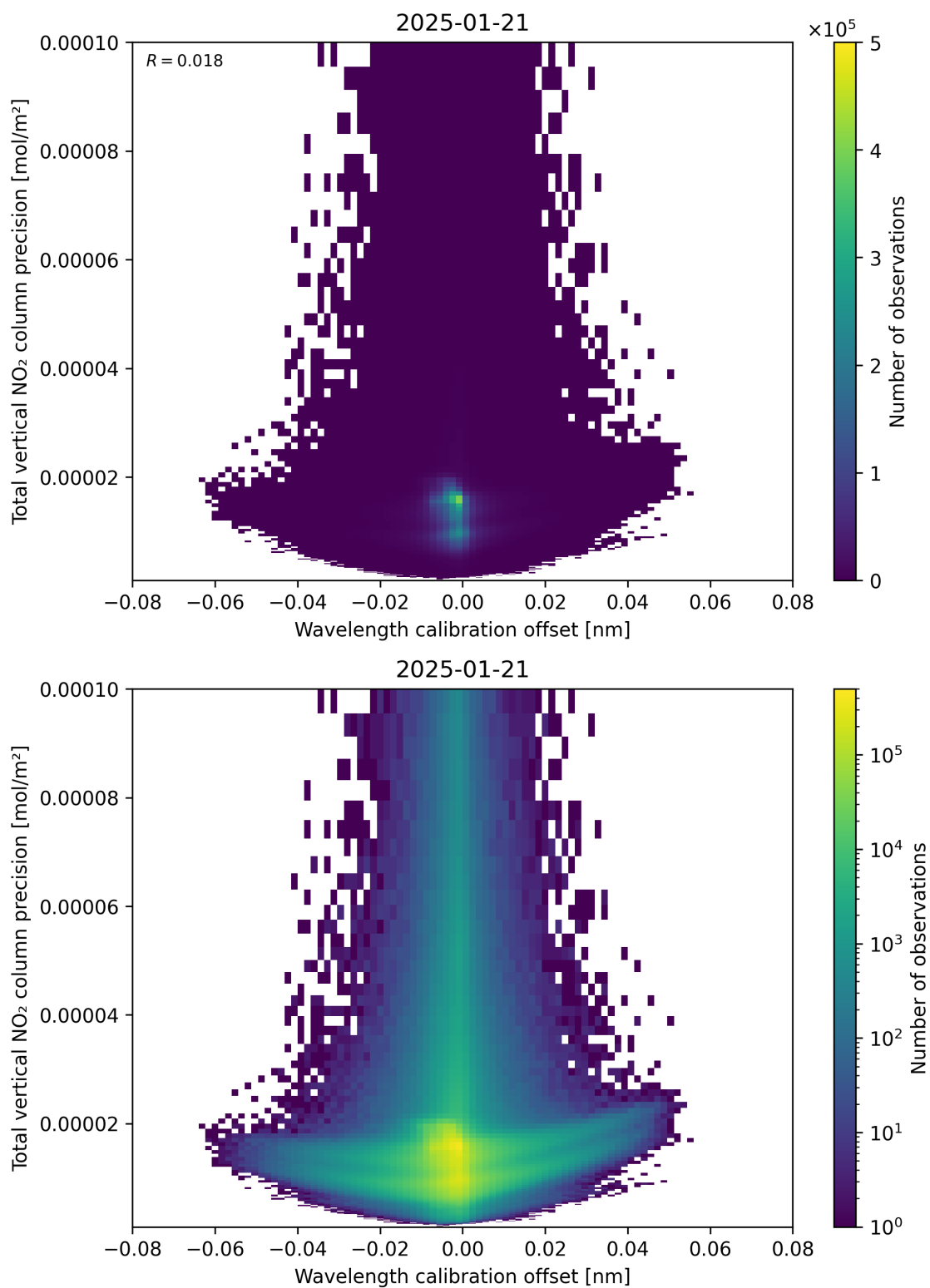
Figure 180: Scatter density plot of “Wavelength calibration offset” against “Total vertical NO 2 column precision” for 2025-01-20 to 2025-01-22.
