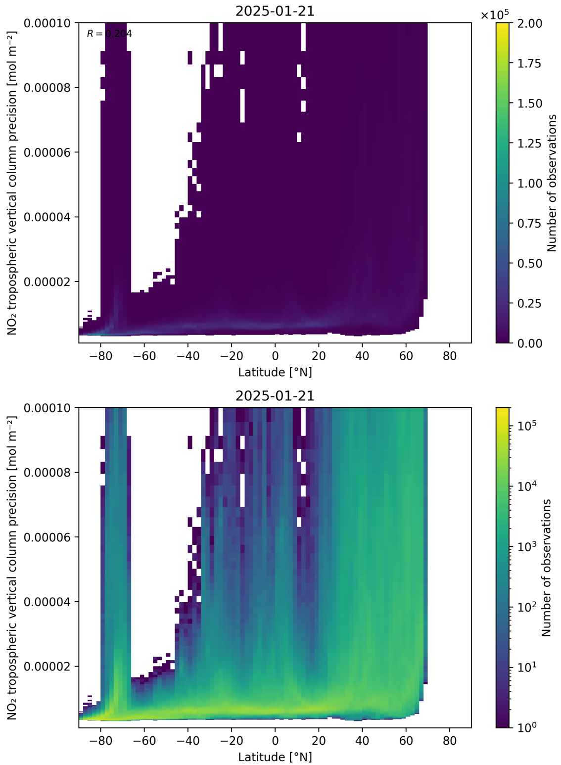
Figure 93: Scatter density plot of “Latitude” against “NO 2 tropospheric vertical column precision” for 2025-01-20 to 2025-01-22.
