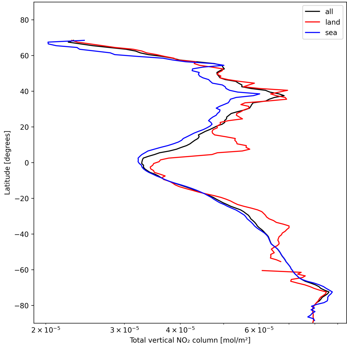
Figure 21: Zonal average of “Total vertical NO 2 column” for 2025-01-20 to 2025-01-22.
