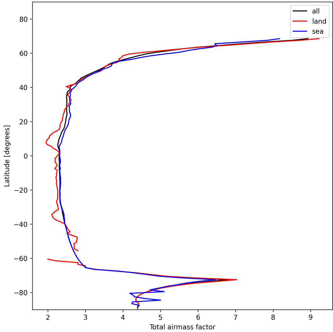
Figure 15: Zonal average of “Total airmass factor” for 2025-01-20 to 2025-01-22.
