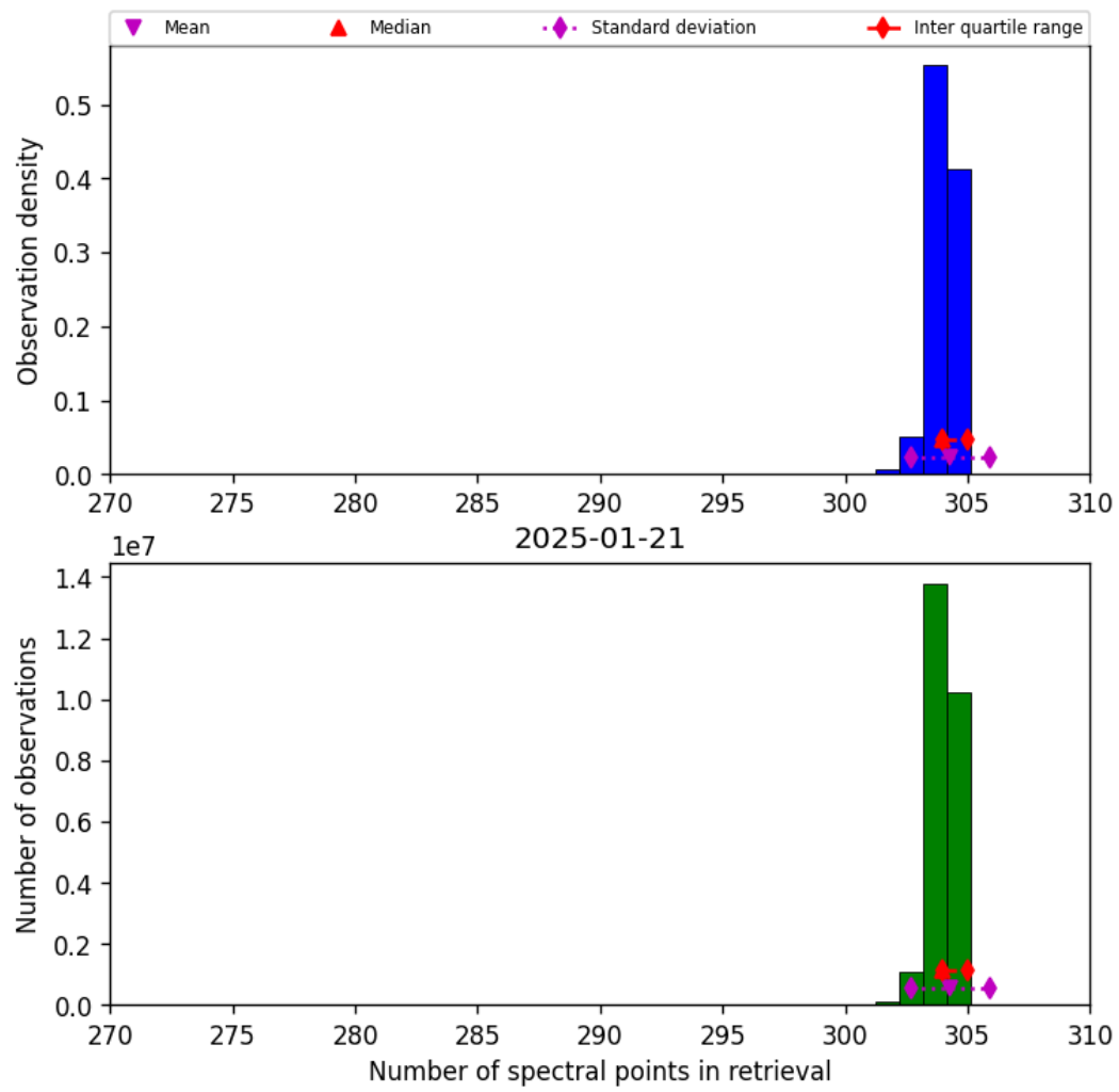
Figure 33: Histogram of “Number of spectral points in retrieval” for 2025-01-20 to 2025-01-22
