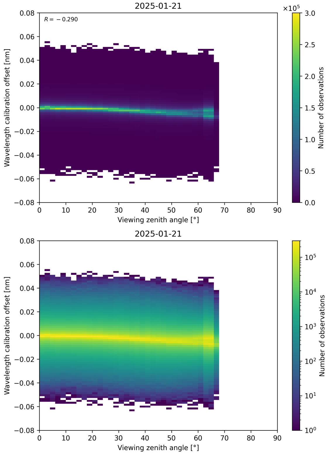
Figure 173: Scatter density plot of “Viewing zenith angle” against “Wavelength calibration offset” for 2025-01-20 to 2025-01-22.
