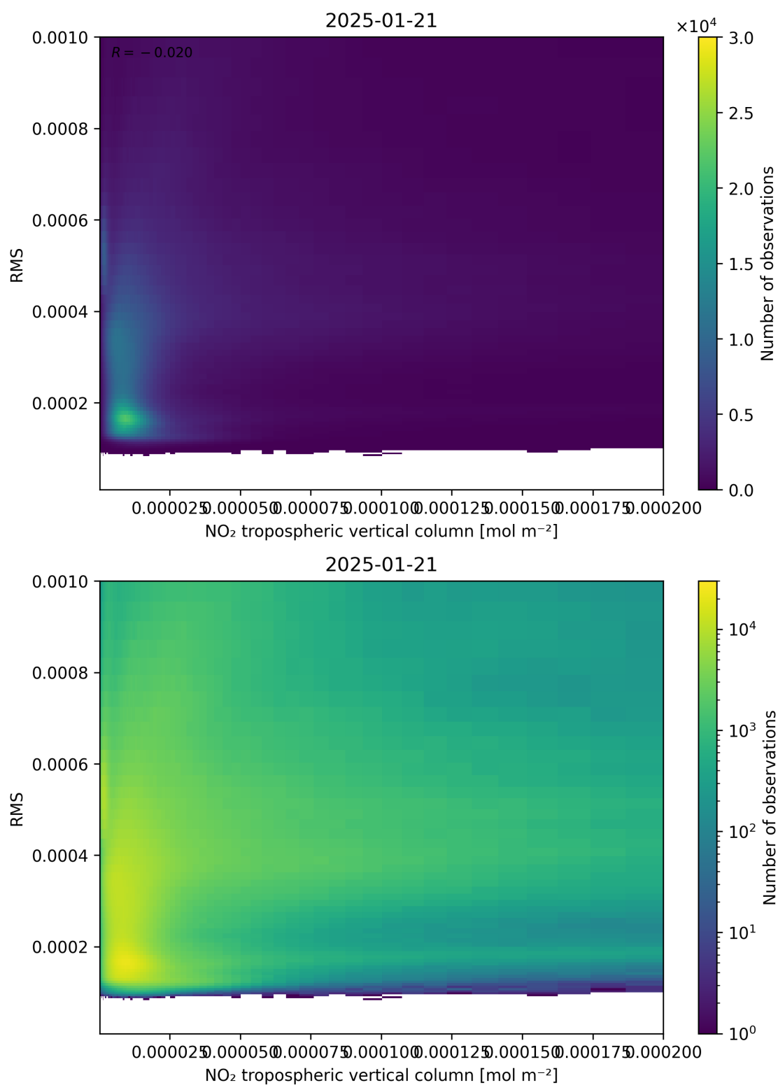
Figure 142: Scatter density plot of “NO 2 tropospheric vertical column” against “RMS” for 2025-01-20 to 2025-01-22.
