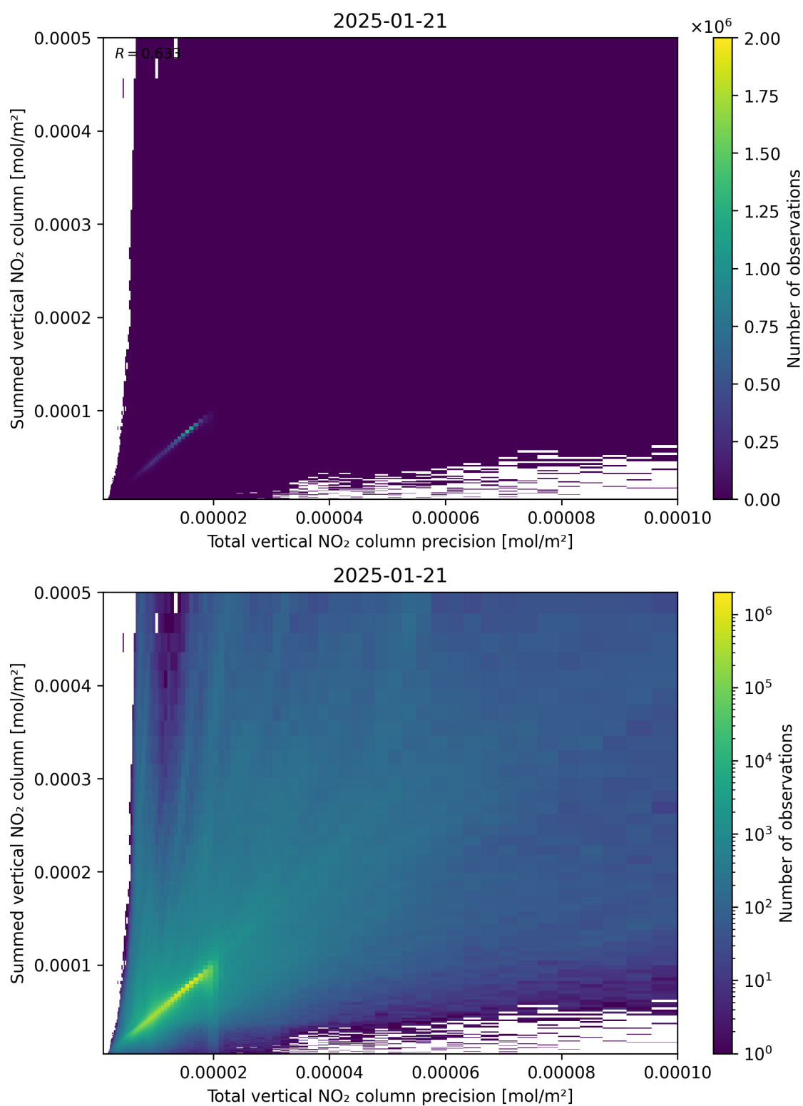
Figure 117: Scatter density plot of “Total vertical NO 2 column precision” against “Summed vertical NO 2 column” for 2025-01-20 to 2025-01-22.
