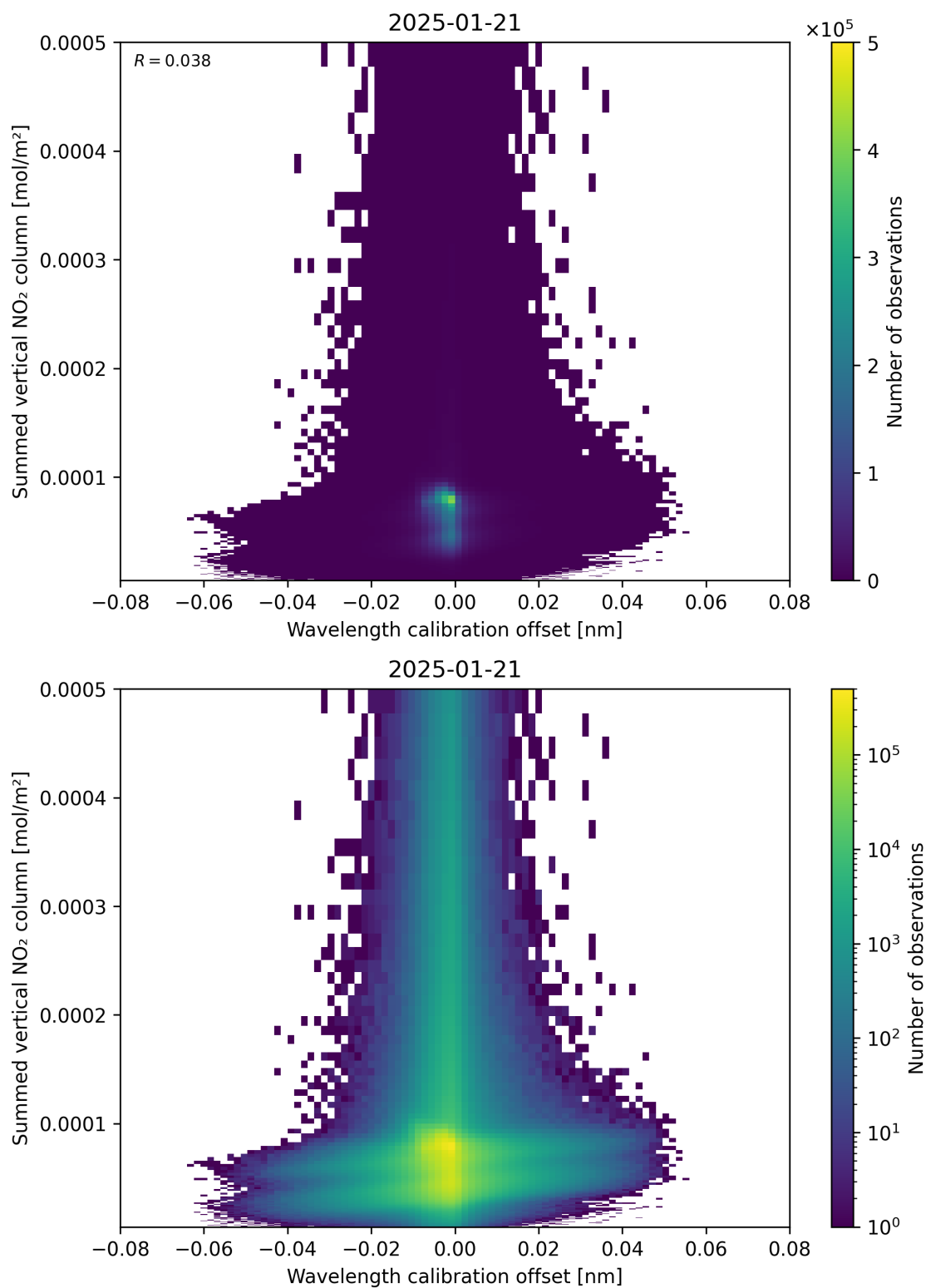
Figure 177: Scatter density plot of “Wavelength calibration offset” against “Summed vertical NO 2 column” for 2025-01-20 to 2025-01-22.
