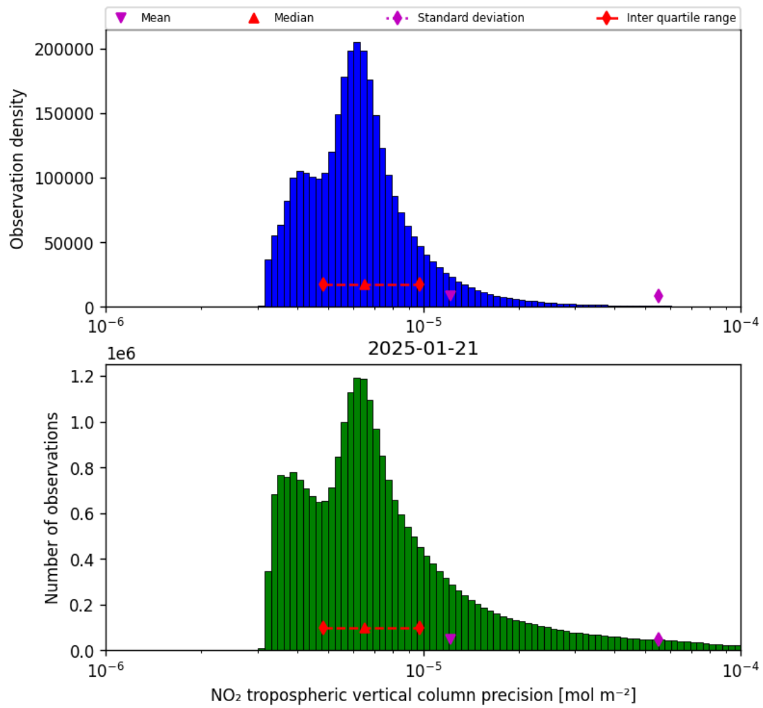
Figure 30: Histogram of “NO 2 tropospheric vertical column precision” for 2025-01-20 to 2025-01-22
