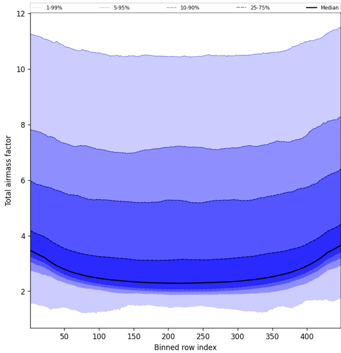
Figure 49: Along track statistics of “Total airmass factor” for 2025-01-20 to 2025-01-22
