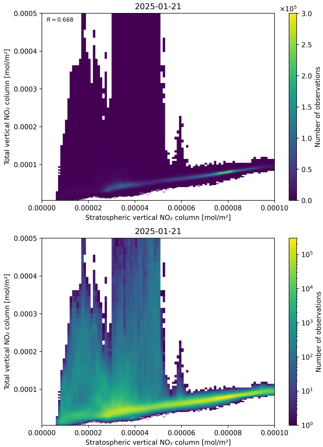
Figure 100: Scatter density plot of “Stratospheric vertical NO 2 column” against “Total vertical NO 2 column” for 2025-01-20 to 2025-01-22.
