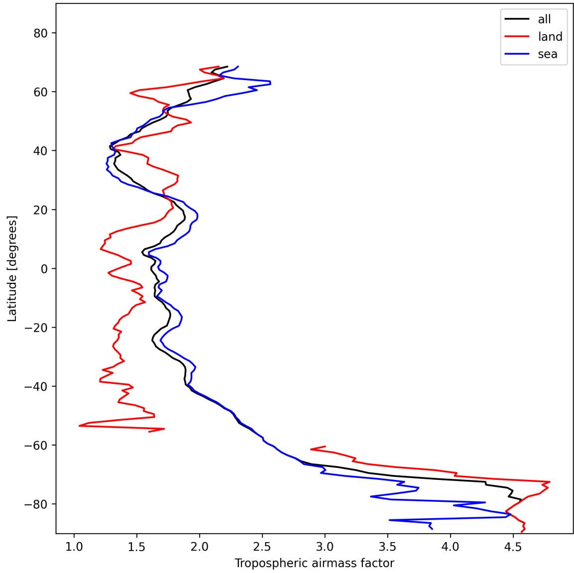
Figure 14: Zonal average of “Tropospheric airmass factor” for 2025-01-20 to 2025-01-22.
