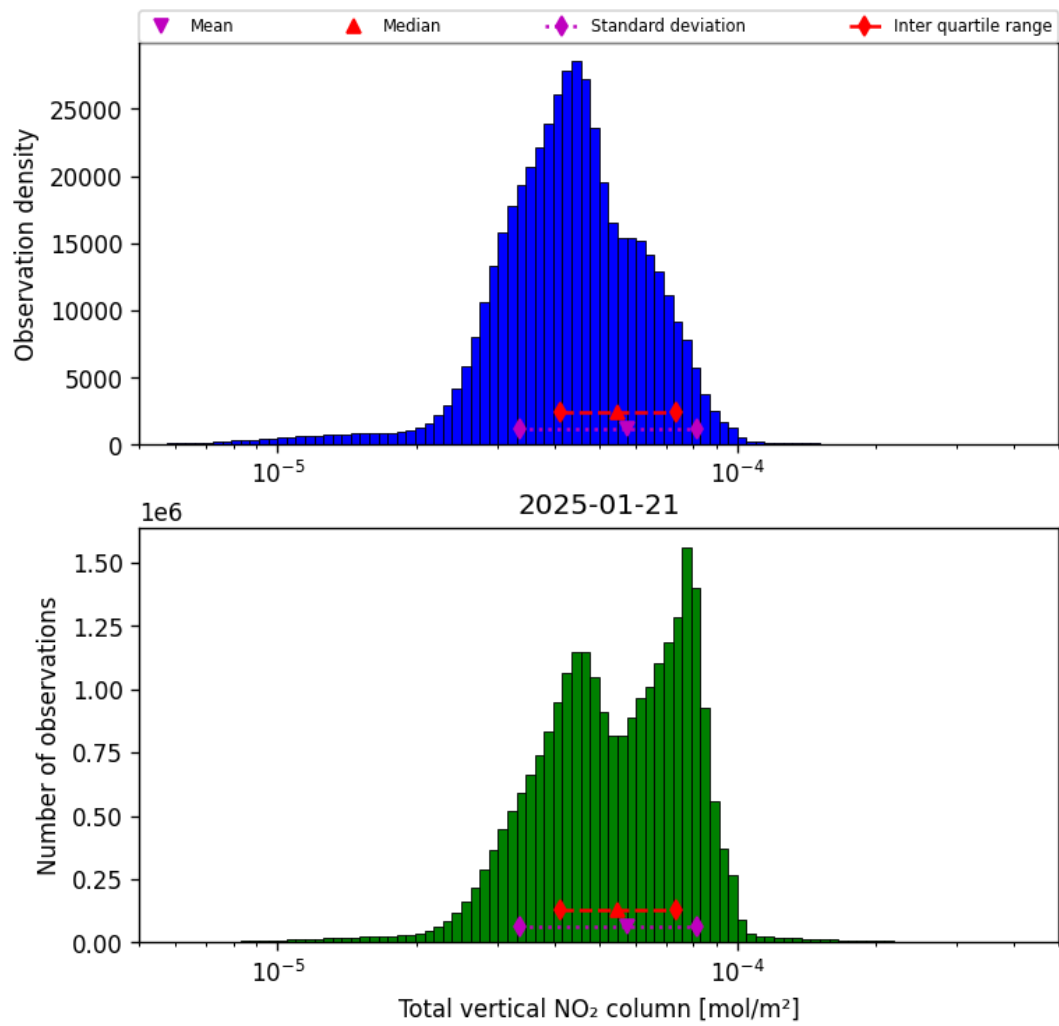
Figure 38: Histogram of “Total vertical NO 2 column” for 2025-01-20 to 2025-01-22
