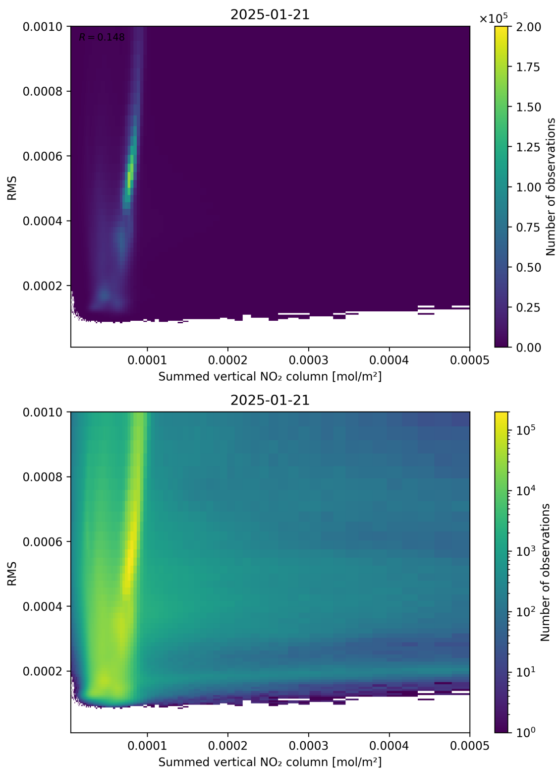
Figure 109: Scatter density plot of “Summed vertical NO 2 column” against “RMS” for 2025-01-20 to 2025-01-22.
