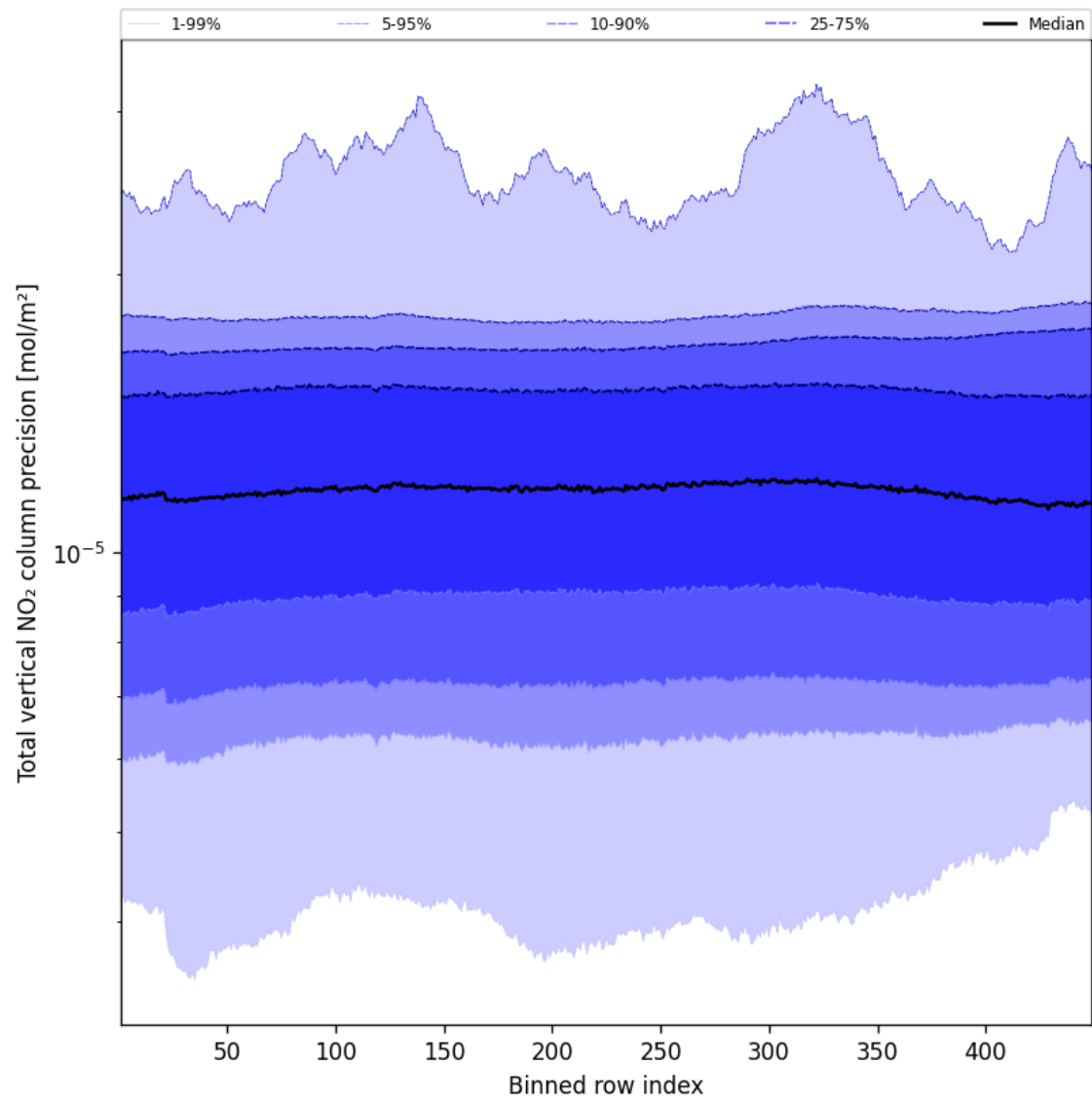
Figure 56: Along track statistics of “Total vertical NO 2 column precision” for 2025-01-20 to 2025-01-22
