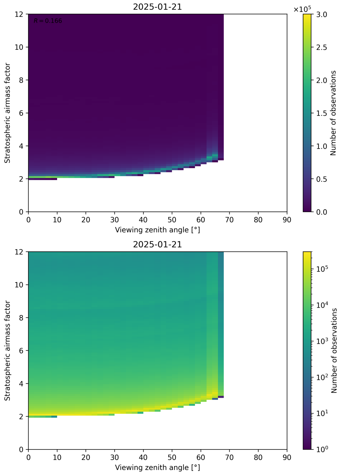
Figure 159: Scatter density plot of “Viewing zenith angle” against “Stratospheric airmass factor” for 2025-01-20 to 2025-01-22.
