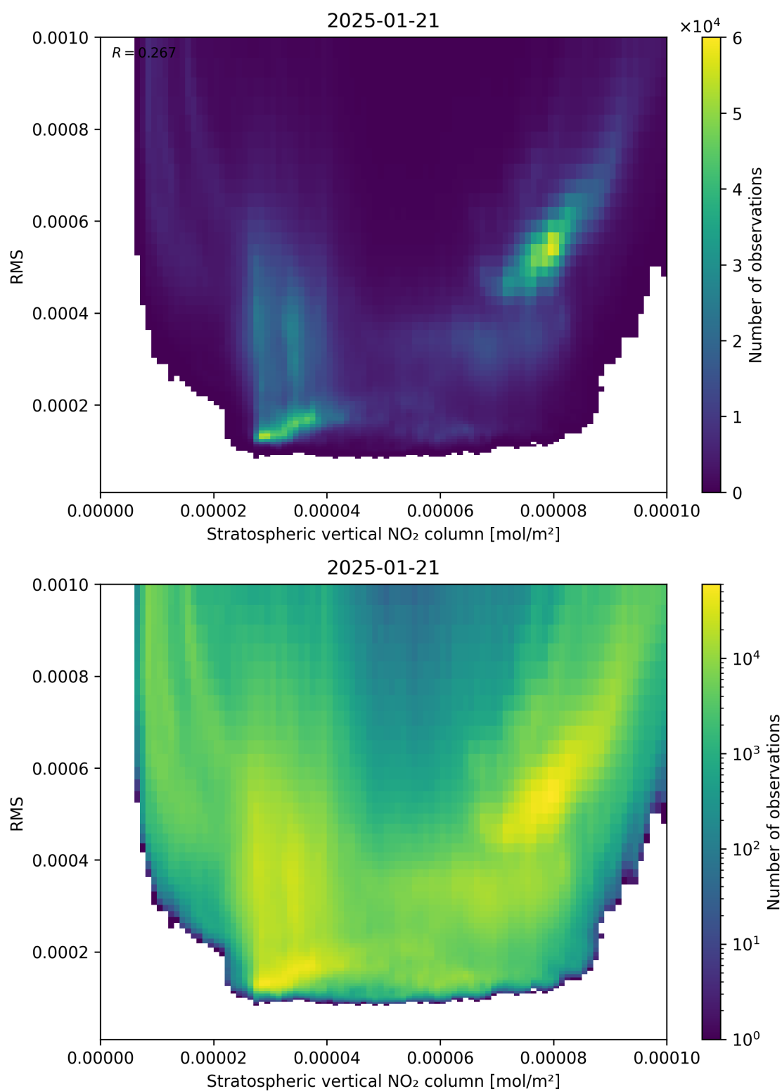
Figure 102: Scatter density plot of “Stratospheric vertical NO 2 column” against “RMS” for 2025-01-20 to 2025-01-22.
