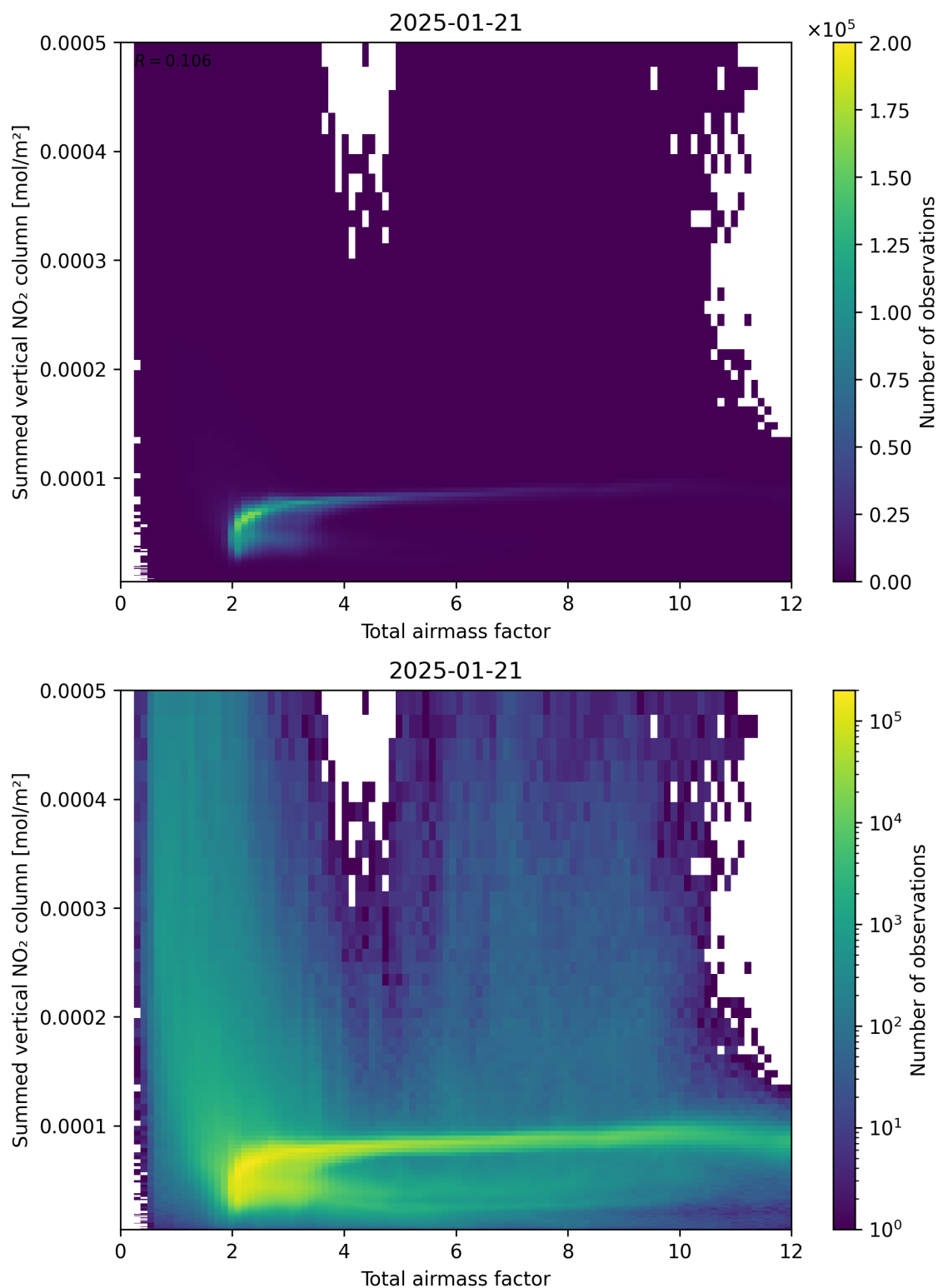
Figure 65: Scatter density plot of “Total airmass factor” against “Summed vertical NO 2 column” for 2025-01-20 to 2025-01-22.
