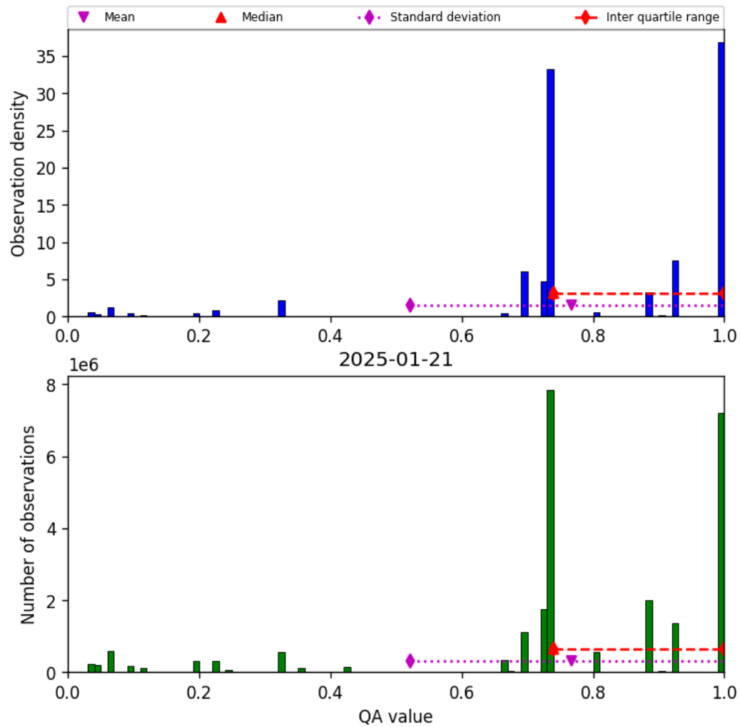
Figure 28: Histogram of “QA value” for 2025-01-20 to 2025-01-22
