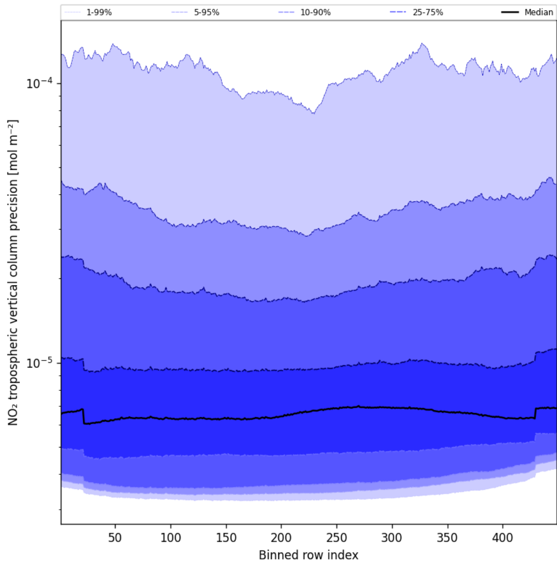
Figure 47: Along track statistics of “NO 2 tropospheric vertical column precision” for 2025-01-20 to 2025-01-22
