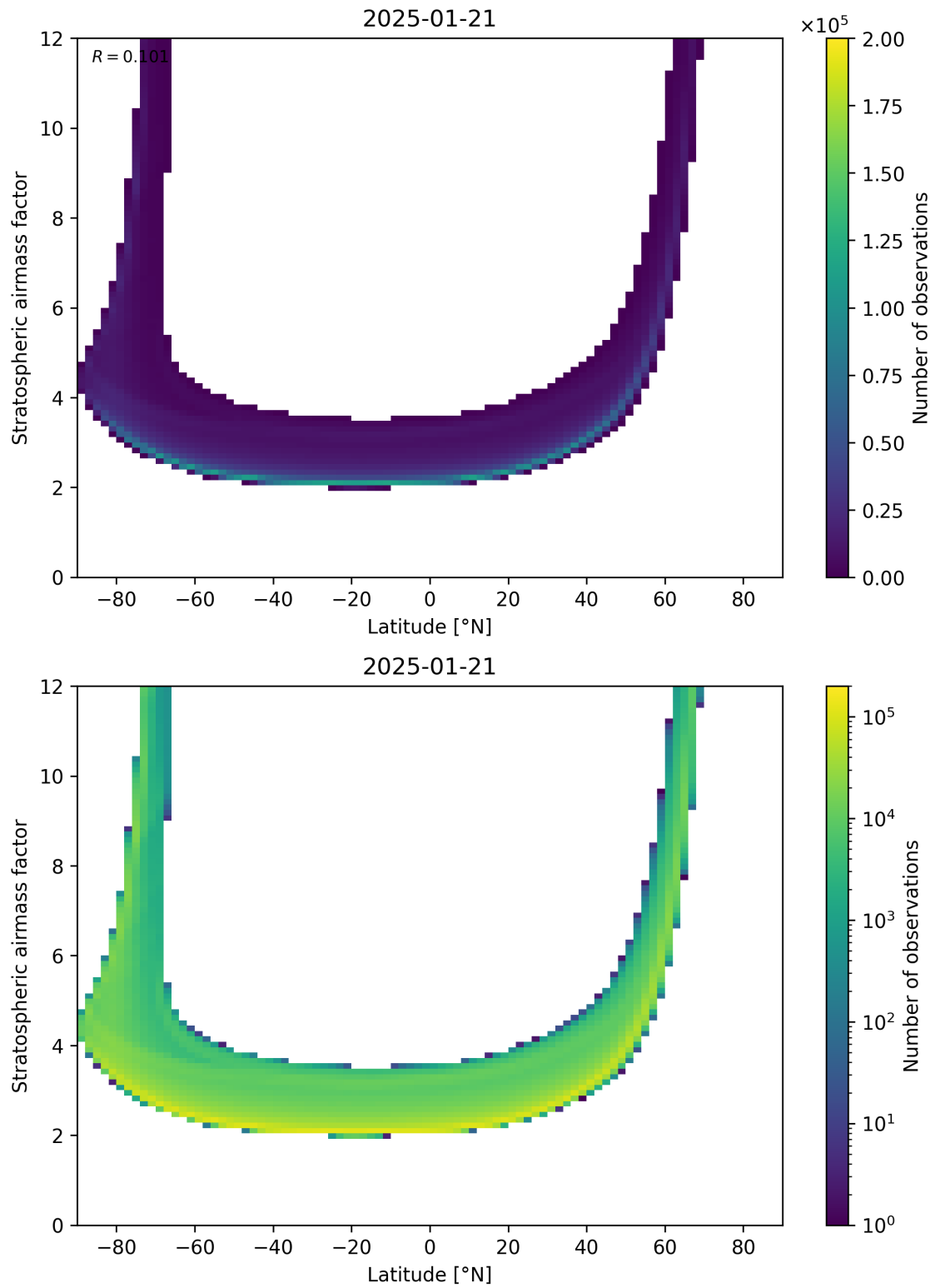
Figure 83: Scatter density plot of “Latitude” against “Stratospheric airmass factor” for 2025-01-20 to 2025-01-22.
