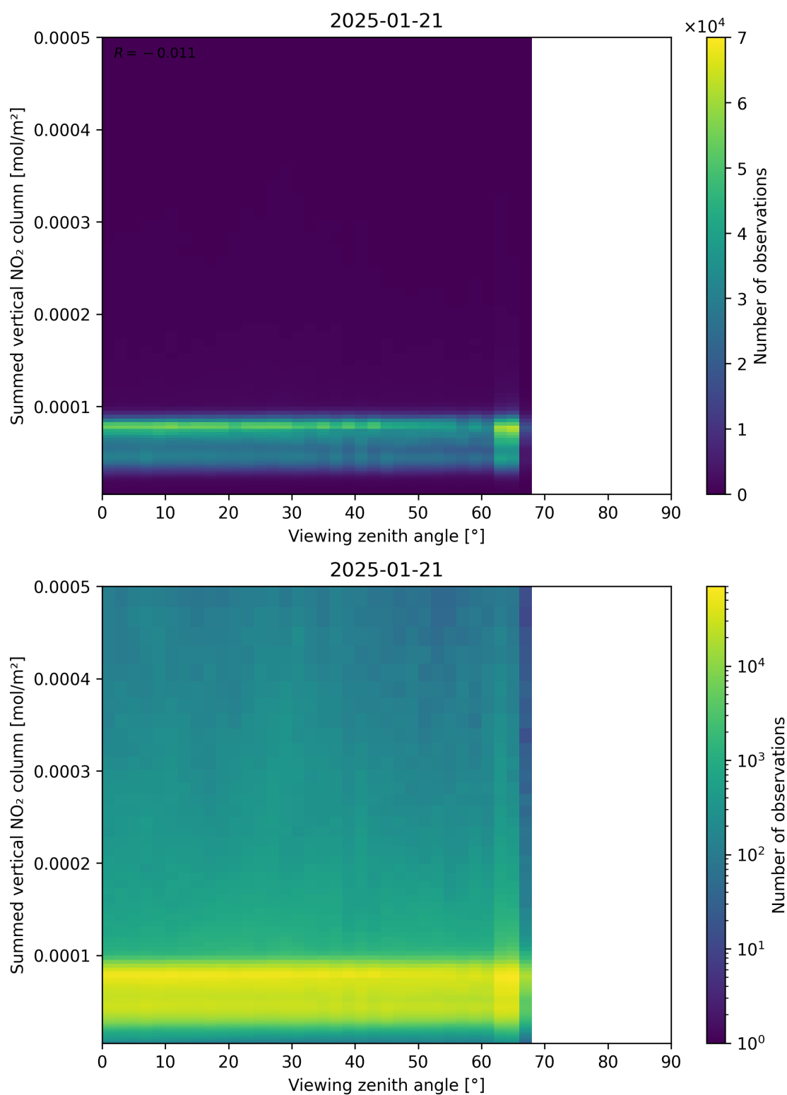
Figure 165: Scatter density plot of “Viewing zenith angle” against “Summed vertical NO 2 column” for 2025-01-20 to 2025-01-22.
