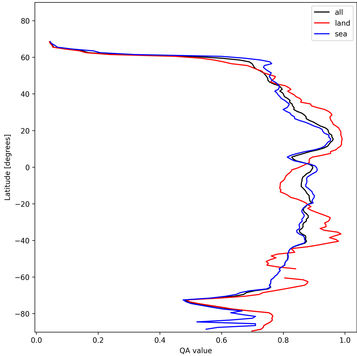
Figure 11: Zonal average of “QA value” for 2025-01-20 to 2025-01-22.
