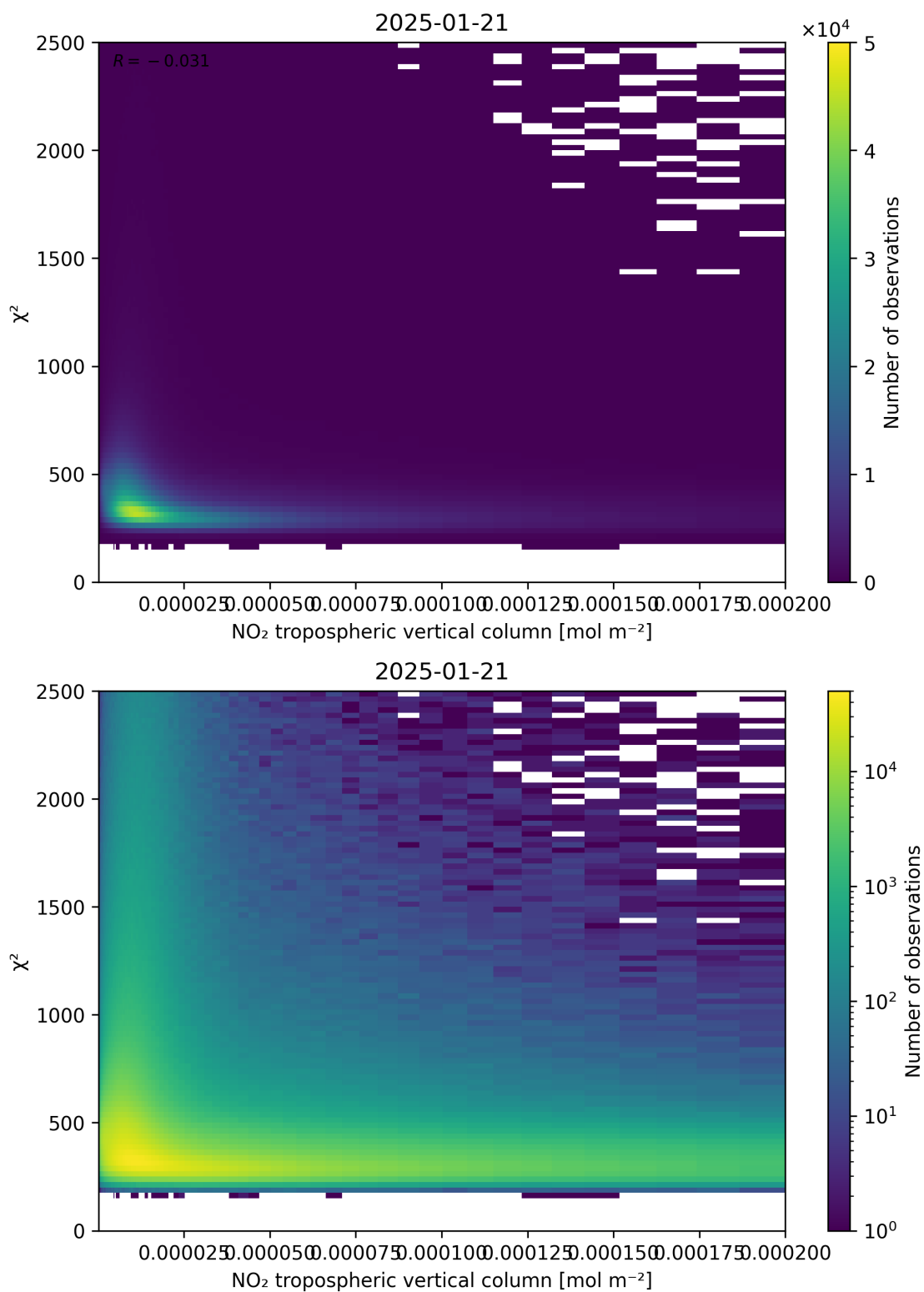
Figure 124: Scatter density plot of “NO 2 tropospheric vertical column” against “ \chi^2 ” for 2025-01-20 to 2025-01-22.
