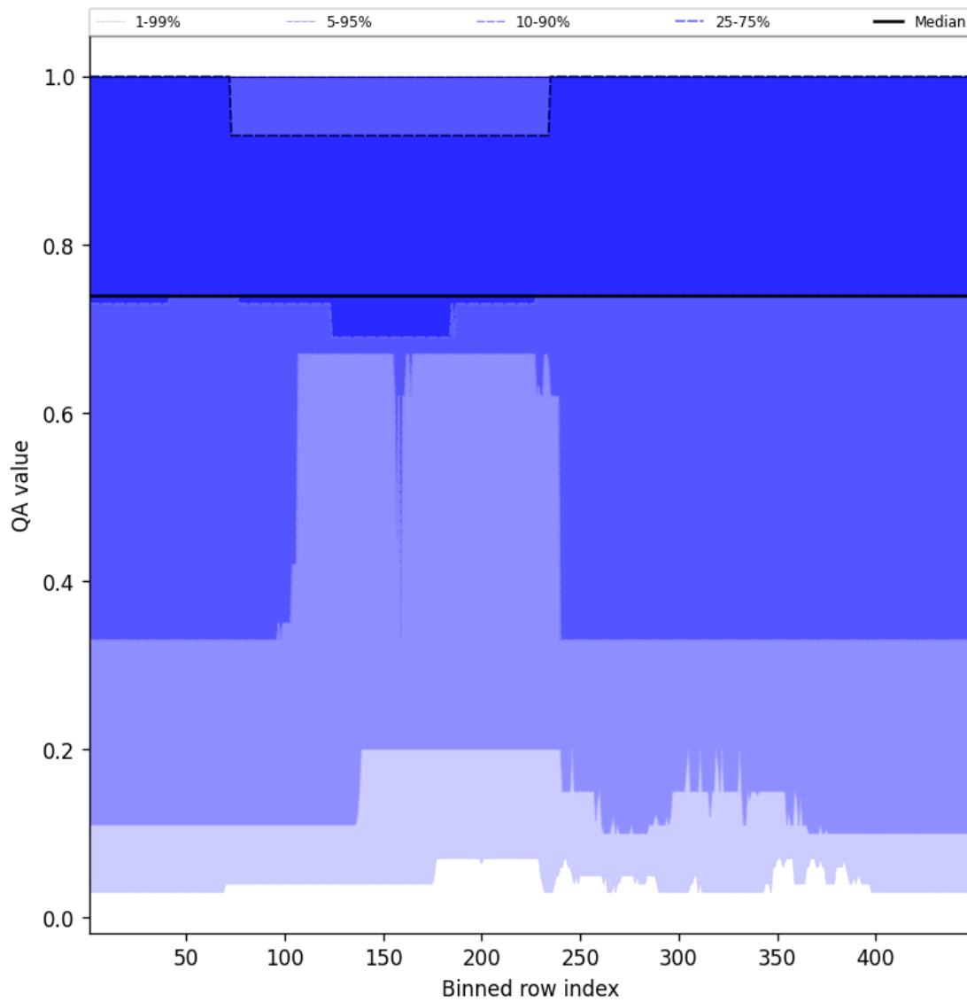
Figure 45: Along track statistics of “QA value” for 2025-01-20 to 2025-01-22
