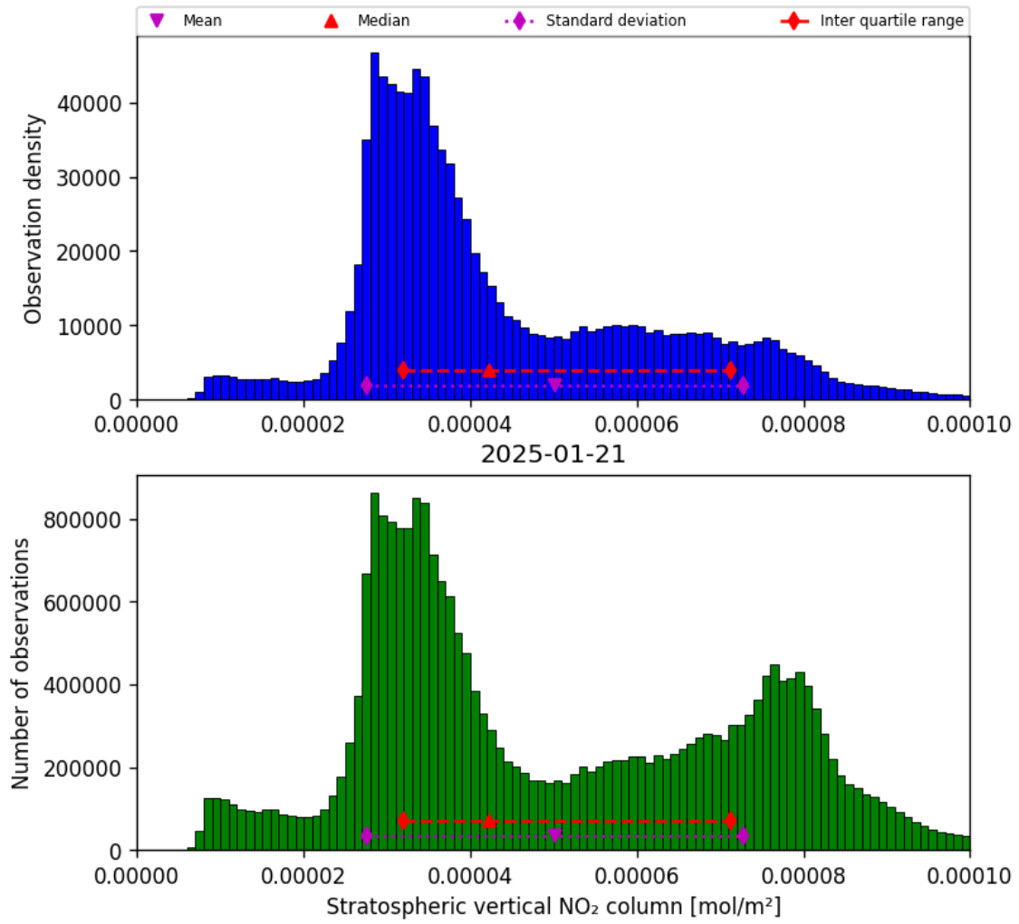
Figure 36: Histogram of “Stratospheric vertical NO 2 column” for 2025-01-20 to 2025-01-22
