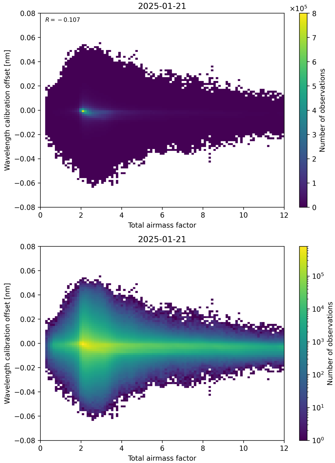
Figure 70: Scatter density plot of “Total airmass factor” against “Wavelength calibration offset” for 2025-01-20 to 2025-01-22.
