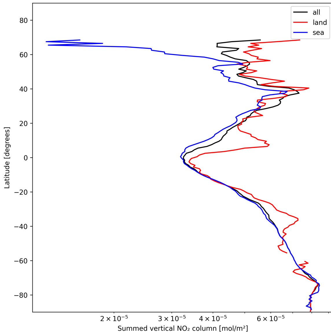
Figure 23: Zonal average of “Summed vertical NO 2 column” for 2025-01-20 to 2025-01-22.
