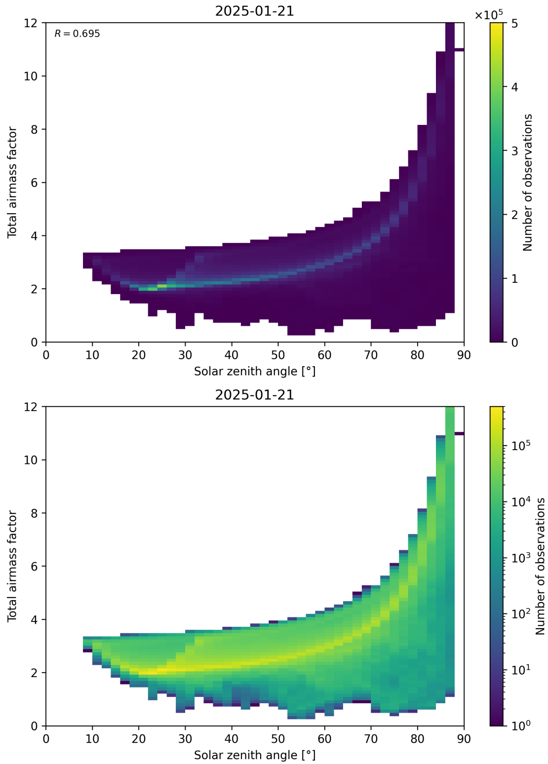
Figure 146: Scatter density plot of “Solar zenith angle” against “Total air mass factor” for 2025-01-20 to 2025-01-22.
