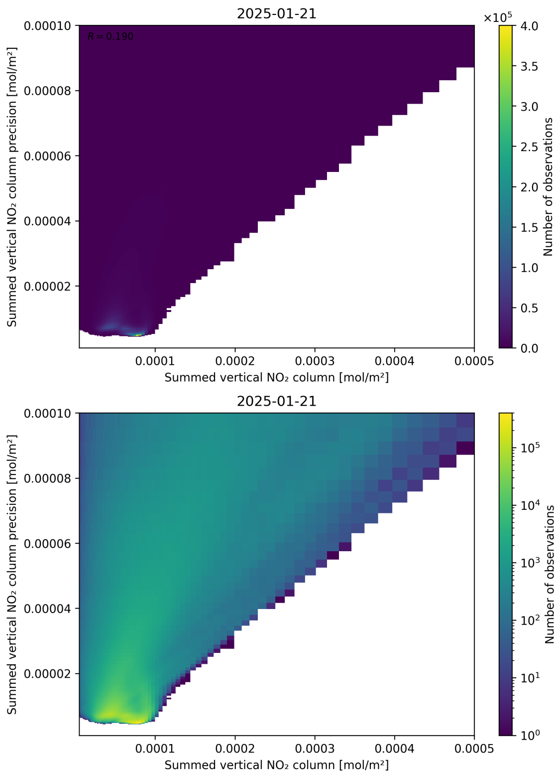
Figure 105: Scatter density plot of “Summed vertical NO 2 column” against “Summed vertical NO 2 column precision” for 2025-01-20 to 2025-01-22.
