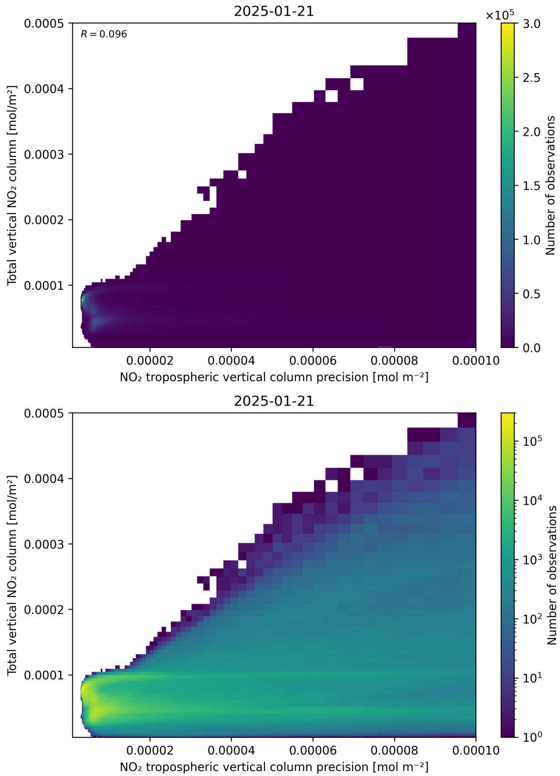
Figure 138: Scatter density plot of “NO 2 tropospheric vertical column precision” against “Total vertical NO 2 column” for 2025-01-20 to 2025-01-22.
