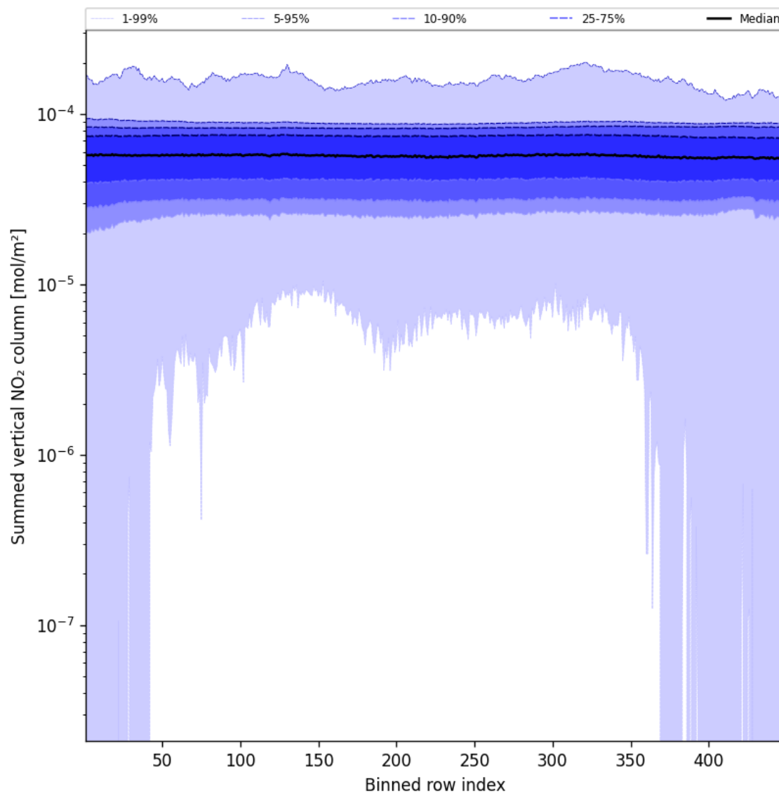
Figure 57: Along track statistics of “Summed vertical NO 2 column” for 2025-01-20 to 2025-01-22
