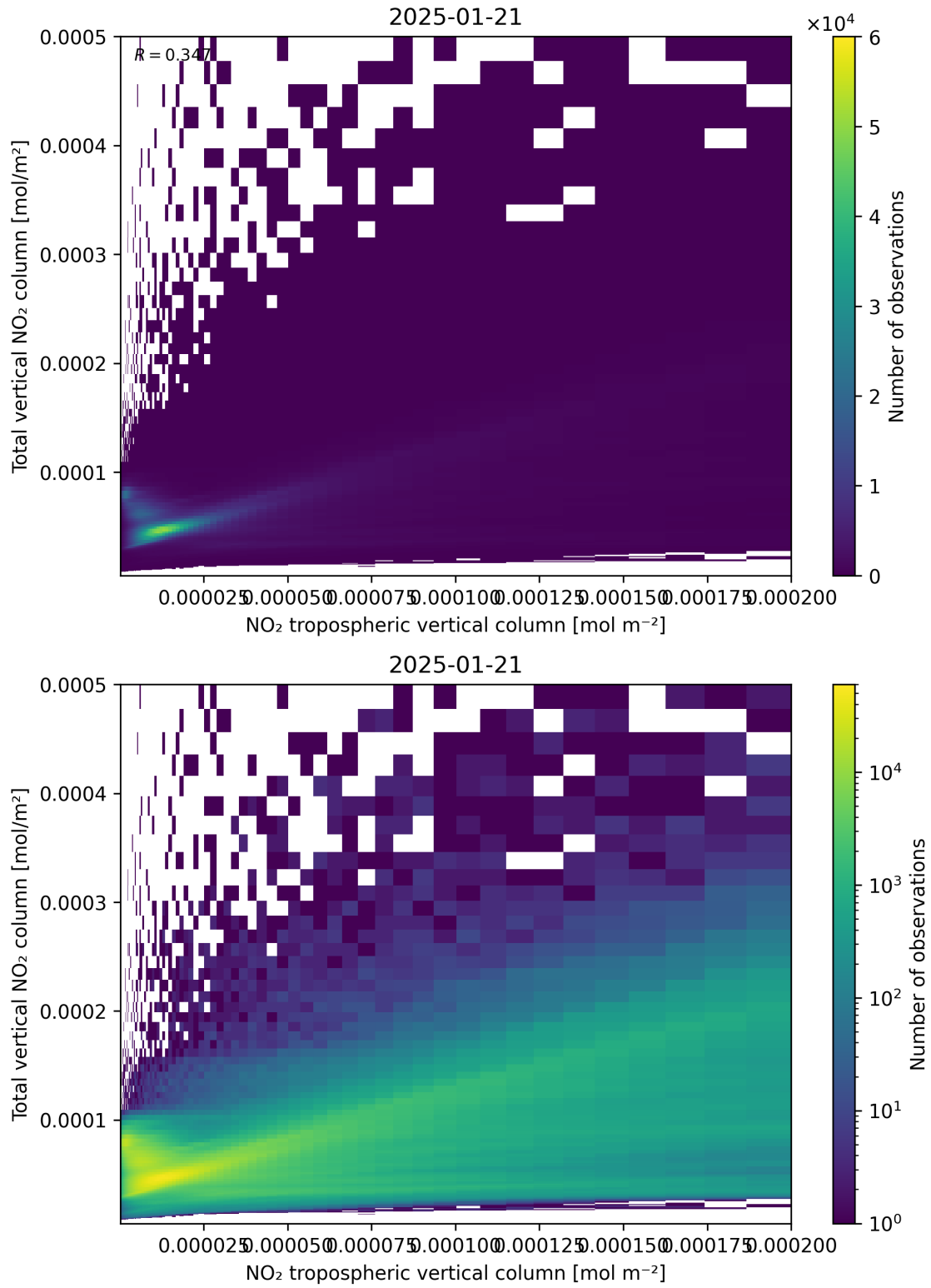
Figure 128: Scatter density plot of “NO 2 tropospheric vertical column” against “Total vertical NO 2 column” for 2025-01-20 to 2025-01-22.
