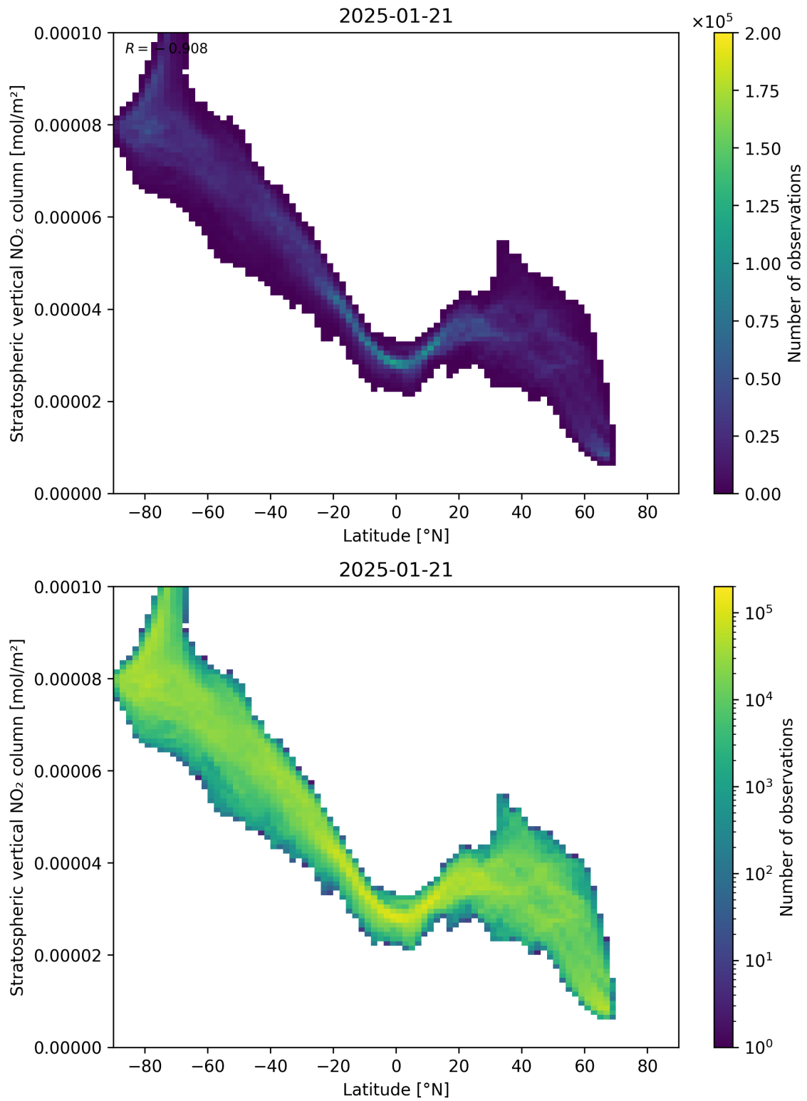
Figure 87: Scatter density plot of “Latitude” against “Stratospheric vertical NO 2 column” for 2025-01-20 to 2025-01-22.
