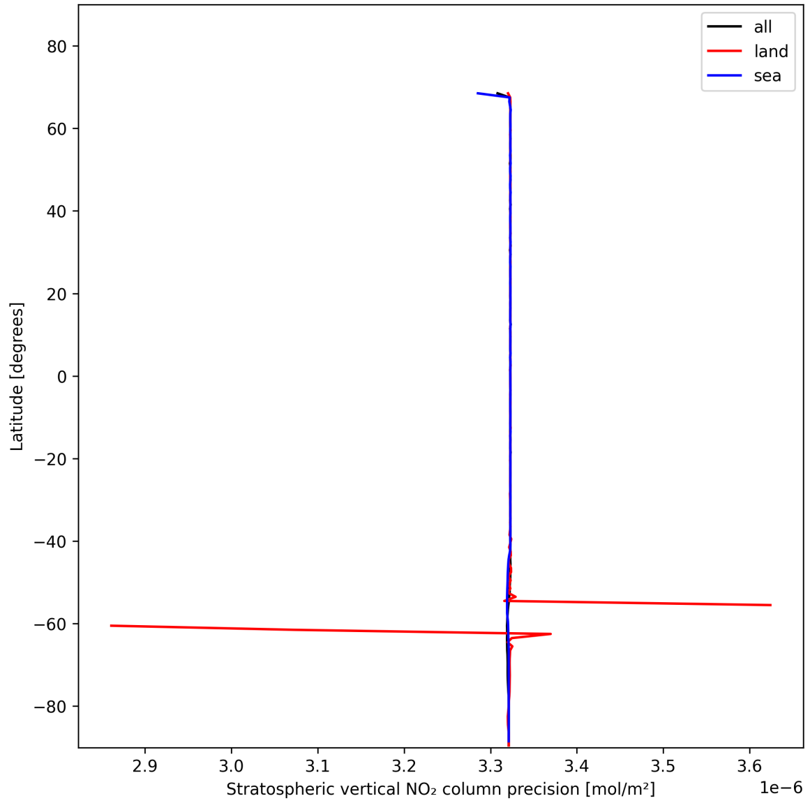
Figure 20: Zonal average of “Stratospheric vertical NO 2 column precision” for 2025-01-20 to 2025-01-22.
