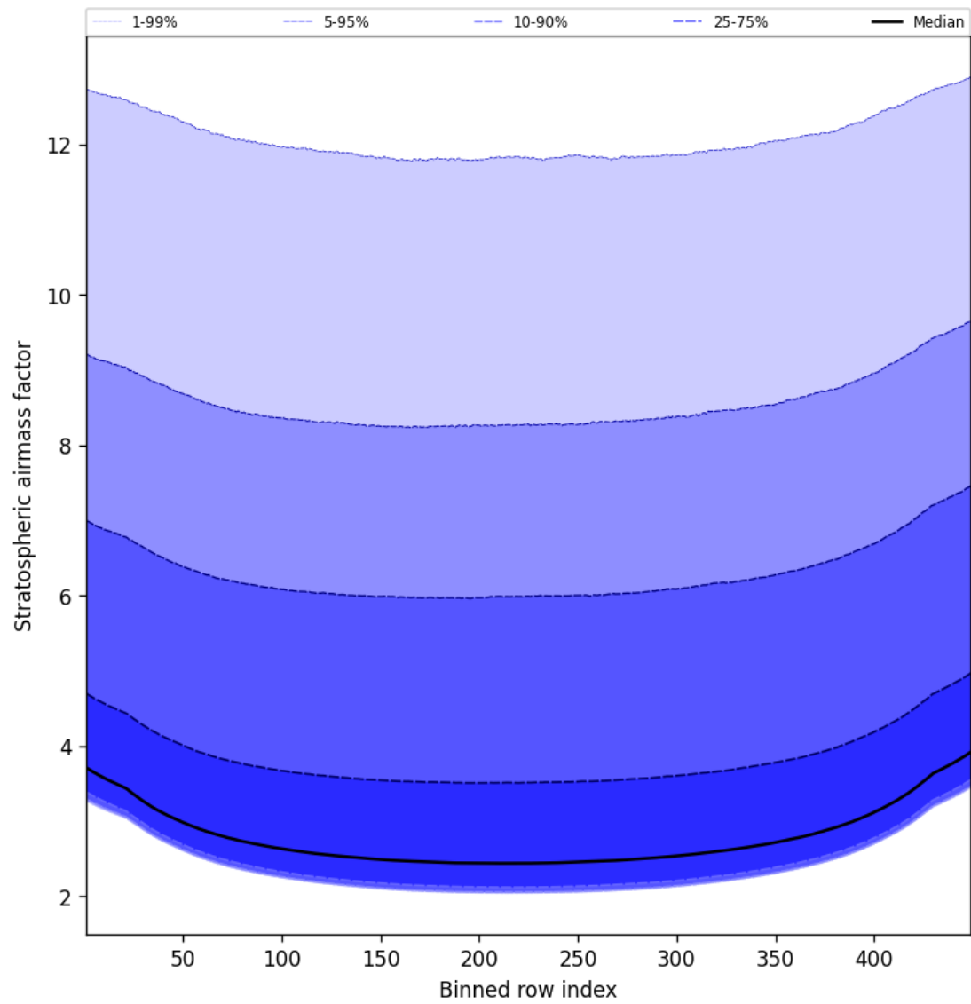
Figure 61: Along track statistics of “Stratospheric air mass factor” for 2025-01-20 to 2025-01-22
