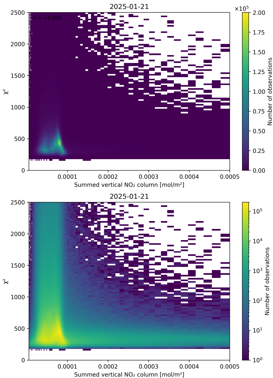
Figure 104: Scatter density plot of “Summed vertical NO 2 column” against “ \chi^2 ” for 2025-01-20 to 2025-01-22.
