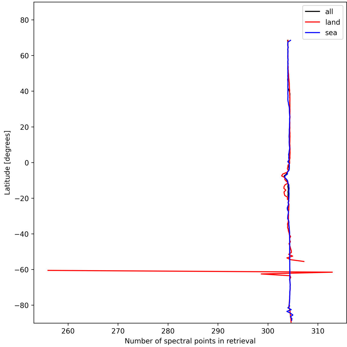
Figure 16: Zonal average of “Number of spectral points in retrieval” for 2025-01-20 to 2025-01-22.
