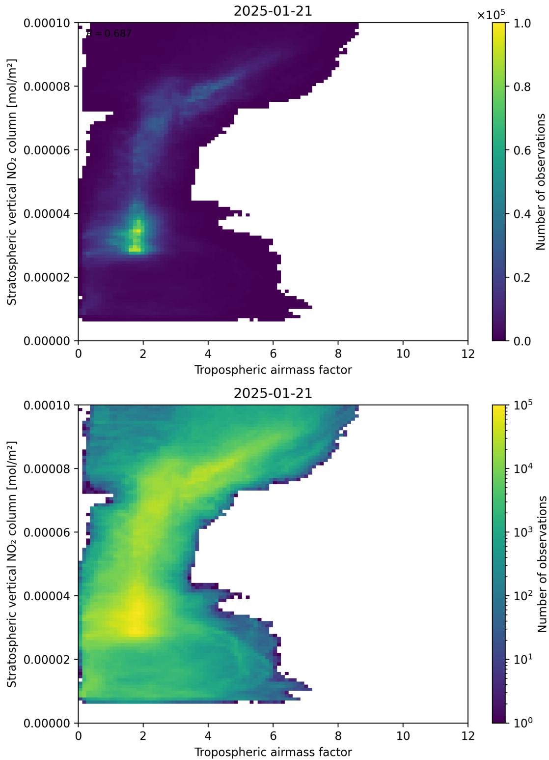
Figure 74: Scatter density plot of “Tropospheric air mass factor” against “Stratospheric vertical NO 2 column” for 2025-01-20 to 2025-01-22.
