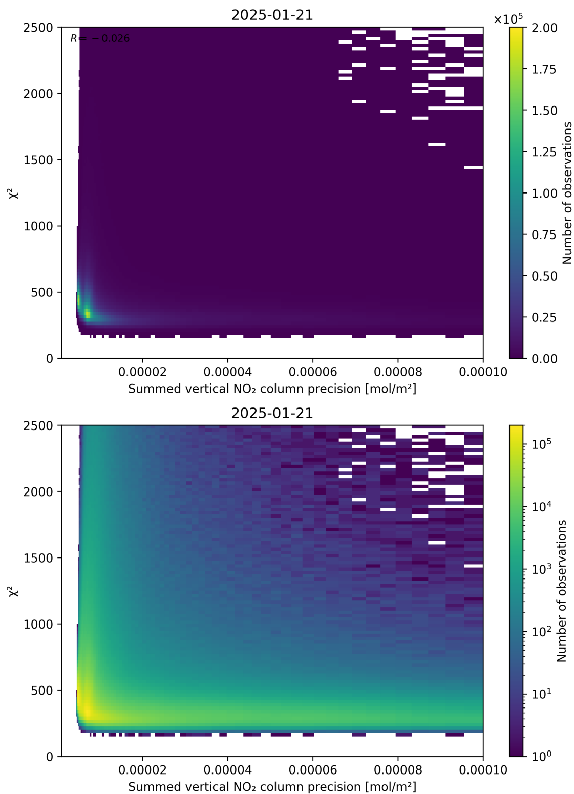
Figure 107: Scatter density plot of “Summed vertical NO 2 column precision” against “ \chi^2 ” for 2025-01-20 to 2025-01-22.
