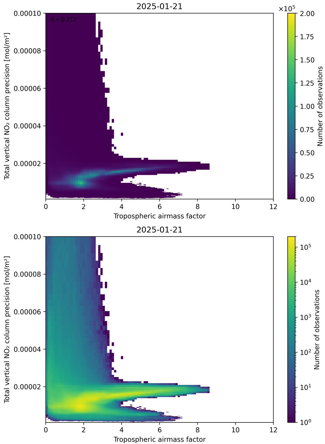
Figure 78: Scatter density plot of “Tropospheric airmass factor” against “Total vertical NO 2 column precision” for 2025-01-20 to 2025-01-22.
