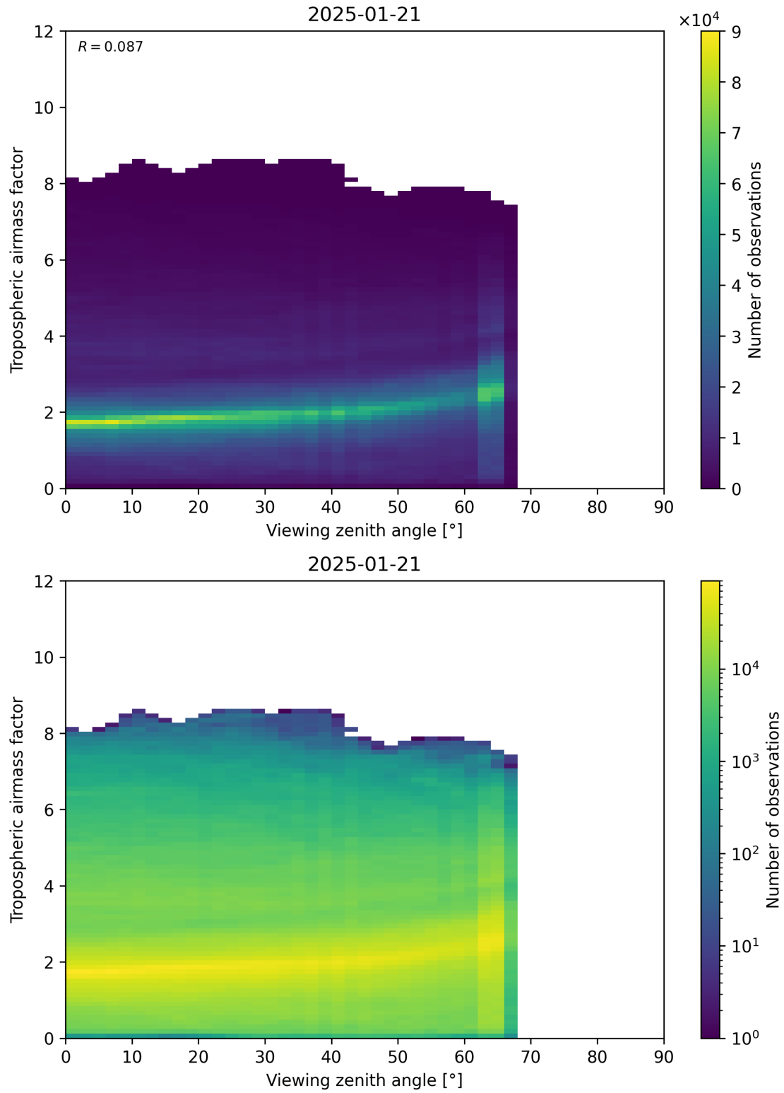
Figure 161: Scatter density plot of “Viewing zenith angle” against “Tropospheric airmass factor” for 2025-01-20 to 2025-01-22.
