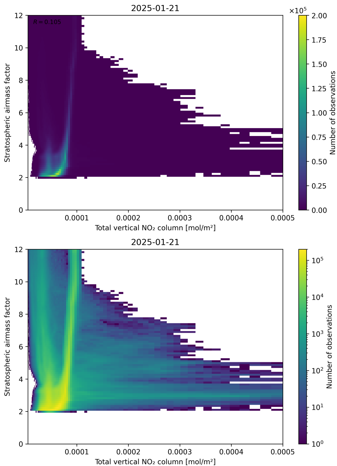
Figure 110: Scatter density plot of “Total vertical NO 2 column” against “Stratospheric airmass factor” for 2025-01-20 to 2025-01-22.
