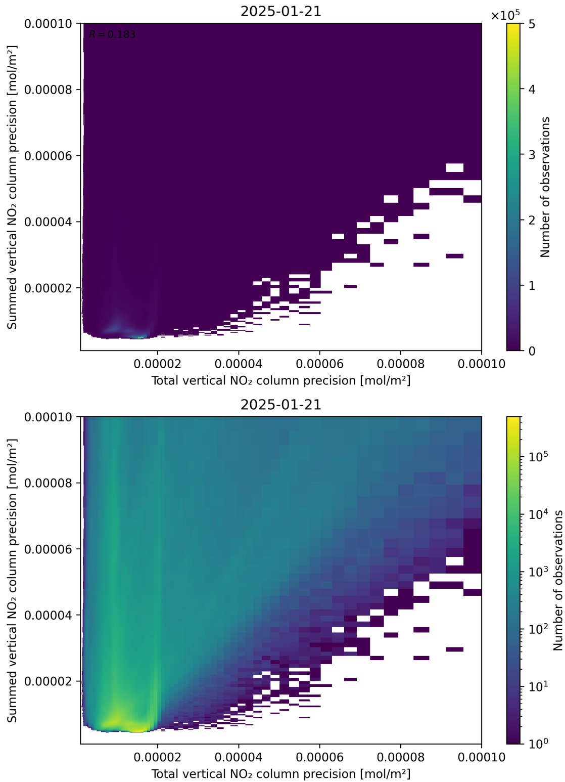
Figure 118: Scatter density plot of “Total vertical NO 2 column precision” against “Summed vertical NO 2 column precision” for 2025-01-20 to 2025-01-22.
