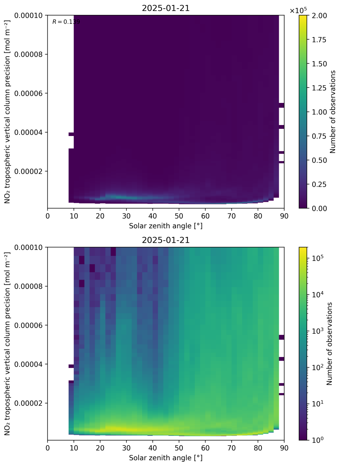
Figure 156: Scatter density plot of “Solar zenith angle” against “NO 2 tropospheric vertical column precision” for 2025-01-20 to 2025-01-22.
