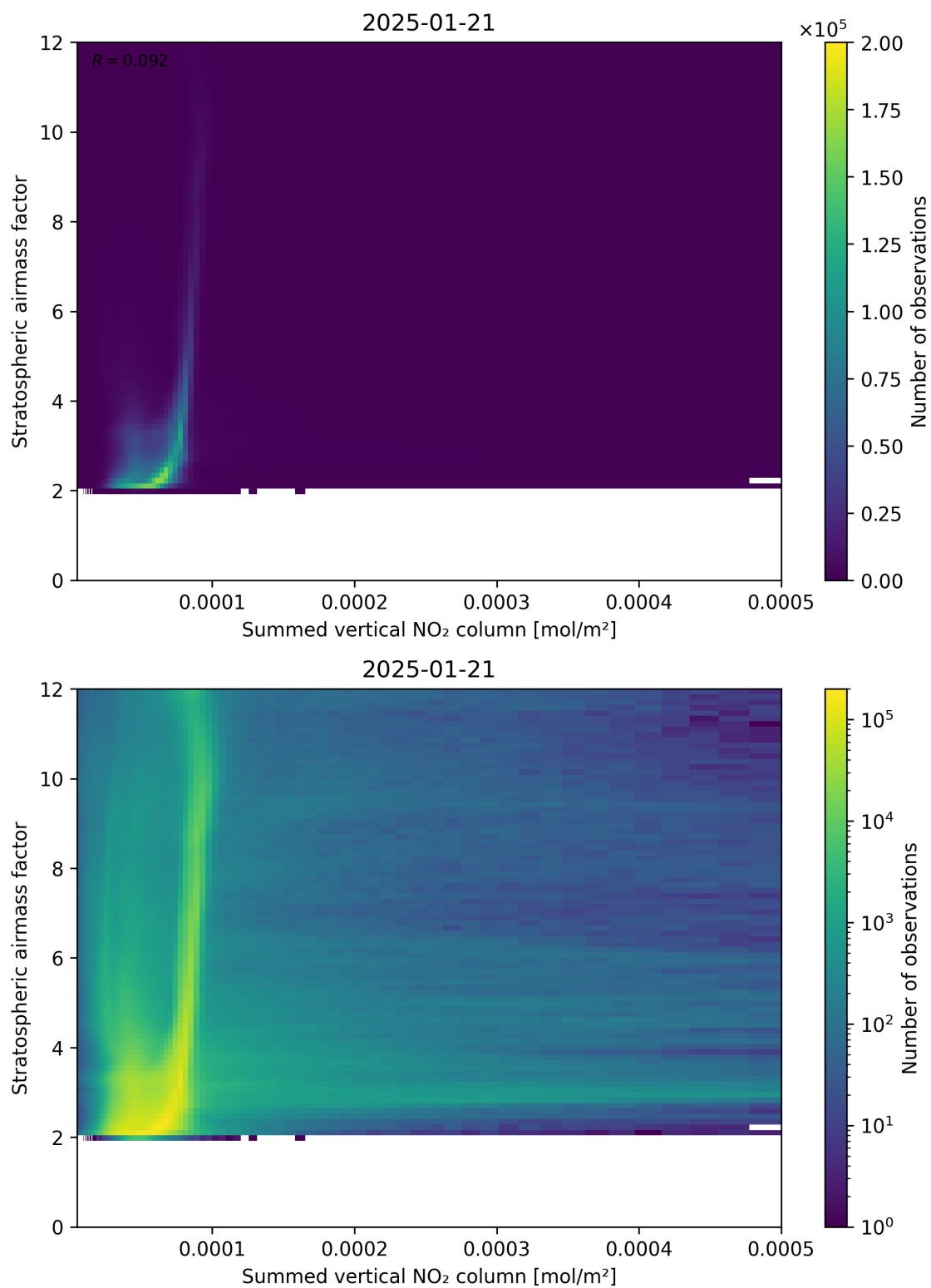
Figure 103: Scatter density plot of “Summed vertical NO 2 column” against “Stratospheric airmass factor” for 2025-01-20 to 2025-01-22.
