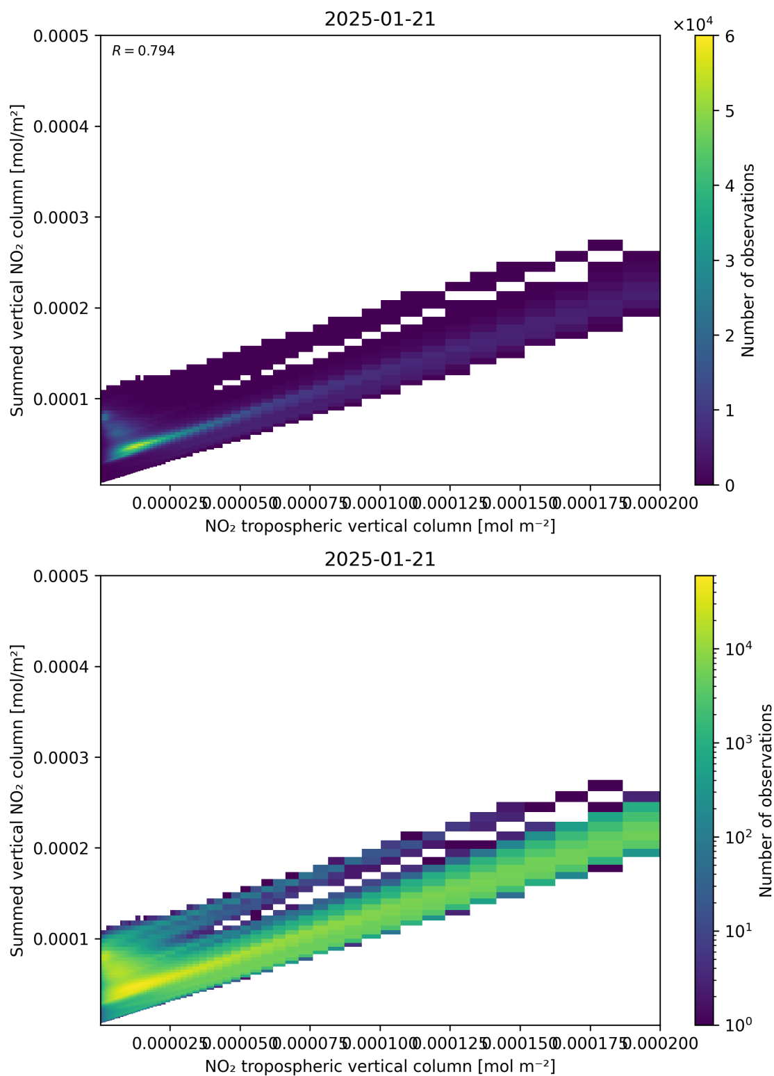
Figure 126: Scatter density plot of “NO 2 tropospheric vertical column” against “Summed vertical NO 2 column” for 2025-01-20 to 2025-01-22.
