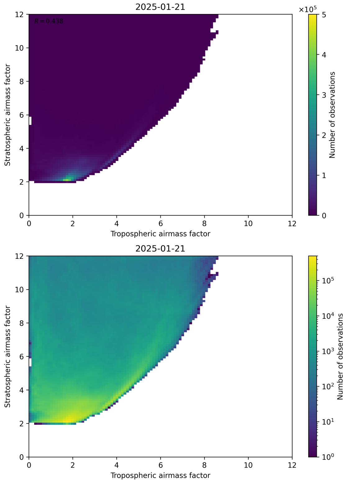
Figure 71: Scatter density plot of “Tropospheric airmass factor” against “Stratospheric airmass factor” for 2025-01-20 to 2025-01-22.
