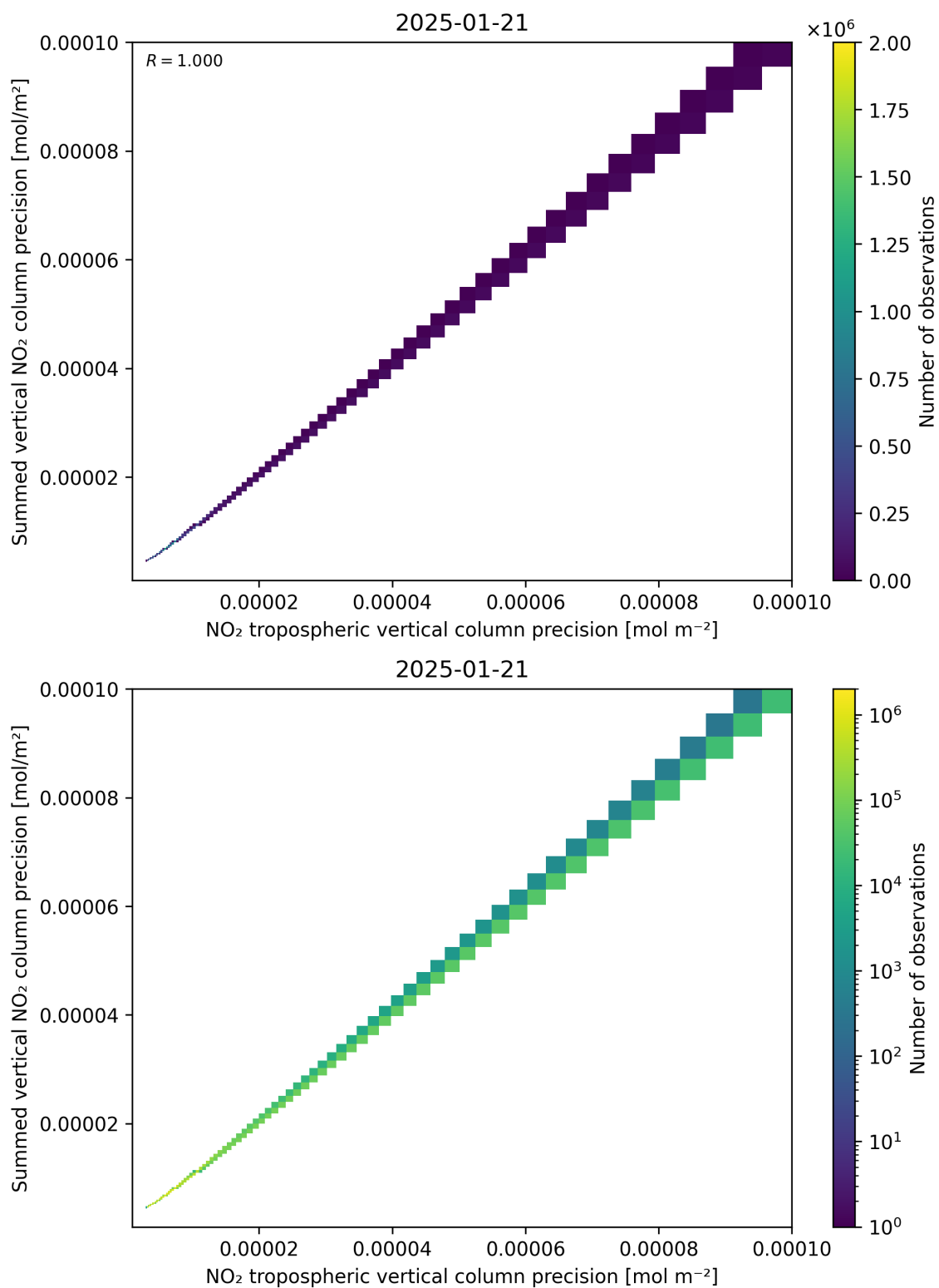
Figure 137: Scatter density plot of “NO 2 tropospheric vertical column precision” against “Summed vertical NO 2 column precision” for 2025-01-20 to 2025-01-22.
