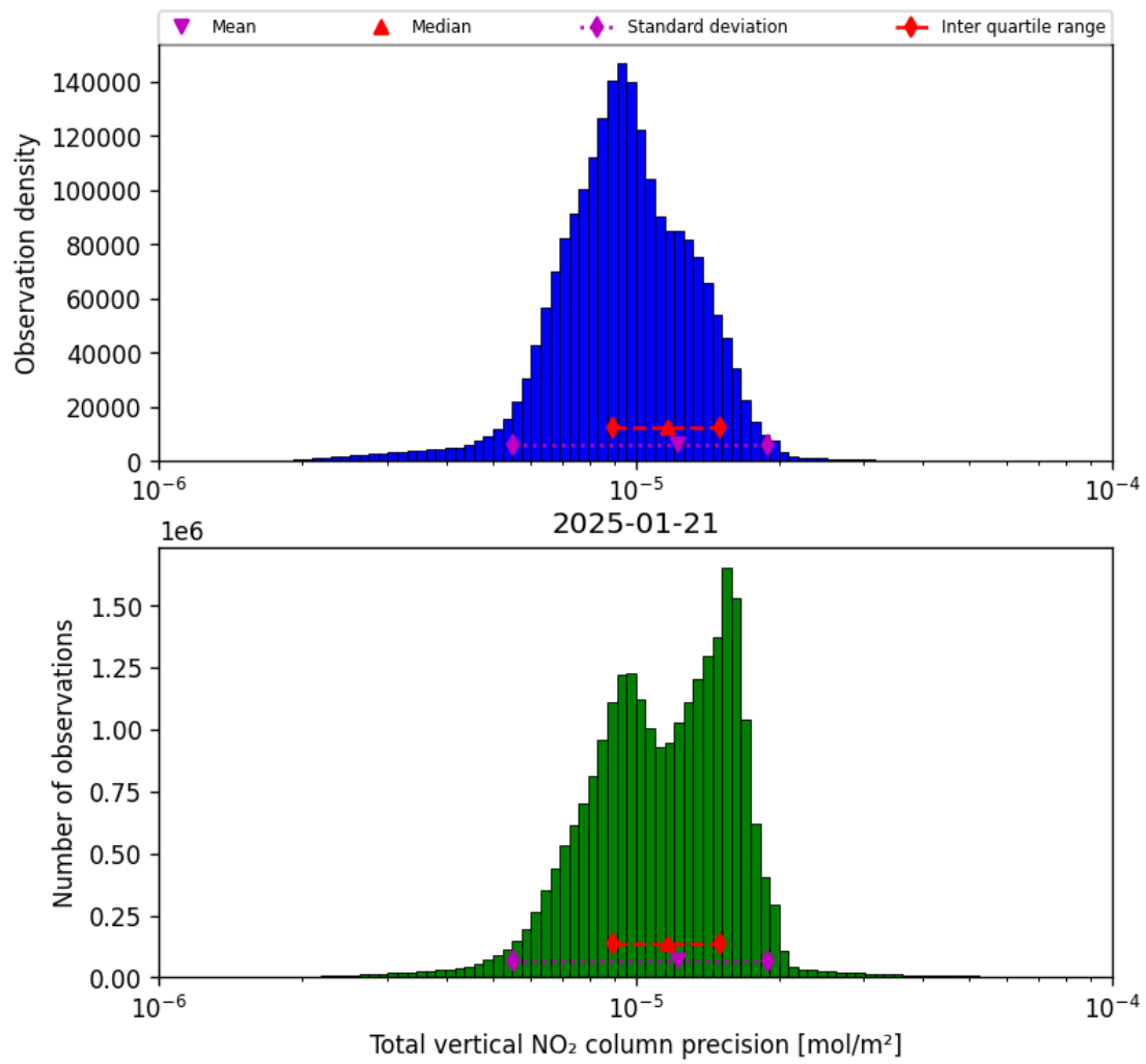
Figure 39: Histogram of “Total vertical NO 2 column precision” for 2025-01-20 to 2025-01-22
