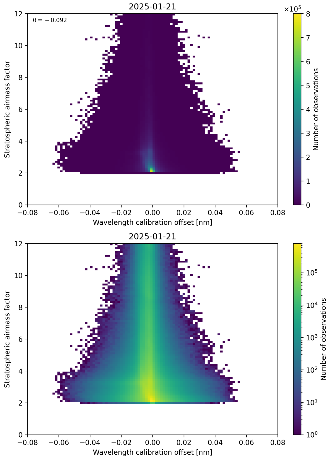
Figure 174: Scatter density plot of “Wavelength calibration offset” against “Stratospheric airmass factor” for 2025-01-20 to 2025-01-22.
