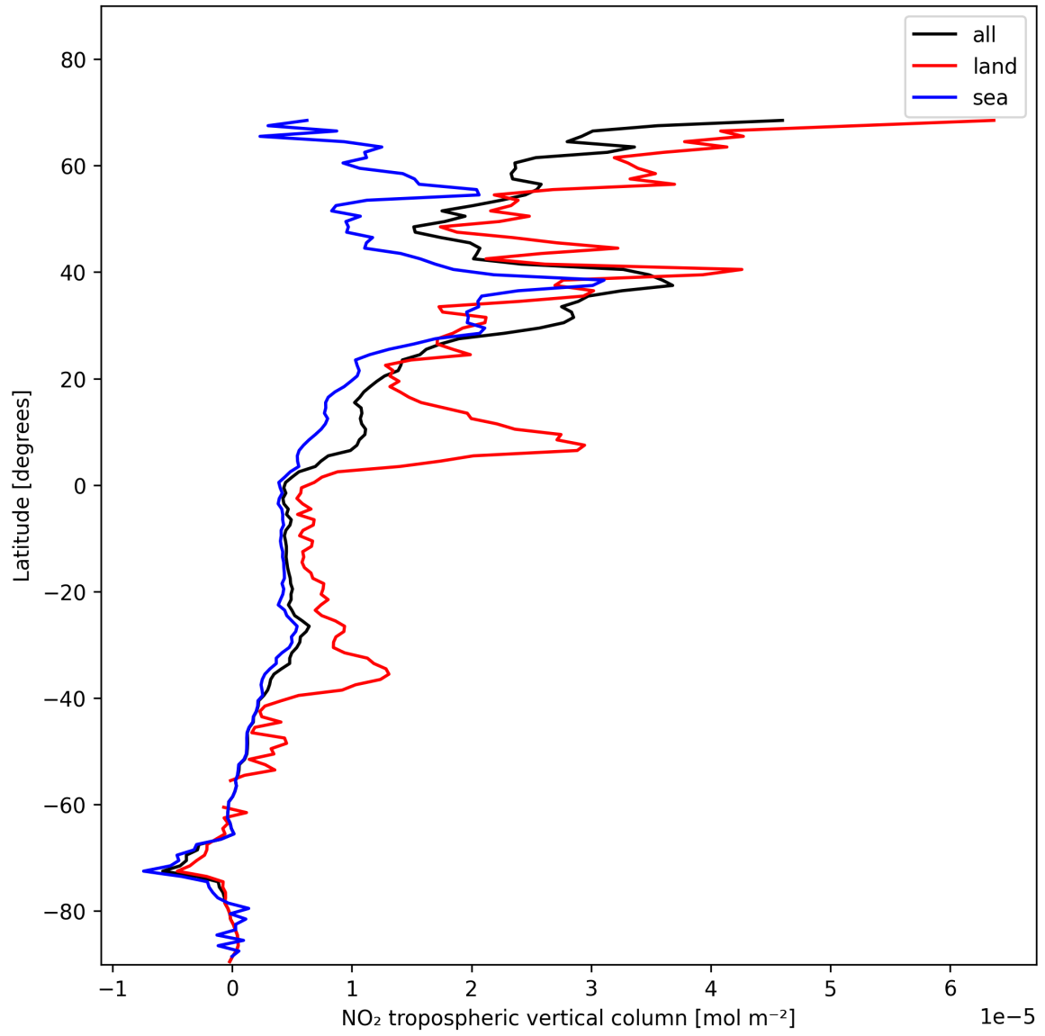
Figure 12: Zonal average of “NO 2 tropospheric vertical column” for 2025-01-20 to 2025-01-22.
