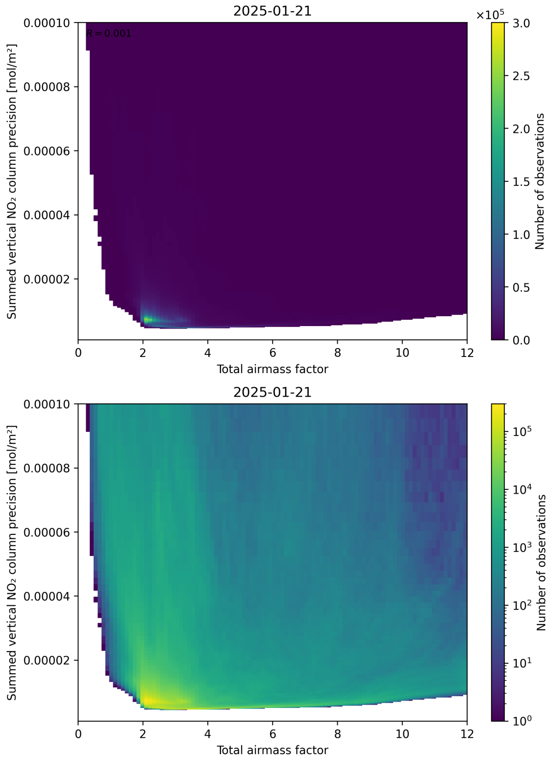
Figure 66: Scatter density plot of “Total airmass factor” against “Summed vertical NO 2 column precision” for 2025-01-20 to 2025-01-22.
