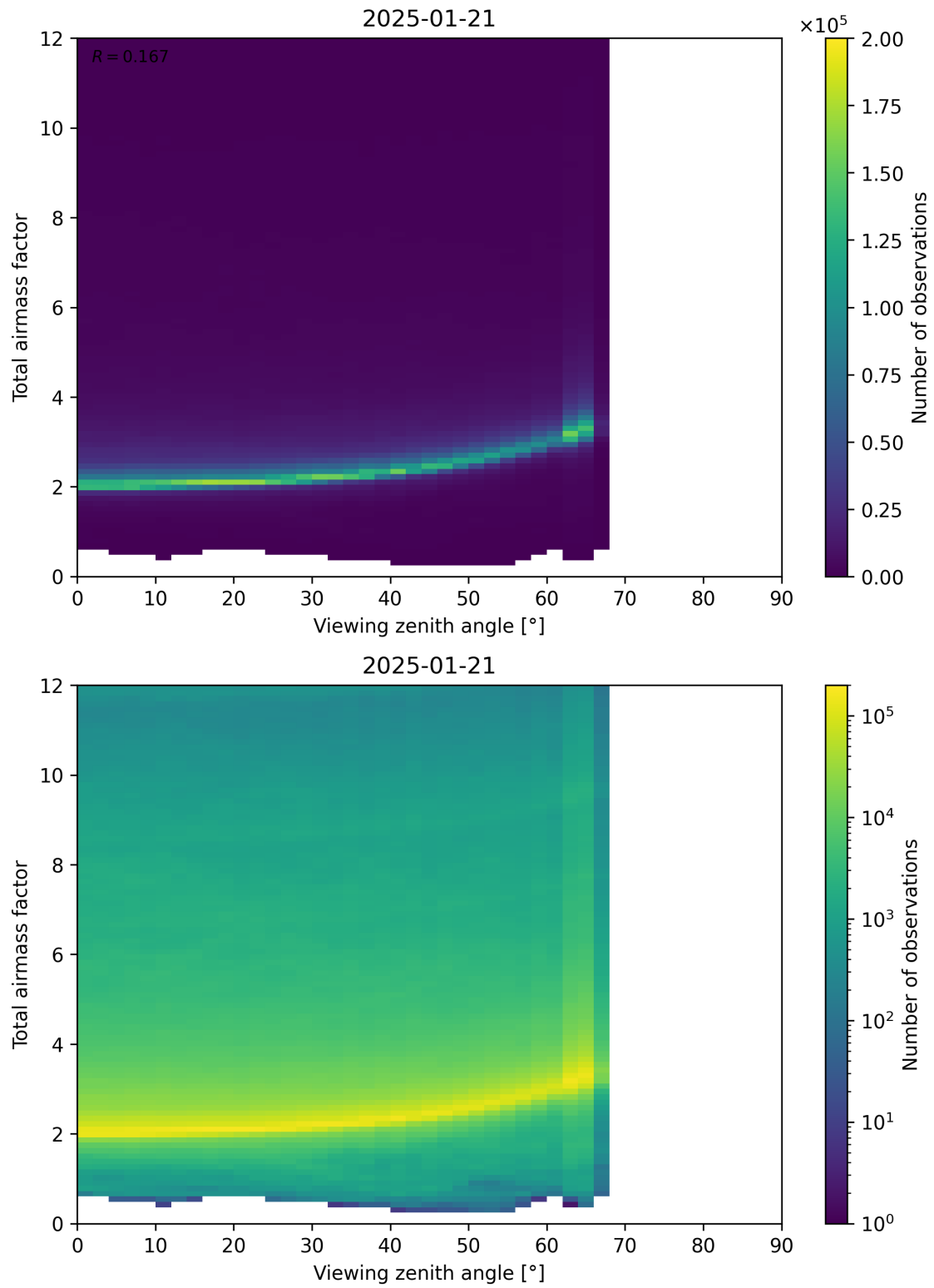
Figure 160: Scatter density plot of “Viewing zenith angle” against “Total airmass factor” for 2025-01-20 to 2025-01-22.
