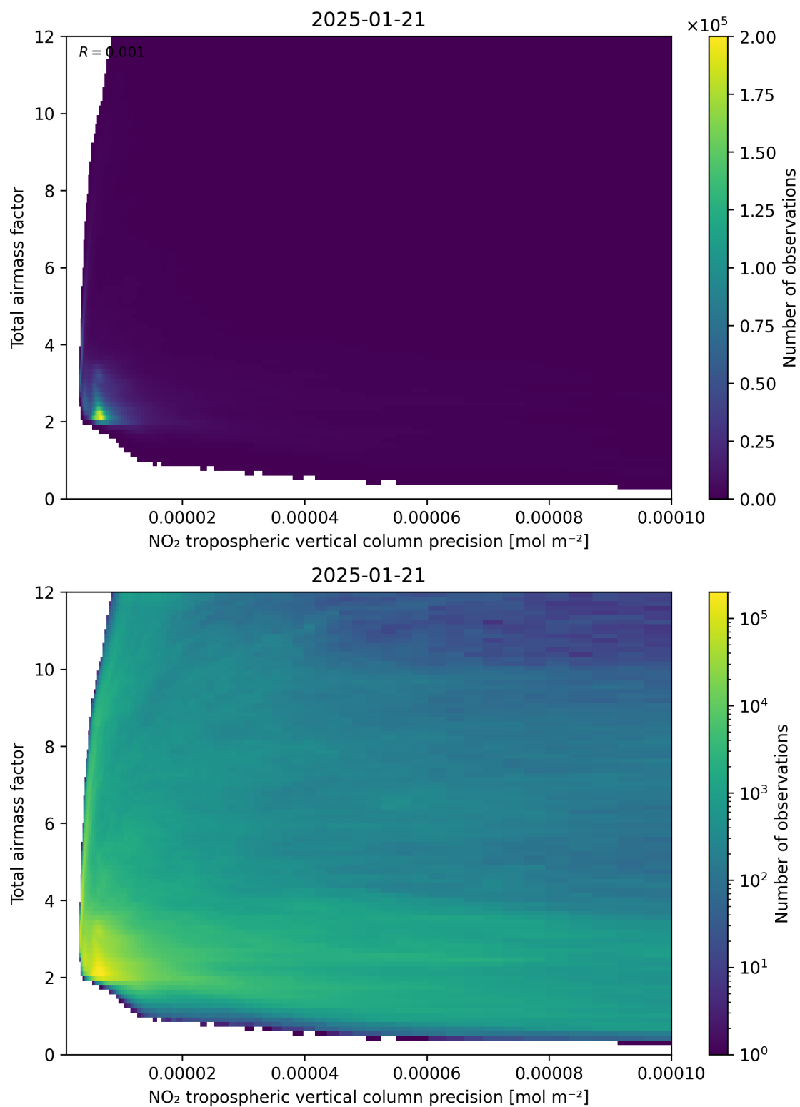
Figure 132: Scatter density plot of “NO 2 tropospheric vertical column precision” against “Total air mass factor” for 2025-01-20 to 2025-01-22.
