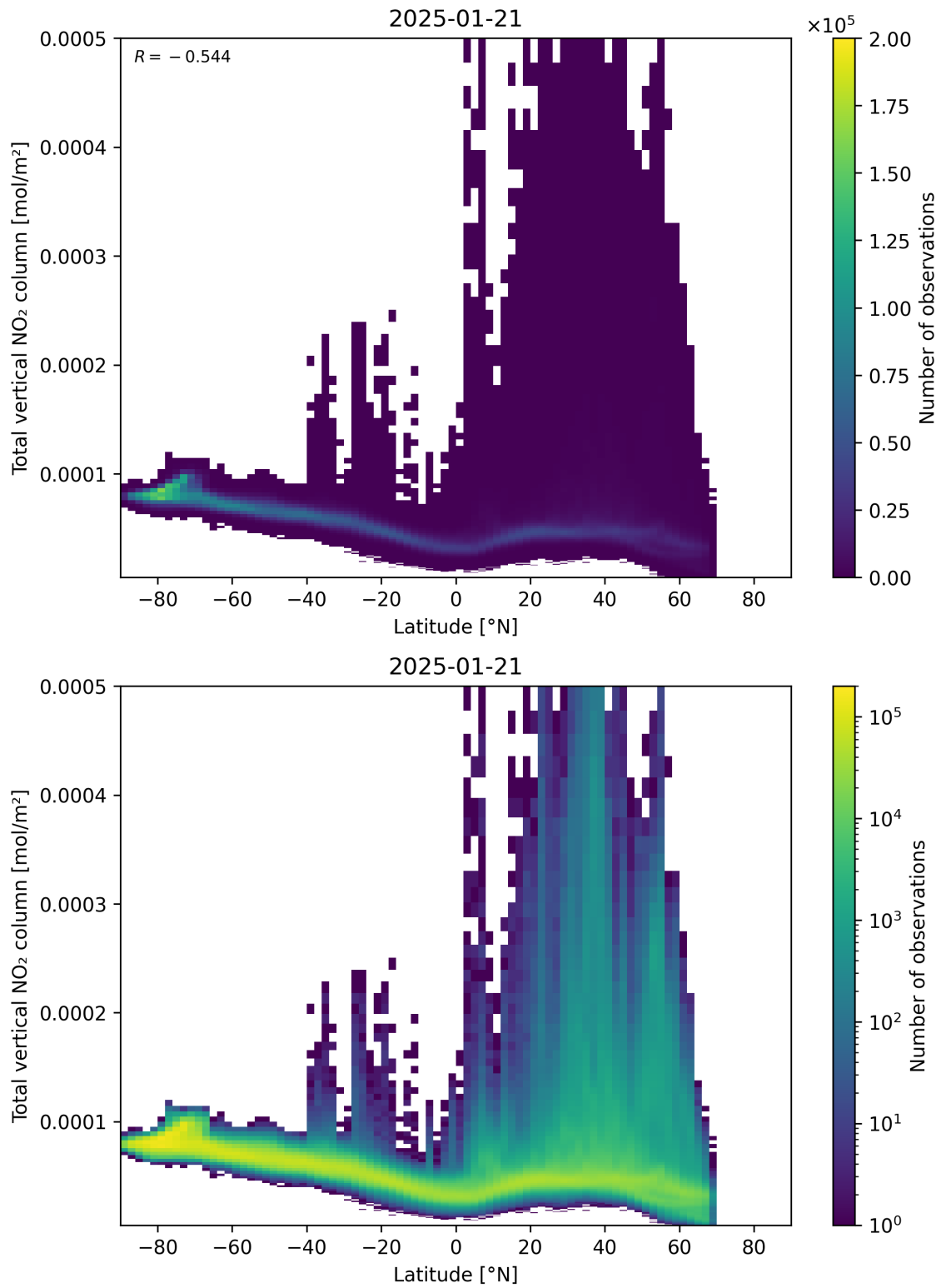
Figure 90: Scatter density plot of “Latitude” against “Total vertical NO 2 column” for 2025-01-20 to 2025-01-22.
