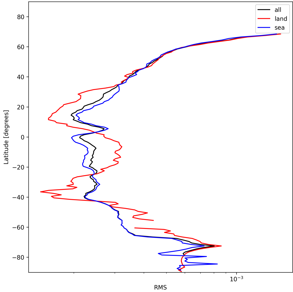
Figure 26: Zonal average of “RMS” for 2025-01-20 to 2025-01-22.
