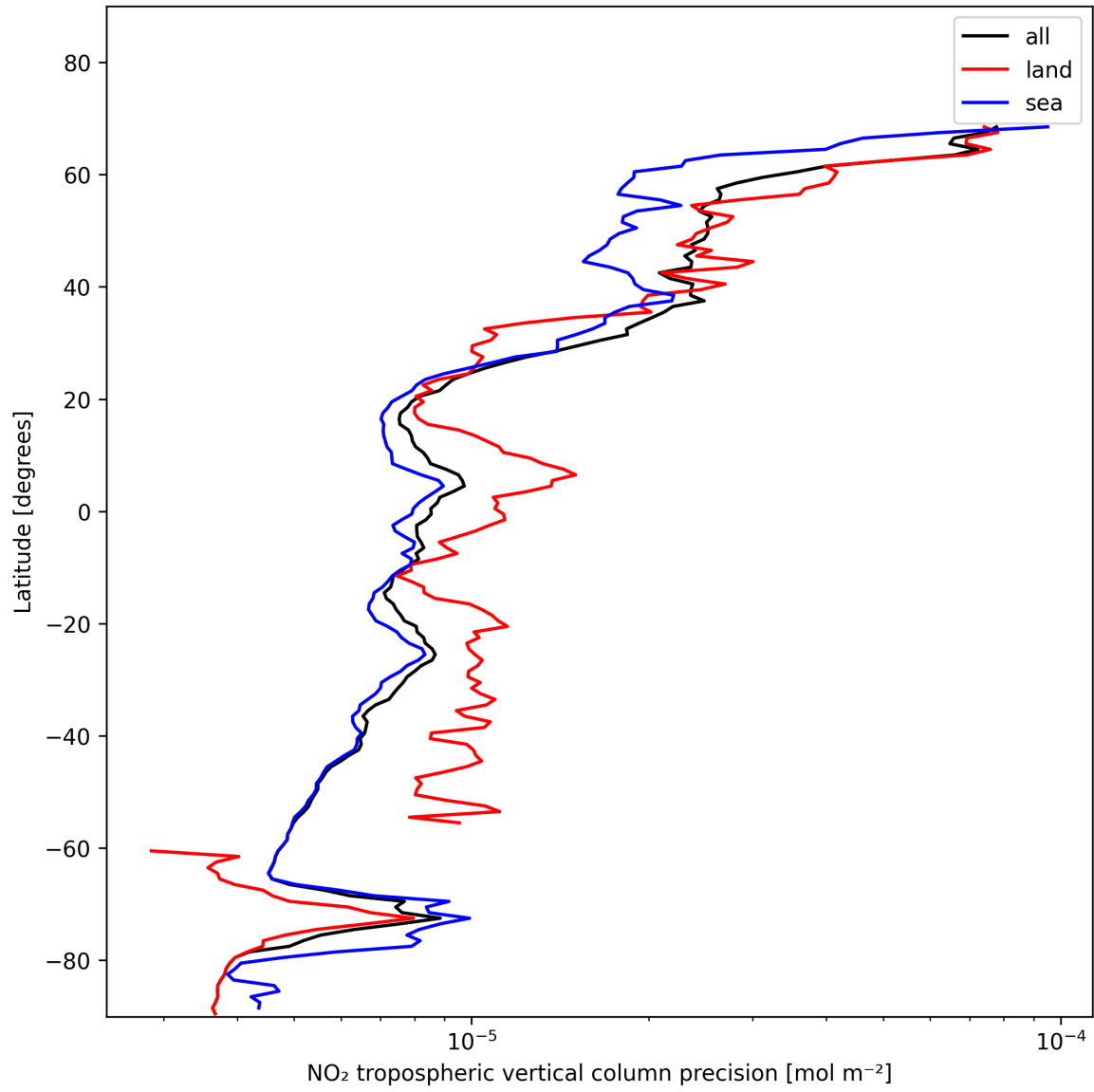
Figure 13: Zonal average of “NO 2 tropospheric vertical column precision” for 2025-01-20 to 2025-01-22.
