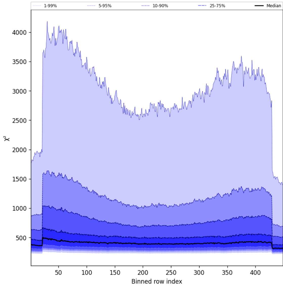
Figure 59: Along track statistics of “ \chi^2 ” for 2025-01-20 to 2025-01-22
