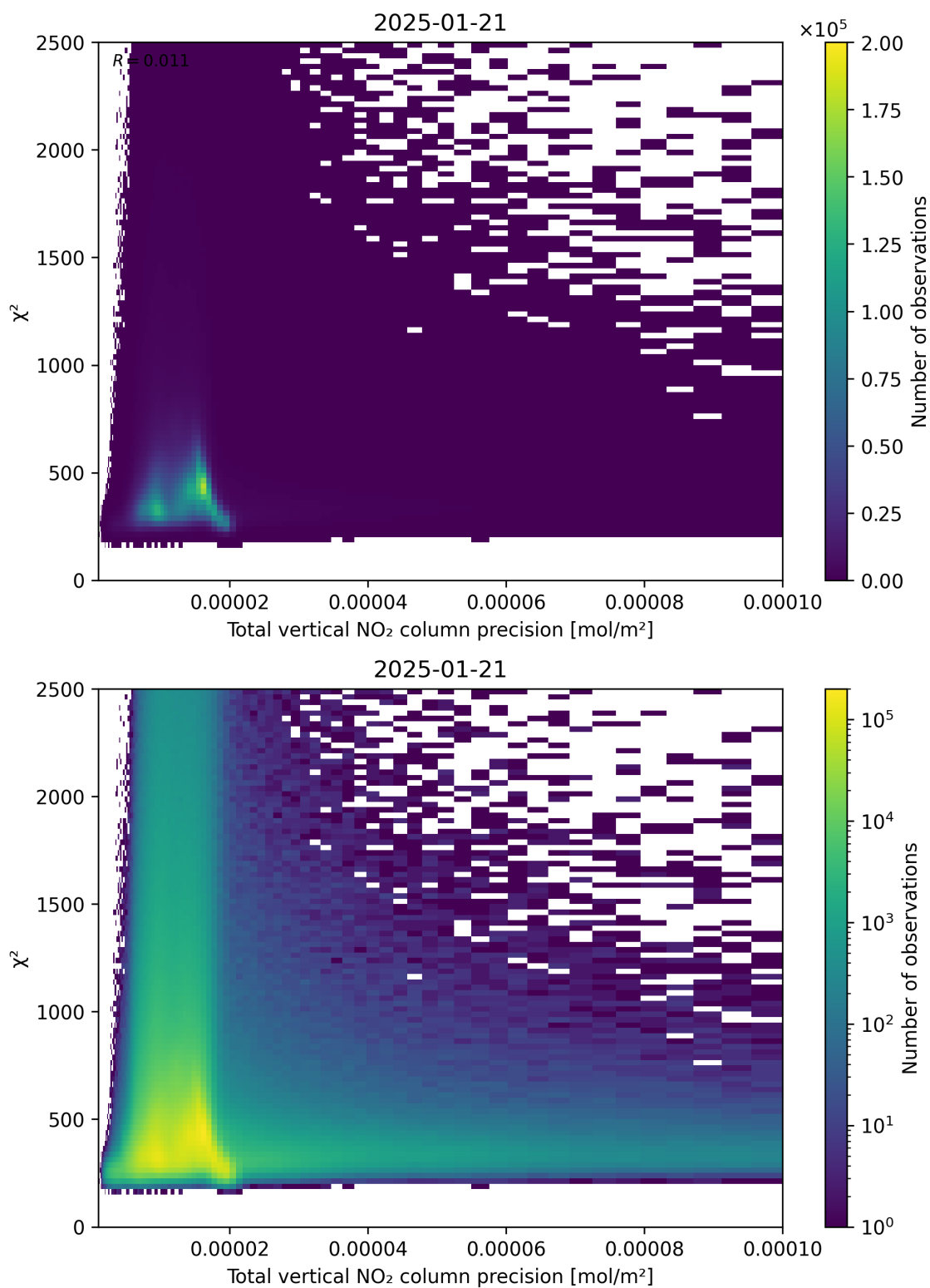
Figure 116: Scatter density plot of “Total vertical NO 2 column precision” against “ \chi^2 ” for 2025-01-20 to 2025-01-22.
