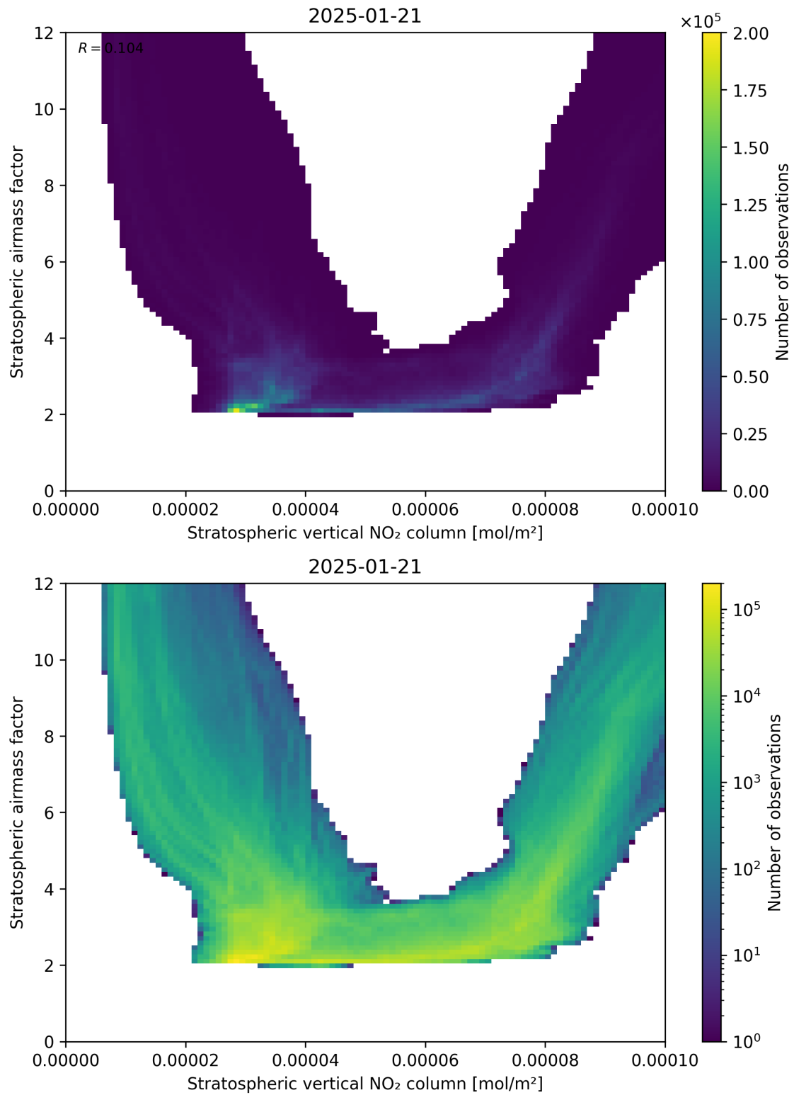
Figure 96: Scatter density plot of “Stratospheric vertical NO 2 column” against “Stratospheric airmass factor” for 2025-01-20 to 2025-01-22.
