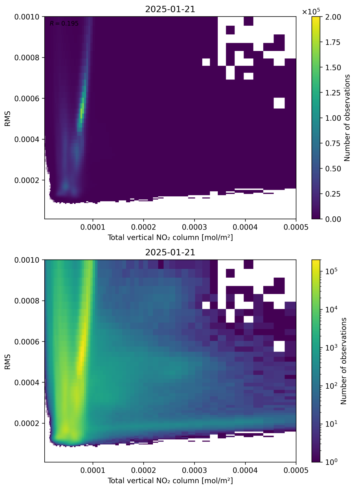
Figure 120: Scatter density plot of “Total vertical NO 2 column” against “RMS” for 2025-01-20 to 2025-01-22.
