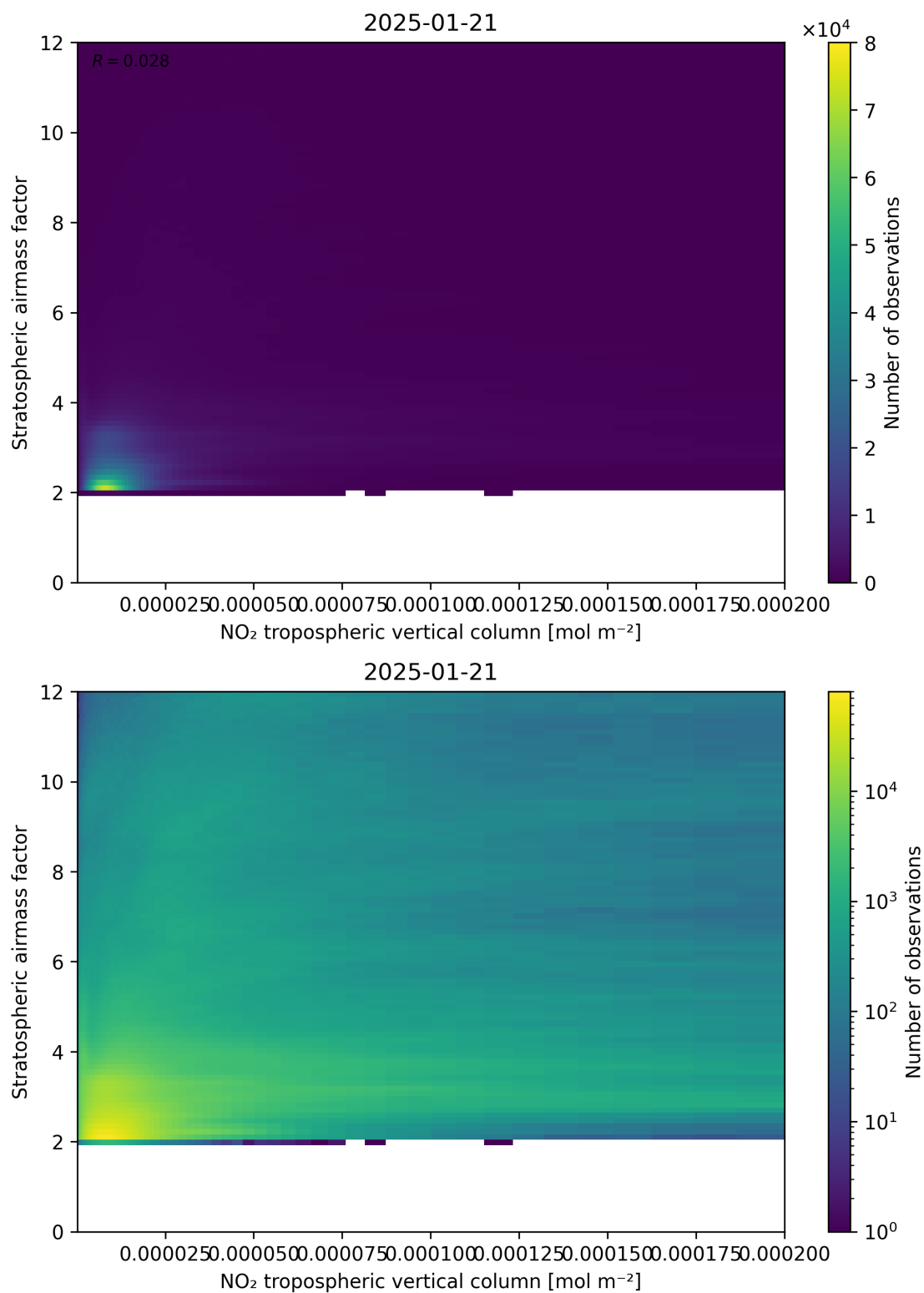
Figure 121: Scatter density plot of “NO 2 tropospheric vertical column” against “Stratospheric airmass factor” for 2025-01-20 to 2025-01-22.
