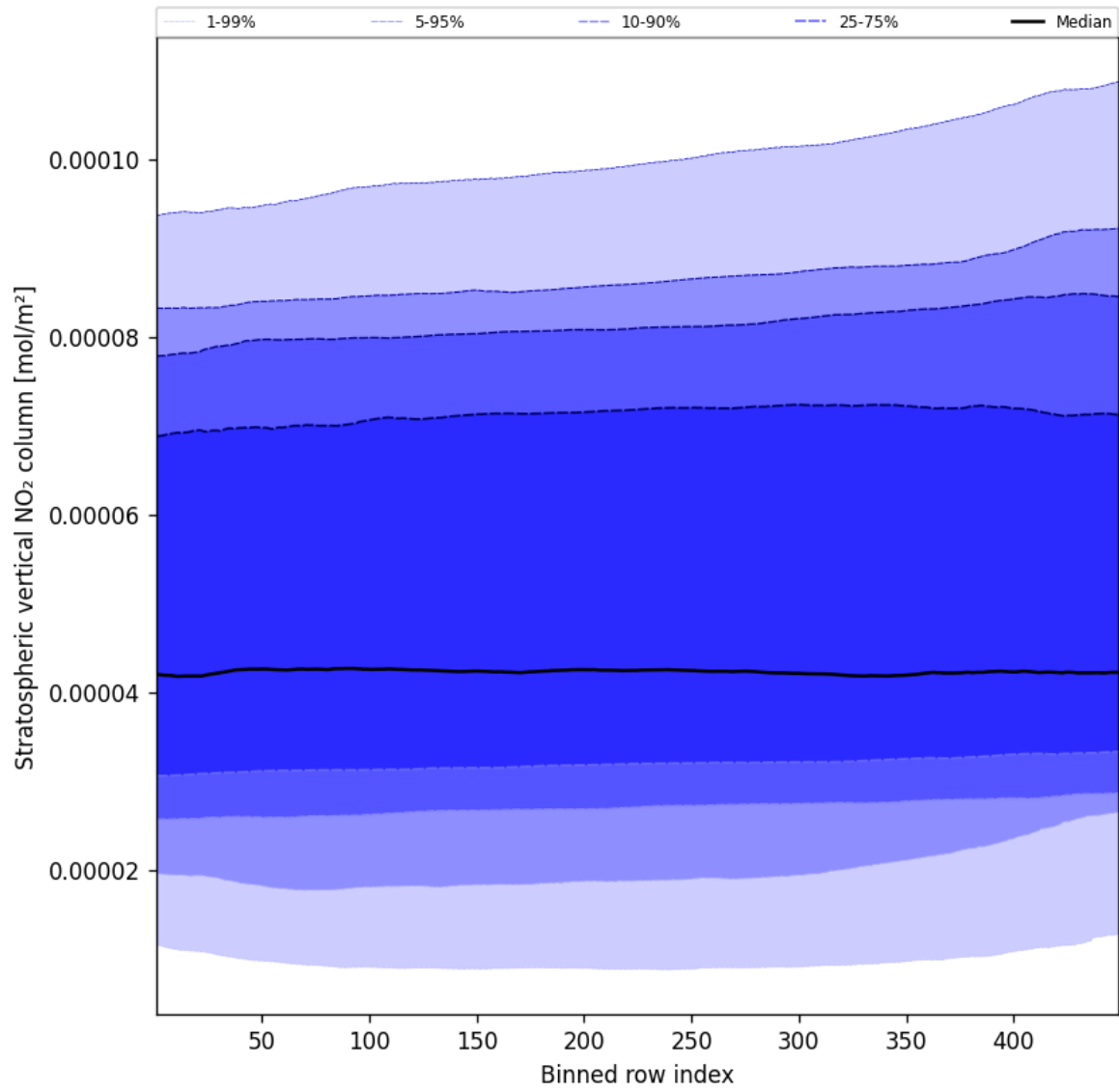
Figure 53: Along track statistics of “Stratospheric vertical NO 2 column” for 2025-01-20 to 2025-01-22
