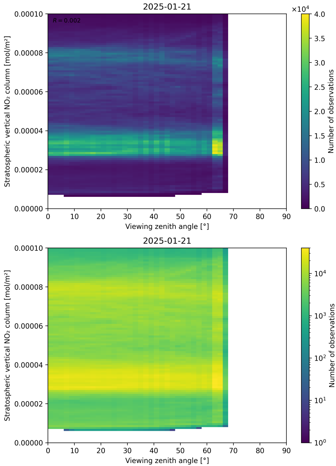
Figure 164: Scatter density plot of “Viewing zenith angle” against “Stratospheric vertical NO 2 column” for 2025-01-20 to 2025-01-22.
