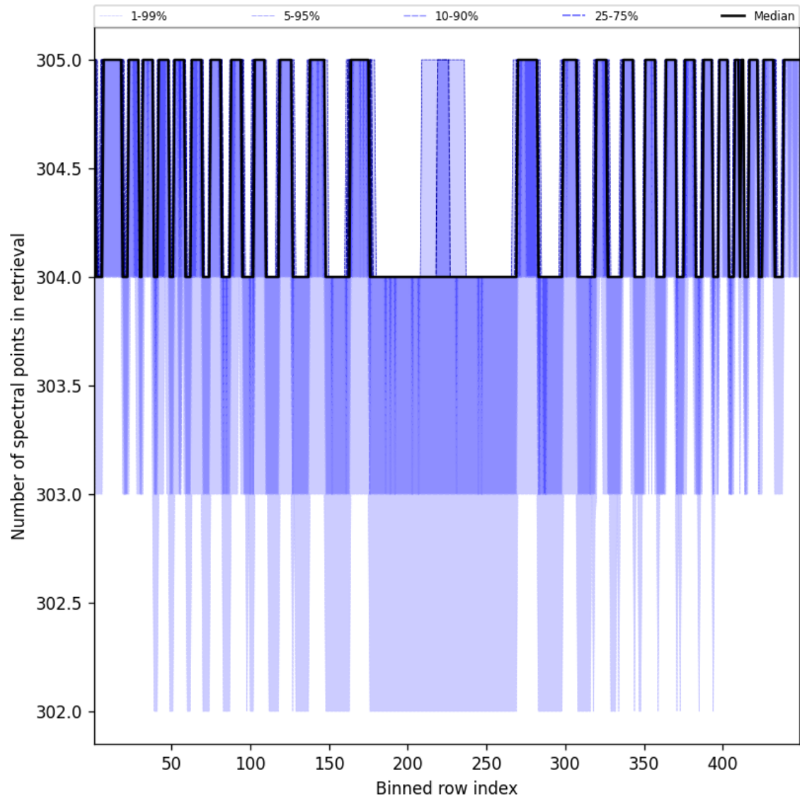
Figure 50: Along track statistics of “Number of spectral points in retrieval” for 2025-01-20 to 2025-01-22
