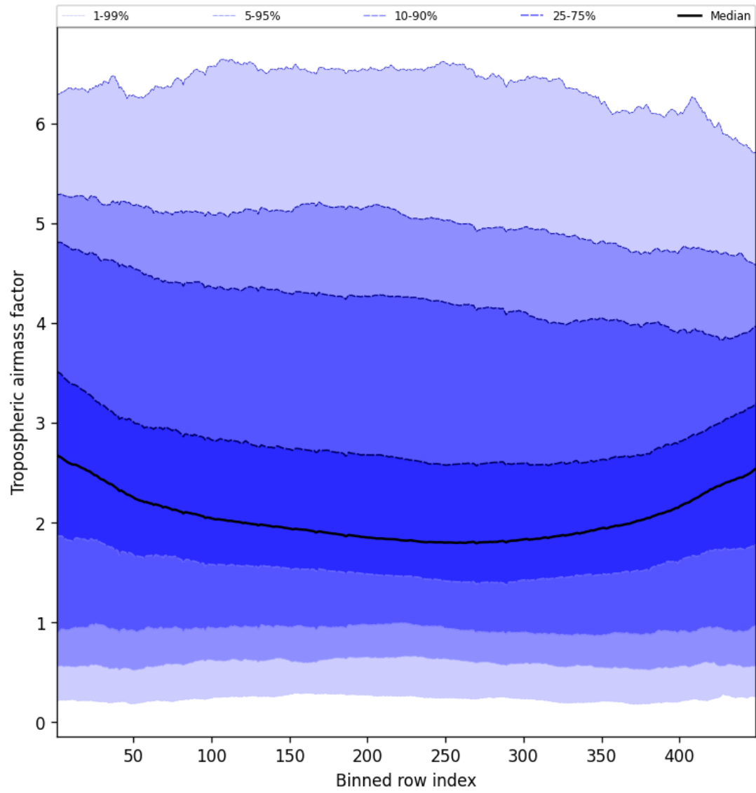
Figure 48: Along track statistics of “Tropospheric airmass factor” for 2025-01-20 to 2025-01-22
