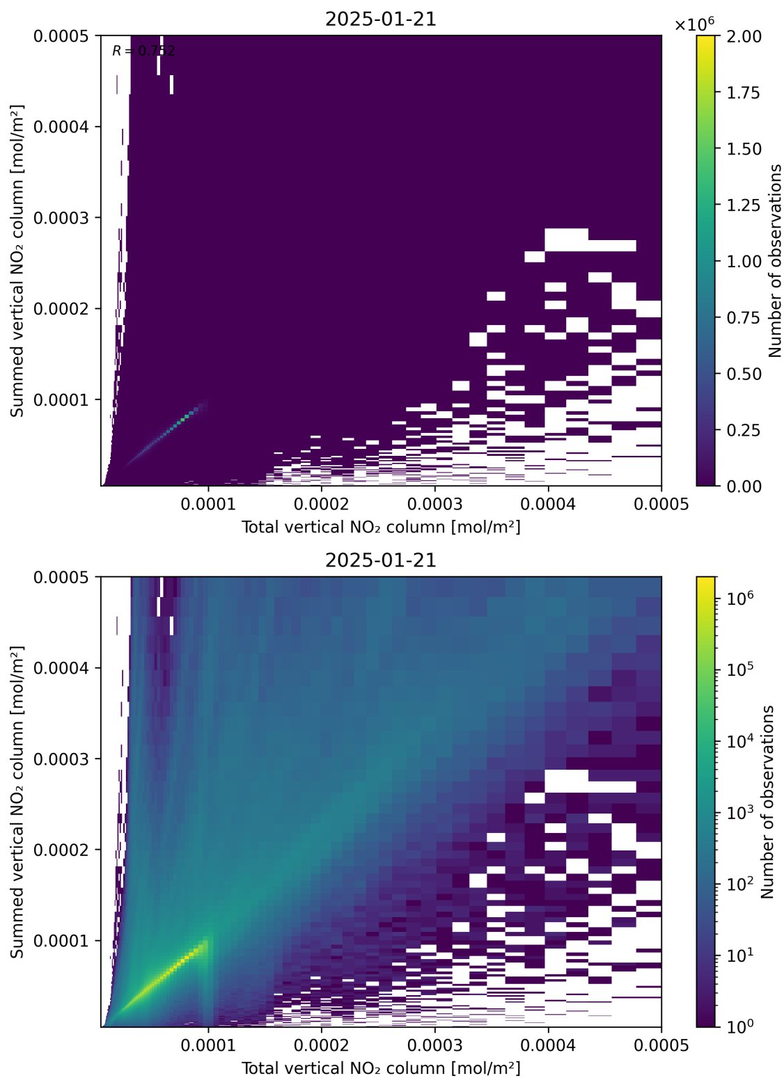
Figure 112: Scatter density plot of “Total vertical NO 2 column” against “Summed vertical NO 2 column” for 2025-01-20 to 2025-01-22.
