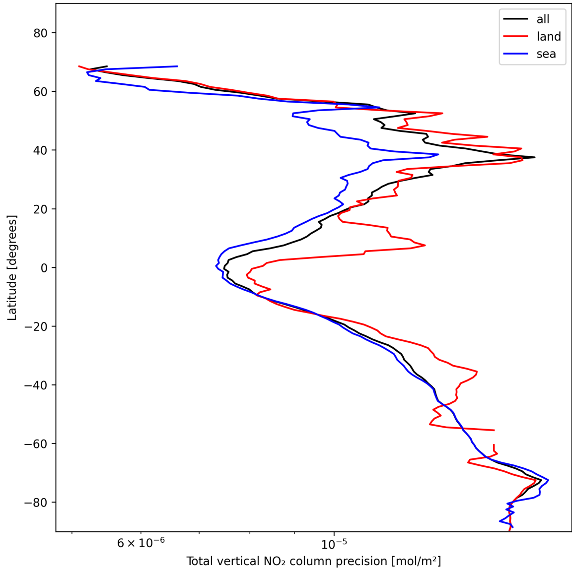
Figure 22: Zonal average of “Total vertical NO 2 column precision” for 2025-01-20 to 2025-01-22.
