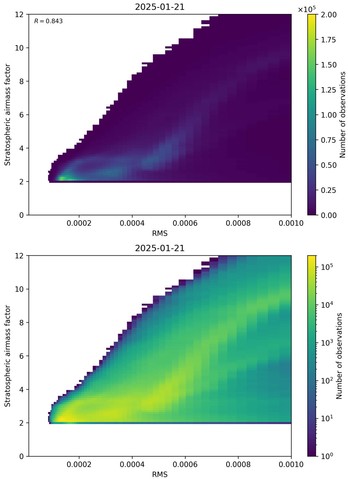
Figure 144: Scatter density plot of “RMS” against “Stratospheric airmass factor” for 2025-01-20 to 2025-01-22.
