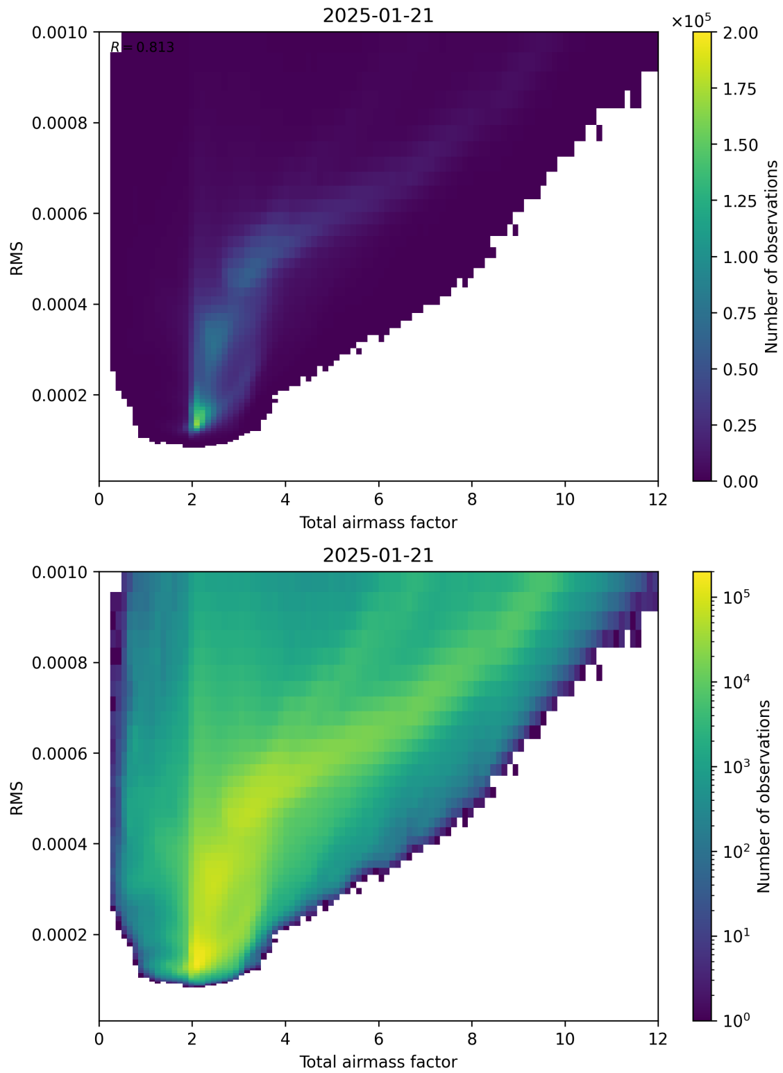
Figure 69: Scatter density plot of “Total airmass factor” against “RMS” for 2025-01-20 to 2025-01-22.
