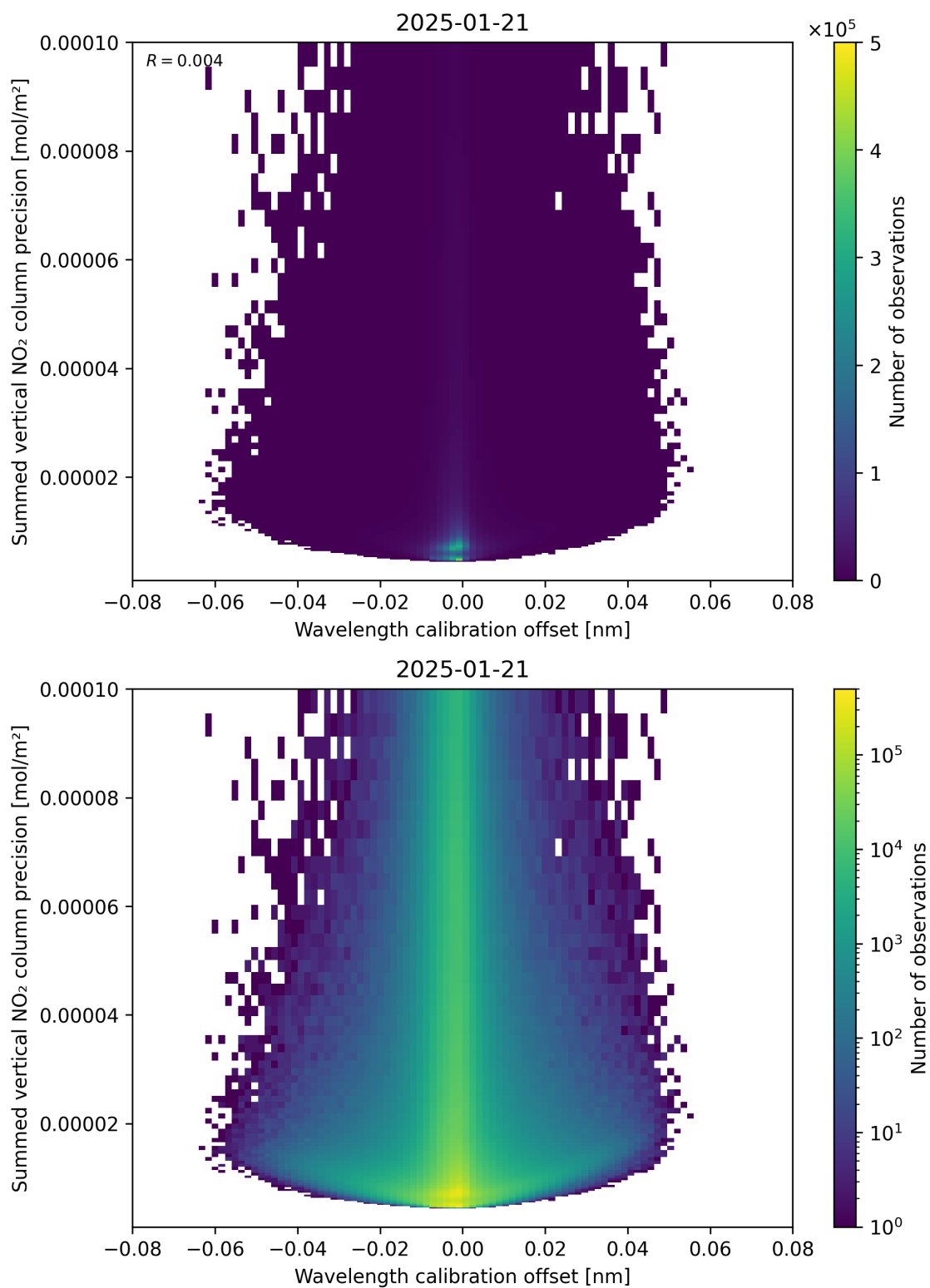
Figure 178: Scatter density plot of “Wavelength calibration offset” against “Summed vertical NO 2 column precision” for 2025-01-20 to 2025-01-22.
