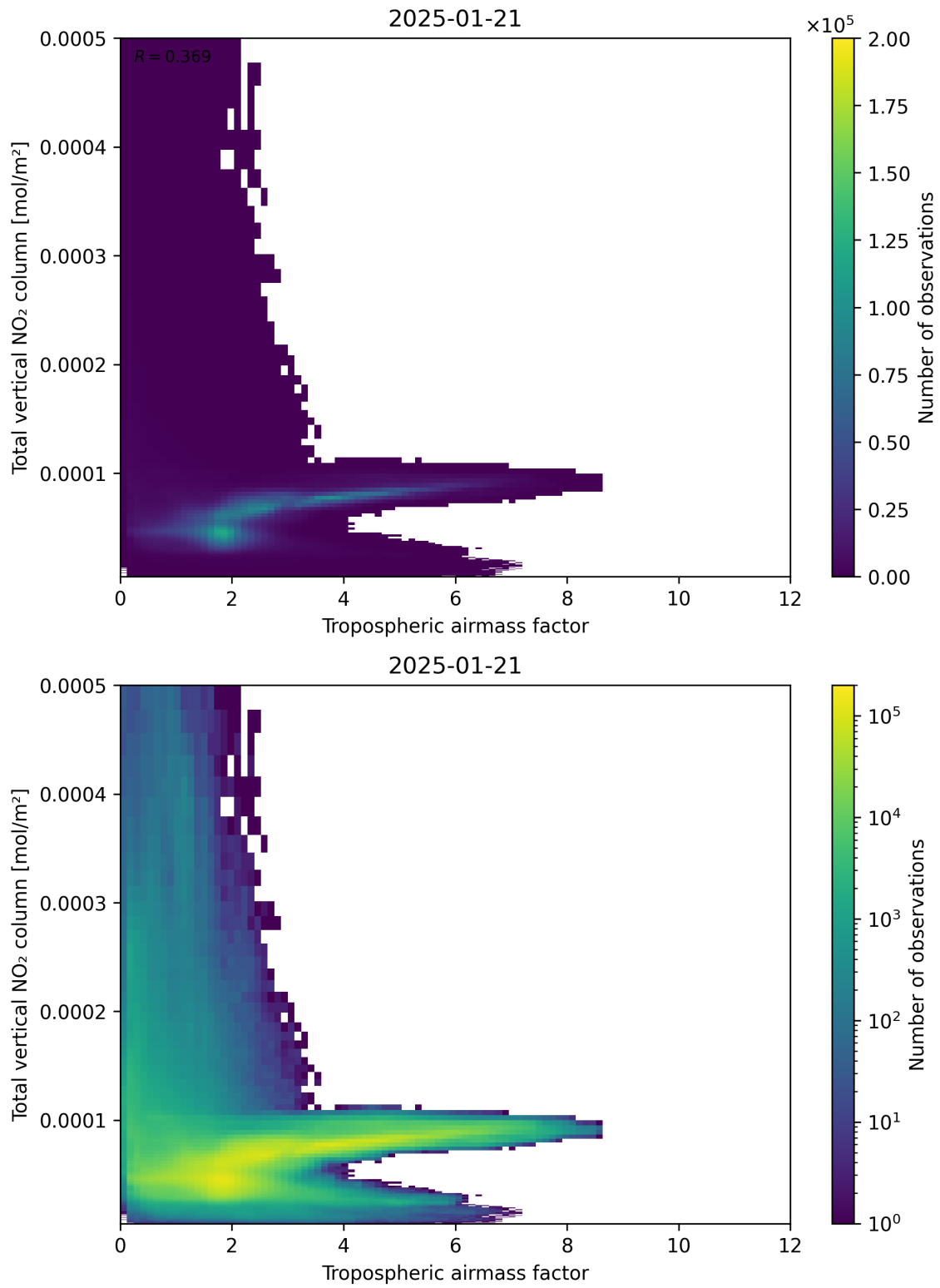
Figure 77: Scatter density plot of “Tropospheric airmass factor” against “Total vertical NO 2 column” for 2025-01-20 to 2025-01-22.
