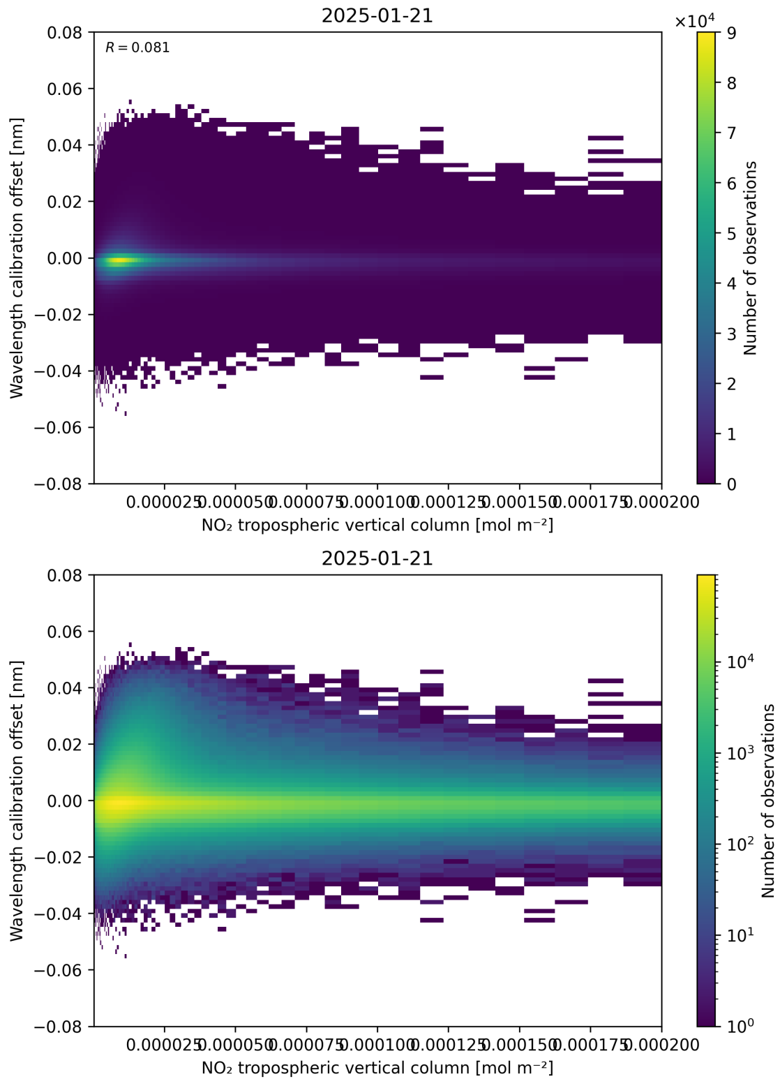
Figure 143: Scatter density plot of “NO 2 tropospheric vertical column” against “Wavelength calibration offset” for 2025-01-20 to 2025-01-22.
