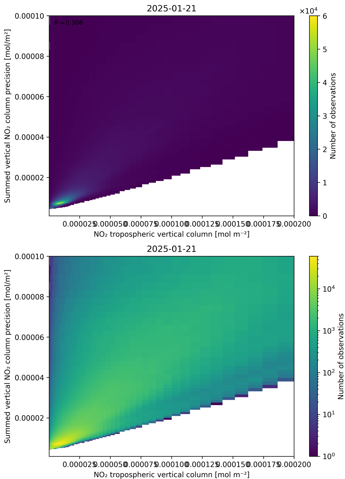
Figure 127: Scatter density plot of “NO 2 tropospheric vertical column” against “Summed vertical NO 2 column precision” for 2025-01-20 to 2025-01-22.
