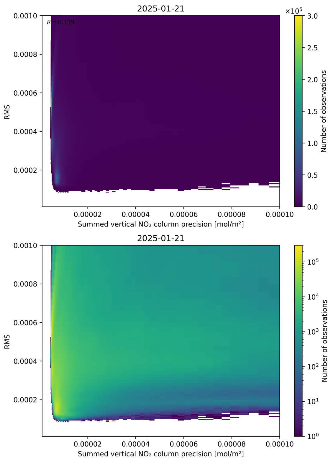
Figure 108: Scatter density plot of “Summed vertical NO 2 column precision” against “RMS” for 2025-01-20 to 2025-01-22.
