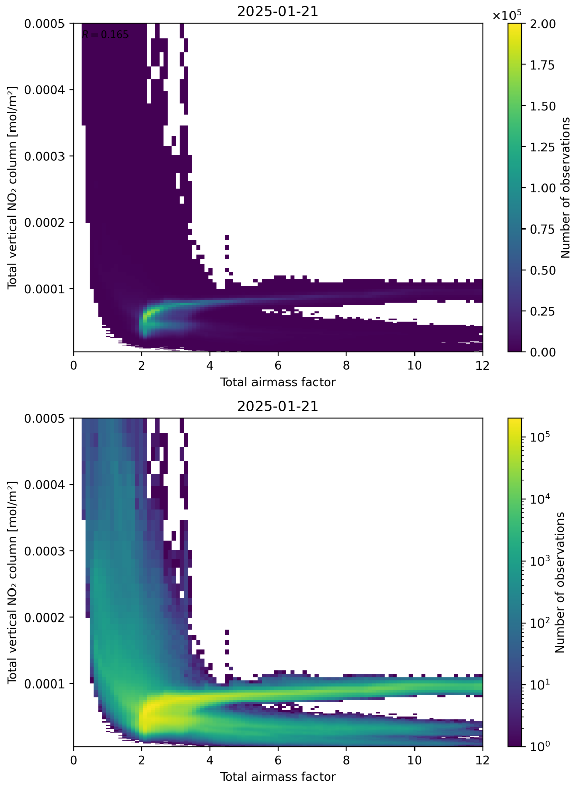
Figure 67: Scatter density plot of “Total airmass factor” against “Total vertical NO 2 column” for 2025-01-20 to 2025-01-22.
