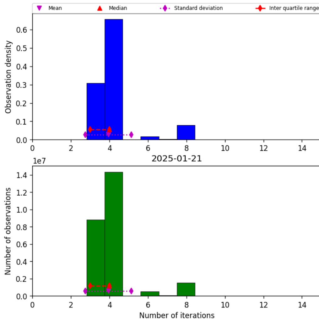
Figure 34: Histogram of “Number of iterations” for 2025-01-20 to 2025-01-22
