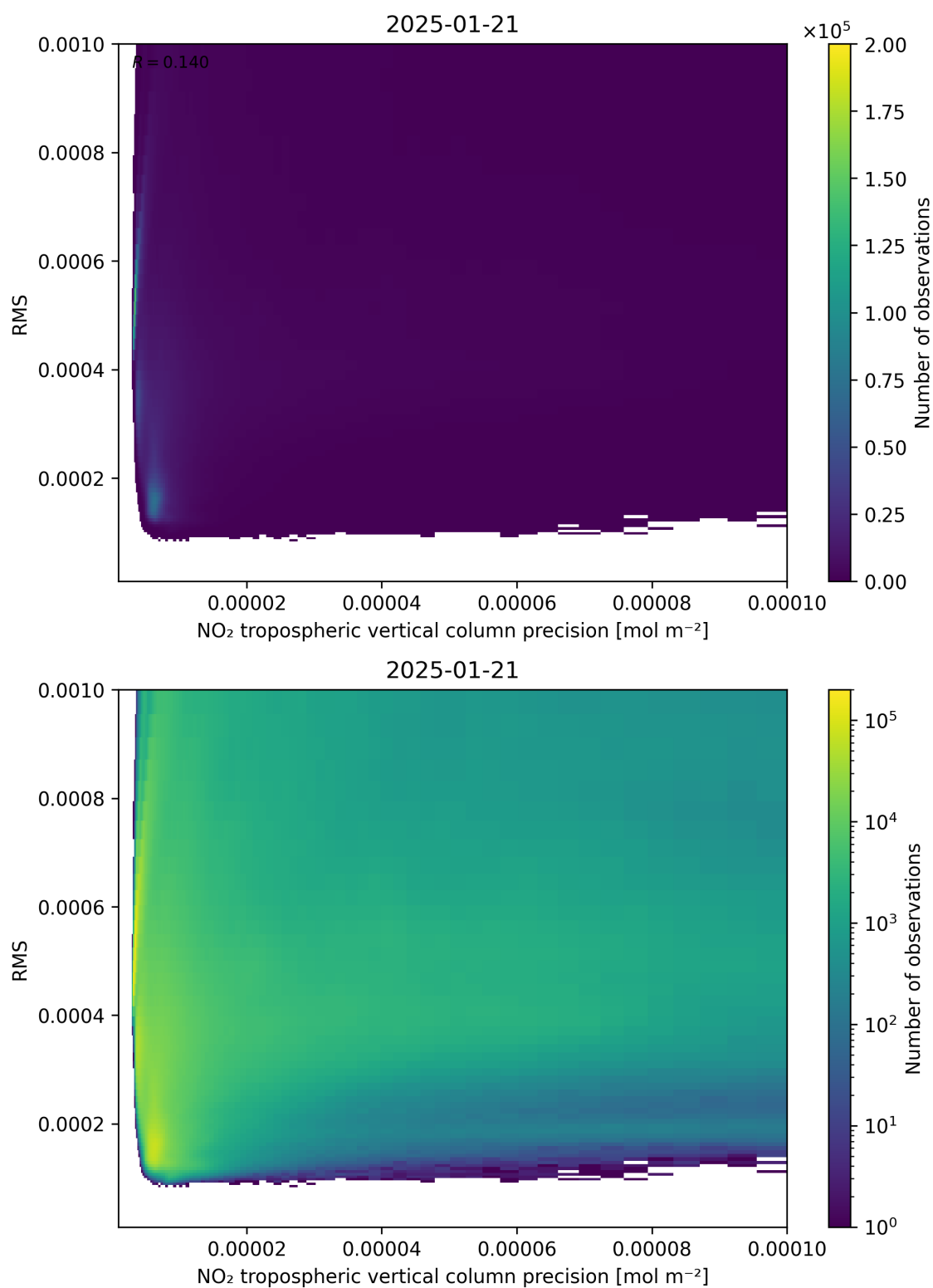
Figure 140: Scatter density plot of “NO 2 tropospheric vertical column precision” against “RMS” for 2025-01-20 to 2025-01-22.
