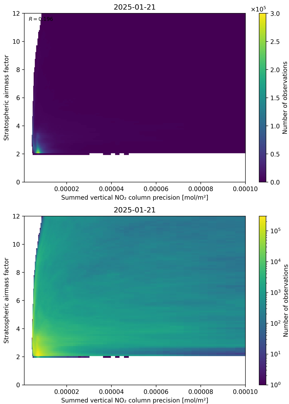
Figure 106: Scatter density plot of “Summed vertical NO 2 column precision” against “Stratospheric airmass factor” for 2025-01-20 to 2025-01-22.
