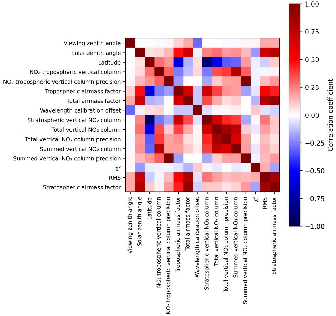
Figure 2: Map of correlation matrix for 2025-01-20 to 2025-01-22.
