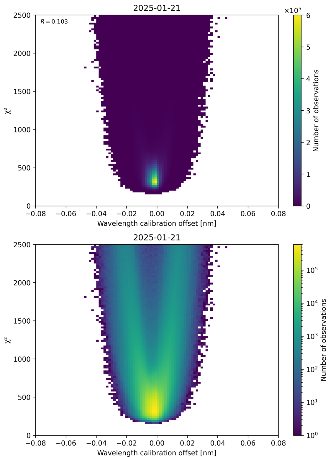
Figure 175: Scatter density plot of “Wavelength calibration offset” against “ \chi^2 ” for 2025-01-20 to 2025-01-22.
