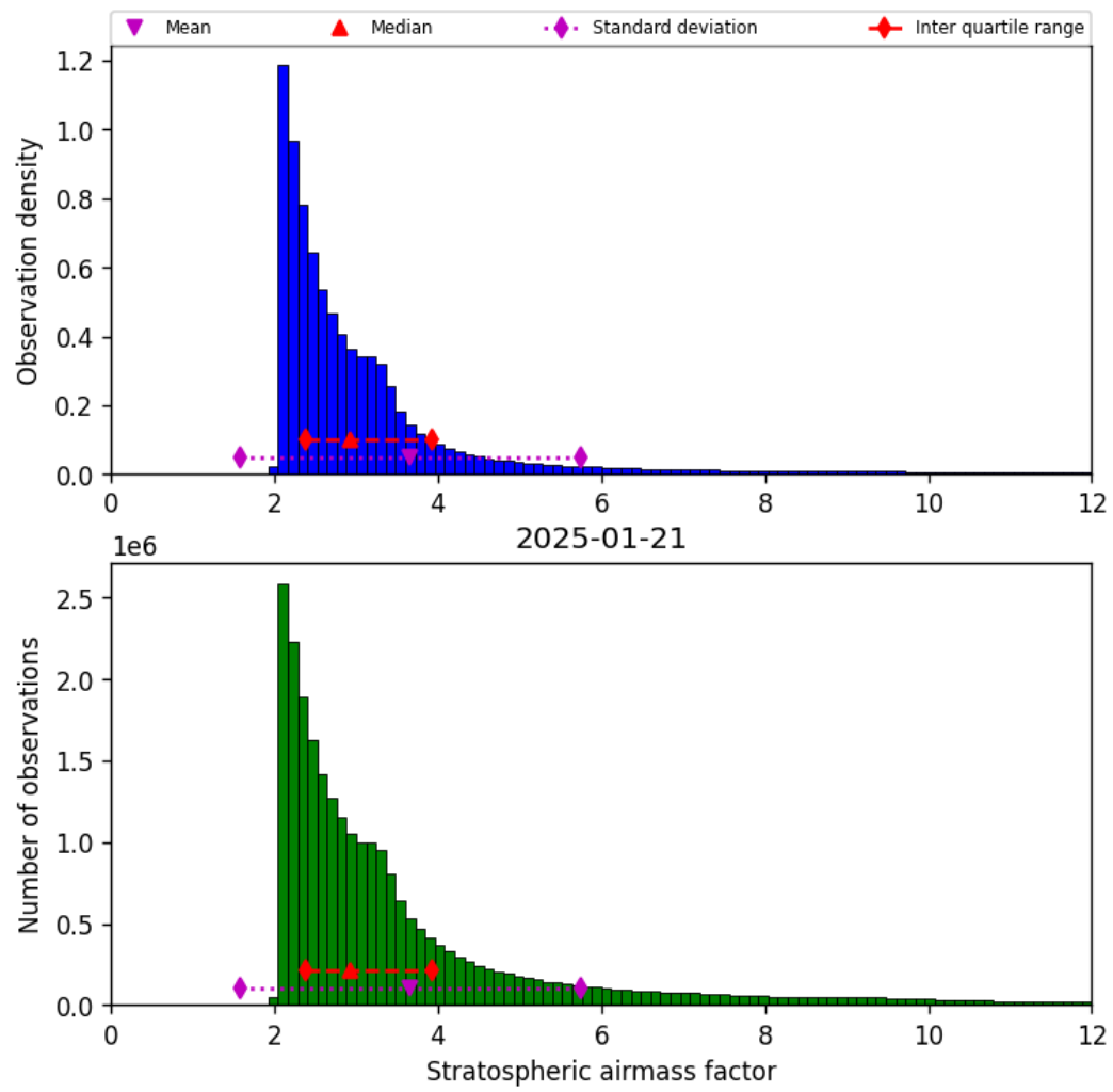
Figure 44: Histogram of “Stratospheric airmass factor” for 2025-01-20 to 2025-01-22
