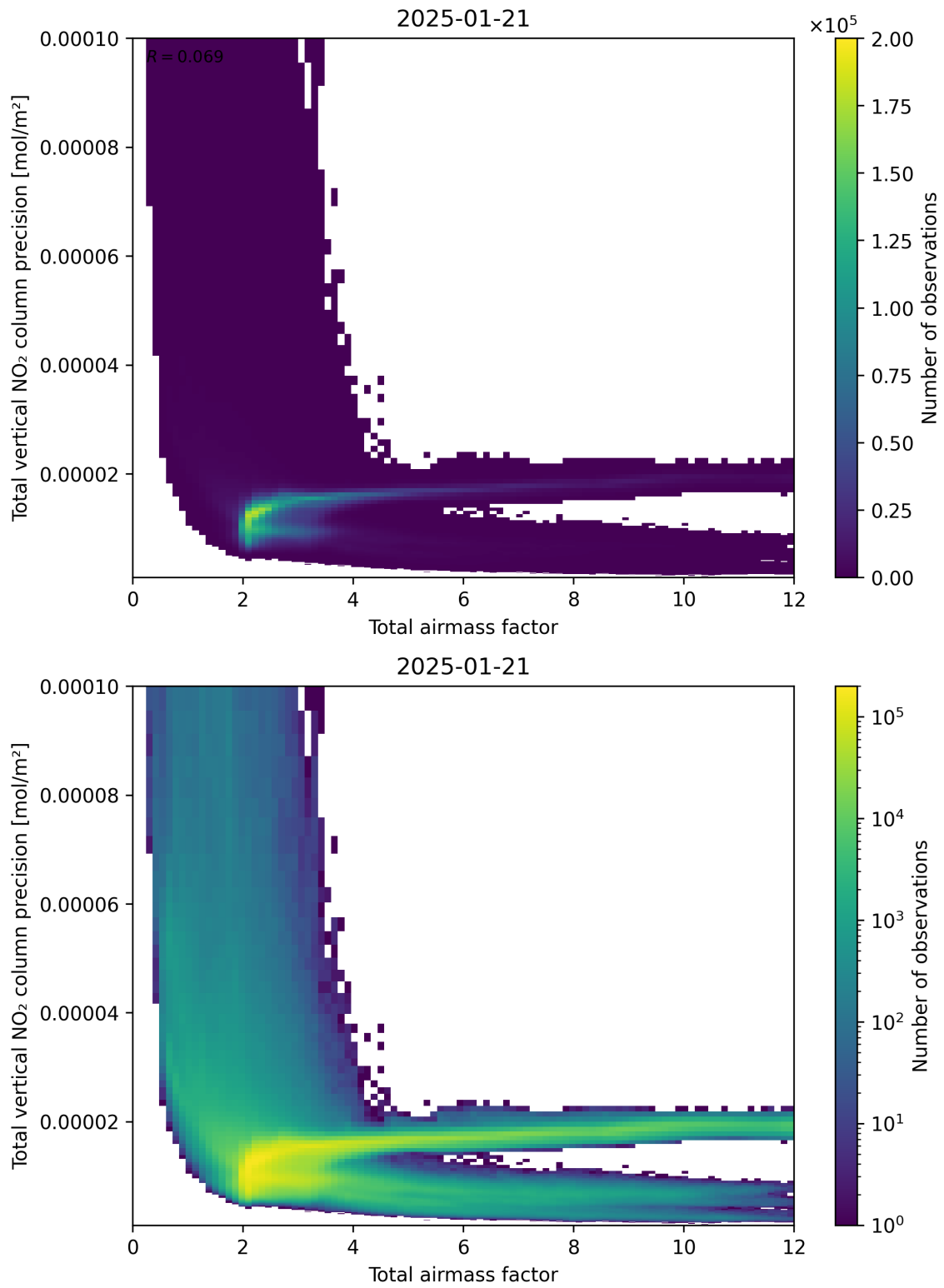
Figure 68: Scatter density plot of “Total airmass factor” against “Total vertical NO 2 column precision” for 2025-01-20 to 2025-01-22.
