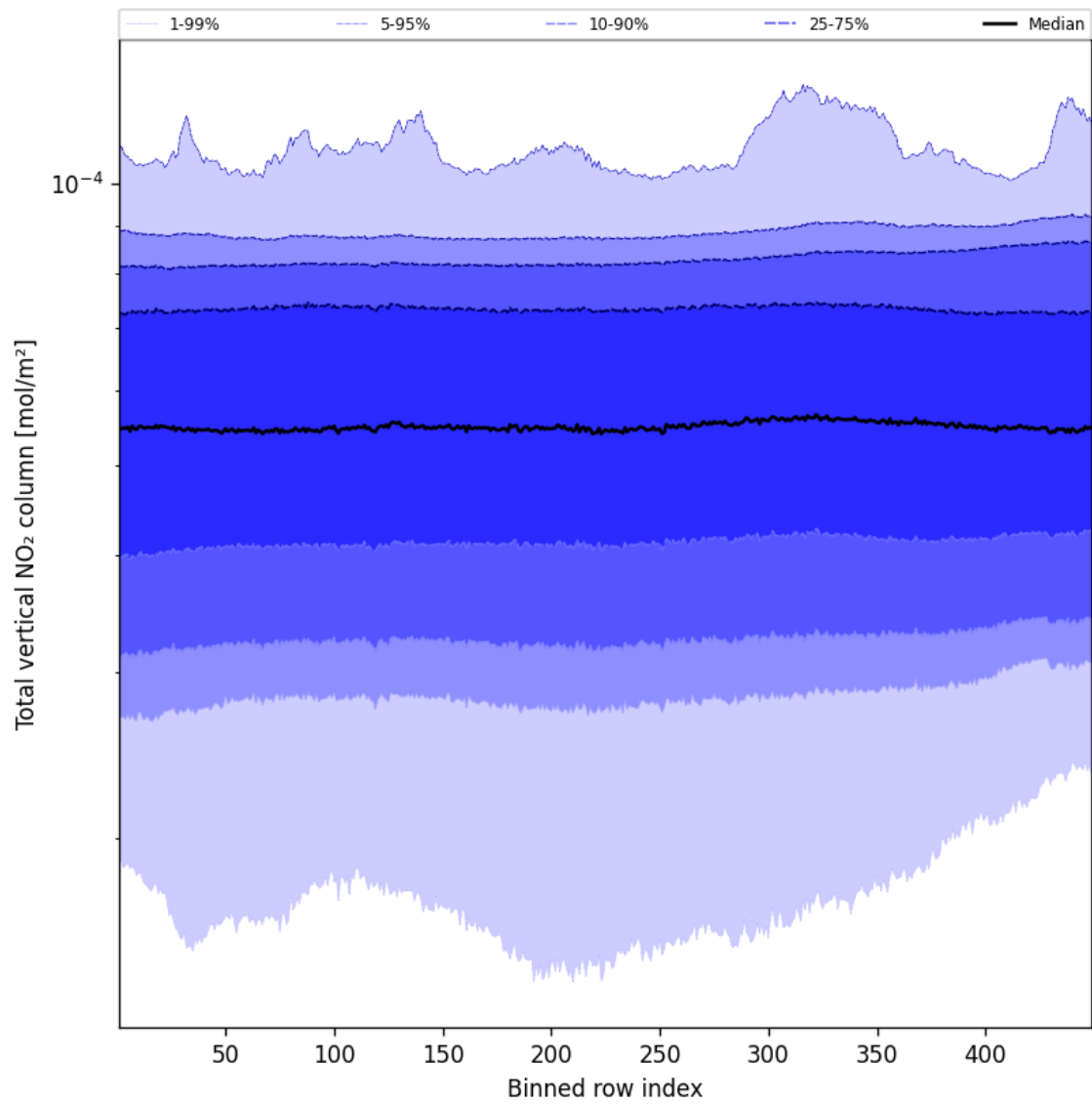
Figure 55: Along track statistics of “Total vertical NO 2 column” for 2025-01-20 to 2025-01-22
