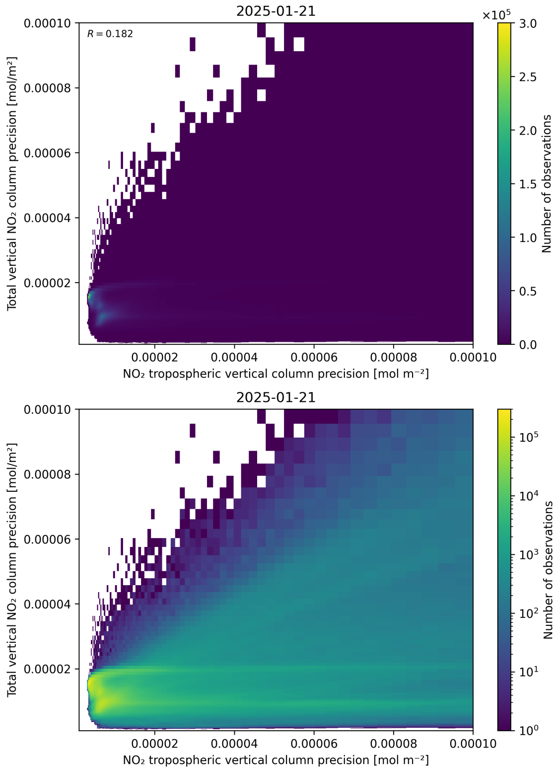
Figure 139: Scatter density plot of “NO 2 tropospheric vertical column precision” against “Total vertical NO 2 column precision” for 2025-01-20 to 2025-01-22.
