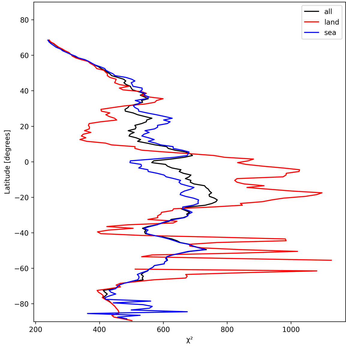
Figure 25: Zonal average of “ \chi^2 ” for 2025-01-20 to 2025-01-22.
