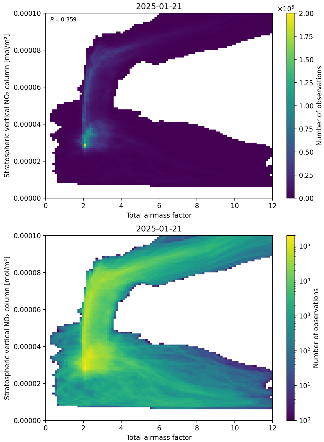
Figure 64: Scatter density plot of “Total airmass factor” against “Stratospheric vertical NO 2 column” for 2025-01-20 to 2025-01-22.
