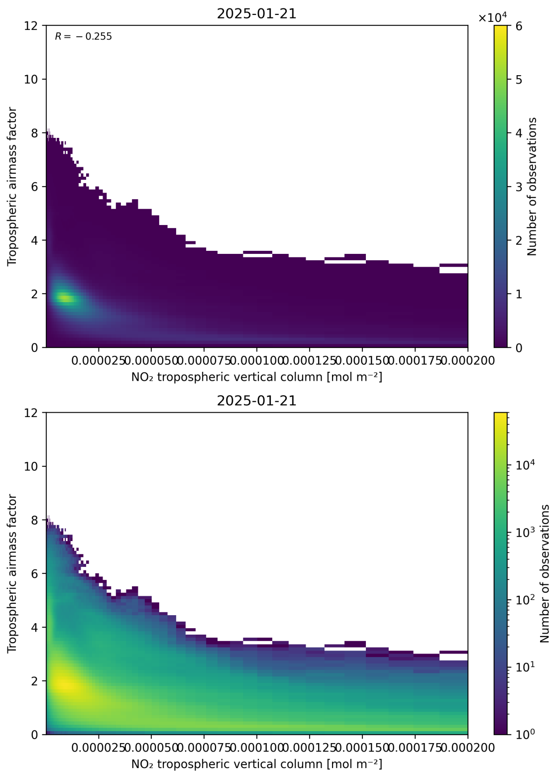
Figure 123: Scatter density plot of “NO 2 tropospheric vertical column” against “Tropospheric airmass factor” for 2025-01-20 to 2025-01-22.
