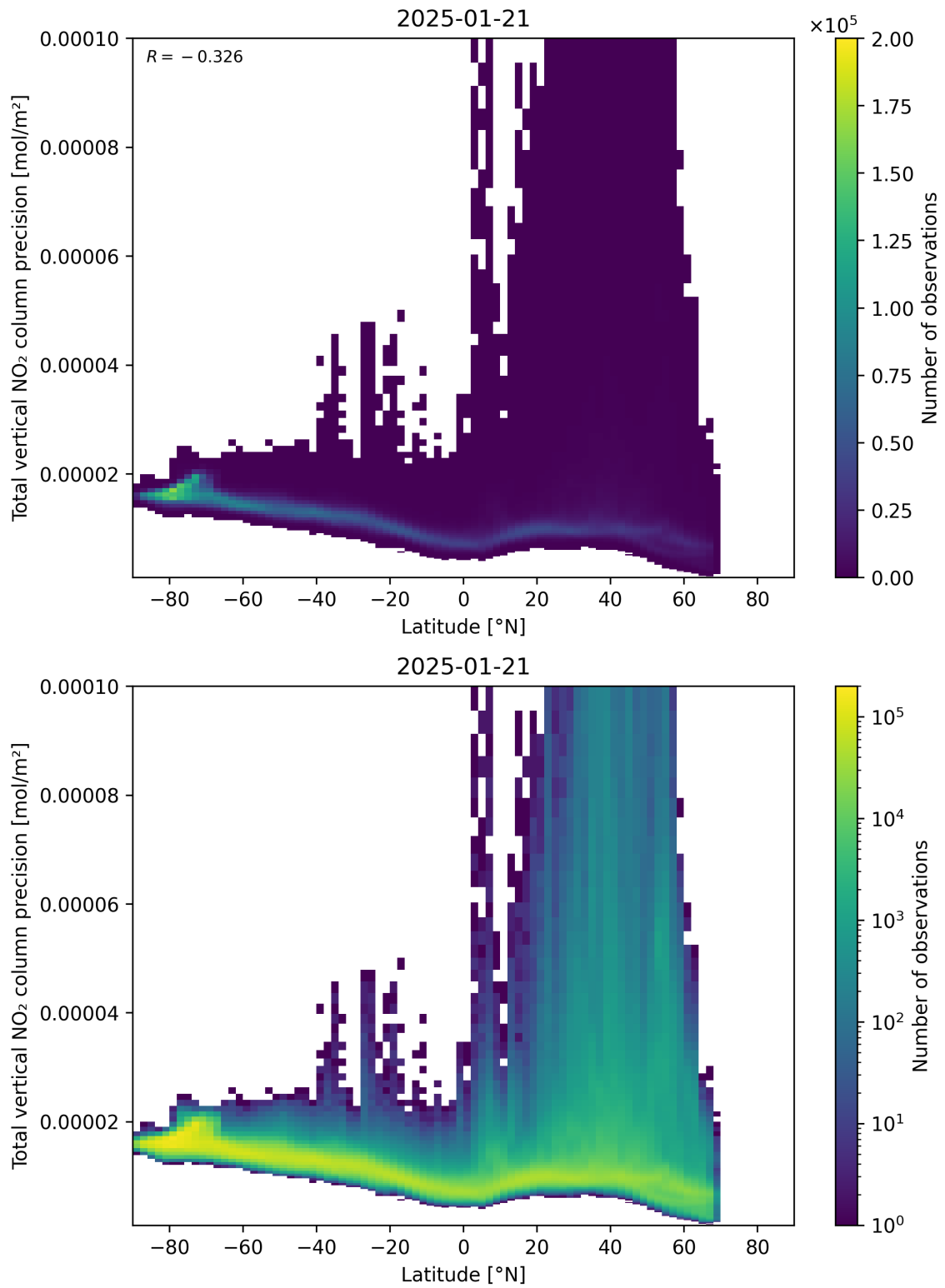
Figure 91: Scatter density plot of “Latitude” against “Total vertical NO 2 column precision” for 2025-01-20 to 2025-01-22.
