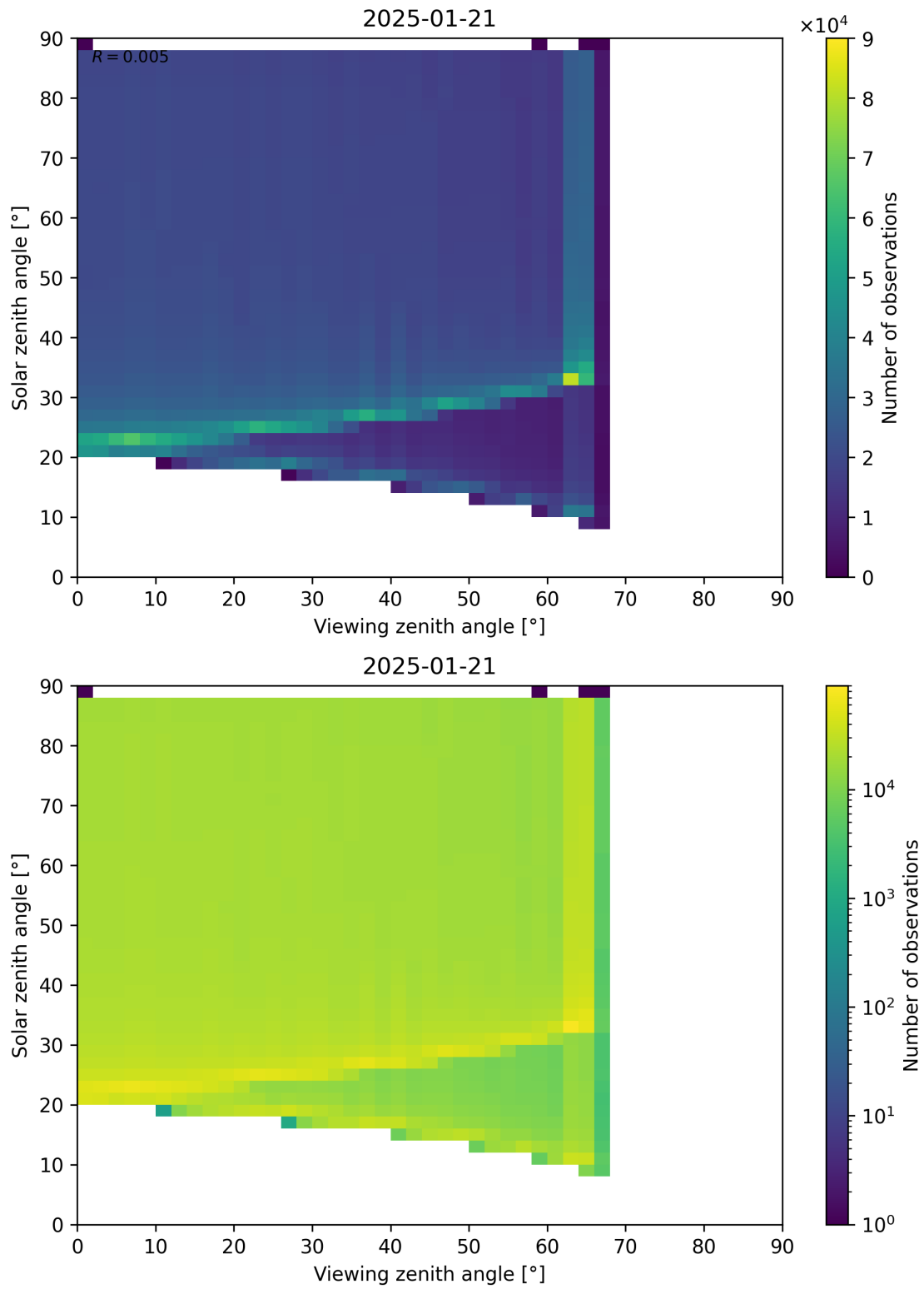
Figure 172: Scatter density plot of “Viewing zenith angle” against “Solar zenith angle” for 2025-01-20 to 2025-01-22.
