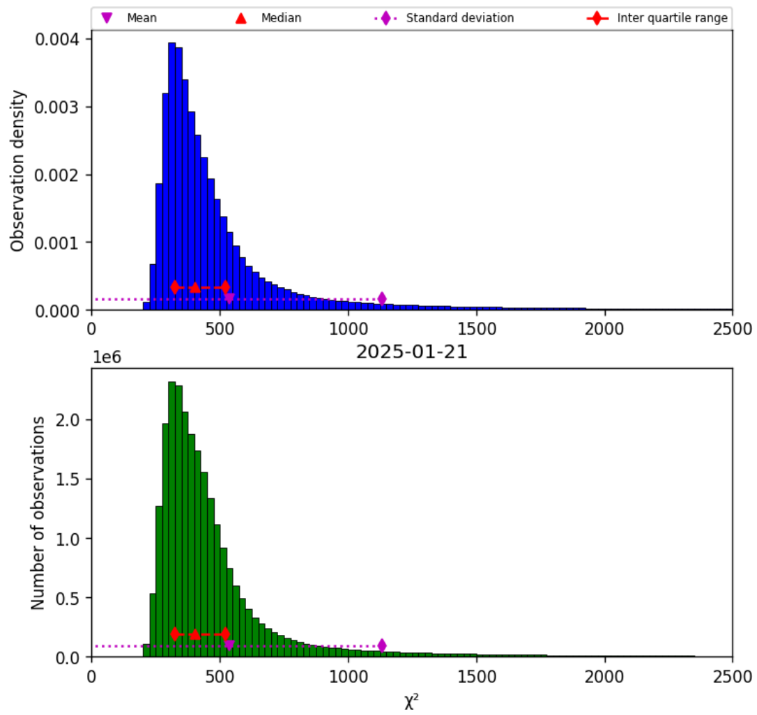
Figure 42: Histogram of “ \chi^2 ” for 2025-01-20 to 2025-01-22
