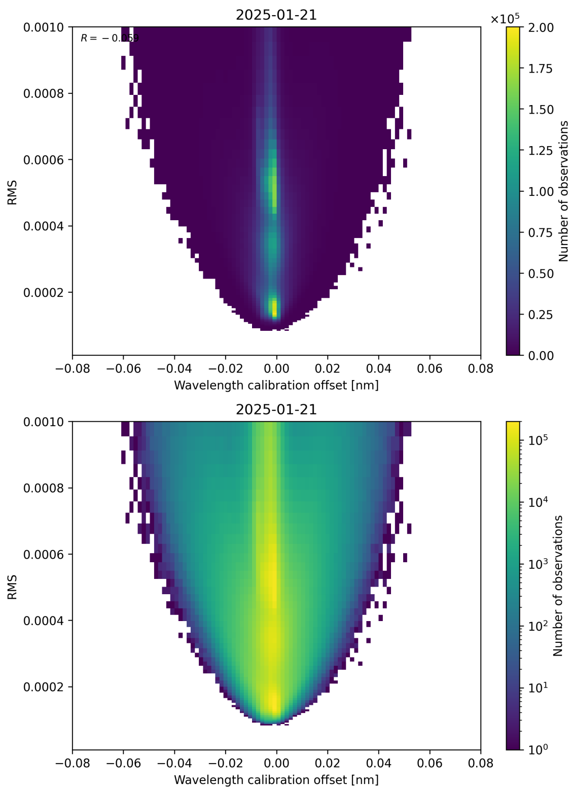
Figure 181: Scatter density plot of “Wavelength calibration offset” against “RMS” for 2025-01-20 to 2025-01-22.
