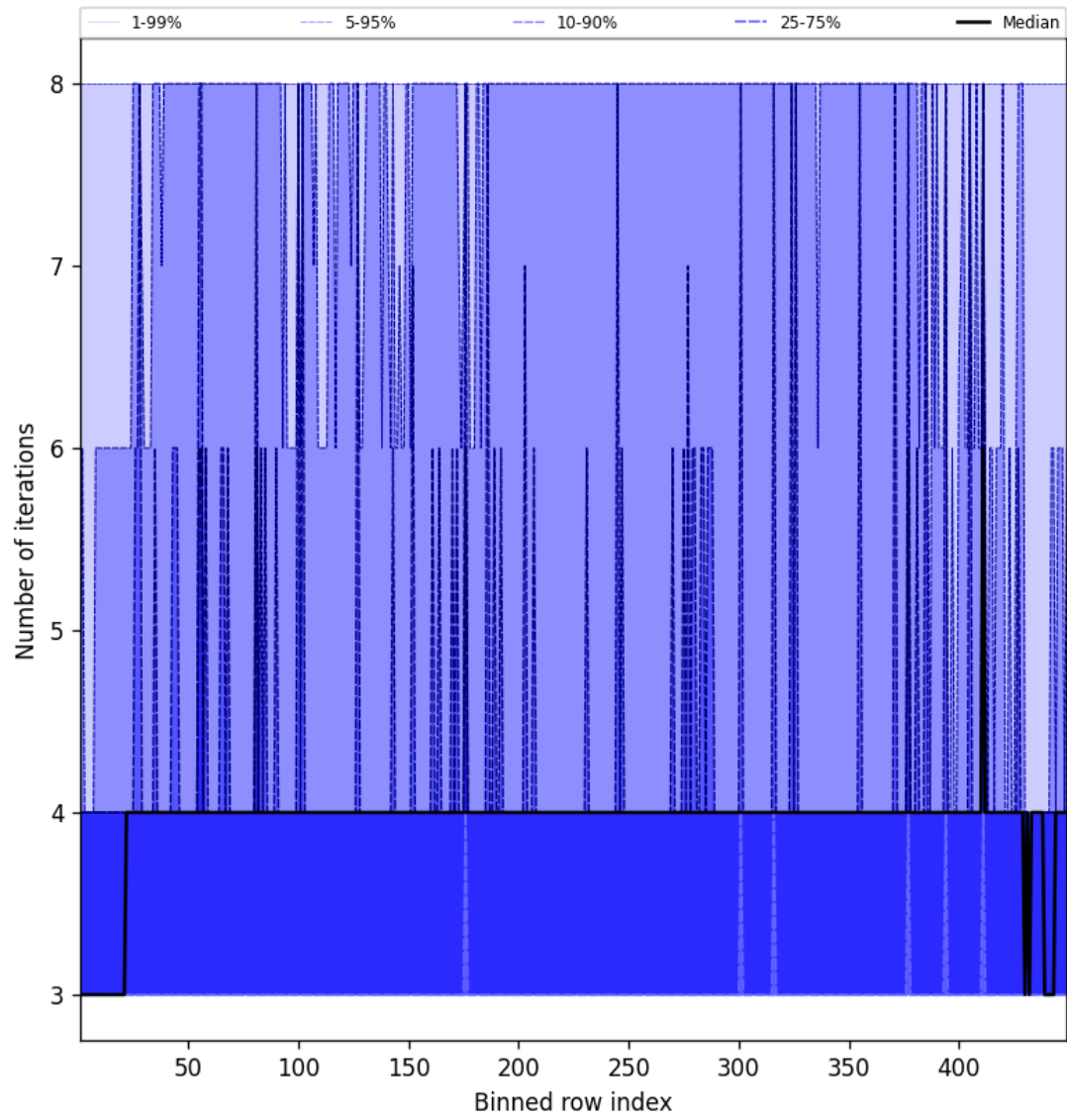
Figure 51: Along track statistics of “Number of iterations” for 2025-01-20 to 2025-01-22
