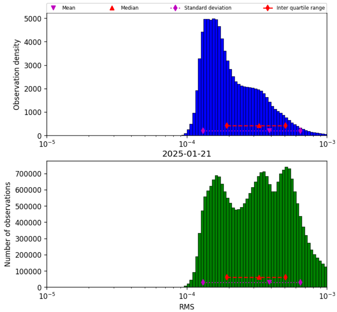
Figure 43: Histogram of “RMS” for 2025-01-20 to 2025-01-22
