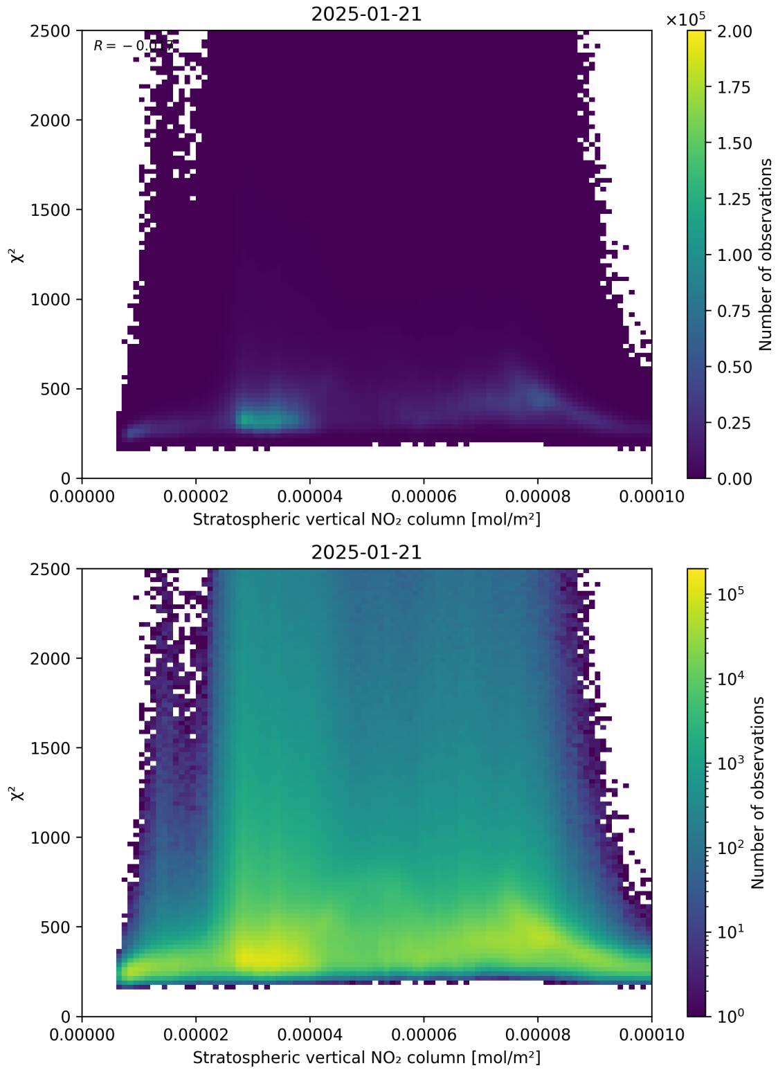
Figure 97: Scatter density plot of “Stratospheric vertical NO 2 column” against “ \chi^2 ” for 2025-01-20 to 2025-01-22.
