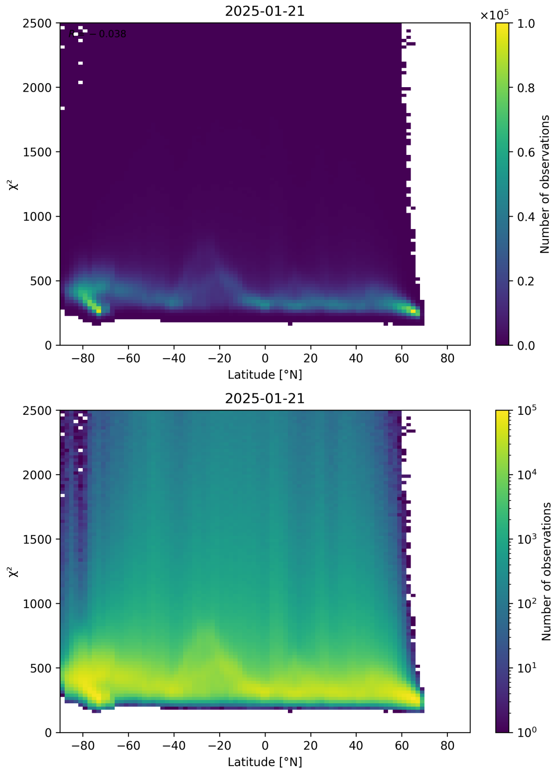
Figure 86: Scatter density plot of “Latitude” against “ \chi^2 ” for 2025-01-20 to 2025-01-22.
