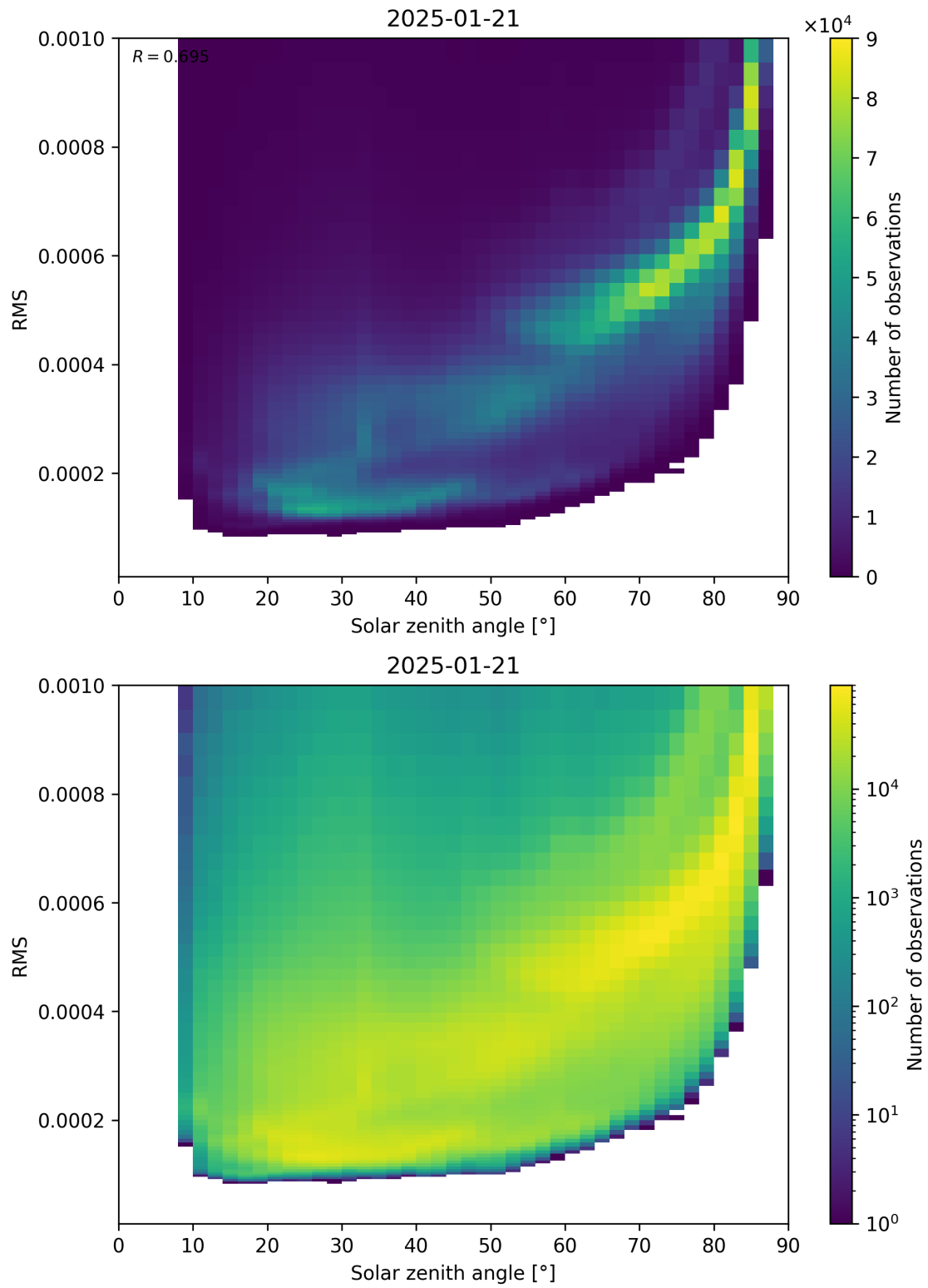
Figure 157: Scatter density plot of “Solar zenith angle” against “RMS” for 2025-01-20 to 2025-01-22.
