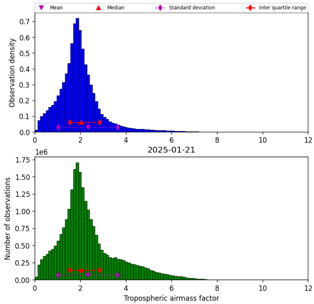
Figure 31: Histogram of “Tropospheric airmass factor” for 2025-01-20 to 2025-01-22
