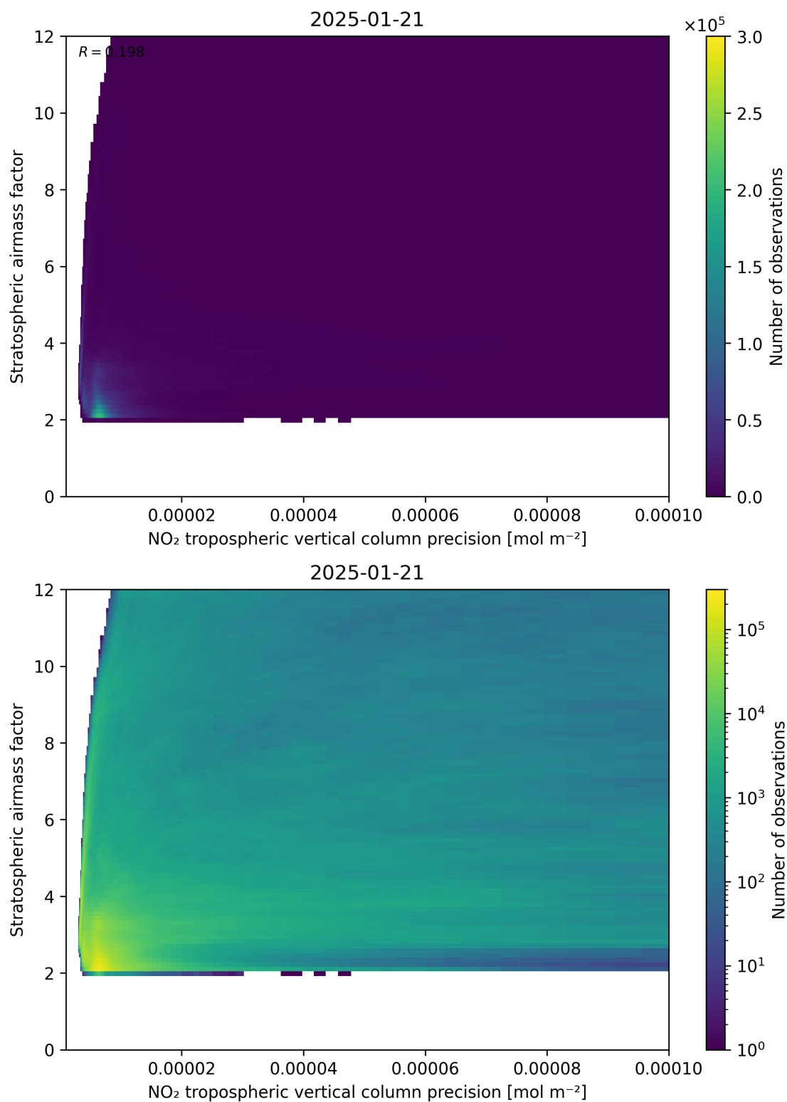
Figure 131: Scatter density plot of “NO 2 tropospheric vertical column precision” against “Stratospheric airmass factor” for 2025-01-20 to 2025-01-22.
