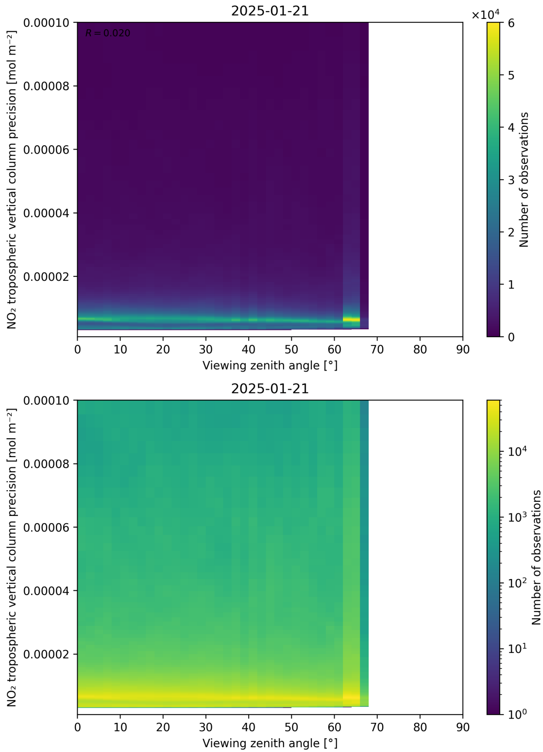
Figure 170: Scatter density plot of “Viewing zenith angle” against “NO 2 tropospheric vertical column precision” for 2025-01-20 to 2025-01-22.
