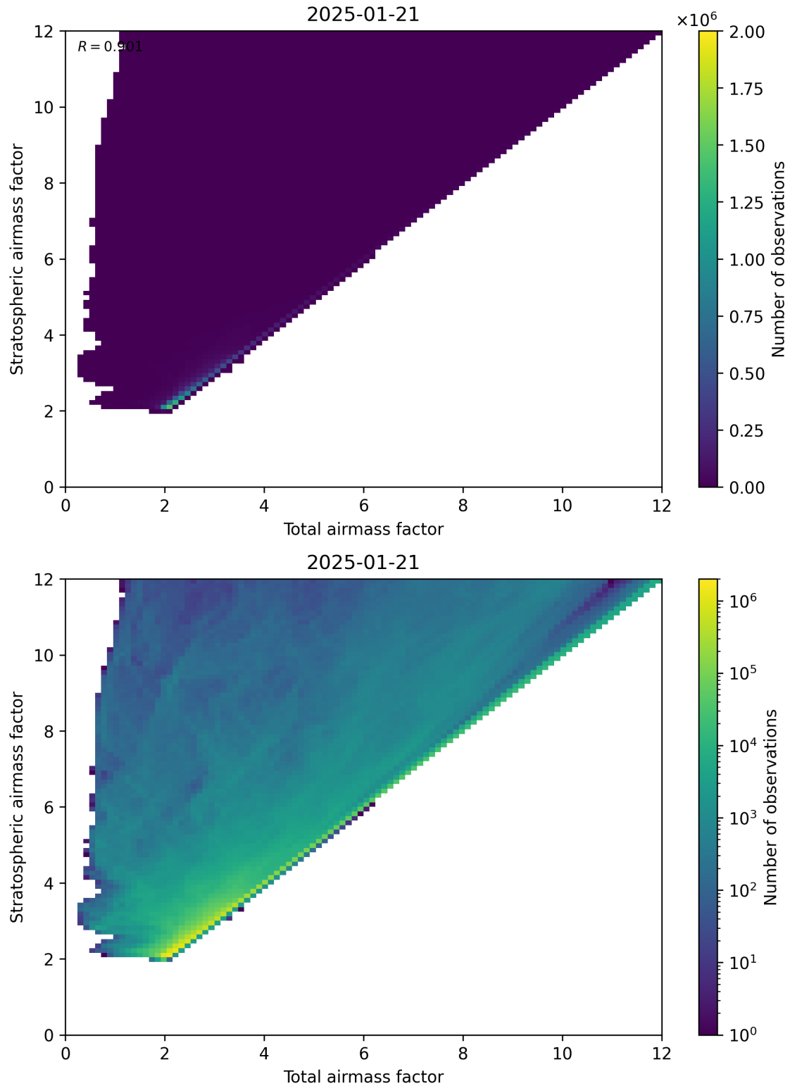
Figure 62: Scatter density plot of “Total airmass factor” against “Stratospheric airmass factor” for 2025-01-20 to 2025-01-22.
