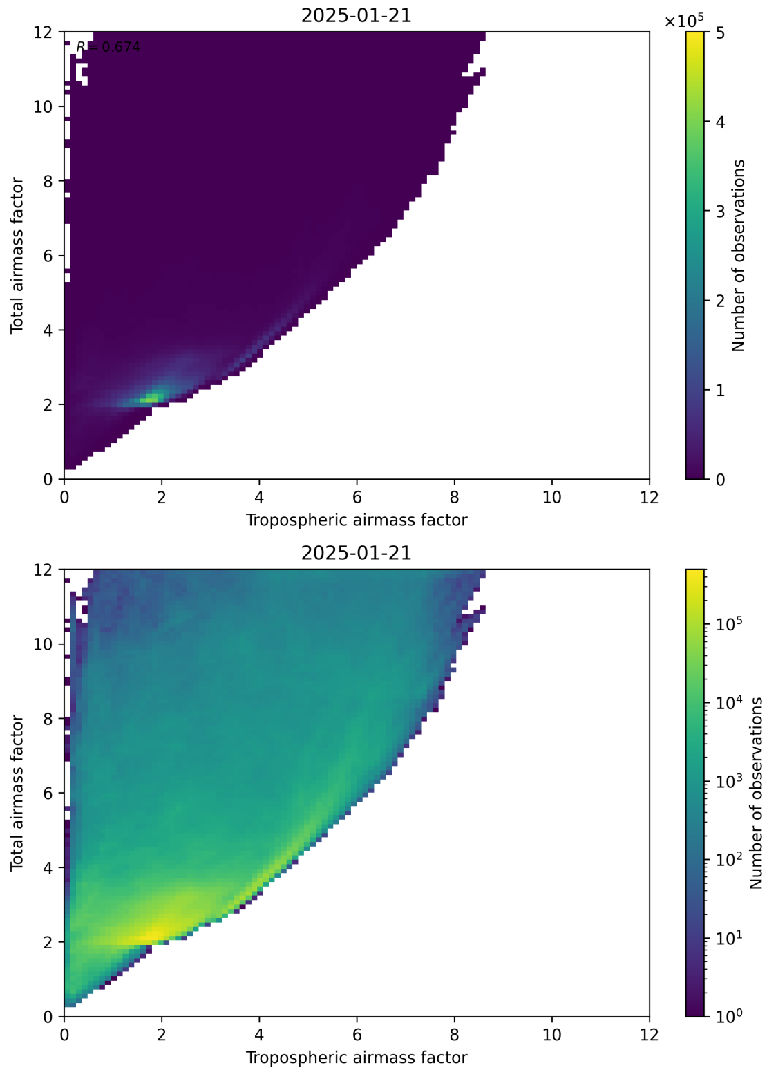
Figure 72: Scatter density plot of “Tropospheric airmass factor” against “Total airmass factor” for 2025-01-20 to 2025-01-22.
