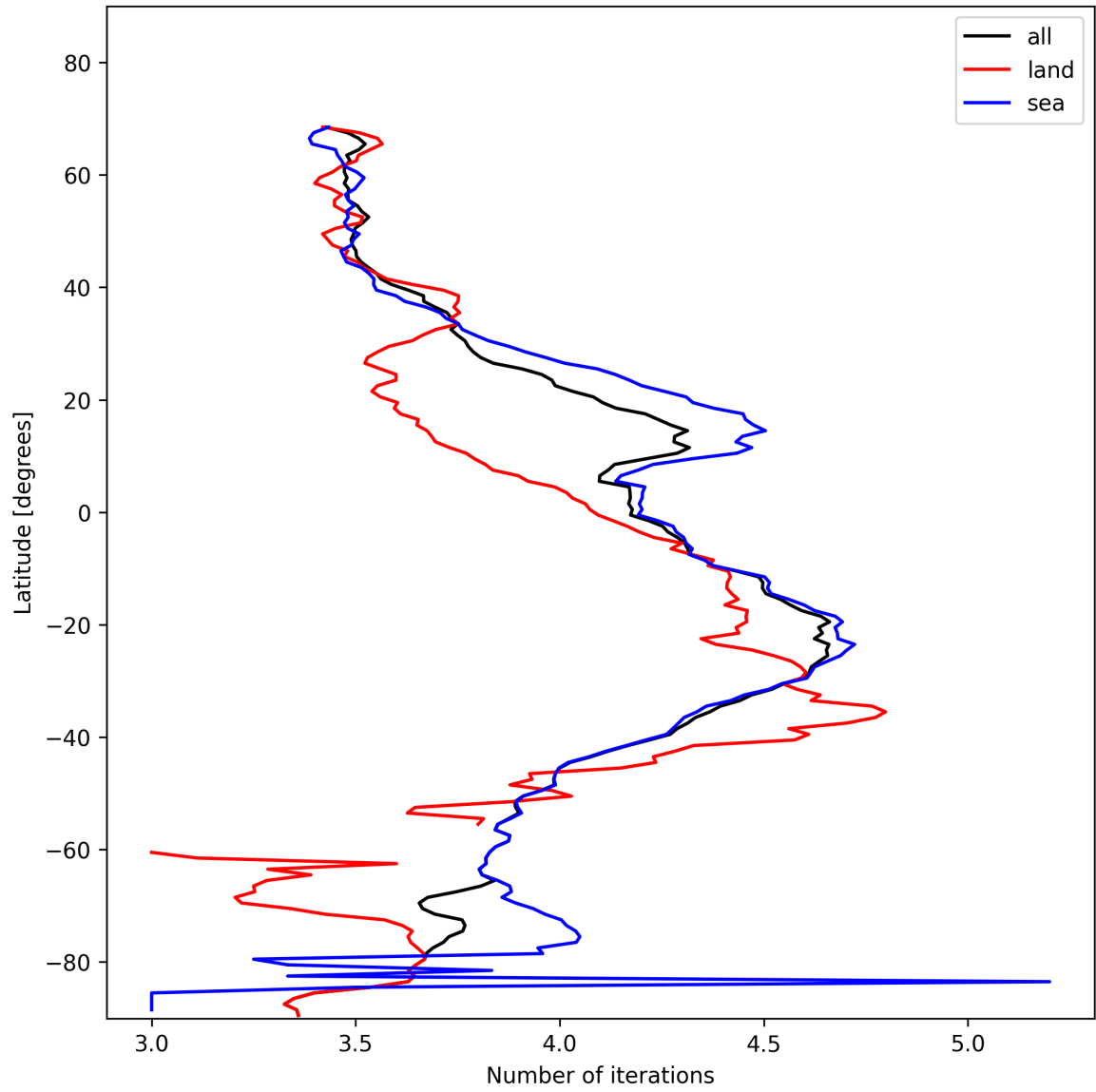
Figure 17: Zonal average of “Number of iterations” for 2025-01-20 to 2025-01-22.
