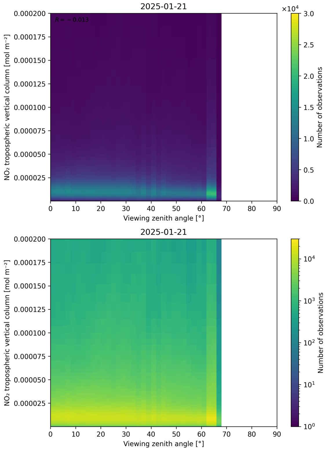
Figure 169: Scatter density plot of “Viewing zenith angle” against “NO 2 tropospheric vertical column” for 2025-01-20 to 2025-01-22.
