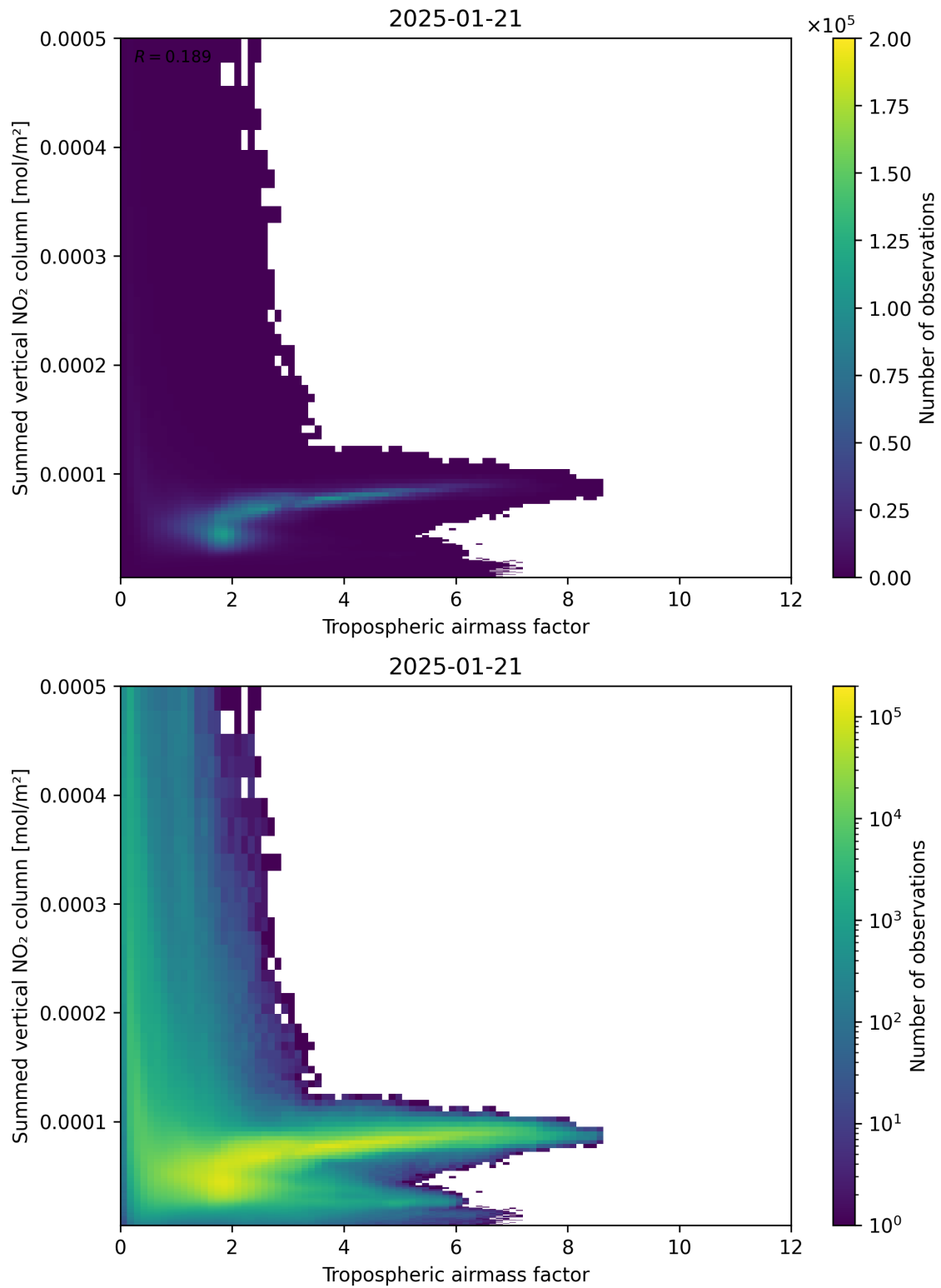
Figure 75: Scatter density plot of “Tropospheric airmass factor” against “Summed vertical NO 2 column” for 2025-01-20 to 2025-01-22.
