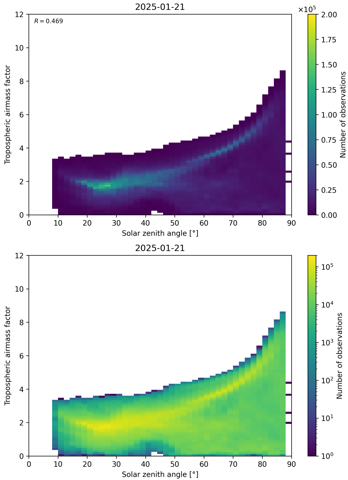
Figure 147: Scatter density plot of “Solar zenith angle” against “Tropospheric airmass factor” for 2025-01-20 to 2025-01-22.
