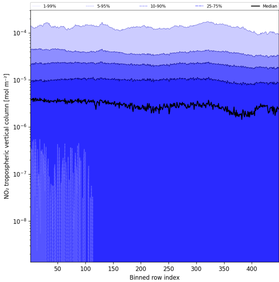
Figure 46: Along track statistics of “NO 2 tropospheric vertical column” for 2025-01-20 to 2025-01-22
