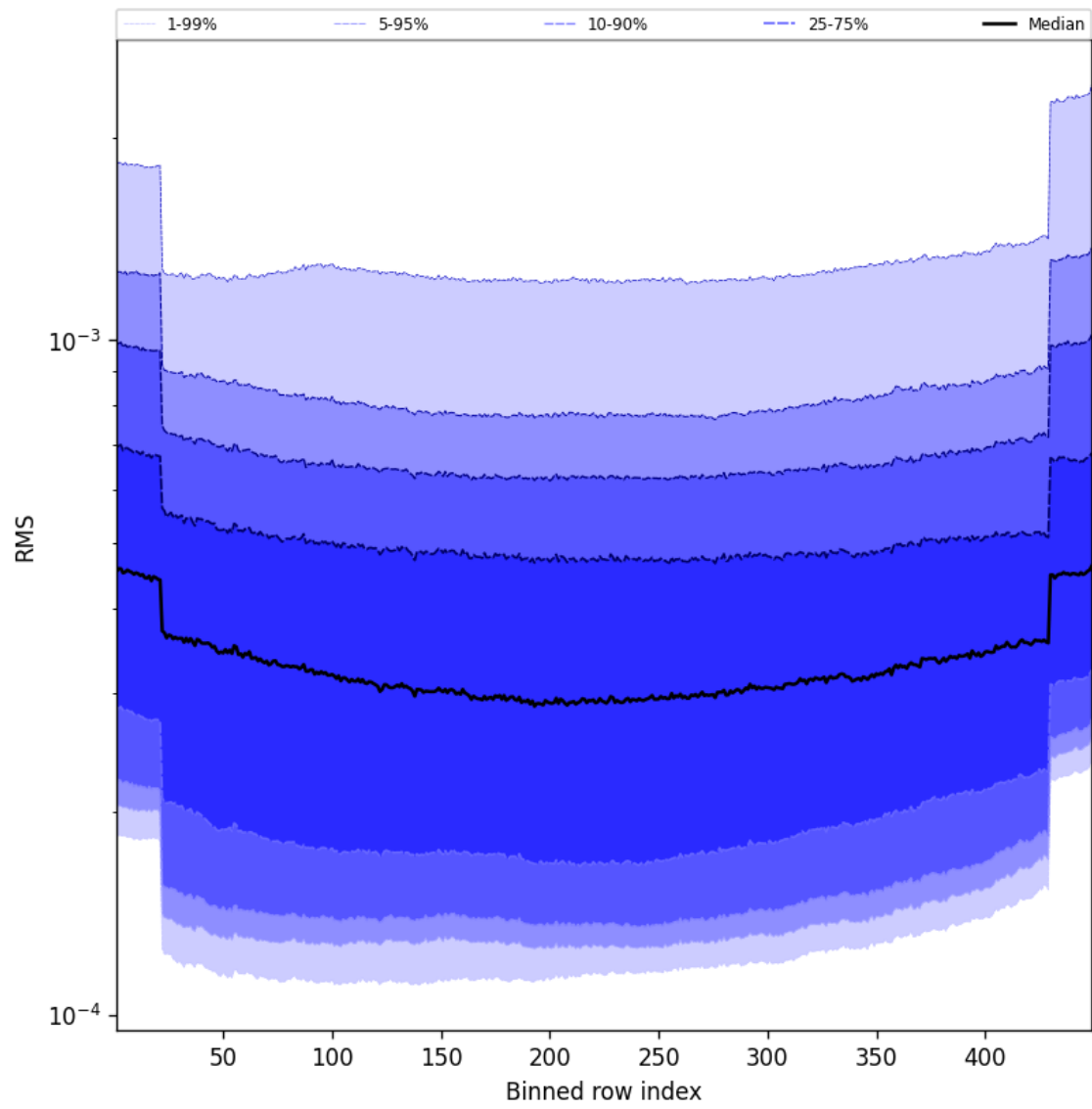
Figure 60: Along track statistics of “RMS” for 2025-01-20 to 2025-01-22
