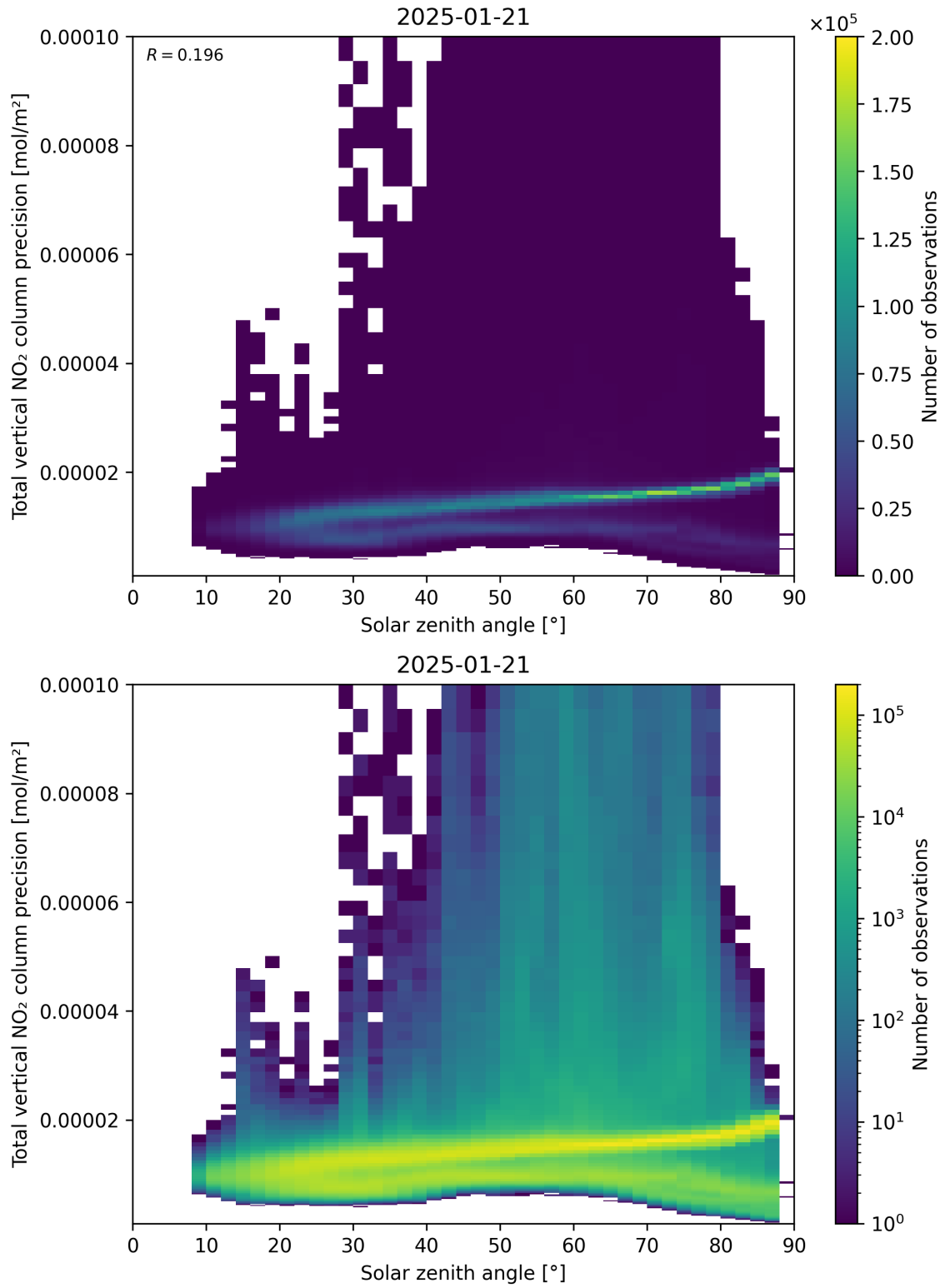
Figure 154: Scatter density plot of “Solar zenith angle” against “Total vertical NO 2 column precision” for 2025-01-20 to 2025-01-22.
