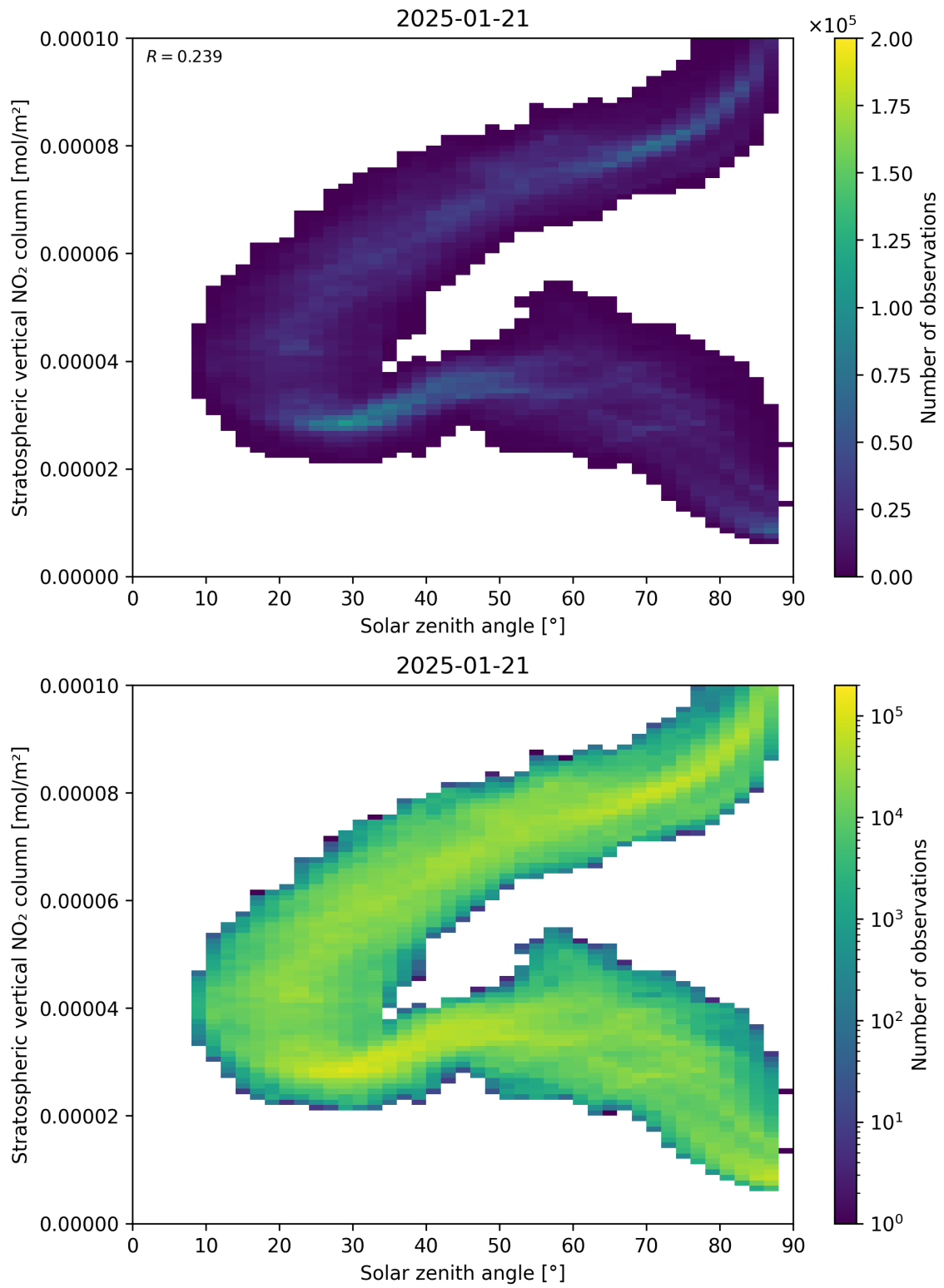
Figure 150: Scatter density plot of “Solar zenith angle” against “Stratospheric vertical NO 2 column” for 2025-01-20 to 2025-01-22.
