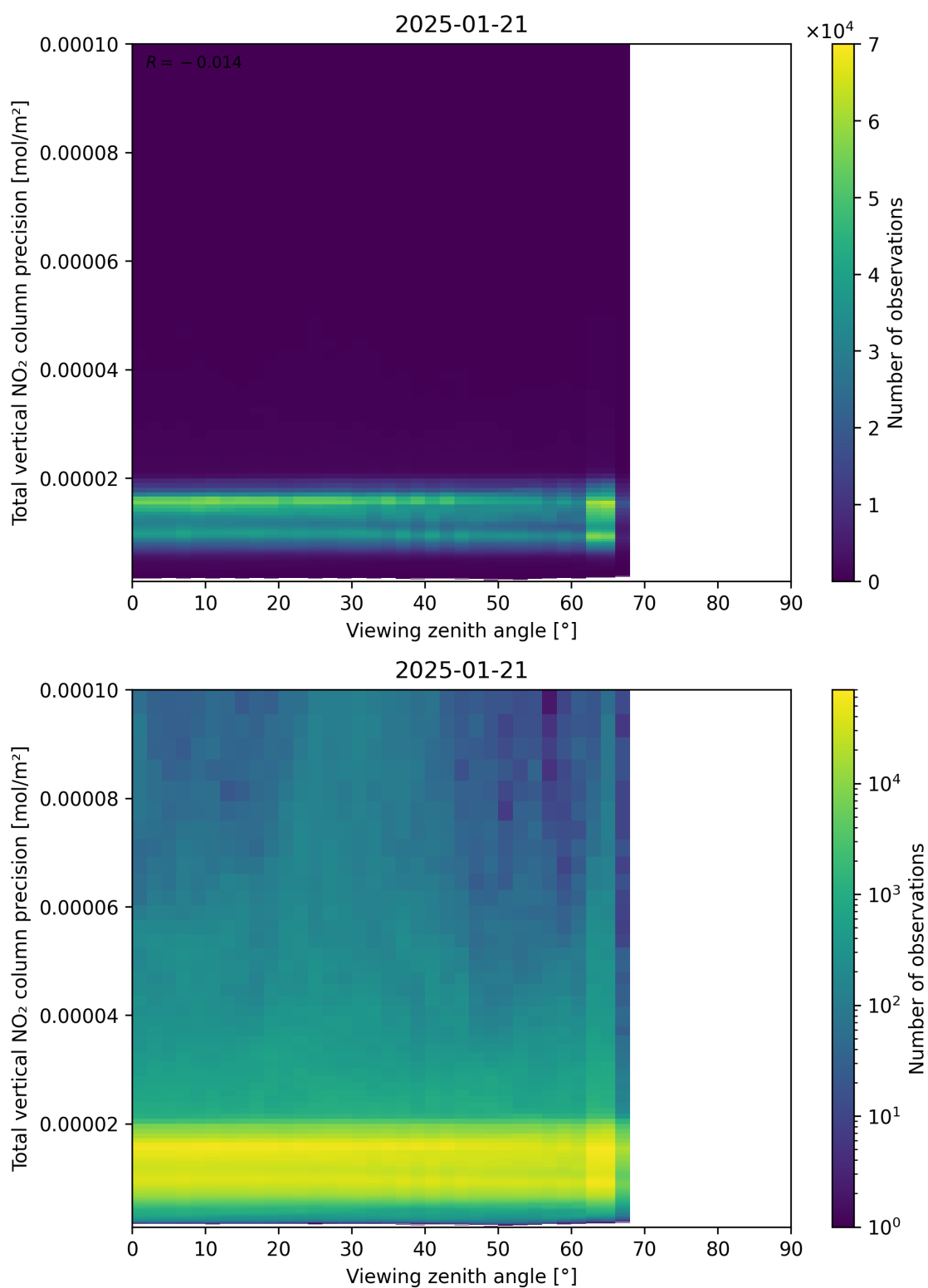
Figure 168: Scatter density plot of “Viewing zenith angle” against “Total vertical NO 2 column precision” for 2025-01-20 to 2025-01-22.
