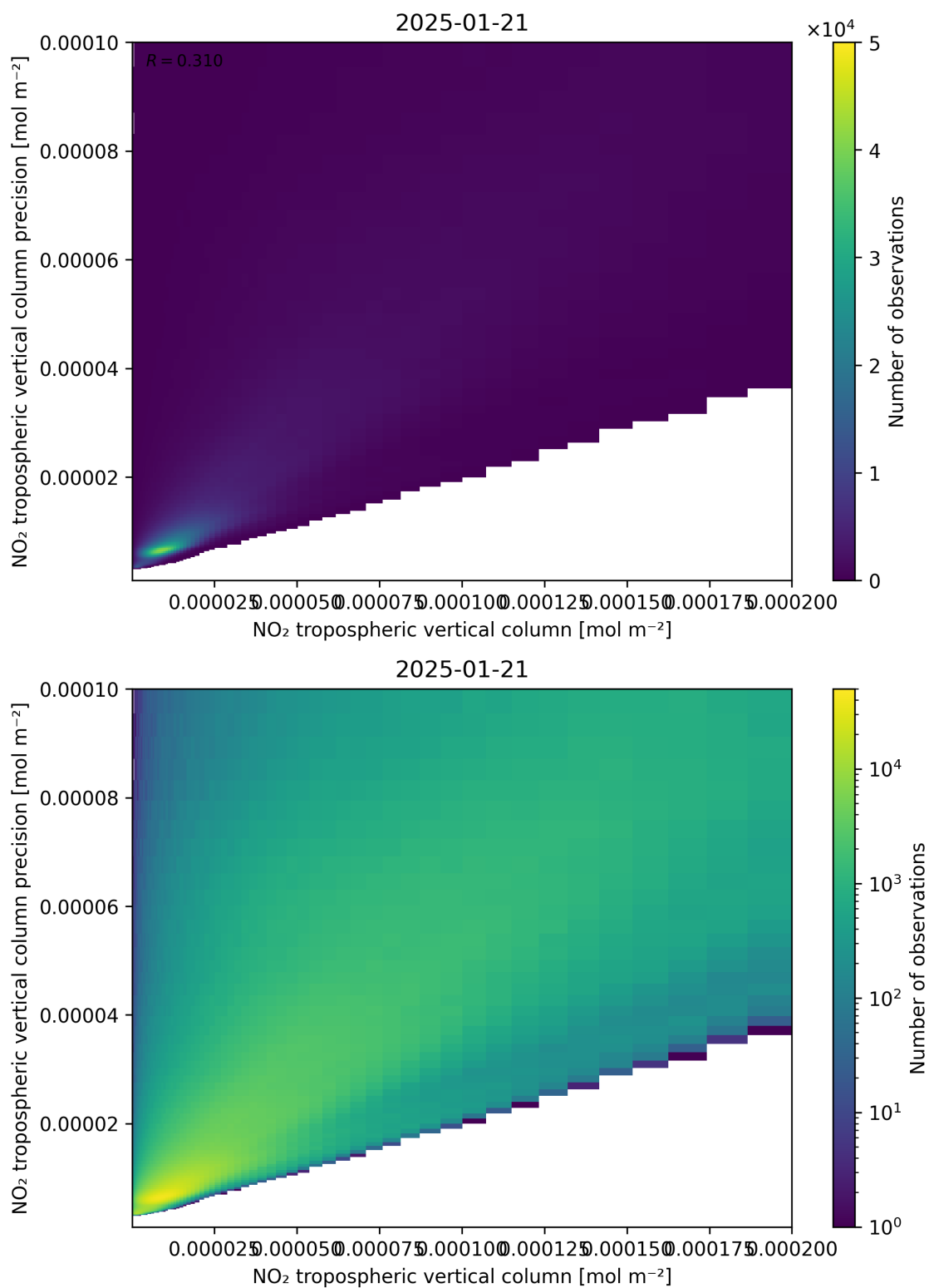
Figure 130: Scatter density plot of “NO 2 tropospheric vertical column” against “NO 2 tropospheric vertical column precision” for 2025-01-20 to 2025-01-22.
