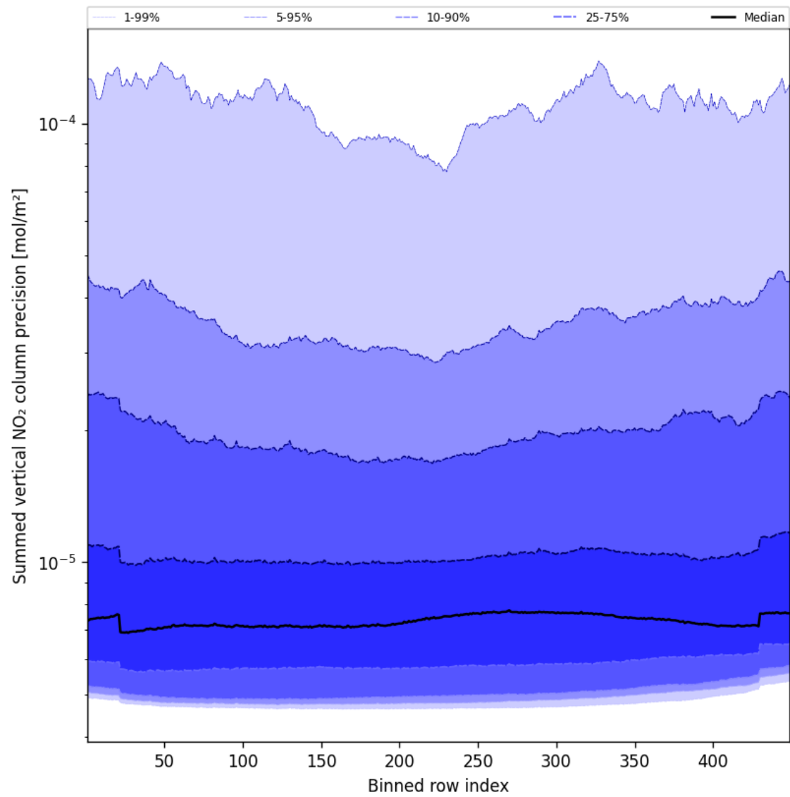
Figure 58: Along track statistics of “Summed vertical NO 2 column precision” for 2025-01-20 to 2025-01-22
