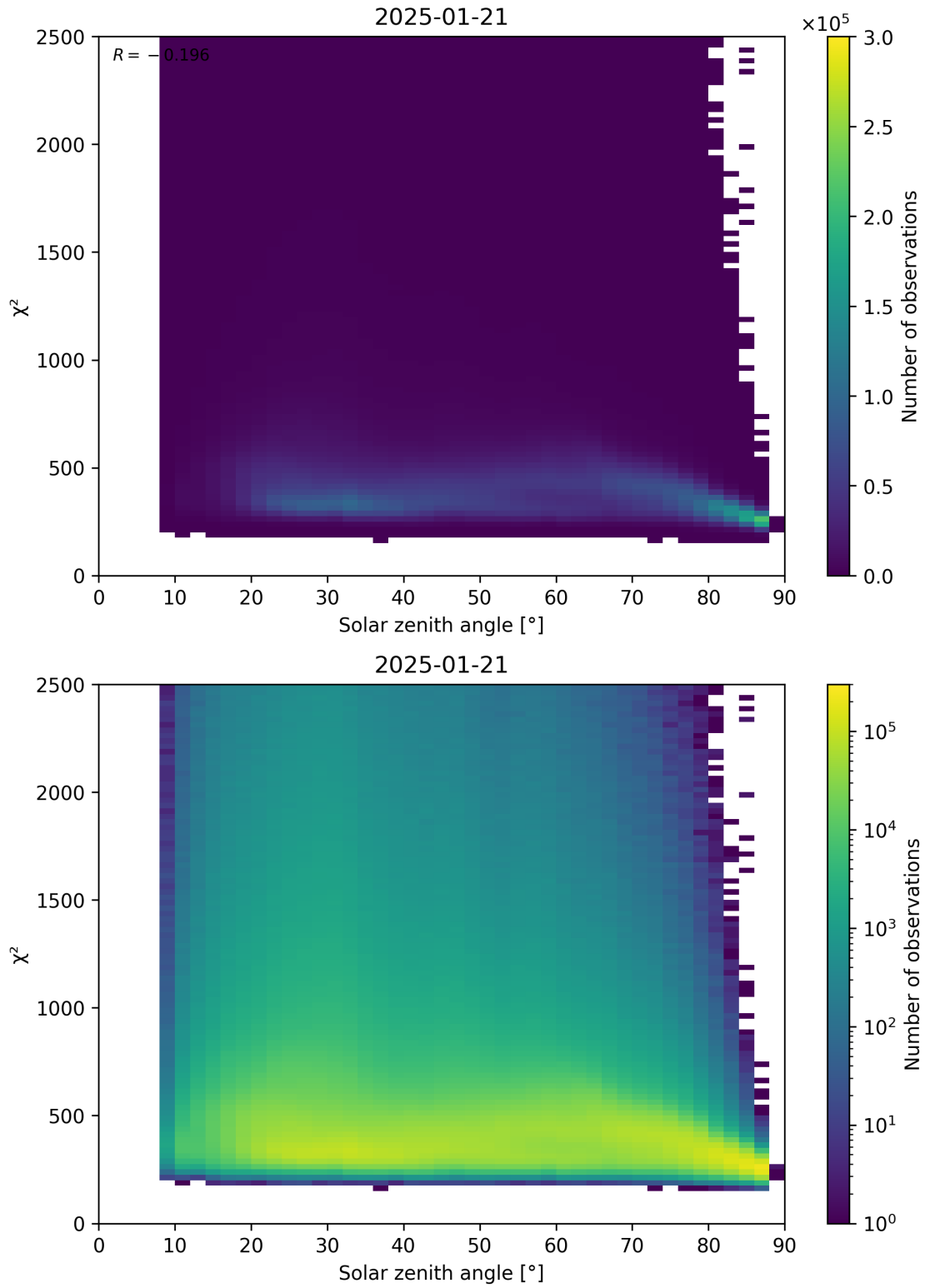
Figure 148: Scatter density plot of “Solar zenith angle” against “ \chi^2 ” for 2025-01-20 to 2025-01-22.
