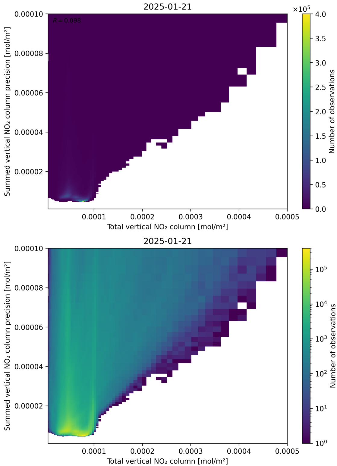
Figure 113: Scatter density plot of “Total vertical NO 2 column” against “Summed vertical NO 2 column precision” for 2025-01-20 to 2025-01-22.
