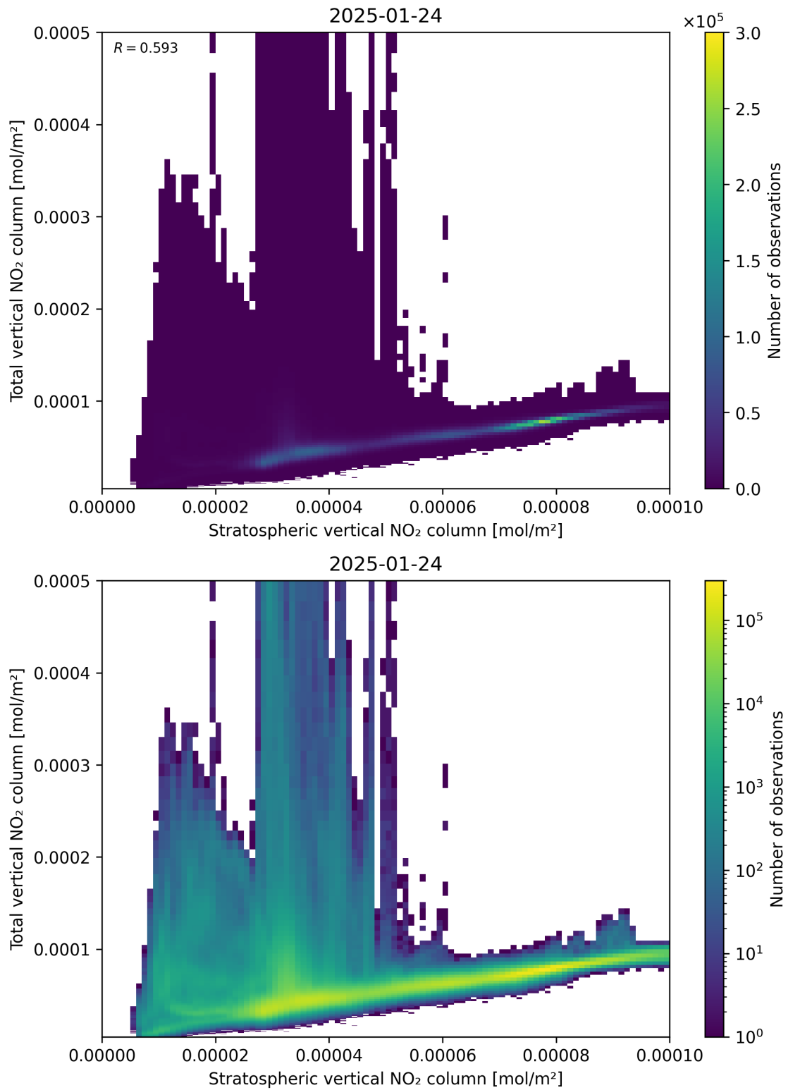
Figure 100: Scatter density plot of “Stratospheric vertical NO 2 column” against “Total vertical NO 2 column” for 2025-01-23 to 2025-01-25.
