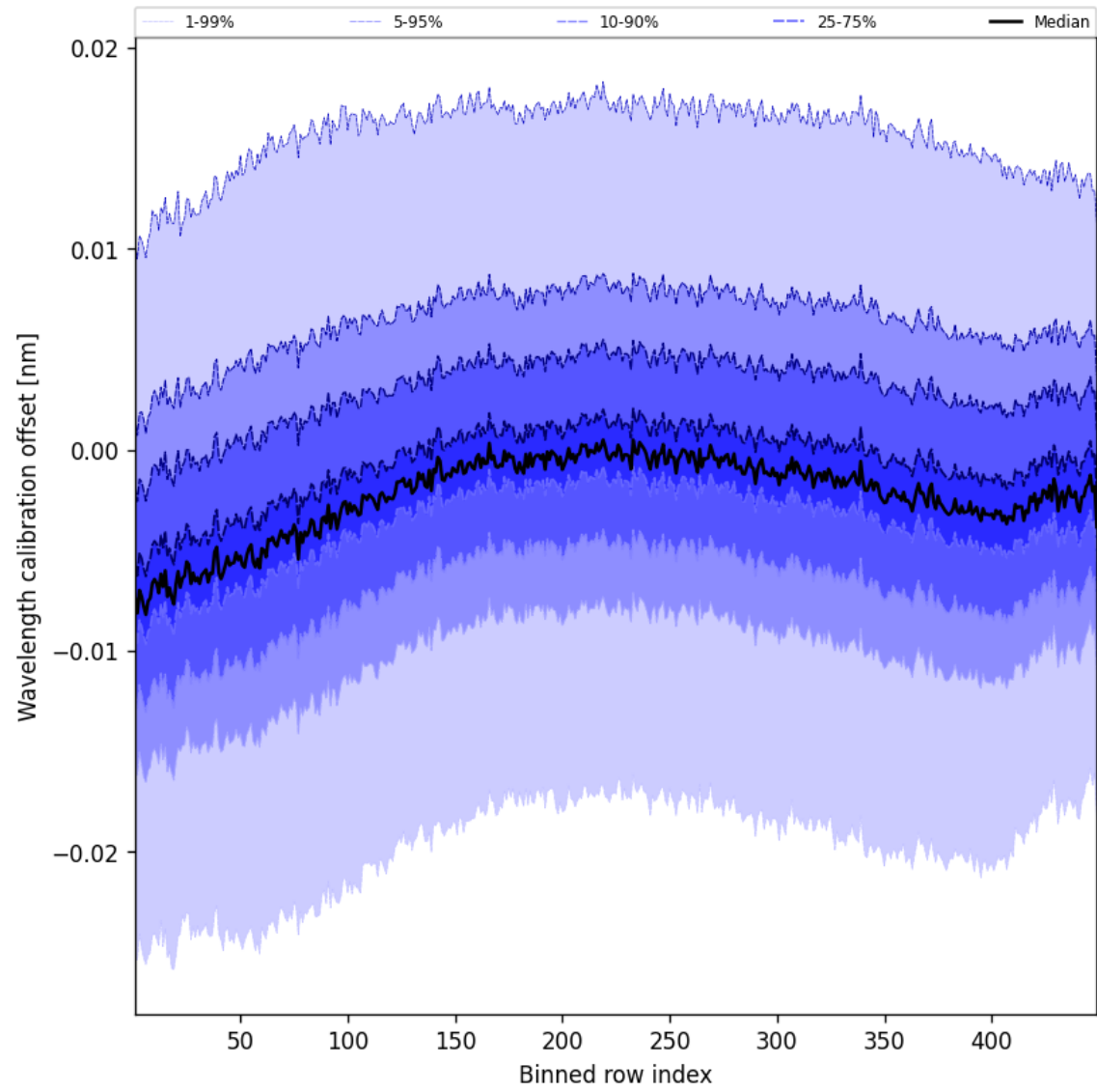
Figure 52: Along track statistics of “Wavelength calibration offset” for 2025-01-23 to 2025-01-25
