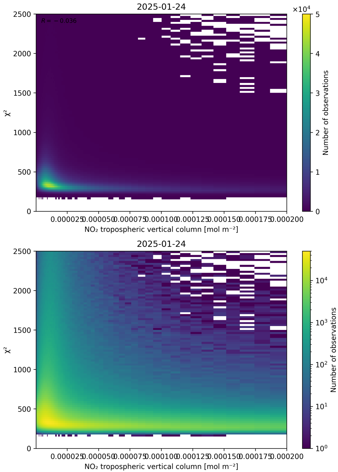
Figure 124: Scatter density plot of “NO 2 tropospheric vertical column” against “ \chi^2 ” for 2025-01-23 to 2025-01-25.
