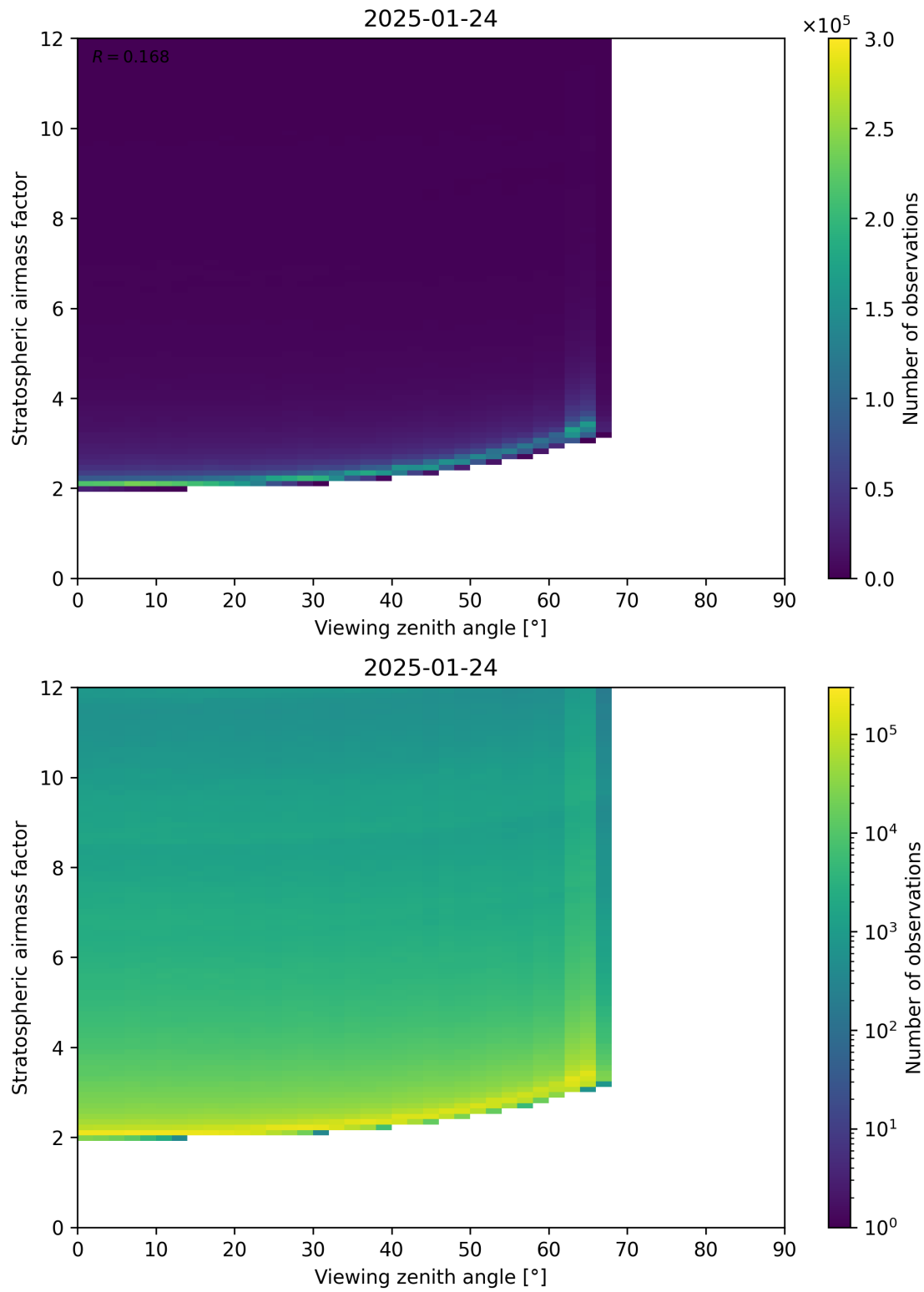
Figure 159: Scatter density plot of “Viewing zenith angle” against “Stratospheric airmass factor” for 2025-01-23 to 2025-01-25.
