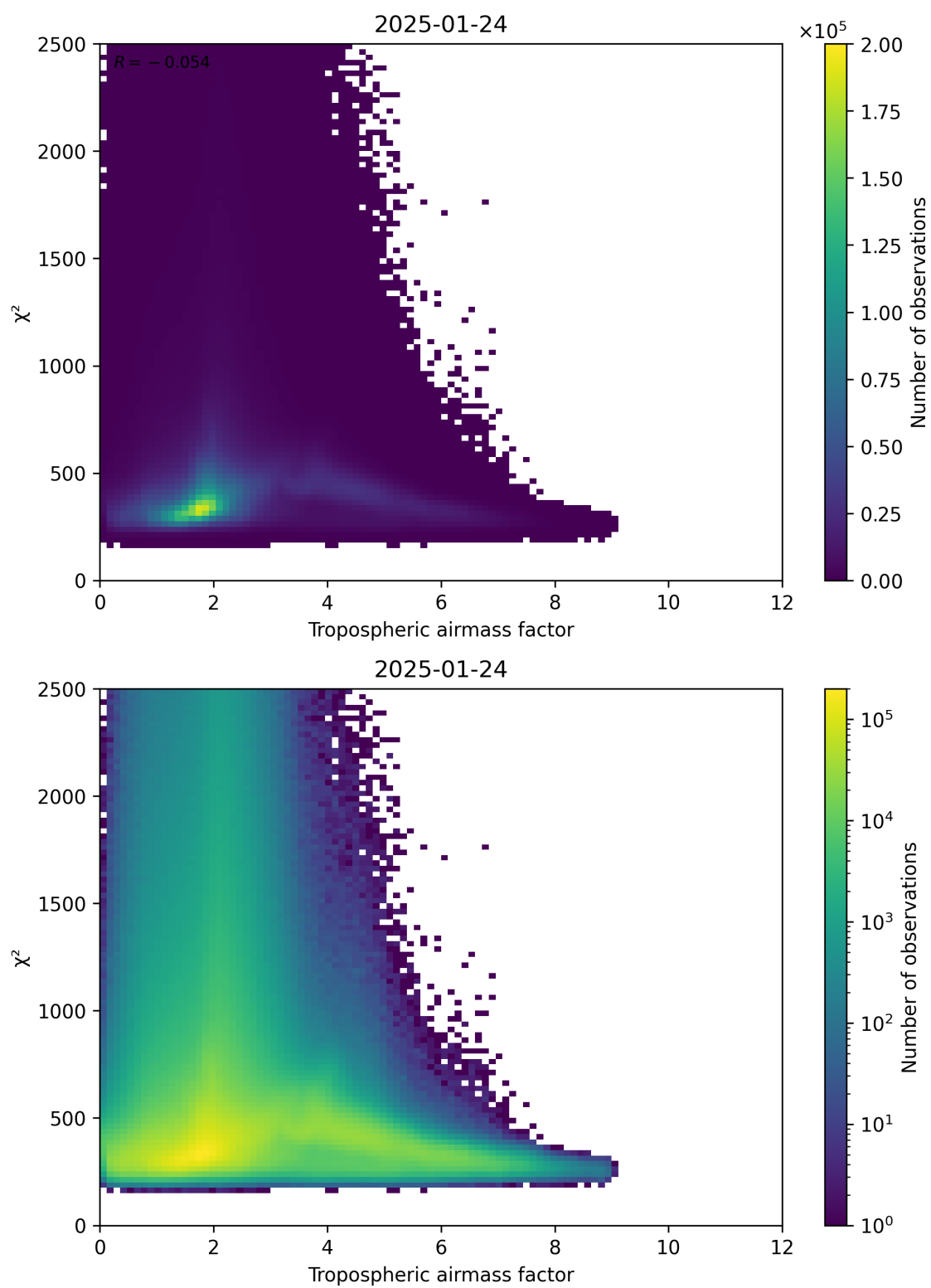
Figure 73: Scatter density plot of “Tropospheric airmass factor” against “ \chi^2 ” for 2025-01-23 to 2025-01-25.
