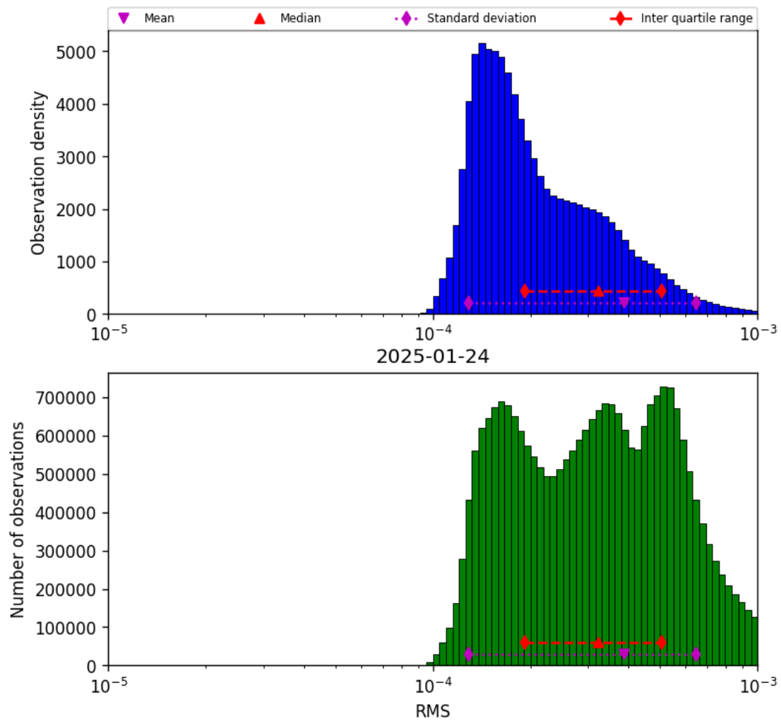
Figure 43: Histogram of “RMS” for 2025-01-23 to 2025-01-25
