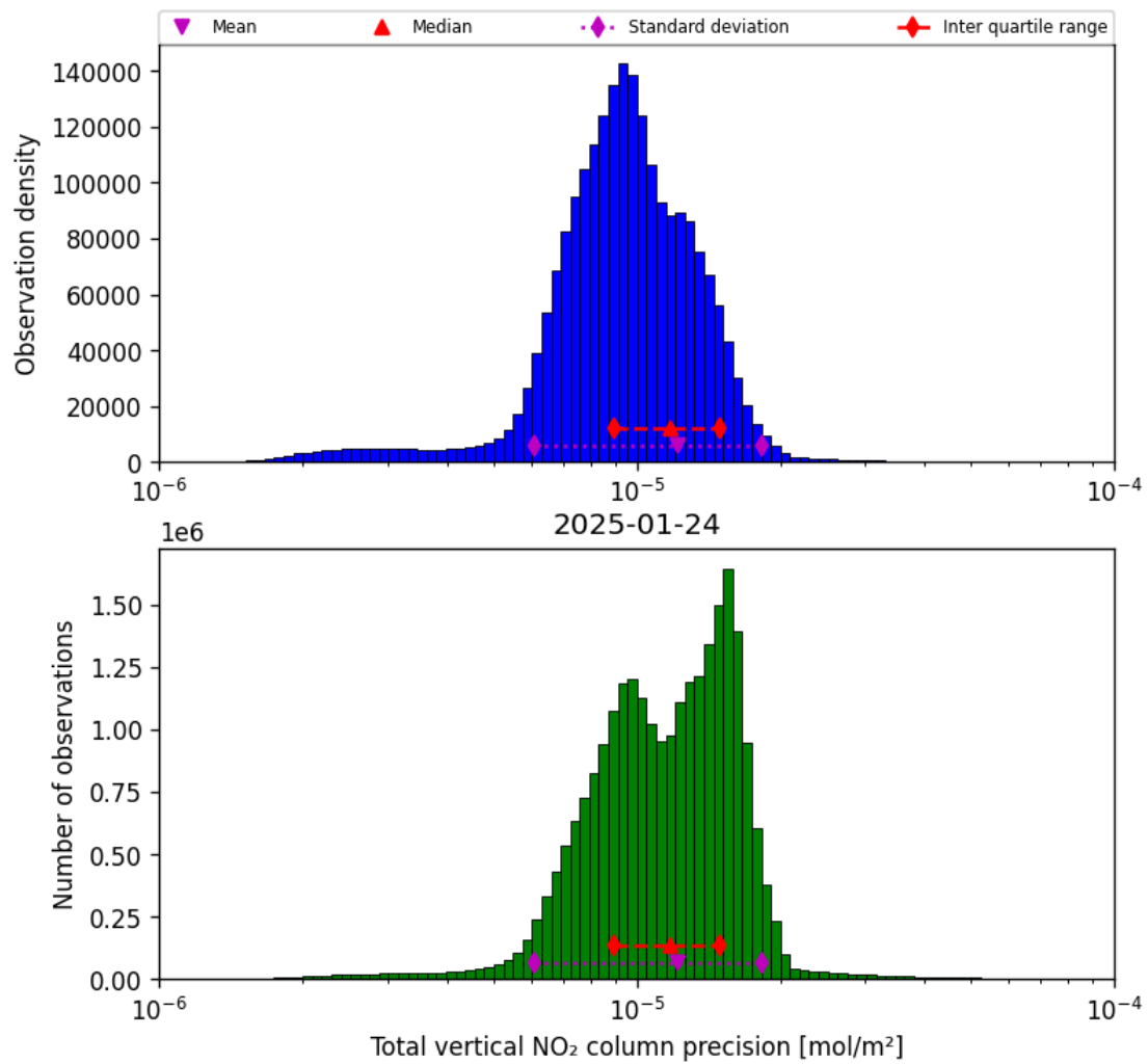
Figure 39: Histogram of “Total vertical NO 2 column precision” for 2025-01-23 to 2025-01-25
