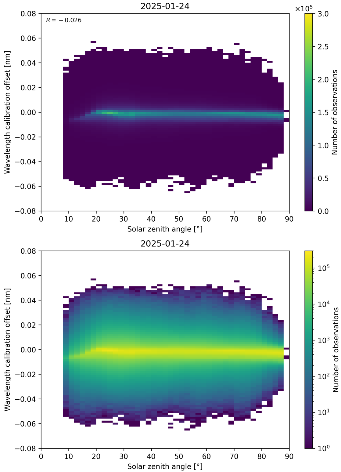
Figure 158: Scatter density plot of “Solar zenith angle” against “Wavelength calibration offset” for 2025-01-23 to 2025-01-25.
