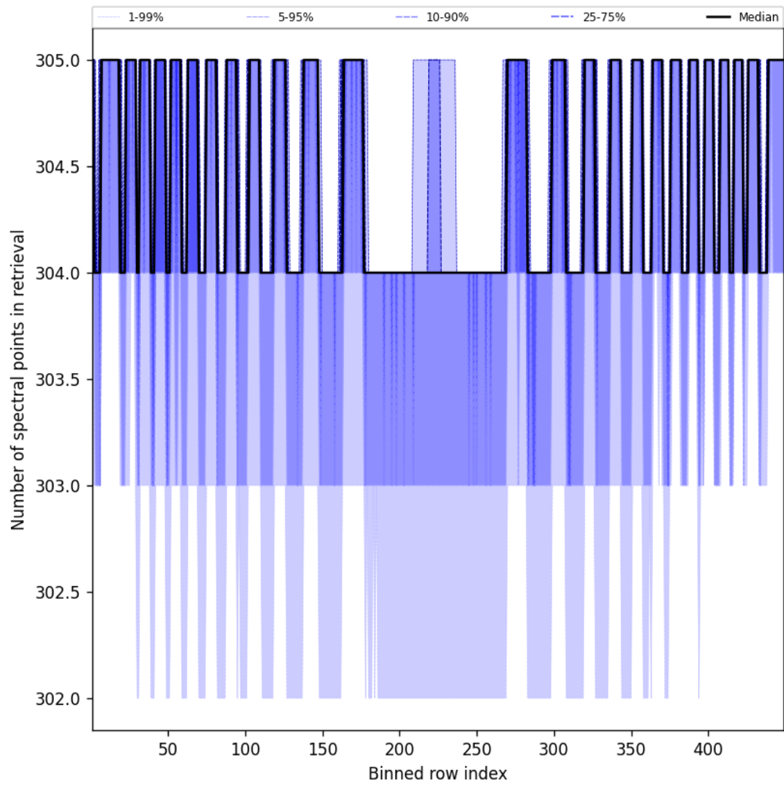
Figure 50: Along track statistics of “Number of spectral points in retrieval” for 2025-01-23 to 2025-01-25
