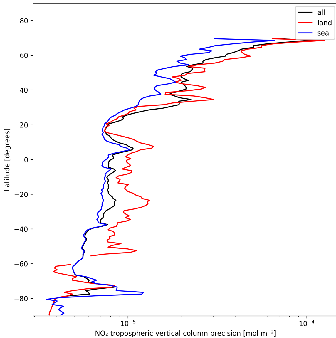
Figure 13: Zonal average of “NO 2 tropospheric vertical column precision” for 2025-01-23 to 2025-01-25.
