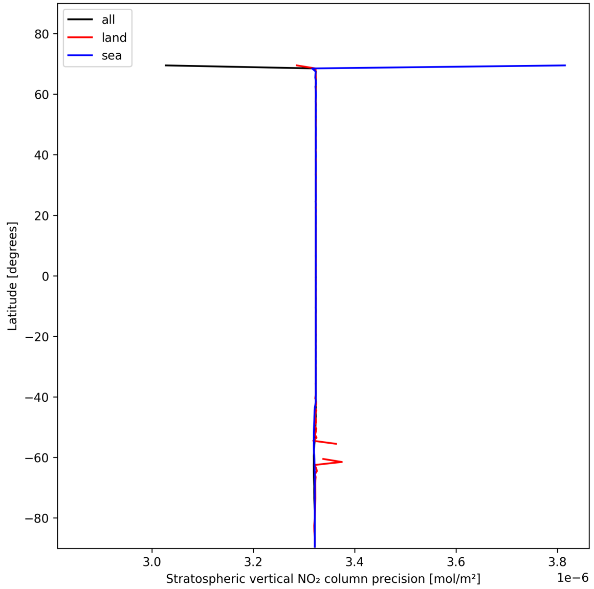
Figure 20: Zonal average of “Stratospheric vertical NO 2 column precision” for 2025-01-23 to 2025-01-25.
