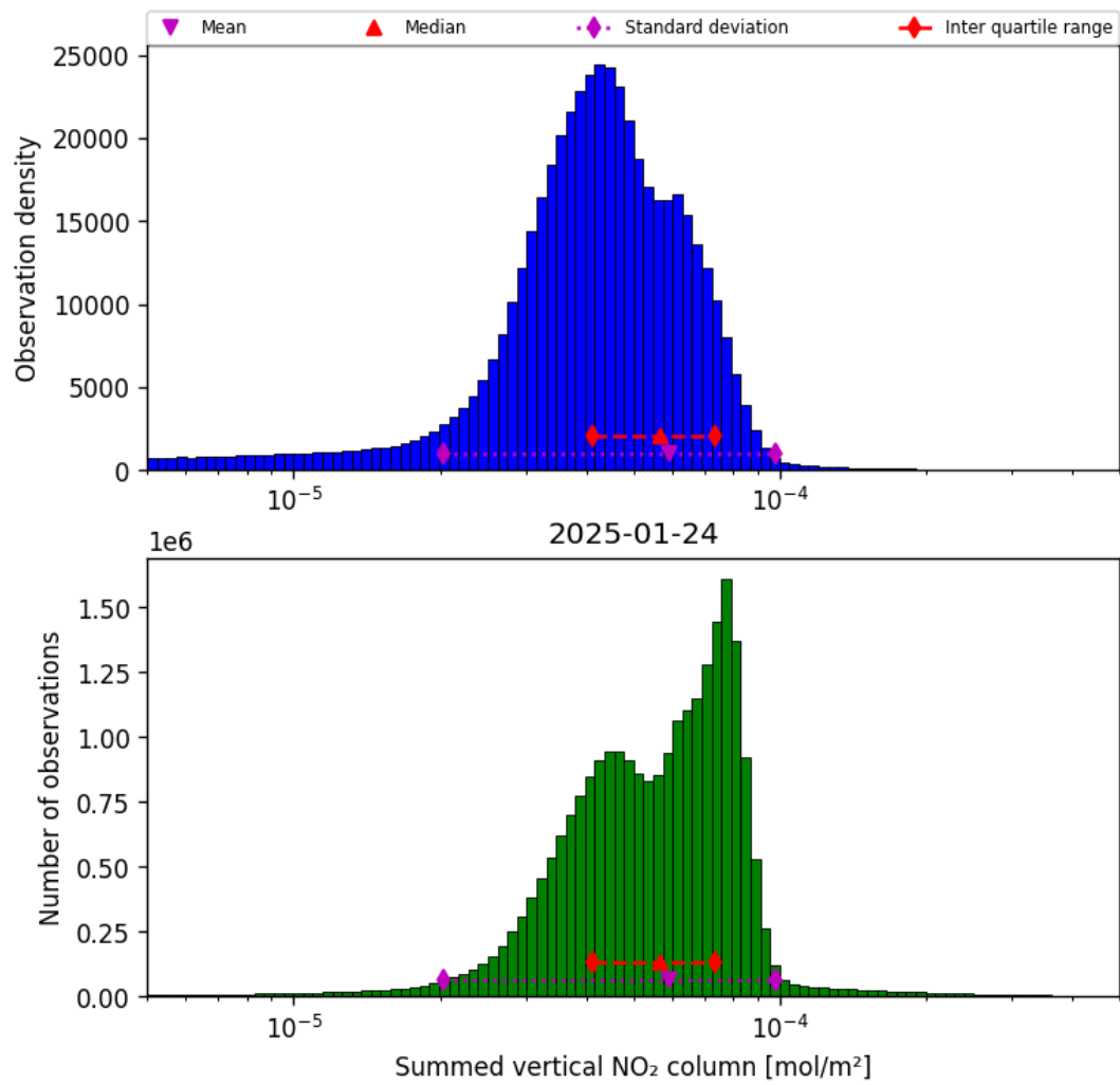
Figure 40: Histogram of “Summed vertical NO 2 column” for 2025-01-23 to 2025-01-25
