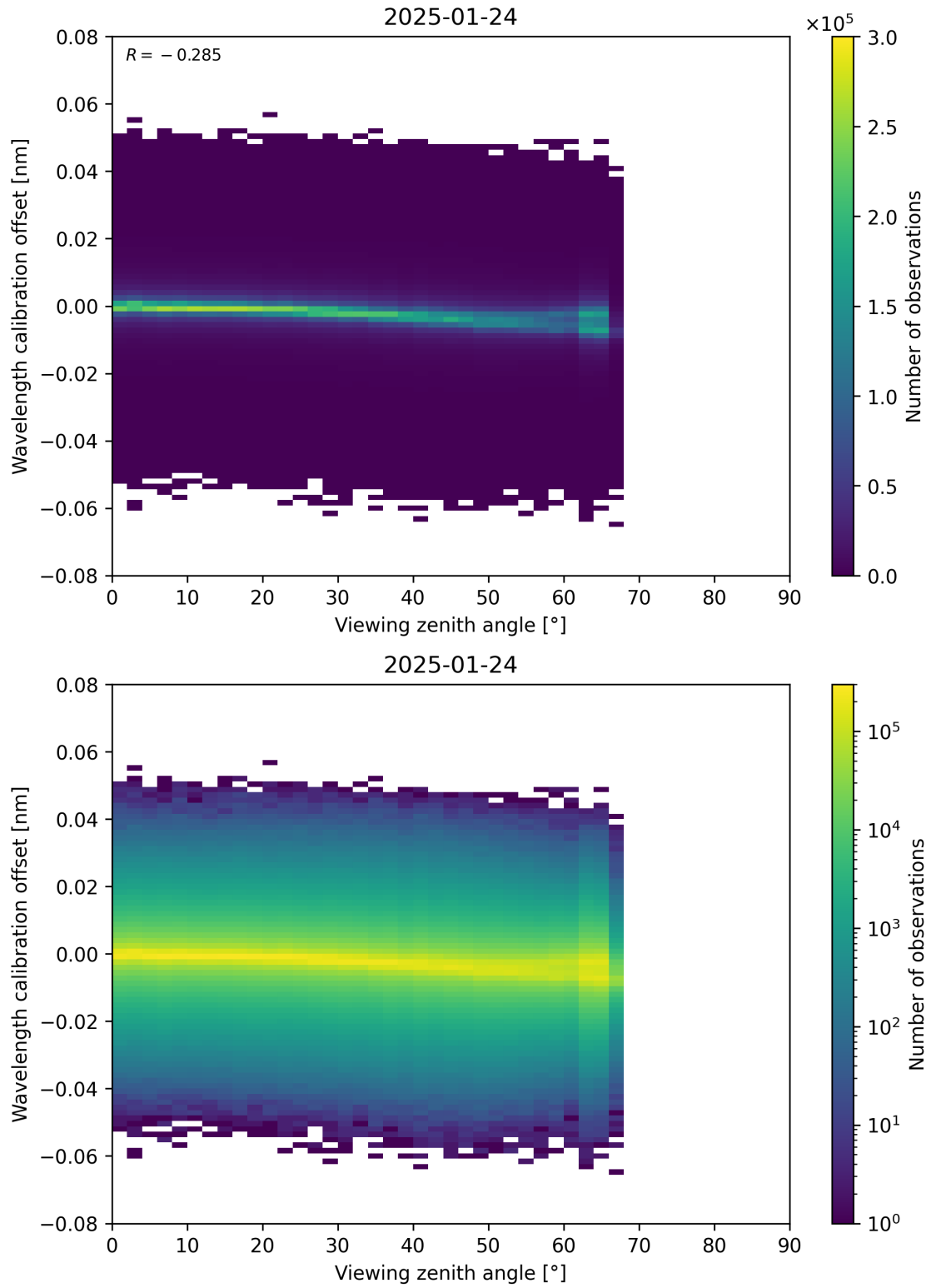
Figure 173: Scatter density plot of “Viewing zenith angle” against “Wavelength calibration offset” for 2025-01-23 to 2025-01-25.
