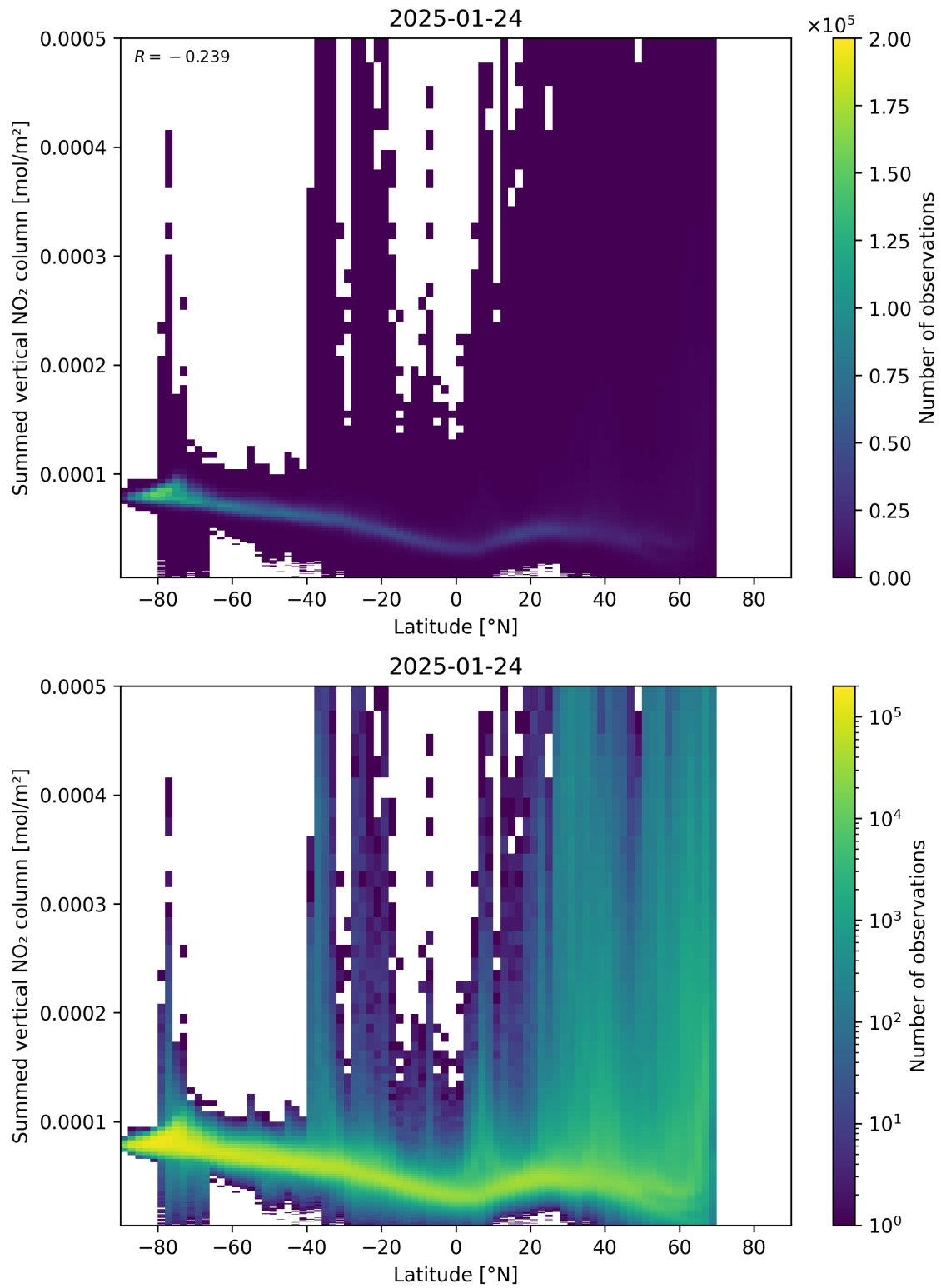
Figure 88: Scatter density plot of “Latitude” against “Summed vertical NO 2 column” for 2025-01-23 to 2025-01-25.
