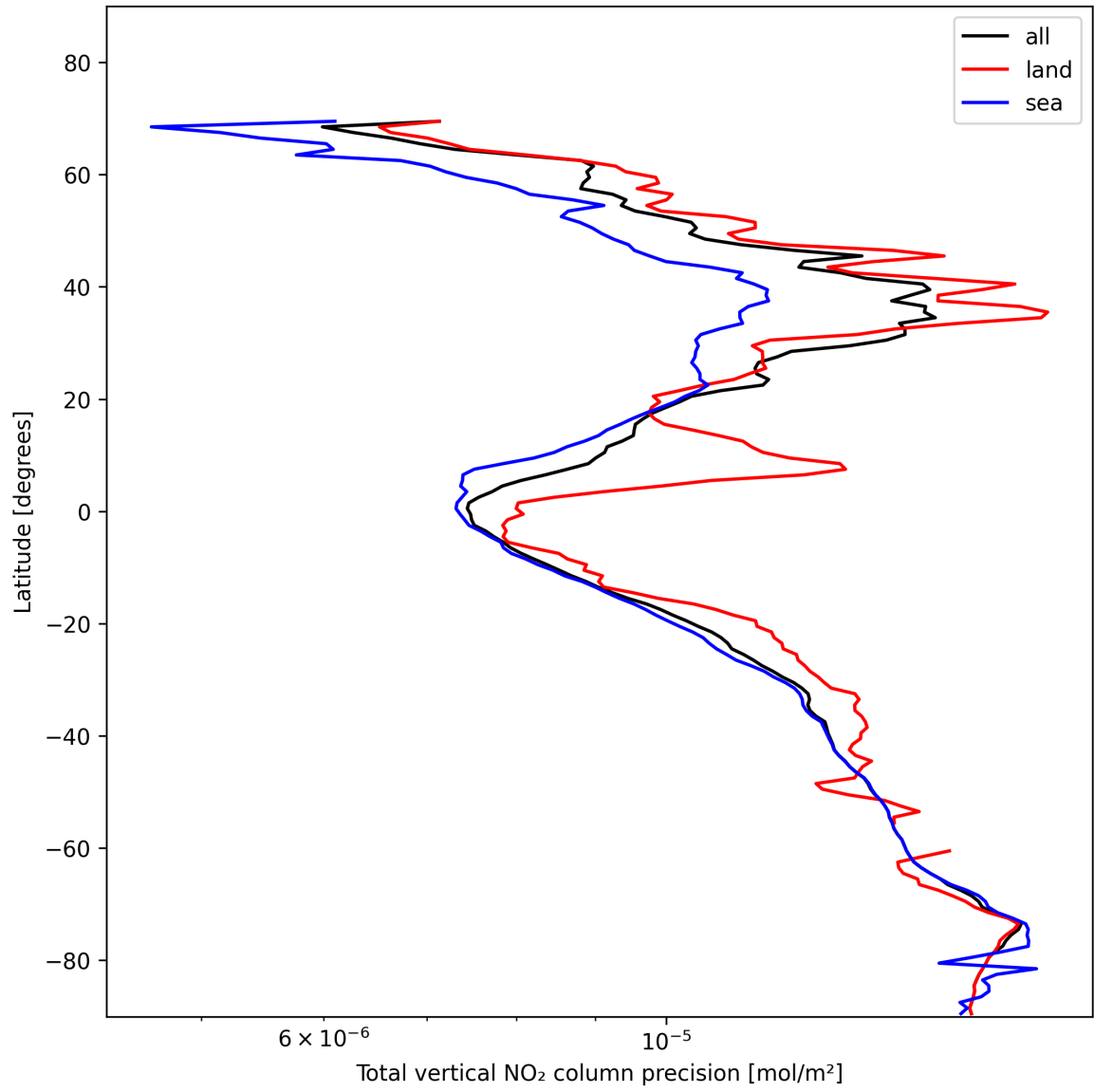
Figure 22: Zonal average of “Total vertical NO 2 column precision” for 2025-01-23 to 2025-01-25.
