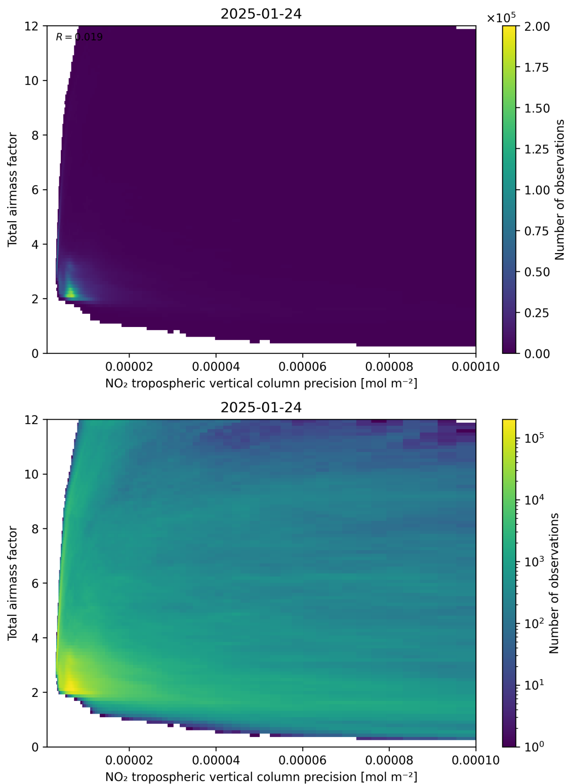
Figure 132: Scatter density plot of “NO 2 tropospheric vertical column precision” against “Total air mass factor” for 2025-01-23 to 2025-01-25.
