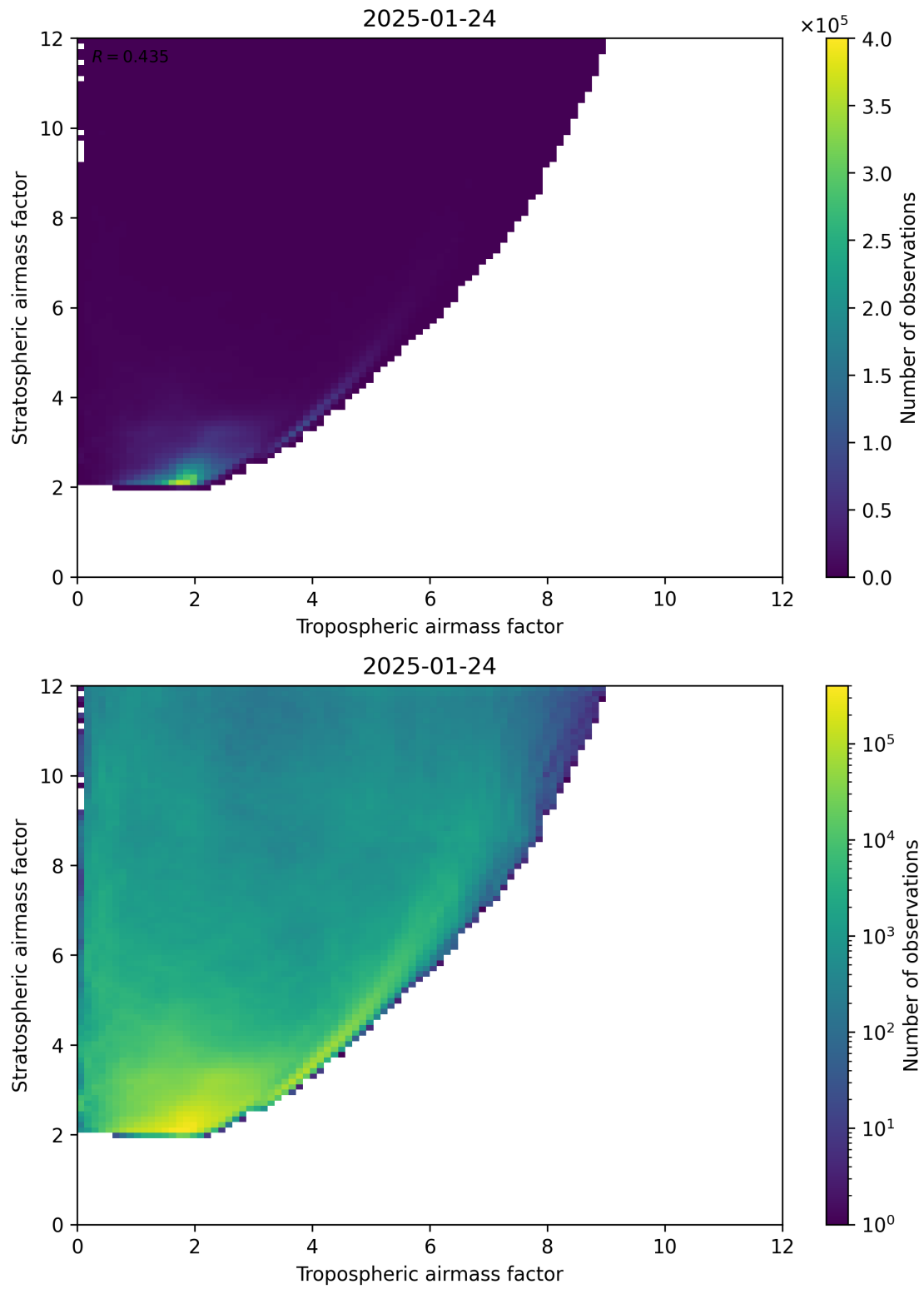
Figure 71: Scatter density plot of “Tropospheric airmass factor” against “Stratospheric airmass factor” for 2025-01-23 to 2025-01-25.
