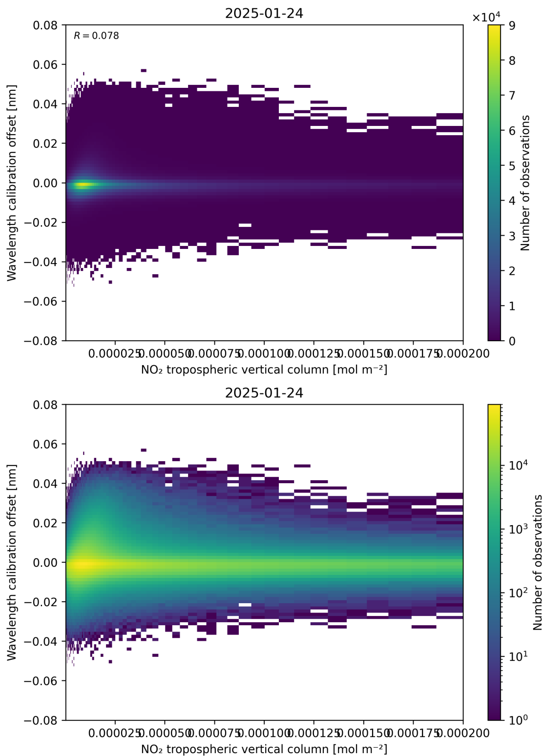
Figure 143: Scatter density plot of “NO 2 tropospheric vertical column” against “Wavelength calibration offset” for 2025-01-23 to 2025-01-25.
