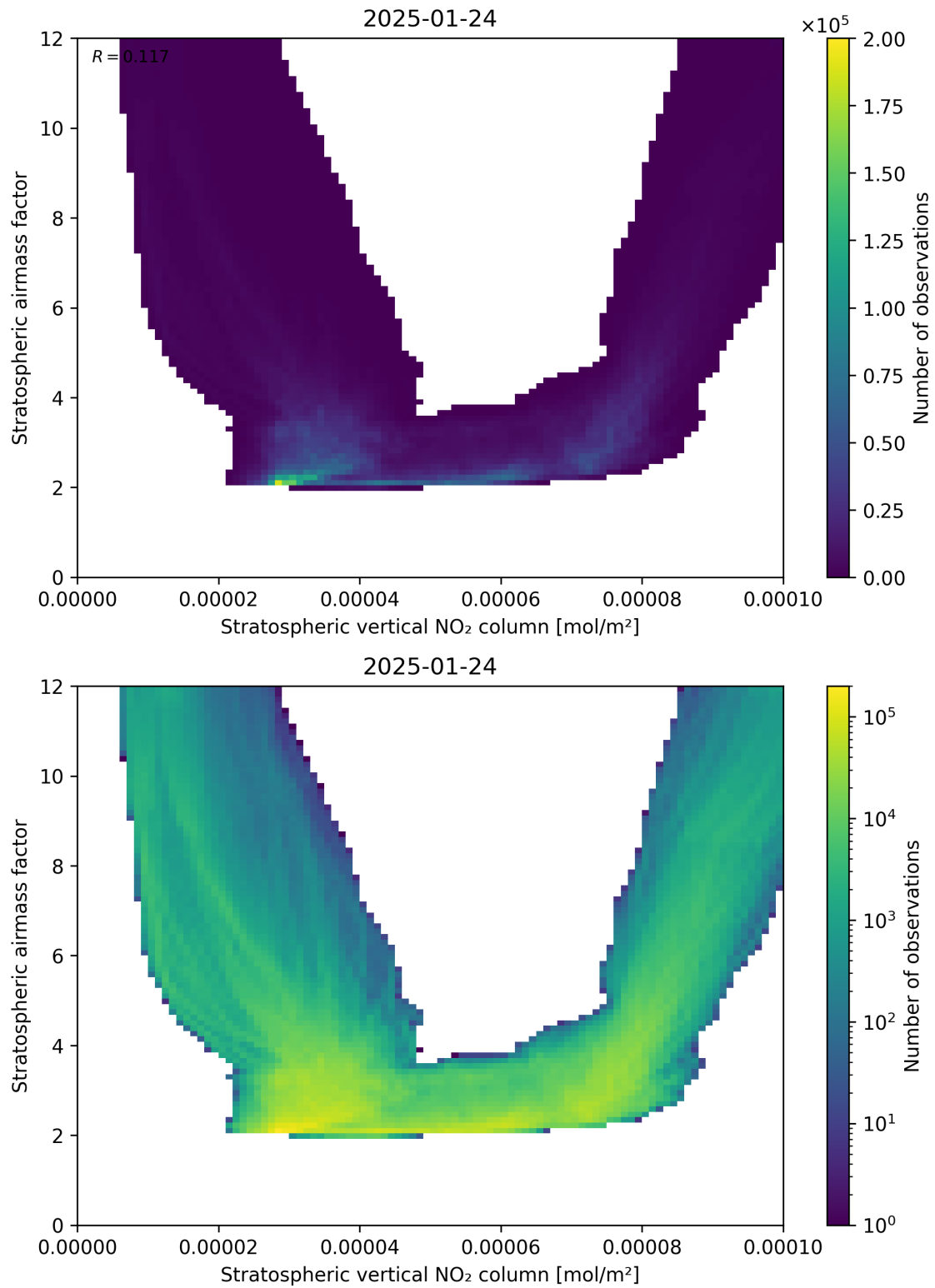
Figure 96: Scatter density plot of “Stratospheric vertical NO 2 column” against “Stratospheric airmass factor” for 2025-01-23 to 2025-01-25.
