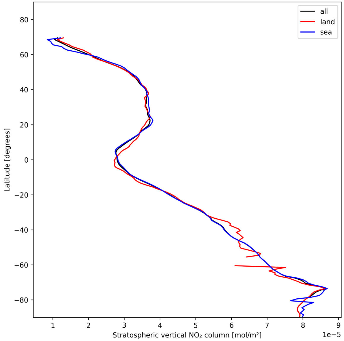
Figure 19: Zonal average of “Stratospheric vertical NO 2 column” for 2025-01-23 to 2025-01-25.
