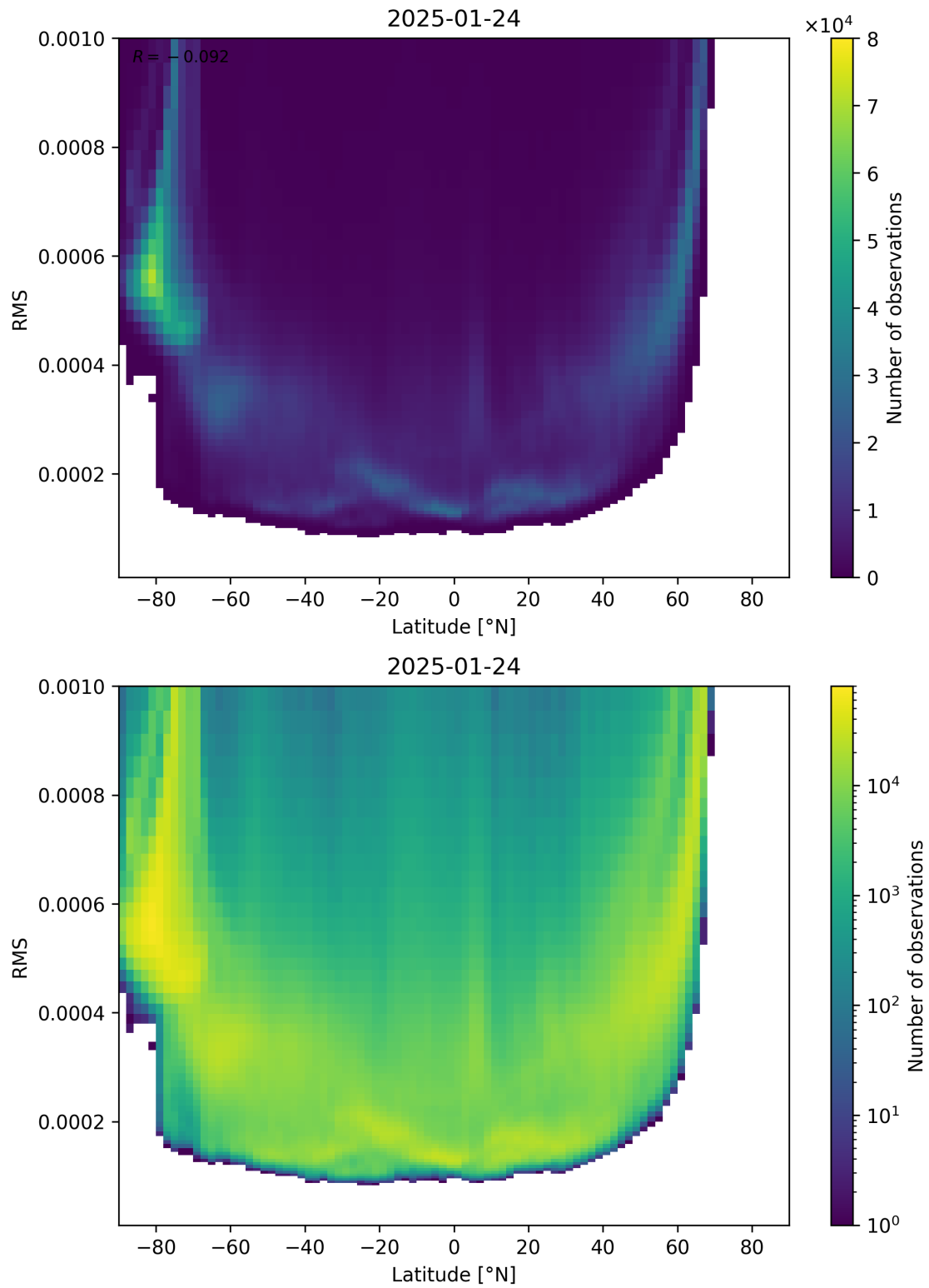
Figure 94: Scatter density plot of “Latitude” against “RMS” for 2025-01-23 to 2025-01-25.
