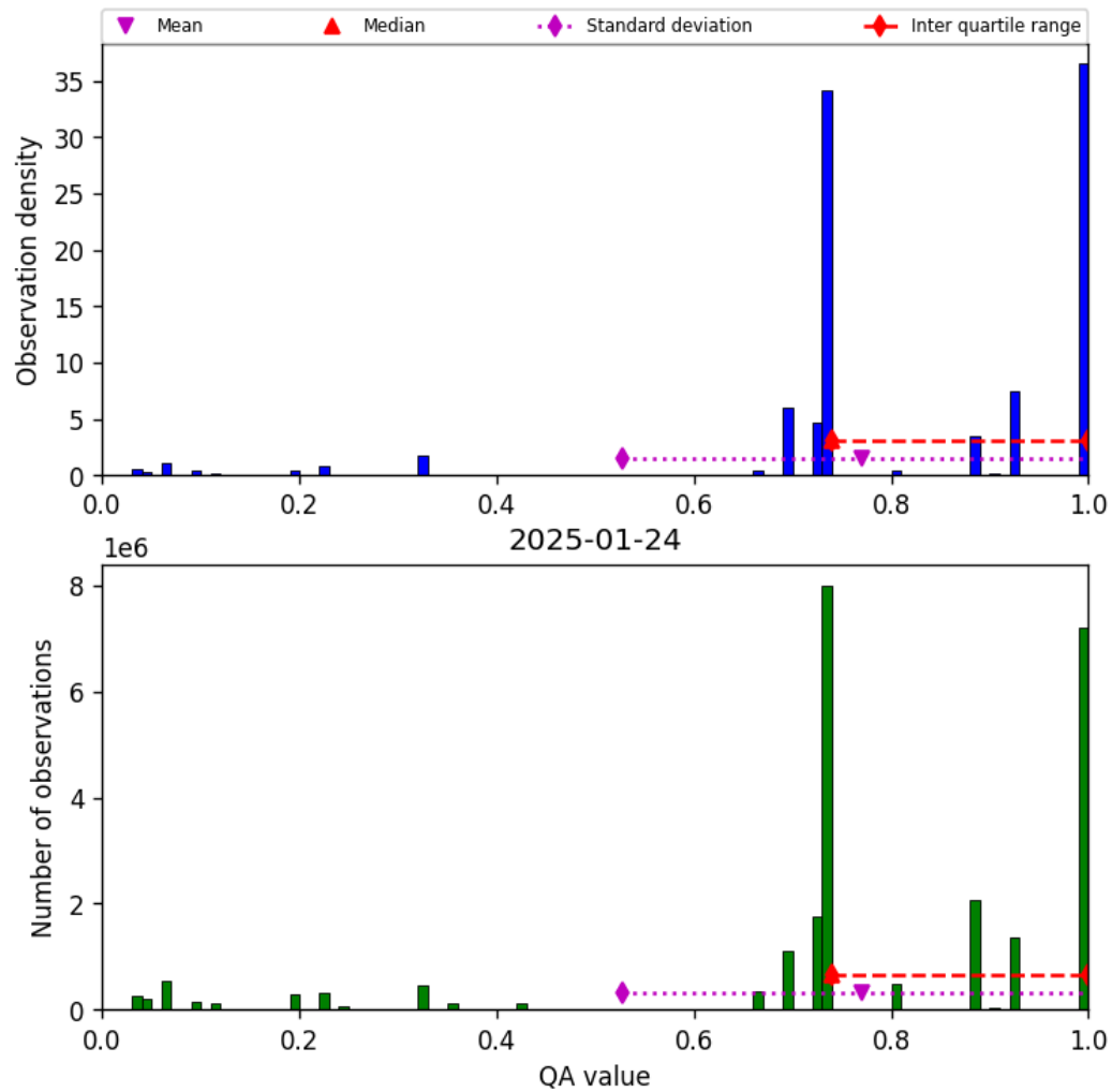
Figure 28: Histogram of “QA value” for 2025-01-23 to 2025-01-25
