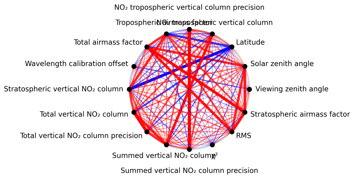
Figure 1: Map of correlation graph for 2025-01-23 to 2025-01-25.
