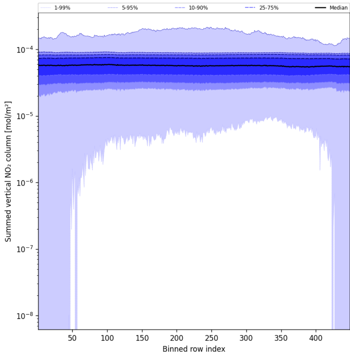
Figure 57: Along track statistics of “Summed vertical NO 2 column” for 2025-01-23 to 2025-01-25
