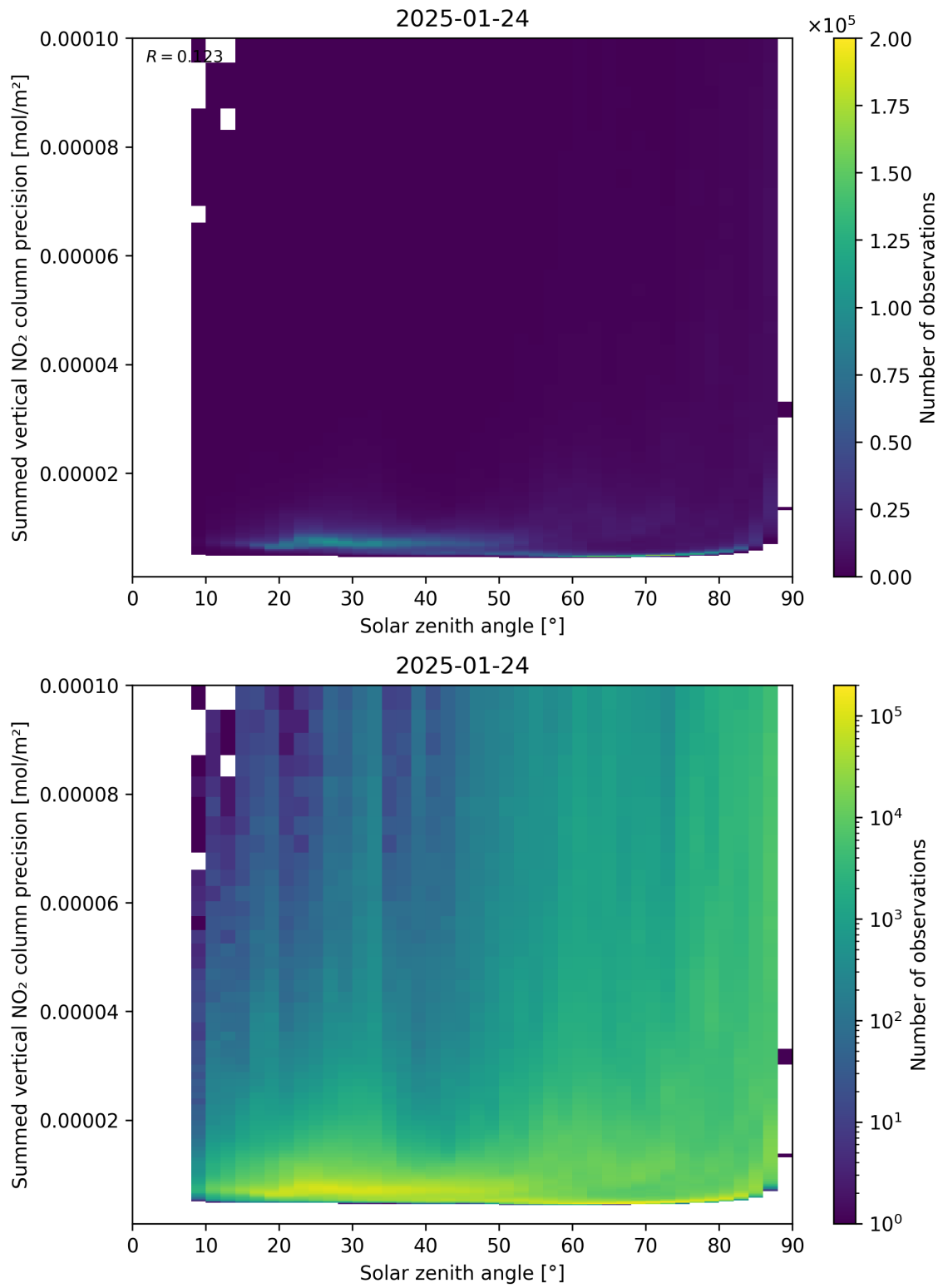
Figure 152: Scatter density plot of “Solar zenith angle” against “Summed vertical NO 2 column precision” for 2025-01-23 to 2025-01-25.
