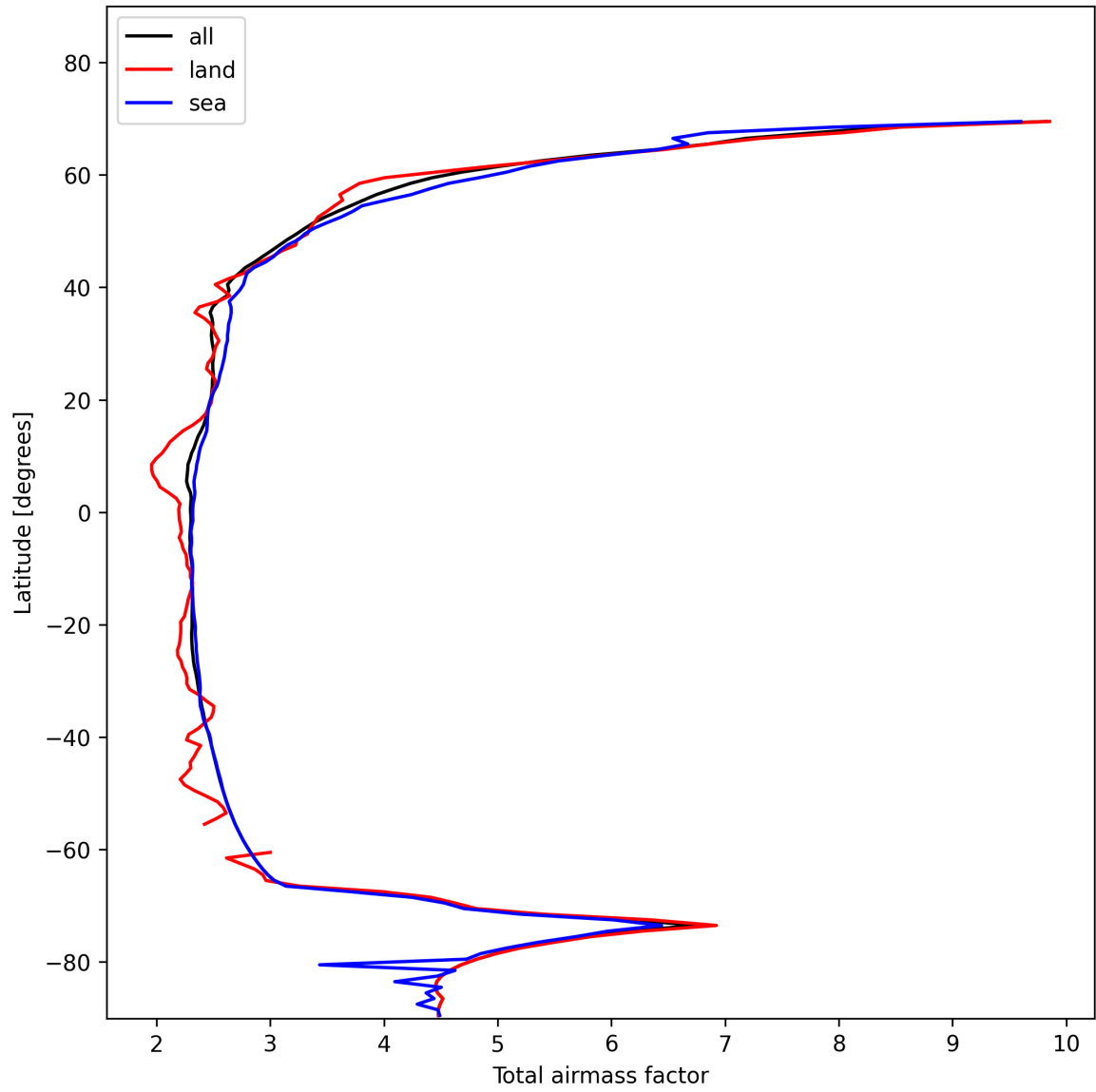
Figure 15: Zonal average of “Total airmass factor” for 2025-01-23 to 2025-01-25.
