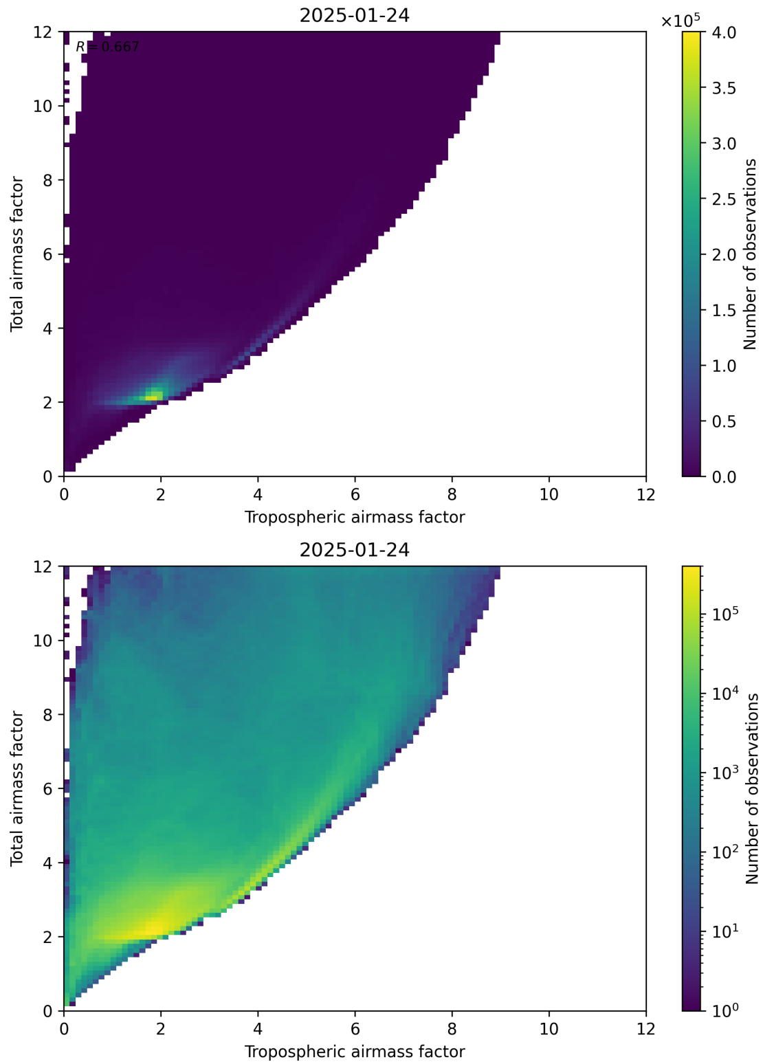
Figure 72: Scatter density plot of “Tropospheric airmass factor” against “Total airmass factor” for 2025-01-23 to 2025-01-25.
