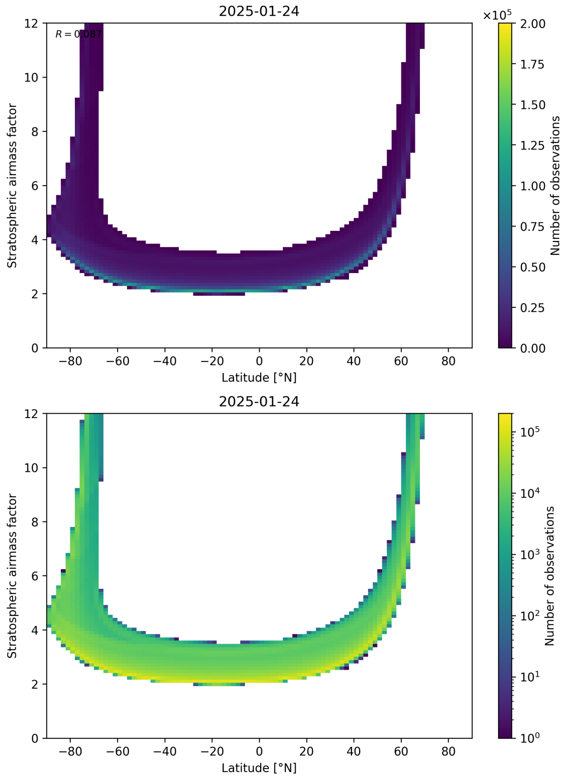
Figure 83: Scatter density plot of “Latitude” against “Stratospheric airmass factor” for 2025-01-23 to 2025-01-25.
