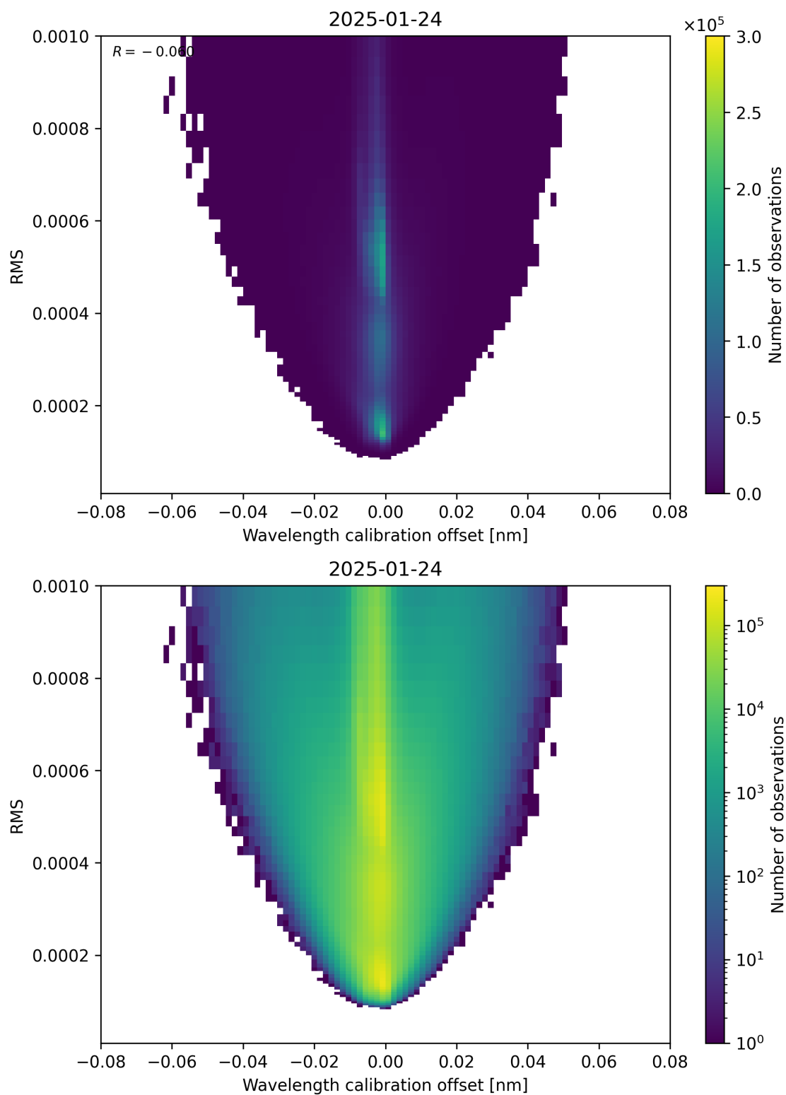
Figure 181: Scatter density plot of “Wavelength calibration offset” against “RMS” for 2025-01-23 to 2025-01-25.
