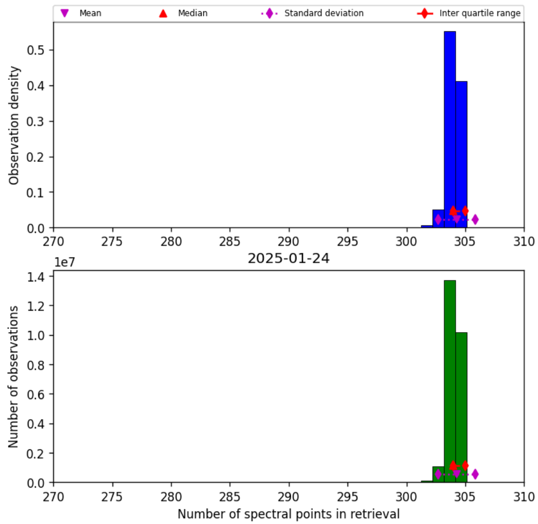
Figure 33: Histogram of “Number of spectral points in retrieval” for 2025-01-23 to 2025-01-25
