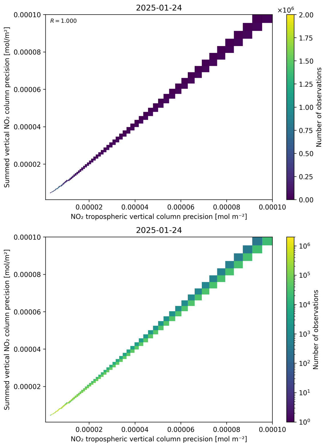
Figure 137: Scatter density plot of “NO 2 tropospheric vertical column precision” against “Summed vertical NO 2 column precision” for 2025-01-23 to 2025-01-25.
