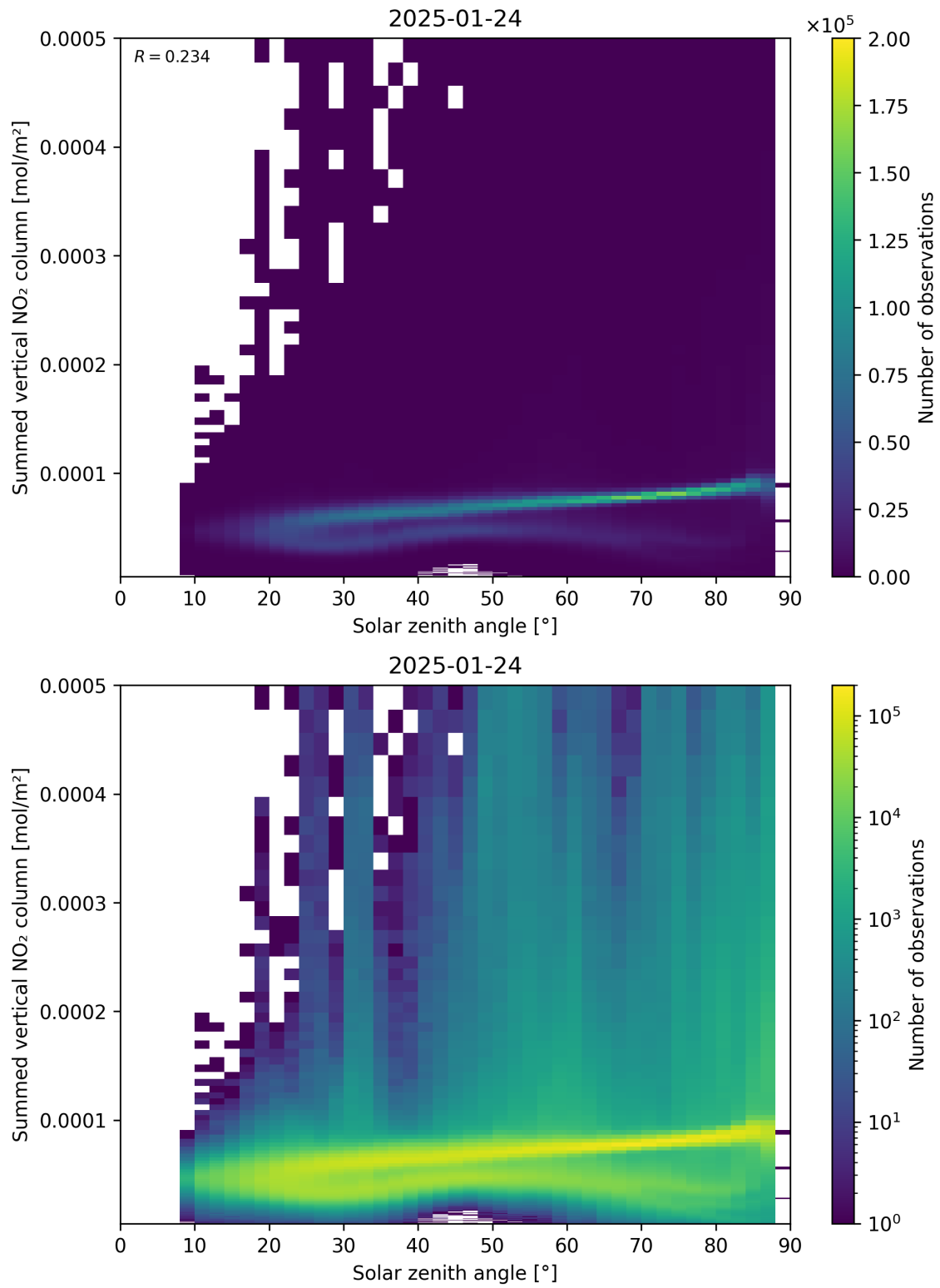
Figure 151: Scatter density plot of “Solar zenith angle” against “Summed vertical NO 2 column” for 2025-01-23 to 2025-01-25.
