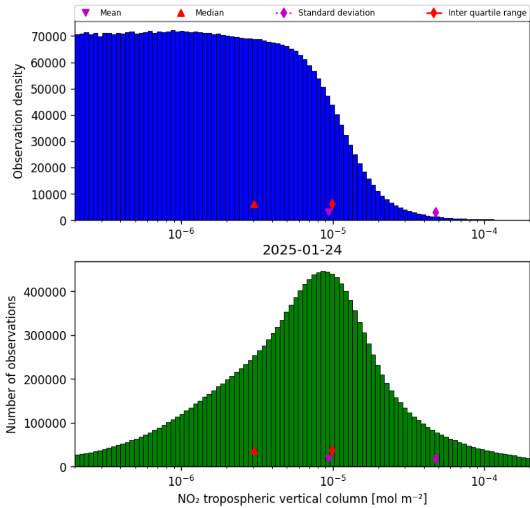
Figure 29: Histogram of “NO 2 tropospheric vertical column” for 2025-01-23 to 2025-01-25
