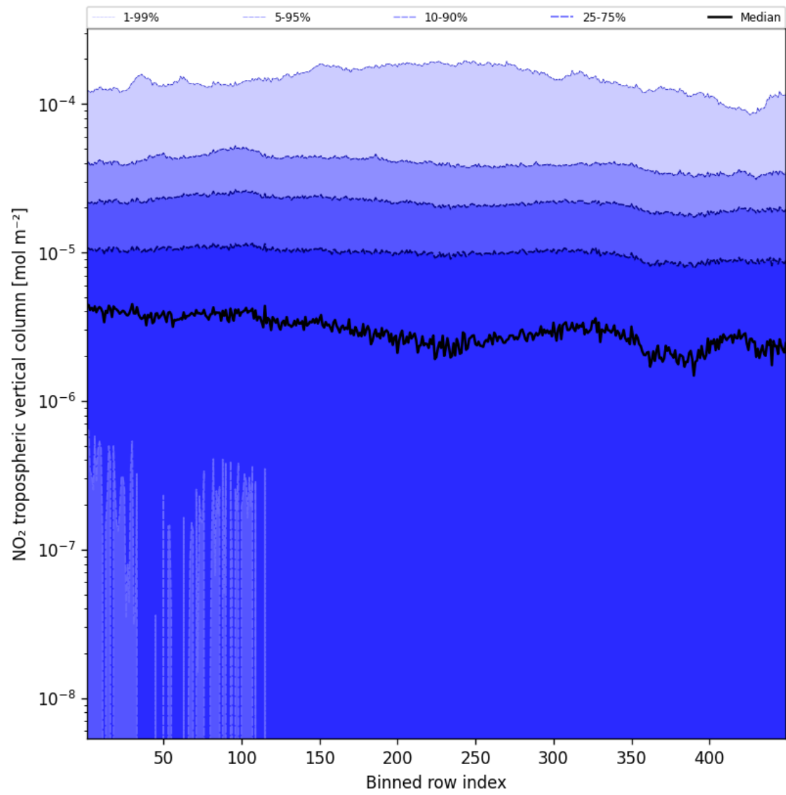
Figure 46: Along track statistics of “NO 2 tropospheric vertical column” for 2025-01-23 to 2025-01-25
