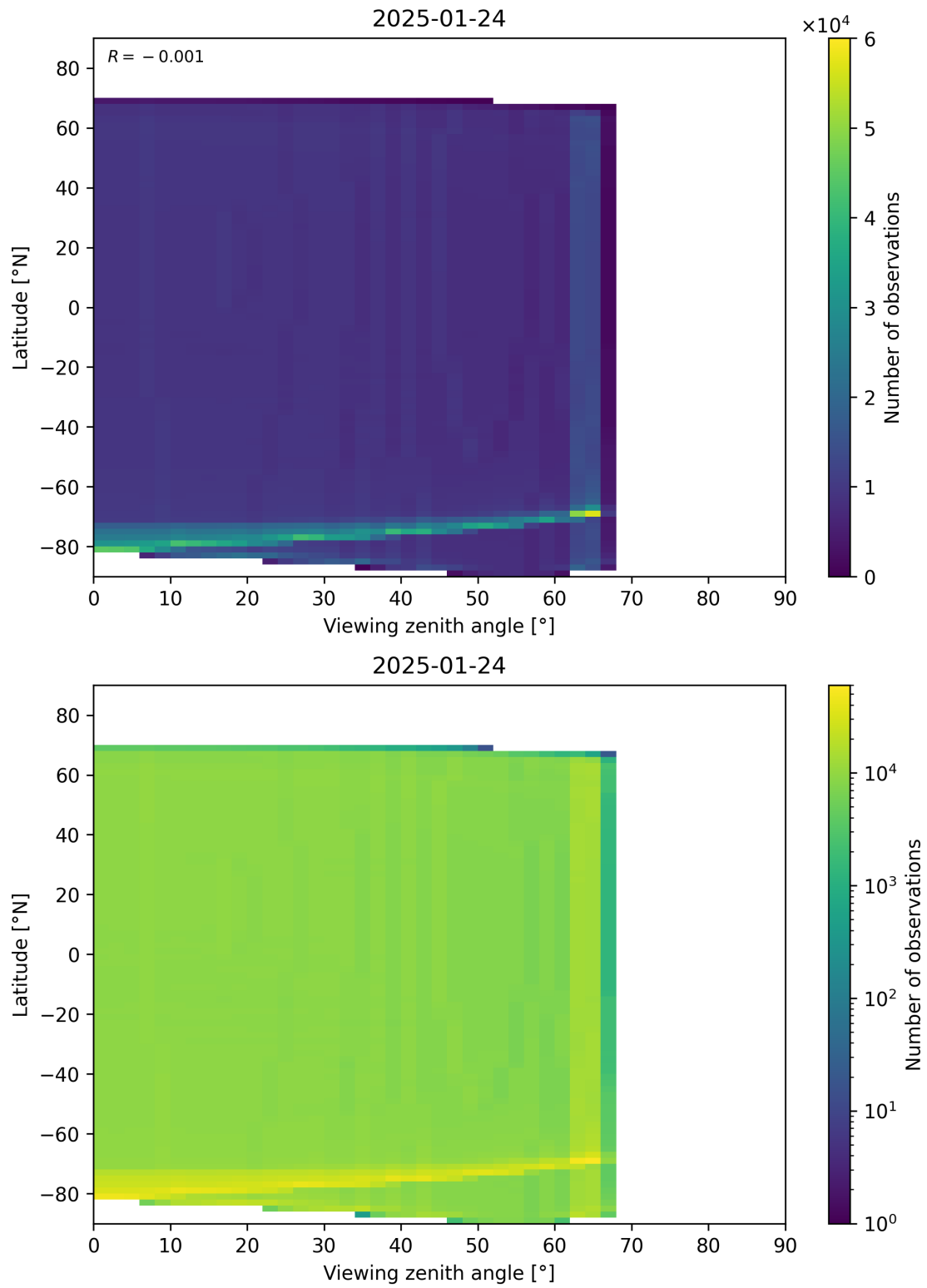
Figure 163: Scatter density plot of “Viewing zenith angle” against “Latitude” for 2025-01-23 to 2025-01-25.
