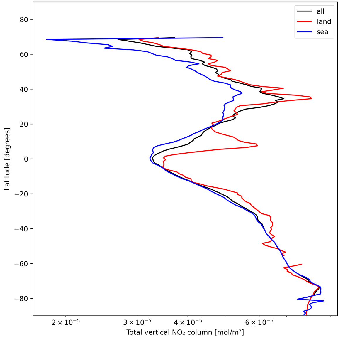
Figure 21: Zonal average of “Total vertical NO 2 column” for 2025-01-23 to 2025-01-25.
