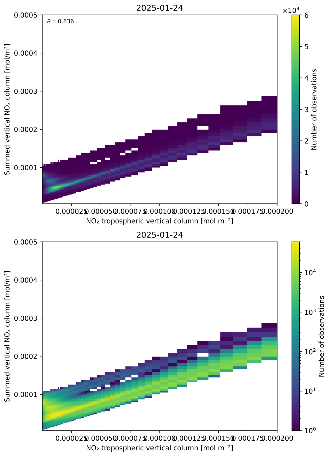
Figure 126: Scatter density plot of “NO 2 tropospheric vertical column” against “Summed vertical NO 2 column” for 2025-01-23 to 2025-01-25.
