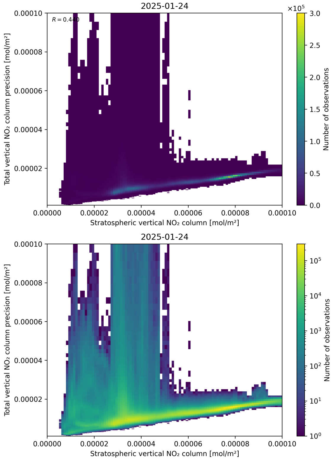
Figure 101: Scatter density plot of “Stratospheric vertical NO 2 column” against “Total vertical NO 2 column precision” for 2025-01-23 to 2025-01-25.
