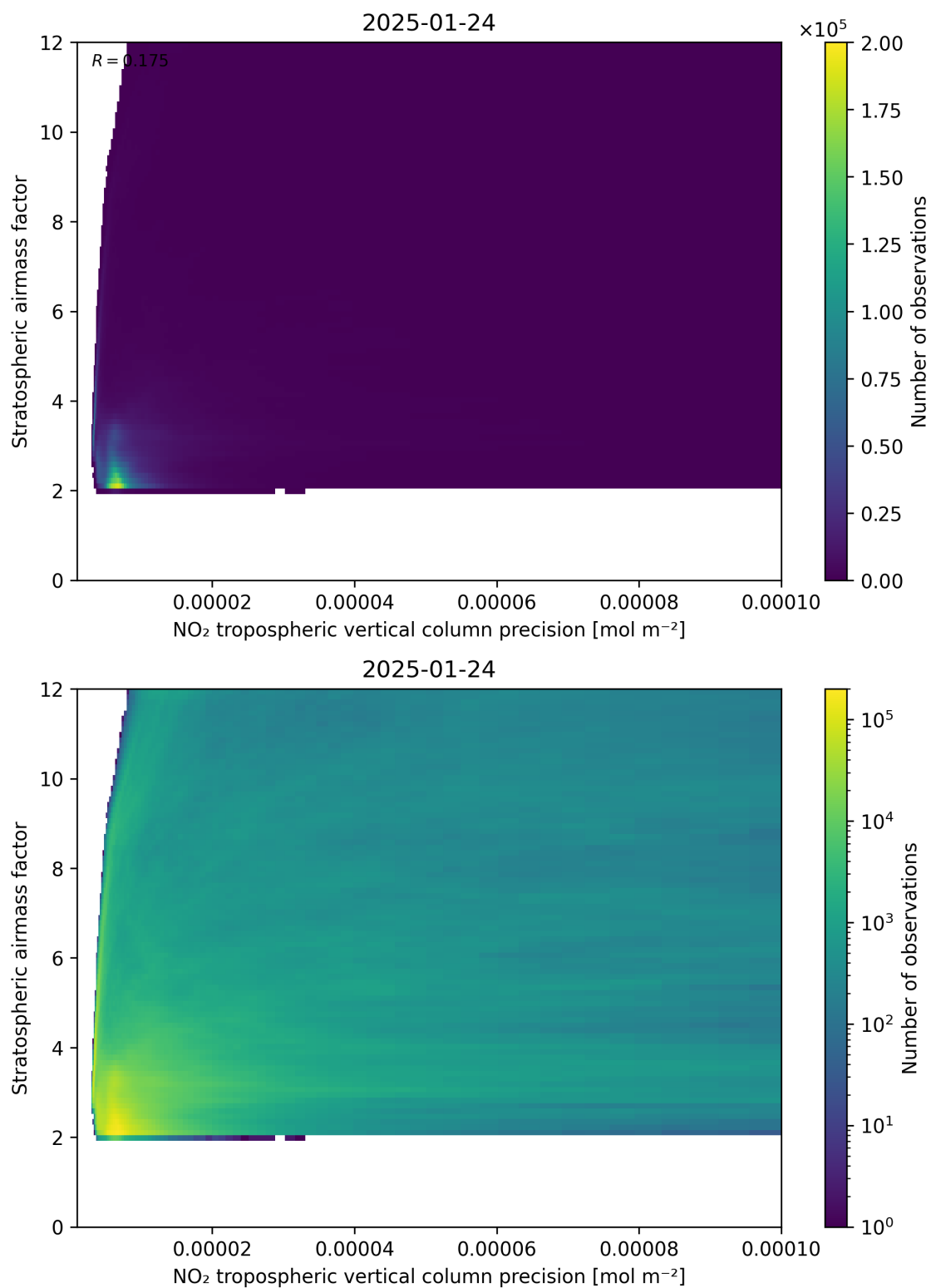
Figure 131: Scatter density plot of “NO 2 tropospheric vertical column precision” against “Stratospheric airmass factor” for 2025-01-23 to 2025-01-25.
