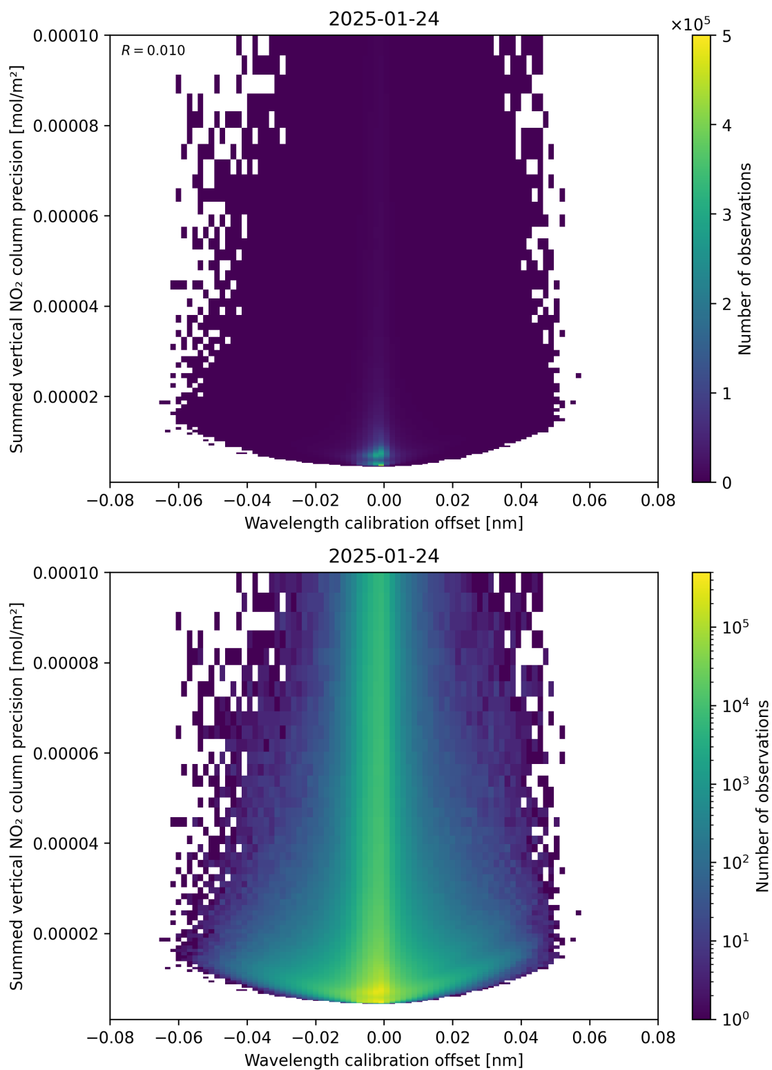
Figure 178: Scatter density plot of “Wavelength calibration offset” against “Summed vertical NO 2 column precision” for 2025-01-23 to 2025-01-25.
