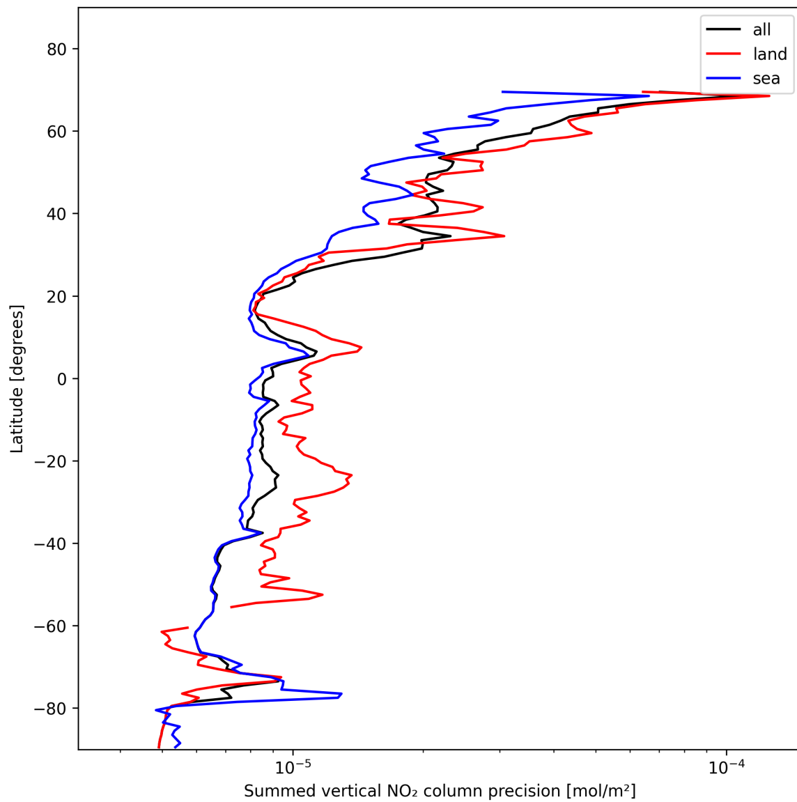
Figure 24: Zonal average of “Summed vertical NO 2 column precision” for 2025-01-23 to 2025-01-25.
