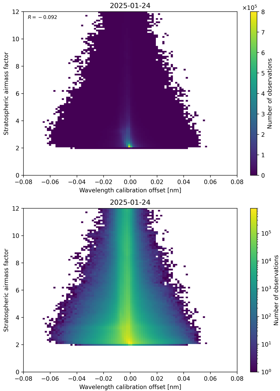
Figure 174: Scatter density plot of “Wavelength calibration offset” against “Stratospheric airmass factor” for 2025-01-23 to 2025-01-25.
