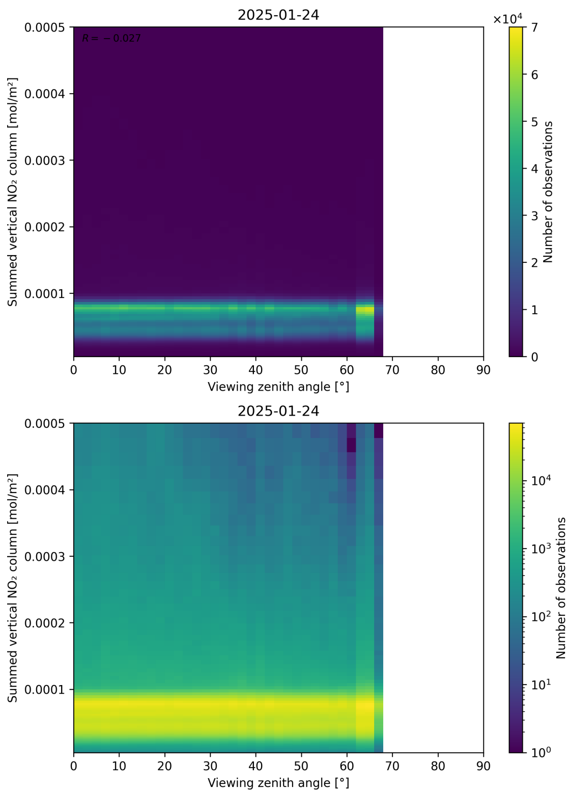
Figure 165: Scatter density plot of “Viewing zenith angle” against “Summed vertical NO 2 column” for 2025-01-23 to 2025-01-25.
