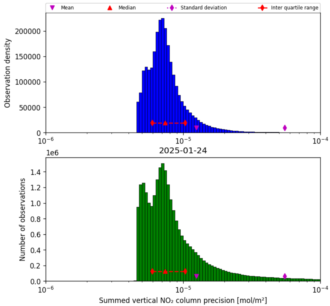
Figure 41: Histogram of "Summed vertical NO 2 column precision" for 2025-01-23 to 2025-01-25
