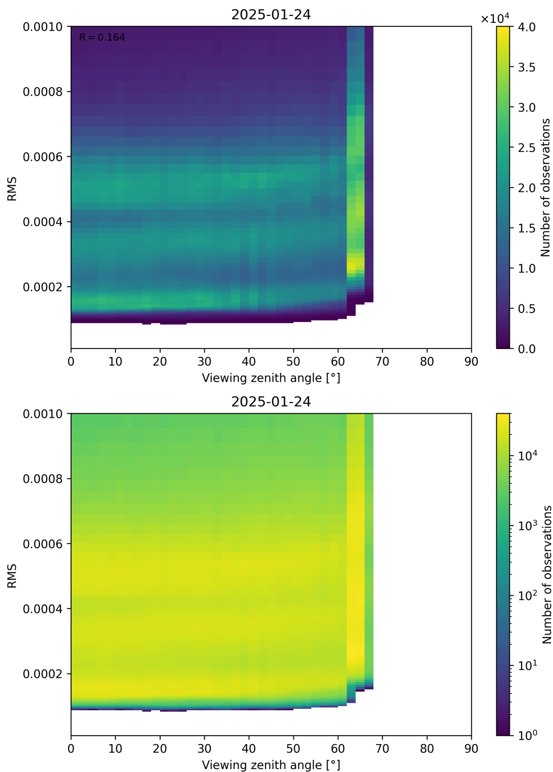
Figure 171: Scatter density plot of “Viewing zenith angle” against “RMS” for 2025-01-23 to 2025-01-25.
