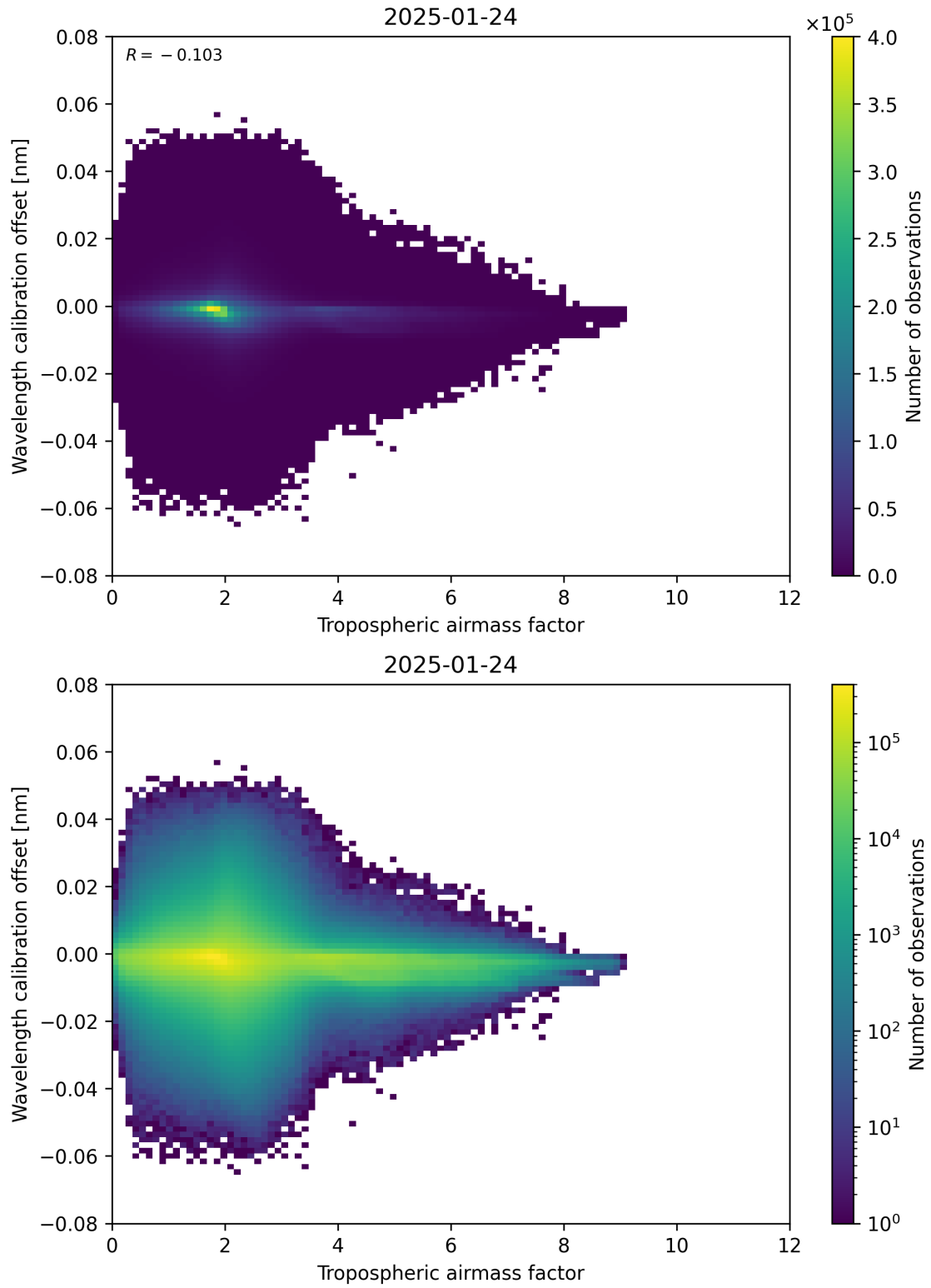
Figure 80: Scatter density plot of “Tropospheric airmass factor” against “Wavelength calibration offset” for 2025-01-23 to 2025-01-25.
