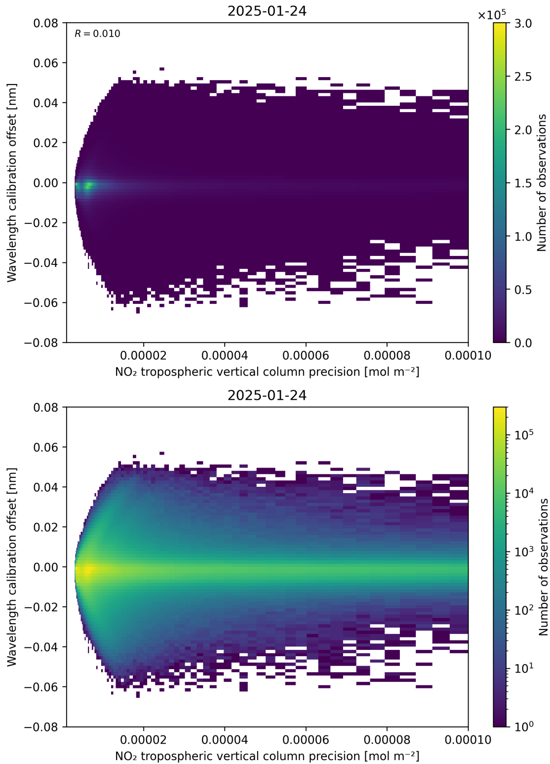
Figure 141: Scatter density plot of “NO 2 tropospheric vertical column precision” against “Wavelength calibration offset” for 2025-01-23 to 2025-01-25.
