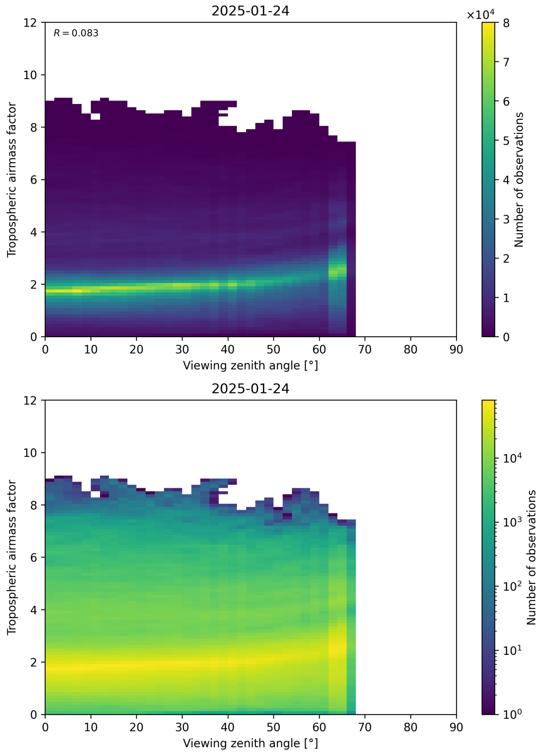
Figure 161: Scatter density plot of “Viewing zenith angle” against “Tropospheric airmass factor” for 2025-01-23 to 2025-01-25.
