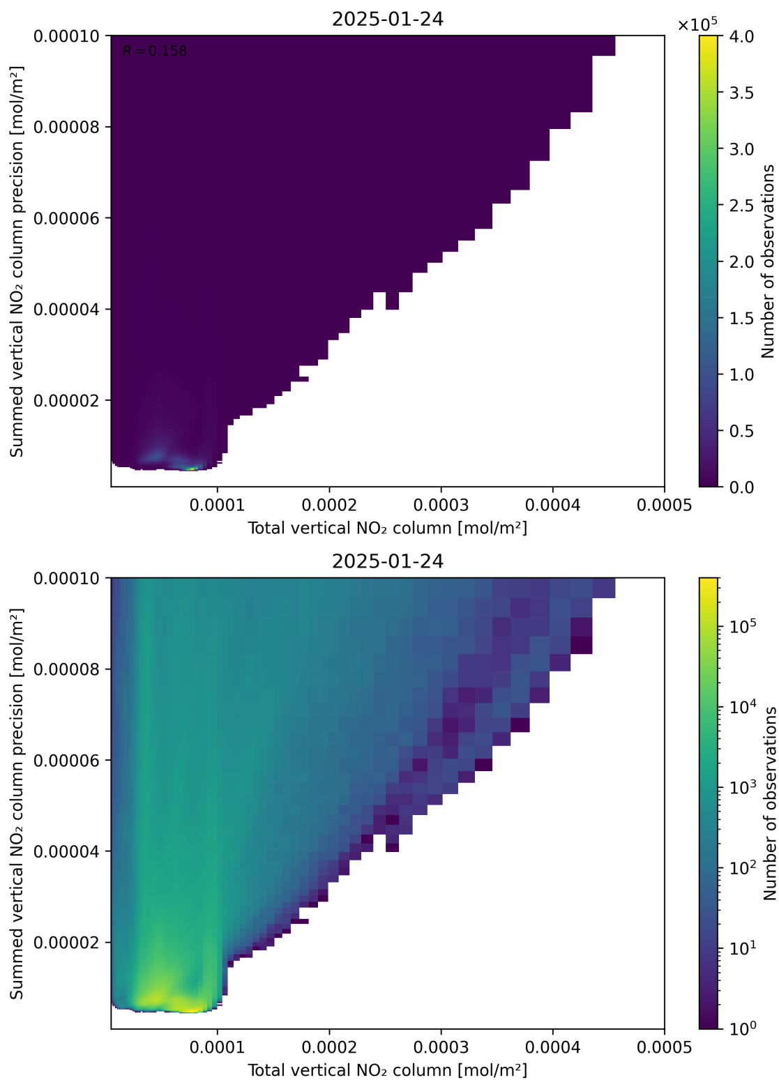
Figure 113: Scatter density plot of “Total vertical NO 2 column” against “Summed vertical NO 2 column precision” for 2025-01-23 to 2025-01-25.
