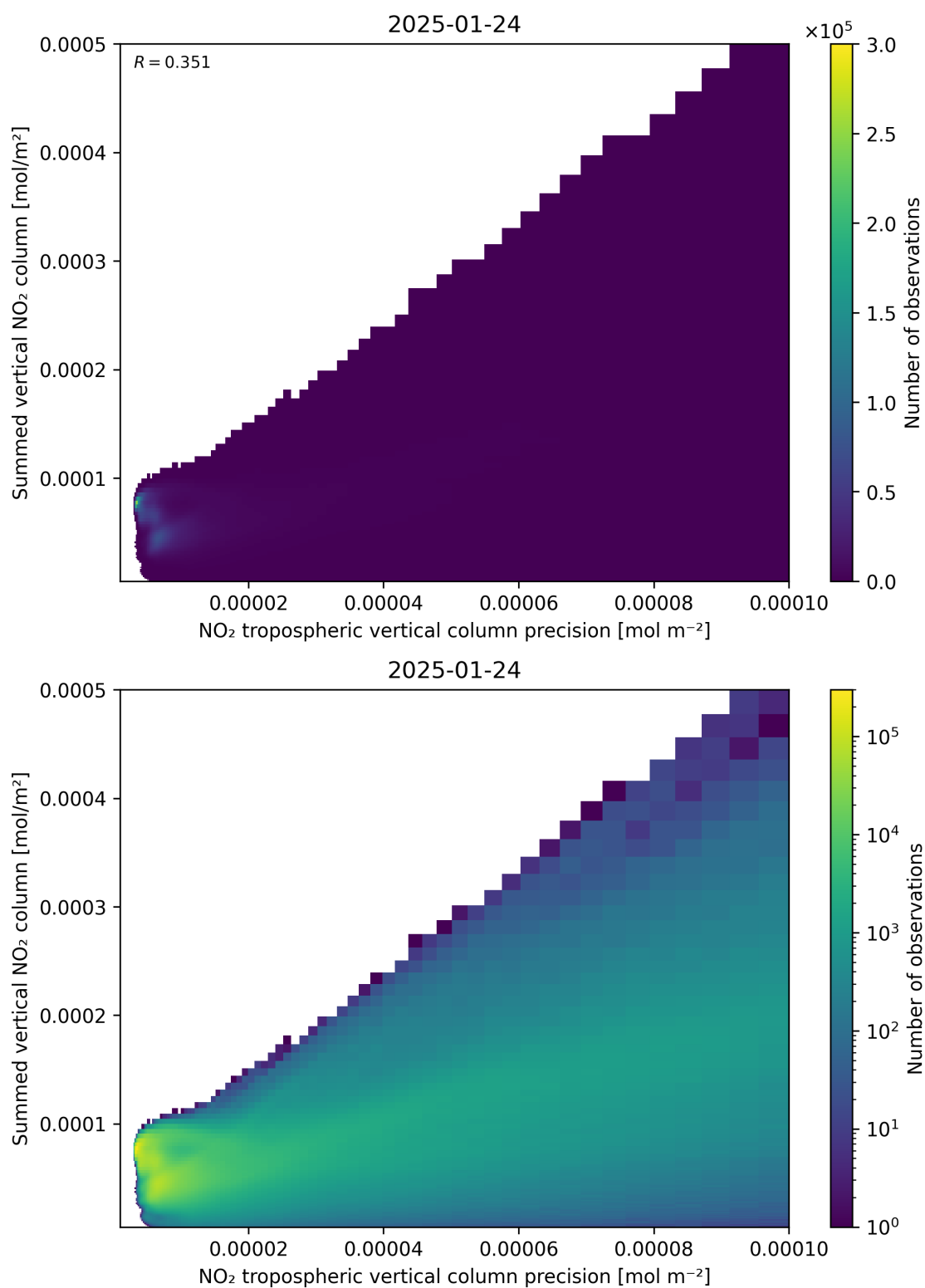
Figure 136: Scatter density plot of “NO 2 tropospheric vertical column precision” against “Summed vertical NO 2 column” for 2025-01-23 to 2025-01-25.
