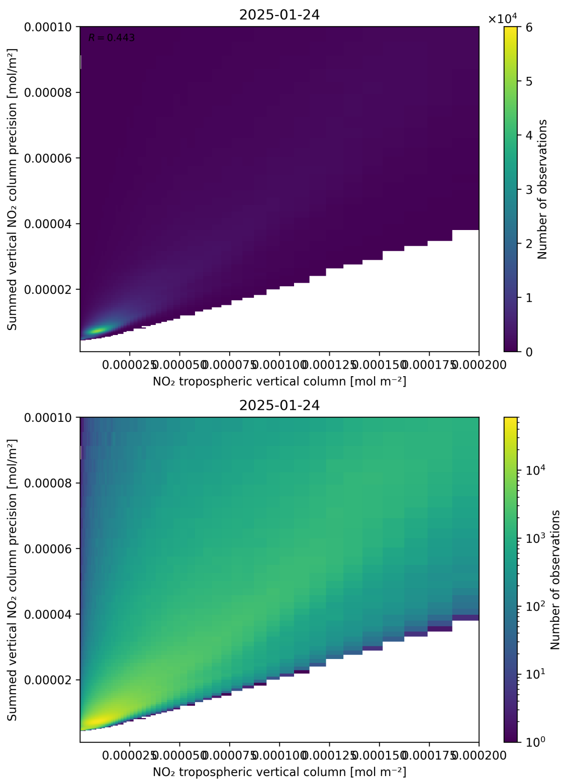
Figure 127: Scatter density plot of “NO 2 tropospheric vertical column” against “Summed vertical NO 2 column precision” for 2025-01-23 to 2025-01-25.
