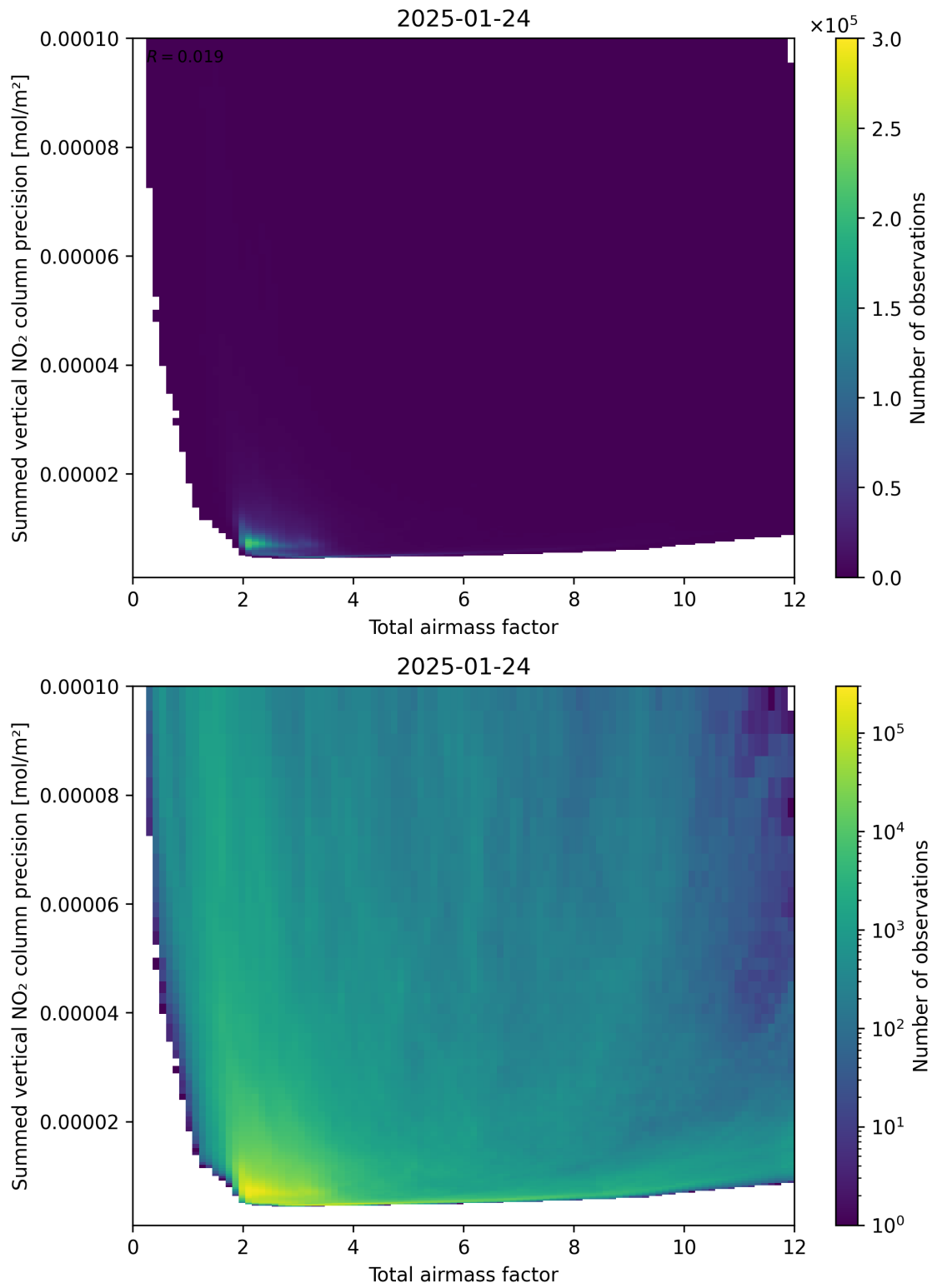
Figure 66: Scatter density plot of “Total airmass factor” against “Summed vertical NO 2 column precision” for 2025-01-23 to 2025-01-25.
