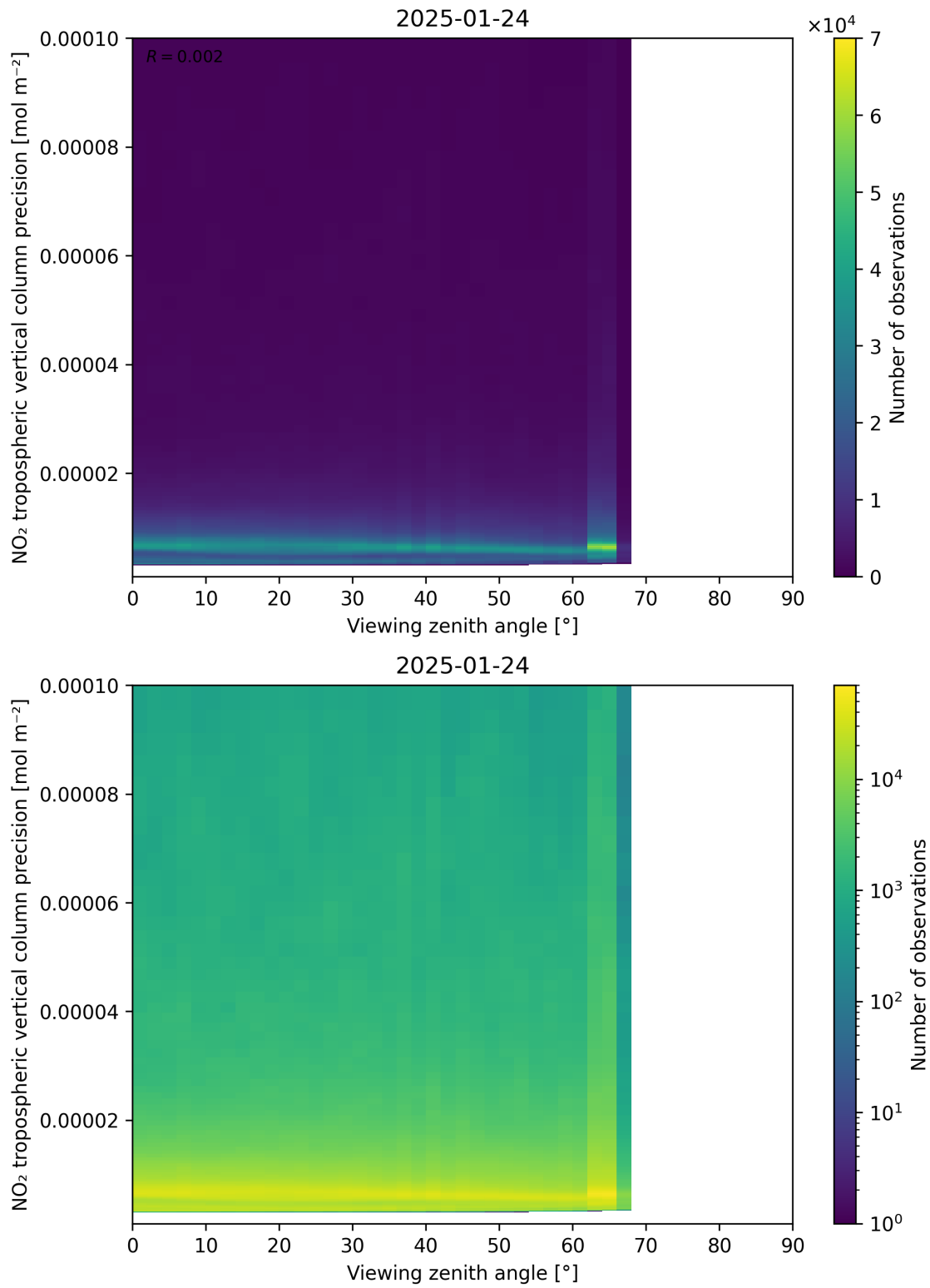
Figure 170: Scatter density plot of “Viewing zenith angle” against “NO 2 tropospheric vertical column precision” for 2025-01-23 to 2025-01-25.
