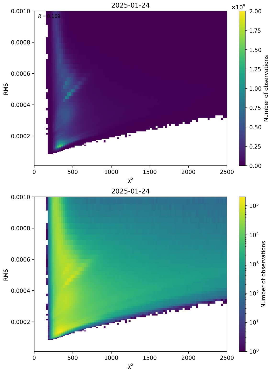
Figure 82: Scatter density plot of “ \chi^2 ” against “RMS” for 2025-01-23 to 2025-01-25.
