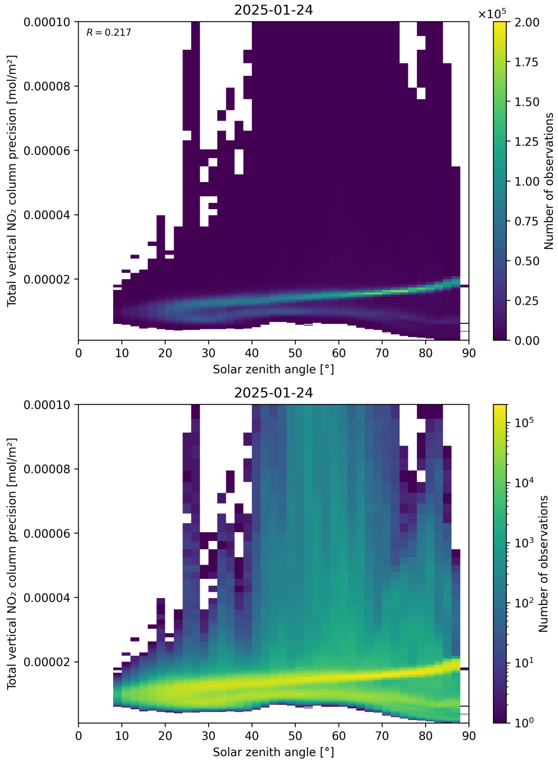
Figure 154: Scatter density plot of “Solar zenith angle” against “Total vertical NO 2 column precision” for 2025-01-23 to 2025-01-25.
