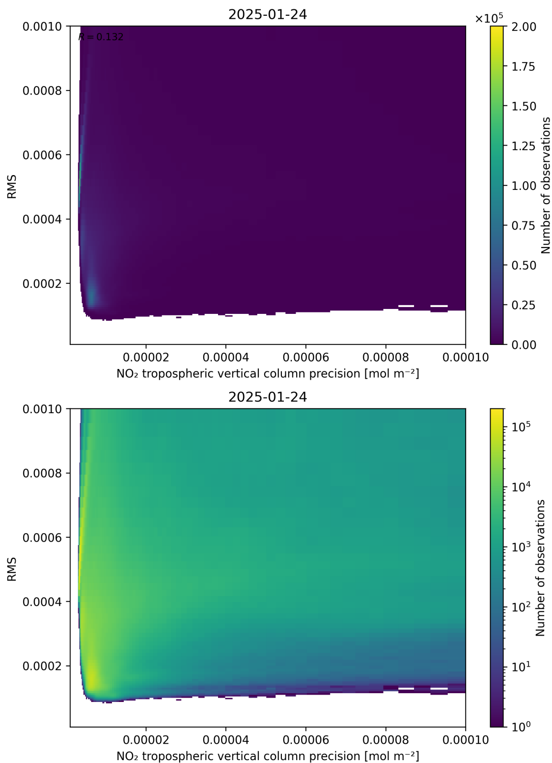
Figure 140: Scatter density plot of “NO 2 tropospheric vertical column precision” against “RMS” for 2025-01-23 to 2025-01-25.
