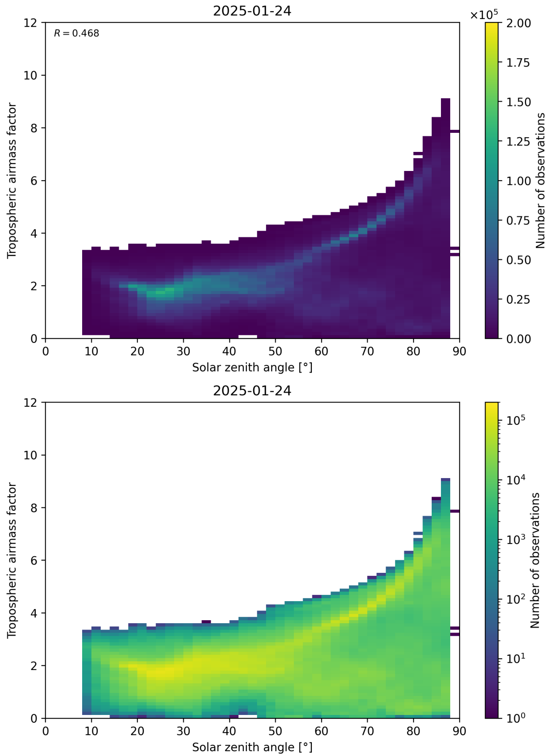
Figure 147: Scatter density plot of “Solar zenith angle” against “Tropospheric airmass factor” for 2025-01-23 to 2025-01-25.
