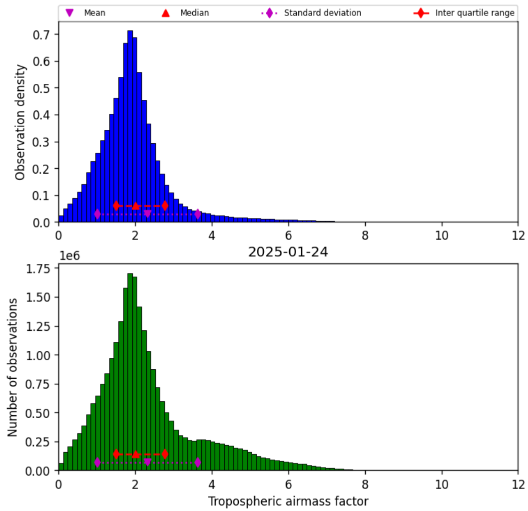
Figure 31: Histogram of “Tropospheric airmass factor” for 2025-01-23 to 2025-01-25
