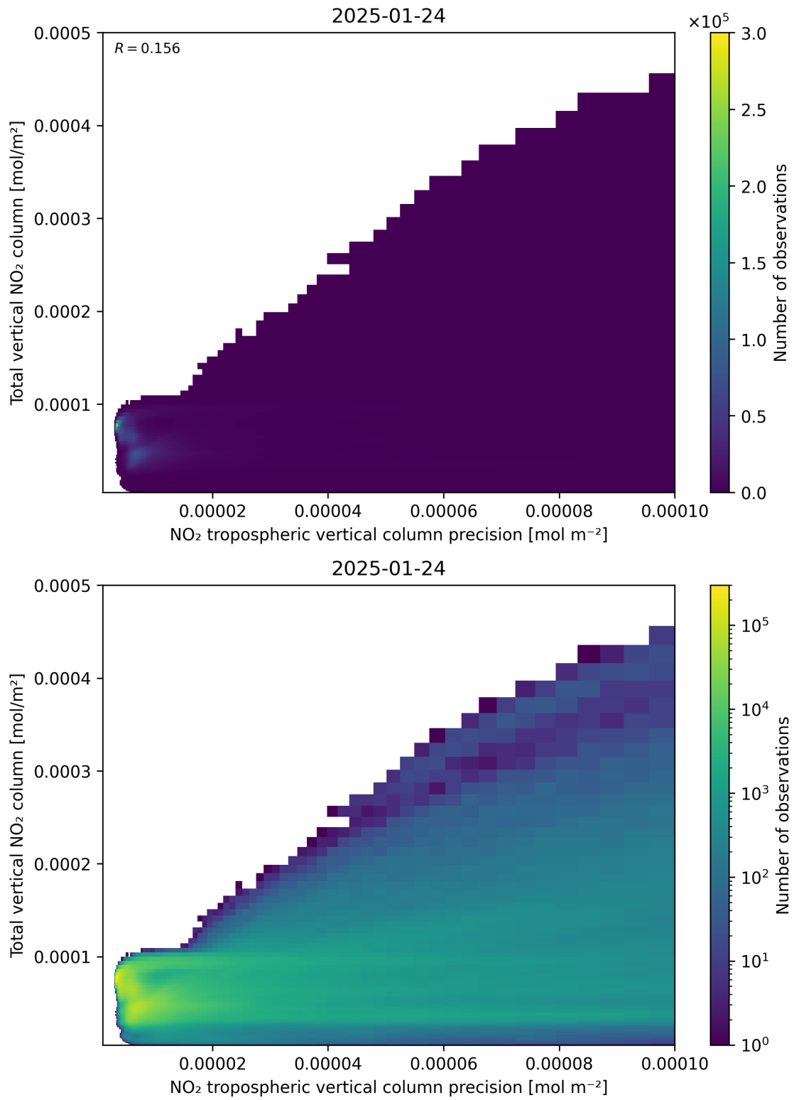
Figure 138: Scatter density plot of “NO 2 tropospheric vertical column precision” against “Total vertical NO 2 column” for 2025-01-23 to 2025-01-25.
