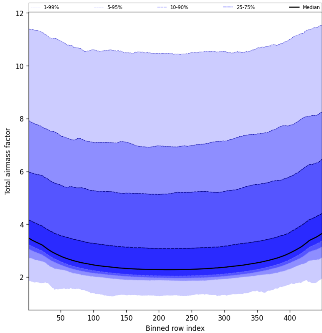
Figure 49: Along track statistics of “Total airmass factor” for 2025-01-23 to 2025-01-25
