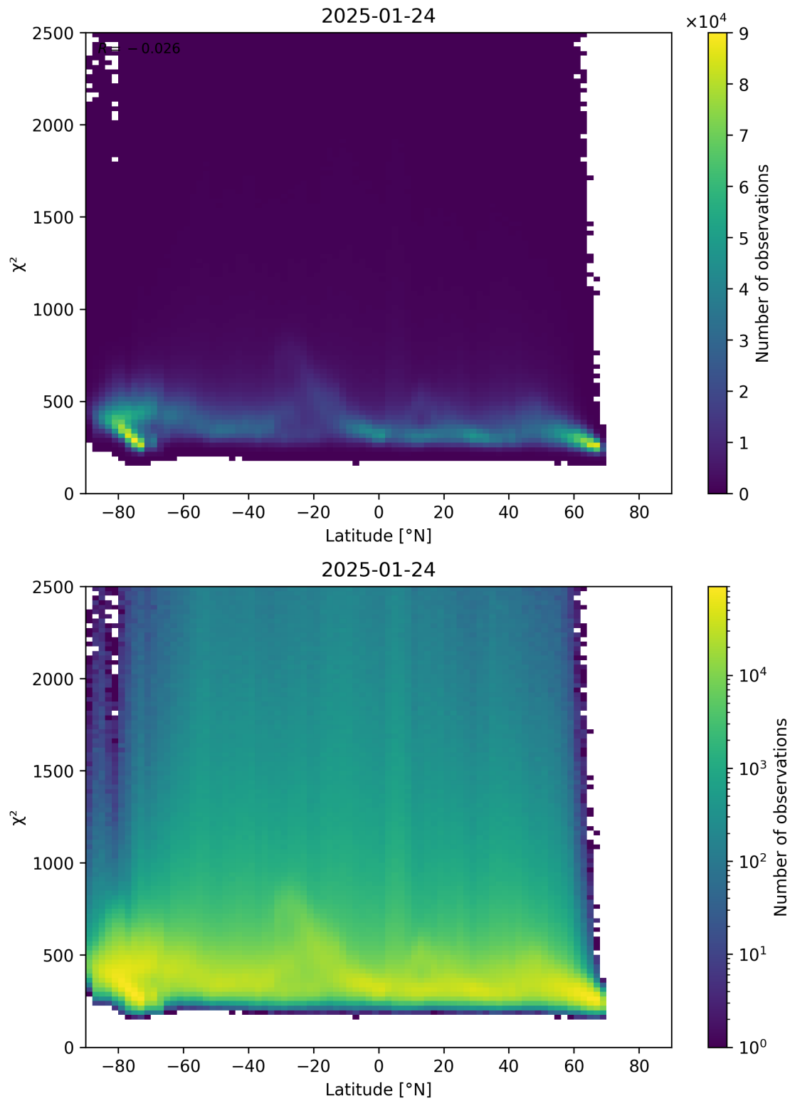
Figure 86: Scatter density plot of “Latitude” against “ \chi^2 ” for 2025-01-23 to 2025-01-25.
