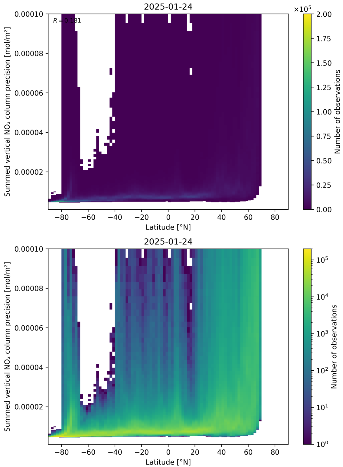
Figure 89: Scatter density plot of “Latitude” against “Summed vertical NO 2 column precision” for 2025-01-23 to 2025-01-25.
