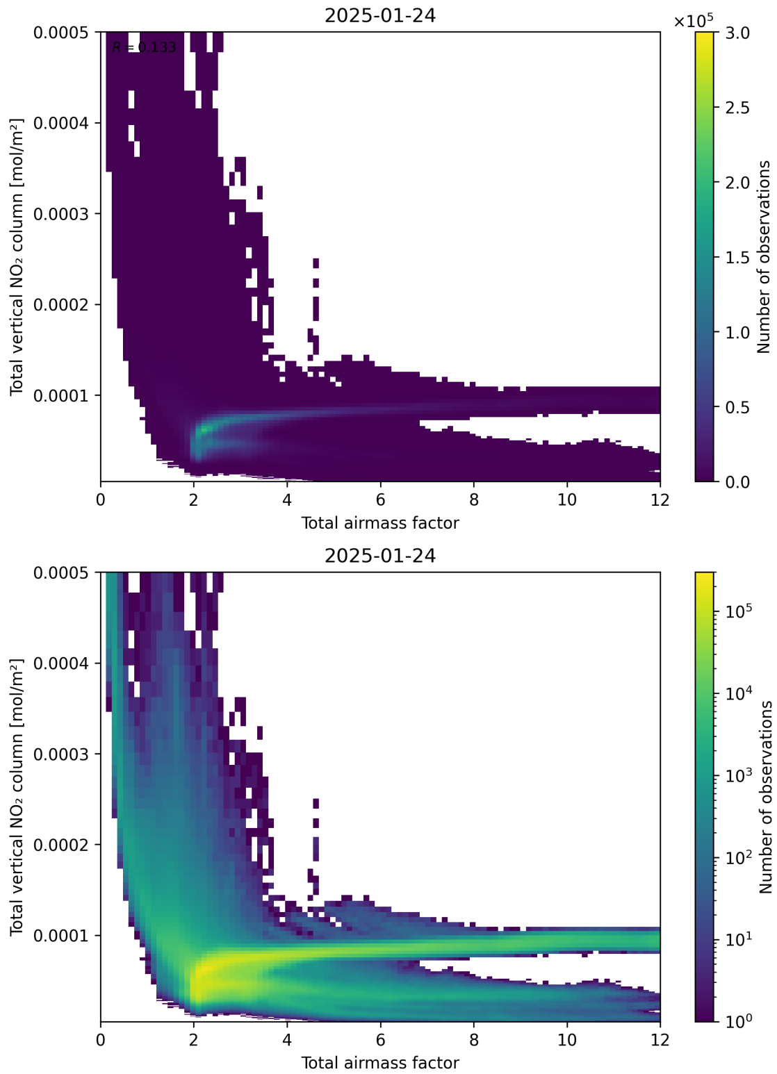
Figure 67: Scatter density plot of “Total air mass factor” against “Total vertical NO 2 column” for 2025-01-23 to 2025-01-25.
