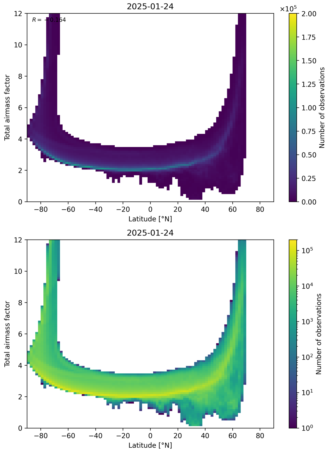
Figure 84: Scatter density plot of “Latitude” against “Total airmass factor” for 2025-01-23 to 2025-01-25.
