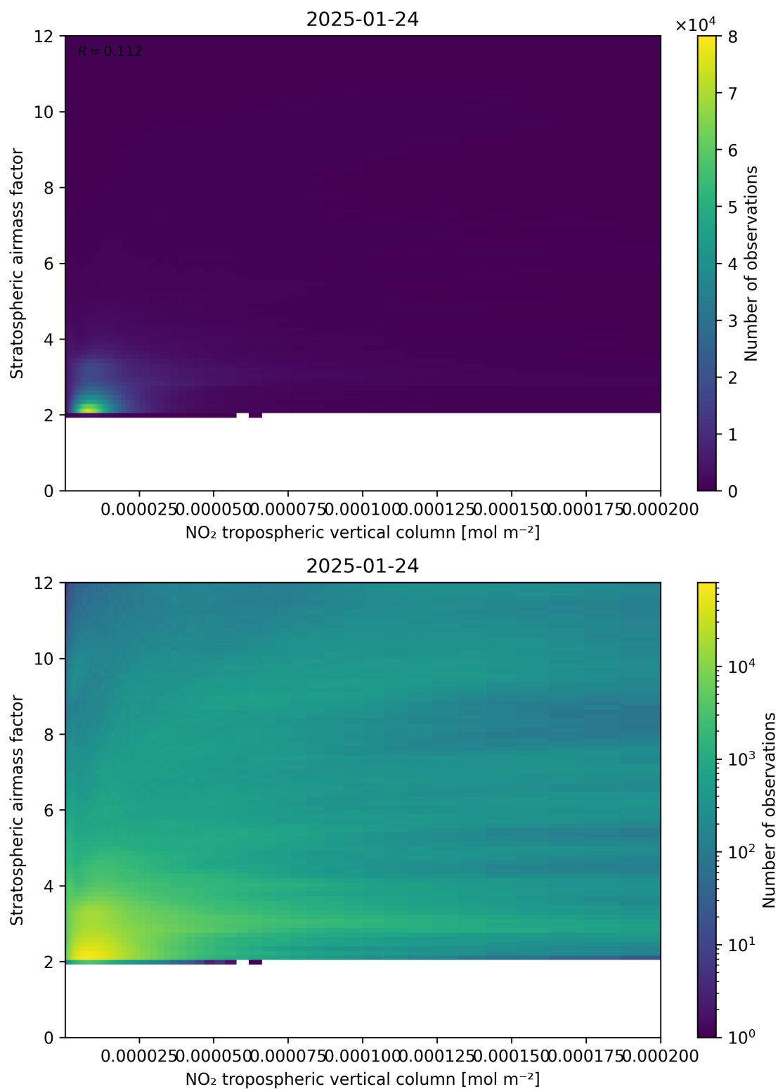
Figure 121: Scatter density plot of “NO 2 tropospheric vertical column” against “Stratospheric airmass factor” for 2025-01-23 to 2025-01-25.
