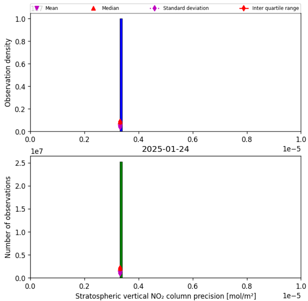
Figure 37: Histogram of “Stratospheric vertical NO 2 column precision” for 2025-01-23 to 2025-01-25
