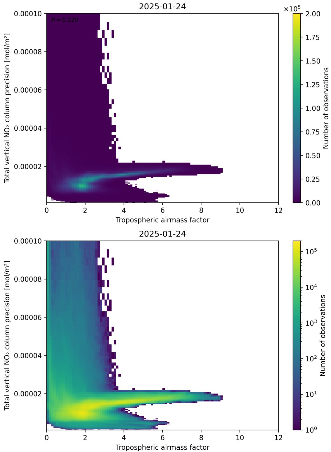
Figure 78: Scatter density plot of “Tropospheric air mass factor” against “Total vertical NO 2 column precision” for 2025-01-23 to 2025-01-25.
