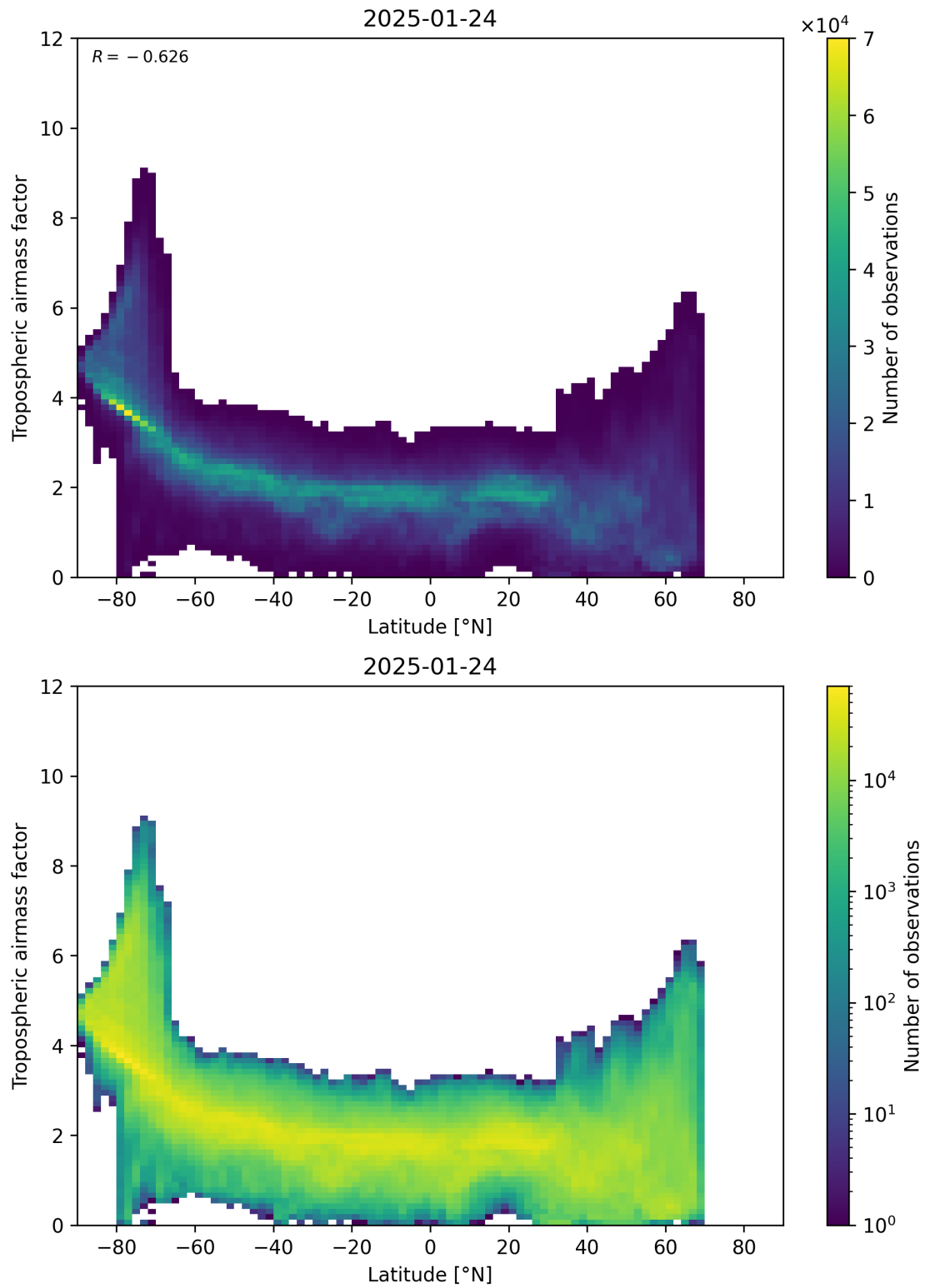
Figure 85: Scatter density plot of “Latitude” against “Tropospheric air mass factor” for 2025-01-23 to 2025-01-25.
