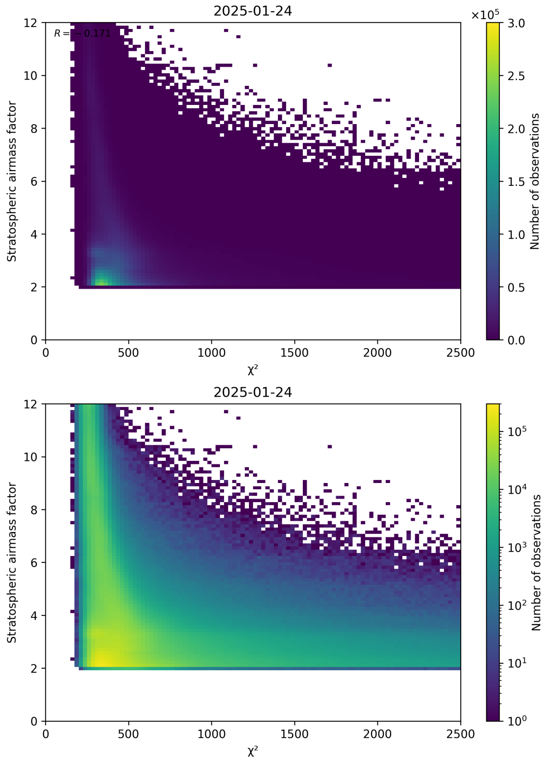
Figure 81: Scatter density plot of “ \chi^2 ” against “Stratospheric airmass factor” for 2025-01-23 to 2025-01-25.
