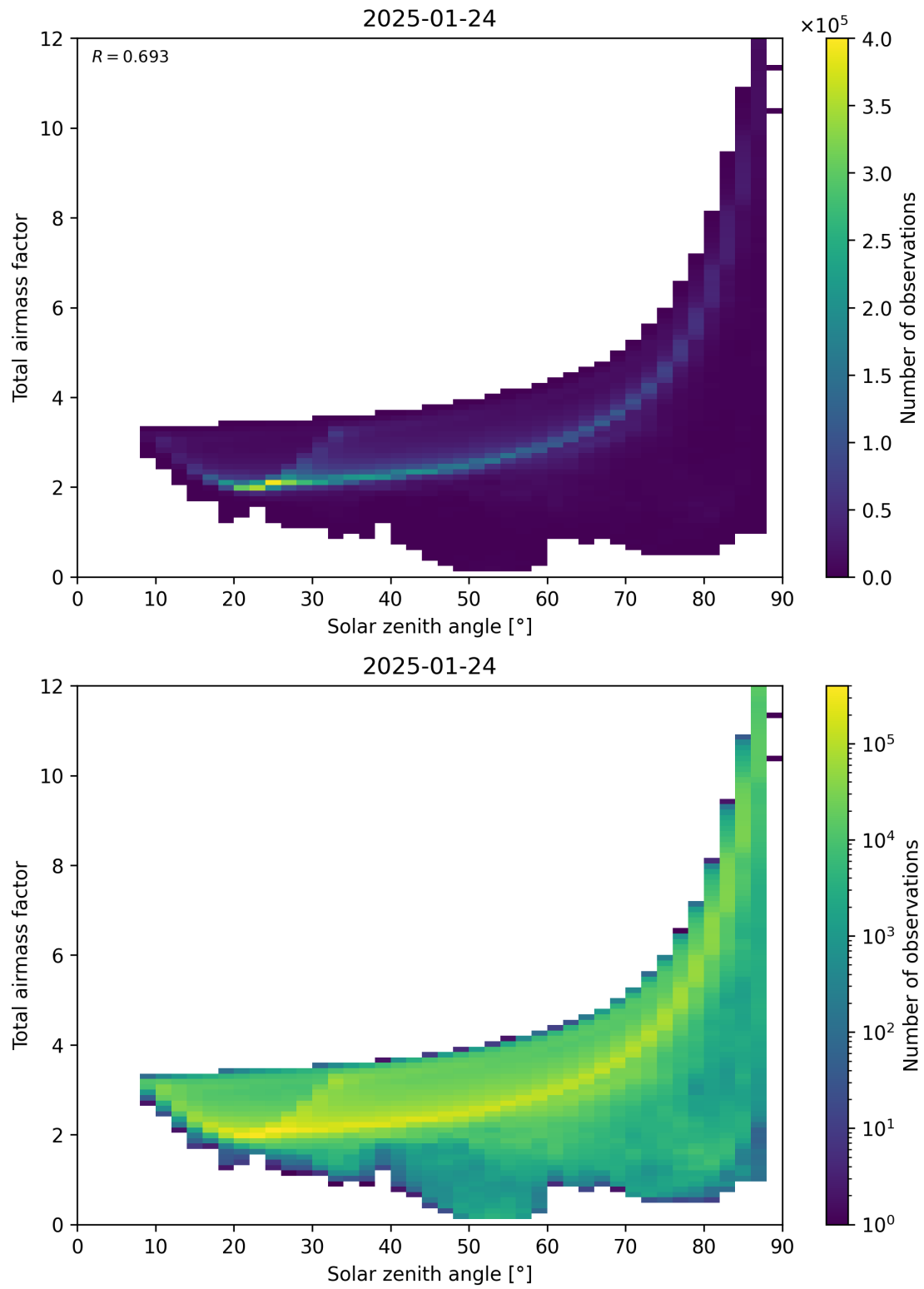
Figure 146: Scatter density plot of “Solar zenith angle” against “Total air mass factor” for 2025-01-23 to 2025-01-25.
