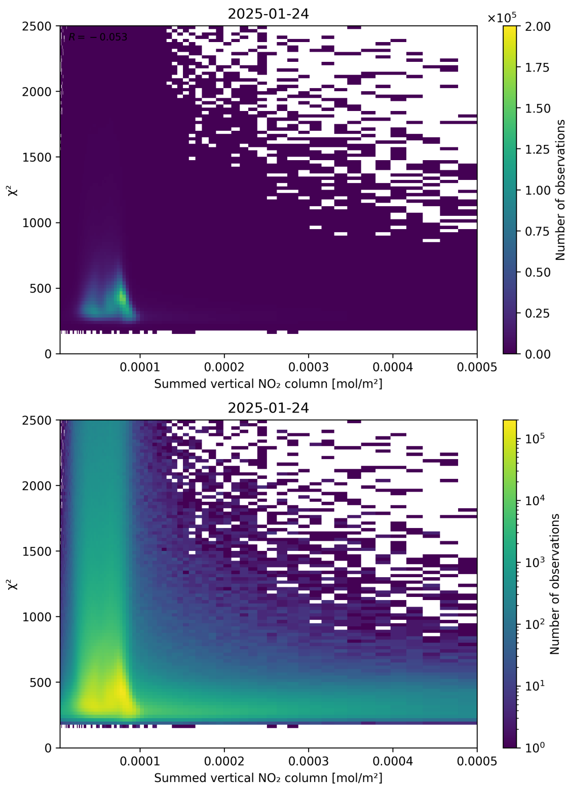
Figure 104: Scatter density plot of “Summed vertical NO 2 column” against “ \chi^2 ” for 2025-01-23 to 2025-01-25.
