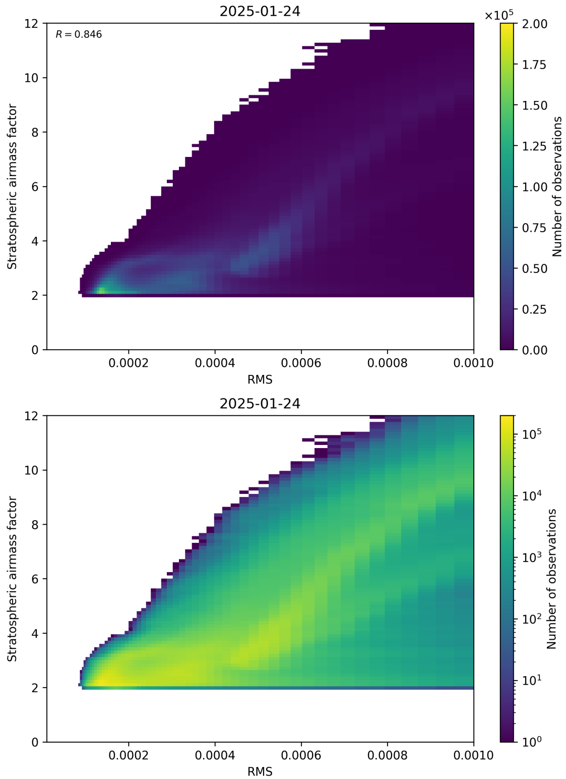
Figure 144: Scatter density plot of “RMS” against “Stratospheric airmass factor” for 2025-01-23 to 2025-01-25.
