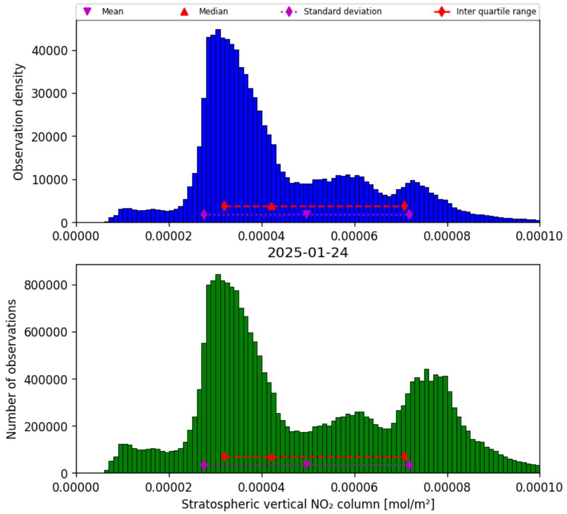
Figure 36: Histogram of “Stratospheric vertical NO 2 column” for 2025-01-23 to 2025-01-25
