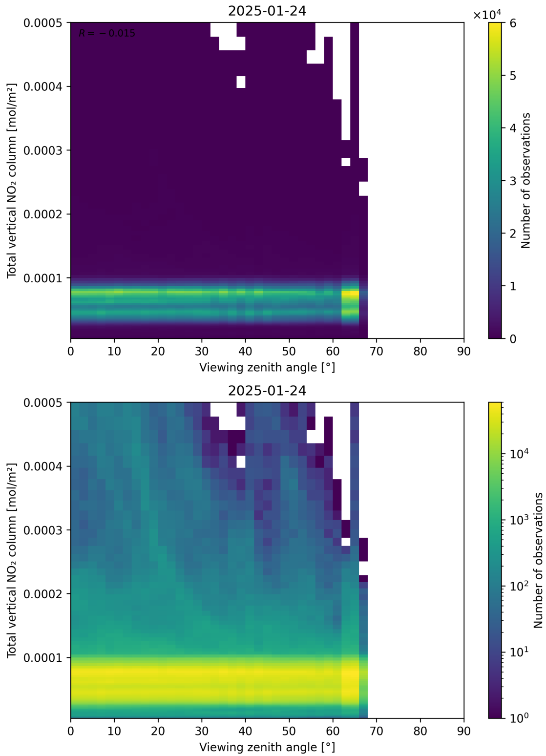
Figure 167: Scatter density plot of “Viewing zenith angle” against “Total vertical NO 2 column” for 2025-01-23 to 2025-01-25.
