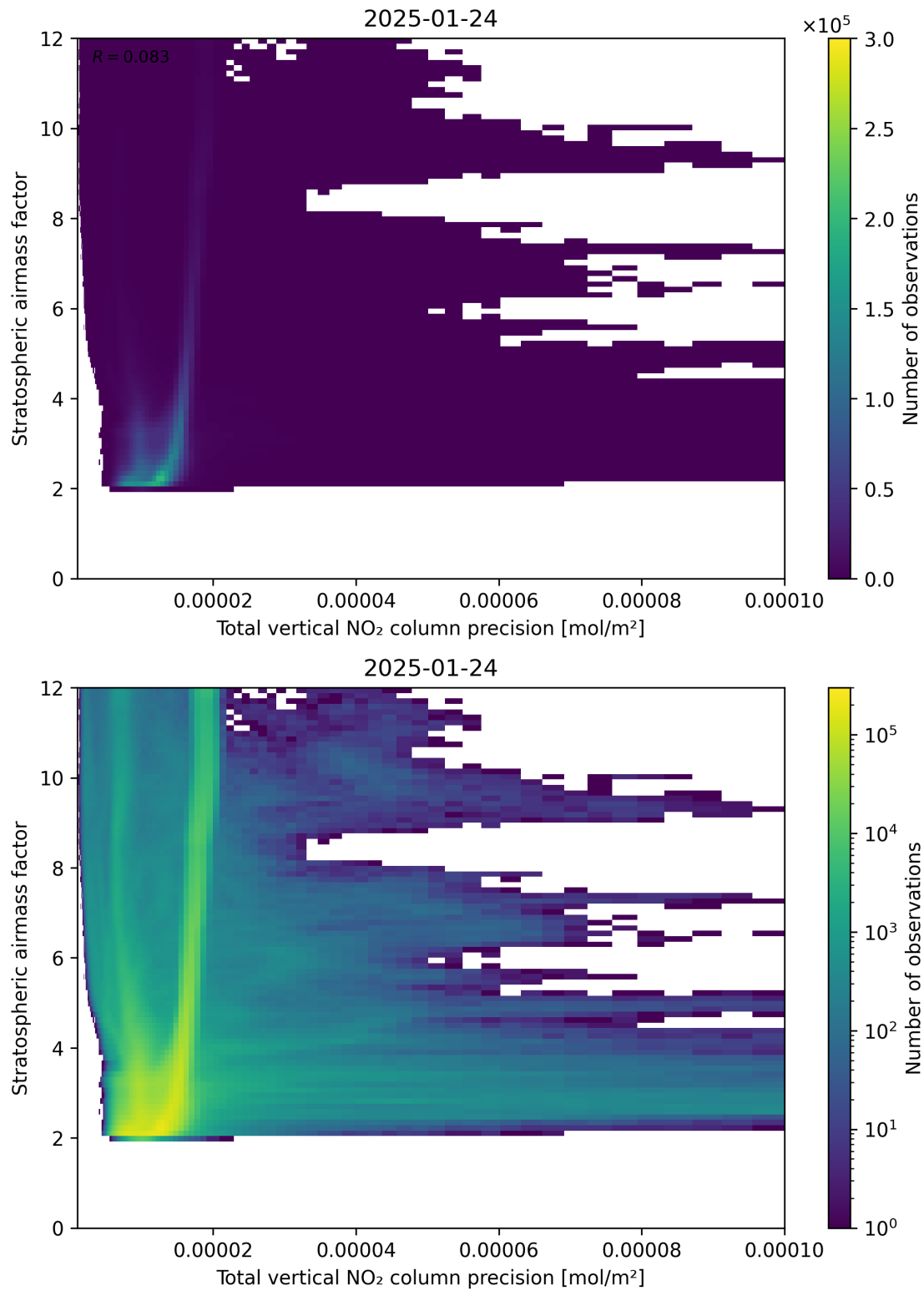
Figure 115: Scatter density plot of “Total vertical NO 2 column precision” against “Stratospheric air mass factor” for 2025-01-23 to 2025-01-25.
