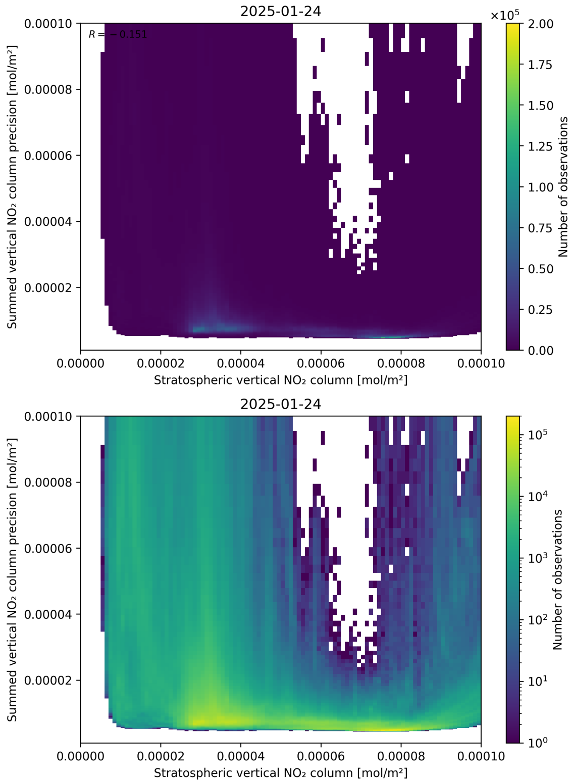
Figure 99: Scatter density plot of “Stratospheric vertical NO 2 column” against “Summed vertical NO 2 column precision” for 2025-01-23 to 2025-01-25.
