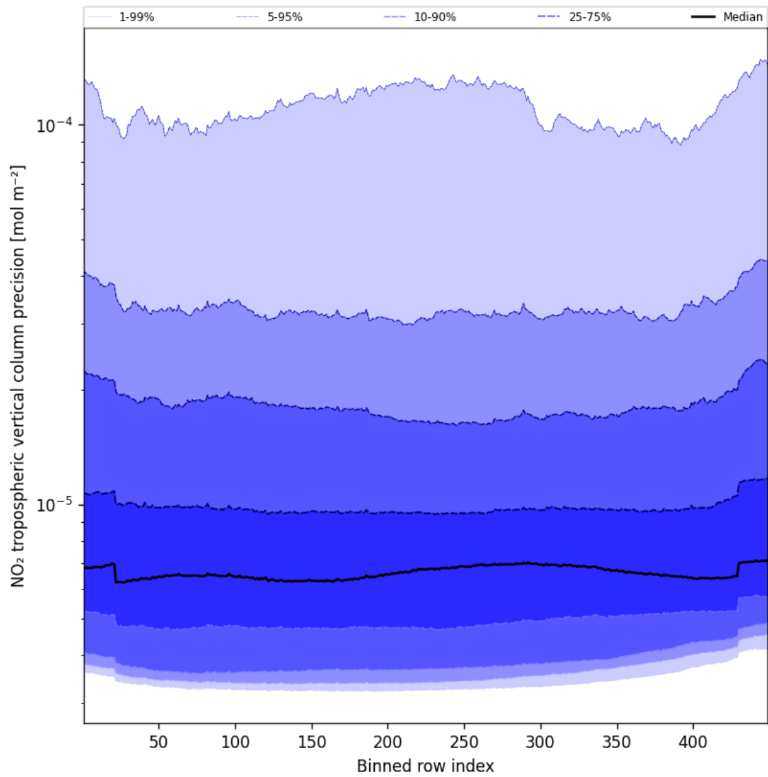
Figure 47: Along track statistics of “NO 2 tropospheric vertical column precision” for 2025-01-23 to 2025-01-25
