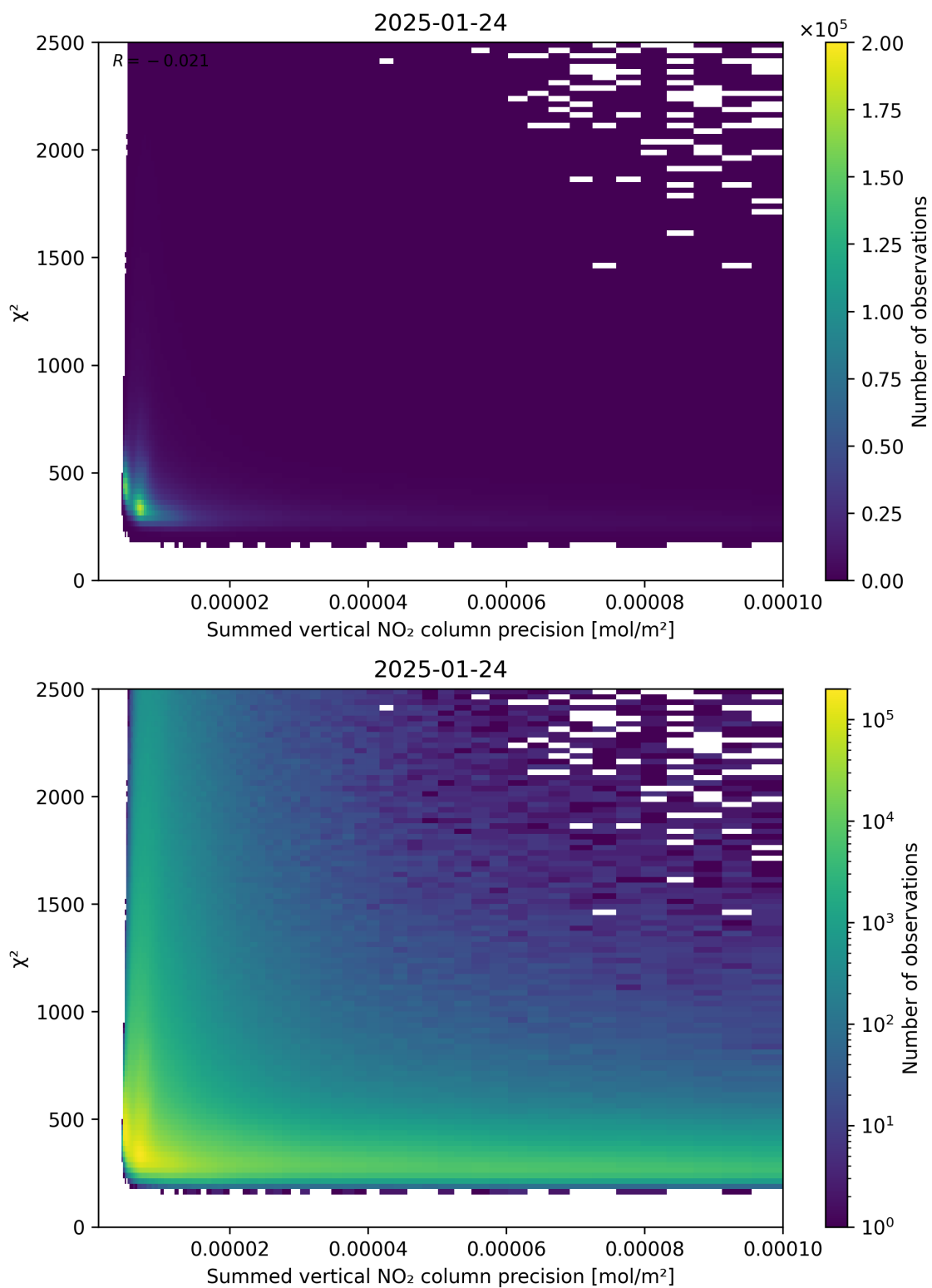
Figure 107: Scatter density plot of “Summed vertical NO 2 column precision” against “ \chi^2 ” for 2025-01-23 to 2025-01-25.
