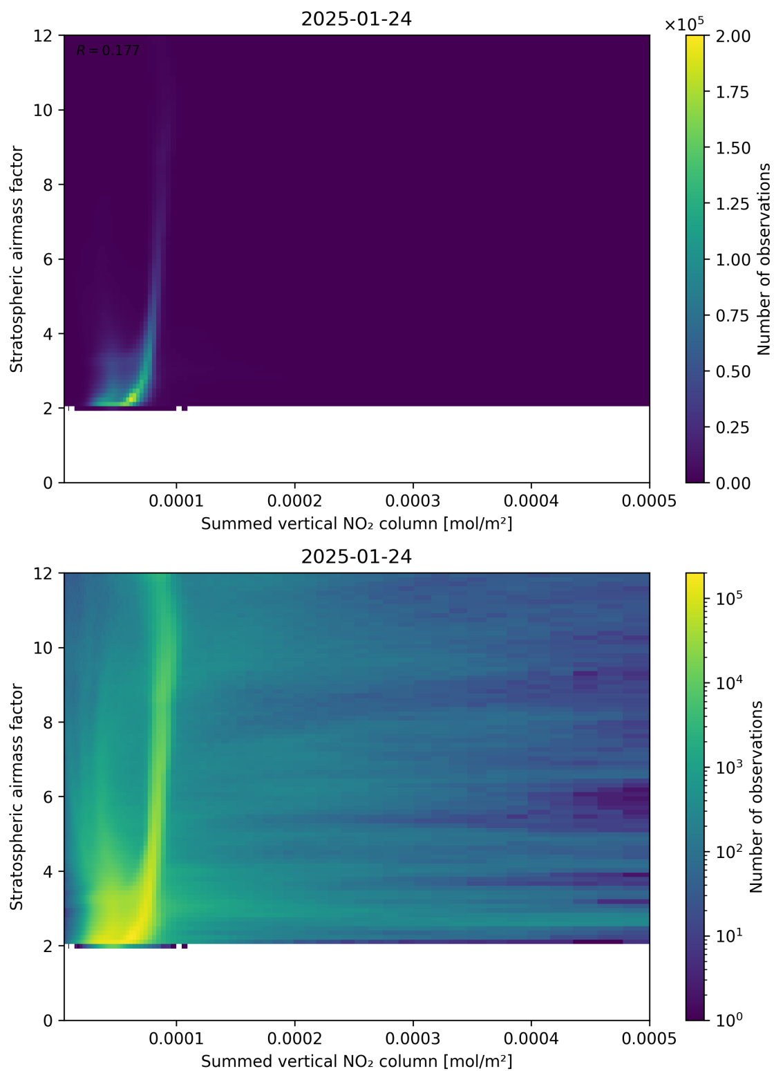
Figure 103: Scatter density plot of “Summed vertical NO 2 column” against “Stratospheric airmass factor” for 2025-01-23 to 2025-01-25.
