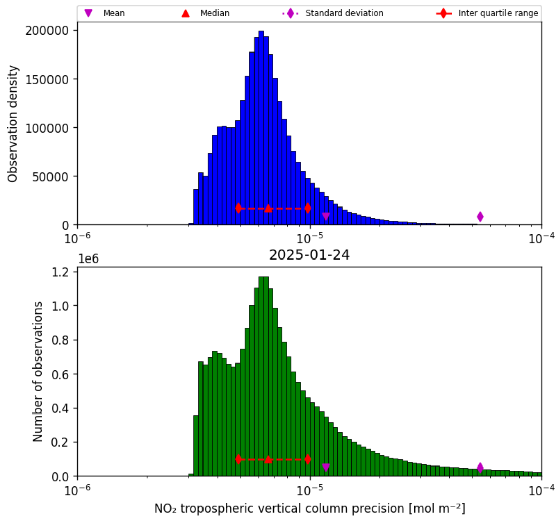
Figure 30: Histogram of “NO 2 tropospheric vertical column precision” for 2025-01-23 to 2025-01-25
