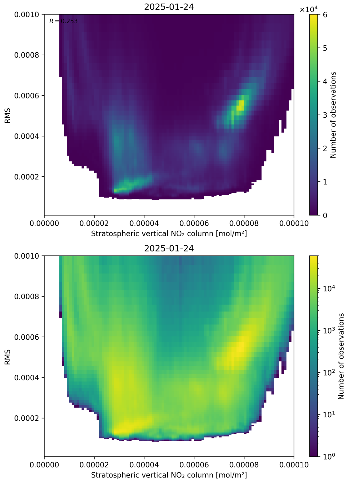
Figure 102: Scatter density plot of “Stratospheric vertical NO 2 column” against “RMS” for 2025-01-23 to 2025-01-25.
