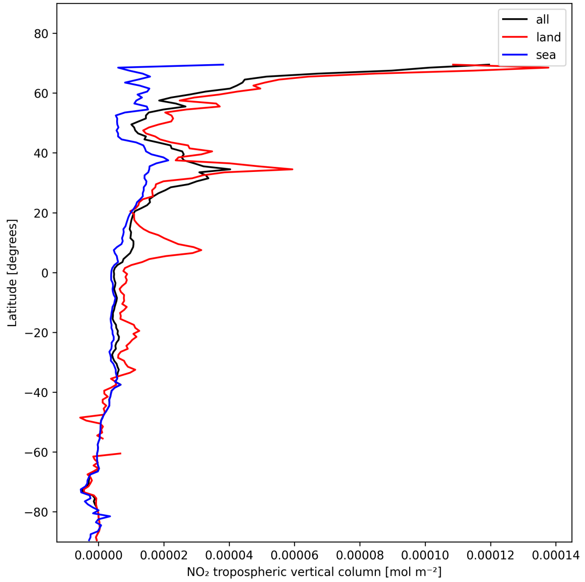
Figure 12: Zonal average of “NO 2 tropospheric vertical column” for 2025-01-23 to 2025-01-25.
