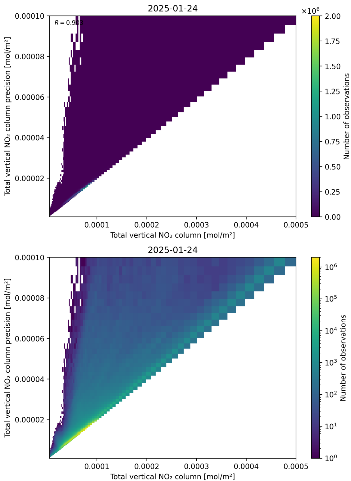
Figure 114: Scatter density plot of “Total vertical NO 2 column” against “Total vertical NO 2 column precision” for 2025-01-23 to 2025-01-25.
