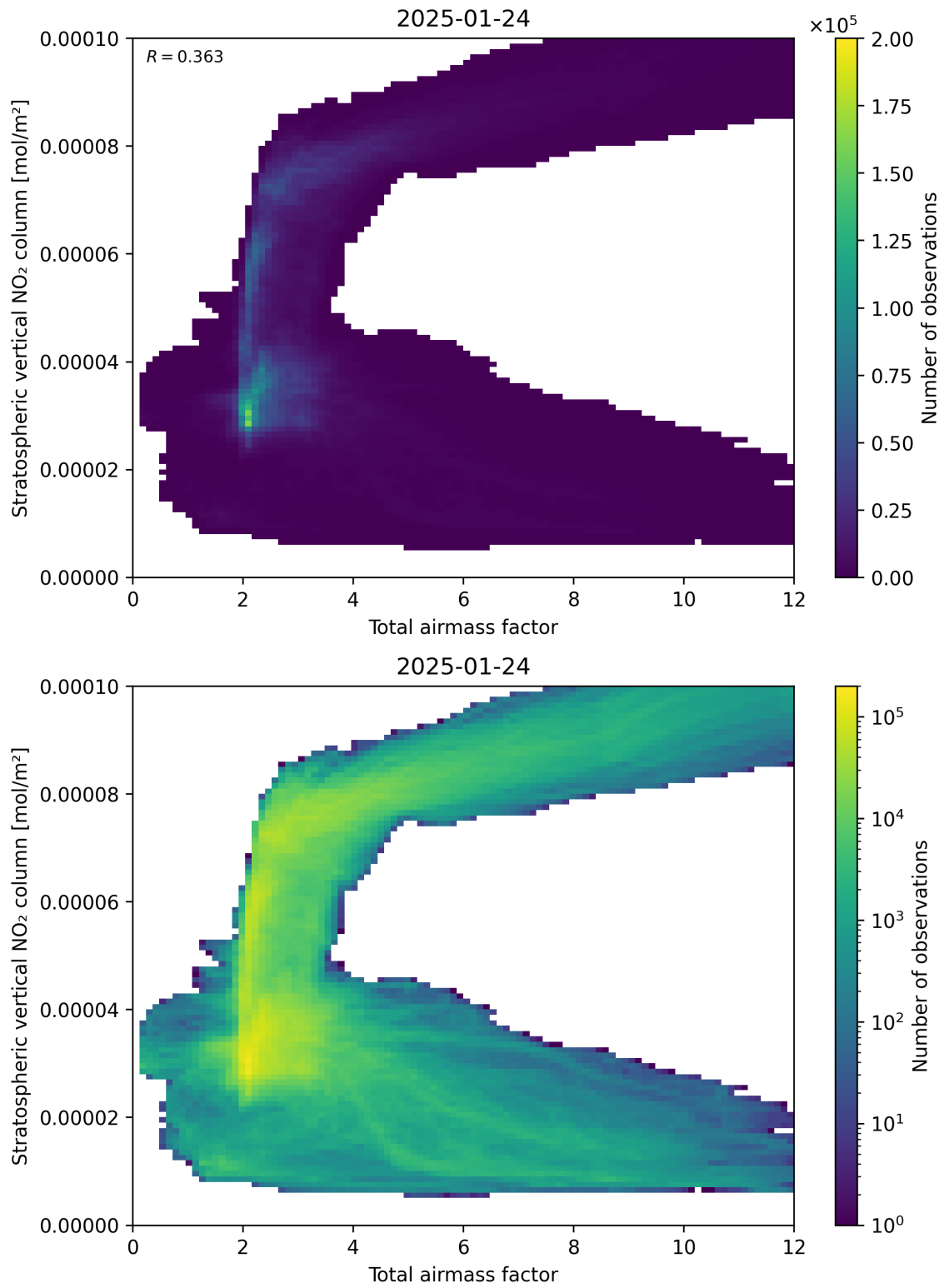
Figure 64: Scatter density plot of “Total airmass factor” against “Stratospheric vertical \text{NO}_2 column” for 2025-01-23 to 2025-01-25.
