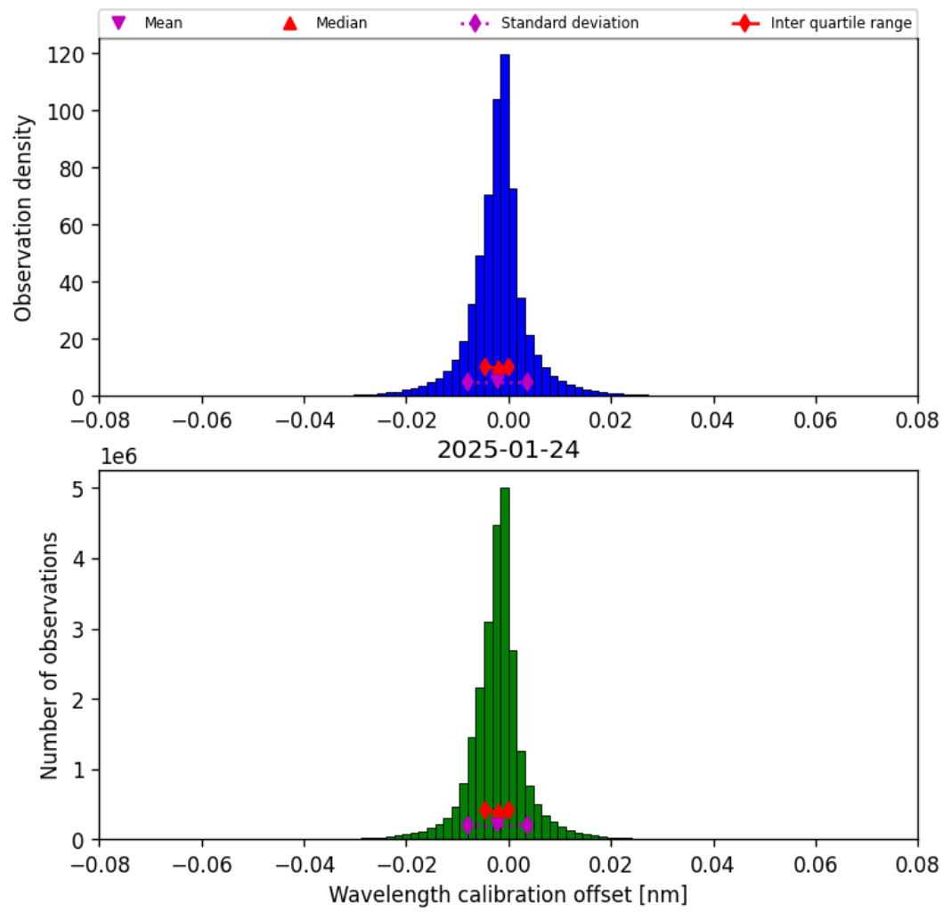
Figure 35: Histogram of “Wavelength calibration offset” for 2025-01-23 to 2025-01-25
