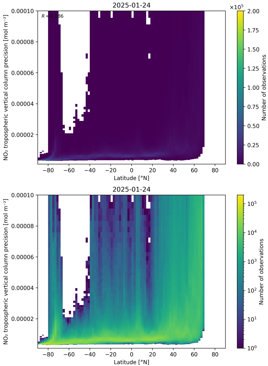
Figure 93: Scatter density plot of “Latitude” against “NO 2 tropospheric vertical column precision” for 2025-01-23 to 2025-01-25.
