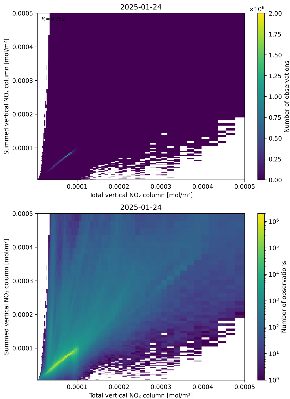
Figure 112: Scatter density plot of “Total vertical NO 2 column” against “Summed vertical NO 2 column” for 2025-01-23 to 2025-01-25.
