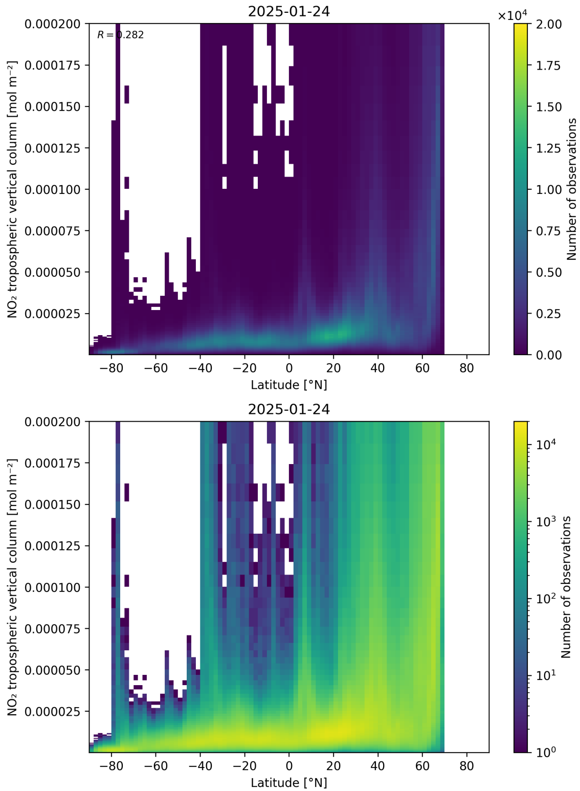
Figure 92: Scatter density plot of “Latitude” against “NO 2 tropospheric vertical column” for 2025-01-23 to 2025-01-25.
