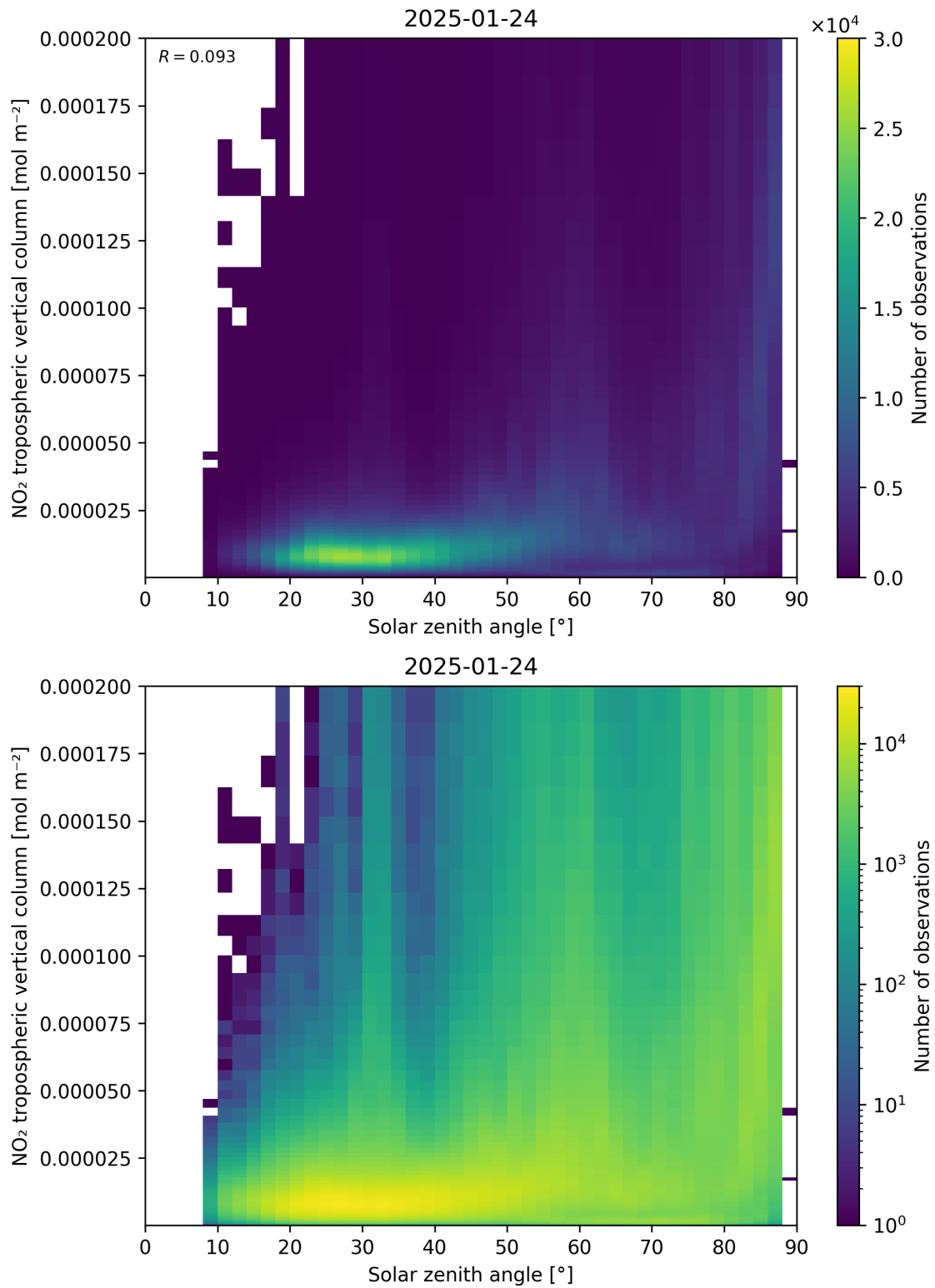
Figure 155: Scatter density plot of “Solar zenith angle” against “NO 2 tropospheric vertical column” for 2025-01-23 to 2025-01-25.
