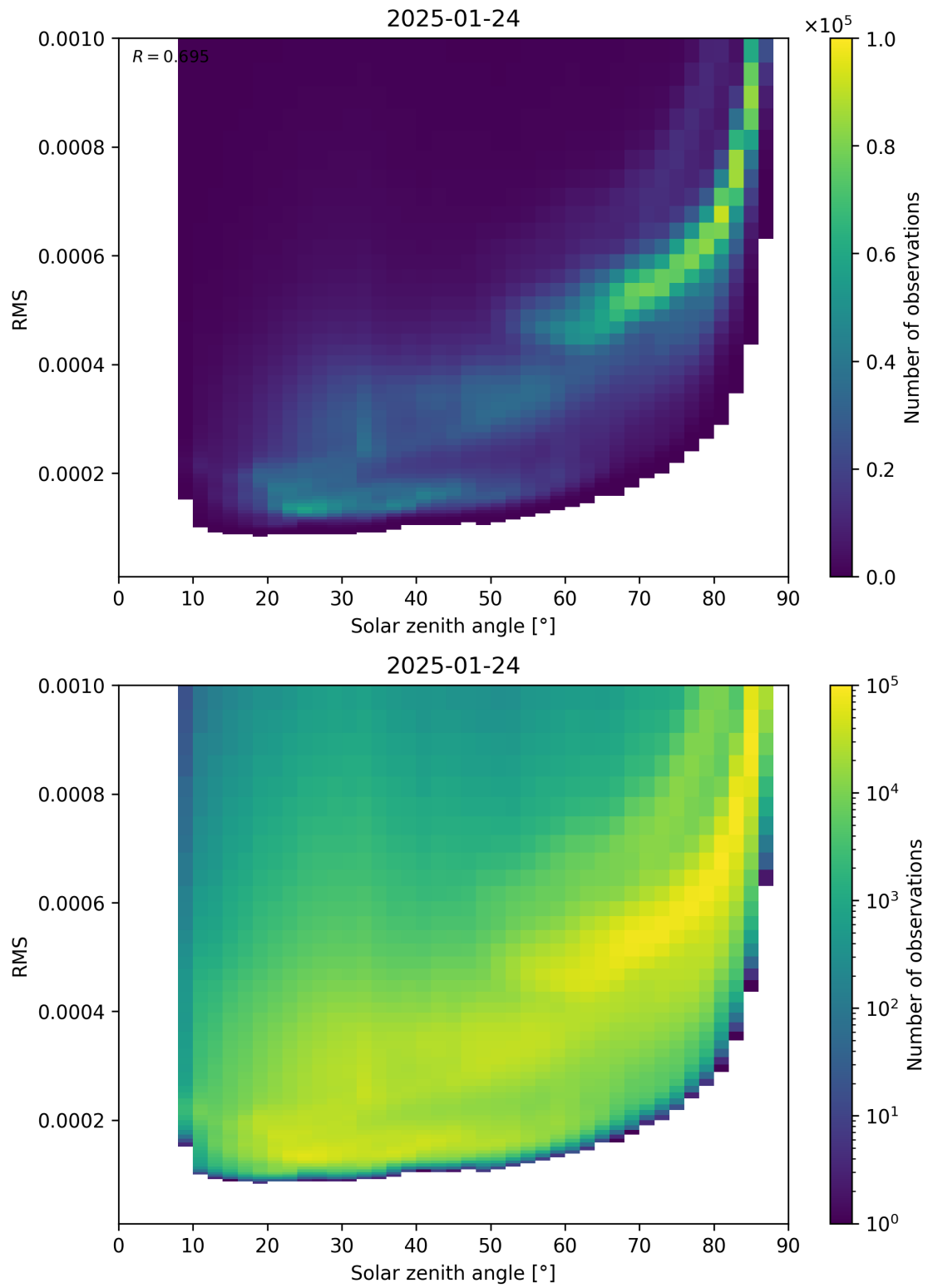
Figure 157: Scatter density plot of “Solar zenith angle” against “RMS” for 2025-01-23 to 2025-01-25.
