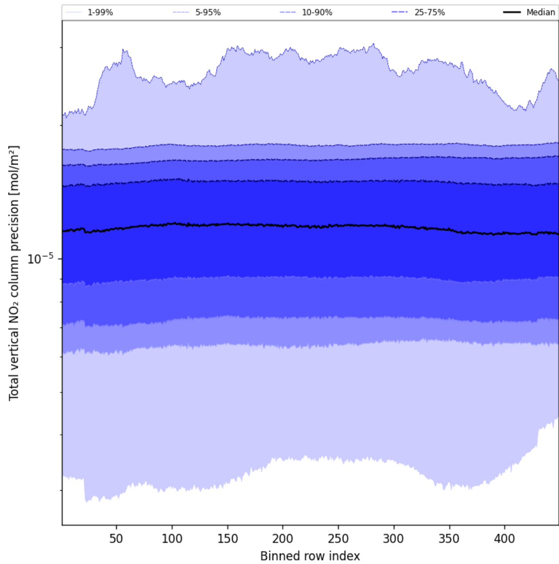
Figure 56: Along track statistics of “Total vertical NO 2 column precision” for 2025-01-23 to 2025-01-25
