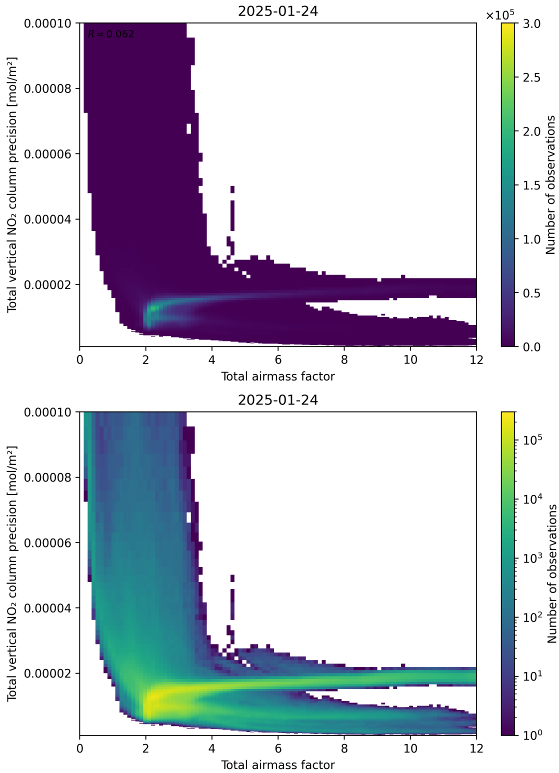
Figure 68: Scatter density plot of “Total airmass factor” against “Total vertical NO 2 column precision” for 2025-01-23 to 2025-01-25.
