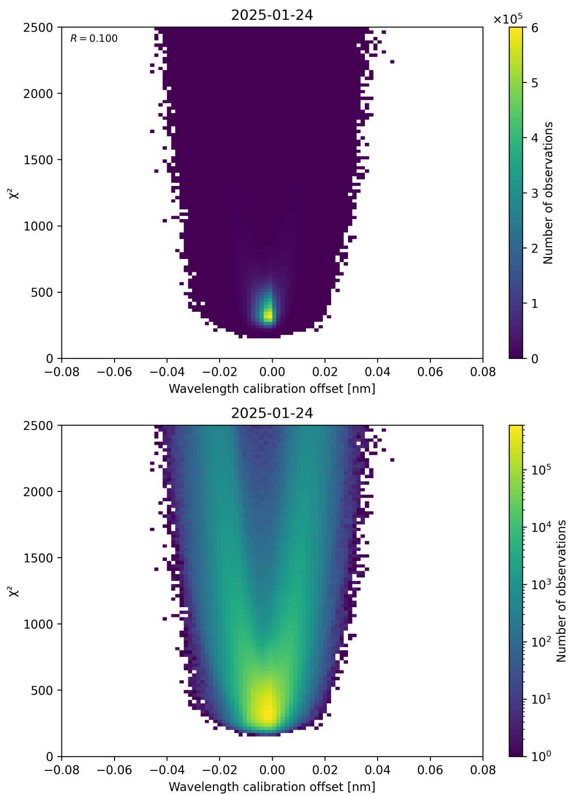
Figure 175: Scatter density plot of “Wavelength calibration offset” against “ \chi^2 ” for 2025-01-23 to 2025-01-25.
