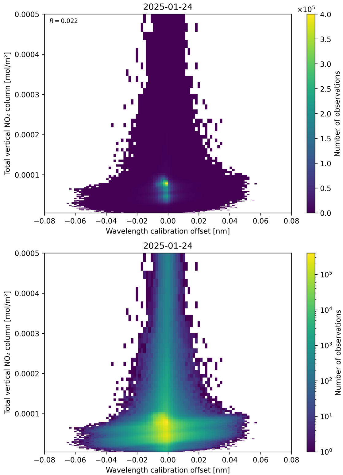
Figure 179: Scatter density plot of “Wavelength calibration offset” against “Total vertical NO 2 column” for 2025-01-23 to 2025-01-25.
