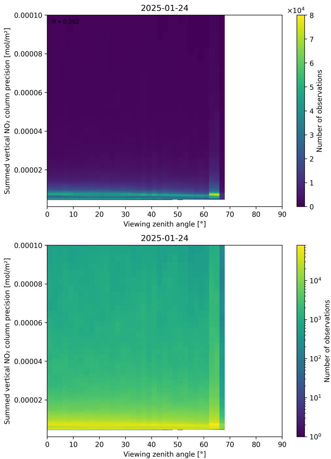
Figure 166: Scatter density plot of “Viewing zenith angle” against “Summed vertical NO 2 column precision” for 2025-01-23 to 2025-01-25.
