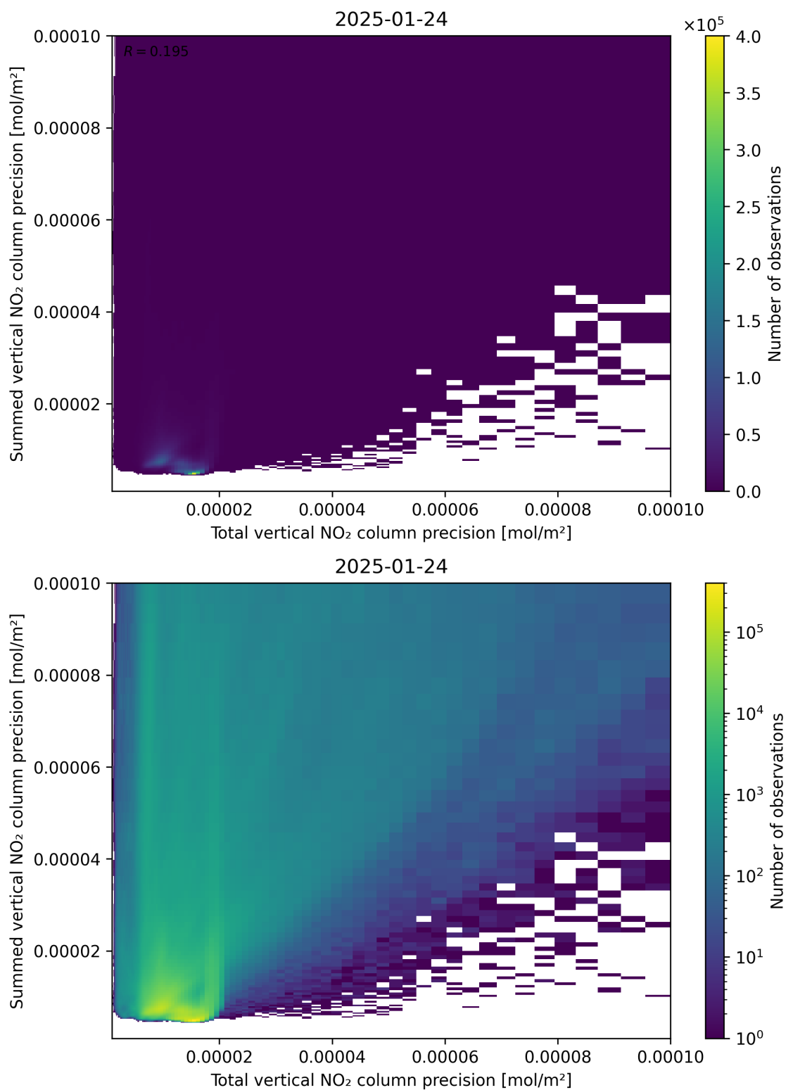
Figure 118: Scatter density plot of “Total vertical NO 2 column precision” against “Summed vertical NO 2 column precision” for 2025-01-23 to 2025-01-25.
