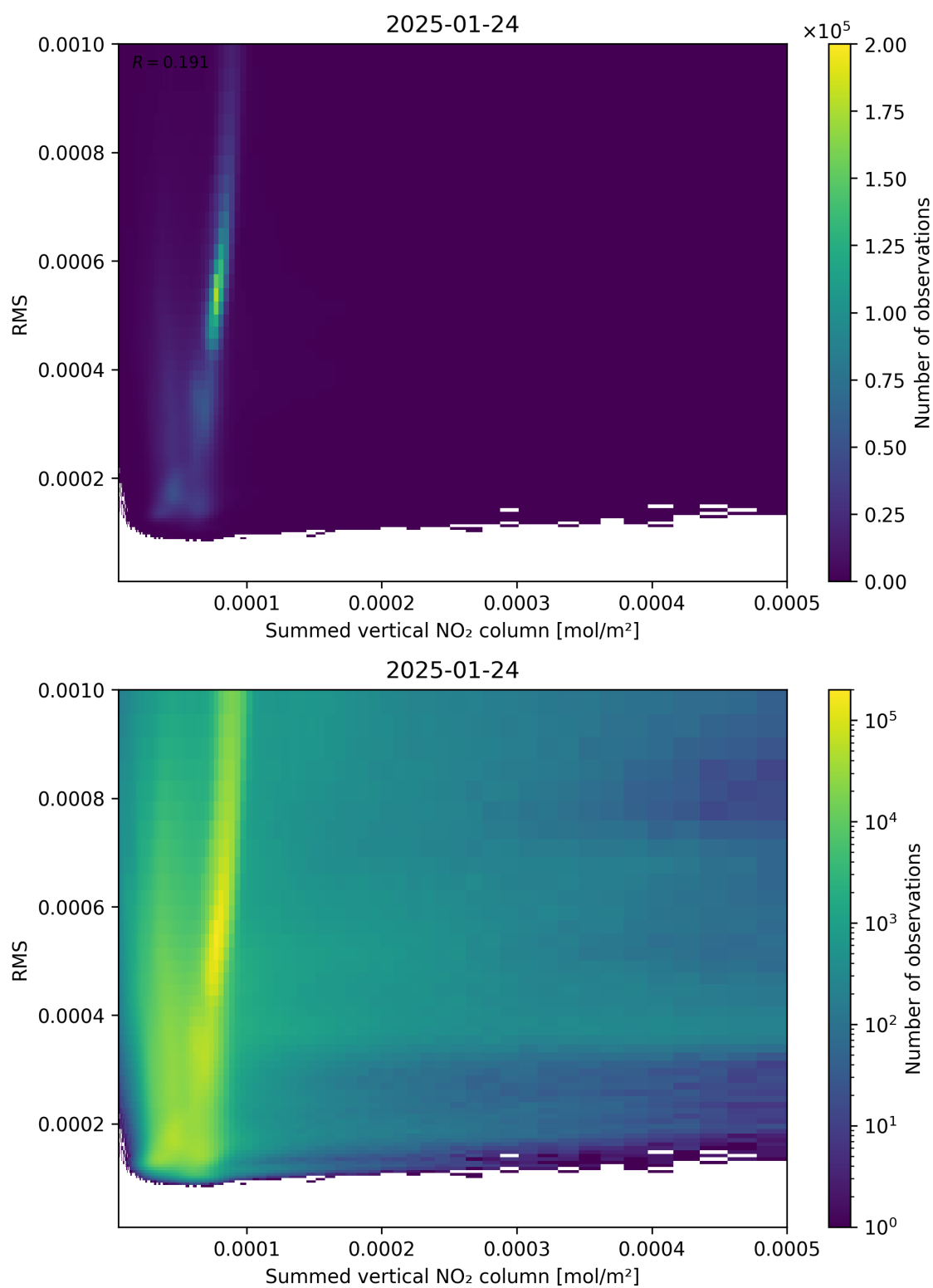
Figure 109: Scatter density plot of “Summed vertical NO 2 column” against “RMS” for 2025-01-23 to 2025-01-25.
