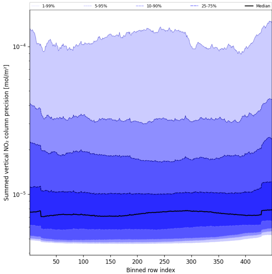
Figure 58: Along track statistics of “Summed vertical NO 2 column precision” for 2025-01-23 to 2025-01-25
