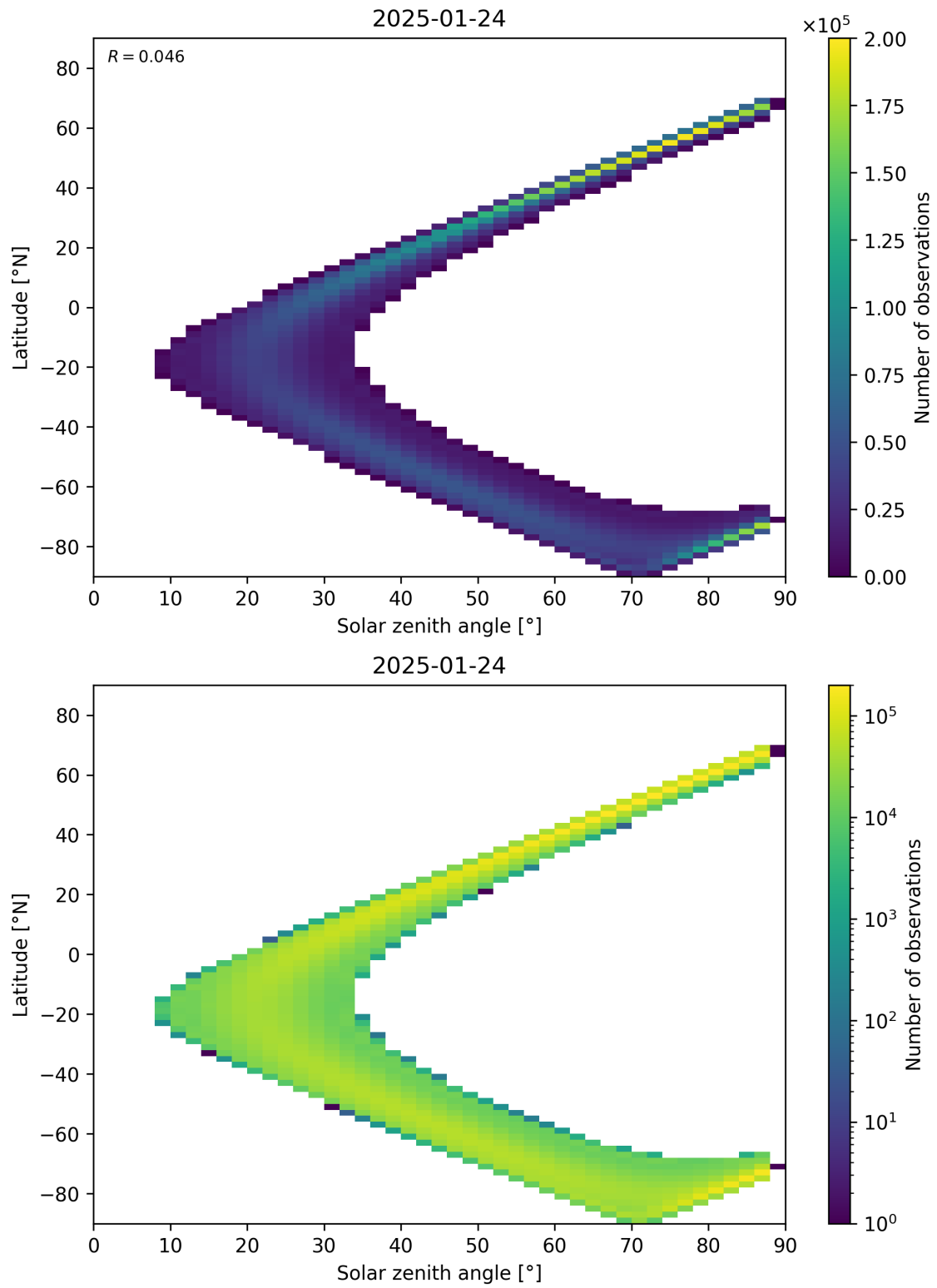
Figure 149: Scatter density plot of “Solar zenith angle” against “Latitude” for 2025-01-23 to 2025-01-25.
