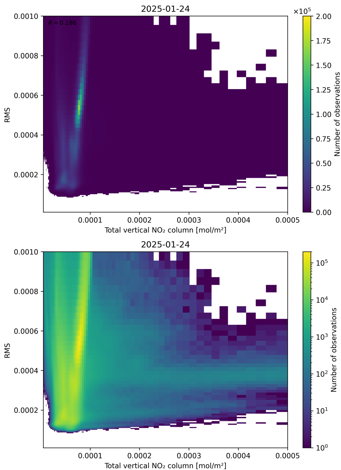
Figure 120: Scatter density plot of “Total vertical NO 2 column” against “RMS” for 2025-01-23 to 2025-01-25.
