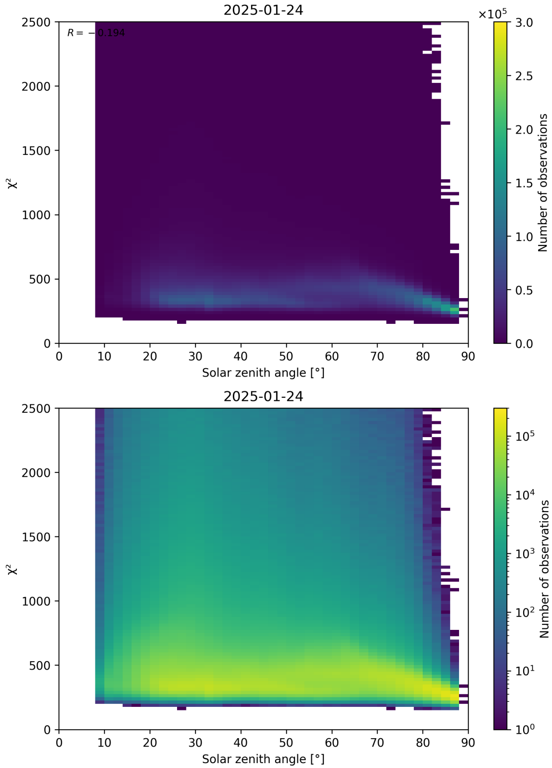
Figure 148: Scatter density plot of “Solar zenith angle” against “ \chi^2 ” for 2025-01-23 to 2025-01-25.
