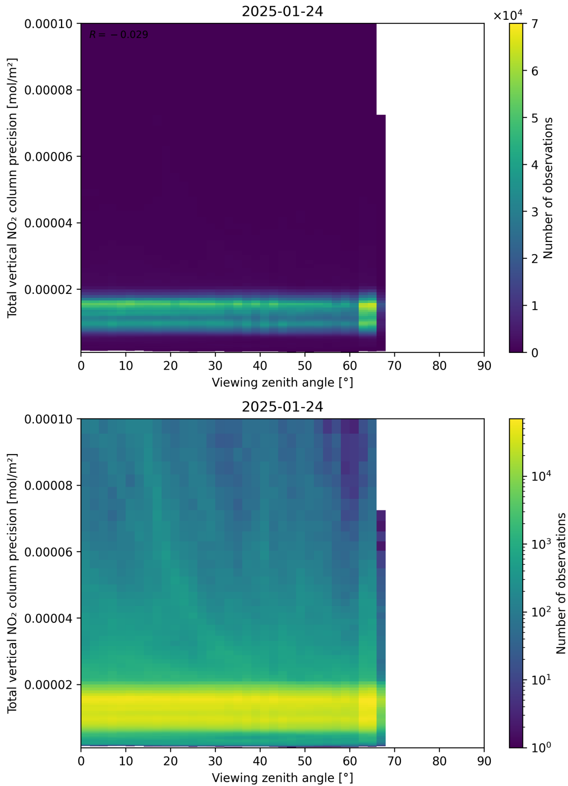
Figure 168: Scatter density plot of “Viewing zenith angle” against “Total vertical NO 2 column precision” for 2025-01-23 to 2025-01-25.
