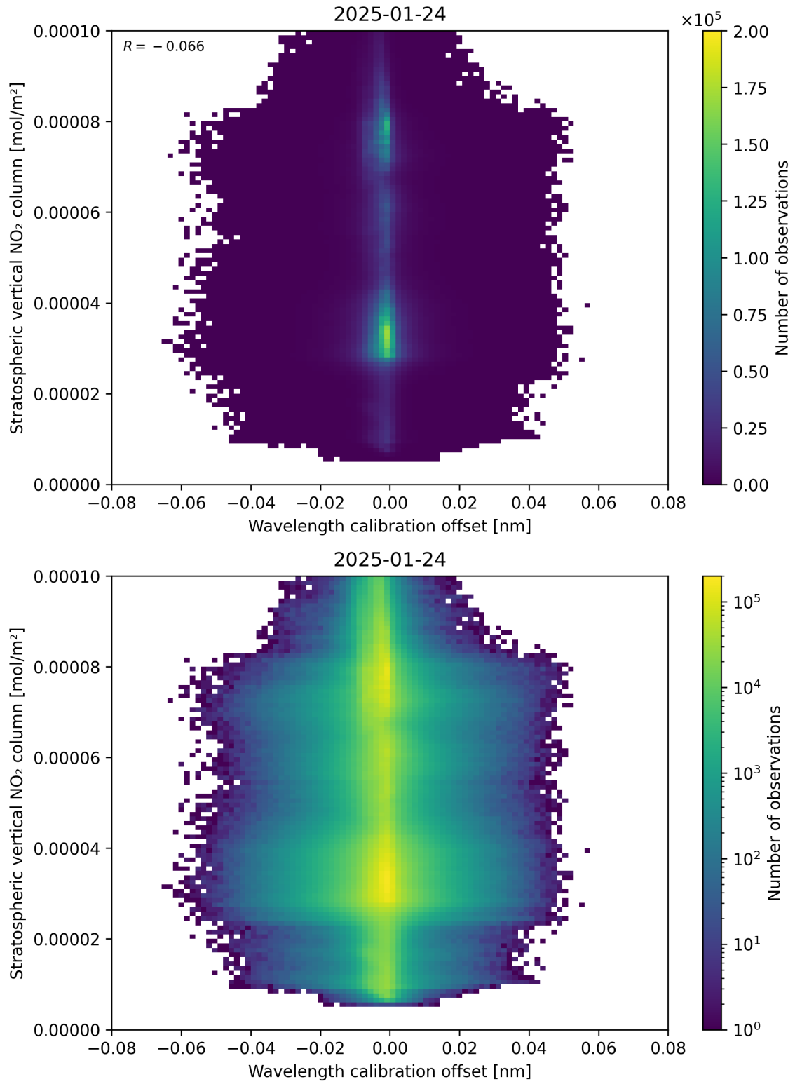
Figure 176: Scatter density plot of “Wavelength calibration offset” against “Stratospheric vertical NO 2 column” for 2025-01-23 to 2025-01-25.
