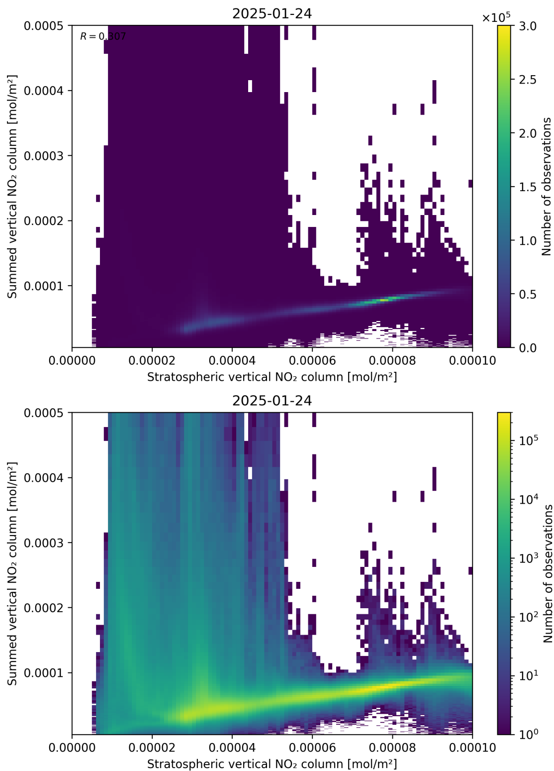
Figure 98: Scatter density plot of “Stratospheric vertical NO 2 column” against “Summed vertical NO 2 column” for 2025-01-23 to 2025-01-25.
