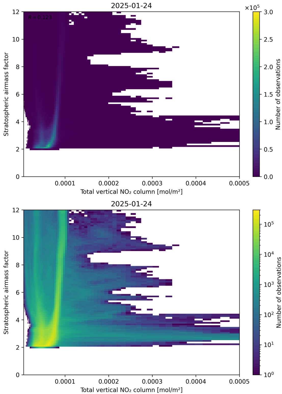
Figure 110: Scatter density plot of “Total vertical NO 2 column” against “Stratospheric airmass factor” for 2025-01-23 to 2025-01-25.
