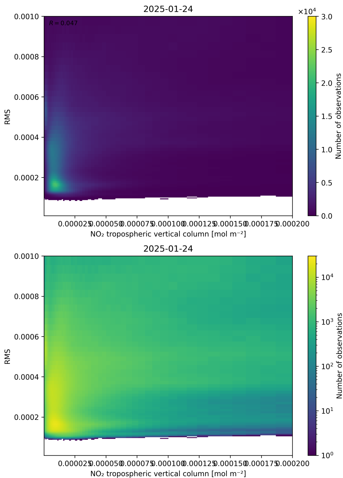
Figure 142: Scatter density plot of “NO 2 tropospheric vertical column” against “RMS” for 2025-01-23 to 2025-01-25.
