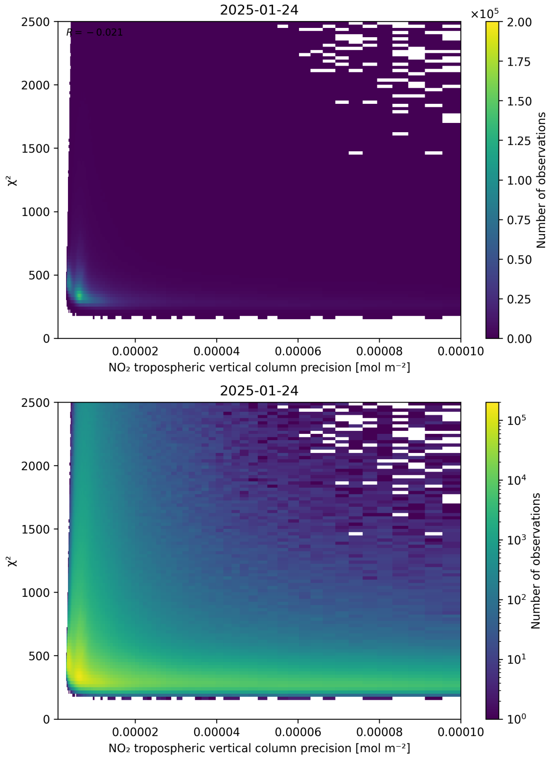
Figure 134: Scatter density plot of “NO 2 tropospheric vertical column precision” against “ \chi^2 ” for 2025-01-23 to 2025-01-25.
