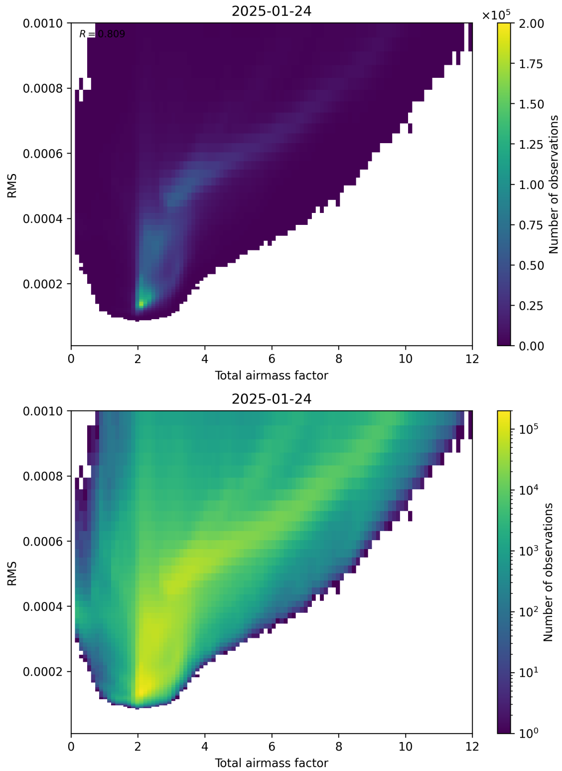
Figure 69: Scatter density plot of “Total airmass factor” against “RMS” for 2025-01-23 to 2025-01-25.
