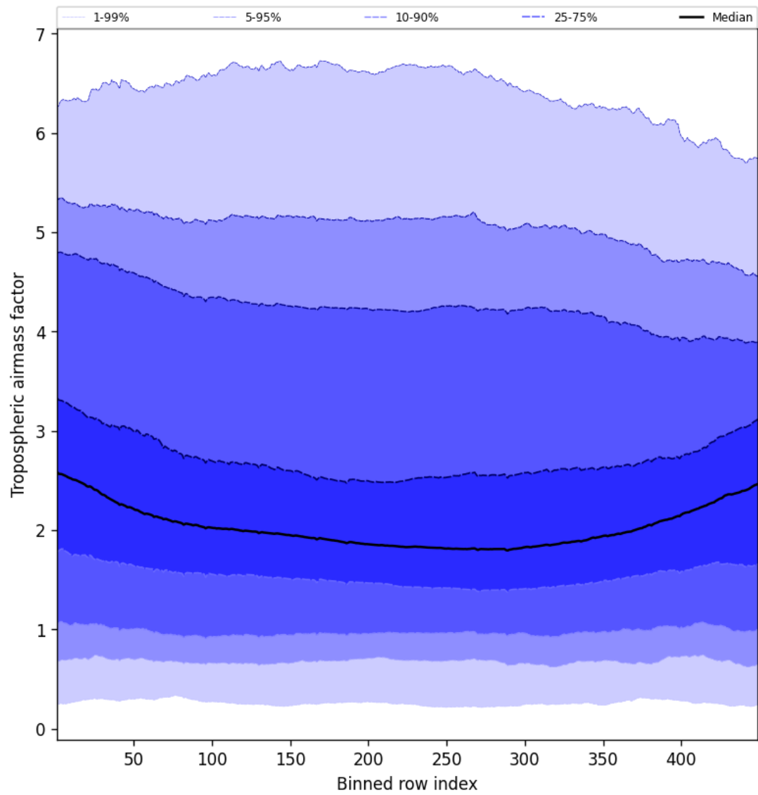
Figure 48: Along track statistics of “Tropospheric airmass factor” for 2025-01-23 to 2025-01-25
