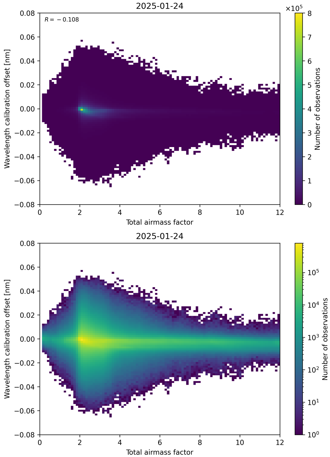
Figure 70: Scatter density plot of “Total airmass factor” against “Wavelength calibration offset” for 2025-01-23 to 2025-01-25.
