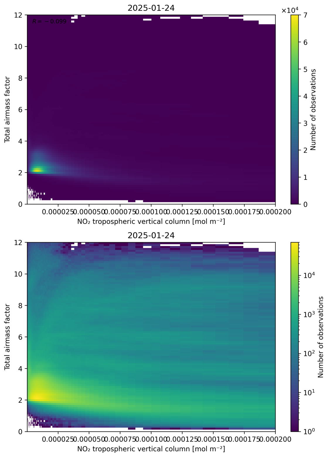
Figure 122: Scatter density plot of “NO 2 tropospheric vertical column” against “Total airmass factor” for 2025-01-23 to 2025-01-25.
