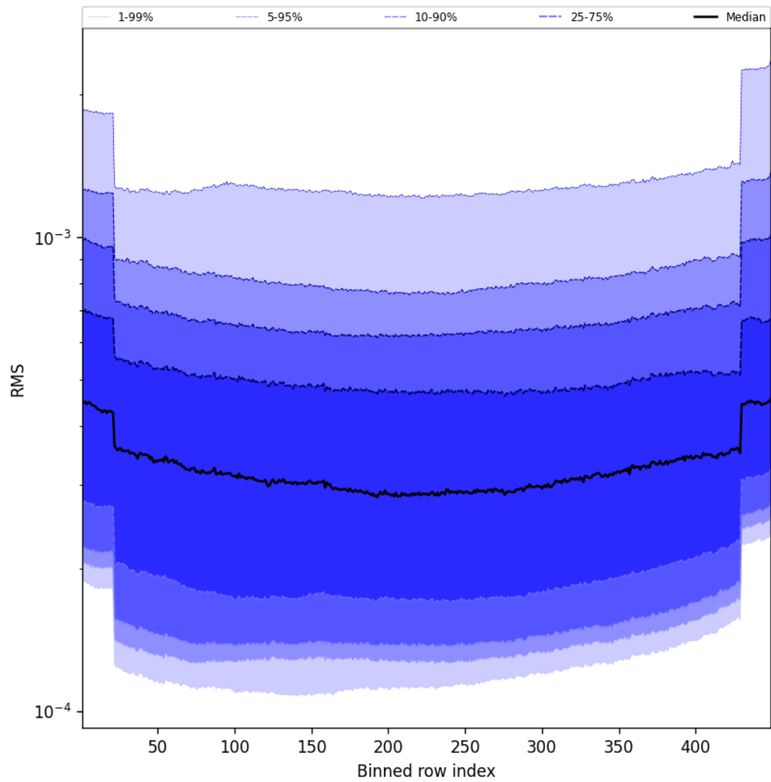
Figure 60: Along track statistics of “RMS” for 2025-01-23 to 2025-01-25
