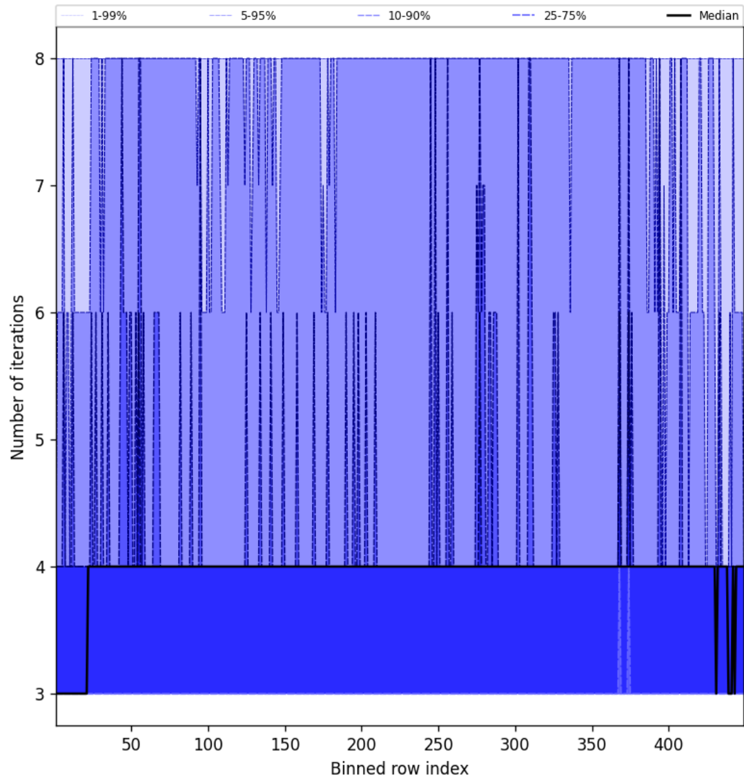
Figure 51: Along track statistics of “Number of iterations” for 2025-01-23 to 2025-01-25
