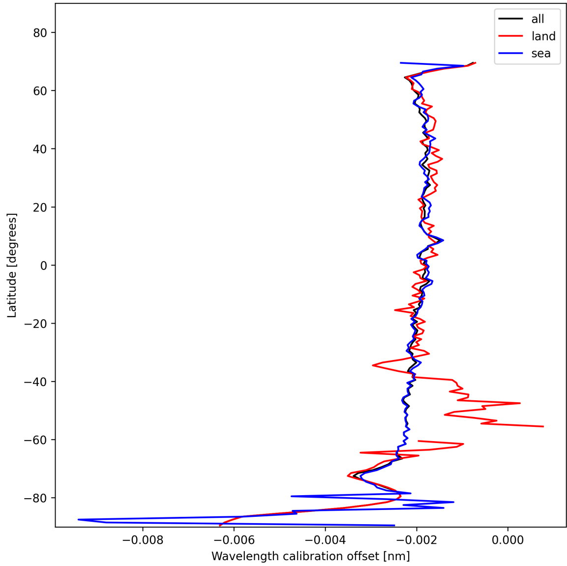
Figure 18: Zonal average of “Wavelength calibration offset” for 2025-01-23 to 2025-01-25.
