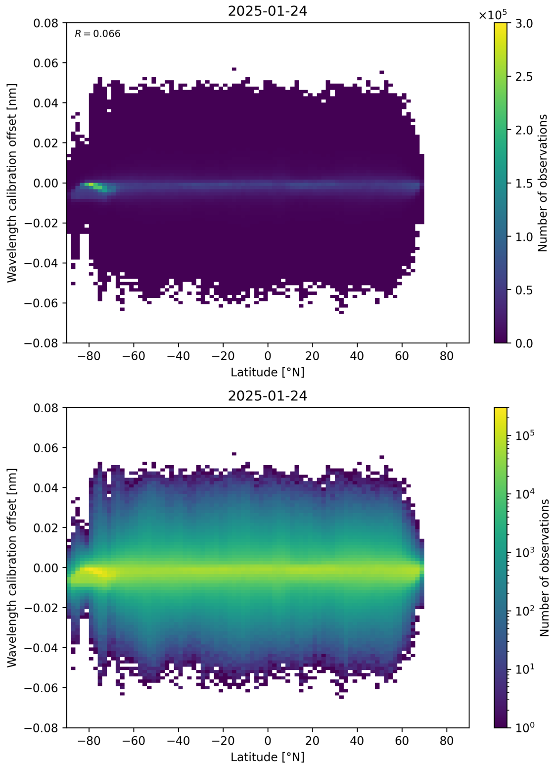
Figure 95: Scatter density plot of “Latitude” against “Wavelength calibration offset” for 2025-01-23 to 2025-01-25.
