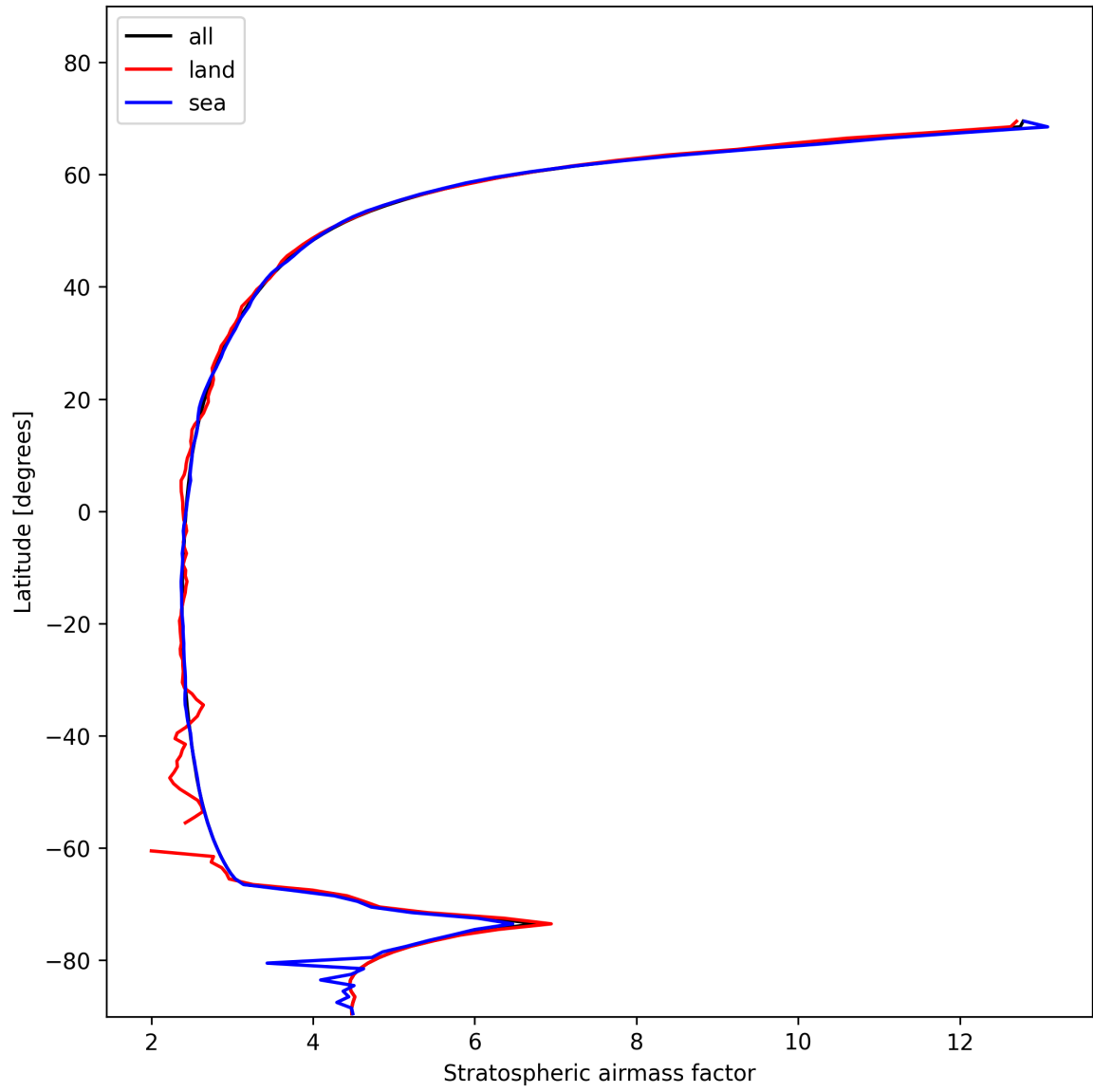
Figure 27: Zonal average of “Stratospheric airmass factor” for 2025-01-23 to 2025-01-25.
