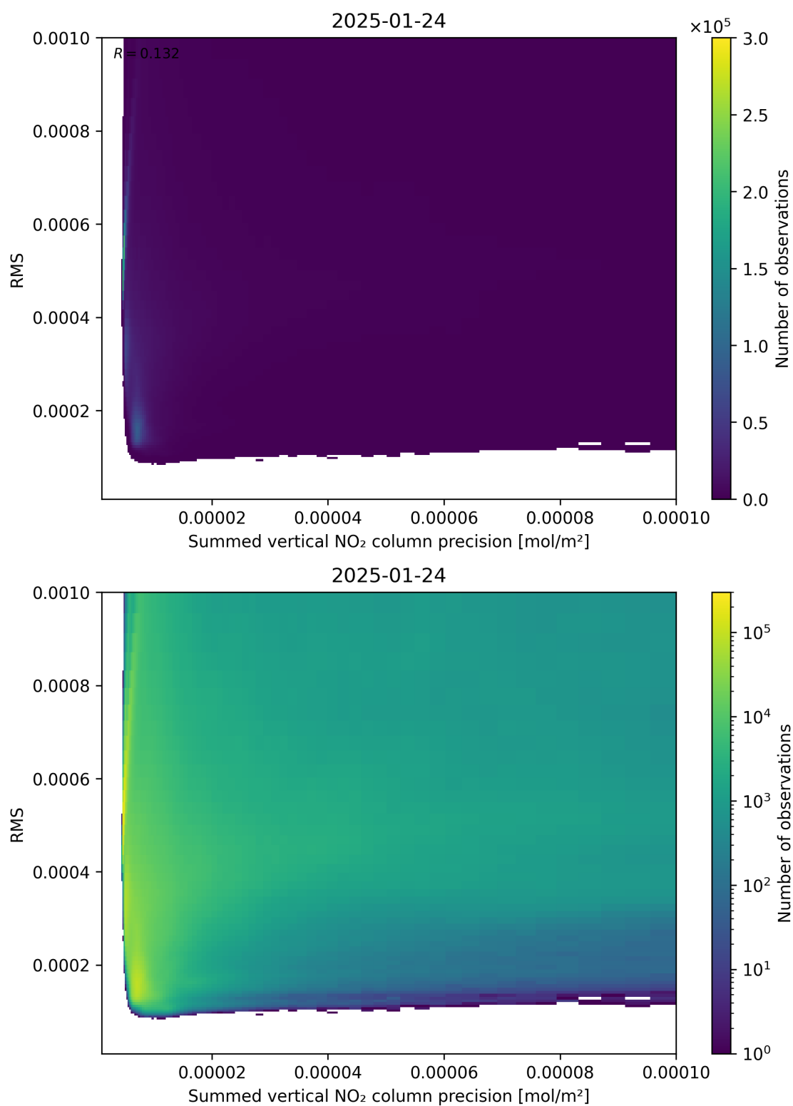
Figure 108: Scatter density plot of “Summed vertical NO 2 column precision” against “RMS” for 2025-01-23 to 2025-01-25.
