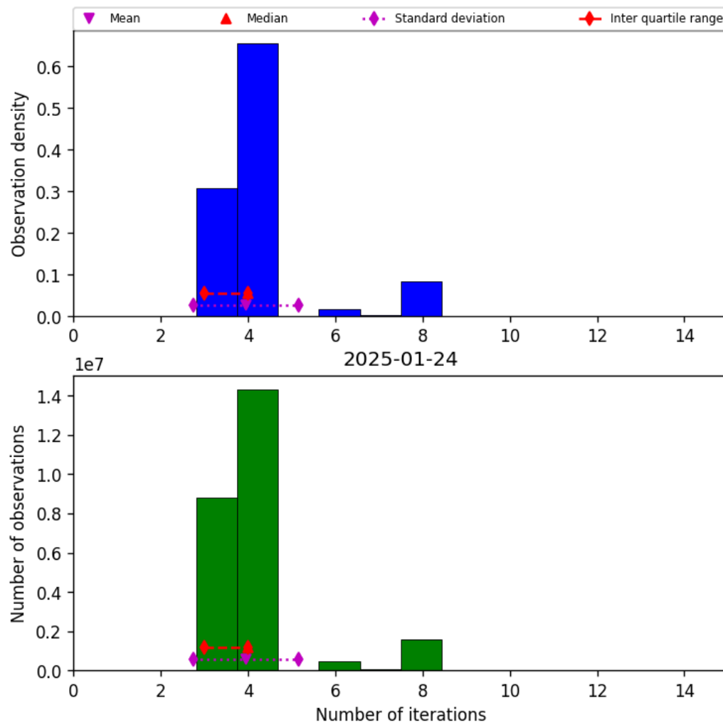
Figure 34: Histogram of “Number of iterations” for 2025-01-23 to 2025-01-25
