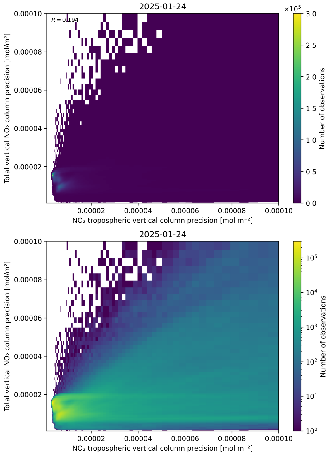
Figure 139: Scatter density plot of “NO 2 tropospheric vertical column precision” against “Total vertical NO 2 column precision” for 2025-01-23 to 2025-01-25.
