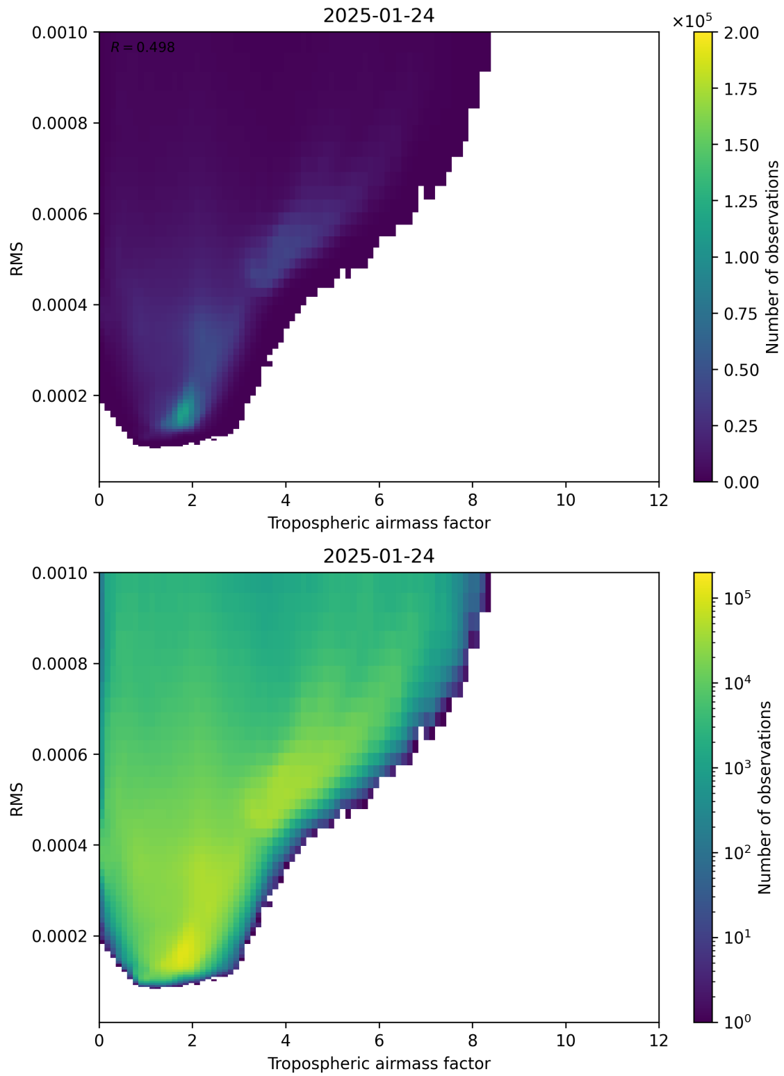
Figure 79: Scatter density plot of “Tropospheric airmass factor” against “RMS” for 2025-01-23 to 2025-01-25.
