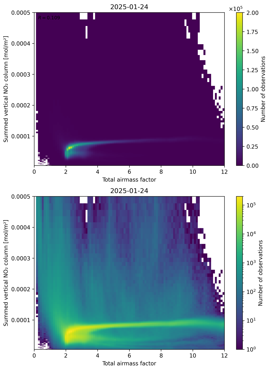
Figure 65: Scatter density plot of “Total airmass factor” against “Summed vertical NO 2 column” for 2025-01-23 to 2025-01-25.
