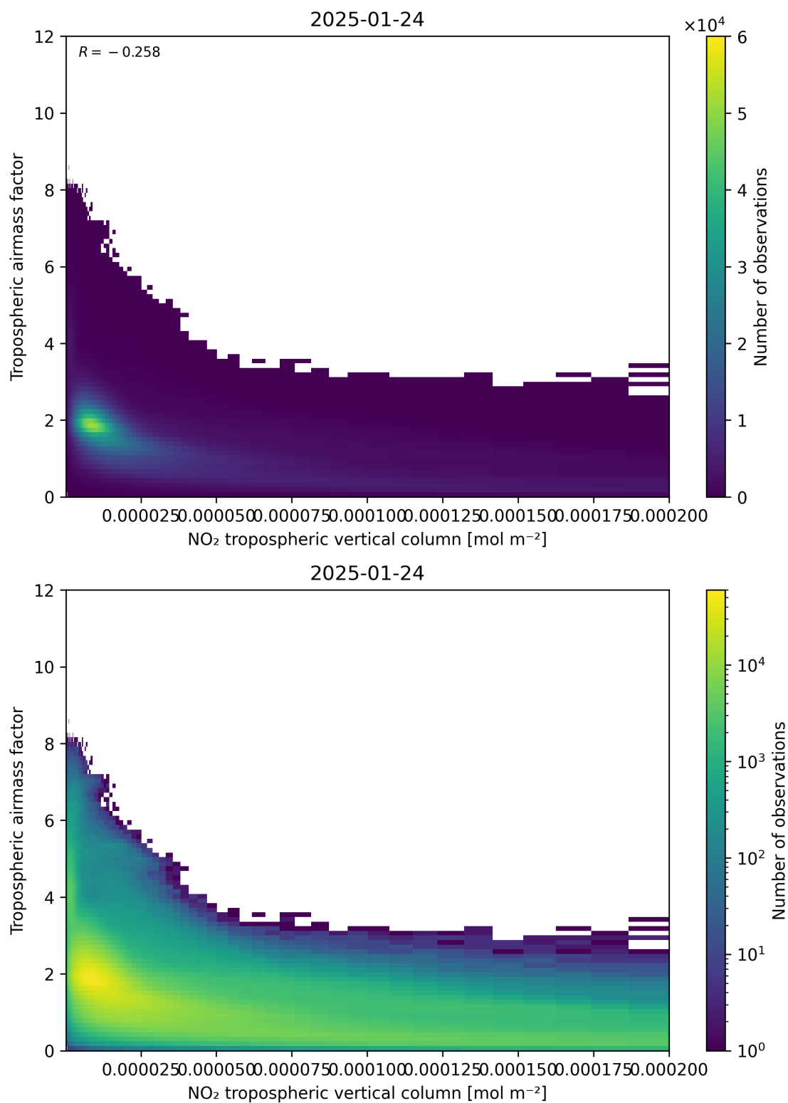
Figure 123: Scatter density plot of “NO 2 tropospheric vertical column” against “Tropospheric air mass factor” for 2025-01-23 to 2025-01-25.
