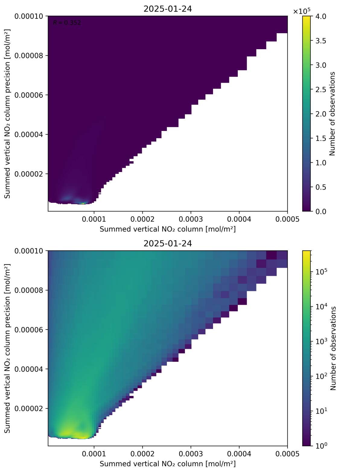
Figure 105: Scatter density plot of “Summed vertical NO 2 column” against “Summed vertical NO 2 column precision” for 2025-01-23 to 2025-01-25.
