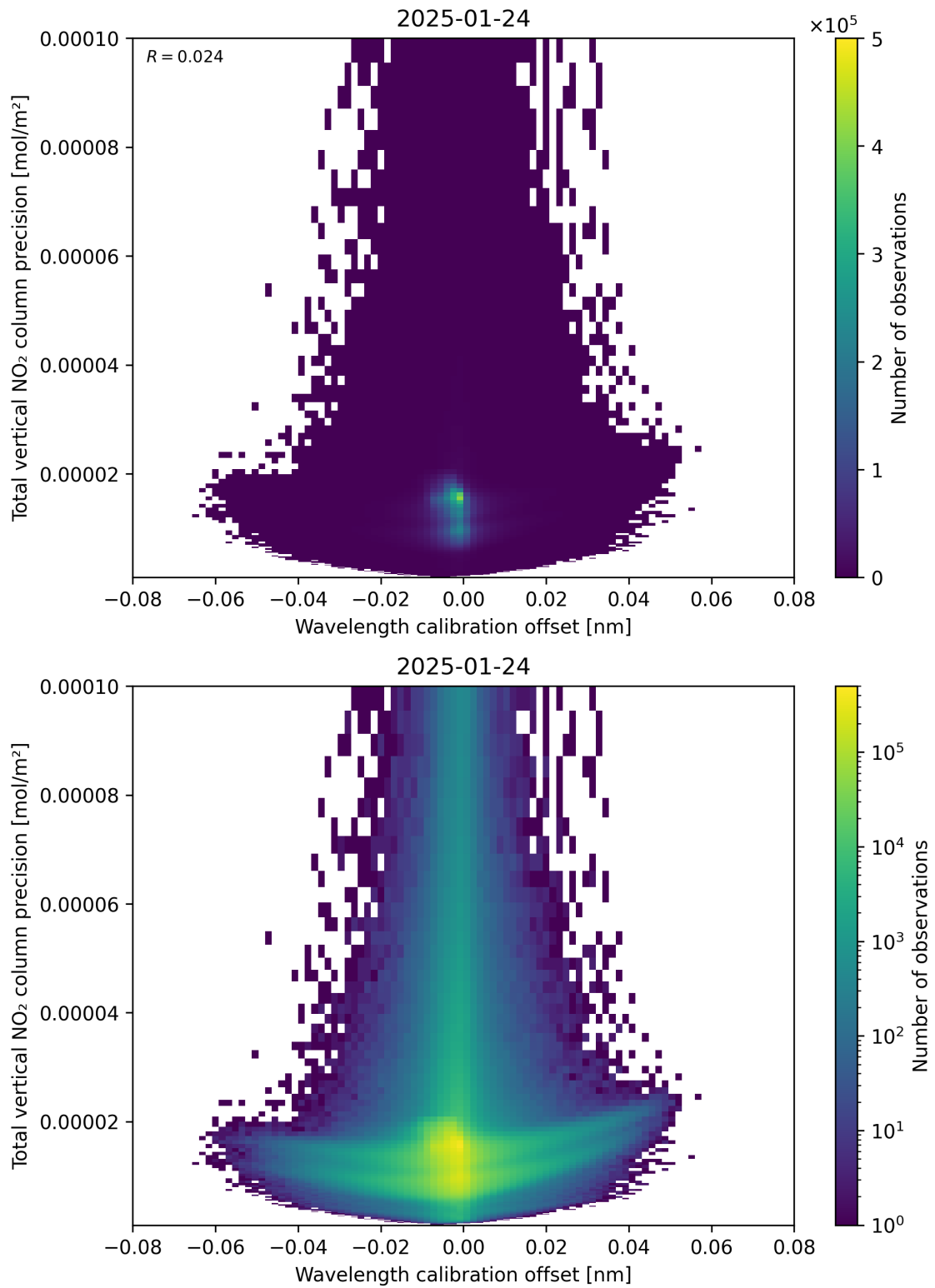
Figure 180: Scatter density plot of “Wavelength calibration offset” against “Total vertical NO 2 column precision” for 2025-01-23 to 2025-01-25.
