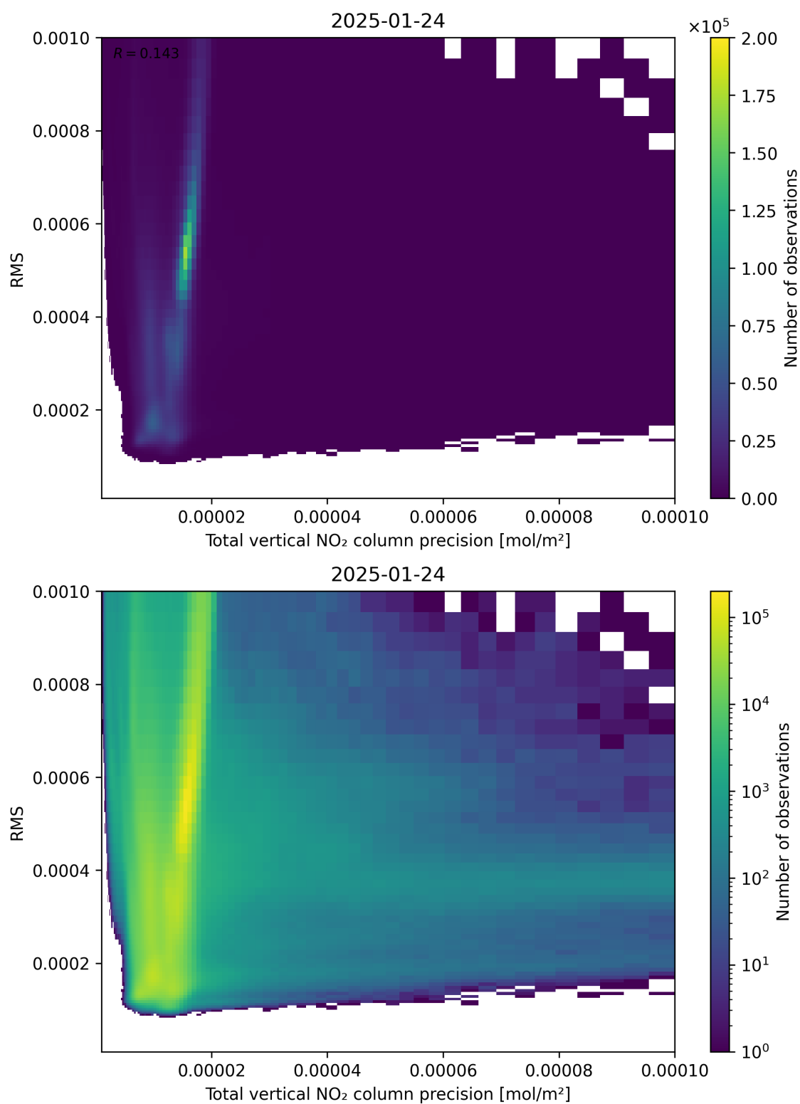
Figure 119: Scatter density plot of “Total vertical NO 2 column precision” against “RMS” for 2025-01-23 to 2025-01-25.
