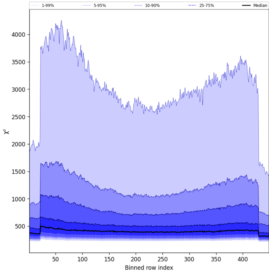
Figure 59: Along track statistics of “ \chi^2 ” for 2025-01-23 to 2025-01-25
