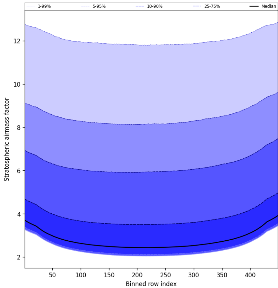
Figure 61: Along track statistics of “Stratospheric airmass factor” for 2025-01-23 to 2025-01-25
