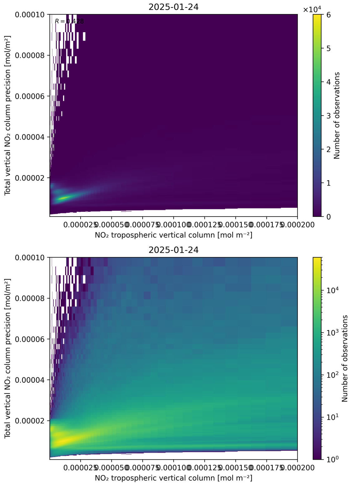
Figure 129: Scatter density plot of “NO 2 tropospheric vertical column” against “Total vertical NO 2 column precision” for 2025-01-23 to 2025-01-25.
