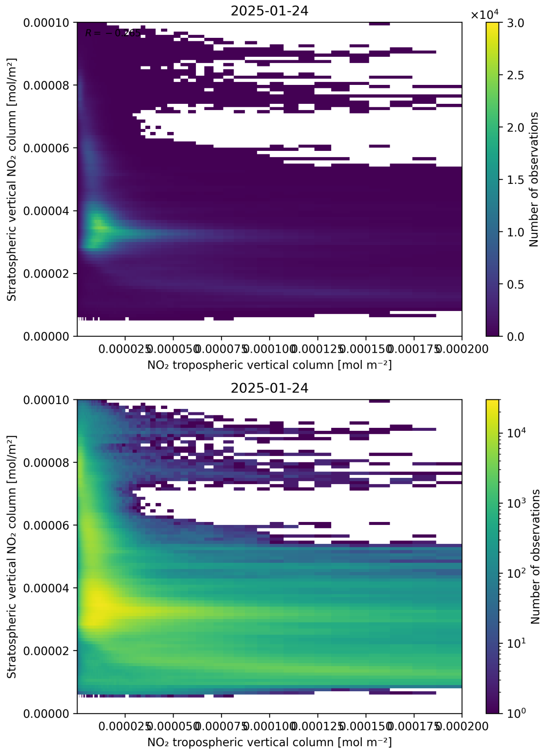
Figure 125: Scatter density plot of “NO 2 tropospheric vertical column” against “Stratospheric vertical NO 2 column” for 2025-01-23 to 2025-01-25.
