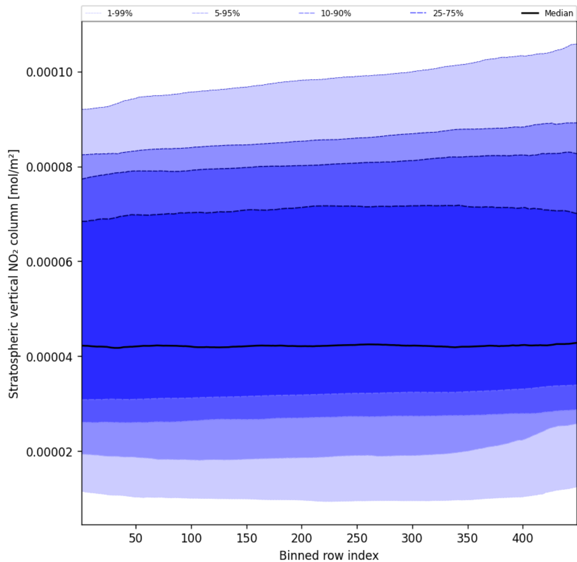
Figure 53: Along track statistics of “Stratospheric vertical NO 2 column” for 2025-01-23 to 2025-01-25
