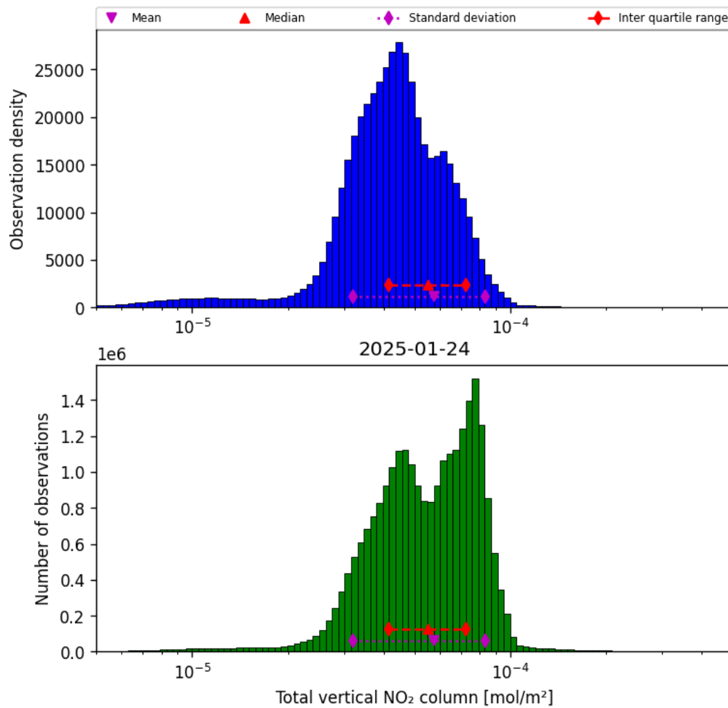
Figure 38: Histogram of “Total vertical NO 2 column” for 2025-01-23 to 2025-01-25
