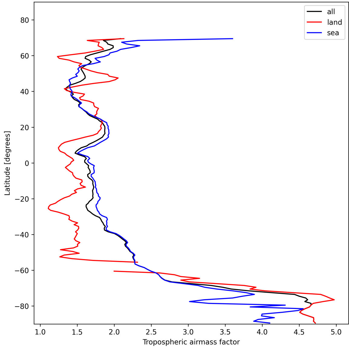
Figure 14: Zonal average of “Tropospheric airmass factor” for 2025-01-23 to 2025-01-25.
