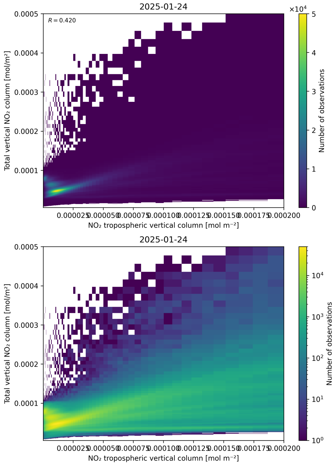
Figure 128: Scatter density plot of “NO 2 tropospheric vertical column” against “Total vertical NO 2 column” for 2025-01-23 to 2025-01-25.
