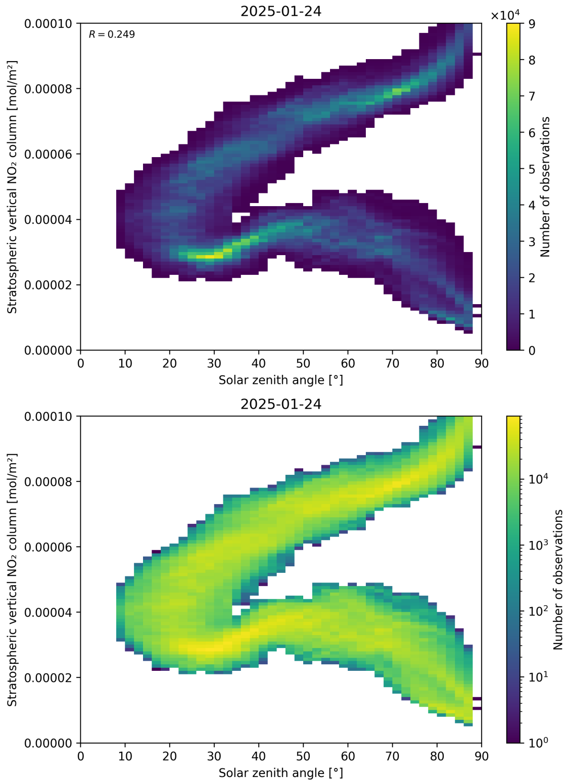
Figure 150: Scatter density plot of “Solar zenith angle” against “Stratospheric vertical NO 2 column” for 2025-01-23 to 2025-01-25.
