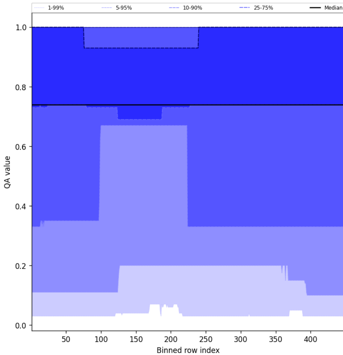
Figure 45: Along track statistics of “QA value” for 2025-01-23 to 2025-01-25
