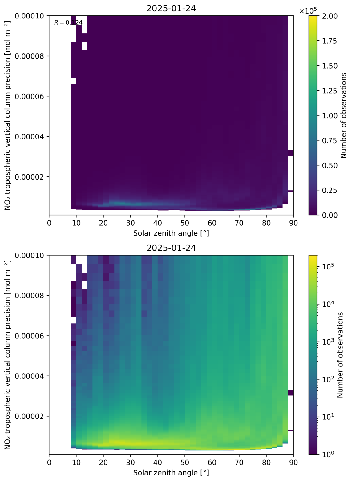
Figure 156: Scatter density plot of “Solar zenith angle” against “NO 2 tropospheric vertical column precision” for 2025-01-23 to 2025-01-25.
