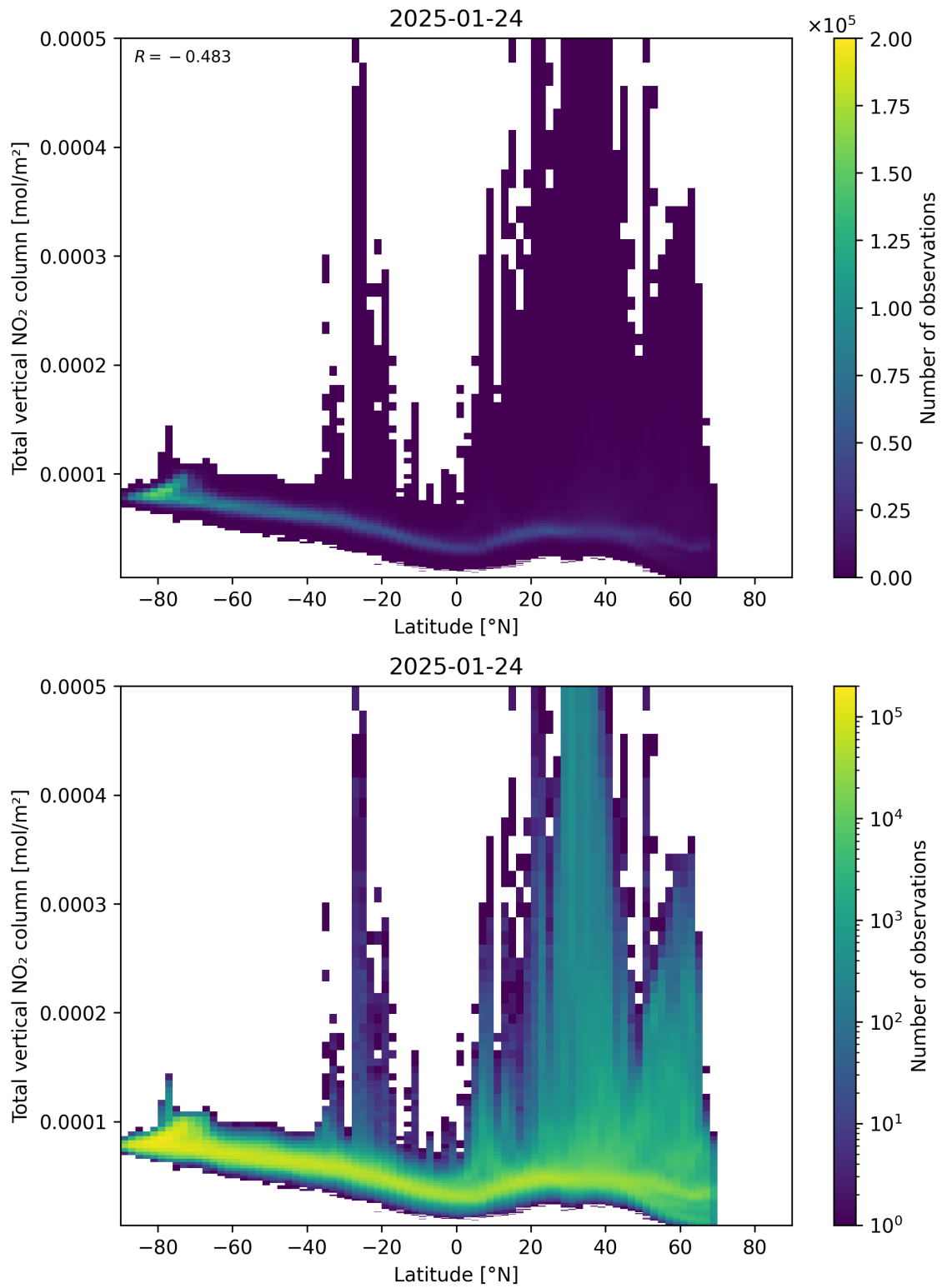
Figure 90: Scatter density plot of “Latitude” against “Total vertical NO 2 column” for 2025-01-23 to 2025-01-25.
