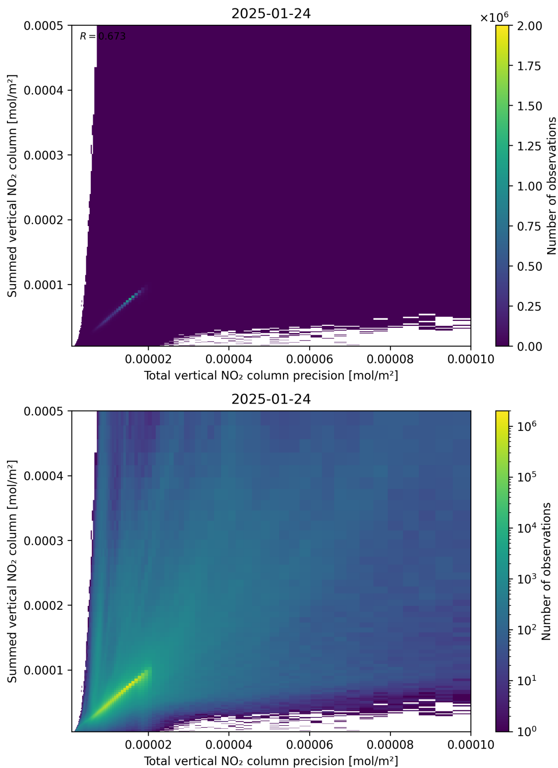
Figure 117: Scatter density plot of “Total vertical NO 2 column precision” against “Summed vertical NO 2 column” for 2025-01-23 to 2025-01-25.
