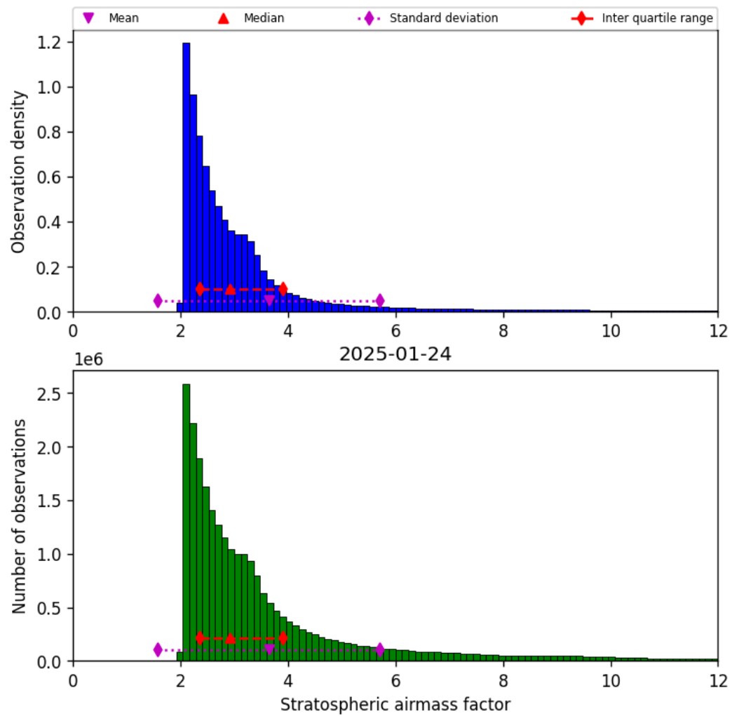
Figure 44: Histogram of “Stratospheric airmass factor” for 2025-01-23 to 2025-01-25
