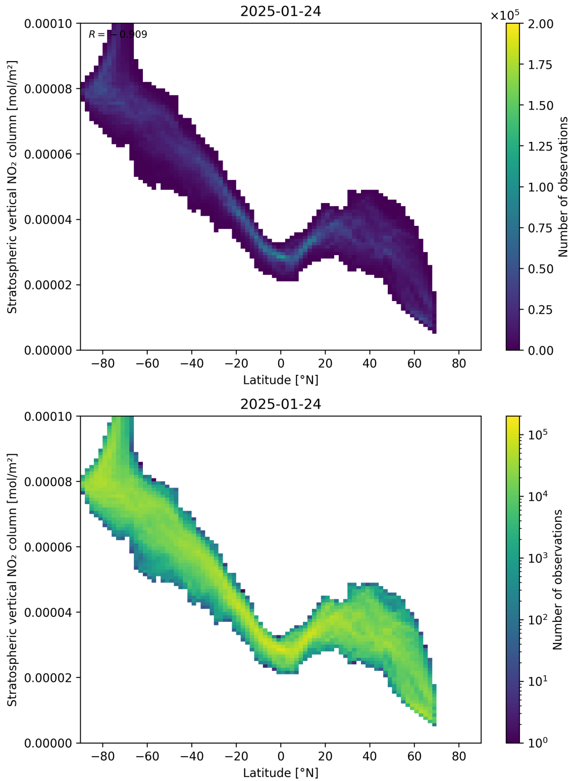
Figure 87: Scatter density plot of “Latitude” against “Stratospheric vertical NO 2 column” for 2025-01-23 to 2025-01-25.
