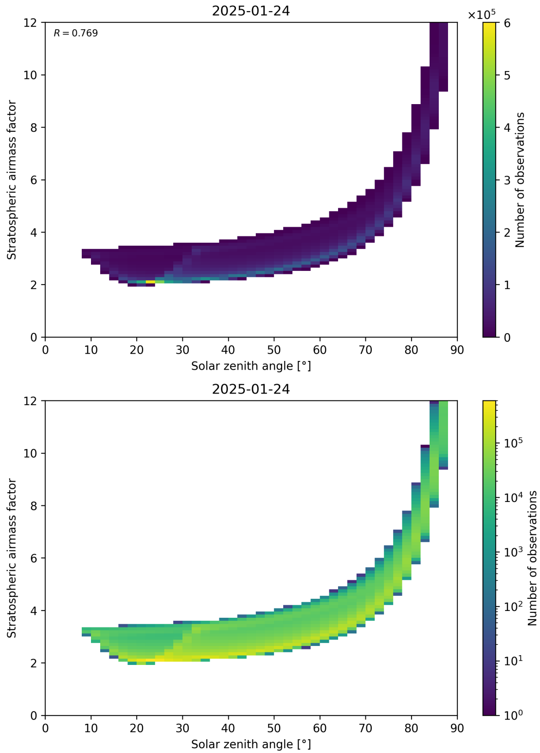
Figure 145: Scatter density plot of “Solar zenith angle” against “Stratospheric airmass factor” for 2025-01-23 to 2025-01-25.
