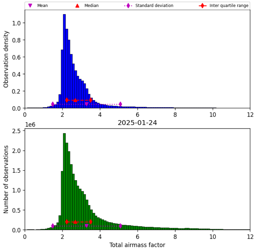
Figure 32: Histogram of “Total airmass factor” for 2025-01-23 to 2025-01-25
