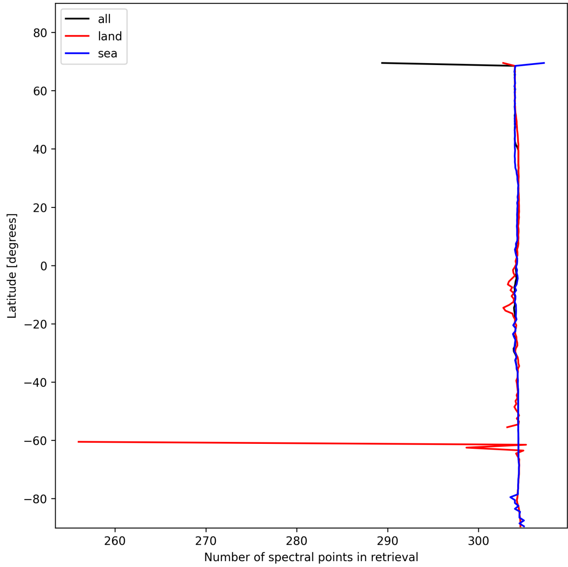
Figure 16: Zonal average of “Number of spectral points in retrieval” for 2025-01-23 to 2025-01-25.
