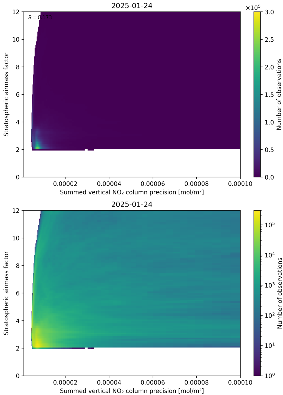
Figure 106: Scatter density plot of “Summed vertical NO 2 column precision” against “Stratospheric airmass factor” for 2025-01-23 to 2025-01-25.
