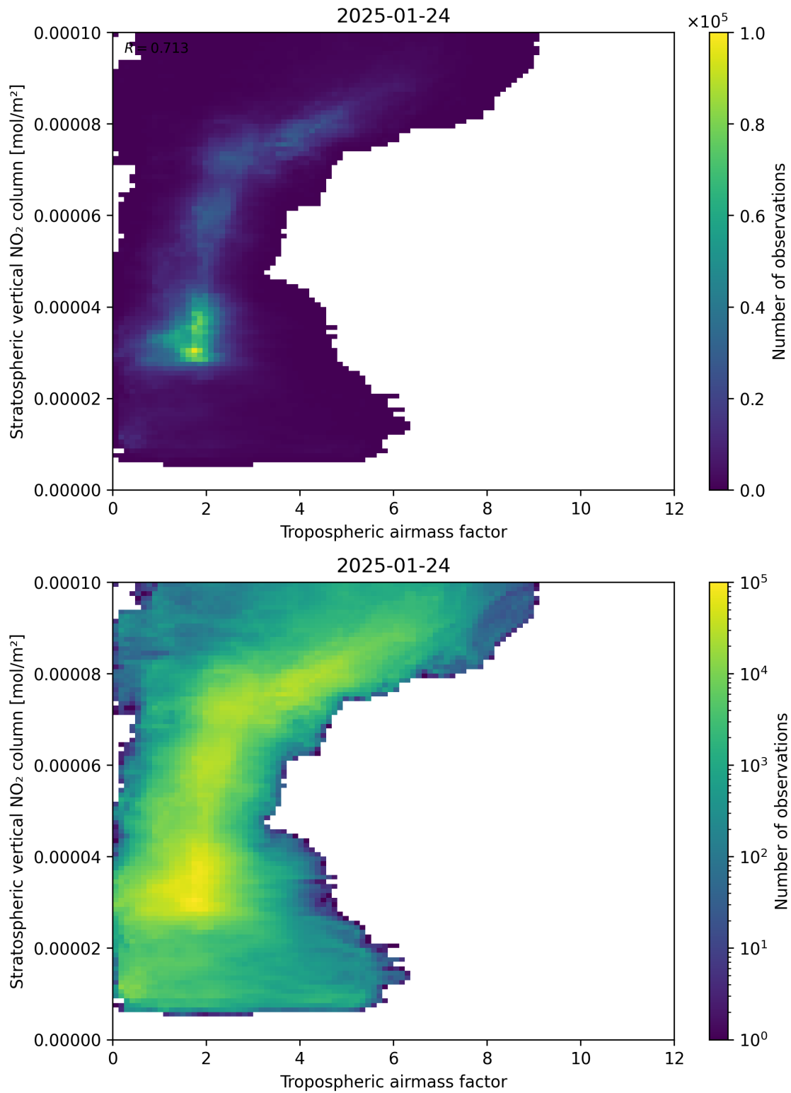
Figure 74: Scatter density plot of “Tropospheric air mass factor” against “Stratospheric vertical NO 2 column” for 2025-01-23 to 2025-01-25.
