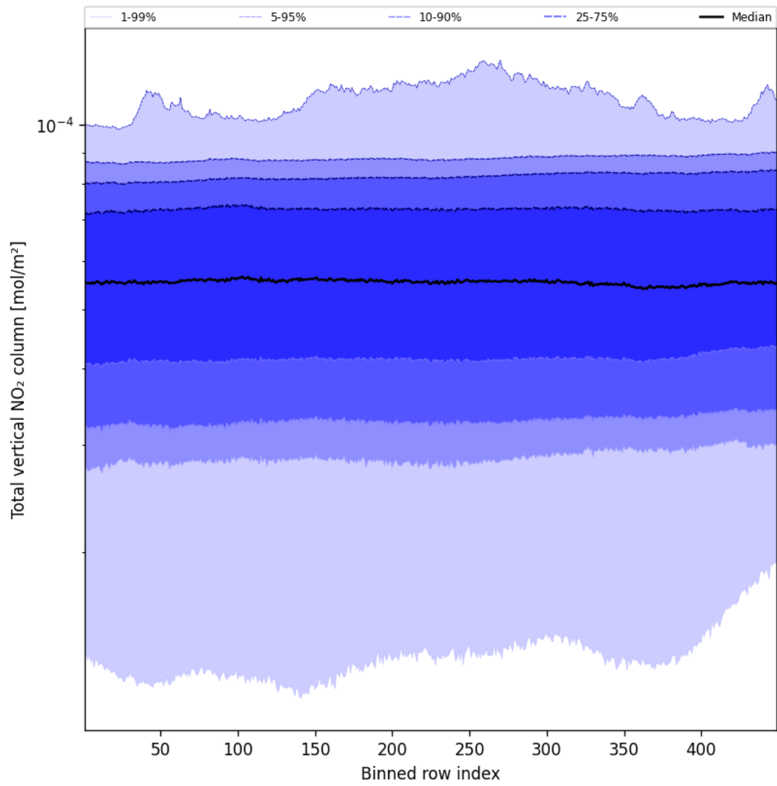
Figure 55: Along track statistics of “Total vertical NO 2 column” for 2025-01-23 to 2025-01-25
