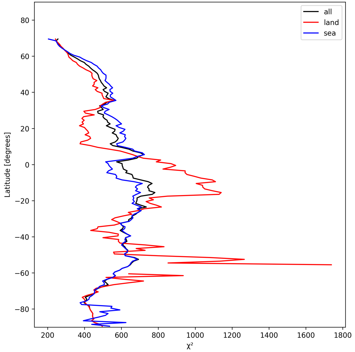
Figure 25: Zonal average of “ \chi^2 ” for 2025-01-23 to 2025-01-25.
