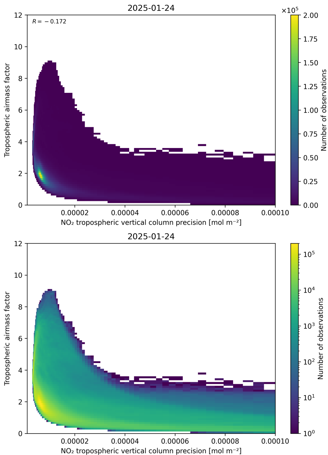
Figure 133: Scatter density plot of “NO 2 tropospheric vertical column precision” against “Tropospheric airmass factor” for 2025-01-23 to 2025-01-25.
