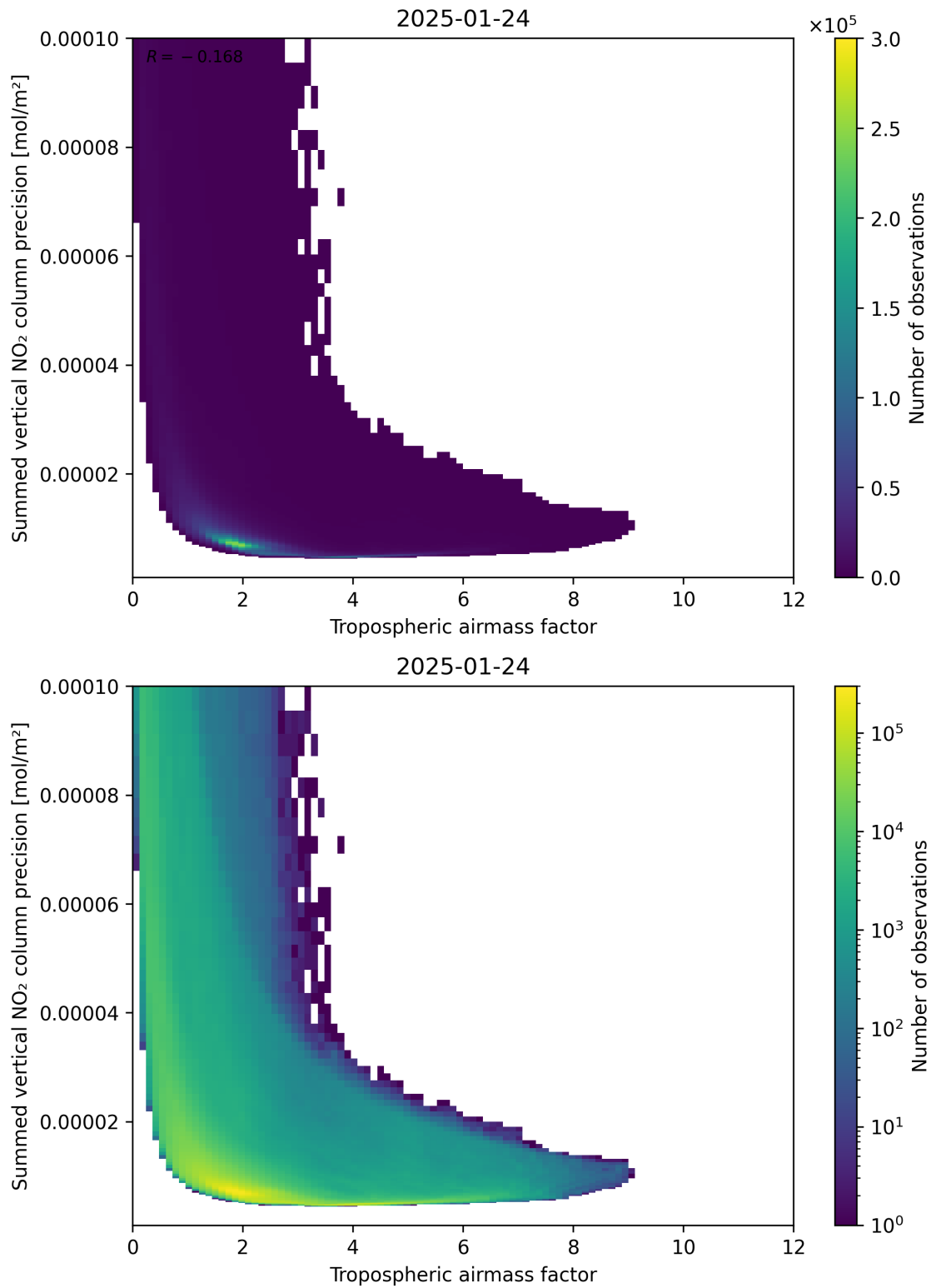
Figure 76: Scatter density plot of “Tropospheric airmass factor” against “Summed vertical NO 2 column precision” for 2025-01-23 to 2025-01-25.
