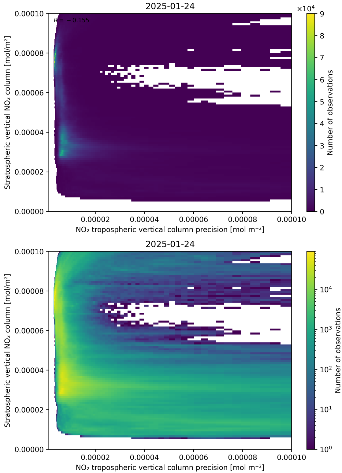
Figure 135: Scatter density plot of “NO 2 tropospheric vertical column precision” against “Stratospheric vertical NO 2 column” for 2025-01-23 to 2025-01-25.
