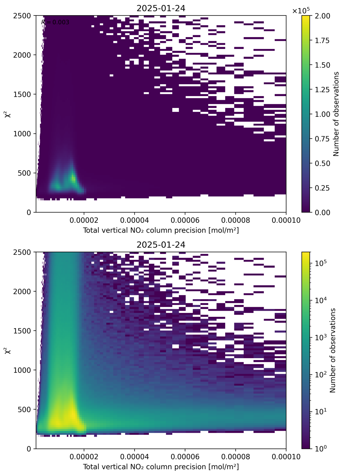
Figure 116: Scatter density plot of “Total vertical NO 2 column precision” against “ \chi^2 ” for 2025-01-23 to 2025-01-25.
