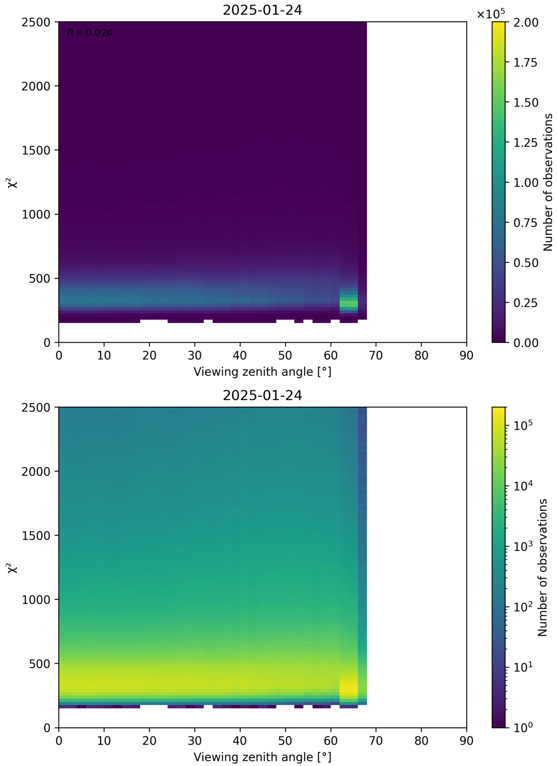
Figure 162: Scatter density plot of “Viewing zenith angle” against “ \chi^2 ” for 2025-01-23 to 2025-01-25.
