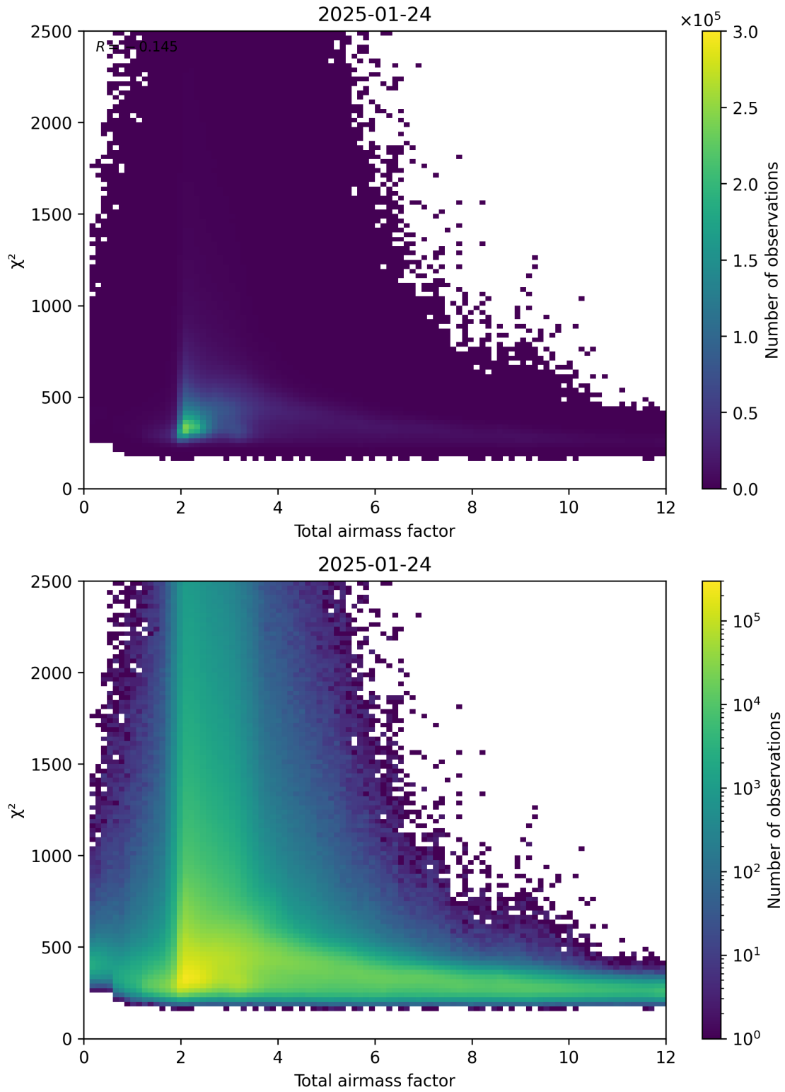
Figure 63: Scatter density plot of “Total airmass factor” against “ \chi^2 ” for 2025-01-23 to 2025-01-25.
