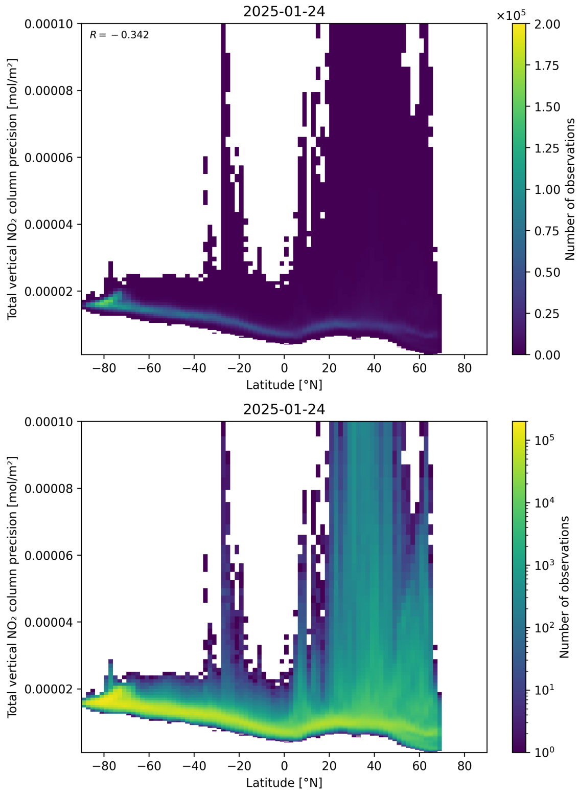
Figure 91: Scatter density plot of “Latitude” against “Total vertical NO 2 column precision” for 2025-01-23 to 2025-01-25.
