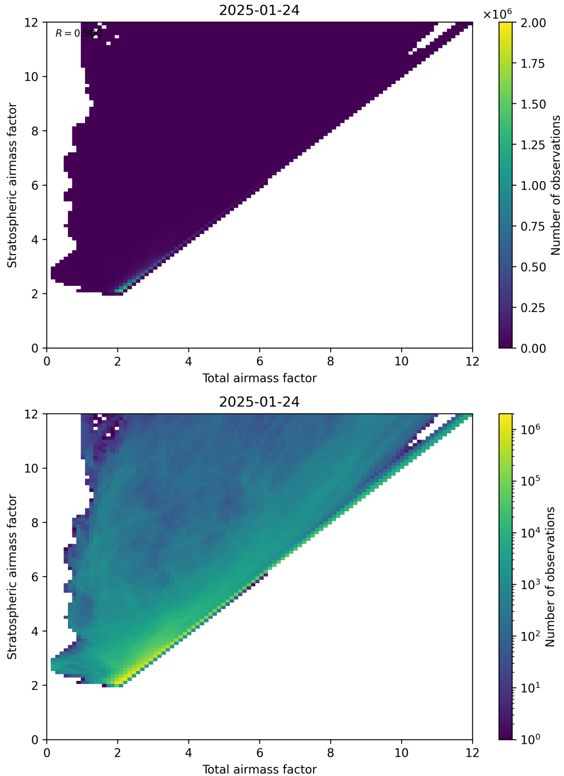
Figure 62: Scatter density plot of “Total airmass factor” against “Stratospheric airmass factor” for 2025-01-23 to 2025-01-25.
