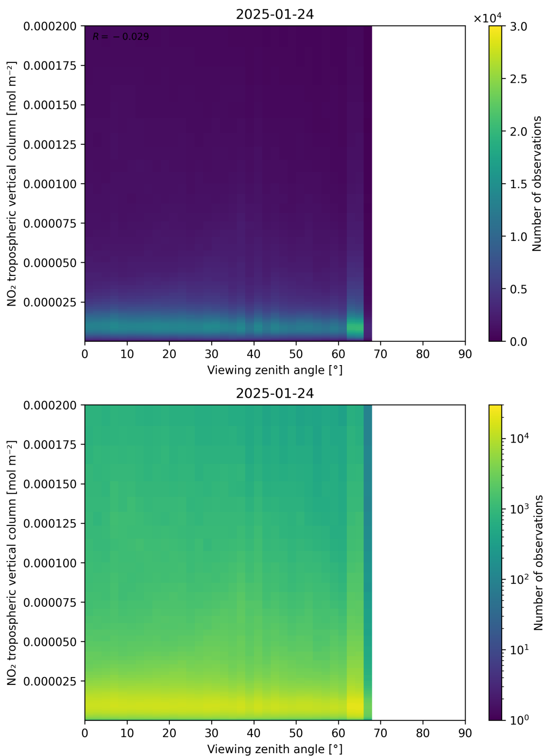
Figure 169: Scatter density plot of “Viewing zenith angle” against “NO 2 tropospheric vertical column” for 2025-01-23 to 2025-01-25.
