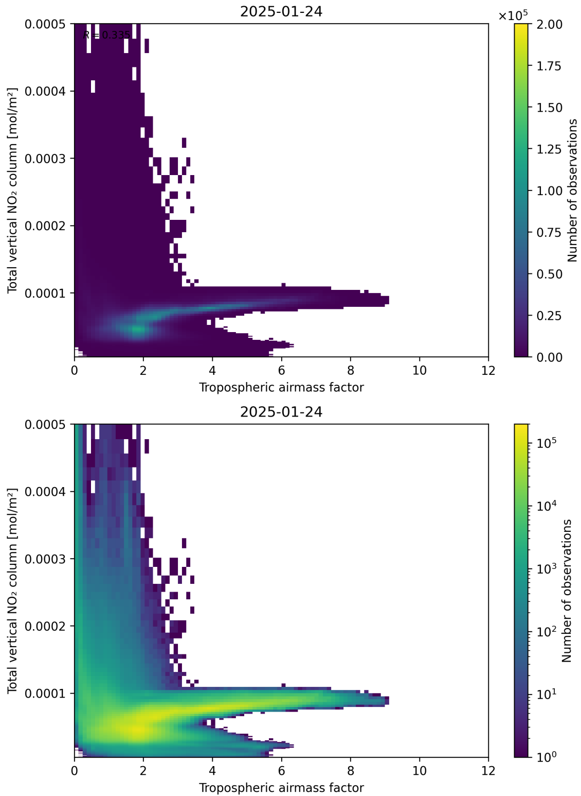
Figure 77: Scatter density plot of “Tropospheric airmass factor” against “Total vertical NO 2 column” for 2025-01-23 to 2025-01-25.
