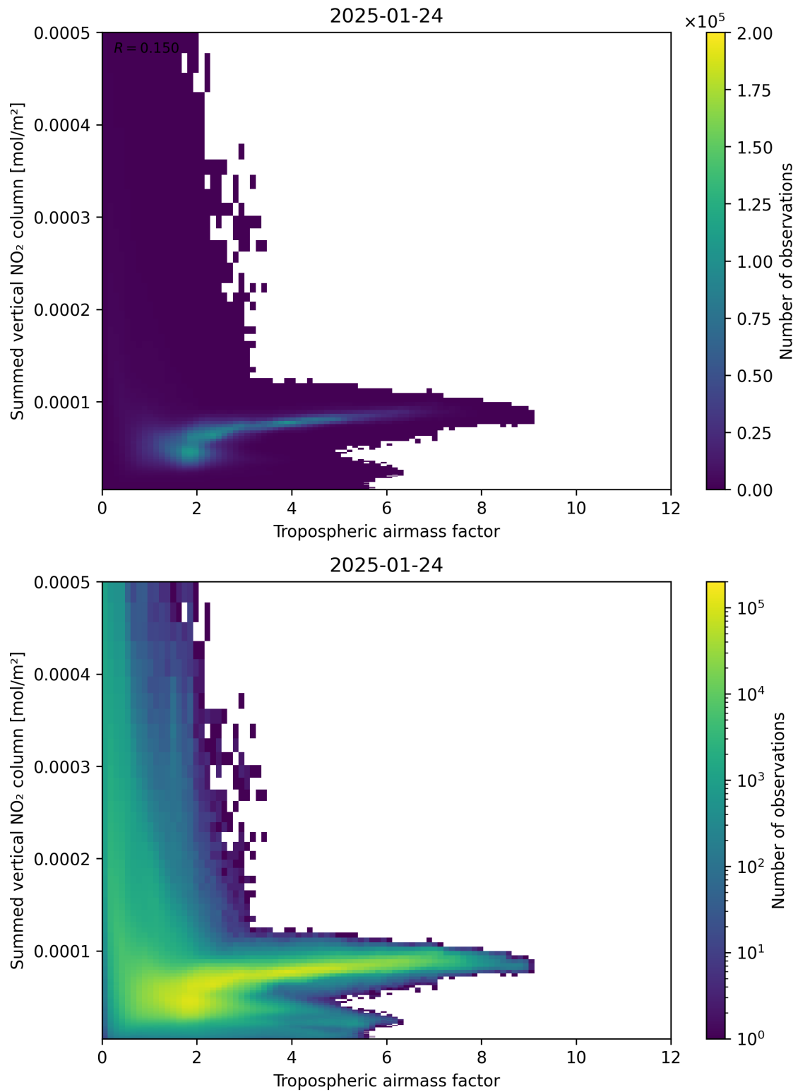
Figure 75: Scatter density plot of “Tropospheric air mass factor” against “Summed vertical NO 2 column” for 2025-01-23 to 2025-01-25.
