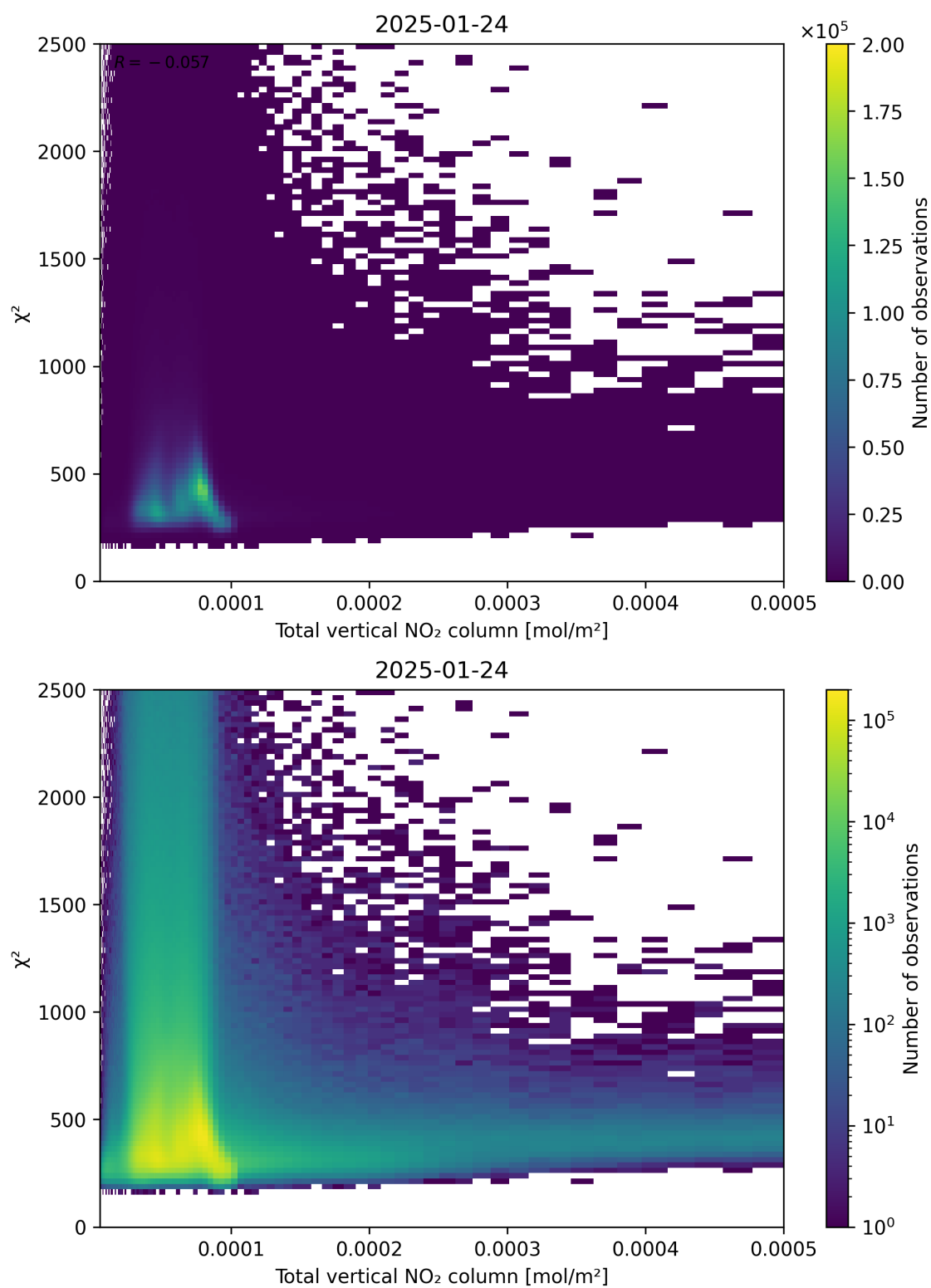
Figure 111: Scatter density plot of “Total vertical NO 2 column” against “ \chi^2 ” for 2025-01-23 to 2025-01-25.
