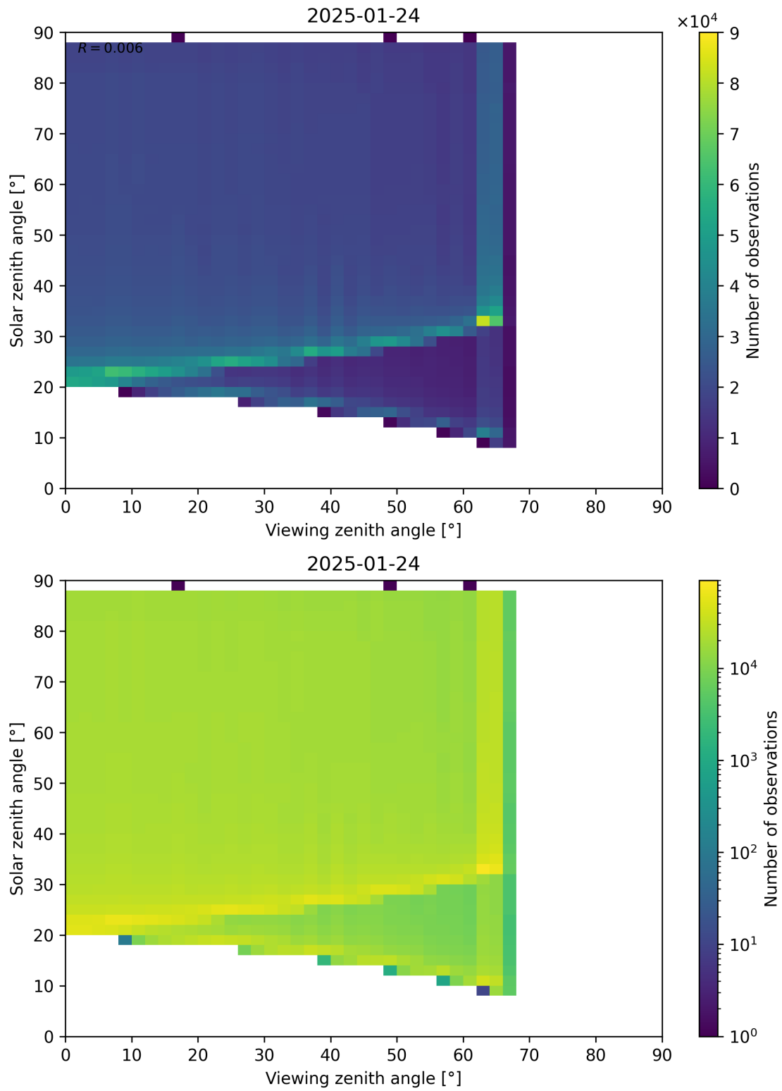
Figure 172: Scatter density plot of “Viewing zenith angle” against “Solar zenith angle” for 2025-01-23 to 2025-01-25.
