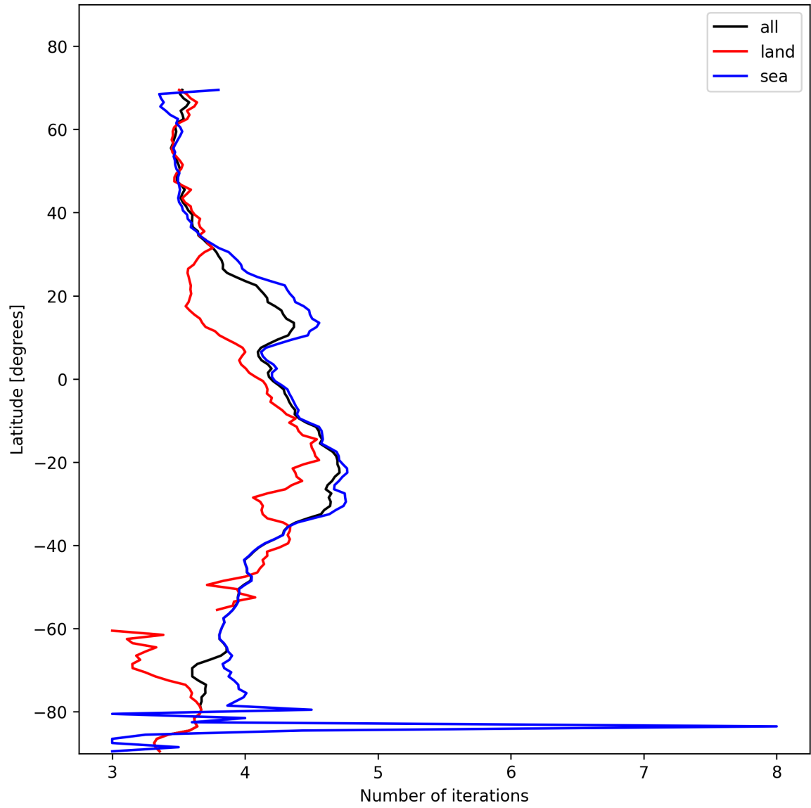
Figure 17: Zonal average of “Number of iterations” for 2025-01-23 to 2025-01-25.
