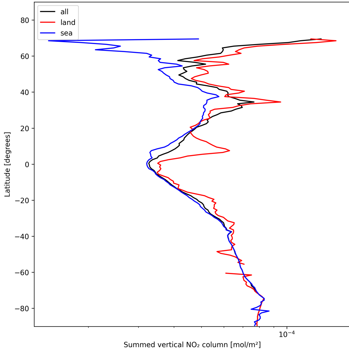
Figure 23: Zonal average of “Summed vertical NO 2 column” for 2025-01-23 to 2025-01-25.
