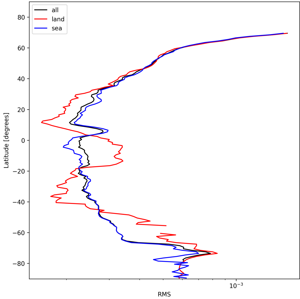
Figure 26: Zonal average of “RMS” for 2025-01-23 to 2025-01-25.
