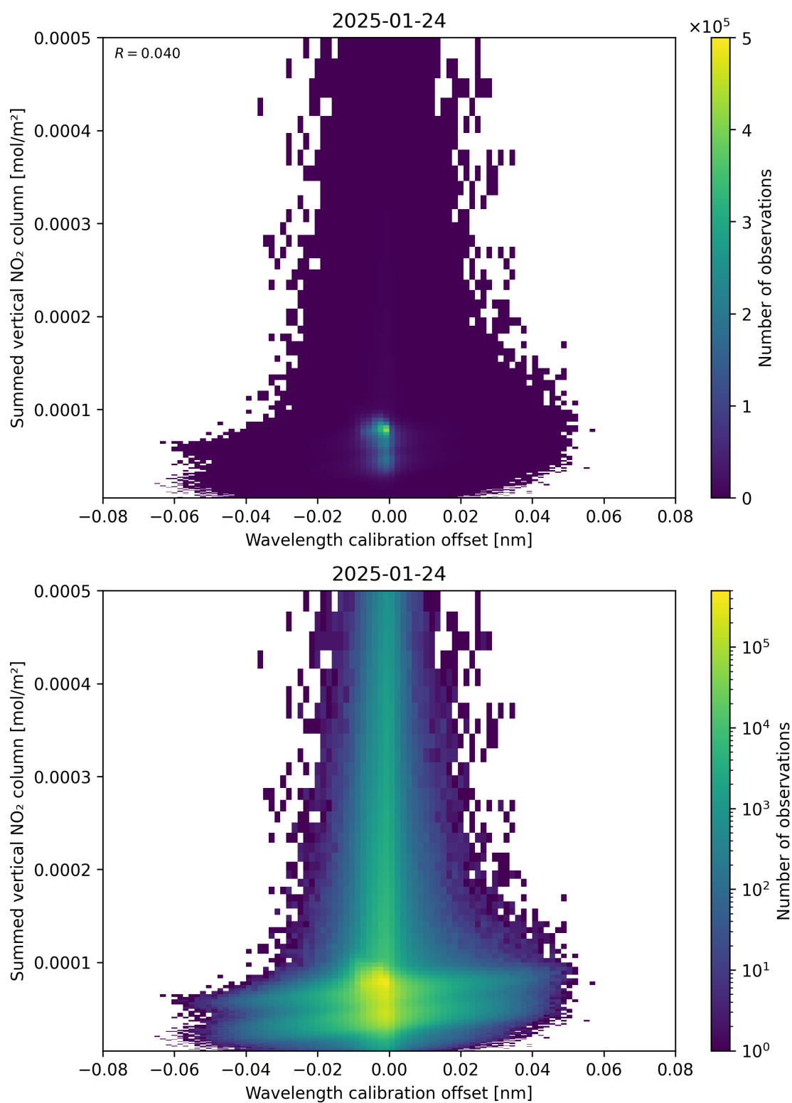
Figure 177: Scatter density plot of “Wavelength calibration offset” against “Summed vertical NO 2 column” for 2025-01-23 to 2025-01-25.
