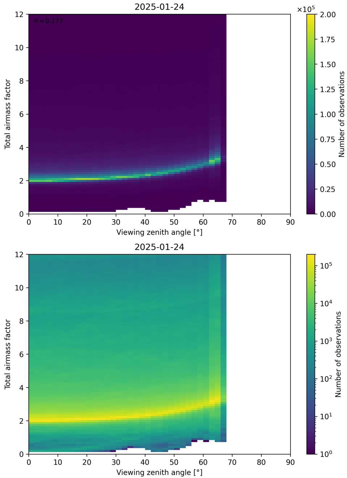
Figure 160: Scatter density plot of “Viewing zenith angle” against “Total airmass factor” for 2025-01-23 to 2025-01-25.
