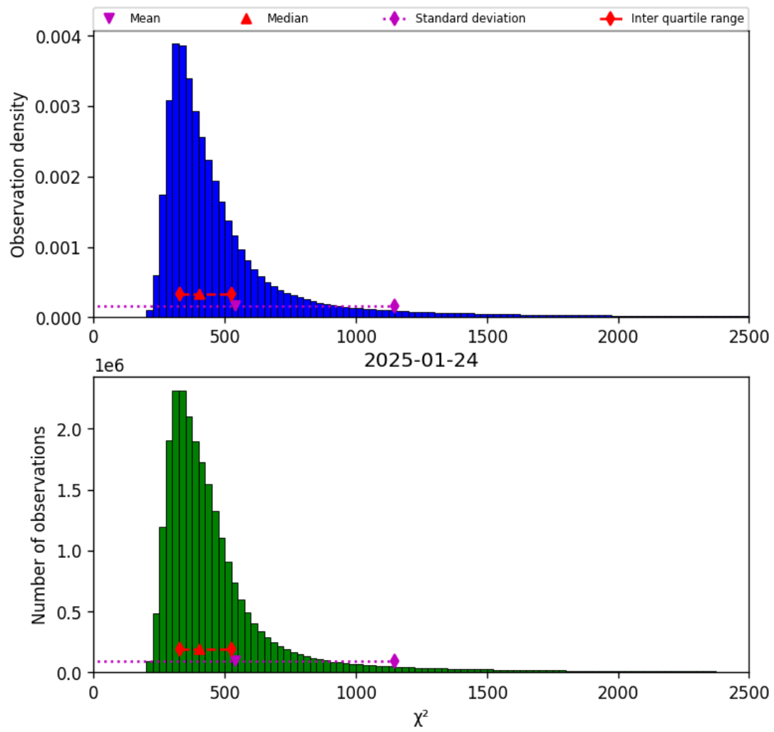
Figure 42: Histogram of “ \chi^2 ” for 2025-01-23 to 2025-01-25
