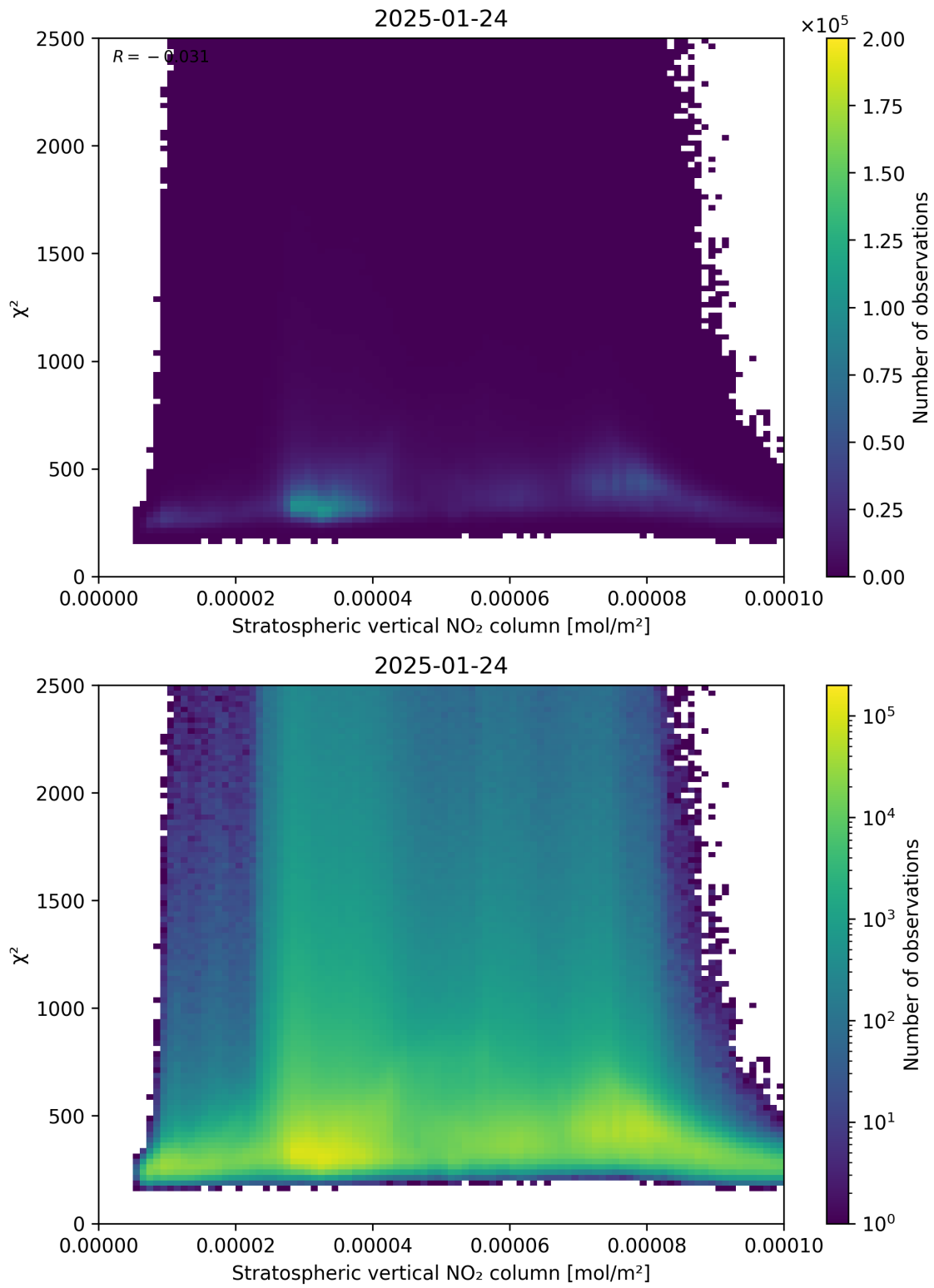
Figure 97: Scatter density plot of “Stratospheric vertical NO 2 column” against “ \chi^2 ” for 2025-01-23 to 2025-01-25.
