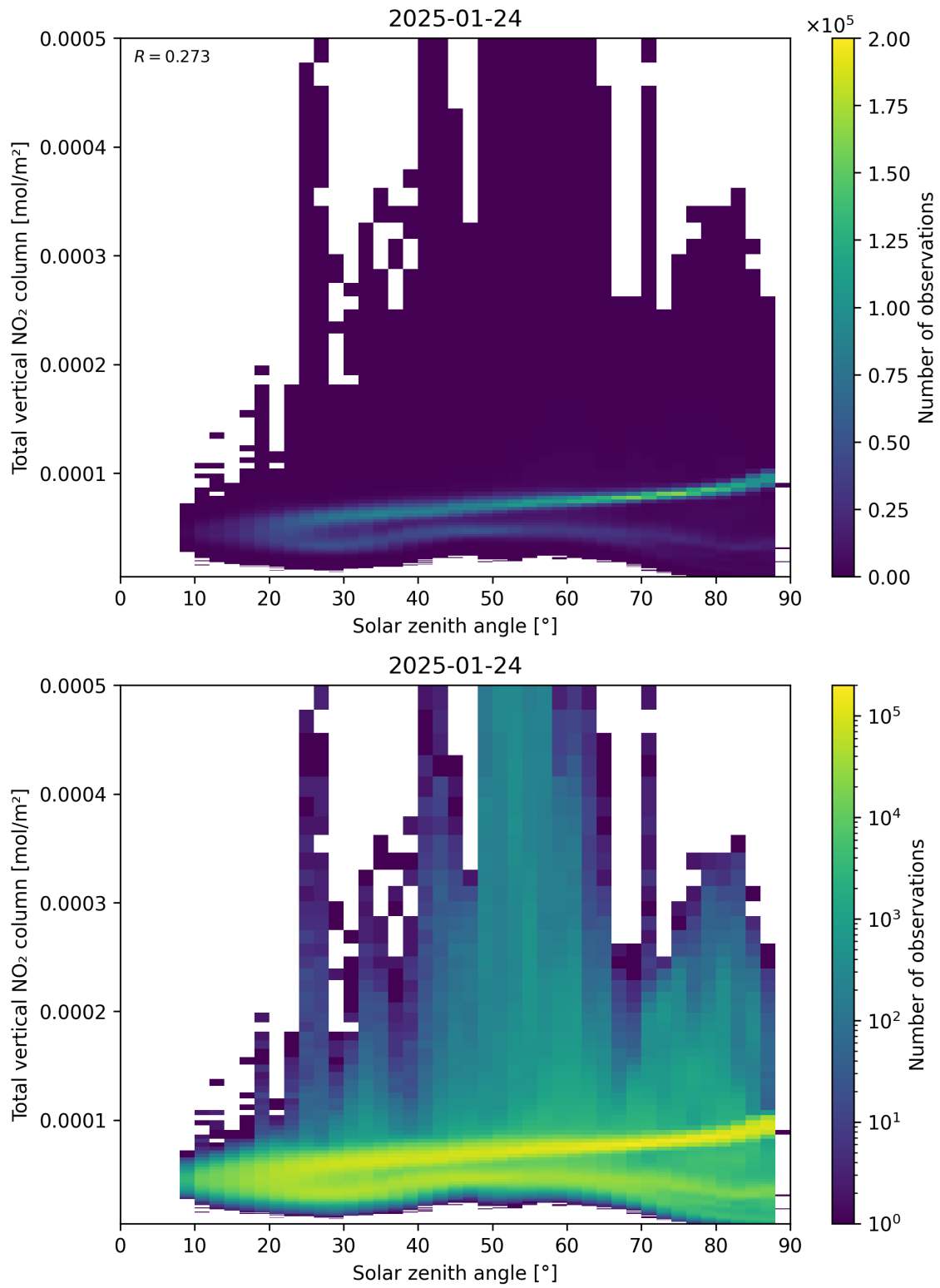
Figure 153: Scatter density plot of “Solar zenith angle” against “Total vertical NO 2 column” for 2025-01-23 to 2025-01-25.
