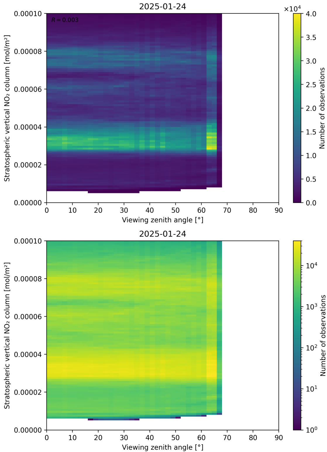
Figure 164: Scatter density plot of “Viewing zenith angle” against “Stratospheric vertical NO 2 column” for 2025-01-23 to 2025-01-25.
