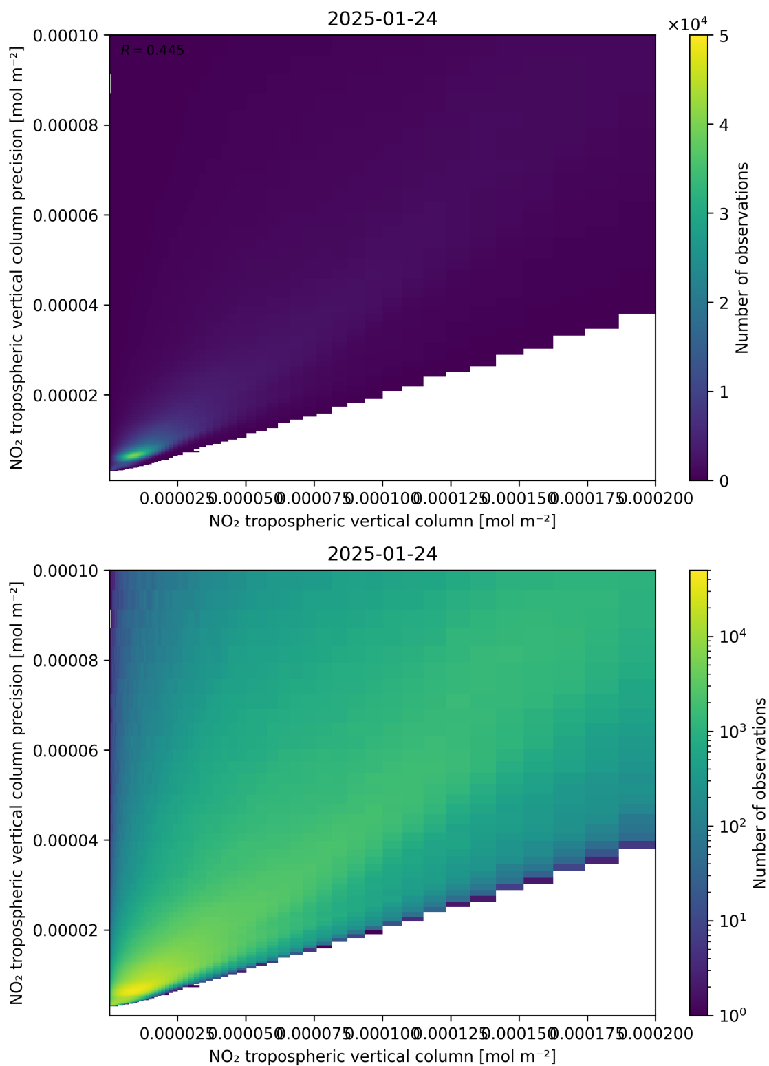
Figure 130: Scatter density plot of “NO 2 tropospheric vertical column” against “NO 2 tropospheric vertical column precision” for 2025-01-23 to 2025-01-25.
