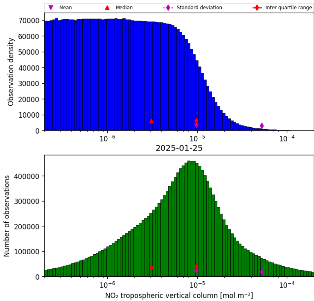
Figure 29: Histogram of “NO 2 tropospheric vertical column” for 2025-01-24 to 2025-01-26
