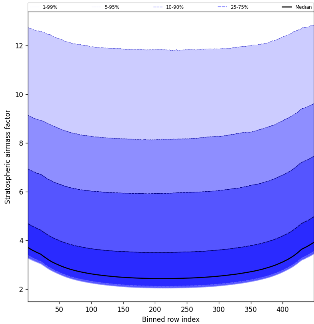
Figure 61: Along track statistics of “Stratospheric airmass factor” for 2025-01-24 to 2025-01-26
