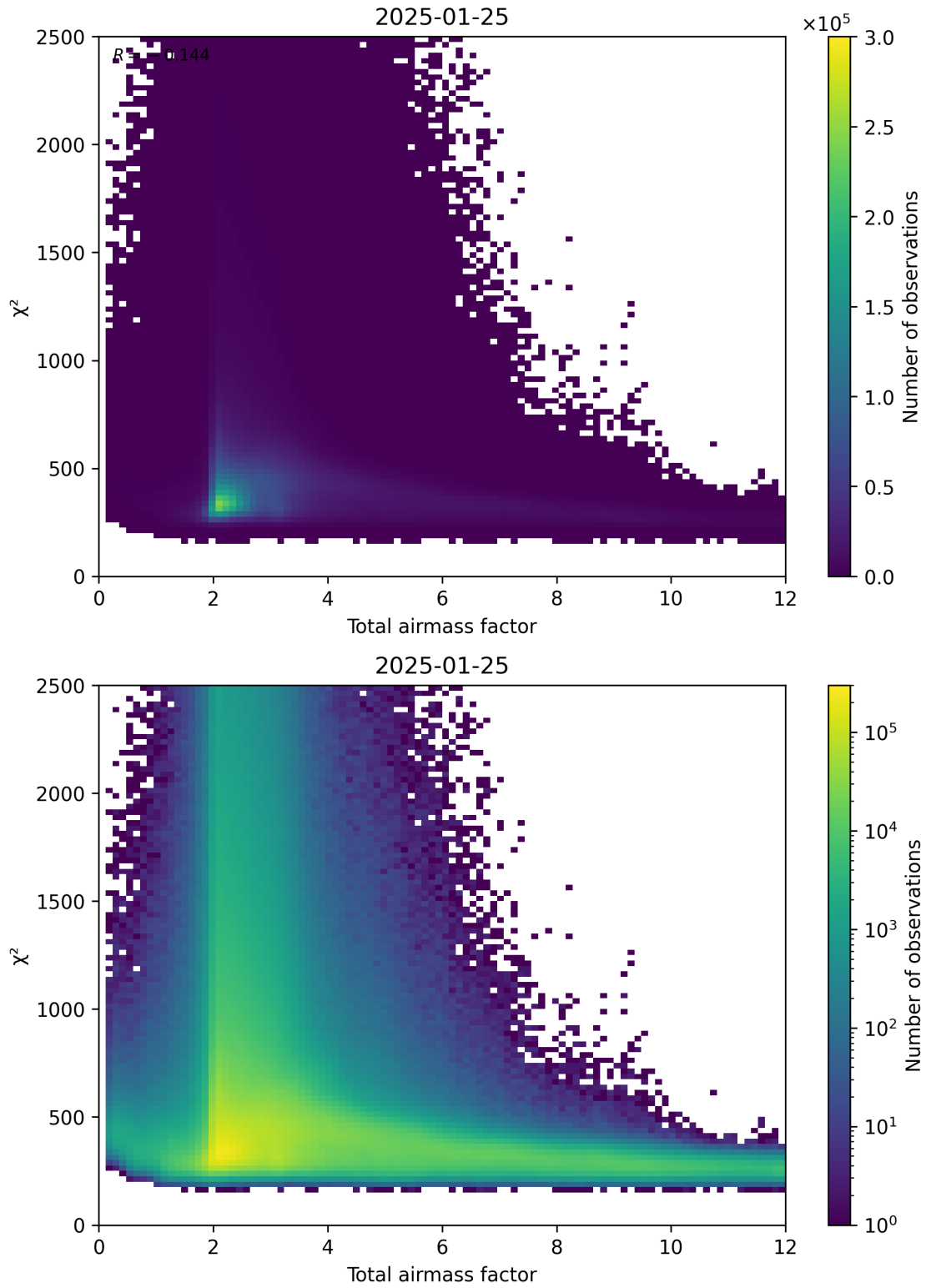
Figure 63: Scatter density plot of “Total airmass factor” against “ \chi^2 ” for 2025-01-24 to 2025-01-26.
