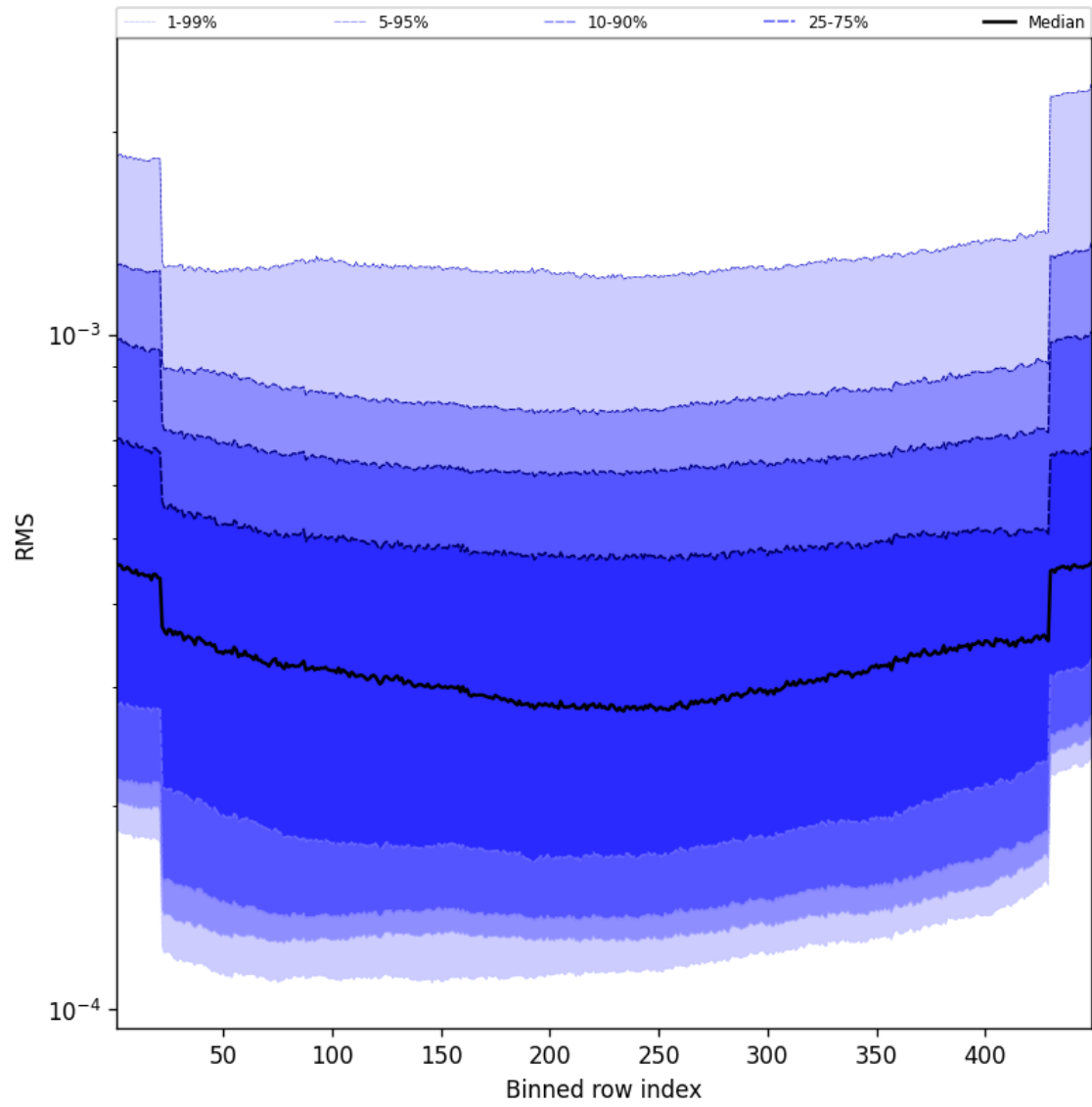
Figure 60: Along track statistics of “RMS” for 2025-01-24 to 2025-01-26
