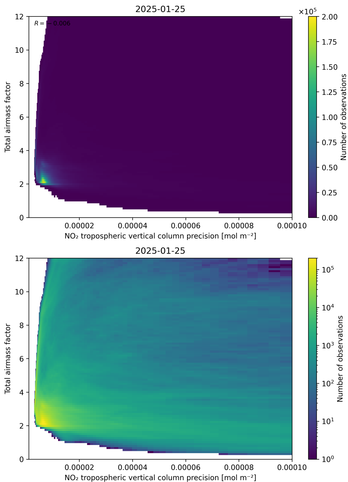
Figure 132: Scatter density plot of “NO 2 tropospheric vertical column precision” against “Total air mass factor” for 2025-01-24 to 2025-01-26.
