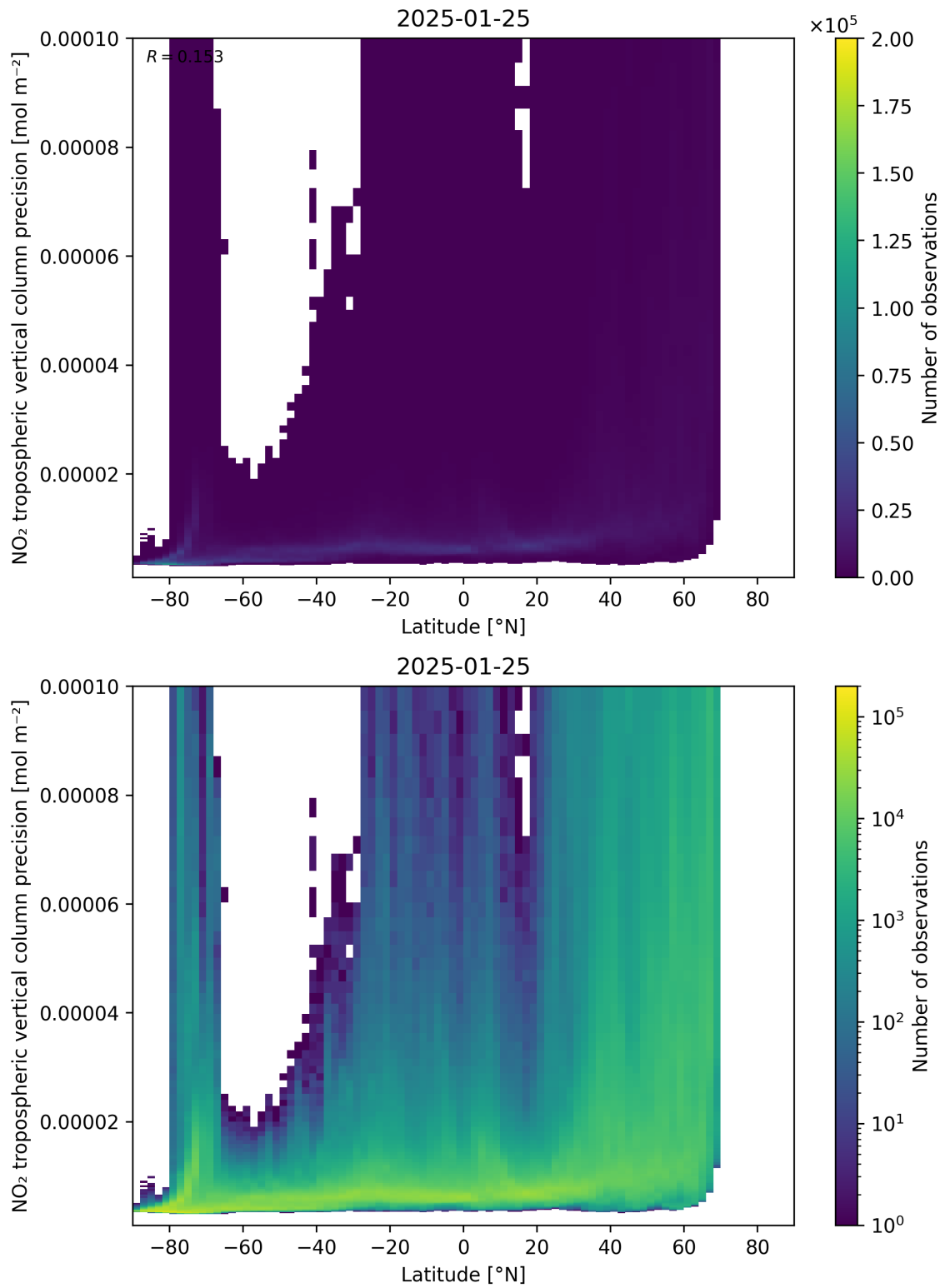
Figure 93: Scatter density plot of “Latitude” against “NO 2 tropospheric vertical column precision” for 2025-01-24 to 2025-01-26.
