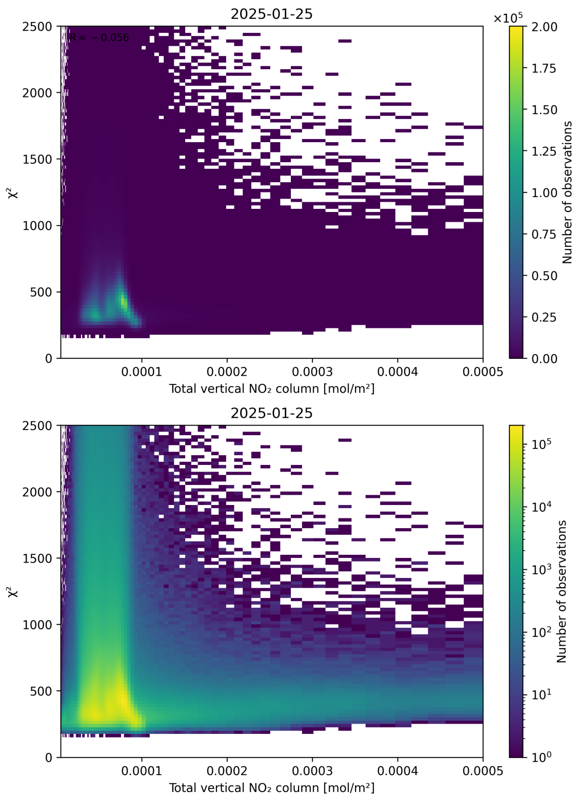
Figure 111: Scatter density plot of “Total vertical NO 2 column” against “ \chi^2 ” for 2025-01-24 to 2025-01-26.
