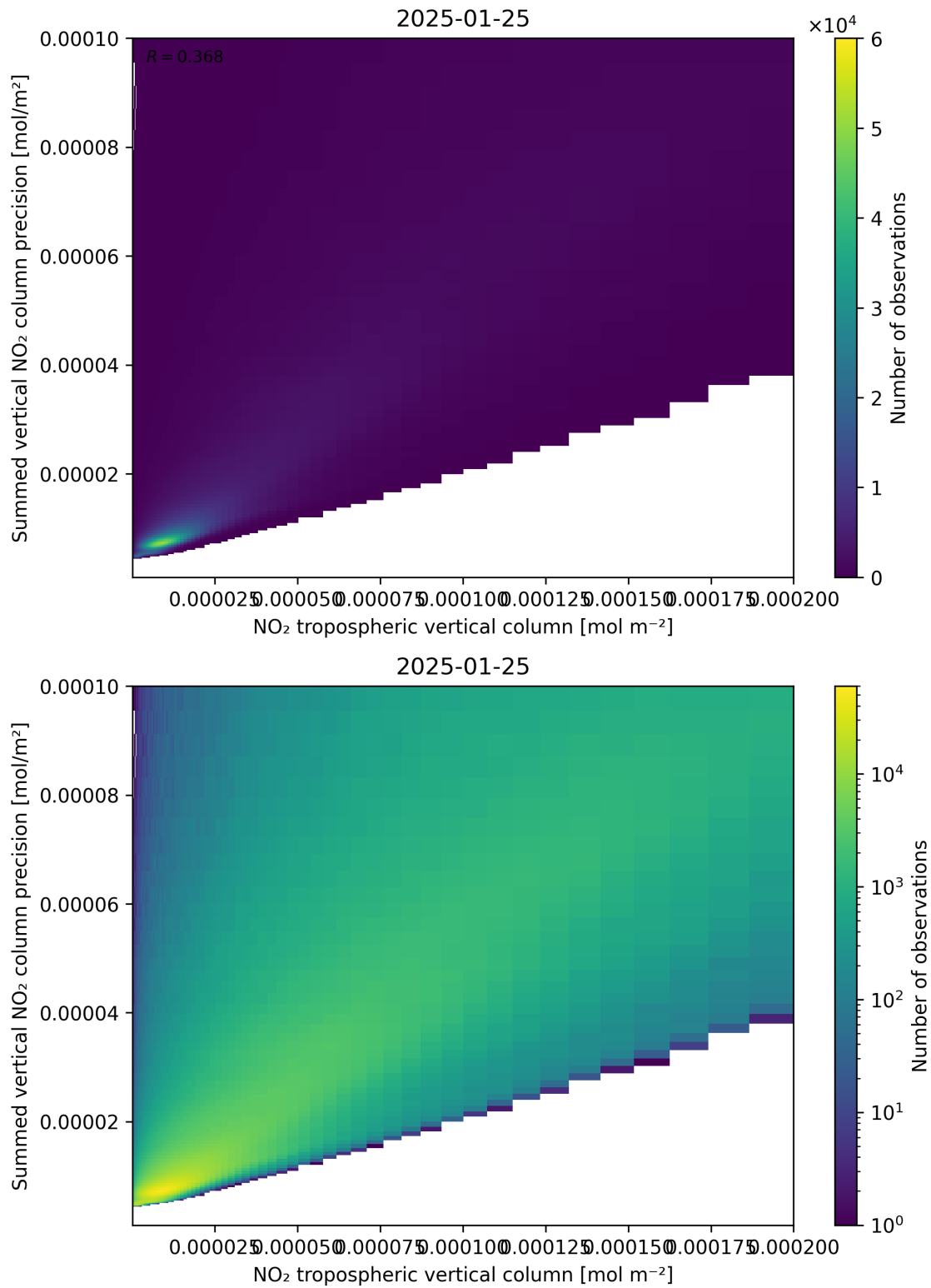
Figure 127: Scatter density plot of “NO 2 tropospheric vertical column” against “Summed vertical NO 2 column precision” for 2025-01-24 to 2025-01-26.
