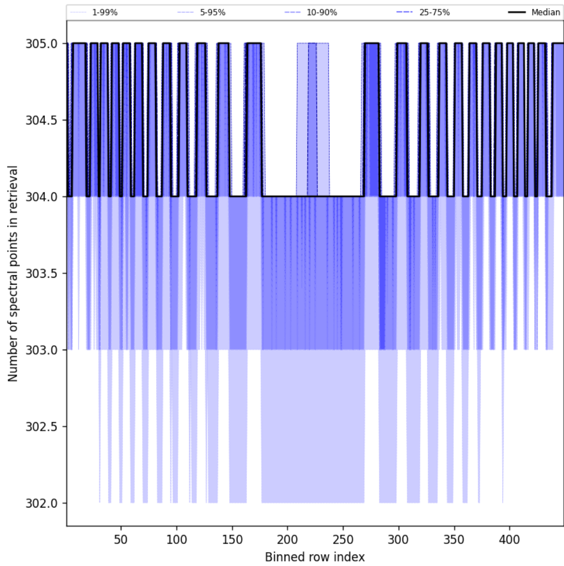
Figure 50: Along track statistics of “Number of spectral points in retrieval” for 2025-01-24 to 2025-01-26
