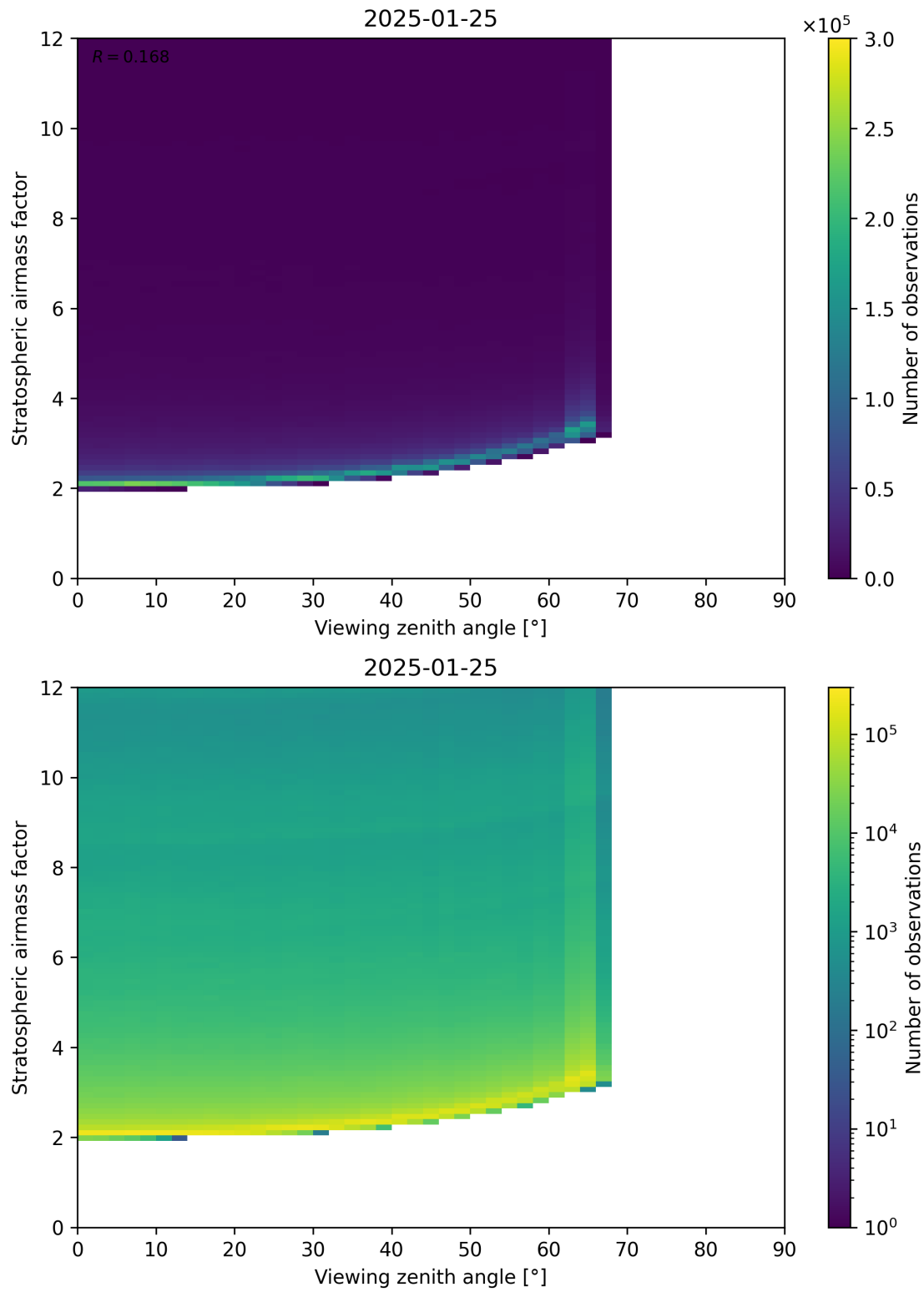
Figure 159: Scatter density plot of “Viewing zenith angle” against “Stratospheric airmass factor” for 2025-01-24 to 2025-01-26.
