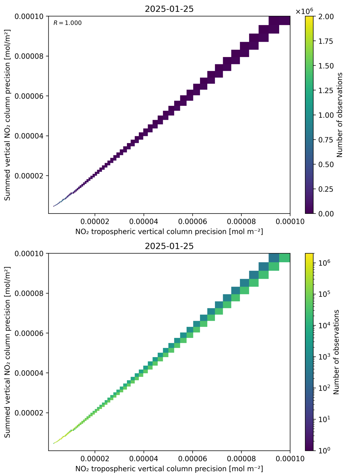
Figure 137: Scatter density plot of “NO 2 tropospheric vertical column precision” against “Summed vertical NO 2 column precision” for 2025-01-24 to 2025-01-26.
