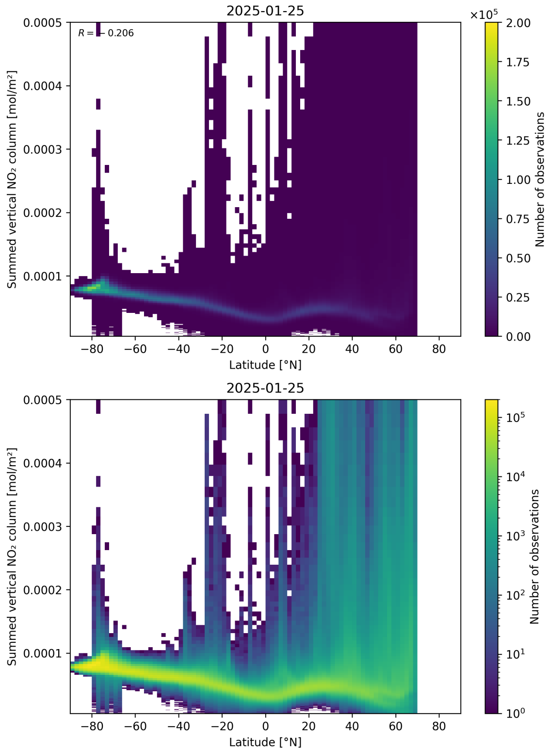
Figure 88: Scatter density plot of “Latitude” against “Summed vertical NO 2 column” for 2025-01-24 to 2025-01-26.
