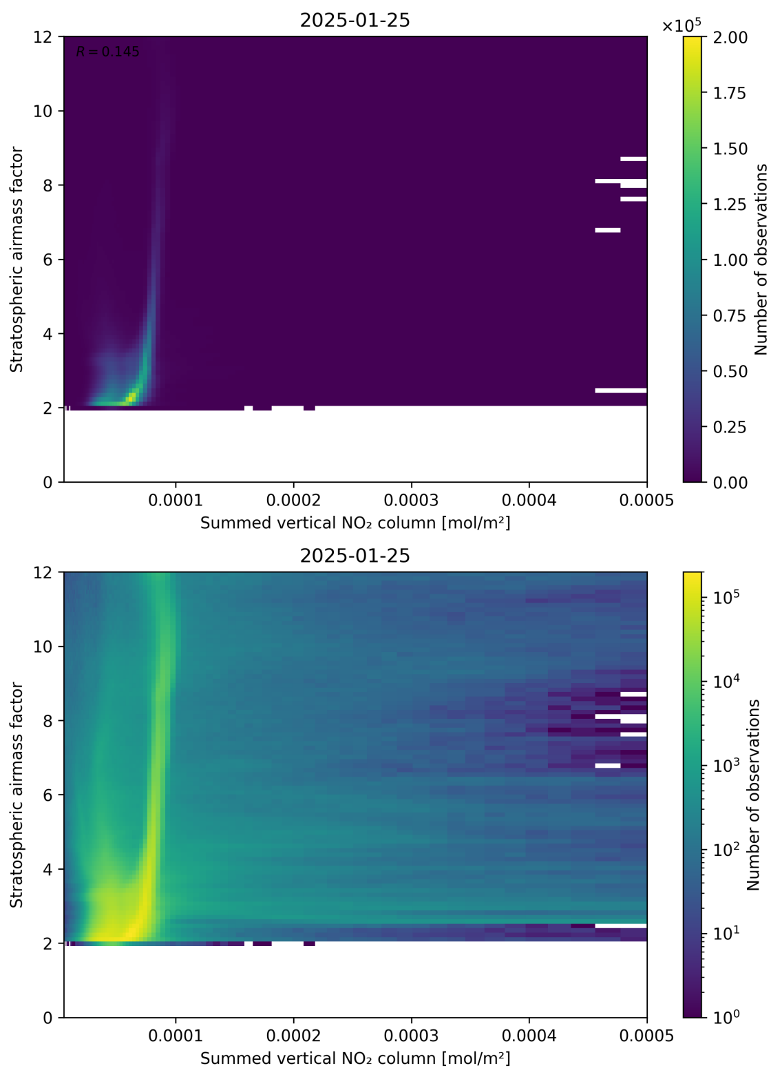
Figure 103: Scatter density plot of “Summed vertical NO 2 column” against “Stratospheric airmass factor” for 2025-01-24 to 2025-01-26.
