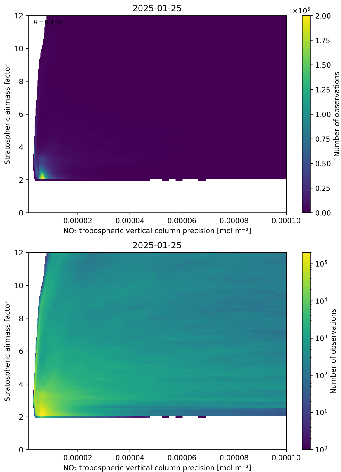
Figure 131: Scatter density plot of “NO 2 tropospheric vertical column precision” against “Stratospheric airmass factor” for 2025-01-24 to 2025-01-26.
