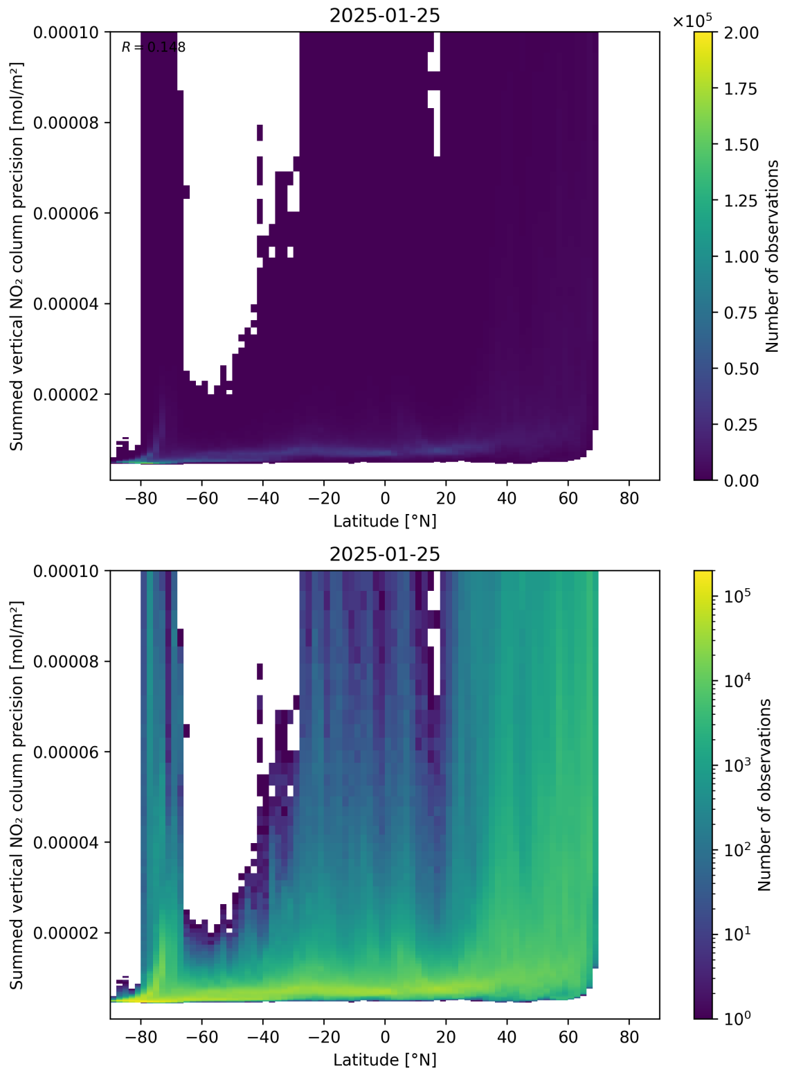
Figure 89: Scatter density plot of “Latitude” against “Summed vertical NO 2 column precision” for 2025-01-24 to 2025-01-26.
