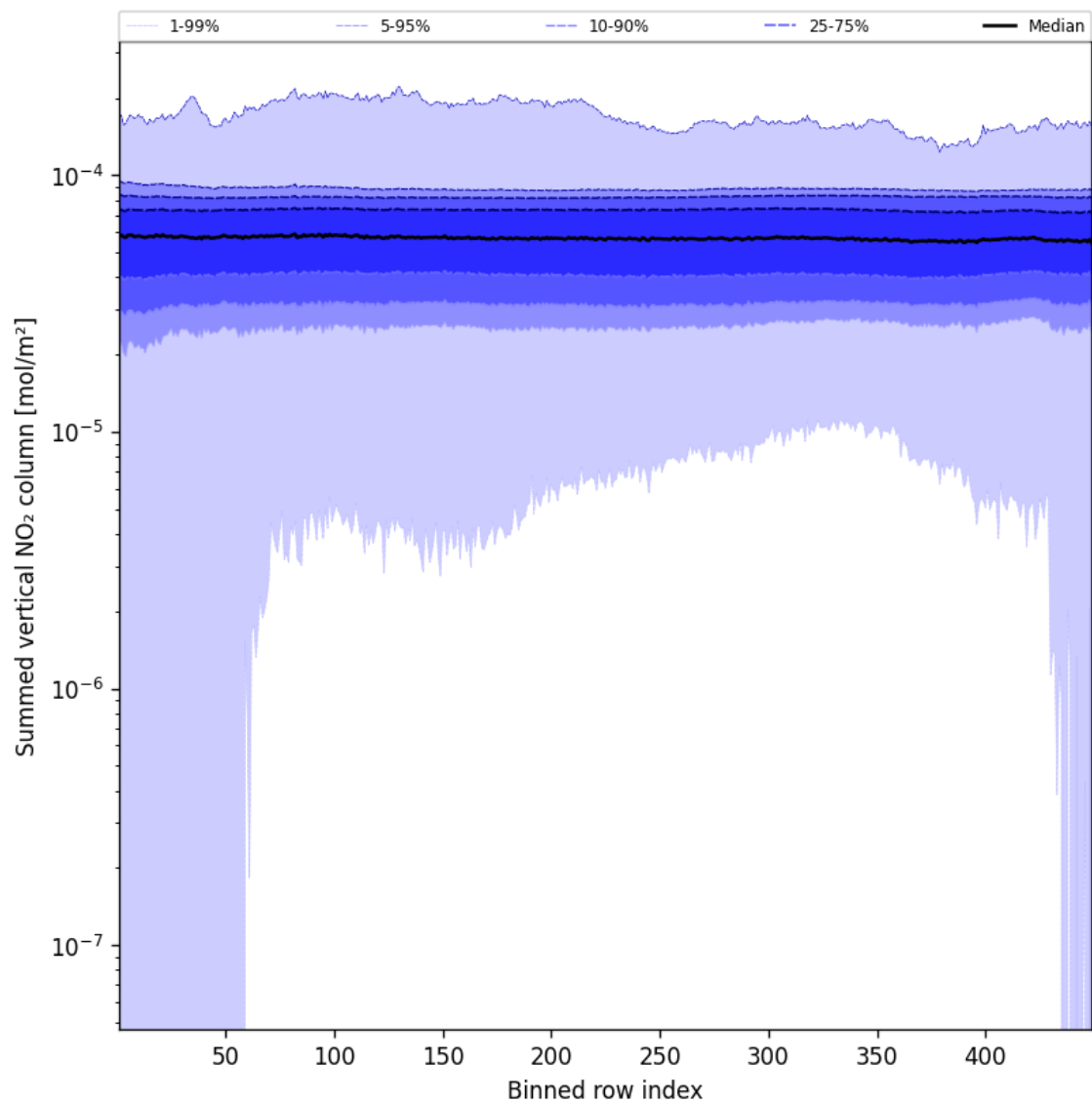
Figure 57: Along track statistics of “Summed vertical NO 2 column” for 2025-01-24 to 2025-01-26
