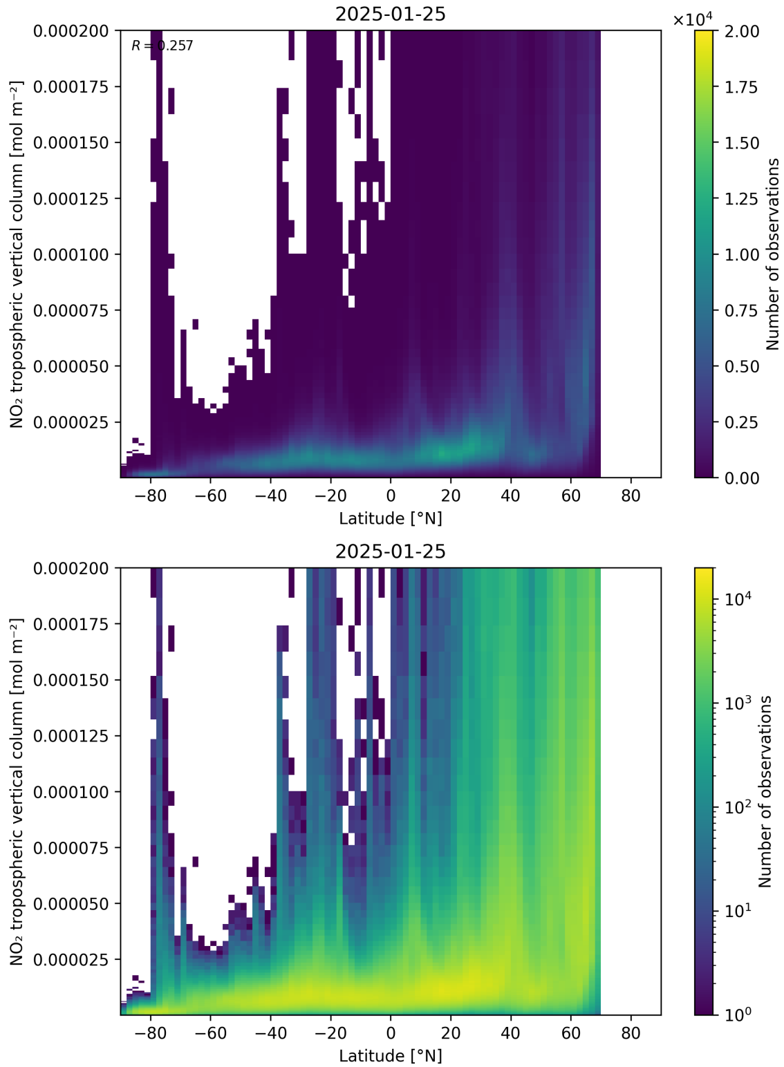
Figure 92: Scatter density plot of “Latitude” against “NO 2 tropospheric vertical column” for 2025-01-24 to 2025-01-26.
