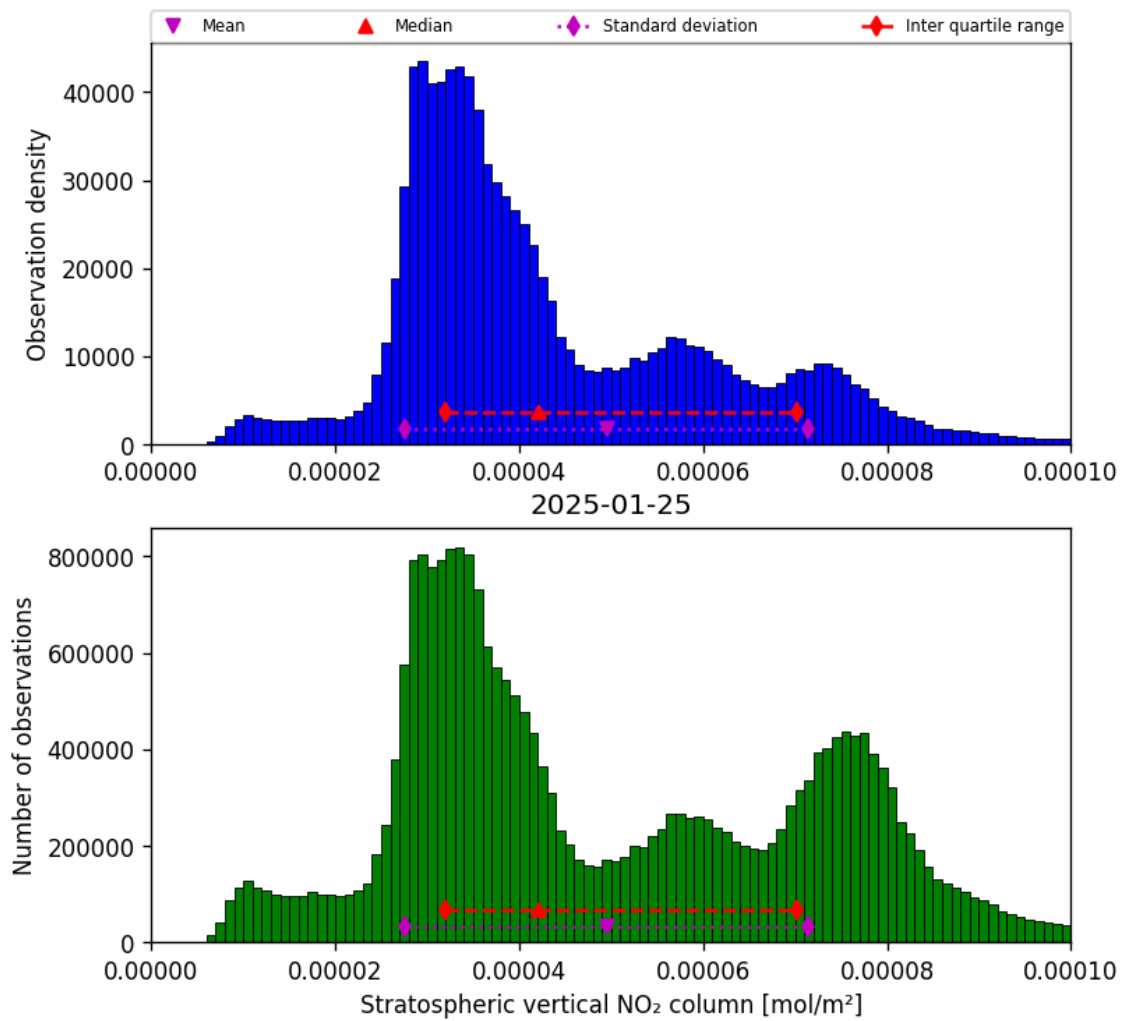
Figure 36: Histogram of “Stratospheric vertical NO 2 column” for 2025-01-24 to 2025-01-26
