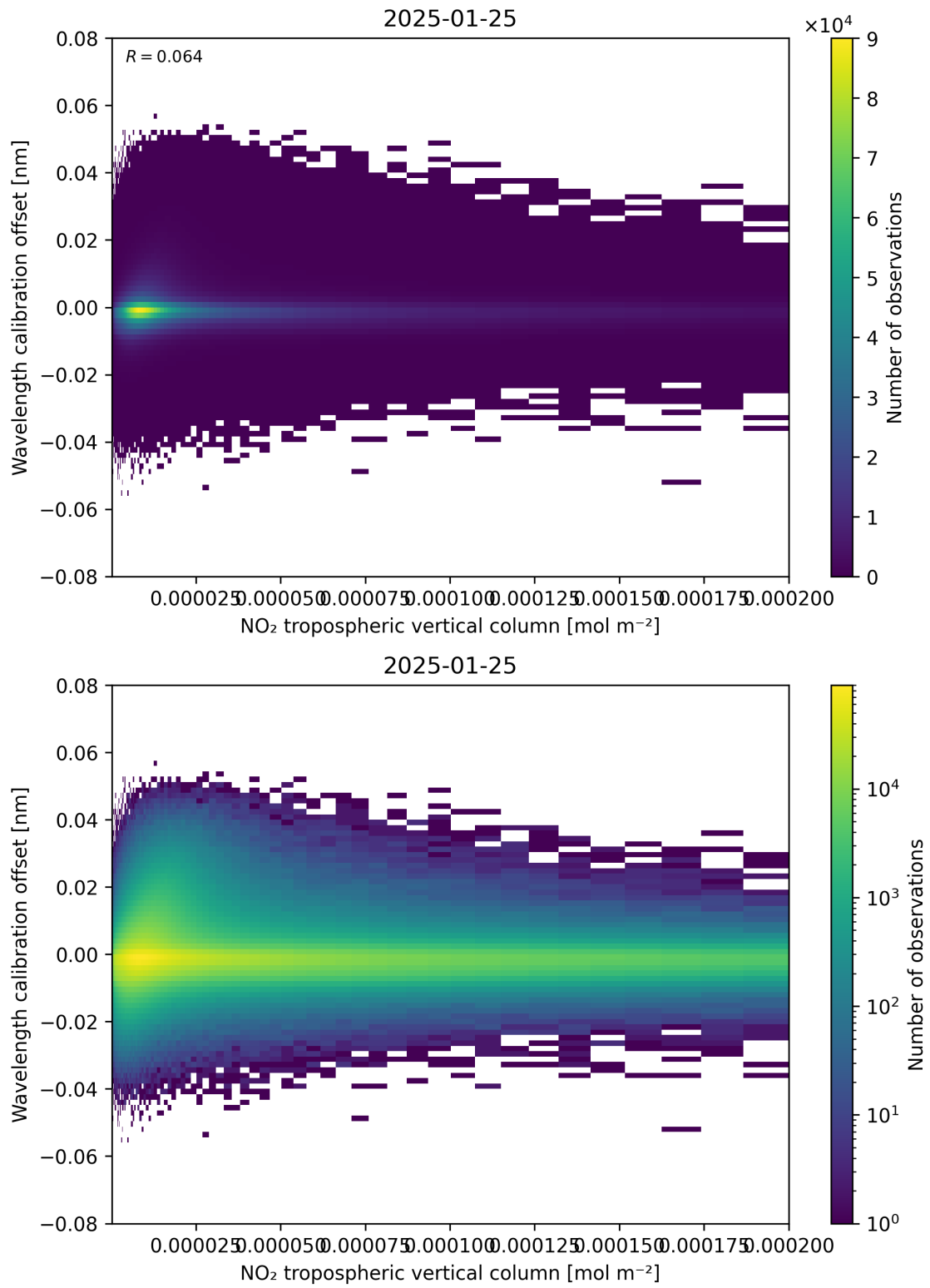
Figure 143: Scatter density plot of “NO 2 tropospheric vertical column” against “Wavelength calibration offset” for 2025-01-24 to 2025-01-26.
