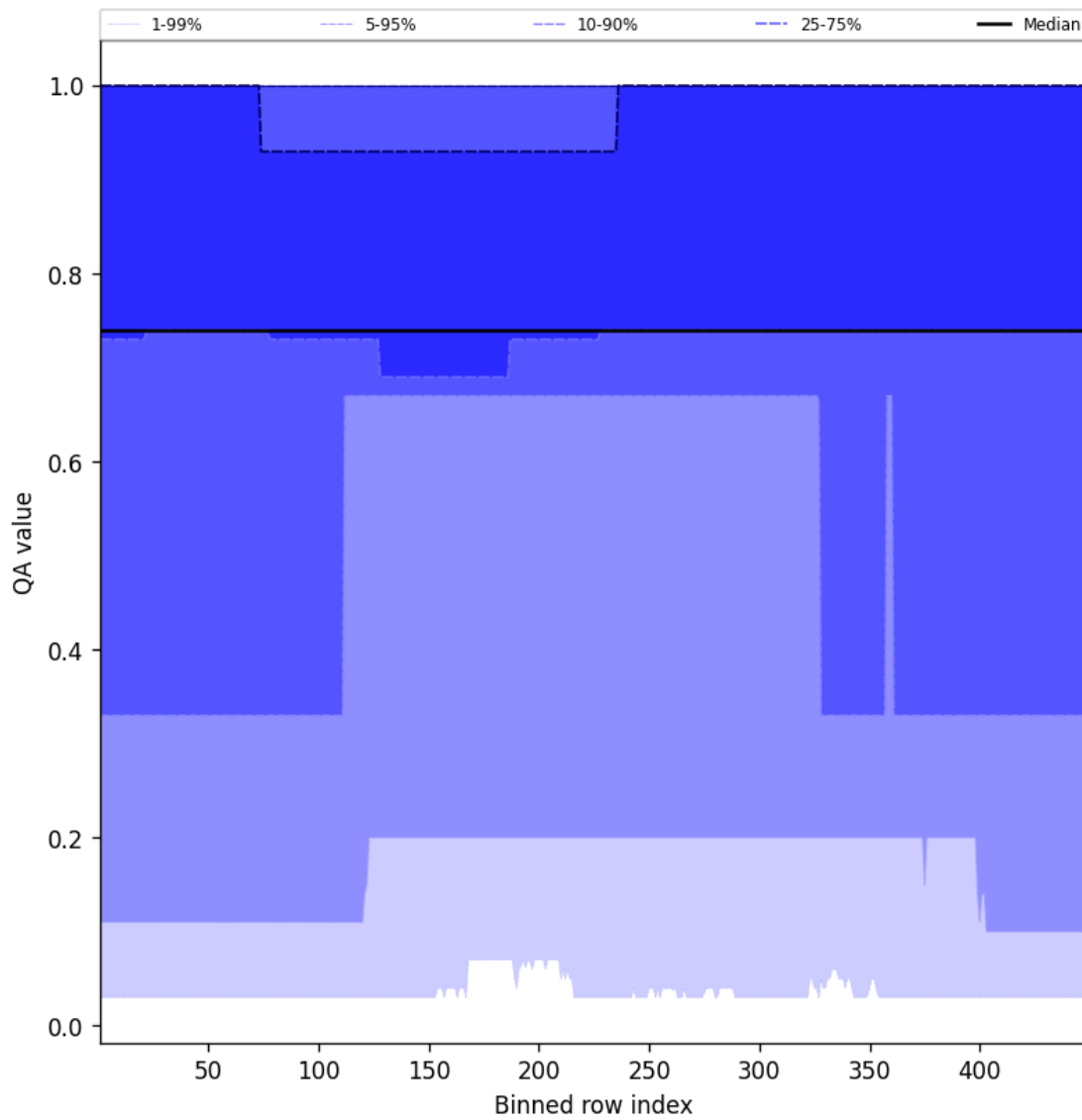
Figure 45: Along track statistics of “QA value” for 2025-01-24 to 2025-01-26
