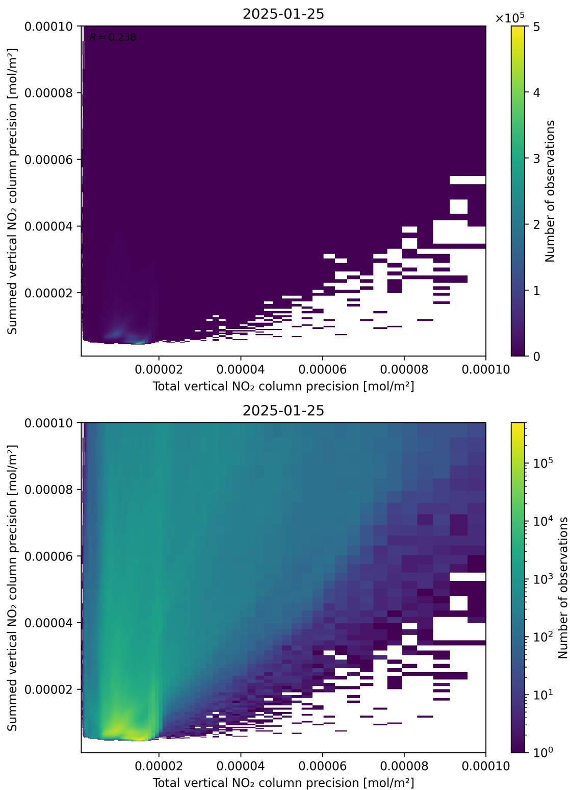
Figure 118: Scatter density plot of “Total vertical NO 2 column precision” against “Summed vertical NO 2 column precision” for 2025-01-24 to 2025-01-26.
