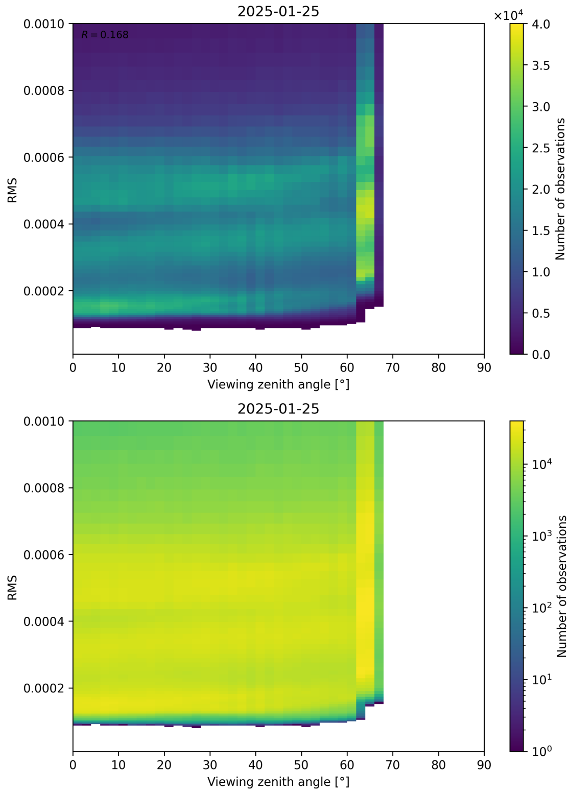
Figure 171: Scatter density plot of “Viewing zenith angle” against “RMS” for 2025-01-24 to 2025-01-26.
