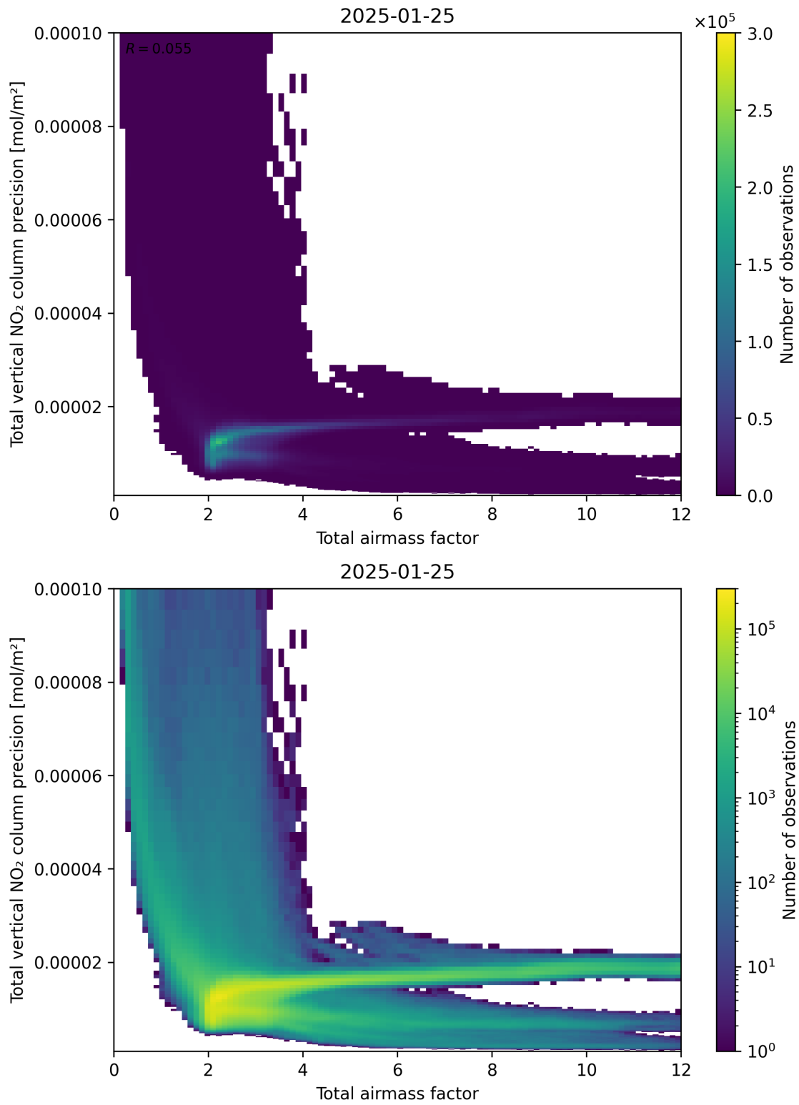
Figure 68: Scatter density plot of “Total airmass factor” against “Total vertical NO 2 column precision” for 2025-01-24 to 2025-01-26.
