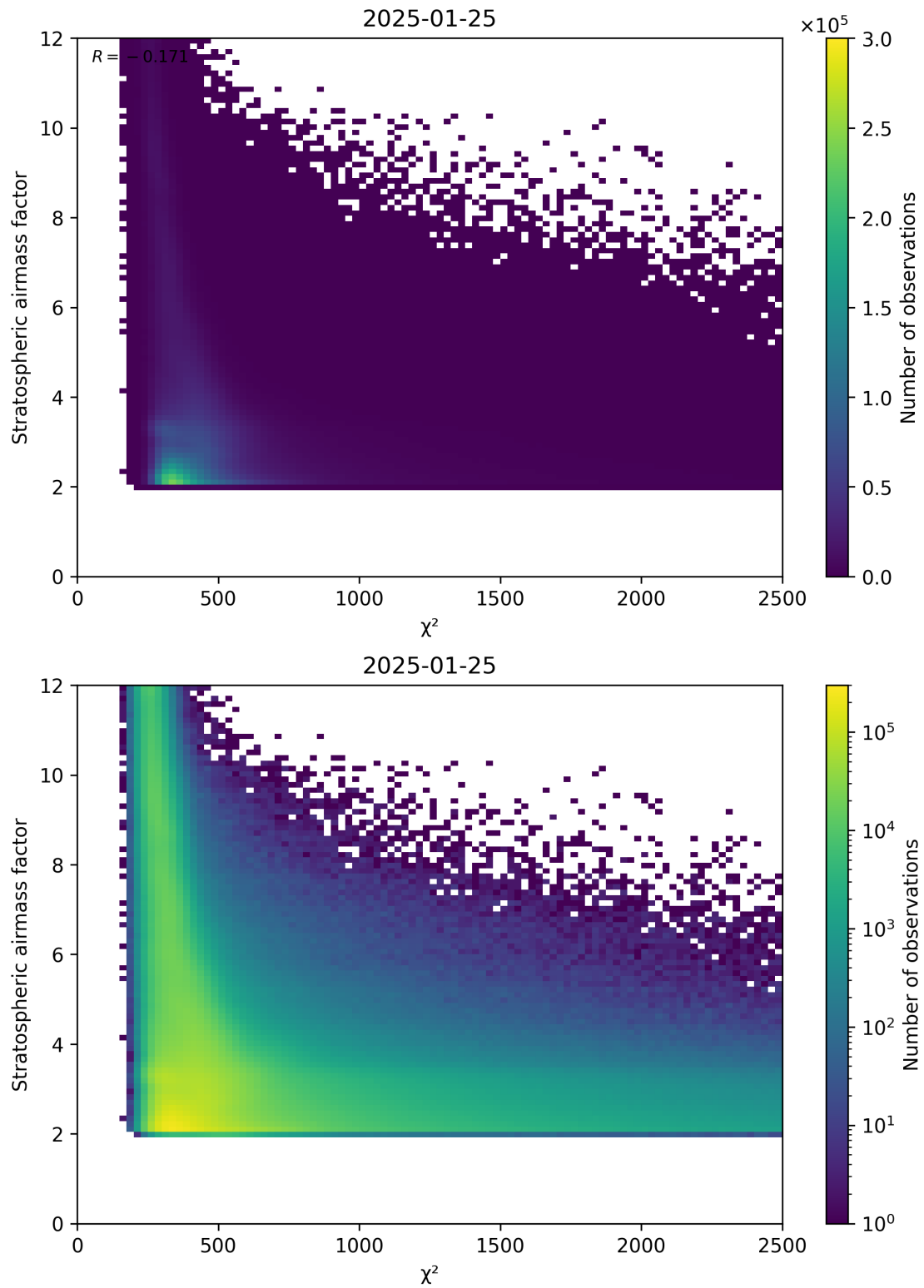
Figure 81: Scatter density plot of “ \chi^2 ” against “Stratospheric airmass factor” for 2025-01-24 to 2025-01-26.
