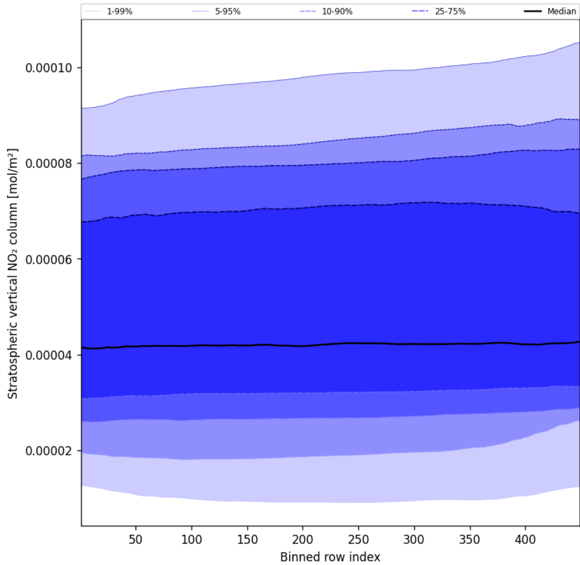
Figure 53: Along track statistics of “Stratospheric vertical NO 2 column” for 2025-01-24 to 2025-01-26
