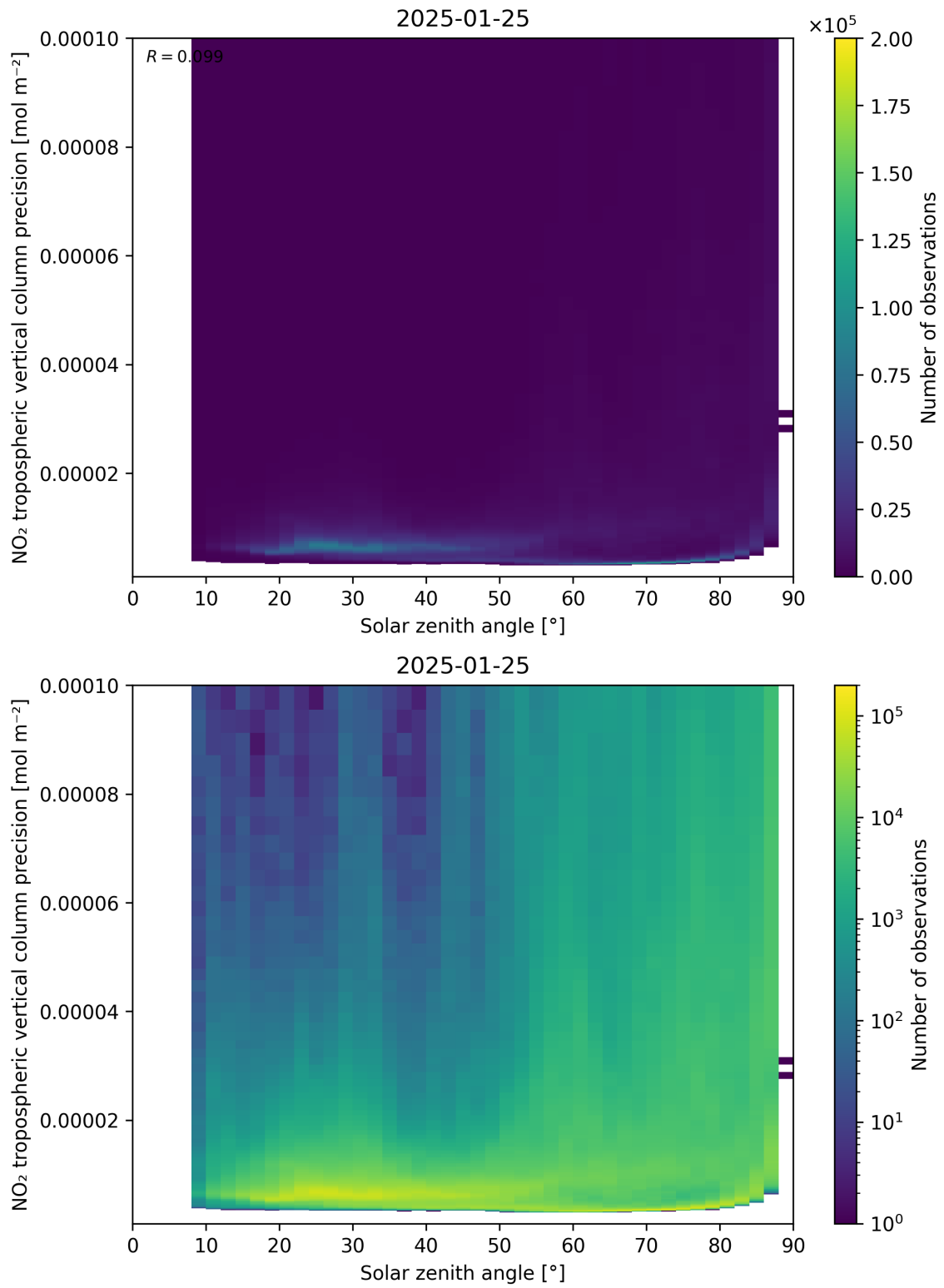
Figure 156: Scatter density plot of “Solar zenith angle” against “NO 2 tropospheric vertical column precision” for 2025-01-24 to 2025-01-26.
