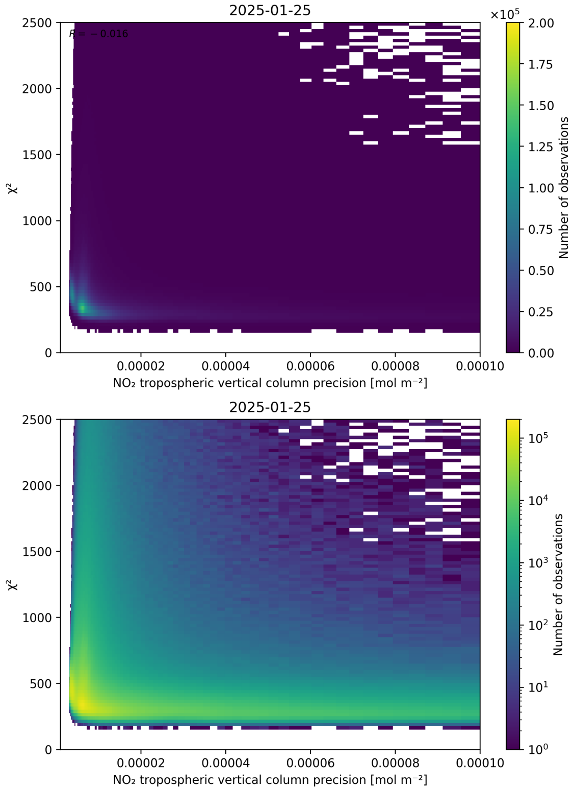
Figure 134: Scatter density plot of “NO 2 tropospheric vertical column precision” against “ \chi^2 ” for 2025-01-24 to 2025-01-26.
