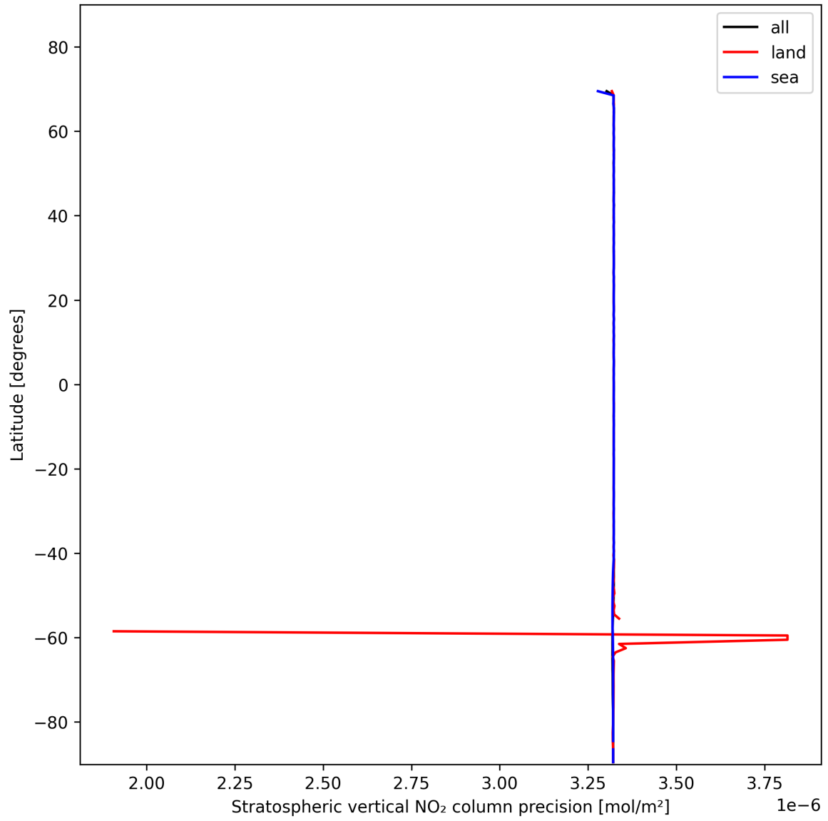
Figure 20: Zonal average of “Stratospheric vertical NO 2 column precision” for 2025-01-24 to 2025-01-26.
