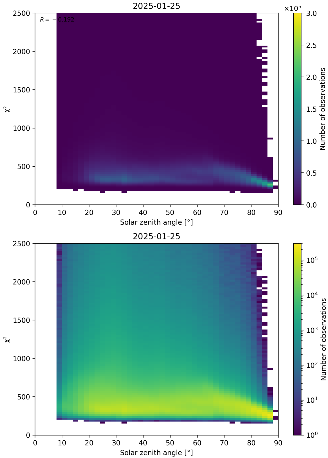
Figure 148: Scatter density plot of “Solar zenith angle” against “ \chi^2 ” for 2025-01-24 to 2025-01-26.
