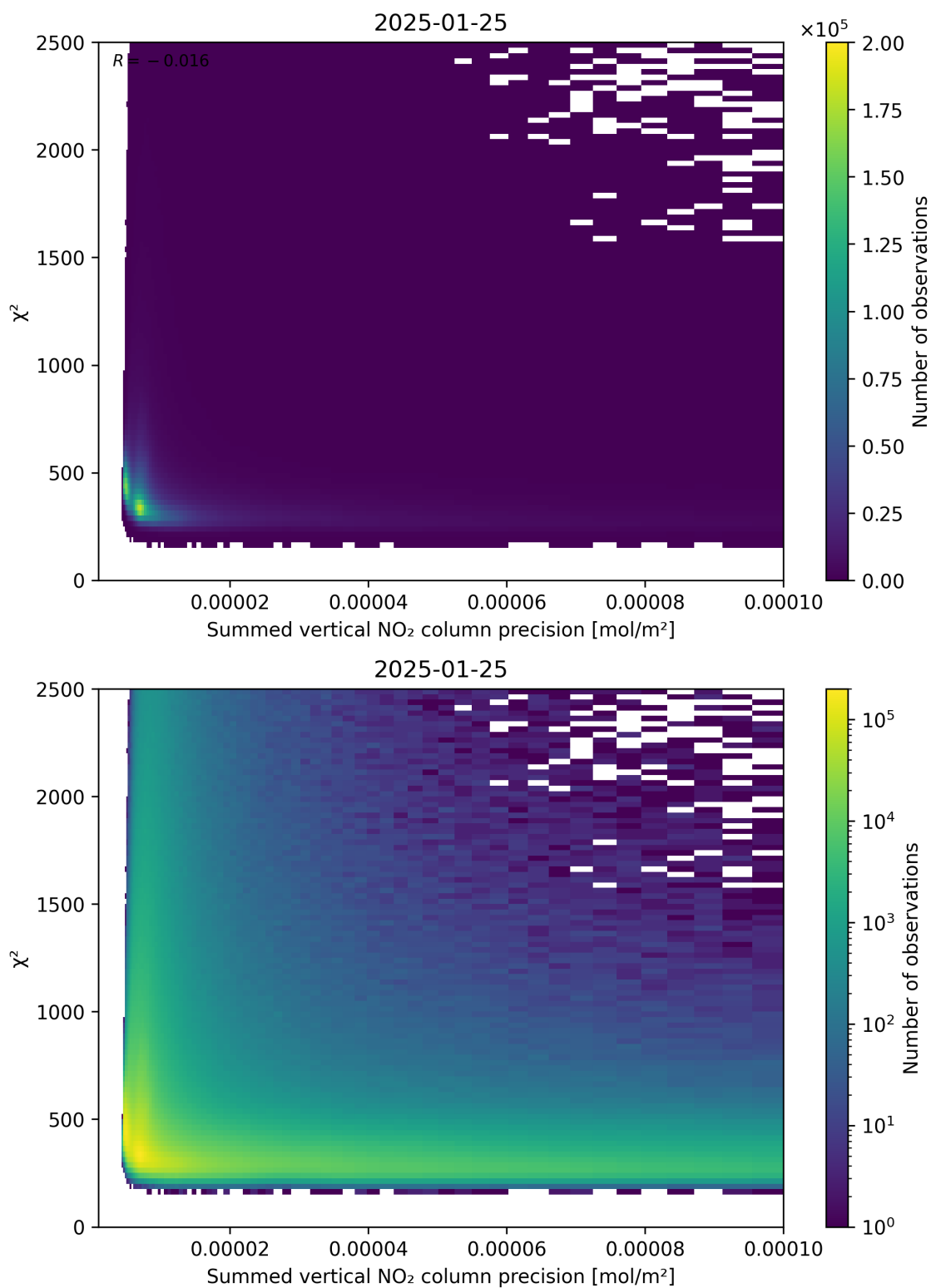
Figure 107: Scatter density plot of “Summed vertical NO 2 column precision” against “ \chi^2 ” for 2025-01-24 to 2025-01-26.
