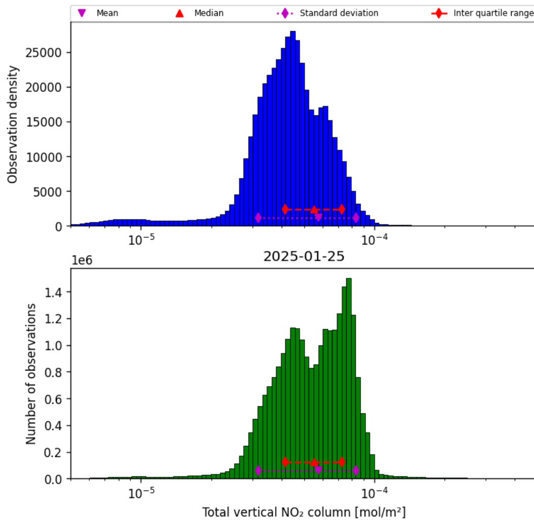
Figure 38: Histogram of “Total vertical NO 2 column” for 2025-01-24 to 2025-01-26
