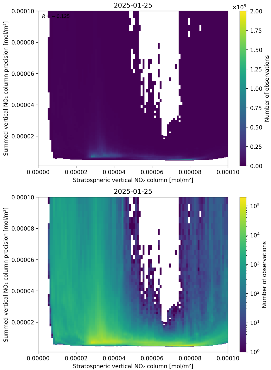
Figure 99: Scatter density plot of “Stratospheric vertical NO 2 column” against “Summed vertical NO 2 column precision” for 2025-01-24 to 2025-01-26.
