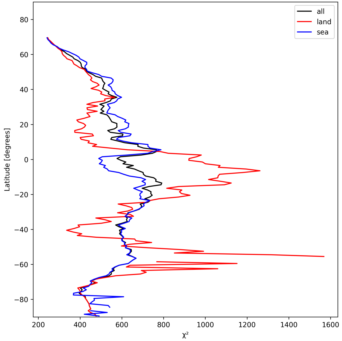
Figure 25: Zonal average of “ \chi^2 ” for 2025-01-24 to 2025-01-26.
