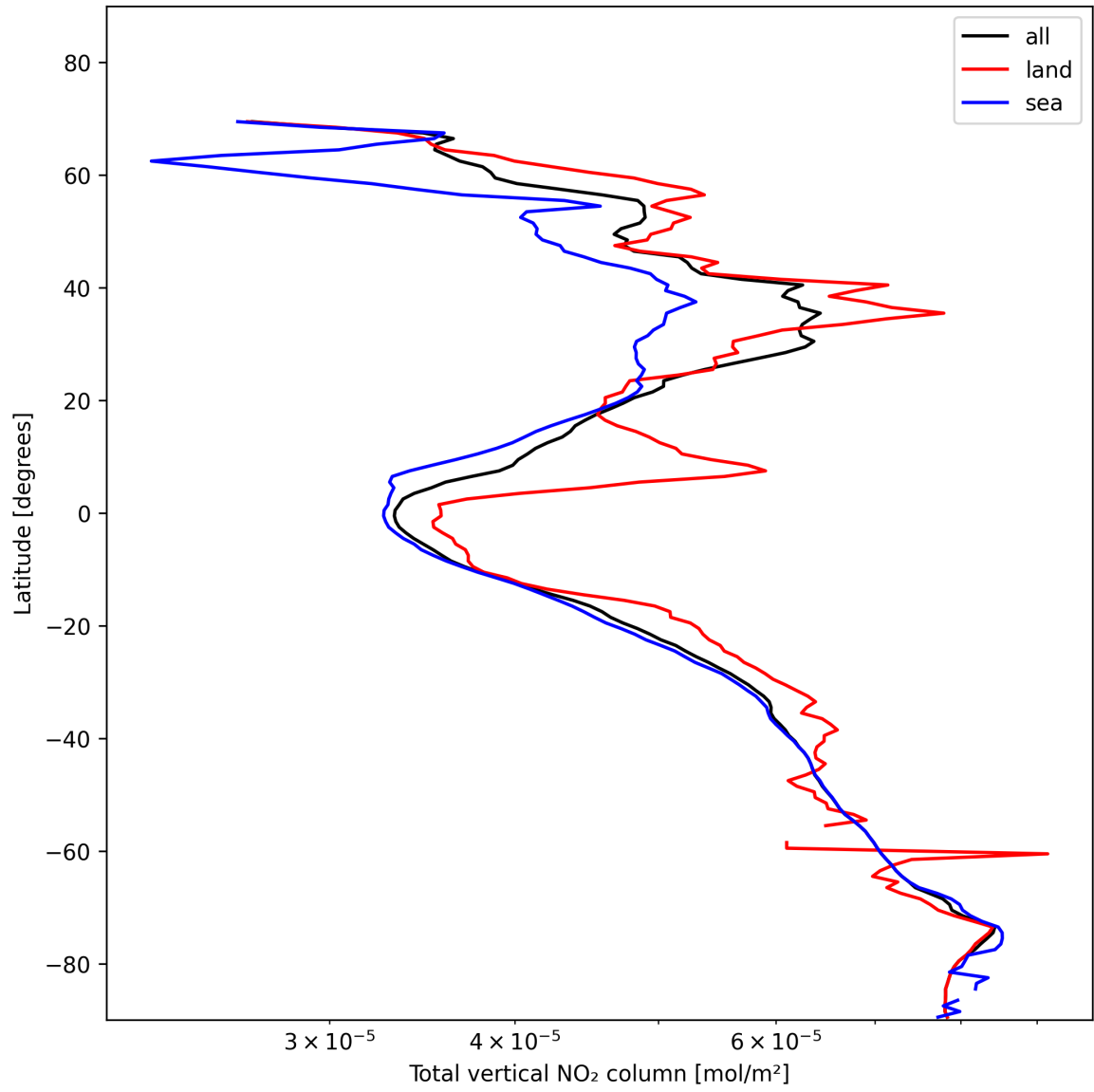
Figure 21: Zonal average of “Total vertical NO 2 column” for 2025-01-24 to 2025-01-26.
