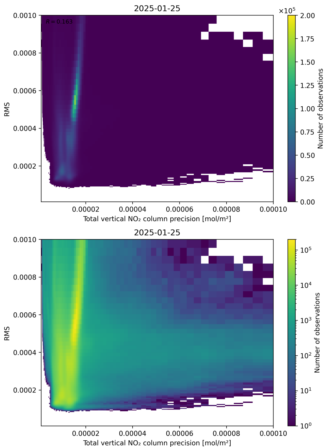
Figure 119: Scatter density plot of “Total vertical NO 2 column precision” against “RMS” for 2025-01-24 to 2025-01-26.
