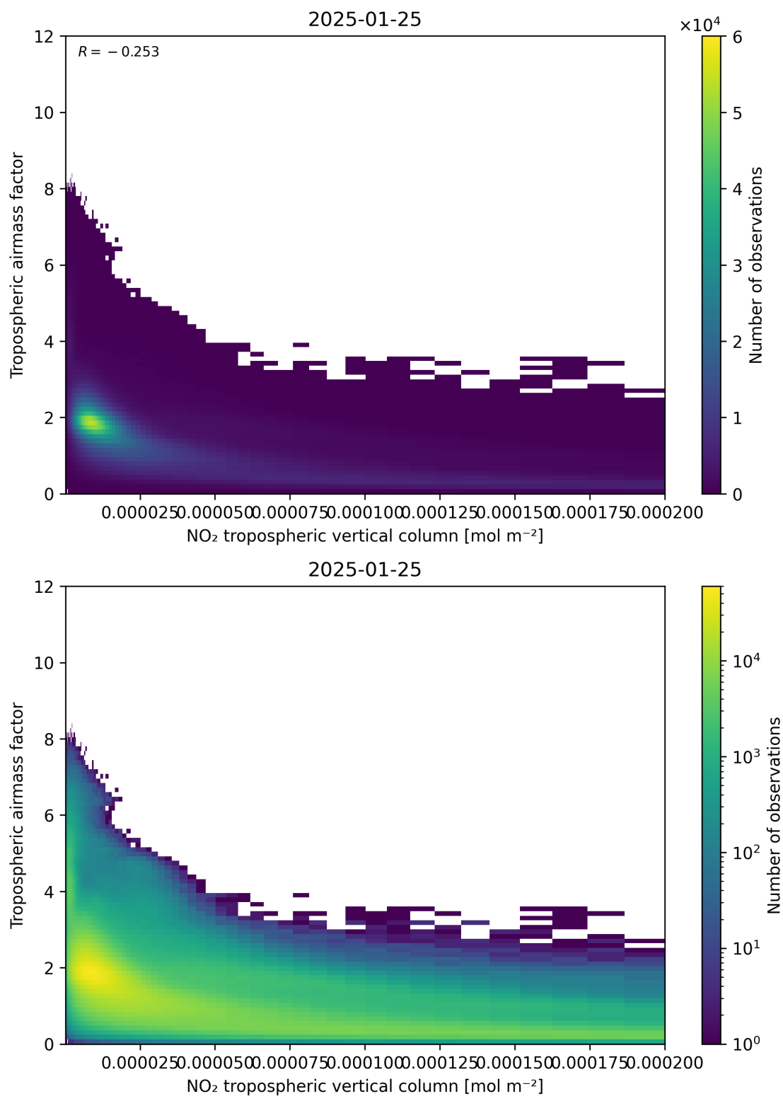
Figure 123: Scatter density plot of “NO 2 tropospheric vertical column” against “Tropospheric air mass factor” for 2025-01-24 to 2025-01-26.
