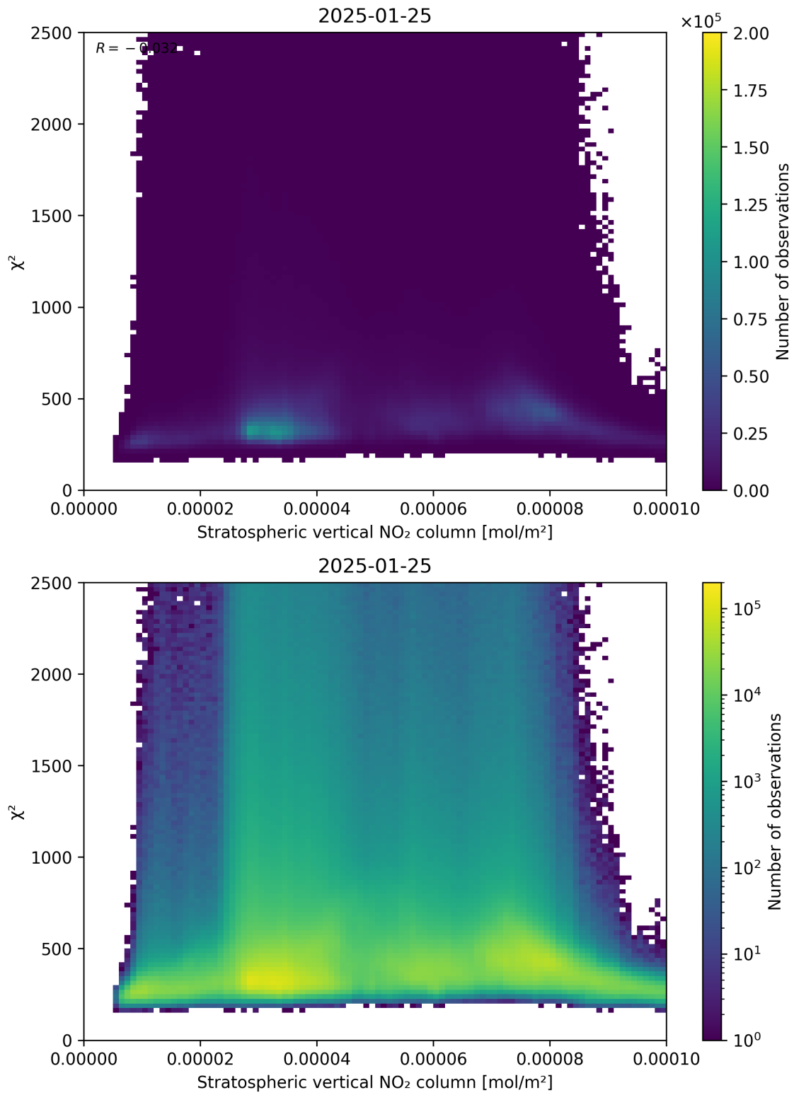
Figure 97: Scatter density plot of “Stratospheric vertical NO 2 column” against “ \chi^2 ” for 2025-01-24 to 2025-01-26.
