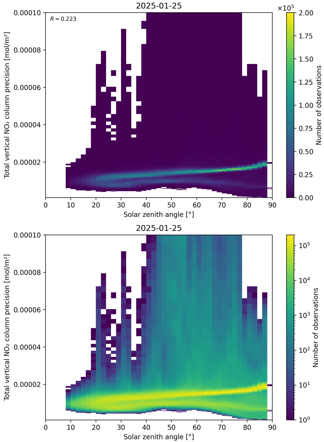
Figure 154: Scatter density plot of “Solar zenith angle” against “Total vertical NO 2 column precision” for 2025-01-24 to 2025-01-26.
