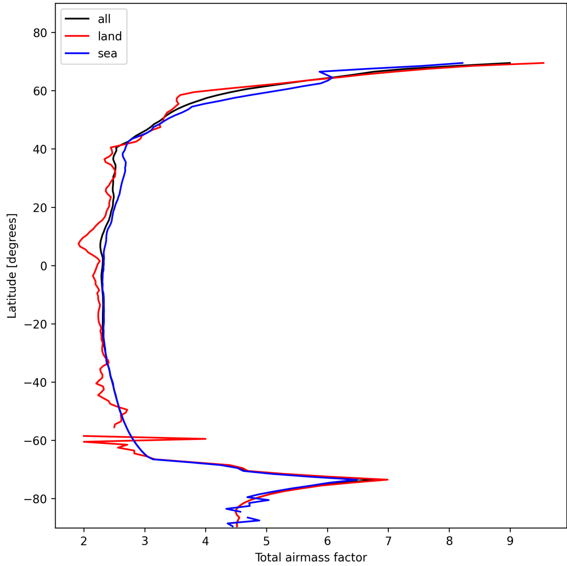
Figure 15: Zonal average of “Total airmass factor” for 2025-01-24 to 2025-01-26.
