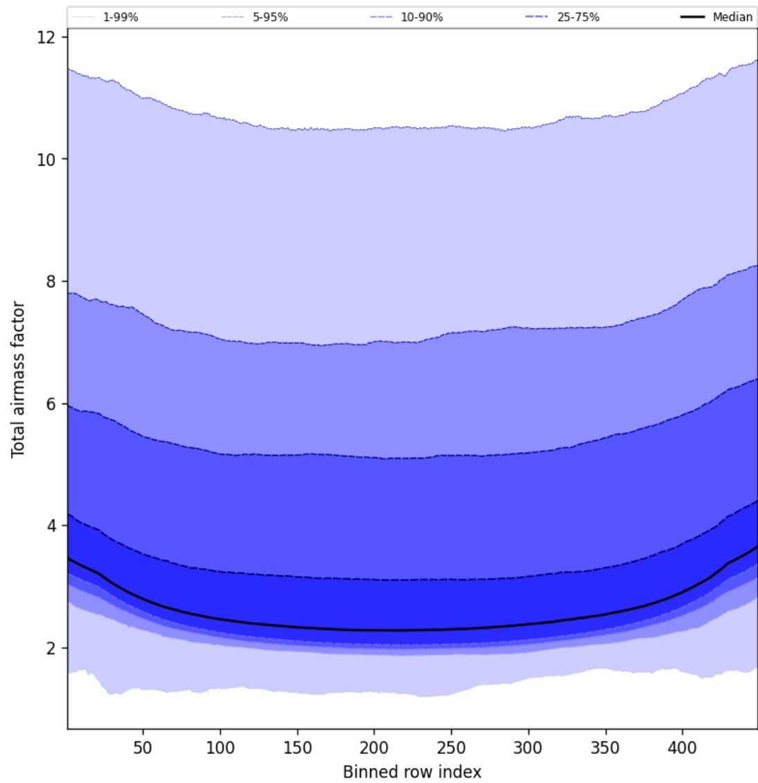
Figure 49: Along track statistics of “Total airmass factor” for 2025-01-24 to 2025-01-26
