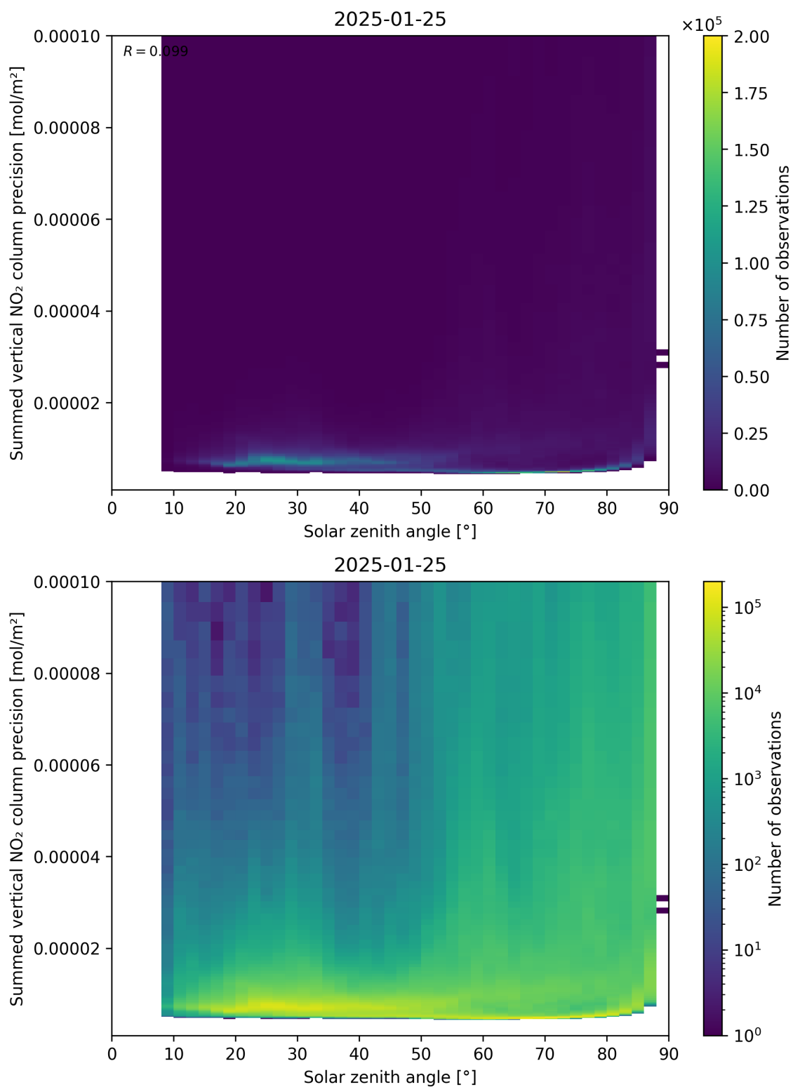
Figure 152: Scatter density plot of “Solar zenith angle” against “Summed vertical NO 2 column precision” for 2025-01-24 to 2025-01-26.
