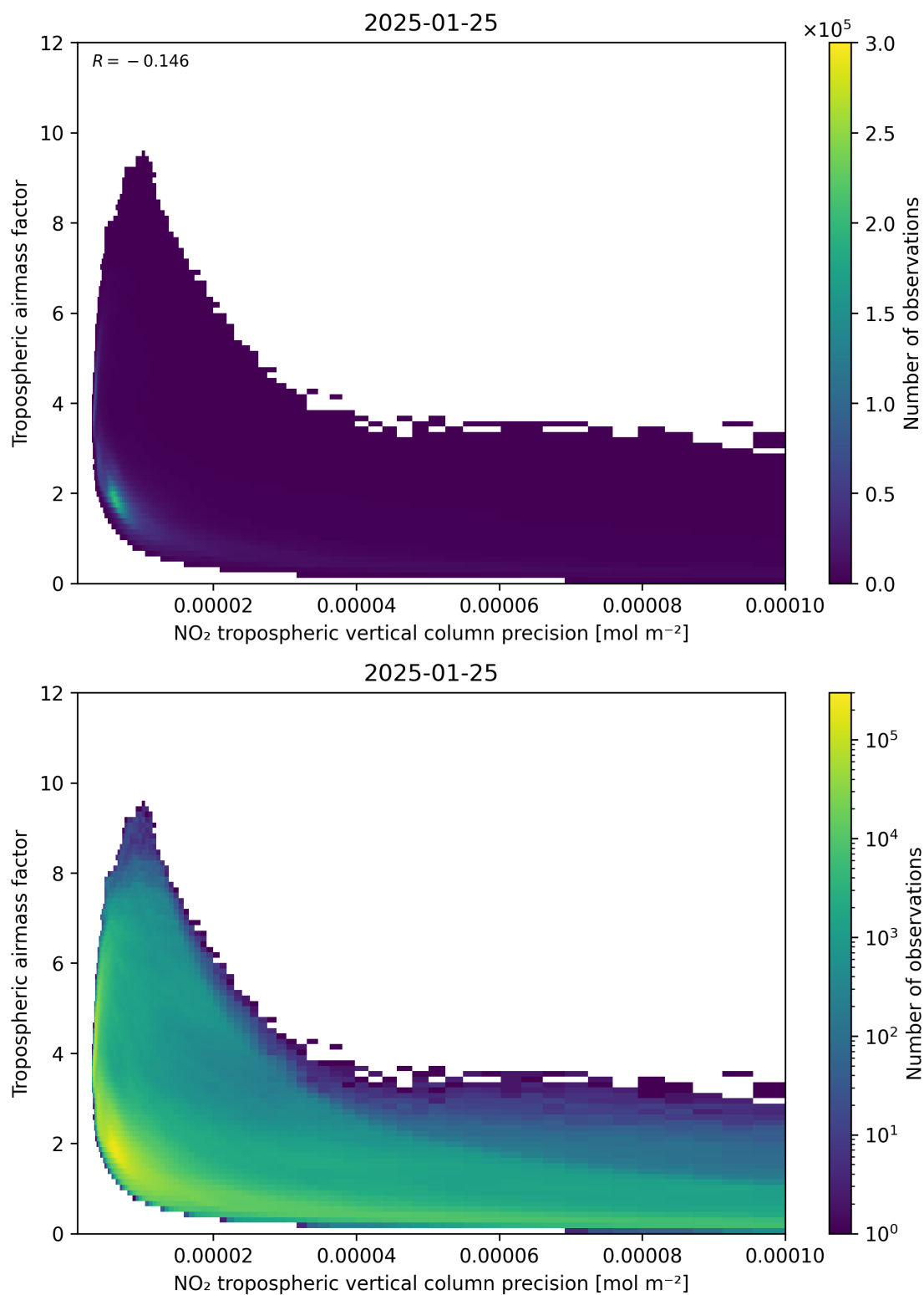
Figure 133: Scatter density plot of “NO 2 tropospheric vertical column precision” against “Tropospheric airmass factor” for 2025-01-24 to 2025-01-26.
