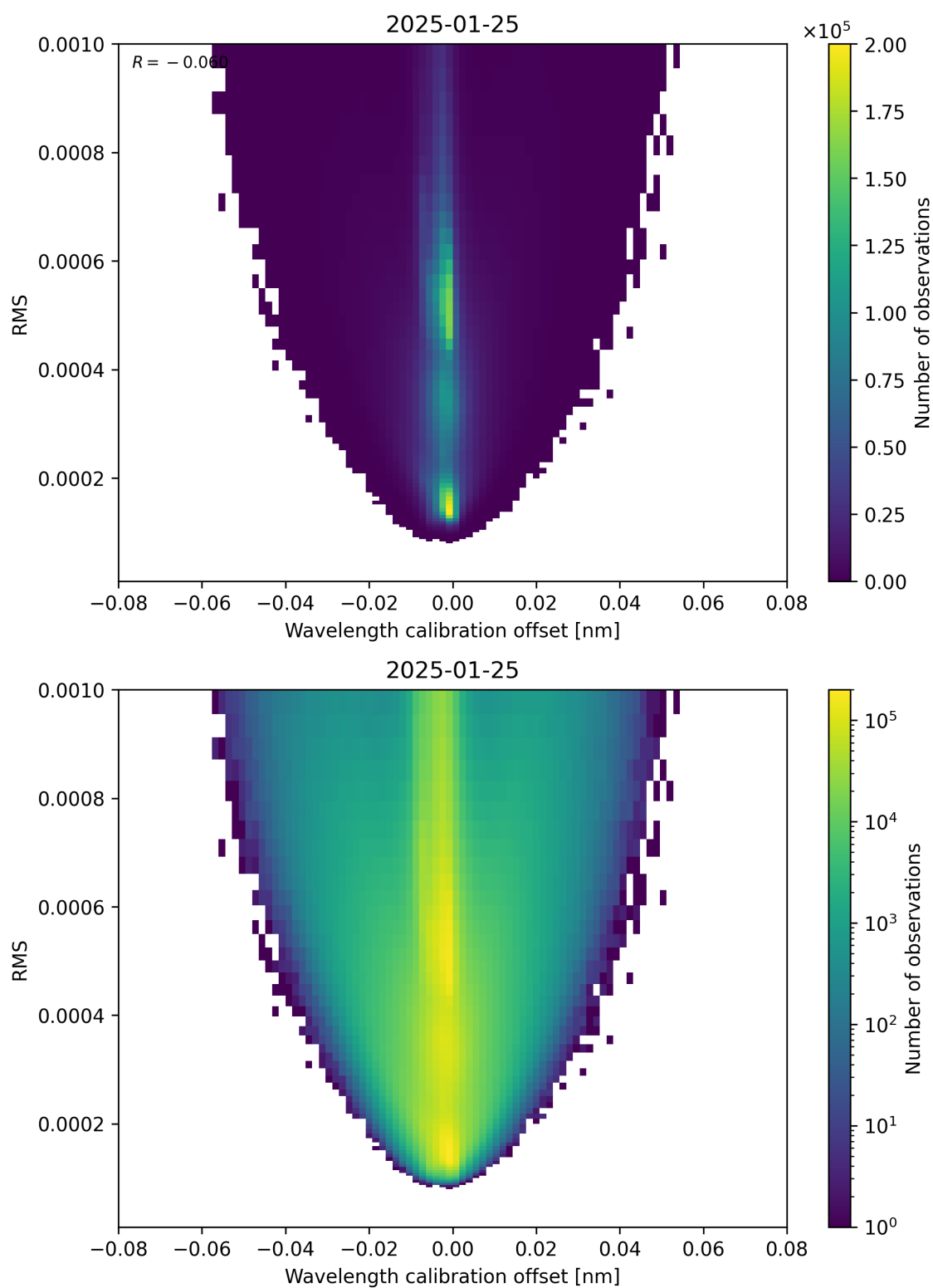
Figure 181: Scatter density plot of “Wavelength calibration offset” against “RMS” for 2025-01-24 to 2025-01-26.
