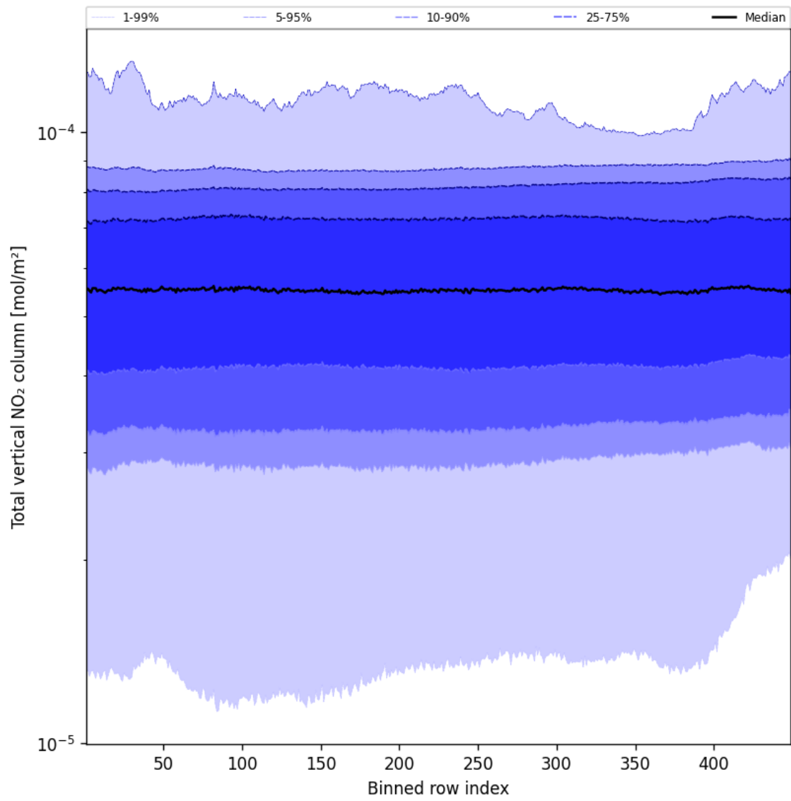
Figure 55: Along track statistics of “Total vertical NO 2 column” for 2025-01-24 to 2025-01-26
