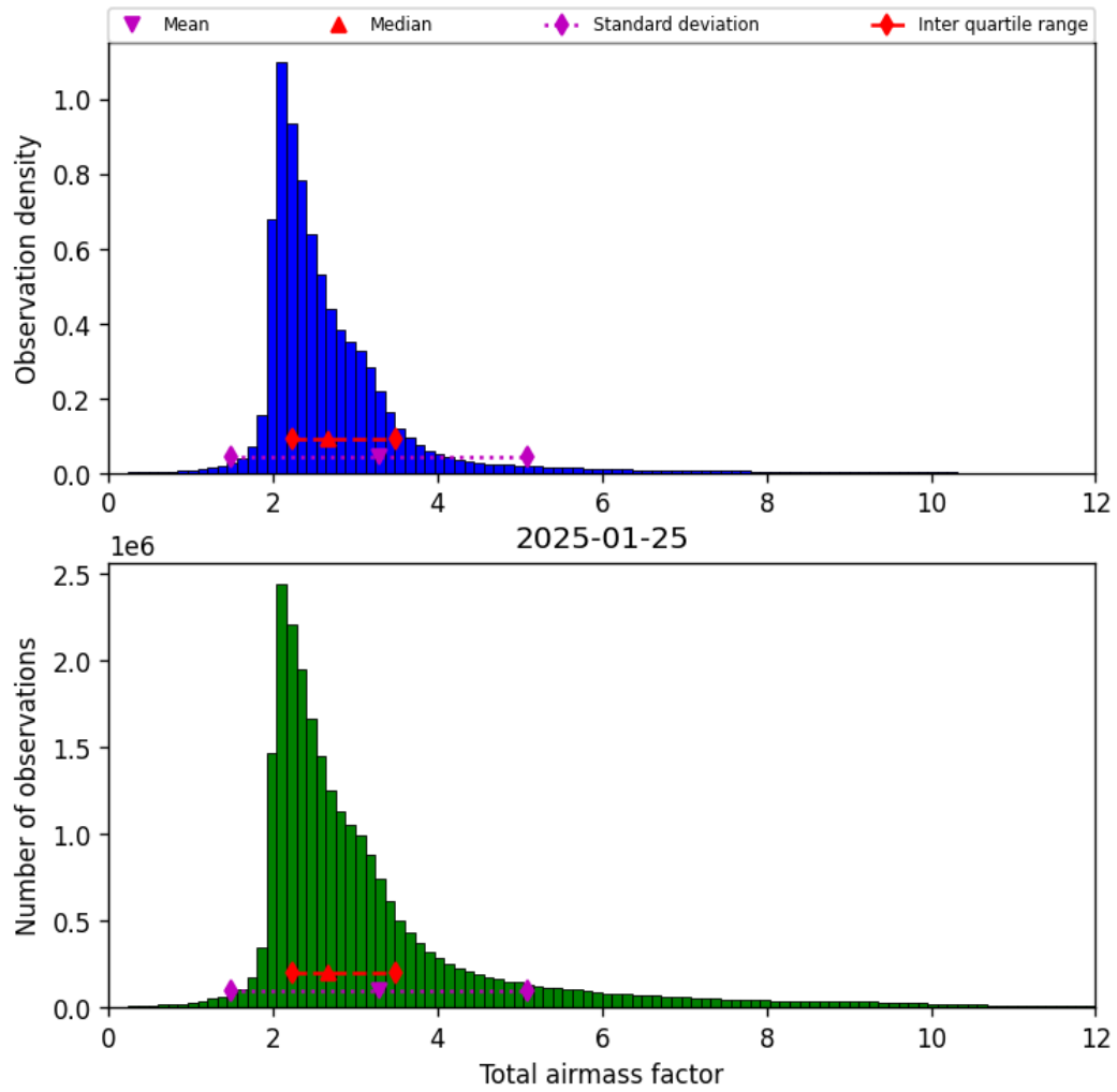
Figure 32: Histogram of “Total airmass factor” for 2025-01-24 to 2025-01-26
