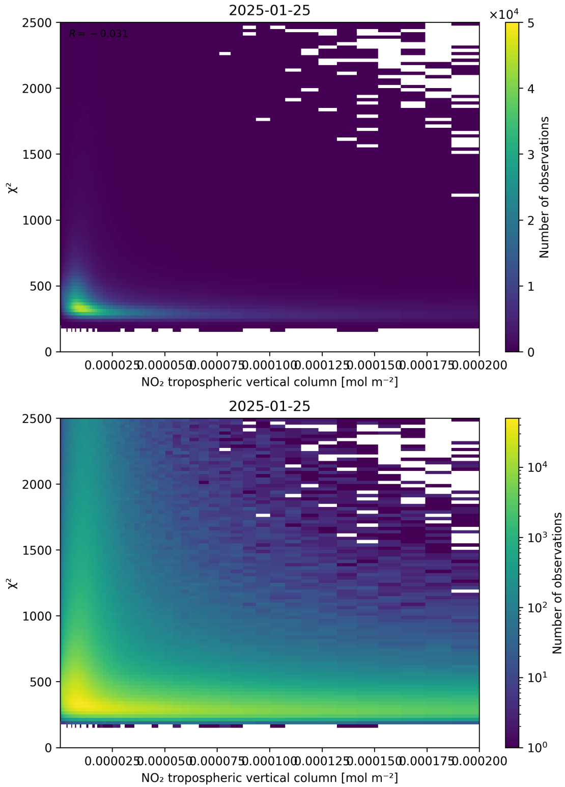
Figure 124: Scatter density plot of “NO 2 tropospheric vertical column” against “ \chi^2 ” for 2025-01-24 to 2025-01-26.
