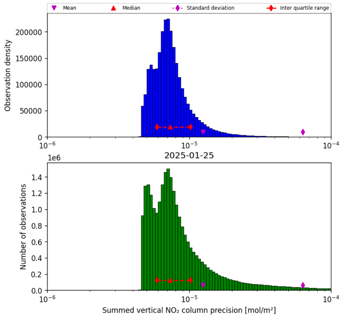
Figure 41: Histogram of "Summed vertical NO 2 column precision" for 2025-01-24 to 2025-01-26
