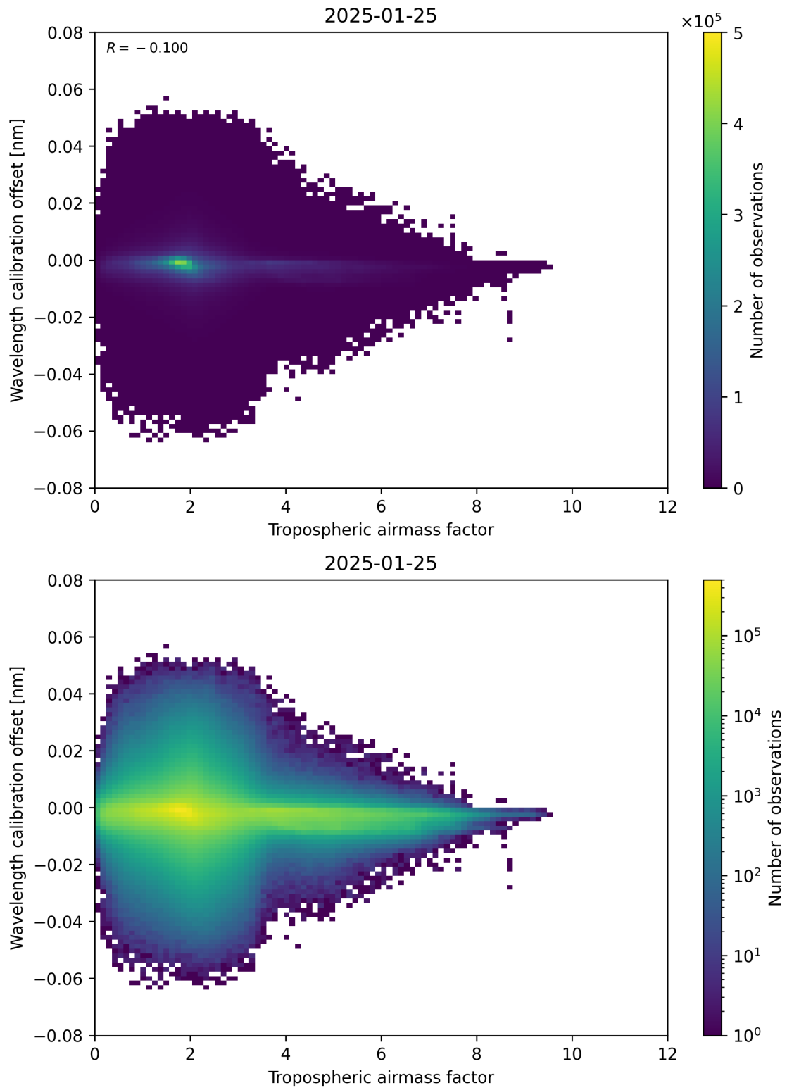
Figure 80: Scatter density plot of “Tropospheric airmass factor” against “Wavelength calibration offset” for 2025-01-24 to 2025-01-26.
