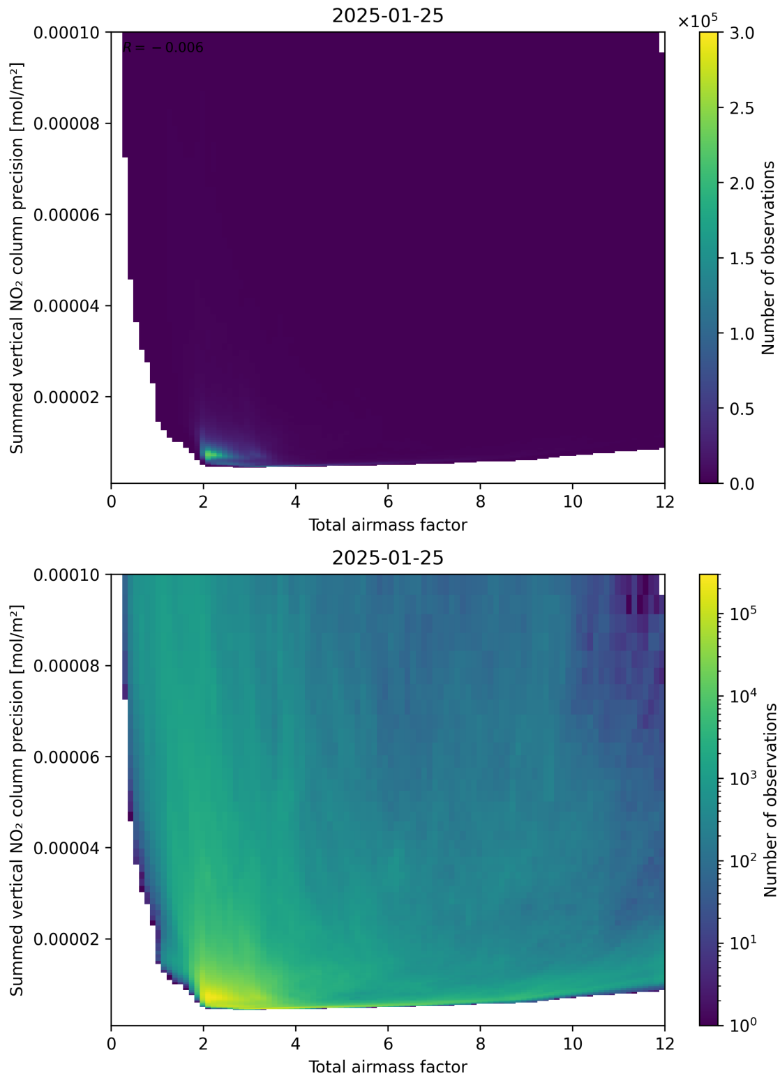
Figure 66: Scatter density plot of “Total airmass factor” against “Summed vertical NO 2 column precision” for 2025-01-24 to 2025-01-26.
