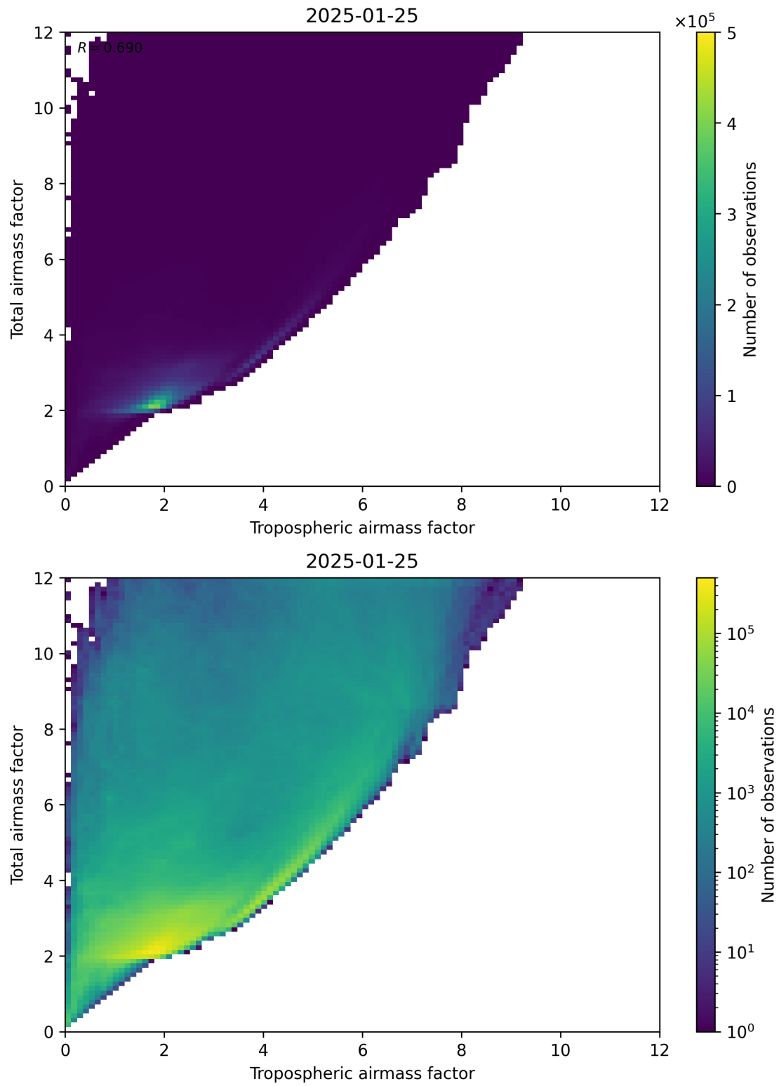
Figure 72: Scatter density plot of “Tropospheric airmass factor” against “Total airmass factor” for 2025-01-24 to 2025-01-26.
