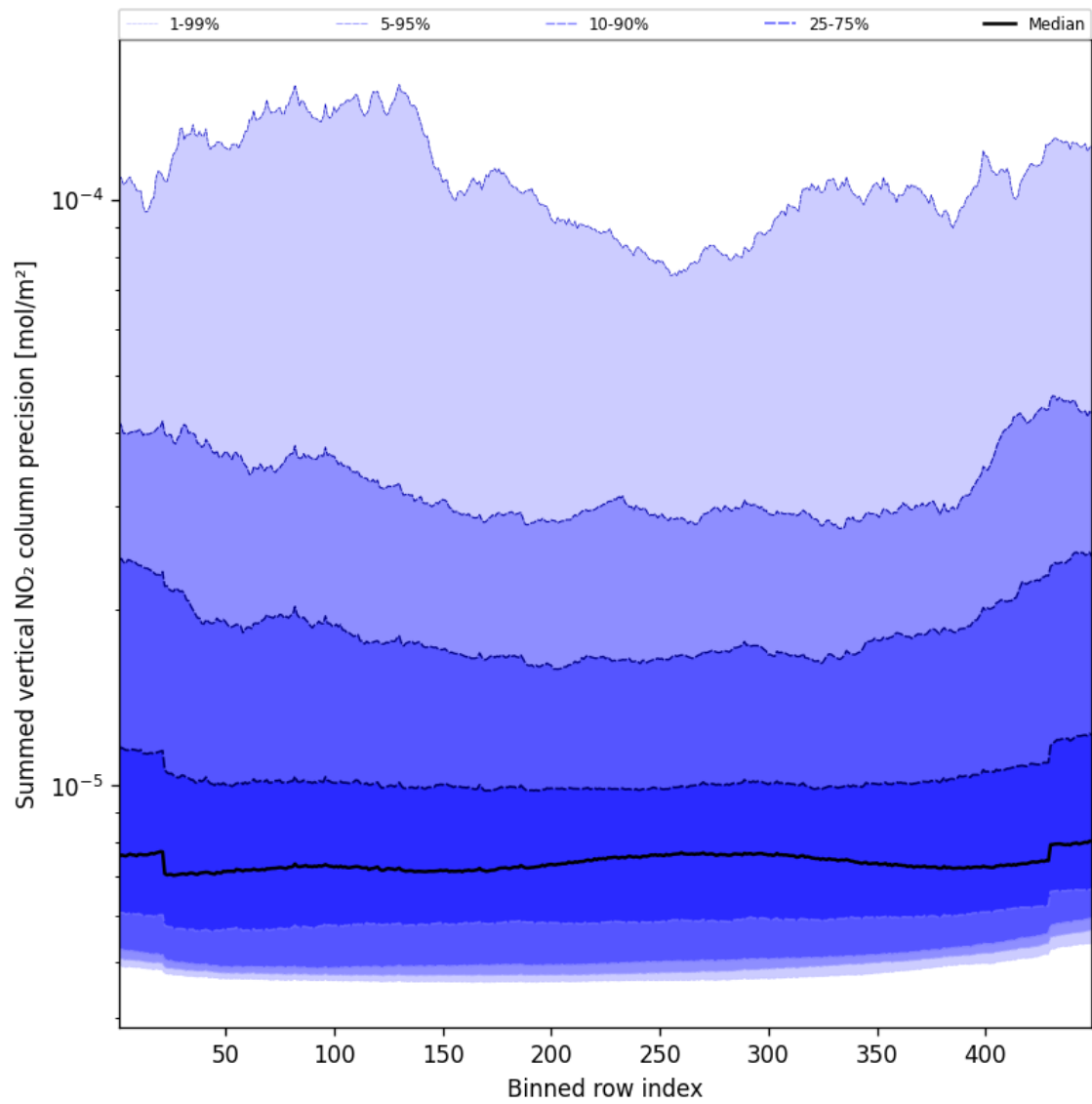
Figure 58: Along track statistics of “Summed vertical NO 2 column precision” for 2025-01-24 to 2025-01-26
