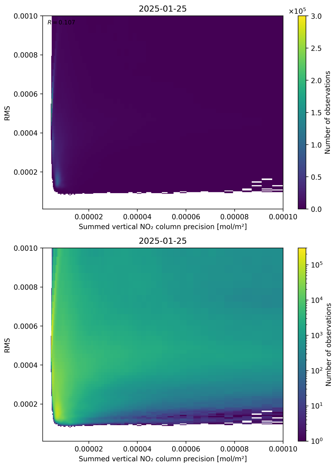
Figure 108: Scatter density plot of “Summed vertical NO 2 column precision” against “RMS” for 2025-01-24 to 2025-01-26.
