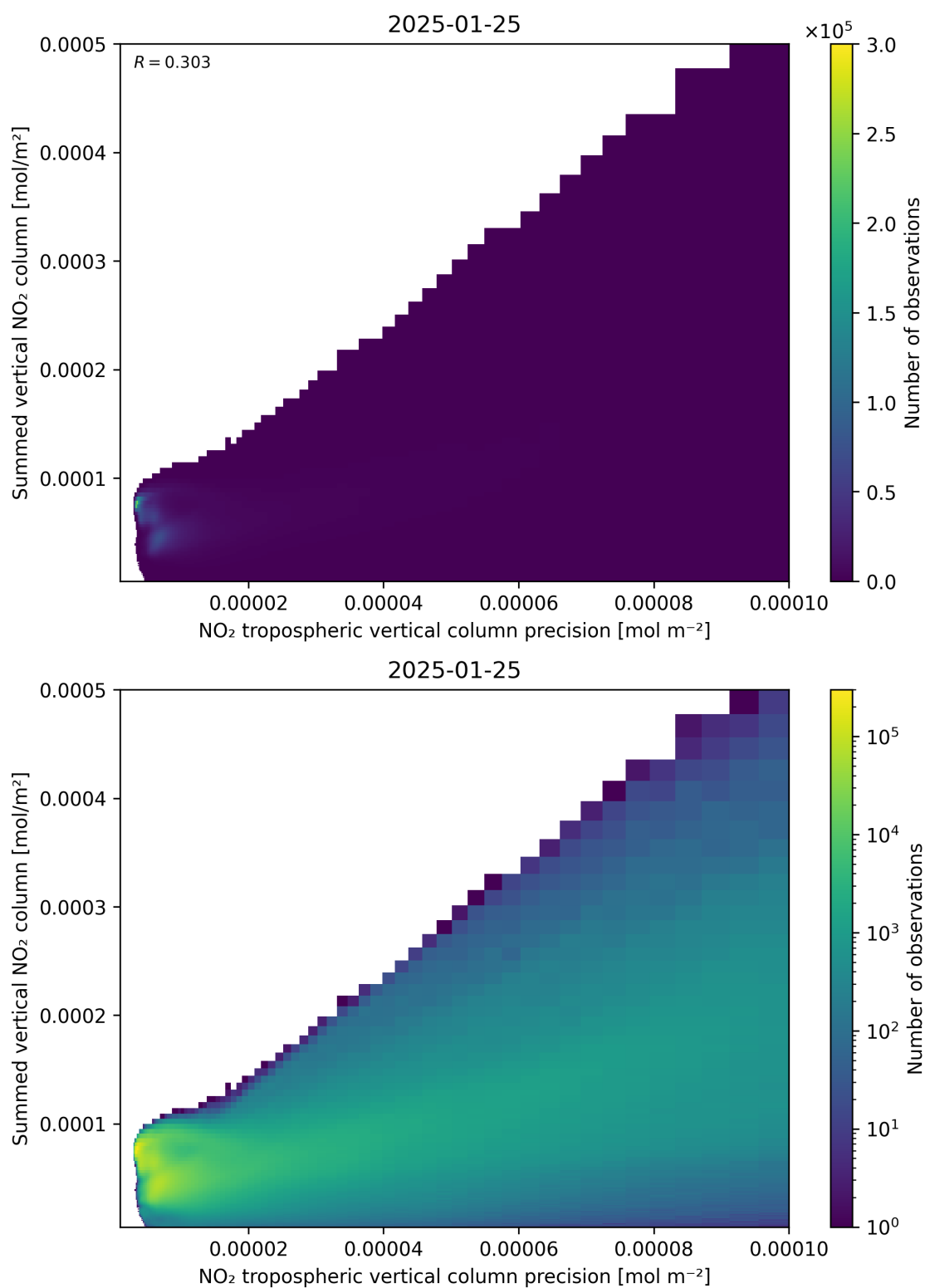
Figure 136: Scatter density plot of “NO 2 tropospheric vertical column precision” against “Summed vertical NO 2 column” for 2025-01-24 to 2025-01-26.
