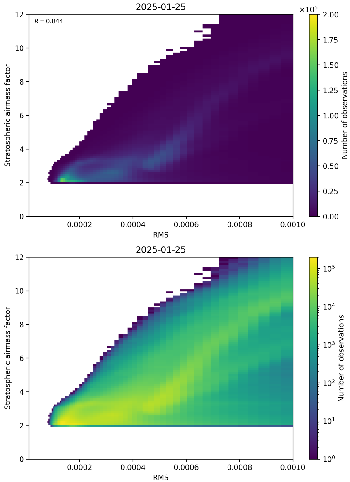
Figure 144: Scatter density plot of “RMS” against “Stratospheric airmass factor” for 2025-01-24 to 2025-01-26.
