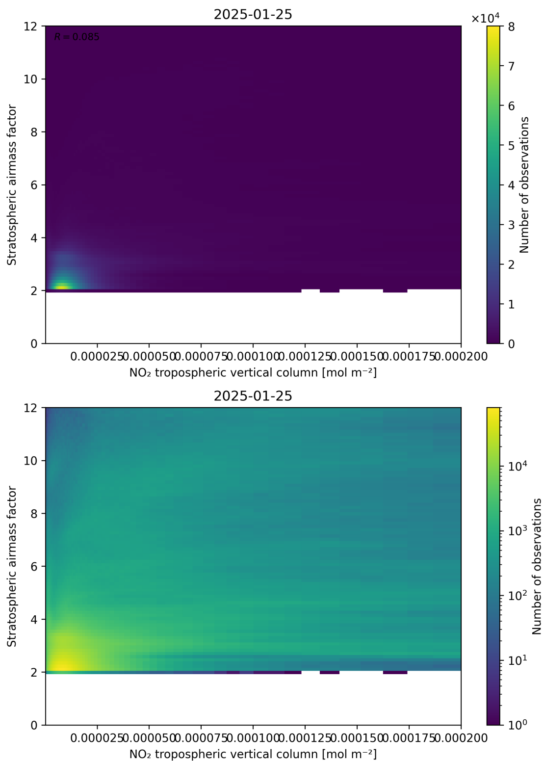
Figure 121: Scatter density plot of “NO 2 tropospheric vertical column” against “Stratospheric airmass factor” for 2025-01-24 to 2025-01-26.
