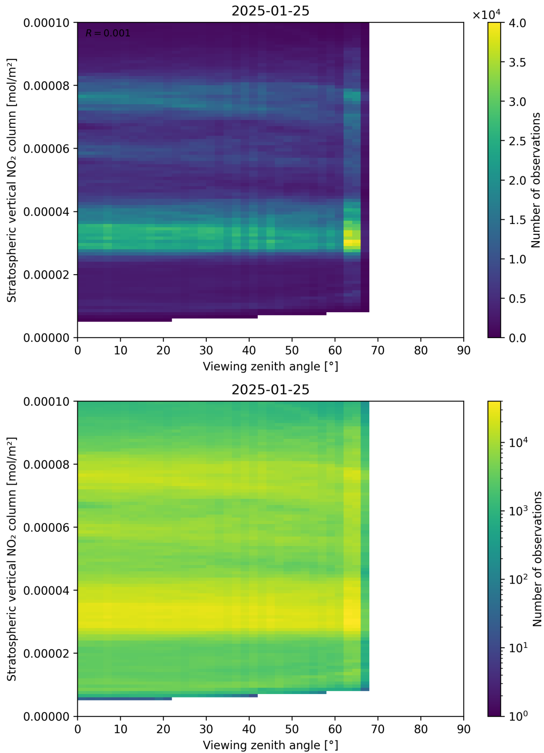
Figure 164: Scatter density plot of “Viewing zenith angle” against “Stratospheric vertical NO 2 column” for 2025-01-24 to 2025-01-26.
