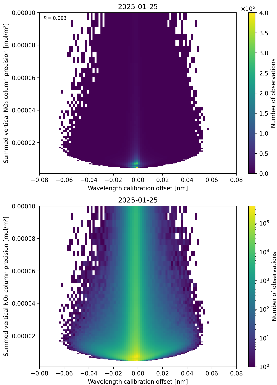
Figure 178: Scatter density plot of “Wavelength calibration offset” against “Summed vertical NO 2 column precision” for 2025-01-24 to 2025-01-26.
