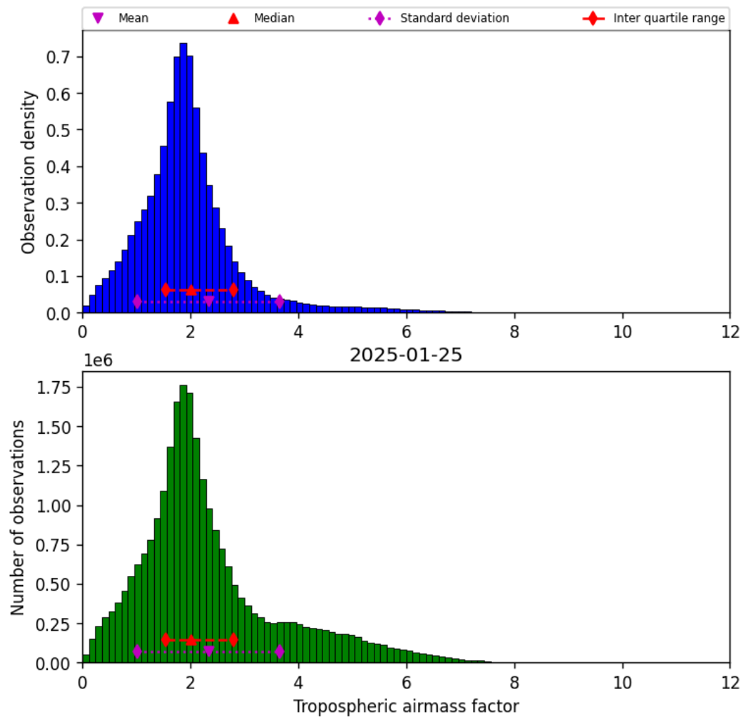
Figure 31: Histogram of “Tropospheric airmass factor” for 2025-01-24 to 2025-01-26
