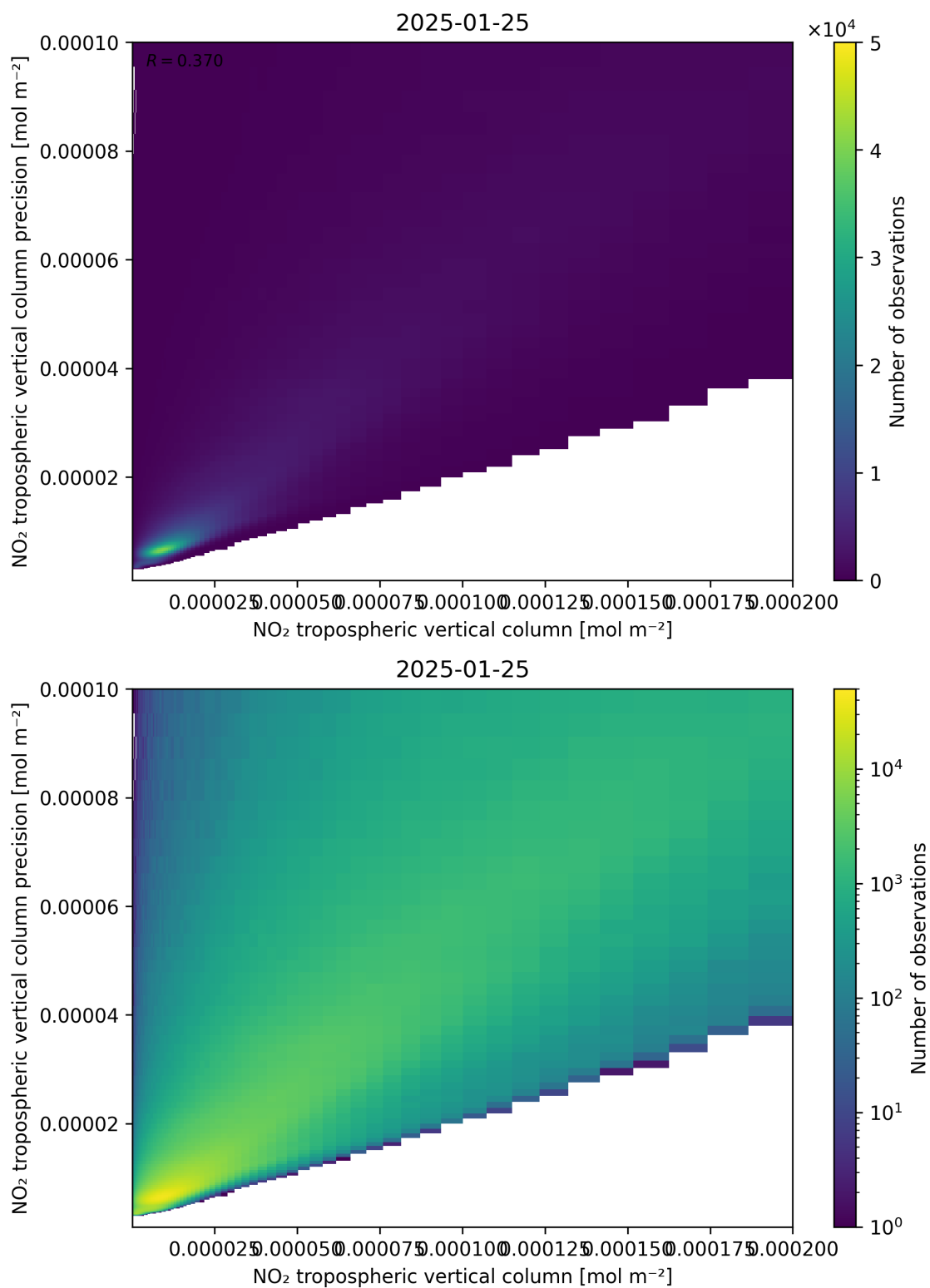
Figure 130: Scatter density plot of “NO 2 tropospheric vertical column” against “NO 2 tropospheric vertical column precision” for 2025-01-24 to 2025-01-26.
