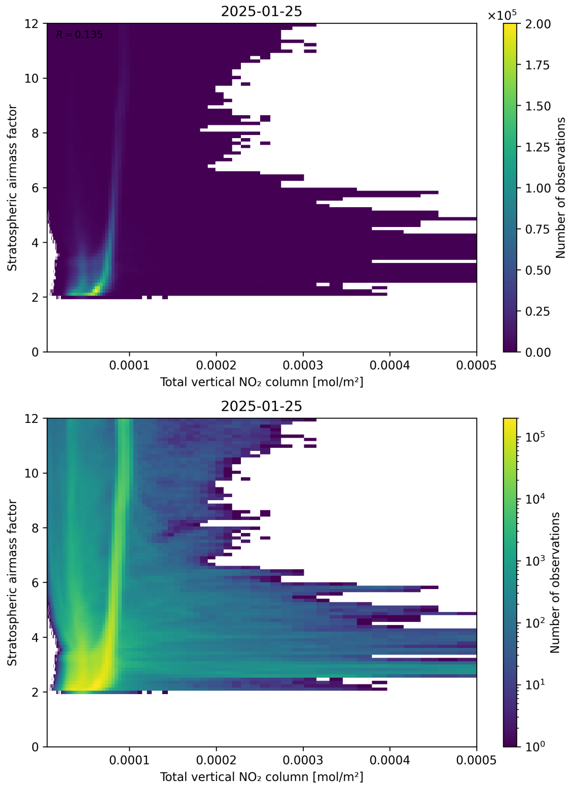
Figure 110: Scatter density plot of “Total vertical NO 2 column” against “Stratospheric airmass factor” for 2025-01-24 to 2025-01-26.
