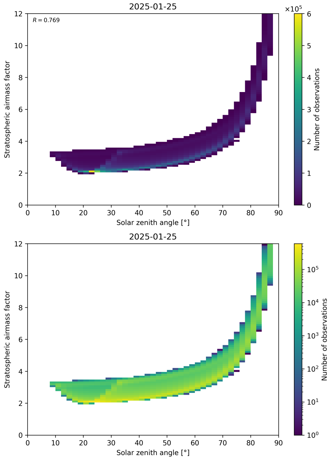
Figure 145: Scatter density plot of “Solar zenith angle” against “Stratospheric airmass factor” for 2025-01-24 to 2025-01-26.
