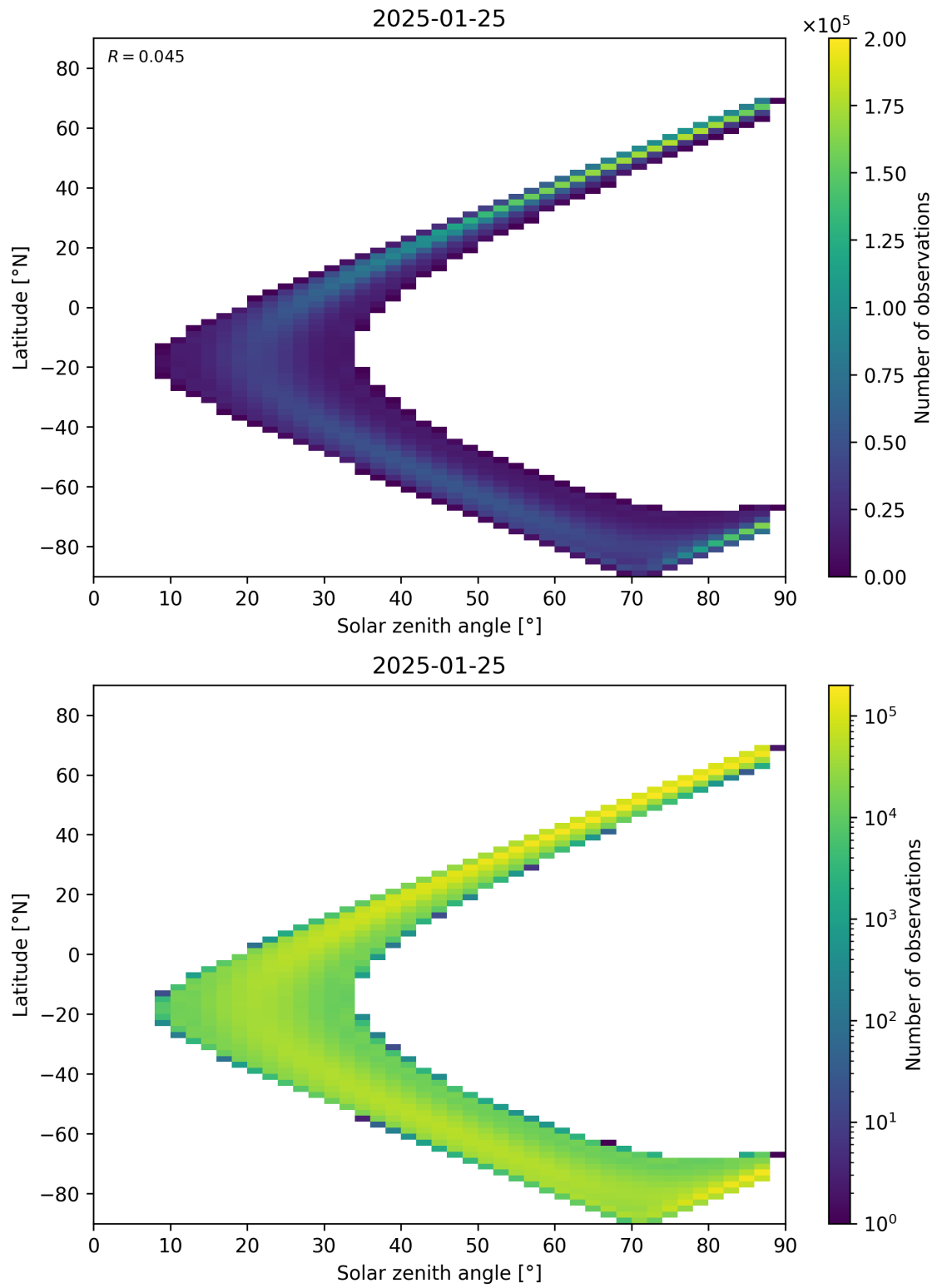
Figure 149: Scatter density plot of “Solar zenith angle” against “Latitude” for 2025-01-24 to 2025-01-26.
