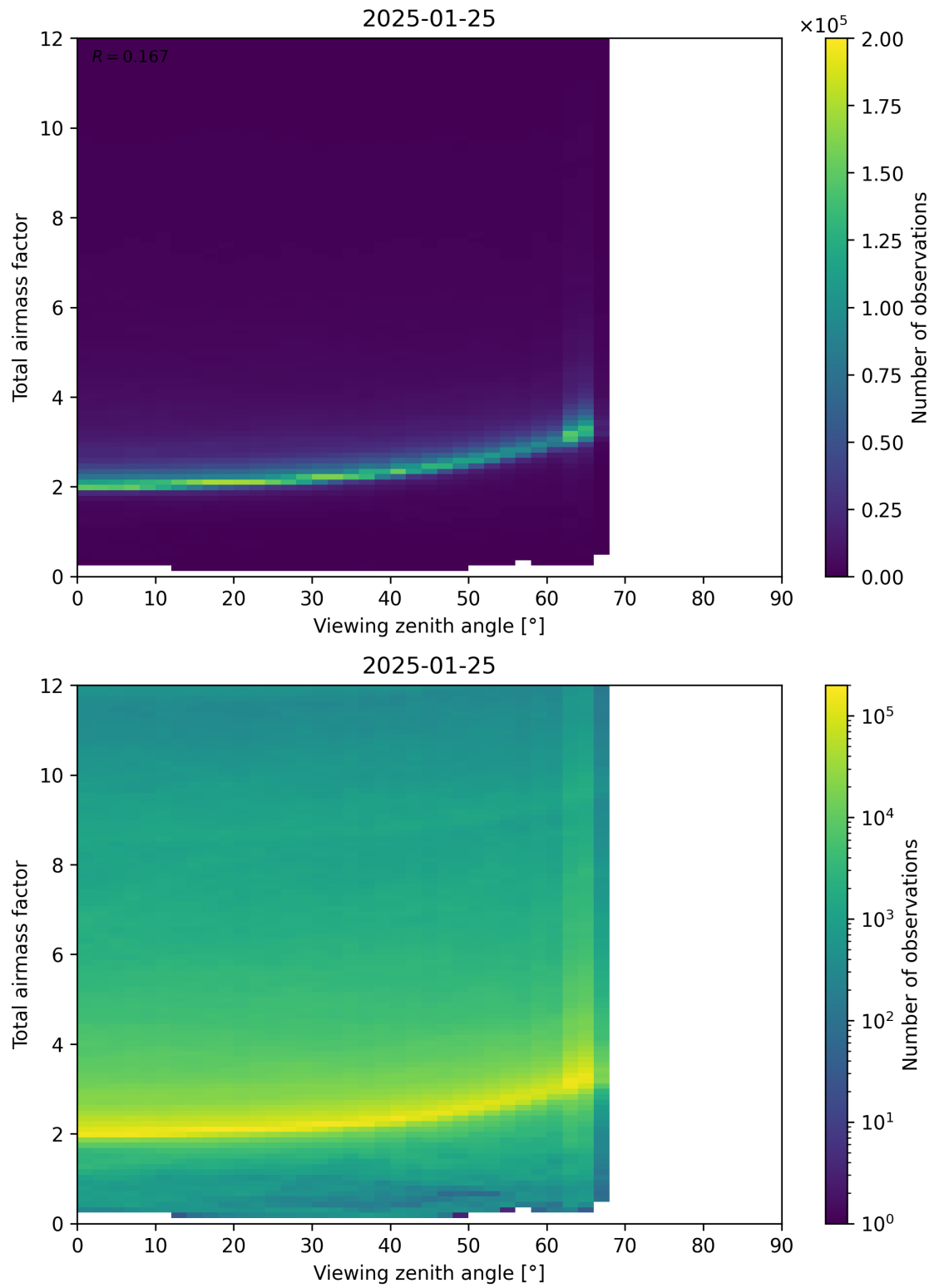
Figure 160: Scatter density plot of “Viewing zenith angle” against “Total airmass factor” for 2025-01-24 to 2025-01-26.
