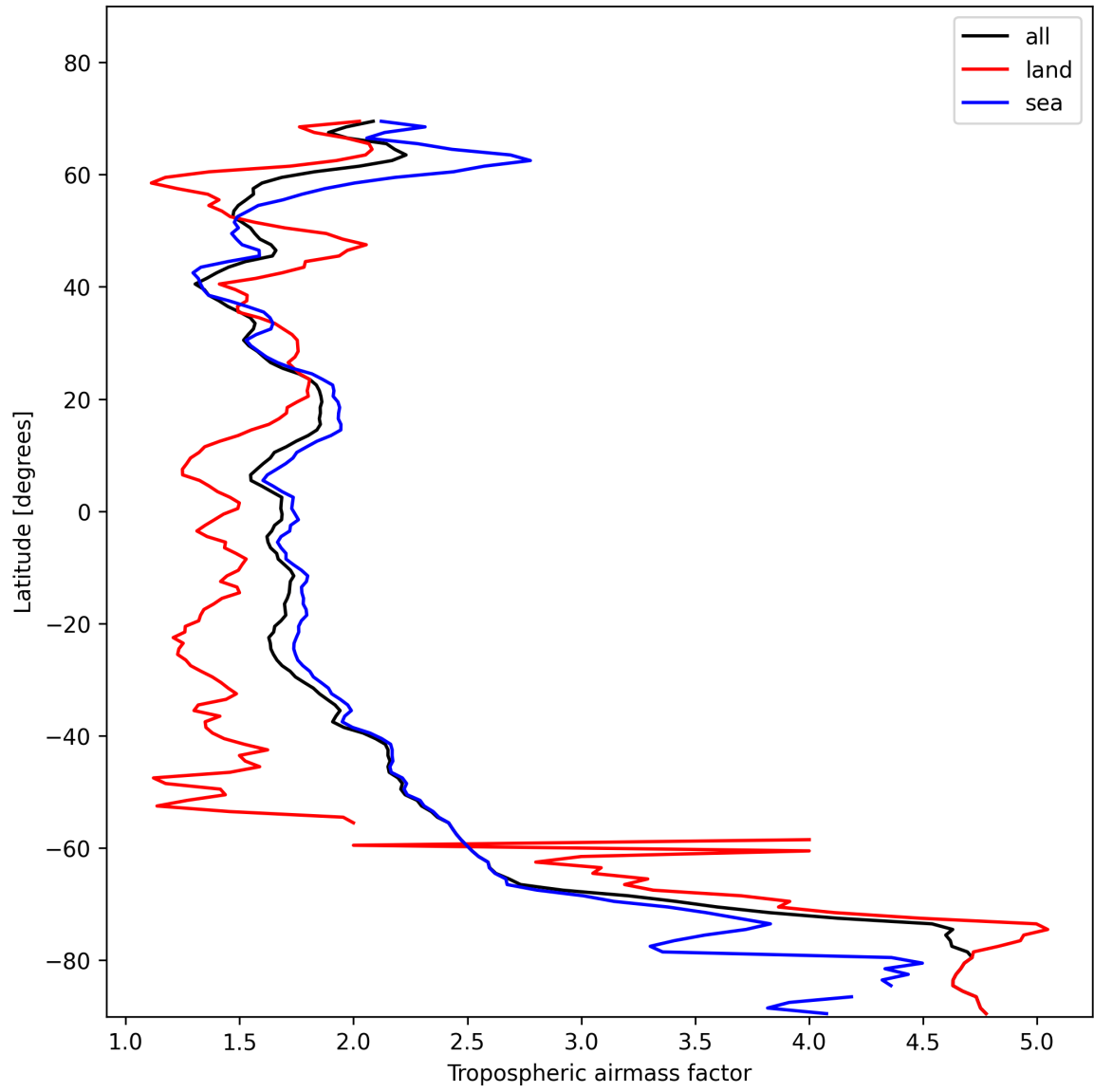
Figure 14: Zonal average of “Tropospheric airmass factor” for 2025-01-24 to 2025-01-26.
