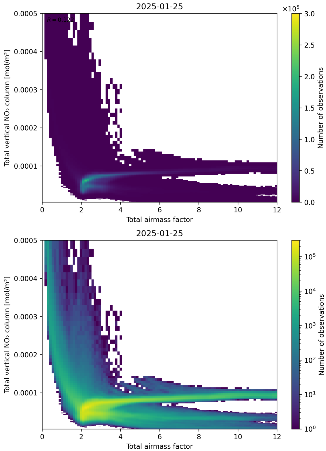
Figure 67: Scatter density plot of “Total airmass factor” against “Total vertical NO 2 column” for 2025-01-24 to 2025-01-26.
