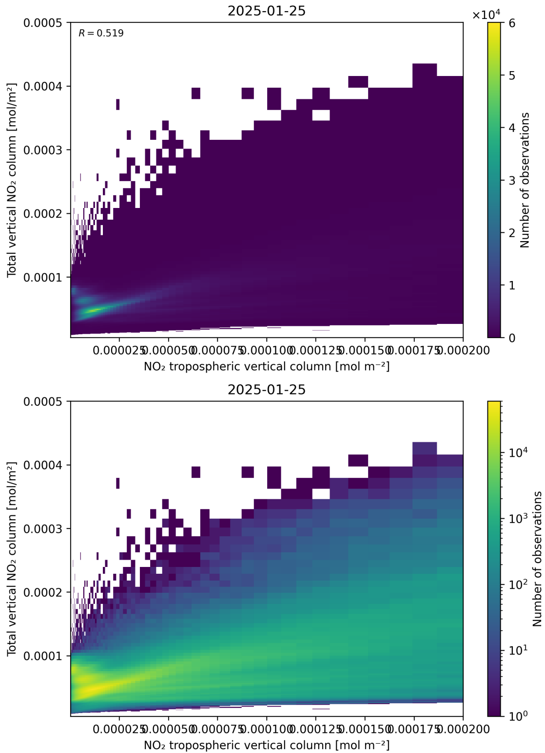
Figure 128: Scatter density plot of “NO 2 tropospheric vertical column” against “Total vertical NO 2 column” for 2025-01-24 to 2025-01-26.
