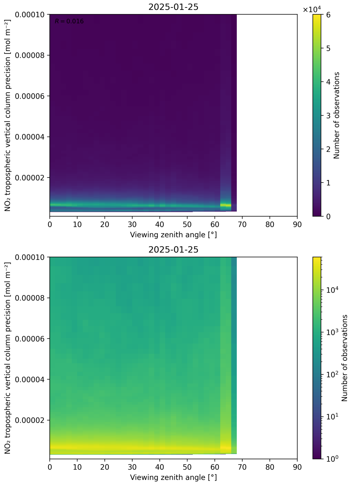
Figure 170: Scatter density plot of “Viewing zenith angle” against “NO 2 tropospheric vertical column precision” for 2025-01-24 to 2025-01-26.
