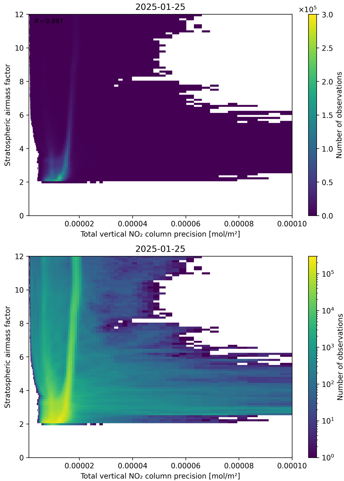
Figure 115: Scatter density plot of “Total vertical NO 2 column precision” against “Stratospheric air mass factor” for 2025-01-24 to 2025-01-26.
