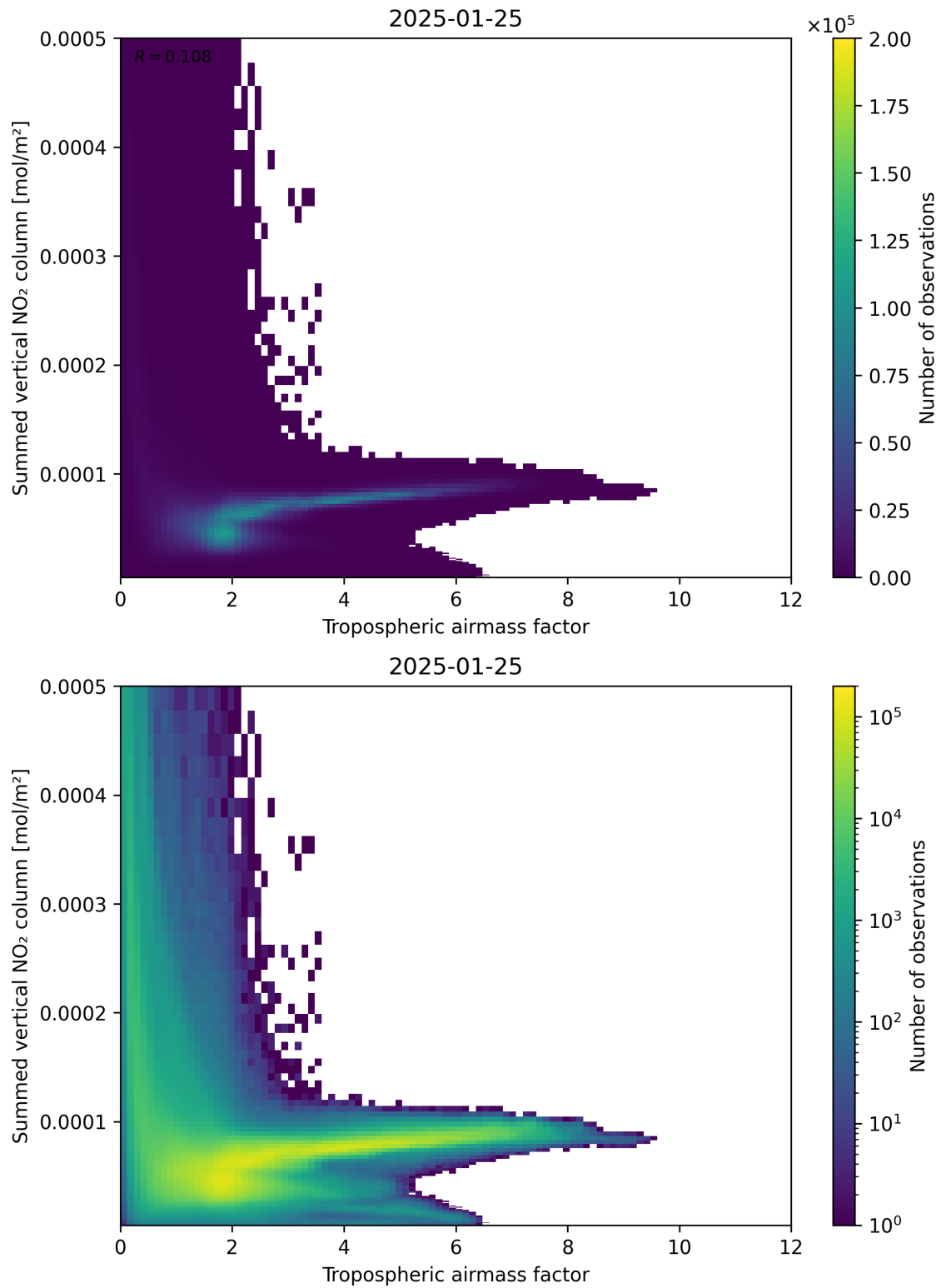
Figure 75: Scatter density plot of “Tropospheric air mass factor” against “Summed vertical NO 2 column” for 2025-01-24 to 2025-01-26.
