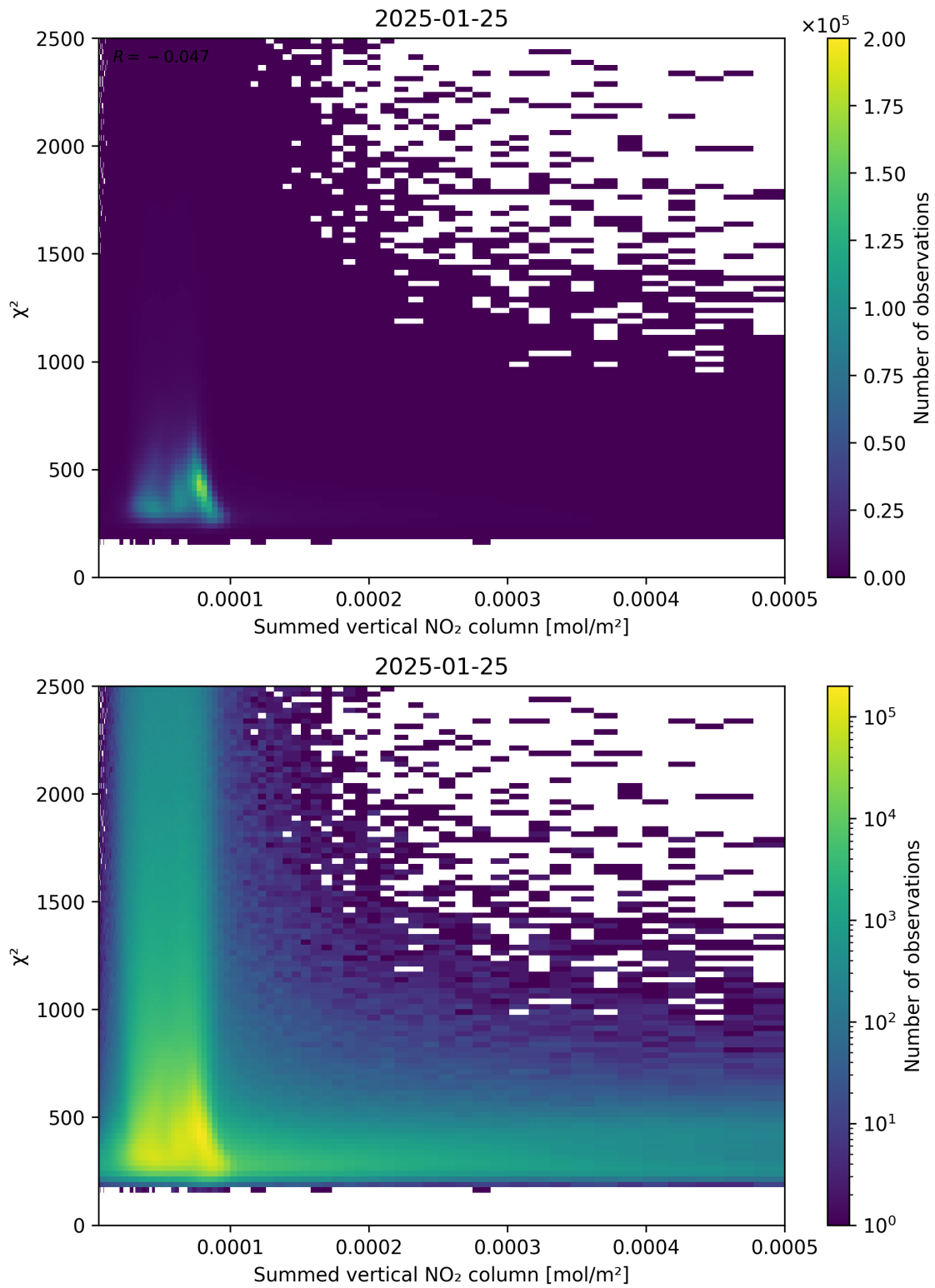
Figure 104: Scatter density plot of “Summed vertical NO 2 column” against “ \chi^2 ” for 2025-01-24 to 2025-01-26.
