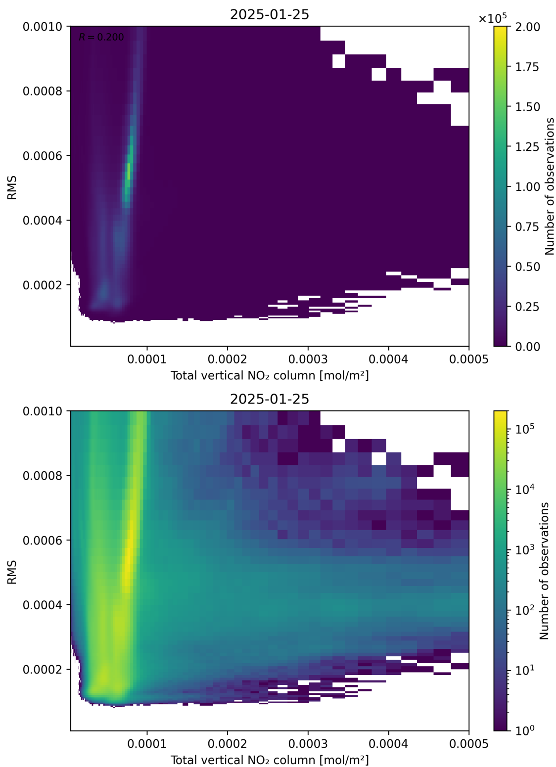
Figure 120: Scatter density plot of “Total vertical NO 2 column” against “RMS” for 2025-01-24 to 2025-01-26.
