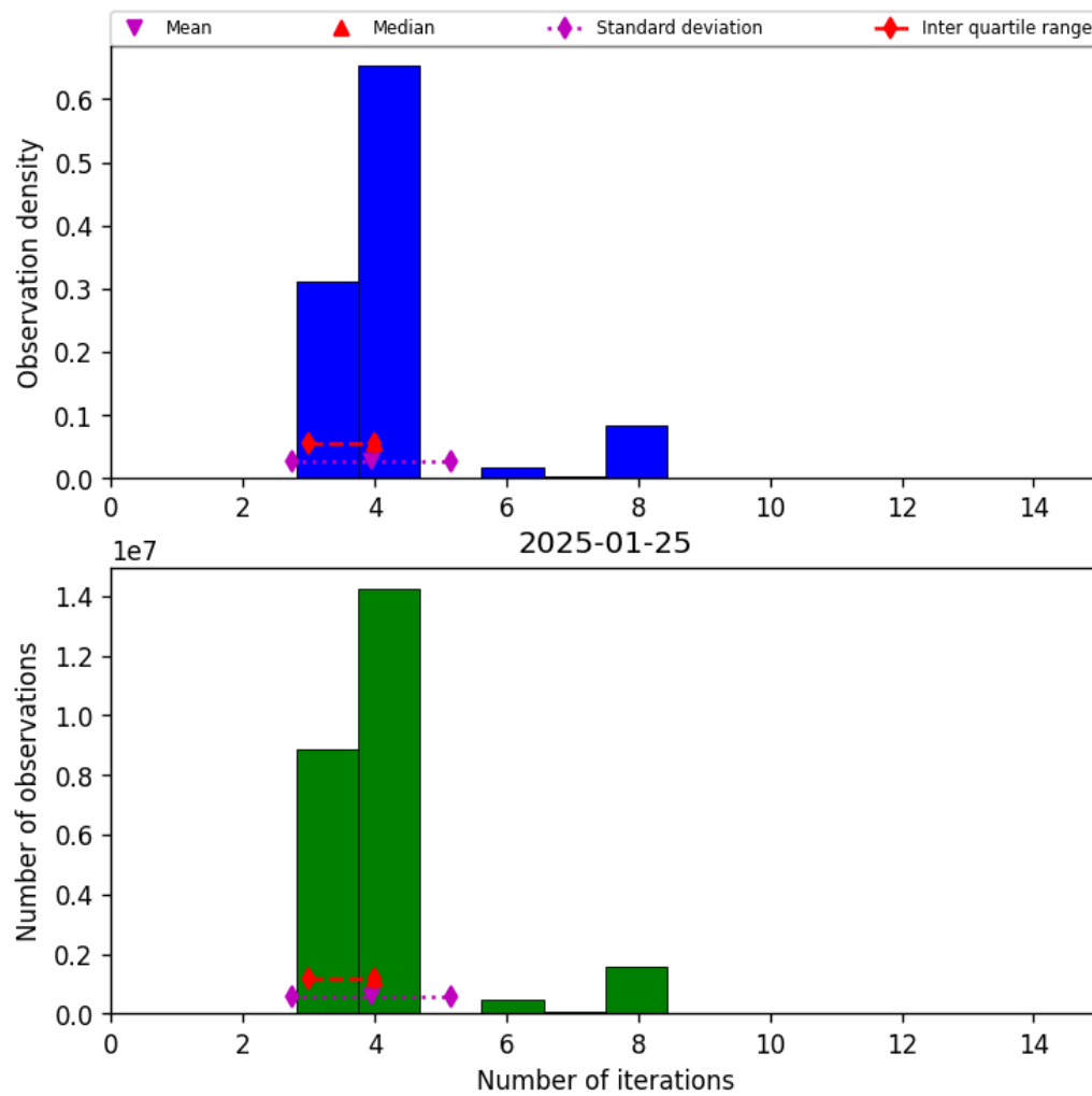
Figure 34: Histogram of “Number of iterations” for 2025-01-24 to 2025-01-26
