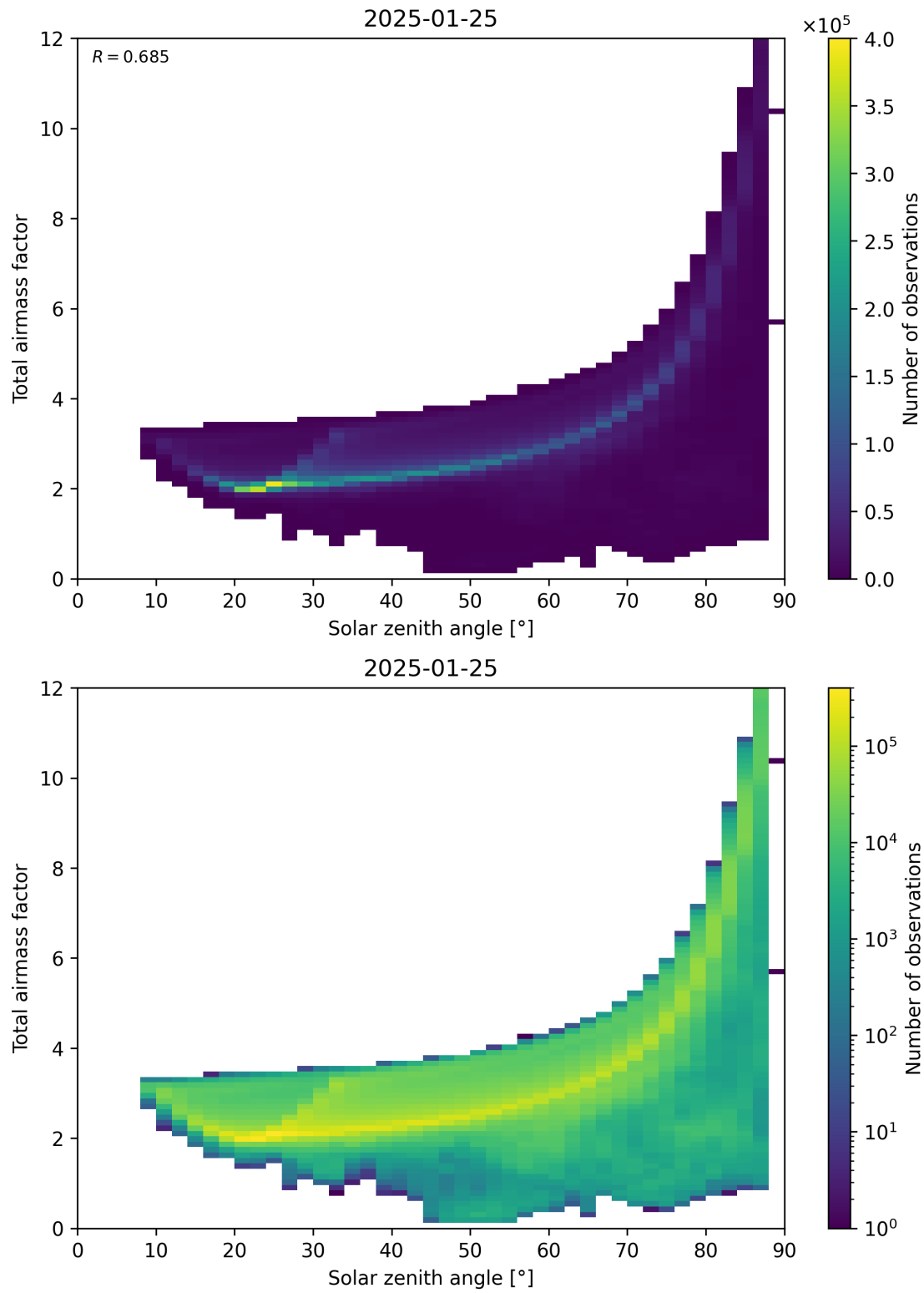
Figure 146: Scatter density plot of “Solar zenith angle” against “Total air mass factor” for 2025-01-24 to 2025-01-26.
