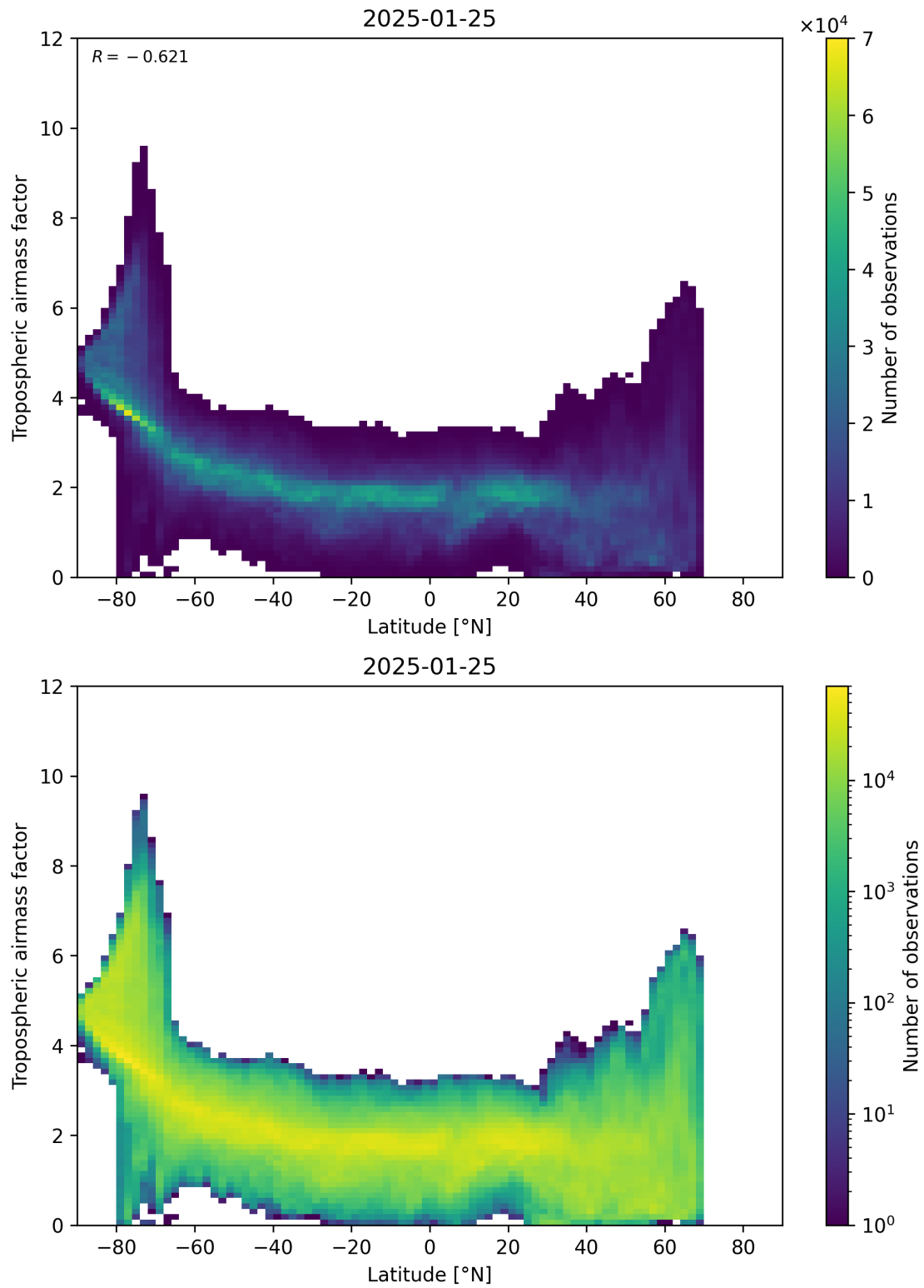
Figure 85: Scatter density plot of “Latitude” against “Tropospheric air mass factor” for 2025-01-24 to 2025-01-26.
