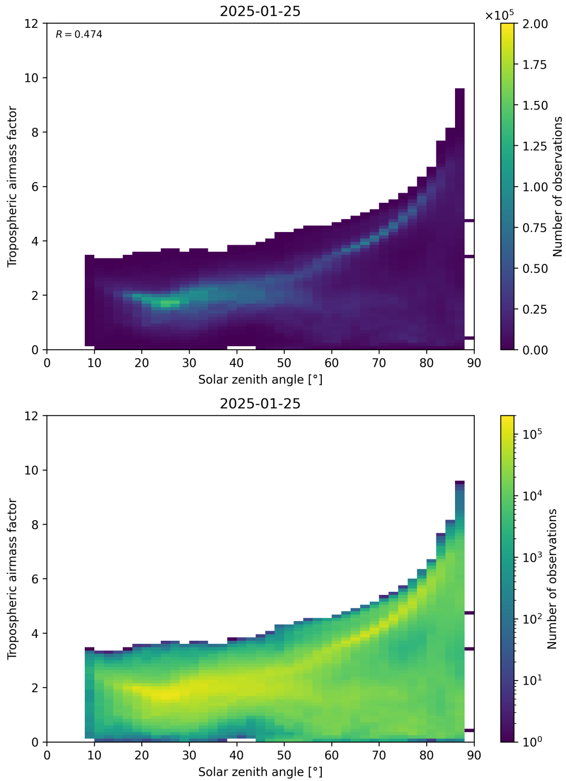
Figure 147: Scatter density plot of “Solar zenith angle” against “Tropospheric airmass factor” for 2025-01-24 to 2025-01-26.
