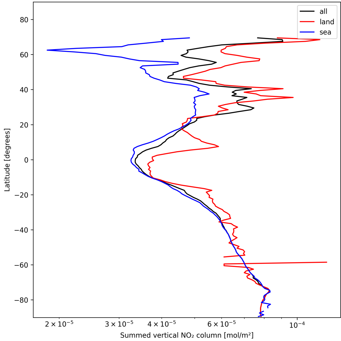
Figure 23: Zonal average of “Summed vertical NO 2 column” for 2025-01-24 to 2025-01-26.
