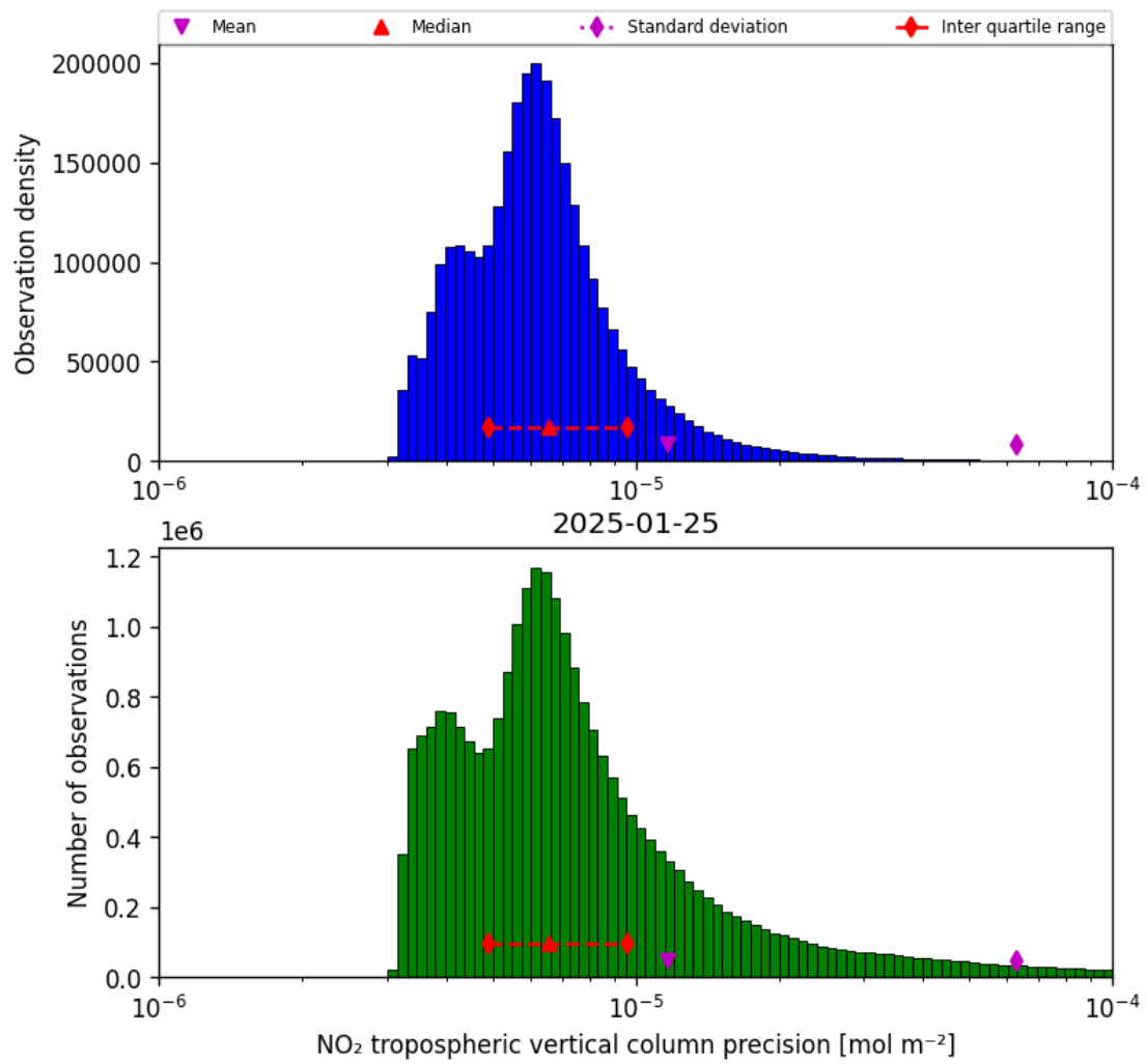
Figure 30: Histogram of “NO 2 tropospheric vertical column precision” for 2025-01-24 to 2025-01-26
