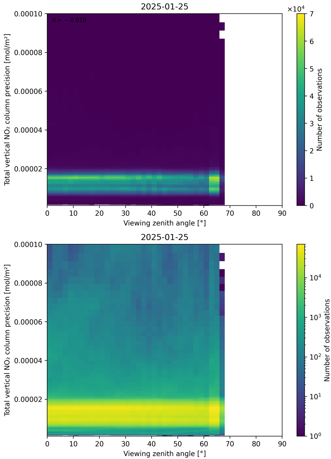
Figure 168: Scatter density plot of “Viewing zenith angle” against “Total vertical NO 2 column precision” for 2025-01-24 to 2025-01-26.
