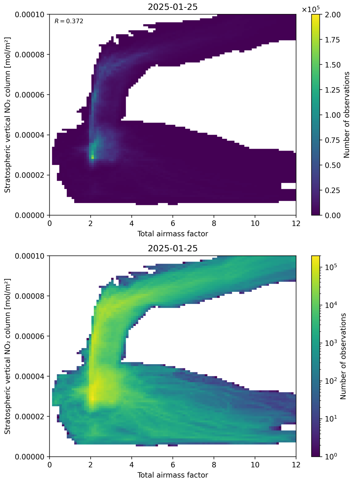
Figure 64: Scatter density plot of “Total airmass factor” against “Stratospheric vertical NO 2 column” for 2025-01-24 to 2025-01-26.
