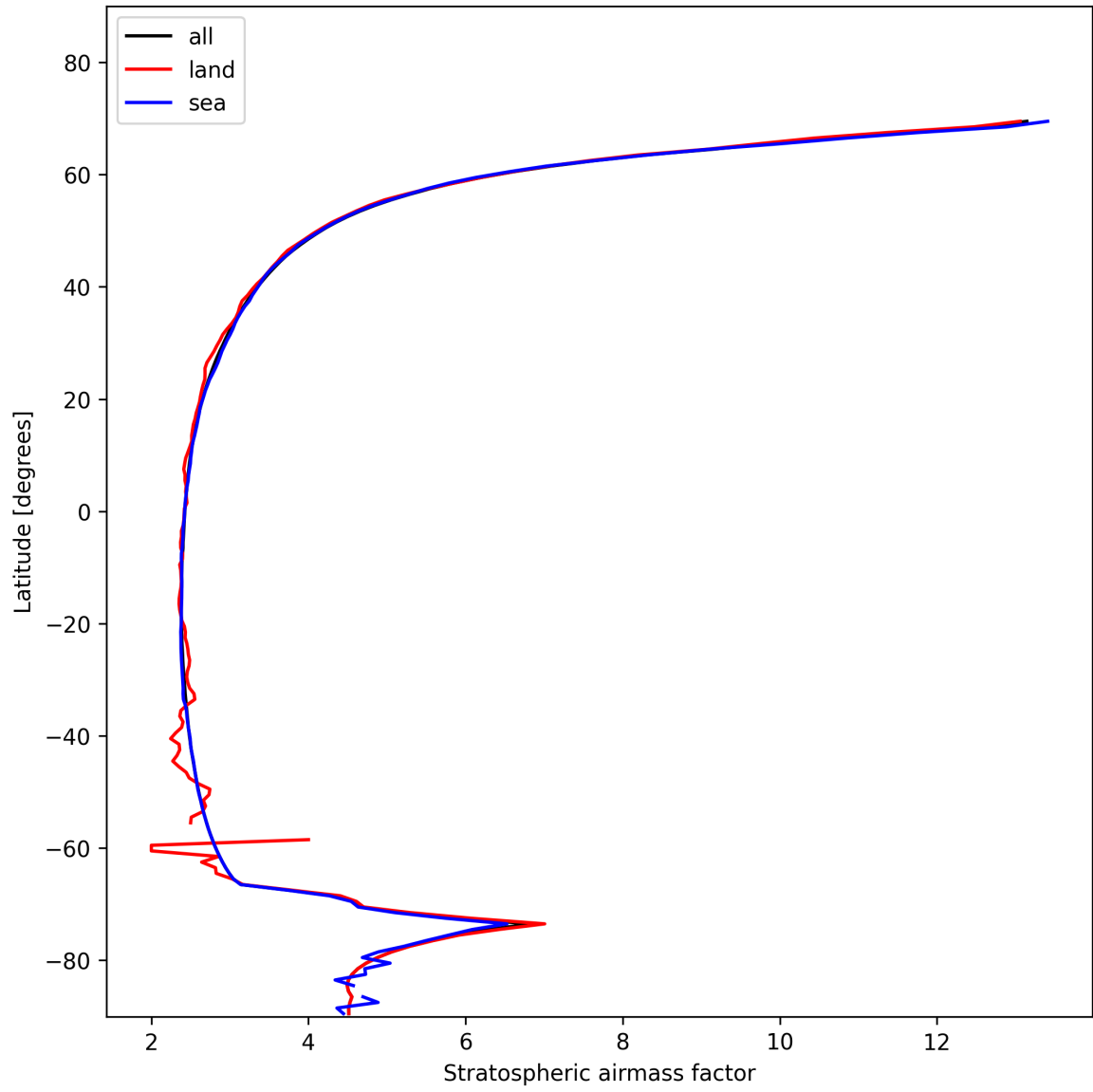
Figure 27: Zonal average of “Stratospheric airmass factor” for 2025-01-24 to 2025-01-26.
