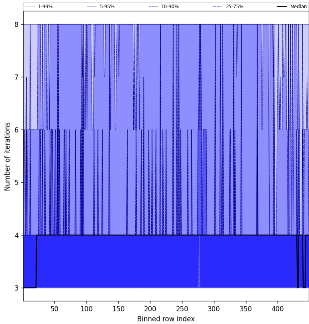
Figure 51: Along track statistics of “Number of iterations” for 2025-01-24 to 2025-01-26
