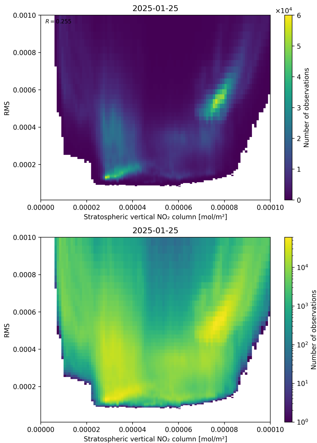
Figure 102: Scatter density plot of “Stratospheric vertical NO 2 column” against “RMS” for 2025-01-24 to 2025-01-26.
