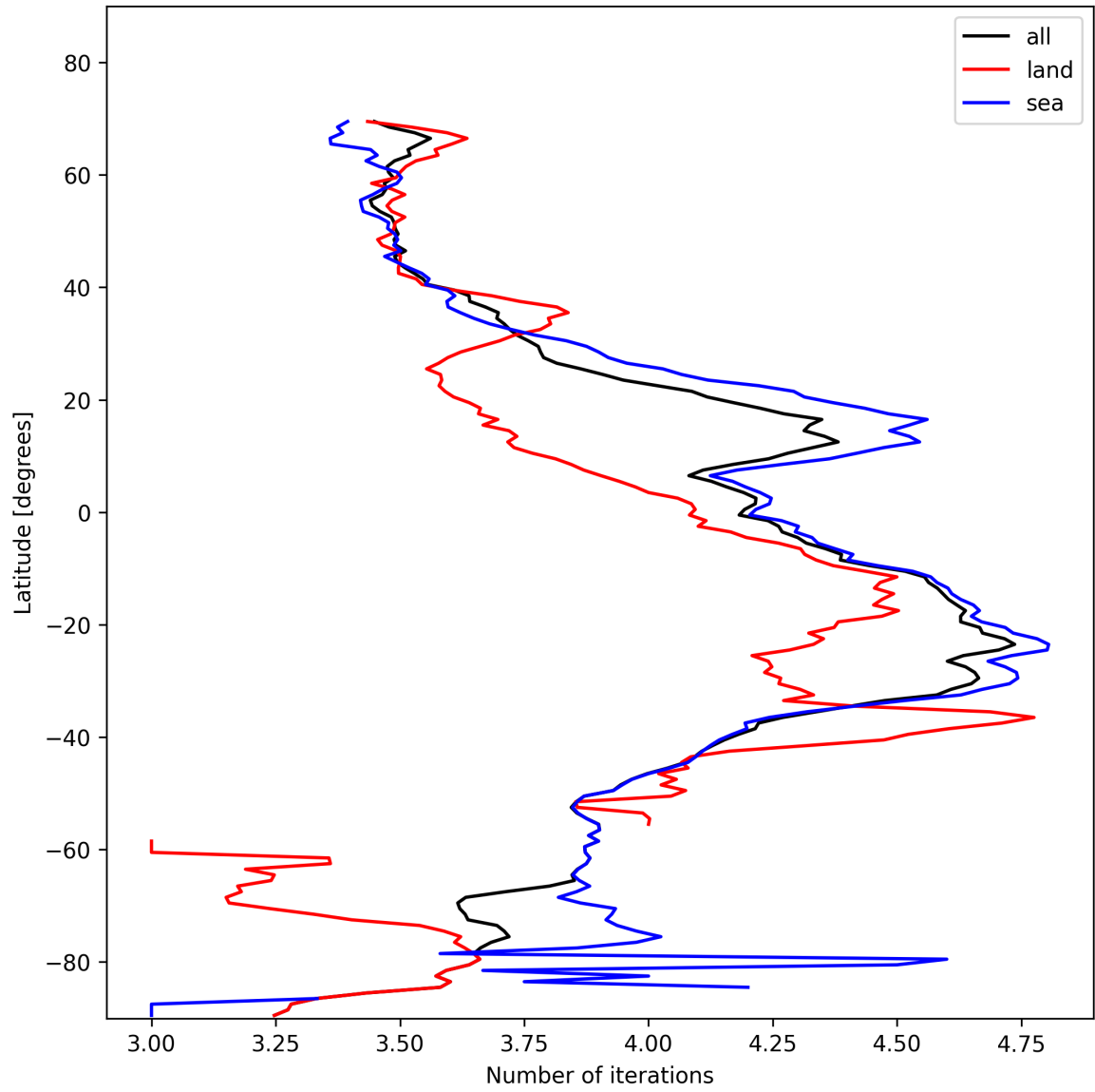
Figure 17: Zonal average of “Number of iterations” for 2025-01-24 to 2025-01-26.
