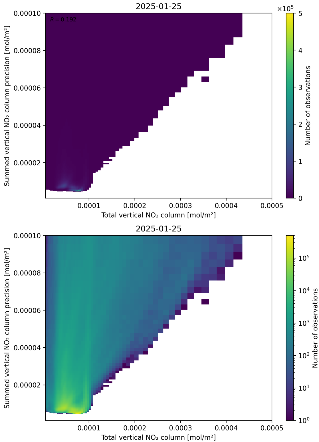
Figure 113: Scatter density plot of “Total vertical NO 2 column” against “Summed vertical NO 2 column precision” for 2025-01-24 to 2025-01-26.
