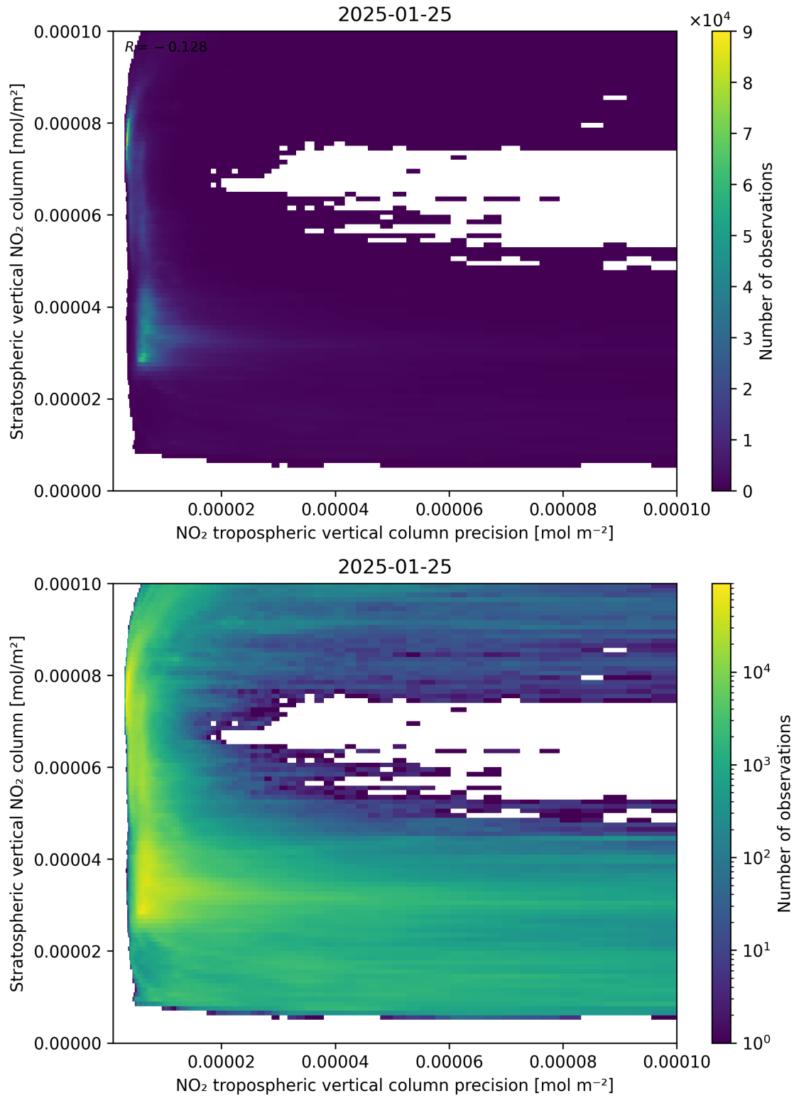
Figure 135: Scatter density plot of “NO 2 tropospheric vertical column precision” against “Stratospheric vertical NO 2 column” for 2025-01-24 to 2025-01-26.
