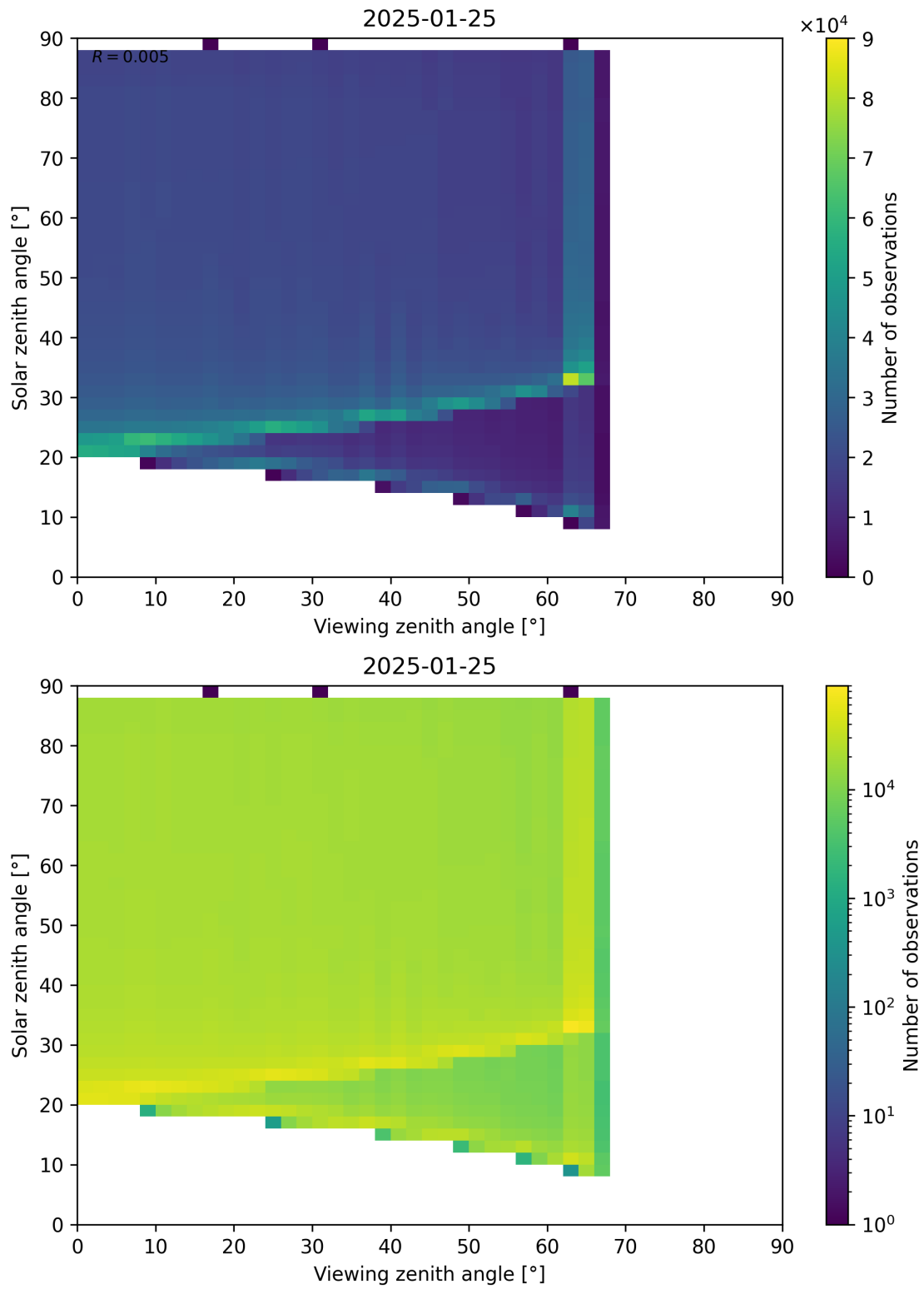
Figure 172: Scatter density plot of “Viewing zenith angle” against “Solar zenith angle” for 2025-01-24 to 2025-01-26.
