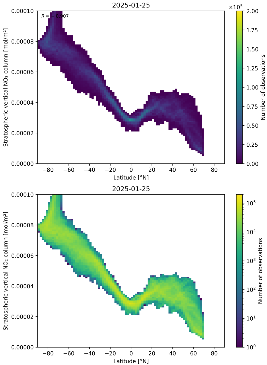
Figure 87: Scatter density plot of “Latitude” against “Stratospheric vertical NO 2 column” for 2025-01-24 to 2025-01-26.
