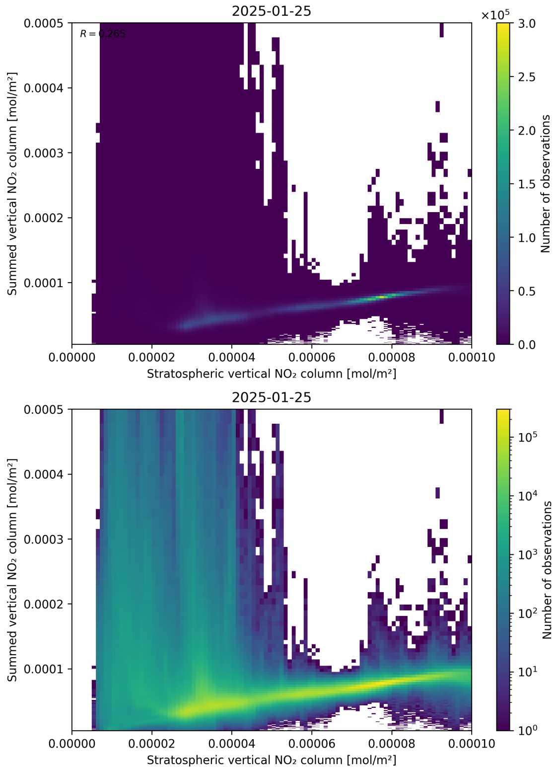
Figure 98: Scatter density plot of “Stratospheric vertical NO 2 column” against “Summed vertical NO 2 column” for 2025-01-24 to 2025-01-26.
