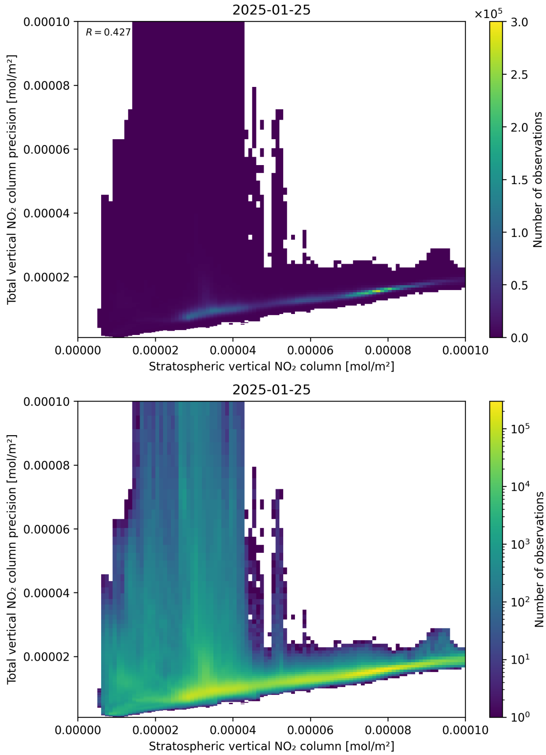
Figure 101: Scatter density plot of “Stratospheric vertical NO 2 column” against “Total vertical NO 2 column precision” for 2025-01-24 to 2025-01-26.
