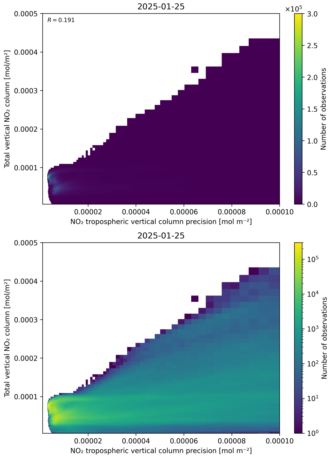
Figure 138: Scatter density plot of “NO 2 tropospheric vertical column precision” against “Total vertical NO 2 column” for 2025-01-24 to 2025-01-26.
