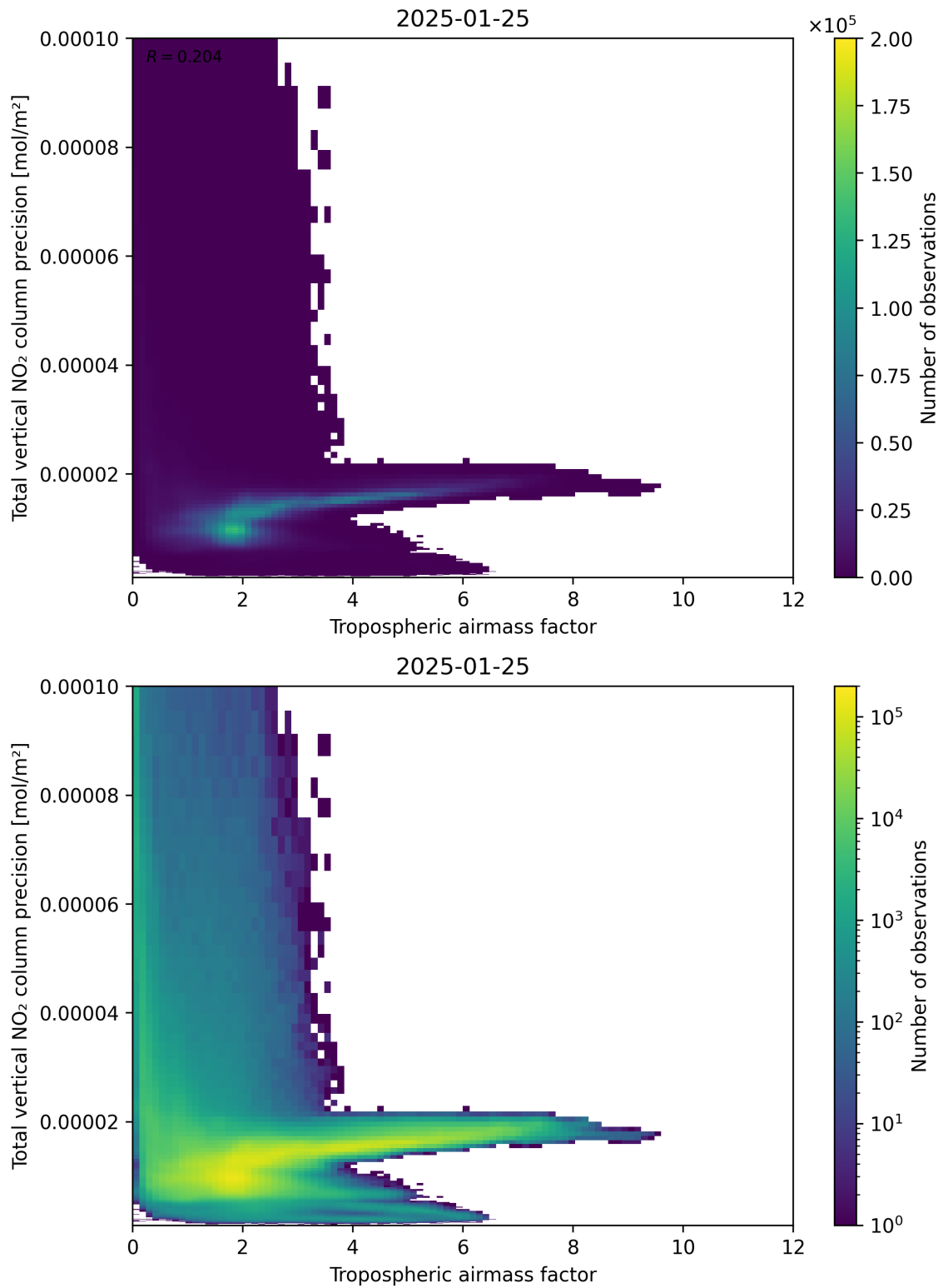
Figure 78: Scatter density plot of “Tropospheric air mass factor” against “Total vertical NO 2 column precision” for 2025-01-24 to 2025-01-26.
