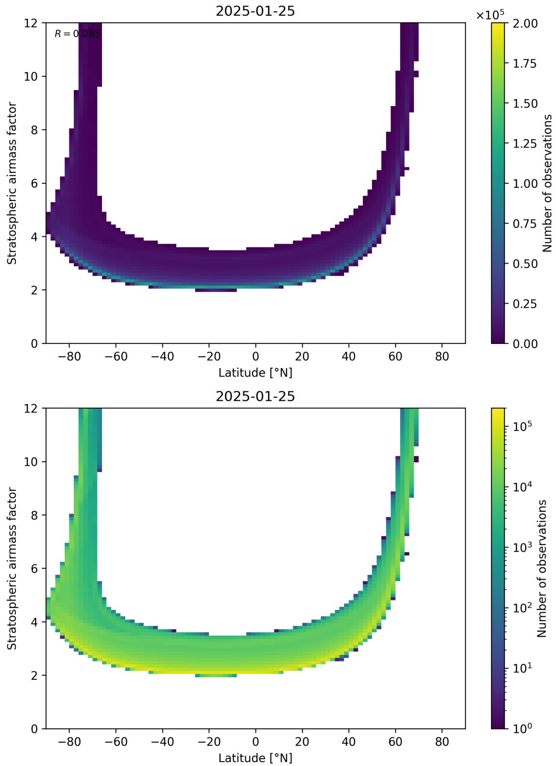
Figure 83: Scatter density plot of “Latitude” against “Stratospheric airmass factor” for 2025-01-24 to 2025-01-26.
