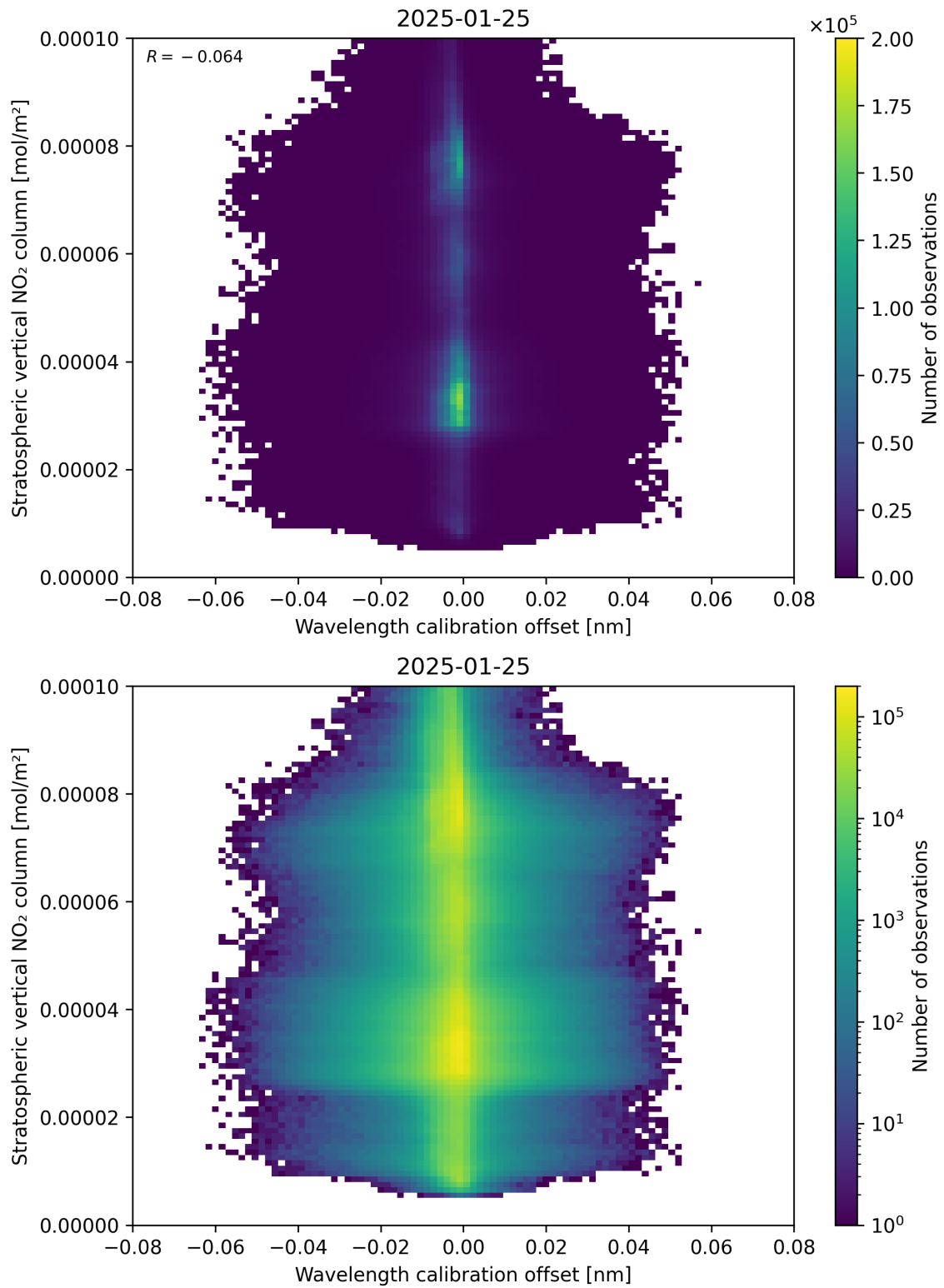
Figure 176: Scatter density plot of “Wavelength calibration offset” against “Stratospheric vertical NO 2 column” for 2025-01-24 to 2025-01-26.
