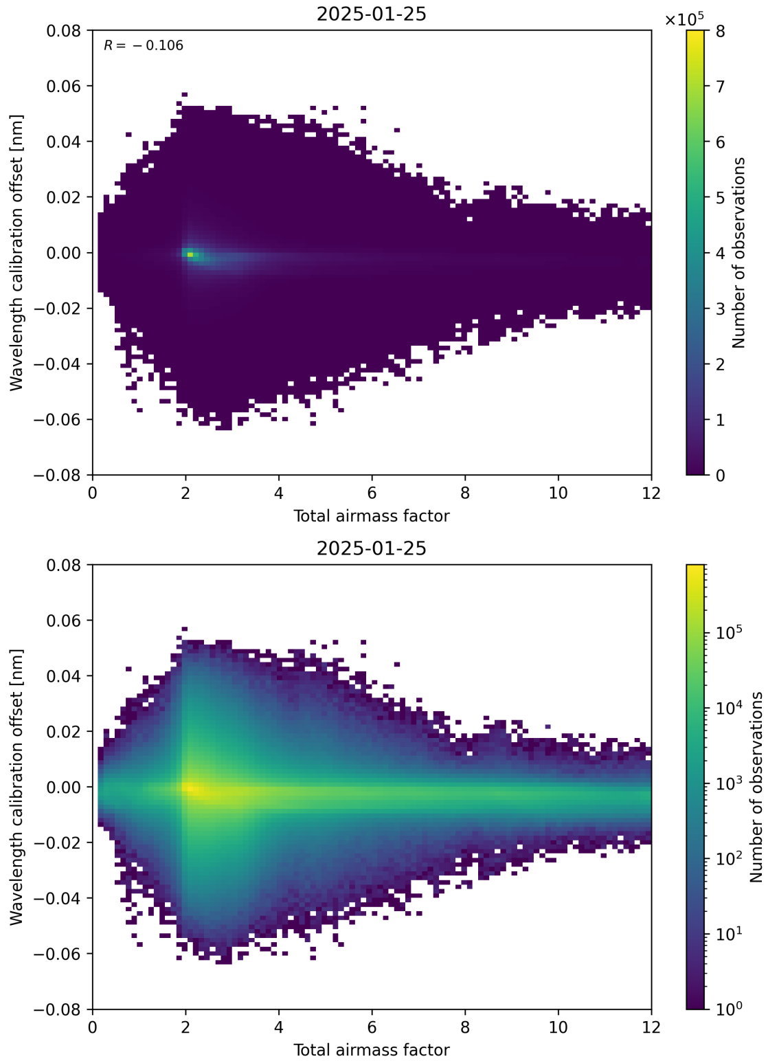
Figure 70: Scatter density plot of “Total airmass factor” against “Wavelength calibration offset” for 2025-01-24 to 2025-01-26.
