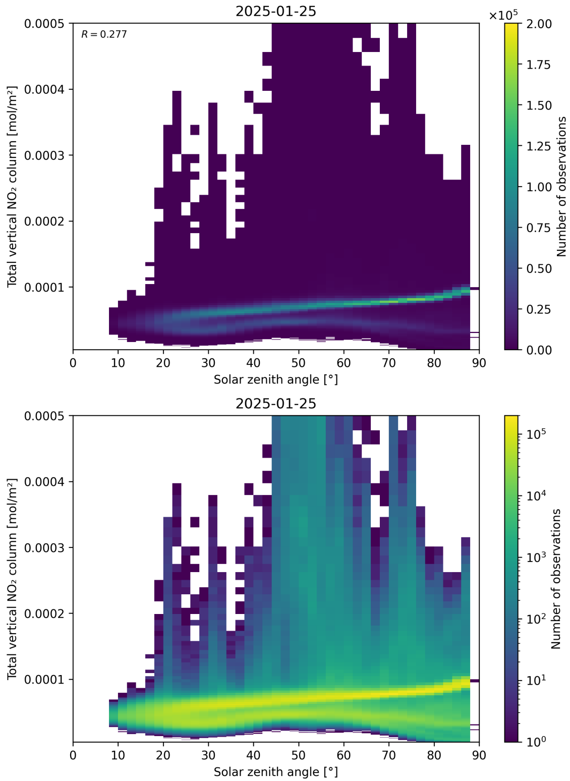
Figure 153: Scatter density plot of “Solar zenith angle” against “Total vertical NO 2 column” for 2025-01-24 to 2025-01-26.
