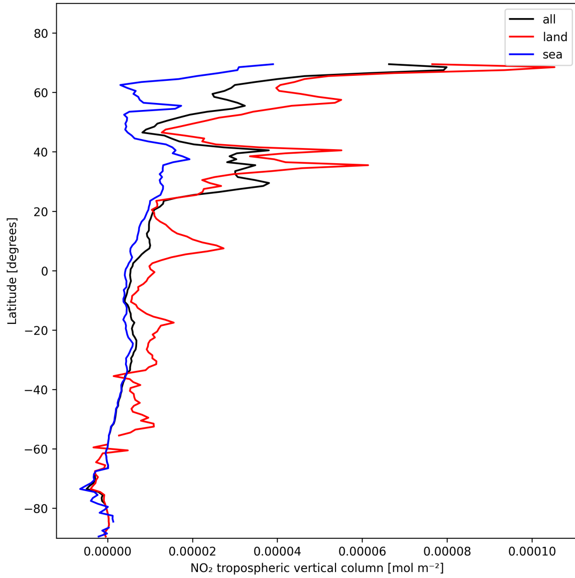
Figure 12: Zonal average of “NO 2 tropospheric vertical column” for 2025-01-24 to 2025-01-26.
