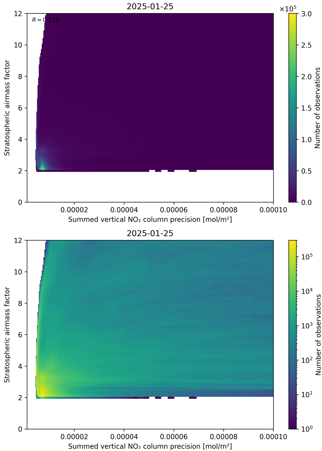
Figure 106: Scatter density plot of “Summed vertical NO 2 column precision” against “Stratospheric airmass factor” for 2025-01-24 to 2025-01-26.
