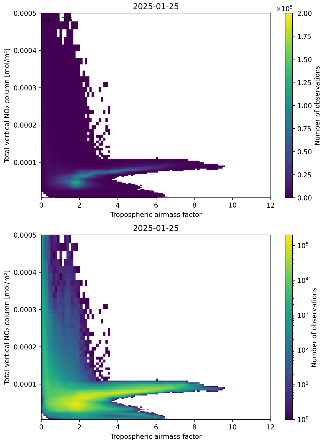
Figure 77: Scatter density plot of “Tropospheric airmass factor” against “Total vertical NO 2 column” for 2025-01-24 to 2025-01-26.
