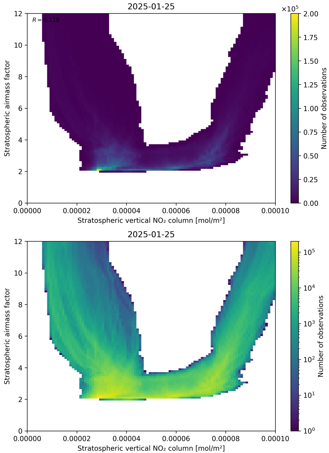
Figure 96: Scatter density plot of “Stratospheric vertical NO 2 column” against “Stratospheric airmass factor” for 2025-01-24 to 2025-01-26.
