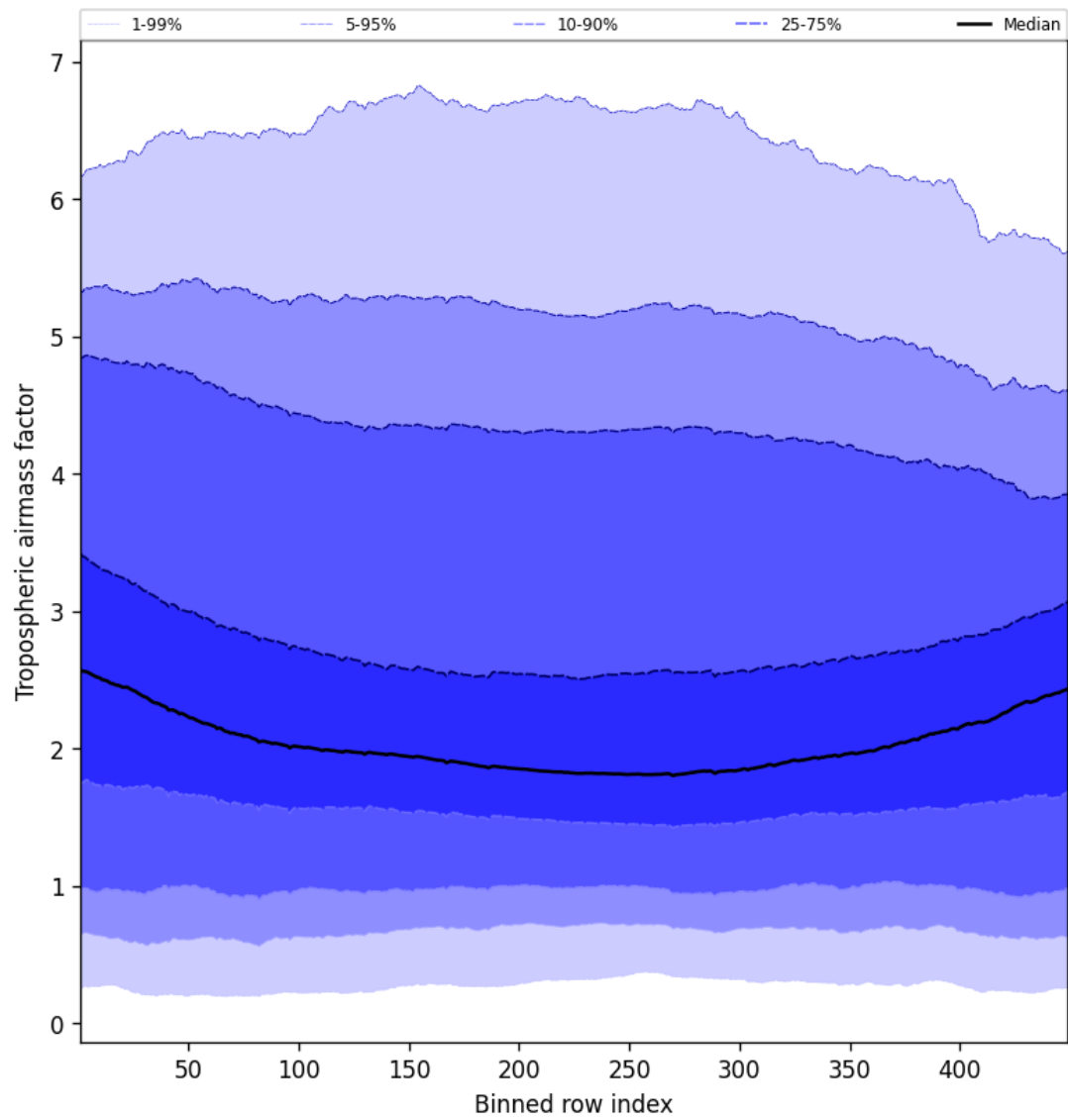
Figure 48: Along track statistics of “Tropospheric airmass factor” for 2025-01-24 to 2025-01-26
