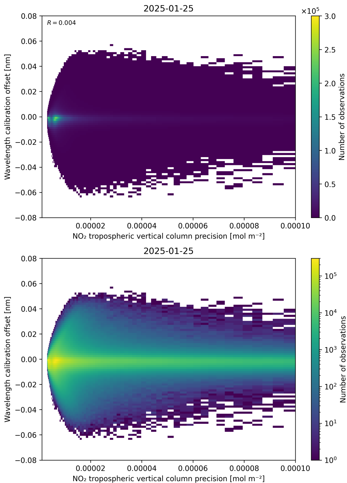
Figure 141: Scatter density plot of “NO 2 tropospheric vertical column precision” against “Wavelength calibration offset” for 2025-01-24 to 2025-01-26.
