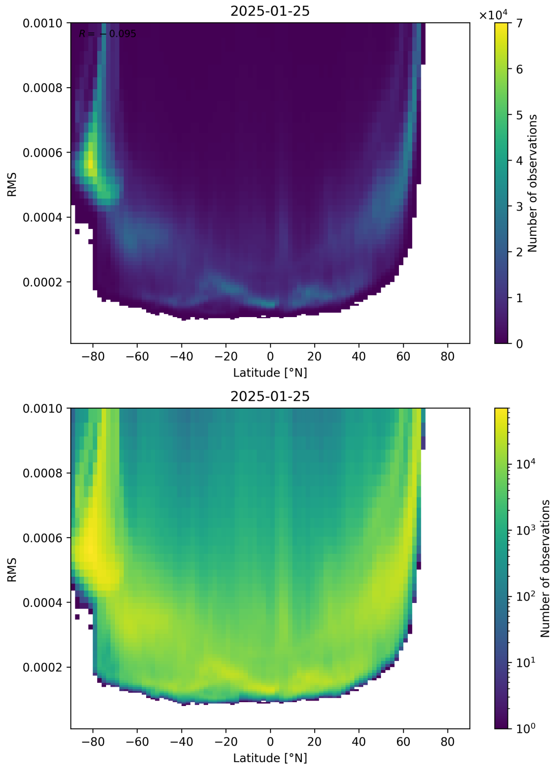
Figure 94: Scatter density plot of “Latitude” against “RMS” for 2025-01-24 to 2025-01-26.
