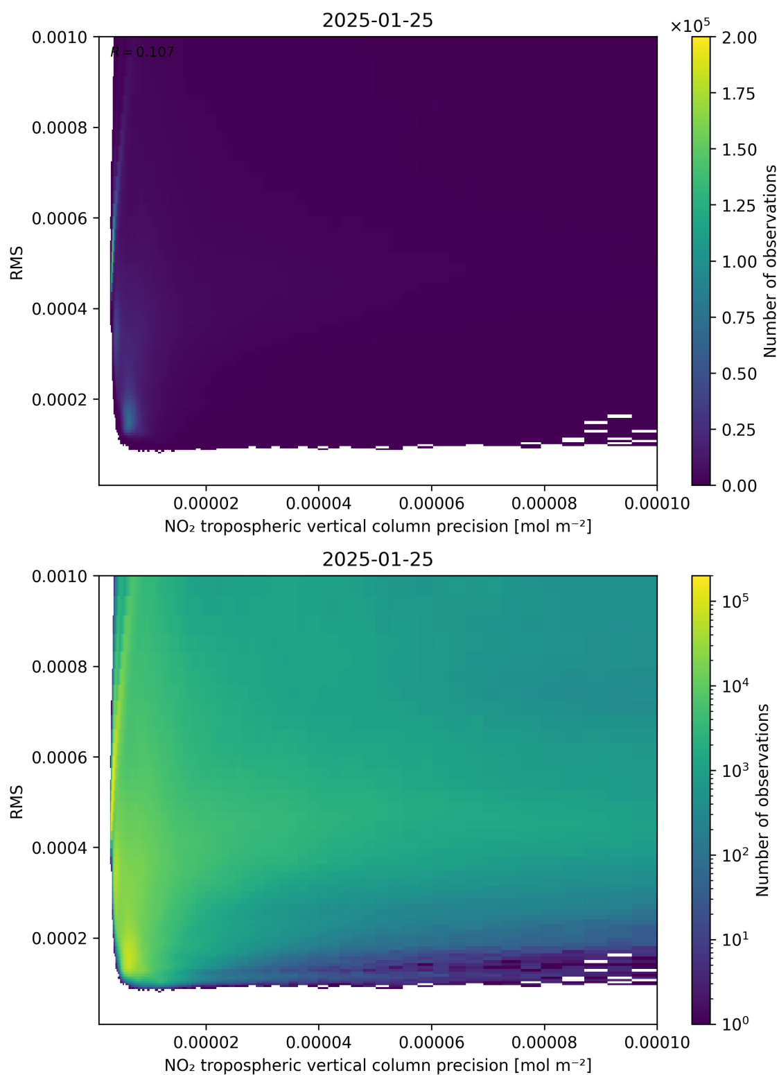
Figure 140: Scatter density plot of “NO 2 tropospheric vertical column precision” against “RMS” for 2025-01-24 to 2025-01-26.
