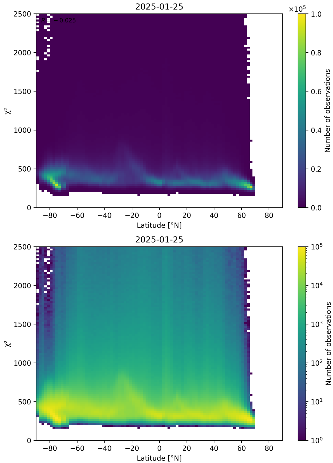
Figure 86: Scatter density plot of “Latitude” against “ \chi^2 ” for 2025-01-24 to 2025-01-26.
