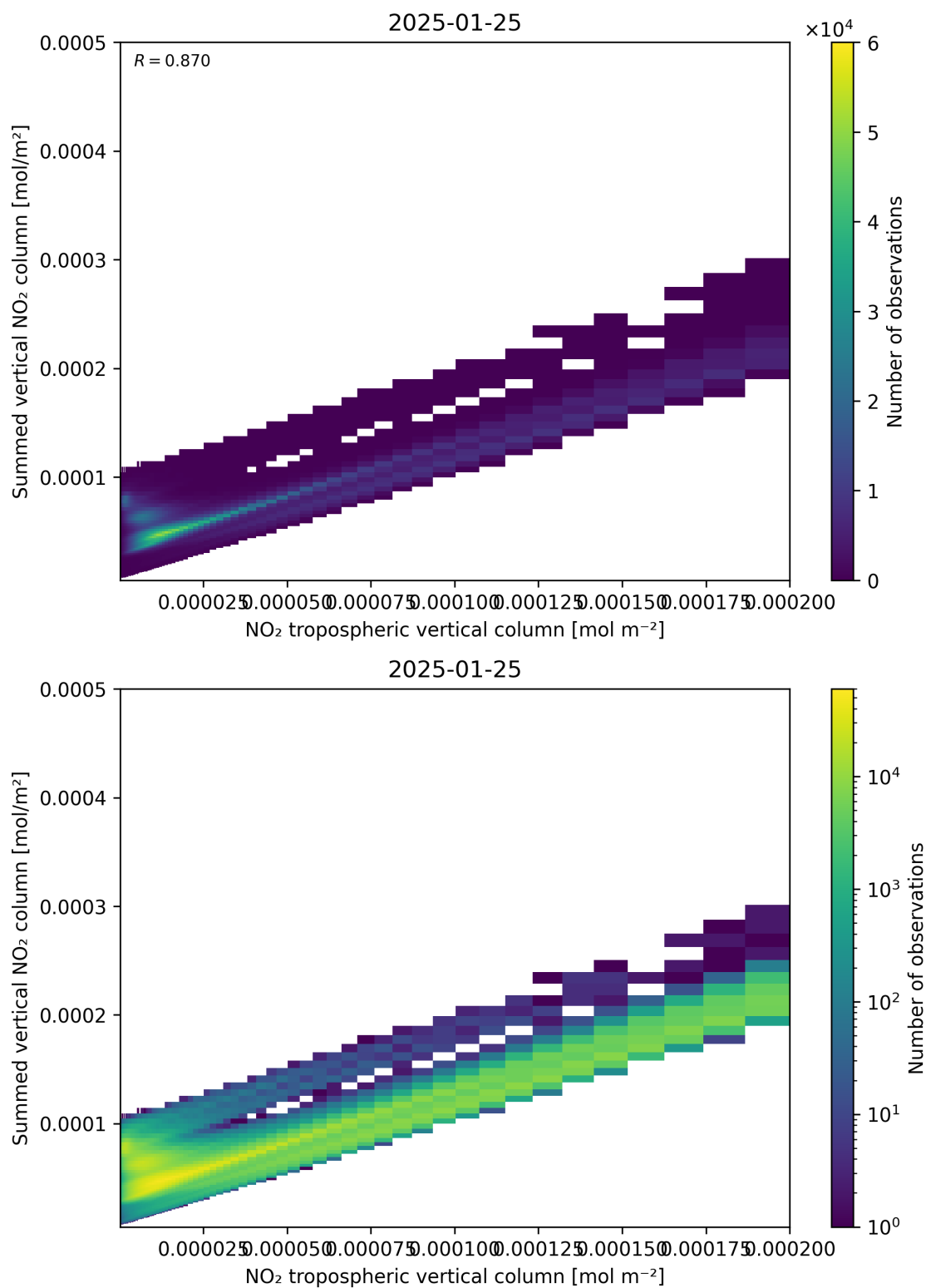
Figure 126: Scatter density plot of “NO 2 tropospheric vertical column” against “Summed vertical NO 2 column” for 2025-01-24 to 2025-01-26.
