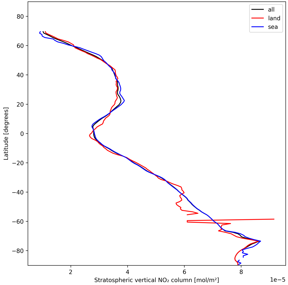
Figure 19: Zonal average of “Stratospheric vertical NO 2 column” for 2025-01-24 to 2025-01-26.
