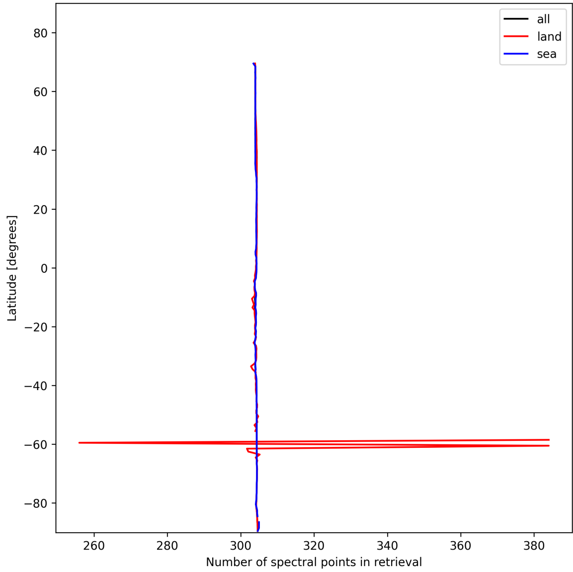
Figure 16: Zonal average of “Number of spectral points in retrieval” for 2025-01-24 to 2025-01-26.
