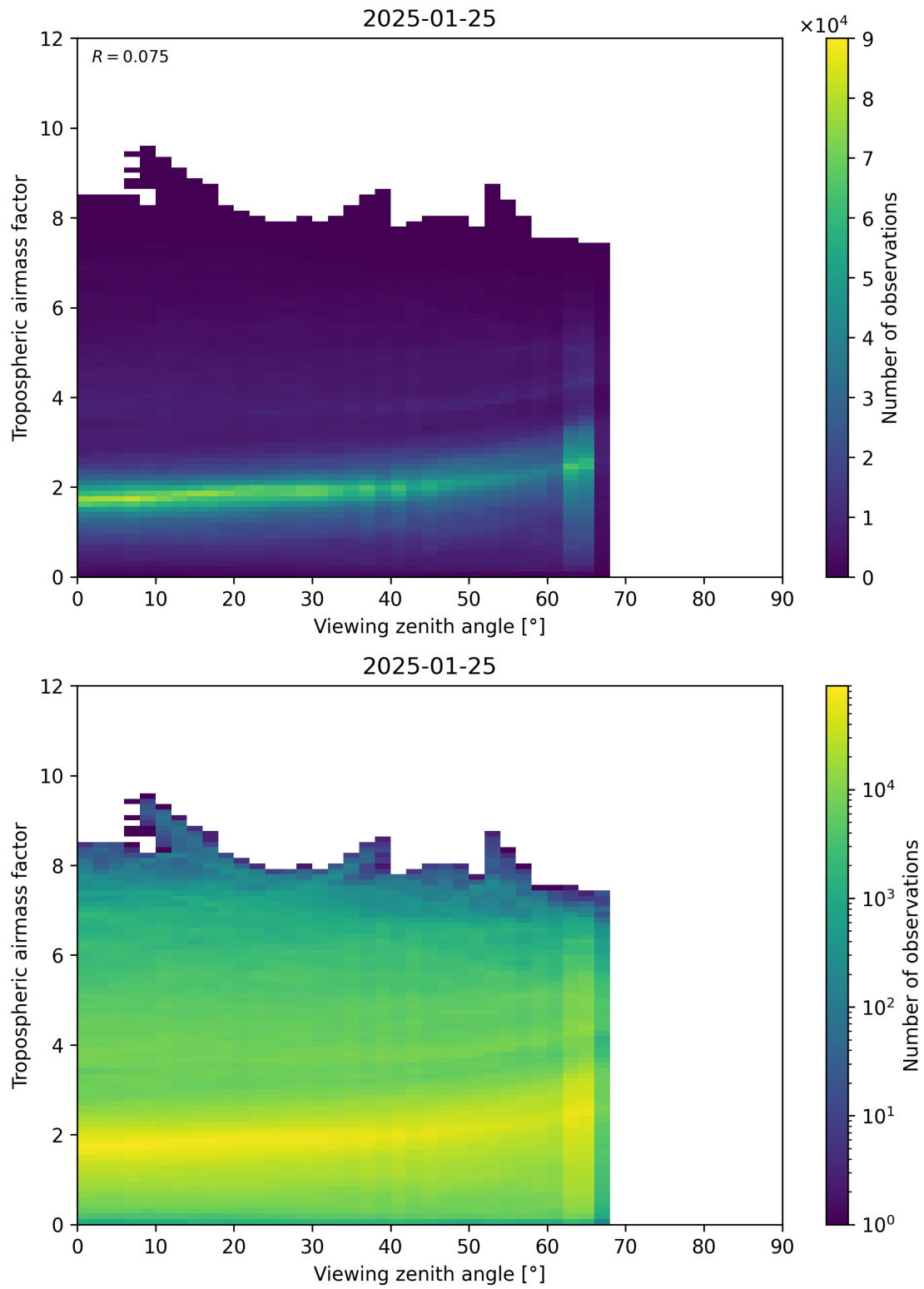
Figure 161: Scatter density plot of “Viewing zenith angle” against “Tropospheric airmass factor” for 2025-01-24 to 2025-01-26.
