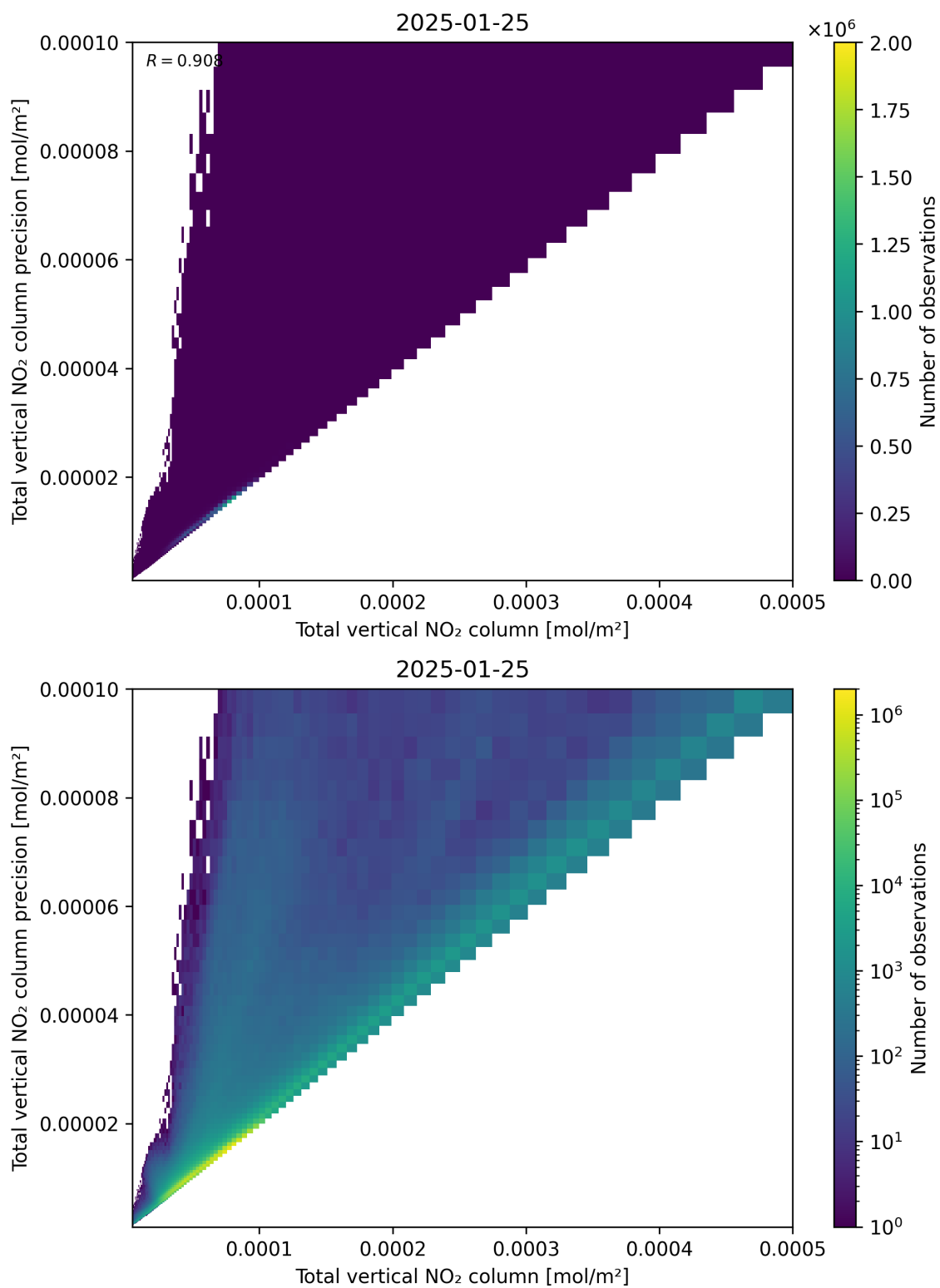
Figure 114: Scatter density plot of “Total vertical NO 2 column” against “Total vertical NO 2 column precision” for 2025-01-24 to 2025-01-26.
