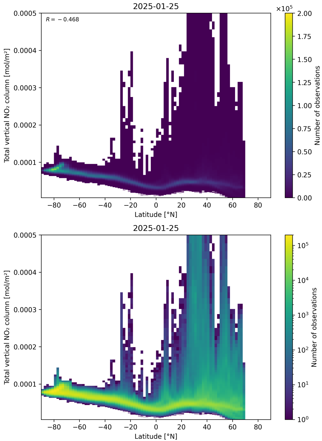
Figure 90: Scatter density plot of “Latitude” against “Total vertical NO 2 column” for 2025-01-24 to 2025-01-26.
