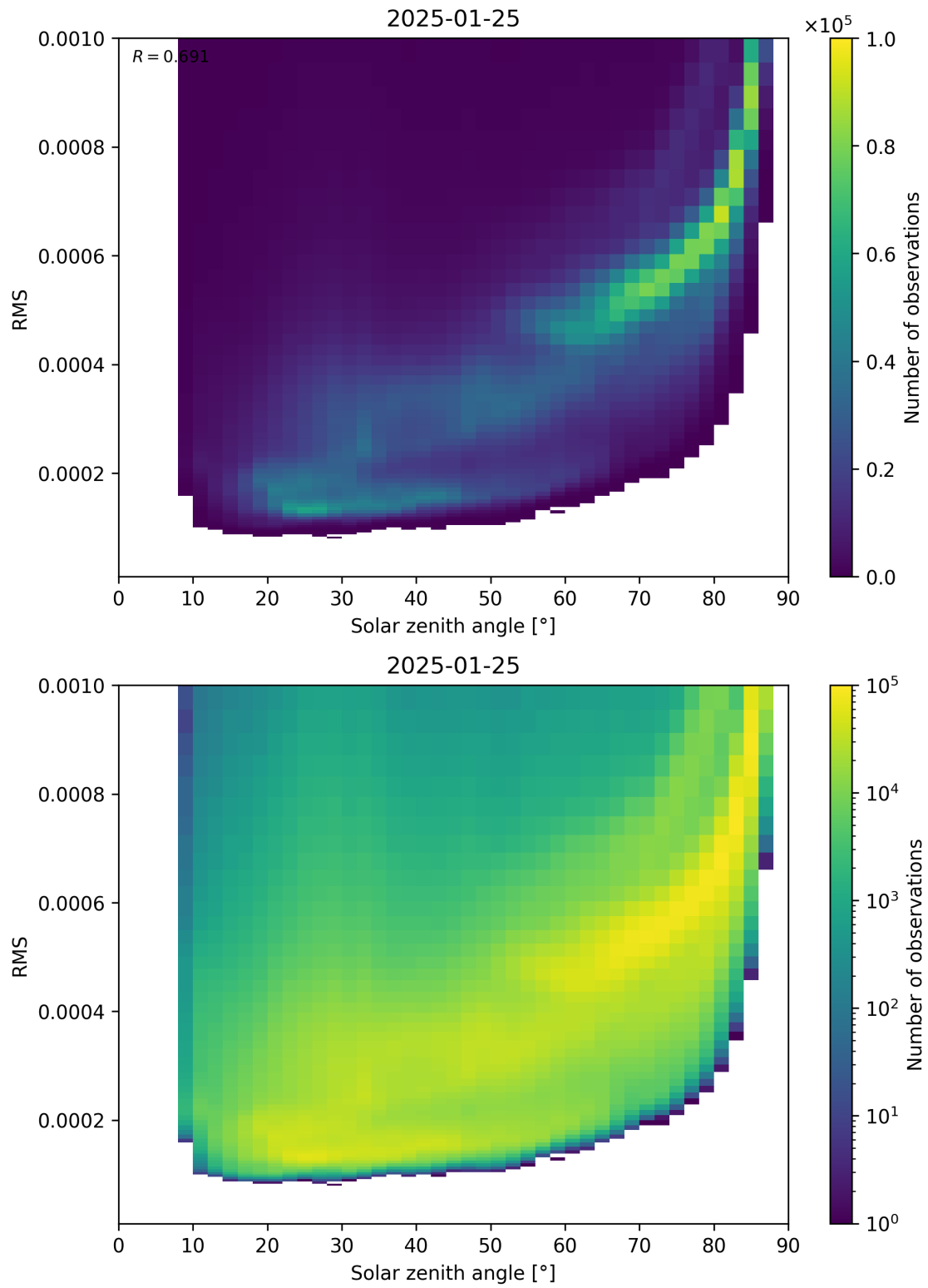
Figure 157: Scatter density plot of “Solar zenith angle” against “RMS” for 2025-01-24 to 2025-01-26.
