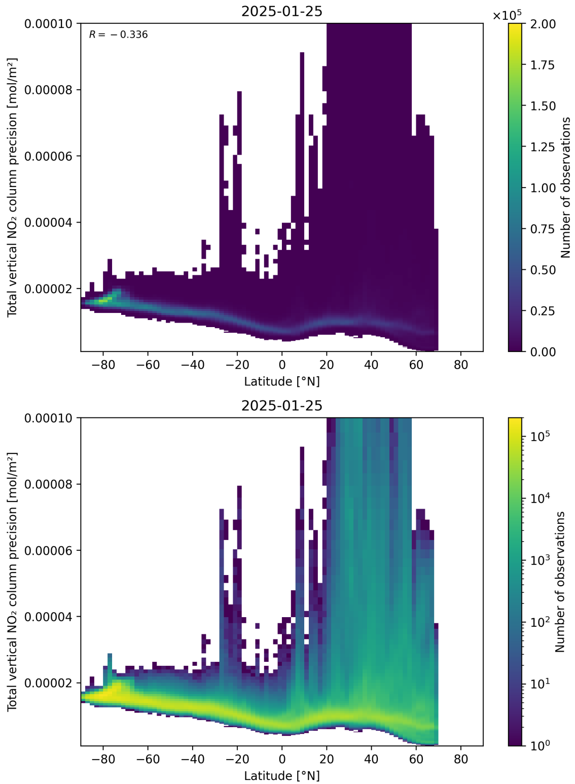
Figure 91: Scatter density plot of “Latitude” against “Total vertical NO 2 column precision” for 2025-01-24 to 2025-01-26.
