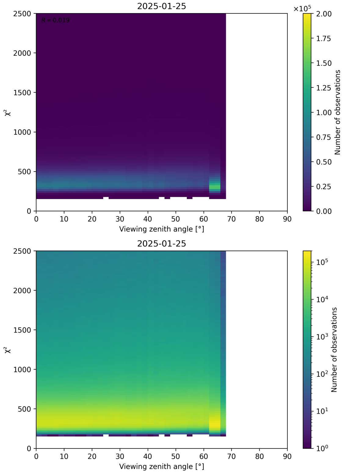
Figure 162: Scatter density plot of “Viewing zenith angle” against “ \chi^2 ” for 2025-01-24 to 2025-01-26.
