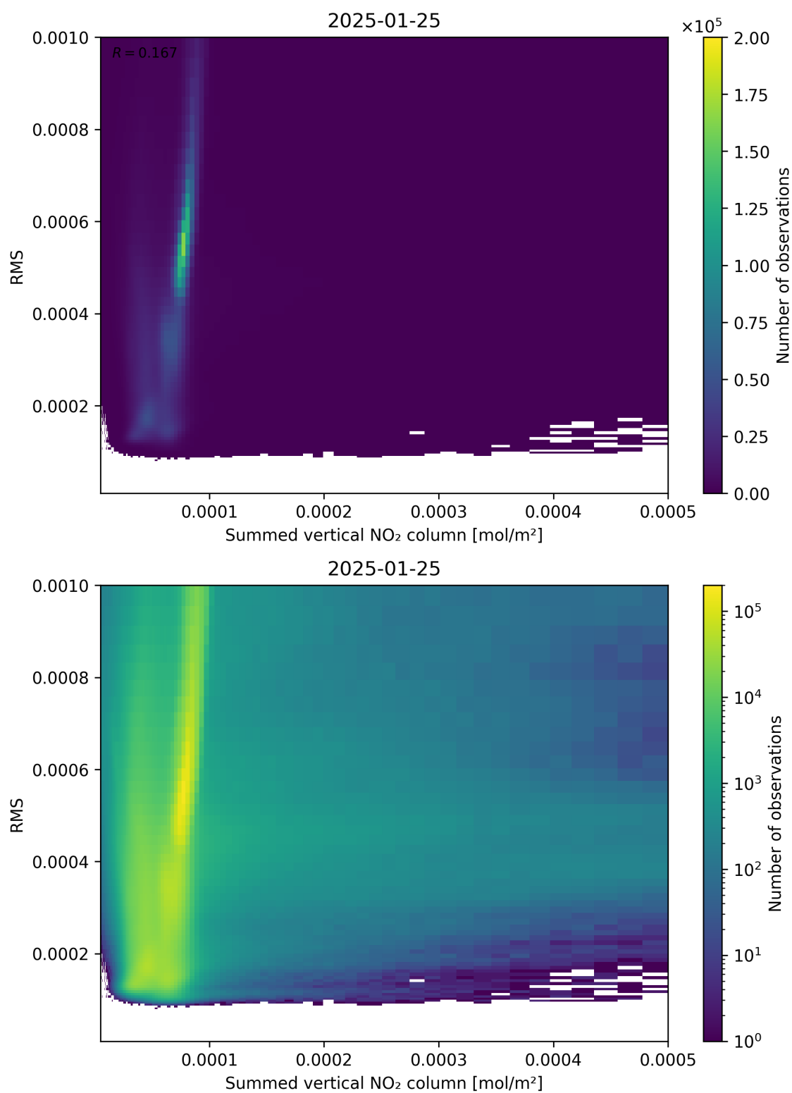
Figure 109: Scatter density plot of “Summed vertical NO 2 column” against “RMS” for 2025-01-24 to 2025-01-26.
