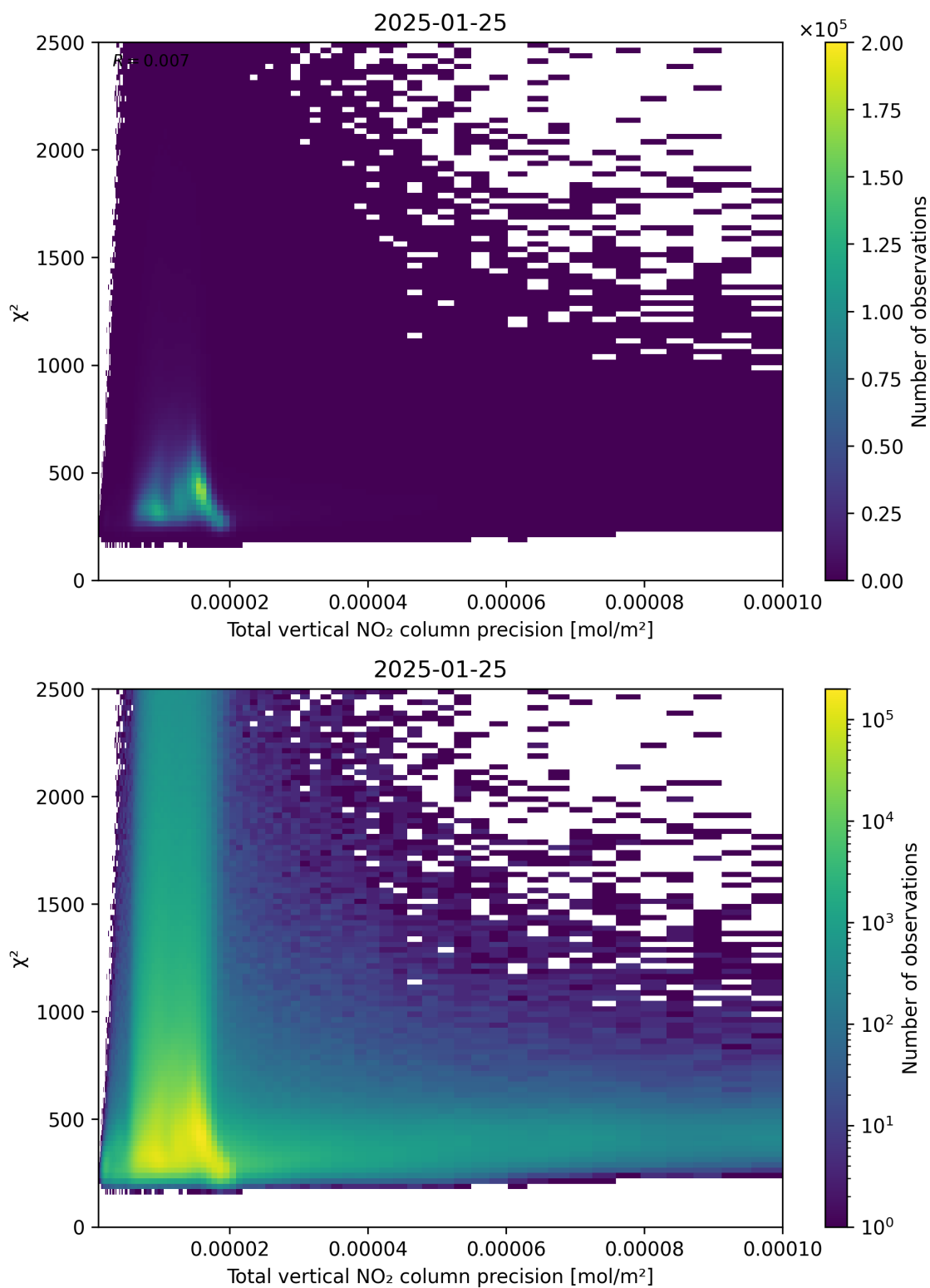
Figure 116: Scatter density plot of “Total vertical NO 2 column precision” against “ \chi^2 ” for 2025-01-24 to 2025-01-26.
