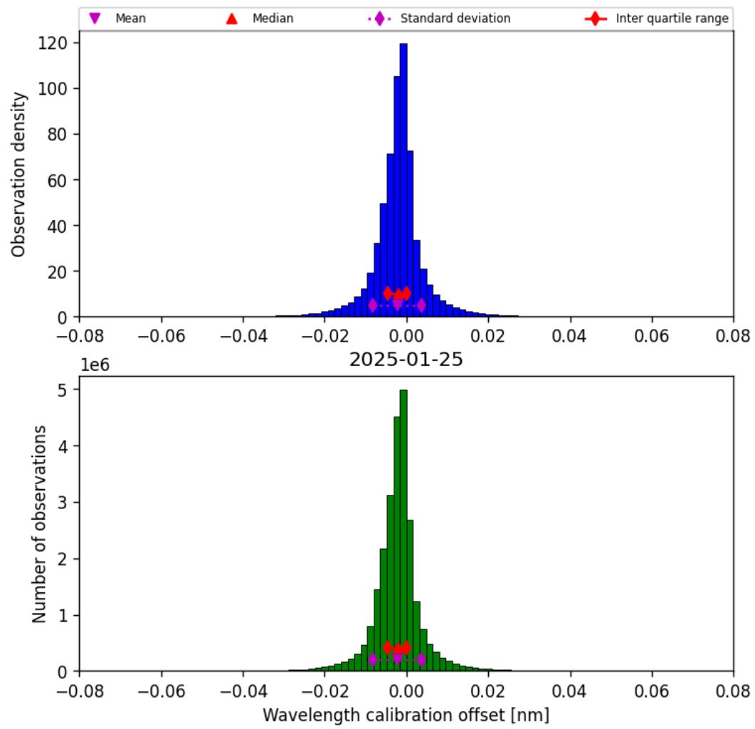
Figure 35: Histogram of “Wavelength calibration offset” for 2025-01-24 to 2025-01-26
