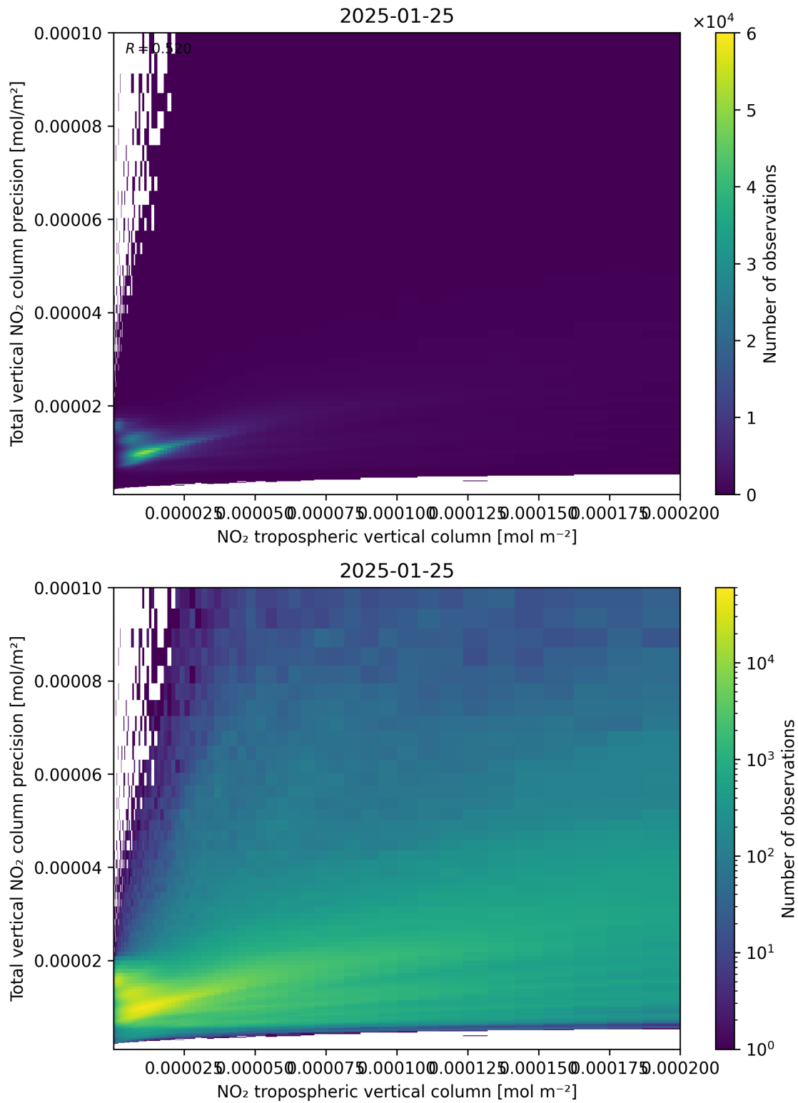
Figure 129: Scatter density plot of “NO 2 tropospheric vertical column” against “Total vertical NO 2 column precision” for 2025-01-24 to 2025-01-26.
