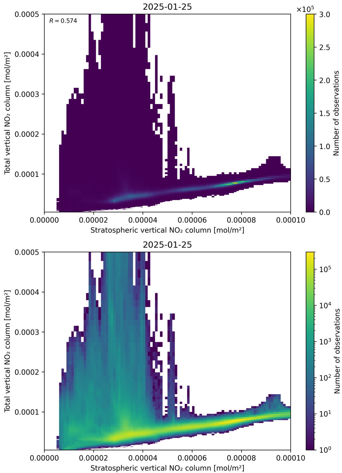
Figure 100: Scatter density plot of “Stratospheric vertical NO 2 column” against “Total vertical NO 2 column” for 2025-01-24 to 2025-01-26.
