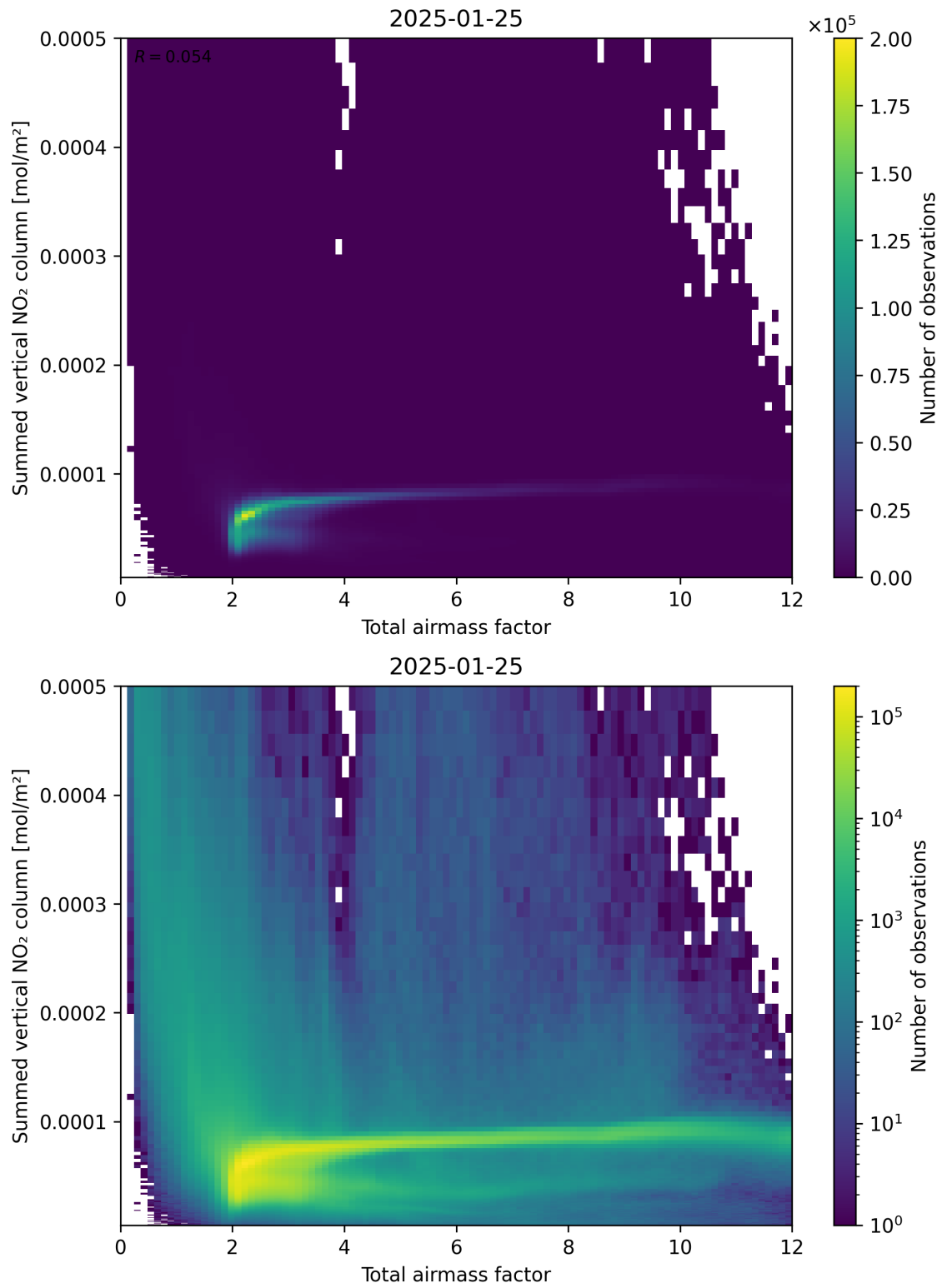
Figure 65: Scatter density plot of “Total airmass factor” against “Summed vertical NO 2 column” for 2025-01-24 to 2025-01-26.
