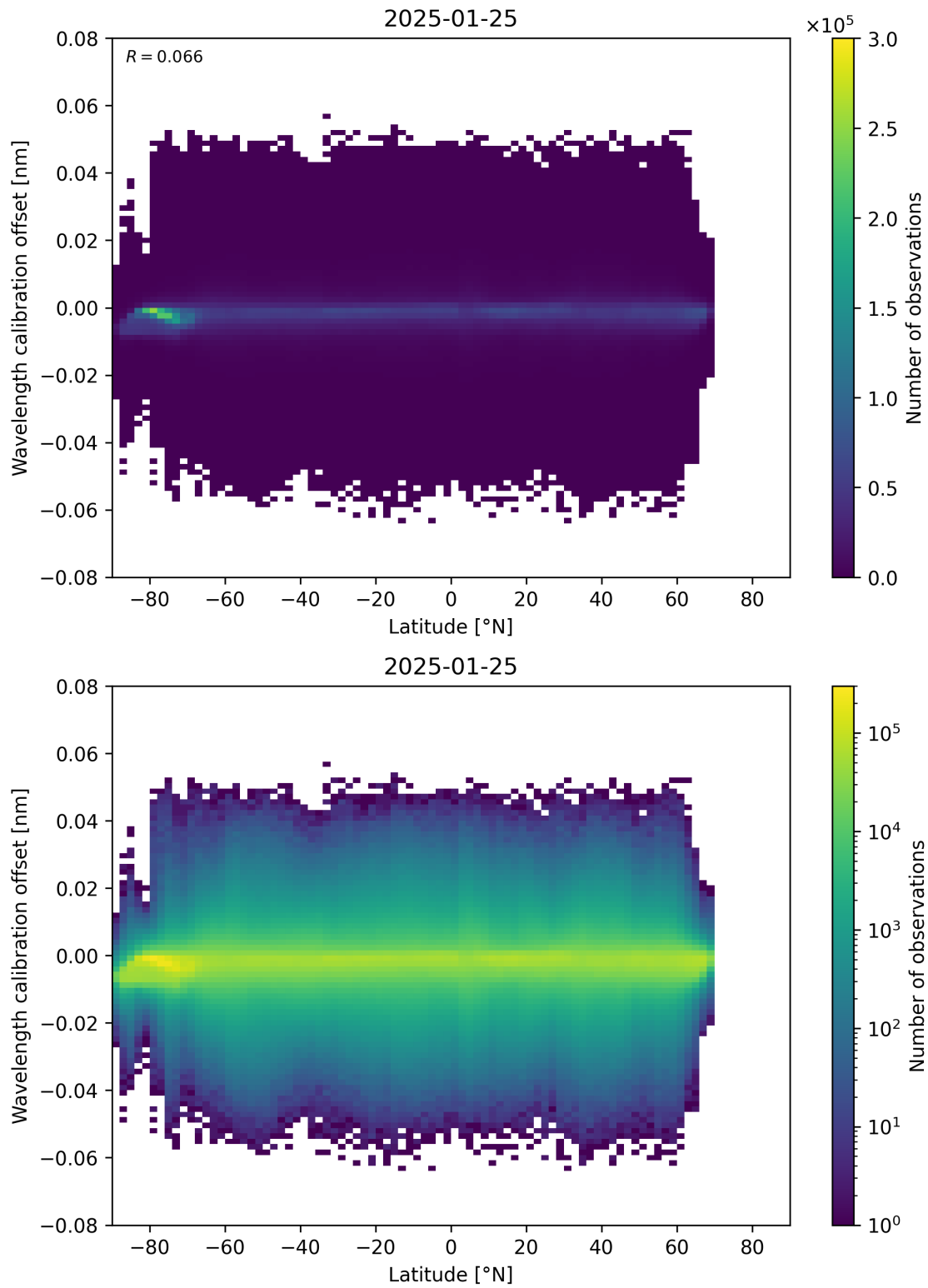
Figure 95: Scatter density plot of “Latitude” against “Wavelength calibration offset” for 2025-01-24 to 2025-01-26.
