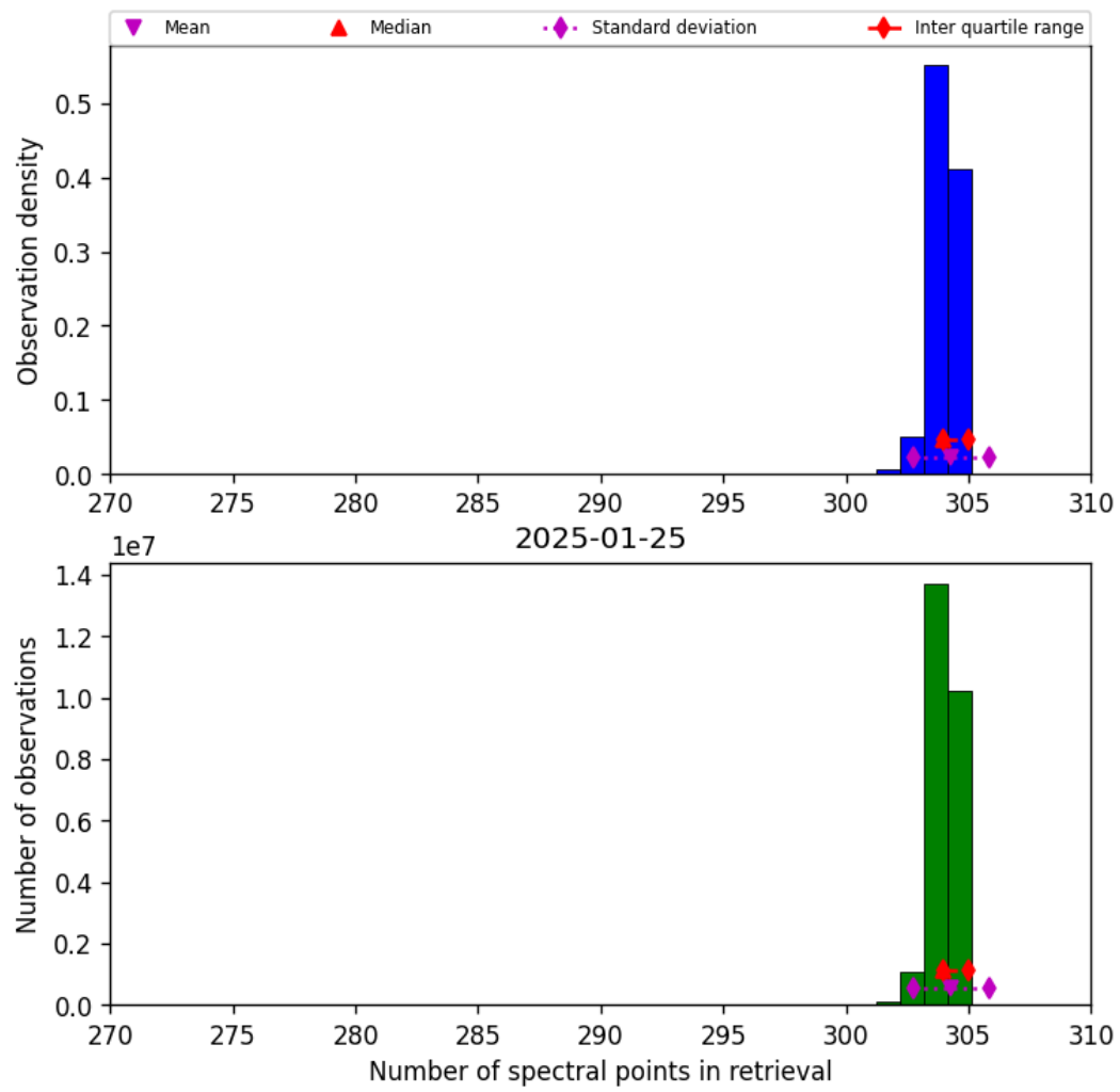
Figure 33: Histogram of “Number of spectral points in retrieval” for 2025-01-24 to 2025-01-26
