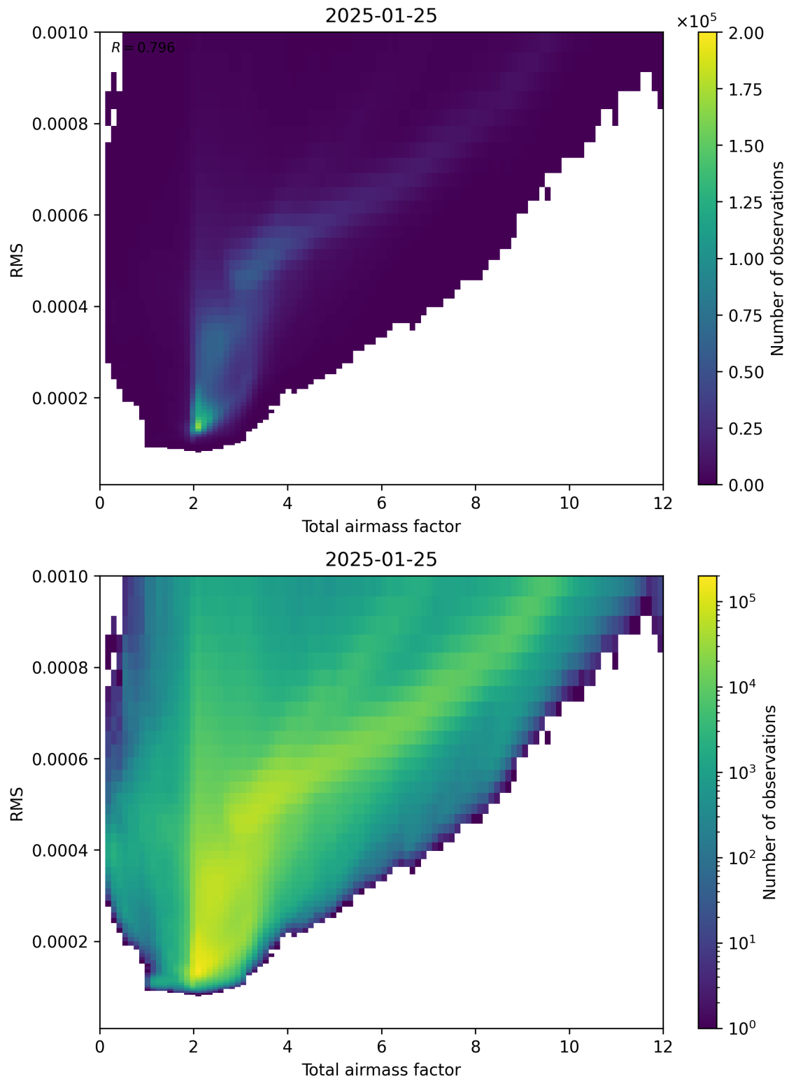
Figure 69: Scatter density plot of “Total airmass factor” against “RMS” for 2025-01-24 to 2025-01-26.
