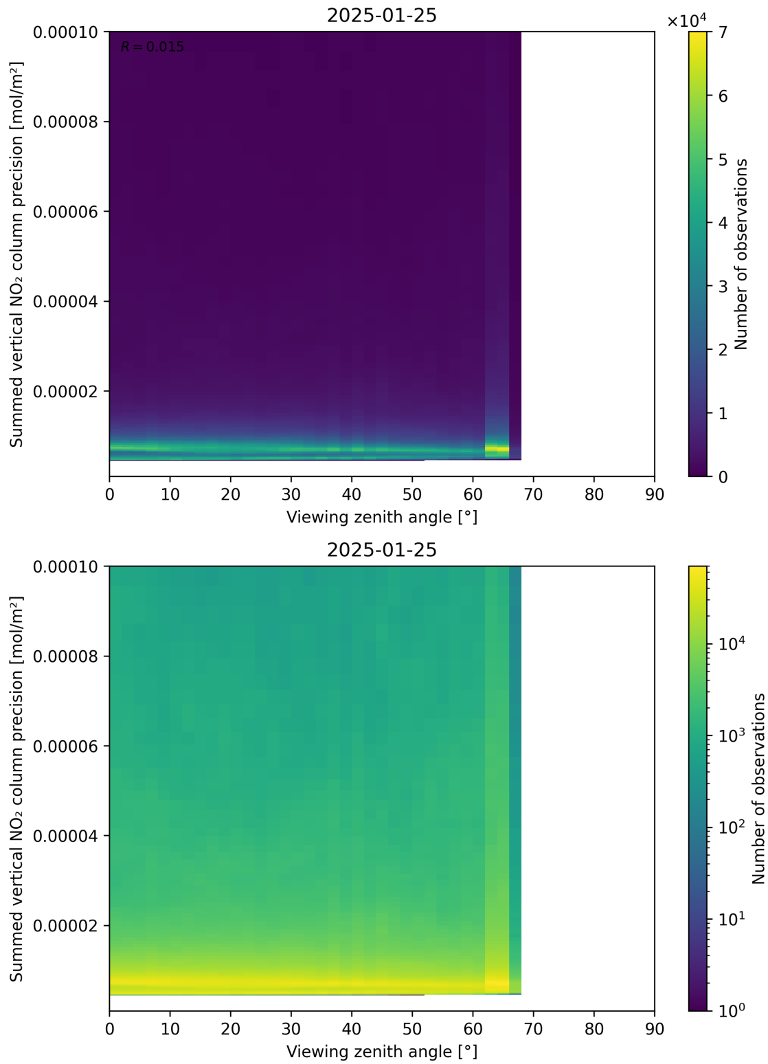
Figure 166: Scatter density plot of “Viewing zenith angle” against “Summed vertical NO 2 column precision” for 2025-01-24 to 2025-01-26.
