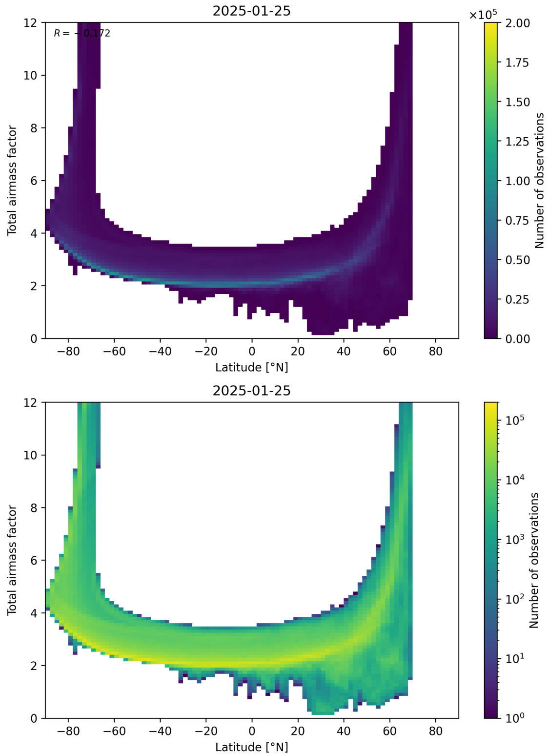
Figure 84: Scatter density plot of “Latitude” against “Total airmass factor” for 2025-01-24 to 2025-01-26.
