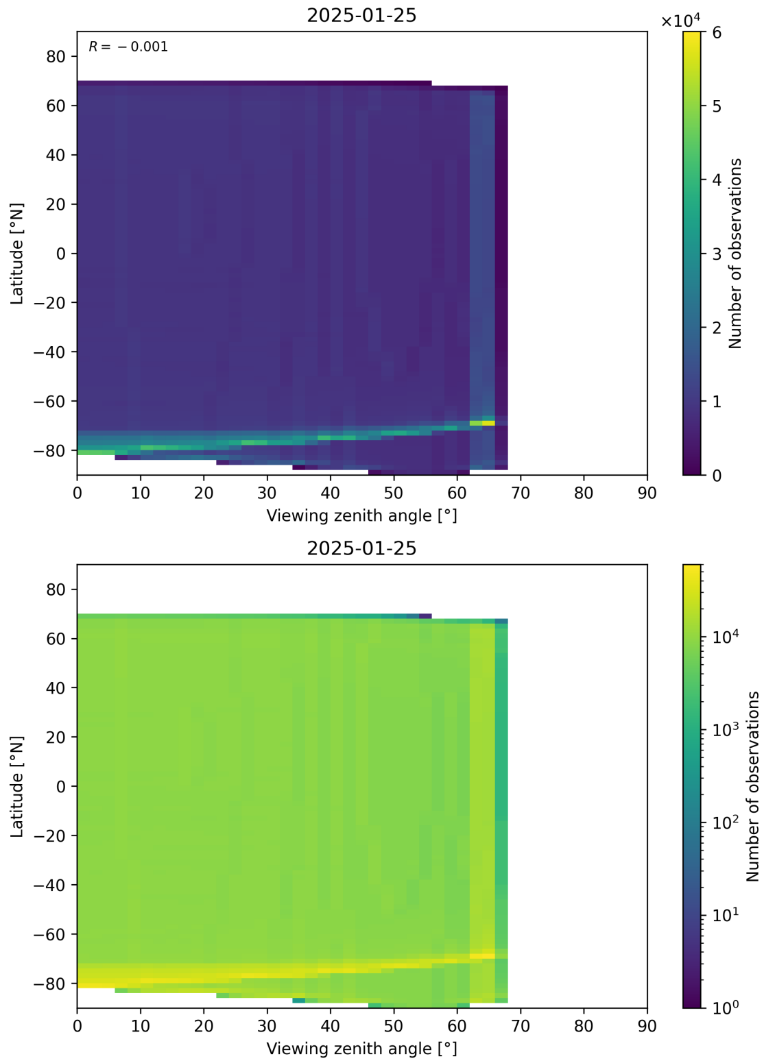
Figure 163: Scatter density plot of “Viewing zenith angle” against “Latitude” for 2025-01-24 to 2025-01-26.
