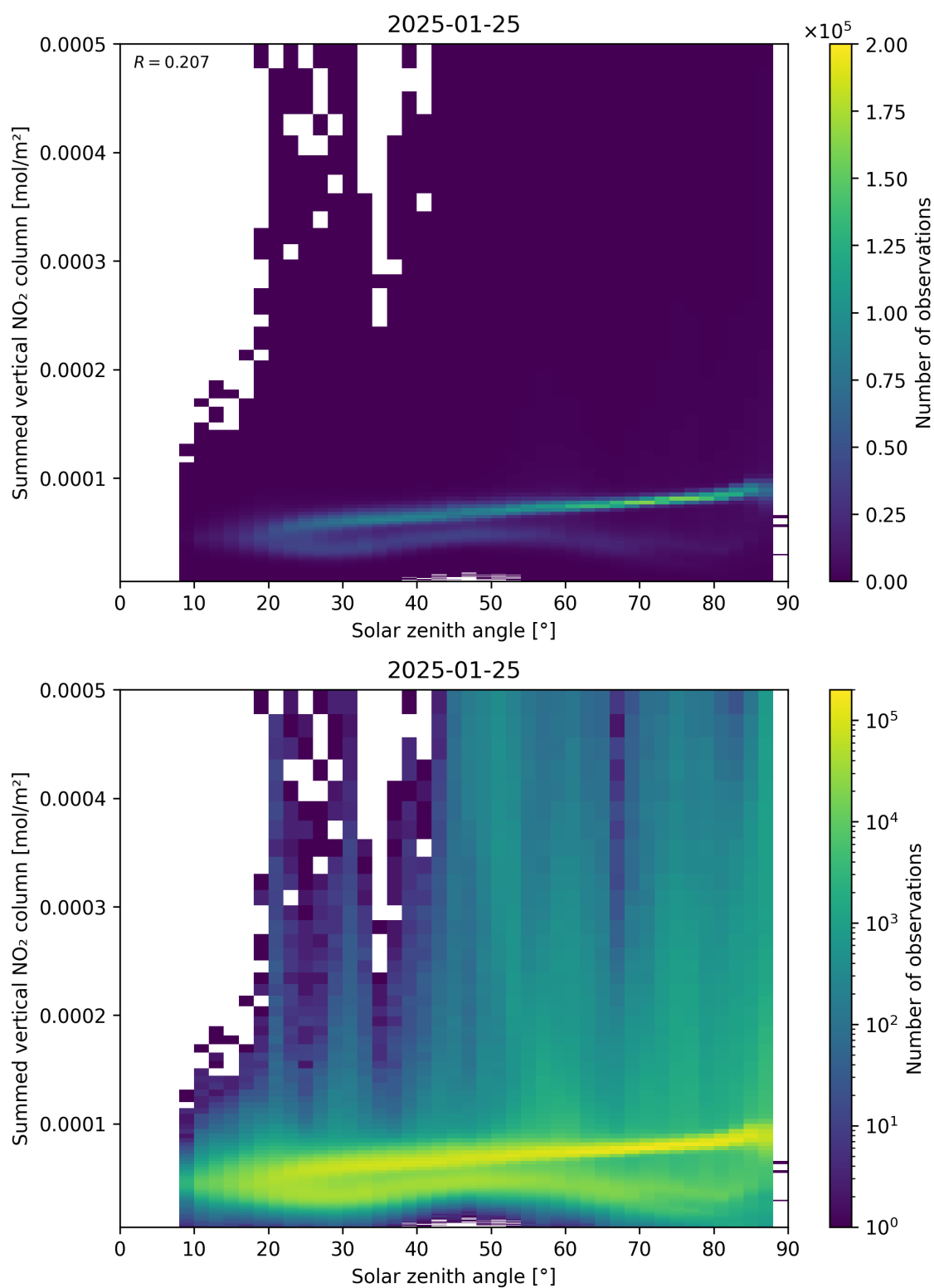
Figure 151: Scatter density plot of “Solar zenith angle” against “Summed vertical NO 2 column” for 2025-01-24 to 2025-01-26.
