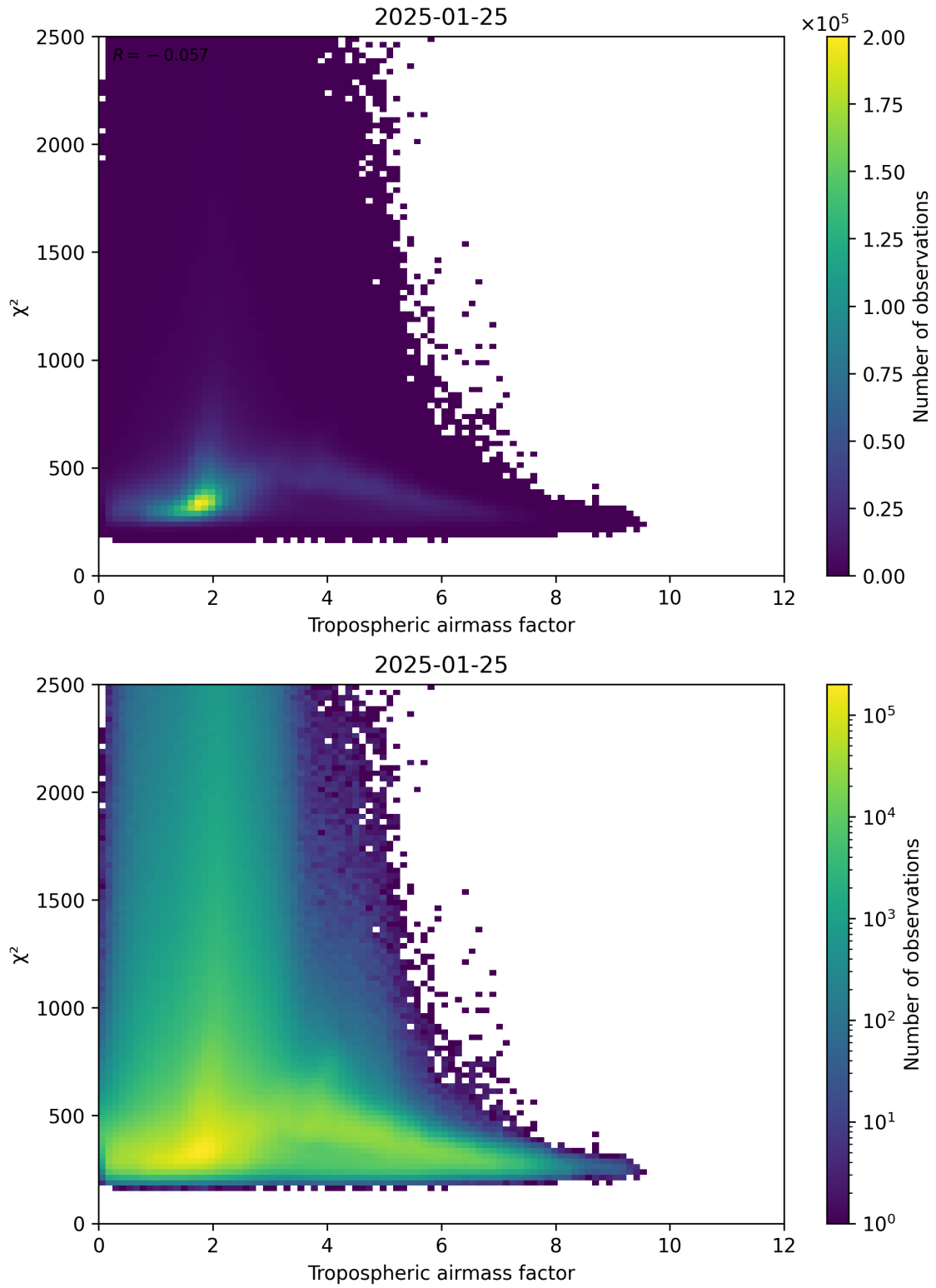
Figure 73: Scatter density plot of “Tropospheric airmass factor” against “ \chi^2 ” for 2025-01-24 to 2025-01-26.
