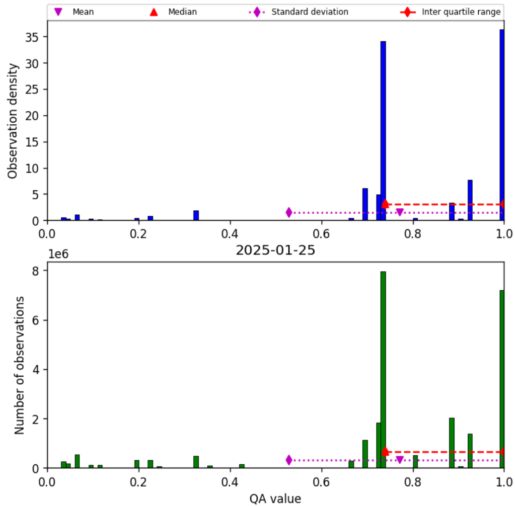
Figure 28: Histogram of “QA value” for 2025-01-24 to 2025-01-26
