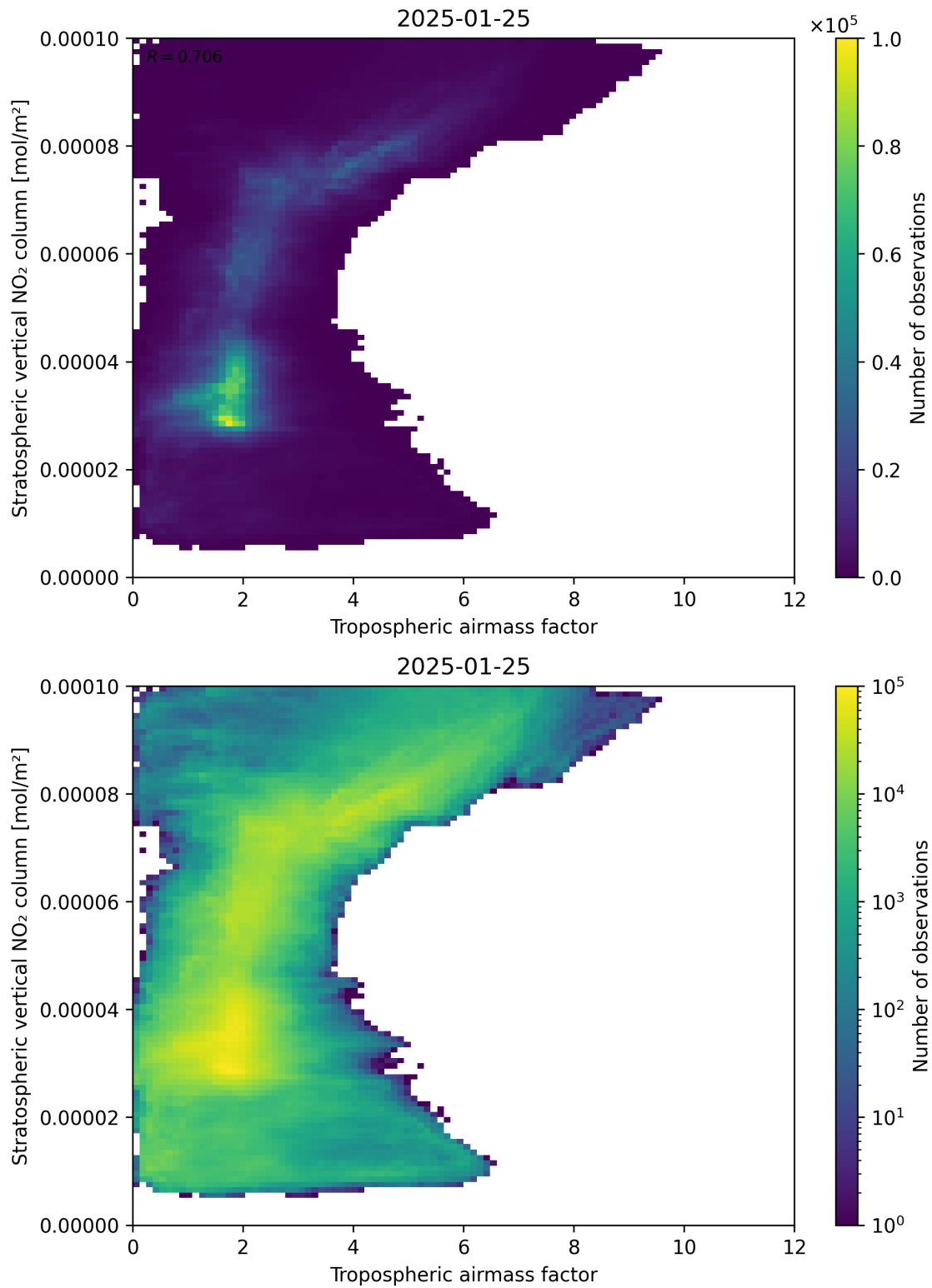
Figure 74: Scatter density plot of “Tropospheric air mass factor” against “Stratospheric vertical NO 2 column” for 2025-01-24 to 2025-01-26.
