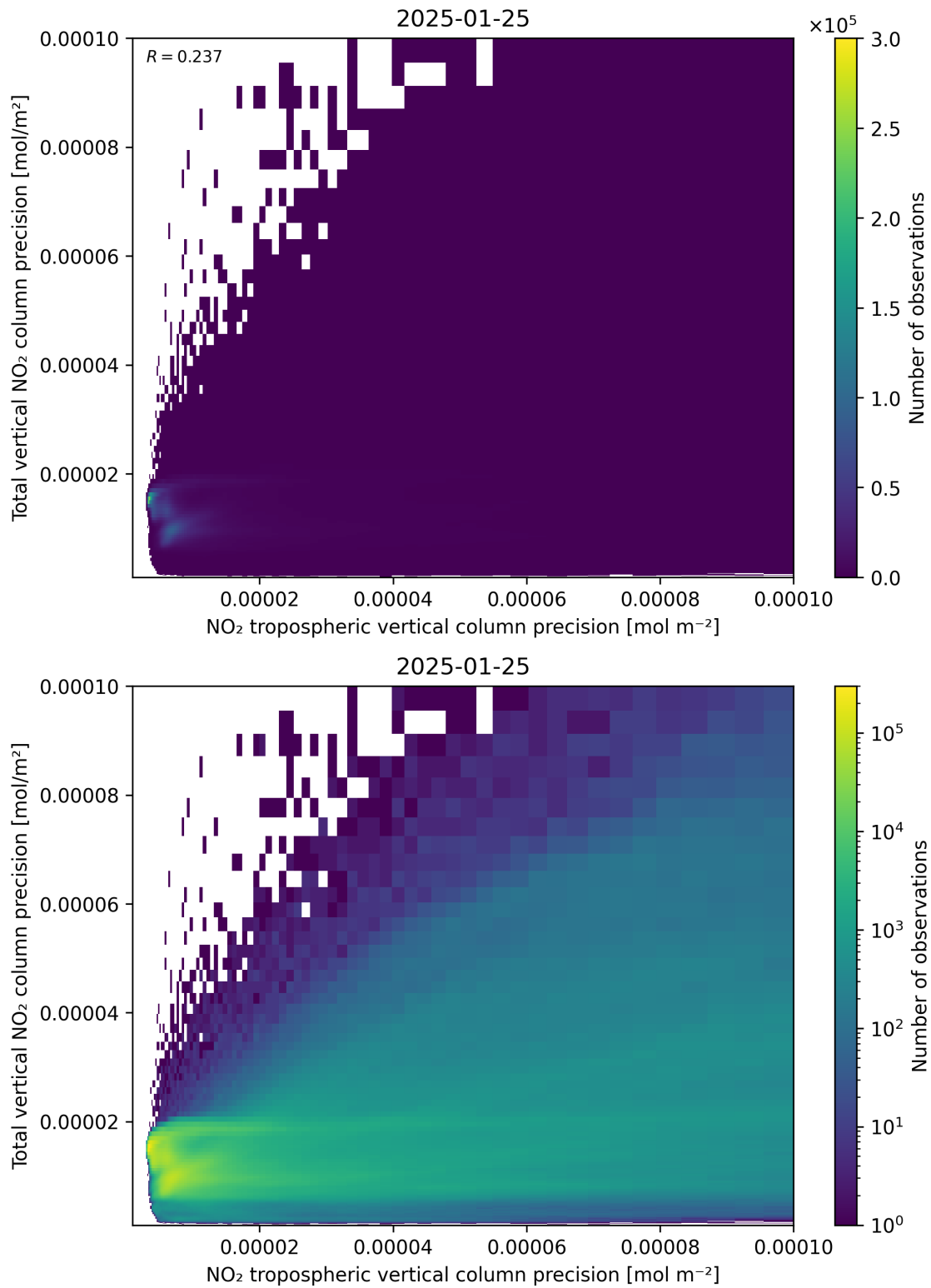
Figure 139: Scatter density plot of “NO 2 tropospheric vertical column precision” against “Total vertical NO 2 column precision” for 2025-01-24 to 2025-01-26.
