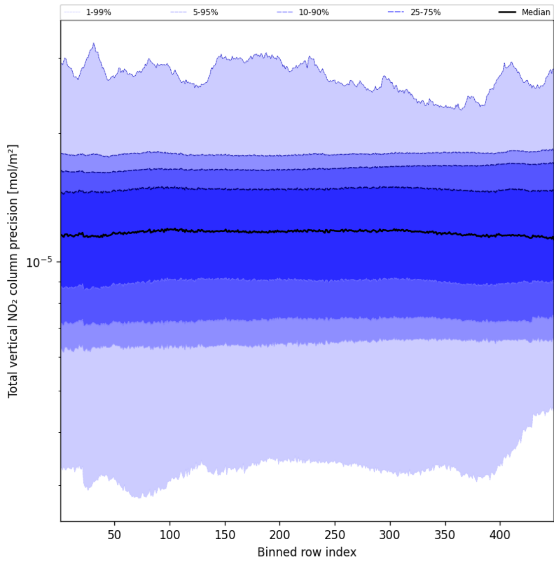
Figure 56: Along track statistics of “Total vertical NO 2 column precision” for 2025-01-24 to 2025-01-26
