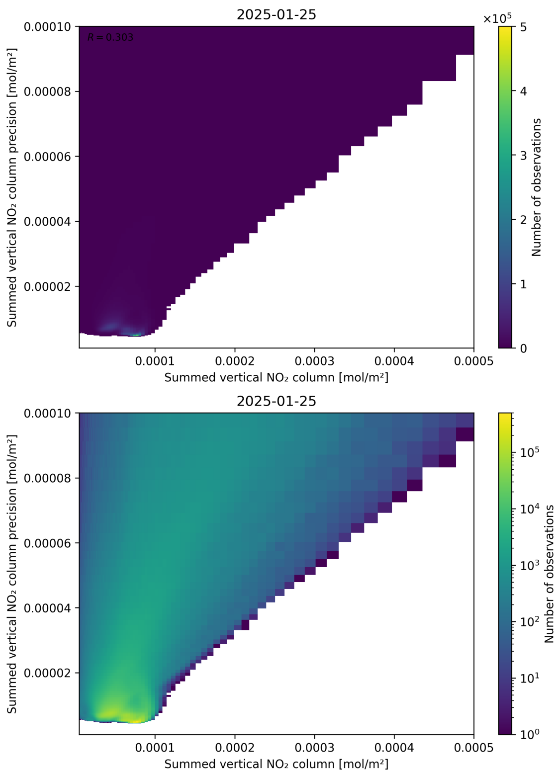
Figure 105: Scatter density plot of “Summed vertical NO 2 column” against “Summed vertical NO 2 column precision” for 2025-01-24 to 2025-01-26.
