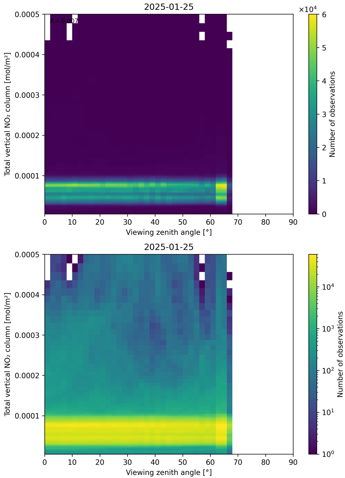
Figure 167: Scatter density plot of “Viewing zenith angle” against “Total vertical NO 2 column” for 2025-01-24 to 2025-01-26.
