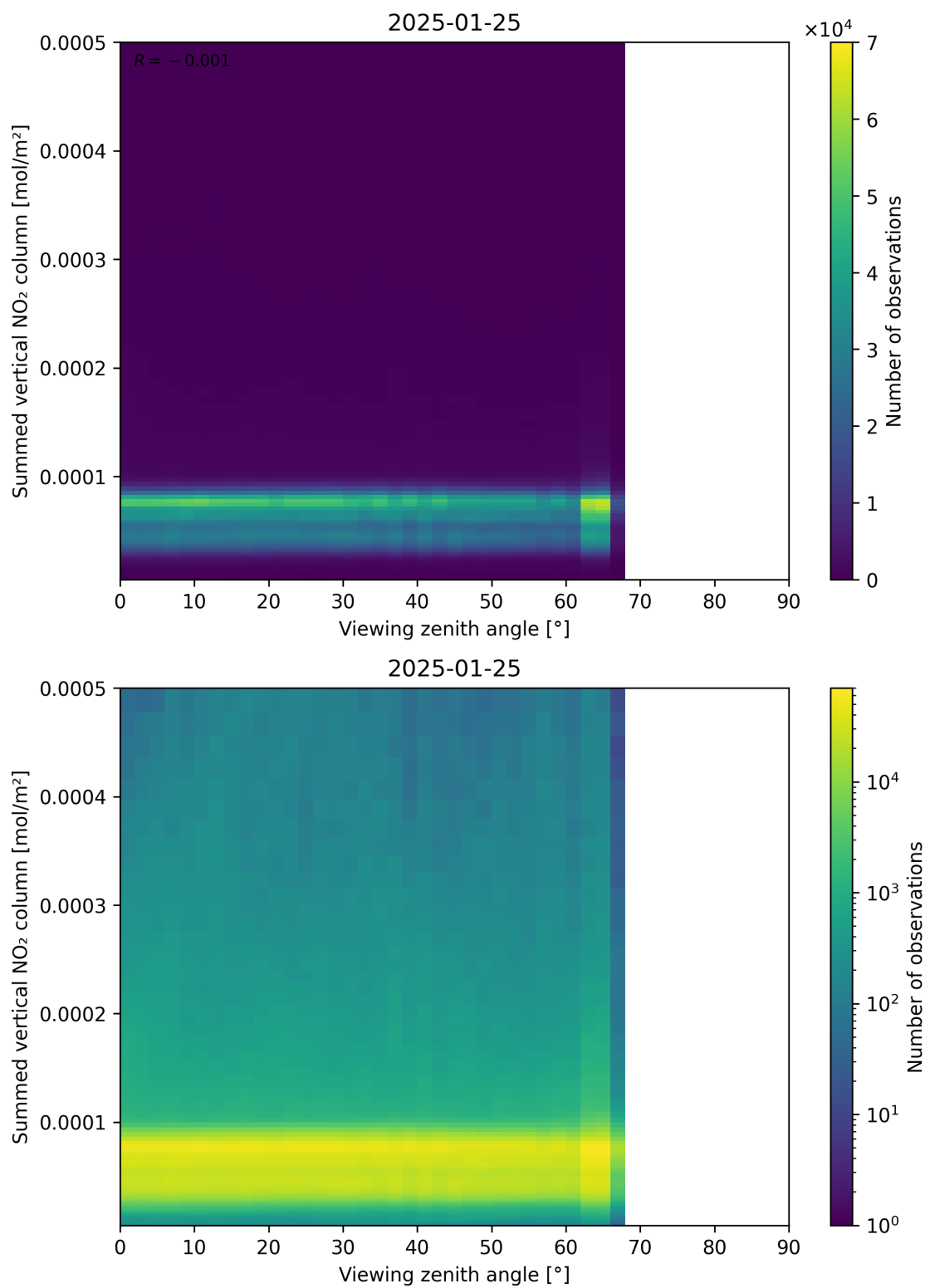
Figure 165: Scatter density plot of “Viewing zenith angle” against “Summed vertical NO 2 column” for 2025-01-24 to 2025-01-26.
