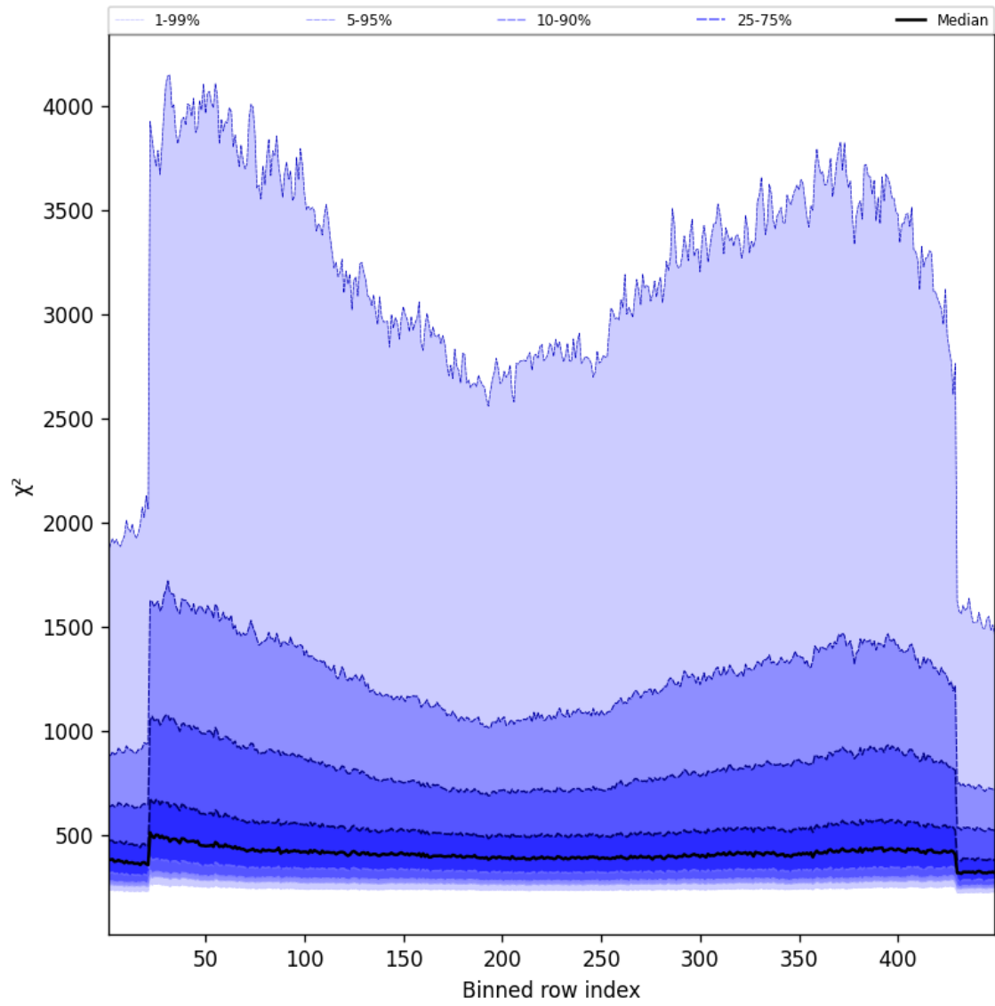
Figure 59: Along track statistics of “ \chi^2 ” for 2025-01-24 to 2025-01-26
