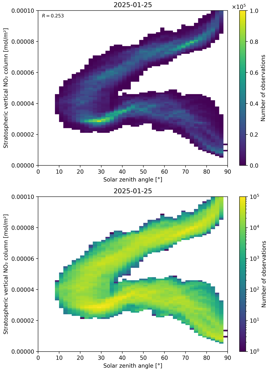
Figure 150: Scatter density plot of “Solar zenith angle” against “Stratospheric vertical NO 2 column” for 2025-01-24 to 2025-01-26.
