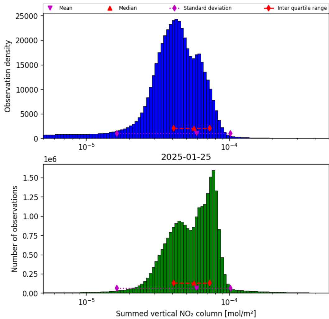
Figure 40: Histogram of “Summed vertical NO 2 column” for 2025-01-24 to 2025-01-26
