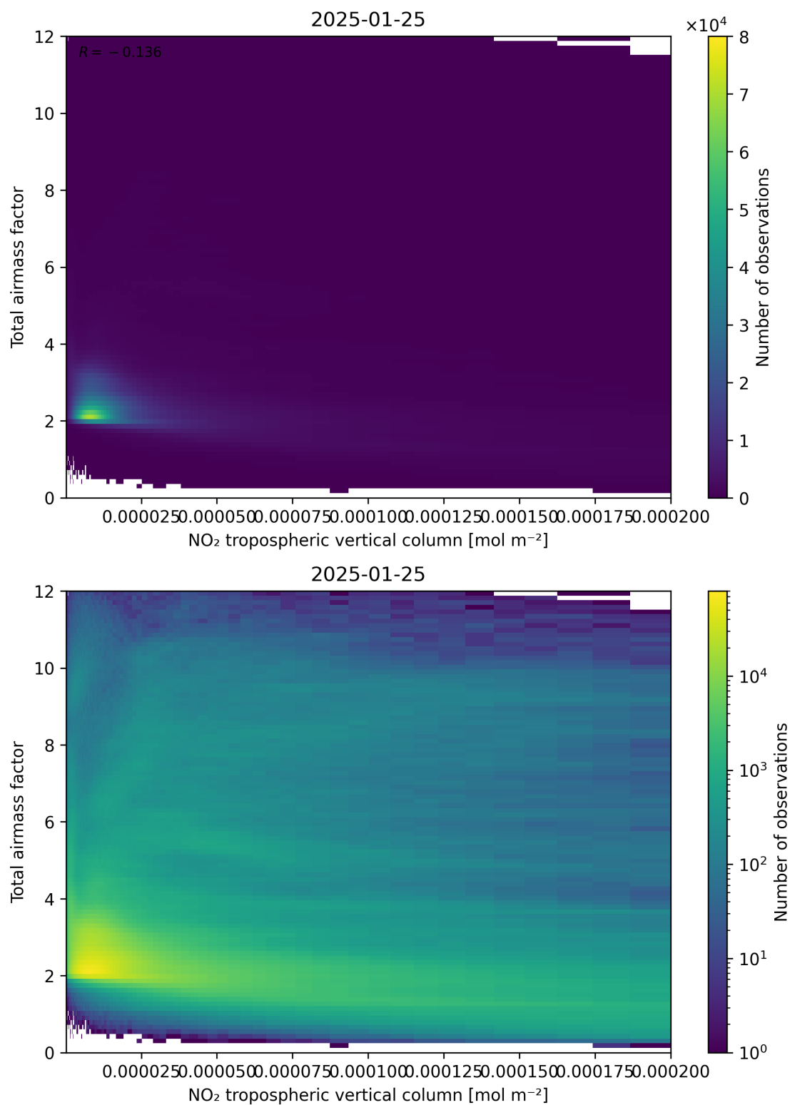
Figure 122: Scatter density plot of “NO 2 tropospheric vertical column” against “Total air mass factor” for 2025-01-24 to 2025-01-26.
