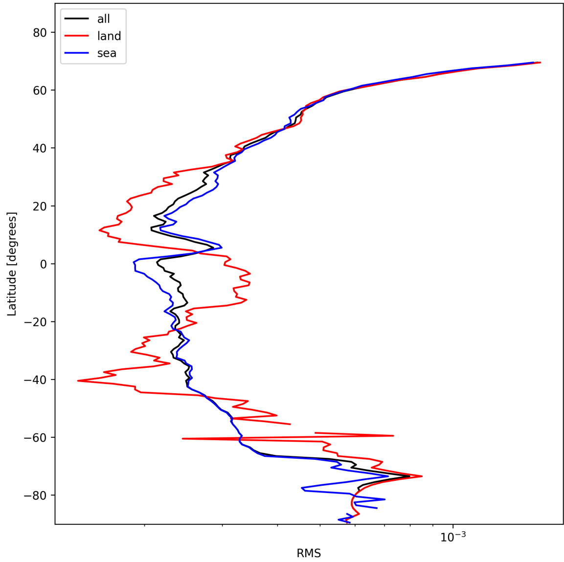
Figure 26: Zonal average of “RMS” for 2025-01-24 to 2025-01-26.
