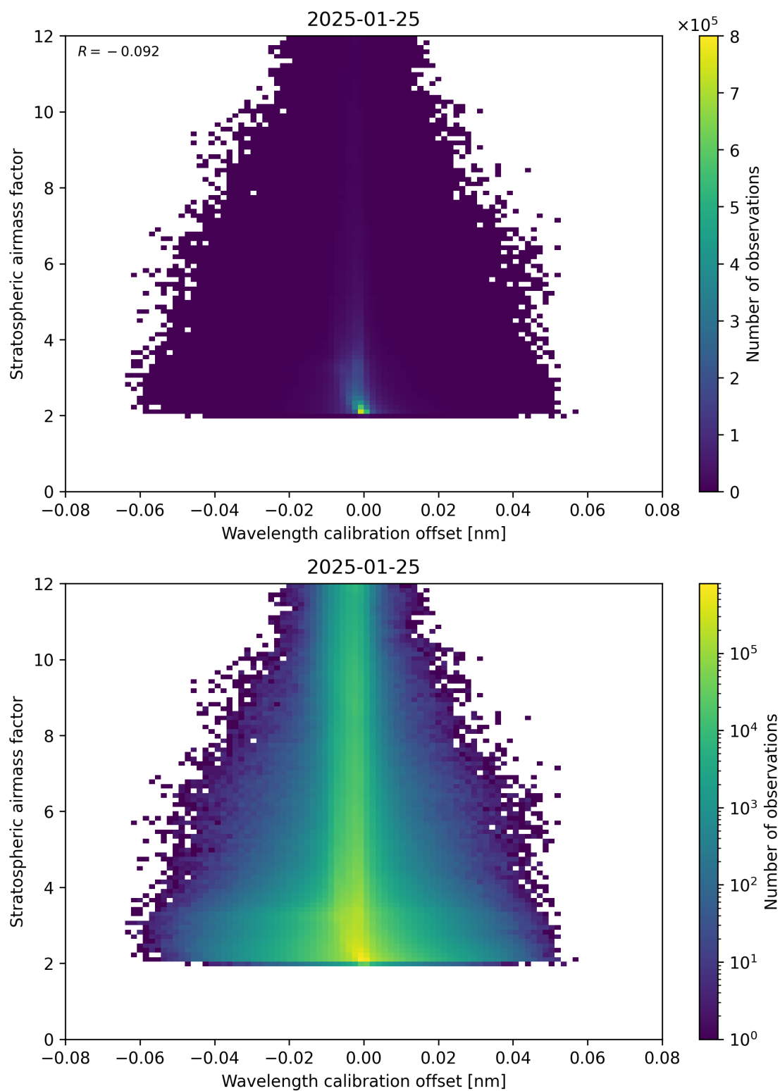
Figure 174: Scatter density plot of “Wavelength calibration offset” against “Stratospheric airmass factor” for 2025-01-24 to 2025-01-26.
