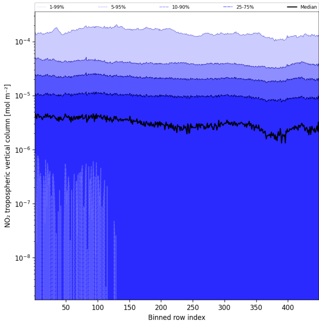
Figure 46: Along track statistics of “NO 2 tropospheric vertical column” for 2025-01-24 to 2025-01-26
