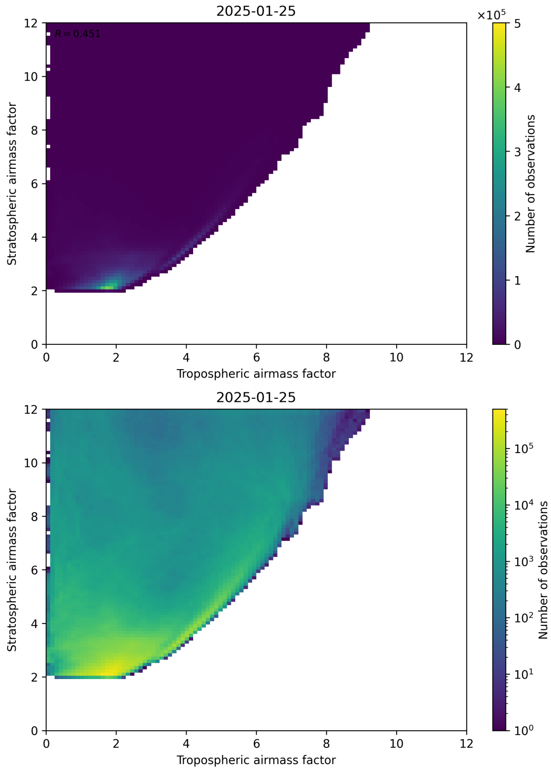
Figure 71: Scatter density plot of “Tropospheric airmass factor” against “Stratospheric airmass factor” for 2025-01-24 to 2025-01-26.
