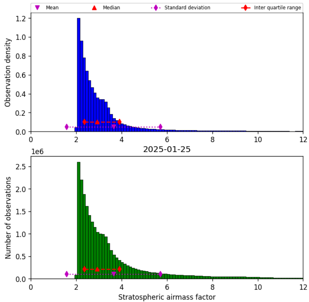
Figure 44: Histogram of “Stratospheric airmass factor” for 2025-01-24 to 2025-01-26
