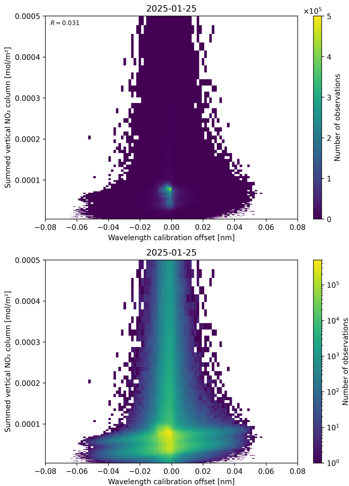
Figure 177: Scatter density plot of “Wavelength calibration offset” against “Summed vertical NO 2 column” for 2025-01-24 to 2025-01-26.
