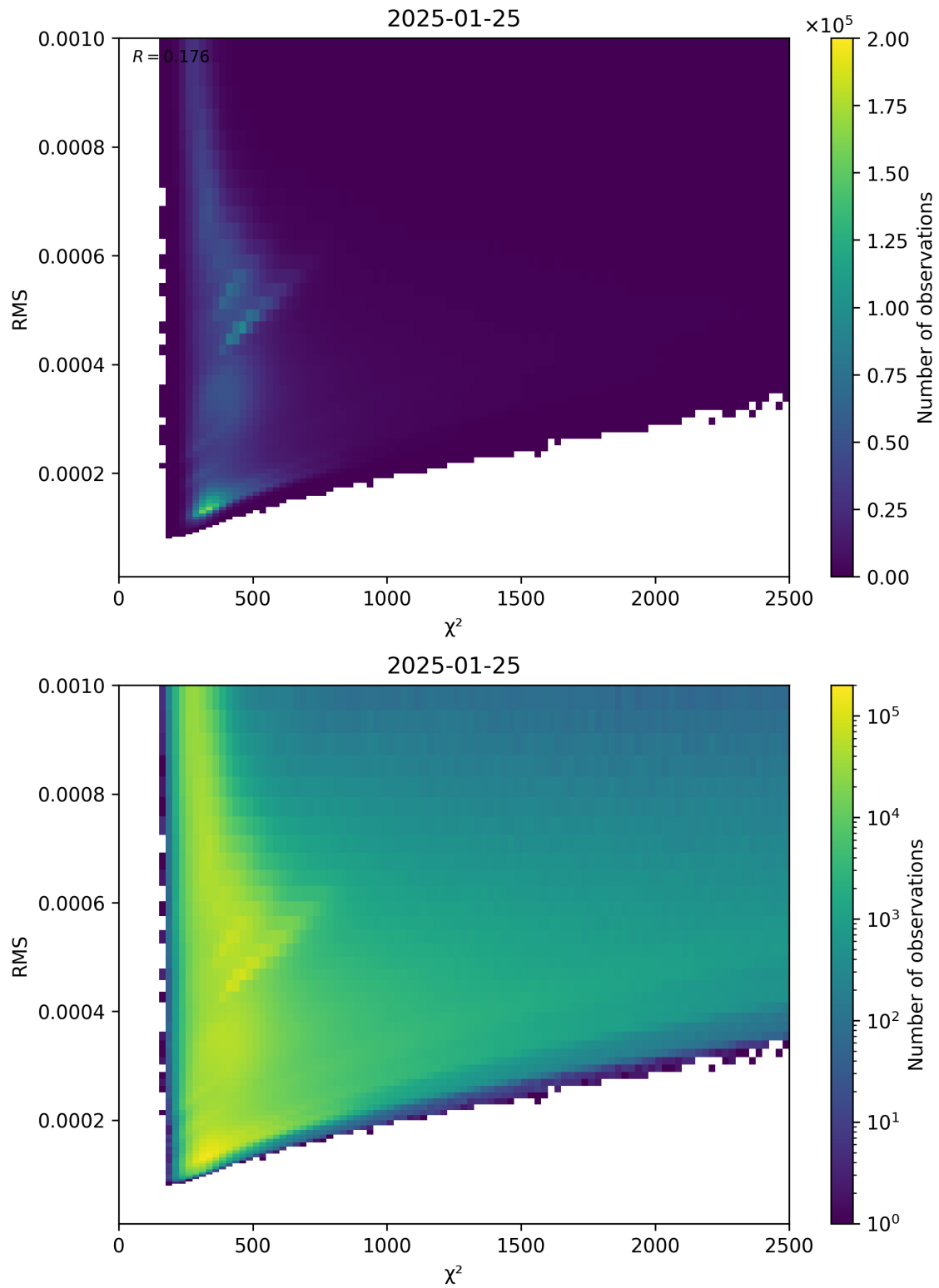
Figure 82: Scatter density plot of “ \chi^2 ” against “RMS” for 2025-01-24 to 2025-01-26.
