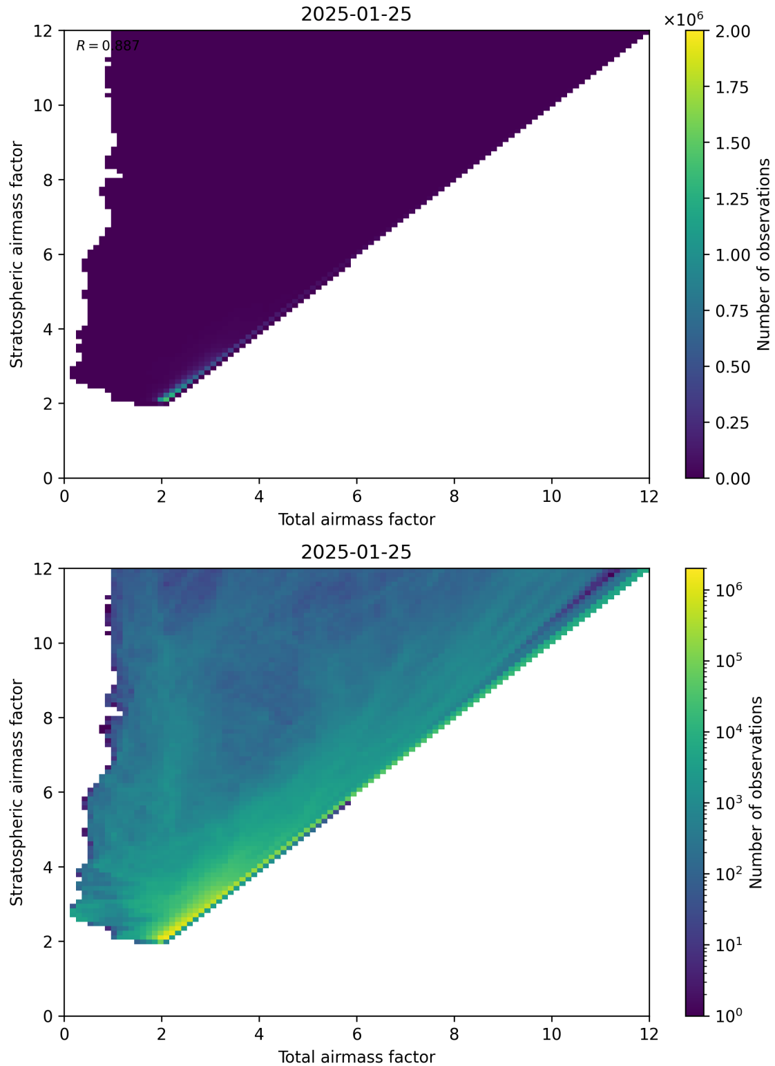
Figure 62: Scatter density plot of “Total airmass factor” against “Stratospheric airmass factor” for 2025-01-24 to 2025-01-26.
