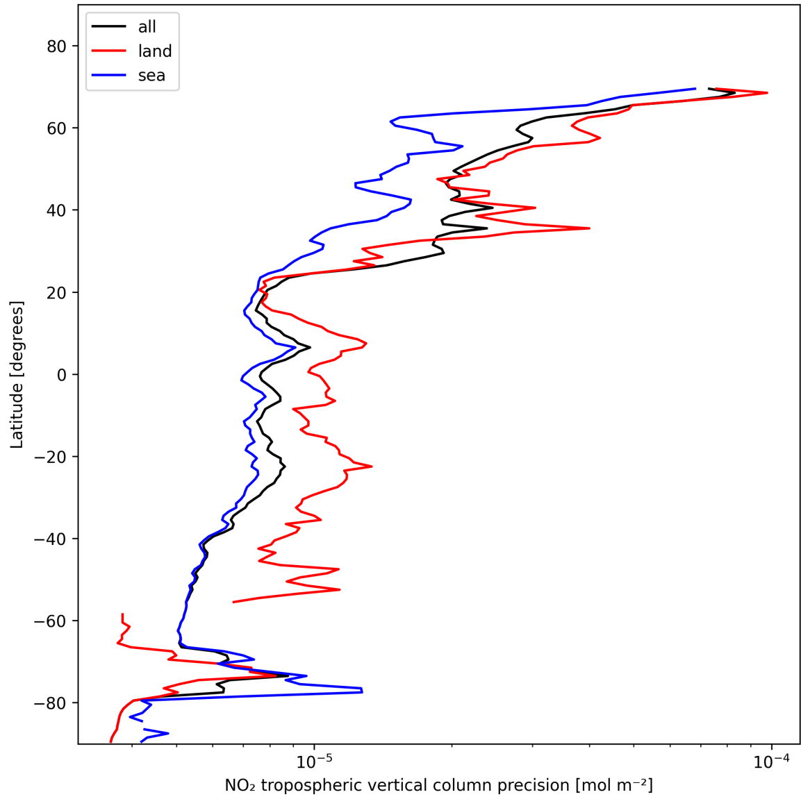
Figure 13: Zonal average of “NO 2 tropospheric vertical column precision” for 2025-01-24 to 2025-01-26.
