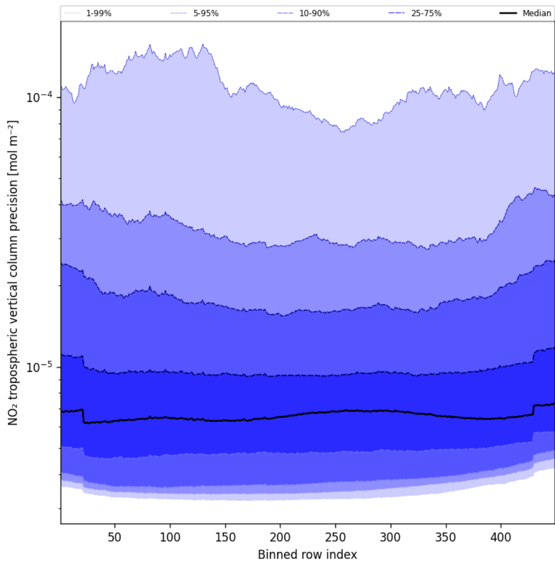
Figure 47: Along track statistics of “NO 2 tropospheric vertical column precision” for 2025-01-24 to 2025-01-26
