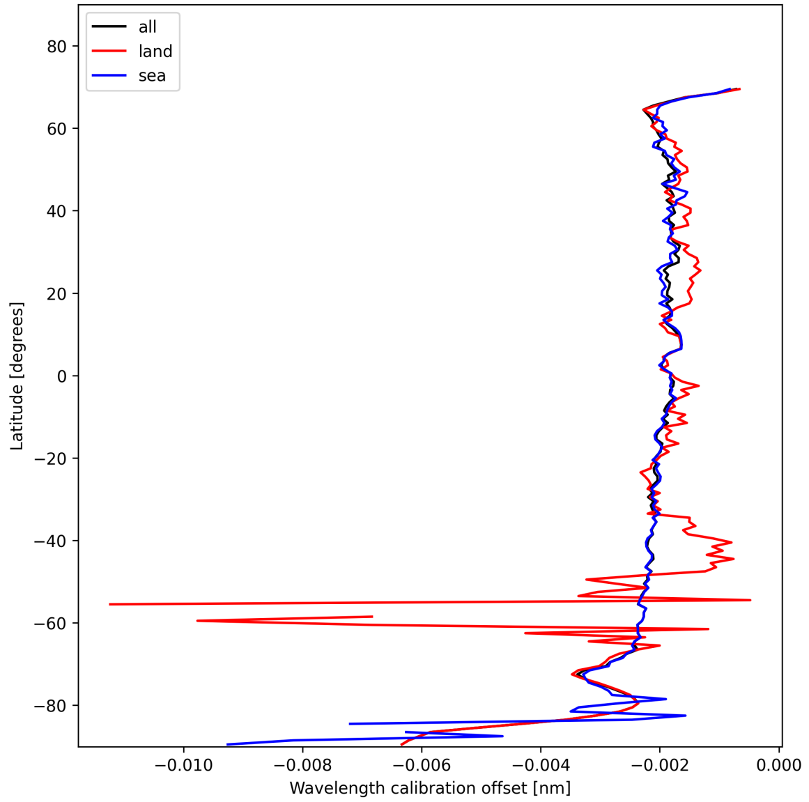
Figure 18: Zonal average of “Wavelength calibration offset” for 2025-01-24 to 2025-01-26.
