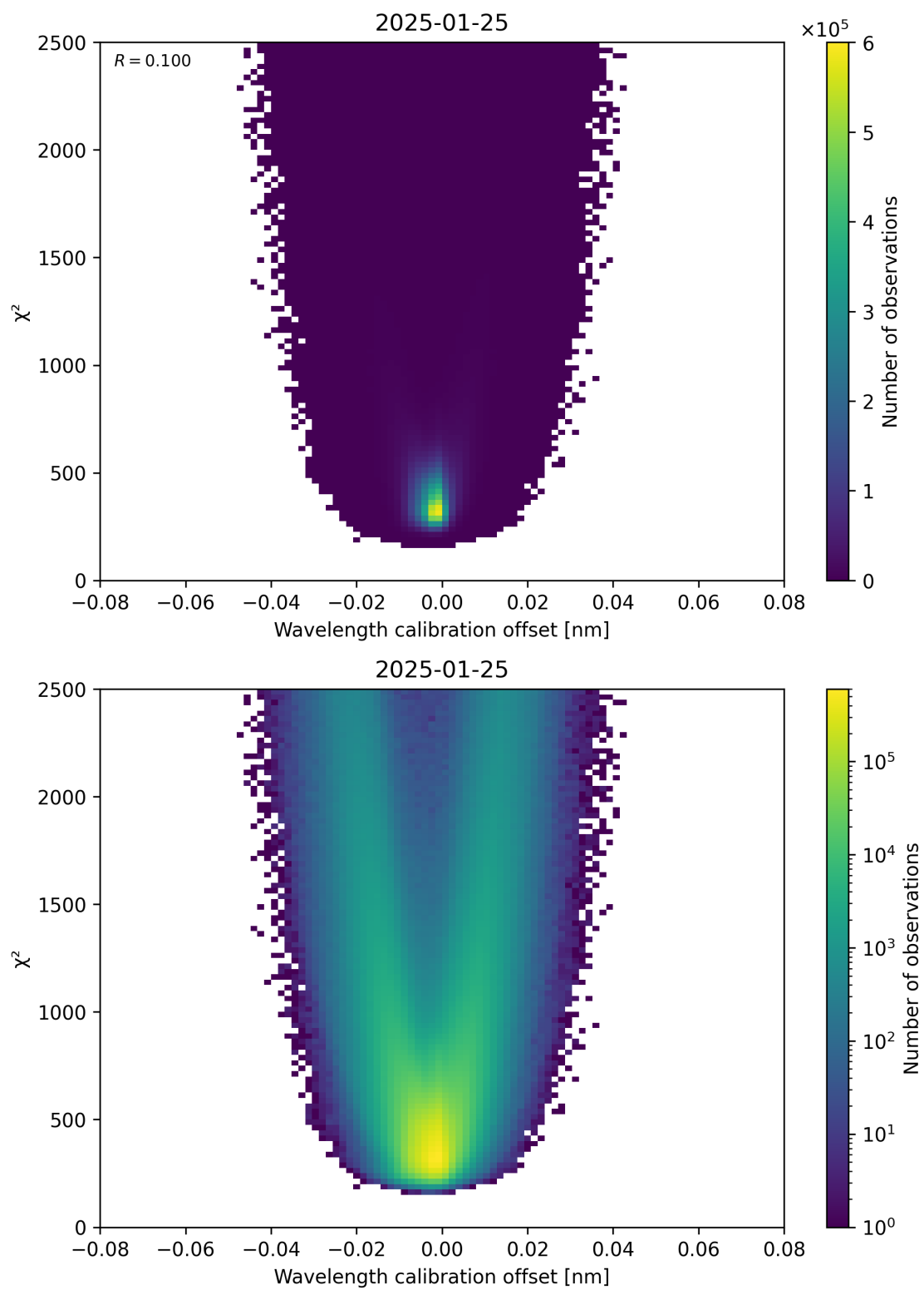
Figure 175: Scatter density plot of “Wavelength calibration offset” against “ \chi^2 ” for 2025-01-24 to 2025-01-26.
