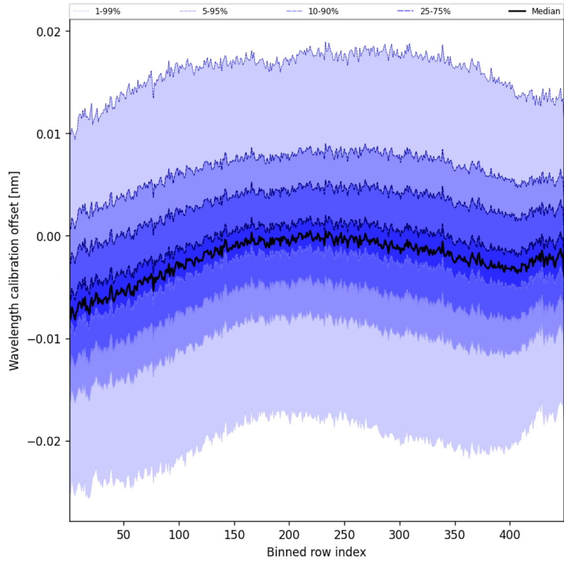
Figure 52: Along track statistics of “Wavelength calibration offset” for 2025-01-24 to 2025-01-26
