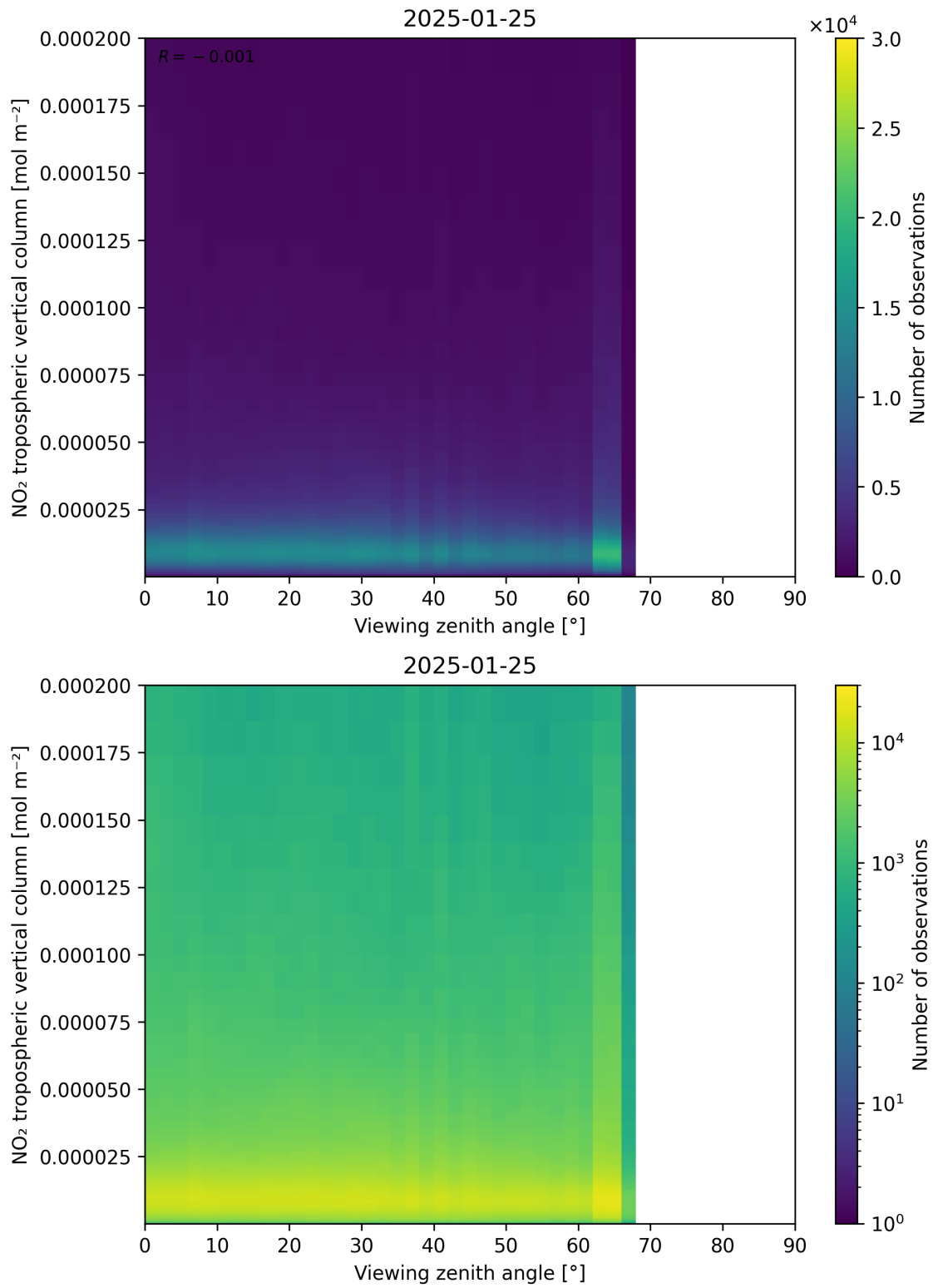
Figure 169: Scatter density plot of “Viewing zenith angle” against “NO 2 tropospheric vertical column” for 2025-01-24 to 2025-01-26.
