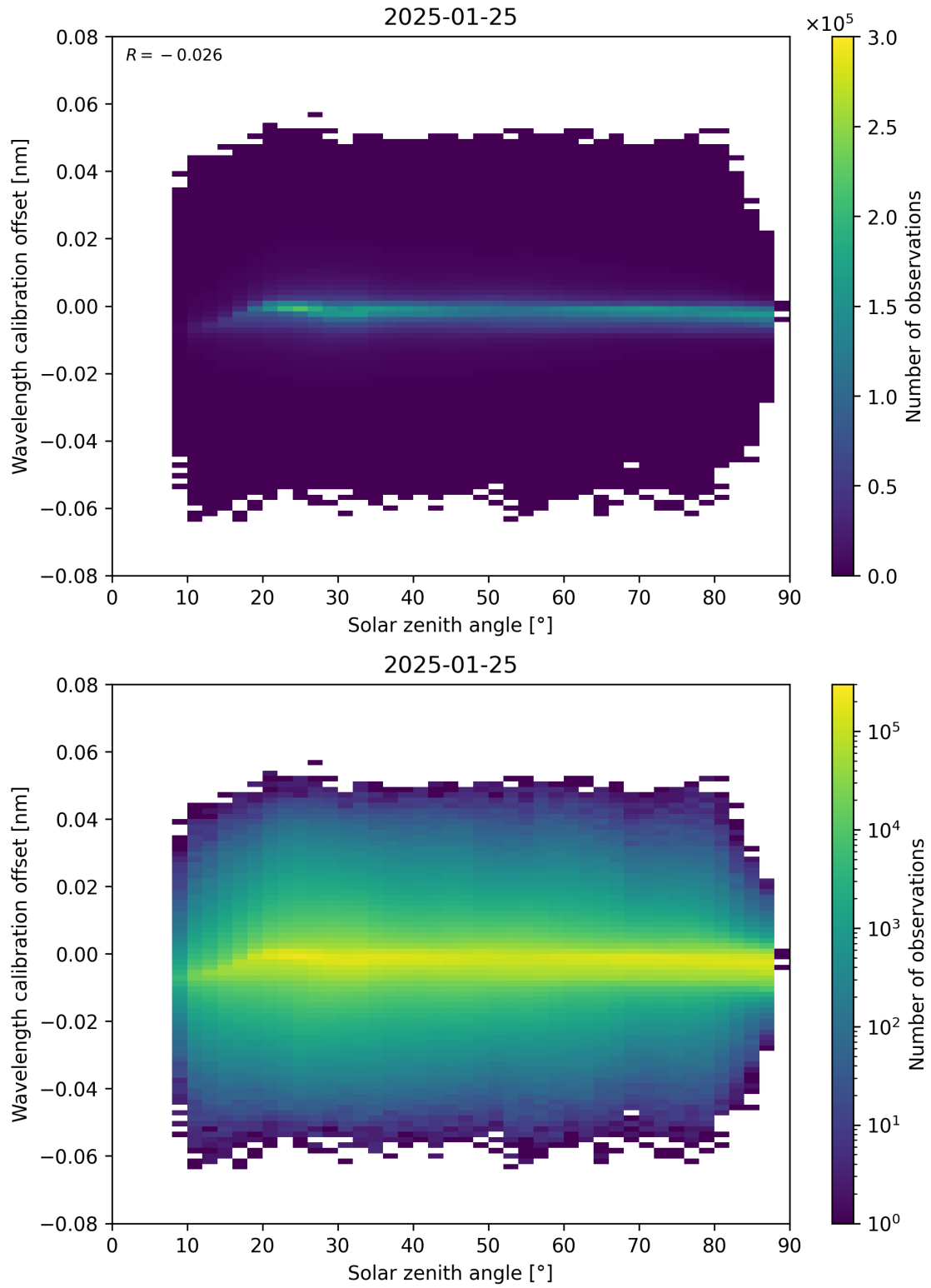
Figure 158: Scatter density plot of “Solar zenith angle” against “Wavelength calibration offset” for 2025-01-24 to 2025-01-26.
