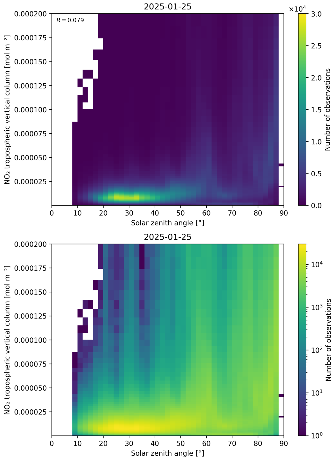
Figure 155: Scatter density plot of “Solar zenith angle” against “NO 2 tropospheric vertical column” for 2025-01-24 to 2025-01-26.
