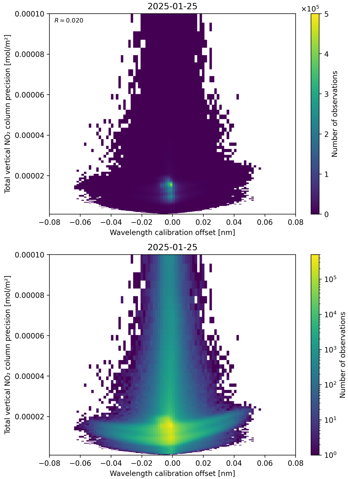
Figure 180: Scatter density plot of “Wavelength calibration offset” against “Total vertical NO 2 column precision” for 2025-01-24 to 2025-01-26.
