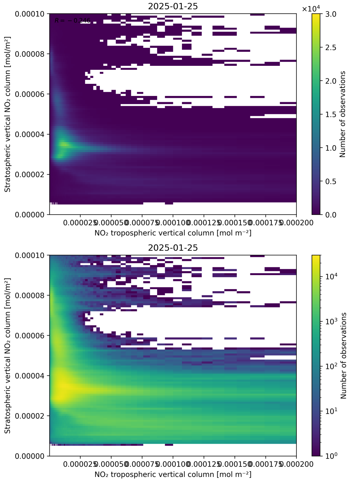
Figure 125: Scatter density plot of “NO 2 tropospheric vertical column” against “Stratospheric vertical NO 2 column” for 2025-01-24 to 2025-01-26.
