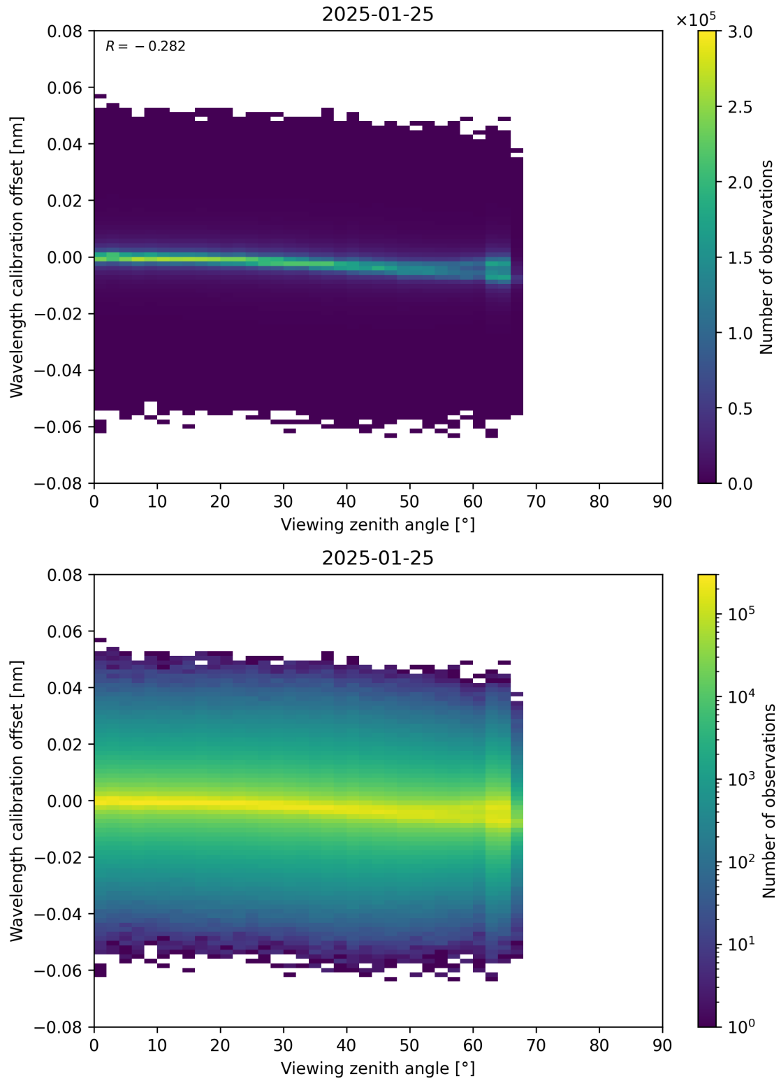
Figure 173: Scatter density plot of “Viewing zenith angle” against “Wavelength calibration offset” for 2025-01-24 to 2025-01-26.
