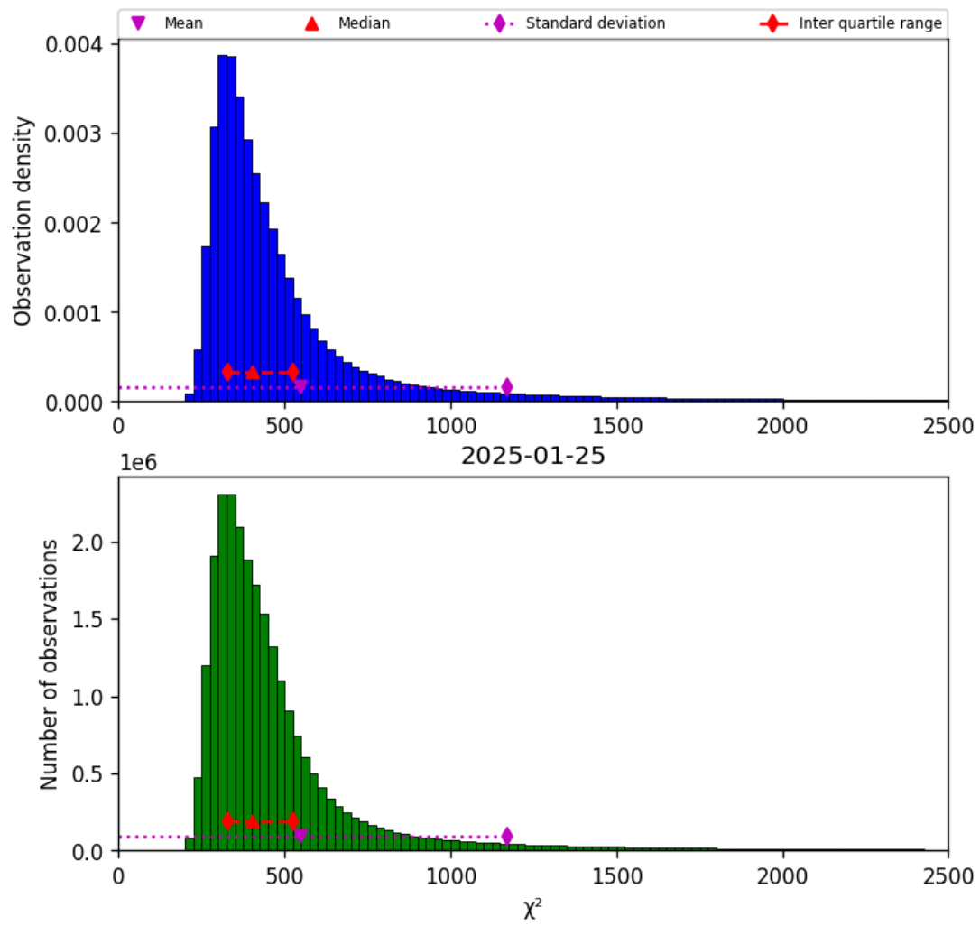
Figure 42: Histogram of " \chi^2 " for 2025-01-24 to 2025-01-26
