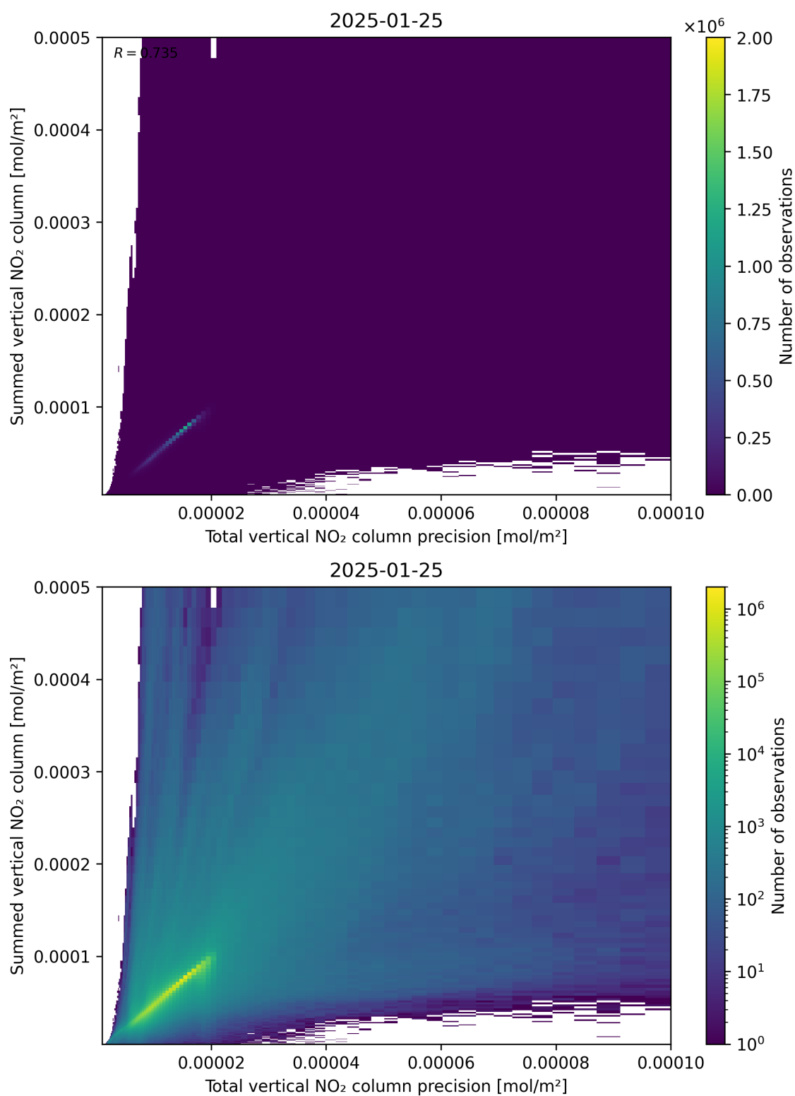
Figure 117: Scatter density plot of “Total vertical NO 2 column precision” against “Summed vertical NO 2 column” for 2025-01-24 to 2025-01-26.
