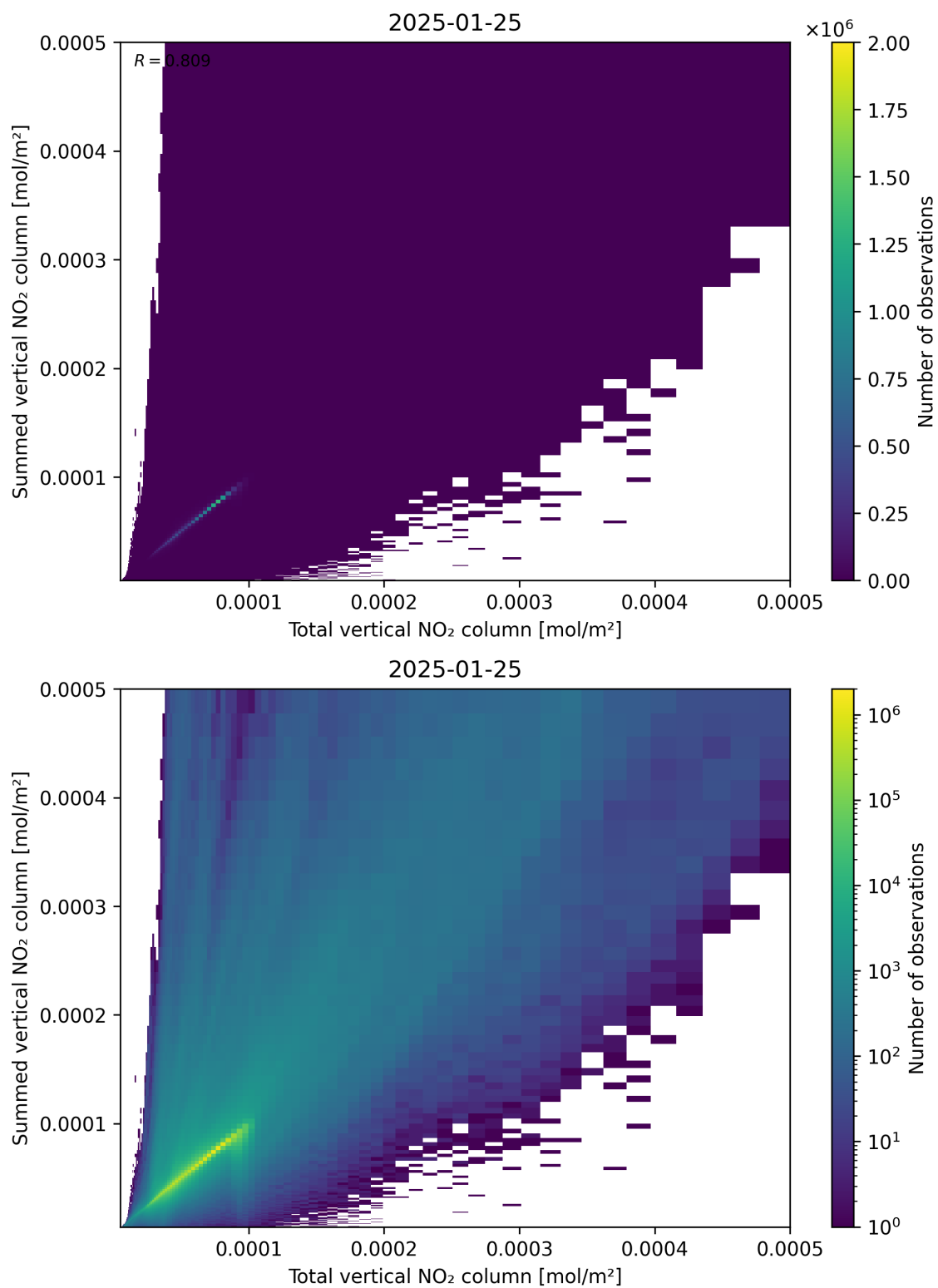
Figure 112: Scatter density plot of “Total vertical NO 2 column” against “Summed vertical NO 2 column” for 2025-01-24 to 2025-01-26.
