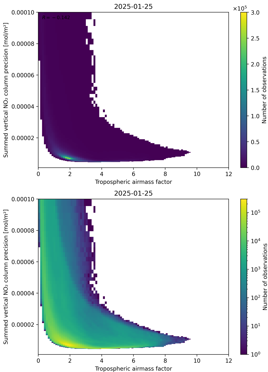
Figure 76: Scatter density plot of “Tropospheric air mass factor” against “Summed vertical NO 2 column precision” for 2025-01-24 to 2025-01-26.
