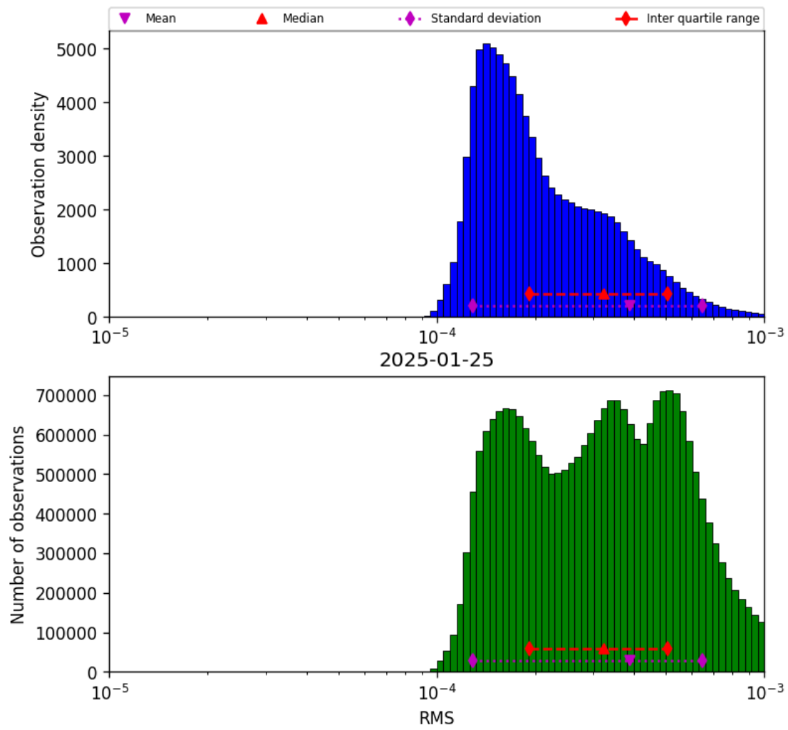
Figure 43: Histogram of “RMS” for 2025-01-24 to 2025-01-26
