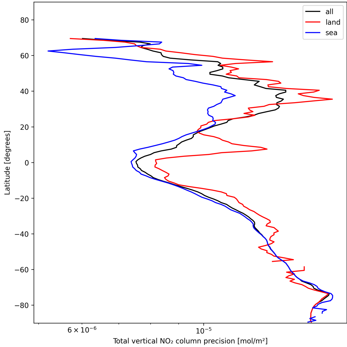
Figure 22: Zonal average of “Total vertical NO 2 column precision” for 2025-01-24 to 2025-01-26.
