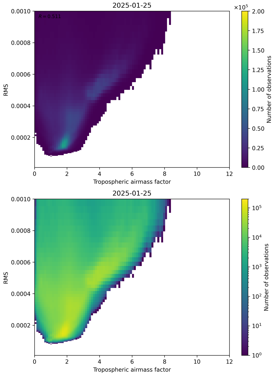
Figure 79: Scatter density plot of “Tropospheric airmass factor” against “RMS” for 2025-01-24 to 2025-01-26.
