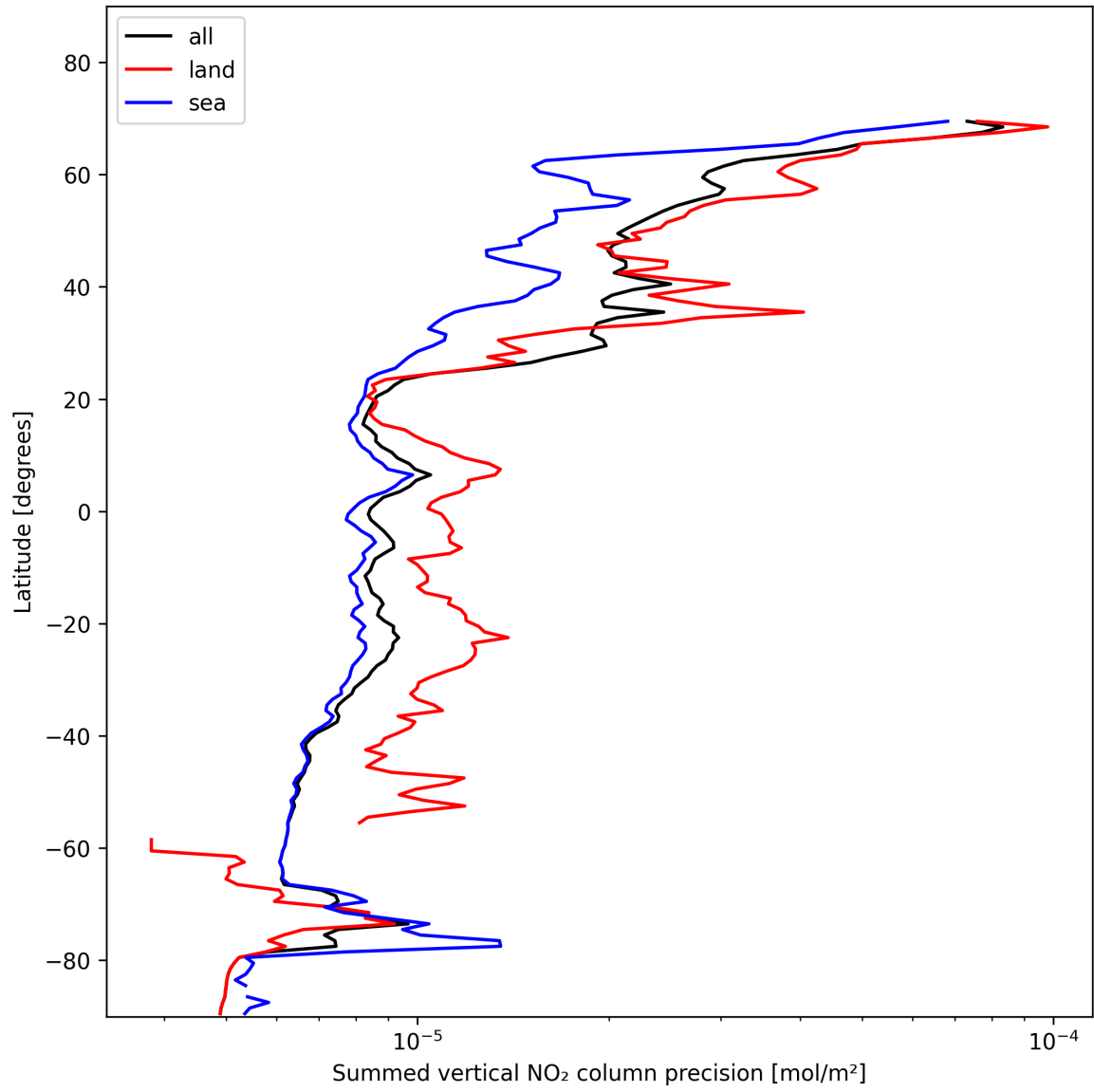
Figure 24: Zonal average of “Summed vertical NO 2 column precision” for 2025-01-24 to 2025-01-26.
