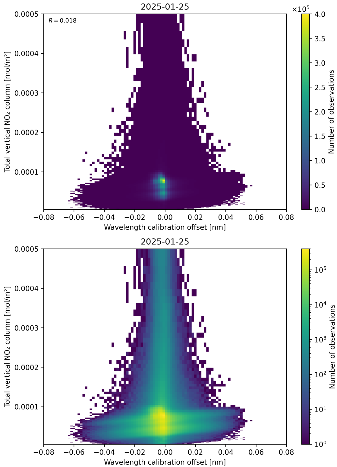
Figure 179: Scatter density plot of “Wavelength calibration offset” against “Total vertical NO 2 column” for 2025-01-24 to 2025-01-26.
