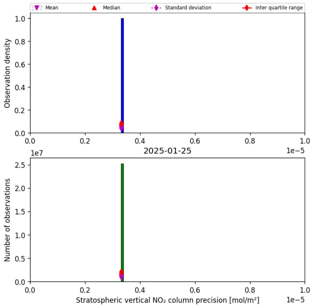
Figure 37: Histogram of “Stratospheric vertical NO 2 column precision” for 2025-01-24 to 2025-01-26
