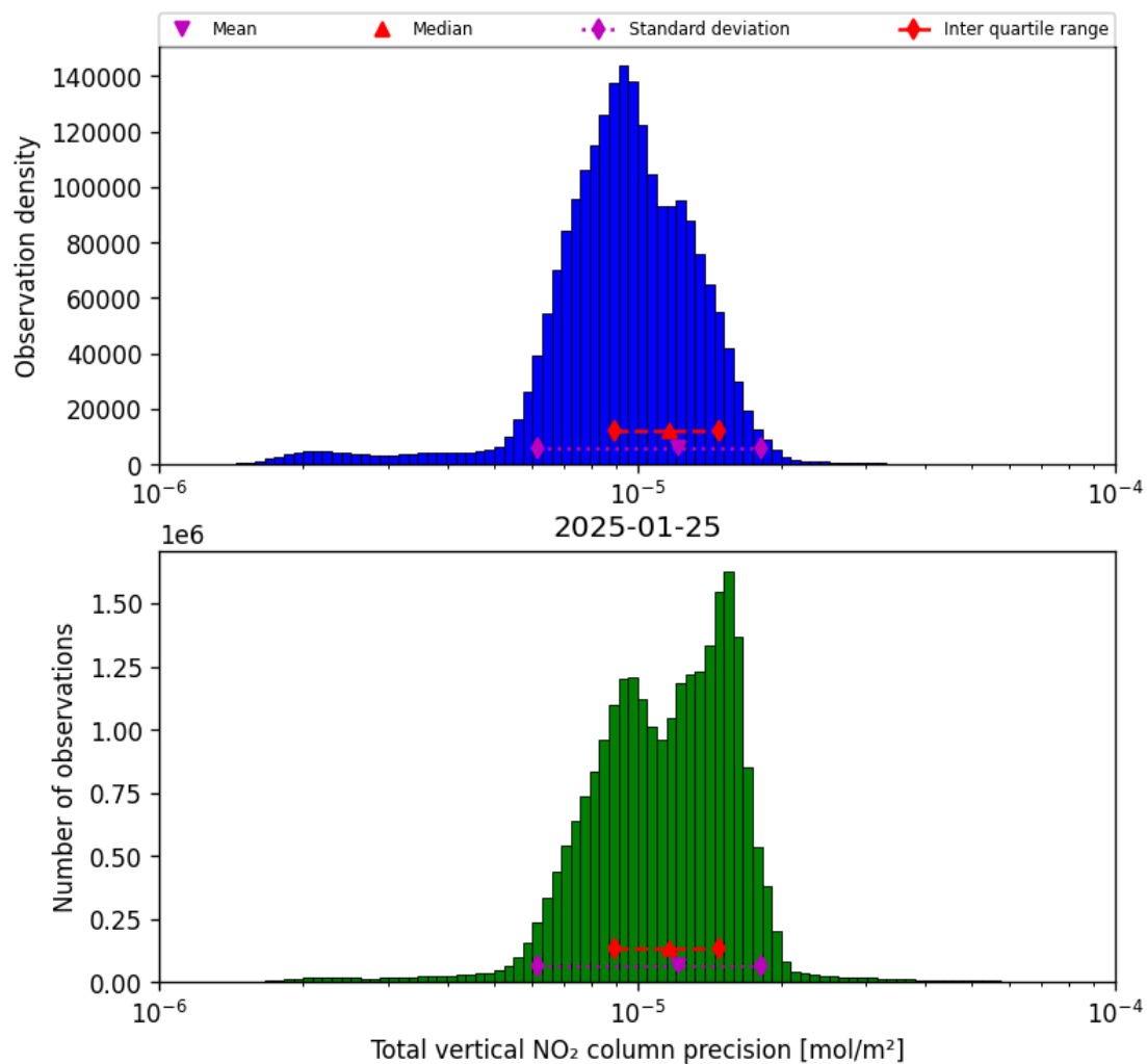
Figure 39: Histogram of “Total vertical NO 2 column precision” for 2025-01-24 to 2025-01-26
