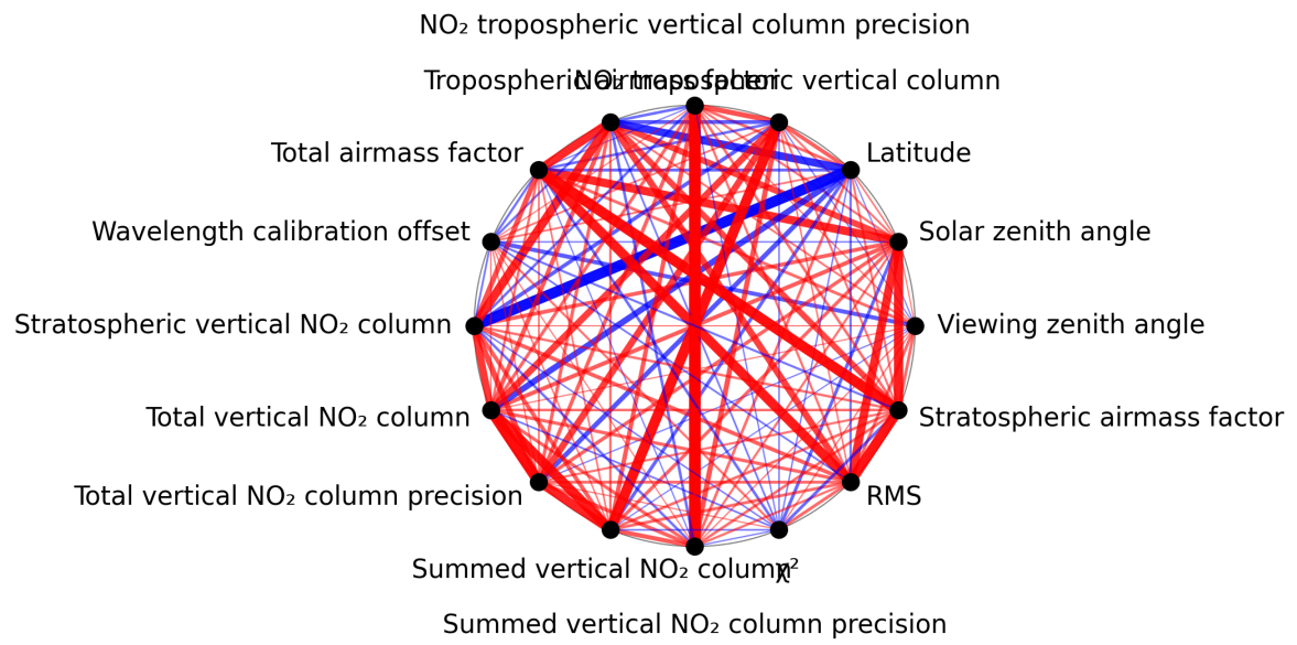
Figure 1: Map of correlation graph for 2025-01-24 to 2025-01-26.
