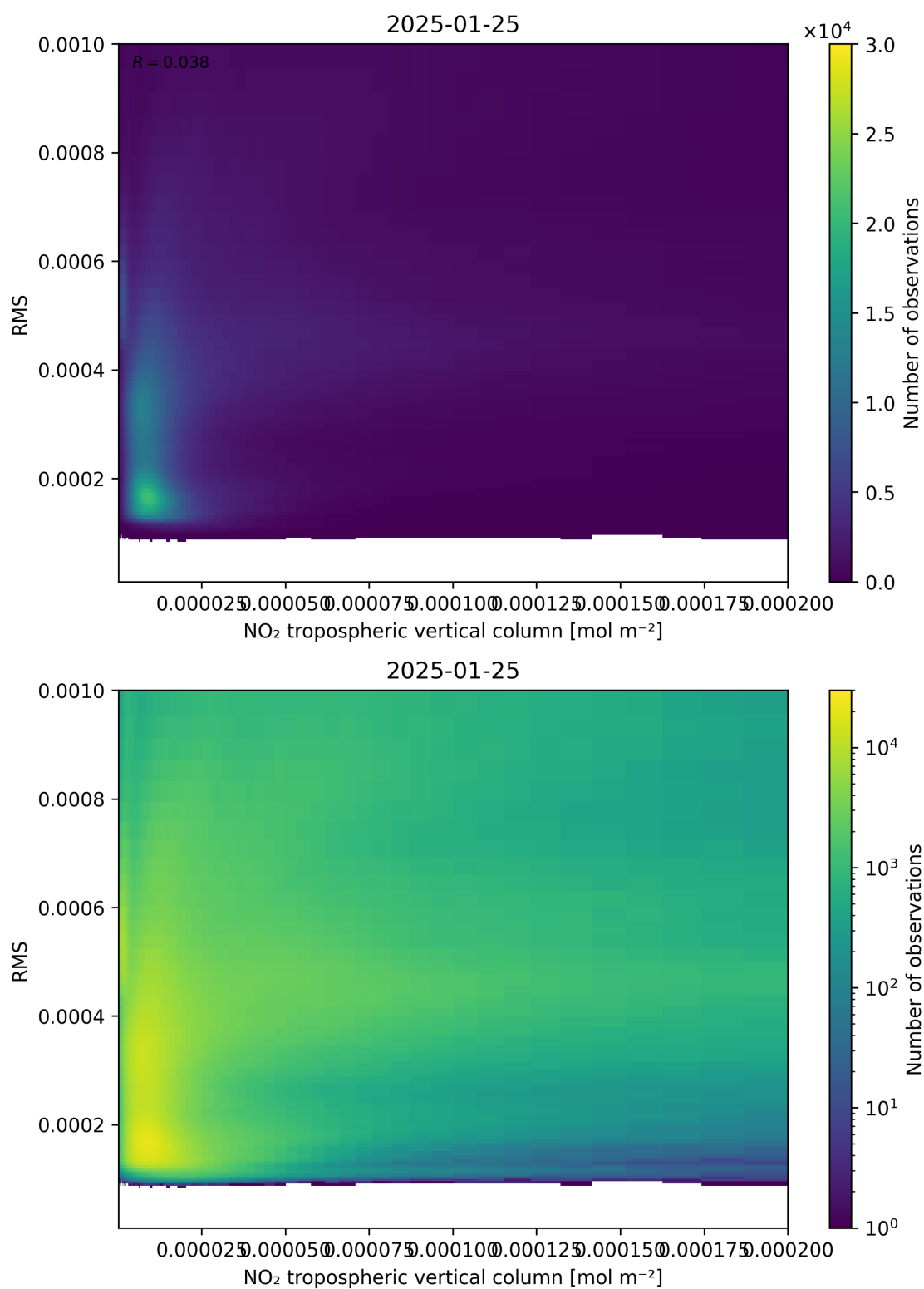
Figure 142: Scatter density plot of “NO 2 tropospheric vertical column” against “RMS” for 2025-01-24 to 2025-01-26.
