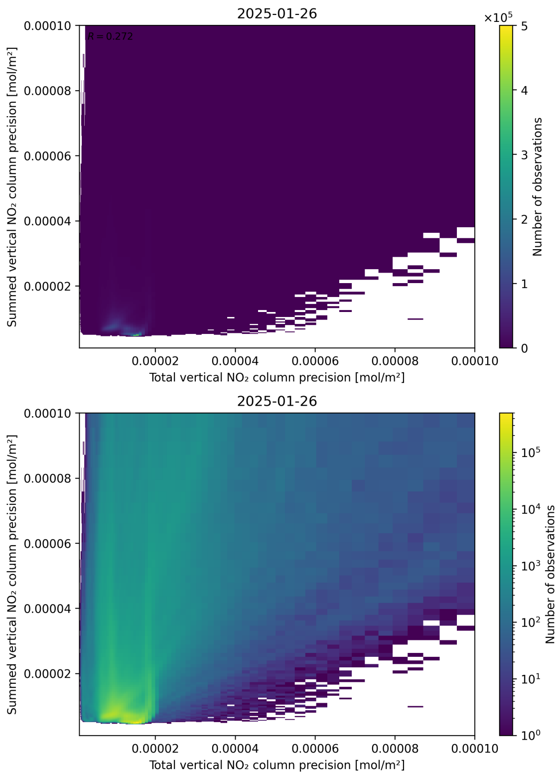
Figure 118: Scatter density plot of “Total vertical NO 2 column precision” against “Summed vertical NO 2 column precision” for 2025-01-25 to 2025-01-27.
