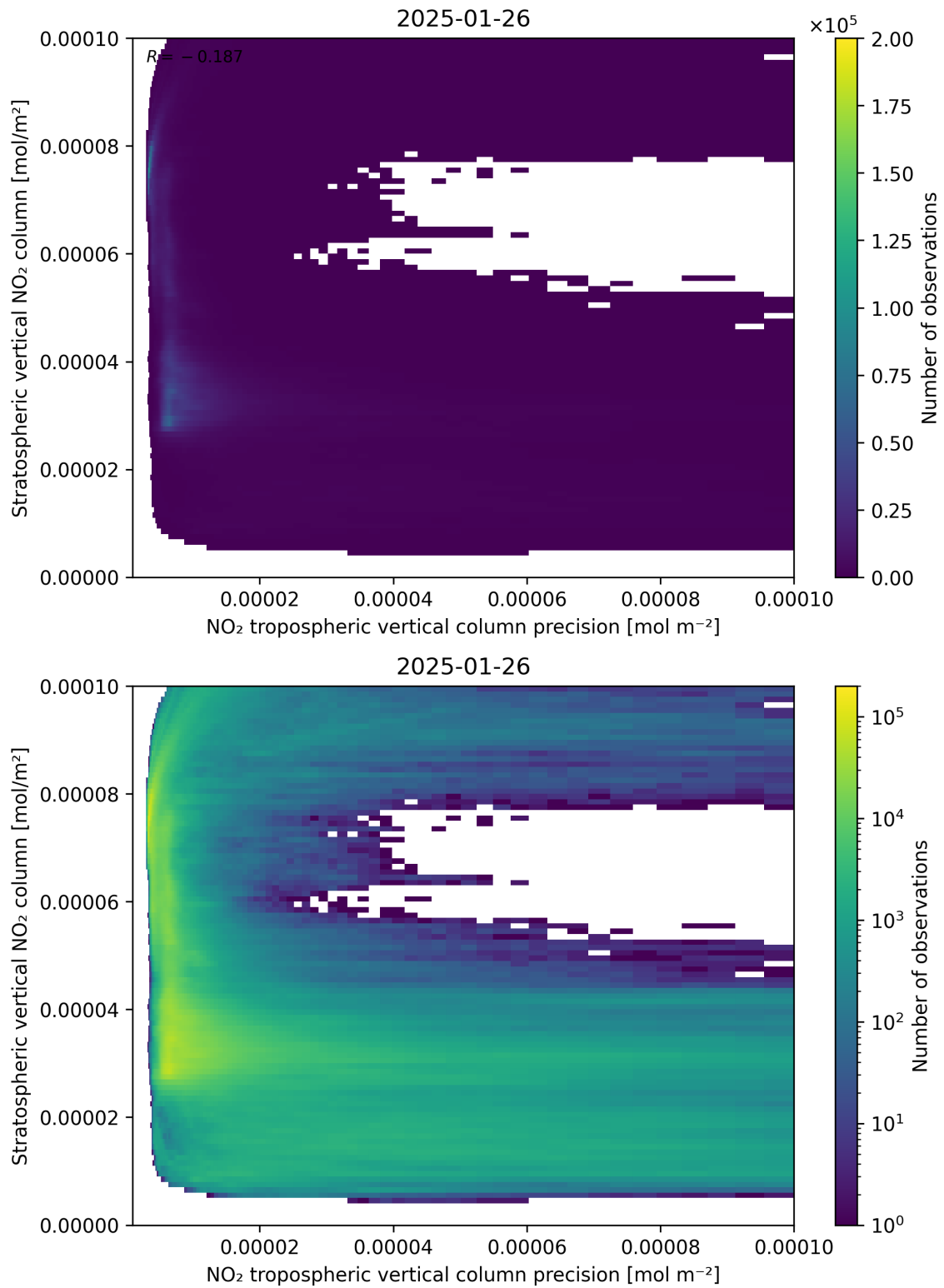
Figure 135: Scatter density plot of “NO 2 tropospheric vertical column precision” against “Stratospheric vertical NO 2 column” for 2025-01-25 to 2025-01-27.
