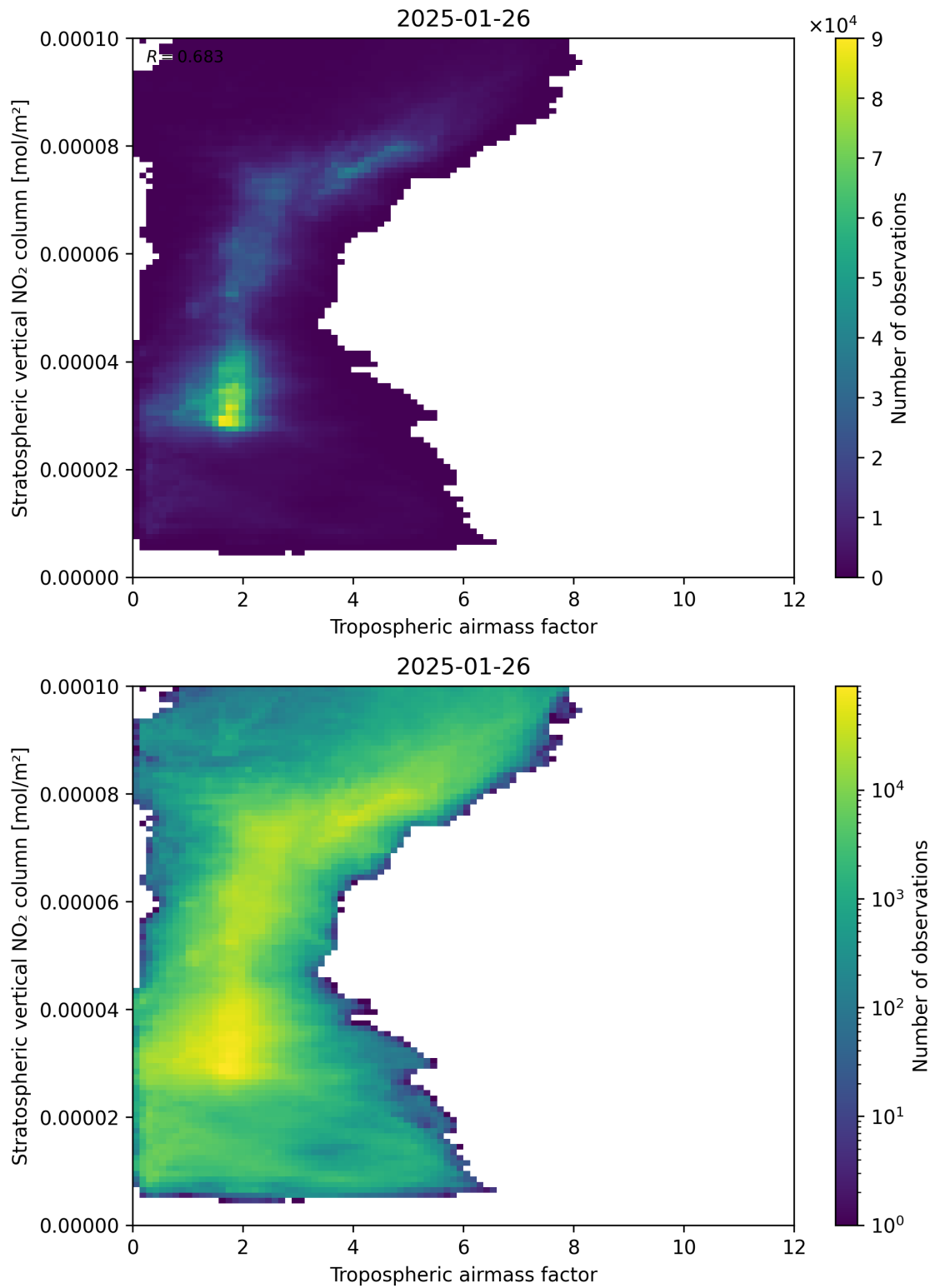
Figure 74: Scatter density plot of “Tropospheric air mass factor” against “Stratospheric vertical NO 2 column” for 2025-01-25 to 2025-01-27.
