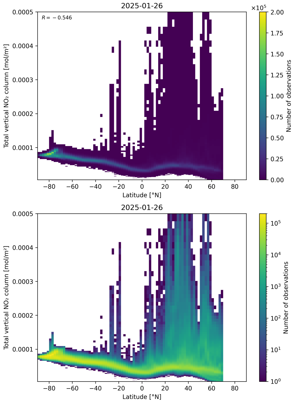
Figure 90: Scatter density plot of “Latitude” against “Total vertical NO 2 column” for 2025-01-25 to 2025-01-27.
