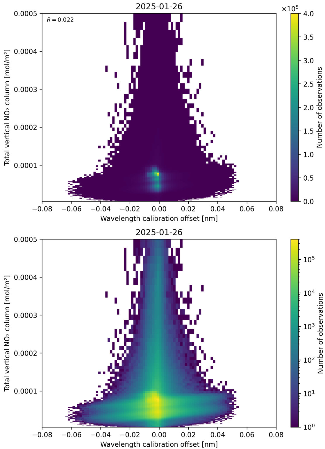
Figure 179: Scatter density plot of “Wavelength calibration offset” against “Total vertical NO 2 column” for 2025-01-25 to 2025-01-27.
