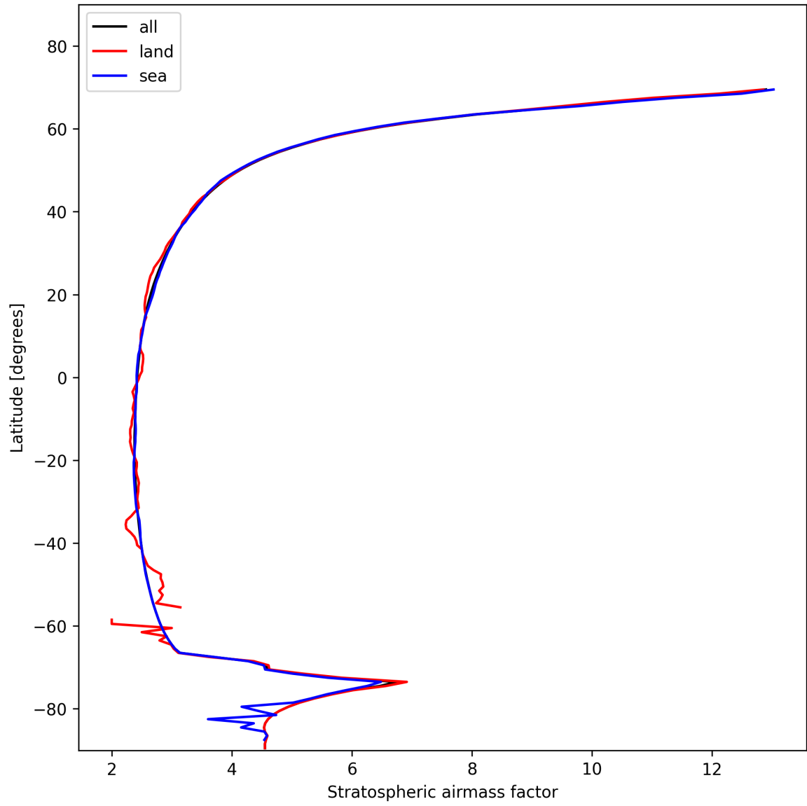
Figure 27: Zonal average of “Stratospheric air mass factor” for 2025-01-25 to 2025-01-27.
