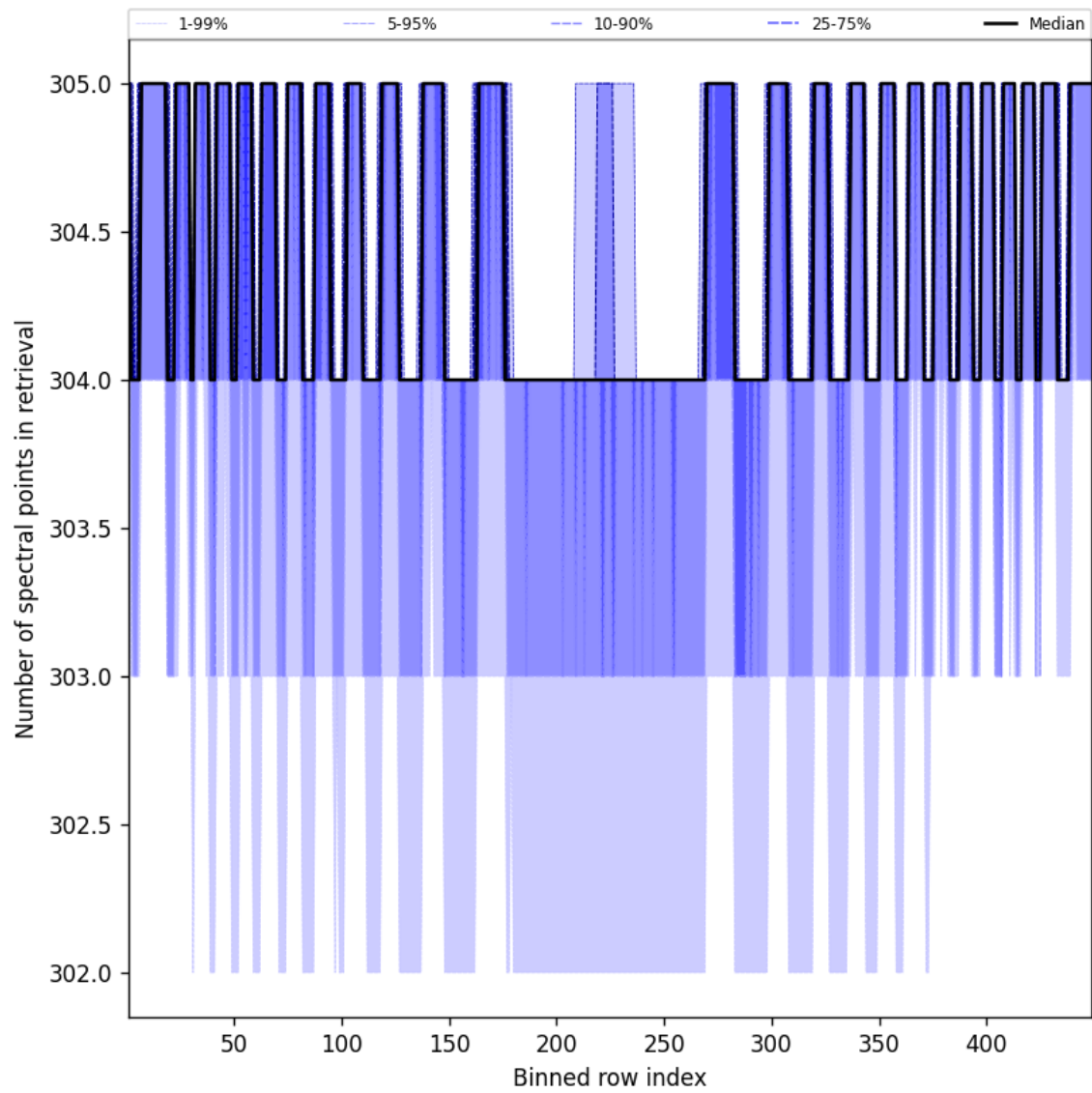
Figure 50: Along track statistics of “Number of spectral points in retrieval” for 2025-01-25 to 2025-01-27
