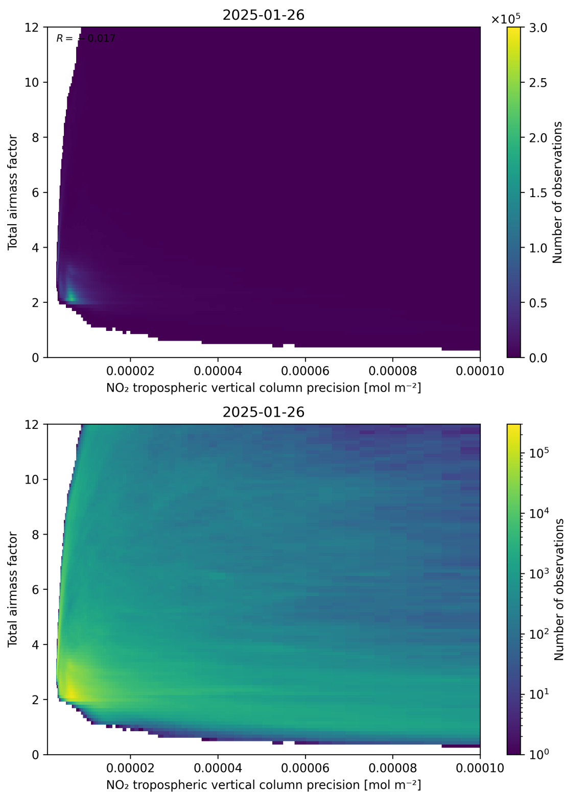
Figure 132: Scatter density plot of “NO 2 tropospheric vertical column precision” against “Total air mass factor” for 2025-01-25 to 2025-01-27.
