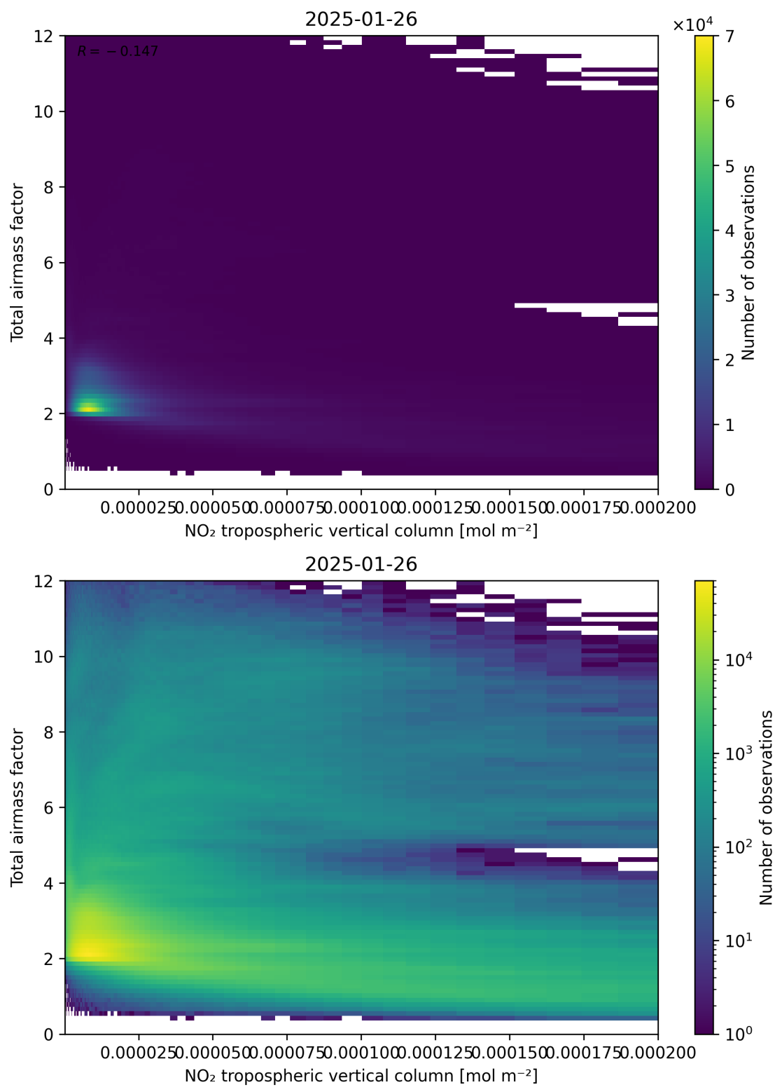
Figure 122: Scatter density plot of “NO 2 tropospheric vertical column” against “Total airmass factor” for 2025-01-25 to 2025-01-27.
