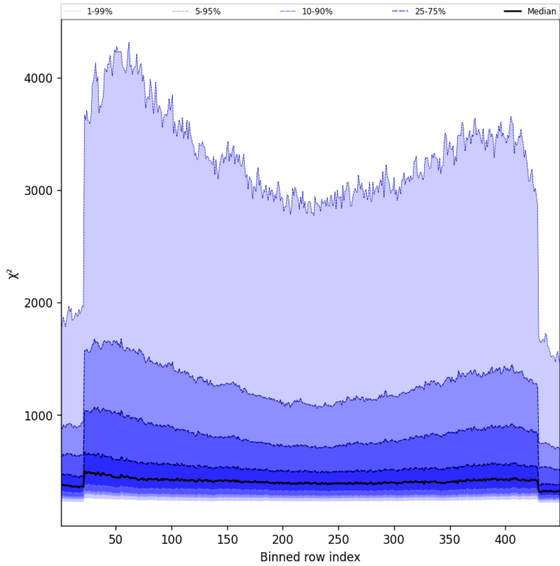
Figure 59: Along track statistics of “ \chi^2 ” for 2025-01-25 to 2025-01-27
