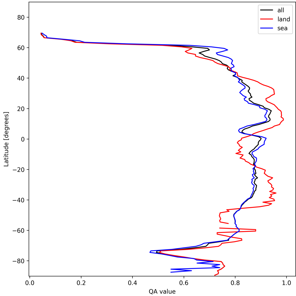
Figure 11: Zonal average of “QA value” for 2025-01-25 to 2025-01-27.
