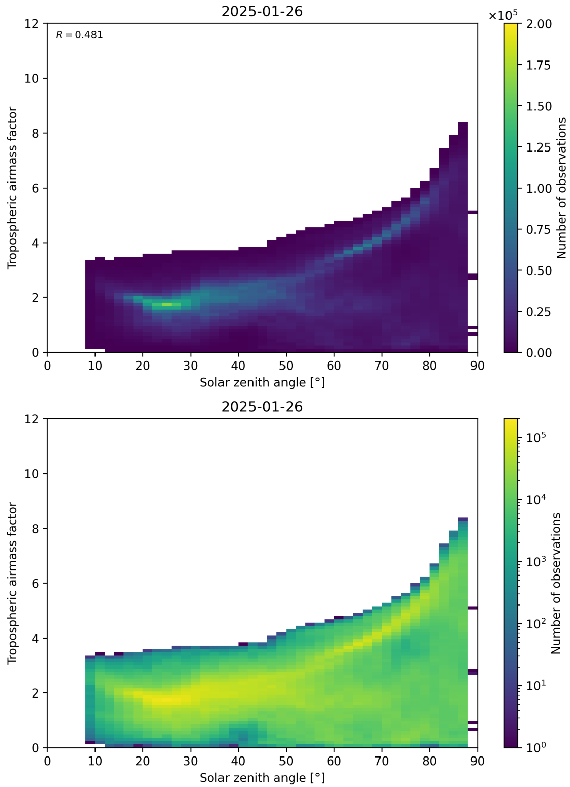
Figure 147: Scatter density plot of “Solar zenith angle” against “Tropospheric airmass factor” for 2025-01-25 to 2025-01-27.
