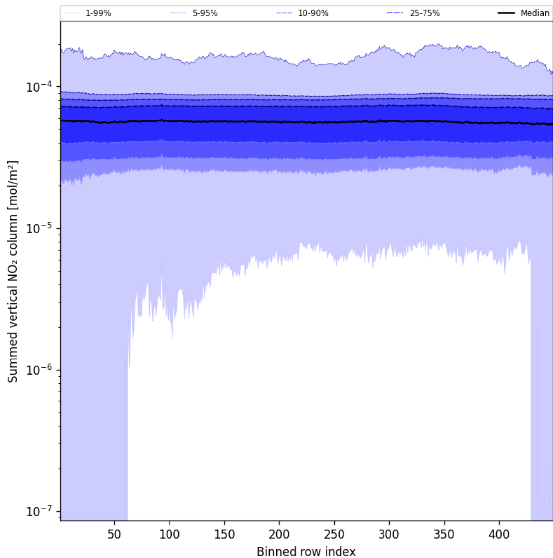
Figure 57: Along track statistics of “Summed vertical NO 2 column” for 2025-01-25 to 2025-01-27
