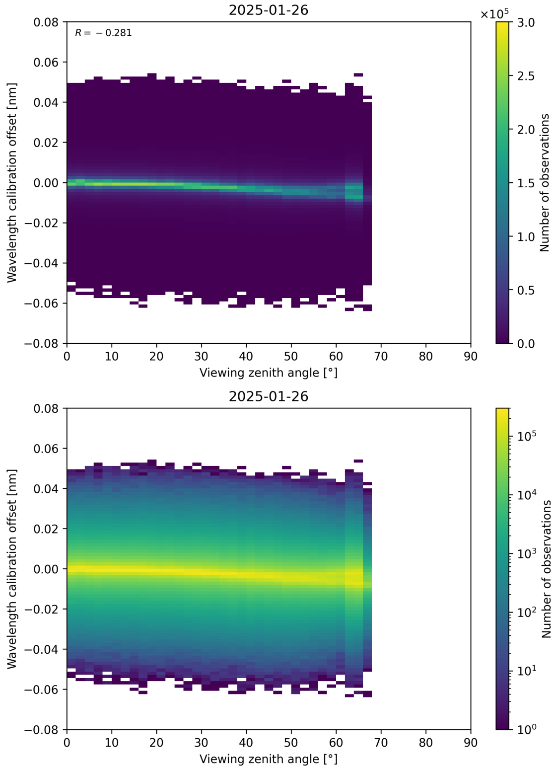
Figure 173: Scatter density plot of “Viewing zenith angle” against “Wavelength calibration offset” for 2025-01-25 to 2025-01-27.
