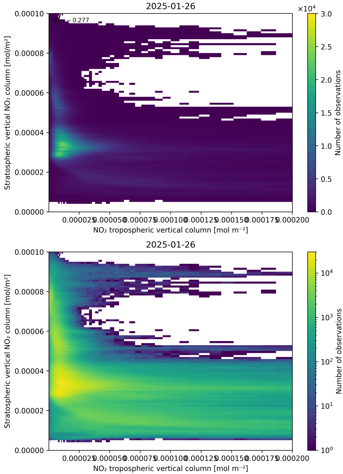
Figure 125: Scatter density plot of “NO 2 tropospheric vertical column” against “Stratospheric vertical NO 2 column” for 2025-01-25 to 2025-01-27.
