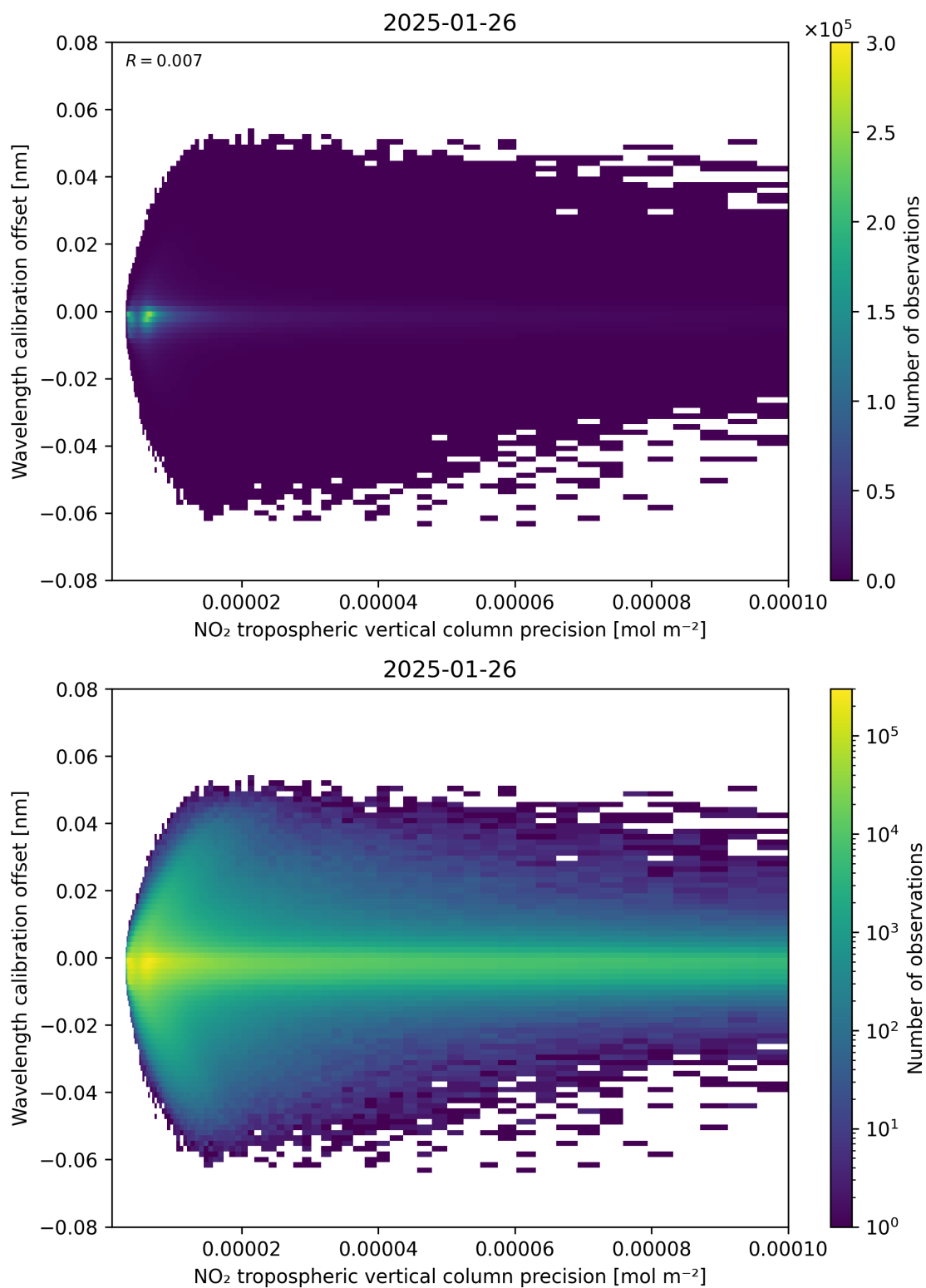
Figure 141: Scatter density plot of “NO 2 tropospheric vertical column precision” against “Wavelength calibration offset” for 2025-01-25 to 2025-01-27.
