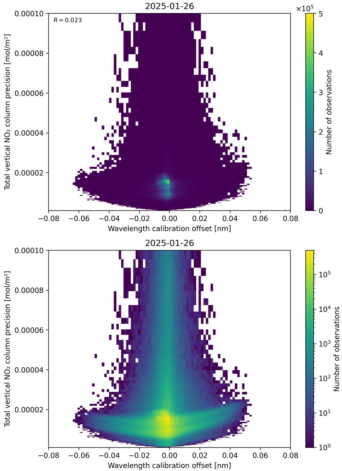
Figure 180: Scatter density plot of “Wavelength calibration offset” against “Total vertical NO 2 column precision” for 2025-01-25 to 2025-01-27.
