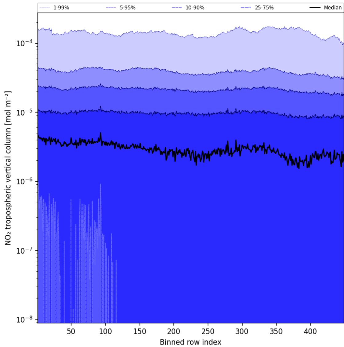
Figure 46: Along track statistics of “NO 2 tropospheric vertical column” for 2025-01-25 to 2025-01-27
