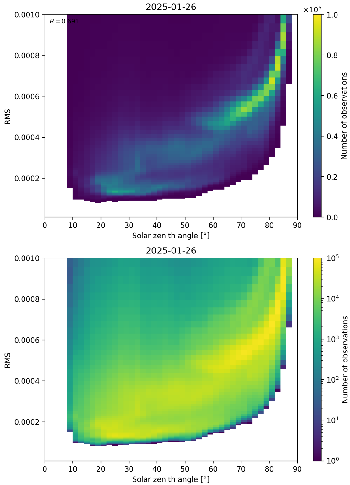
Figure 157: Scatter density plot of “Solar zenith angle” against “RMS” for 2025-01-25 to 2025-01-27.
