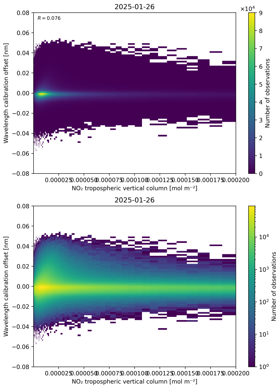
Figure 143: Scatter density plot of “NO 2 tropospheric vertical column” against “Wavelength calibration offset” for 2025-01-25 to 2025-01-27.
