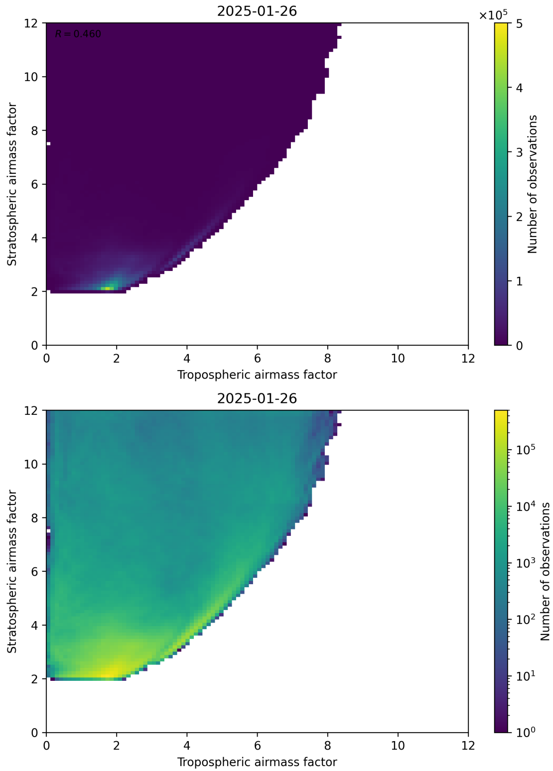
Figure 71: Scatter density plot of “Tropospheric airmass factor” against “Stratospheric airmass factor” for 2025-01-25 to 2025-01-27.
