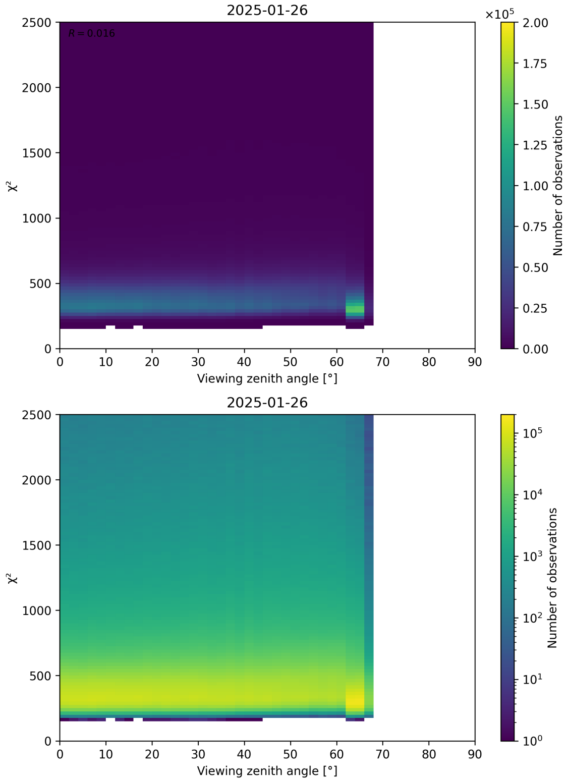
Figure 162: Scatter density plot of “Viewing zenith angle” against “ \chi^2 ” for 2025-01-25 to 2025-01-27.
