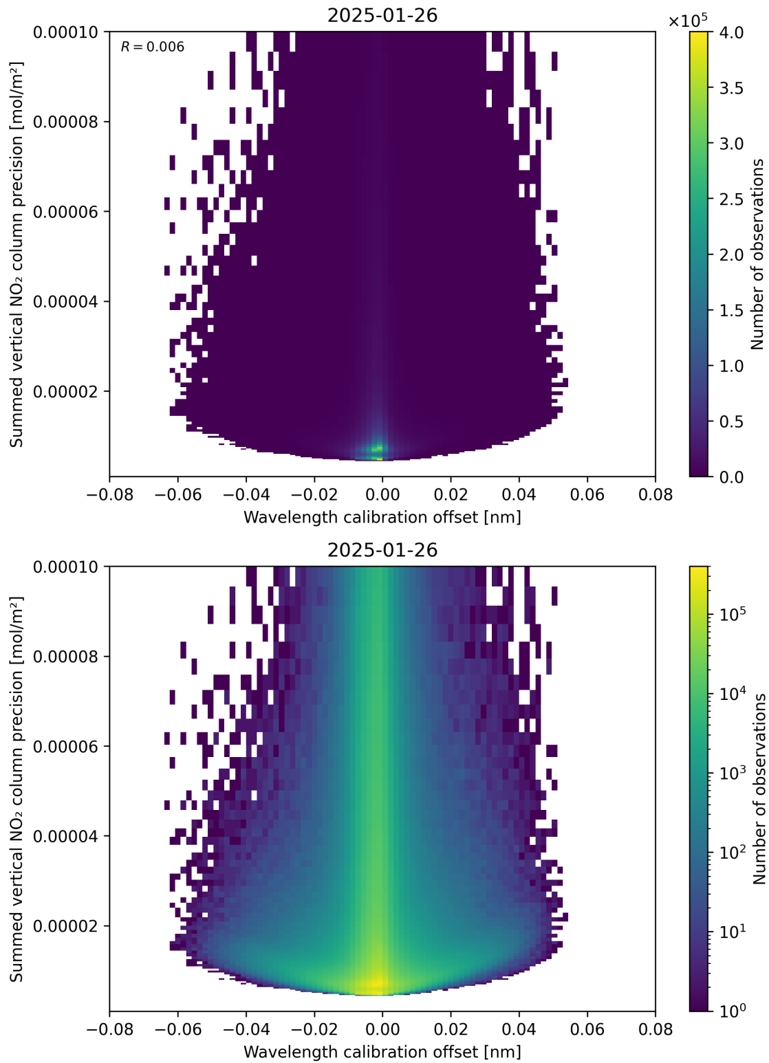
Figure 178: Scatter density plot of “Wavelength calibration offset” against “Summed vertical NO 2 column precision” for 2025-01-25 to 2025-01-27.
