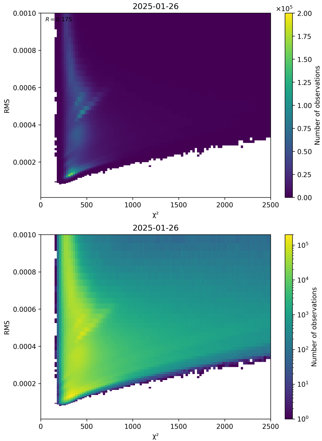
Figure 82: Scatter density plot of “ \chi^2 ” against “RMS” for 2025-01-25 to 2025-01-27.
