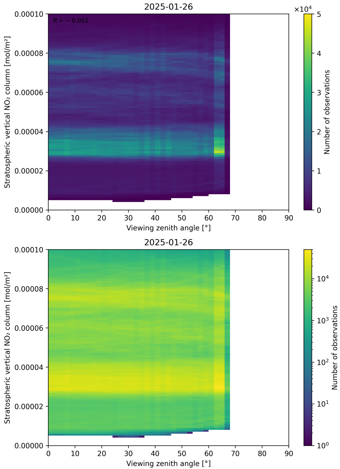
Figure 164: Scatter density plot of “Viewing zenith angle” against “Stratospheric vertical NO 2 column” for 2025-01-25 to 2025-01-27.
