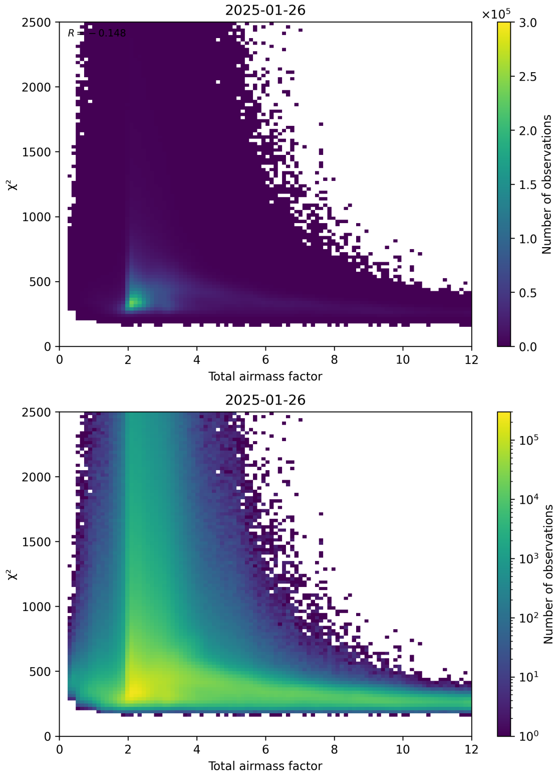
Figure 63: Scatter density plot of “Total airmass factor” against “ \chi^2 ” for 2025-01-25 to 2025-01-27.
