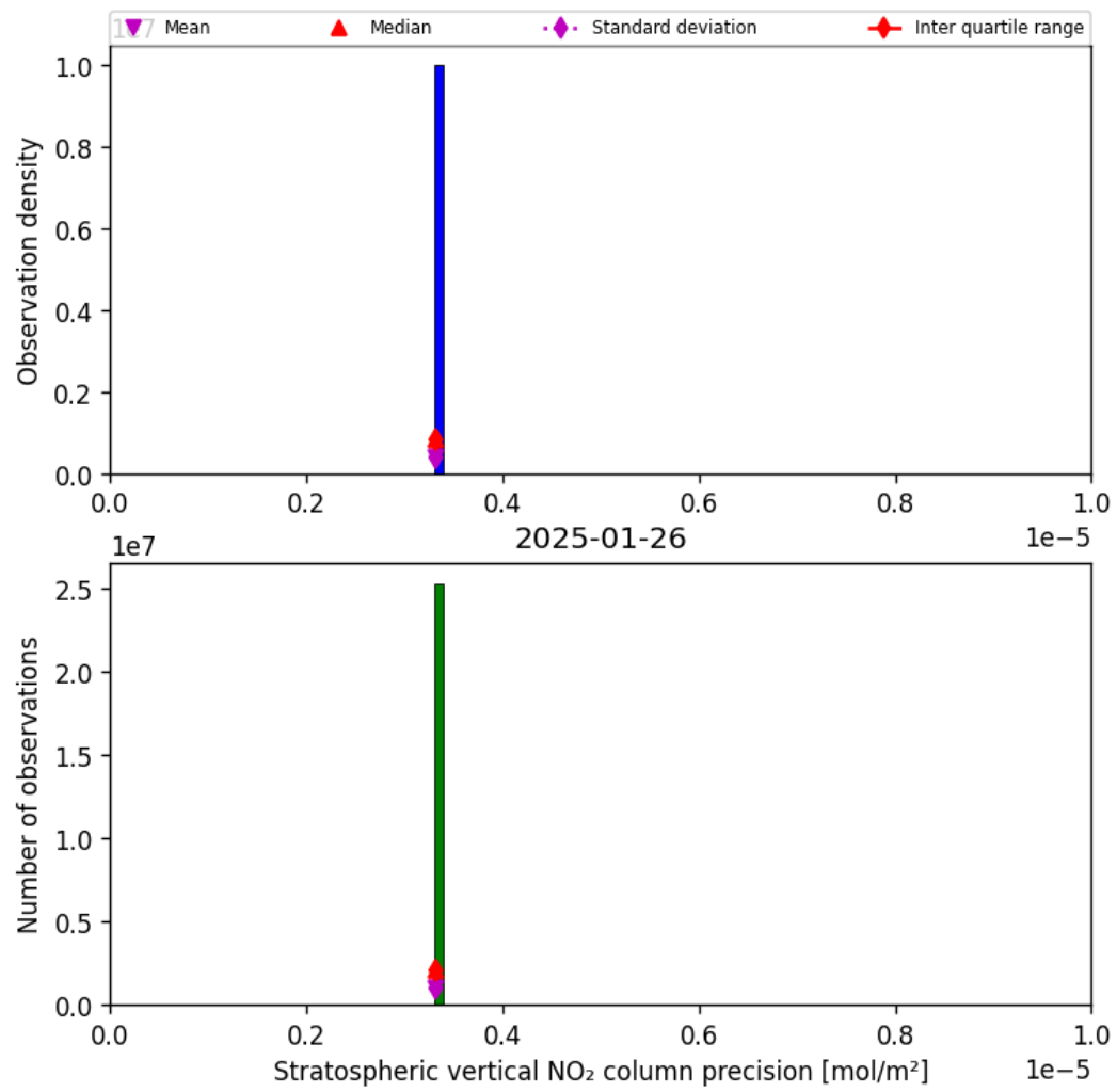
Figure 37: Histogram of “Stratospheric vertical NO 2 column precision” for 2025-01-25 to 2025-01-27
