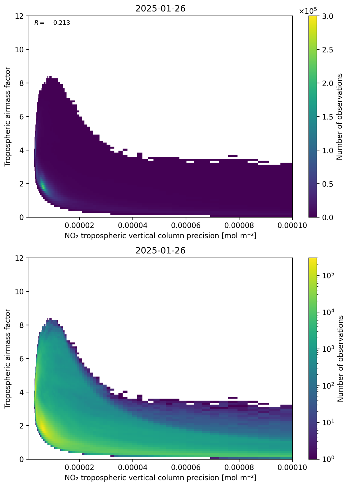
Figure 133: Scatter density plot of “NO 2 tropospheric vertical column precision” against “Tropospheric air mass factor” for 2025-01-25 to 2025-01-27.
