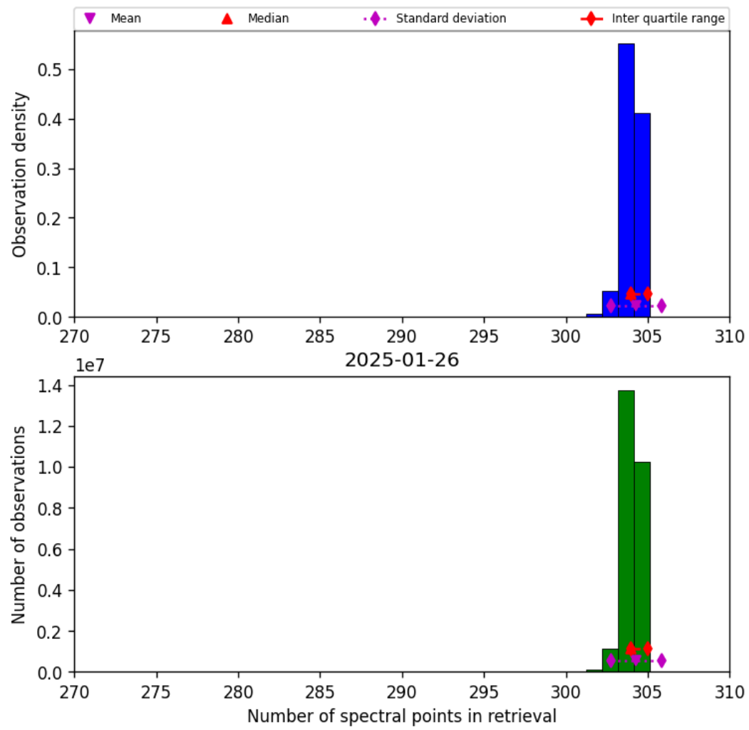
Figure 33: Histogram of “Number of spectral points in retrieval” for 2025-01-25 to 2025-01-27
