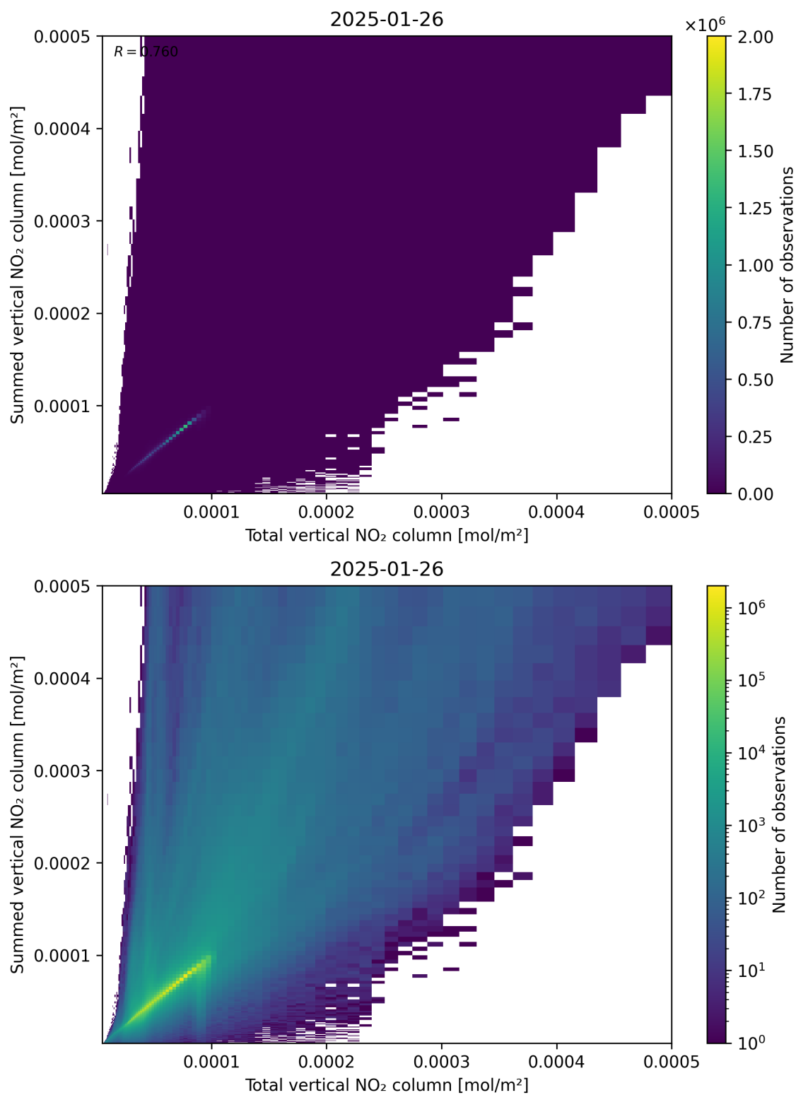
Figure 112: Scatter density plot of “Total vertical NO 2 column” against “Summed vertical NO 2 column” for 2025-01-25 to 2025-01-27.
