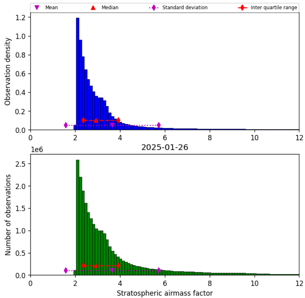
Figure 44: Histogram of “Stratospheric airmass factor” for 2025-01-25 to 2025-01-27
