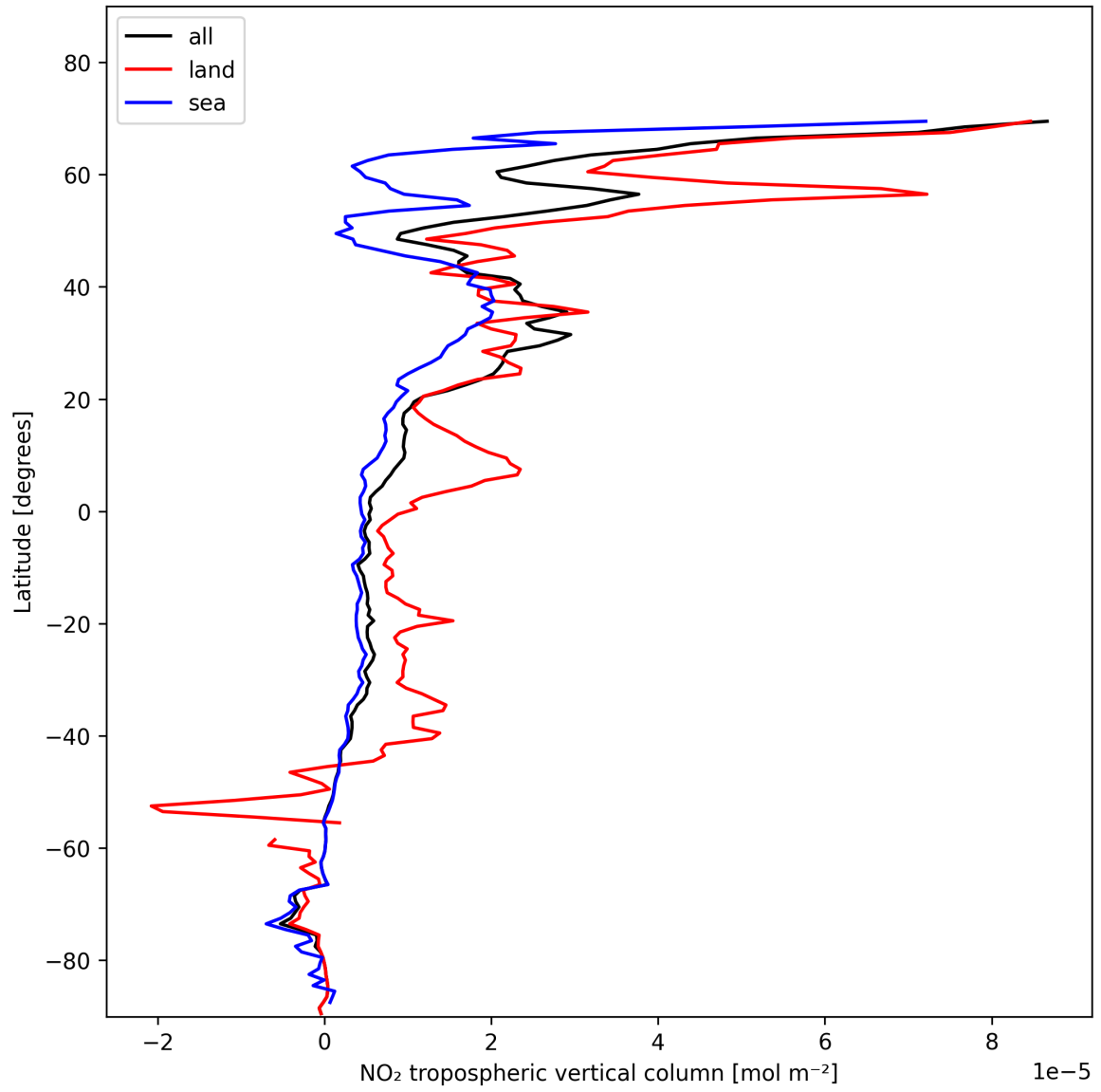
Figure 12: Zonal average of “NO 2 tropospheric vertical column” for 2025-01-25 to 2025-01-27.
