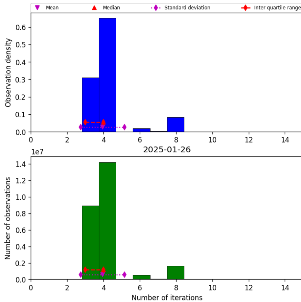
Figure 34: Histogram of “Number of iterations” for 2025-01-25 to 2025-01-27
