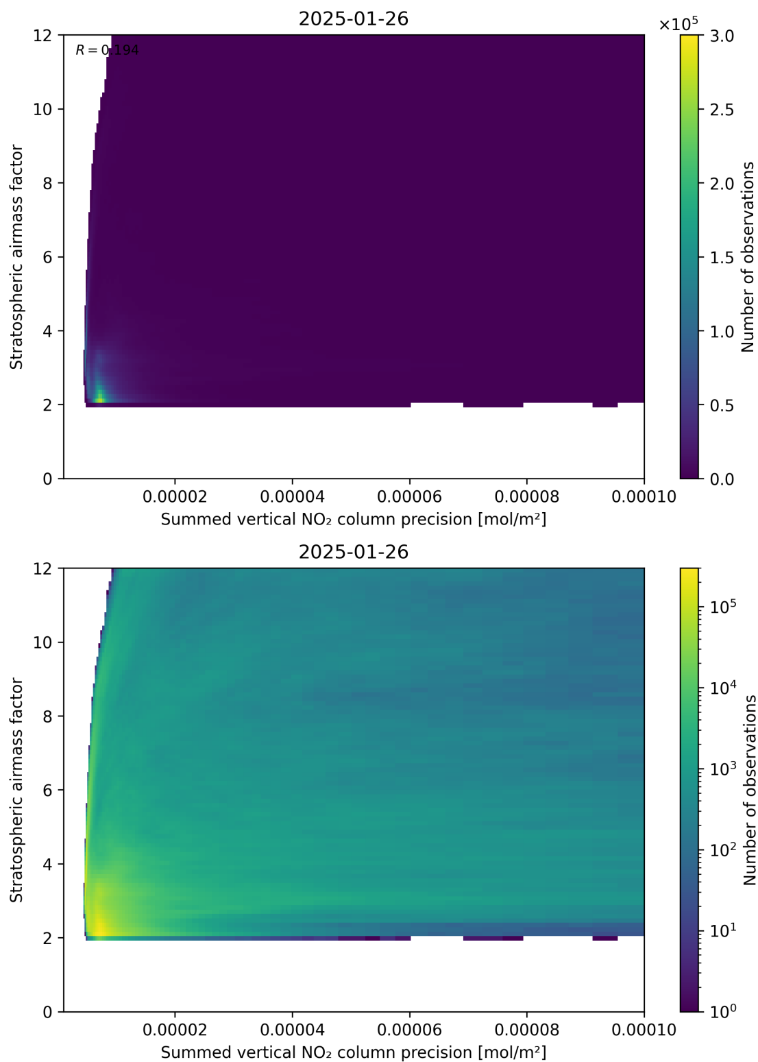
Figure 106: Scatter density plot of “Summed vertical NO 2 column precision” against “Stratospheric airmass factor” for 2025-01-25 to 2025-01-27.
