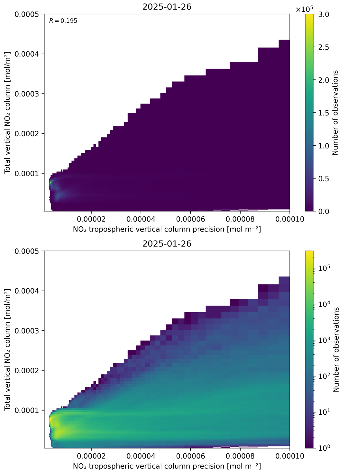
Figure 138: Scatter density plot of “NO 2 tropospheric vertical column precision” against “Total vertical NO 2 column” for 2025-01-25 to 2025-01-27.
