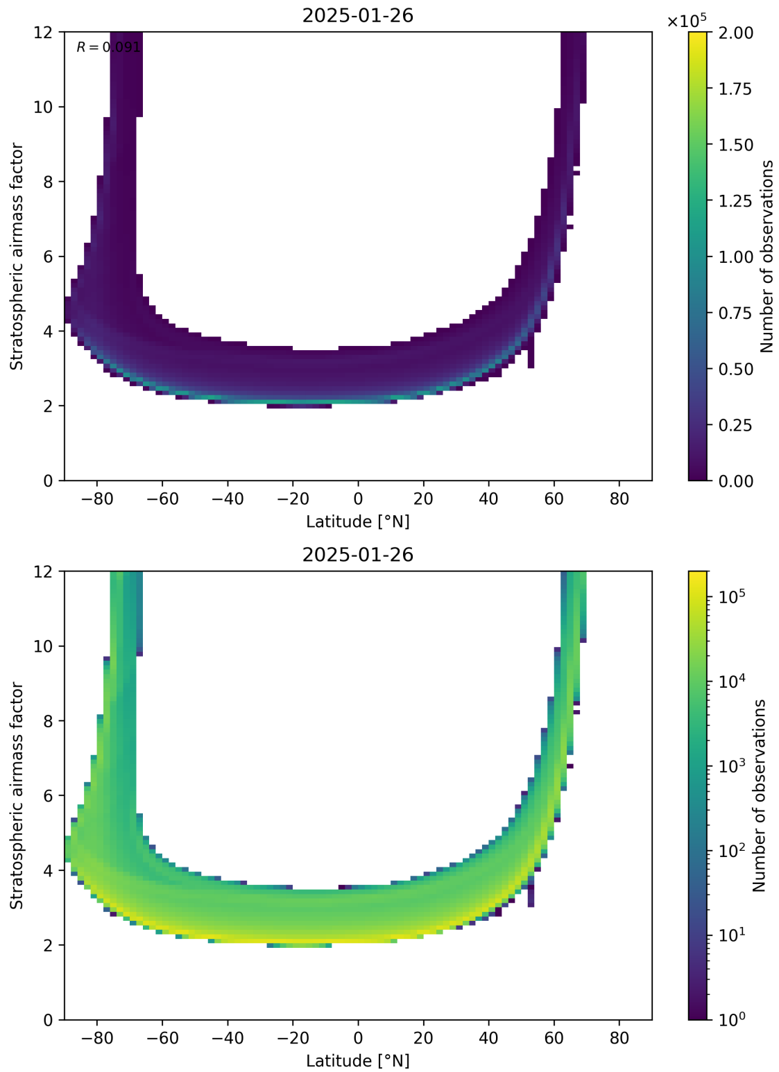
Figure 83: Scatter density plot of “Latitude” against “Stratospheric air mass factor” for 2025-01-25 to 2025-01-27.
