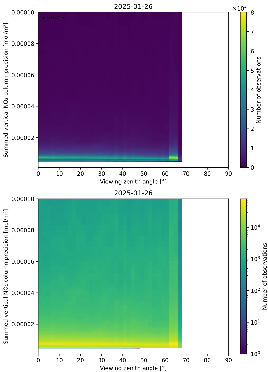
Figure 166: Scatter density plot of “Viewing zenith angle” against “Summed vertical NO 2 column precision” for 2025-01-25 to 2025-01-27.
