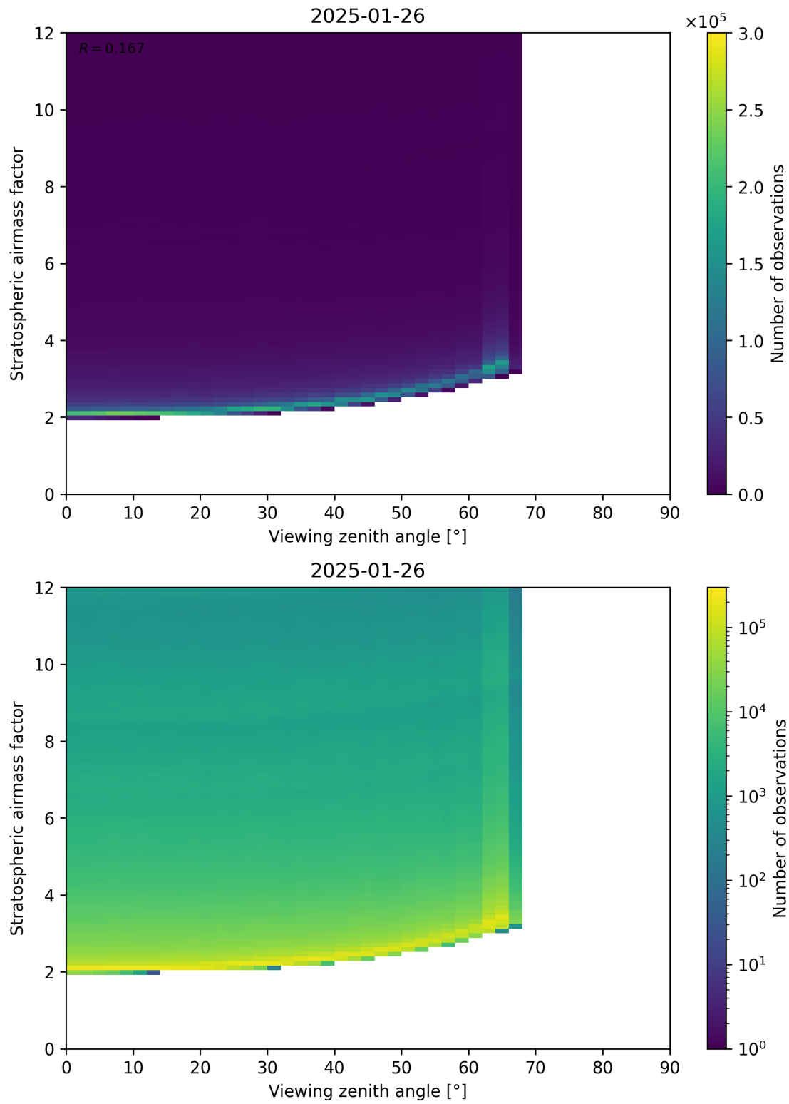
Figure 159: Scatter density plot of “Viewing zenith angle” against “Stratospheric airmass factor” for 2025-01-25 to 2025-01-27.
