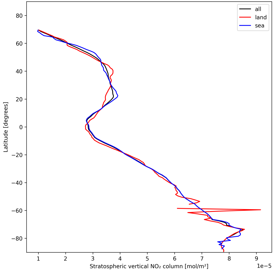
Figure 19: Zonal average of “Stratospheric vertical NO 2 column” for 2025-01-25 to 2025-01-27.
