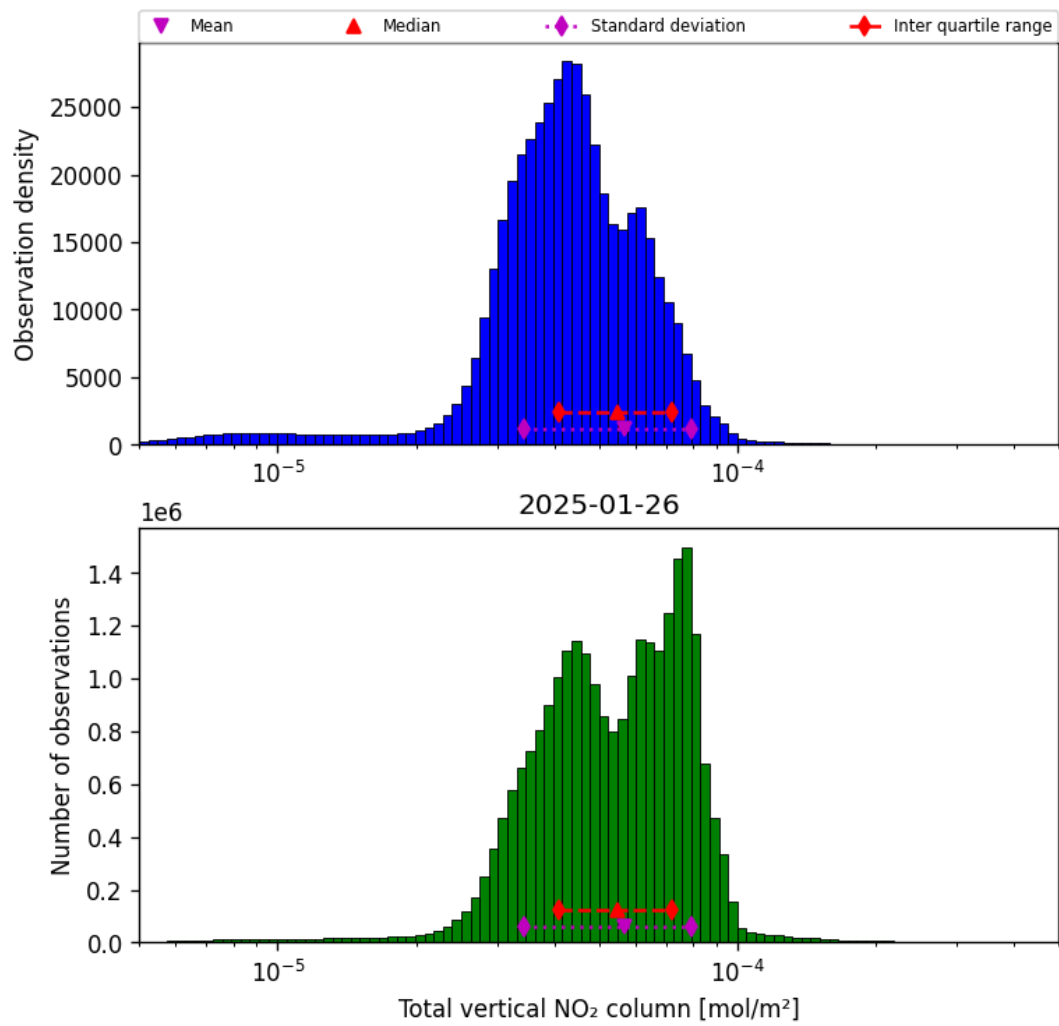
Figure 38: Histogram of “Total vertical NO 2 column” for 2025-01-25 to 2025-01-27
