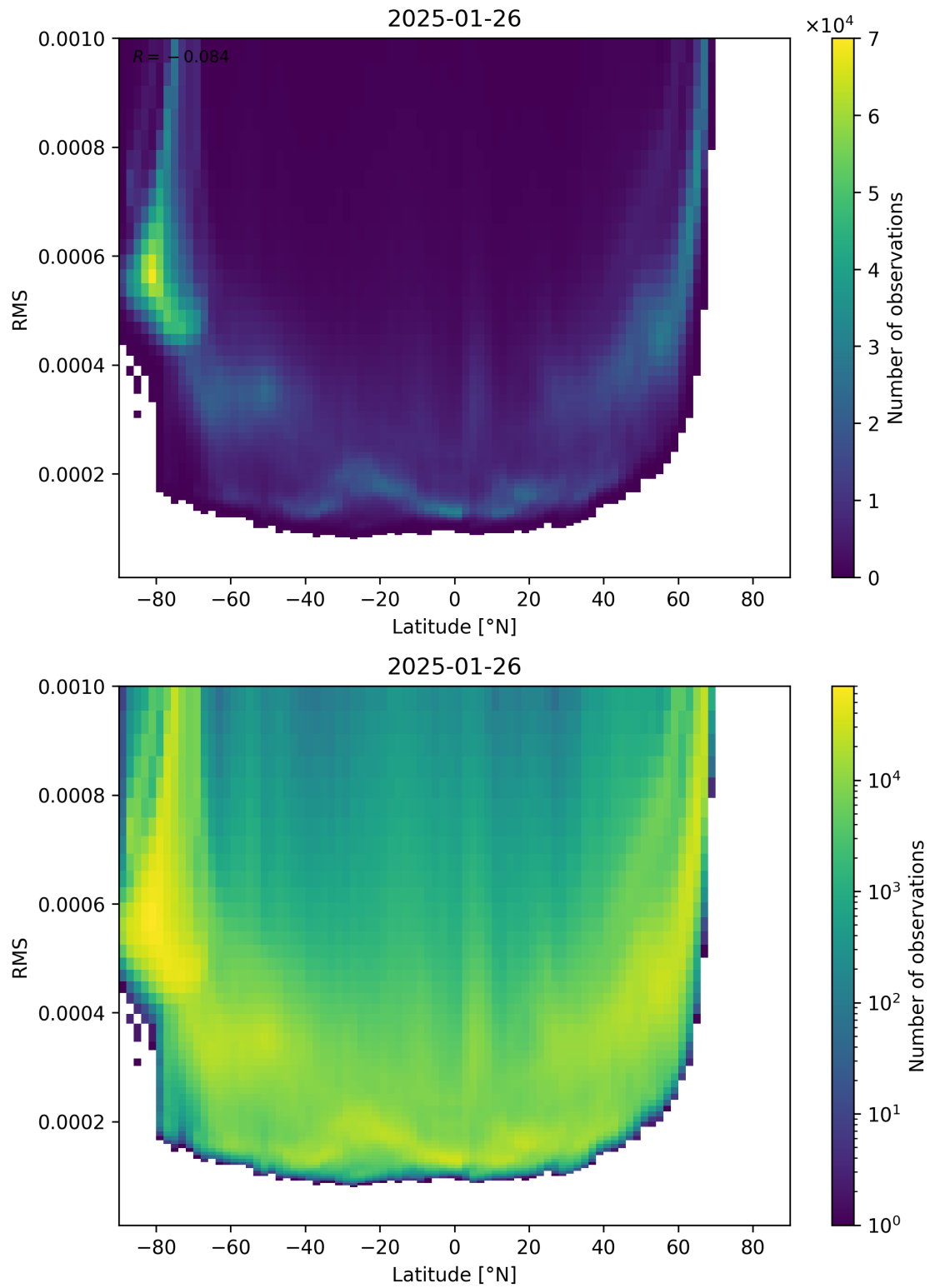
Figure 94: Scatter density plot of “Latitude” against “RMS” for 2025-01-25 to 2025-01-27.
