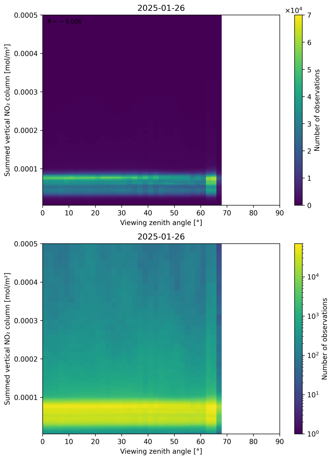
Figure 165: Scatter density plot of “Viewing zenith angle” against “Summed vertical NO 2 column” for 2025-01-25 to 2025-01-27.
