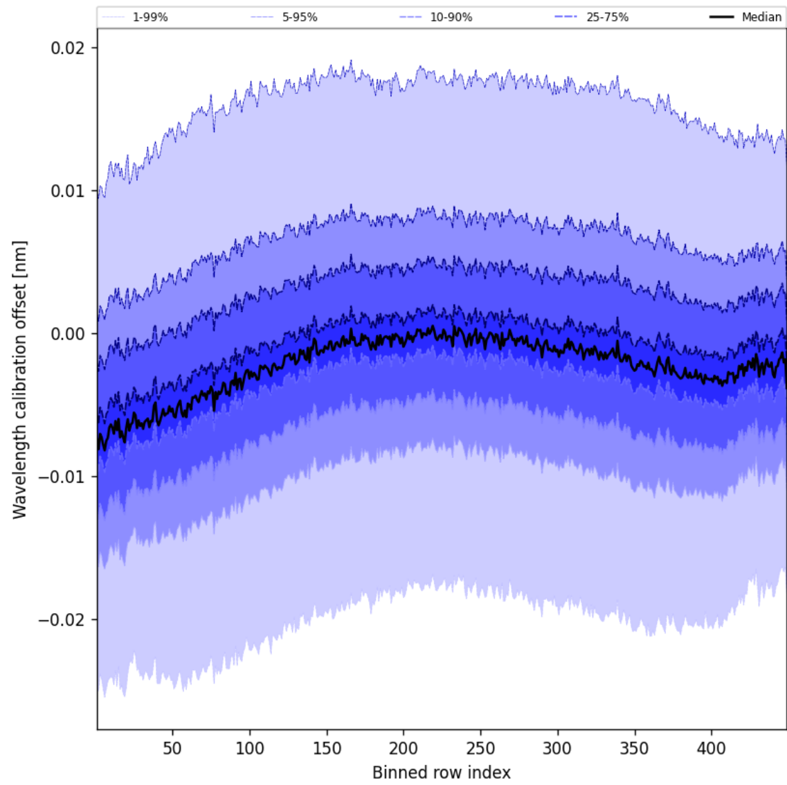
Figure 52: Along track statistics of “Wavelength calibration offset” for 2025-01-25 to 2025-01-27
