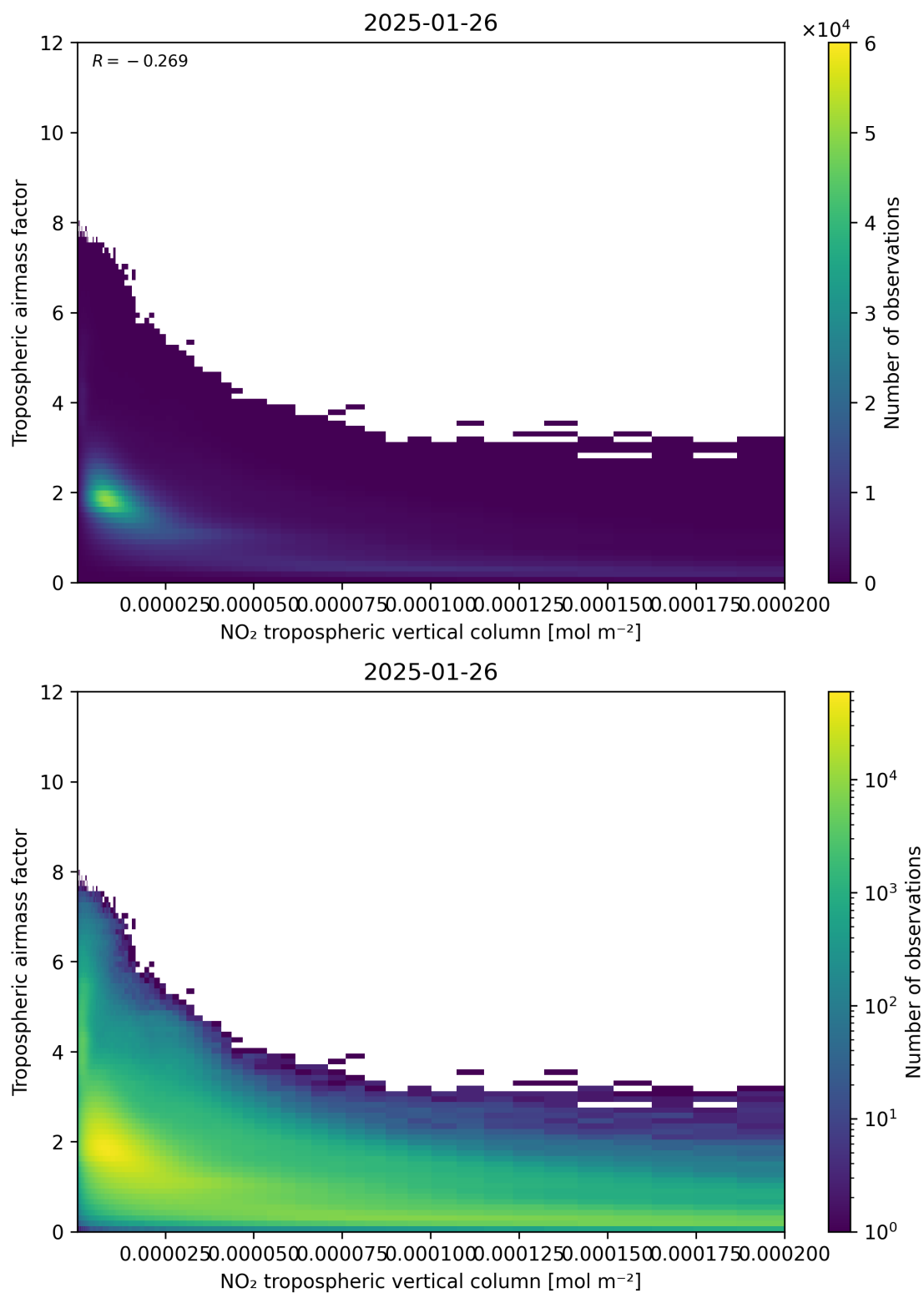
Figure 123: Scatter density plot of “NO 2 tropospheric vertical column” against “Tropospheric air mass factor” for 2025-01-25 to 2025-01-27.
