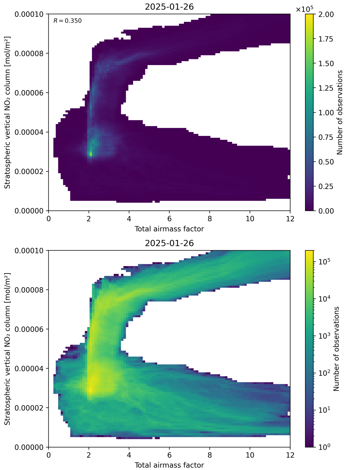
Figure 64: Scatter density plot of “Total airmass factor” against “Stratospheric vertical NO 2 column” for 2025-01-25 to 2025-01-27.
