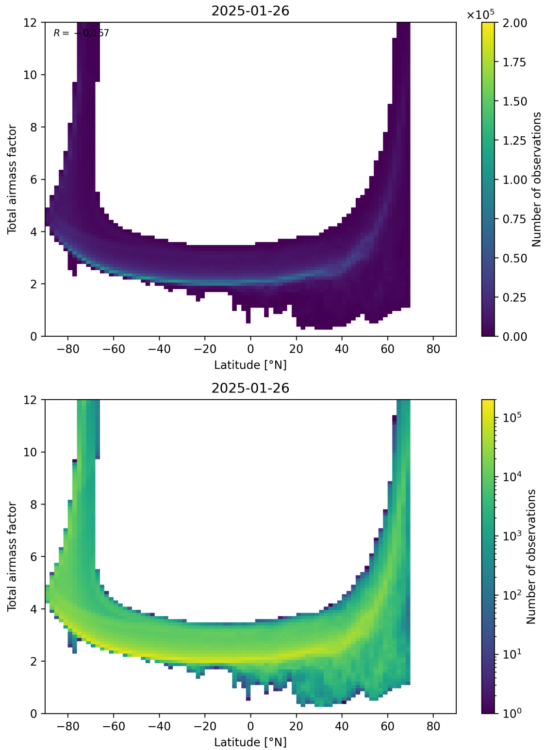
Figure 84: Scatter density plot of “Latitude” against “Total airmass factor” for 2025-01-25 to 2025-01-27.
