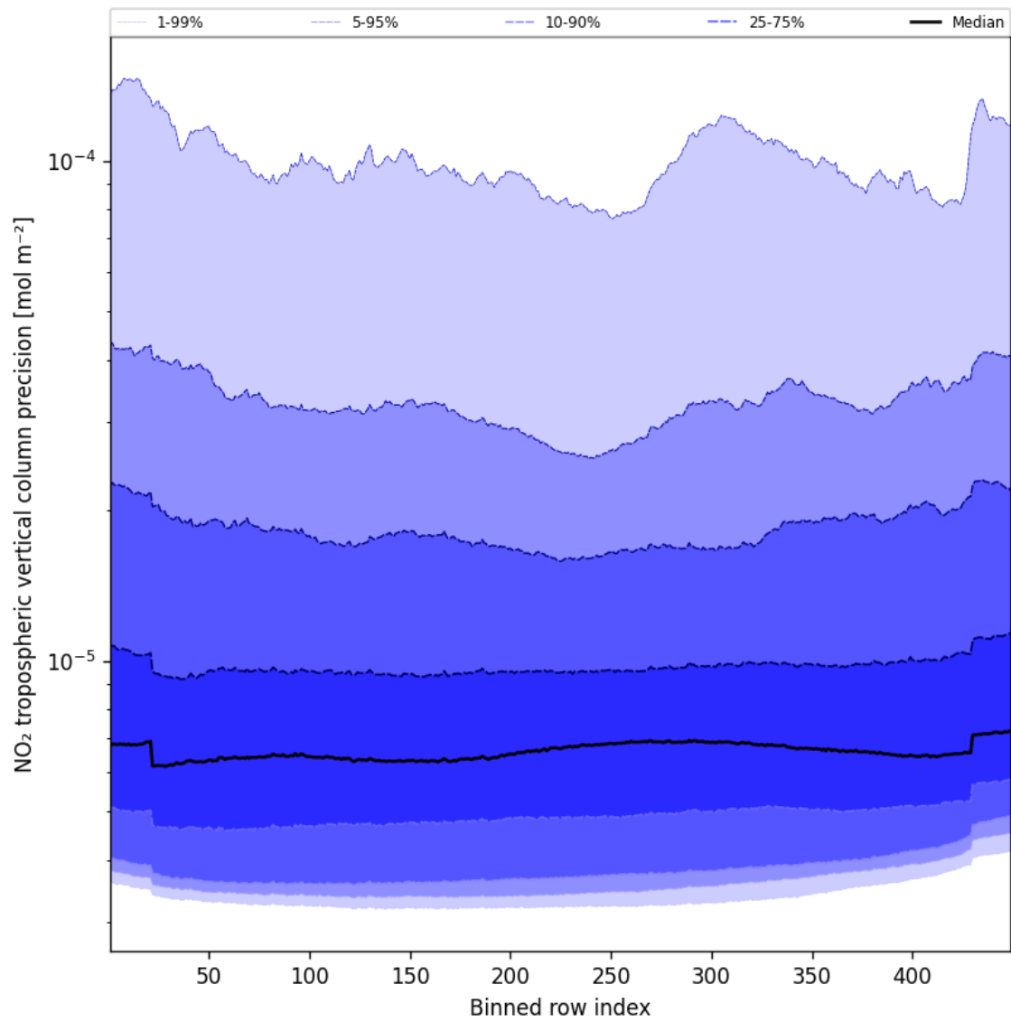
Figure 47: Along track statistics of “NO 2 tropospheric vertical column precision” for 2025-01-25 to 2025-01-27
