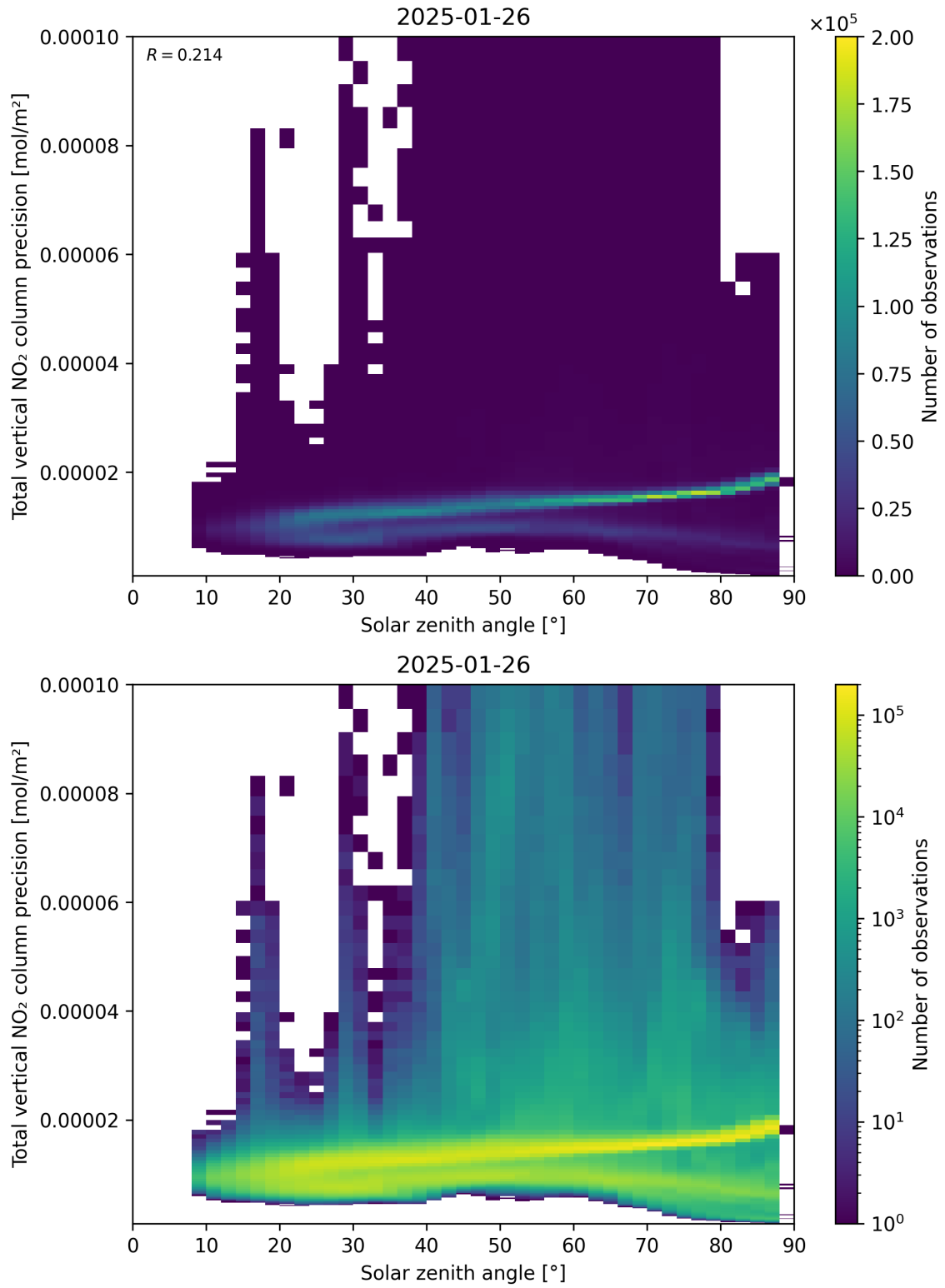
Figure 154: Scatter density plot of “Solar zenith angle” against “Total vertical NO 2 column precision” for 2025-01-25 to 2025-01-27.
