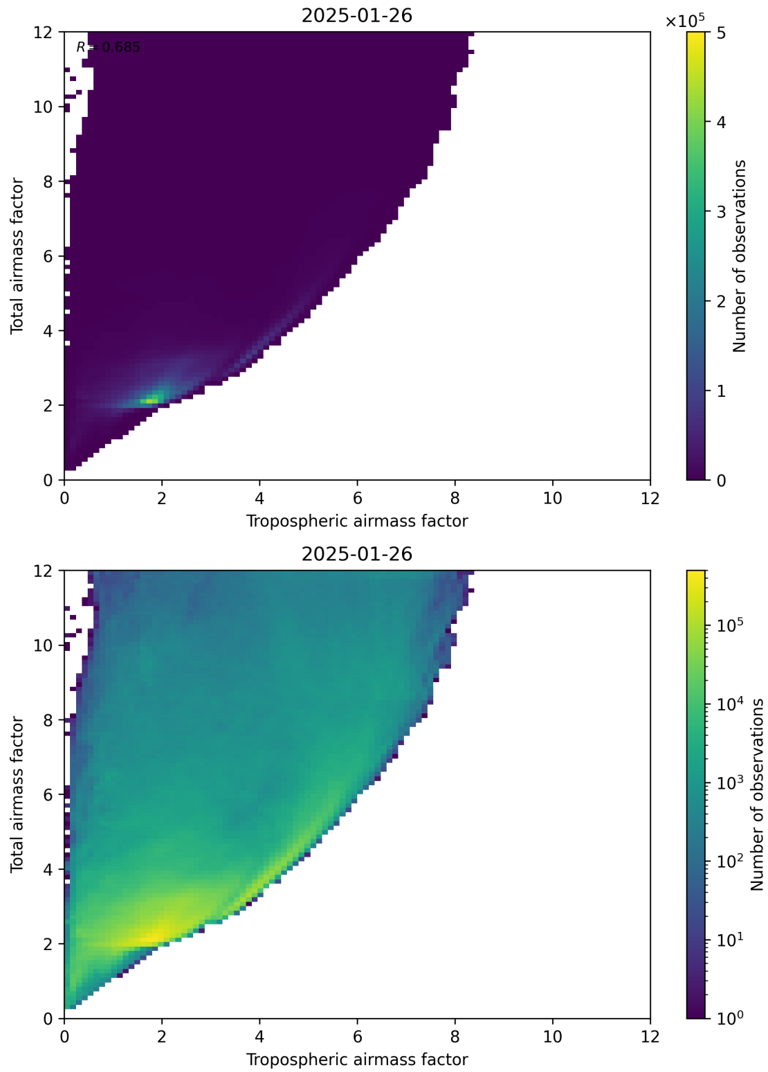
Figure 72: Scatter density plot of “Tropospheric airmass factor” against “Total airmass factor” for 2025-01-25 to 2025-01-27.
