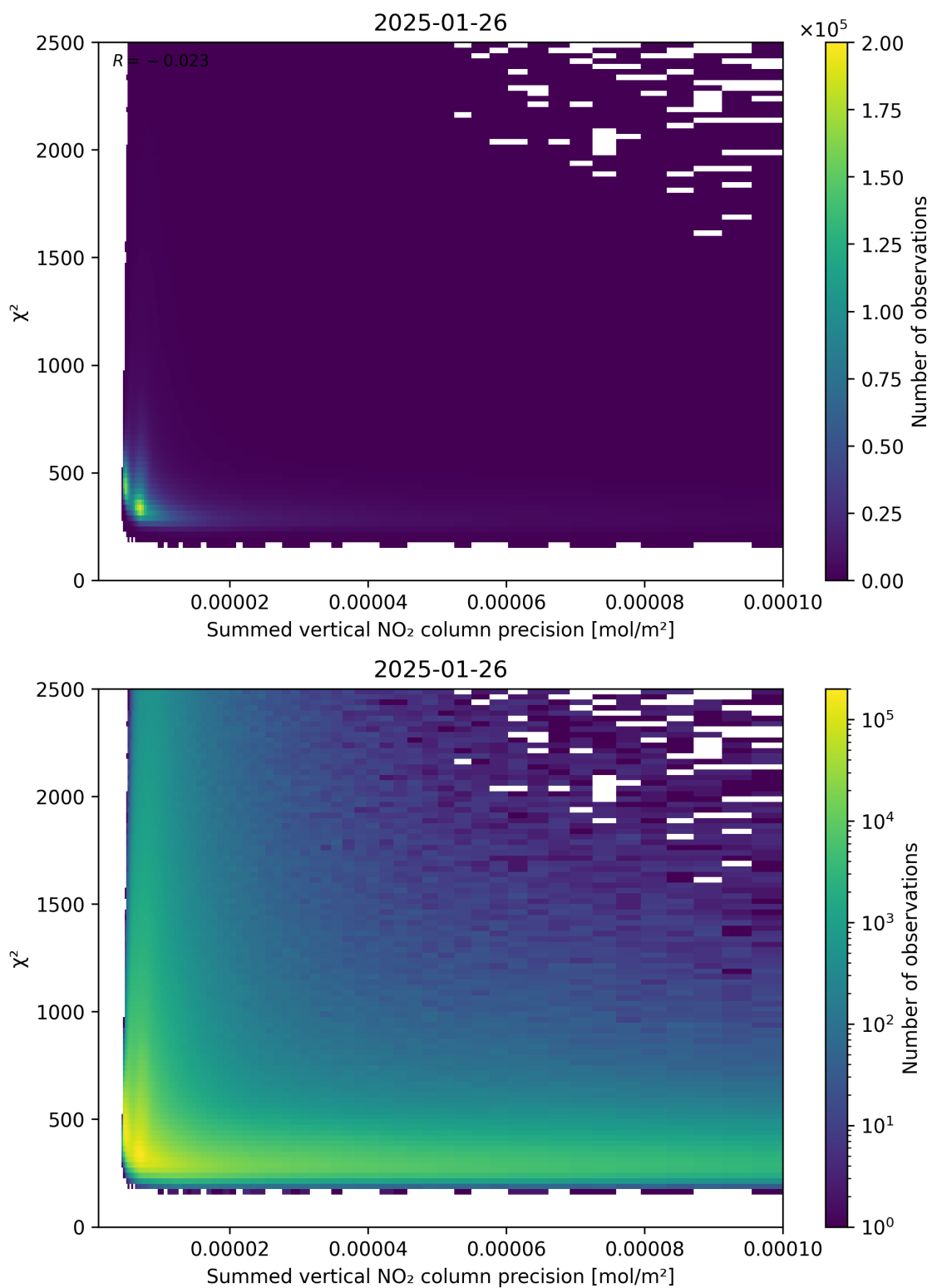
Figure 107: Scatter density plot of “Summed vertical NO 2 column precision” against “ \chi^2 ” for 2025-01-25 to 2025-01-27.
