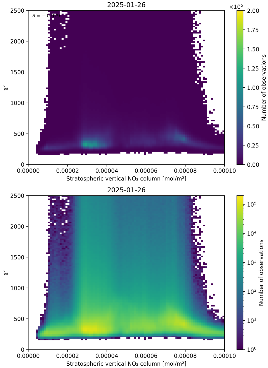
Figure 97: Scatter density plot of “Stratospheric vertical NO 2 column” against “ \chi^2 ” for 2025-01-25 to 2025-01-27.
