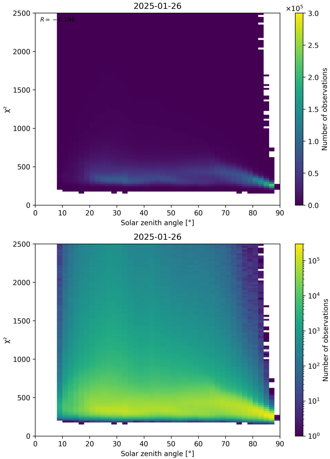
Figure 148: Scatter density plot of “Solar zenith angle” against “ \chi^2 ” for 2025-01-25 to 2025-01-27.
