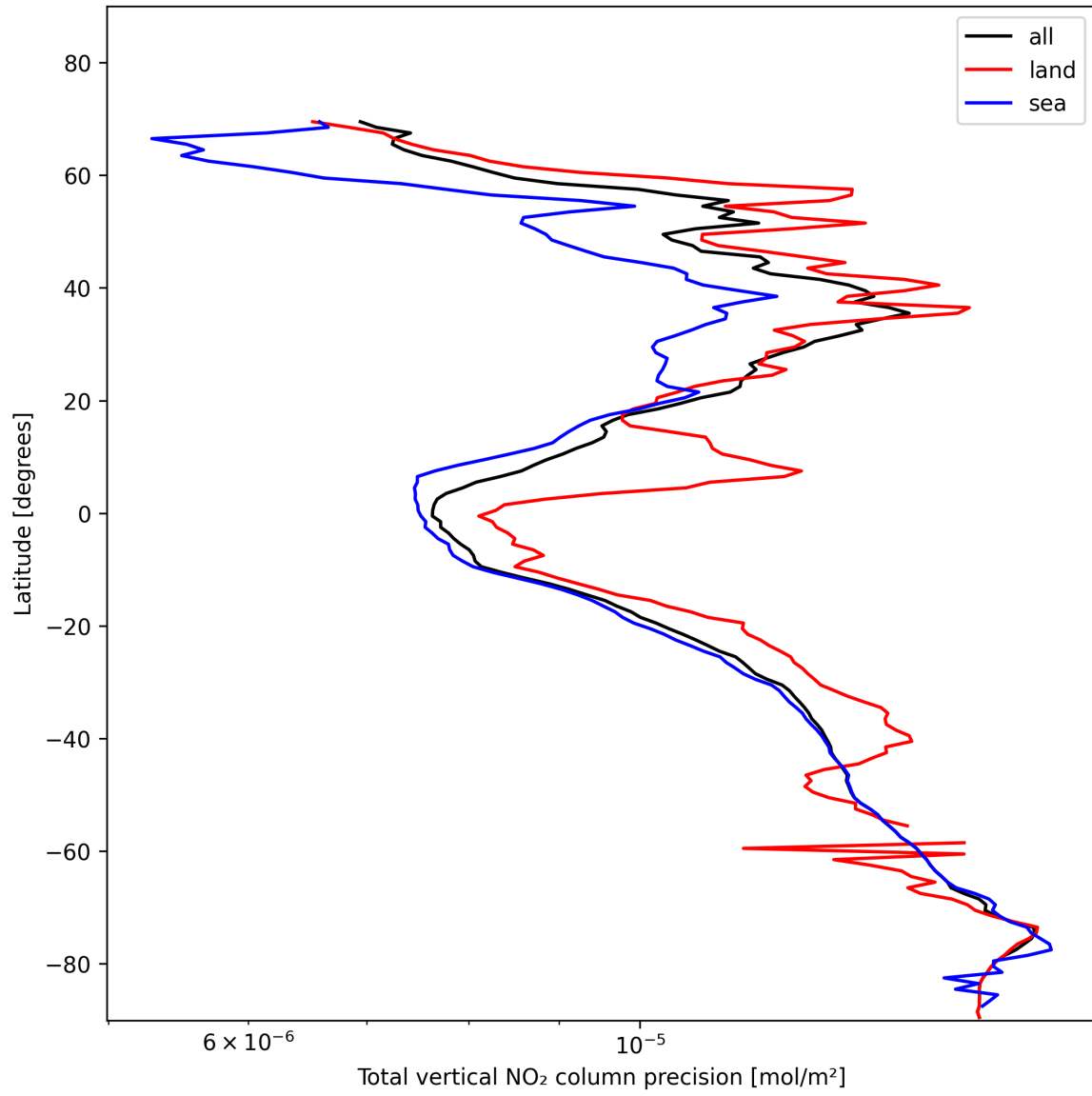
Figure 22: Zonal average of “Total vertical NO 2 column precision” for 2025-01-25 to 2025-01-27.
