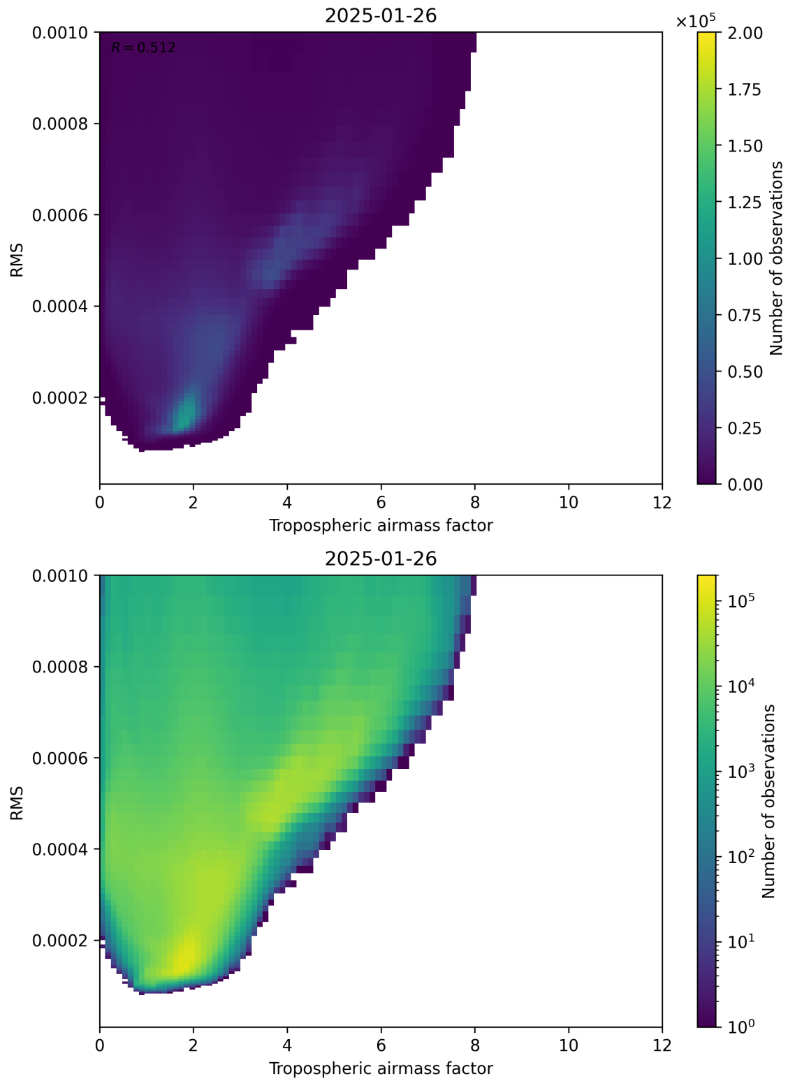
Figure 79: Scatter density plot of “Tropospheric airmass factor” against “RMS” for 2025-01-25 to 2025-01-27.
