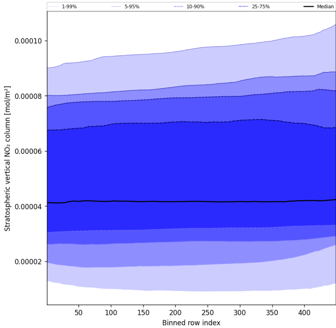
Figure 53: Along track statistics of “Stratospheric vertical NO 2 column” for 2025-01-25 to 2025-01-27
