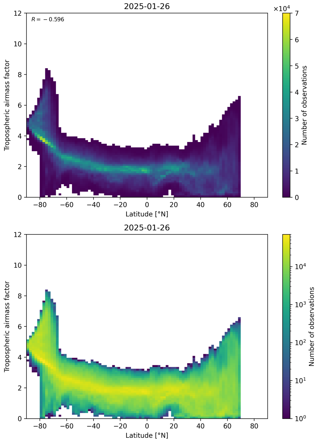
Figure 85: Scatter density plot of “Latitude” against “Tropospheric airmass factor” for 2025-01-25 to 2025-01-27.
