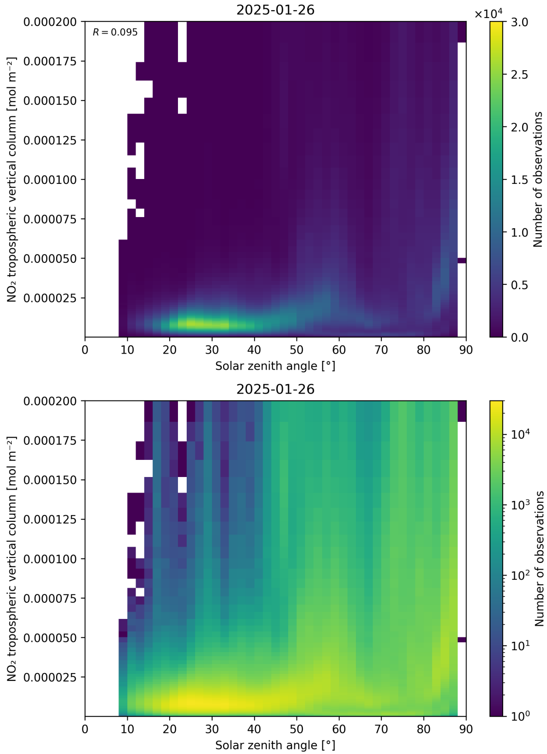
Figure 155: Scatter density plot of “Solar zenith angle” against “NO 2 tropospheric vertical column” for 2025-01-25 to 2025-01-27.
