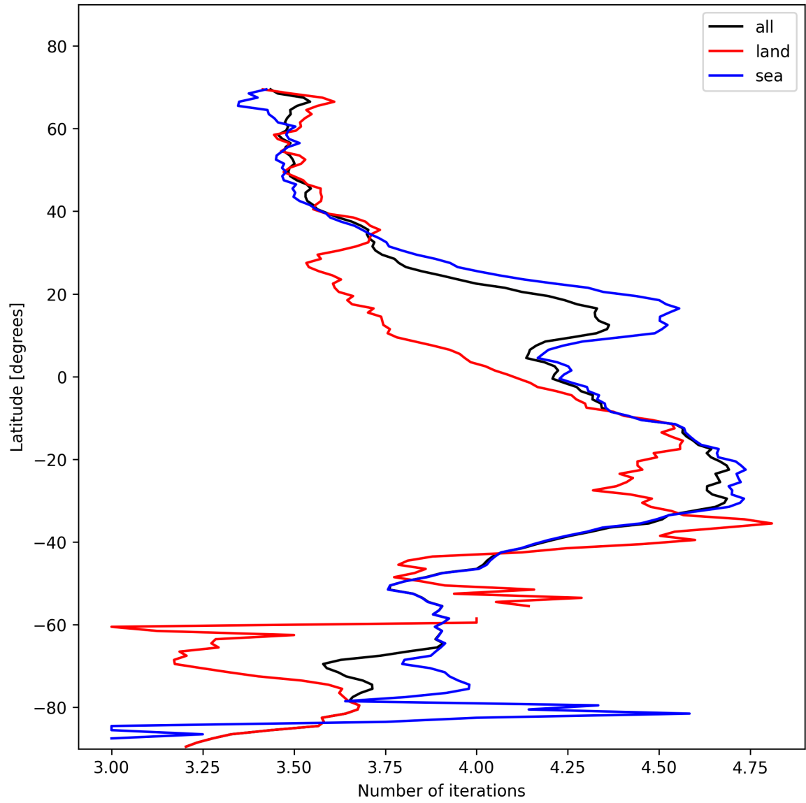
Figure 17: Zonal average of “Number of iterations” for 2025-01-25 to 2025-01-27.
