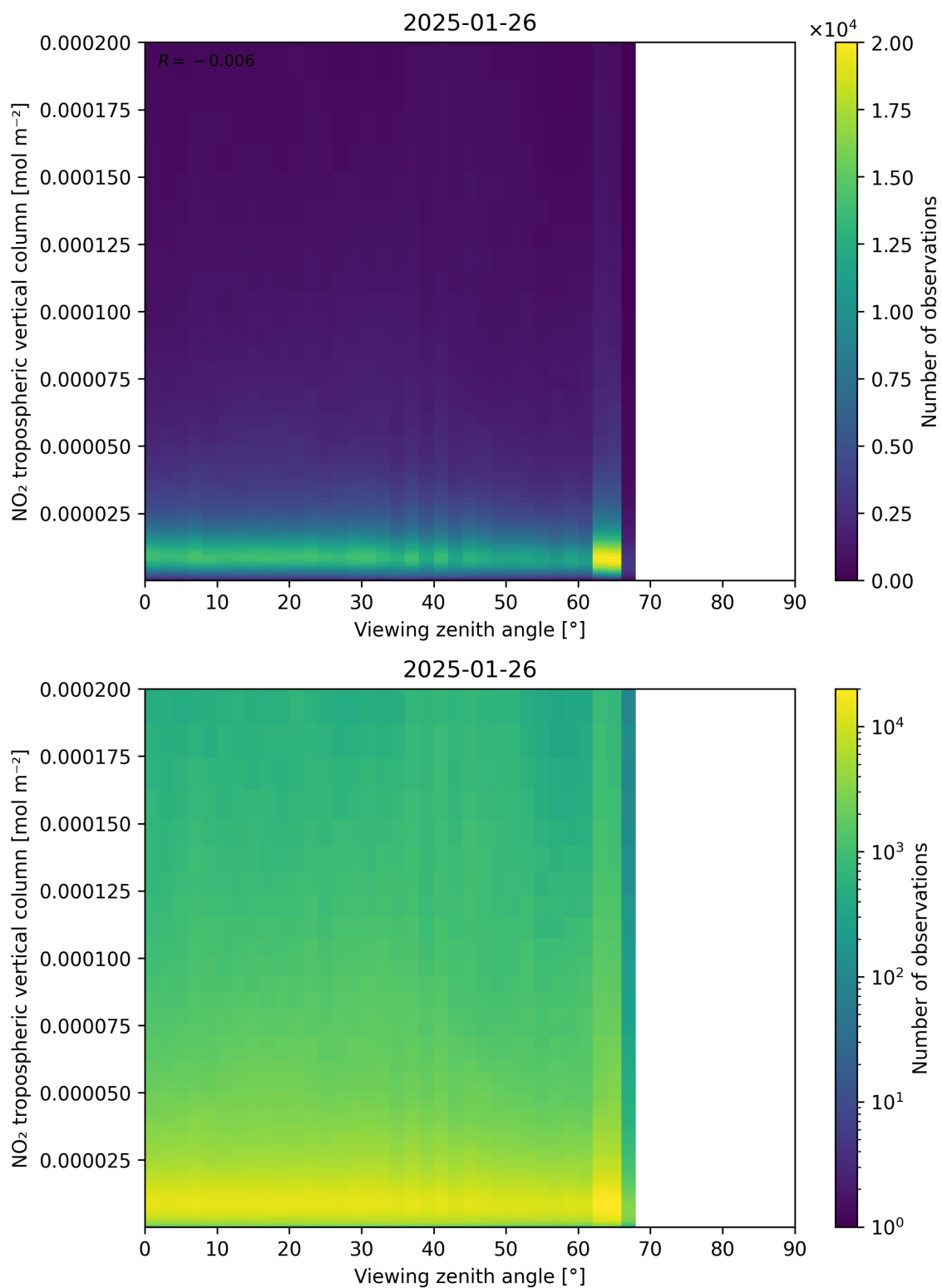
Figure 169: Scatter density plot of “Viewing zenith angle” against “NO 2 tropospheric vertical column” for 2025-01-25 to 2025-01-27.
