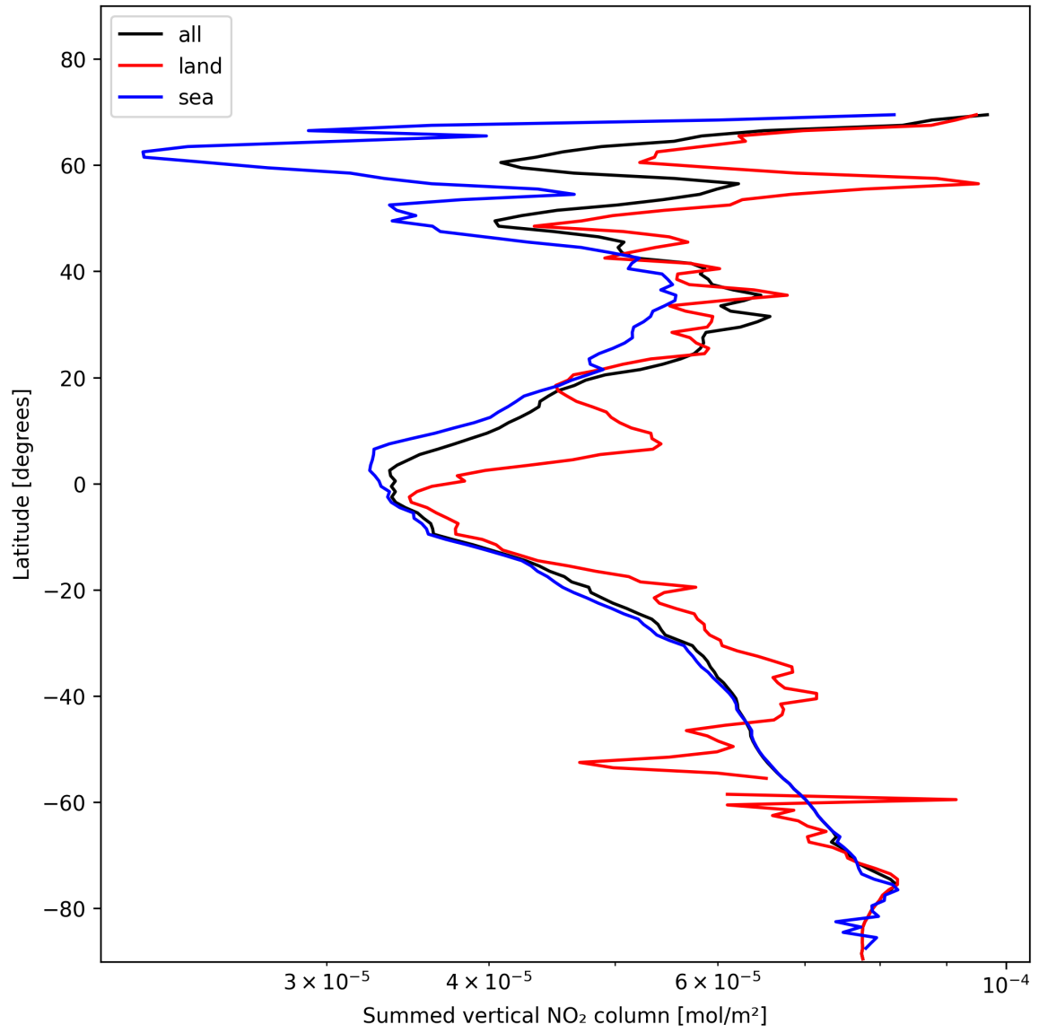
Figure 23: Zonal average of “Summed vertical NO 2 column” for 2025-01-25 to 2025-01-27.
