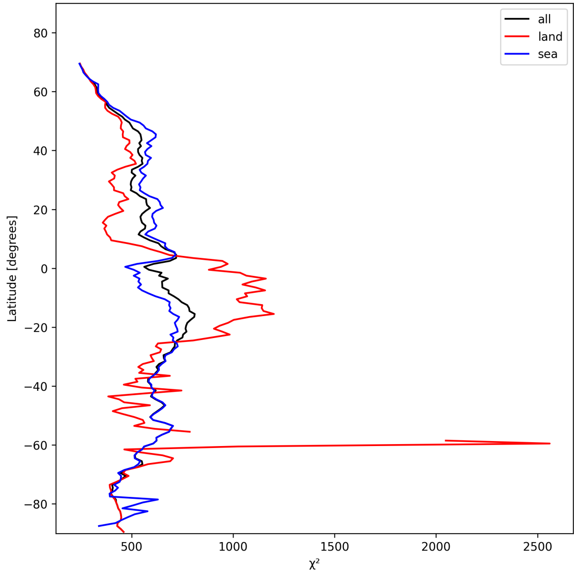
Figure 25: Zonal average of “ \chi^2 ” for 2025-01-25 to 2025-01-27.
