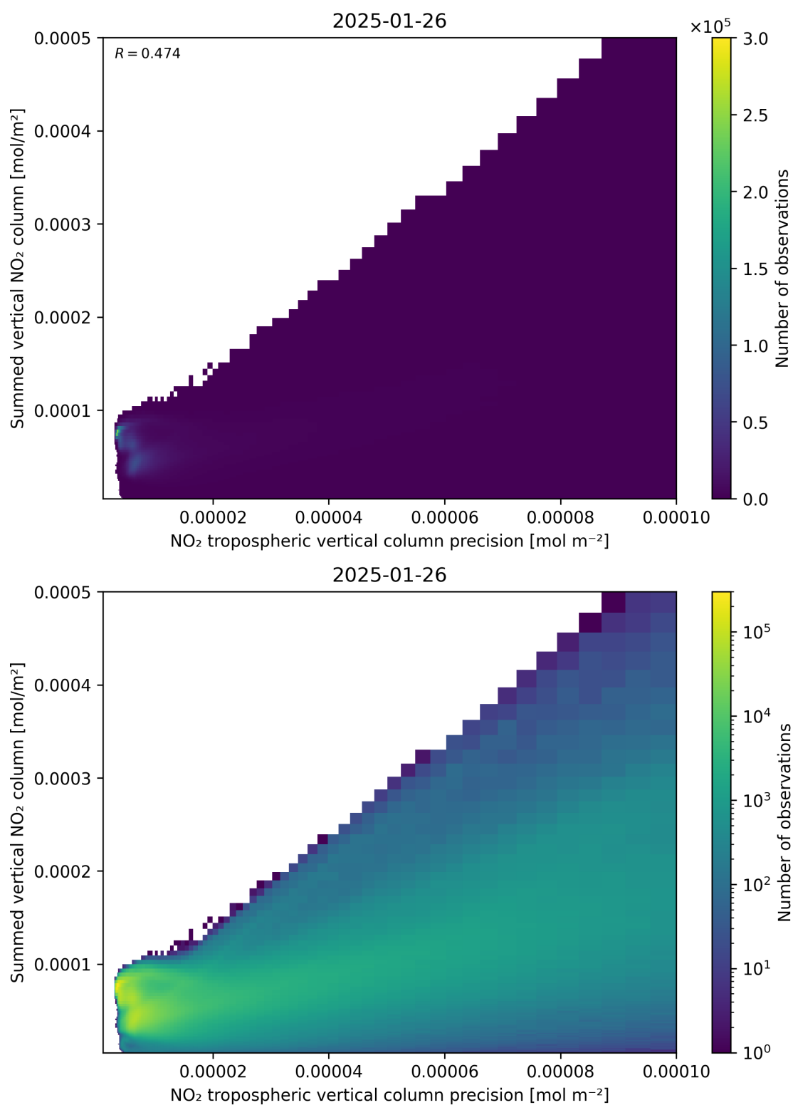
Figure 136: Scatter density plot of “NO 2 tropospheric vertical column precision” against “Summed vertical NO 2 column” for 2025-01-25 to 2025-01-27.
