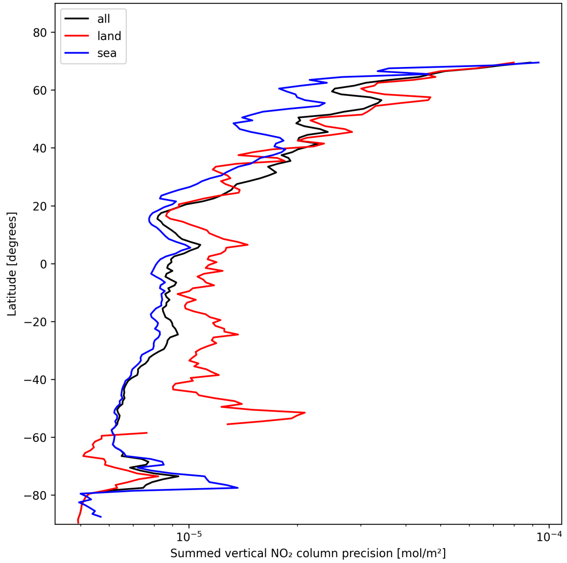
Figure 24: Zonal average of “Summed vertical NO 2 column precision” for 2025-01-25 to 2025-01-27.
