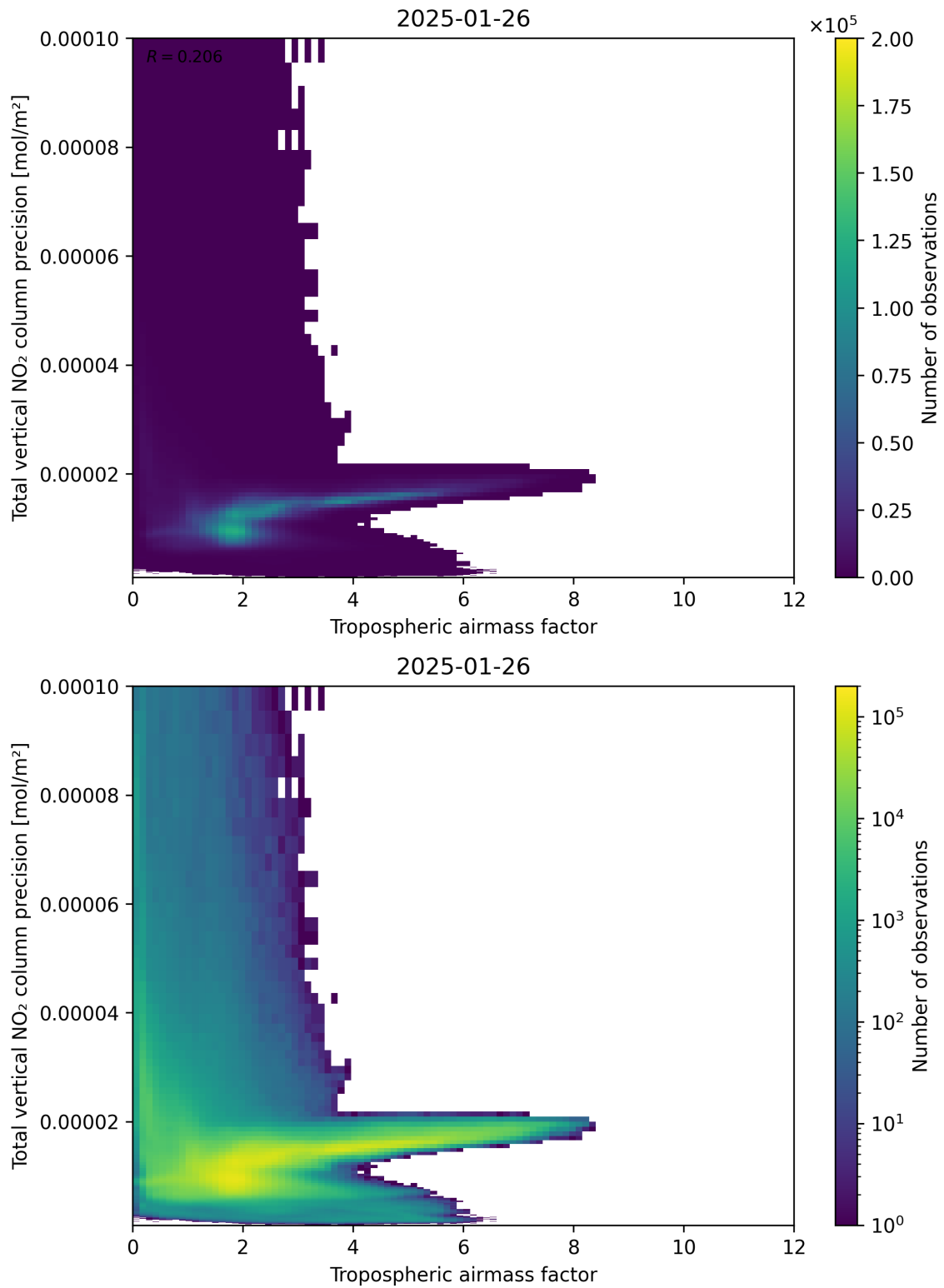
Figure 78: Scatter density plot of “Tropospheric air mass factor” against “Total vertical NO 2 column precision” for 2025-01-25 to 2025-01-27.
