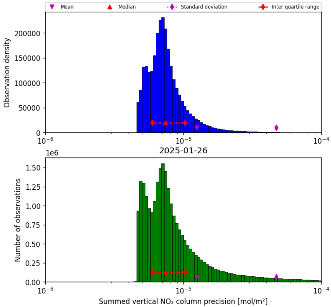
Figure 41: Histogram of "Summed vertical NO 2 column precision" for 2025-01-25 to 2025-01-27
