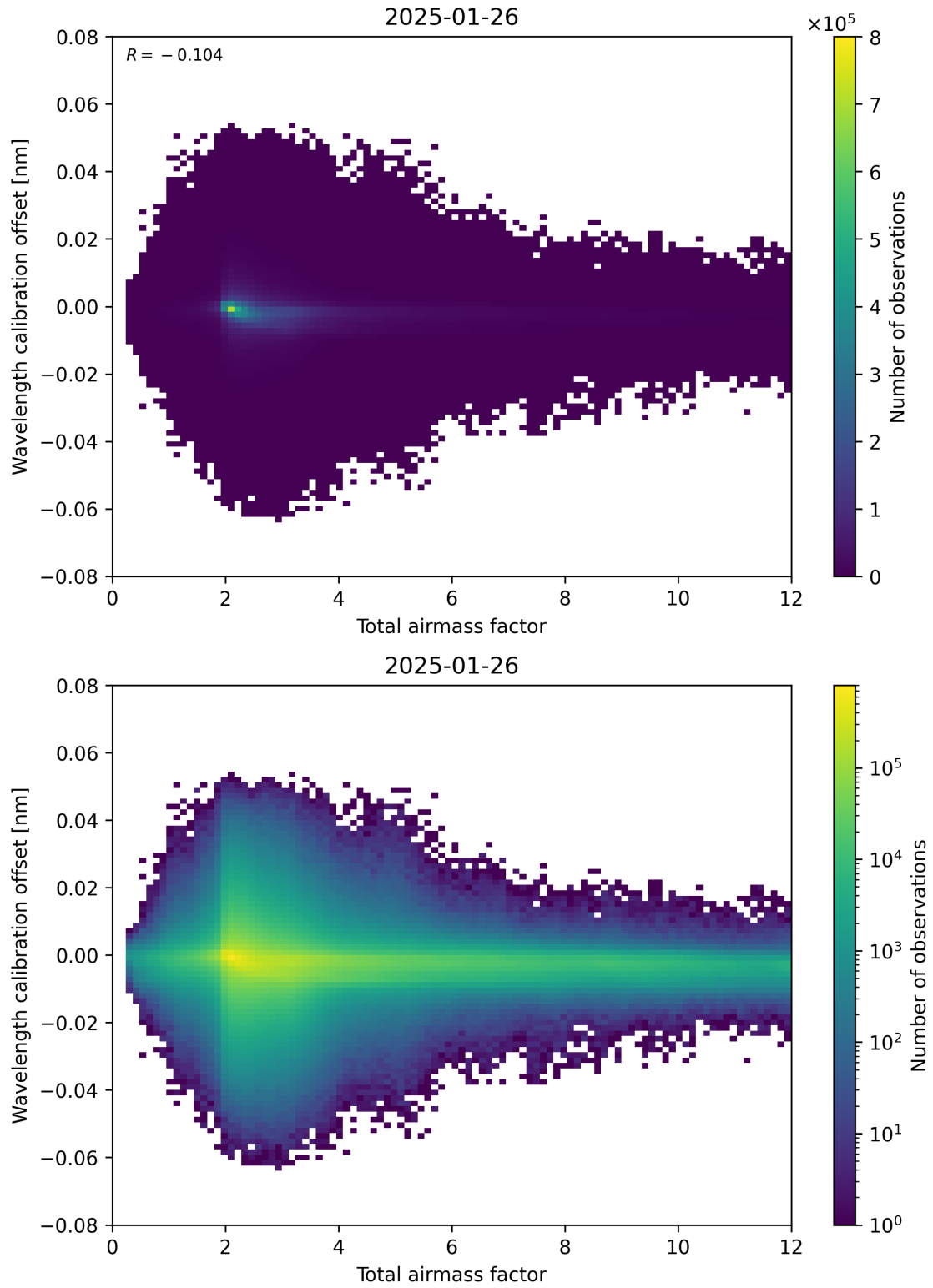
Figure 70: Scatter density plot of “Total airmass factor” against “Wavelength calibration offset” for 2025-01-25 to 2025-01-27.
