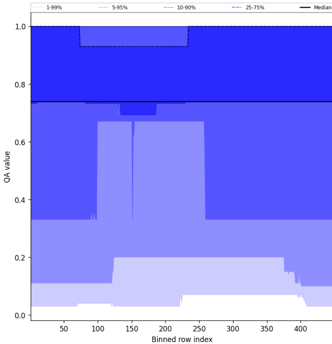
Figure 45: Along track statistics of “QA value” for 2025-01-25 to 2025-01-27
