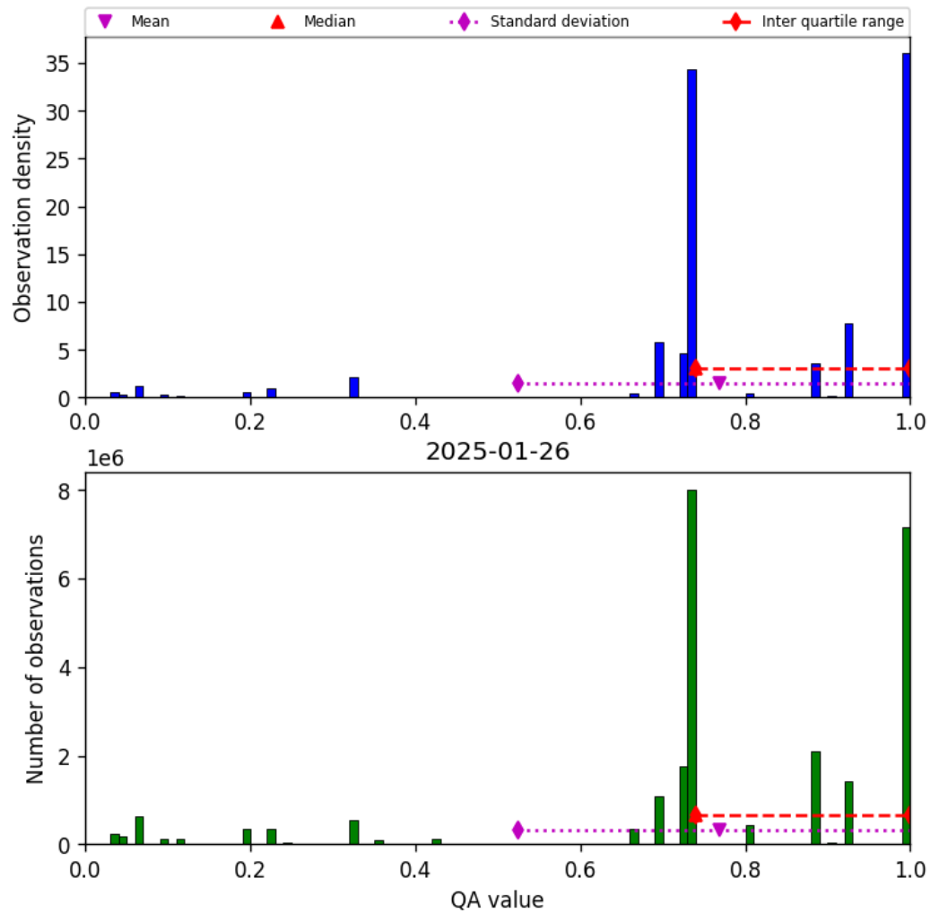
Figure 28: Histogram of “QA value” for 2025-01-25 to 2025-01-27
