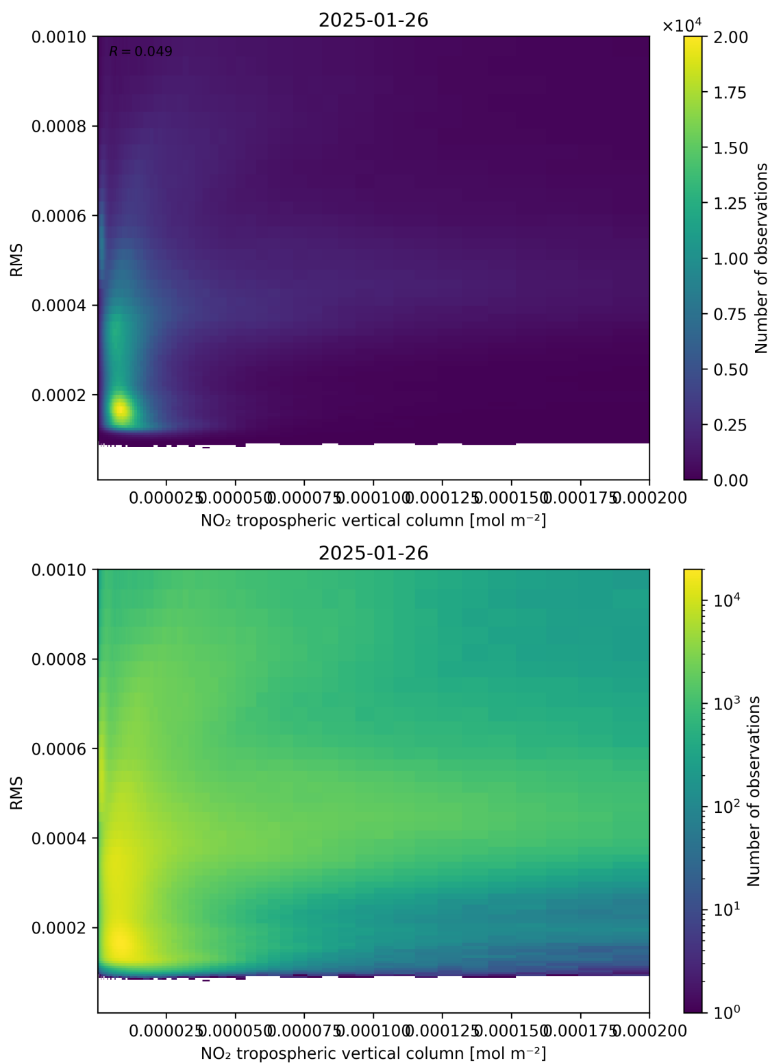
Figure 142: Scatter density plot of “NO 2 tropospheric vertical column” against “RMS” for 2025-01-25 to 2025-01-27.
