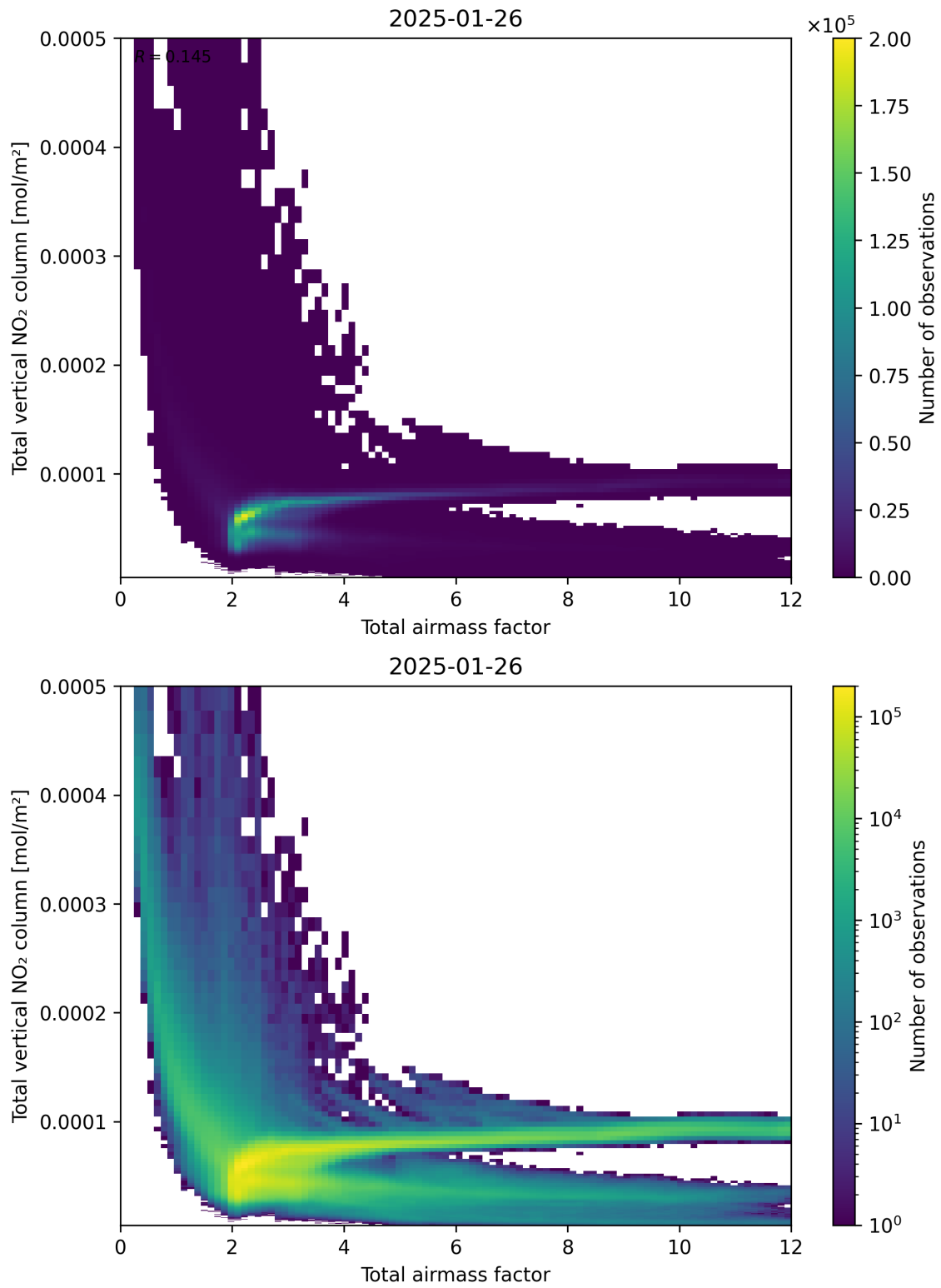
Figure 67: Scatter density plot of “Total airmass factor” against “Total vertical NO 2 column” for 2025-01-25 to 2025-01-27.
