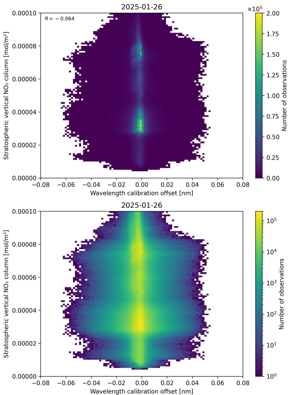
Figure 176: Scatter density plot of “Wavelength calibration offset” against “Stratospheric vertical NO 2 column” for 2025-01-25 to 2025-01-27.
