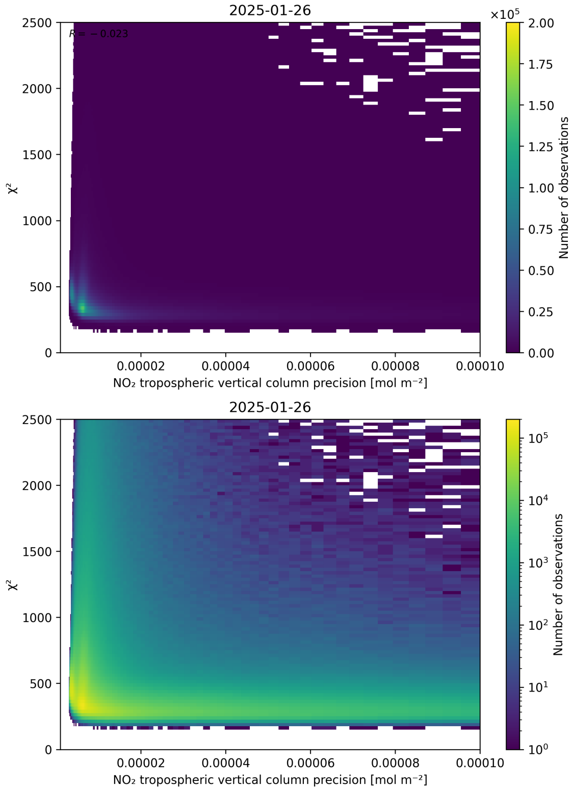
Figure 134: Scatter density plot of “NO 2 tropospheric vertical column precision” against “ \chi^2 ” for 2025-01-25 to 2025-01-27.
