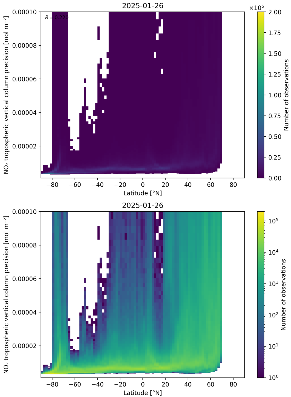
Figure 93: Scatter density plot of “Latitude” against “NO 2 tropospheric vertical column precision” for 2025-01-25 to 2025-01-27.
