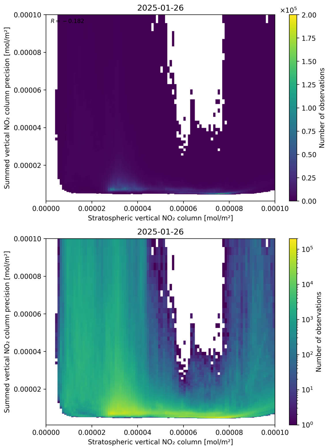
Figure 99: Scatter density plot of “Stratospheric vertical NO 2 column” against “Summed vertical NO 2 column precision” for 2025-01-25 to 2025-01-27.
