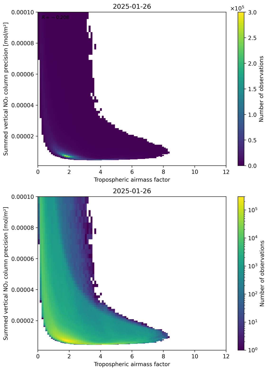
Figure 76: Scatter density plot of “Tropospheric air mass factor” against “Summed vertical NO 2 column precision” for 2025-01-25 to 2025-01-27.
