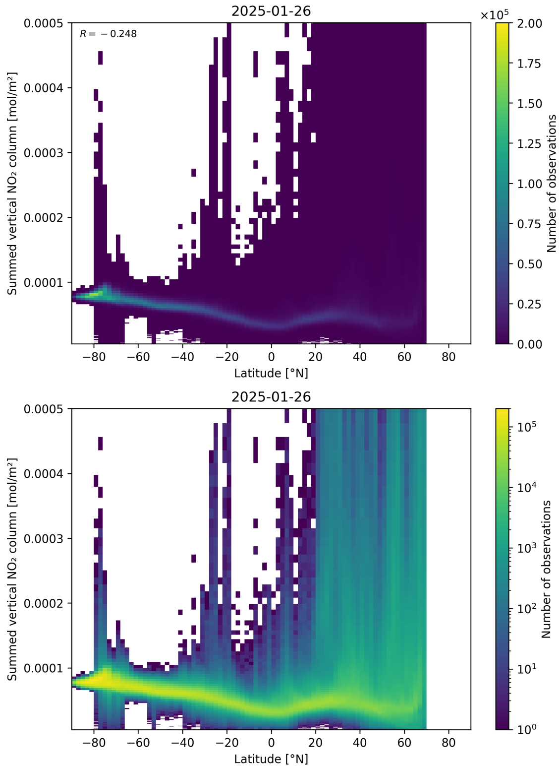
Figure 88: Scatter density plot of “Latitude” against “Summed vertical NO 2 column” for 2025-01-25 to 2025-01-27.
