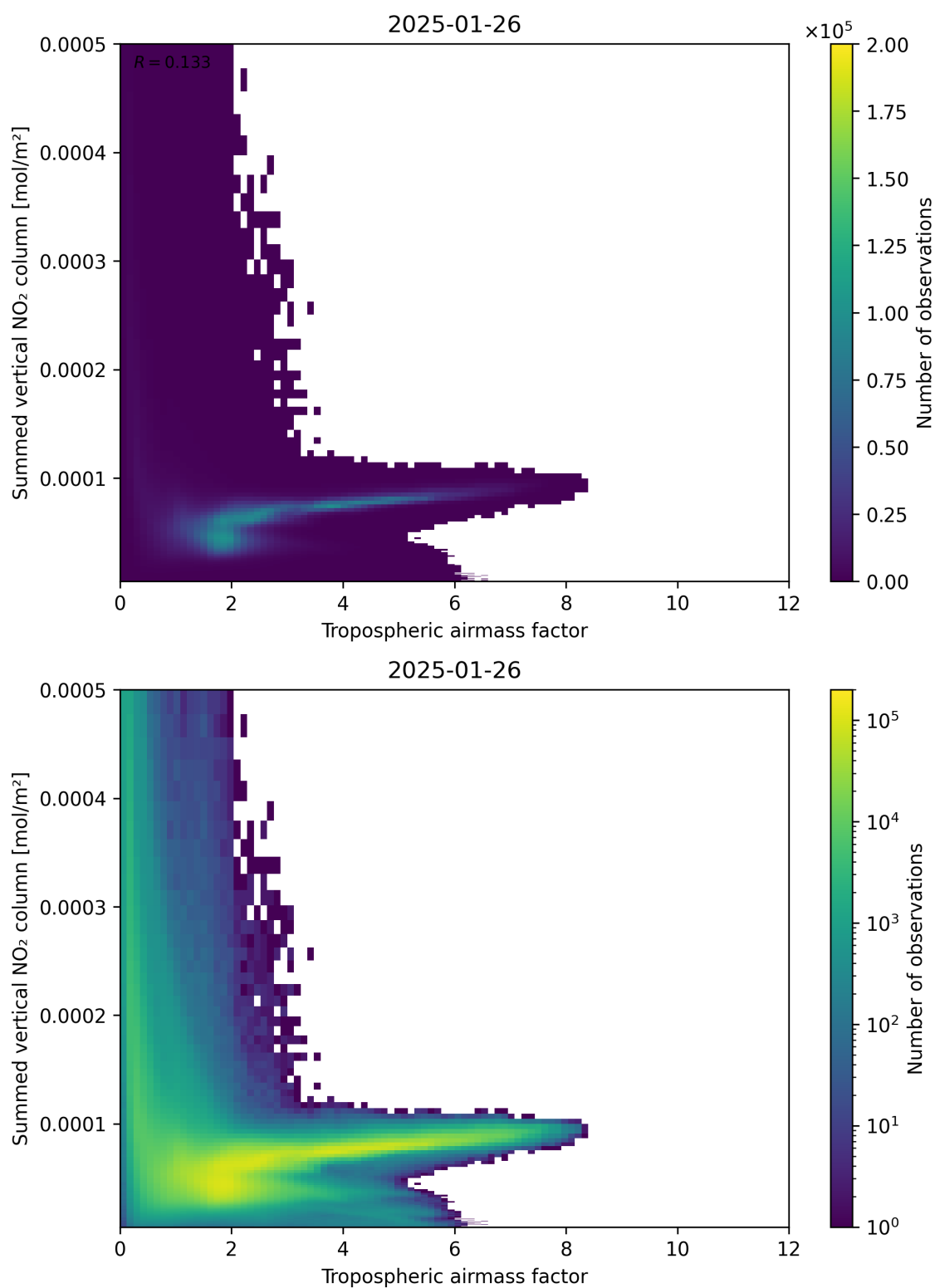
Figure 75: Scatter density plot of “Tropospheric air mass factor” against “Summed vertical NO 2 column” for 2025-01-25 to 2025-01-27.
