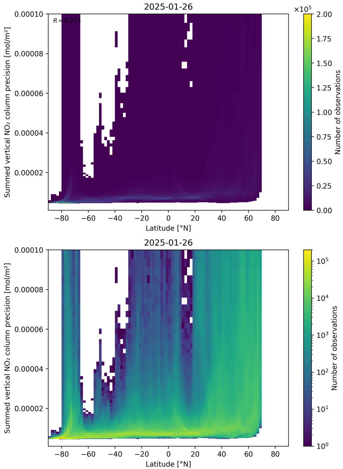
Figure 89: Scatter density plot of “Latitude” against “Summed vertical NO 2 column precision” for 2025-01-25 to 2025-01-27.
