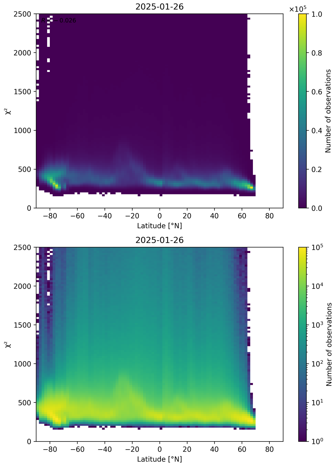
Figure 86: Scatter density plot of “Latitude” against “ \chi^2 ” for 2025-01-25 to 2025-01-27.
