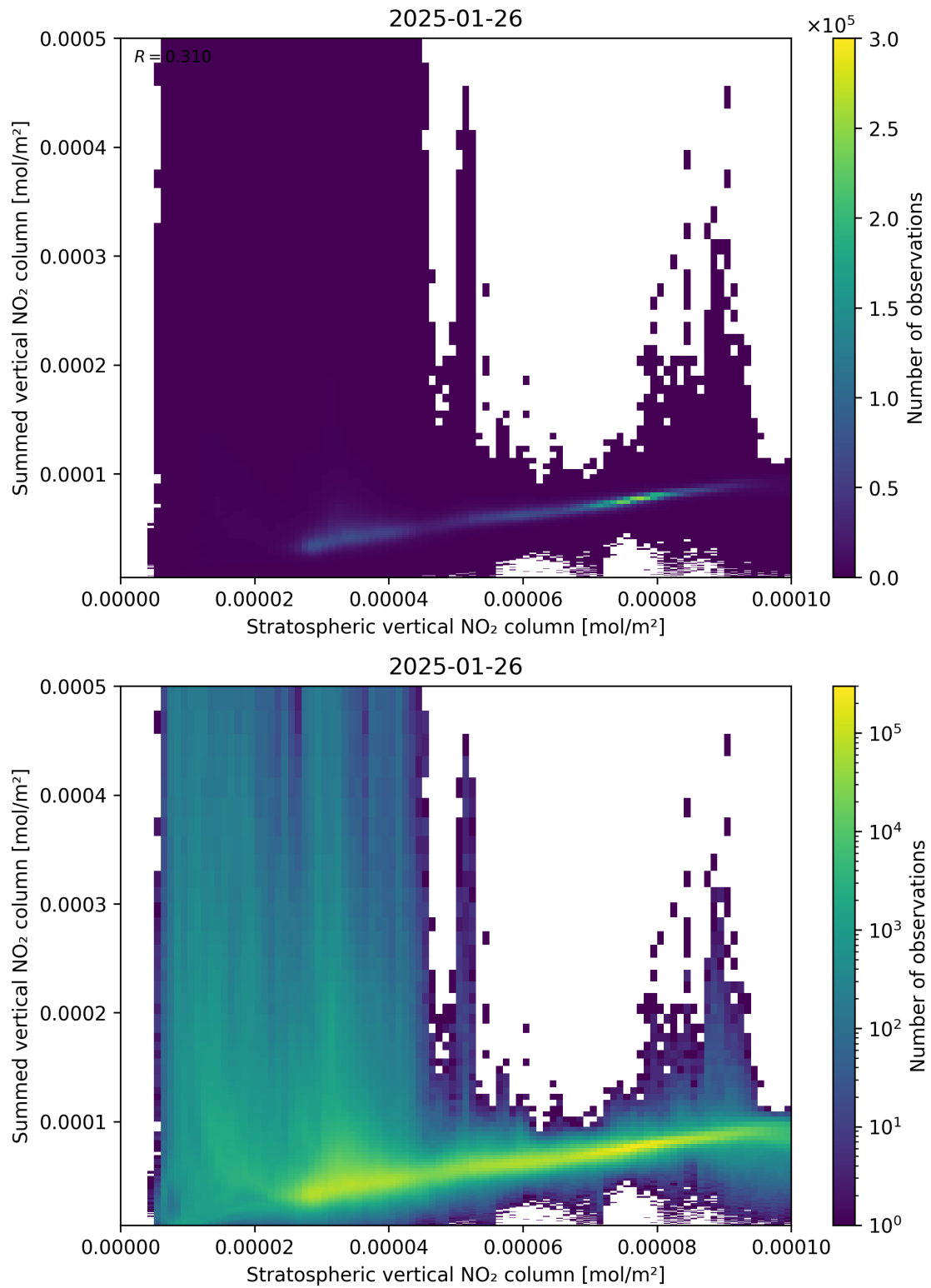
Figure 98: Scatter density plot of “Stratospheric vertical NO 2 column” against “Summed vertical NO 2 column” for 2025-01-25 to 2025-01-27.
