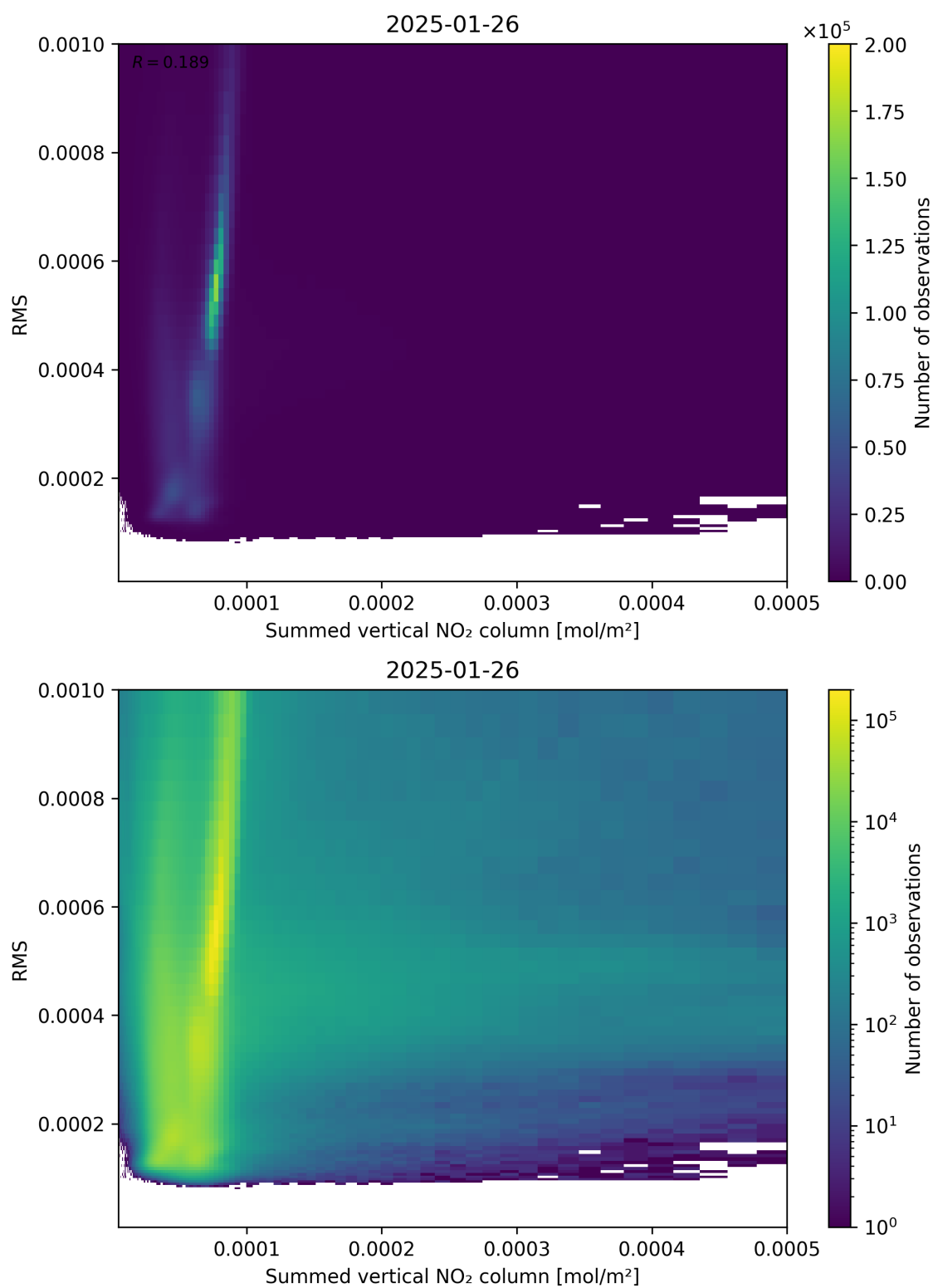
Figure 109: Scatter density plot of “Summed vertical NO 2 column” against “RMS” for 2025-01-25 to 2025-01-27.
