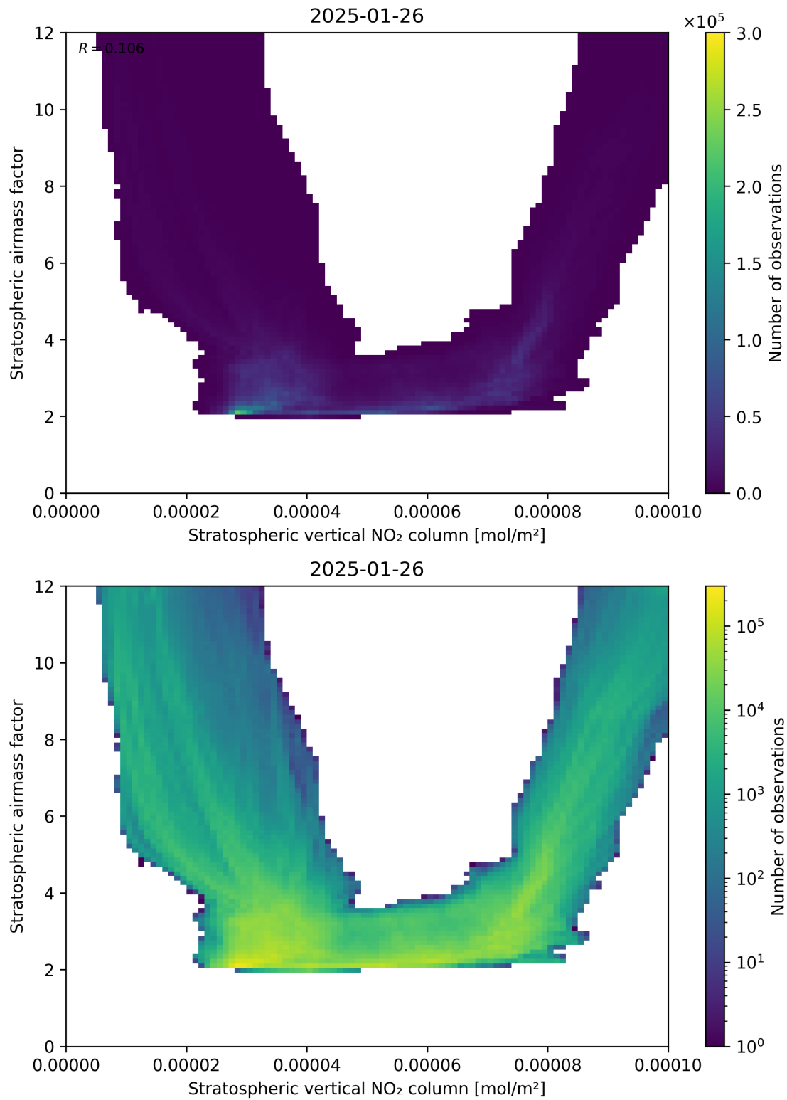
Figure 96: Scatter density plot of “Stratospheric vertical NO 2 column” against “Stratospheric airmass factor” for 2025-01-25 to 2025-01-27.
