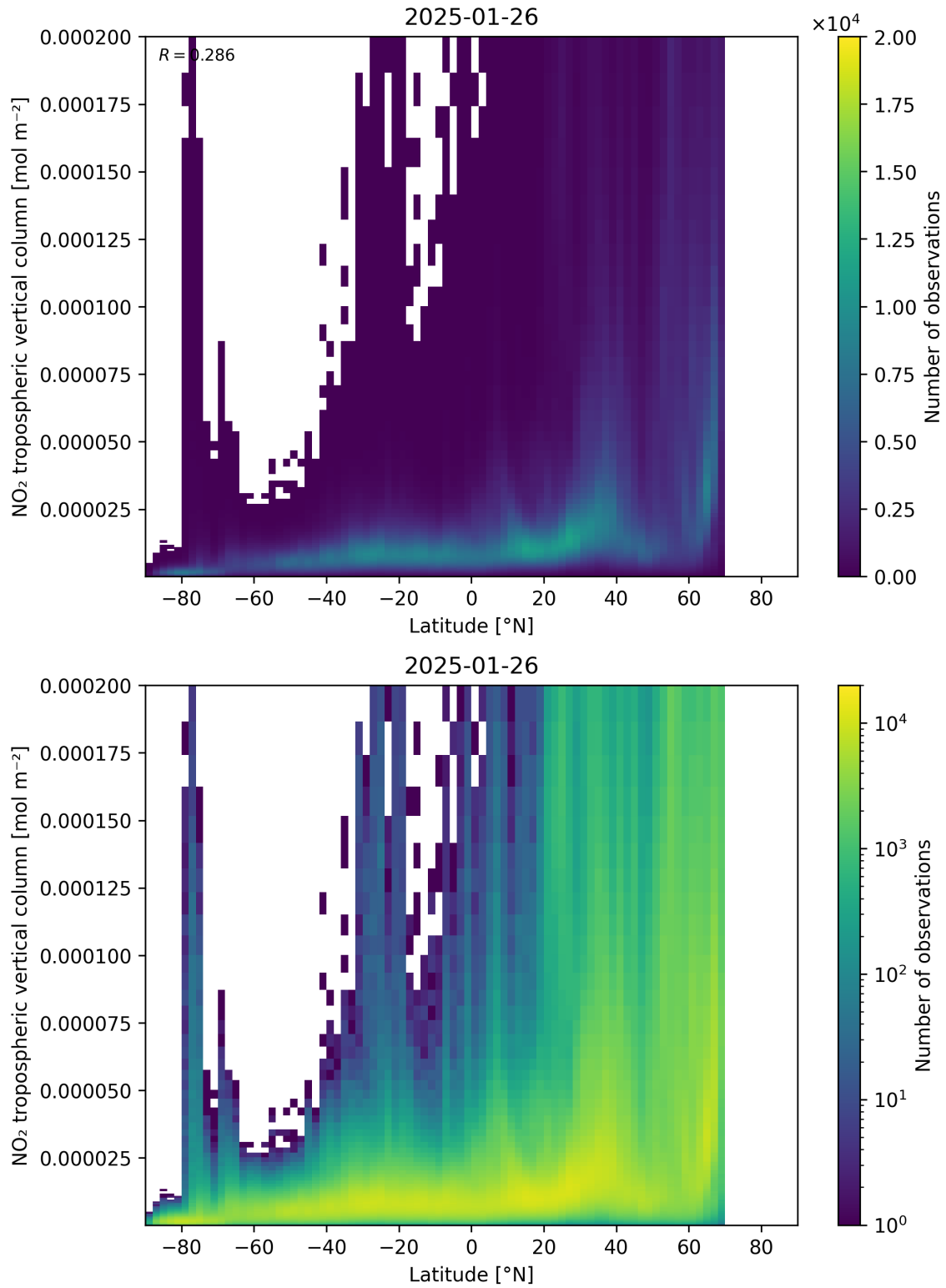
Figure 92: Scatter density plot of “Latitude” against “NO 2 tropospheric vertical column” for 2025-01-25 to 2025-01-27.
