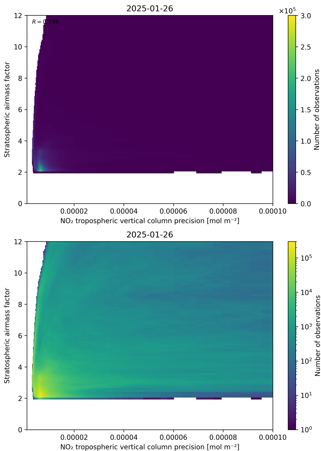
Figure 131: Scatter density plot of “NO 2 tropospheric vertical column precision” against “Stratospheric airmass factor” for 2025-01-25 to 2025-01-27.
