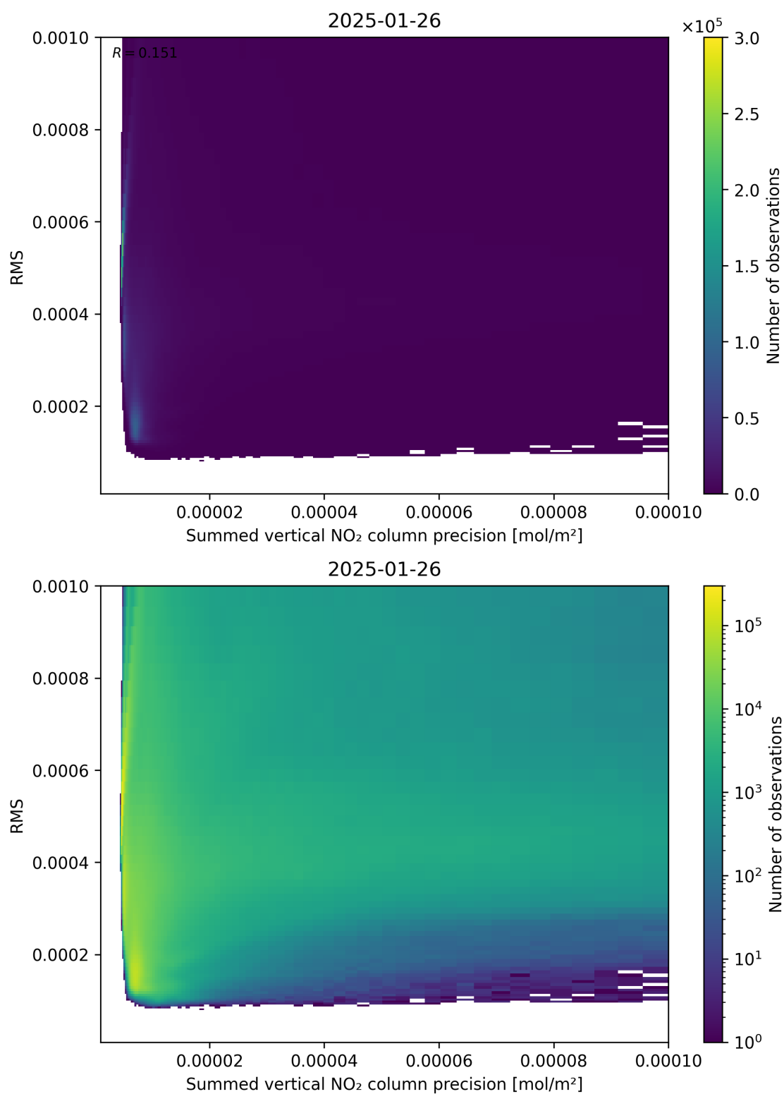
Figure 108: Scatter density plot of “Summed vertical NO 2 column precision” against “RMS” for 2025-01-25 to 2025-01-27.
