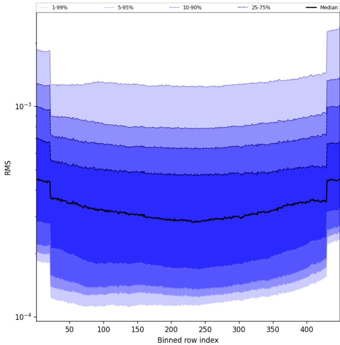
Figure 60: Along track statistics of “RMS” for 2025-01-25 to 2025-01-27
