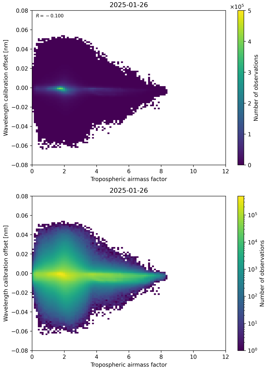
Figure 80: Scatter density plot of “Tropospheric airmass factor” against “Wavelength calibration offset” for 2025-01-25 to 2025-01-27.
