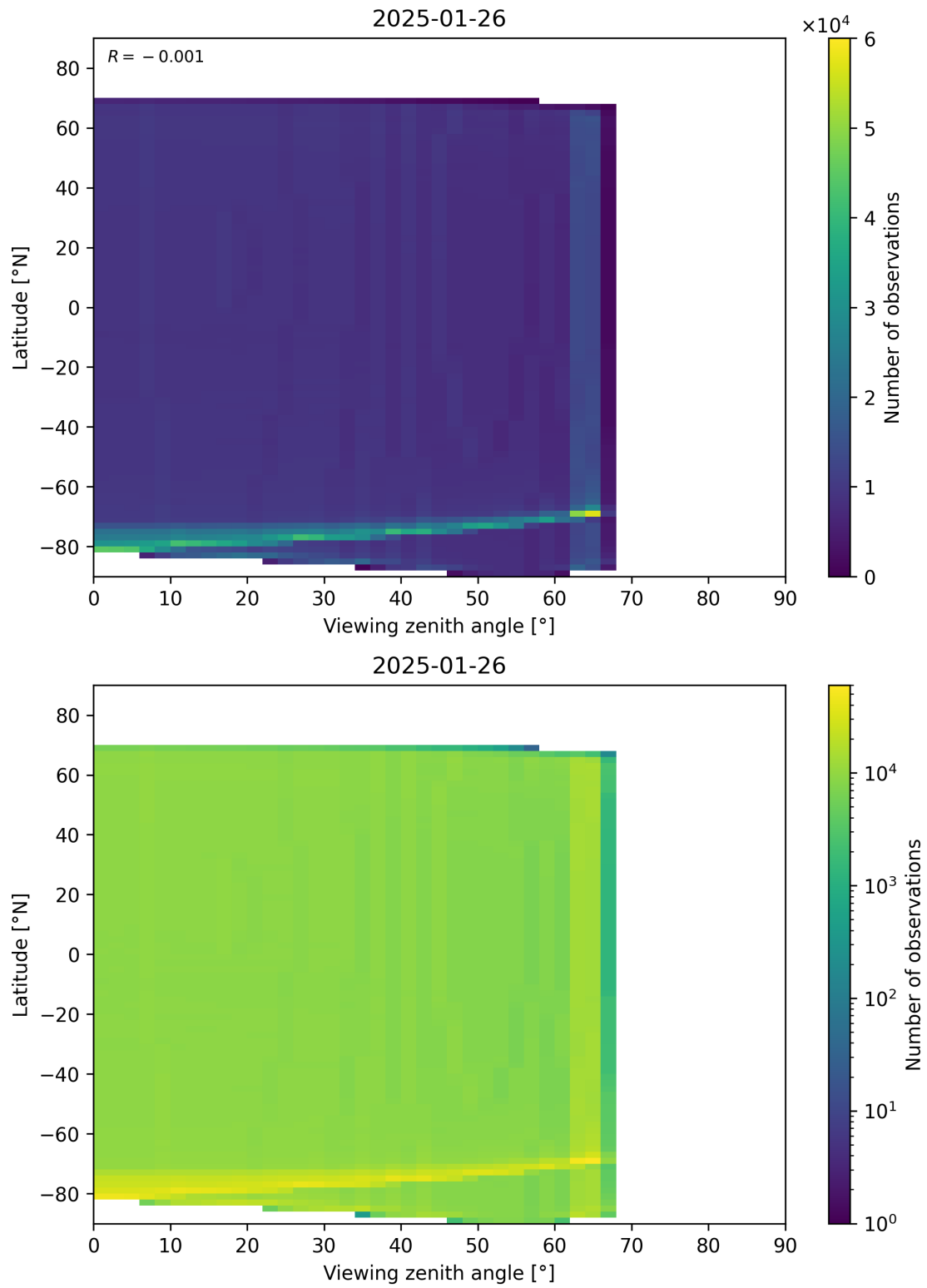
Figure 163: Scatter density plot of “Viewing zenith angle” against “Latitude” for 2025-01-25 to 2025-01-27.
