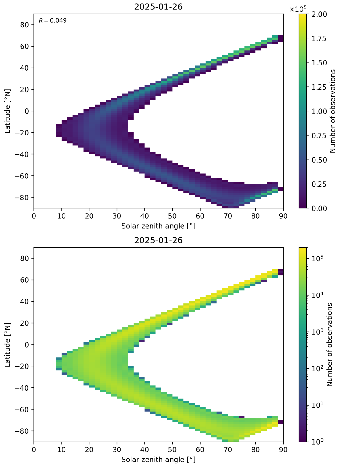
Figure 149: Scatter density plot of “Solar zenith angle” against “Latitude” for 2025-01-25 to 2025-01-27.
