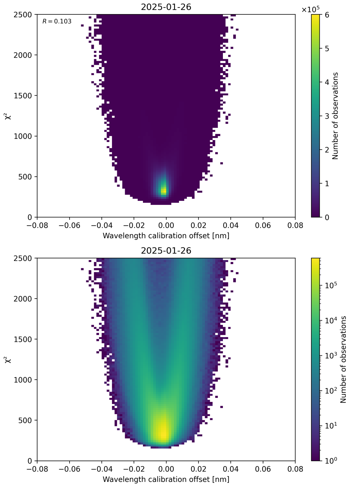
Figure 175: Scatter density plot of “Wavelength calibration offset” against “ \chi^2 ” for 2025-01-25 to 2025-01-27.
