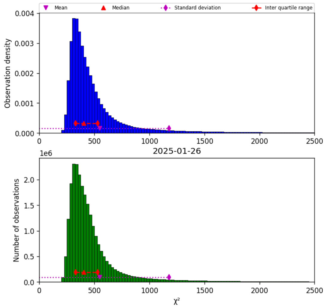
Figure 42: Histogram of “ \chi^2 ” for 2025-01-25 to 2025-01-27
