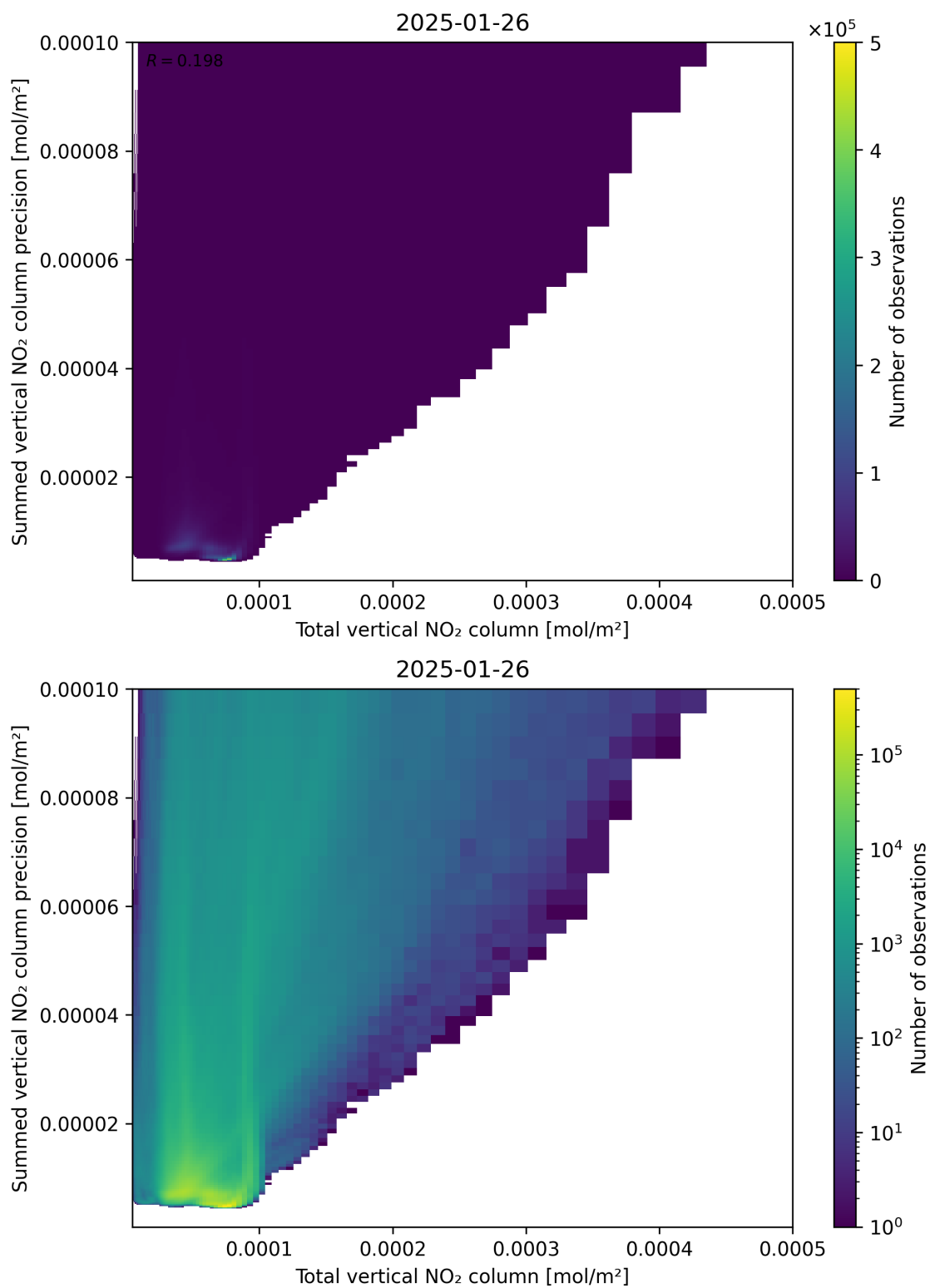
Figure 113: Scatter density plot of “Total vertical NO 2 column” against “Summed vertical NO 2 column precision” for 2025-01-25 to 2025-01-27.
