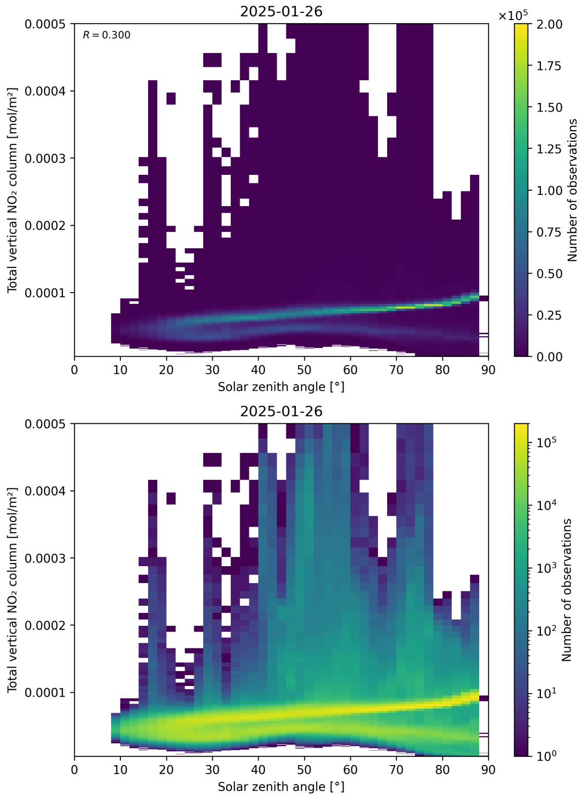
Figure 153: Scatter density plot of “Solar zenith angle” against “Total vertical NO 2 column” for 2025-01-25 to 2025-01-27.
