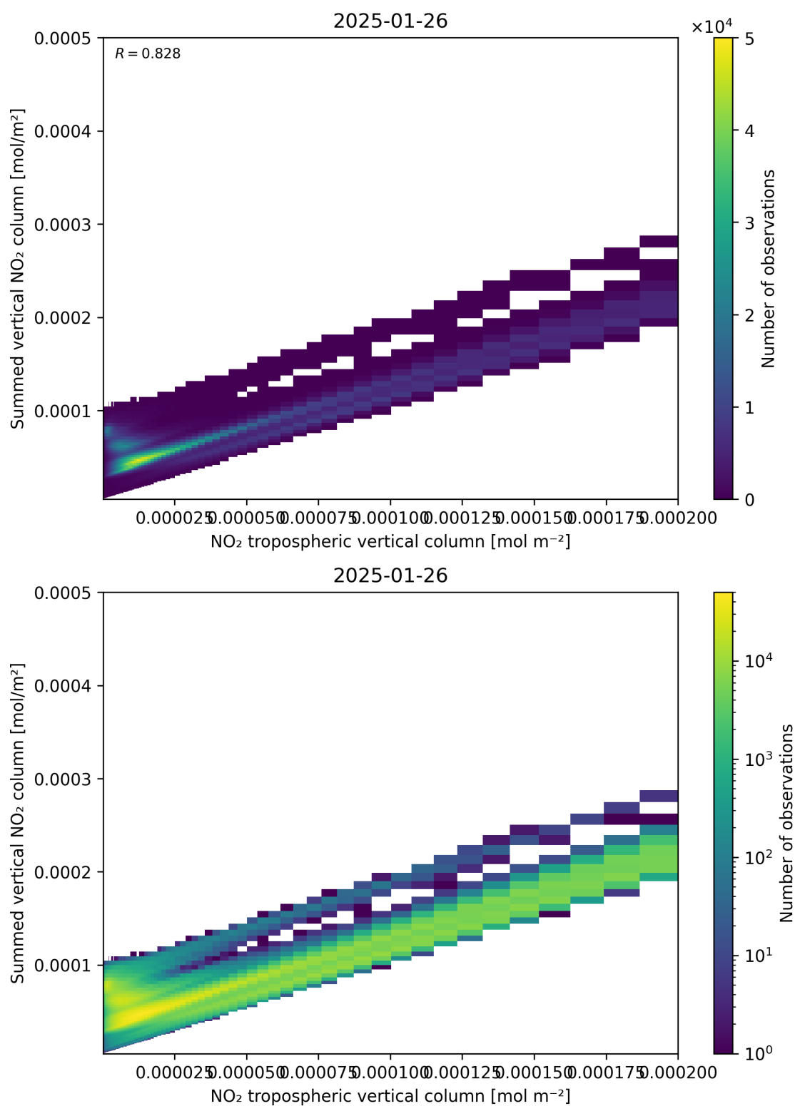
Figure 126: Scatter density plot of “NO 2 tropospheric vertical column” against “Summed vertical NO 2 column” for 2025-01-25 to 2025-01-27.
