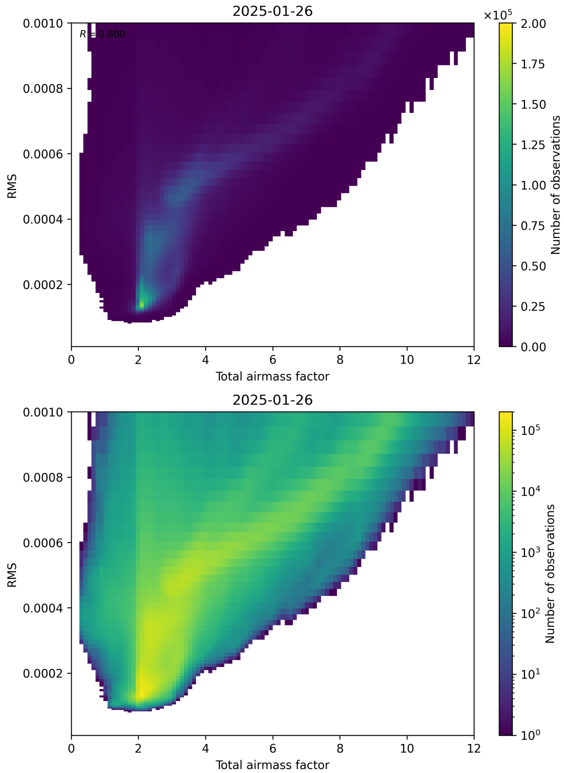
Figure 69: Scatter density plot of “Total airmass factor” against “RMS” for 2025-01-25 to 2025-01-27.
