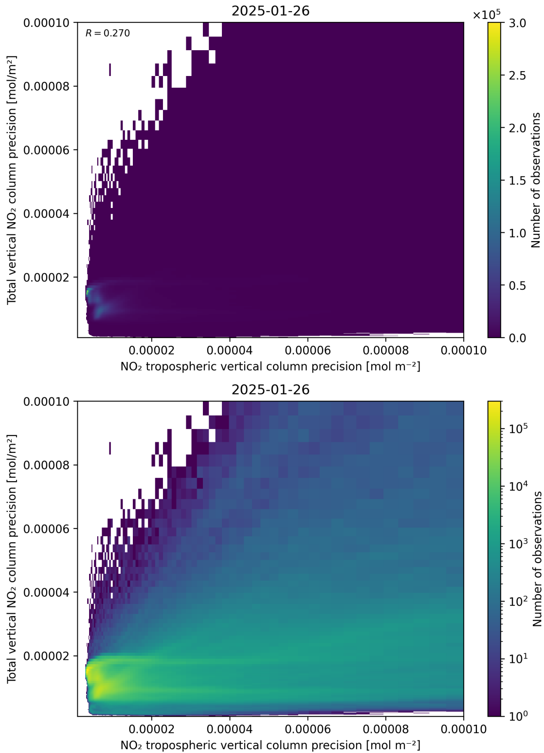
Figure 139: Scatter density plot of “NO 2 tropospheric vertical column precision” against “Total vertical NO 2 column precision” for 2025-01-25 to 2025-01-27.
