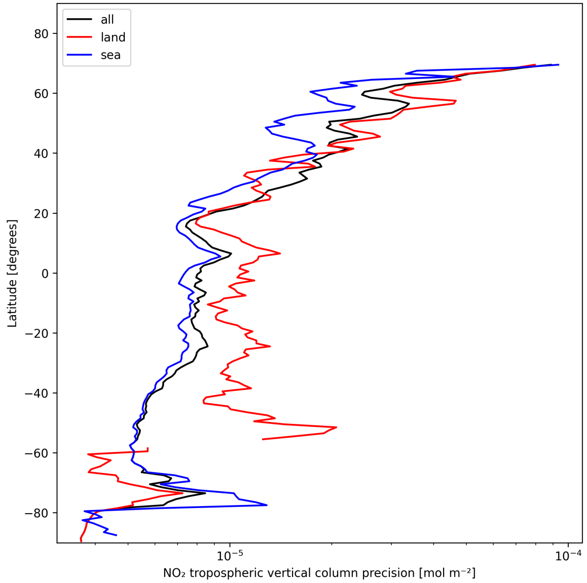
Figure 13: Zonal average of “NO 2 tropospheric vertical column precision” for 2025-01-25 to 2025-01-27.
