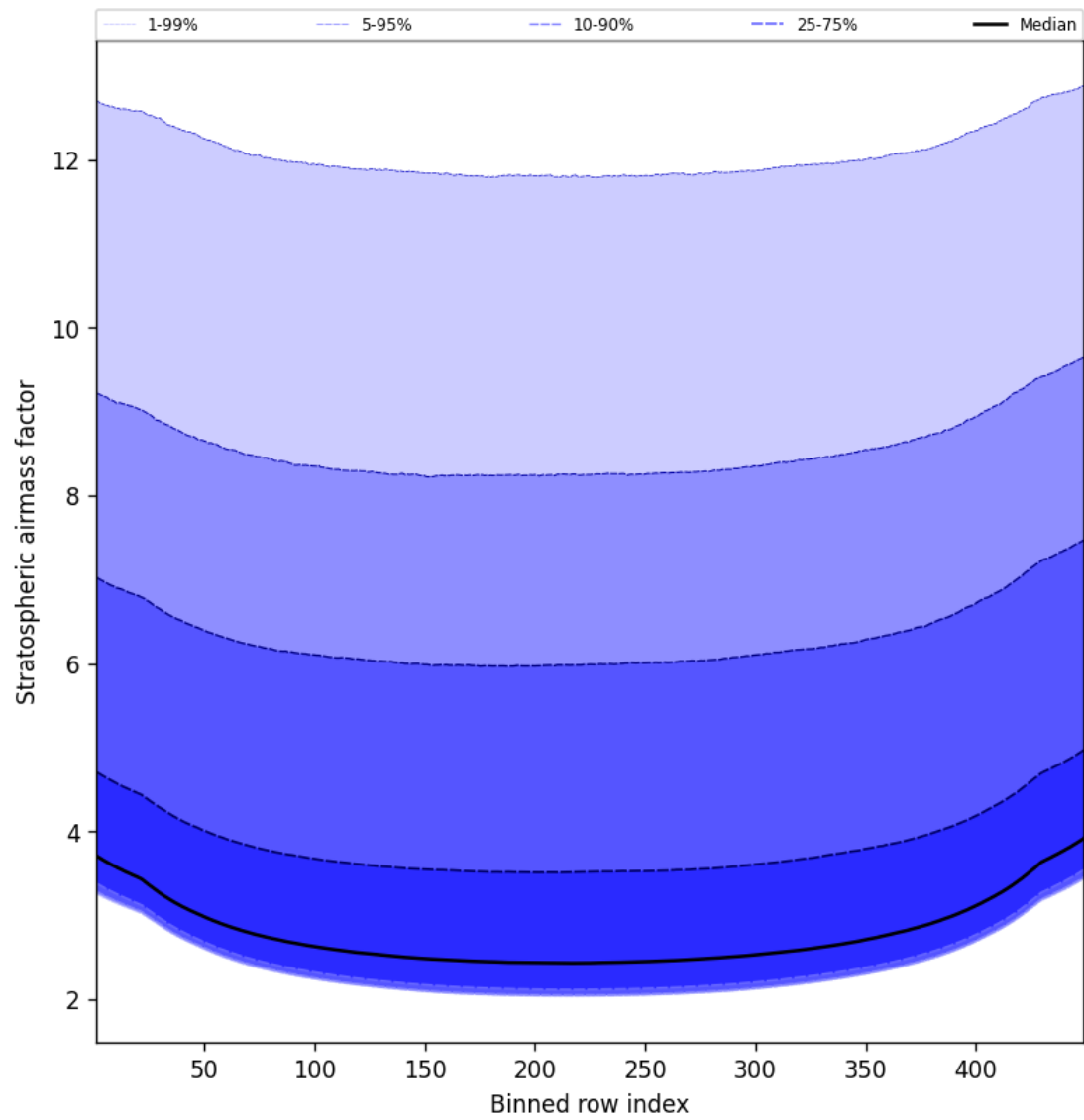
Figure 61: Along track statistics of “Stratospheric airmass factor” for 2025-01-25 to 2025-01-27
