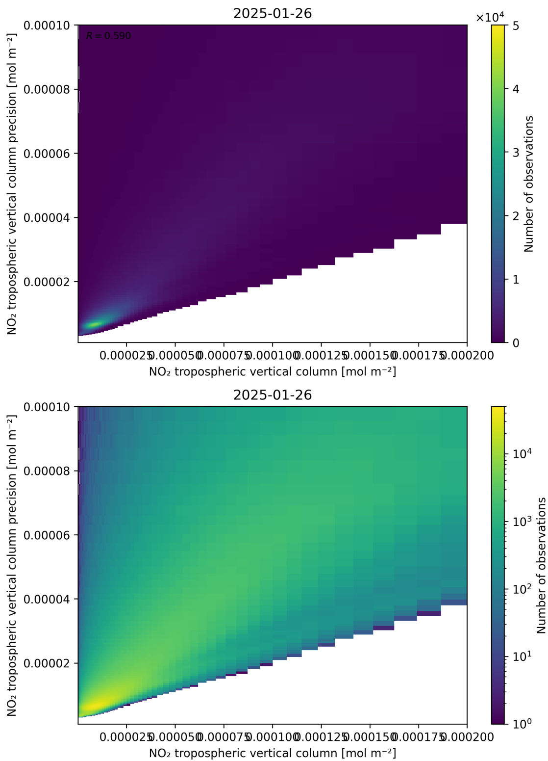
Figure 130: Scatter density plot of “NO 2 tropospheric vertical column” against “NO 2 tropospheric vertical column precision” for 2025-01-25 to 2025-01-27.
