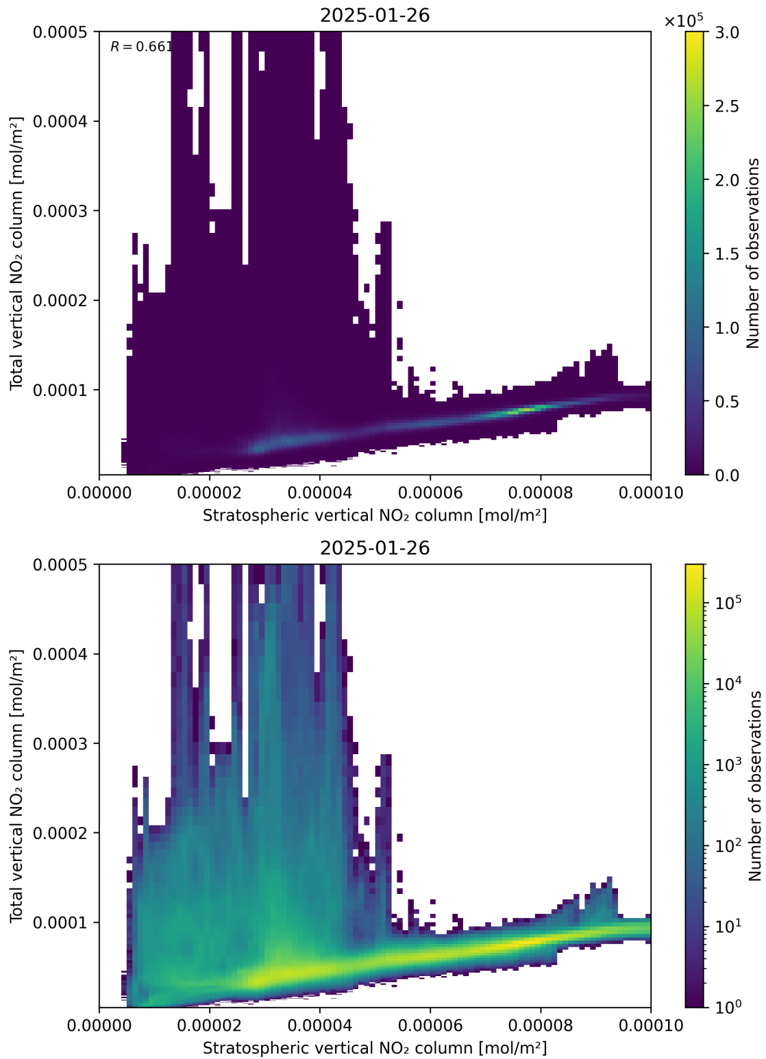
Figure 100: Scatter density plot of “Stratospheric vertical NO 2 column” against “Total vertical NO 2 column” for 2025-01-25 to 2025-01-27.
