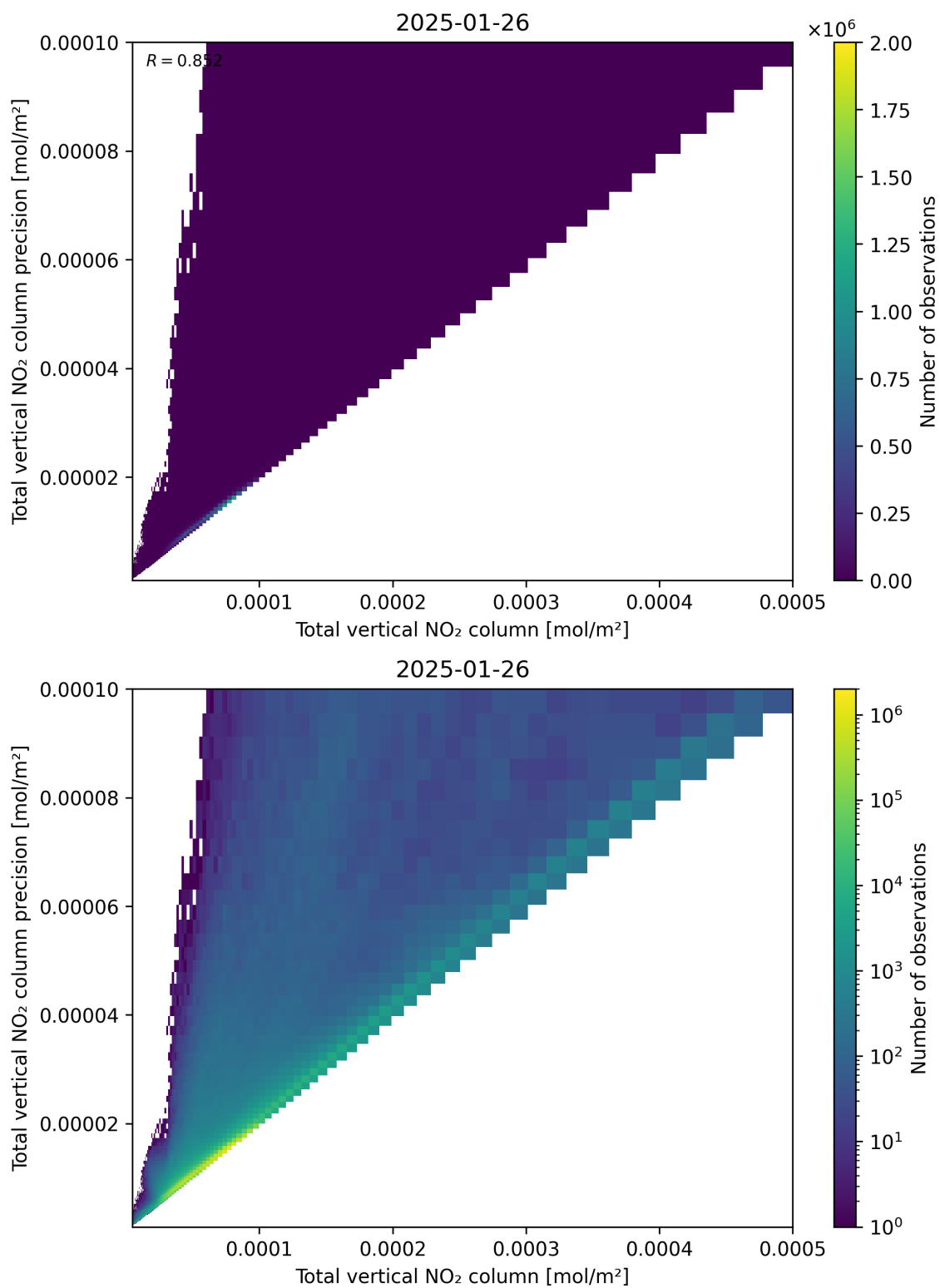
Figure 114: Scatter density plot of “Total vertical NO 2 column” against “Total vertical NO 2 column precision” for 2025-01-25 to 2025-01-27.
