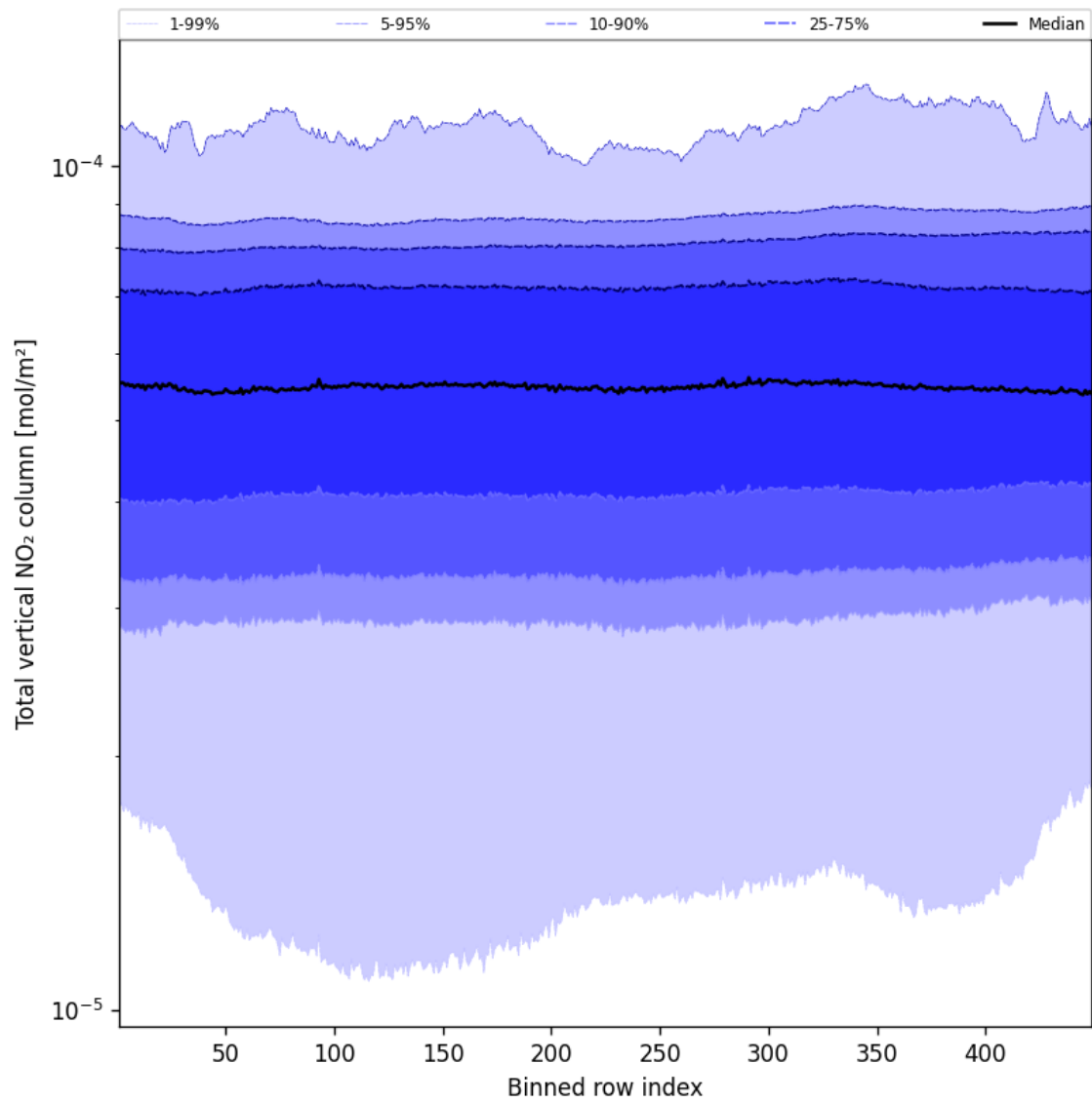
Figure 55: Along track statistics of “Total vertical NO 2 column” for 2025-01-25 to 2025-01-27
