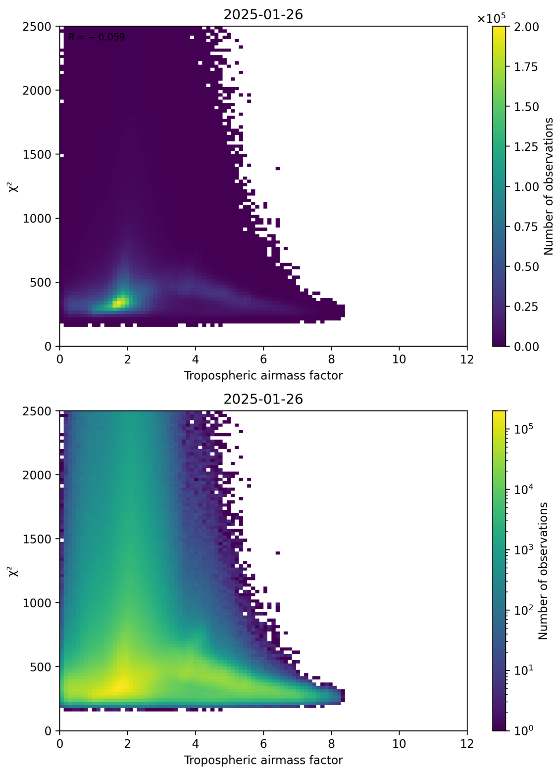
Figure 73: Scatter density plot of “Tropospheric airmass factor” against “ \chi^2 ” for 2025-01-25 to 2025-01-27.
