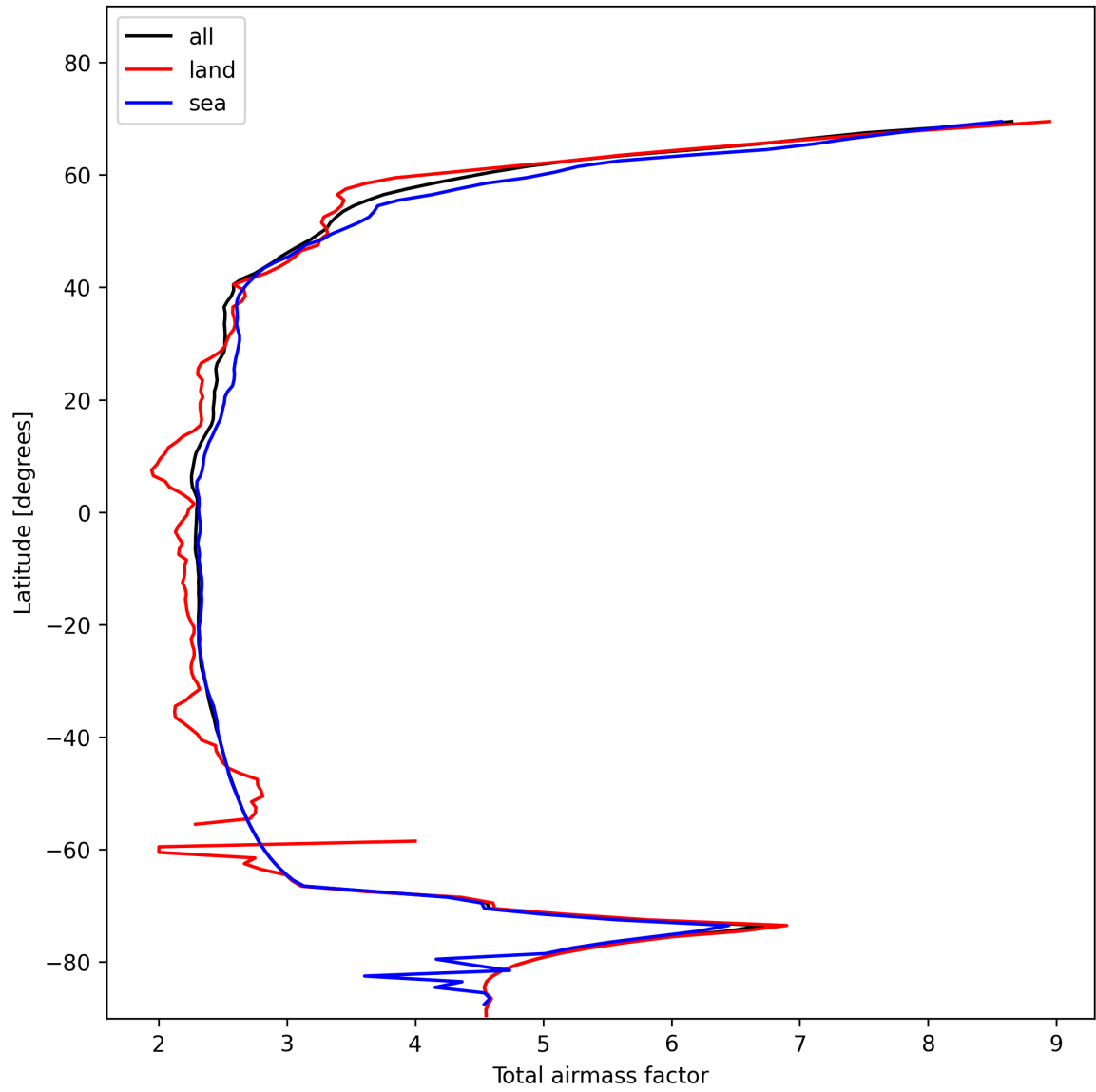
Figure 15: Zonal average of “Total airmass factor” for 2025-01-25 to 2025-01-27.
