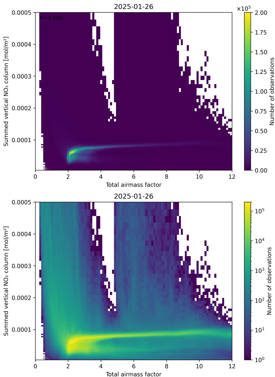
Figure 65: Scatter density plot of “Total airmass factor” against “Summed vertical NO 2 column” for 2025-01-25 to 2025-01-27.
