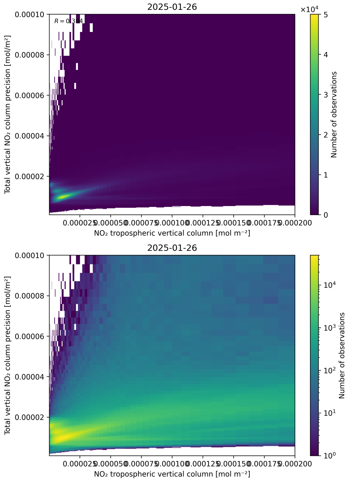
Figure 129: Scatter density plot of “NO 2 tropospheric vertical column” against “Total vertical NO 2 column precision” for 2025-01-25 to 2025-01-27.
