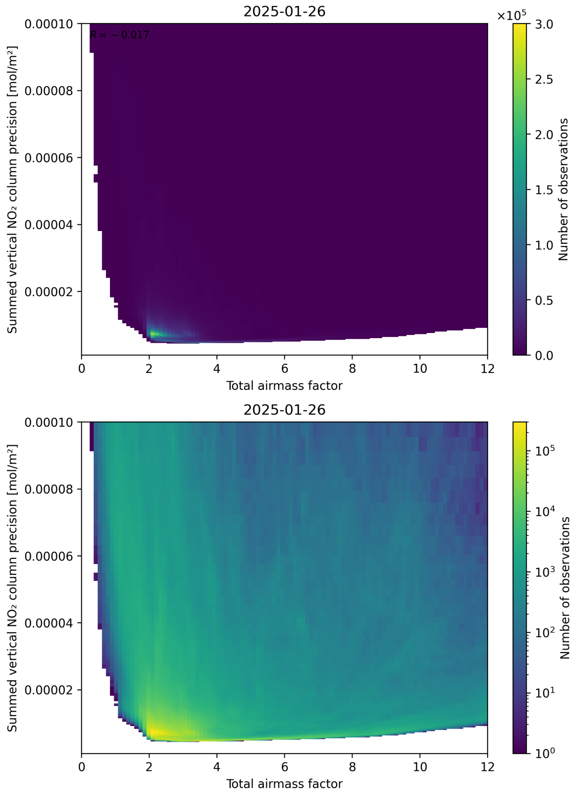
Figure 66: Scatter density plot of “Total airmass factor” against “Summed vertical NO 2 column precision” for 2025-01-25 to 2025-01-27.
