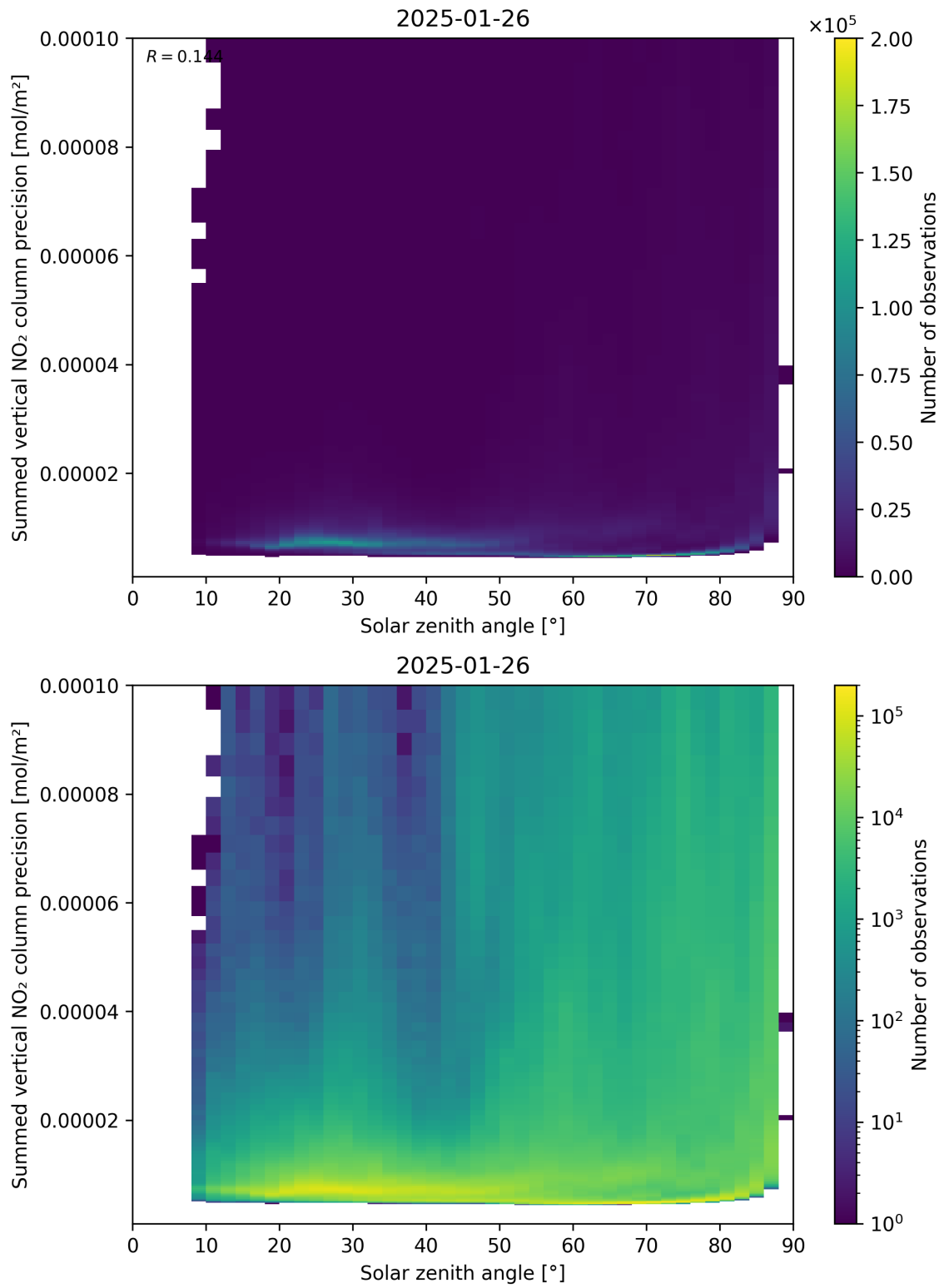
Figure 152: Scatter density plot of “Solar zenith angle” against “Summed vertical NO 2 column precision” for 2025-01-25 to 2025-01-27.
