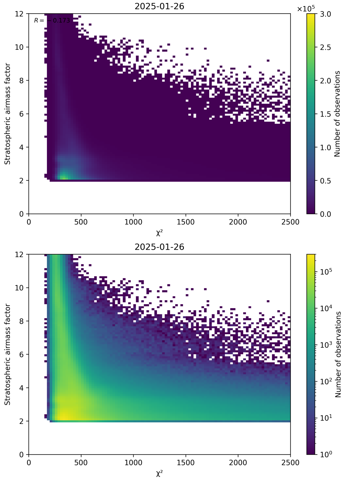
Figure 81: Scatter density plot of “ \chi^2 ” against “Stratospheric airmass factor” for 2025-01-25 to 2025-01-27.
