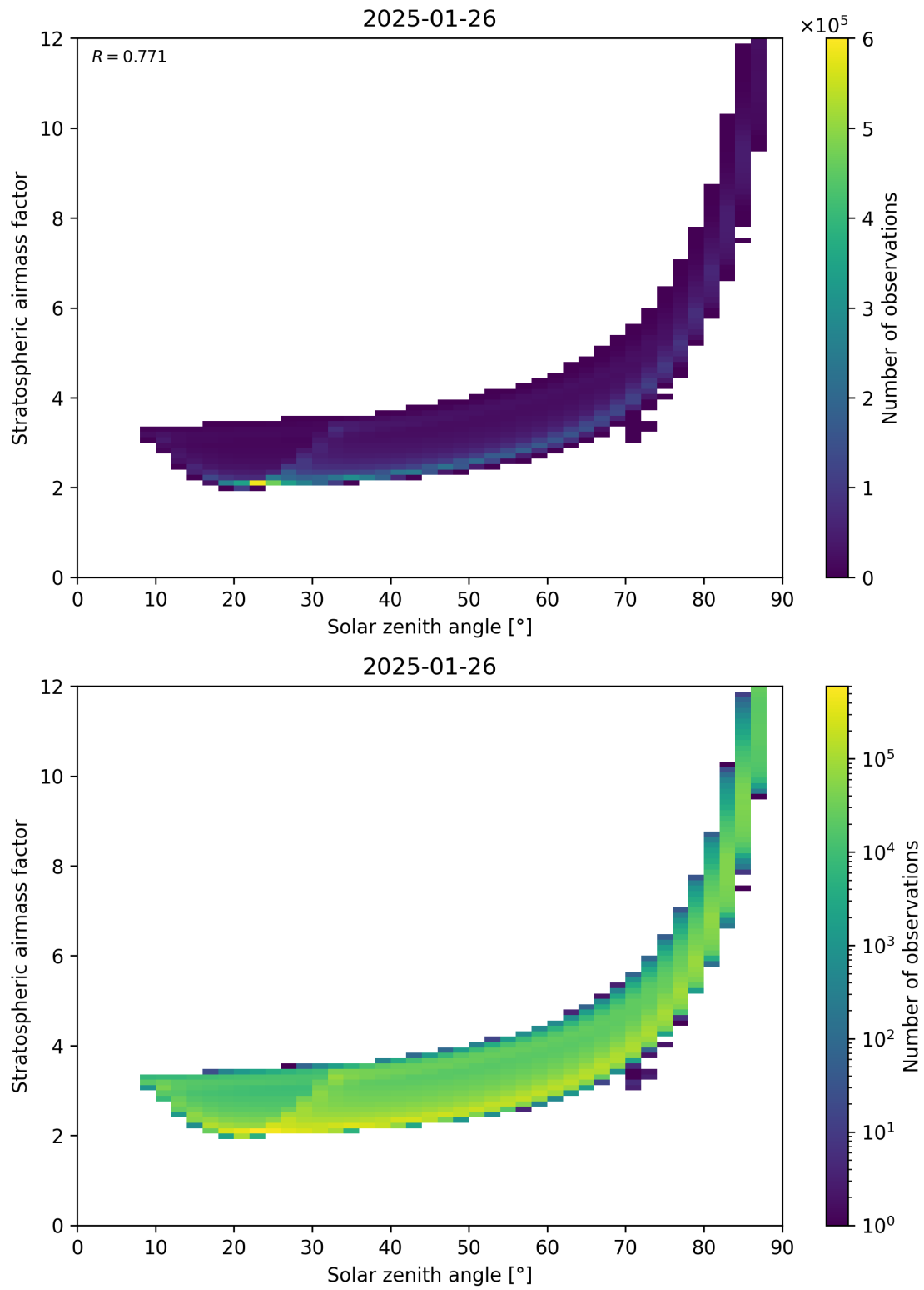
Figure 145: Scatter density plot of “Solar zenith angle” against “Stratospheric airmass factor” for 2025-01-25 to 2025-01-27.
