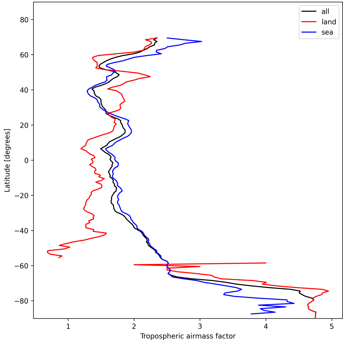
Figure 14: Zonal average of “Tropospheric air mass factor” for 2025-01-25 to 2025-01-27.
