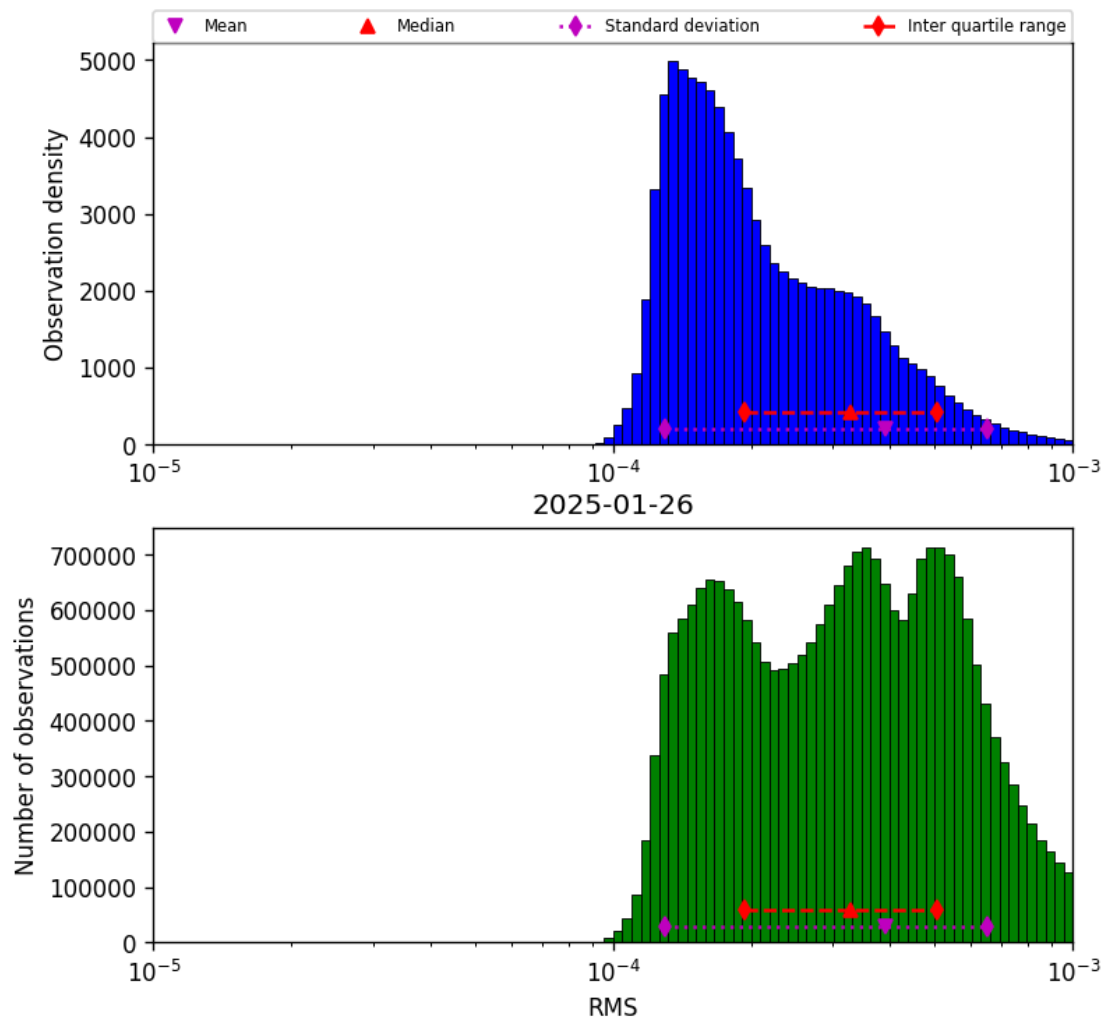
Figure 43: Histogram of “RMS” for 2025-01-25 to 2025-01-27
