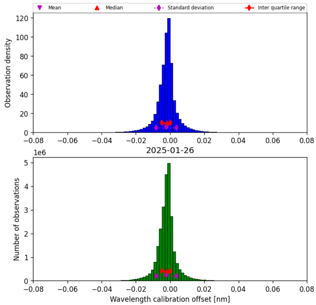
Figure 35: Histogram of “Wavelength calibration offset” for 2025-01-25 to 2025-01-27
