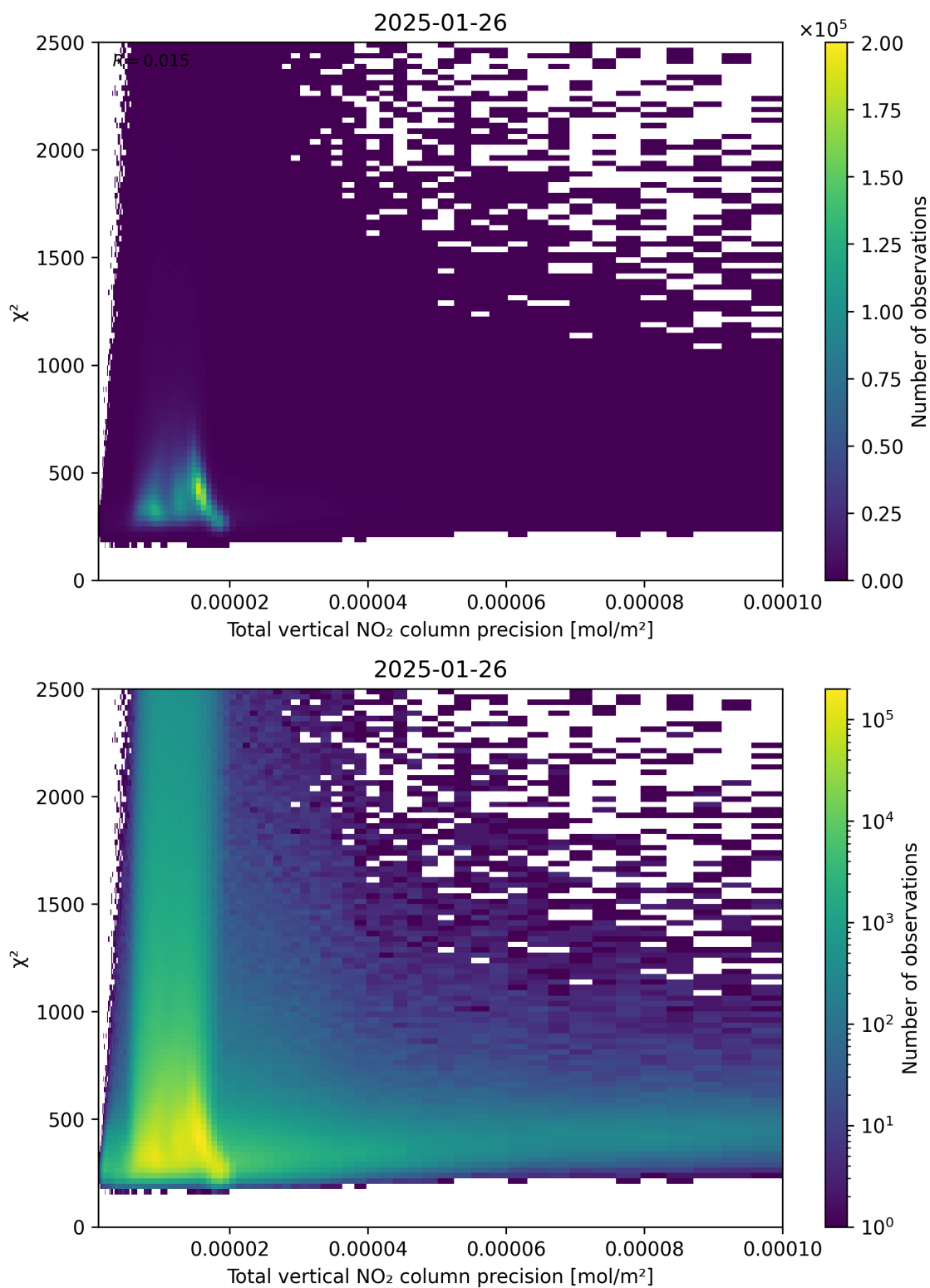
Figure 116: Scatter density plot of “Total vertical NO 2 column precision” against “ \chi^2 ” for 2025-01-25 to 2025-01-27.
