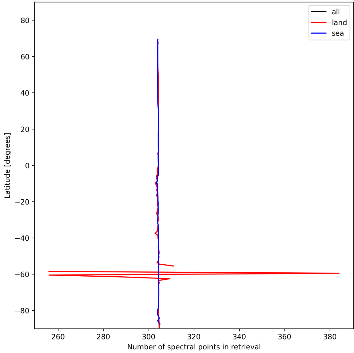
Figure 16: Zonal average of “Number of spectral points in retrieval” for 2025-01-25 to 2025-01-27.
