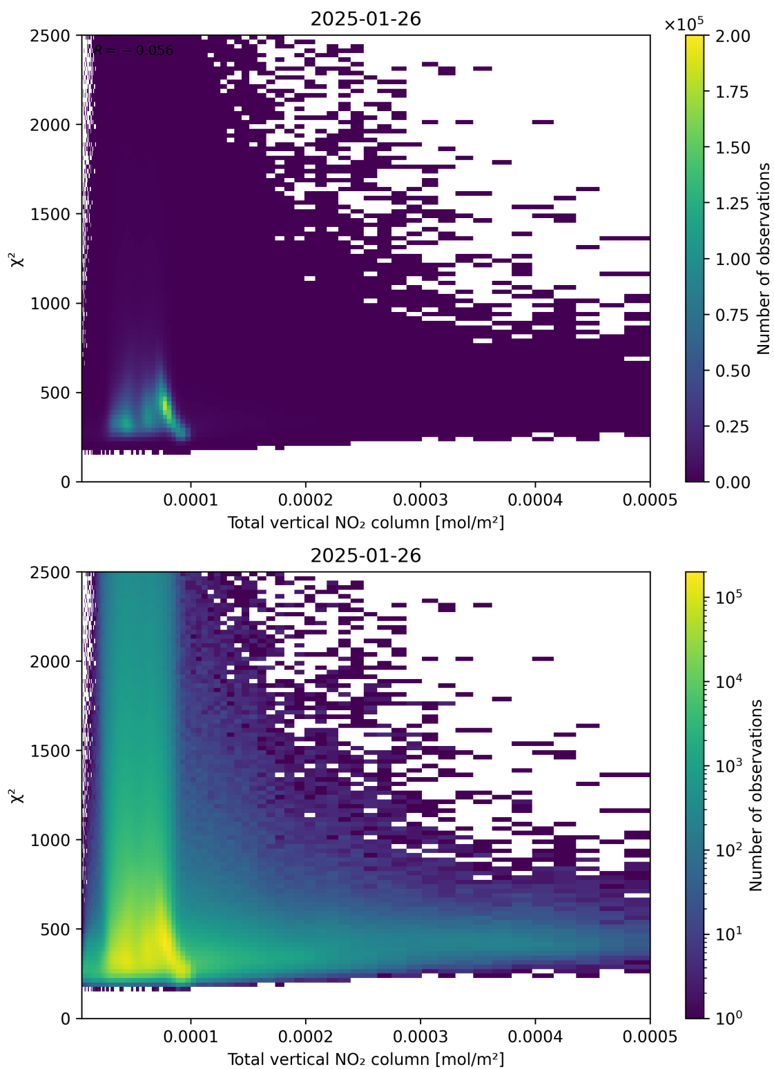
Figure 111: Scatter density plot of “Total vertical NO 2 column” against “ \chi^2 ” for 2025-01-25 to 2025-01-27.
