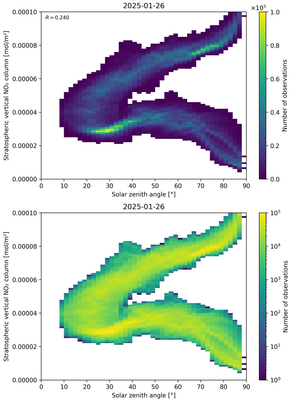
Figure 150: Scatter density plot of “Solar zenith angle” against “Stratospheric vertical NO 2 column” for 2025-01-25 to 2025-01-27.
