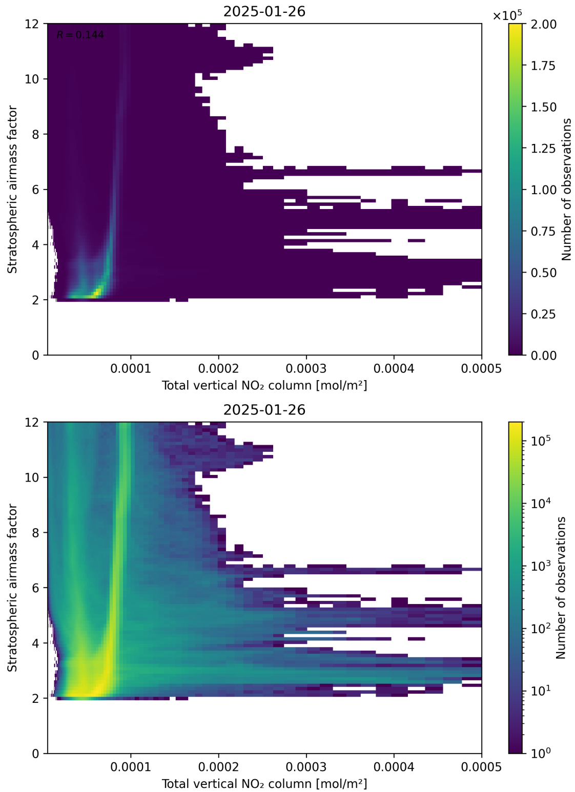
Figure 110: Scatter density plot of “Total vertical NO 2 column” against “Stratospheric airmass factor” for 2025-01-25 to 2025-01-27.
