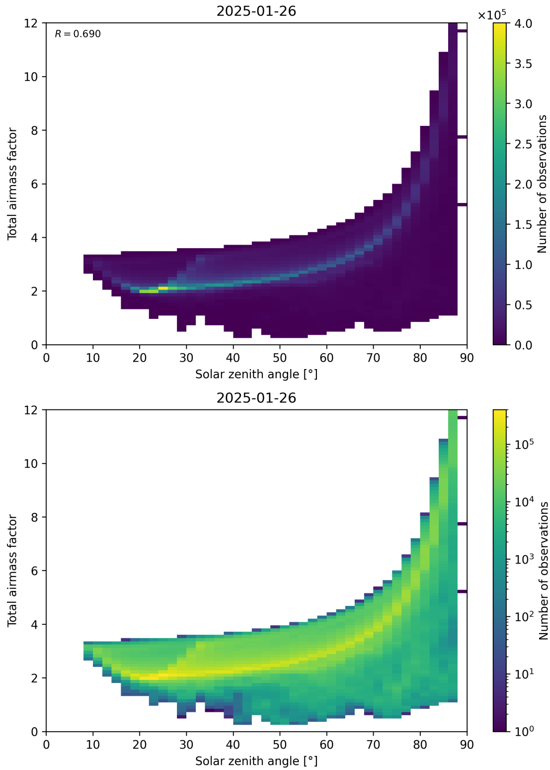
Figure 146: Scatter density plot of “Solar zenith angle” against “Total air mass factor” for 2025-01-25 to 2025-01-27.
