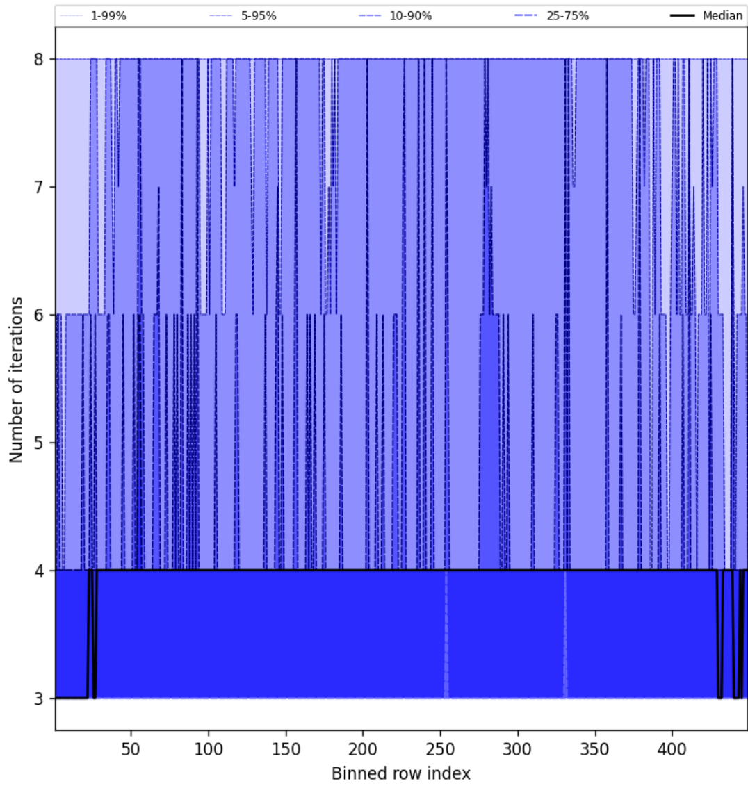
Figure 51: Along track statistics of “Number of iterations” for 2025-01-25 to 2025-01-27
