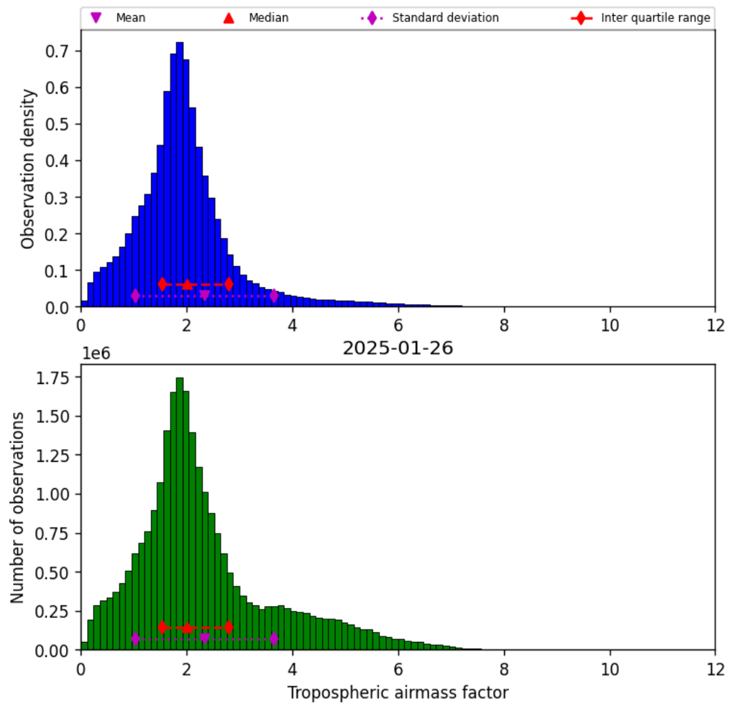
Figure 31: Histogram of “Tropospheric airmass factor” for 2025-01-25 to 2025-01-27
