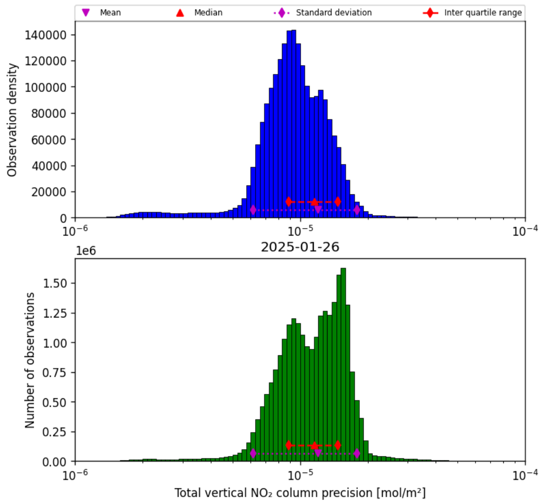
Figure 39: Histogram of “Total vertical NO 2 column precision” for 2025-01-25 to 2025-01-27
