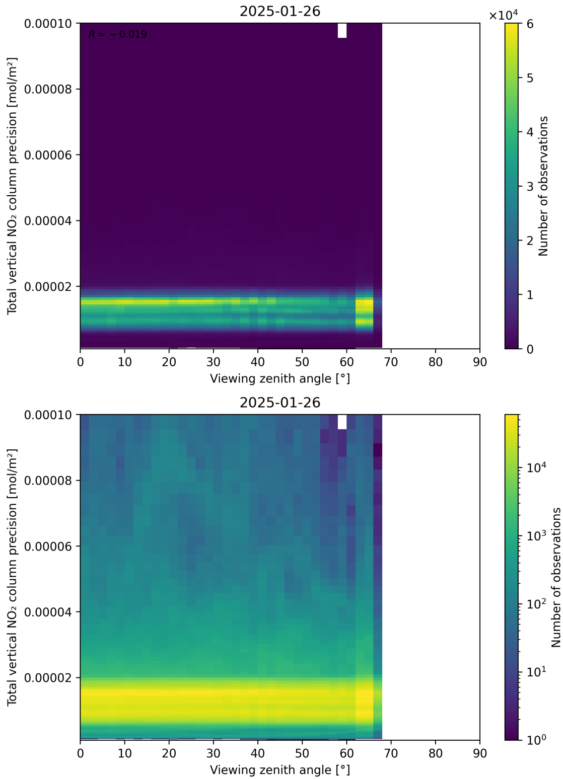
Figure 168: Scatter density plot of “Viewing zenith angle” against “Total vertical NO 2 column precision” for 2025-01-25 to 2025-01-27.
