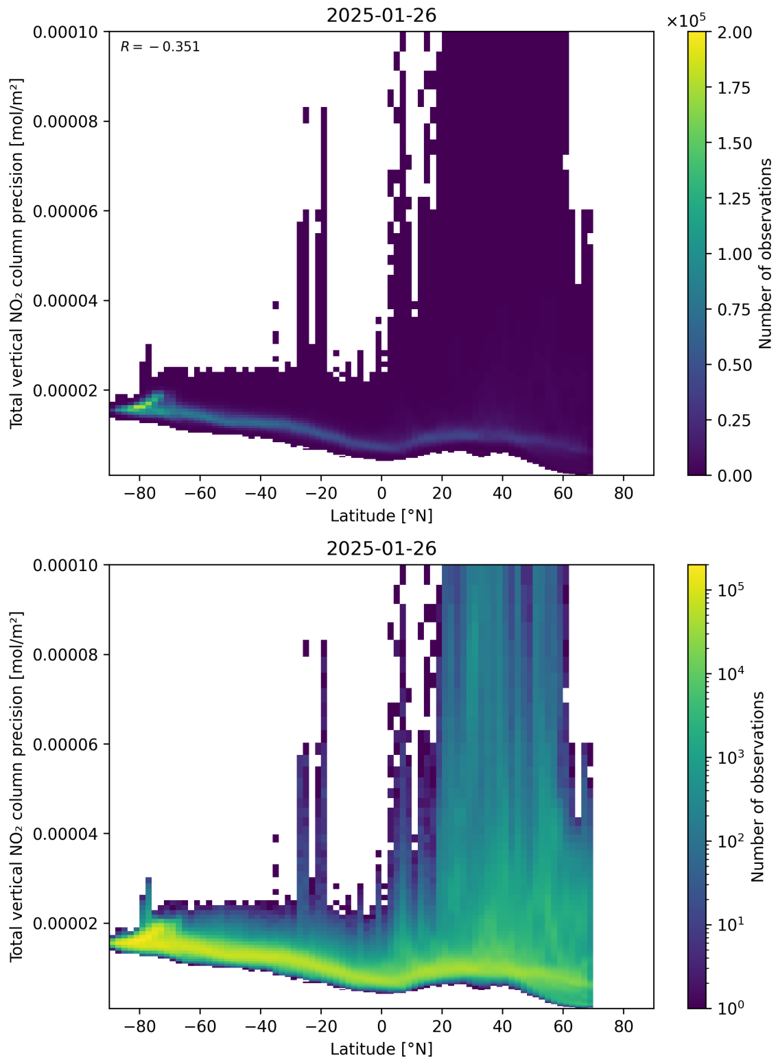
Figure 91: Scatter density plot of “Latitude” against “Total vertical NO 2 column precision” for 2025-01-25 to 2025-01-27.
