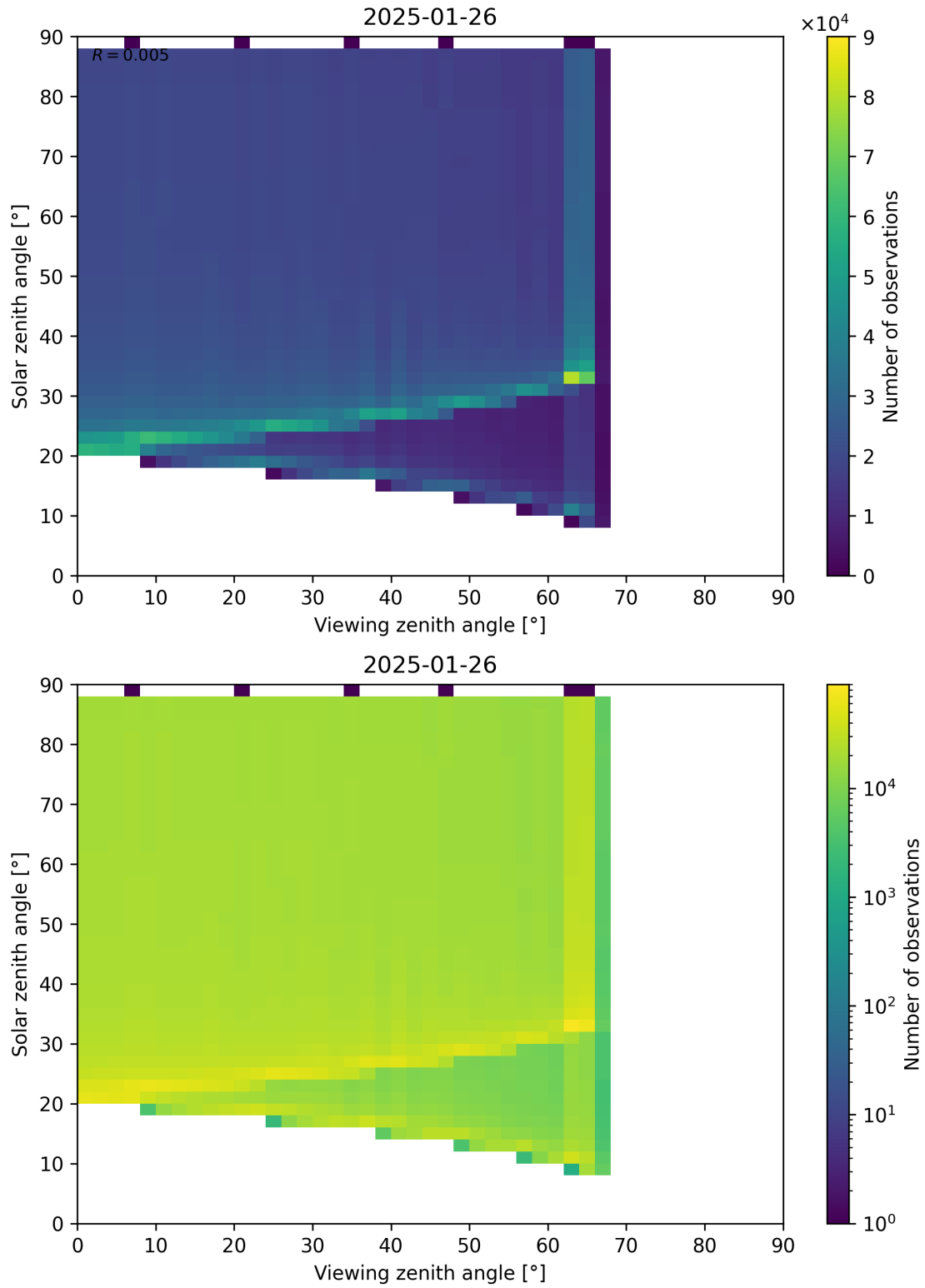
Figure 172: Scatter density plot of “Viewing zenith angle” against “Solar zenith angle” for 2025-01-25 to 2025-01-27.
