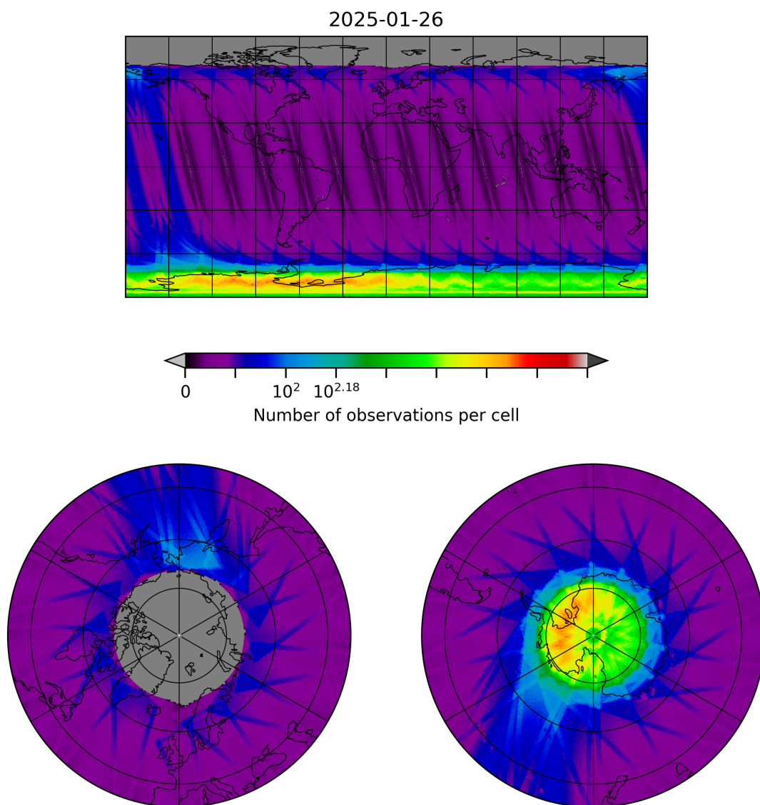
Figure 10: Map of the number of observations for 2025-01-25 to 2025-01-27
