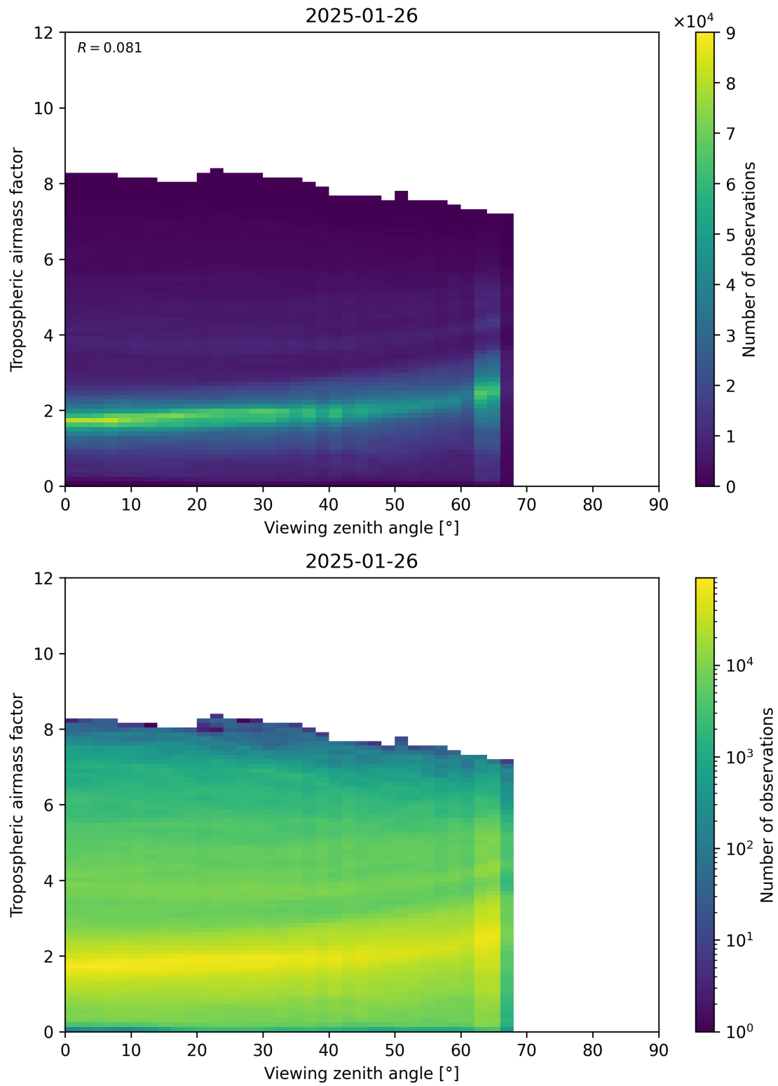
Figure 161: Scatter density plot of “Viewing zenith angle” against “Tropospheric airmass factor” for 2025-01-25 to 2025-01-27.
