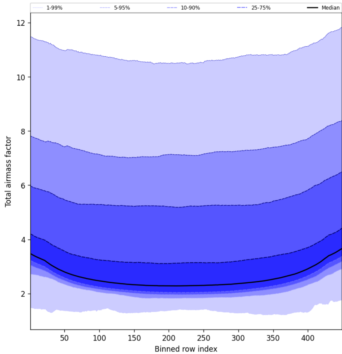
Figure 49: Along track statistics of “Total airmass factor” for 2025-01-25 to 2025-01-27
