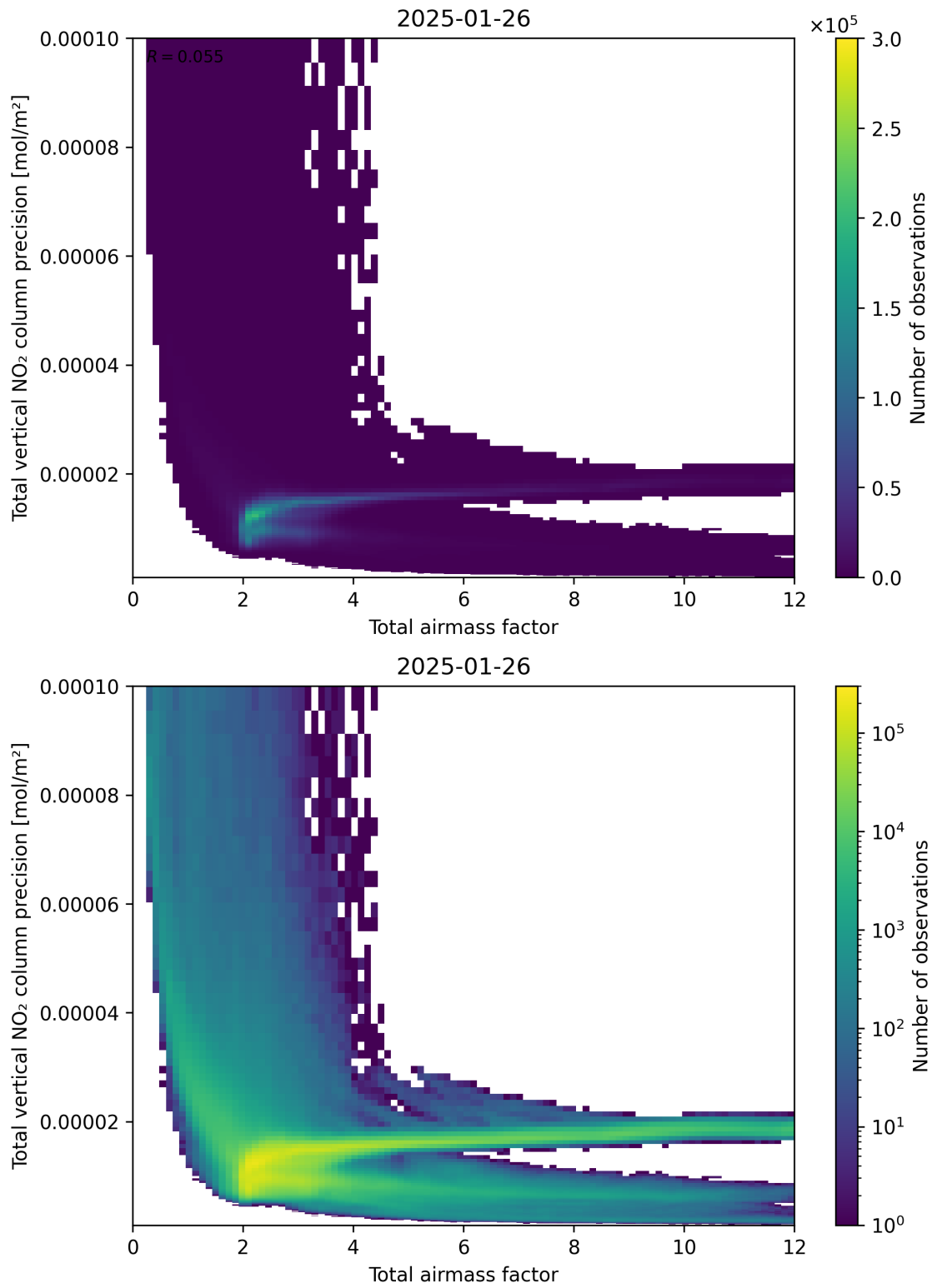
Figure 68: Scatter density plot of “Total airmass factor” against “Total vertical NO 2 column precision” for 2025-01-25 to 2025-01-27.
