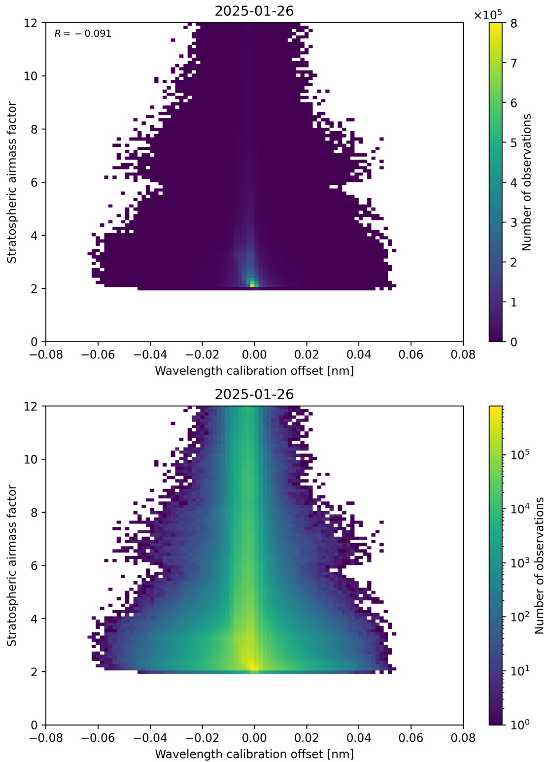
Figure 174: Scatter density plot of “Wavelength calibration offset” against “Stratospheric airmass factor” for 2025-01-25 to 2025-01-27.
