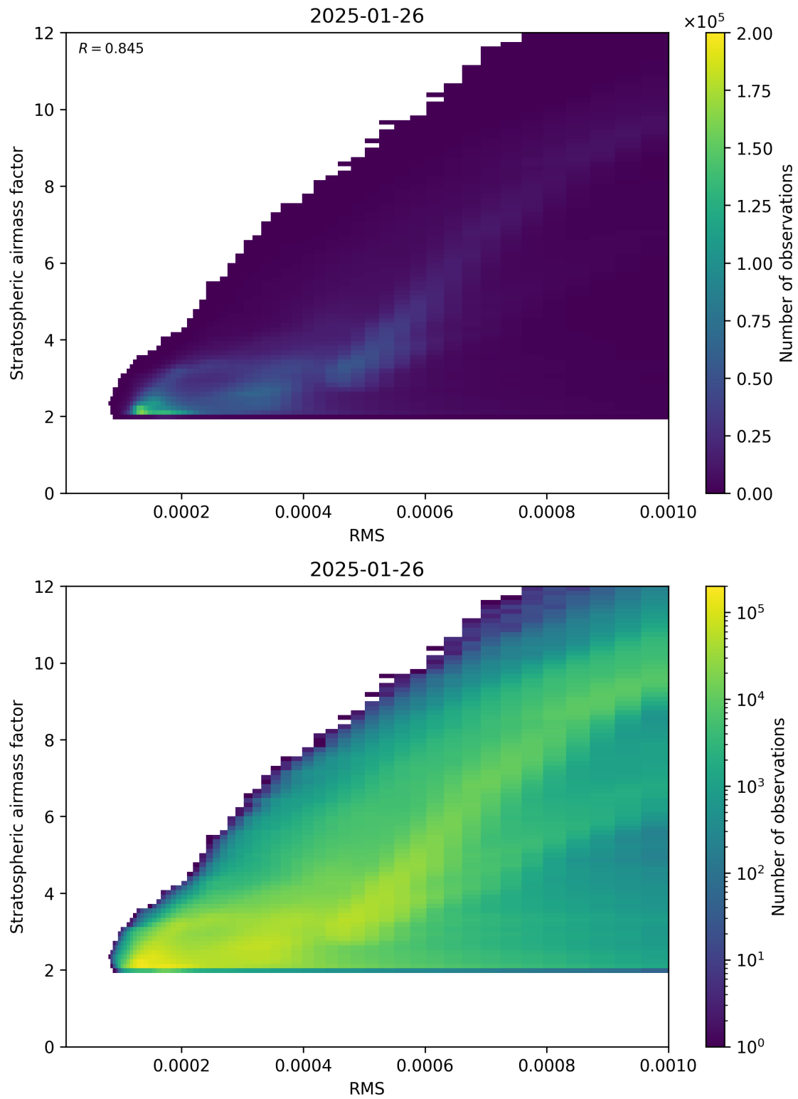
Figure 144: Scatter density plot of “RMS” against “Stratospheric airmass factor” for 2025-01-25 to 2025-01-27.
