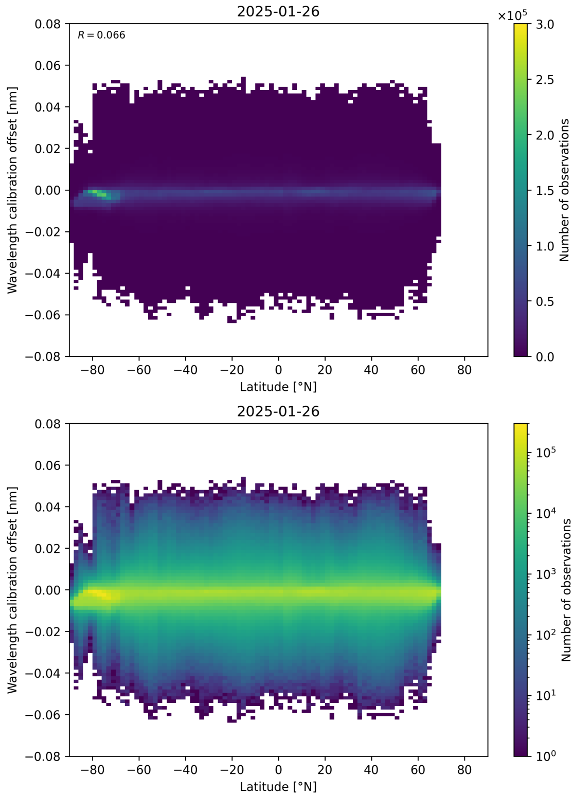
Figure 95: Scatter density plot of “Latitude” against “Wavelength calibration offset” for 2025-01-25 to 2025-01-27.
