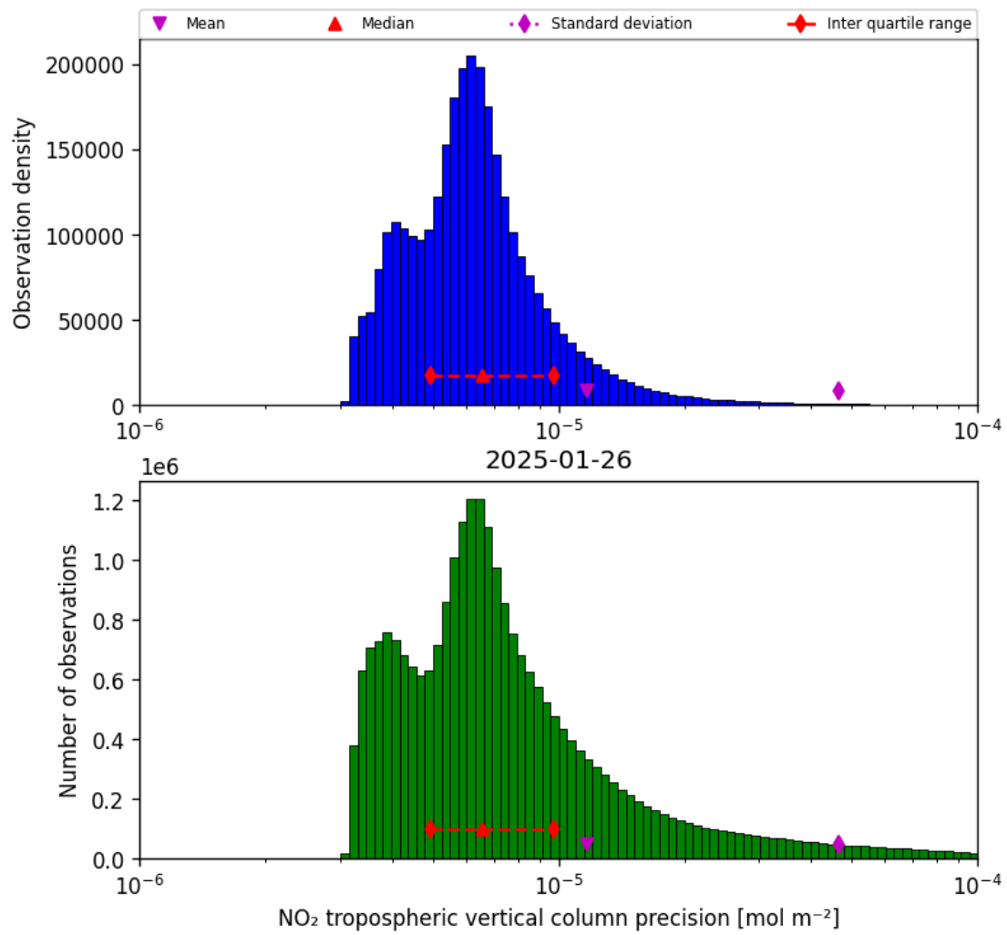
Figure 30: Histogram of “NO 2 tropospheric vertical column precision” for 2025-01-25 to 2025-01-27
