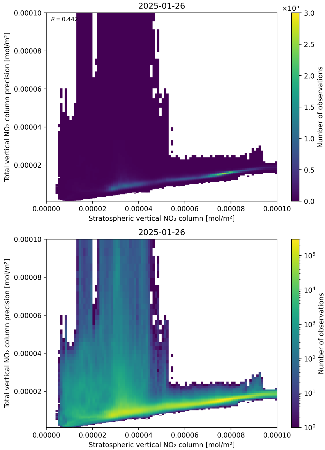
Figure 101: Scatter density plot of “Stratospheric vertical NO 2 column” against “Total vertical NO 2 column precision” for 2025-01-25 to 2025-01-27.
