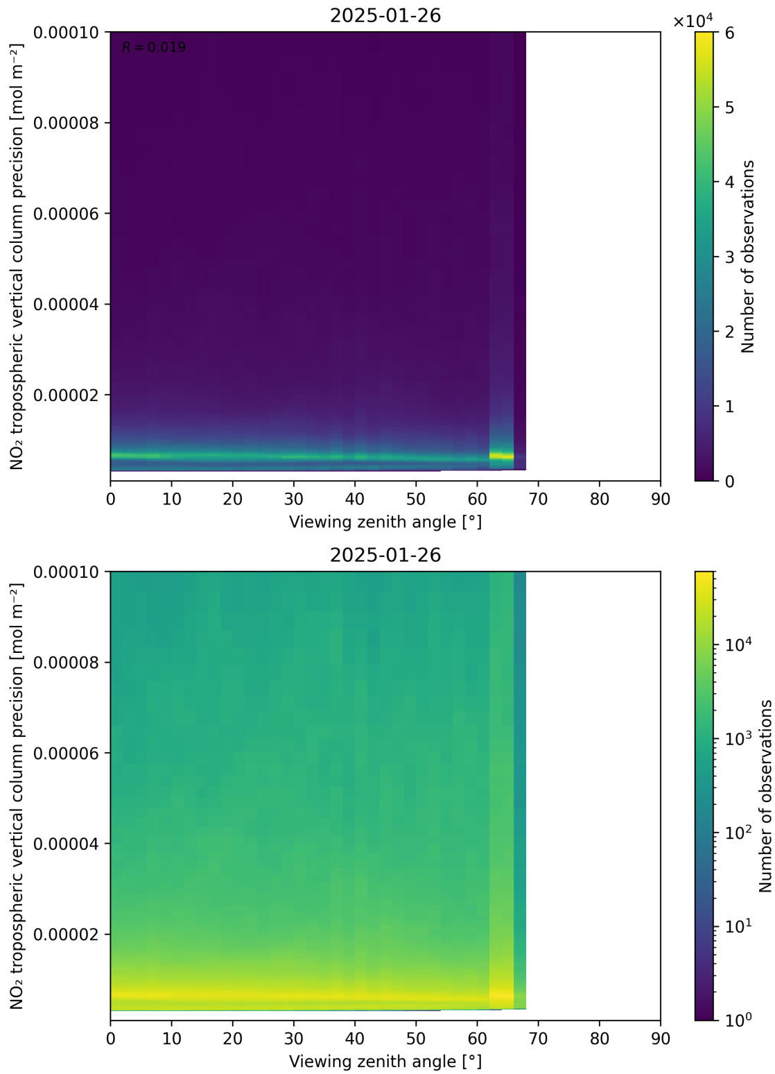
Figure 170: Scatter density plot of “Viewing zenith angle” against “NO 2 tropospheric vertical column precision” for 2025-01-25 to 2025-01-27.
