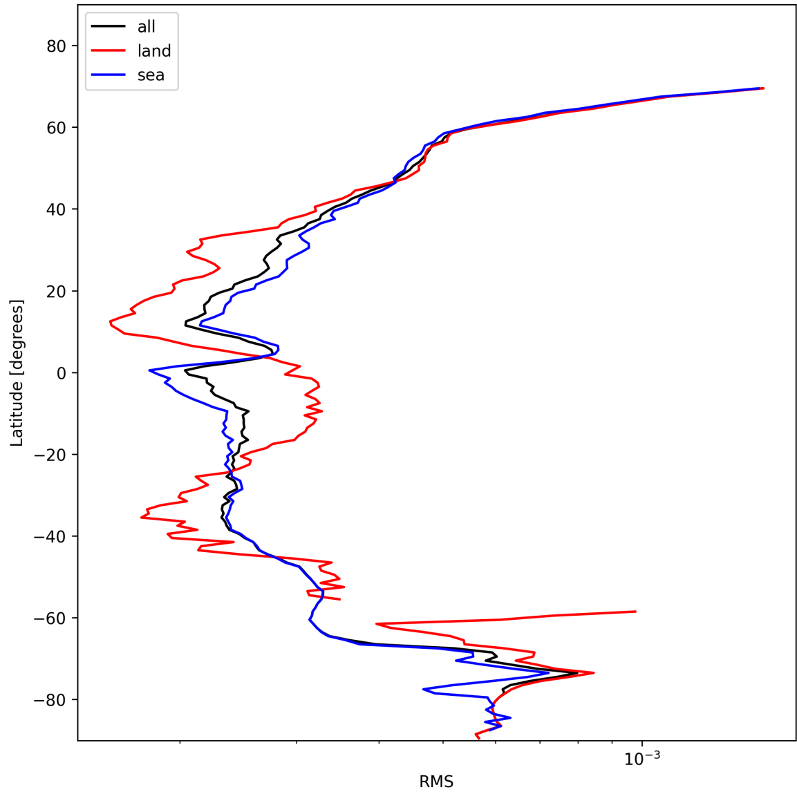
Figure 26: Zonal average of “RMS” for 2025-01-25 to 2025-01-27.
