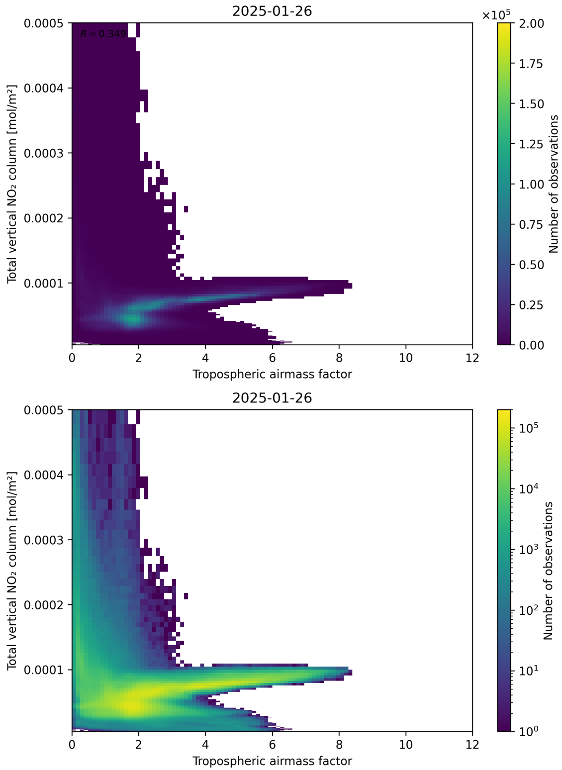
Figure 77: Scatter density plot of “Tropospheric airmass factor” against “Total vertical \text{NO}_2 column” for 2025-01-25 to 2025-01-27.
