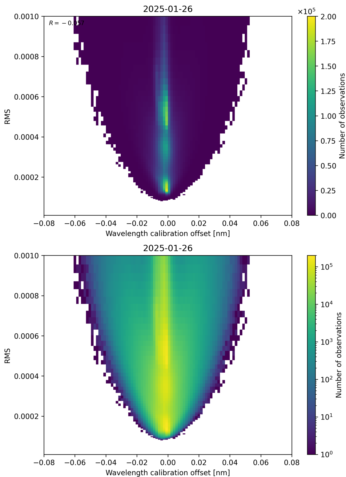
Figure 181: Scatter density plot of “Wavelength calibration offset” against “RMS” for 2025-01-25 to 2025-01-27.
