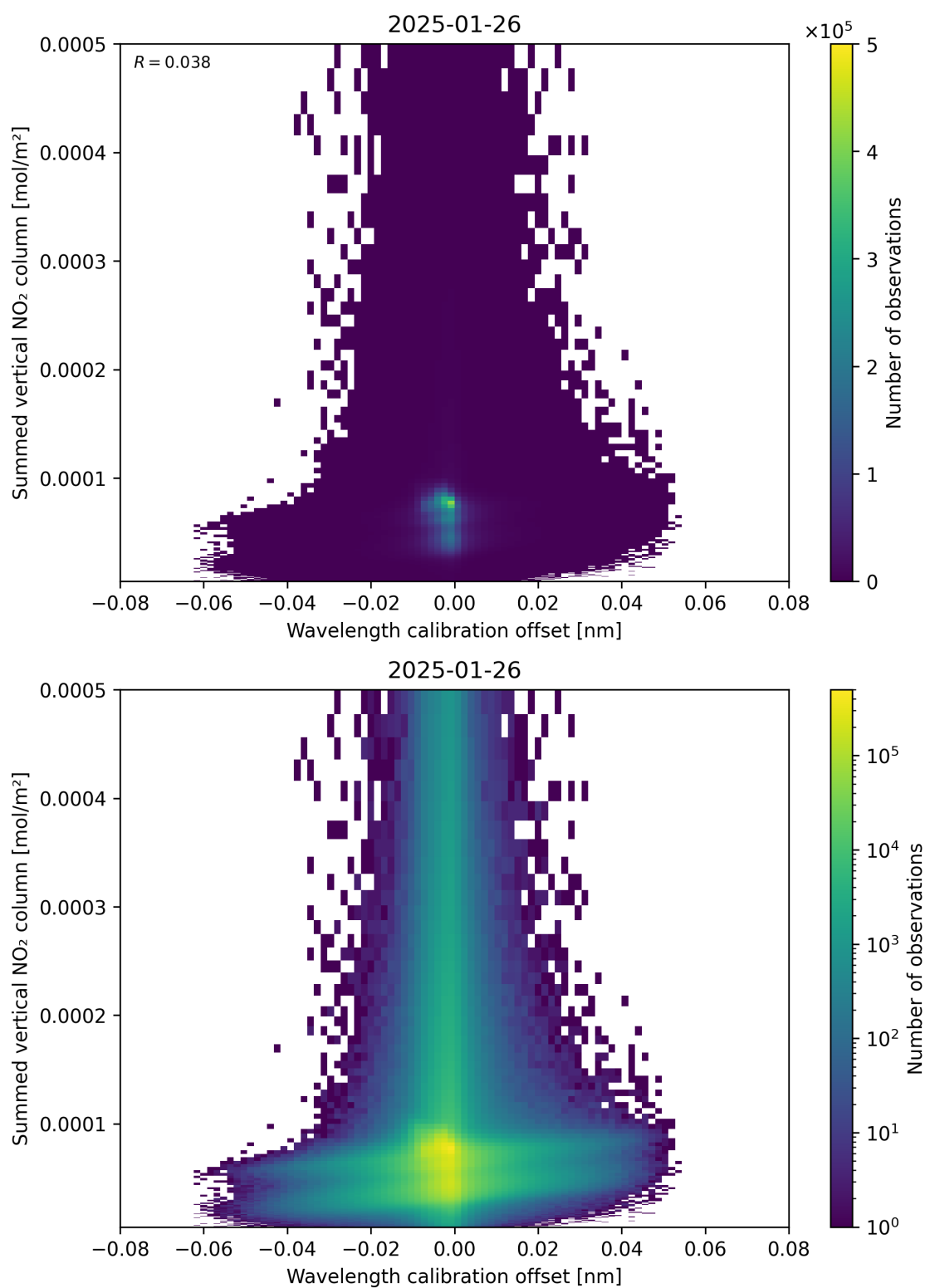
Figure 177: Scatter density plot of “Wavelength calibration offset” against “Summed vertical NO 2 column” for 2025-01-25 to 2025-01-27.
