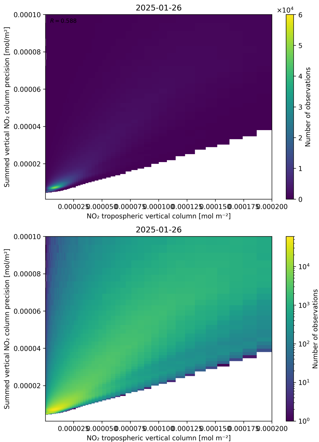
Figure 127: Scatter density plot of “NO 2 tropospheric vertical column” against “Summed vertical NO 2 column precision” for 2025-01-25 to 2025-01-27.
