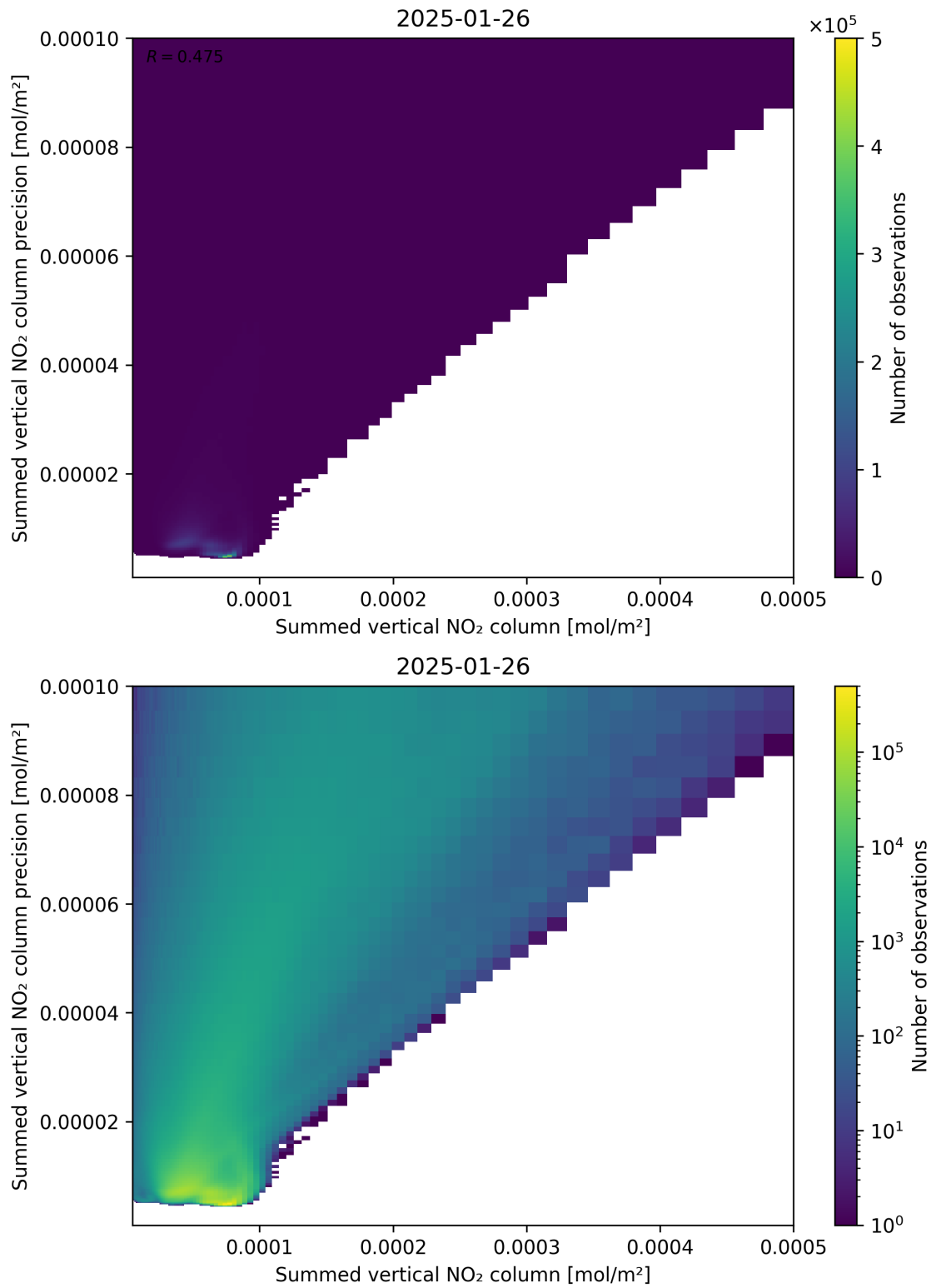
Figure 105: Scatter density plot of “Summed vertical NO 2 column” against “Summed vertical NO 2 column precision” for 2025-01-25 to 2025-01-27.
