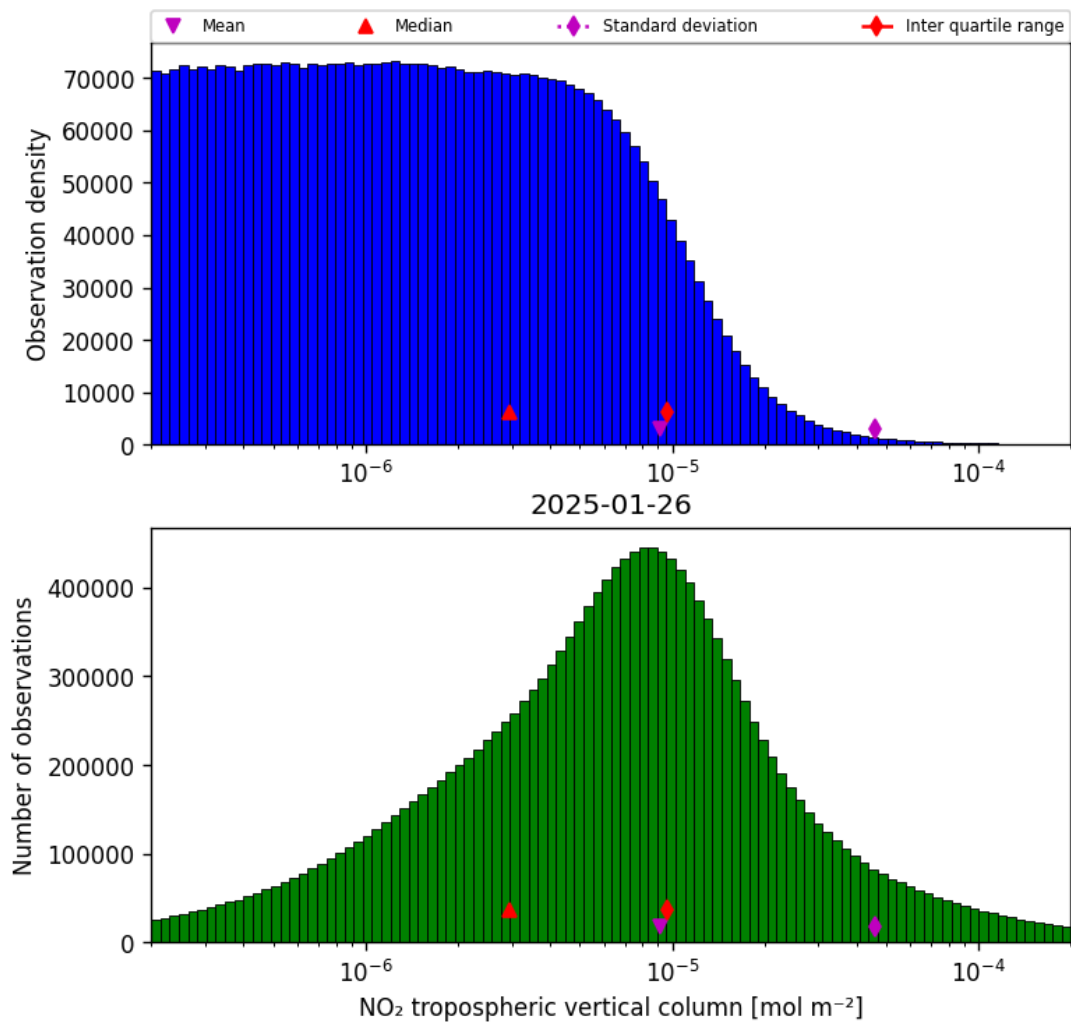
Figure 29: Histogram of “NO 2 tropospheric vertical column” for 2025-01-25 to 2025-01-27
