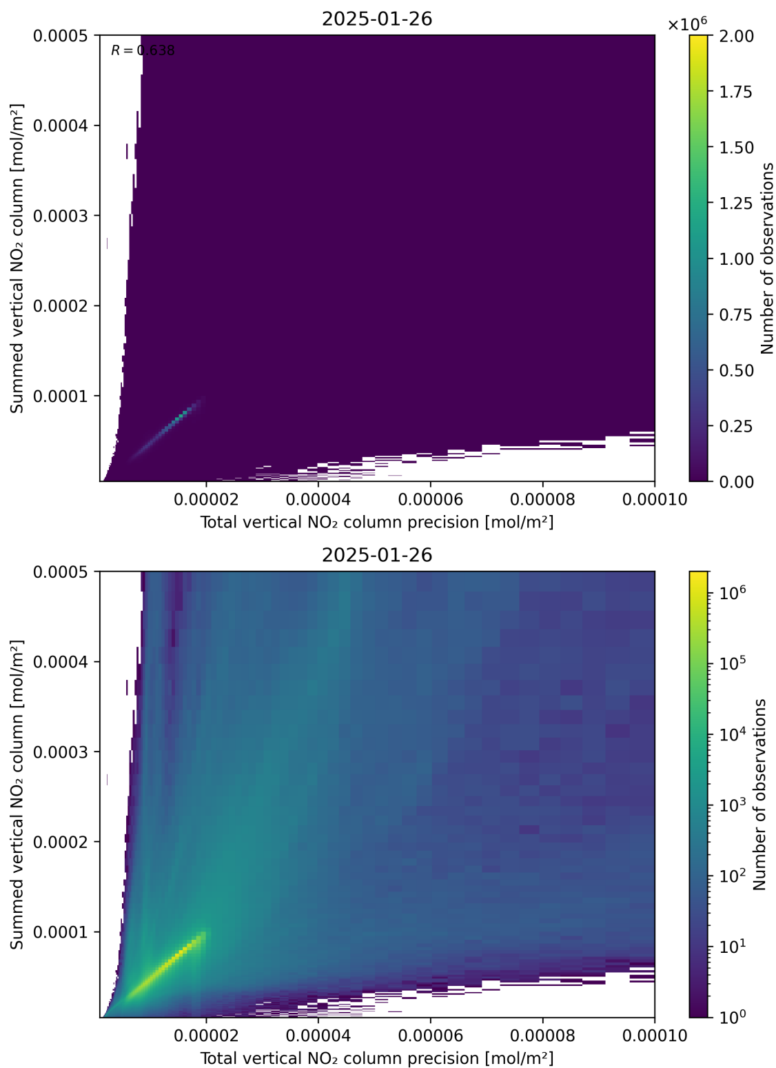
Figure 117: Scatter density plot of “Total vertical NO 2 column precision” against “Summed vertical NO 2 column” for 2025-01-25 to 2025-01-27.
