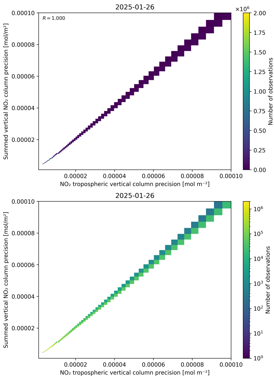
Figure 137: Scatter density plot of “NO 2 tropospheric vertical column precision” against “Summed vertical NO 2 column precision” for 2025-01-25 to 2025-01-27.
