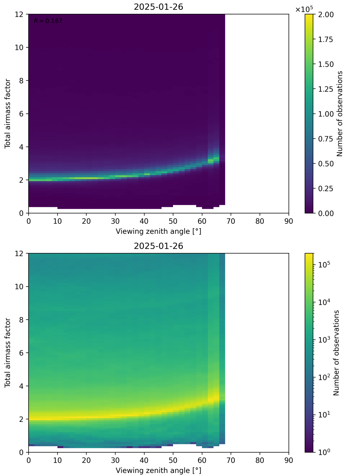
Figure 160: Scatter density plot of “Viewing zenith angle” against “Total airmass factor” for 2025-01-25 to 2025-01-27.
