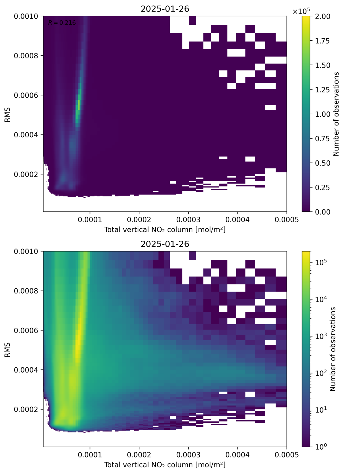
Figure 120: Scatter density plot of “Total vertical NO 2 column” against “RMS” for 2025-01-25 to 2025-01-27.
