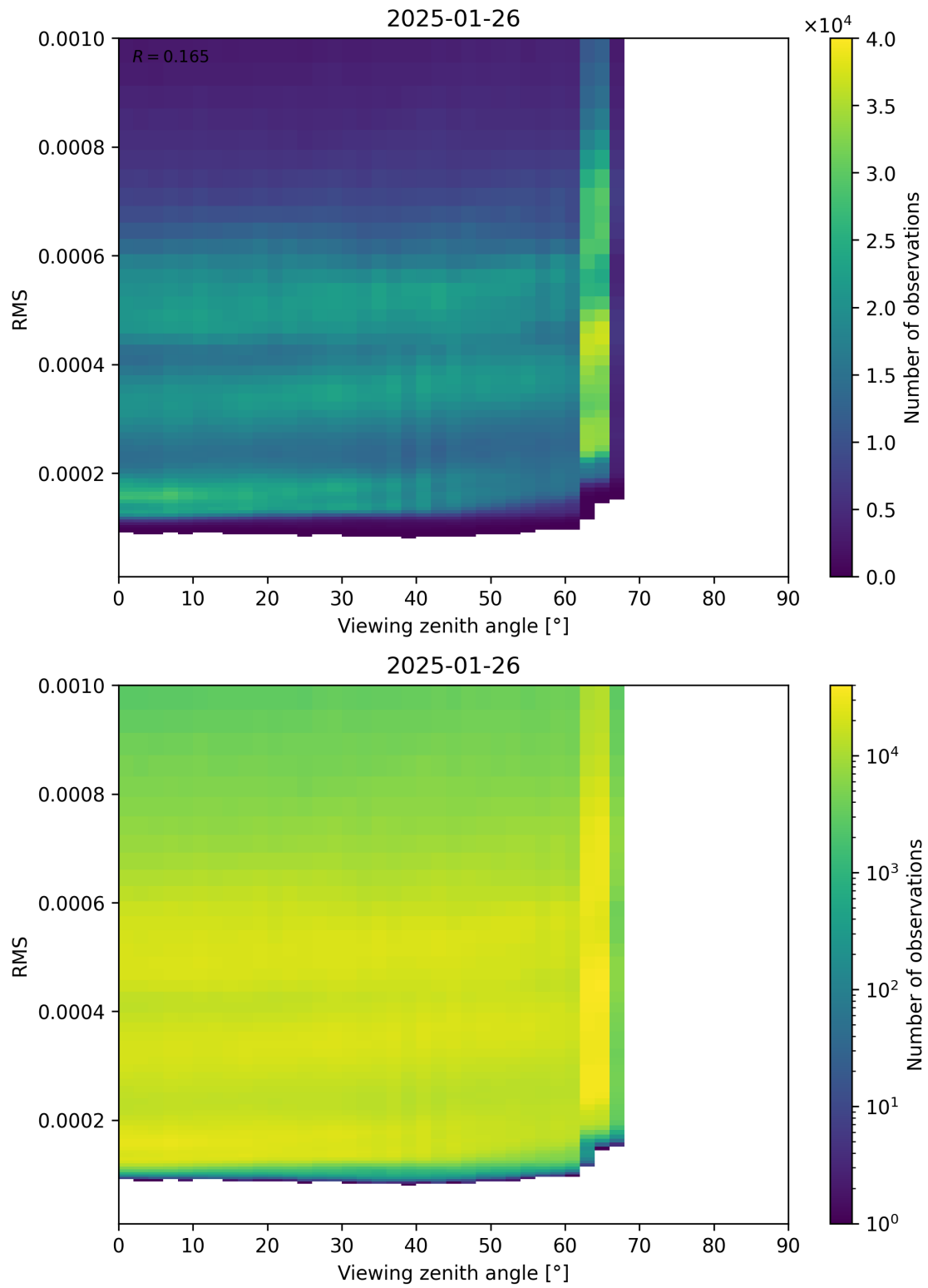
Figure 171: Scatter density plot of “Viewing zenith angle” against “RMS” for 2025-01-25 to 2025-01-27.
