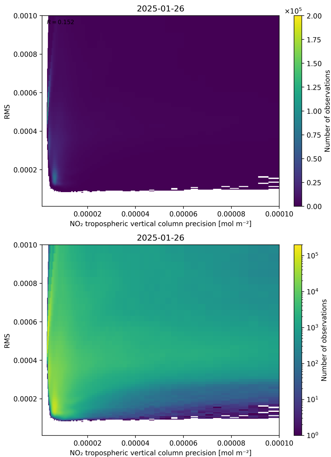
Figure 140: Scatter density plot of “NO 2 tropospheric vertical column precision” against “RMS” for 2025-01-25 to 2025-01-27.
