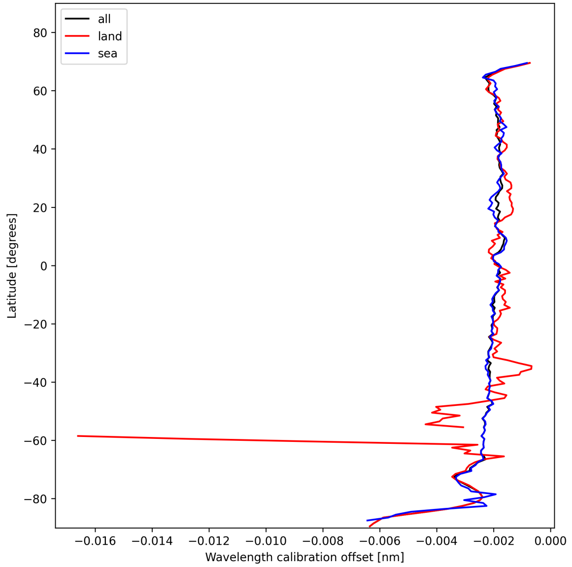
Figure 18: Zonal average of “Wavelength calibration offset” for 2025-01-25 to 2025-01-27.
