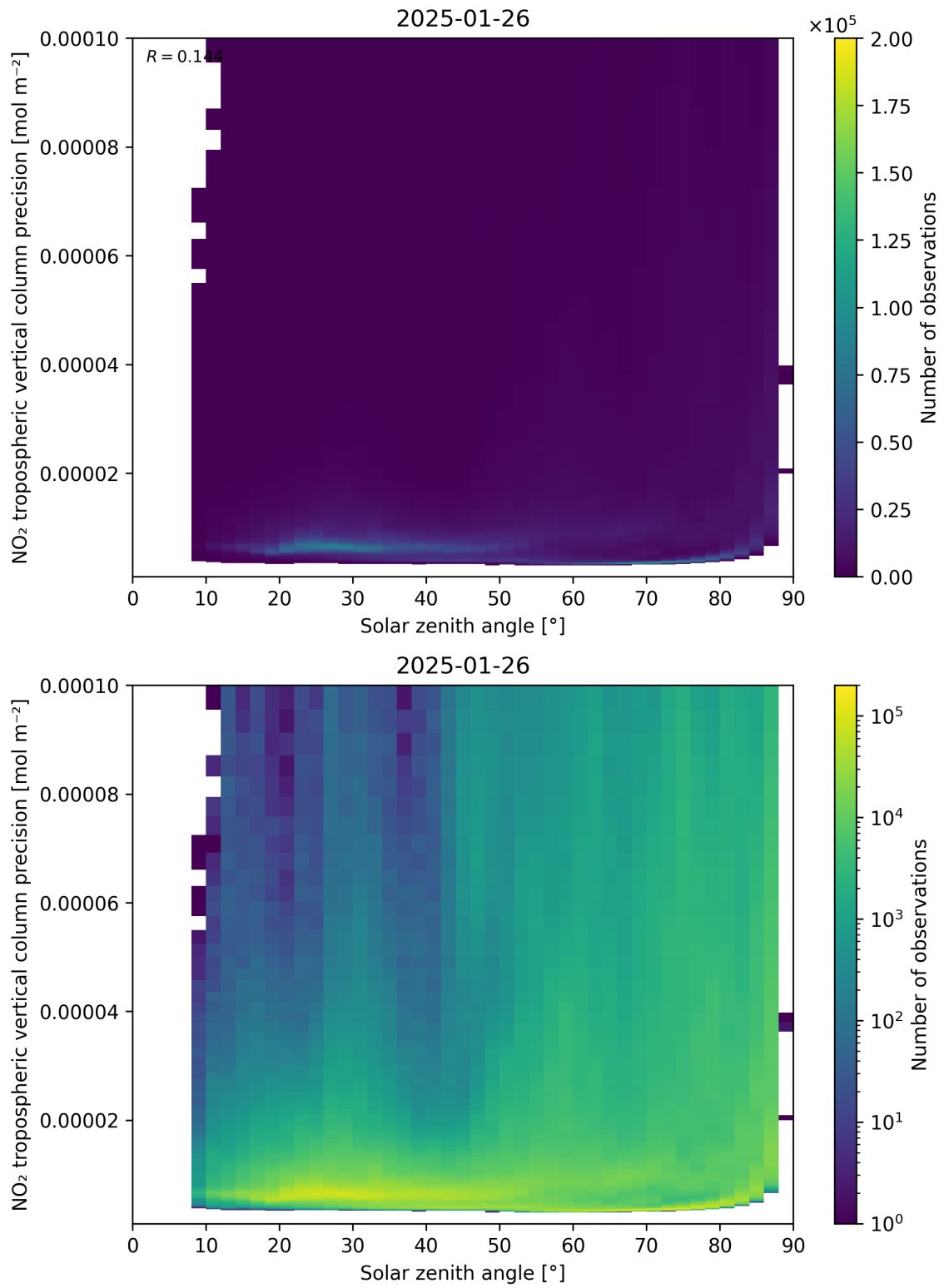
Figure 156: Scatter density plot of “Solar zenith angle” against “NO 2 tropospheric vertical column precision” for 2025-01-25 to 2025-01-27.
