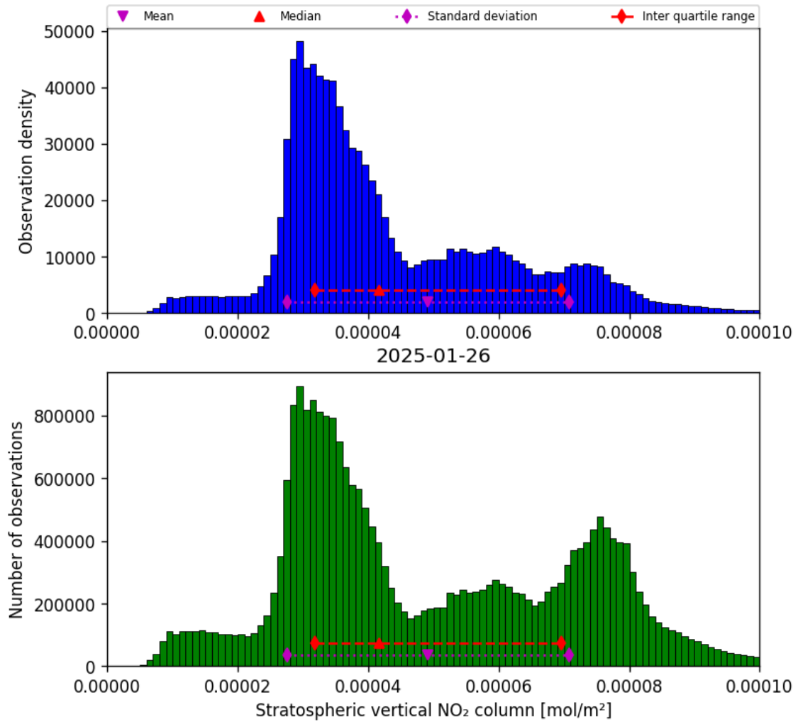
Figure 36: Histogram of “Stratospheric vertical NO 2 column” for 2025-01-25 to 2025-01-27
