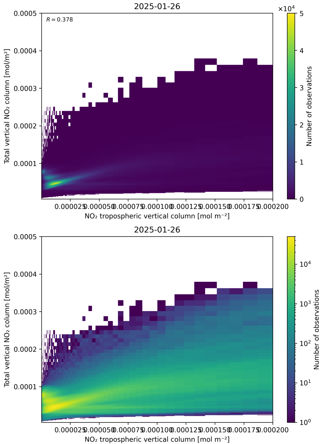
Figure 128: Scatter density plot of “NO 2 tropospheric vertical column” against “Total vertical NO 2 column” for 2025-01-25 to 2025-01-27.
