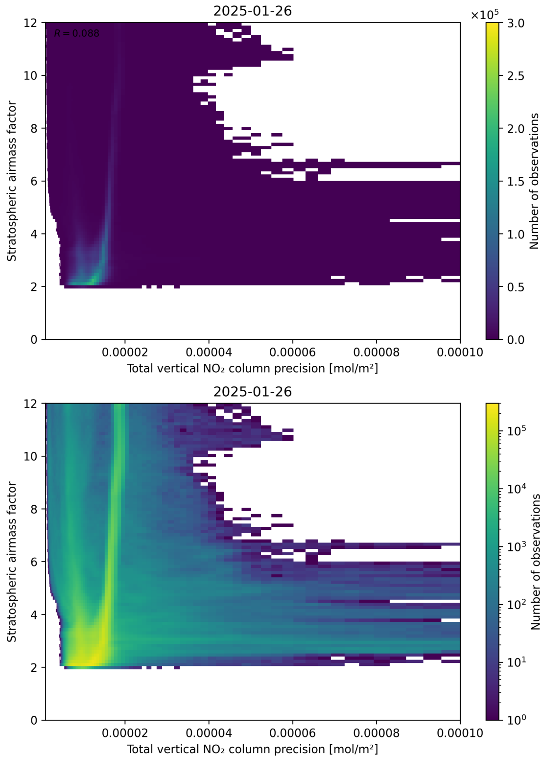
Figure 115: Scatter density plot of “Total vertical NO 2 column precision” against “Stratospheric air mass factor” for 2025-01-25 to 2025-01-27.
