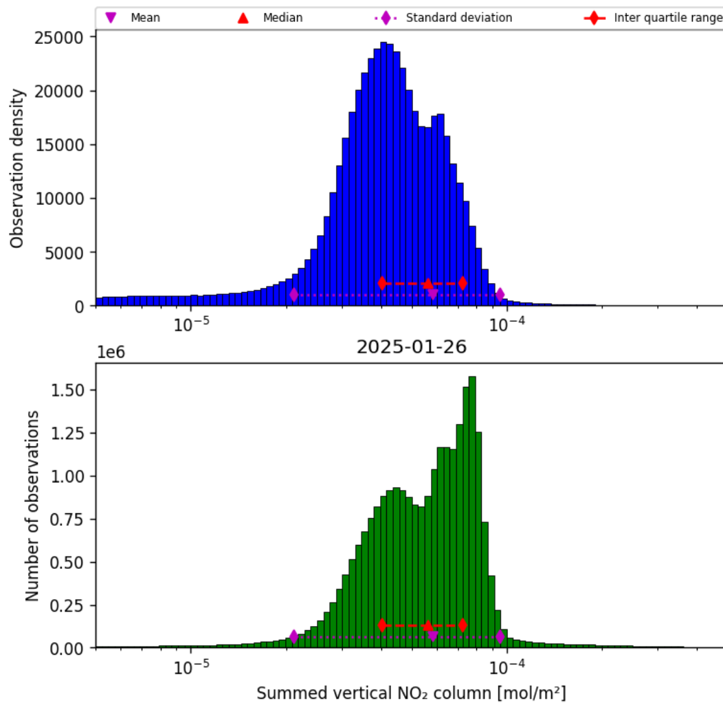
Figure 40: Histogram of “Summed vertical NO 2 column” for 2025-01-25 to 2025-01-27
