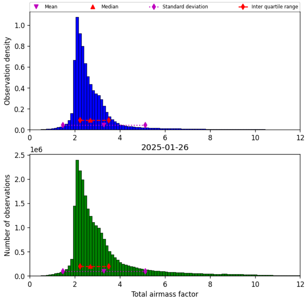
Figure 32: Histogram of “Total airmass factor” for 2025-01-25 to 2025-01-27
