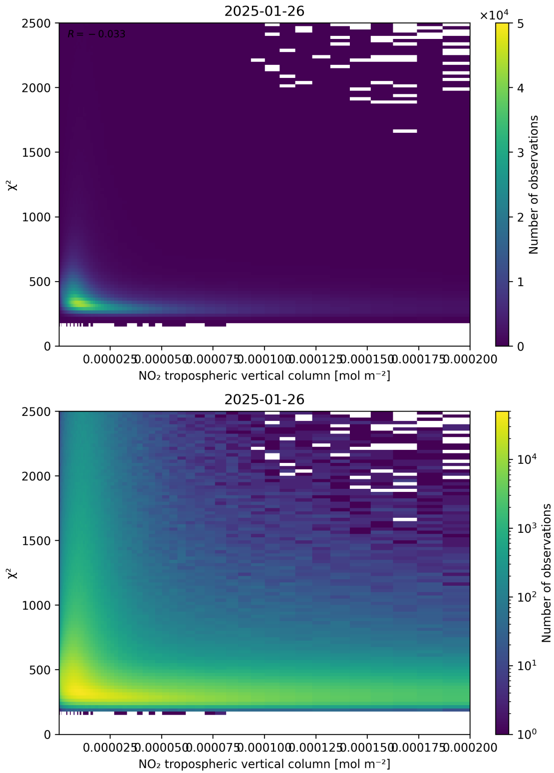
Figure 124: Scatter density plot of “NO 2 tropospheric vertical column” against “ \chi^2 ” for 2025-01-25 to 2025-01-27.
