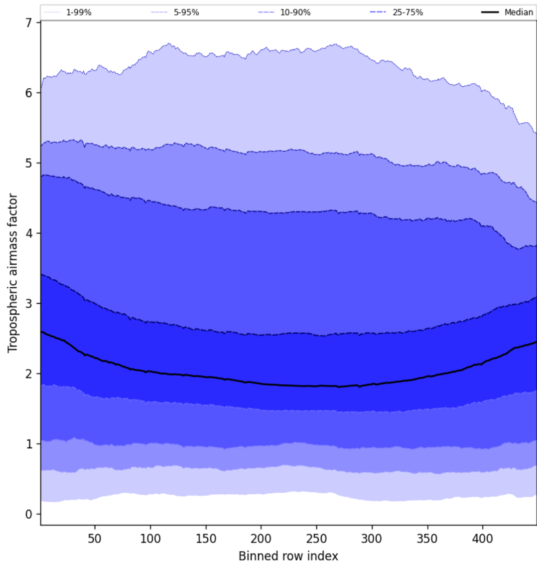
Figure 48: Along track statistics of “Tropospheric airmass factor” for 2025-01-25 to 2025-01-27
