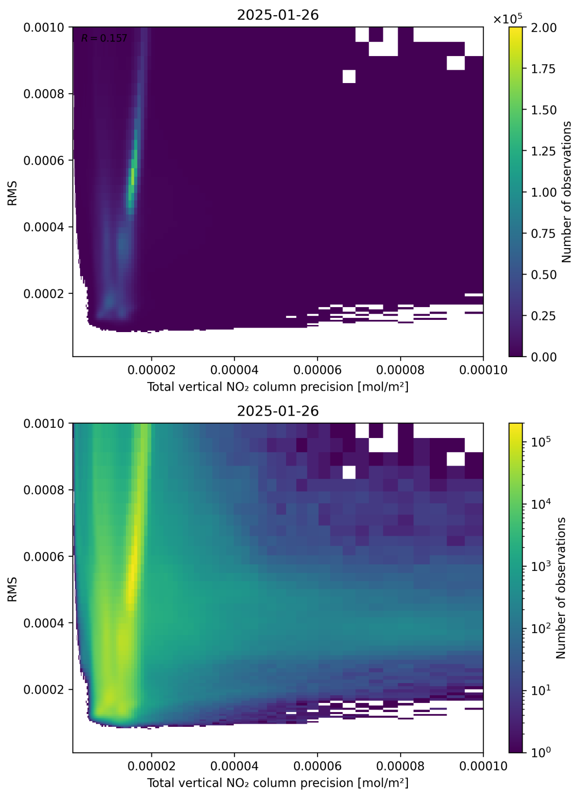
Figure 119: Scatter density plot of “Total vertical NO 2 column precision” against “RMS” for 2025-01-25 to 2025-01-27.
