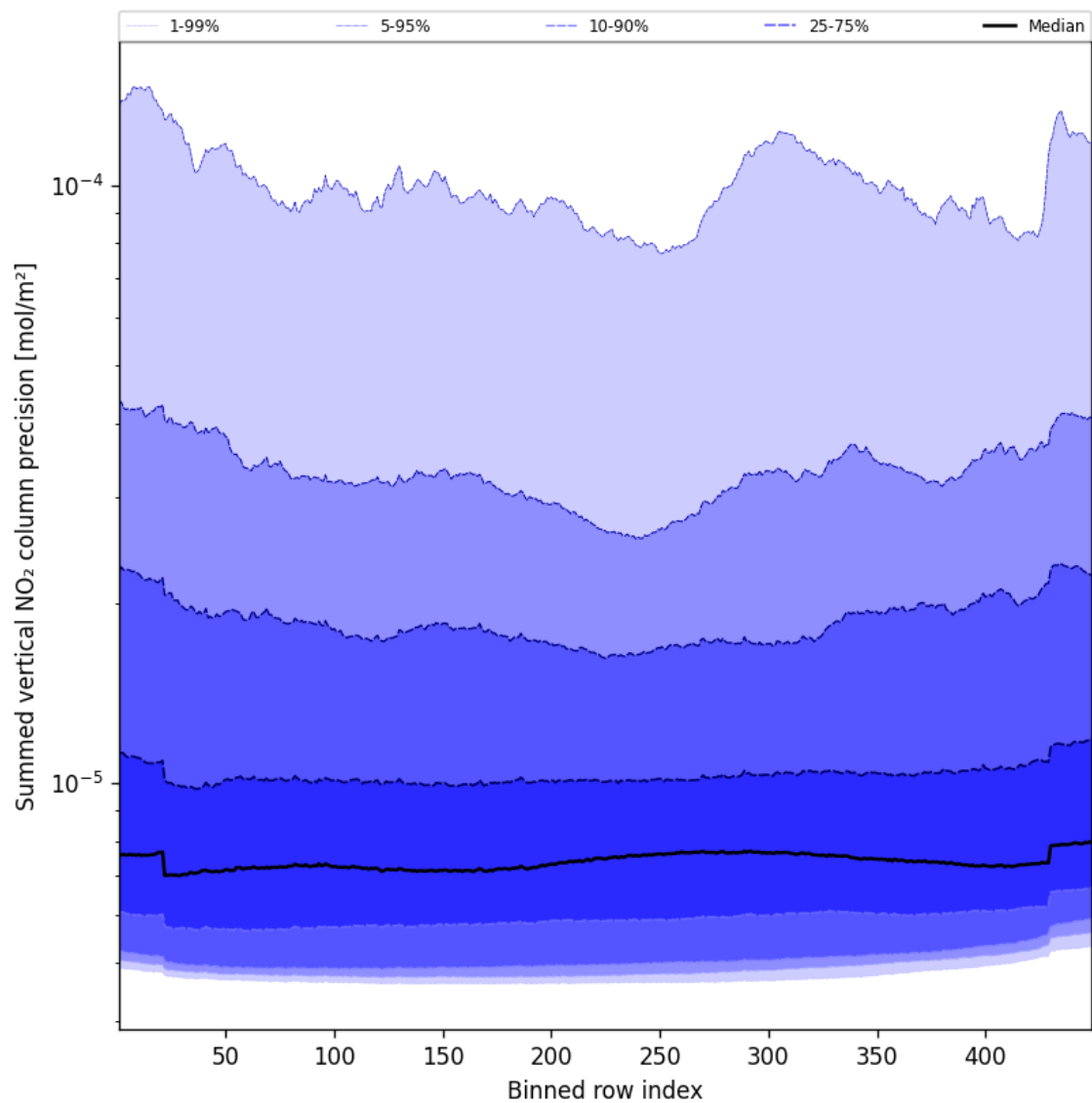
Figure 58: Along track statistics of “Summed vertical NO 2 column precision” for 2025-01-25 to 2025-01-27
