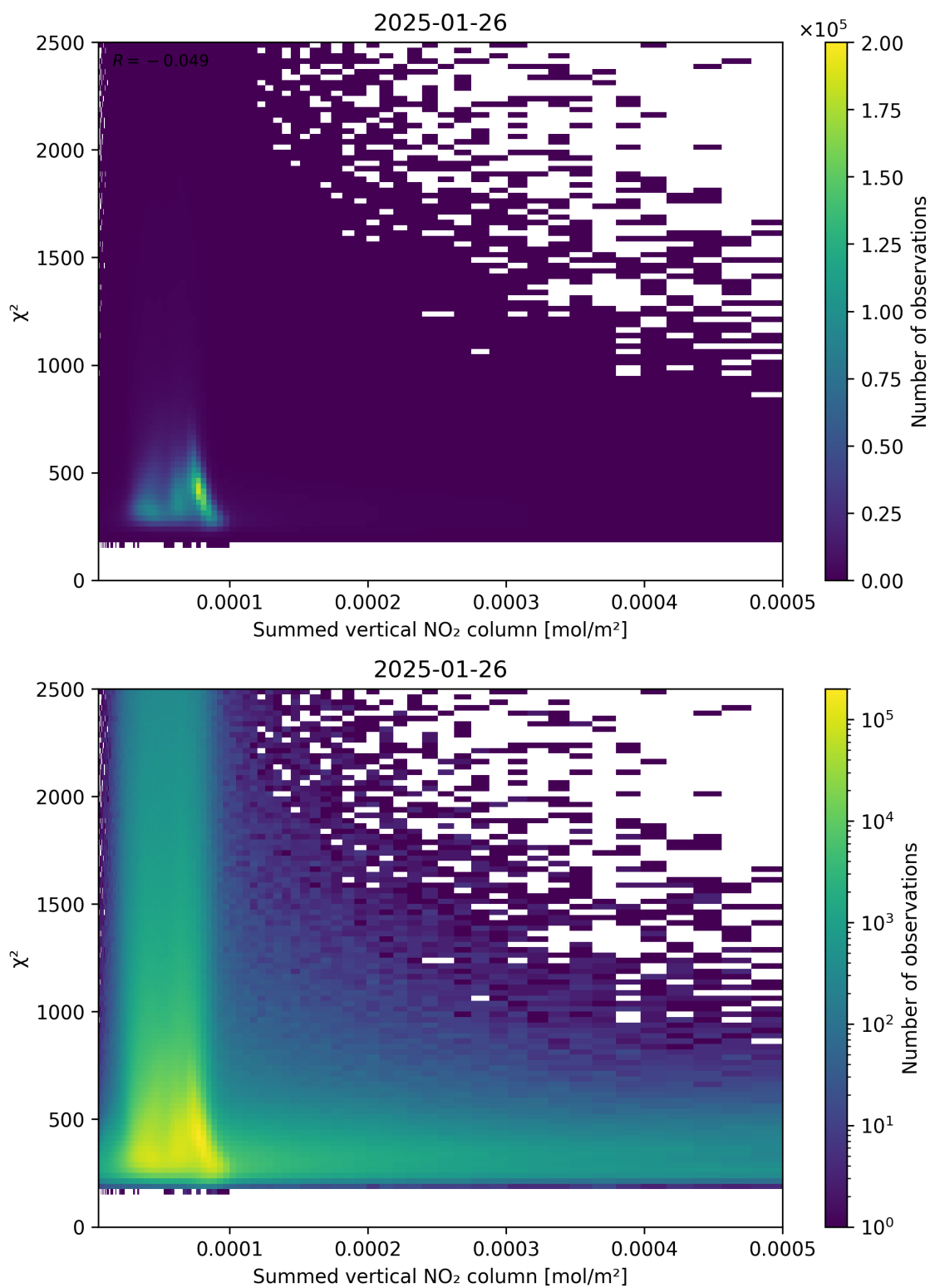
Figure 104: Scatter density plot of “Summed vertical NO 2 column” against “ \chi^2 ” for 2025-01-25 to 2025-01-27.
