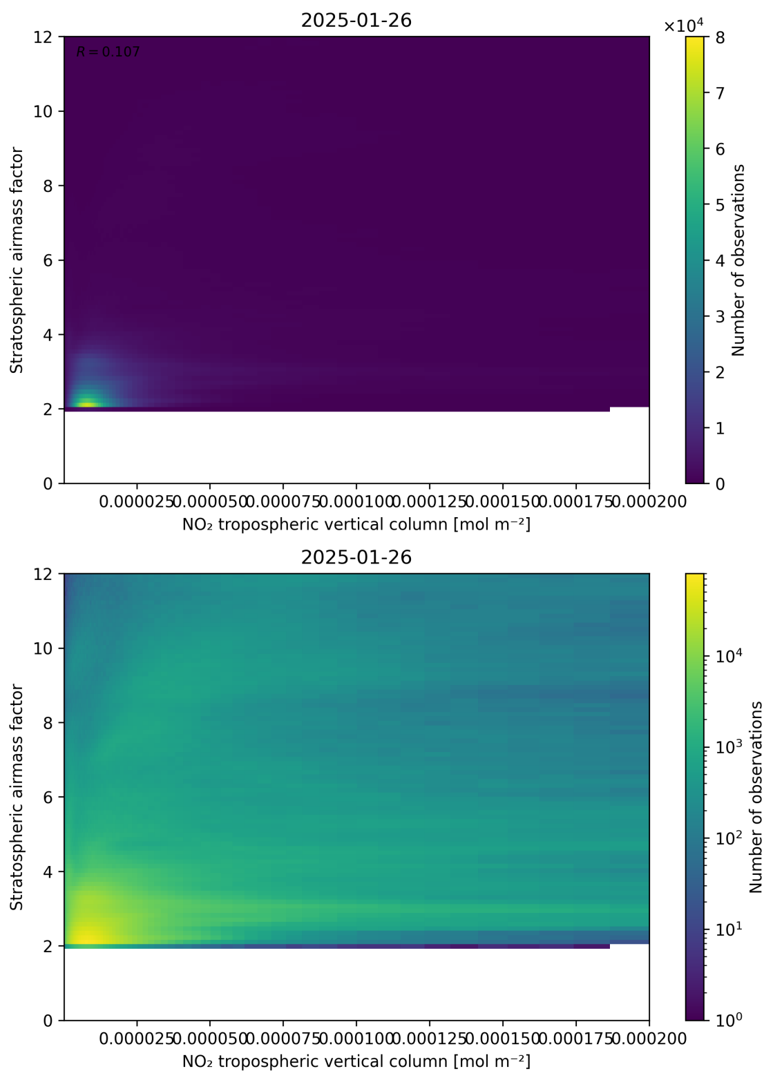
Figure 121: Scatter density plot of “NO 2 tropospheric vertical column” against “Stratospheric airmass factor” for 2025-01-25 to 2025-01-27.
