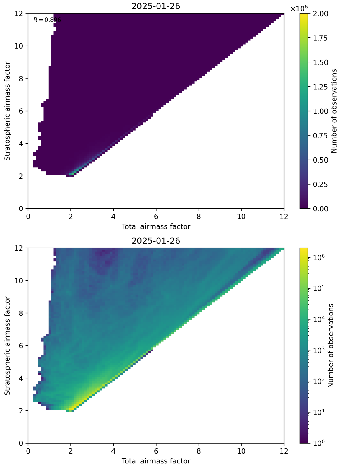
Figure 62: Scatter density plot of “Total air mass factor” against “Stratospheric air mass factor” for 2025-01-25 to 2025-01-27.
