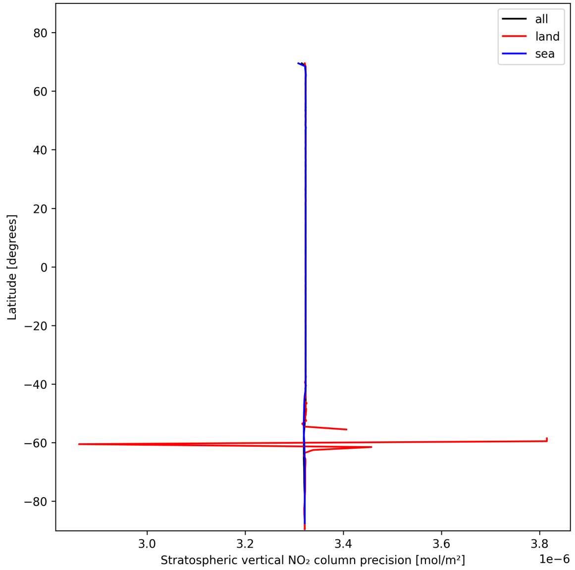
Figure 20: Zonal average of “Stratospheric vertical NO 2 column precision” for 2025-01-25 to 2025-01-27.
