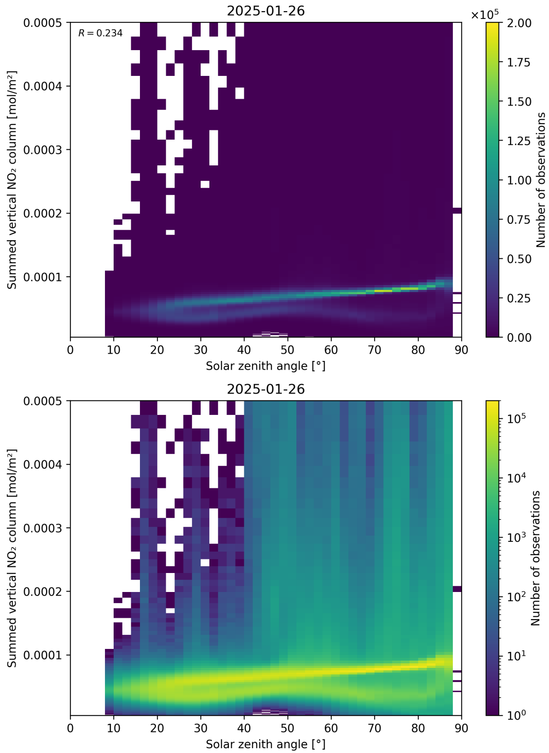
Figure 151: Scatter density plot of “Solar zenith angle” against “Summed vertical NO 2 column” for 2025-01-25 to 2025-01-27.
