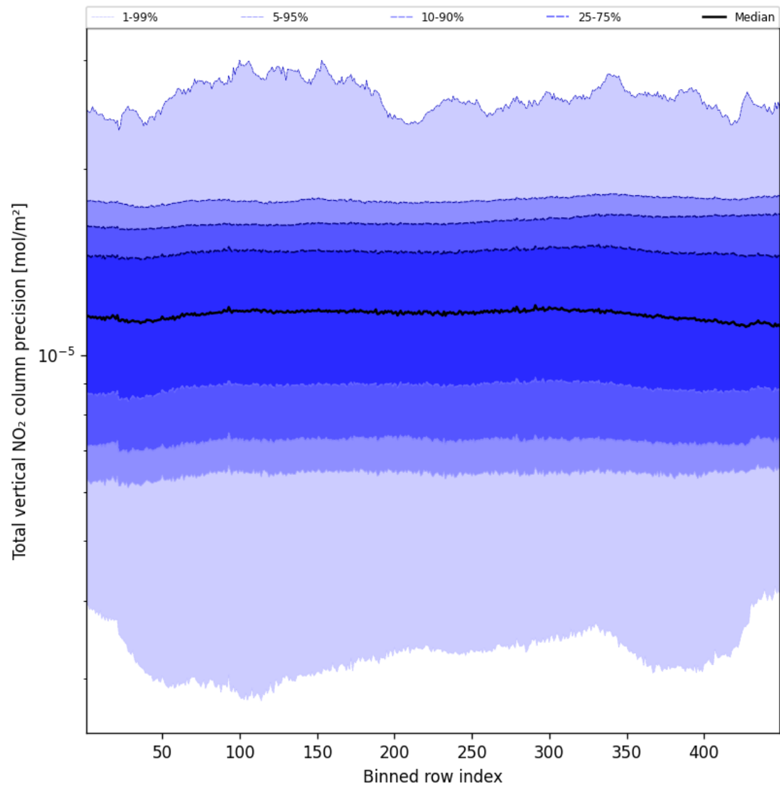
Figure 56: Along track statistics of “Total vertical NO 2 column precision” for 2025-01-25 to 2025-01-27
