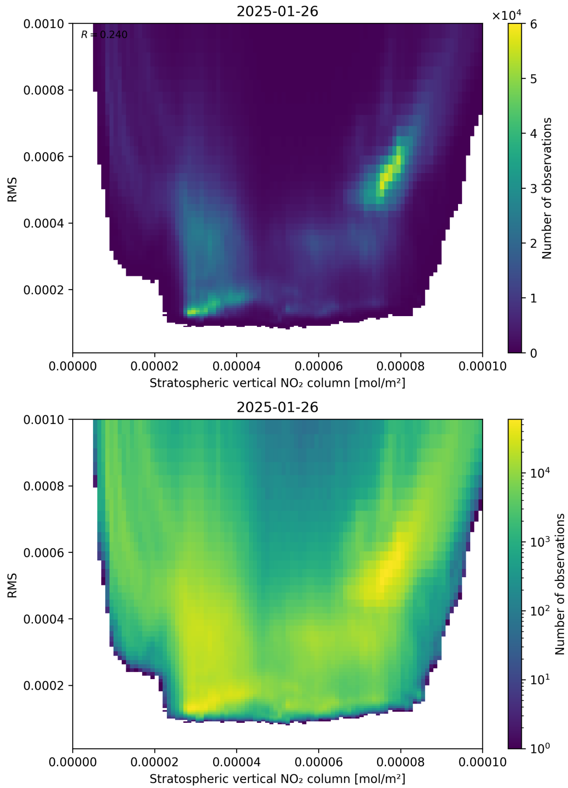
Figure 102: Scatter density plot of “Stratospheric vertical NO 2 column” against “RMS” for 2025-01-25 to 2025-01-27.
