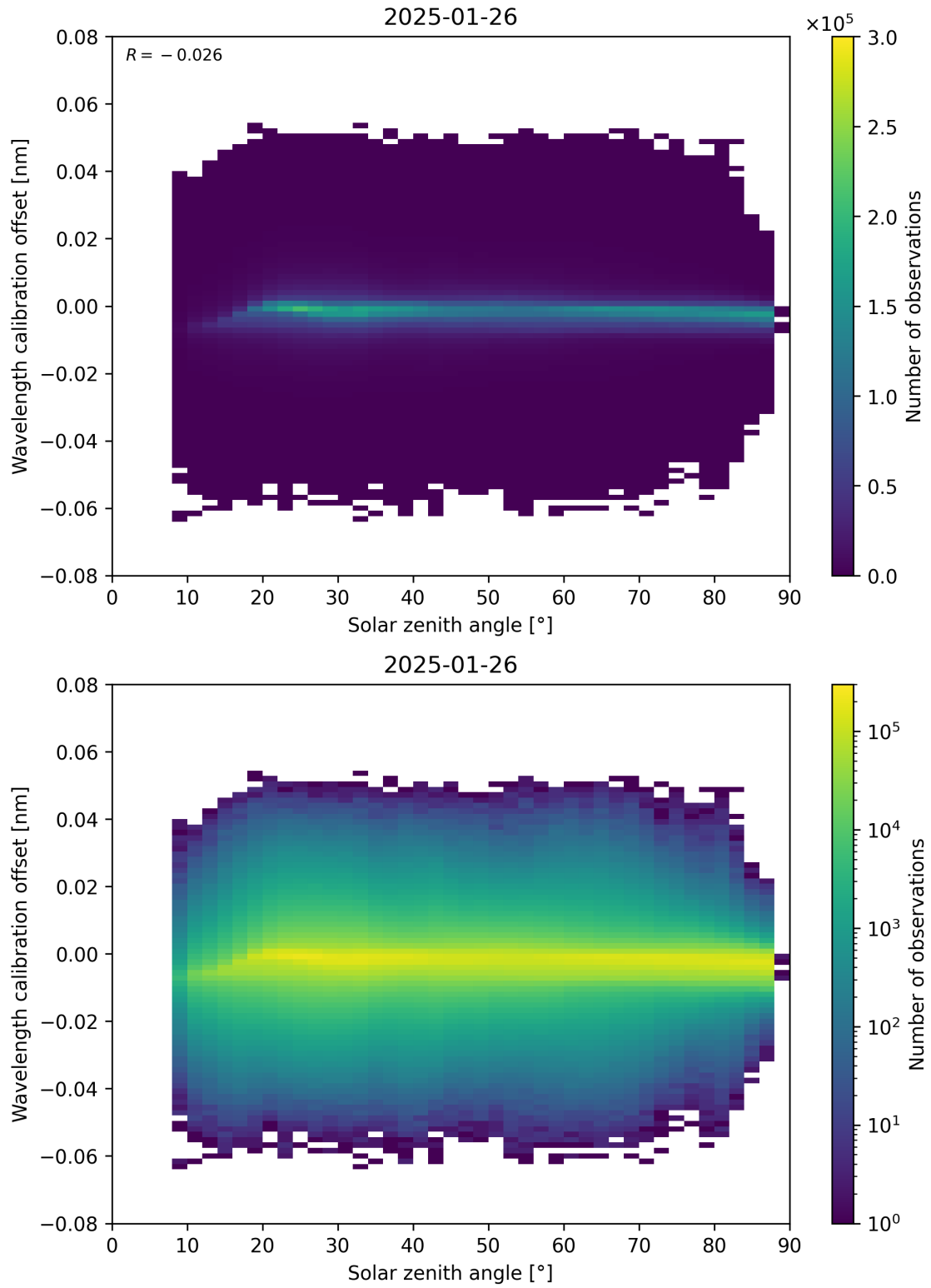
Figure 158: Scatter density plot of “Solar zenith angle” against “Wavelength calibration offset” for 2025-01-25 to 2025-01-27.
