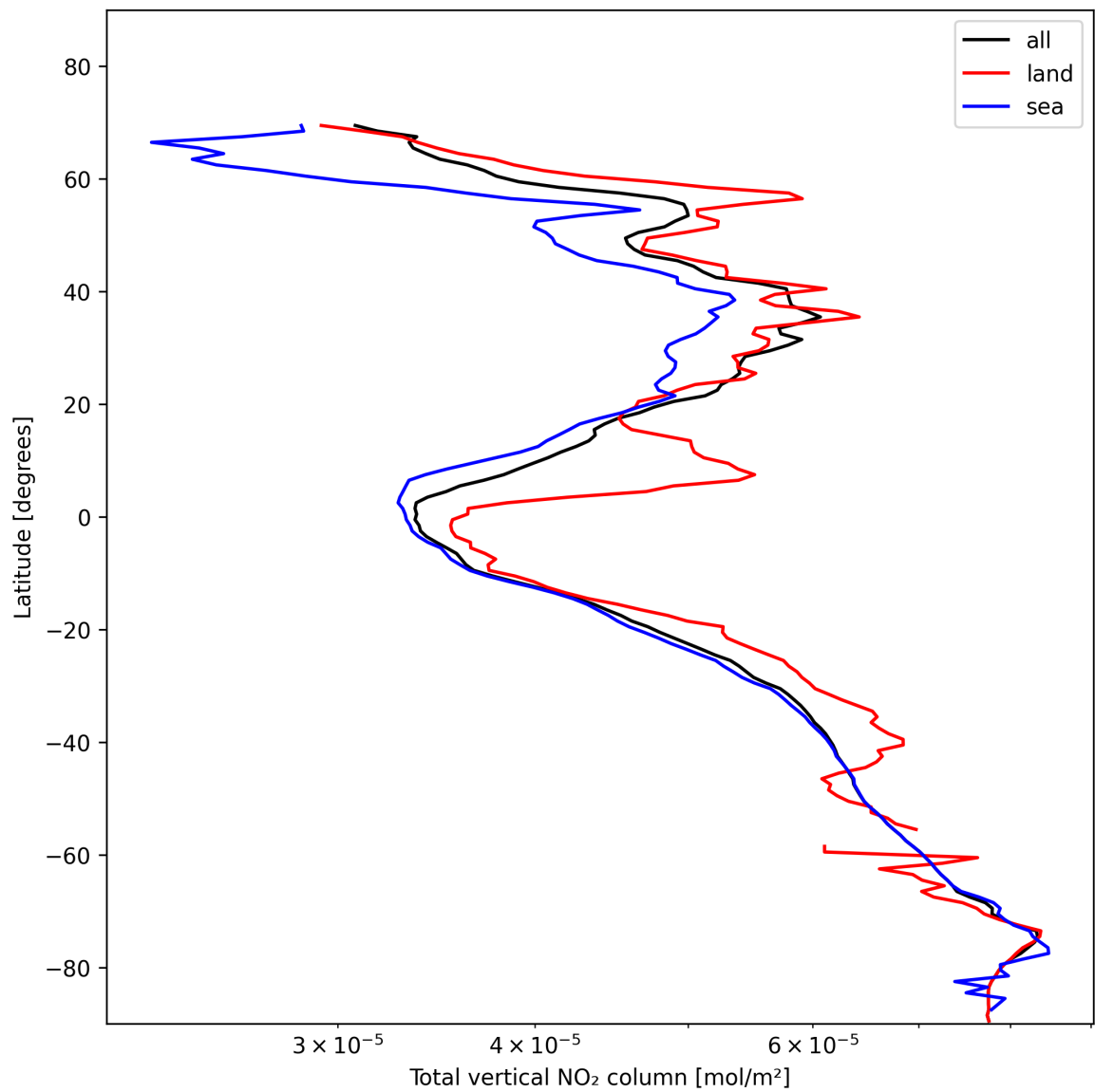
Figure 21: Zonal average of “Total vertical NO 2 column” for 2025-01-25 to 2025-01-27.
