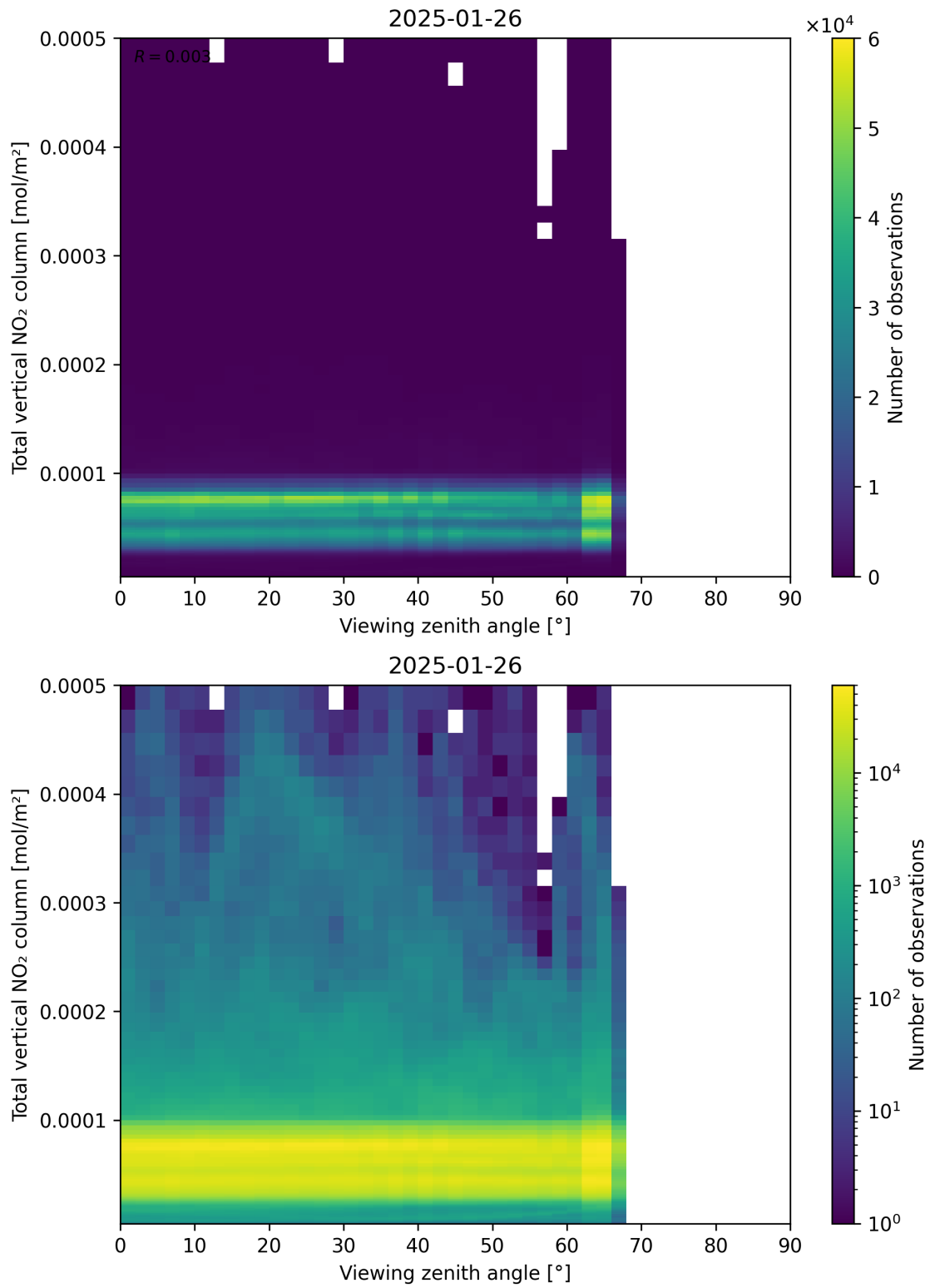
Figure 167: Scatter density plot of “Viewing zenith angle” against “Total vertical NO 2 column” for 2025-01-25 to 2025-01-27.
