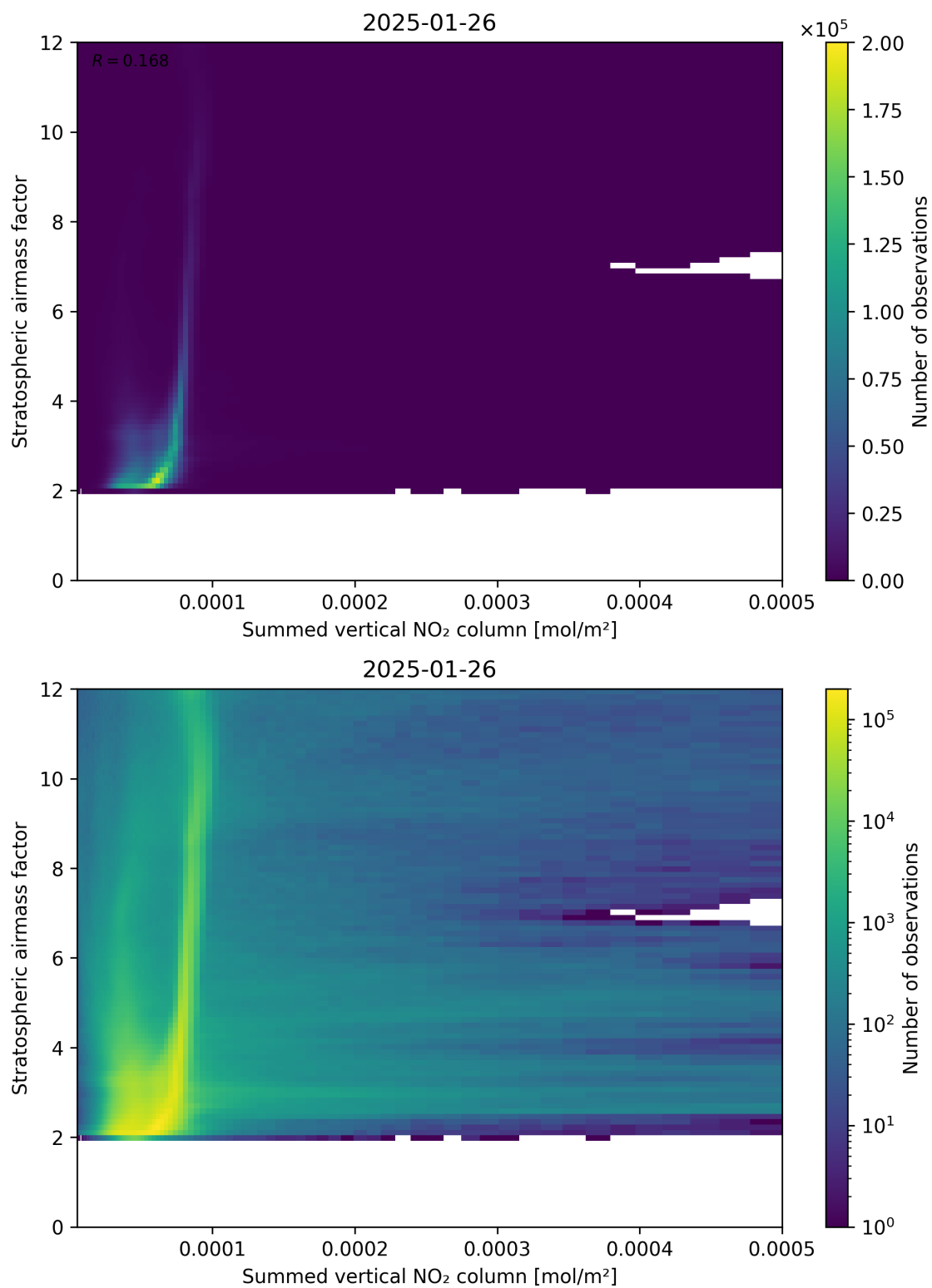
Figure 103: Scatter density plot of “Summed vertical NO 2 column” against “Stratospheric airmass factor” for 2025-01-25 to 2025-01-27.
