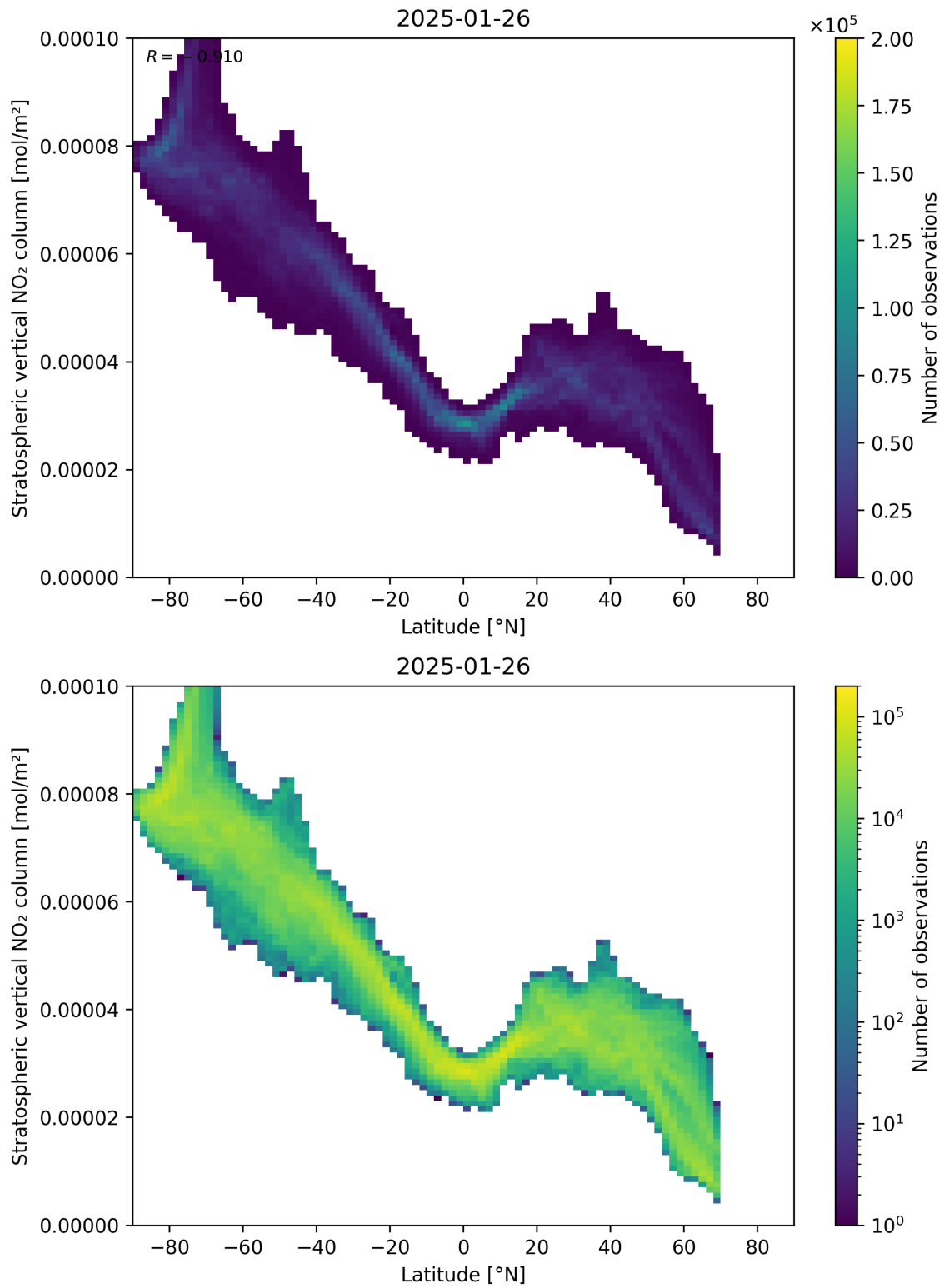
Figure 87: Scatter density plot of “Latitude” against “Stratospheric vertical NO 2 column” for 2025-01-25 to 2025-01-27.
