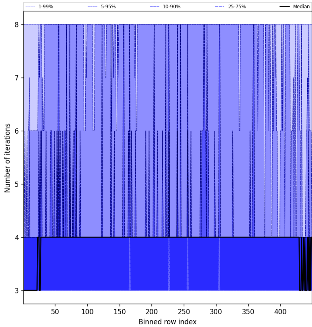
Figure 51: Along track statistics of “Number of iterations” for 2025-01-26 to 2025-01-28
