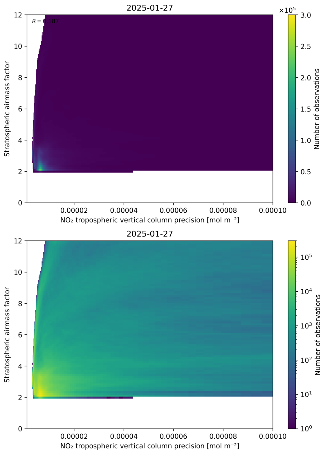
Figure 131: Scatter density plot of “NO 2 tropospheric vertical column precision” against “Stratospheric airmass factor” for 2025-01-26 to 2025-01-28.
