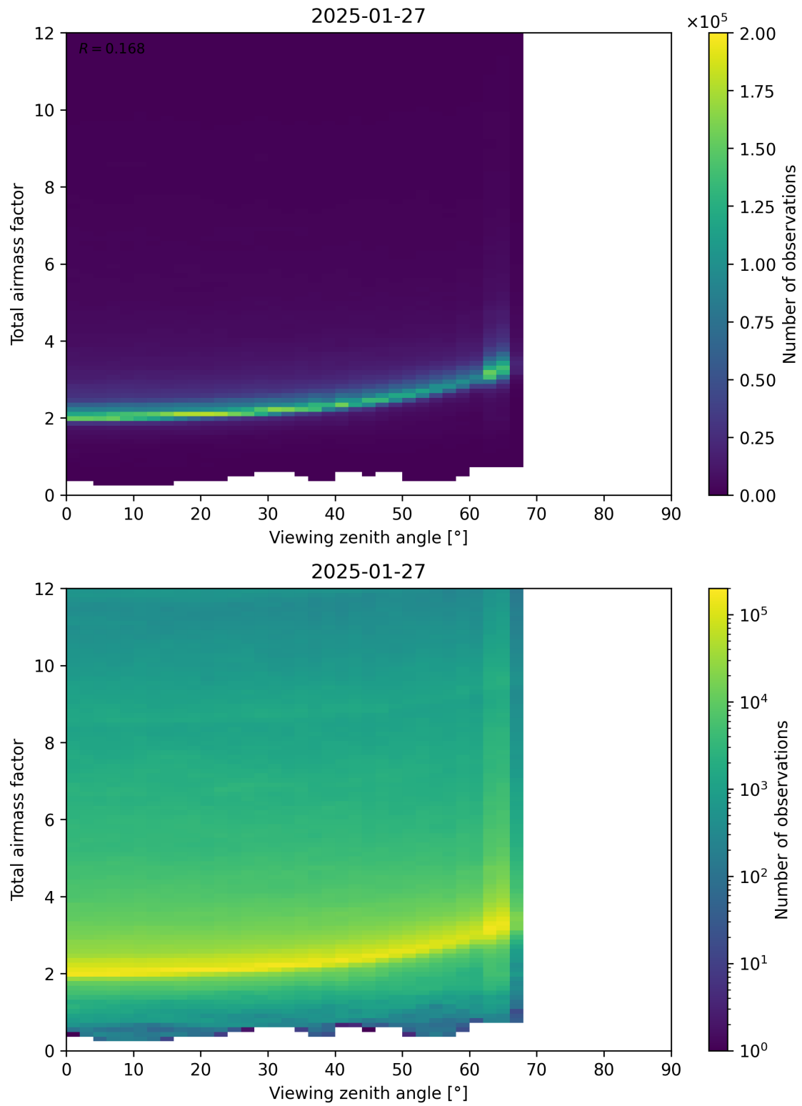
Figure 160: Scatter density plot of “Viewing zenith angle” against “Total airmass factor” for 2025-01-26 to 2025-01-28.
