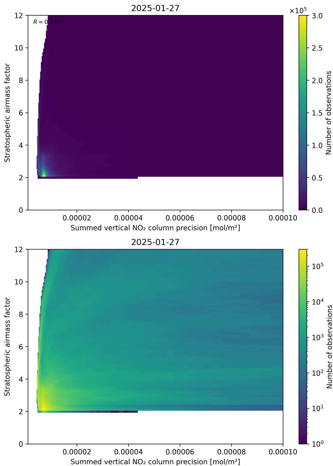
Figure 106: Scatter density plot of “Summed vertical NO 2 column precision” against “Stratospheric airmass factor” for 2025-01-26 to 2025-01-28.
