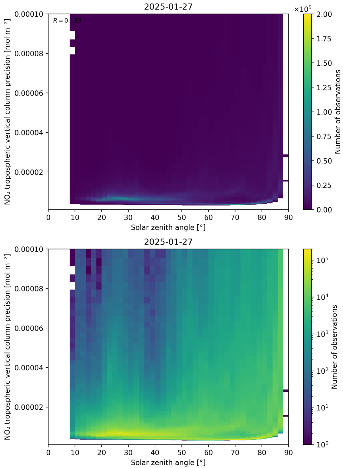
Figure 156: Scatter density plot of “Solar zenith angle” against “NO 2 tropospheric vertical column precision” for 2025-01-26 to 2025-01-28.
