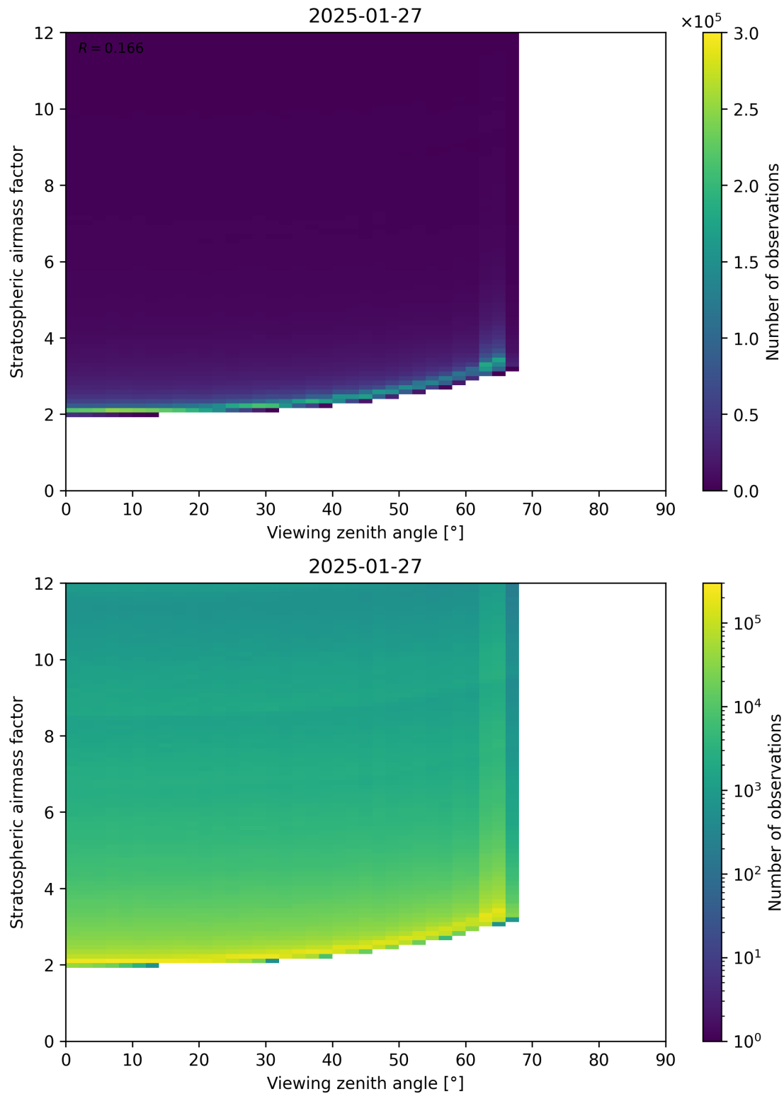
Figure 159: Scatter density plot of “Viewing zenith angle” against “Stratospheric airmass factor” for 2025-01-26 to 2025-01-28.
