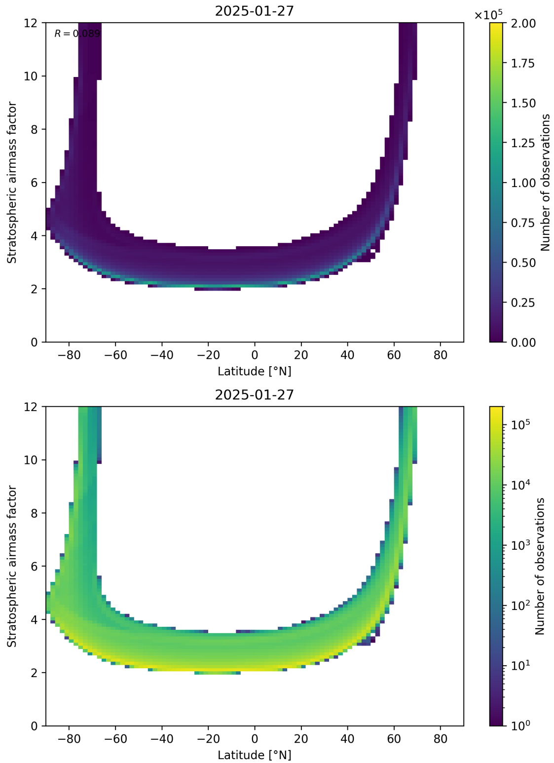
Figure 83: Scatter density plot of “Latitude” against “Stratospheric air mass factor” for 2025-01-26 to 2025-01-28.
