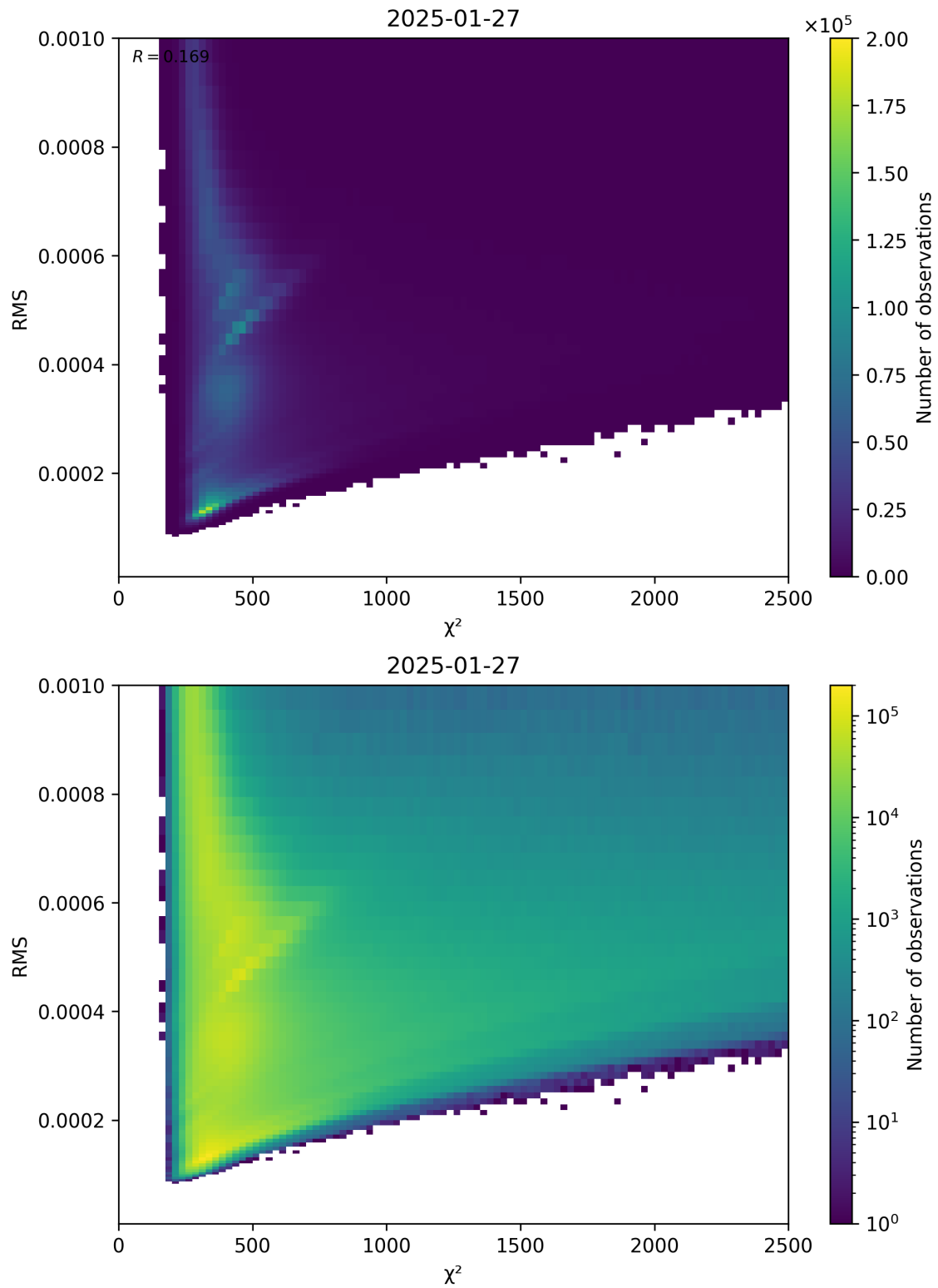
Figure 82: Scatter density plot of “ \chi^2 ” against “RMS” for 2025-01-26 to 2025-01-28.
