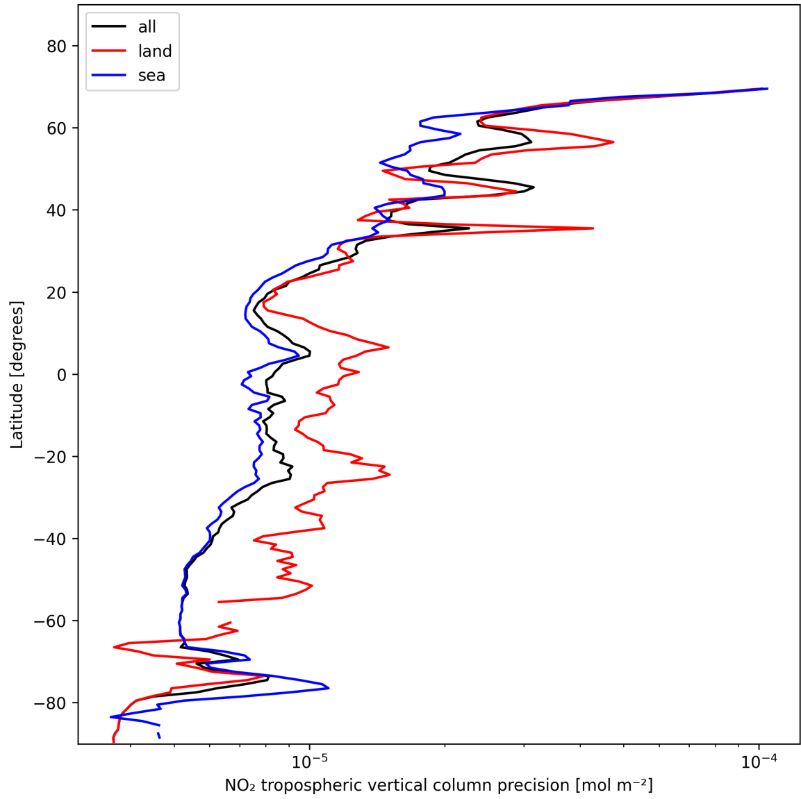
Figure 13: Zonal average of “NO 2 tropospheric vertical column precision” for 2025-01-26 to 2025-01-28.
