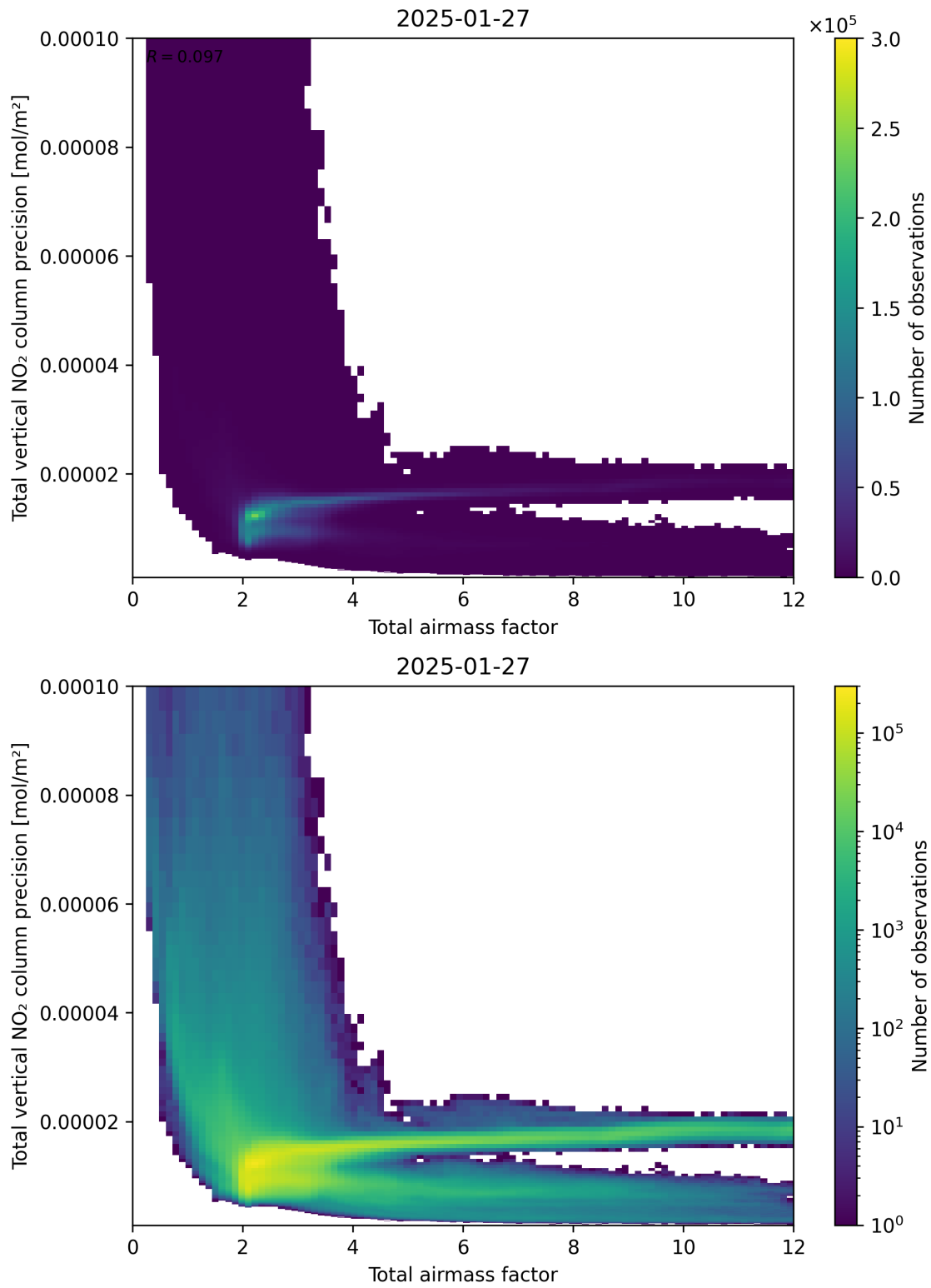
Figure 68: Scatter density plot of “Total airmass factor” against “Total vertical NO 2 column precision” for 2025-01-26 to 2025-01-28.
