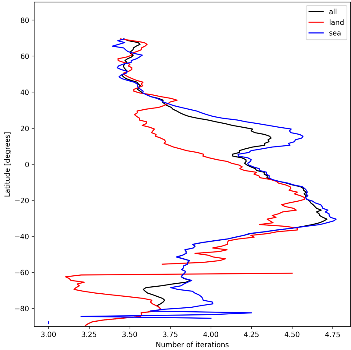
Figure 17: Zonal average of “Number of iterations” for 2025-01-26 to 2025-01-28.
