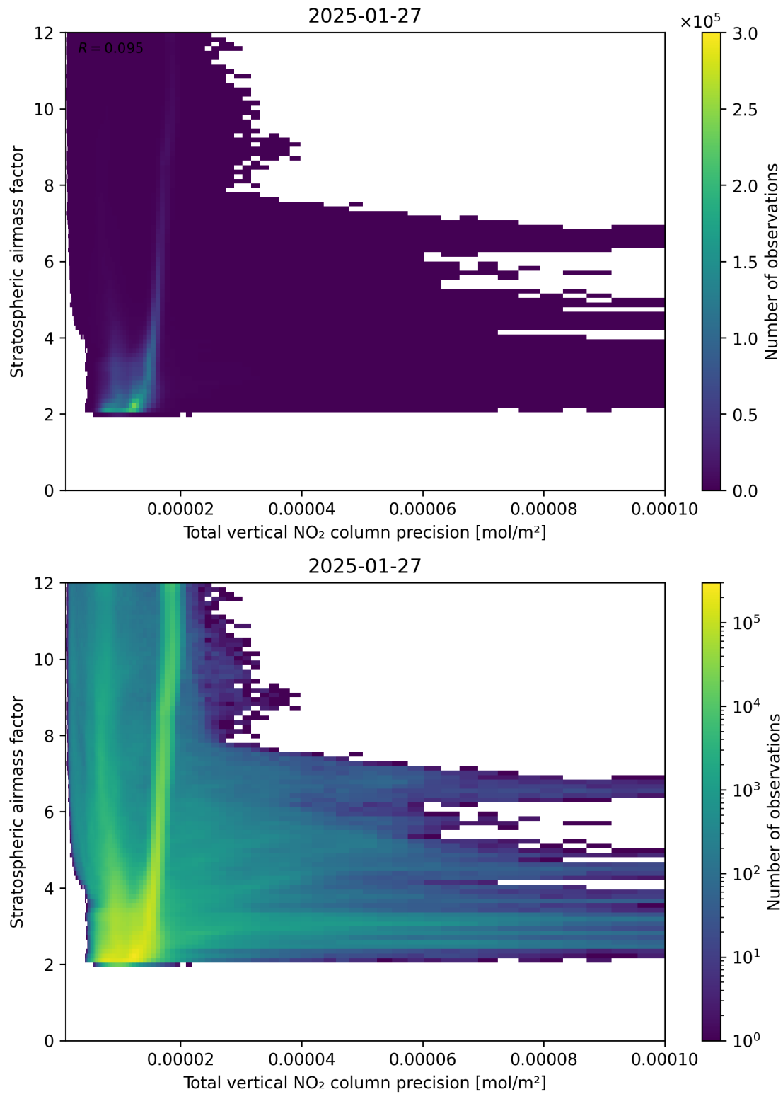
Figure 115: Scatter density plot of “Total vertical NO 2 column precision” against “Stratospheric airmass factor” for 2025-01-26 to 2025-01-28.
