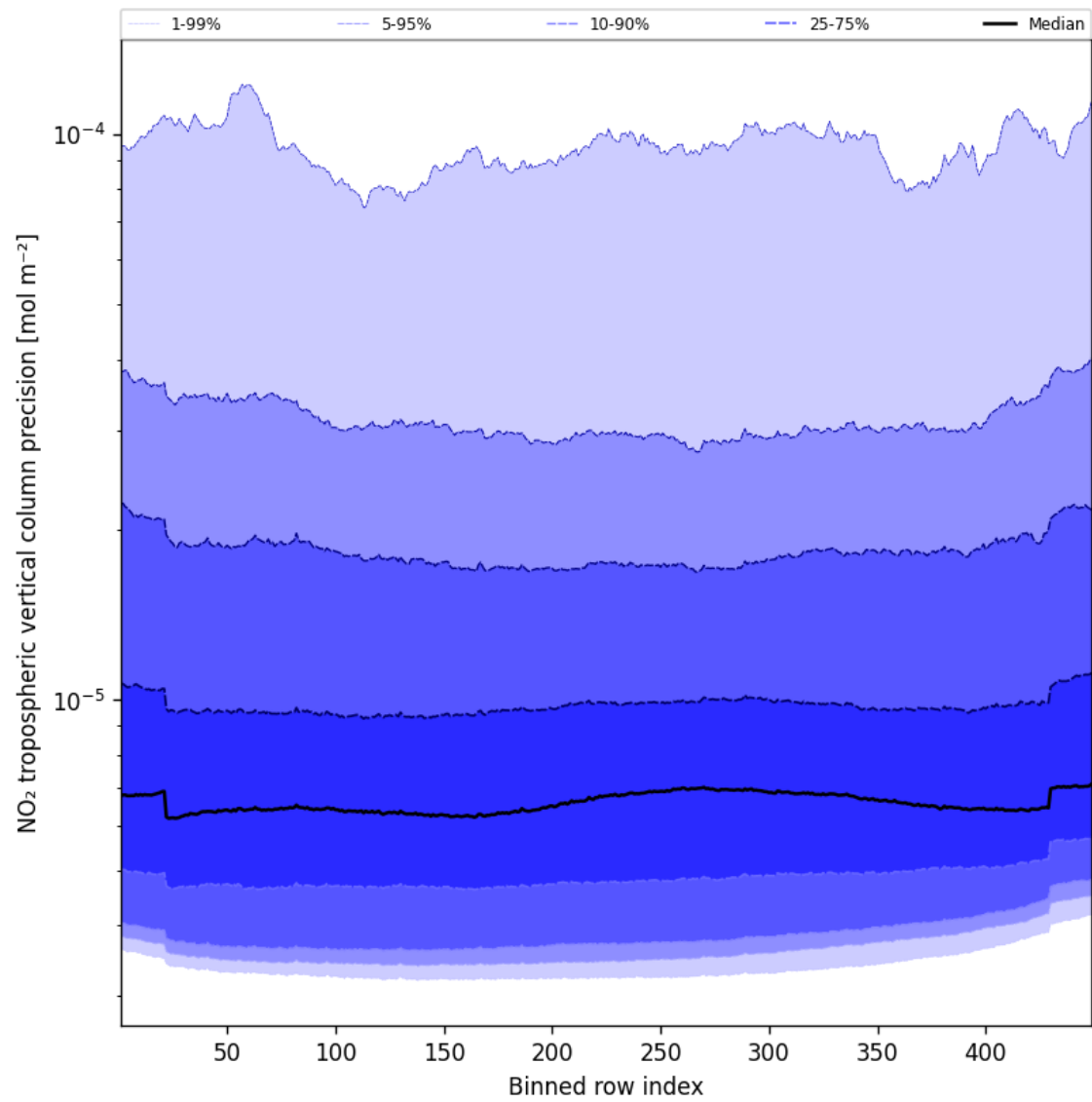
Figure 47: Along track statistics of “NO 2 tropospheric vertical column precision” for 2025-01-26 to 2025-01-28
