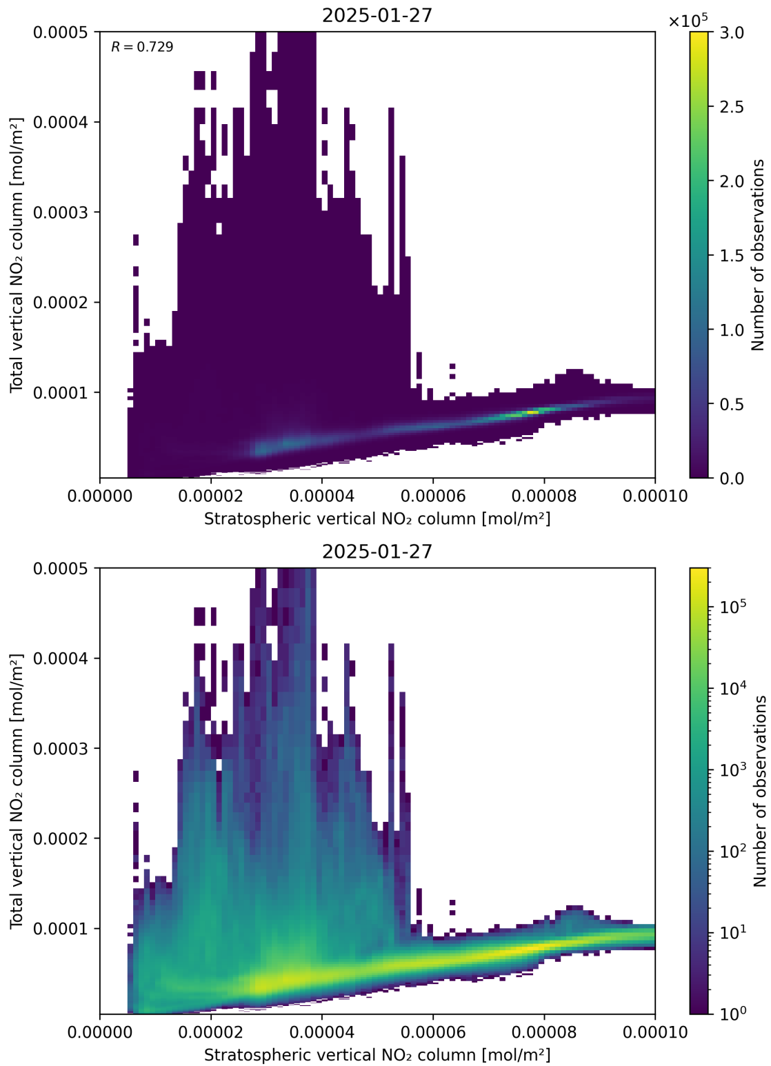
Figure 100: Scatter density plot of “Stratospheric vertical NO 2 column” against “Total vertical NO 2 column” for 2025-01-26 to 2025-01-28.
