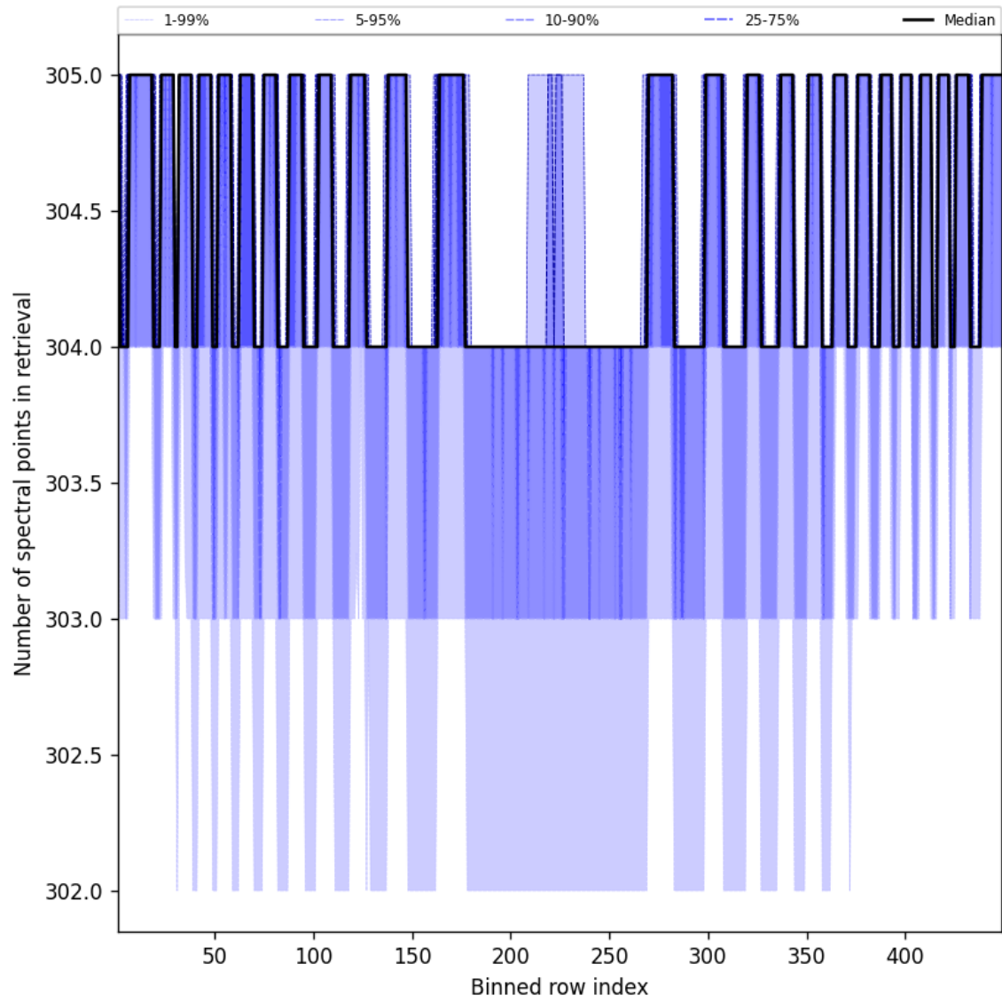
Figure 50: Along track statistics of “Number of spectral points in retrieval” for 2025-01-26 to 2025-01-28
