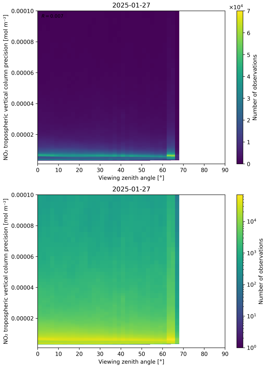
Figure 170: Scatter density plot of “Viewing zenith angle” against “NO 2 tropospheric vertical column precision” for 2025-01-26 to 2025-01-28.
