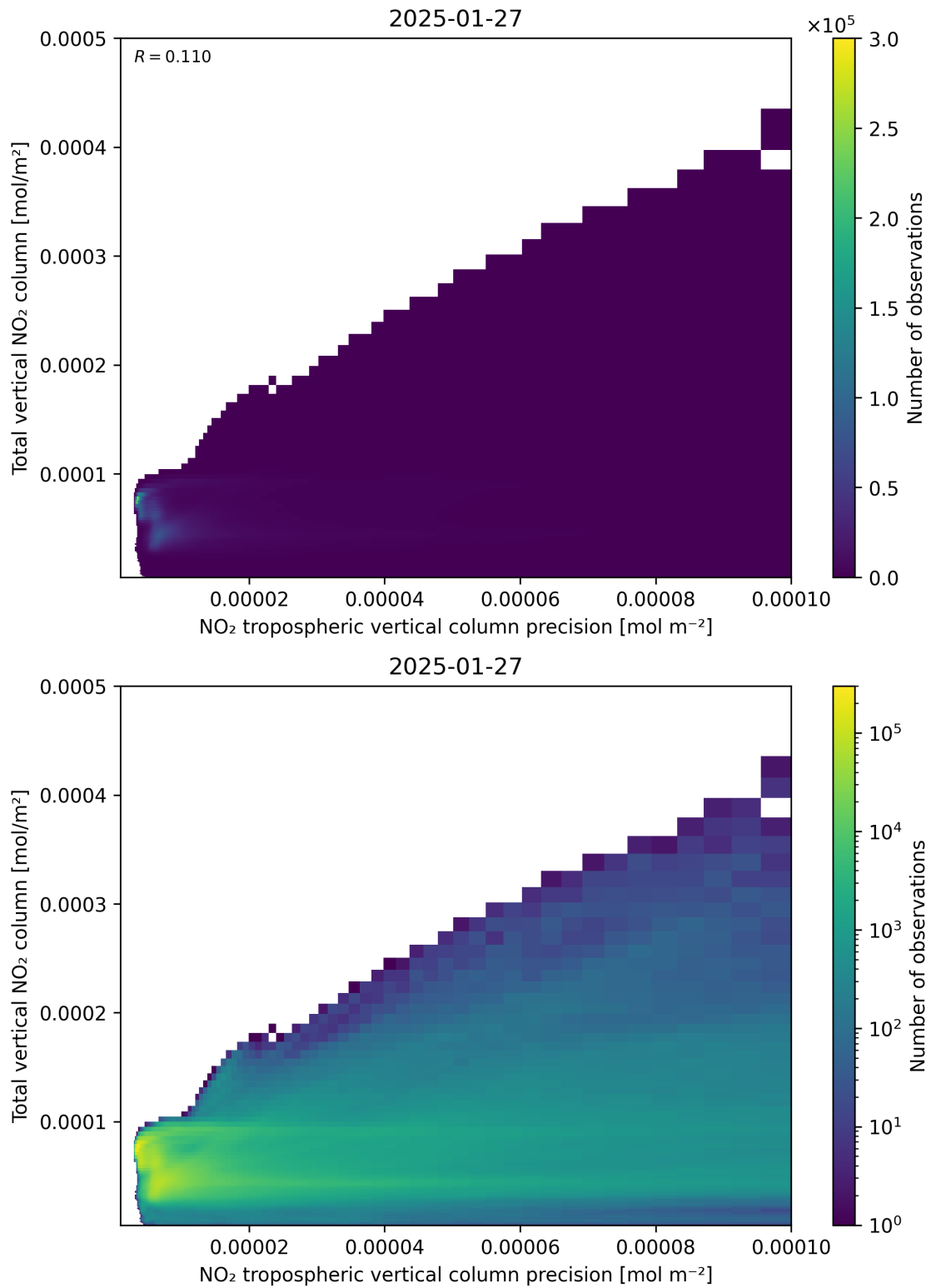
Figure 138: Scatter density plot of “NO 2 tropospheric vertical column precision” against “Total vertical NO 2 column” for 2025-01-26 to 2025-01-28.
