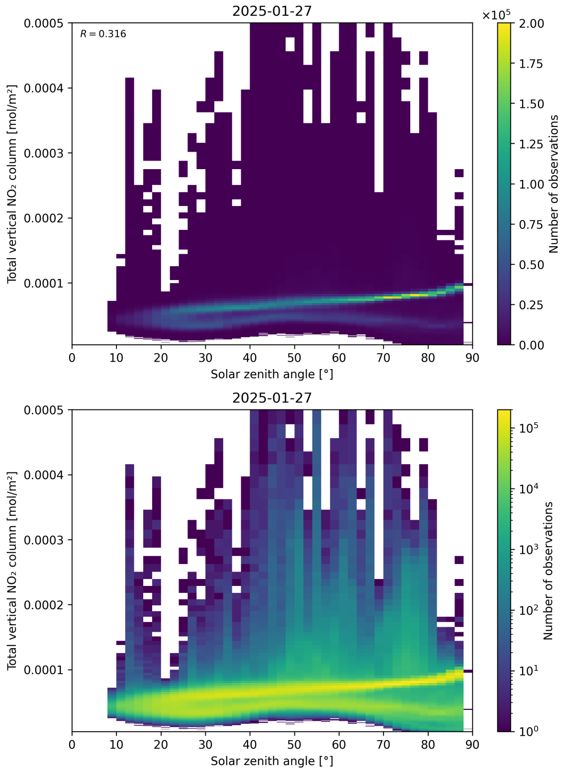
Figure 153: Scatter density plot of “Solar zenith angle” against “Total vertical NO 2 column” for 2025-01-26 to 2025-01-28.
