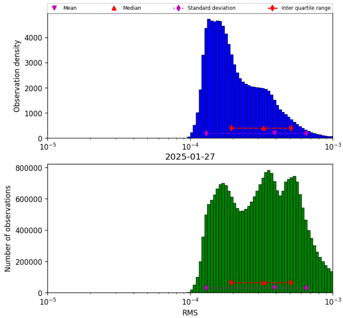
Figure 43: Histogram of “RMS” for 2025-01-26 to 2025-01-28
