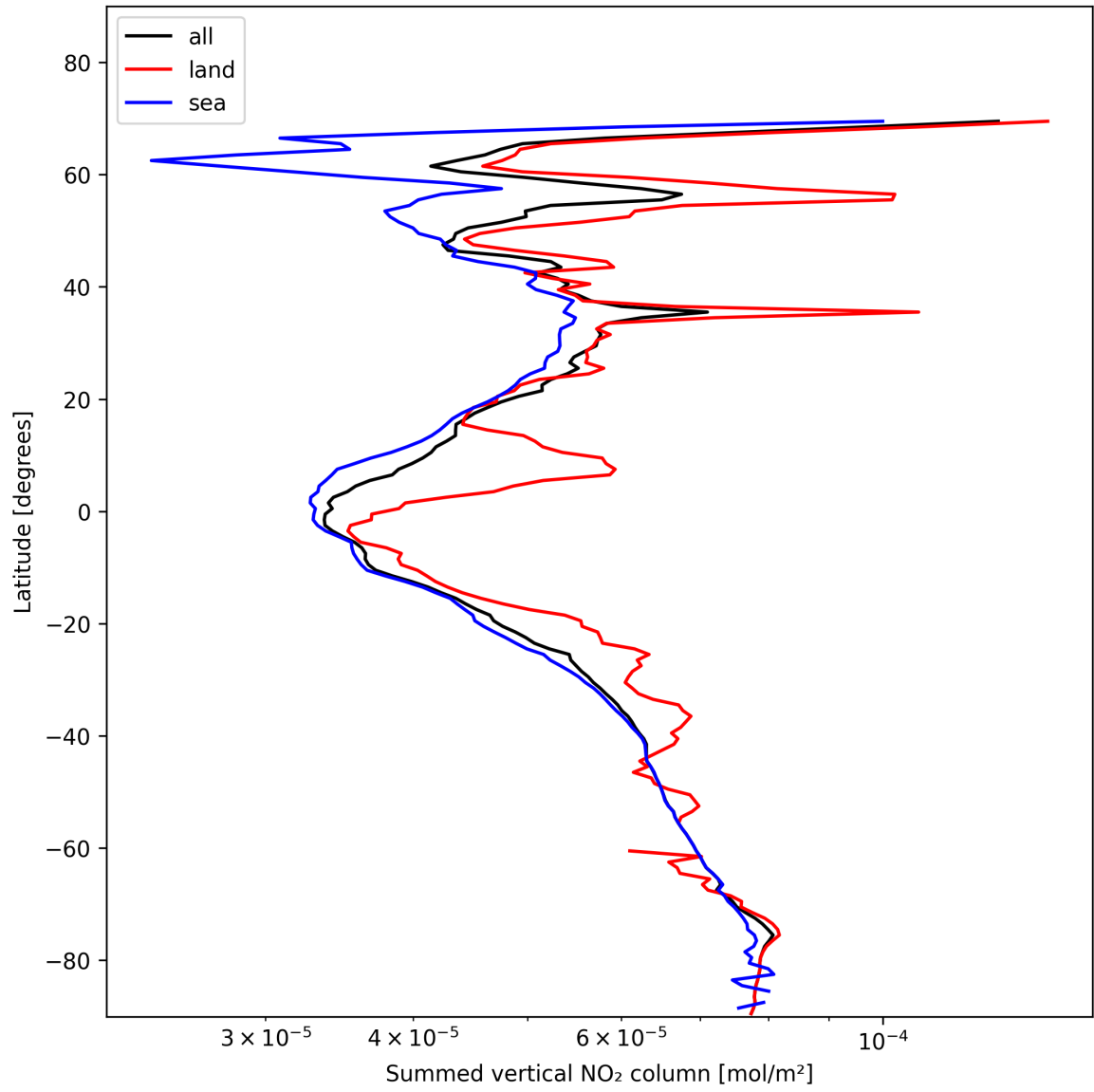
Figure 23: Zonal average of “Summed vertical NO 2 column” for 2025-01-26 to 2025-01-28.
