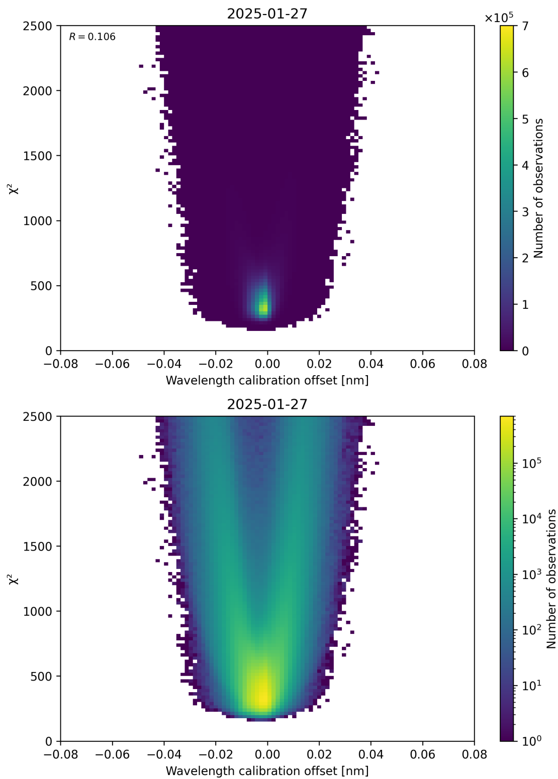
Figure 175: Scatter density plot of “Wavelength calibration offset” against “ \chi^2 ” for 2025-01-26 to 2025-01-28.
