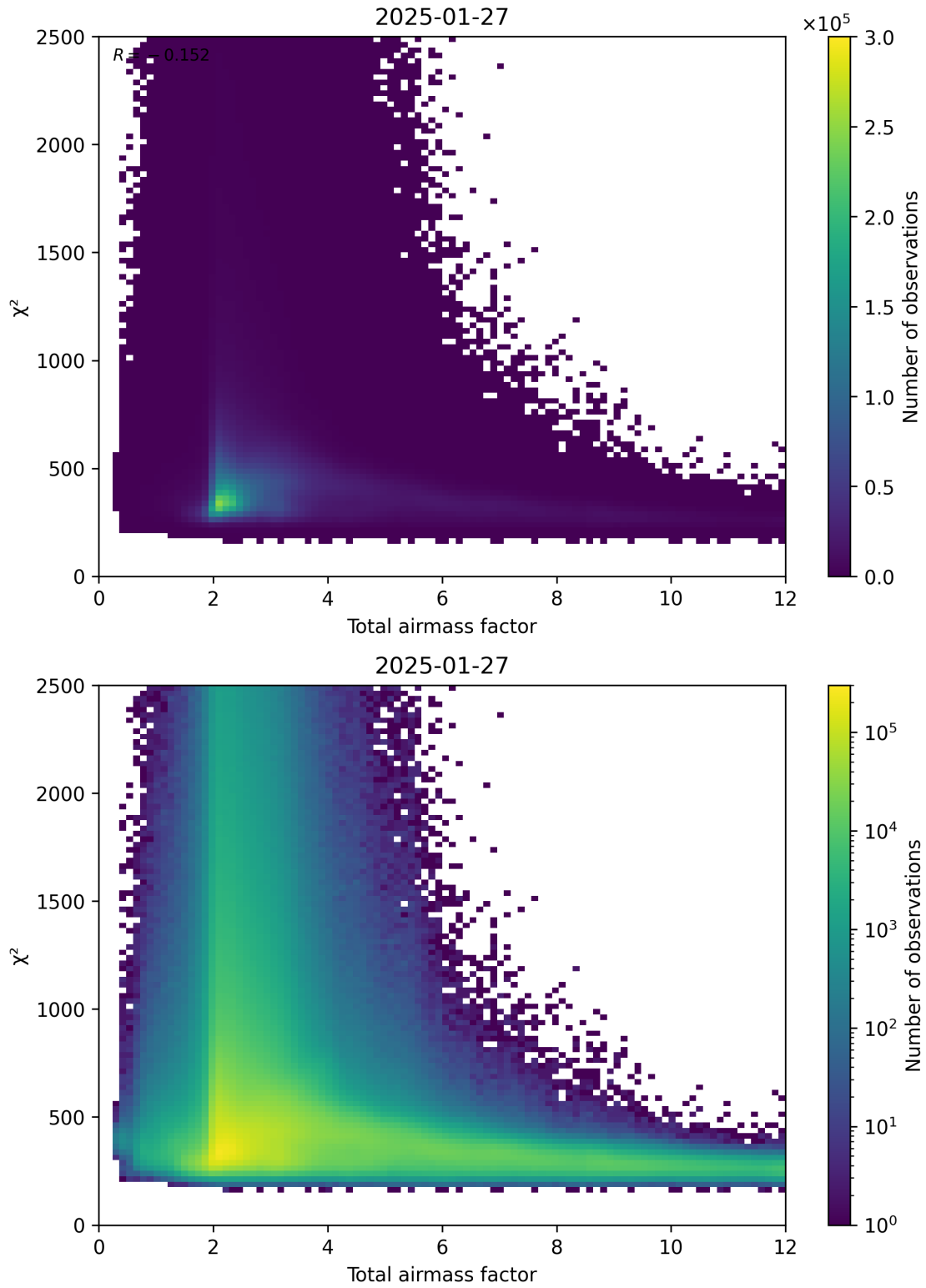
Figure 63: Scatter density plot of “Total airmass factor” against “ \chi^2 ” for 2025-01-26 to 2025-01-28.
