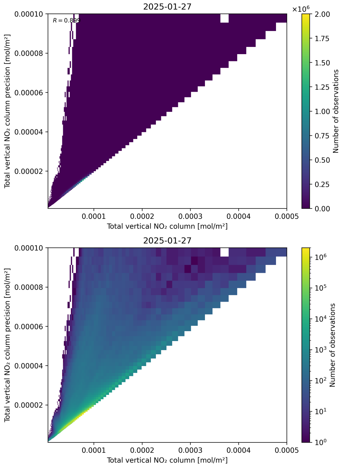
Figure 114: Scatter density plot of “Total vertical NO 2 column” against “Total vertical NO 2 column precision” for 2025-01-26 to 2025-01-28.
