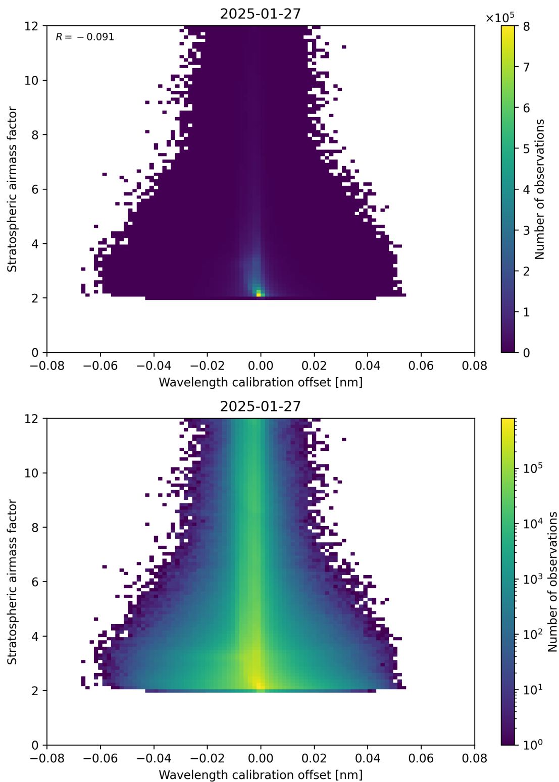
Figure 174: Scatter density plot of “Wavelength calibration offset” against “Stratospheric airmass factor” for 2025-01-26 to 2025-01-28.
