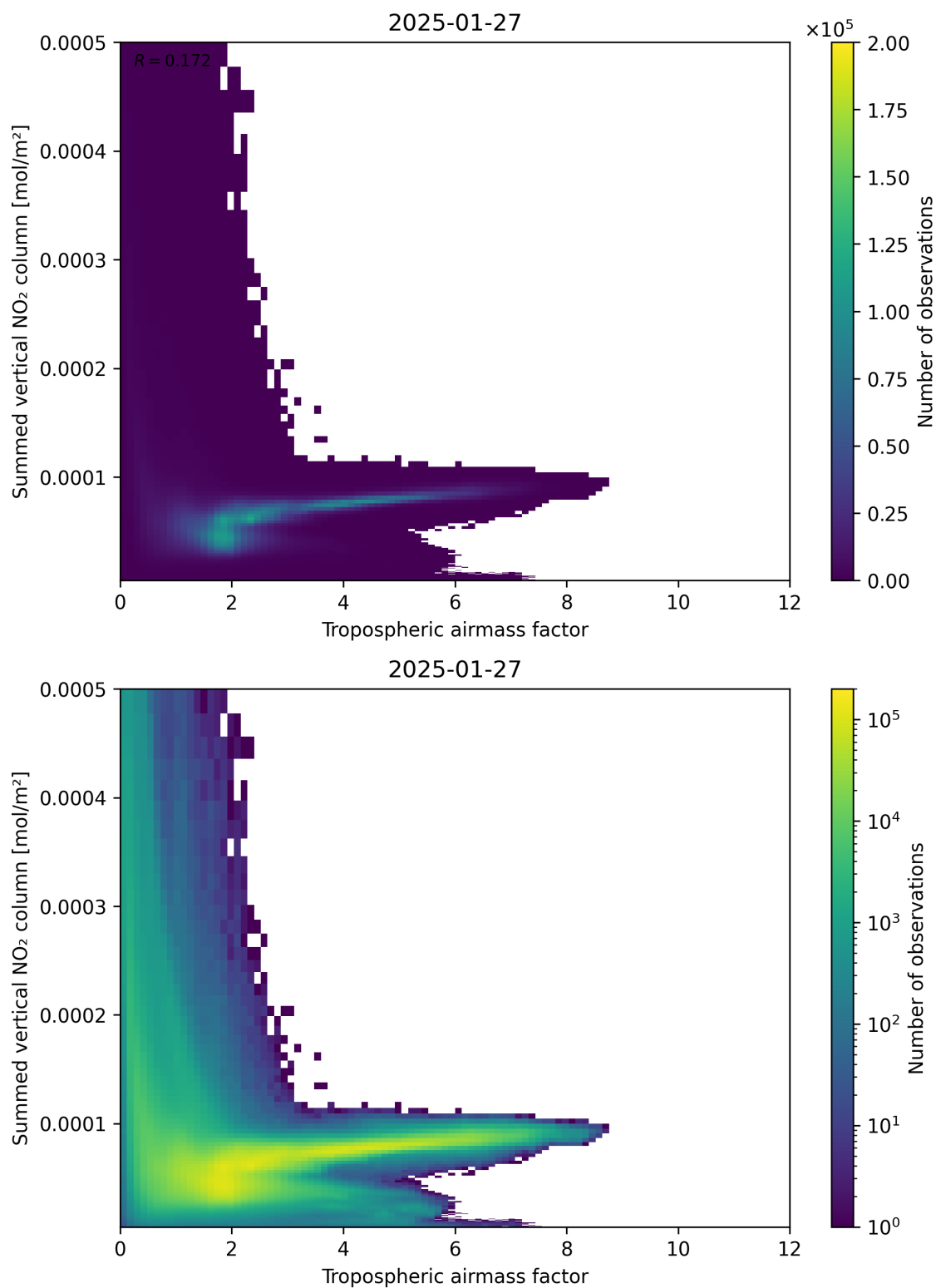
Figure 75: Scatter density plot of “Tropospheric airmass factor” against “Summed vertical NO 2 column” for 2025-01-26 to 2025-01-28.
