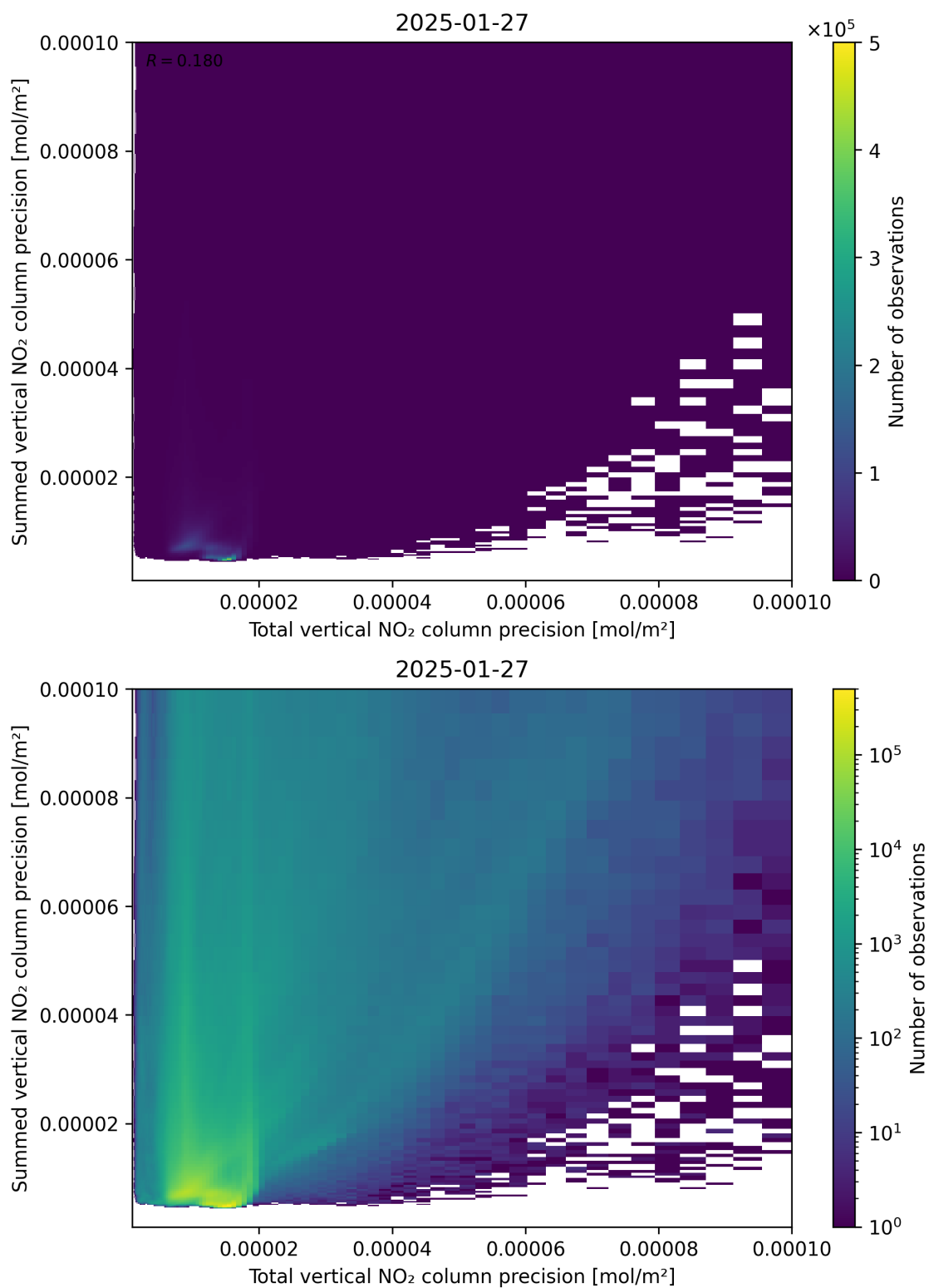
Figure 118: Scatter density plot of “Total vertical NO 2 column precision” against “Summed vertical NO 2 column precision” for 2025-01-26 to 2025-01-28.
