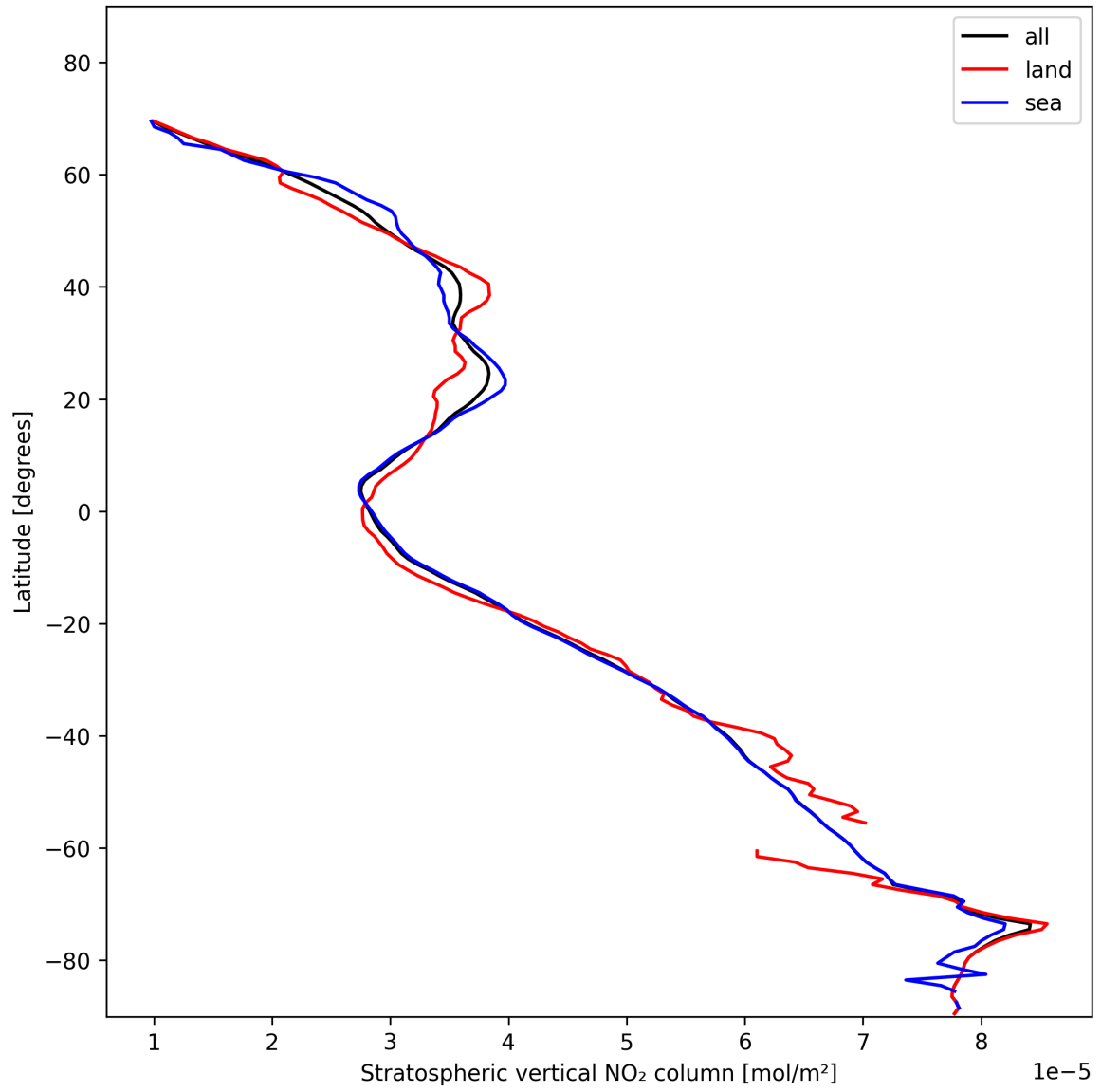
Figure 19: Zonal average of “Stratospheric vertical NO 2 column” for 2025-01-26 to 2025-01-28.
