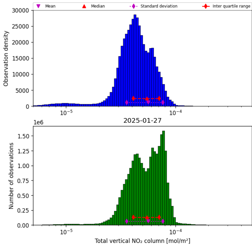
Figure 38: Histogram of “Total vertical NO 2 column” for 2025-01-26 to 2025-01-28
