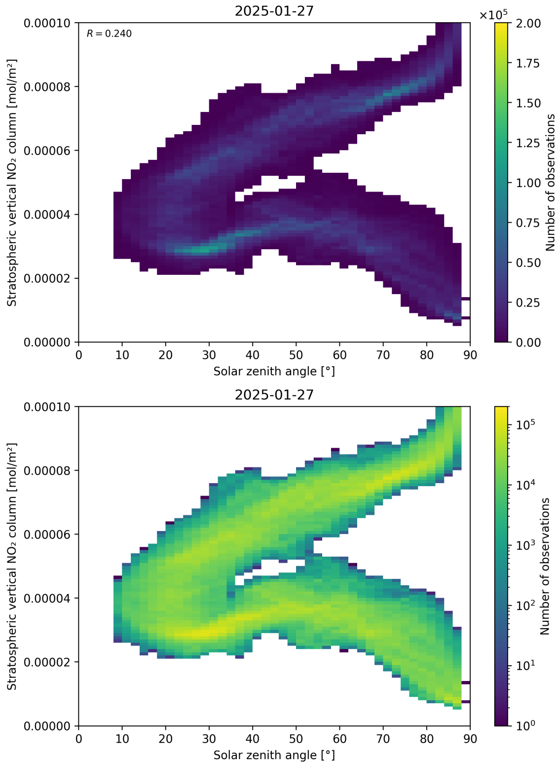
Figure 150: Scatter density plot of “Solar zenith angle” against “Stratospheric vertical NO 2 column” for 2025-01-26 to 2025-01-28.
