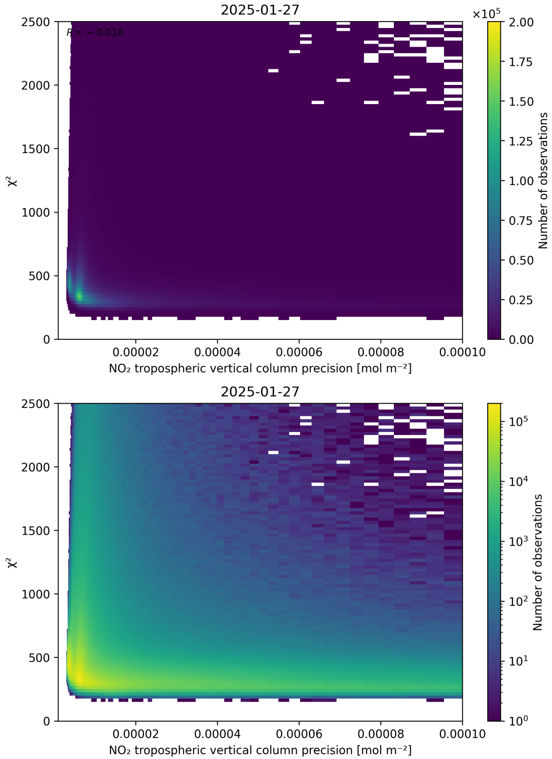
Figure 134: Scatter density plot of “NO 2 tropospheric vertical column precision” against “ \chi^2 ” for 2025-01-26 to 2025-01-28.
