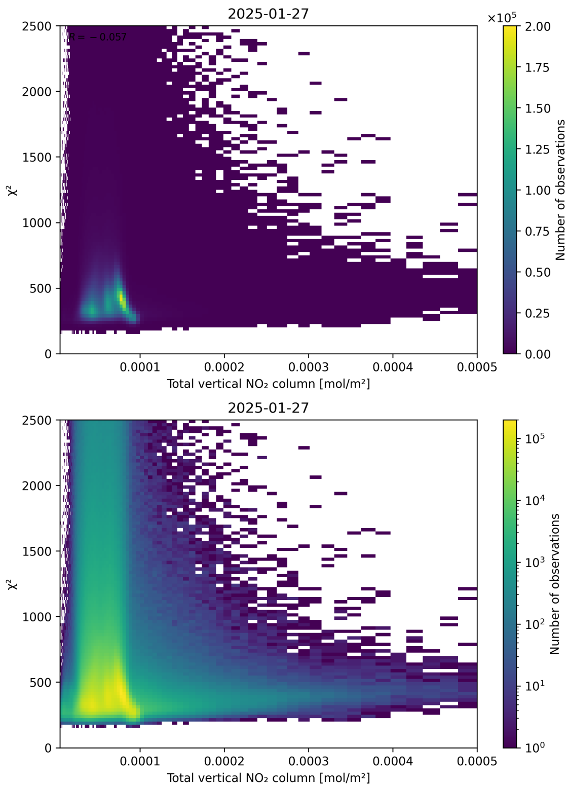
Figure 111: Scatter density plot of “Total vertical NO 2 column” against “ \chi^2 ” for 2025-01-26 to 2025-01-28.
