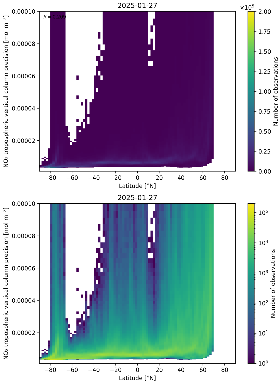
Figure 93: Scatter density plot of “Latitude” against “NO 2 tropospheric vertical column precision” for 2025-01-26 to 2025-01-28.
