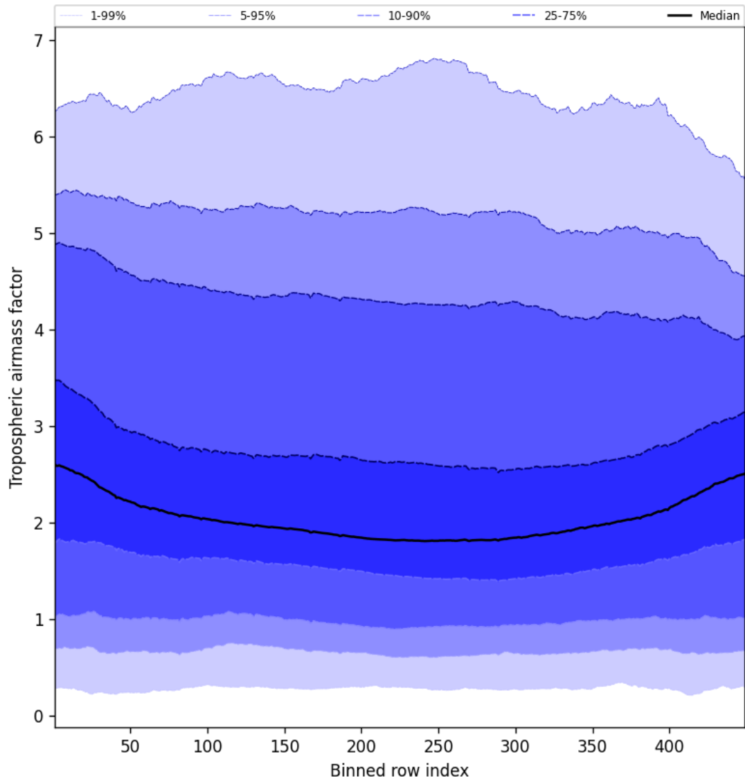
Figure 48: Along track statistics of “Tropospheric airmass factor” for 2025-01-26 to 2025-01-28
