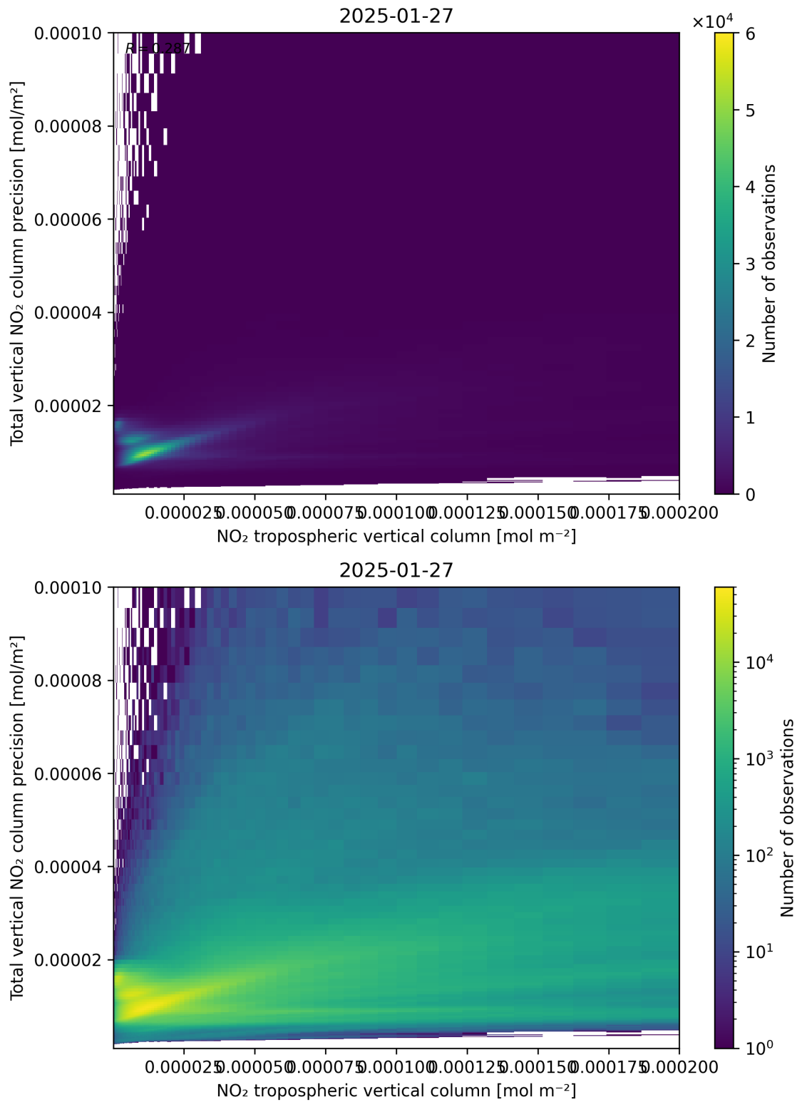
Figure 129: Scatter density plot of “NO 2 tropospheric vertical column” against “Total vertical NO 2 column precision” for 2025-01-26 to 2025-01-28.
