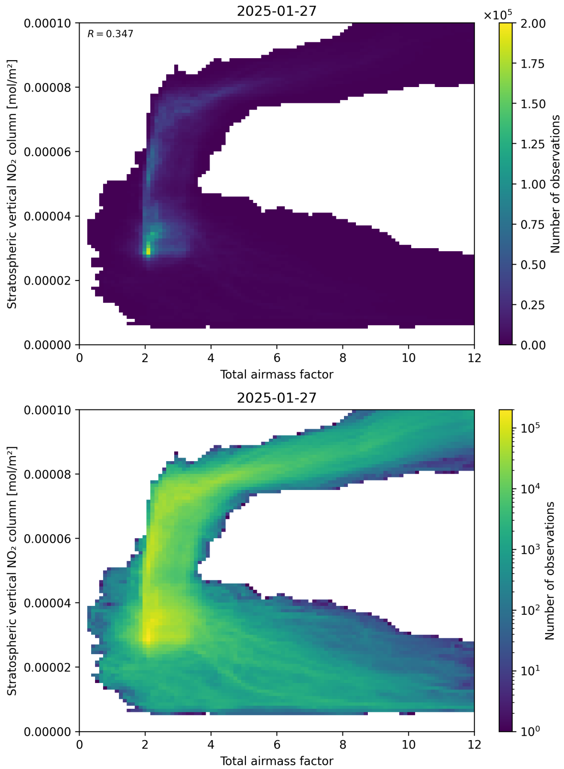
Figure 64: Scatter density plot of “Total airmass factor” against “Stratospheric vertical NO 2 column” for 2025-01-26 to 2025-01-28.
