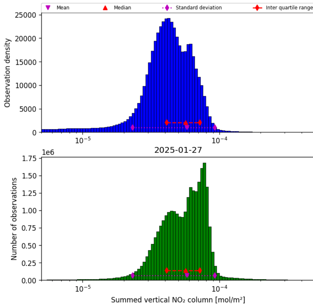
Figure 40: Histogram of “Summed vertical NO 2 column” for 2025-01-26 to 2025-01-28
