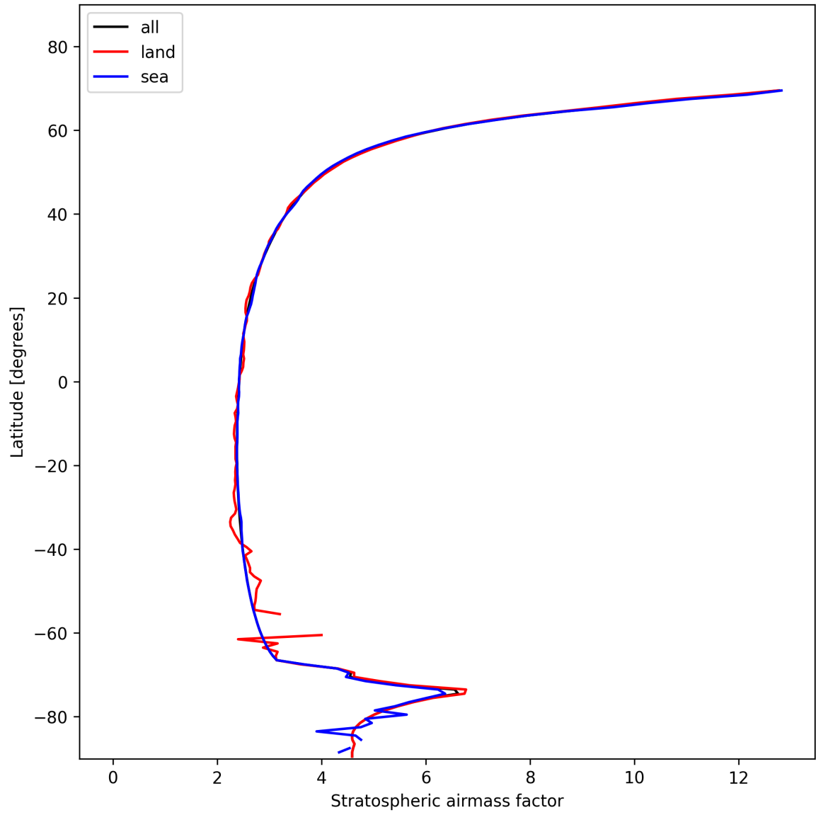
Figure 27: Zonal average of “Stratospheric airmass factor” for 2025-01-26 to 2025-01-28.
