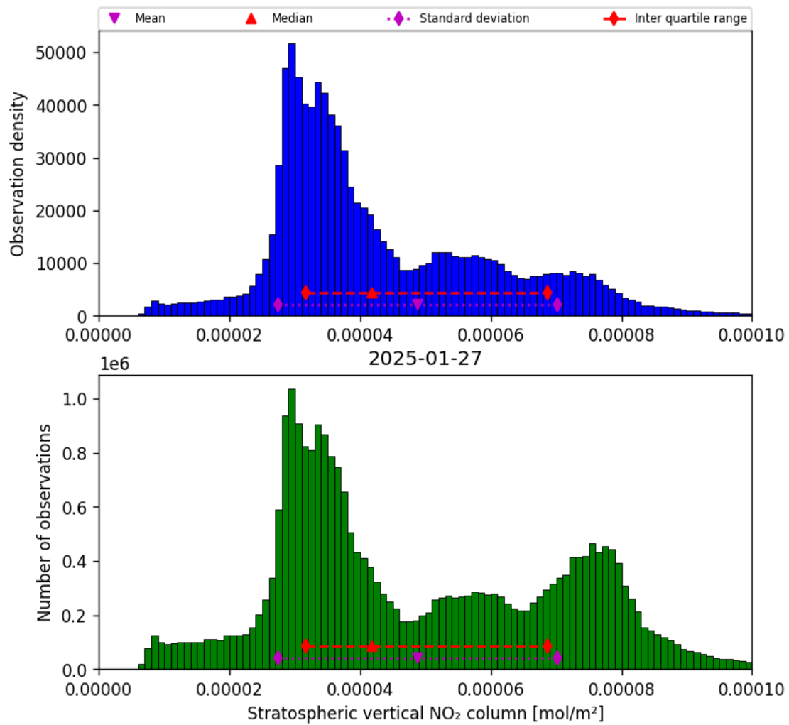
Figure 36: Histogram of “Stratospheric vertical NO 2 column” for 2025-01-26 to 2025-01-28
