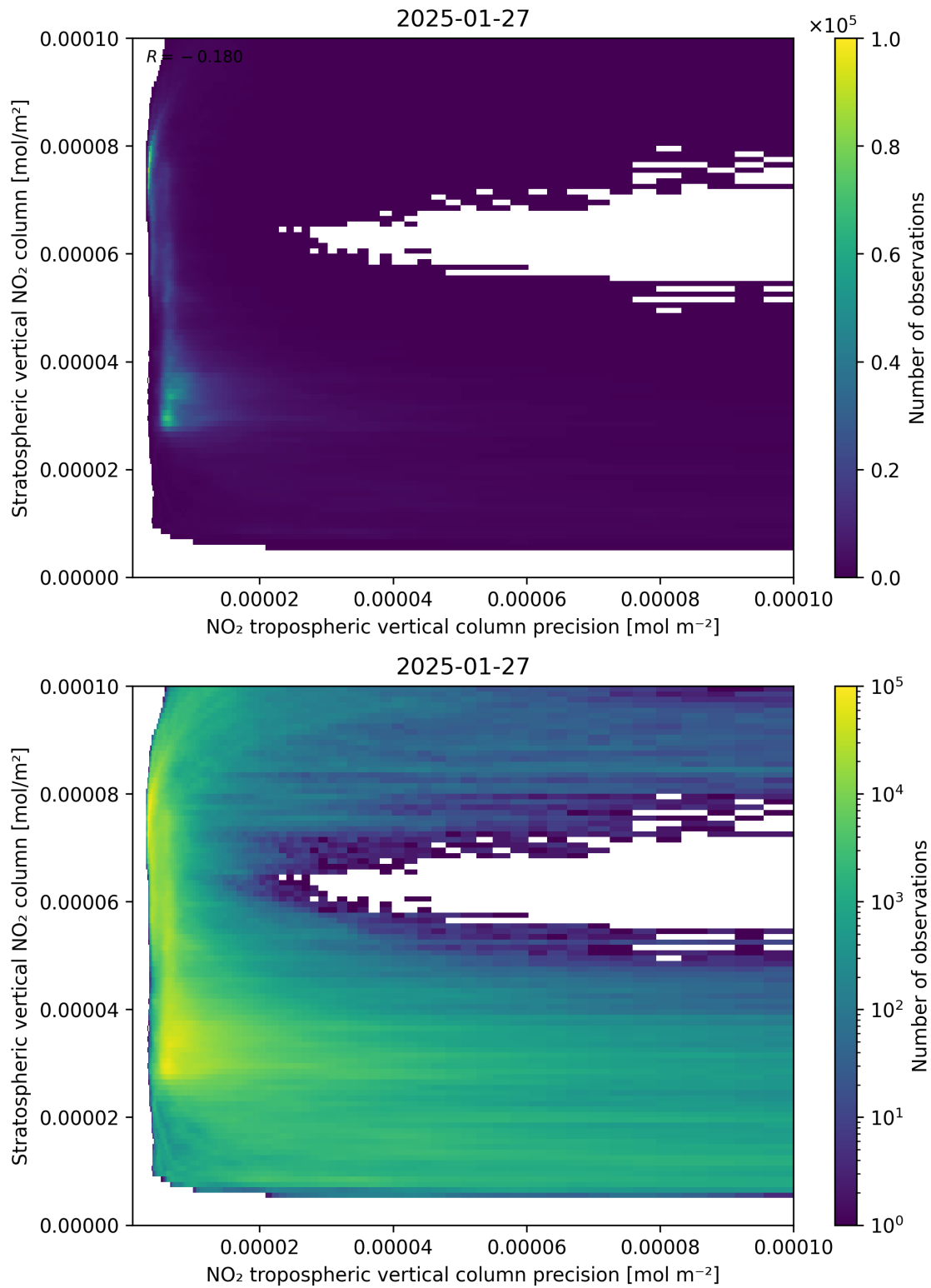
Figure 135: Scatter density plot of “NO 2 tropospheric vertical column precision” against “Stratospheric vertical NO 2 column” for 2025-01-26 to 2025-01-28.
