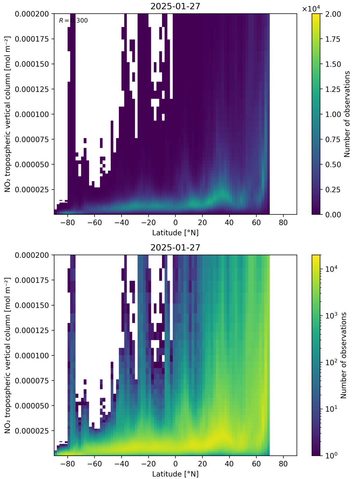
Figure 92: Scatter density plot of “Latitude” against “NO 2 tropospheric vertical column” for 2025-01-26 to 2025-01-28.
