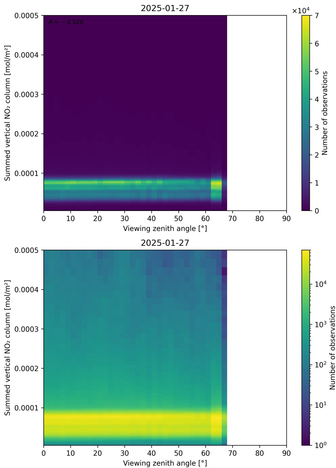
Figure 165: Scatter density plot of “Viewing zenith angle” against “Summed vertical NO 2 column” for 2025-01-26 to 2025-01-28.
