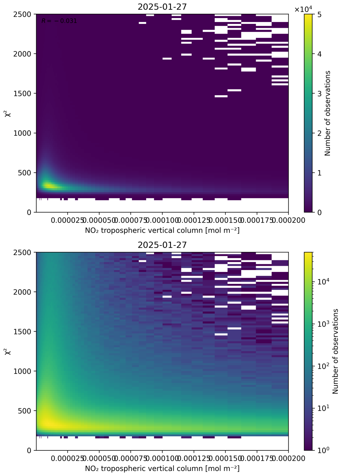
Figure 124: Scatter density plot of “NO 2 tropospheric vertical column” against “ \chi^2 ” for 2025-01-26 to 2025-01-28.
