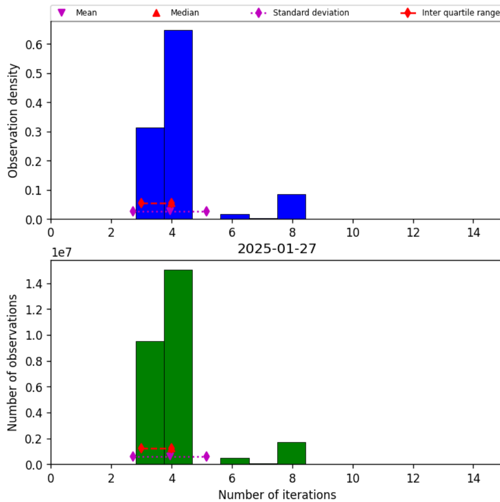
Figure 34: Histogram of “Number of iterations” for 2025-01-26 to 2025-01-28
