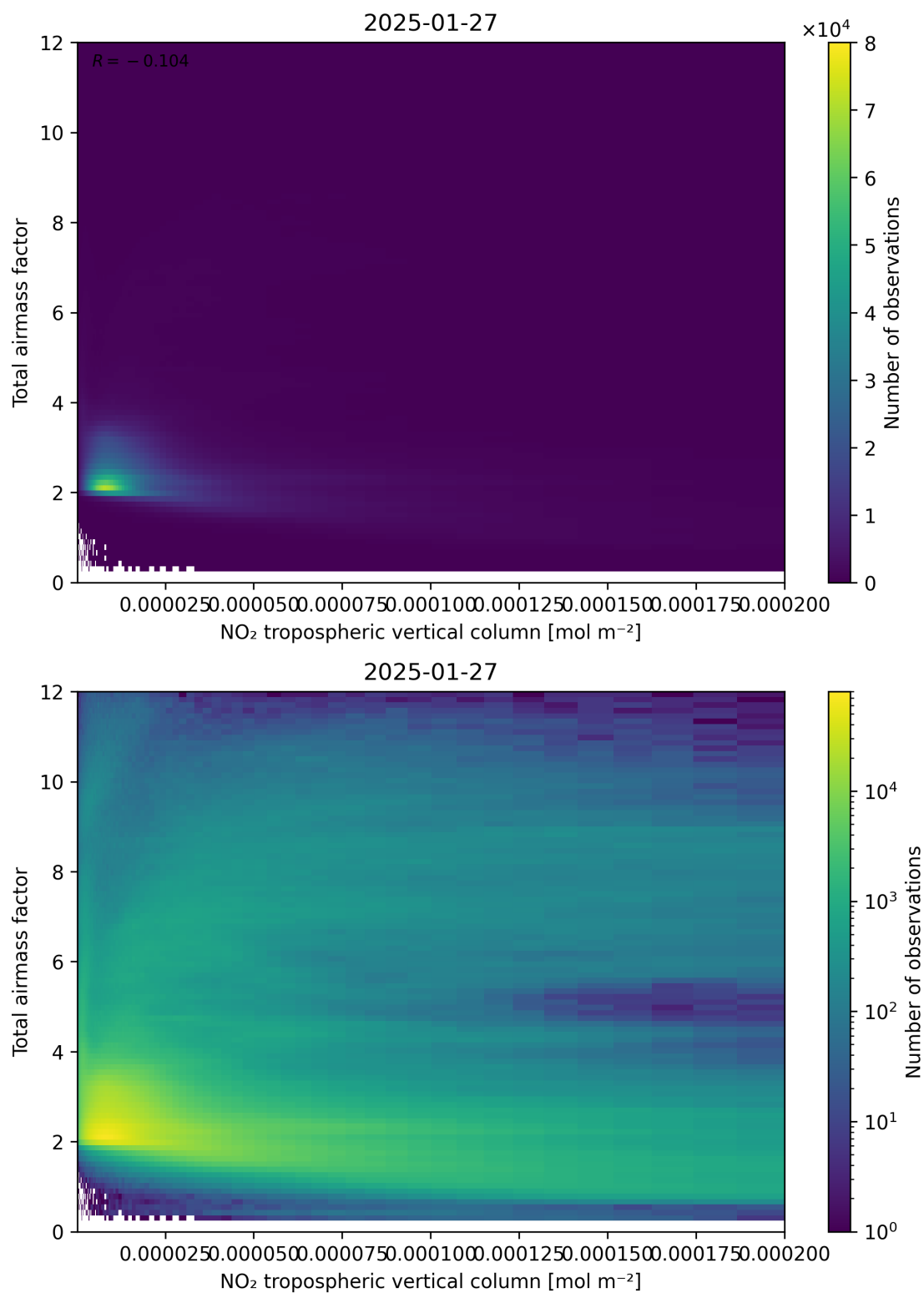
Figure 122: Scatter density plot of “NO 2 tropospheric vertical column” against “Total air mass factor” for 2025-01-26 to 2025-01-28.
