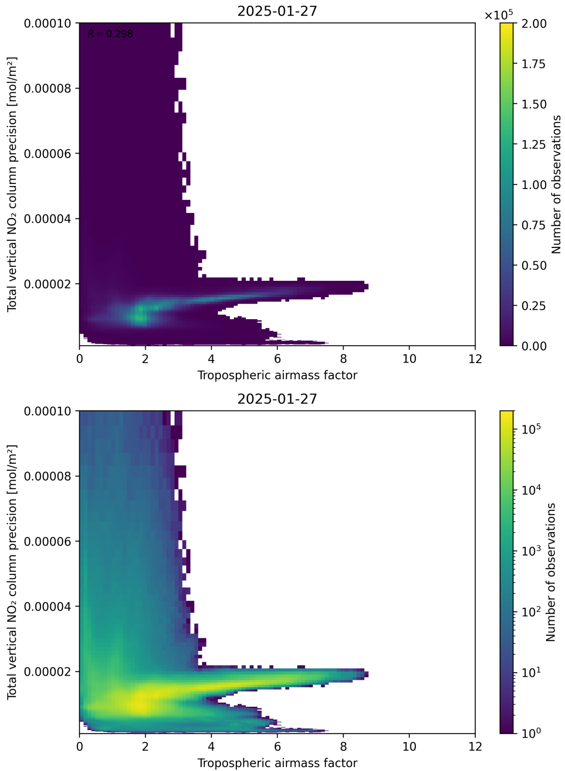
Figure 78: Scatter density plot of “Tropospheric air mass factor” against “Total vertical NO 2 column precision” for 2025-01-26 to 2025-01-28.
