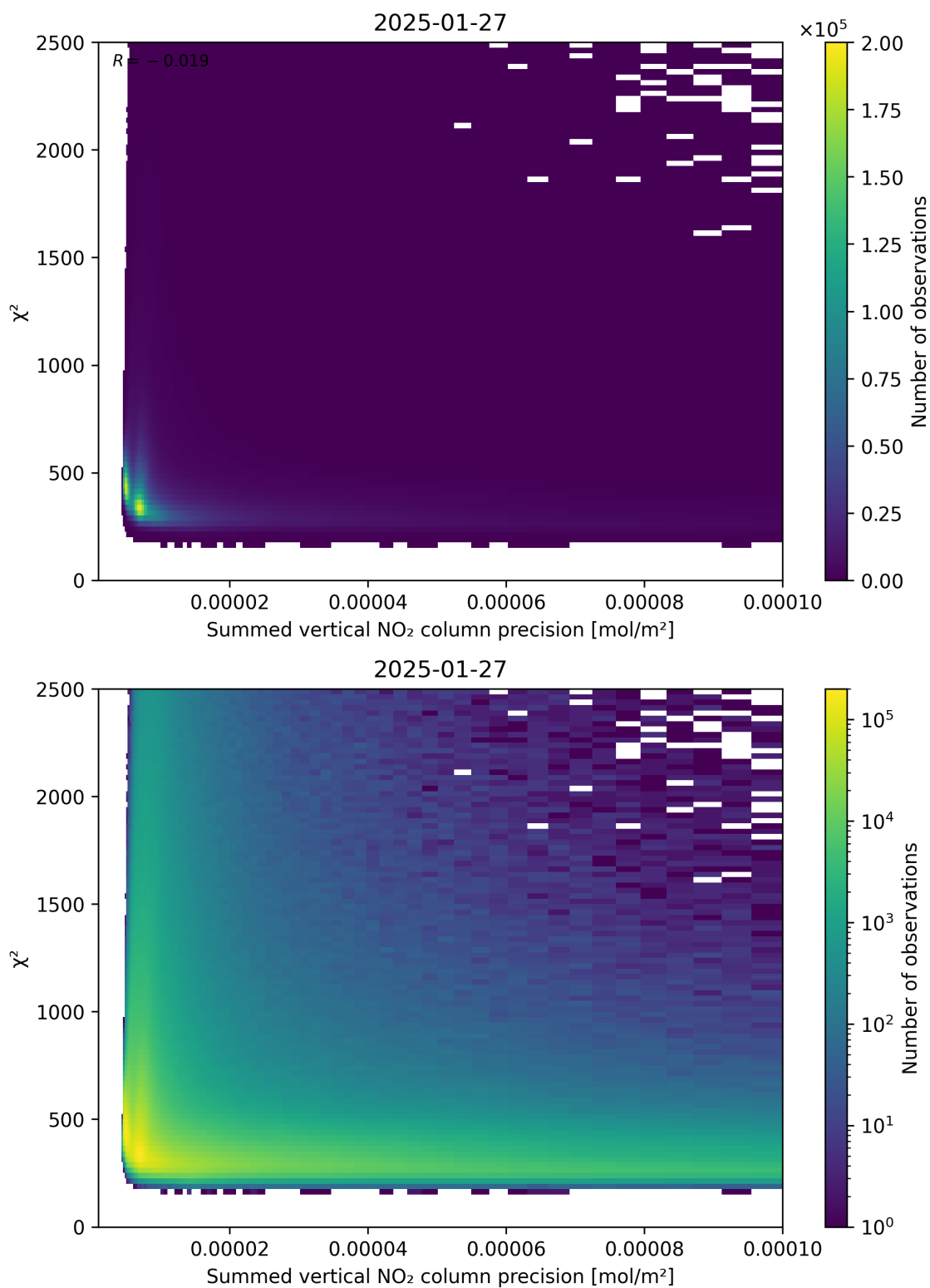
Figure 107: Scatter density plot of “Summed vertical NO 2 column precision” against “ \chi^2 ” for 2025-01-26 to 2025-01-28.
