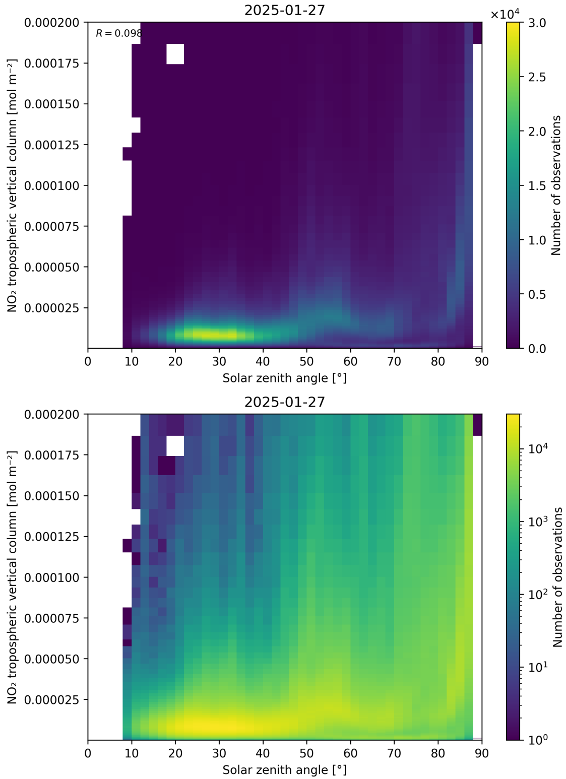
Figure 155: Scatter density plot of “Solar zenith angle” against “NO 2 tropospheric vertical column” for 2025-01-26 to 2025-01-28.
