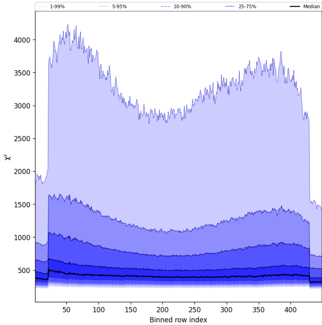
Figure 59: Along track statistics of “ \chi^2 ” for 2025-01-26 to 2025-01-28
