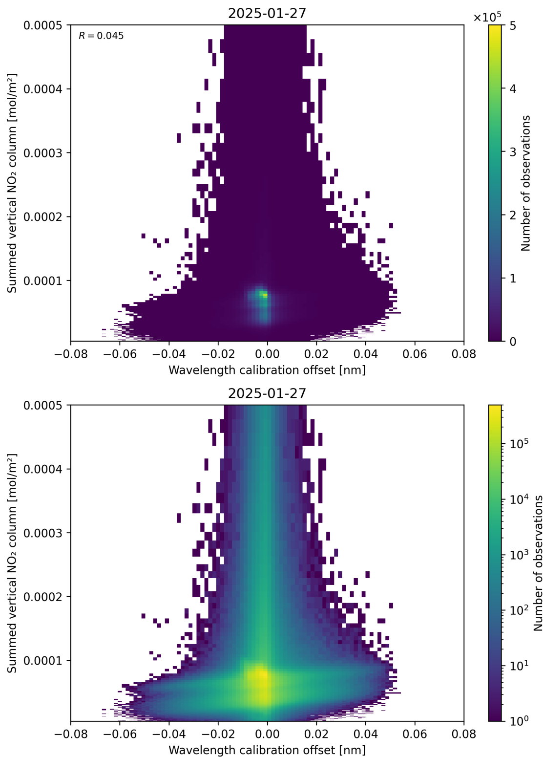
Figure 177: Scatter density plot of “Wavelength calibration offset” against “Summed vertical NO 2 column” for 2025-01-26 to 2025-01-28.
