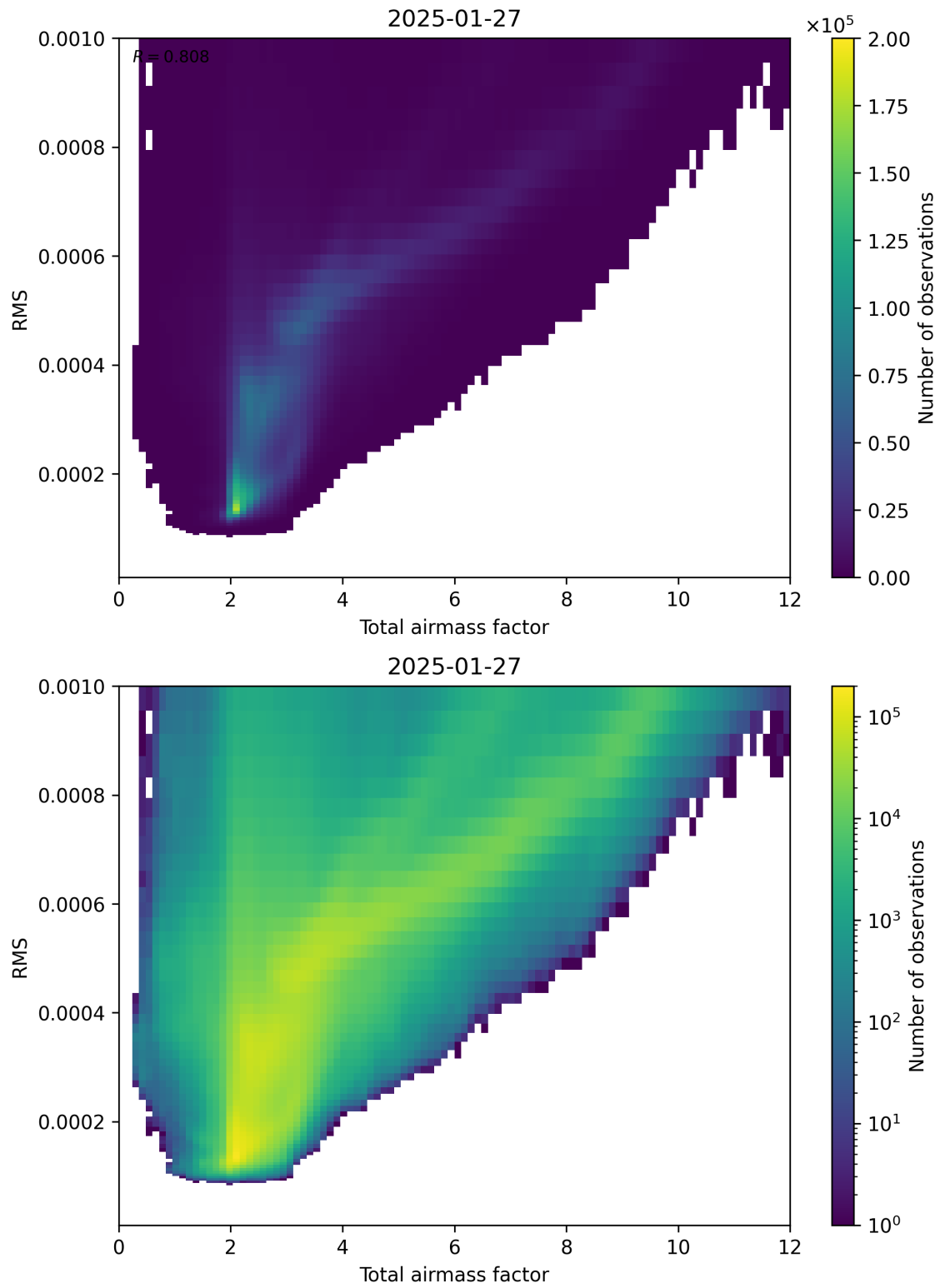
Figure 69: Scatter density plot of “Total airmass factor” against “RMS” for 2025-01-26 to 2025-01-28.
