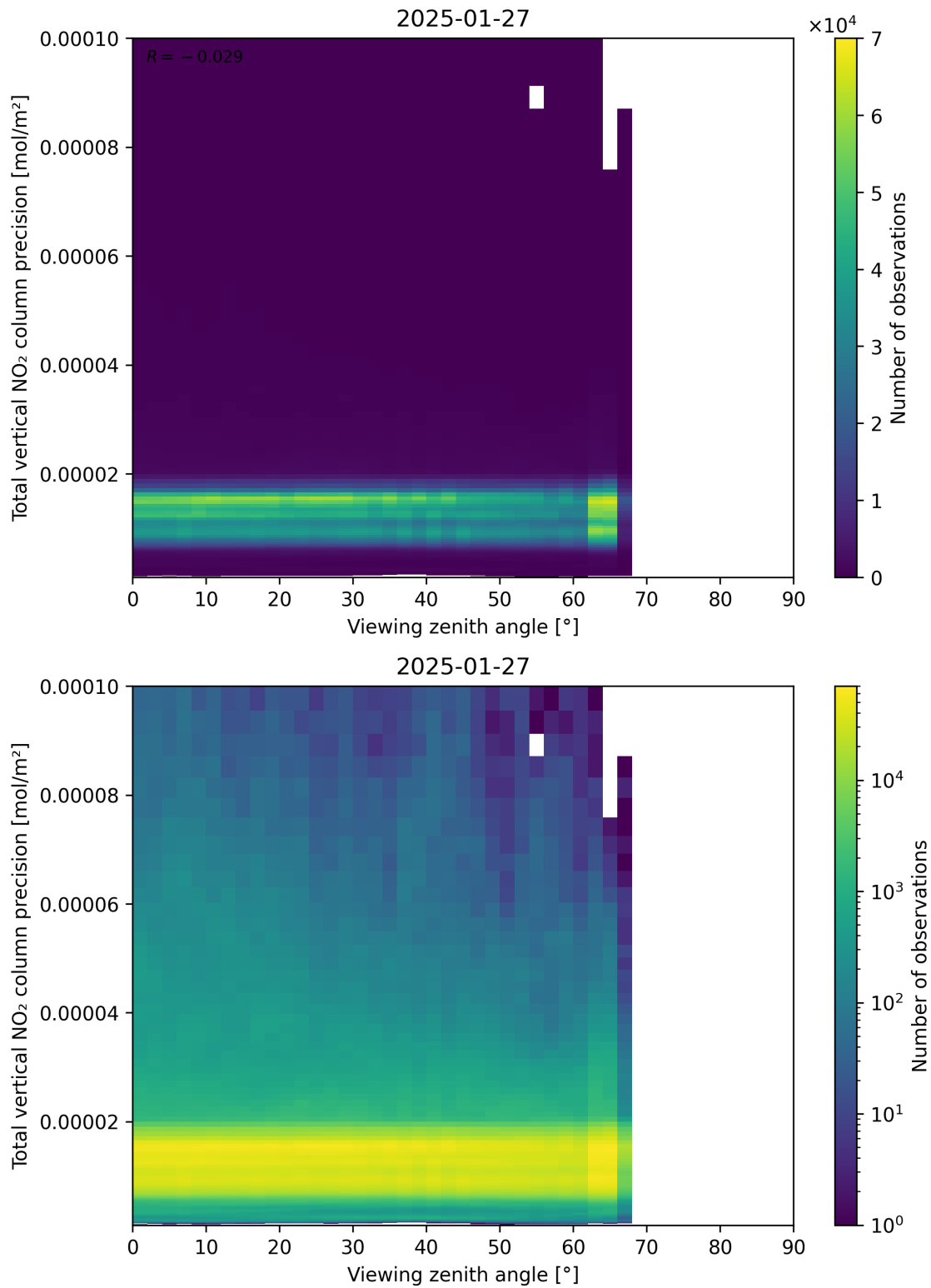
Figure 168: Scatter density plot of “Viewing zenith angle” against “Total vertical NO 2 column precision” for 2025-01-26 to 2025-01-28.
