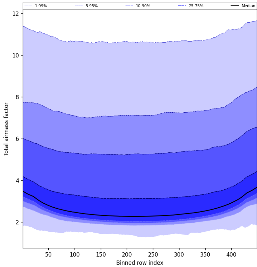
Figure 49: Along track statistics of “Total airmass factor” for 2025-01-26 to 2025-01-28
