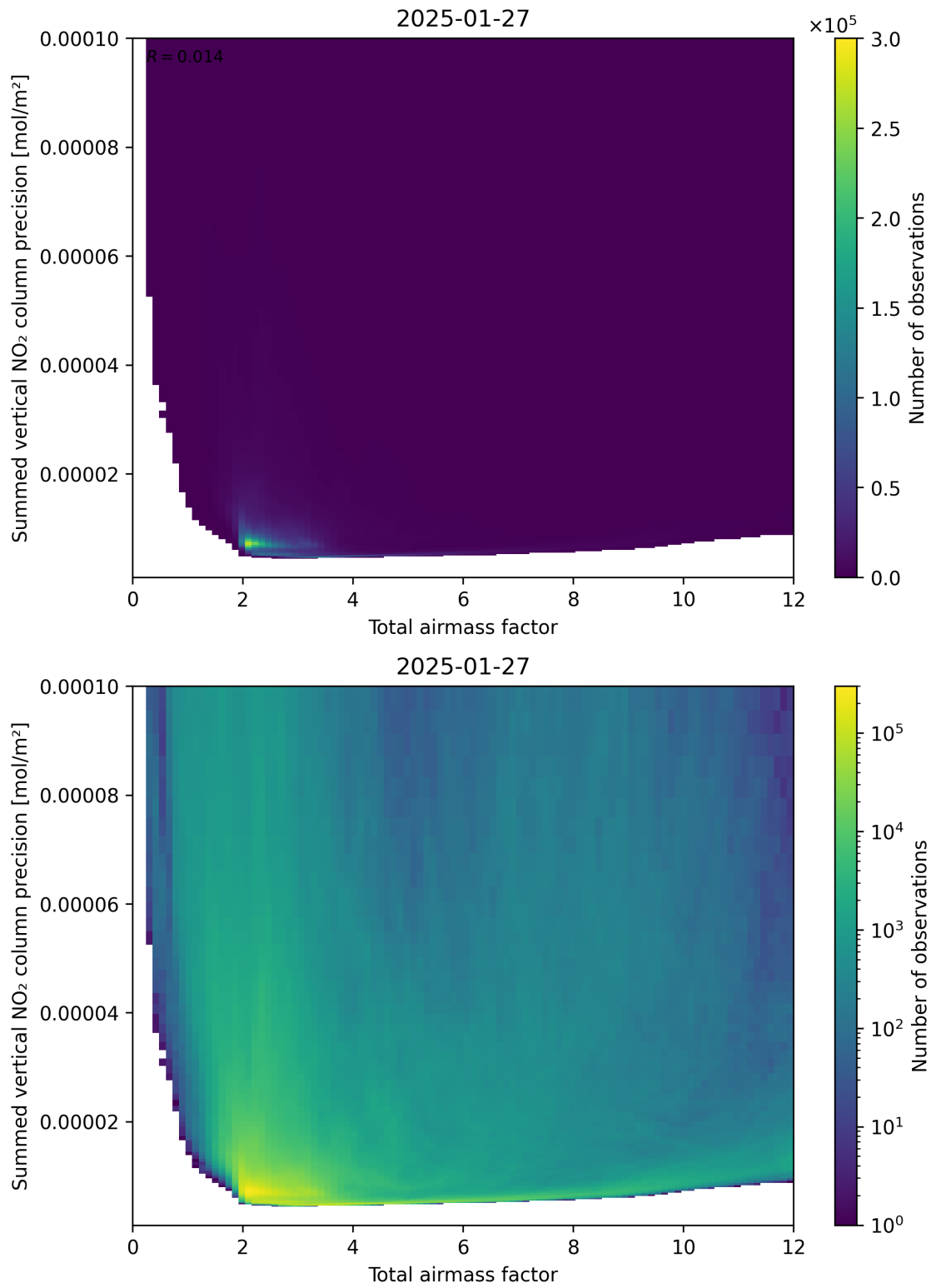
Figure 66: Scatter density plot of “Total airmass factor” against “Summed vertical NO 2 column precision” for 2025-01-26 to 2025-01-28.
