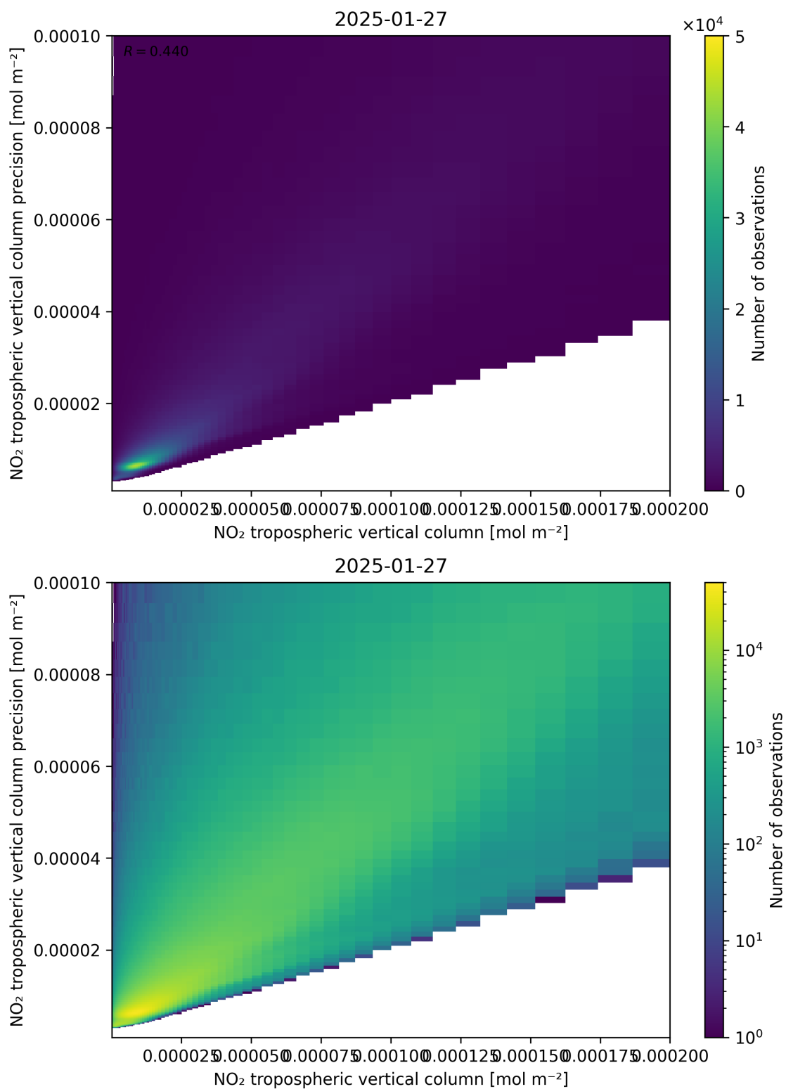
Figure 130: Scatter density plot of “NO 2 tropospheric vertical column” against “NO 2 tropospheric vertical column precision” for 2025-01-26 to 2025-01-28.
