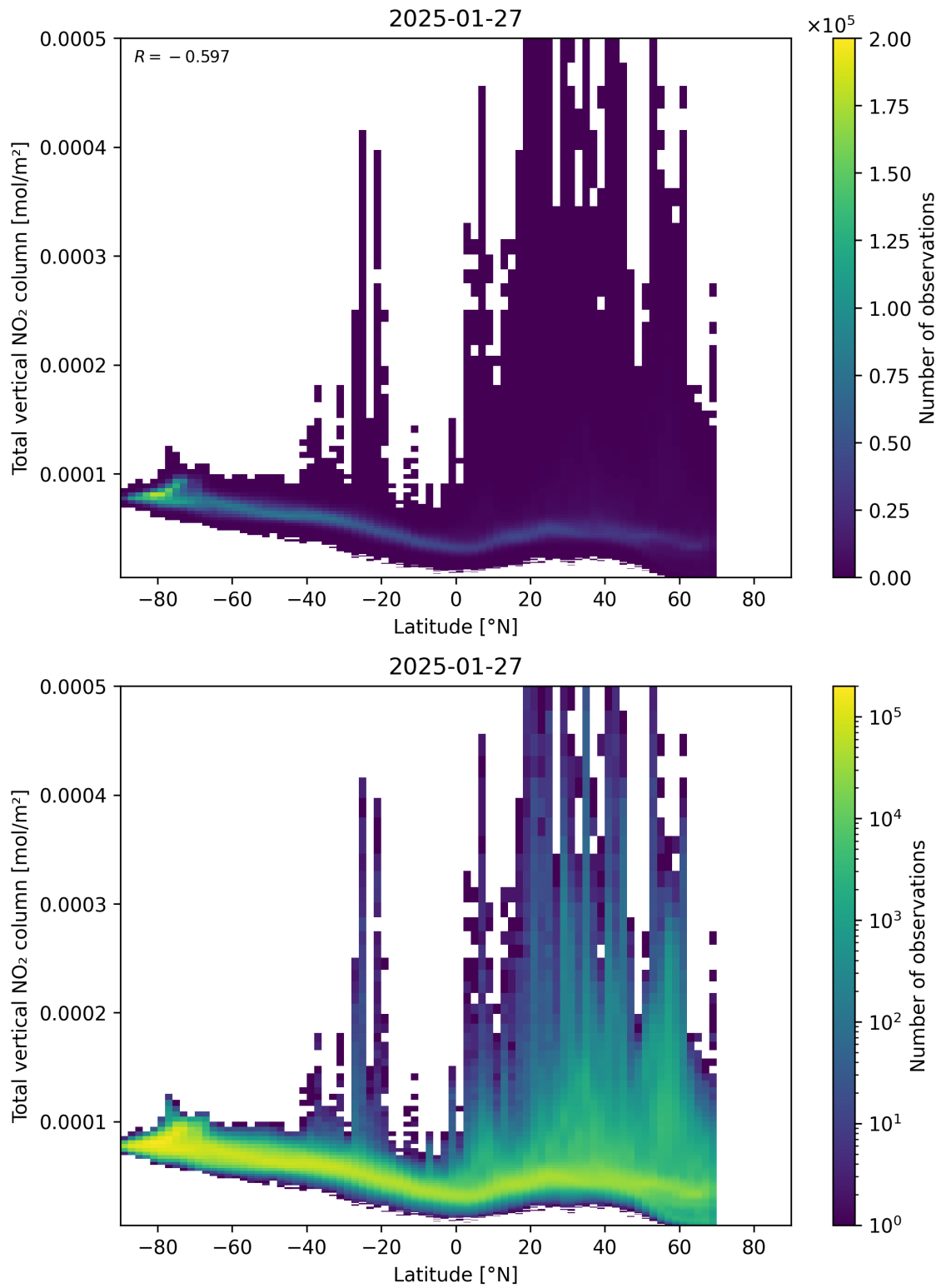
Figure 90: Scatter density plot of “Latitude” against “Total vertical NO 2 column” for 2025-01-26 to 2025-01-28.
