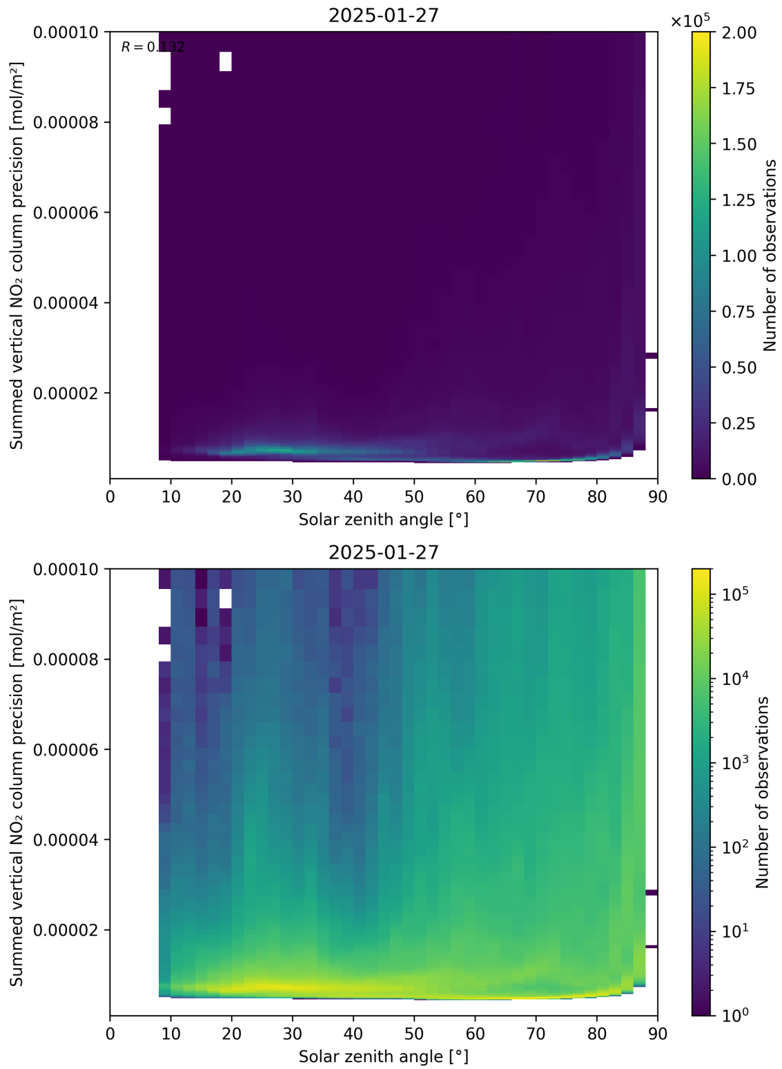
Figure 152: Scatter density plot of “Solar zenith angle” against “Summed vertical NO 2 column precision” for 2025-01-26 to 2025-01-28.
