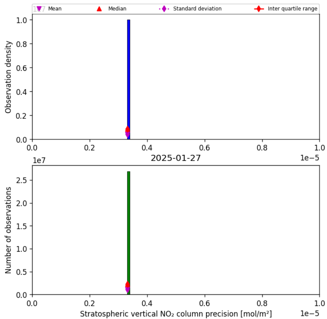
Figure 37: Histogram of “Stratospheric vertical NO 2 column precision” for 2025-01-26 to 2025-01-28
