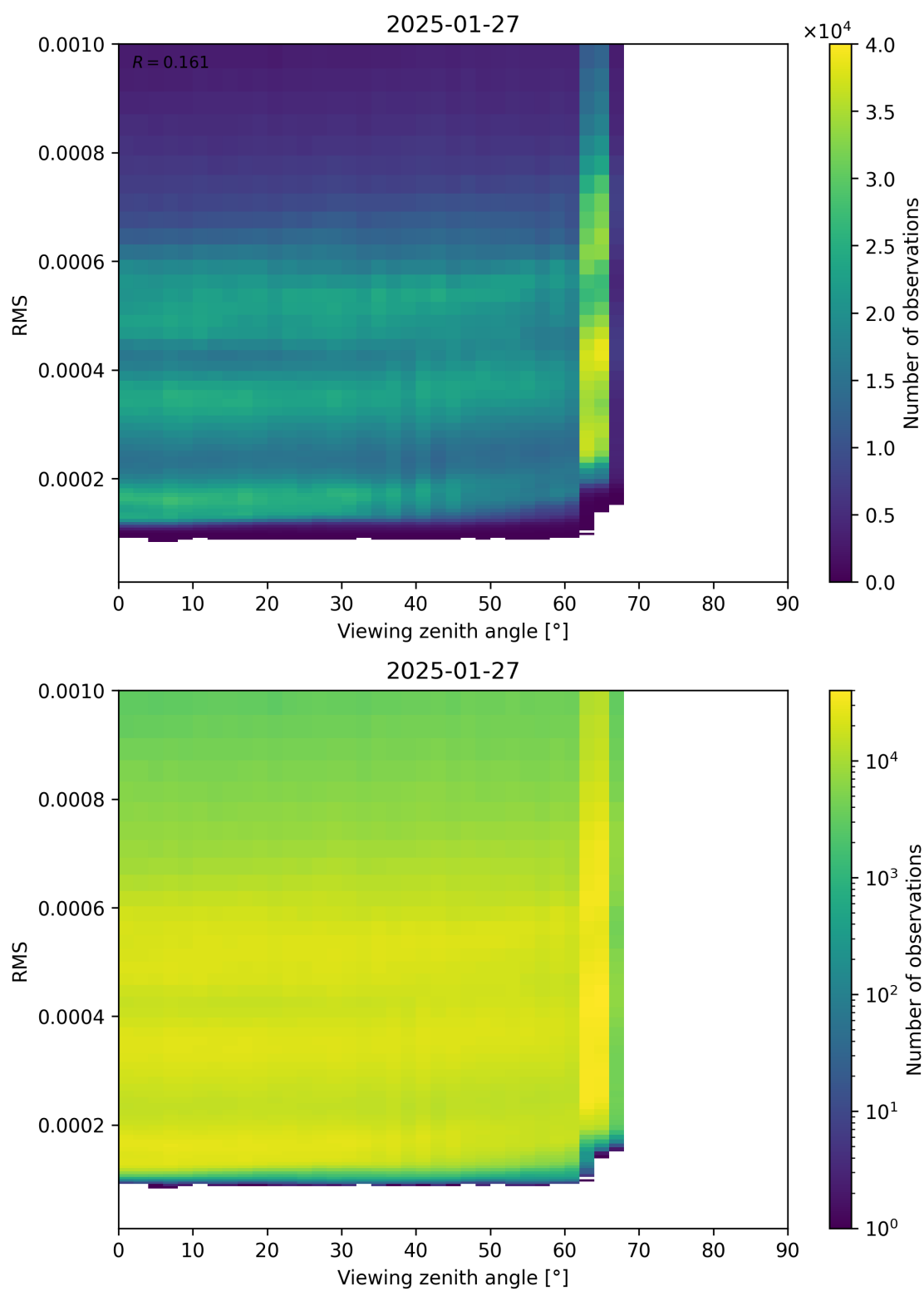
Figure 171: Scatter density plot of “Viewing zenith angle” against “RMS” for 2025-01-26 to 2025-01-28.
