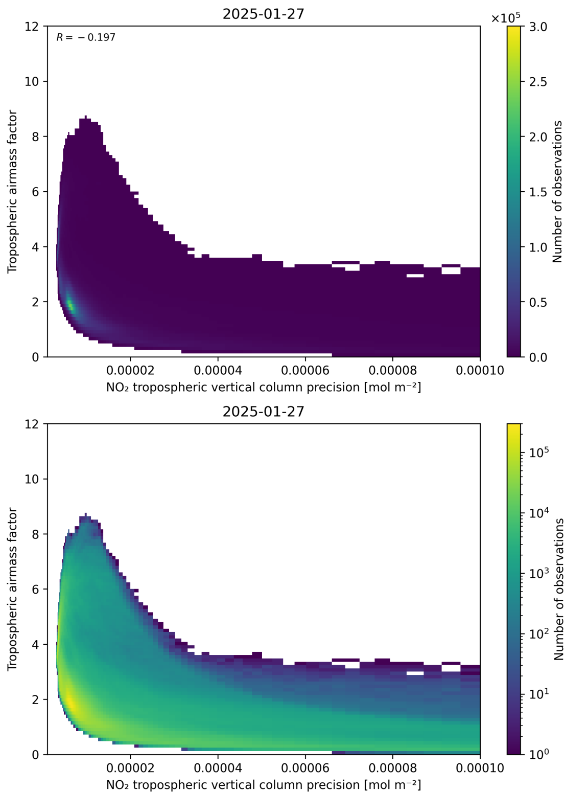
Figure 133: Scatter density plot of “NO 2 tropospheric vertical column precision” against “Tropospheric airmass factor” for 2025-01-26 to 2025-01-28.
