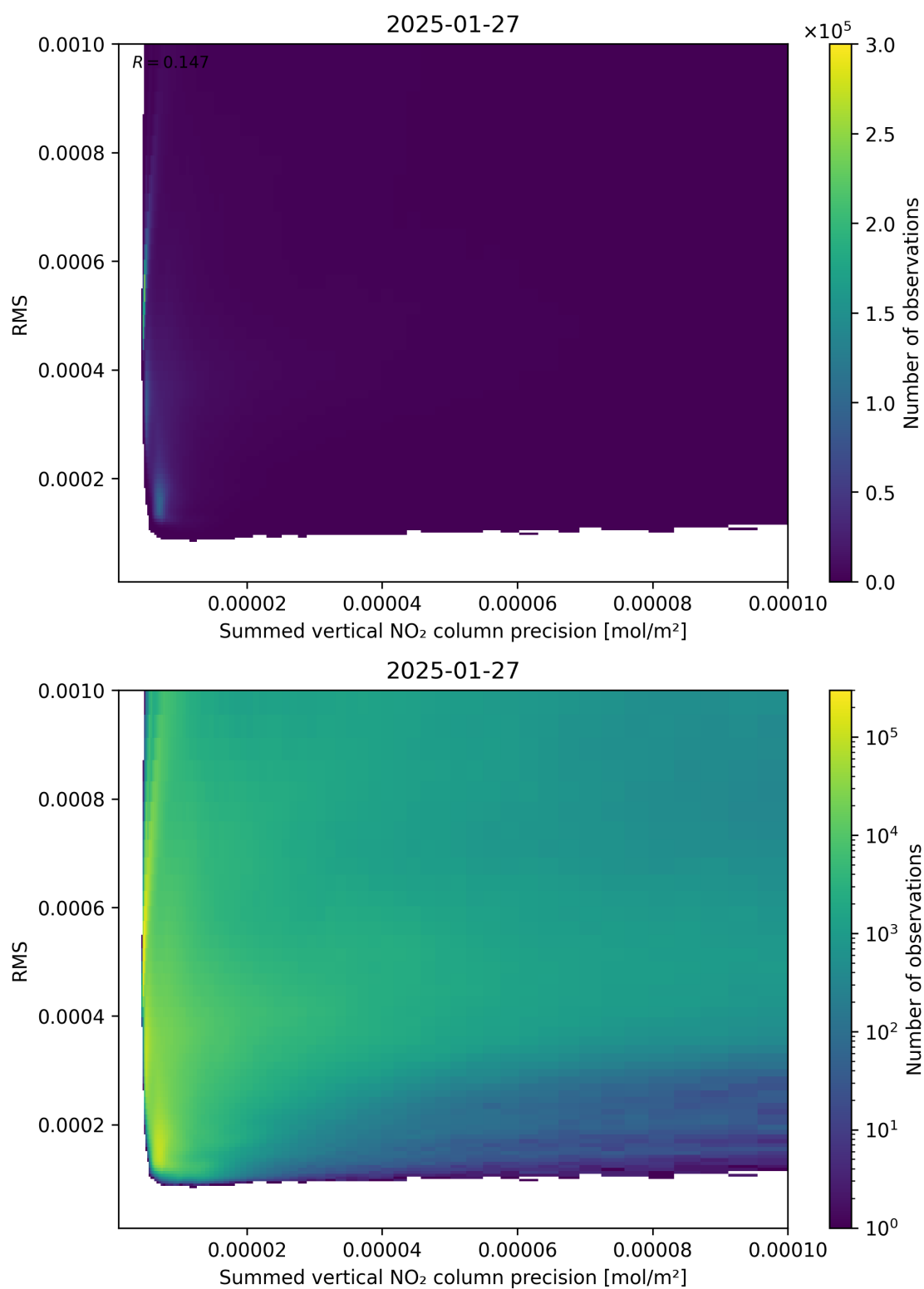
Figure 108: Scatter density plot of “Summed vertical NO 2 column precision” against “RMS” for 2025-01-26 to 2025-01-28.
