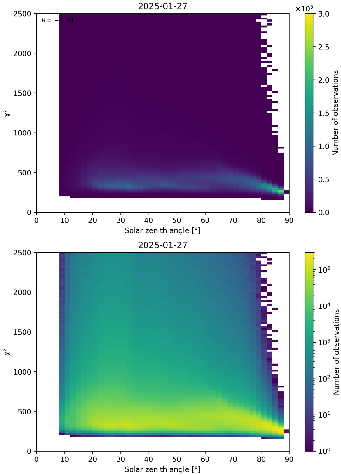
Figure 148: Scatter density plot of “Solar zenith angle” against “ \chi^2 ” for 2025-01-26 to 2025-01-28.
