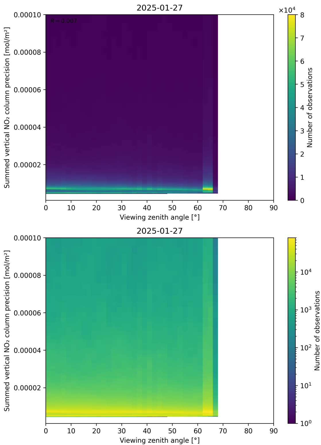
Figure 166: Scatter density plot of “Viewing zenith angle” against “Summed vertical NO 2 column precision” for 2025-01-26 to 2025-01-28.
