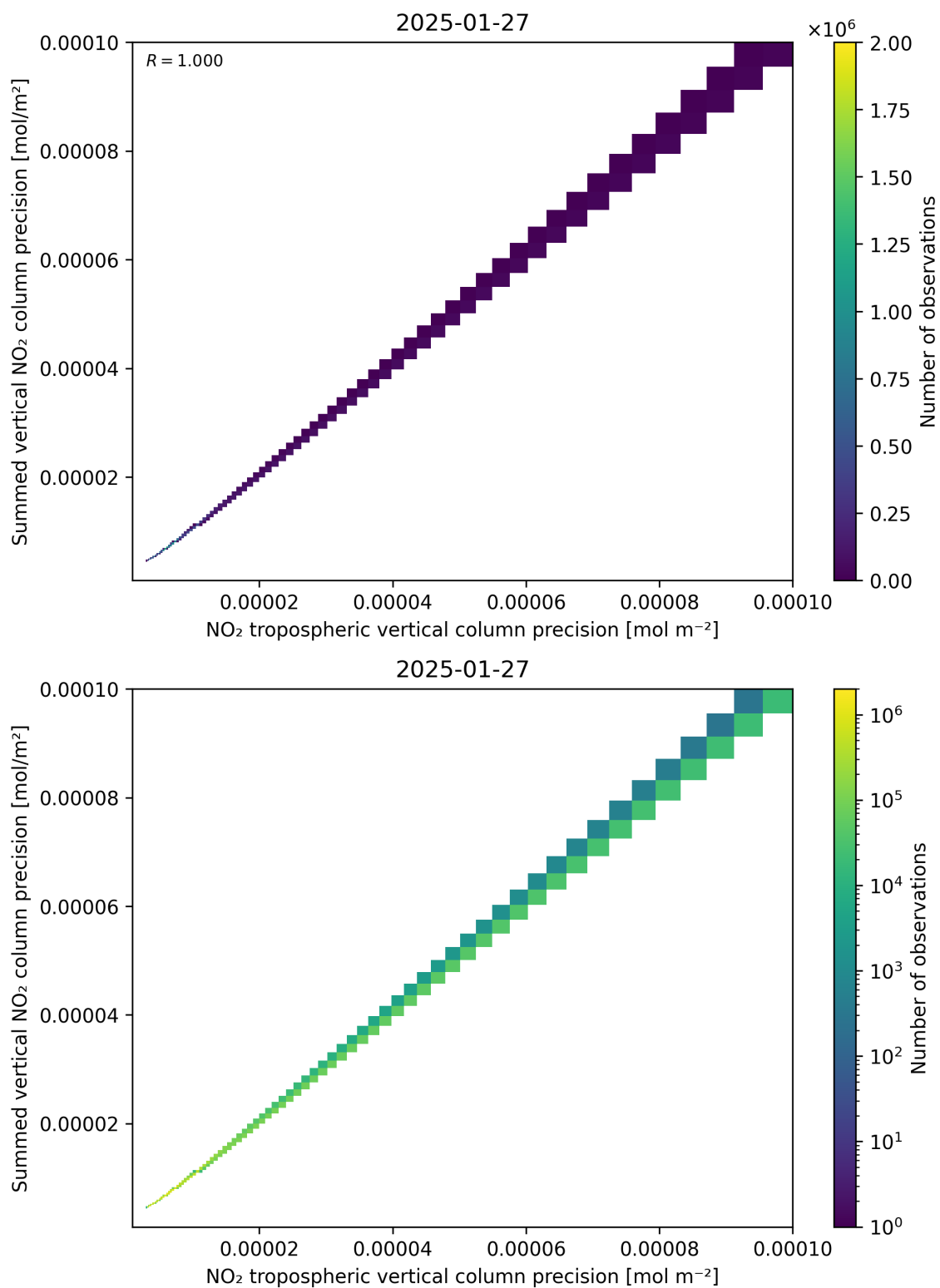
Figure 137: Scatter density plot of “NO 2 tropospheric vertical column precision” against “Summed vertical NO 2 column precision” for 2025-01-26 to 2025-01-28.
