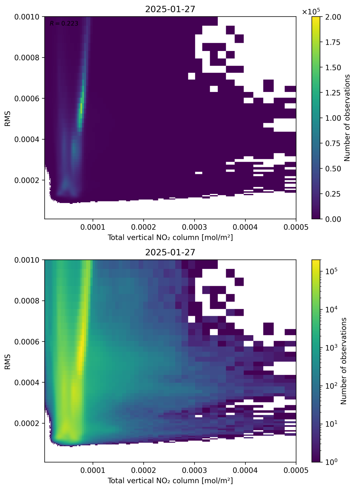
Figure 120: Scatter density plot of “Total vertical NO 2 column” against “RMS” for 2025-01-26 to 2025-01-28.
