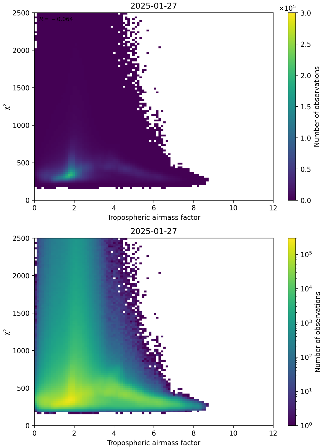
Figure 73: Scatter density plot of “Tropospheric airmass factor” against “ \chi^2 ” for 2025-01-26 to 2025-01-28.
