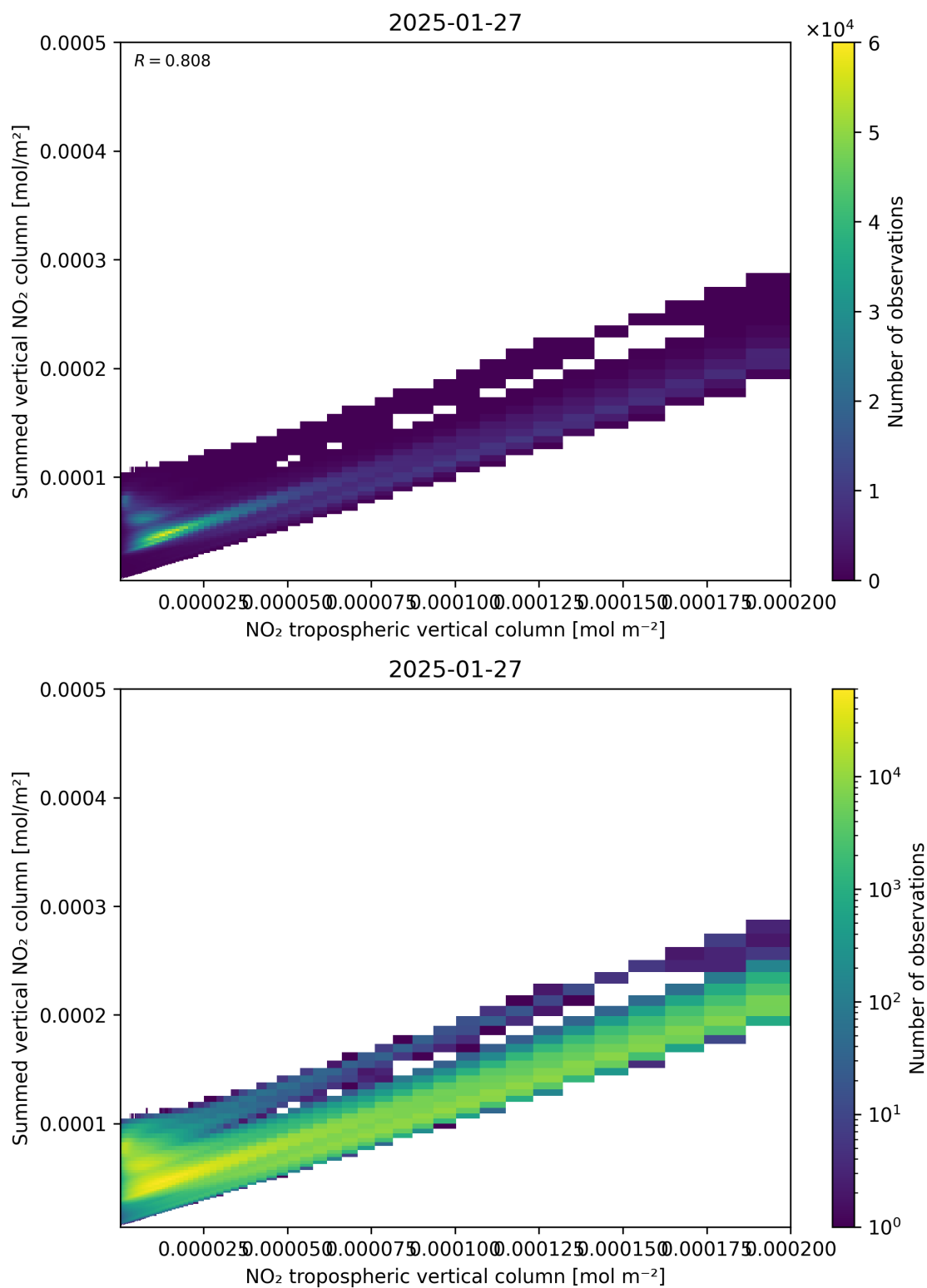
Figure 126: Scatter density plot of “NO 2 tropospheric vertical column” against “Summed vertical NO 2 column” for 2025-01-26 to 2025-01-28.
