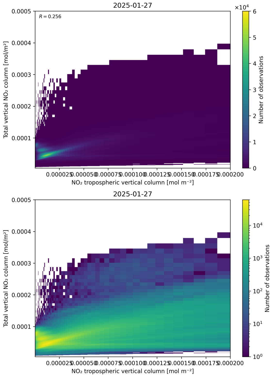
Figure 128: Scatter density plot of “NO 2 tropospheric vertical column” against “Total vertical NO 2 column” for 2025-01-26 to 2025-01-28.
