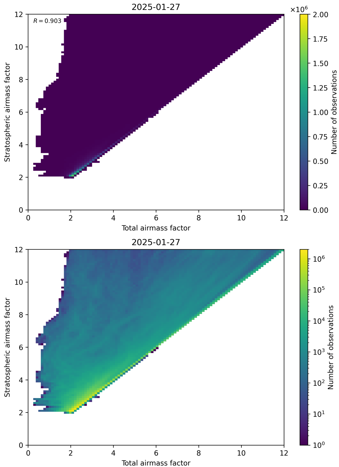
Figure 62: Scatter density plot of “Total airmass factor” against “Stratospheric airmass factor” for 2025-01-26 to 2025-01-28.
