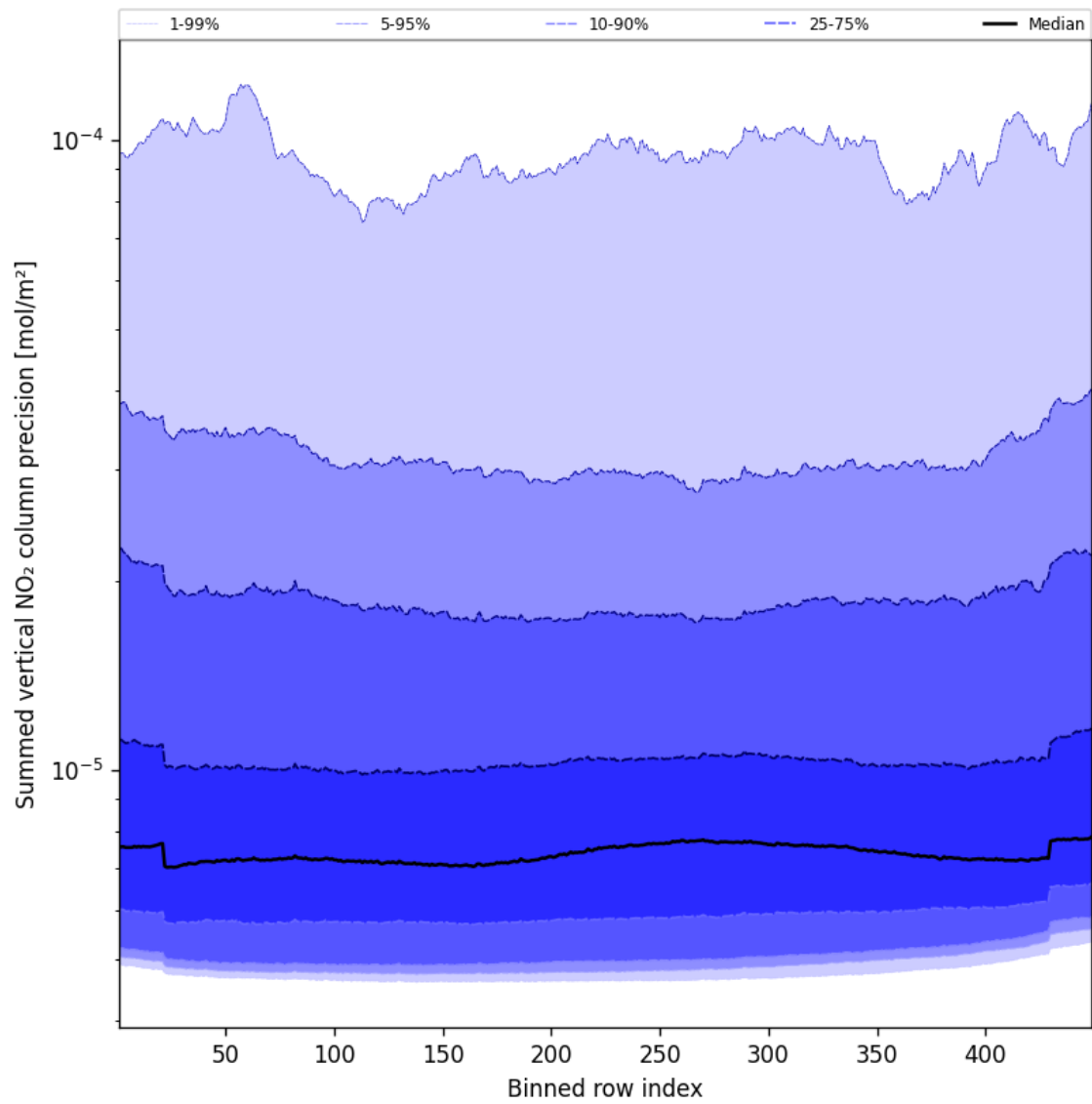
Figure 58: Along track statistics of “Summed vertical NO 2 column precision” for 2025-01-26 to 2025-01-28
