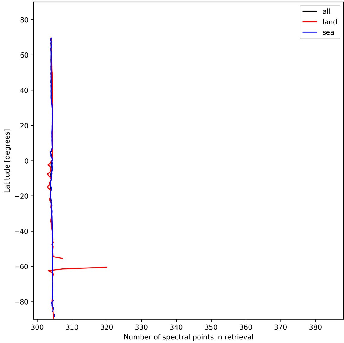
Figure 16: Zonal average of “Number of spectral points in retrieval” for 2025-01-26 to 2025-01-28.
