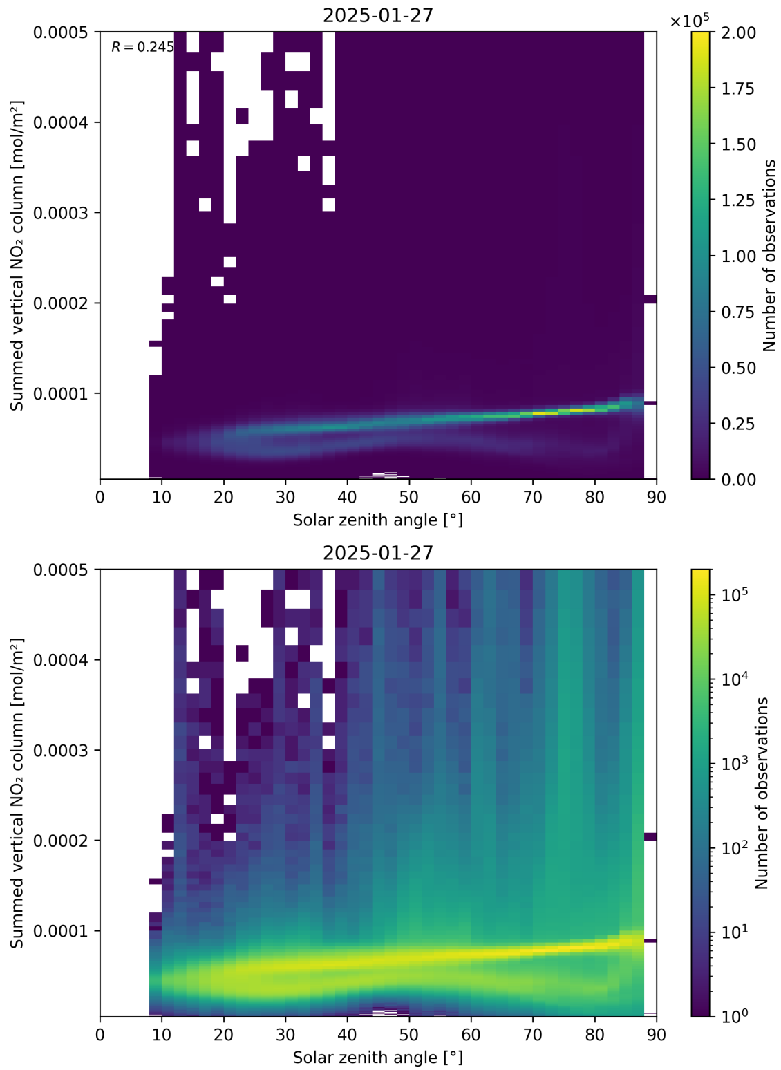
Figure 151: Scatter density plot of “Solar zenith angle” against “Summed vertical NO 2 column” for 2025-01-26 to 2025-01-28.
