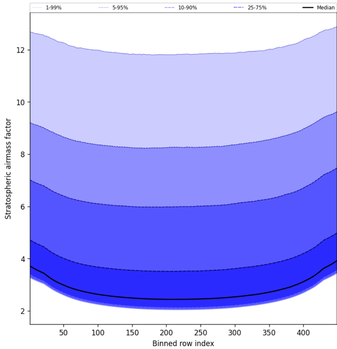
Figure 61: Along track statistics of “Stratospheric airmass factor” for 2025-01-26 to 2025-01-28
