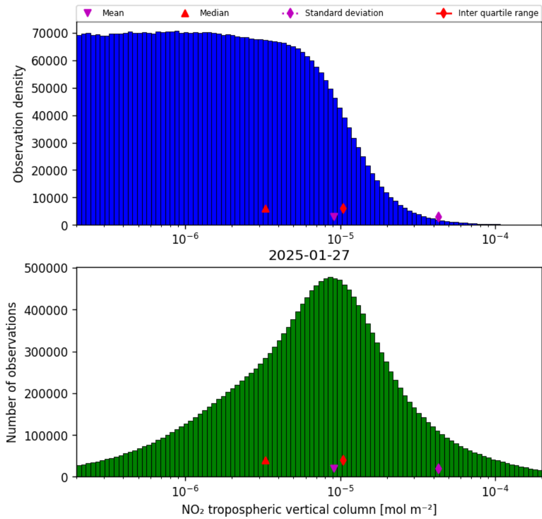
Figure 29: Histogram of “NO 2 tropospheric vertical column” for 2025-01-26 to 2025-01-28
