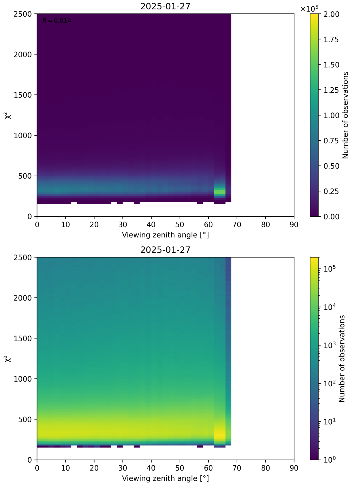
Figure 162: Scatter density plot of “Viewing zenith angle” against “ \chi^2 ” for 2025-01-26 to 2025-01-28.
