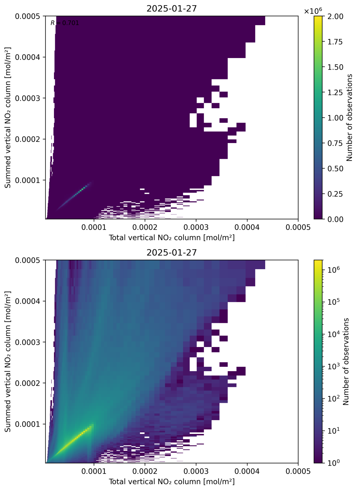
Figure 112: Scatter density plot of “Total vertical NO 2 column” against “Summed vertical NO 2 column” for 2025-01-26 to 2025-01-28.
