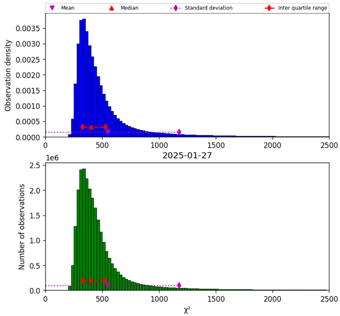
Figure 42: Histogram of “ \chi^2 ” for 2025-01-26 to 2025-01-28
