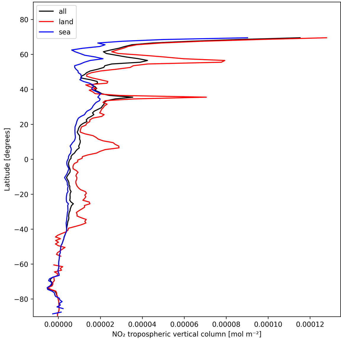
Figure 12: Zonal average of “NO 2 tropospheric vertical column” for 2025-01-26 to 2025-01-28.
