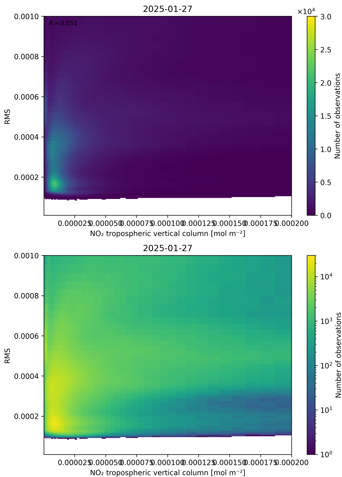
Figure 142: Scatter density plot of “NO 2 tropospheric vertical column” against “RMS” for 2025-01-26 to 2025-01-28.
