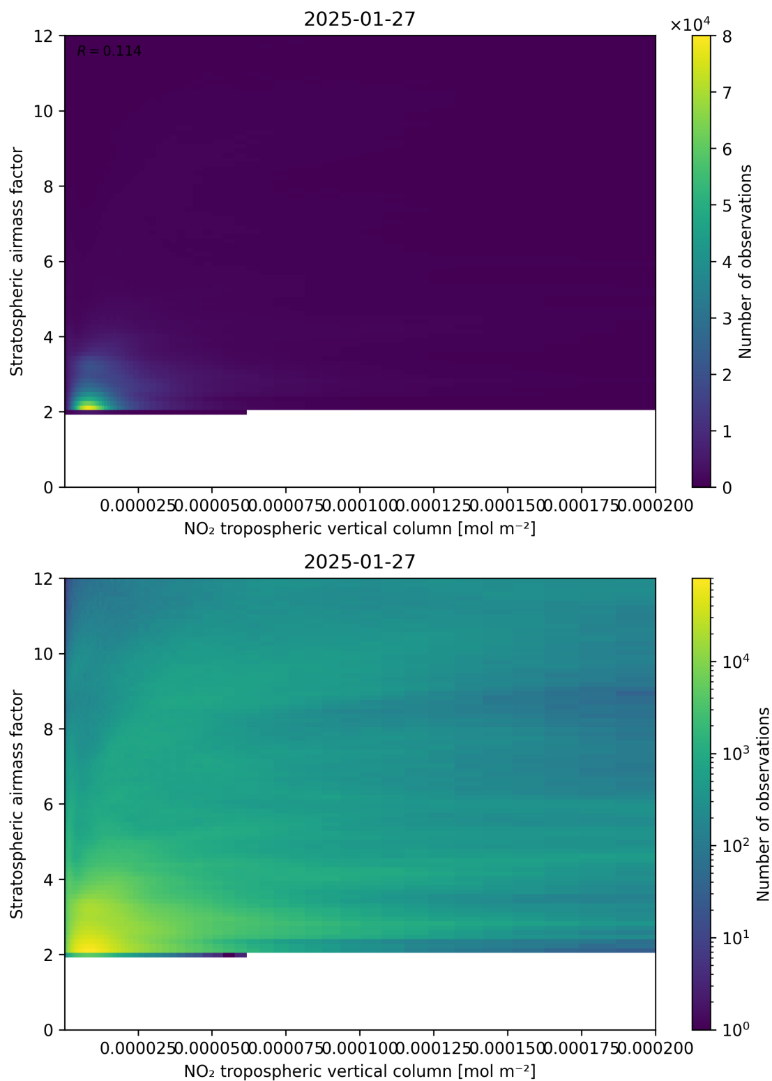
Figure 121: Scatter density plot of “NO 2 tropospheric vertical column” against “Stratospheric airmass factor” for 2025-01-26 to 2025-01-28.
