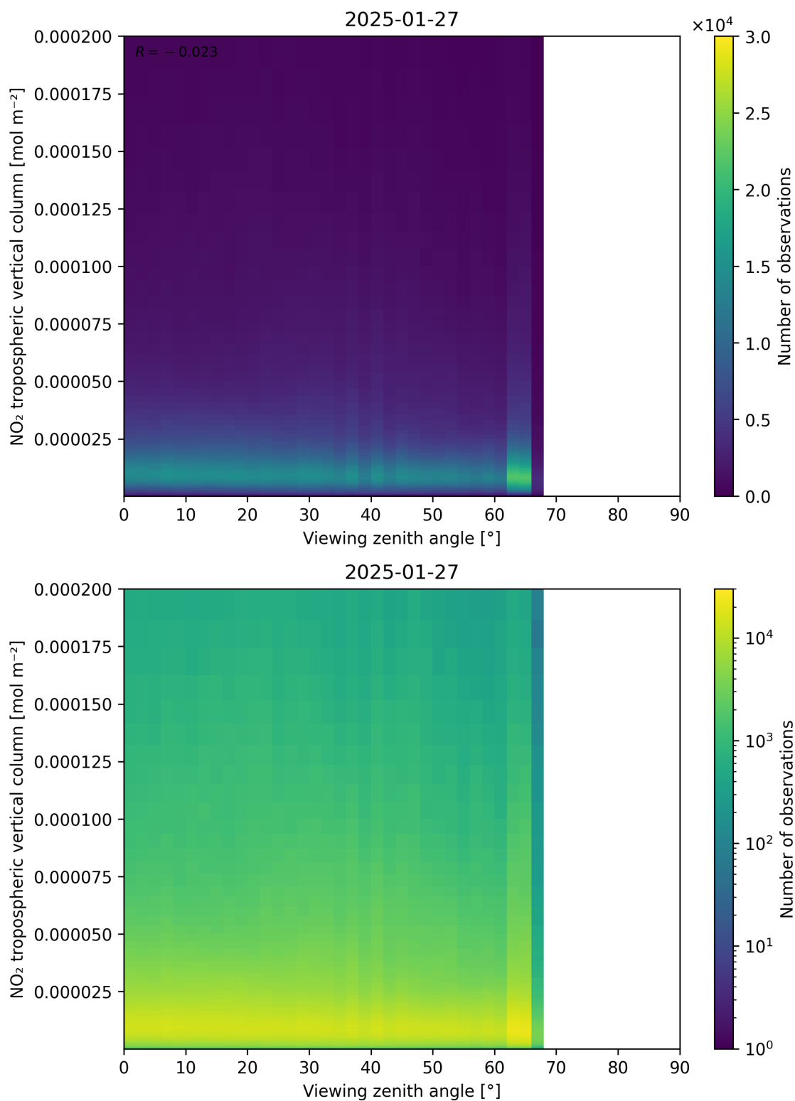
Figure 169: Scatter density plot of “Viewing zenith angle” against “NO 2 tropospheric vertical column” for 2025-01-26 to 2025-01-28.
