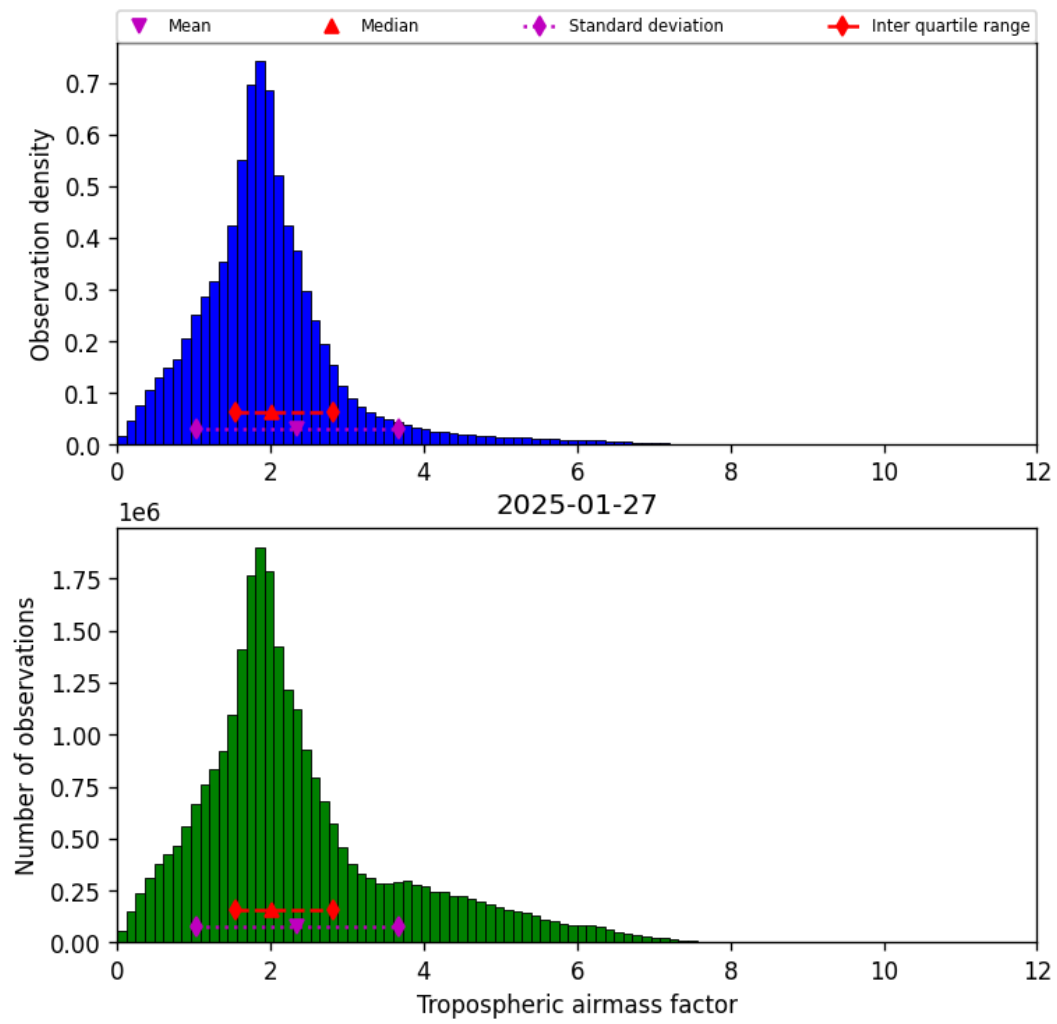
Figure 31: Histogram of “Tropospheric airmass factor” for 2025-01-26 to 2025-01-28
