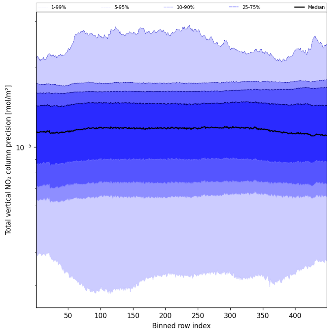
Figure 56: Along track statistics of “Total vertical NO 2 column precision” for 2025-01-26 to 2025-01-28
