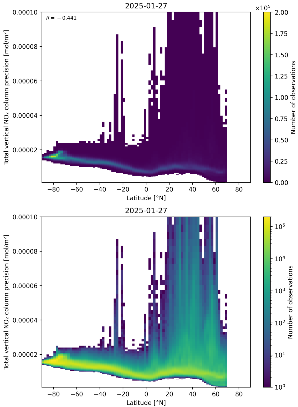
Figure 91: Scatter density plot of “Latitude” against “Total vertical NO 2 column precision” for 2025-01-26 to 2025-01-28.
