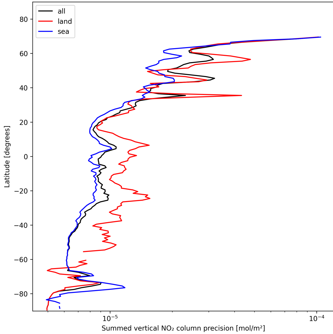
Figure 24: Zonal average of “Summed vertical NO 2 column precision” for 2025-01-26 to 2025-01-28.
