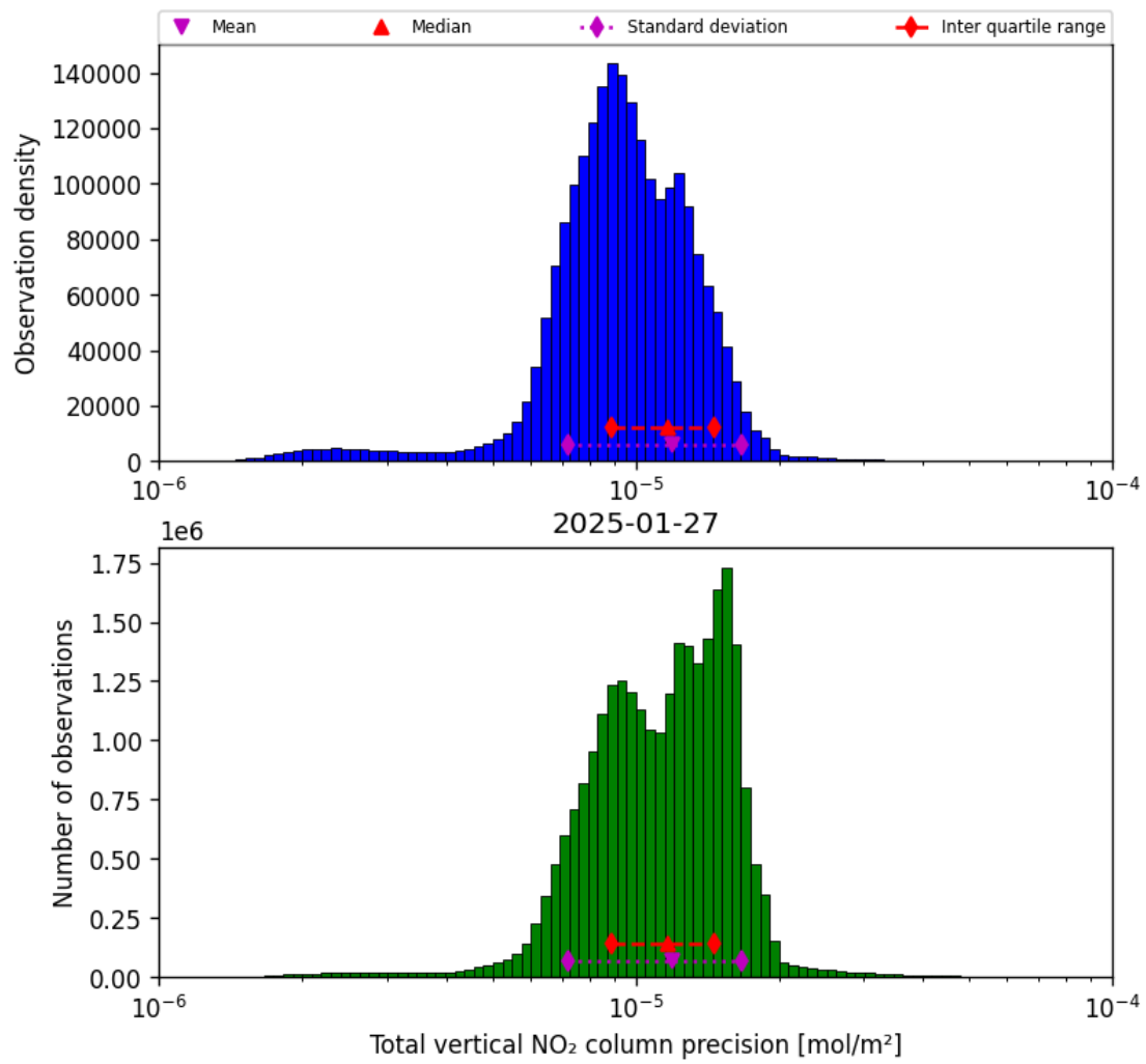
Figure 39: Histogram of “Total vertical NO 2 column precision” for 2025-01-26 to 2025-01-28
