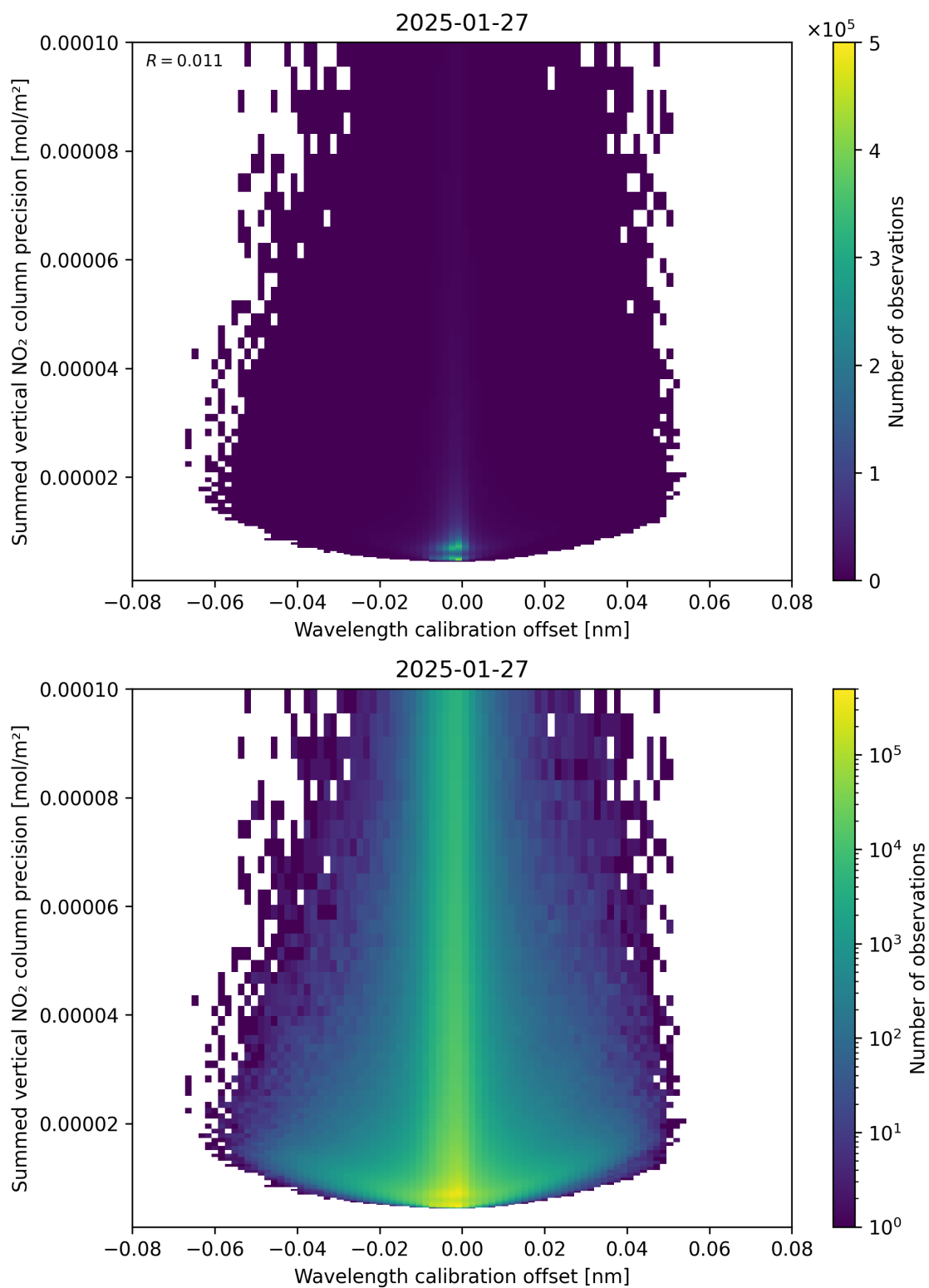
Figure 178: Scatter density plot of “Wavelength calibration offset” against “Summed vertical NO 2 column precision” for 2025-01-26 to 2025-01-28.
