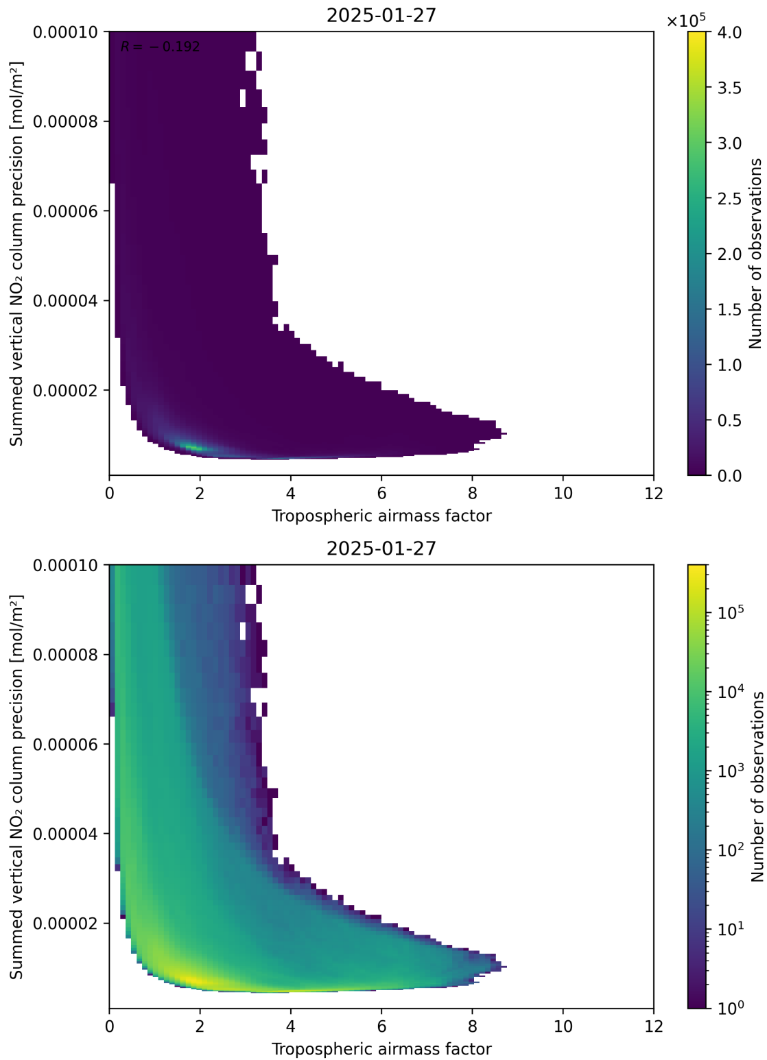
Figure 76: Scatter density plot of “Tropospheric airmass factor” against “Summed vertical NO 2 column precision” for 2025-01-26 to 2025-01-28.
