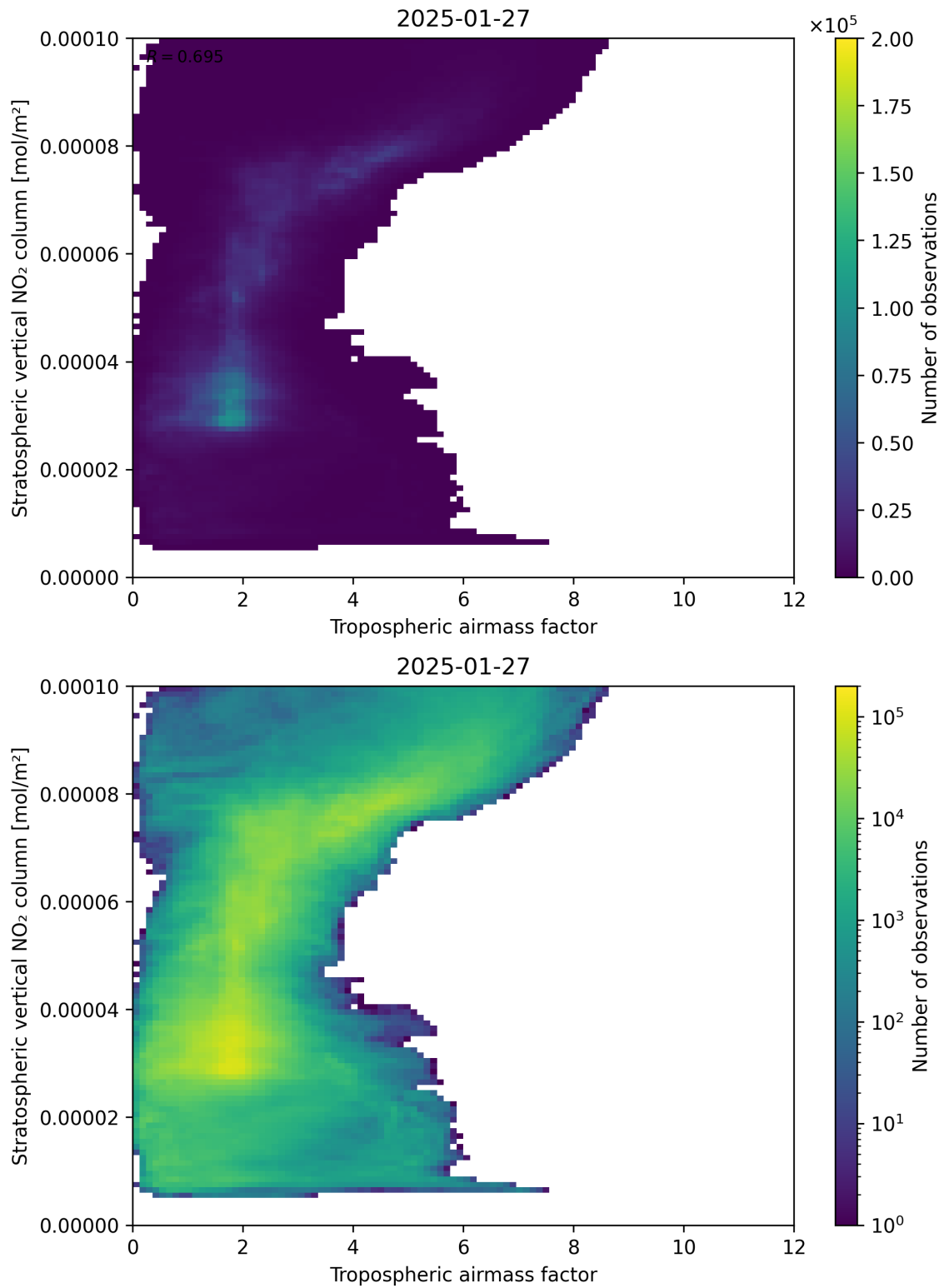
Figure 74: Scatter density plot of “Tropospheric air mass factor” against “Stratospheric vertical NO 2 column” for 2025-01-26 to 2025-01-28.
