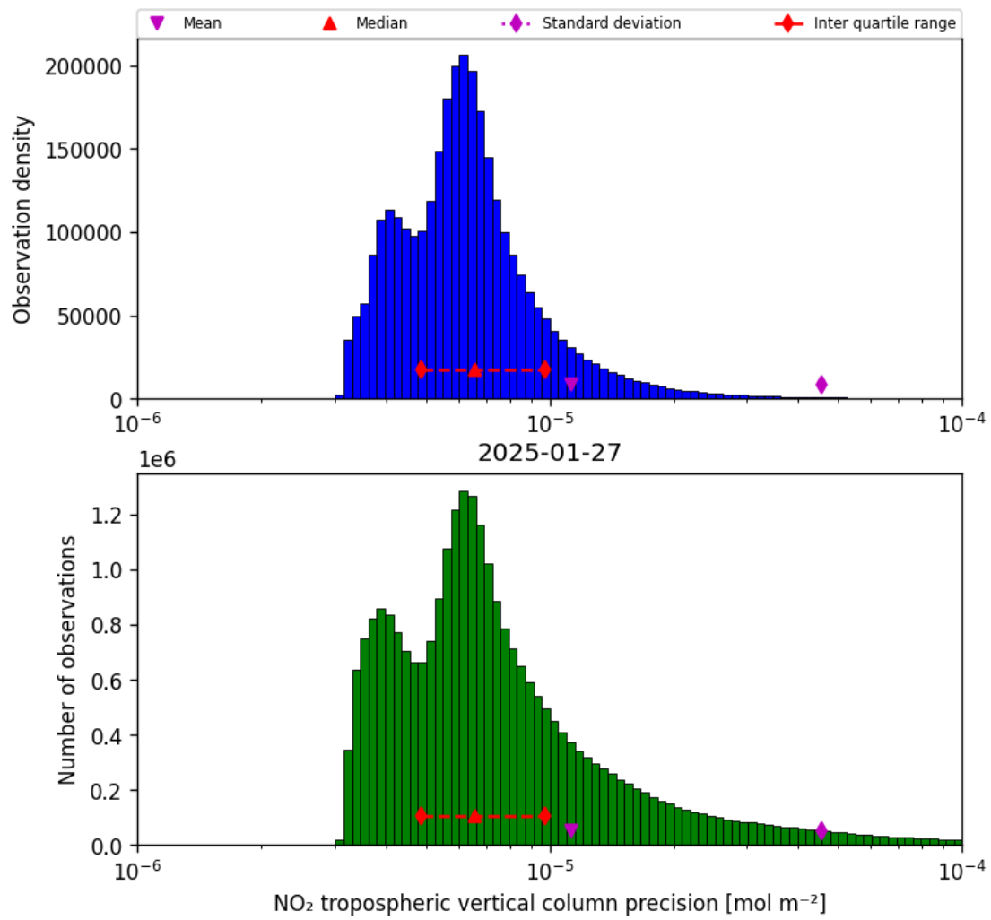
Figure 30: Histogram of “NO 2 tropospheric vertical column precision” for 2025-01-26 to 2025-01-28
