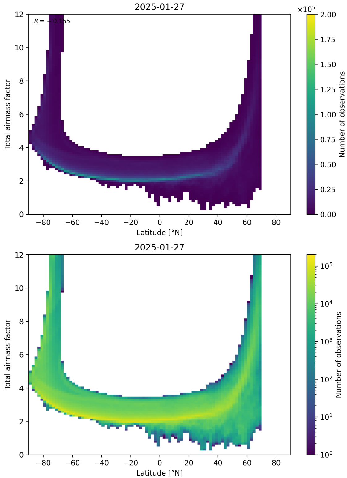
Figure 84: Scatter density plot of “Latitude” against “Total airmass factor” for 2025-01-26 to 2025-01-28.
