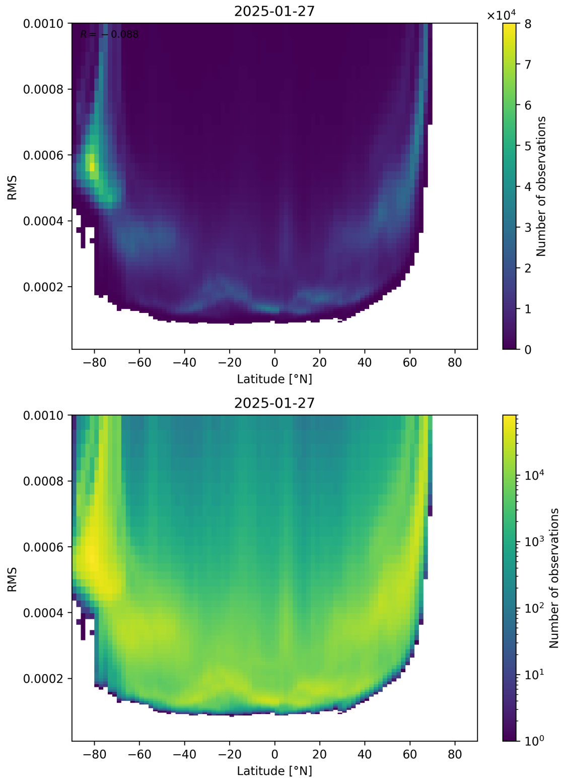
Figure 94: Scatter density plot of “Latitude” against “RMS” for 2025-01-26 to 2025-01-28.
