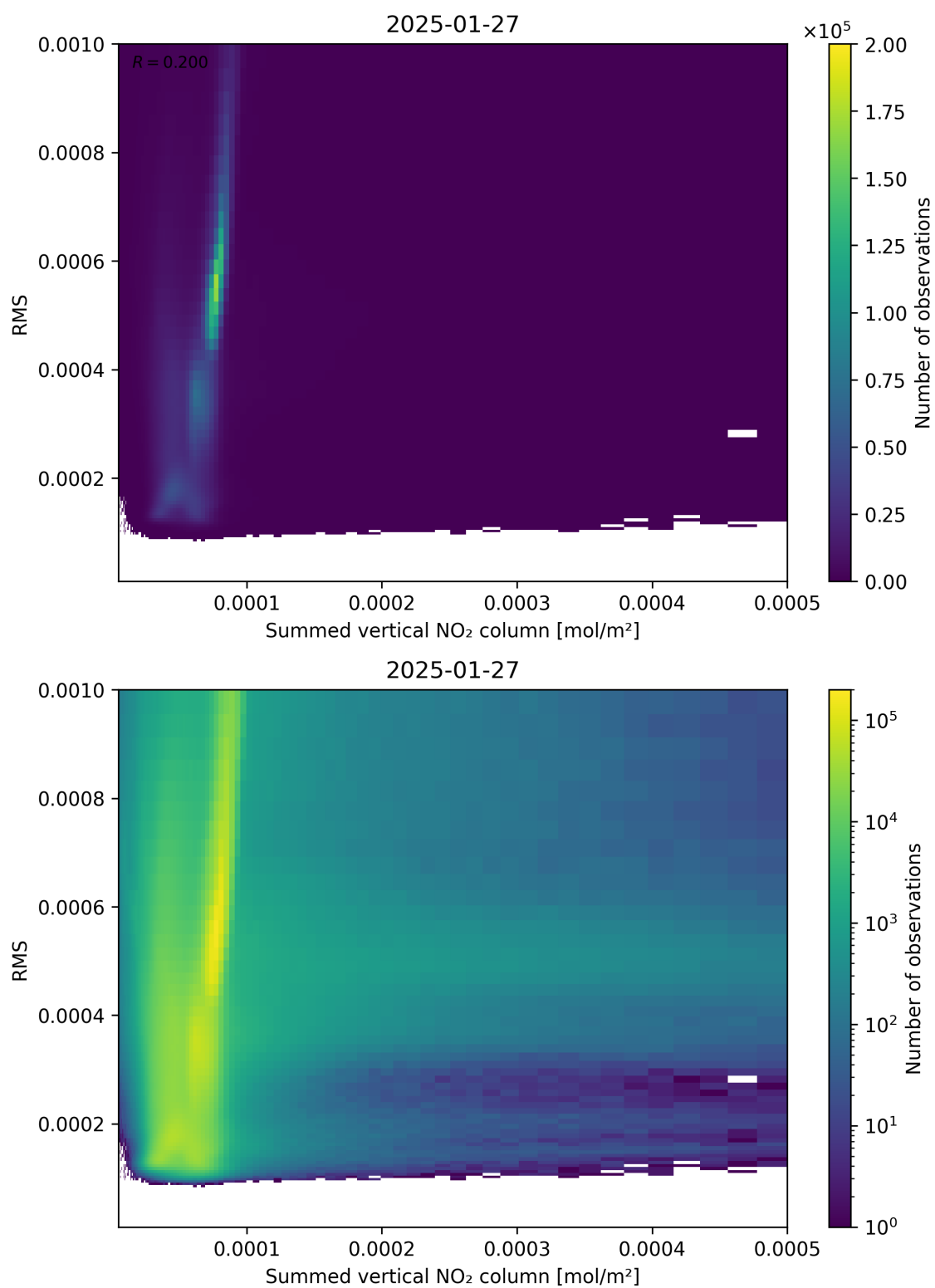
Figure 109: Scatter density plot of “Summed vertical NO 2 column” against “RMS” for 2025-01-26 to 2025-01-28.
