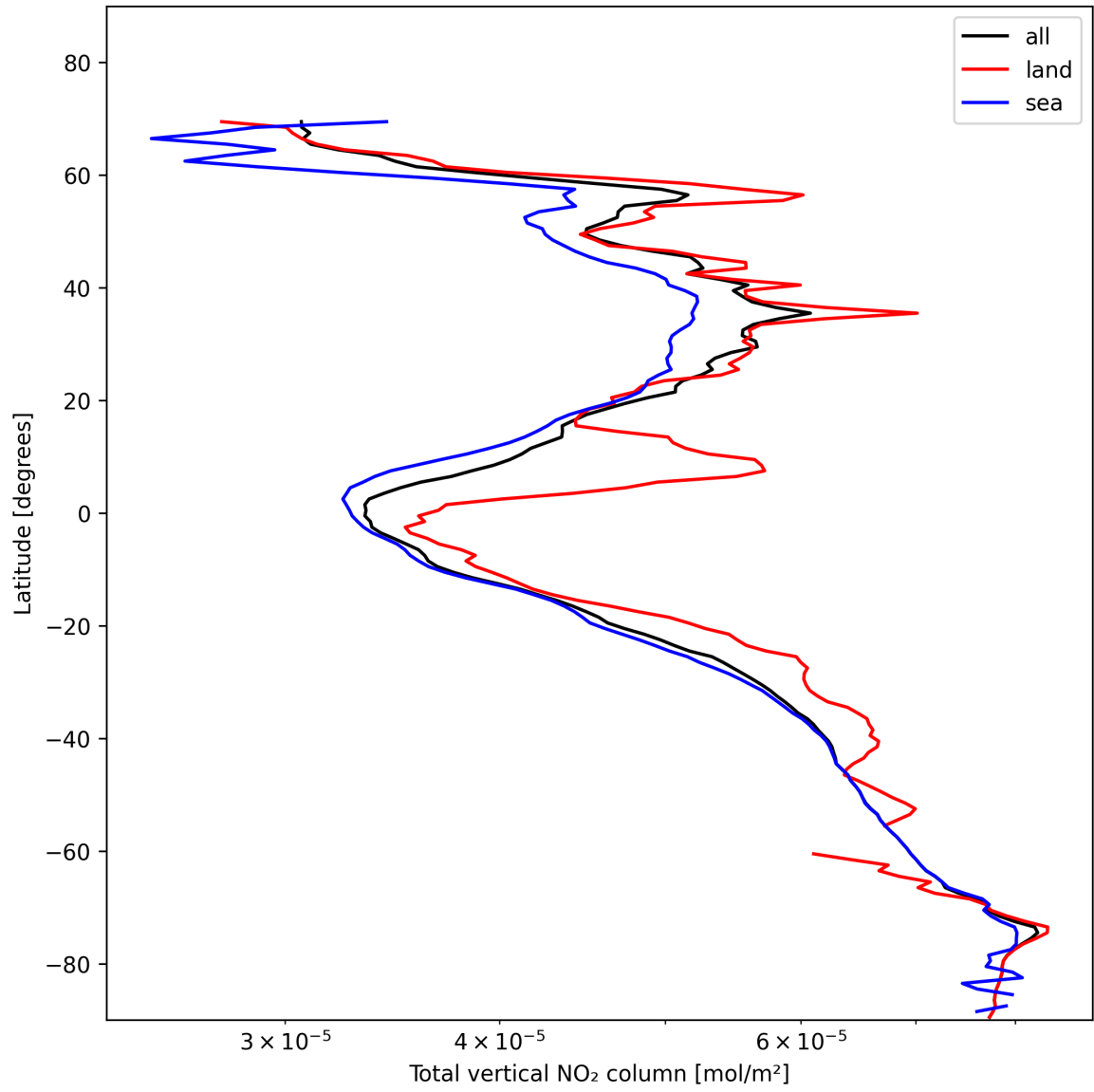
Figure 21: Zonal average of “Total vertical NO 2 column” for 2025-01-26 to 2025-01-28.
