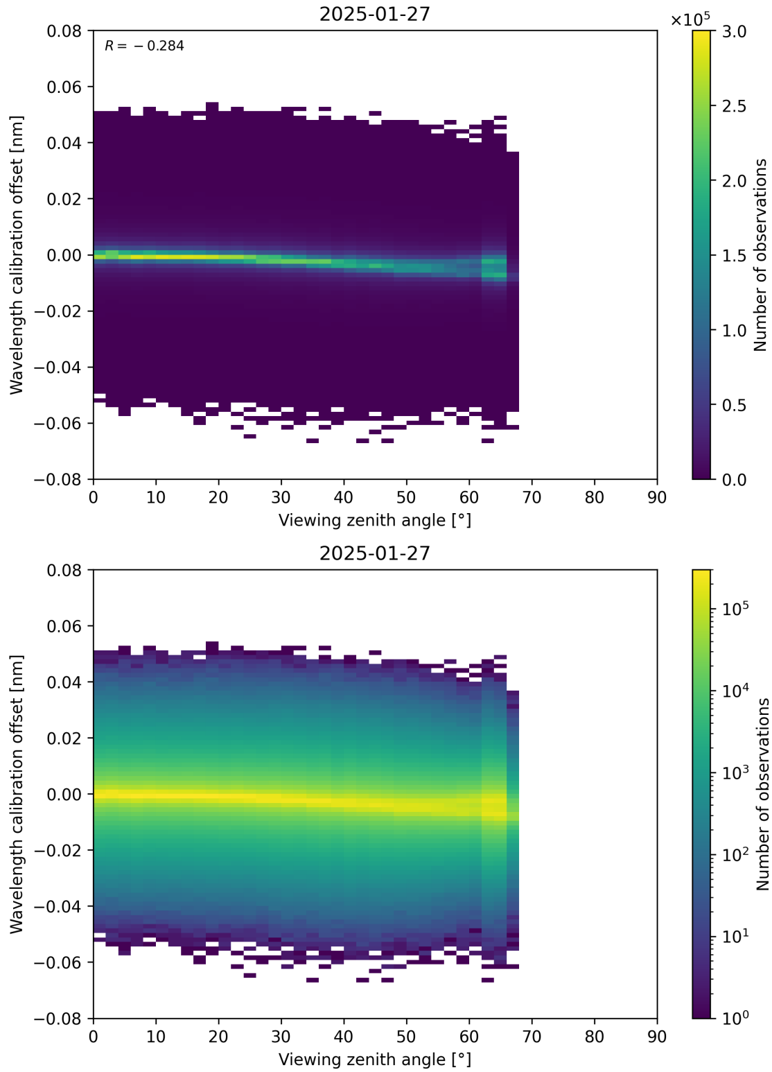
Figure 173: Scatter density plot of “Viewing zenith angle” against “Wavelength calibration offset” for 2025-01-26 to 2025-01-28.
