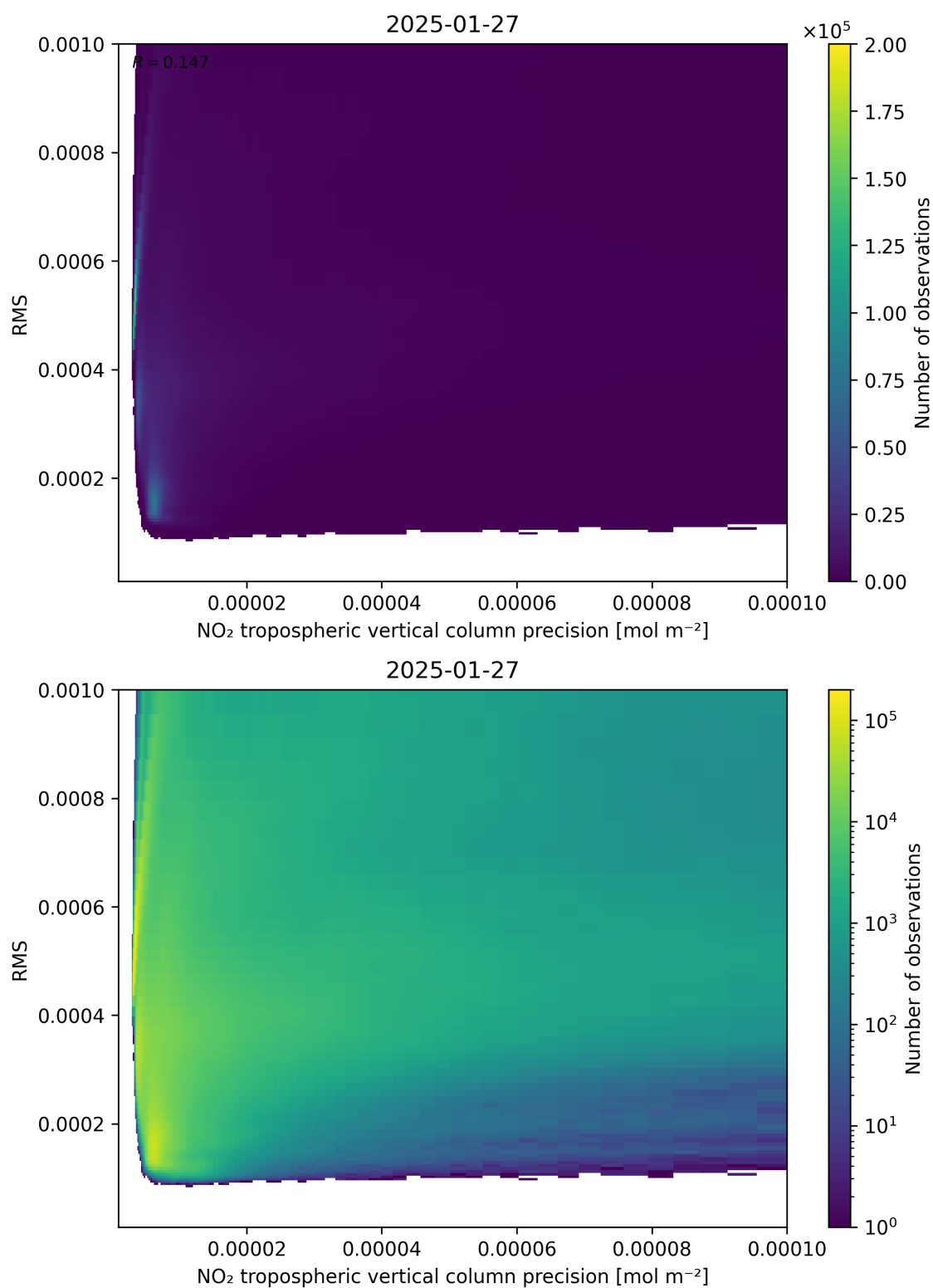
Figure 140: Scatter density plot of “NO 2 tropospheric vertical column precision” against “RMS” for 2025-01-26 to 2025-01-28.
