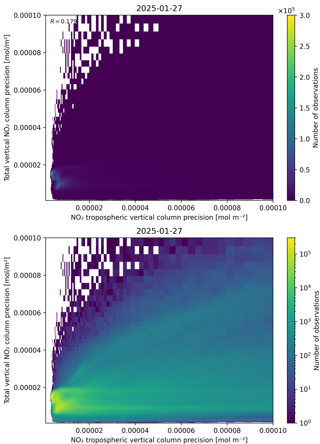
Figure 139: Scatter density plot of “NO 2 tropospheric vertical column precision” against “Total vertical NO 2 column precision” for 2025-01-26 to 2025-01-28.
