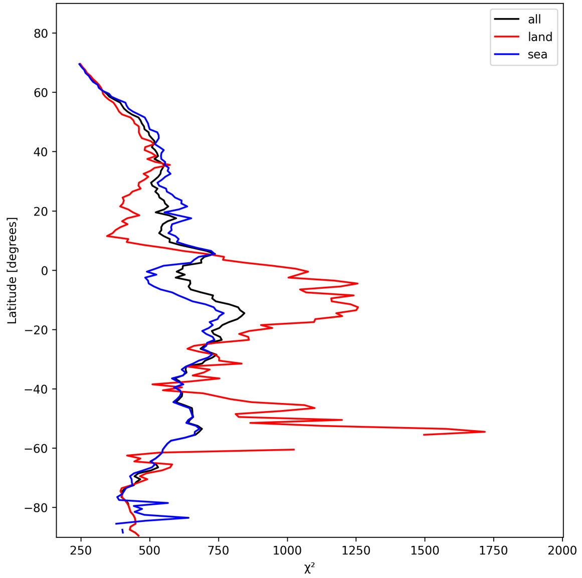
Figure 25: Zonal average of “ \chi^2 ” for 2025-01-26 to 2025-01-28.
