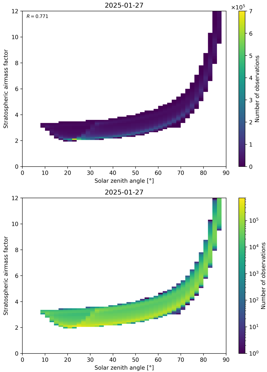
Figure 145: Scatter density plot of “Solar zenith angle” against “Stratospheric airmass factor” for 2025-01-26 to 2025-01-28.
