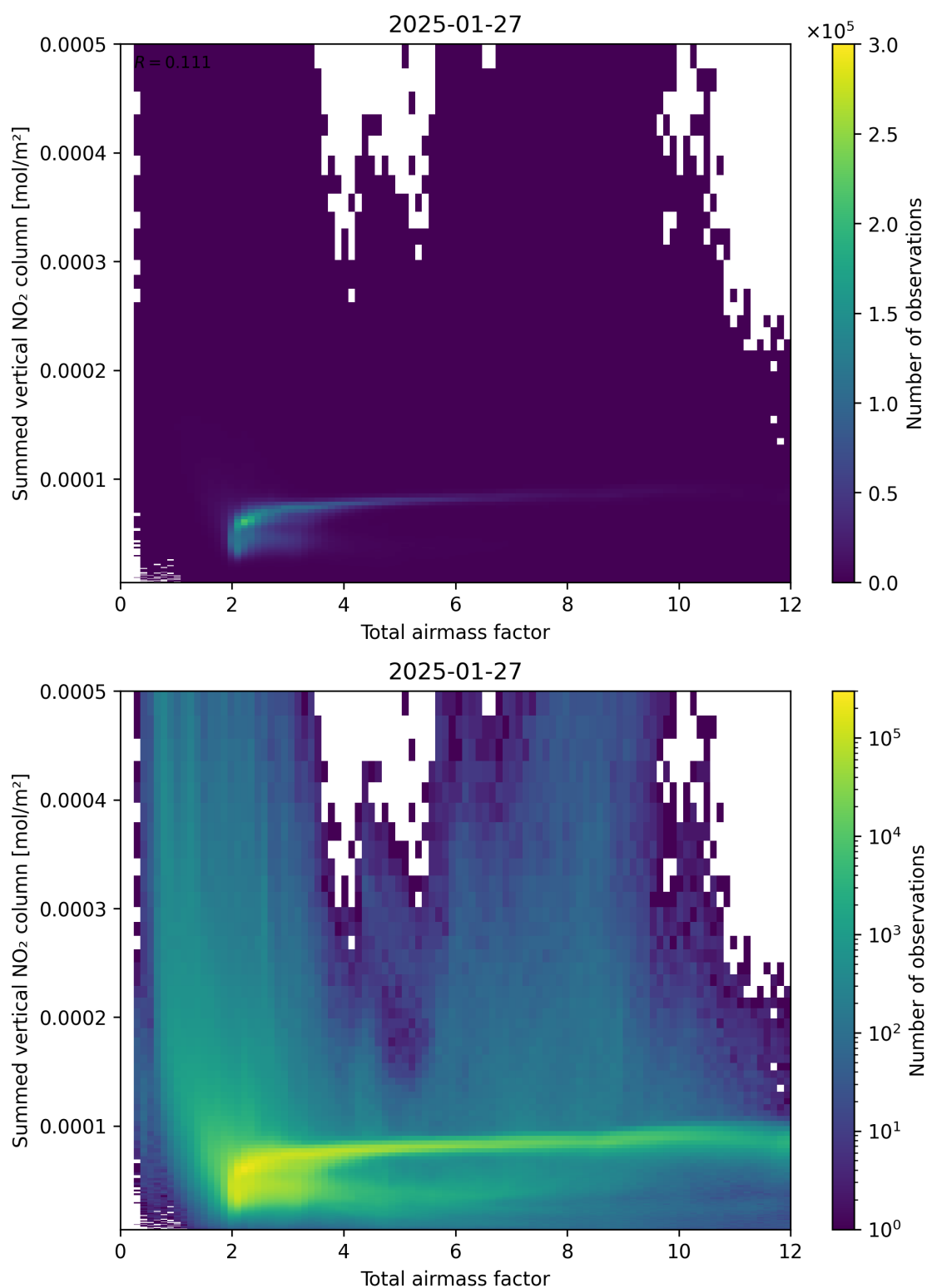
Figure 65: Scatter density plot of “Total airmass factor” against “Summed vertical NO 2 column” for 2025-01-26 to 2025-01-28.
