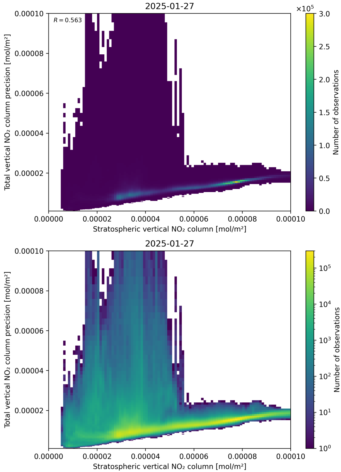
Figure 101: Scatter density plot of “Stratospheric vertical NO 2 column” against “Total vertical NO 2 column precision” for 2025-01-26 to 2025-01-28.
