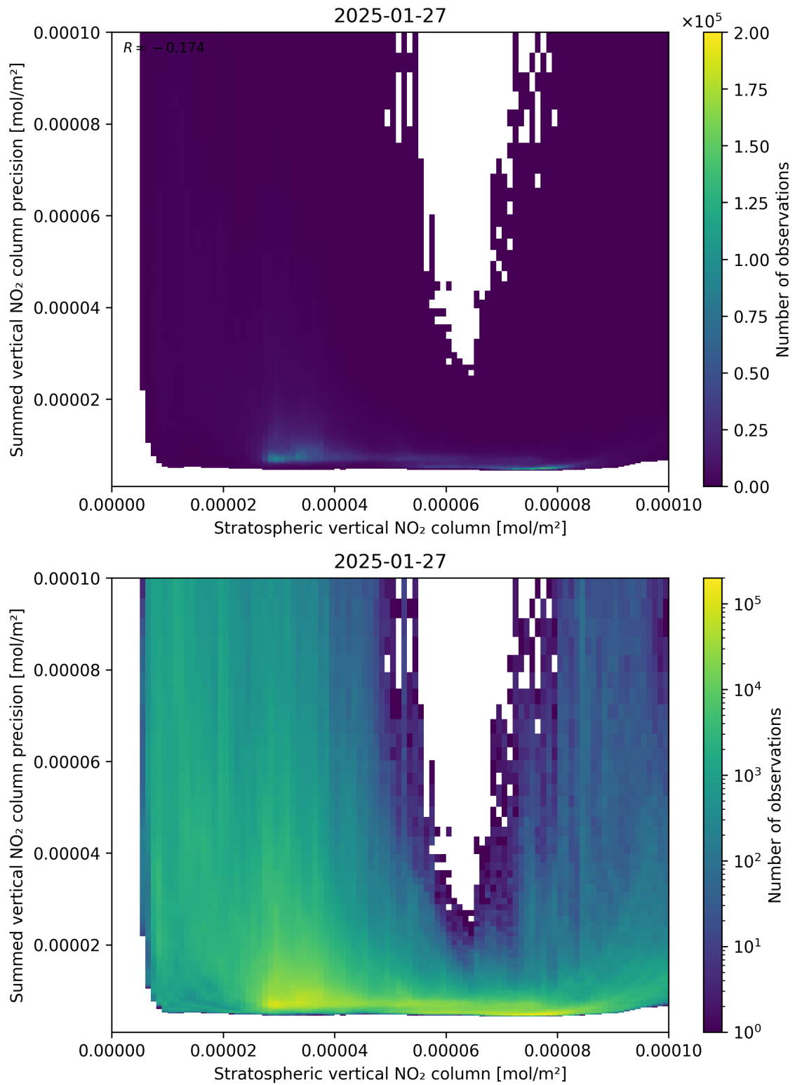
Figure 99: Scatter density plot of “Stratospheric vertical NO 2 column” against “Summed vertical NO 2 column precision” for 2025-01-26 to 2025-01-28.
