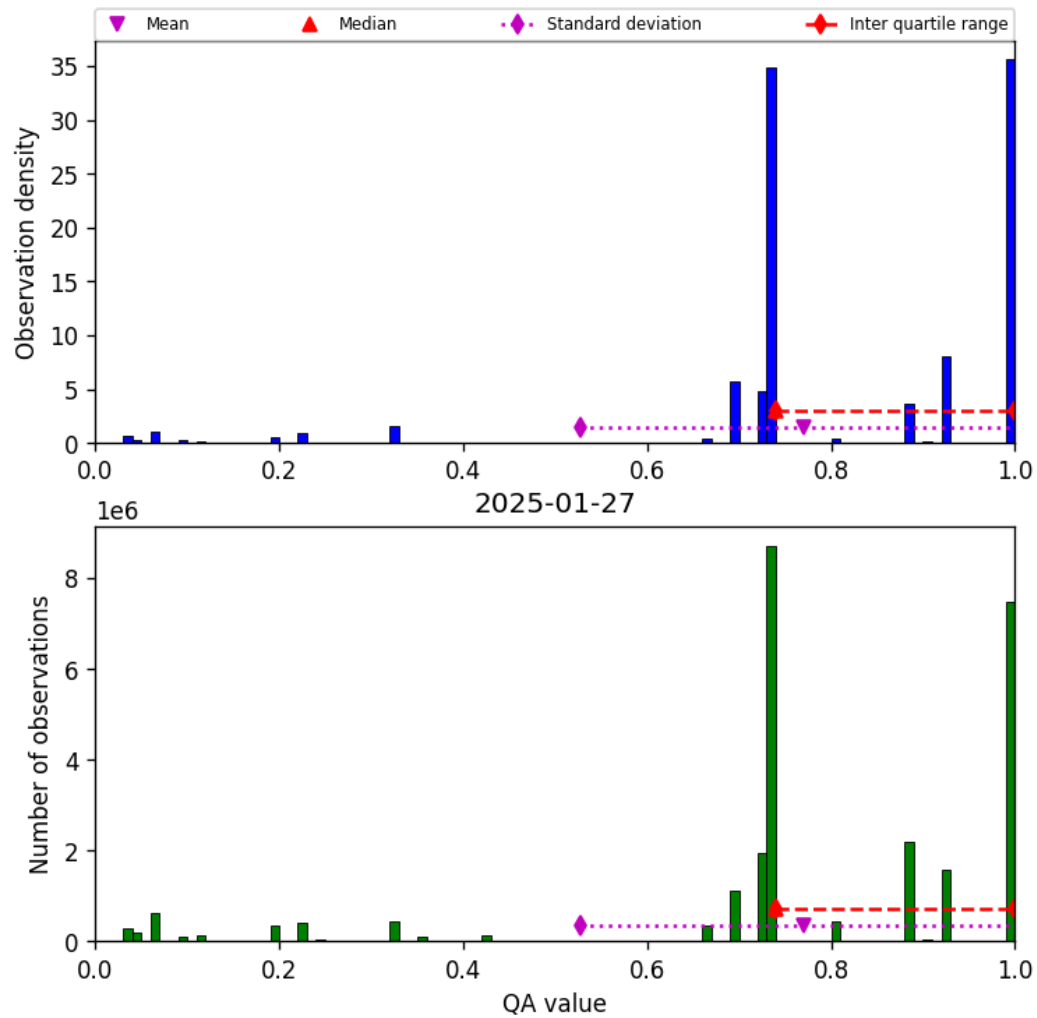
Figure 28: Histogram of “QA value” for 2025-01-26 to 2025-01-28
