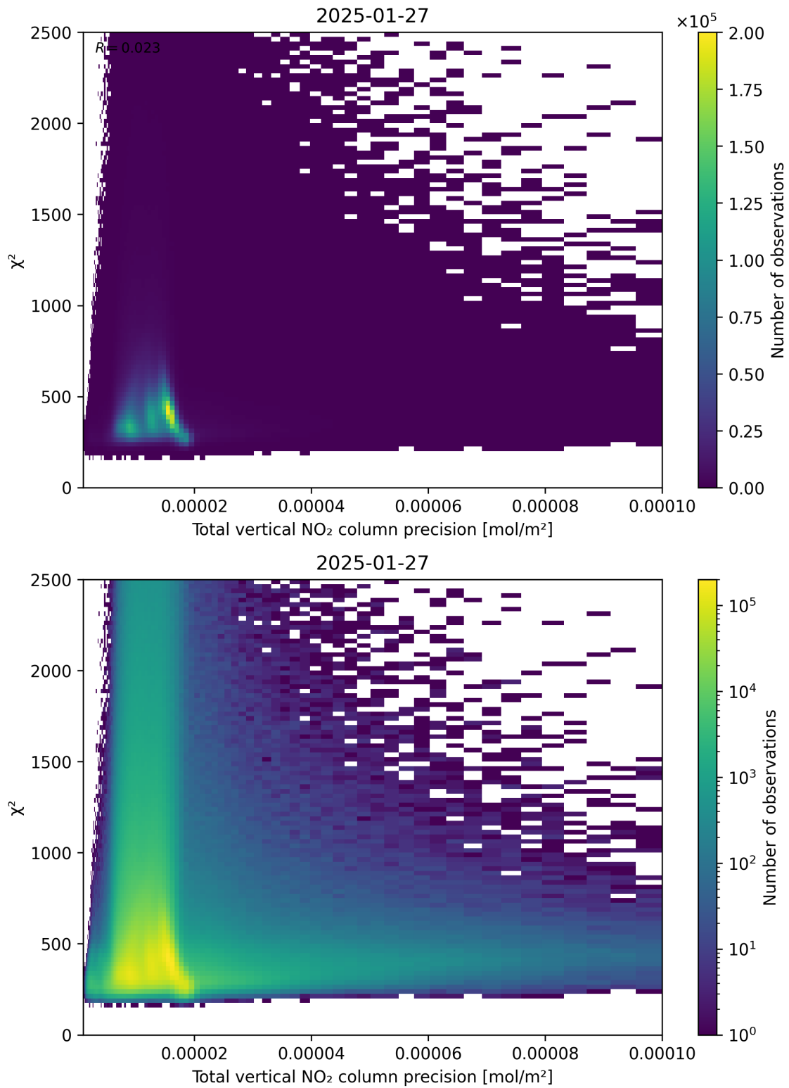
Figure 116: Scatter density plot of “Total vertical NO 2 column precision” against “ \chi^2 ” for 2025-01-26 to 2025-01-28.
