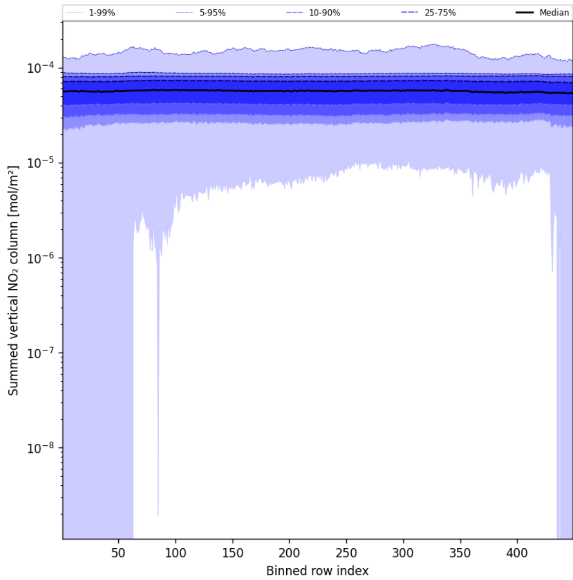
Figure 57: Along track statistics of “Summed vertical NO 2 column” for 2025-01-26 to 2025-01-28
