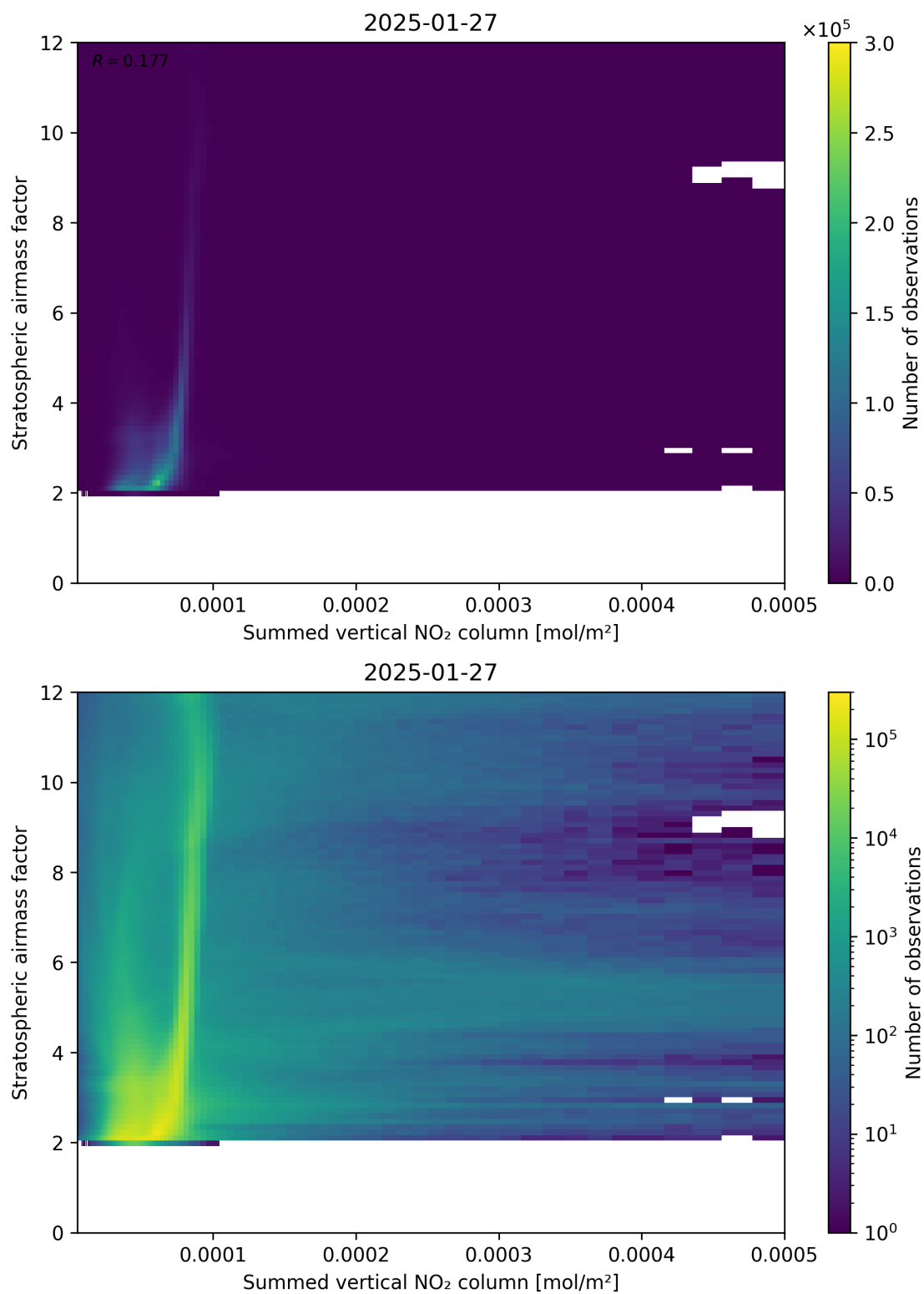
Figure 103: Scatter density plot of “Summed vertical NO 2 column” against “Stratospheric airmass factor” for 2025-01-26 to 2025-01-28.
