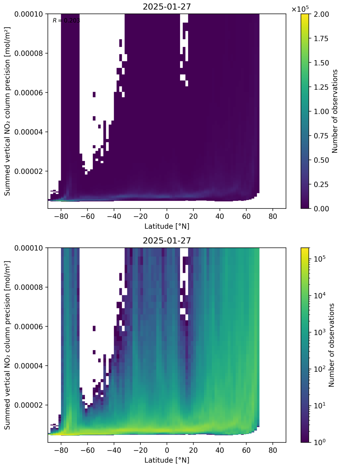
Figure 89: Scatter density plot of “Latitude” against “Summed vertical NO 2 column precision” for 2025-01-26 to 2025-01-28.
