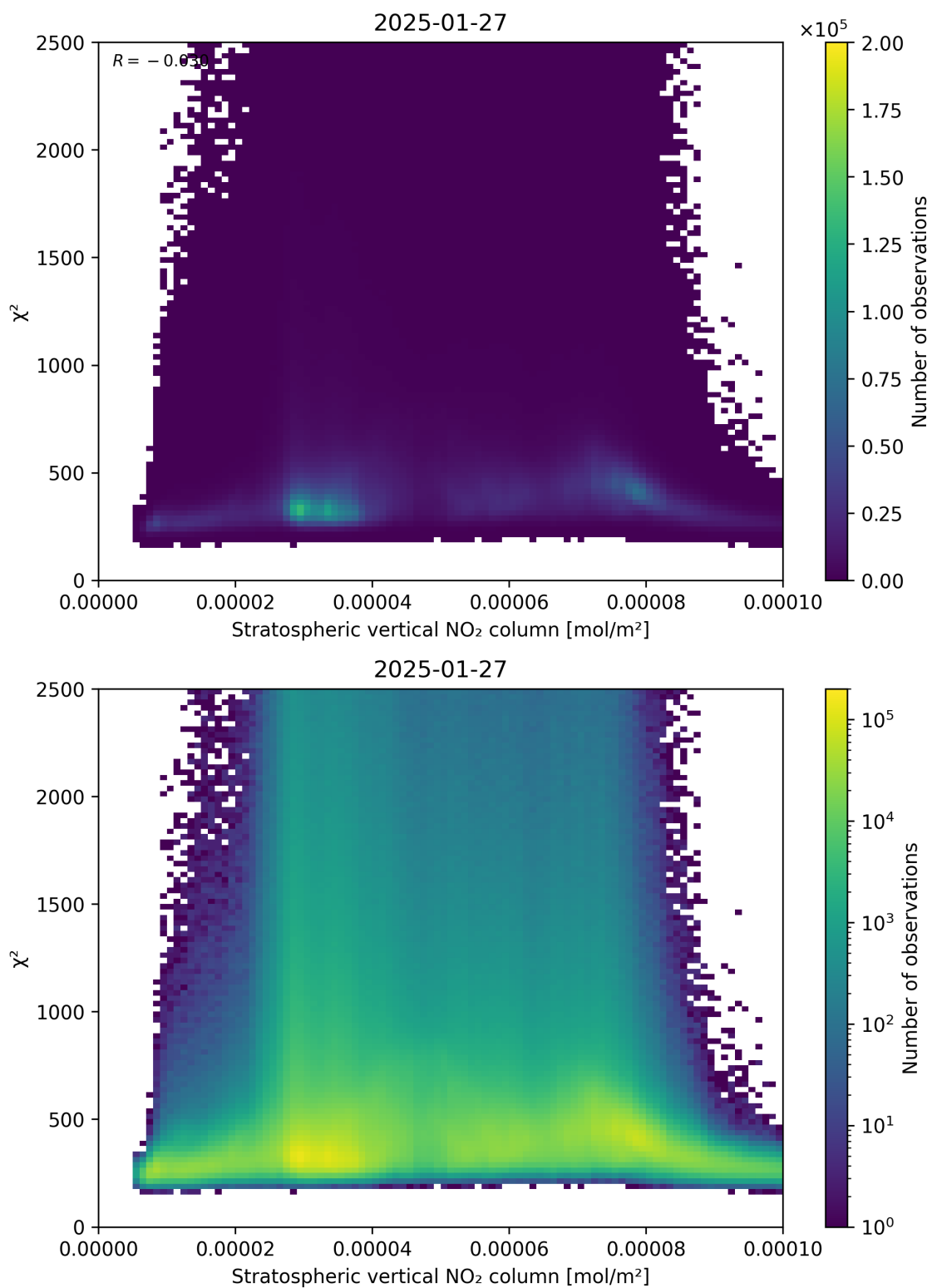
Figure 97: Scatter density plot of “Stratospheric vertical NO 2 column” against “ \chi^2 ” for 2025-01-26 to 2025-01-28.
