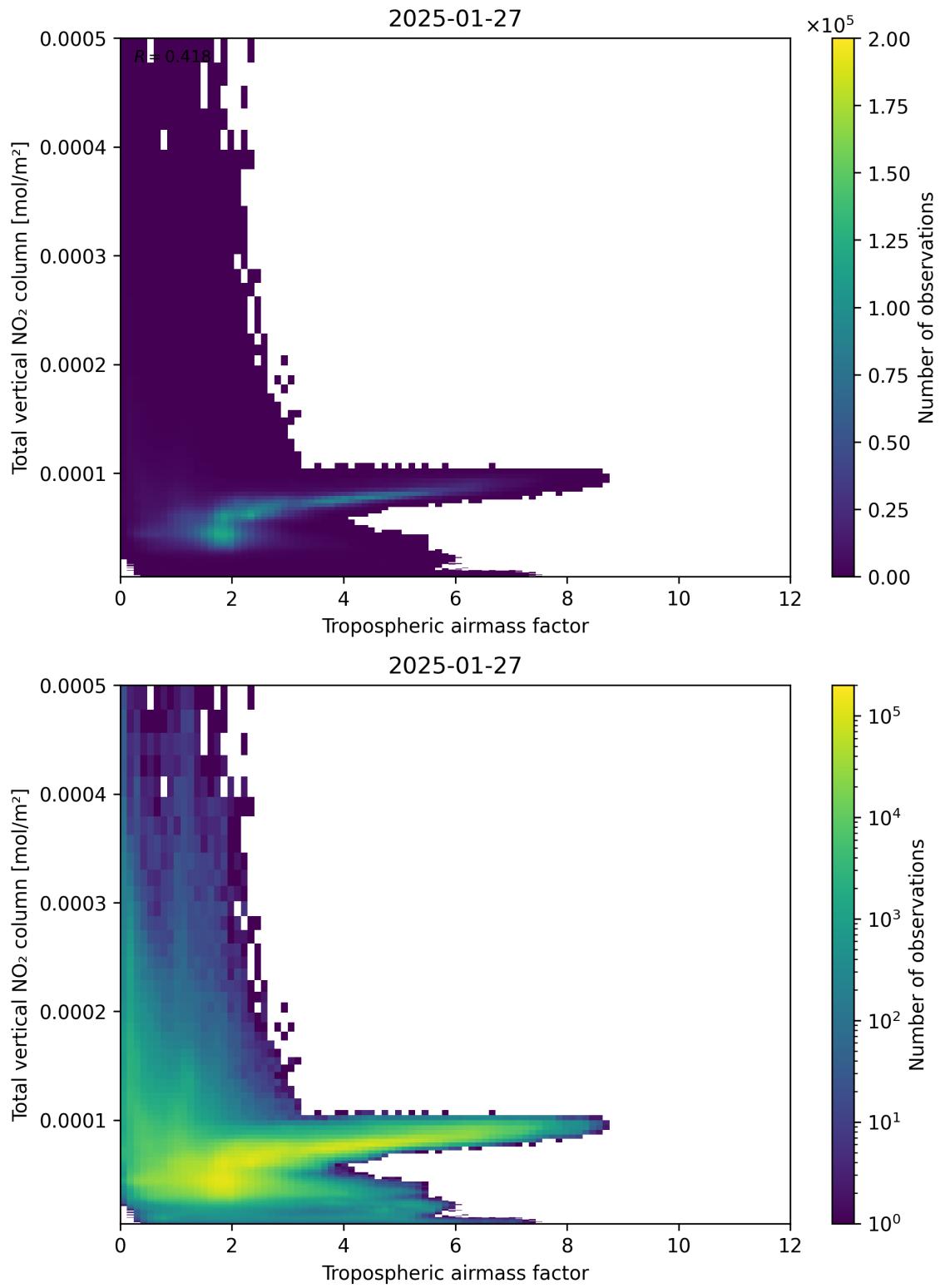
Figure 77: Scatter density plot of “Tropospheric airmass factor” against “Total vertical NO 2 column” for 2025-01-26 to 2025-01-28.
