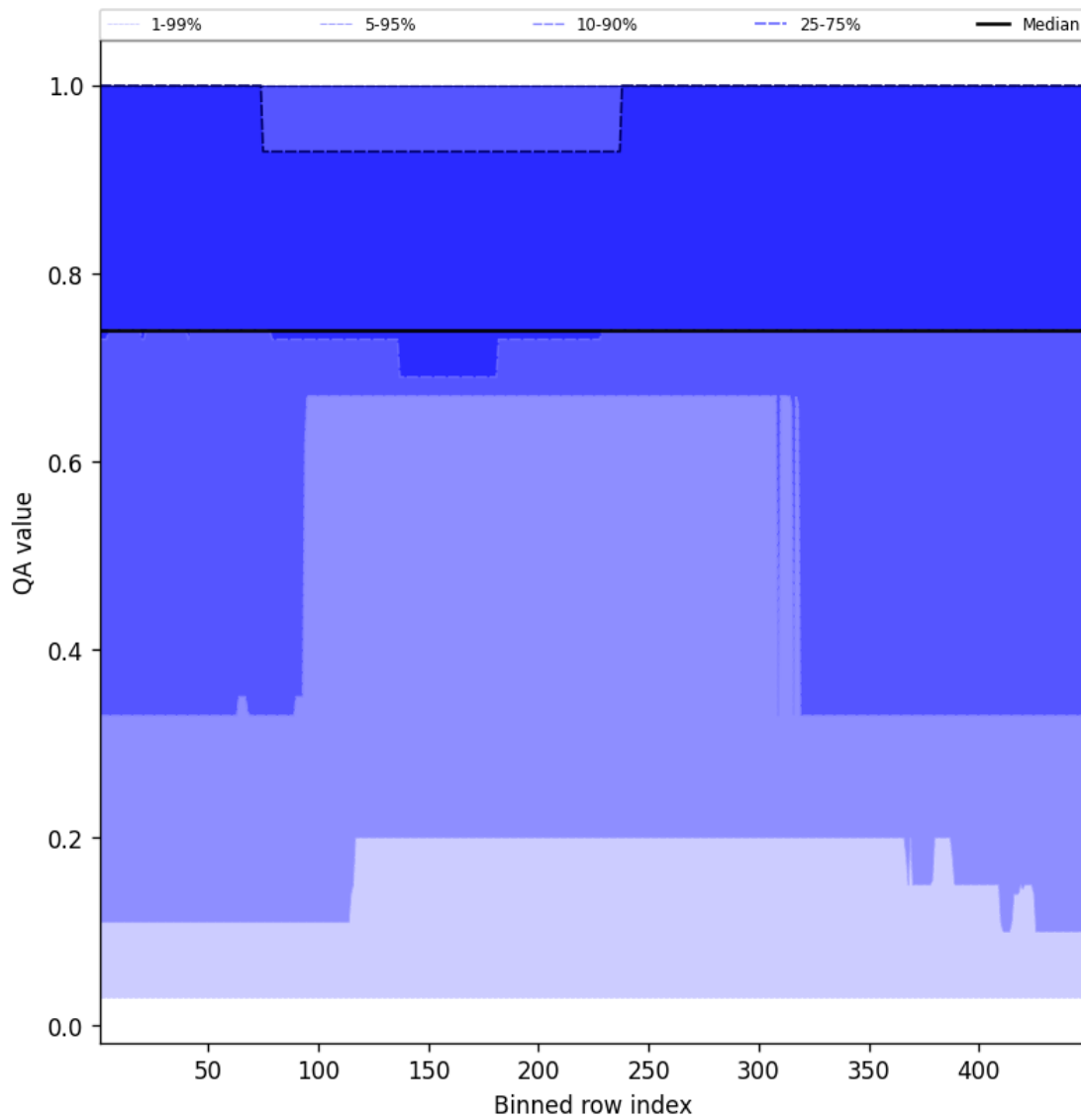
Figure 45: Along track statistics of “QA value” for 2025-01-26 to 2025-01-28
