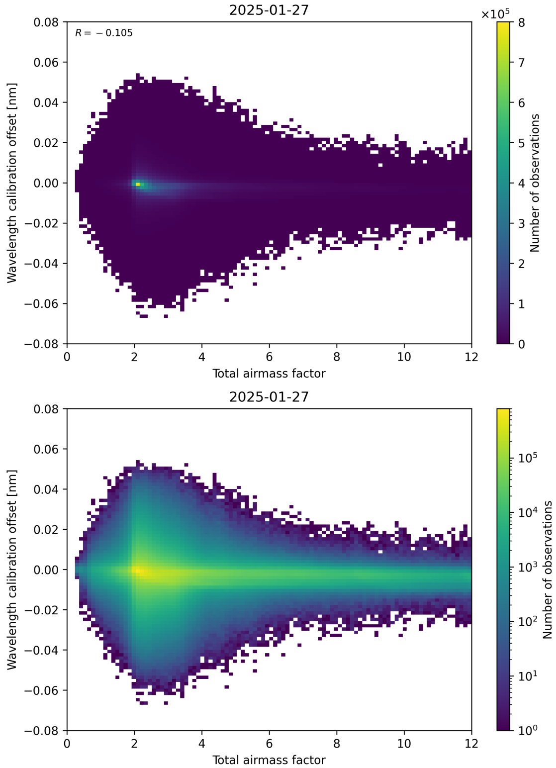
Figure 70: Scatter density plot of “Total airmass factor” against “Wavelength calibration offset” for 2025-01-26 to 2025-01-28.
