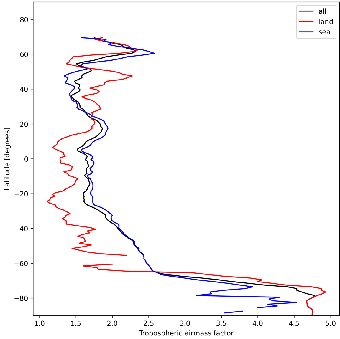
Figure 14: Zonal average of “Tropospheric airmass factor” for 2025-01-26 to 2025-01-28.
