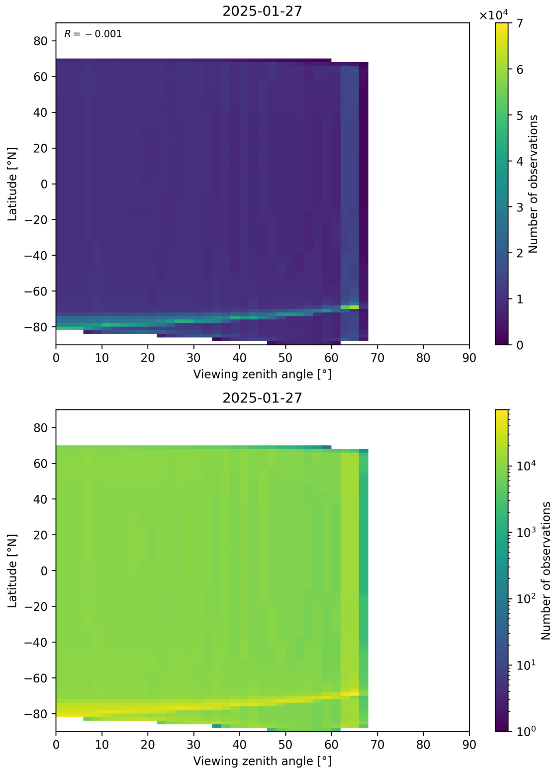
Figure 163: Scatter density plot of “Viewing zenith angle” against “Latitude” for 2025-01-26 to 2025-01-28.
