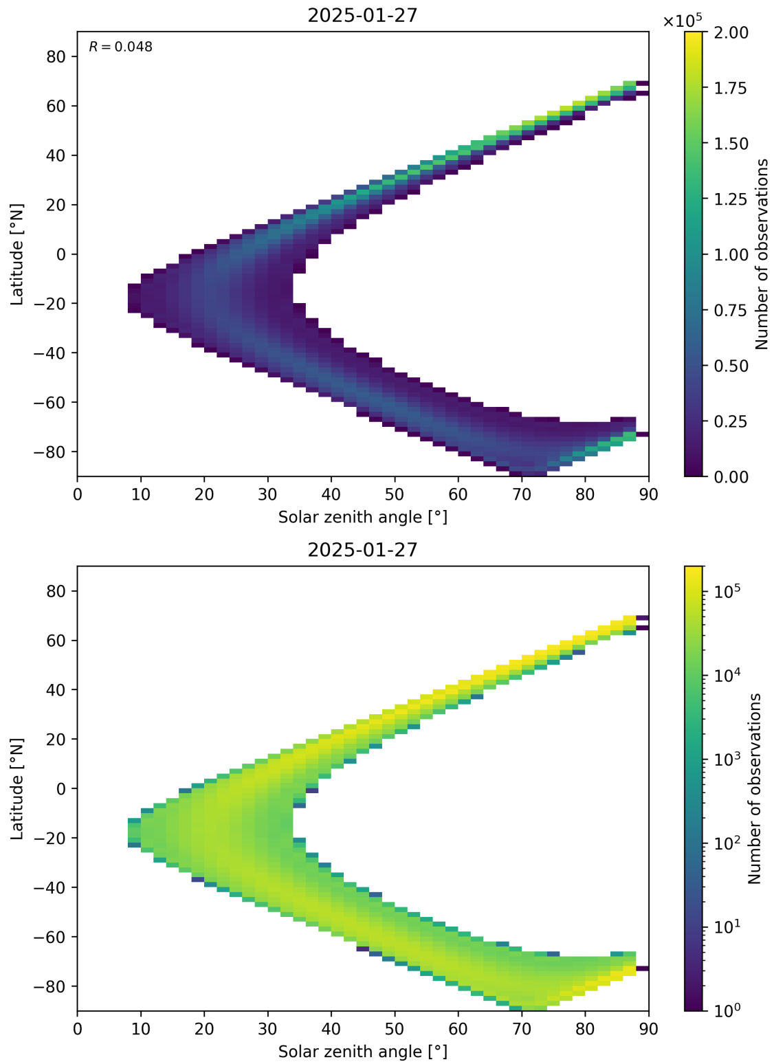
Figure 149: Scatter density plot of “Solar zenith angle” against “Latitude” for 2025-01-26 to 2025-01-28.
