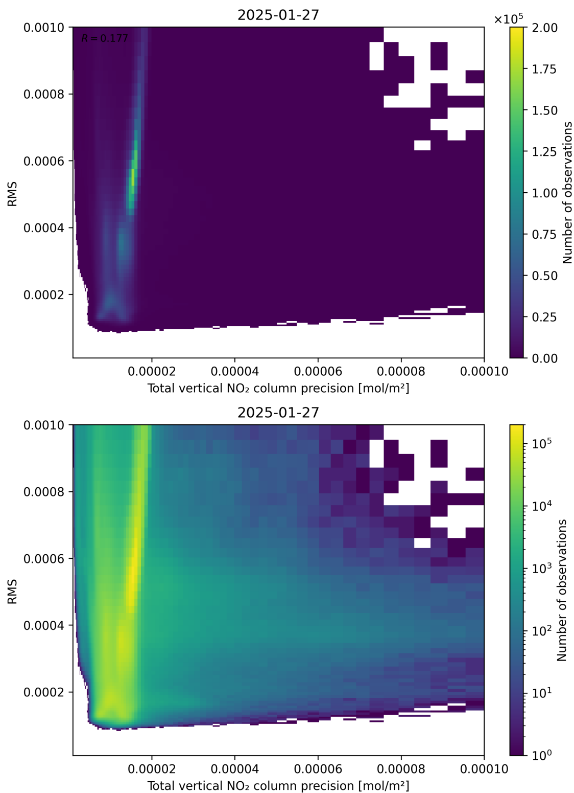
Figure 119: Scatter density plot of “Total vertical NO 2 column precision” against “RMS” for 2025-01-26 to 2025-01-28.
