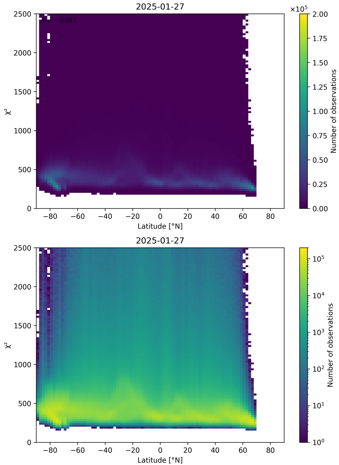
Figure 86: Scatter density plot of “Latitude” against “ \chi^2 ” for 2025-01-26 to 2025-01-28.
