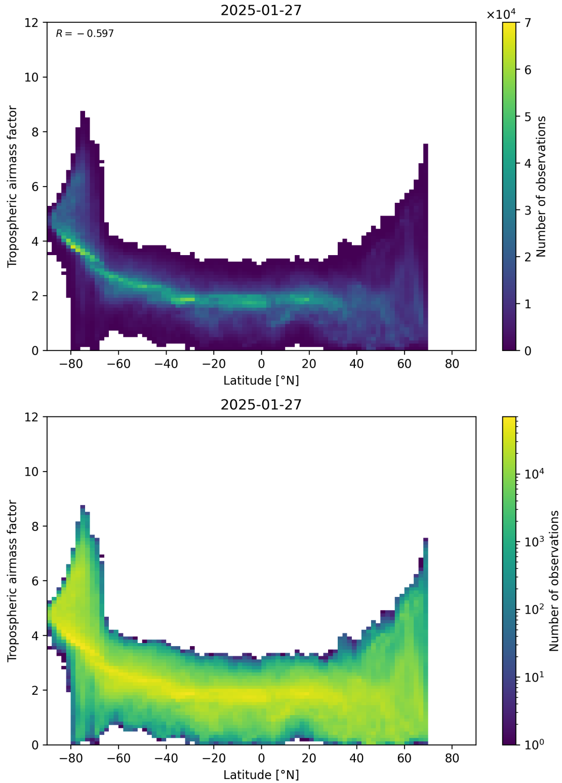
Figure 85: Scatter density plot of “Latitude” against “Tropospheric air mass factor” for 2025-01-26 to 2025-01-28.
