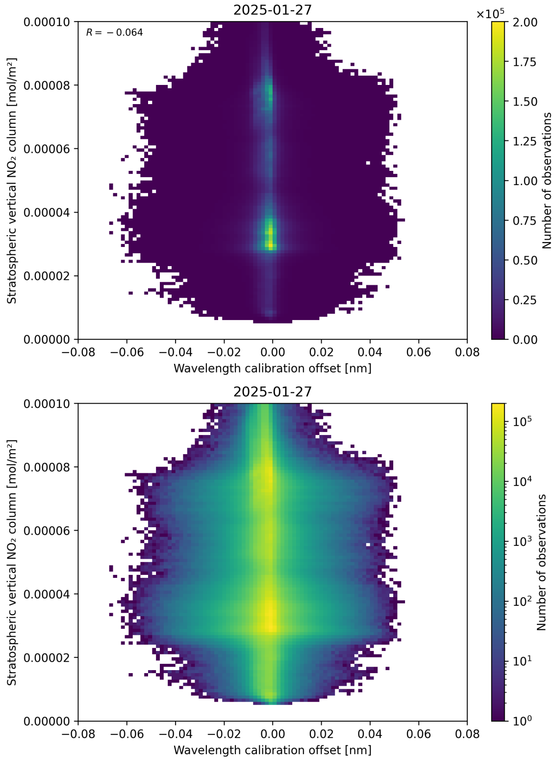
Figure 176: Scatter density plot of “Wavelength calibration offset” against “Stratospheric vertical NO 2 column” for 2025-01-26 to 2025-01-28.
