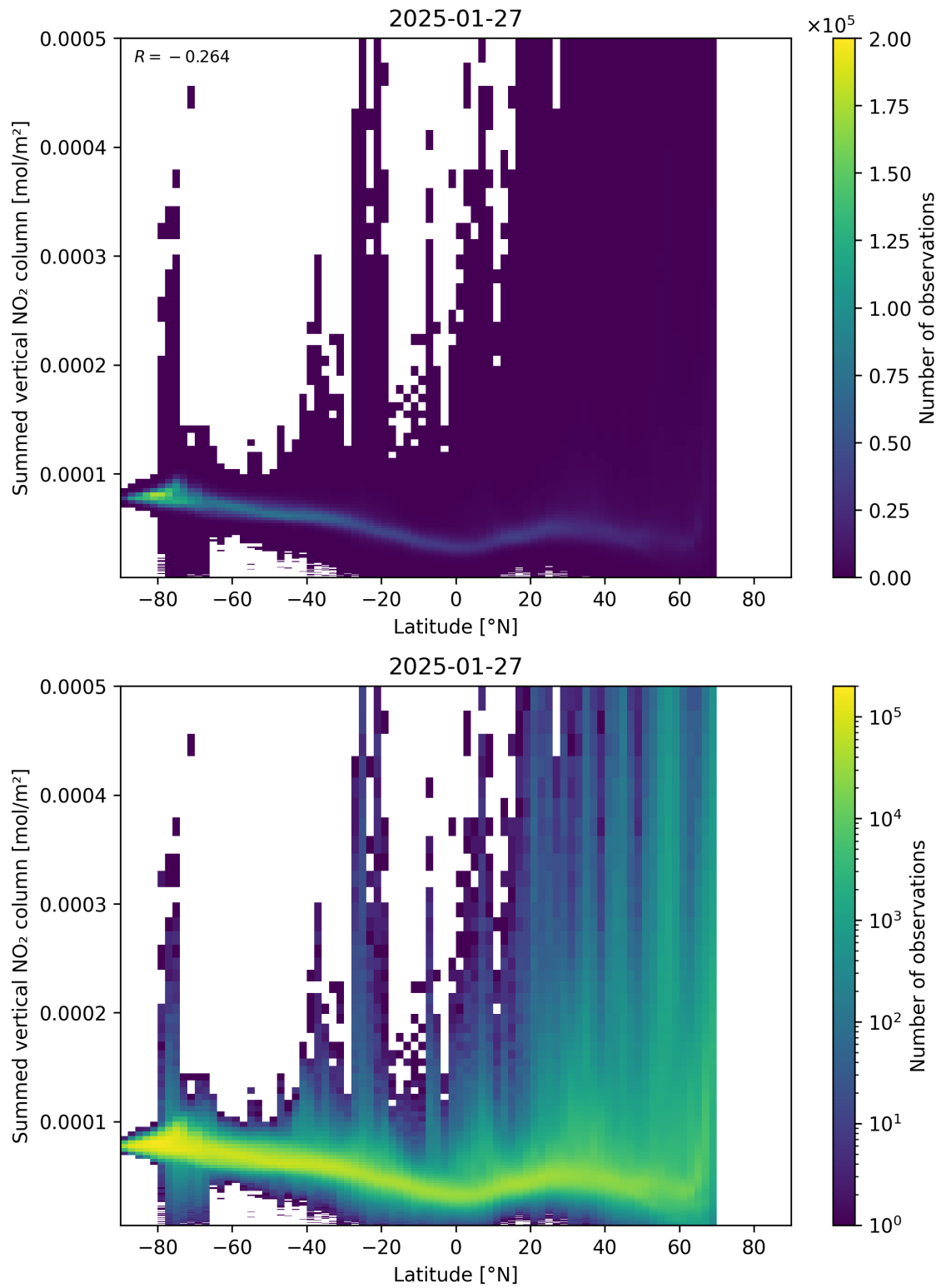
Figure 88: Scatter density plot of “Latitude” against “Summed vertical NO 2 column” for 2025-01-26 to 2025-01-28.
