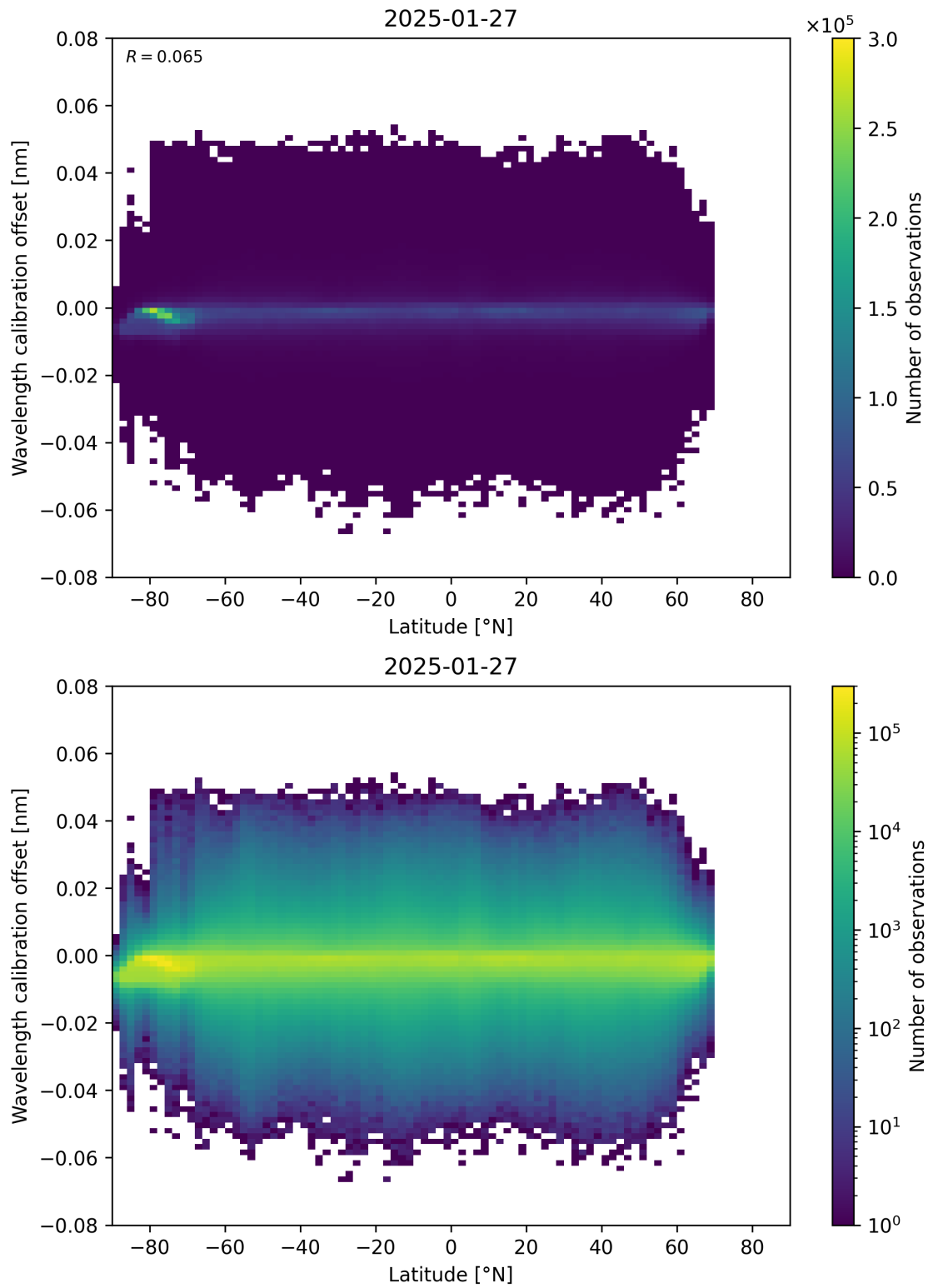
Figure 95: Scatter density plot of “Latitude” against “Wavelength calibration offset” for 2025-01-26 to 2025-01-28.
