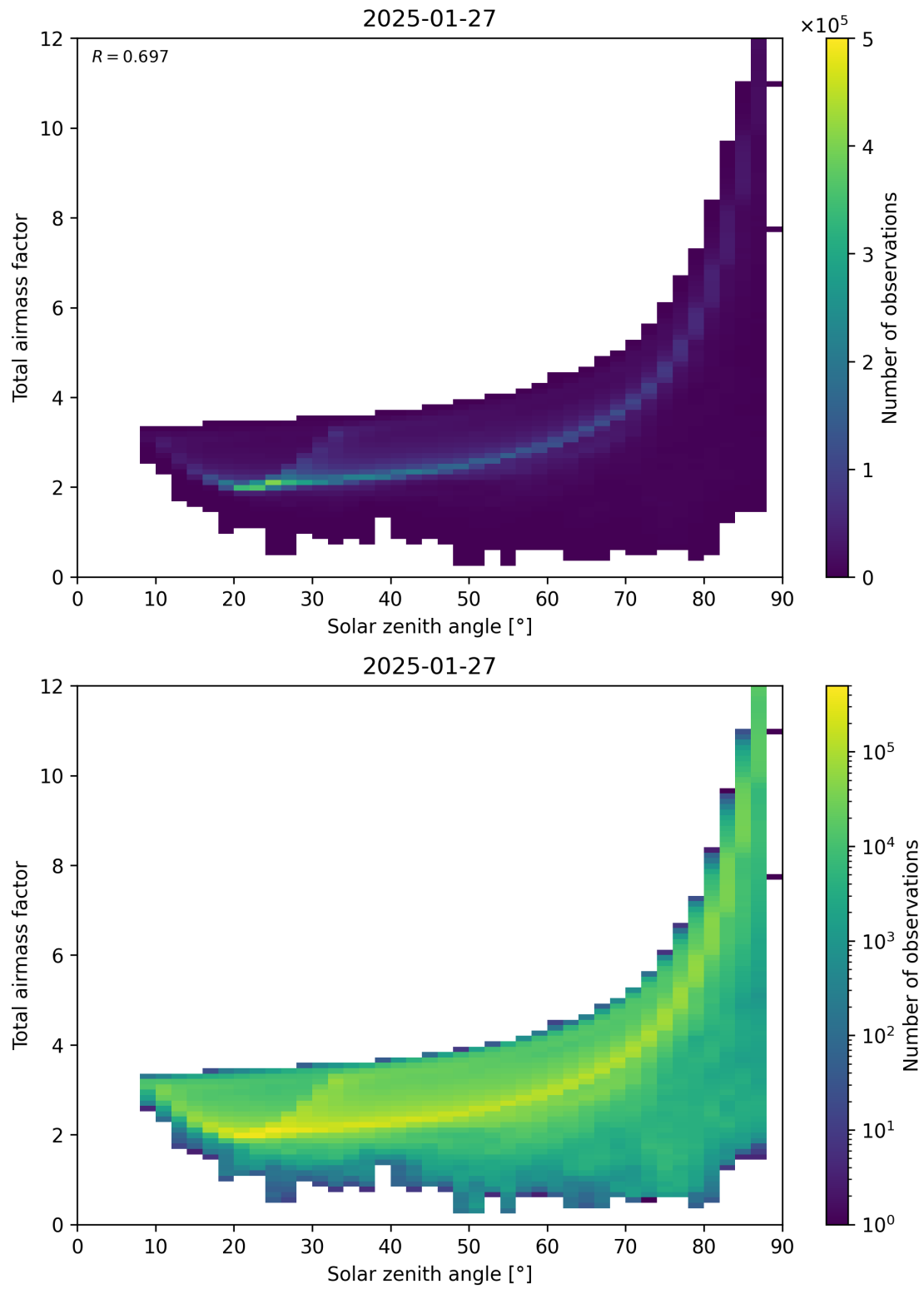
Figure 146: Scatter density plot of “Solar zenith angle” against “Total air mass factor” for 2025-01-26 to 2025-01-28.
