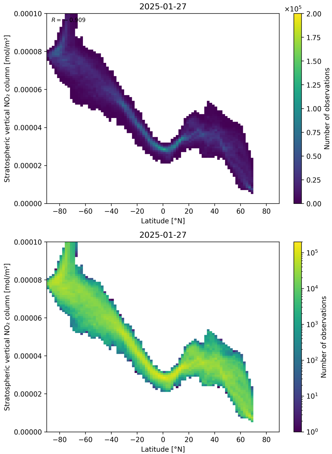
Figure 87: Scatter density plot of “Latitude” against “Stratospheric vertical NO 2 column” for 2025-01-26 to 2025-01-28.
