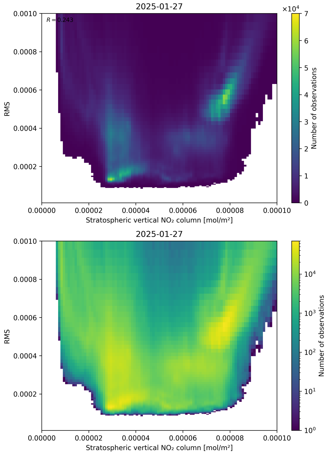
Figure 102: Scatter density plot of “Stratospheric vertical NO 2 column” against “RMS” for 2025-01-26 to 2025-01-28.
