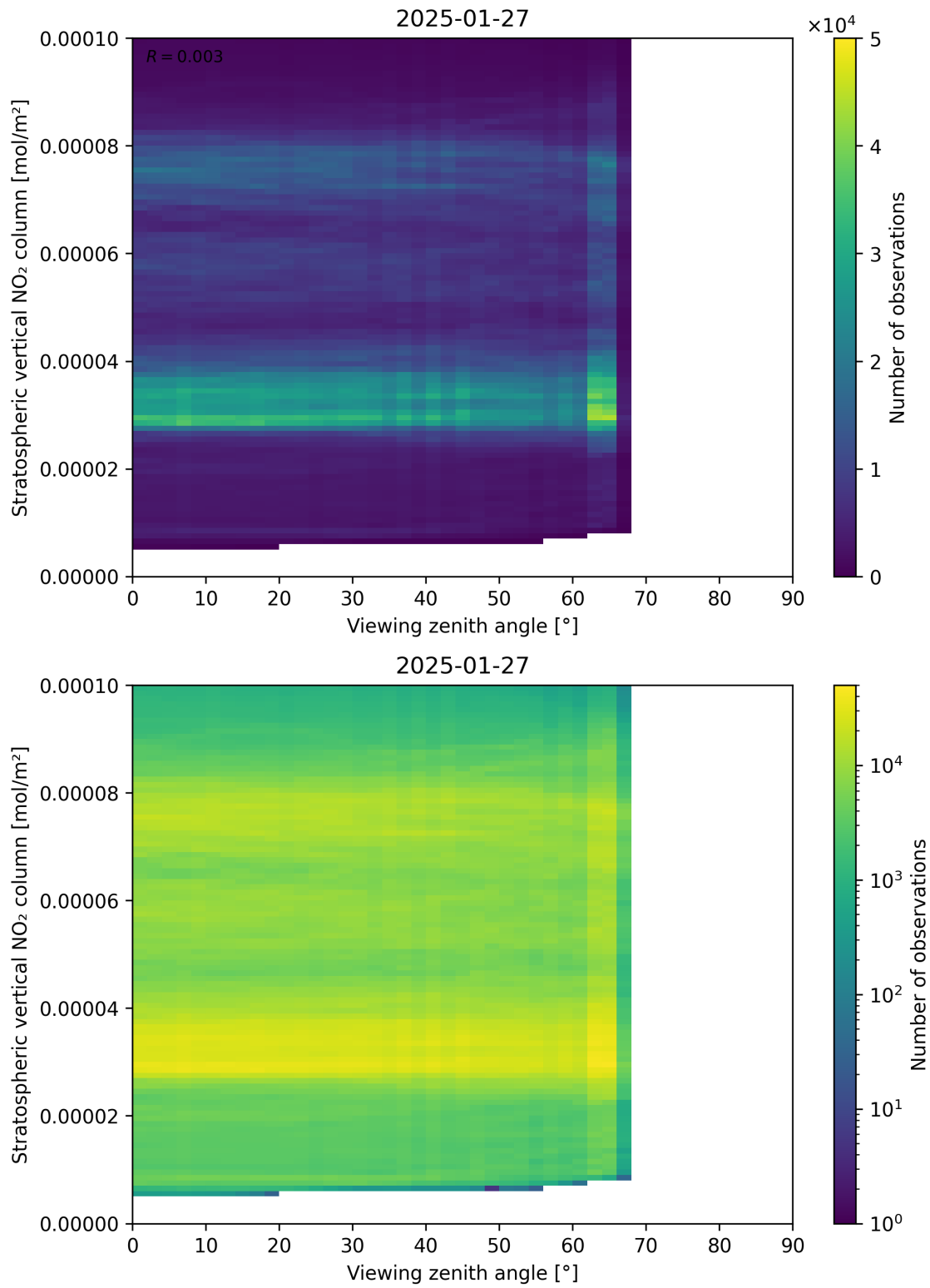
Figure 164: Scatter density plot of “Viewing zenith angle” against “Stratospheric vertical NO 2 column” for 2025-01-26 to 2025-01-28.
