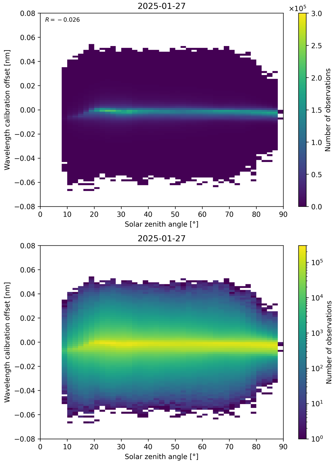
Figure 158: Scatter density plot of “Solar zenith angle” against “Wavelength calibration offset” for 2025-01-26 to 2025-01-28.
