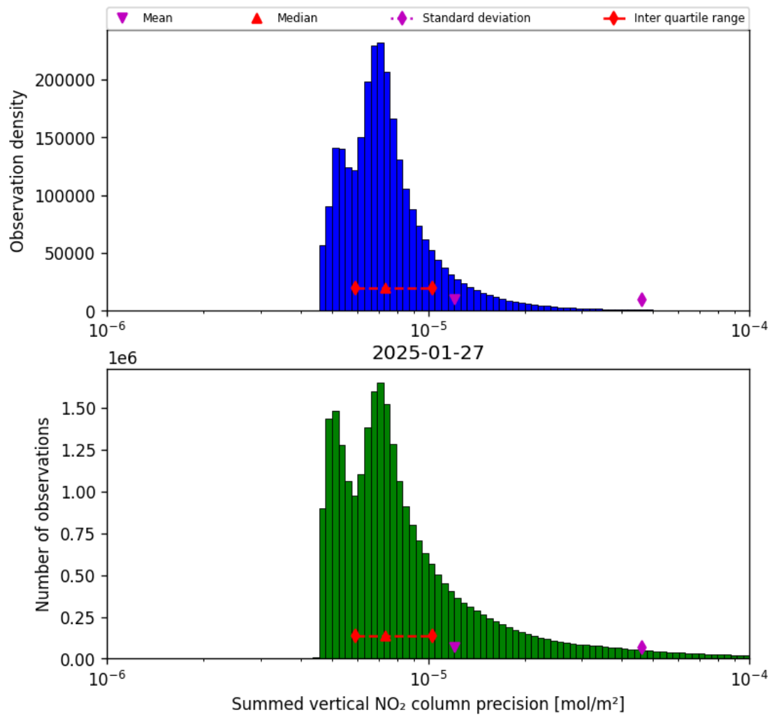
Figure 41: Histogram of “Summed vertical NO 2 column precision” for 2025-01-26 to 2025-01-28
