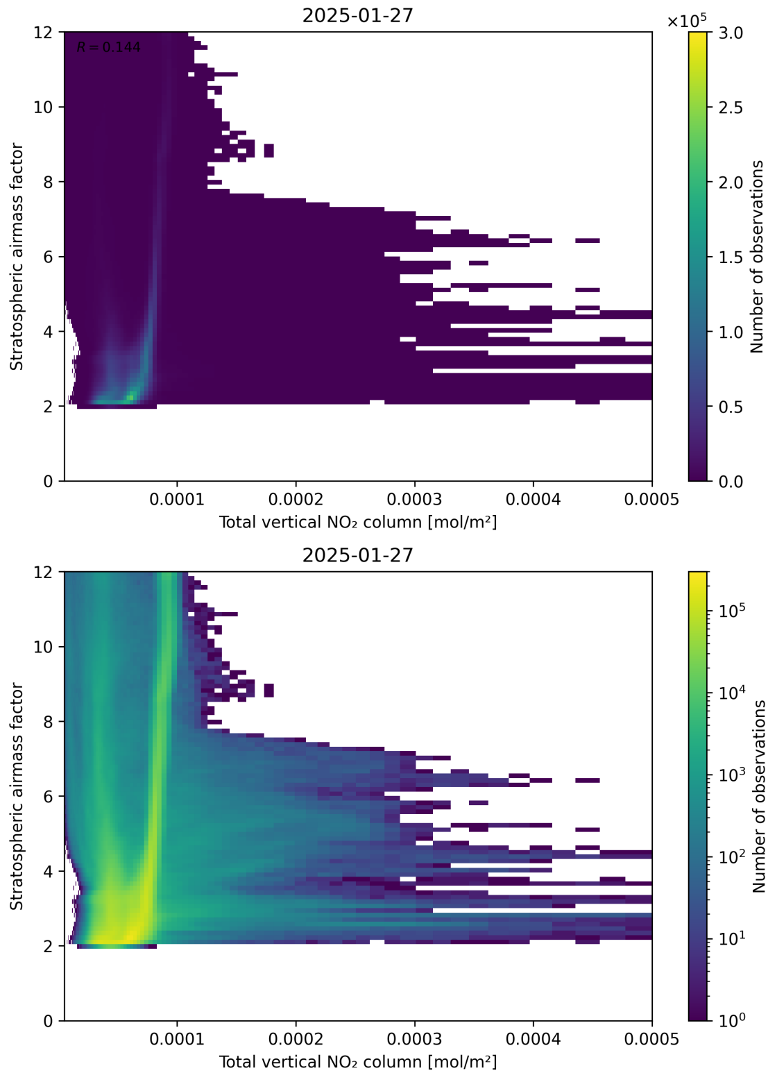
Figure 110: Scatter density plot of “Total vertical NO 2 column” against “Stratospheric airmass factor” for 2025-01-26 to 2025-01-28.
