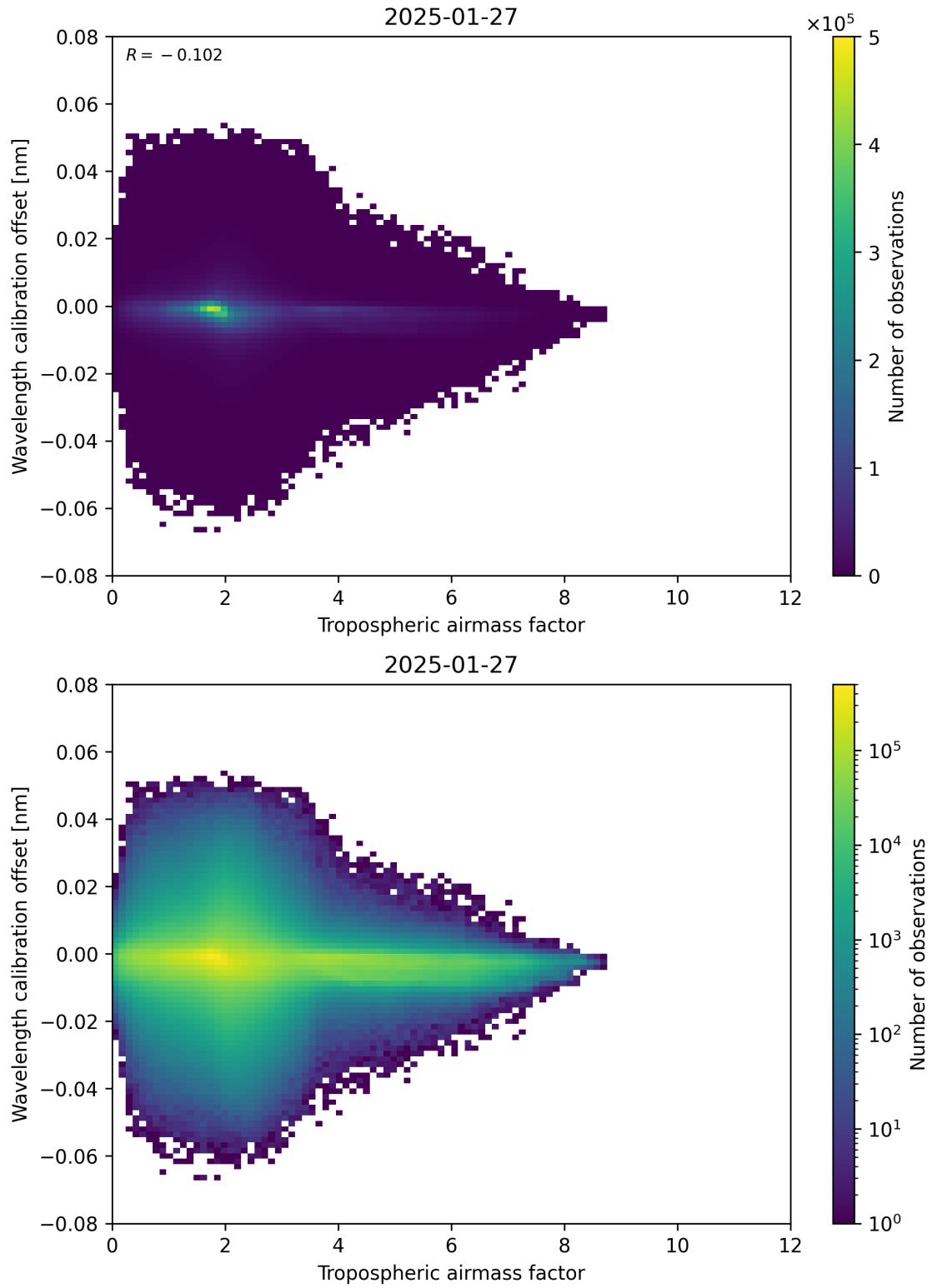
Figure 80: Scatter density plot of “Tropospheric airmass factor” against “Wavelength calibration offset” for 2025-01-26 to 2025-01-28.
