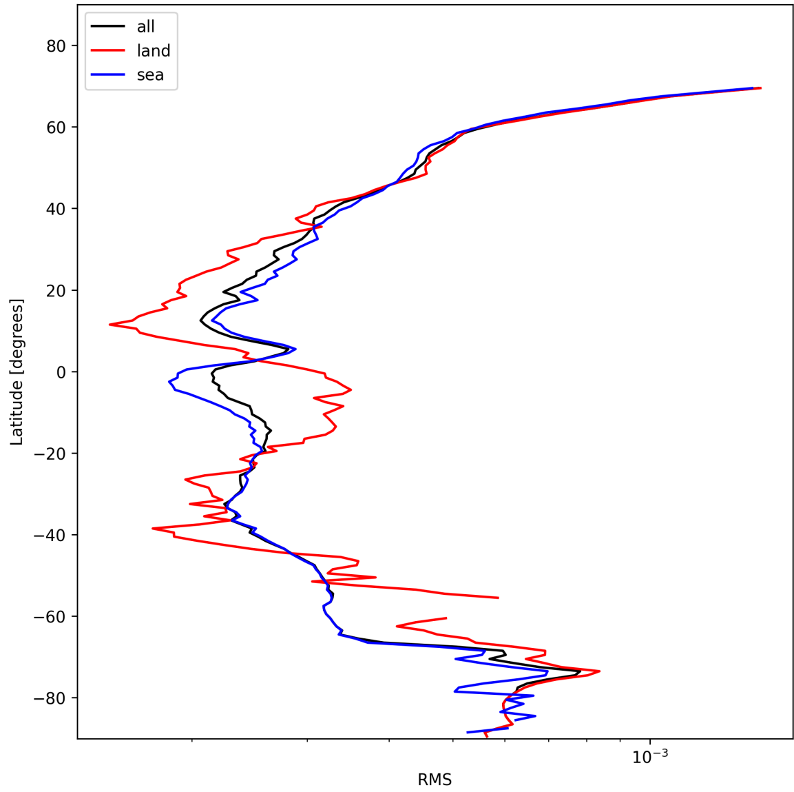
Figure 26: Zonal average of “RMS” for 2025-01-26 to 2025-01-28.
