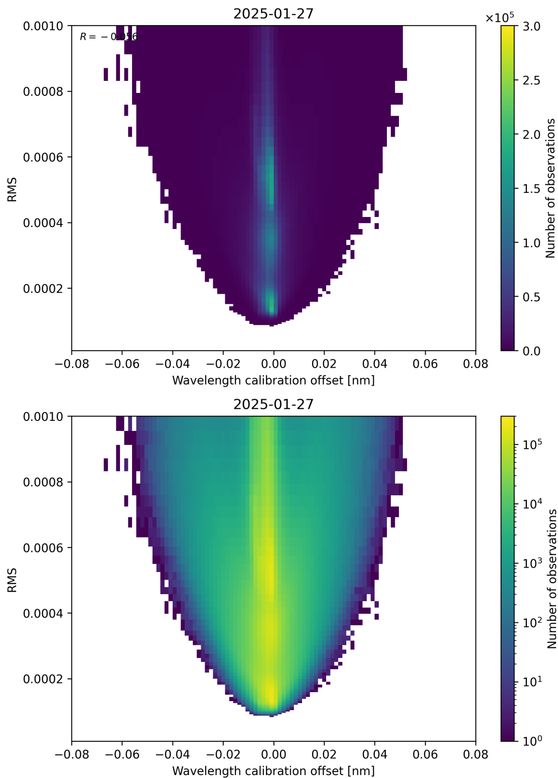
Figure 181: Scatter density plot of “Wavelength calibration offset” against “RMS” for 2025-01-26 to 2025-01-28.
