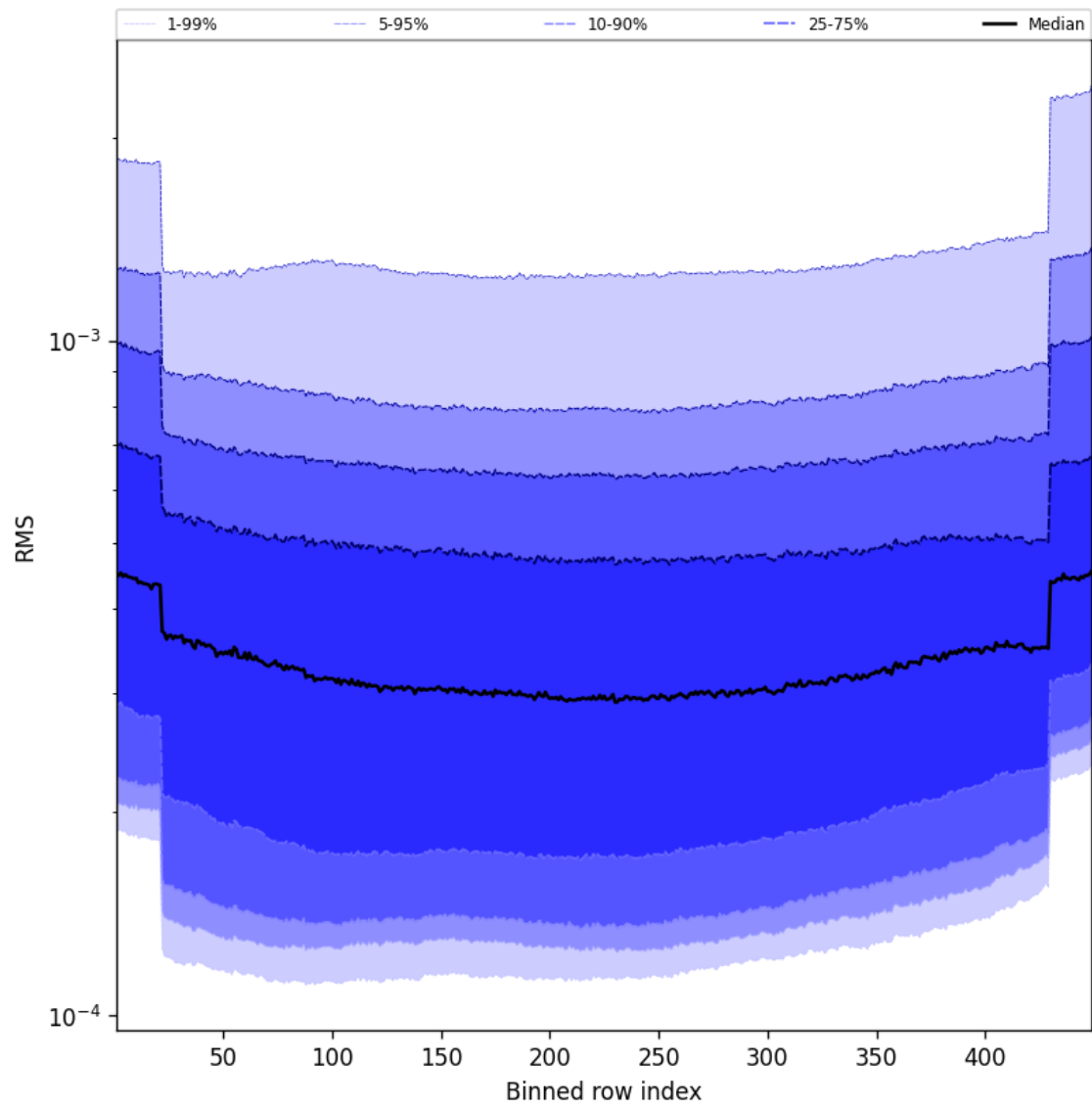
Figure 60: Along track statistics of “RMS” for 2025-01-26 to 2025-01-28
