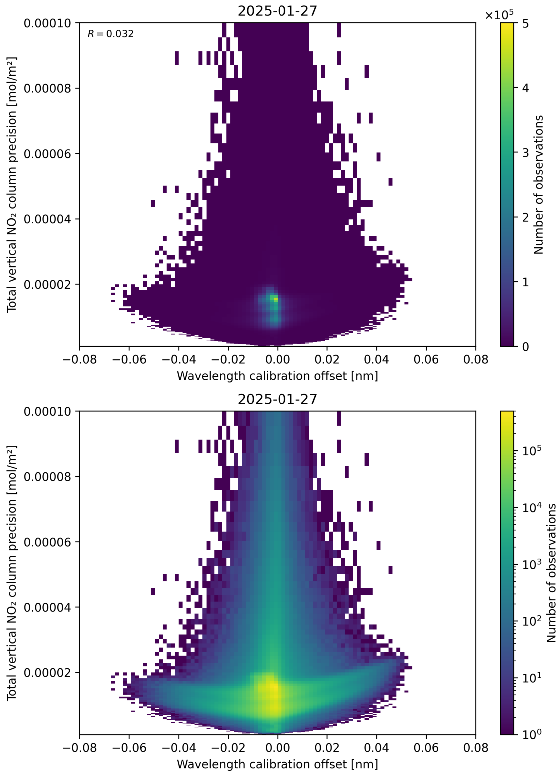
Figure 180: Scatter density plot of “Wavelength calibration offset” against “Total vertical NO 2 column precision” for 2025-01-26 to 2025-01-28.
