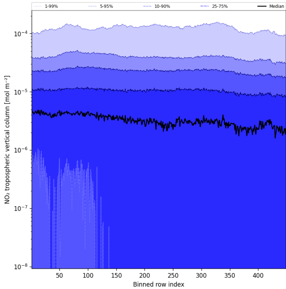
Figure 46: Along track statistics of “NO 2 tropospheric vertical column” for 2025-01-26 to 2025-01-28
