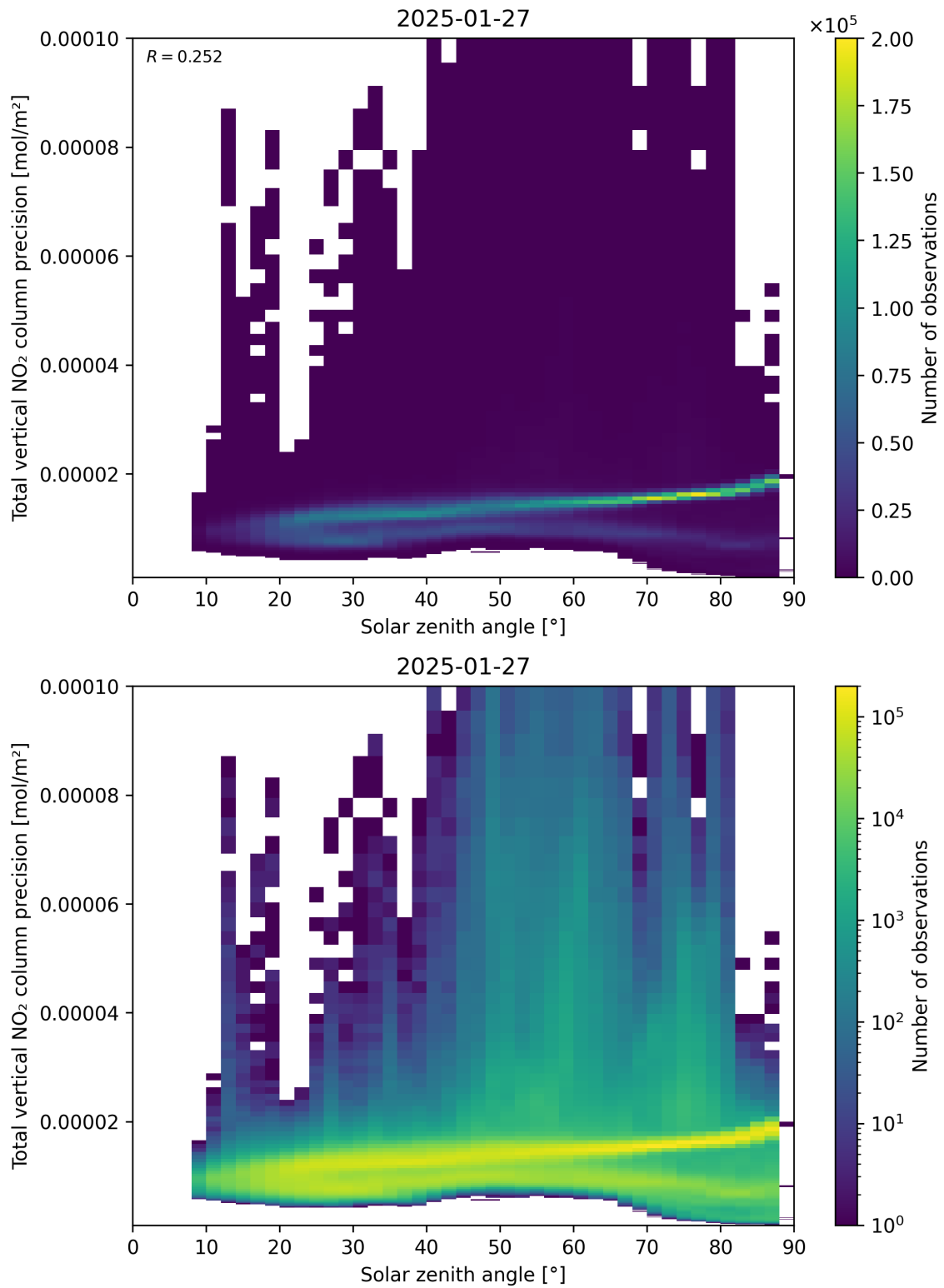
Figure 154: Scatter density plot of “Solar zenith angle” against “Total vertical NO 2 column precision” for 2025-01-26 to 2025-01-28.
