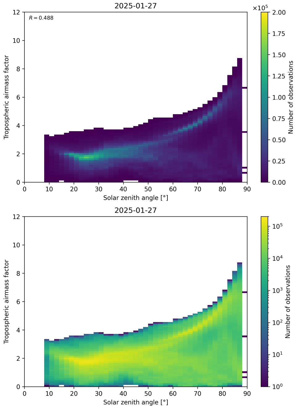
Figure 147: Scatter density plot of “Solar zenith angle” against “Tropospheric airmass factor” for 2025-01-26 to 2025-01-28.
