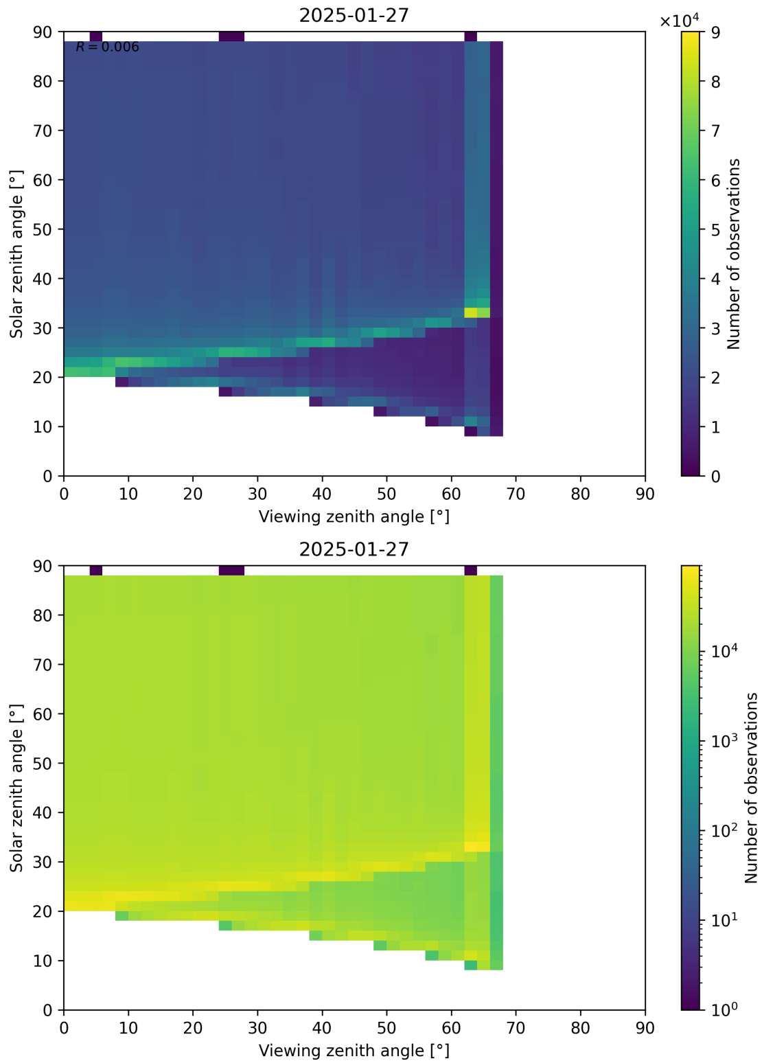
Figure 172: Scatter density plot of “Viewing zenith angle” against “Solar zenith angle” for 2025-01-26 to 2025-01-28.
