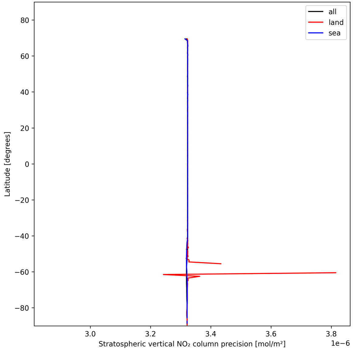
Figure 20: Zonal average of “Stratospheric vertical NO 2 column precision” for 2025-01-26 to 2025-01-28.
