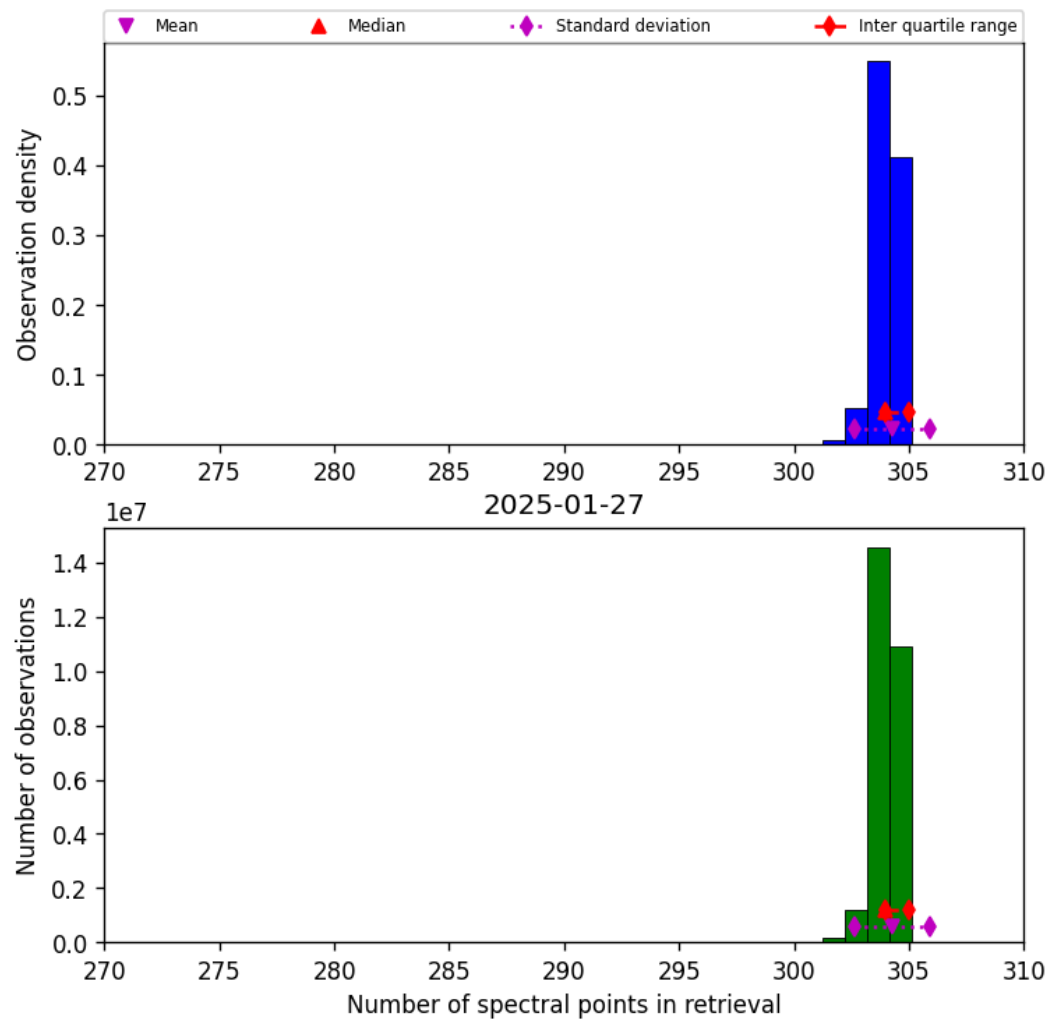
Figure 33: Histogram of “Number of spectral points in retrieval” for 2025-01-26 to 2025-01-28
