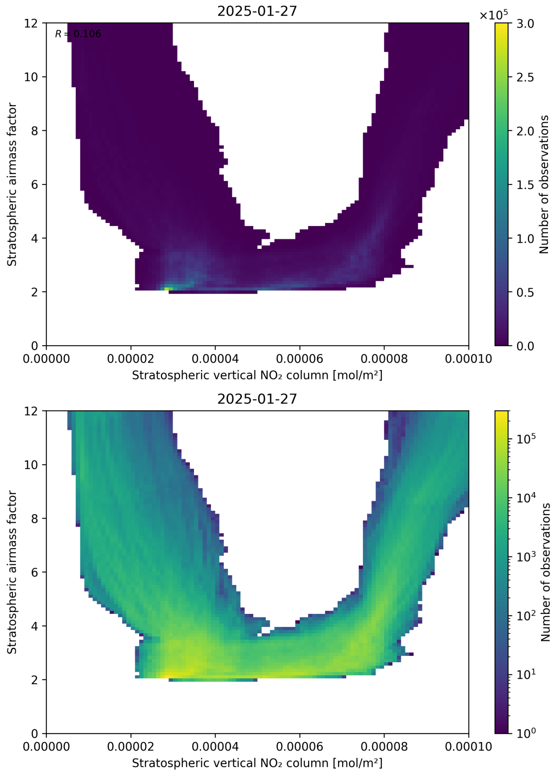
Figure 96: Scatter density plot of “Stratospheric vertical NO 2 column” against “Stratospheric airmass factor” for 2025-01-26 to 2025-01-28.
