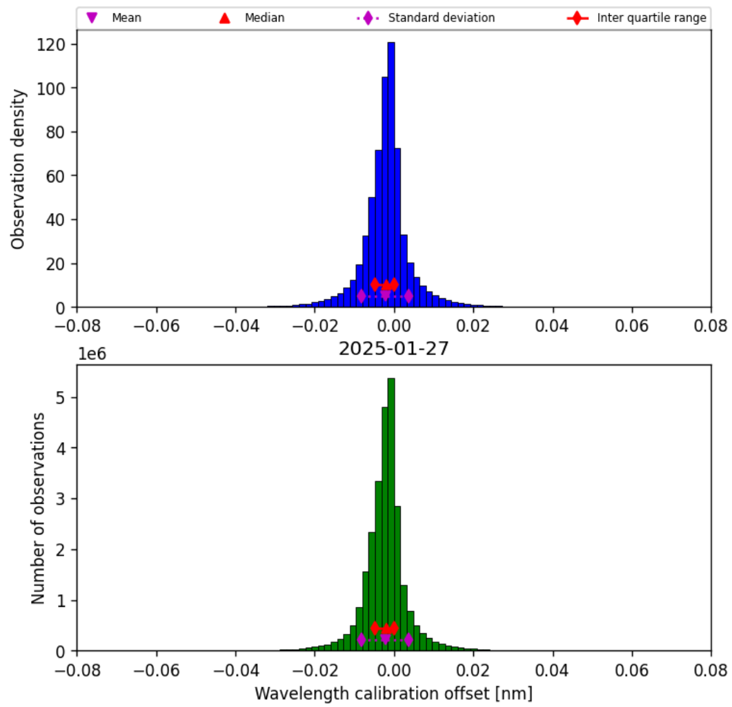
Figure 35: Histogram of “Wavelength calibration offset” for 2025-01-26 to 2025-01-28
