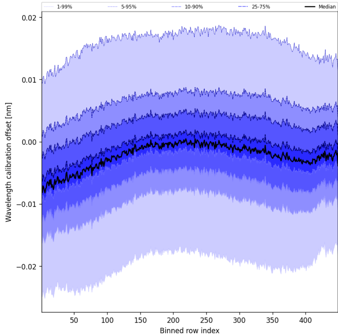
Figure 52: Along track statistics of “Wavelength calibration offset” for 2025-01-26 to 2025-01-28
