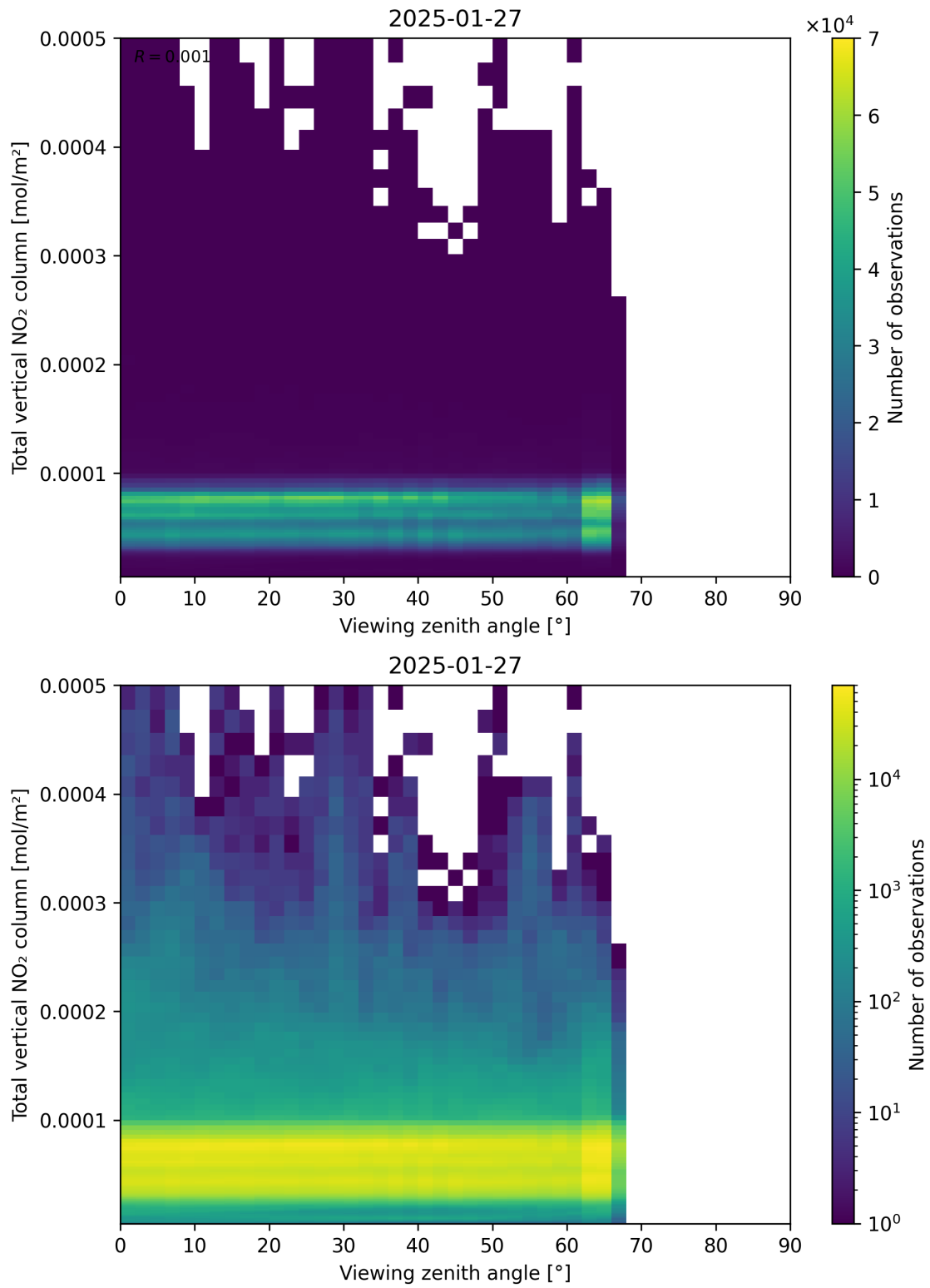
Figure 167: Scatter density plot of “Viewing zenith angle” against “Total vertical NO 2 column” for 2025-01-26 to 2025-01-28.
