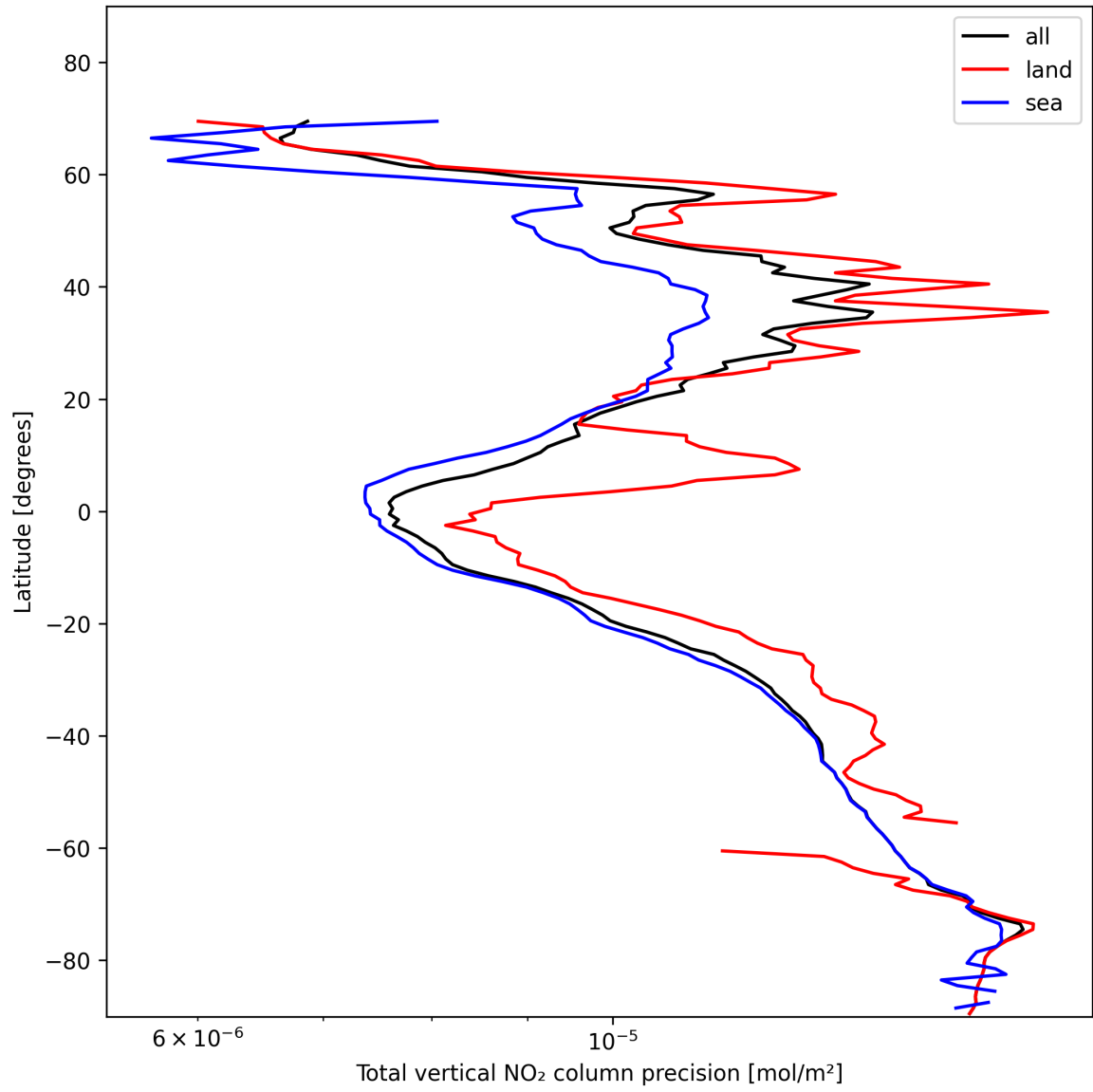
Figure 22: Zonal average of “Total vertical NO 2 column precision” for 2025-01-26 to 2025-01-28.
