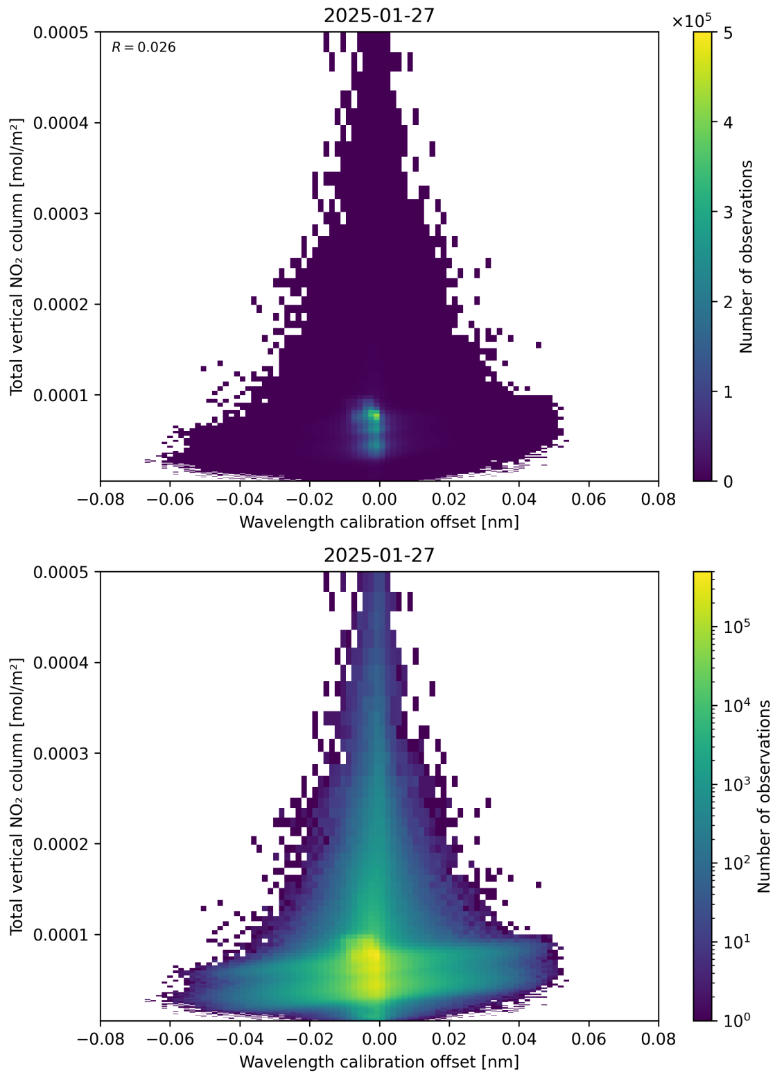
Figure 179: Scatter density plot of “Wavelength calibration offset” against “Total vertical NO 2 column” for 2025-01-26 to 2025-01-28.
