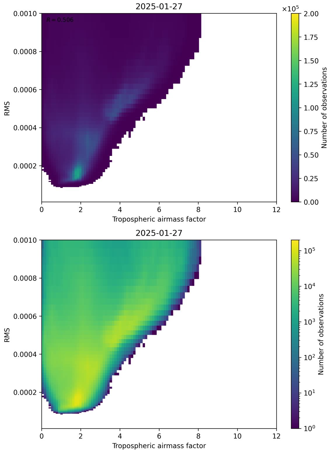
Figure 79: Scatter density plot of “Tropospheric airmass factor” against “RMS” for 2025-01-26 to 2025-01-28.
