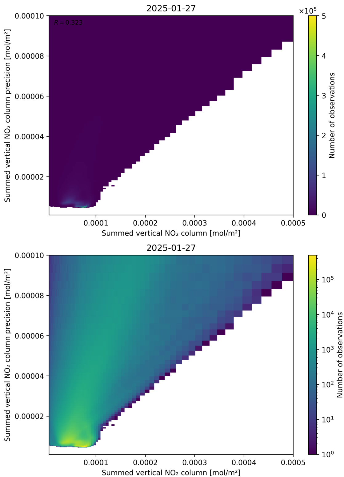
Figure 105: Scatter density plot of “Summed vertical NO 2 column” against “Summed vertical NO 2 column precision” for 2025-01-26 to 2025-01-28.
