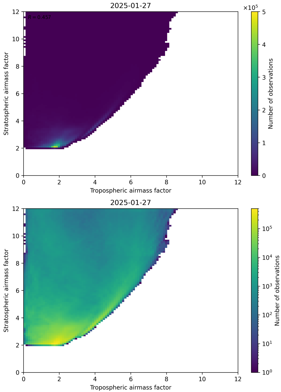
Figure 71: Scatter density plot of “Tropospheric airmass factor” against “Stratospheric airmass factor” for 2025-01-26 to 2025-01-28.
