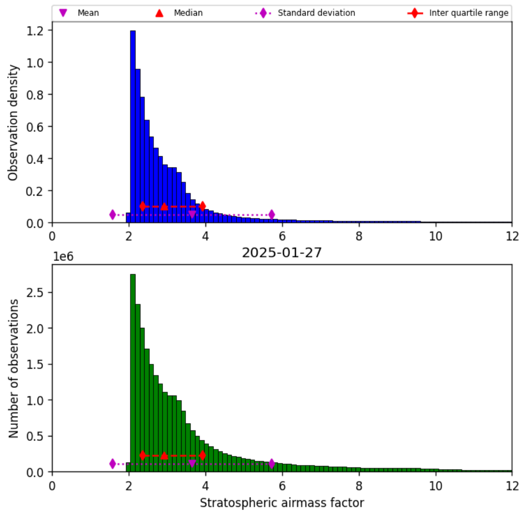
Figure 44: Histogram of “Stratospheric airmass factor” for 2025-01-26 to 2025-01-28
