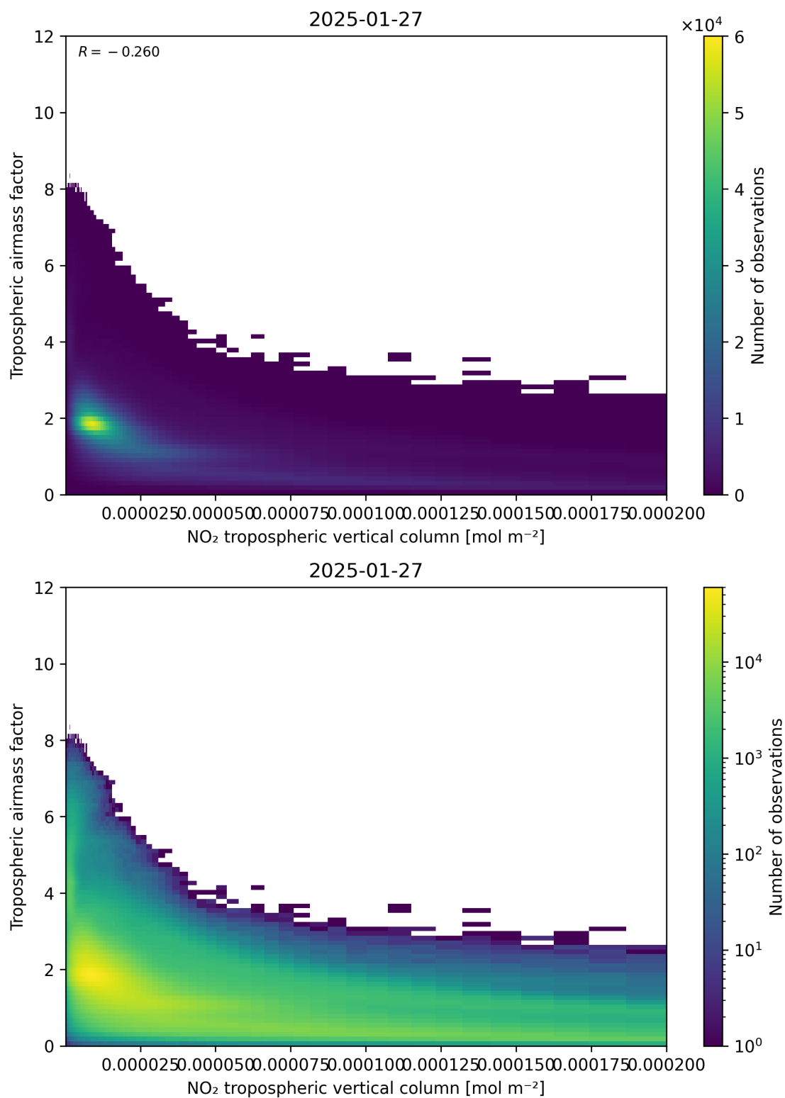
Figure 123: Scatter density plot of “NO 2 tropospheric vertical column” against “Tropospheric air mass factor” for 2025-01-26 to 2025-01-28.
