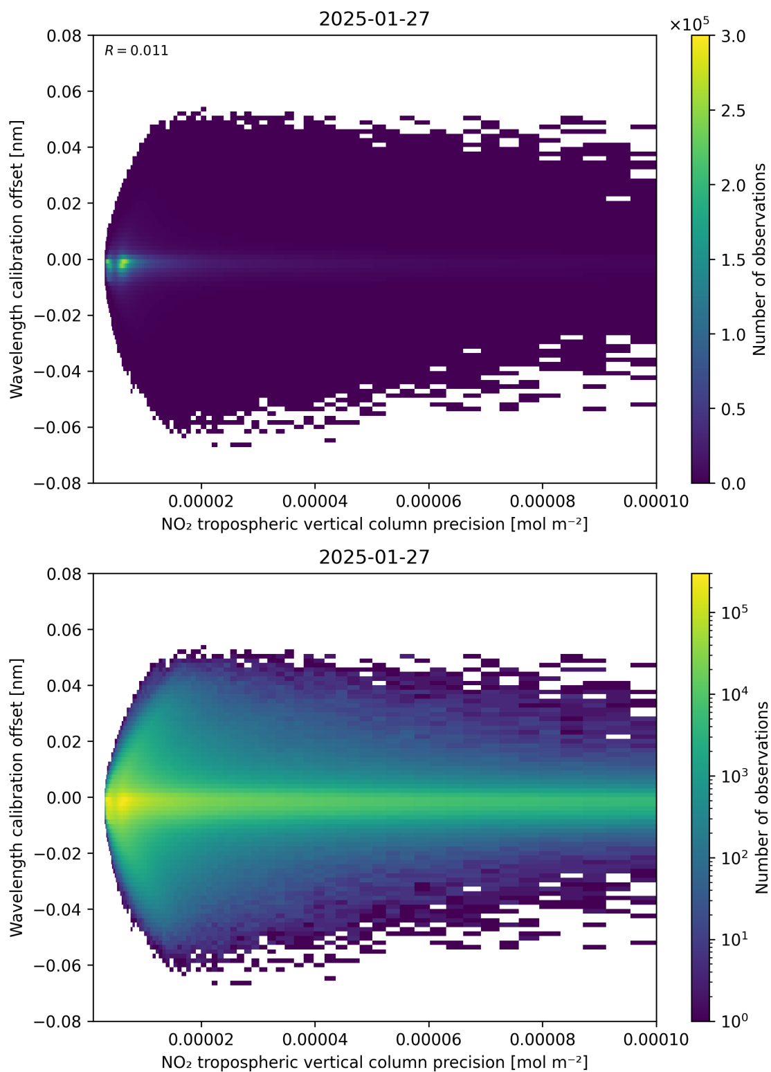
Figure 141: Scatter density plot of “NO 2 tropospheric vertical column precision” against “Wavelength calibration offset” for 2025-01-26 to 2025-01-28.
