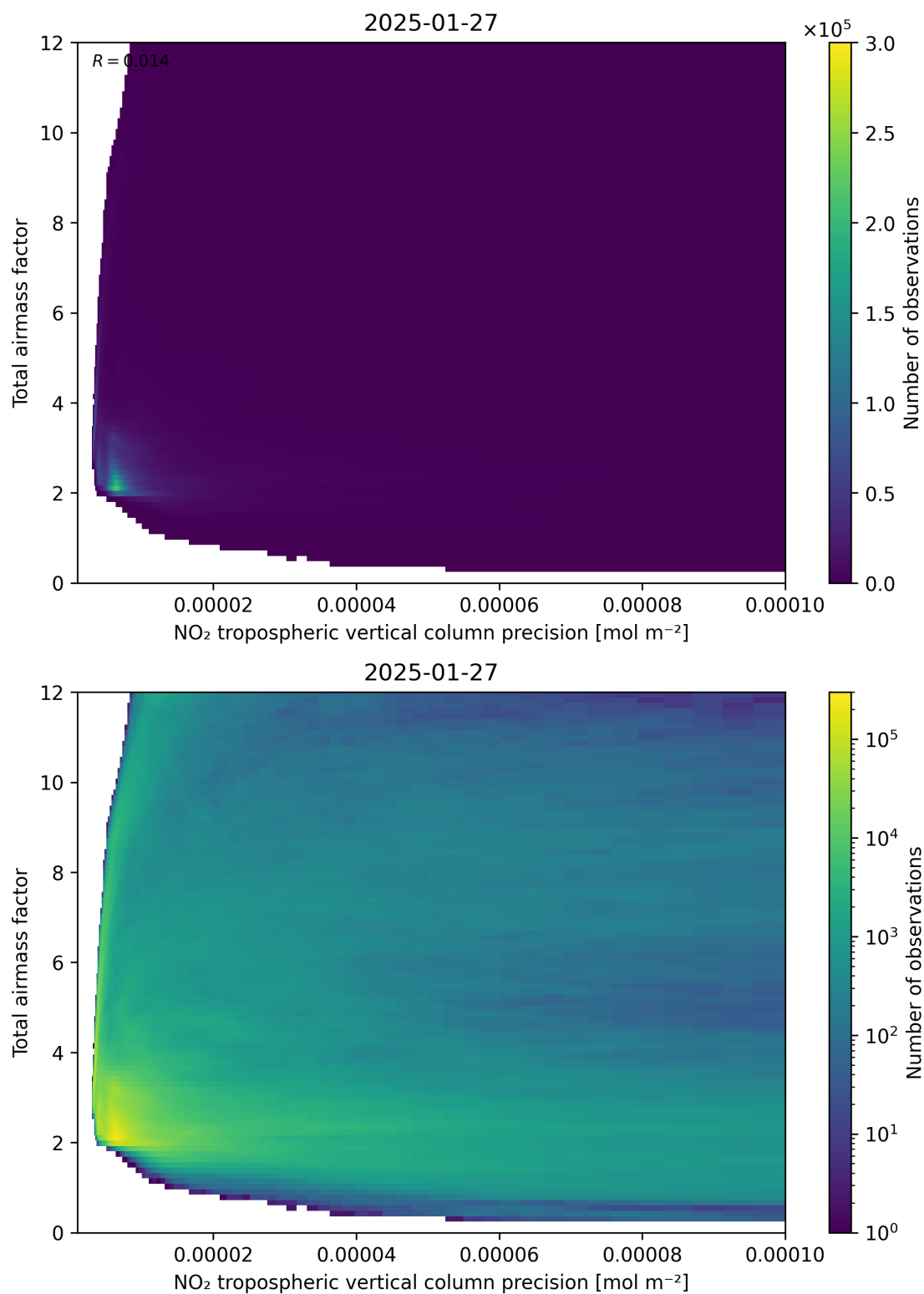
Figure 132: Scatter density plot of “NO 2 tropospheric vertical column precision” against “Total air mass factor” for 2025-01-26 to 2025-01-28.
