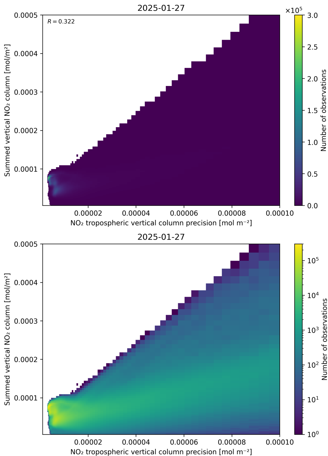
Figure 136: Scatter density plot of “NO 2 tropospheric vertical column precision” against “Summed vertical NO 2 column” for 2025-01-26 to 2025-01-28.
