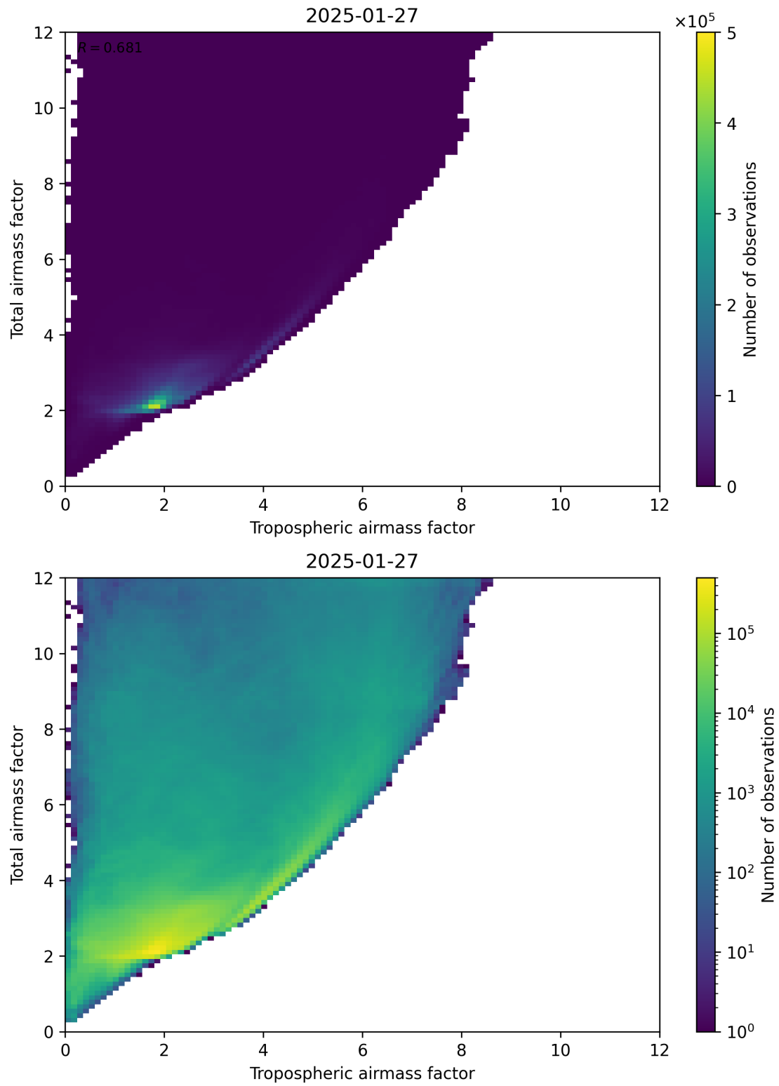
Figure 72: Scatter density plot of “Tropospheric airmass factor” against “Total airmass factor” for 2025-01-26 to 2025-01-28.
