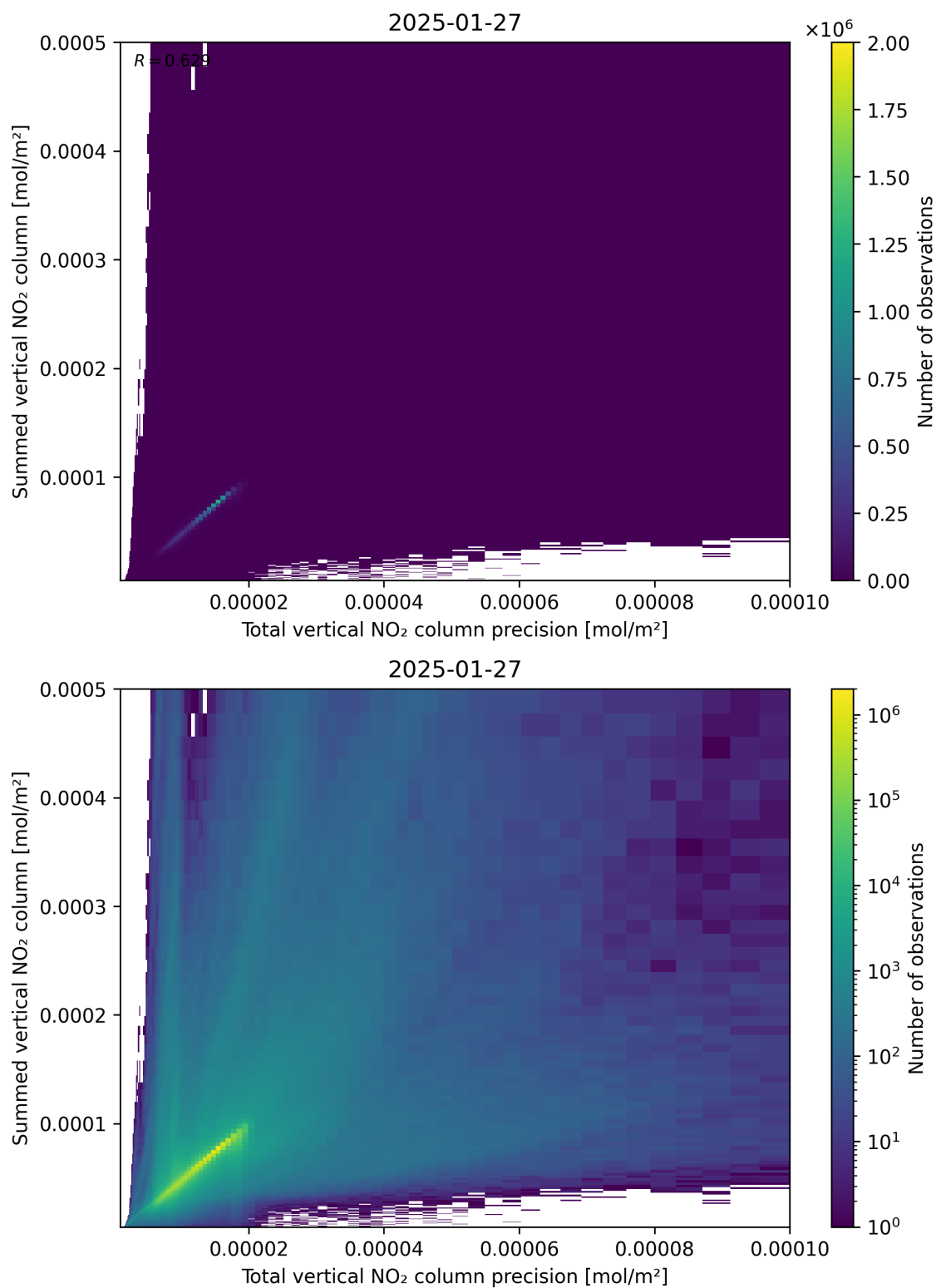
Figure 117: Scatter density plot of “Total vertical NO 2 column precision” against “Summed vertical NO 2 column” for 2025-01-26 to 2025-01-28.
