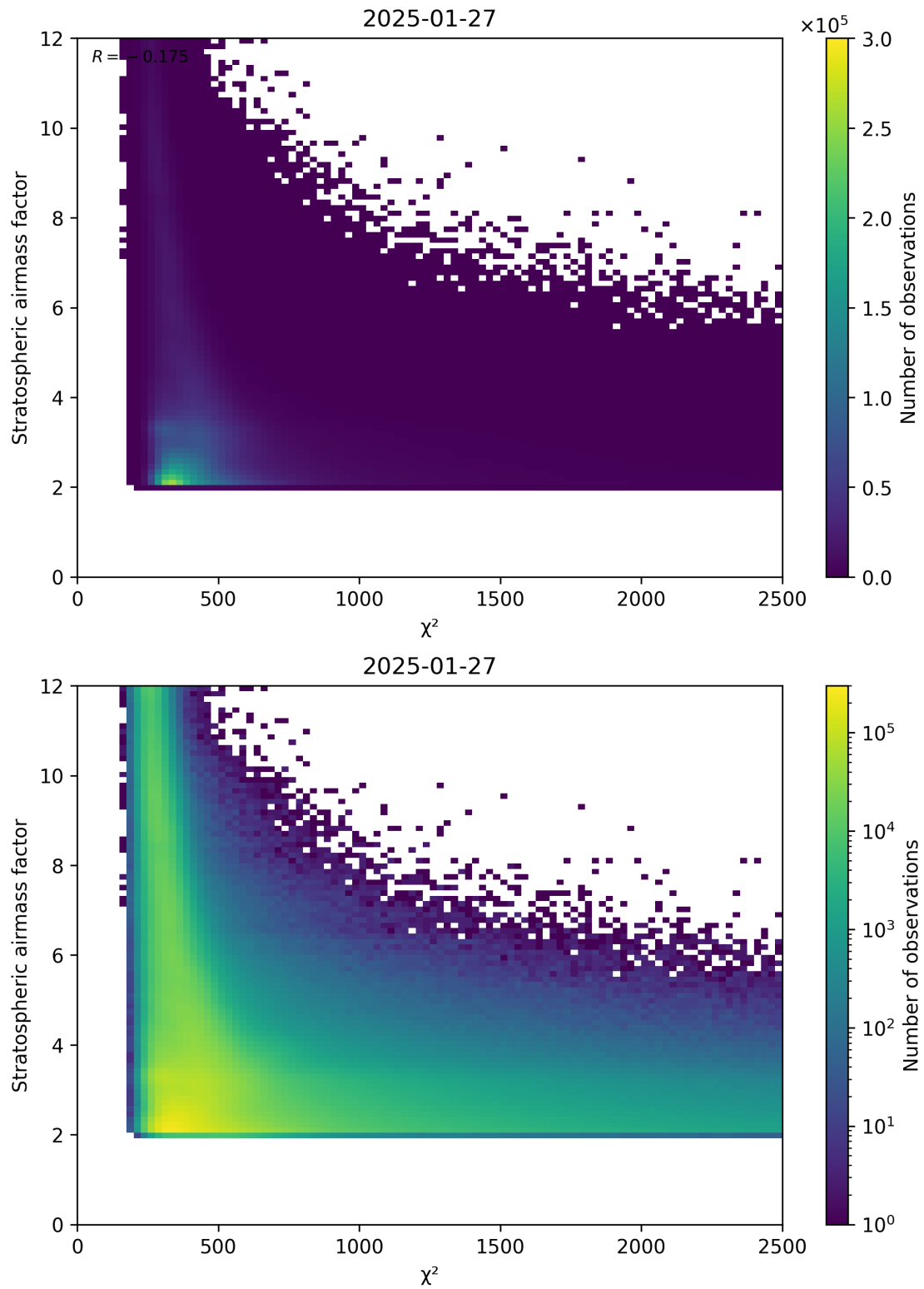
Figure 81: Scatter density plot of “ \chi^2 ” against “Stratospheric airmass factor” for 2025-01-26 to 2025-01-28.
