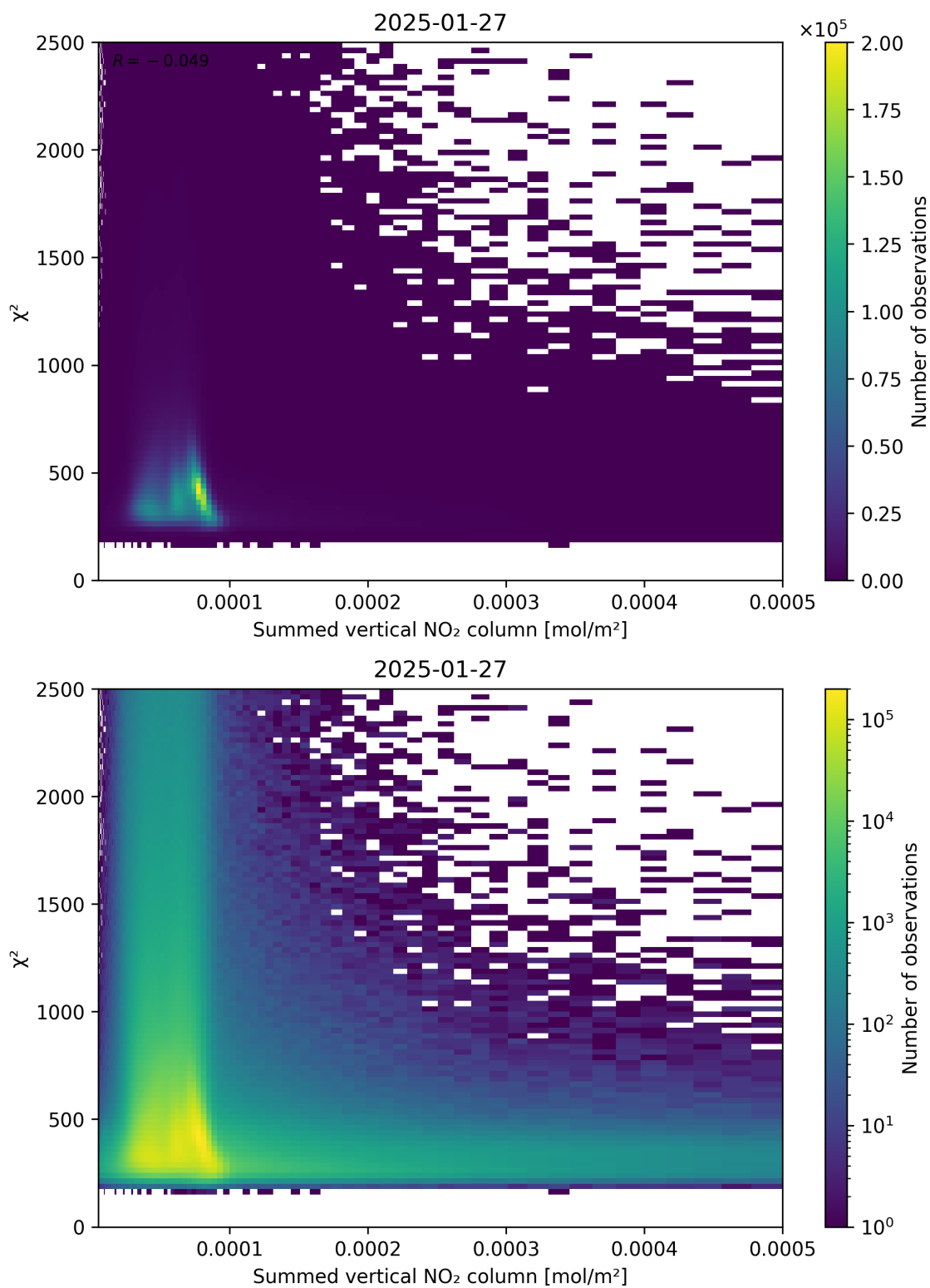
Figure 104: Scatter density plot of “Summed vertical NO 2 column” against “ \chi^2 ” for 2025-01-26 to 2025-01-28.
