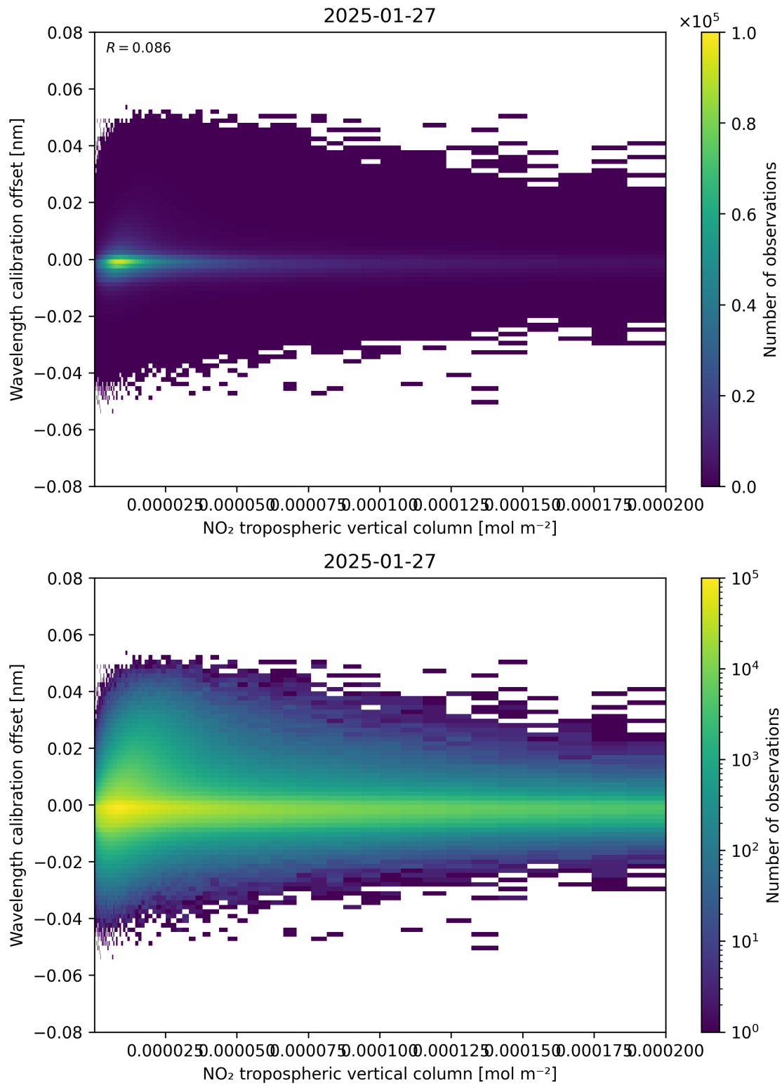
Figure 143: Scatter density plot of “NO 2 tropospheric vertical column” against “Wavelength calibration offset” for 2025-01-26 to 2025-01-28.
