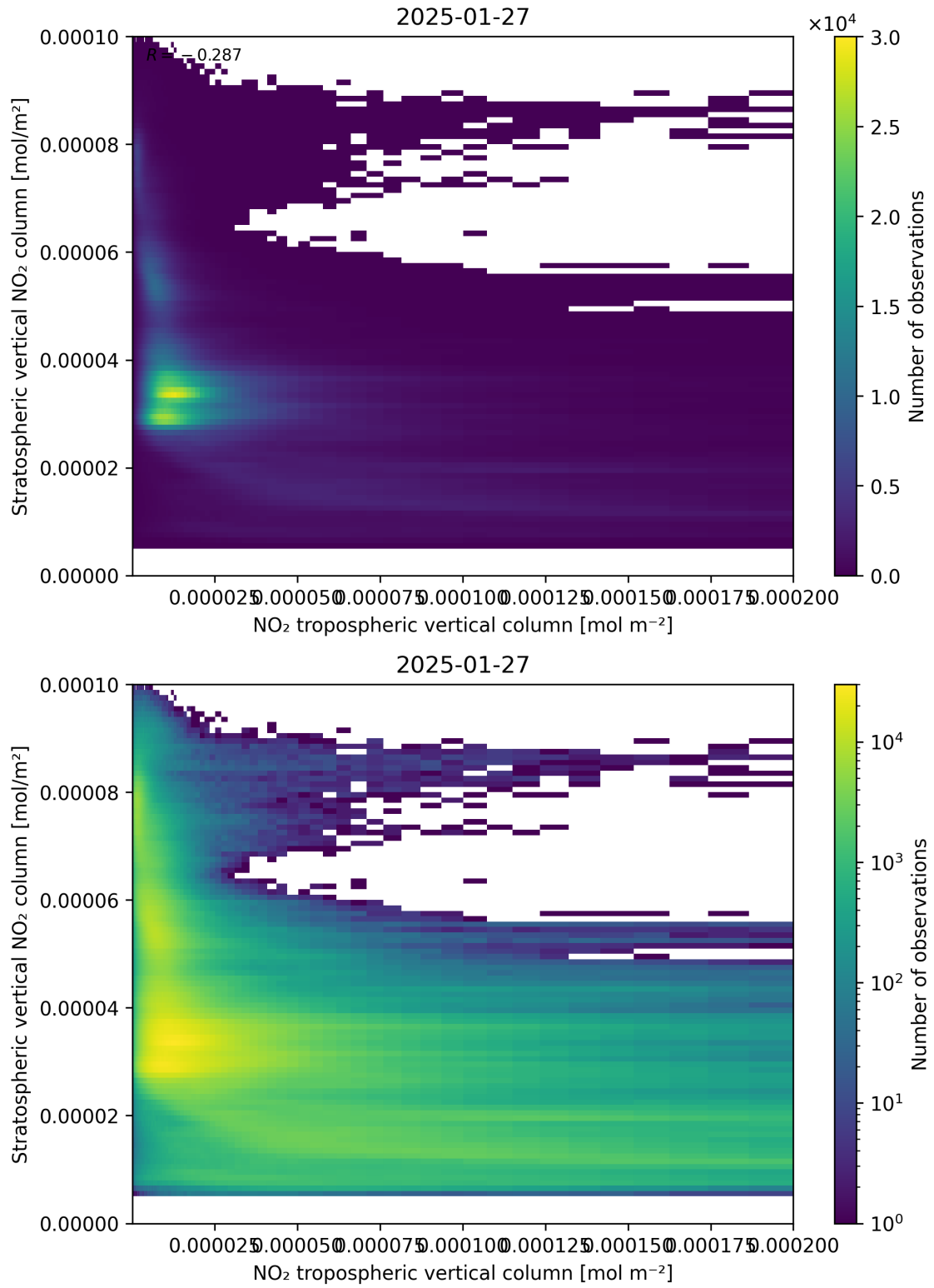
Figure 125: Scatter density plot of “NO 2 tropospheric vertical column” against “Stratospheric vertical NO 2 column” for 2025-01-26 to 2025-01-28.
