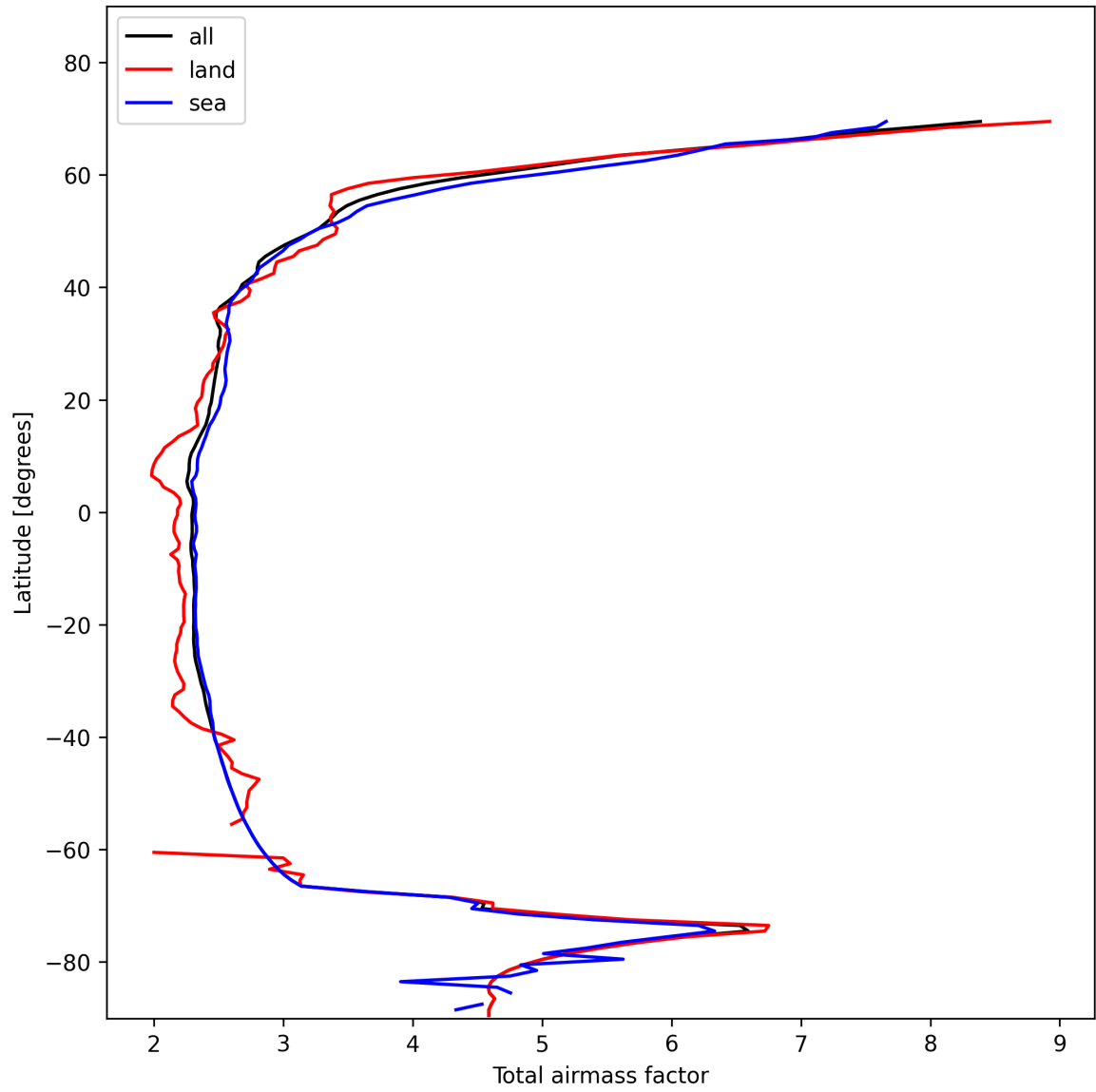
Figure 15: Zonal average of “Total airmass factor” for 2025-01-26 to 2025-01-28.
