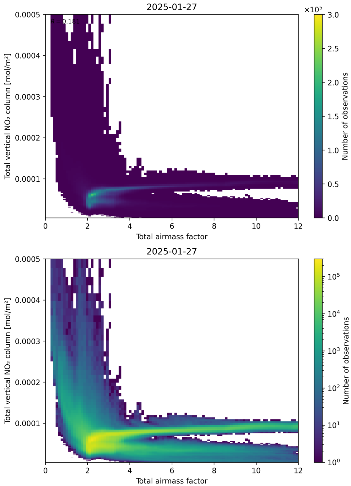
Figure 67: Scatter density plot of “Total airmass factor” against “Total vertical NO 2 column” for 2025-01-26 to 2025-01-28.
