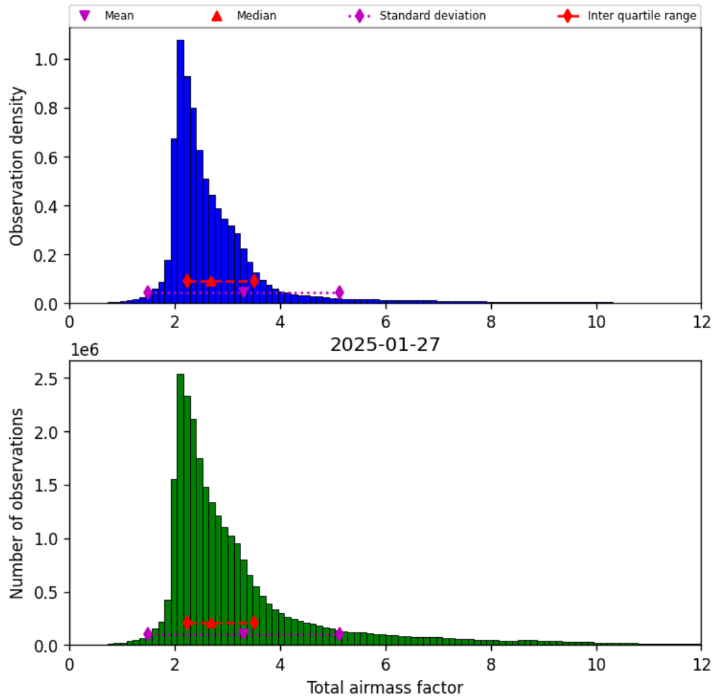
Figure 32: Histogram of “Total airmass factor” for 2025-01-26 to 2025-01-28
