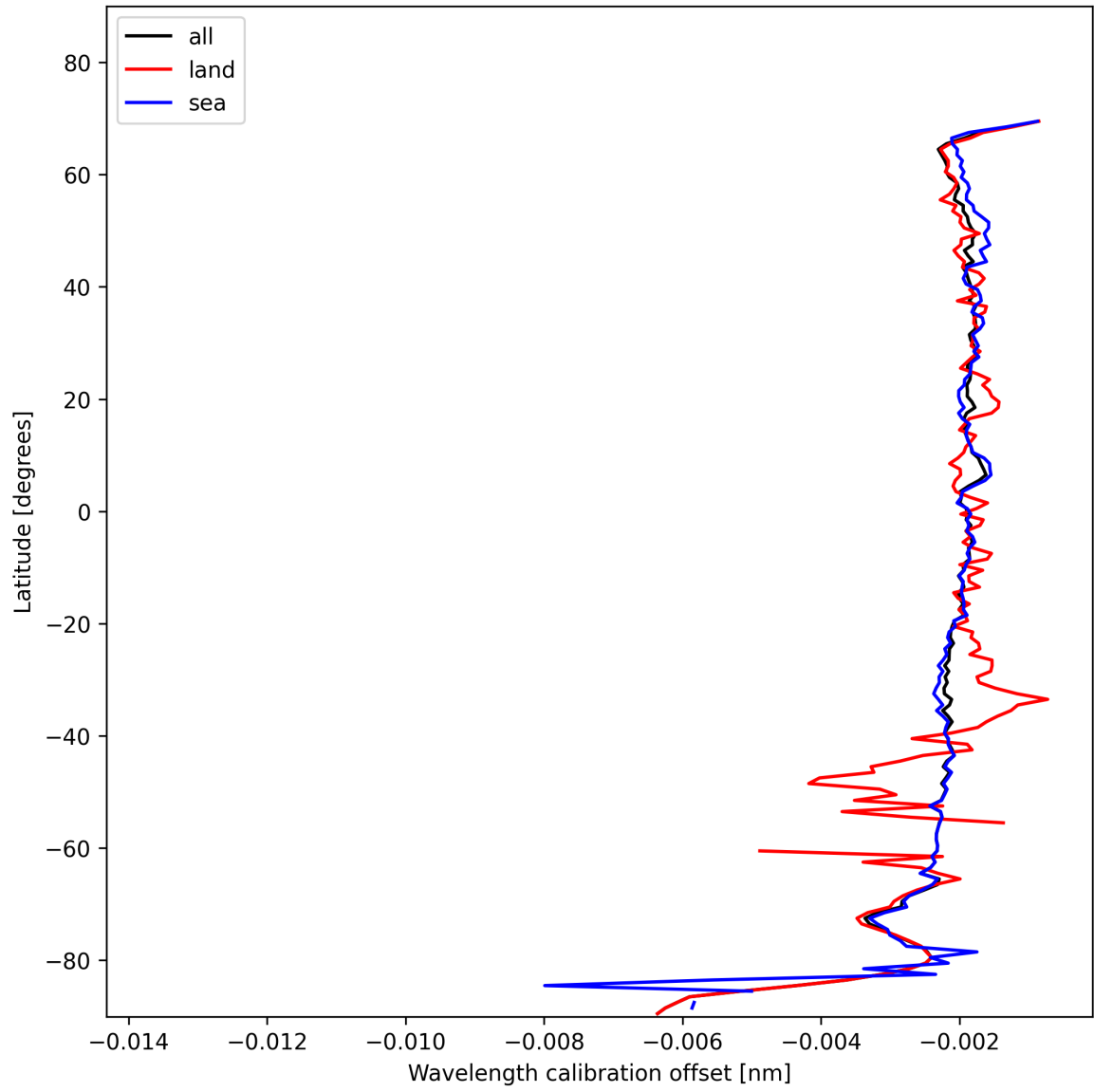
Figure 18: Zonal average of “Wavelength calibration offset” for 2025-01-26 to 2025-01-28.
