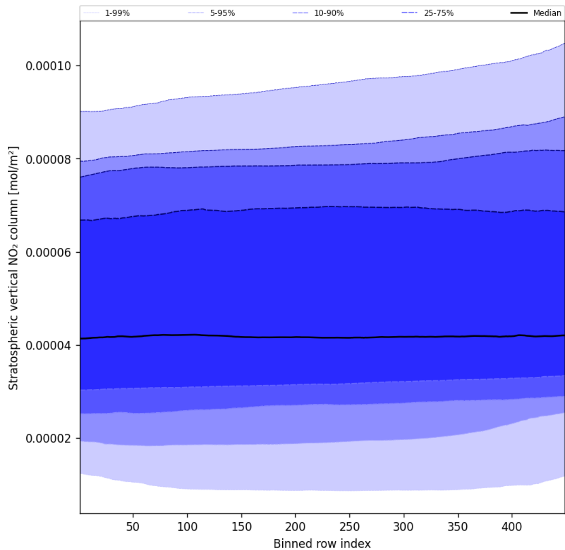
Figure 53: Along track statistics of “Stratospheric vertical NO 2 column” for 2025-01-26 to 2025-01-28
