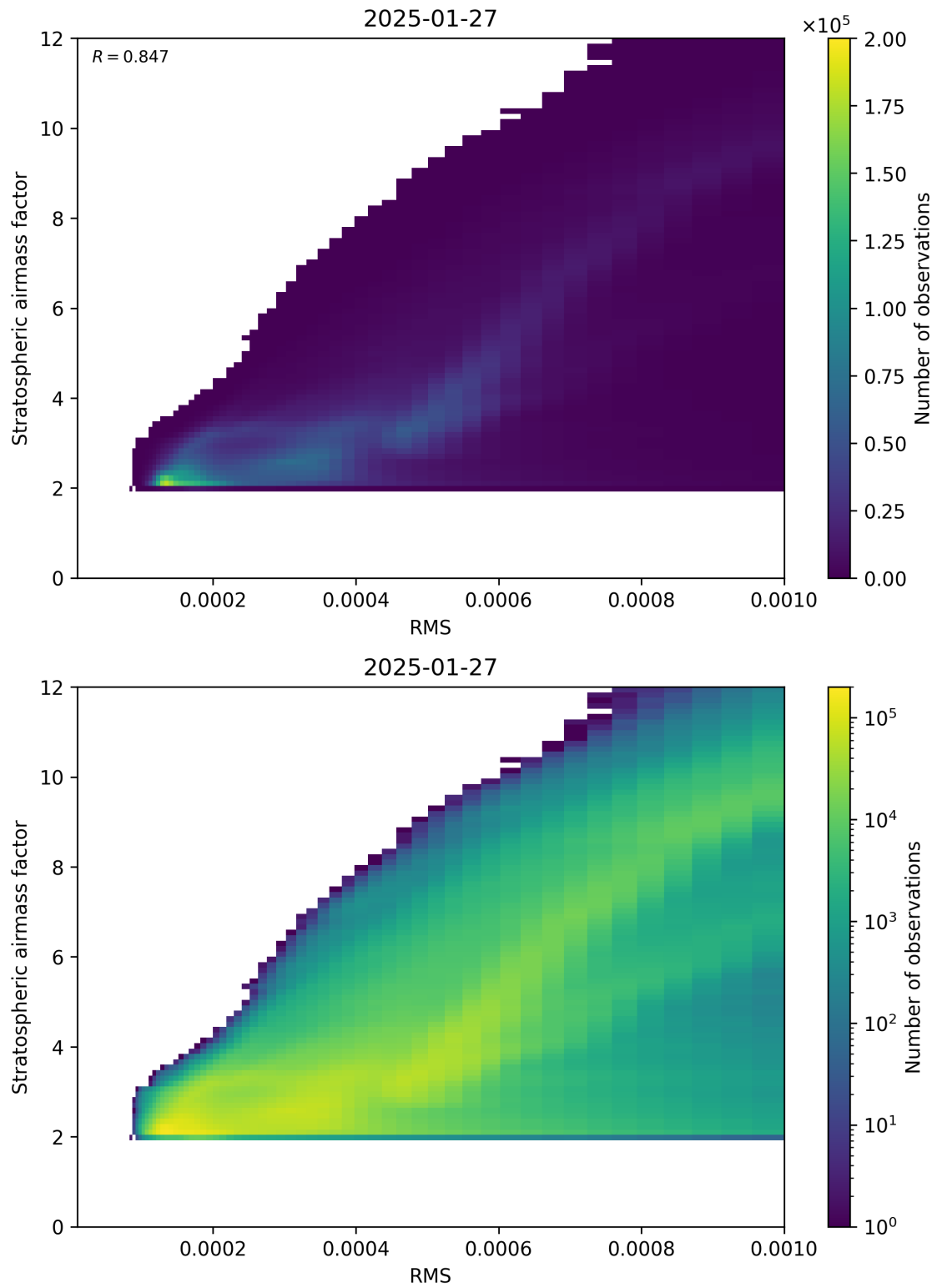
Figure 144: Scatter density plot of “RMS” against “Stratospheric airmass factor” for 2025-01-26 to 2025-01-28.
