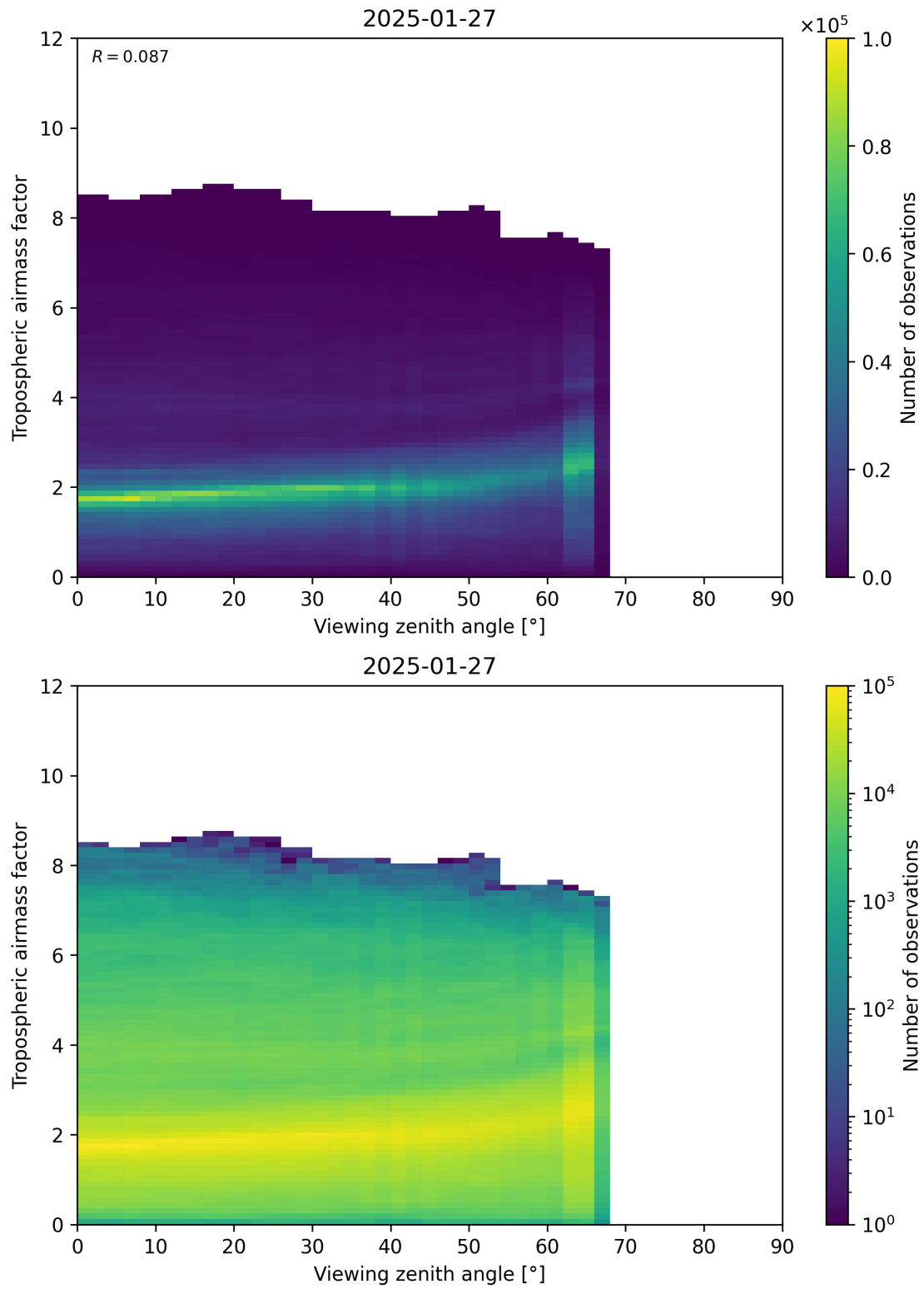
Figure 161: Scatter density plot of “Viewing zenith angle” against “Tropospheric airmass factor” for 2025-01-26 to 2025-01-28.
