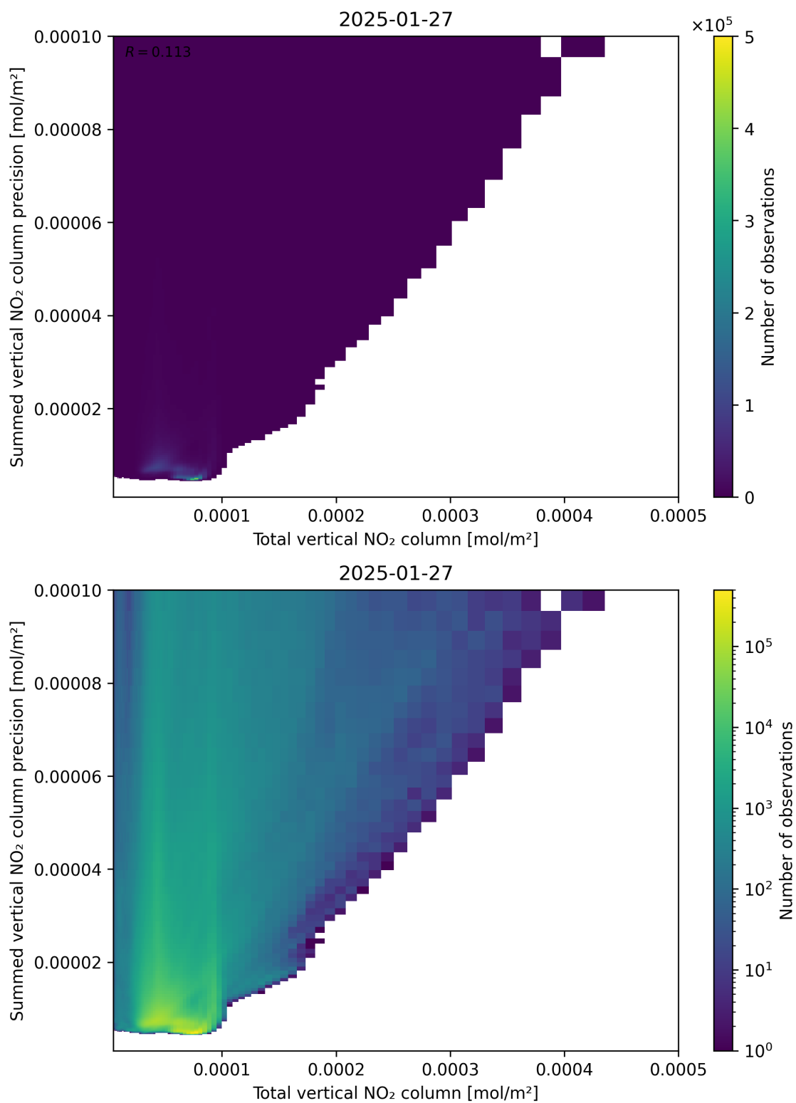
Figure 113: Scatter density plot of “Total vertical NO 2 column” against “Summed vertical NO 2 column precision” for 2025-01-26 to 2025-01-28.
