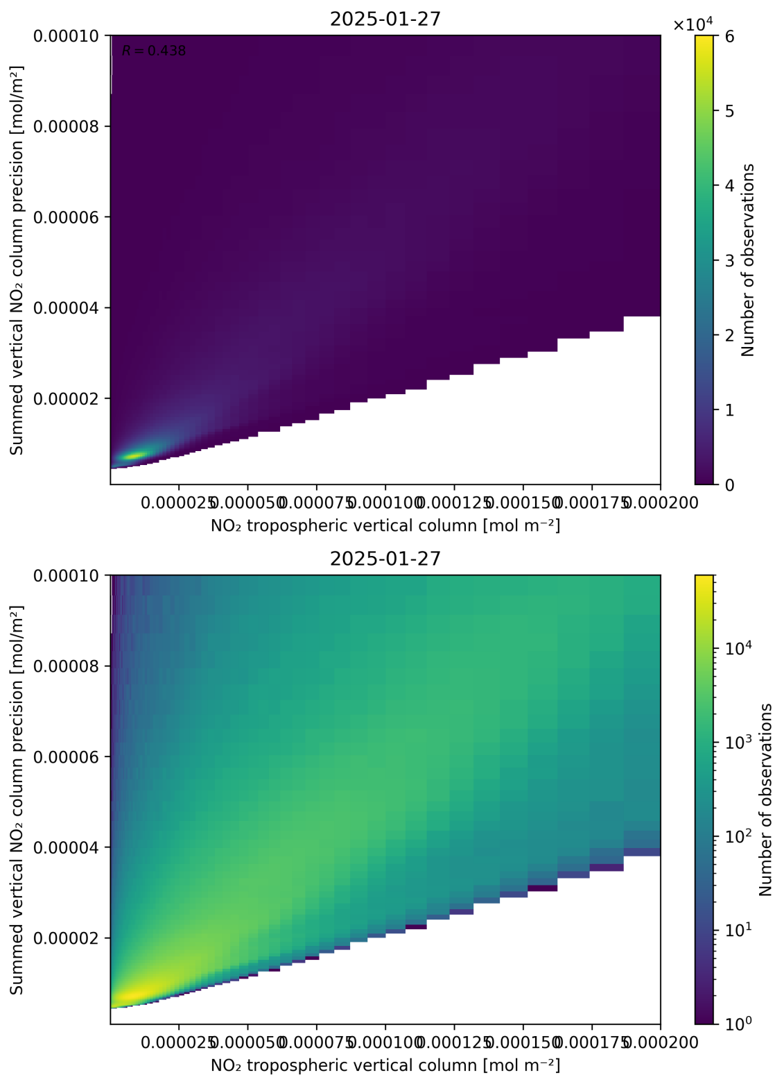
Figure 127: Scatter density plot of “NO 2 tropospheric vertical column” against “Summed vertical NO 2 column precision” for 2025-01-26 to 2025-01-28.
