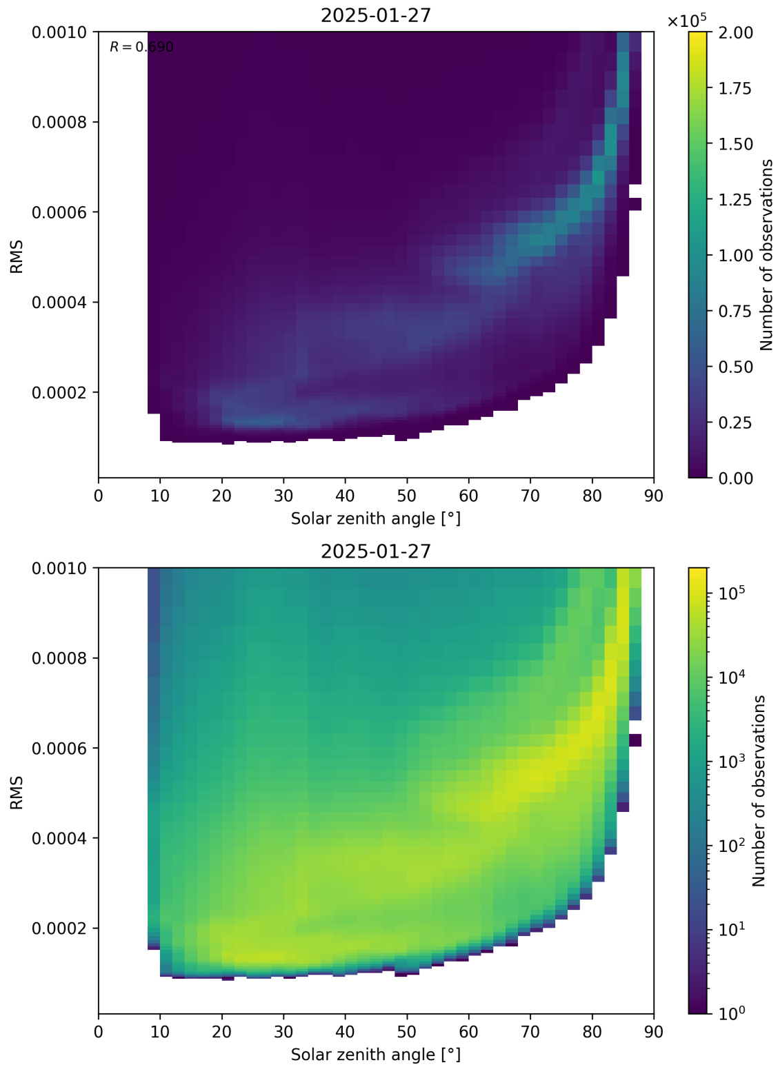
Figure 157: Scatter density plot of “Solar zenith angle” against “RMS” for 2025-01-26 to 2025-01-28.
