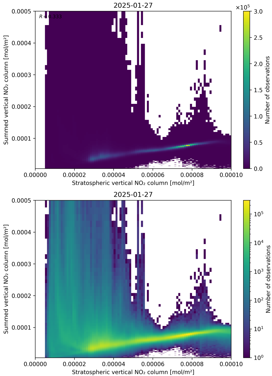
Figure 98: Scatter density plot of “Stratospheric vertical NO 2 column” against “Summed vertical NO 2 column” for 2025-01-26 to 2025-01-28.
