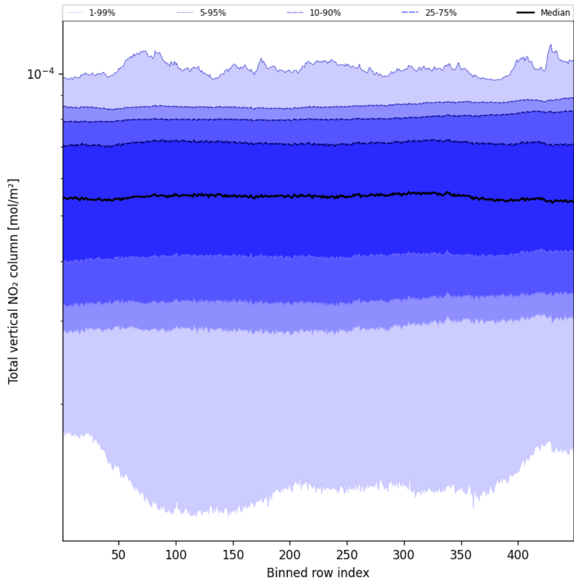
Figure 55: Along track statistics of “Total vertical NO 2 column” for 2025-01-26 to 2025-01-28
