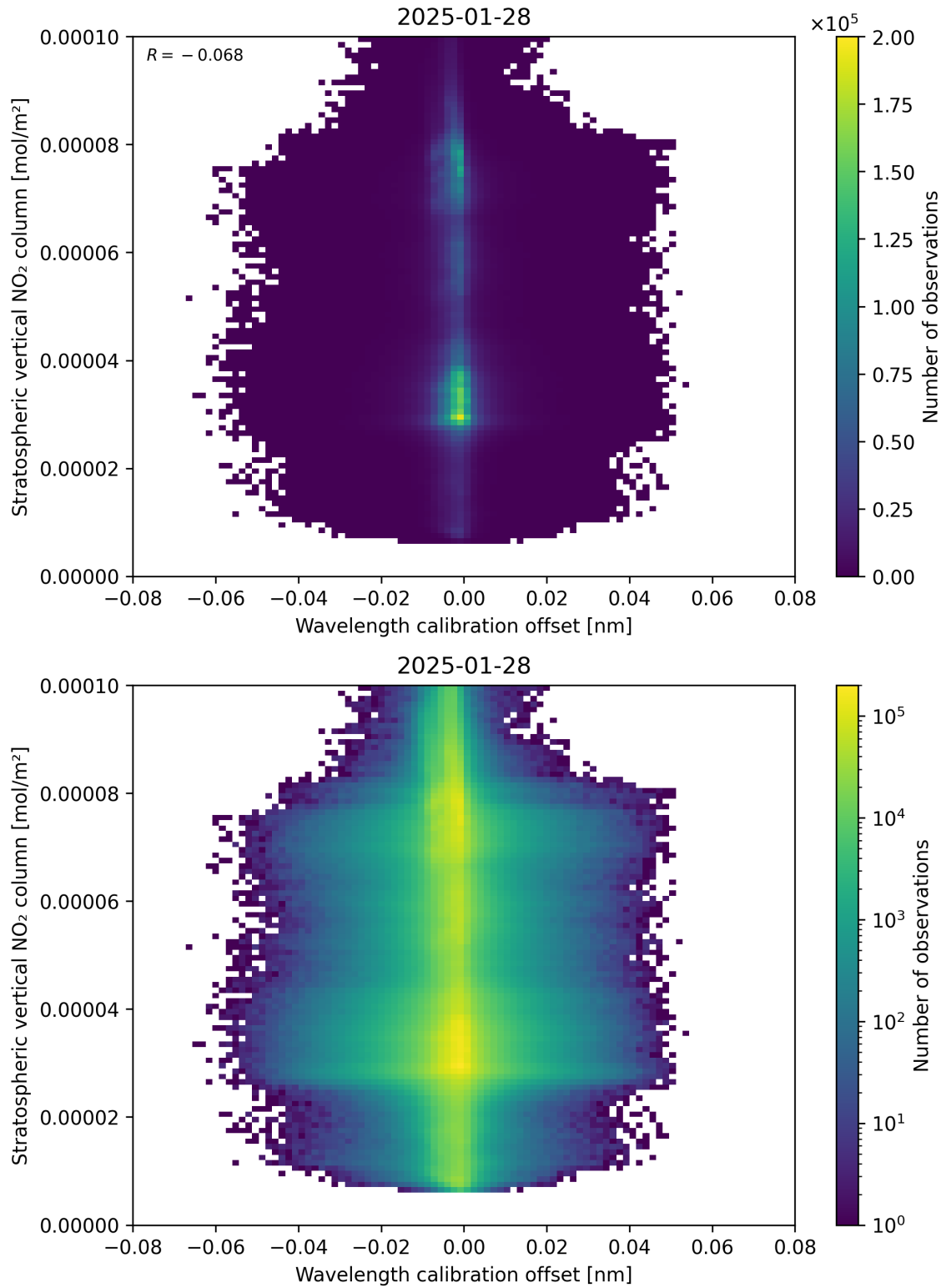
Figure 176: Scatter density plot of “Wavelength calibration offset” against “Stratospheric vertical NO 2 column” for 2025-01-28 to 2025-01-29.
