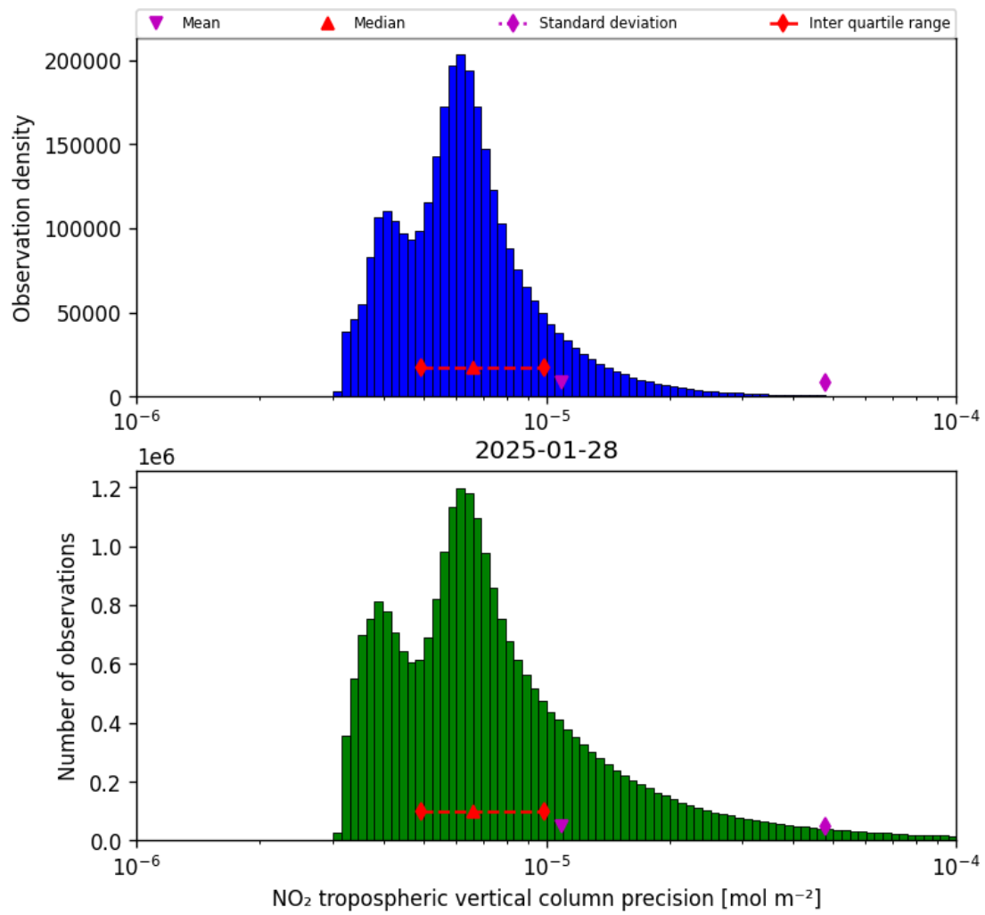
Figure 30: Histogram of “NO 2 tropospheric vertical column precision” for 2025-01-28 to 2025-01-29
