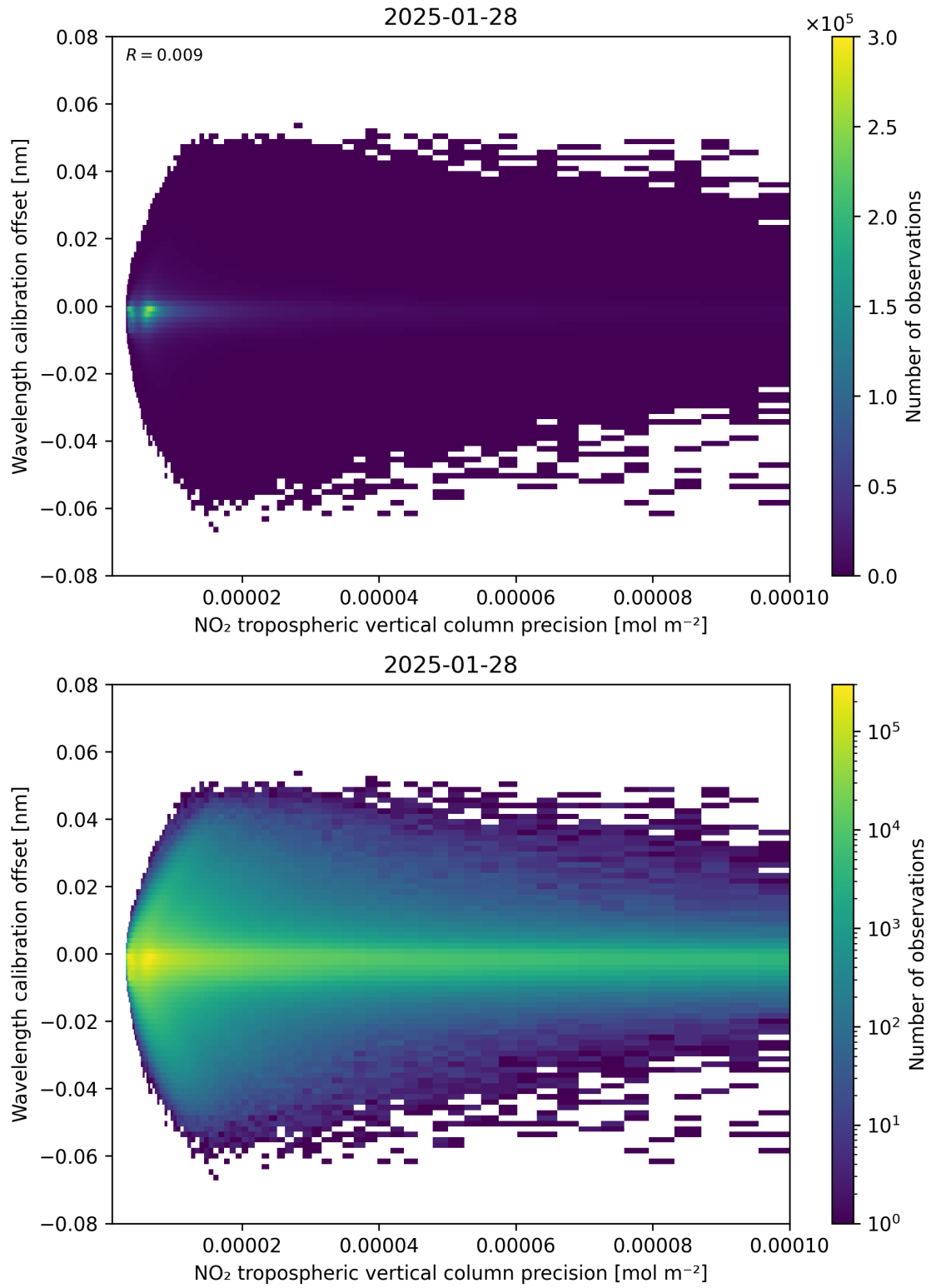
Figure 141: Scatter density plot of “NO 2 tropospheric vertical column precision” against “Wavelength calibration offset” for 2025-01-28 to 2025-01-29.
