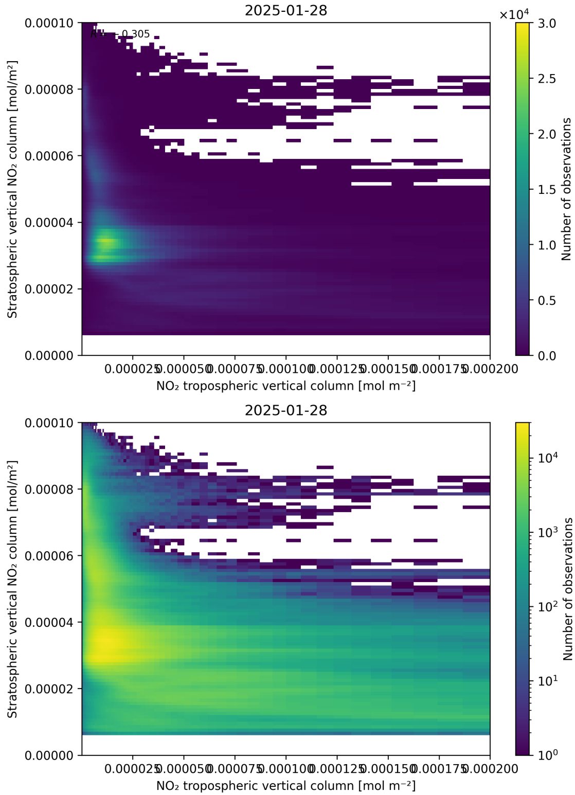
Figure 125: Scatter density plot of “NO 2 tropospheric vertical column” against “Stratospheric vertical NO 2 column” for 2025-01-28 to 2025-01-29.
