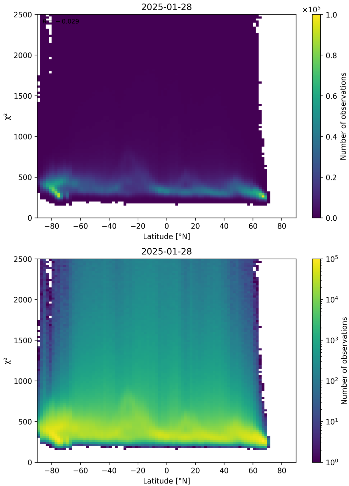
Figure 86: Scatter density plot of “Latitude” against “ \chi^2 ” for 2025-01-28 to 2025-01-29.
