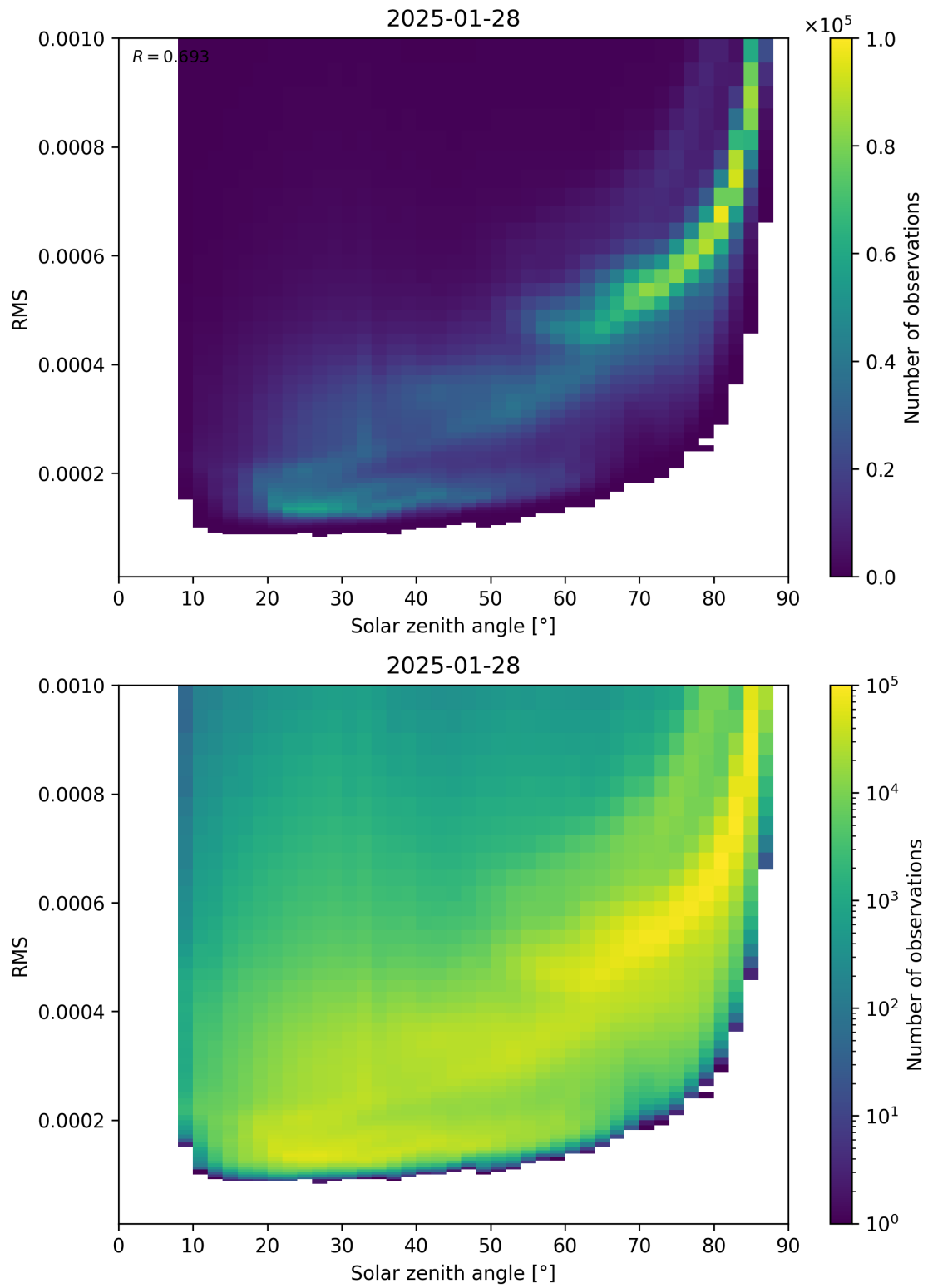
Figure 157: Scatter density plot of “Solar zenith angle” against “RMS” for 2025-01-28 to 2025-01-29.
