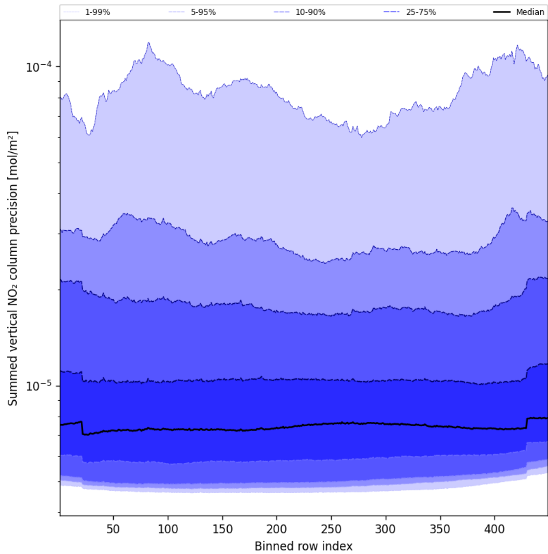
Figure 58: Along track statistics of “Summed vertical NO 2 column precision” for 2025-01-28 to 2025-01-29
