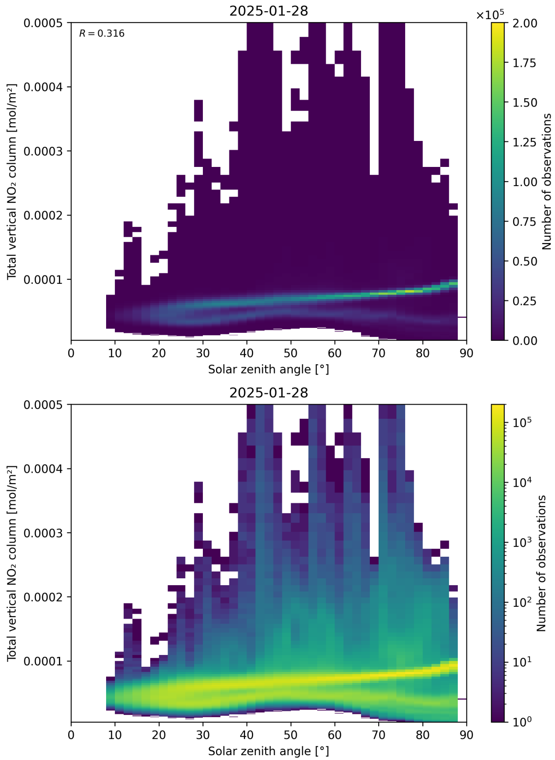
Figure 153: Scatter density plot of “Solar zenith angle” against “Total vertical NO 2 column” for 2025-01-28 to 2025-01-29.
