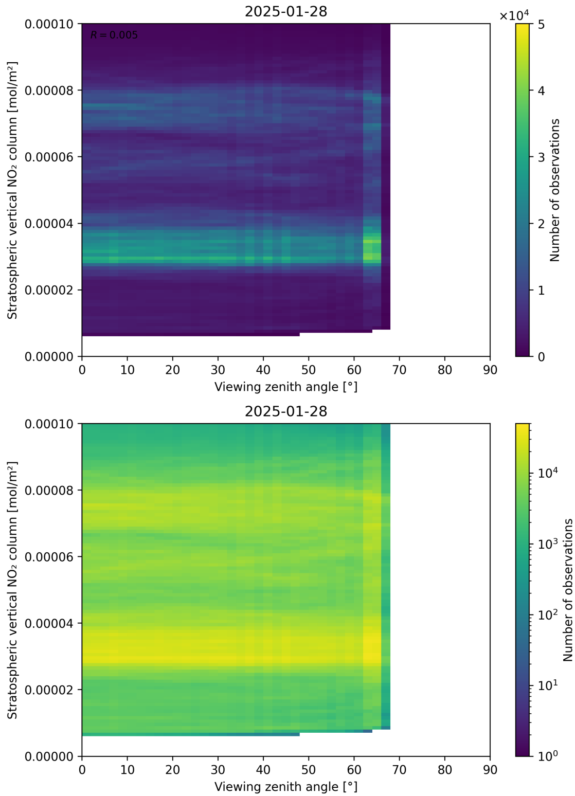
Figure 164: Scatter density plot of “Viewing zenith angle” against “Stratospheric vertical NO 2 column” for 2025-01-28 to 2025-01-29.
