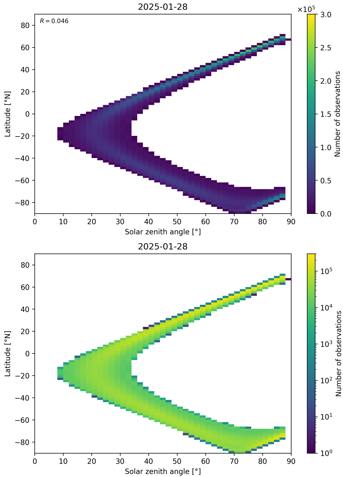
Figure 149: Scatter density plot of “Solar zenith angle” against “Latitude” for 2025-01-28 to 2025-01-29.
