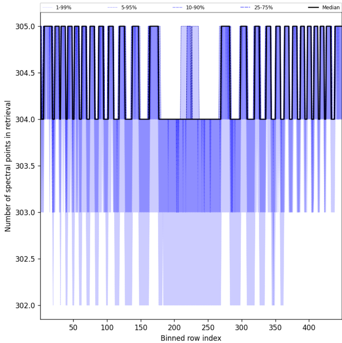
Figure 50: Along track statistics of “Number of spectral points in retrieval” for 2025-01-28 to 2025-01-29
