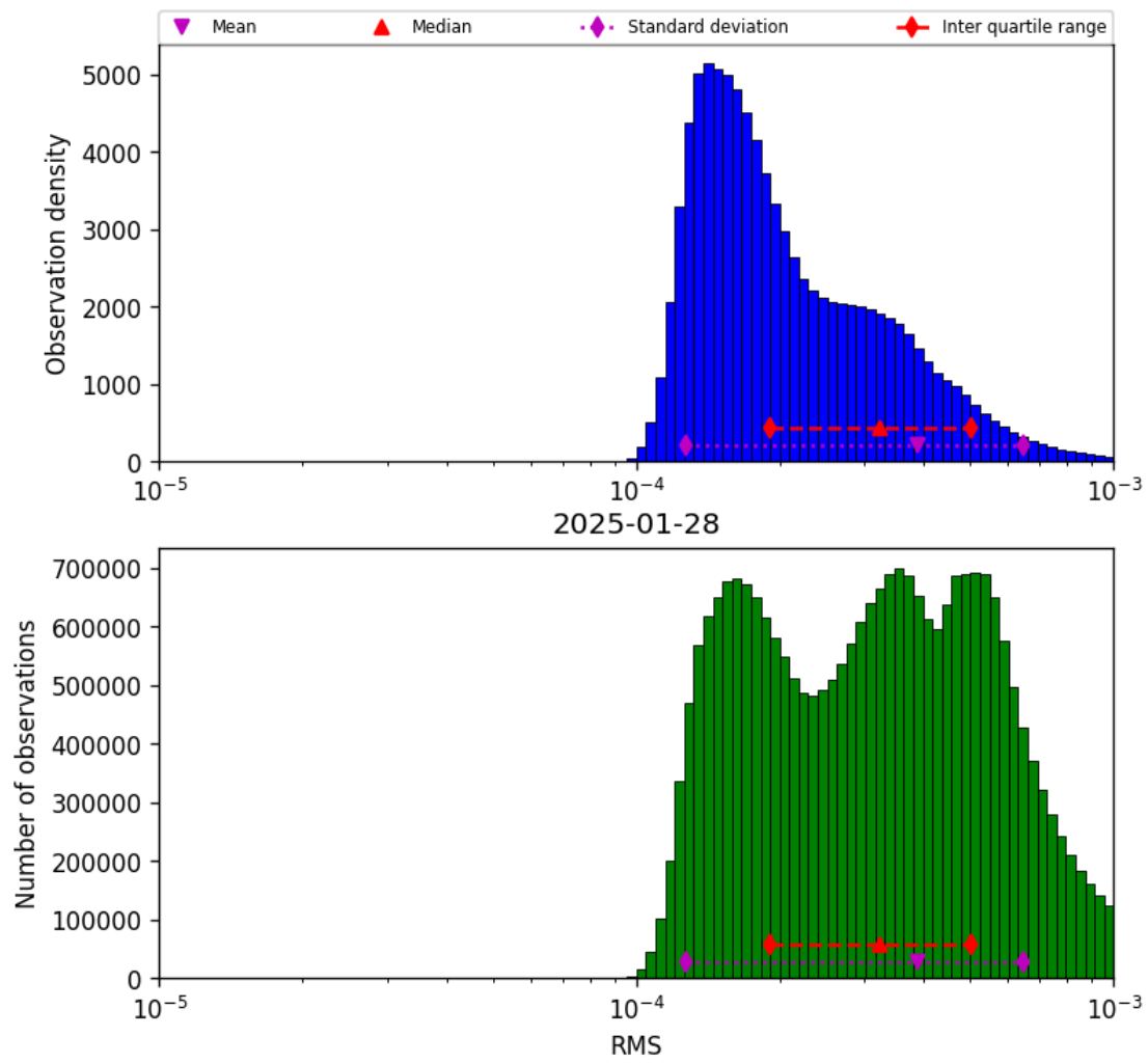
Figure 43: Histogram of “RMS” for 2025-01-28 to 2025-01-29
