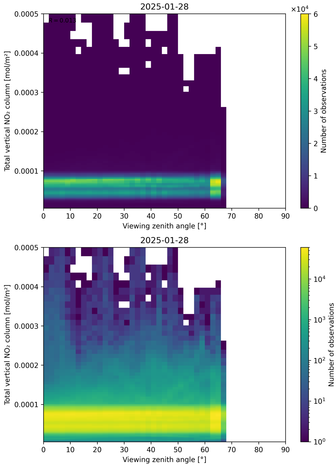
Figure 167: Scatter density plot of “Viewing zenith angle” against “Total vertical NO 2 column” for 2025-01-28 to 2025-01-29.
