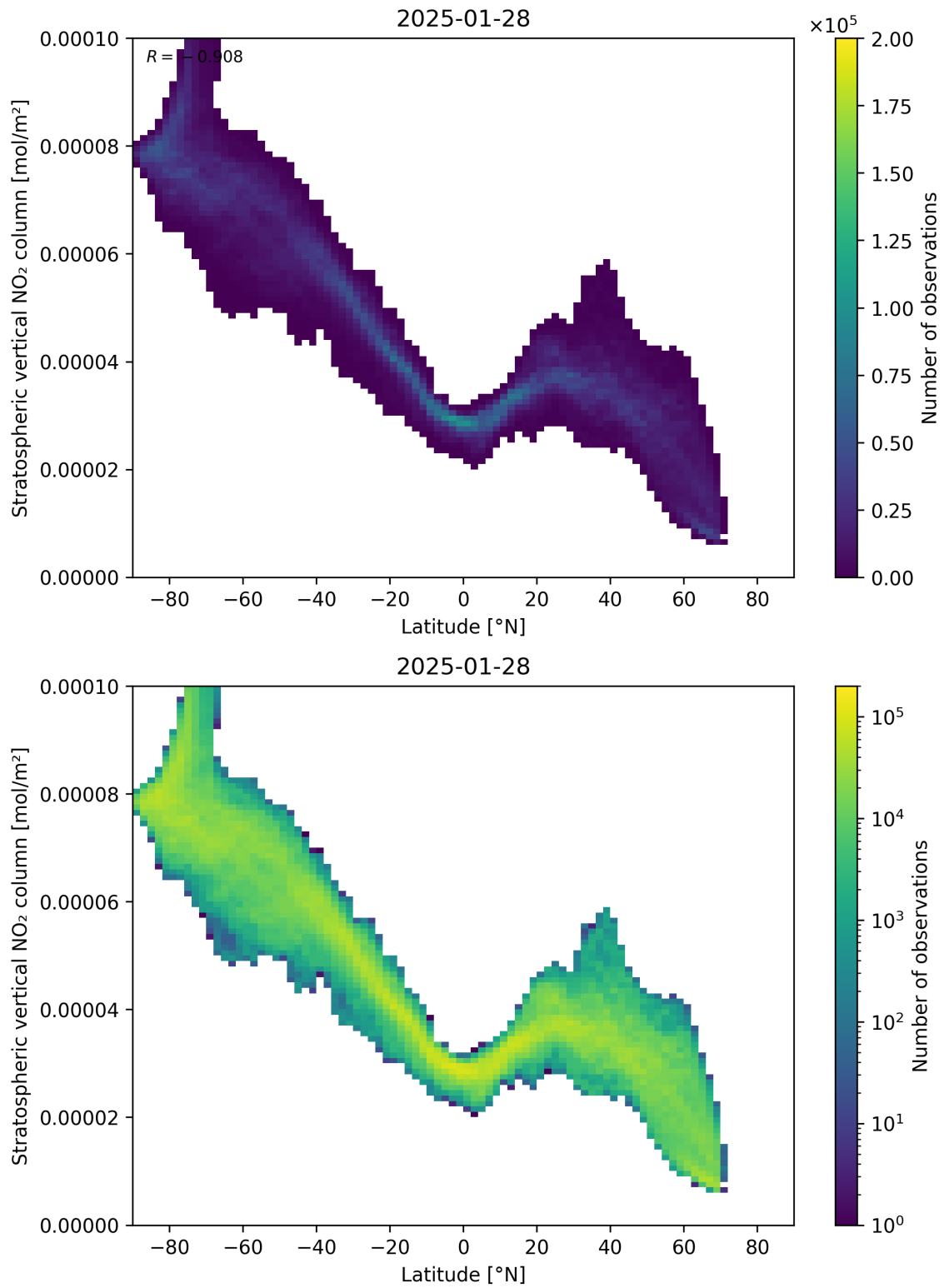
Figure 87: Scatter density plot of “Latitude” against “Stratospheric vertical NO 2 column” for 2025-01-28 to 2025-01-29.
