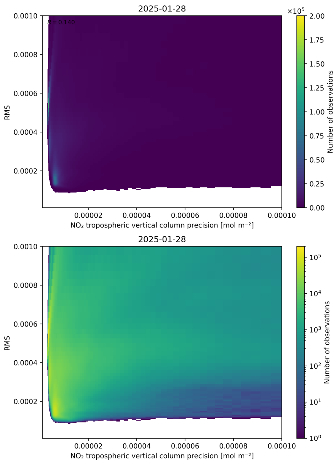
Figure 140: Scatter density plot of “NO 2 tropospheric vertical column precision” against “RMS” for 2025-01-28 to 2025-01-29.
