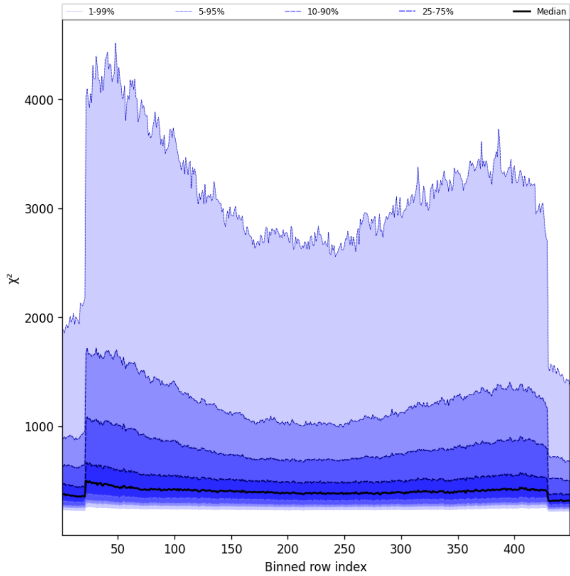
Figure 59: Along track statistics of “ \chi^2 ” for 2025-01-28 to 2025-01-29
