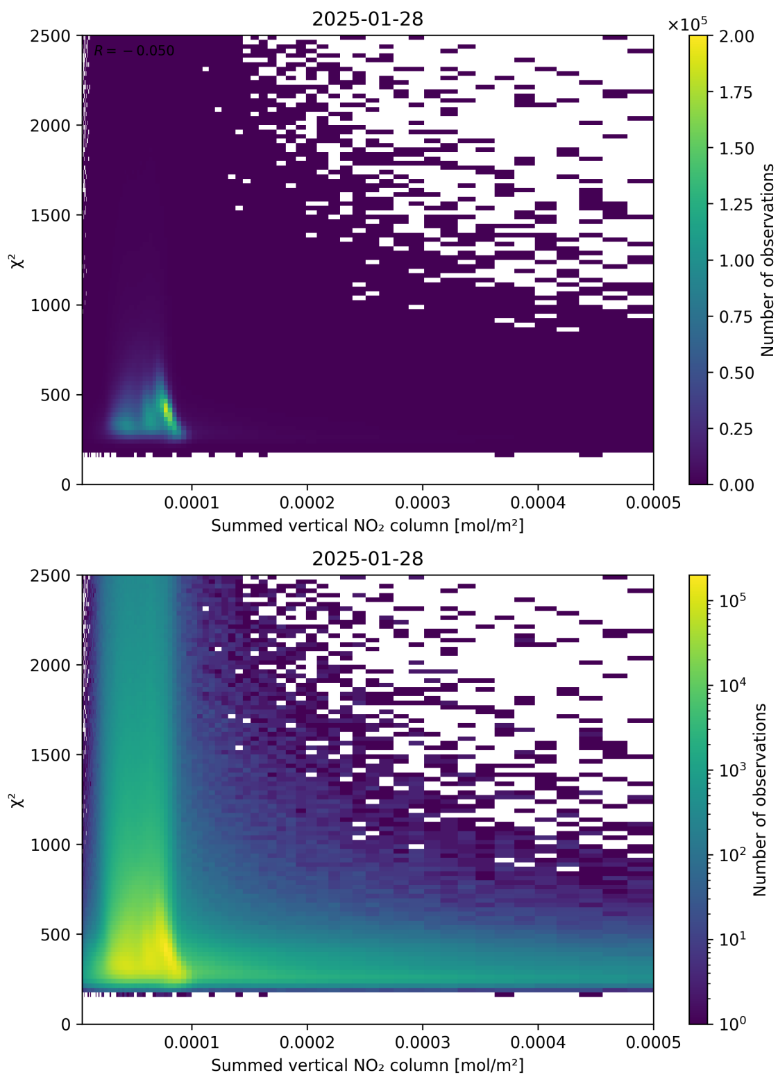
Figure 104: Scatter density plot of “Summed vertical NO 2 column” against “ \chi^2 ” for 2025-01-28 to 2025-01-29.
