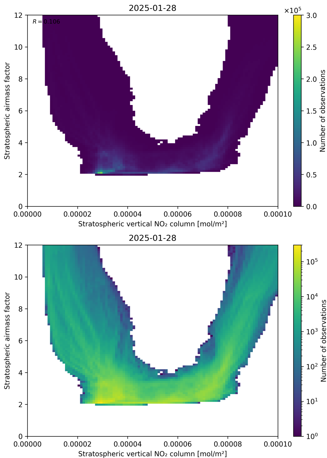
Figure 96: Scatter density plot of “Stratospheric vertical NO 2 column” against “Stratospheric airmass factor” for 2025-01-28 to 2025-01-29.
