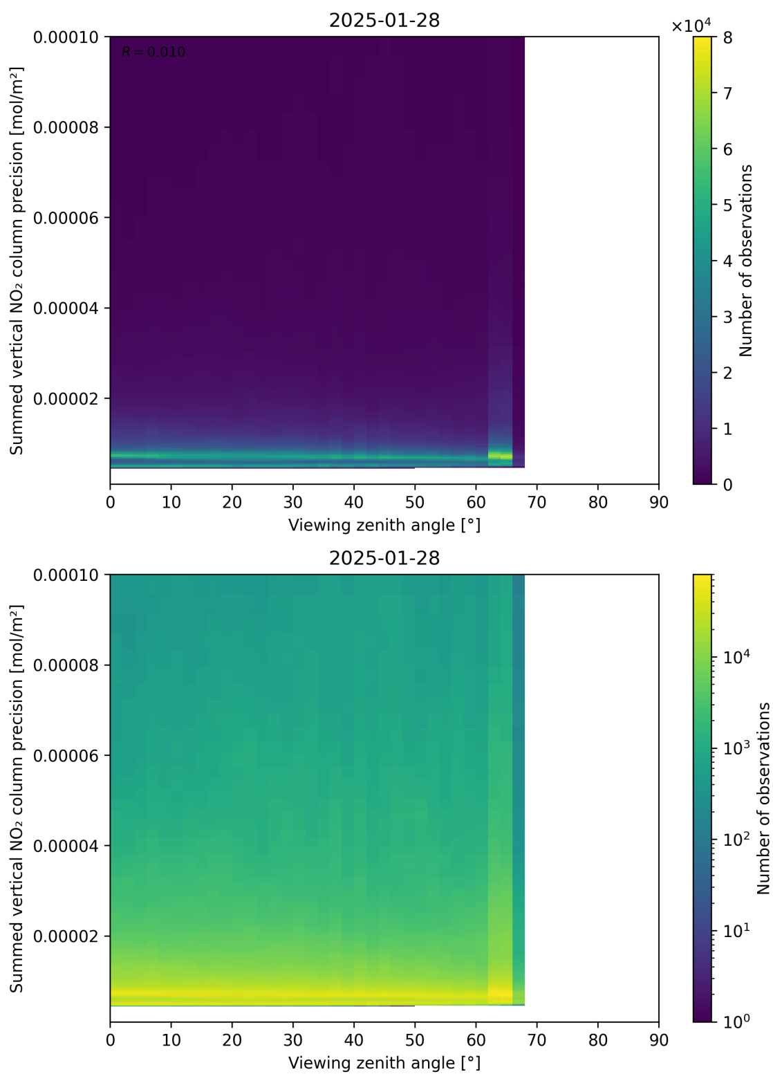
Figure 166: Scatter density plot of “Viewing zenith angle” against “Summed vertical NO 2 column precision” for 2025-01-28 to 2025-01-29.
