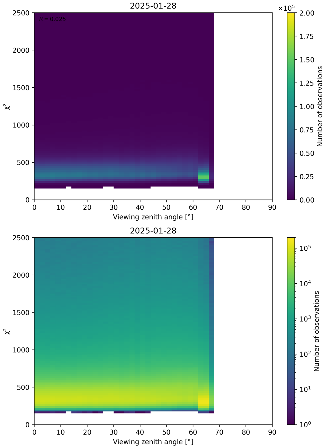
Figure 162: Scatter density plot of “Viewing zenith angle” against “ \chi^2 ” for 2025-01-28 to 2025-01-29.
