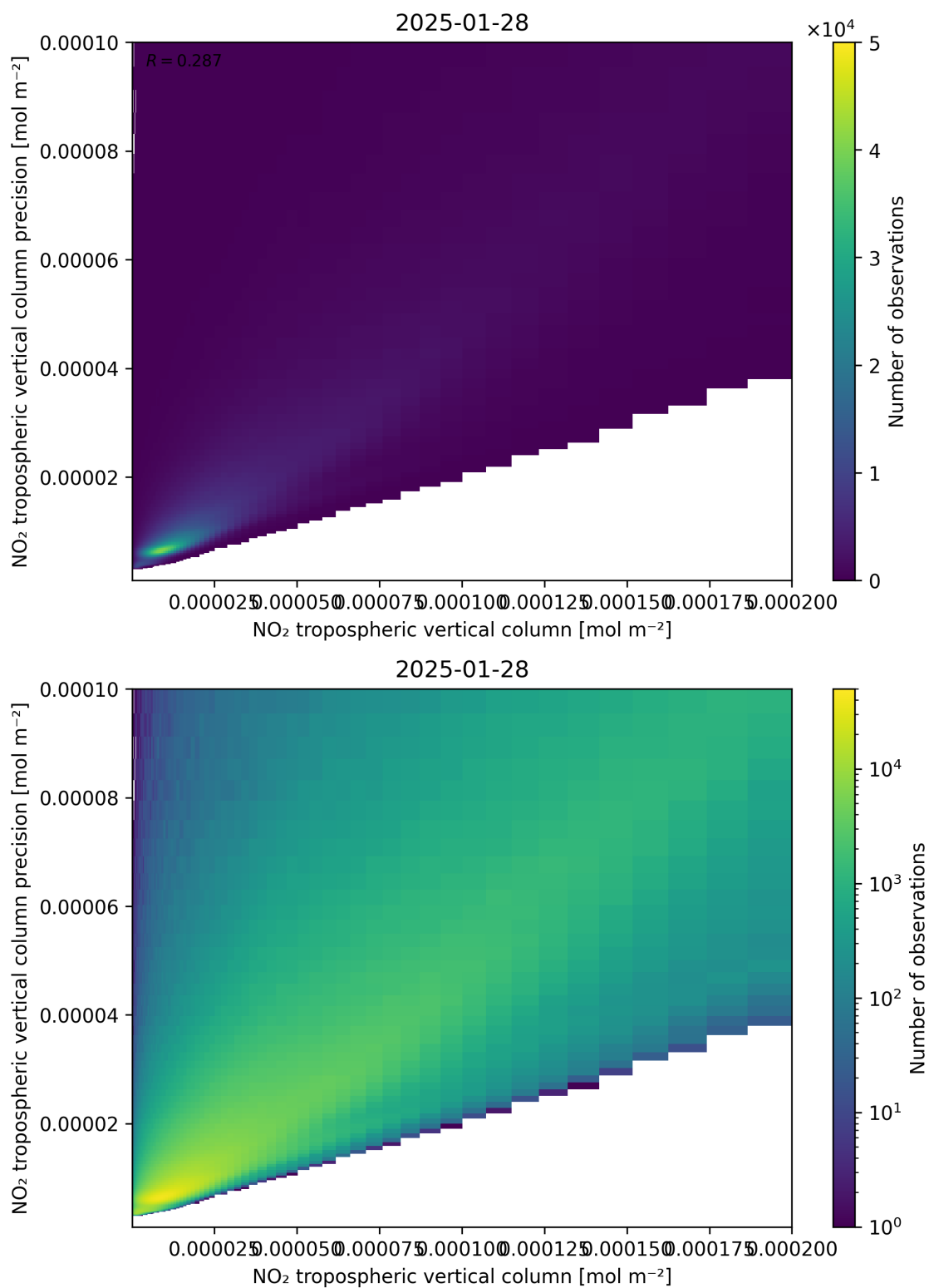
Figure 130: Scatter density plot of “NO 2 tropospheric vertical column” against “NO 2 tropospheric vertical column precision” for 2025-01-28 to 2025-01-29.
