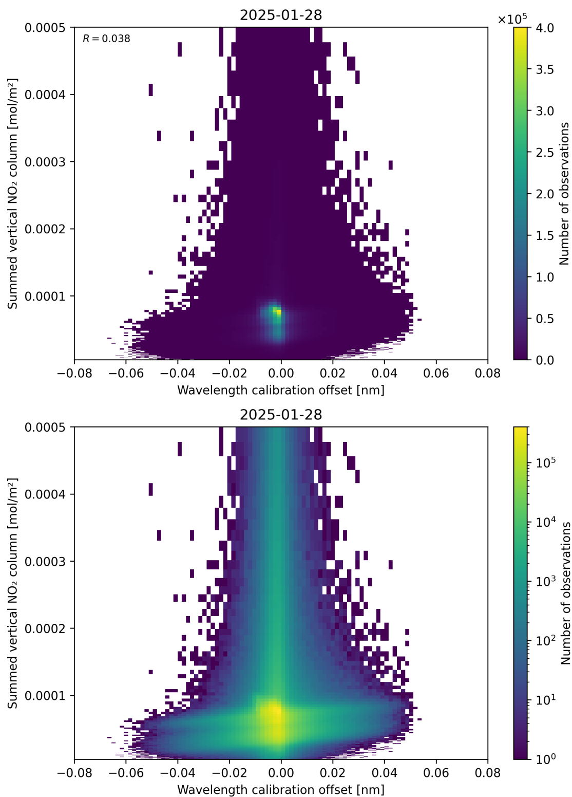
Figure 177: Scatter density plot of “Wavelength calibration offset” against “Summed vertical NO 2 column” for 2025-01-28 to 2025-01-29.
