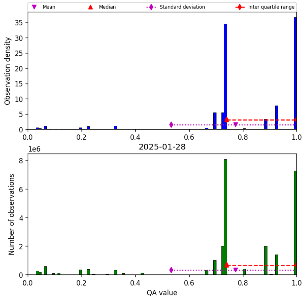
Figure 28: Histogram of “QA value” for 2025-01-28 to 2025-01-29
