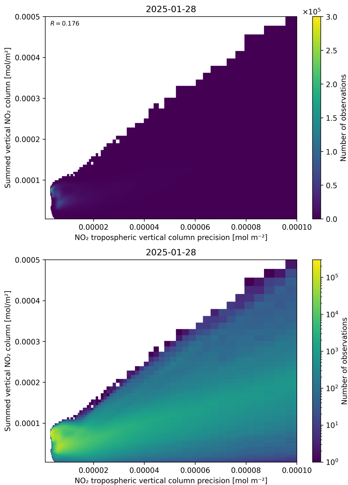
Figure 136: Scatter density plot of “NO 2 tropospheric vertical column precision” against “Summed vertical NO 2 column” for 2025-01-28 to 2025-01-29.
