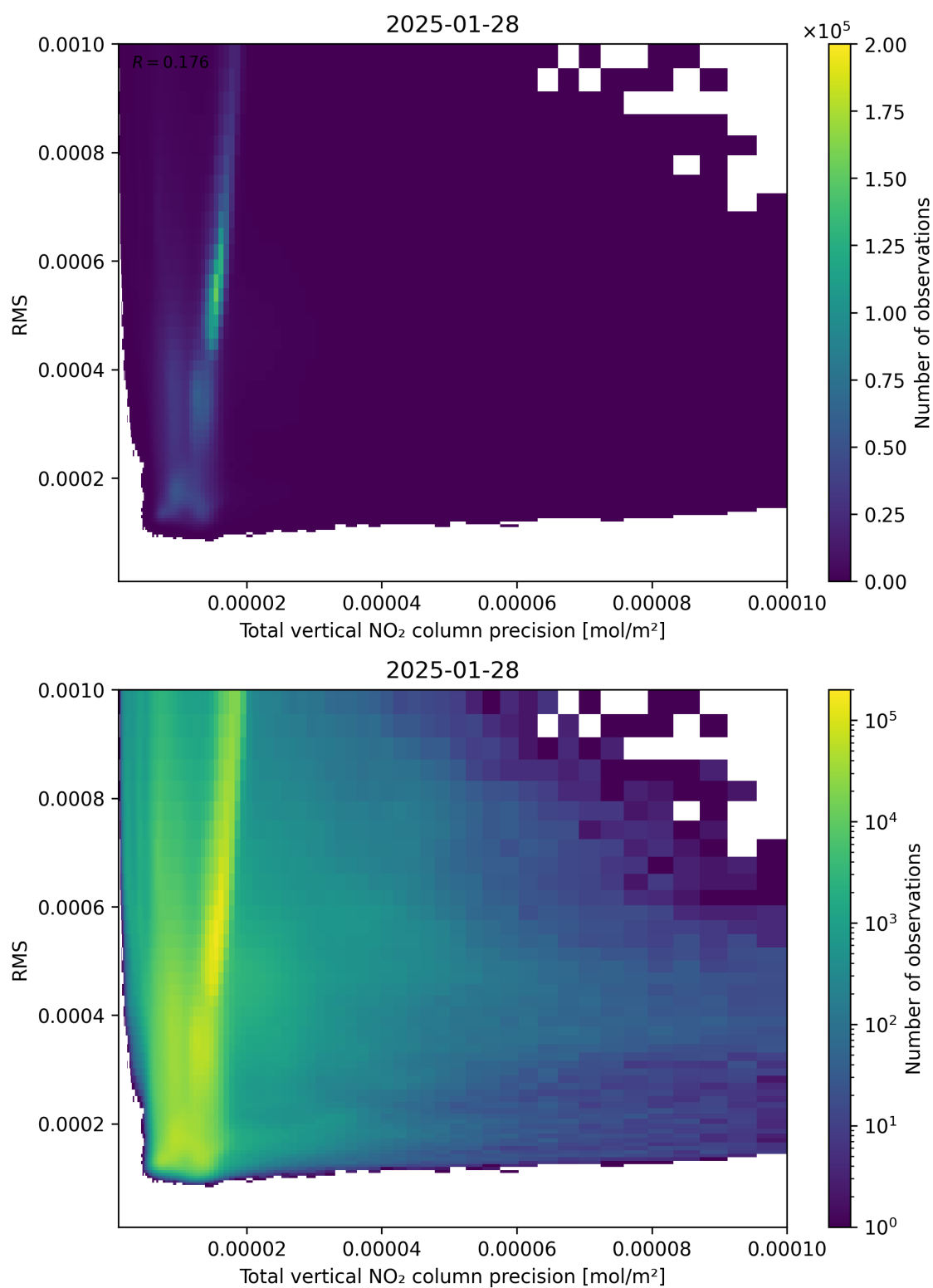
Figure 119: Scatter density plot of “Total vertical NO 2 column precision” against “RMS” for 2025-01-28 to 2025-01-29.
