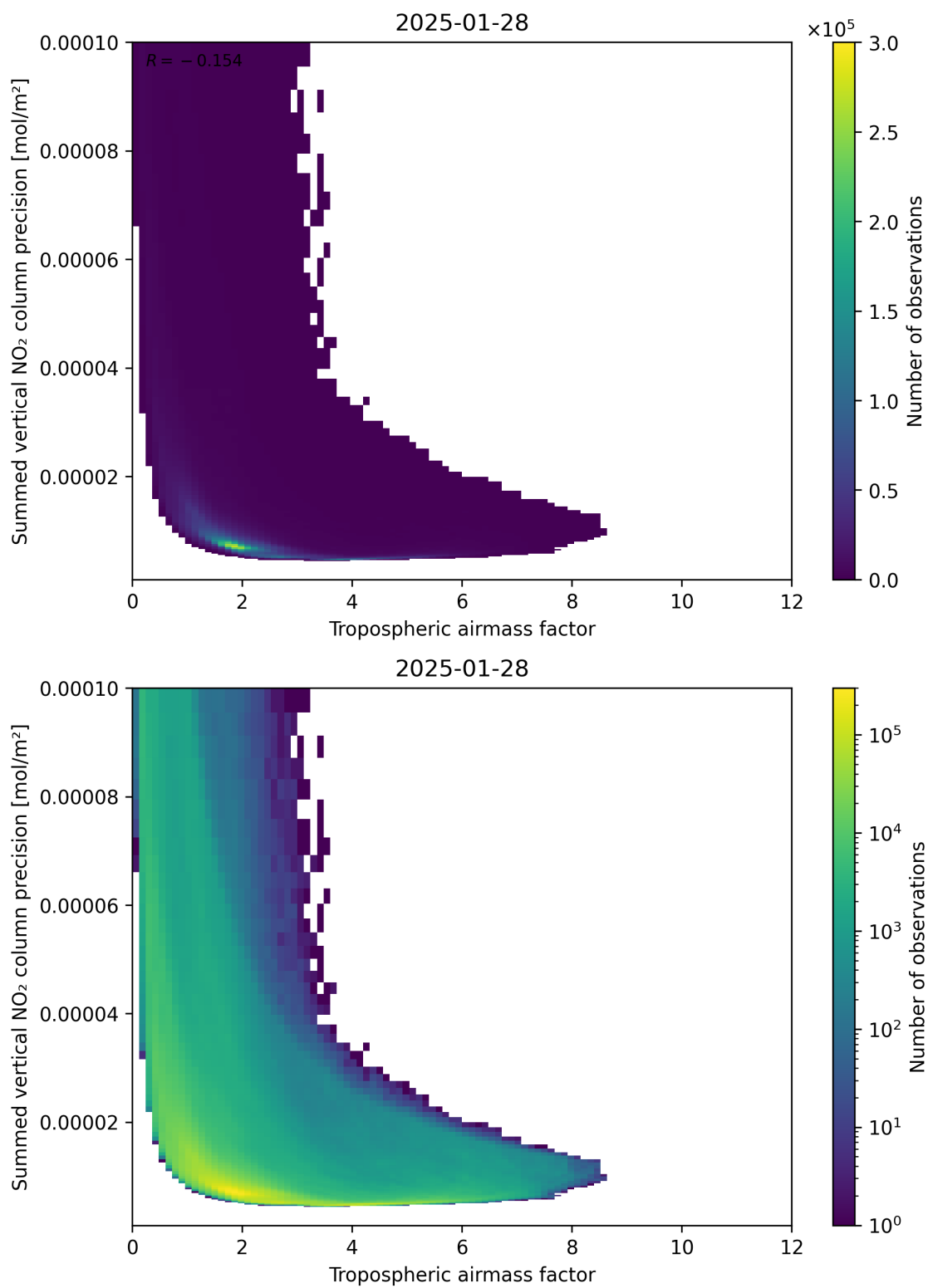
Figure 76: Scatter density plot of “Tropospheric air mass factor” against “Summed vertical NO 2 column precision” for 2025-01-28 to 2025-01-29.
