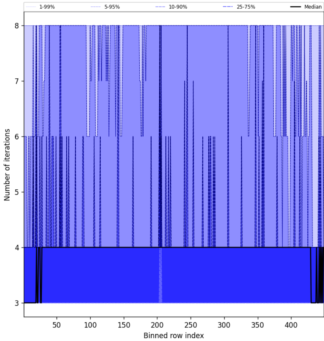
Figure 51: Along track statistics of “Number of iterations” for 2025-01-28 to 2025-01-29
