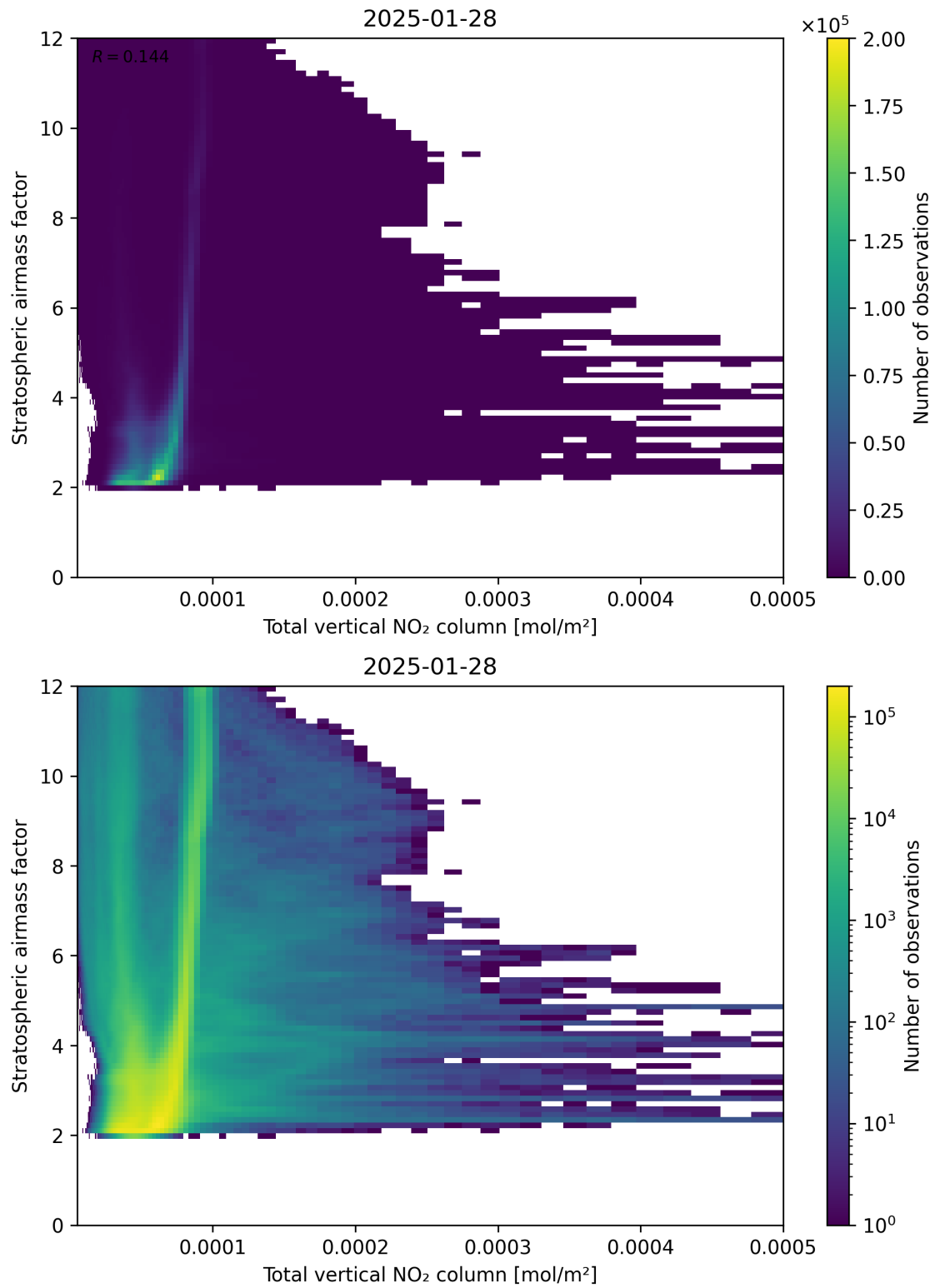
Figure 110: Scatter density plot of “Total vertical NO 2 column” against “Stratospheric airmass factor” for 2025-01-28 to 2025-01-29.
