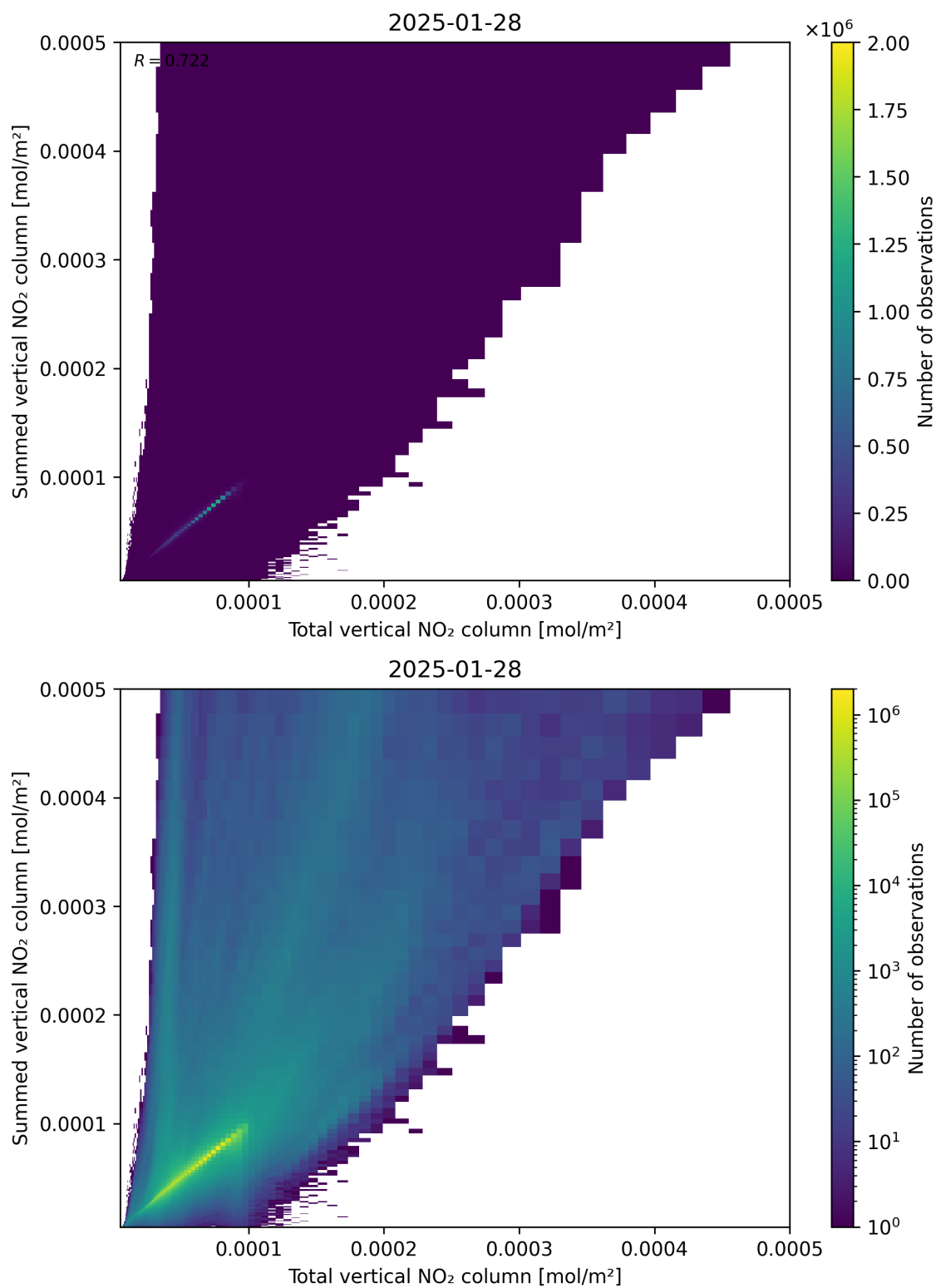
Figure 112: Scatter density plot of “Total vertical NO 2 column” against “Summed vertical NO 2 column” for 2025-01-28 to 2025-01-29.
