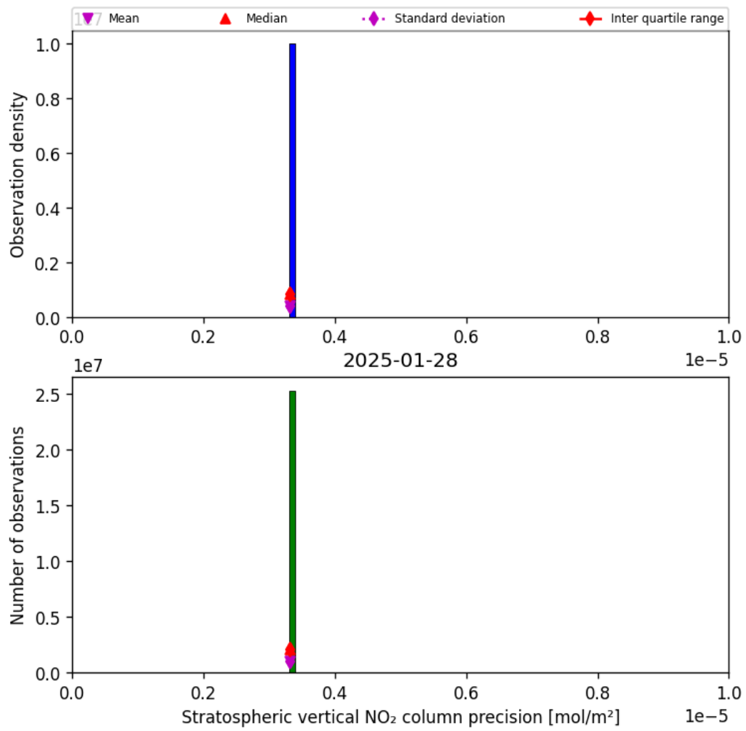
Figure 37: Histogram of “Stratospheric vertical NO 2 column precision” for 2025-01-28 to 2025-01-29
