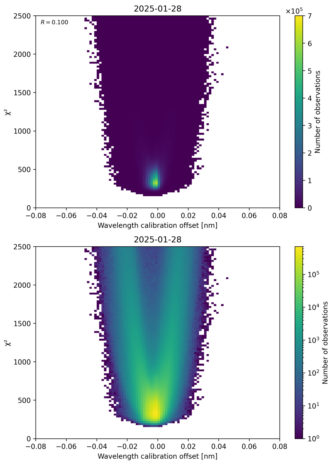
Figure 175: Scatter density plot of “Wavelength calibration offset” against “ \chi^2 ” for 2025-01-28 to 2025-01-29.
