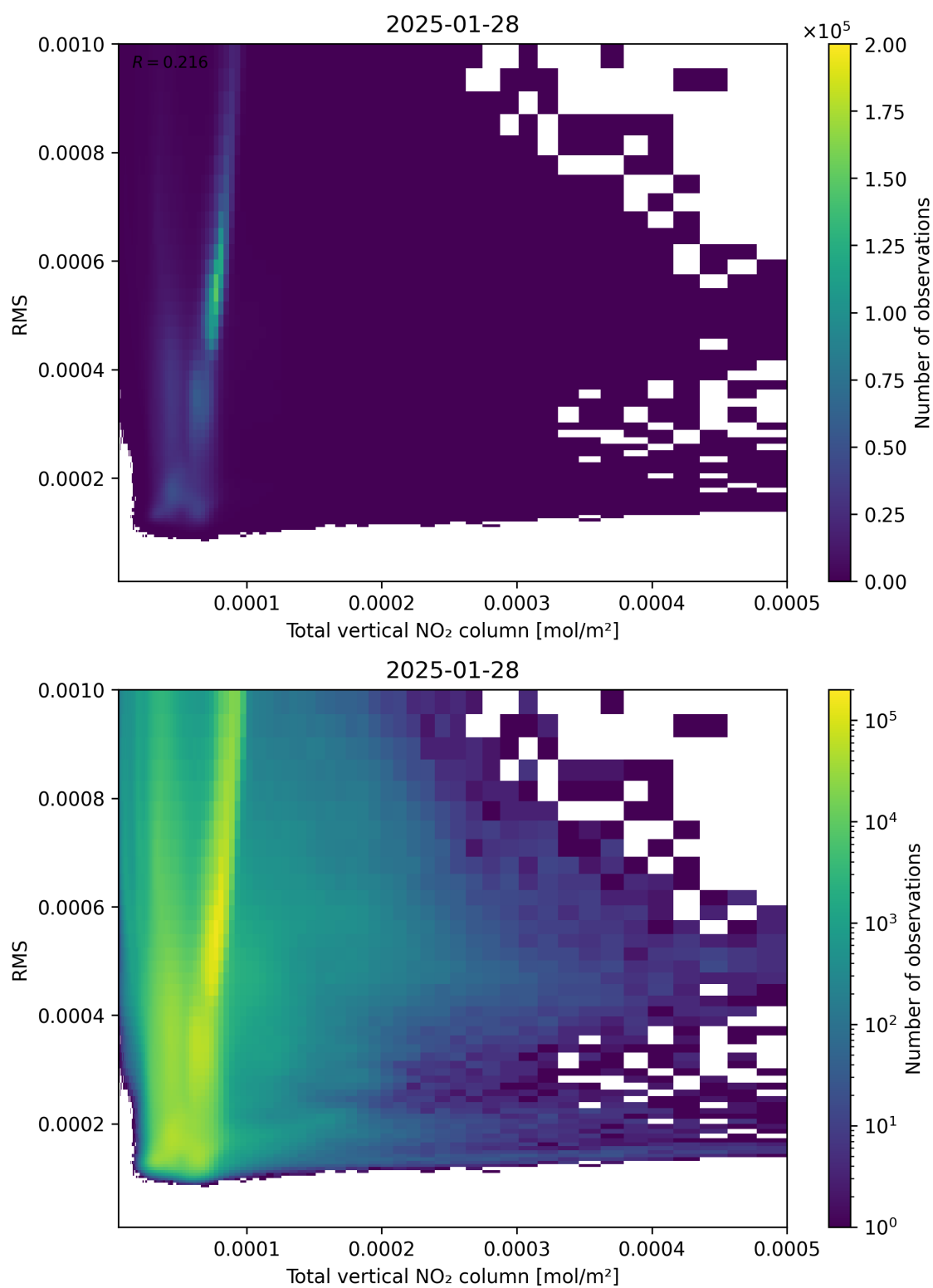
Figure 120: Scatter density plot of “Total vertical NO 2 column” against “RMS” for 2025-01-28 to 2025-01-29.
