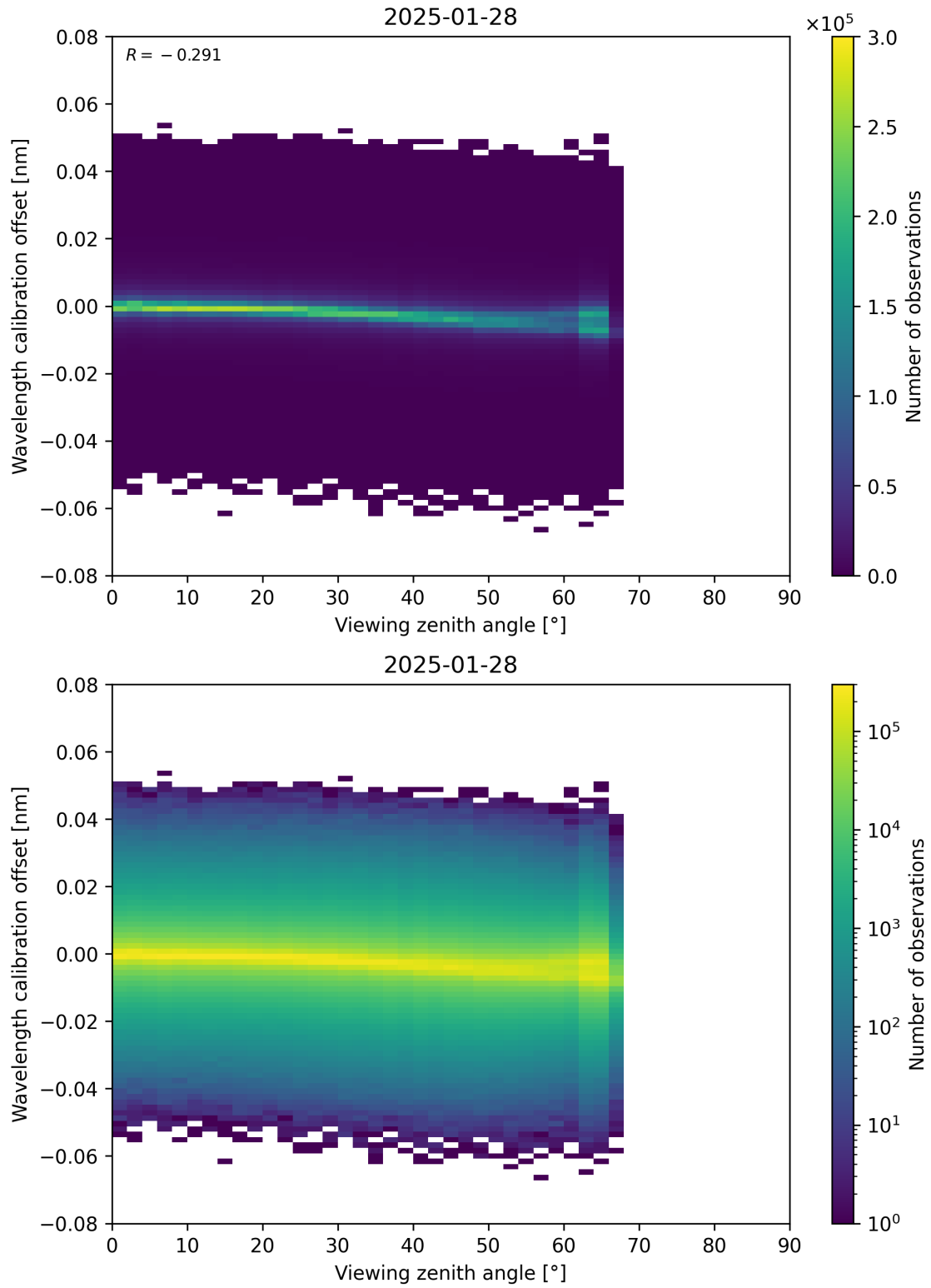
Figure 173: Scatter density plot of “Viewing zenith angle” against “Wavelength calibration offset” for 2025-01-28 to 2025-01-29.
