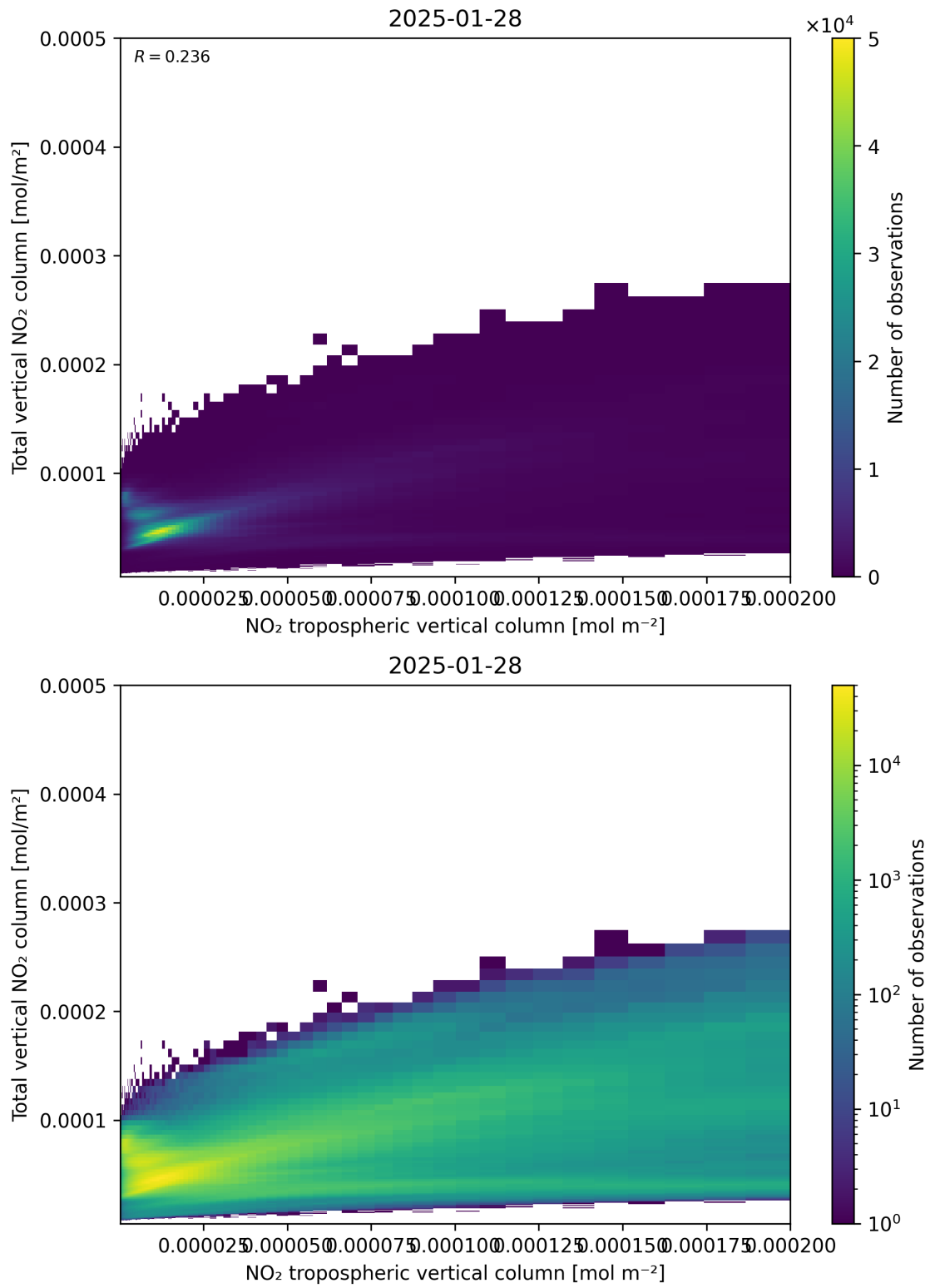
Figure 128: Scatter density plot of “NO 2 tropospheric vertical column” against “Total vertical NO 2 column” for 2025-01-28 to 2025-01-29.
