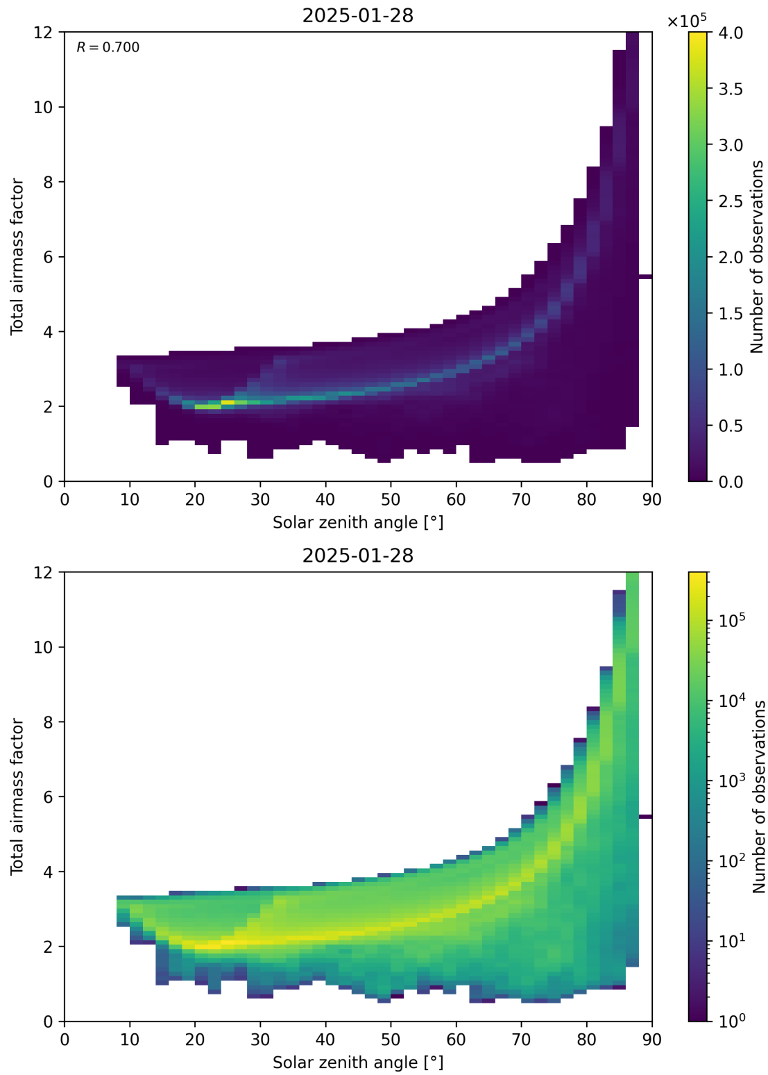
Figure 146: Scatter density plot of “Solar zenith angle” against “Total air mass factor” for 2025-01-28 to 2025-01-29.
