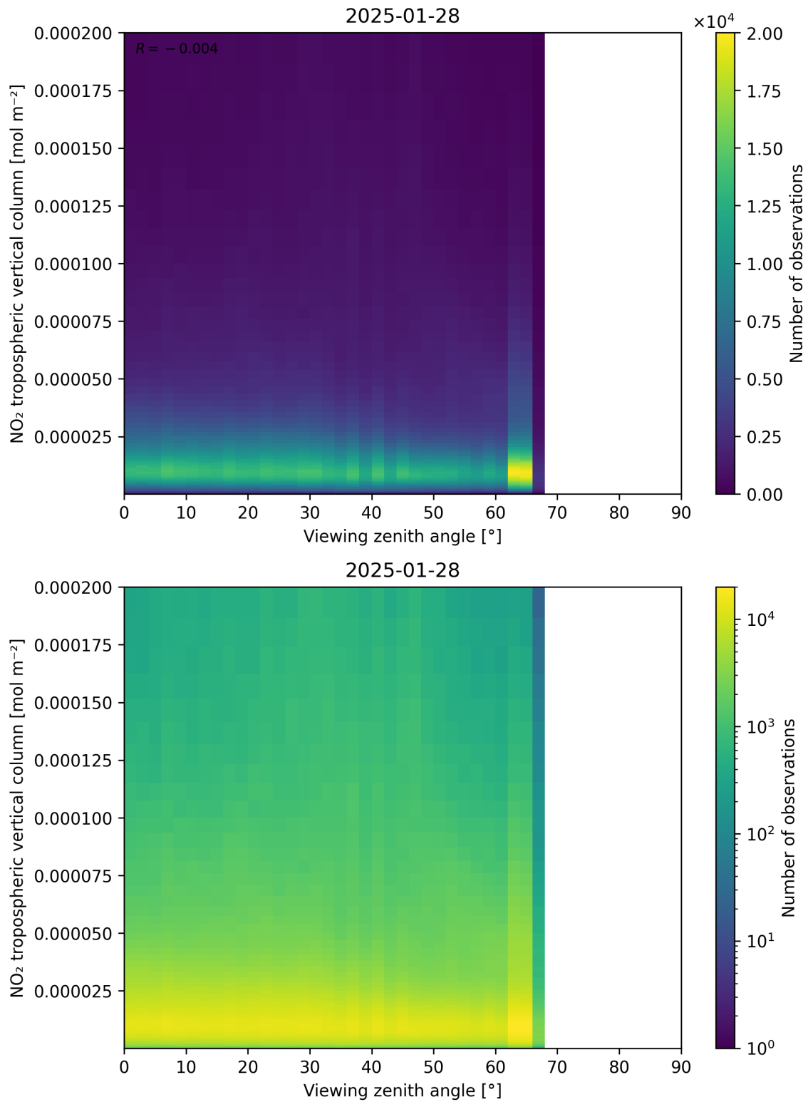
Figure 169: Scatter density plot of “Viewing zenith angle” against “NO 2 tropospheric vertical column” for 2025-01-28 to 2025-01-29.
