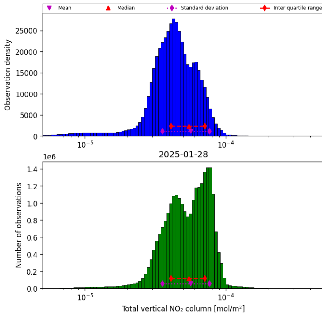
Figure 38: Histogram of “Total vertical NO 2 column” for 2025-01-28 to 2025-01-29
