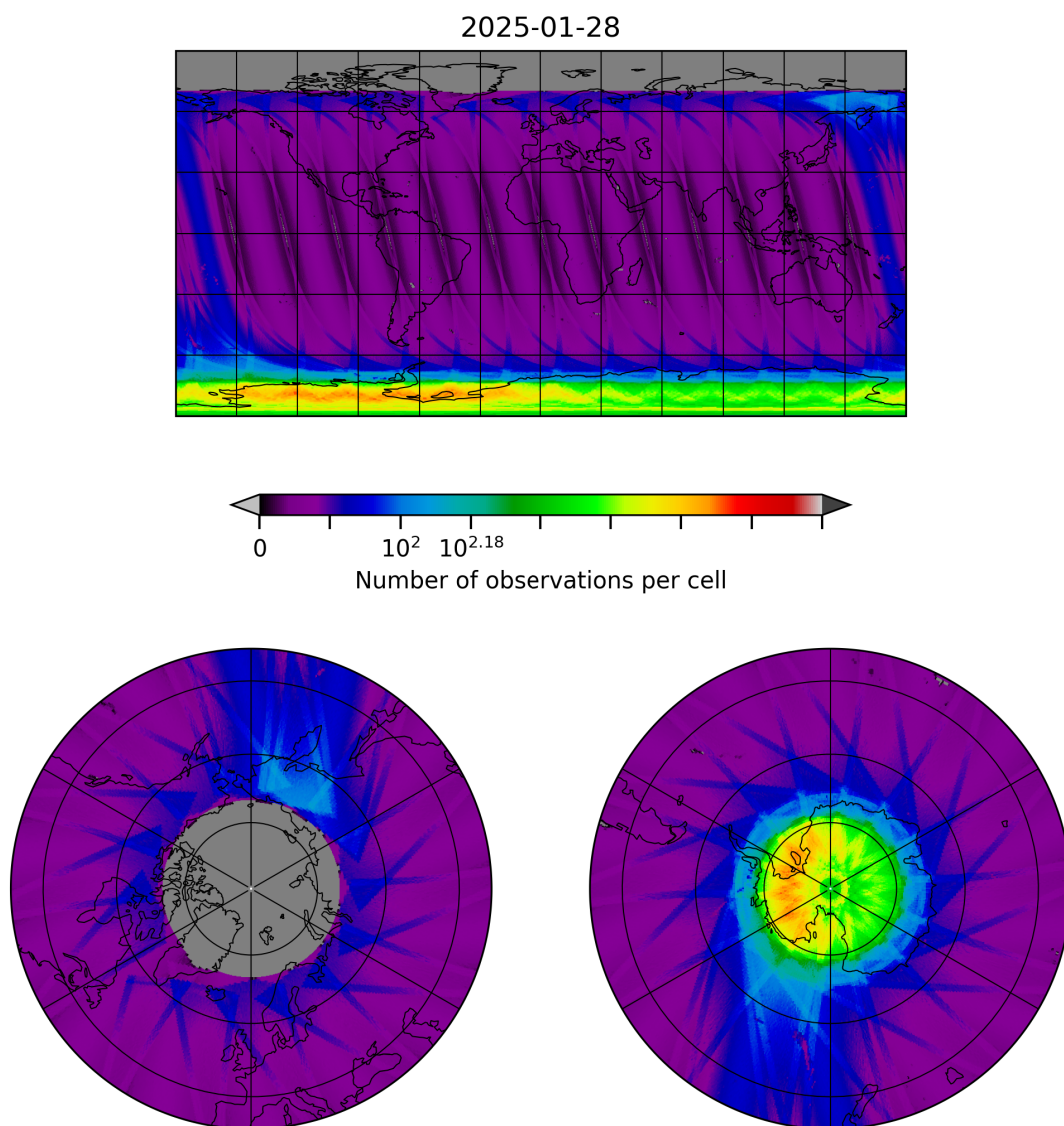
Figure 10: Map of the number of observations for 2025-01-28 to 2025-01-29
