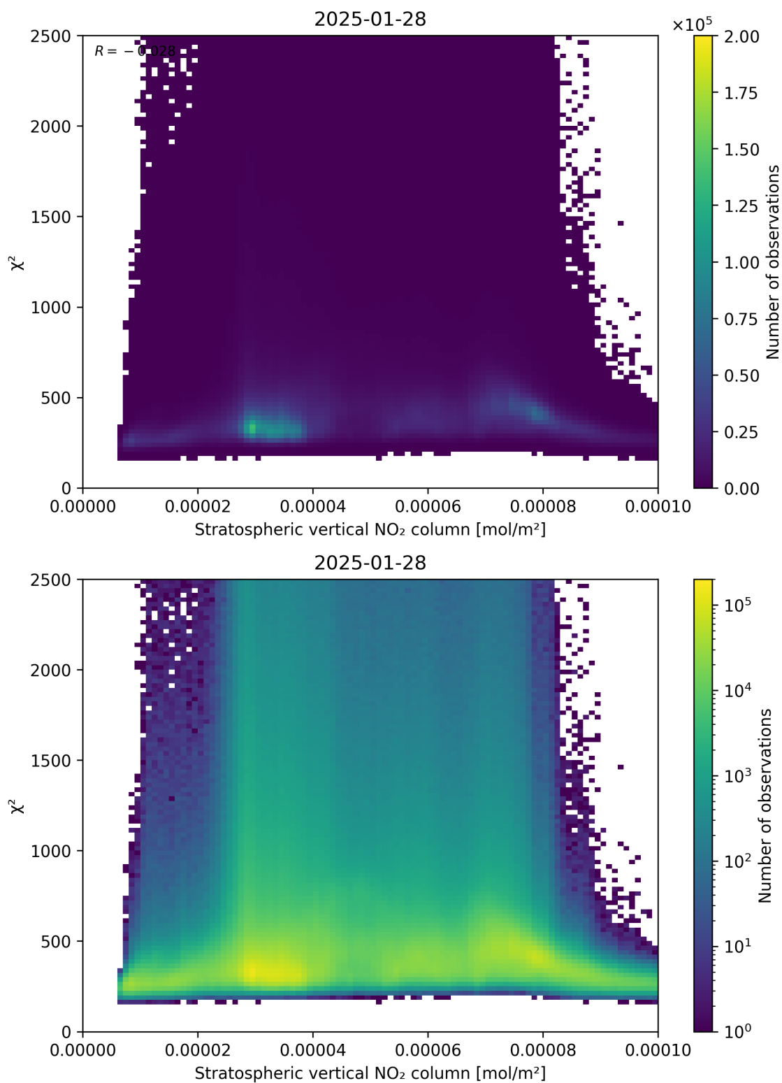
Figure 97: Scatter density plot of “Stratospheric vertical NO 2 column” against “ \chi^2 ” for 2025-01-28 to 2025-01-29.
