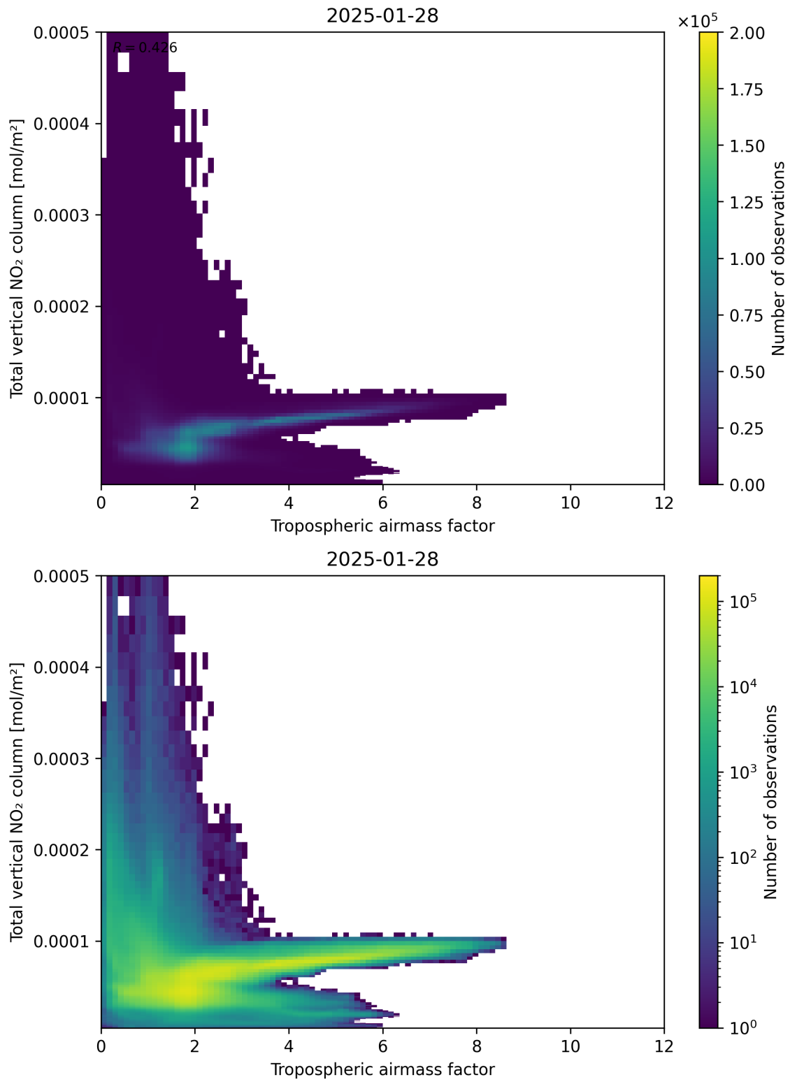
Figure 77: Scatter density plot of “Tropospheric airmass factor” against “Total vertical NO 2 column” for 2025-01-28 to 2025-01-29.
