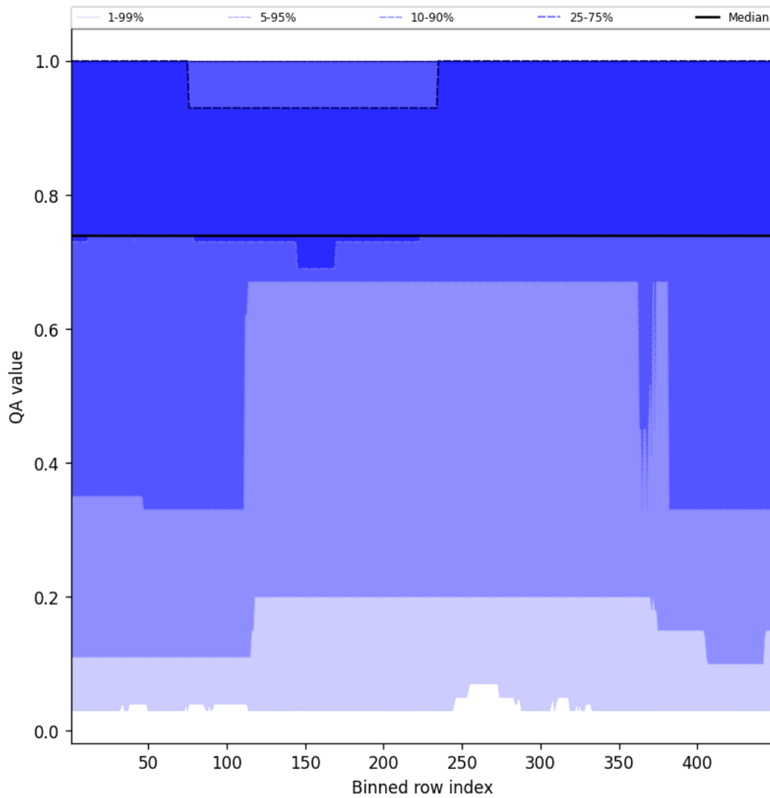
Figure 45: Along track statistics of "QA value" for 2025-01-28 to 2025-01-29
