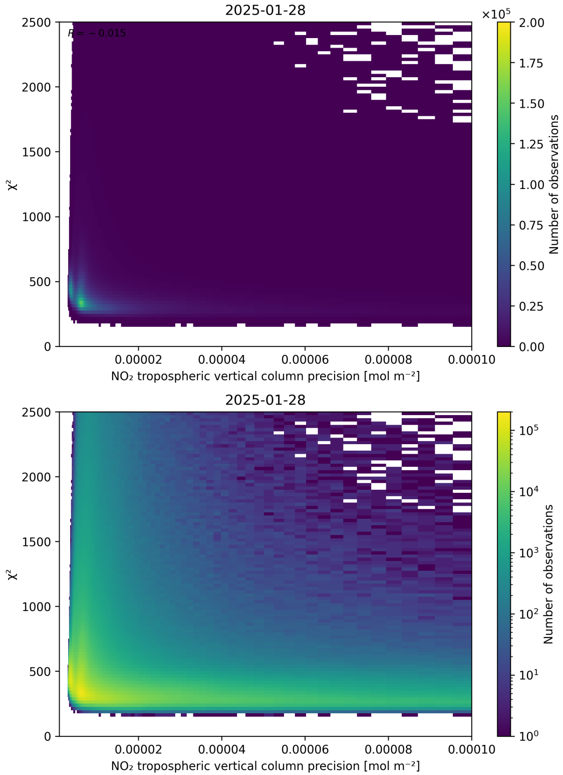
Figure 134: Scatter density plot of “NO 2 tropospheric vertical column precision” against “ \chi^2 ” for 2025-01-28 to 2025-01-29.
