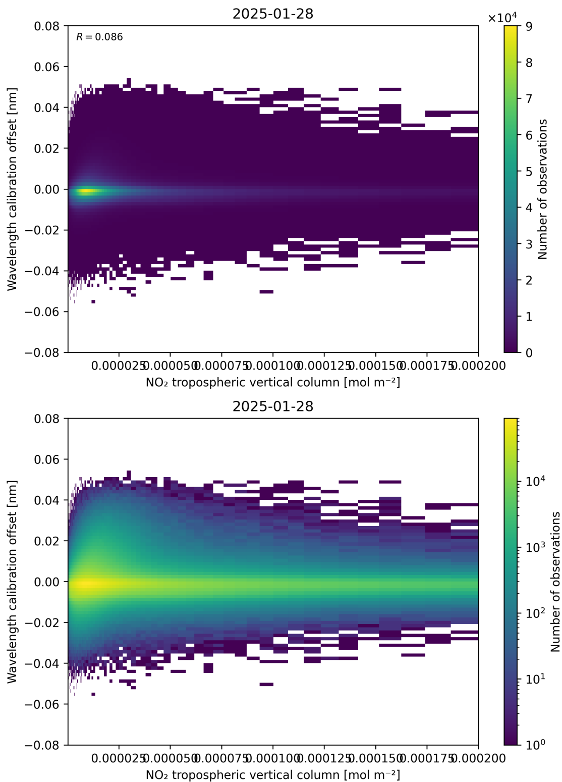
Figure 143: Scatter density plot of “NO 2 tropospheric vertical column” against “Wavelength calibration offset” for 2025-01-28 to 2025-01-29.
