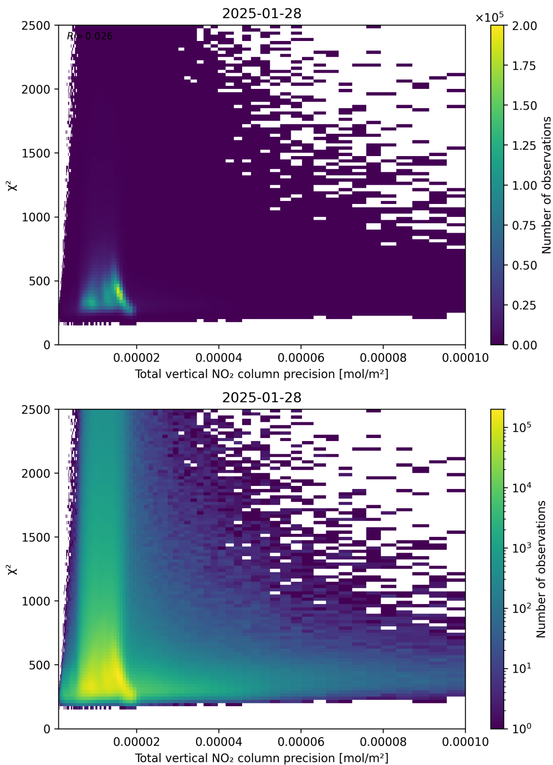
Figure 116: Scatter density plot of “Total vertical NO 2 column precision” against “ \chi^2 ” for 2025-01-28 to 2025-01-29.
