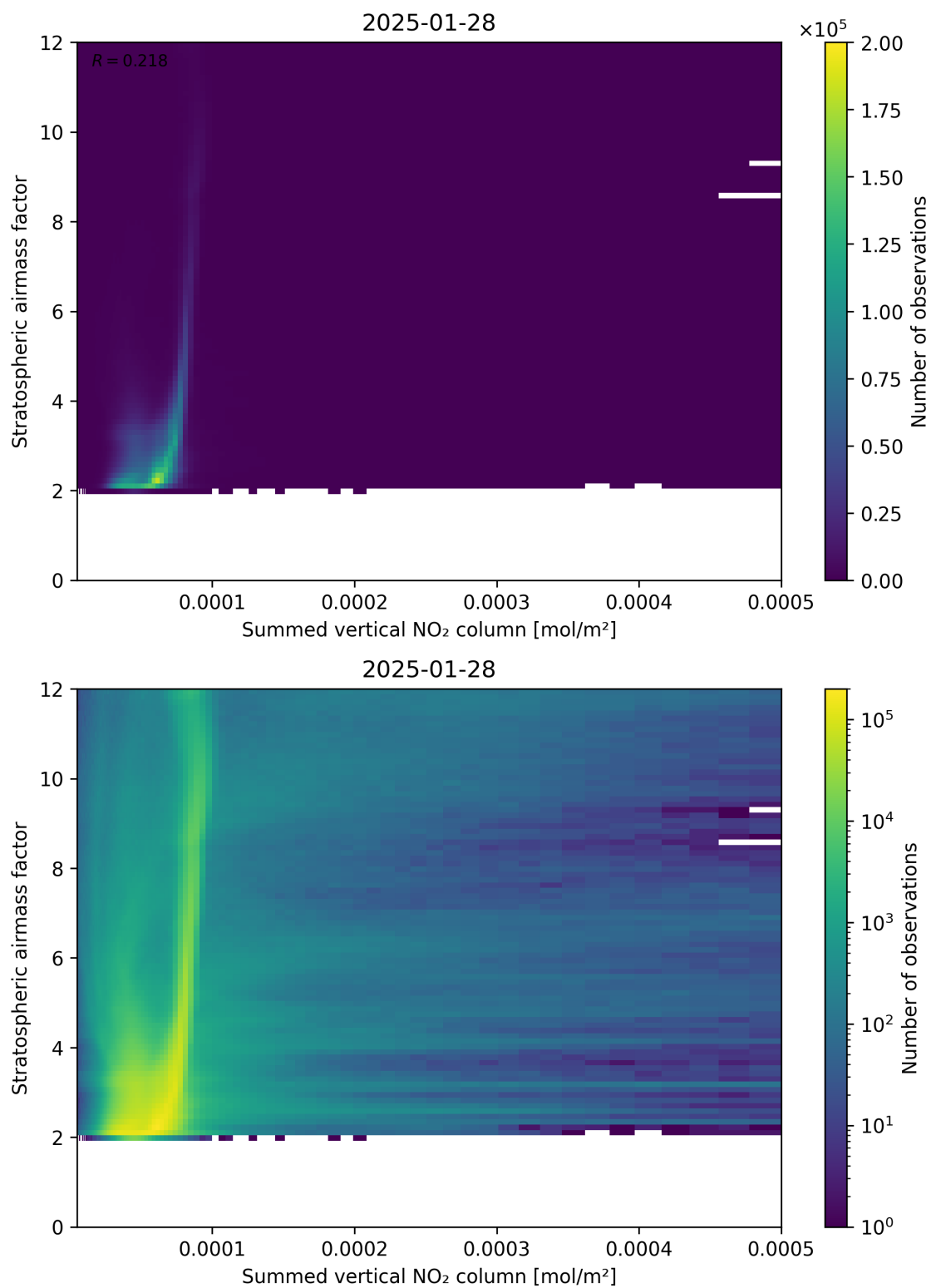
Figure 103: Scatter density plot of “Summed vertical NO 2 column” against “Stratospheric airmass factor” for 2025-01-28 to 2025-01-29.
