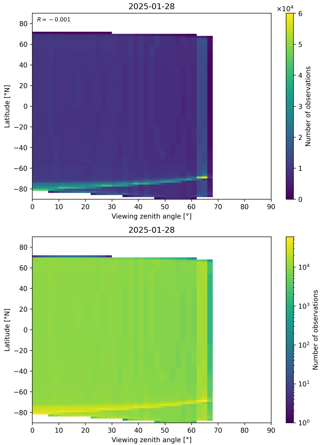
Figure 163: Scatter density plot of “Viewing zenith angle” against “Latitude” for 2025-01-28 to 2025-01-29.
