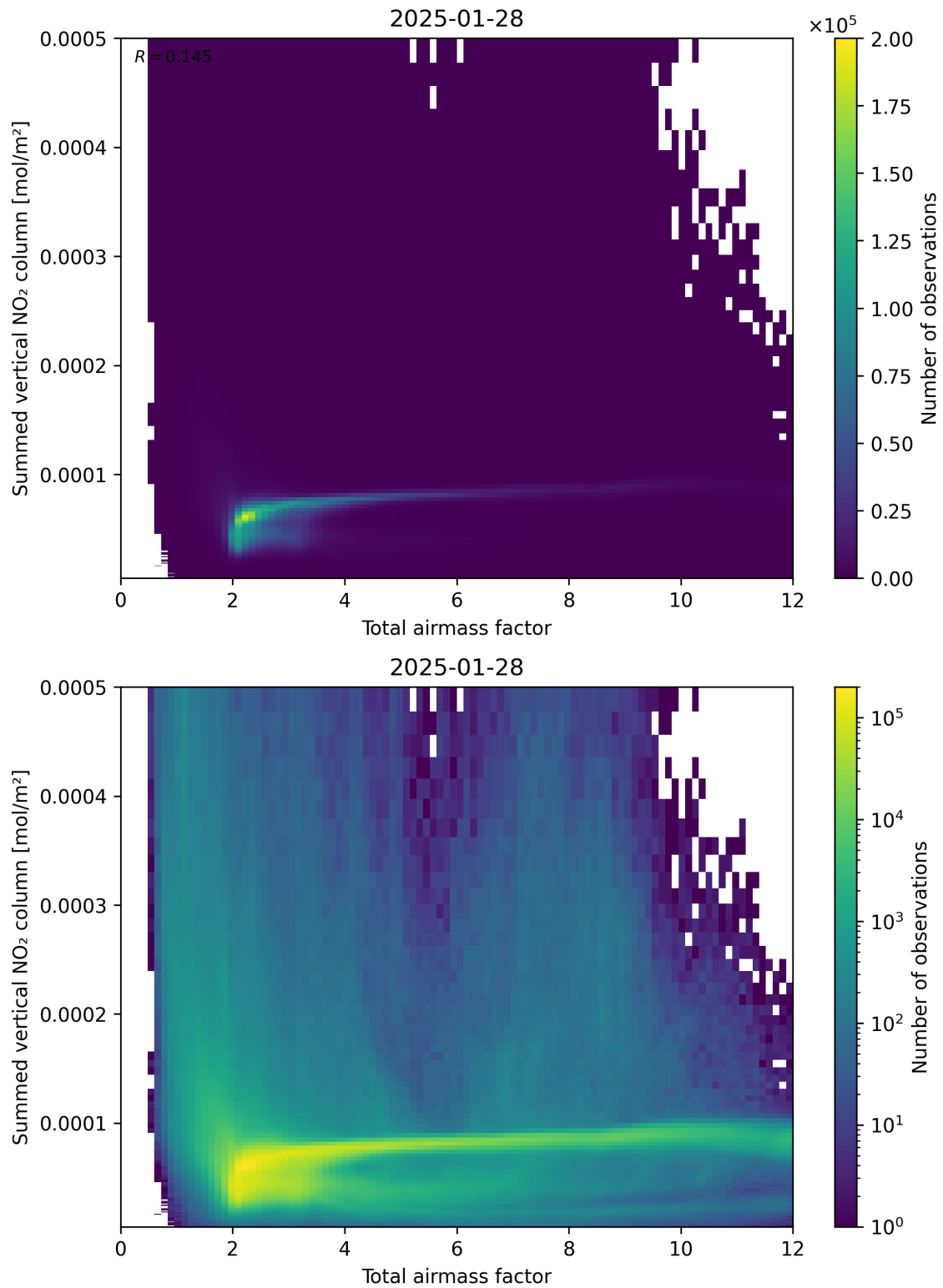
Figure 65: Scatter density plot of “Total airmass factor” against “Summed vertical NO 2 column” for 2025-01-28 to 2025-01-29.
