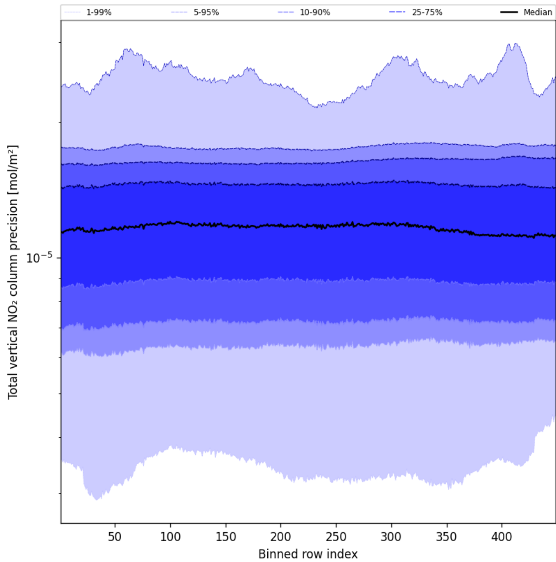
Figure 56: Along track statistics of “Total vertical NO 2 column precision” for 2025-01-28 to 2025-01-29
