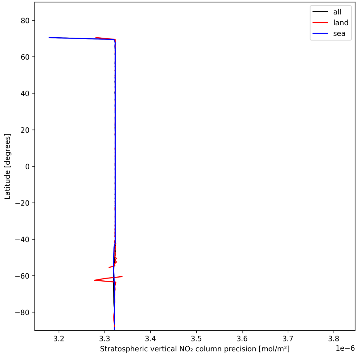
Figure 20: Zonal average of “Stratospheric vertical NO 2 column precision” for 2025-01-28 to 2025-01-29.
