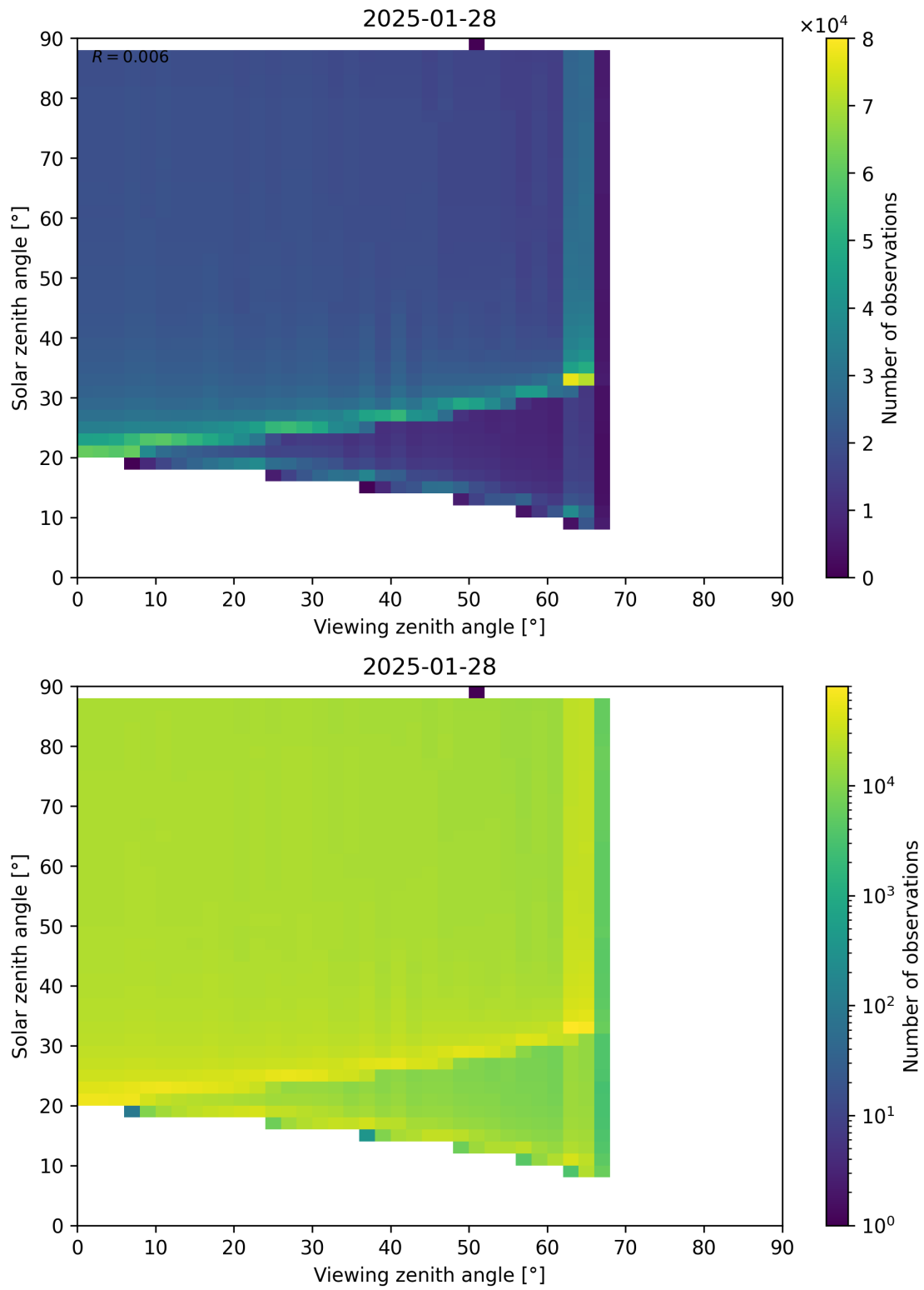
Figure 172: Scatter density plot of “Viewing zenith angle” against “Solar zenith angle” for 2025-01-28 to 2025-01-29.
