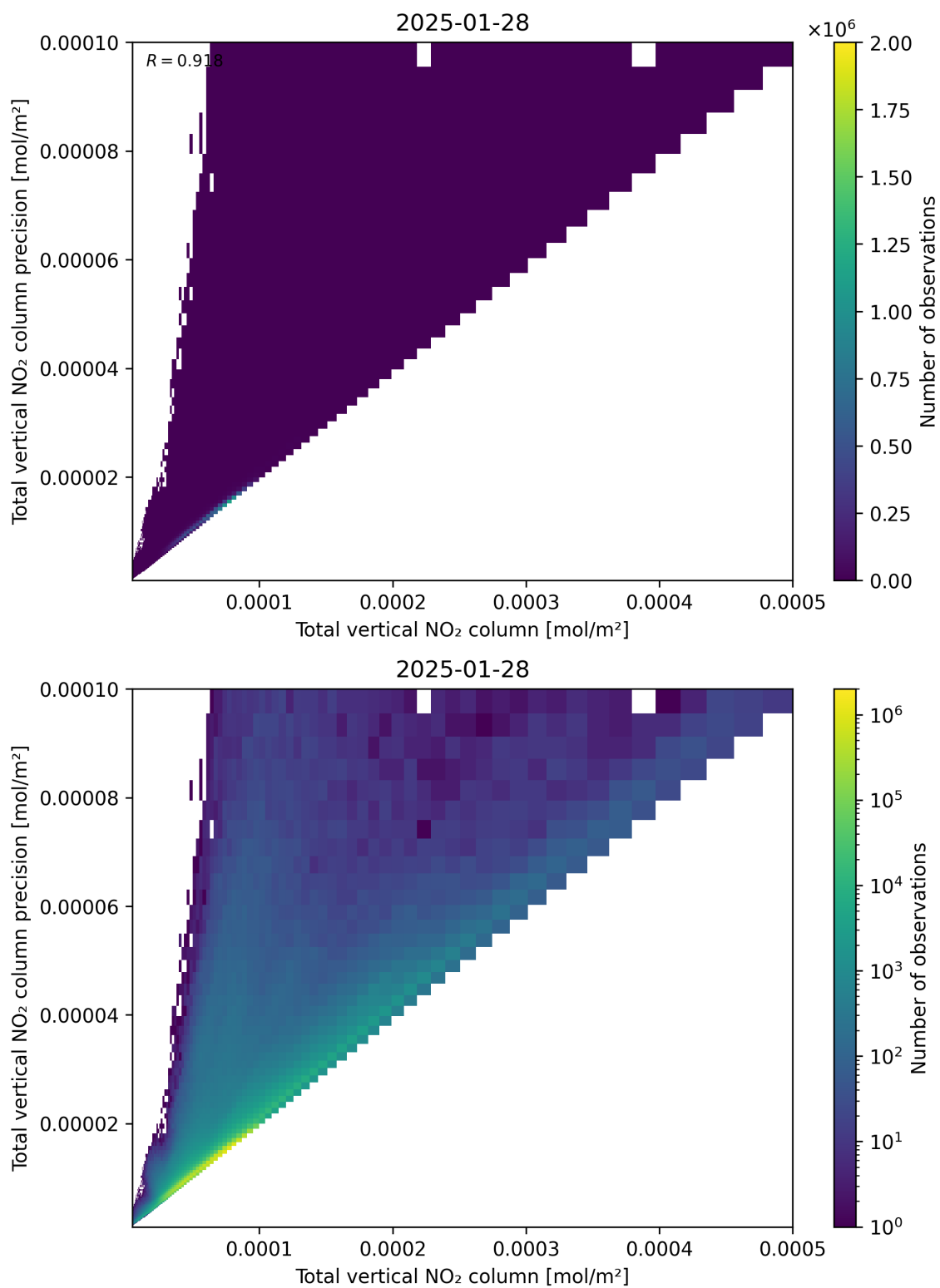
Figure 114: Scatter density plot of “Total vertical NO 2 column” against “Total vertical NO 2 column precision” for 2025-01-28 to 2025-01-29.
