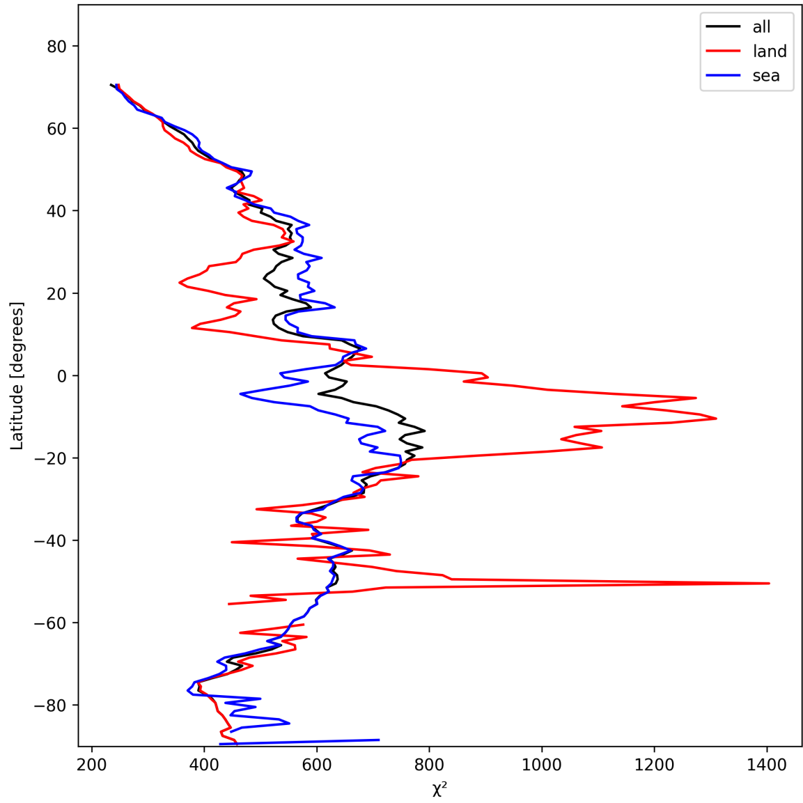
Figure 25: Zonal average of “ \chi^2 ” for 2025-01-28 to 2025-01-29.
