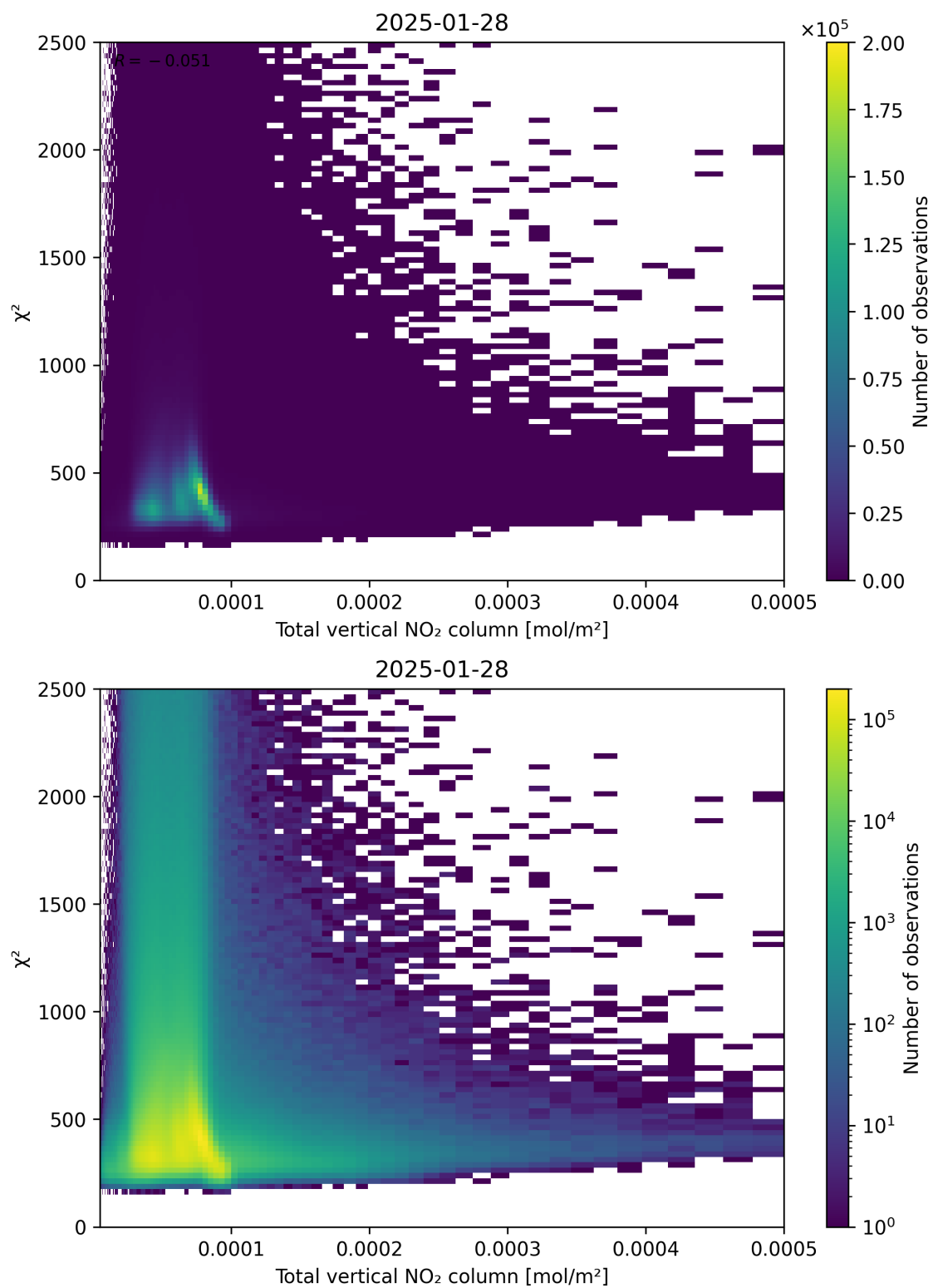
Figure 111: Scatter density plot of “Total vertical NO 2 column” against “ \chi^2 ” for 2025-01-28 to 2025-01-29.
