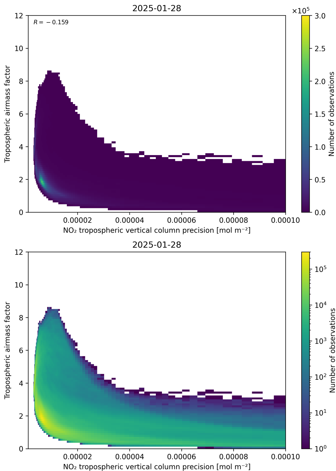
Figure 133: Scatter density plot of “NO 2 tropospheric vertical column precision” against “Tropospheric air mass factor” for 2025-01-28 to 2025-01-29.
