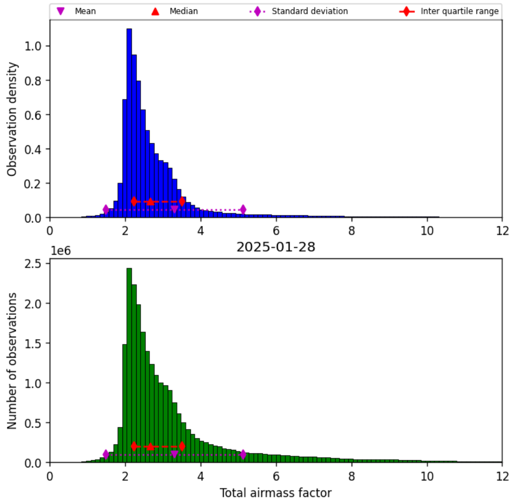
Figure 32: Histogram of “Total airmass factor” for 2025-01-28 to 2025-01-29
