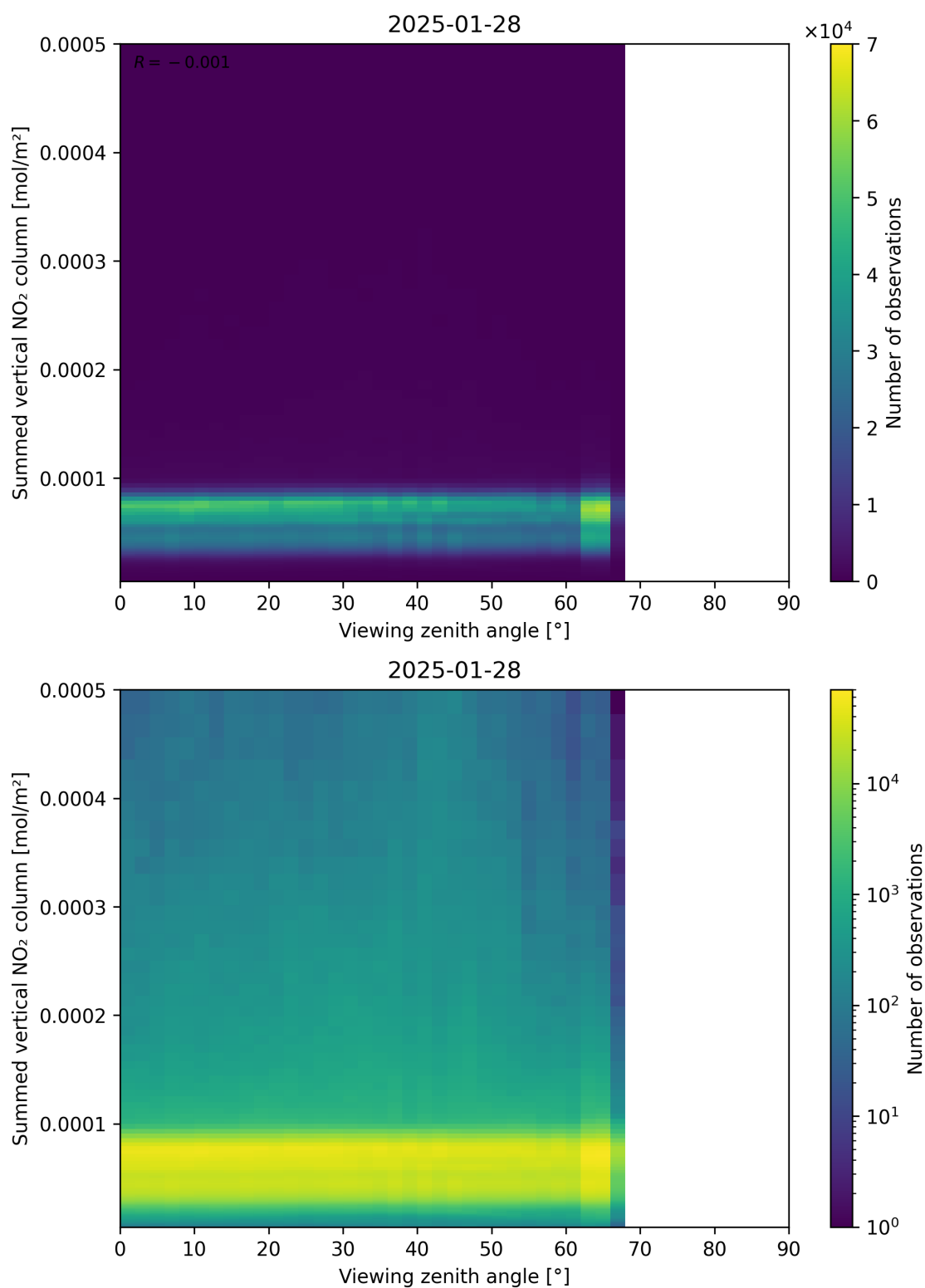
Figure 165: Scatter density plot of “Viewing zenith angle” against “Summed vertical NO 2 column” for 2025-01-28 to 2025-01-29.
