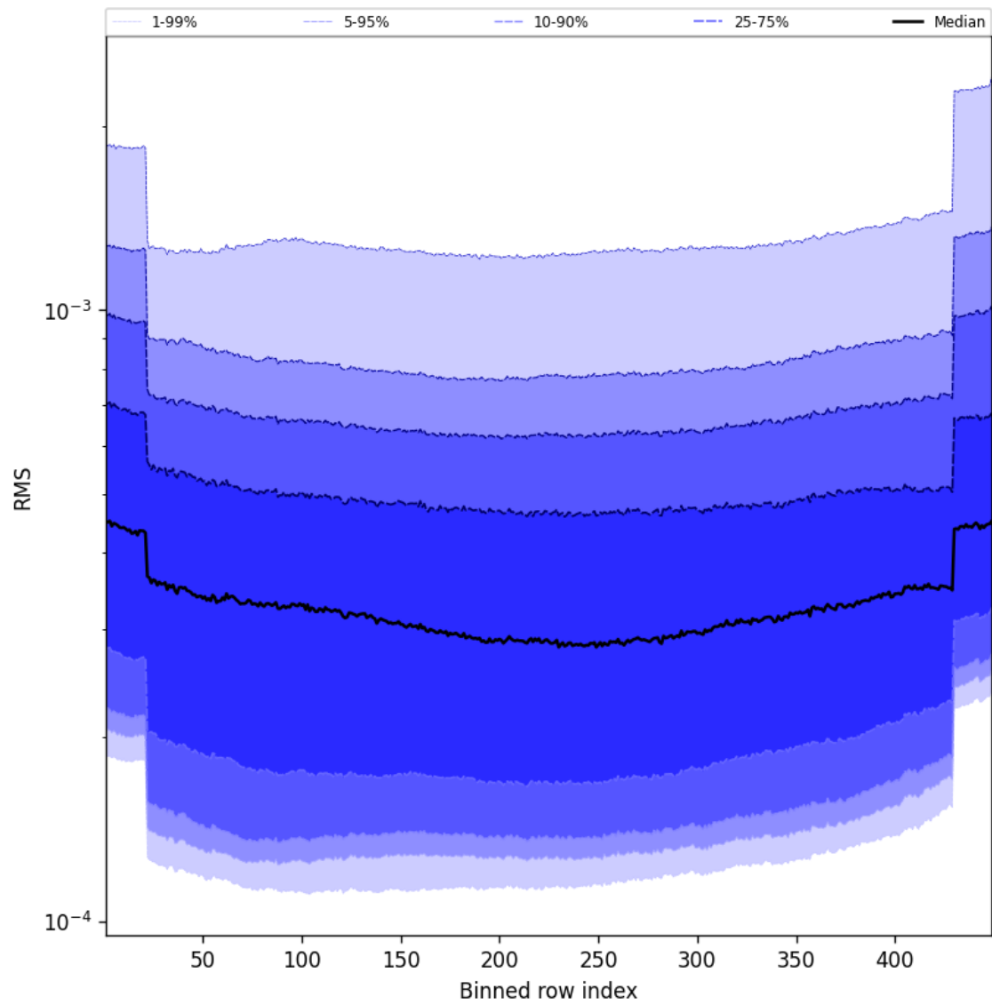
Figure 60: Along track statistics of “RMS” for 2025-01-28 to 2025-01-29
