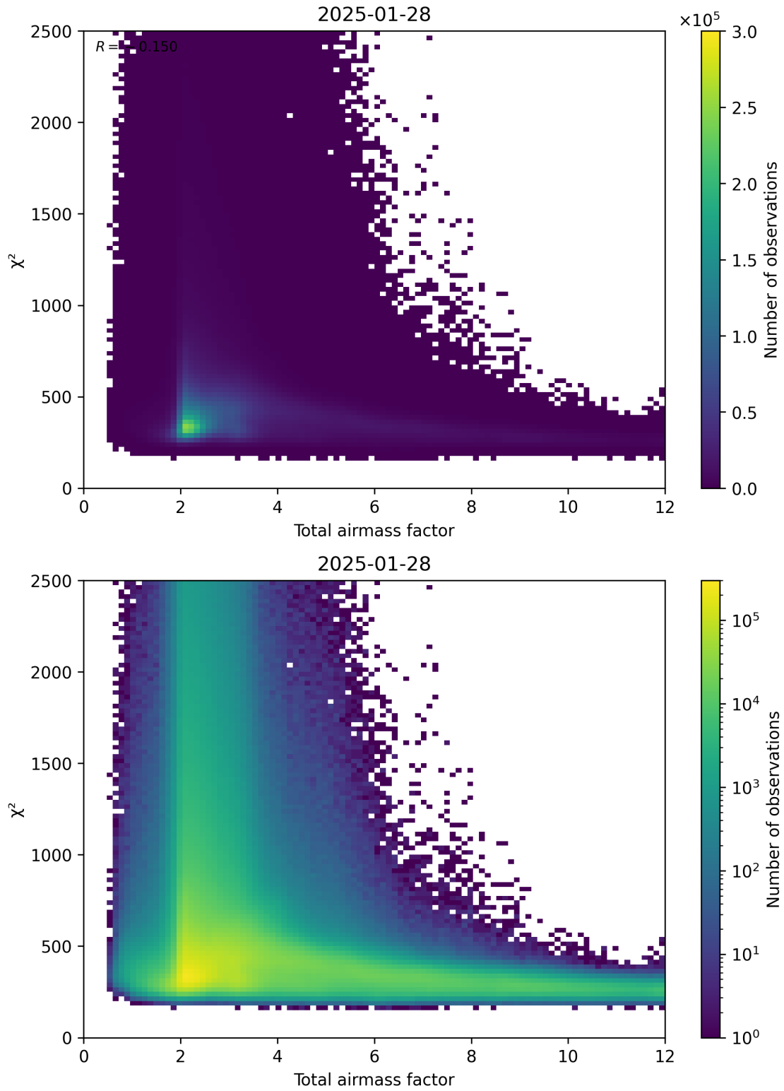
Figure 63: Scatter density plot of “Total airmass factor” against “ \chi^2 ” for 2025-01-28 to 2025-01-29.
