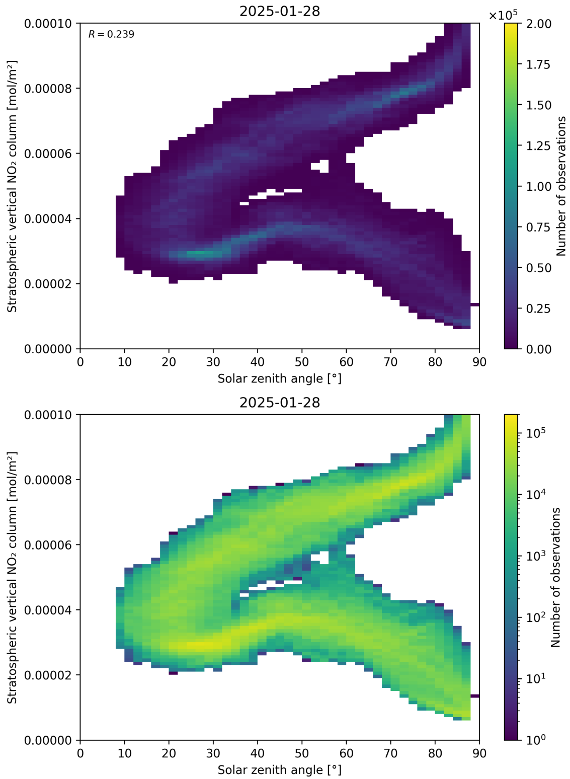
Figure 150: Scatter density plot of “Solar zenith angle” against “Stratospheric vertical NO 2 column” for 2025-01-28 to 2025-01-29.
