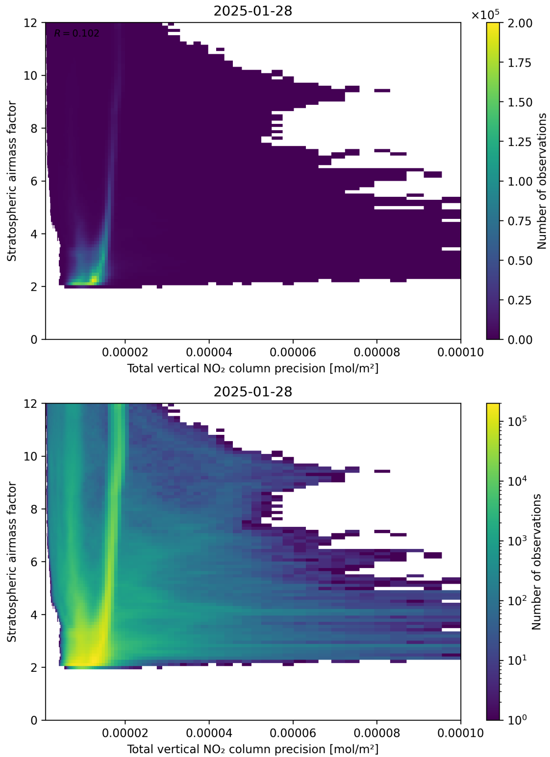
Figure 115: Scatter density plot of “Total vertical NO 2 column precision” against “Stratospheric air mass factor” for 2025-01-28 to 2025-01-29.
