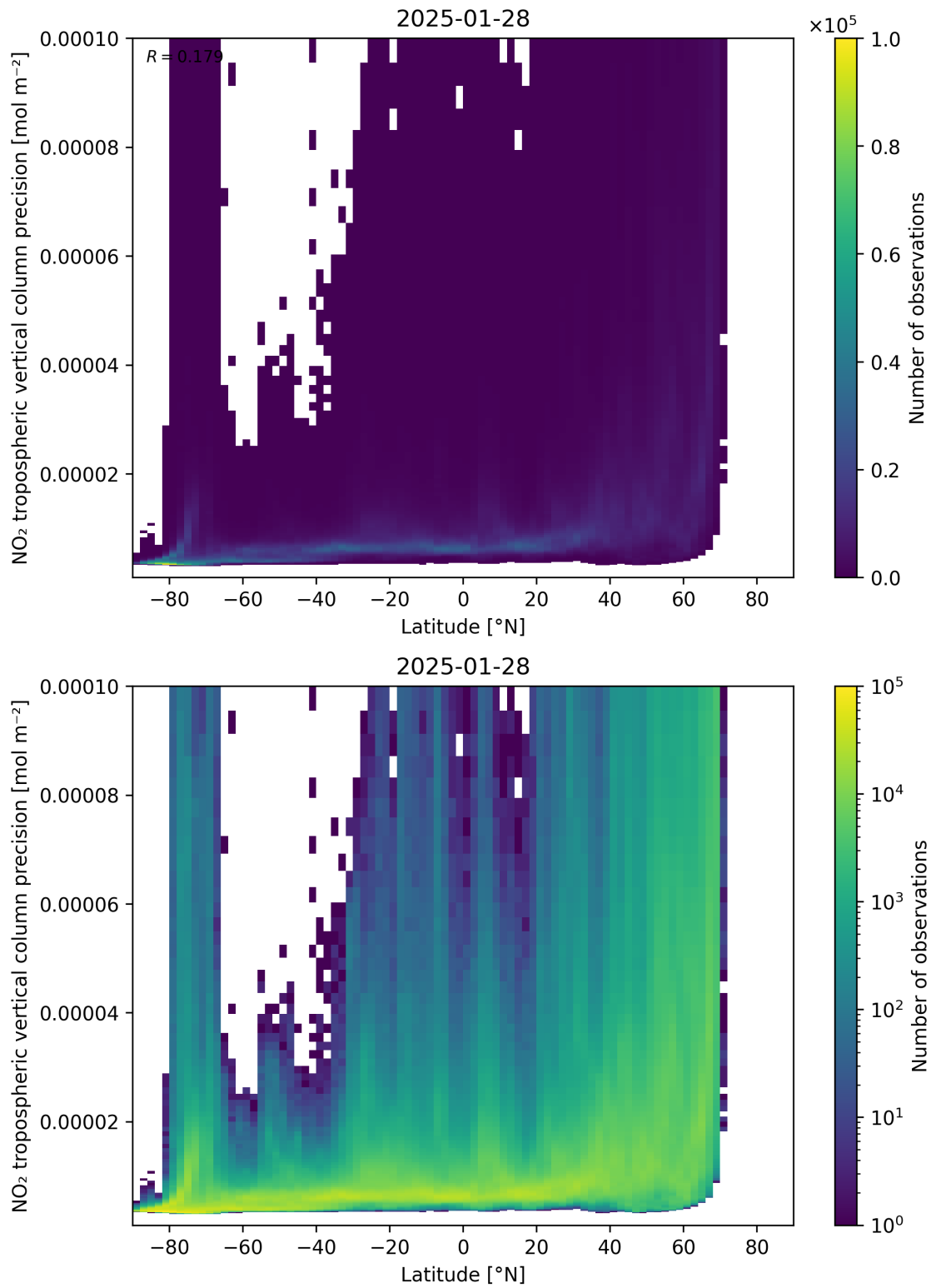
Figure 93: Scatter density plot of “Latitude” against “NO 2 tropospheric vertical column precision” for 2025-01-28 to 2025-01-29.
