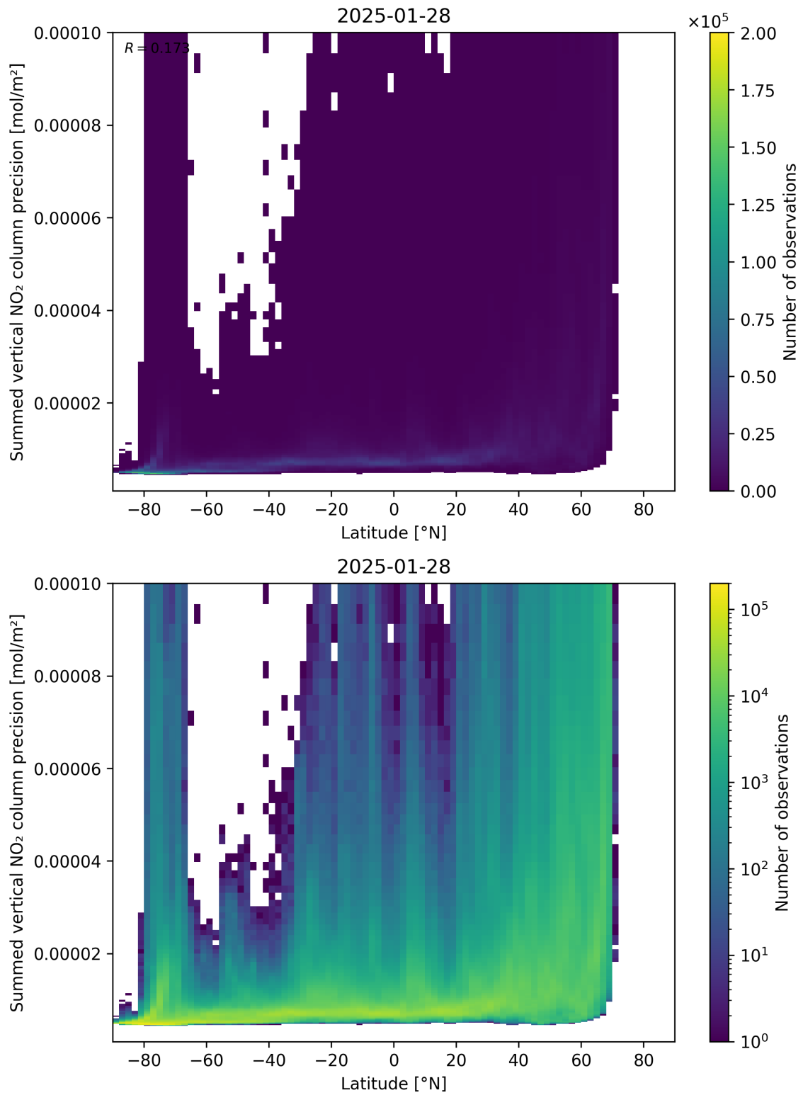
Figure 89: Scatter density plot of “Latitude” against “Summed vertical NO 2 column precision” for 2025-01-28 to 2025-01-29.
