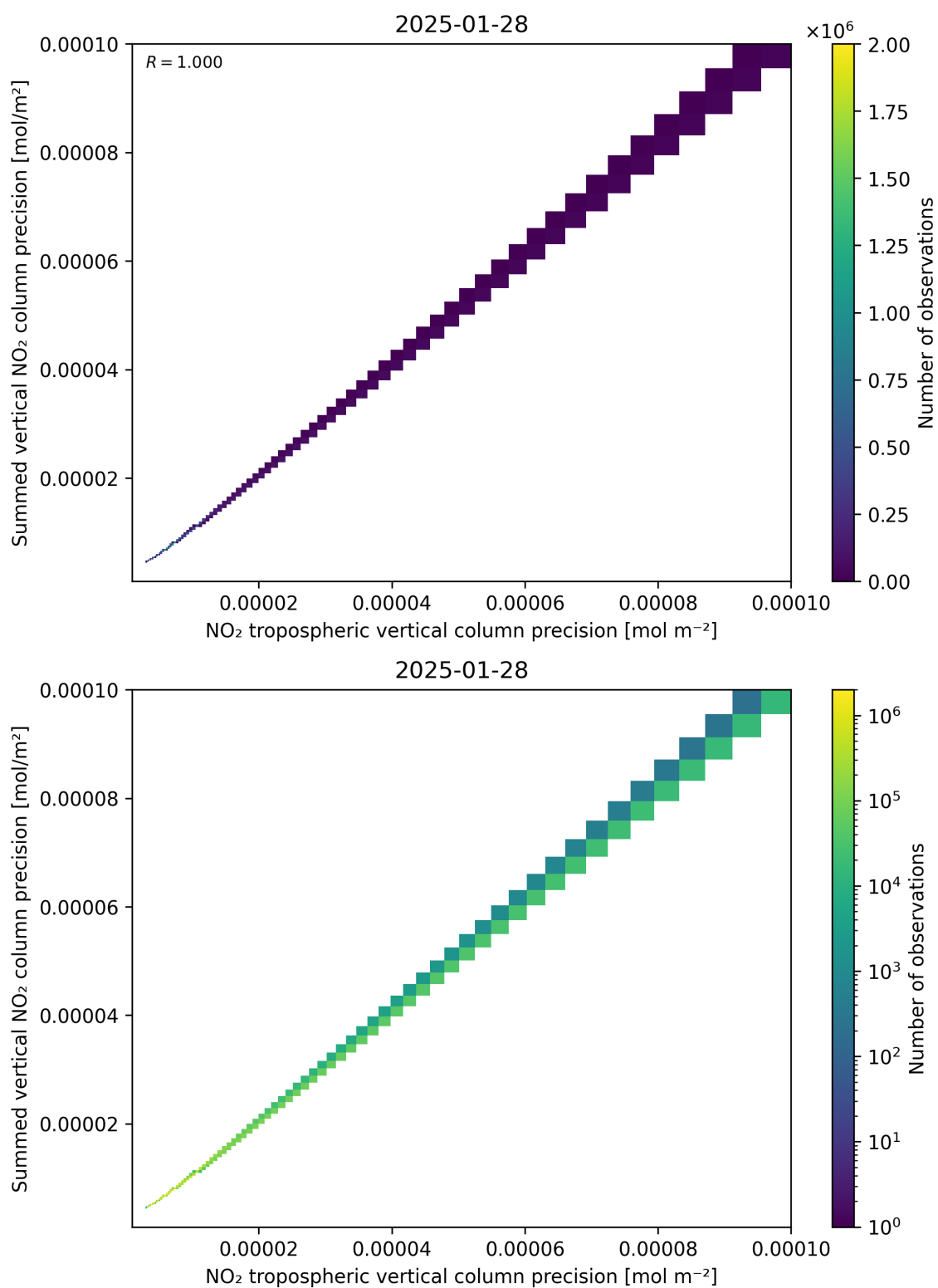
Figure 137: Scatter density plot of “NO 2 tropospheric vertical column precision” against “Summed vertical NO 2 column precision” for 2025-01-28 to 2025-01-29.
