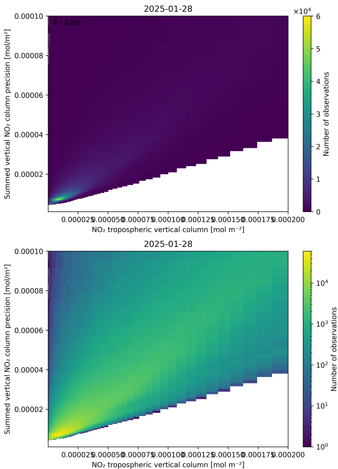
Figure 127: Scatter density plot of “NO 2 tropospheric vertical column” against “Summed vertical NO 2 column precision” for 2025-01-28 to 2025-01-29.
