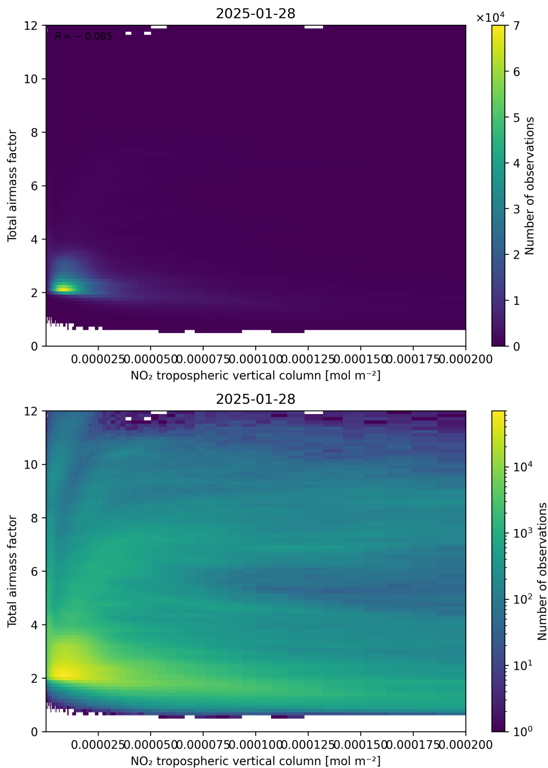
Figure 122: Scatter density plot of “NO 2 tropospheric vertical column” against “Total air mass factor” for 2025-01-28 to 2025-01-29.
