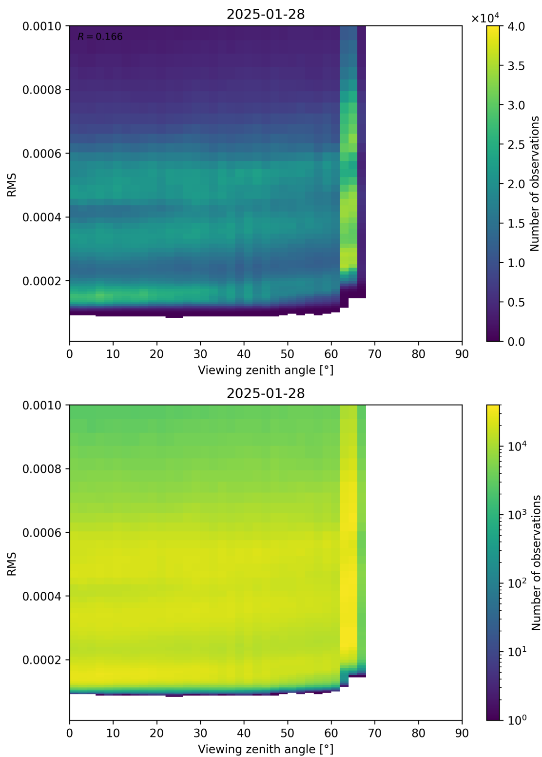
Figure 171: Scatter density plot of “Viewing zenith angle” against “RMS” for 2025-01-28 to 2025-01-29.
