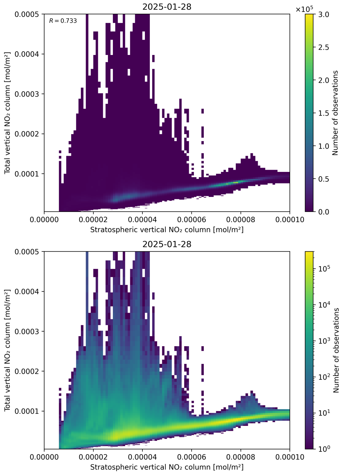
Figure 100: Scatter density plot of “Stratospheric vertical NO 2 column” against “Total vertical NO 2 column” for 2025-01-28 to 2025-01-29.
