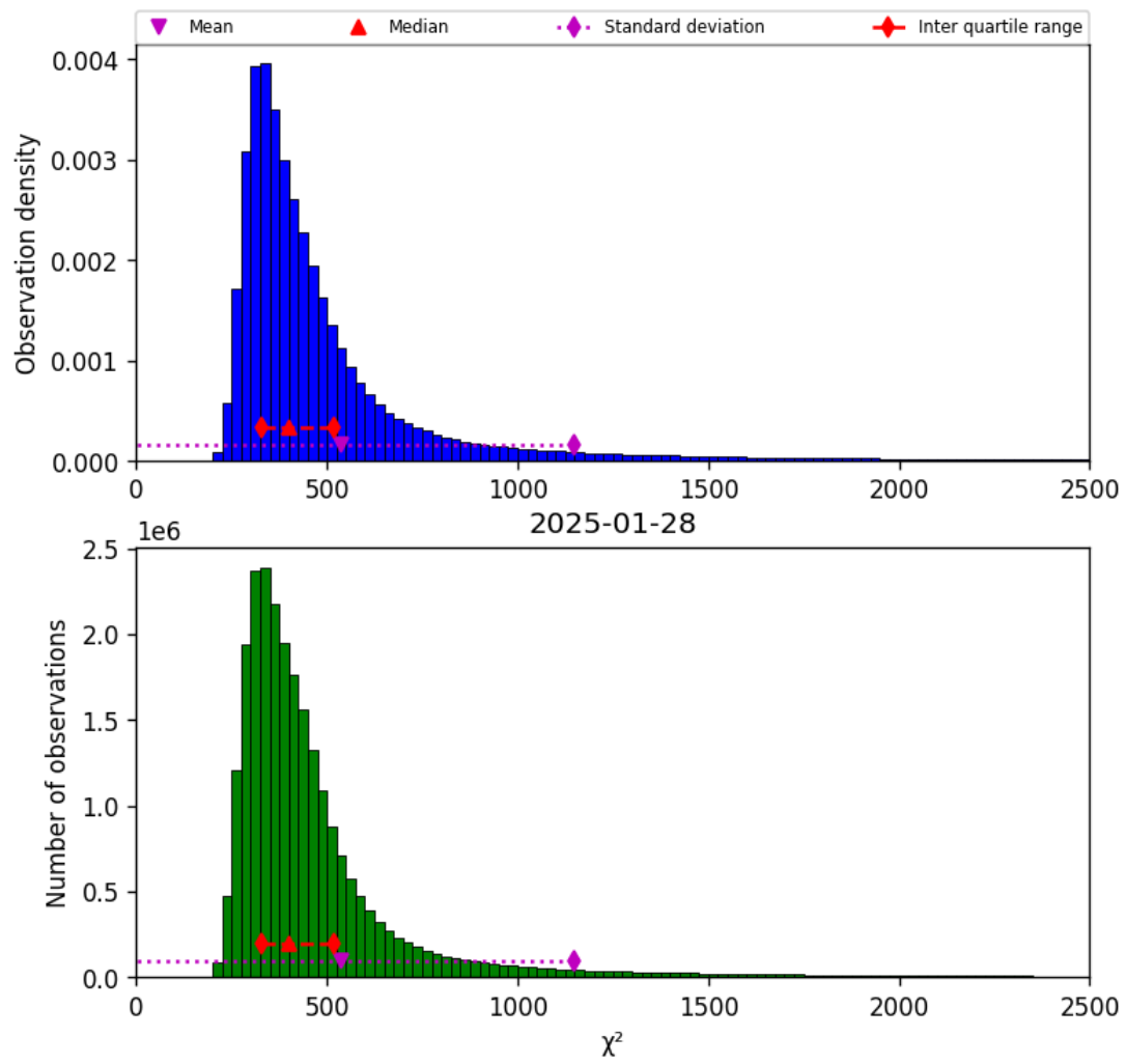
Figure 42: Histogram of " \chi^2 " for 2025-01-28 to 2025-01-29
