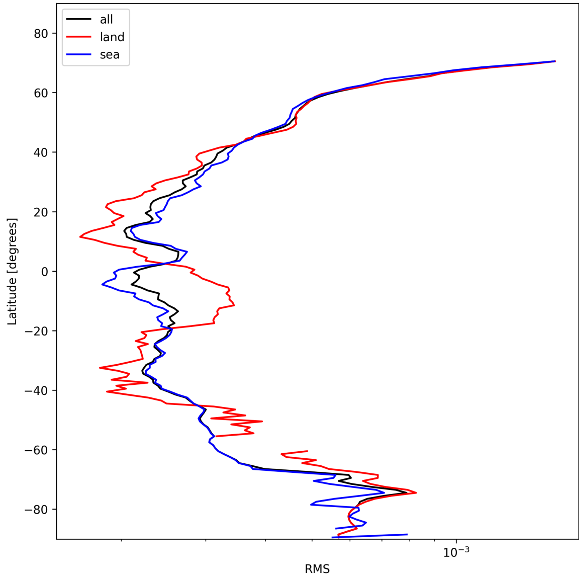
Figure 26: Zonal average of “RMS” for 2025-01-28 to 2025-01-29.
