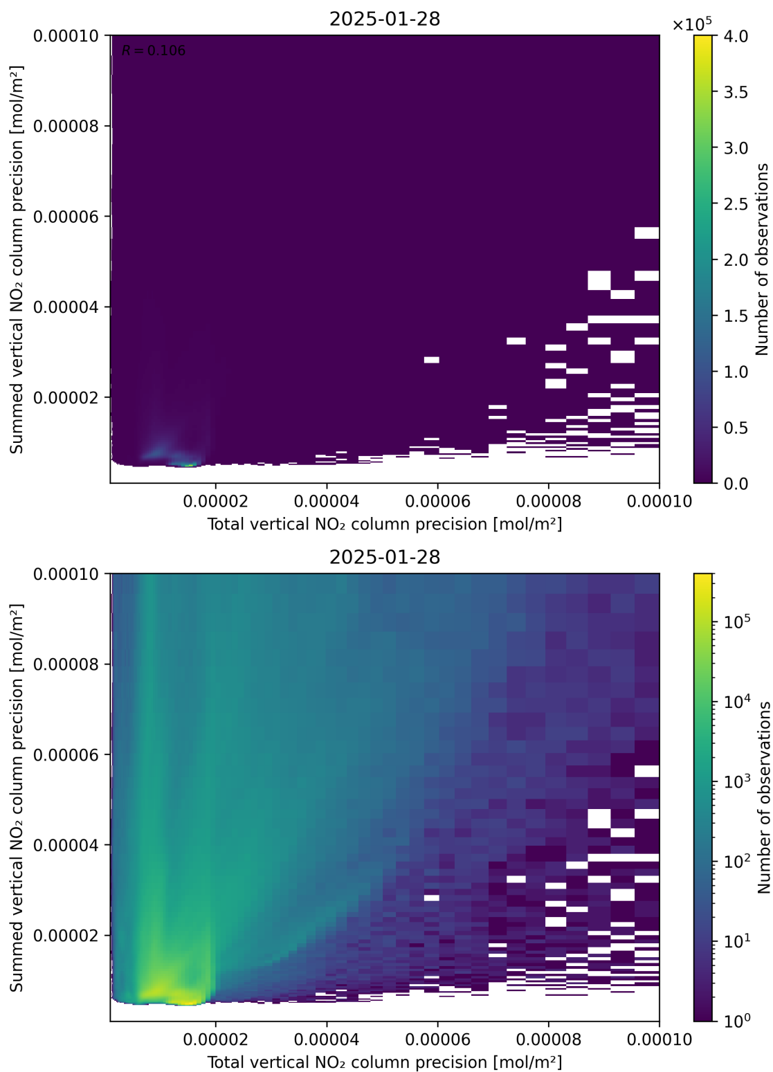
Figure 118: Scatter density plot of “Total vertical NO 2 column precision” against “Summed vertical NO 2 column precision” for 2025-01-28 to 2025-01-29.
