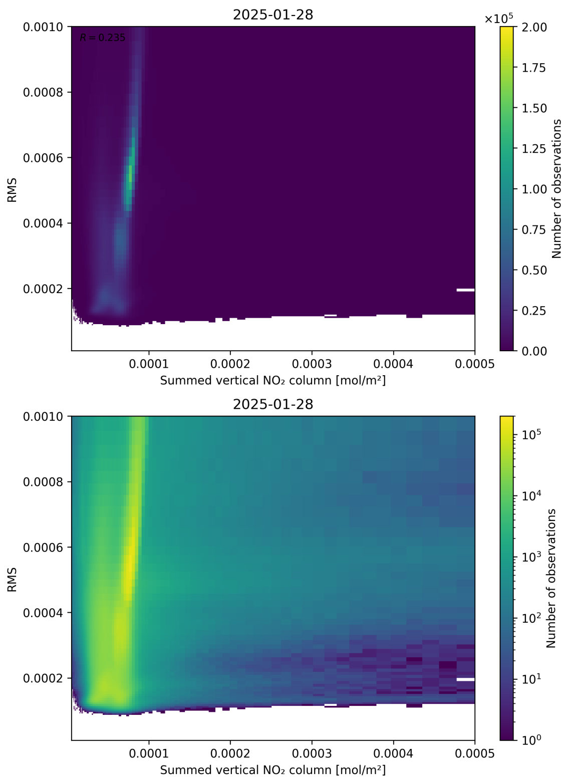
Figure 109: Scatter density plot of “Summed vertical NO 2 column” against “RMS” for 2025-01-28 to 2025-01-29.
