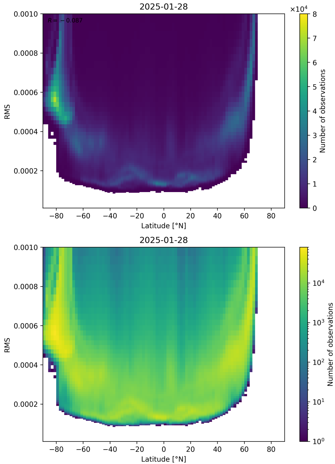
Figure 94: Scatter density plot of “Latitude” against “RMS” for 2025-01-28 to 2025-01-29.
