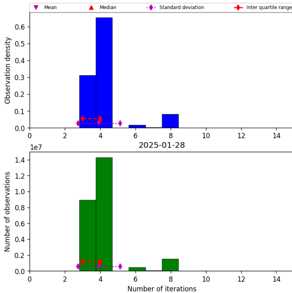
Figure 34: Histogram of “Number of iterations” for 2025-01-28 to 2025-01-29
