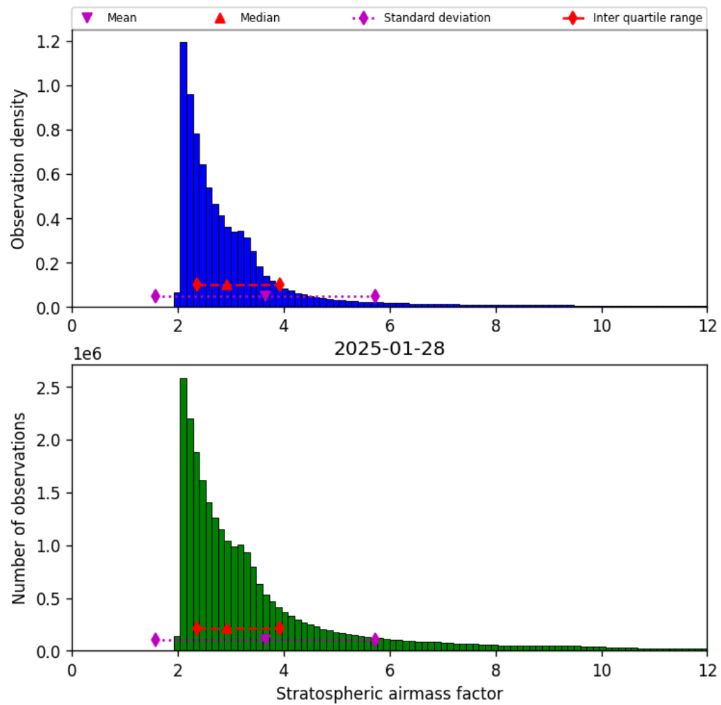
Figure 44: Histogram of “Stratospheric airmass factor” for 2025-01-28 to 2025-01-29
