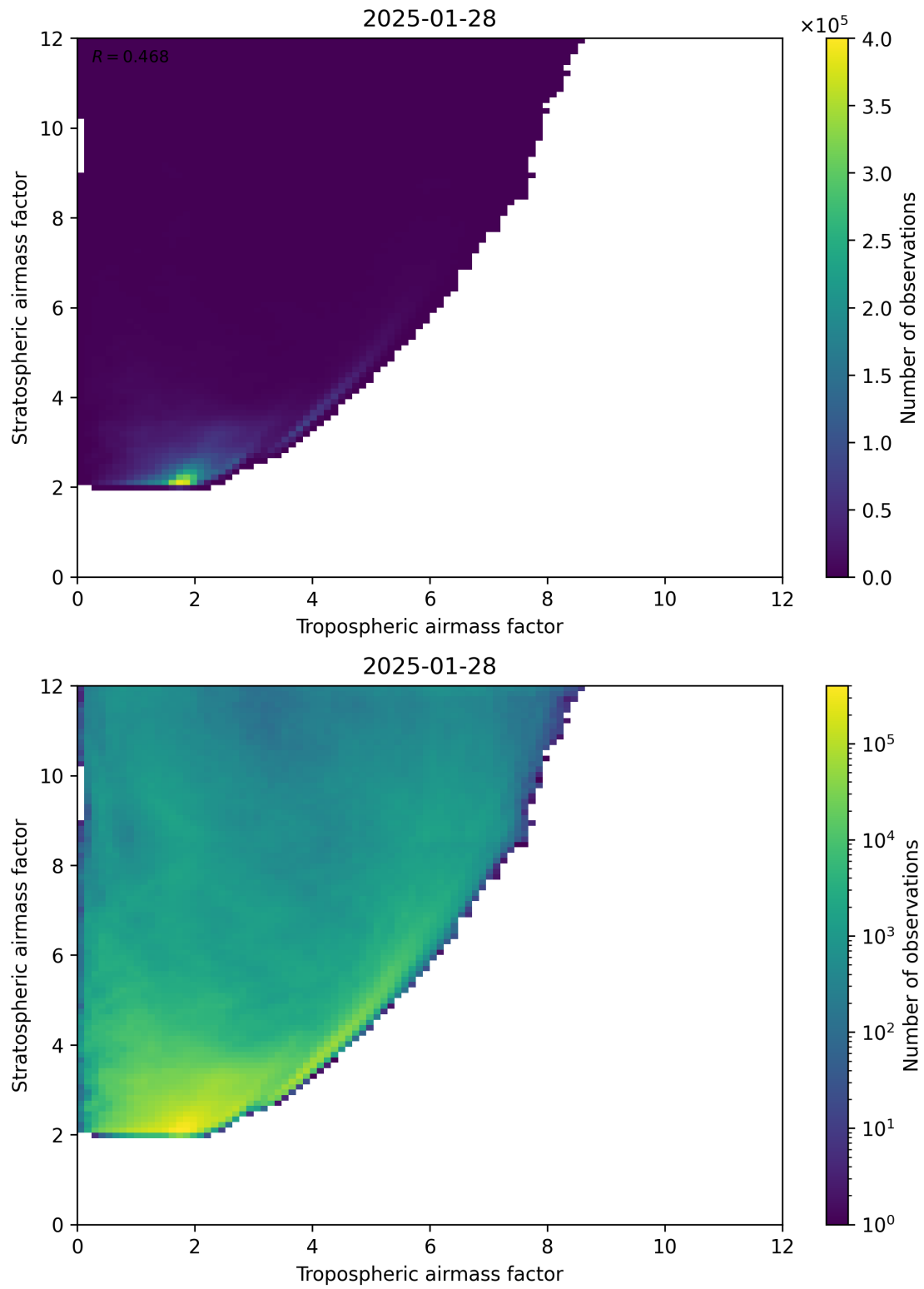
Figure 71: Scatter density plot of “Tropospheric airmass factor” against “Stratospheric airmass factor” for 2025-01-28 to 2025-01-29.
