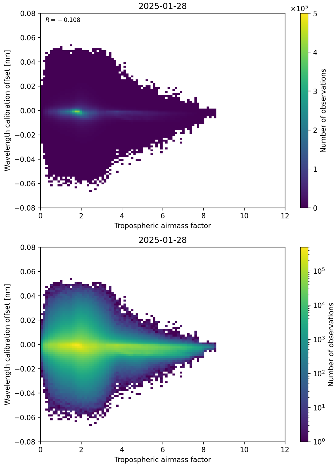
Figure 80: Scatter density plot of “Tropospheric airmass factor” against “Wavelength calibration offset” for 2025-01-28 to 2025-01-29.
