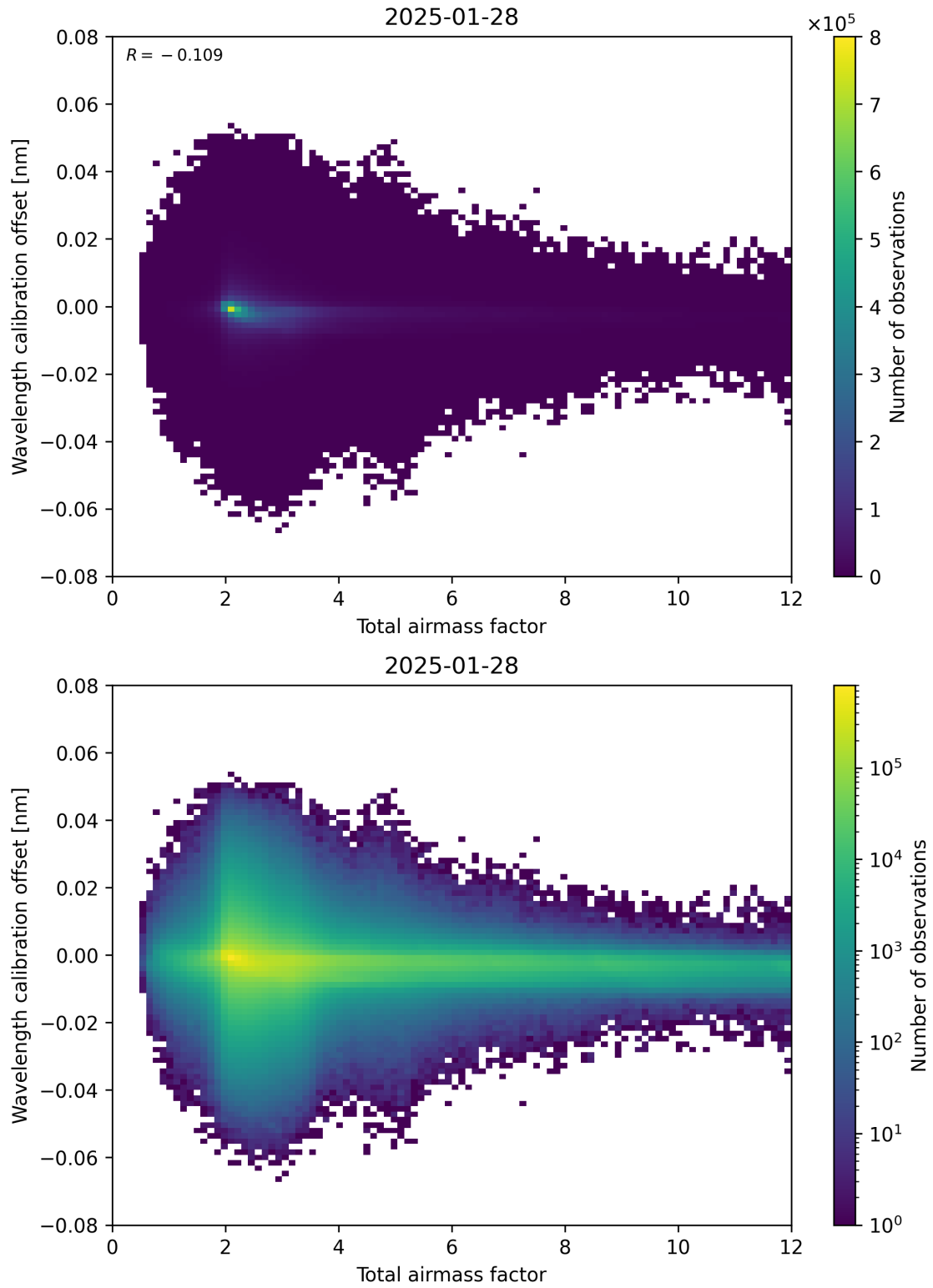
Figure 70: Scatter density plot of “Total airmass factor” against “Wavelength calibration offset” for 2025-01-28 to 2025-01-29.
