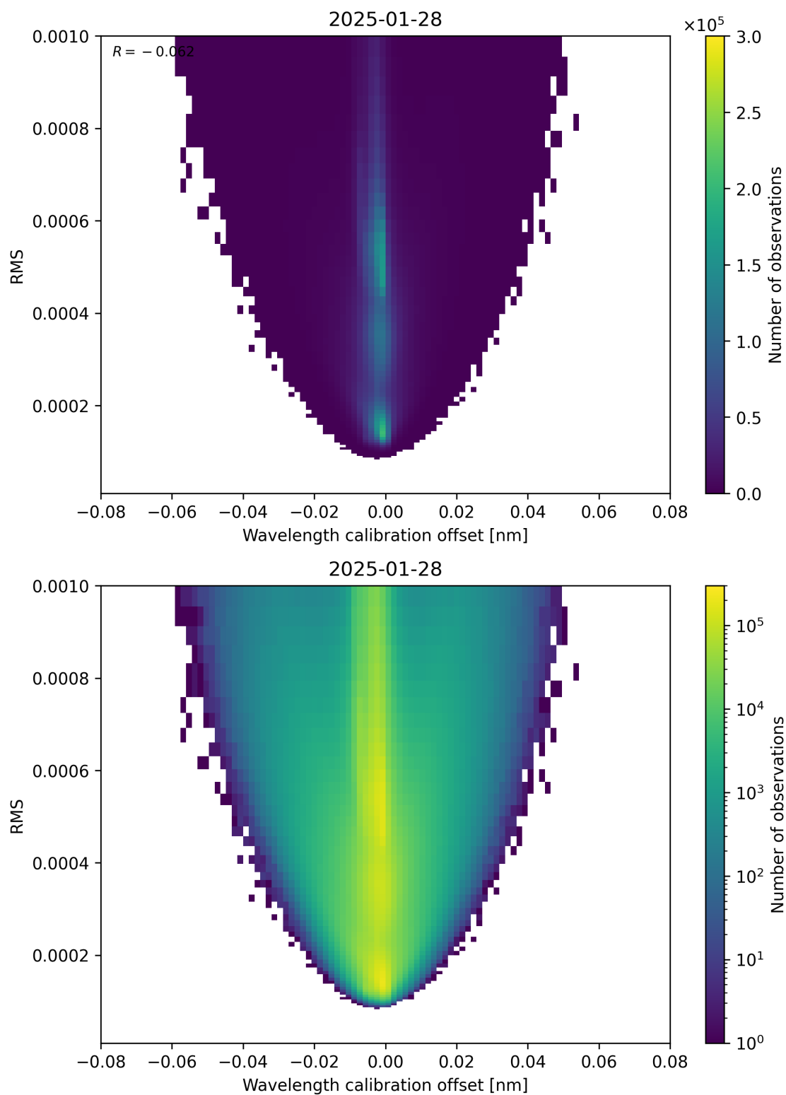
Figure 181: Scatter density plot of “Wavelength calibration offset” against “RMS” for 2025-01-28 to 2025-01-29.
