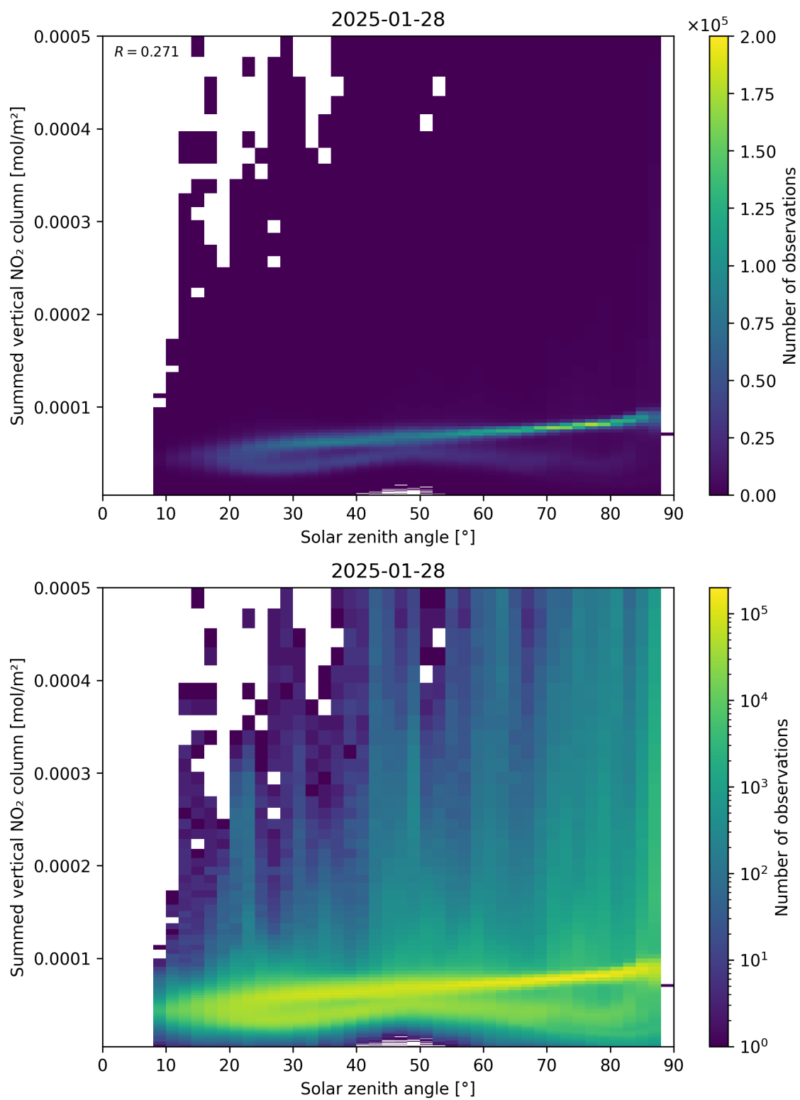
Figure 151: Scatter density plot of “Solar zenith angle” against “Summed vertical NO 2 column” for 2025-01-28 to 2025-01-29.
