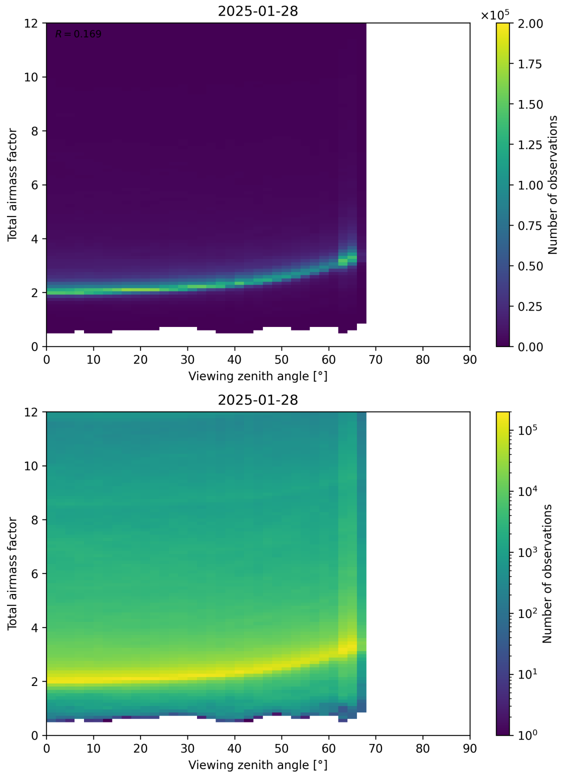
Figure 160: Scatter density plot of “Viewing zenith angle” against “Total airmass factor” for 2025-01-28 to 2025-01-29.
