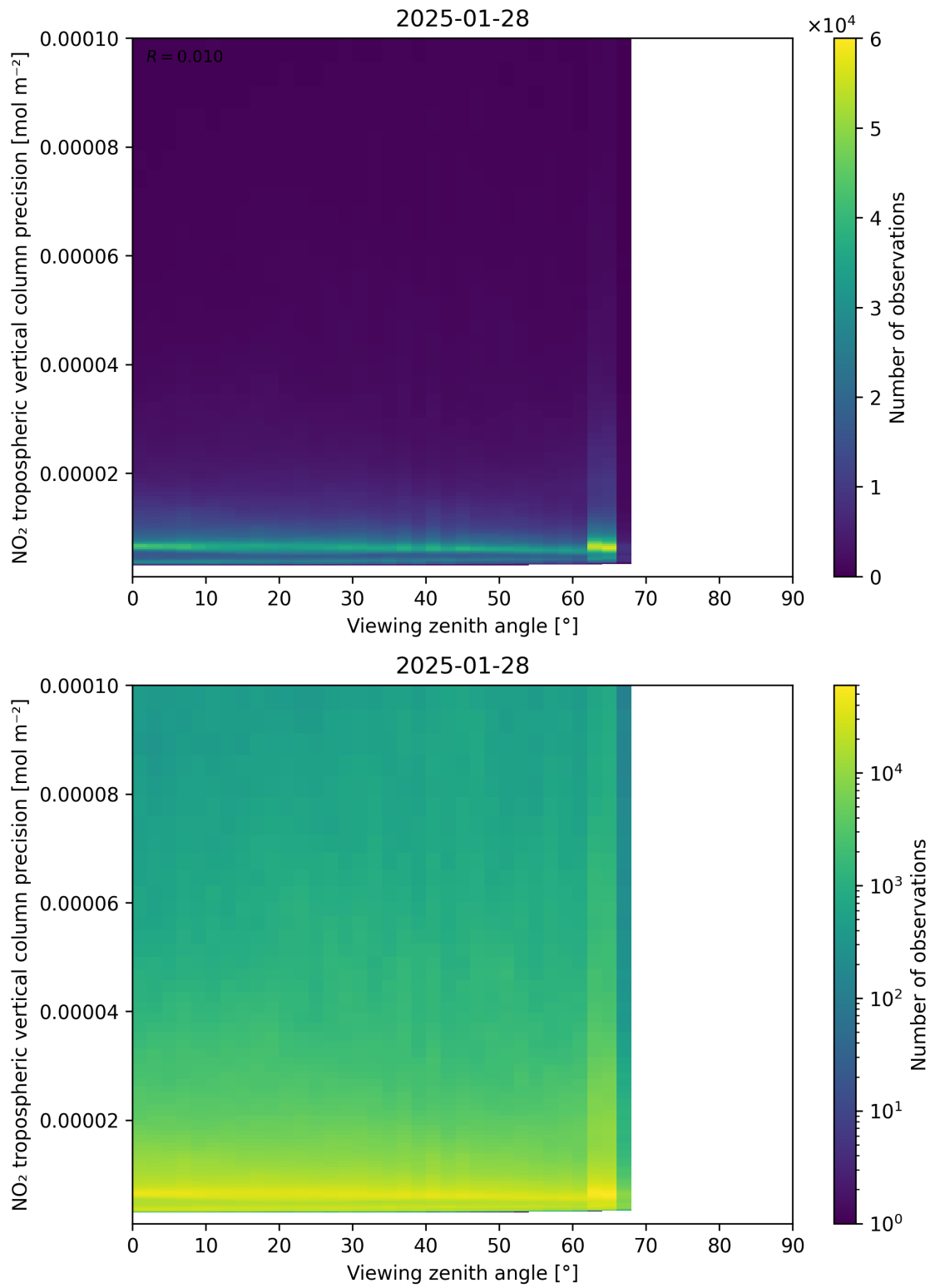
Figure 170: Scatter density plot of “Viewing zenith angle” against “NO 2 tropospheric vertical column precision” for 2025-01-28 to 2025-01-29.
