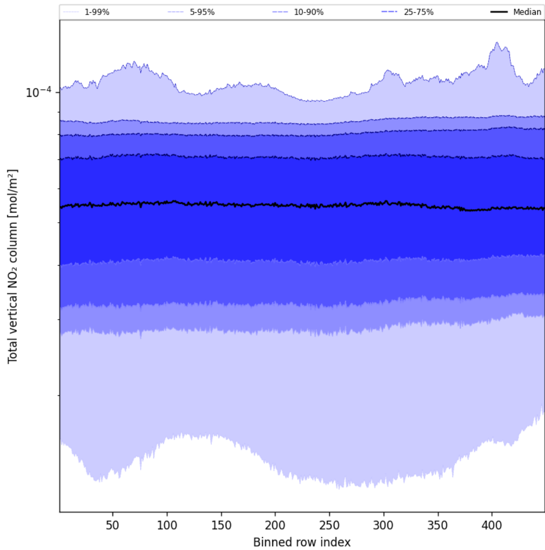
Figure 55: Along track statistics of “Total vertical NO 2 column” for 2025-01-28 to 2025-01-29
