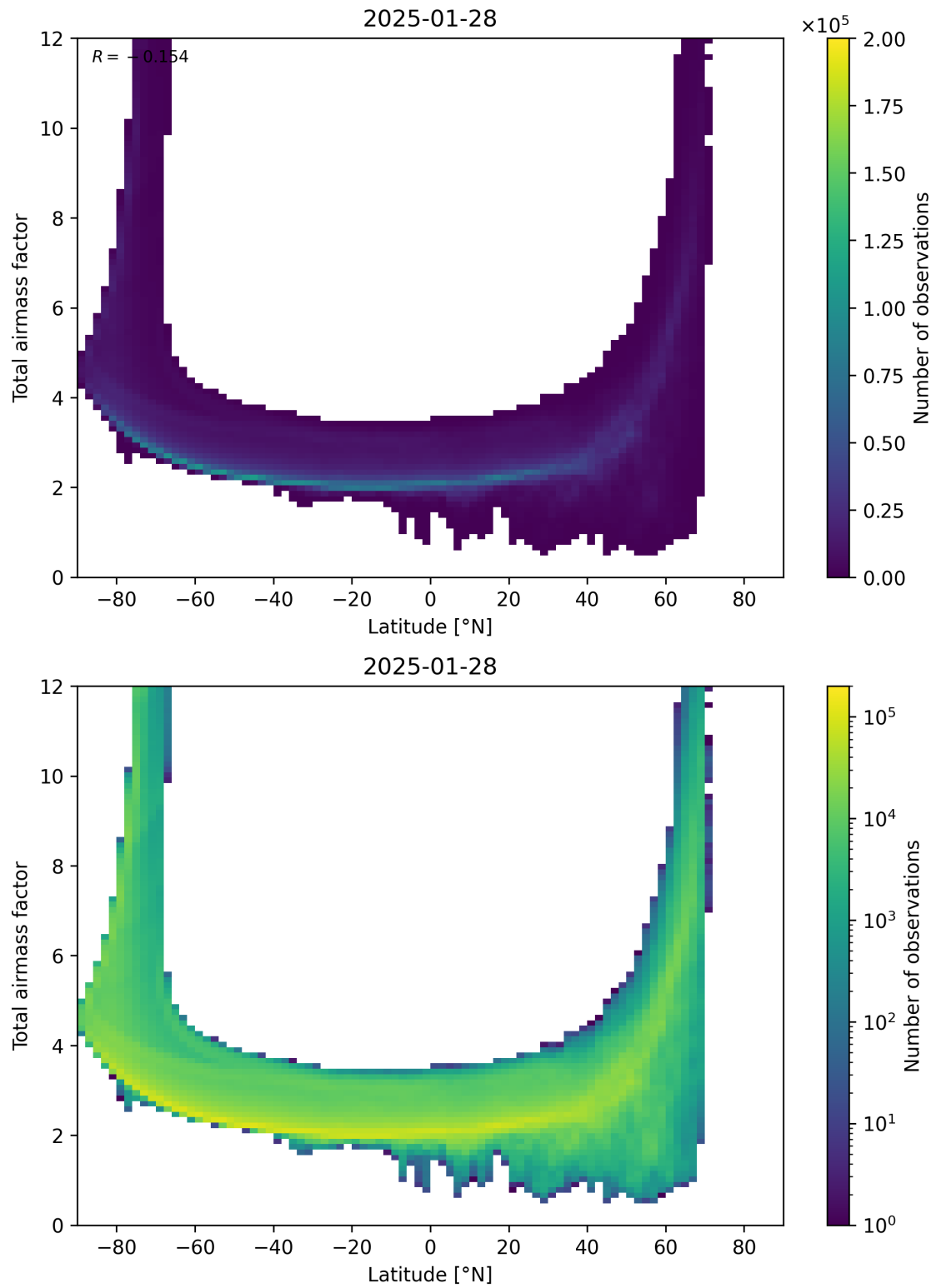
Figure 84: Scatter density plot of “Latitude” against “Total airmass factor” for 2025-01-28 to 2025-01-29.
