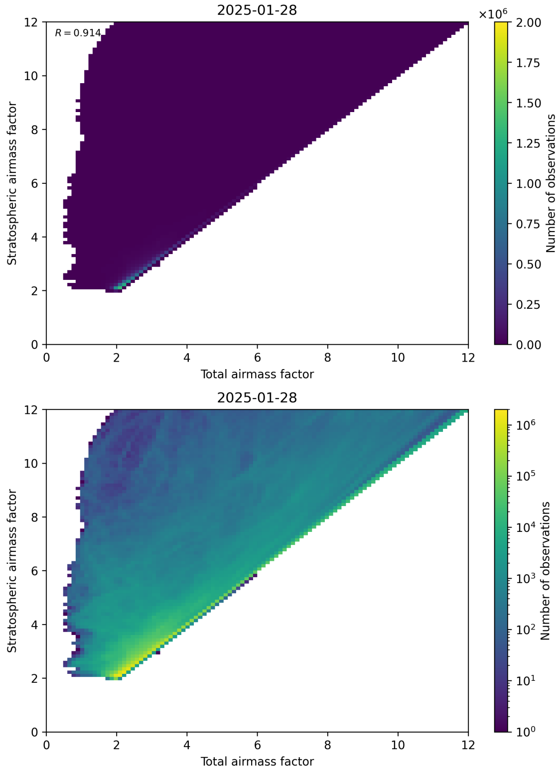
Figure 62: Scatter density plot of “Total airmass factor” against “Stratospheric airmass factor” for 2025-01-28 to 2025-01-29.
