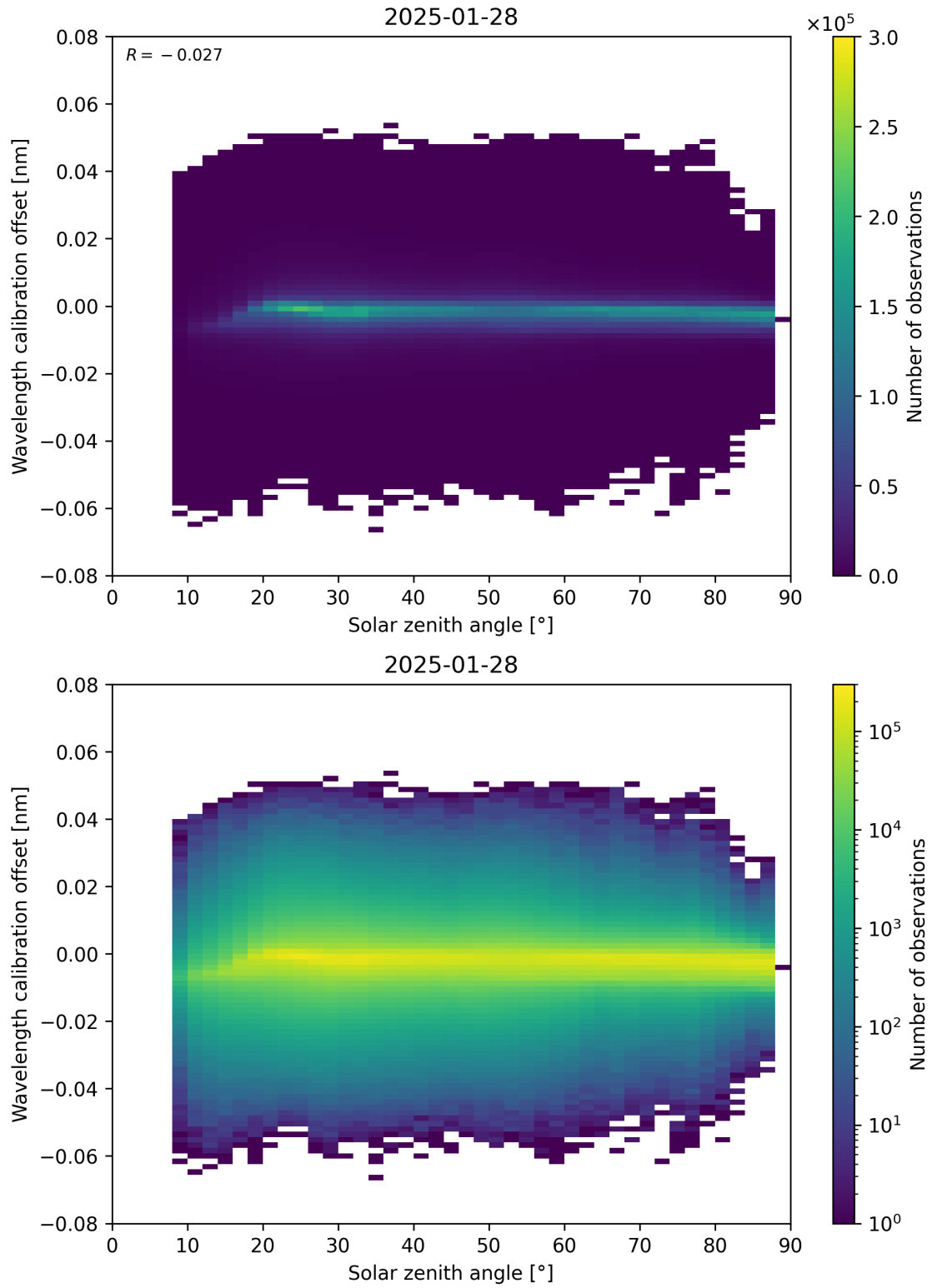
Figure 158: Scatter density plot of “Solar zenith angle” against “Wavelength calibration offset” for 2025-01-28 to 2025-01-29.
