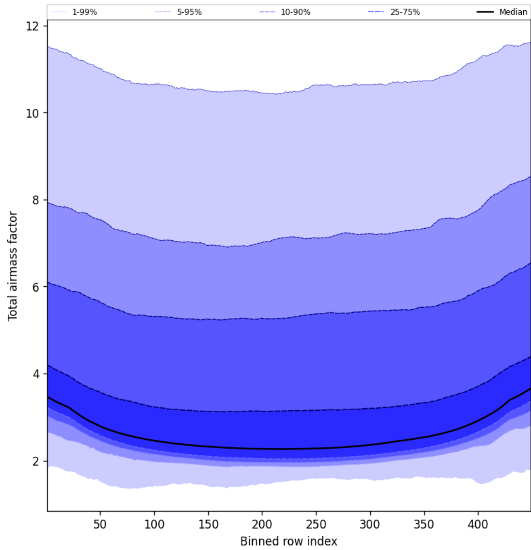
Figure 49: Along track statistics of “Total airmass factor” for 2025-01-28 to 2025-01-29
