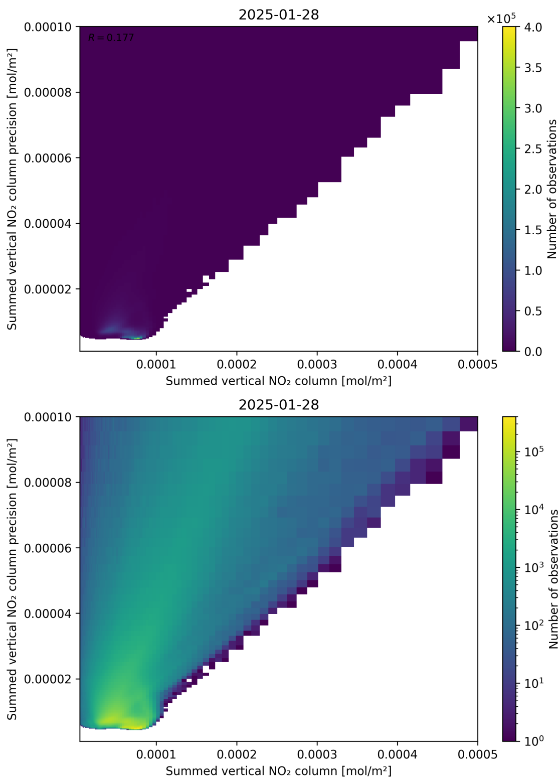
Figure 105: Scatter density plot of “Summed vertical NO 2 column” against “Summed vertical NO 2 column precision” for 2025-01-28 to 2025-01-29.
