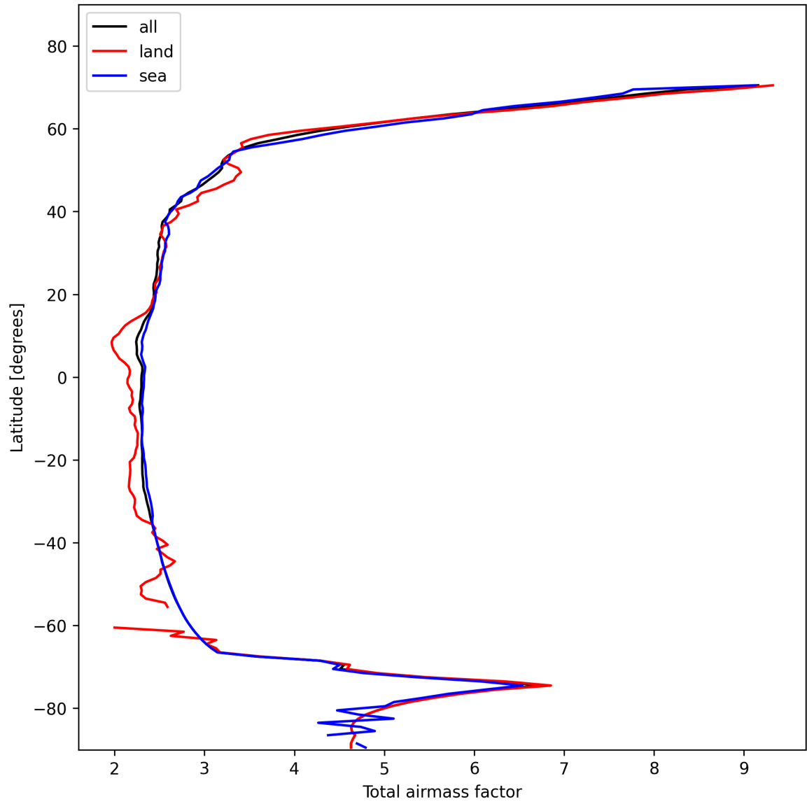
Figure 15: Zonal average of “Total airmass factor” for 2025-01-28 to 2025-01-29.
