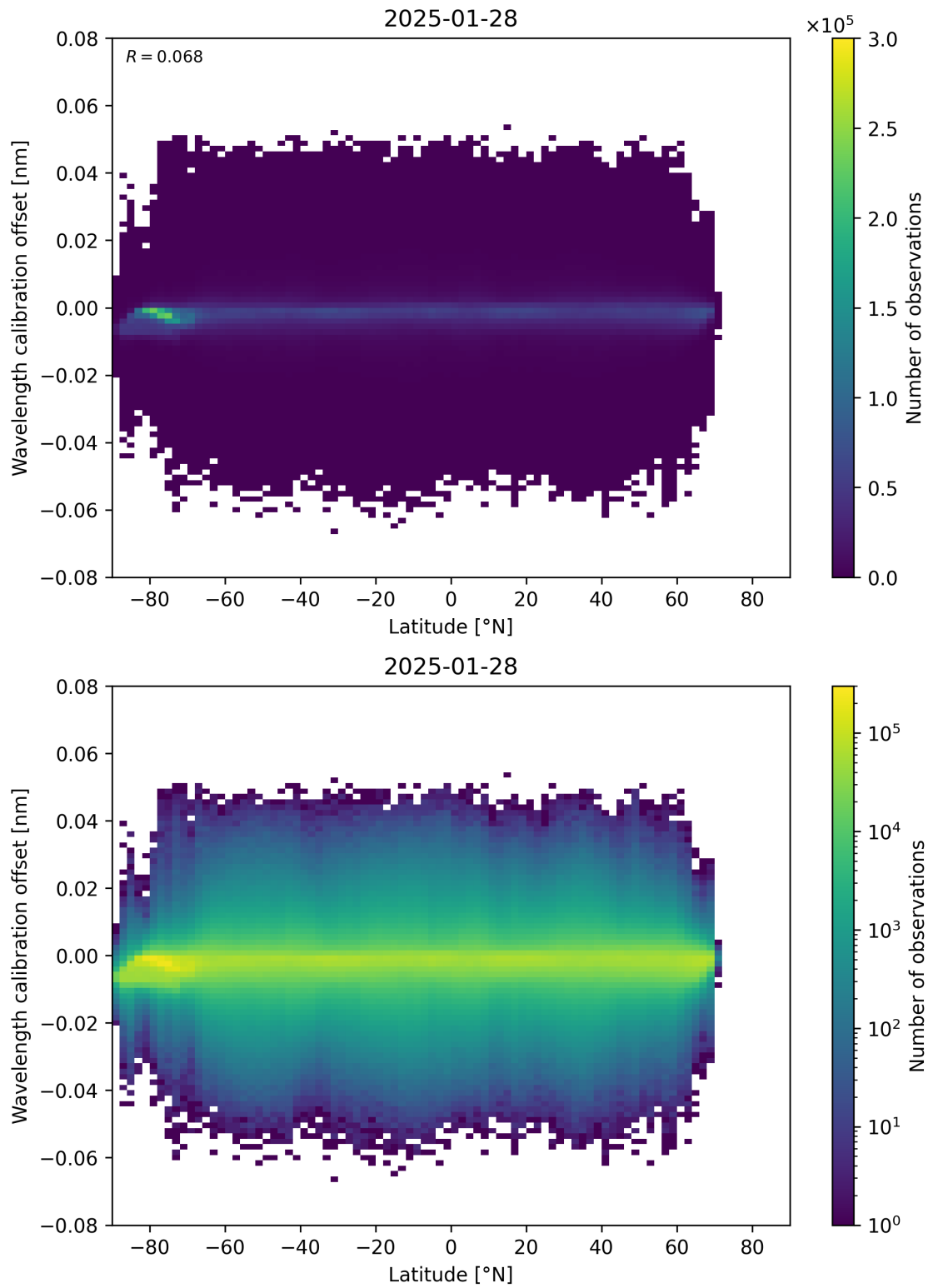
Figure 95: Scatter density plot of “Latitude” against “Wavelength calibration offset” for 2025-01-28 to 2025-01-29.
