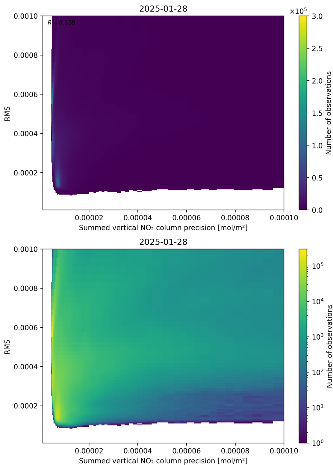
Figure 108: Scatter density plot of “Summed vertical NO 2 column precision” against “RMS” for 2025-01-28 to 2025-01-29.
