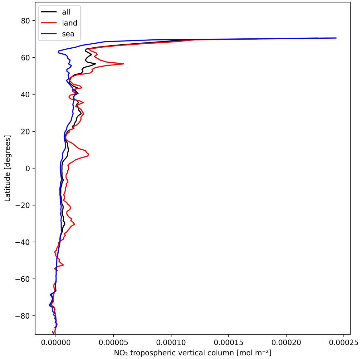
Figure 12: Zonal average of “NO 2 tropospheric vertical column” for 2025-01-28 to 2025-01-29.
