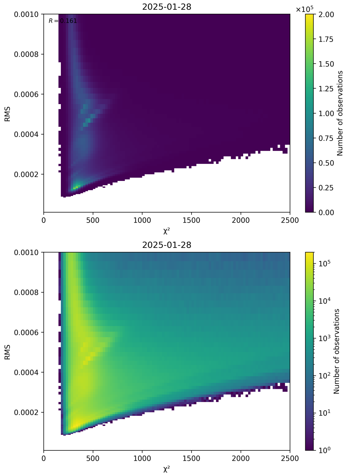
Figure 82: Scatter density plot of “ \chi^2 ” against “RMS” for 2025-01-28 to 2025-01-29.
