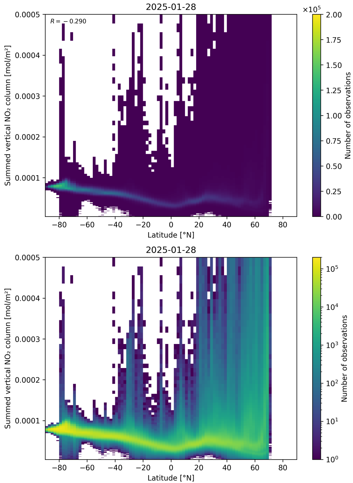
Figure 88: Scatter density plot of “Latitude” against “Summed vertical NO 2 column” for 2025-01-28 to 2025-01-29.
