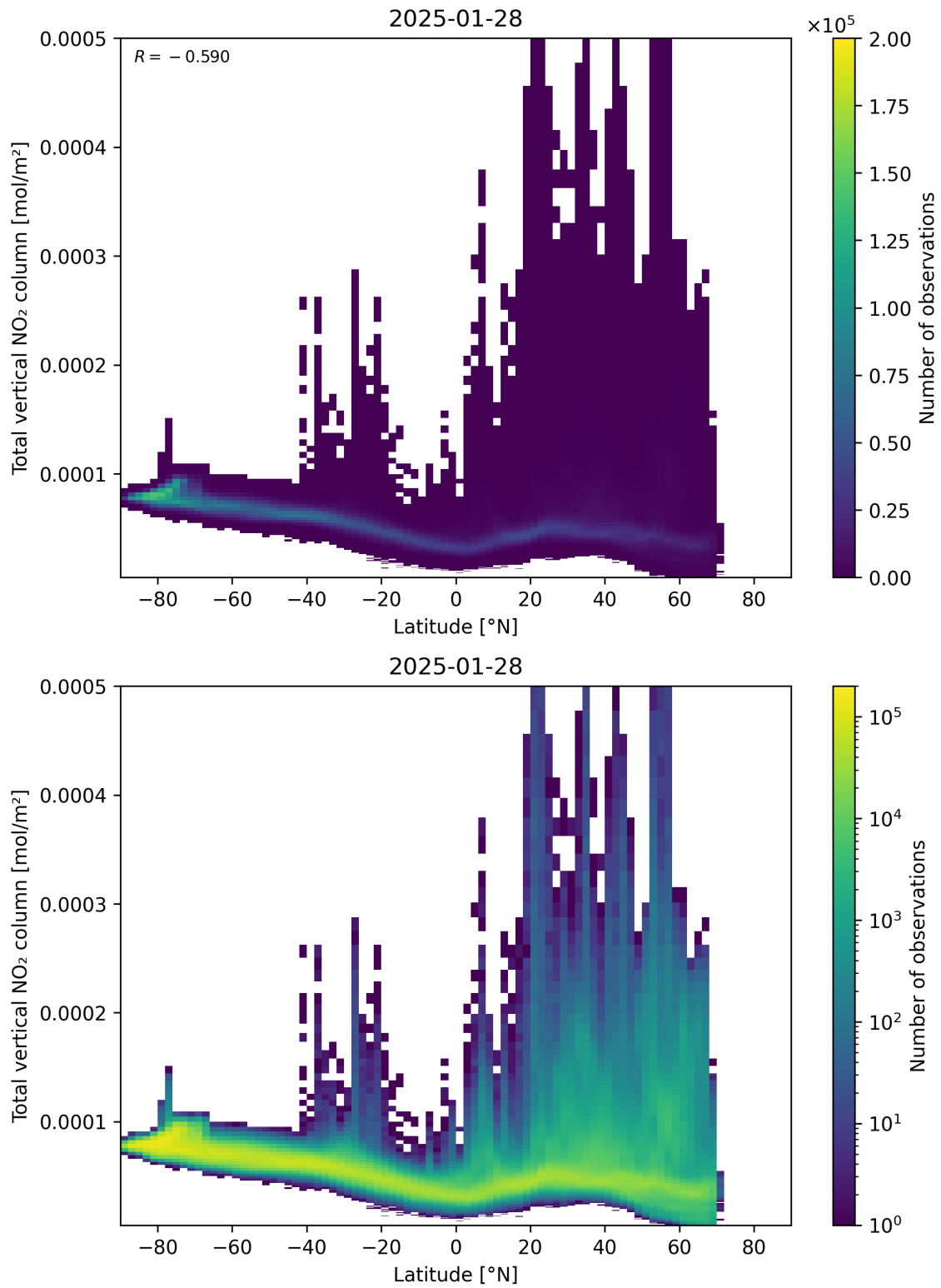
Figure 90: Scatter density plot of “Latitude” against “Total vertical NO 2 column” for 2025-01-28 to 2025-01-29.
