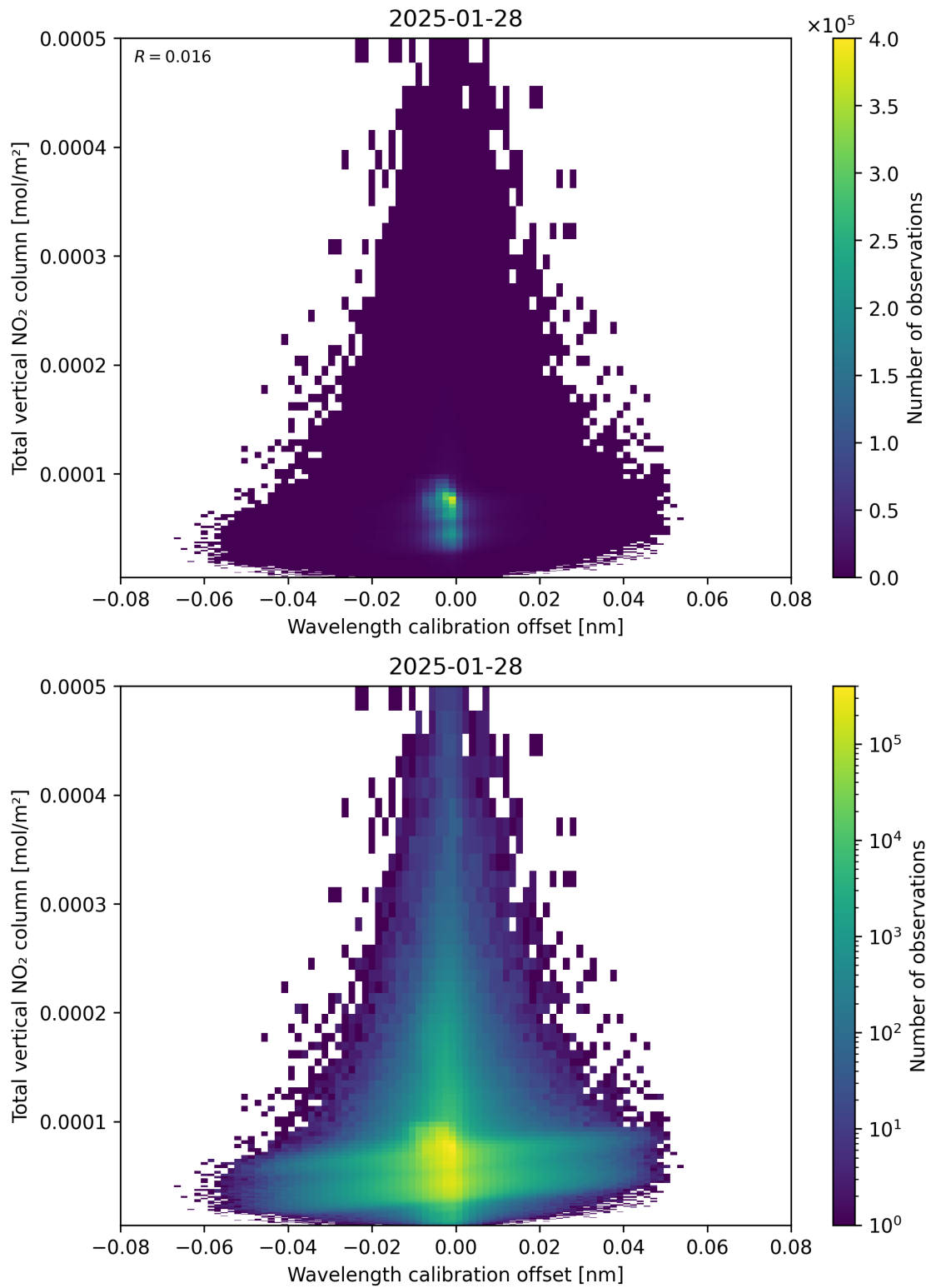
Figure 179: Scatter density plot of “Wavelength calibration offset” against “Total vertical NO 2 column” for 2025-01-28 to 2025-01-29.
