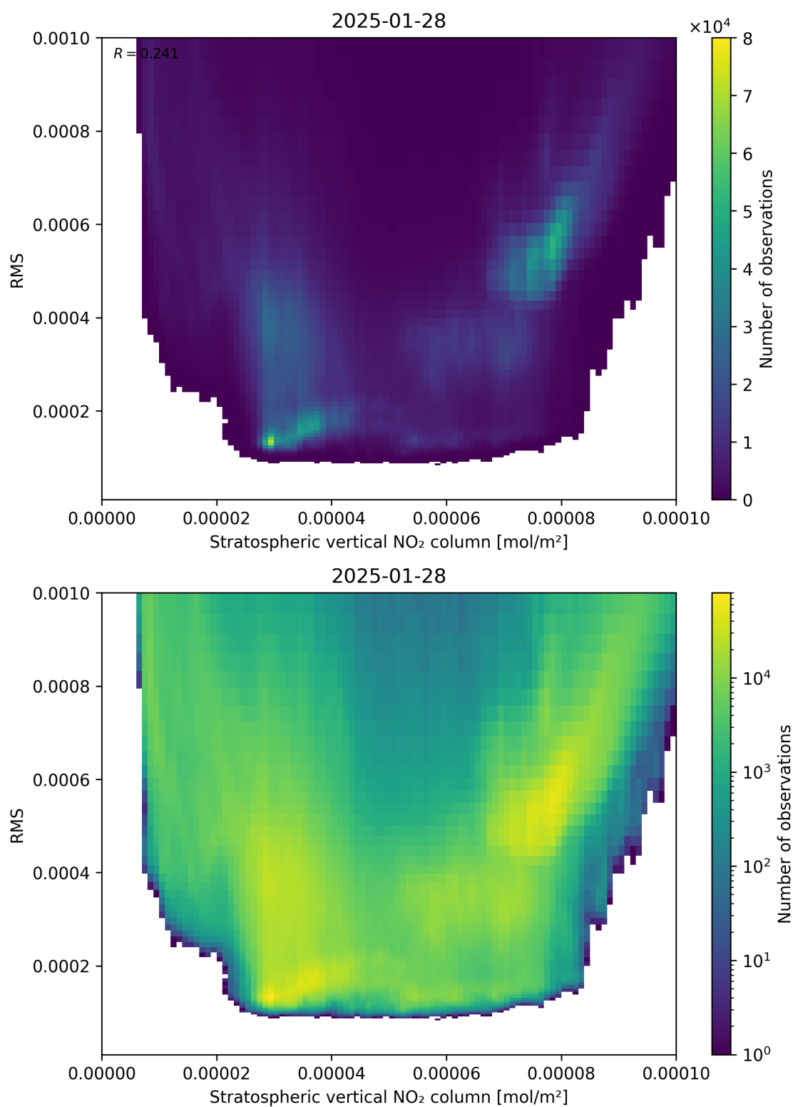
Figure 102: Scatter density plot of “Stratospheric vertical NO 2 column” against “RMS” for 2025-01-28 to 2025-01-29.
