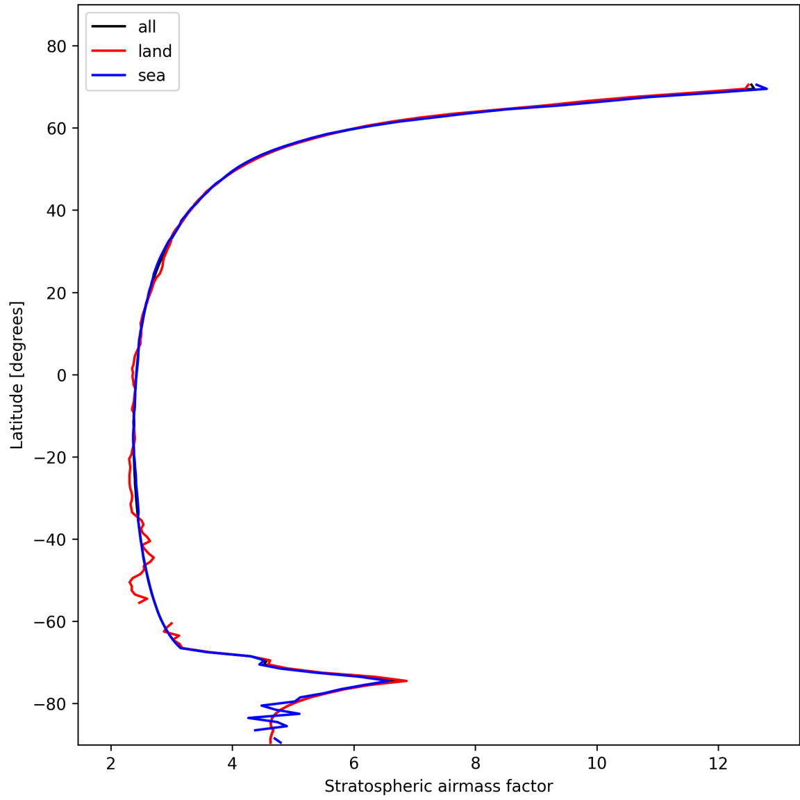
Figure 27: Zonal average of “Stratospheric air mass factor” for 2025-01-28 to 2025-01-29.
