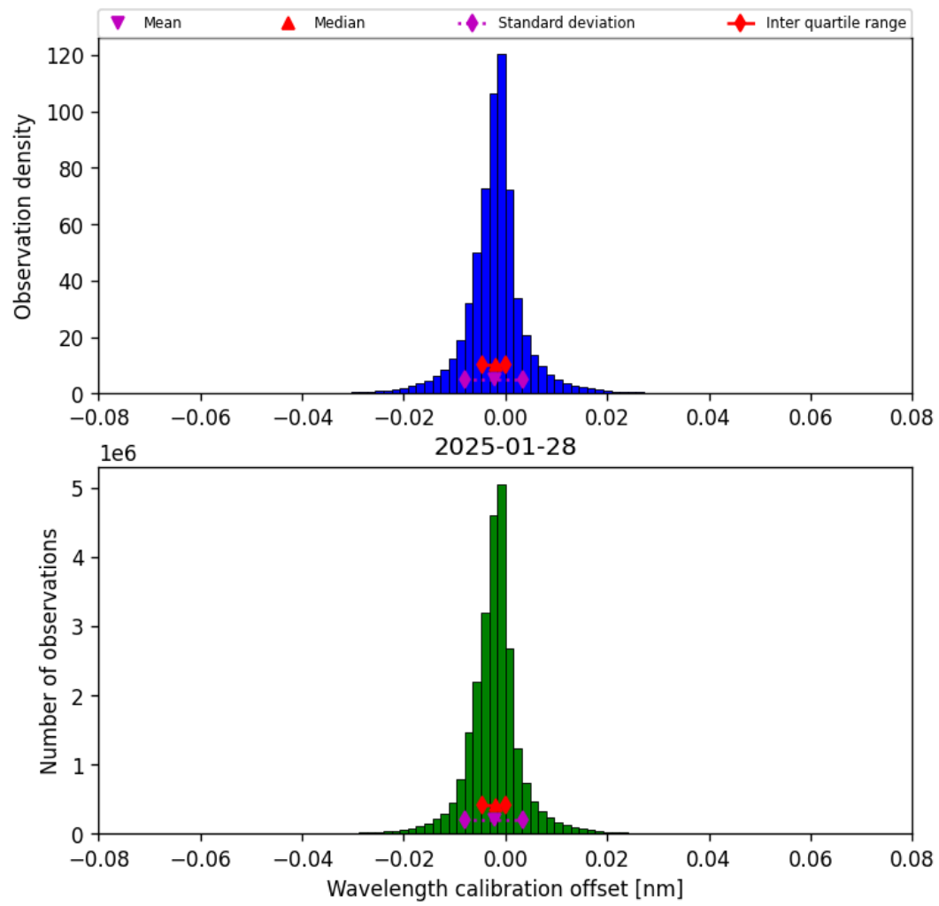
Figure 35: Histogram of “Wavelength calibration offset” for 2025-01-28 to 2025-01-29
