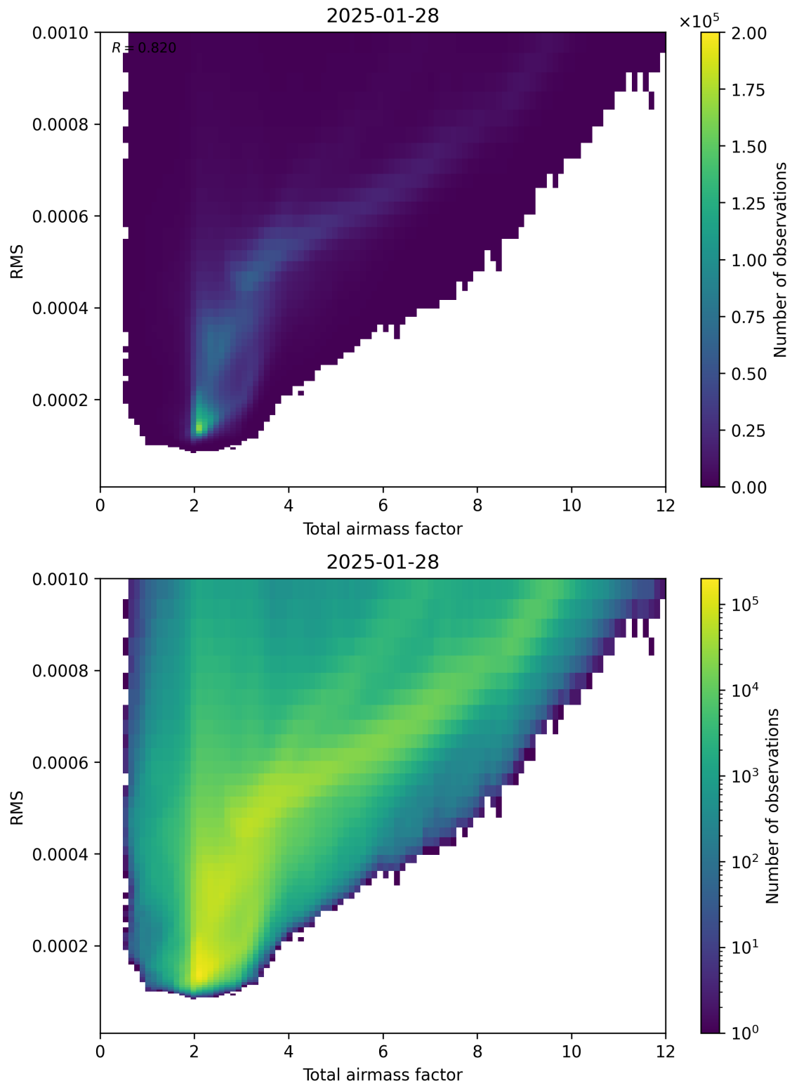
Figure 69: Scatter density plot of “Total airmass factor” against “RMS” for 2025-01-28 to 2025-01-29.
