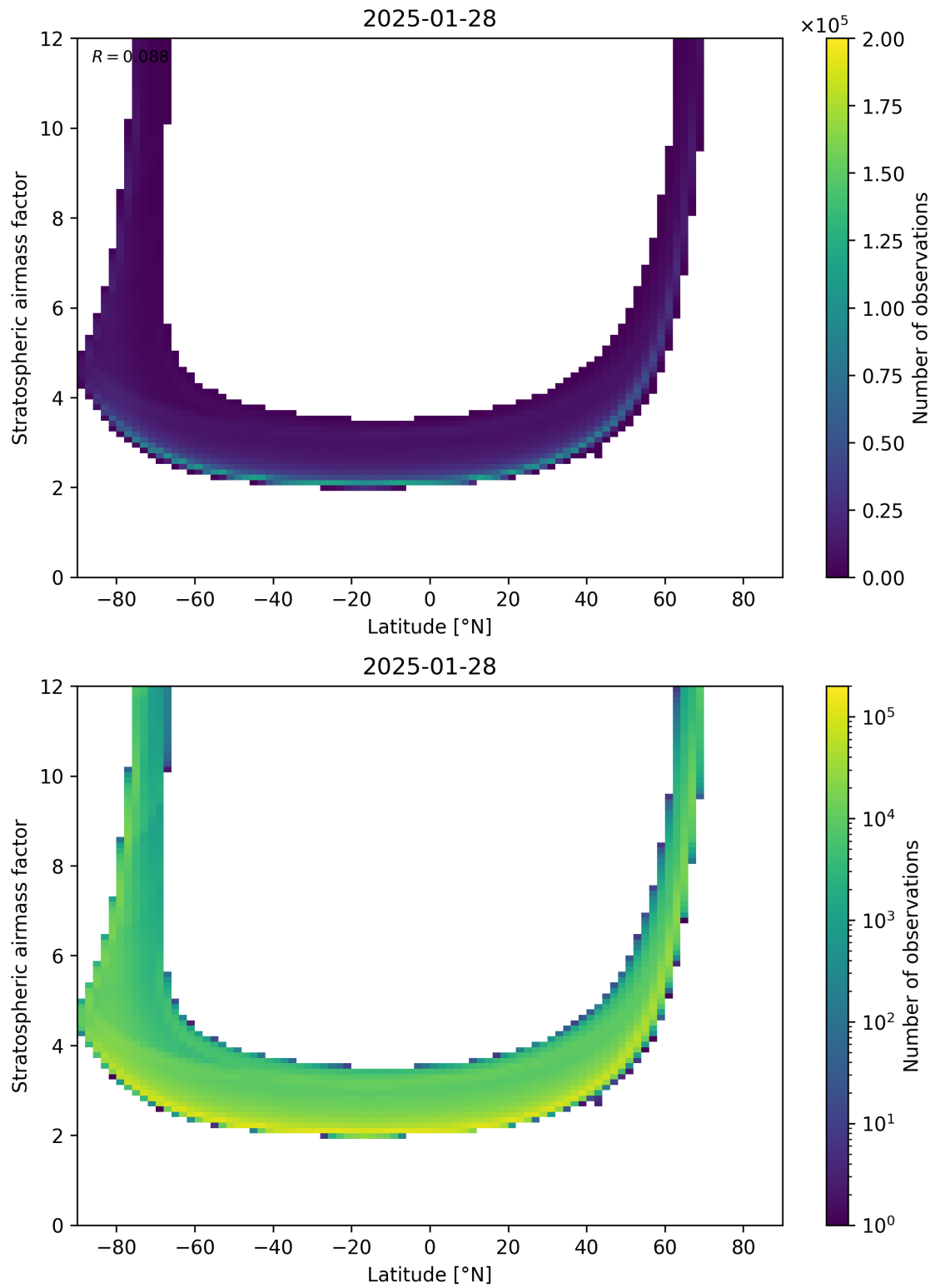
Figure 83: Scatter density plot of “Latitude” against “Stratospheric airmass factor” for 2025-01-28 to 2025-01-29.
