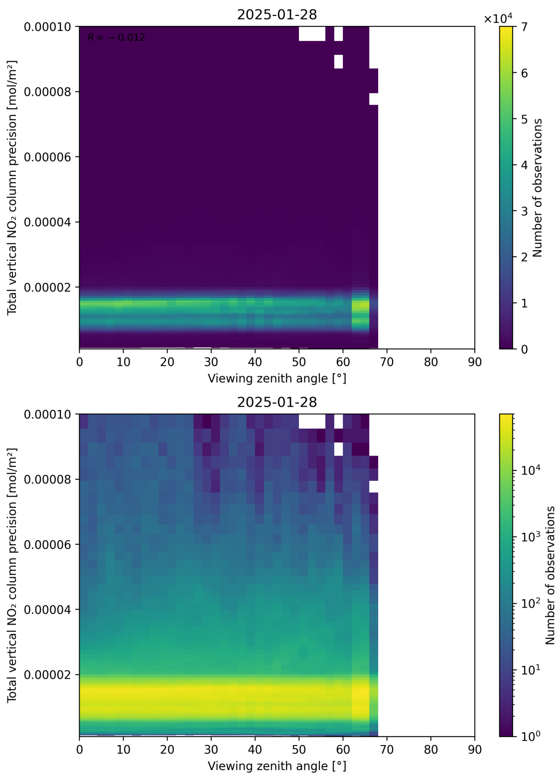
Figure 168: Scatter density plot of “Viewing zenith angle” against “Total vertical NO 2 column precision” for 2025-01-28 to 2025-01-29.
