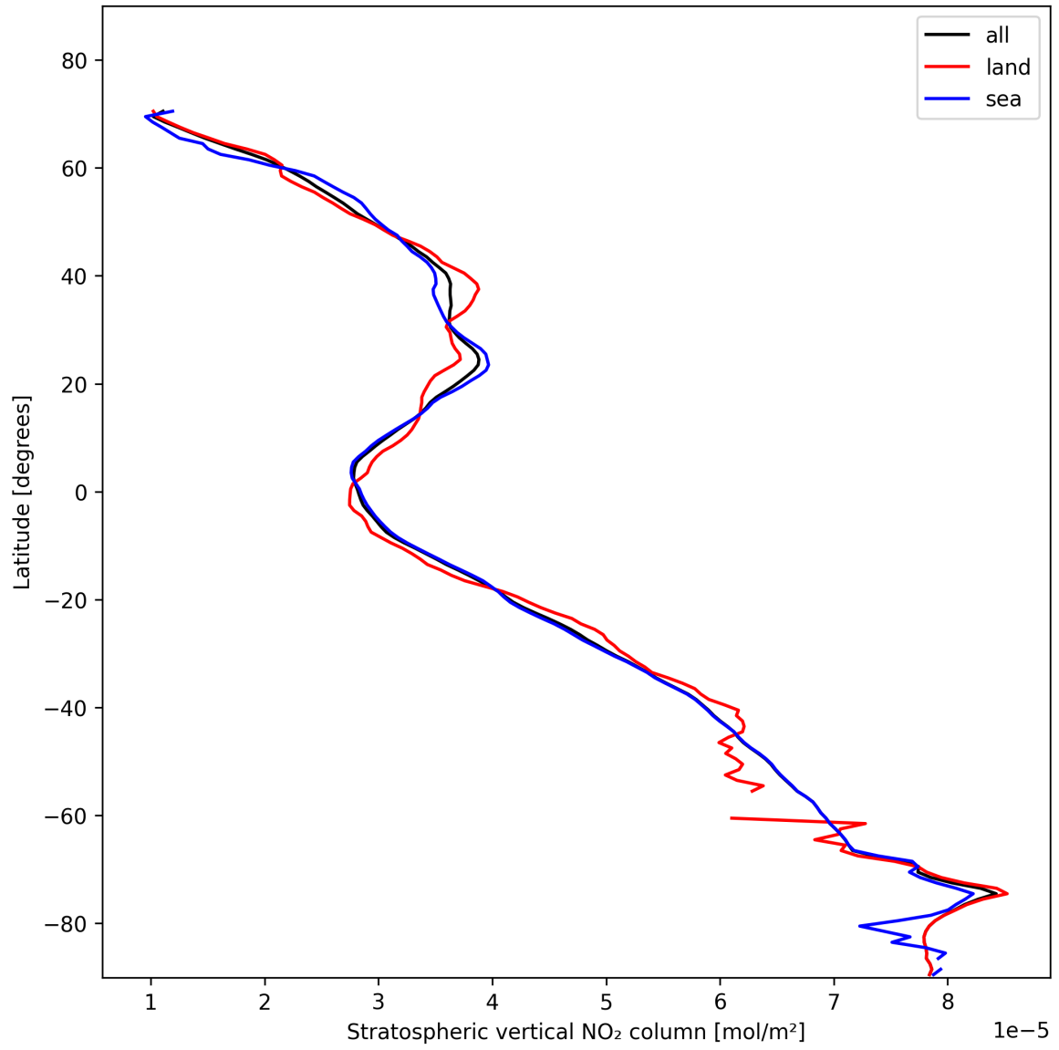
Figure 19: Zonal average of “Stratospheric vertical NO 2 column” for 2025-01-28 to 2025-01-29.
