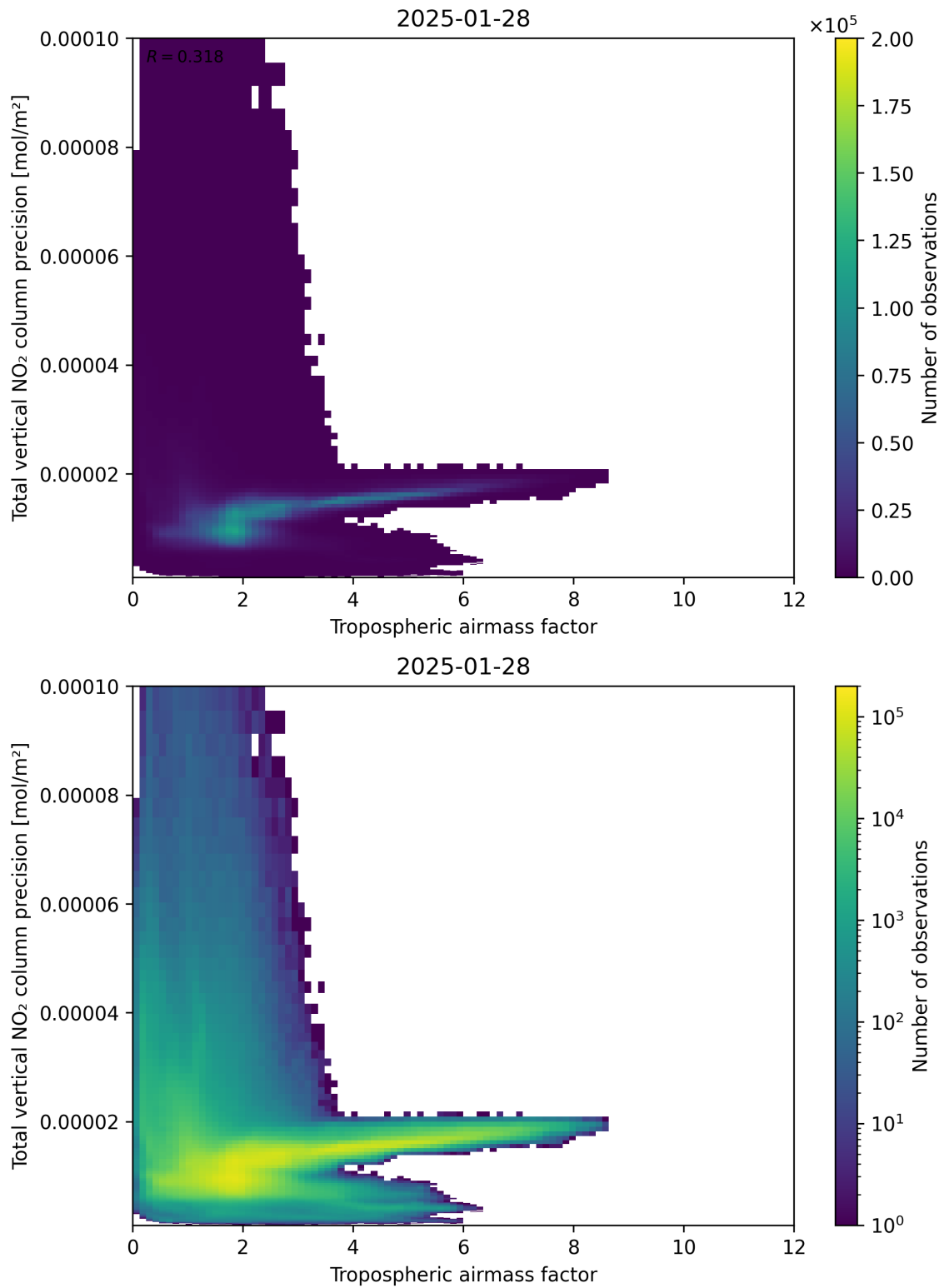
Figure 78: Scatter density plot of “Tropospheric airmass factor” against “Total vertical NO 2 column precision” for 2025-01-28 to 2025-01-29.
