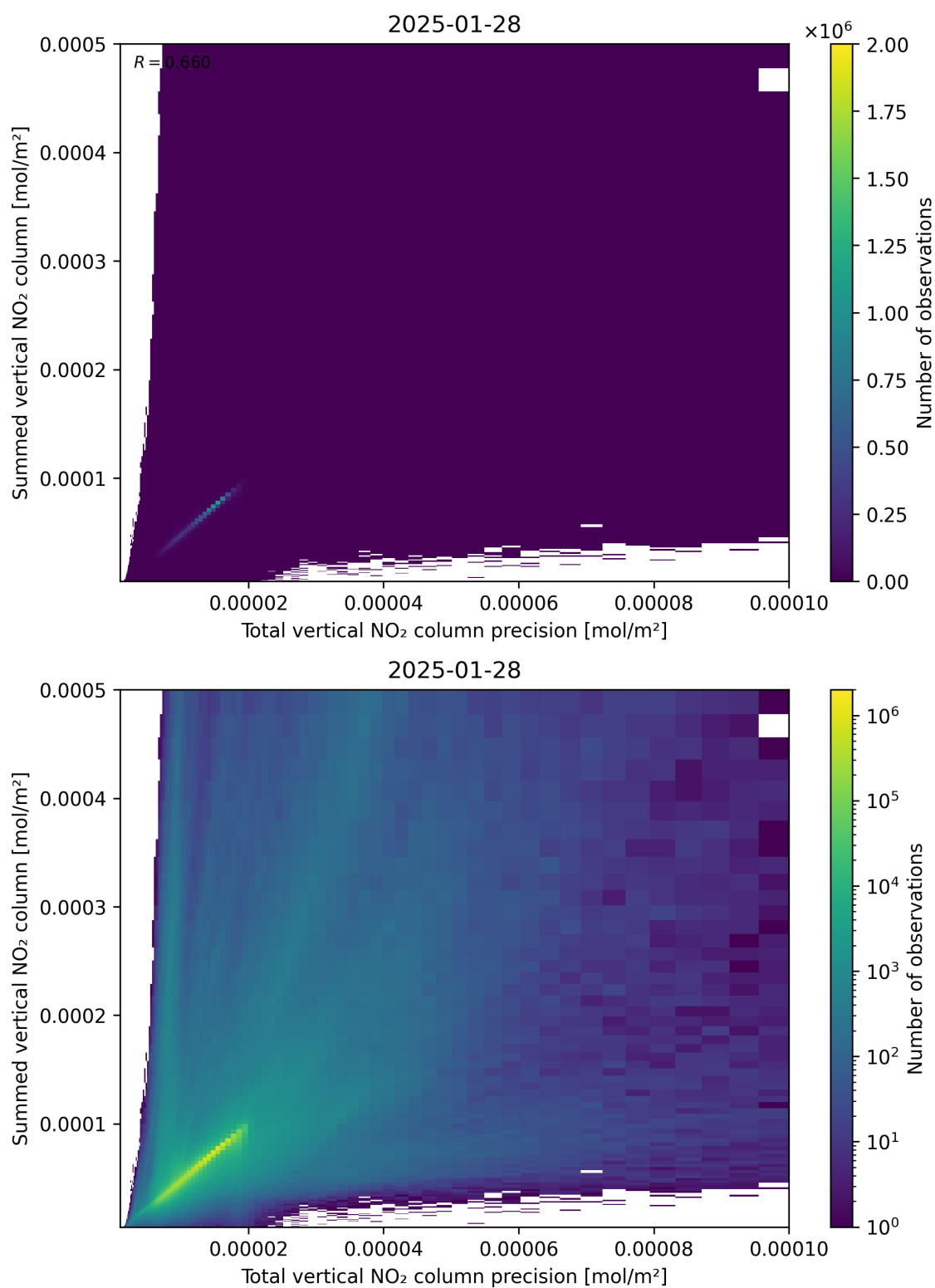
Figure 117: Scatter density plot of “Total vertical NO 2 column precision” against “Summed vertical NO 2 column” for 2025-01-28 to 2025-01-29.
