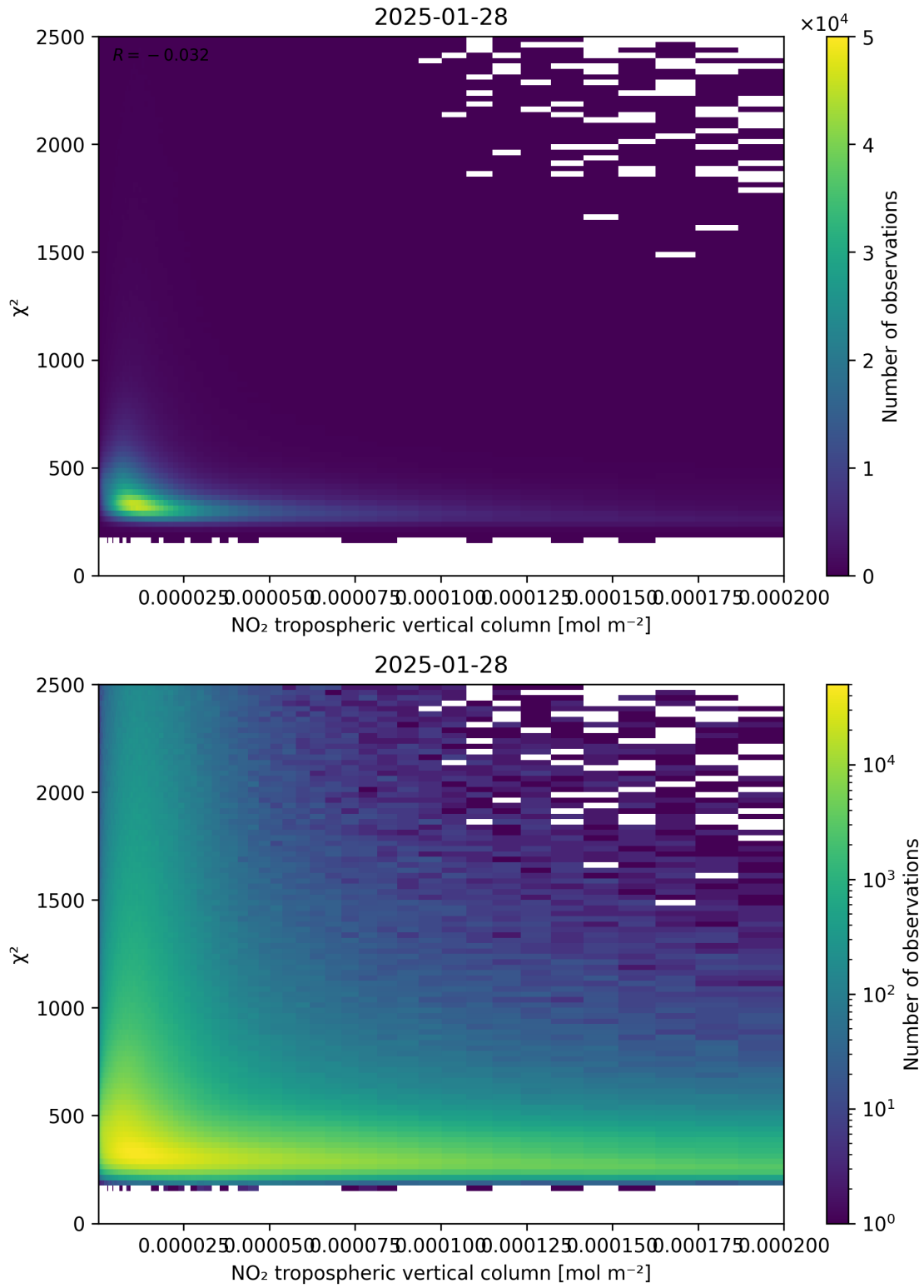
Figure 124: Scatter density plot of “NO 2 tropospheric vertical column” against “ \chi^2 ” for 2025-01-28 to 2025-01-29.
