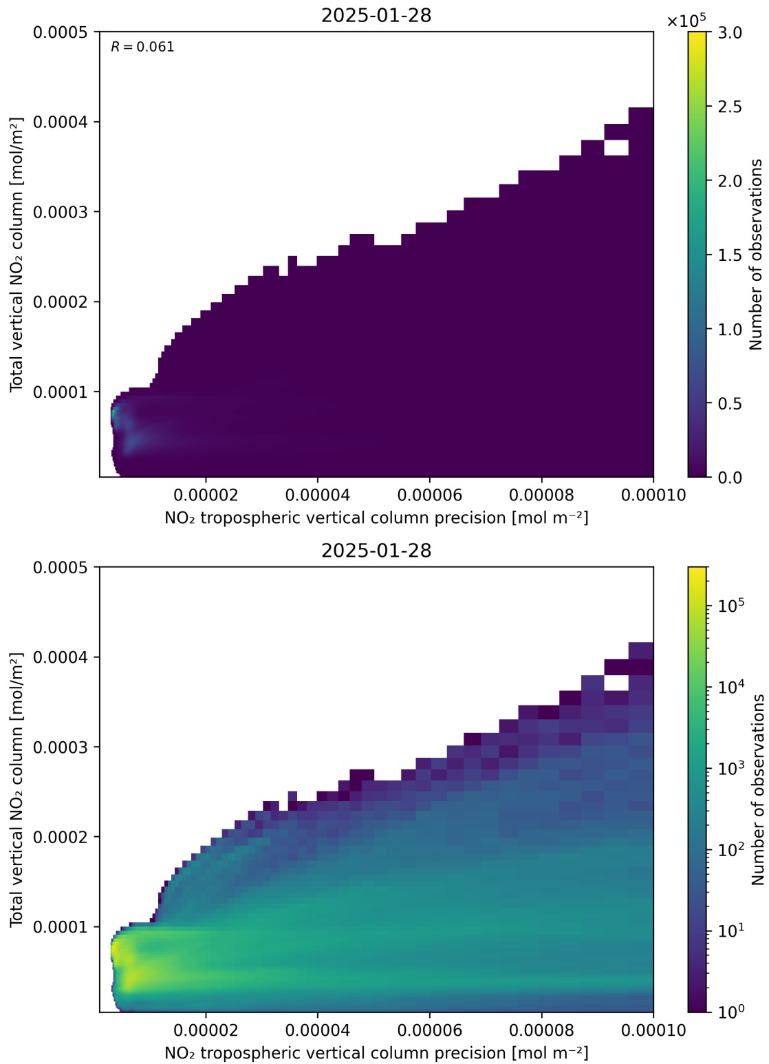
Figure 138: Scatter density plot of “NO 2 tropospheric vertical column precision” against “Total vertical NO 2 column” for 2025-01-28 to 2025-01-29.
