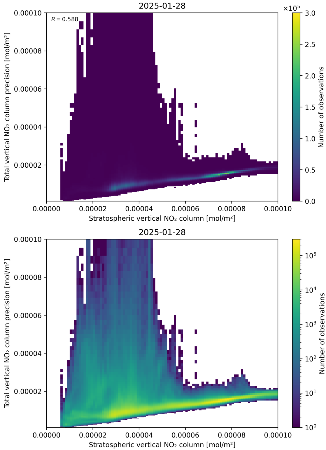
Figure 101: Scatter density plot of “Stratospheric vertical NO 2 column” against “Total vertical NO 2 column precision” for 2025-01-28 to 2025-01-29.
