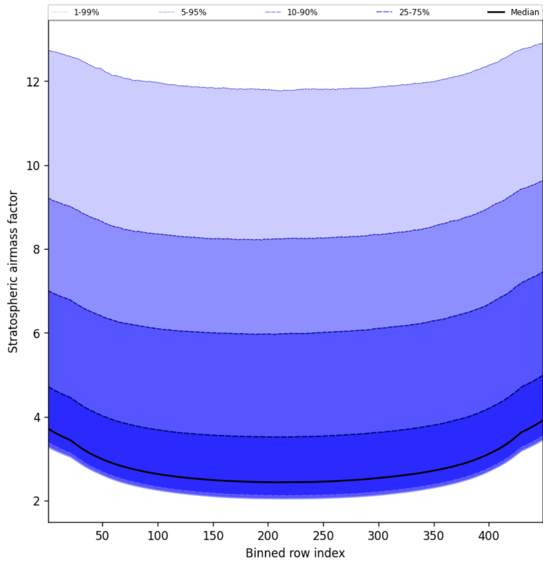
Figure 61: Along track statistics of “Stratospheric air mass factor” for 2025-01-28 to 2025-01-29
