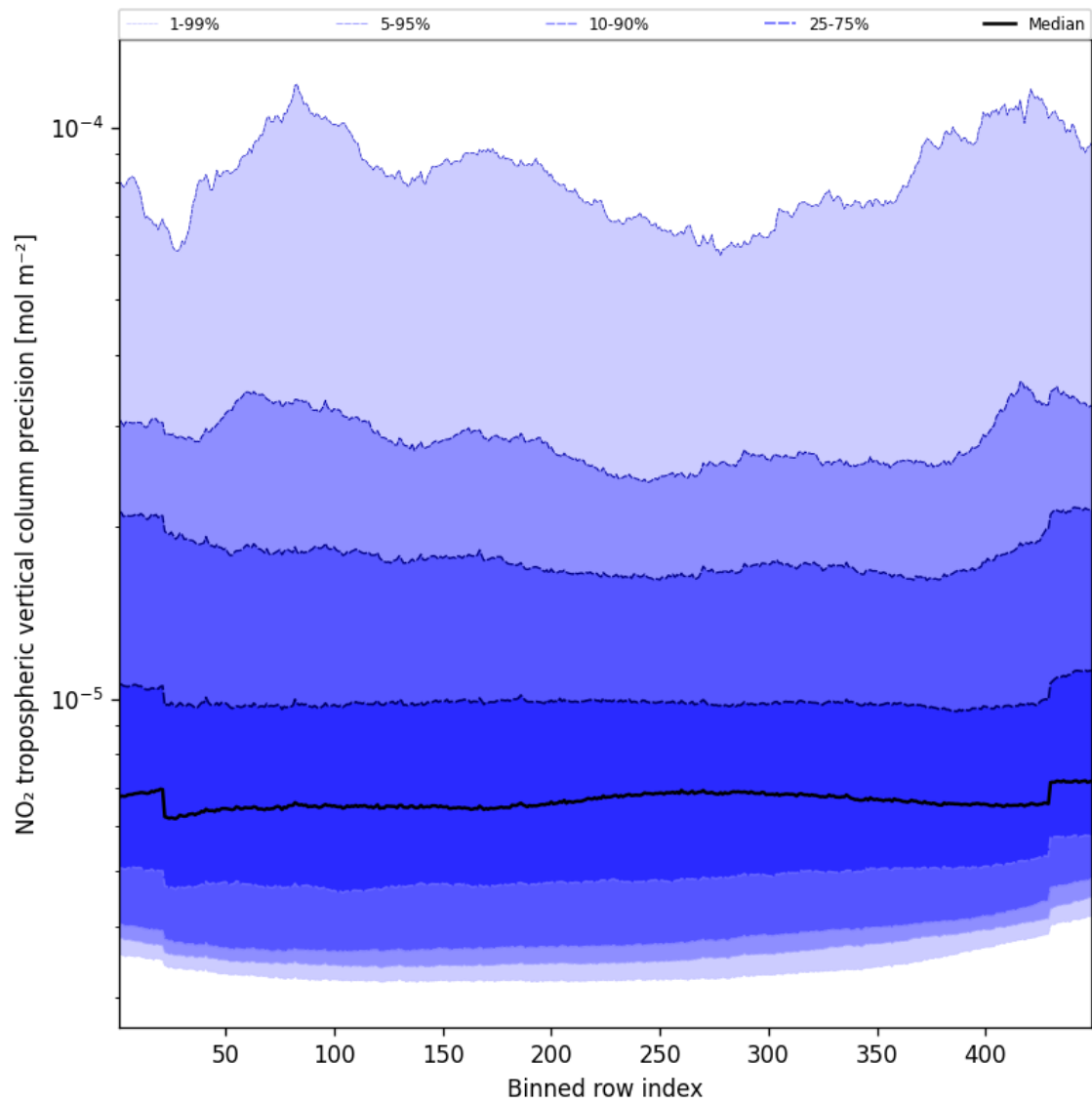
Figure 47: Along track statistics of “NO 2 tropospheric vertical column precision” for 2025-01-28 to 2025-01-29
