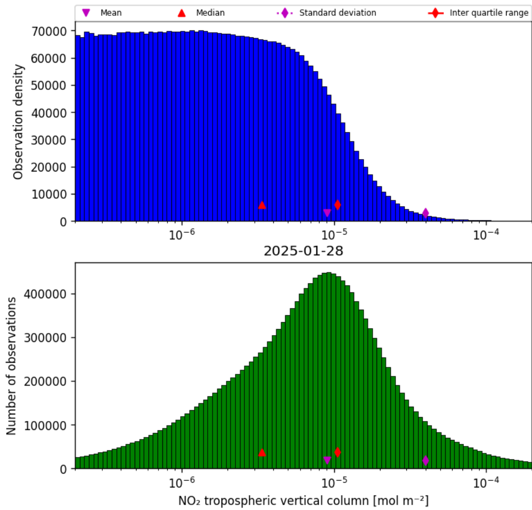
Figure 29: Histogram of “NO 2 tropospheric vertical column” for 2025-01-28 to 2025-01-29
