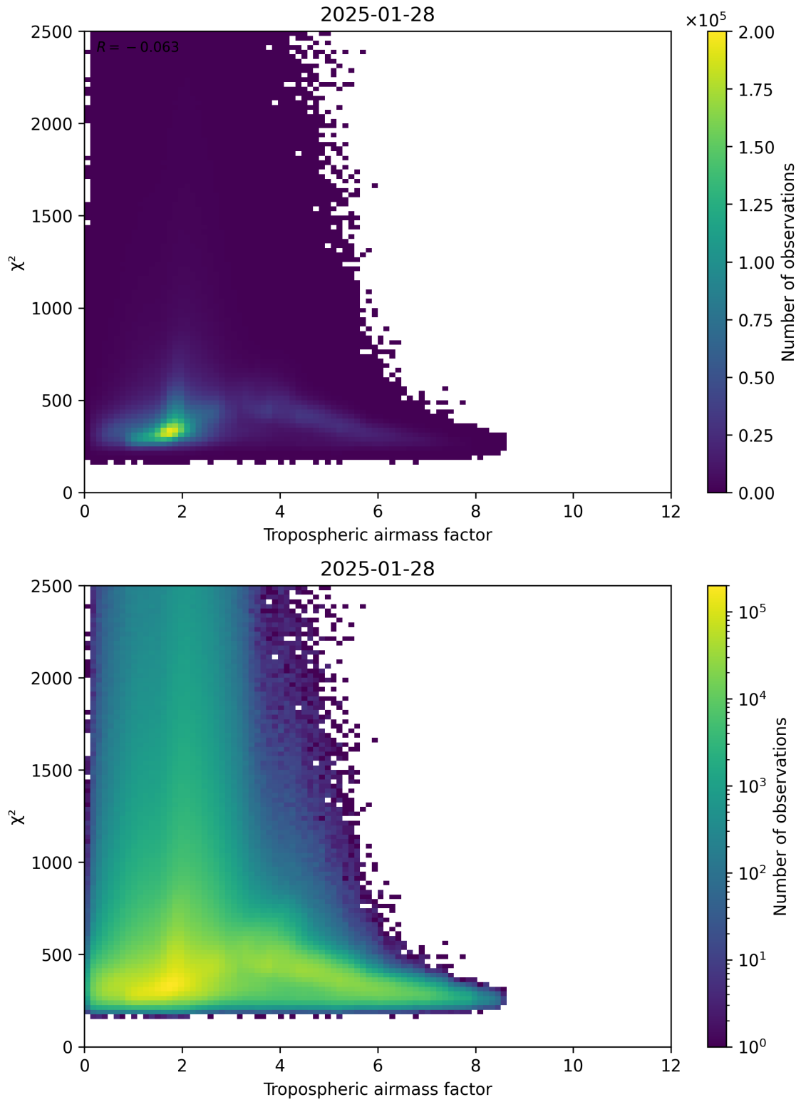
Figure 73: Scatter density plot of “Tropospheric airmass factor” against “ \chi^2 ” for 2025-01-28 to 2025-01-29.
