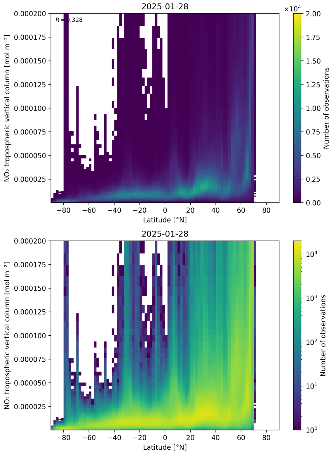
Figure 92: Scatter density plot of “Latitude” against “NO 2 tropospheric vertical column” for 2025-01-28 to 2025-01-29.
