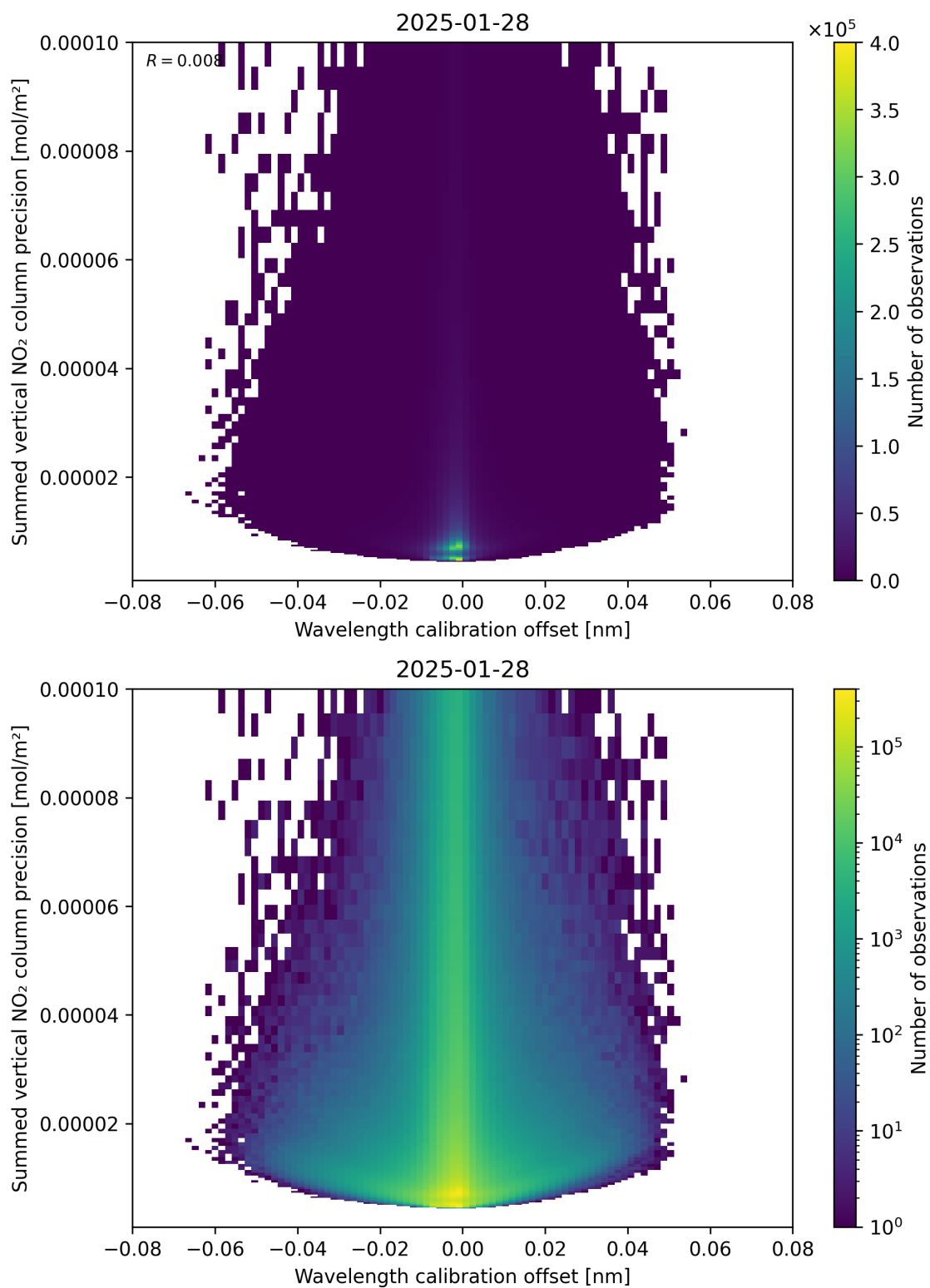
Figure 178: Scatter density plot of “Wavelength calibration offset” against “Summed vertical NO 2 column precision” for 2025-01-28 to 2025-01-29.
