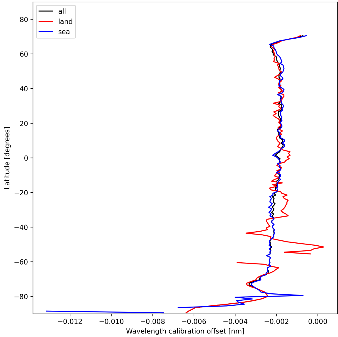
Figure 18: Zonal average of “Wavelength calibration offset” for 2025-01-28 to 2025-01-29.
