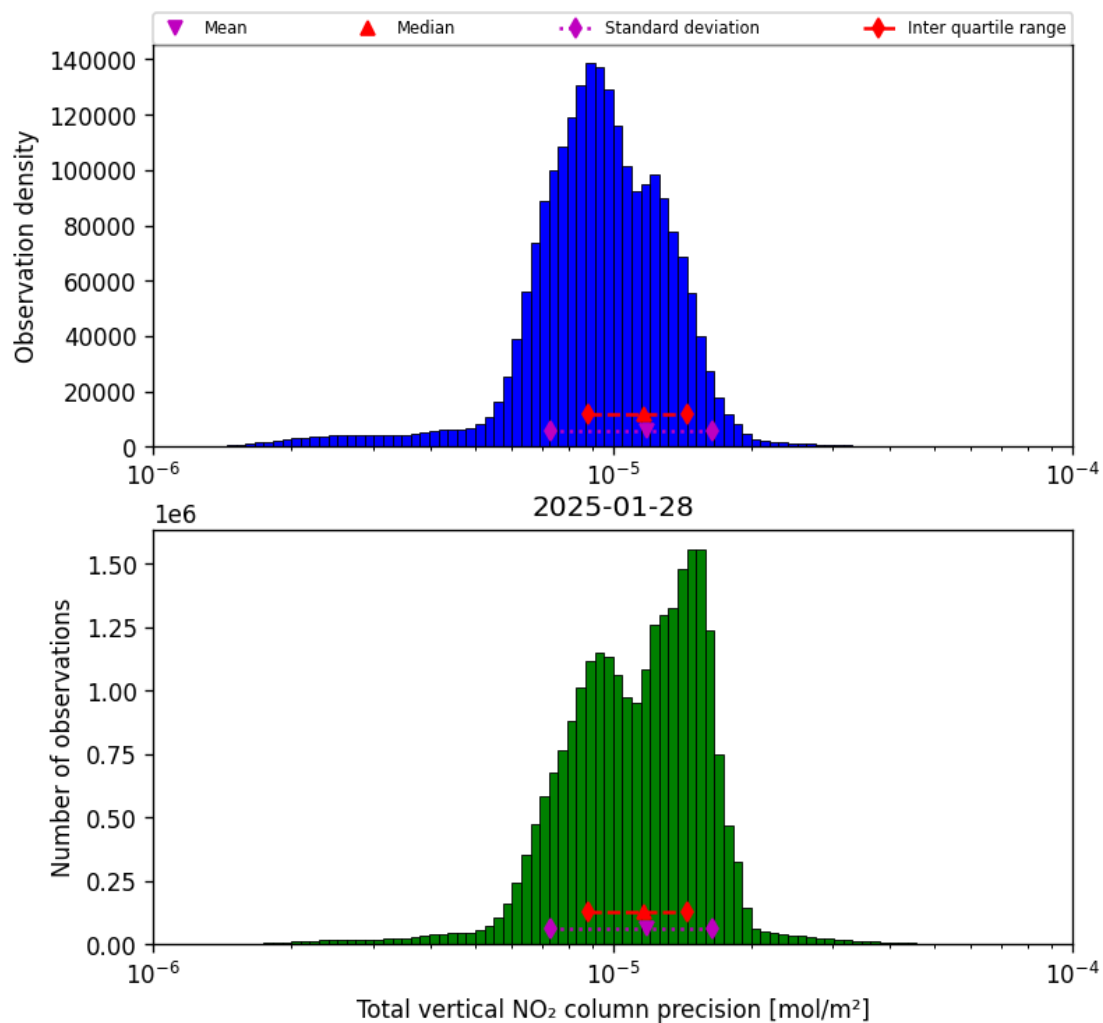
Figure 39: Histogram of “Total vertical NO 2 column precision” for 2025-01-28 to 2025-01-29
