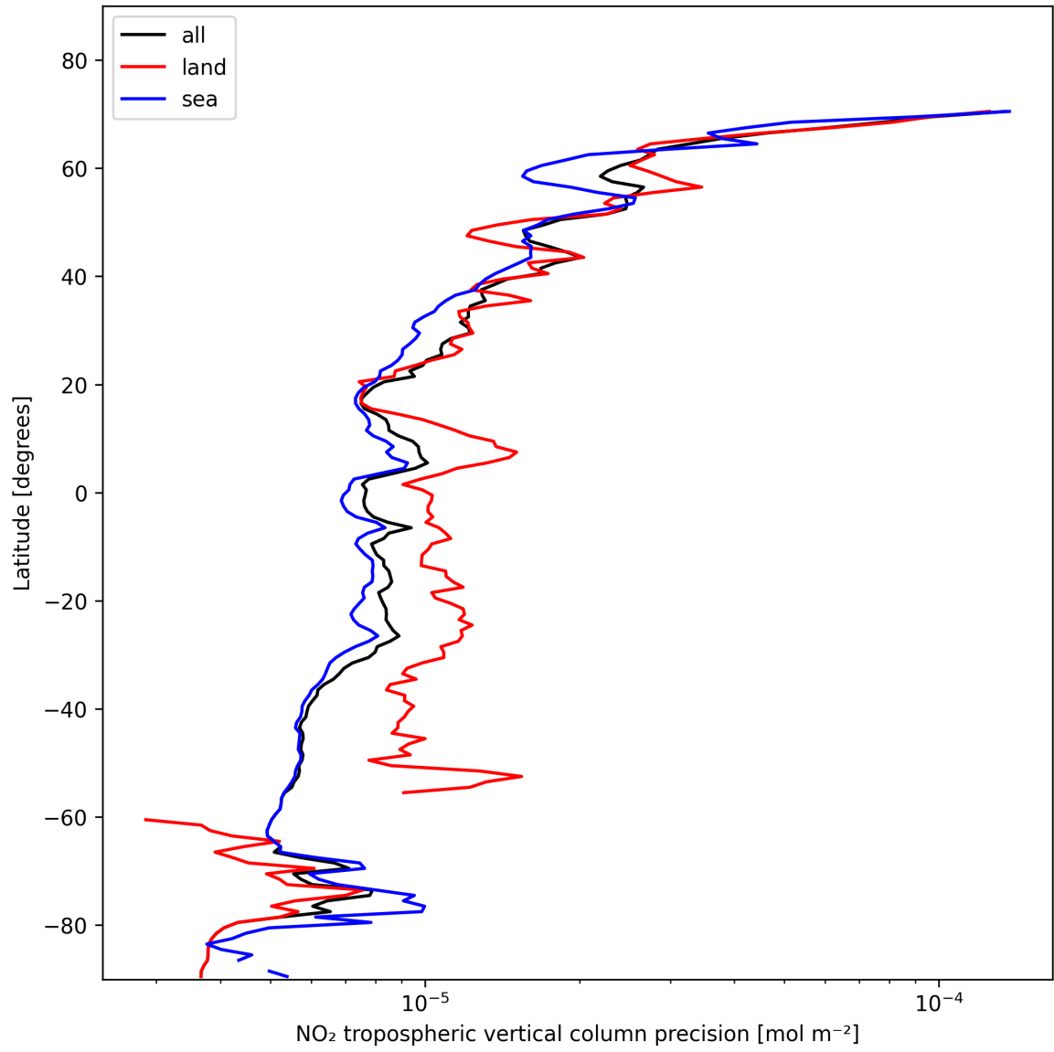
Figure 13: Zonal average of “NO 2 tropospheric vertical column precision” for 2025-01-28 to 2025-01-29.
