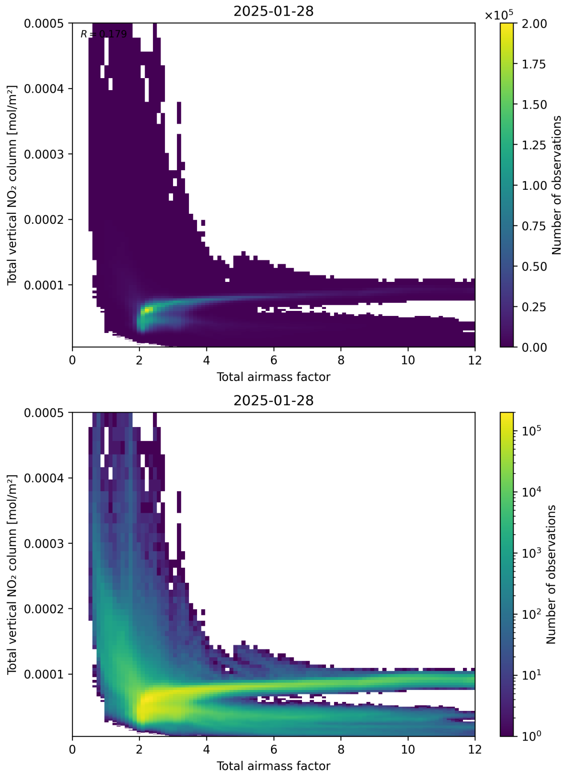
Figure 67: Scatter density plot of “Total airmass factor” against “Total vertical NO 2 column” for 2025-01-28 to 2025-01-29.
