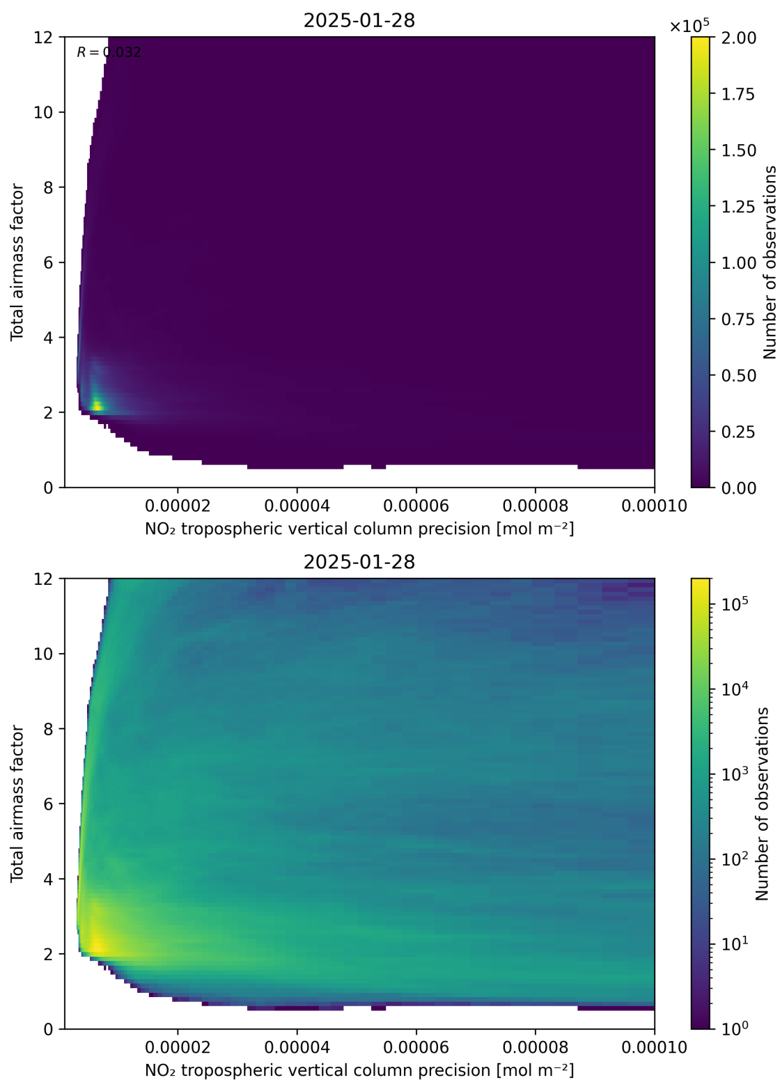
Figure 132: Scatter density plot of “NO 2 tropospheric vertical column precision” against “Total air mass factor” for 2025-01-28 to 2025-01-29.
