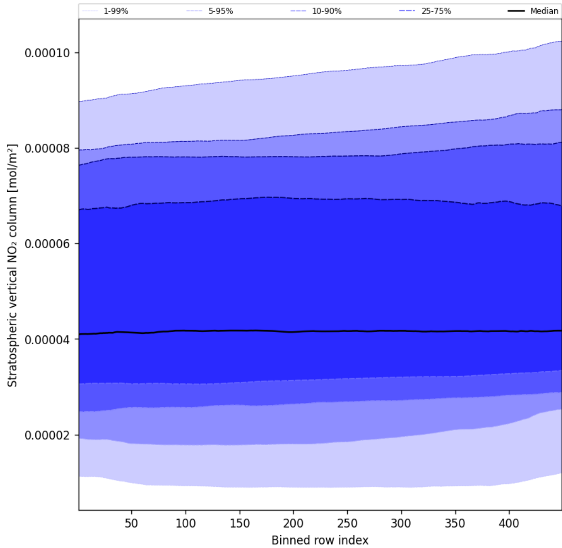
Figure 53: Along track statistics of “Stratospheric vertical NO 2 column” for 2025-01-28 to 2025-01-29
