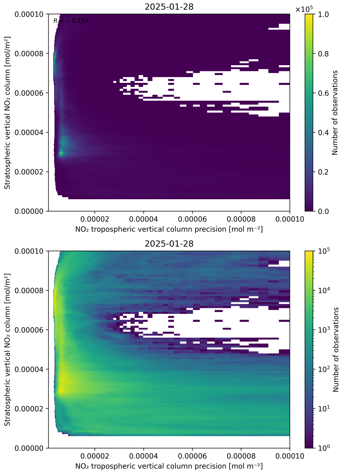
Figure 135: Scatter density plot of “NO 2 tropospheric vertical column precision” against “Stratospheric vertical NO 2 column” for 2025-01-28 to 2025-01-29.
