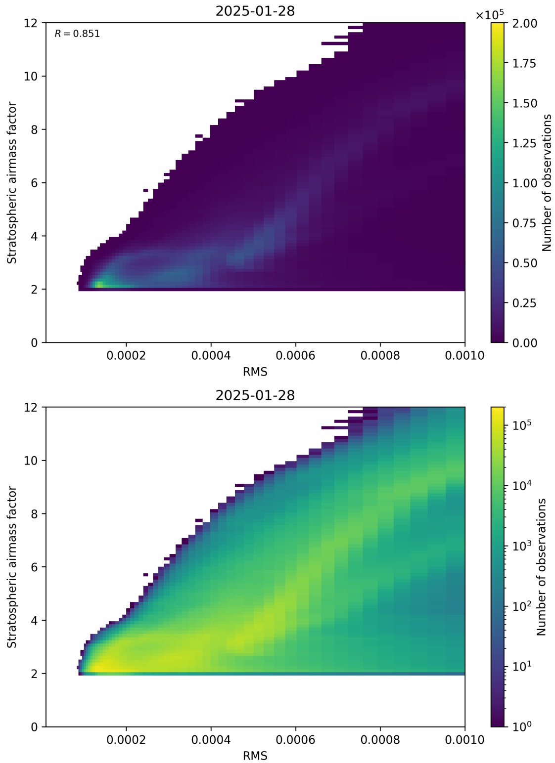
Figure 144: Scatter density plot of “RMS” against “Stratospheric airmass factor” for 2025-01-28 to 2025-01-29.
