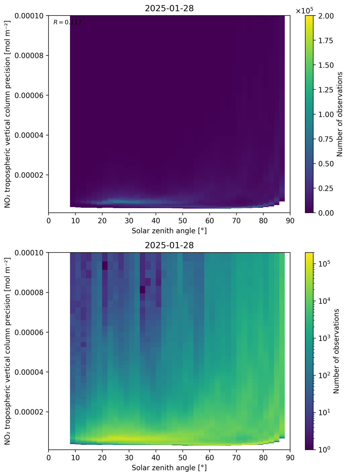
Figure 156: Scatter density plot of “Solar zenith angle” against “NO 2 tropospheric vertical column precision” for 2025-01-28 to 2025-01-29.
