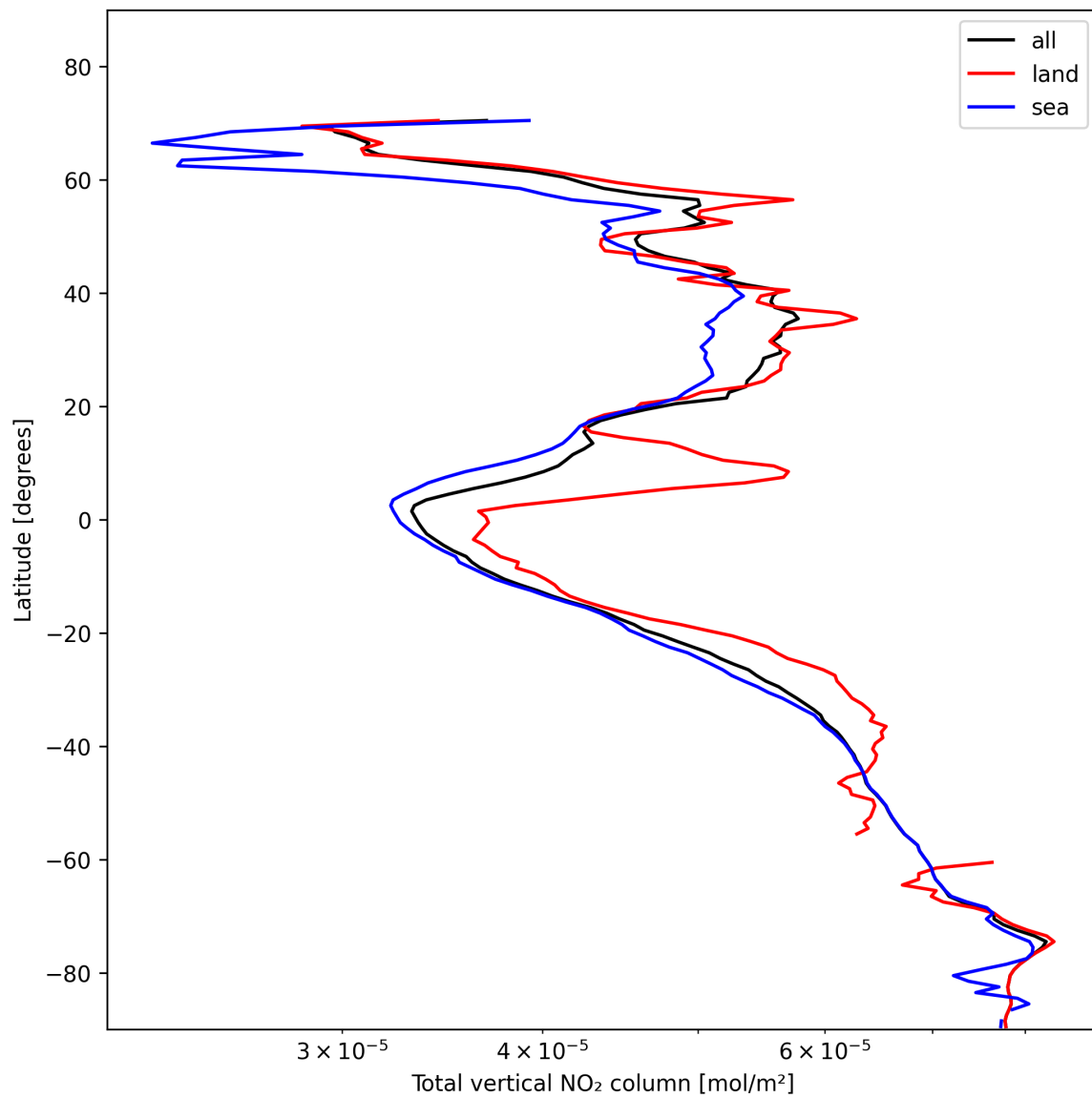
Figure 21: Zonal average of “Total vertical NO 2 column” for 2025-01-28 to 2025-01-29.
