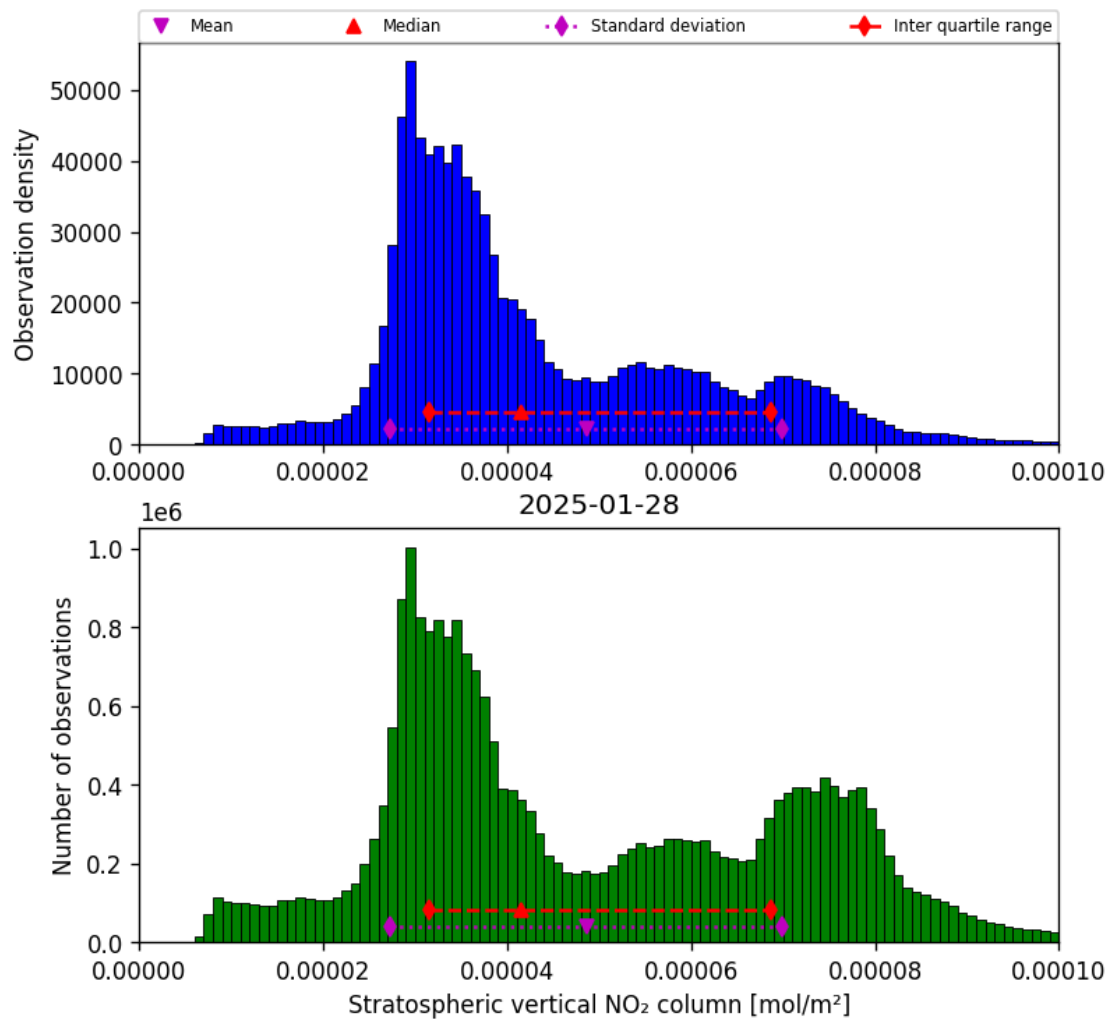
Figure 36: Histogram of “Stratospheric vertical NO 2 column” for 2025-01-28 to 2025-01-29
