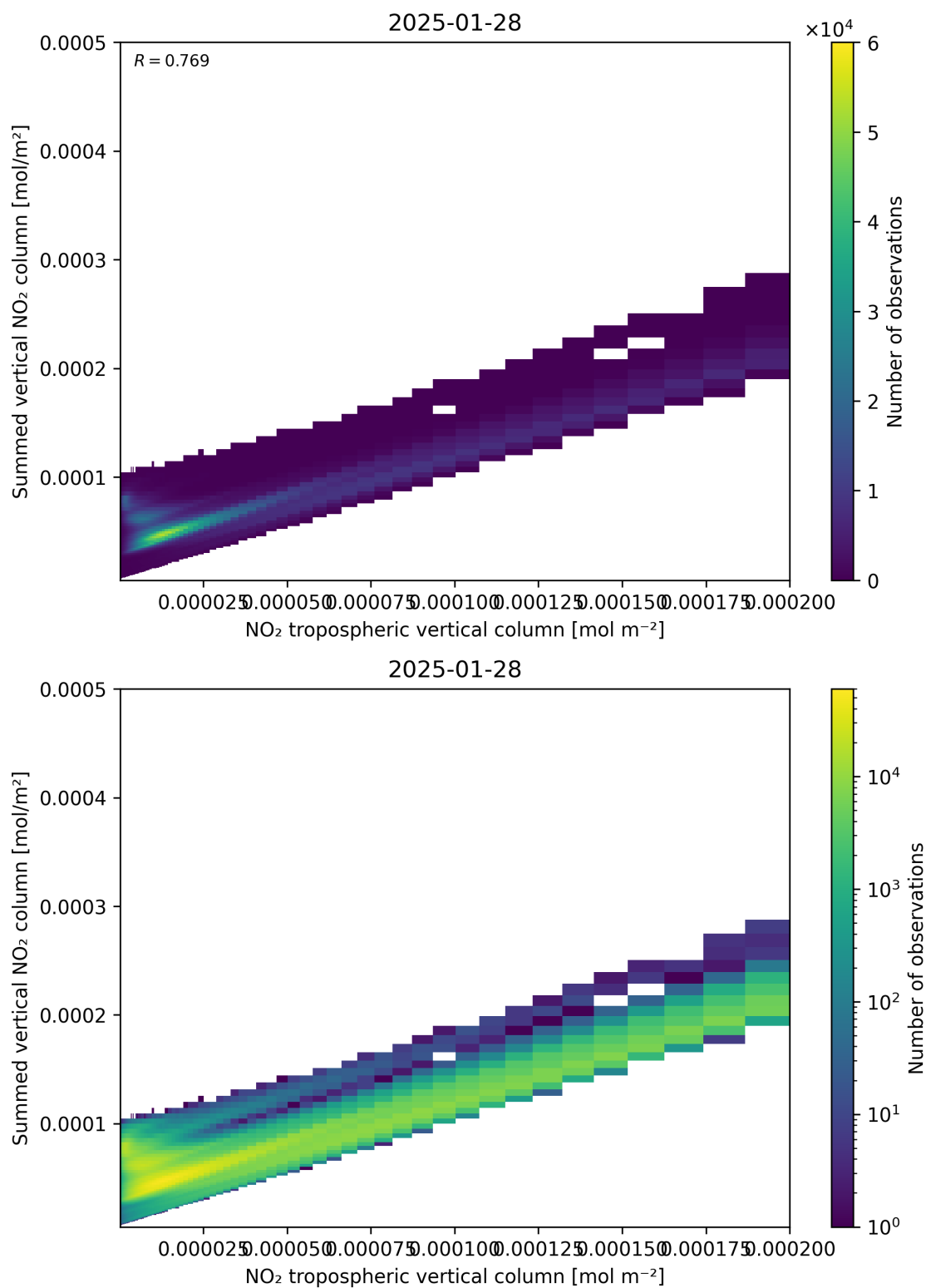
Figure 126: Scatter density plot of “NO 2 tropospheric vertical column” against “Summed vertical NO 2 column” for 2025-01-28 to 2025-01-29.
