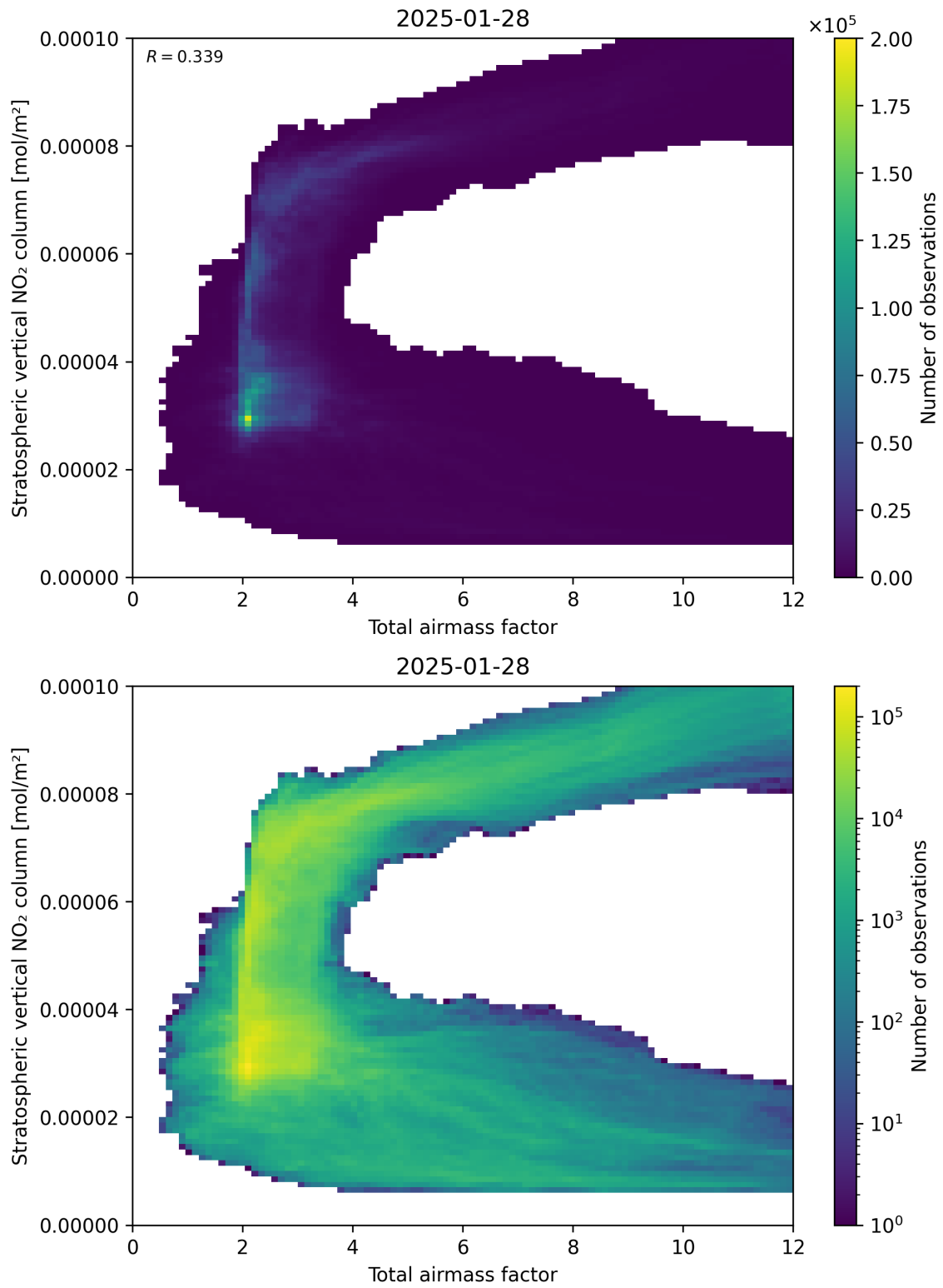
Figure 64: Scatter density plot of “Total airmass factor” against “Stratospheric vertical \text{NO}_2 column” for 2025-01-28 to 2025-01-29.
