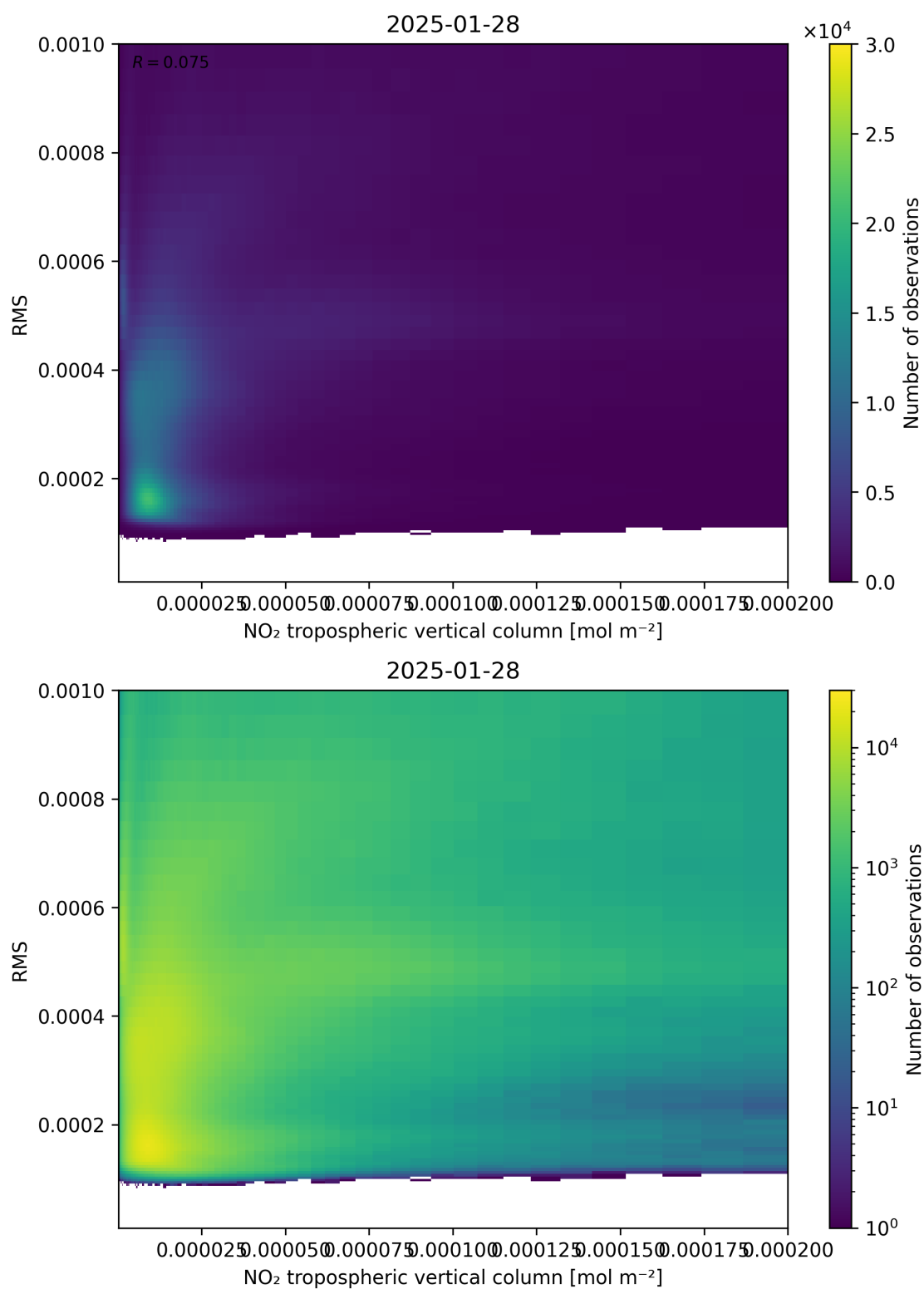
Figure 142: Scatter density plot of “NO 2 tropospheric vertical column” against “RMS” for 2025-01-28 to 2025-01-29.
