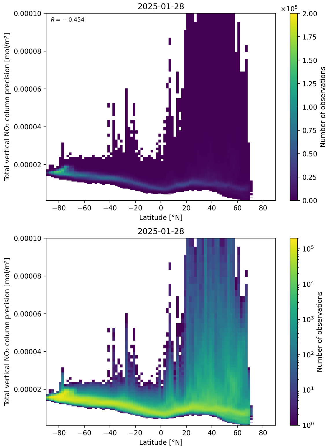
Figure 91: Scatter density plot of “Latitude” against “Total vertical NO 2 column precision” for 2025-01-28 to 2025-01-29.
