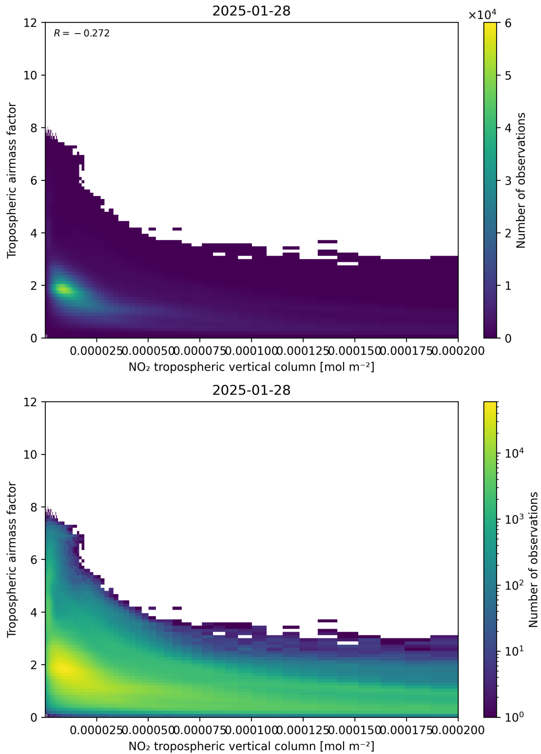
Figure 123: Scatter density plot of “NO 2 tropospheric vertical column” against “Tropospheric air mass factor” for 2025-01-28 to 2025-01-29.
