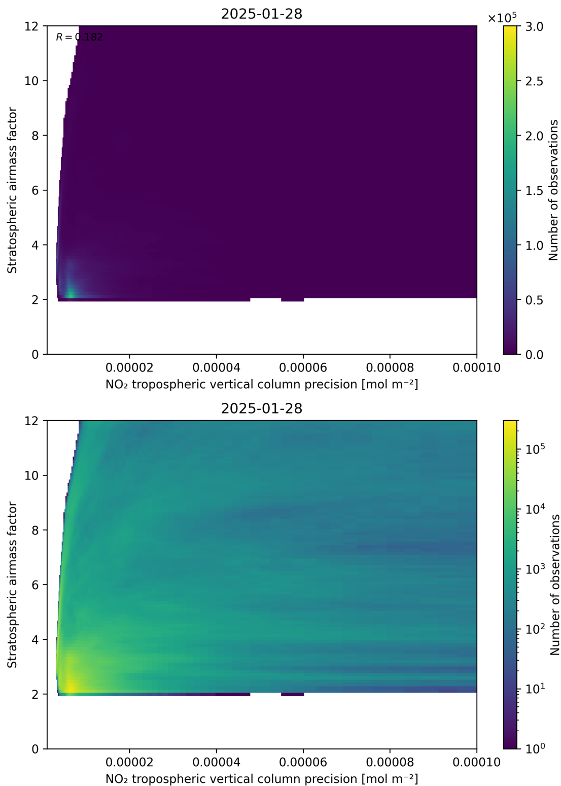
Figure 131: Scatter density plot of “NO 2 tropospheric vertical column precision” against “Stratospheric airmass factor” for 2025-01-28 to 2025-01-29.
