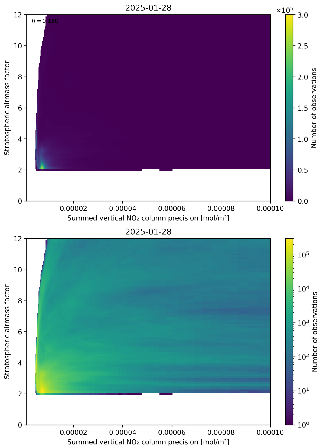
Figure 106: Scatter density plot of “Summed vertical NO 2 column precision” against “Stratospheric airmass factor” for 2025-01-28 to 2025-01-29.
