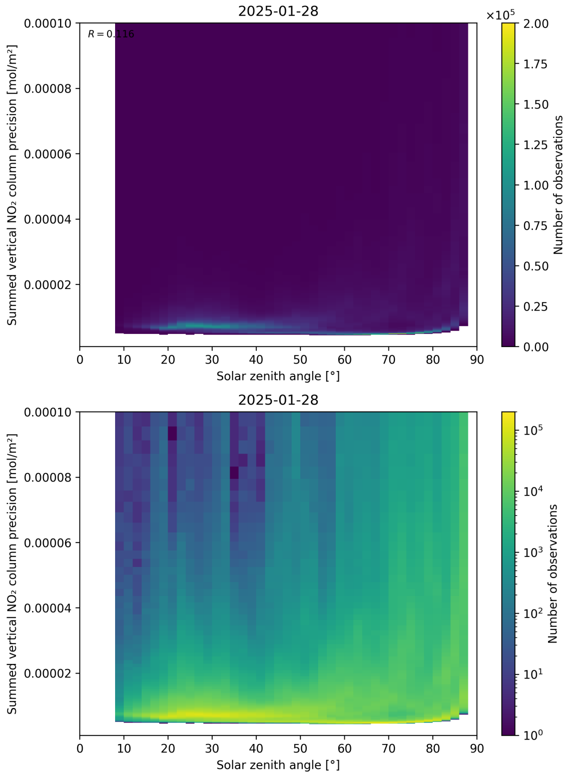
Figure 152: Scatter density plot of “Solar zenith angle” against “Summed vertical NO 2 column precision” for 2025-01-28 to 2025-01-29.
