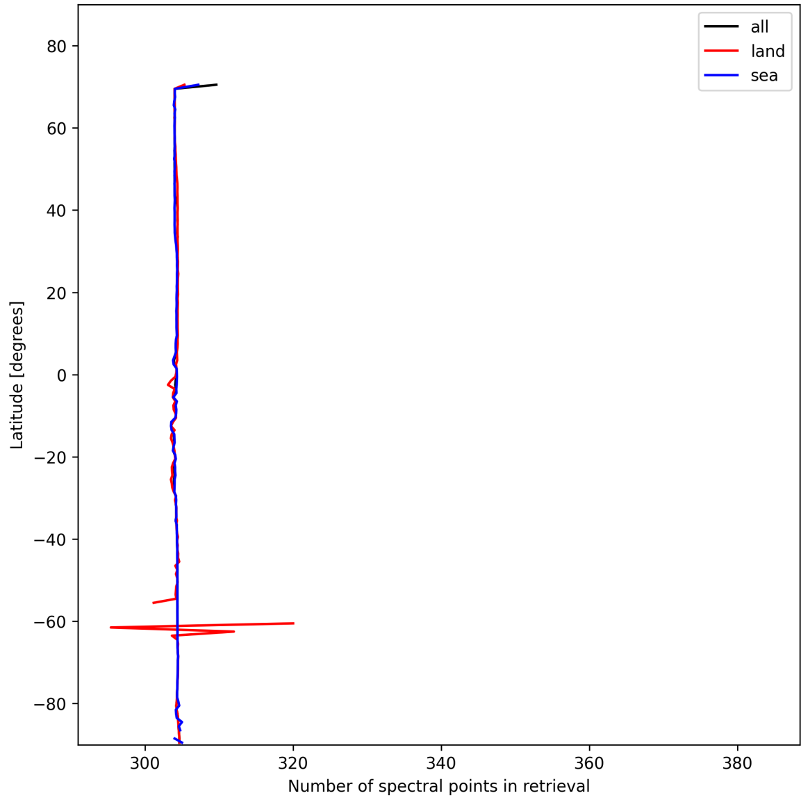
Figure 16: Zonal average of “Number of spectral points in retrieval” for 2025-01-28 to 2025-01-29.
