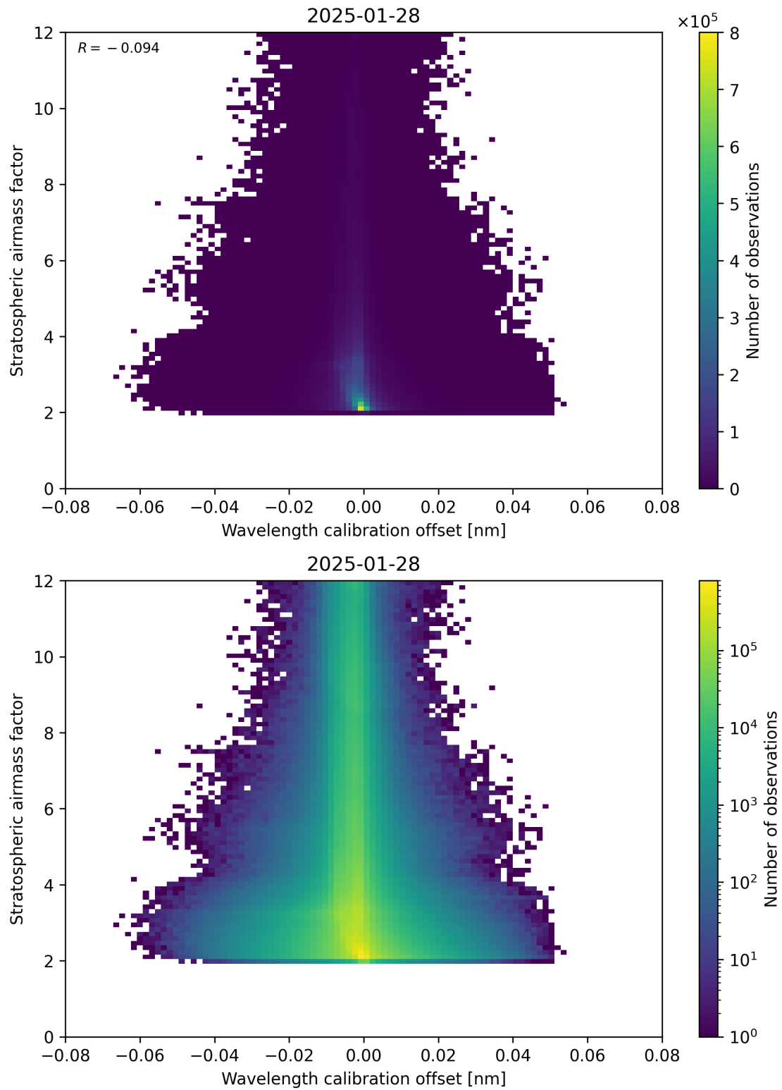
Figure 174: Scatter density plot of “Wavelength calibration offset” against “Stratospheric airmass factor” for 2025-01-28 to 2025-01-29.
