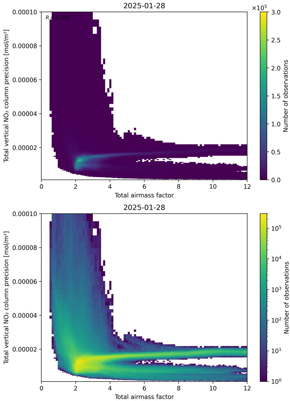
Figure 68: Scatter density plot of “Total airmass factor” against “Total vertical NO 2 column precision” for 2025-01-28 to 2025-01-29.
