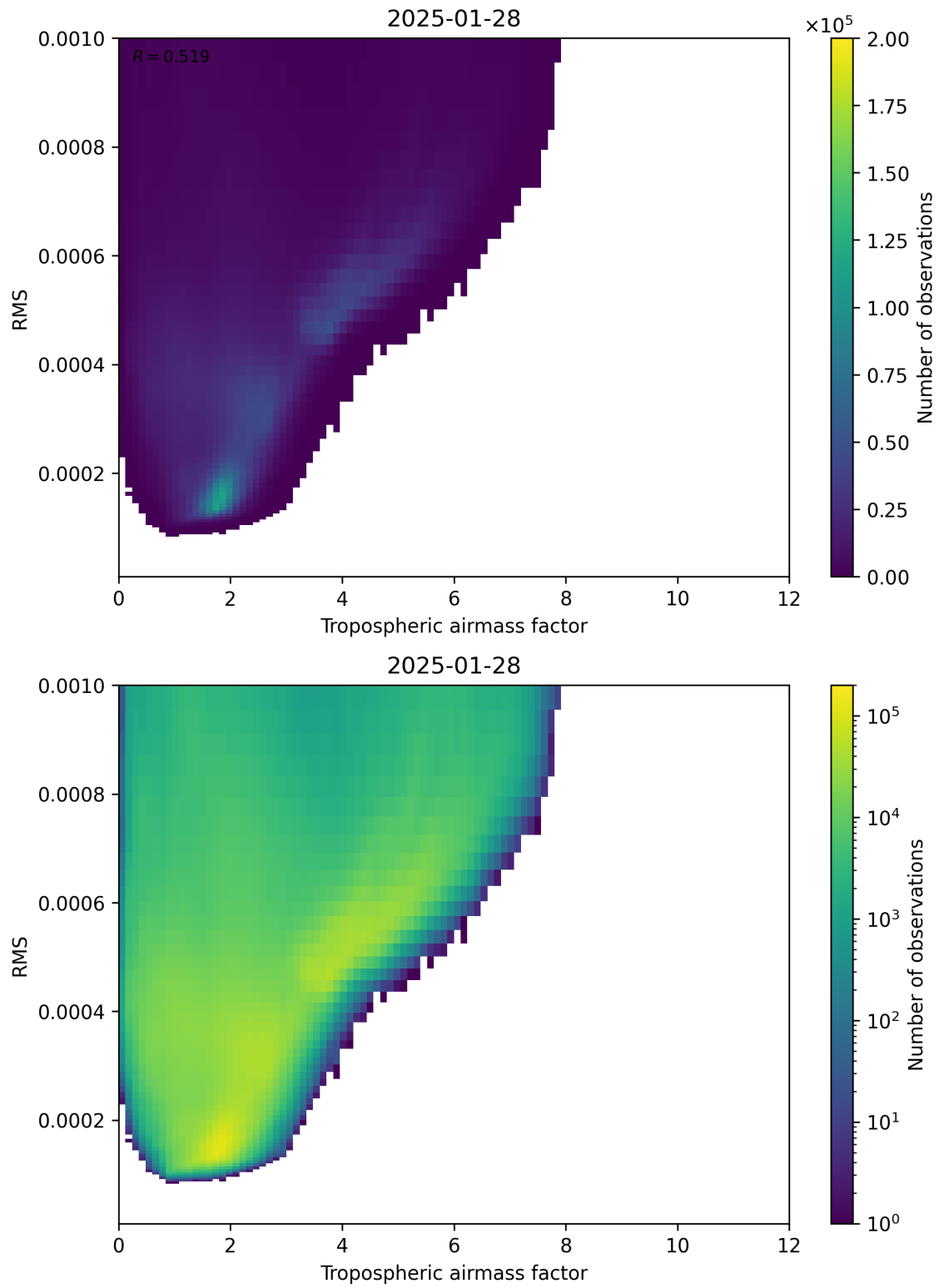
Figure 79: Scatter density plot of “Tropospheric airmass factor” against “RMS” for 2025-01-28 to 2025-01-29.
