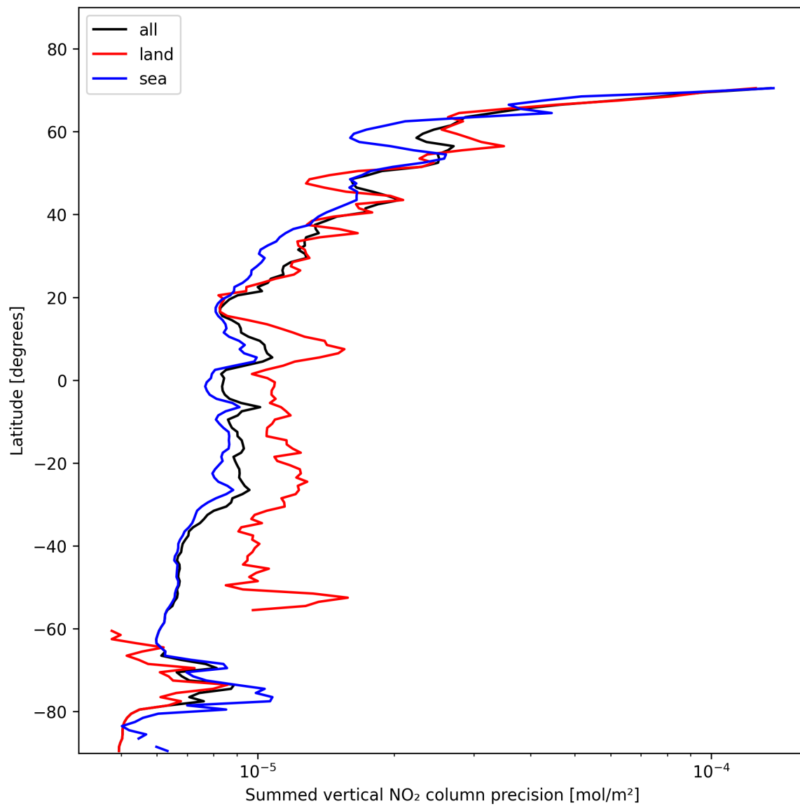
Figure 24: Zonal average of “Summed vertical NO 2 column precision” for 2025-01-28 to 2025-01-29.
