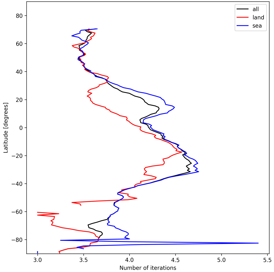
Figure 17: Zonal average of “Number of iterations” for 2025-01-28 to 2025-01-29.
