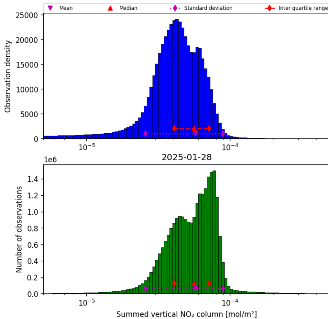
Figure 40: Histogram of “Summed vertical NO 2 column” for 2025-01-28 to 2025-01-29
