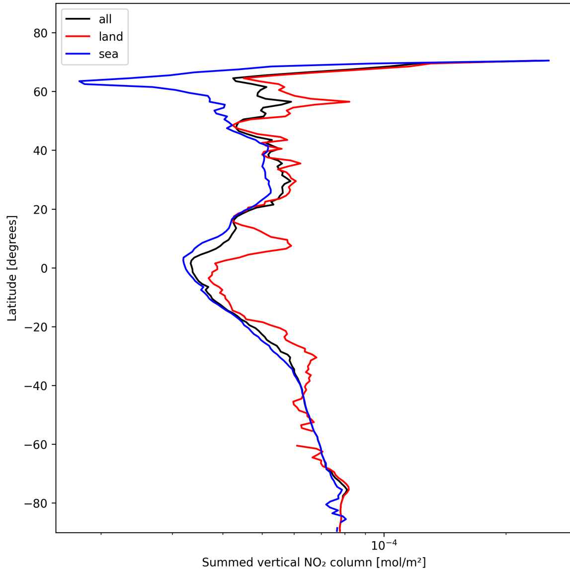
Figure 23: Zonal average of “Summed vertical NO 2 column” for 2025-01-28 to 2025-01-29.
