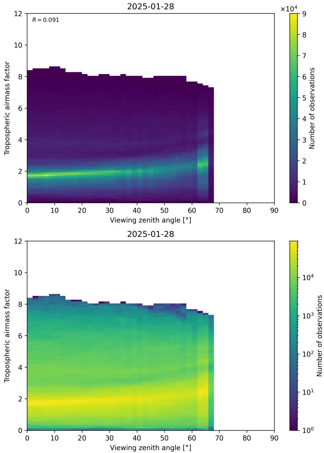
Figure 161: Scatter density plot of “Viewing zenith angle” against “Tropospheric airmass factor” for 2025-01-28 to 2025-01-29.
