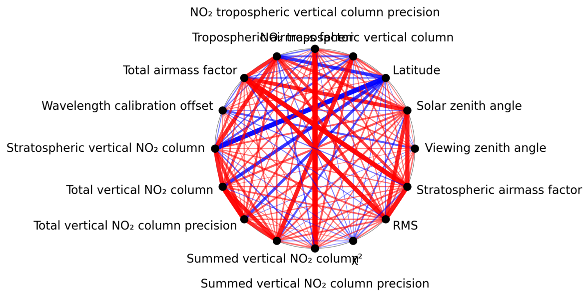
Figure 1: Map of correlation graph for 2025-01-28 to 2025-01-29.
