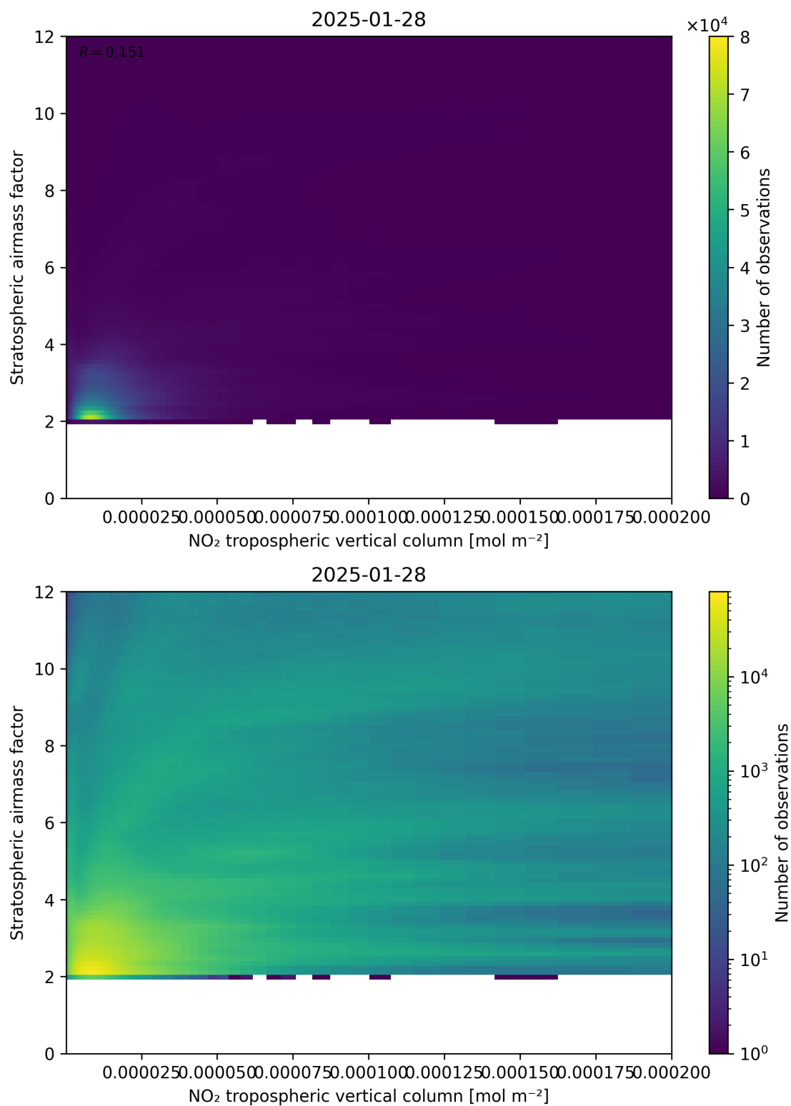
Figure 121: Scatter density plot of “NO 2 tropospheric vertical column” against “Stratospheric airmass factor” for 2025-01-28 to 2025-01-29.
