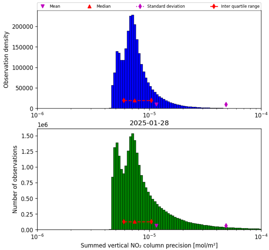
Figure 41: Histogram of “Summed vertical NO 2 column precision” for 2025-01-28 to 2025-01-29
