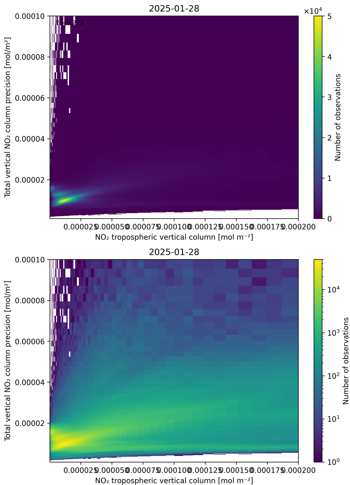
Figure 129: Scatter density plot of “NO 2 tropospheric vertical column” against “Total vertical NO 2 column precision” for 2025-01-28 to 2025-01-29.
