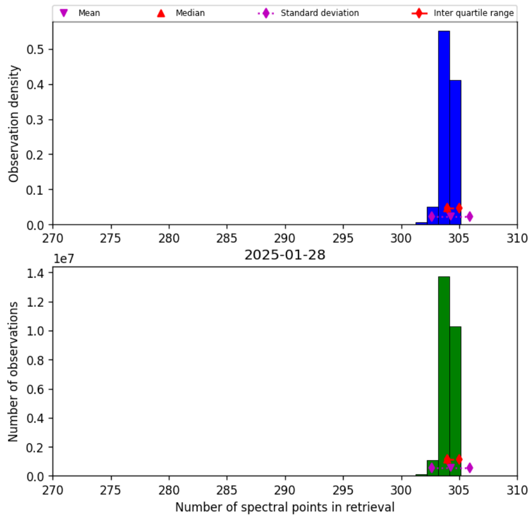
Figure 33: Histogram of “Number of spectral points in retrieval” for 2025-01-28 to 2025-01-29
