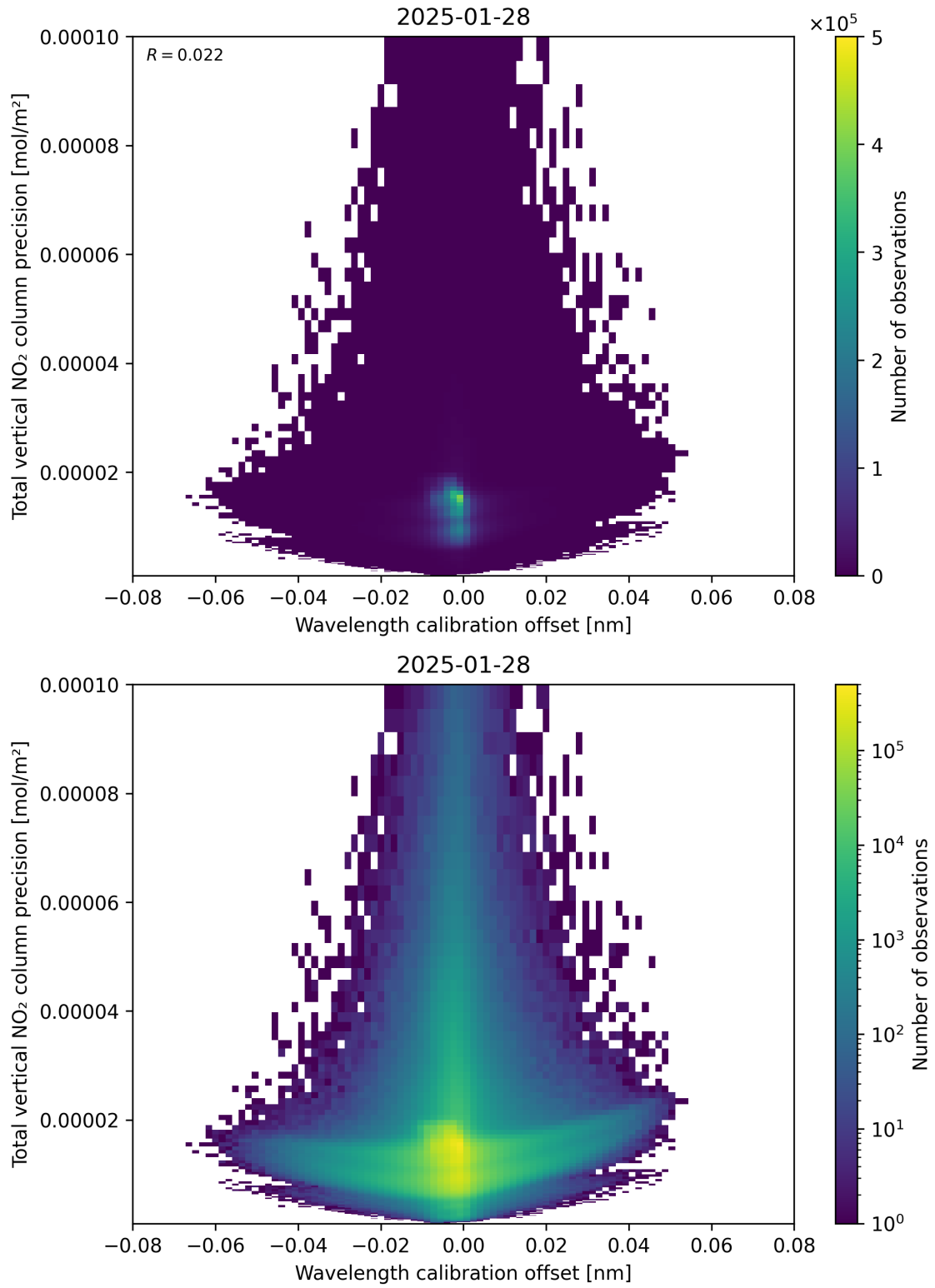
Figure 180: Scatter density plot of “Wavelength calibration offset” against “Total vertical NO 2 column precision” for 2025-01-28 to 2025-01-29.
