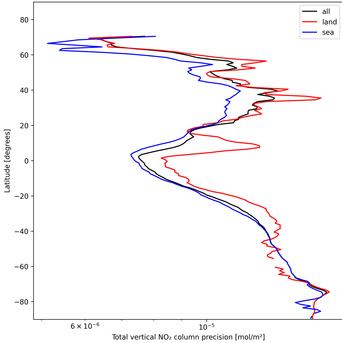
Figure 22: Zonal average of “Total vertical NO 2 column precision” for 2025-01-28 to 2025-01-29.
