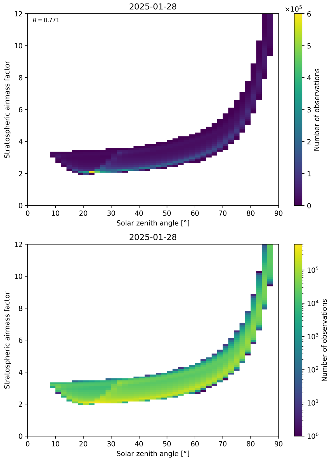
Figure 145: Scatter density plot of “Solar zenith angle” against “Stratospheric airmass factor” for 2025-01-28 to 2025-01-29.
