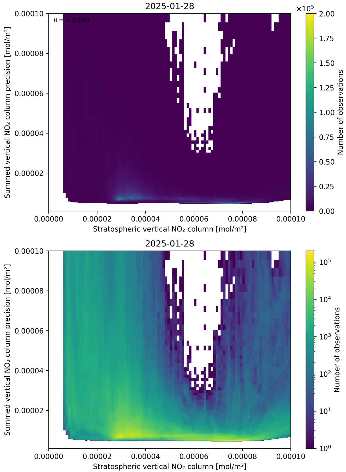
Figure 99: Scatter density plot of “Stratospheric vertical NO 2 column” against “Summed vertical NO 2 column precision” for 2025-01-28 to 2025-01-29.
