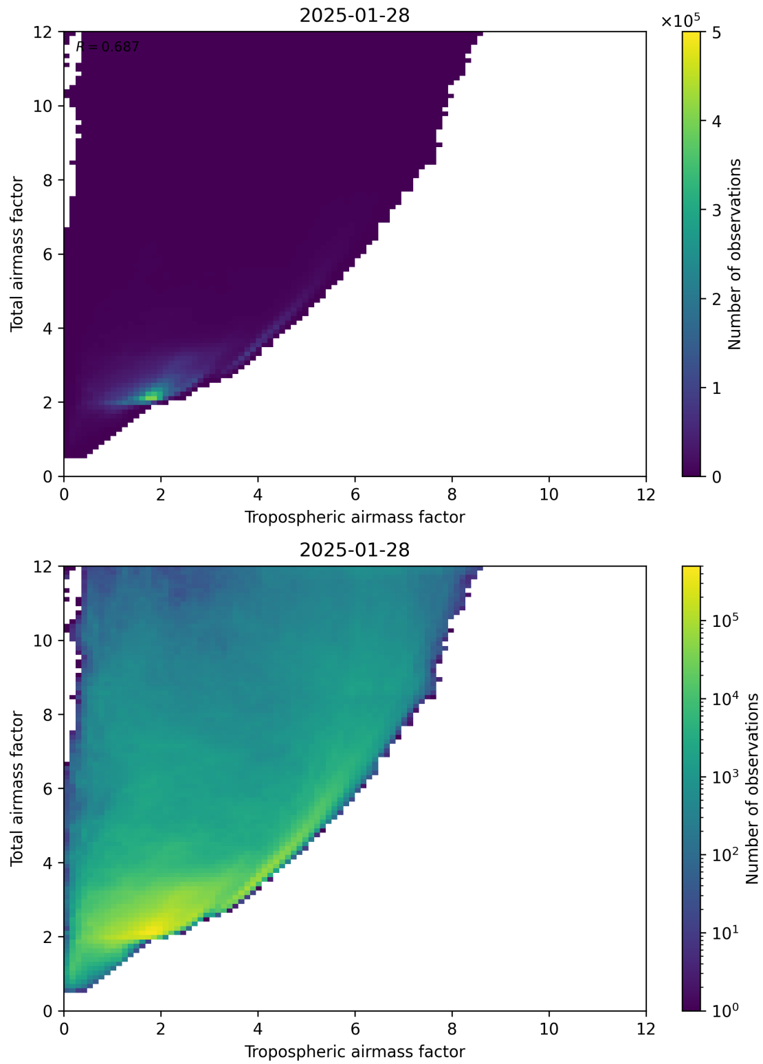
Figure 72: Scatter density plot of “Tropospheric airmass factor” against “Total airmass factor” for 2025-01-28 to 2025-01-29.
