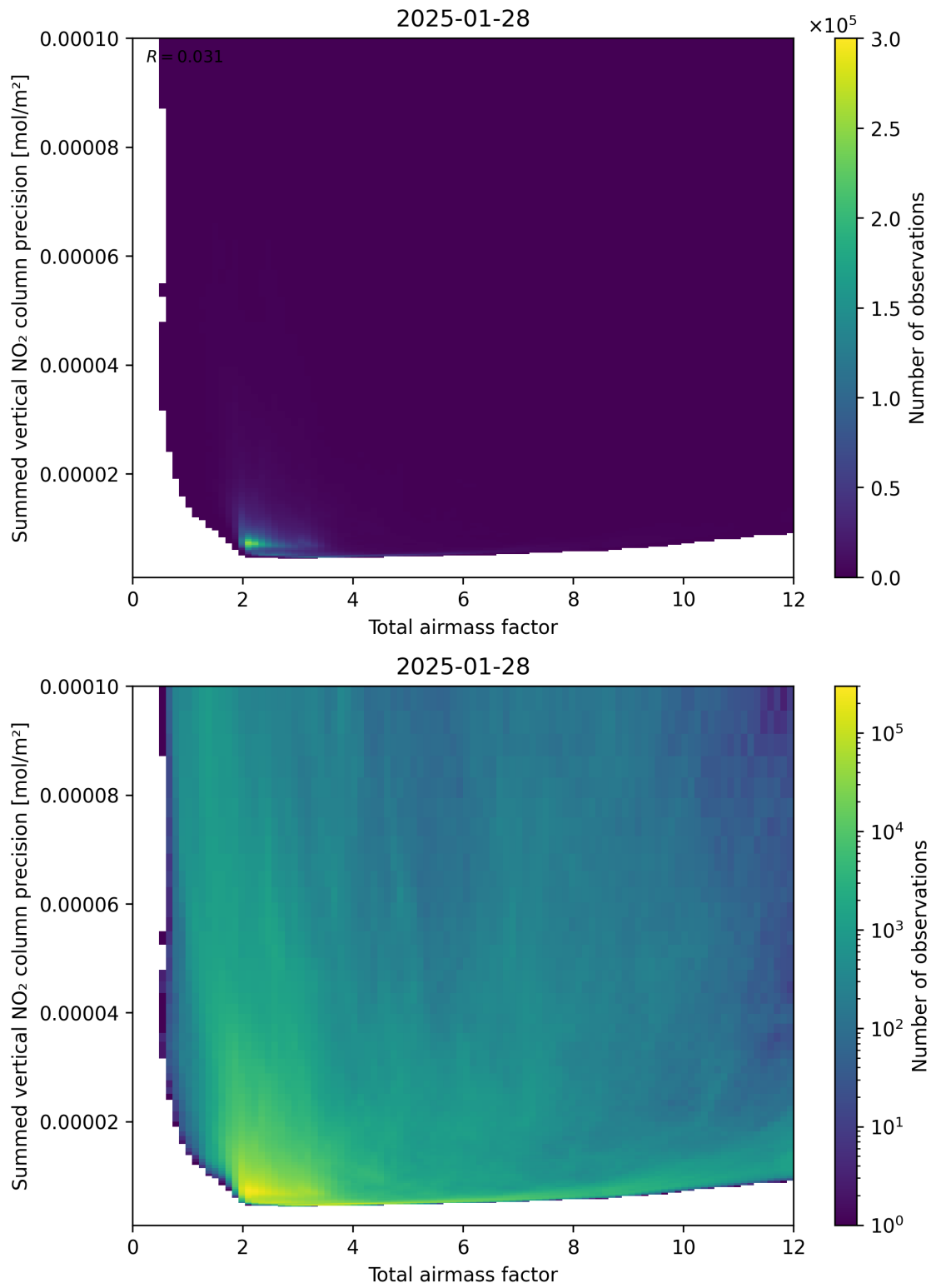
Figure 66: Scatter density plot of “Total airmass factor” against “Summed vertical NO 2 column precision” for 2025-01-28 to 2025-01-29.
