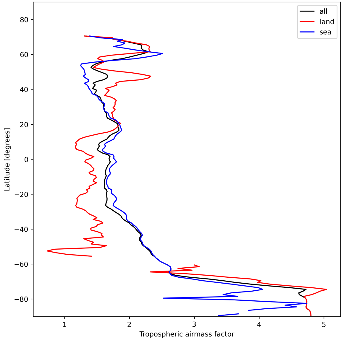
Figure 14: Zonal average of “Tropospheric airmass factor” for 2025-01-28 to 2025-01-29.
