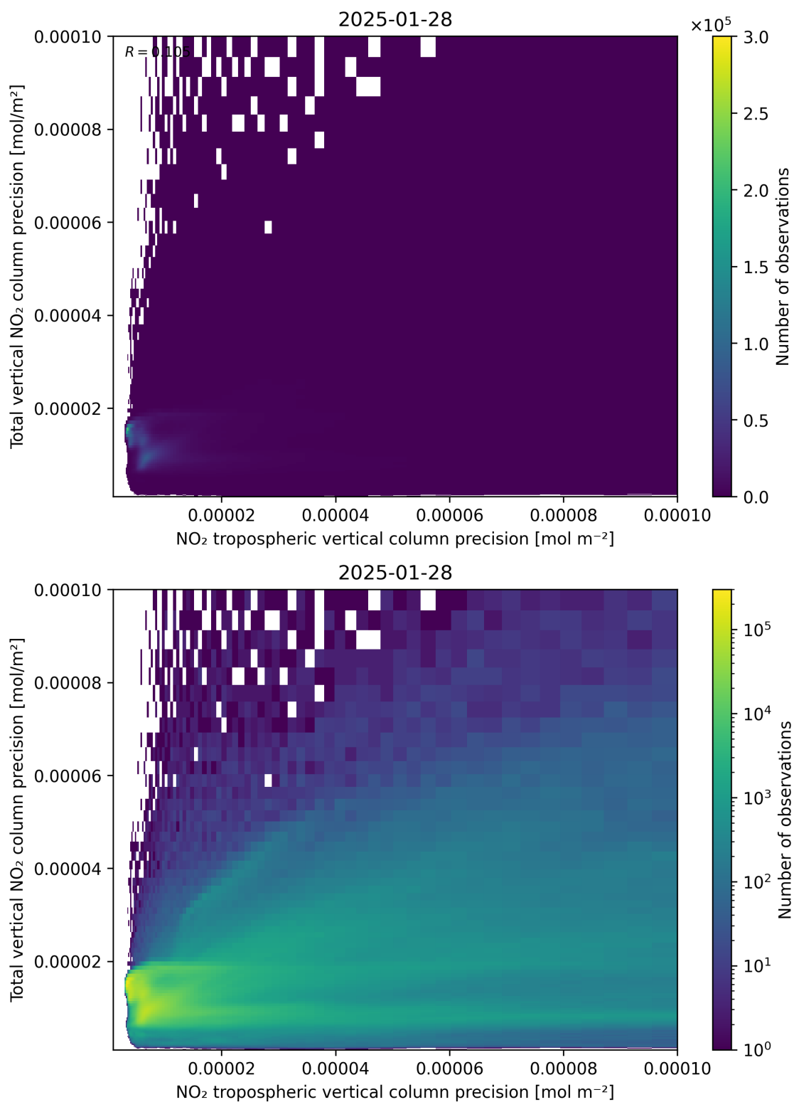
Figure 139: Scatter density plot of “NO 2 tropospheric vertical column precision” against “Total vertical NO 2 column precision” for 2025-01-28 to 2025-01-29.
