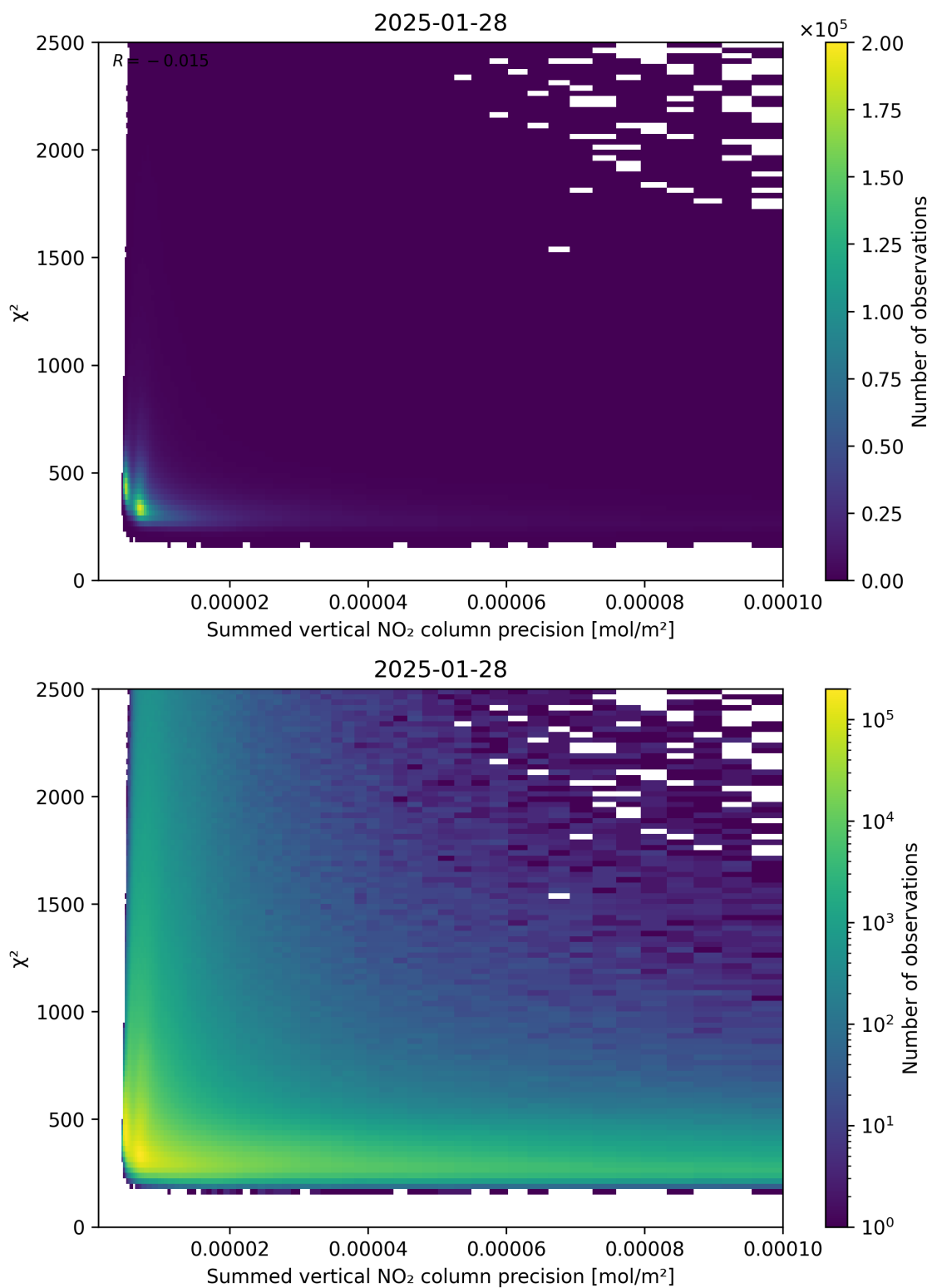
Figure 107: Scatter density plot of “Summed vertical NO 2 column precision” against “ \chi^2 ” for 2025-01-28 to 2025-01-29.
