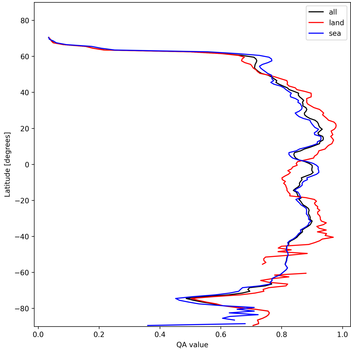
Figure 11: Zonal average of “QA value” for 2025-01-28 to 2025-01-29.
