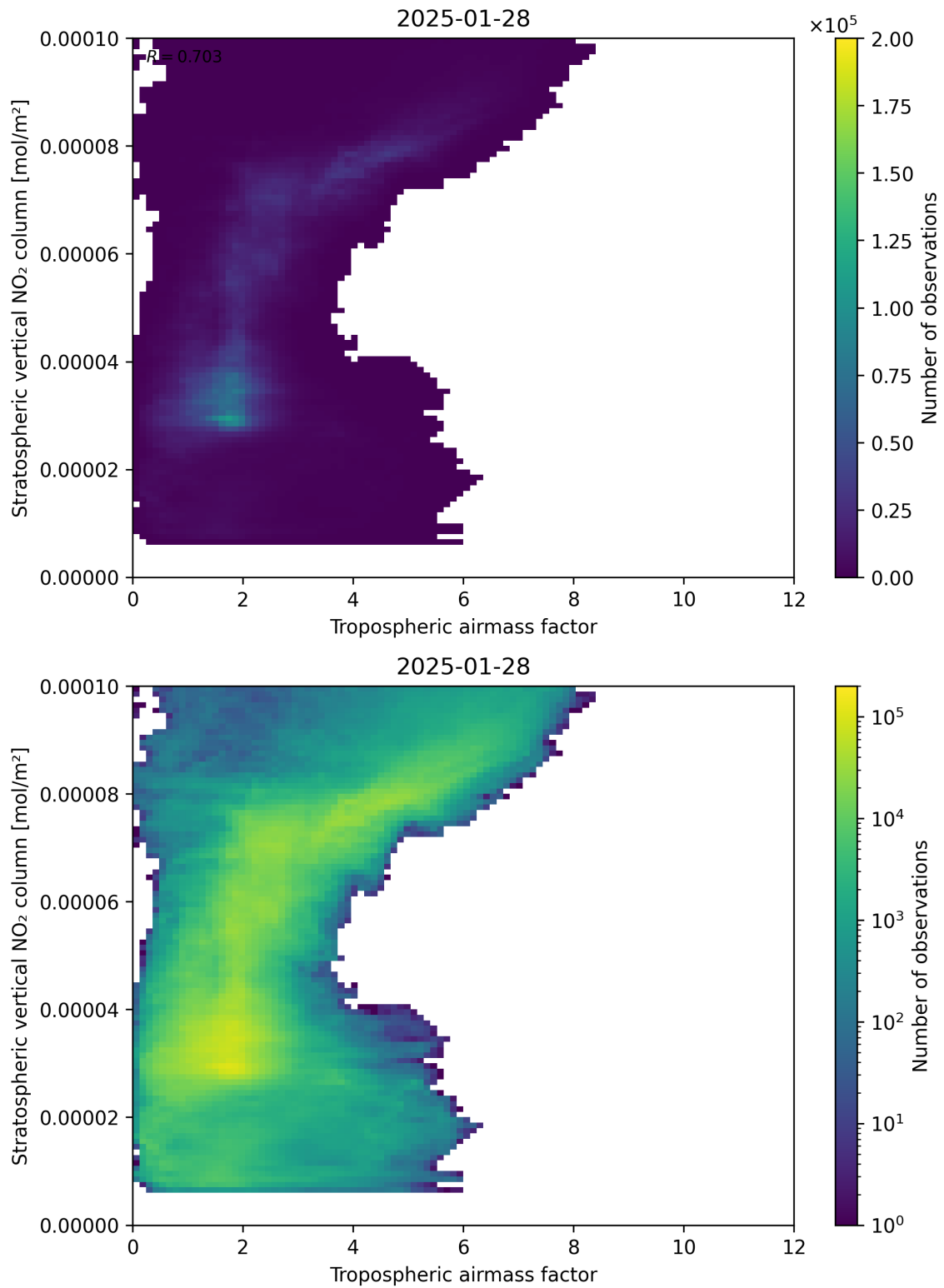
Figure 74: Scatter density plot of “Tropospheric airmass factor” against “Stratospheric vertical NO 2 column” for 2025-01-28 to 2025-01-29.
