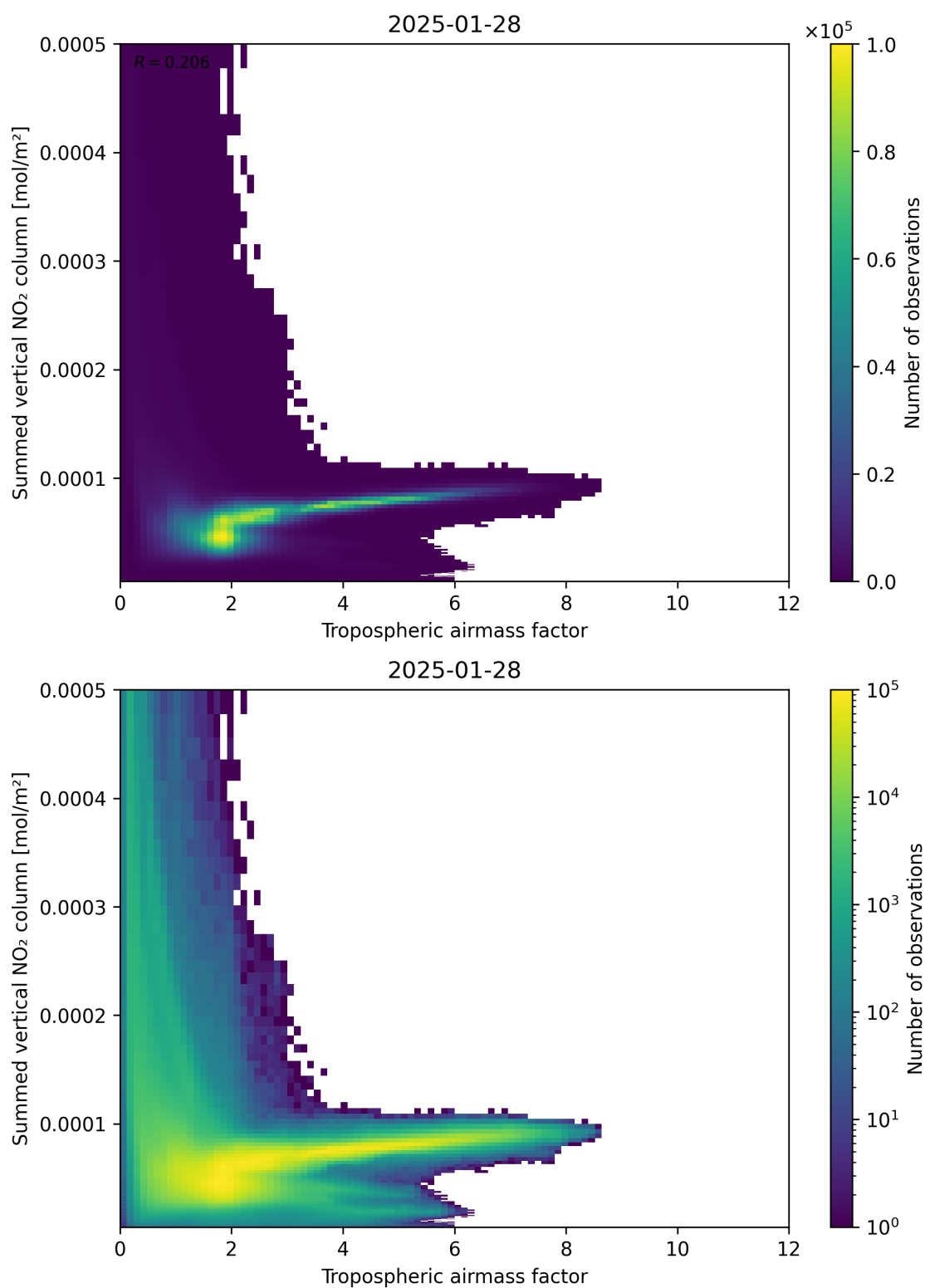
Figure 75: Scatter density plot of “Tropospheric air mass factor” against “Summed vertical NO 2 column” for 2025-01-28 to 2025-01-29.
