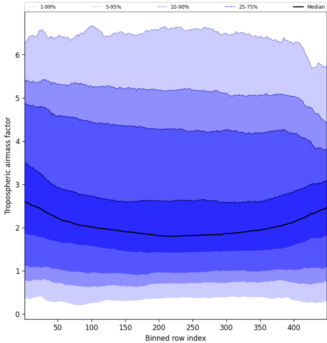
Figure 48: Along track statistics of “Tropospheric airmass factor” for 2025-01-28 to 2025-01-29
