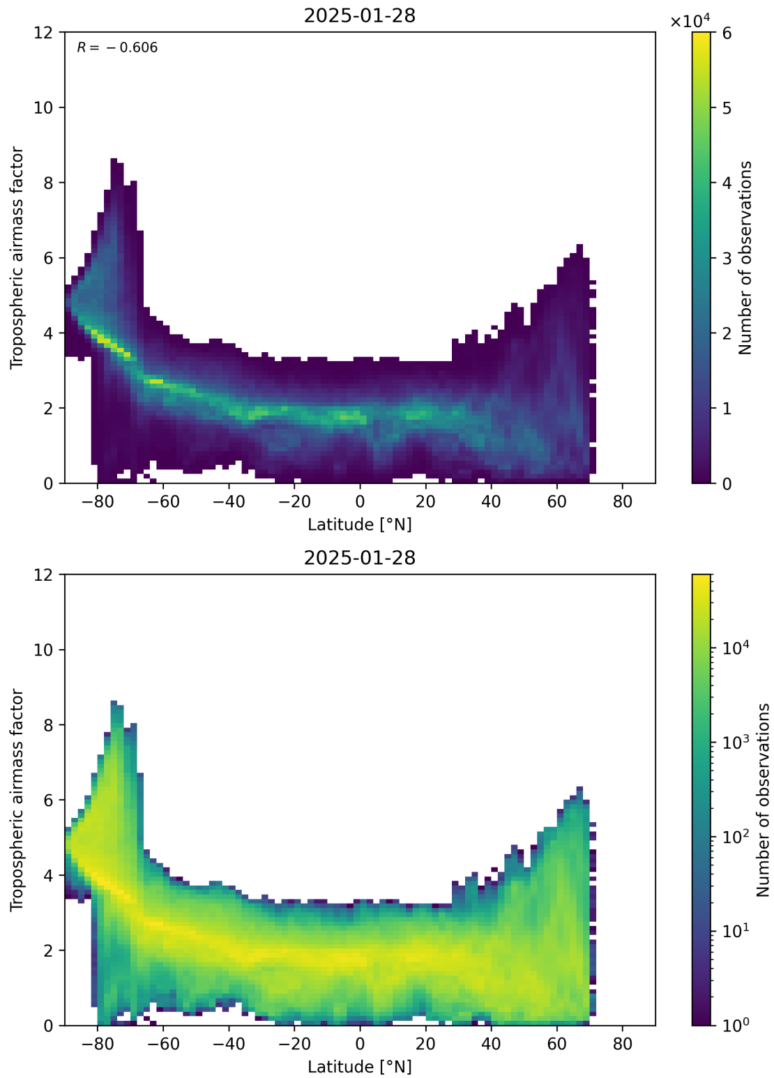
Figure 85: Scatter density plot of “Latitude” against “Tropospheric airmass factor” for 2025-01-28 to 2025-01-29.
