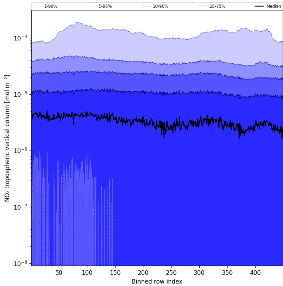
Figure 46: Along track statistics of “NO 2 tropospheric vertical column” for 2025-01-28 to 2025-01-29
