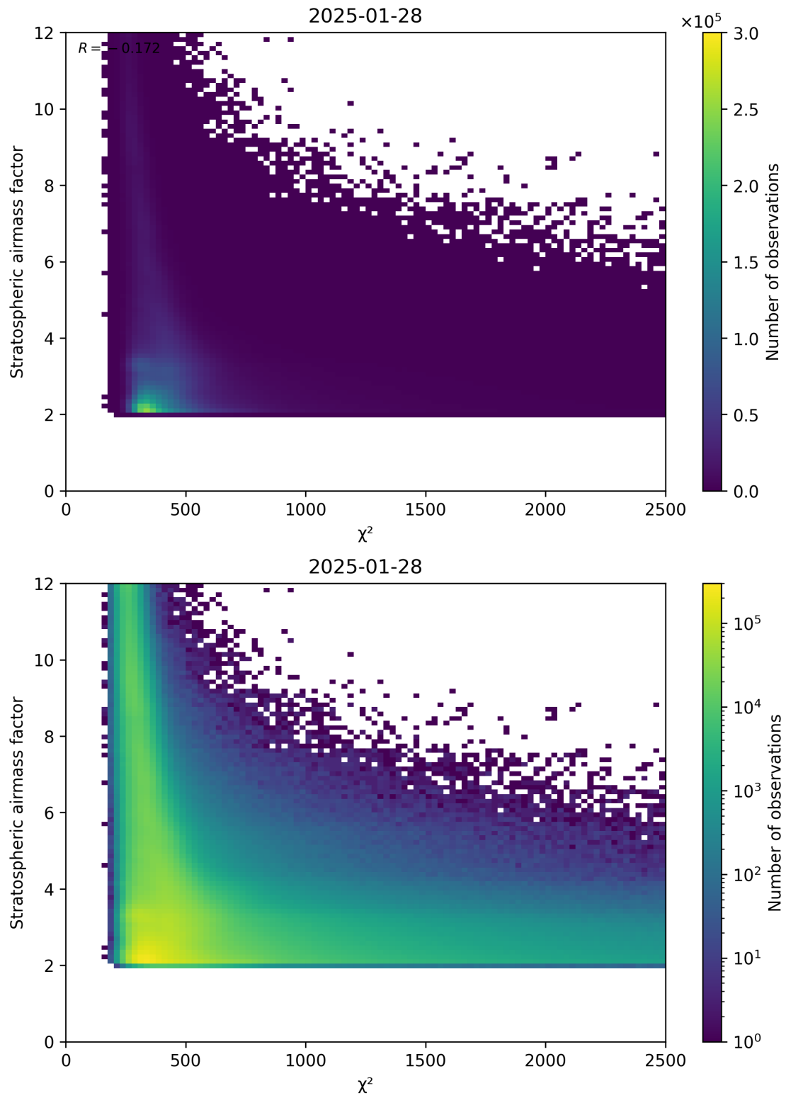
Figure 81: Scatter density plot of “ \chi^2 ” against “Stratospheric airmass factor” for 2025-01-28 to 2025-01-29.
