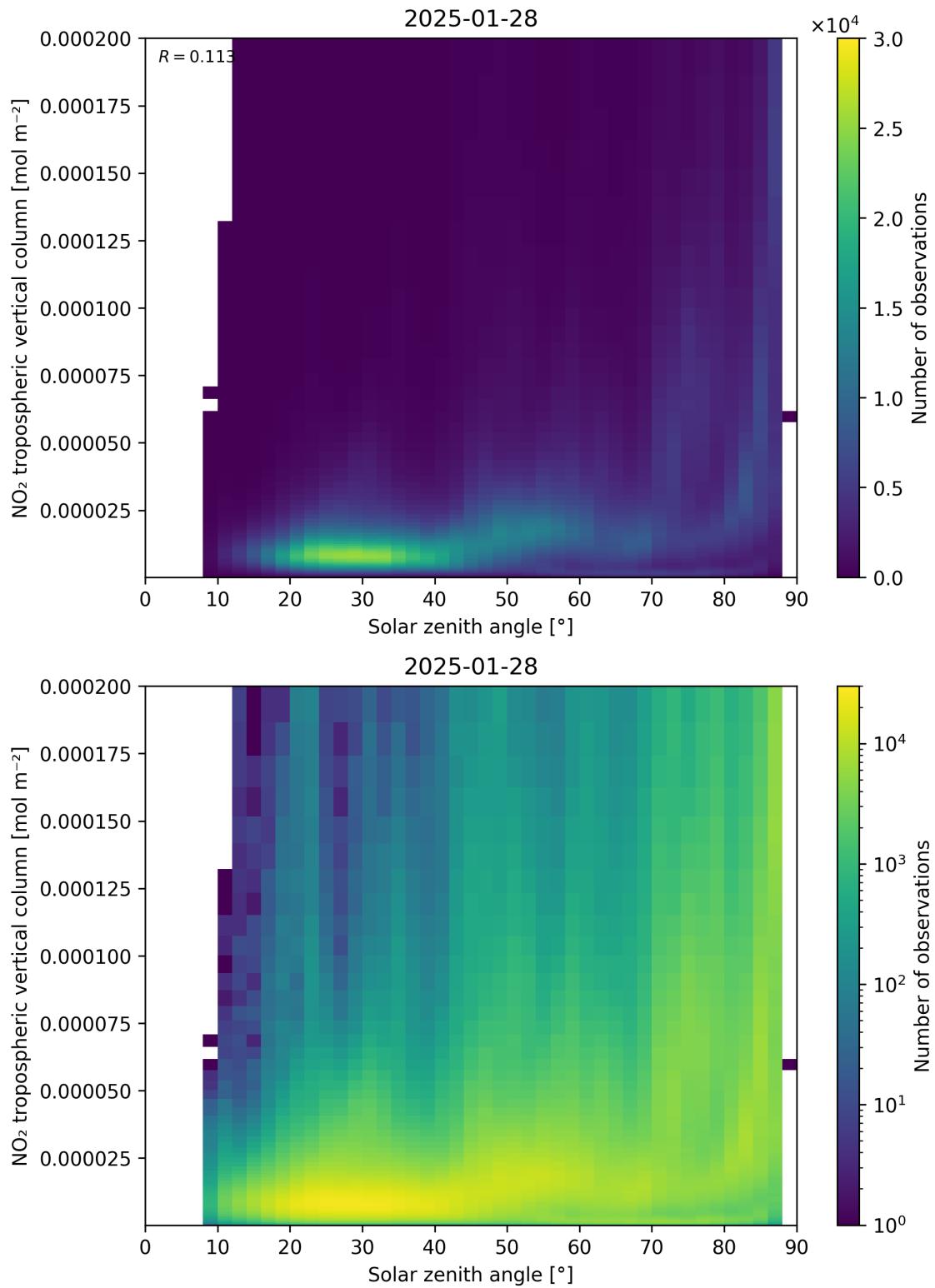
Figure 155: Scatter density plot of “Solar zenith angle” against “NO 2 tropospheric vertical column” for 2025-01-28 to 2025-01-29.
