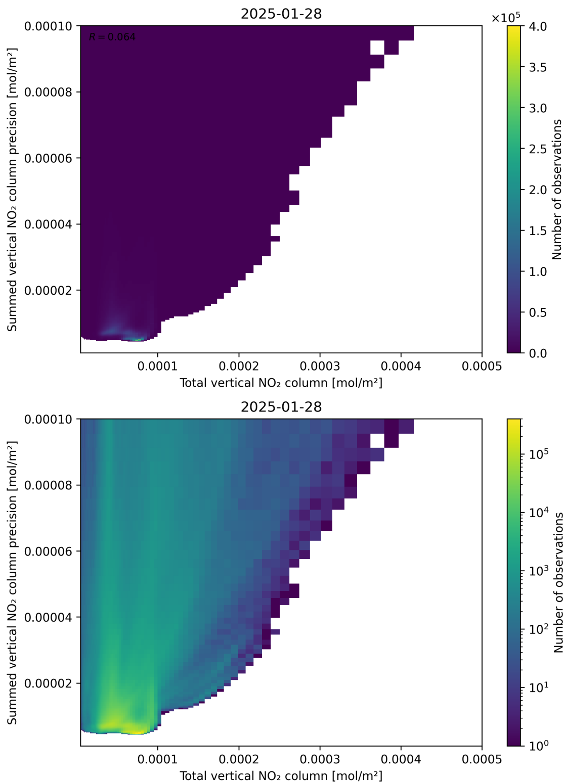
Figure 113: Scatter density plot of “Total vertical NO 2 column” against “Summed vertical NO 2 column precision” for 2025-01-28 to 2025-01-29.
