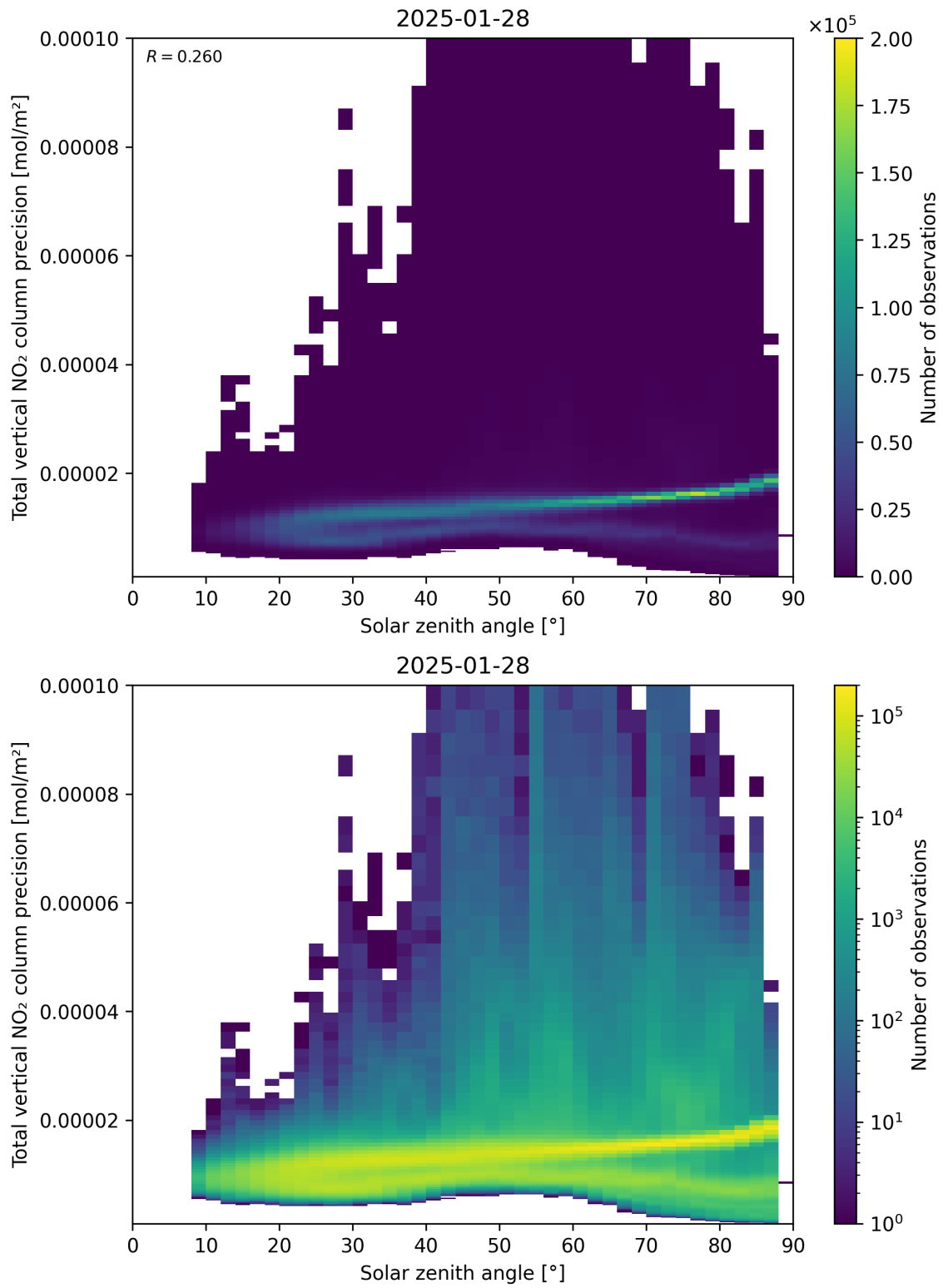
Figure 154: Scatter density plot of “Solar zenith angle” against “Total vertical NO 2 column precision” for 2025-01-28 to 2025-01-29.
