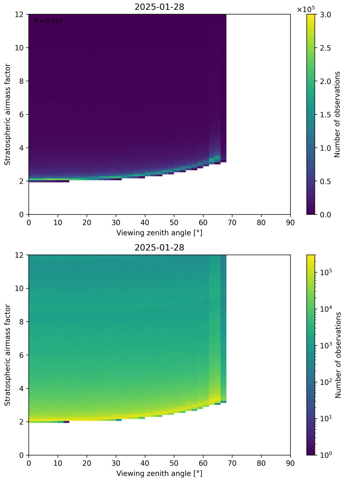
Figure 159: Scatter density plot of “Viewing zenith angle” against “Stratospheric airmass factor” for 2025-01-28 to 2025-01-29.
