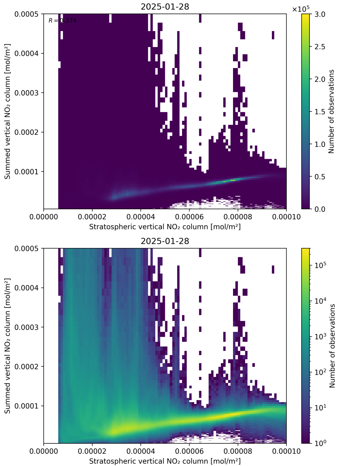
Figure 98: Scatter density plot of “Stratospheric vertical NO 2 column” against “Summed vertical NO 2 column” for 2025-01-28 to 2025-01-29.
