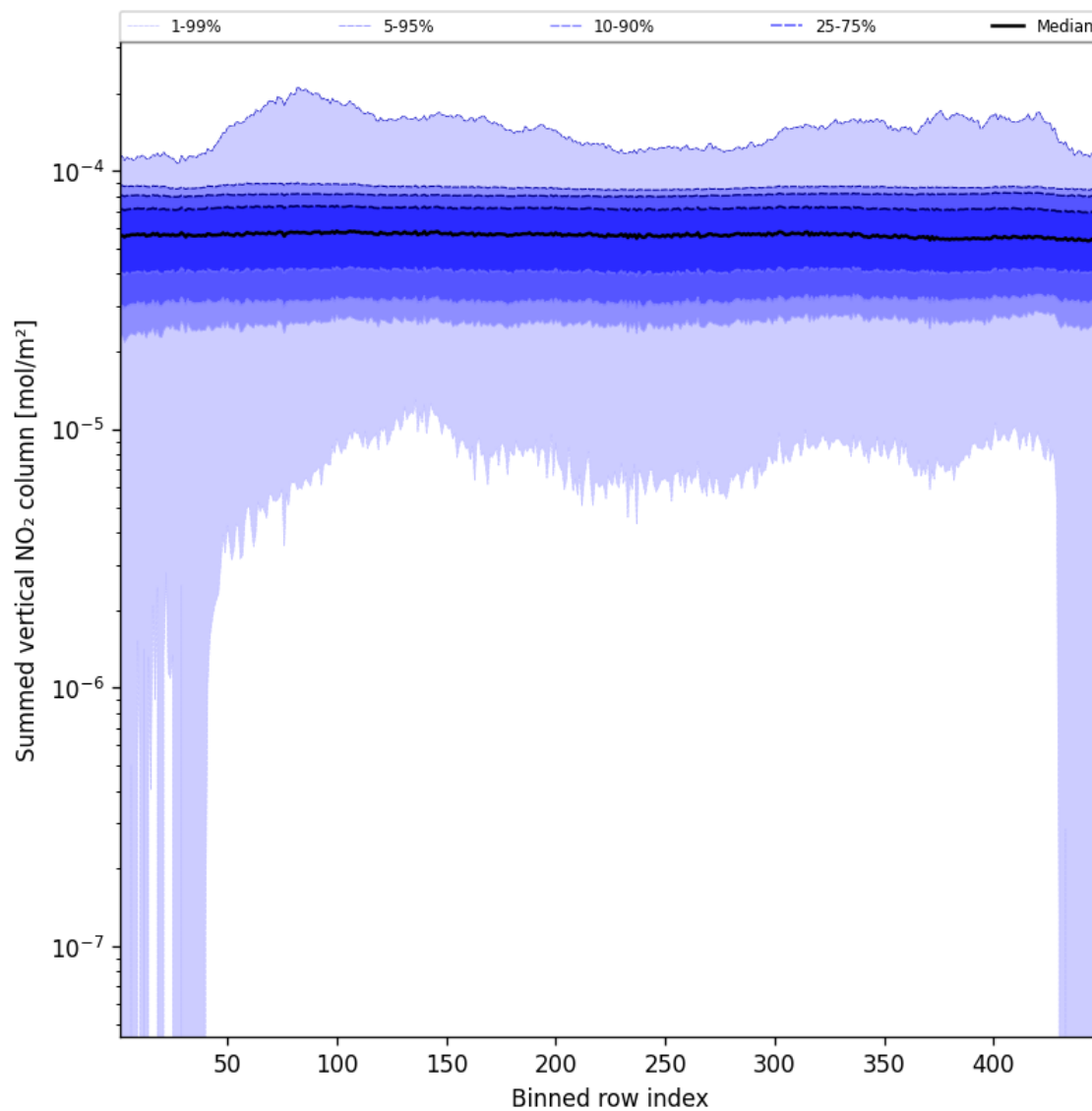
Figure 57: Along track statistics of “Summed vertical NO 2 column” for 2025-01-28 to 2025-01-29
