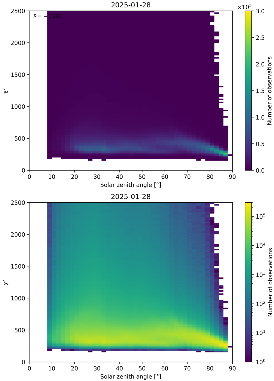
Figure 148: Scatter density plot of “Solar zenith angle” against “ \chi^2 ” for 2025-01-28 to 2025-01-29.
