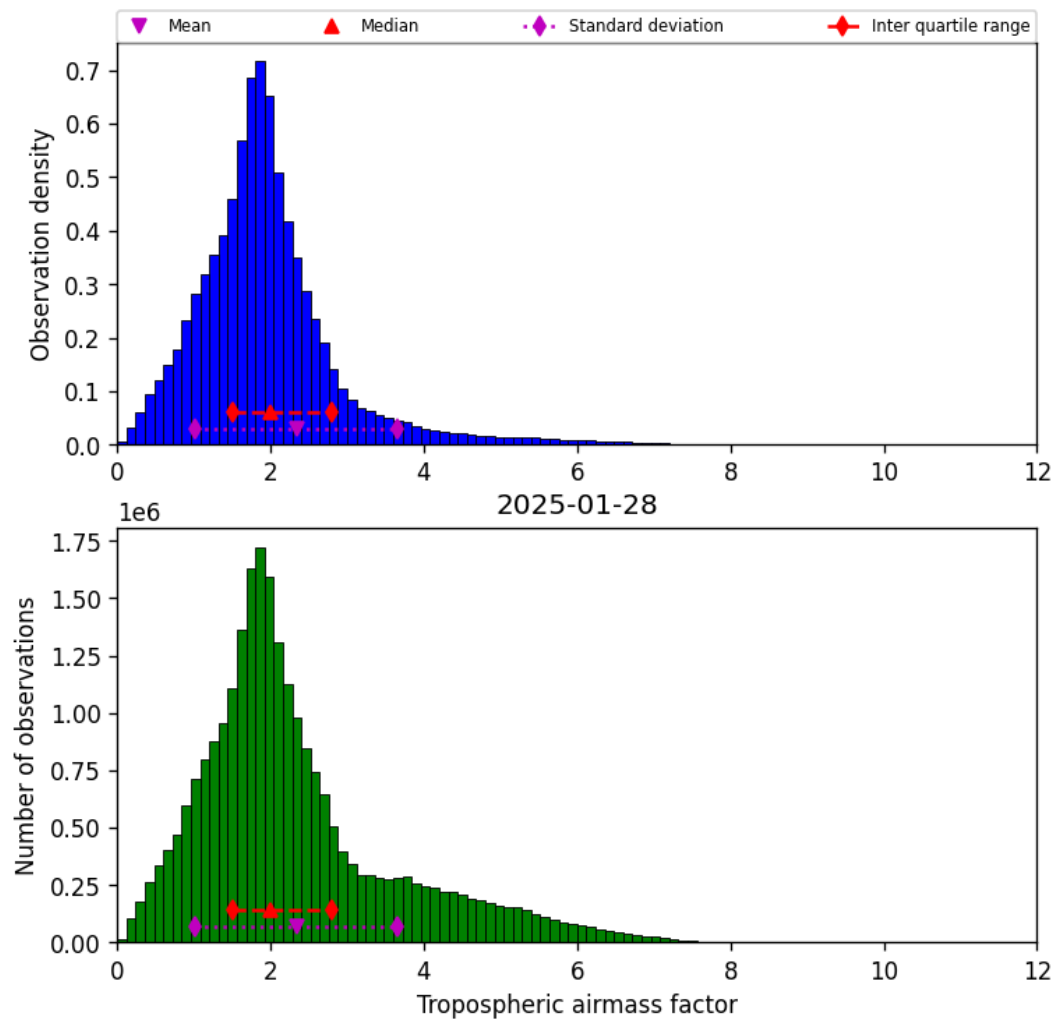
Figure 31: Histogram of “Tropospheric airmass factor” for 2025-01-28 to 2025-01-29
