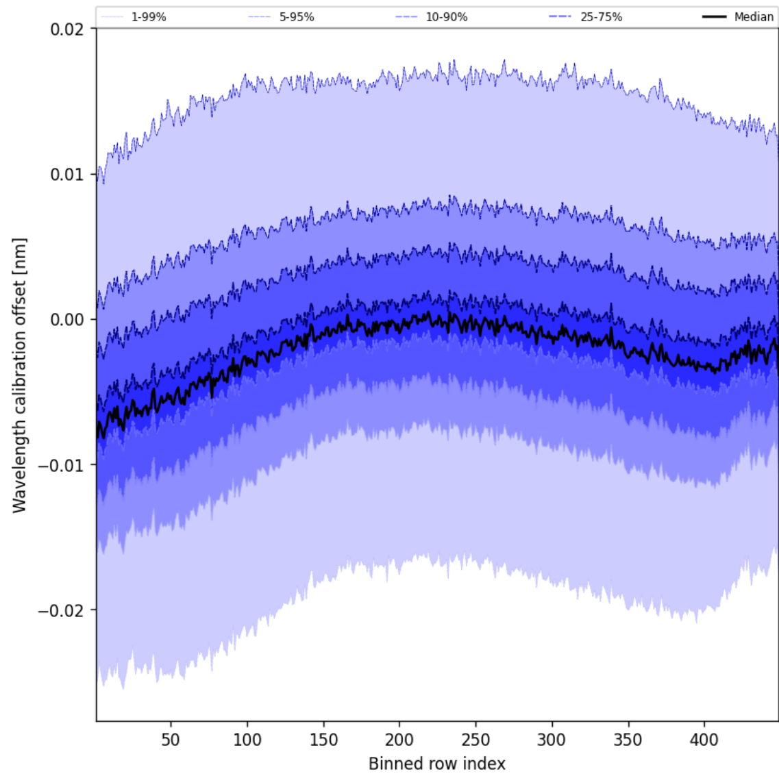
Figure 52: Along track statistics of “Wavelength calibration offset” for 2025-01-28 to 2025-01-29
