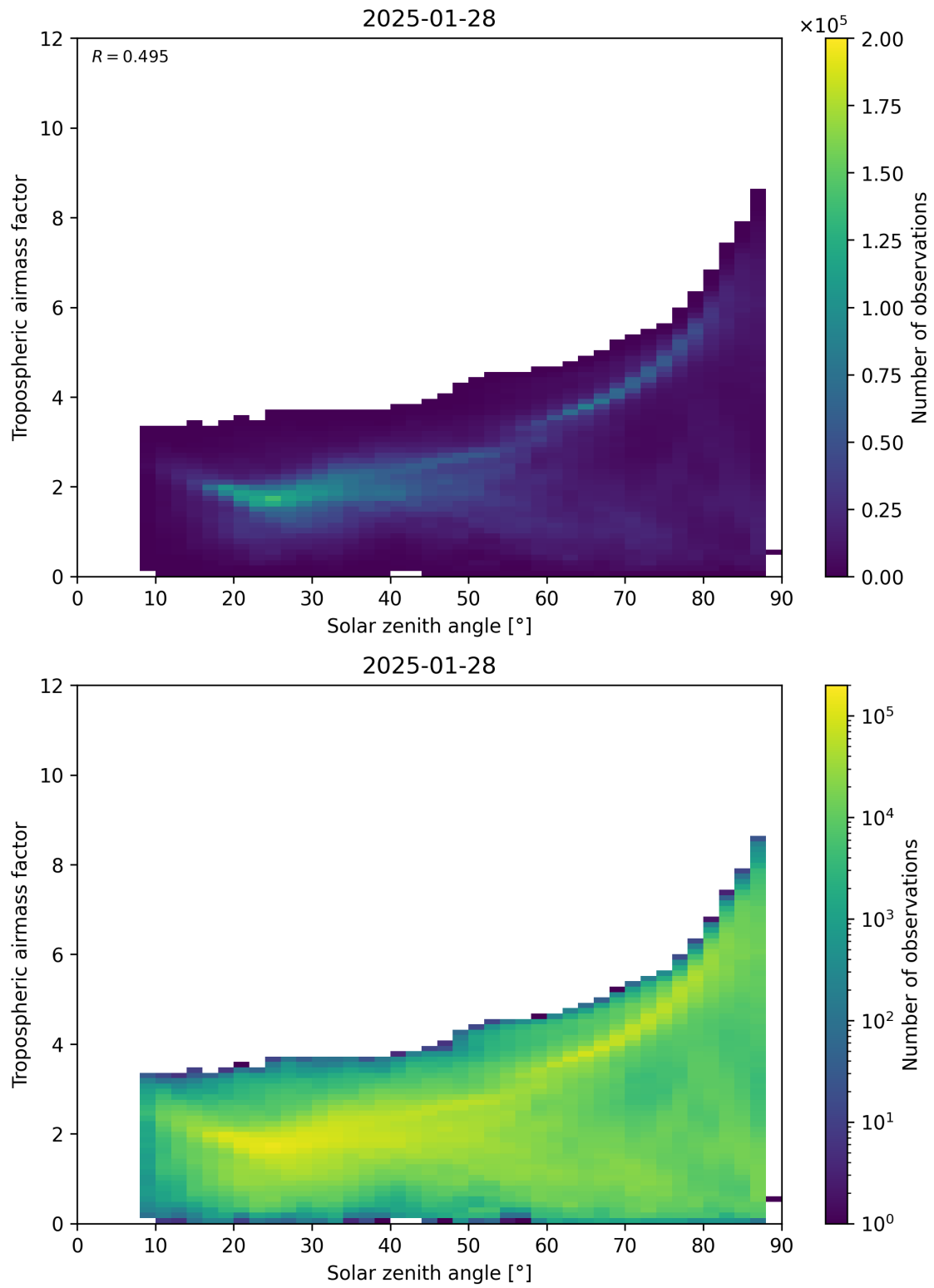
Figure 147: Scatter density plot of “Solar zenith angle” against “Tropospheric airmass factor” for 2025-01-28 to 2025-01-29.
