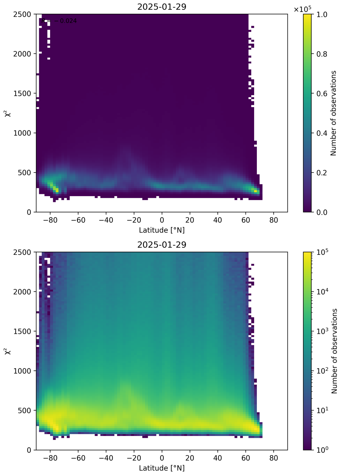
Figure 86: Scatter density plot of “Latitude” against “ \chi^2 ” for 2025-01-28 to 2025-01-30.
