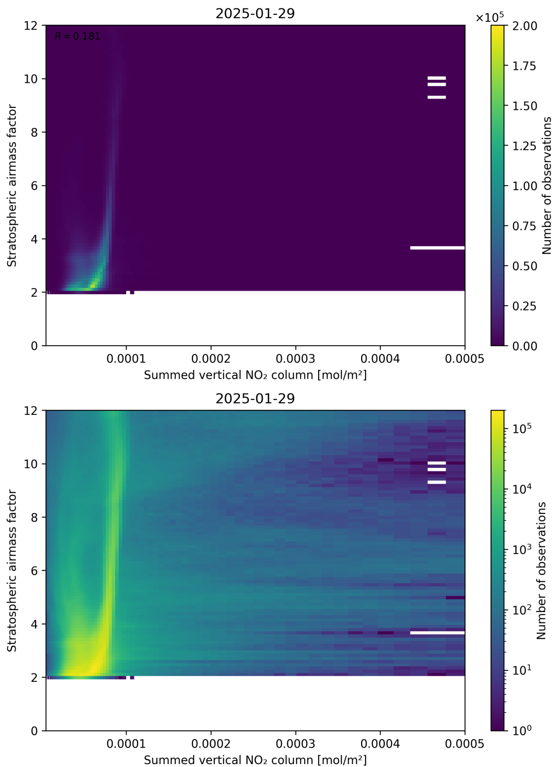
Figure 103: Scatter density plot of “Summed vertical NO 2 column” against “Stratospheric airmass factor” for 2025-01-28 to 2025-01-30.
