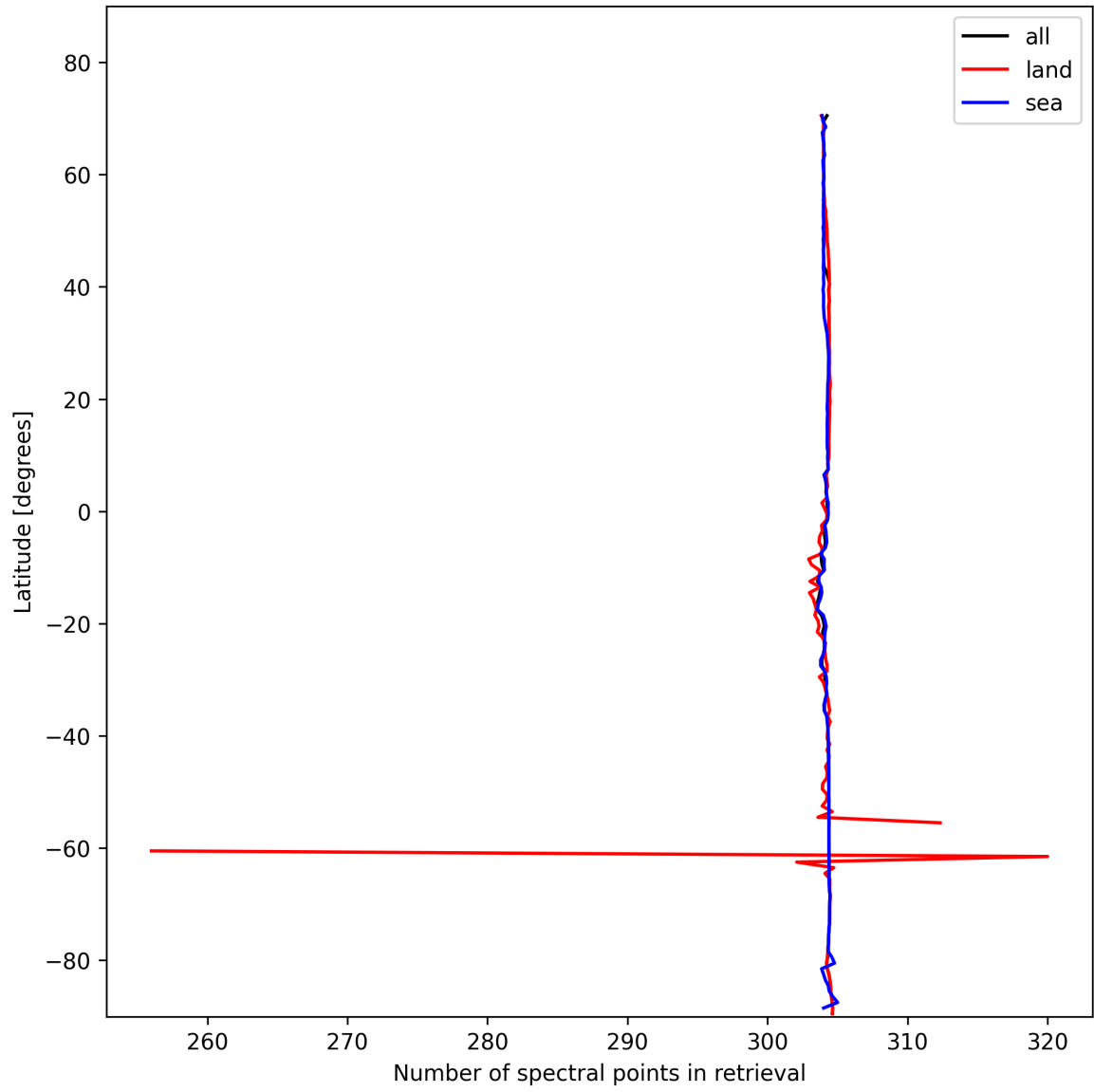
Figure 16: Zonal average of “Number of spectral points in retrieval” for 2025-01-28 to 2025-01-30.
