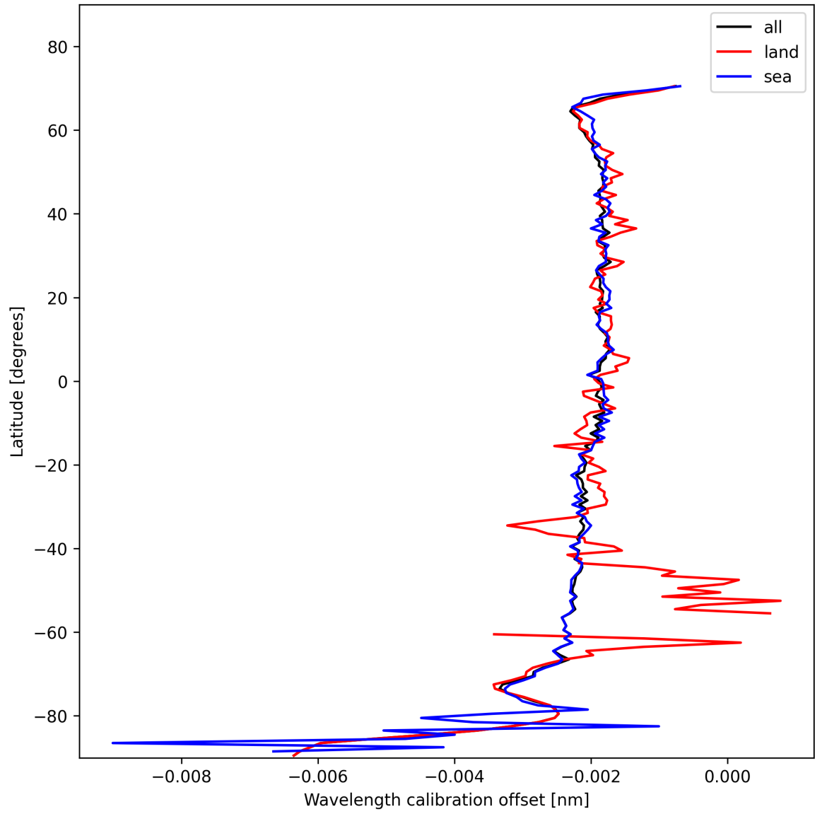
Figure 18: Zonal average of “Wavelength calibration offset” for 2025-01-28 to 2025-01-30.
