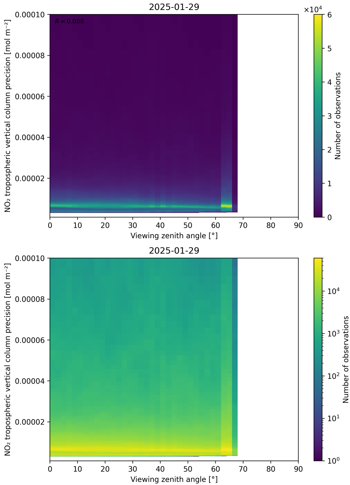
Figure 170: Scatter density plot of “Viewing zenith angle” against “NO 2 tropospheric vertical column precision” for 2025-01-28 to 2025-01-30.
