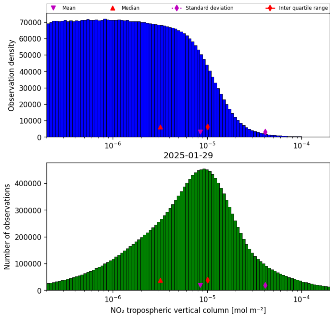
Figure 29: Histogram of “NO 2 tropospheric vertical column” for 2025-01-28 to 2025-01-30
