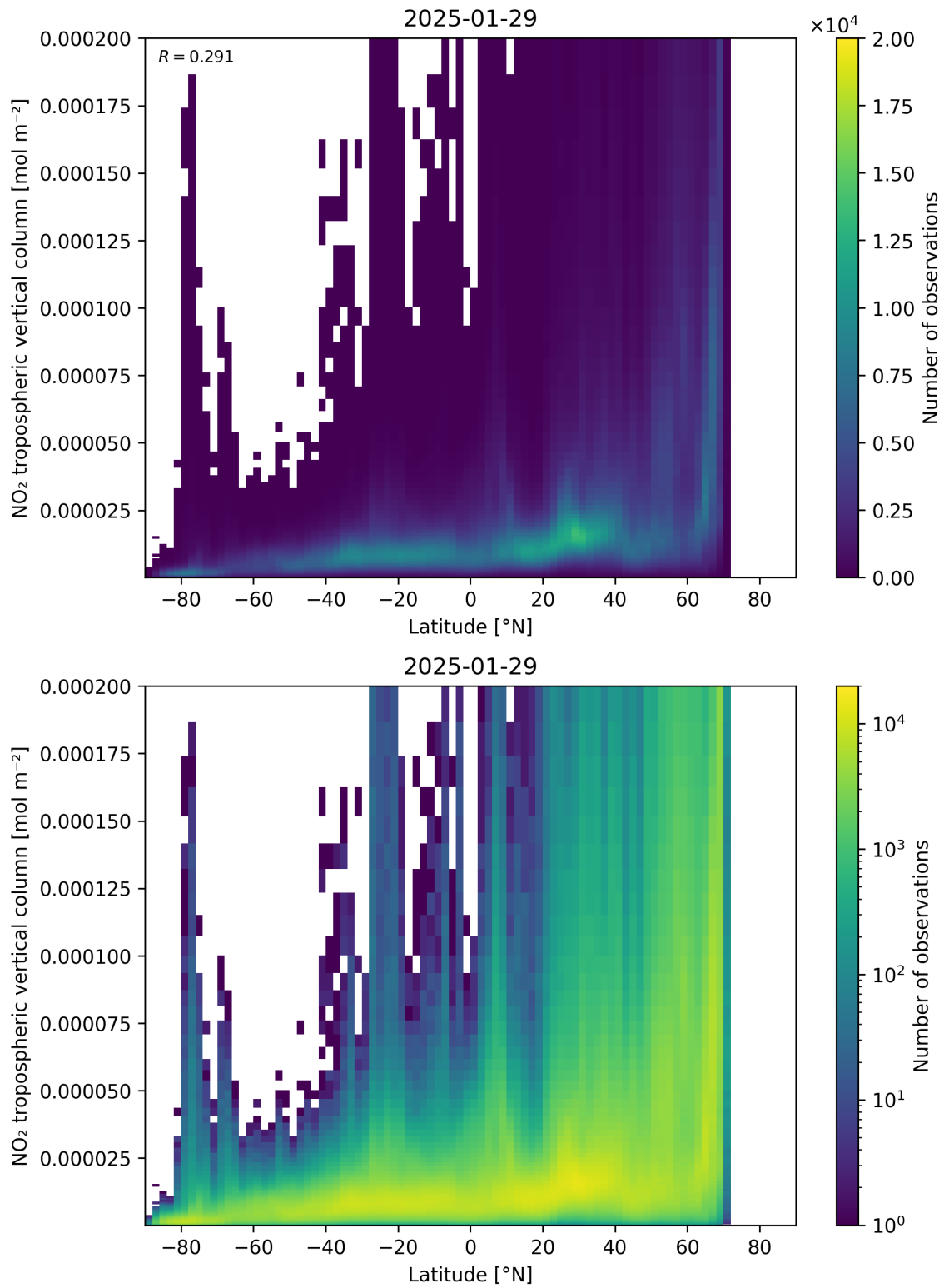
Figure 92: Scatter density plot of “Latitude” against “NO 2 tropospheric vertical column” for 2025-01-28 to 2025-01-30.
