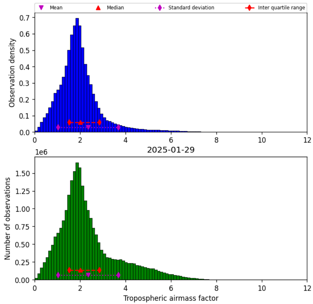
Figure 31: Histogram of “Tropospheric airmass factor” for 2025-01-28 to 2025-01-30
