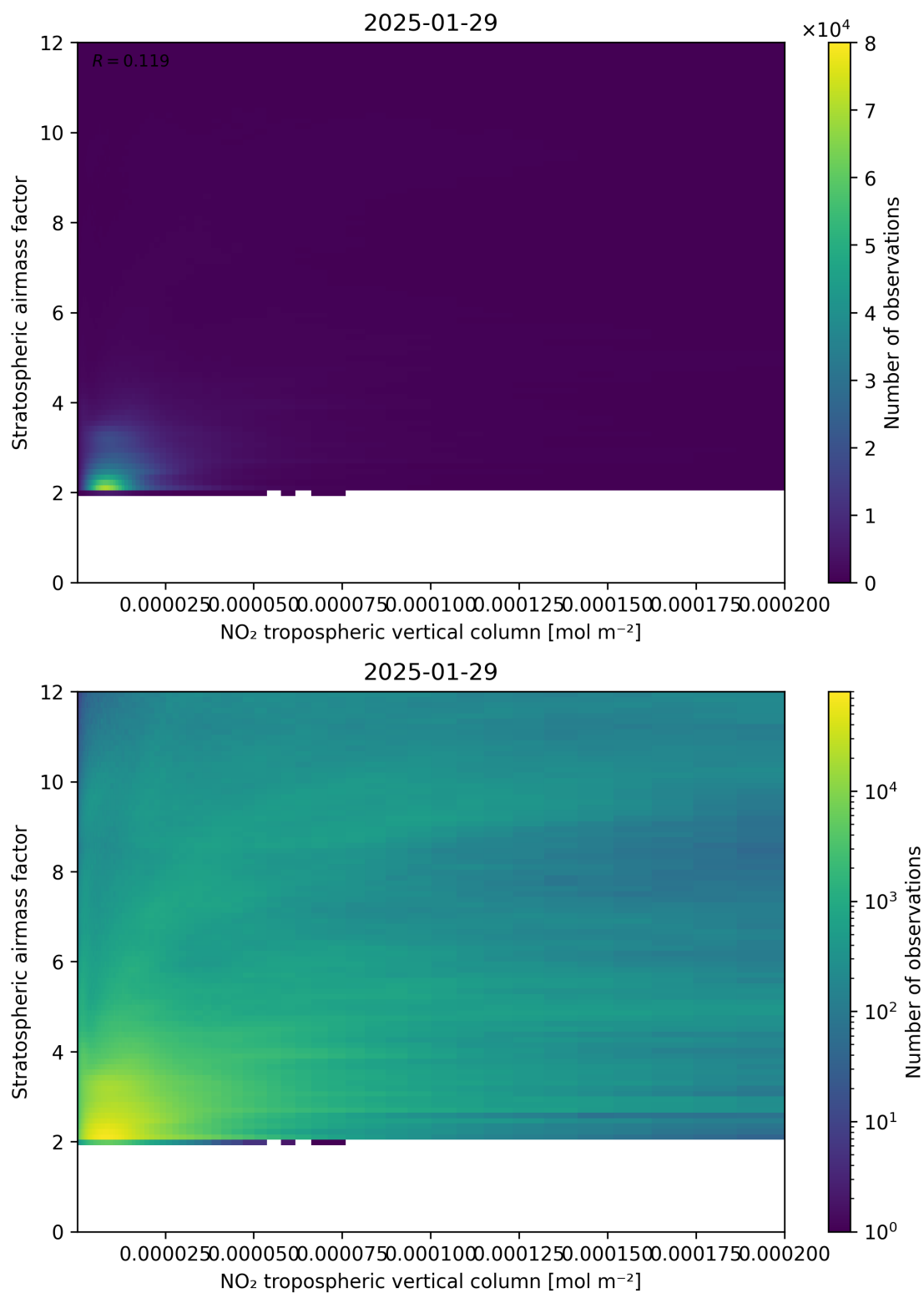
Figure 121: Scatter density plot of “NO 2 tropospheric vertical column” against “Stratospheric airmass factor” for 2025-01-28 to 2025-01-30.
