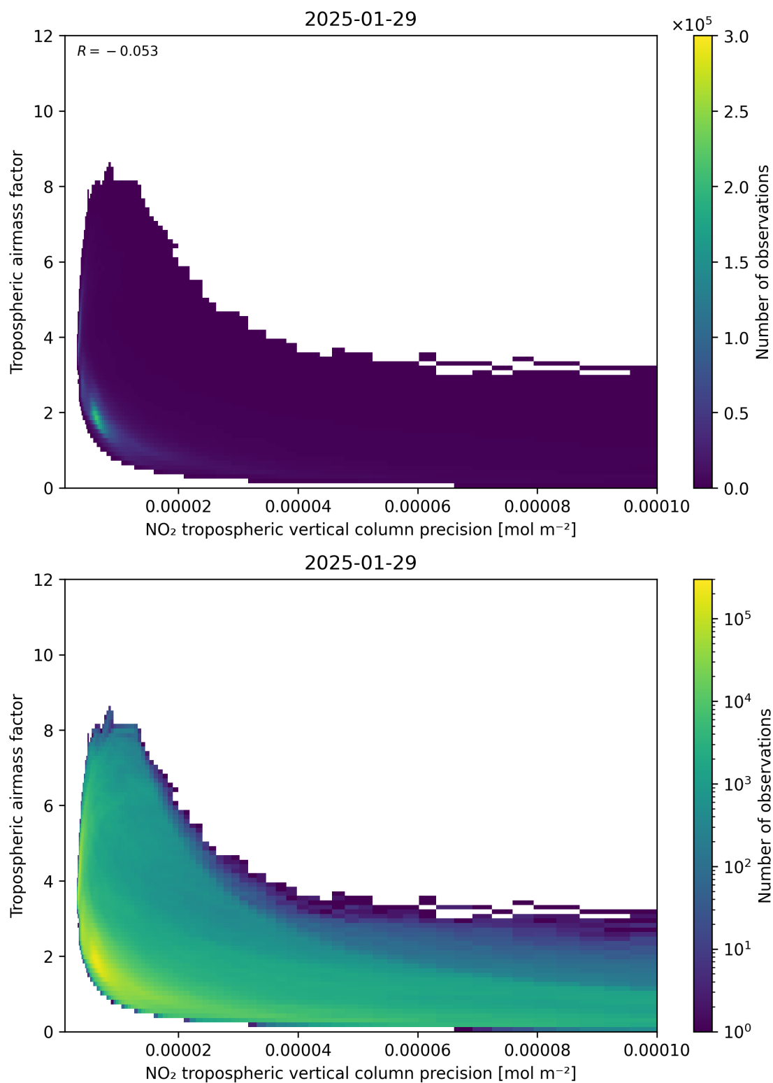
Figure 133: Scatter density plot of “NO 2 tropospheric vertical column precision” against “Tropospheric airmass factor” for 2025-01-28 to 2025-01-30.
