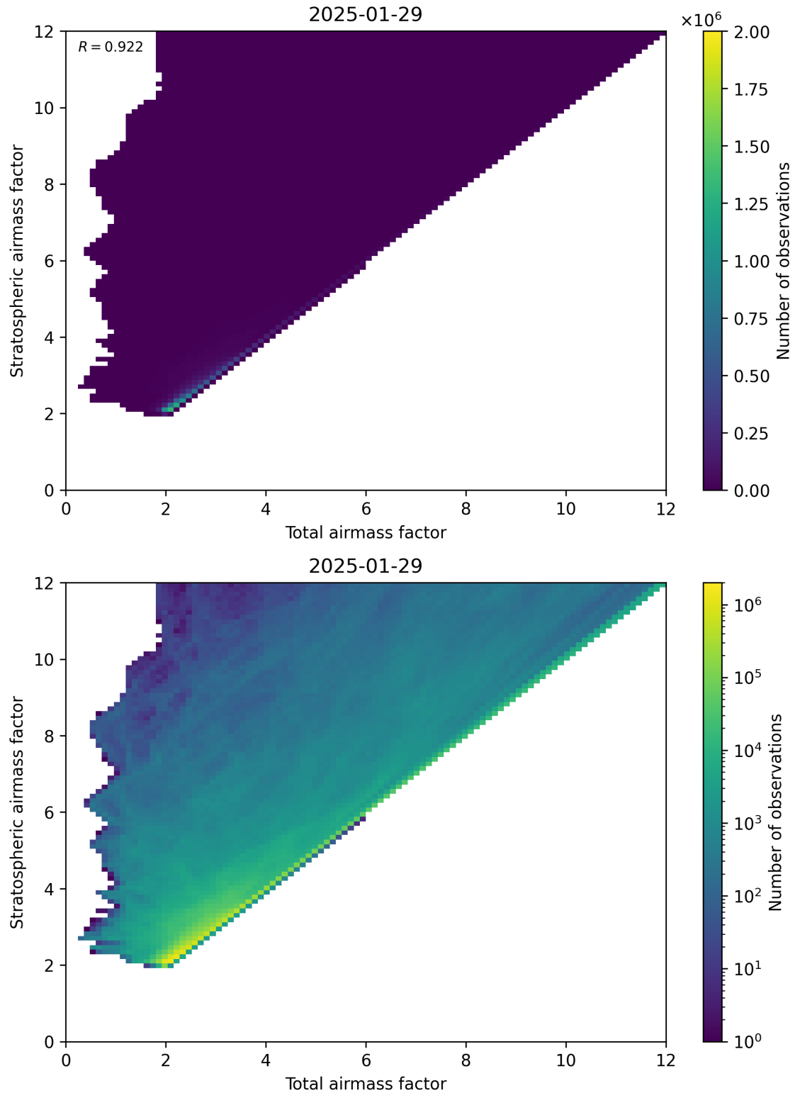
Figure 62: Scatter density plot of “Total air mass factor” against “Stratospheric air mass factor” for 2025-01-28 to 2025-01-30.
