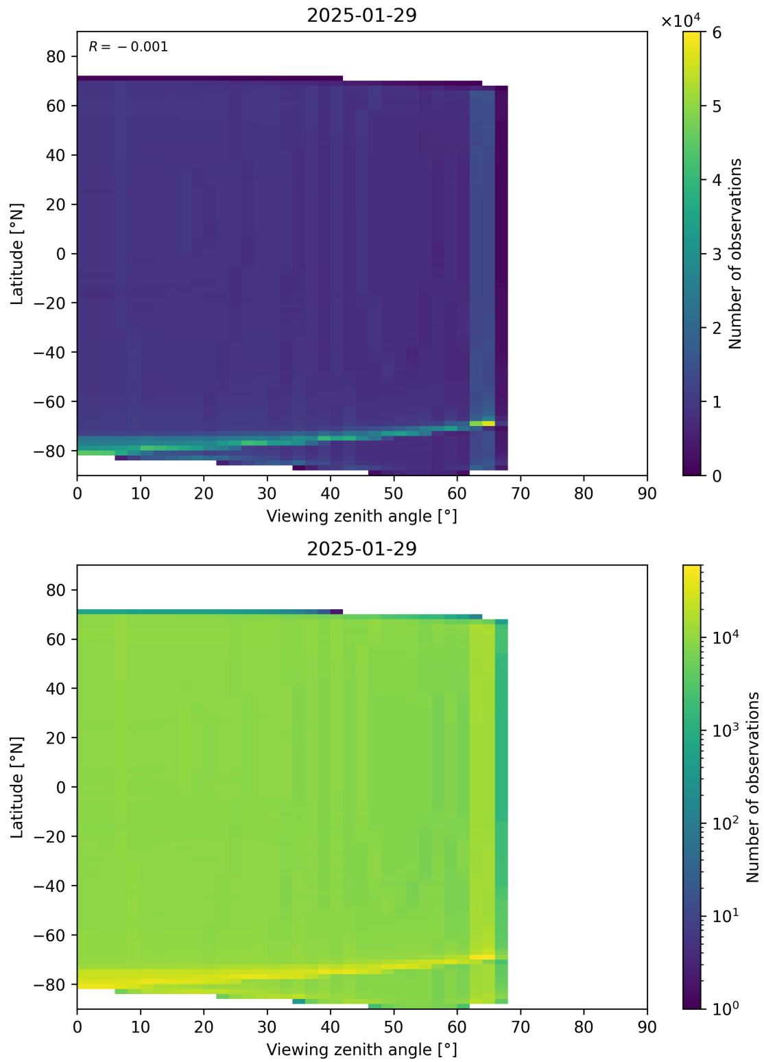
Figure 163: Scatter density plot of “Viewing zenith angle” against “Latitude” for 2025-01-28 to 2025-01-30.
