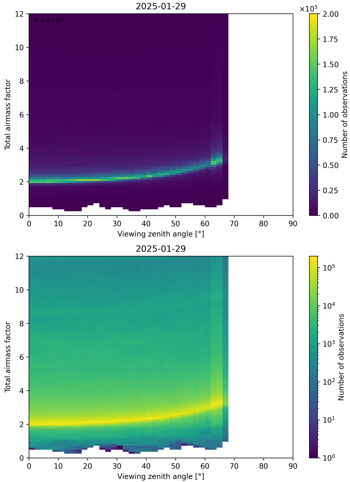
Figure 160: Scatter density plot of “Viewing zenith angle” against “Total airmass factor” for 2025-01-28 to 2025-01-30.
