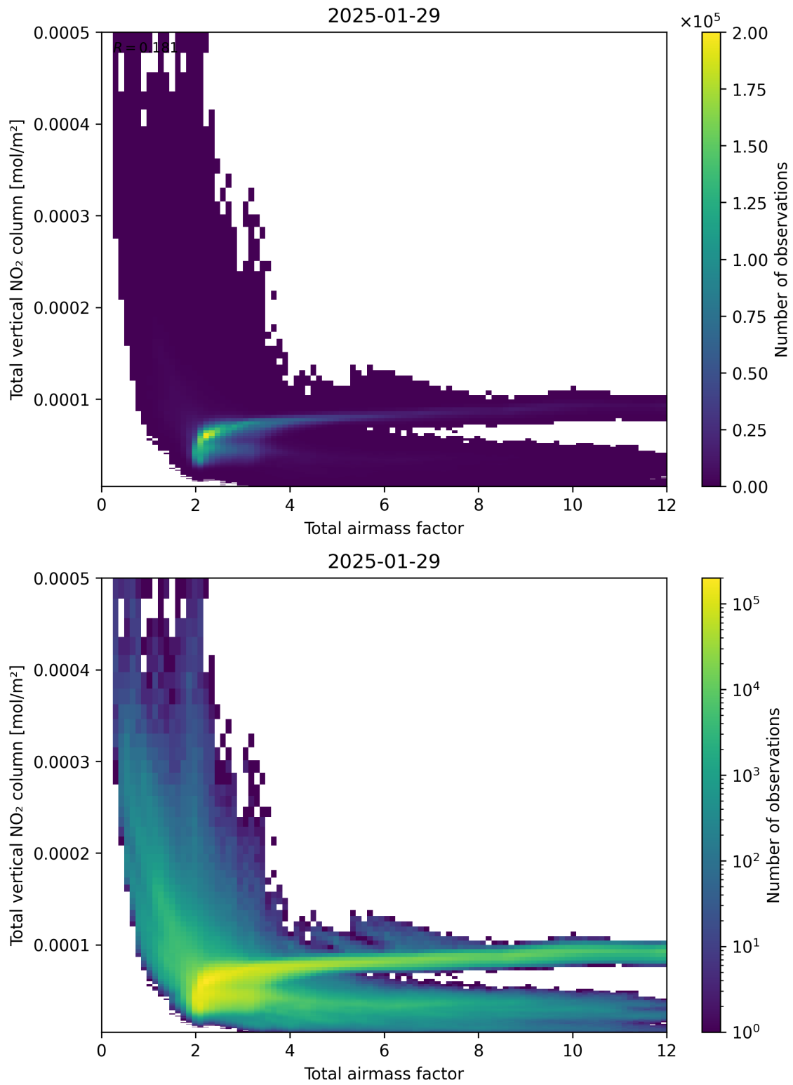
Figure 67: Scatter density plot of “Total airmass factor” against “Total vertical NO 2 column” for 2025-01-28 to 2025-01-30.
