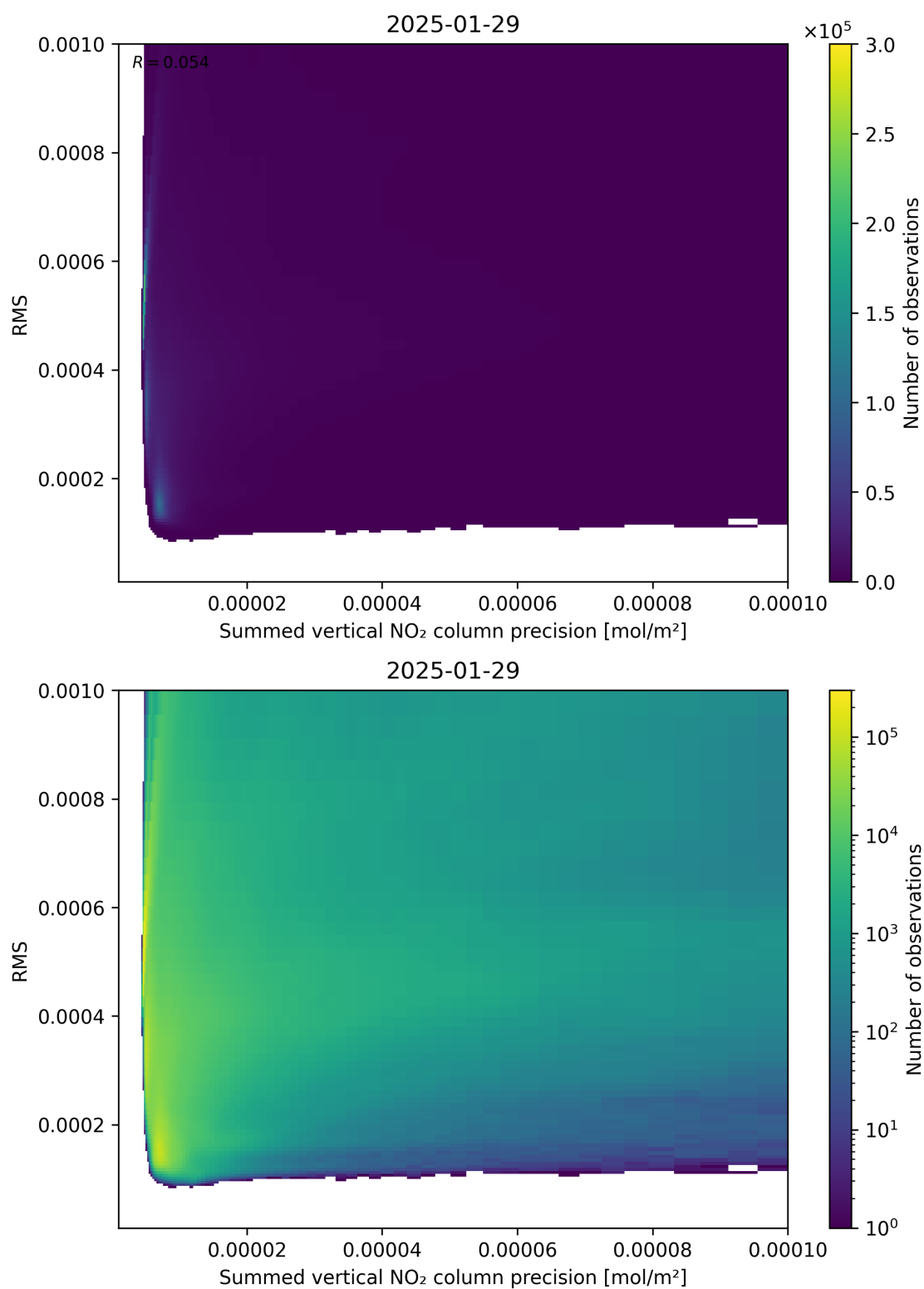
Figure 108: Scatter density plot of “Summed vertical NO 2 column precision” against “RMS” for 2025-01-28 to 2025-01-30.
