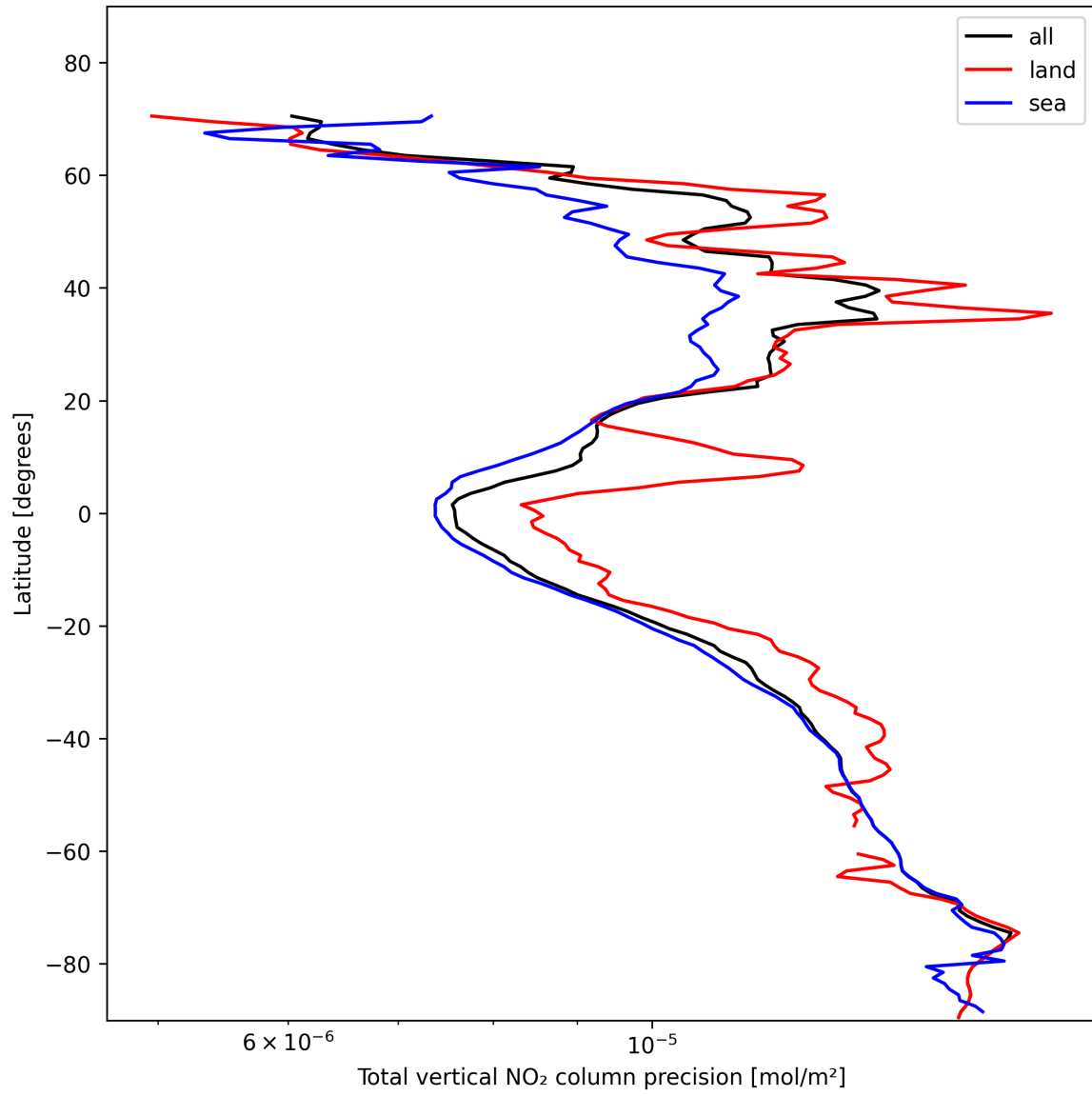
Figure 22: Zonal average of “Total vertical NO 2 column precision” for 2025-01-28 to 2025-01-30.
