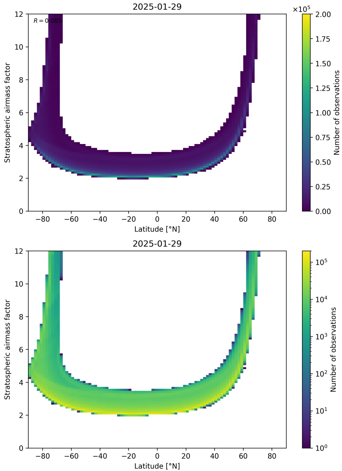
Figure 83: Scatter density plot of “Latitude” against “Stratospheric airmass factor” for 2025-01-28 to 2025-01-30.
