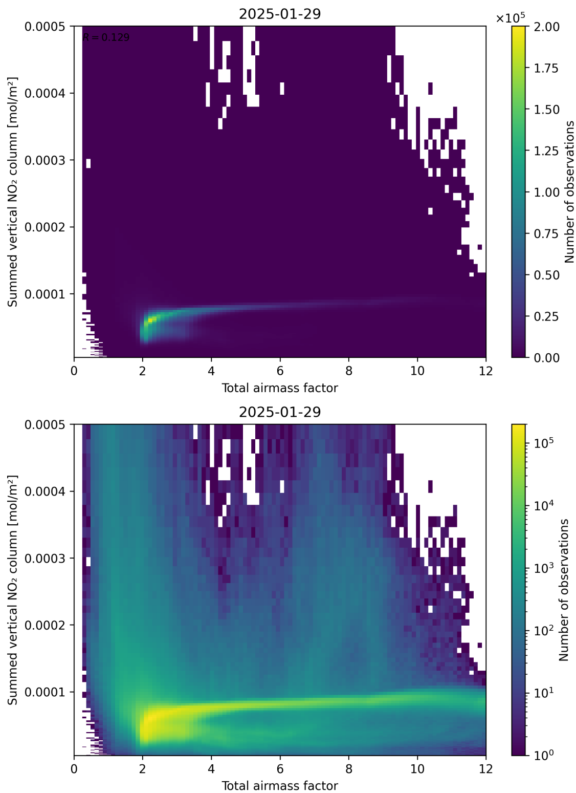
Figure 65: Scatter density plot of “Total airmass factor” against “Summed vertical NO 2 column” for 2025-01-28 to 2025-01-30.
