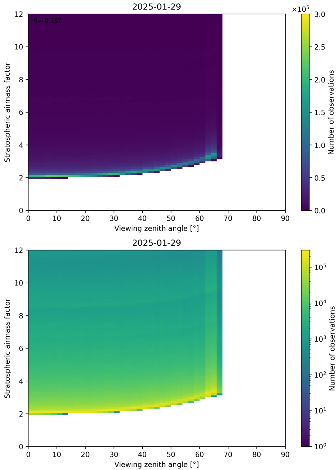
Figure 159: Scatter density plot of “Viewing zenith angle” against “Stratospheric airmass factor” for 2025-01-28 to 2025-01-30.
