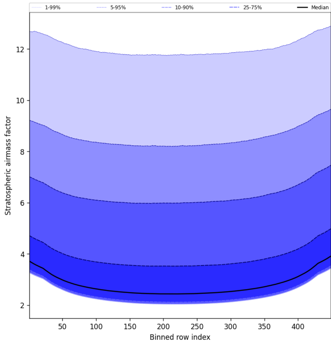
Figure 61: Along track statistics of “Stratospheric airmass factor” for 2025-01-28 to 2025-01-30
