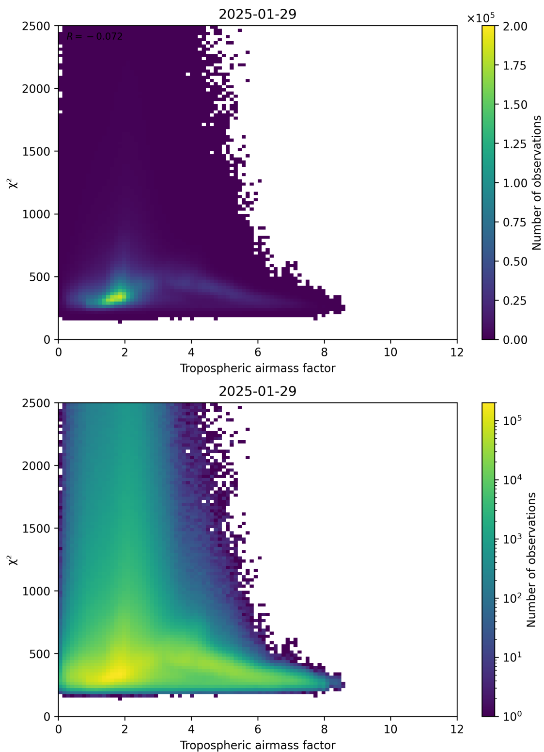
Figure 73: Scatter density plot of “Tropospheric airmass factor” against “ \chi^2 ” for 2025-01-28 to 2025-01-30.
