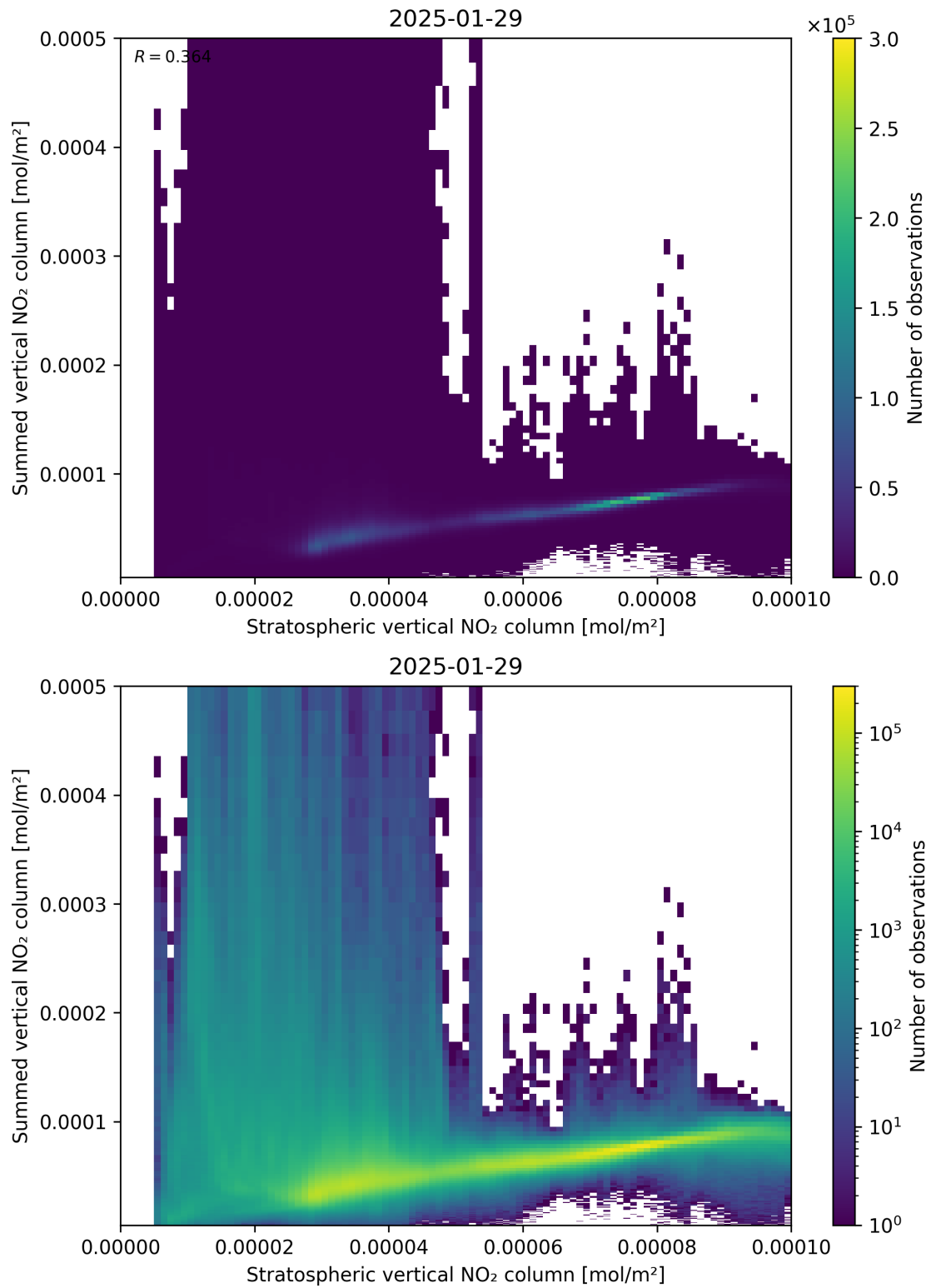
Figure 98: Scatter density plot of “Stratospheric vertical NO 2 column” against “Summed vertical NO 2 column” for 2025-01-28 to 2025-01-30.
