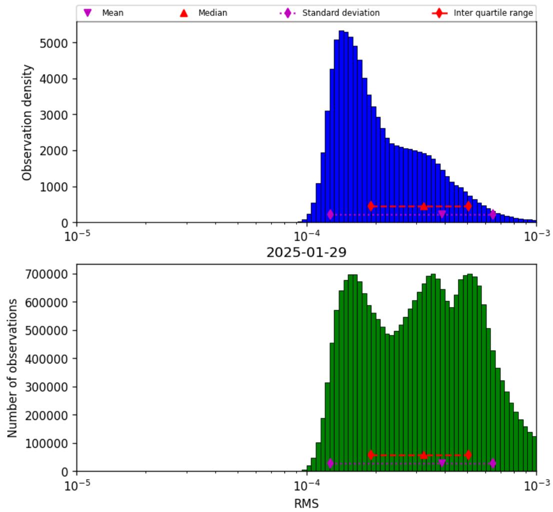
Figure 43: Histogram of “RMS” for 2025-01-28 to 2025-01-30
