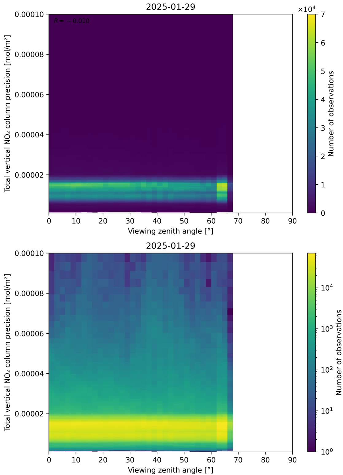
Figure 168: Scatter density plot of “Viewing zenith angle” against “Total vertical NO 2 column precision” for 2025-01-28 to 2025-01-30.
