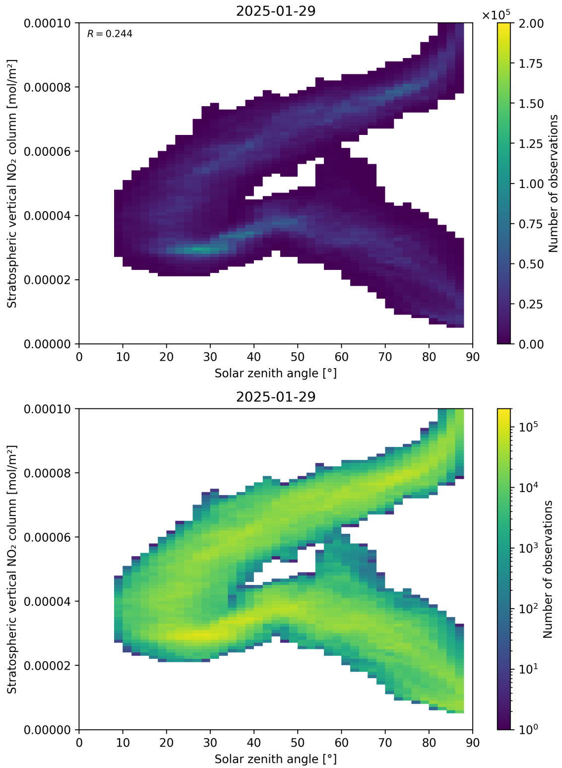
Figure 150: Scatter density plot of “Solar zenith angle” against “Stratospheric vertical NO 2 column” for 2025-01-28 to 2025-01-30.
