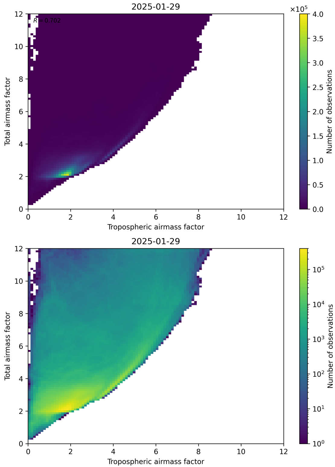
Figure 72: Scatter density plot of “Tropospheric airmass factor” against “Total airmass factor” for 2025-01-28 to 2025-01-30.
