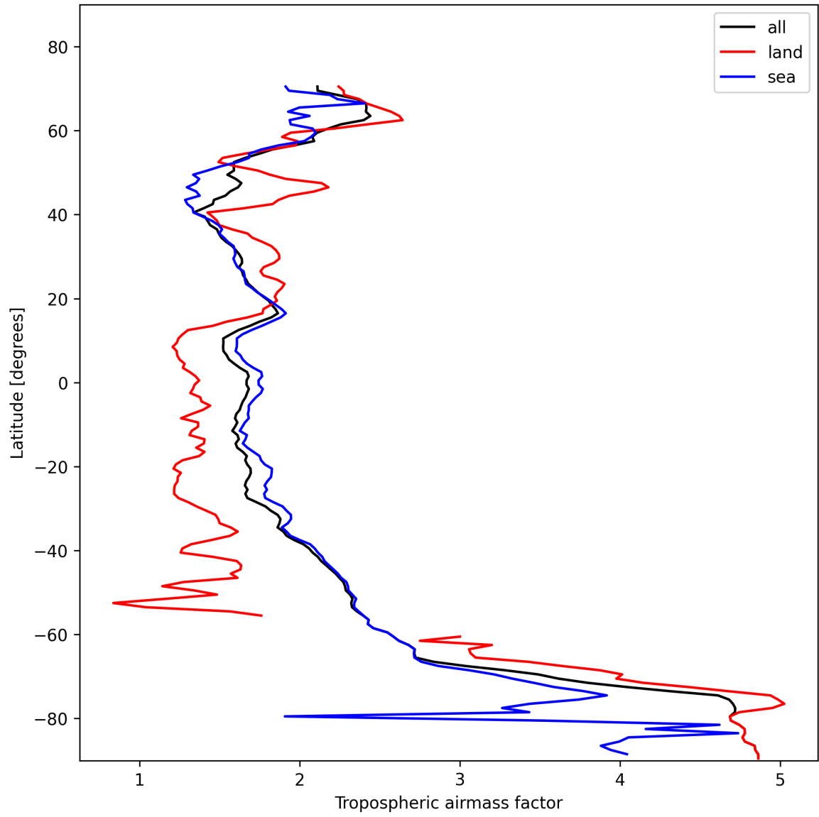
Figure 14: Zonal average of “Tropospheric air mass factor” for 2025-01-28 to 2025-01-30.
