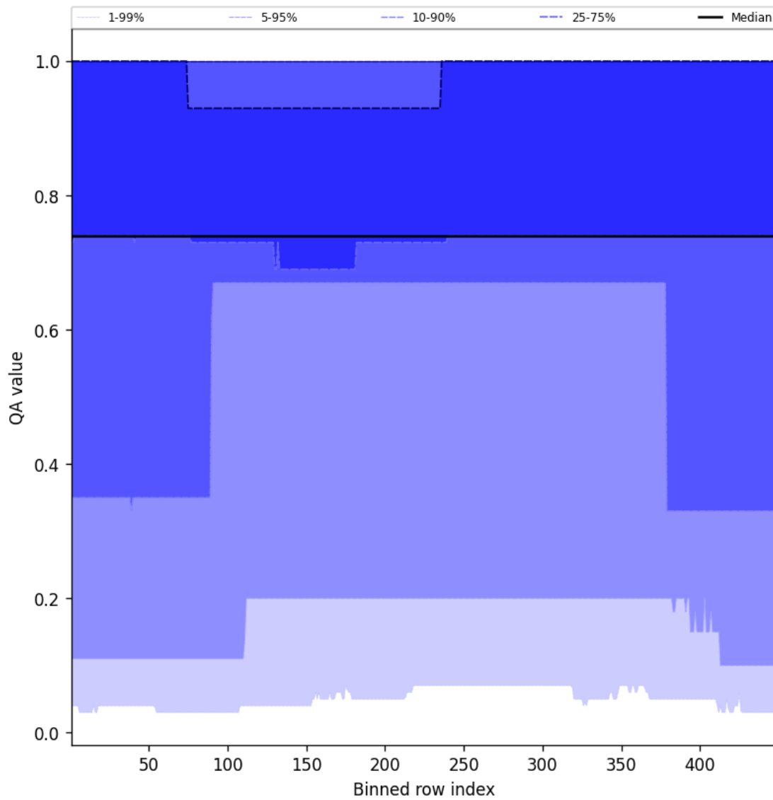
Figure 45: Along track statistics of “QA value” for 2025-01-28 to 2025-01-30
