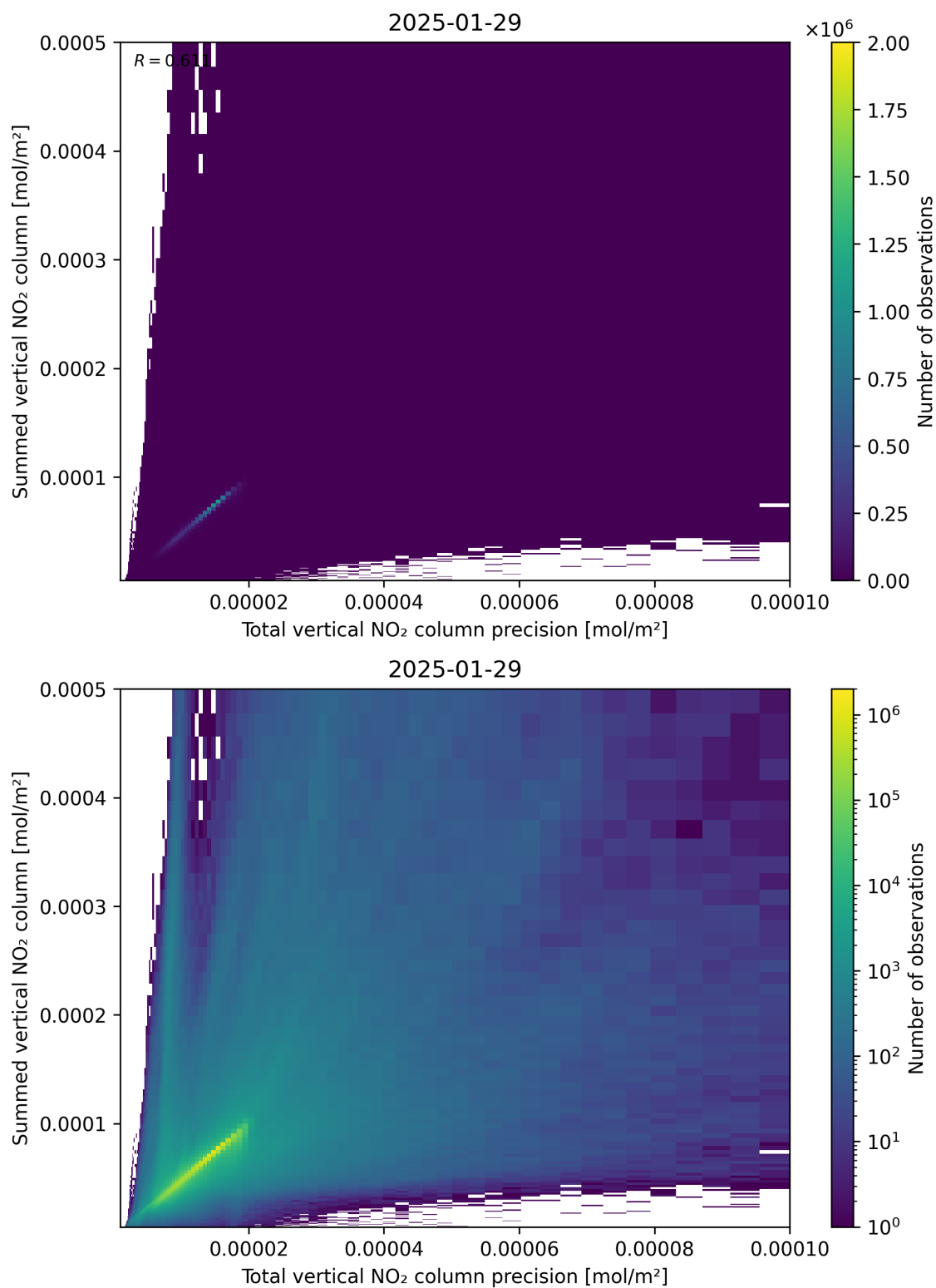
Figure 117: Scatter density plot of “Total vertical NO 2 column precision” against “Summed vertical NO 2 column” for 2025-01-28 to 2025-01-30.
