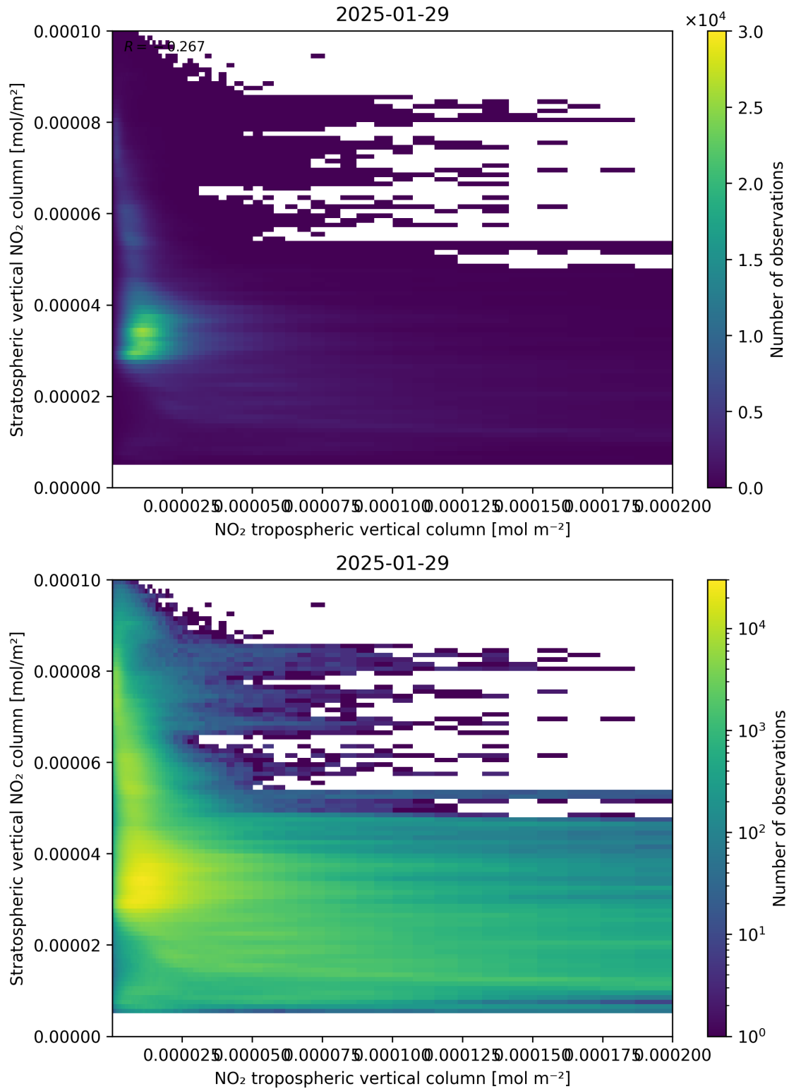
Figure 125: Scatter density plot of “NO 2 tropospheric vertical column” against “Stratospheric vertical NO 2 column” for 2025-01-28 to 2025-01-30.
