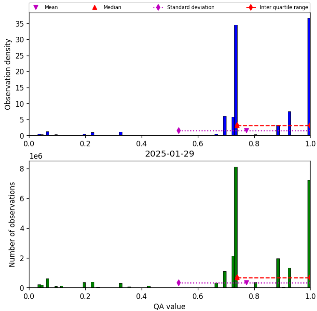
Figure 28: Histogram of “QA value” for 2025-01-28 to 2025-01-30
