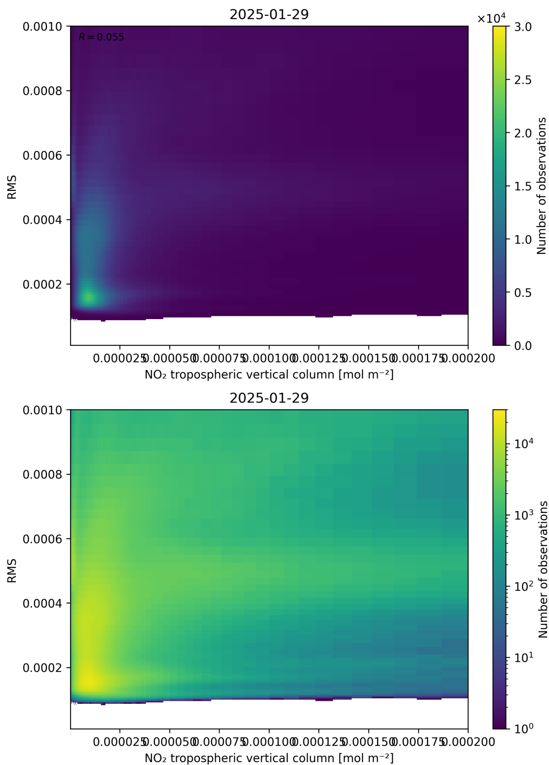
Figure 142: Scatter density plot of “NO 2 tropospheric vertical column” against “RMS” for 2025-01-28 to 2025-01-30.
