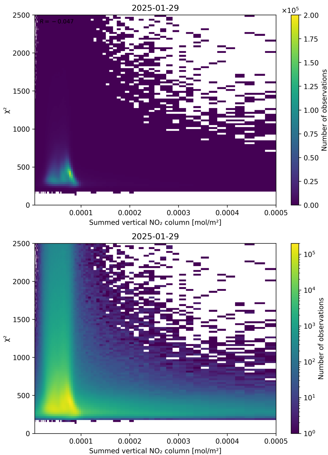
Figure 104: Scatter density plot of “Summed vertical NO 2 column” against “ \chi^2 ” for 2025-01-28 to 2025-01-30.
