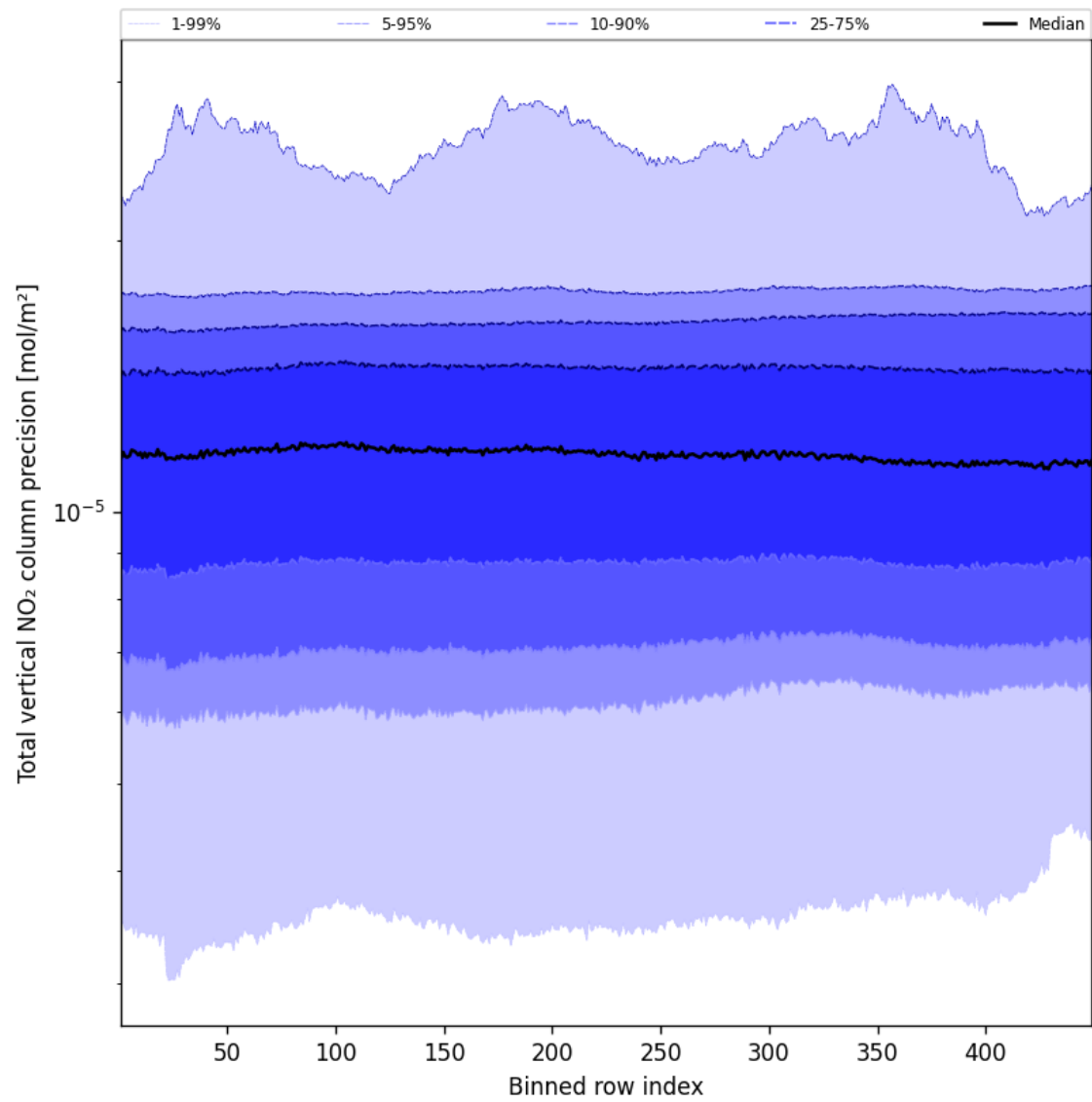
Figure 56: Along track statistics of “Total vertical NO 2 column precision” for 2025-01-28 to 2025-01-30
