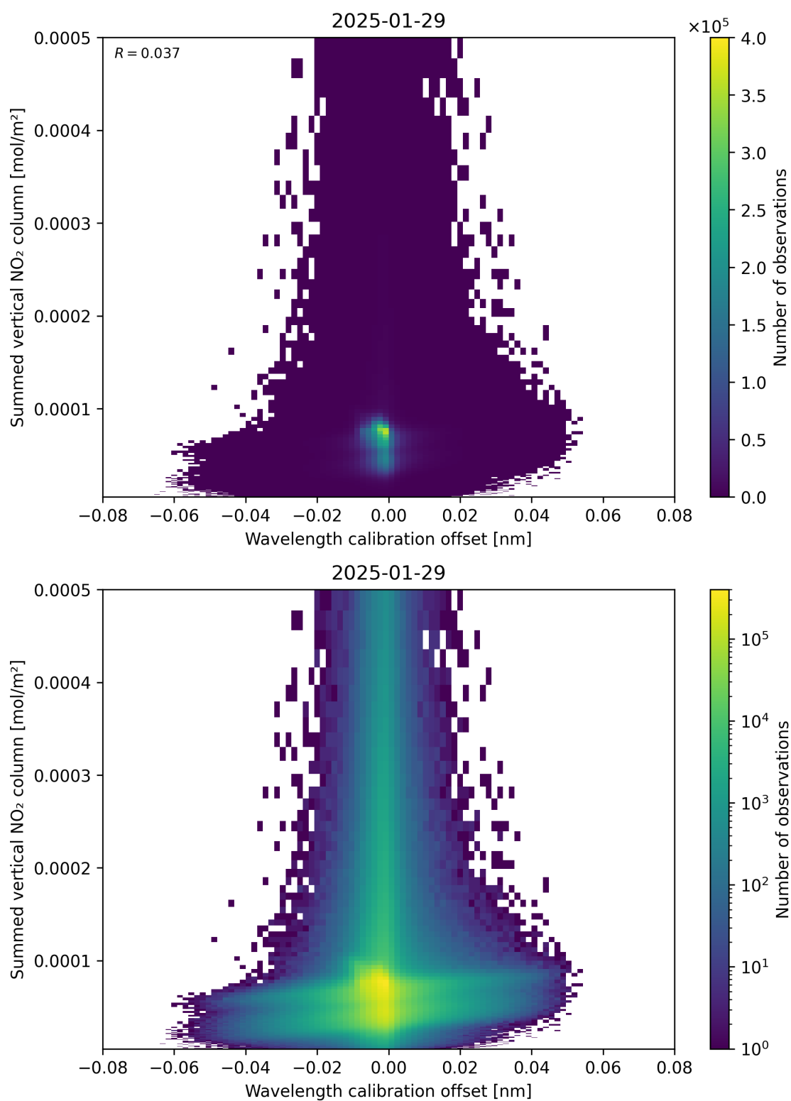
Figure 177: Scatter density plot of “Wavelength calibration offset” against “Summed vertical NO 2 column” for 2025-01-28 to 2025-01-30.
