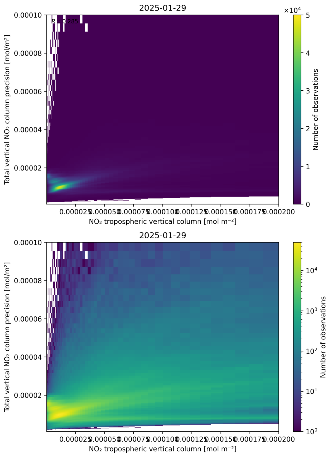
Figure 129: Scatter density plot of “NO 2 tropospheric vertical column” against “Total vertical NO 2 column precision” for 2025-01-28 to 2025-01-30.
