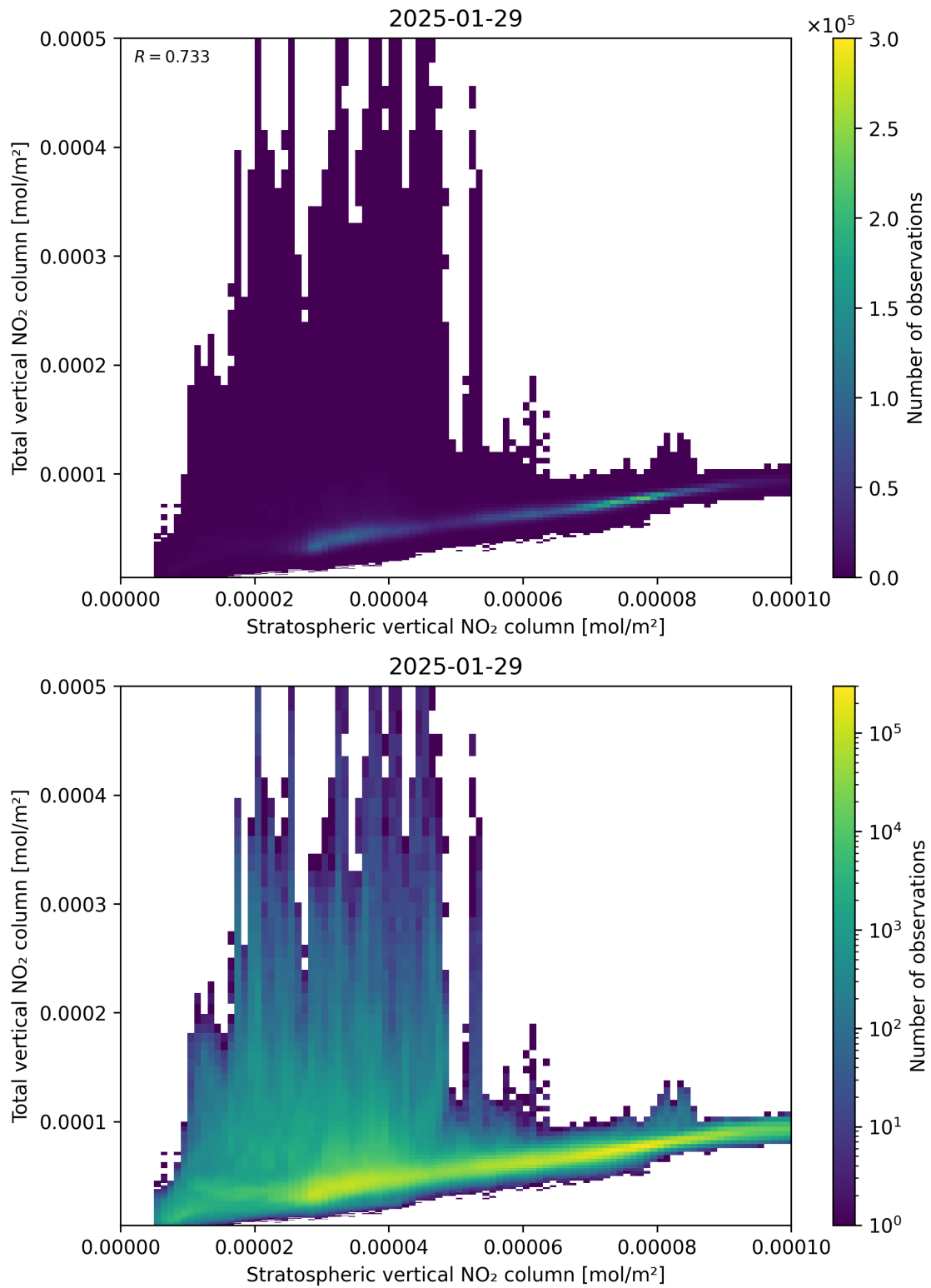
Figure 100: Scatter density plot of “Stratospheric vertical NO 2 column” against “Total vertical NO 2 column” for 2025-01-28 to 2025-01-30.
