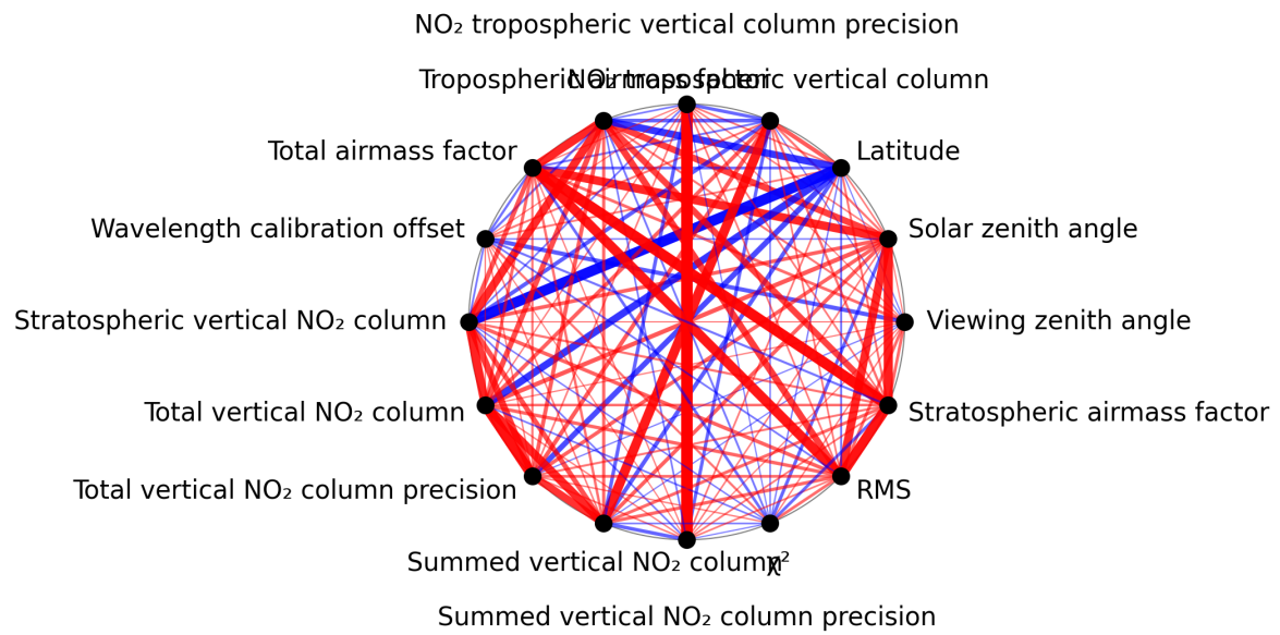
Figure 1: Map of correlation graph for 2025-01-28 to 2025-01-30.
