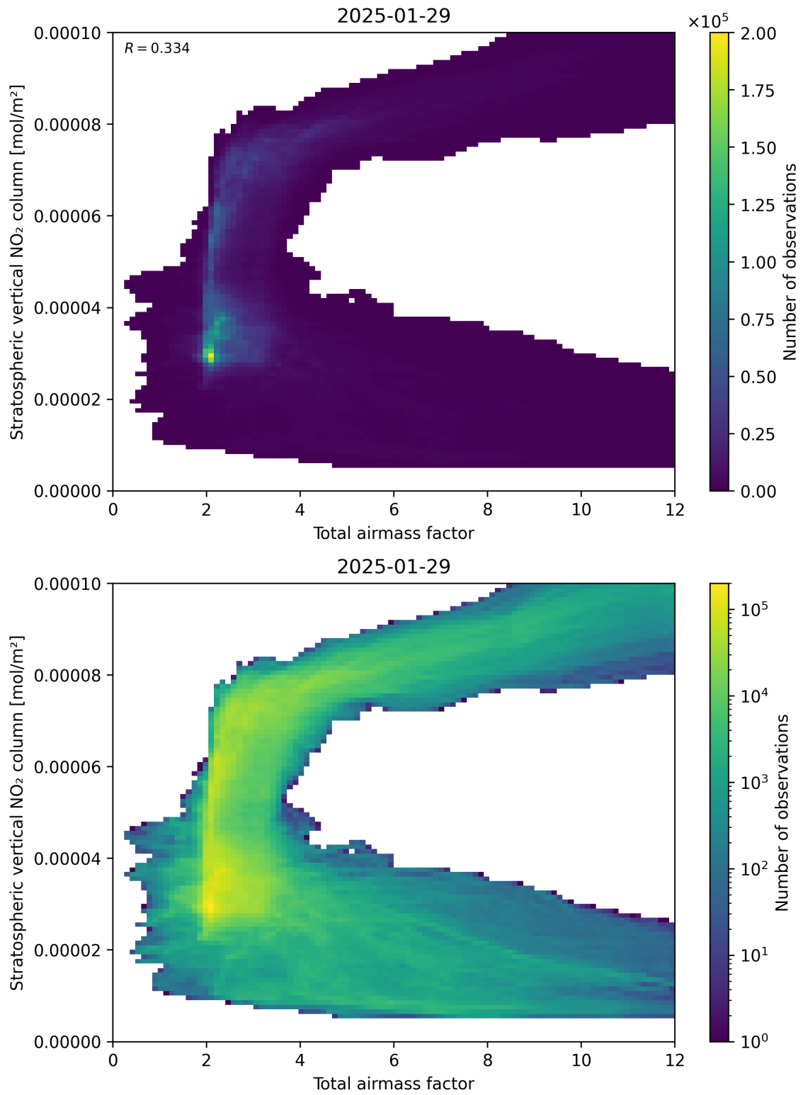
Figure 64: Scatter density plot of “Total airmass factor” against “Stratospheric vertical NO 2 column” for 2025-01-28 to 2025-01-30.
