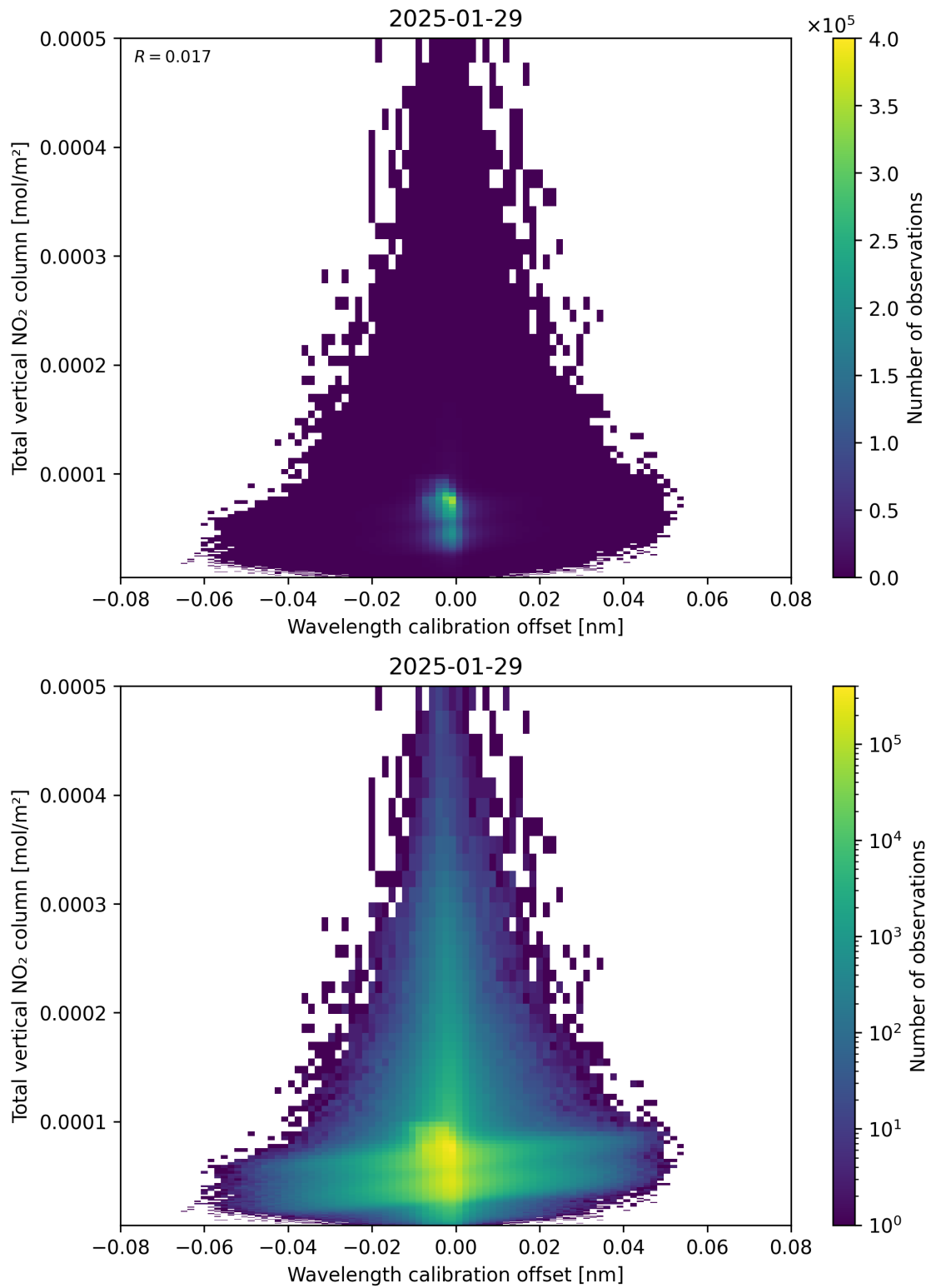
Figure 179: Scatter density plot of “Wavelength calibration offset” against “Total vertical NO 2 column” for 2025-01-28 to 2025-01-30.
