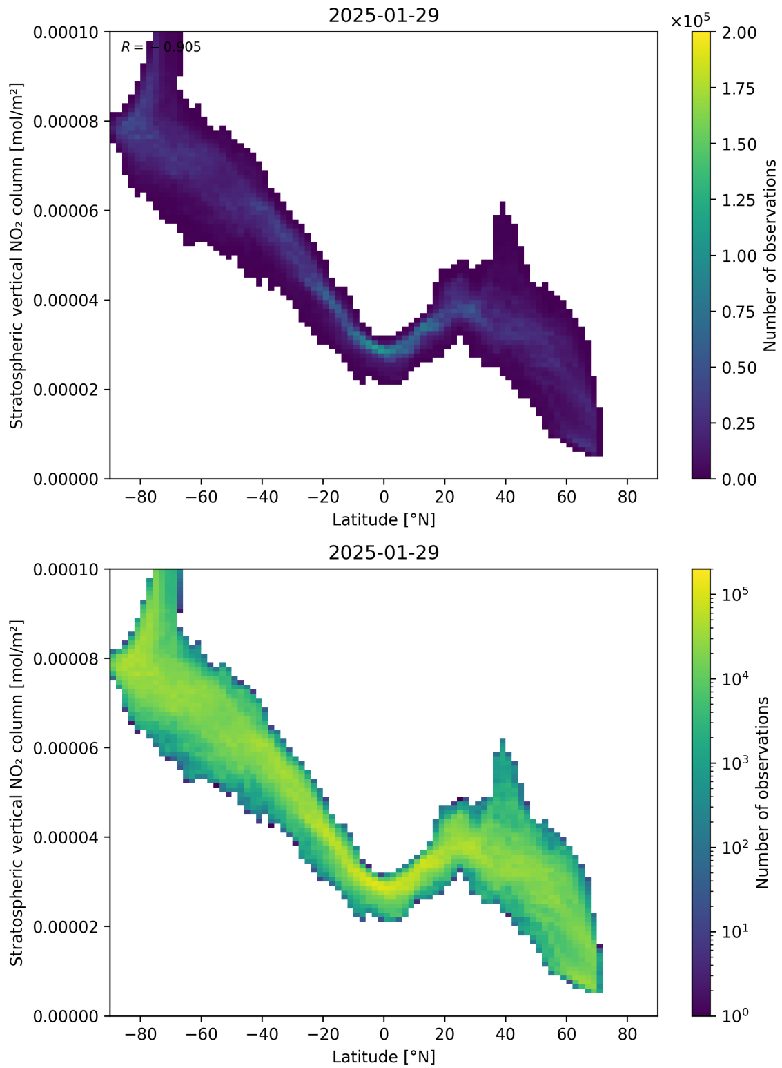
Figure 87: Scatter density plot of “Latitude” against “Stratospheric vertical NO 2 column” for 2025-01-28 to 2025-01-30.
