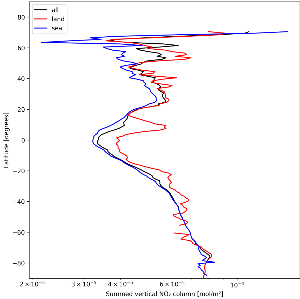
Figure 23: Zonal average of “Summed vertical NO 2 column” for 2025-01-28 to 2025-01-30.
