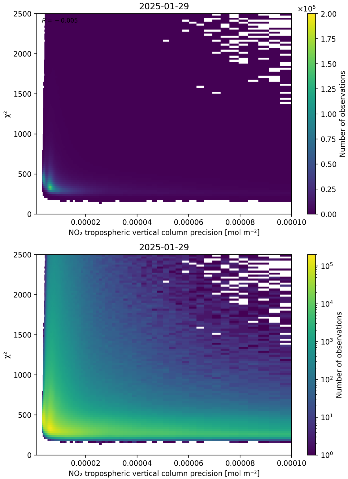
Figure 134: Scatter density plot of “NO 2 tropospheric vertical column precision” against “ \chi^2 ” for 2025-01-28 to 2025-01-30.
