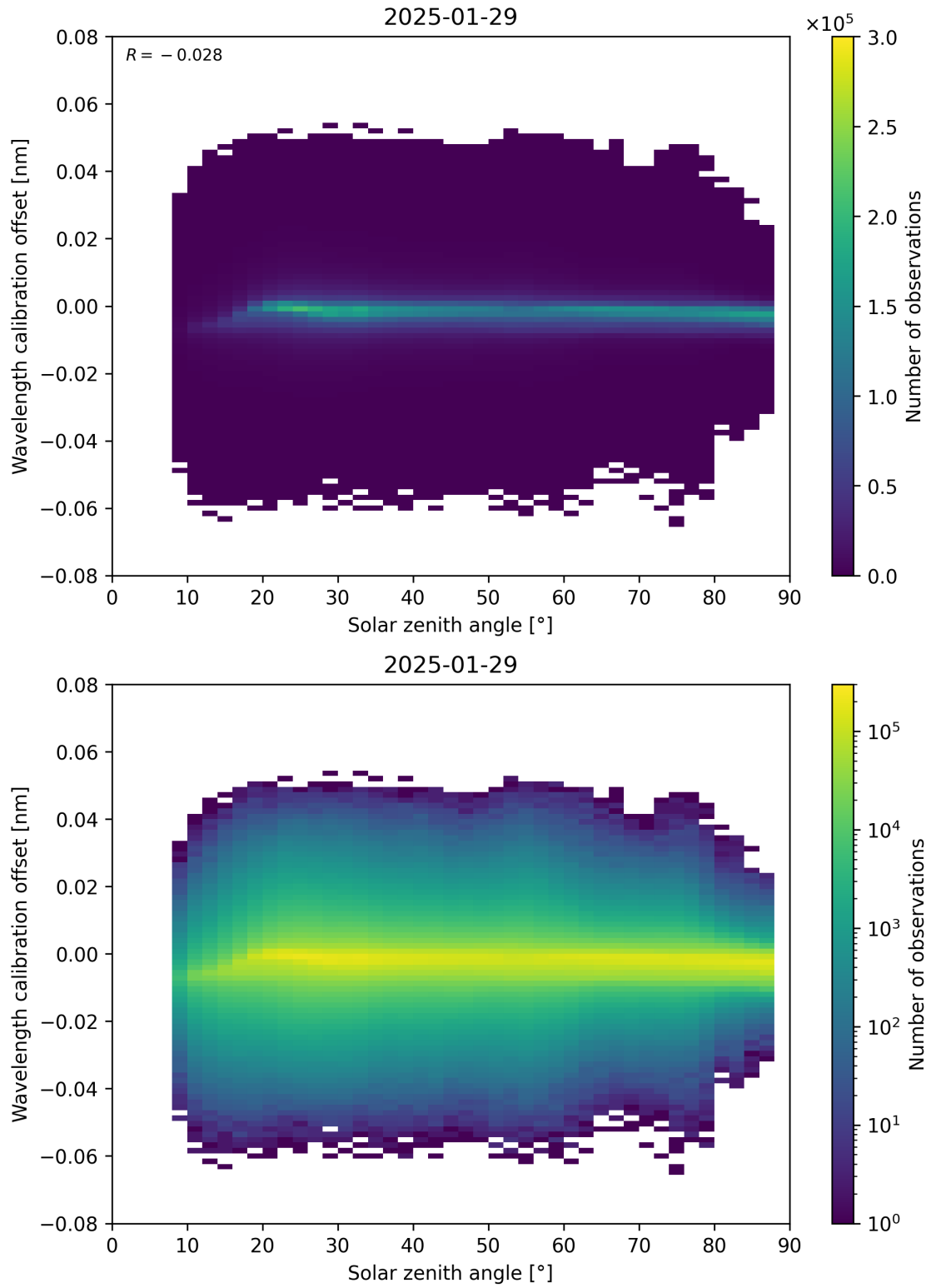
Figure 158: Scatter density plot of “Solar zenith angle” against “Wavelength calibration offset” for 2025-01-28 to 2025-01-30.
