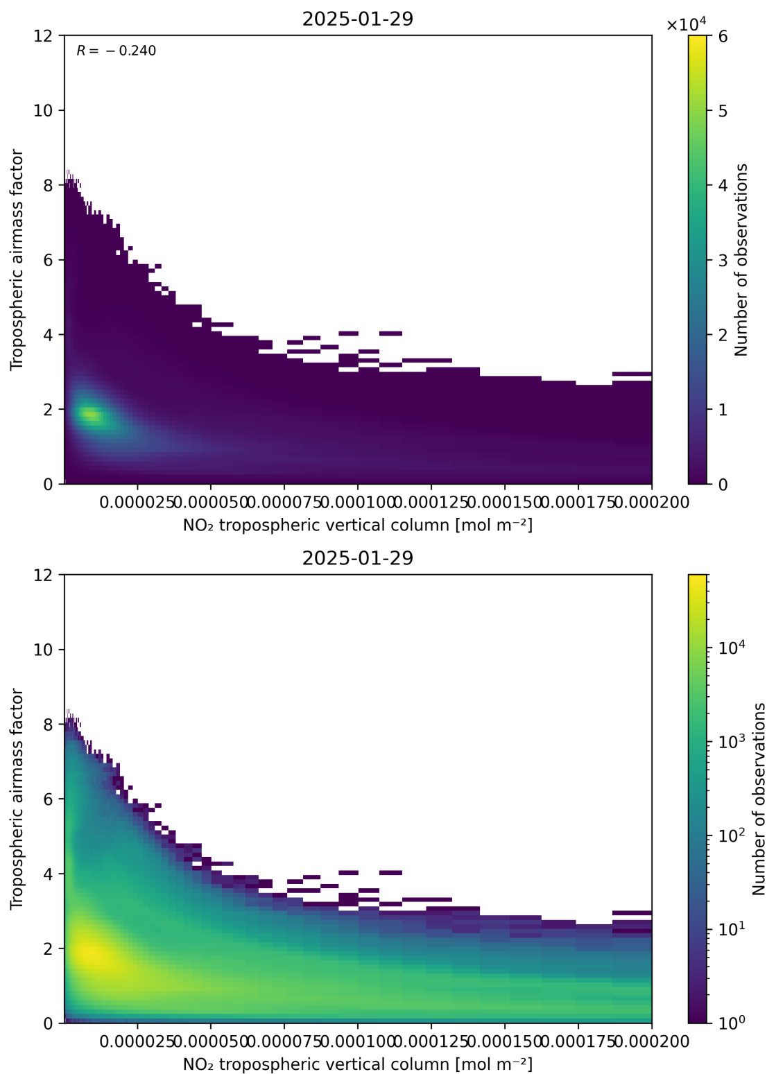
Figure 123: Scatter density plot of “NO 2 tropospheric vertical column” against “Tropospheric air mass factor” for 2025-01-28 to 2025-01-30.
