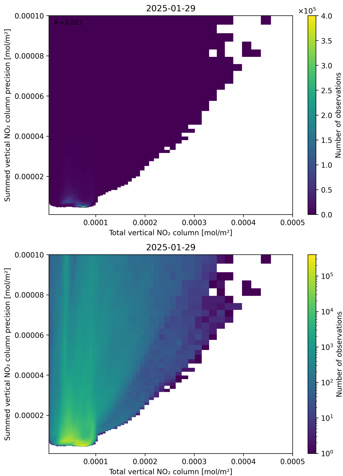
Figure 113: Scatter density plot of “Total vertical NO 2 column” against “Summed vertical NO 2 column precision” for 2025-01-28 to 2025-01-30.
