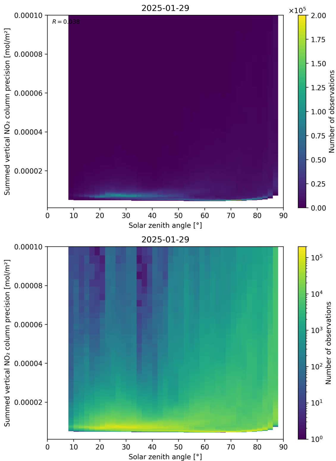
Figure 152: Scatter density plot of “Solar zenith angle” against “Summed vertical NO 2 column precision” for 2025-01-28 to 2025-01-30.
