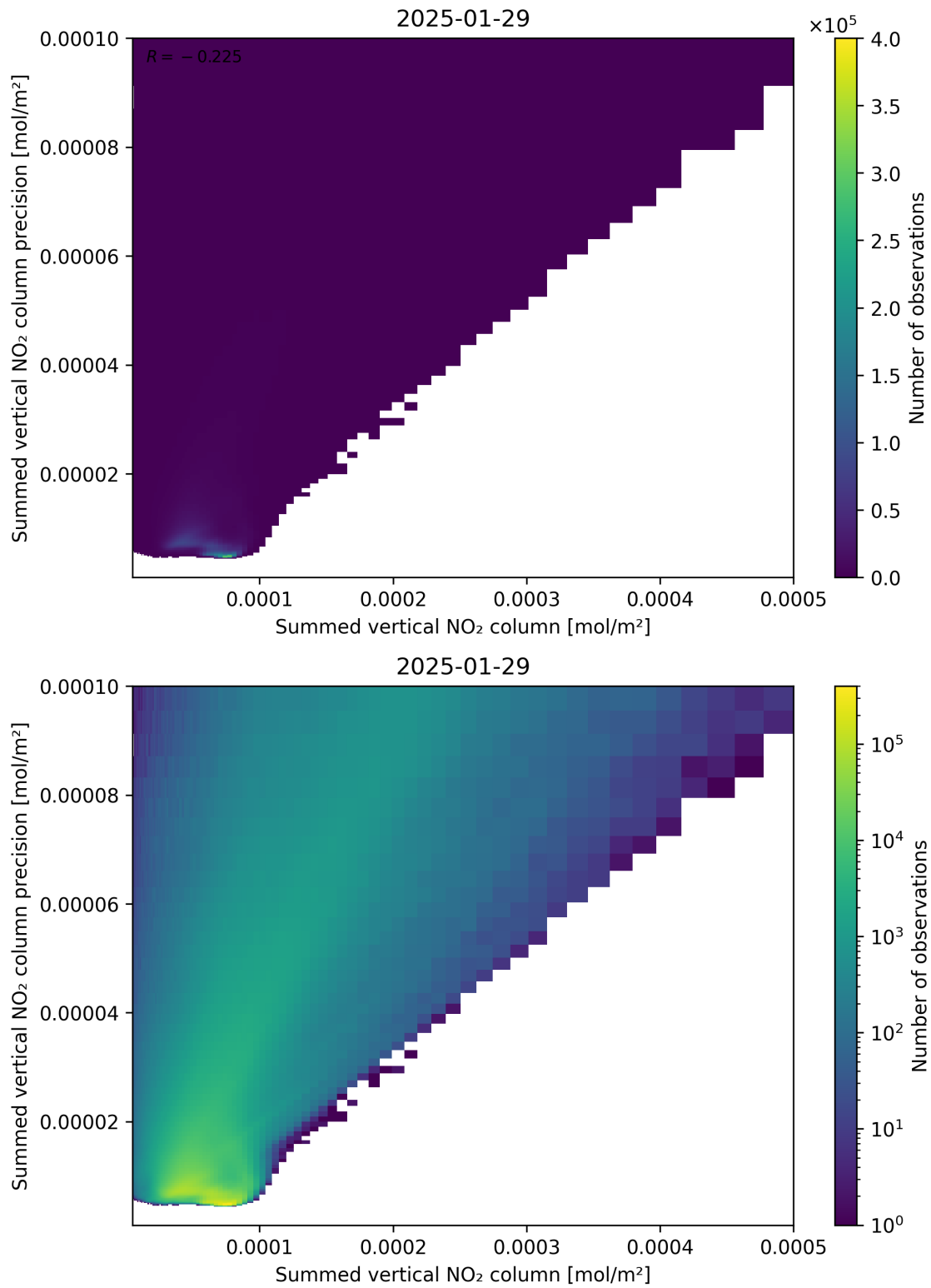
Figure 105: Scatter density plot of “Summed vertical NO 2 column” against “Summed vertical NO 2 column precision” for 2025-01-28 to 2025-01-30.
