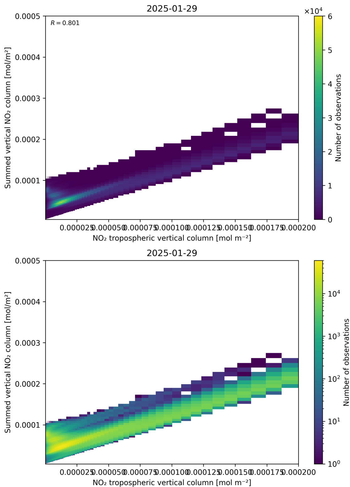
Figure 126: Scatter density plot of “NO 2 tropospheric vertical column” against “Summed vertical NO 2 column” for 2025-01-28 to 2025-01-30.
