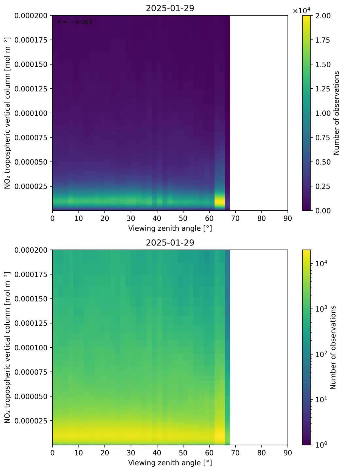
Figure 169: Scatter density plot of “Viewing zenith angle” against “NO 2 tropospheric vertical column” for 2025-01-28 to 2025-01-30.
