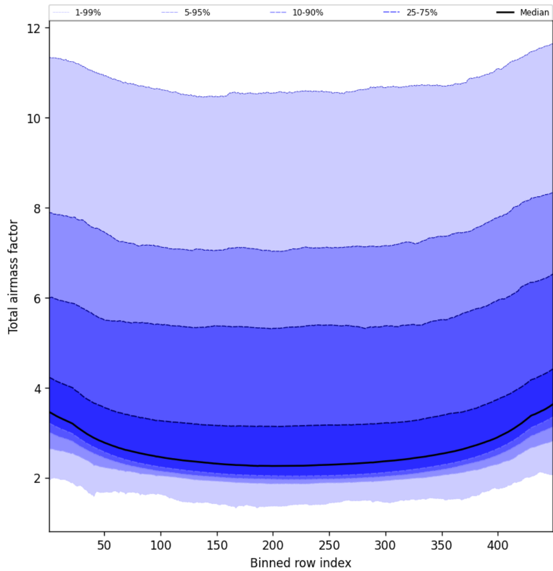
Figure 49: Along track statistics of “Total airmass factor” for 2025-01-28 to 2025-01-30
