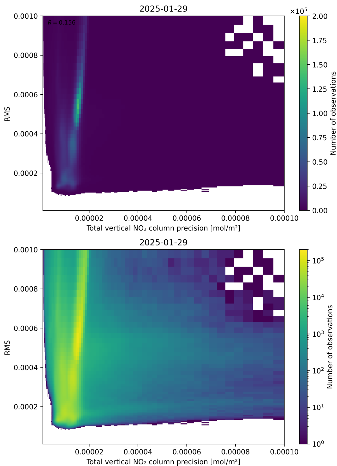
Figure 119: Scatter density plot of “Total vertical NO 2 column precision” against “RMS” for 2025-01-28 to 2025-01-30.
