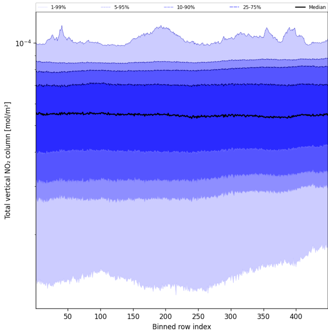
Figure 55: Along track statistics of “Total vertical NO 2 column” for 2025-01-28 to 2025-01-30
