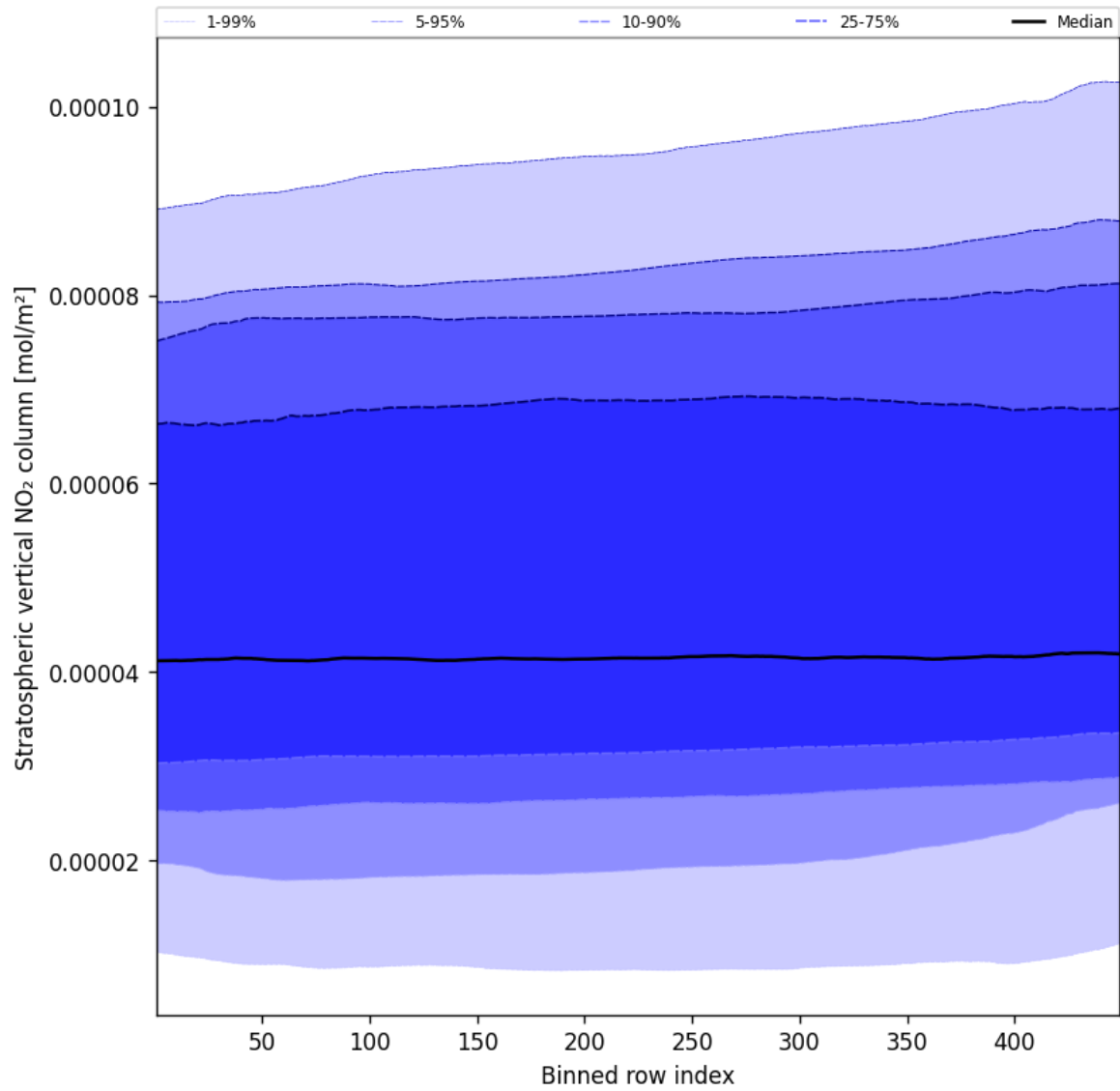
Figure 53: Along track statistics of “Stratospheric vertical NO 2 column” for 2025-01-28 to 2025-01-30
