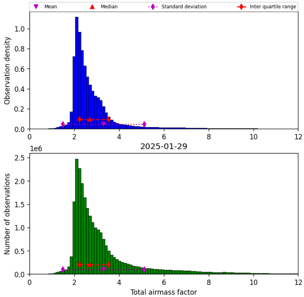
Figure 32: Histogram of “Total airmass factor” for 2025-01-28 to 2025-01-30
