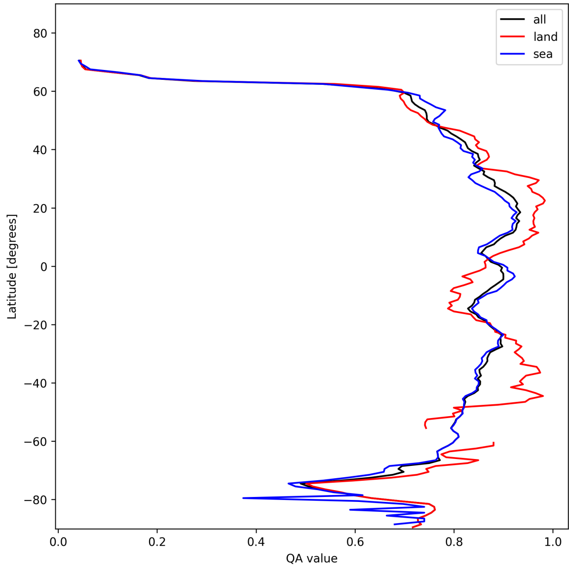
Figure 11: Zonal average of “QA value” for 2025-01-28 to 2025-01-30.
