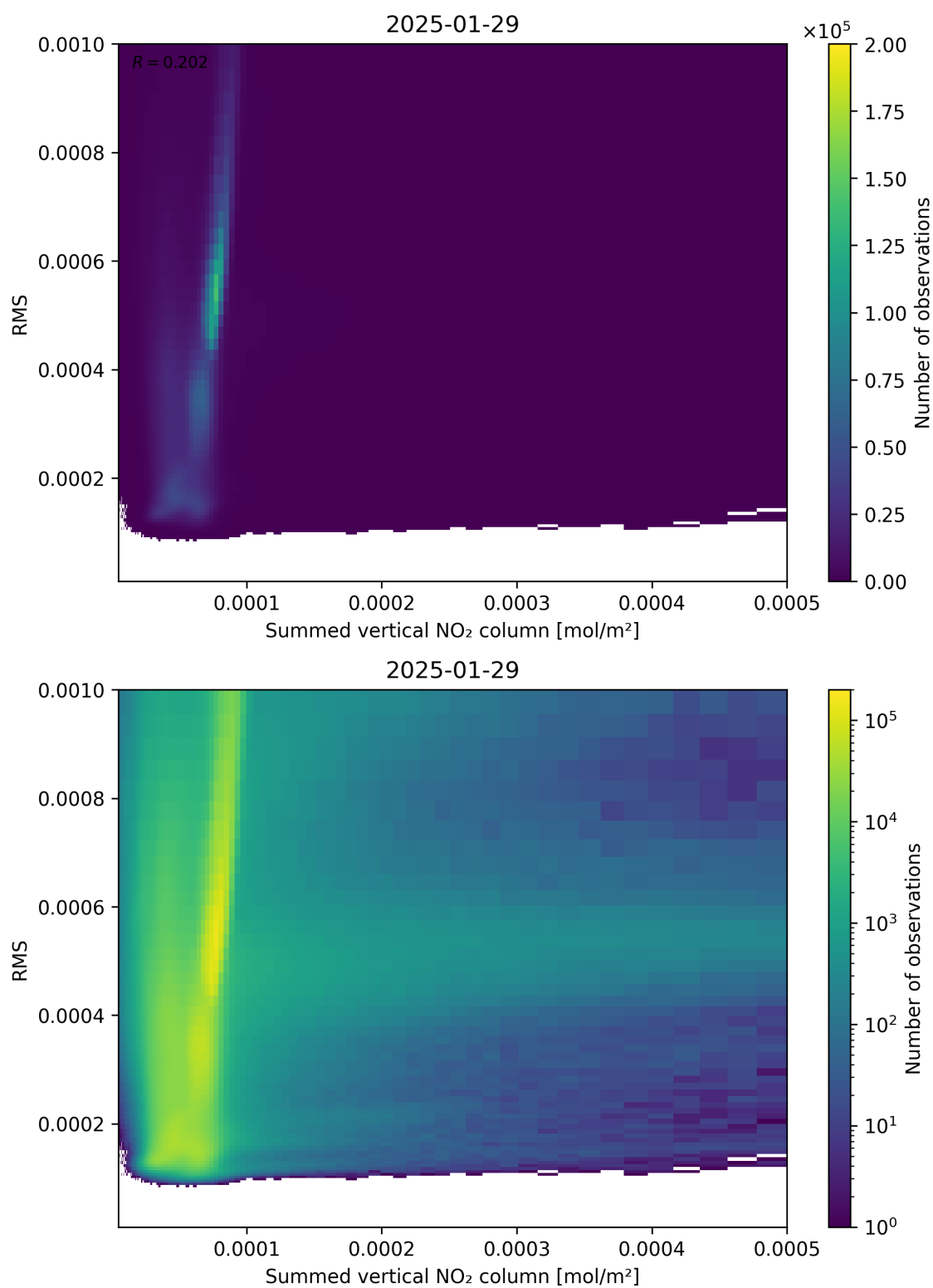
Figure 109: Scatter density plot of “Summed vertical NO 2 column” against “RMS” for 2025-01-28 to 2025-01-30.
