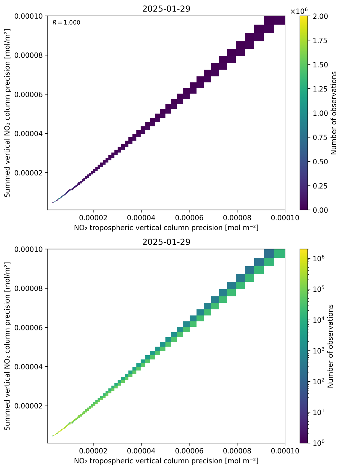
Figure 137: Scatter density plot of “NO 2 tropospheric vertical column precision” against “Summed vertical NO 2 column precision” for 2025-01-28 to 2025-01-30.
