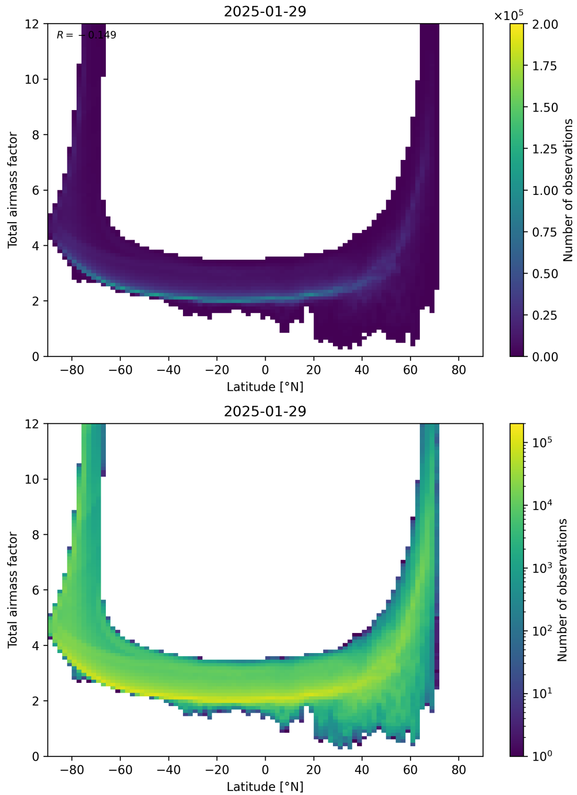
Figure 84: Scatter density plot of “Latitude” against “Total airmass factor” for 2025-01-28 to 2025-01-30.
