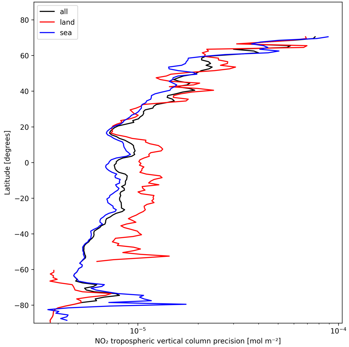
Figure 13: Zonal average of “NO 2 tropospheric vertical column precision” for 2025-01-28 to 2025-01-30.
