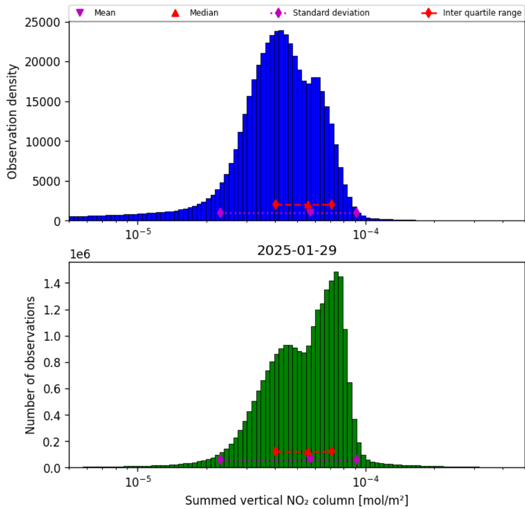
Figure 40: Histogram of “Summed vertical NO 2 column” for 2025-01-28 to 2025-01-30
