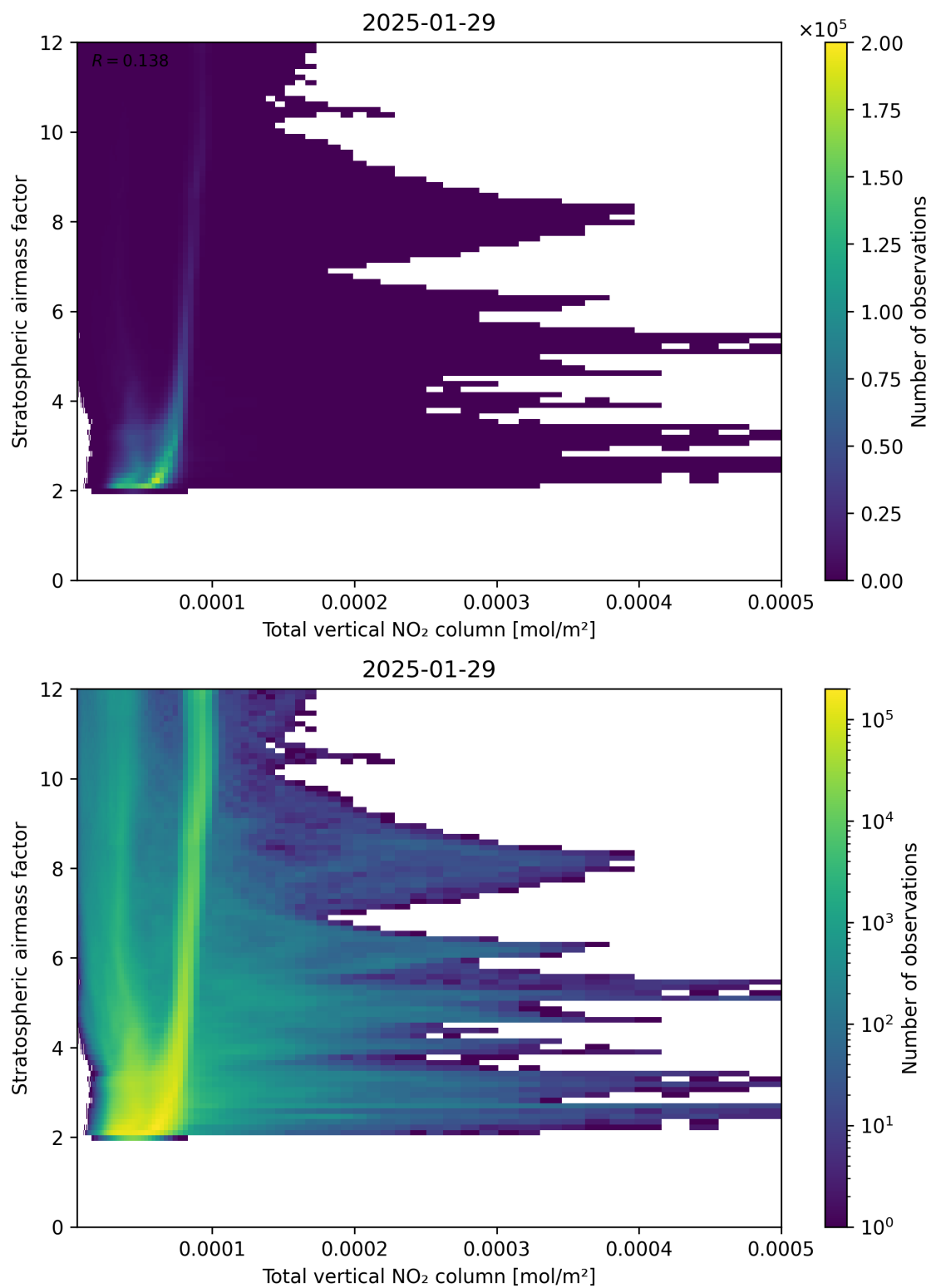
Figure 110: Scatter density plot of “Total vertical NO 2 column” against “Stratospheric airmass factor” for 2025-01-28 to 2025-01-30.
