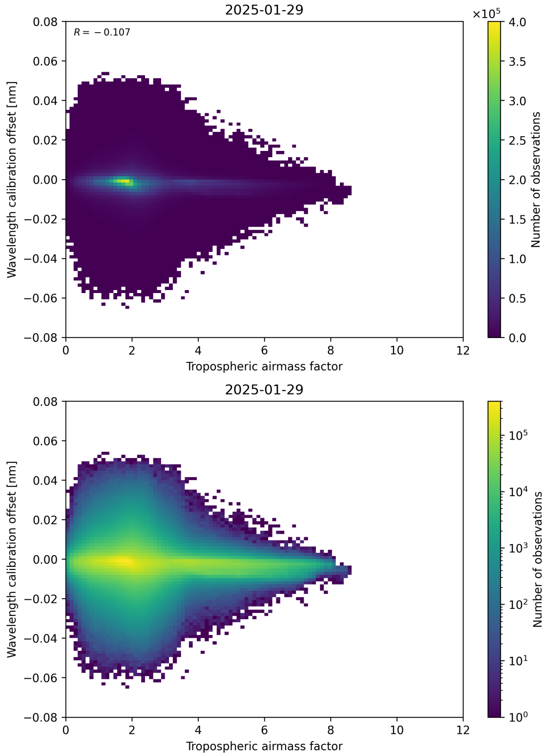
Figure 80: Scatter density plot of “Tropospheric airmass factor” against “Wavelength calibration offset” for 2025-01-28 to 2025-01-30.
