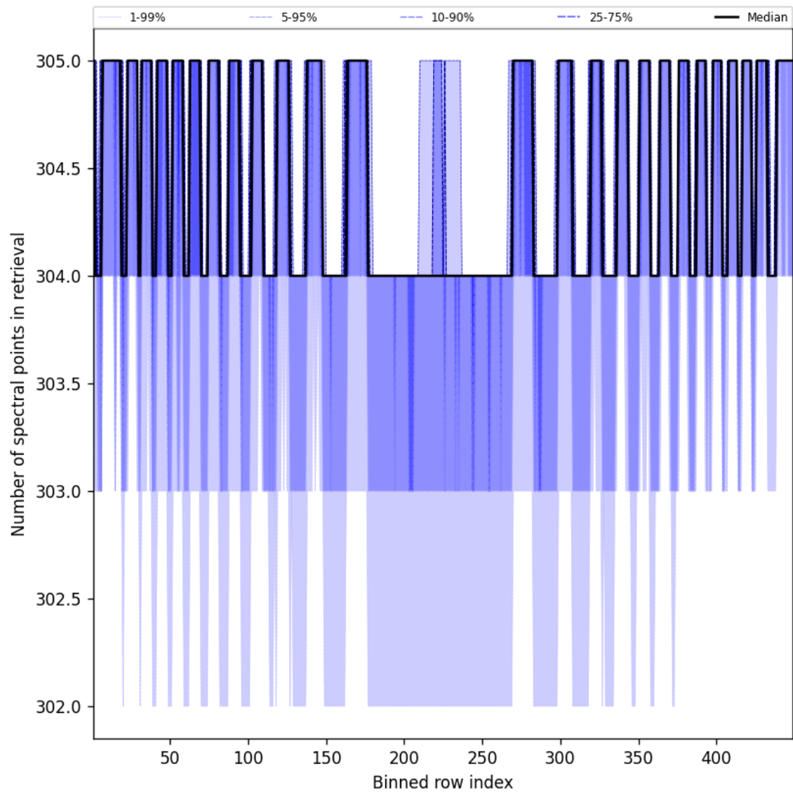
Figure 50: Along track statistics of “Number of spectral points in retrieval” for 2025-01-28 to 2025-01-30
