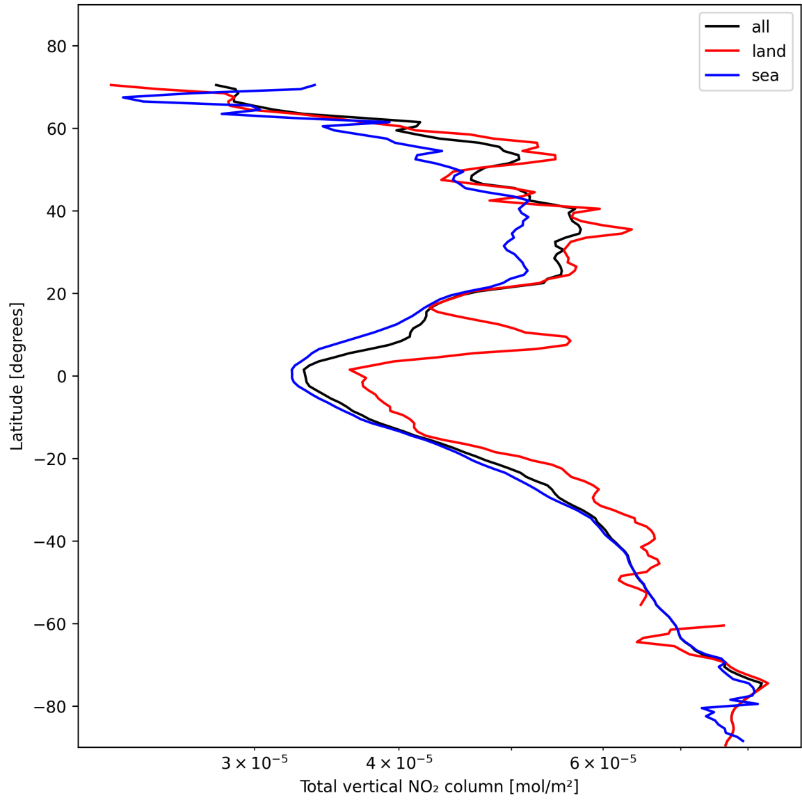
Figure 21: Zonal average of “Total vertical NO 2 column” for 2025-01-28 to 2025-01-30.
