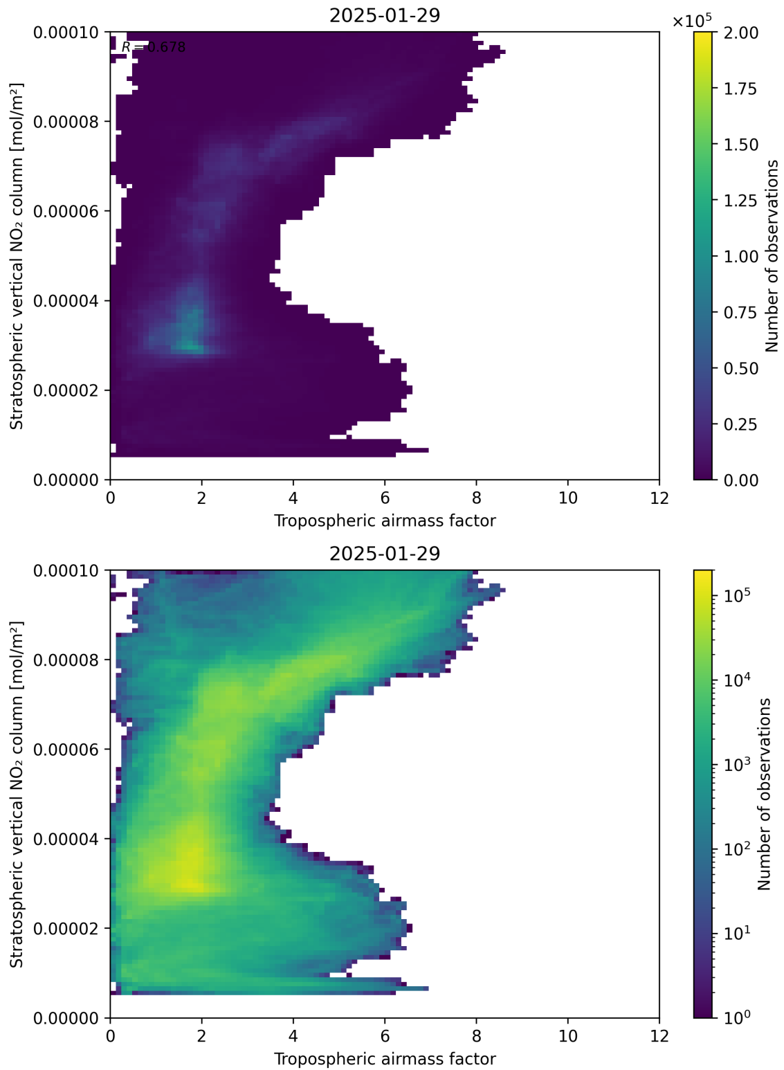
Figure 74: Scatter density plot of “Tropospheric air mass factor” against “Stratospheric vertical NO 2 column” for 2025-01-28 to 2025-01-30.
