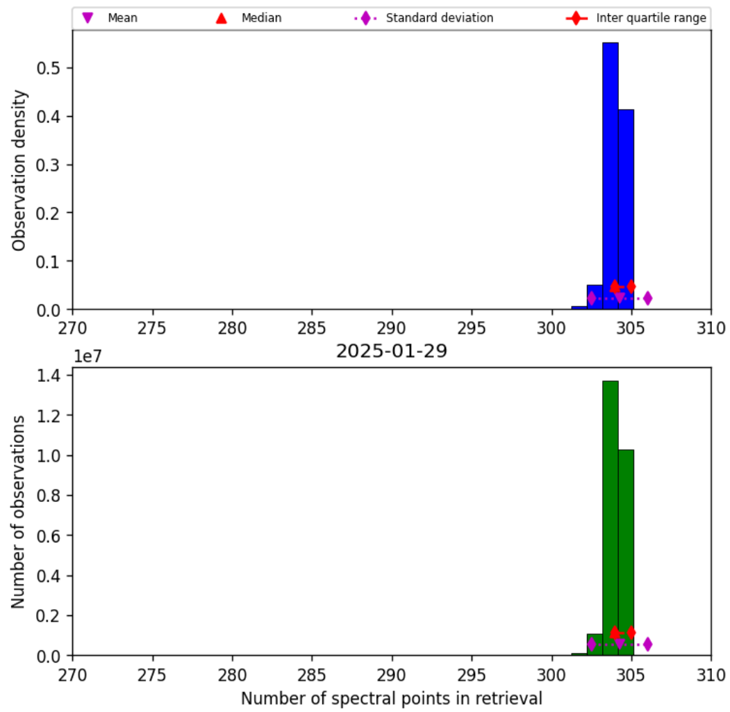
Figure 33: Histogram of “Number of spectral points in retrieval” for 2025-01-28 to 2025-01-30
