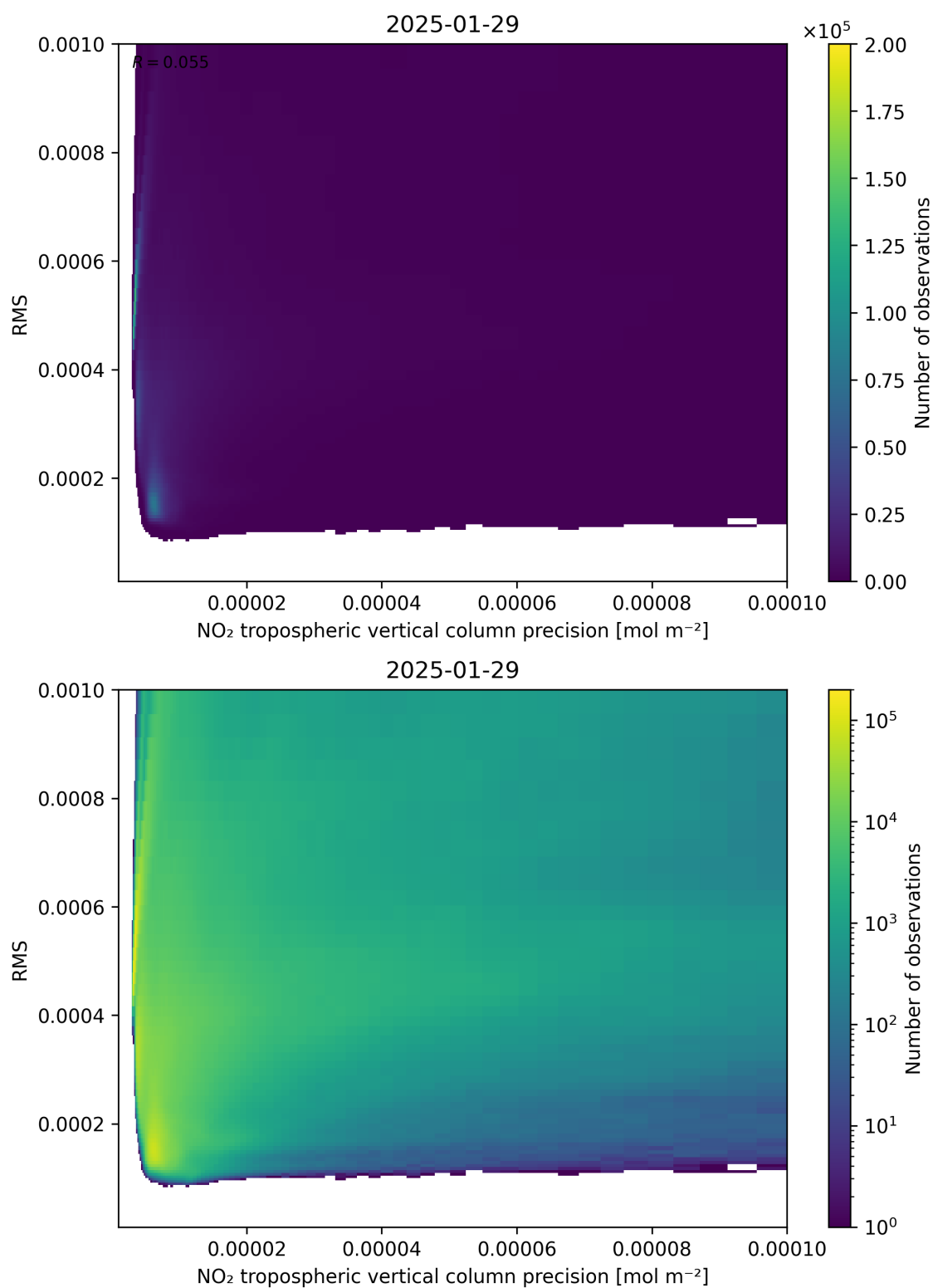
Figure 140: Scatter density plot of “NO 2 tropospheric vertical column precision” against “RMS” for 2025-01-28 to 2025-01-30.
