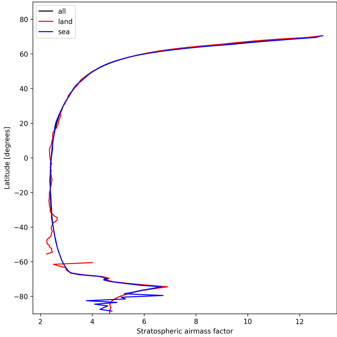
Figure 27: Zonal average of “Stratospheric airmass factor” for 2025-01-28 to 2025-01-30.
