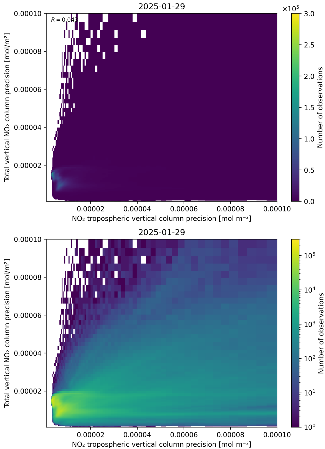
Figure 139: Scatter density plot of “NO 2 tropospheric vertical column precision” against “Total vertical NO 2 column precision” for 2025-01-28 to 2025-01-30.
