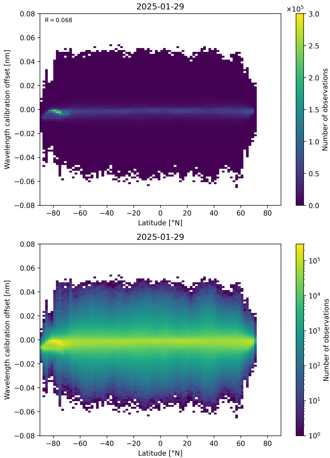
Figure 95: Scatter density plot of “Latitude” against “Wavelength calibration offset” for 2025-01-28 to 2025-01-30.
