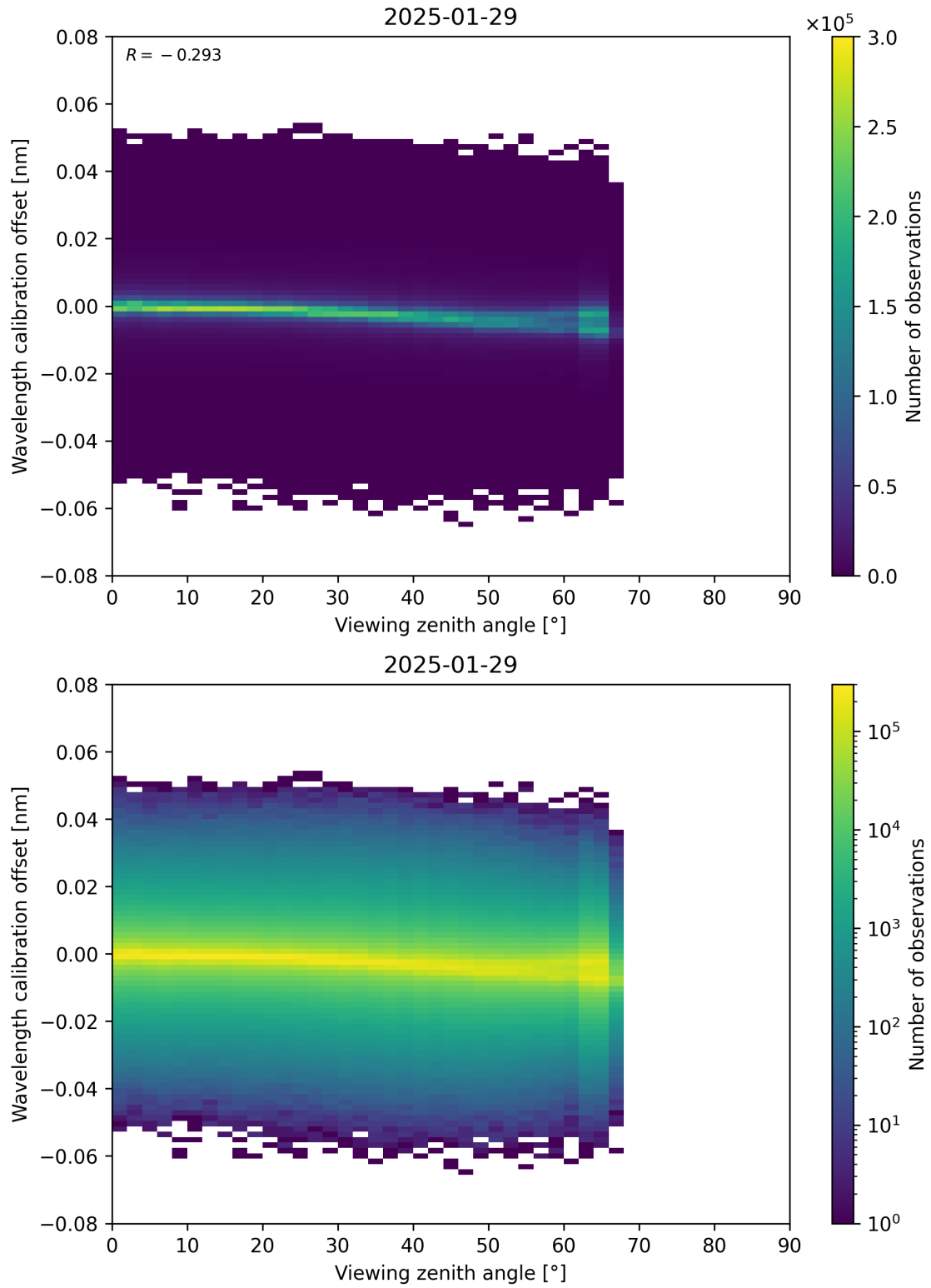
Figure 173: Scatter density plot of “Viewing zenith angle” against “Wavelength calibration offset” for 2025-01-28 to 2025-01-30.
