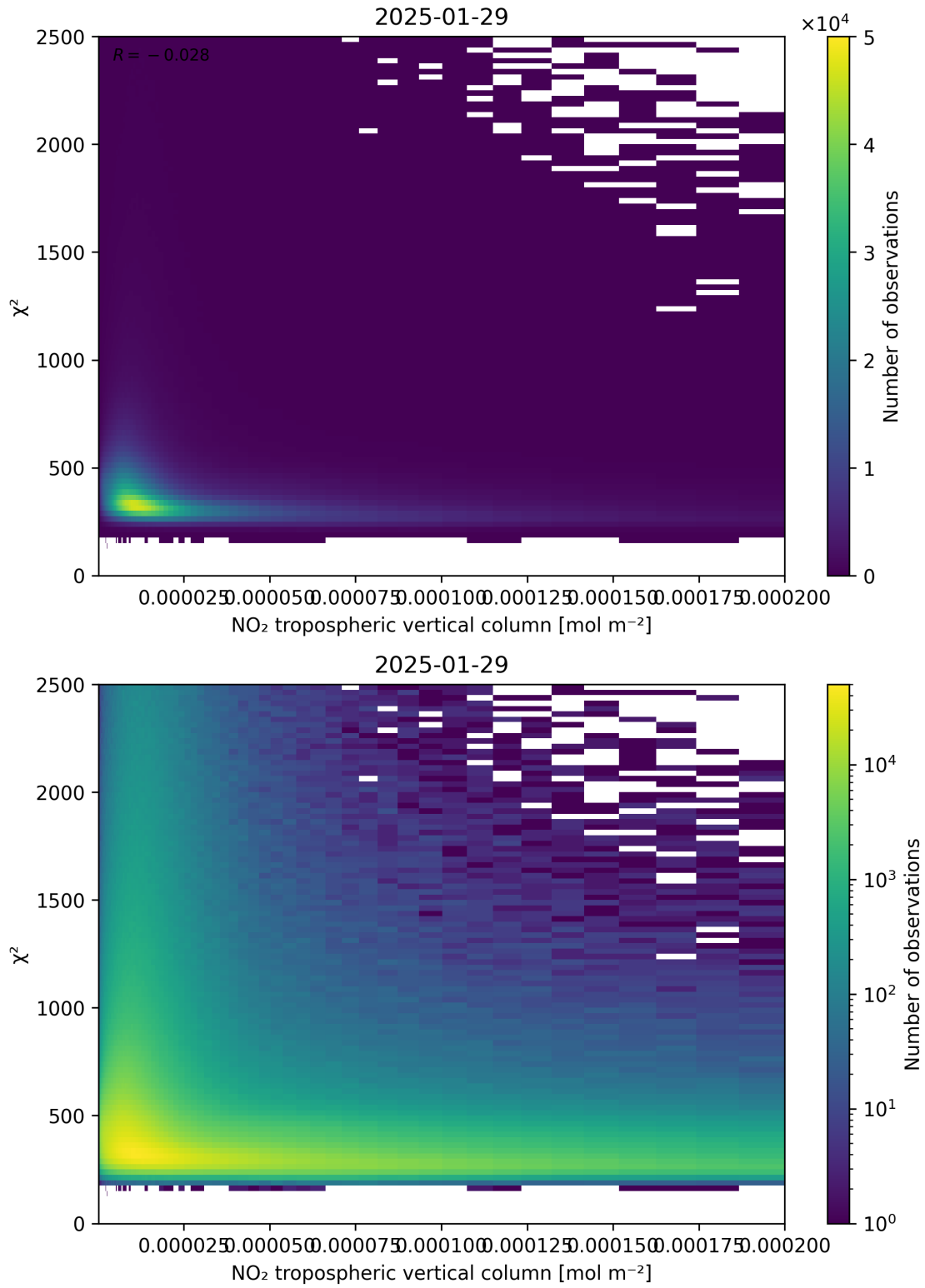
Figure 124: Scatter density plot of “NO 2 tropospheric vertical column” against “ \chi^2 ” for 2025-01-28 to 2025-01-30.
