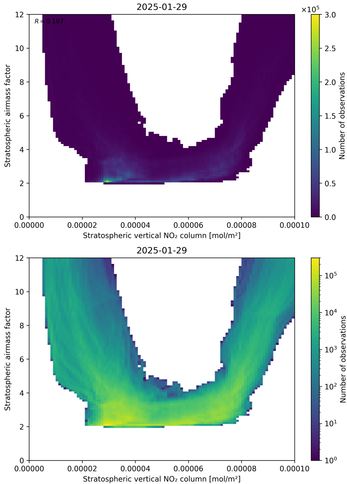
Figure 96: Scatter density plot of “Stratospheric vertical NO 2 column” against “Stratospheric airmass factor” for 2025-01-28 to 2025-01-30.
