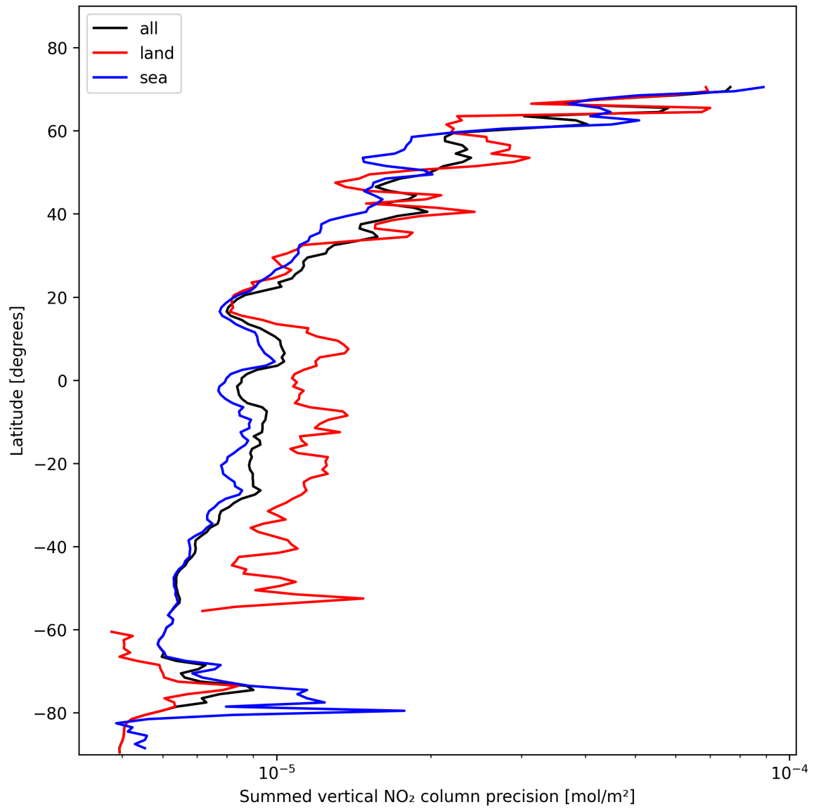
Figure 24: Zonal average of “Summed vertical NO 2 column precision” for 2025-01-28 to 2025-01-30.
