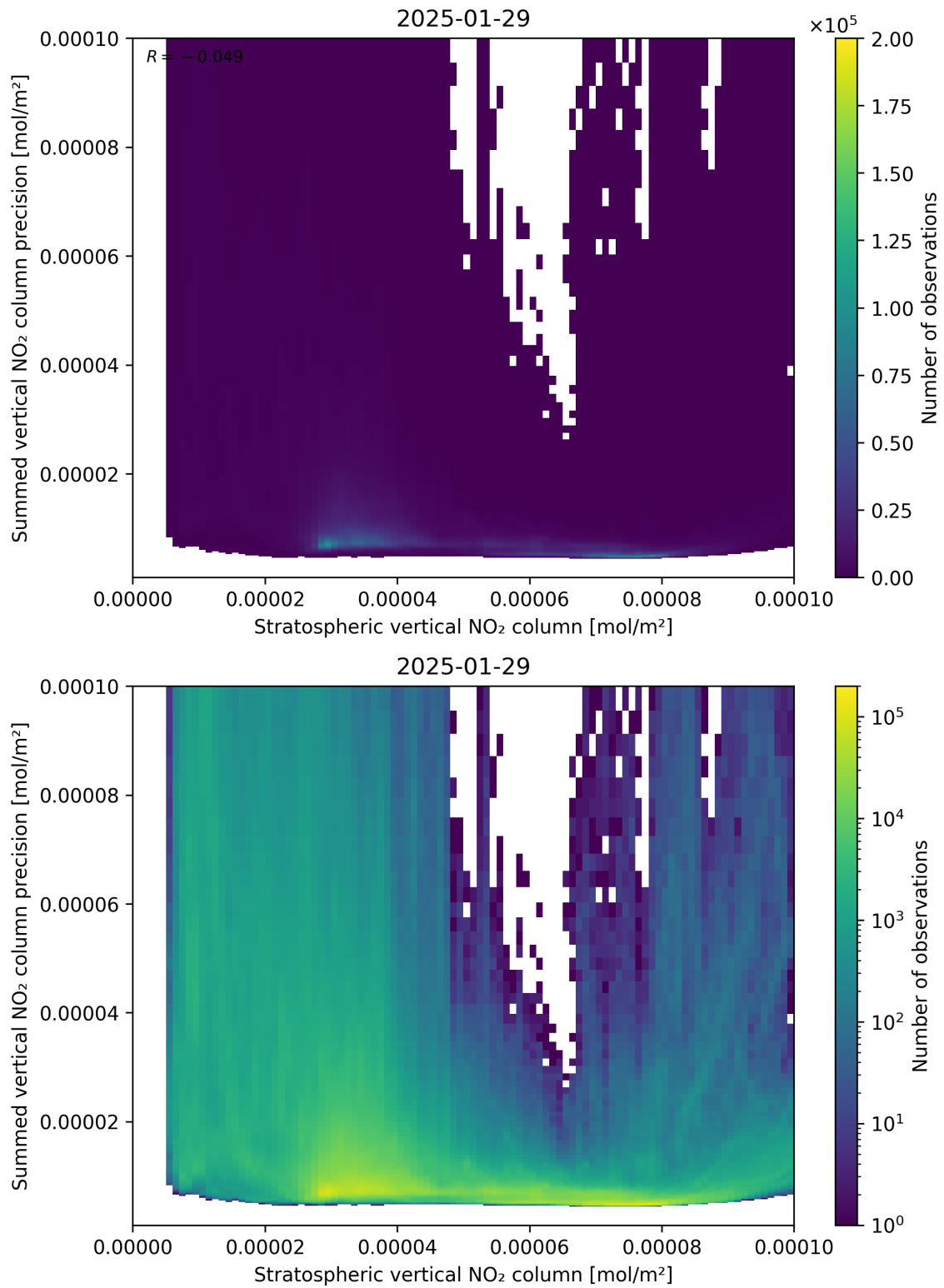
Figure 99: Scatter density plot of “Stratospheric vertical NO 2 column” against “Summed vertical NO 2 column precision” for 2025-01-28 to 2025-01-30.
