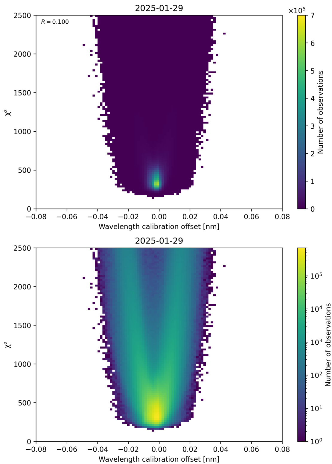
Figure 175: Scatter density plot of “Wavelength calibration offset” against “ \chi^2 ” for 2025-01-28 to 2025-01-30.
