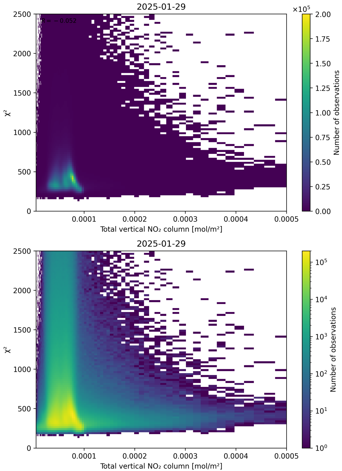
Figure 111: Scatter density plot of “Total vertical NO 2 column” against “ \chi^2 ” for 2025-01-28 to 2025-01-30.
