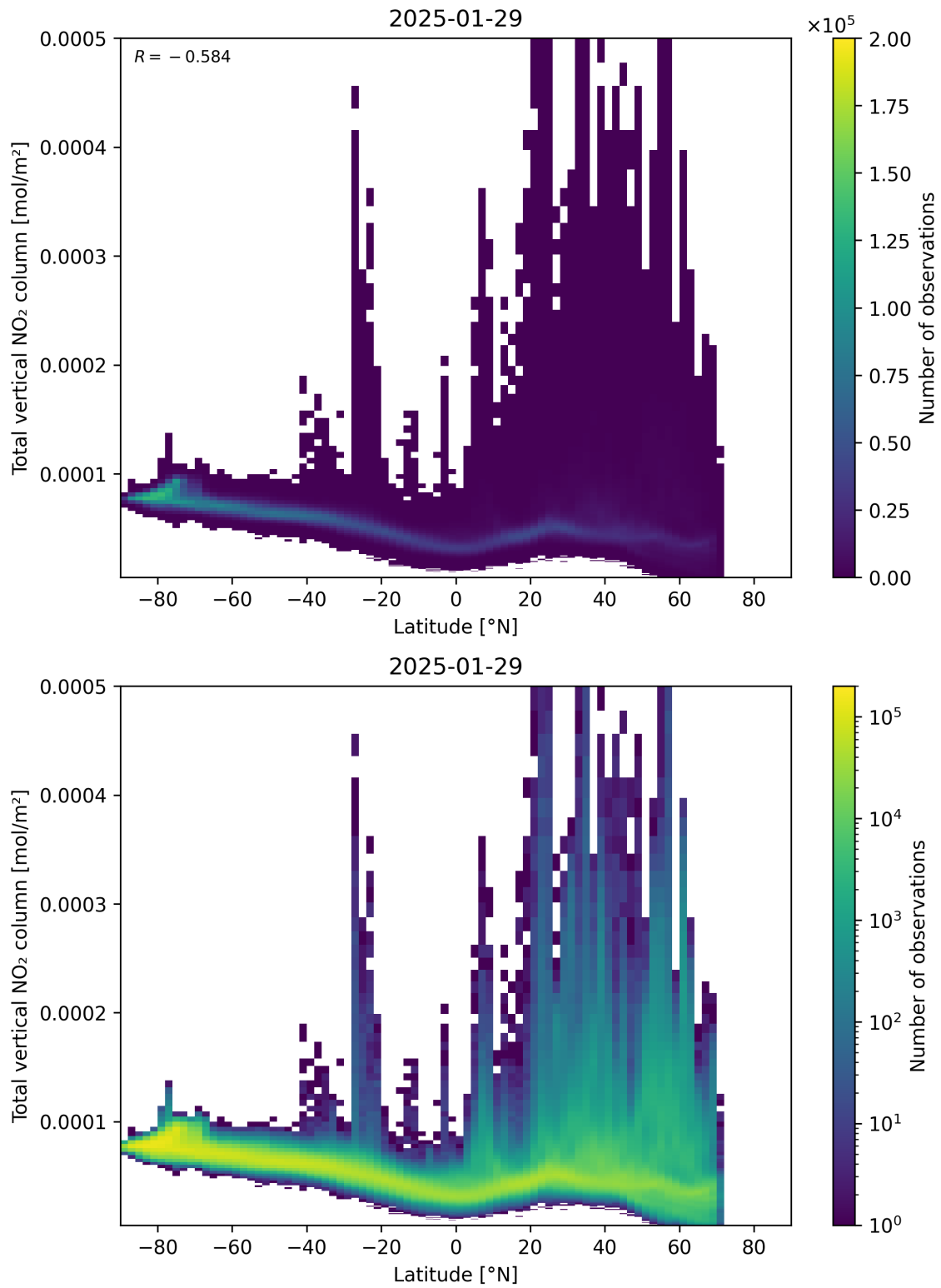
Figure 90: Scatter density plot of “Latitude” against “Total vertical NO 2 column” for 2025-01-28 to 2025-01-30.
