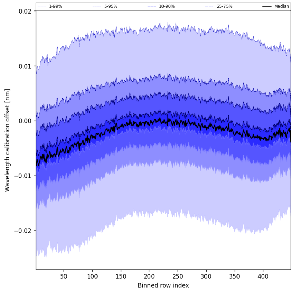
Figure 52: Along track statistics of “Wavelength calibration offset” for 2025-01-28 to 2025-01-30
