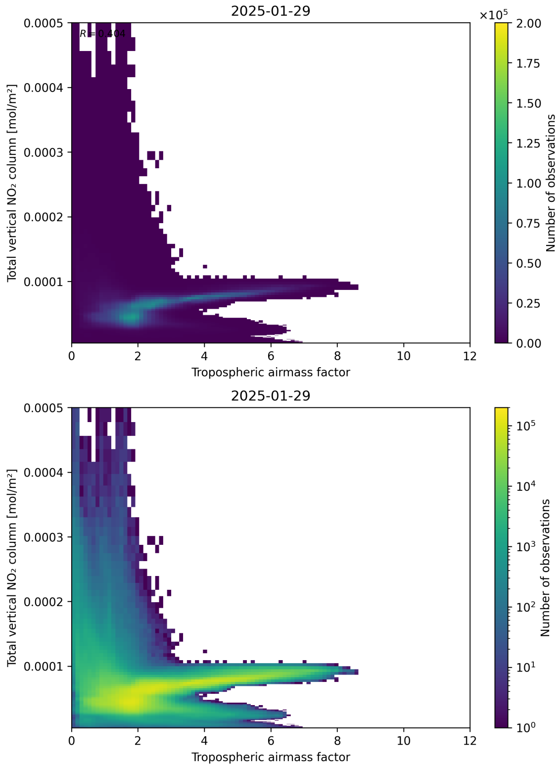
Figure 77: Scatter density plot of “Tropospheric airmass factor” against “Total vertical NO 2 column” for 2025-01-28 to 2025-01-30.
