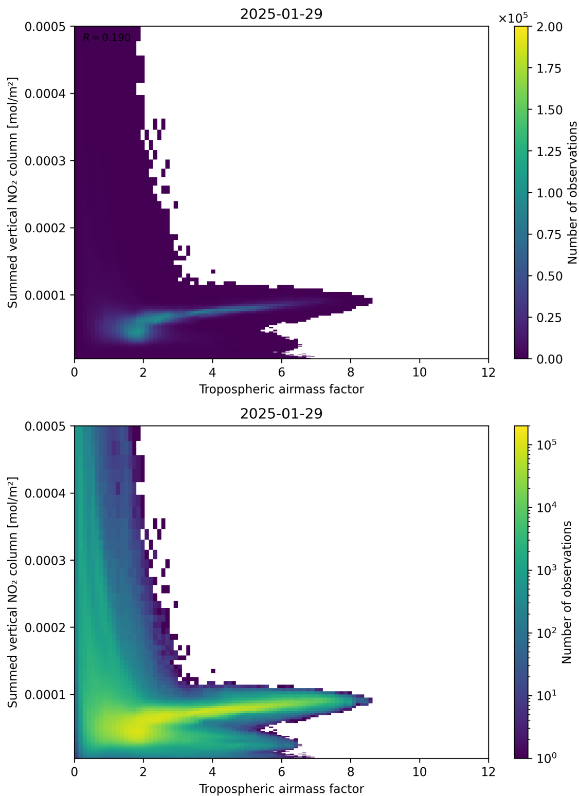
Figure 75: Scatter density plot of “Tropospheric airmass factor” against “Summed vertical NO 2 column” for 2025-01-28 to 2025-01-30.
