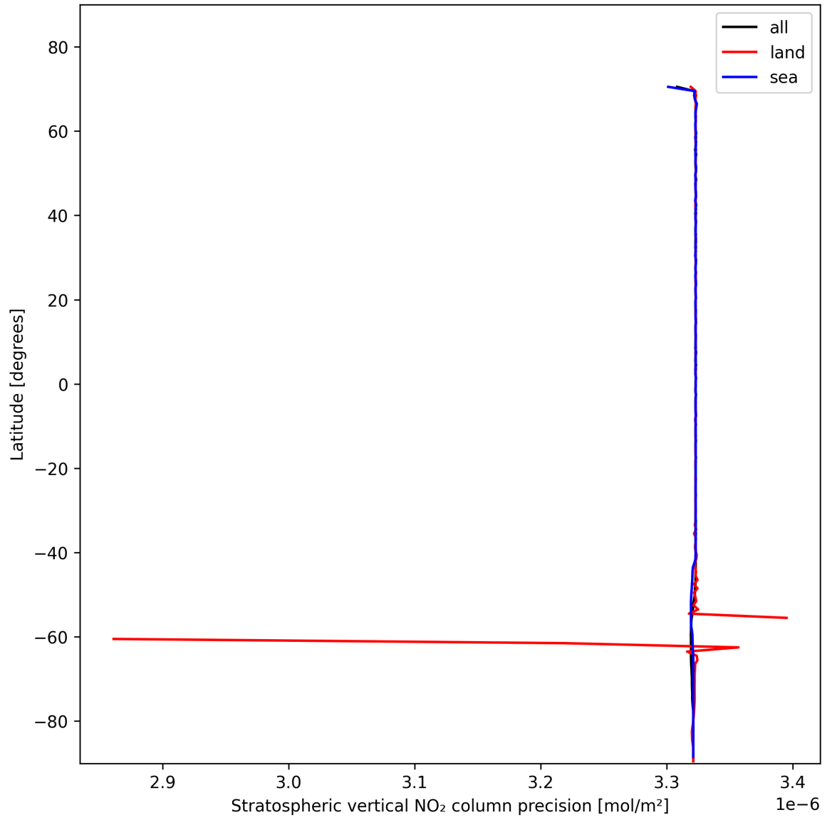
Figure 20: Zonal average of “Stratospheric vertical NO 2 column precision” for 2025-01-28 to 2025-01-30.
