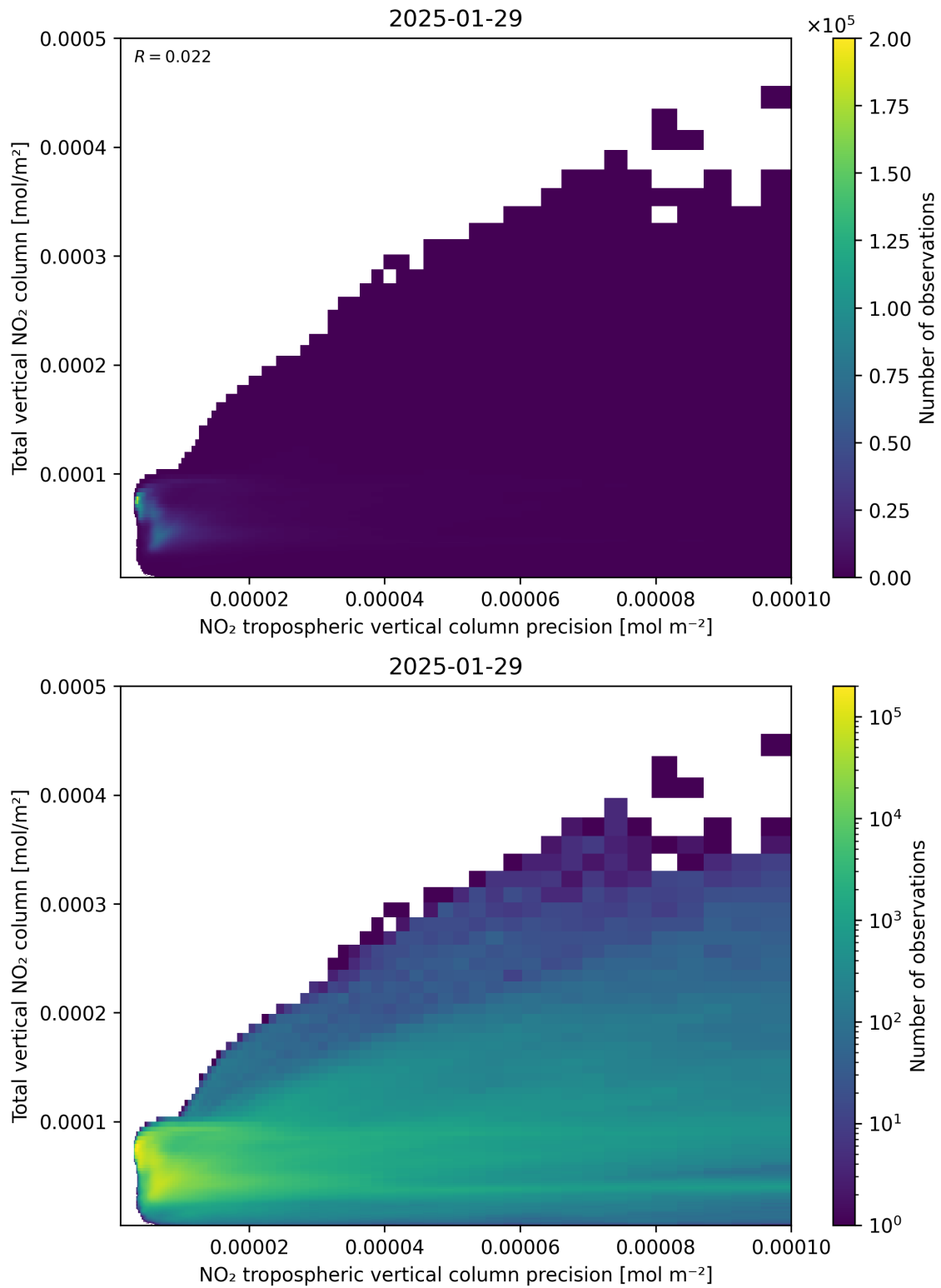
Figure 138: Scatter density plot of “NO 2 tropospheric vertical column precision” against “Total vertical NO 2 column” for 2025-01-28 to 2025-01-30.
