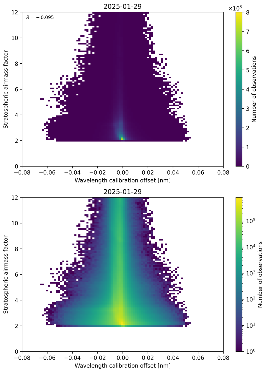
Figure 174: Scatter density plot of “Wavelength calibration offset” against “Stratospheric airmass factor” for 2025-01-28 to 2025-01-30.
