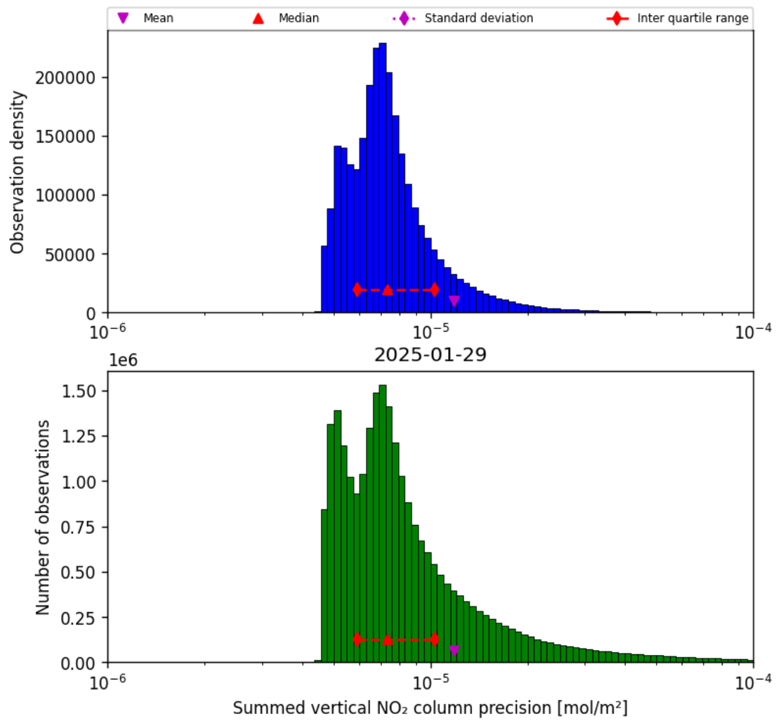
Figure 41: Histogram of "Summed vertical NO 2 column precision" for 2025-01-28 to 2025-01-30
