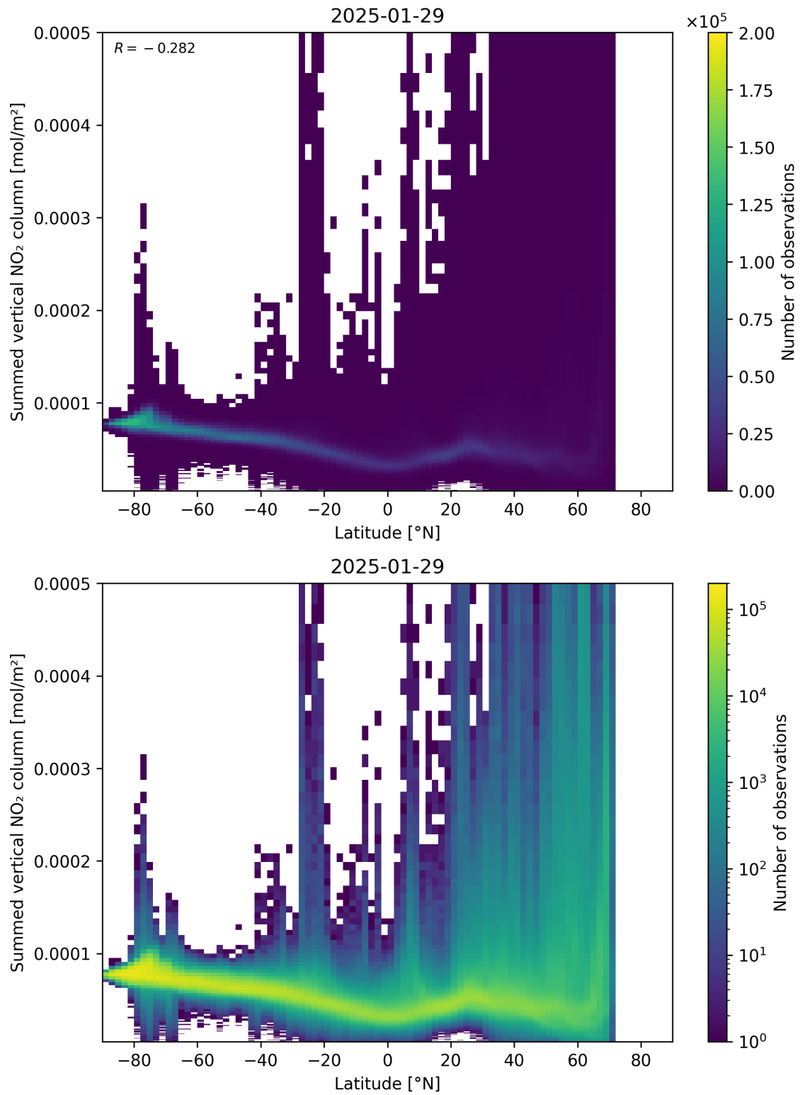
Figure 88: Scatter density plot of “Latitude” against “Summed vertical NO 2 column” for 2025-01-28 to 2025-01-30.
