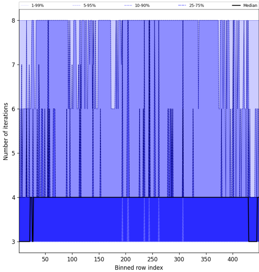
Figure 51: Along track statistics of “Number of iterations” for 2025-01-28 to 2025-01-30
