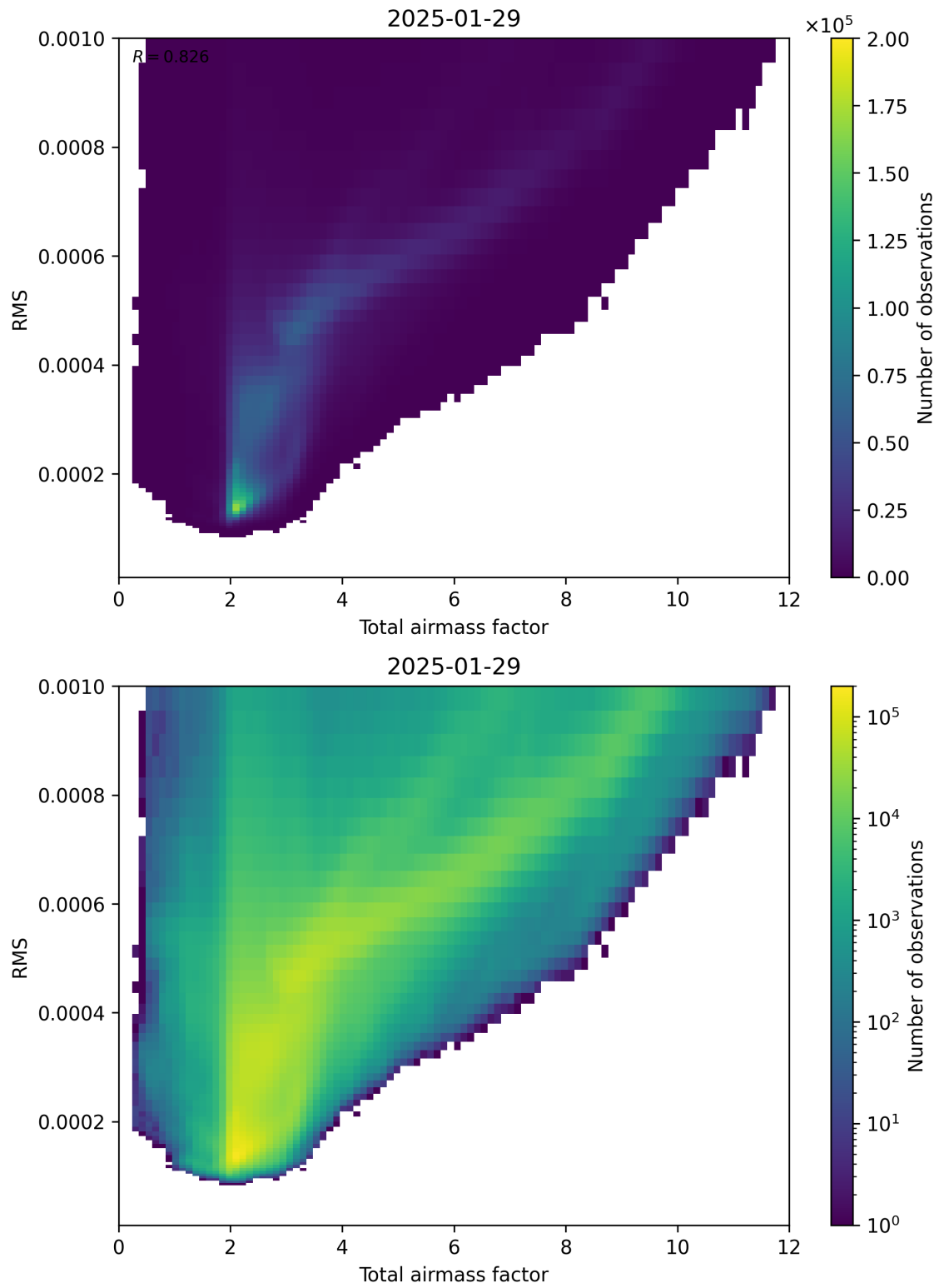
Figure 69: Scatter density plot of “Total airmass factor” against “RMS” for 2025-01-28 to 2025-01-30.
