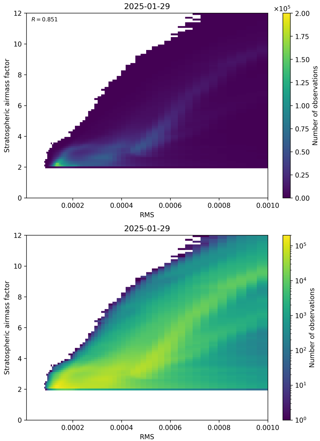
Figure 144: Scatter density plot of “RMS” against “Stratospheric airmass factor” for 2025-01-28 to 2025-01-30.
