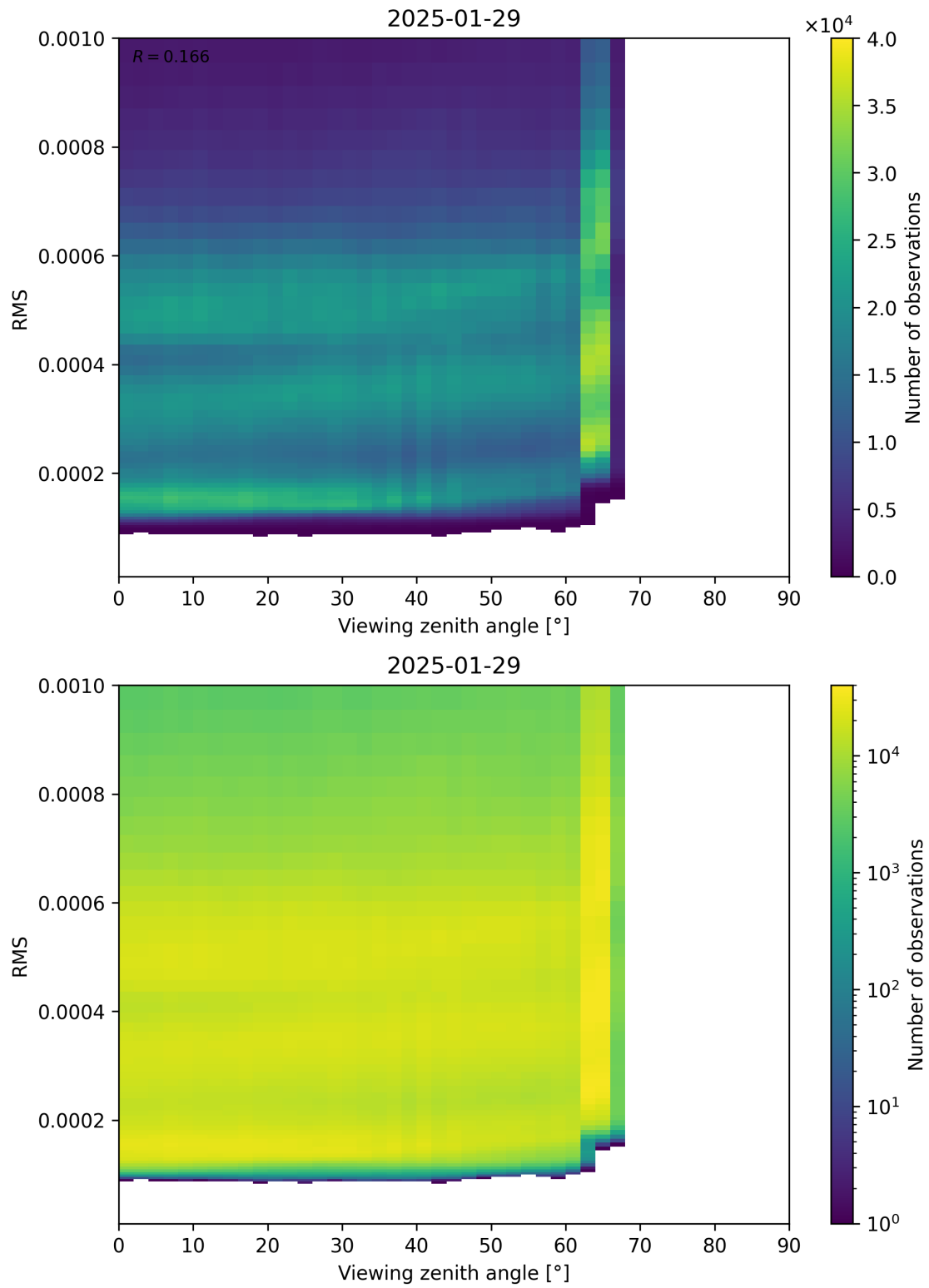
Figure 171: Scatter density plot of “Viewing zenith angle” against “RMS” for 2025-01-28 to 2025-01-30.
