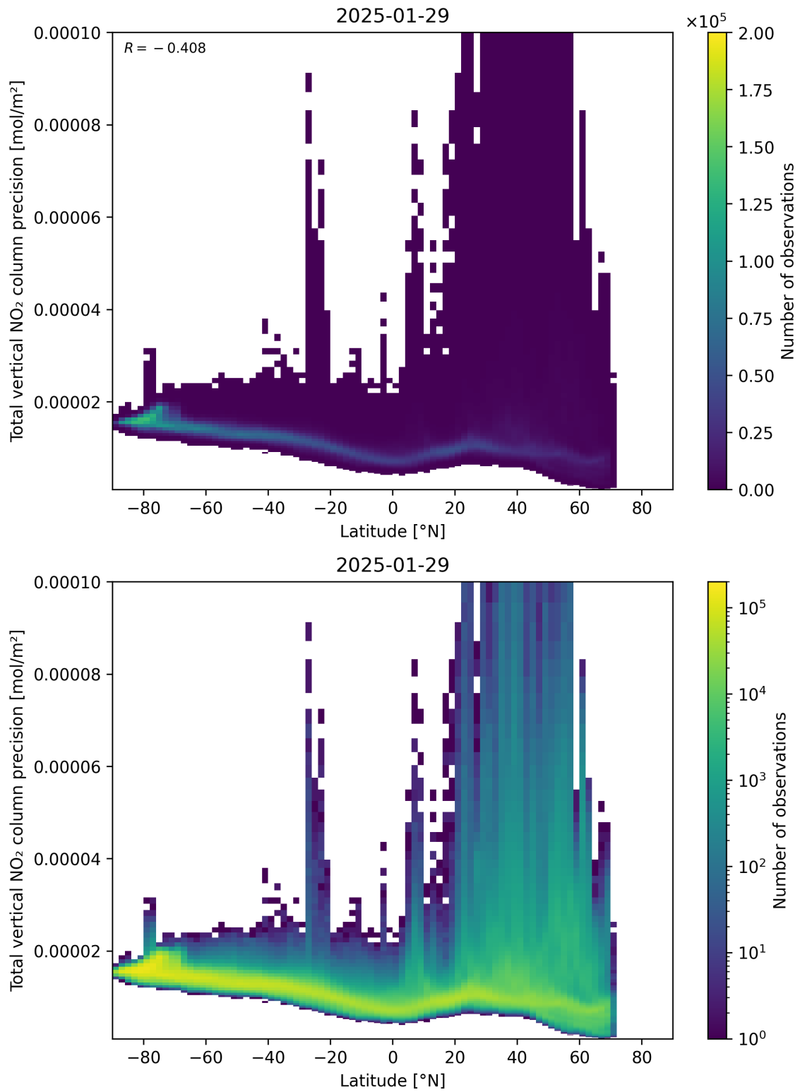
Figure 91: Scatter density plot of “Latitude” against “Total vertical NO 2 column precision” for 2025-01-28 to 2025-01-30.
