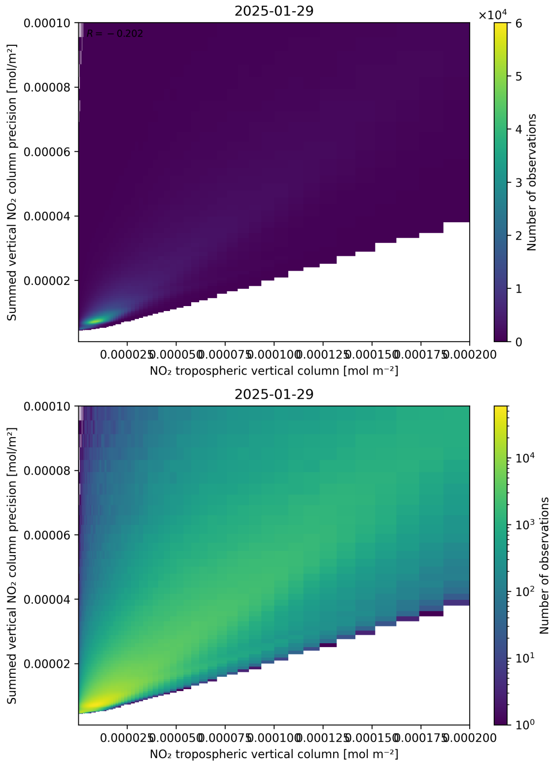
Figure 127: Scatter density plot of “NO 2 tropospheric vertical column” against “Summed vertical NO 2 column precision” for 2025-01-28 to 2025-01-30.
