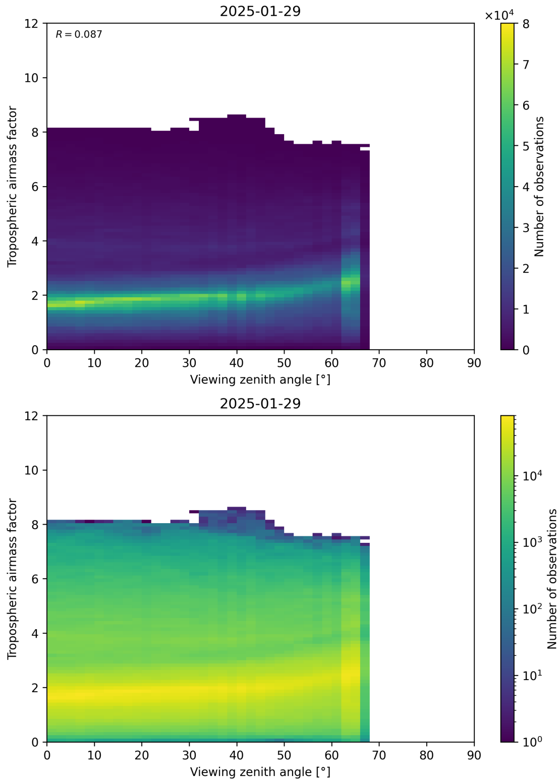
Figure 161: Scatter density plot of “Viewing zenith angle” against “Tropospheric airmass factor” for 2025-01-28 to 2025-01-30.
