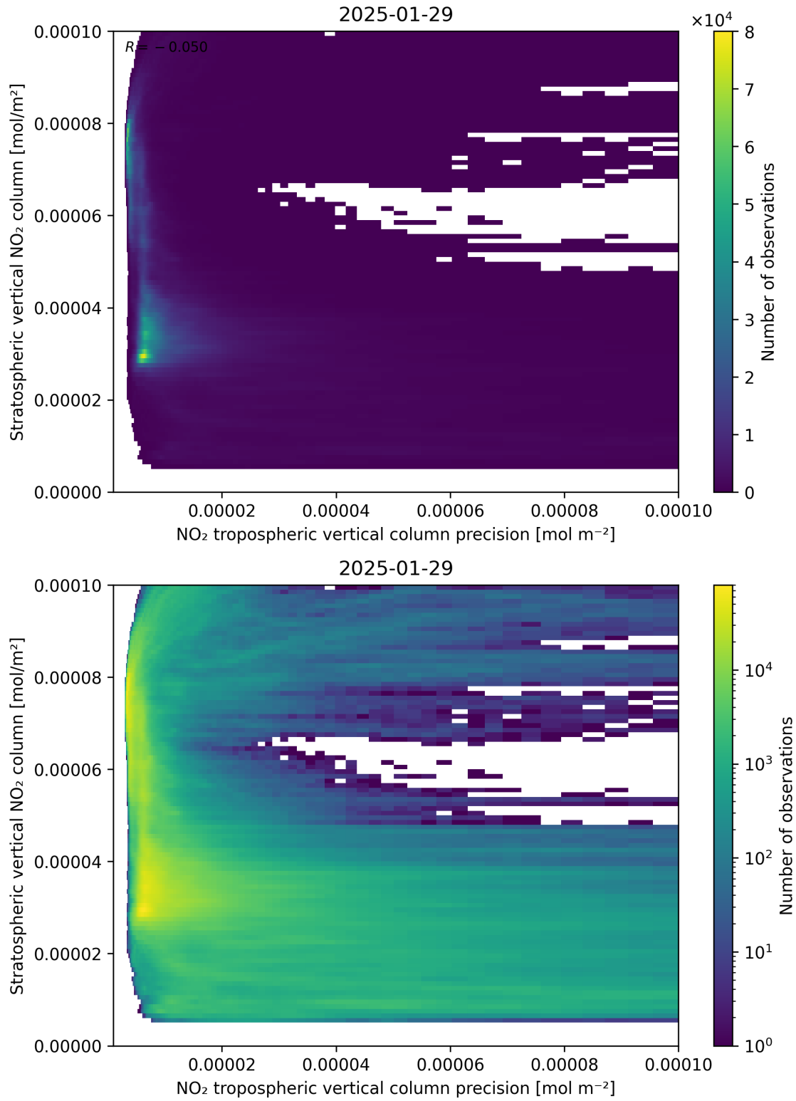
Figure 135: Scatter density plot of “NO 2 tropospheric vertical column precision” against “Stratospheric vertical NO 2 column” for 2025-01-28 to 2025-01-30.
