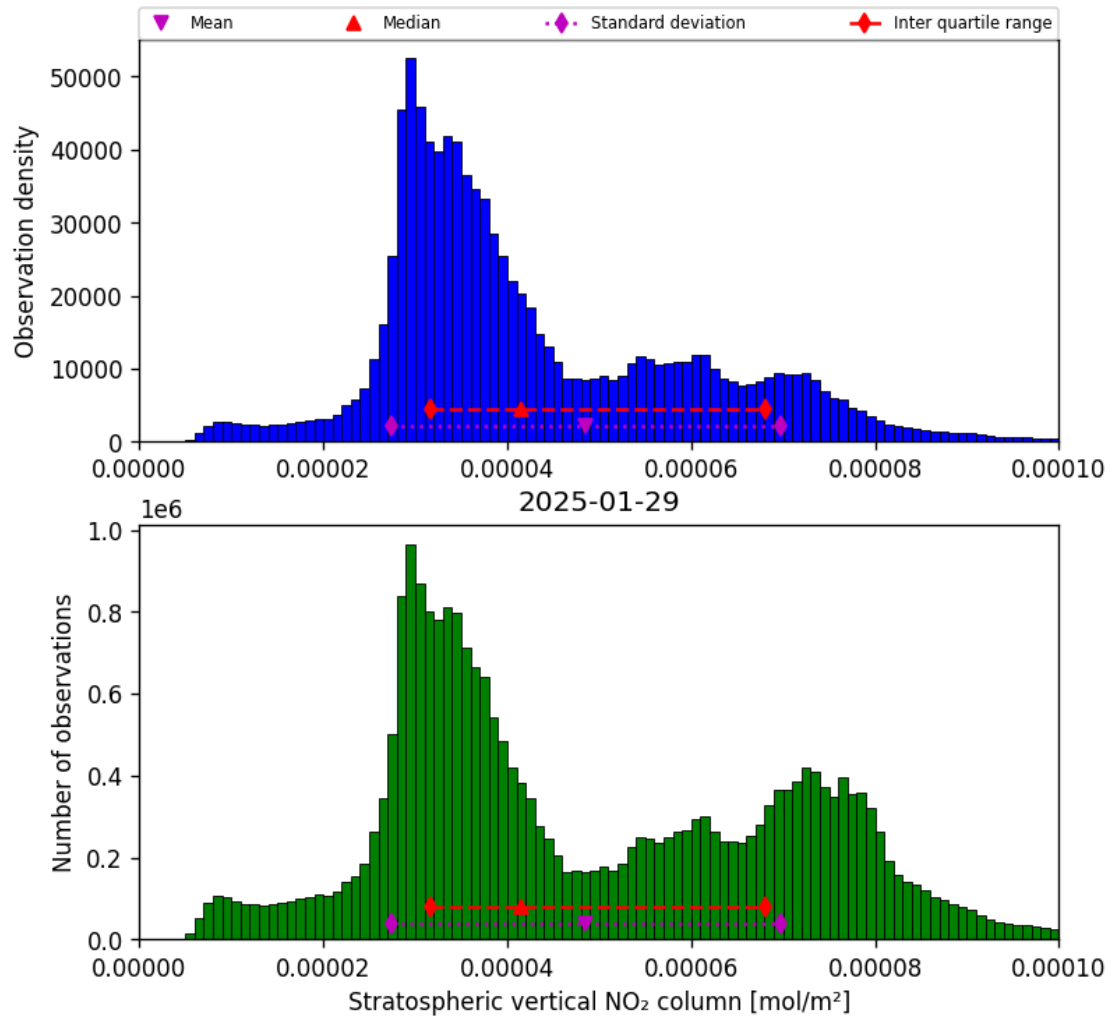
Figure 36: Histogram of “Stratospheric vertical NO 2 column” for 2025-01-28 to 2025-01-30
