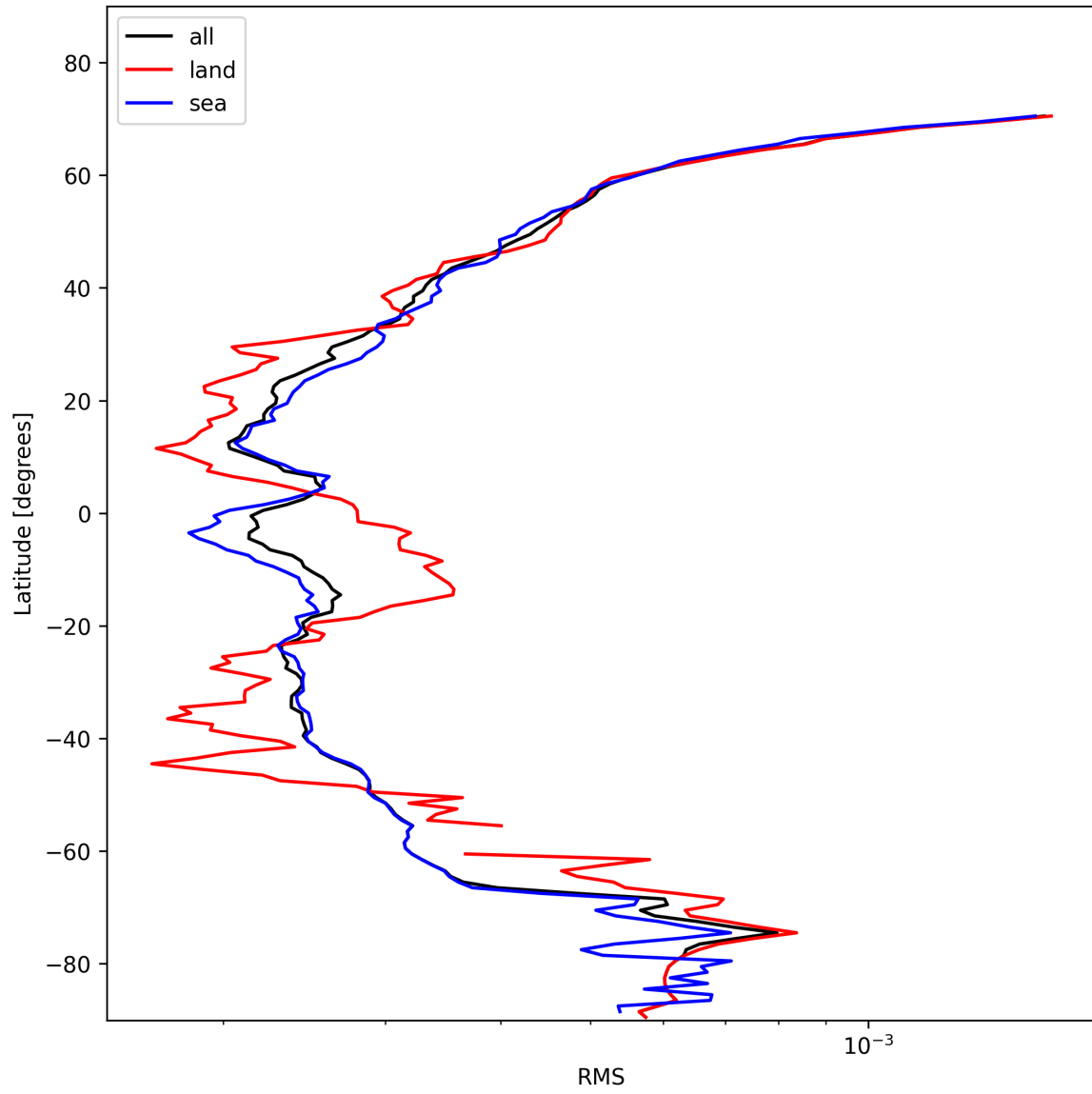
Figure 26: Zonal average of “RMS” for 2025-01-28 to 2025-01-30.
