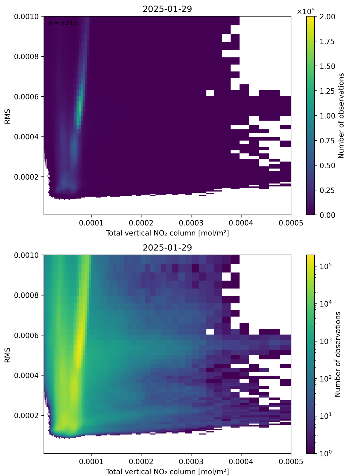
Figure 120: Scatter density plot of “Total vertical NO 2 column” against “RMS” for 2025-01-28 to 2025-01-30.
