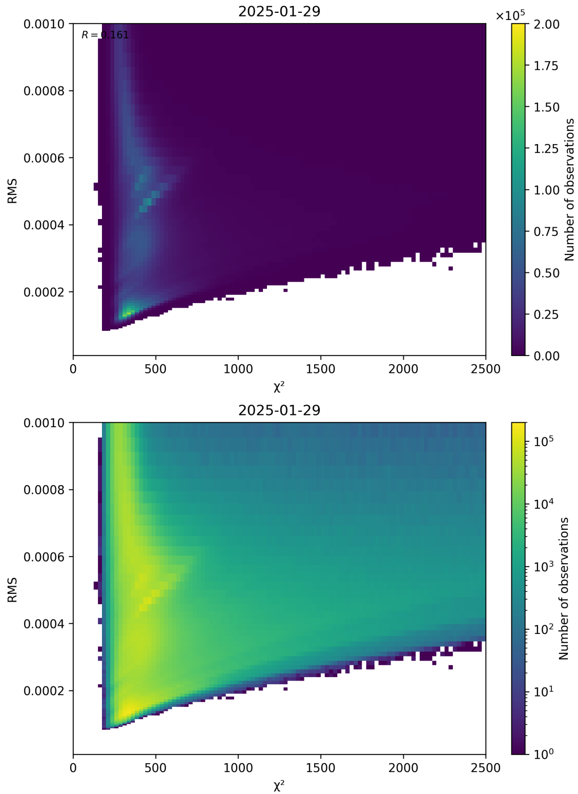
Figure 82: Scatter density plot of “ \chi^2 ” against “RMS” for 2025-01-28 to 2025-01-30.
