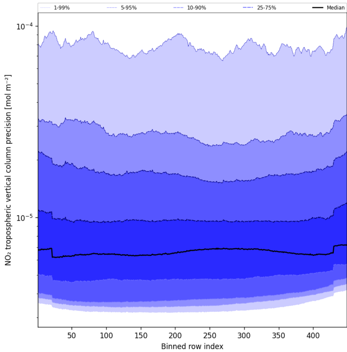
Figure 47: Along track statistics of “NO 2 tropospheric vertical column precision” for 2025-01-28 to 2025-01-30
