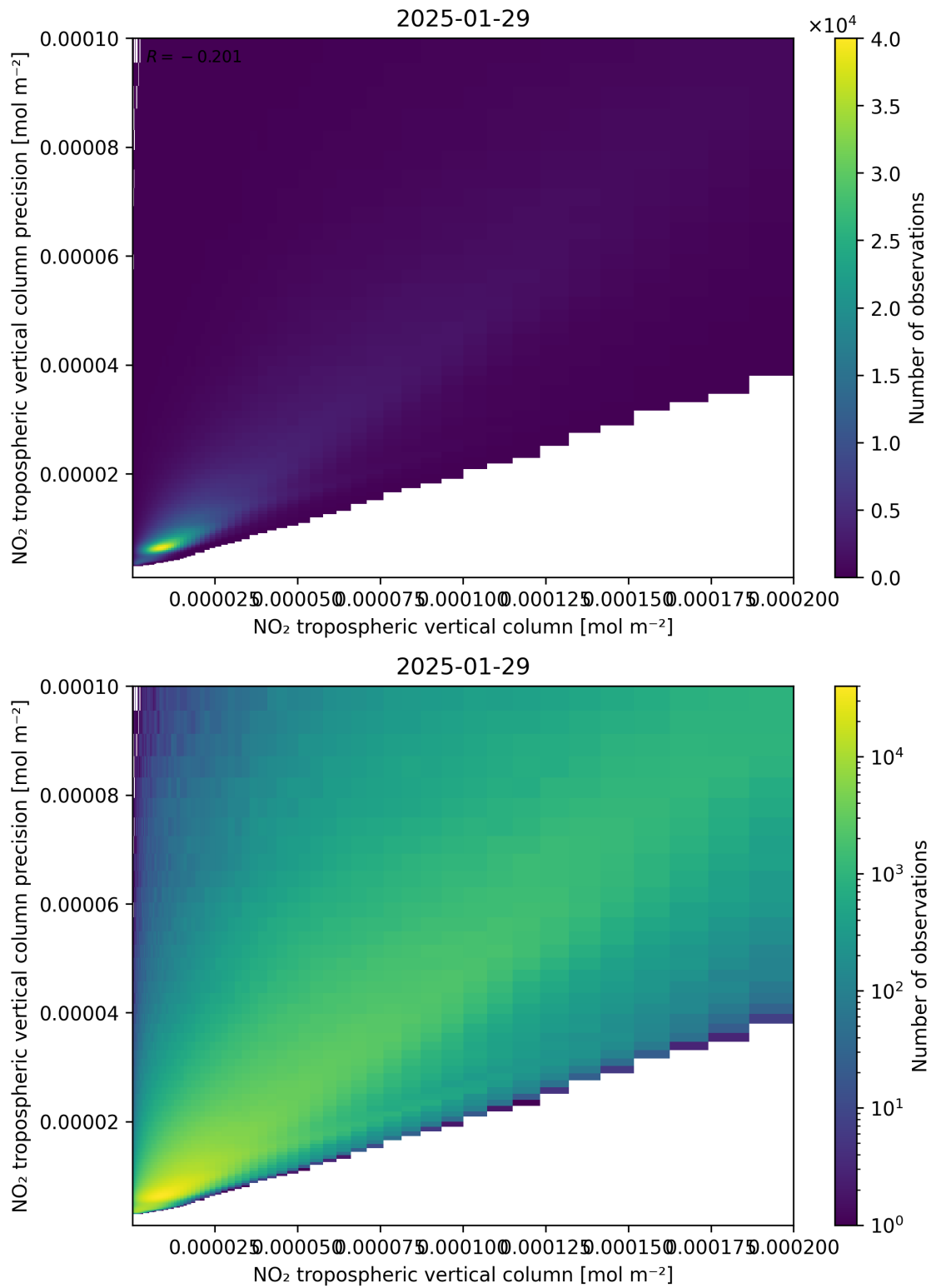
Figure 130: Scatter density plot of “NO 2 tropospheric vertical column” against “NO 2 tropospheric vertical column precision” for 2025-01-28 to 2025-01-30.
