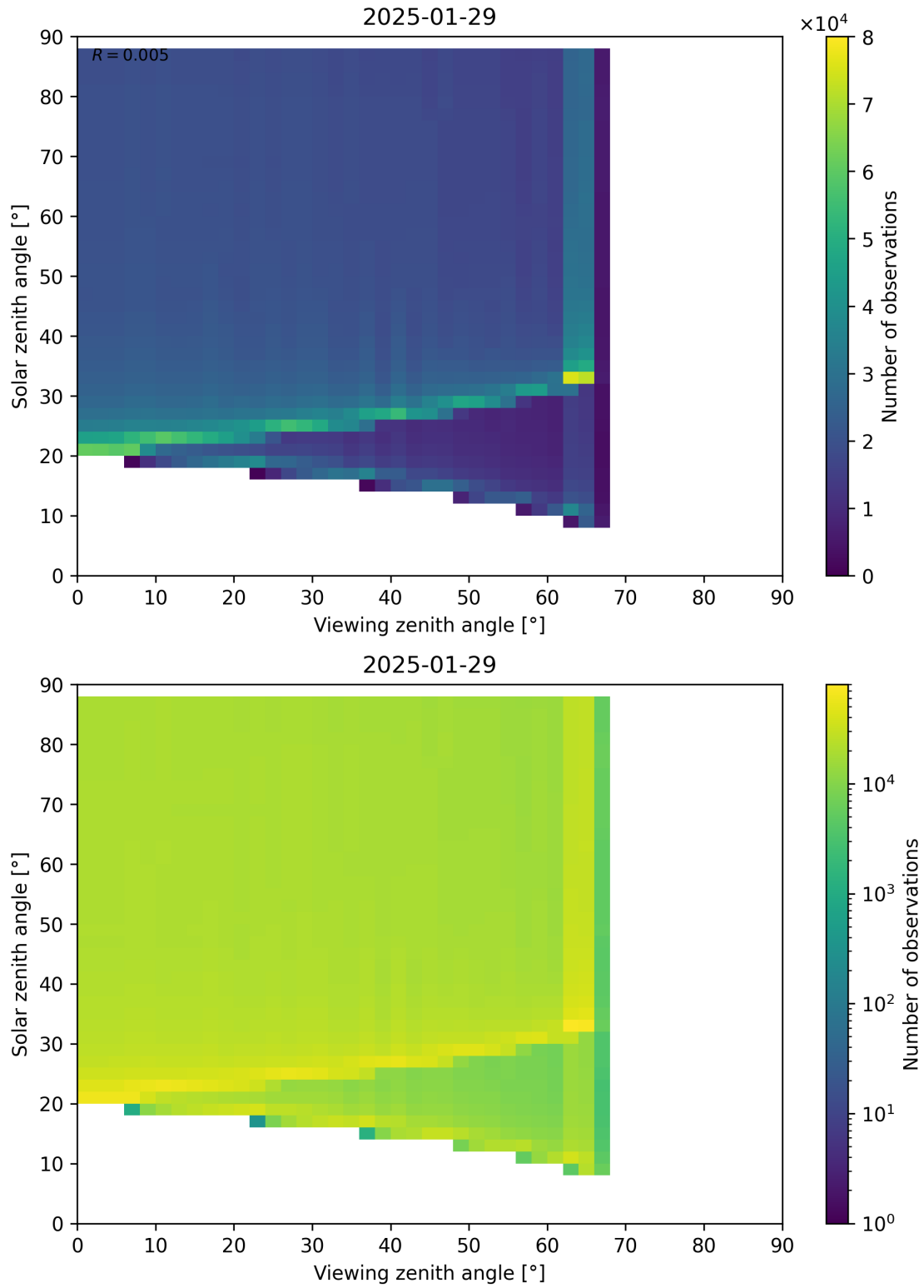
Figure 172: Scatter density plot of “Viewing zenith angle” against “Solar zenith angle” for 2025-01-28 to 2025-01-30.
