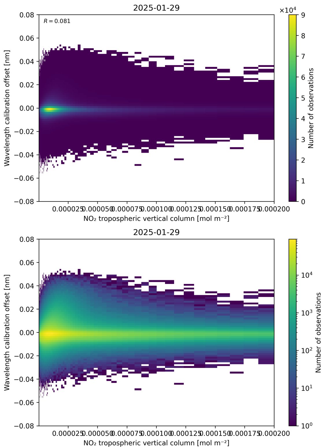
Figure 143: Scatter density plot of “NO 2 tropospheric vertical column” against “Wavelength calibration offset” for 2025-01-28 to 2025-01-30.
