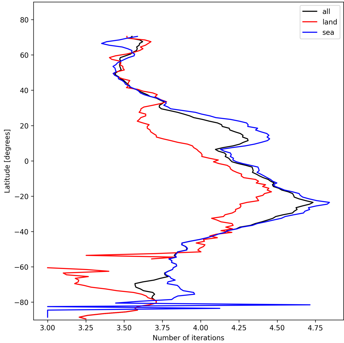
Figure 17: Zonal average of “Number of iterations” for 2025-01-28 to 2025-01-30.
