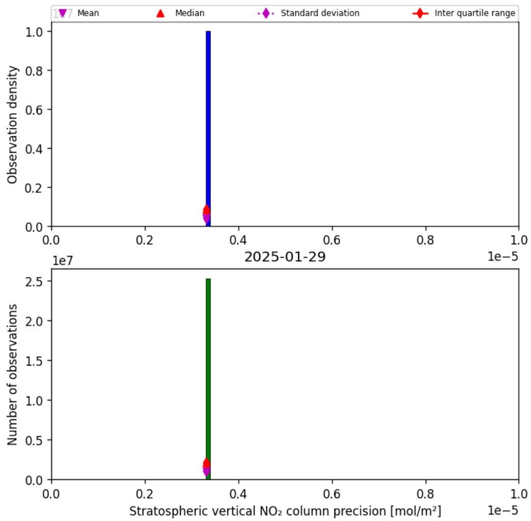
Figure 37: Histogram of “Stratospheric vertical NO 2 column precision” for 2025-01-28 to 2025-01-30
