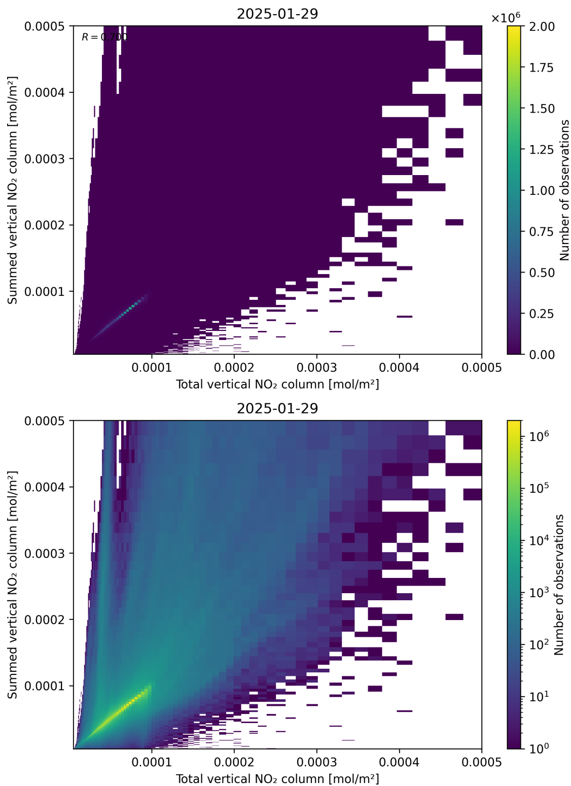
Figure 112: Scatter density plot of “Total vertical NO 2 column” against “Summed vertical NO 2 column” for 2025-01-28 to 2025-01-30.
