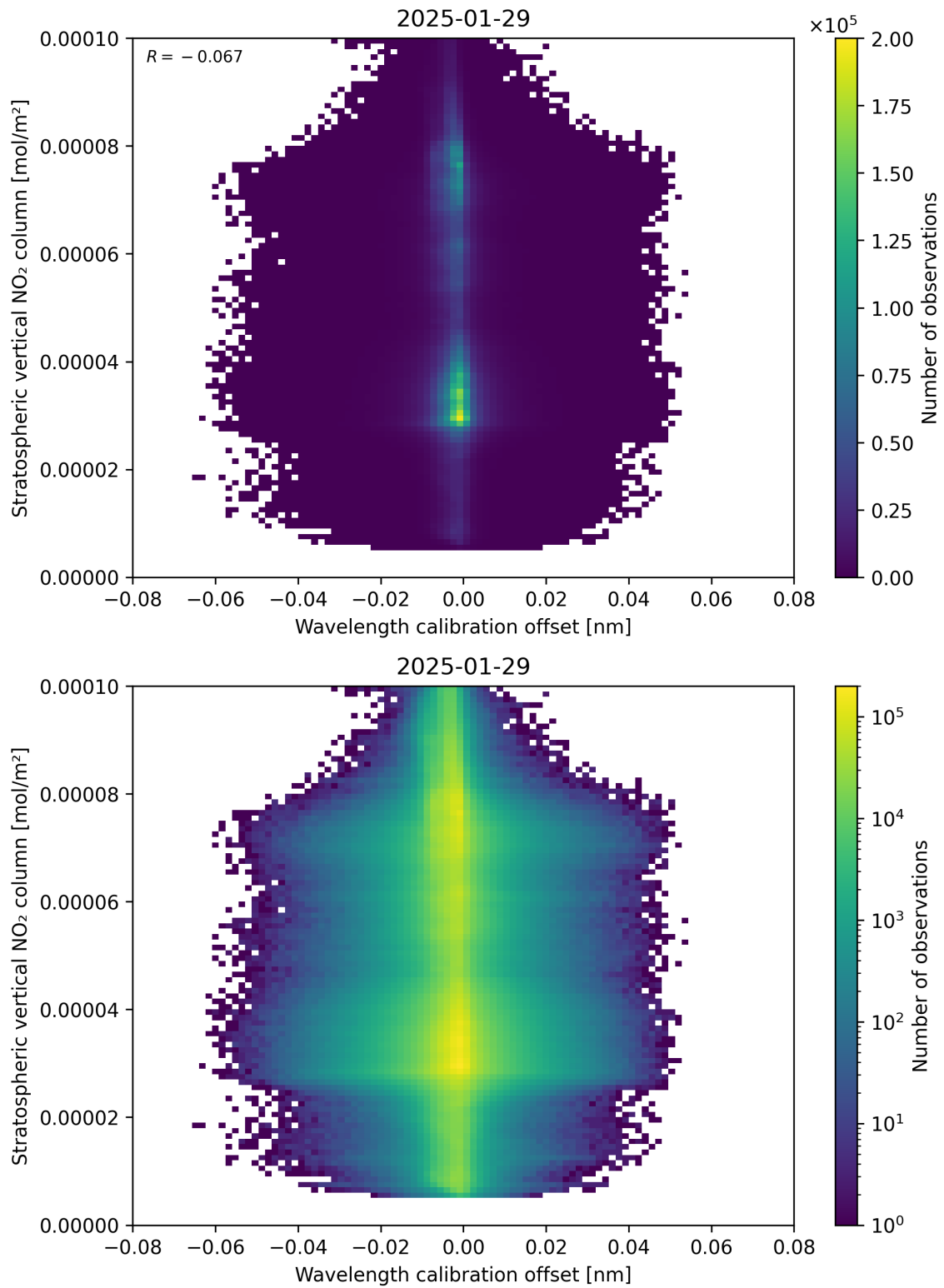
Figure 176: Scatter density plot of “Wavelength calibration offset” against “Stratospheric vertical NO 2 column” for 2025-01-28 to 2025-01-30.
