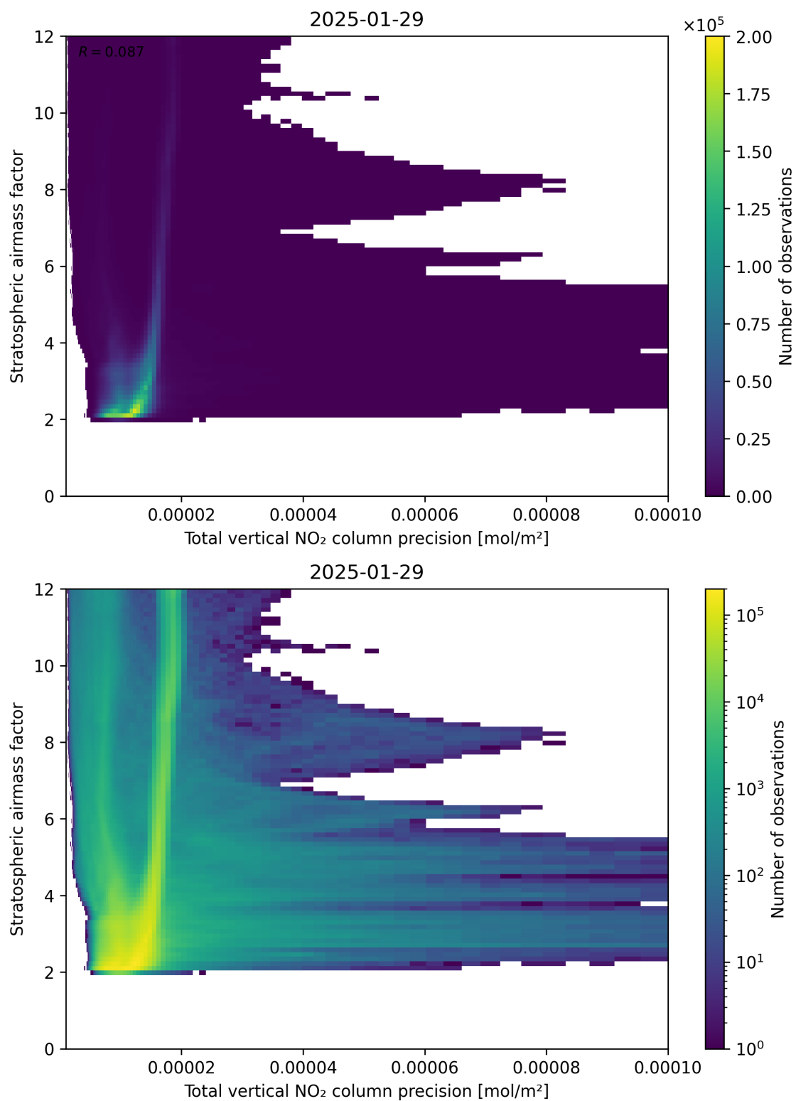
Figure 115: Scatter density plot of “Total vertical NO 2 column precision” against “Stratospheric air mass factor” for 2025-01-28 to 2025-01-30.
