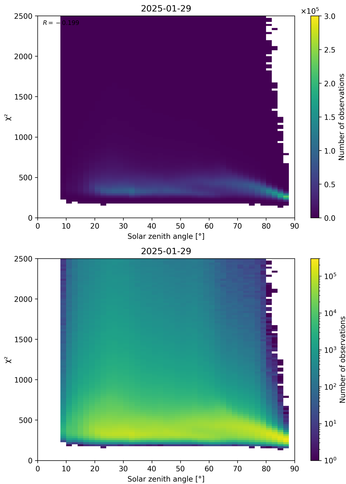
Figure 148: Scatter density plot of “Solar zenith angle” against “ \chi^2 ” for 2025-01-28 to 2025-01-30.
