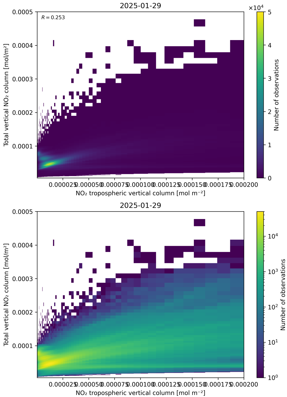
Figure 128: Scatter density plot of “NO 2 tropospheric vertical column” against “Total vertical NO 2 column” for 2025-01-28 to 2025-01-30.
