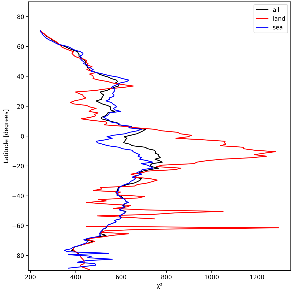
Figure 25: Zonal average of “ \chi^2 ” for 2025-01-28 to 2025-01-30.
