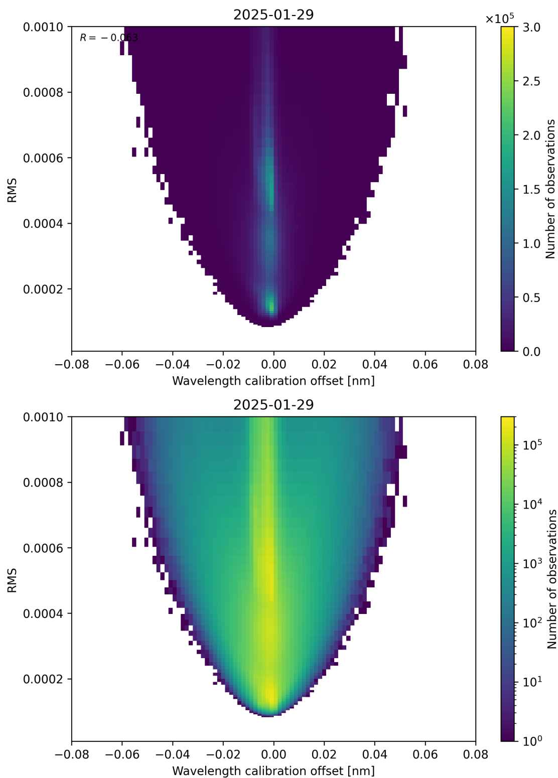
Figure 181: Scatter density plot of “Wavelength calibration offset” against “RMS” for 2025-01-28 to 2025-01-30.
