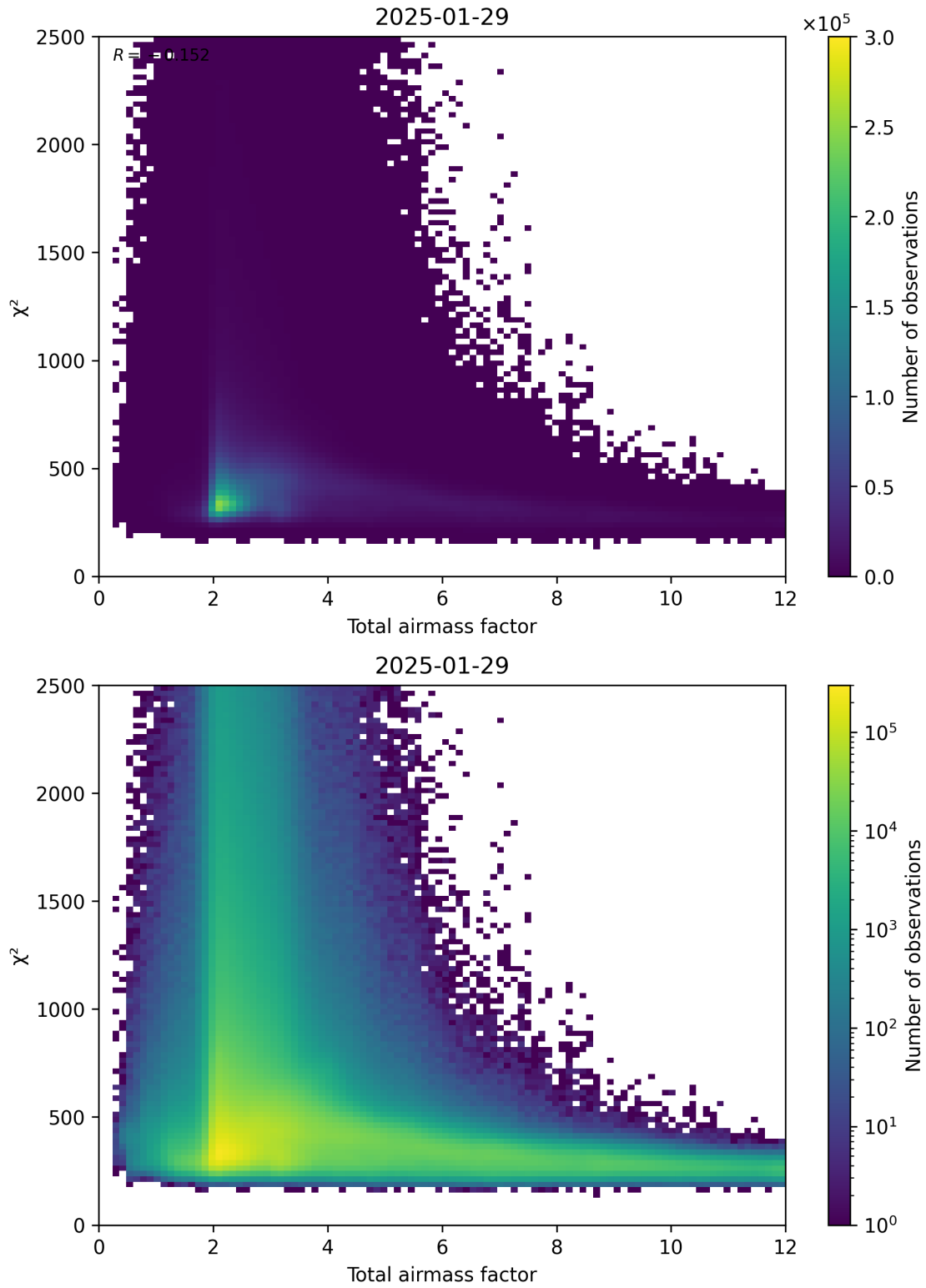
Figure 63: Scatter density plot of “Total airmass factor” against “ \chi^2 ” for 2025-01-28 to 2025-01-30.
