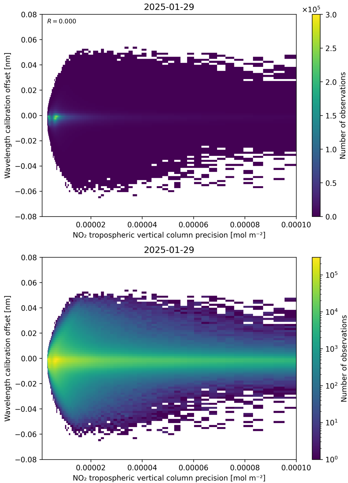
Figure 141: Scatter density plot of “NO 2 tropospheric vertical column precision” against “Wavelength calibration offset” for 2025-01-28 to 2025-01-30.
