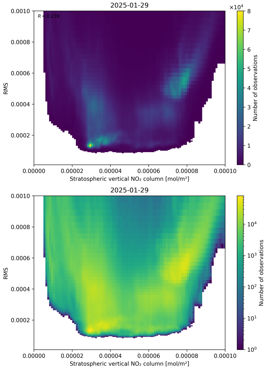
Figure 102: Scatter density plot of “Stratospheric vertical NO 2 column” against “RMS” for 2025-01-28 to 2025-01-30.
