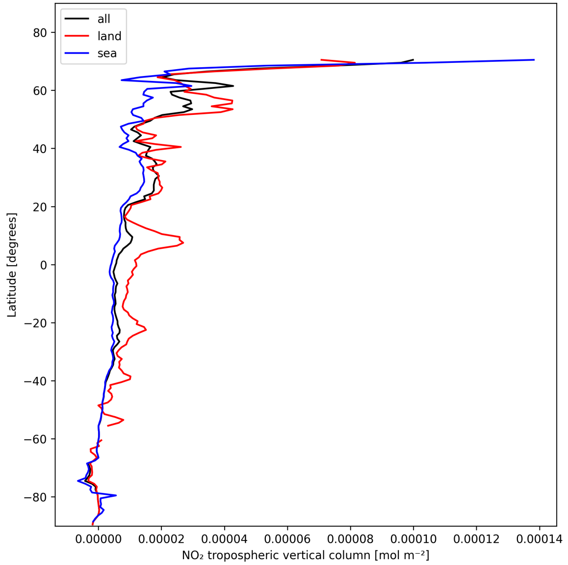
Figure 12: Zonal average of “NO 2 tropospheric vertical column” for 2025-01-28 to 2025-01-30.
