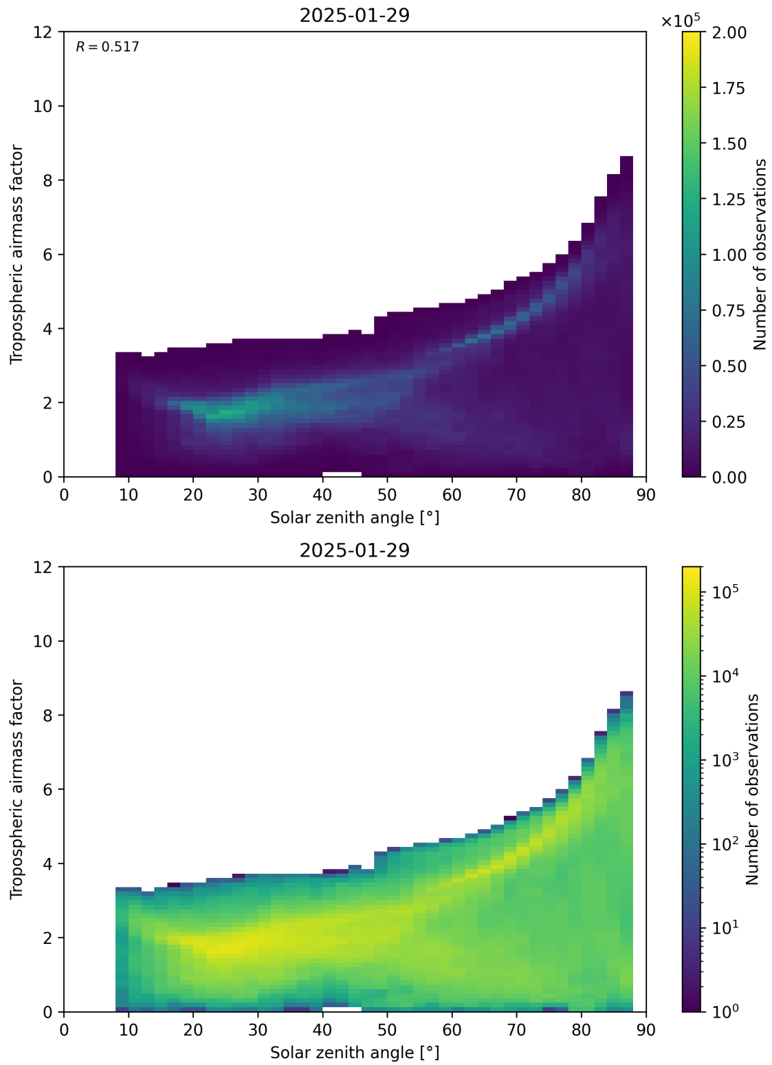
Figure 147: Scatter density plot of “Solar zenith angle” against “Tropospheric airmass factor” for 2025-01-28 to 2025-01-30.
