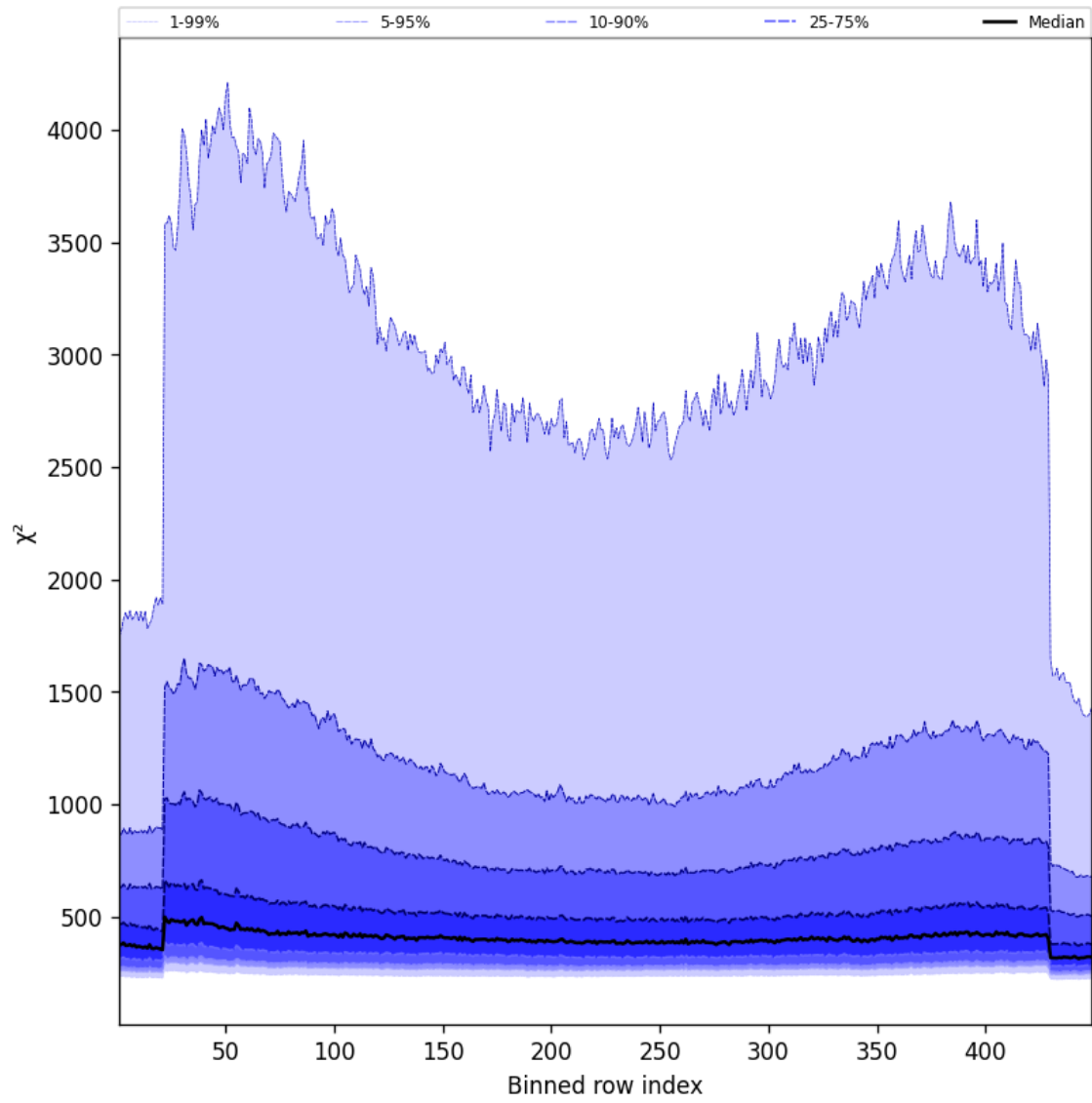
Figure 59: Along track statistics of “ \chi^2 ” for 2025-01-28 to 2025-01-30
