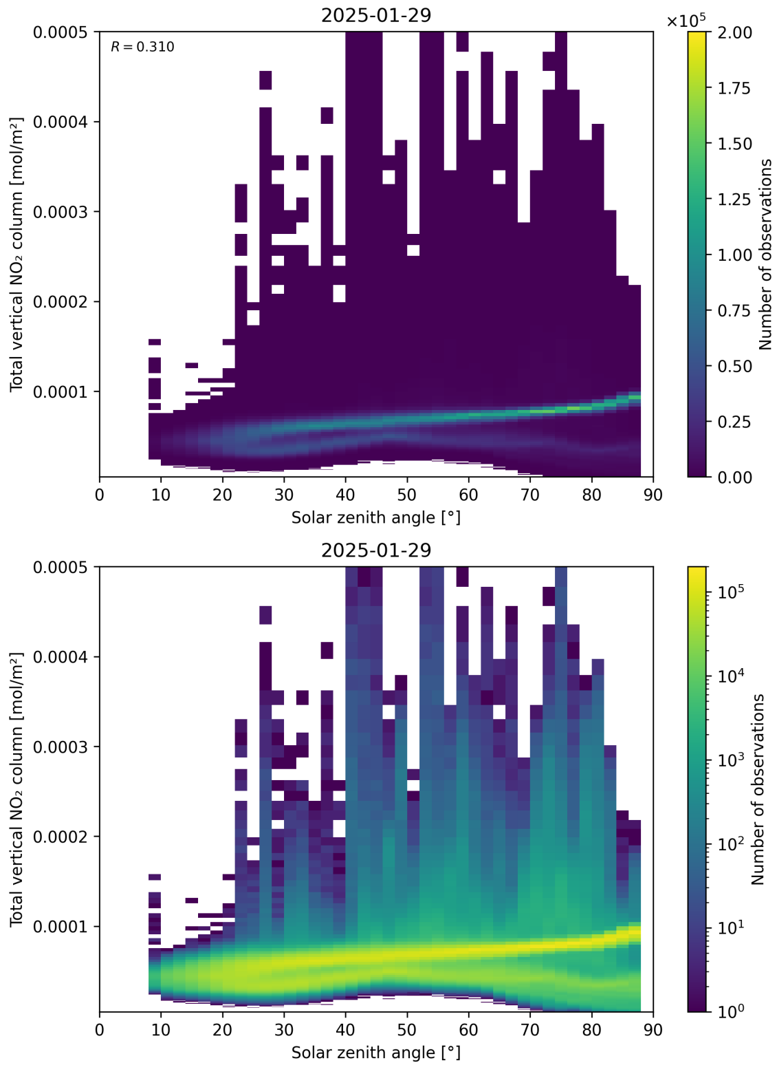
Figure 153: Scatter density plot of “Solar zenith angle” against “Total vertical NO 2 column” for 2025-01-28 to 2025-01-30.
