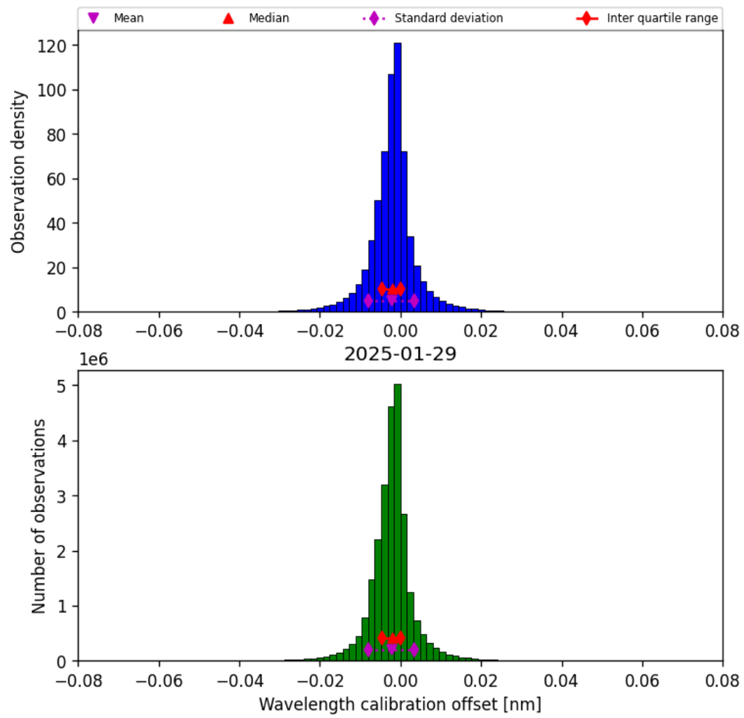
Figure 35: Histogram of “Wavelength calibration offset” for 2025-01-28 to 2025-01-30
