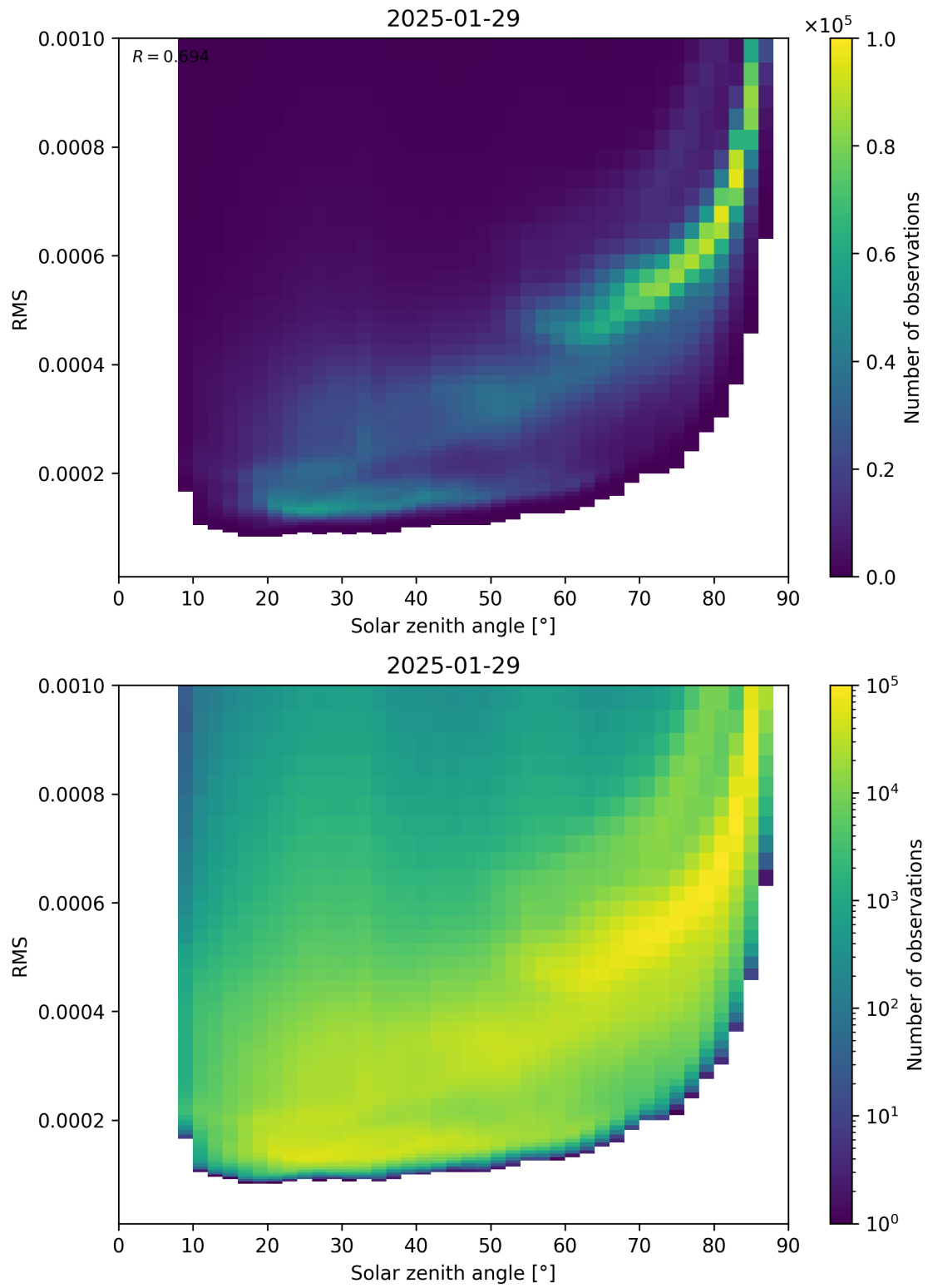
Figure 157: Scatter density plot of “Solar zenith angle” against “RMS” for 2025-01-28 to 2025-01-30.
