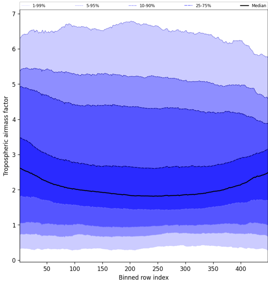
Figure 48: Along track statistics of “Tropospheric airmass factor” for 2025-01-28 to 2025-01-30
