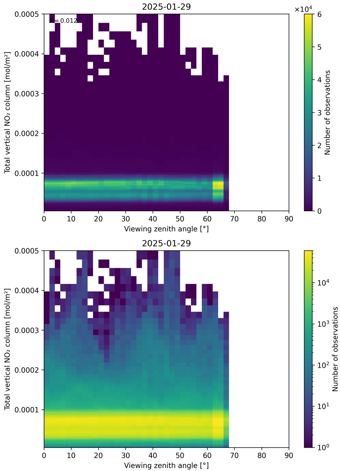
Figure 167: Scatter density plot of “Viewing zenith angle” against “Total vertical NO 2 column” for 2025-01-28 to 2025-01-30.
