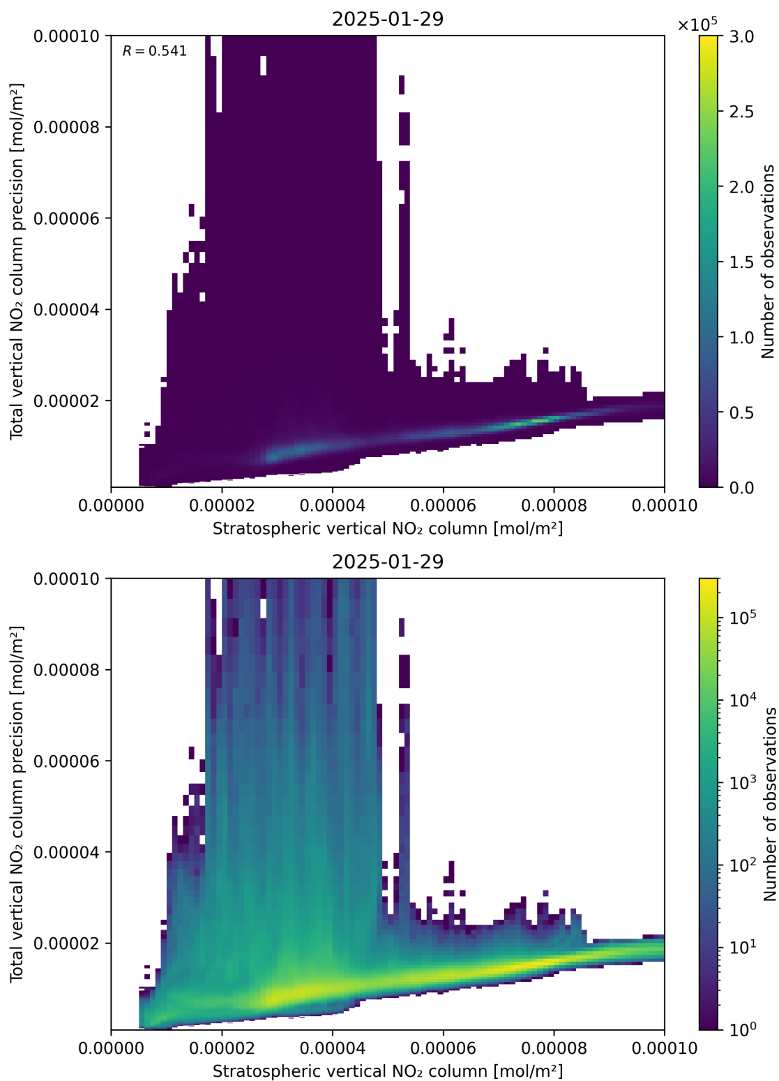
Figure 101: Scatter density plot of “Stratospheric vertical NO 2 column” against “Total vertical NO 2 column precision” for 2025-01-28 to 2025-01-30.
