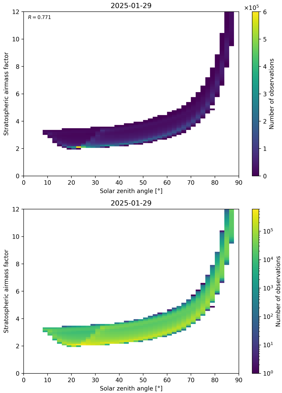
Figure 145: Scatter density plot of “Solar zenith angle” against “Stratospheric airmass factor” for 2025-01-28 to 2025-01-30.
