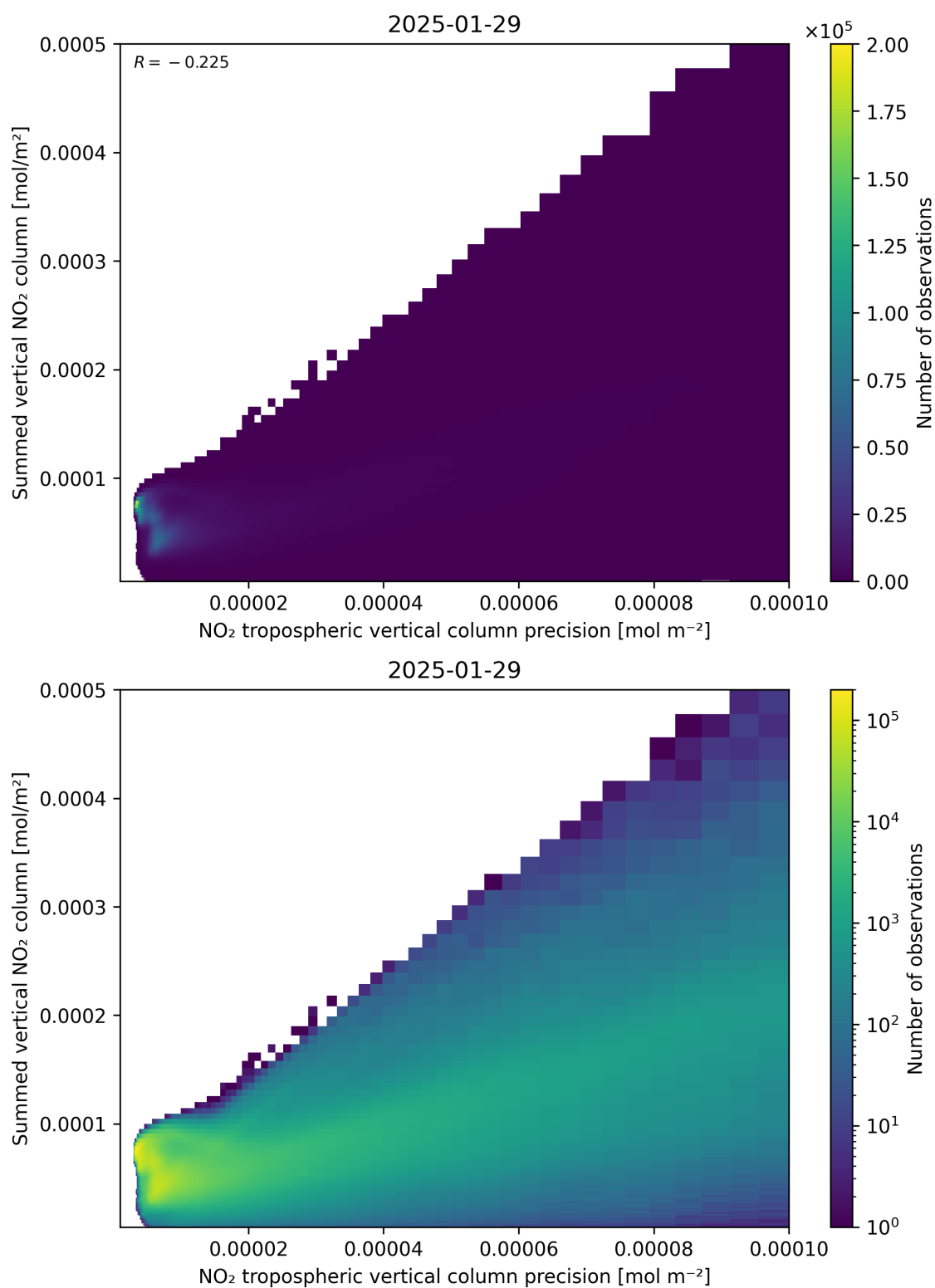
Figure 136: Scatter density plot of “NO 2 tropospheric vertical column precision” against “Summed vertical NO 2 column” for 2025-01-28 to 2025-01-30.
