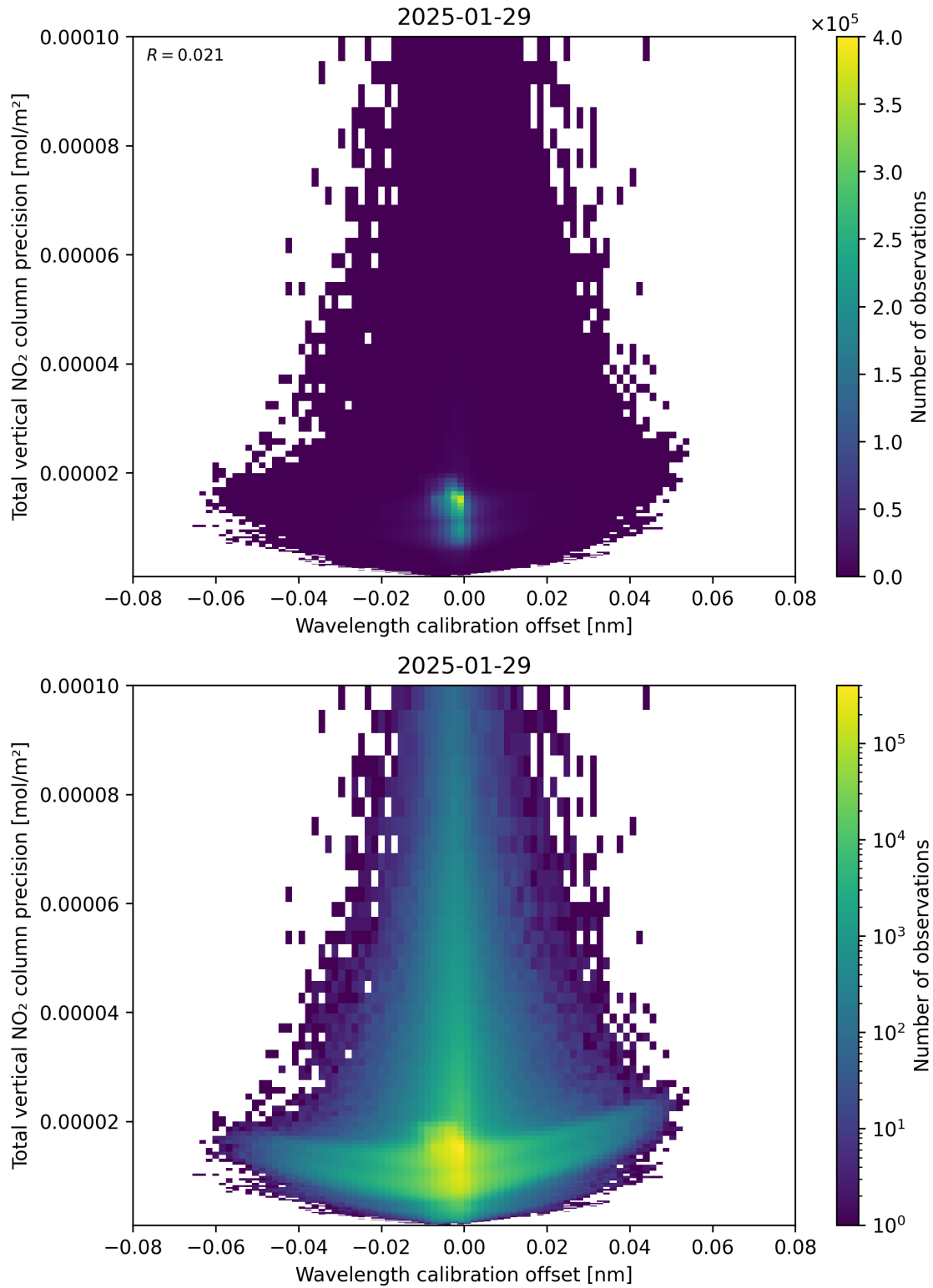
Figure 180: Scatter density plot of “Wavelength calibration offset” against “Total vertical NO 2 column precision” for 2025-01-28 to 2025-01-30.
