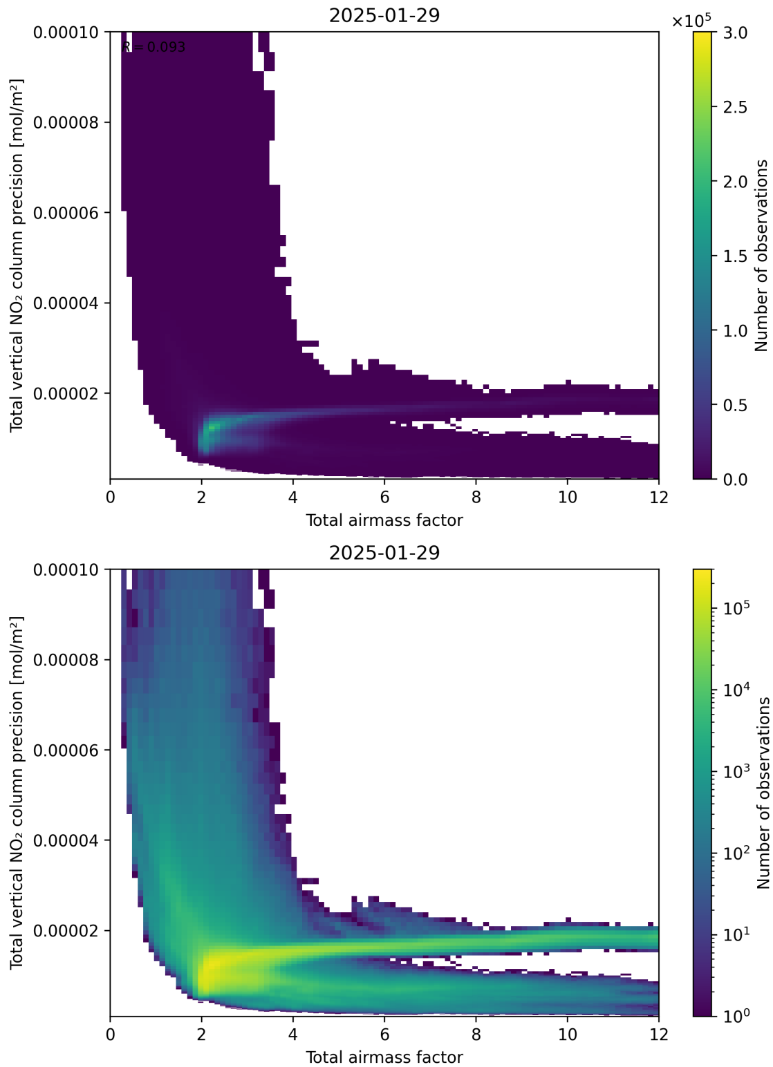
Figure 68: Scatter density plot of “Total airmass factor” against “Total vertical NO 2 column precision” for 2025-01-28 to 2025-01-30.
