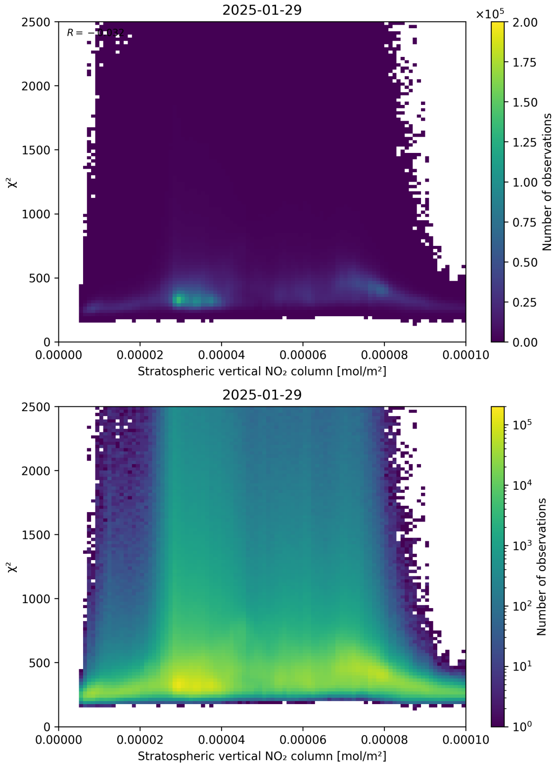
Figure 97: Scatter density plot of “Stratospheric vertical NO 2 column” against “ \chi^2 ” for 2025-01-28 to 2025-01-30.
