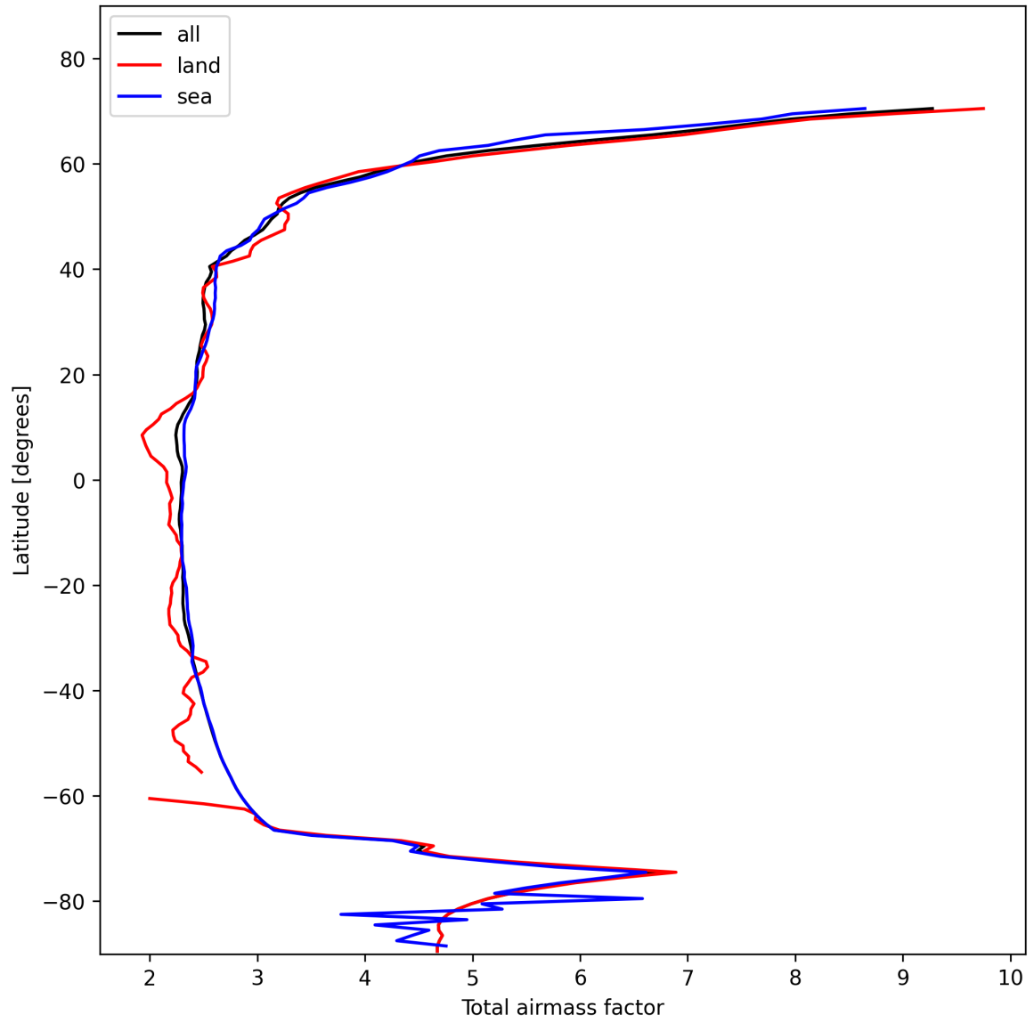
Figure 15: Zonal average of “Total airmass factor” for 2025-01-28 to 2025-01-30.
