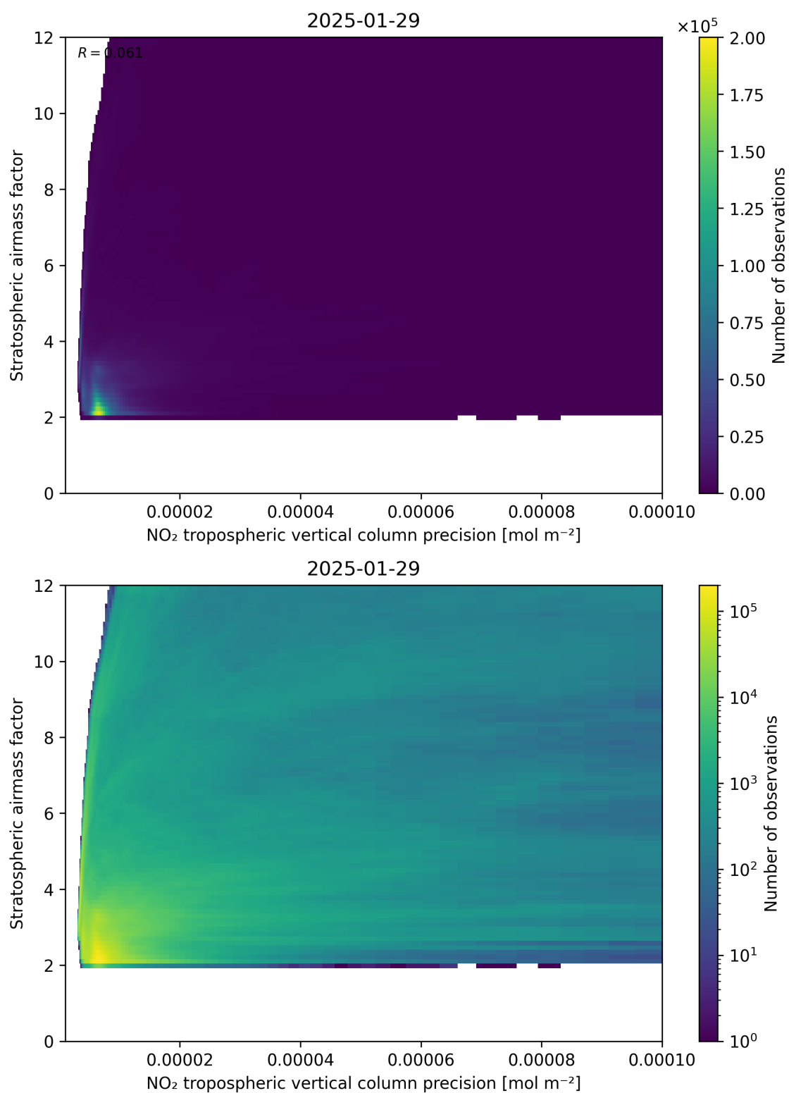
Figure 131: Scatter density plot of “NO 2 tropospheric vertical column precision” against “Stratospheric airmass factor” for 2025-01-28 to 2025-01-30.
