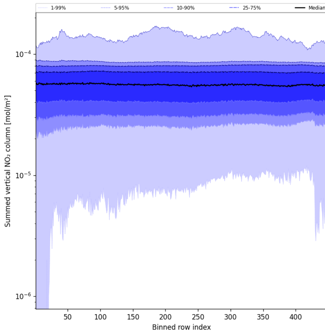
Figure 57: Along track statistics of “Summed vertical NO 2 column” for 2025-01-28 to 2025-01-30
