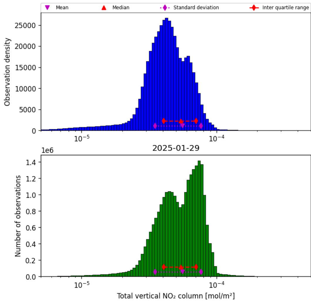
Figure 38: Histogram of “Total vertical NO 2 column” for 2025-01-28 to 2025-01-30
