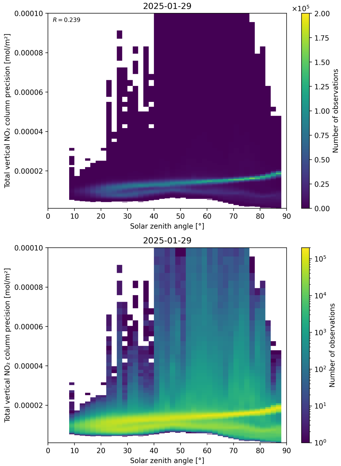
Figure 154: Scatter density plot of “Solar zenith angle” against “Total vertical NO 2 column precision” for 2025-01-28 to 2025-01-30.
