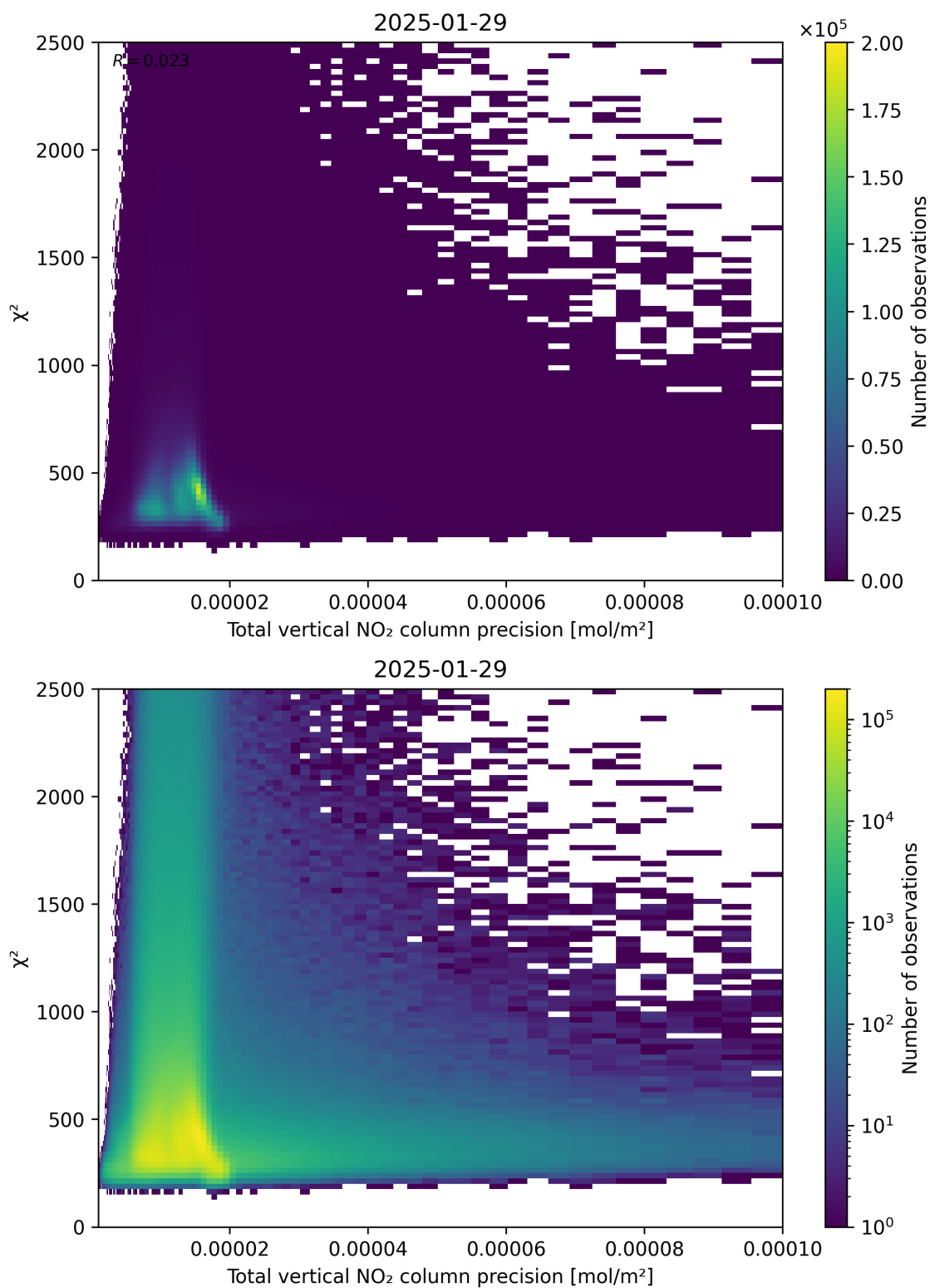
Figure 116: Scatter density plot of “Total vertical NO 2 column precision” against “ \chi^2 ” for 2025-01-28 to 2025-01-30.
