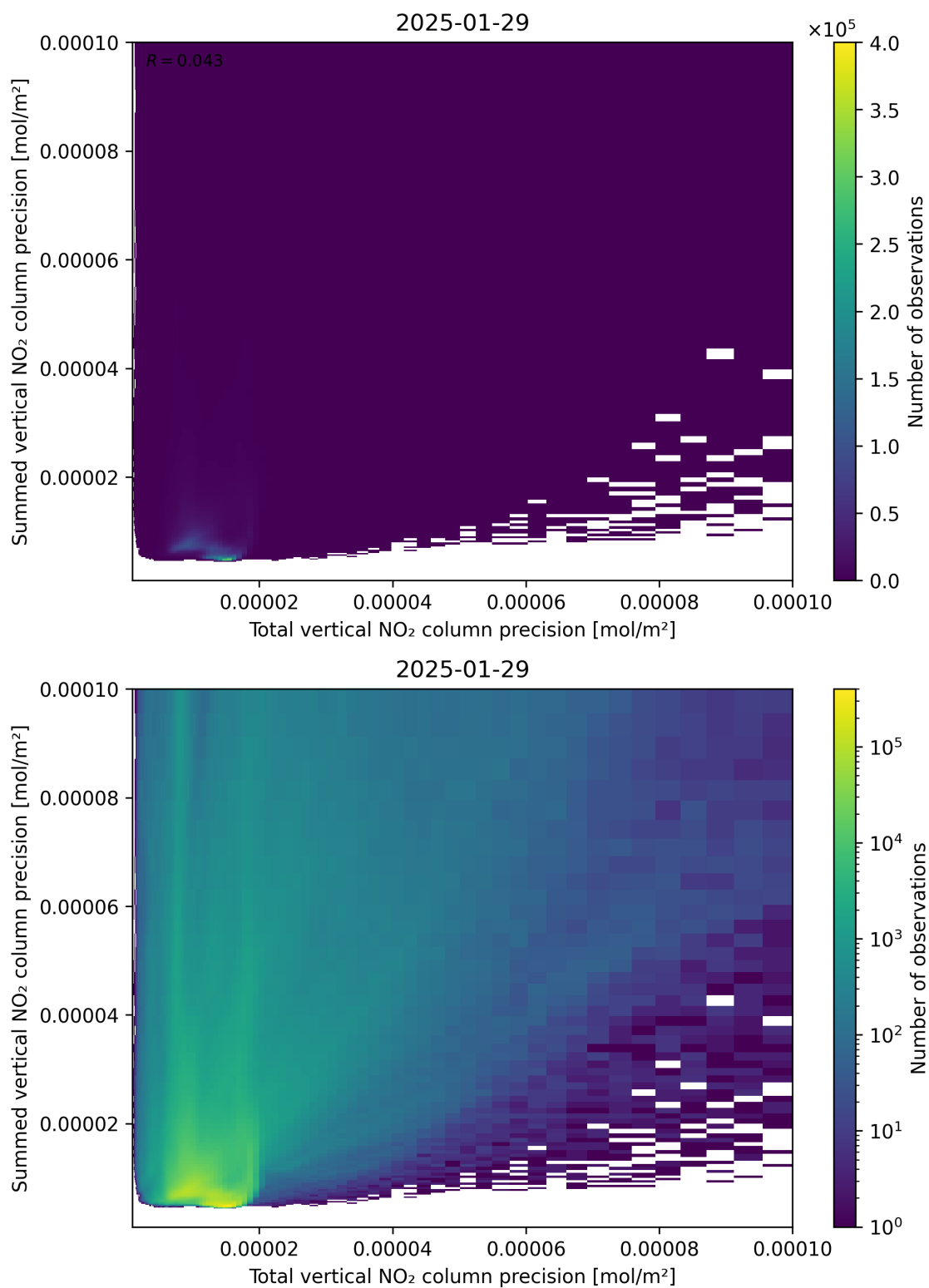
Figure 118: Scatter density plot of “Total vertical NO 2 column precision” against “Summed vertical NO 2 column precision” for 2025-01-28 to 2025-01-30.
