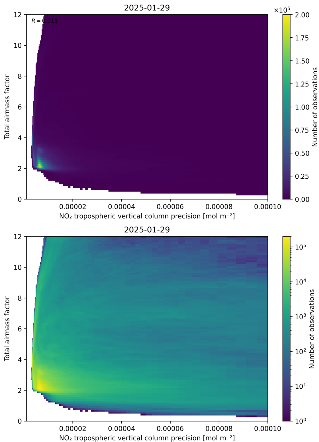
Figure 132: Scatter density plot of “NO 2 tropospheric vertical column precision” against “Total air mass factor” for 2025-01-28 to 2025-01-30.
