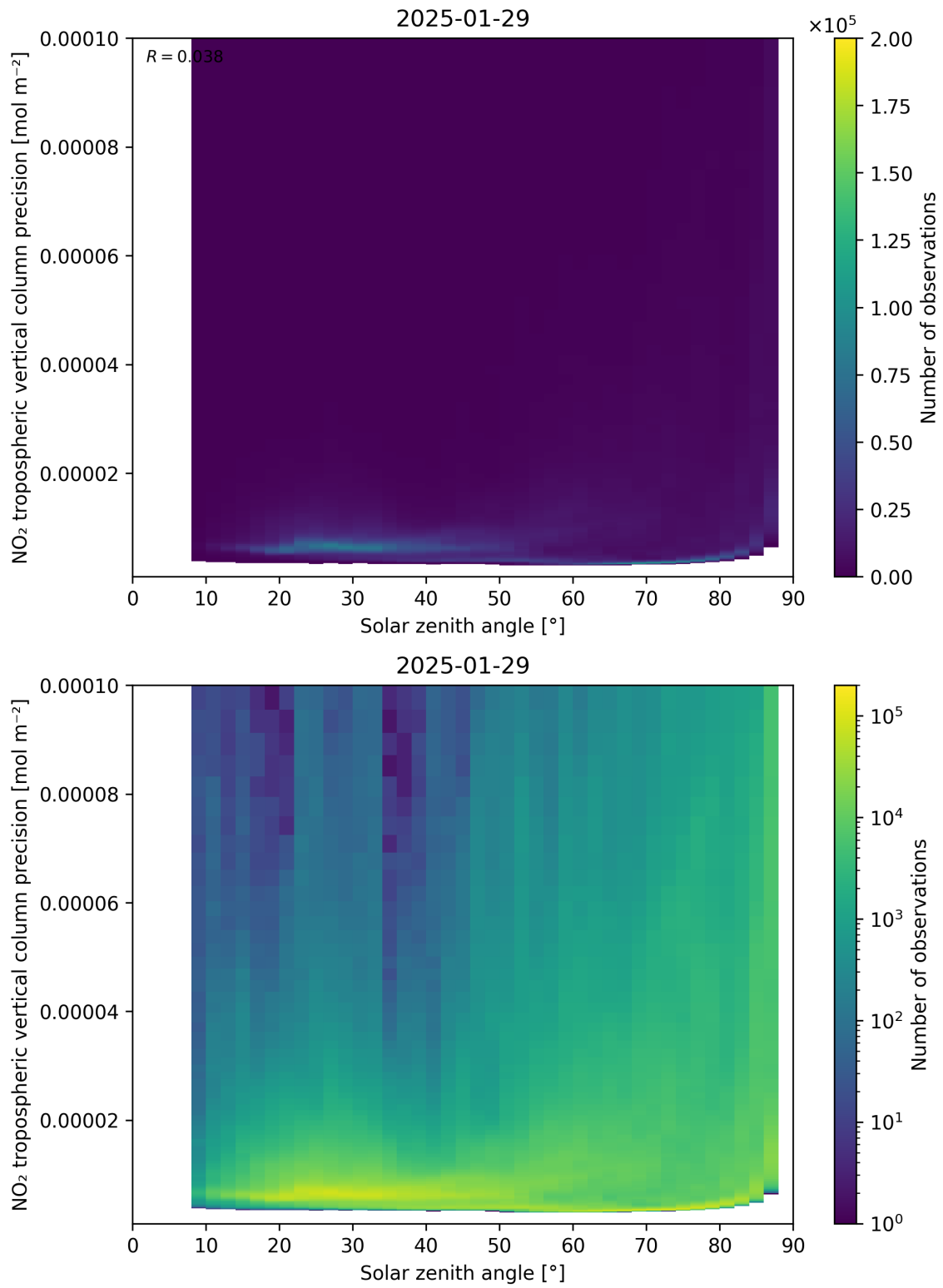
Figure 156: Scatter density plot of “Solar zenith angle” against “NO 2 tropospheric vertical column precision” for 2025-01-28 to 2025-01-30.
