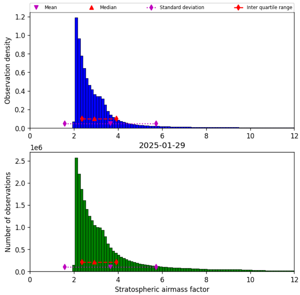
Figure 44: Histogram of “Stratospheric airmass factor” for 2025-01-28 to 2025-01-30
