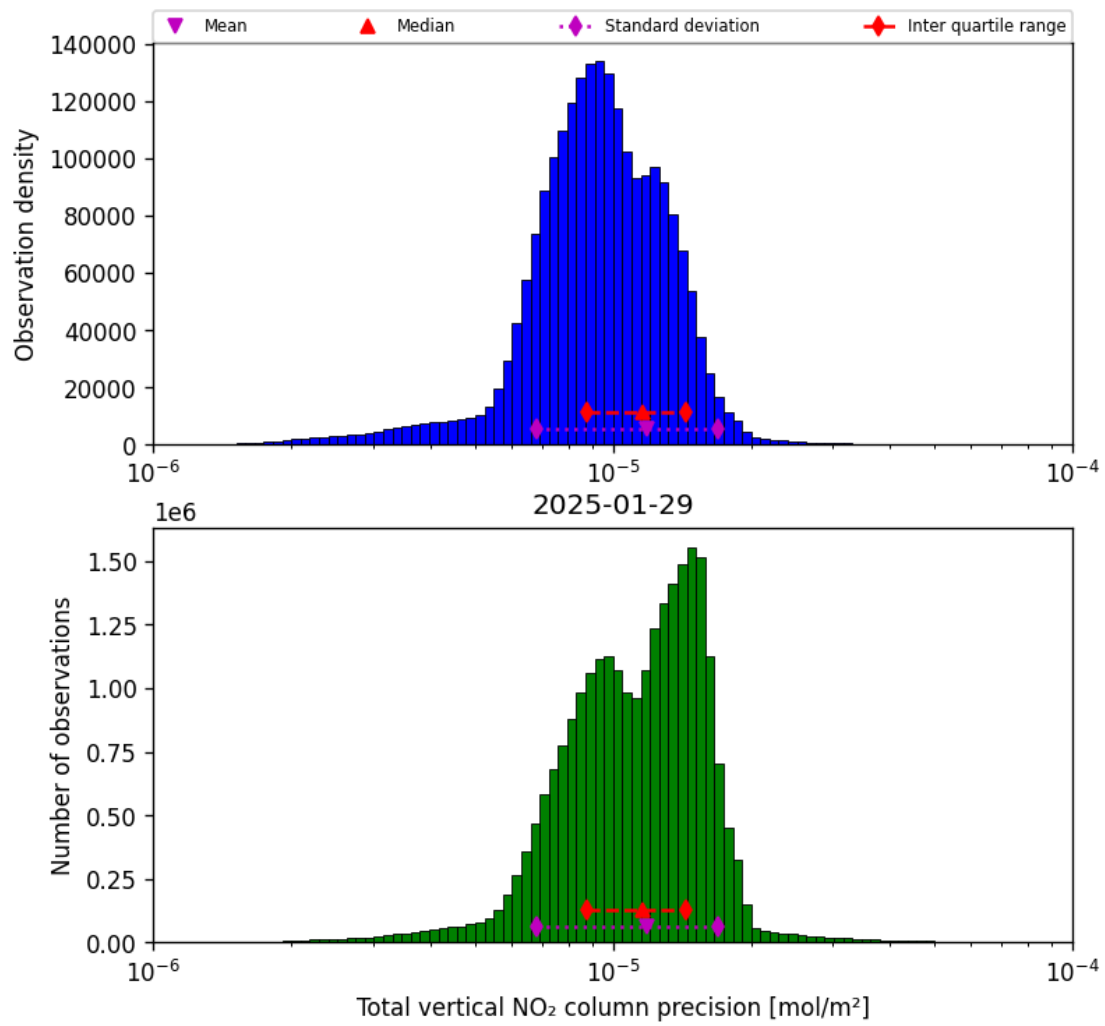
Figure 39: Histogram of “Total vertical NO 2 column precision” for 2025-01-28 to 2025-01-30
