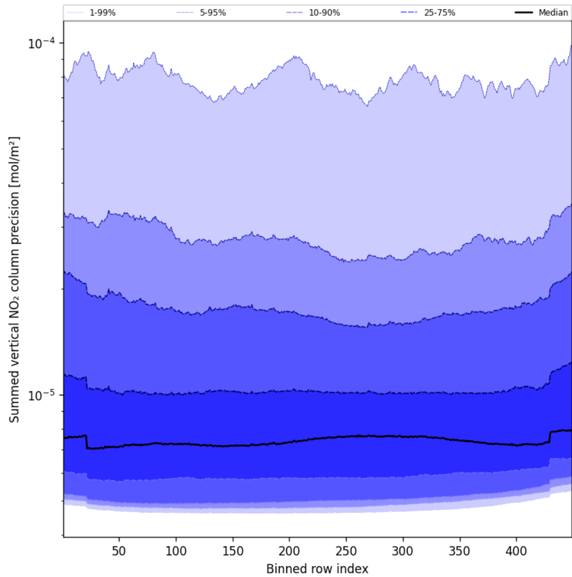
Figure 58: Along track statistics of “Summed vertical NO 2 column precision” for 2025-01-28 to 2025-01-30
