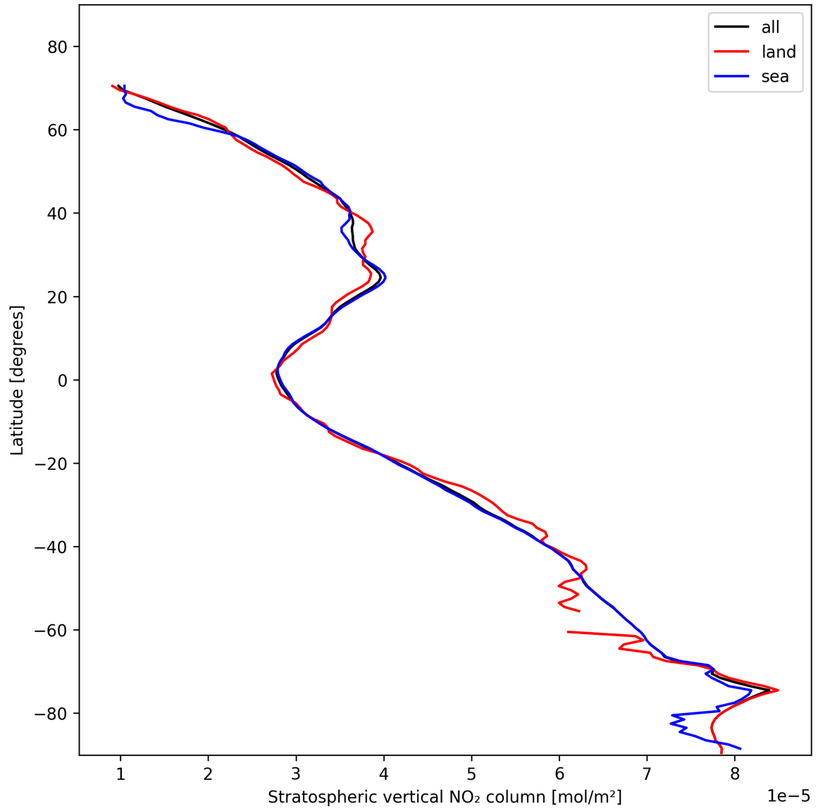
Figure 19: Zonal average of “Stratospheric vertical NO 2 column” for 2025-01-28 to 2025-01-30.
