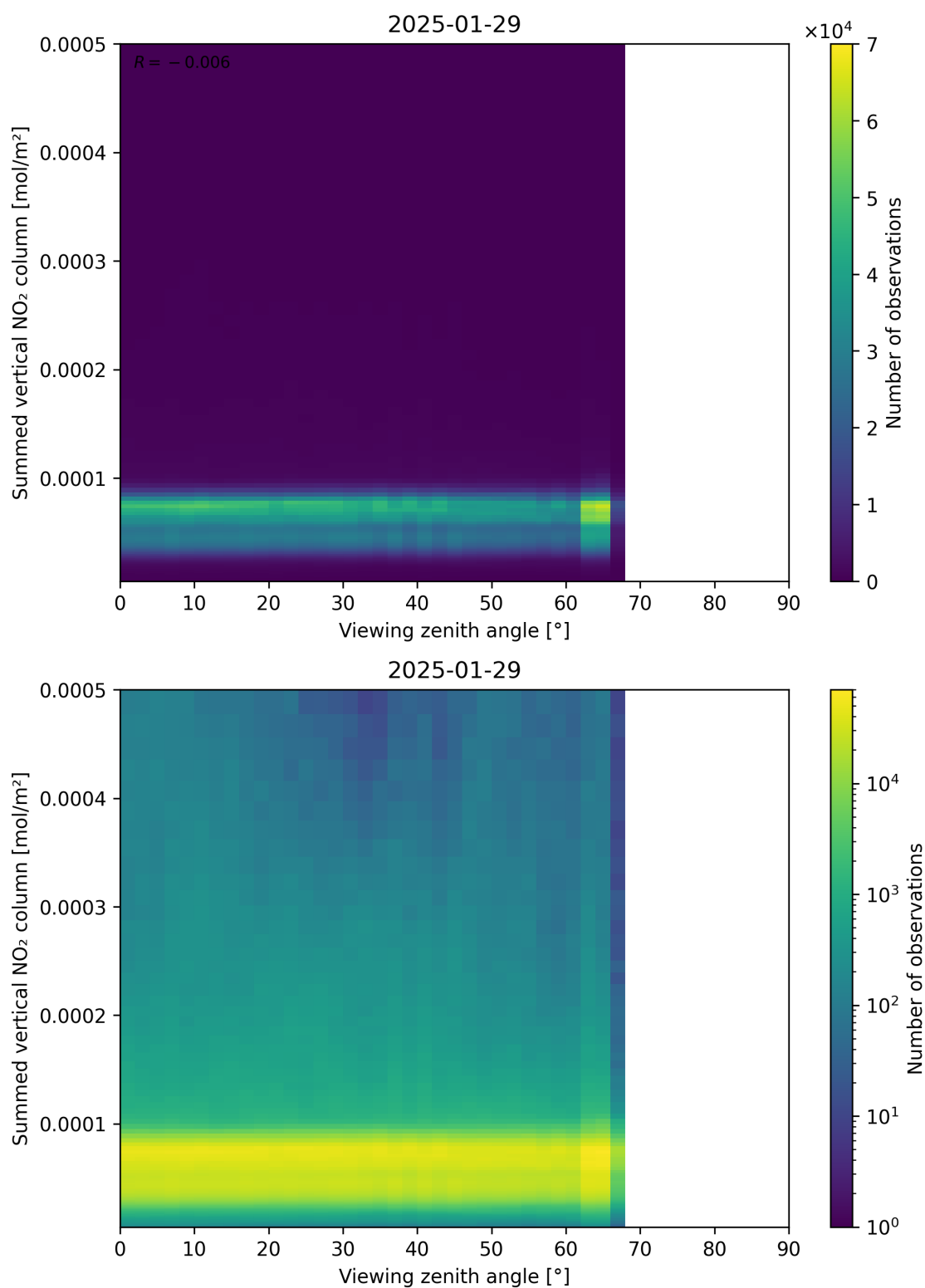
Figure 165: Scatter density plot of “Viewing zenith angle” against “Summed vertical NO 2 column” for 2025-01-28 to 2025-01-30.
