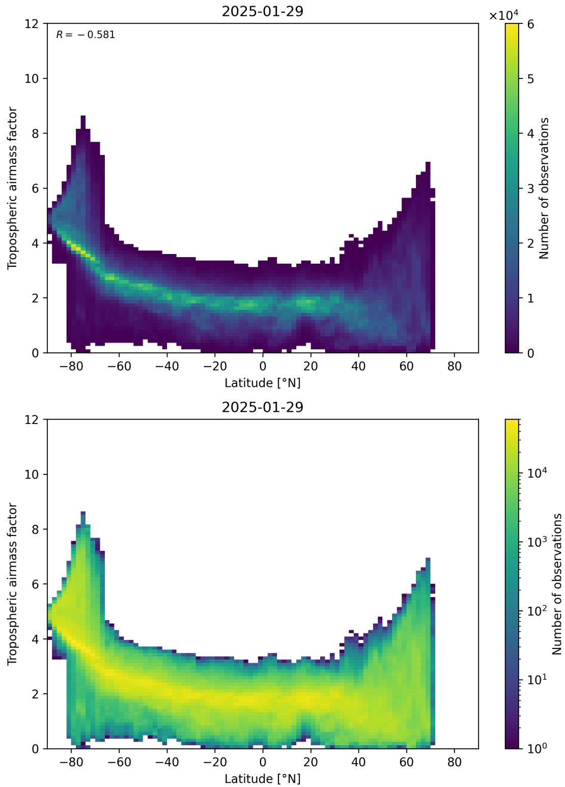
Figure 85: Scatter density plot of “Latitude” against “Tropospheric airmass factor” for 2025-01-28 to 2025-01-30.
