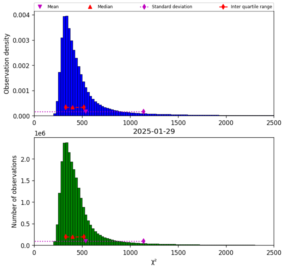
Figure 42: Histogram of “ \chi^2 ” for 2025-01-28 to 2025-01-30
