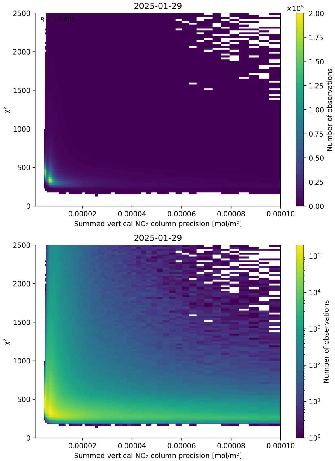
Figure 107: Scatter density plot of “Summed vertical NO 2 column precision” against “ \chi^2 ” for 2025-01-28 to 2025-01-30.
