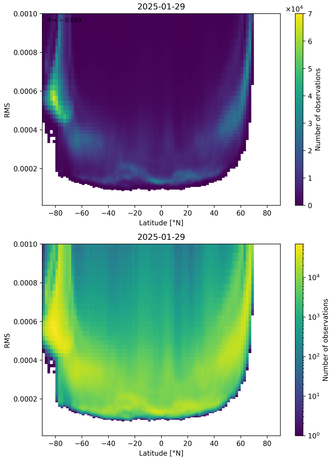
Figure 94: Scatter density plot of “Latitude” against “RMS” for 2025-01-28 to 2025-01-30.
