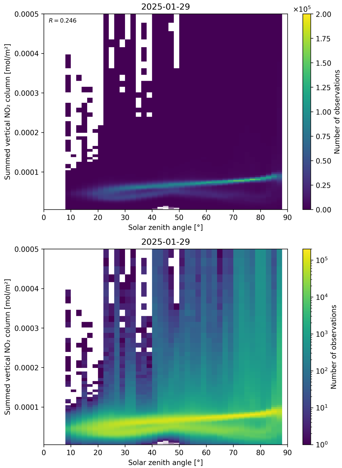
Figure 151: Scatter density plot of “Solar zenith angle” against “Summed vertical NO 2 column” for 2025-01-28 to 2025-01-30.
