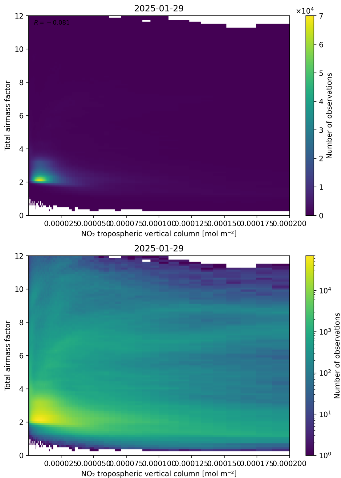
Figure 122: Scatter density plot of “NO 2 tropospheric vertical column” against “Total air mass factor” for 2025-01-28 to 2025-01-30.
