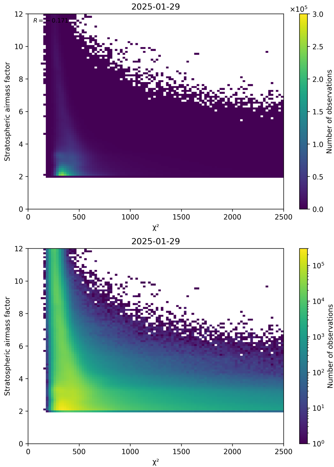
Figure 81: Scatter density plot of “ \chi^2 ” against “Stratospheric airmass factor” for 2025-01-28 to 2025-01-30.
