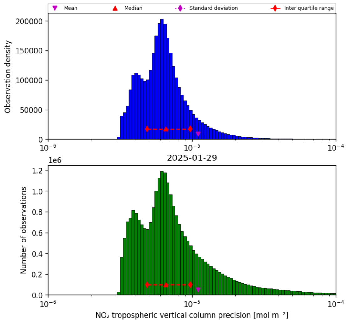
Figure 30: Histogram of “NO 2 tropospheric vertical column precision” for 2025-01-28 to 2025-01-30
