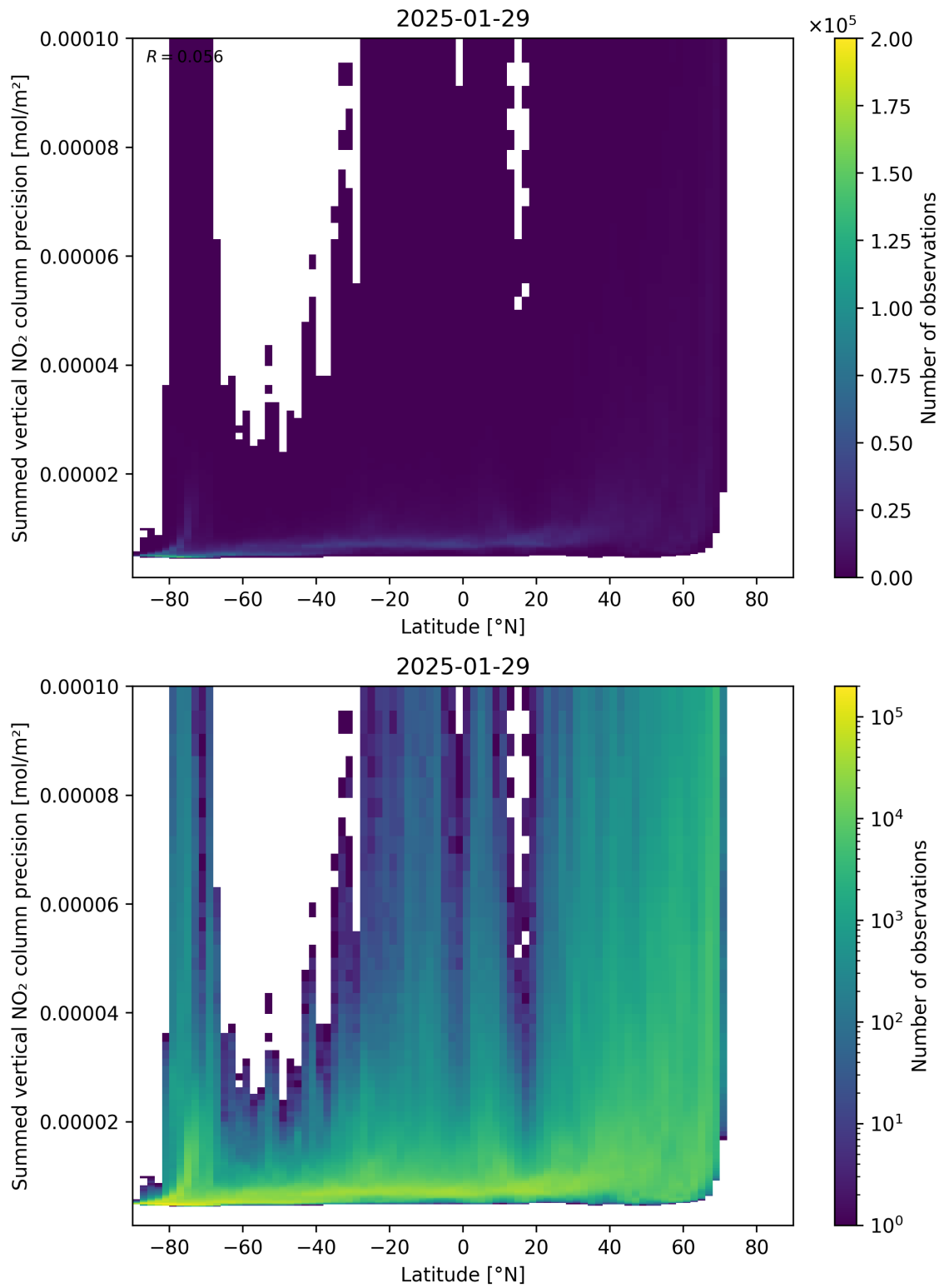
Figure 89: Scatter density plot of “Latitude” against “Summed vertical NO 2 column precision” for 2025-01-28 to 2025-01-30.
