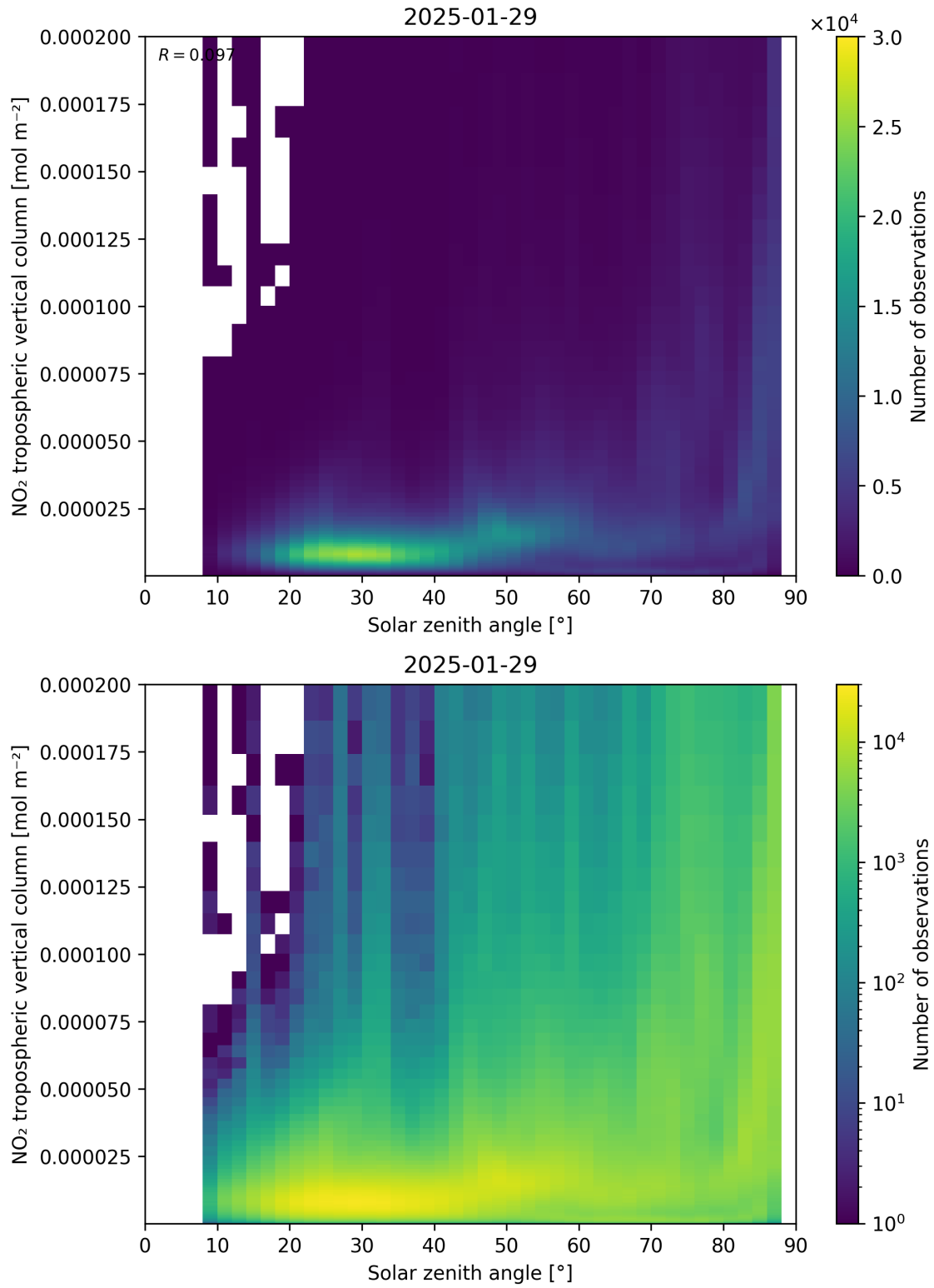
Figure 155: Scatter density plot of “Solar zenith angle” against “NO 2 tropospheric vertical column” for 2025-01-28 to 2025-01-30.
