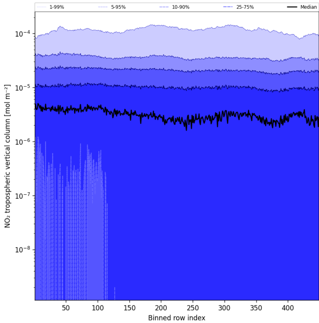
Figure 46: Along track statistics of “NO 2 tropospheric vertical column” for 2025-01-28 to 2025-01-30
