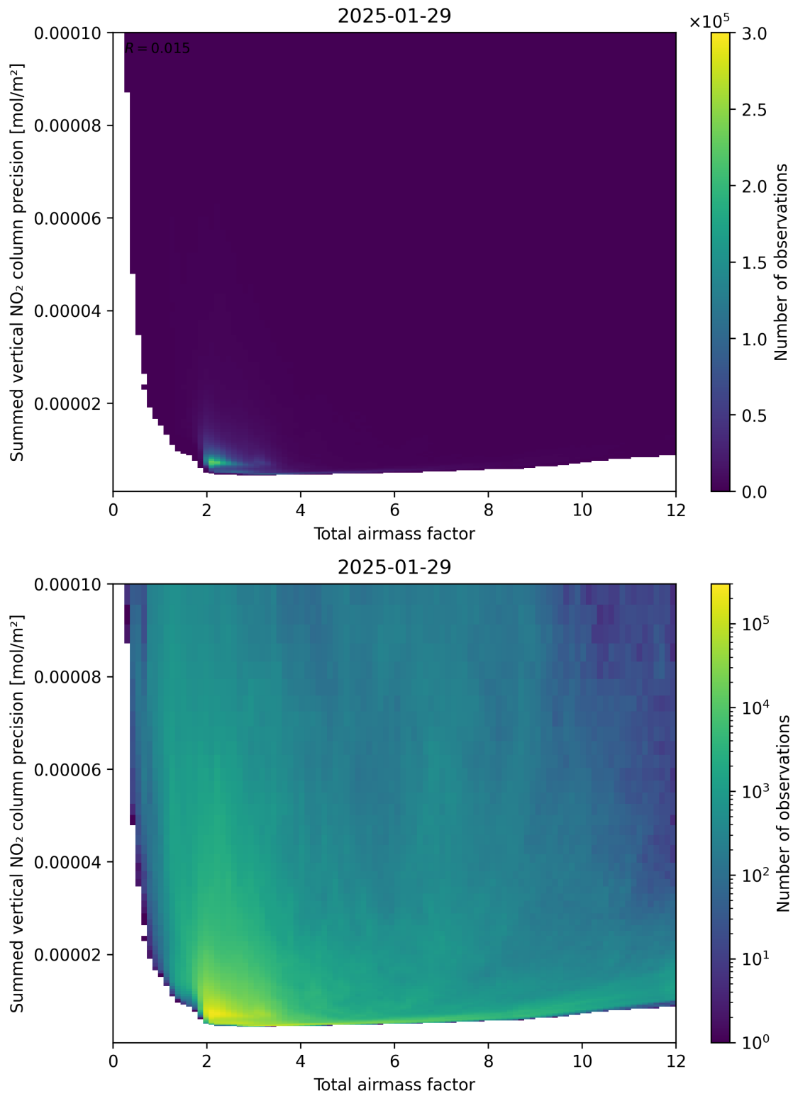
Figure 66: Scatter density plot of “Total airmass factor” against “Summed vertical NO 2 column precision” for 2025-01-28 to 2025-01-30.
