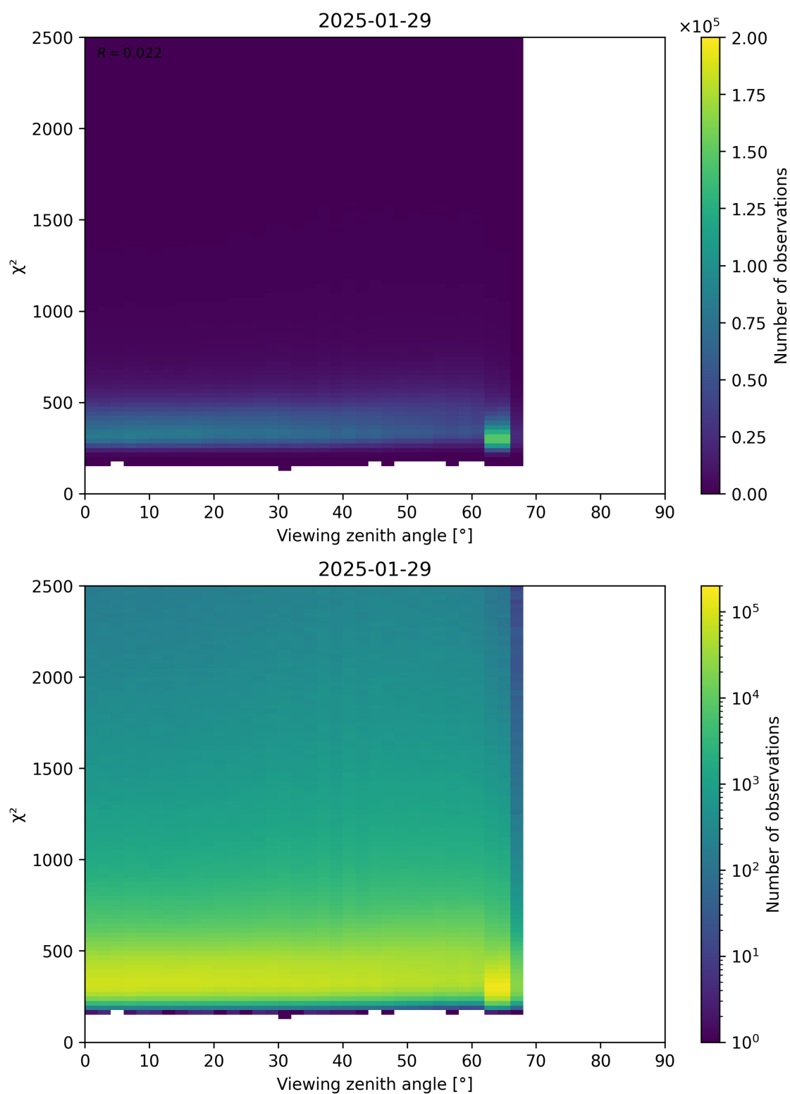
Figure 162: Scatter density plot of “Viewing zenith angle” against “ \chi^2 ” for 2025-01-28 to 2025-01-30.
