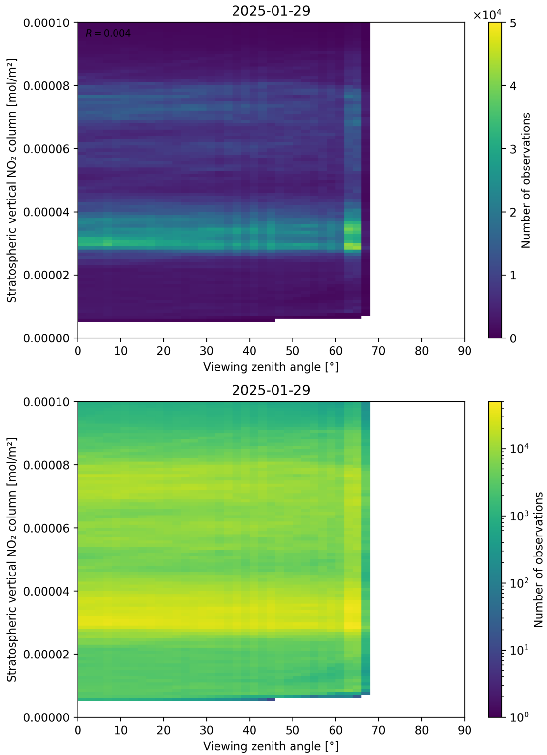
Figure 164: Scatter density plot of “Viewing zenith angle” against “Stratospheric vertical NO 2 column” for 2025-01-28 to 2025-01-30.
