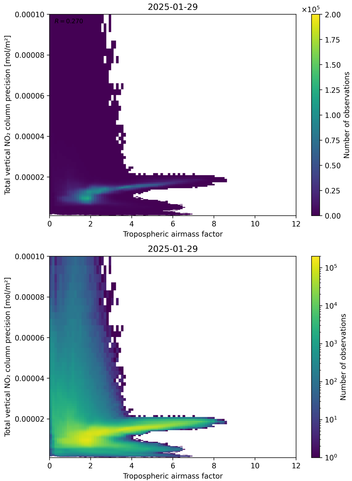
Figure 78: Scatter density plot of “Tropospheric air mass factor” against “Total vertical NO 2 column precision” for 2025-01-28 to 2025-01-30.
