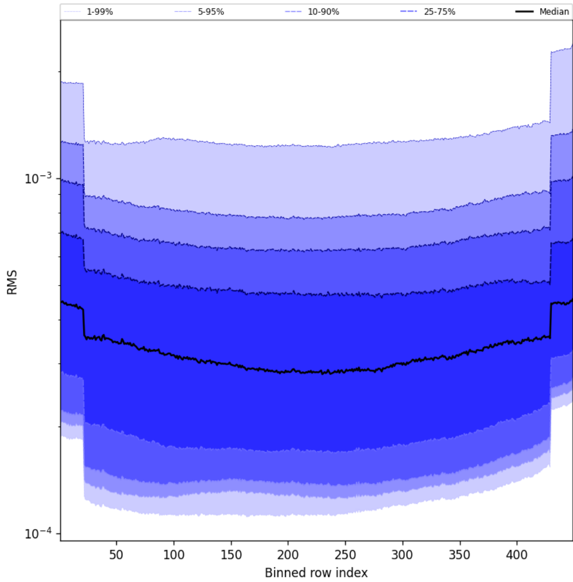
Figure 60: Along track statistics of “RMS” for 2025-01-28 to 2025-01-30
