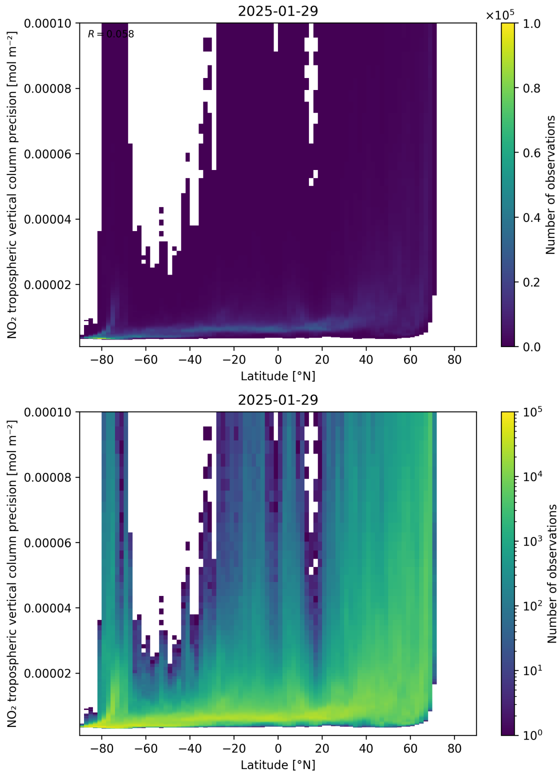
Figure 93: Scatter density plot of “Latitude” against “NO 2 tropospheric vertical column precision” for 2025-01-28 to 2025-01-30.
