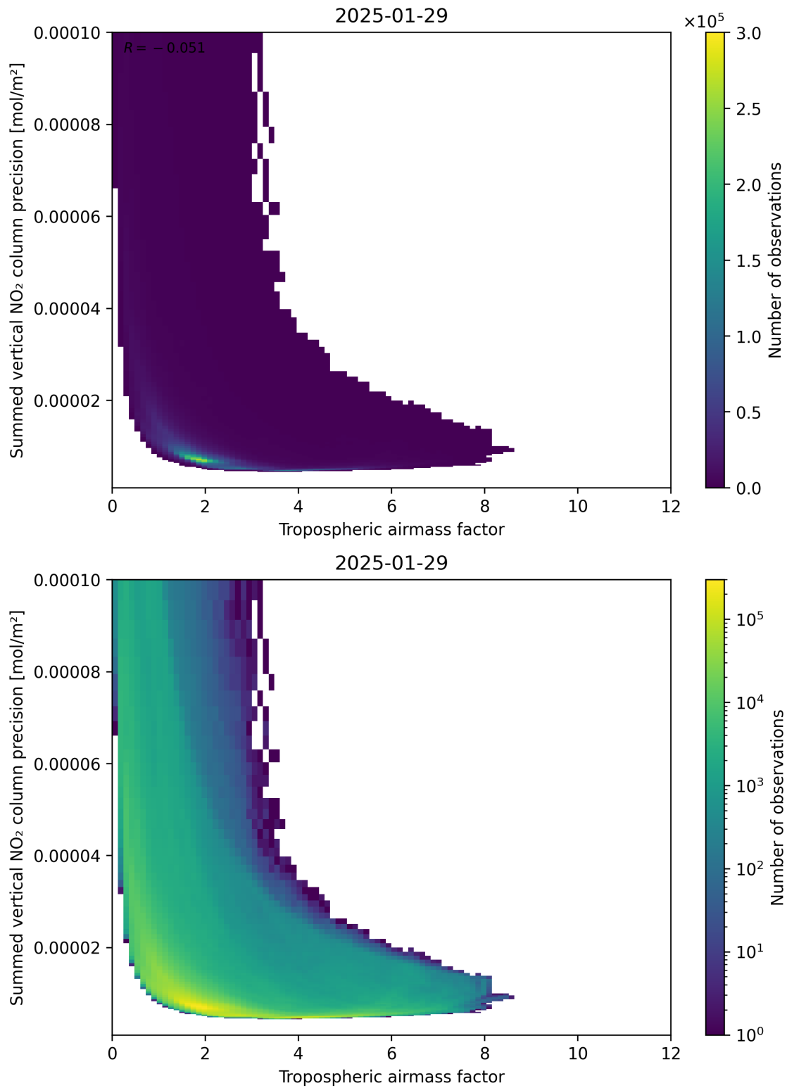
Figure 76: Scatter density plot of “Tropospheric air mass factor” against “Summed vertical NO 2 column precision” for 2025-01-28 to 2025-01-30.
