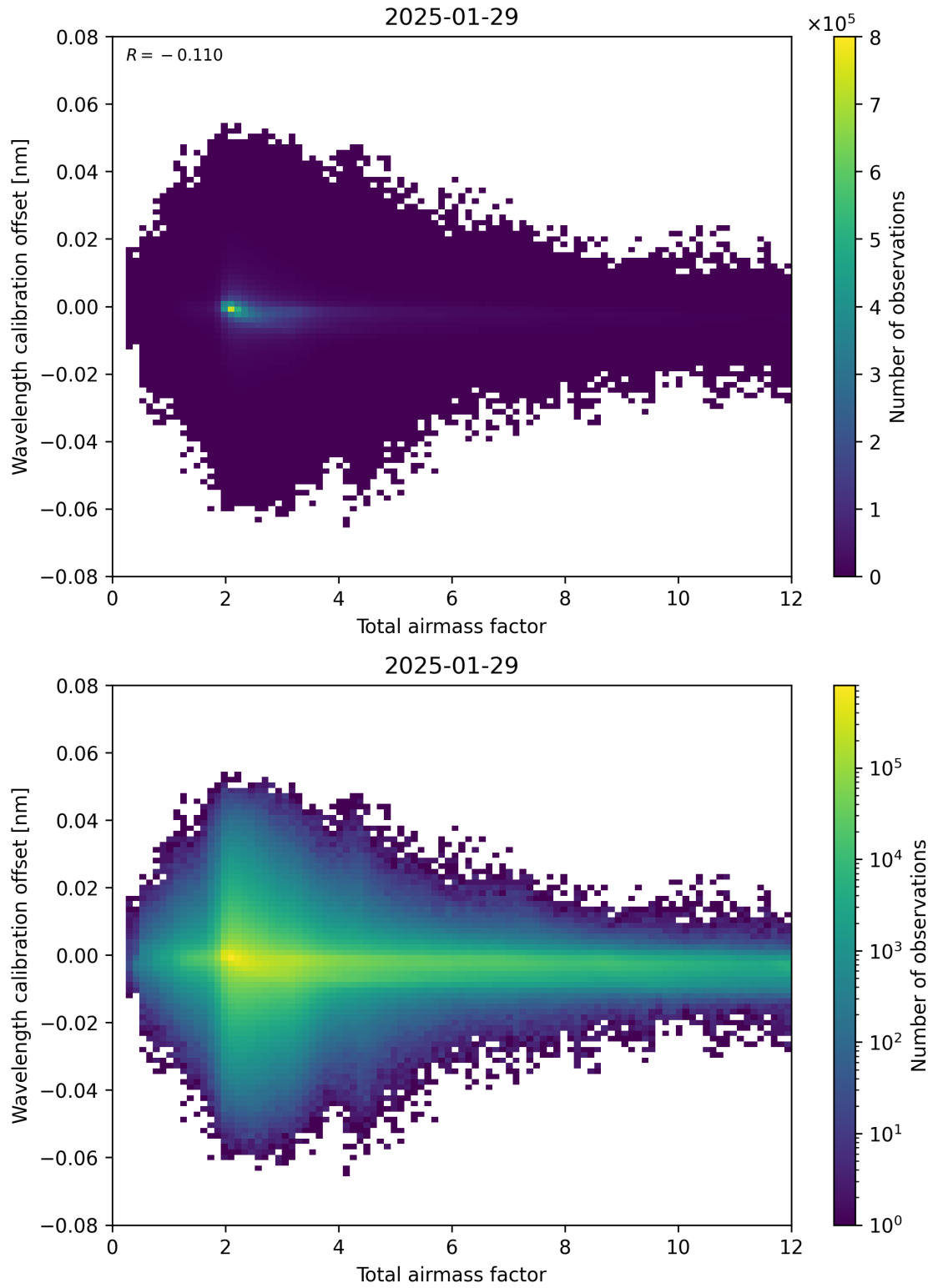
Figure 70: Scatter density plot of “Total airmass factor” against “Wavelength calibration offset” for 2025-01-28 to 2025-01-30.
