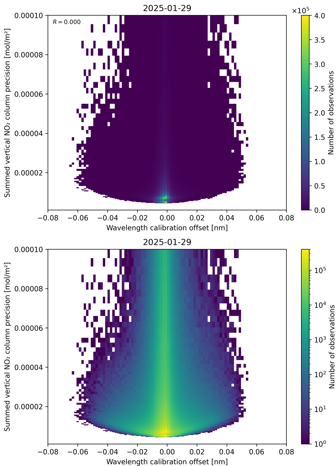
Figure 178: Scatter density plot of “Wavelength calibration offset” against “Summed vertical NO 2 column precision” for 2025-01-28 to 2025-01-30.
