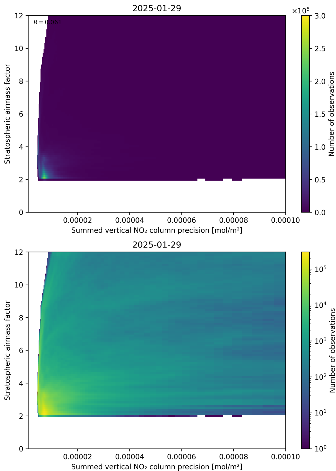
Figure 106: Scatter density plot of “Summed vertical NO 2 column precision” against “Stratospheric airmass factor” for 2025-01-28 to 2025-01-30.
