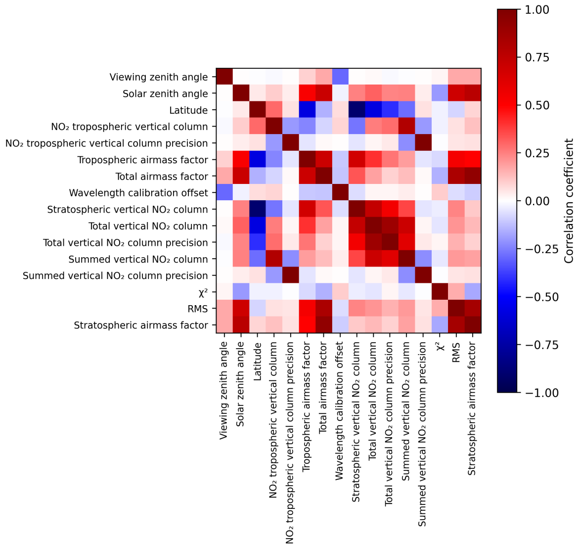
Figure 2: Map of correlation matrix for 2025-01-28 to 2025-01-30.
