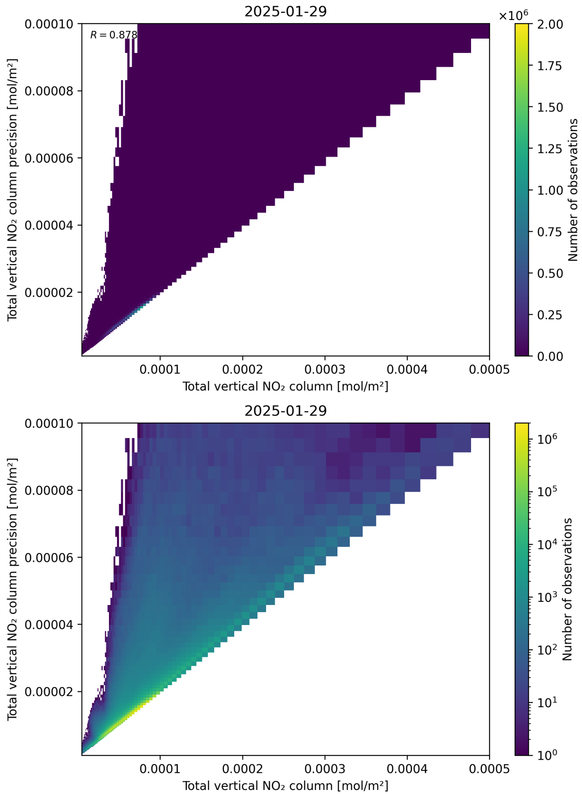
Figure 114: Scatter density plot of “Total vertical NO 2 column” against “Total vertical NO 2 column precision” for 2025-01-28 to 2025-01-30.
