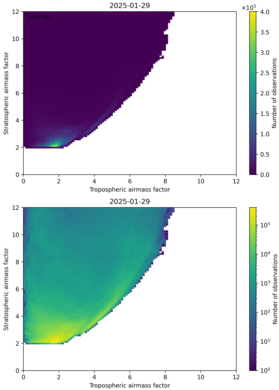
Figure 71: Scatter density plot of “Tropospheric airmass factor” against “Stratospheric airmass factor” for 2025-01-28 to 2025-01-30.
