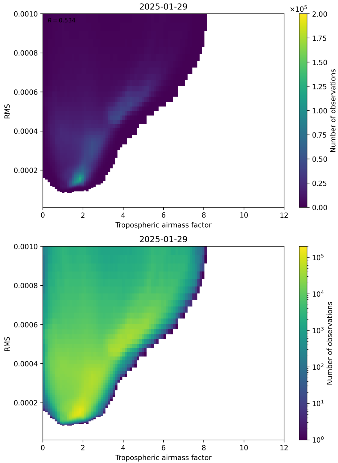
Figure 79: Scatter density plot of “Tropospheric airmass factor” against “RMS” for 2025-01-28 to 2025-01-30.
