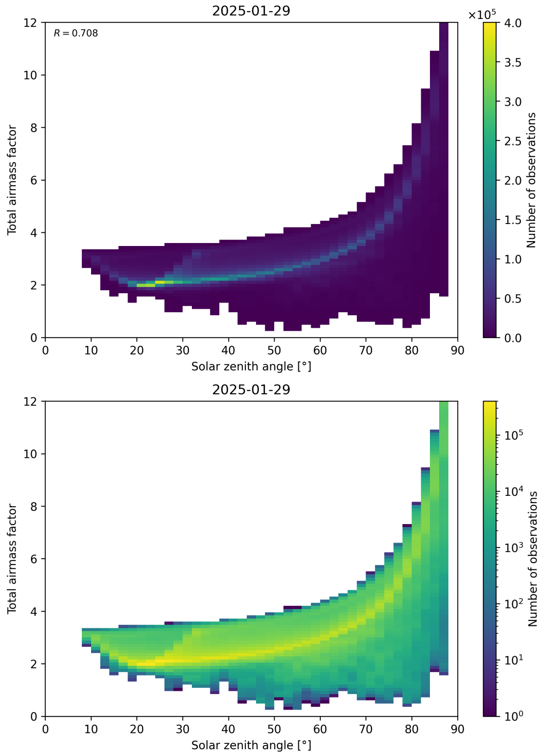
Figure 146: Scatter density plot of “Solar zenith angle” against “Total air mass factor” for 2025-01-28 to 2025-01-30.
