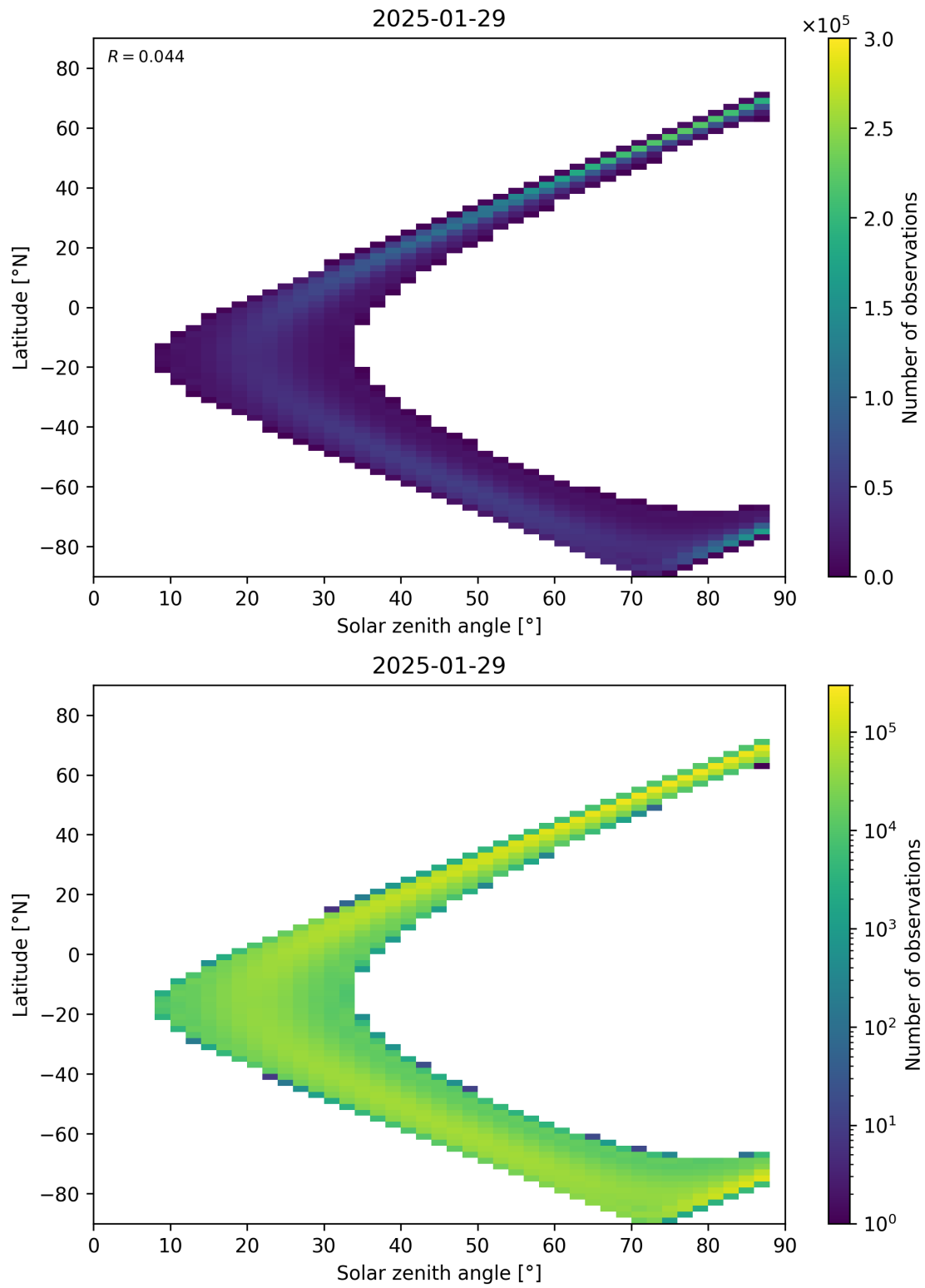
Figure 149: Scatter density plot of “Solar zenith angle” against “Latitude” for 2025-01-28 to 2025-01-30.
