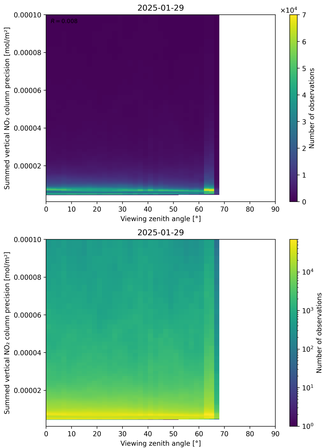
Figure 166: Scatter density plot of “Viewing zenith angle” against “Summed vertical NO 2 column precision” for 2025-01-28 to 2025-01-30.
