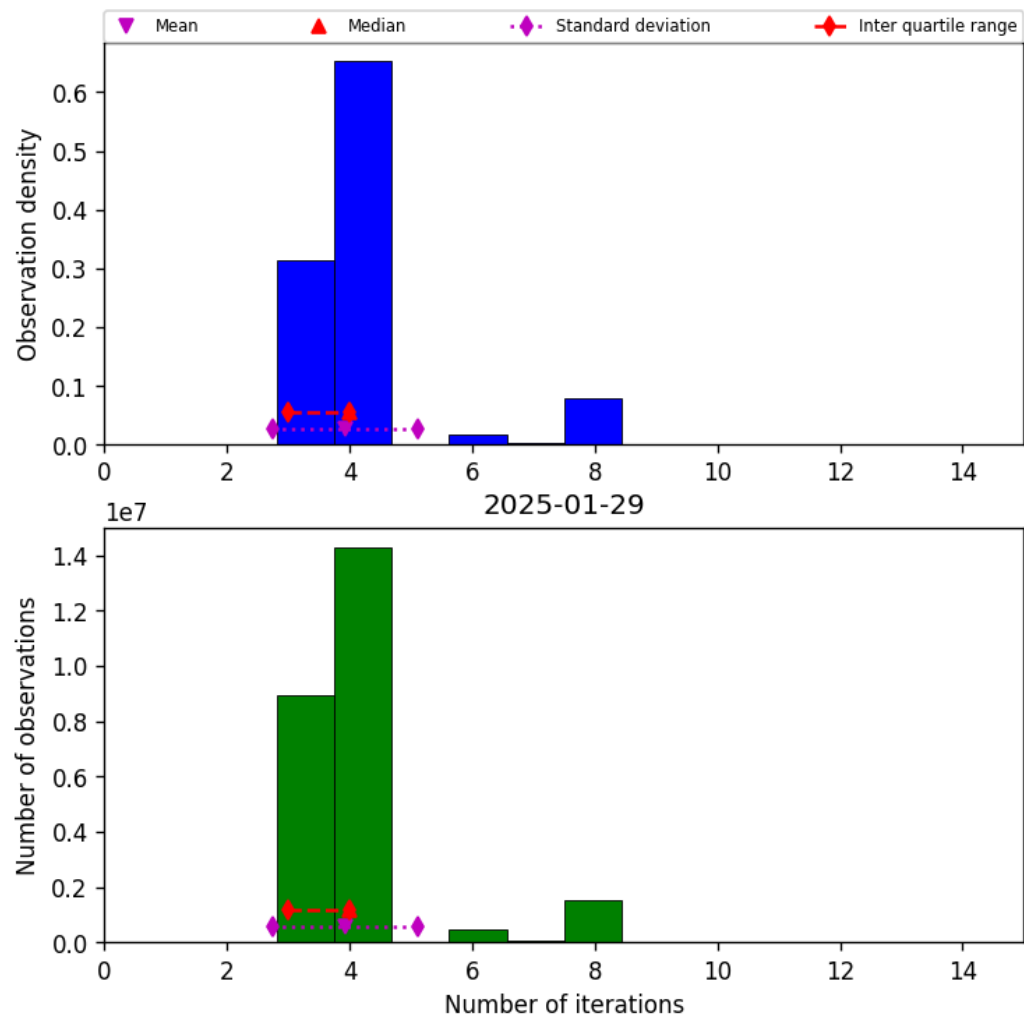
Figure 34: Histogram of “Number of iterations” for 2025-01-28 to 2025-01-30
