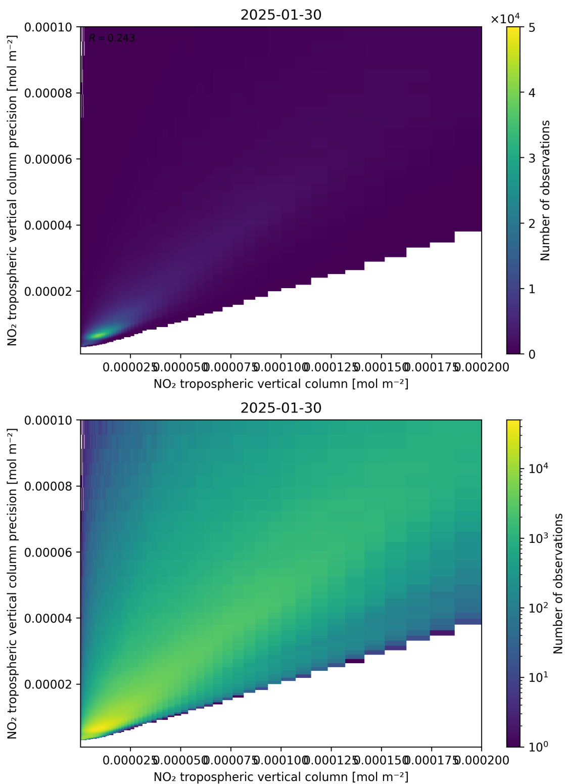
Figure 130: Scatter density plot of “NO 2 tropospheric vertical column” against “NO 2 tropospheric vertical column precision” for 2025-01-29 to 2025-01-31.
