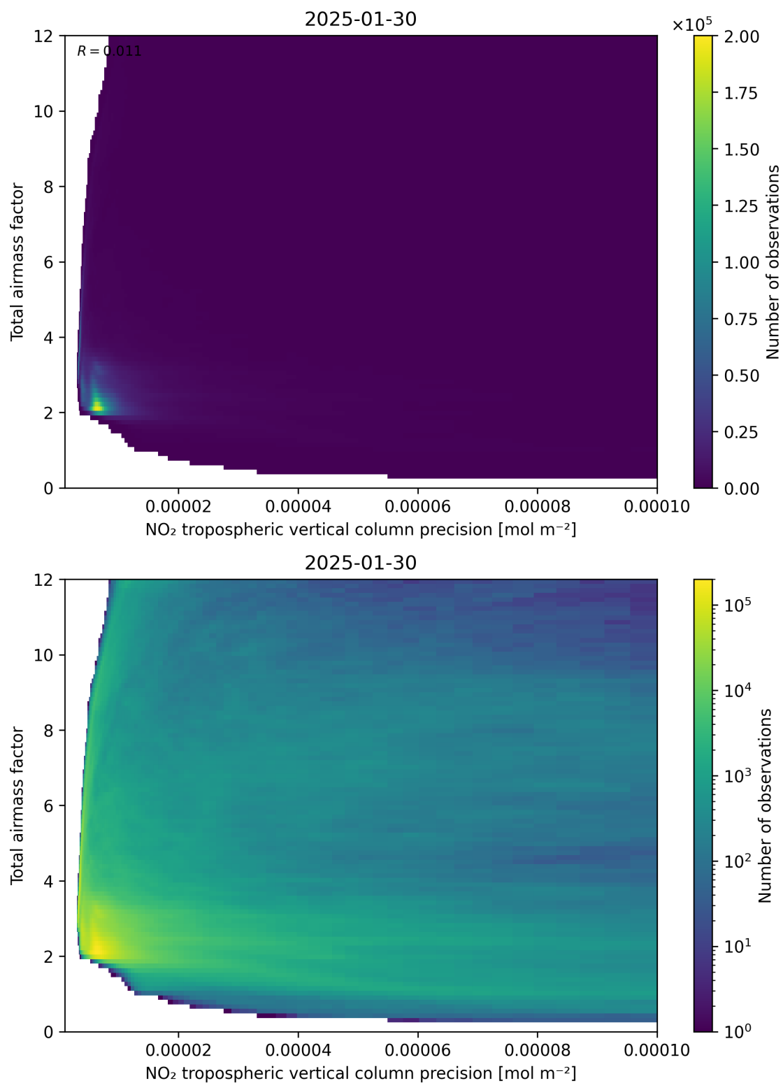
Figure 132: Scatter density plot of “NO 2 tropospheric vertical column precision” against “Total air mass factor” for 2025-01-29 to 2025-01-31.
