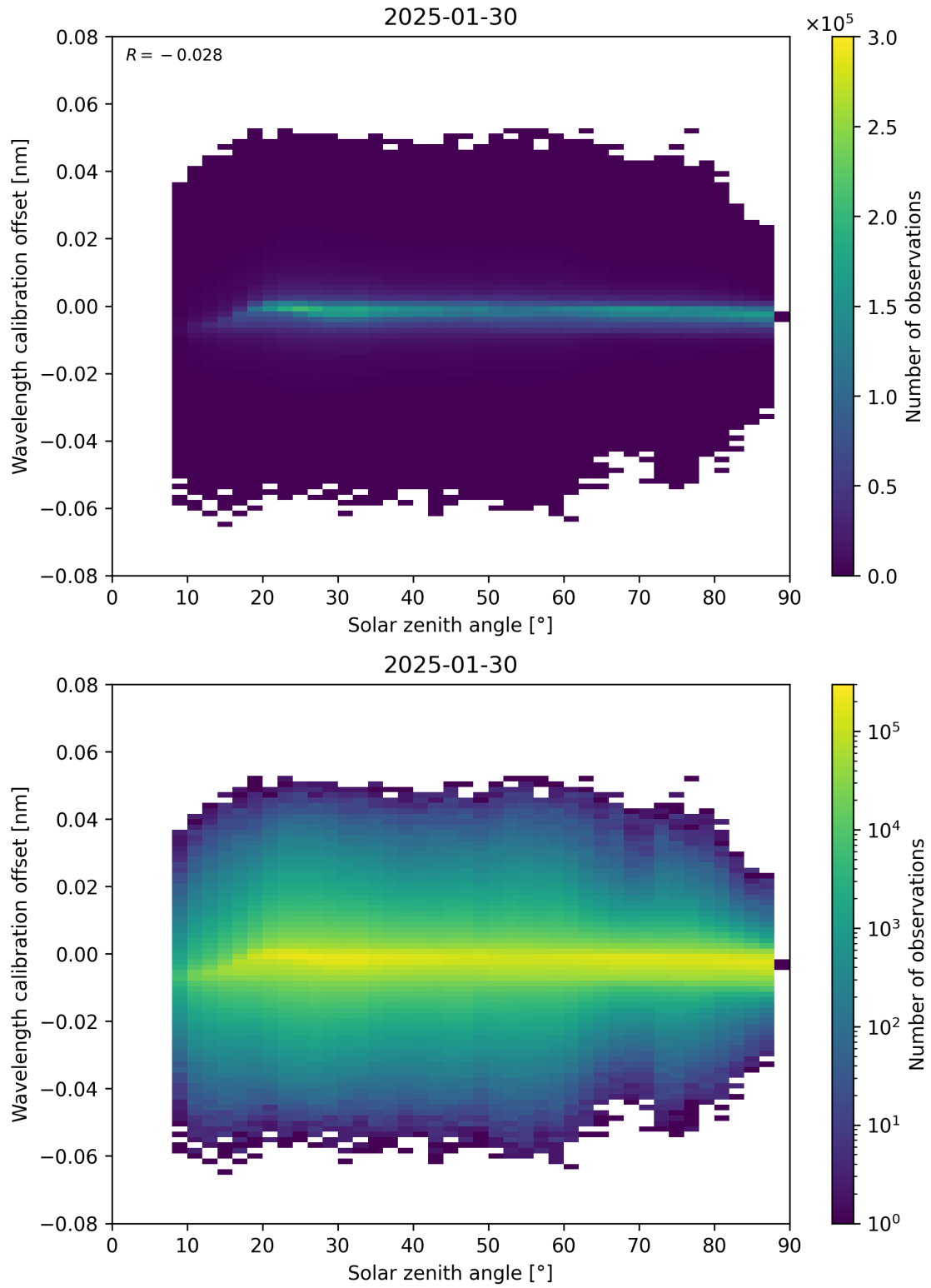
Figure 158: Scatter density plot of “Solar zenith angle” against “Wavelength calibration offset” for 2025-01-29 to 2025-01-31.
