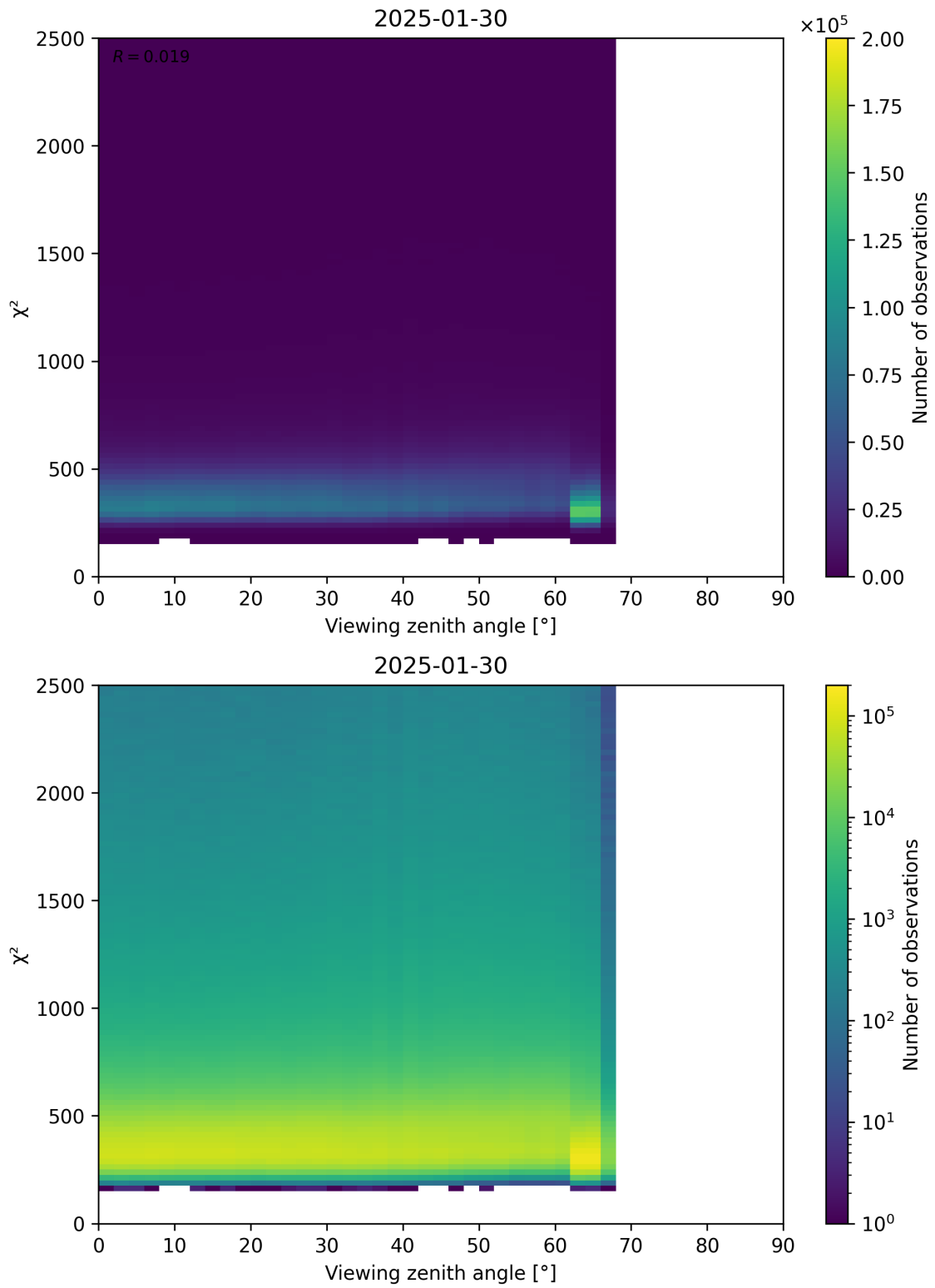
Figure 162: Scatter density plot of “Viewing zenith angle” against “ \chi^2 ” for 2025-01-29 to 2025-01-31.
