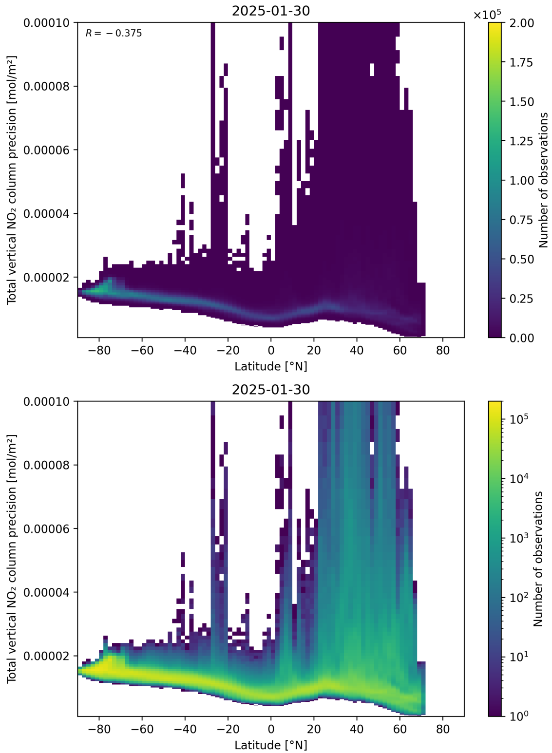
Figure 91: Scatter density plot of “Latitude” against “Total vertical NO 2 column precision” for 2025-01-29 to 2025-01-31.
