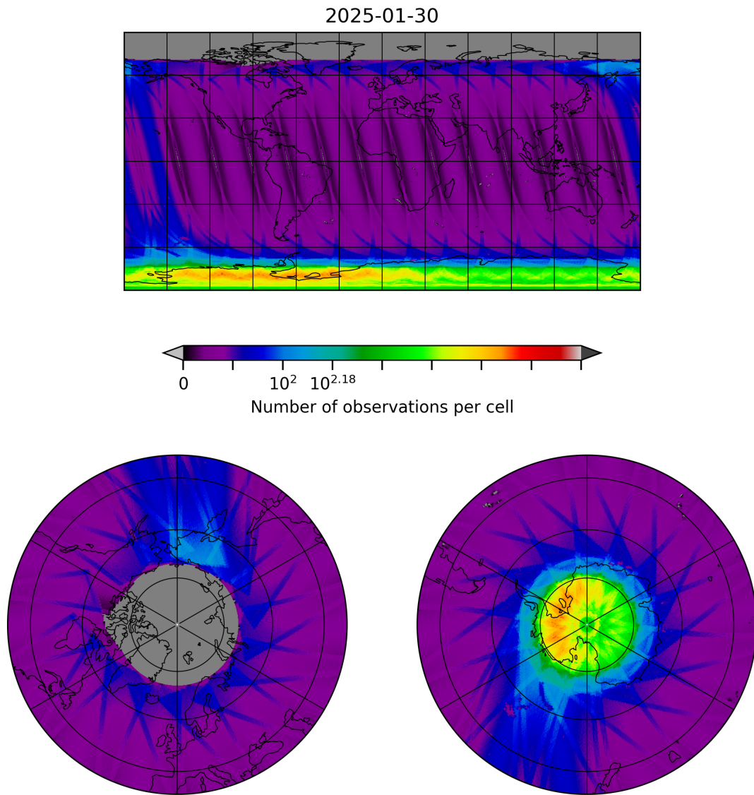
Figure 10: Map of the number of observations for 2025-01-29 to 2025-01-31
