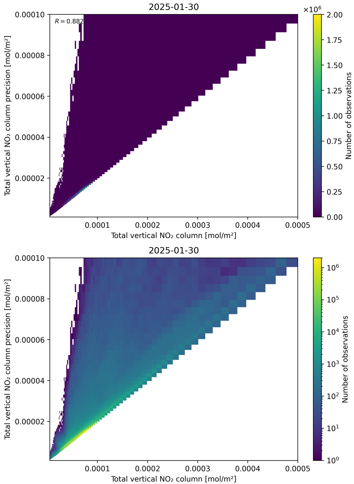
Figure 114: Scatter density plot of “Total vertical NO 2 column” against “Total vertical NO 2 column precision” for 2025-01-29 to 2025-01-31.
