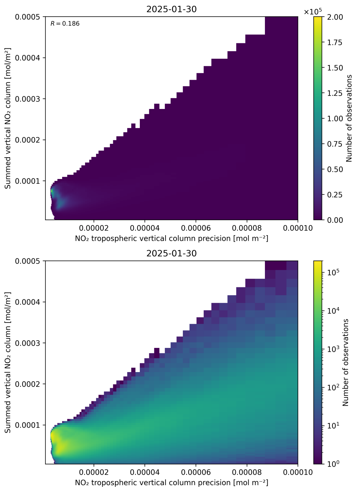
Figure 136: Scatter density plot of “NO 2 tropospheric vertical column precision” against “Summed vertical NO 2 column” for 2025-01-29 to 2025-01-31.
