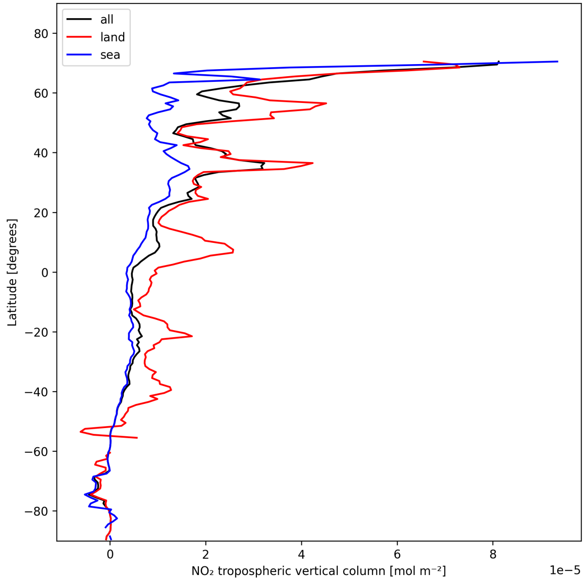
Figure 12: Zonal average of “NO 2 tropospheric vertical column” for 2025-01-29 to 2025-01-31.
