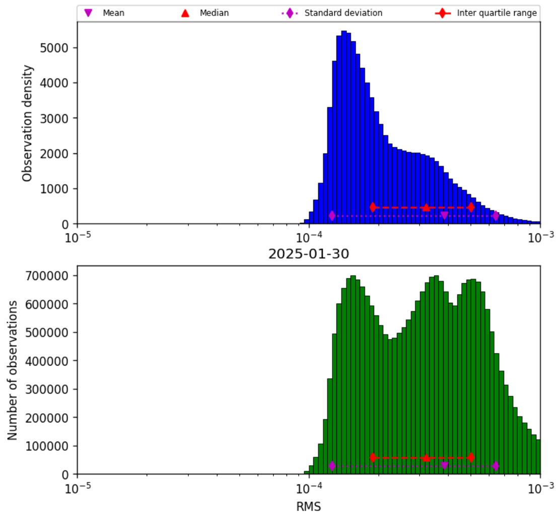
Figure 43: Histogram of “RMS” for 2025-01-29 to 2025-01-31
