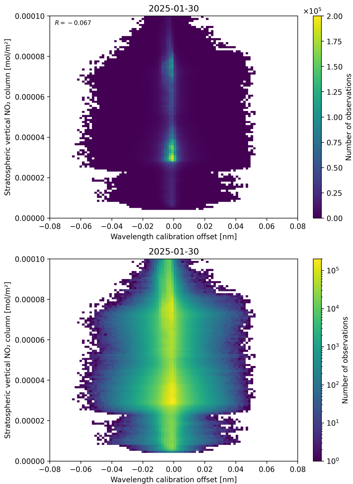
Figure 176: Scatter density plot of “Wavelength calibration offset” against “Stratospheric vertical NO 2 column” for 2025-01-29 to 2025-01-31.
