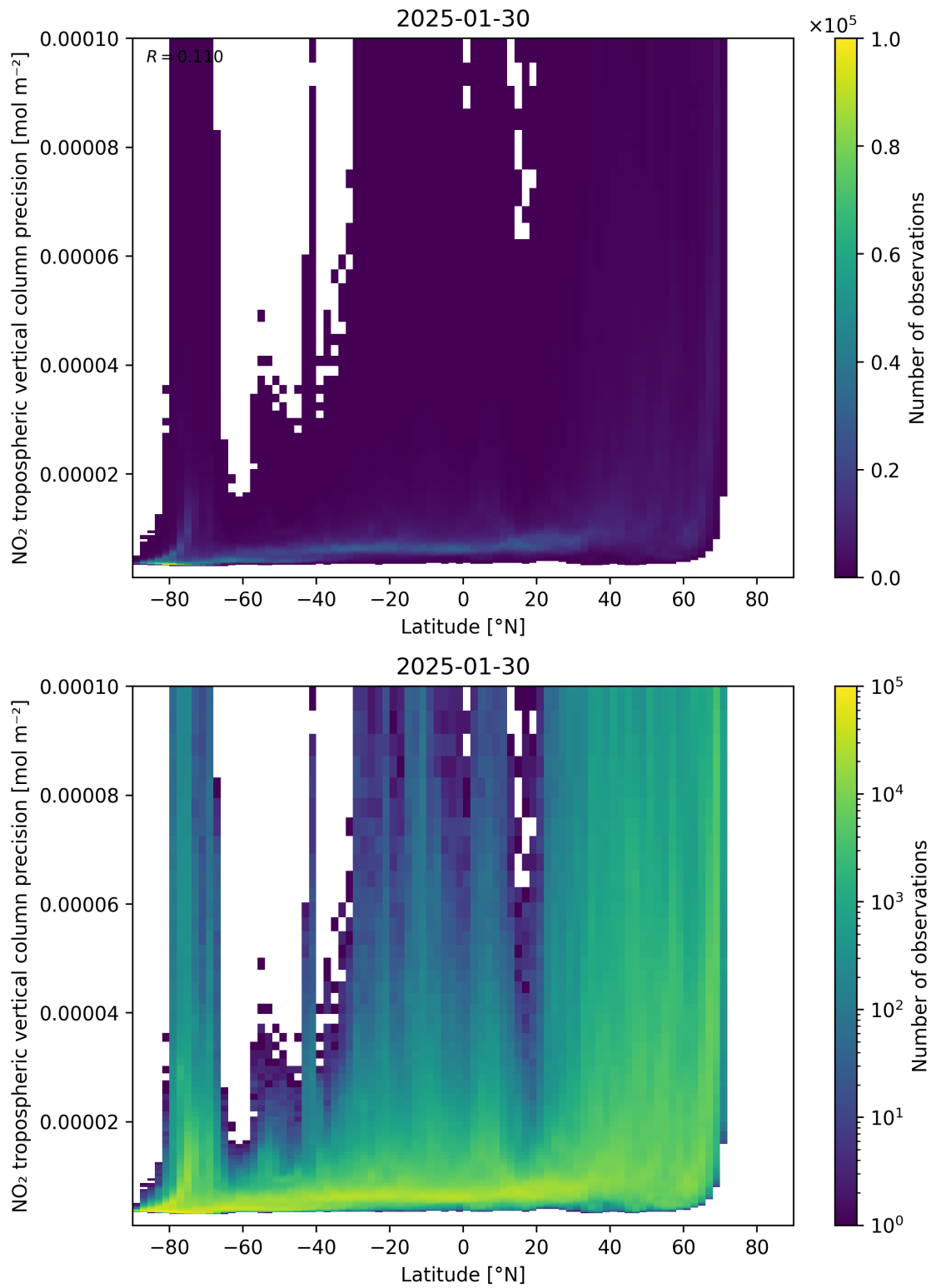
Figure 93: Scatter density plot of “Latitude” against “NO 2 tropospheric vertical column precision” for 2025-01-29 to 2025-01-31.
