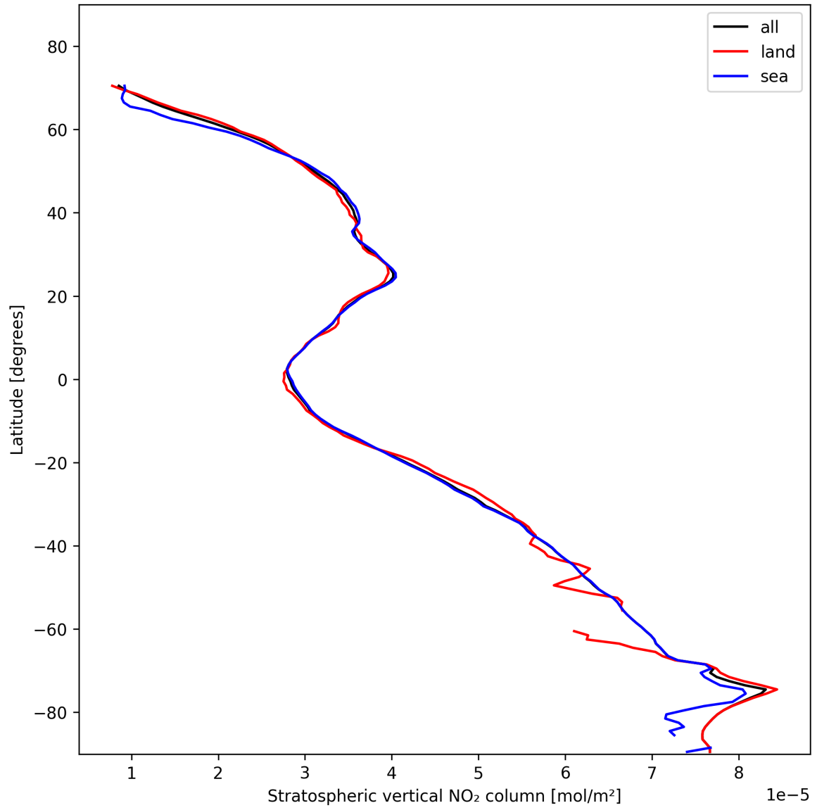
Figure 19: Zonal average of “Stratospheric vertical NO 2 column” for 2025-01-29 to 2025-01-31.
