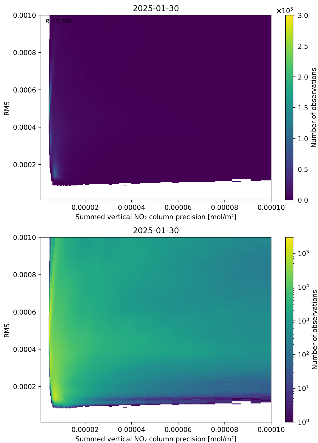
Figure 108: Scatter density plot of “Summed vertical NO 2 column precision” against “RMS” for 2025-01-29 to 2025-01-31.
