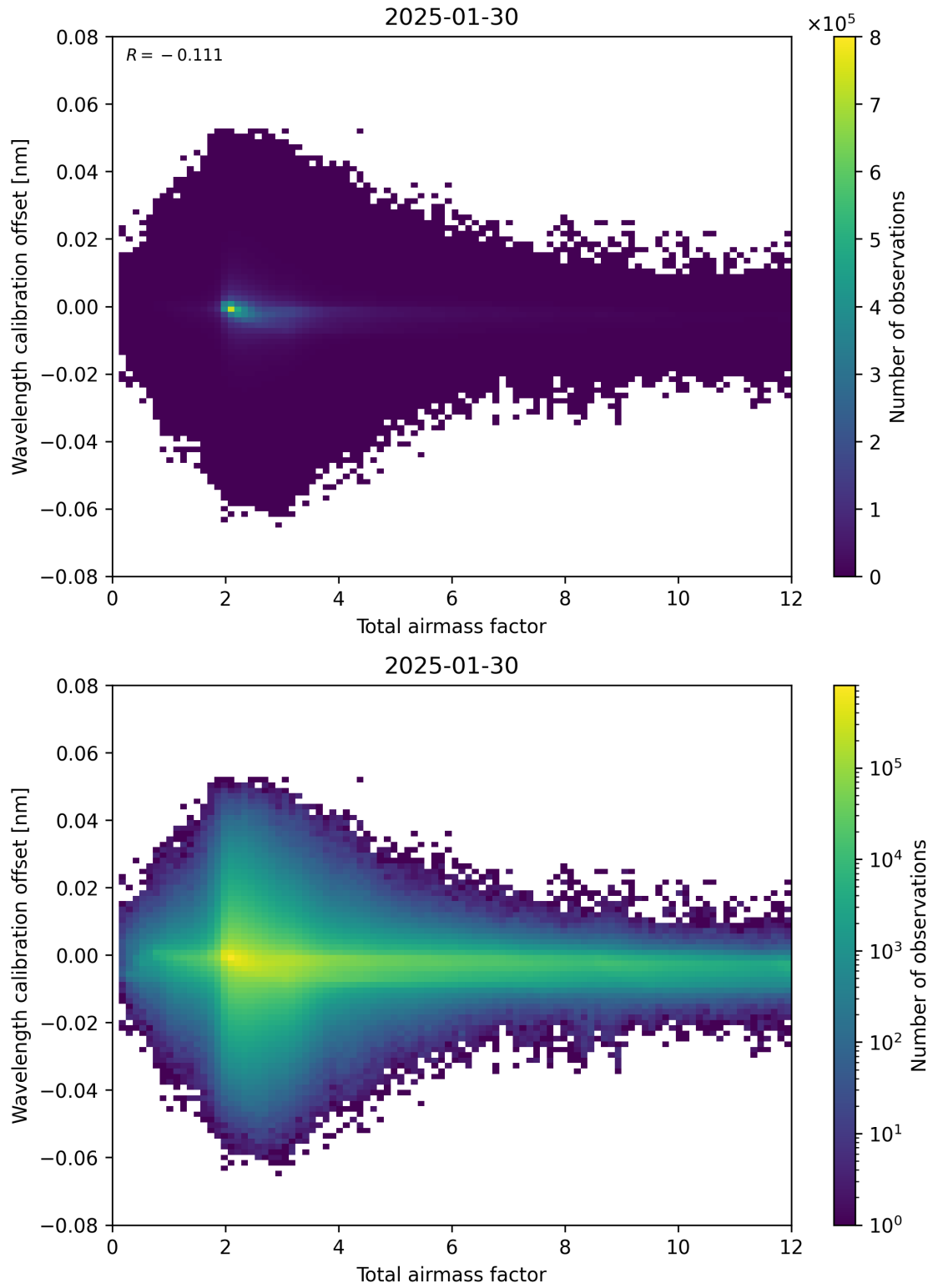
Figure 70: Scatter density plot of “Total airmass factor” against “Wavelength calibration offset” for 2025-01-29 to 2025-01-31.
