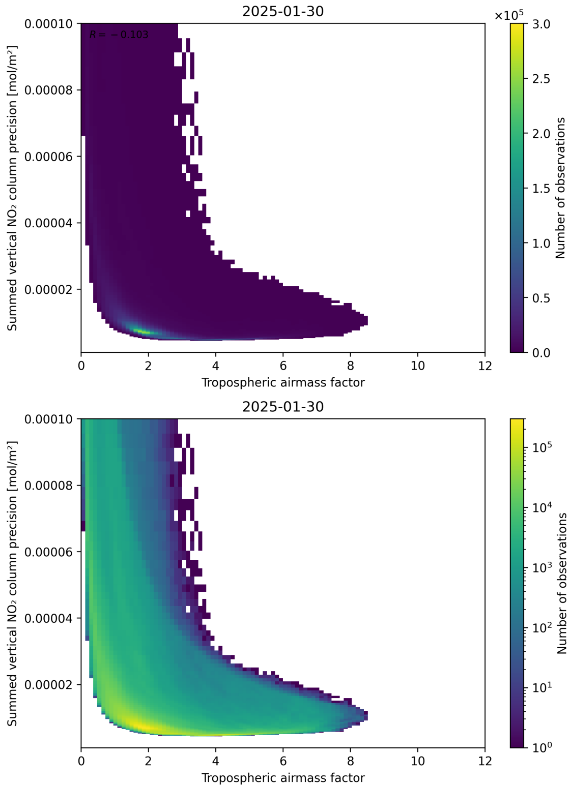
Figure 76: Scatter density plot of “Tropospheric air mass factor” against “Summed vertical NO 2 column precision” for 2025-01-29 to 2025-01-31.
