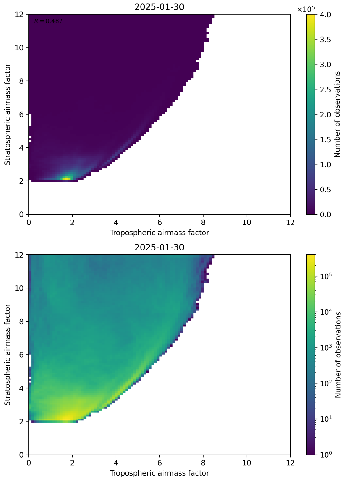
Figure 71: Scatter density plot of “Tropospheric airmass factor” against “Stratospheric airmass factor” for 2025-01-29 to 2025-01-31.
