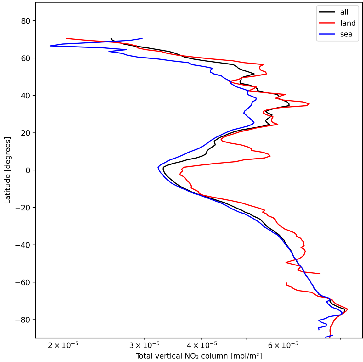
Figure 21: Zonal average of “Total vertical NO 2 column” for 2025-01-29 to 2025-01-31.
