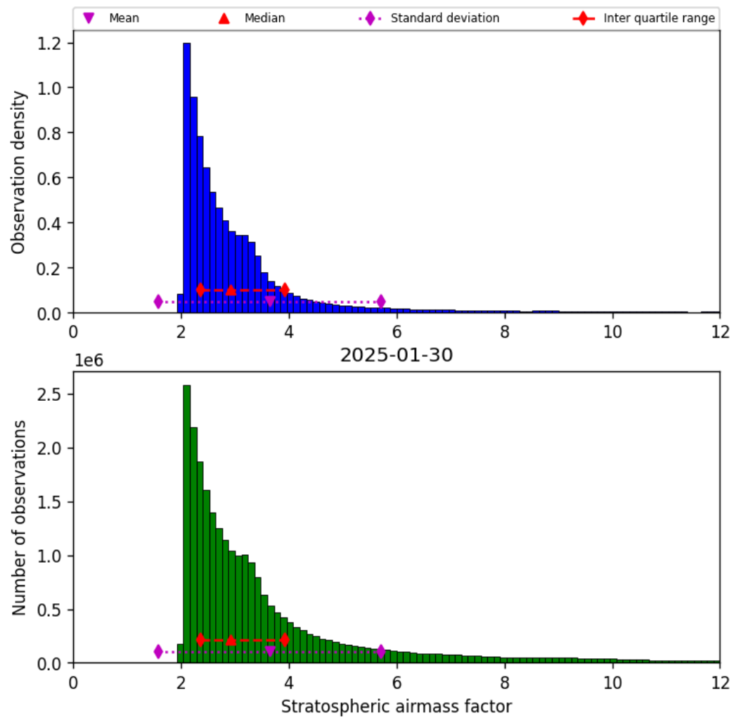
Figure 44: Histogram of “Stratospheric airmass factor” for 2025-01-29 to 2025-01-31
