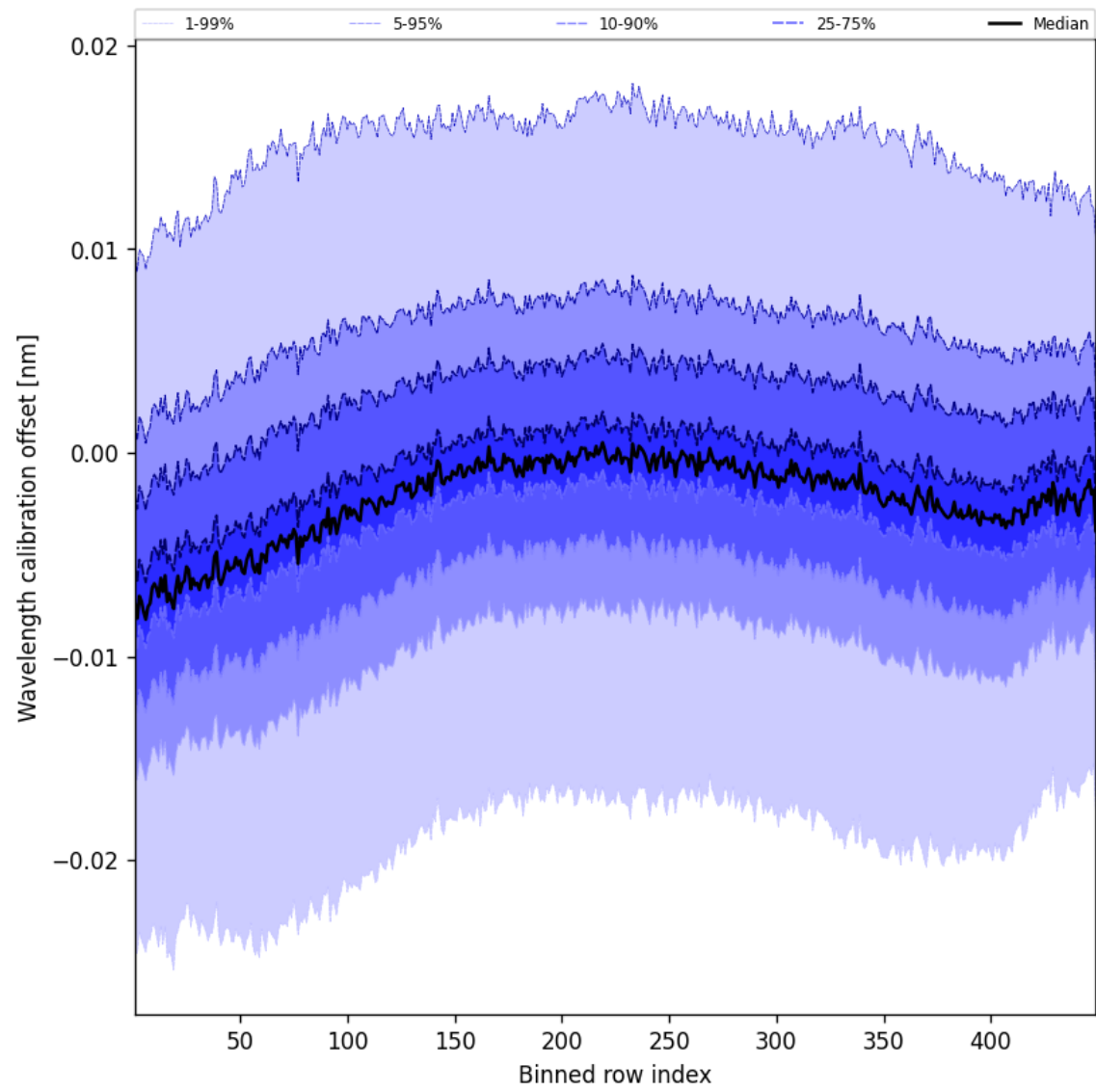
Figure 52: Along track statistics of “Wavelength calibration offset” for 2025-01-29 to 2025-01-31
