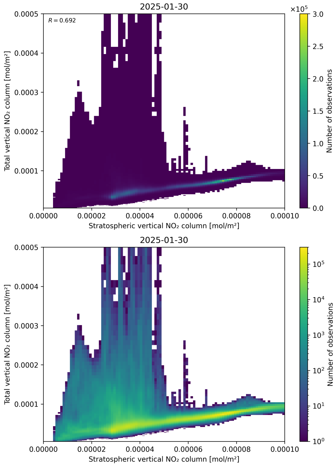
Figure 100: Scatter density plot of “Stratospheric vertical NO 2 column” against “Total vertical NO 2 column” for 2025-01-29 to 2025-01-31.
