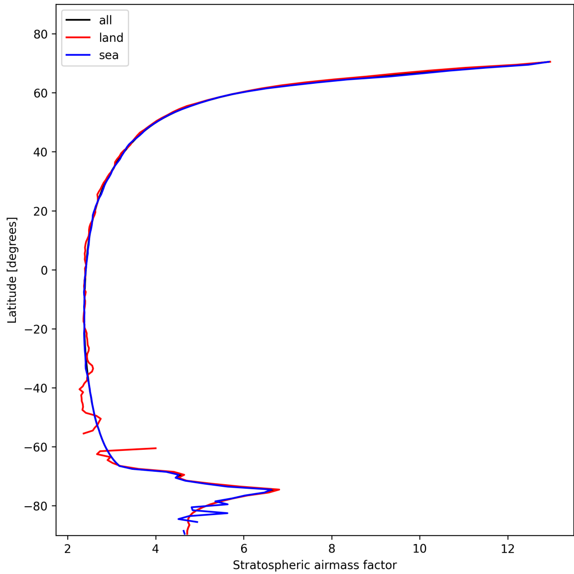
Figure 27: Zonal average of “Stratospheric airmass factor” for 2025-01-29 to 2025-01-31.
