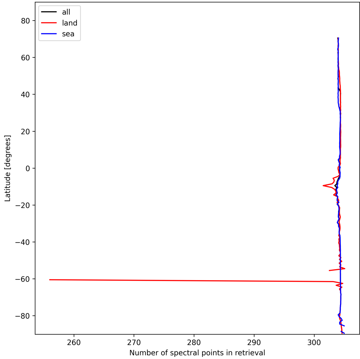
Figure 16: Zonal average of “Number of spectral points in retrieval” for 2025-01-29 to 2025-01-31.
