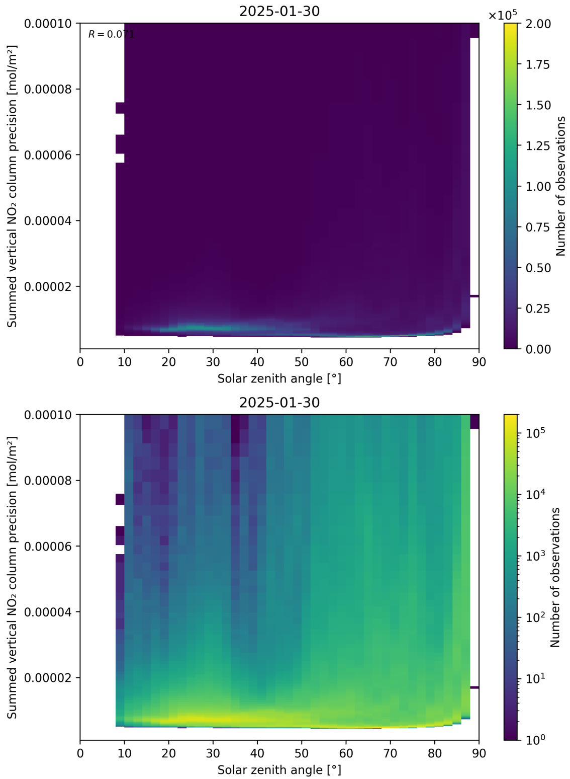
Figure 152: Scatter density plot of “Solar zenith angle” against “Summed vertical NO 2 column precision” for 2025-01-29 to 2025-01-31.
