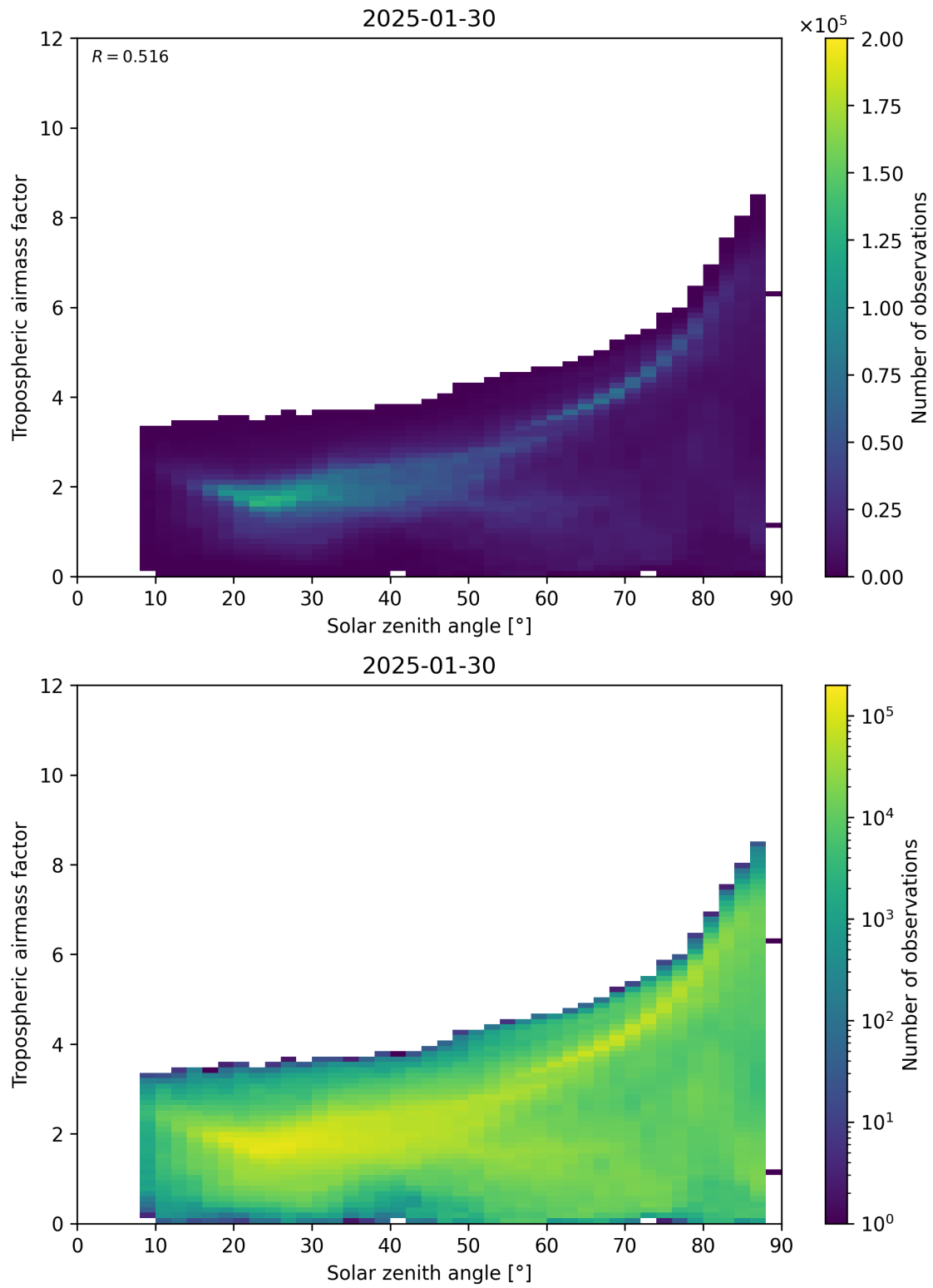
Figure 147: Scatter density plot of “Solar zenith angle” against “Tropospheric airmass factor” for 2025-01-29 to 2025-01-31.
