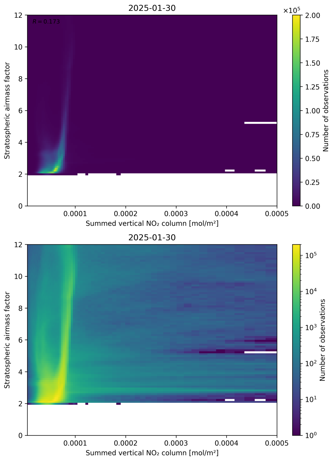
Figure 103: Scatter density plot of “Summed vertical NO 2 column” against “Stratospheric airmass factor” for 2025-01-29 to 2025-01-31.
