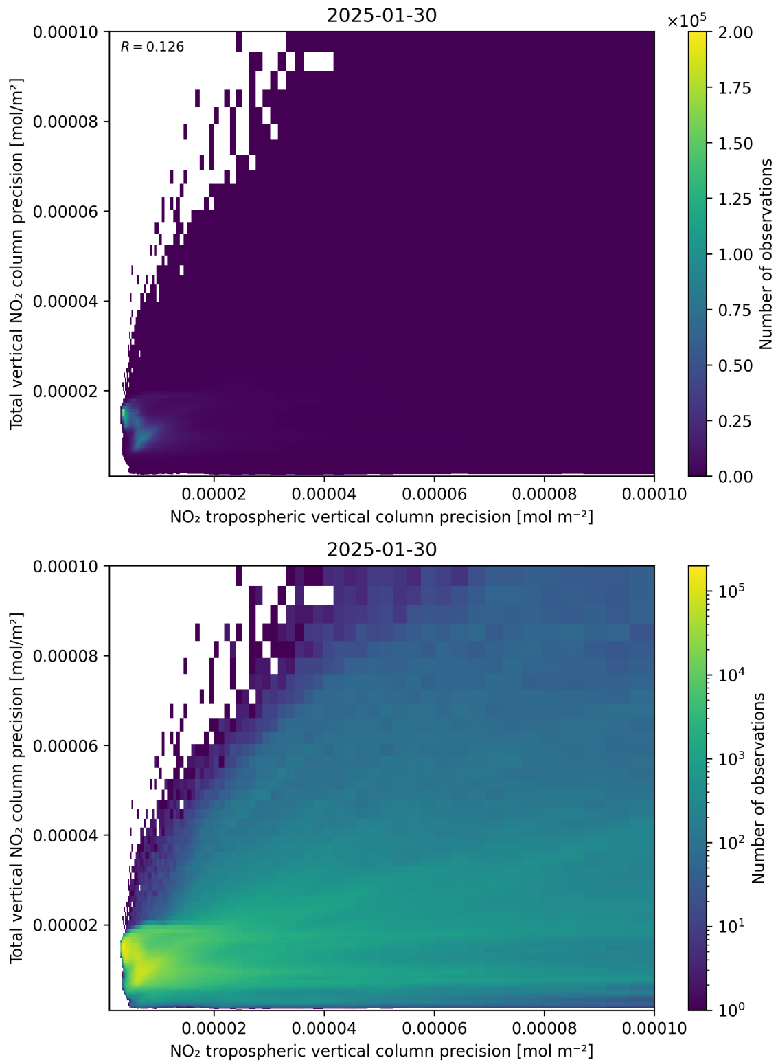
Figure 139: Scatter density plot of “NO 2 tropospheric vertical column precision” against “Total vertical NO 2 column precision” for 2025-01-29 to 2025-01-31.
