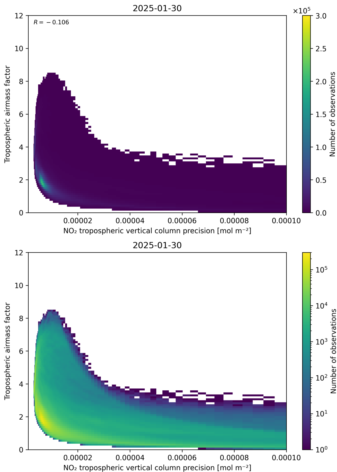
Figure 133: Scatter density plot of “NO 2 tropospheric vertical column precision” against “Tropospheric air mass factor” for 2025-01-29 to 2025-01-31.
