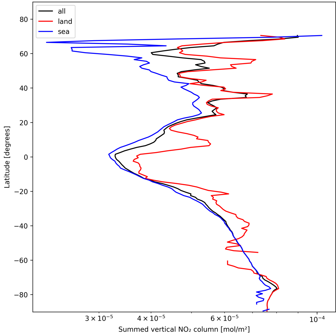
Figure 23: Zonal average of “Summed vertical NO 2 column” for 2025-01-29 to 2025-01-31.
