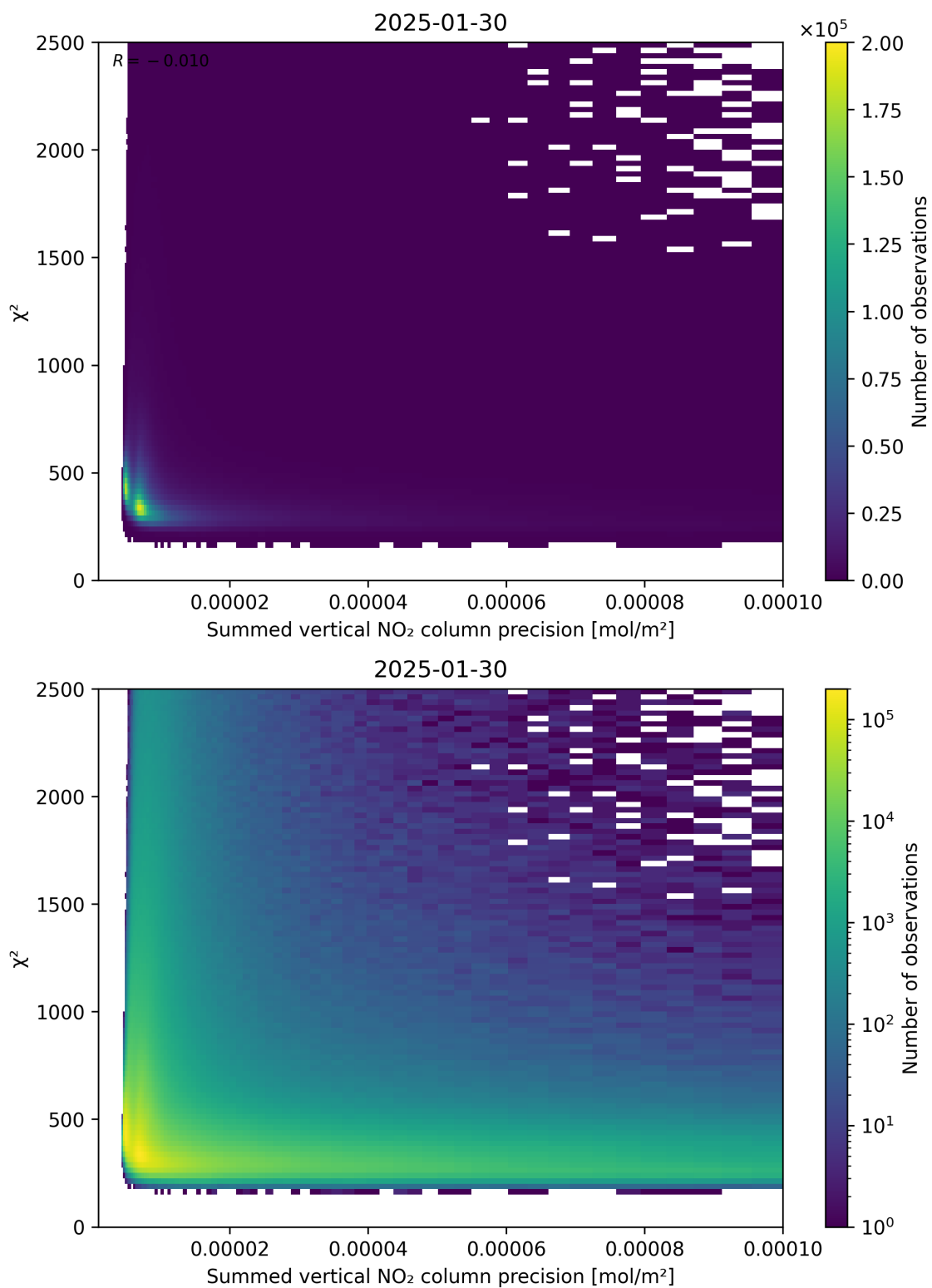
Figure 107: Scatter density plot of “Summed vertical NO 2 column precision” against “ \chi^2 ” for 2025-01-29 to 2025-01-31.
