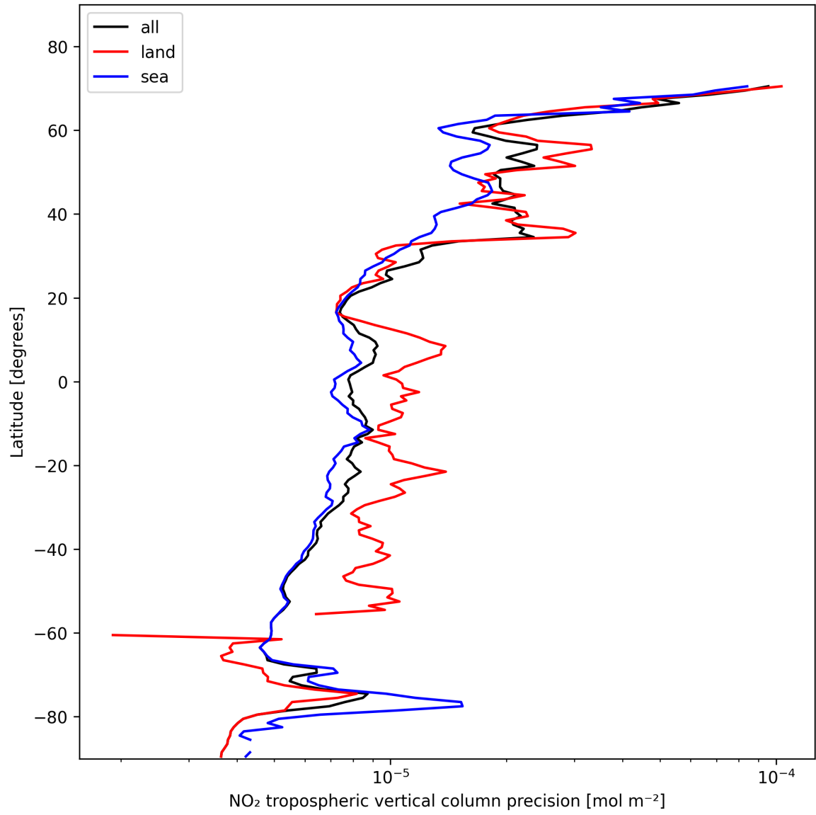
Figure 13: Zonal average of “NO 2 tropospheric vertical column precision” for 2025-01-29 to 2025-01-31.
