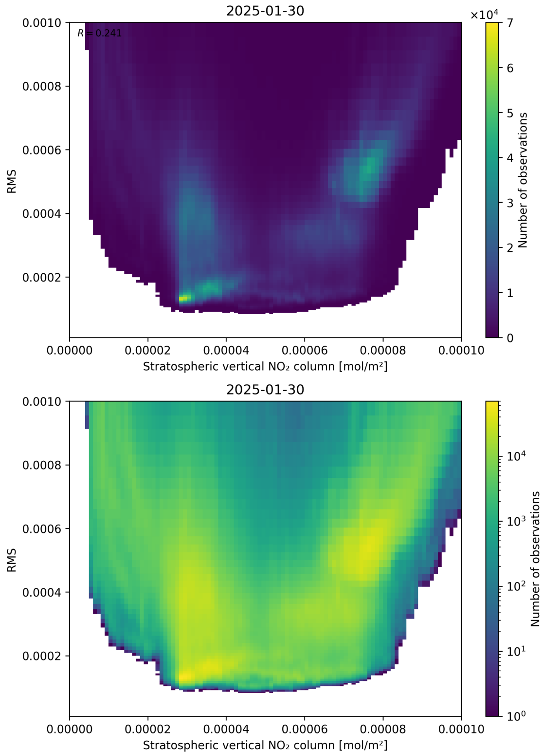
Figure 102: Scatter density plot of “Stratospheric vertical NO 2 column” against “RMS” for 2025-01-29 to 2025-01-31.
