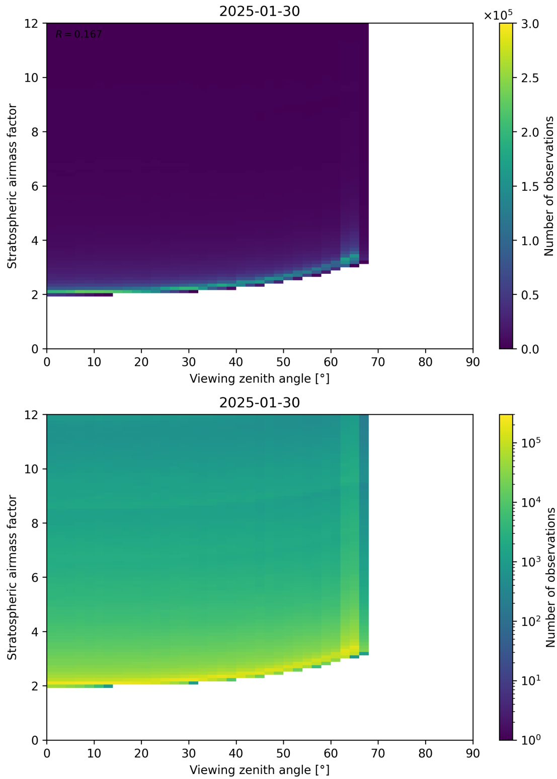
Figure 159: Scatter density plot of “Viewing zenith angle” against “Stratospheric airmass factor” for 2025-01-29 to 2025-01-31.
