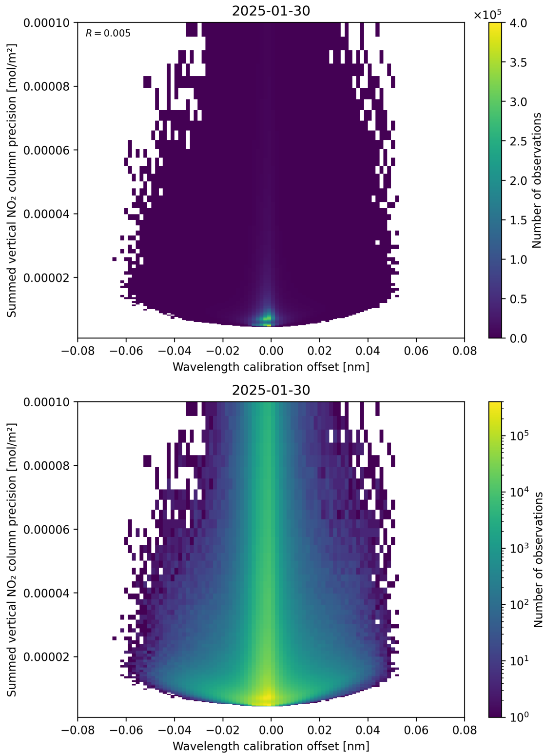
Figure 178: Scatter density plot of “Wavelength calibration offset” against “Summed vertical NO 2 column precision” for 2025-01-29 to 2025-01-31.
