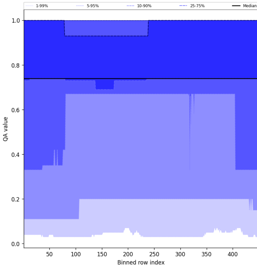
Figure 45: Along track statistics of “QA value” for 2025-01-29 to 2025-01-31
