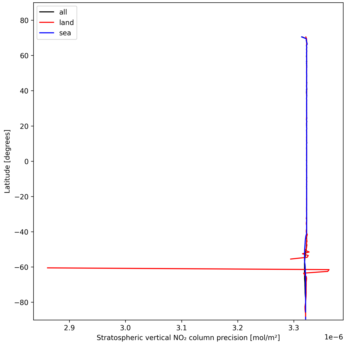
Figure 20: Zonal average of “Stratospheric vertical NO 2 column precision” for 2025-01-29 to 2025-01-31.
