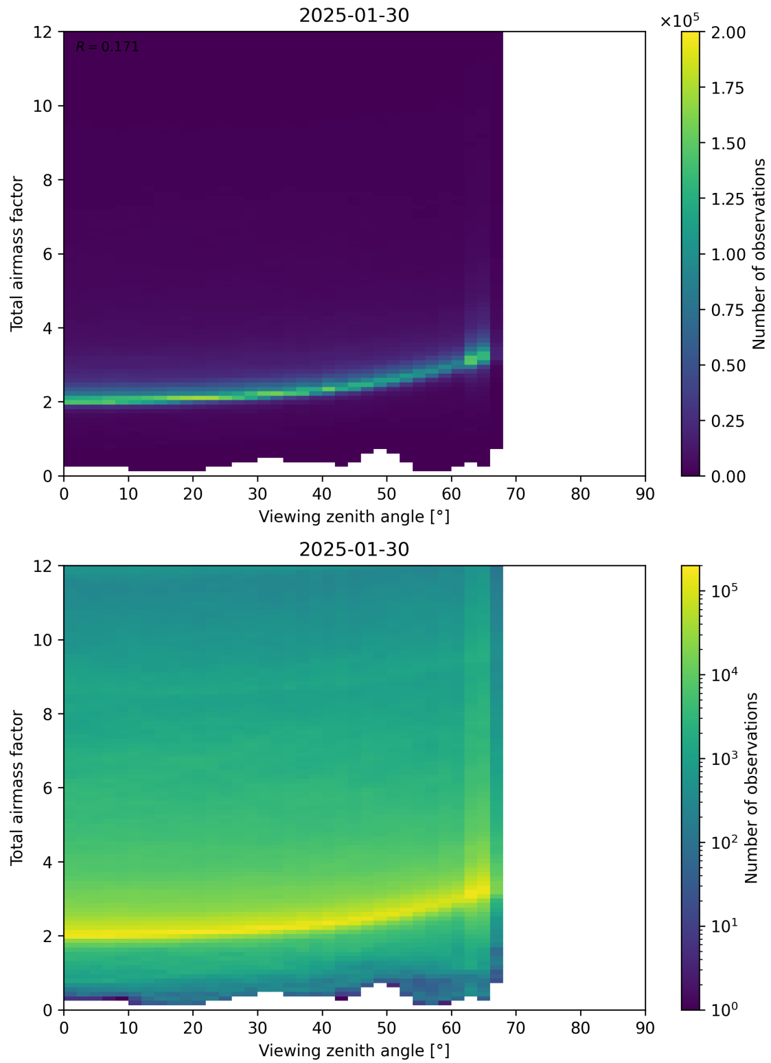
Figure 160: Scatter density plot of “Viewing zenith angle” against “Total airmass factor” for 2025-01-29 to 2025-01-31.
