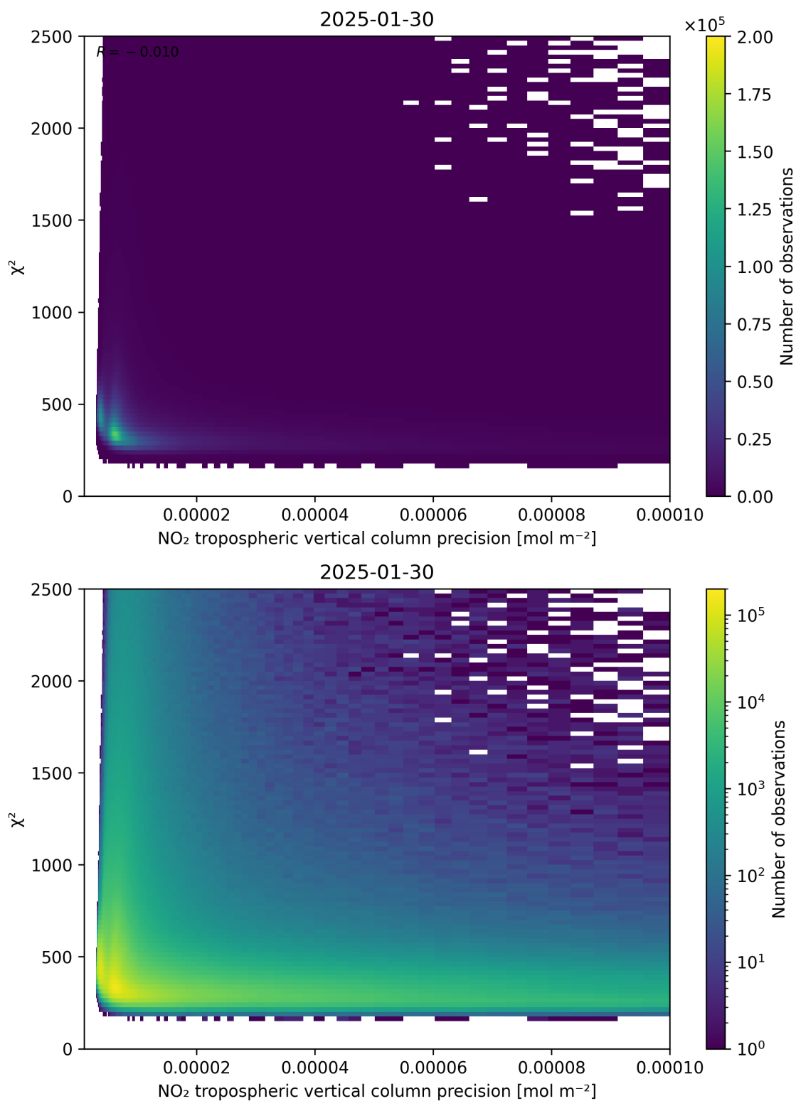
Figure 134: Scatter density plot of “NO 2 tropospheric vertical column precision” against “ \chi^2 ” for 2025-01-29 to 2025-01-31.
