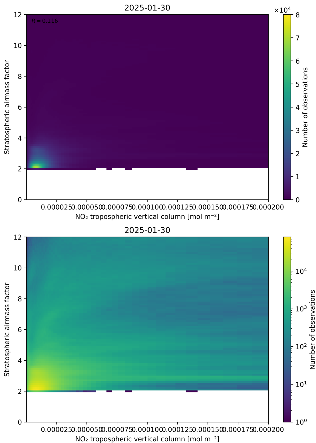
Figure 121: Scatter density plot of “NO 2 tropospheric vertical column” against “Stratospheric air mass factor” for 2025-01-29 to 2025-01-31.
