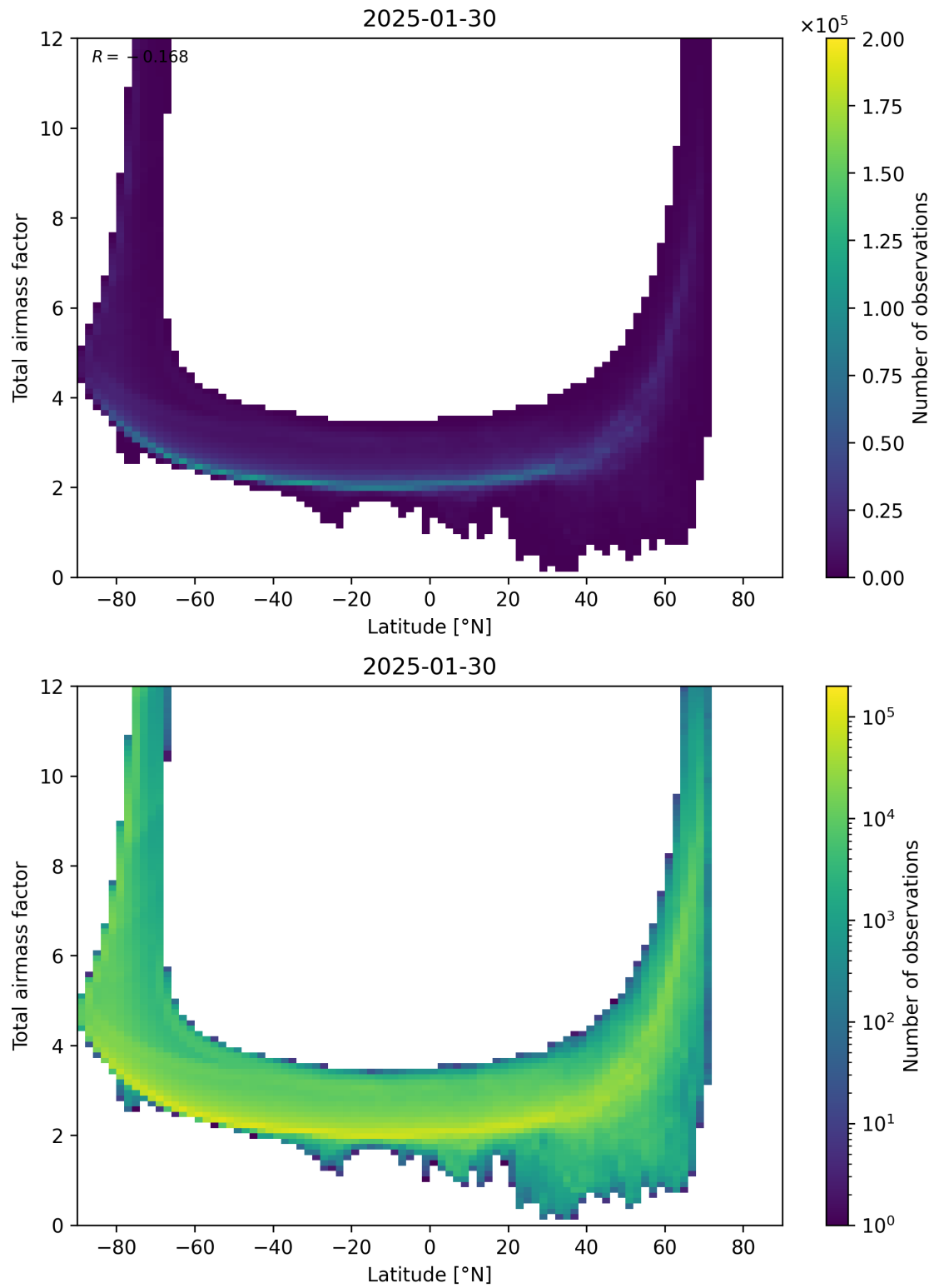
Figure 84: Scatter density plot of “Latitude” against “Total airmass factor” for 2025-01-29 to 2025-01-31.
