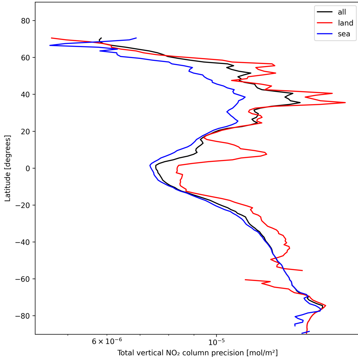
Figure 22: Zonal average of "Total vertical NO 2 column precision" for 2025-01-29 to 2025-01-31.
