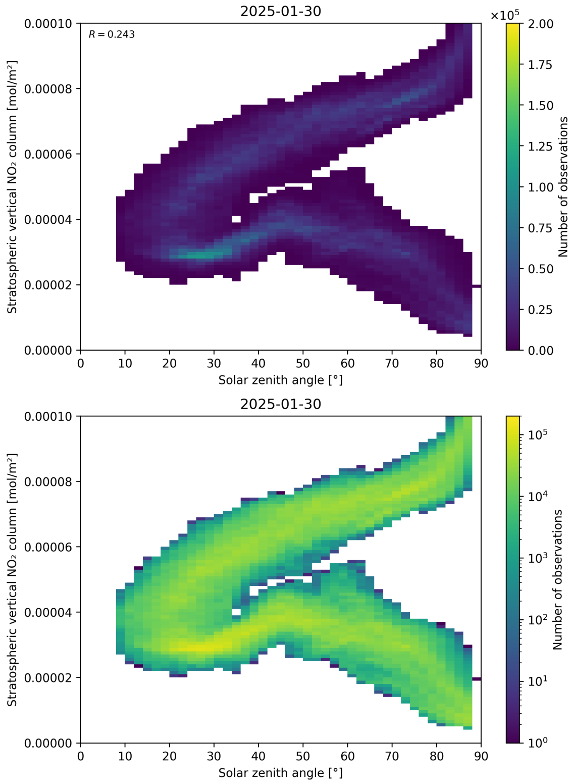
Figure 150: Scatter density plot of “Solar zenith angle” against “Stratospheric vertical NO 2 column” for 2025-01-29 to 2025-01-31.
