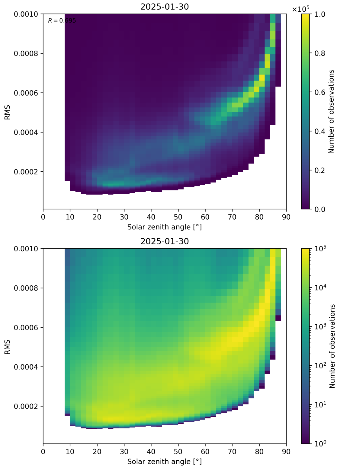
Figure 157: Scatter density plot of “Solar zenith angle” against “RMS” for 2025-01-29 to 2025-01-31.
