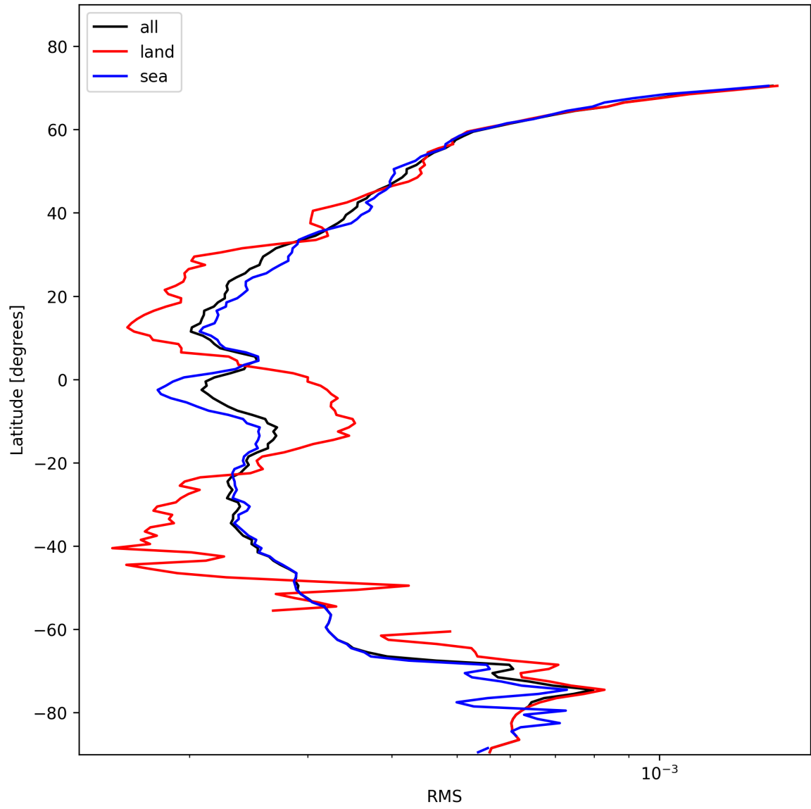
Figure 26: Zonal average of “RMS” for 2025-01-29 to 2025-01-31.
