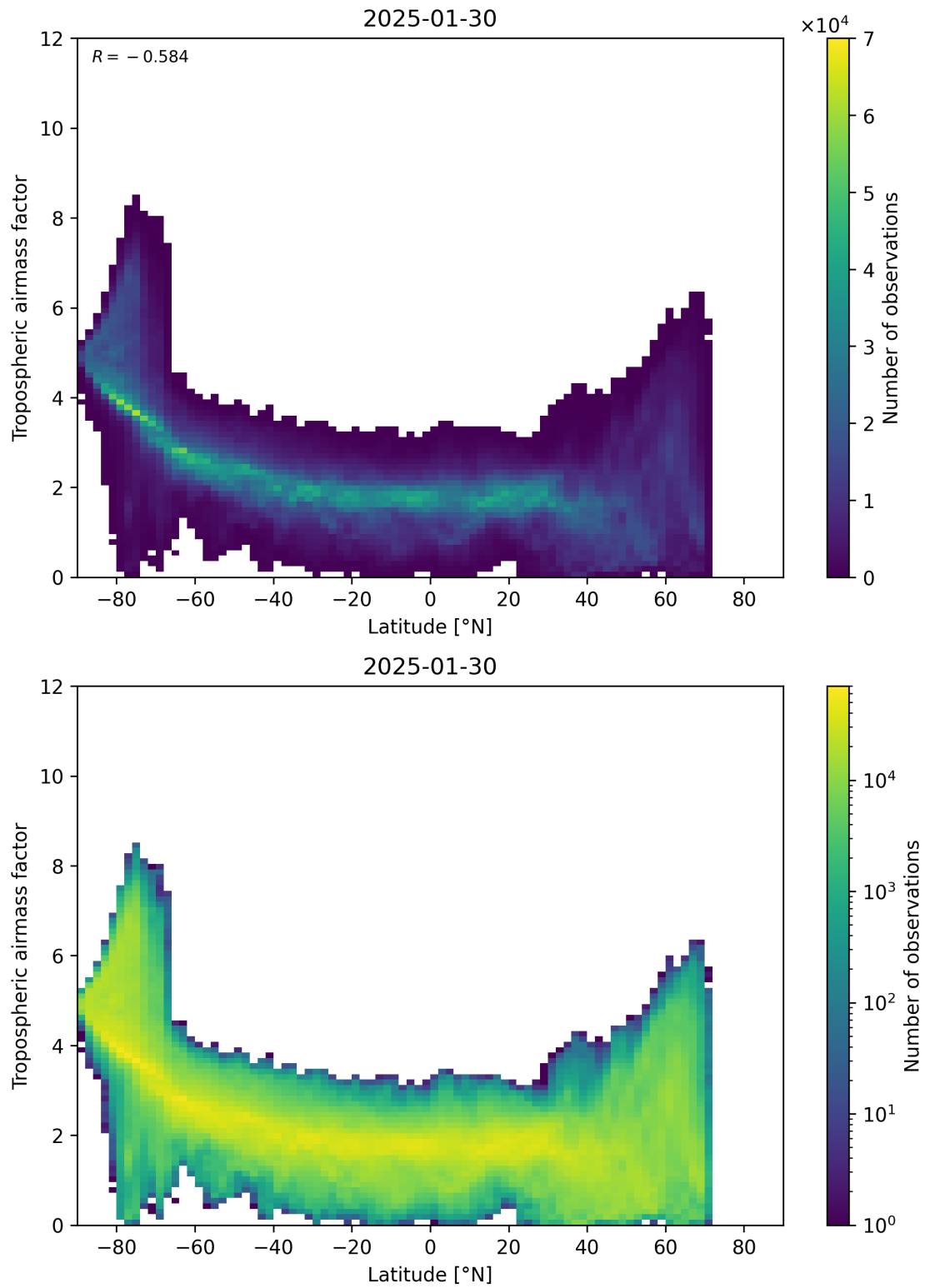
Figure 85: Scatter density plot of “Latitude” against “Tropospheric air mass factor” for 2025-01-29 to 2025-01-31.
