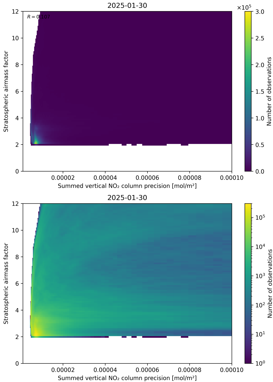
Figure 106: Scatter density plot of “Summed vertical NO 2 column precision” against “Stratospheric airmass factor” for 2025-01-29 to 2025-01-31.
