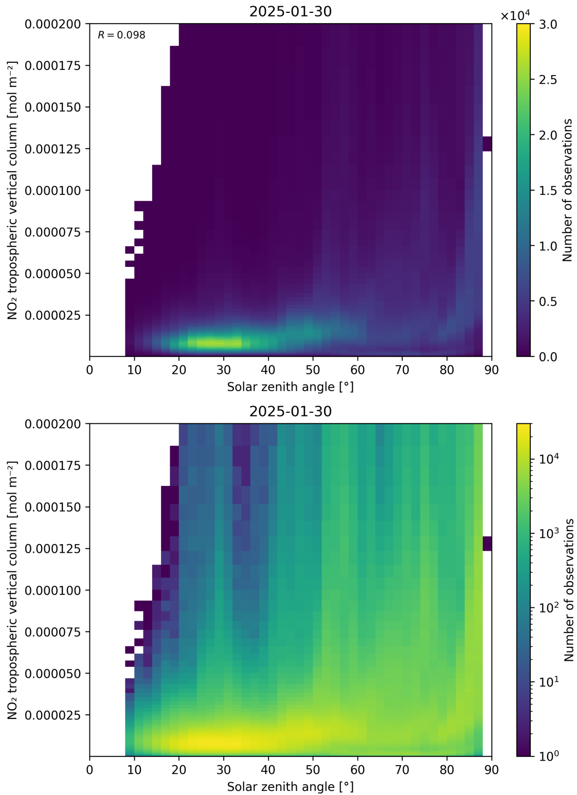
Figure 155: Scatter density plot of “Solar zenith angle” against “NO 2 tropospheric vertical column” for 2025-01-29 to 2025-01-31.
