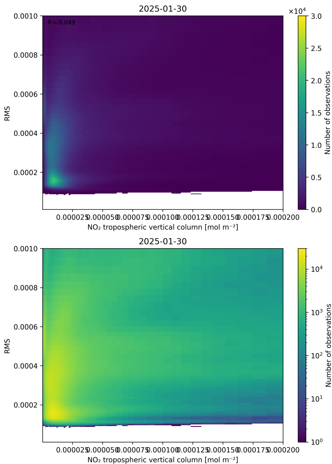
Figure 142: Scatter density plot of “NO 2 tropospheric vertical column” against “RMS” for 2025-01-29 to 2025-01-31.
