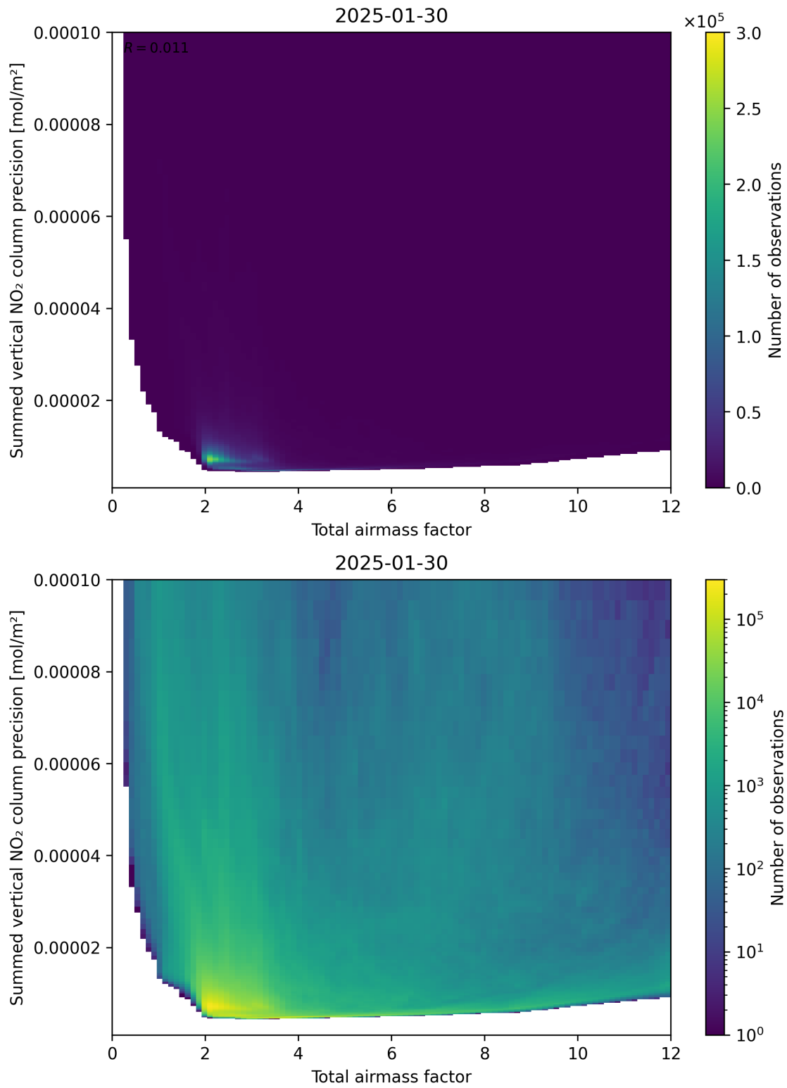
Figure 66: Scatter density plot of “Total airmass factor” against “Summed vertical NO 2 column precision” for 2025-01-29 to 2025-01-31.
