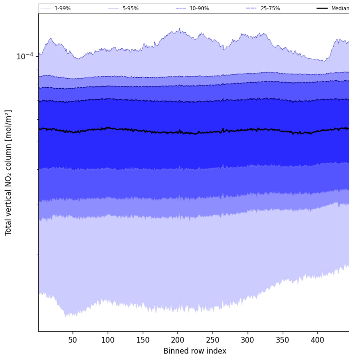
Figure 55: Along track statistics of “Total vertical NO 2 column” for 2025-01-29 to 2025-01-31
