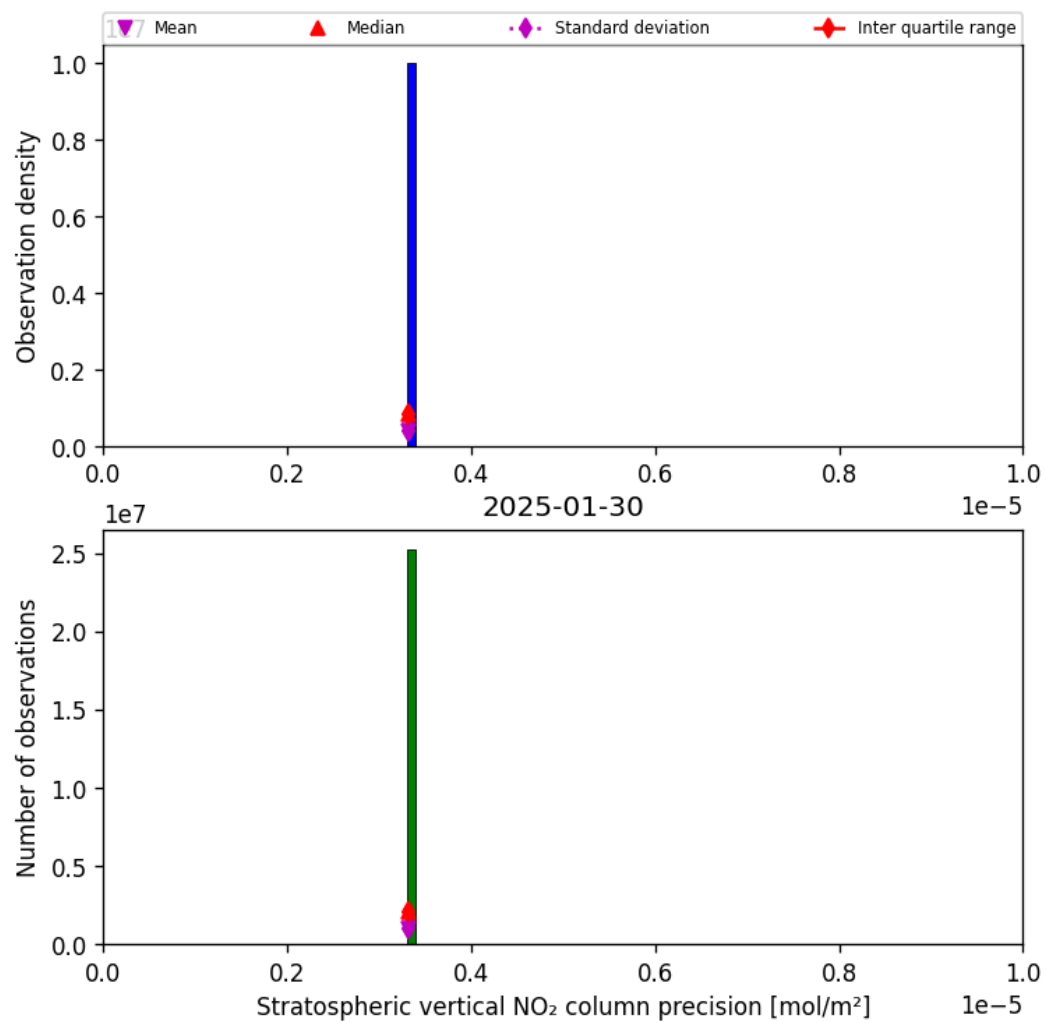
Figure 37: Histogram of “Stratospheric vertical NO 2 column precision” for 2025-01-29 to 2025-01-31
