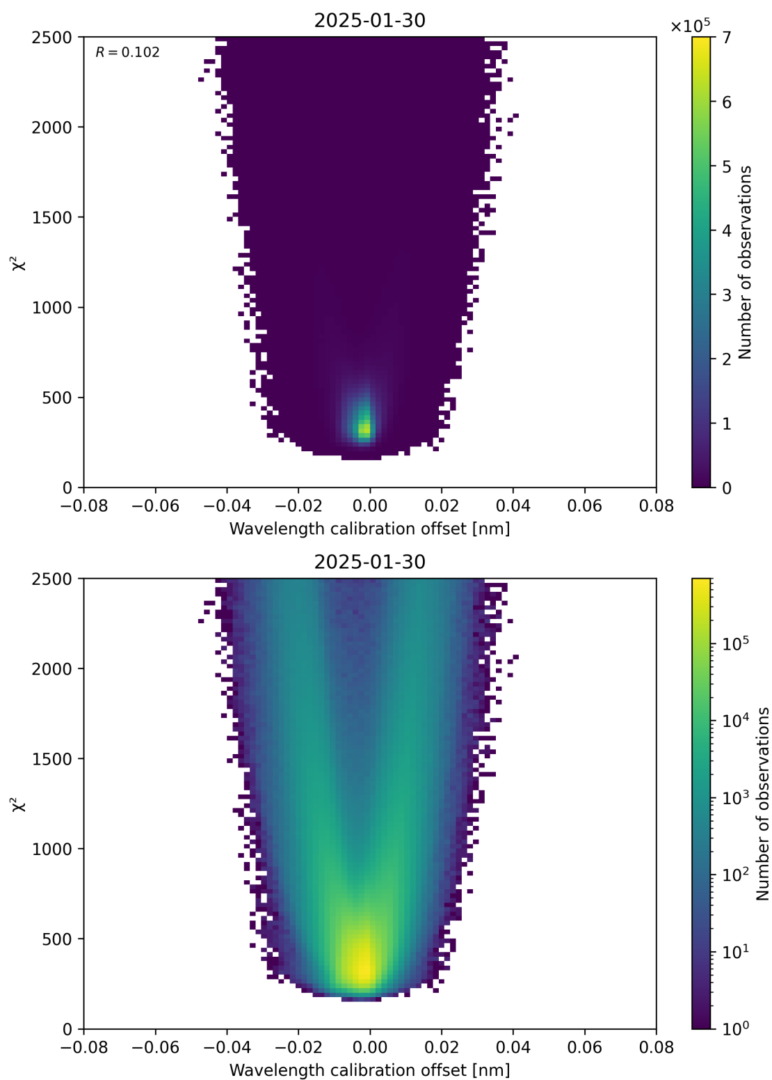
Figure 175: Scatter density plot of “Wavelength calibration offset” against “ \chi^2 ” for 2025-01-29 to 2025-01-31.
