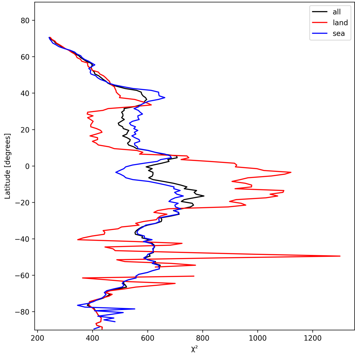
Figure 25: Zonal average of “ \chi^2 ” for 2025-01-29 to 2025-01-31.
