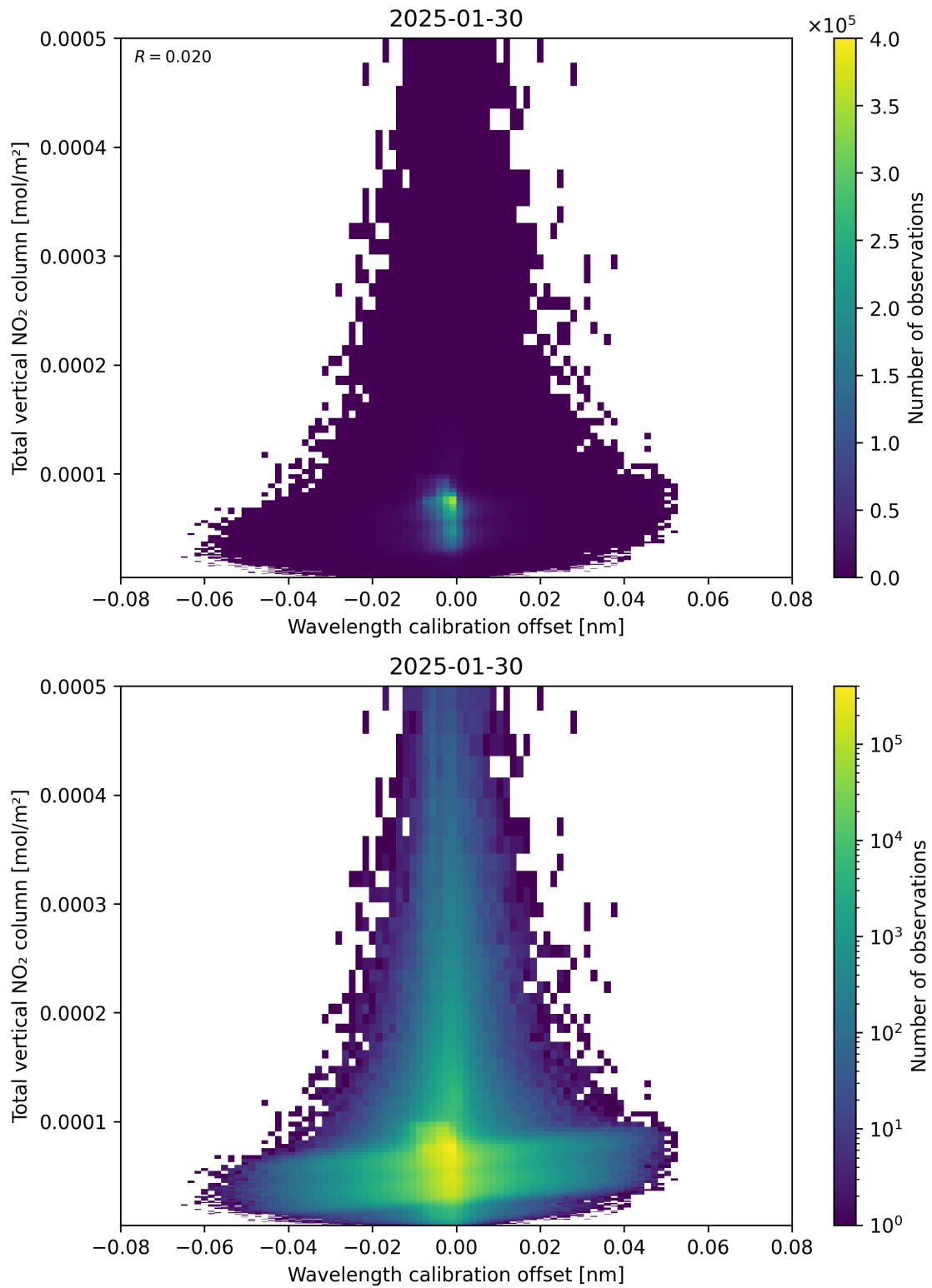
Figure 179: Scatter density plot of “Wavelength calibration offset” against “Total vertical NO 2 column” for 2025-01-29 to 2025-01-31.
