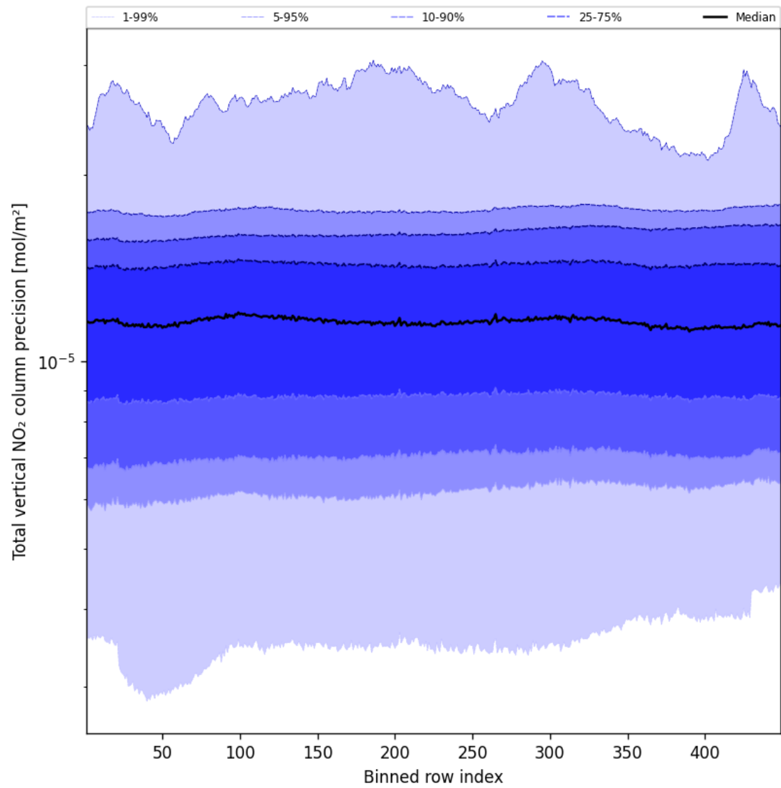
Figure 56: Along track statistics of “Total vertical NO 2 column precision” for 2025-01-29 to 2025-01-31
