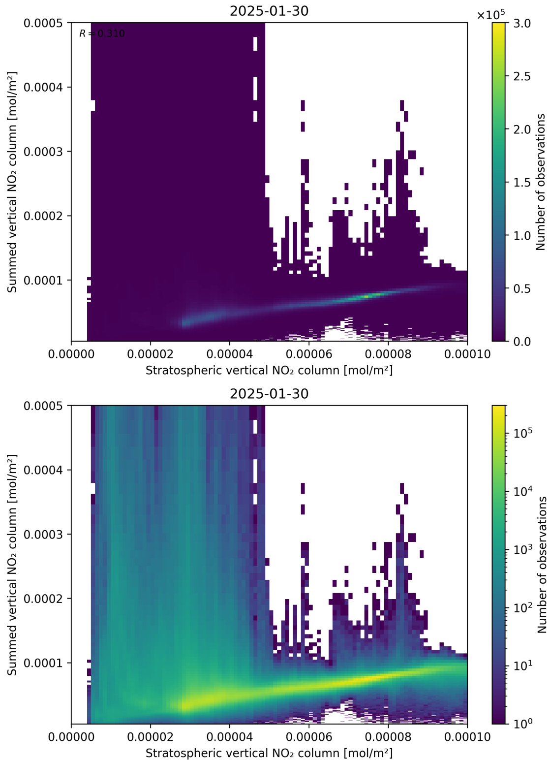
Figure 98: Scatter density plot of “Stratospheric vertical NO 2 column” against “Summed vertical NO 2 column” for 2025-01-29 to 2025-01-31.
