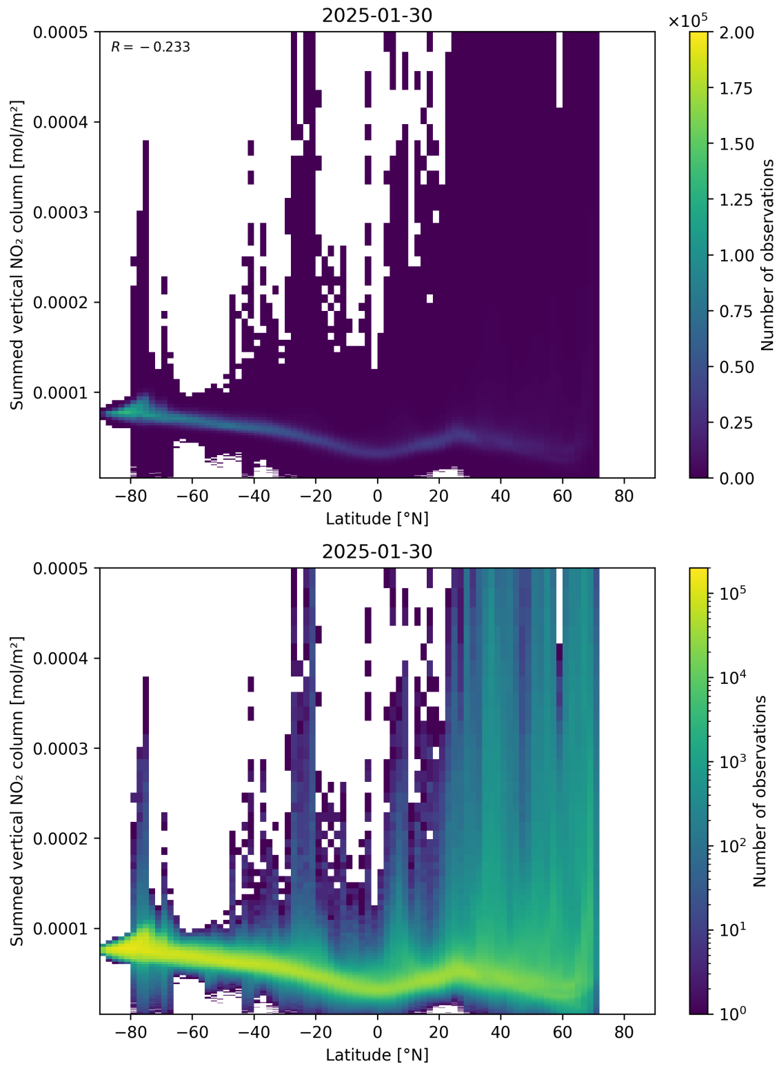
Figure 88: Scatter density plot of “Latitude” against “Summed vertical NO 2 column” for 2025-01-29 to 2025-01-31.
