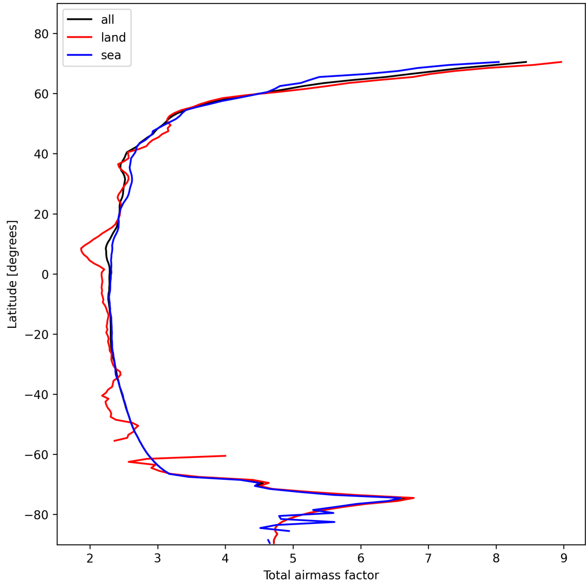
Figure 15: Zonal average of “Total airmass factor” for 2025-01-29 to 2025-01-31.
