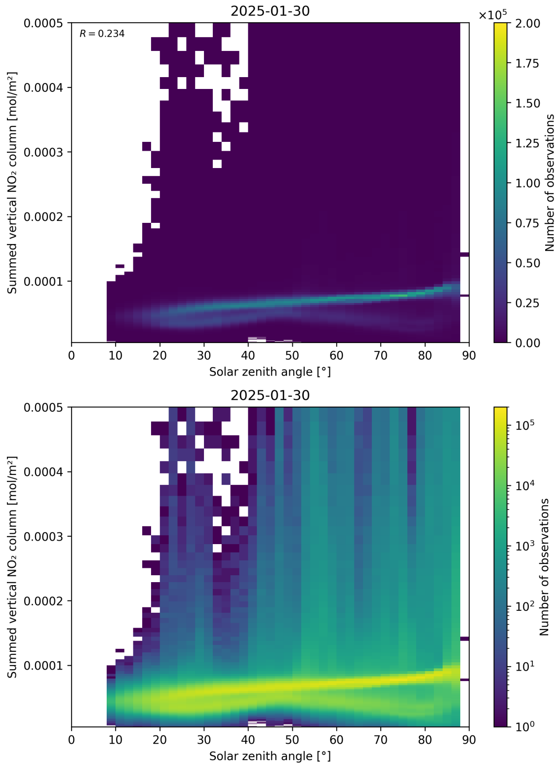
Figure 151: Scatter density plot of “Solar zenith angle” against “Summed vertical NO 2 column” for 2025-01-29 to 2025-01-31.
