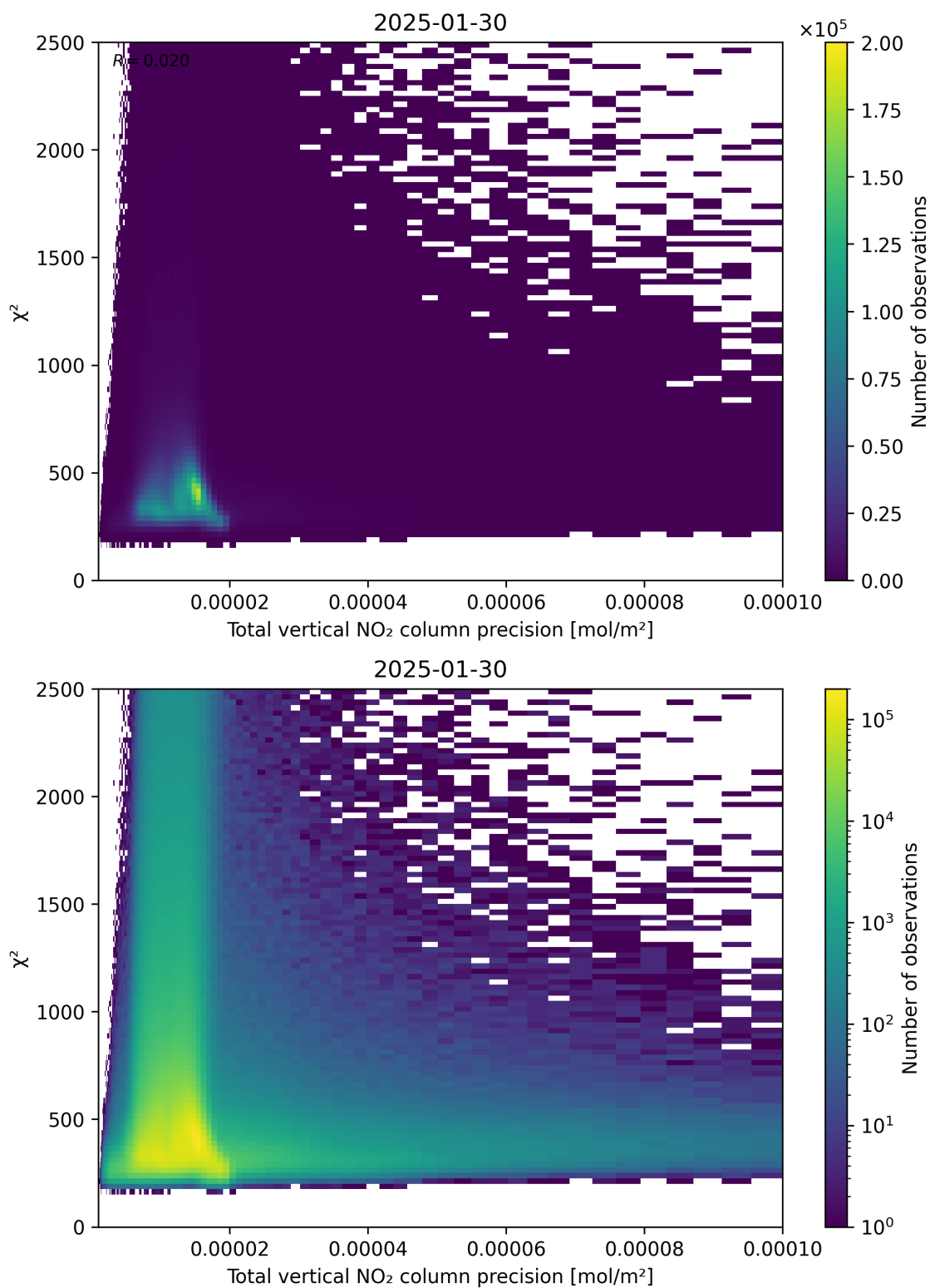
Figure 116: Scatter density plot of “Total vertical NO 2 column precision” against “ \chi^2 ” for 2025-01-29 to 2025-01-31.
