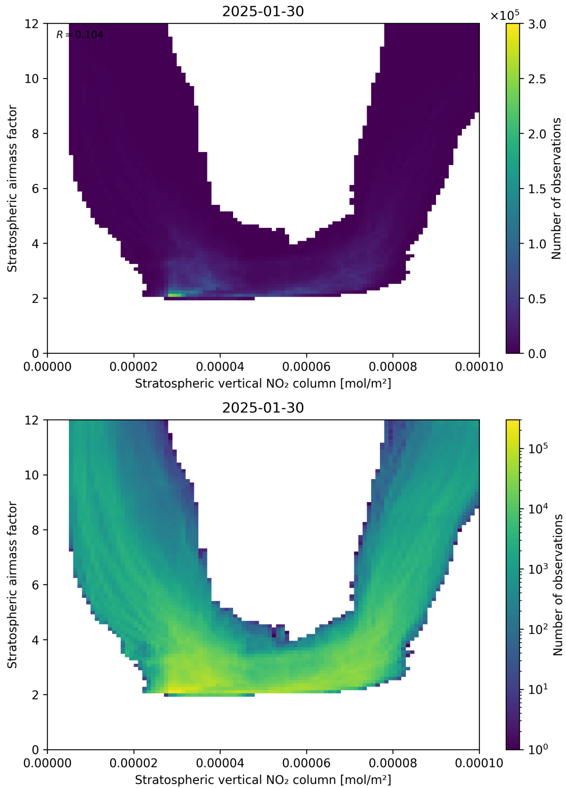
Figure 96: Scatter density plot of “Stratospheric vertical NO 2 column” against “Stratospheric airmass factor” for 2025-01-29 to 2025-01-31.
