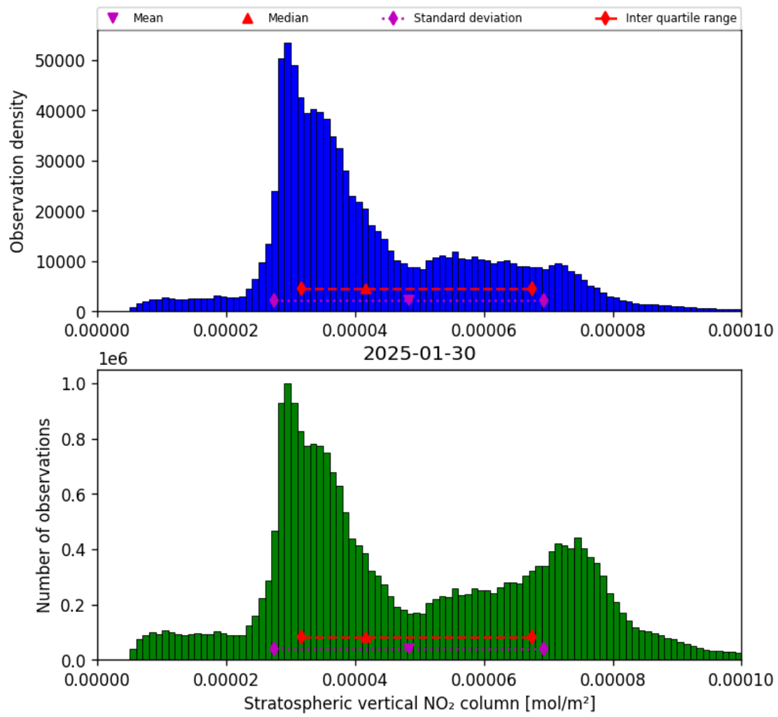
Figure 36: Histogram of “Stratospheric vertical NO 2 column” for 2025-01-29 to 2025-01-31
