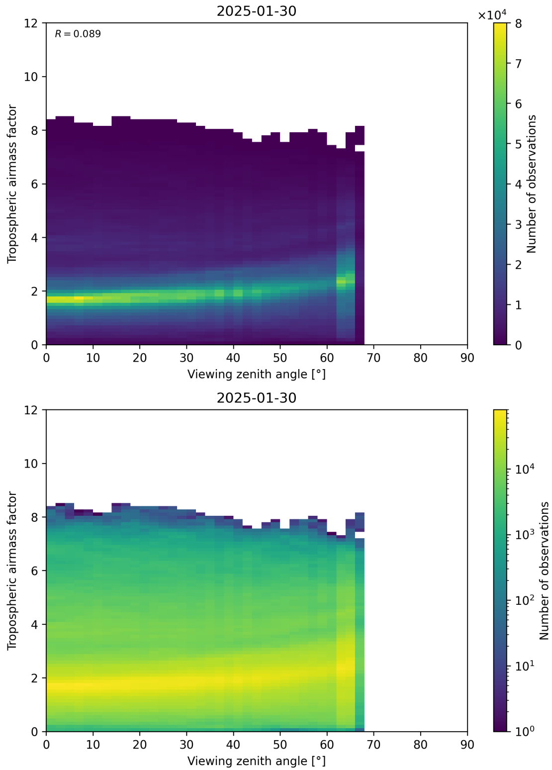
Figure 161: Scatter density plot of “Viewing zenith angle” against “Tropospheric airmass factor” for 2025-01-29 to 2025-01-31.
