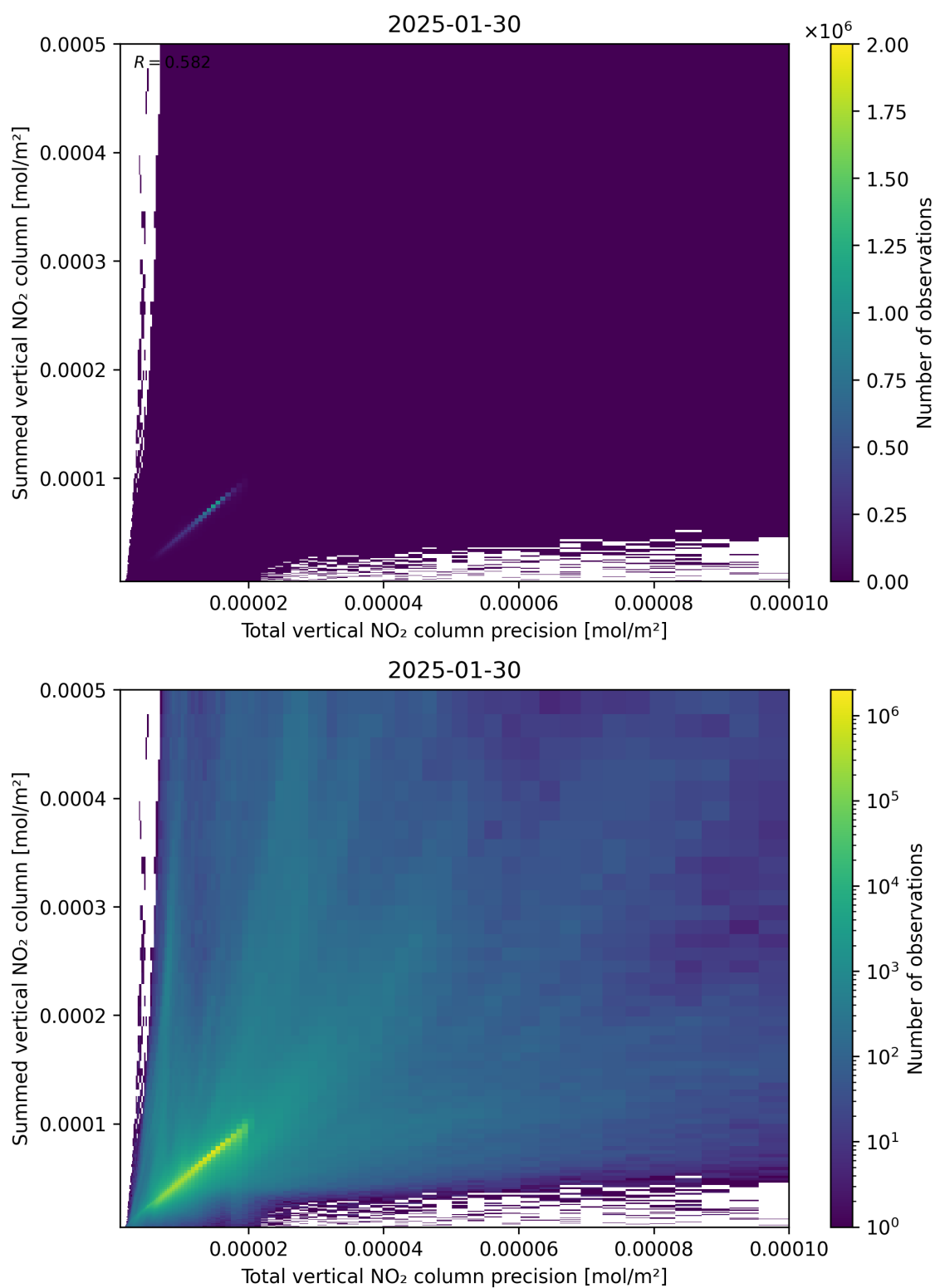
Figure 117: Scatter density plot of “Total vertical NO 2 column precision” against “Summed vertical NO 2 column” for 2025-01-29 to 2025-01-31.
