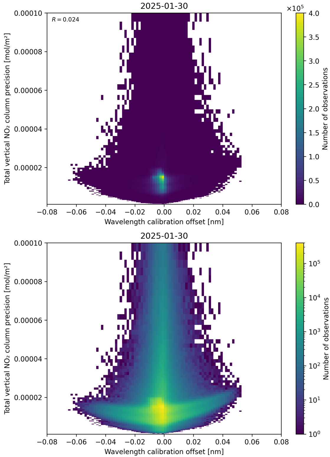
Figure 180: Scatter density plot of “Wavelength calibration offset” against “Total vertical NO 2 column precision” for 2025-01-29 to 2025-01-31.
