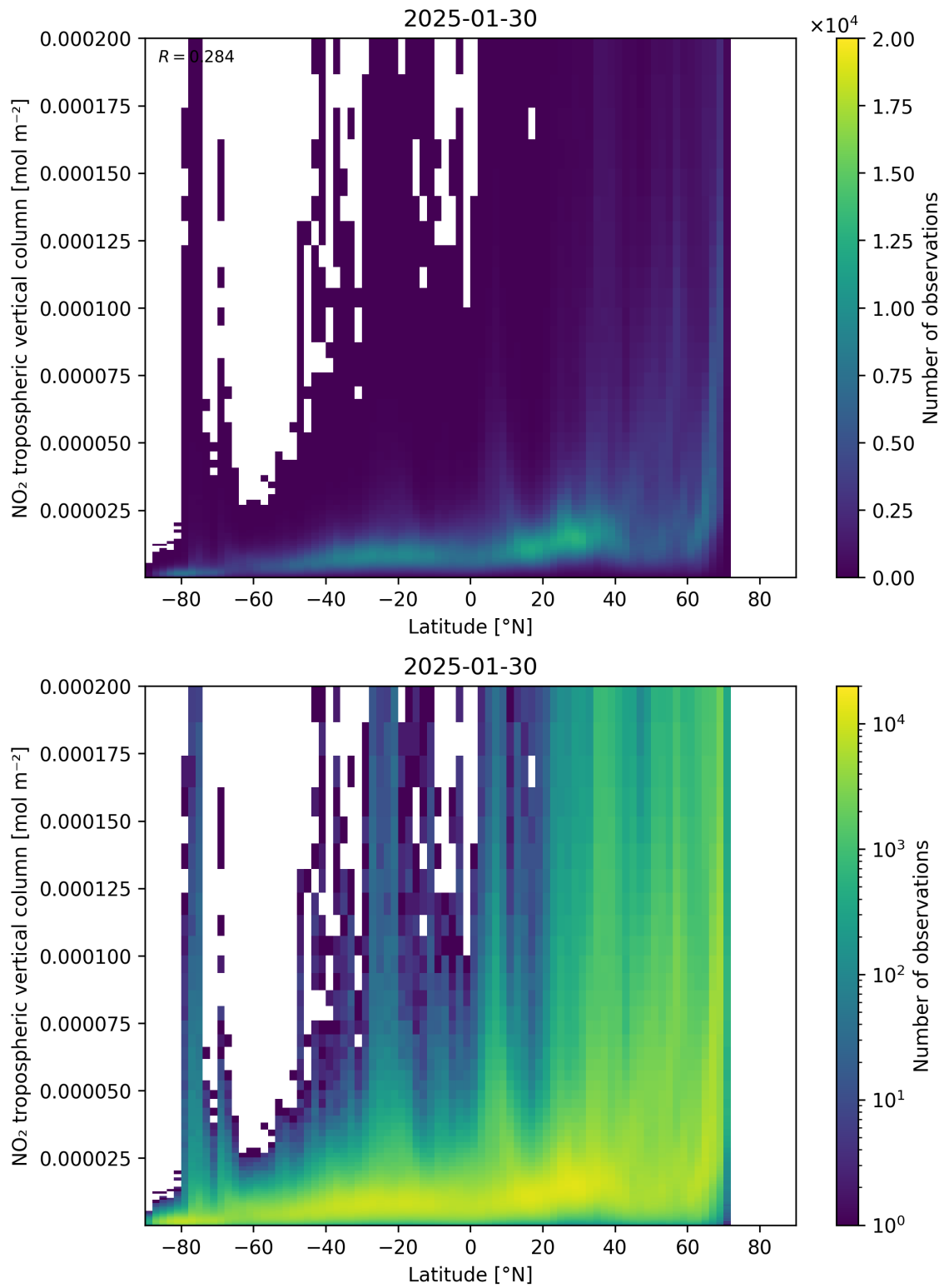
Figure 92: Scatter density plot of “Latitude” against “NO 2 tropospheric vertical column” for 2025-01-29 to 2025-01-31.
