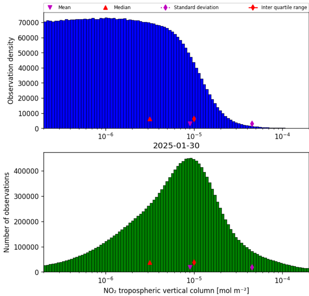
Figure 29: Histogram of “NO 2 tropospheric vertical column” for 2025-01-29 to 2025-01-31
