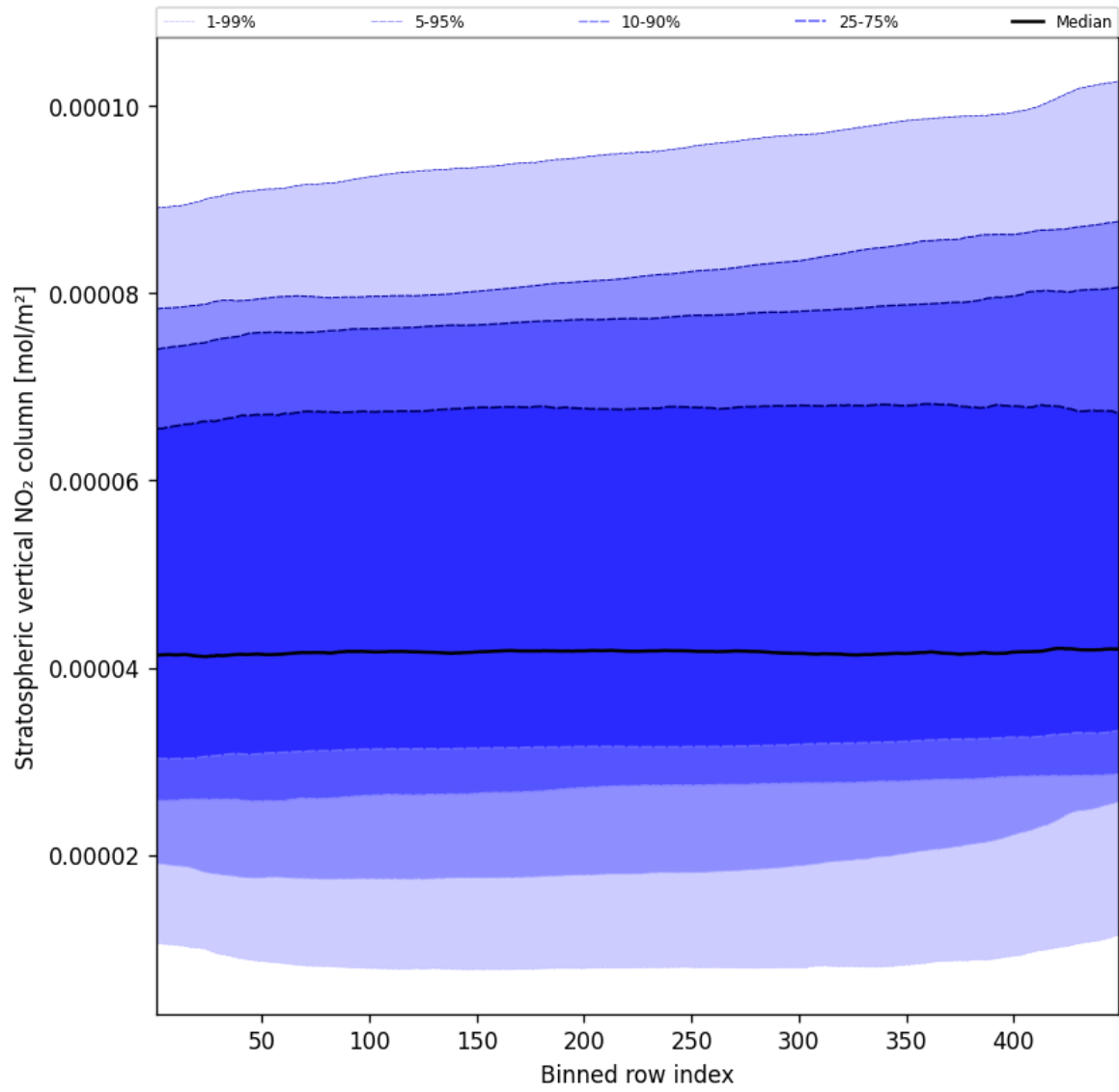
Figure 53: Along track statistics of “Stratospheric vertical NO 2 column” for 2025-01-29 to 2025-01-31
