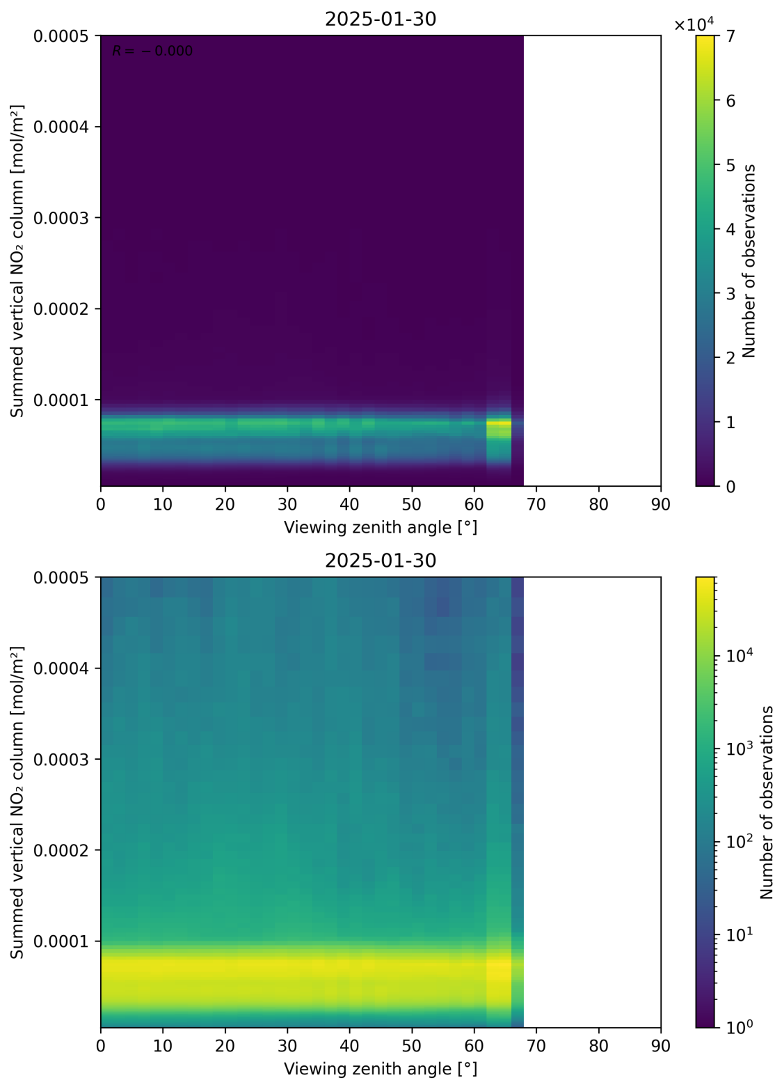
Figure 165: Scatter density plot of “Viewing zenith angle” against “Summed vertical NO 2 column” for 2025-01-29 to 2025-01-31.
