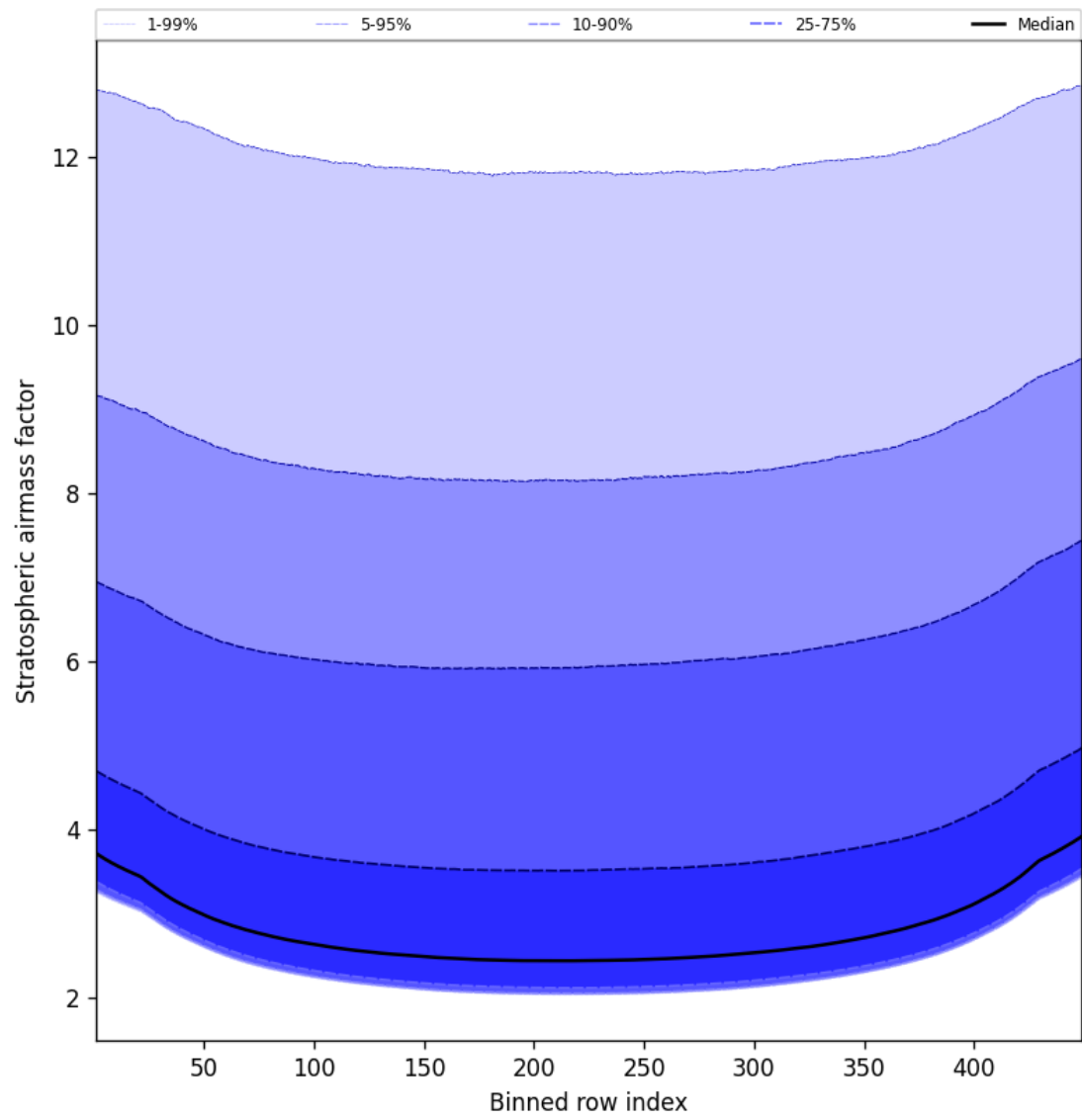
Figure 61: Along track statistics of “Stratospheric airmass factor” for 2025-01-29 to 2025-01-31
