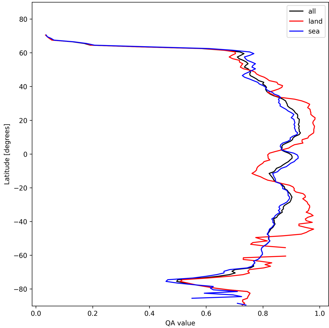
Figure 11: Zonal average of “QA value” for 2025-01-29 to 2025-01-31.
