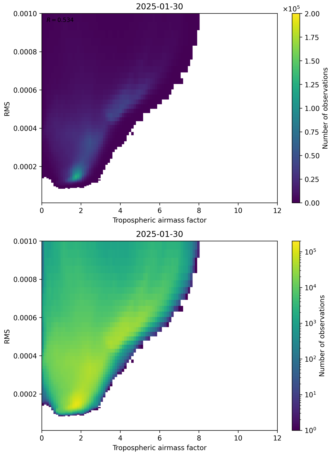
Figure 79: Scatter density plot of “Tropospheric airmass factor” against “RMS” for 2025-01-29 to 2025-01-31.
