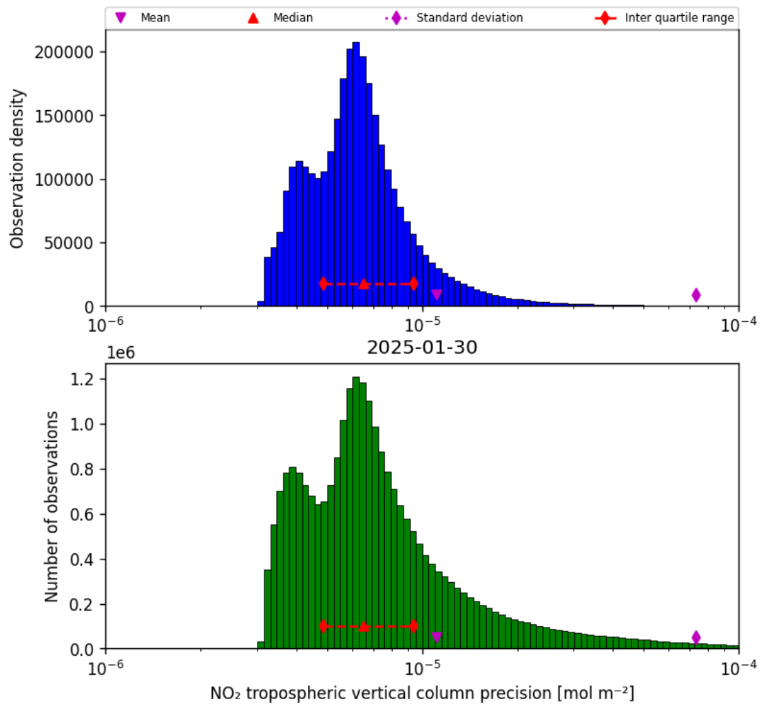
Figure 30: Histogram of “NO 2 tropospheric vertical column precision” for 2025-01-29 to 2025-01-31
