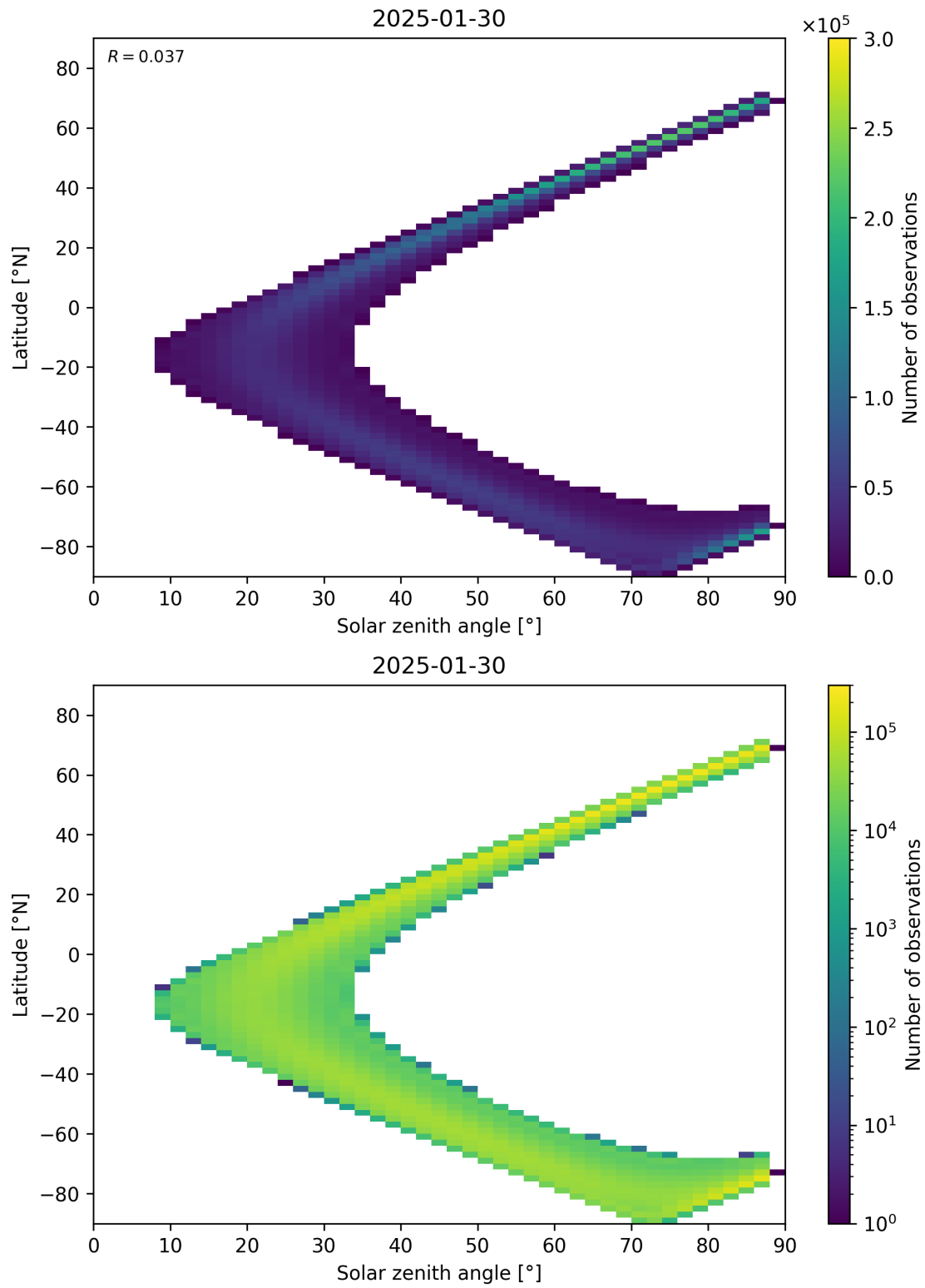
Figure 149: Scatter density plot of “Solar zenith angle” against “Latitude” for 2025-01-29 to 2025-01-31.
