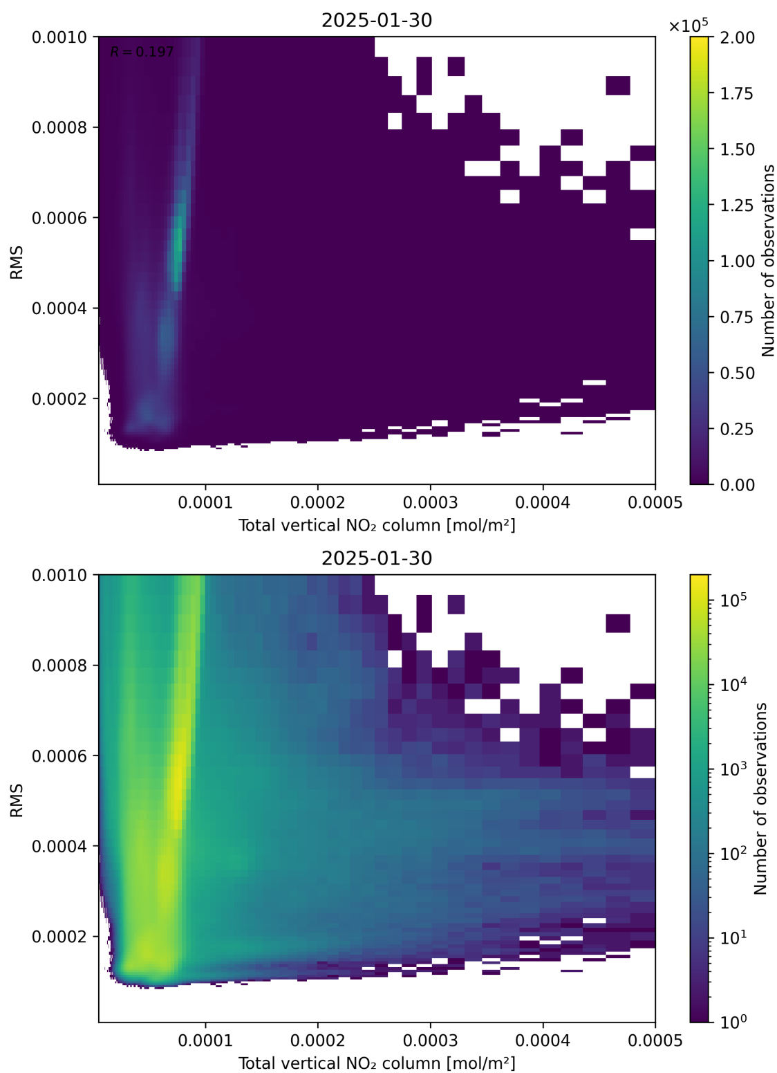
Figure 120: Scatter density plot of “Total vertical NO 2 column” against “RMS” for 2025-01-29 to 2025-01-31.
