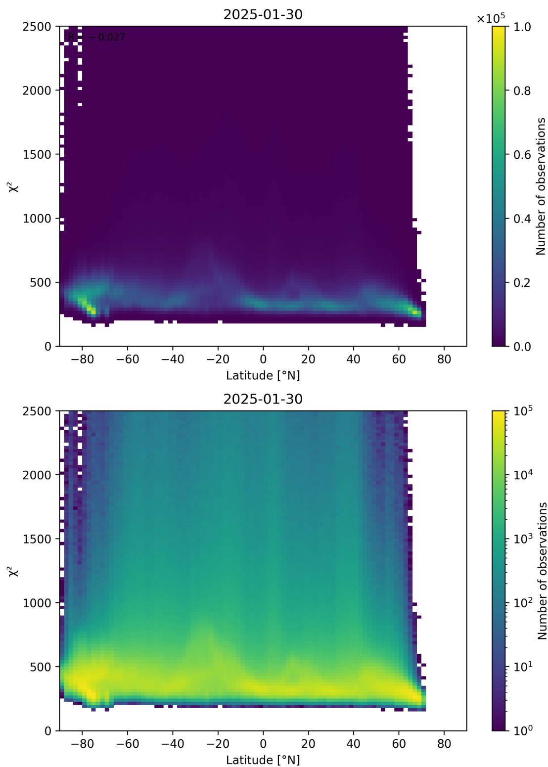
Figure 86: Scatter density plot of “Latitude” against “ \chi^2 ” for 2025-01-29 to 2025-01-31.
