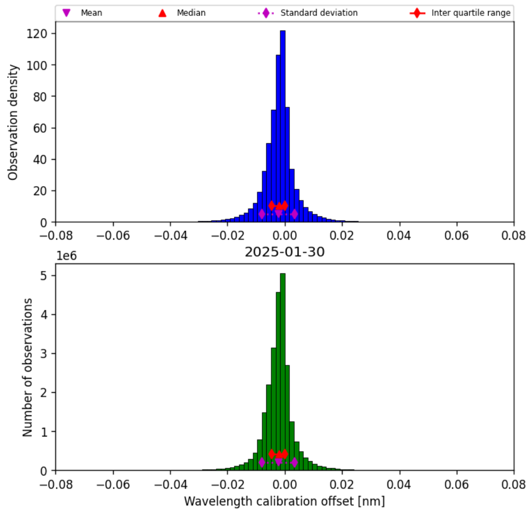
Figure 35: Histogram of “Wavelength calibration offset” for 2025-01-29 to 2025-01-31
