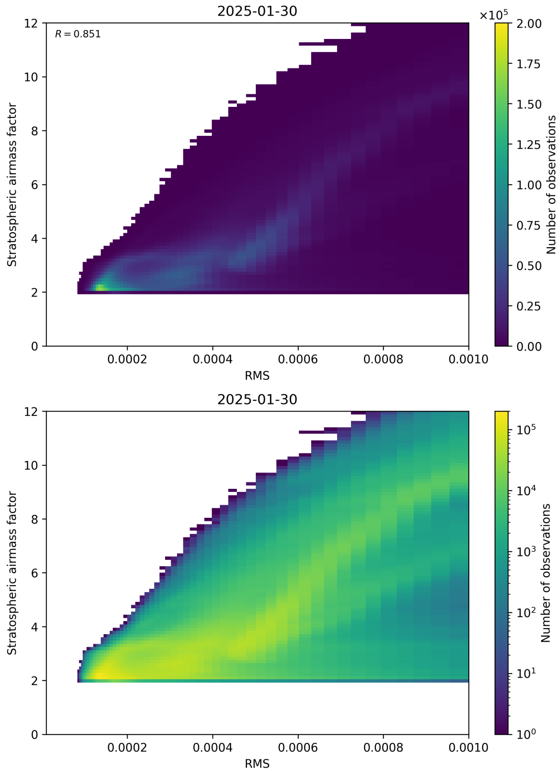
Figure 144: Scatter density plot of “RMS” against “Stratospheric airmass factor” for 2025-01-29 to 2025-01-31.
