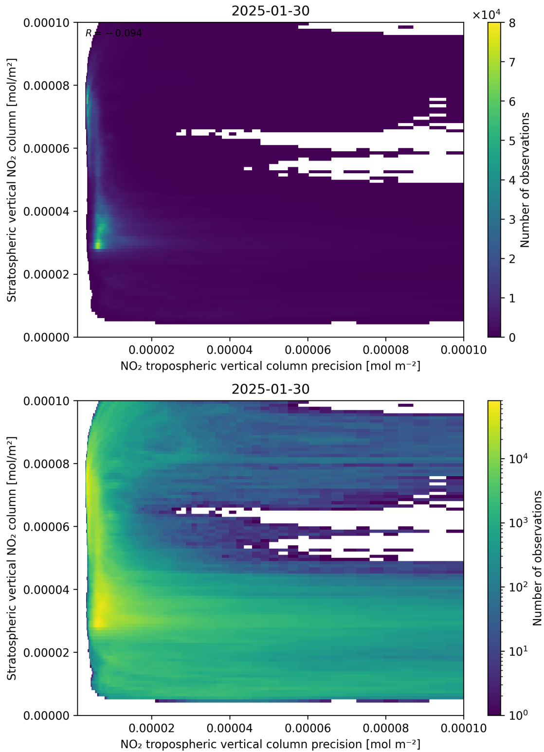
Figure 135: Scatter density plot of “NO 2 tropospheric vertical column precision” against “Stratospheric vertical NO 2 column” for 2025-01-29 to 2025-01-31.
