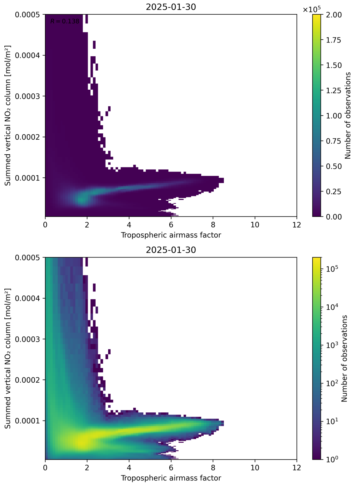
Figure 75: Scatter density plot of “Tropospheric air mass factor” against “Summed vertical NO 2 column” for 2025-01-29 to 2025-01-31.
