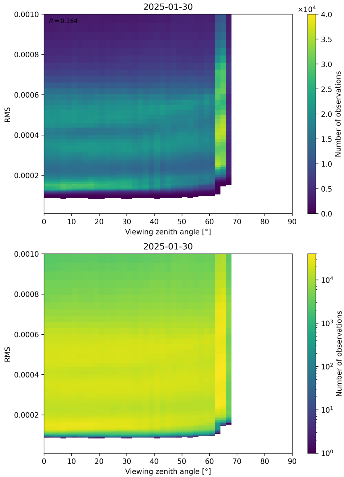
Figure 171: Scatter density plot of “Viewing zenith angle” against “RMS” for 2025-01-29 to 2025-01-31.
