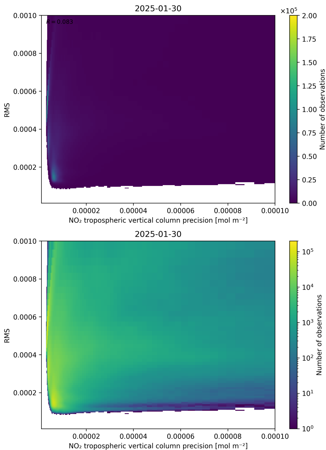
Figure 140: Scatter density plot of “NO 2 tropospheric vertical column precision” against “RMS” for 2025-01-29 to 2025-01-31.
