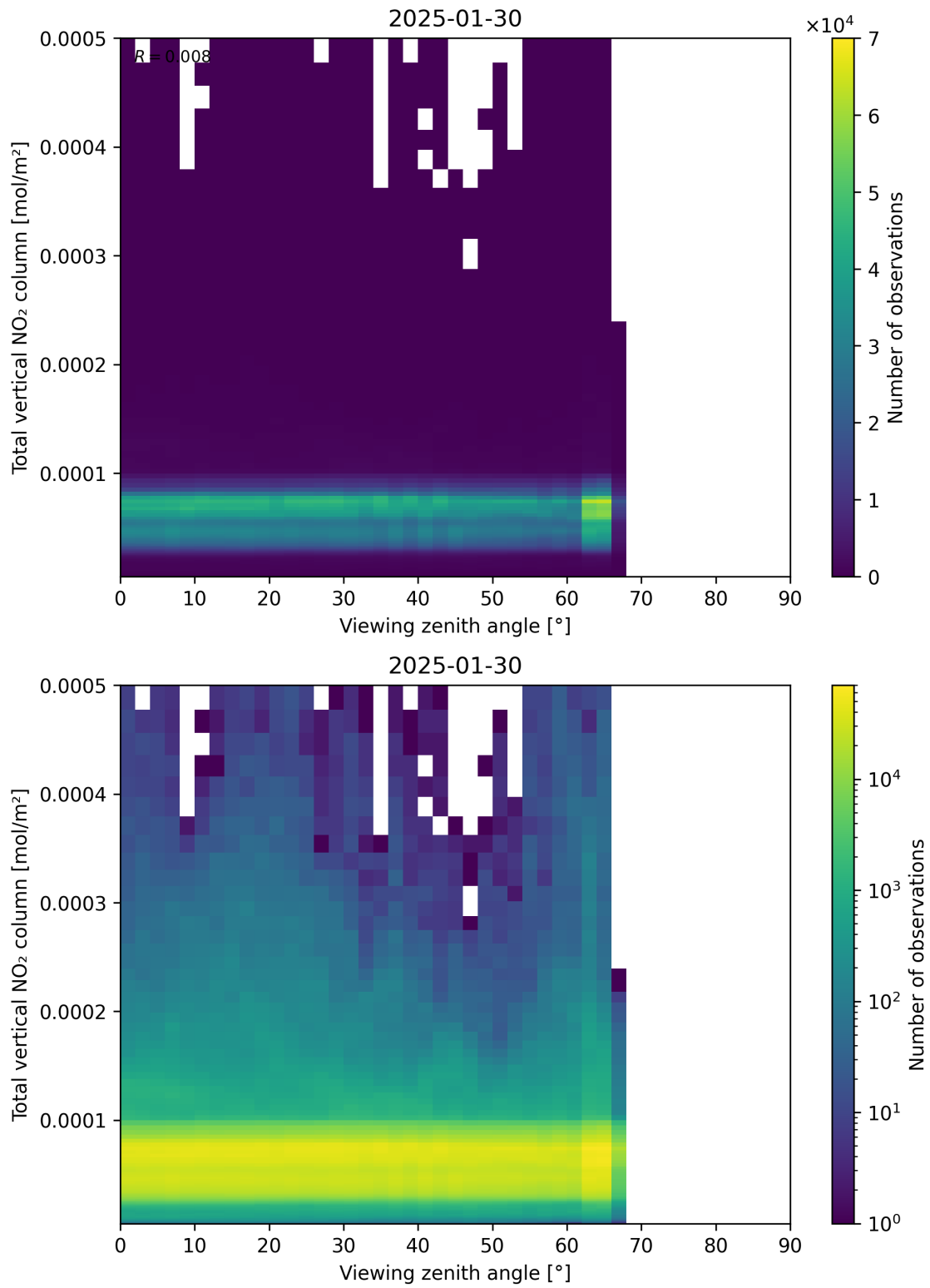
Figure 167: Scatter density plot of “Viewing zenith angle” against “Total vertical NO 2 column” for 2025-01-29 to 2025-01-31.
