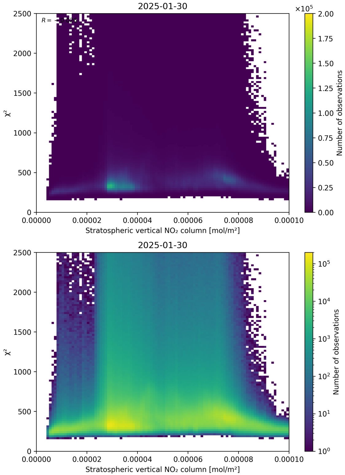
Figure 97: Scatter density plot of “Stratospheric vertical NO 2 column” against “ \chi^2 ” for 2025-01-29 to 2025-01-31.
