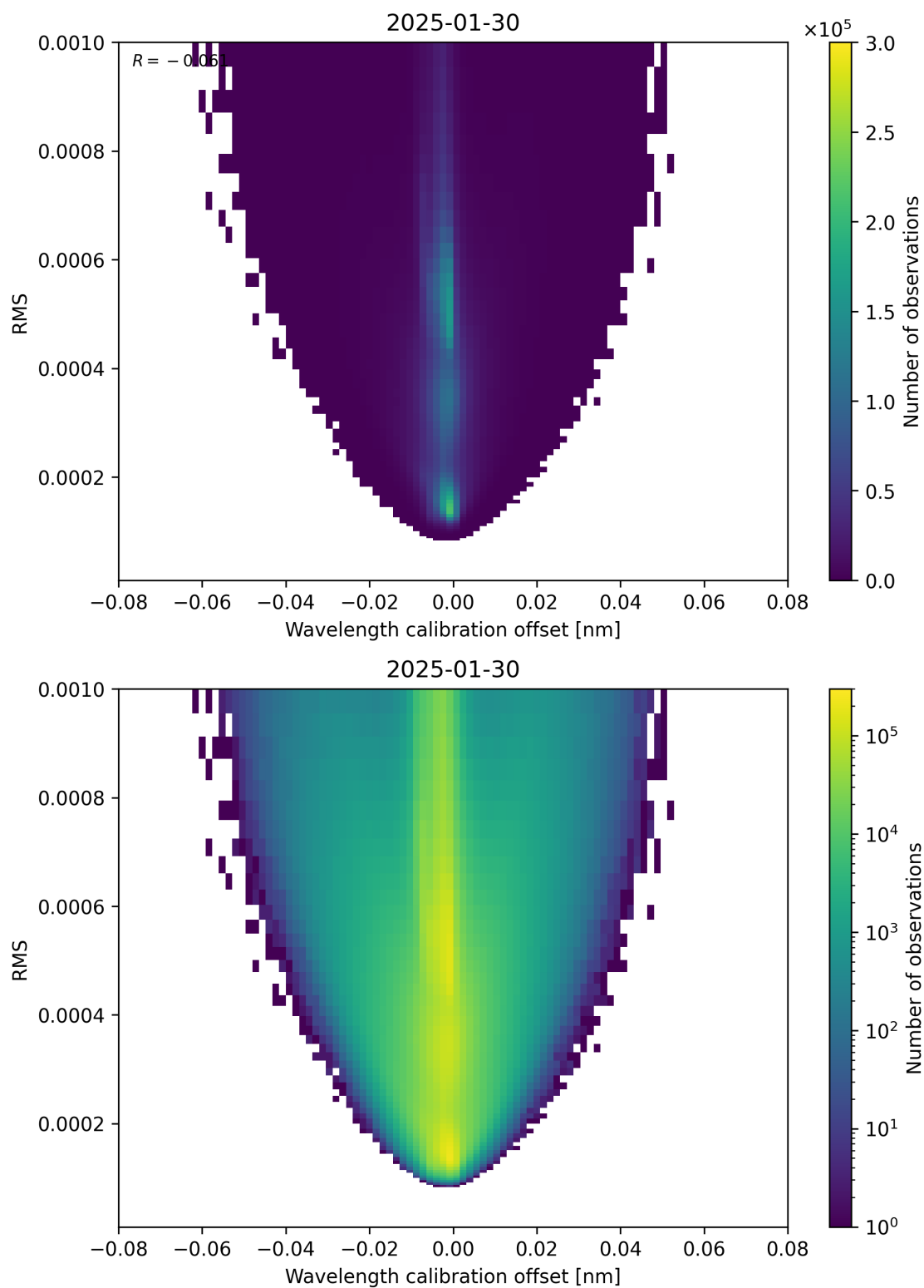
Figure 181: Scatter density plot of “Wavelength calibration offset” against “RMS” for 2025-01-29 to 2025-01-31.
