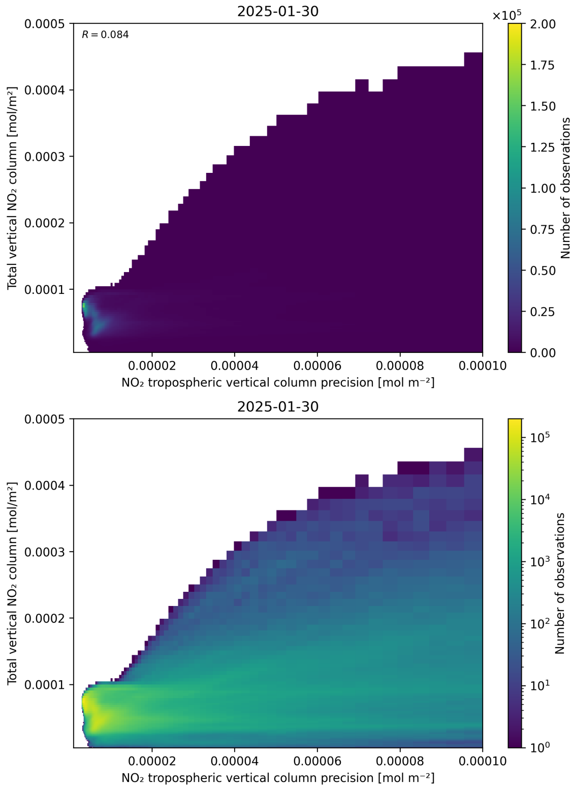
Figure 138: Scatter density plot of “NO 2 tropospheric vertical column precision” against “Total vertical NO 2 column” for 2025-01-29 to 2025-01-31.
