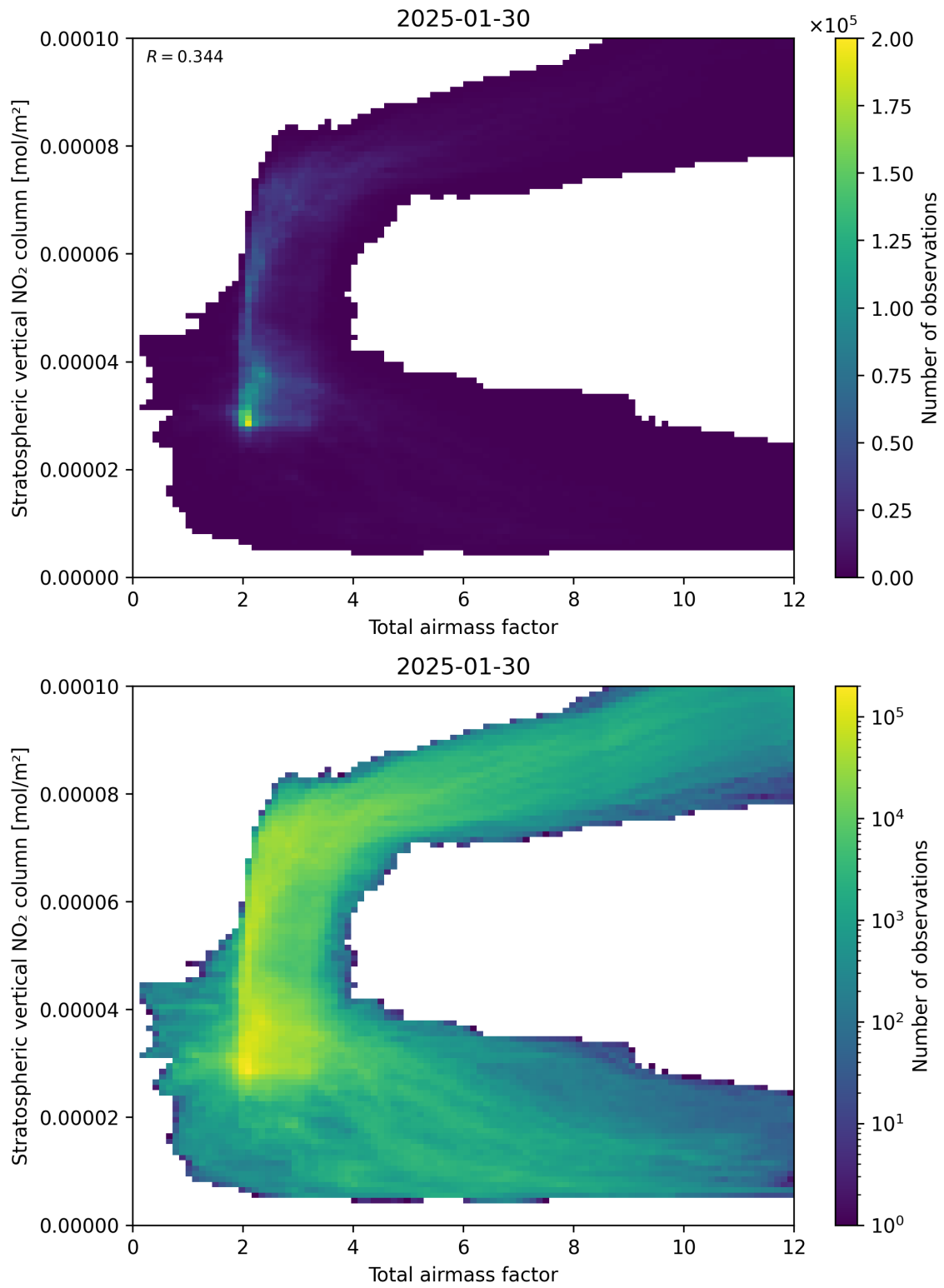
Figure 64: Scatter density plot of “Total airmass factor” against “Stratospheric vertical \text{NO}_2 column” for 2025-01-29 to 2025-01-31.
