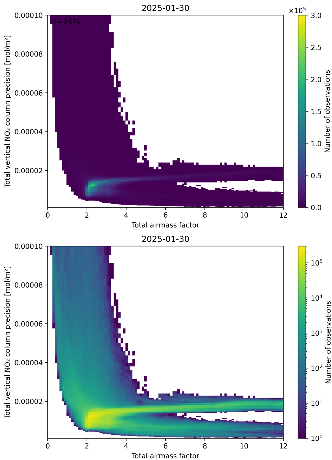
Figure 68: Scatter density plot of “Total airmass factor” against “Total vertical NO 2 column precision” for 2025-01-29 to 2025-01-31.
