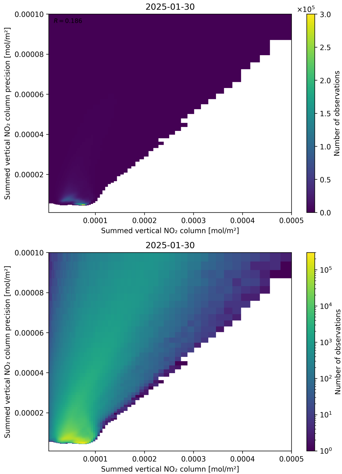
Figure 105: Scatter density plot of “Summed vertical NO 2 column” against “Summed vertical NO 2 column precision” for 2025-01-29 to 2025-01-31.
