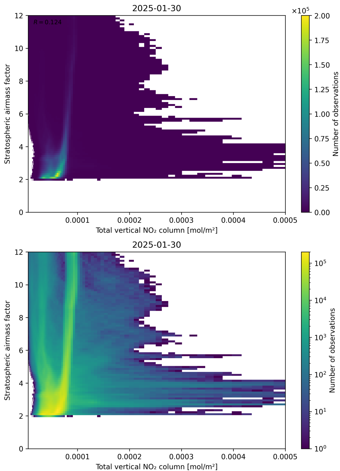
Figure 110: Scatter density plot of “Total vertical NO 2 column” against “Stratospheric airmass factor” for 2025-01-29 to 2025-01-31.
