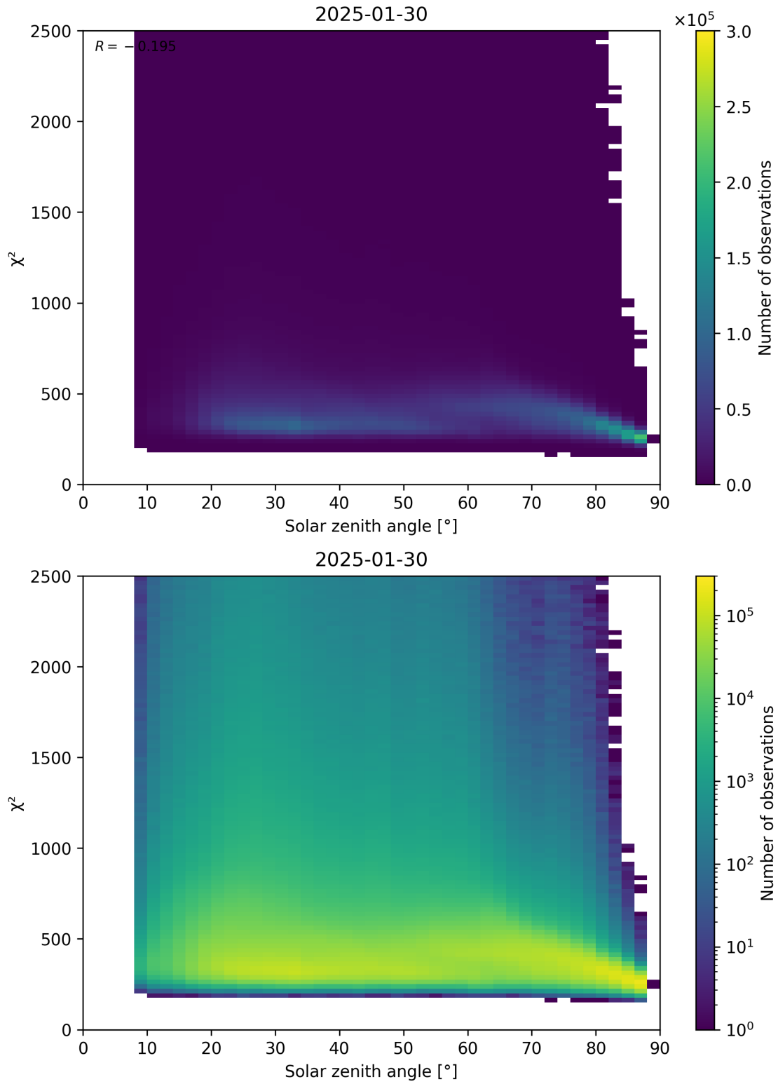
Figure 148: Scatter density plot of “Solar zenith angle” against “ \chi^2 ” for 2025-01-29 to 2025-01-31.
