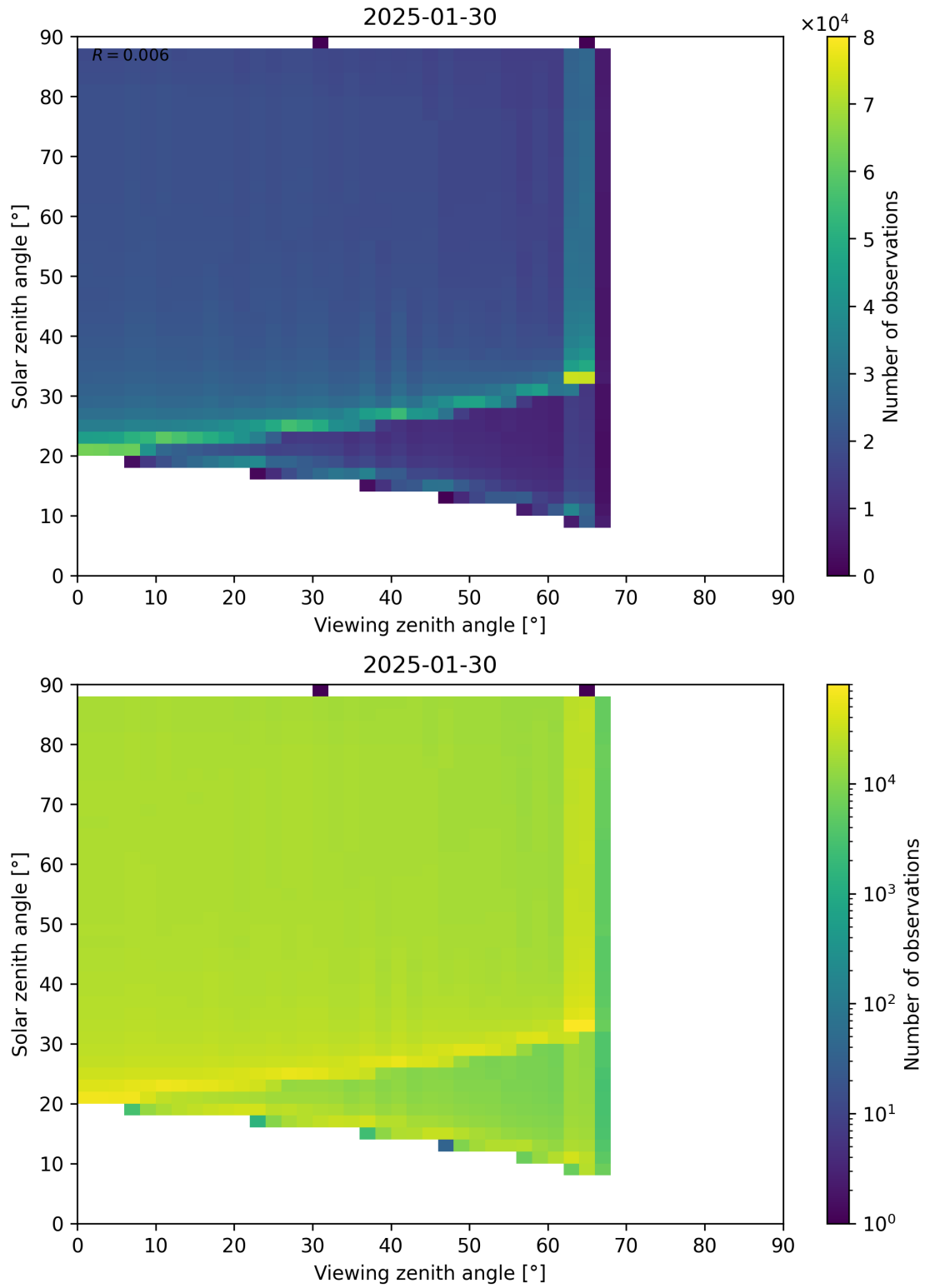
Figure 172: Scatter density plot of “Viewing zenith angle” against “Solar zenith angle” for 2025-01-29 to 2025-01-31.
