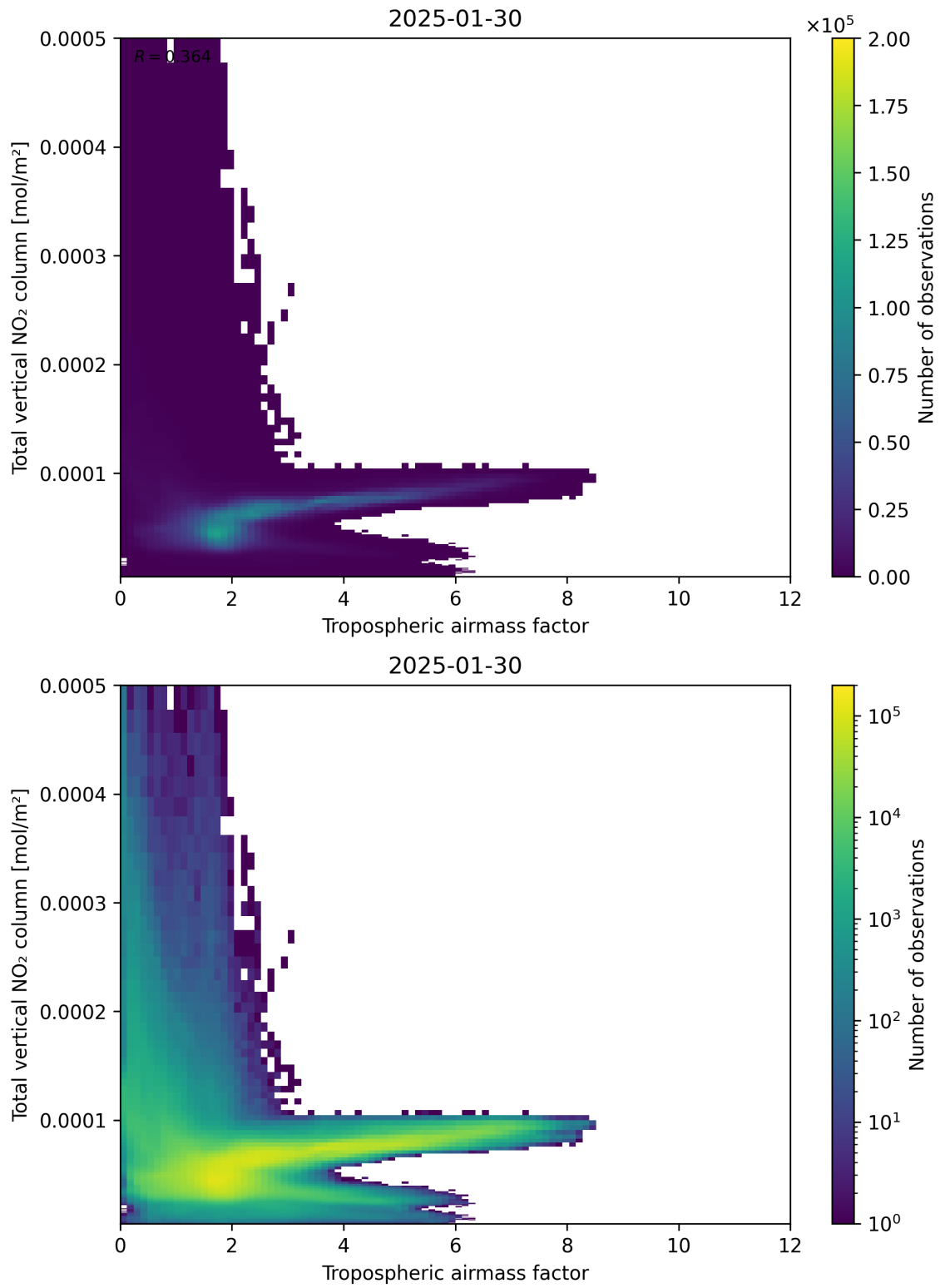
Figure 77: Scatter density plot of “Tropospheric airmass factor” against “Total vertical NO 2 column” for 2025-01-29 to 2025-01-31.
