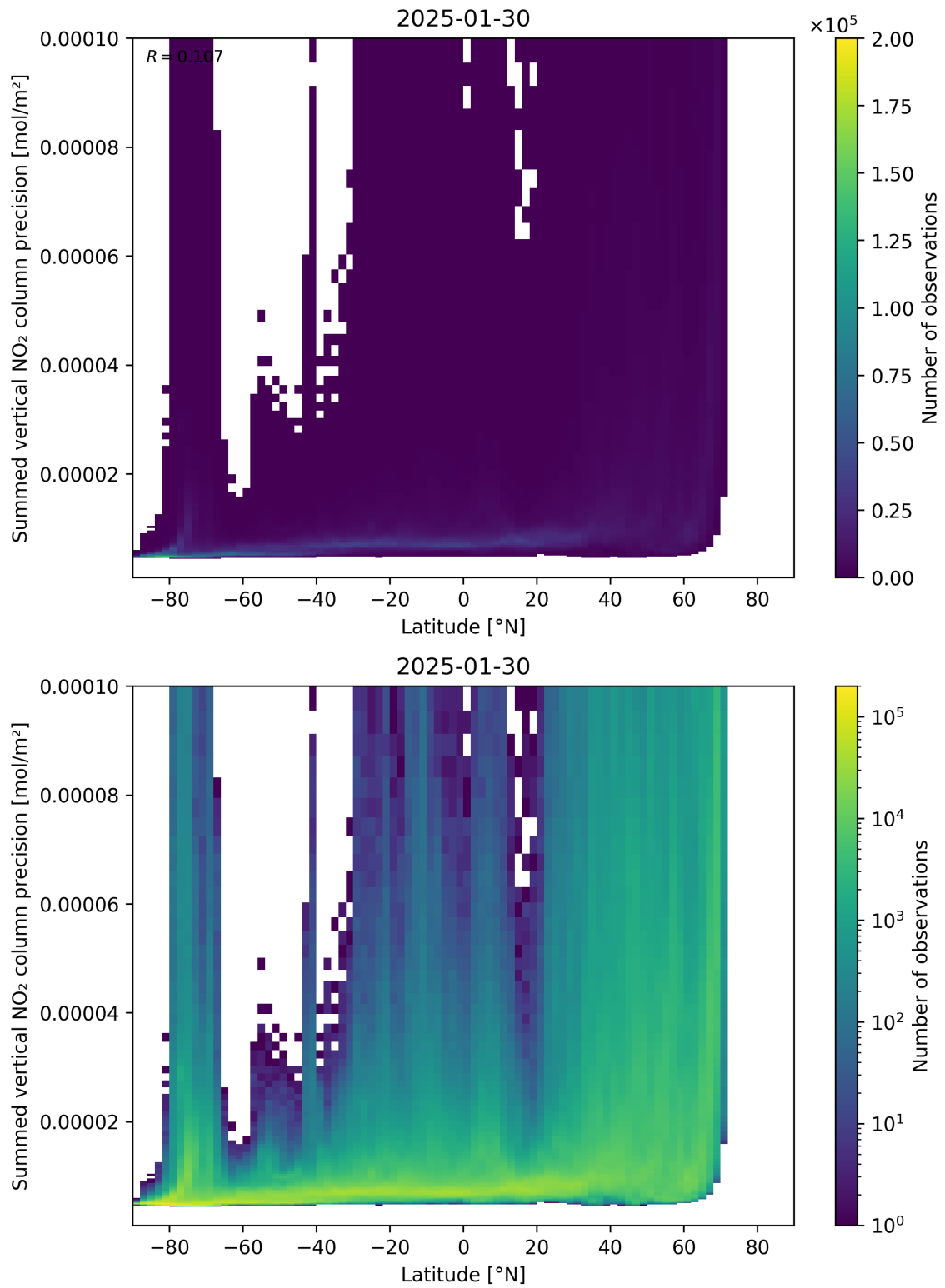
Figure 89: Scatter density plot of “Latitude” against “Summed vertical NO 2 column precision” for 2025-01-29 to 2025-01-31.
