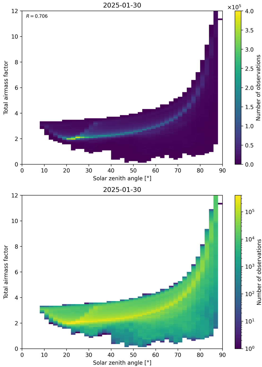
Figure 146: Scatter density plot of “Solar zenith angle” against “Total air mass factor” for 2025-01-29 to 2025-01-31.
