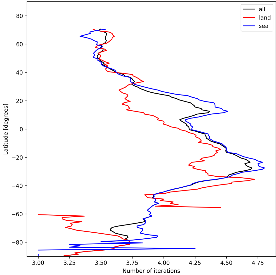
Figure 17: Zonal average of “Number of iterations” for 2025-01-29 to 2025-01-31.
