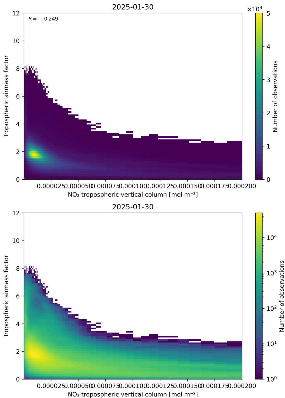
Figure 123: Scatter density plot of “NO 2 tropospheric vertical column” against “Tropospheric air mass factor” for 2025-01-29 to 2025-01-31.
