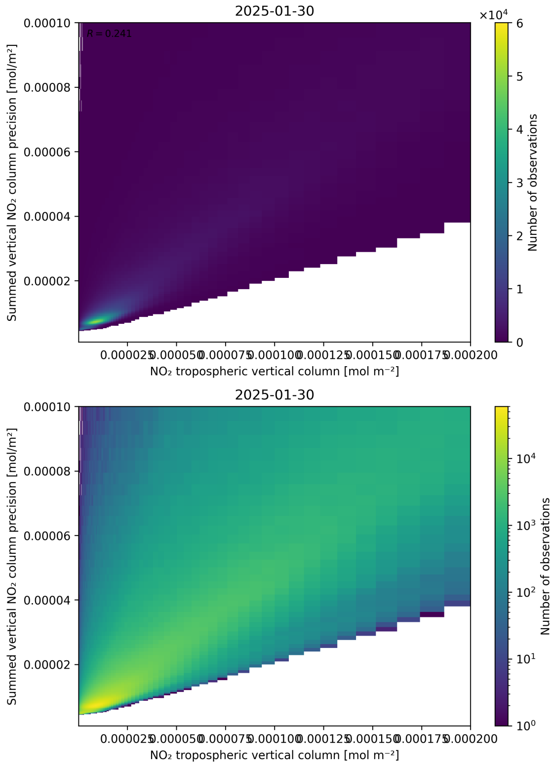
Figure 127: Scatter density plot of “NO 2 tropospheric vertical column” against “Summed vertical NO 2 column precision” for 2025-01-29 to 2025-01-31.
