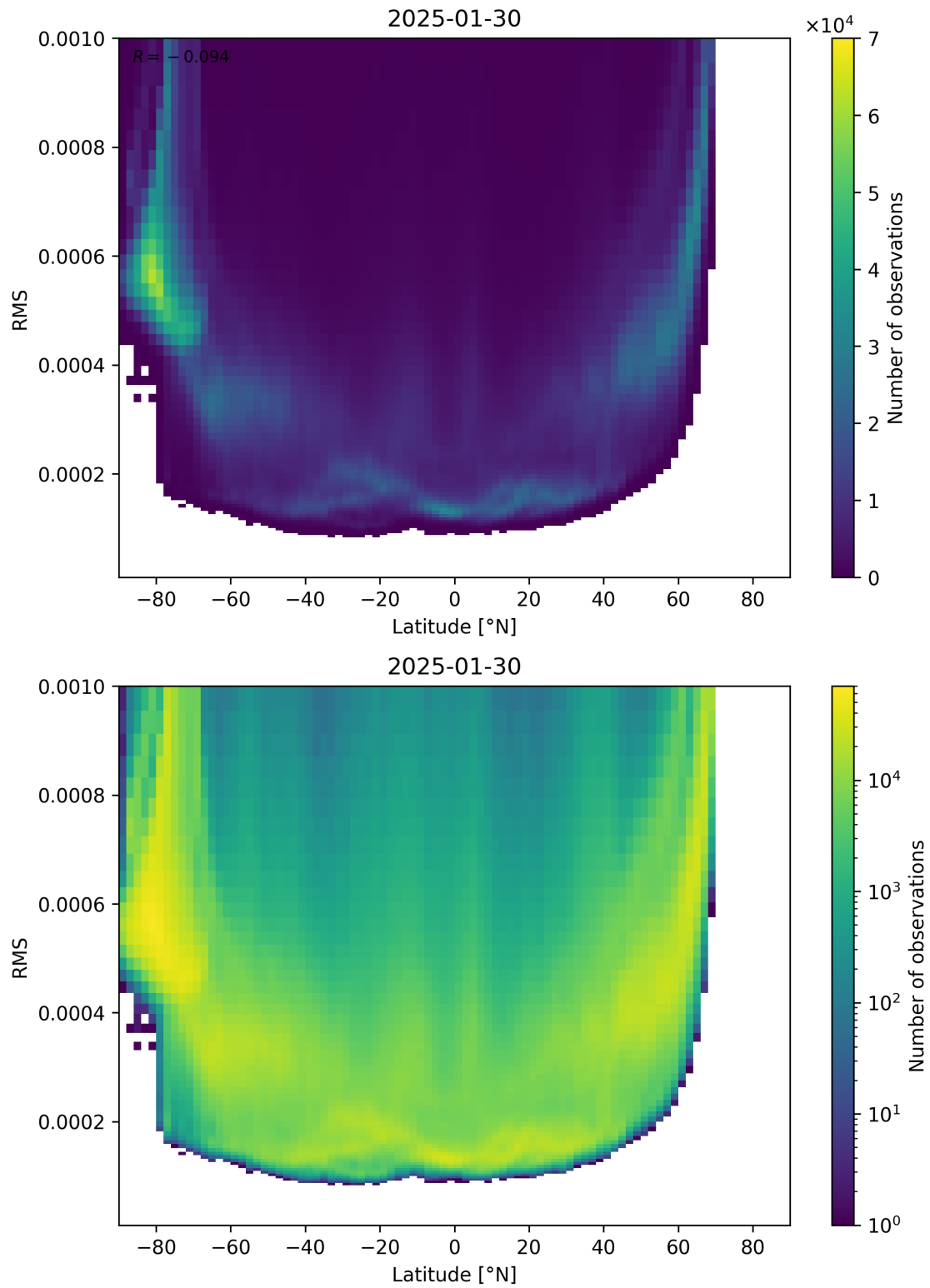
Figure 94: Scatter density plot of “Latitude” against “RMS” for 2025-01-29 to 2025-01-31.
