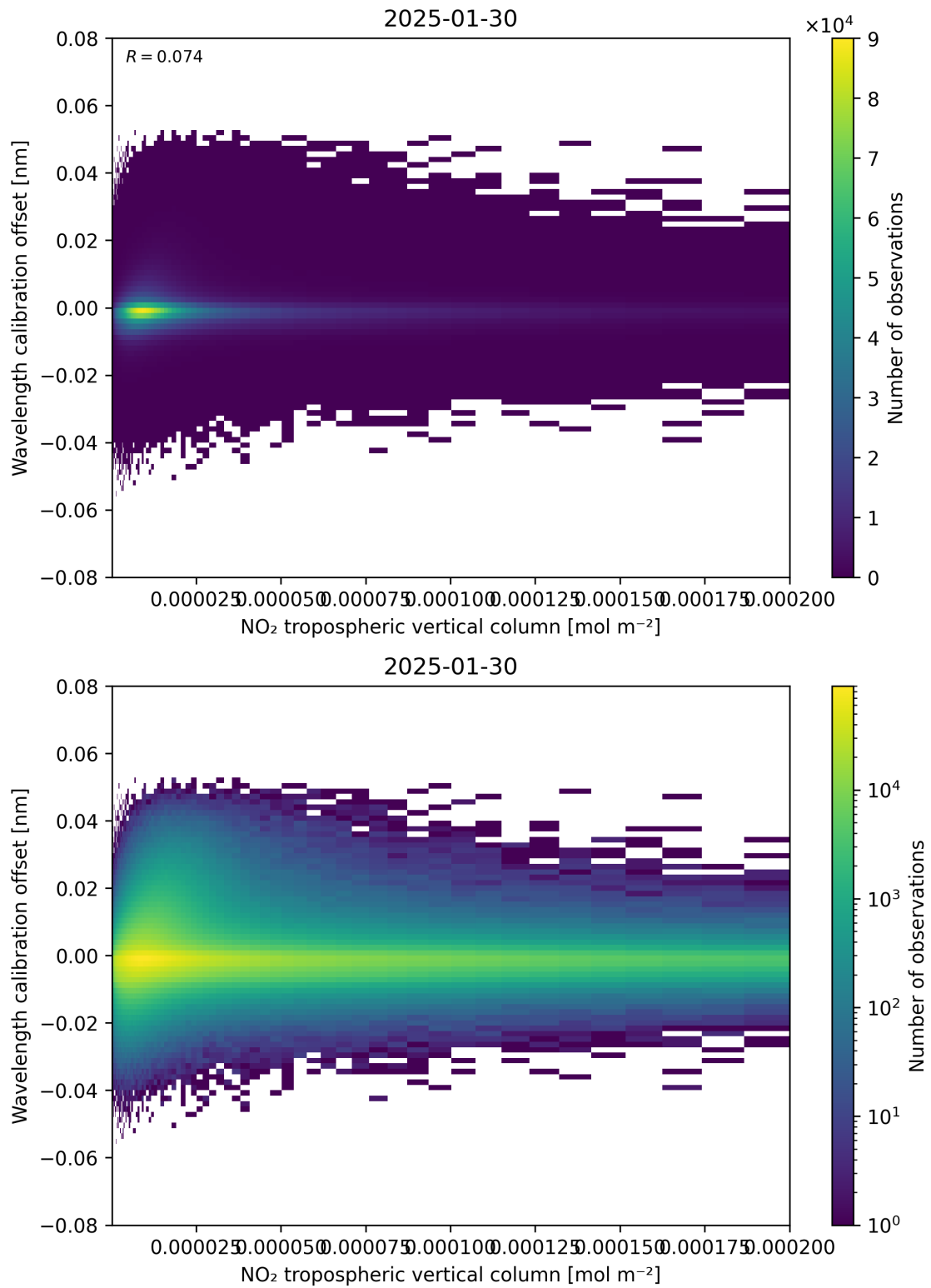
Figure 143: Scatter density plot of “NO 2 tropospheric vertical column” against “Wavelength calibration offset” for 2025-01-29 to 2025-01-31.
