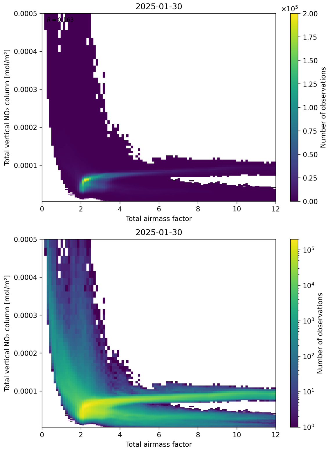
Figure 67: Scatter density plot of “Total airmass factor” against “Total vertical NO 2 column” for 2025-01-29 to 2025-01-31.
