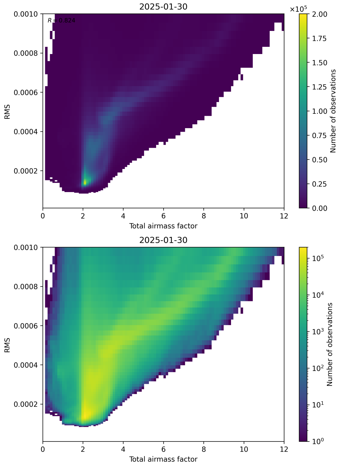
Figure 69: Scatter density plot of “Total airmass factor” against “RMS” for 2025-01-29 to 2025-01-31.
