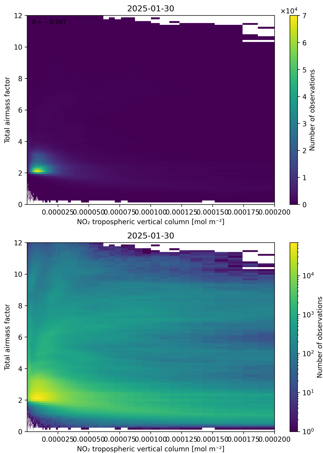
Figure 122: Scatter density plot of “NO 2 tropospheric vertical column” against “Total air mass factor” for 2025-01-29 to 2025-01-31.
