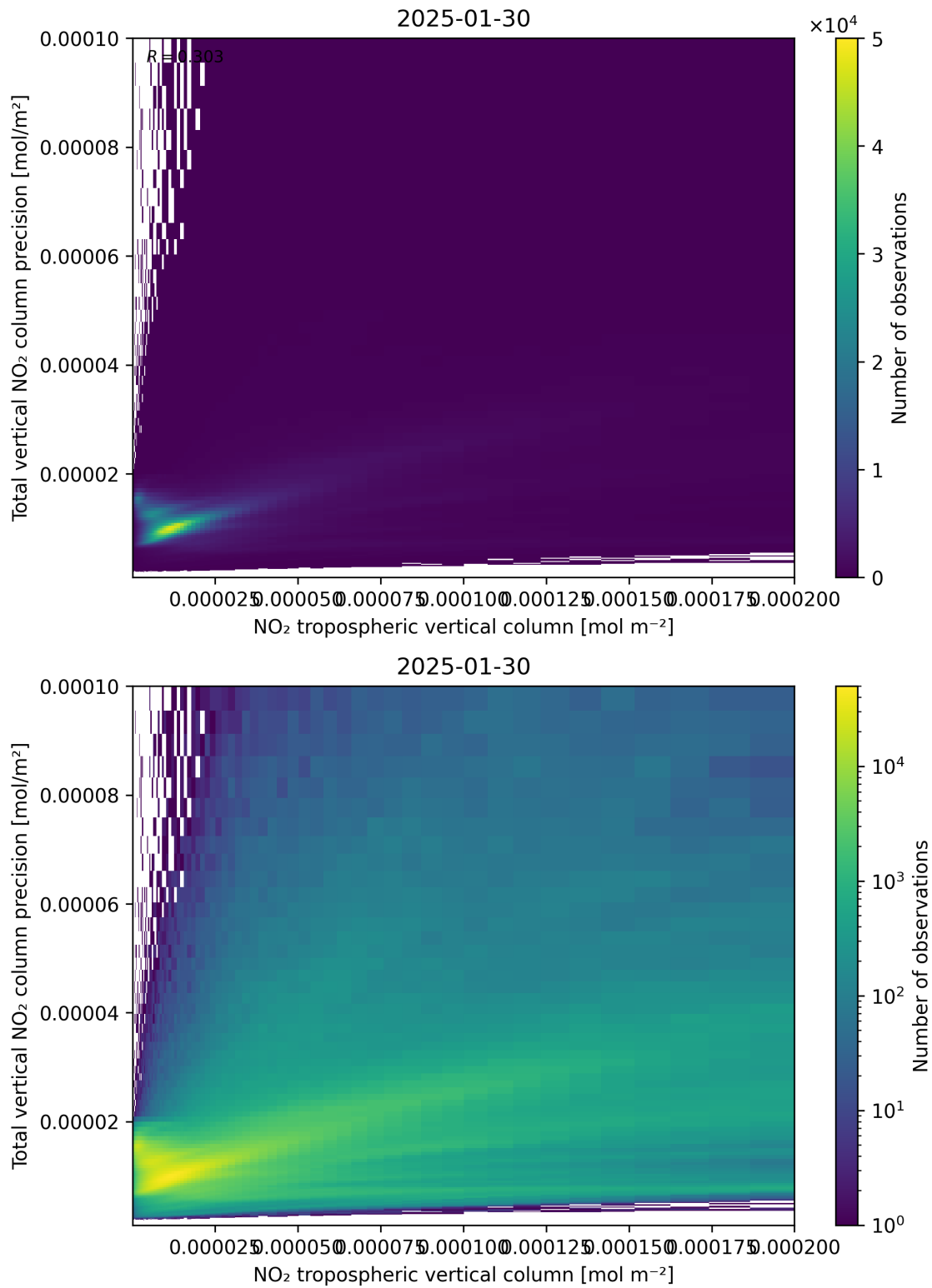
Figure 129: Scatter density plot of “NO 2 tropospheric vertical column” against “Total vertical NO 2 column precision” for 2025-01-29 to 2025-01-31.
