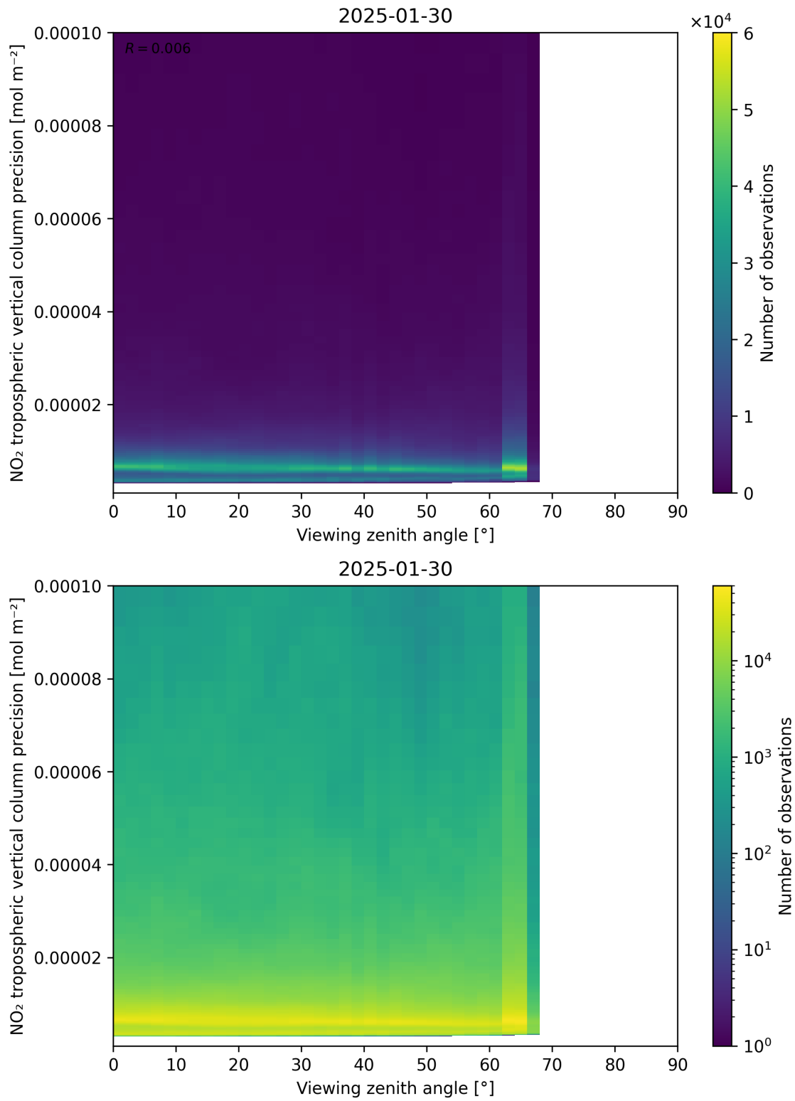
Figure 170: Scatter density plot of “Viewing zenith angle” against “NO 2 tropospheric vertical column precision” for 2025-01-29 to 2025-01-31.
