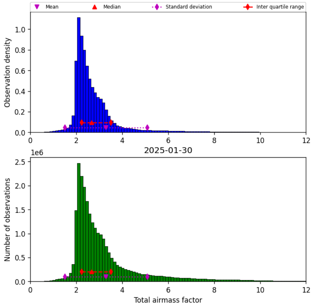
Figure 32: Histogram of “Total airmass factor” for 2025-01-29 to 2025-01-31
