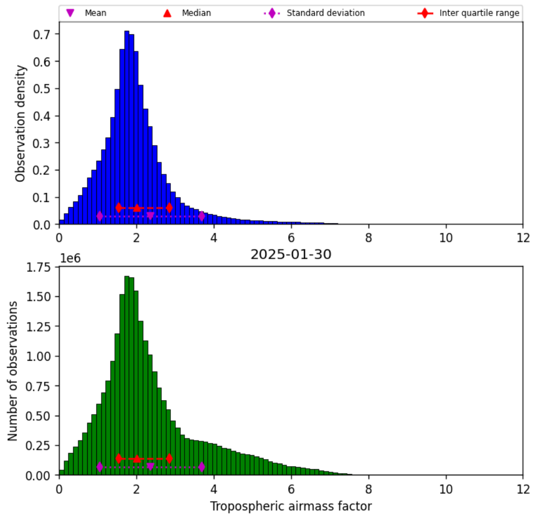
Figure 31: Histogram of “Tropospheric airmass factor” for 2025-01-29 to 2025-01-31
