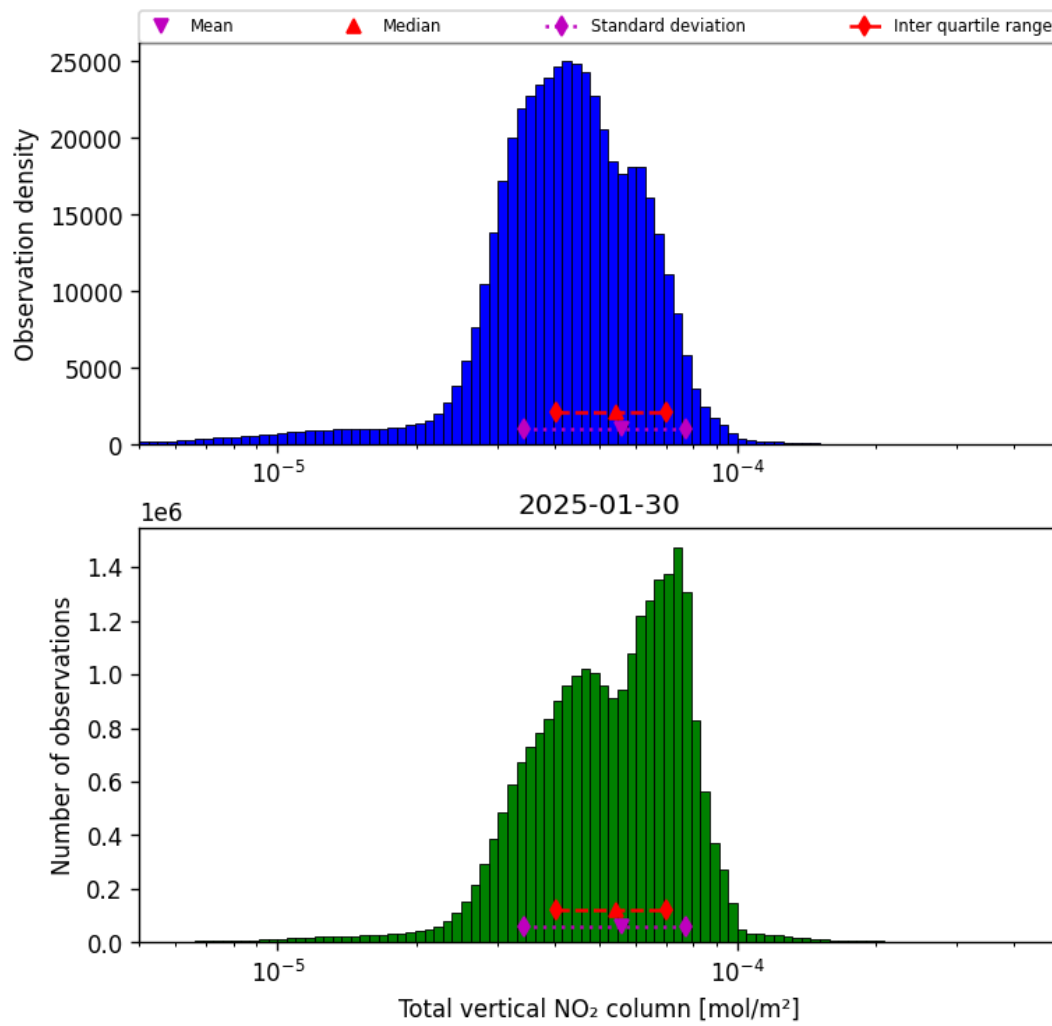
Figure 38: Histogram of “Total vertical NO 2 column” for 2025-01-29 to 2025-01-31
