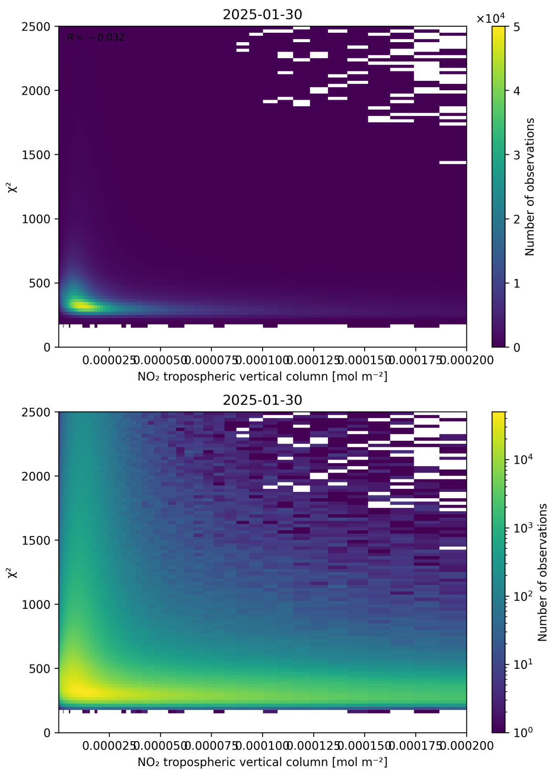
Figure 124: Scatter density plot of “NO 2 tropospheric vertical column” against “ \chi^2 ” for 2025-01-29 to 2025-01-31.
