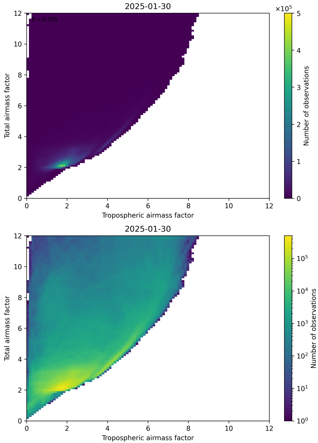
Figure 72: Scatter density plot of “Tropospheric airmass factor” against “Total airmass factor” for 2025-01-29 to 2025-01-31.
