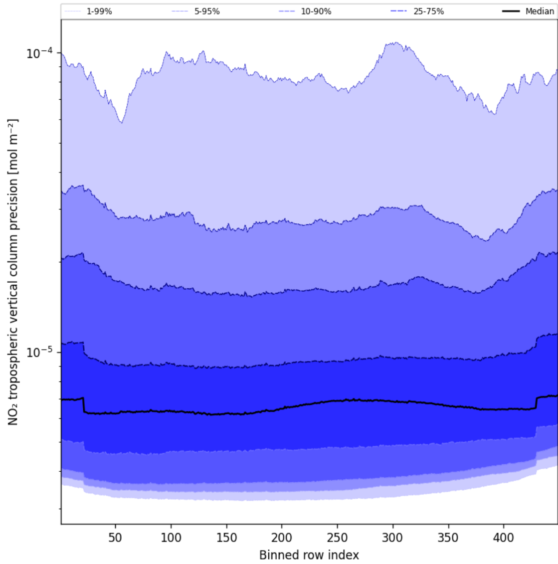
Figure 47: Along track statistics of “NO 2 tropospheric vertical column precision” for 2025-01-29 to 2025-01-31
