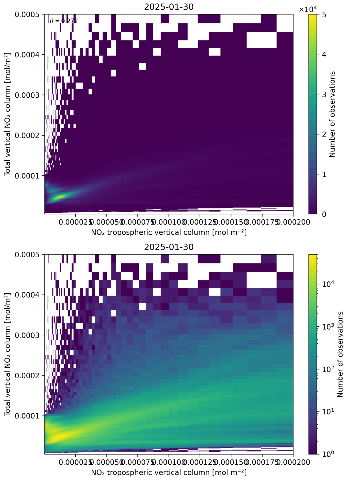
Figure 128: Scatter density plot of “NO 2 tropospheric vertical column” against “Total vertical NO 2 column” for 2025-01-29 to 2025-01-31.
