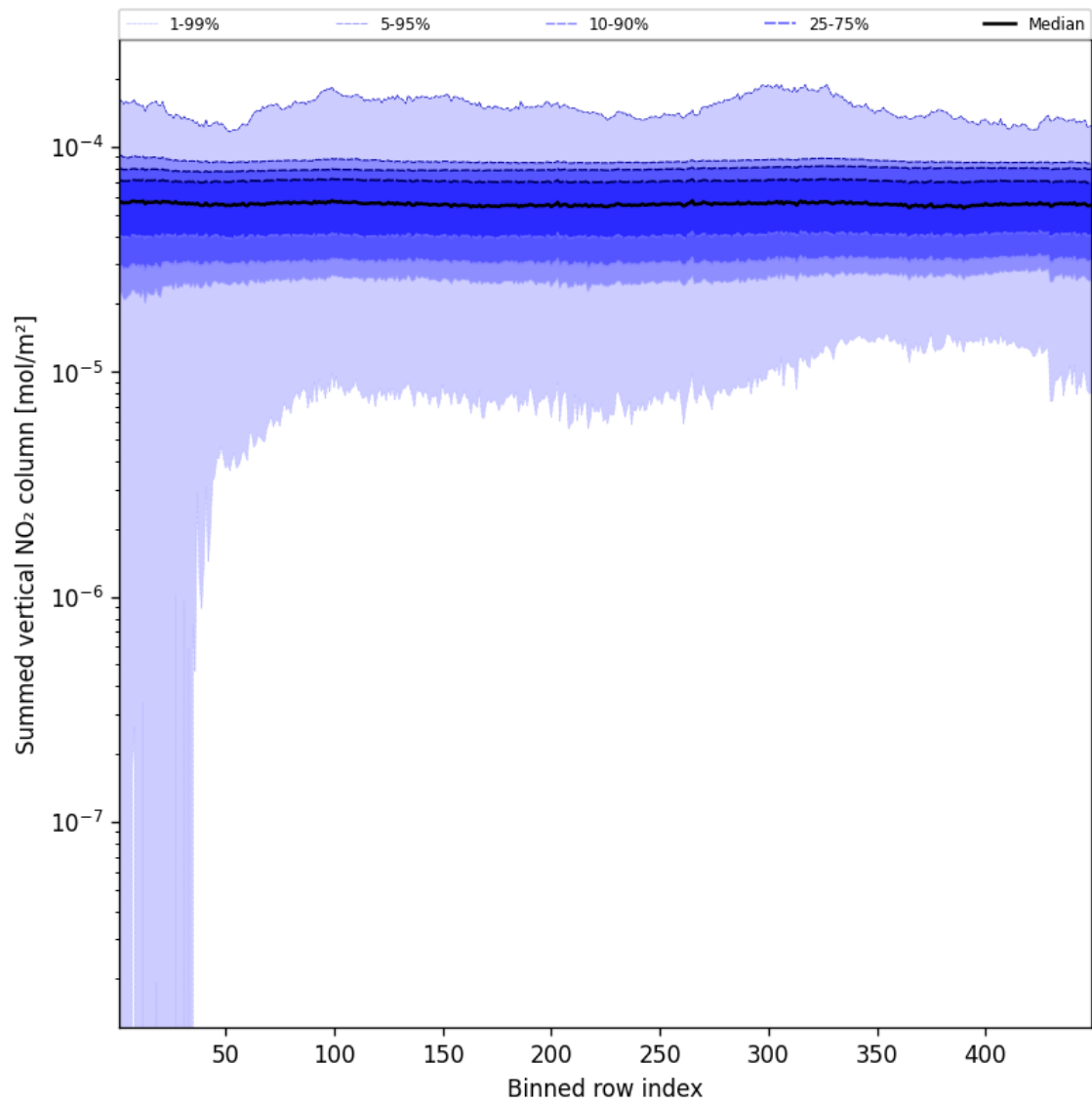
Figure 57: Along track statistics of “Summed vertical NO 2 column” for 2025-01-29 to 2025-01-31
