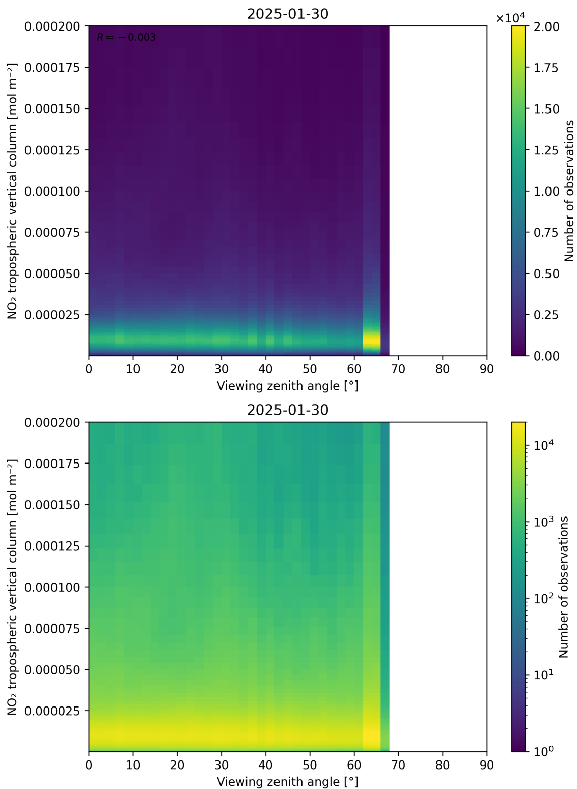
Figure 169: Scatter density plot of “Viewing zenith angle” against “NO 2 tropospheric vertical column” for 2025-01-29 to 2025-01-31.
