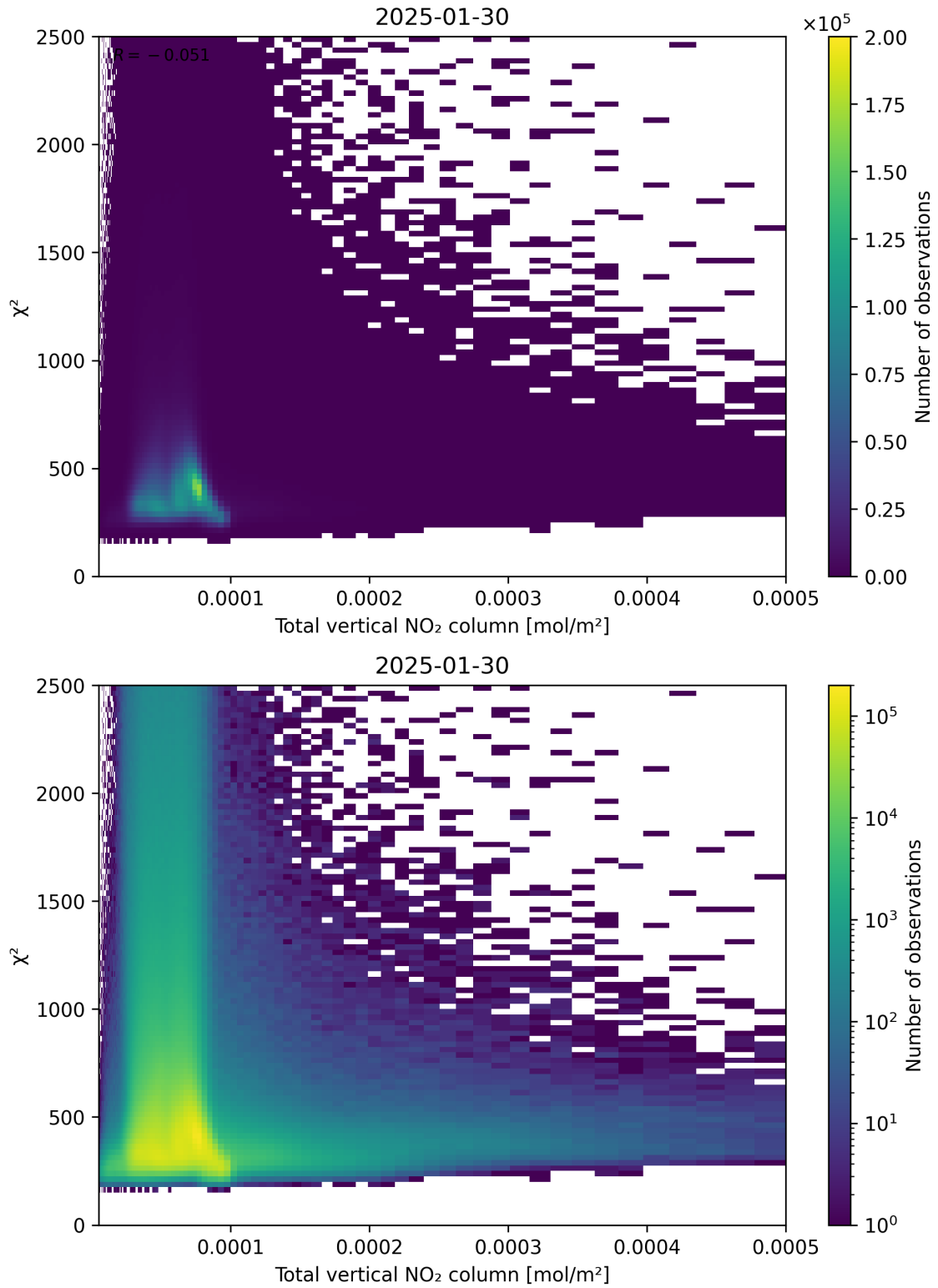
Figure 111: Scatter density plot of “Total vertical NO 2 column” against “ \chi^2 ” for 2025-01-29 to 2025-01-31.
