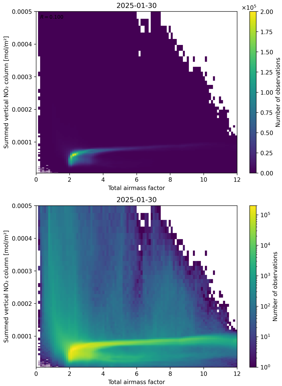
Figure 65: Scatter density plot of “Total airmass factor” against “Summed vertical NO 2 column” for 2025-01-29 to 2025-01-31.
