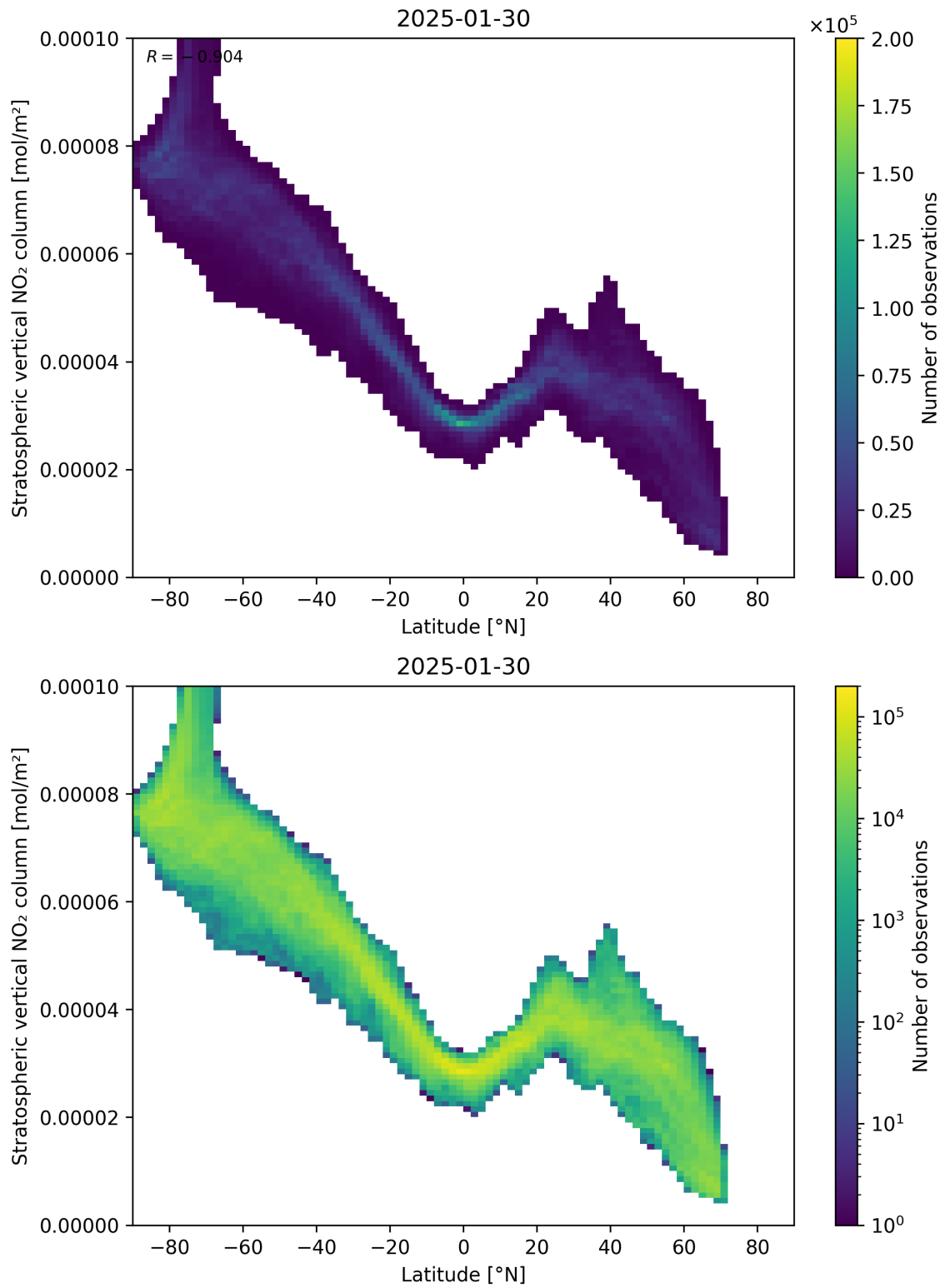
Figure 87: Scatter density plot of “Latitude” against “Stratospheric vertical NO 2 column” for 2025-01-29 to 2025-01-31.
