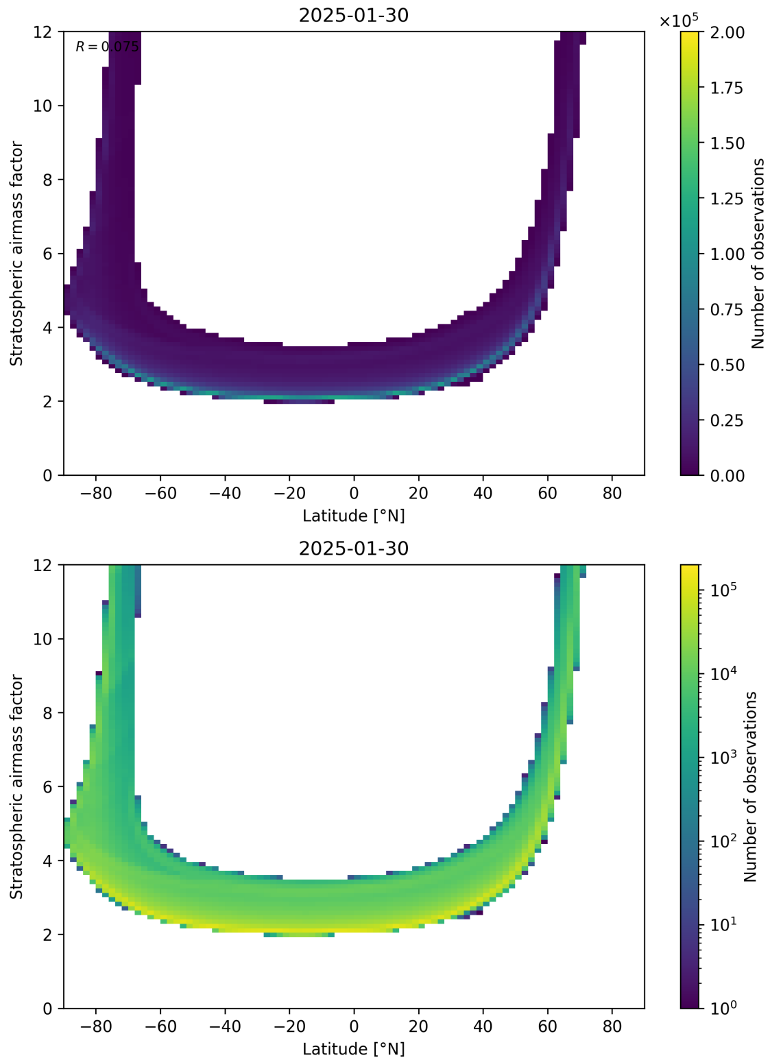
Figure 83: Scatter density plot of “Latitude” against “Stratospheric air mass factor” for 2025-01-29 to 2025-01-31.
