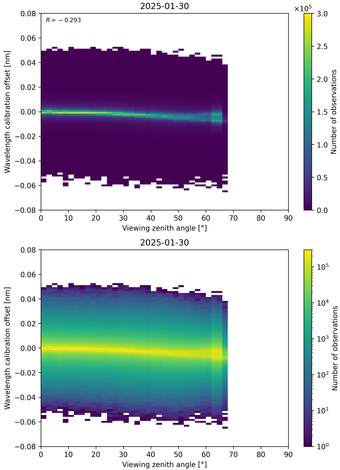
Figure 173: Scatter density plot of “Viewing zenith angle” against “Wavelength calibration offset” for 2025-01-29 to 2025-01-31.
