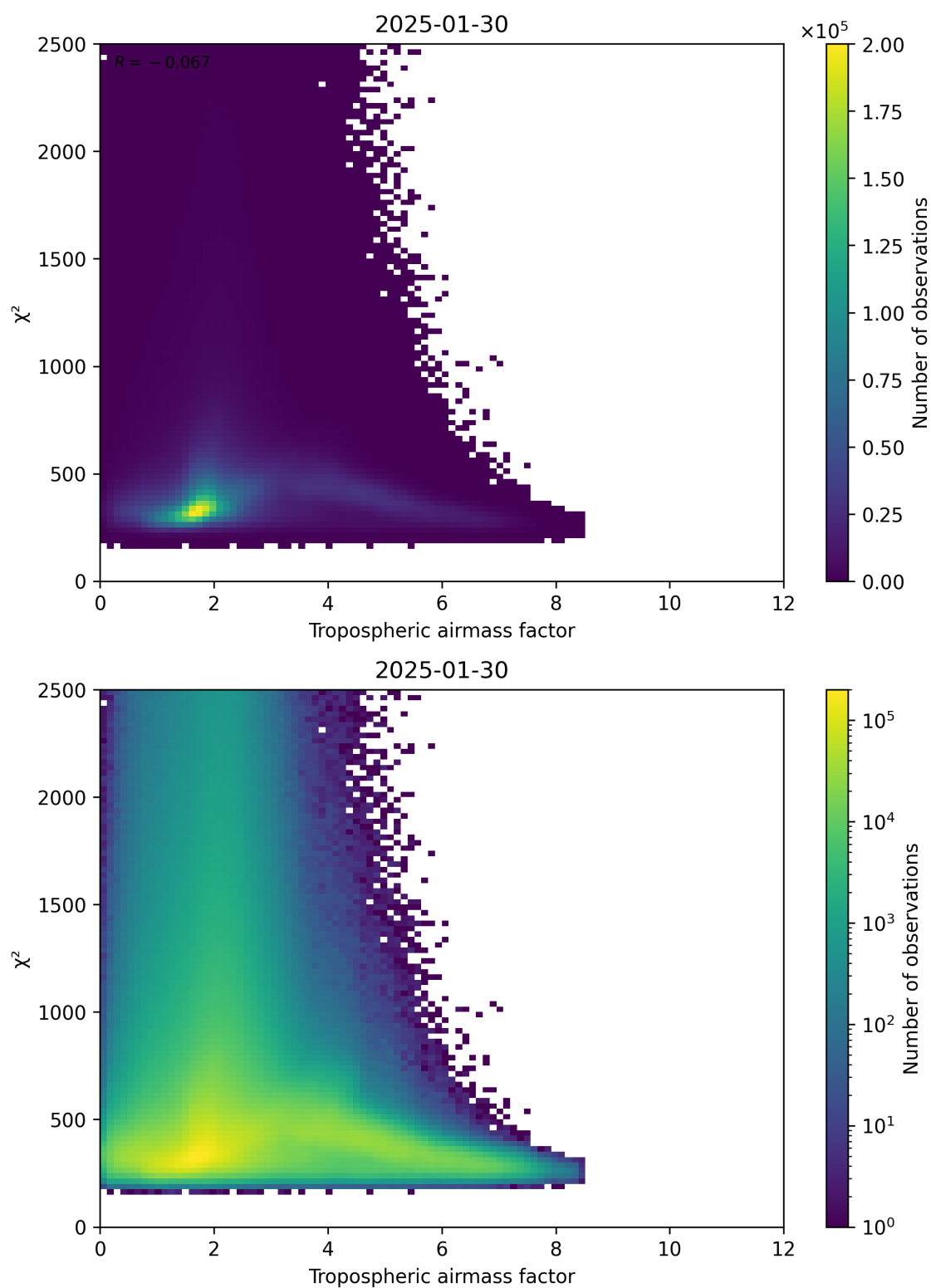
Figure 73: Scatter density plot of “Tropospheric airmass factor” against “ \chi^2 ” for 2025-01-29 to 2025-01-31.
