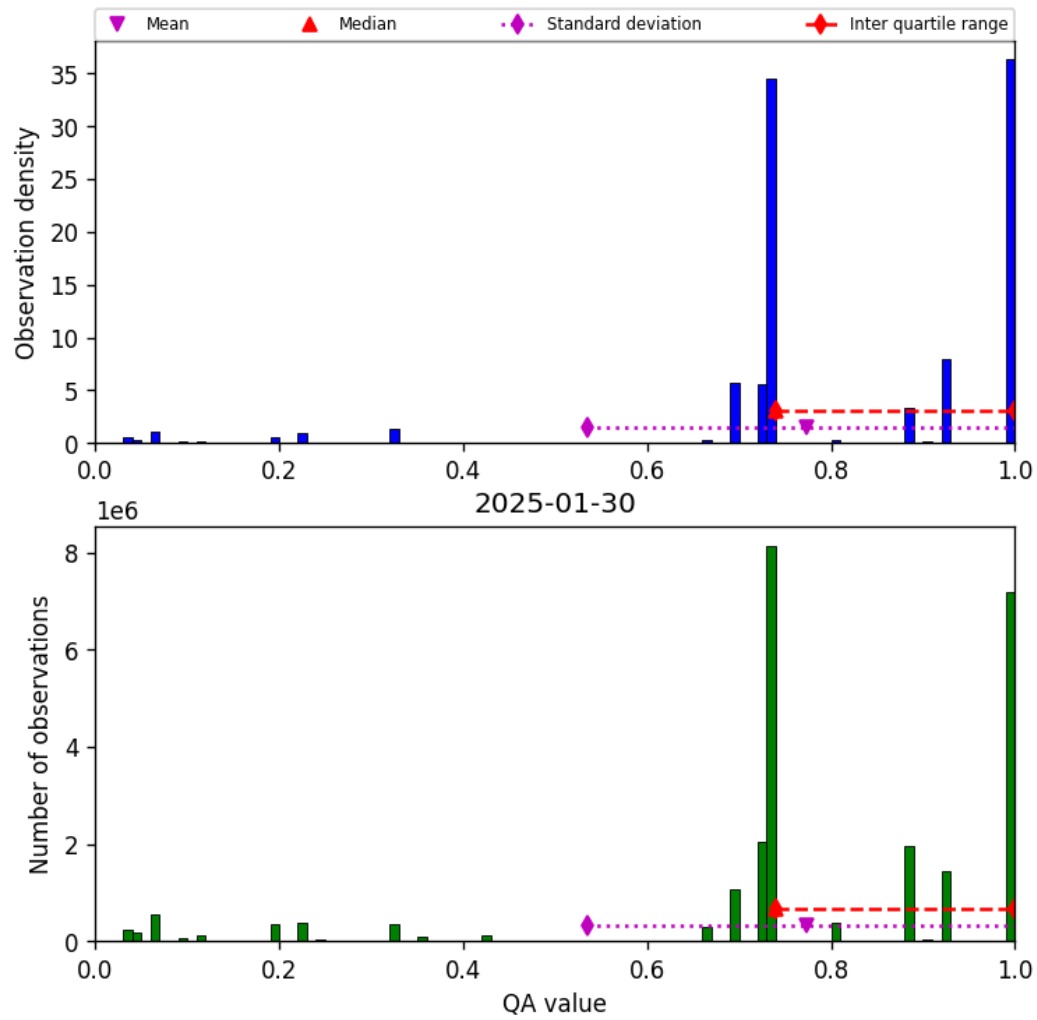
Figure 28: Histogram of “QA value” for 2025-01-29 to 2025-01-31
