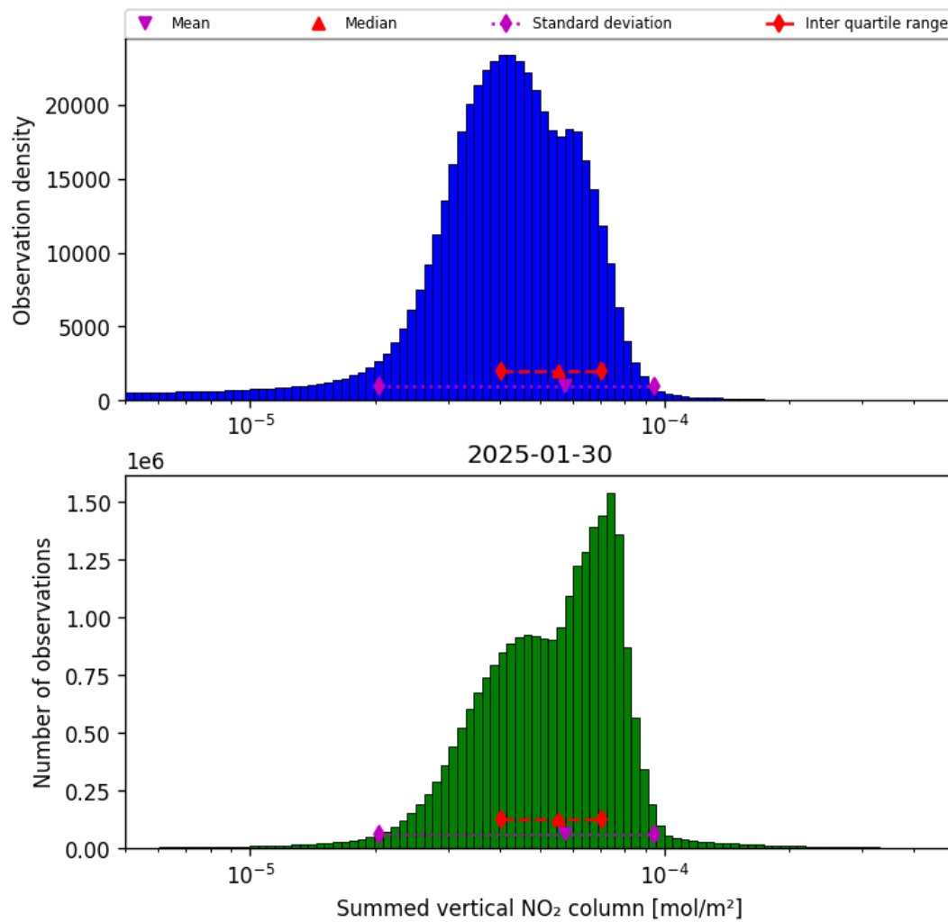
Figure 40: Histogram of “Summed vertical NO 2 column” for 2025-01-29 to 2025-01-31
