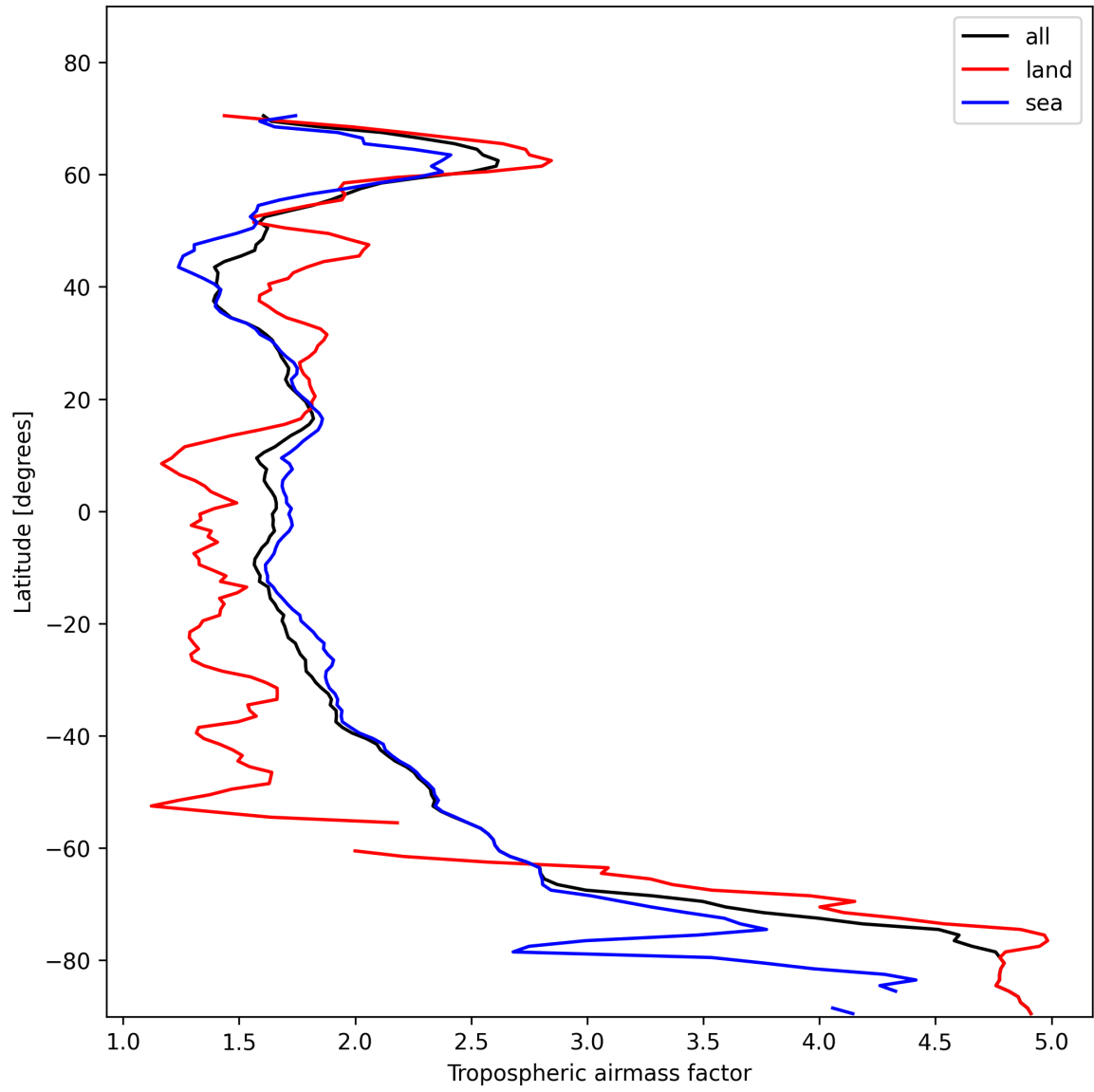
Figure 14: Zonal average of “Tropospheric airmass factor” for 2025-01-29 to 2025-01-31.
