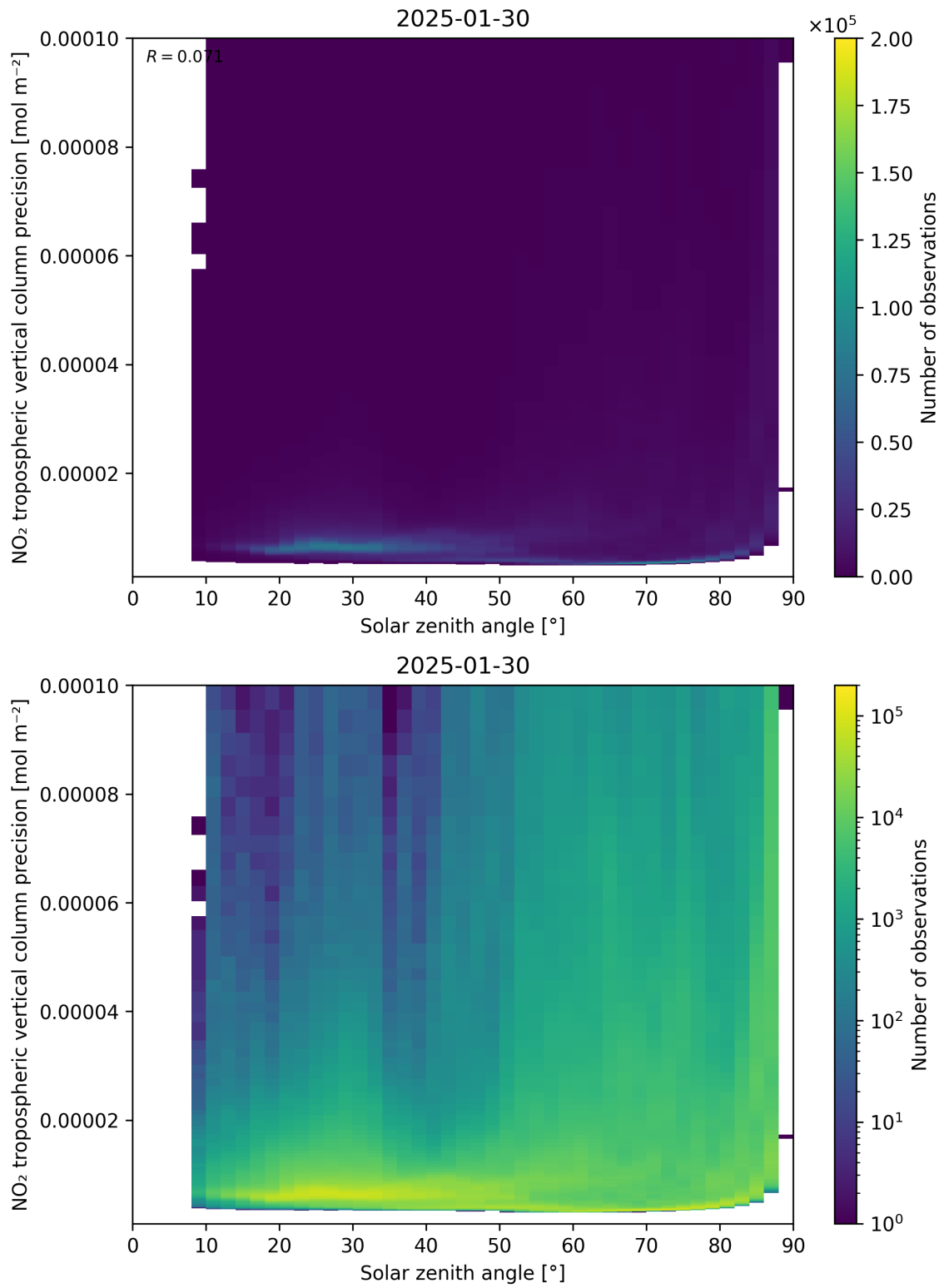
Figure 156: Scatter density plot of “Solar zenith angle” against “NO 2 tropospheric vertical column precision” for 2025-01-29 to 2025-01-31.
