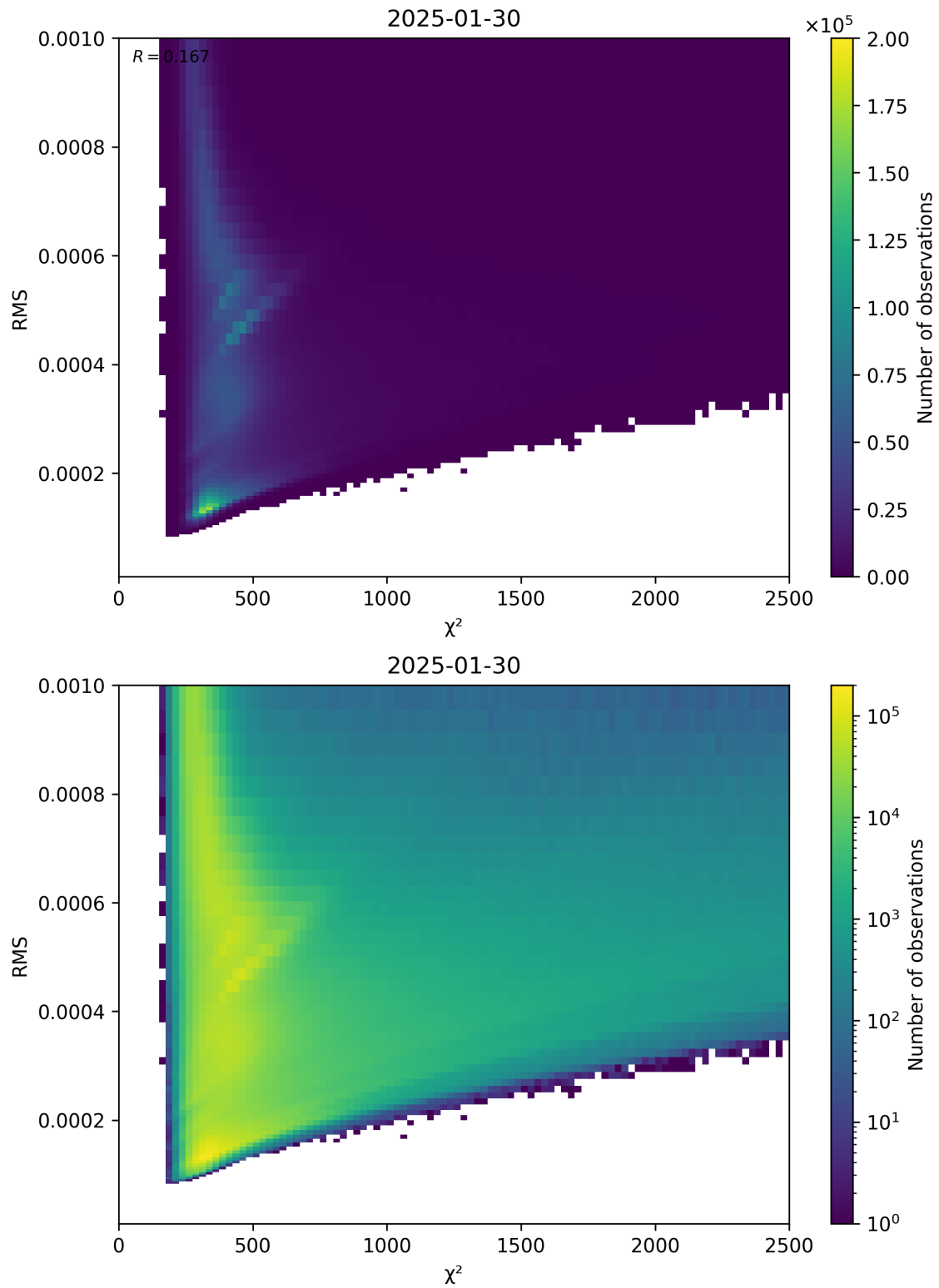
Figure 82: Scatter density plot of “ \chi^2 ” against “RMS” for 2025-01-29 to 2025-01-31.
