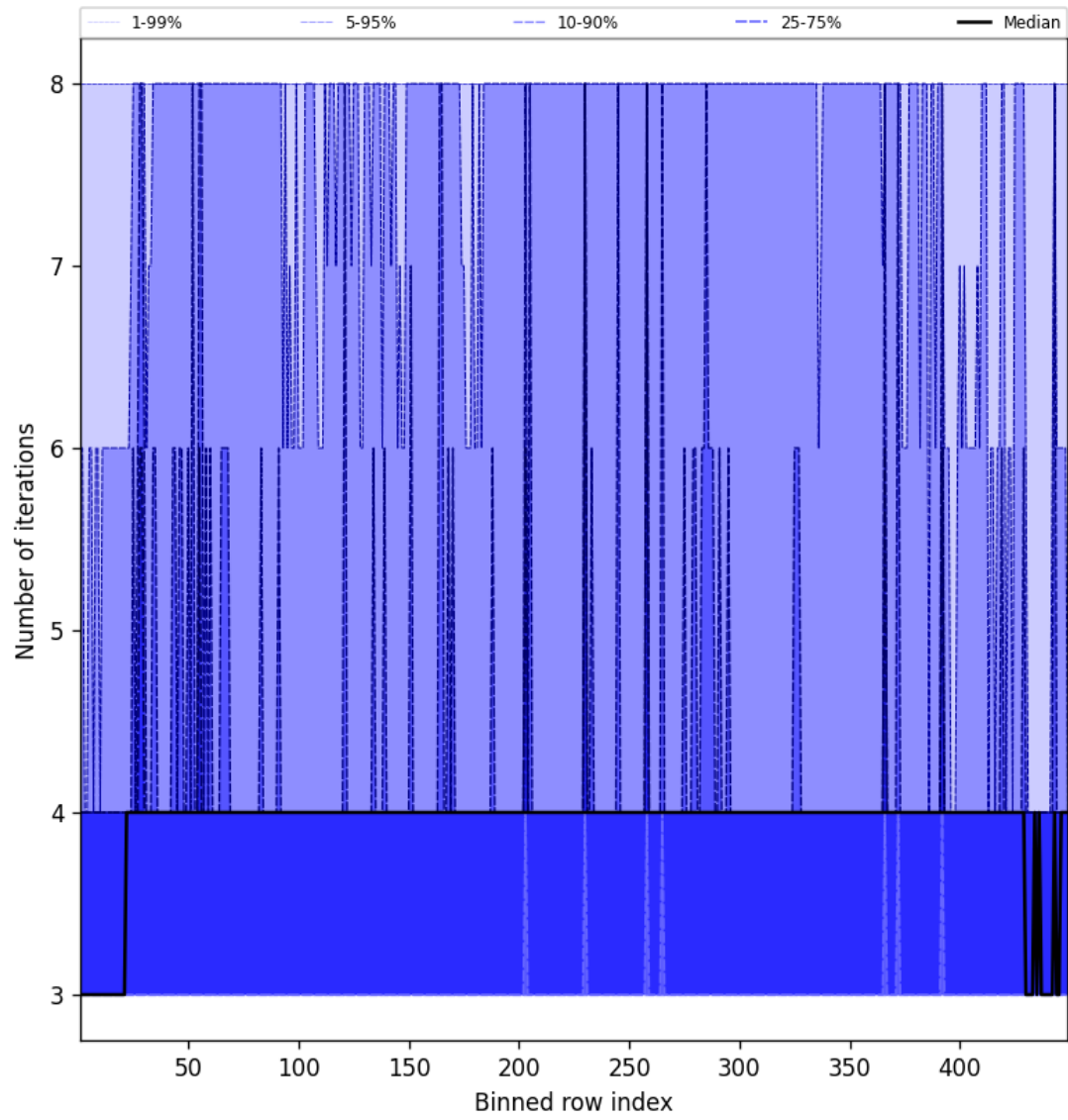
Figure 51: Along track statistics of “Number of iterations” for 2025-01-29 to 2025-01-31
