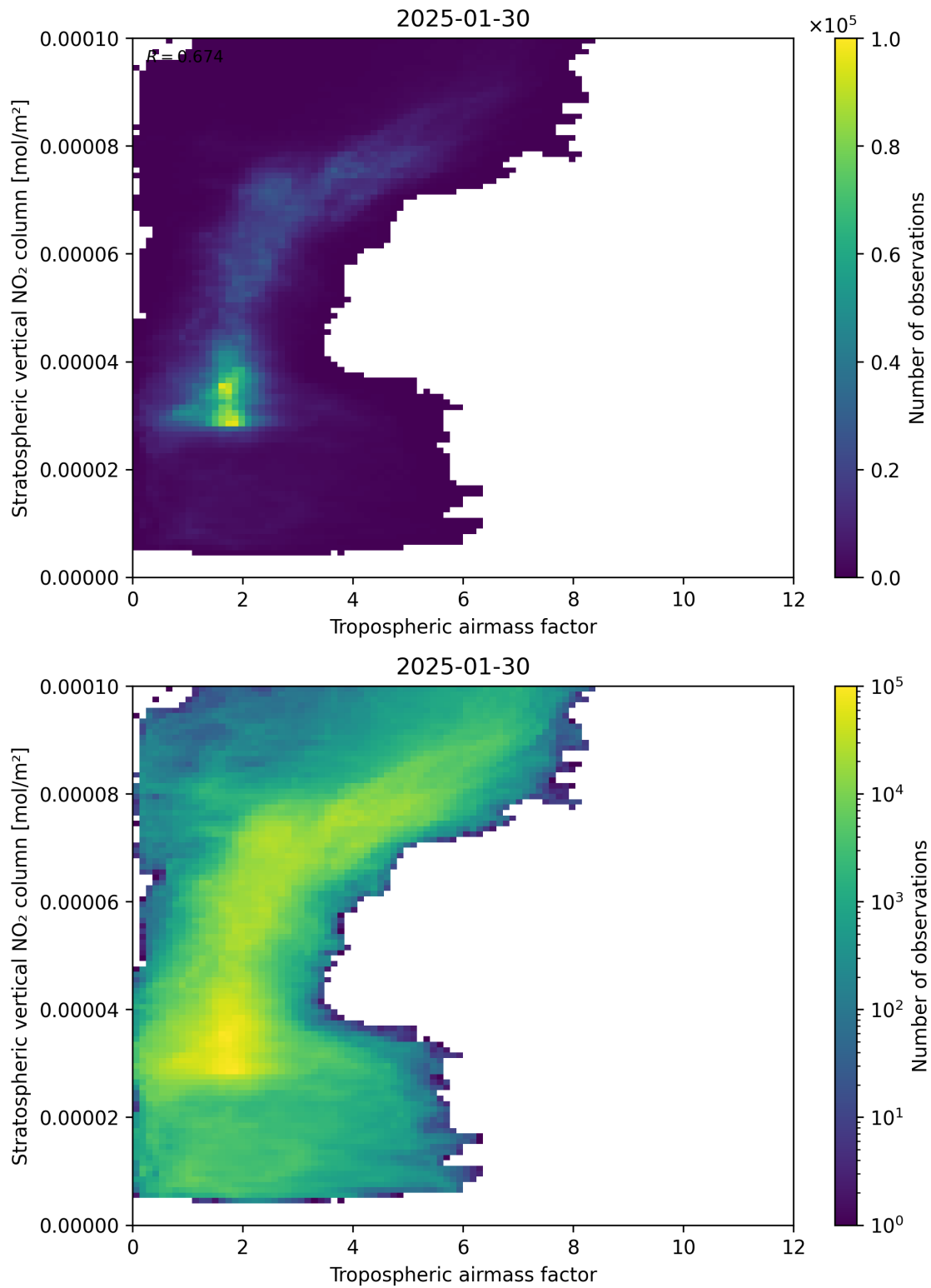
Figure 74: Scatter density plot of “Tropospheric air mass factor” against “Stratospheric vertical NO 2 column” for 2025-01-29 to 2025-01-31.
