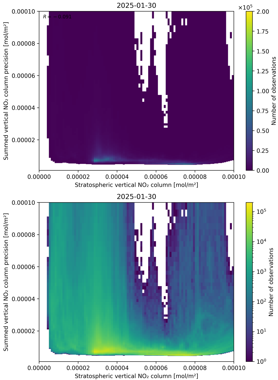
Figure 99: Scatter density plot of “Stratospheric vertical NO 2 column” against “Summed vertical NO 2 column precision” for 2025-01-29 to 2025-01-31.
