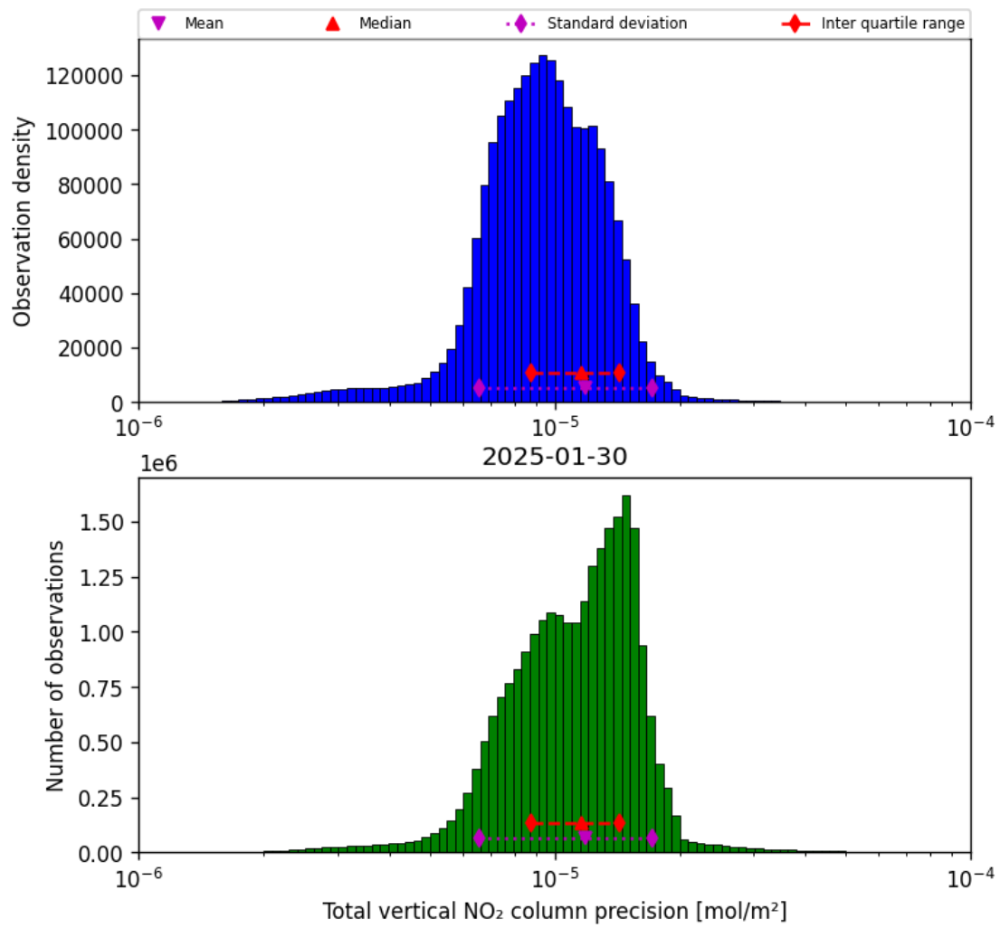
Figure 39: Histogram of “Total vertical NO 2 column precision” for 2025-01-29 to 2025-01-31
