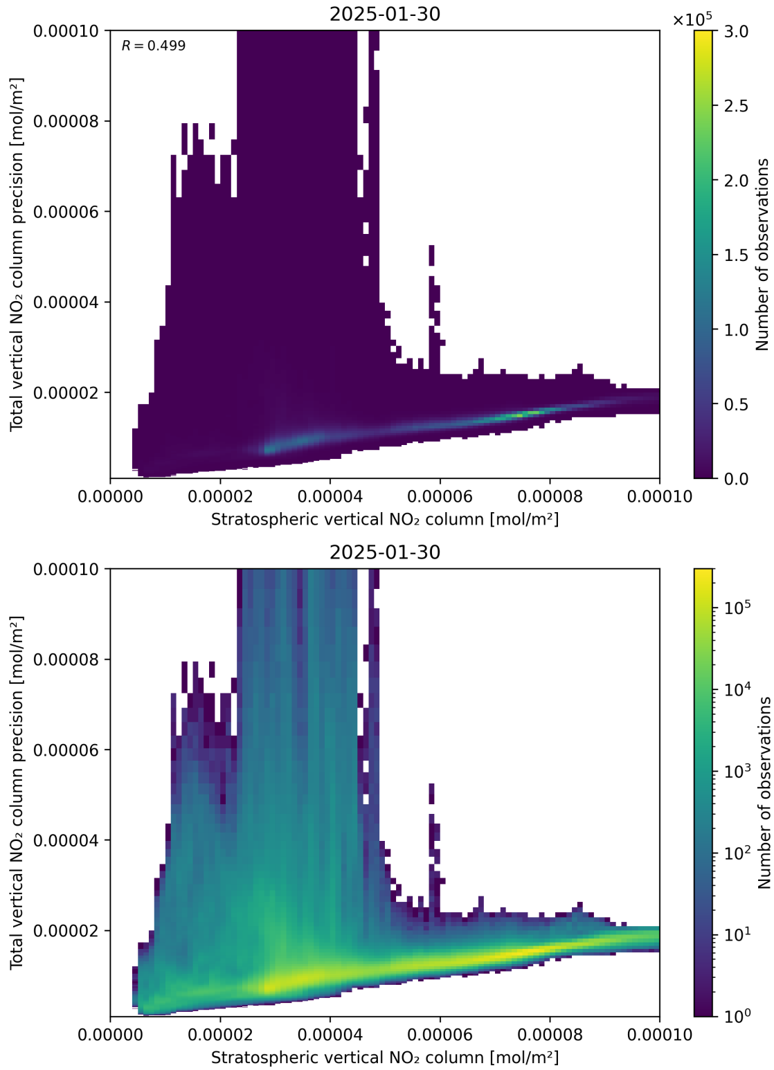
Figure 101: Scatter density plot of “Stratospheric vertical NO 2 column” against “Total vertical NO 2 column precision” for 2025-01-29 to 2025-01-31.
