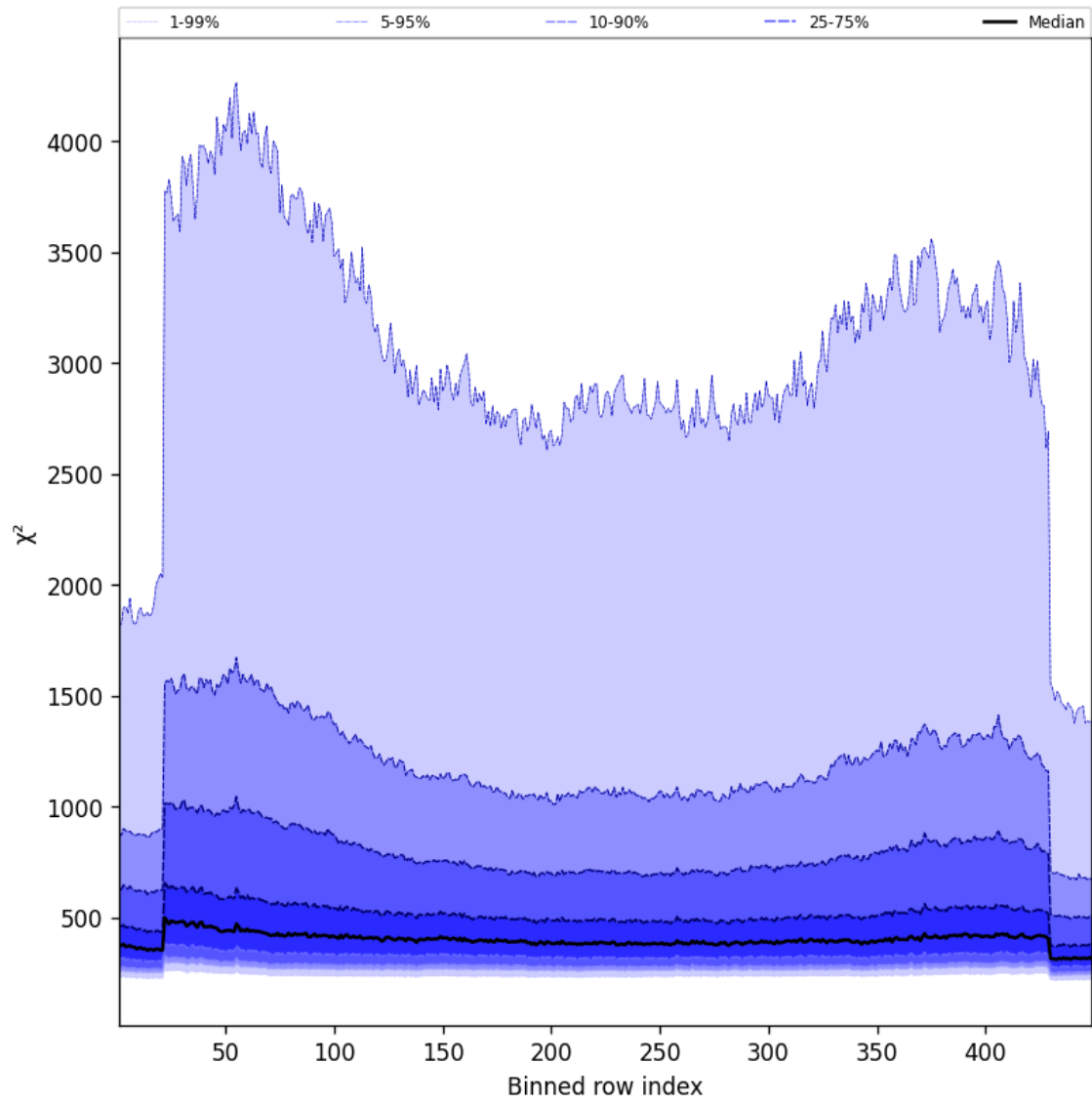
Figure 59: Along track statistics of “ \chi^2 ” for 2025-01-29 to 2025-01-31
