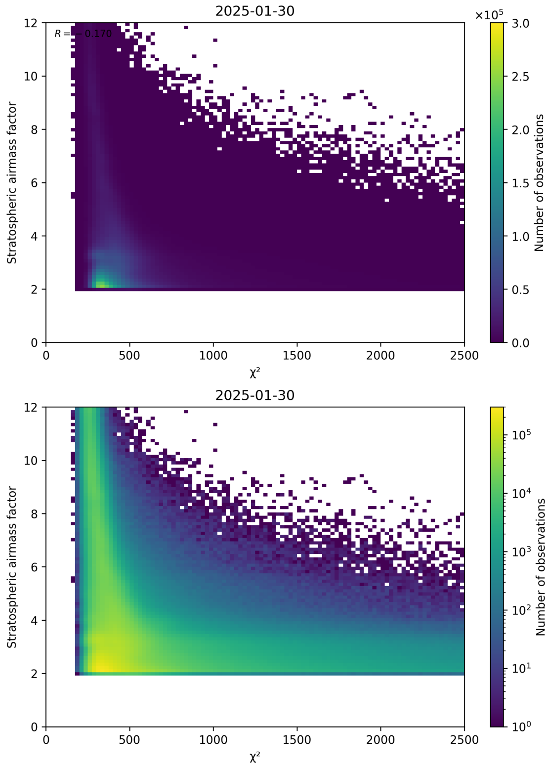
Figure 81: Scatter density plot of “ \chi^2 ” against “Stratospheric airmass factor” for 2025-01-29 to 2025-01-31.
