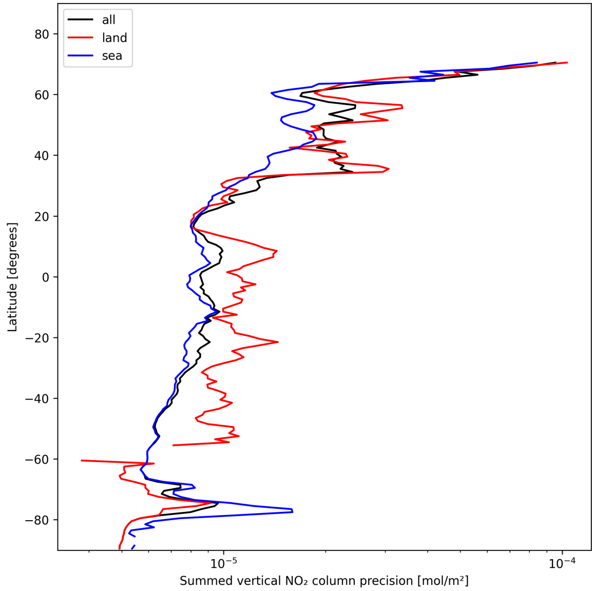
Figure 24: Zonal average of “Summed vertical NO 2 column precision” for 2025-01-29 to 2025-01-31.
