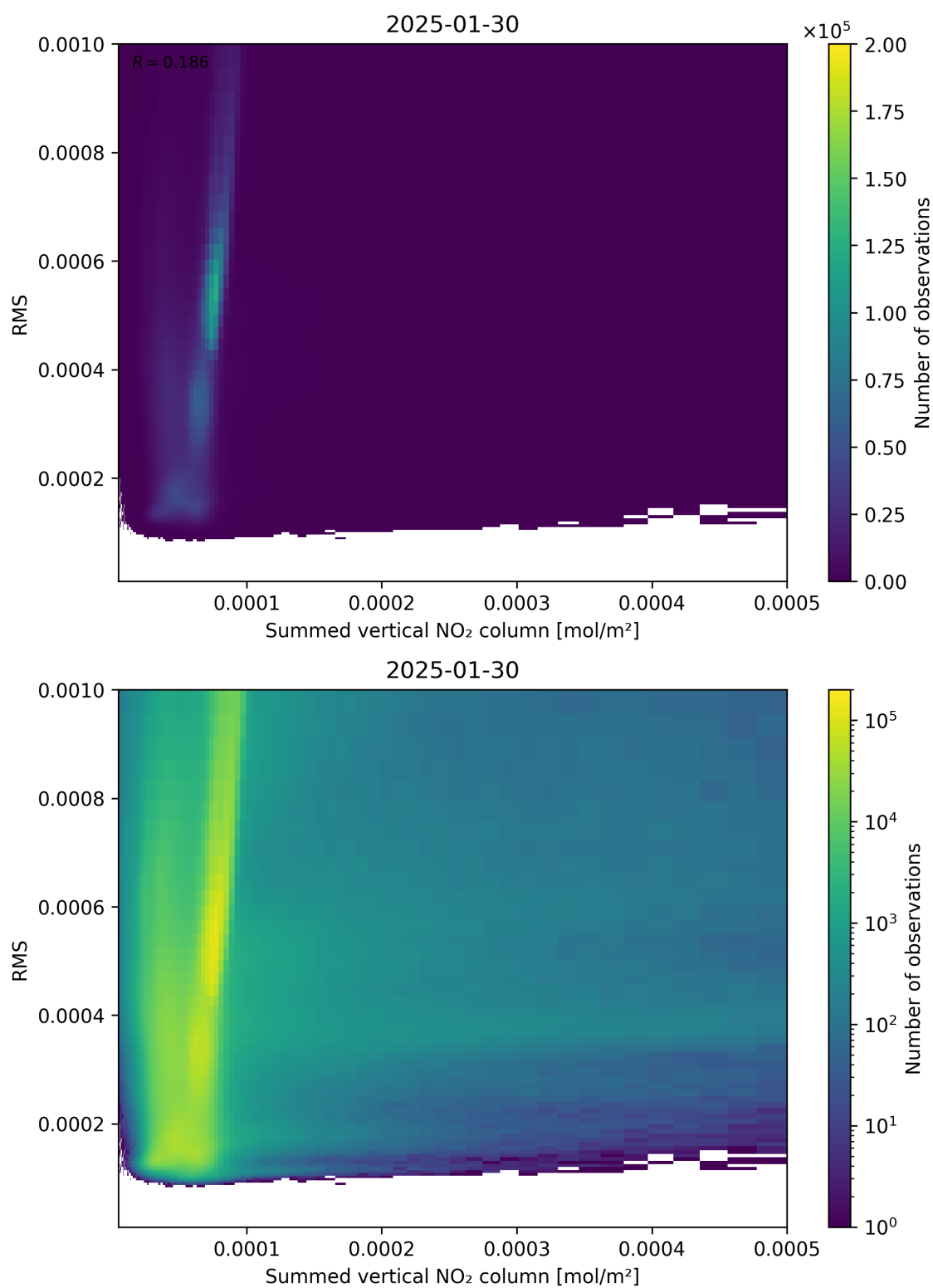
Figure 109: Scatter density plot of “Summed vertical NO 2 column” against “RMS” for 2025-01-29 to 2025-01-31.
