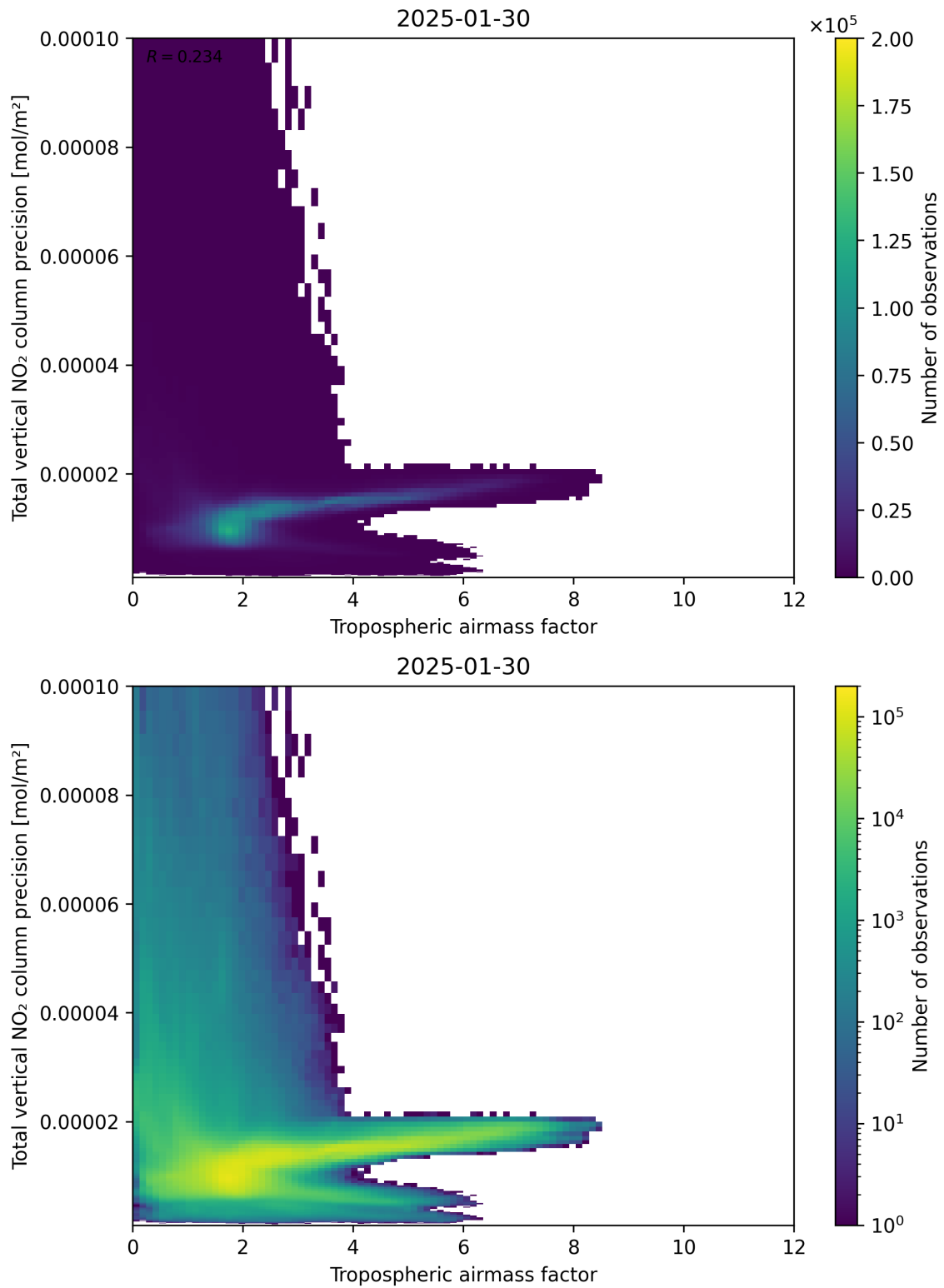
Figure 78: Scatter density plot of “Tropospheric airmass factor” against “Total vertical NO 2 column precision” for 2025-01-29 to 2025-01-31.
