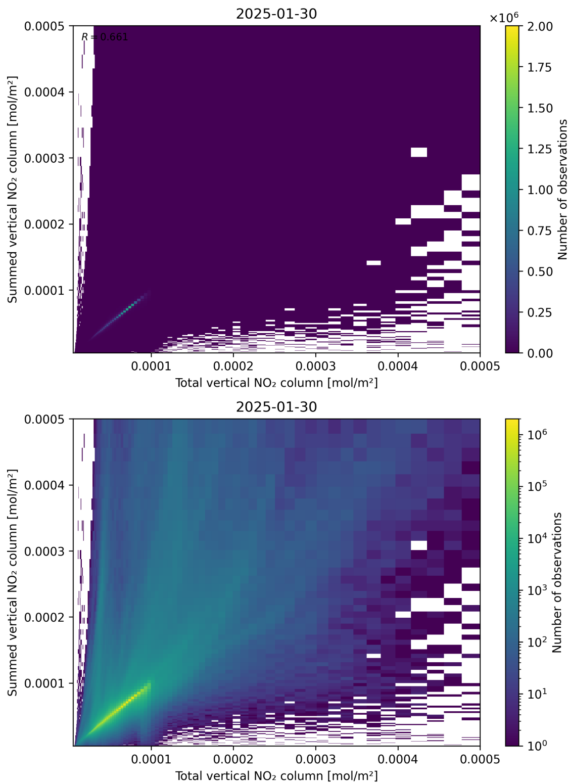
Figure 112: Scatter density plot of “Total vertical NO 2 column” against “Summed vertical NO 2 column” for 2025-01-29 to 2025-01-31.
