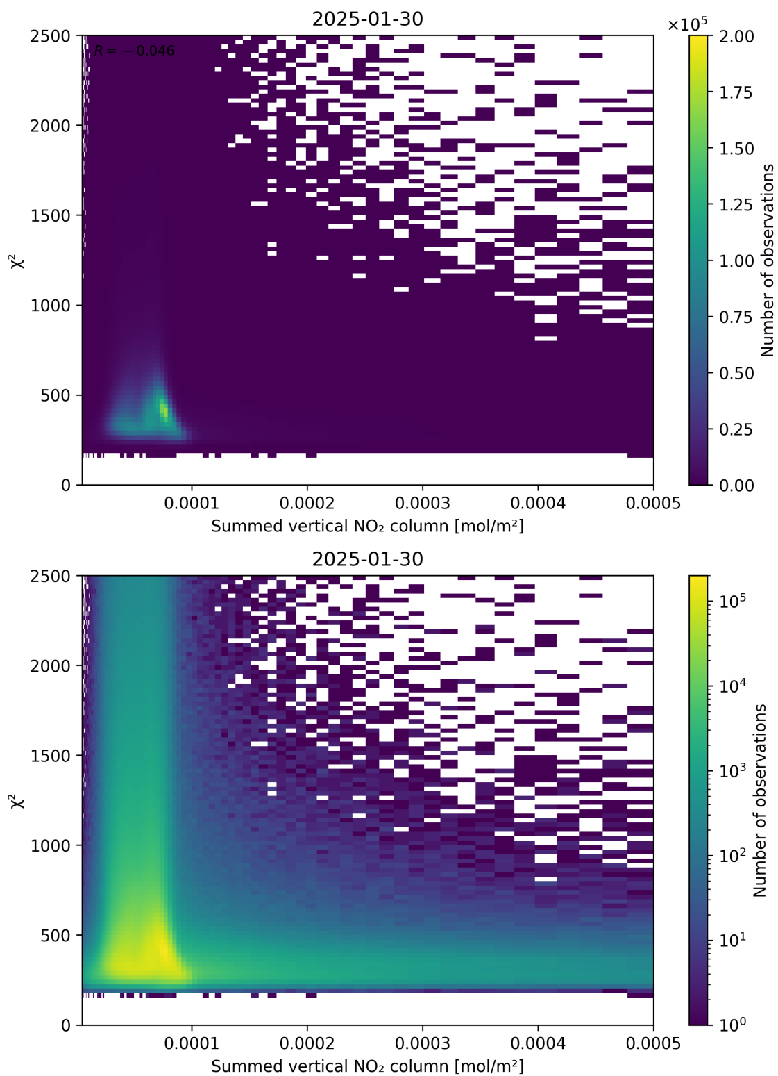
Figure 104: Scatter density plot of “Summed vertical NO 2 column” against “ \chi^2 ” for 2025-01-29 to 2025-01-31.
