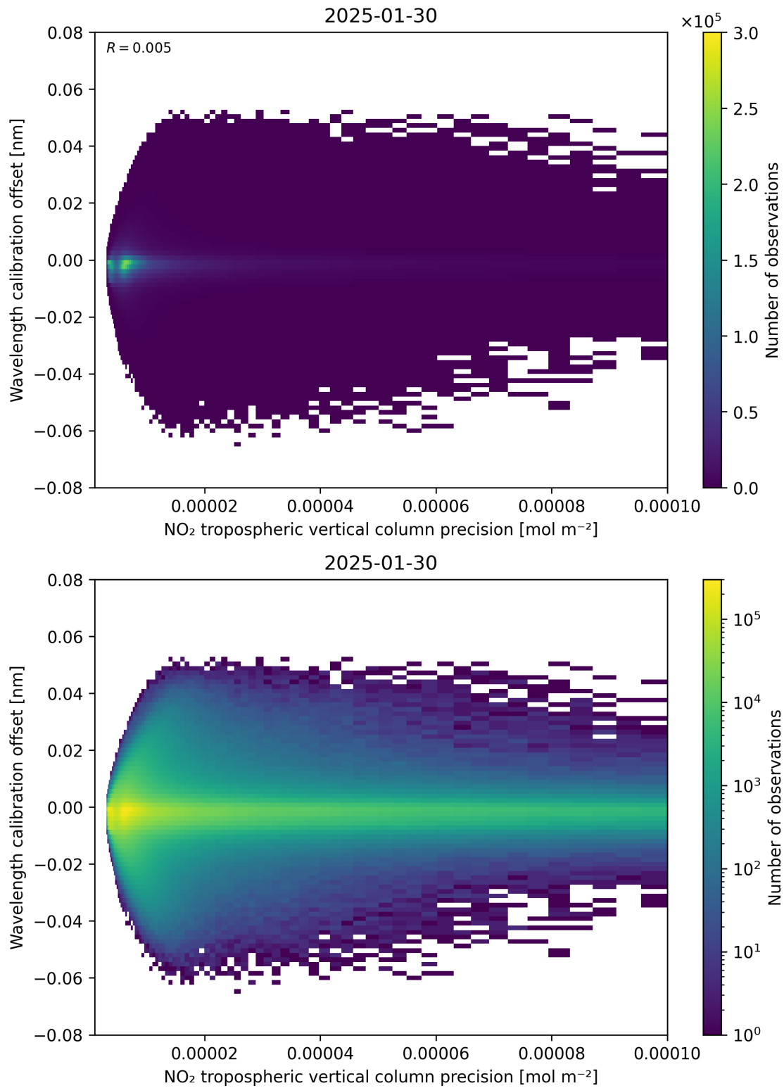
Figure 141: Scatter density plot of “NO 2 tropospheric vertical column precision” against “Wavelength calibration offset” for 2025-01-29 to 2025-01-31.
