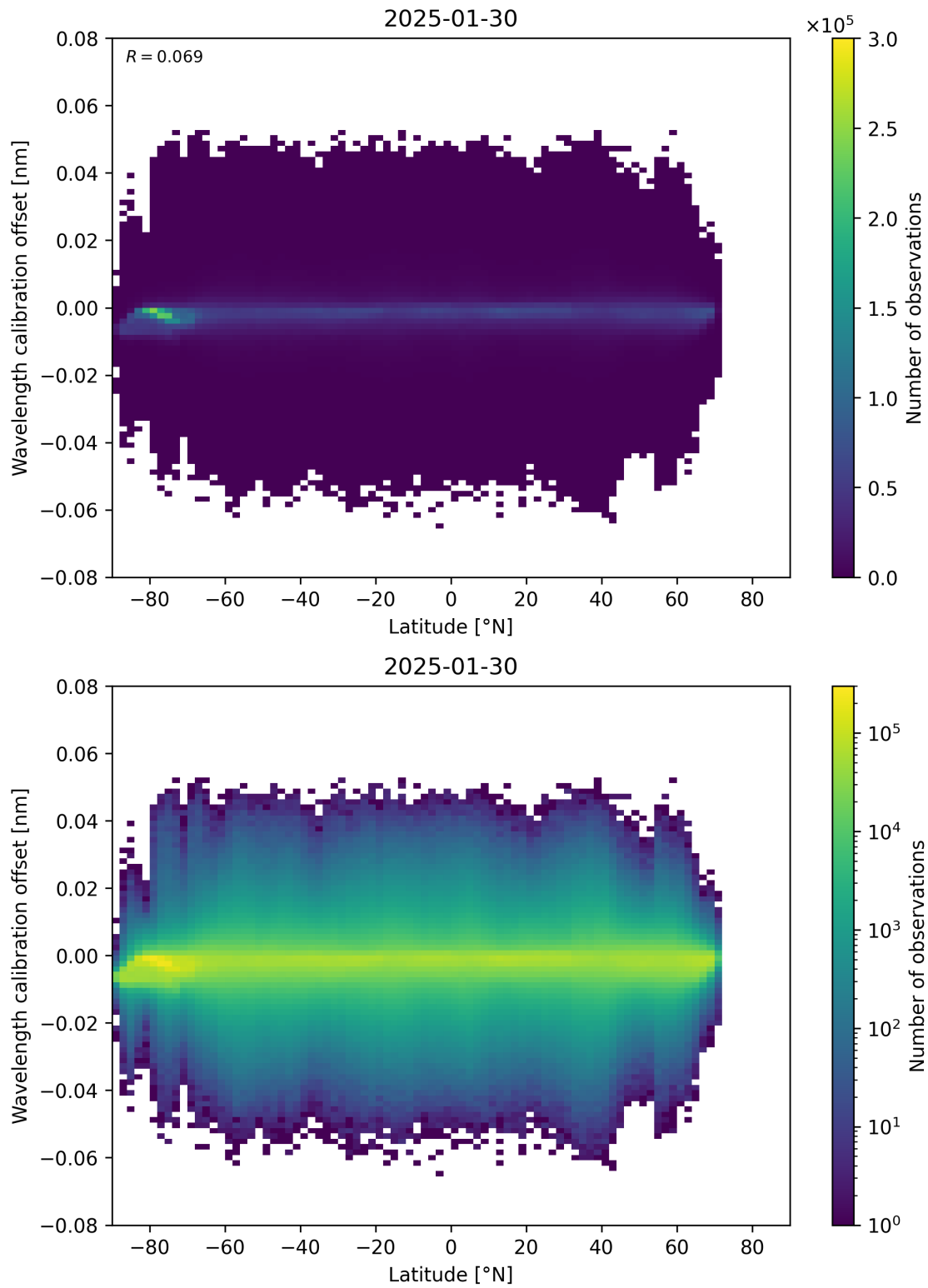
Figure 95: Scatter density plot of “Latitude” against “Wavelength calibration offset” for 2025-01-29 to 2025-01-31.
