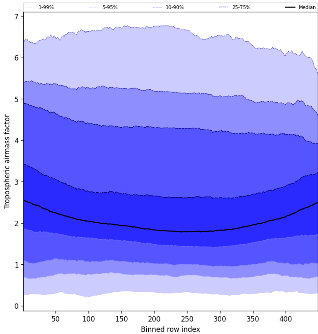
Figure 48: Along track statistics of “Tropospheric airmass factor” for 2025-01-29 to 2025-01-31
