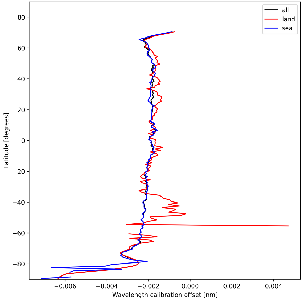
Figure 18: Zonal average of “Wavelength calibration offset” for 2025-01-29 to 2025-01-31.
