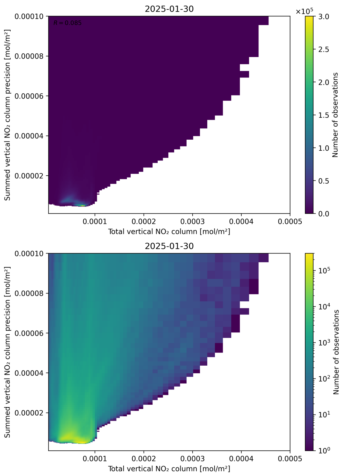
Figure 113: Scatter density plot of “Total vertical NO 2 column” against “Summed vertical NO 2 column precision” for 2025-01-29 to 2025-01-31.
