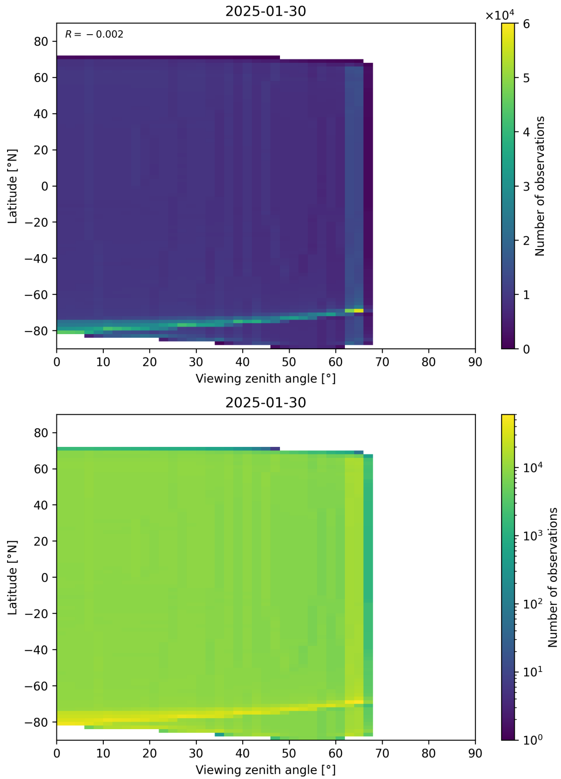
Figure 163: Scatter density plot of “Viewing zenith angle” against “Latitude” for 2025-01-29 to 2025-01-31.
