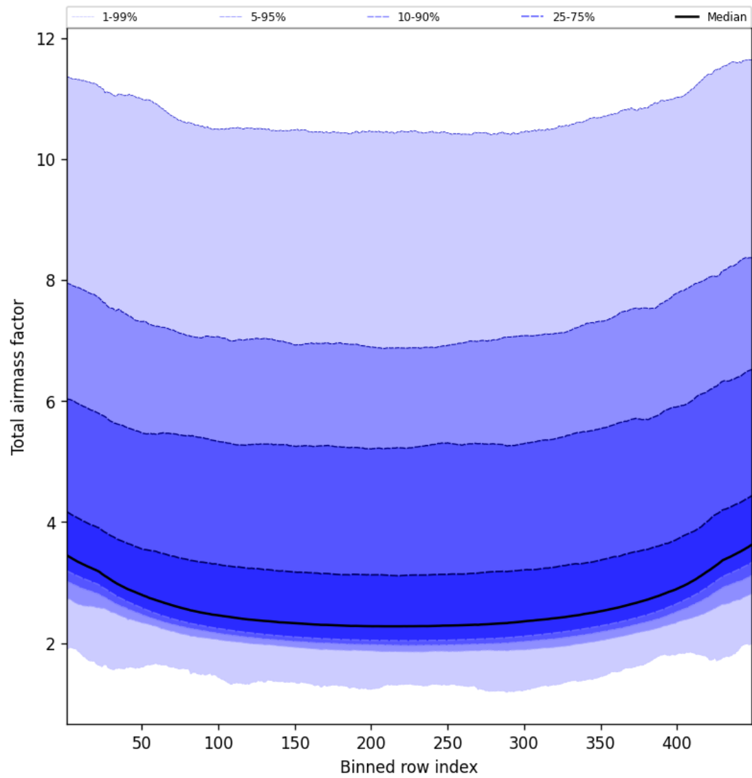
Figure 49: Along track statistics of “Total airmass factor” for 2025-01-29 to 2025-01-31
