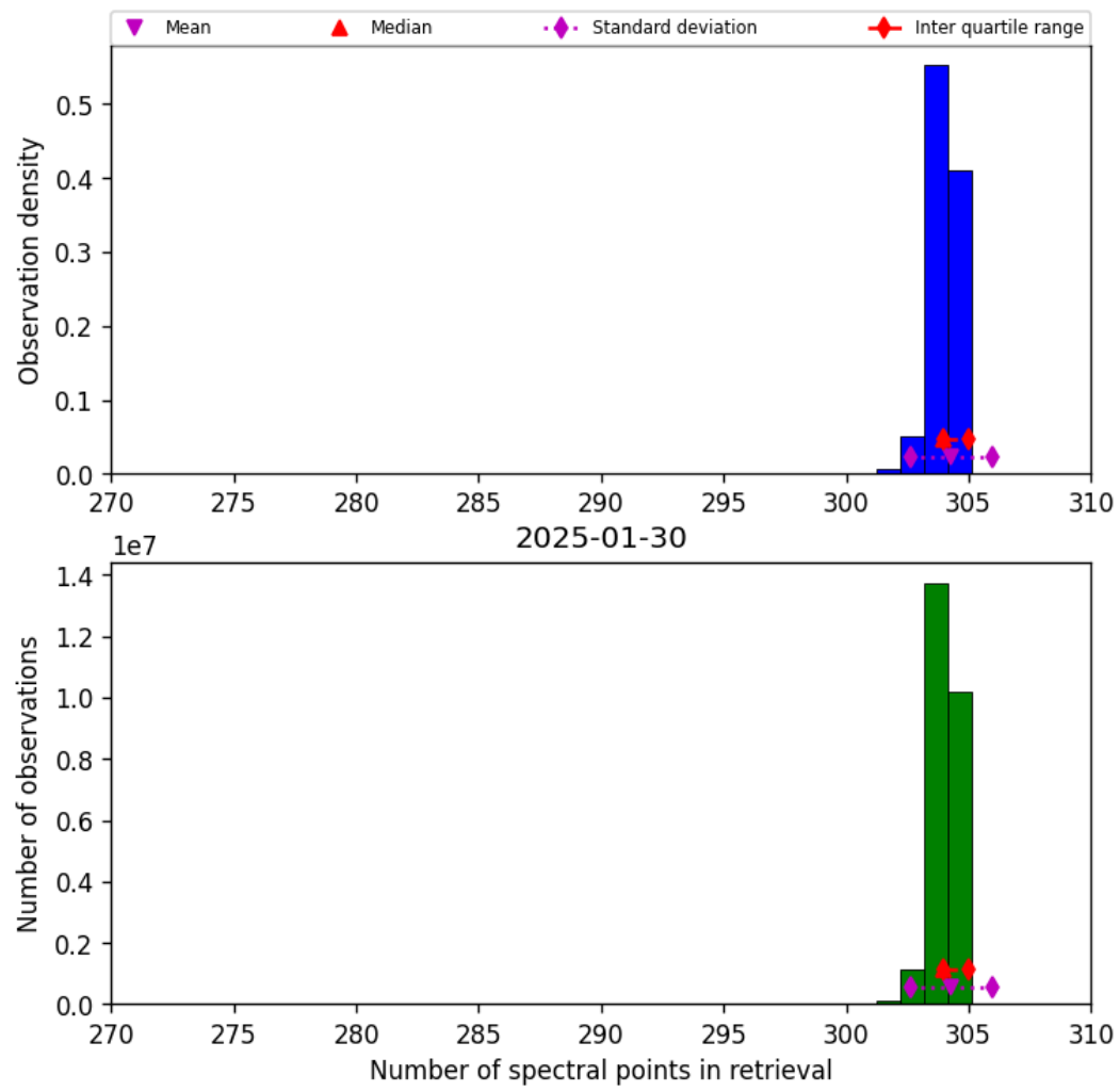
Figure 33: Histogram of “Number of spectral points in retrieval” for 2025-01-29 to 2025-01-31
