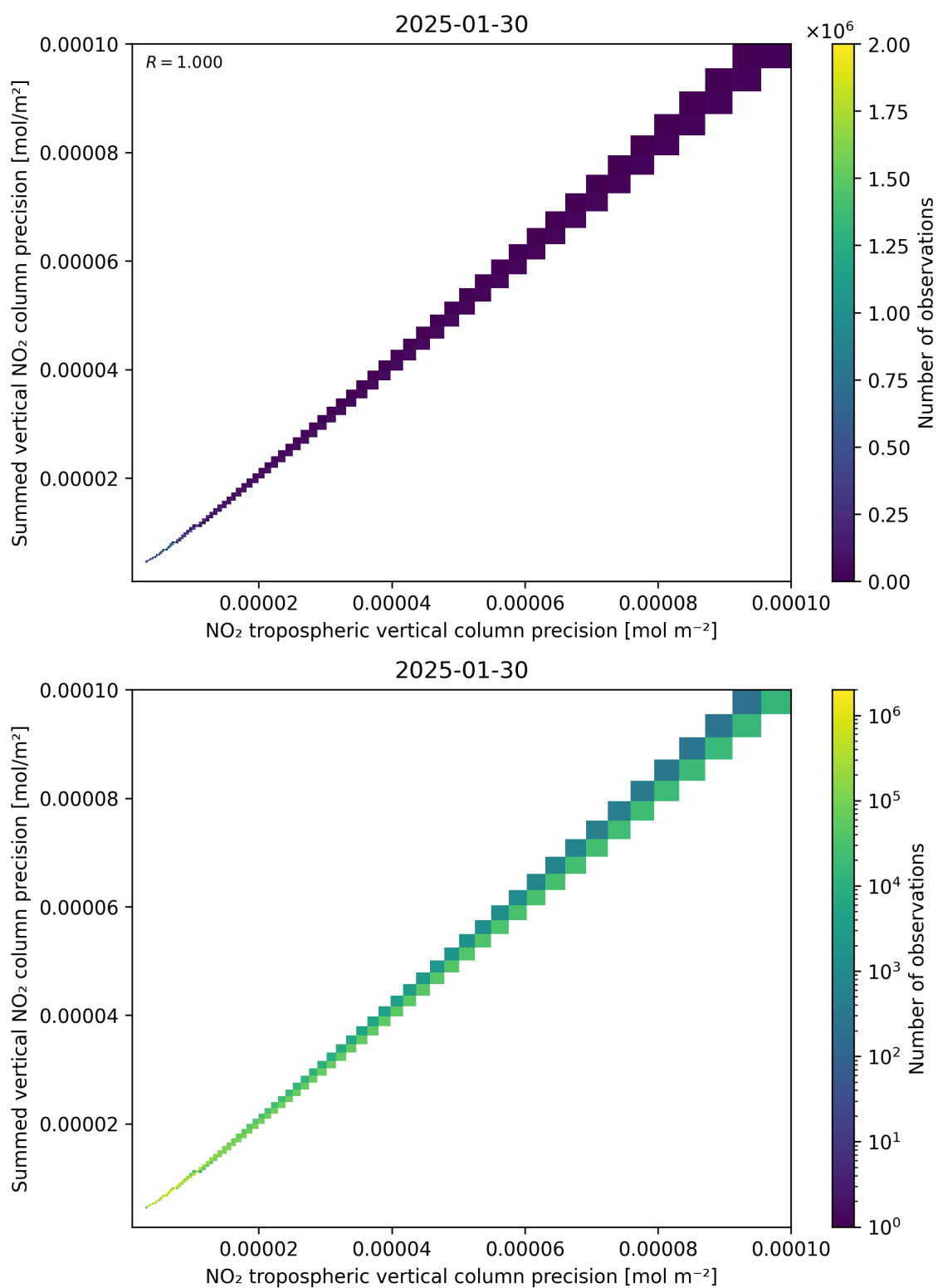
Figure 137: Scatter density plot of “NO 2 tropospheric vertical column precision” against “Summed vertical NO 2 column precision” for 2025-01-29 to 2025-01-31.
