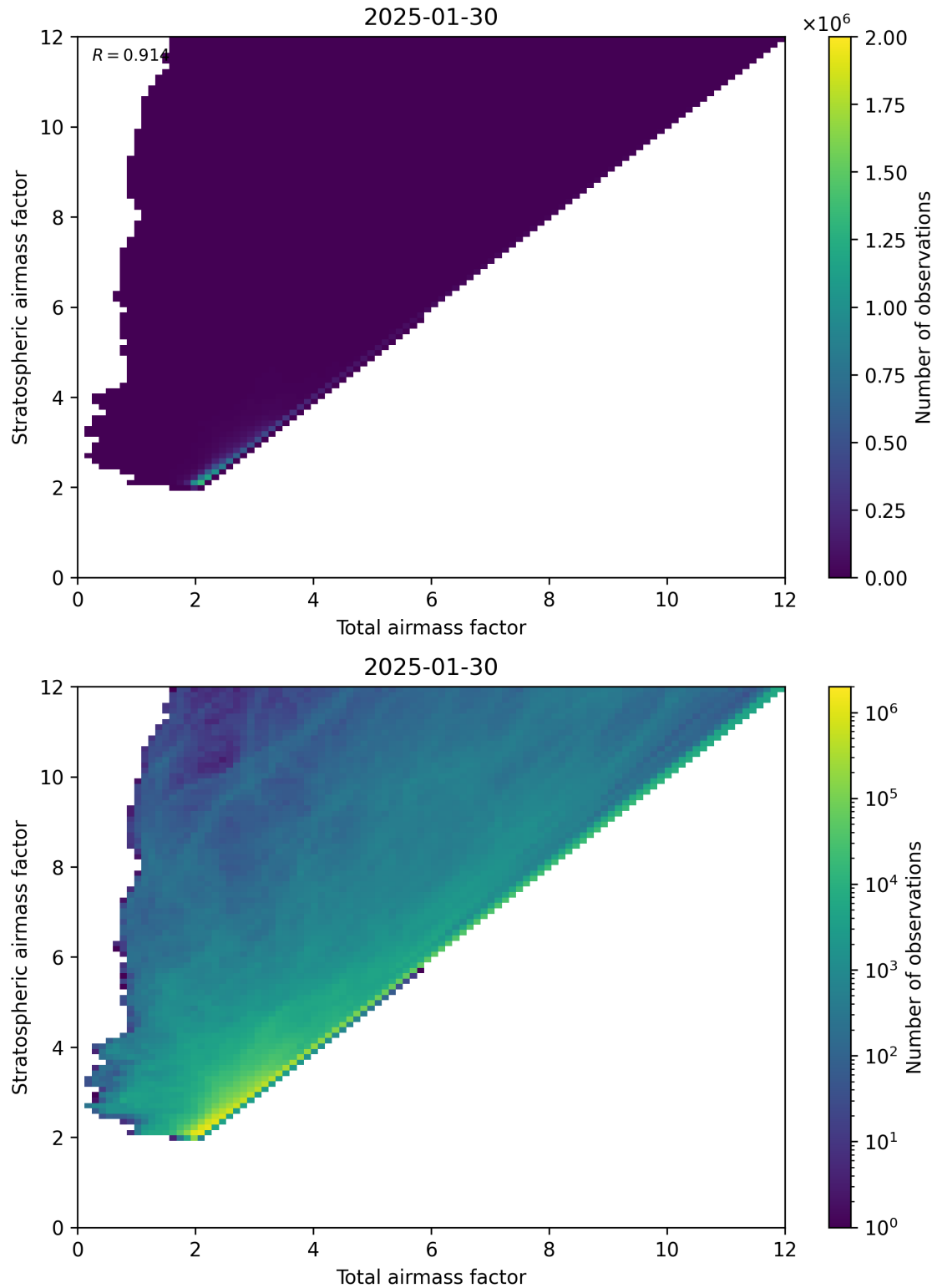
Figure 62: Scatter density plot of “Total airmass factor” against “Stratospheric airmass factor” for 2025-01-29 to 2025-01-31.
