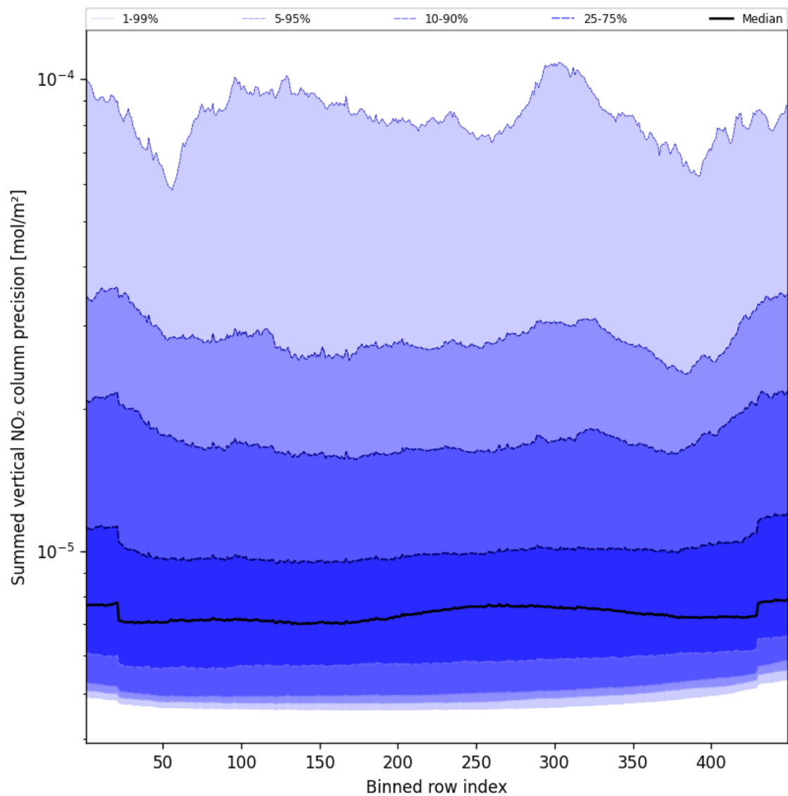
Figure 58: Along track statistics of “Summed vertical NO 2 column precision” for 2025-01-29 to 2025-01-31
