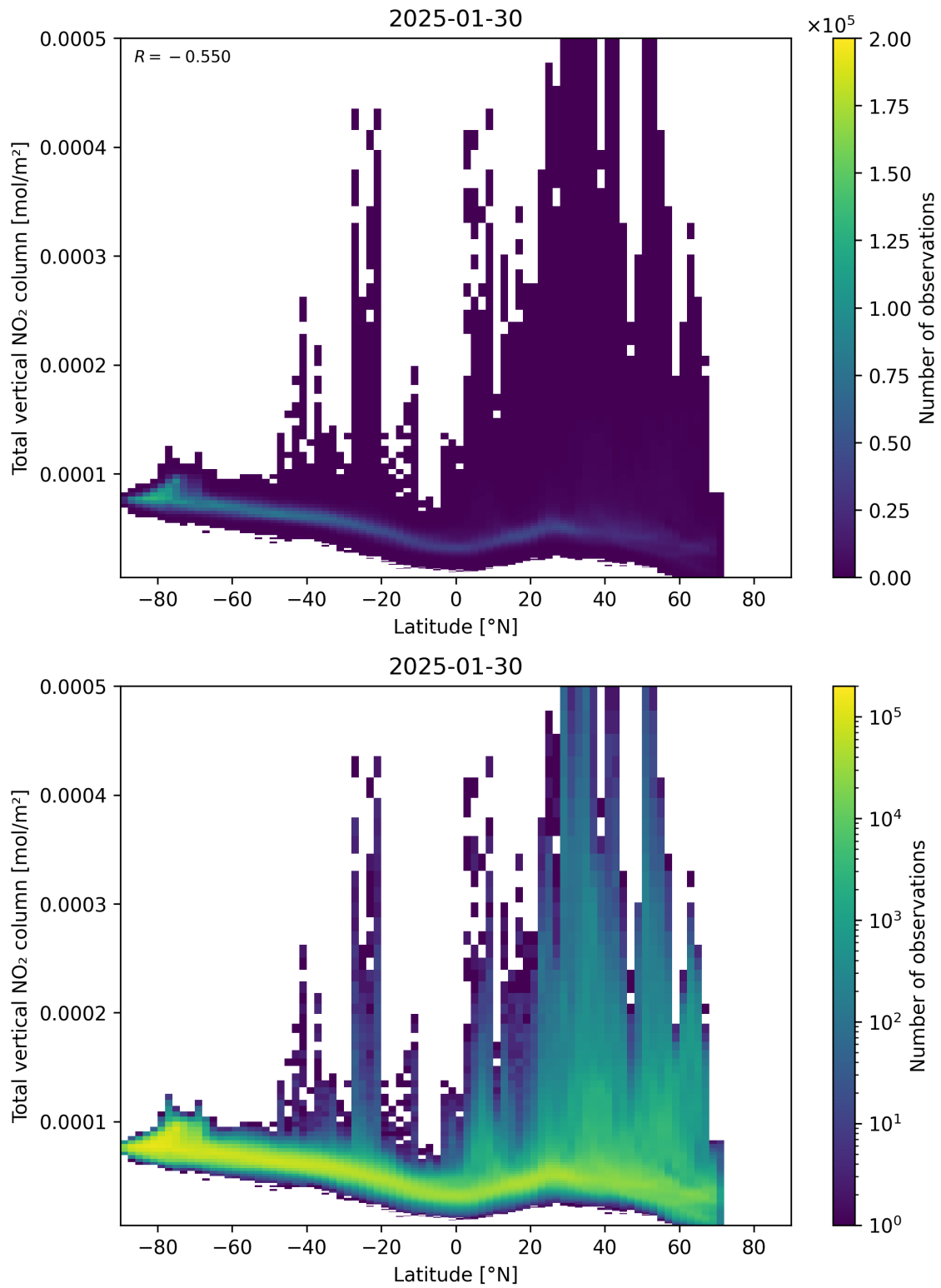
Figure 90: Scatter density plot of “Latitude” against “Total vertical NO 2 column” for 2025-01-29 to 2025-01-31.
