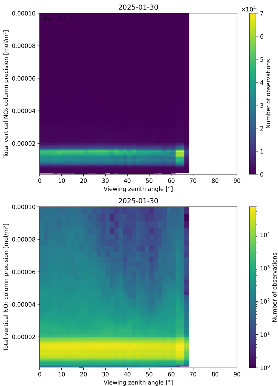
Figure 168: Scatter density plot of “Viewing zenith angle” against “Total vertical NO 2 column precision” for 2025-01-29 to 2025-01-31.
