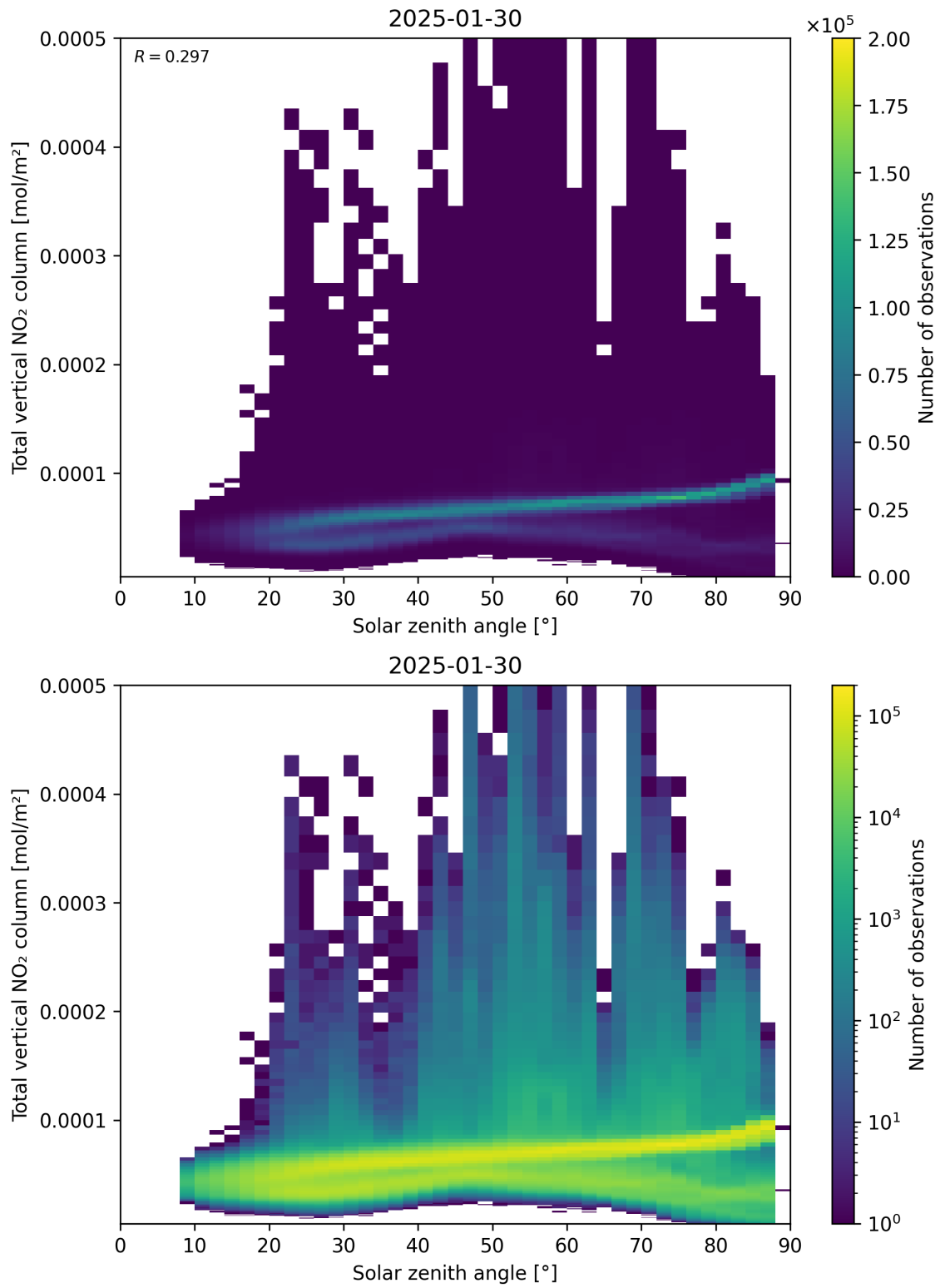
Figure 153: Scatter density plot of “Solar zenith angle” against “Total vertical NO 2 column” for 2025-01-29 to 2025-01-31.
