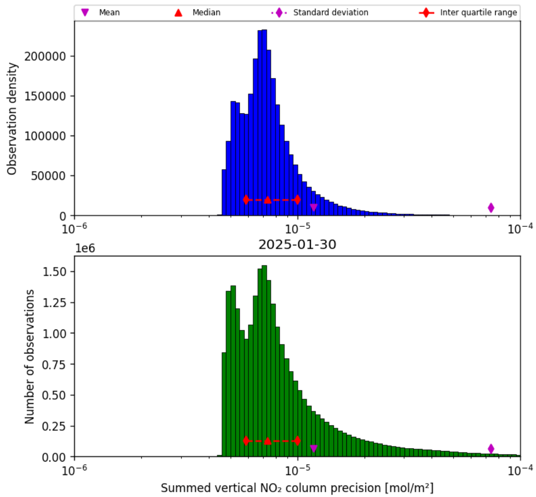
Figure 41: Histogram of “Summed vertical NO 2 column precision” for 2025-01-29 to 2025-01-31
