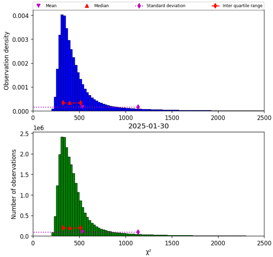
Figure 42: Histogram of " \chi^2 " for 2025-01-29 to 2025-01-31
