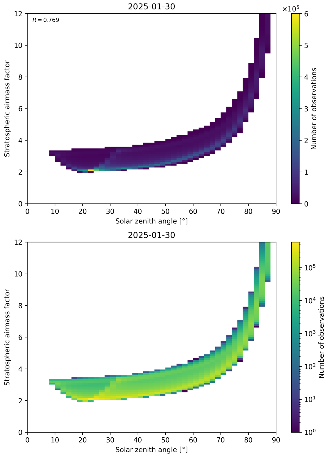
Figure 145: Scatter density plot of “Solar zenith angle” against “Stratospheric airmass factor” for 2025-01-29 to 2025-01-31.
