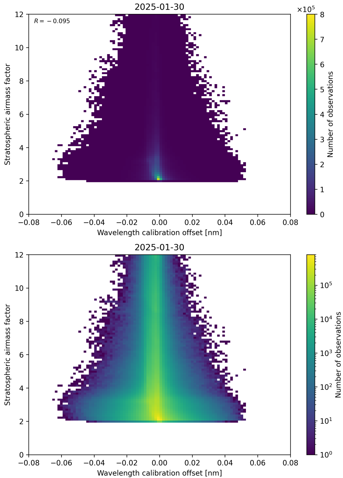
Figure 174: Scatter density plot of “Wavelength calibration offset” against “Stratospheric airmass factor” for 2025-01-29 to 2025-01-31.
