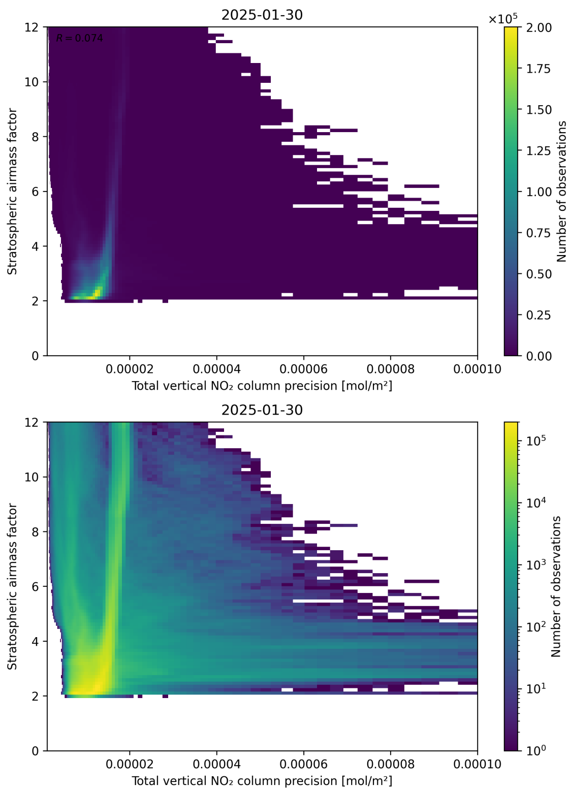
Figure 115: Scatter density plot of “Total vertical NO 2 column precision” against “Stratospheric air mass factor” for 2025-01-29 to 2025-01-31.
