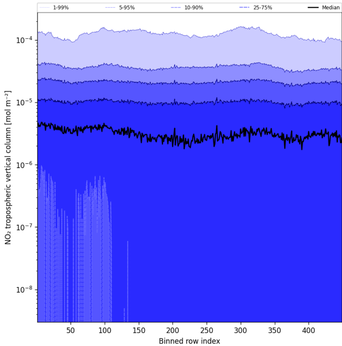
Figure 46: Along track statistics of “NO 2 tropospheric vertical column” for 2025-01-29 to 2025-01-31
