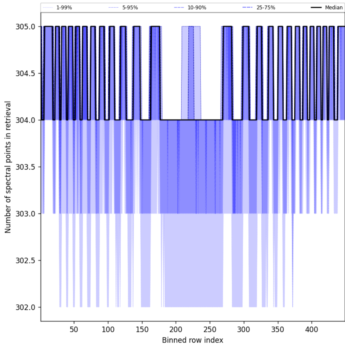
Figure 50: Along track statistics of “Number of spectral points in retrieval” for 2025-01-29 to 2025-01-31
