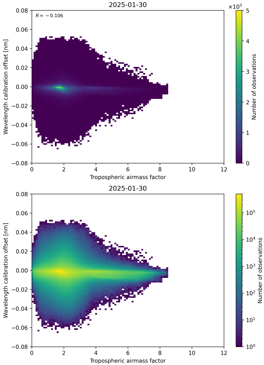
Figure 80: Scatter density plot of “Tropospheric airmass factor” against “Wavelength calibration offset” for 2025-01-29 to 2025-01-31.
