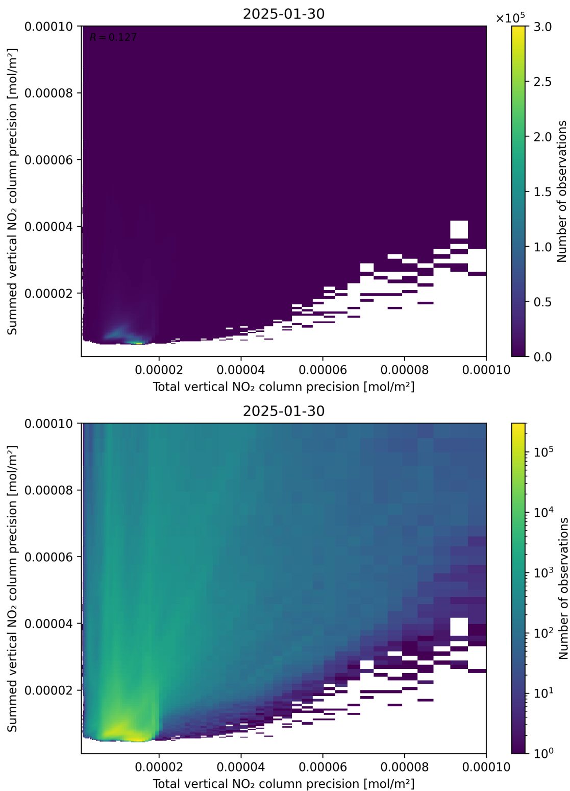
Figure 118: Scatter density plot of “Total vertical NO 2 column precision” against “Summed vertical NO 2 column precision” for 2025-01-29 to 2025-01-31.
