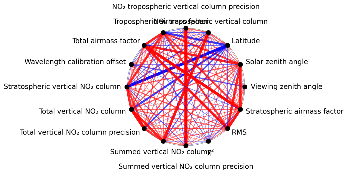
Figure 1: Map of correlation graph for 2025-01-29 to 2025-01-31.
