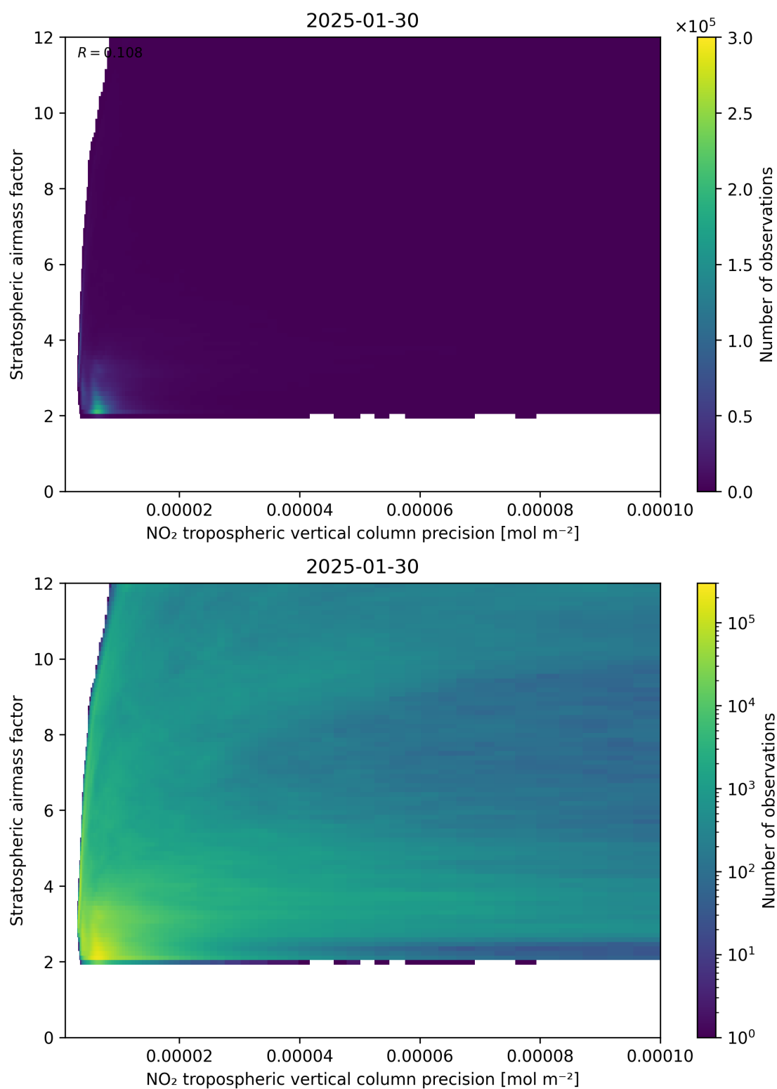
Figure 131: Scatter density plot of “NO 2 tropospheric vertical column precision” against “Stratospheric airmass factor” for 2025-01-29 to 2025-01-31.
