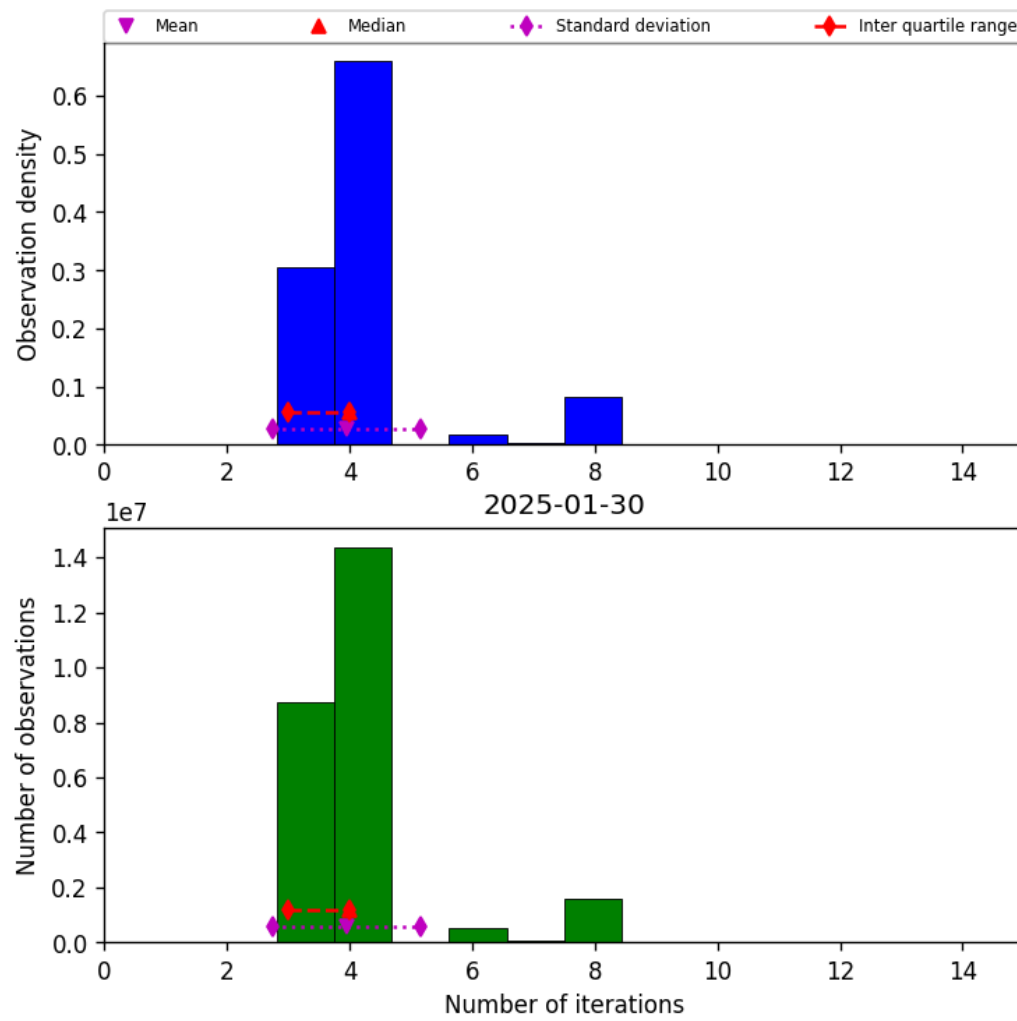
Figure 34: Histogram of “Number of iterations” for 2025-01-29 to 2025-01-31
