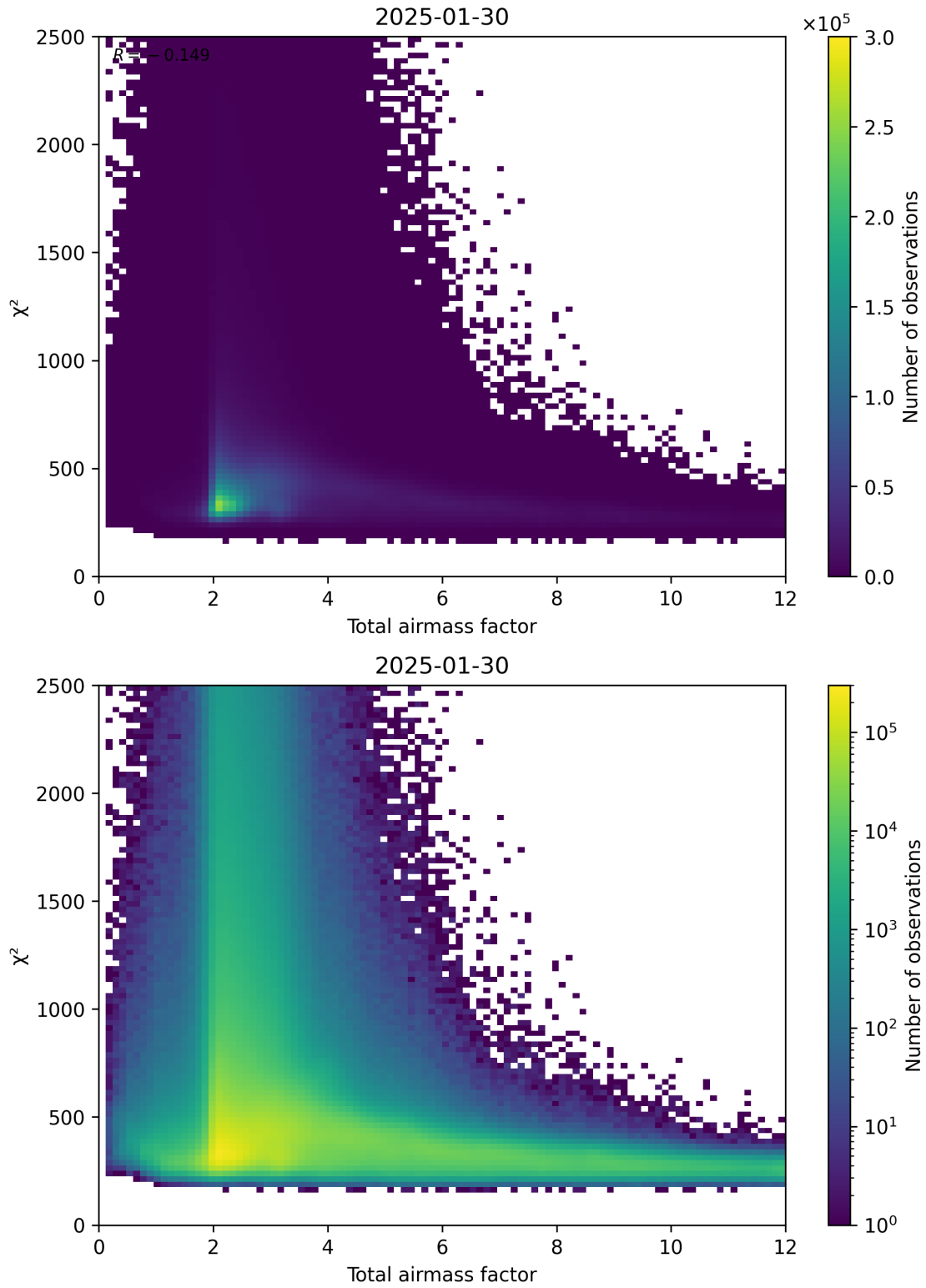
Figure 63: Scatter density plot of “Total airmass factor” against “ \chi^2 ” for 2025-01-29 to 2025-01-31.
