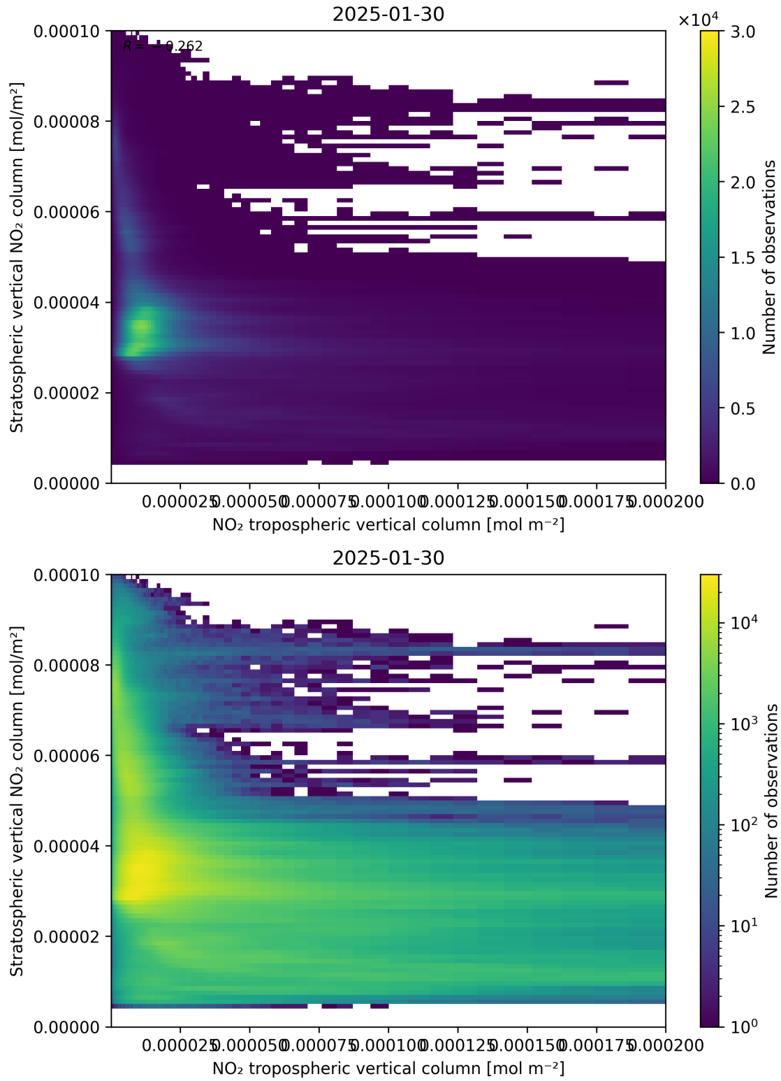
Figure 125: Scatter density plot of “NO 2 tropospheric vertical column” against “Stratospheric vertical NO 2 column” for 2025-01-29 to 2025-01-31.
