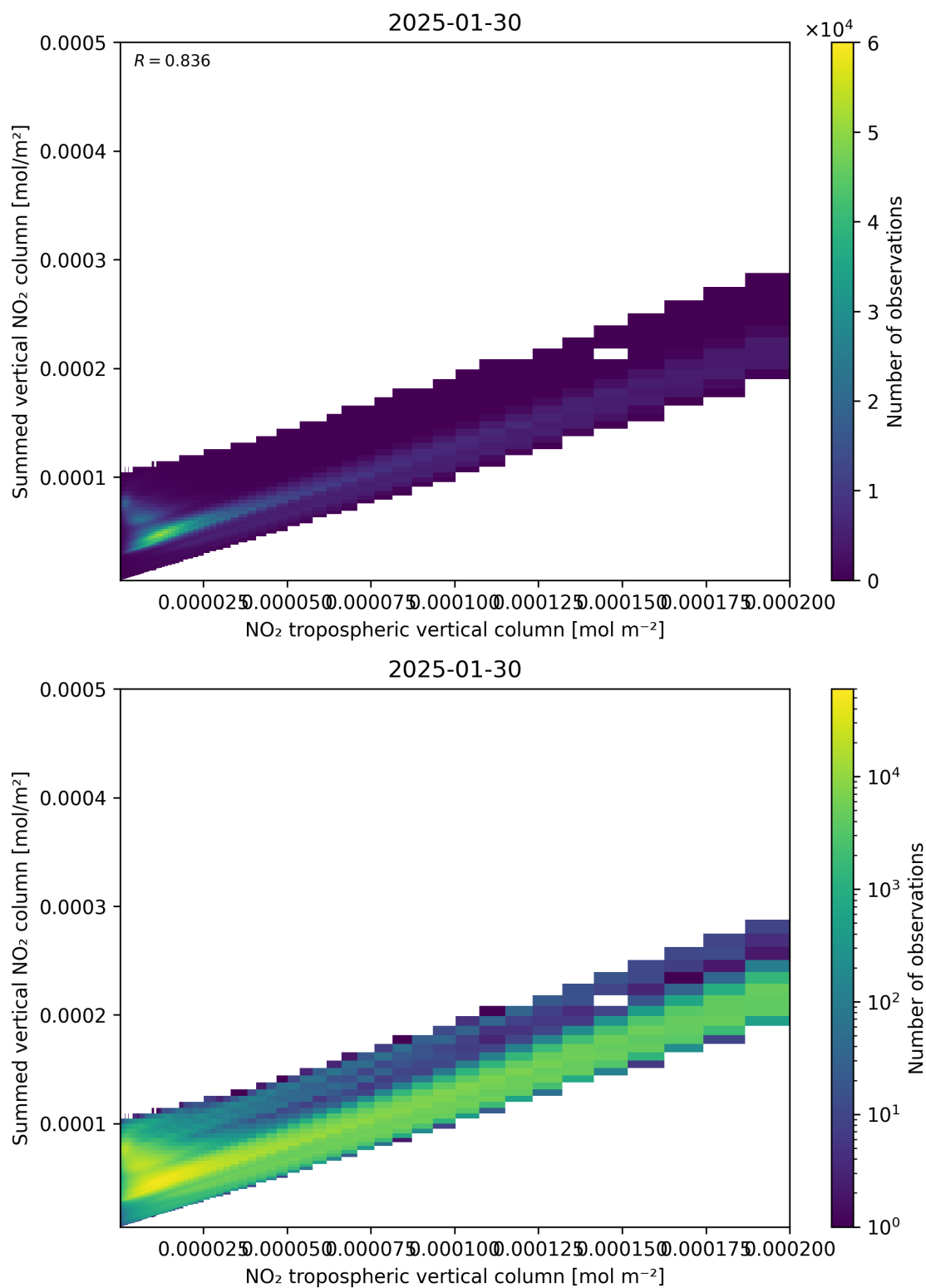
Figure 126: Scatter density plot of “NO 2 tropospheric vertical column” against “Summed vertical NO 2 column” for 2025-01-29 to 2025-01-31.
