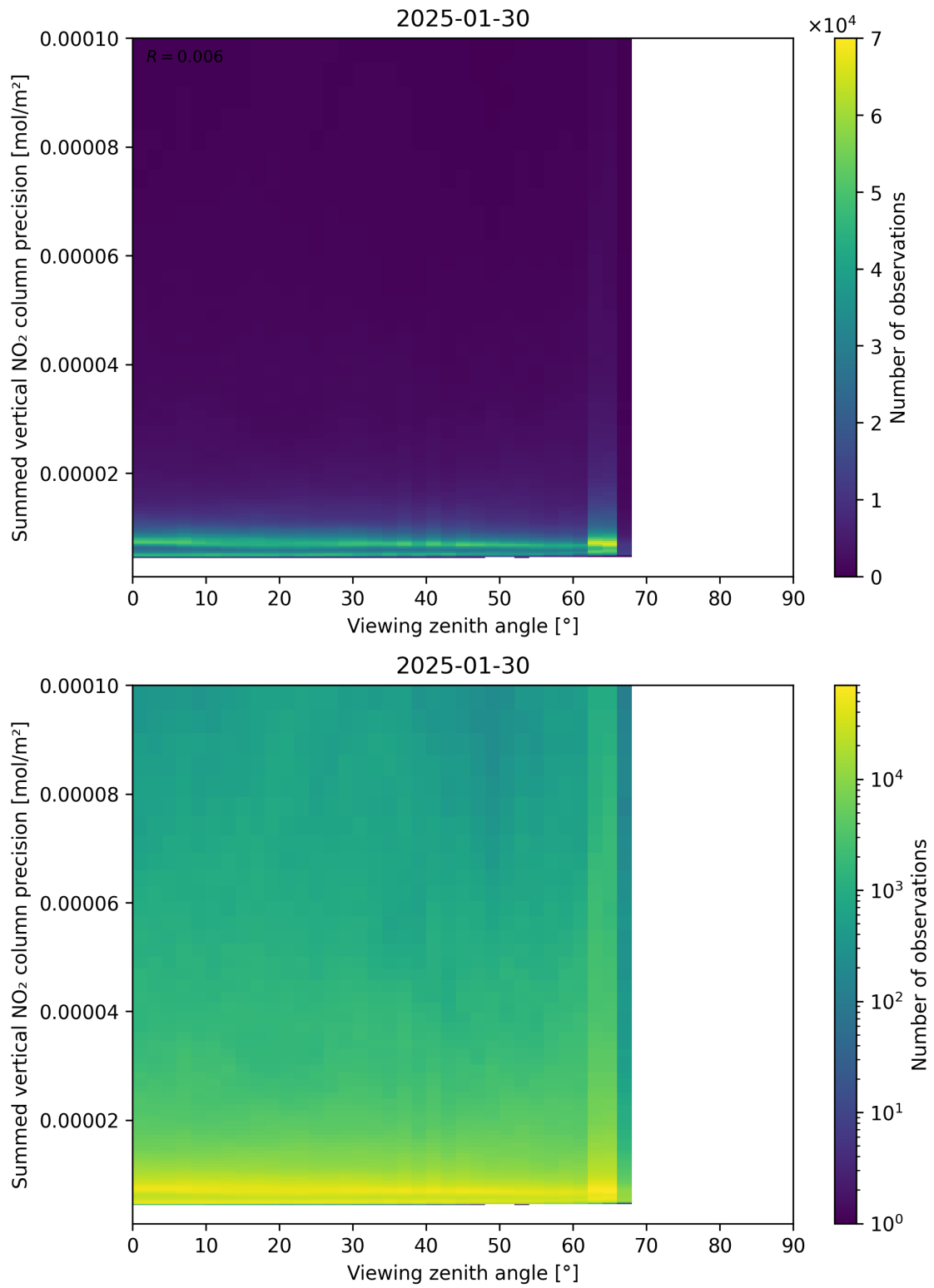
Figure 166: Scatter density plot of “Viewing zenith angle” against “Summed vertical NO 2 column precision” for 2025-01-29 to 2025-01-31.
