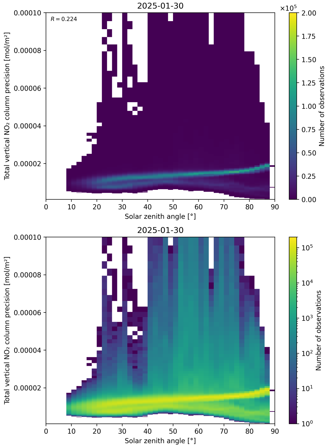
Figure 154: Scatter density plot of “Solar zenith angle” against “Total vertical NO 2 column precision” for 2025-01-29 to 2025-01-31.
