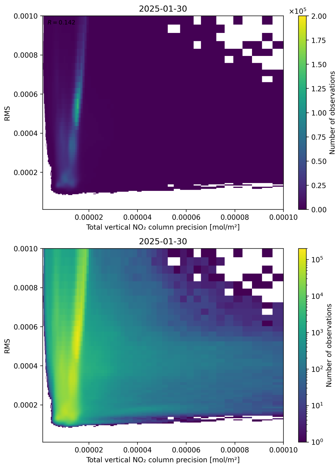
Figure 119: Scatter density plot of “Total vertical NO 2 column precision” against “RMS” for 2025-01-29 to 2025-01-31.
