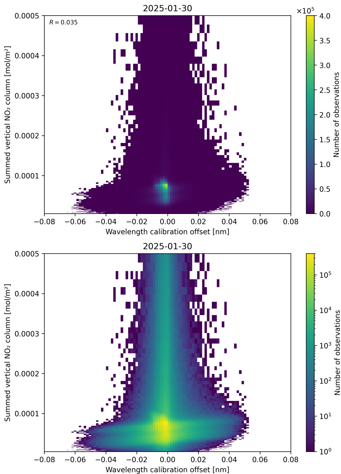
Figure 177: Scatter density plot of “Wavelength calibration offset” against “Summed vertical NO 2 column” for 2025-01-29 to 2025-01-31.
