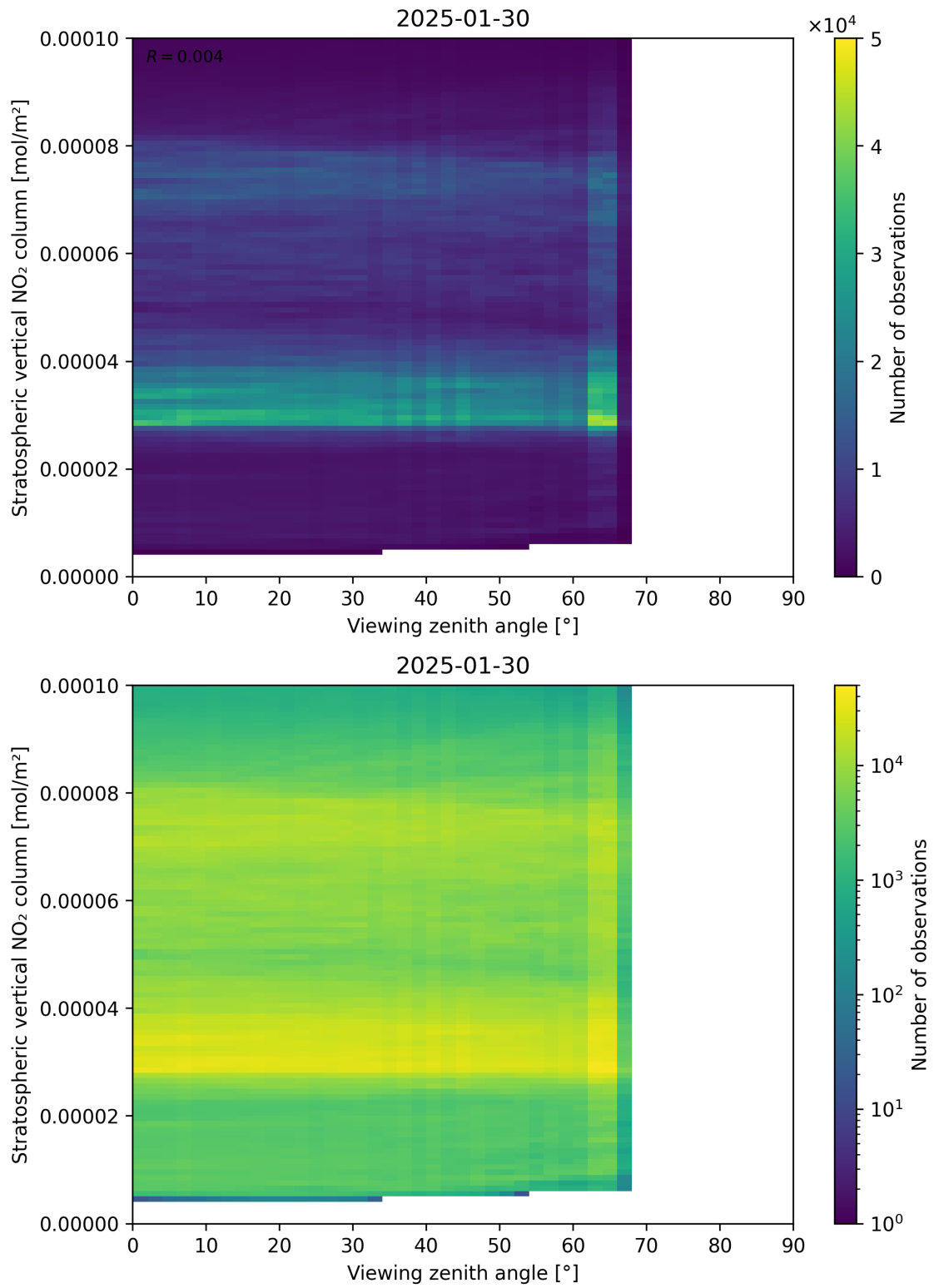
Figure 164: Scatter density plot of “Viewing zenith angle” against “Stratospheric vertical NO 2 column” for 2025-01-29 to 2025-01-31.
