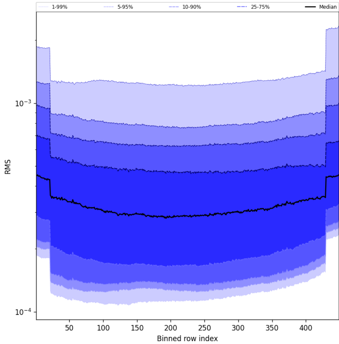
Figure 60: Along track statistics of “RMS” for 2025-01-29 to 2025-01-31
