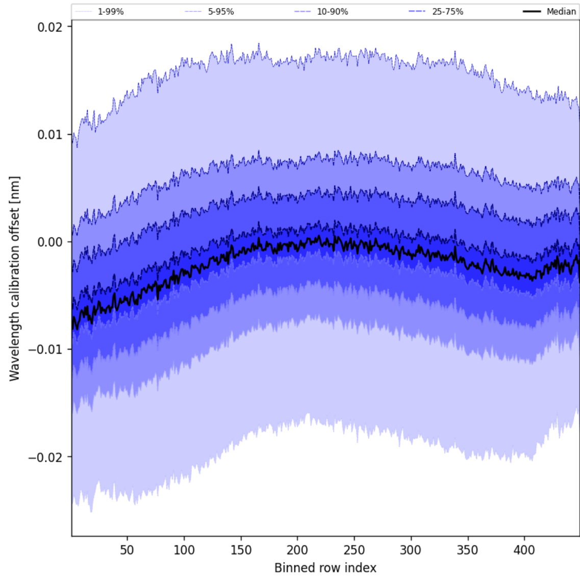
Figure 52: Along track statistics of “Wavelength calibration offset” for 2025-01-31 to 2025-02-02
