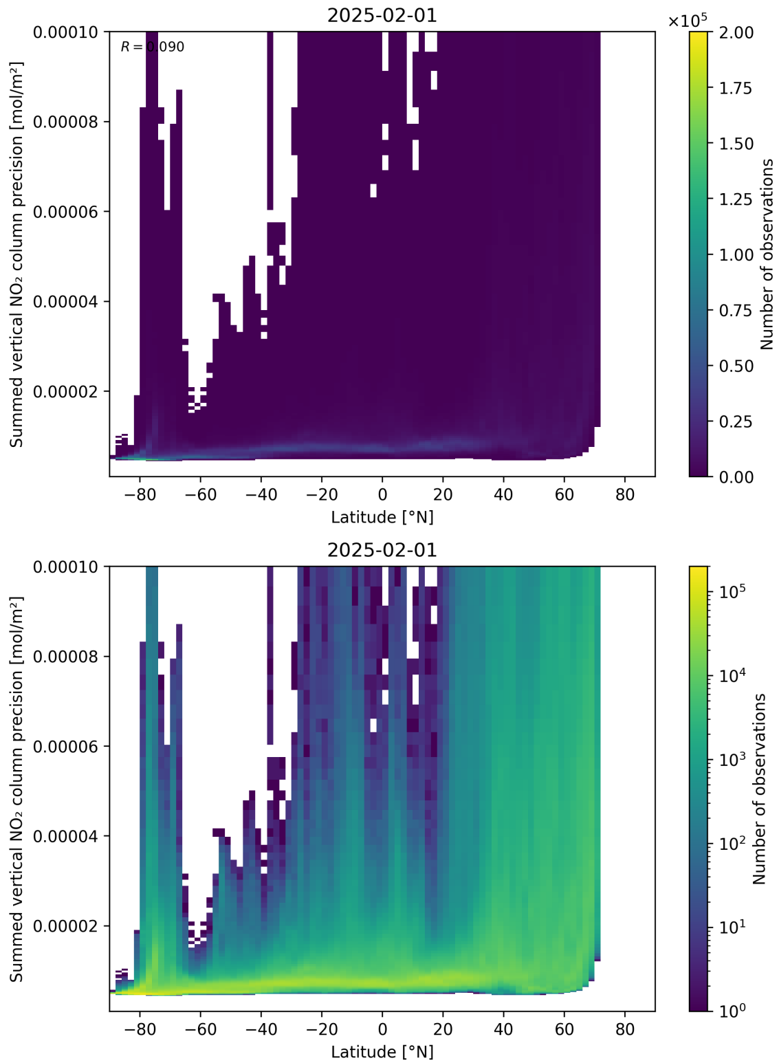
Figure 89: Scatter density plot of “Latitude” against “Summed vertical NO 2 column precision” for 2025-01-31 to 2025-02-02.
