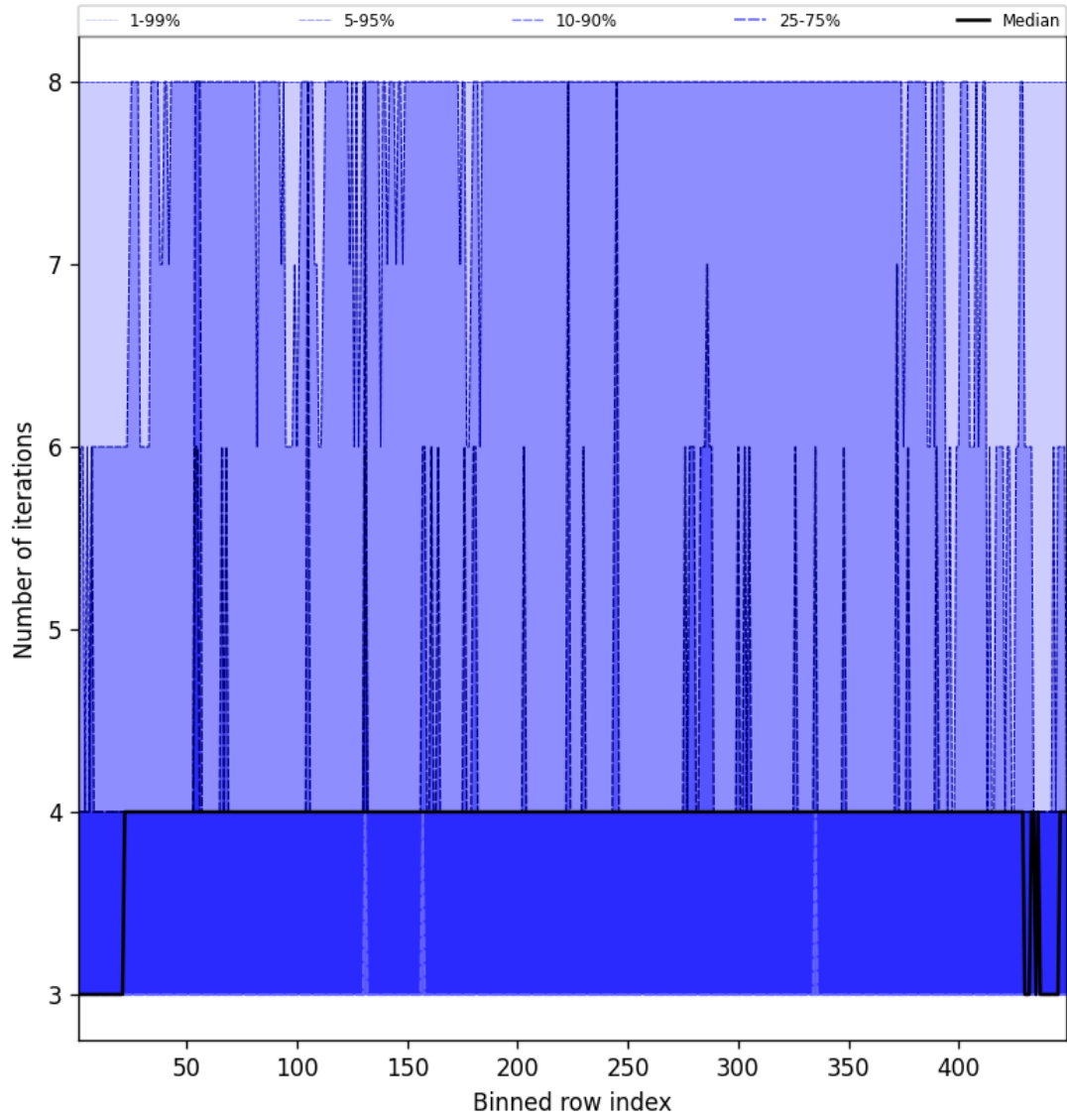
Figure 51: Along track statistics of “Number of iterations” for 2025-01-31 to 2025-02-02
