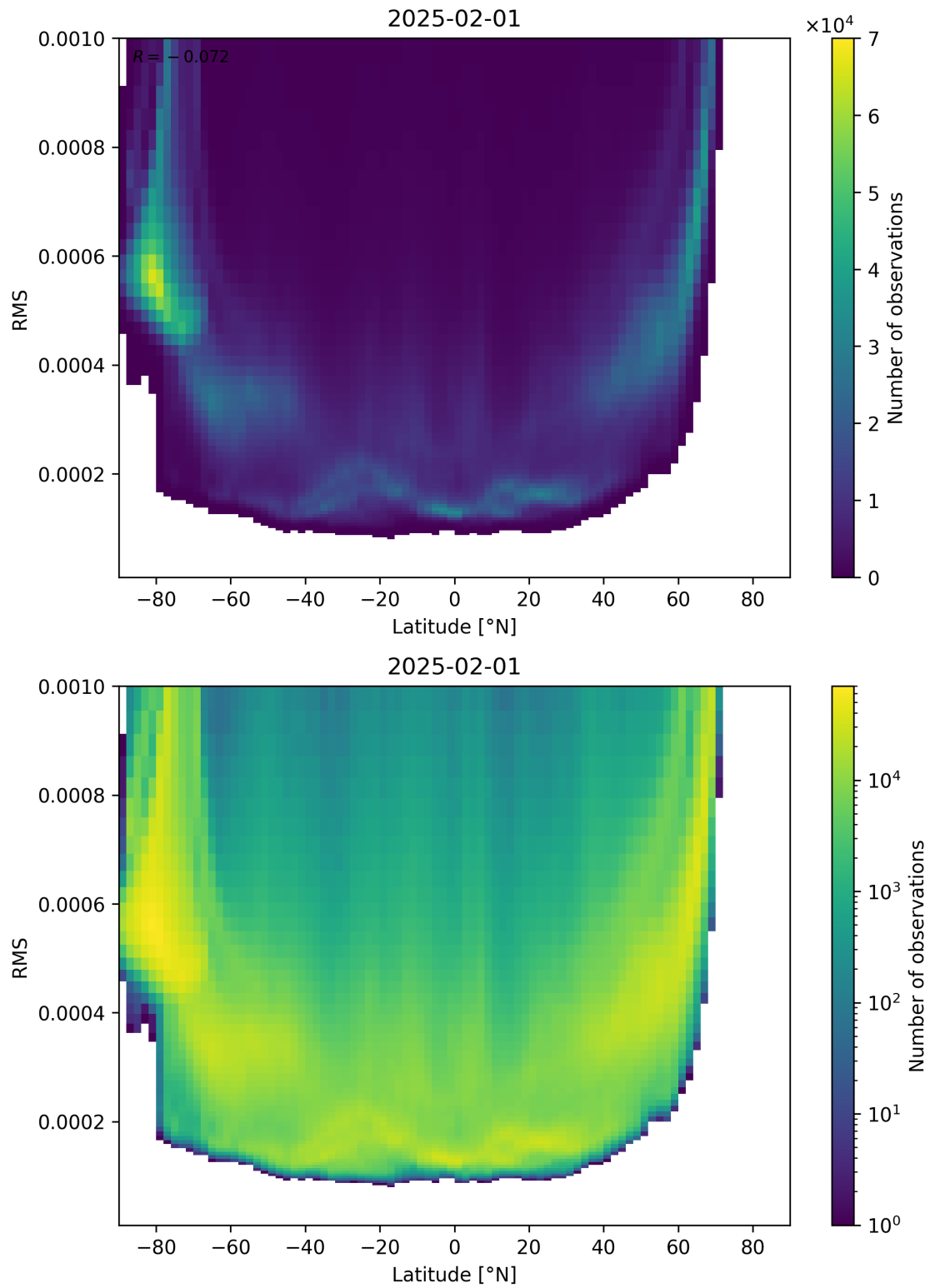
Figure 94: Scatter density plot of “Latitude” against “RMS” for 2025-01-31 to 2025-02-02.
