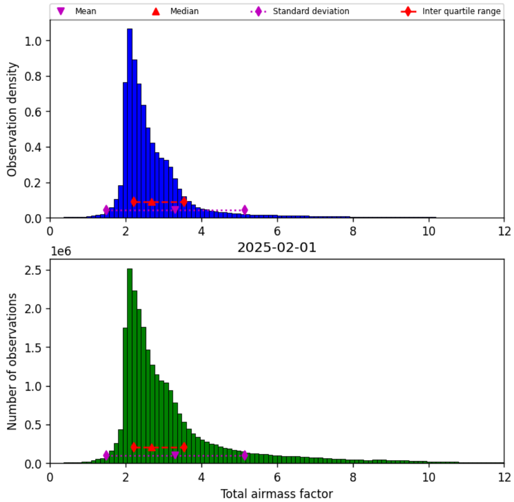
Figure 32: Histogram of “Total airmass factor” for 2025-01-31 to 2025-02-02
