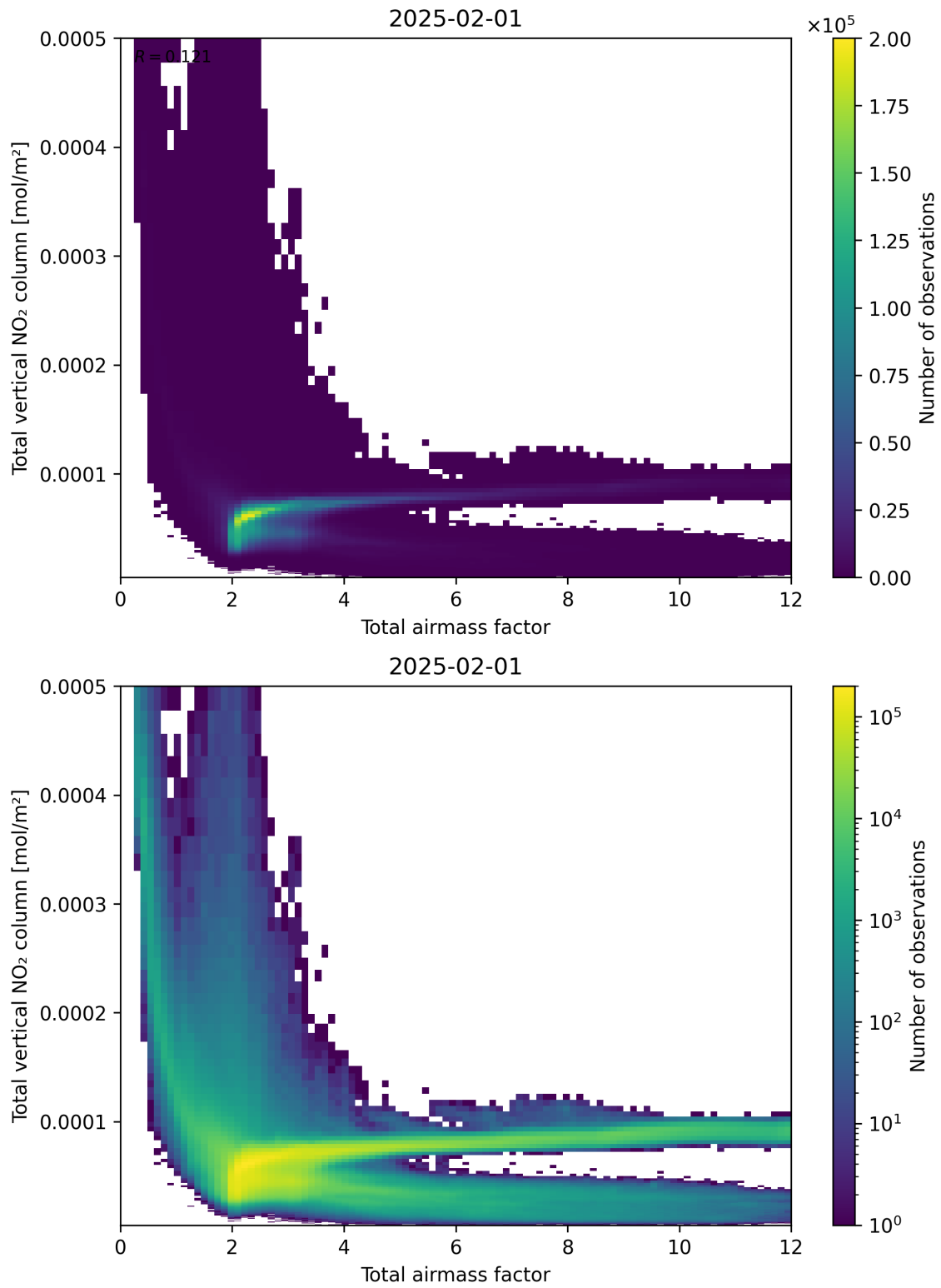
Figure 67: Scatter density plot of “Total airmass factor” against “Total vertical NO 2 column” for 2025-01-31 to 2025-02-02.
