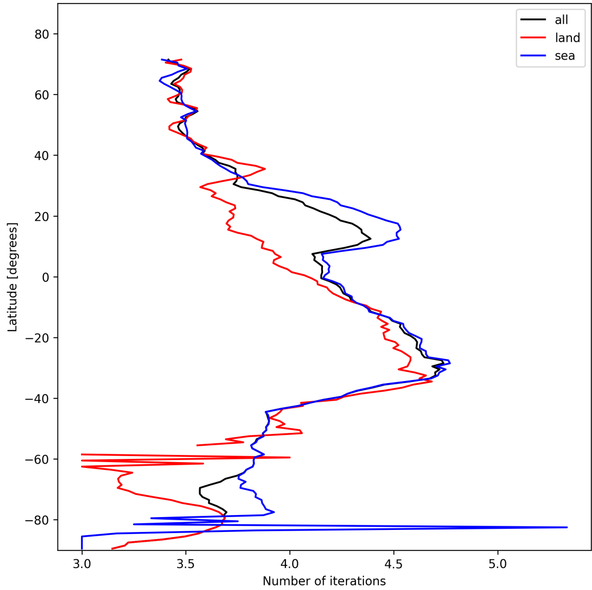
Figure 17: Zonal average of “Number of iterations” for 2025-01-31 to 2025-02-02.
