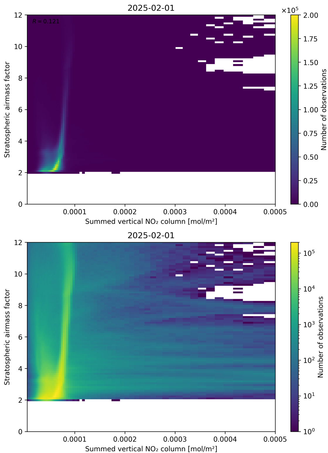
Figure 103: Scatter density plot of “Summed vertical NO 2 column” against “Stratospheric airmass factor” for 2025-01-31 to 2025-02-02.
