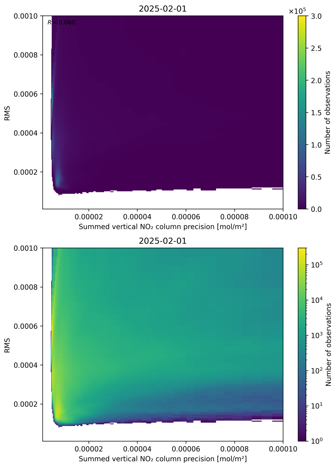
Figure 108: Scatter density plot of “Summed vertical NO 2 column precision” against “RMS” for 2025-01-31 to 2025-02-02.
