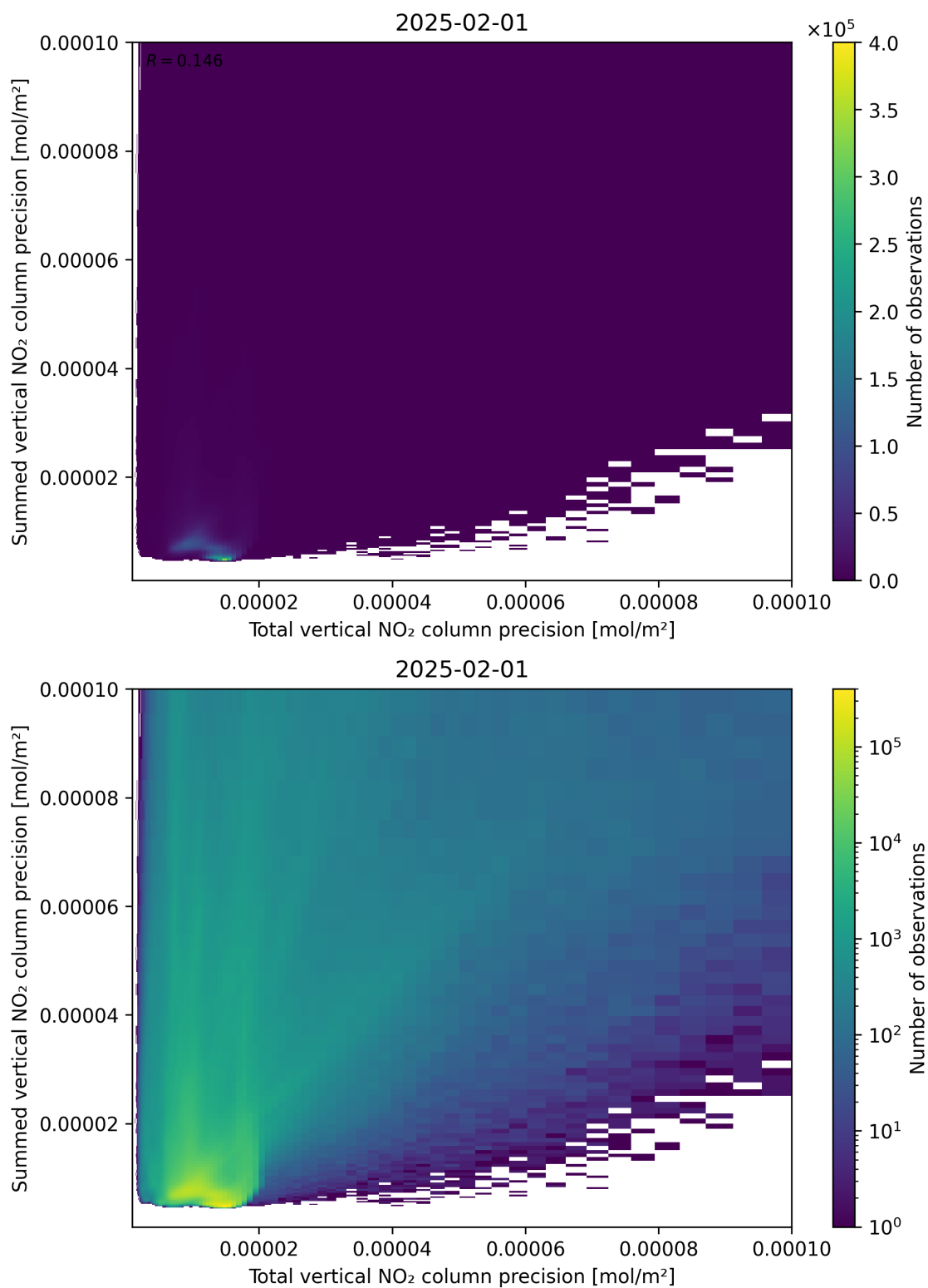
Figure 118: Scatter density plot of “Total vertical NO 2 column precision” against “Summed vertical NO 2 column precision” for 2025-01-31 to 2025-02-02.
