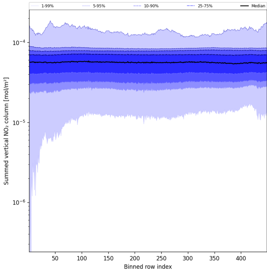
Figure 57: Along track statistics of “Summed vertical NO 2 column” for 2025-01-31 to 2025-02-02
