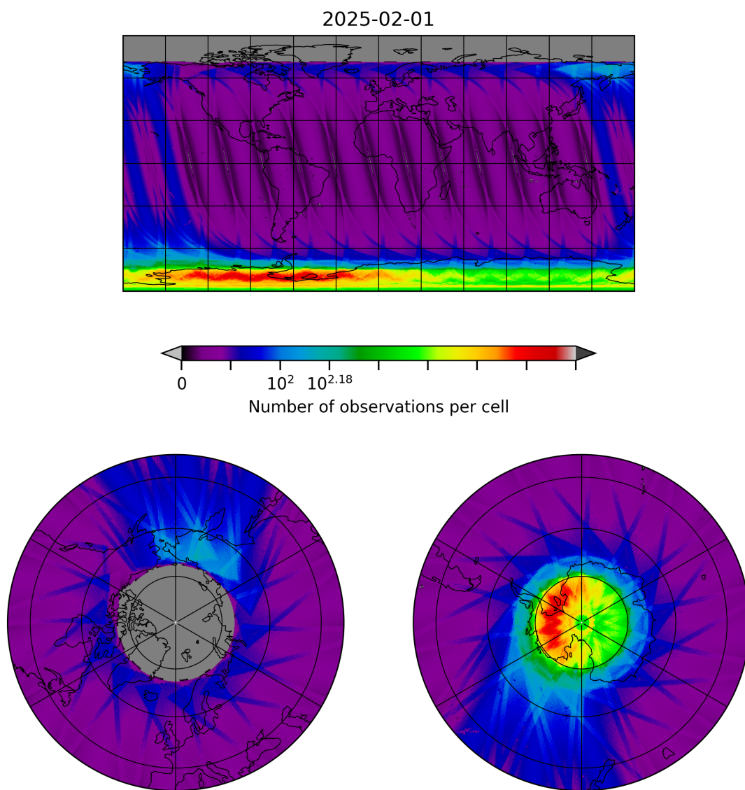
Figure 10: Map of the number of observations for 2025-01-31 to 2025-02-02
