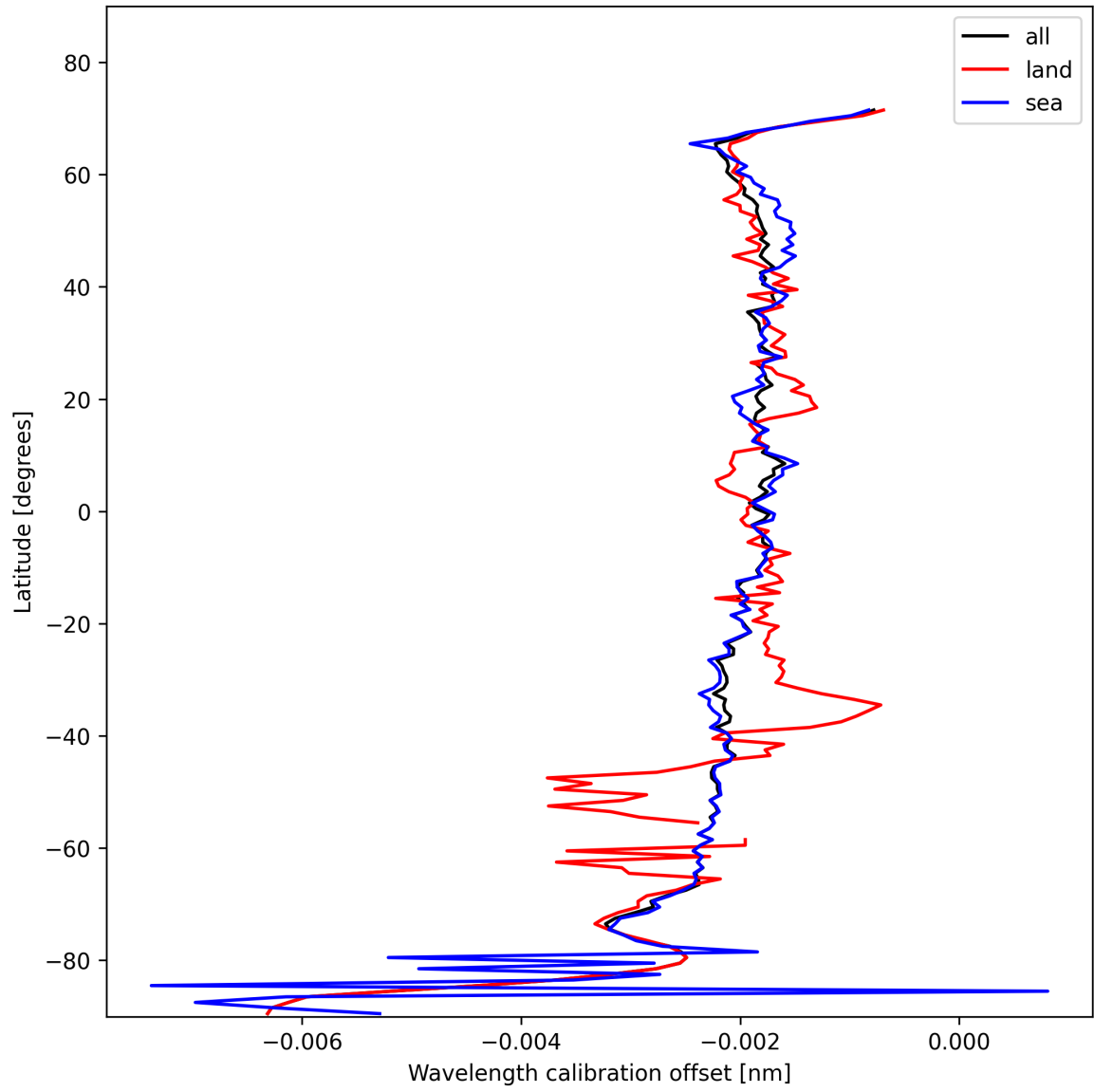
Figure 18: Zonal average of “Wavelength calibration offset” for 2025-01-31 to 2025-02-02.
