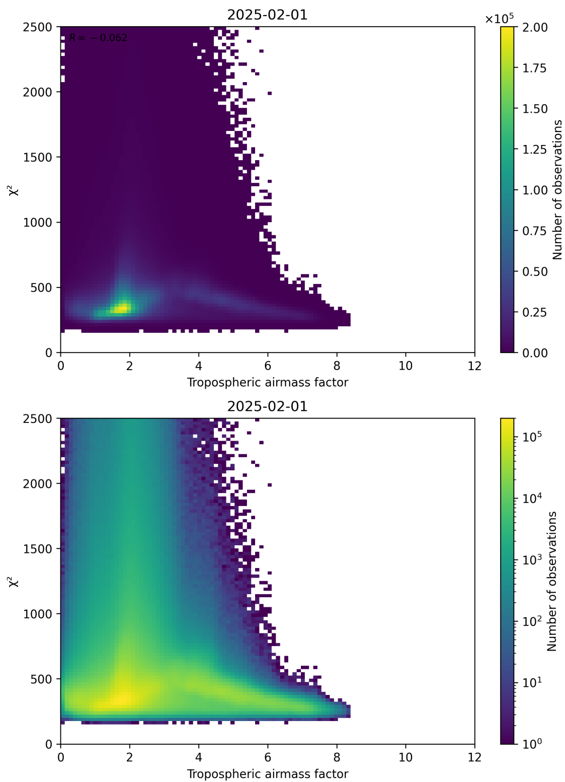
Figure 73: Scatter density plot of “Tropospheric airmass factor” against “ \chi^2 ” for 2025-01-31 to 2025-02-02.
