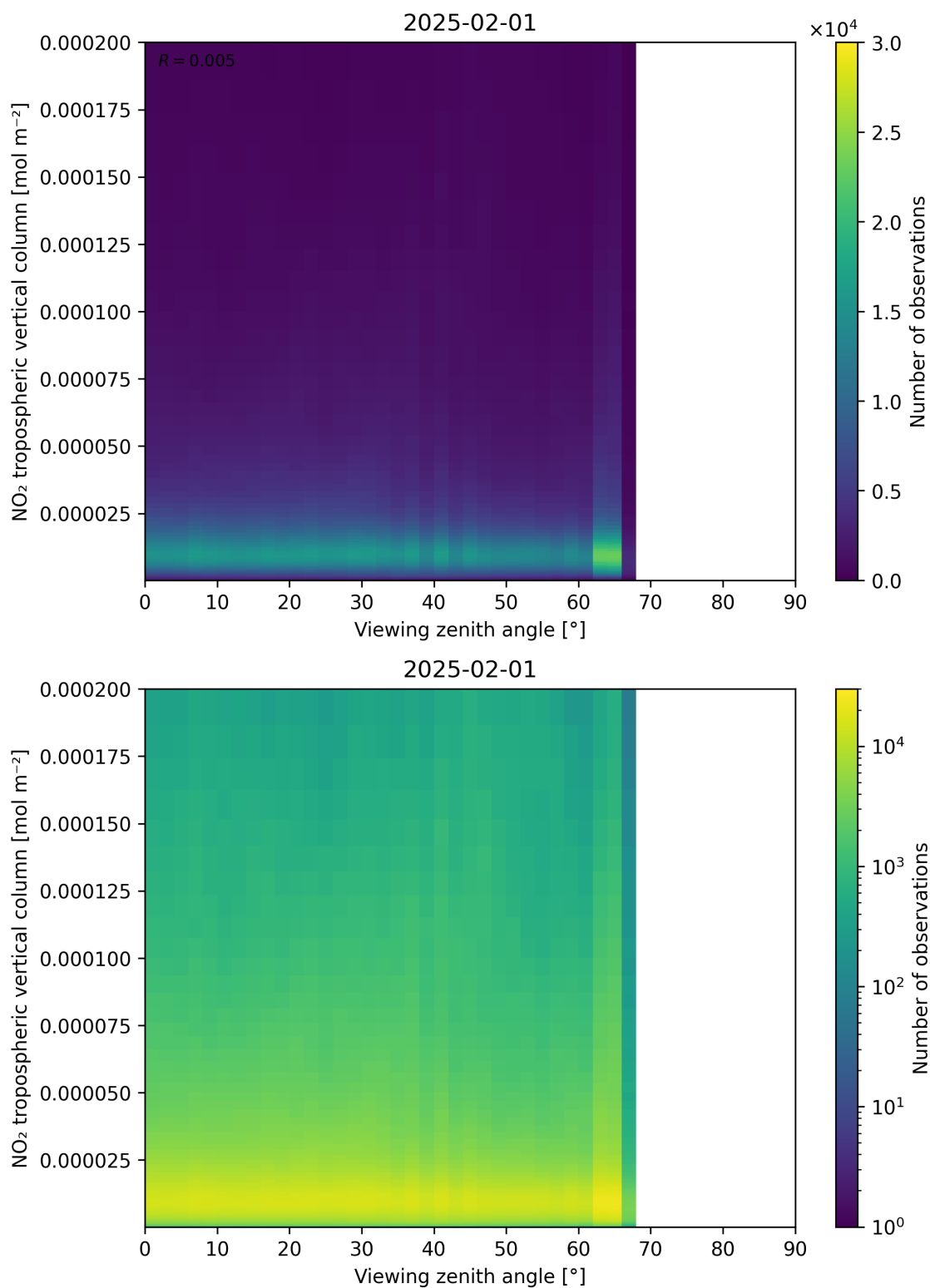
Figure 169: Scatter density plot of “Viewing zenith angle” against “NO 2 tropospheric vertical column” for 2025-01-31 to 2025-02-02.
