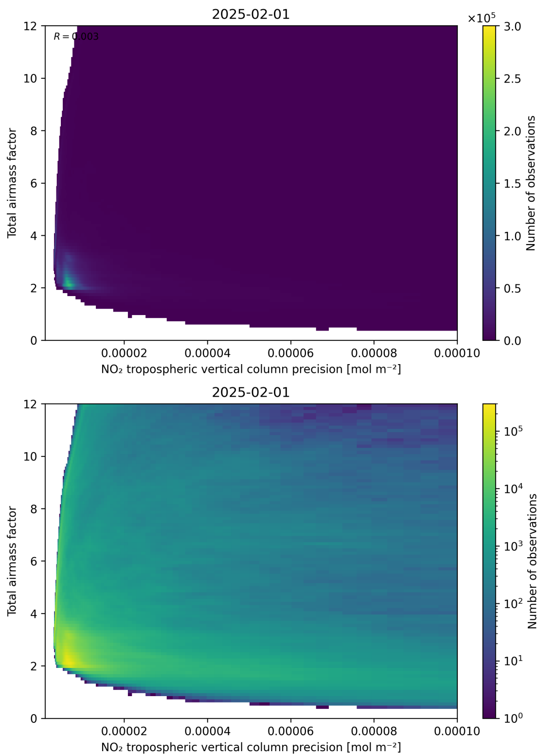
Figure 132: Scatter density plot of “NO 2 tropospheric vertical column precision” against “Total air mass factor” for 2025-01-31 to 2025-02-02.
