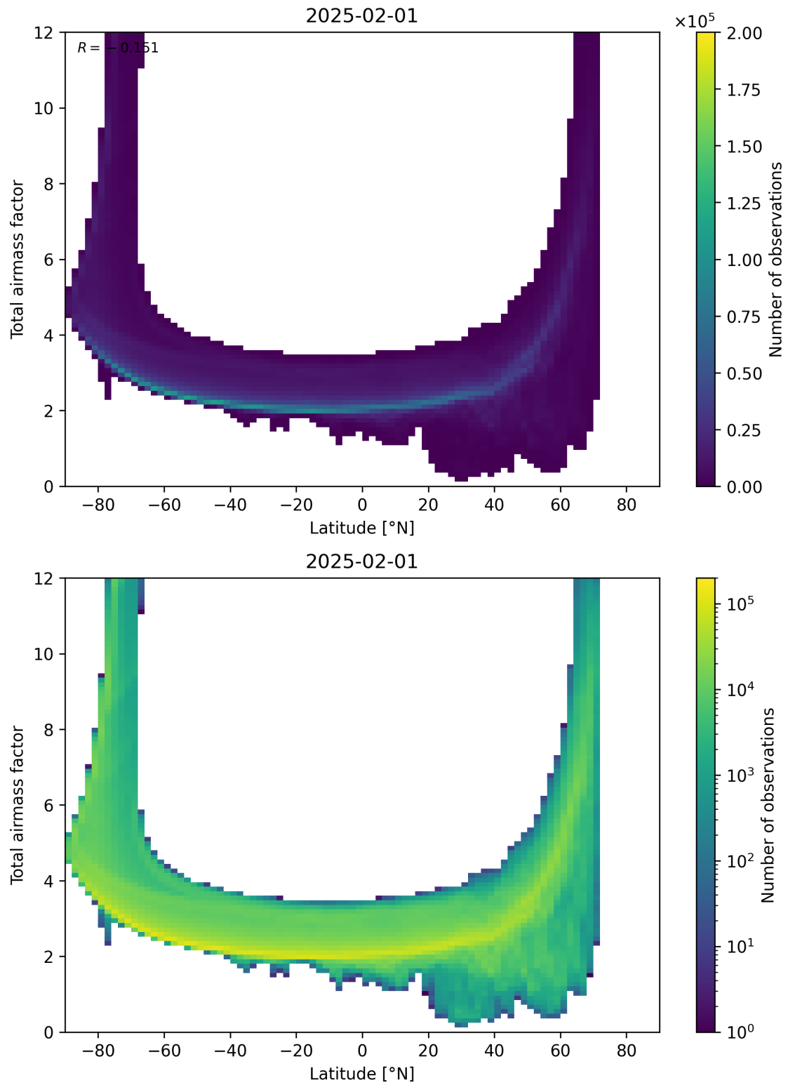
Figure 84: Scatter density plot of “Latitude” against “Total airmass factor” for 2025-01-31 to 2025-02-02.
