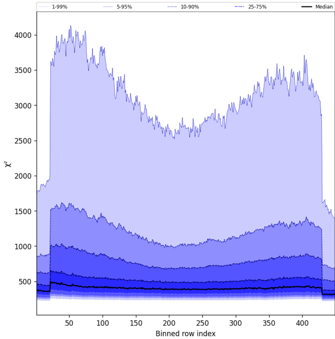
Figure 59: Along track statistics of “ \chi^2 ” for 2025-01-31 to 2025-02-02
