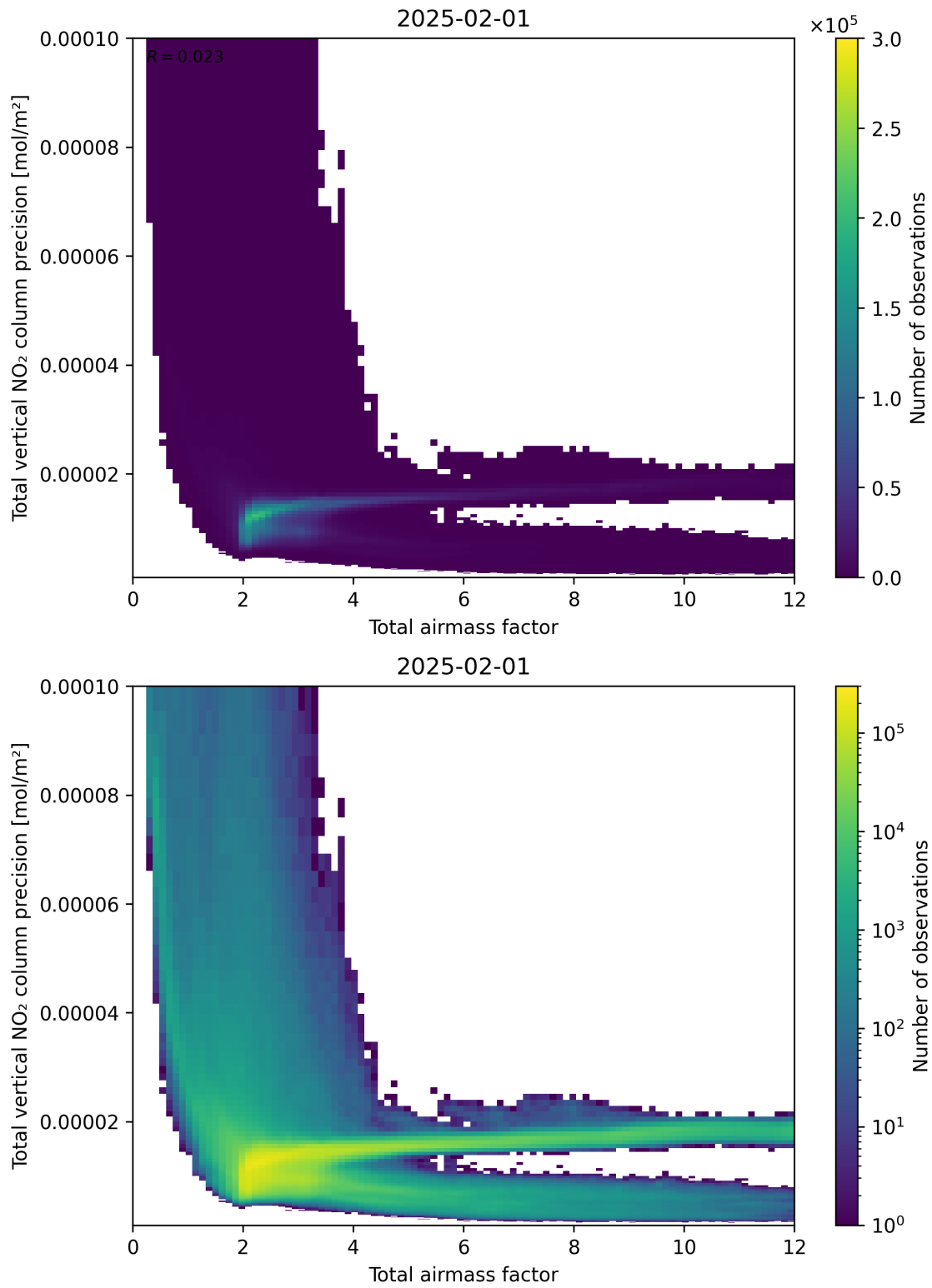
Figure 68: Scatter density plot of “Total airmass factor” against “Total vertical NO 2 column precision” for 2025-01-31 to 2025-02-02.
