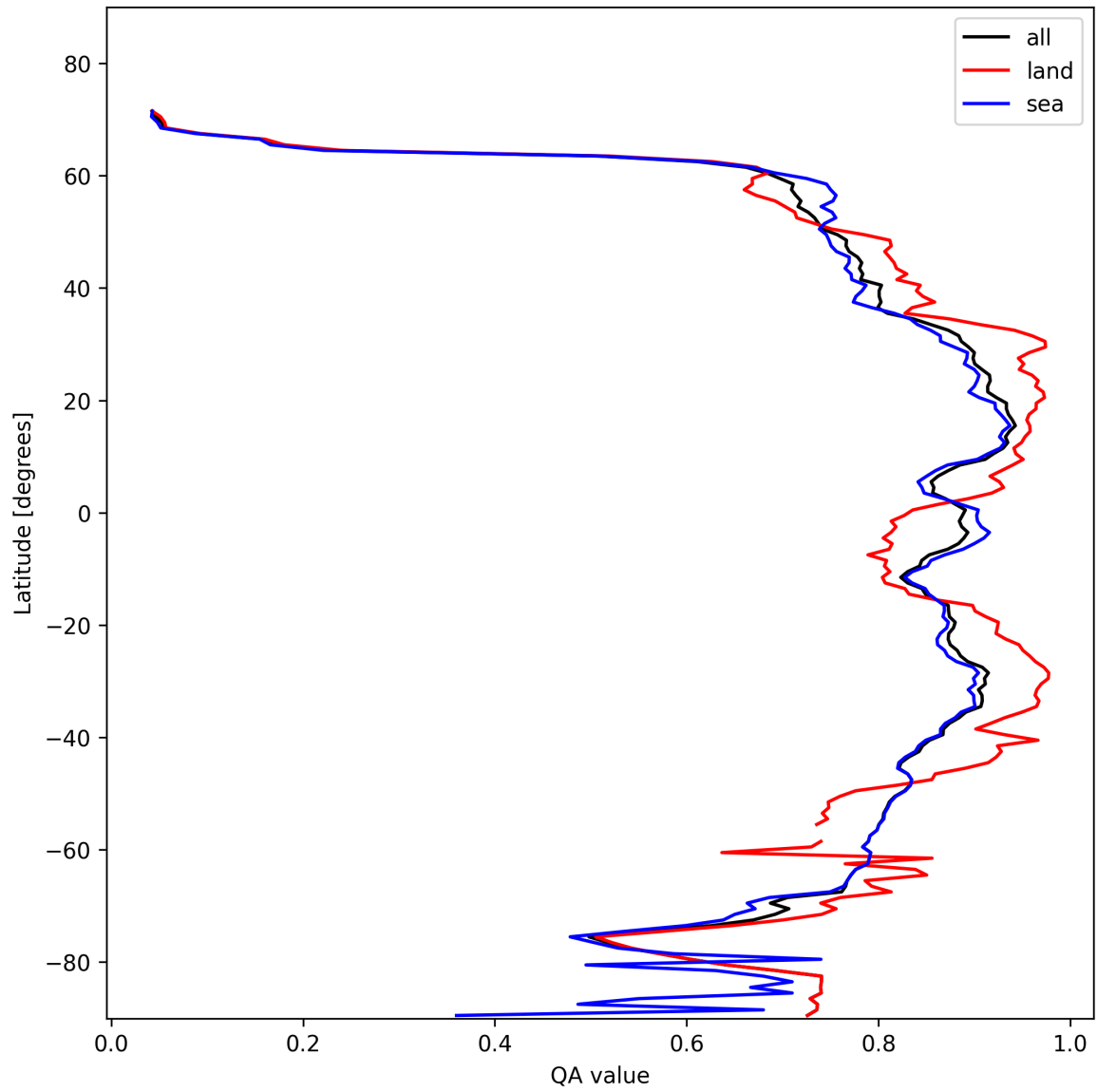
Figure 11: Zonal average of “QA value” for 2025-01-31 to 2025-02-02.
