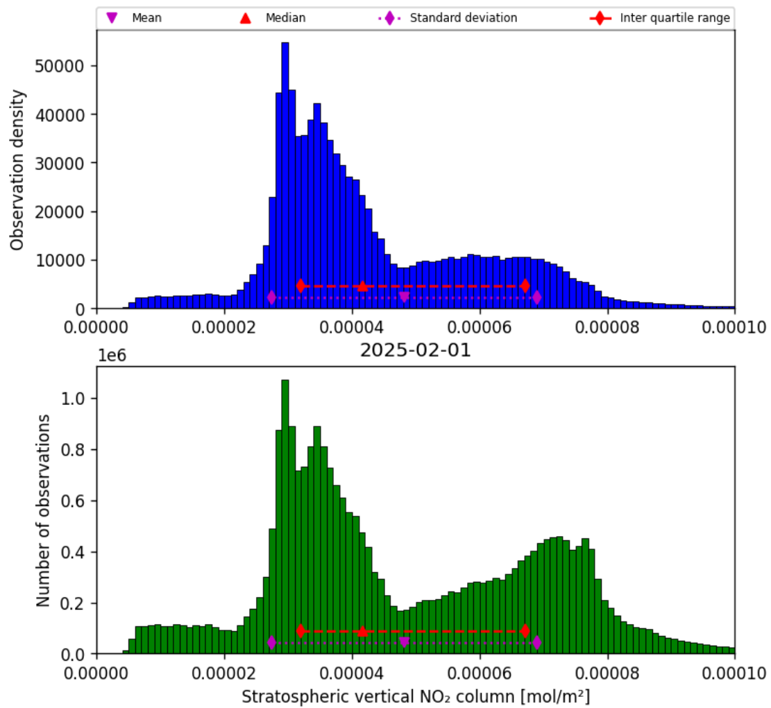
Figure 36: Histogram of “Stratospheric vertical NO 2 column” for 2025-01-31 to 2025-02-02
