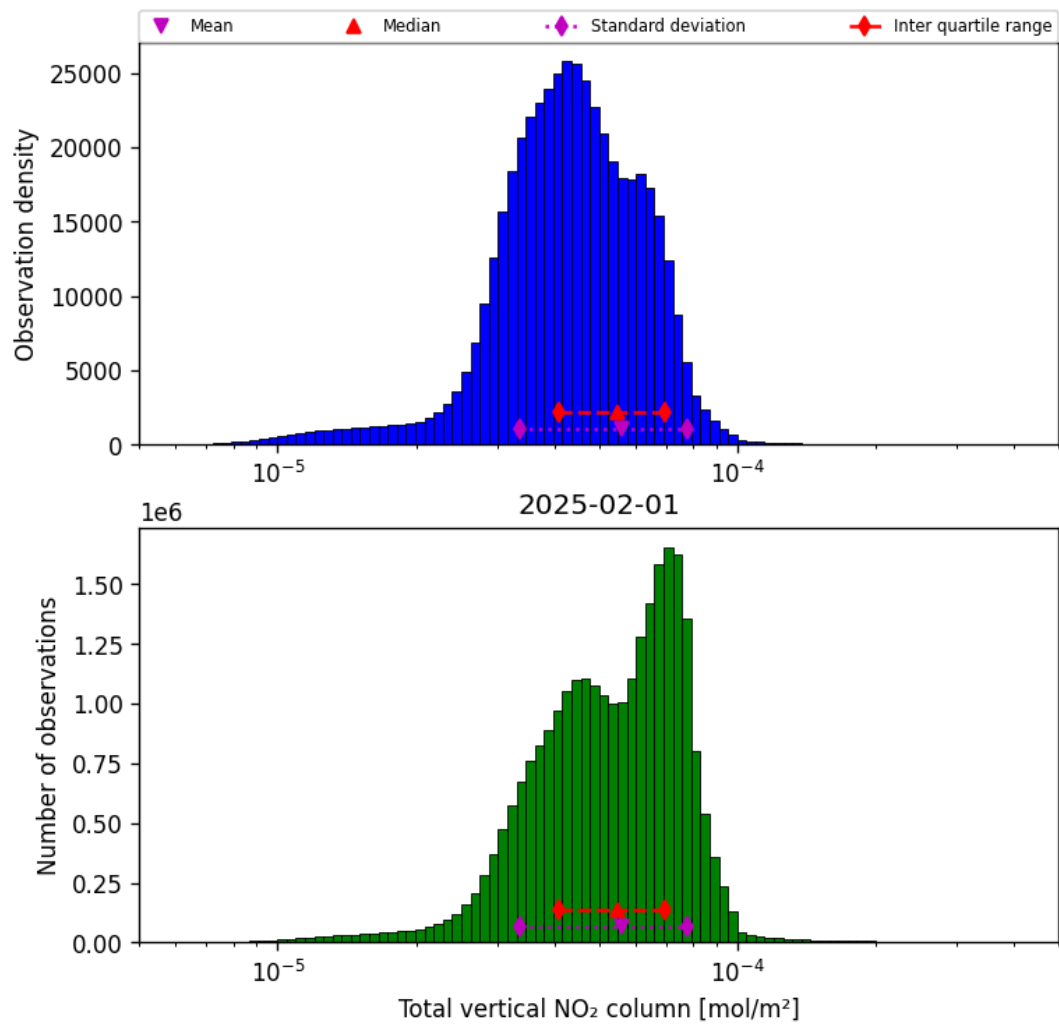
Figure 38: Histogram of “Total vertical NO 2 column” for 2025-01-31 to 2025-02-02
