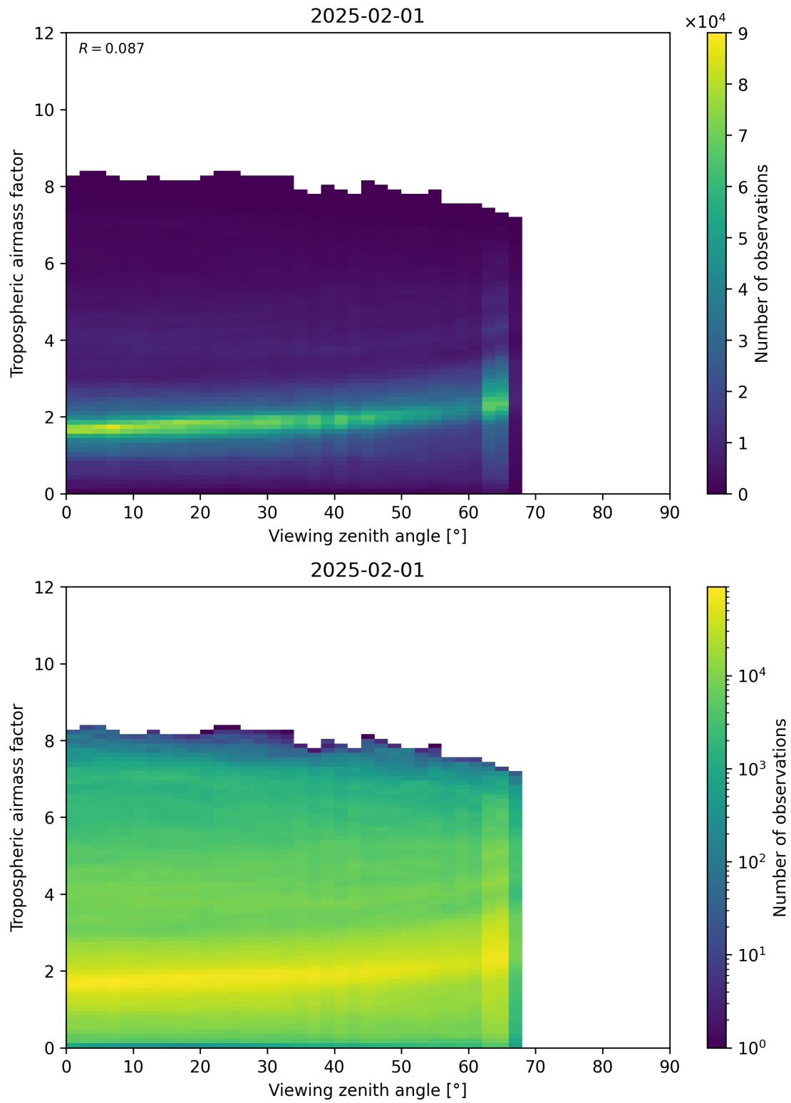
Figure 161: Scatter density plot of “Viewing zenith angle” against “Tropospheric airmass factor” for 2025-01-31 to 2025-02-02.
