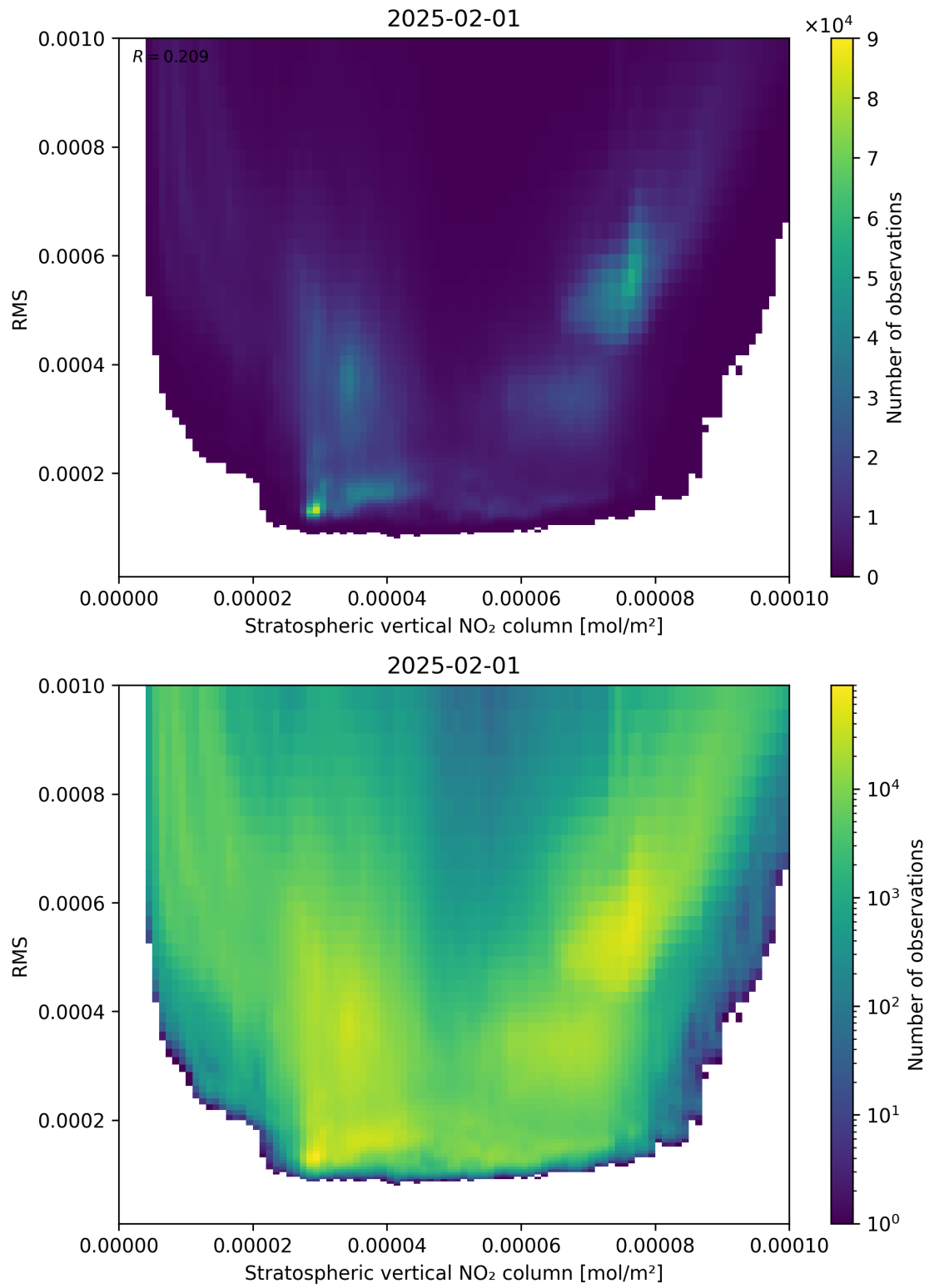
Figure 102: Scatter density plot of “Stratospheric vertical NO 2 column” against “RMS” for 2025-01-31 to 2025-02-02.
