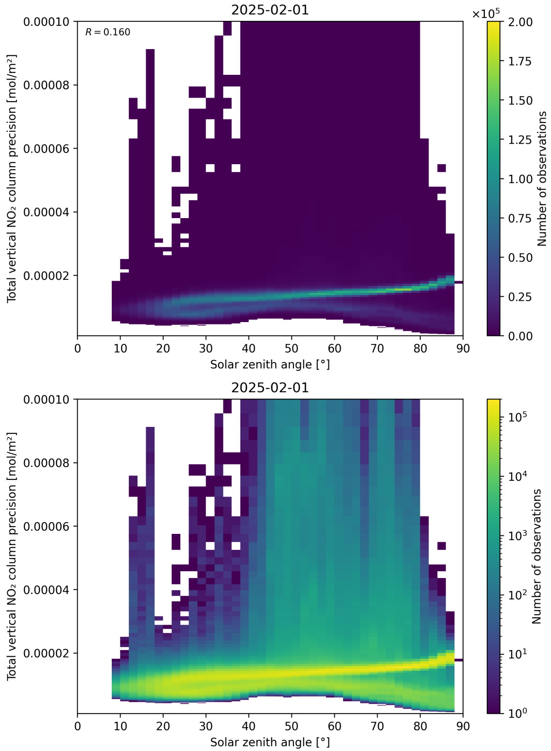
Figure 154: Scatter density plot of “Solar zenith angle” against “Total vertical NO 2 column precision” for 2025-01-31 to 2025-02-02.
