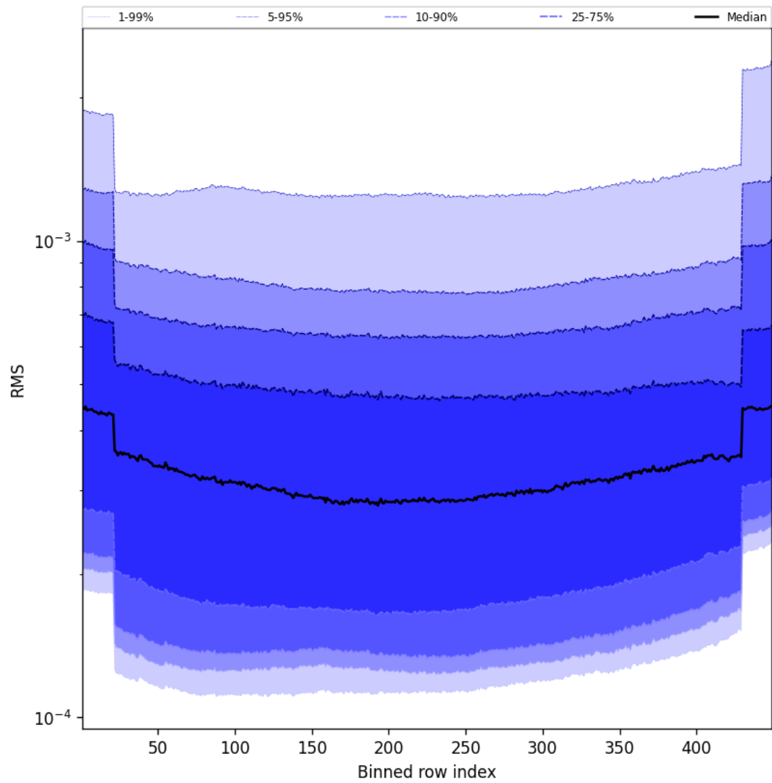
Figure 60: Along track statistics of “RMS” for 2025-01-31 to 2025-02-02
