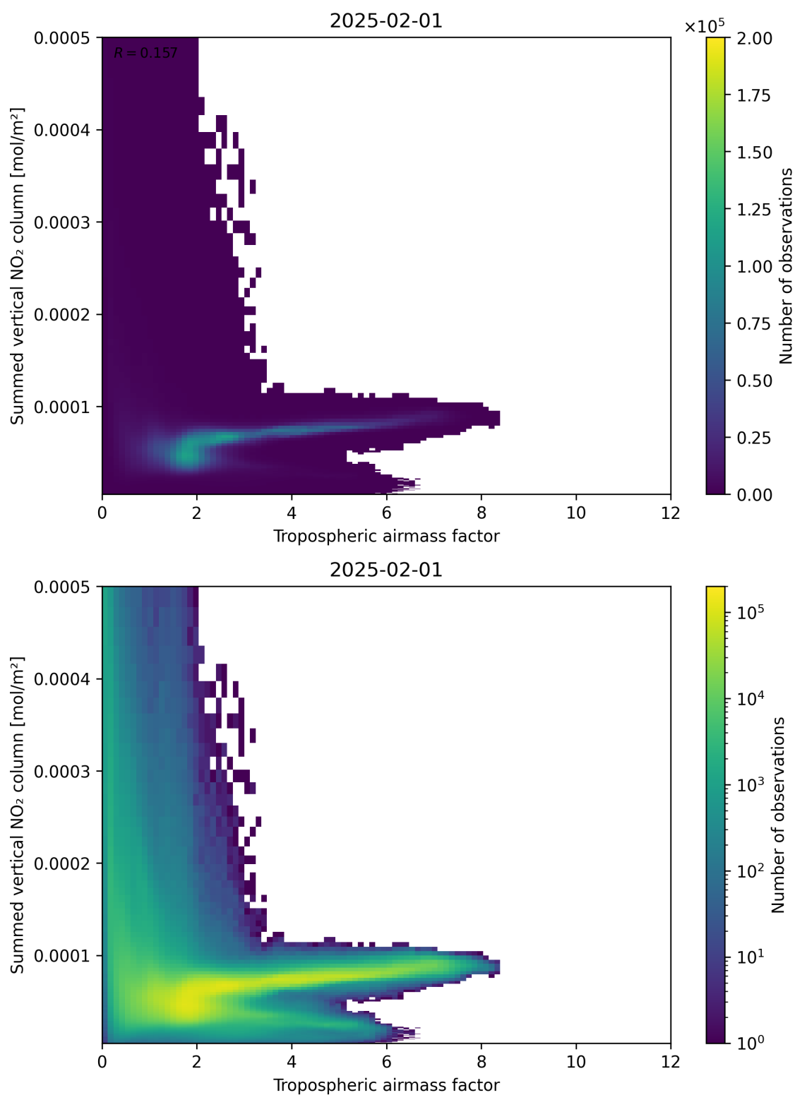
Figure 75: Scatter density plot of “Tropospheric airmass factor” against “Summed vertical NO 2 column” for 2025-01-31 to 2025-02-02.
