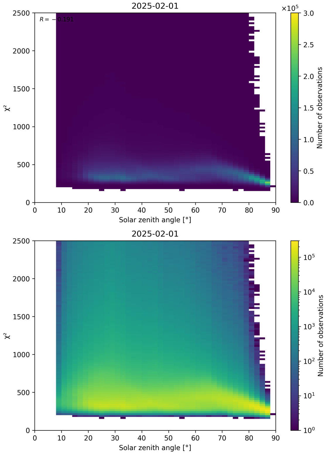
Figure 148: Scatter density plot of “Solar zenith angle” against “ \chi^2 ” for 2025-01-31 to 2025-02-02.
