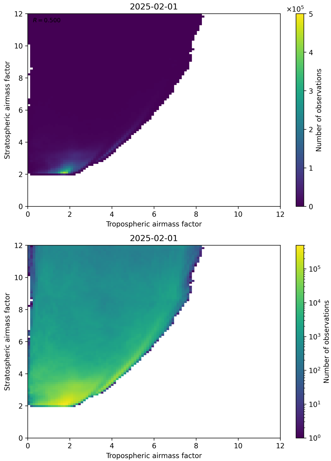
Figure 71: Scatter density plot of “Tropospheric airmass factor” against “Stratospheric airmass factor” for 2025-01-31 to 2025-02-02.
