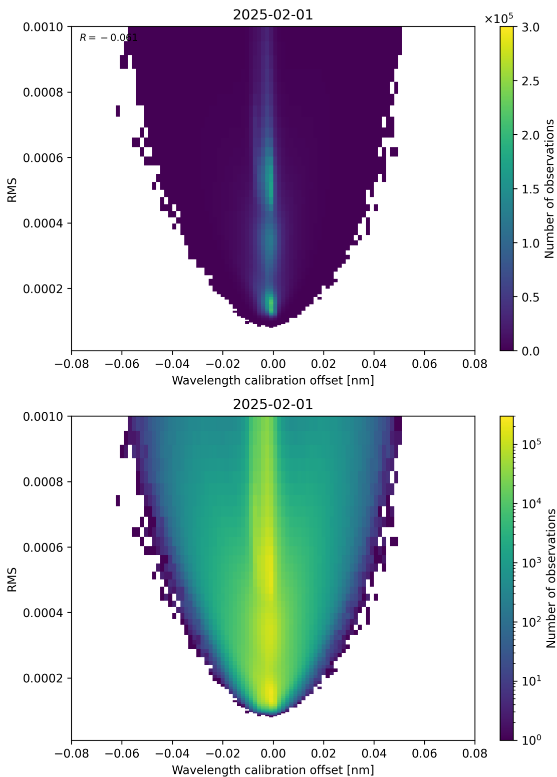
Figure 181: Scatter density plot of “Wavelength calibration offset” against “RMS” for 2025-01-31 to 2025-02-02.
