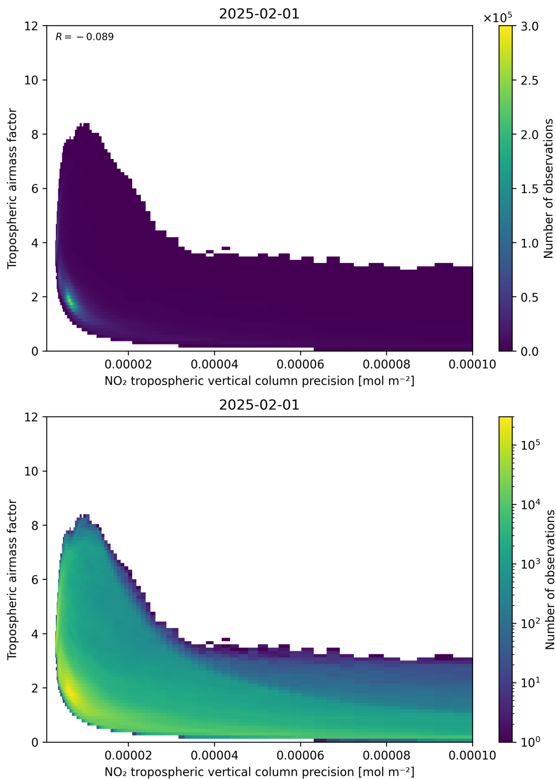
Figure 133: Scatter density plot of “NO 2 tropospheric vertical column precision” against “Tropospheric air mass factor” for 2025-01-31 to 2025-02-02.
