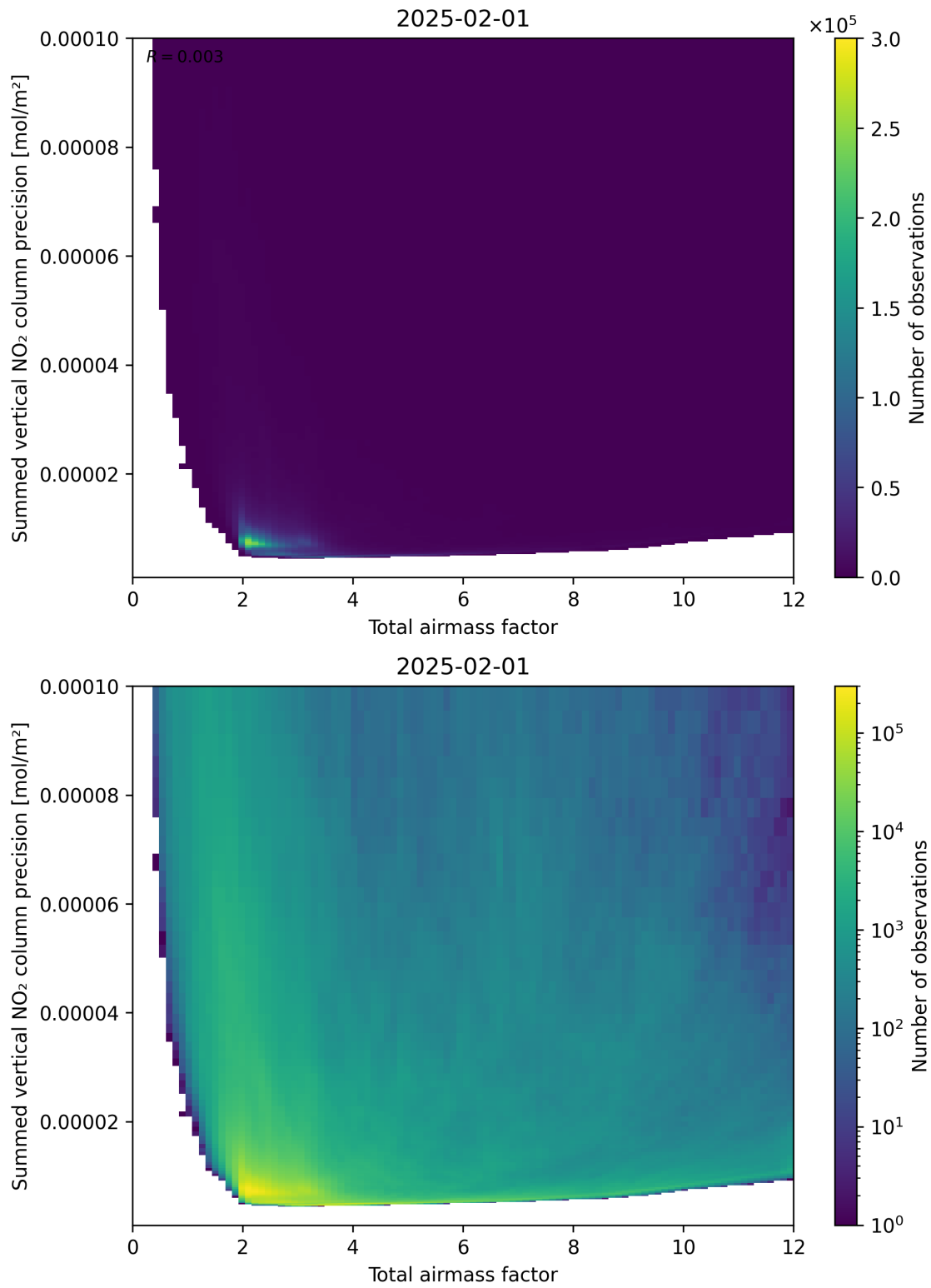
Figure 66: Scatter density plot of “Total airmass factor” against “Summed vertical NO 2 column precision” for 2025-01-31 to 2025-02-02.
