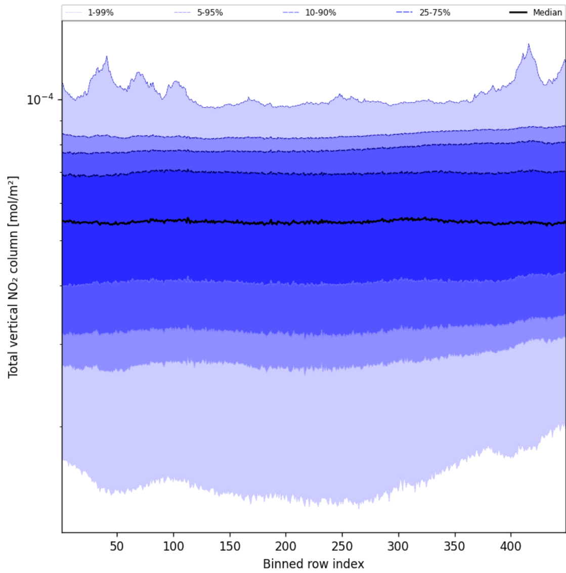
Figure 55: Along track statistics of “Total vertical NO 2 column” for 2025-01-31 to 2025-02-02
