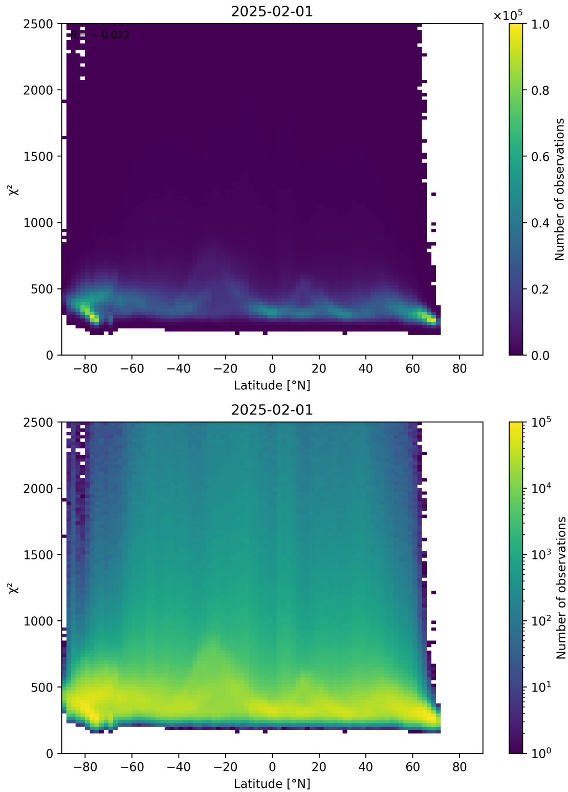
Figure 86: Scatter density plot of “Latitude” against “ \chi^2 ” for 2025-01-31 to 2025-02-02.
