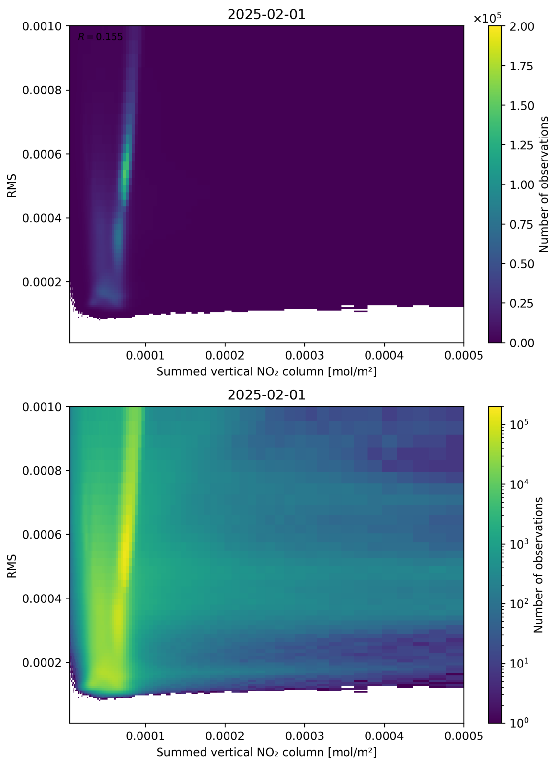
Figure 109: Scatter density plot of “Summed vertical NO 2 column” against “RMS” for 2025-01-31 to 2025-02-02.
