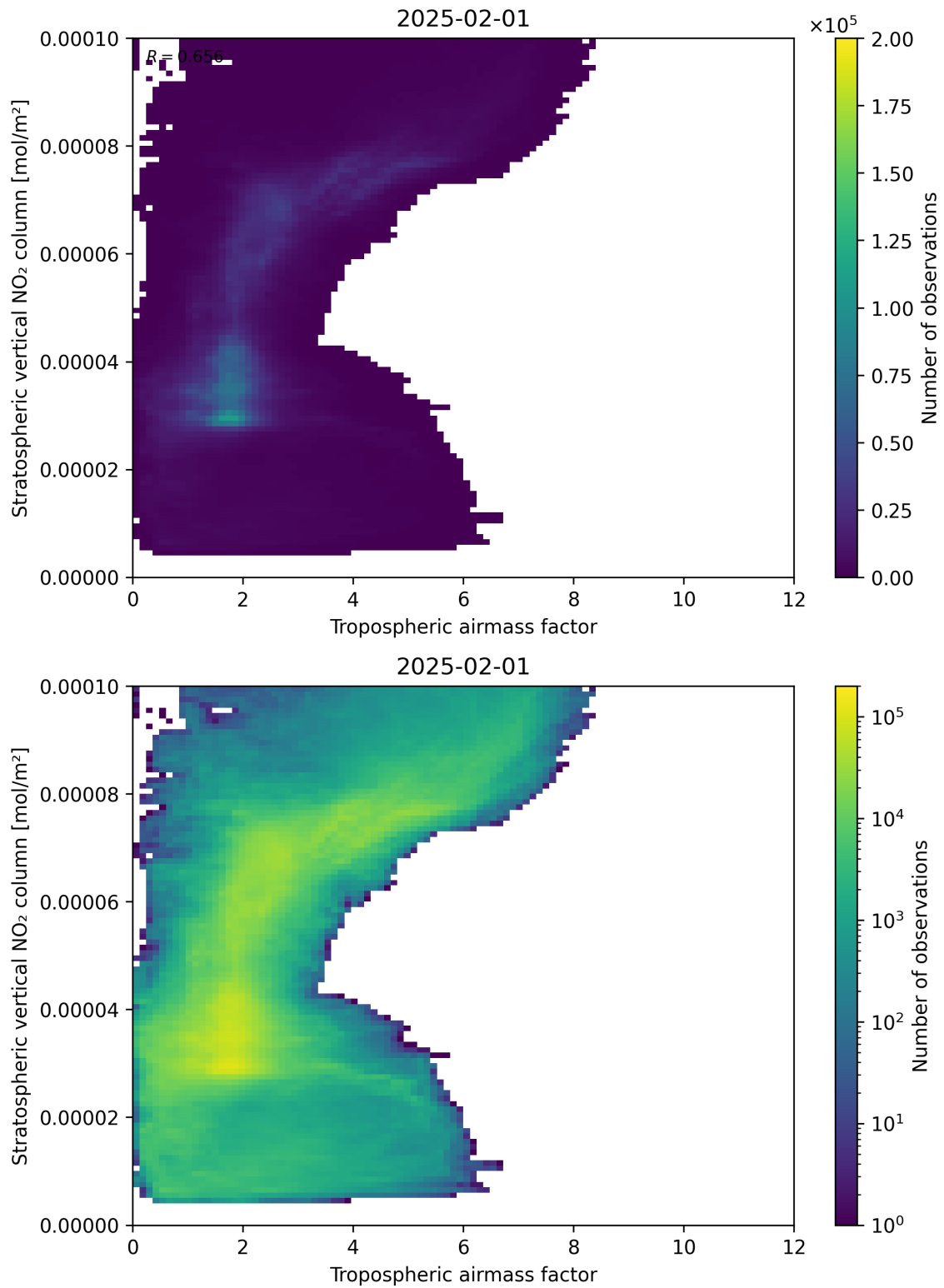
Figure 74: Scatter density plot of “Tropospheric airmass factor” against “Stratospheric vertical NO 2 column” for 2025-01-31 to 2025-02-02.
