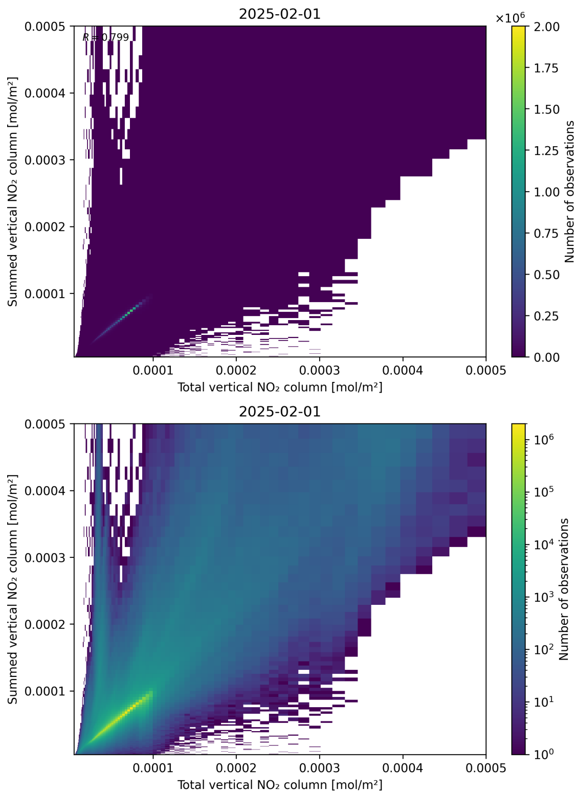
Figure 112: Scatter density plot of “Total vertical NO 2 column” against “Summed vertical NO 2 column” for 2025-01-31 to 2025-02-02.
