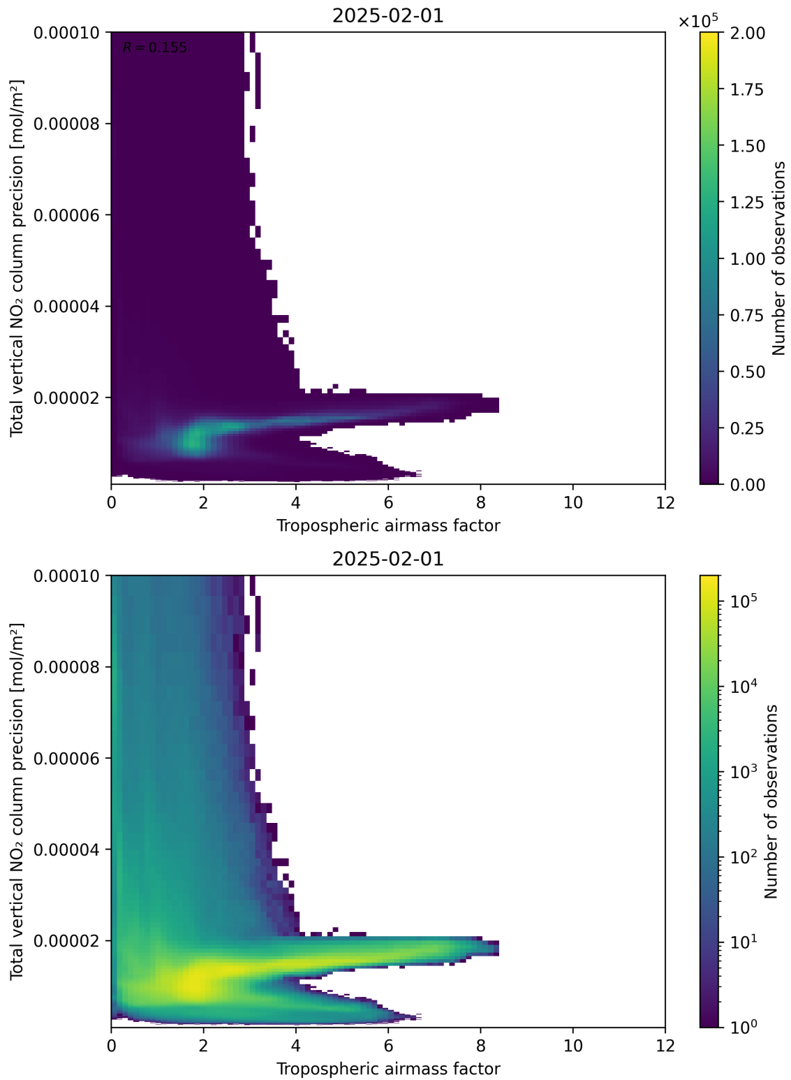
Figure 78: Scatter density plot of “Tropospheric air mass factor” against “Total vertical NO 2 column precision” for 2025-01-31 to 2025-02-02.
