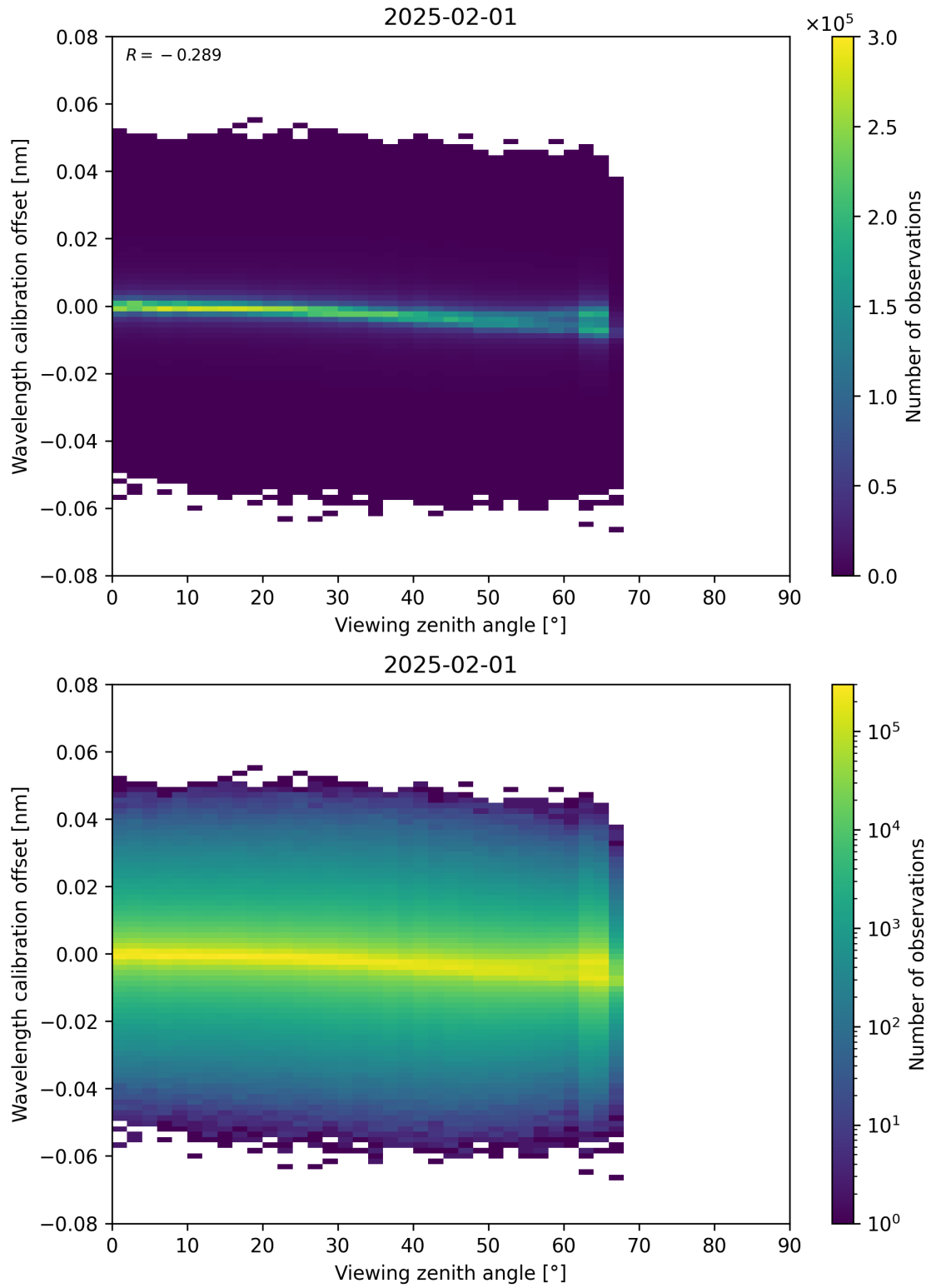
Figure 173: Scatter density plot of “Viewing zenith angle” against “Wavelength calibration offset” for 2025-01-31 to 2025-02-02.
