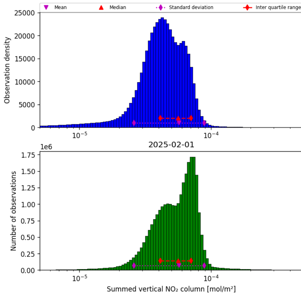
Figure 40: Histogram of “Summed vertical NO 2 column” for 2025-01-31 to 2025-02-02
