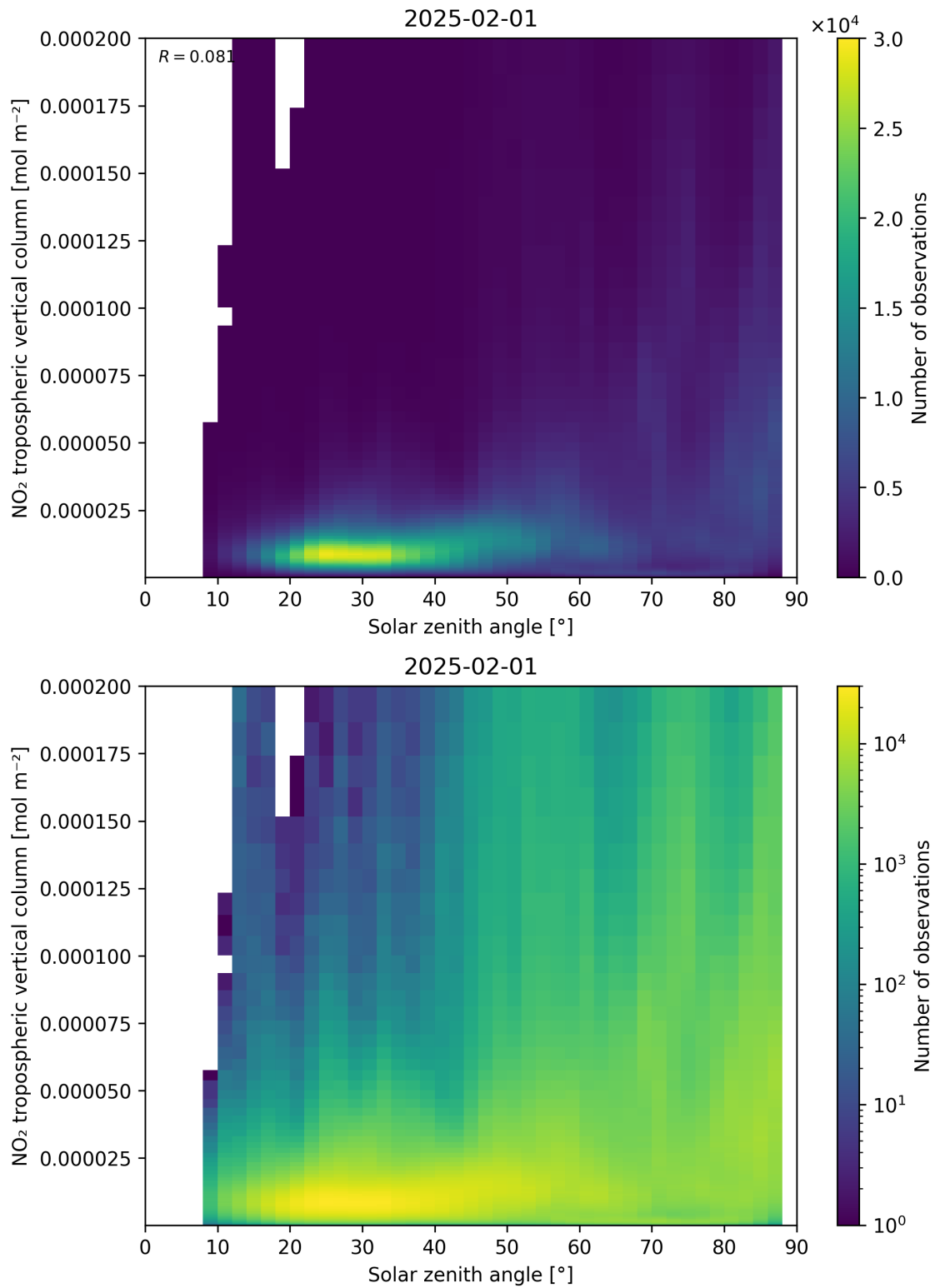
Figure 155: Scatter density plot of “Solar zenith angle” against “NO 2 tropospheric vertical column” for 2025-01-31 to 2025-02-02.
