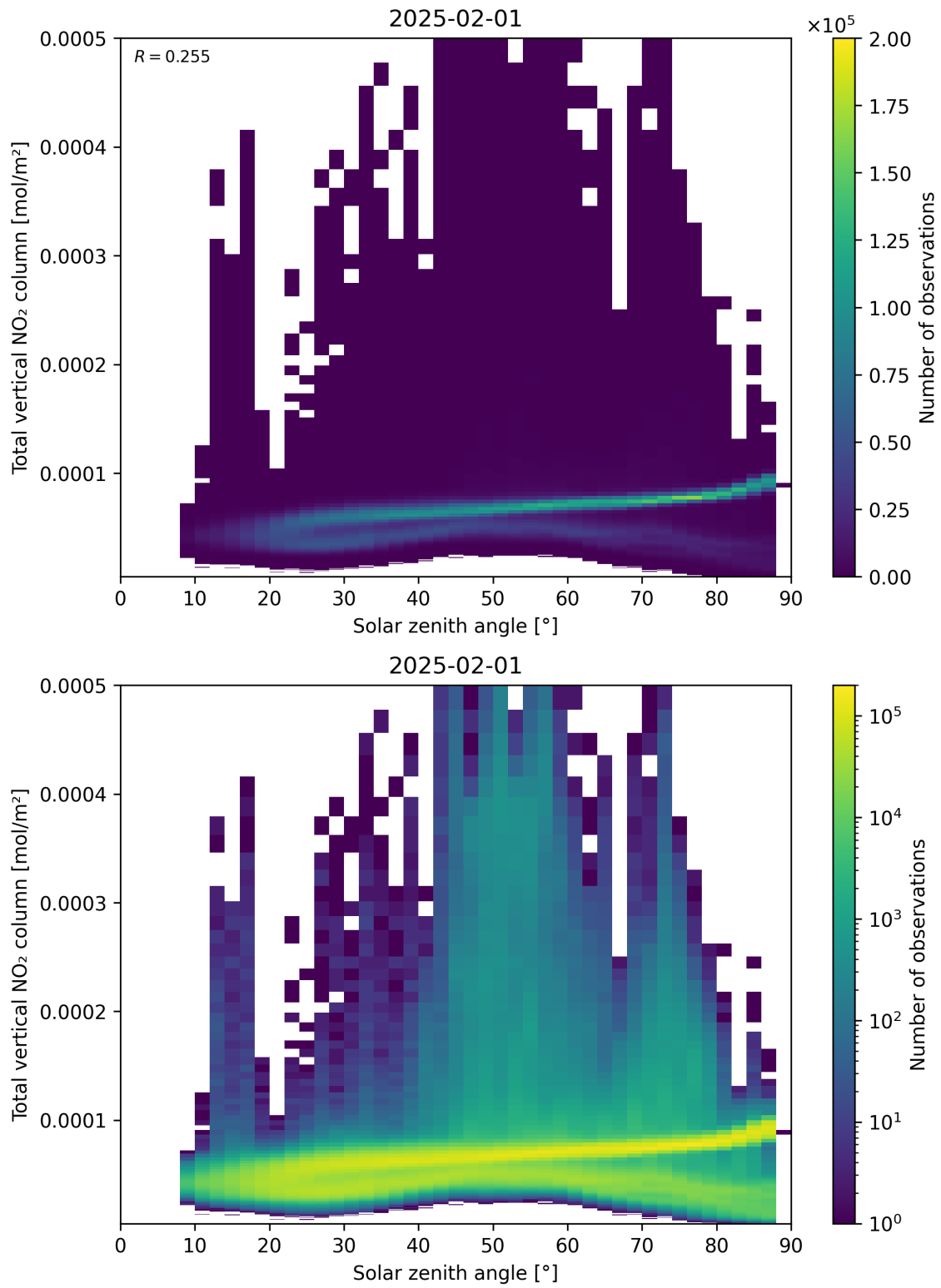
Figure 153: Scatter density plot of “Solar zenith angle” against “Total vertical NO 2 column” for 2025-01-31 to 2025-02-02.
