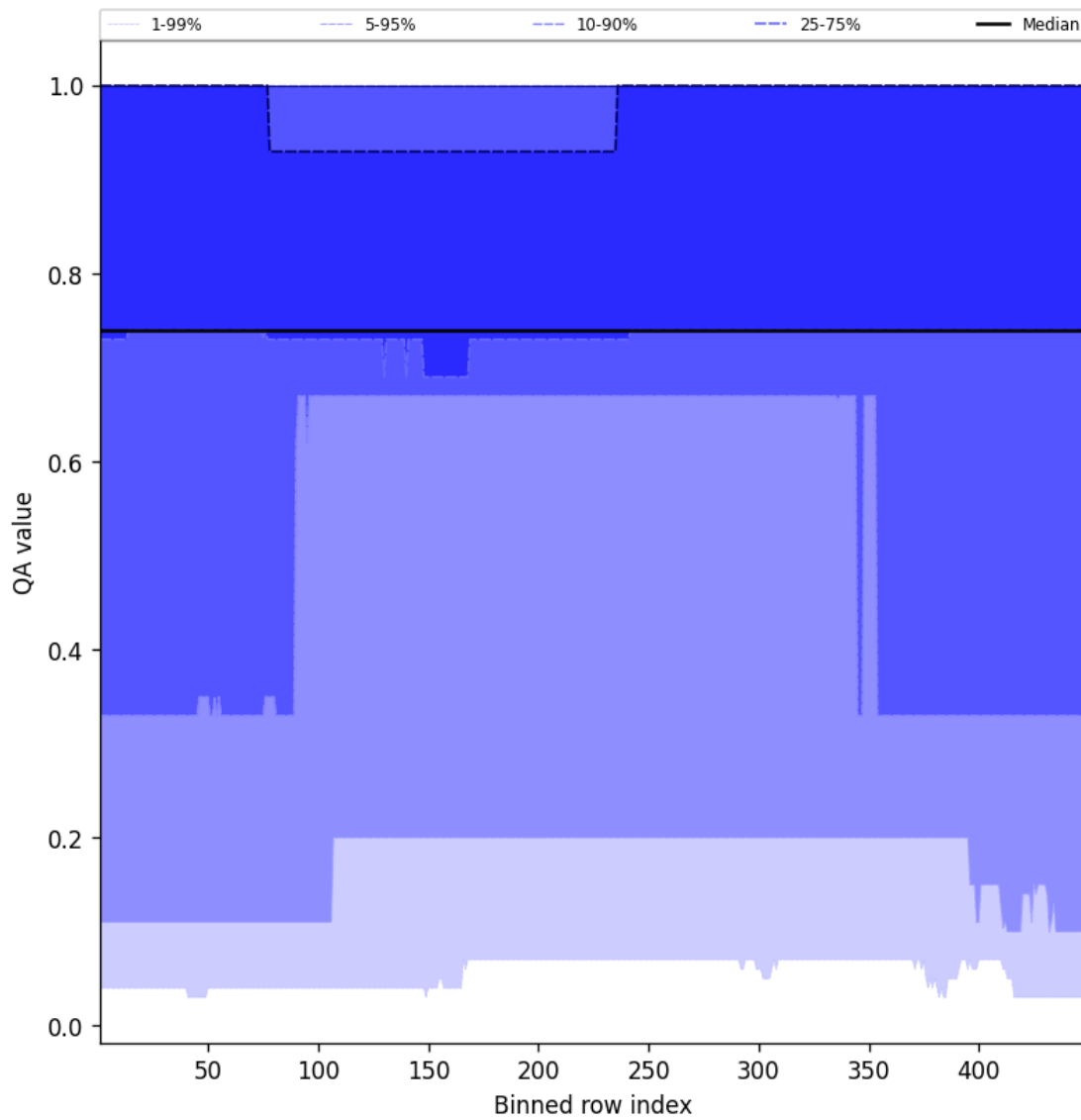
Figure 45: Along track statistics of “QA value” for 2025-01-31 to 2025-02-02
