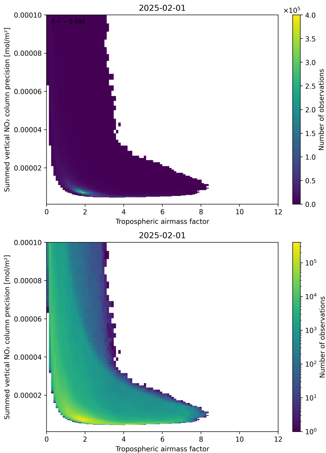
Figure 76: Scatter density plot of “Tropospheric air mass factor” against “Summed vertical NO 2 column precision” for 2025-01-31 to 2025-02-02.
