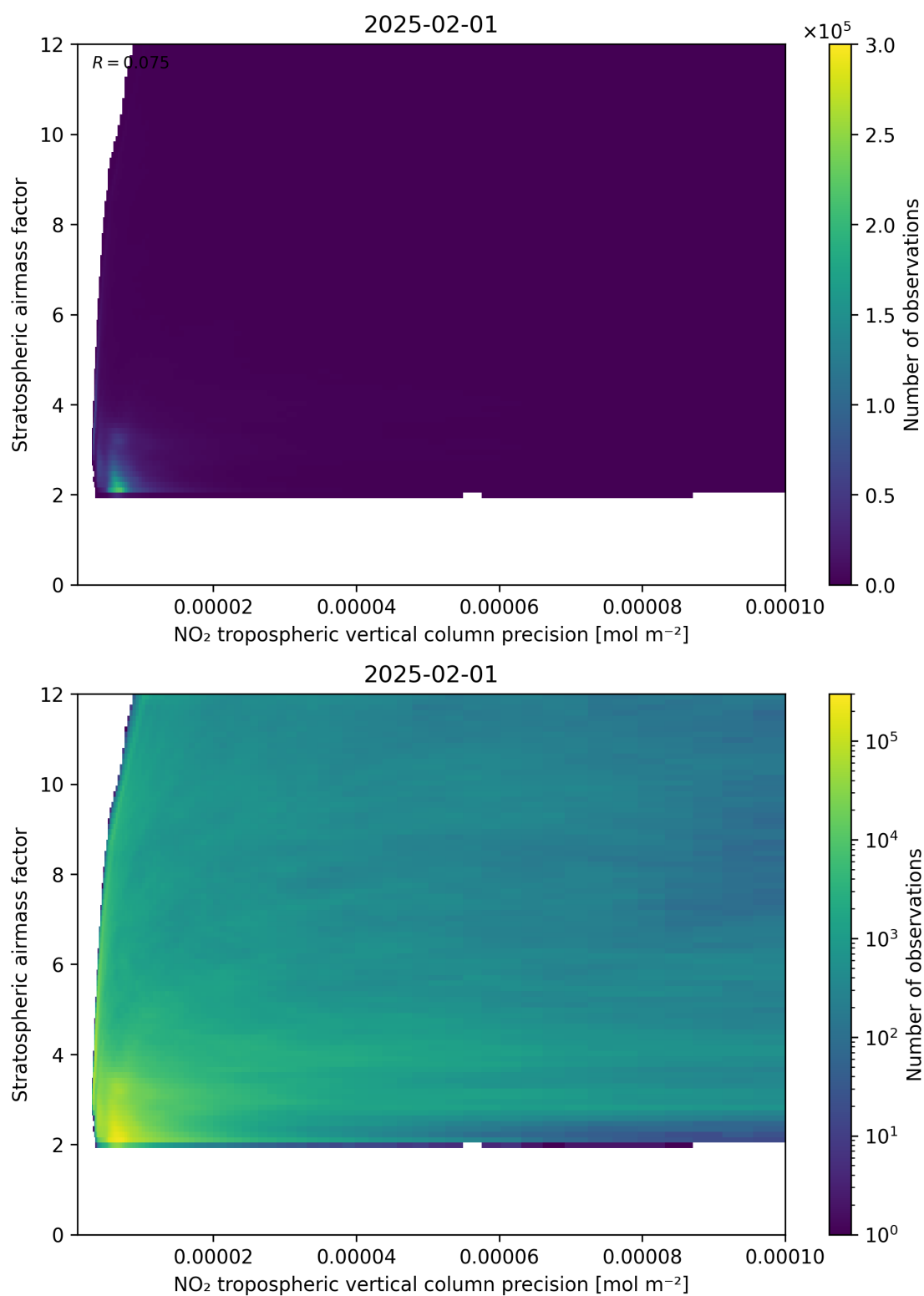
Figure 131: Scatter density plot of “NO 2 tropospheric vertical column precision” against “Stratospheric airmass factor” for 2025-01-31 to 2025-02-02.
