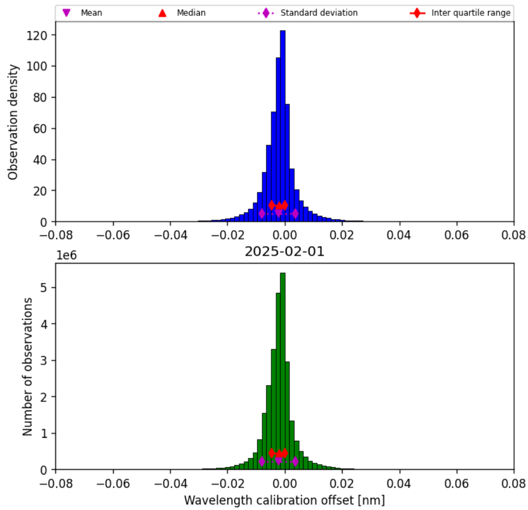
Figure 35: Histogram of “Wavelength calibration offset” for 2025-01-31 to 2025-02-02
