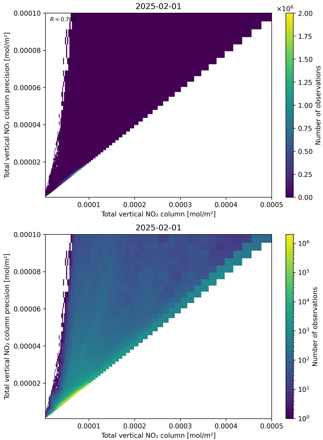
Figure 114: Scatter density plot of “Total vertical NO 2 column” against “Total vertical NO 2 column precision” for 2025-01-31 to 2025-02-02.
