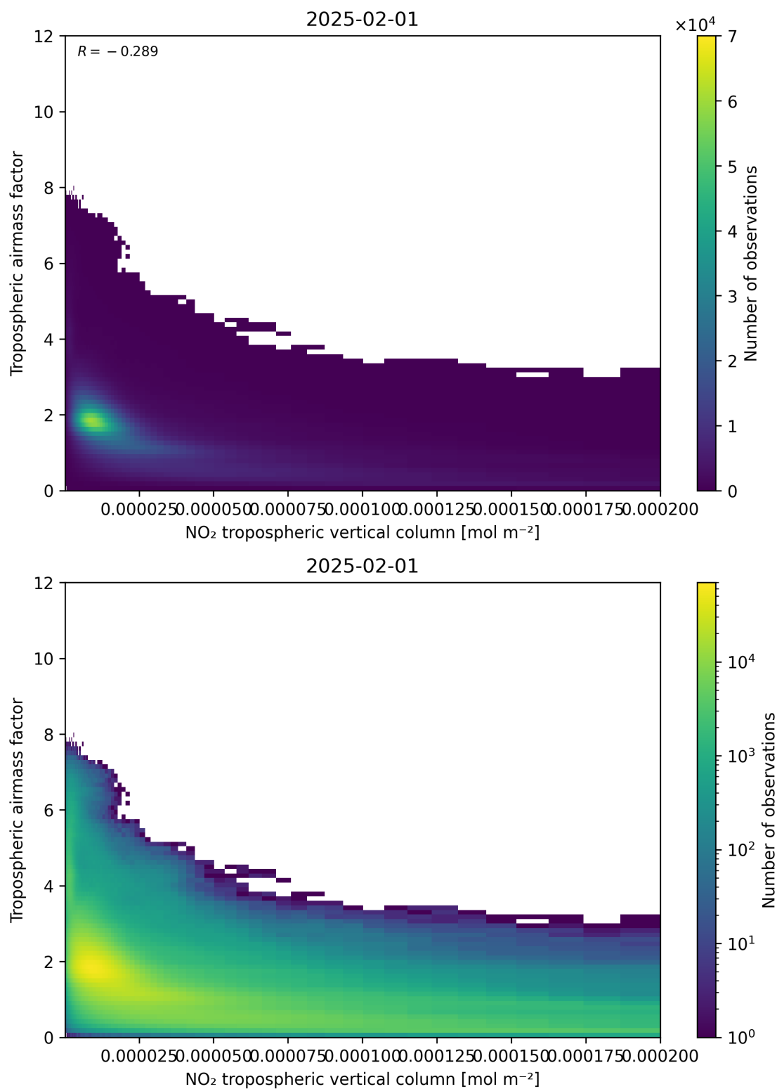
Figure 123: Scatter density plot of “NO 2 tropospheric vertical column” against “Tropospheric air mass factor” for 2025-01-31 to 2025-02-02.
