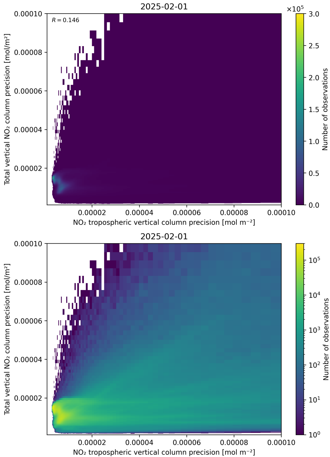
Figure 139: Scatter density plot of “NO 2 tropospheric vertical column precision” against “Total vertical NO 2 column precision” for 2025-01-31 to 2025-02-02.
