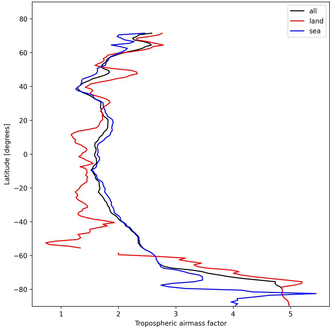
Figure 14: Zonal average of “Tropospheric airmass factor” for 2025-01-31 to 2025-02-02.
