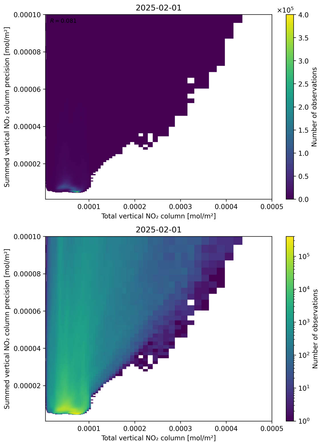
Figure 113: Scatter density plot of “Total vertical NO 2 column” against “Summed vertical NO 2 column precision” for 2025-01-31 to 2025-02-02.
