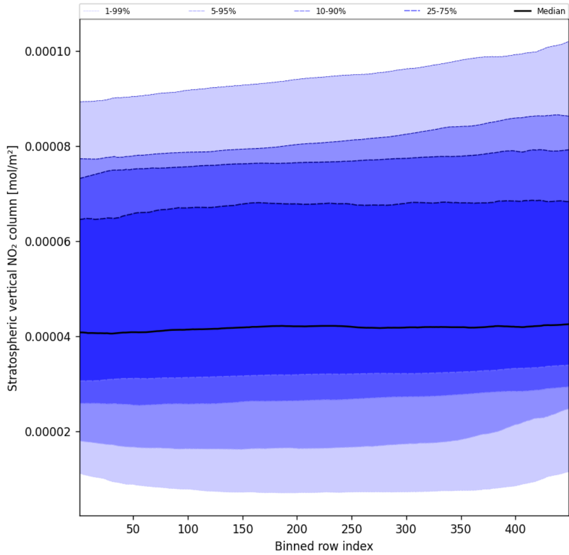
Figure 53: Along track statistics of “Stratospheric vertical NO 2 column” for 2025-01-31 to 2025-02-02
