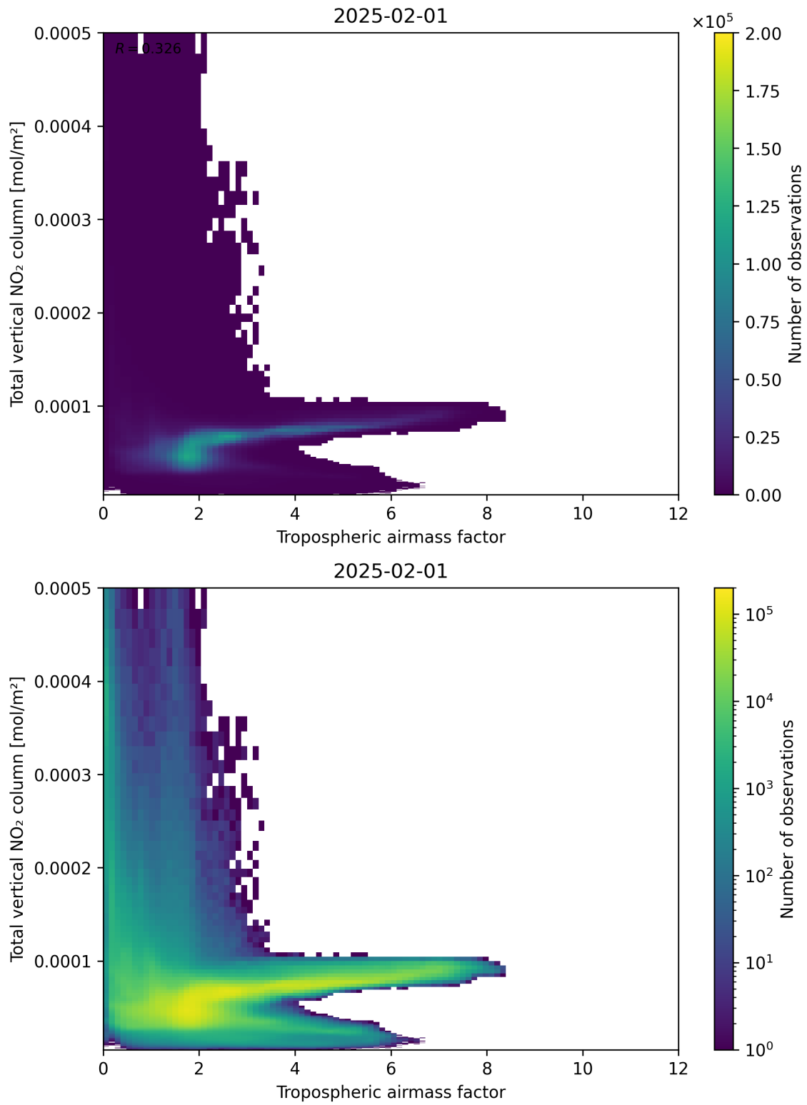
Figure 77: Scatter density plot of “Tropospheric airmass factor” against “Total vertical NO 2 column” for 2025-01-31 to 2025-02-02.
