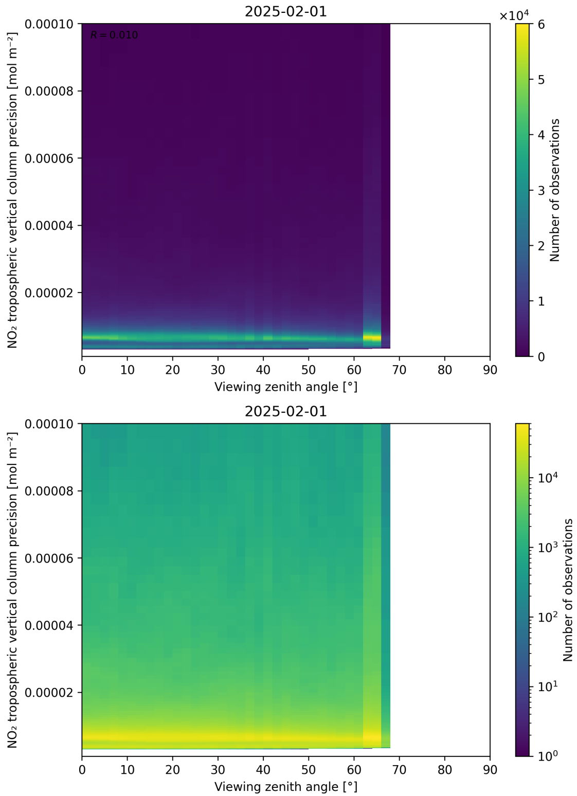
Figure 170: Scatter density plot of “Viewing zenith angle” against “NO 2 tropospheric vertical column precision” for 2025-01-31 to 2025-02-02.
