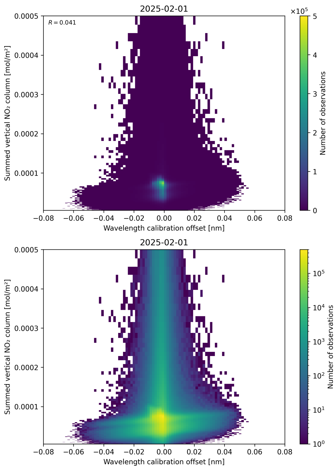
Figure 177: Scatter density plot of “Wavelength calibration offset” against “Summed vertical NO 2 column” for 2025-01-31 to 2025-02-02.
