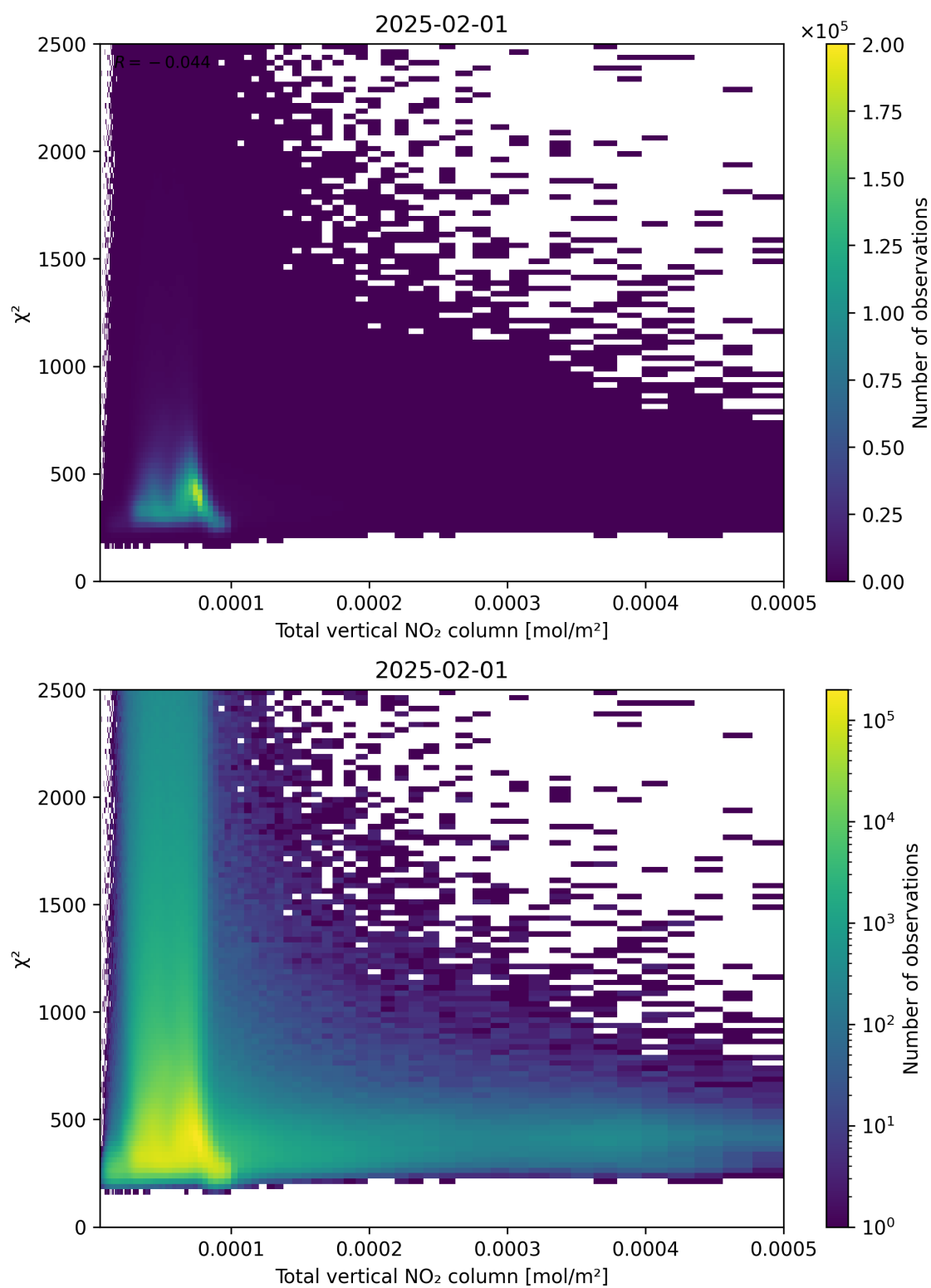
Figure 111: Scatter density plot of “Total vertical NO 2 column” against “ \chi^2 ” for 2025-01-31 to 2025-02-02.
