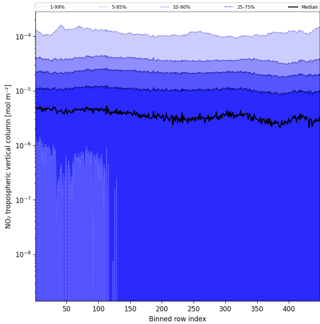
Figure 46: Along track statistics of “NO 2 tropospheric vertical column” for 2025-01-31 to 2025-02-02
