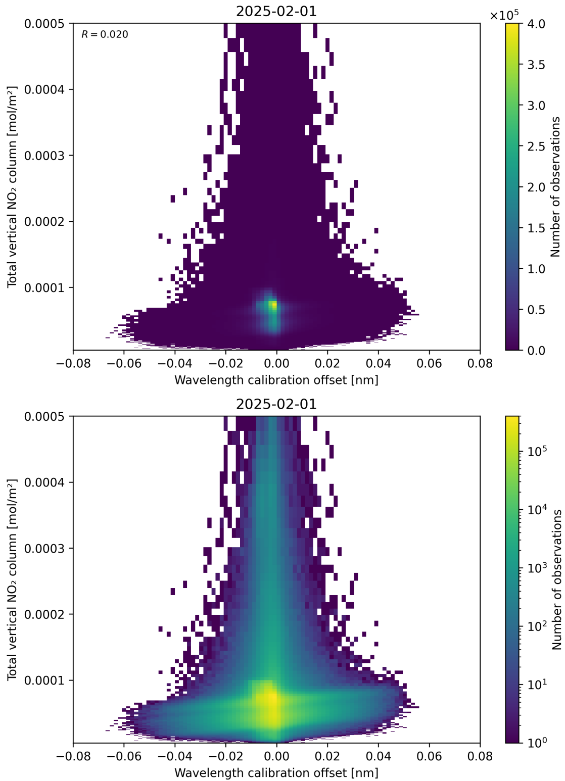
Figure 179: Scatter density plot of “Wavelength calibration offset” against “Total vertical NO 2 column” for 2025-01-31 to 2025-02-02.
