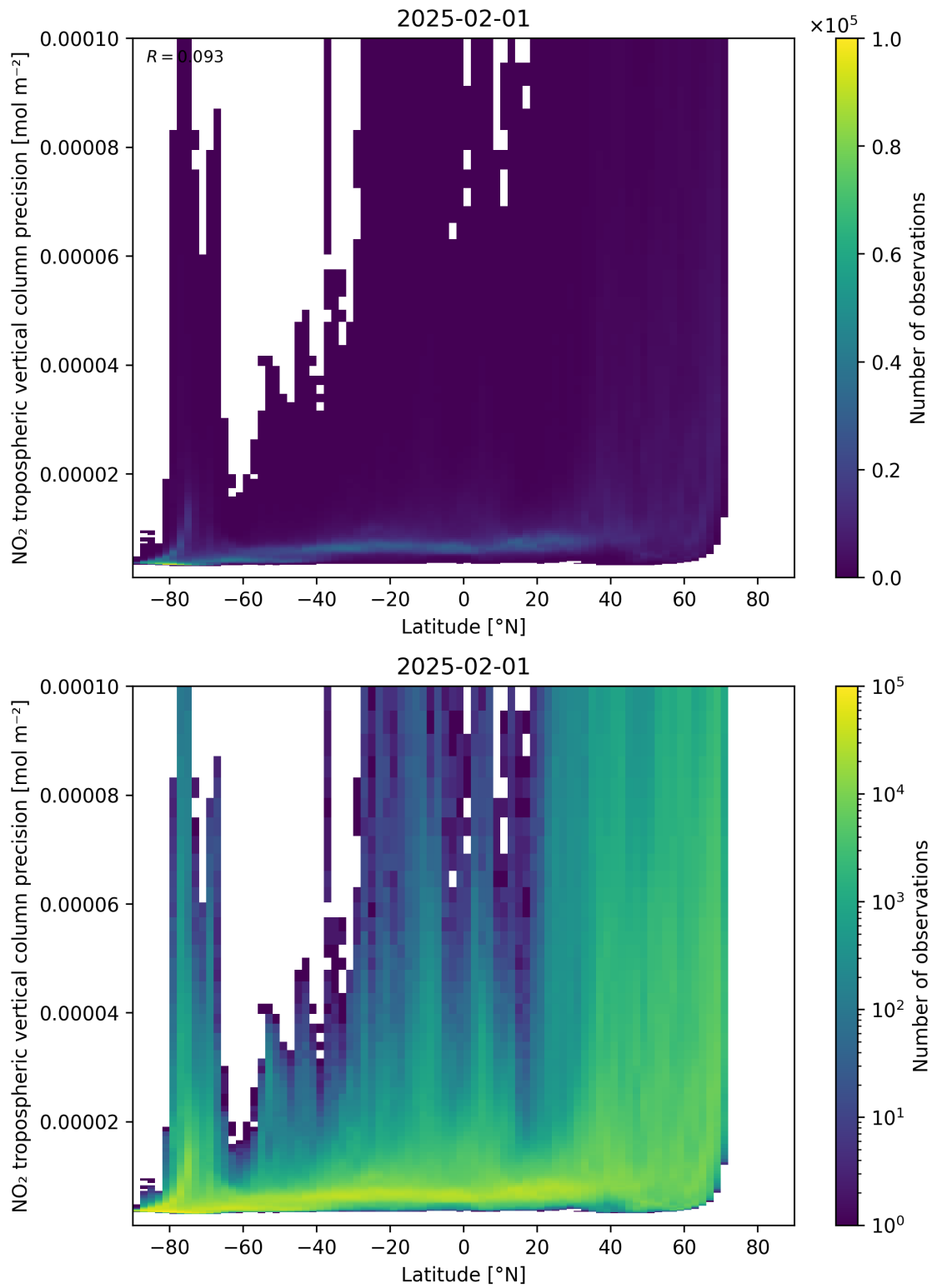
Figure 93: Scatter density plot of “Latitude” against “NO 2 tropospheric vertical column precision” for 2025-01-31 to 2025-02-02.
