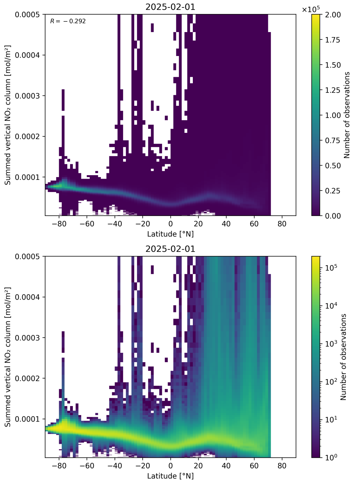
Figure 88: Scatter density plot of “Latitude” against “Summed vertical NO 2 column” for 2025-01-31 to 2025-02-02.
