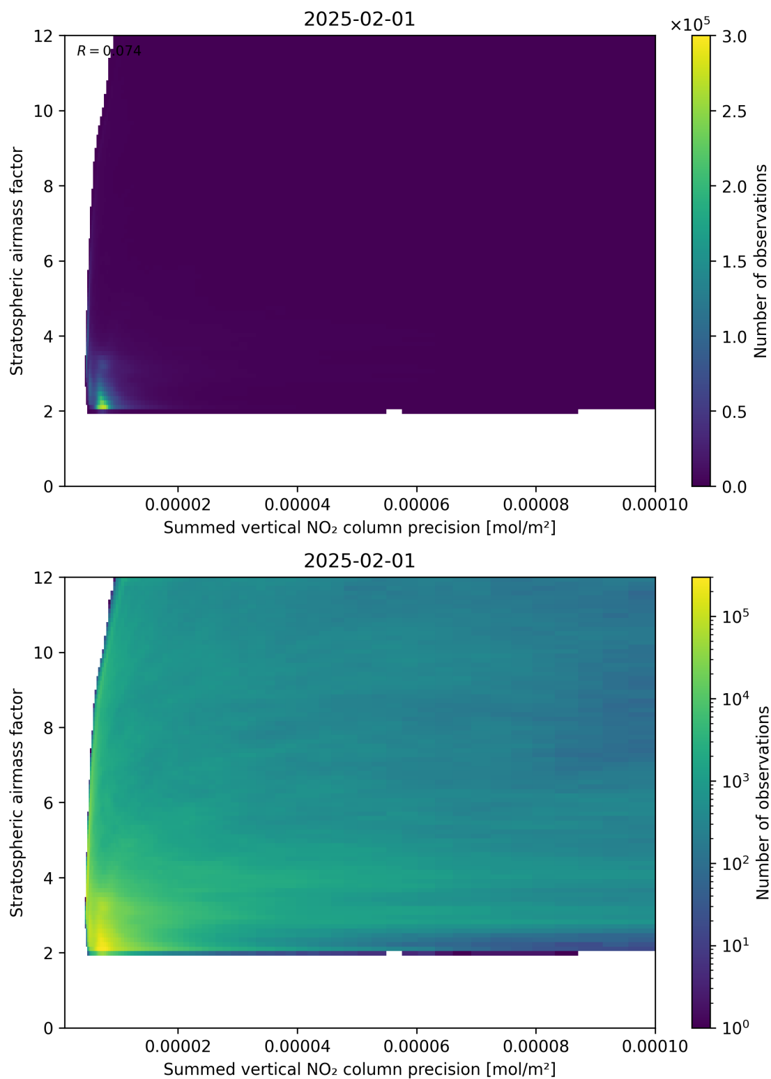
Figure 106: Scatter density plot of “Summed vertical NO 2 column precision” against “Stratospheric airmass factor” for 2025-01-31 to 2025-02-02.
