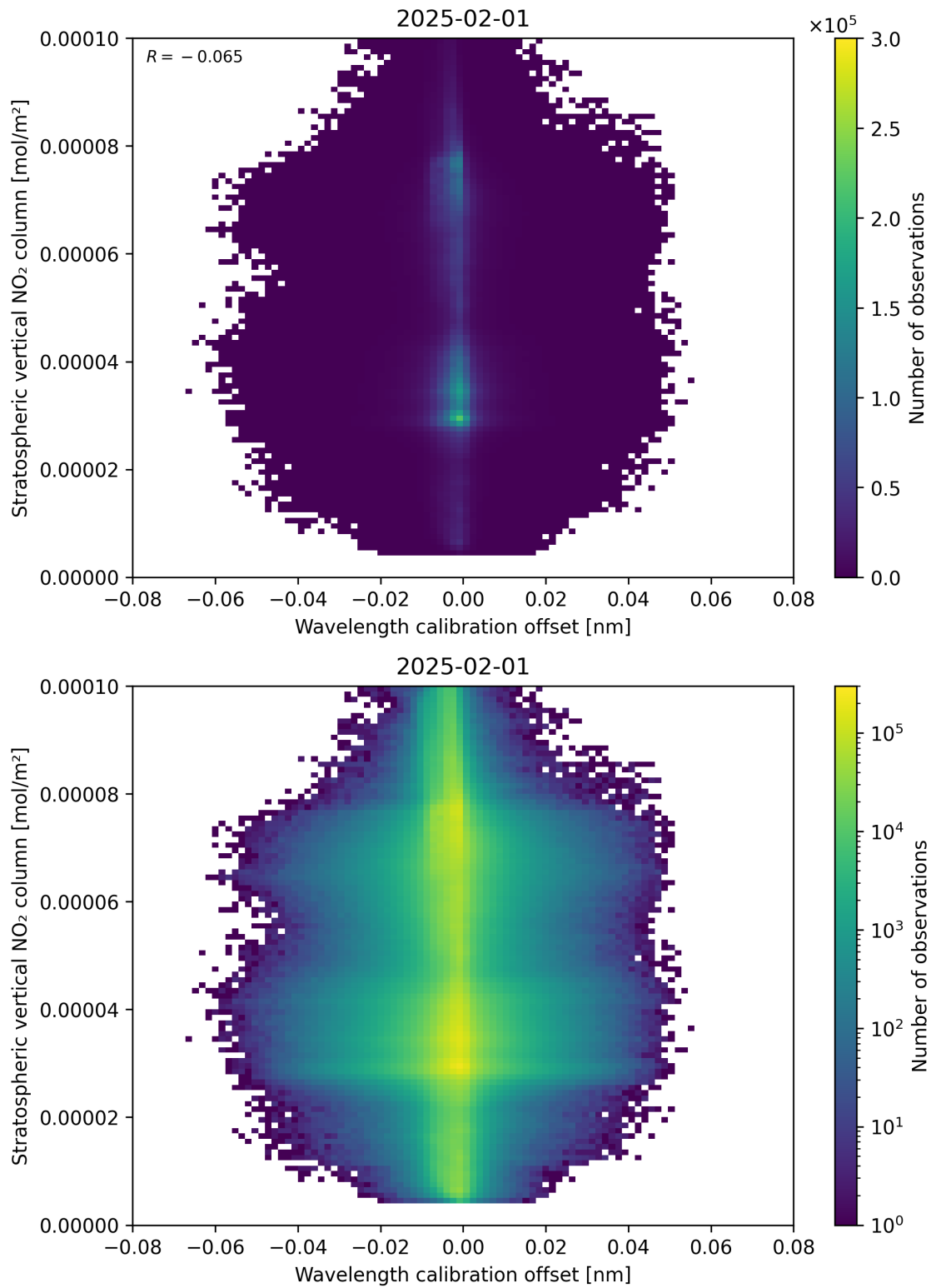
Figure 176: Scatter density plot of “Wavelength calibration offset” against “Stratospheric vertical NO 2 column” for 2025-01-31 to 2025-02-02.
