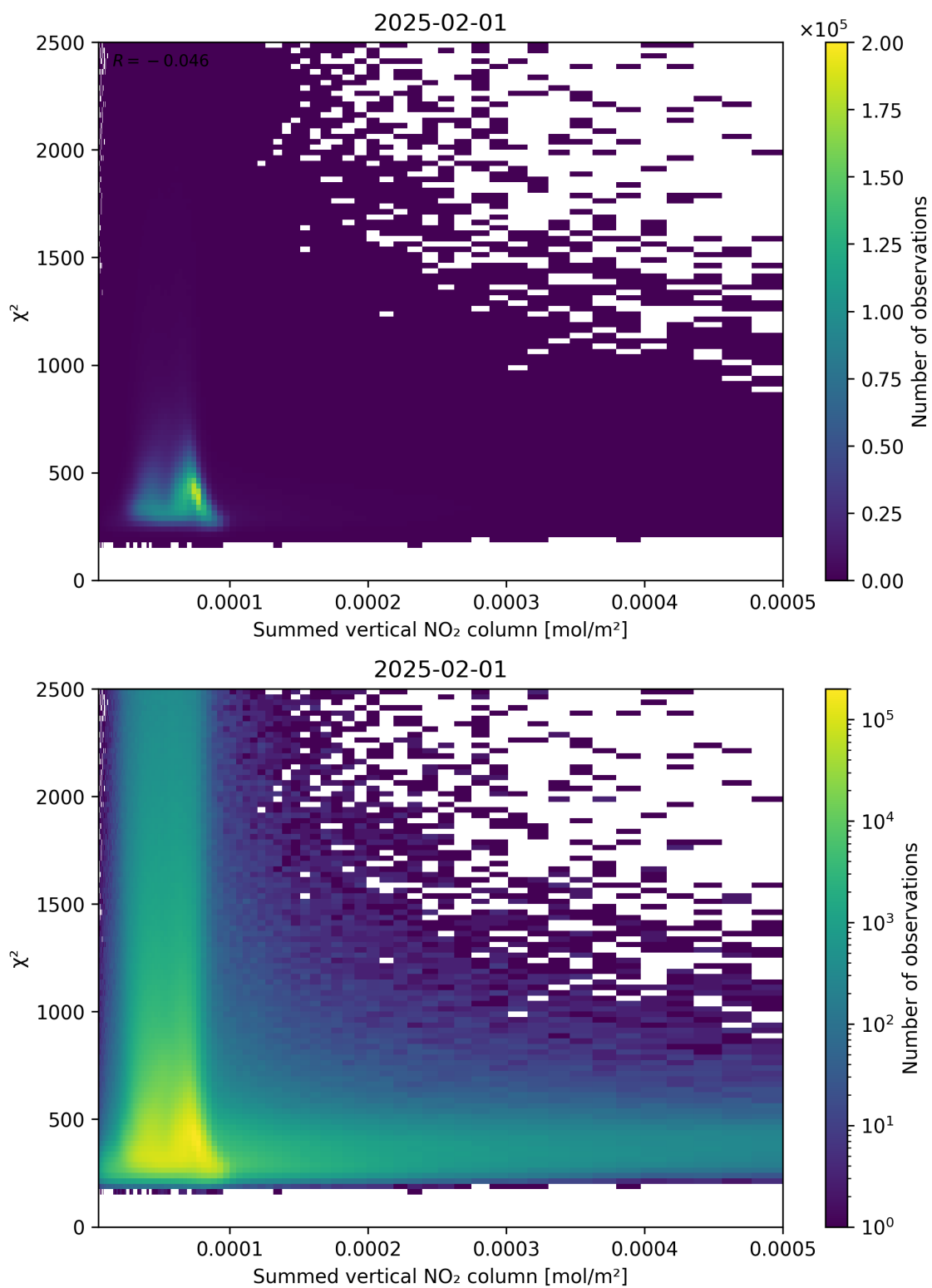
Figure 104: Scatter density plot of “Summed vertical NO 2 column” against “ \chi^2 ” for 2025-01-31 to 2025-02-02.
