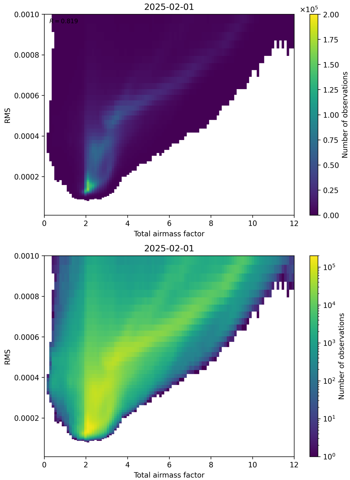
Figure 69: Scatter density plot of “Total airmass factor” against “RMS” for 2025-01-31 to 2025-02-02.
