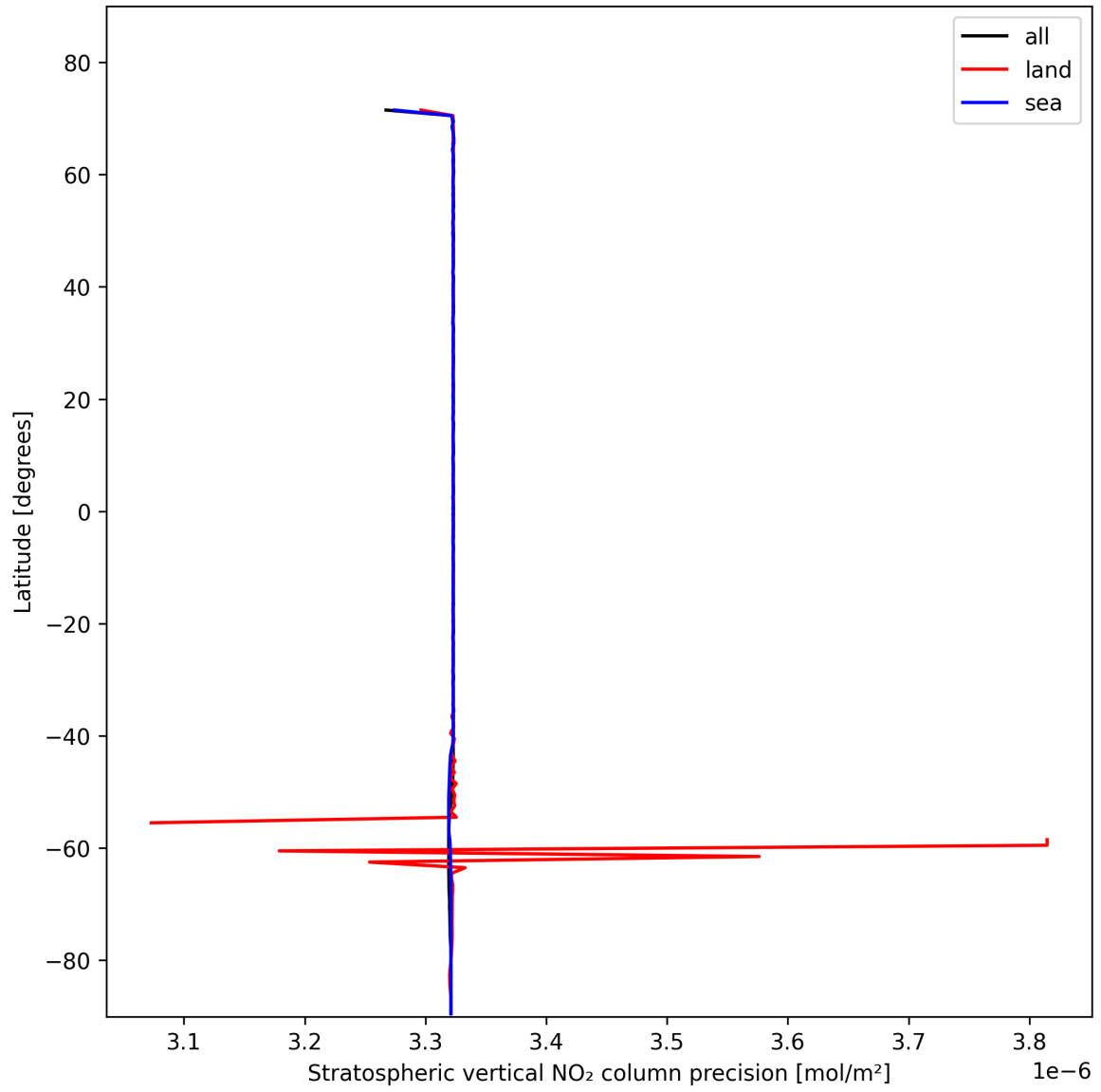
Figure 20: Zonal average of “Stratospheric vertical NO 2 column precision” for 2025-01-31 to 2025-02-02.
