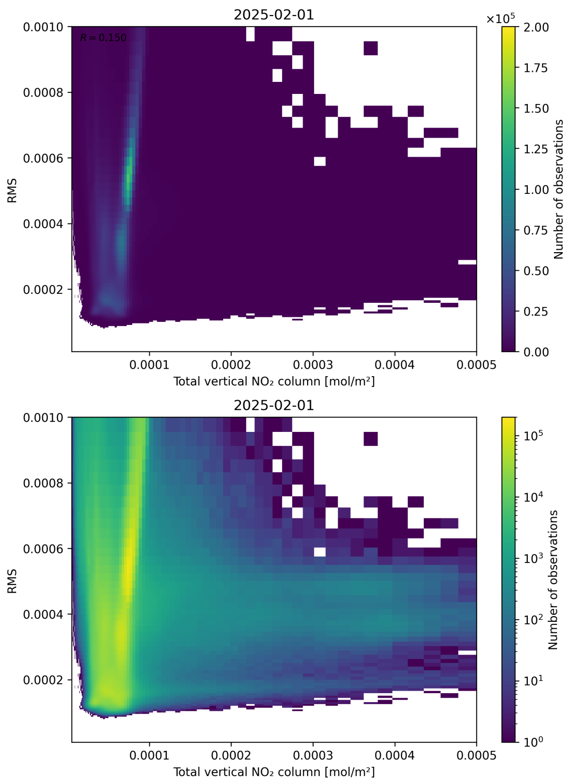
Figure 120: Scatter density plot of “Total vertical NO 2 column” against “RMS” for 2025-01-31 to 2025-02-02.
