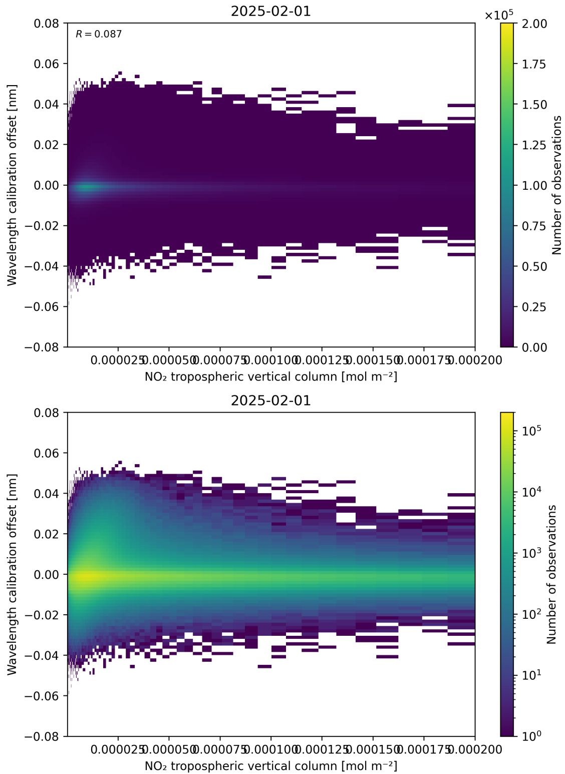
Figure 143: Scatter density plot of “NO 2 tropospheric vertical column” against “Wavelength calibration offset” for 2025-01-31 to 2025-02-02.
