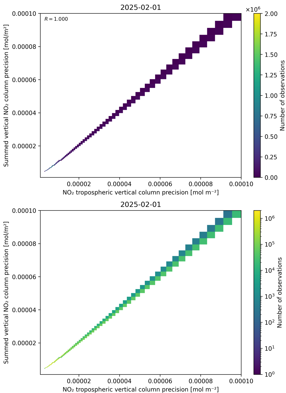
Figure 137: Scatter density plot of “NO 2 tropospheric vertical column precision” against “Summed vertical NO 2 column precision” for 2025-01-31 to 2025-02-02.
