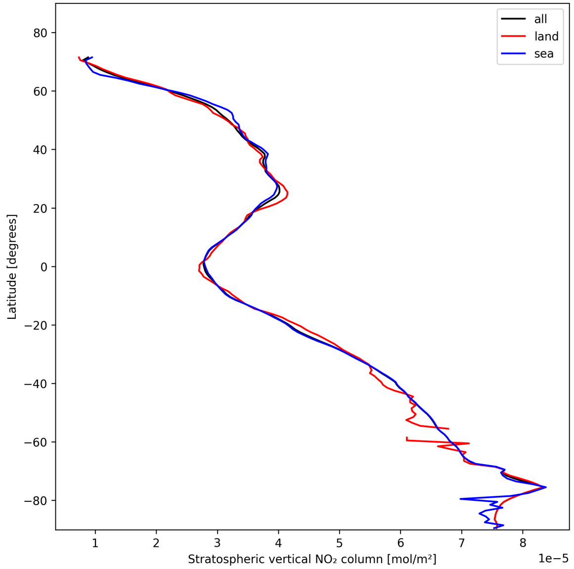
Figure 19: Zonal average of “Stratospheric vertical NO 2 column” for 2025-01-31 to 2025-02-02.
