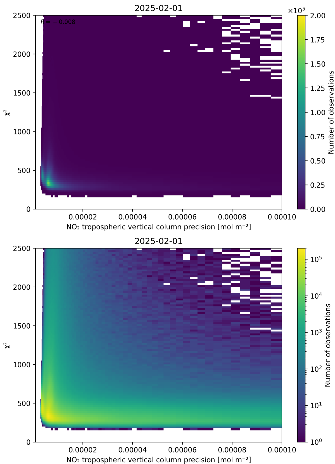
Figure 134: Scatter density plot of “NO 2 tropospheric vertical column precision” against “ \chi^2 ” for 2025-01-31 to 2025-02-02.
