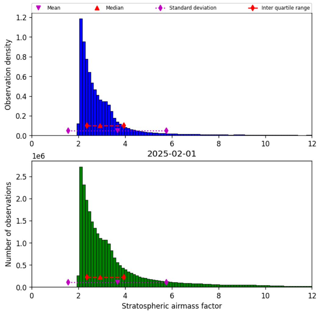
Figure 44: Histogram of “Stratospheric airmass factor” for 2025-01-31 to 2025-02-02
