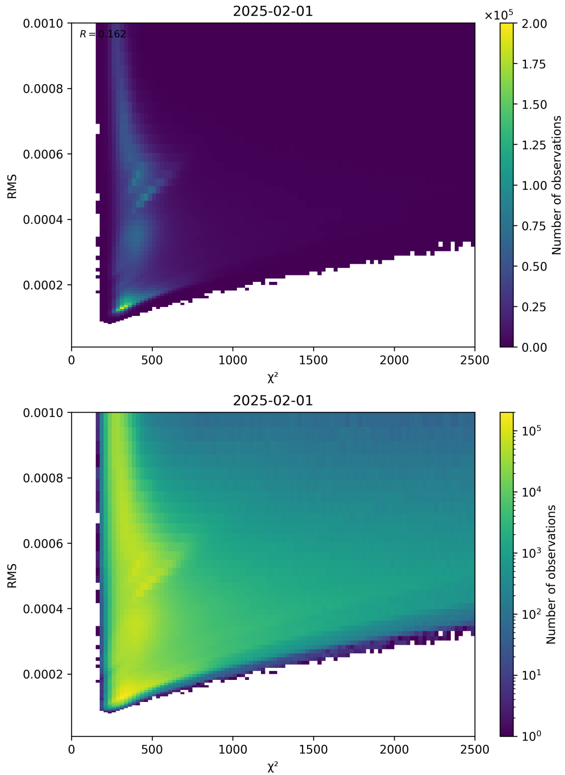
Figure 82: Scatter density plot of “ \chi^2 ” against “RMS” for 2025-01-31 to 2025-02-02.
