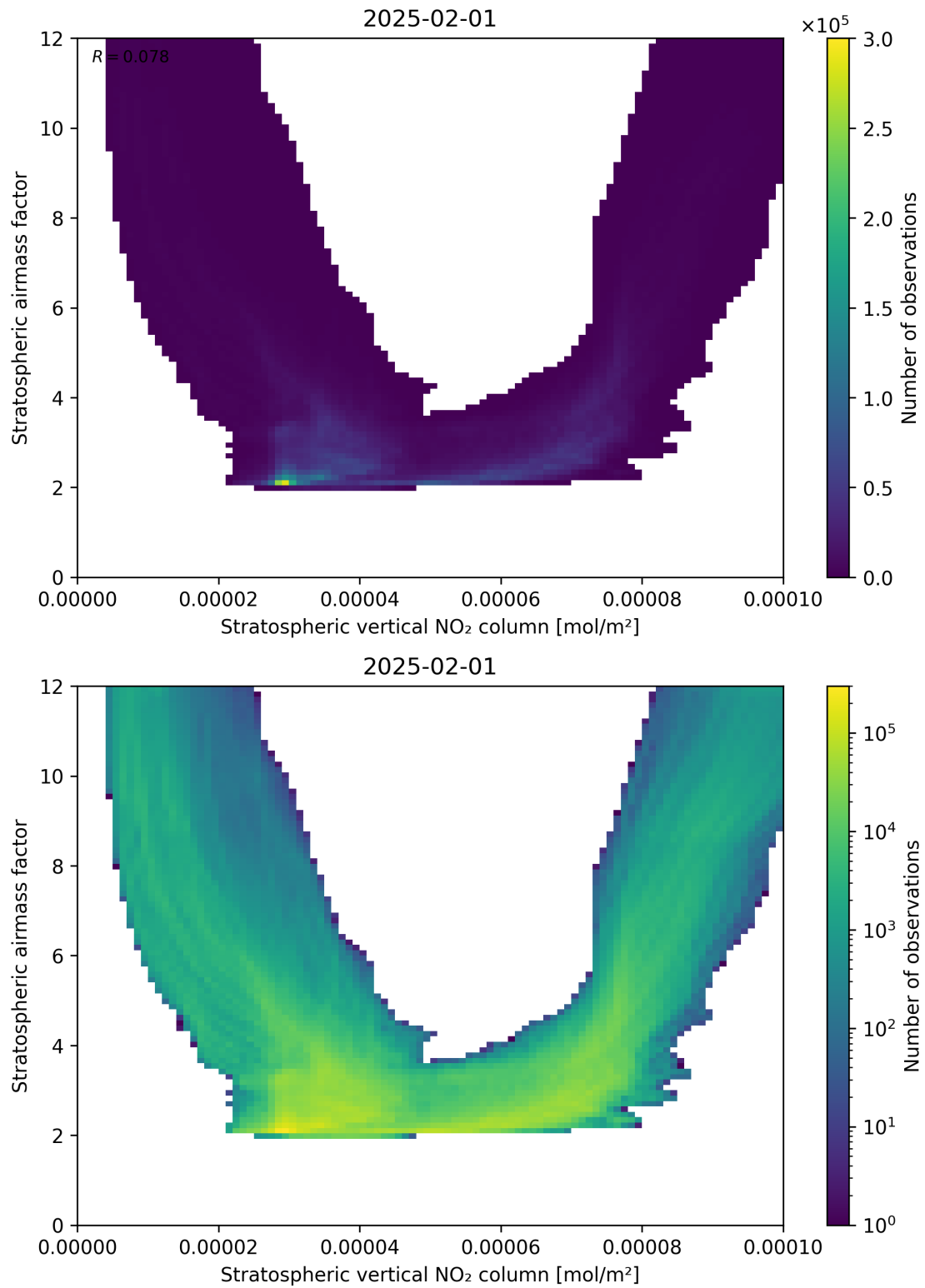
Figure 96: Scatter density plot of “Stratospheric vertical NO 2 column” against “Stratospheric airmass factor” for 2025-01-31 to 2025-02-02.
