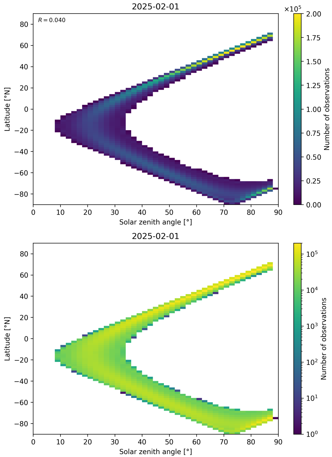
Figure 149: Scatter density plot of “Solar zenith angle” against “Latitude” for 2025-01-31 to 2025-02-02.
