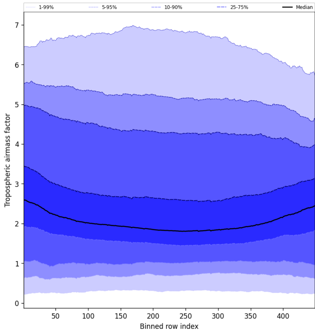
Figure 48: Along track statistics of “Tropospheric air mass factor” for 2025-01-31 to 2025-02-02
