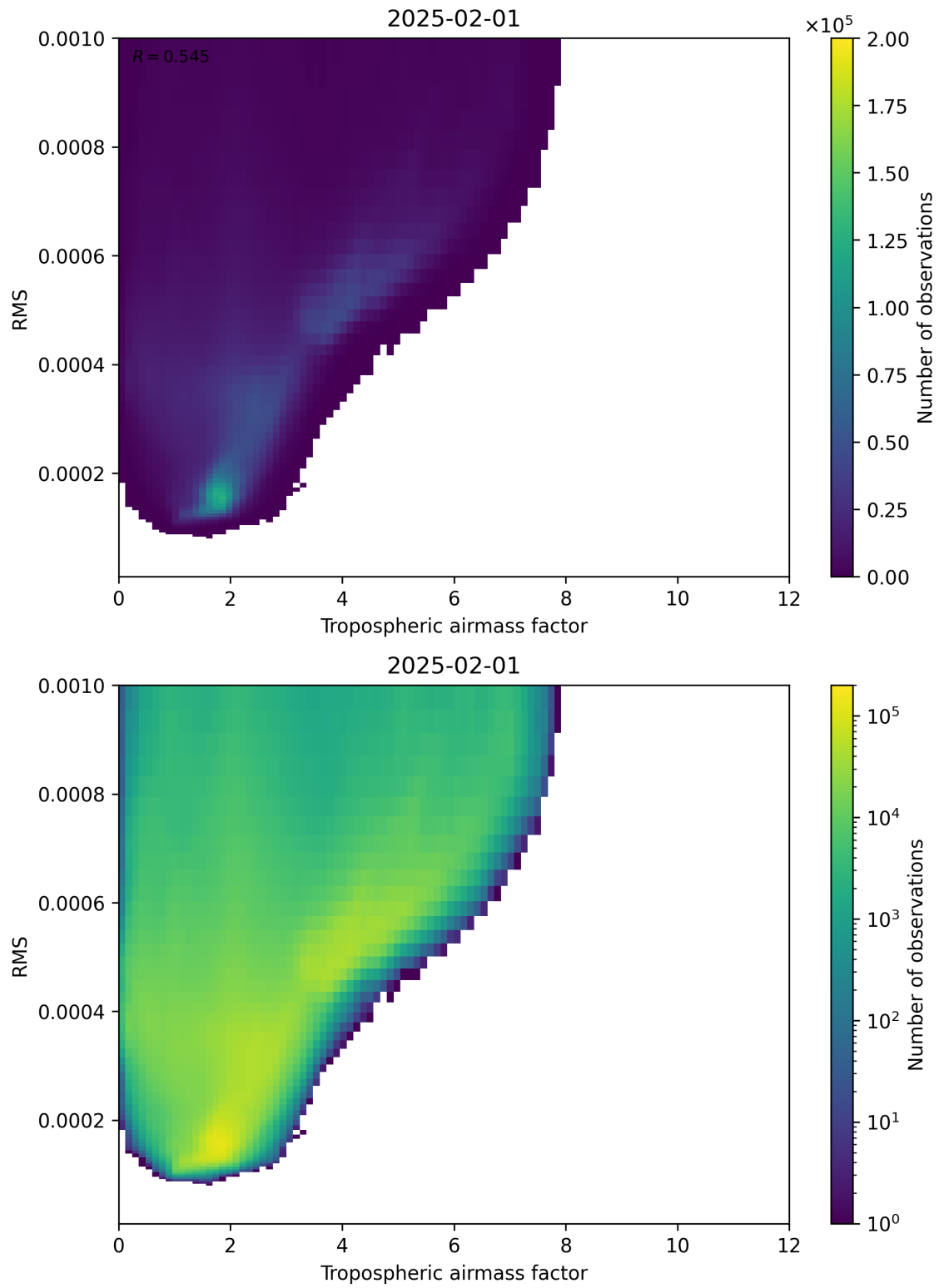
Figure 79: Scatter density plot of “Tropospheric airmass factor” against “RMS” for 2025-01-31 to 2025-02-02.
