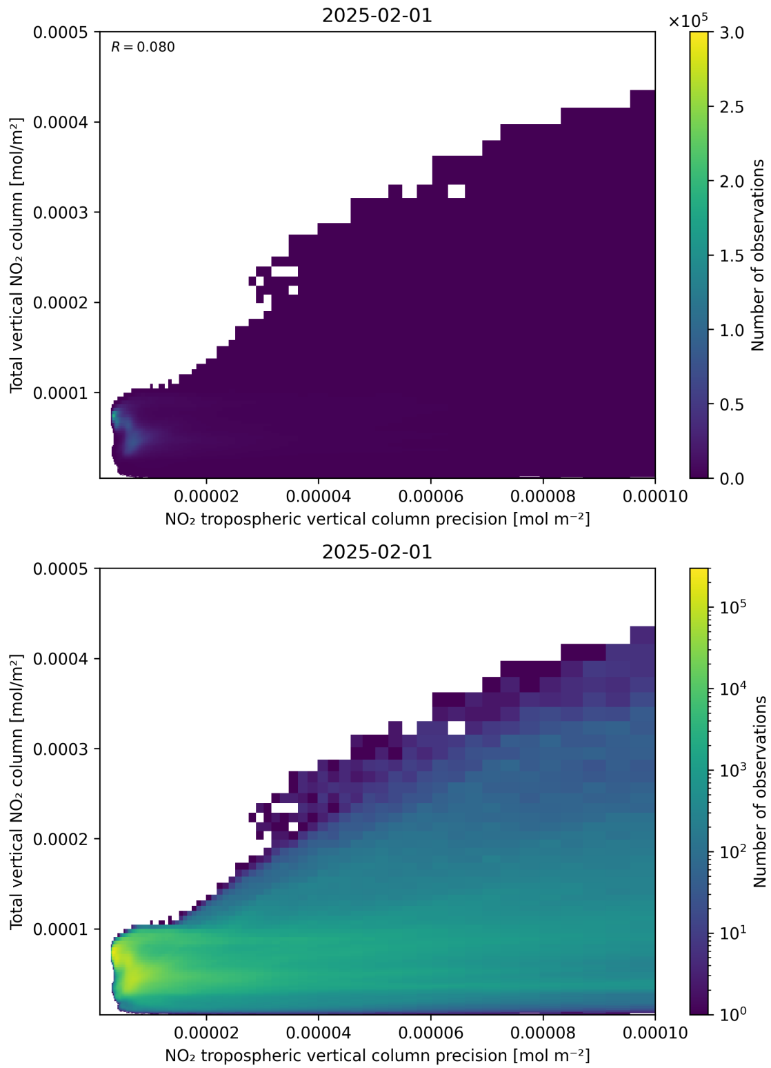
Figure 138: Scatter density plot of “NO 2 tropospheric vertical column precision” against “Total vertical NO 2 column” for 2025-01-31 to 2025-02-02.
