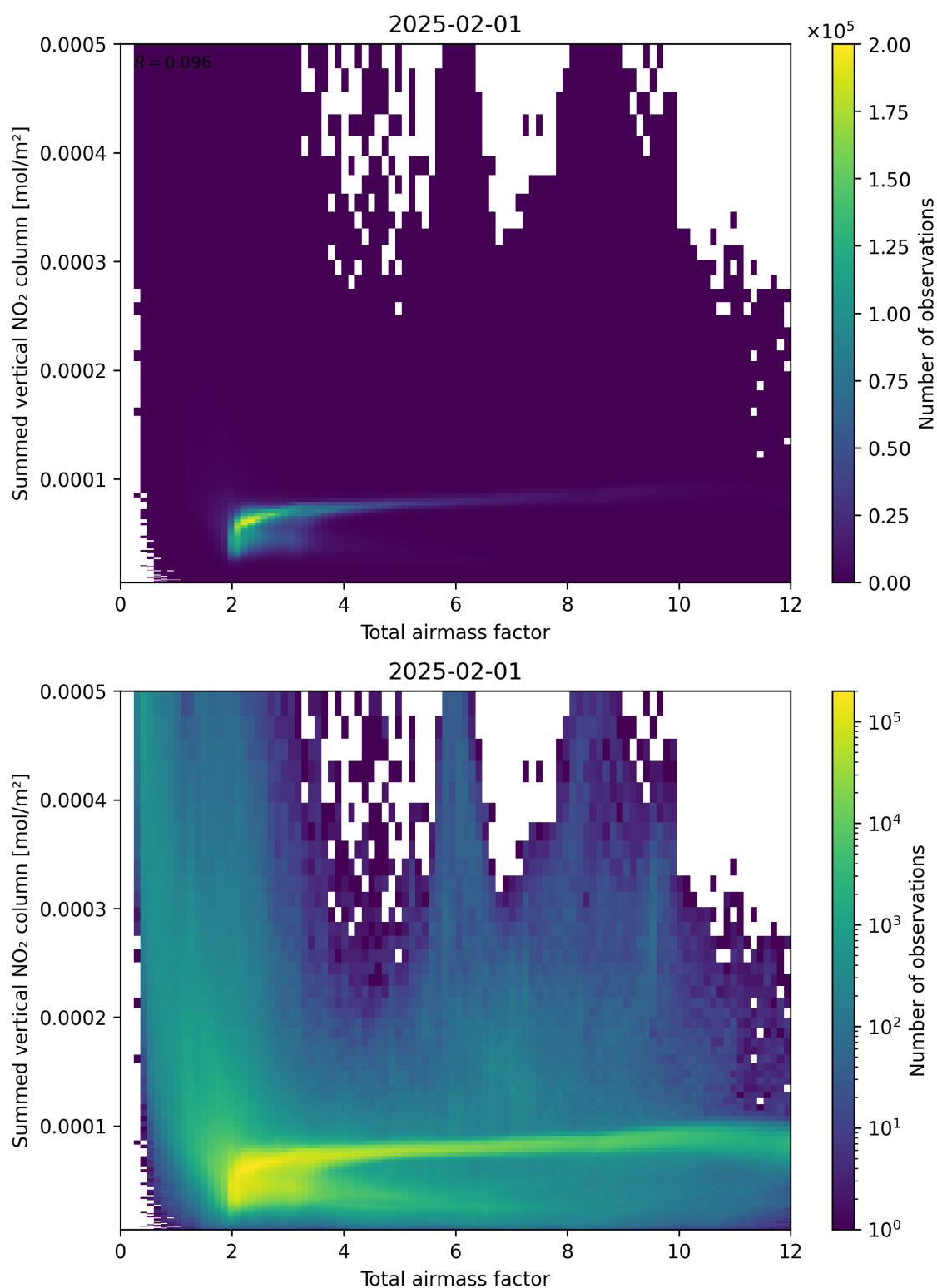
Figure 65: Scatter density plot of “Total airmass factor” against “Summed vertical NO 2 column” for 2025-01-31 to 2025-02-02.
