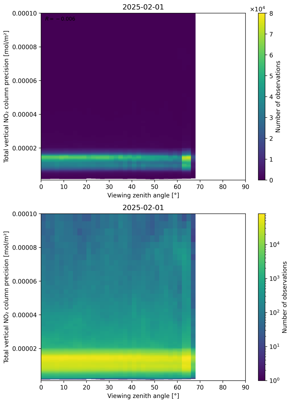
Figure 168: Scatter density plot of “Viewing zenith angle” against “Total vertical NO 2 column precision” for 2025-01-31 to 2025-02-02.
