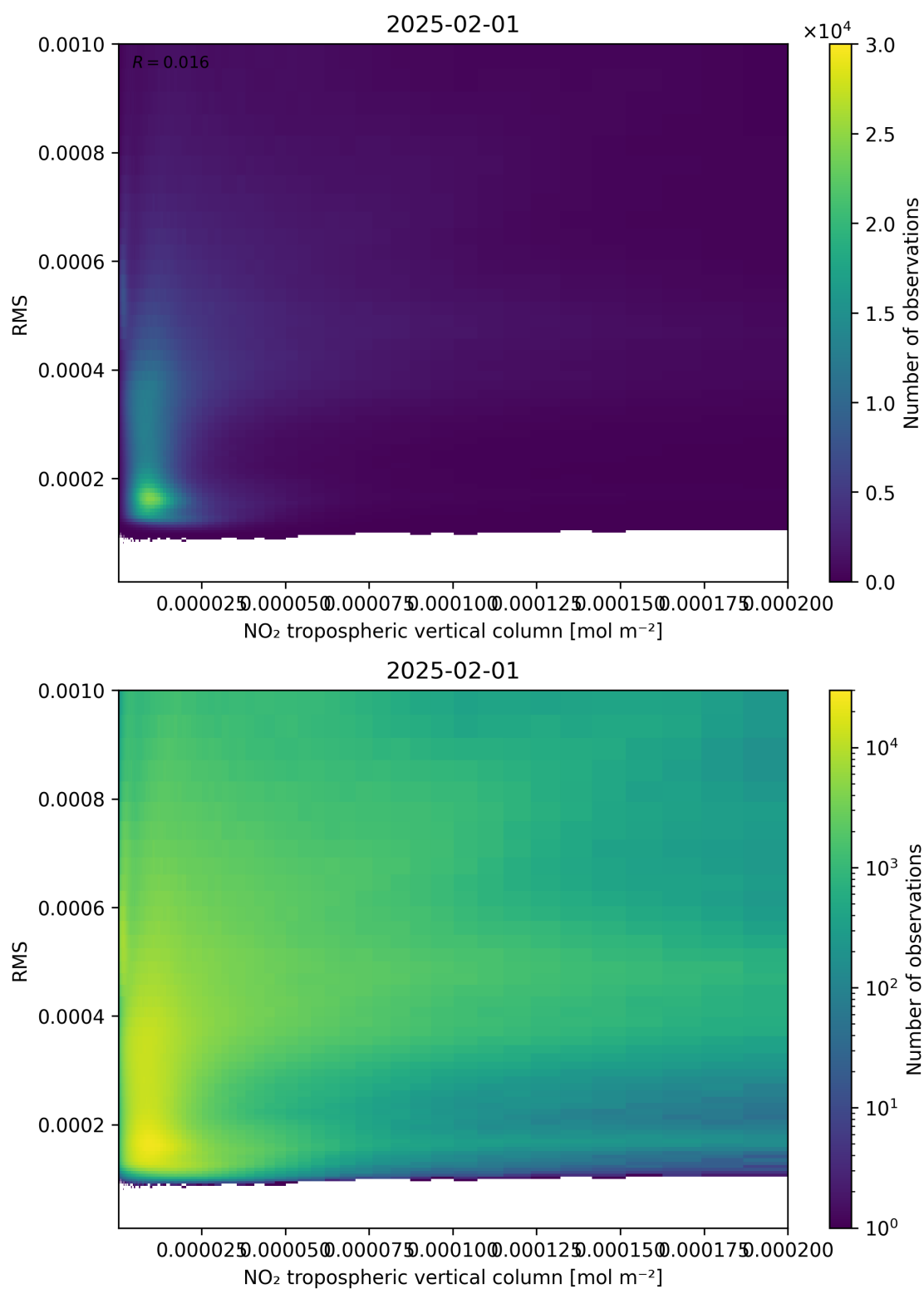
Figure 142: Scatter density plot of “NO 2 tropospheric vertical column” against “RMS” for 2025-01-31 to 2025-02-02.
