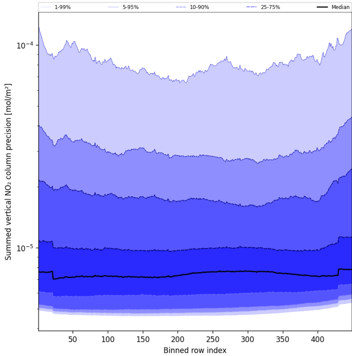
Figure 58: Along track statistics of “Summed vertical NO 2 column precision” for 2025-01-31 to 2025-02-02
