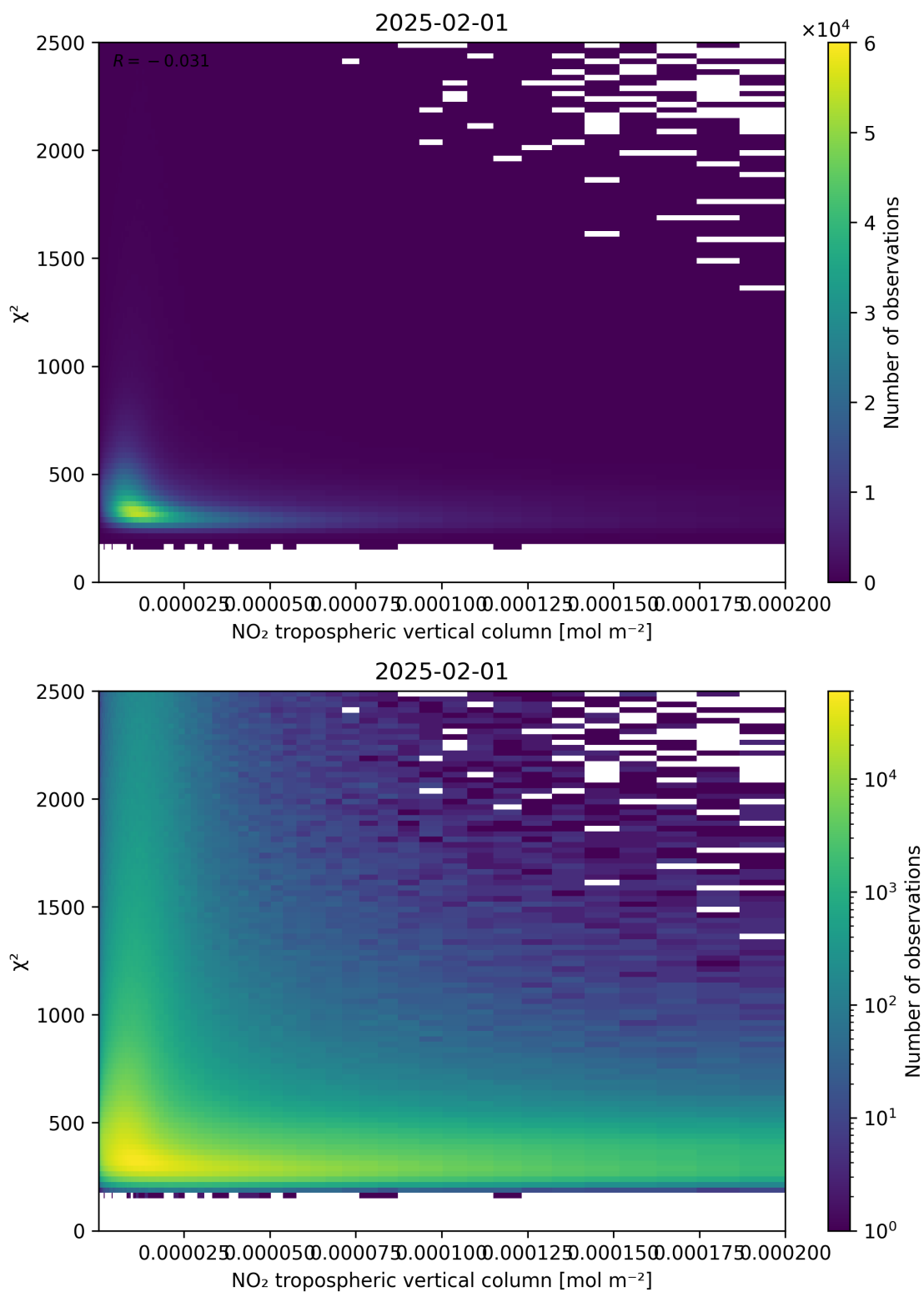
Figure 124: Scatter density plot of “NO 2 tropospheric vertical column” against “ \chi^2 ” for 2025-01-31 to 2025-02-02.
