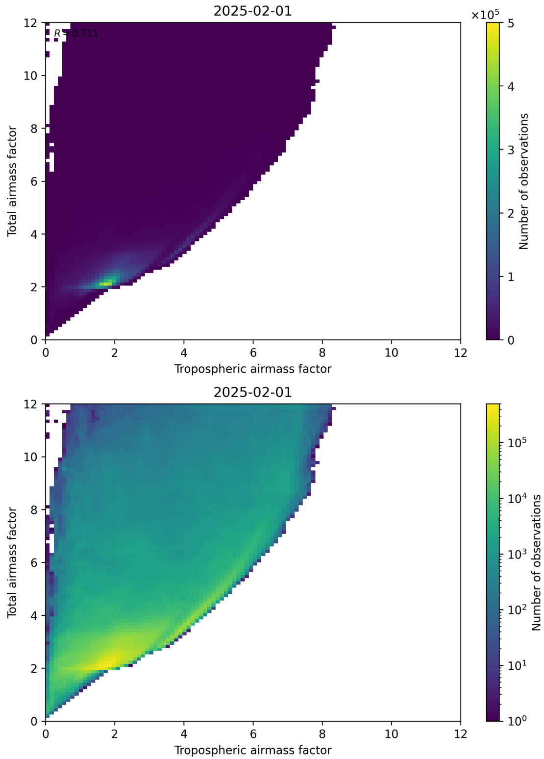
Figure 72: Scatter density plot of “Tropospheric airmass factor” against “Total airmass factor” for 2025-01-31 to 2025-02-02.
