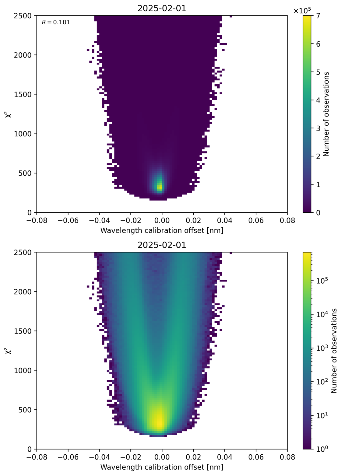
Figure 175: Scatter density plot of “Wavelength calibration offset” against “ \chi^2 ” for 2025-01-31 to 2025-02-02.
