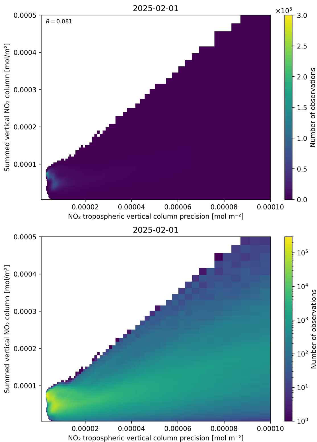
Figure 136: Scatter density plot of “NO 2 tropospheric vertical column precision” against “Summed vertical NO 2 column” for 2025-01-31 to 2025-02-02.
