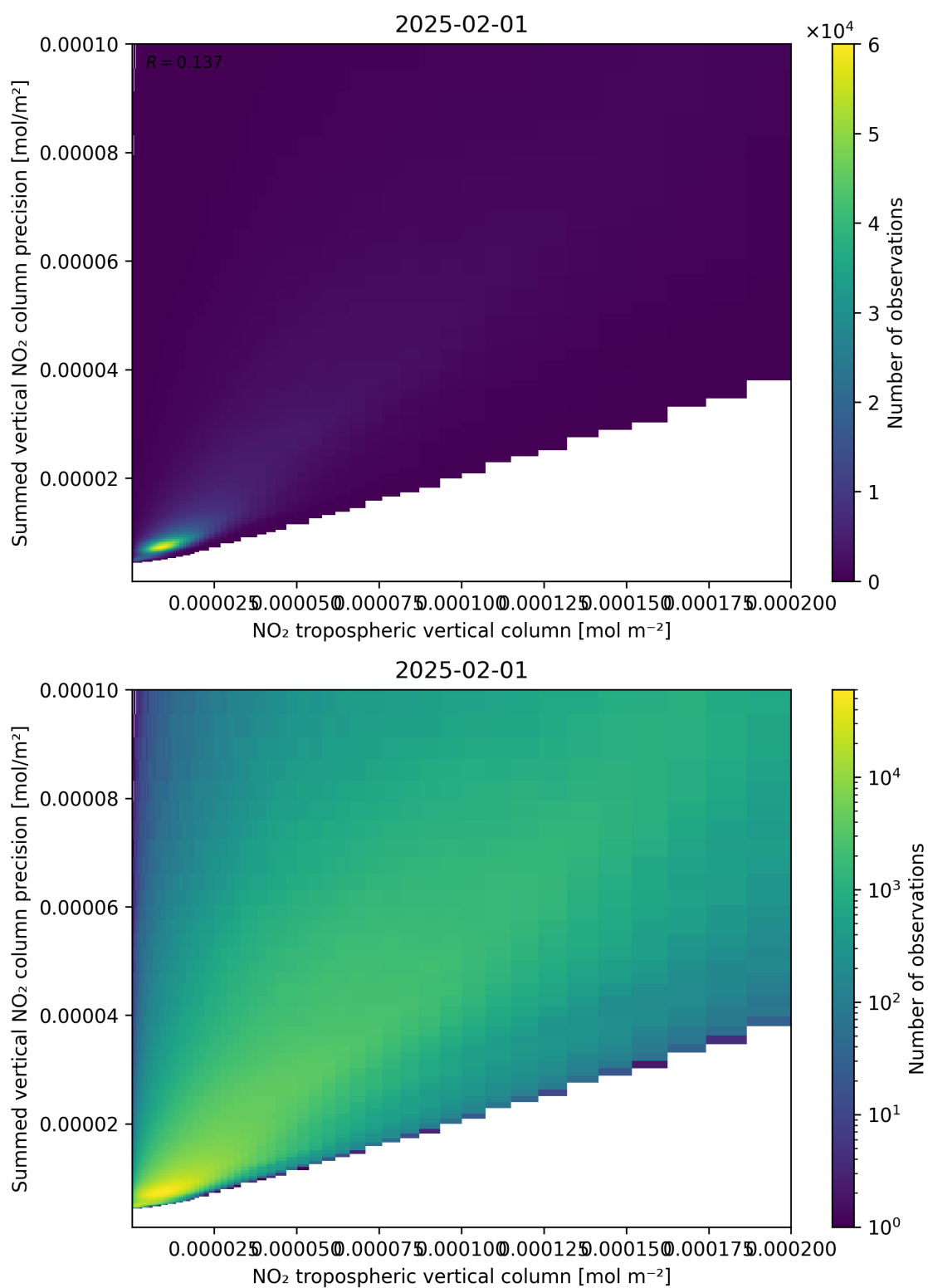
Figure 127: Scatter density plot of “NO 2 tropospheric vertical column” against “Summed vertical NO 2 column precision” for 2025-01-31 to 2025-02-02.
