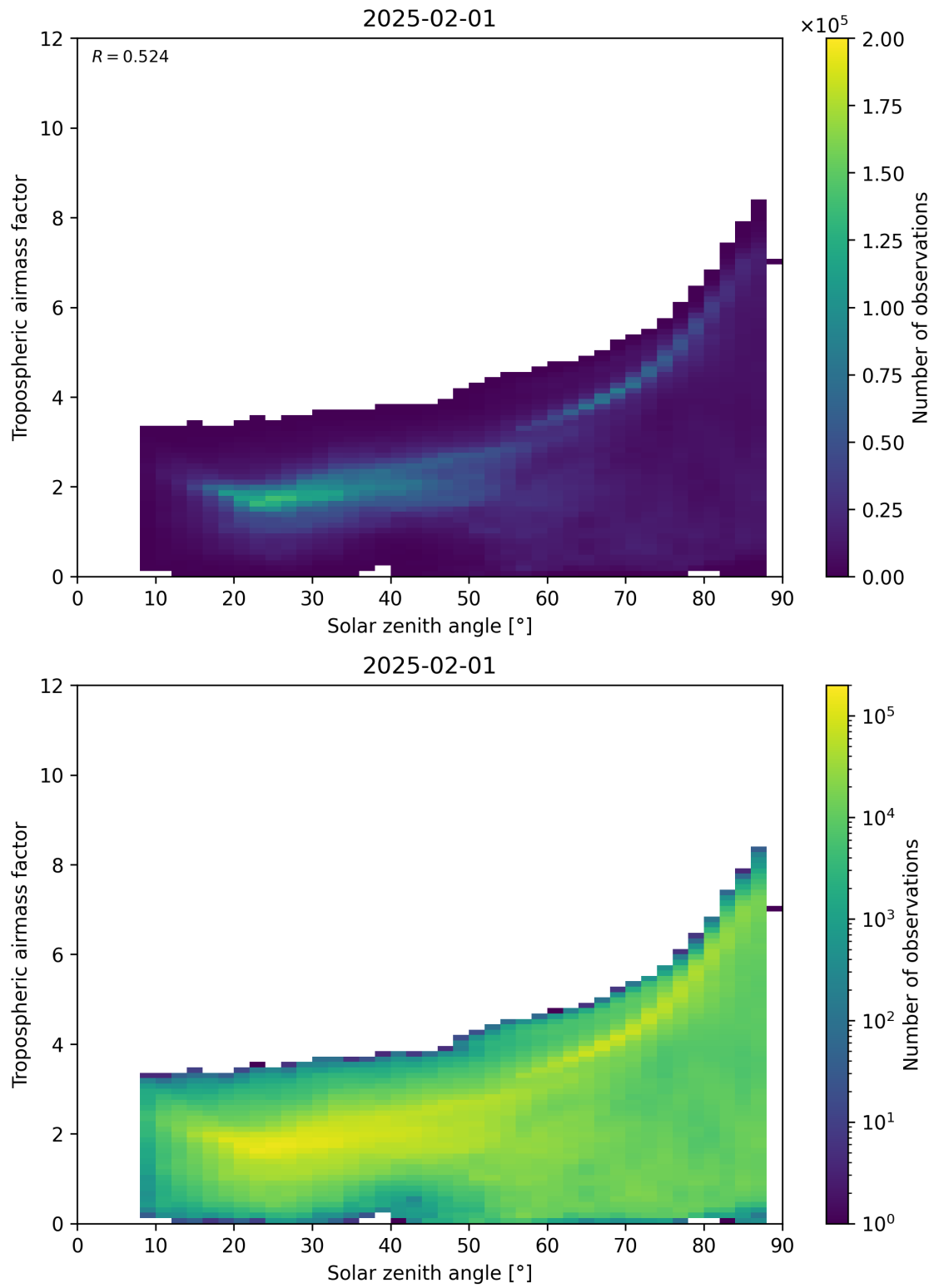
Figure 147: Scatter density plot of “Solar zenith angle” against “Tropospheric airmass factor” for 2025-01-31 to 2025-02-02.
