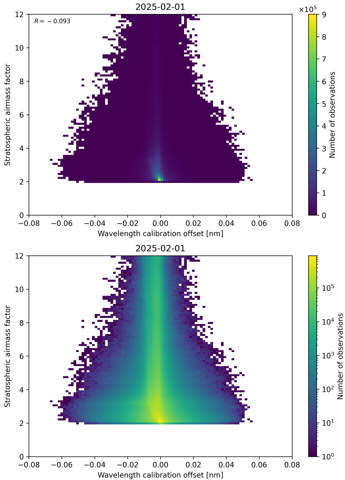
Figure 174: Scatter density plot of “Wavelength calibration offset” against “Stratospheric airmass factor” for 2025-01-31 to 2025-02-02.
