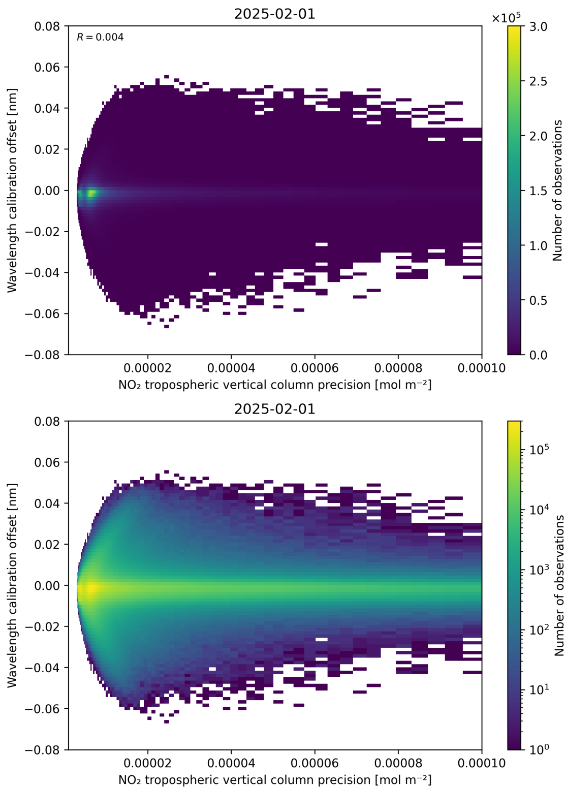
Figure 141: Scatter density plot of “NO 2 tropospheric vertical column precision” against “Wavelength calibration offset” for 2025-01-31 to 2025-02-02.
