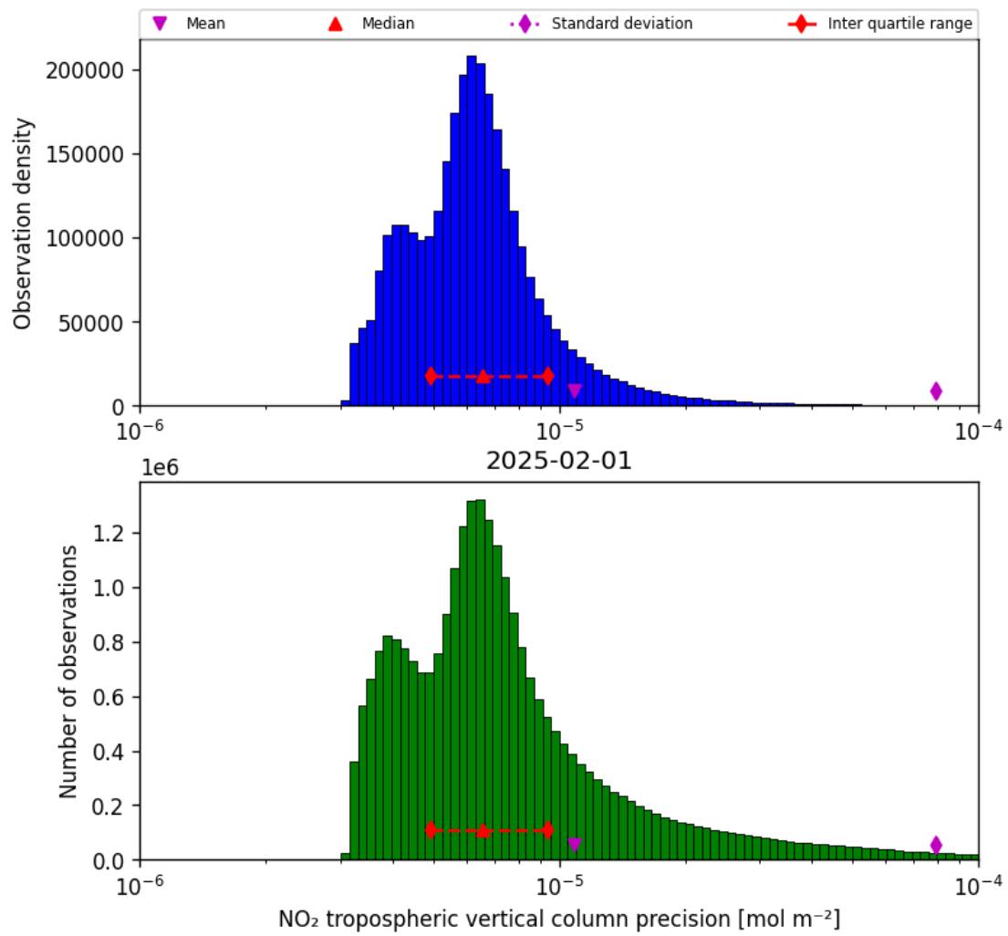
Figure 30: Histogram of “NO 2 tropospheric vertical column precision” for 2025-01-31 to 2025-02-02
