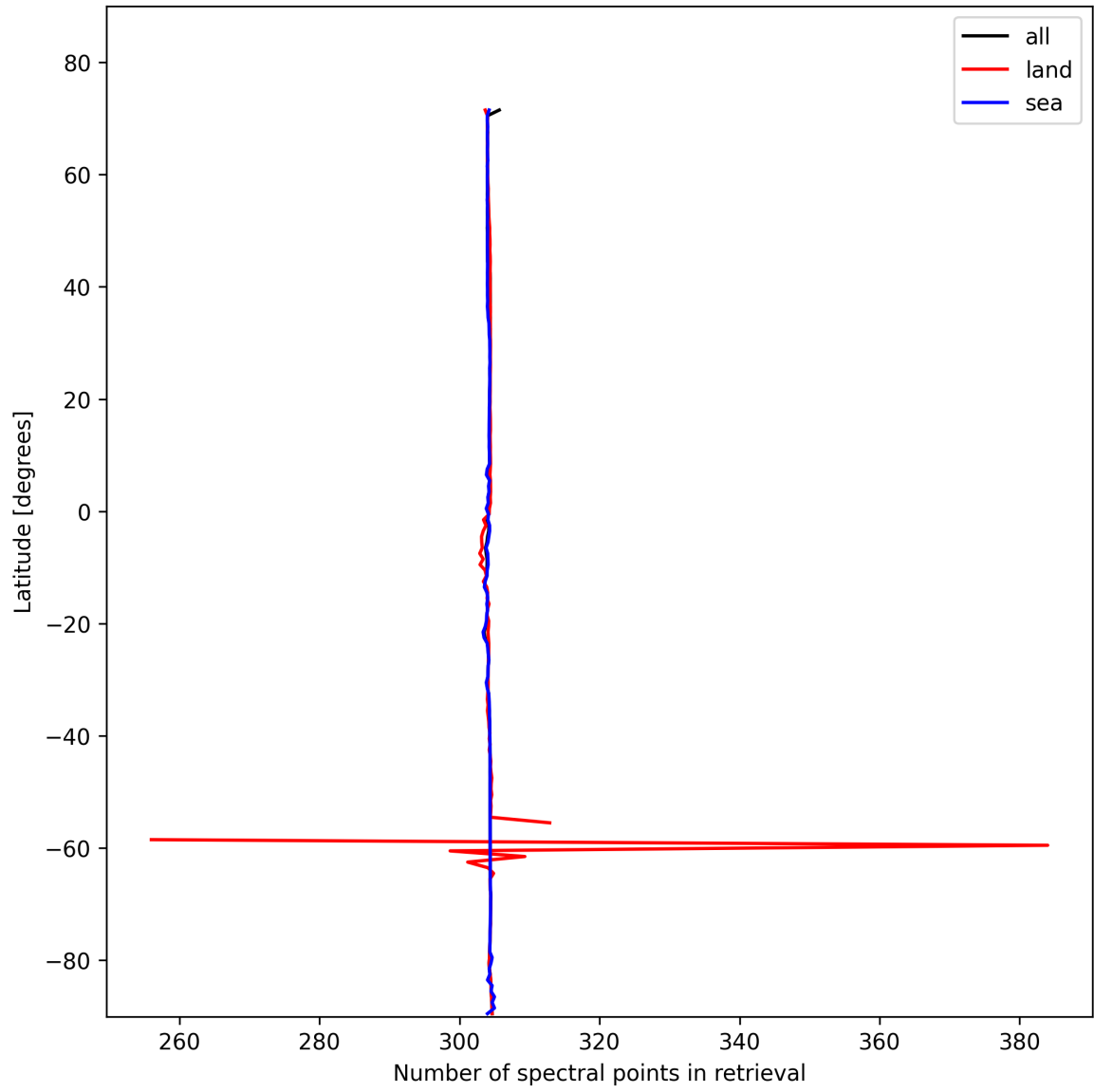
Figure 16: Zonal average of “Number of spectral points in retrieval” for 2025-01-31 to 2025-02-02.
