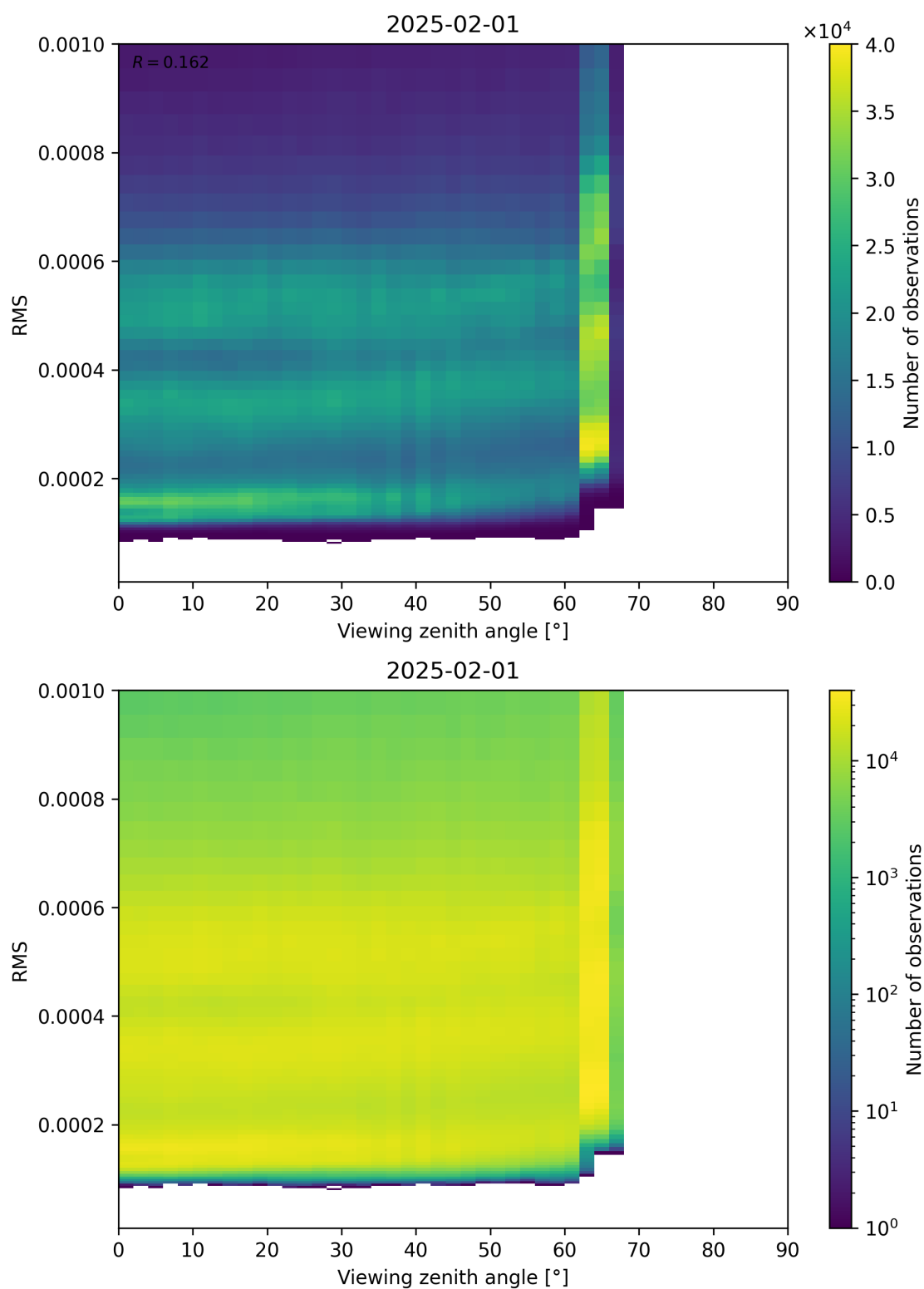
Figure 171: Scatter density plot of “Viewing zenith angle” against “RMS” for 2025-01-31 to 2025-02-02.
