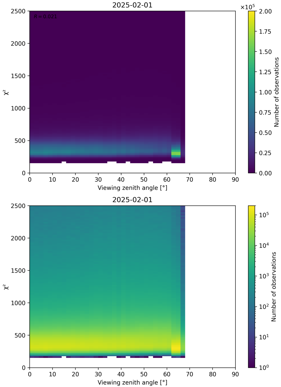
Figure 162: Scatter density plot of “Viewing zenith angle” against “ \chi^2 ” for 2025-01-31 to 2025-02-02.
