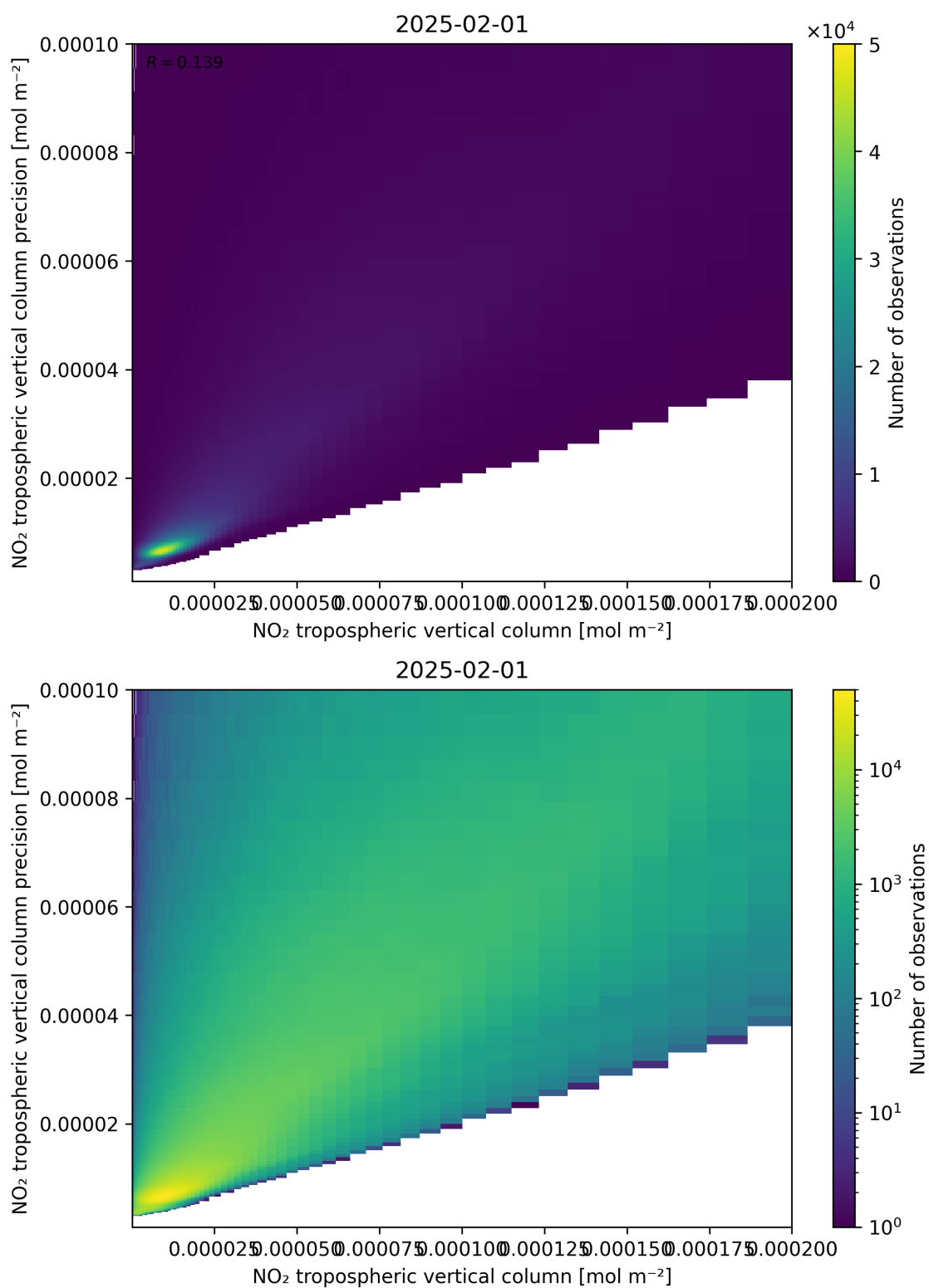
Figure 130: Scatter density plot of “NO 2 tropospheric vertical column” against “NO 2 tropospheric vertical column precision” for 2025-01-31 to 2025-02-02.
