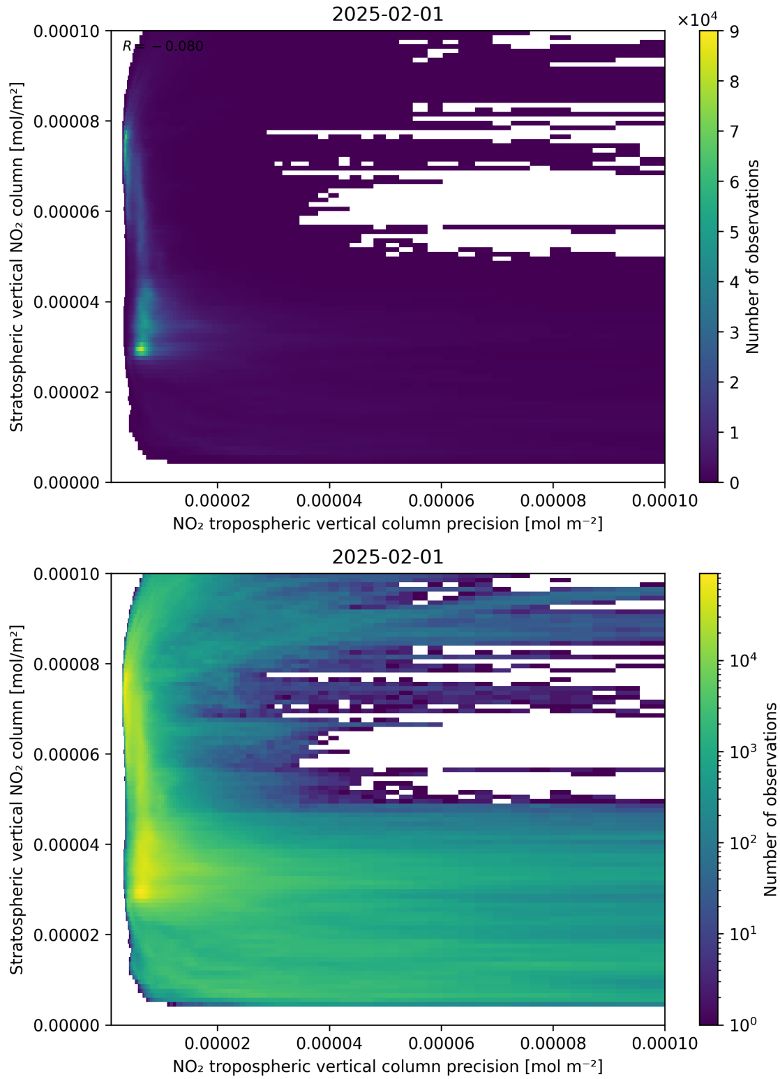
Figure 135: Scatter density plot of “NO 2 tropospheric vertical column precision” against “Stratospheric vertical NO 2 column” for 2025-01-31 to 2025-02-02.
