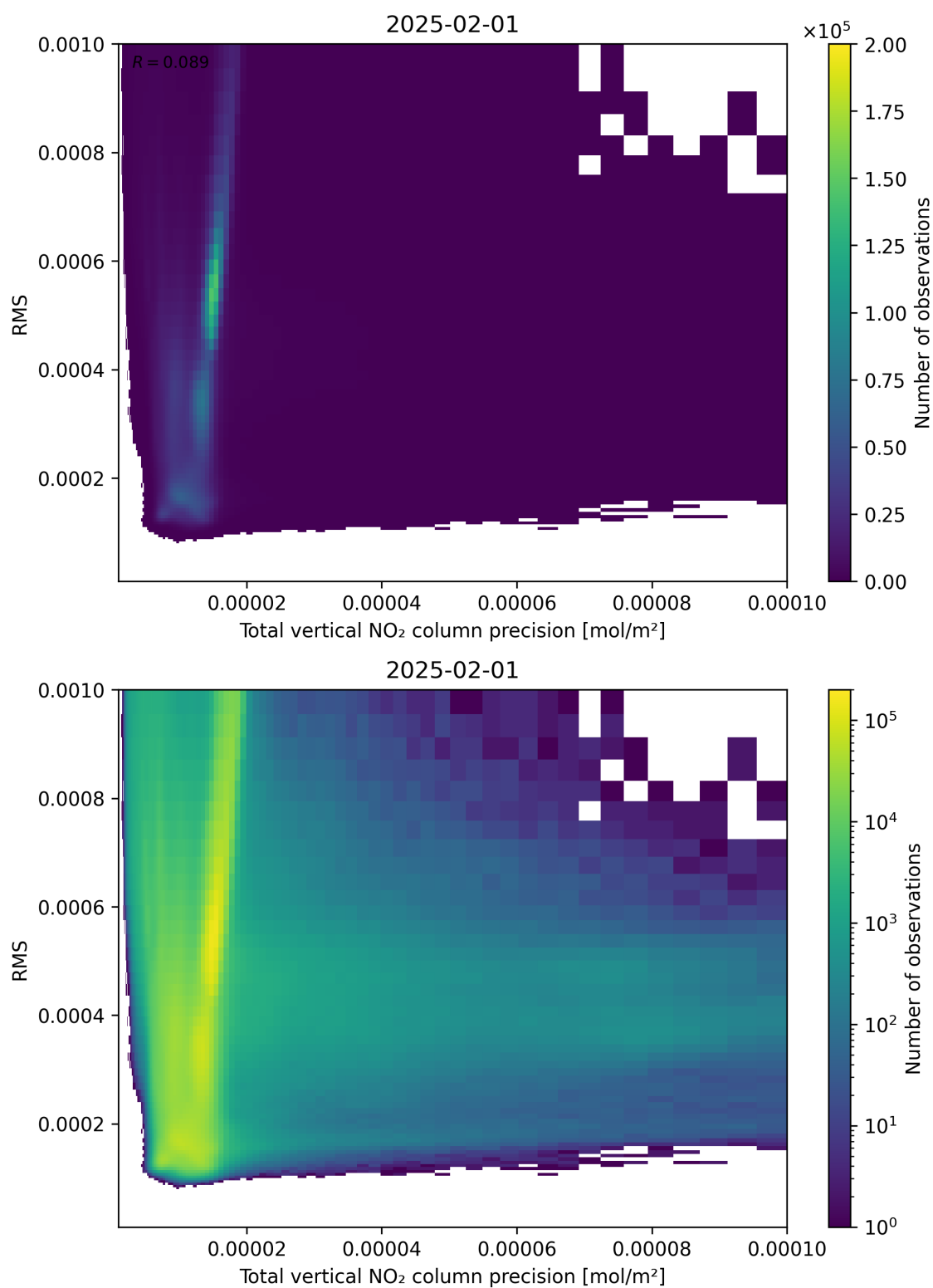
Figure 119: Scatter density plot of “Total vertical NO 2 column precision” against “RMS” for 2025-01-31 to 2025-02-02.
