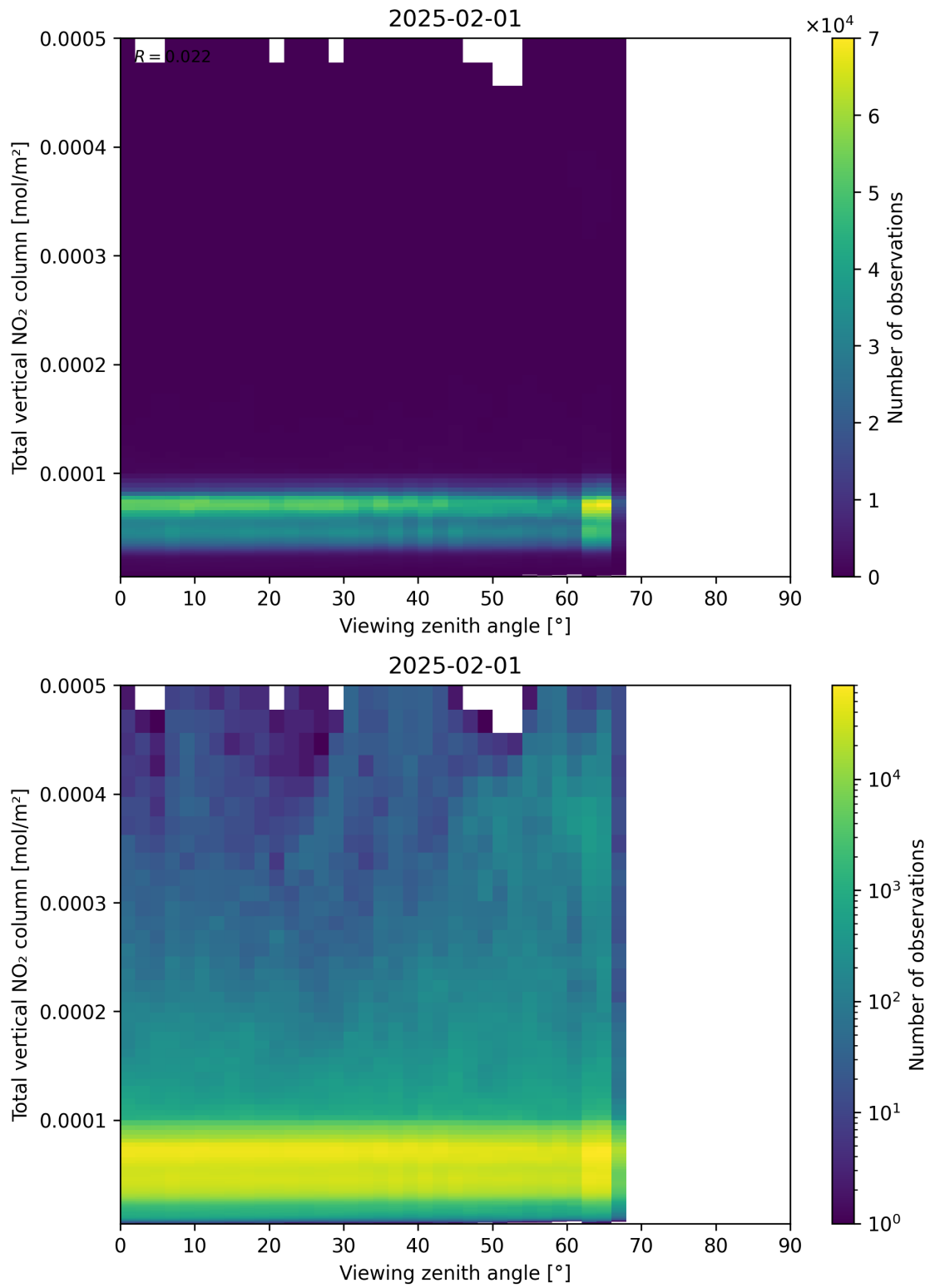
Figure 167: Scatter density plot of “Viewing zenith angle” against “Total vertical NO 2 column” for 2025-01-31 to 2025-02-02.
