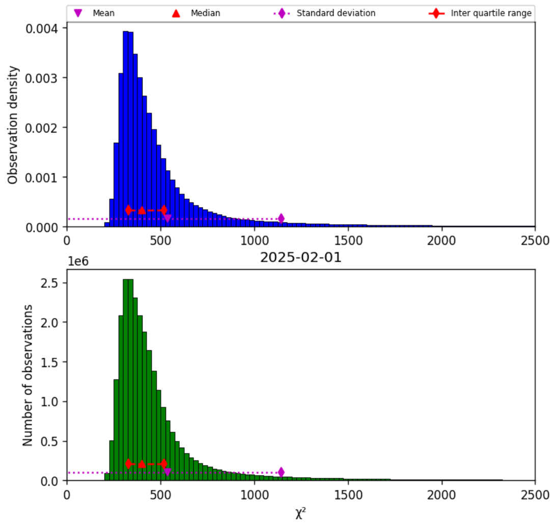
Figure 42: Histogram of “ \chi^2 ” for 2025-01-31 to 2025-02-02
