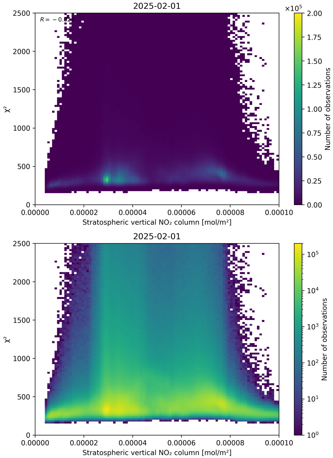
Figure 97: Scatter density plot of “Stratospheric vertical NO 2 column” against “ \chi^2 ” for 2025-01-31 to 2025-02-02.
