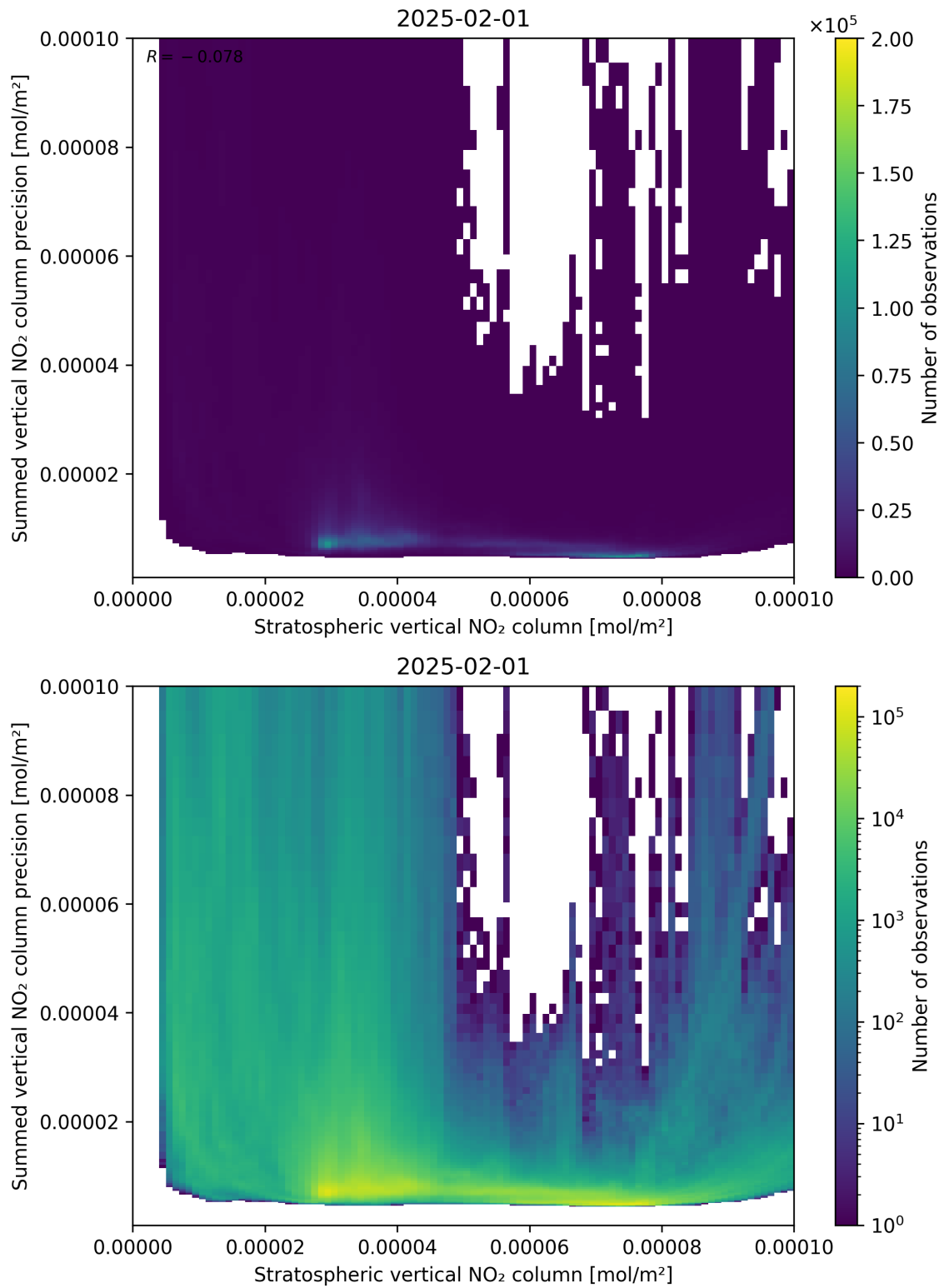
Figure 99: Scatter density plot of “Stratospheric vertical NO 2 column” against “Summed vertical NO 2 column precision” for 2025-01-31 to 2025-02-02.
