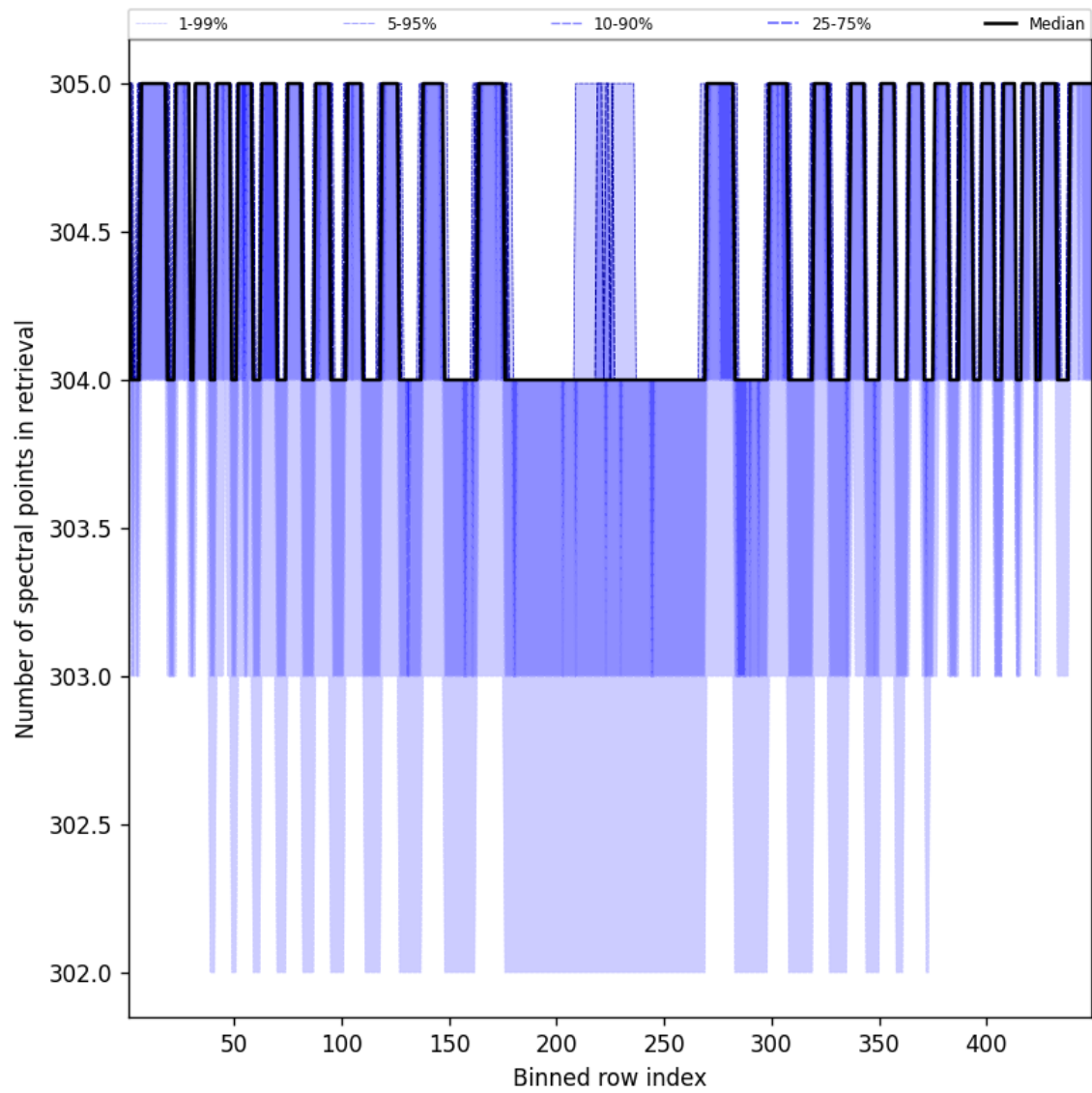
Figure 50: Along track statistics of “Number of spectral points in retrieval” for 2025-01-31 to 2025-02-02
