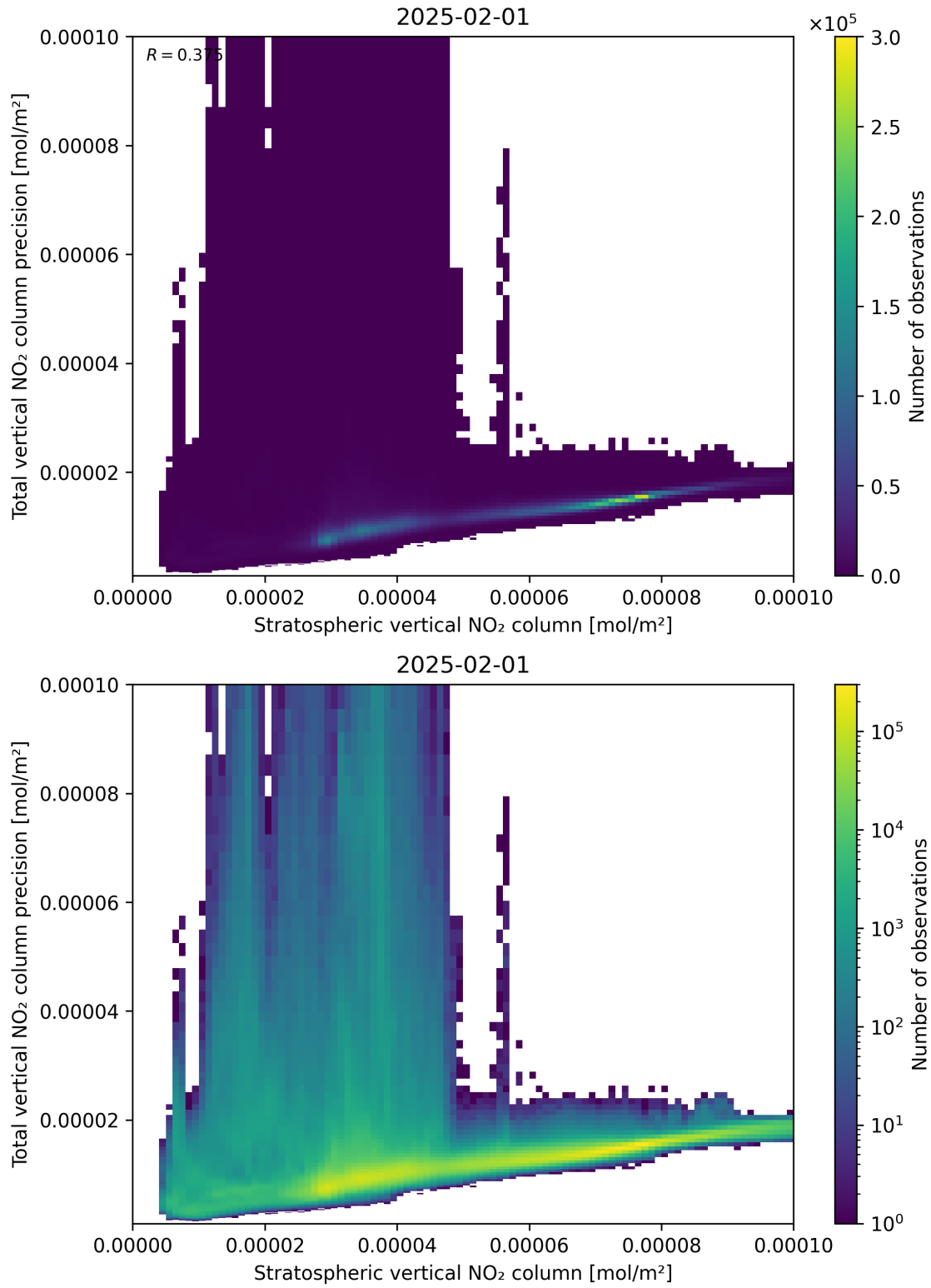
Figure 101: Scatter density plot of “Stratospheric vertical NO 2 column” against “Total vertical NO 2 column precision” for 2025-01-31 to 2025-02-02.
