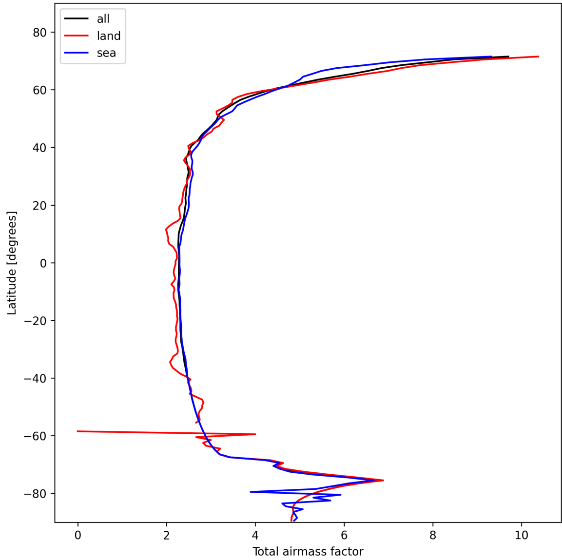
Figure 15: Zonal average of “Total airmass factor” for 2025-01-31 to 2025-02-02.
