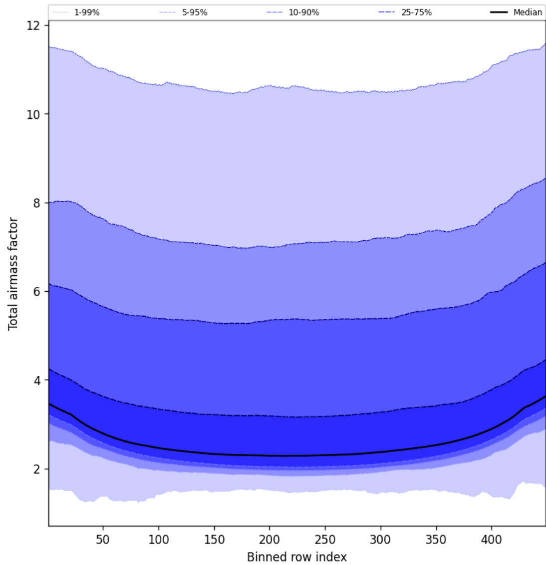
Figure 49: Along track statistics of “Total airmass factor” for 2025-01-31 to 2025-02-02
