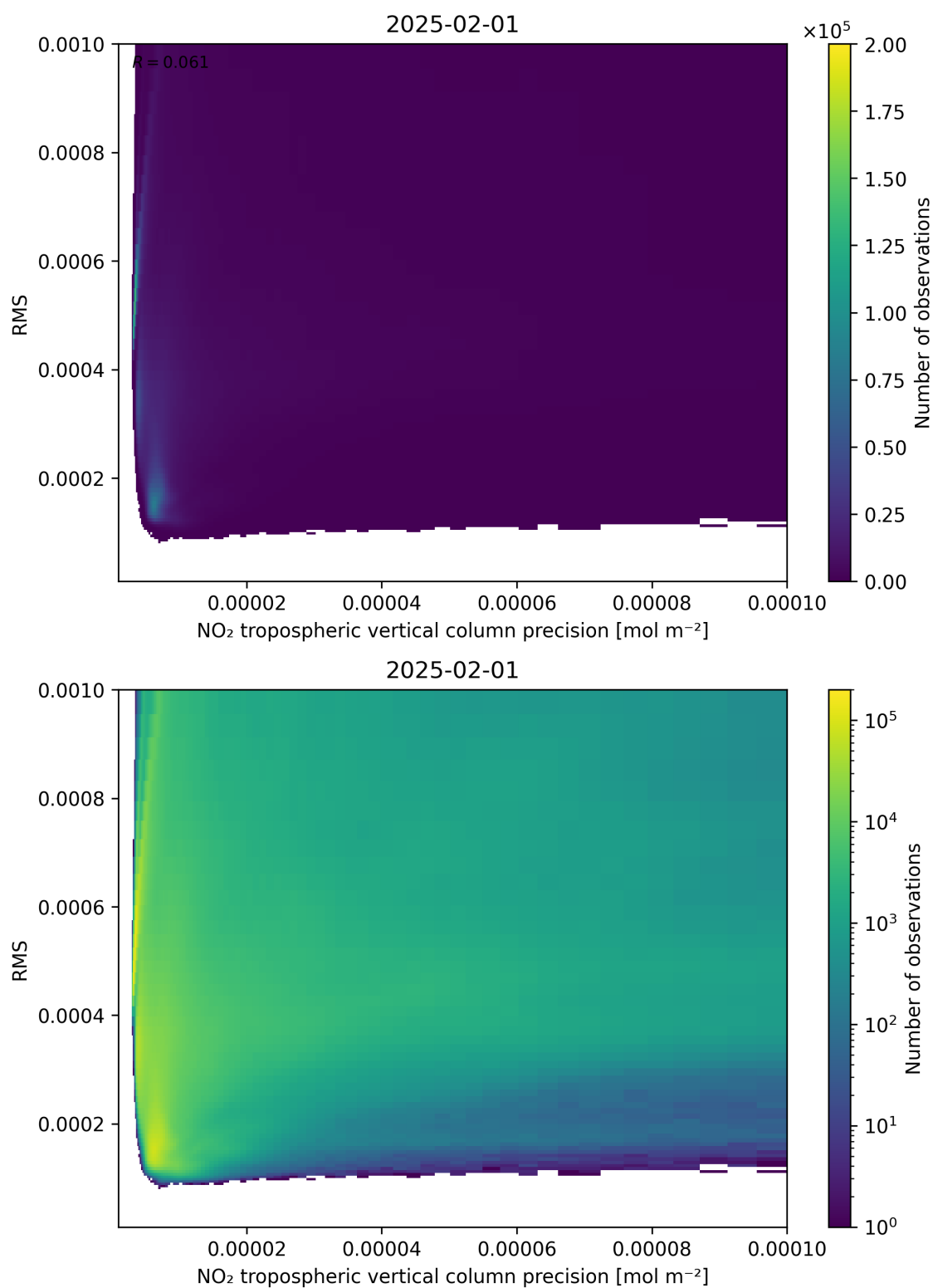
Figure 140: Scatter density plot of “NO 2 tropospheric vertical column precision” against “RMS” for 2025-01-31 to 2025-02-02.
