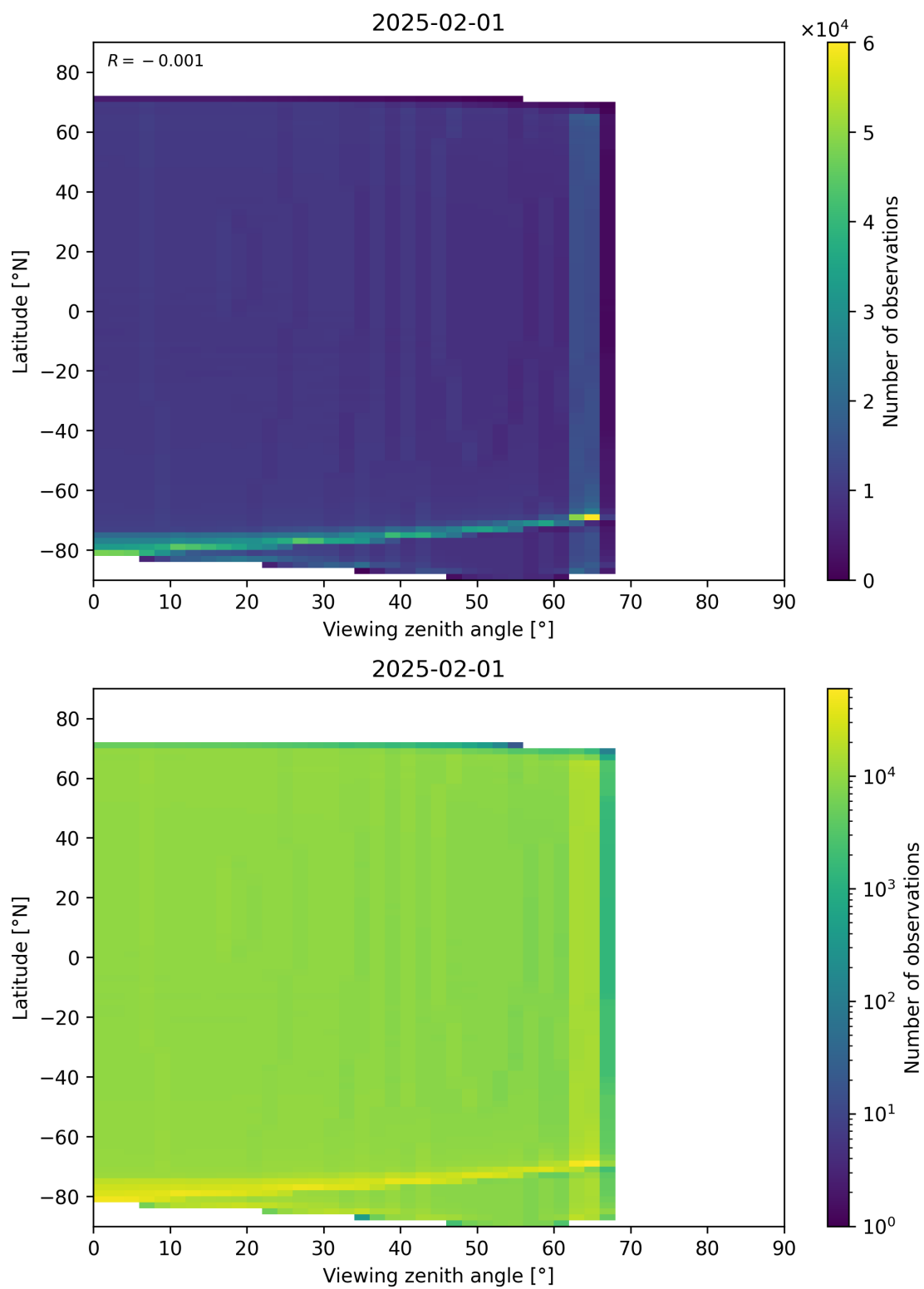
Figure 163: Scatter density plot of “Viewing zenith angle” against “Latitude” for 2025-01-31 to 2025-02-02.
