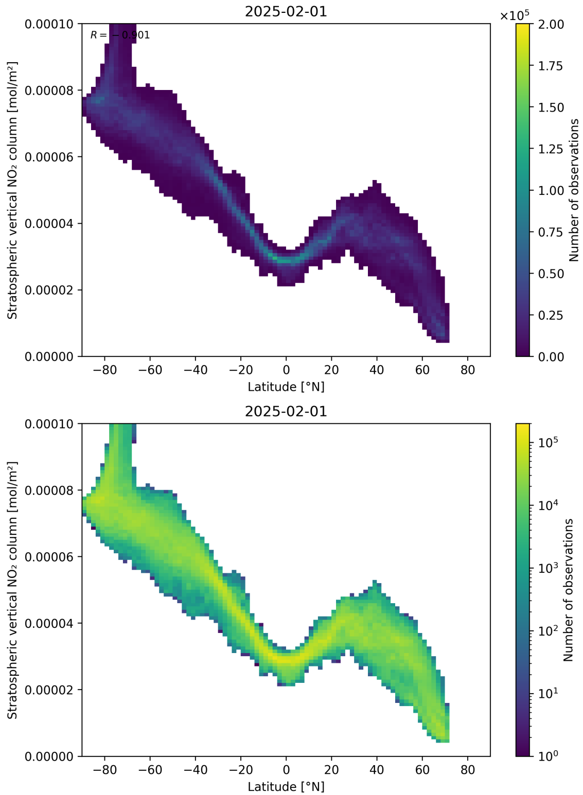
Figure 87: Scatter density plot of “Latitude” against “Stratospheric vertical NO 2 column” for 2025-01-31 to 2025-02-02.
