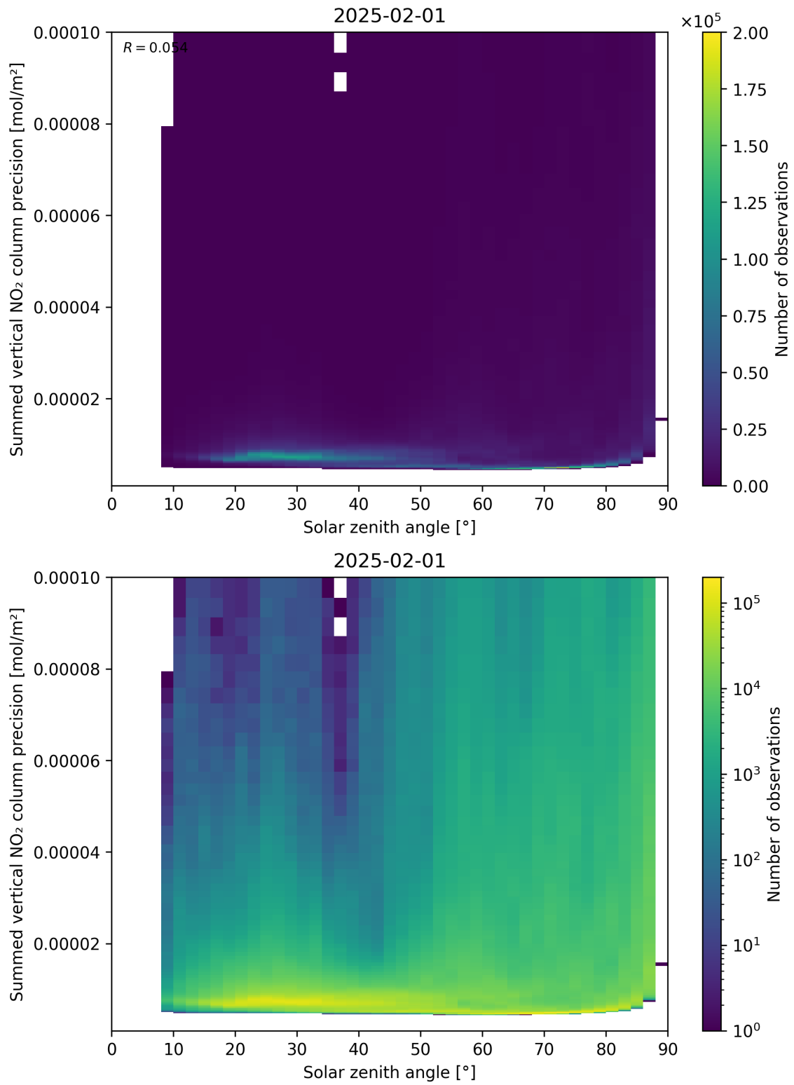
Figure 152: Scatter density plot of “Solar zenith angle” against “Summed vertical NO 2 column precision” for 2025-01-31 to 2025-02-02.
