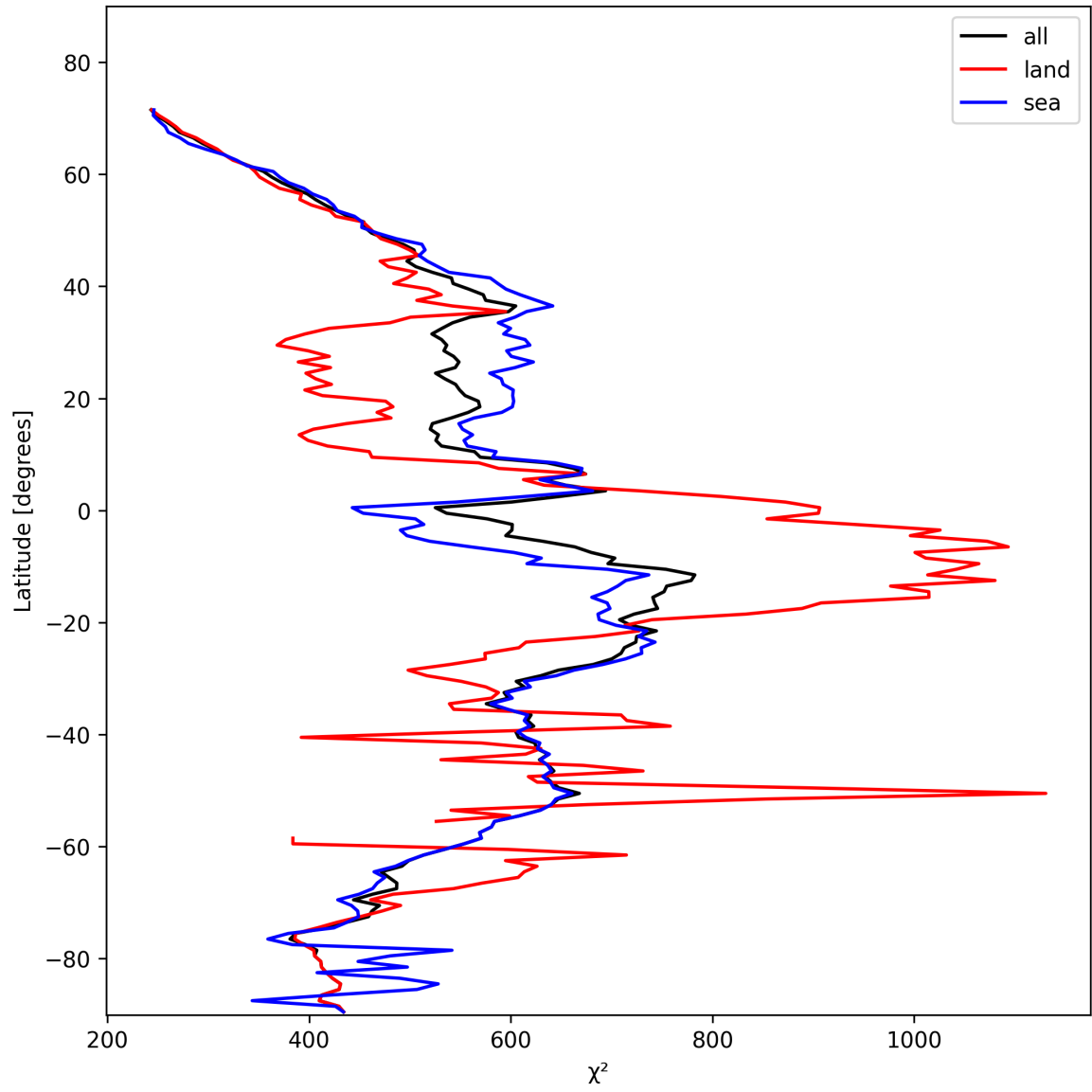
Figure 25: Zonal average of “ \chi^2 ” for 2025-01-31 to 2025-02-02.
