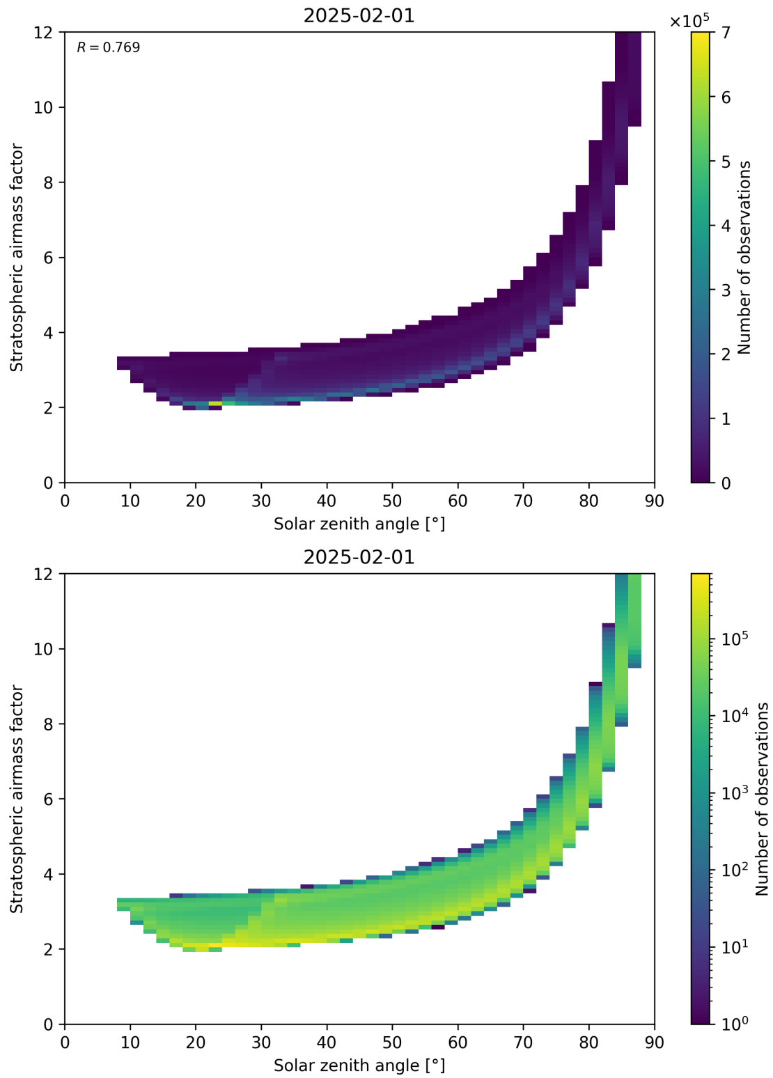
Figure 145: Scatter density plot of “Solar zenith angle” against “Stratospheric airmass factor” for 2025-01-31 to 2025-02-02.
