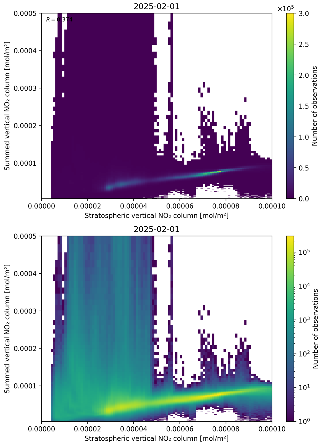
Figure 98: Scatter density plot of “Stratospheric vertical NO 2 column” against “Summed vertical NO 2 column” for 2025-01-31 to 2025-02-02.
