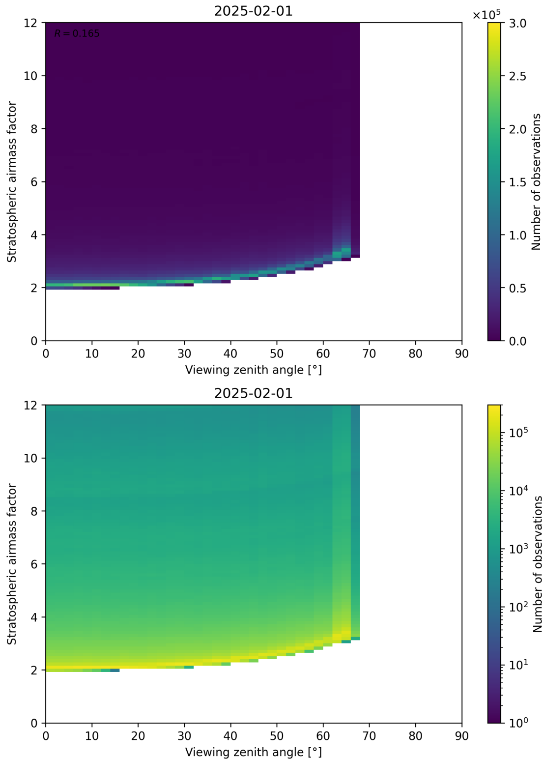
Figure 159: Scatter density plot of “Viewing zenith angle” against “Stratospheric airmass factor” for 2025-01-31 to 2025-02-02.
