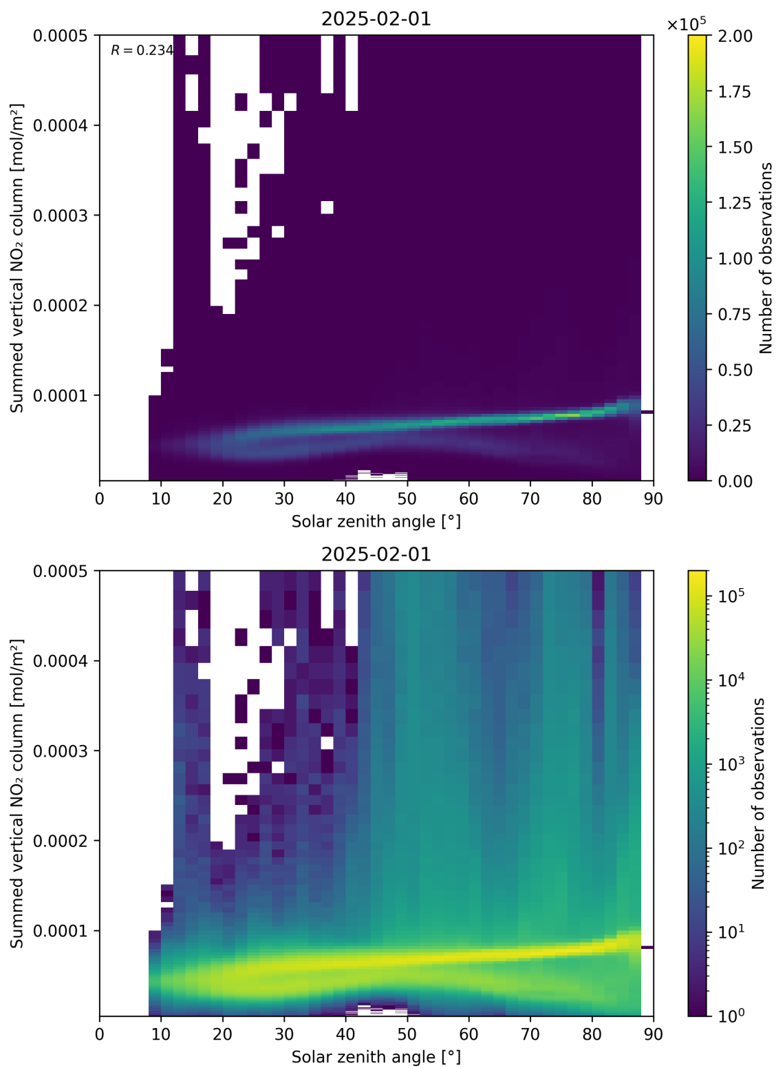
Figure 151: Scatter density plot of “Solar zenith angle” against “Summed vertical NO 2 column” for 2025-01-31 to 2025-02-02.
