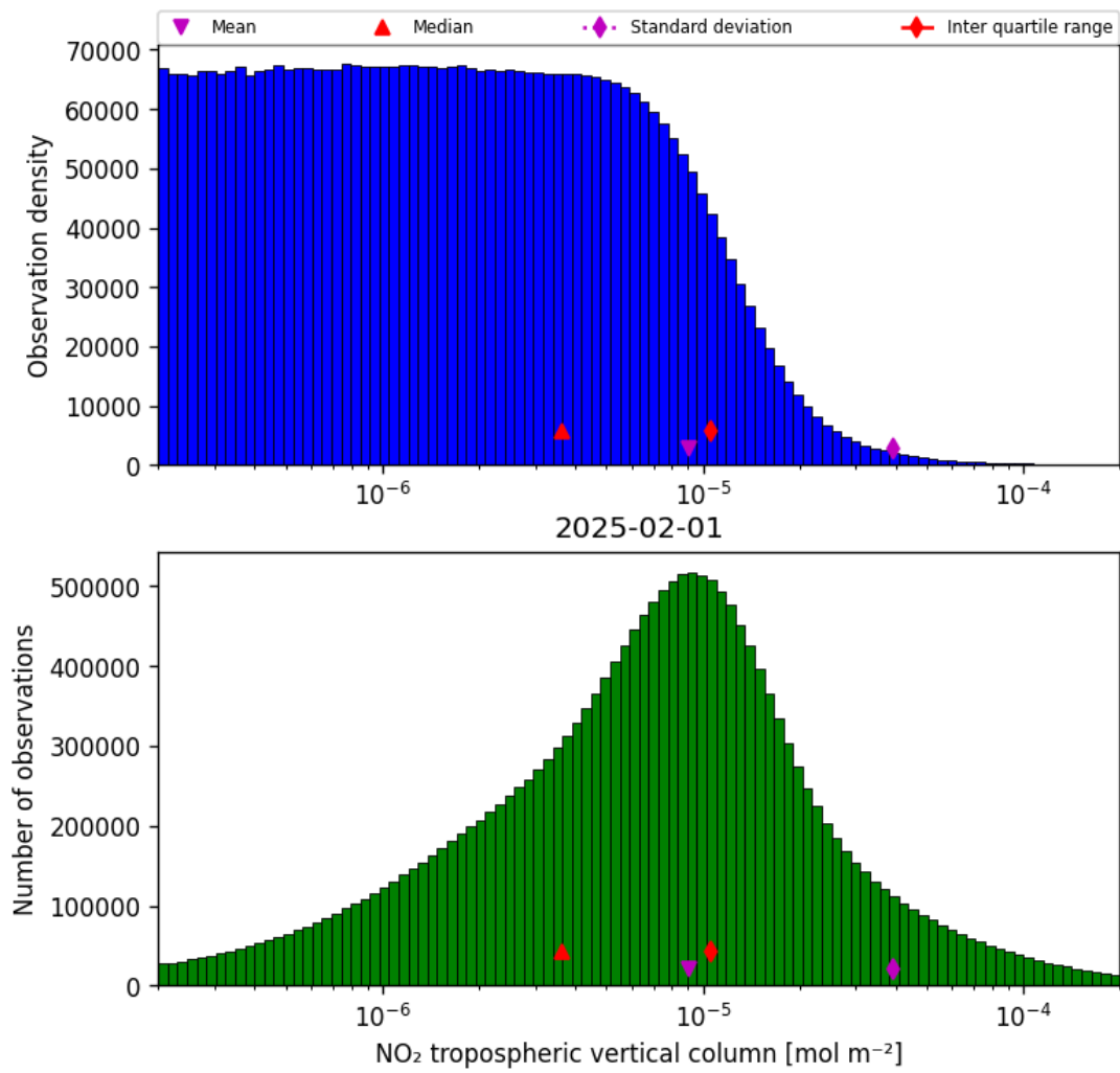
Figure 29: Histogram of “NO 2 tropospheric vertical column” for 2025-01-31 to 2025-02-02
