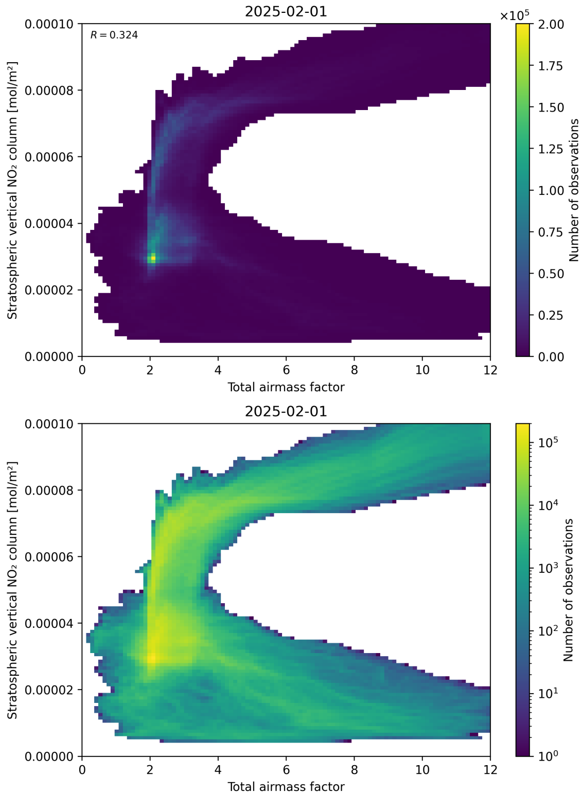
Figure 64: Scatter density plot of “Total airmass factor” against “Stratospheric vertical NO 2 column” for 2025-01-31 to 2025-02-02.
