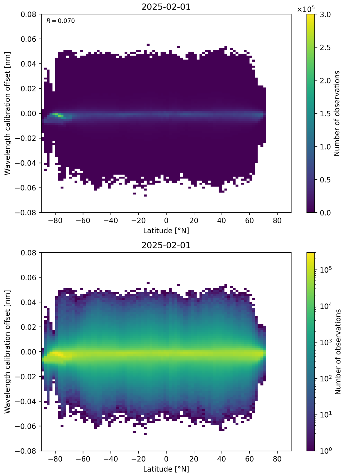
Figure 95: Scatter density plot of “Latitude” against “Wavelength calibration offset” for 2025-01-31 to 2025-02-02.
