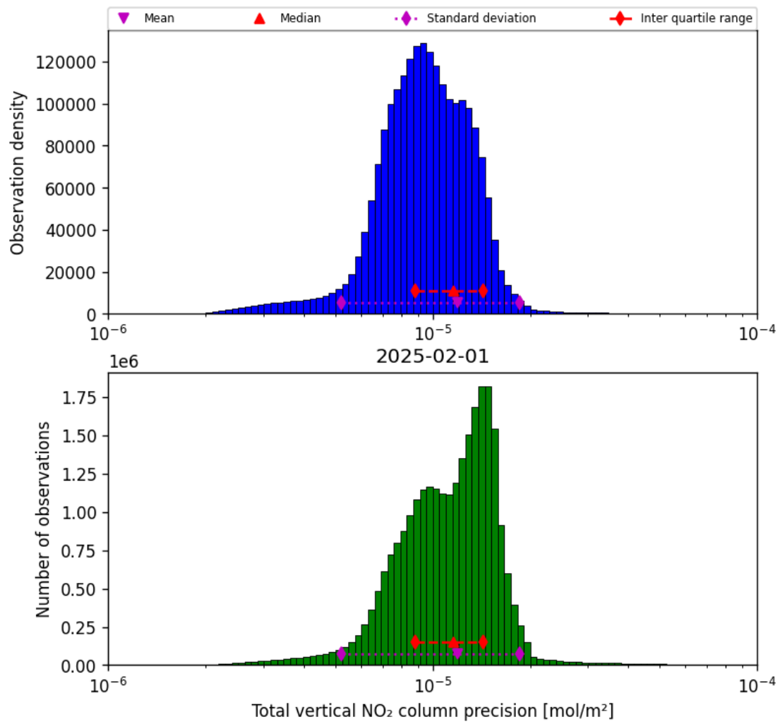
Figure 39: Histogram of “Total vertical NO 2 column precision” for 2025-01-31 to 2025-02-02
