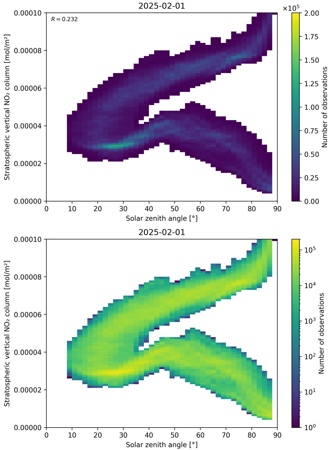
Figure 150: Scatter density plot of “Solar zenith angle” against “Stratospheric vertical NO 2 column” for 2025-01-31 to 2025-02-02.
