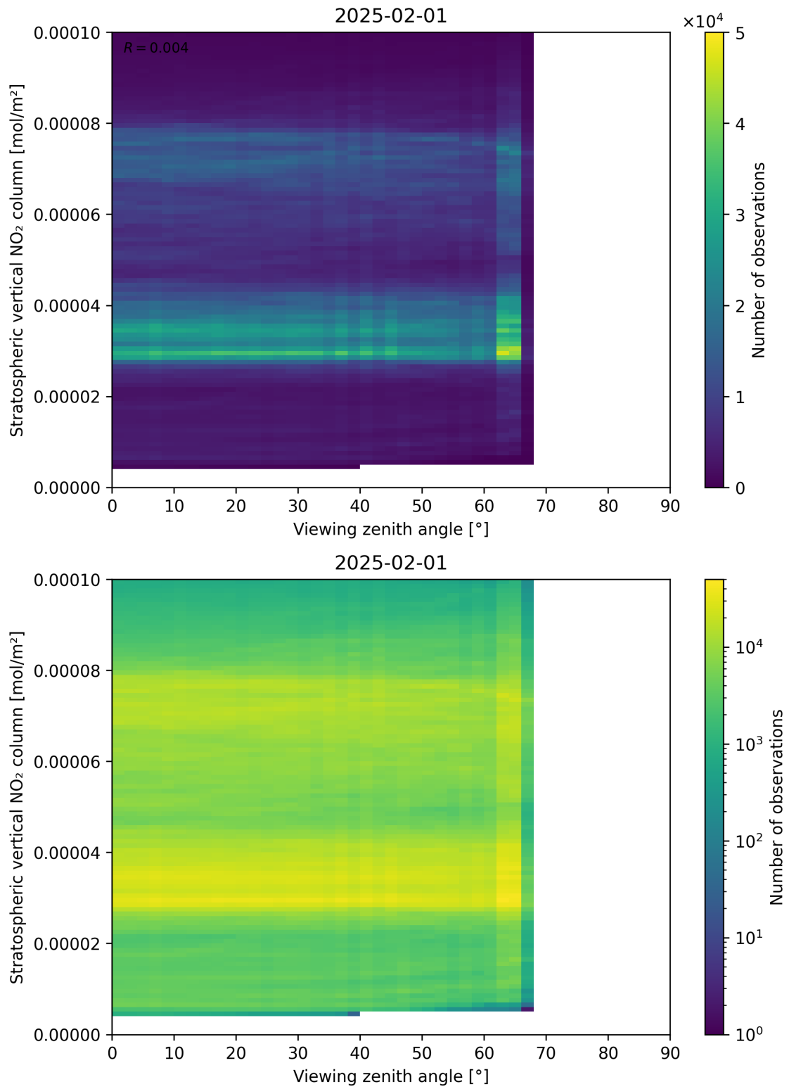
Figure 164: Scatter density plot of “Viewing zenith angle” against “Stratospheric vertical NO 2 column” for 2025-01-31 to 2025-02-02.
