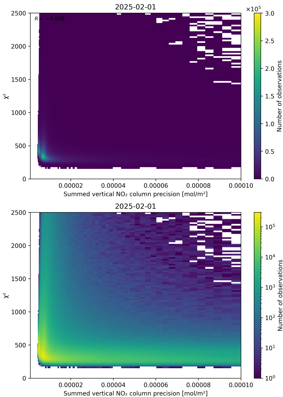
Figure 107: Scatter density plot of “Summed vertical NO 2 column precision” against “ \chi^2 ” for 2025-01-31 to 2025-02-02.
