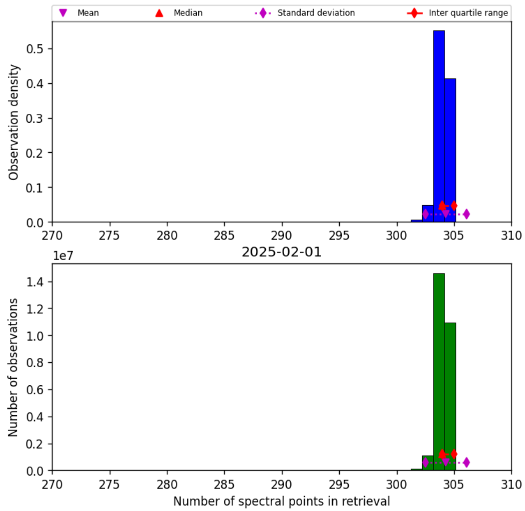
Figure 33: Histogram of “Number of spectral points in retrieval” for 2025-01-31 to 2025-02-02
