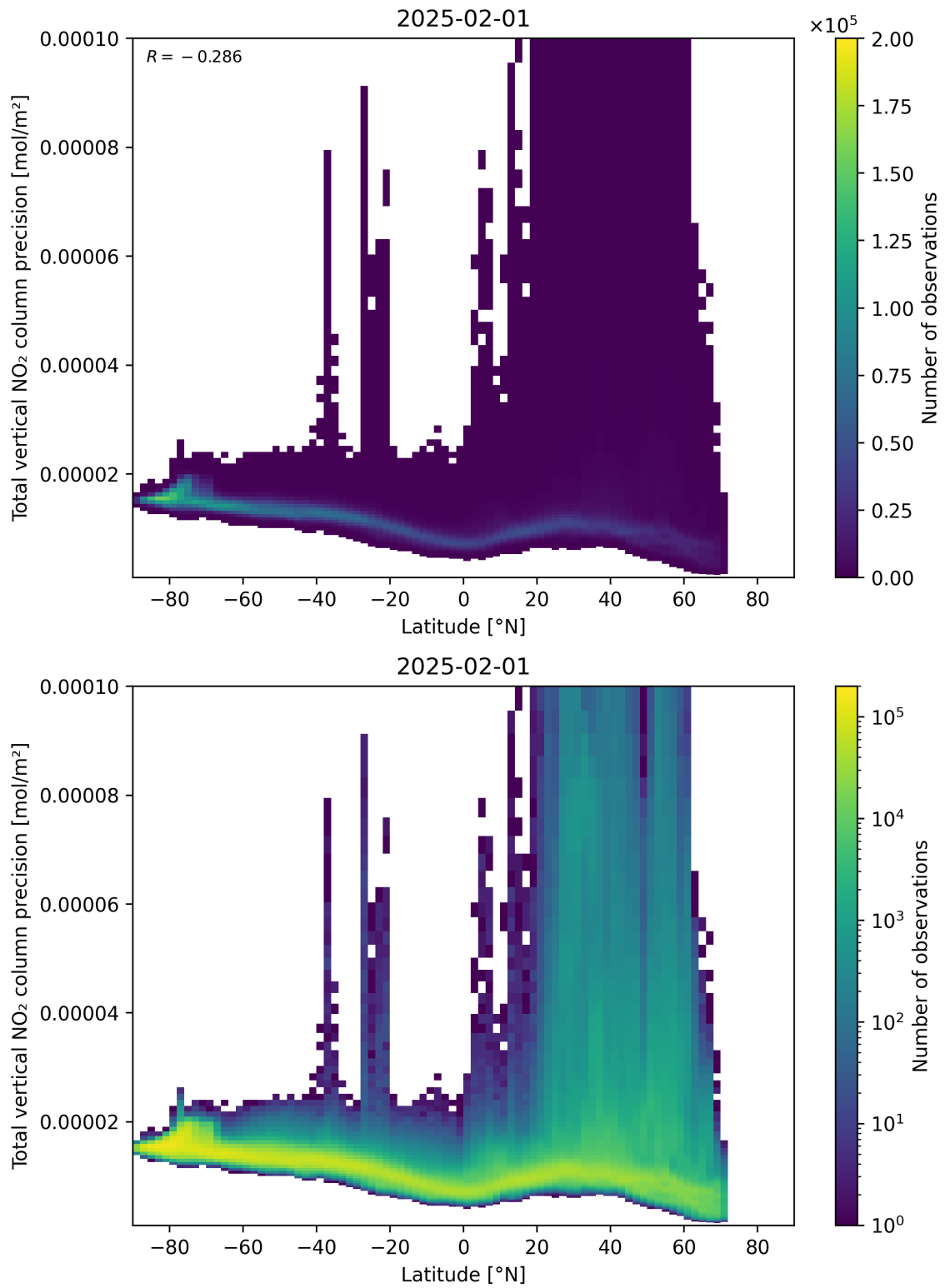
Figure 91: Scatter density plot of “Latitude” against “Total vertical NO 2 column precision” for 2025-01-31 to 2025-02-02.
