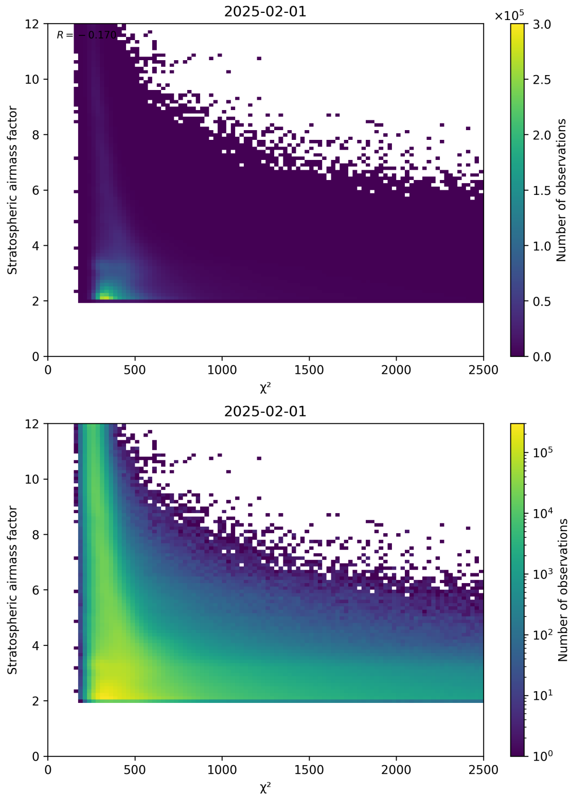
Figure 81: Scatter density plot of “ \chi^2 ” against “Stratospheric airmass factor” for 2025-01-31 to 2025-02-02.
