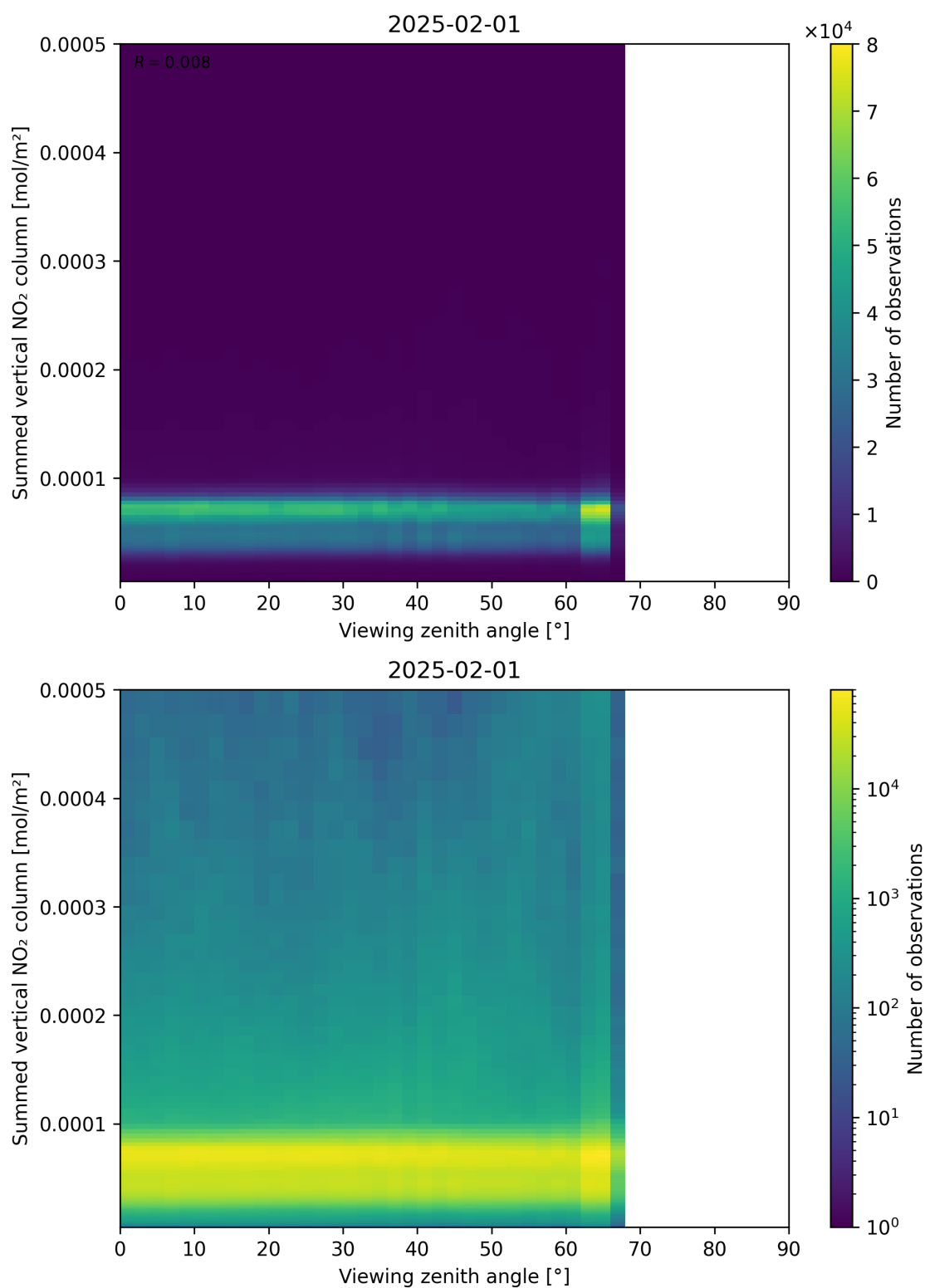
Figure 165: Scatter density plot of “Viewing zenith angle” against “Summed vertical NO 2 column” for 2025-01-31 to 2025-02-02.
