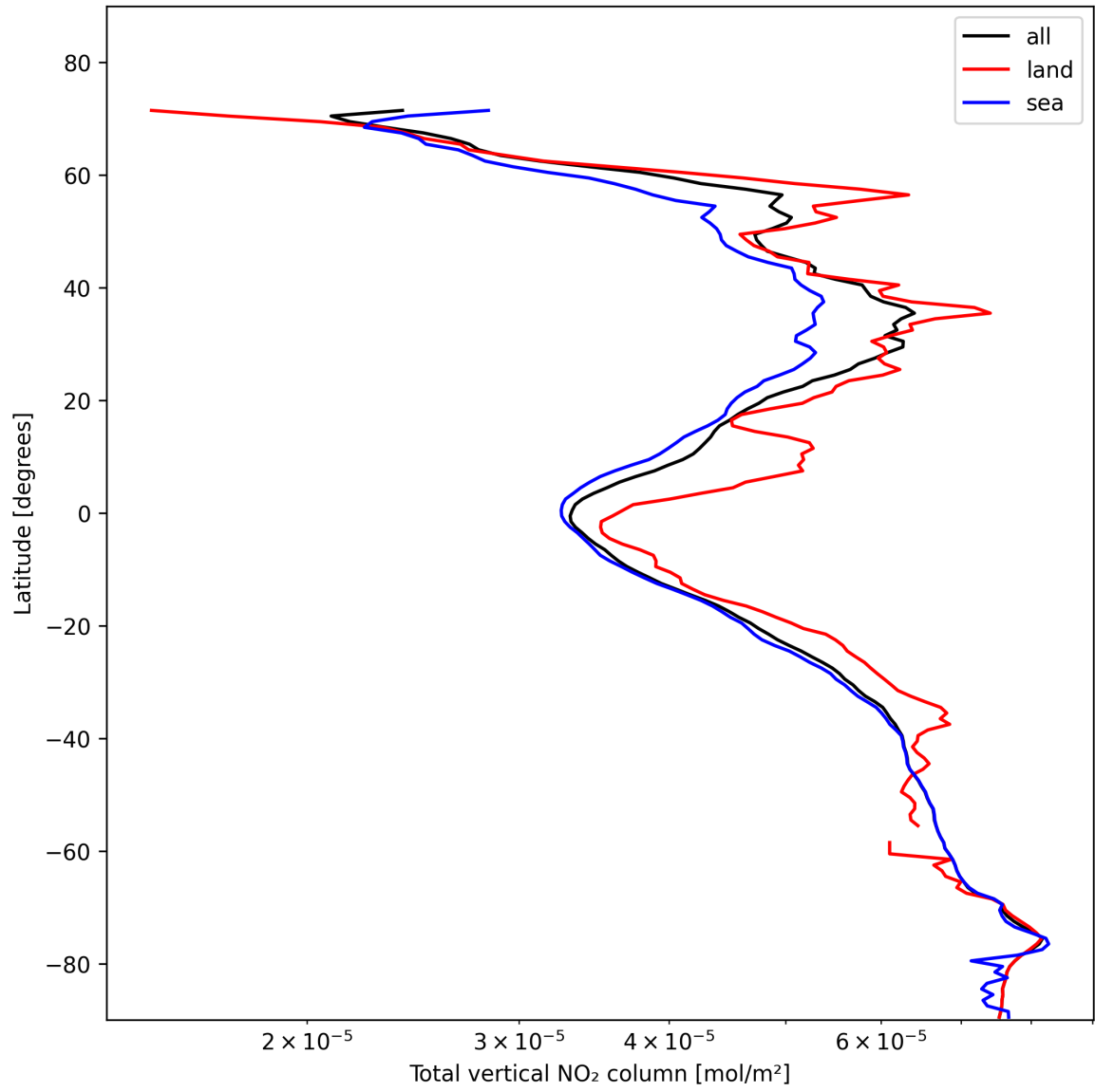
Figure 21: Zonal average of “Total vertical NO 2 column” for 2025-01-31 to 2025-02-02.
