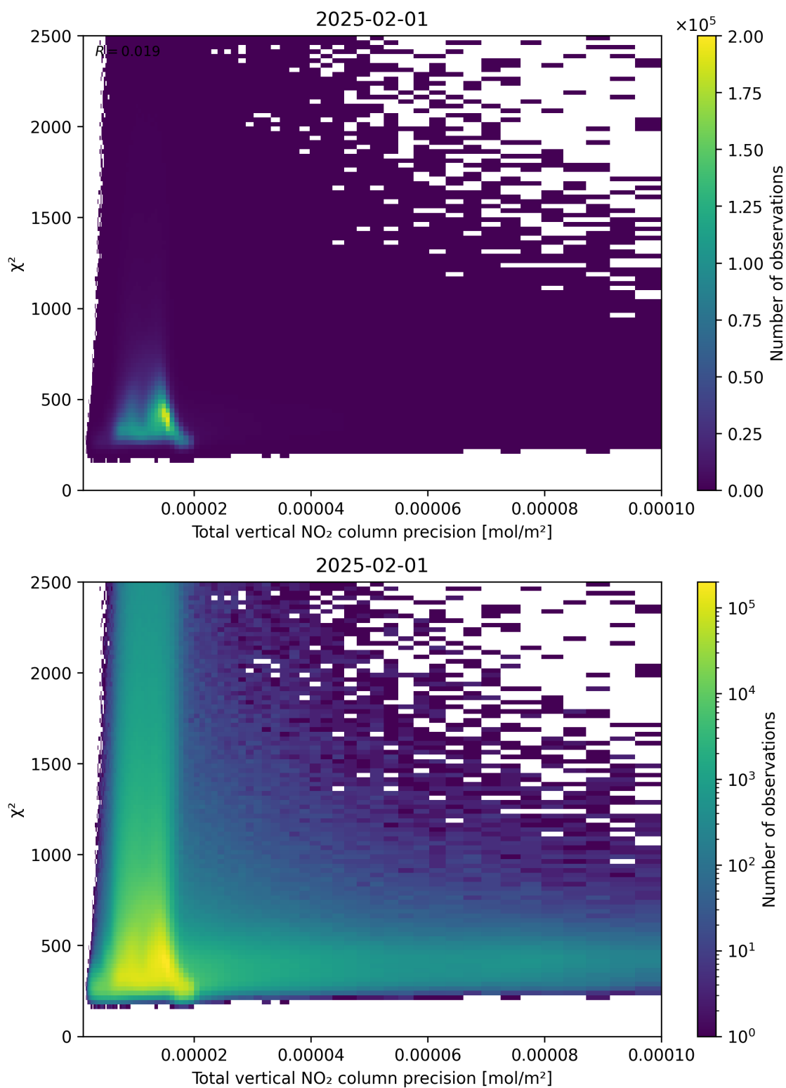
Figure 116: Scatter density plot of “Total vertical NO 2 column precision” against “ \chi^2 ” for 2025-01-31 to 2025-02-02.
