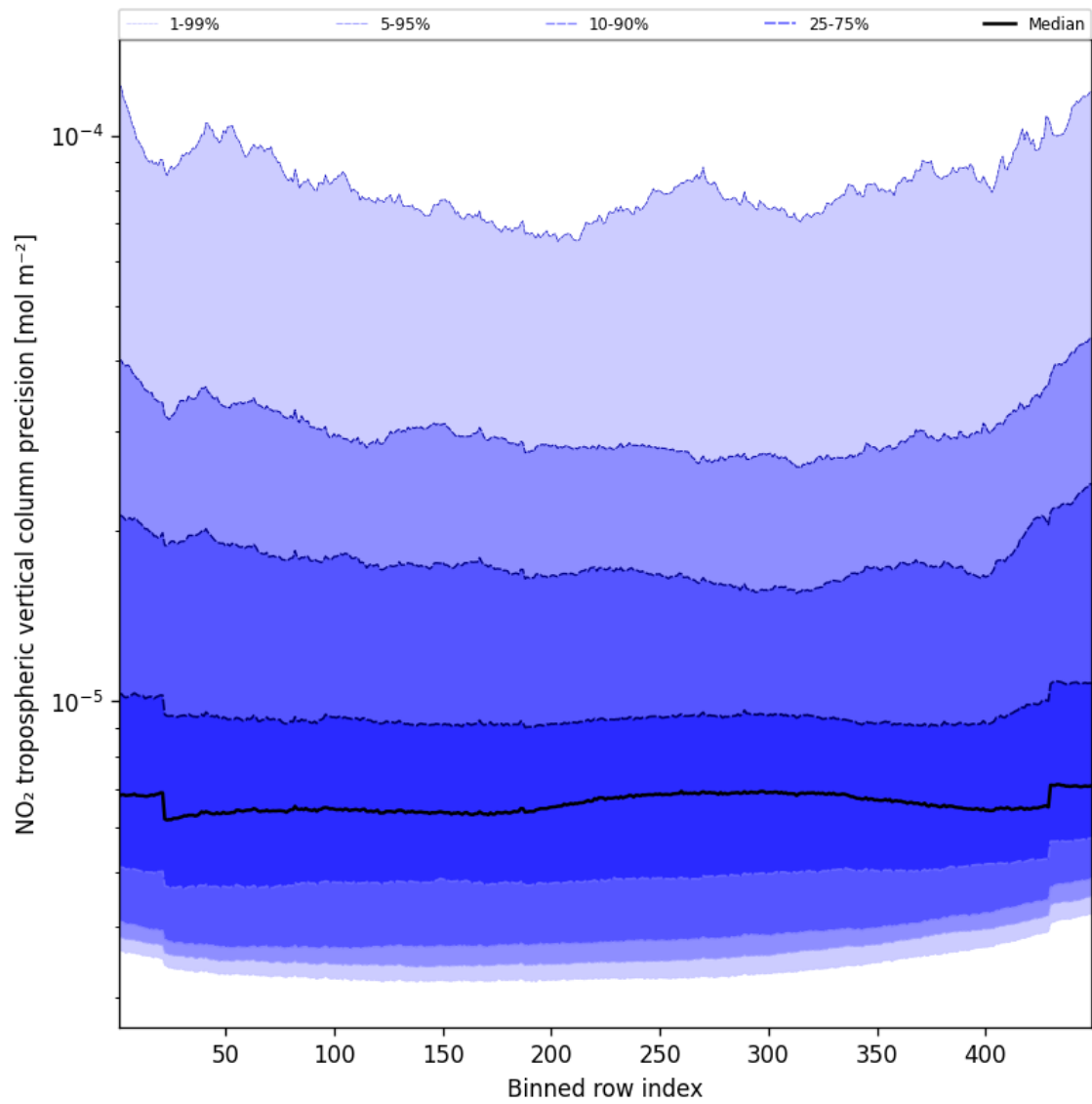
Figure 47: Along track statistics of “NO 2 tropospheric vertical column precision” for 2025-01-31 to 2025-02-02
