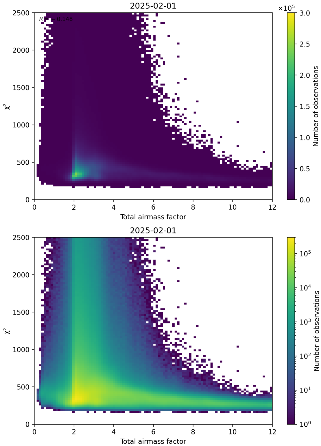
Figure 63: Scatter density plot of “Total airmass factor” against “ \chi^2 ” for 2025-01-31 to 2025-02-02.
