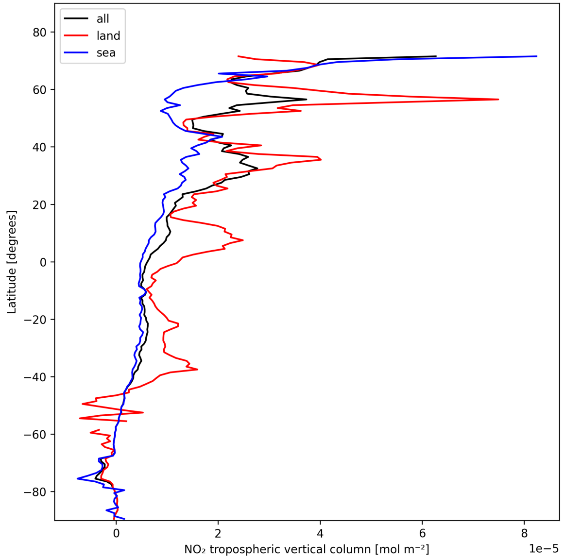
Figure 12: Zonal average of “NO 2 tropospheric vertical column” for 2025-01-31 to 2025-02-02.
