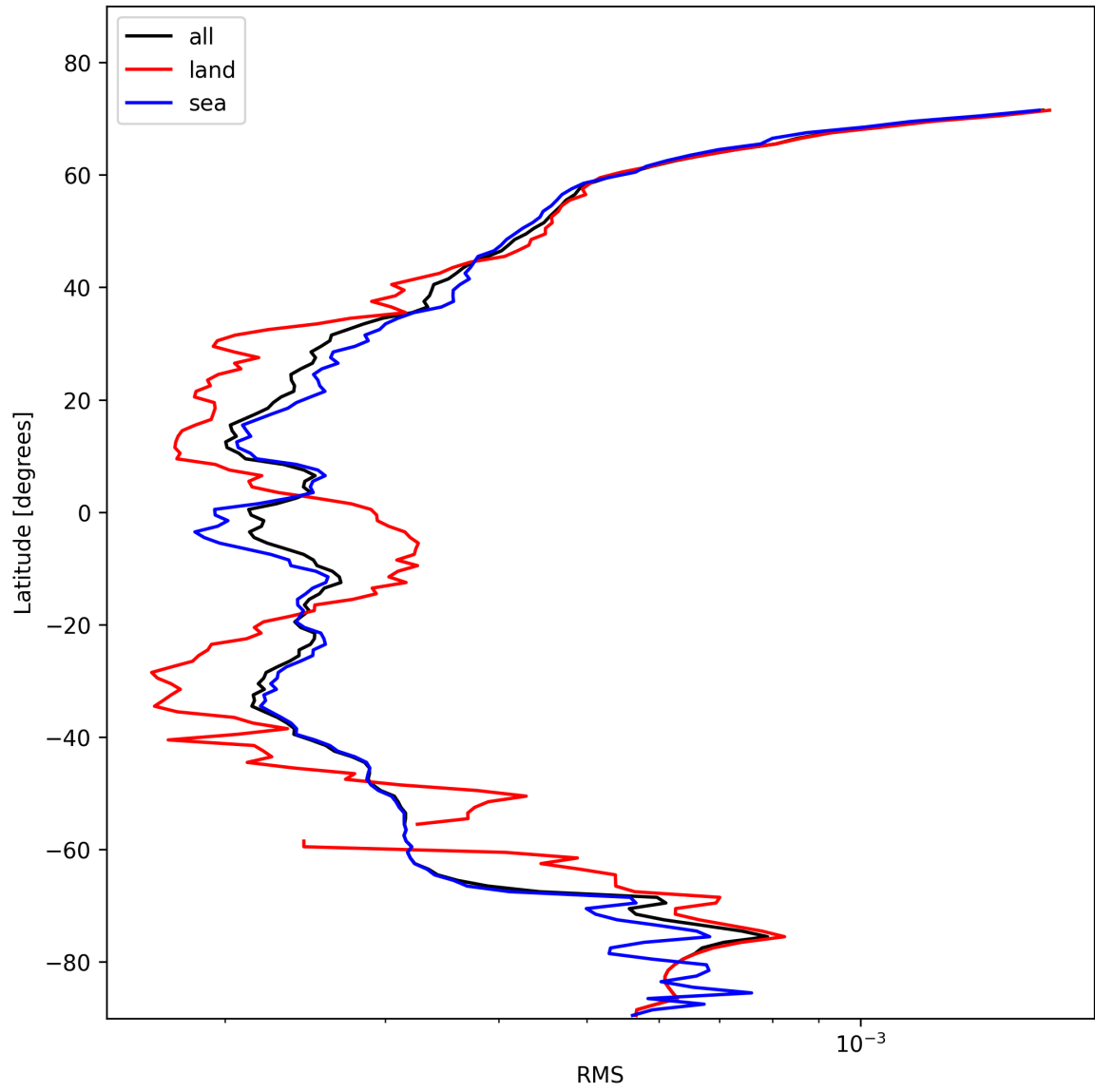
Figure 26: Zonal average of “RMS” for 2025-01-31 to 2025-02-02.
