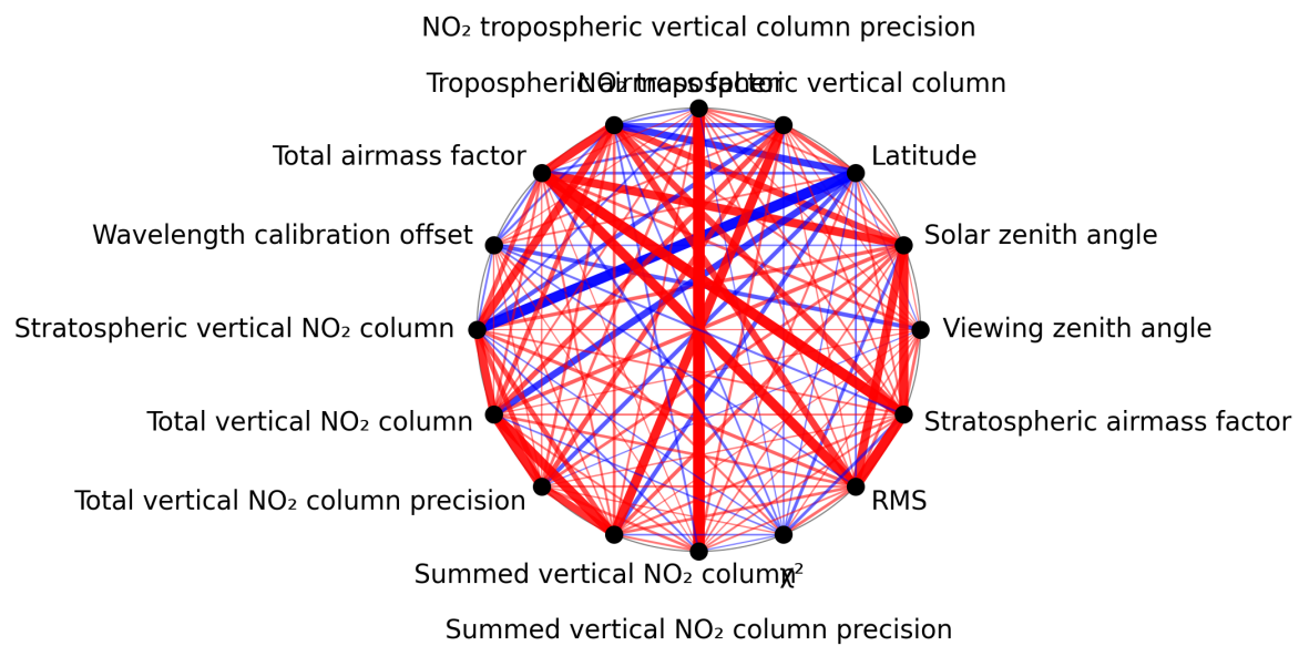
Figure 1: Map of correlation graph for 2025-01-31 to 2025-02-02.
