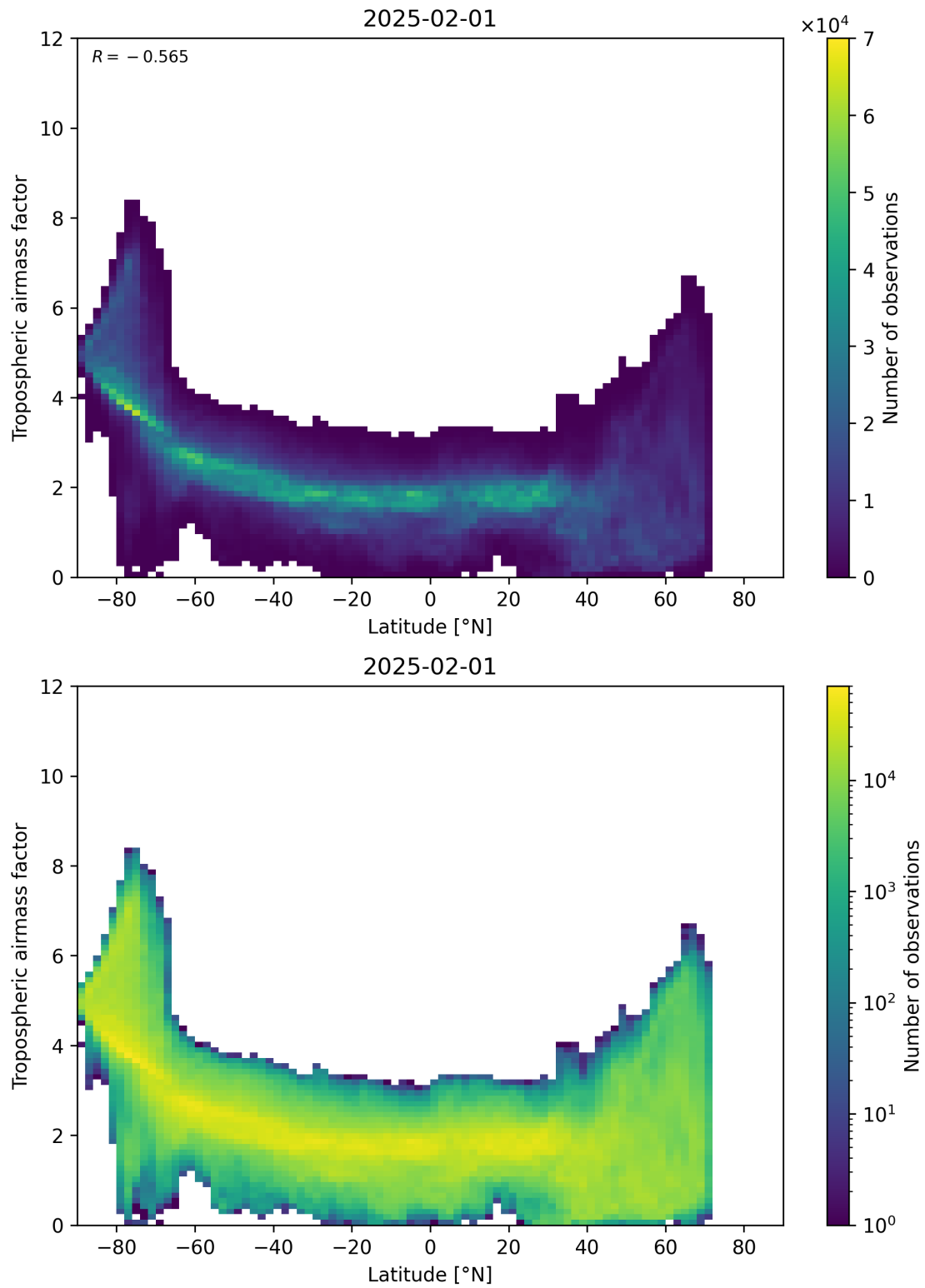
Figure 85: Scatter density plot of “Latitude” against “Tropospheric airmass factor” for 2025-01-31 to 2025-02-02.
