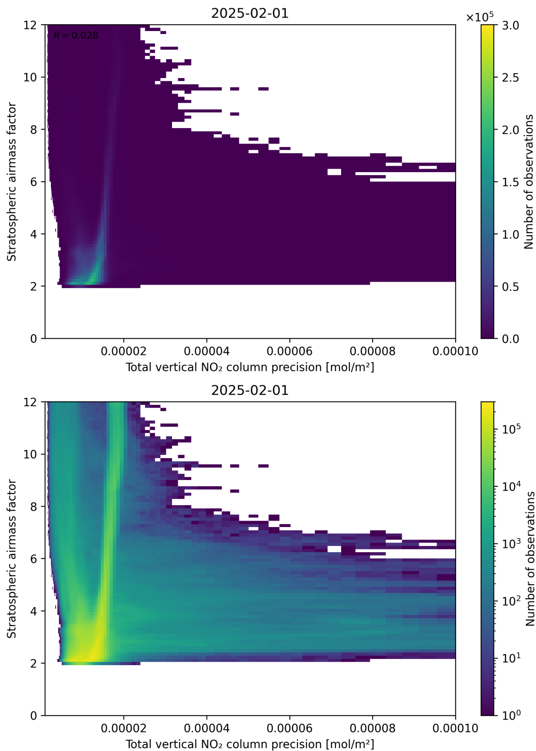
Figure 115: Scatter density plot of “Total vertical NO 2 column precision” against “Stratospheric air mass factor” for 2025-01-31 to 2025-02-02.
