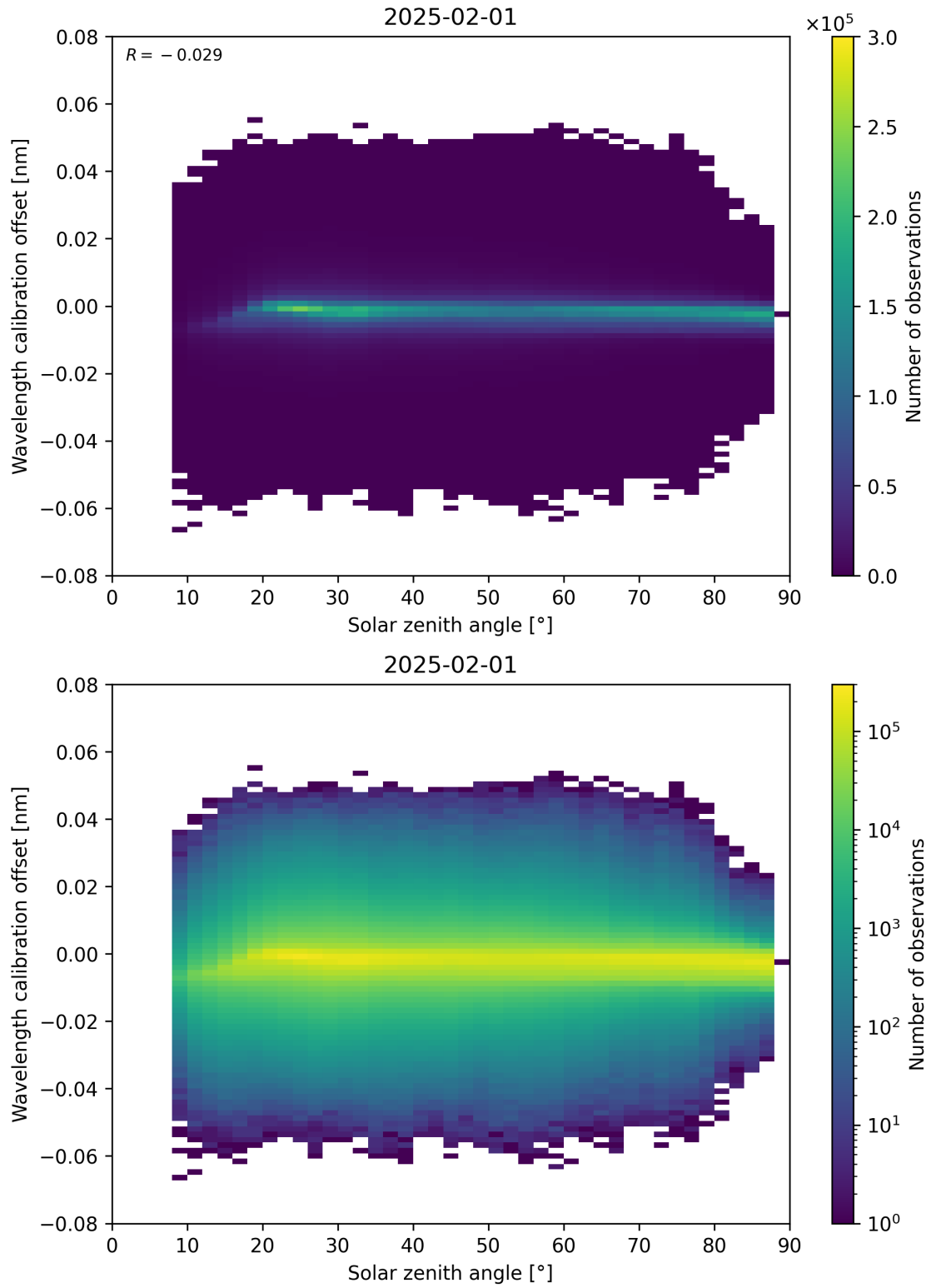
Figure 158: Scatter density plot of “Solar zenith angle” against “Wavelength calibration offset” for 2025-01-31 to 2025-02-02.
