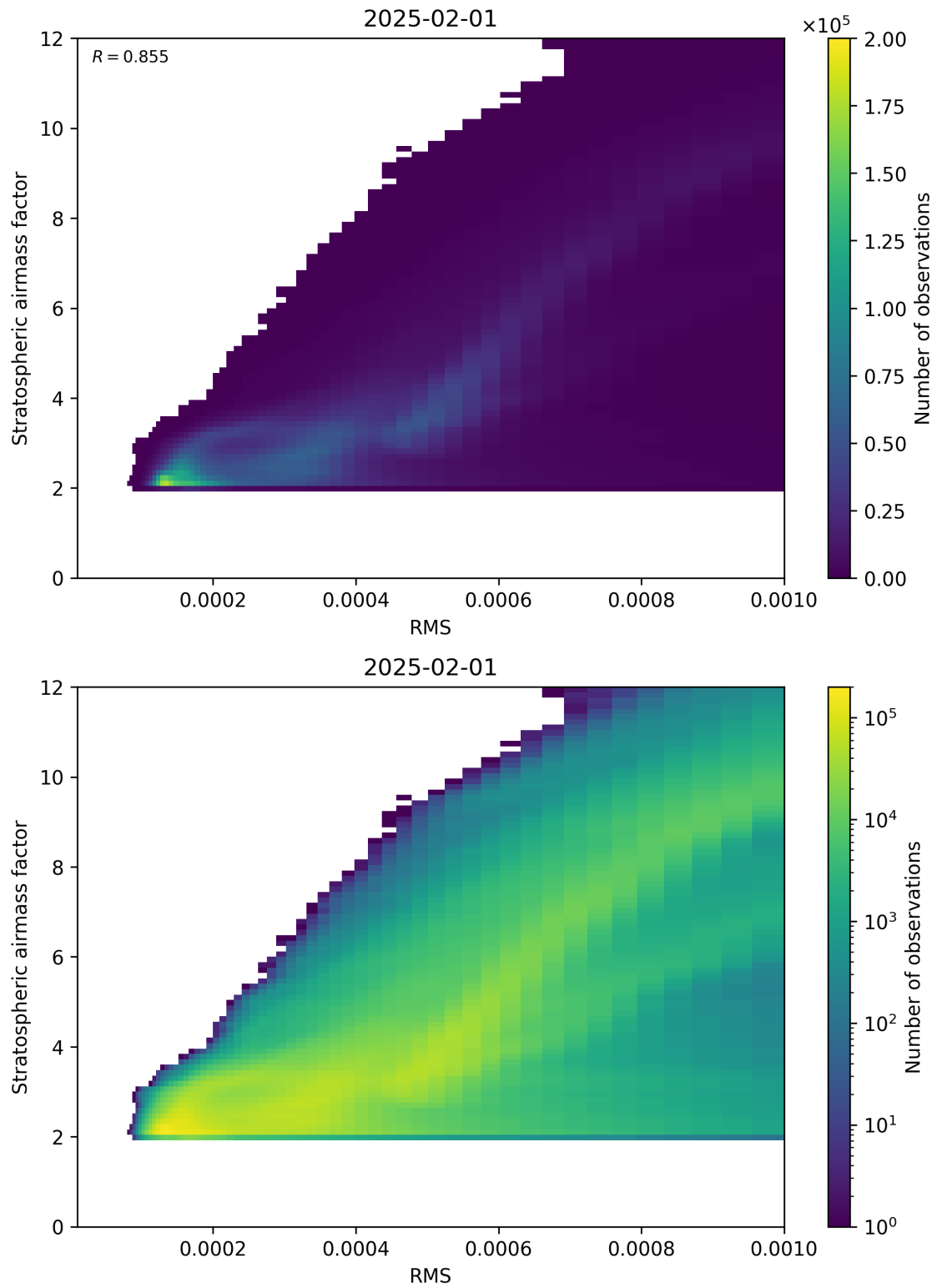
Figure 144: Scatter density plot of “RMS” against “Stratospheric airmass factor” for 2025-01-31 to 2025-02-02.
