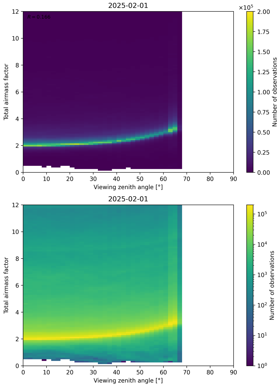
Figure 160: Scatter density plot of “Viewing zenith angle” against “Total airmass factor” for 2025-01-31 to 2025-02-02.
