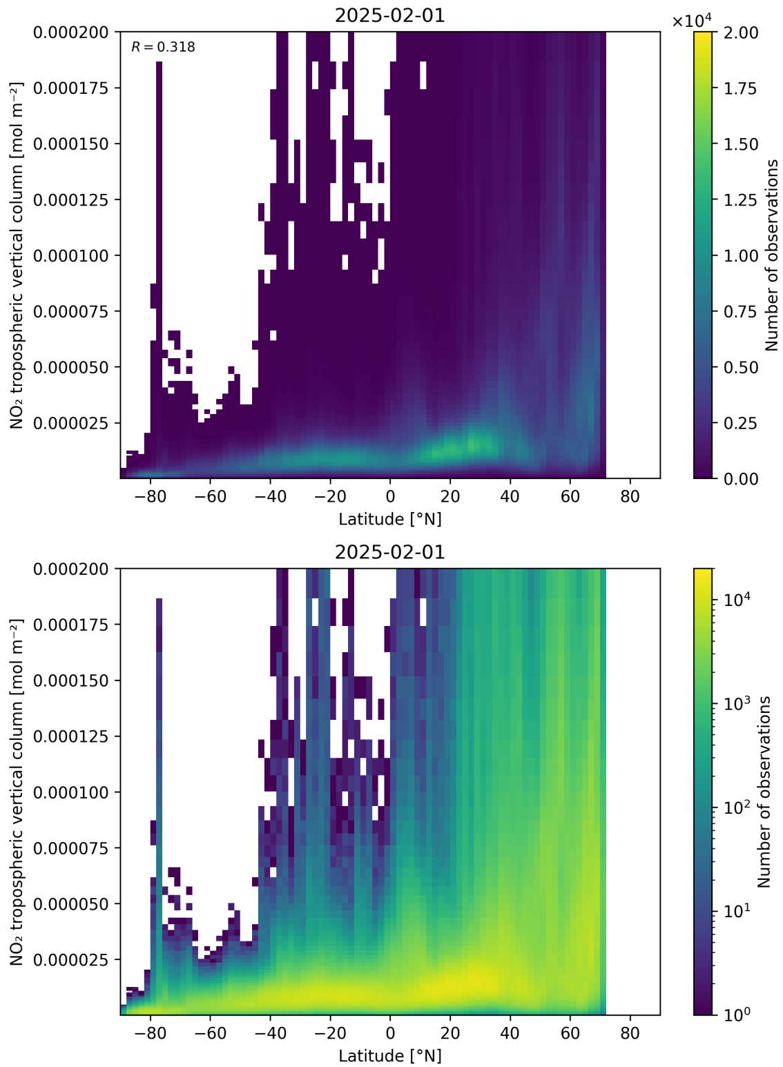
Figure 92: Scatter density plot of “Latitude” against “NO 2 tropospheric vertical column” for 2025-01-31 to 2025-02-02.
