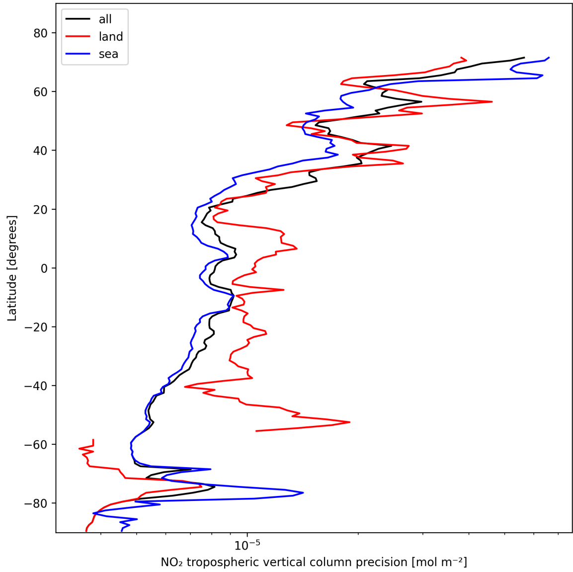
Figure 13: Zonal average of “NO 2 tropospheric vertical column precision” for 2025-01-31 to 2025-02-02.
