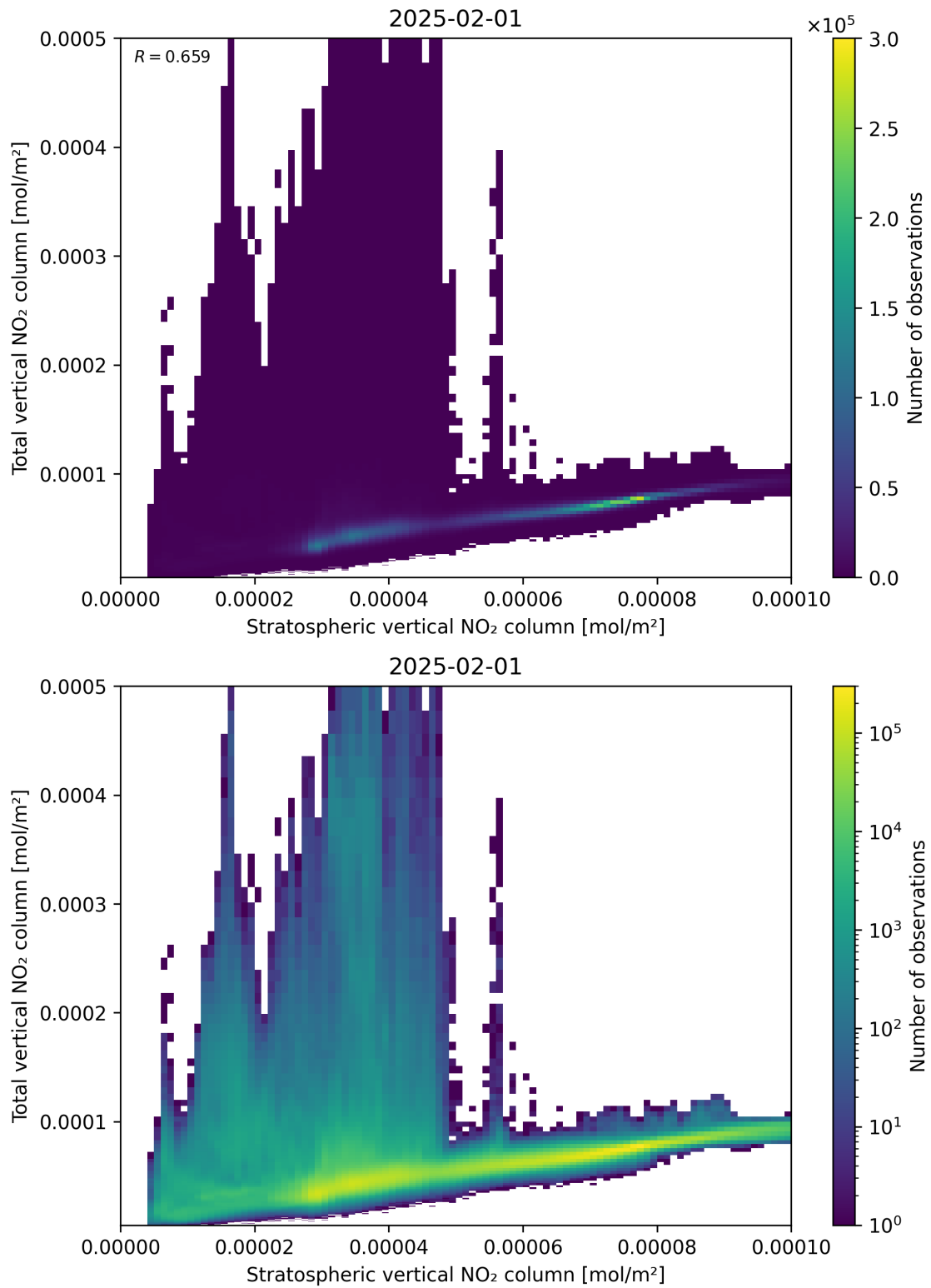
Figure 100: Scatter density plot of “Stratospheric vertical NO 2 column” against “Total vertical NO 2 column” for 2025-01-31 to 2025-02-02.
