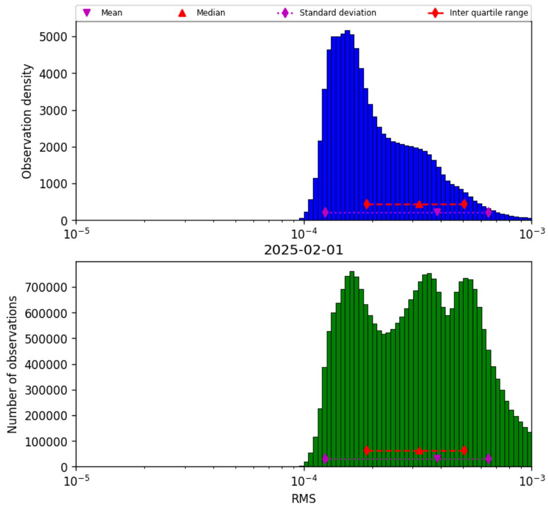
Figure 43: Histogram of “RMS” for 2025-01-31 to 2025-02-02
