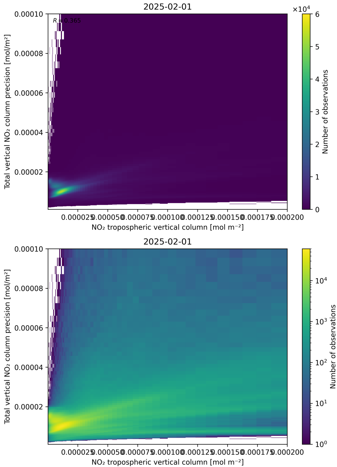
Figure 129: Scatter density plot of “NO 2 tropospheric vertical column” against “Total vertical NO 2 column precision” for 2025-01-31 to 2025-02-02.
