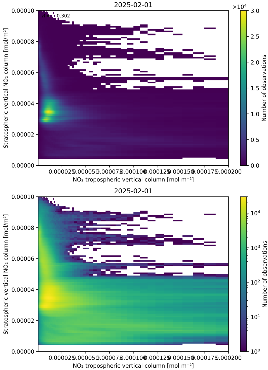
Figure 125: Scatter density plot of “NO 2 tropospheric vertical column” against “Stratospheric vertical NO 2 column” for 2025-01-31 to 2025-02-02.
