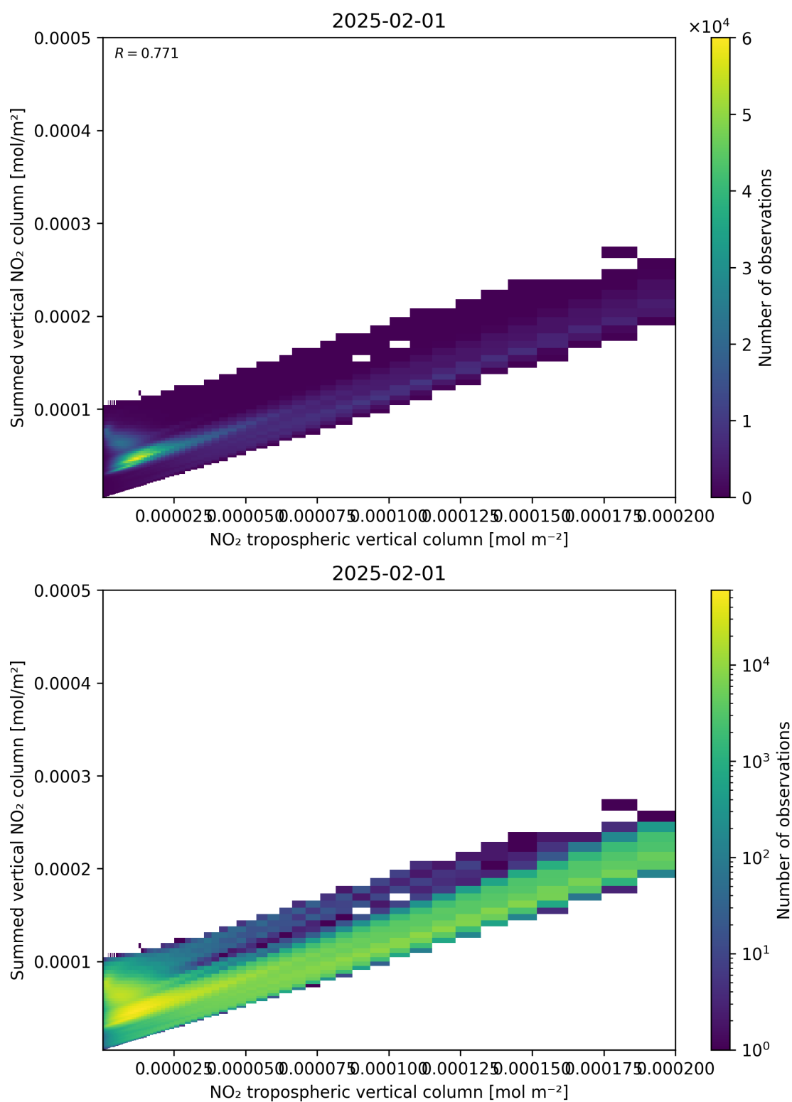
Figure 126: Scatter density plot of “NO 2 tropospheric vertical column” against “Summed vertical NO 2 column” for 2025-01-31 to 2025-02-02.
