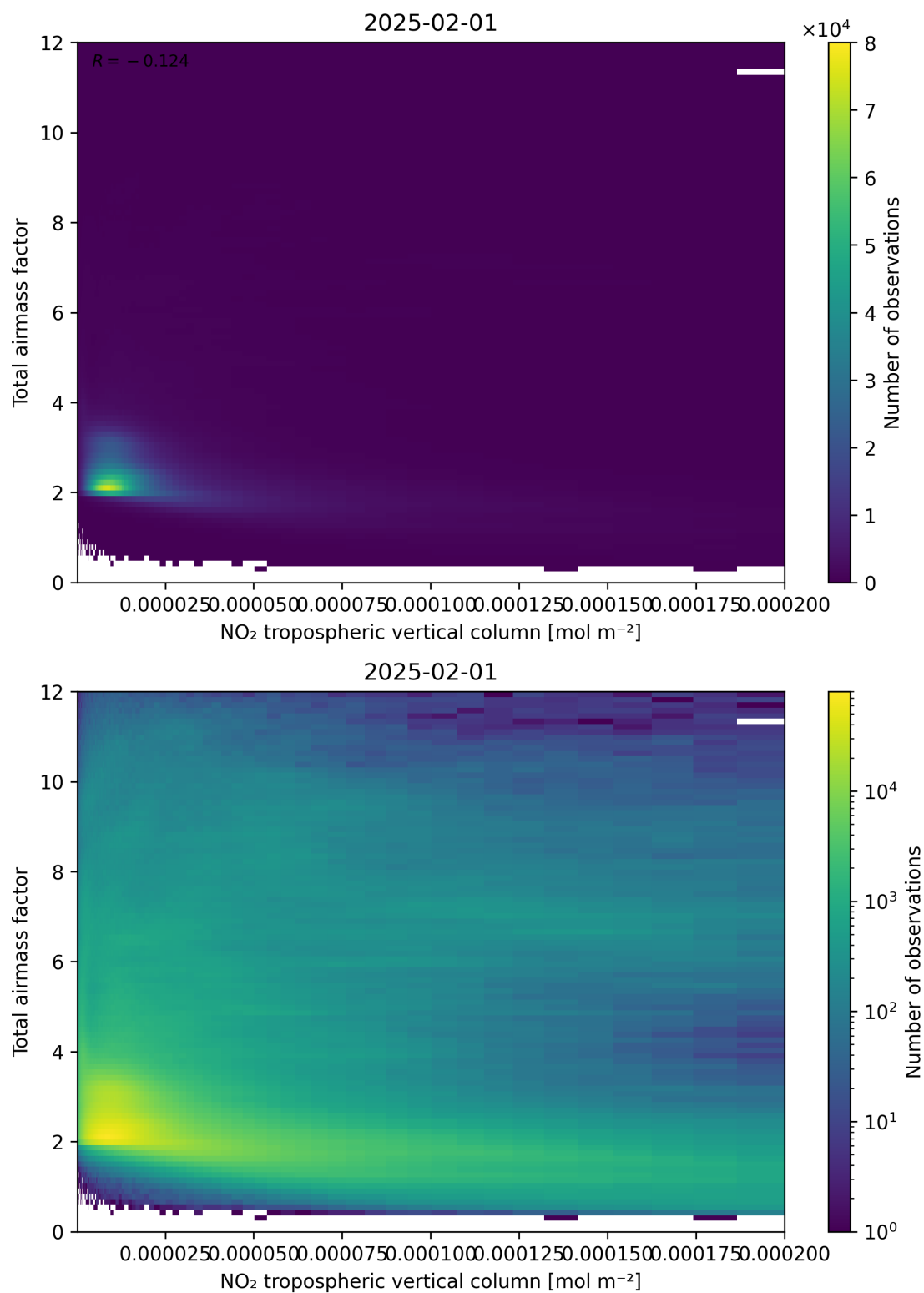
Figure 122: Scatter density plot of “NO 2 tropospheric vertical column” against “Total air mass factor” for 2025-01-31 to 2025-02-02.
