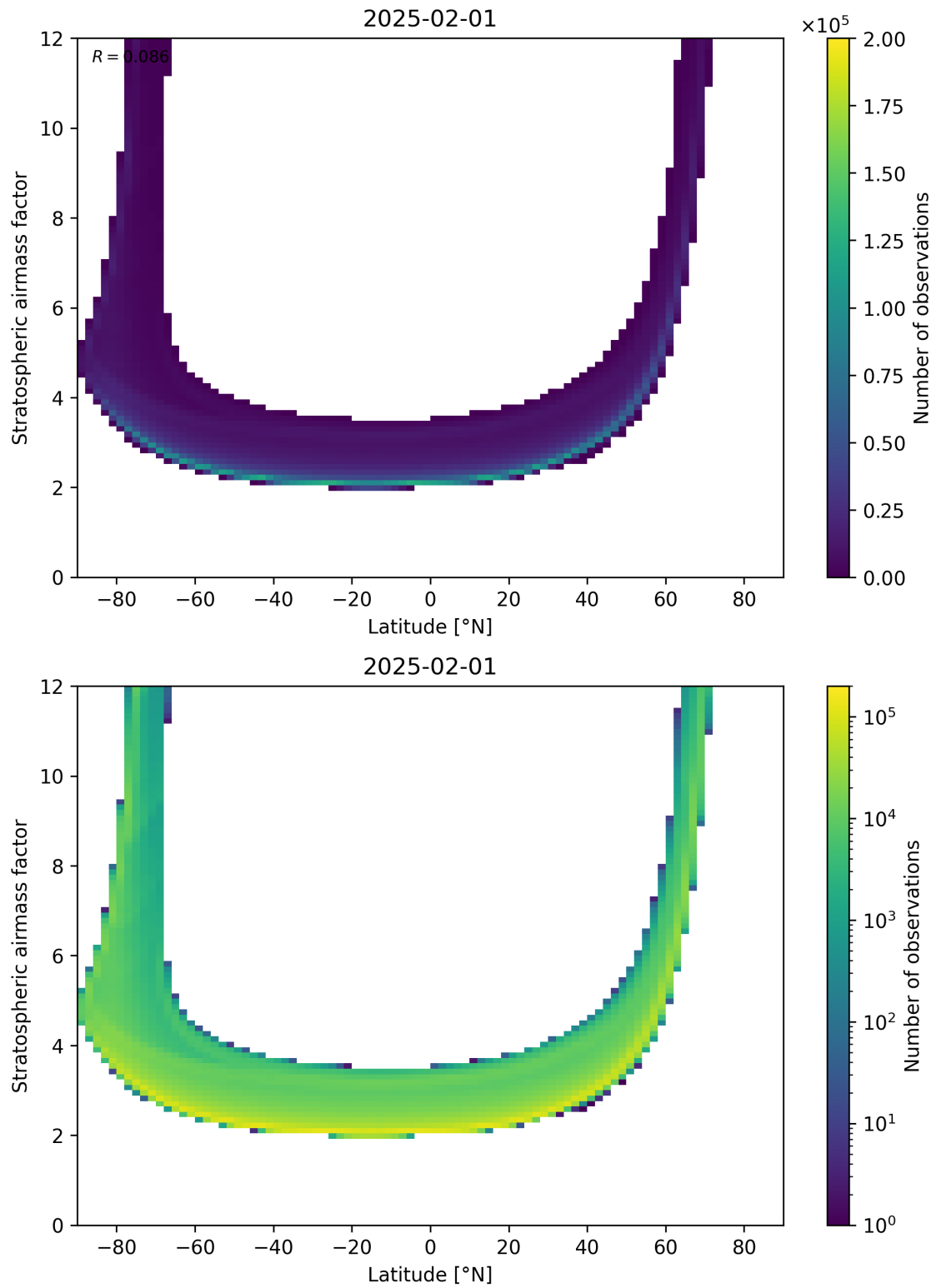
Figure 83: Scatter density plot of “Latitude” against “Stratospheric air mass factor” for 2025-01-31 to 2025-02-02.
