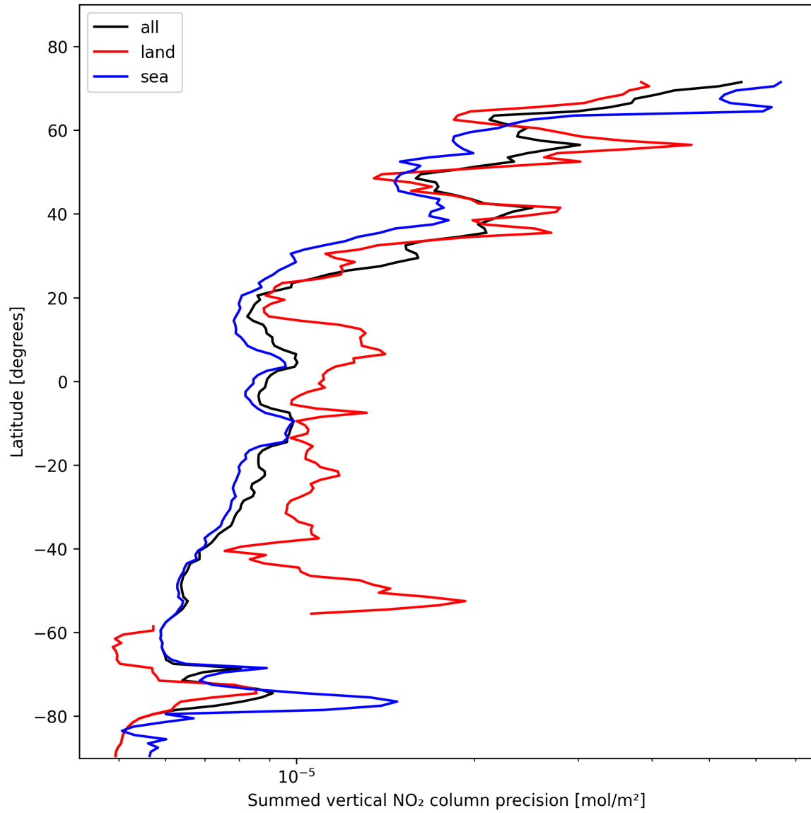
Figure 24: Zonal average of “Summed vertical NO 2 column precision” for 2025-01-31 to 2025-02-02.
