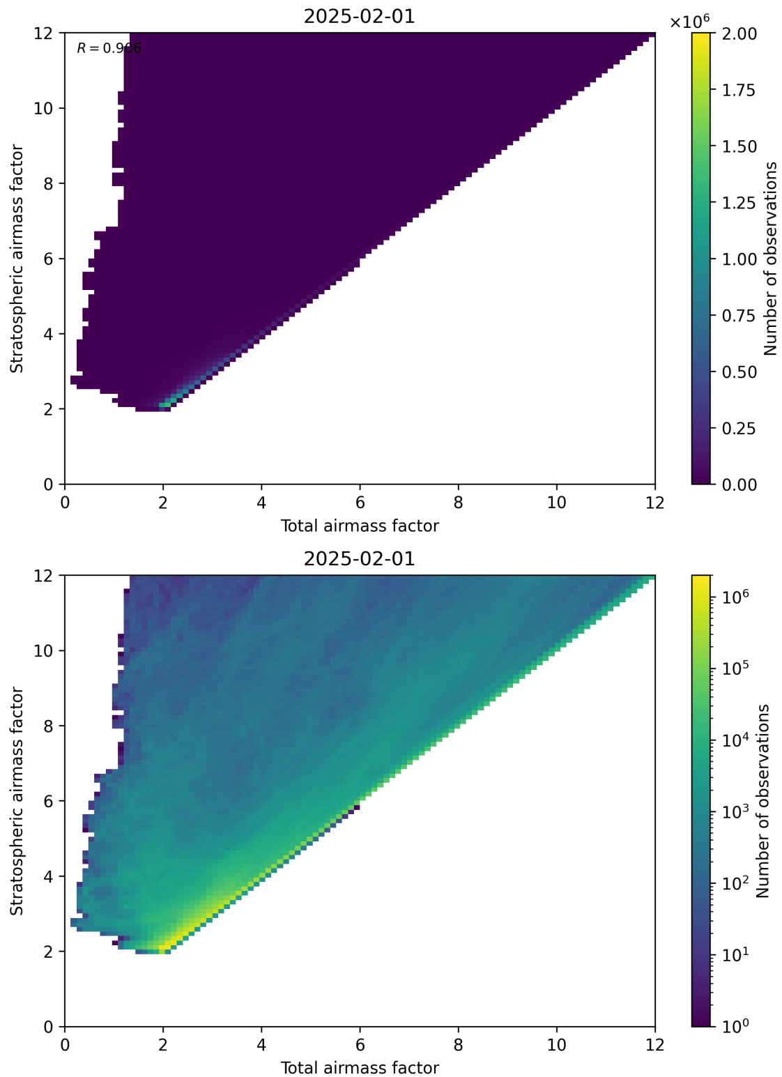
Figure 62: Scatter density plot of “Total air mass factor” against “Stratospheric air mass factor” for 2025-01-31 to 2025-02-02.
