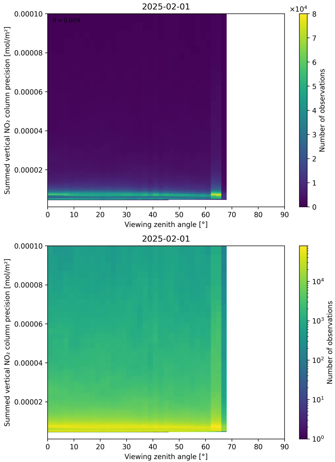
Figure 166: Scatter density plot of “Viewing zenith angle” against “Summed vertical NO 2 column precision” for 2025-01-31 to 2025-02-02.
