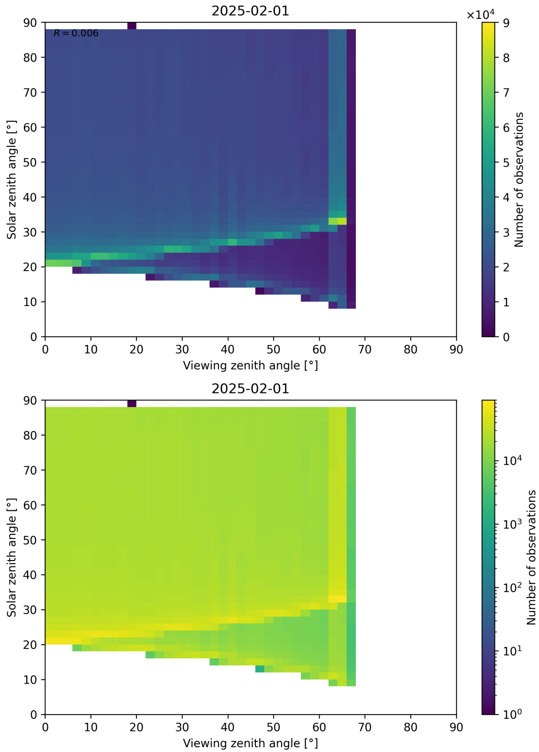
Figure 172: Scatter density plot of “Viewing zenith angle” against “Solar zenith angle” for 2025-01-31 to 2025-02-02.
