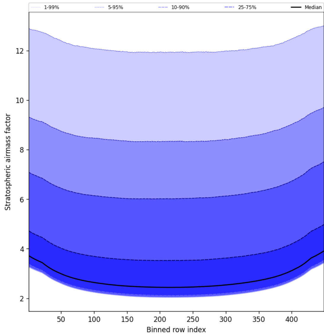
Figure 61: Along track statistics of “Stratospheric airmass factor” for 2025-01-31 to 2025-02-02
