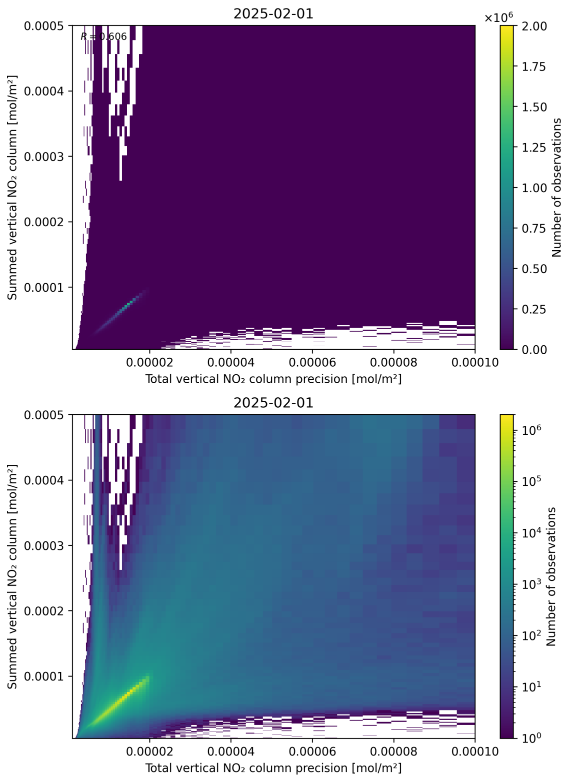
Figure 117: Scatter density plot of “Total vertical NO 2 column precision” against “Summed vertical NO 2 column” for 2025-01-31 to 2025-02-02.
