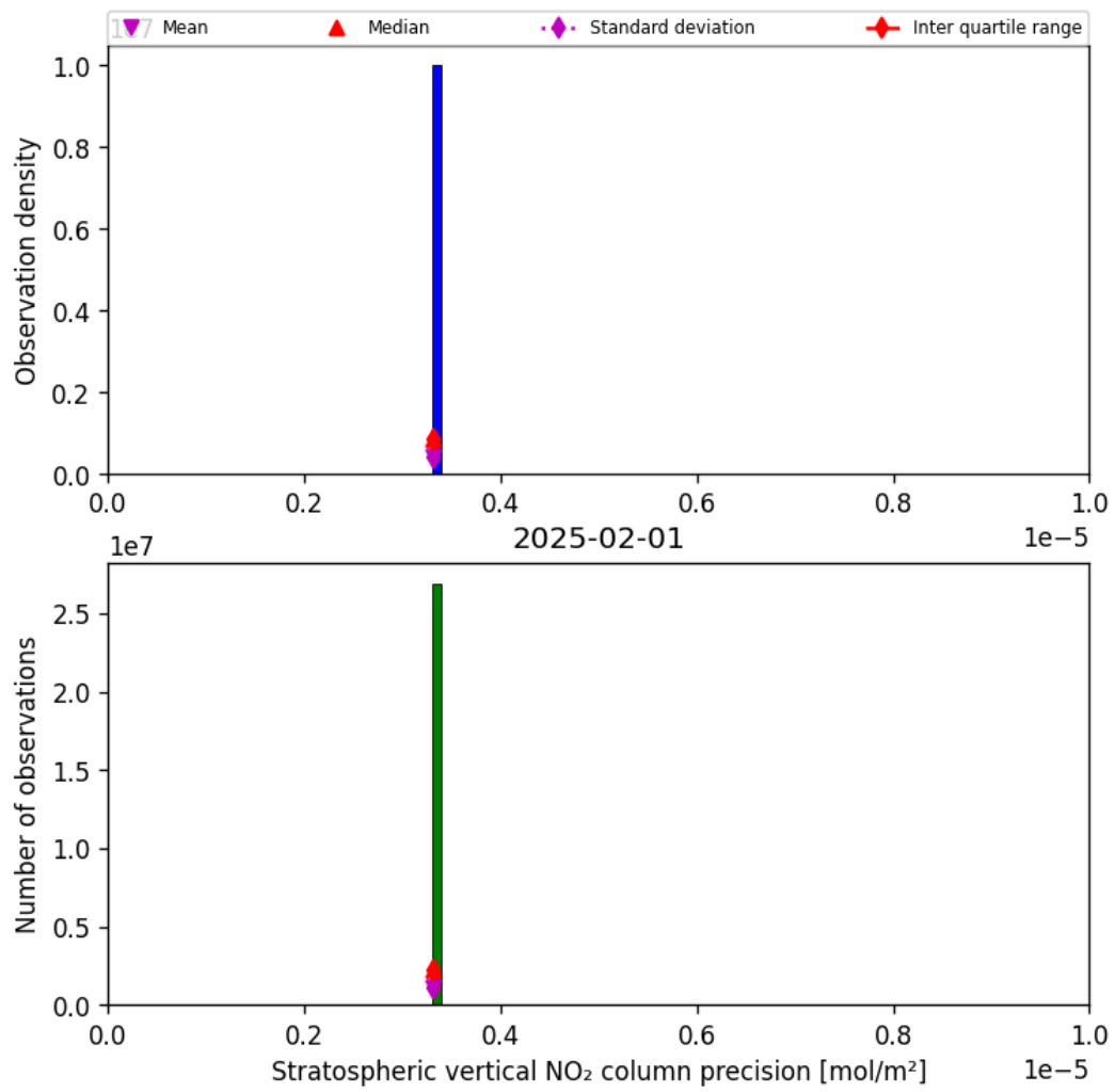
Figure 37: Histogram of “Stratospheric vertical NO 2 column precision” for 2025-01-31 to 2025-02-02
