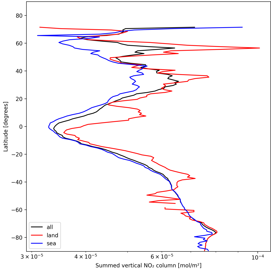
Figure 23: Zonal average of “Summed vertical NO 2 column” for 2025-01-31 to 2025-02-02.
