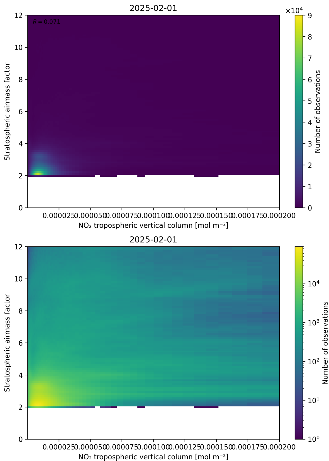
Figure 121: Scatter density plot of “NO 2 tropospheric vertical column” against “Stratospheric airmass factor” for 2025-01-31 to 2025-02-02.
