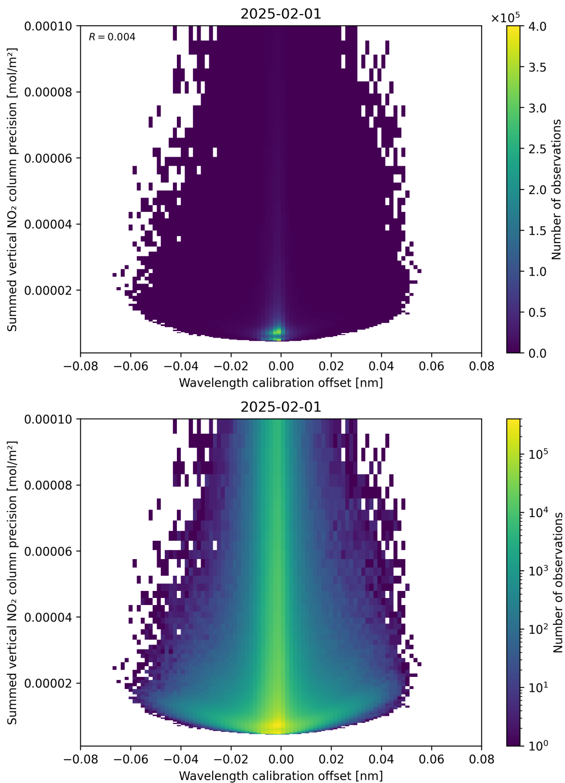
Figure 178: Scatter density plot of “Wavelength calibration offset” against “Summed vertical NO 2 column precision” for 2025-01-31 to 2025-02-02.
