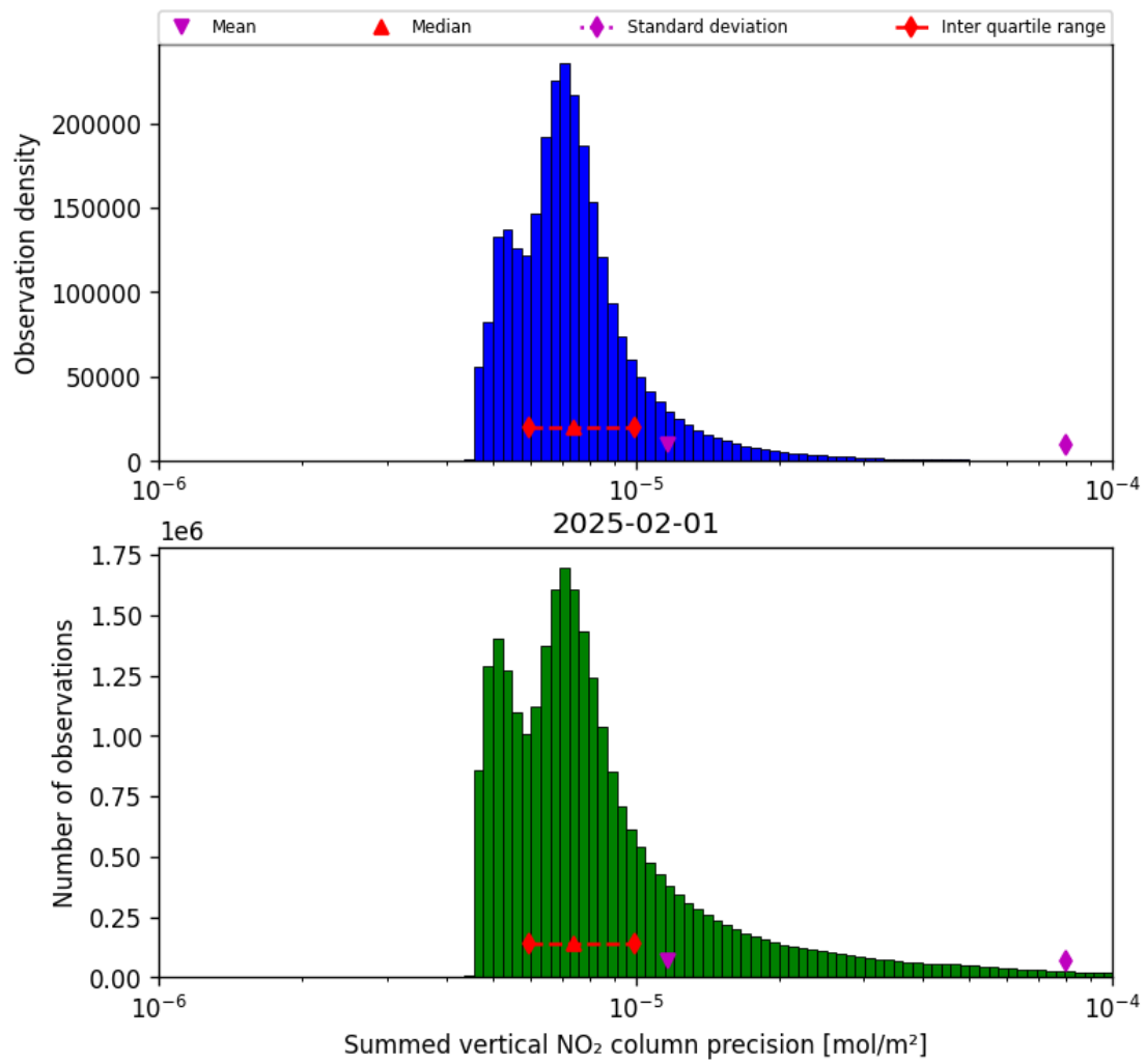
Figure 41: Histogram of “Summed vertical NO 2 column precision” for 2025-01-31 to 2025-02-02
