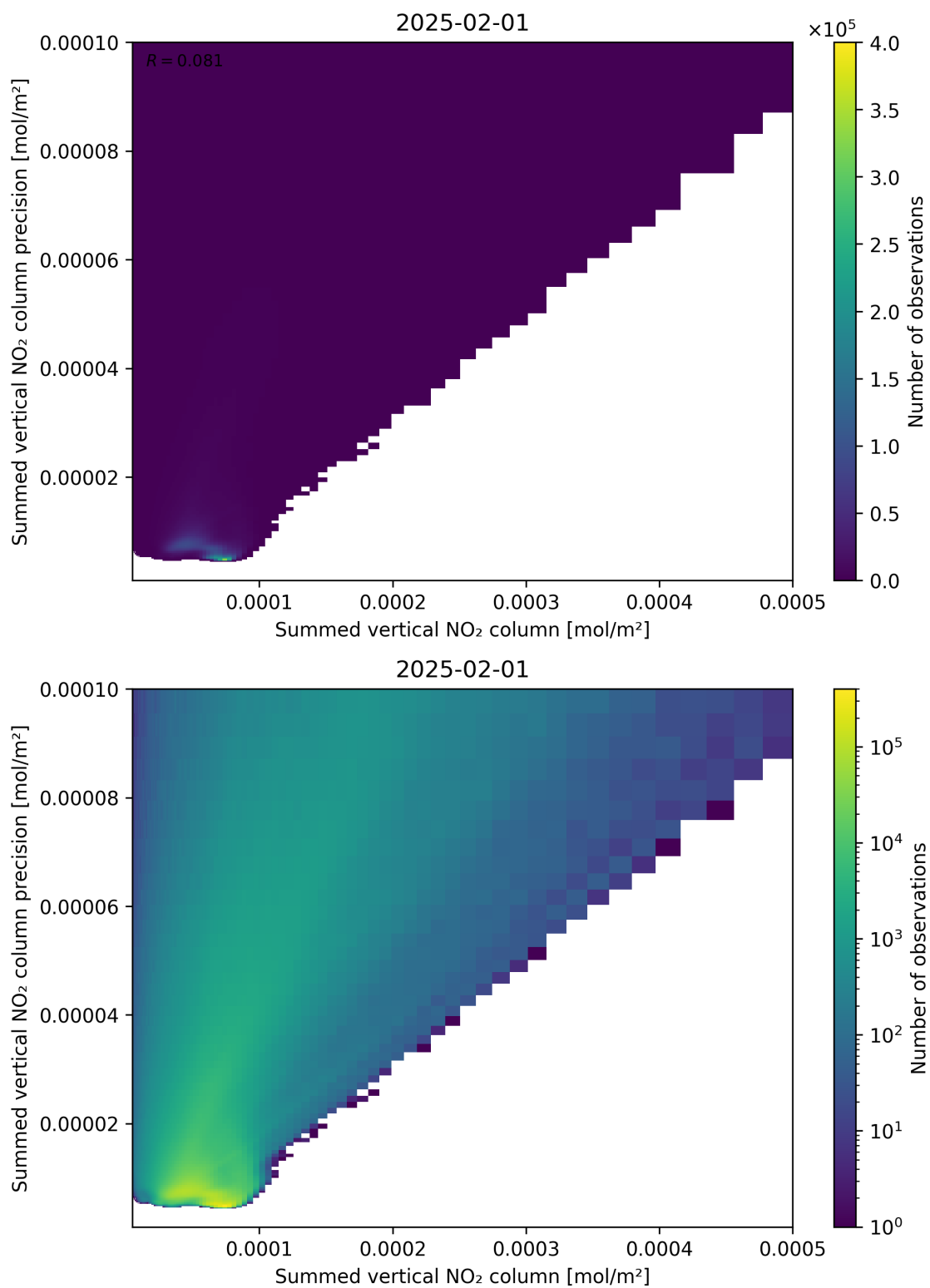
Figure 105: Scatter density plot of “Summed vertical NO 2 column” against “Summed vertical NO 2 column precision” for 2025-01-31 to 2025-02-02.
