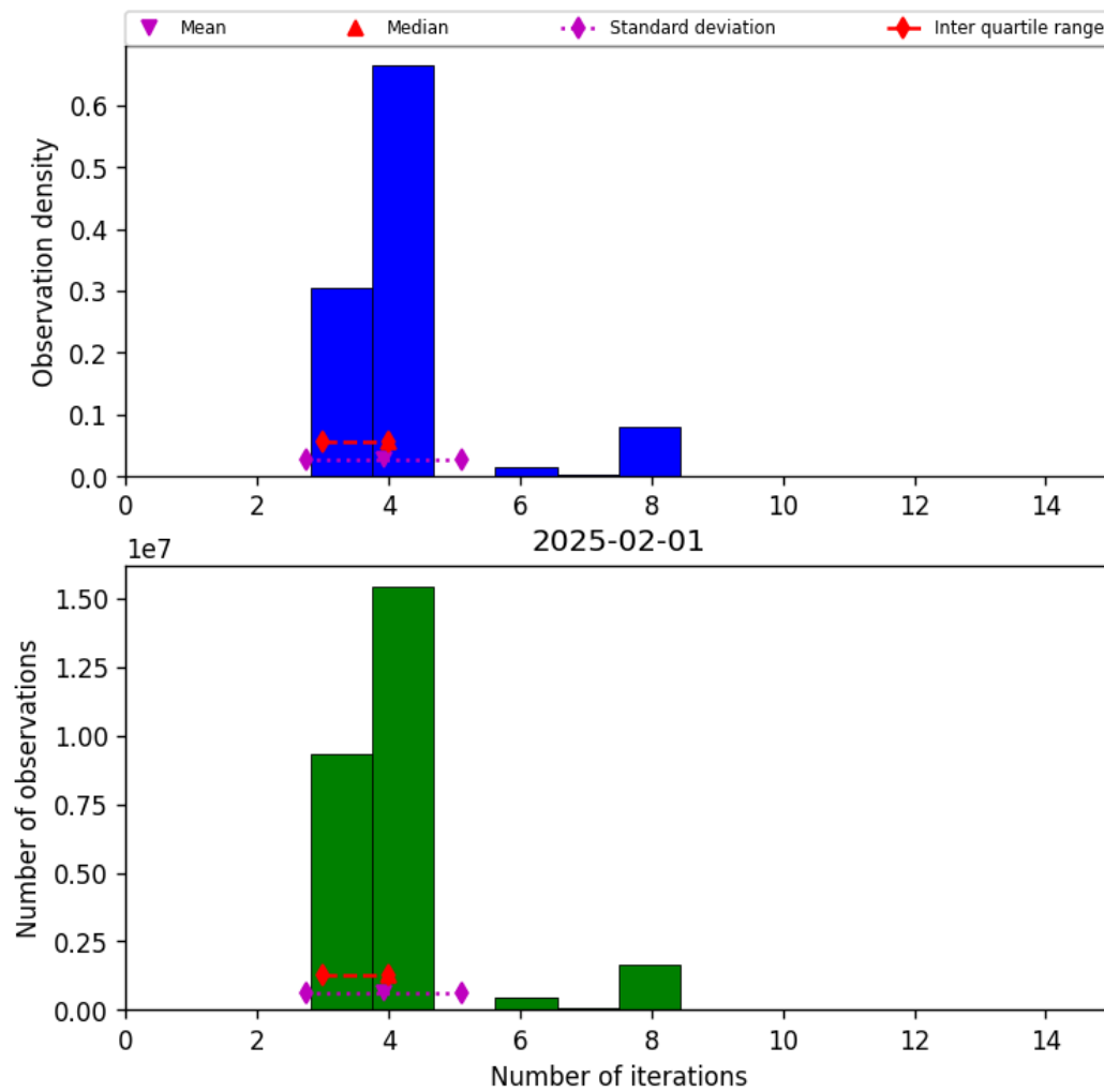
Figure 34: Histogram of “Number of iterations” for 2025-01-31 to 2025-02-02
