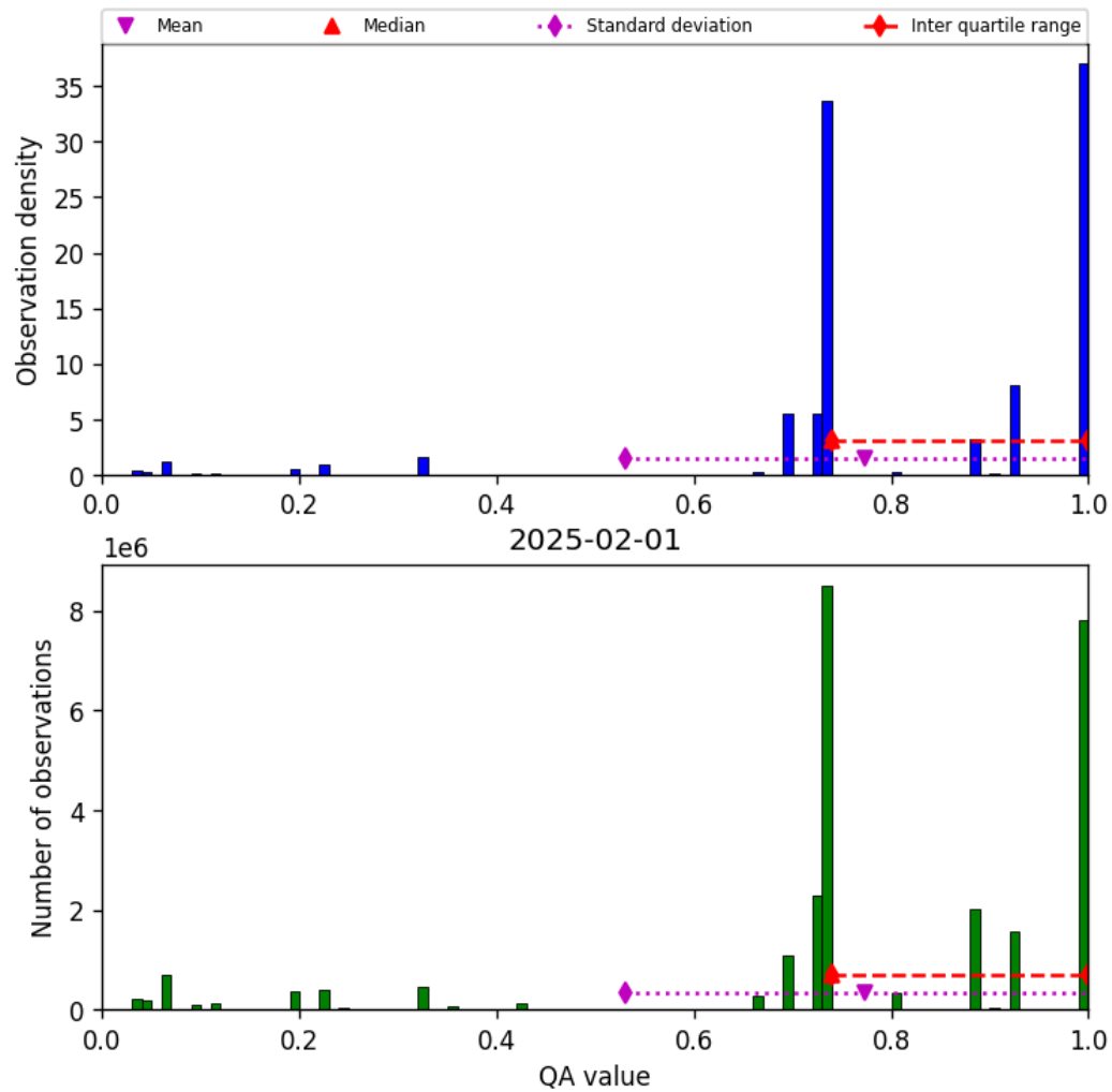
Figure 28: Histogram of “QA value” for 2025-01-31 to 2025-02-02
