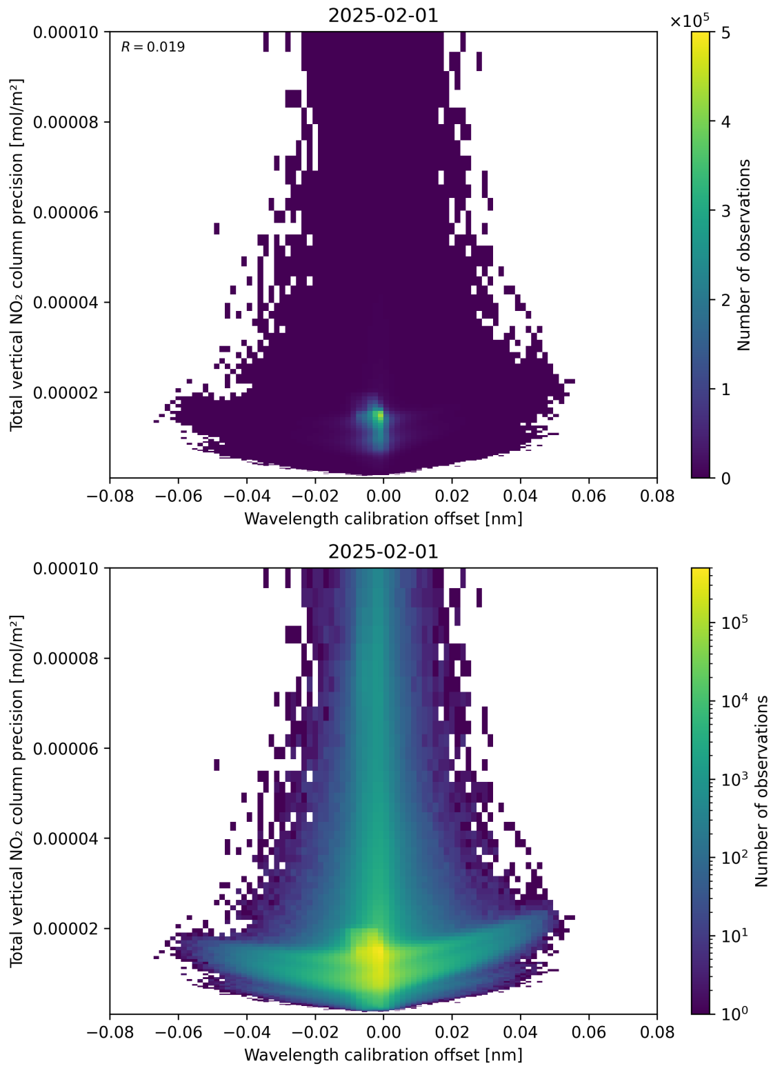
Figure 180: Scatter density plot of “Wavelength calibration offset” against “Total vertical NO 2 column precision” for 2025-01-31 to 2025-02-02.
