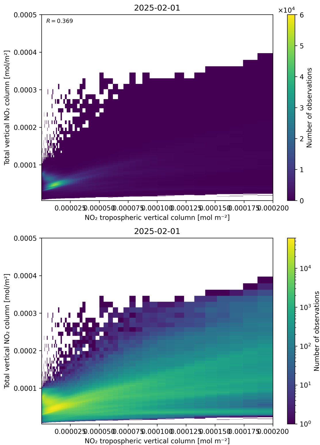
Figure 128: Scatter density plot of “NO 2 tropospheric vertical column” against “Total vertical NO 2 column” for 2025-01-31 to 2025-02-02.
