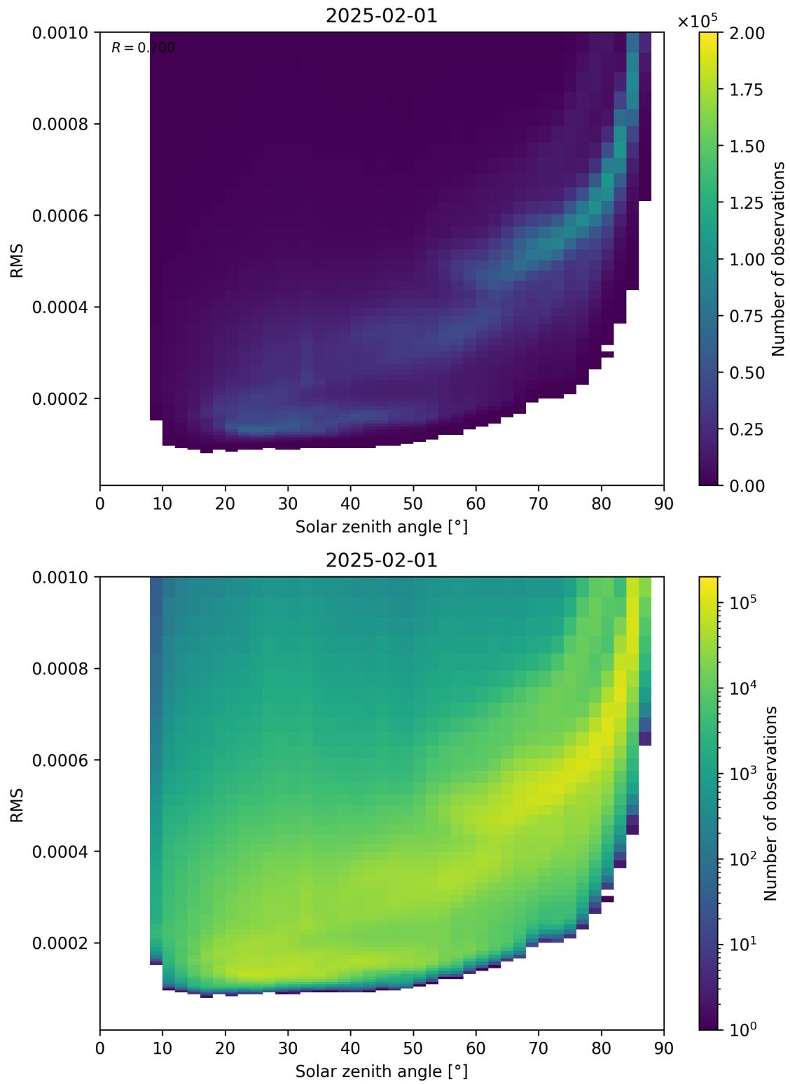
Figure 157: Scatter density plot of “Solar zenith angle” against “RMS” for 2025-01-31 to 2025-02-02.
