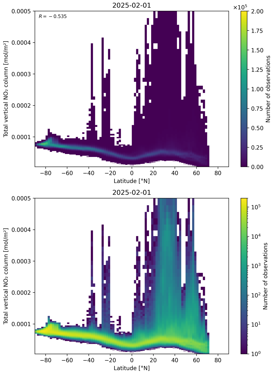
Figure 90: Scatter density plot of “Latitude” against “Total vertical NO 2 column” for 2025-01-31 to 2025-02-02.
