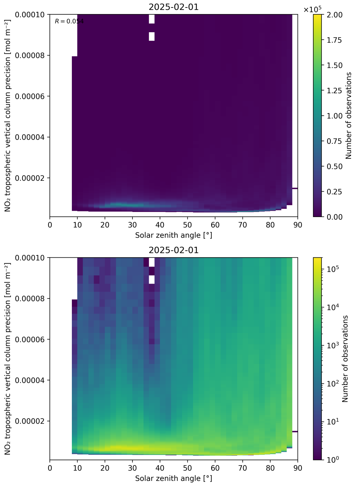
Figure 156: Scatter density plot of “Solar zenith angle” against “NO 2 tropospheric vertical column precision” for 2025-01-31 to 2025-02-02.
