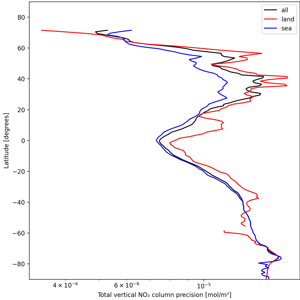
Figure 22: Zonal average of “Total vertical NO 2 column precision” for 2025-01-31 to 2025-02-02.
