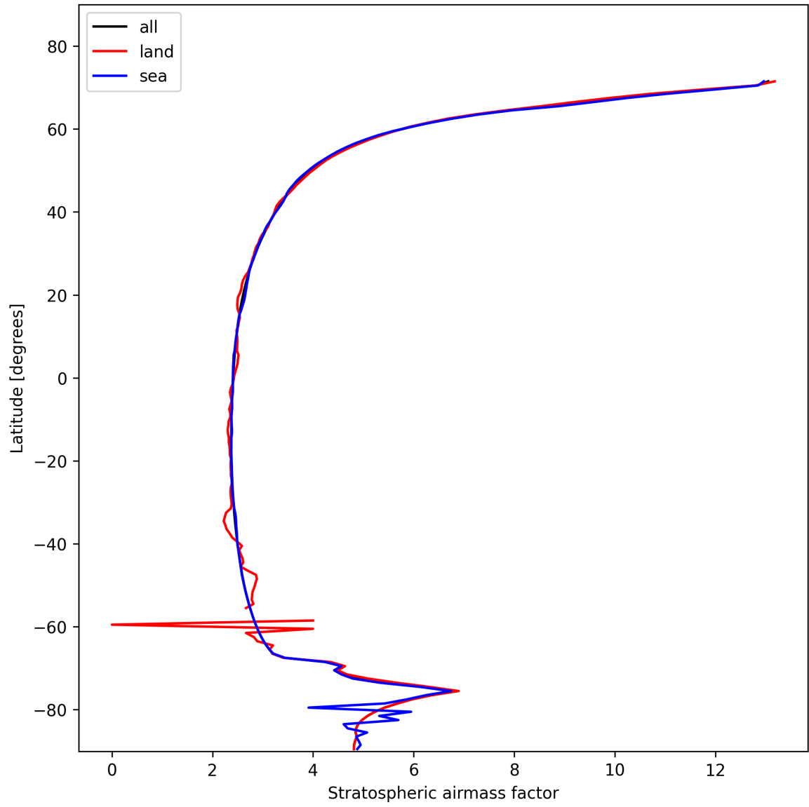
Figure 27: Zonal average of “Stratospheric air mass factor” for 2025-01-31 to 2025-02-02.
