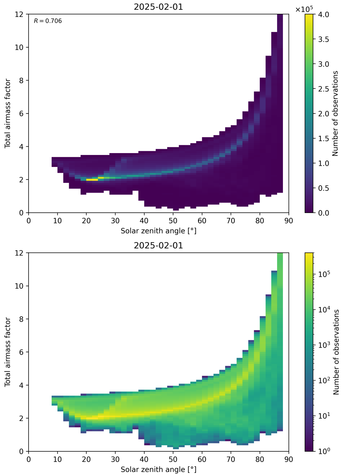
Figure 146: Scatter density plot of “Solar zenith angle” against “Total air mass factor” for 2025-01-31 to 2025-02-02.
