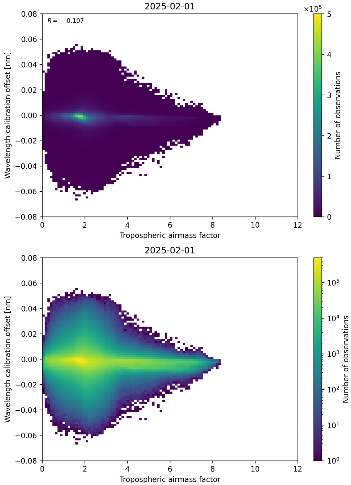
Figure 80: Scatter density plot of “Tropospheric airmass factor” against “Wavelength calibration offset” for 2025-01-31 to 2025-02-02.
