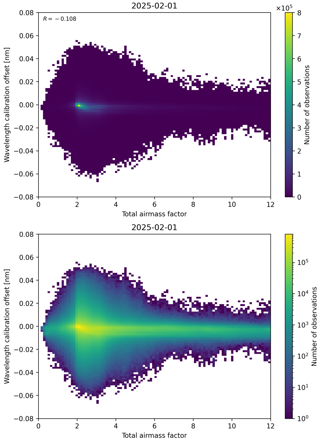
Figure 70: Scatter density plot of “Total airmass factor” against “Wavelength calibration offset” for 2025-01-31 to 2025-02-02.
