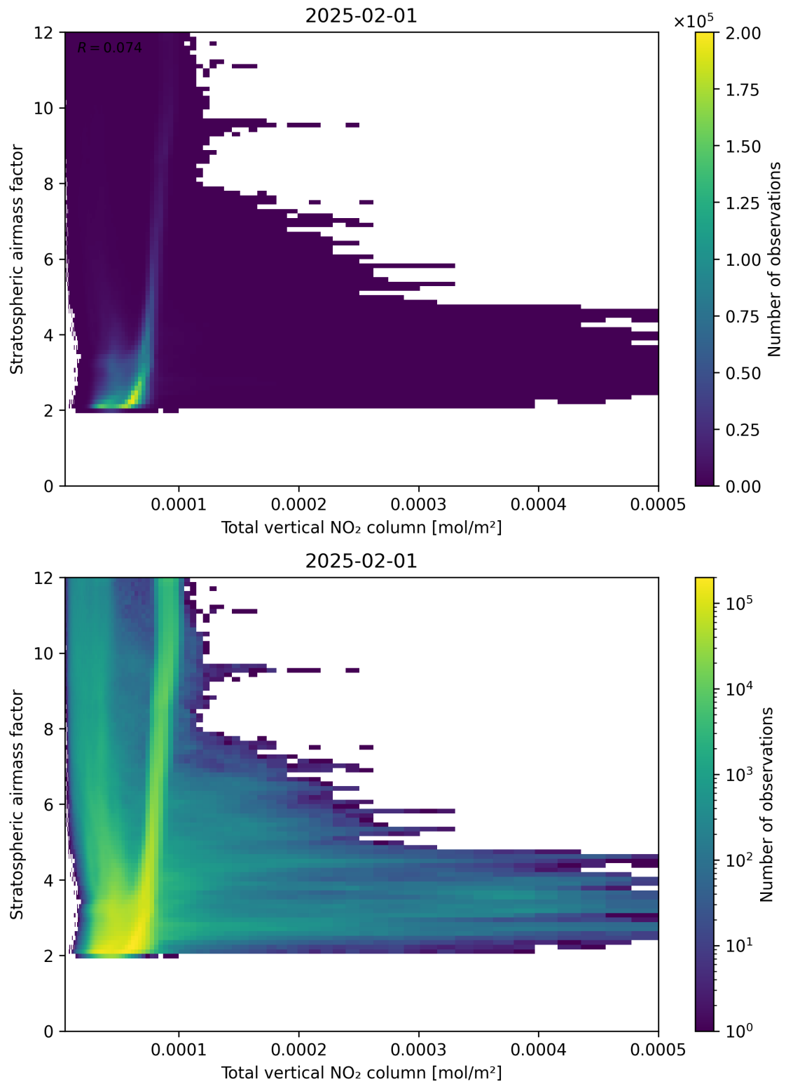
Figure 110: Scatter density plot of “Total vertical NO 2 column” against “Stratospheric airmass factor” for 2025-01-31 to 2025-02-02.
