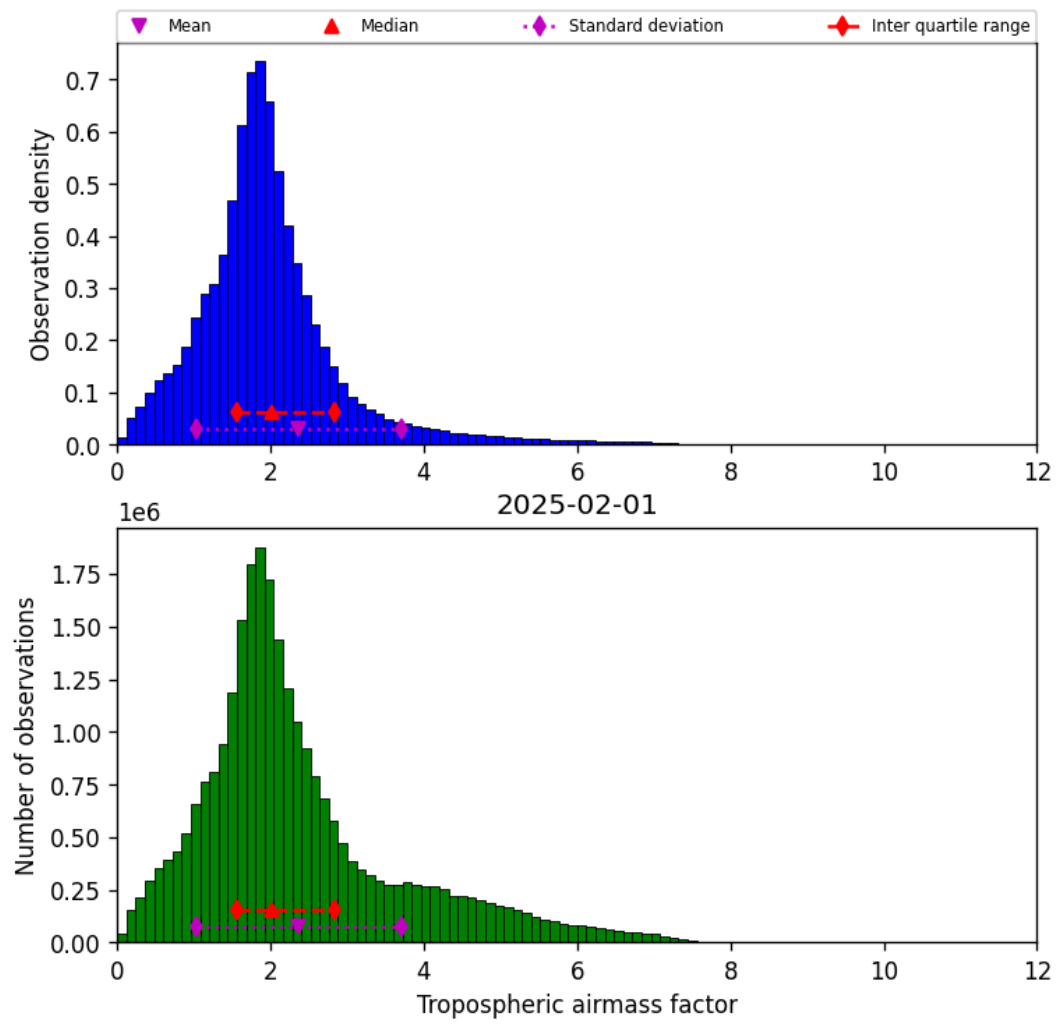
Figure 31: Histogram of “Tropospheric airmass factor” for 2025-01-31 to 2025-02-02
