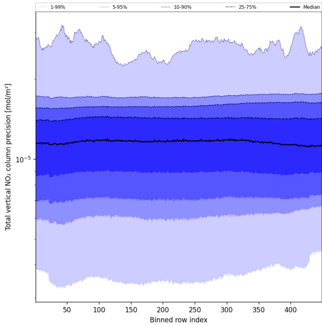
Figure 56: Along track statistics of “Total vertical NO 2 column precision” for 2025-01-31 to 2025-02-02
