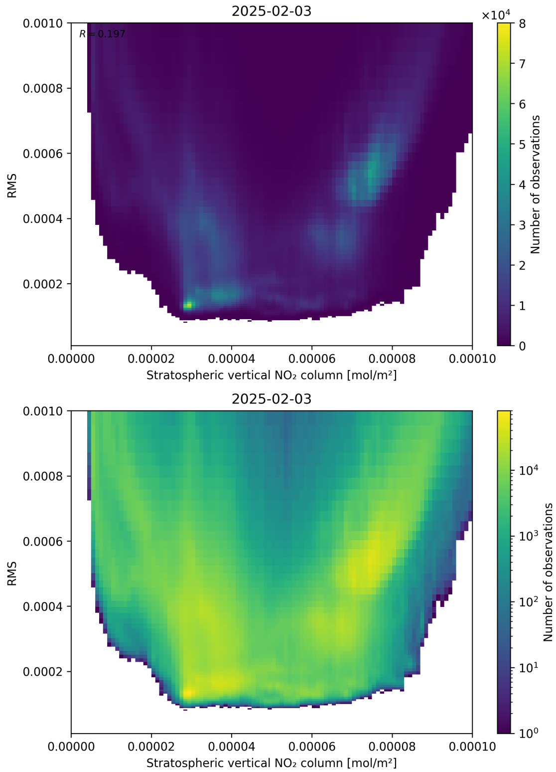
Figure 102: Scatter density plot of “Stratospheric vertical NO 2 column” against “RMS” for 2025-02-03 to 2025-02-04.
