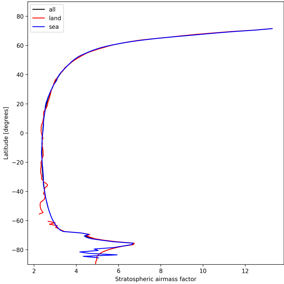
Figure 27: Zonal average of “Stratospheric air mass factor” for 2025-02-03 to 2025-02-04.
