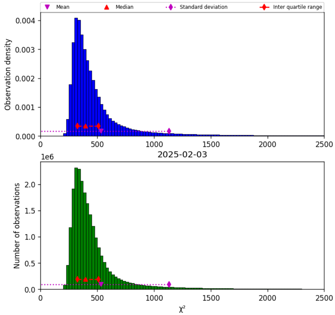
Figure 42: Histogram of “ \chi^2 ” for 2025-02-03 to 2025-02-04
