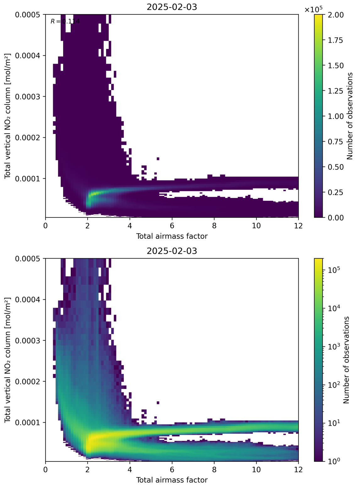
Figure 67: Scatter density plot of “Total airmass factor” against “Total vertical NO 2 column” for 2025-02-03 to 2025-02-04.
