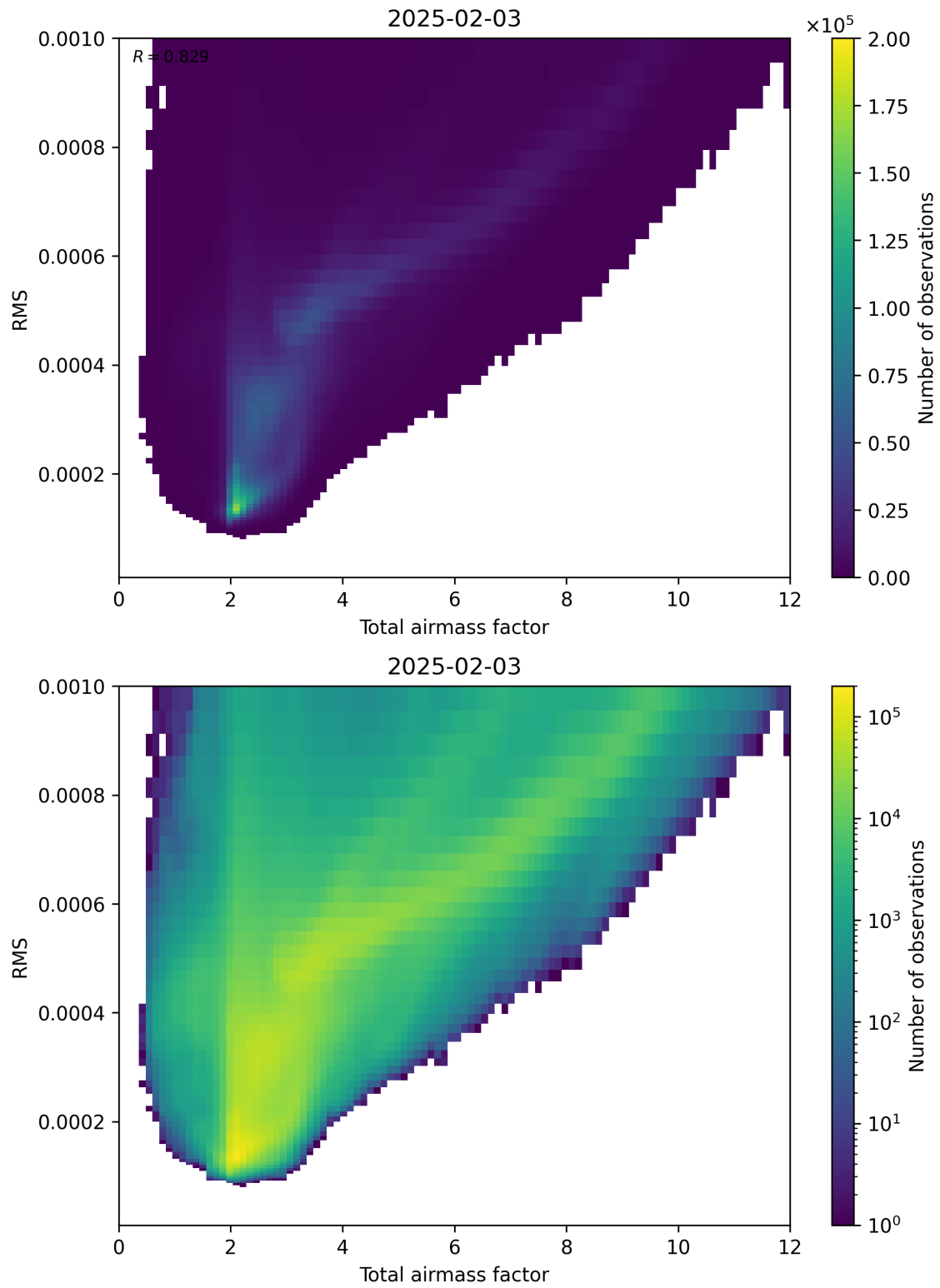
Figure 69: Scatter density plot of “Total airmass factor” against “RMS” for 2025-02-03 to 2025-02-04.
