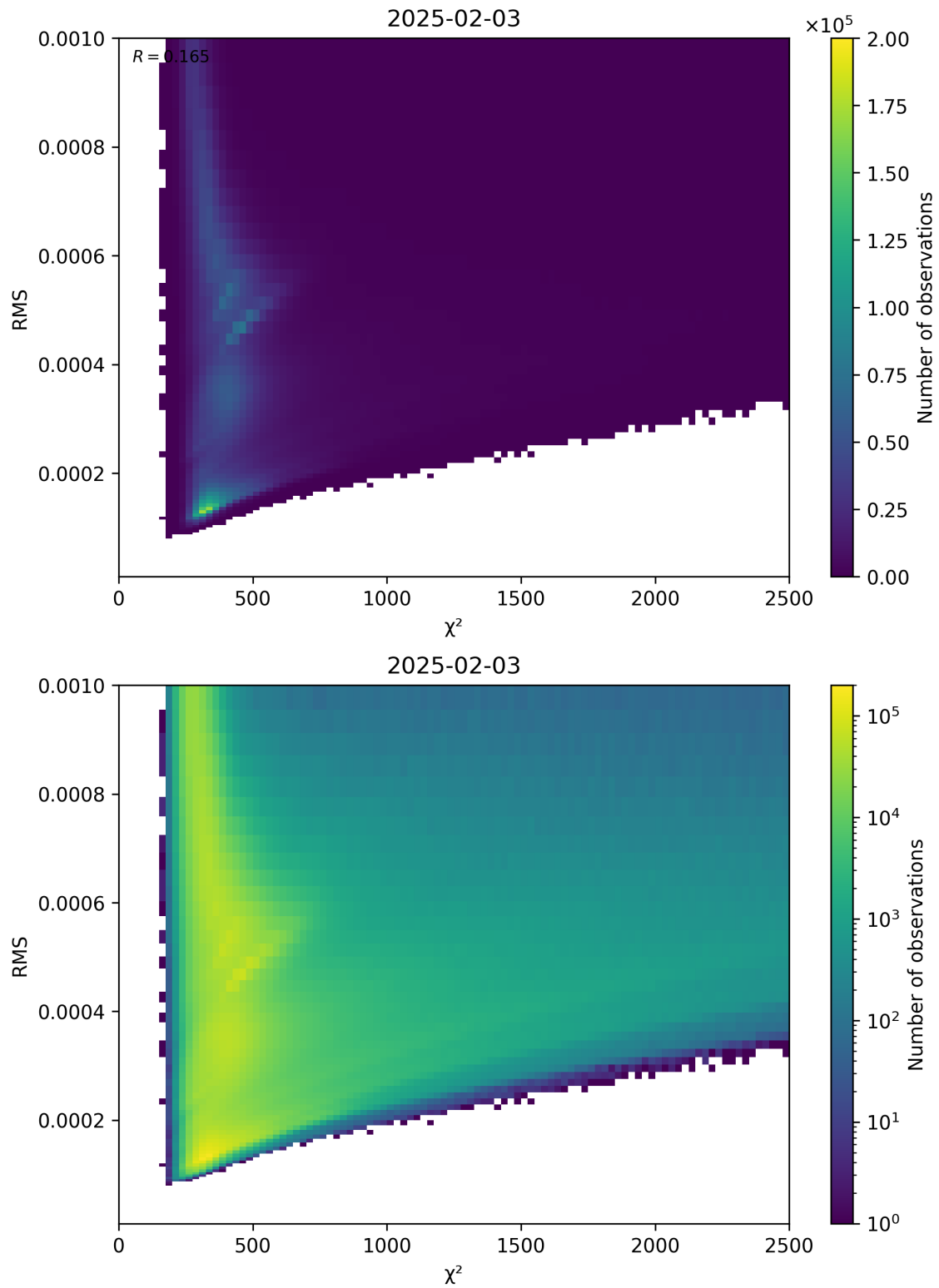
Figure 82: Scatter density plot of “ \chi^2 ” against “RMS” for 2025-02-03 to 2025-02-04.
