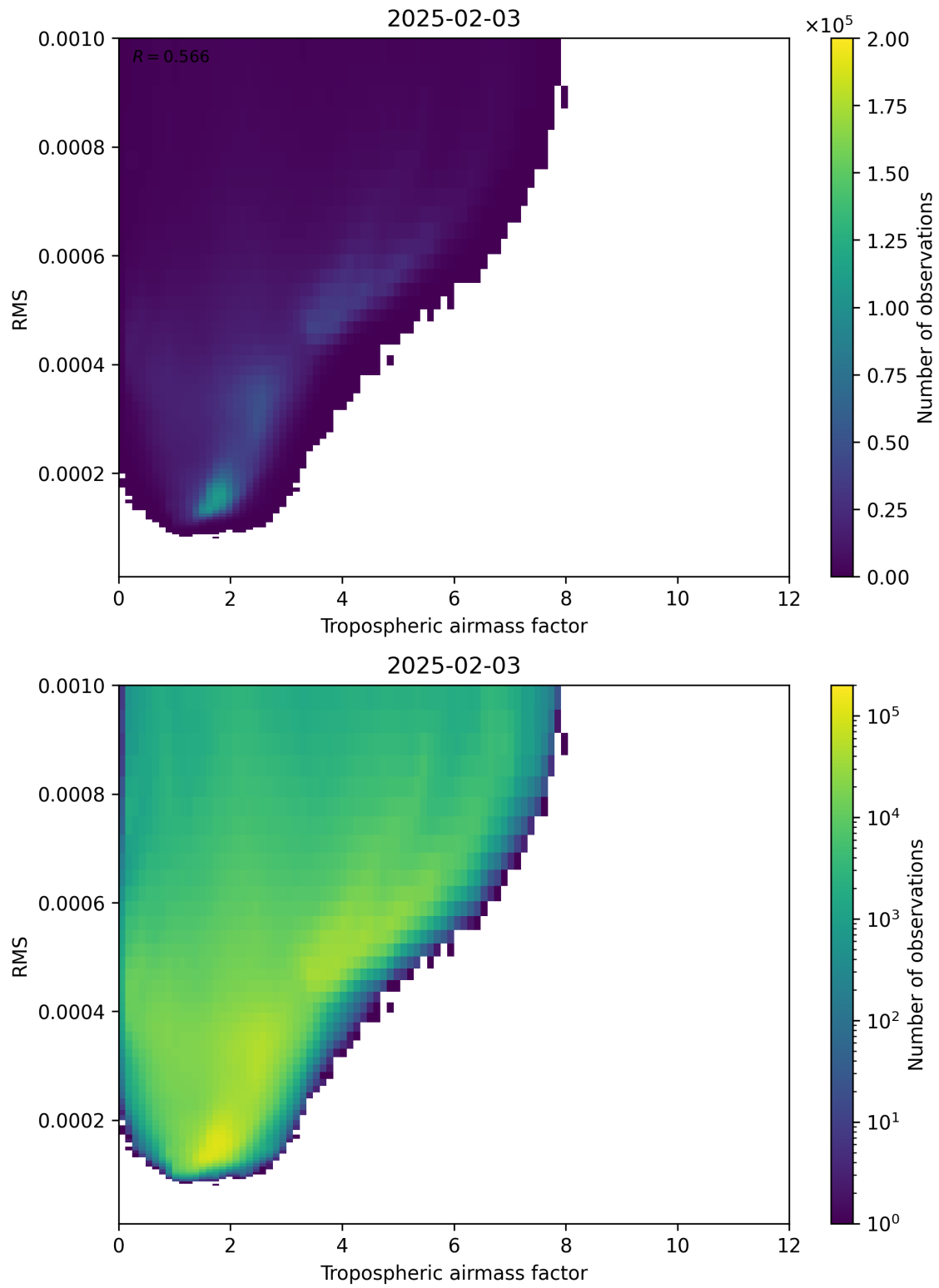
Figure 79: Scatter density plot of “Tropospheric airmass factor” against “RMS” for 2025-02-03 to 2025-02-04.
