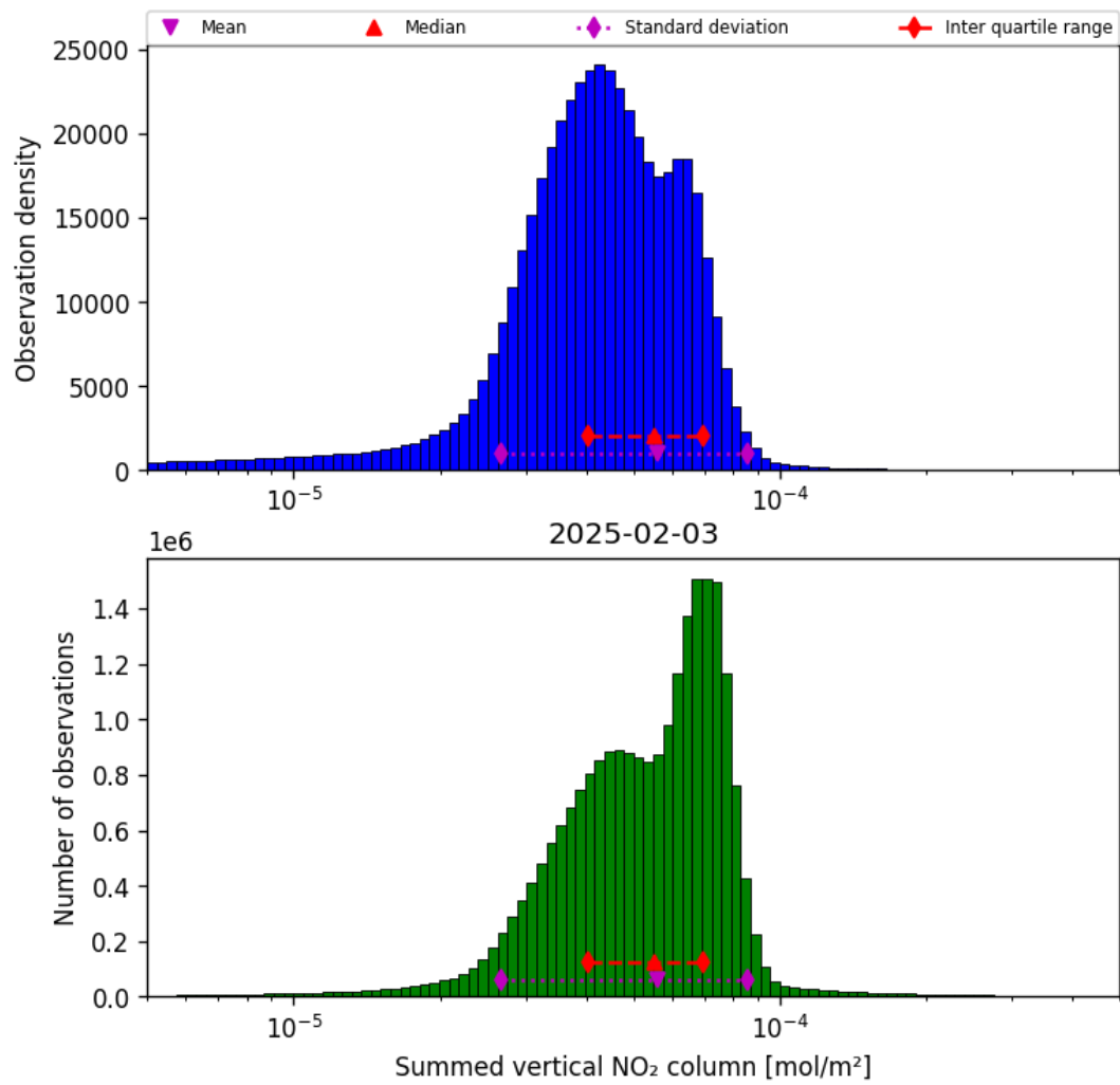
Figure 40: Histogram of “Summed vertical NO 2 column” for 2025-02-03 to 2025-02-04
