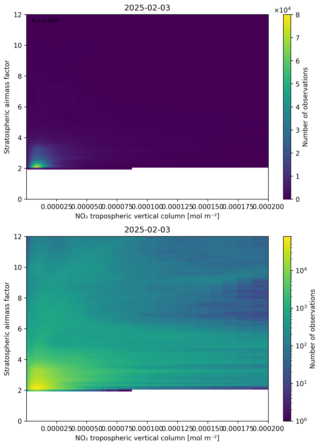
Figure 121: Scatter density plot of “NO 2 tropospheric vertical column” against “Stratospheric airmass factor” for 2025-02-03 to 2025-02-04.
