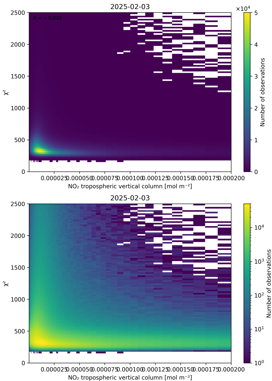
Figure 124: Scatter density plot of “NO 2 tropospheric vertical column” against “ \chi^2 ” for 2025-02-03 to 2025-02-04.
