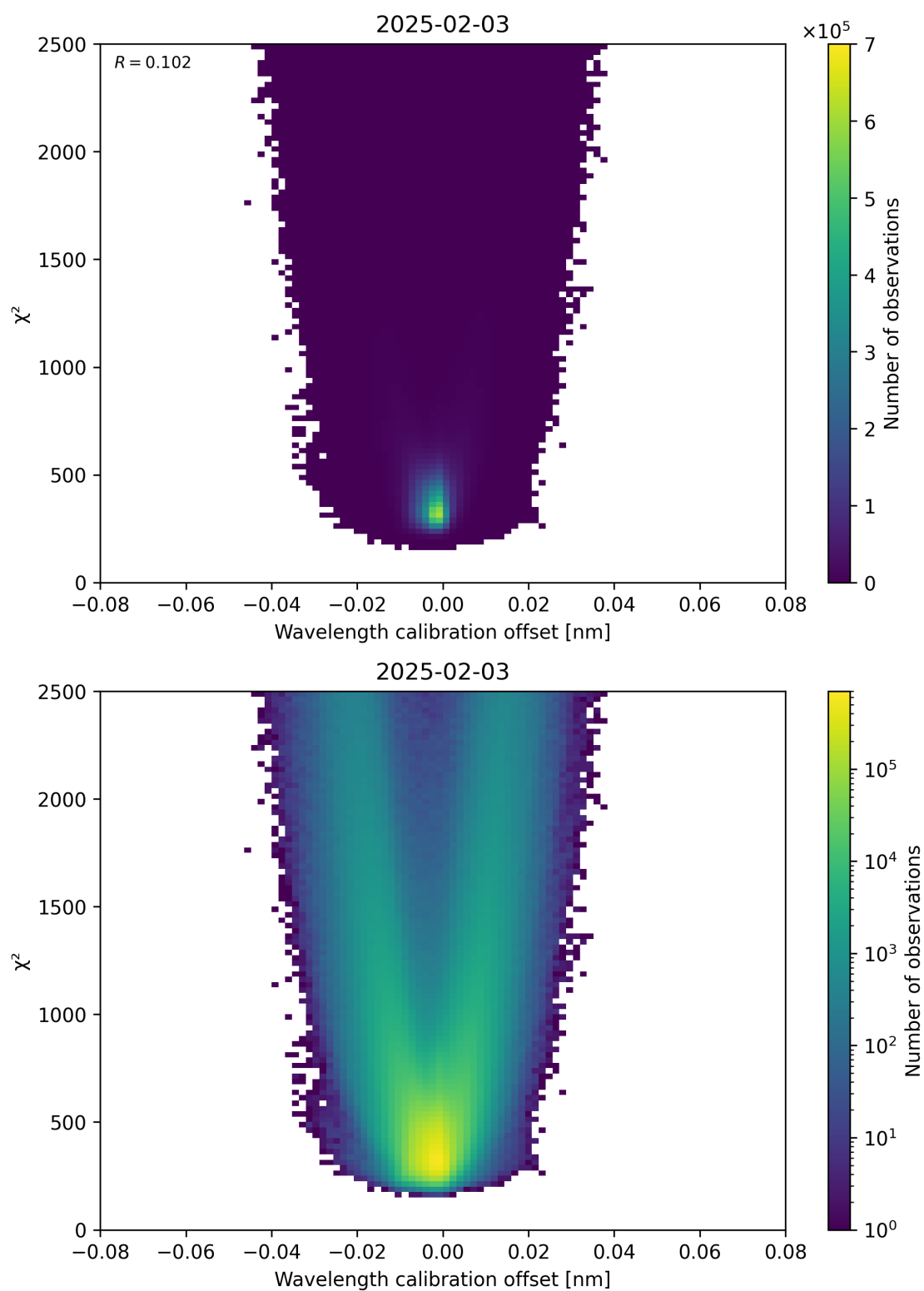
Figure 175: Scatter density plot of “Wavelength calibration offset” against “ \chi^2 ” for 2025-02-03 to 2025-02-04.
