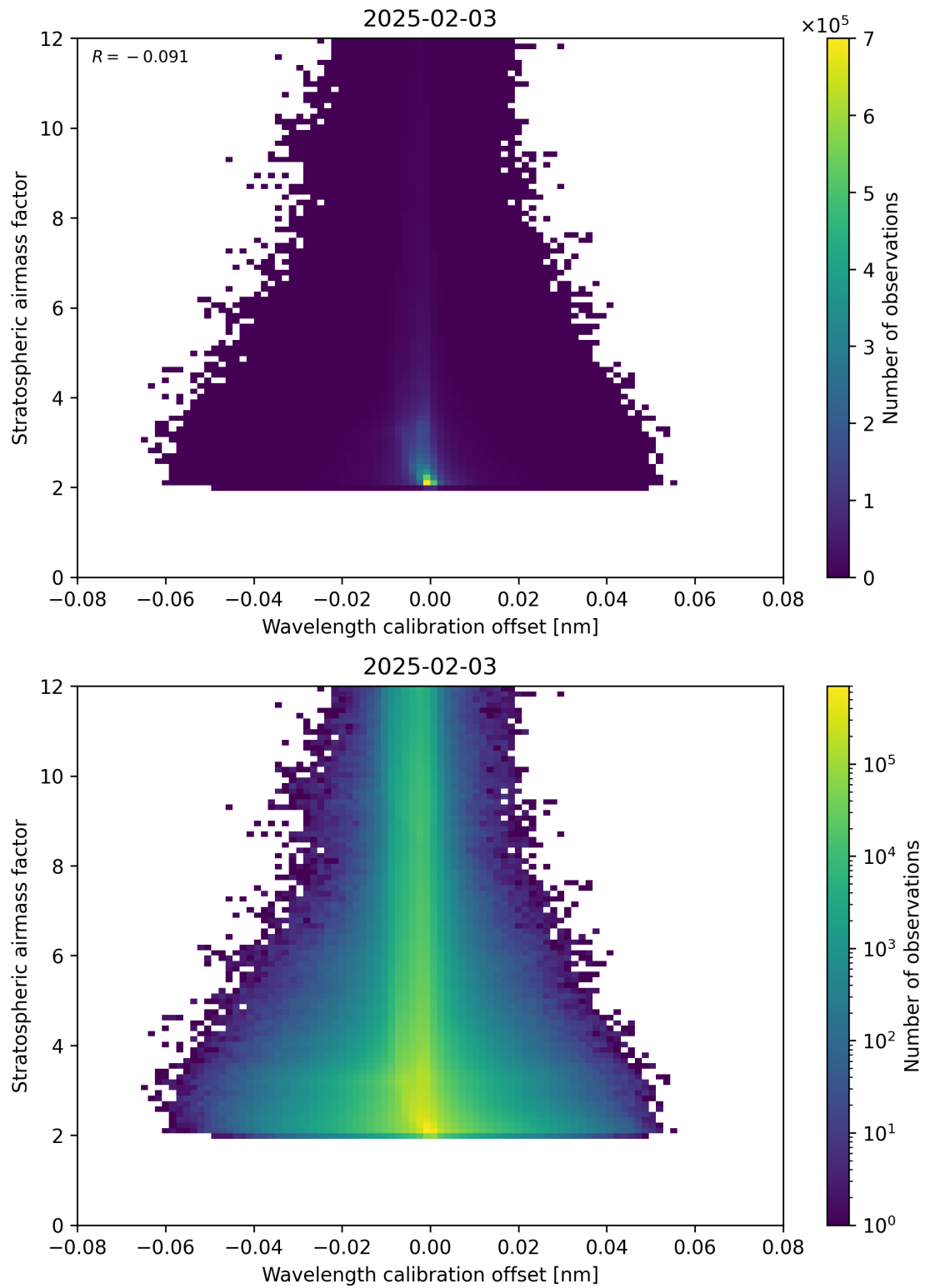
Figure 174: Scatter density plot of “Wavelength calibration offset” against “Stratospheric airmass factor” for 2025-02-03 to 2025-02-04.
