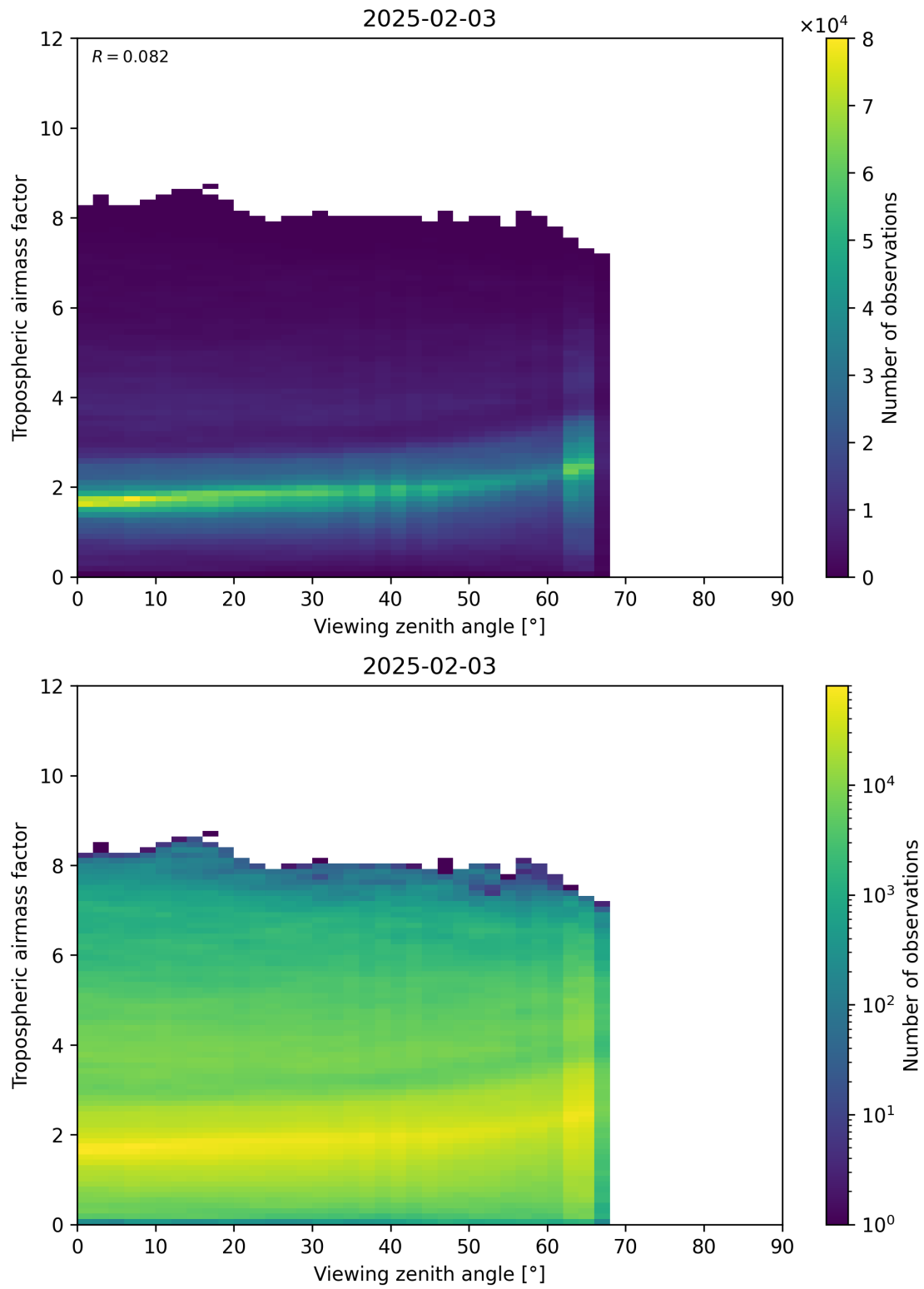
Figure 161: Scatter density plot of “Viewing zenith angle” against “Tropospheric airmass factor” for 2025-02-03 to 2025-02-04.
