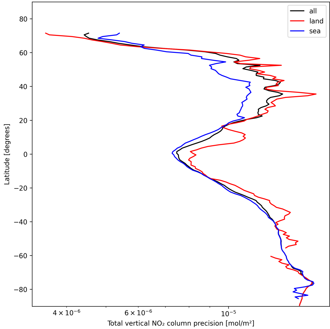
Figure 22: Zonal average of “Total vertical NO 2 column precision” for 2025-02-03 to 2025-02-04.
