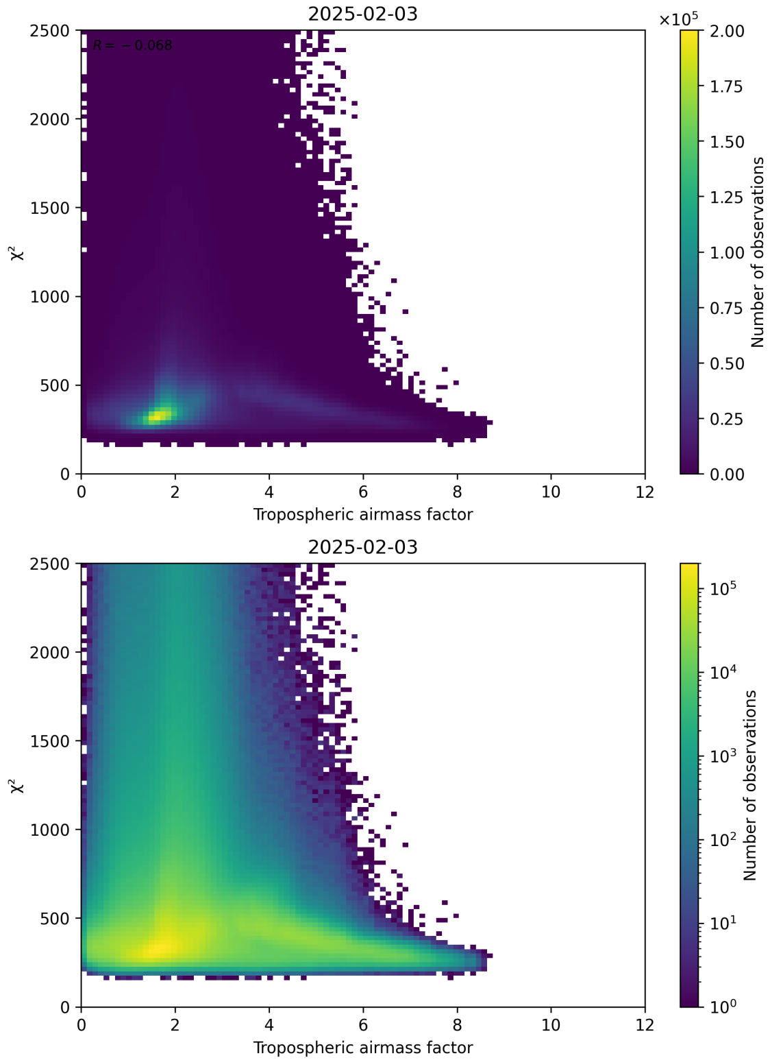
Figure 73: Scatter density plot of “Tropospheric airmass factor” against “ \chi^2 ” for 2025-02-03 to 2025-02-04.
