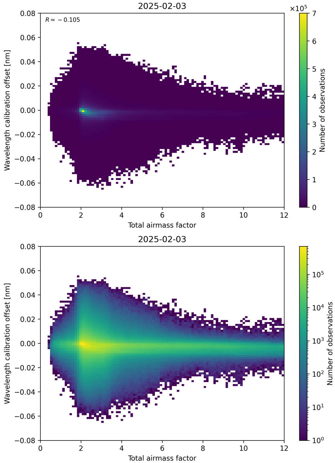
Figure 70: Scatter density plot of “Total airmass factor” against “Wavelength calibration offset” for 2025-02-03 to 2025-02-04.
