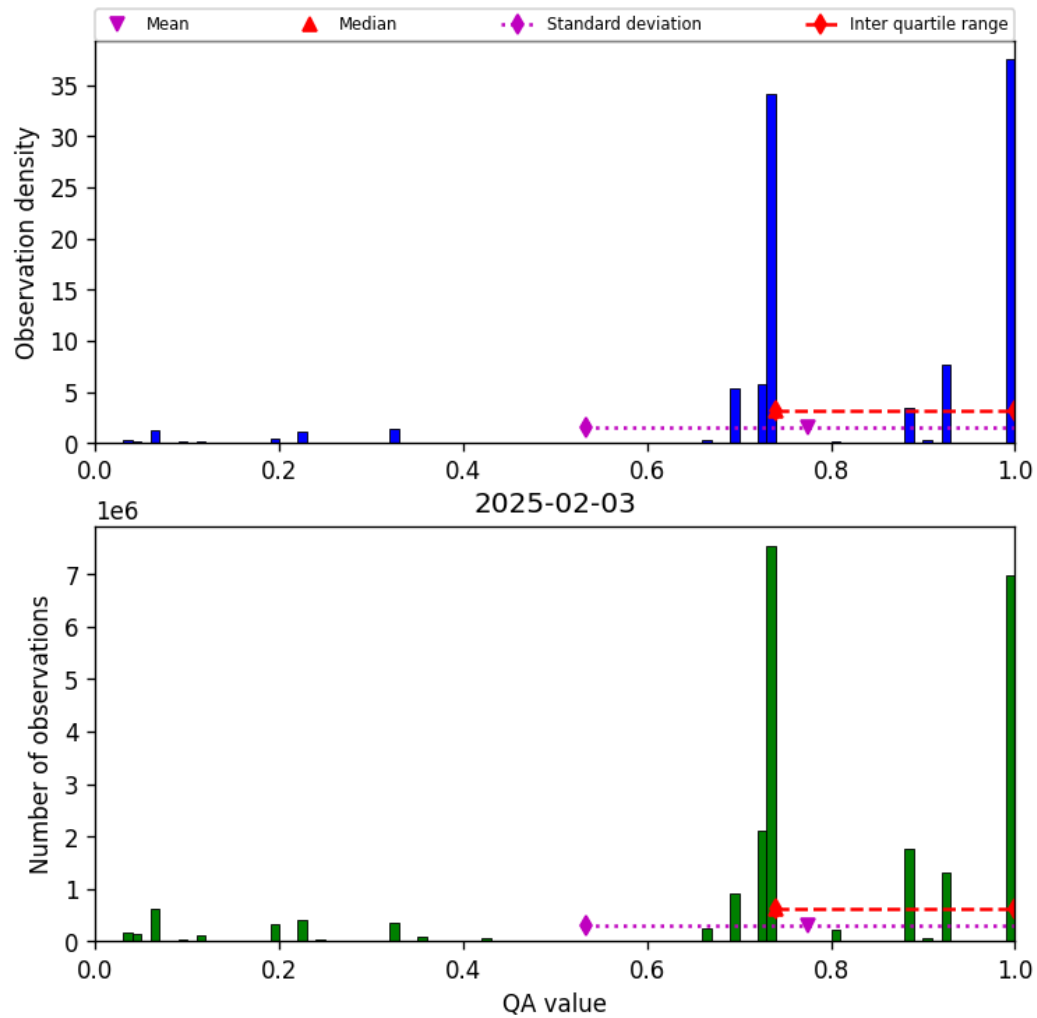
Figure 28: Histogram of “QA value” for 2025-02-03 to 2025-02-04
