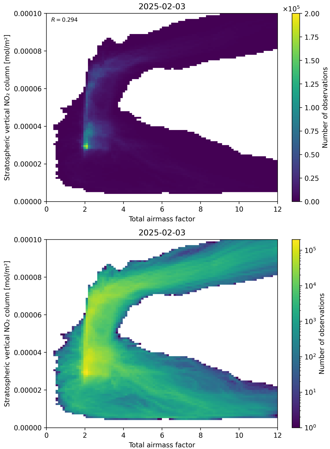
Figure 64: Scatter density plot of “Total airmass factor” against “Stratospheric vertical NO 2 column” for 2025-02-03 to 2025-02-04.
