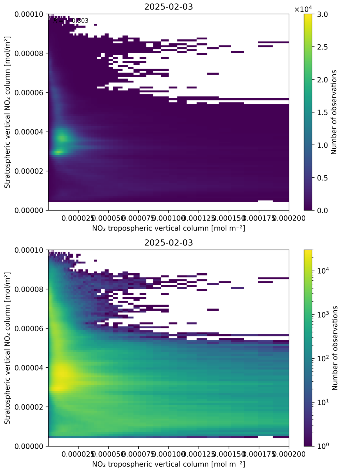
Figure 125: Scatter density plot of “NO 2 tropospheric vertical column” against “Stratospheric vertical NO 2 column” for 2025-02-03 to 2025-02-04.
