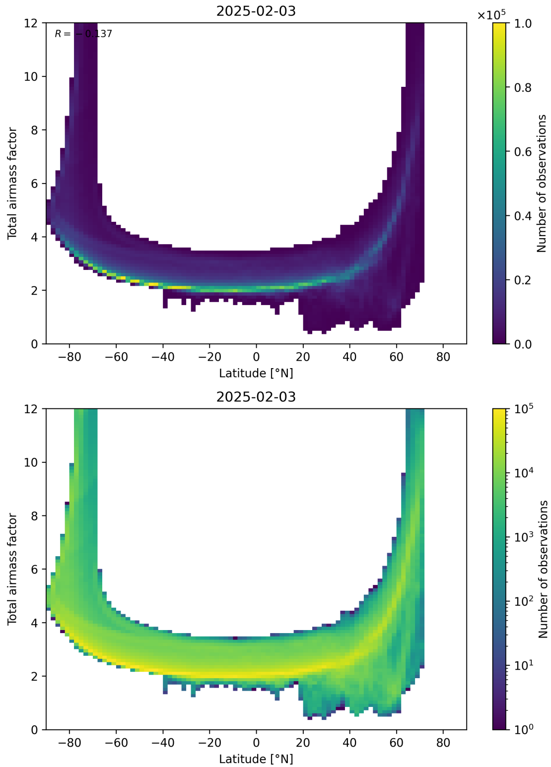
Figure 84: Scatter density plot of “Latitude” against “Total airmass factor” for 2025-02-03 to 2025-02-04.
