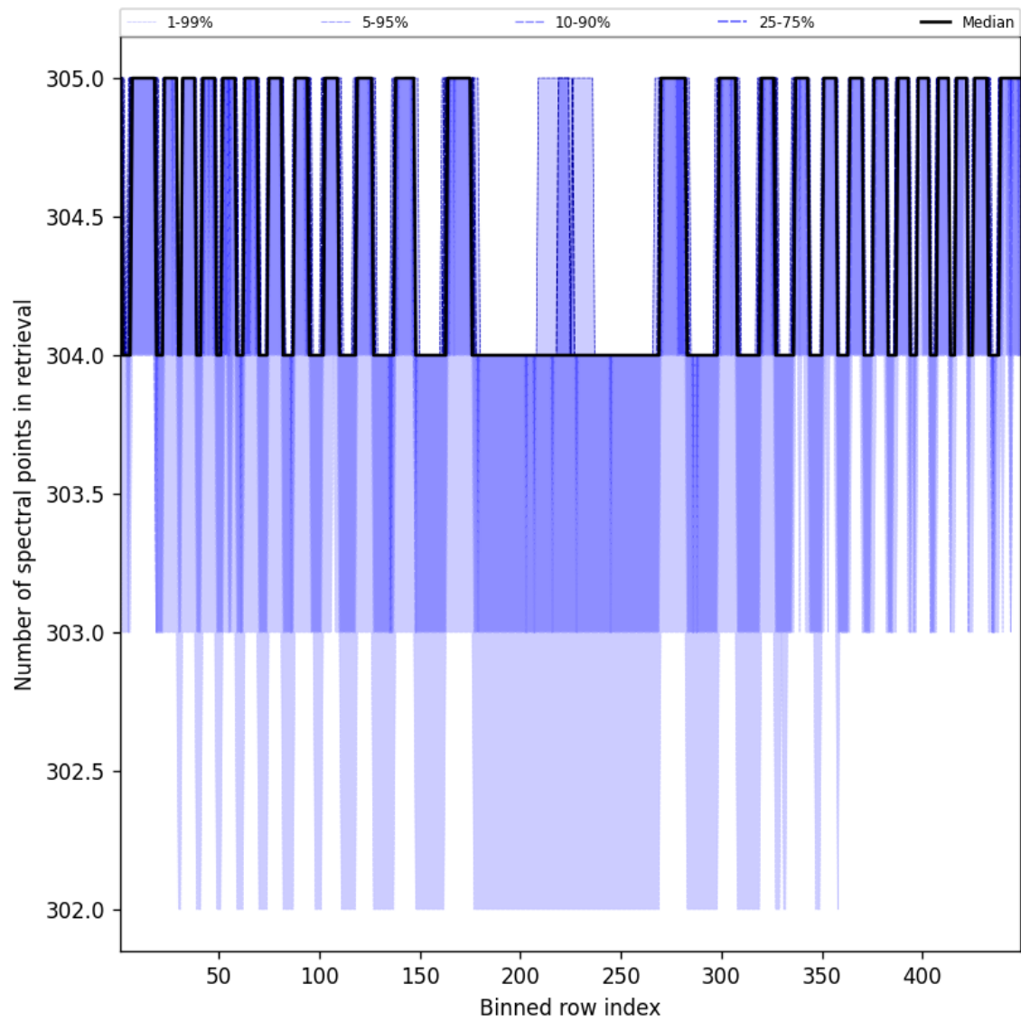
Figure 50: Along track statistics of “Number of spectral points in retrieval” for 2025-02-03 to 2025-02-04
