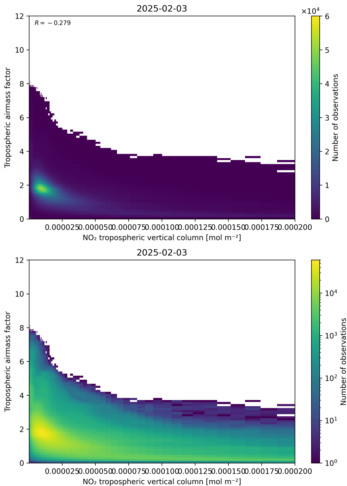
Figure 123: Scatter density plot of “NO 2 tropospheric vertical column” against “Tropospheric air mass factor” for 2025-02-03 to 2025-02-04.
