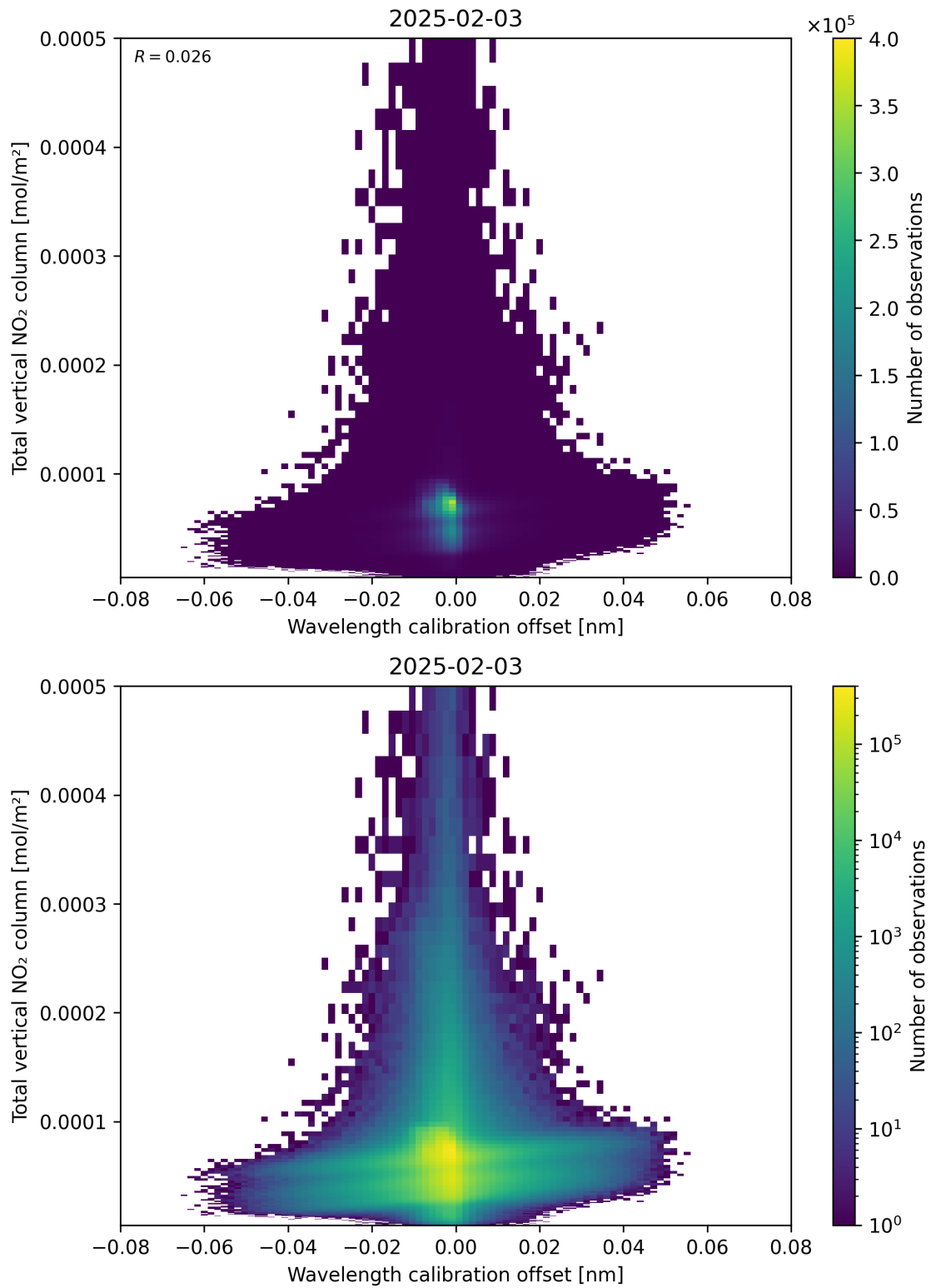
Figure 179: Scatter density plot of “Wavelength calibration offset” against “Total vertical NO 2 column” for 2025-02-03 to 2025-02-04.
