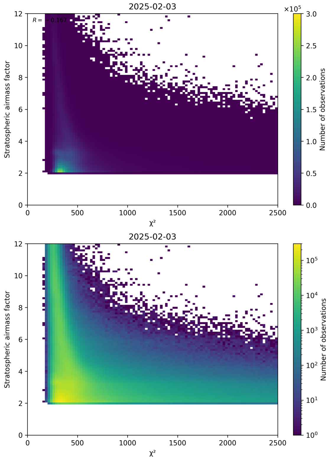
Figure 81: Scatter density plot of “ \chi^2 ” against “Stratospheric airmass factor” for 2025-02-03 to 2025-02-04.
