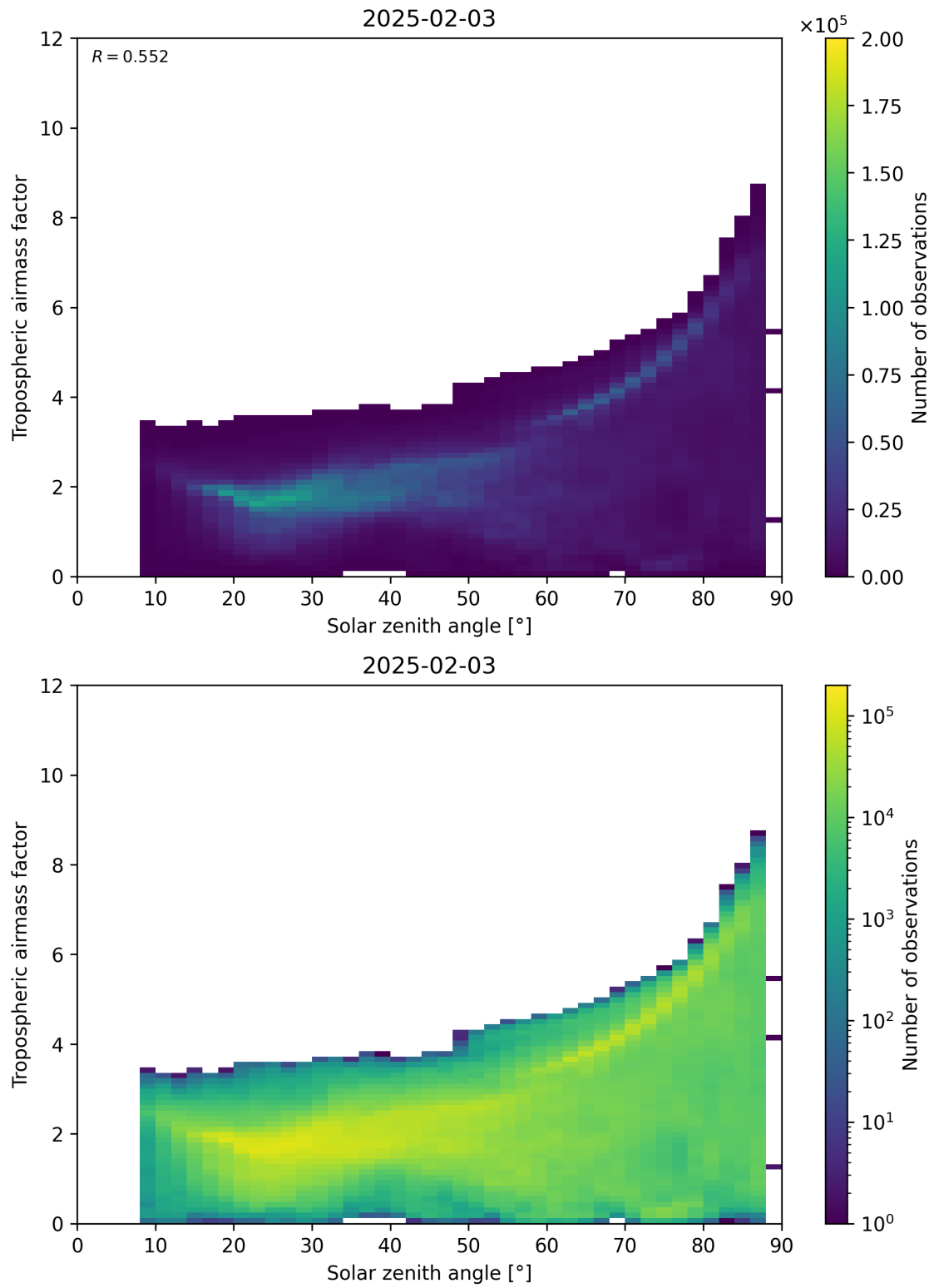
Figure 147: Scatter density plot of “Solar zenith angle” against “Tropospheric airmass factor” for 2025-02-03 to 2025-02-04.
