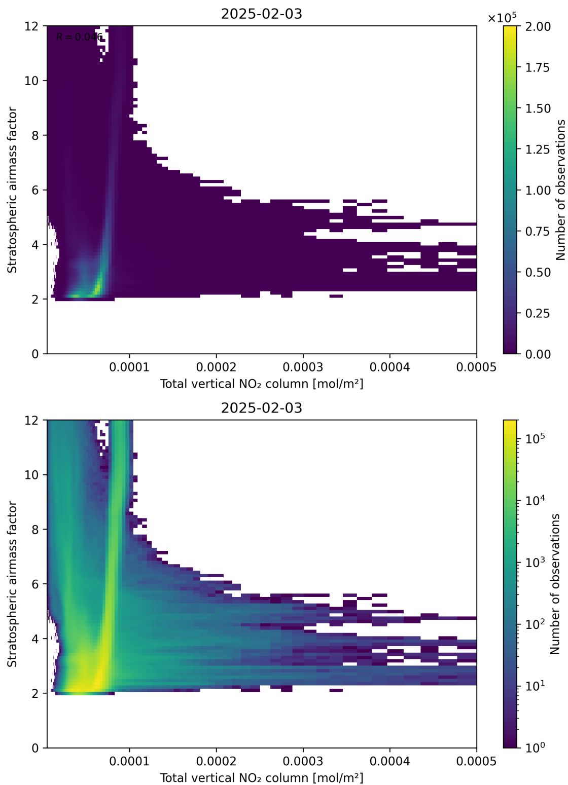
Figure 110: Scatter density plot of “Total vertical NO 2 column” against “Stratospheric air mass factor” for 2025-02-03 to 2025-02-04.
