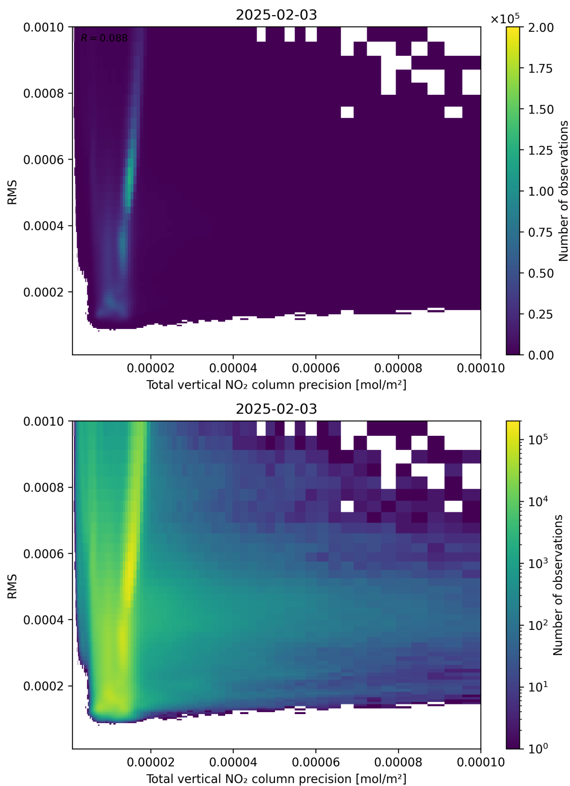
Figure 119: Scatter density plot of “Total vertical NO 2 column precision” against “RMS” for 2025-02-03 to 2025-02-04.
