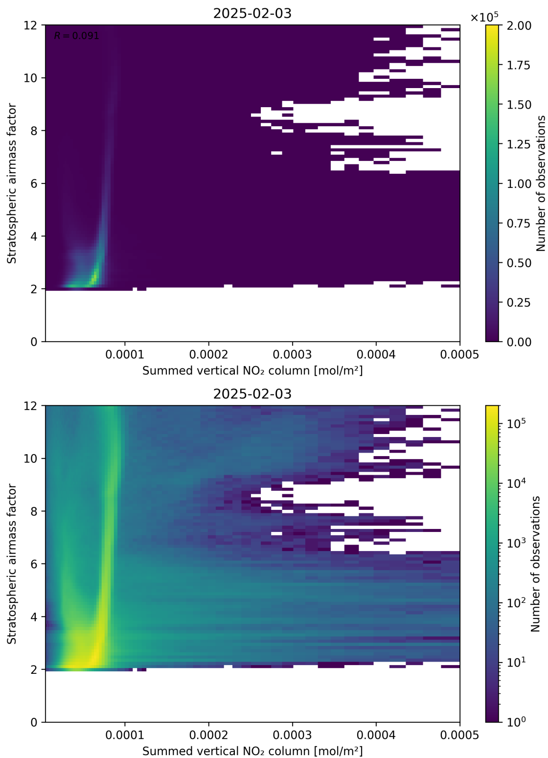
Figure 103: Scatter density plot of “Summed vertical NO 2 column” against “Stratospheric airmass factor” for 2025-02-03 to 2025-02-04.
