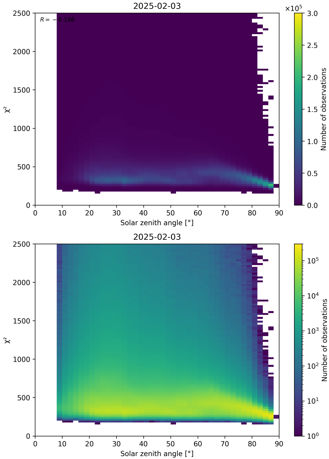
Figure 148: Scatter density plot of “Solar zenith angle” against “ \chi^2 ” for 2025-02-03 to 2025-02-04.
