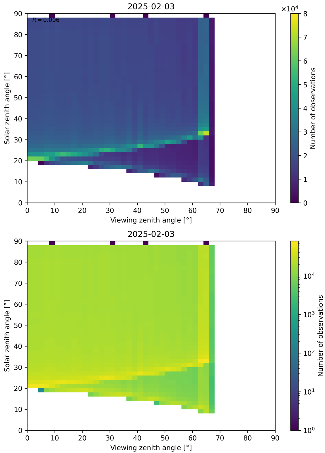
Figure 172: Scatter density plot of “Viewing zenith angle” against “Solar zenith angle” for 2025-02-03 to 2025-02-04.
