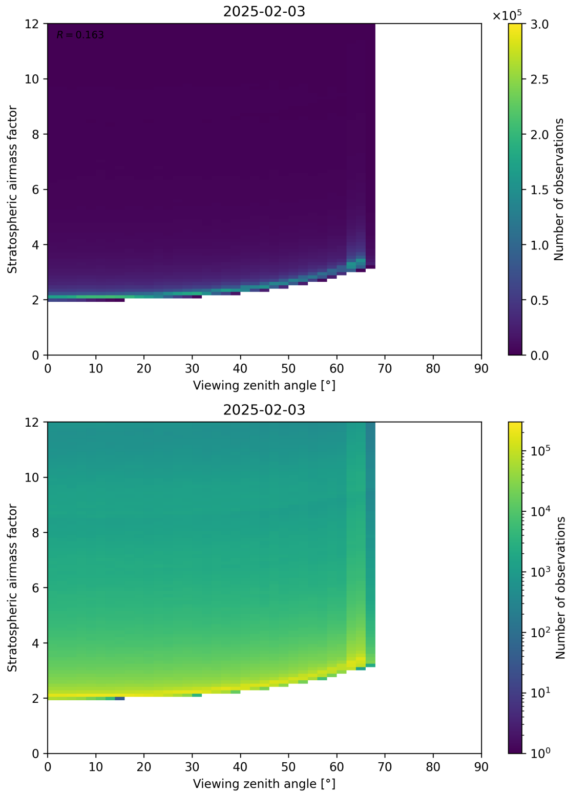
Figure 159: Scatter density plot of “Viewing zenith angle” against “Stratospheric airmass factor” for 2025-02-03 to 2025-02-04.
