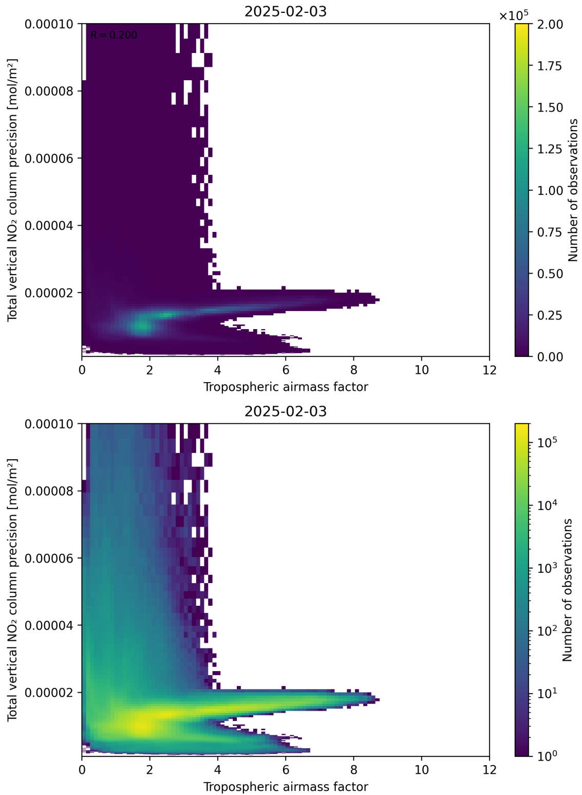
Figure 78: Scatter density plot of “Tropospheric air mass factor” against “Total vertical NO 2 column precision” for 2025-02-03 to 2025-02-04.
