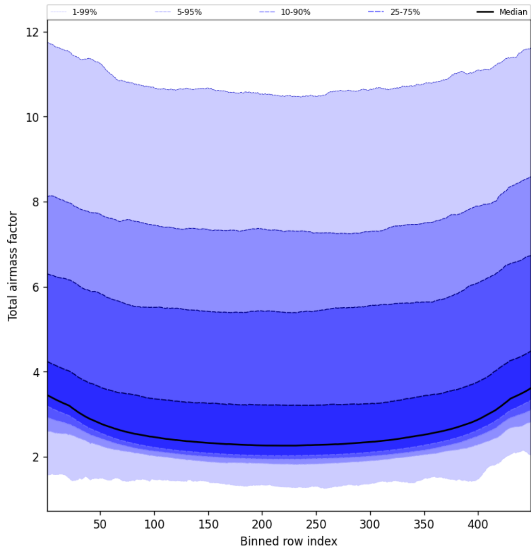
Figure 49: Along track statistics of “Total airmass factor” for 2025-02-03 to 2025-02-04
