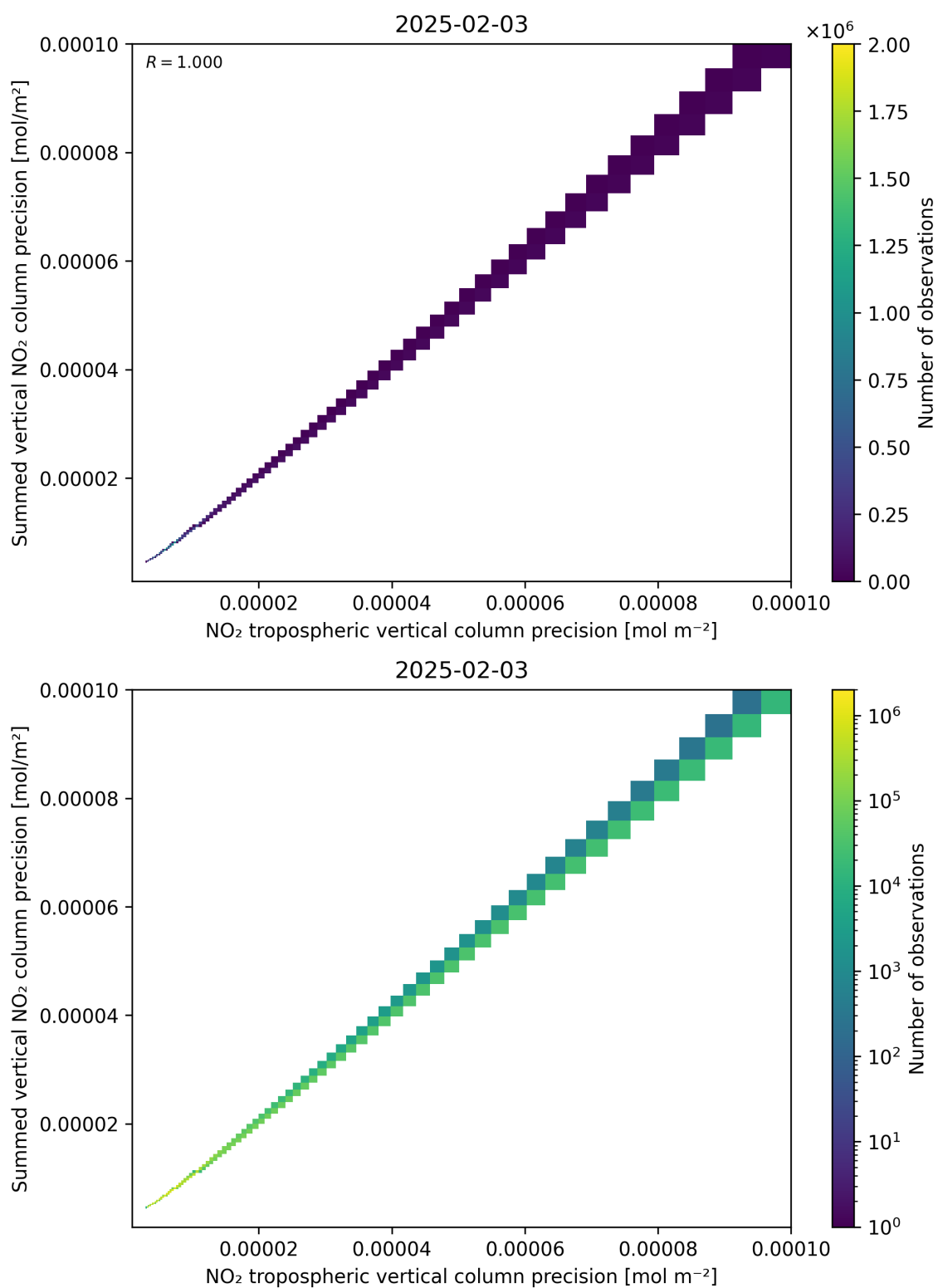
Figure 137: Scatter density plot of “NO 2 tropospheric vertical column precision” against “Summed vertical NO 2 column precision” for 2025-02-03 to 2025-02-04.
