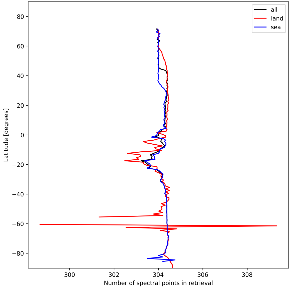
Figure 16: Zonal average of “Number of spectral points in retrieval” for 2025-02-03 to 2025-02-04.
