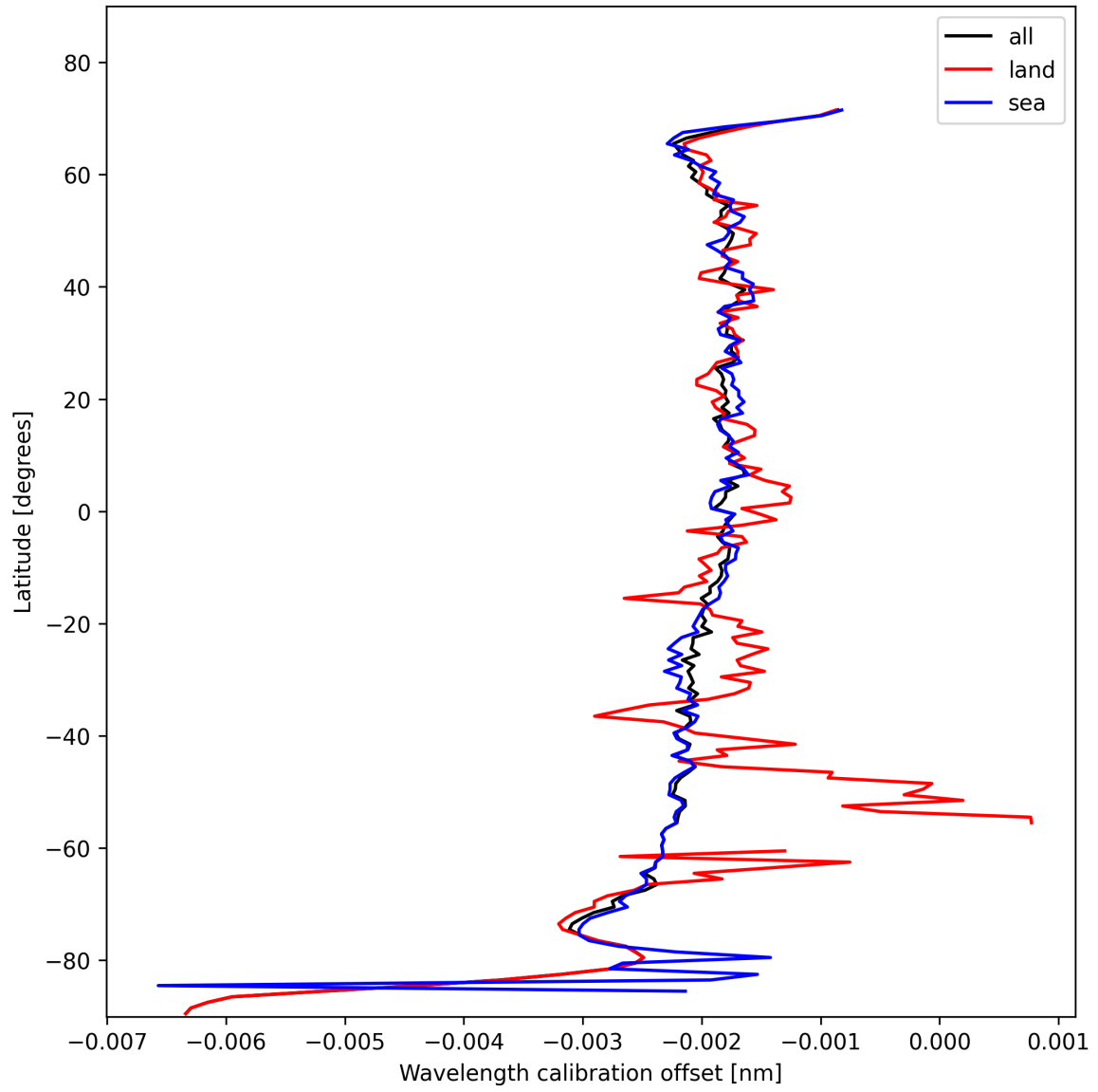
Figure 18: Zonal average of “Wavelength calibration offset” for 2025-02-03 to 2025-02-04.
