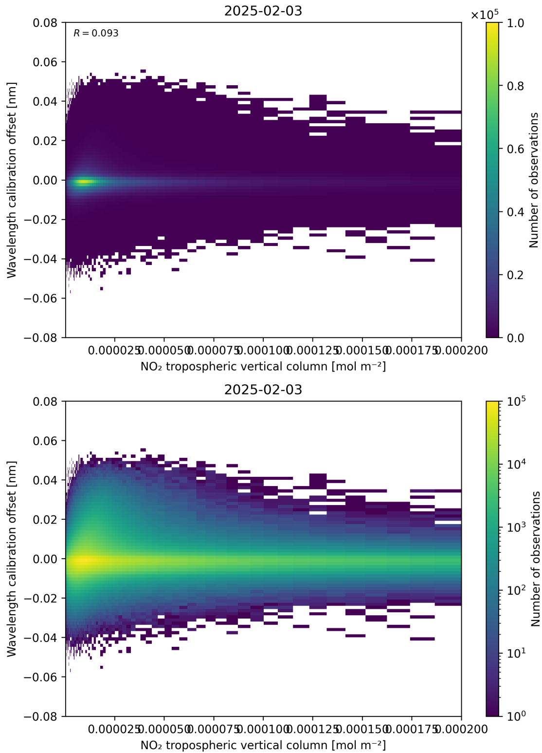
Figure 143: Scatter density plot of “NO 2 tropospheric vertical column” against “Wavelength calibration offset” for 2025-02-03 to 2025-02-04.
