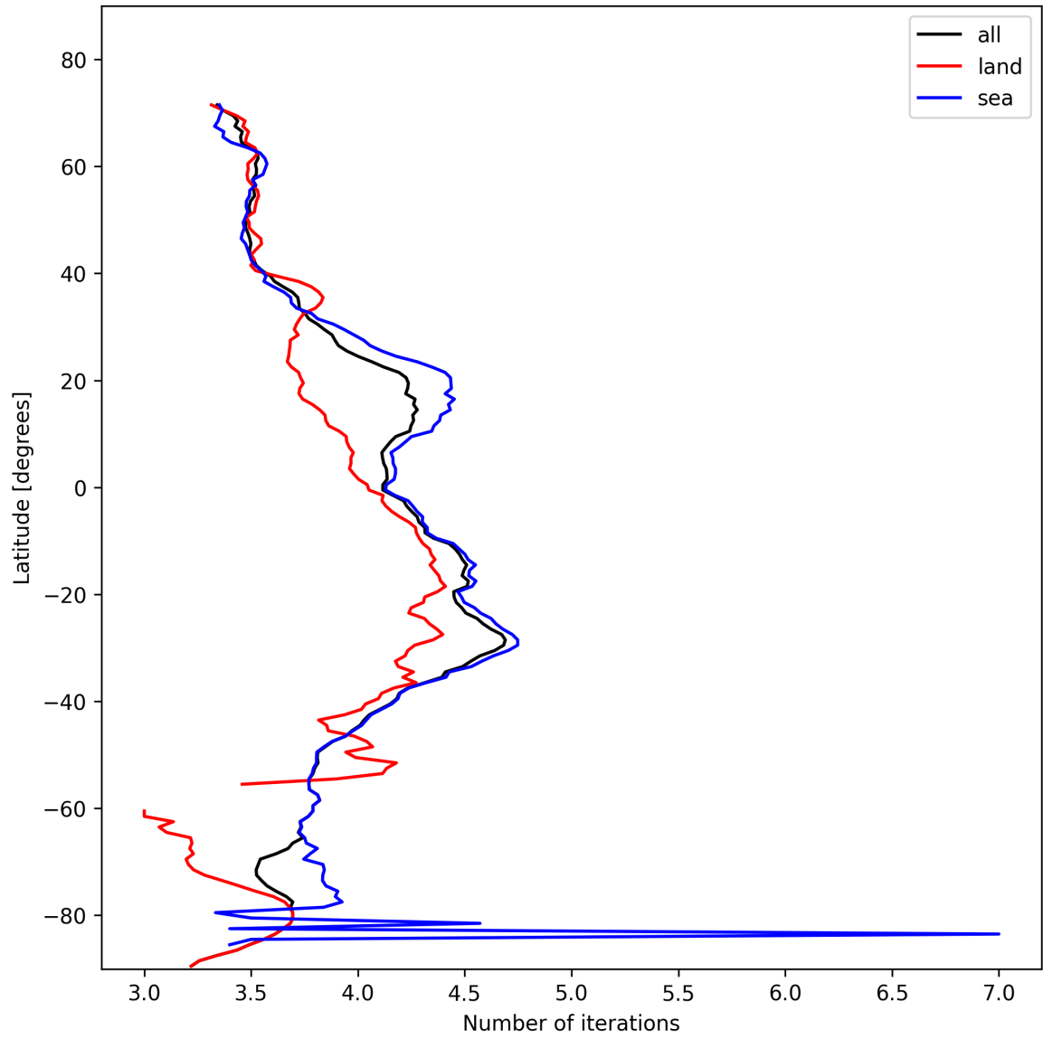
Figure 17: Zonal average of “Number of iterations” for 2025-02-03 to 2025-02-04.
