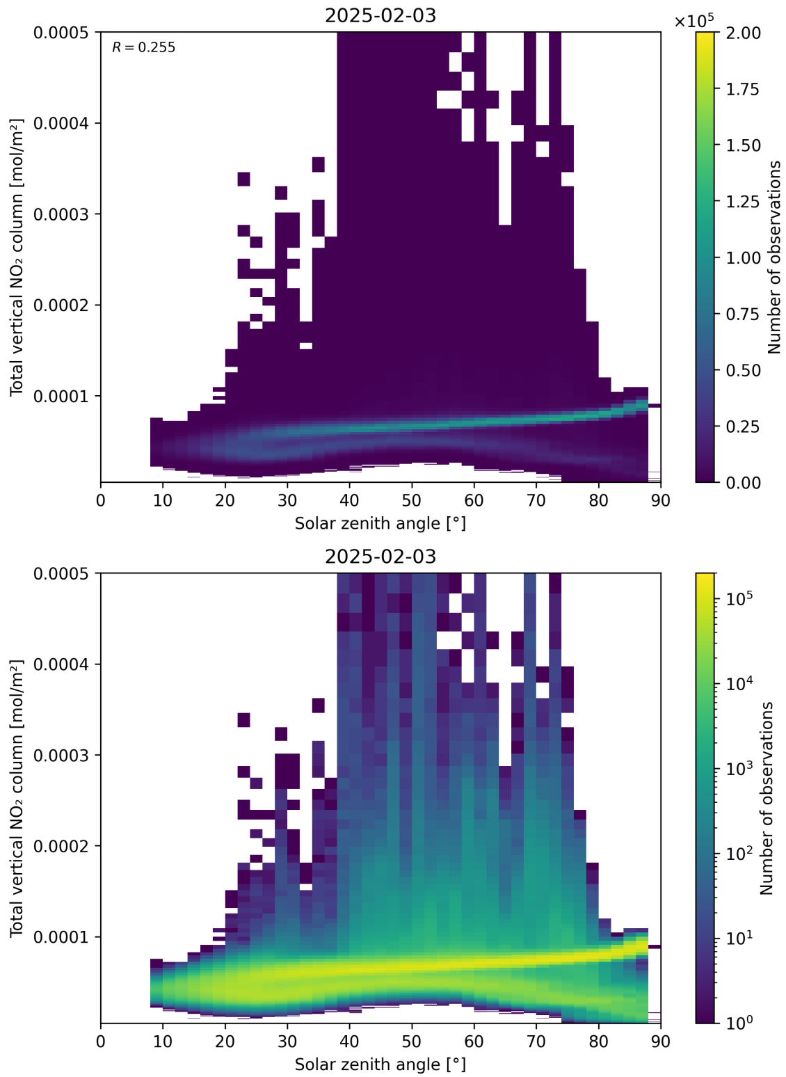
Figure 153: Scatter density plot of “Solar zenith angle” against “Total vertical NO 2 column” for 2025-02-03 to 2025-02-04.
