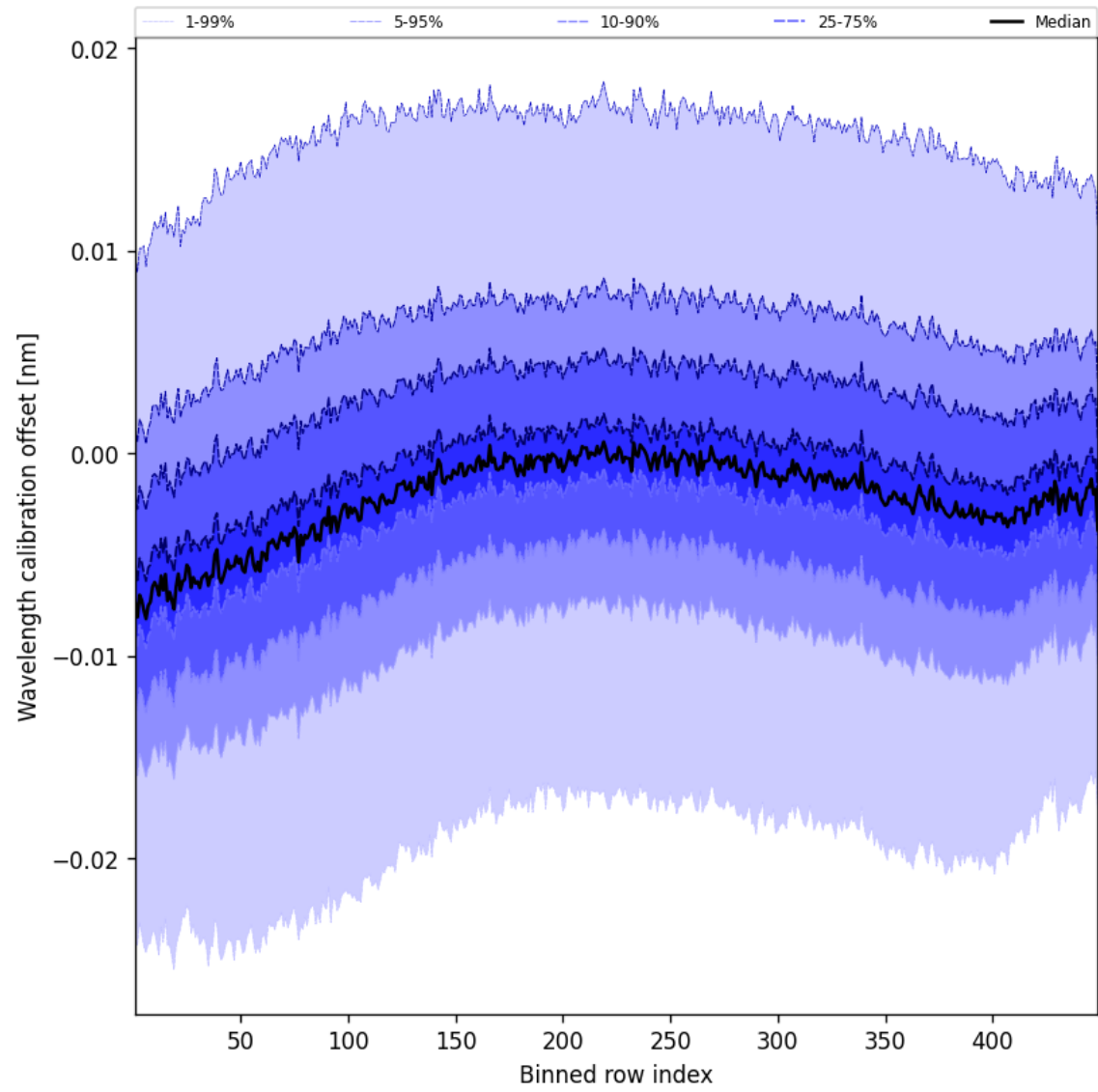
Figure 52: Along track statistics of “Wavelength calibration offset” for 2025-02-03 to 2025-02-04
