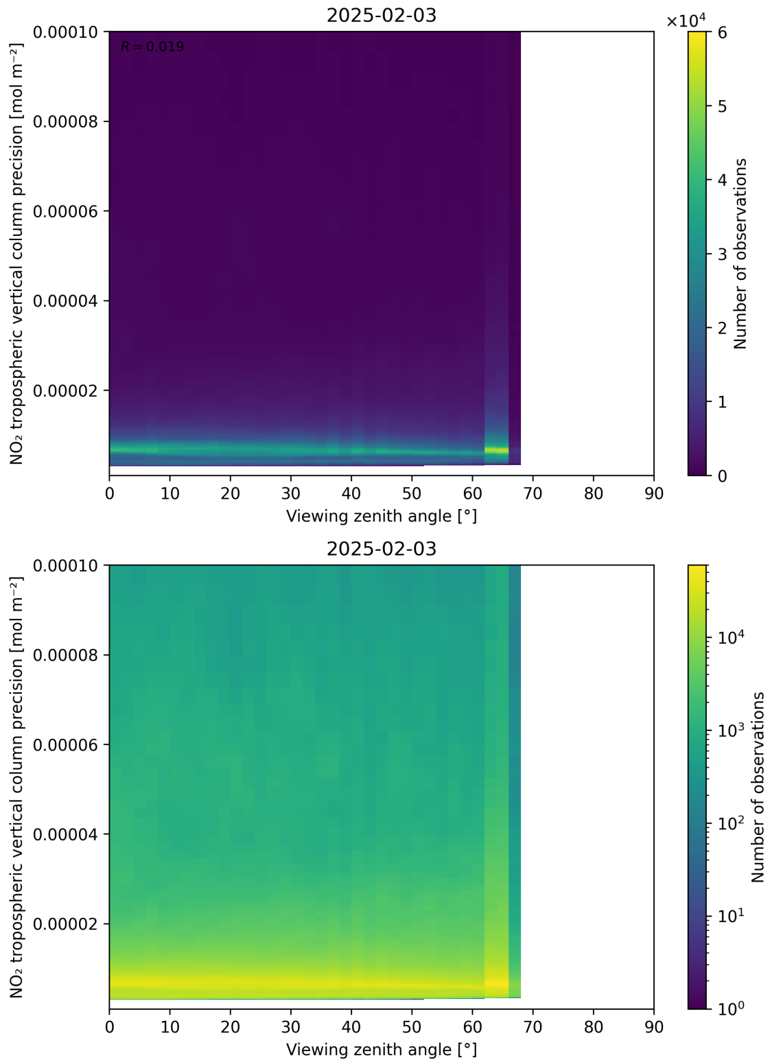
Figure 170: Scatter density plot of “Viewing zenith angle” against “NO 2 tropospheric vertical column precision” for 2025-02-03 to 2025-02-04.
