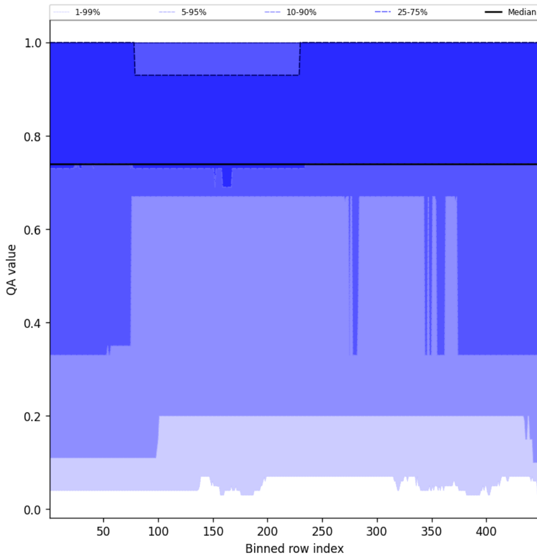
Figure 45: Along track statistics of “QA value” for 2025-02-03 to 2025-02-04
