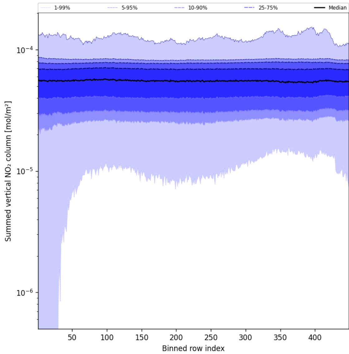
Figure 57: Along track statistics of “Summed vertical NO 2 column” for 2025-02-03 to 2025-02-04
