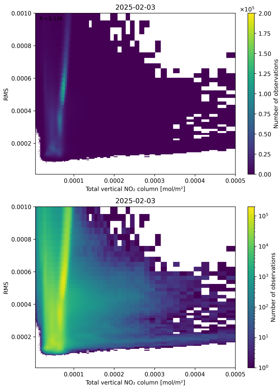
Figure 120: Scatter density plot of “Total vertical NO 2 column” against “RMS” for 2025-02-03 to 2025-02-04.
