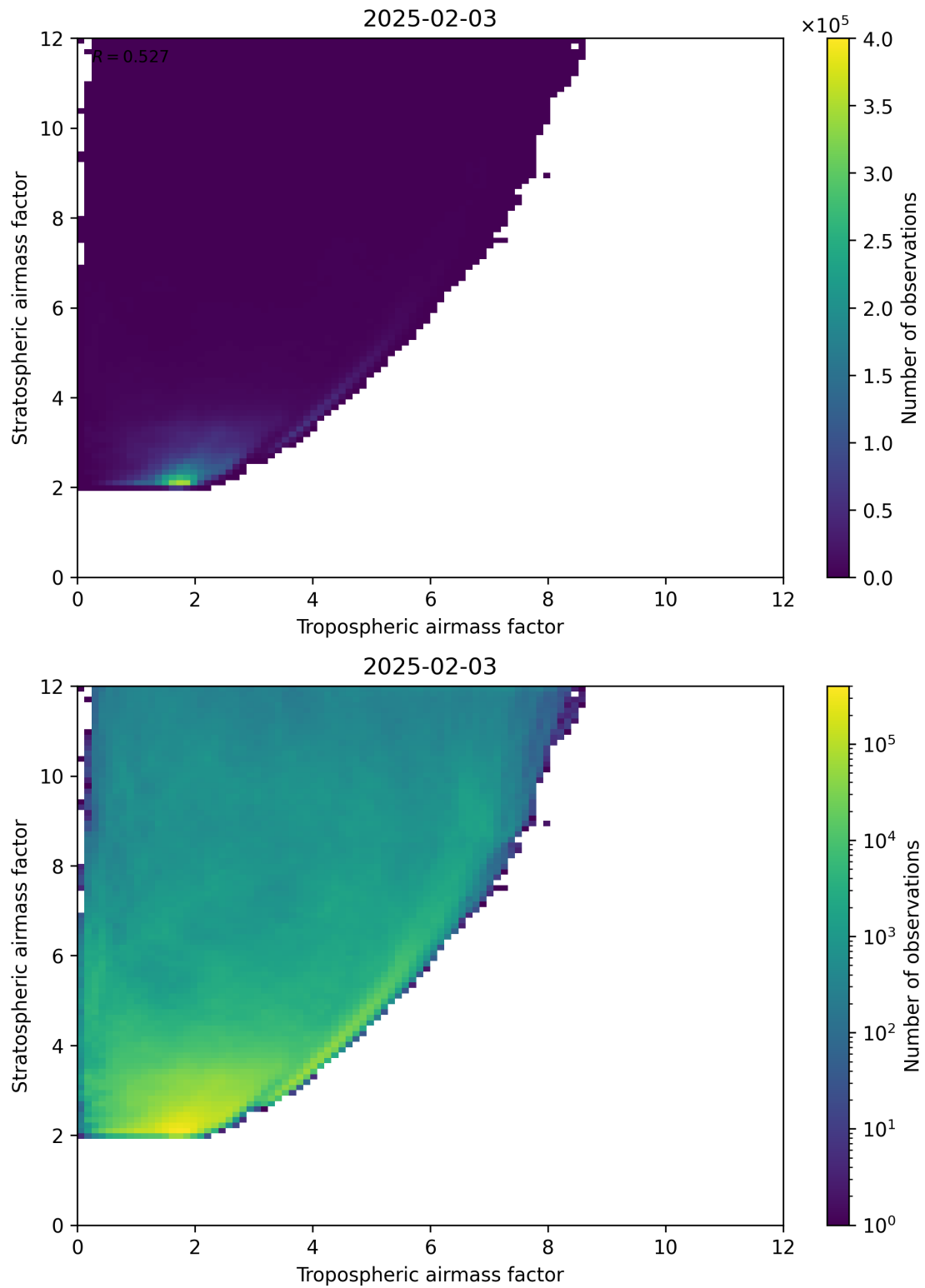
Figure 71: Scatter density plot of “Tropospheric airmass factor” against “Stratospheric airmass factor” for 2025-02-03 to 2025-02-04.
