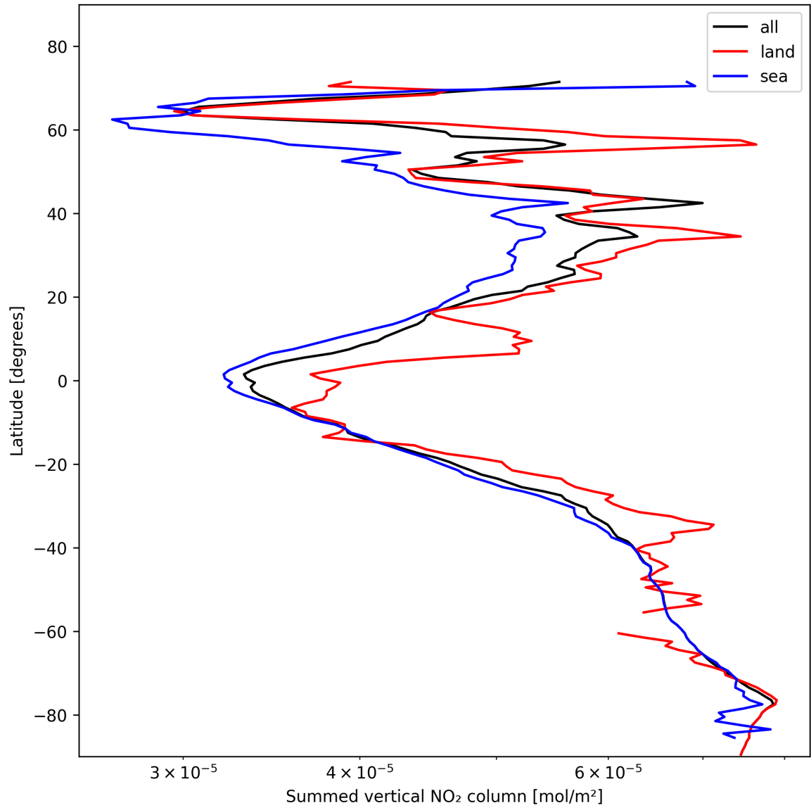
Figure 23: Zonal average of “Summed vertical NO 2 column” for 2025-02-03 to 2025-02-04.
