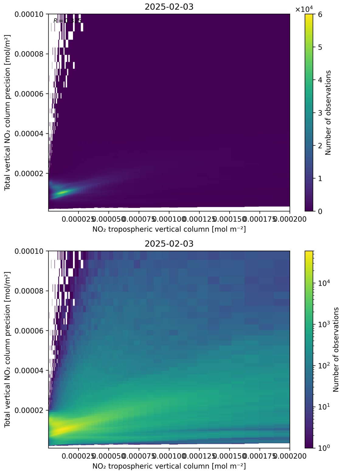
Figure 129: Scatter density plot of “NO 2 tropospheric vertical column” against “Total vertical NO 2 column precision” for 2025-02-03 to 2025-02-04.
