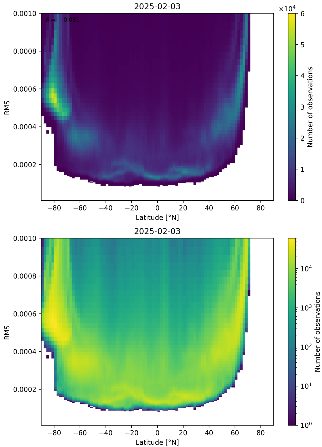
Figure 94: Scatter density plot of “Latitude” against “RMS” for 2025-02-03 to 2025-02-04.
