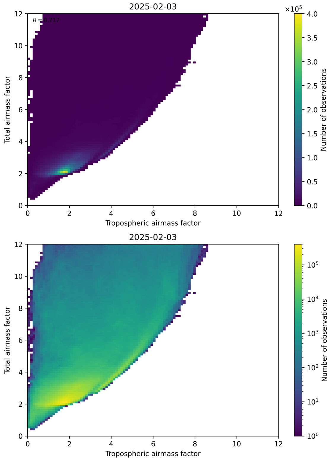
Figure 72: Scatter density plot of “Tropospheric airmass factor” against “Total airmass factor” for 2025-02-03 to 2025-02-04.
