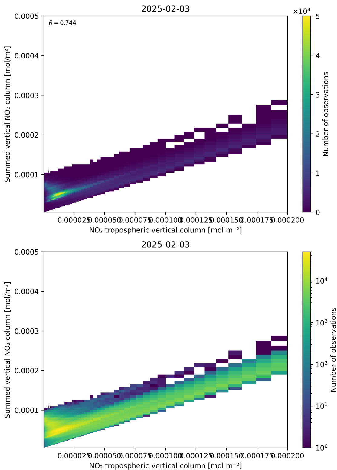
Figure 126: Scatter density plot of “NO 2 tropospheric vertical column” against “Summed vertical NO 2 column” for 2025-02-03 to 2025-02-04.
