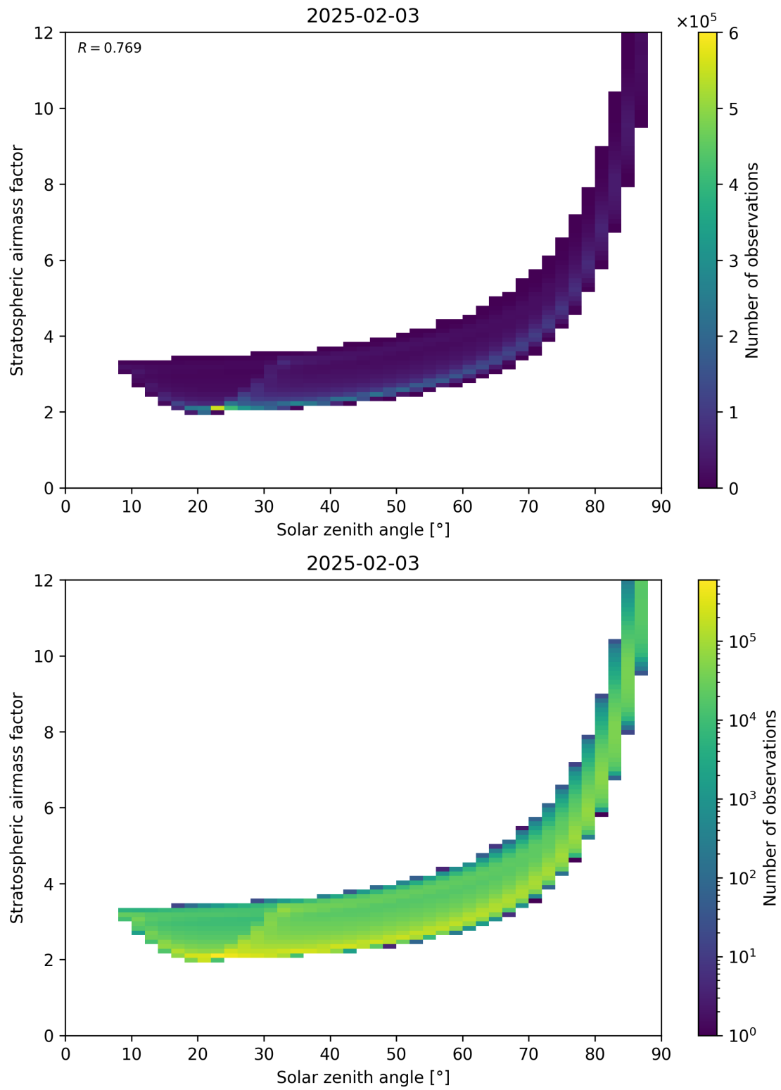
Figure 145: Scatter density plot of “Solar zenith angle” against “Stratospheric airmass factor” for 2025-02-03 to 2025-02-04.
