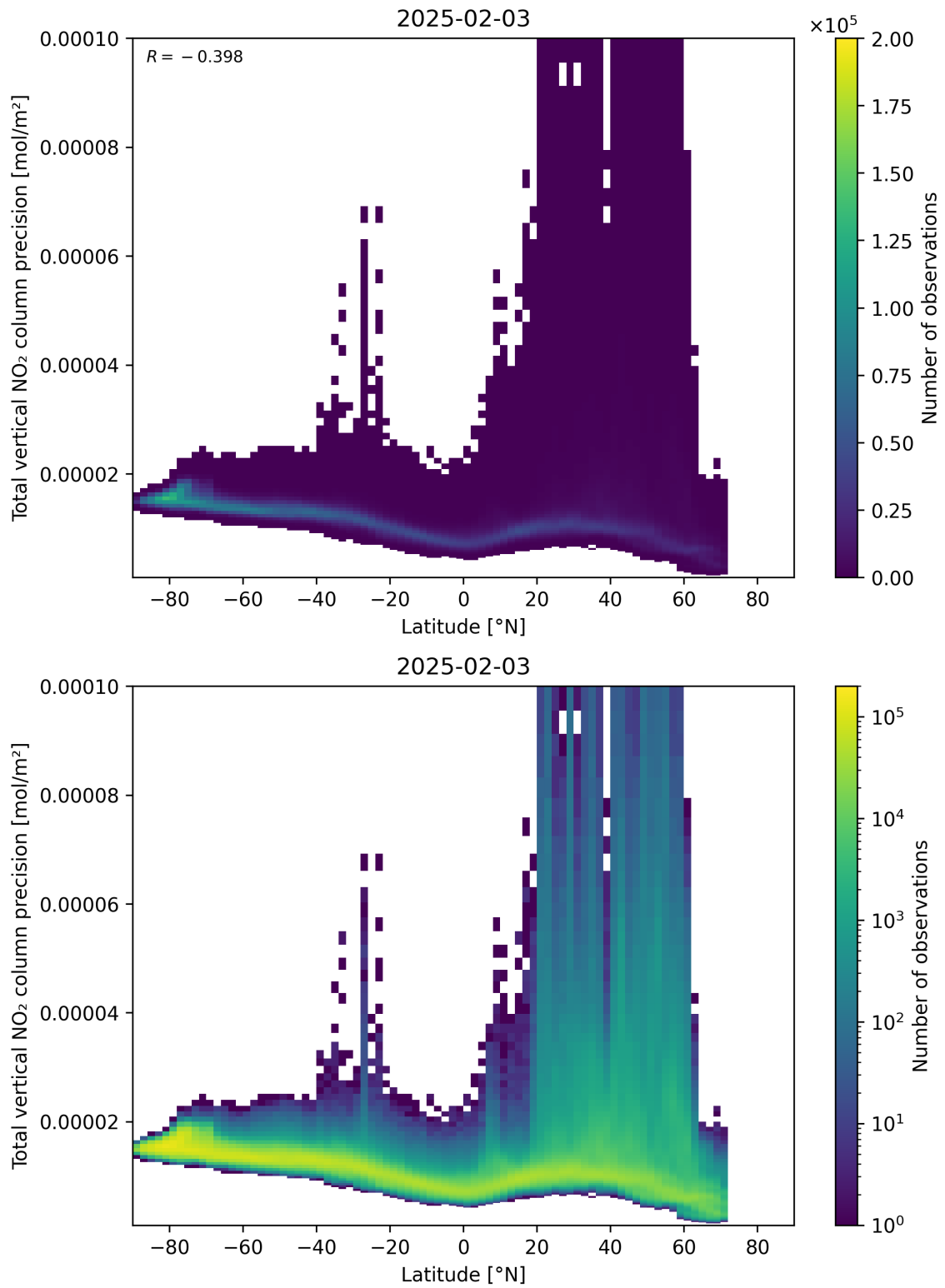
Figure 91: Scatter density plot of “Latitude” against “Total vertical NO 2 column precision” for 2025-02-03 to 2025-02-04.
