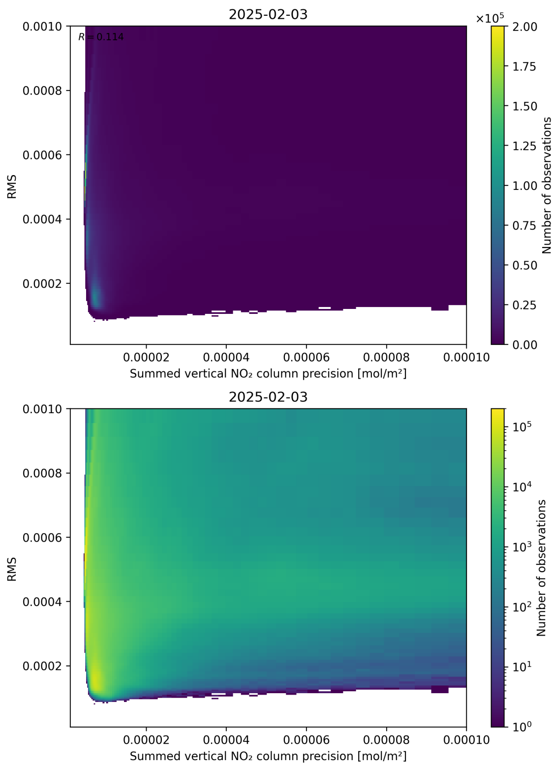
Figure 108: Scatter density plot of “Summed vertical NO 2 column precision” against “RMS” for 2025-02-03 to 2025-02-04.
