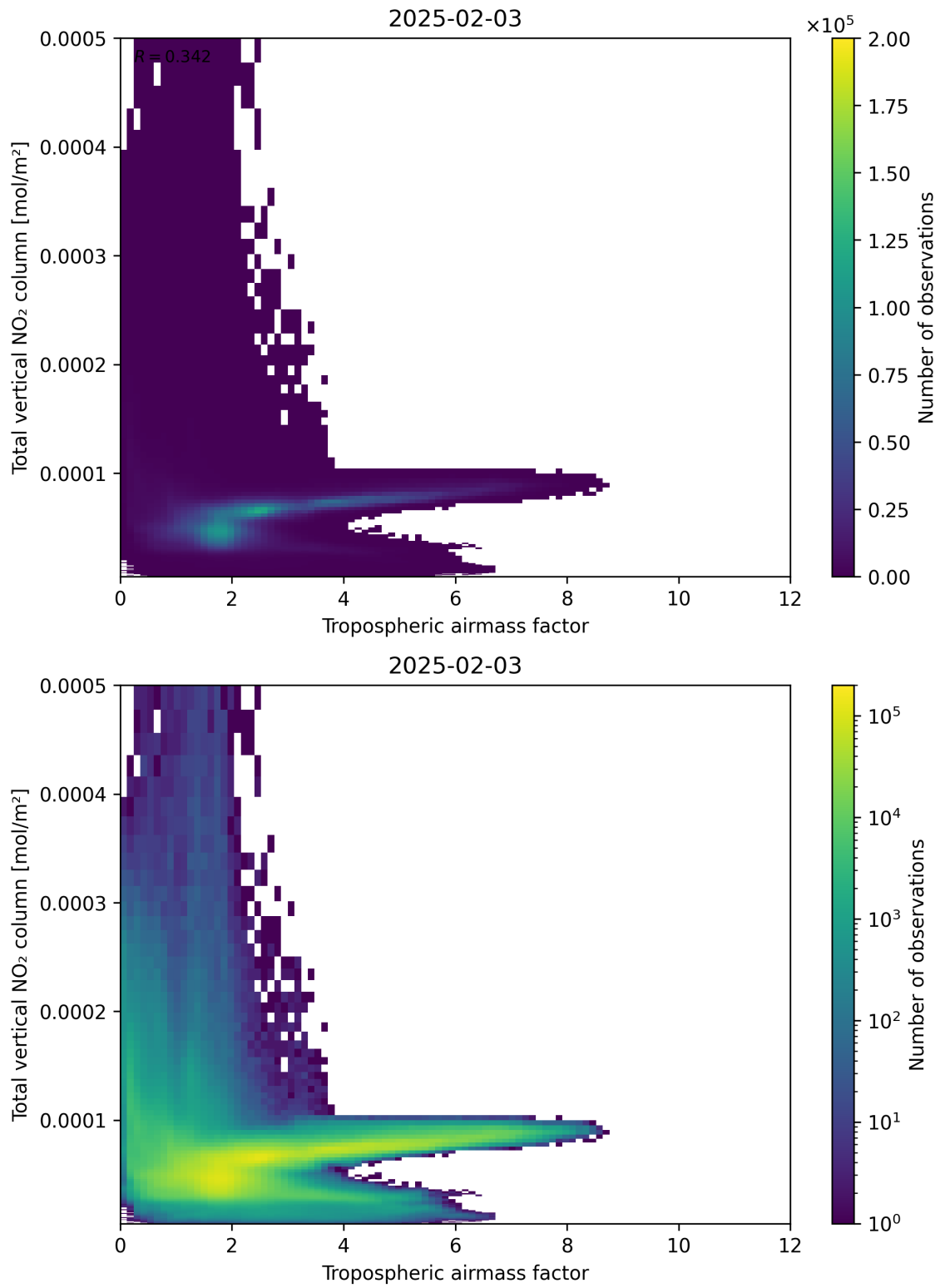
Figure 77: Scatter density plot of “Tropospheric airmass factor” against “Total vertical NO 2 column” for 2025-02-03 to 2025-02-04.
