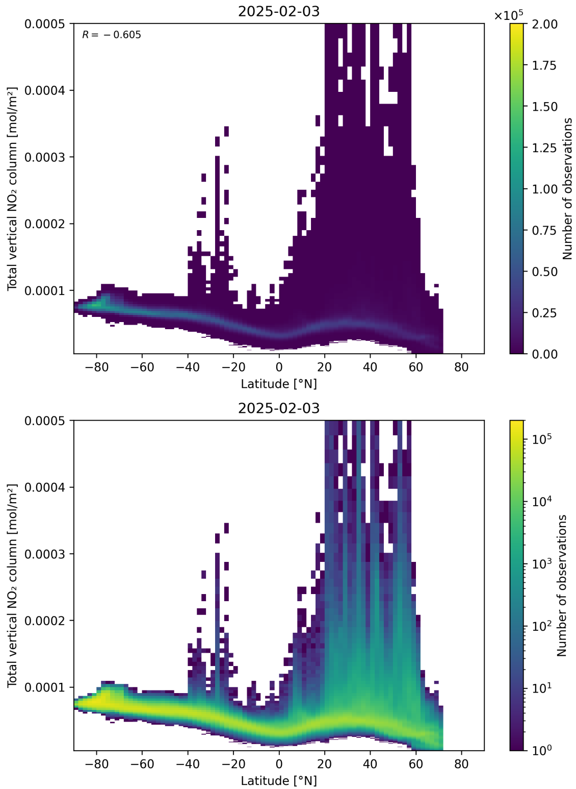
Figure 90: Scatter density plot of “Latitude” against “Total vertical NO 2 column” for 2025-02-03 to 2025-02-04.
