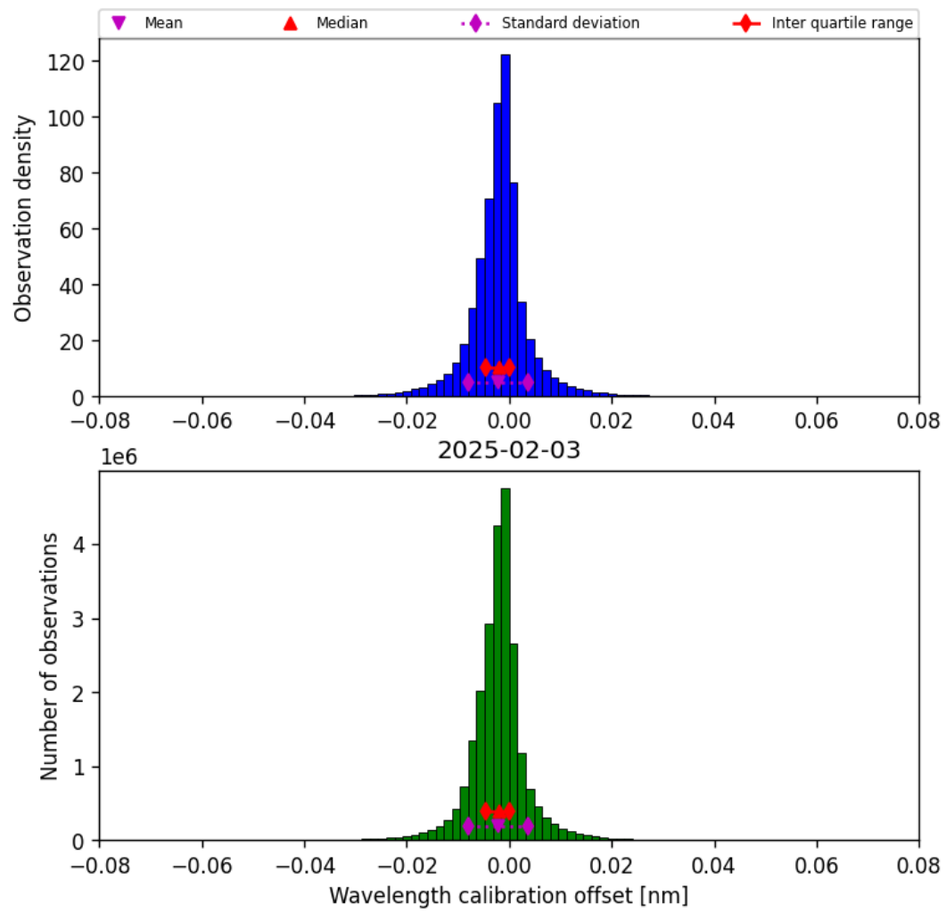
Figure 35: Histogram of “Wavelength calibration offset” for 2025-02-03 to 2025-02-04
