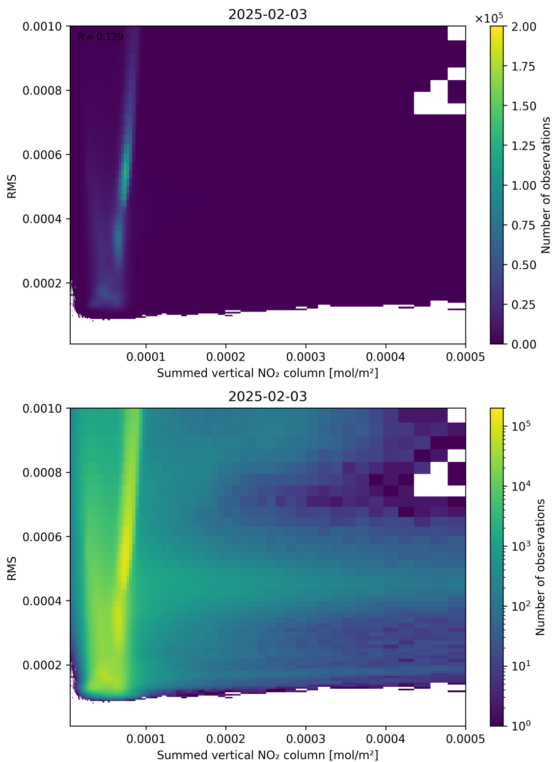
Figure 109: Scatter density plot of “Summed vertical NO 2 column” against “RMS” for 2025-02-03 to 2025-02-04.
