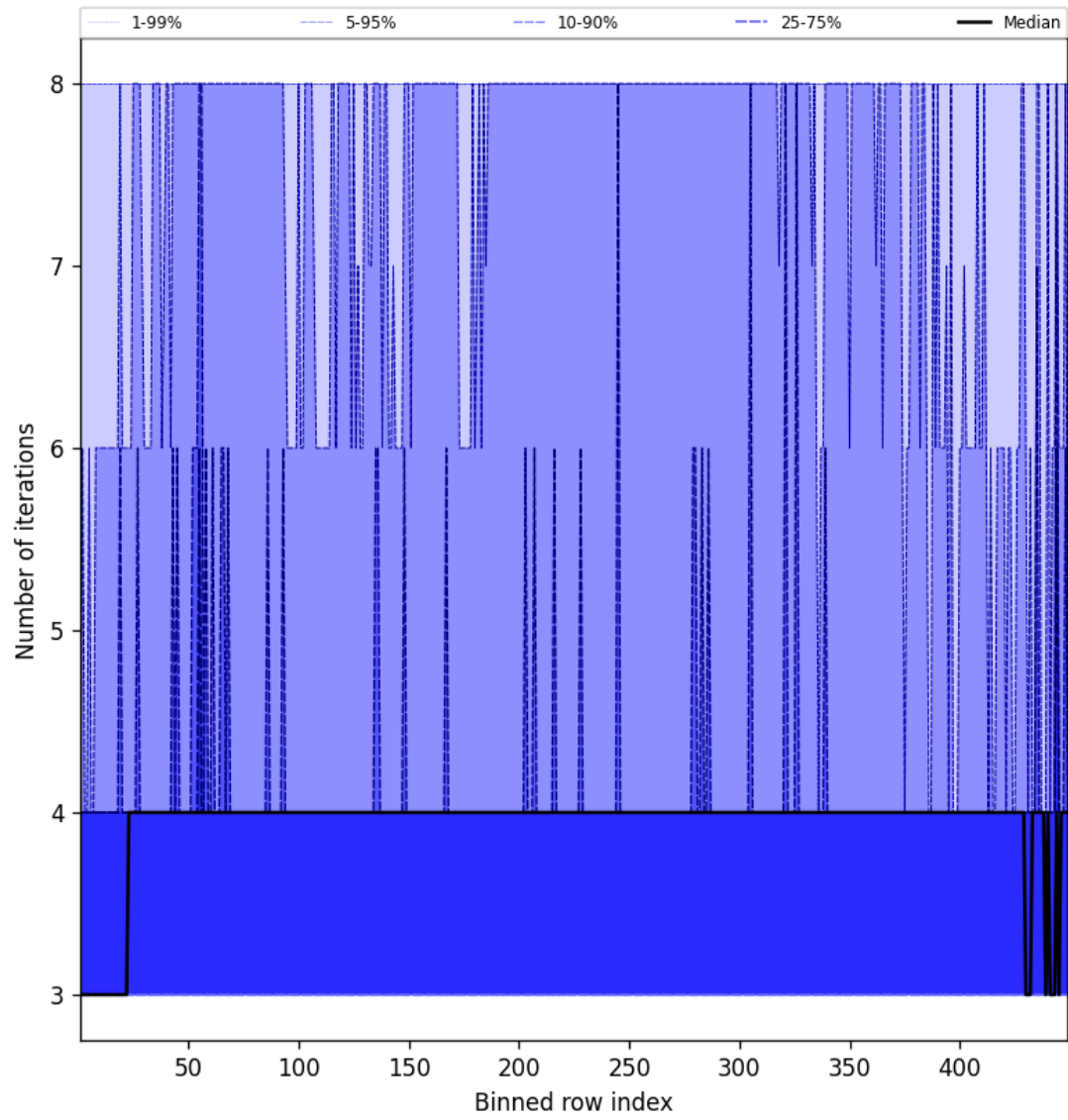
Figure 51: Along track statistics of “Number of iterations” for 2025-02-03 to 2025-02-04
