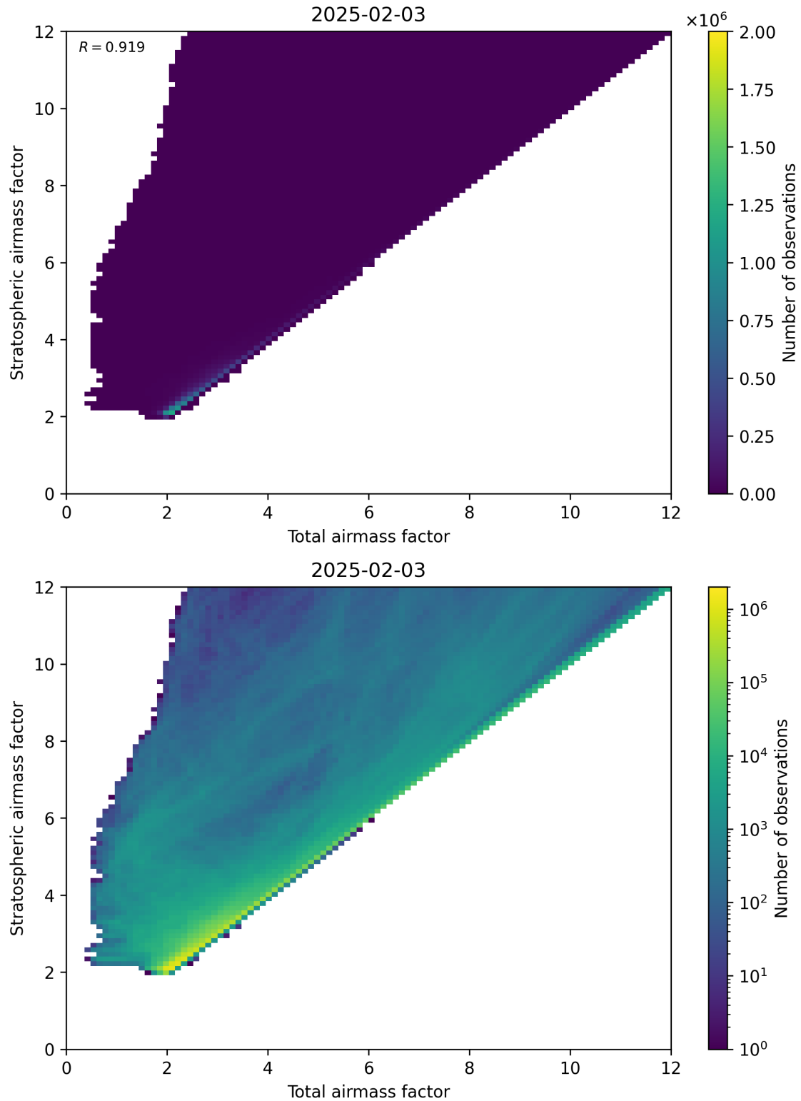
Figure 62: Scatter density plot of “Total airmass factor” against “Stratospheric airmass factor” for 2025-02-03 to 2025-02-04.
