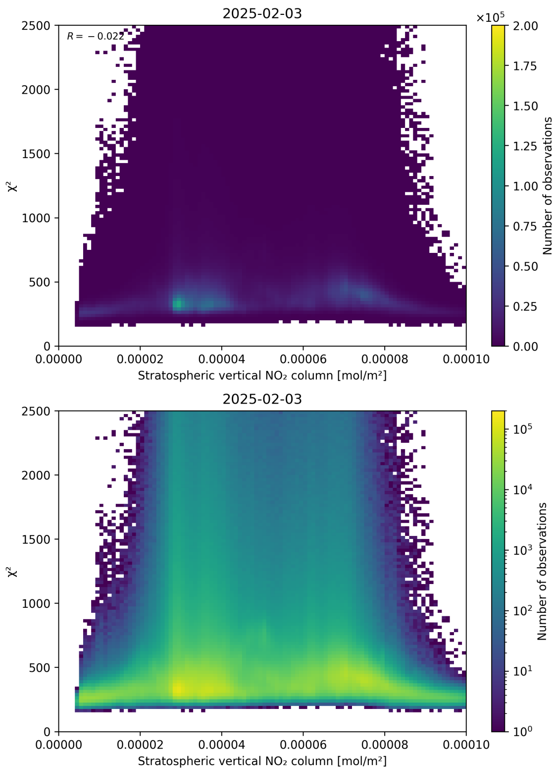
Figure 97: Scatter density plot of “Stratospheric vertical NO 2 column” against “ \chi^2 ” for 2025-02-03 to 2025-02-04.
