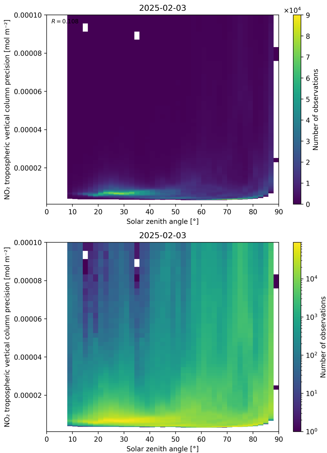
Figure 156: Scatter density plot of “Solar zenith angle” against “NO 2 tropospheric vertical column precision” for 2025-02-03 to 2025-02-04.
