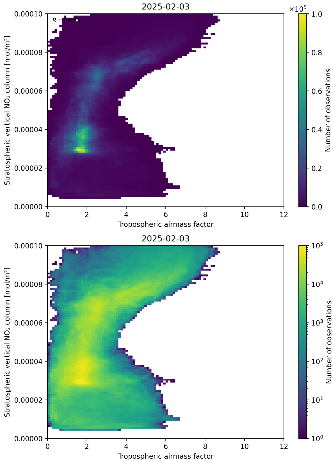
Figure 74: Scatter density plot of “Tropospheric air mass factor” against “Stratospheric vertical NO 2 column” for 2025-02-03 to 2025-02-04.
