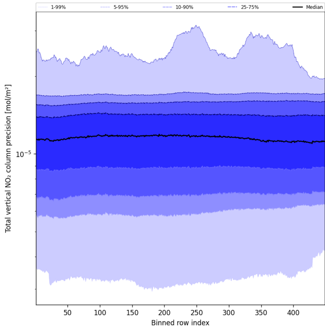
Figure 56: Along track statistics of "Total vertical NO 2 column precision" for 2025-02-03 to 2025-02-04
