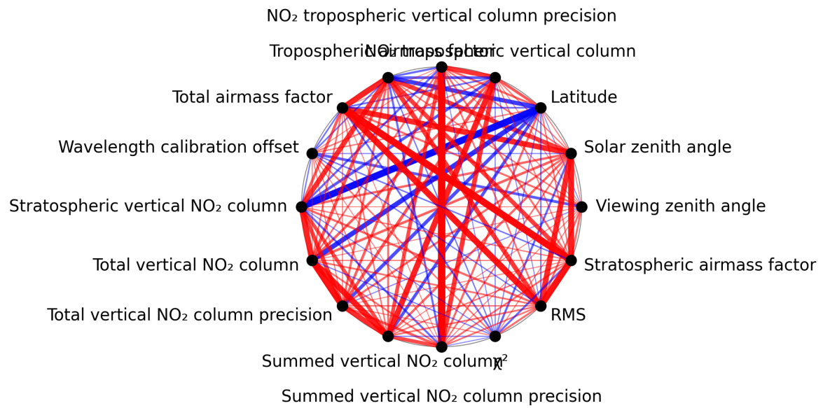
Figure 1: Map of correlation graph for 2025-02-03 to 2025-02-04.
