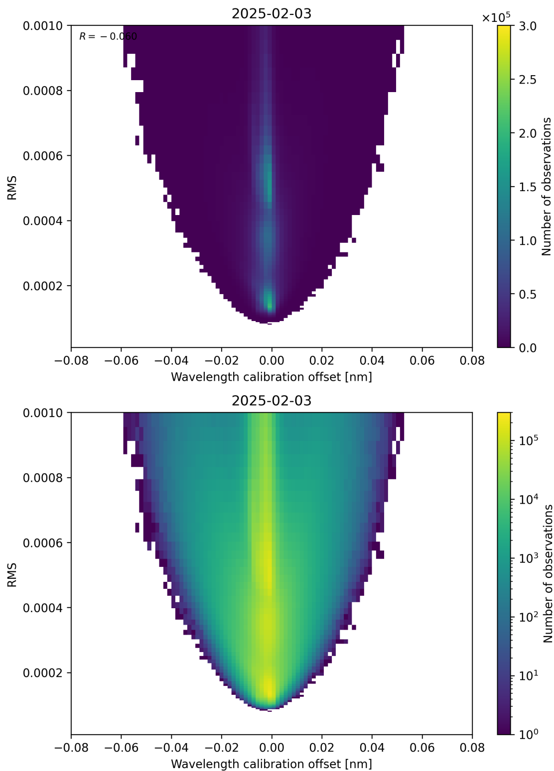
Figure 181: Scatter density plot of “Wavelength calibration offset” against “RMS” for 2025-02-03 to 2025-02-04.
