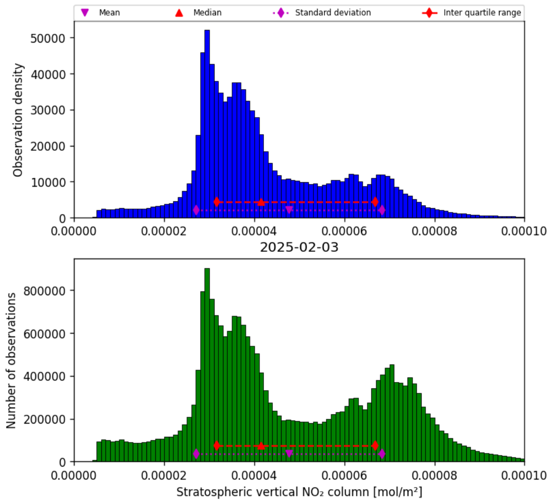
Figure 36: Histogram of “Stratospheric vertical NO 2 column” for 2025-02-03 to 2025-02-04
