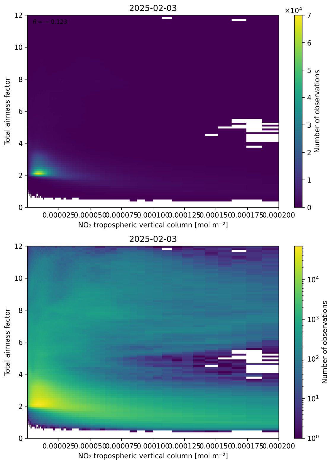
Figure 122: Scatter density plot of “NO 2 tropospheric vertical column” against “Total air mass factor” for 2025-02-03 to 2025-02-04.
