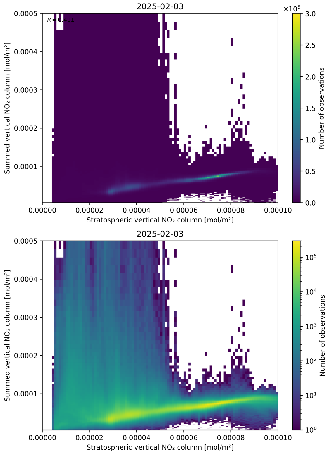
Figure 98: Scatter density plot of “Stratospheric vertical NO 2 column” against “Summed vertical NO 2 column” for 2025-02-03 to 2025-02-04.
