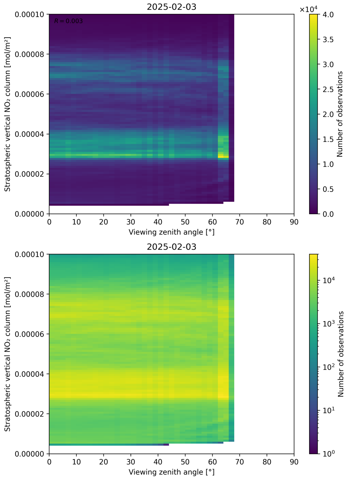
Figure 164: Scatter density plot of “Viewing zenith angle” against “Stratospheric vertical NO 2 column” for 2025-02-03 to 2025-02-04.
