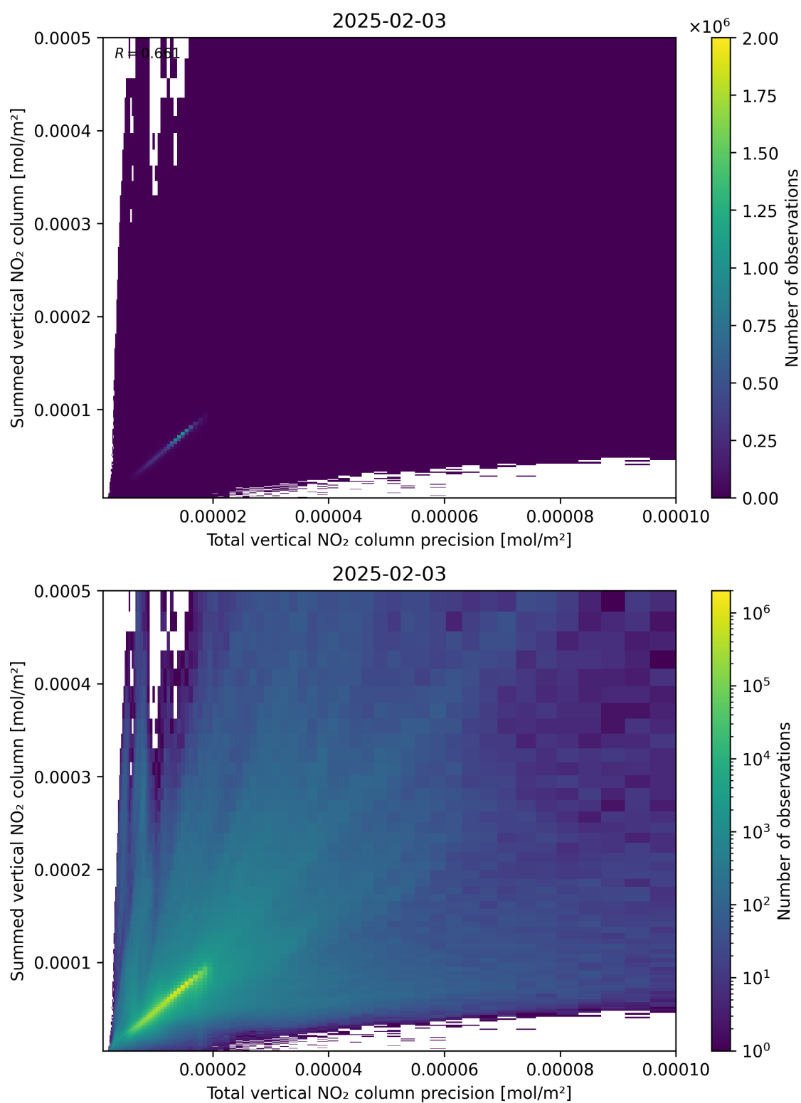
Figure 117: Scatter density plot of “Total vertical NO 2 column precision” against “Summed vertical NO 2 column” for 2025-02-03 to 2025-02-04.
