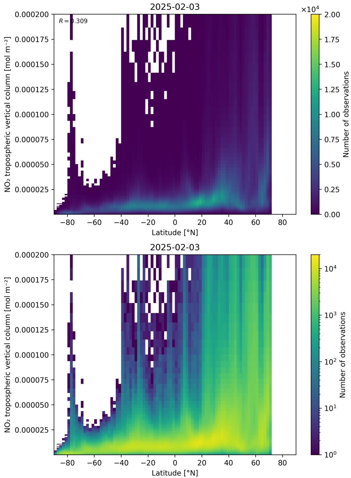
Figure 92: Scatter density plot of “Latitude” against “NO 2 tropospheric vertical column” for 2025-02-03 to 2025-02-04.
