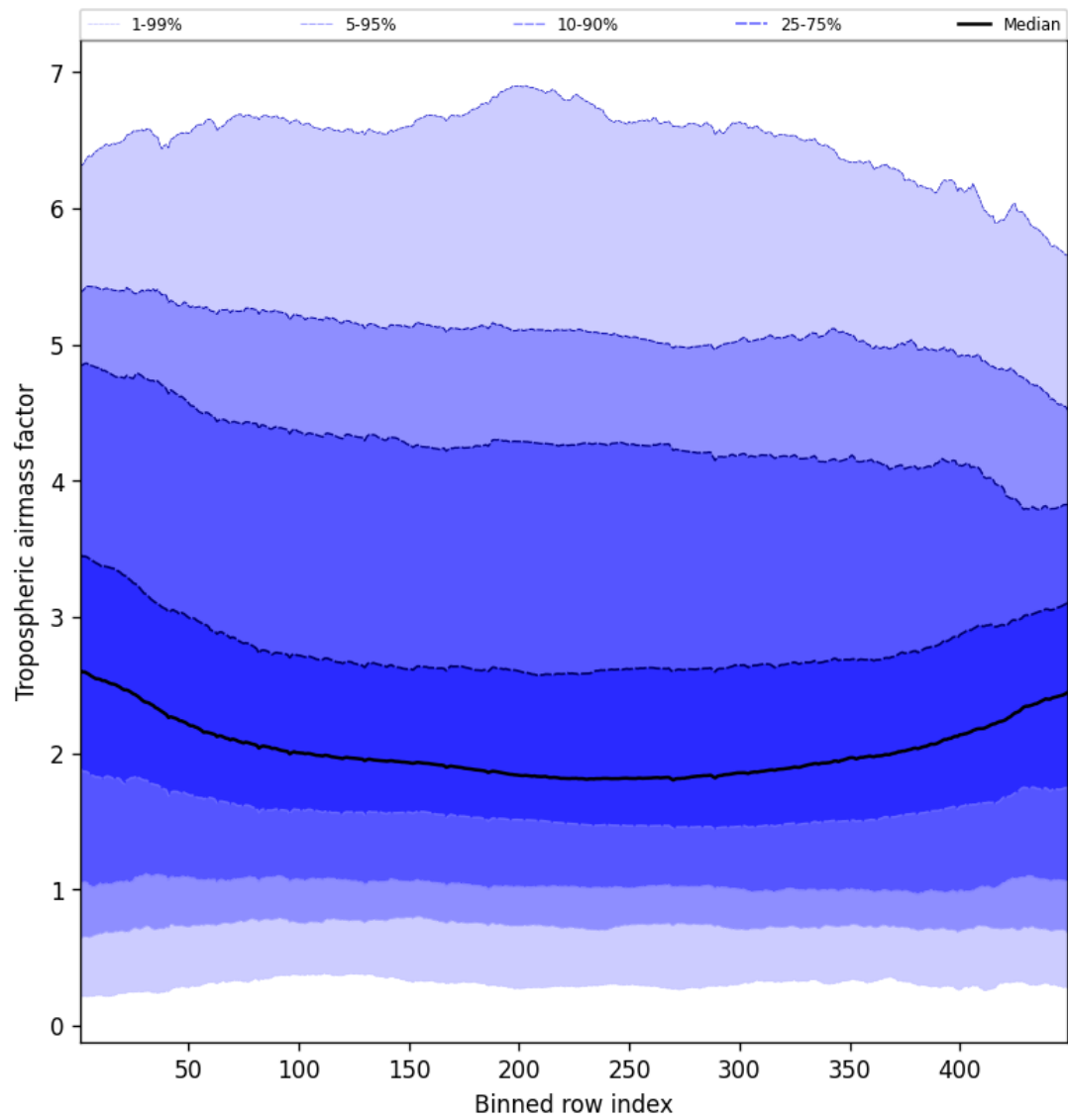
Figure 48: Along track statistics of “Tropospheric airmass factor” for 2025-02-03 to 2025-02-04
