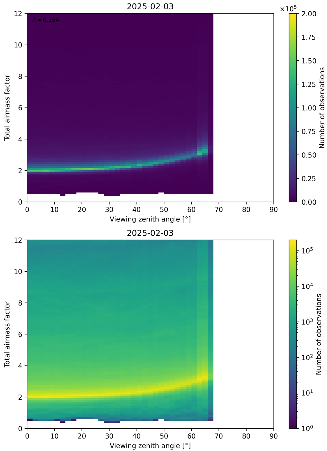
Figure 160: Scatter density plot of “Viewing zenith angle” against “Total airmass factor” for 2025-02-03 to 2025-02-04.
