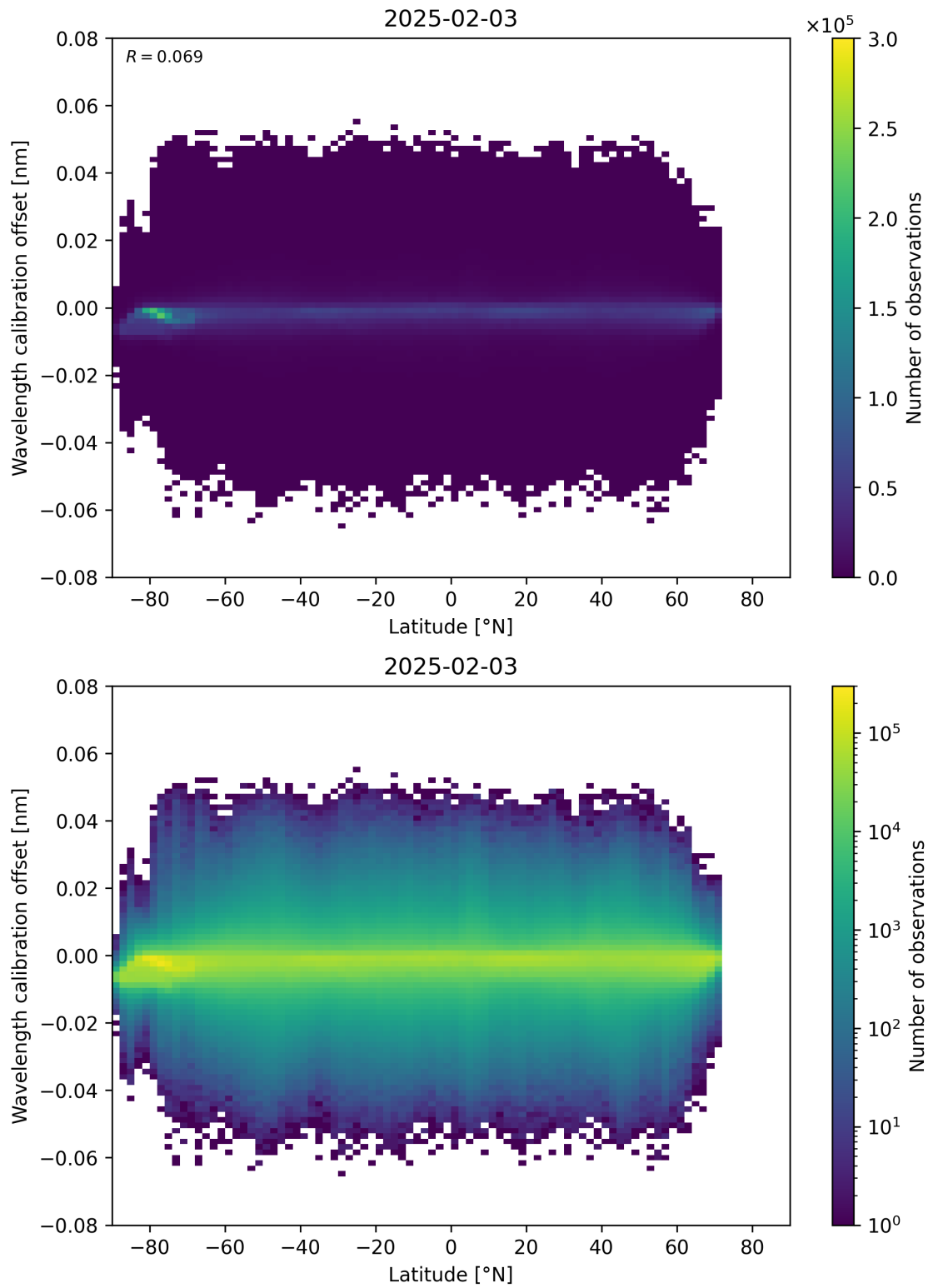
Figure 95: Scatter density plot of “Latitude” against “Wavelength calibration offset” for 2025-02-03 to 2025-02-04.
