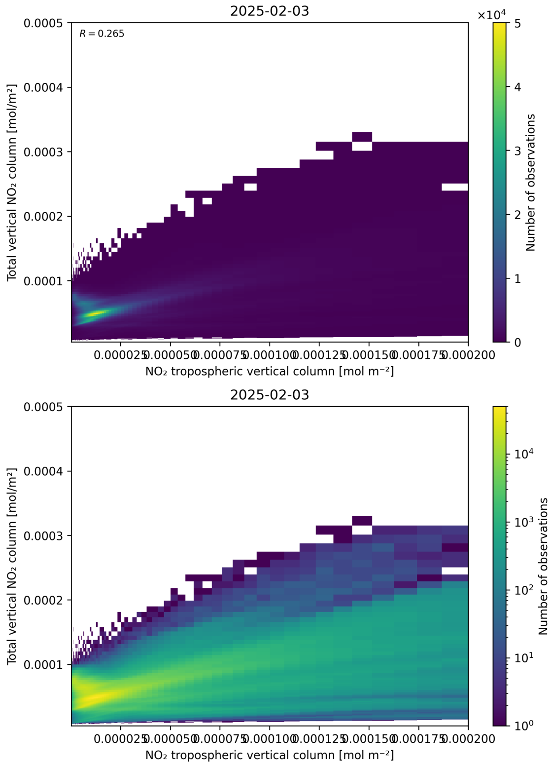
Figure 128: Scatter density plot of “NO 2 tropospheric vertical column” against “Total vertical NO 2 column” for 2025-02-03 to 2025-02-04.
