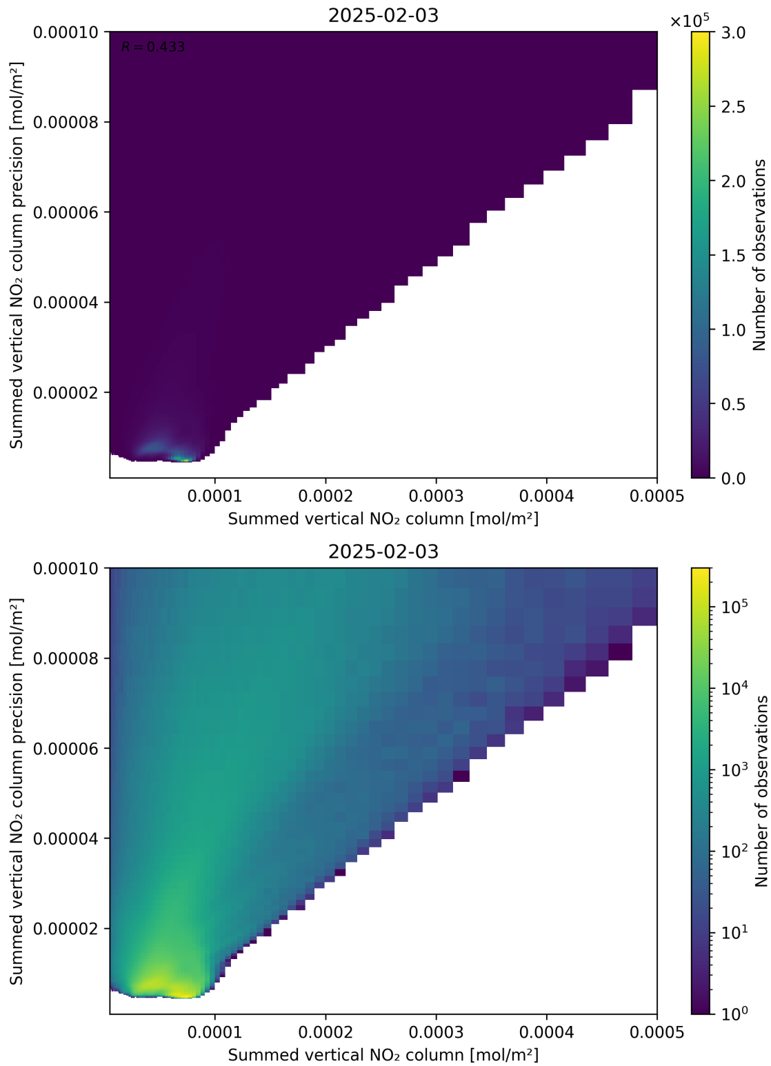
Figure 105: Scatter density plot of “Summed vertical NO 2 column” against “Summed vertical NO 2 column precision” for 2025-02-03 to 2025-02-04.
