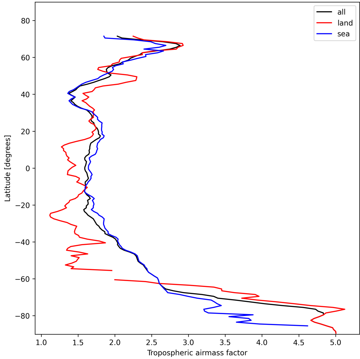
Figure 14: Zonal average of “Tropospheric airmass factor” for 2025-02-03 to 2025-02-04.
