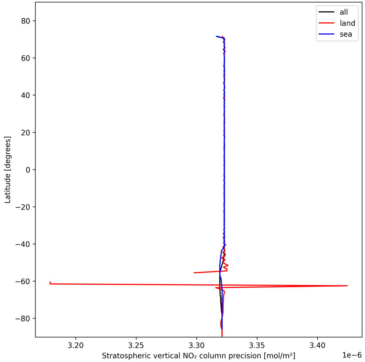
Figure 20: Zonal average of “Stratospheric vertical NO 2 column precision” for 2025-02-03 to 2025-02-04.
