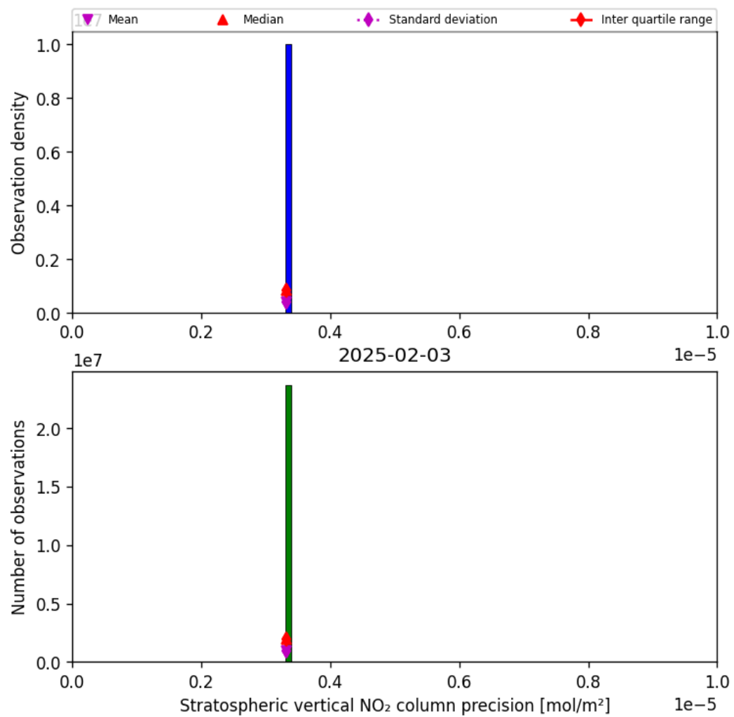
Figure 37: Histogram of “Stratospheric vertical NO 2 column precision” for 2025-02-03 to 2025-02-04
