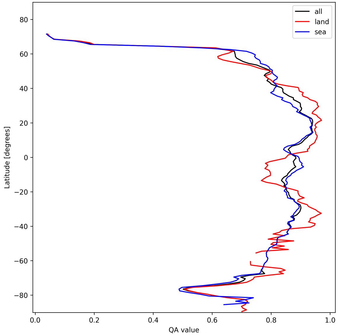
Figure 11: Zonal average of “QA value” for 2025-02-03 to 2025-02-04.
