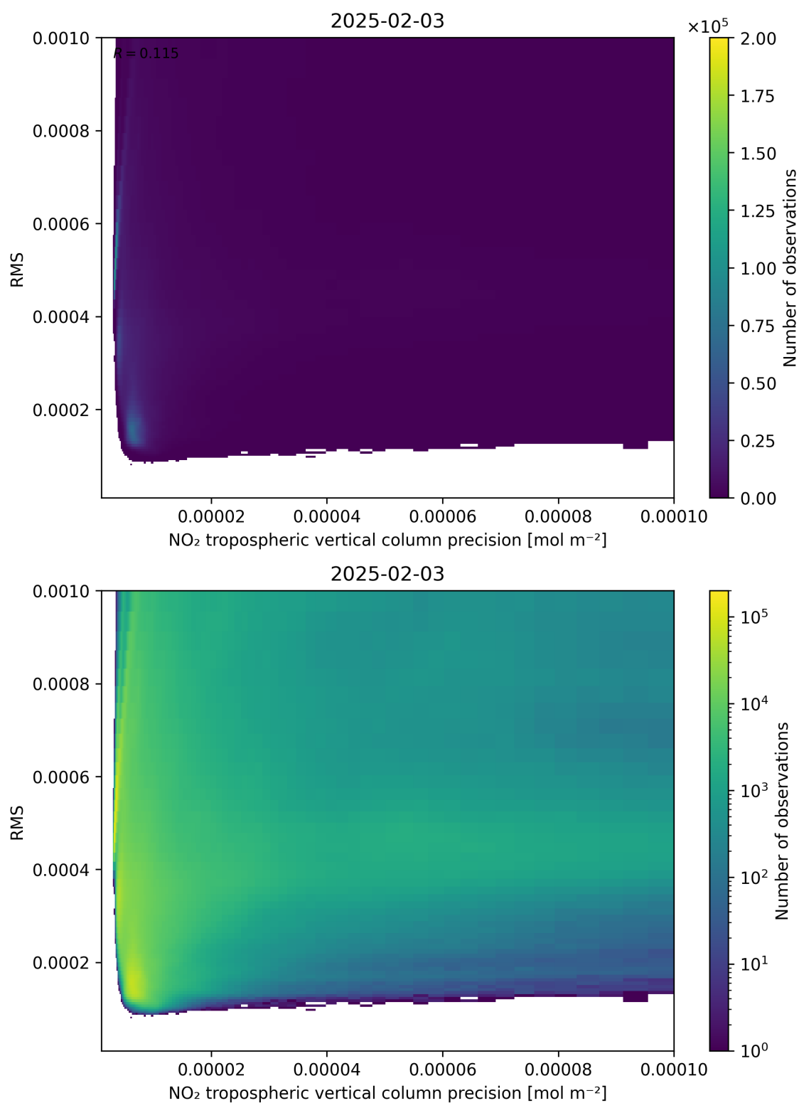
Figure 140: Scatter density plot of “NO 2 tropospheric vertical column precision” against “RMS” for 2025-02-03 to 2025-02-04.
