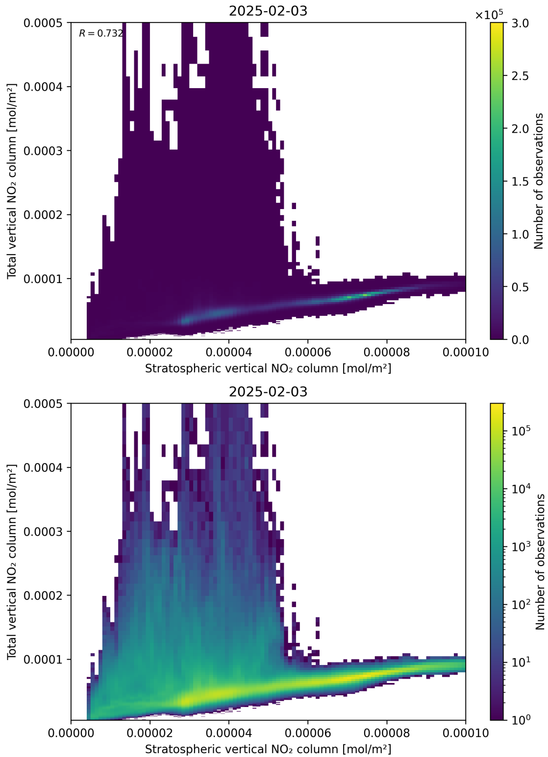
Figure 100: Scatter density plot of “Stratospheric vertical NO 2 column” against “Total vertical NO 2 column” for 2025-02-03 to 2025-02-04.
