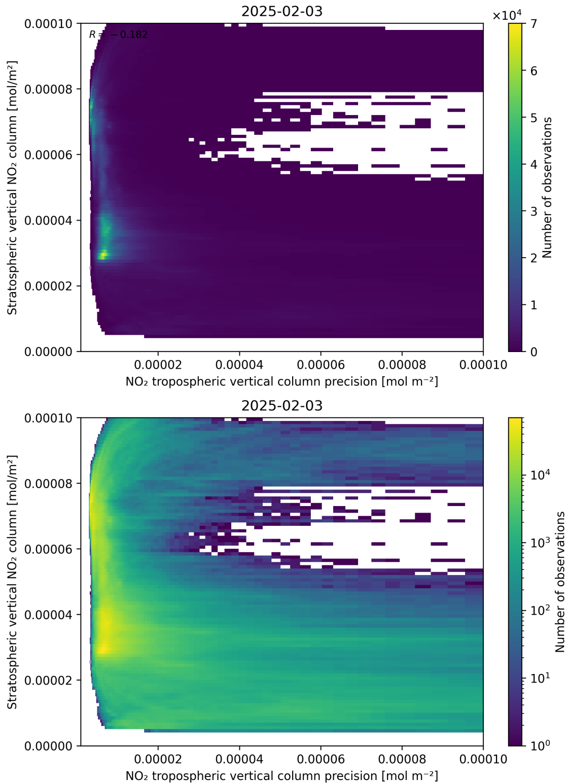
Figure 135: Scatter density plot of “NO 2 tropospheric vertical column precision” against “Stratospheric vertical NO 2 column” for 2025-02-03 to 2025-02-04.
