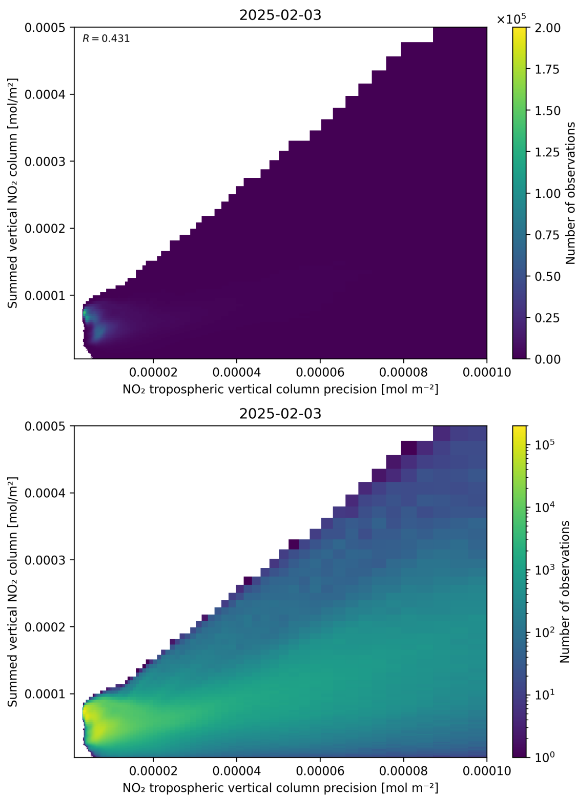
Figure 136: Scatter density plot of “NO 2 tropospheric vertical column precision” against “Summed vertical NO 2 column” for 2025-02-03 to 2025-02-04.
