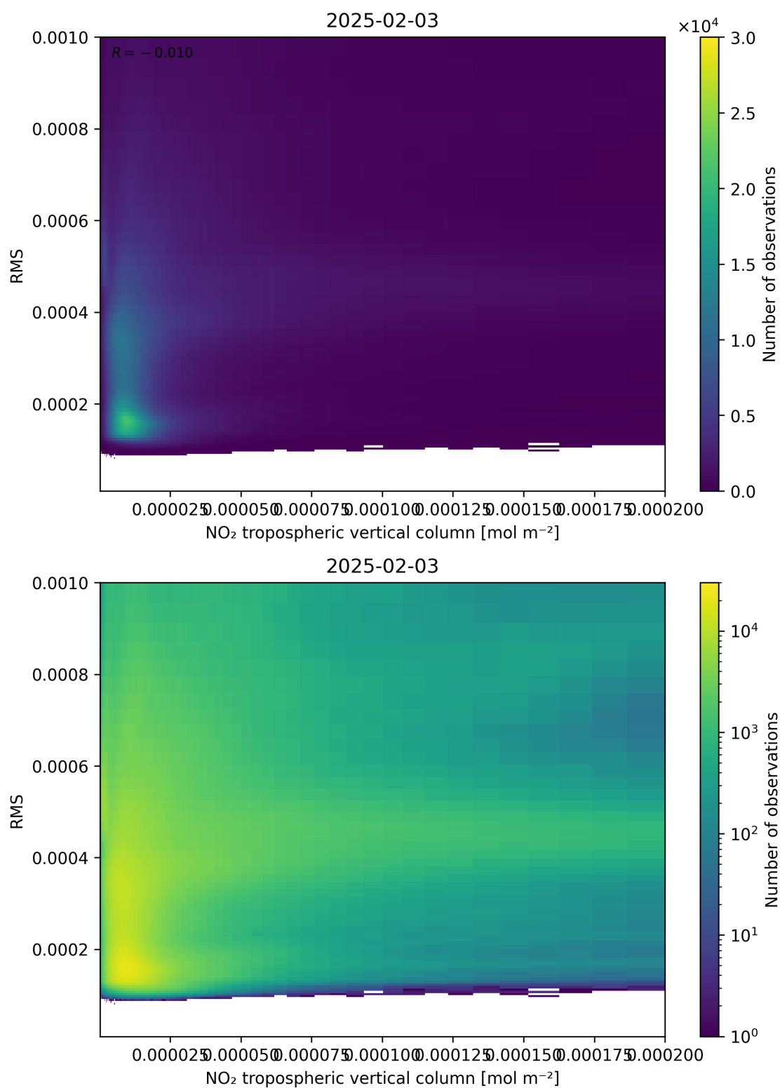
Figure 142: Scatter density plot of “NO 2 tropospheric vertical column” against “RMS” for 2025-02-03 to 2025-02-04.
