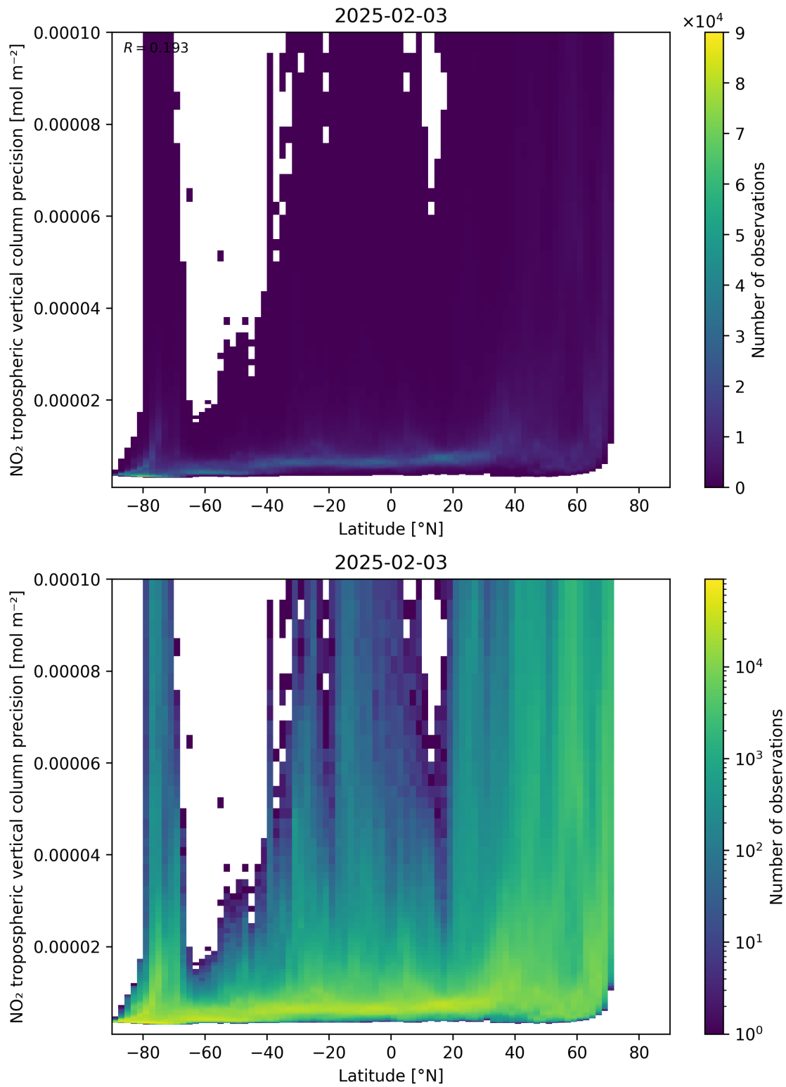
Figure 93: Scatter density plot of “Latitude” against “NO 2 tropospheric vertical column precision” for 2025-02-03 to 2025-02-04.
