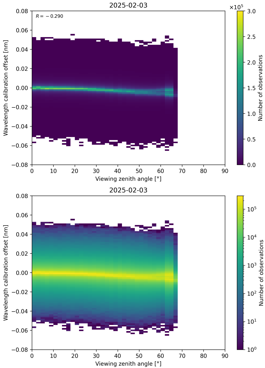
Figure 173: Scatter density plot of “Viewing zenith angle” against “Wavelength calibration offset” for 2025-02-03 to 2025-02-04.
