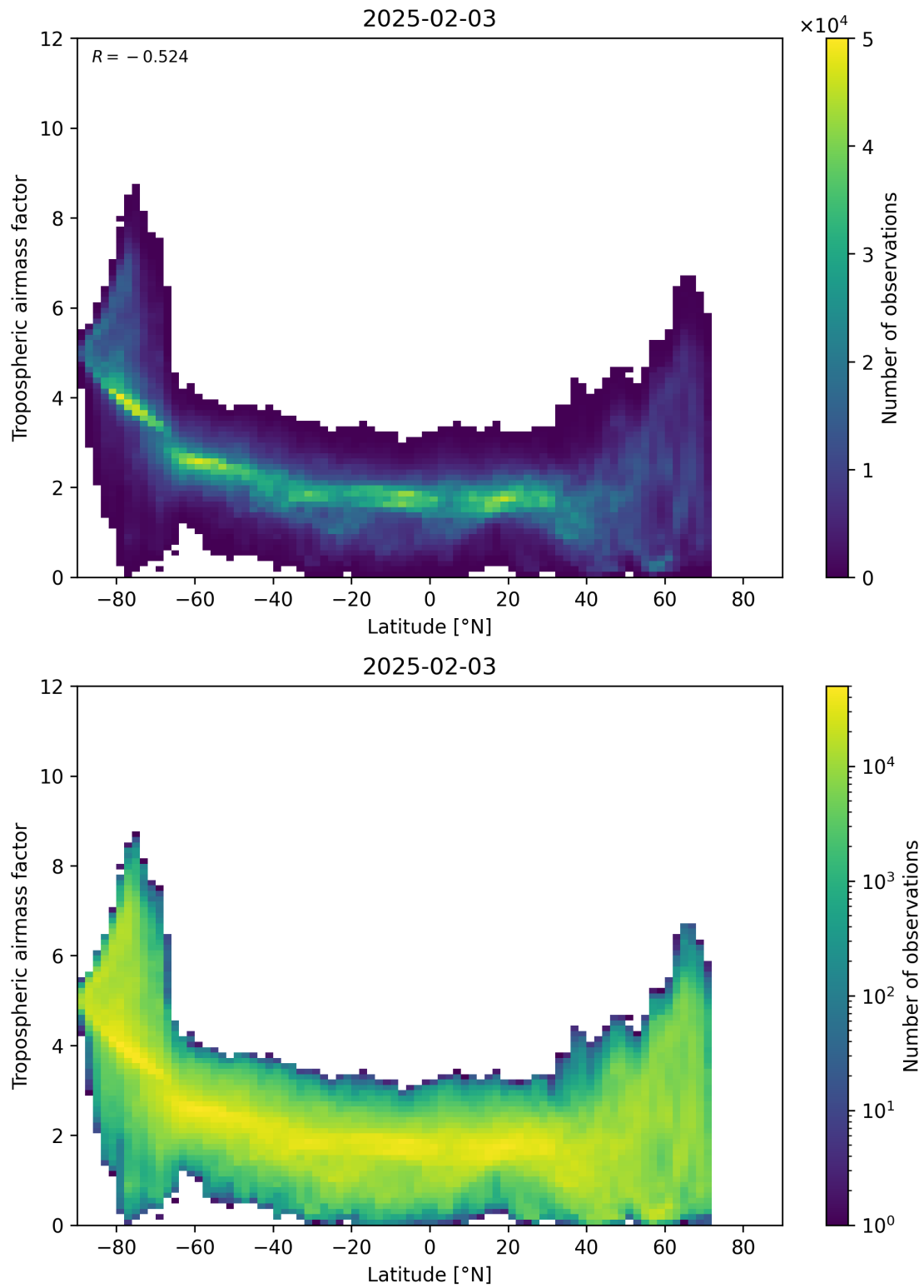
Figure 85: Scatter density plot of “Latitude” against “Tropospheric airmass factor” for 2025-02-03 to 2025-02-04.
