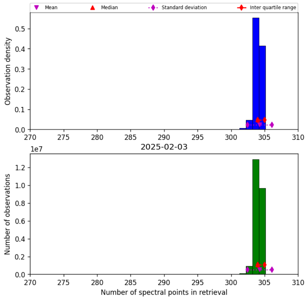
Figure 33: Histogram of “Number of spectral points in retrieval” for 2025-02-03 to 2025-02-04
