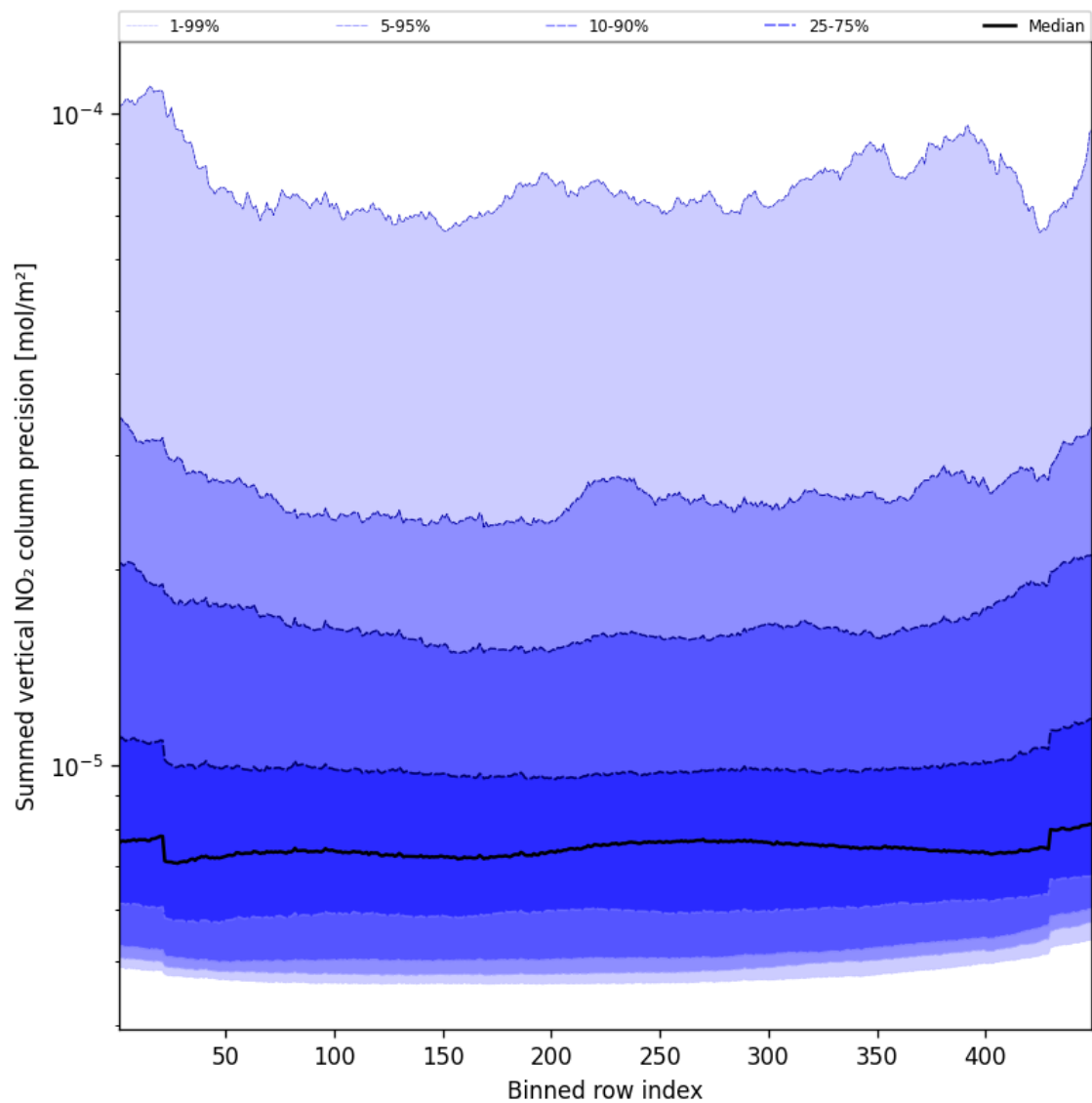
Figure 58: Along track statistics of “Summed vertical NO 2 column precision” for 2025-02-03 to 2025-02-04
