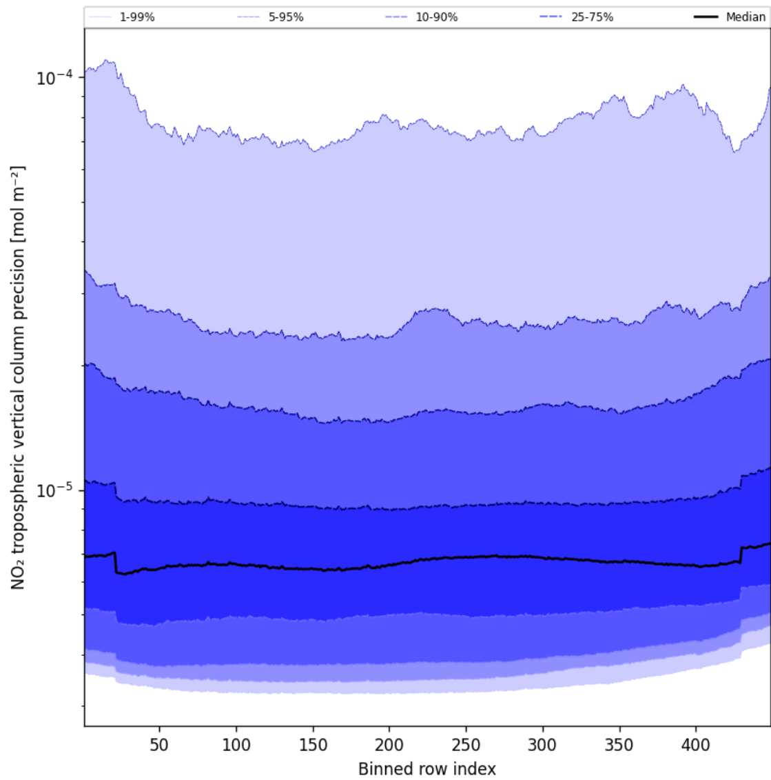
Figure 47: Along track statistics of “NO 2 tropospheric vertical column precision” for 2025-02-03 to 2025-02-04
