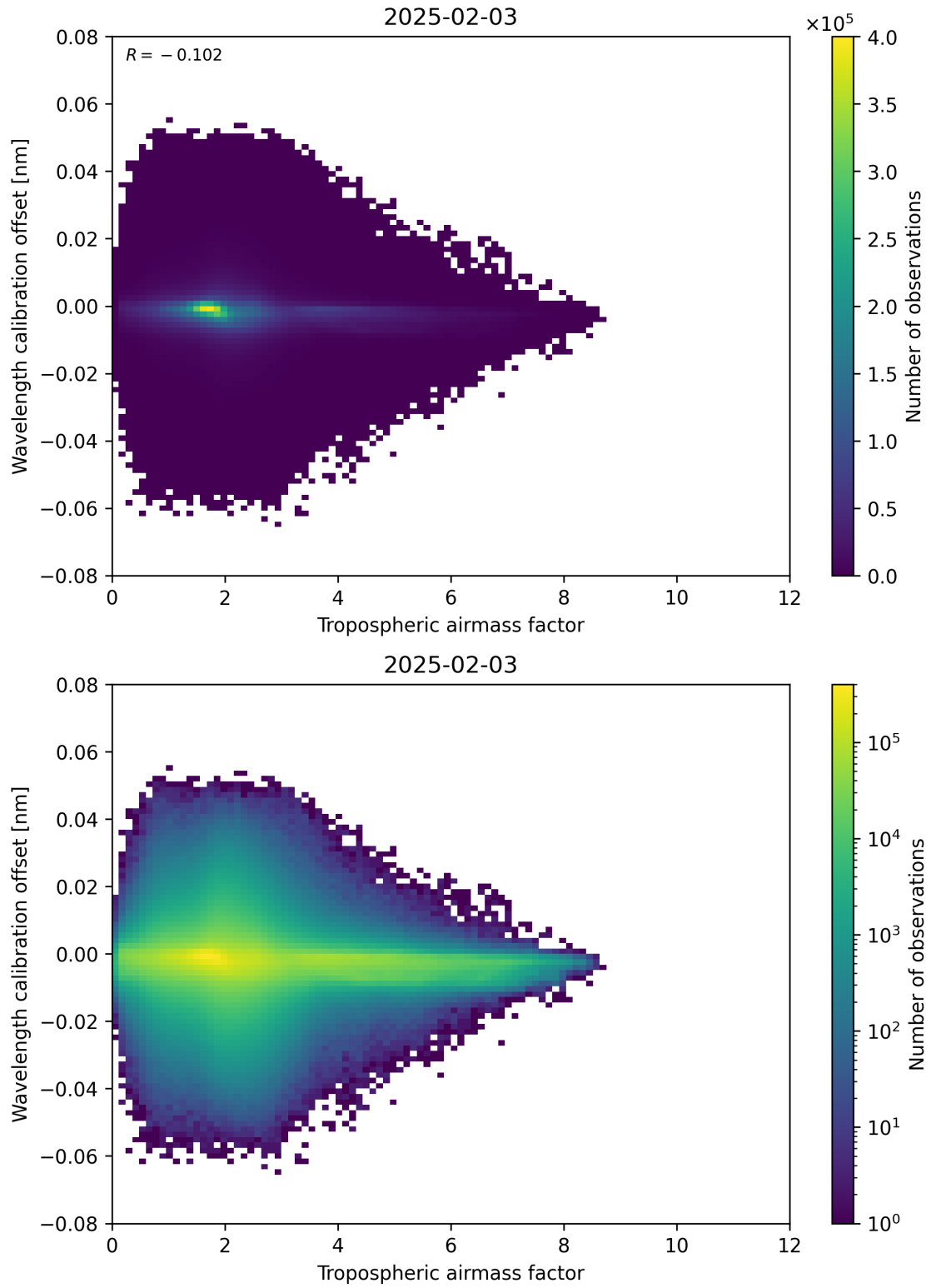
Figure 80: Scatter density plot of “Tropospheric airmass factor” against “Wavelength calibration offset” for 2025-02-03 to 2025-02-04.
