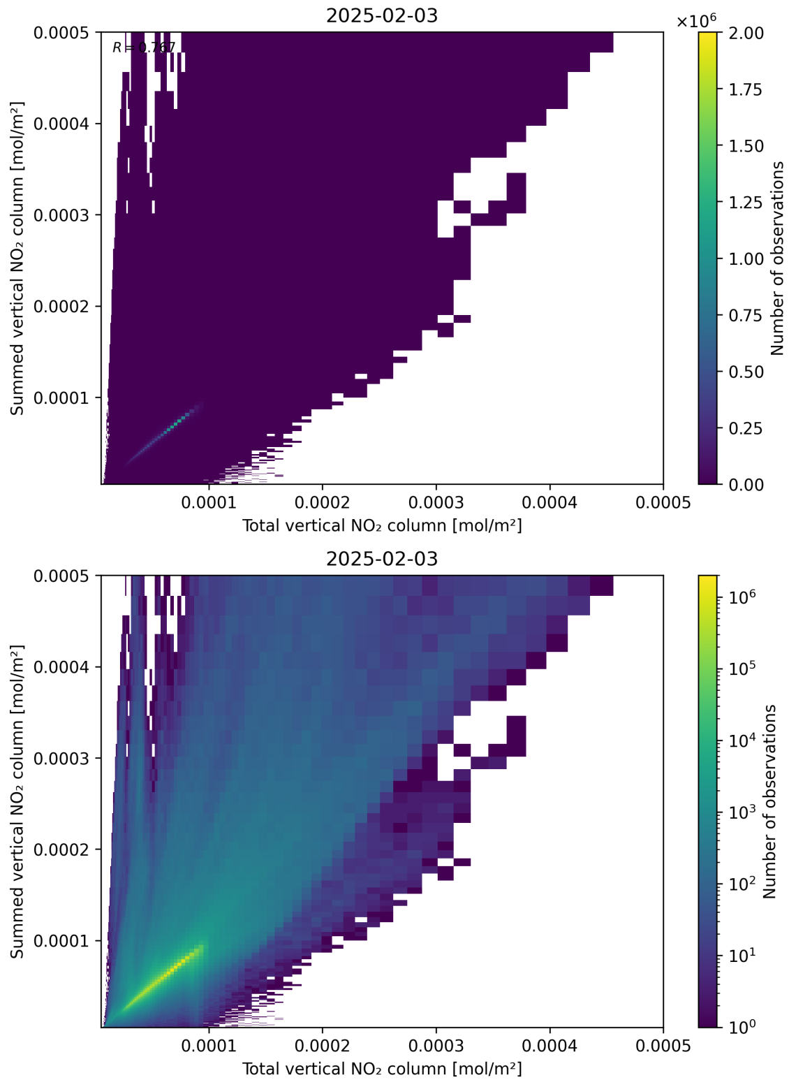
Figure 112: Scatter density plot of “Total vertical NO 2 column” against “Summed vertical NO 2 column” for 2025-02-03 to 2025-02-04.
