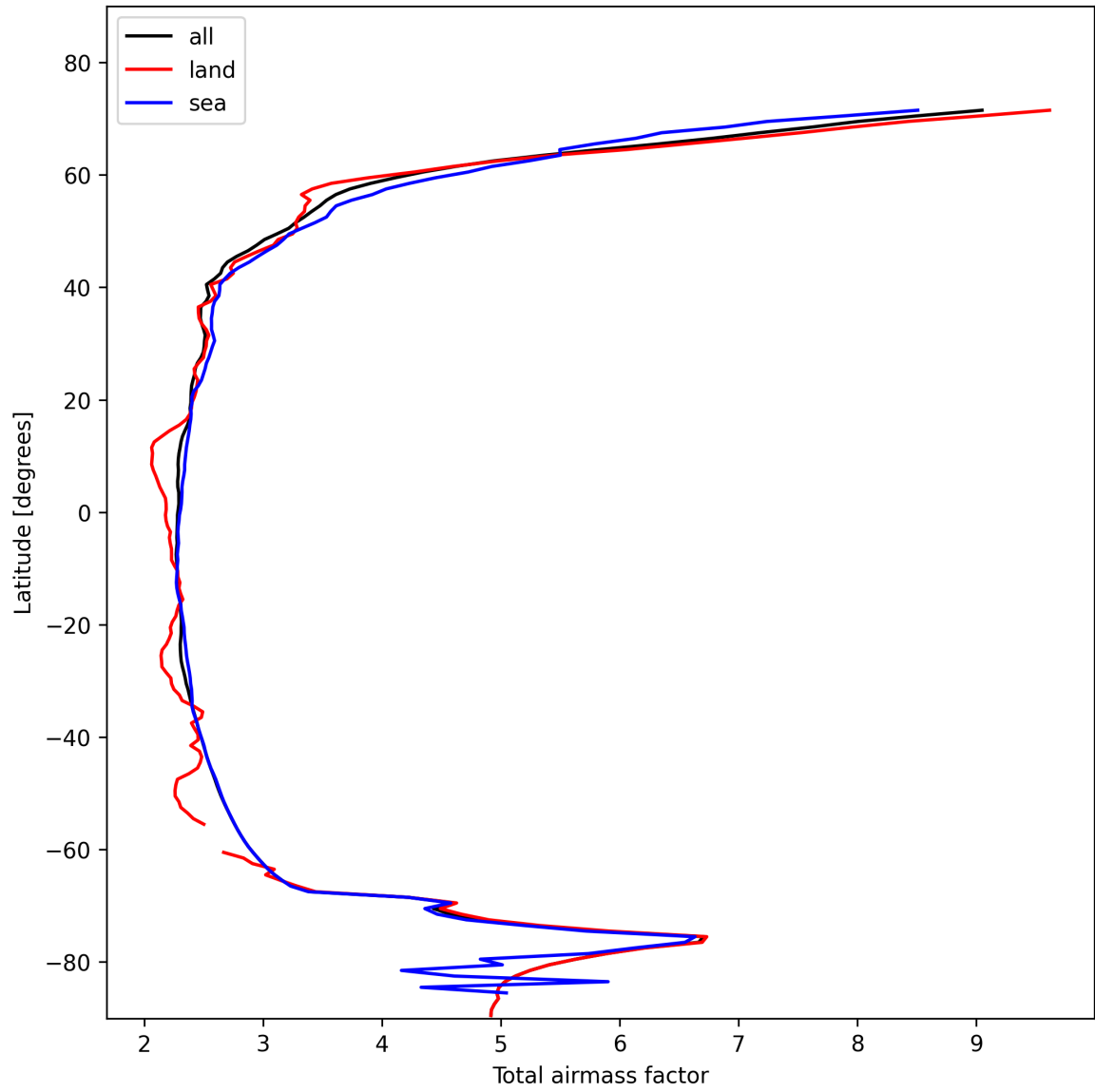
Figure 15: Zonal average of “Total airmass factor” for 2025-02-03 to 2025-02-04.
