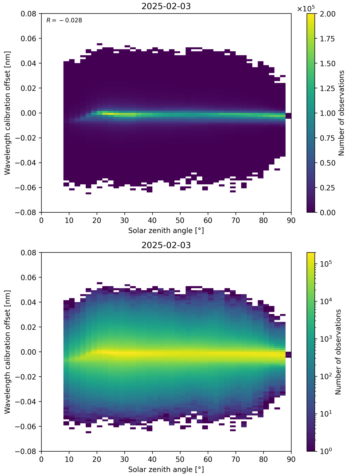
Figure 158: Scatter density plot of “Solar zenith angle” against “Wavelength calibration offset” for 2025-02-03 to 2025-02-04.
