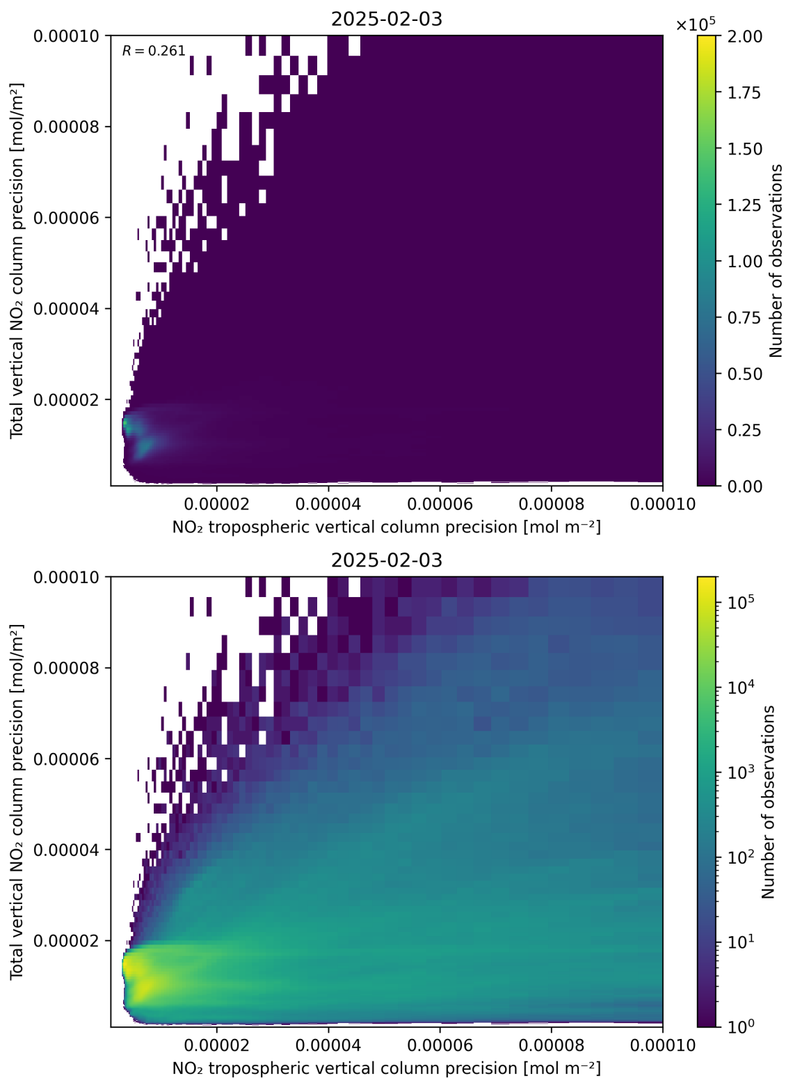
Figure 139: Scatter density plot of “NO 2 tropospheric vertical column precision” against “Total vertical NO 2 column precision” for 2025-02-03 to 2025-02-04.
