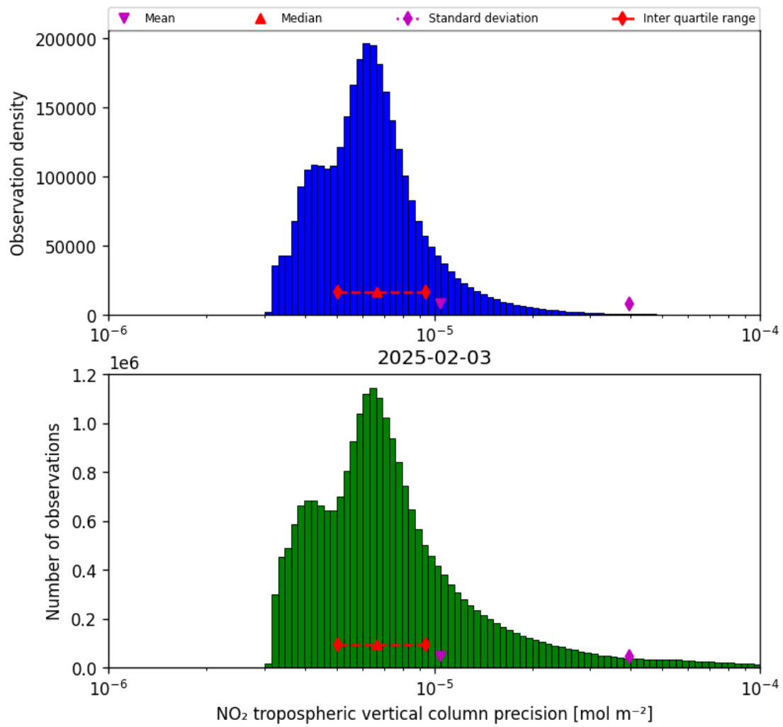
Figure 30: Histogram of “NO 2 tropospheric vertical column precision” for 2025-02-03 to 2025-02-04
