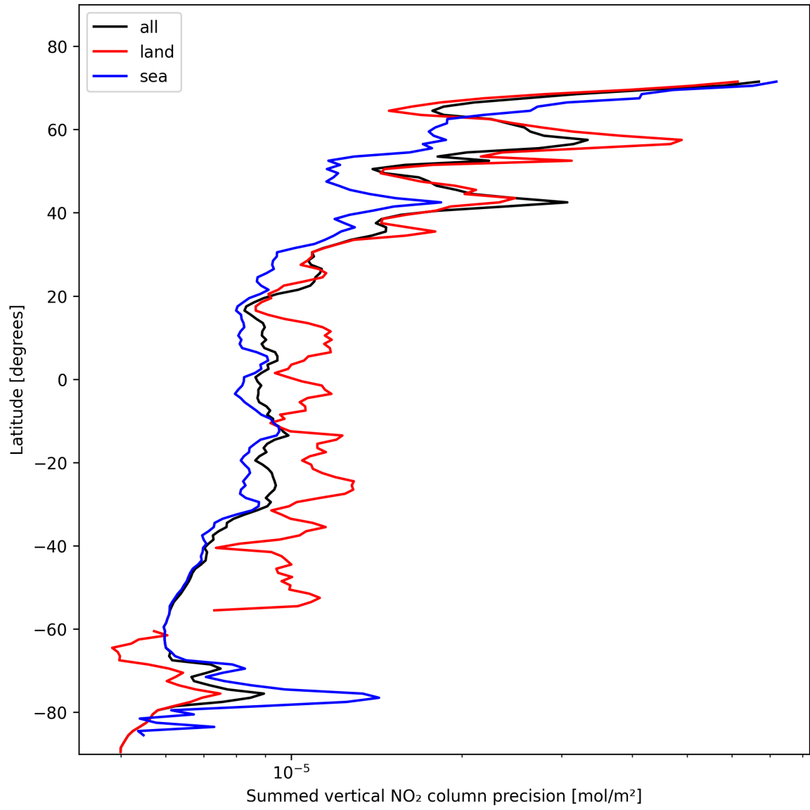
Figure 24: Zonal average of “Summed vertical NO 2 column precision” for 2025-02-03 to 2025-02-04.
