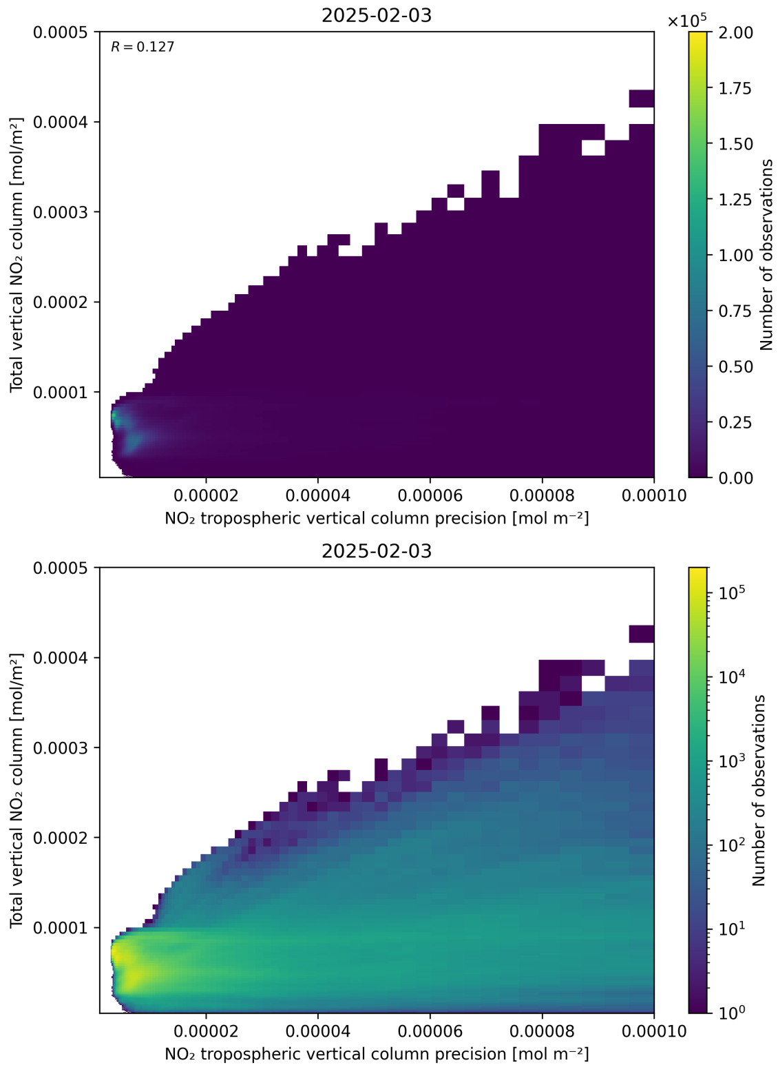
Figure 138: Scatter density plot of “NO 2 tropospheric vertical column precision” against “Total vertical NO 2 column” for 2025-02-03 to 2025-02-04.
