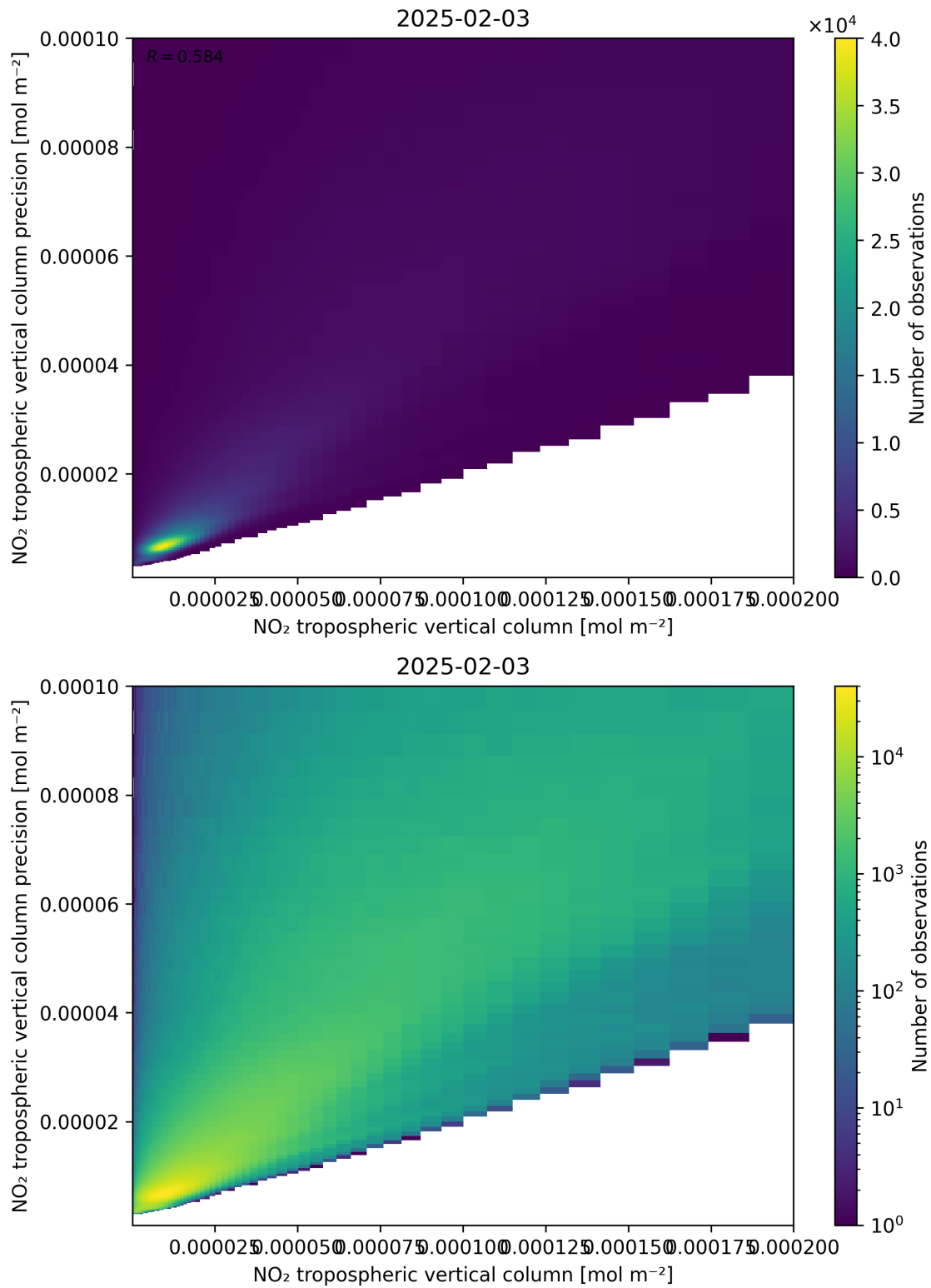
Figure 130: Scatter density plot of “NO 2 tropospheric vertical column” against “NO 2 tropospheric vertical column precision” for 2025-02-03 to 2025-02-04.
