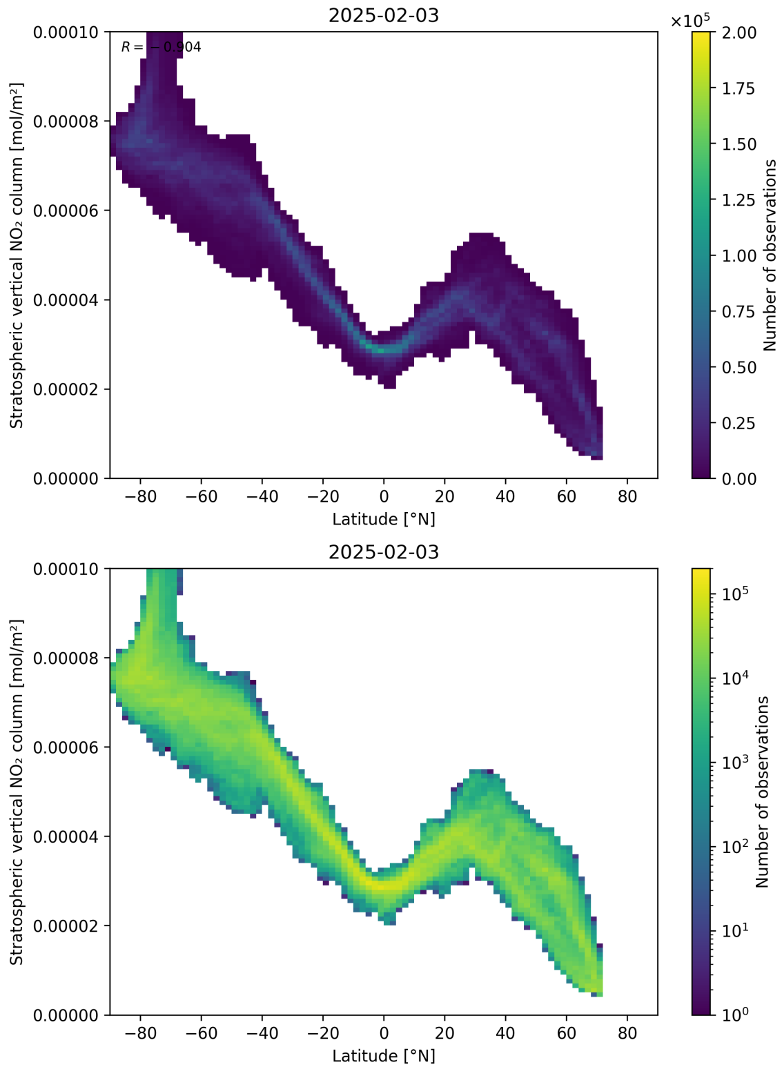
Figure 87: Scatter density plot of “Latitude” against “Stratospheric vertical NO 2 column” for 2025-02-03 to 2025-02-04.
