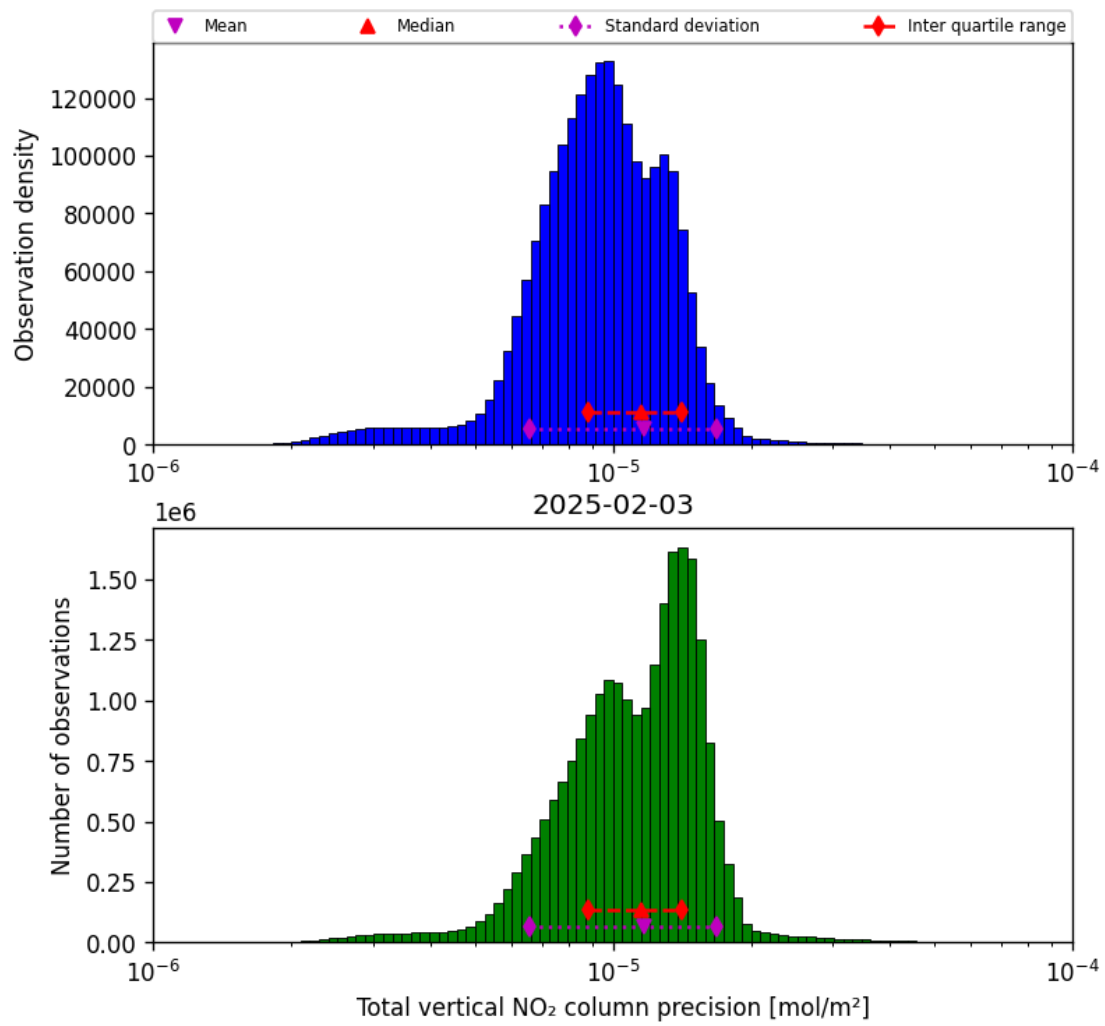
Figure 39: Histogram of “Total vertical NO 2 column precision” for 2025-02-03 to 2025-02-04
