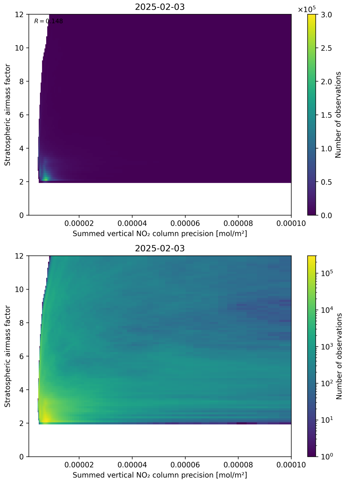
Figure 106: Scatter density plot of “Summed vertical NO 2 column precision” against “Stratospheric airmass factor” for 2025-02-03 to 2025-02-04.
