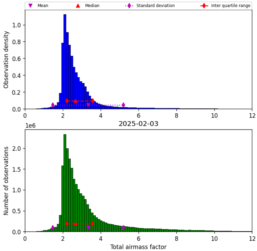
Figure 32: Histogram of “Total airmass factor” for 2025-02-03 to 2025-02-04
