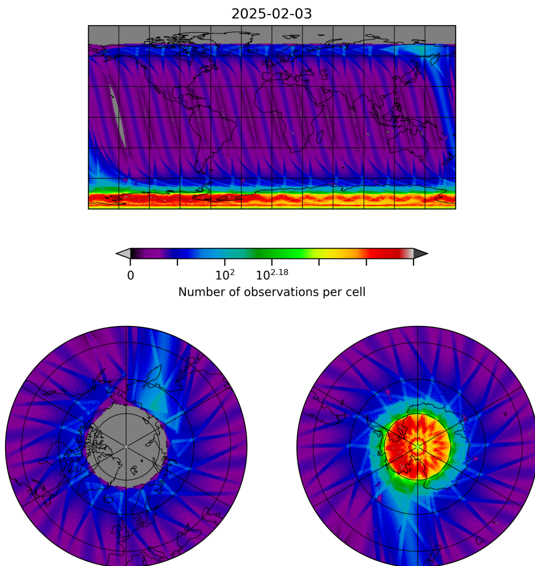
Figure 10: Map of the number of observations for 2025-02-03 to 2025-02-04
