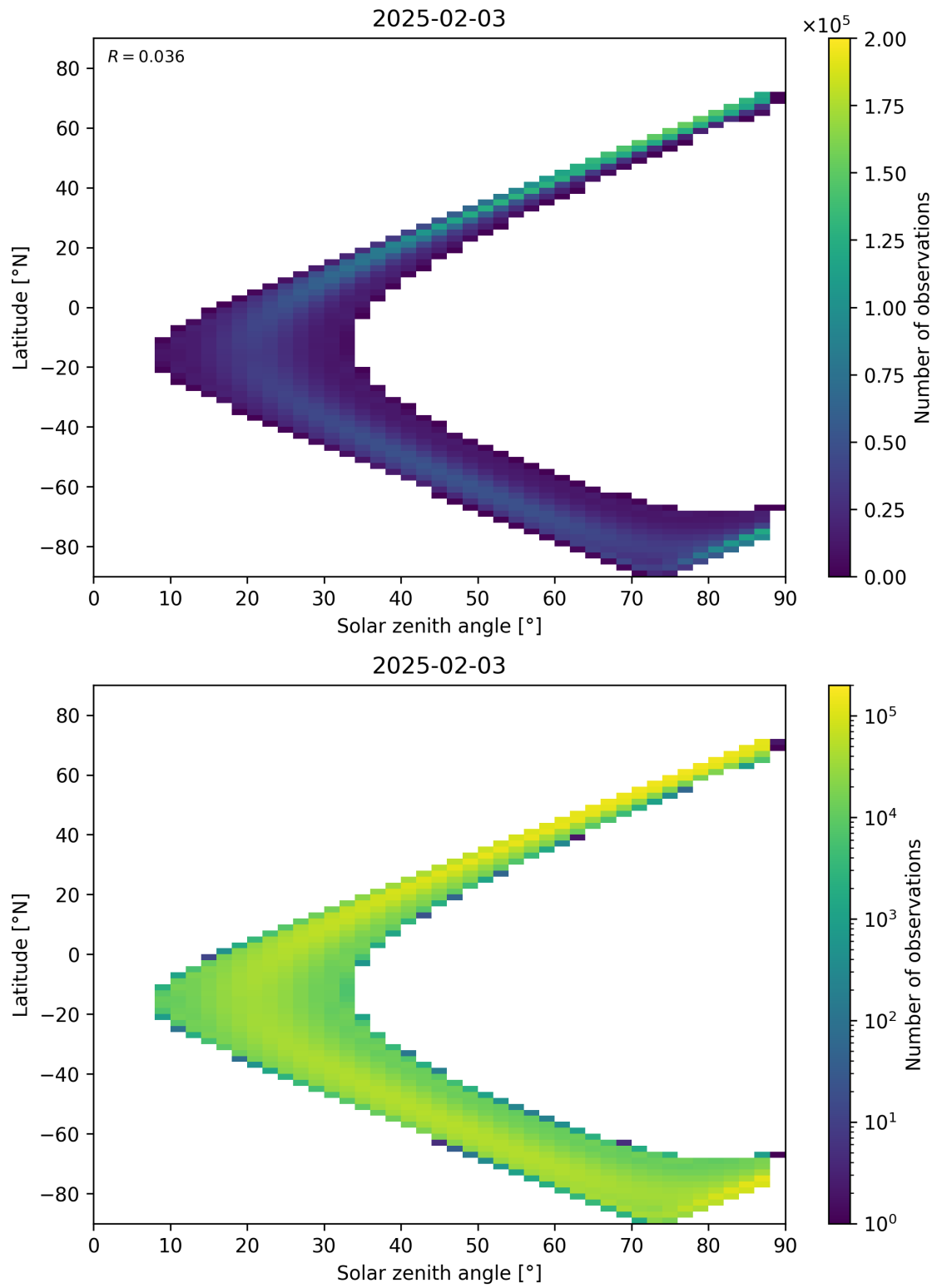
Figure 149: Scatter density plot of “Solar zenith angle” against “Latitude” for 2025-02-03 to 2025-02-04.
