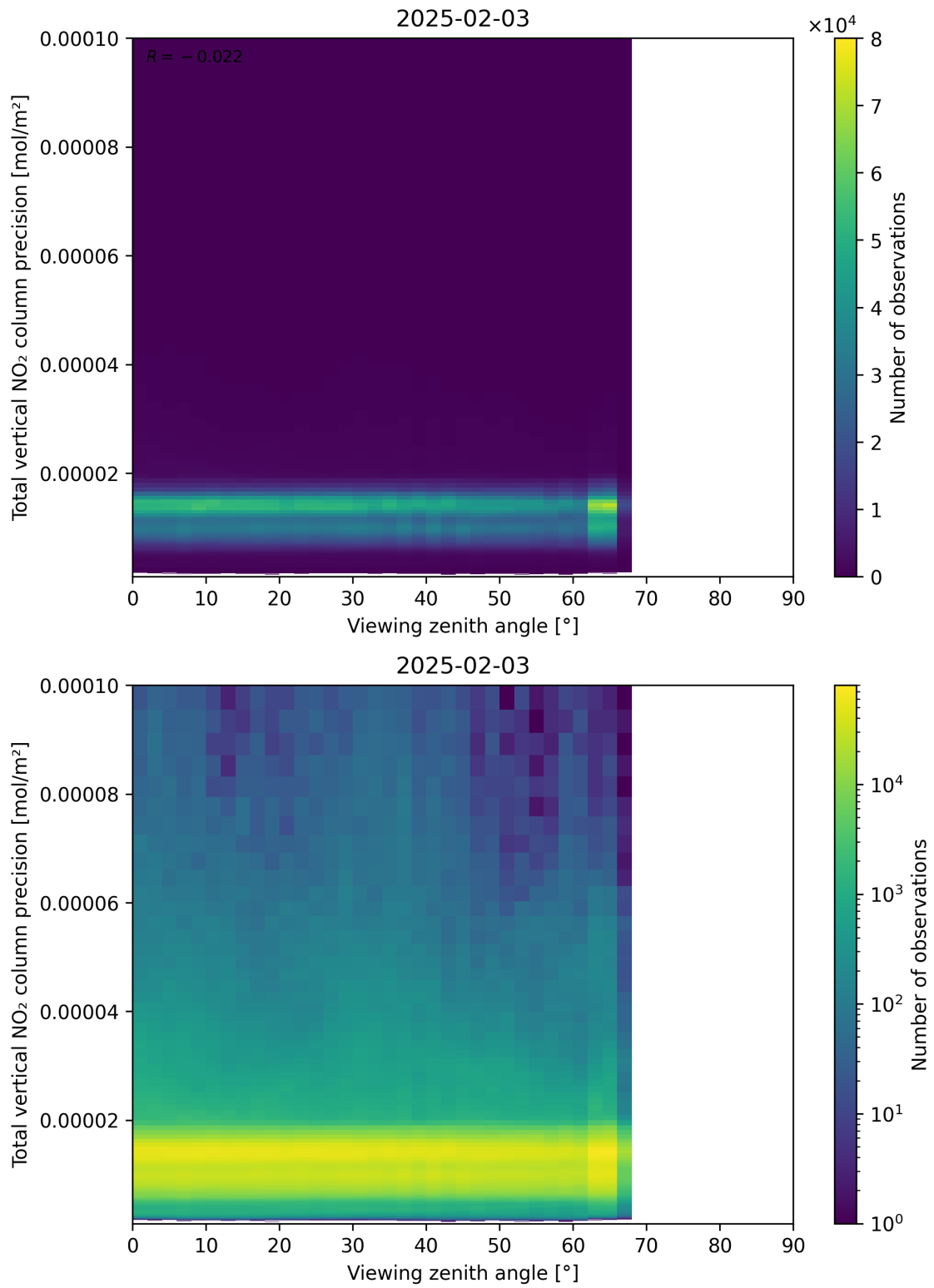
Figure 168: Scatter density plot of “Viewing zenith angle” against “Total vertical NO 2 column precision” for 2025-02-03 to 2025-02-04.
