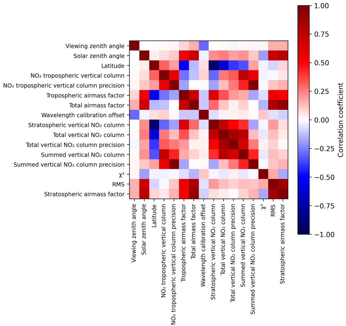
Figure 2: Map of correlation matrix for 2025-02-03 to 2025-02-04.
