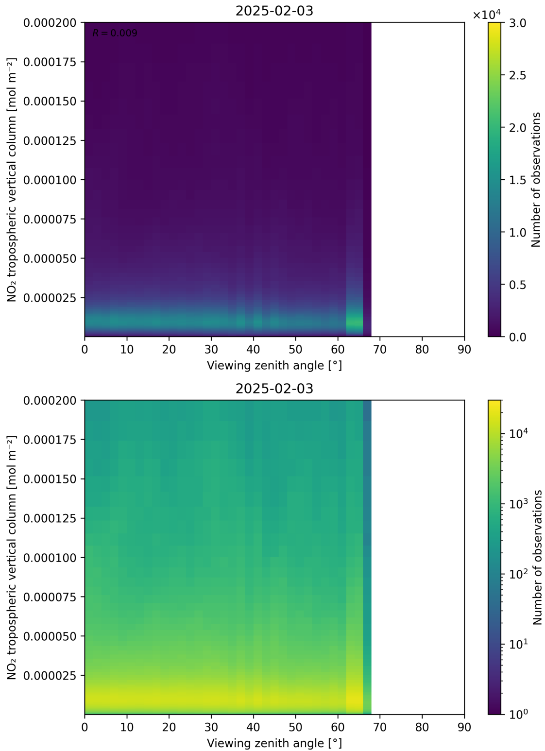
Figure 169: Scatter density plot of “Viewing zenith angle” against “NO 2 tropospheric vertical column” for 2025-02-03 to 2025-02-04.
