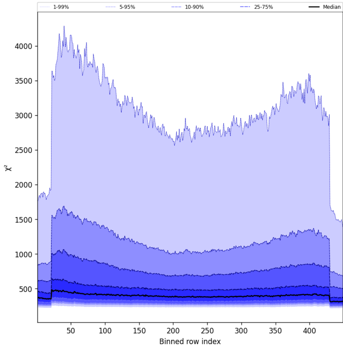
Figure 59: Along track statistics of “ \chi^2 ” for 2025-02-03 to 2025-02-04
