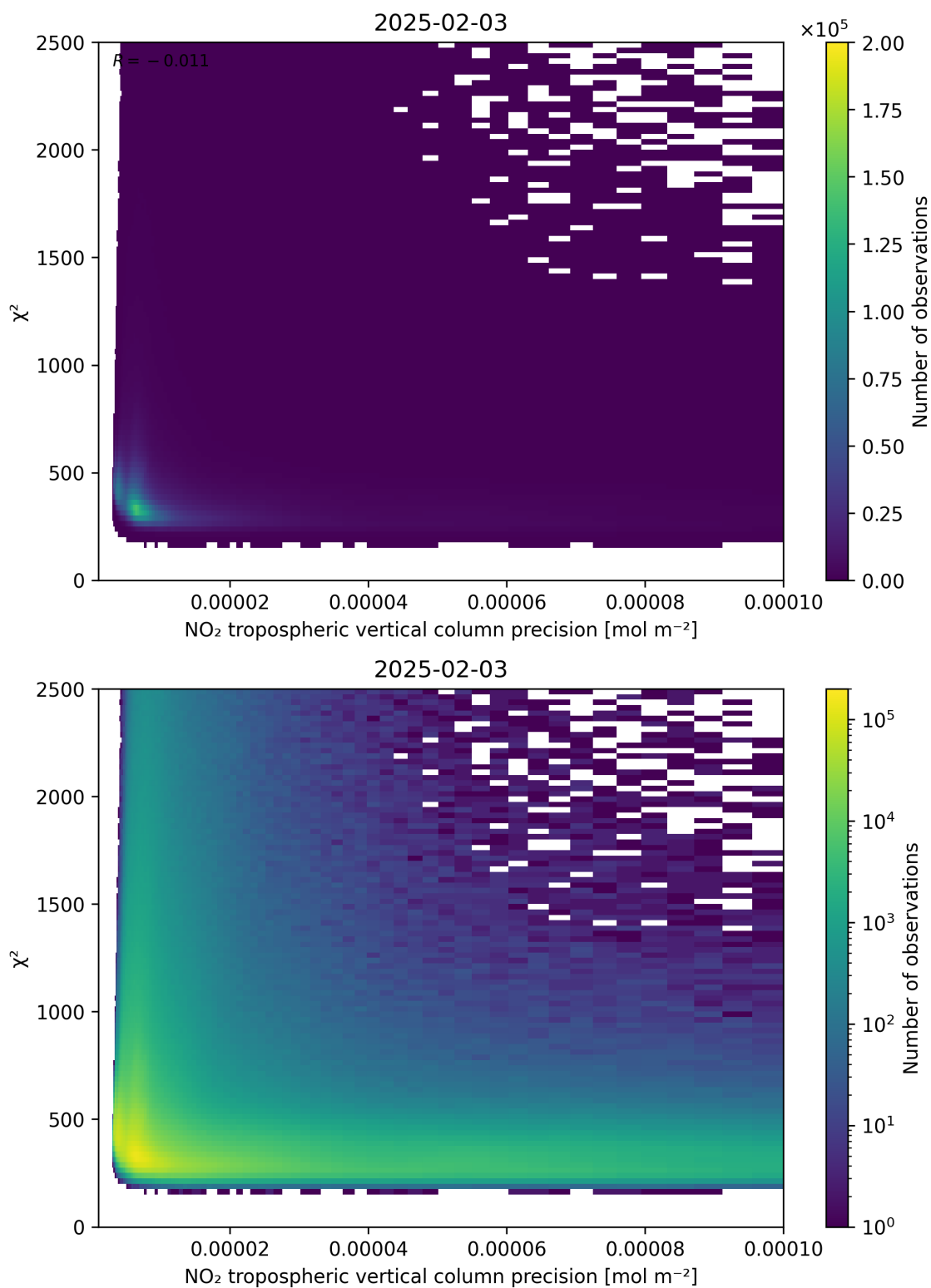
Figure 134: Scatter density plot of “NO 2 tropospheric vertical column precision” against “ \chi^2 ” for 2025-02-03 to 2025-02-04.
