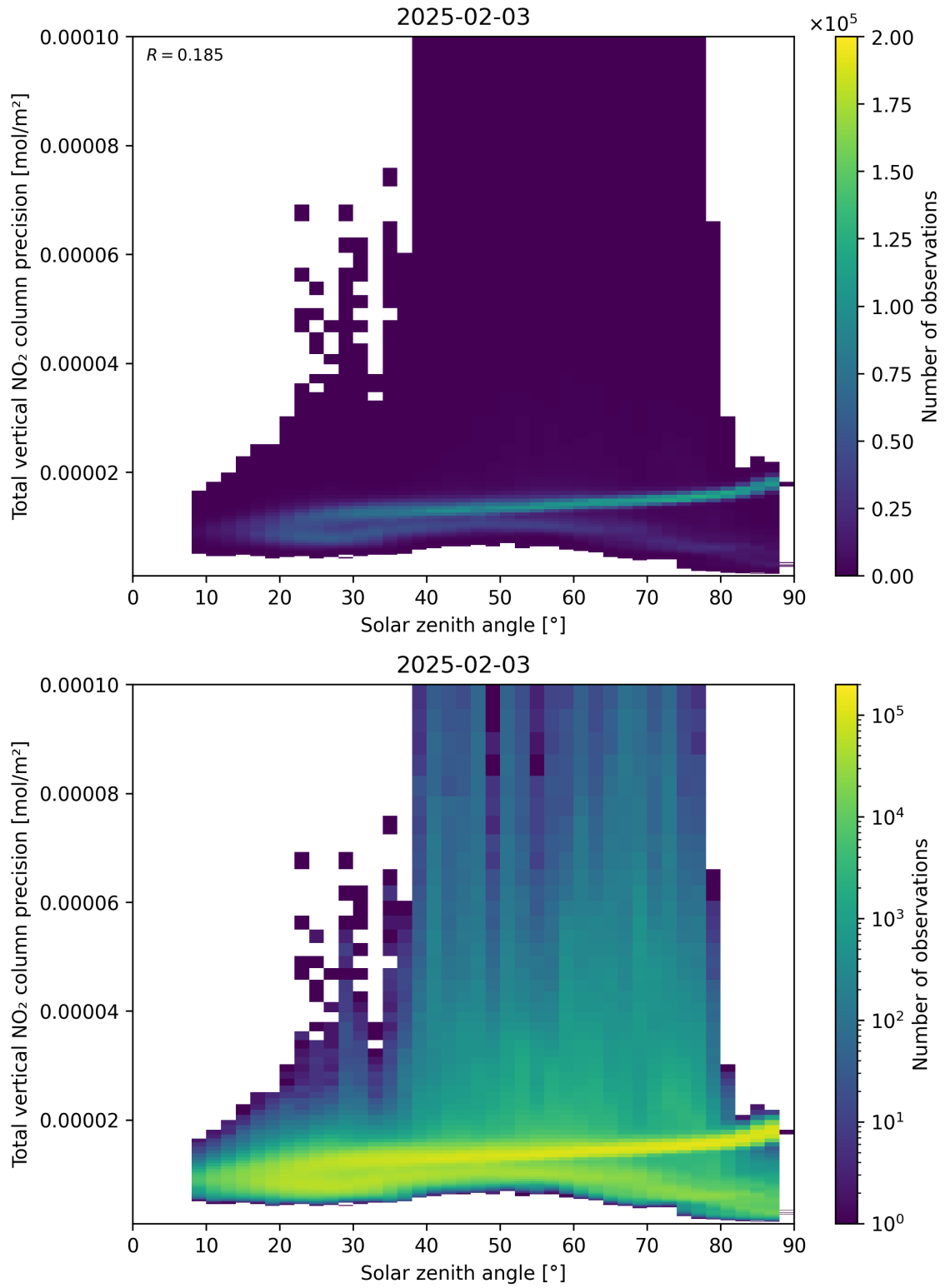
Figure 154: Scatter density plot of “Solar zenith angle” against “Total vertical NO 2 column precision” for 2025-02-03 to 2025-02-04.
