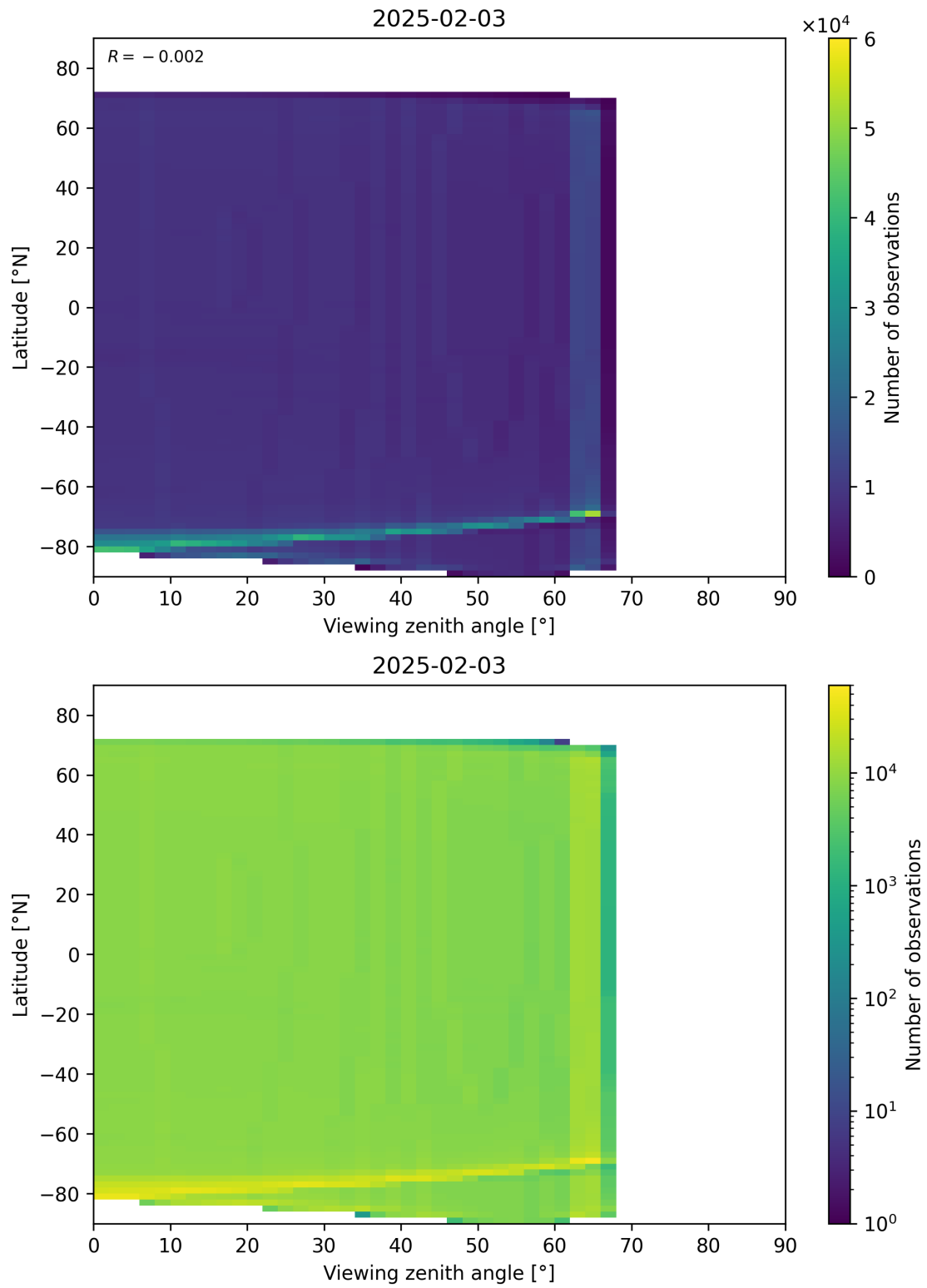
Figure 163: Scatter density plot of “Viewing zenith angle” against “Latitude” for 2025-02-03 to 2025-02-04.
