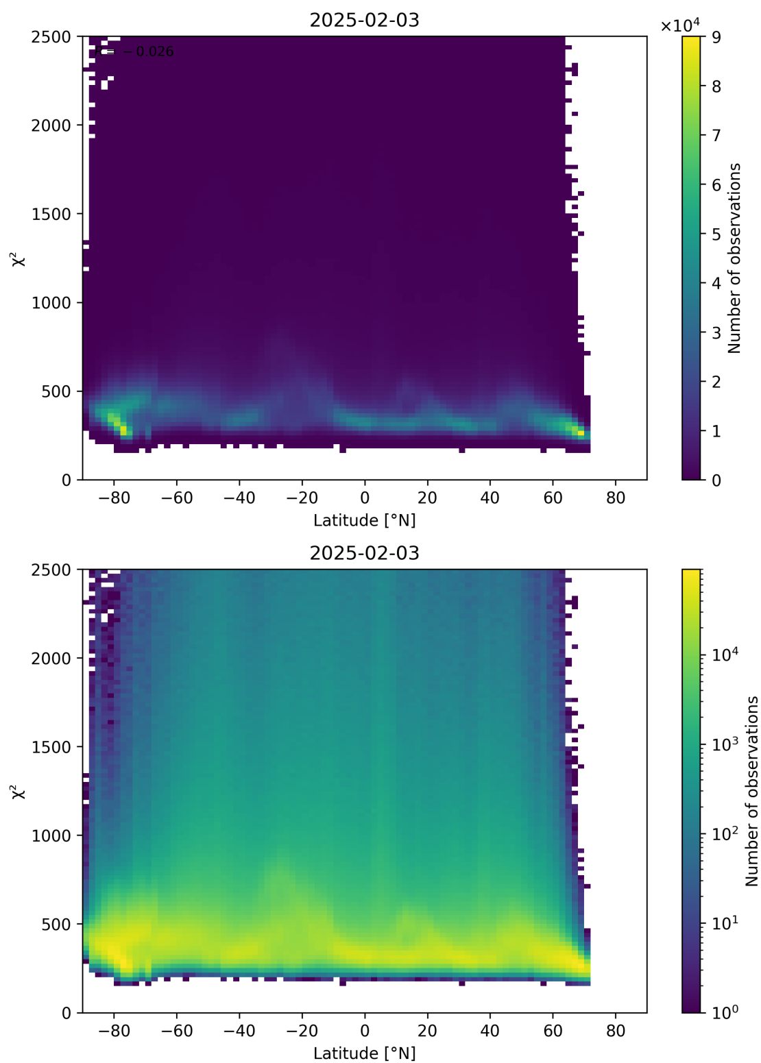
Figure 86: Scatter density plot of “Latitude” against “ \chi^2 ” for 2025-02-03 to 2025-02-04.
