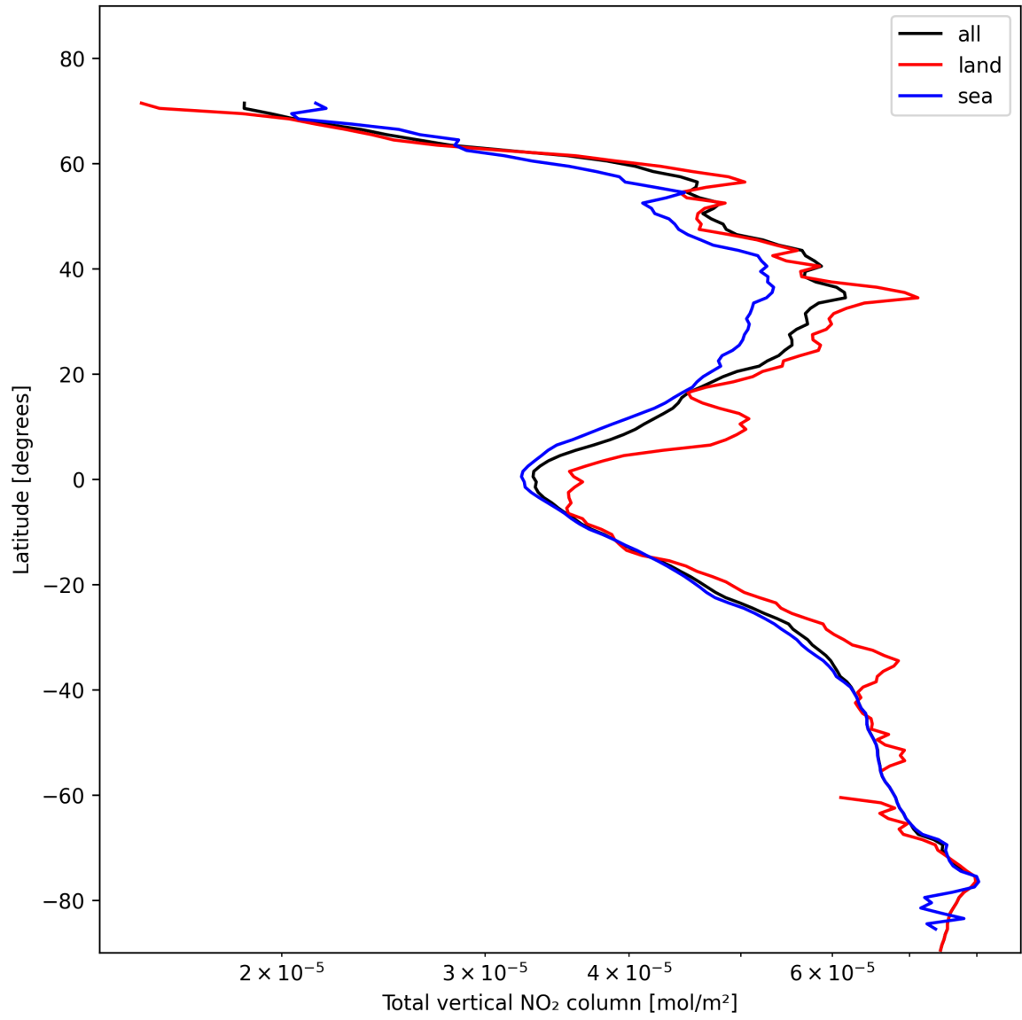
Figure 21: Zonal average of “Total vertical NO 2 column” for 2025-02-03 to 2025-02-04.
