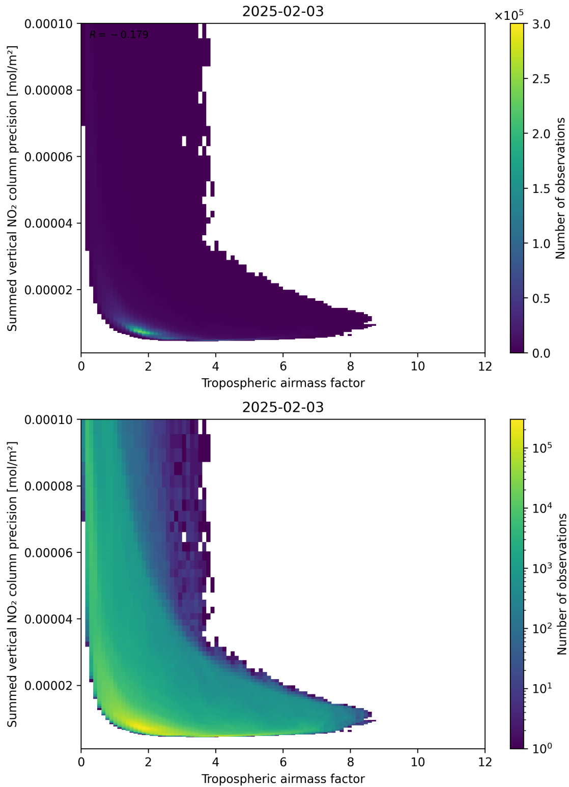
Figure 76: Scatter density plot of “Tropospheric airmass factor” against “Summed vertical NO 2 column precision” for 2025-02-03 to 2025-02-04.
