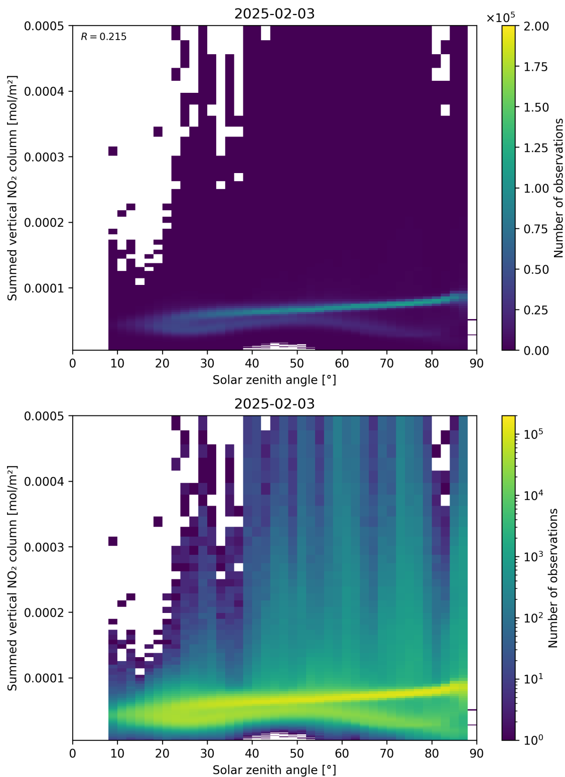
Figure 151: Scatter density plot of “Solar zenith angle” against “Summed vertical NO 2 column” for 2025-02-03 to 2025-02-04.
