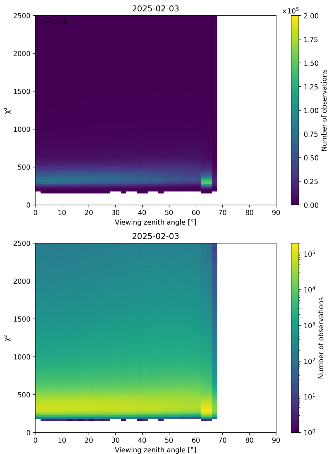
Figure 162: Scatter density plot of “Viewing zenith angle” against “ \chi^2 ” for 2025-02-03 to 2025-02-04.
