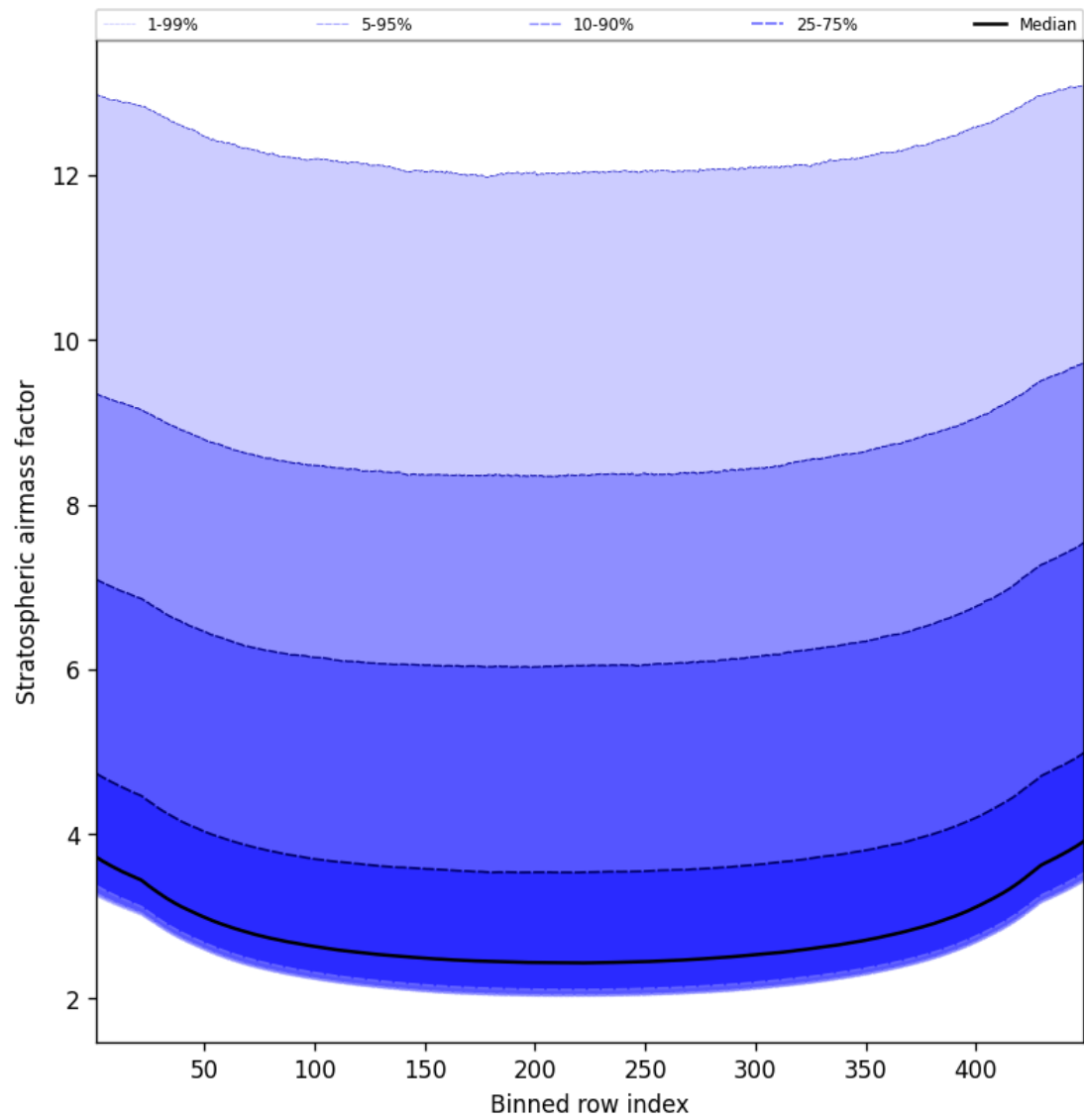
Figure 61: Along track statistics of “Stratospheric airmass factor” for 2025-02-03 to 2025-02-04
