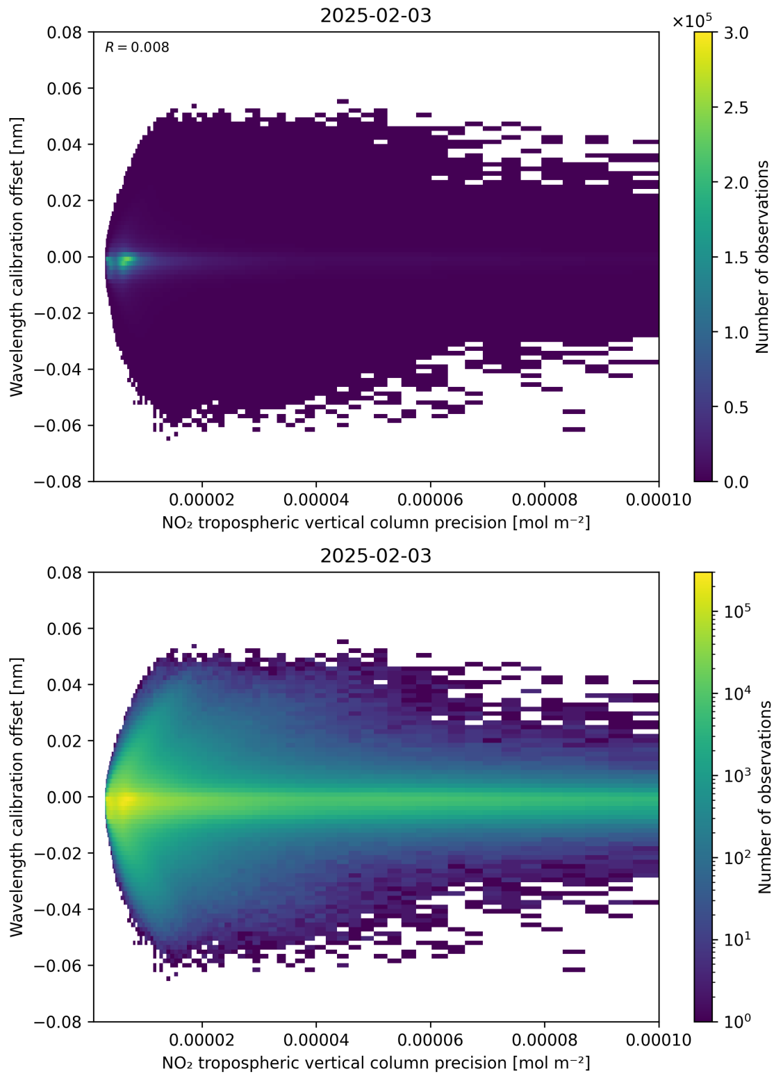
Figure 141: Scatter density plot of “NO 2 tropospheric vertical column precision” against “Wavelength calibration offset” for 2025-02-03 to 2025-02-04.
