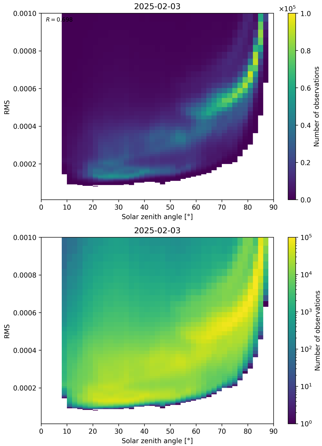
Figure 157: Scatter density plot of “Solar zenith angle” against “RMS” for 2025-02-03 to 2025-02-04.
