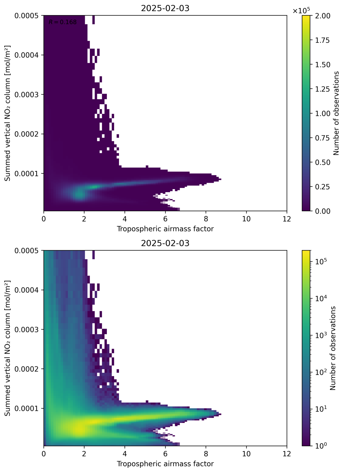
Figure 75: Scatter density plot of “Tropospheric air mass factor” against “Summed vertical NO 2 column” for 2025-02-03 to 2025-02-04.
