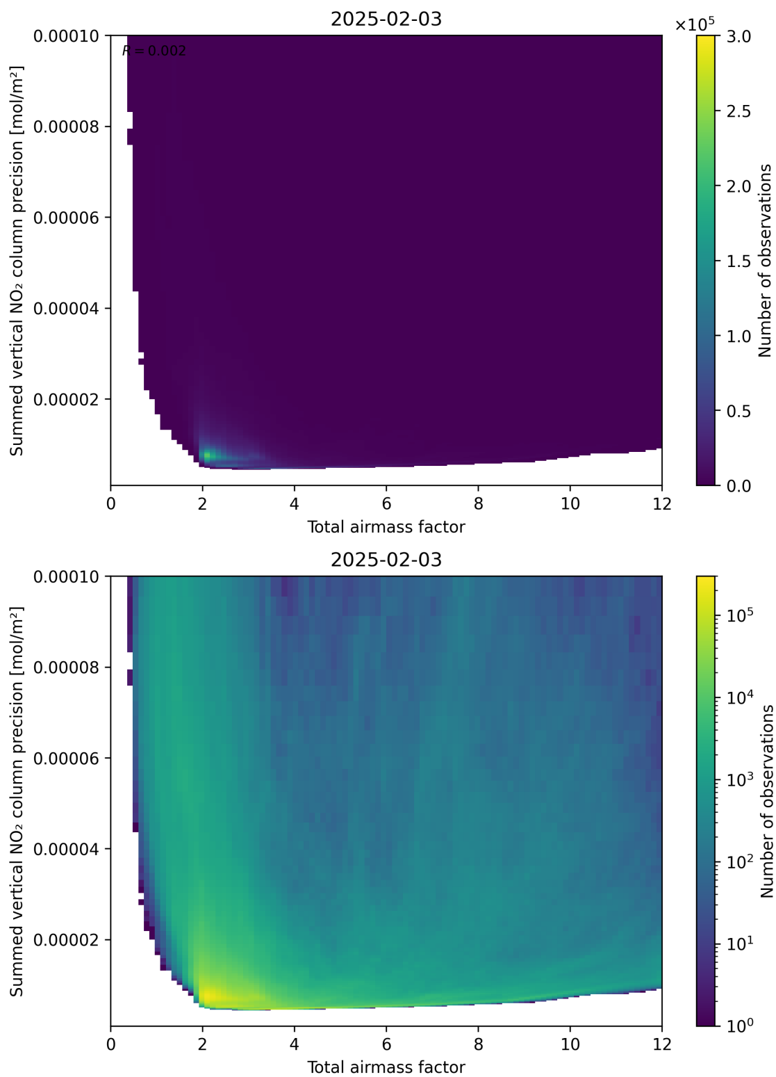
Figure 66: Scatter density plot of “Total airmass factor” against “Summed vertical NO 2 column precision” for 2025-02-03 to 2025-02-04.
