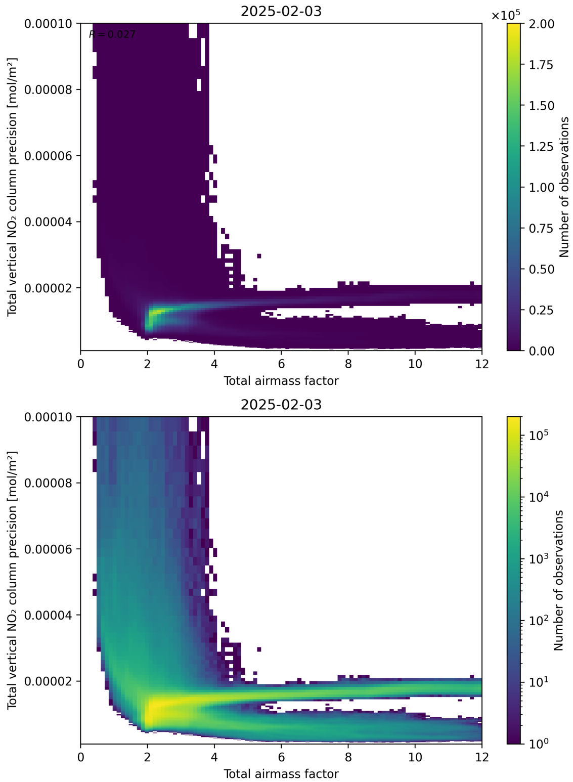
Figure 68: Scatter density plot of “Total airmass factor” against “Total vertical NO 2 column precision” for 2025-02-03 to 2025-02-04.
