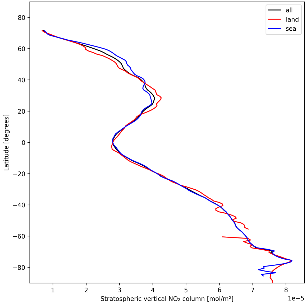
Figure 19: Zonal average of “Stratospheric vertical NO 2 column” for 2025-02-03 to 2025-02-04.
