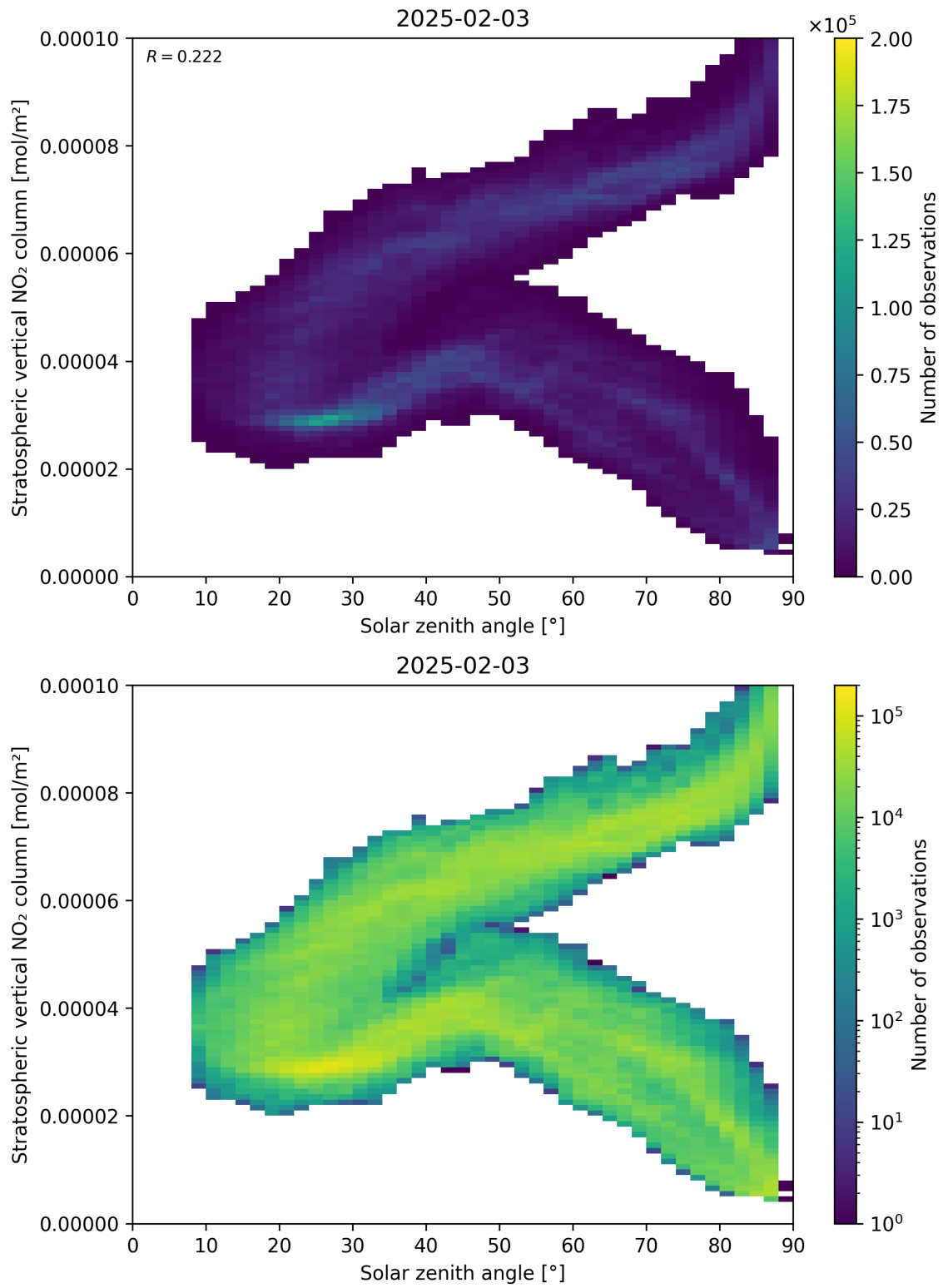
Figure 150: Scatter density plot of “Solar zenith angle” against “Stratospheric vertical NO 2 column” for 2025-02-03 to 2025-02-04.
