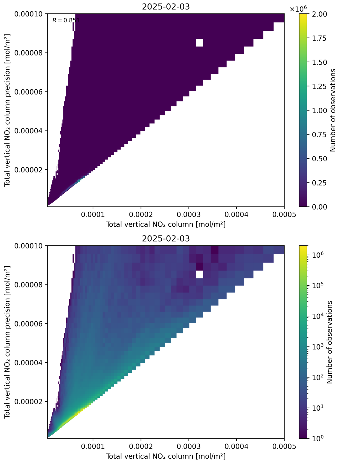
Figure 114: Scatter density plot of “Total vertical NO 2 column” against “Total vertical NO 2 column precision” for 2025-02-03 to 2025-02-04.
