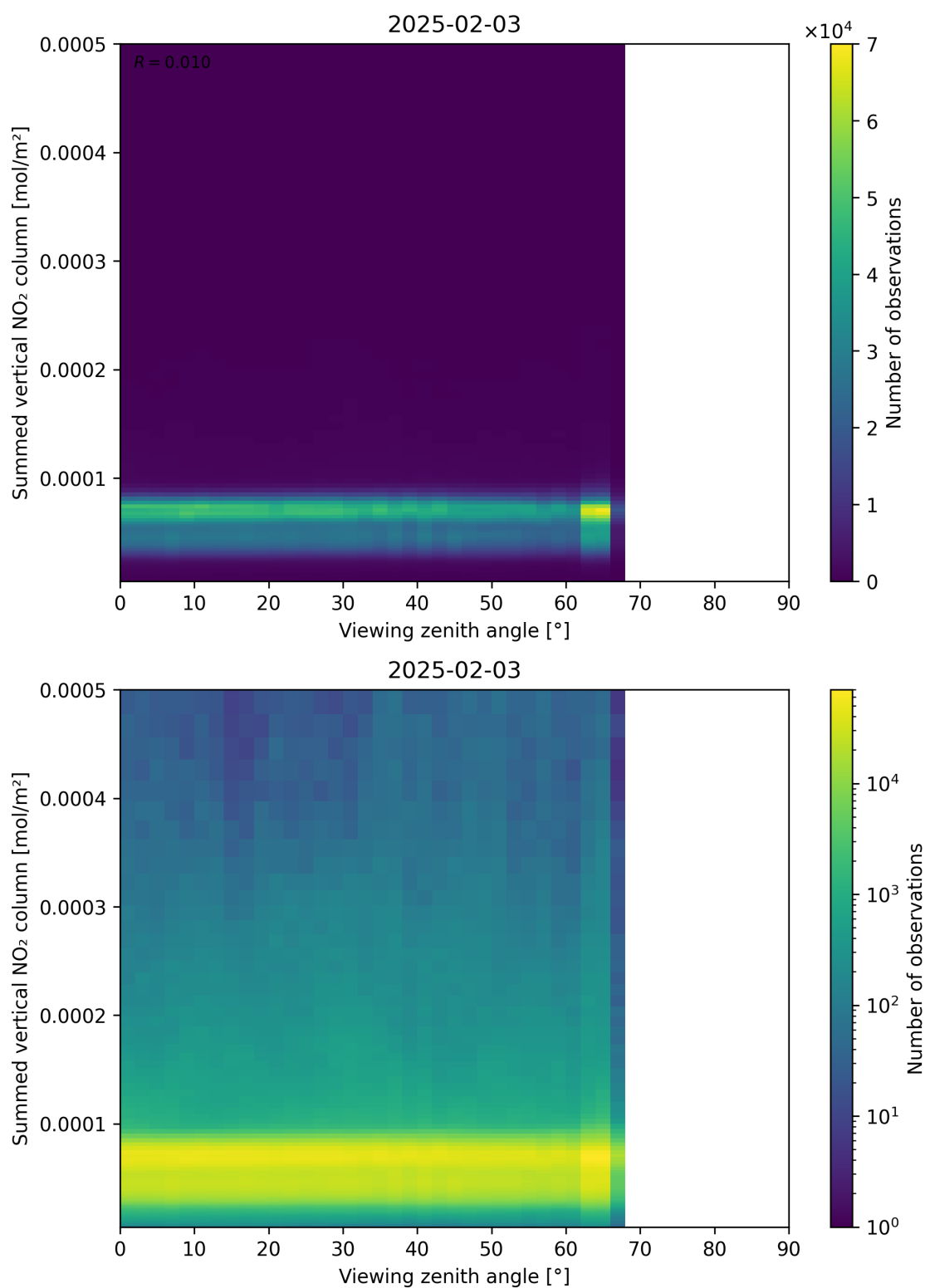
Figure 165: Scatter density plot of “Viewing zenith angle” against “Summed vertical NO 2 column” for 2025-02-03 to 2025-02-04.
