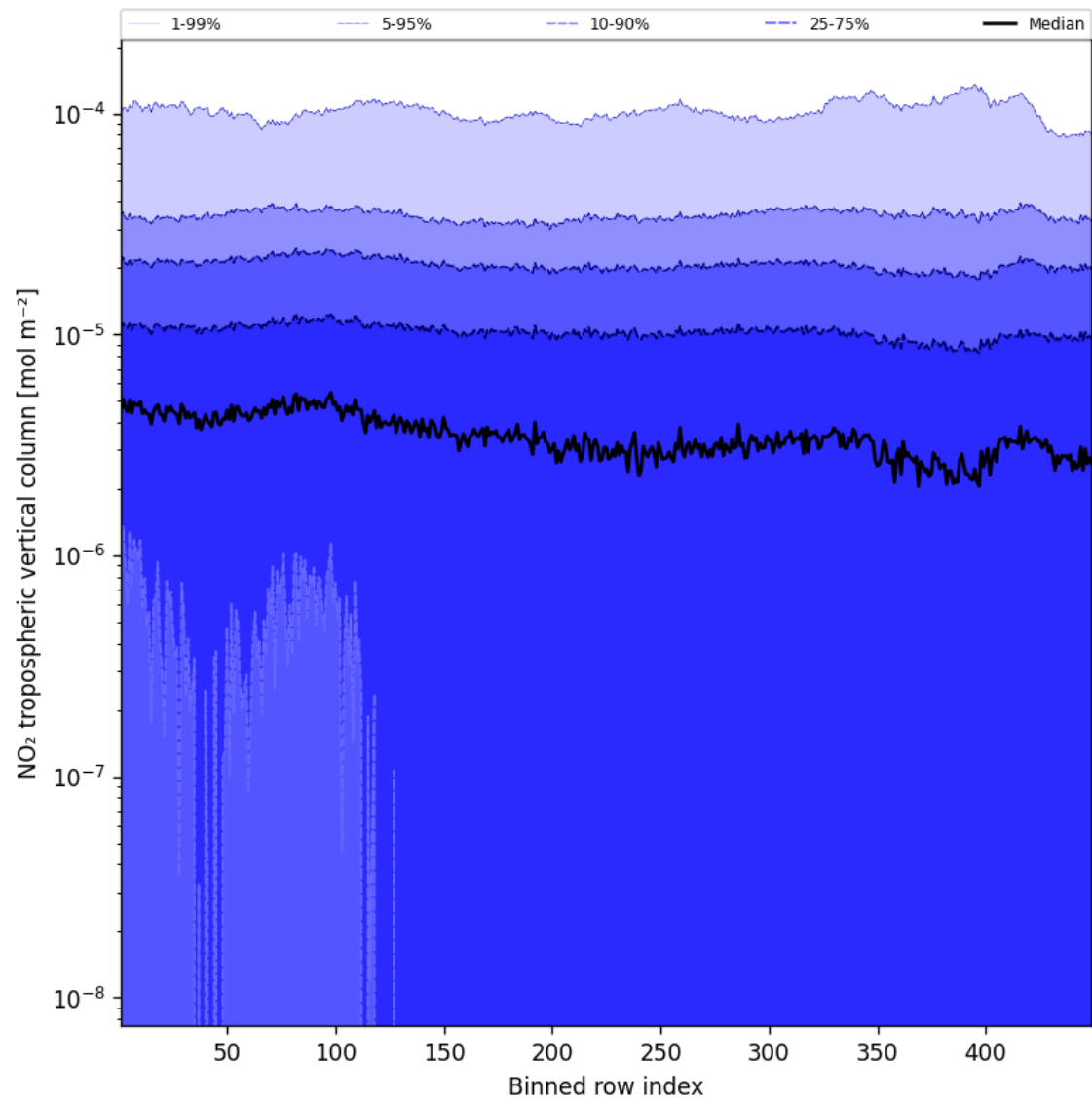
Figure 46: Along track statistics of “NO 2 tropospheric vertical column” for 2025-02-03 to 2025-02-04
