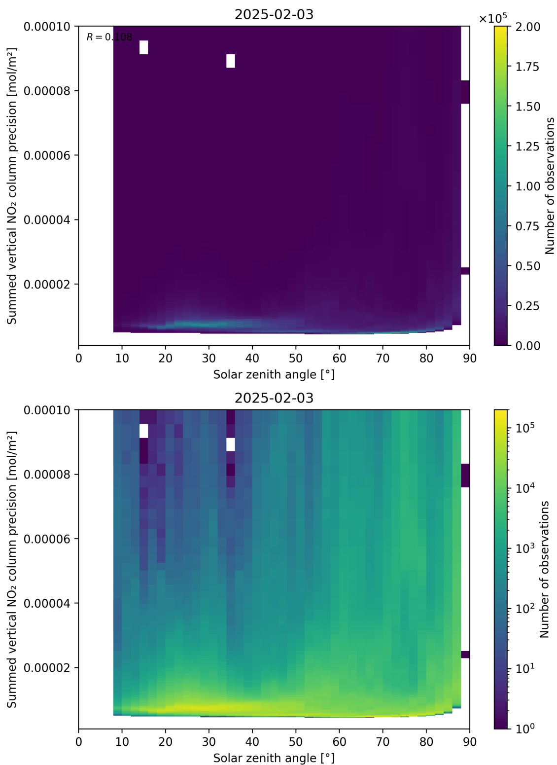
Figure 152: Scatter density plot of “Solar zenith angle” against “Summed vertical NO 2 column precision” for 2025-02-03 to 2025-02-04.
