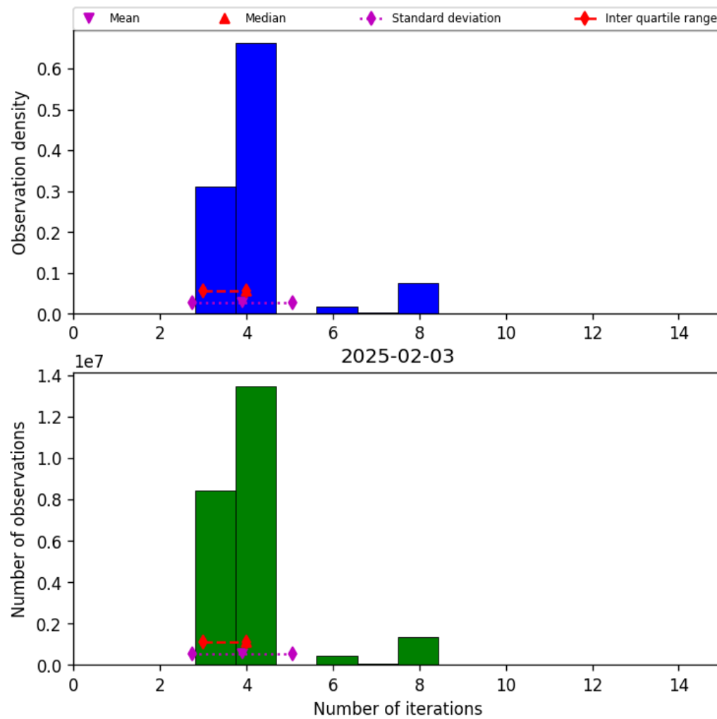
Figure 34: Histogram of “Number of iterations” for 2025-02-03 to 2025-02-04
