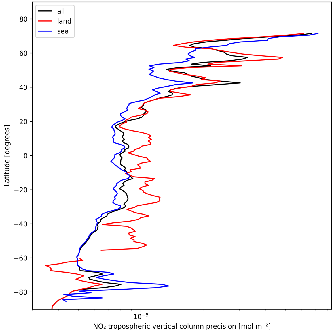
Figure 13: Zonal average of “NO 2 tropospheric vertical column precision” for 2025-02-03 to 2025-02-04.
