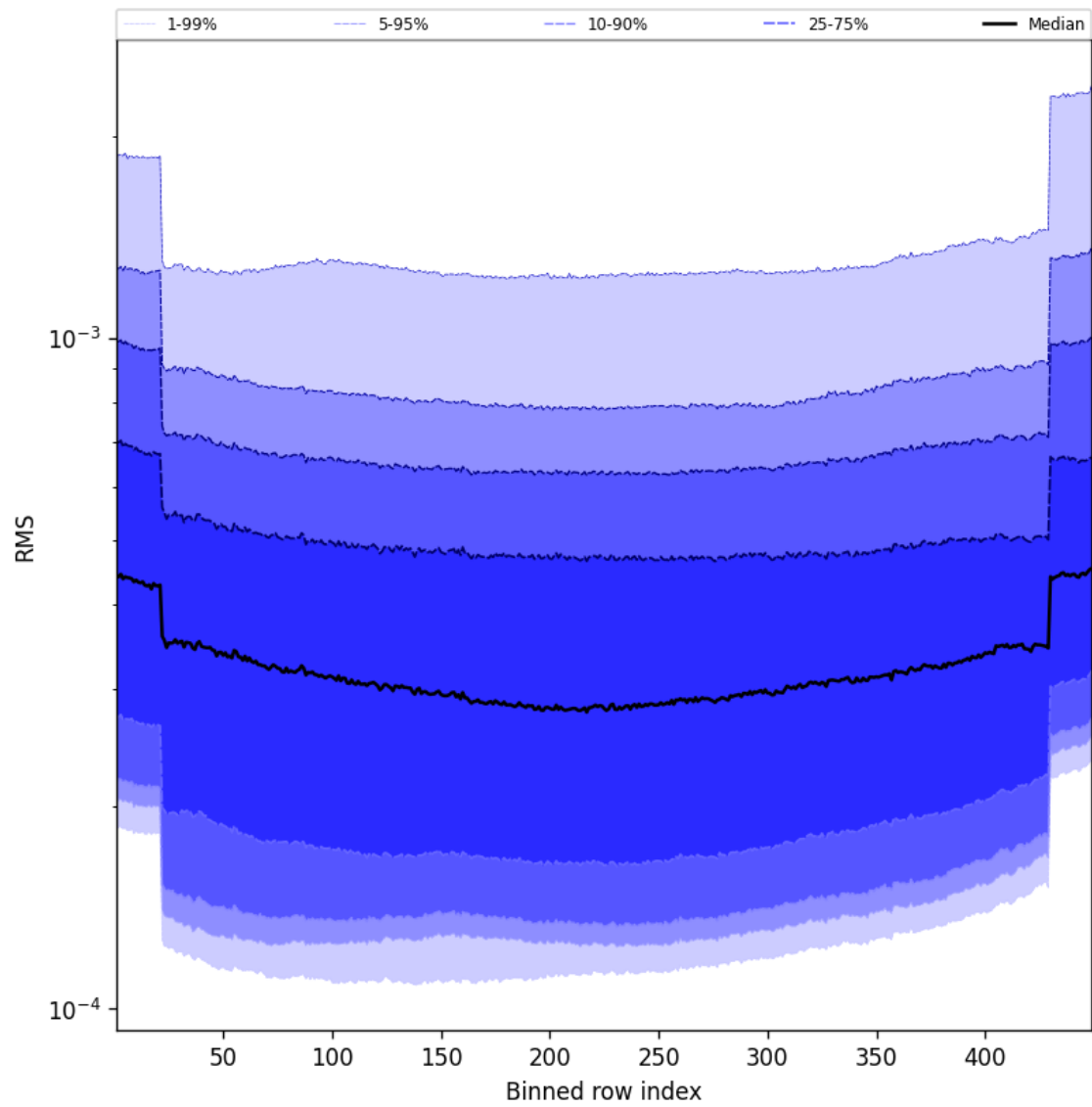
Figure 60: Along track statistics of “RMS” for 2025-02-03 to 2025-02-04
