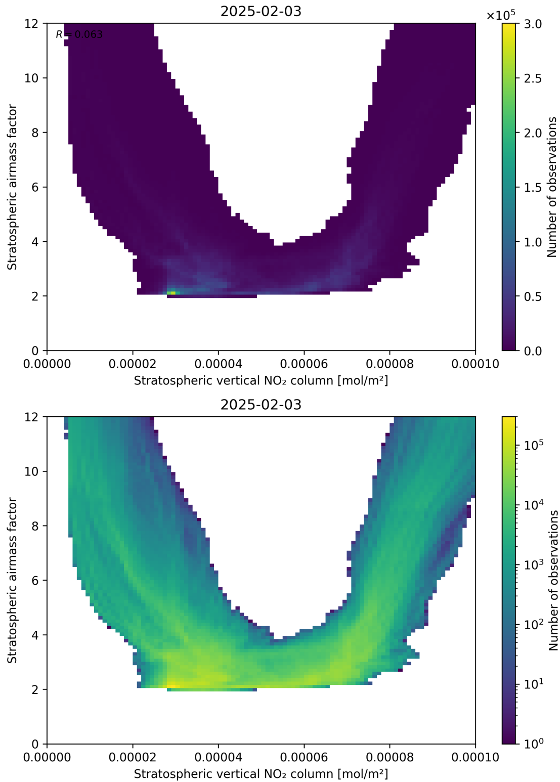
Figure 96: Scatter density plot of “Stratospheric vertical NO 2 column” against “Stratospheric airmass factor” for 2025-02-03 to 2025-02-04.
