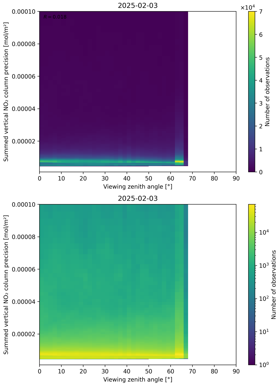
Figure 166: Scatter density plot of “Viewing zenith angle” against “Summed vertical NO 2 column precision” for 2025-02-03 to 2025-02-04.
