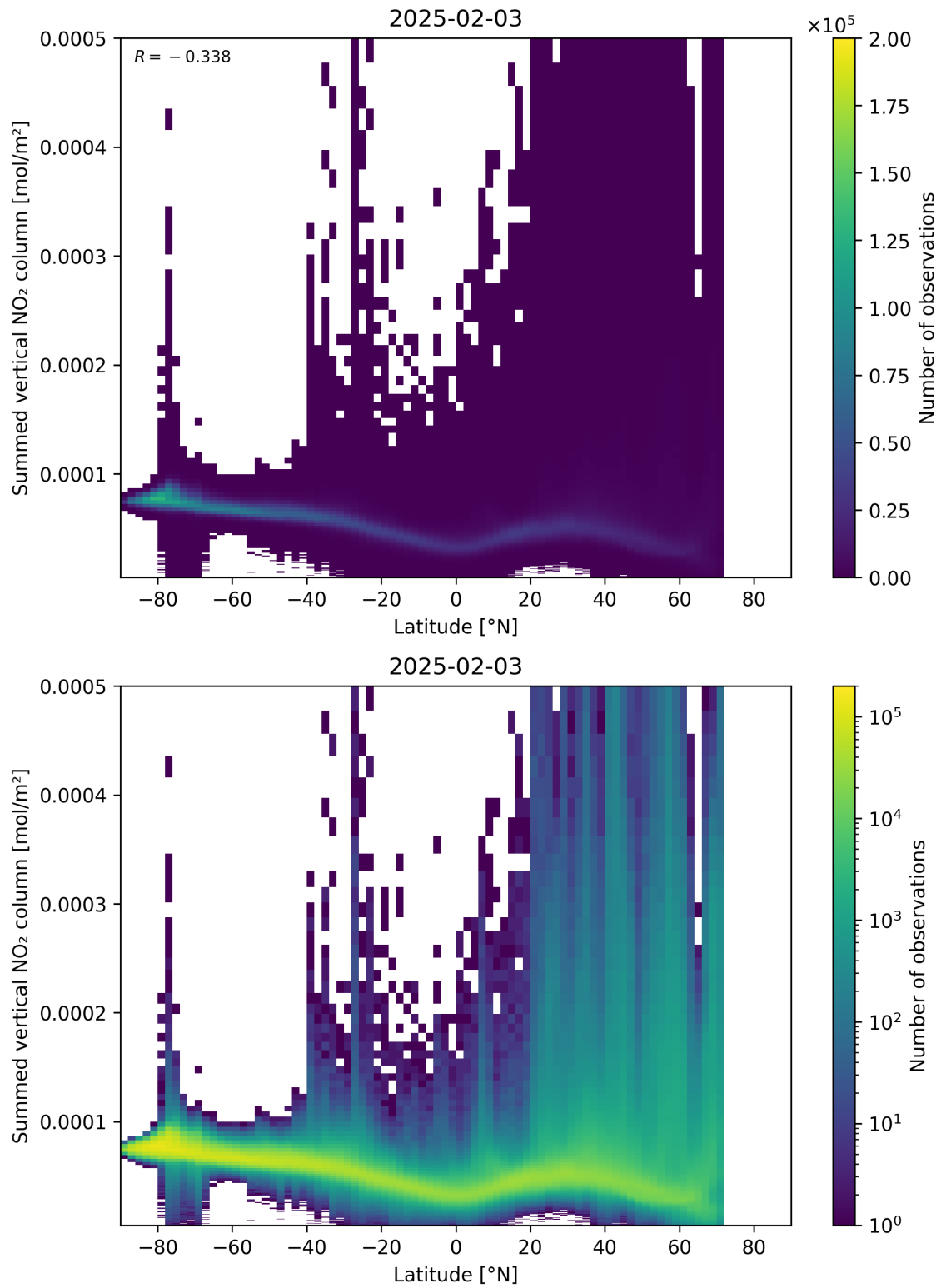
Figure 88: Scatter density plot of “Latitude” against “Summed vertical NO 2 column” for 2025-02-03 to 2025-02-04.
