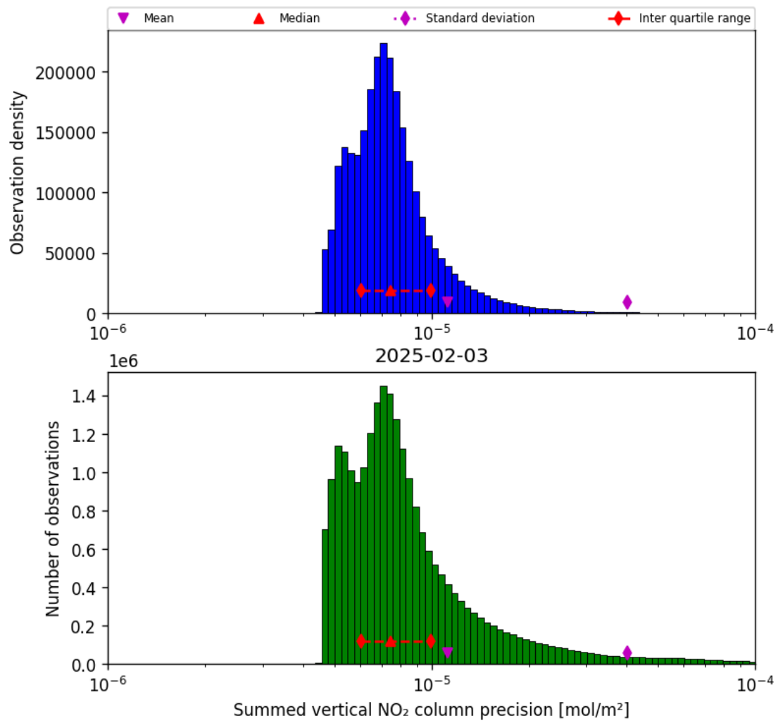
Figure 41: Histogram of "Summed vertical NO 2 column precision" for 2025-02-03 to 2025-02-04
