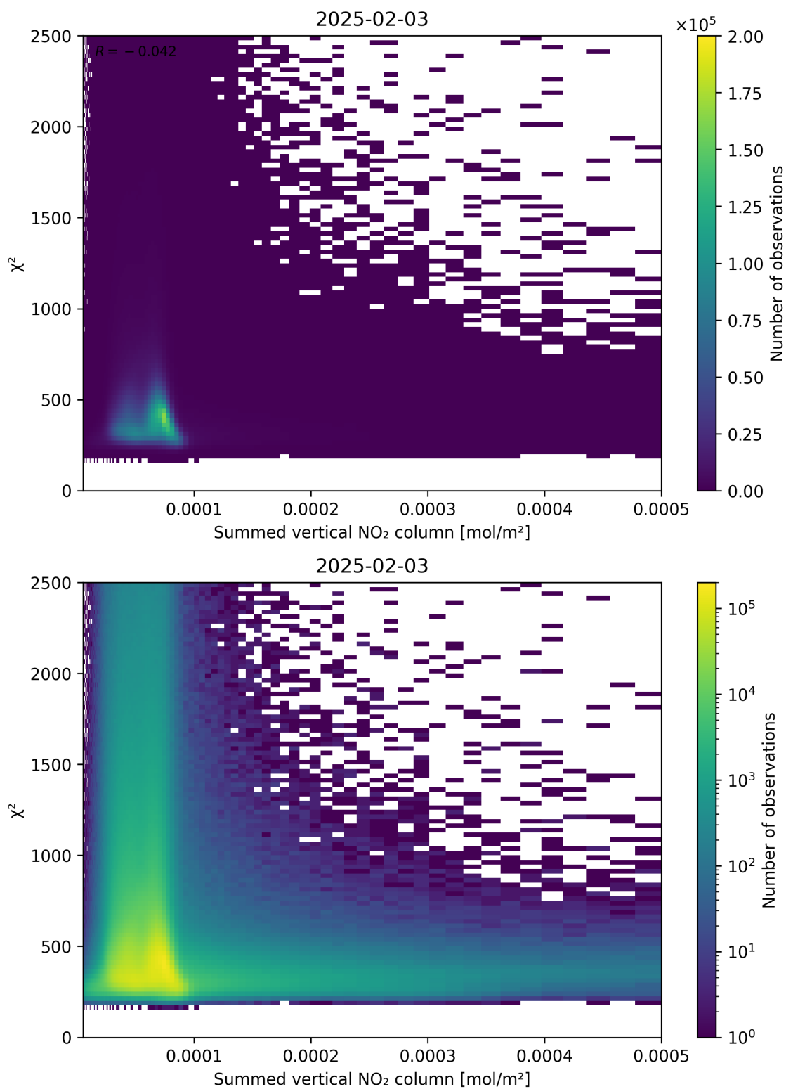
Figure 104: Scatter density plot of “Summed vertical NO 2 column” against “ \chi^2 ” for 2025-02-03 to 2025-02-04.
