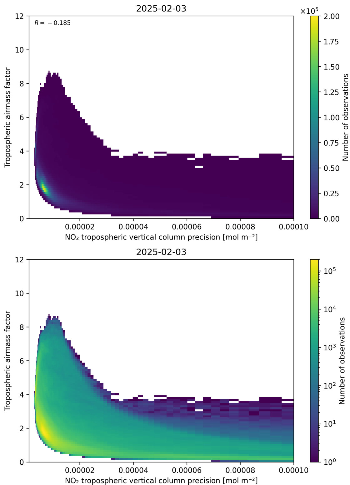
Figure 133: Scatter density plot of “NO 2 tropospheric vertical column precision” against “Tropospheric air mass factor” for 2025-02-03 to 2025-02-04.
