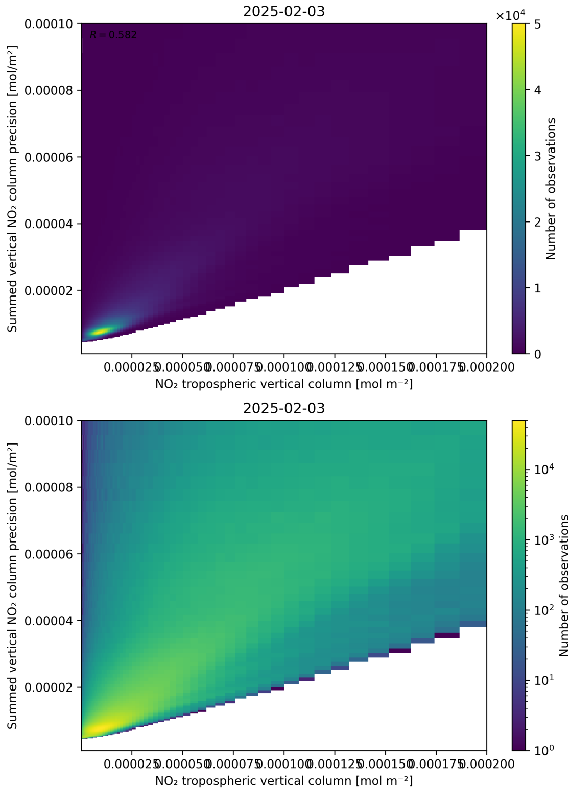
Figure 127: Scatter density plot of “NO 2 tropospheric vertical column” against “Summed vertical NO 2 column precision” for 2025-02-03 to 2025-02-04.
