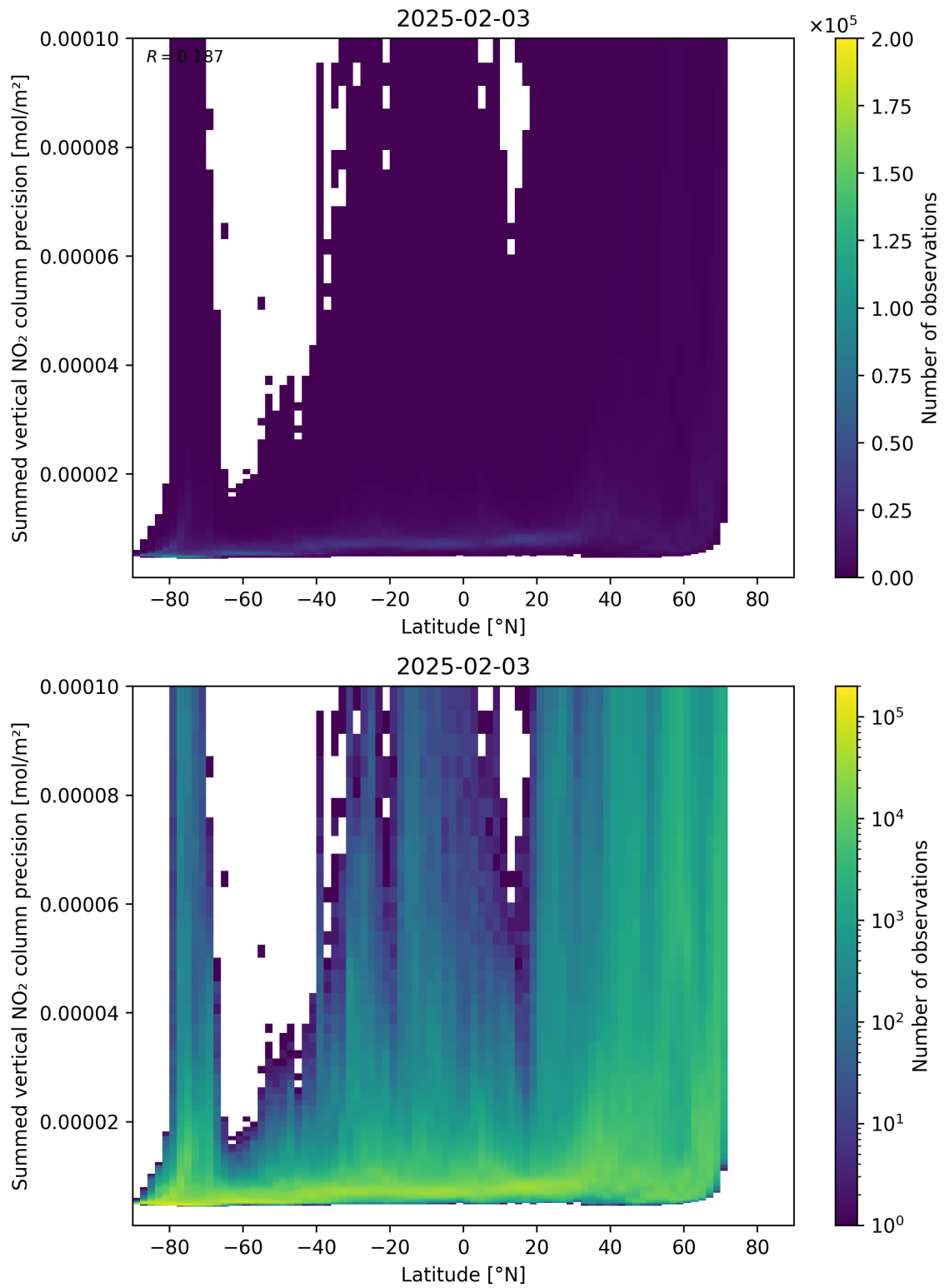
Figure 89: Scatter density plot of “Latitude” against “Summed vertical NO 2 column precision” for 2025-02-03 to 2025-02-04.
