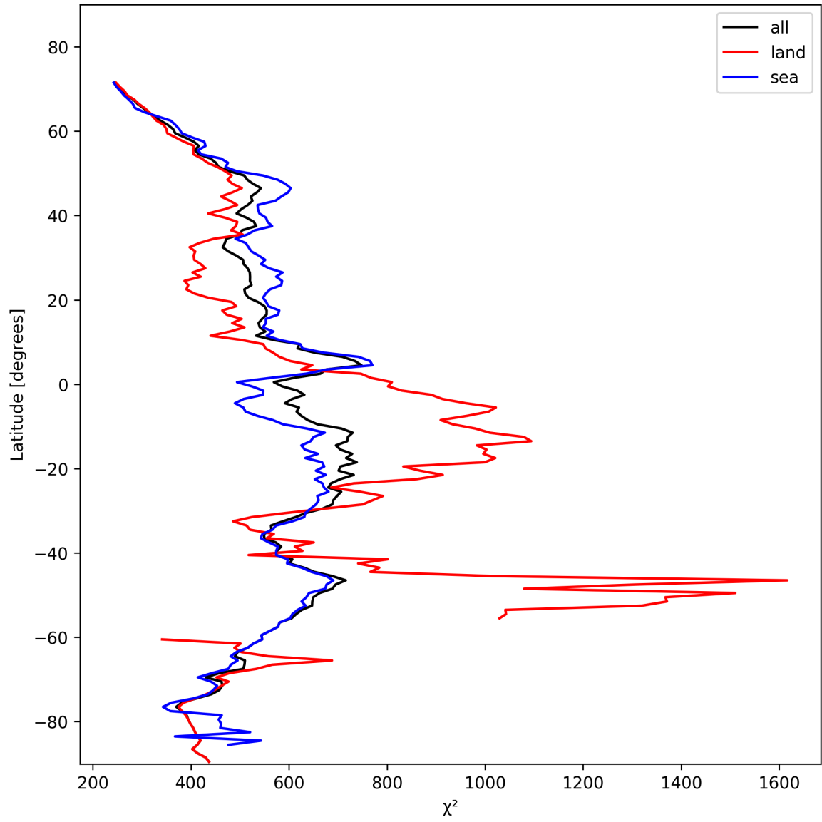
Figure 25: Zonal average of “ \chi^2 ” for 2025-02-03 to 2025-02-04.
