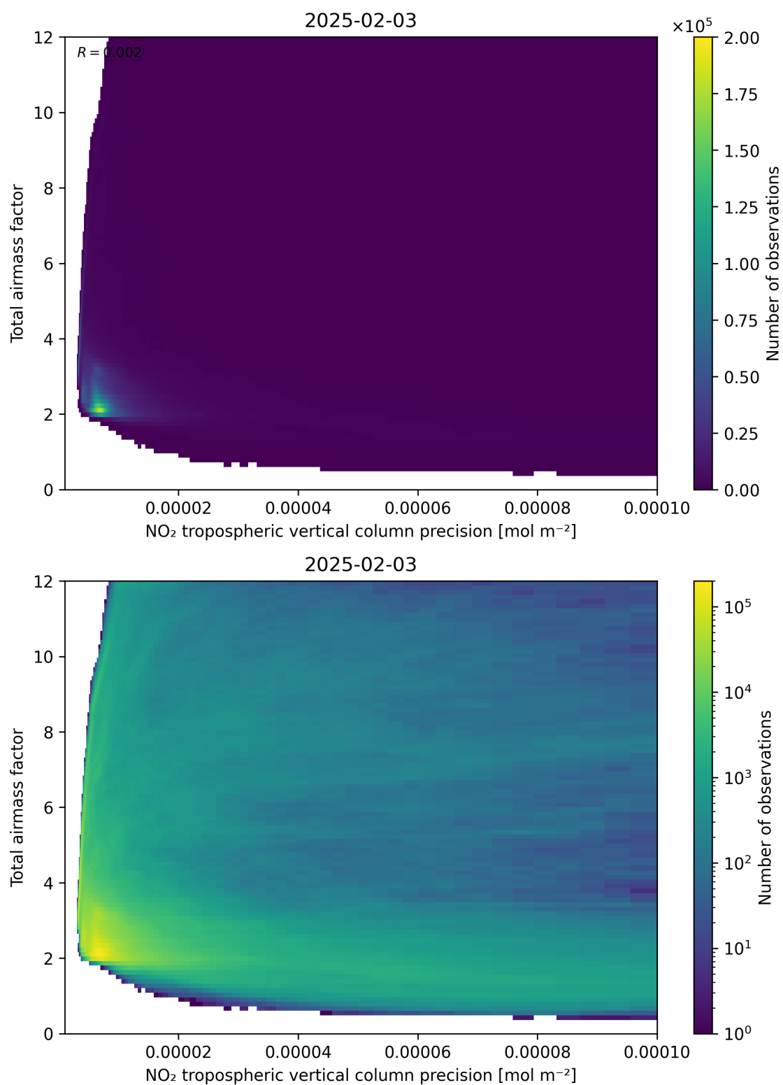
Figure 132: Scatter density plot of “NO 2 tropospheric vertical column precision” against “Total air mass factor” for 2025-02-03 to 2025-02-04.
