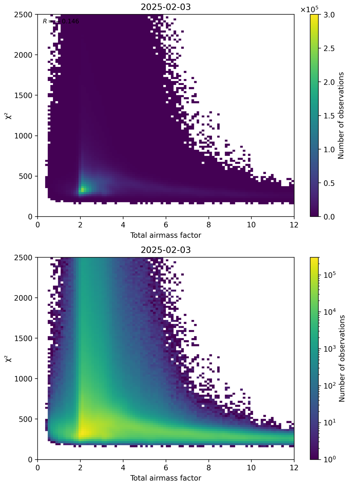
Figure 63: Scatter density plot of “Total airmass factor” against “ \chi^2 ” for 2025-02-03 to 2025-02-04.
