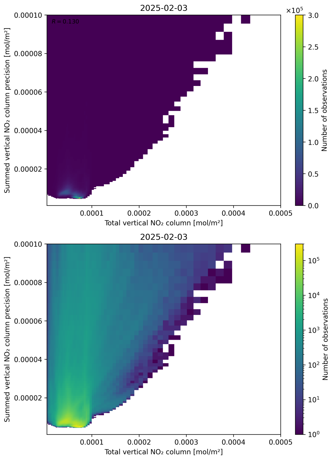
Figure 113: Scatter density plot of “Total vertical NO 2 column” against “Summed vertical NO 2 column precision” for 2025-02-03 to 2025-02-04.
