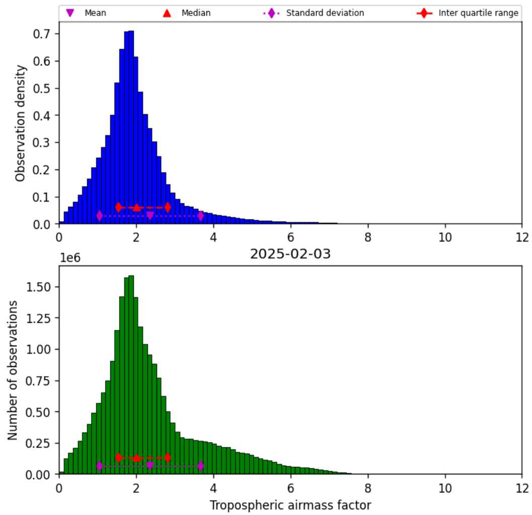
Figure 31: Histogram of “Tropospheric airmass factor” for 2025-02-03 to 2025-02-04
