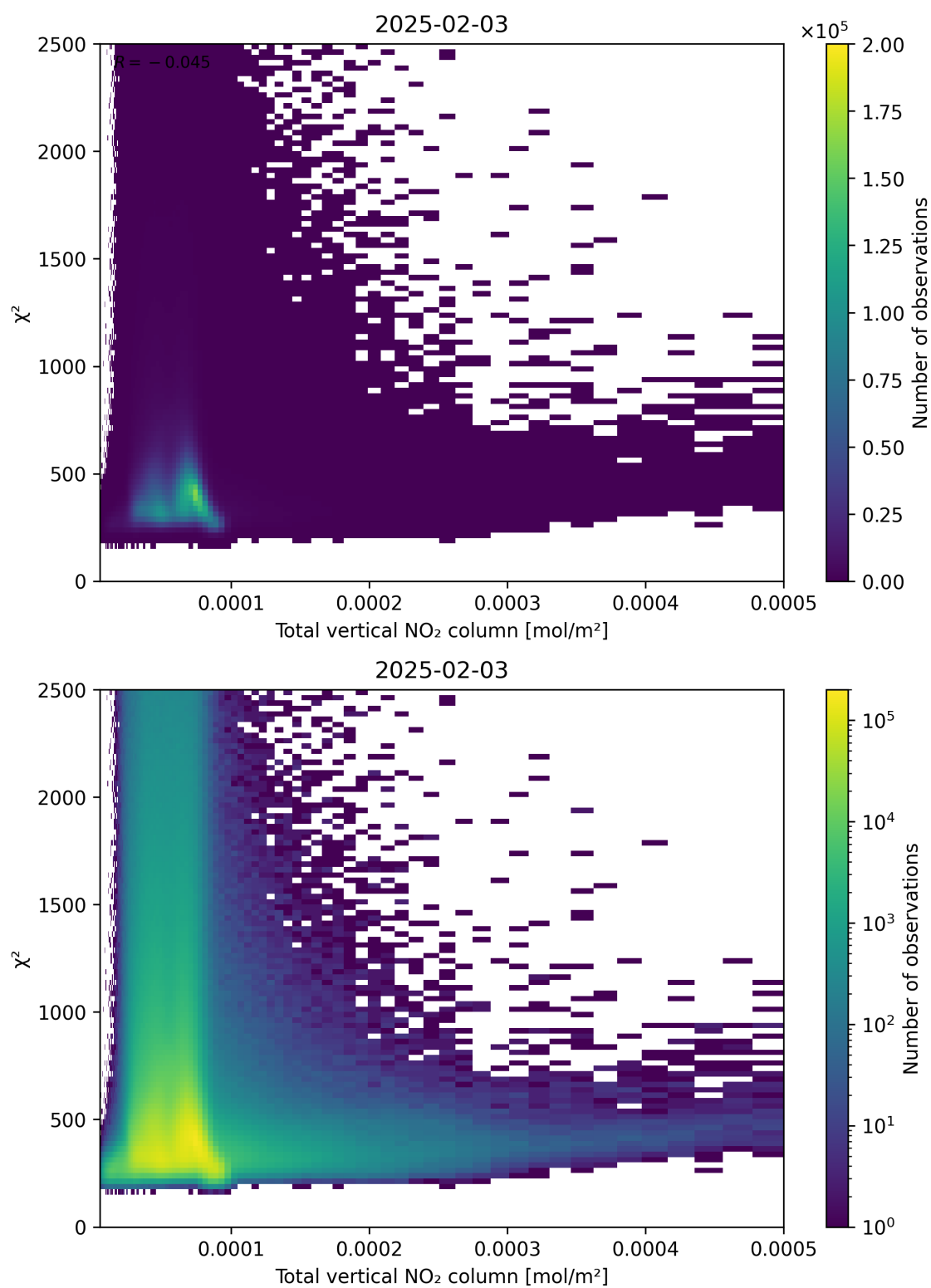
Figure 111: Scatter density plot of “Total vertical NO 2 column” against “ \chi^2 ” for 2025-02-03 to 2025-02-04.
