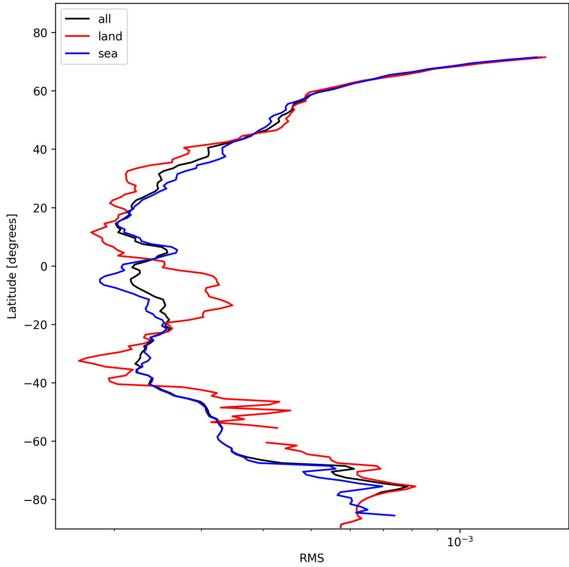
Figure 26: Zonal average of “RMS” for 2025-02-03 to 2025-02-04.
