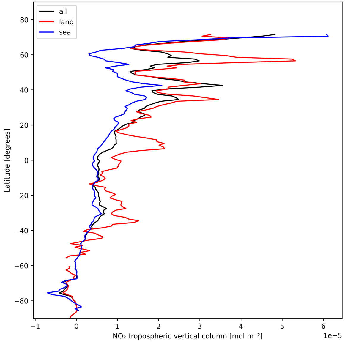
Figure 12: Zonal average of “NO 2 tropospheric vertical column” for 2025-02-03 to 2025-02-04.
