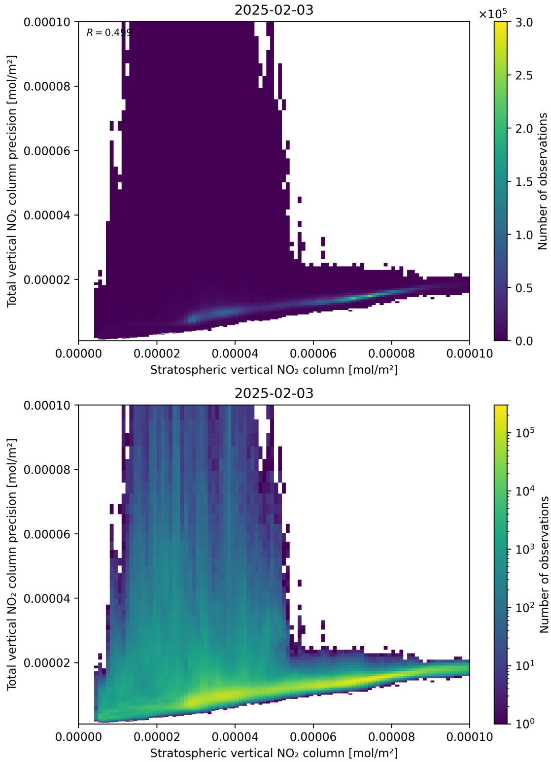
Figure 101: Scatter density plot of “Stratospheric vertical NO 2 column” against “Total vertical NO 2 column precision” for 2025-02-03 to 2025-02-04.
