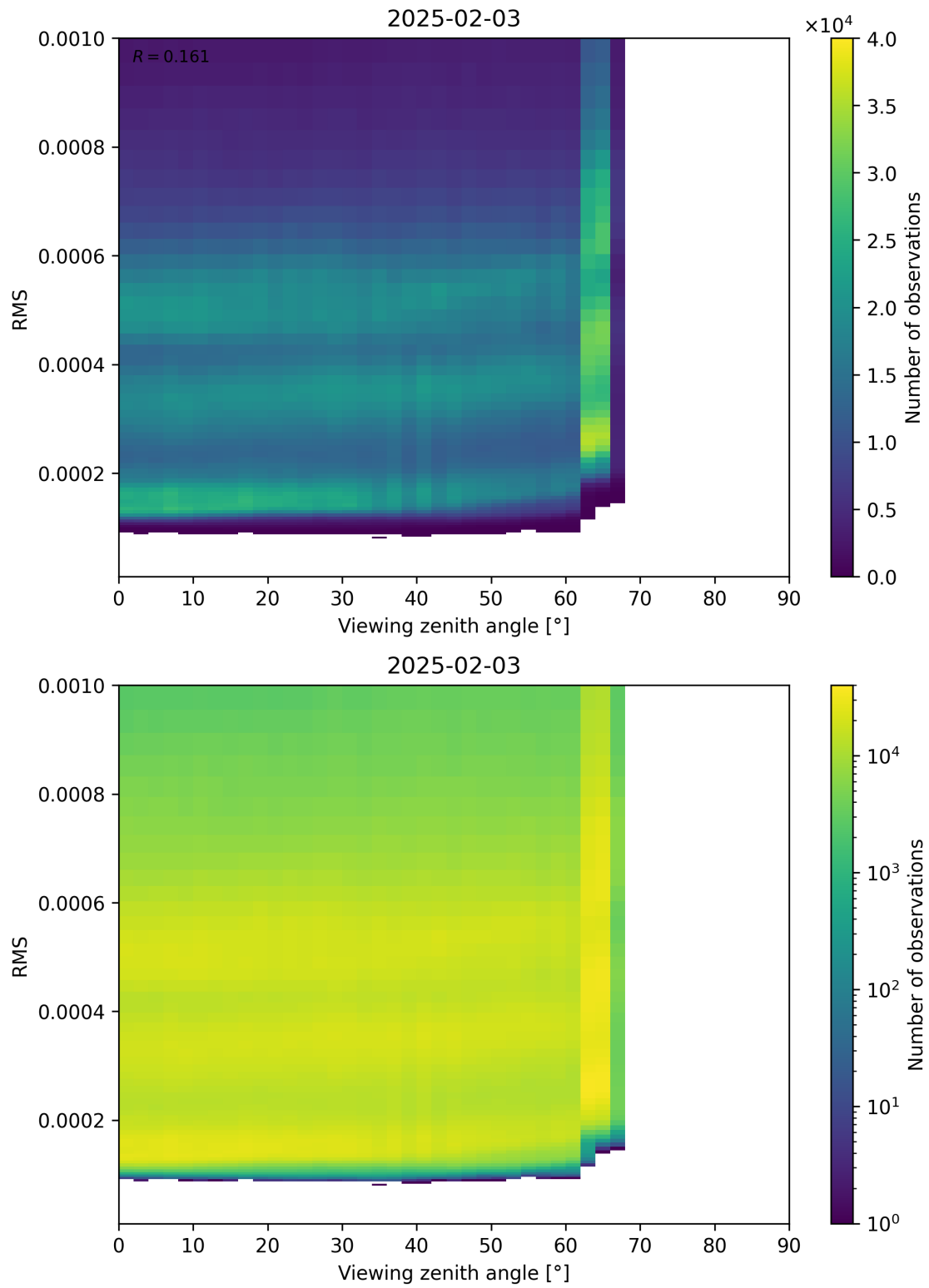
Figure 171: Scatter density plot of “Viewing zenith angle” against “RMS” for 2025-02-03 to 2025-02-04.
