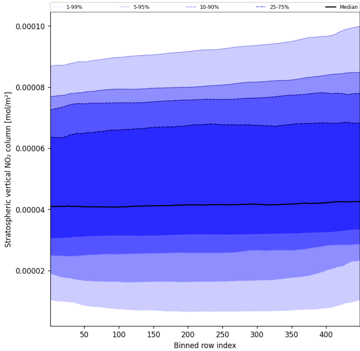
Figure 53: Along track statistics of “Stratospheric vertical NO 2 column” for 2025-02-03 to 2025-02-04
