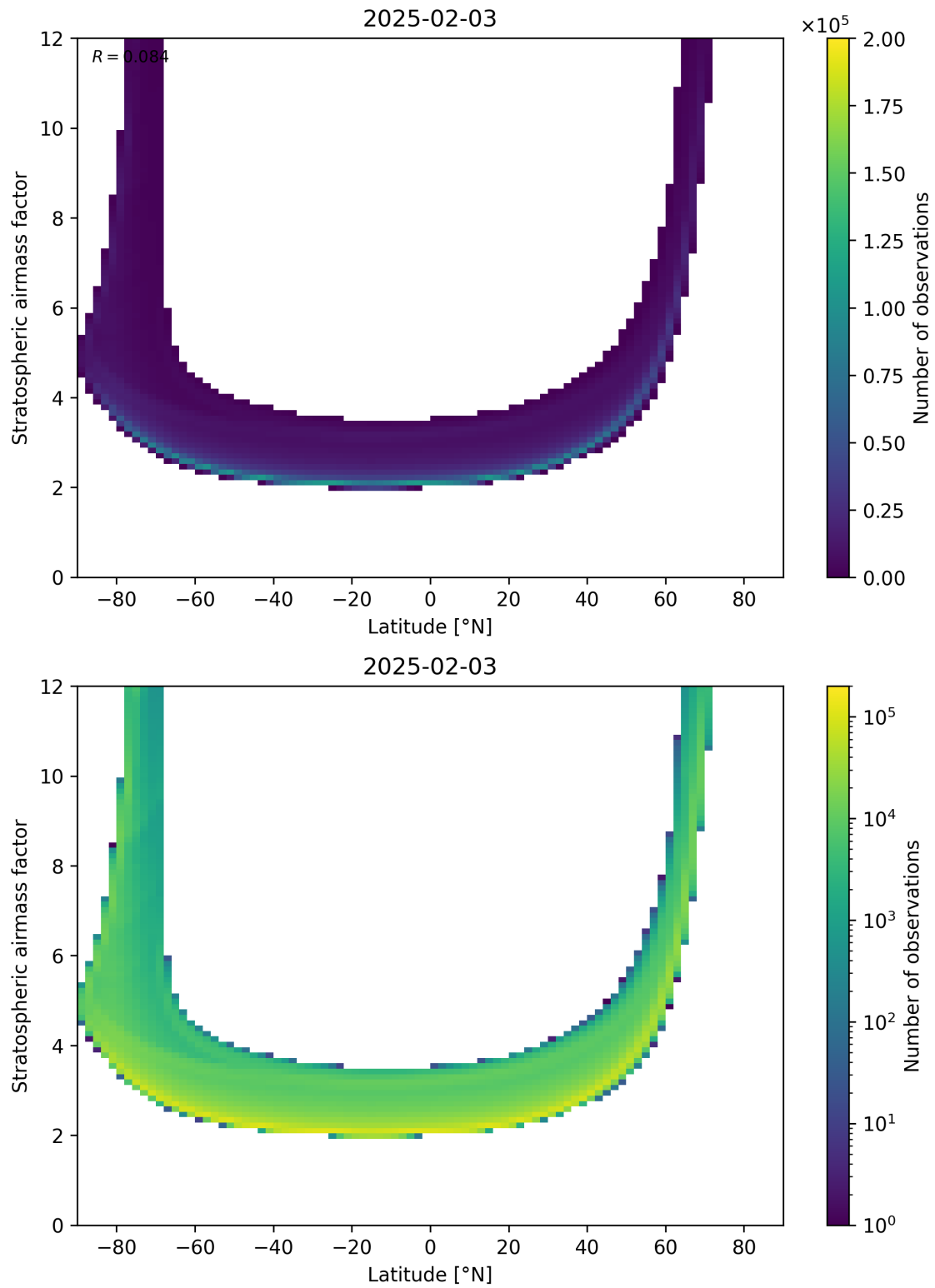
Figure 83: Scatter density plot of “Latitude” against “Stratospheric air mass factor” for 2025-02-03 to 2025-02-04.
