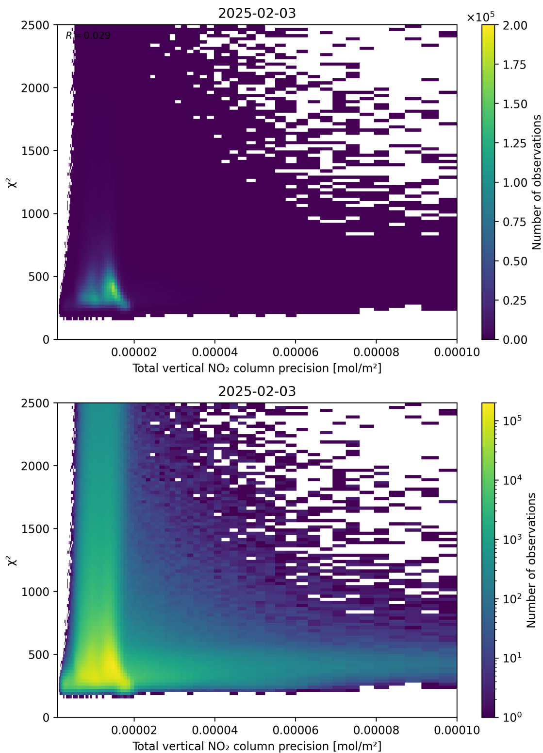
Figure 116: Scatter density plot of “Total vertical NO 2 column precision” against “ \chi^2 ” for 2025-02-03 to 2025-02-04.
