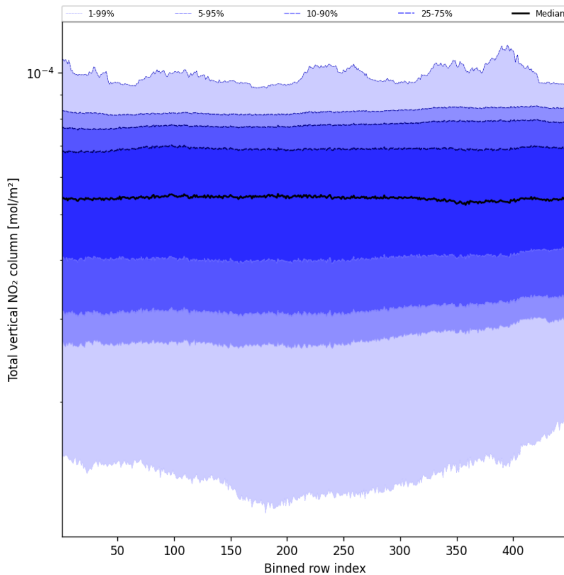
Figure 55: Along track statistics of “Total vertical NO 2 column” for 2025-02-03 to 2025-02-04
