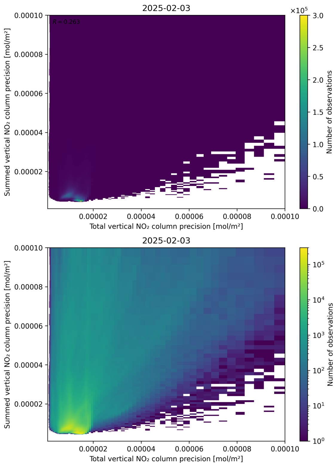
Figure 118: Scatter density plot of “Total vertical NO 2 column precision” against “Summed vertical NO 2 column precision” for 2025-02-03 to 2025-02-04.
