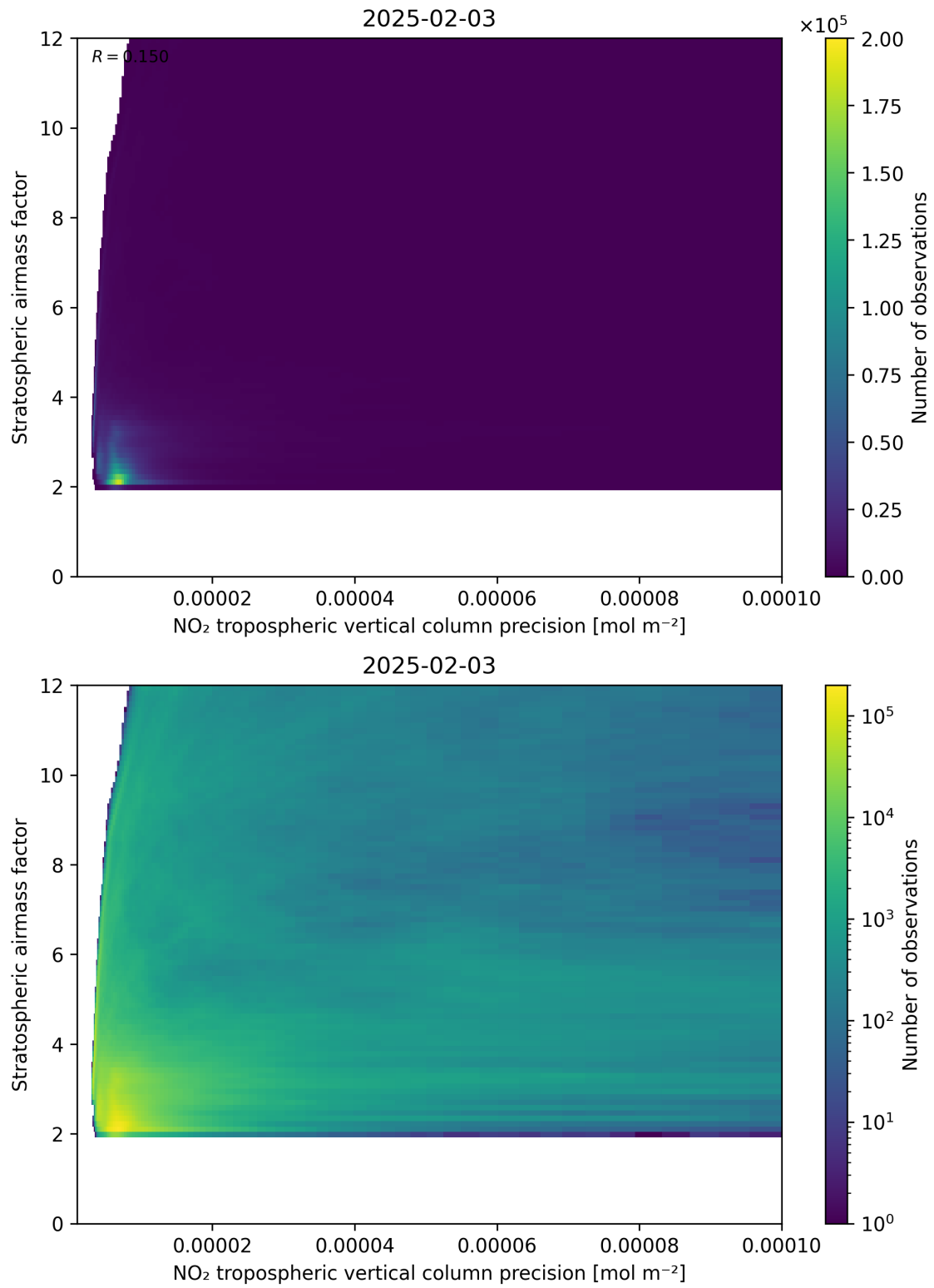
Figure 131: Scatter density plot of “NO 2 tropospheric vertical column precision” against “Stratospheric airmass factor” for 2025-02-03 to 2025-02-04.
