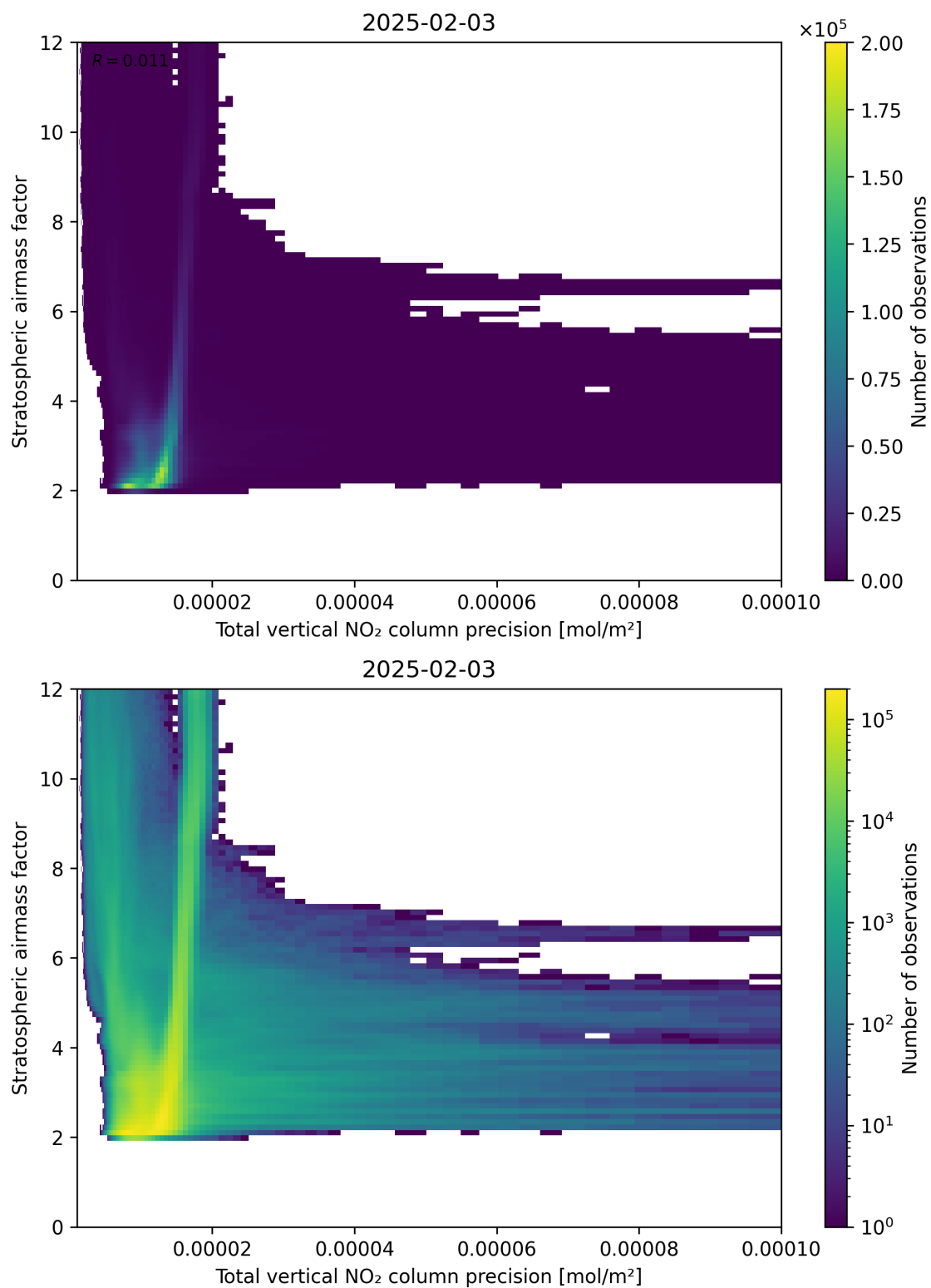
Figure 115: Scatter density plot of “Total vertical NO 2 column precision” against “Stratospheric air mass factor” for 2025-02-03 to 2025-02-04.
