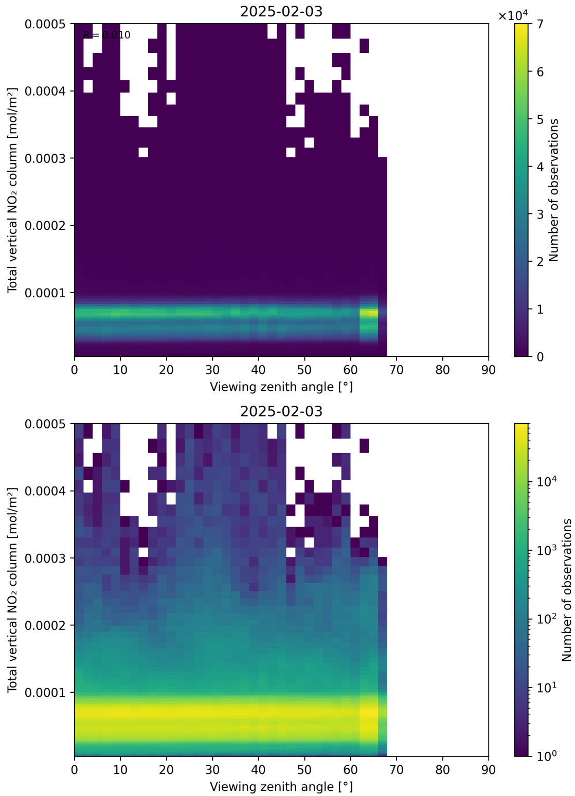
Figure 167: Scatter density plot of “Viewing zenith angle” against “Total vertical NO 2 column” for 2025-02-03 to 2025-02-04.
