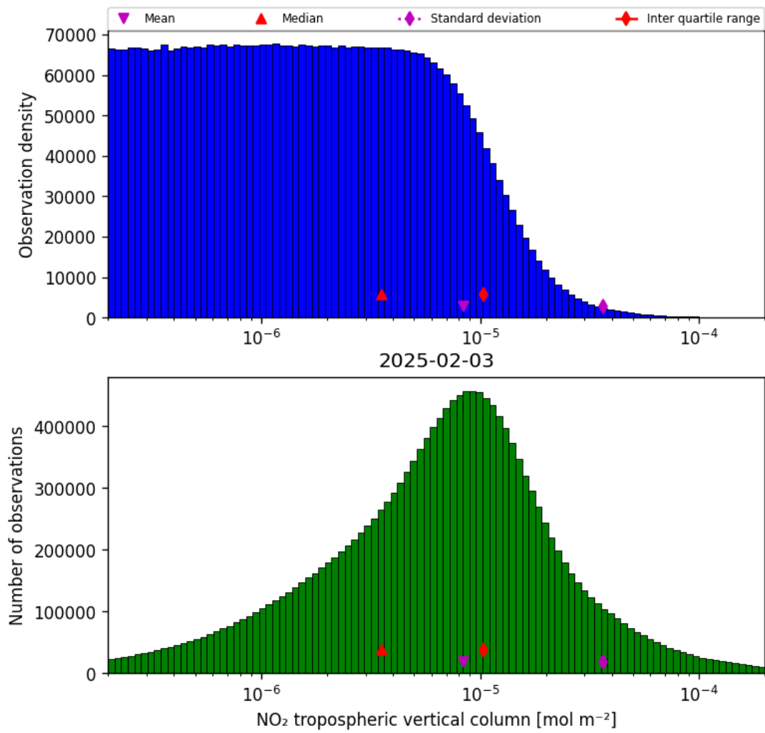
Figure 29: Histogram of “NO 2 tropospheric vertical column” for 2025-02-03 to 2025-02-04
