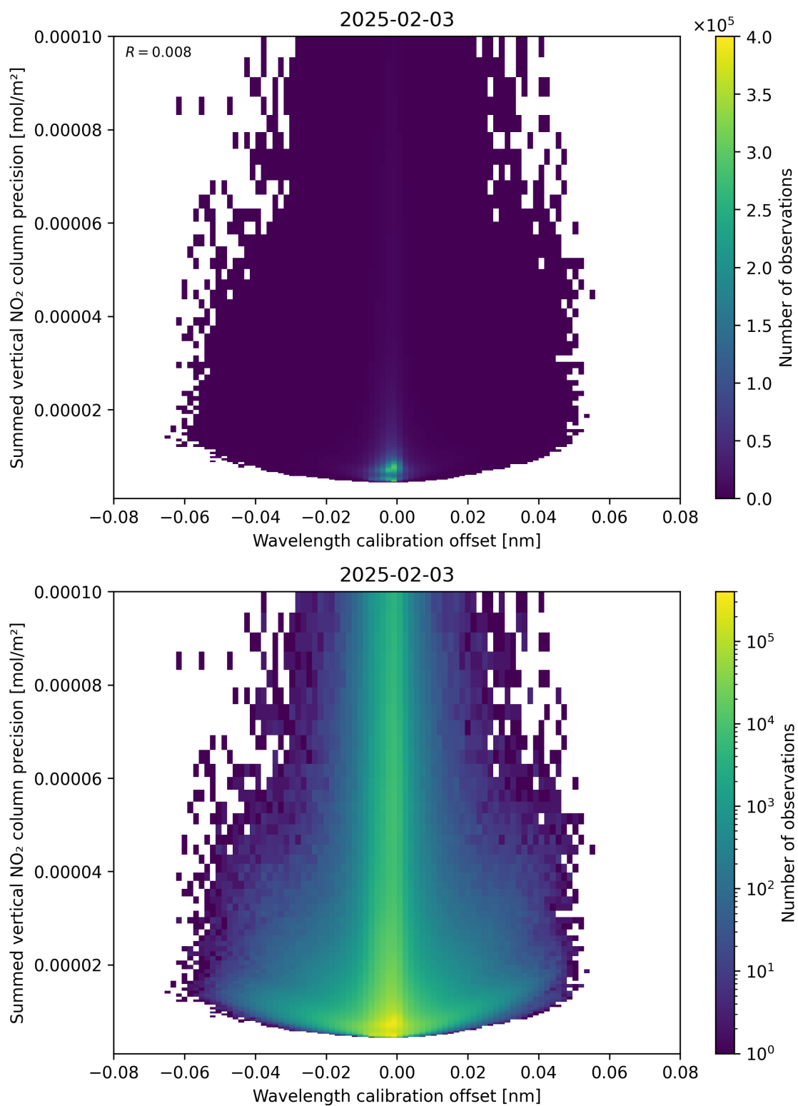
Figure 178: Scatter density plot of “Wavelength calibration offset” against “Summed vertical NO 2 column precision” for 2025-02-03 to 2025-02-04.
