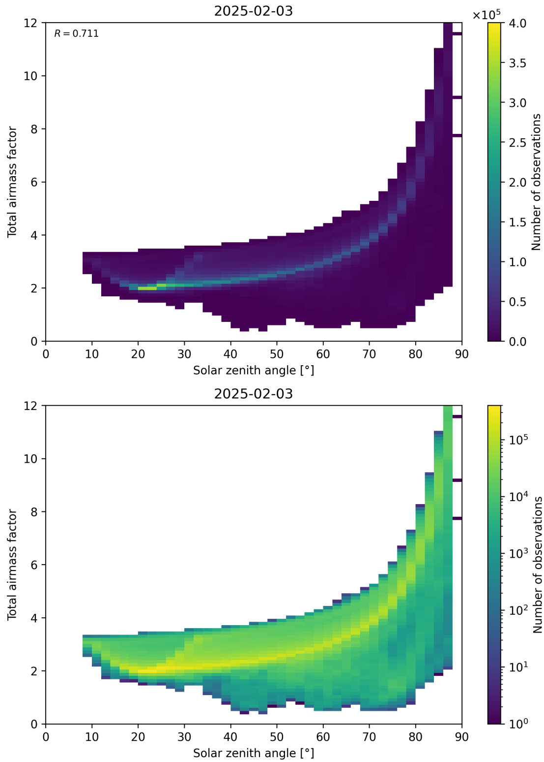
Figure 146: Scatter density plot of “Solar zenith angle” against “Total airmass factor” for 2025-02-03 to 2025-02-04.
