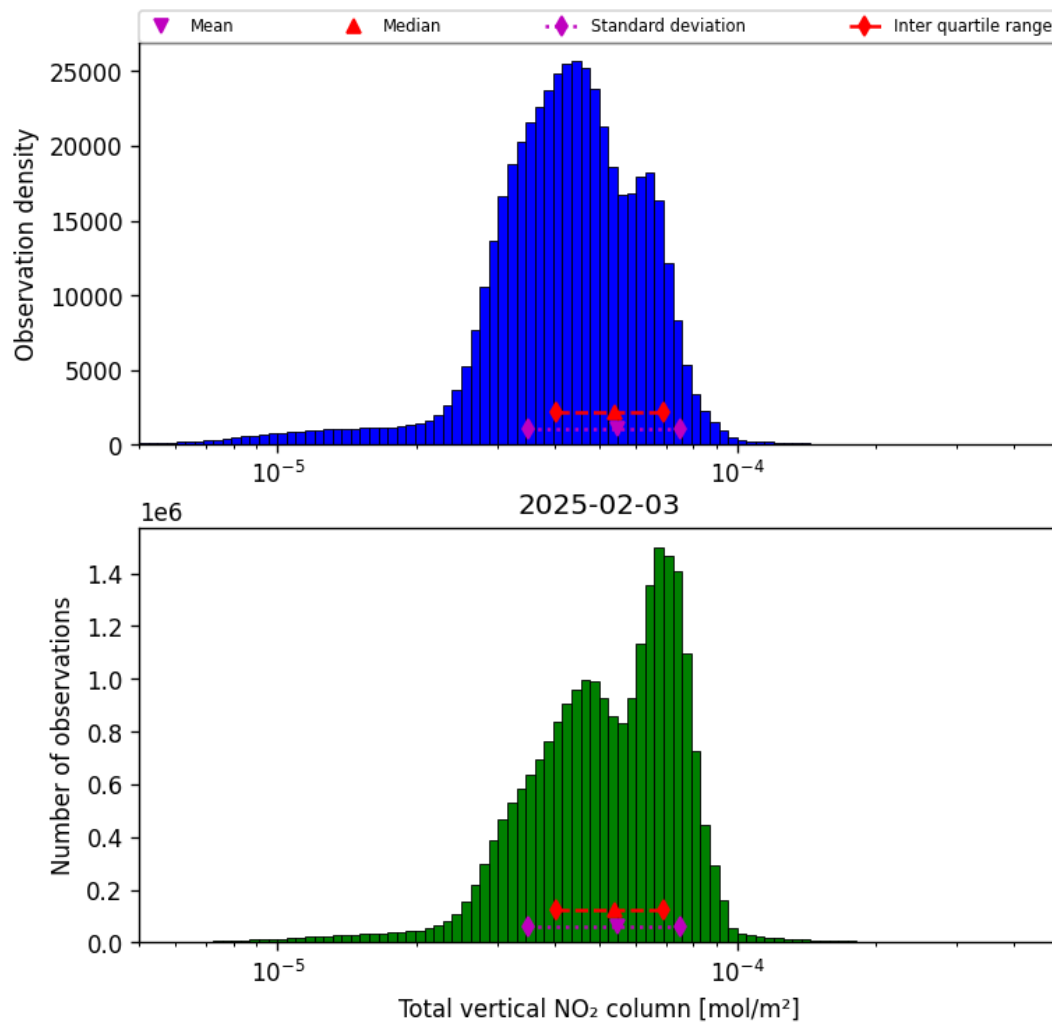
Figure 38: Histogram of “Total vertical NO 2 column” for 2025-02-03 to 2025-02-04
