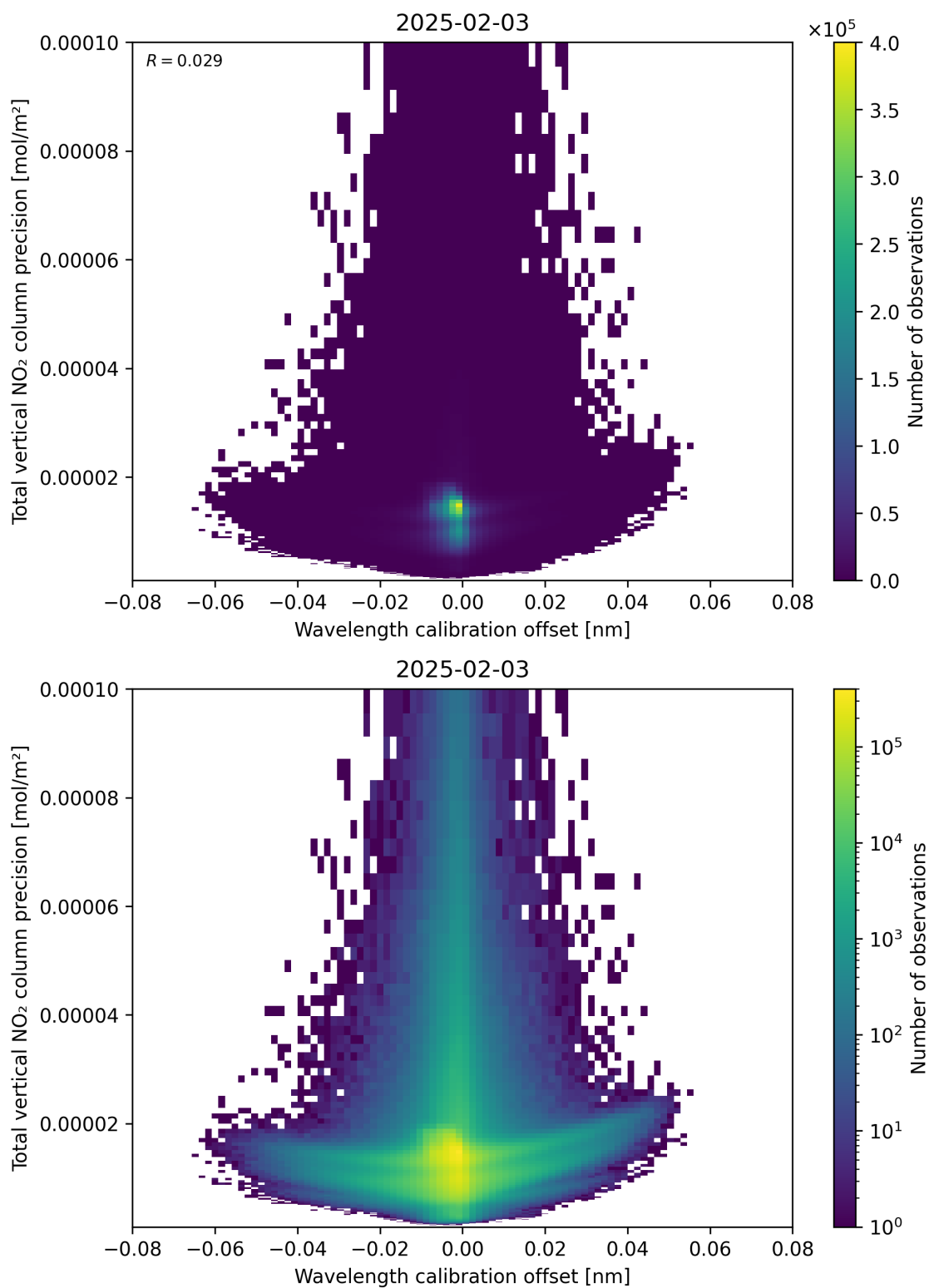
Figure 180: Scatter density plot of “Wavelength calibration offset” against “Total vertical NO 2 column precision” for 2025-02-03 to 2025-02-04.
