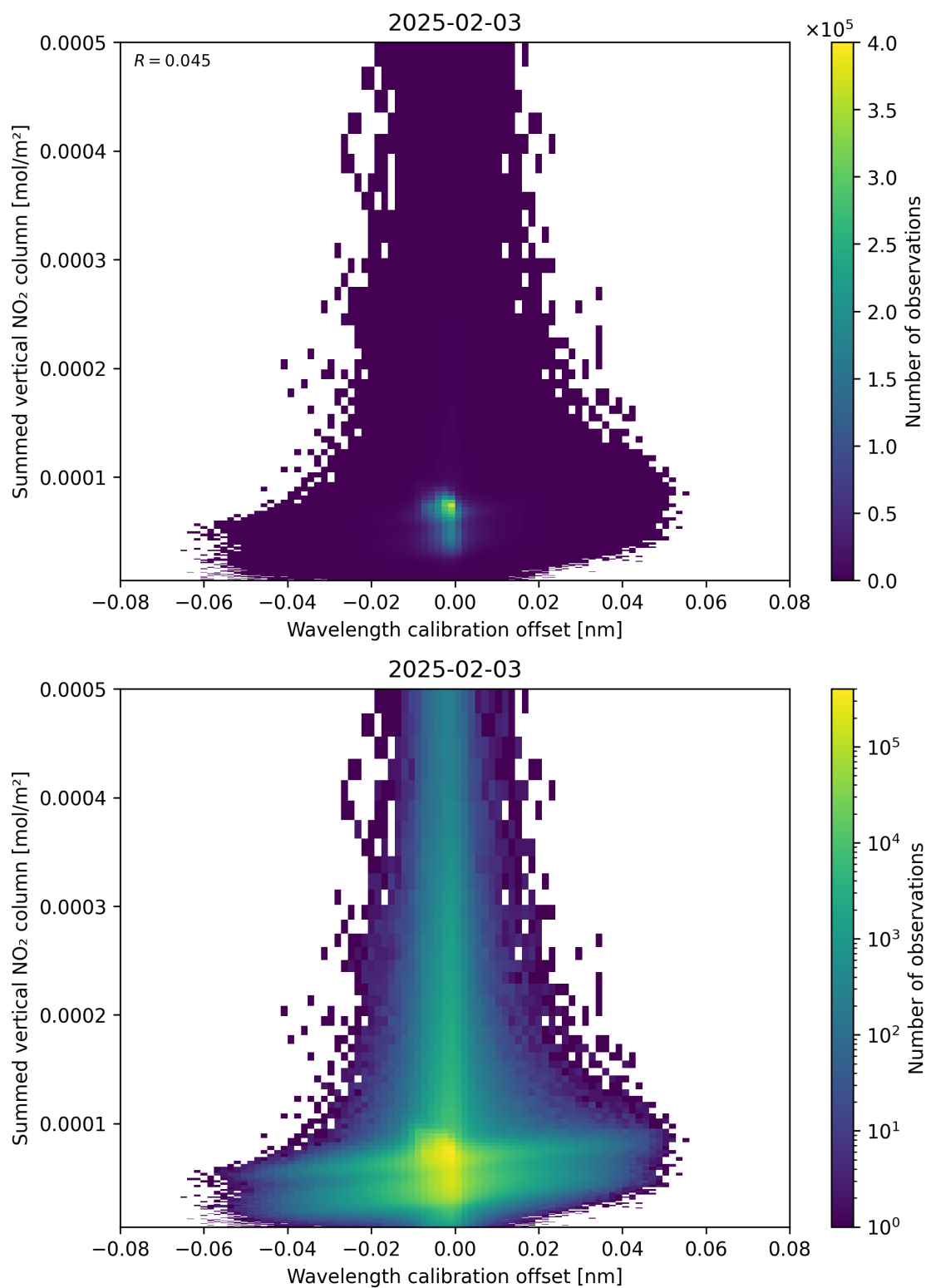
Figure 177: Scatter density plot of “Wavelength calibration offset” against “Summed vertical NO 2 column” for 2025-02-03 to 2025-02-04.
