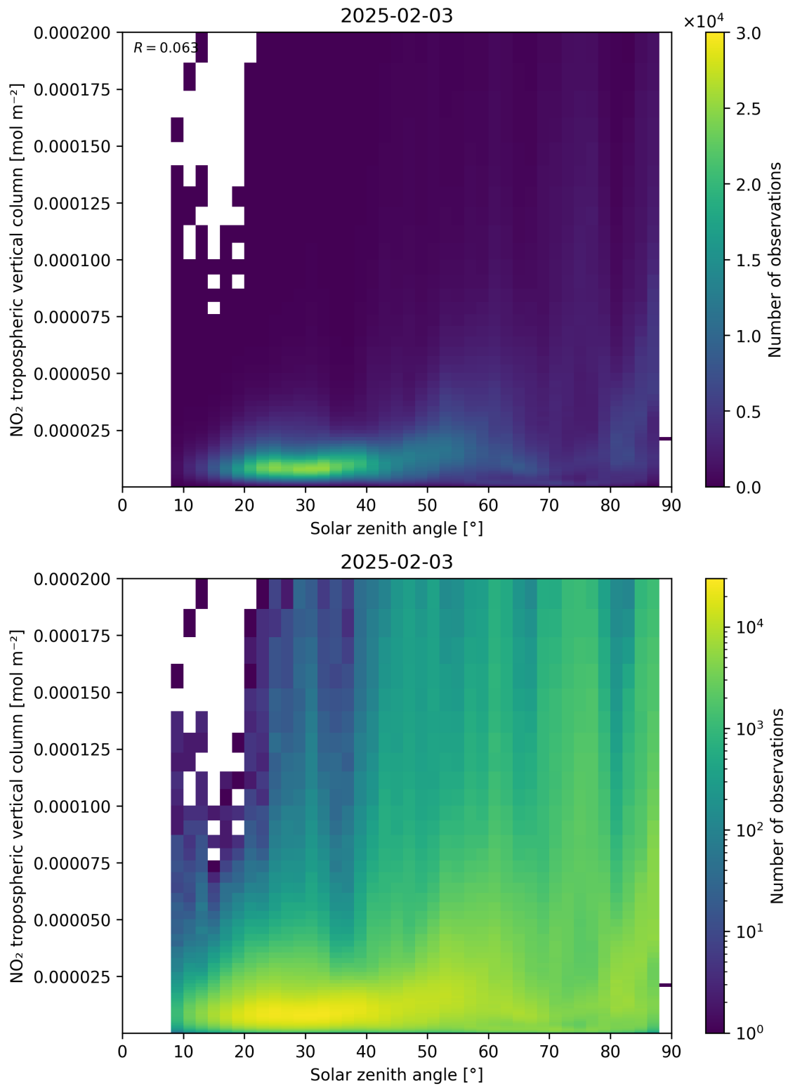
Figure 155: Scatter density plot of “Solar zenith angle” against “NO 2 tropospheric vertical column” for 2025-02-03 to 2025-02-04.
