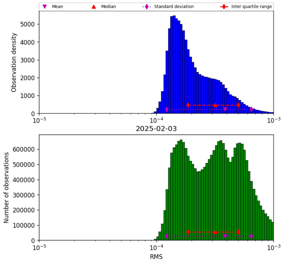
Figure 43: Histogram of “RMS” for 2025-02-03 to 2025-02-04
