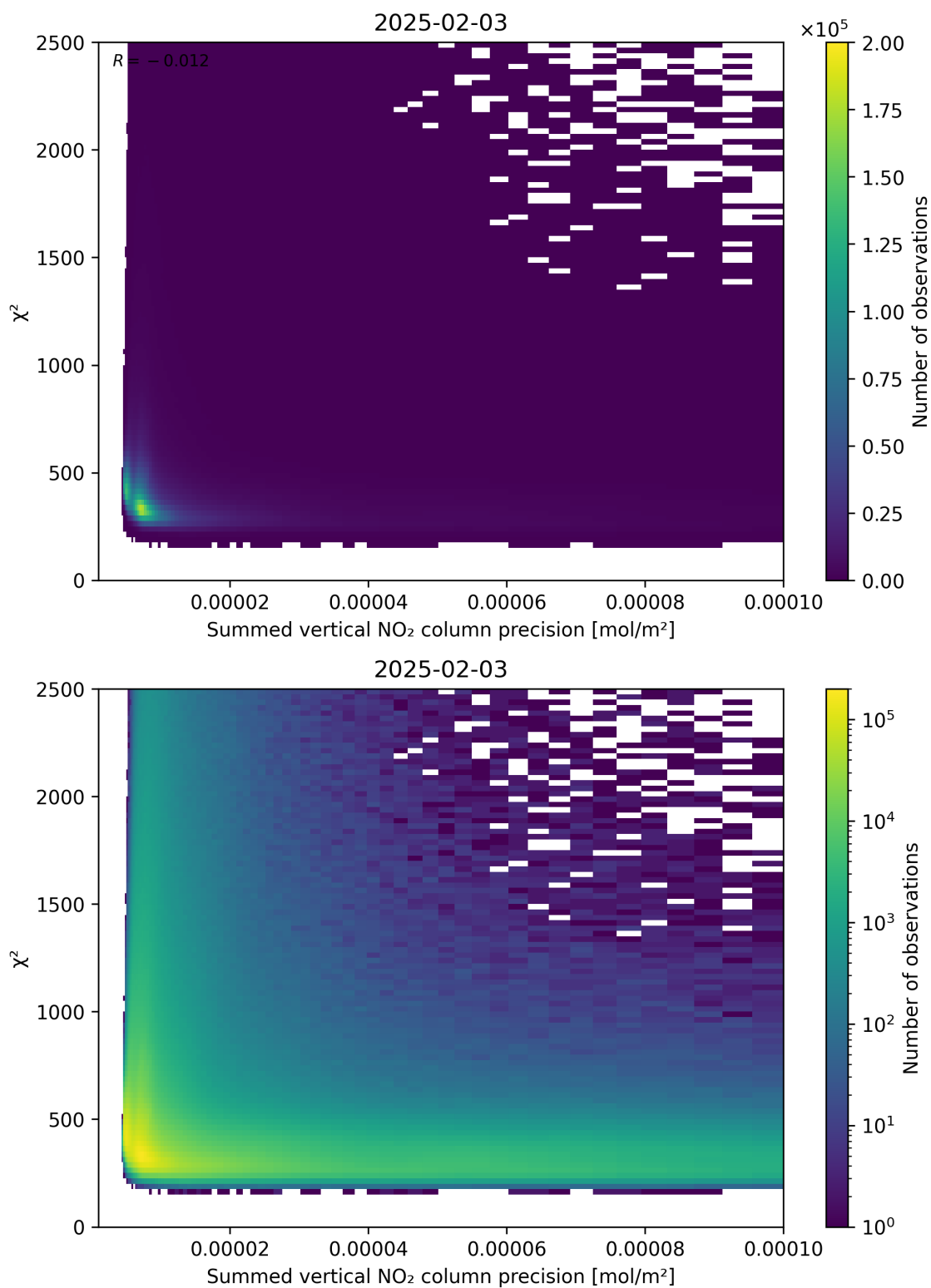
Figure 107: Scatter density plot of “Summed vertical NO 2 column precision” against “ \chi^2 ” for 2025-02-03 to 2025-02-04.
