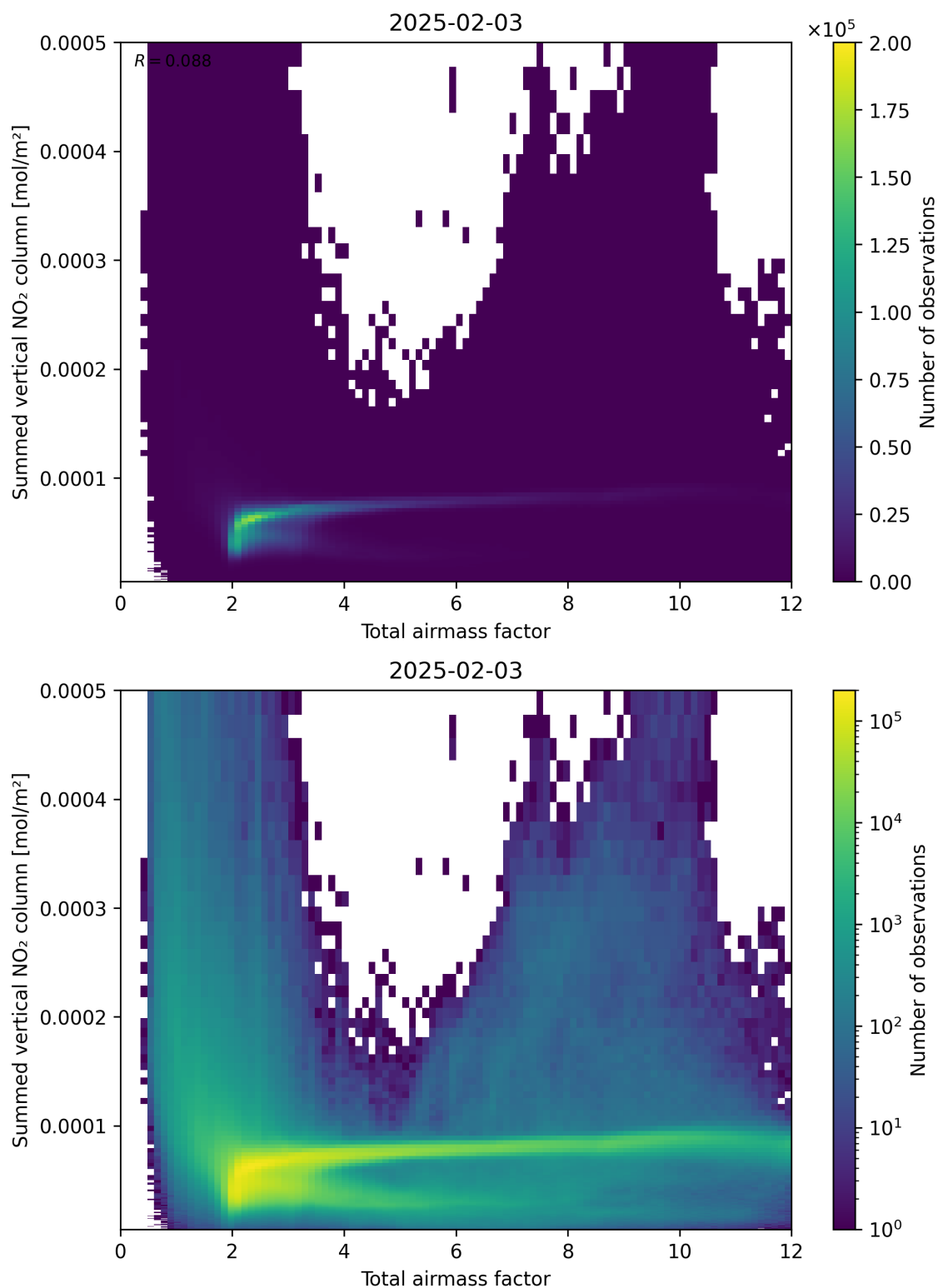
Figure 65: Scatter density plot of “Total airmass factor” against “Summed vertical NO 2 column” for 2025-02-03 to 2025-02-04.
