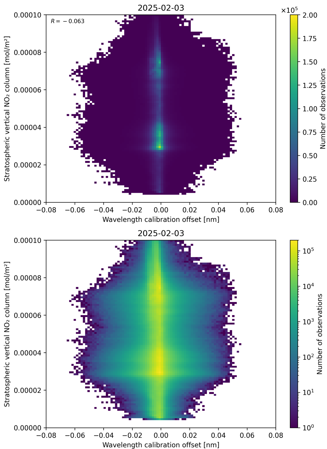
Figure 176: Scatter density plot of “Wavelength calibration offset” against “Stratospheric vertical NO 2 column” for 2025-02-03 to 2025-02-04.
