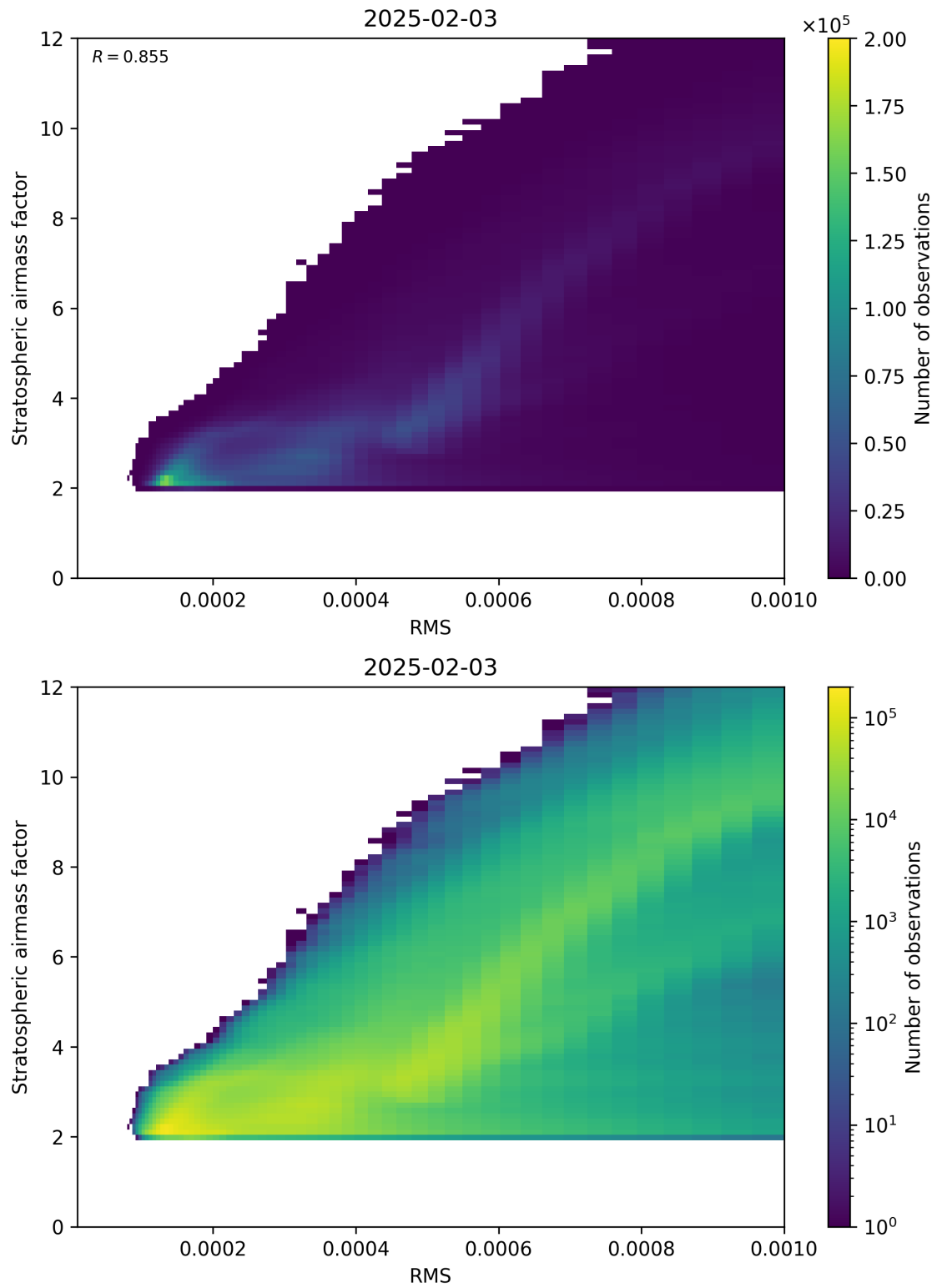
Figure 144: Scatter density plot of “RMS” against “Stratospheric airmass factor” for 2025-02-03 to 2025-02-04.
