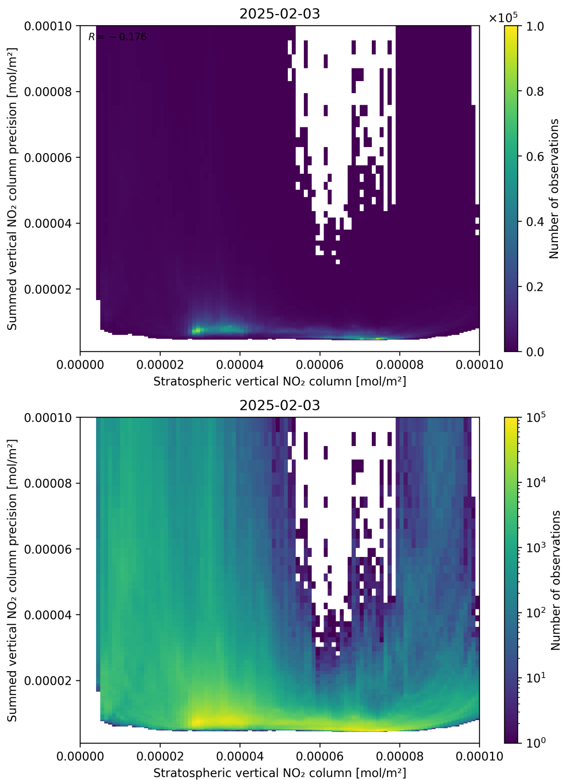
Figure 99: Scatter density plot of “Stratospheric vertical NO 2 column” against “Summed vertical NO 2 column precision” for 2025-02-03 to 2025-02-04.
