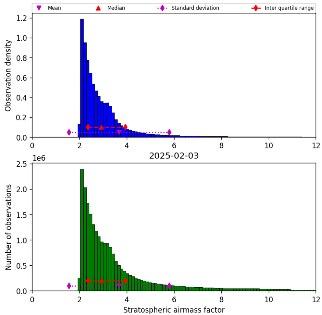
Figure 44: Histogram of “Stratospheric airmass factor” for 2025-02-03 to 2025-02-04
