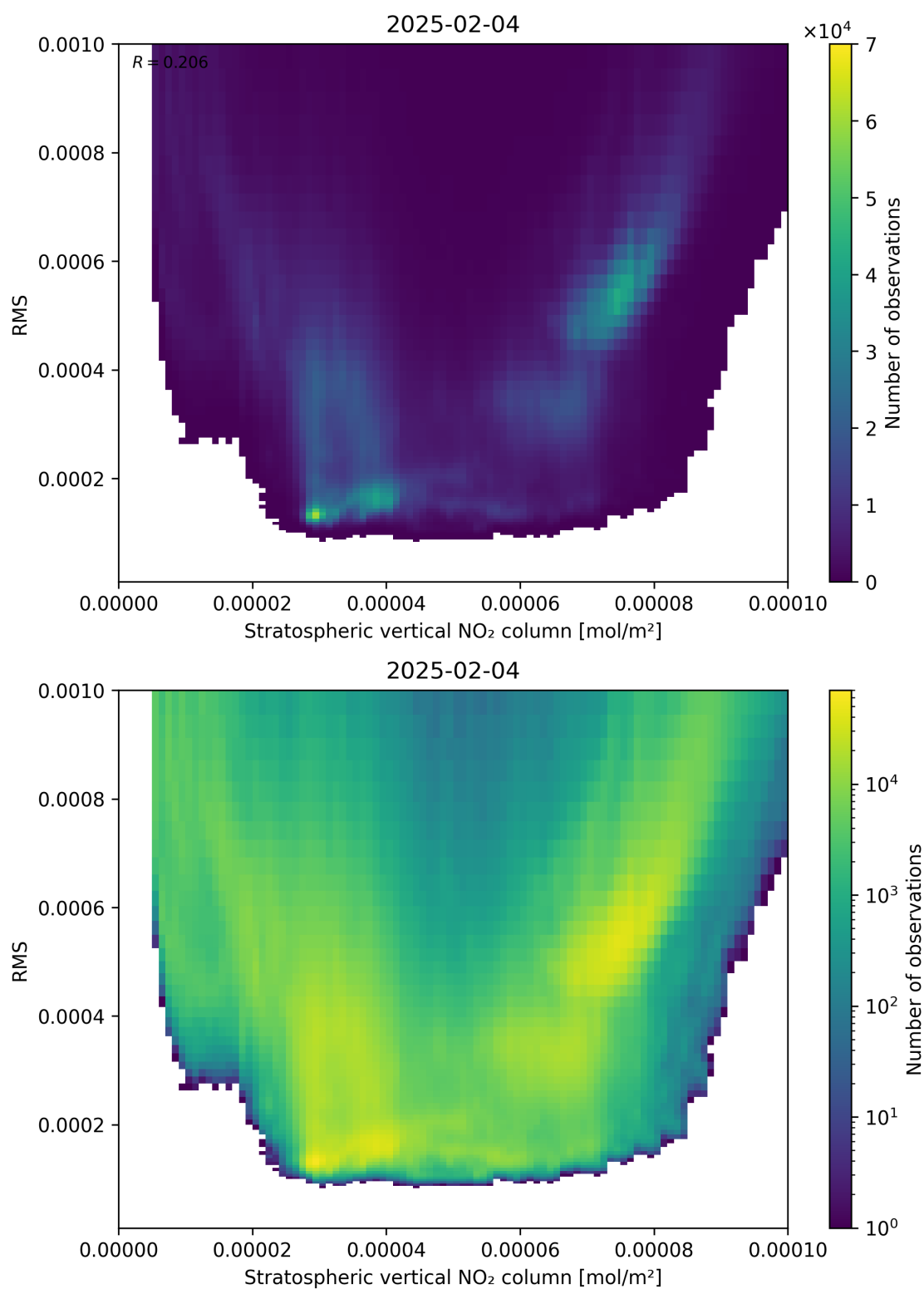
Figure 102: Scatter density plot of “Stratospheric vertical NO 2 column” against “RMS” for 2025-02-04 to 2025-02-05.
