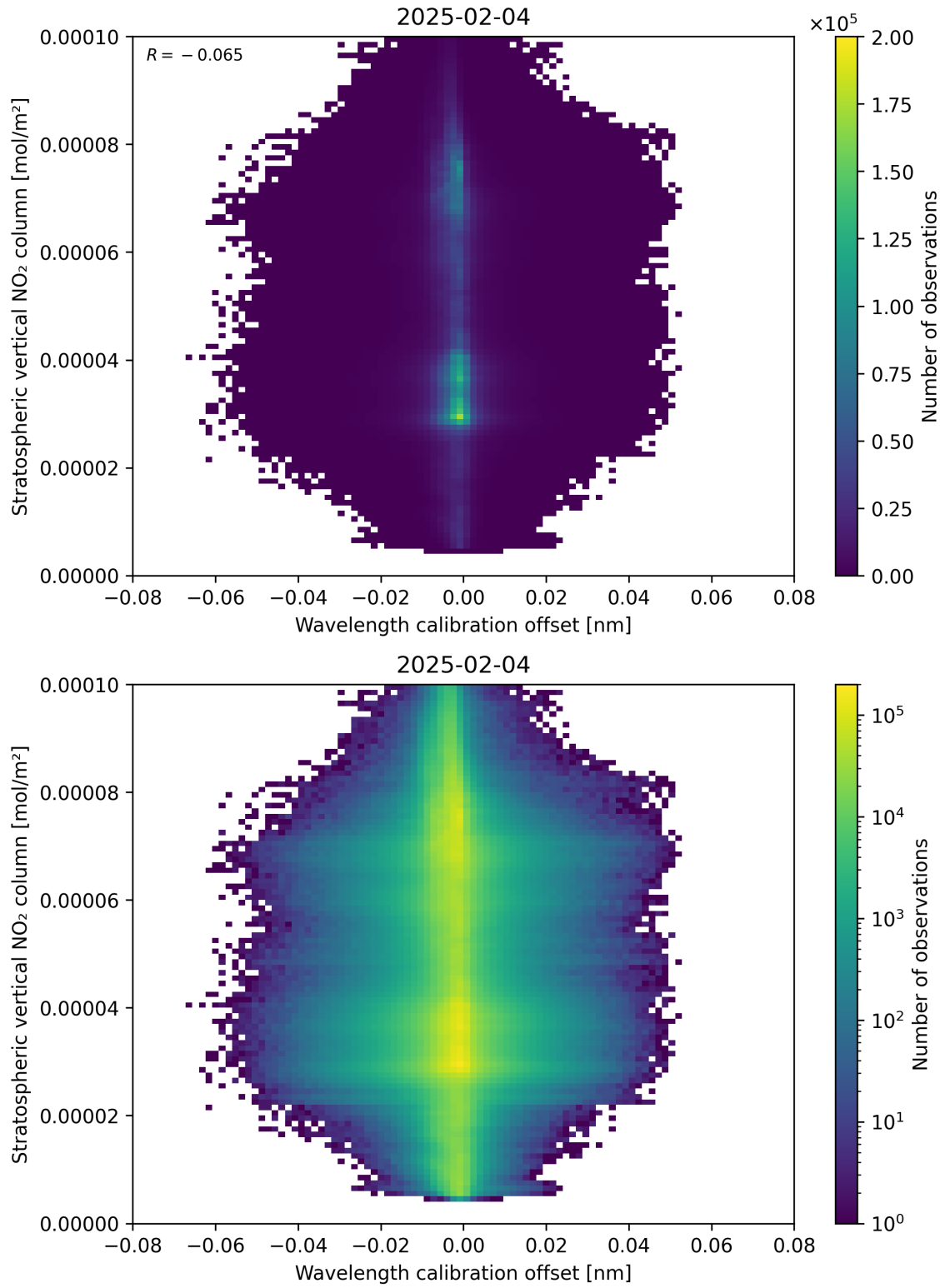
Figure 176: Scatter density plot of “Wavelength calibration offset” against “Stratospheric vertical NO 2 column” for 2025-02-04 to 2025-02-05.
