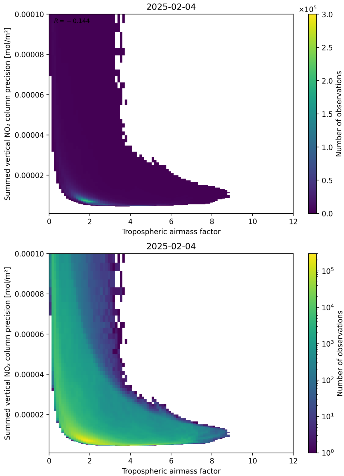
Figure 76: Scatter density plot of “Tropospheric air mass factor” against “Summed vertical NO 2 column precision” for 2025-02-04 to 2025-02-05.
