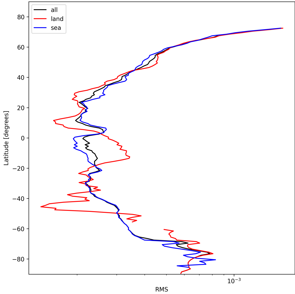
Figure 26: Zonal average of “RMS” for 2025-02-04 to 2025-02-05.
