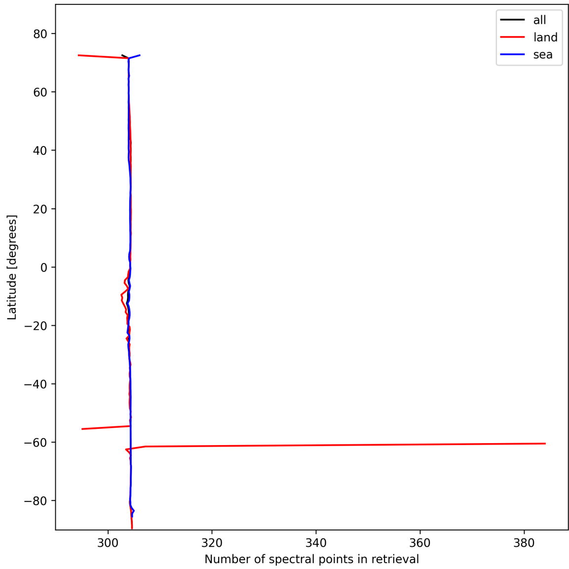
Figure 16: Zonal average of “Number of spectral points in retrieval” for 2025-02-04 to 2025-02-05.
