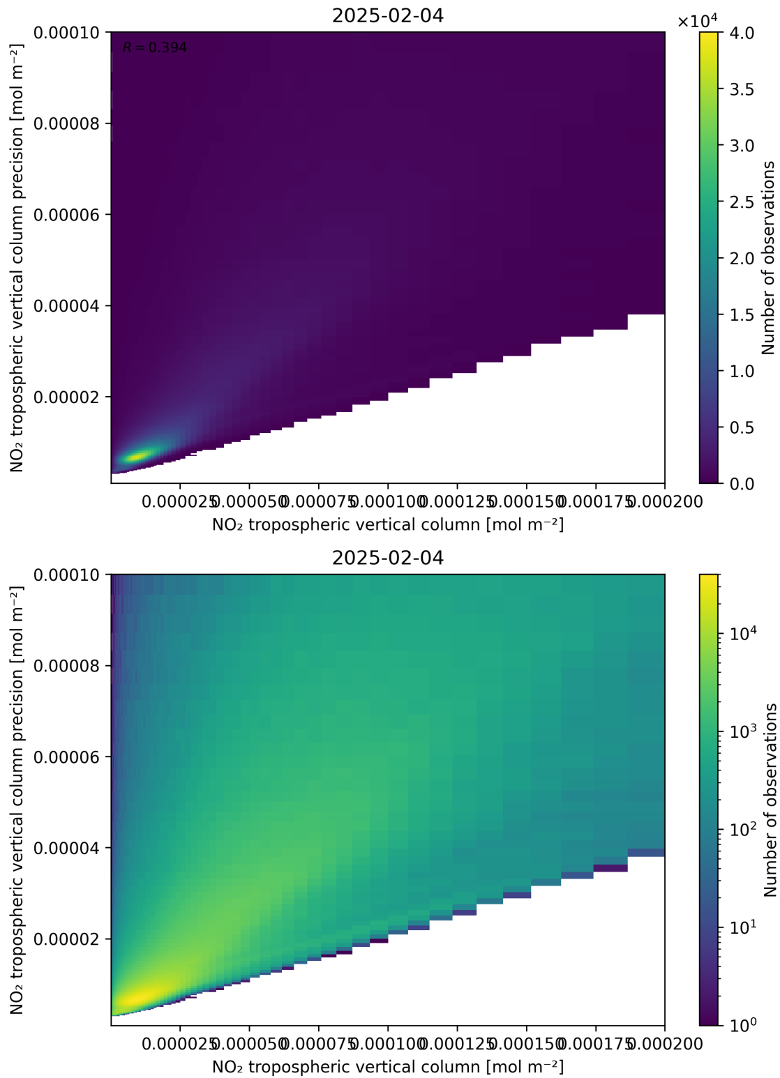
Figure 130: Scatter density plot of “NO 2 tropospheric vertical column” against “NO 2 tropospheric vertical column precision” for 2025-02-04 to 2025-02-05.
