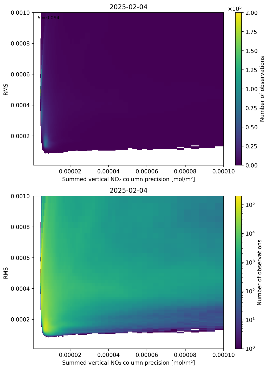
Figure 108: Scatter density plot of “Summed vertical NO 2 column precision” against “RMS” for 2025-02-04 to 2025-02-05.
