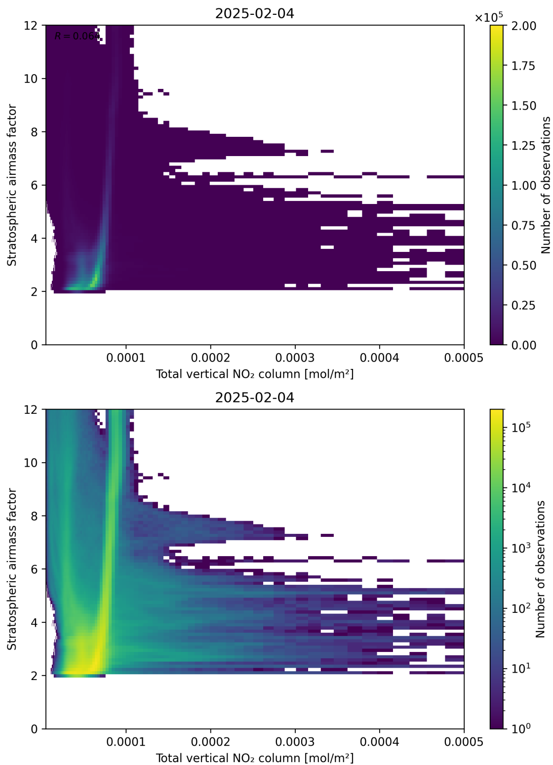
Figure 110: Scatter density plot of “Total vertical NO 2 column” against “Stratospheric air mass factor” for 2025-02-04 to 2025-02-05.
