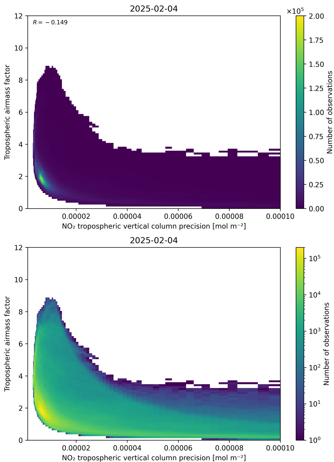
Figure 133: Scatter density plot of “NO 2 tropospheric vertical column precision” against “Tropospheric air mass factor” for 2025-02-04 to 2025-02-05.
