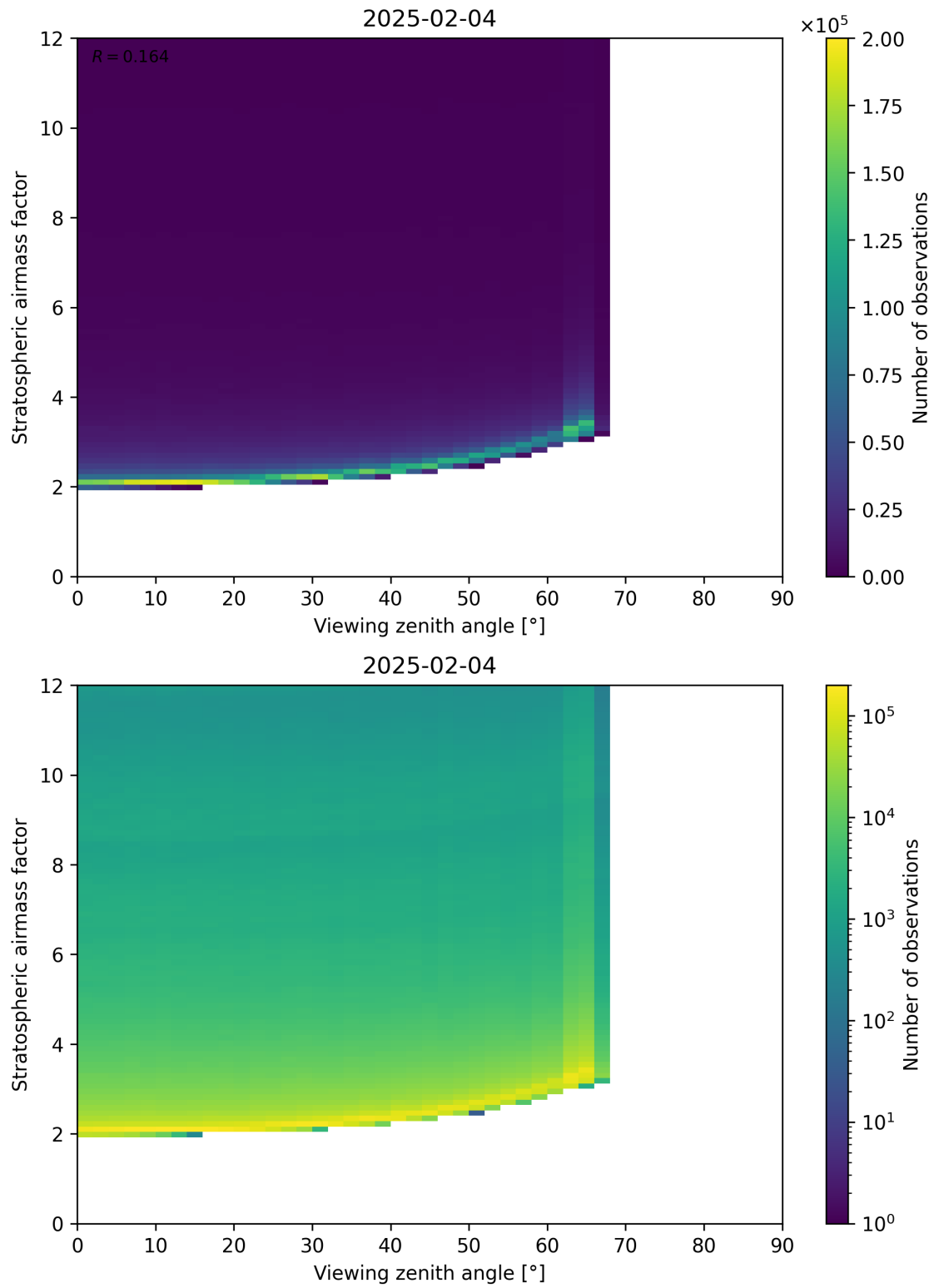
Figure 159: Scatter density plot of “Viewing zenith angle” against “Stratospheric airmass factor” for 2025-02-04 to 2025-02-05.
