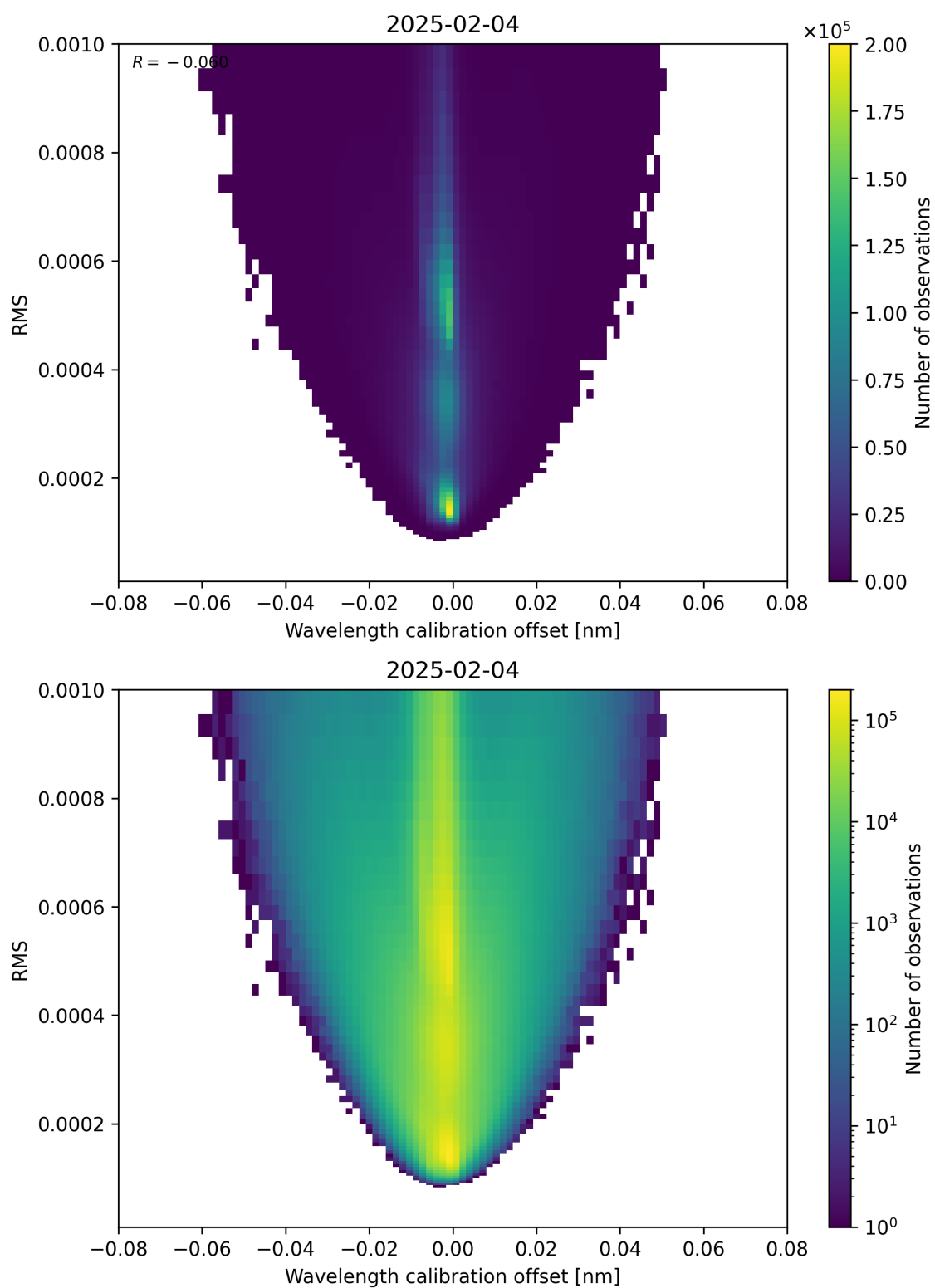
Figure 181: Scatter density plot of “Wavelength calibration offset” against “RMS” for 2025-02-04 to 2025-02-05.
