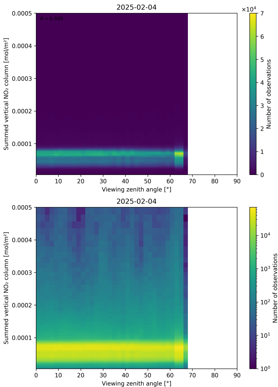
Figure 165: Scatter density plot of “Viewing zenith angle” against “Summed vertical NO 2 column” for 2025-02-04 to 2025-02-05.
