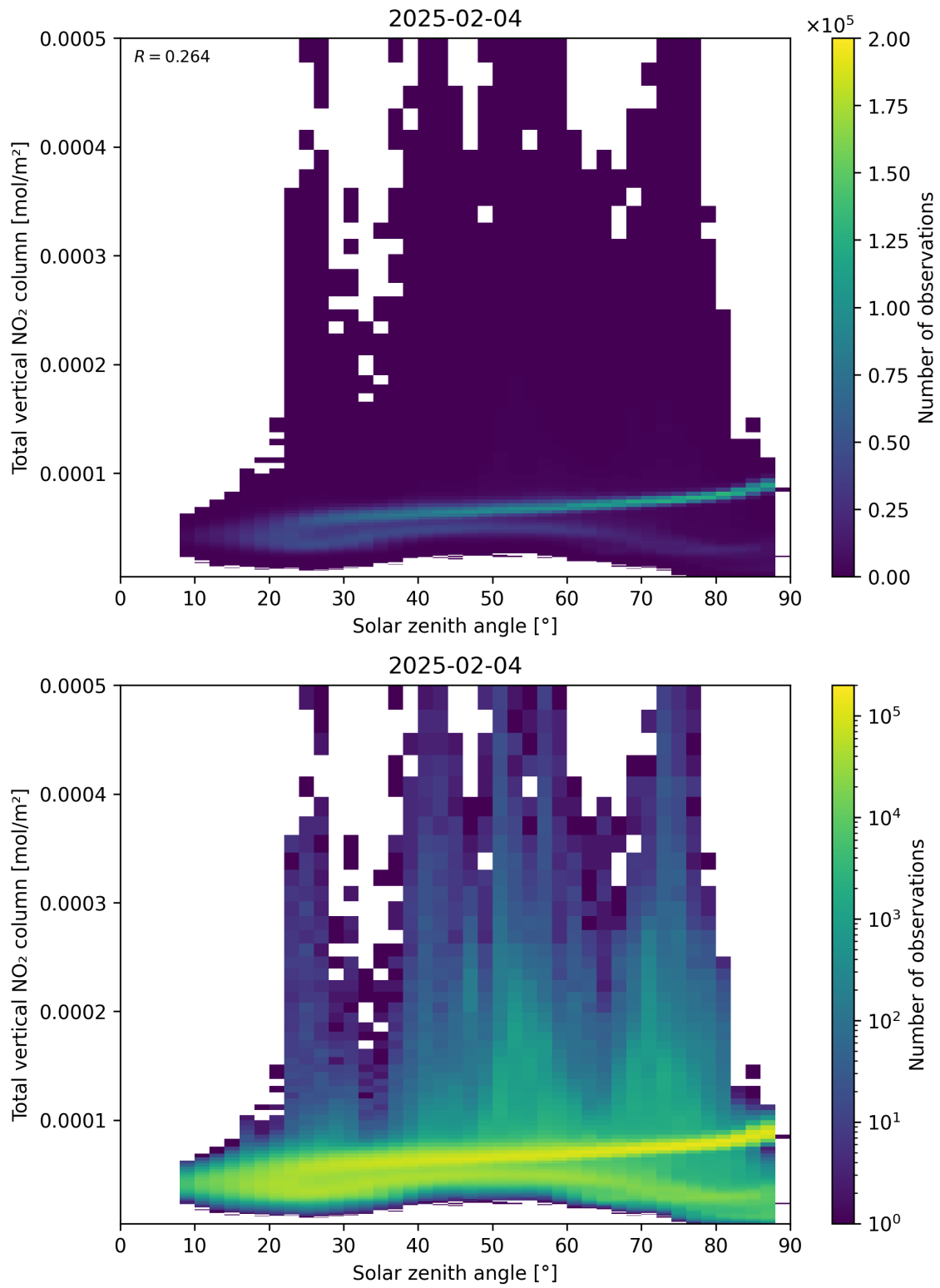
Figure 153: Scatter density plot of “Solar zenith angle” against “Total vertical NO 2 column” for 2025-02-04 to 2025-02-05.
