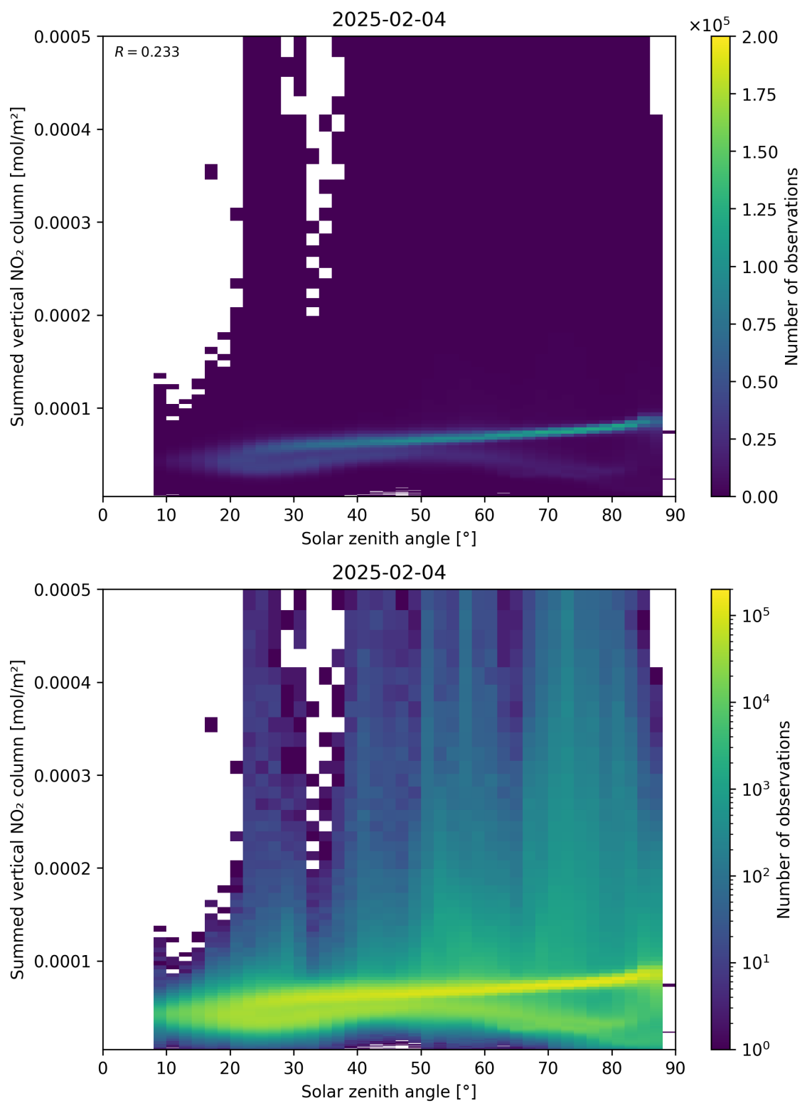
Figure 151: Scatter density plot of “Solar zenith angle” against “Summed vertical NO 2 column” for 2025-02-04 to 2025-02-05.
