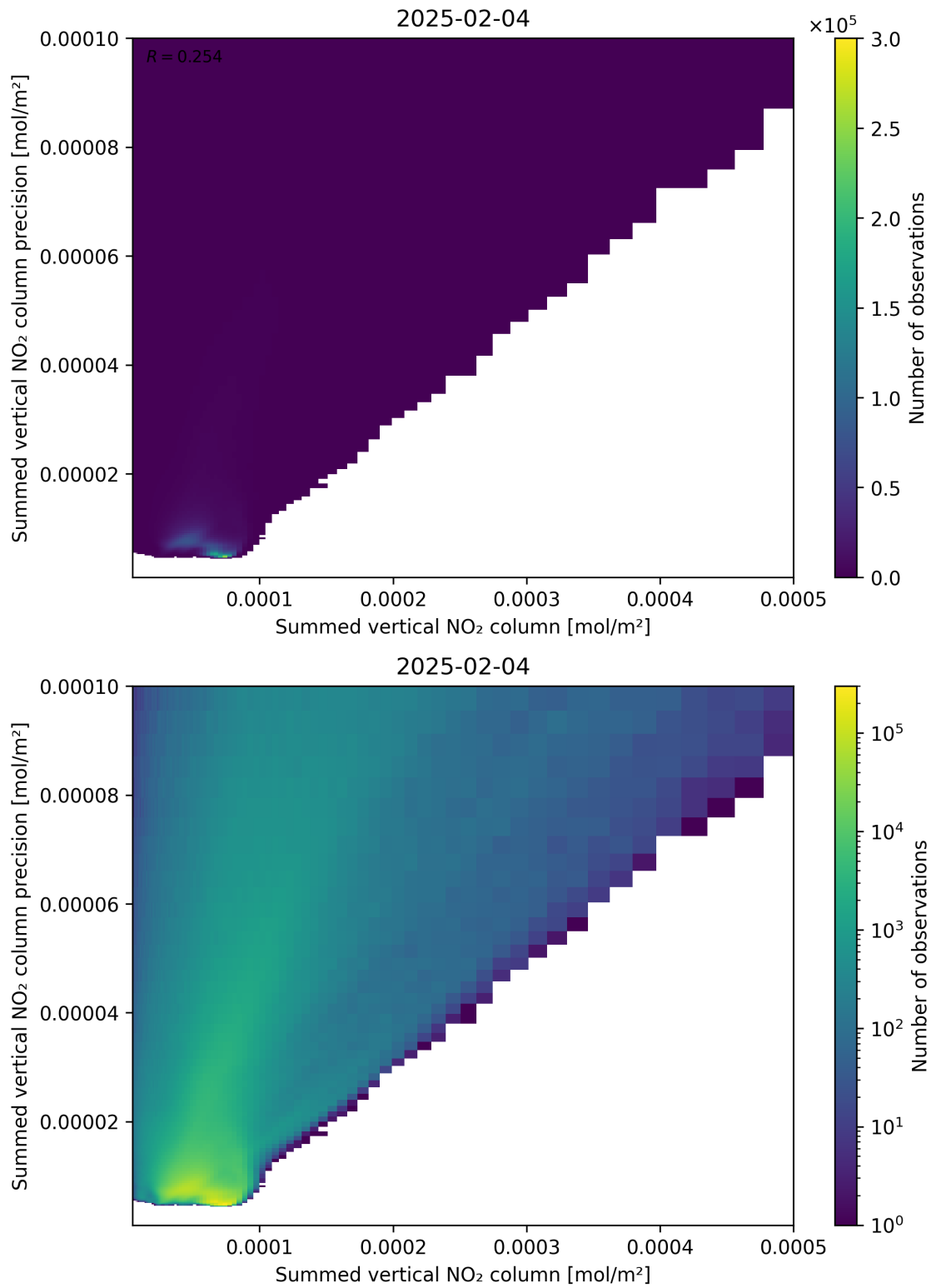
Figure 105: Scatter density plot of “Summed vertical NO 2 column” against “Summed vertical NO 2 column precision” for 2025-02-04 to 2025-02-05.
