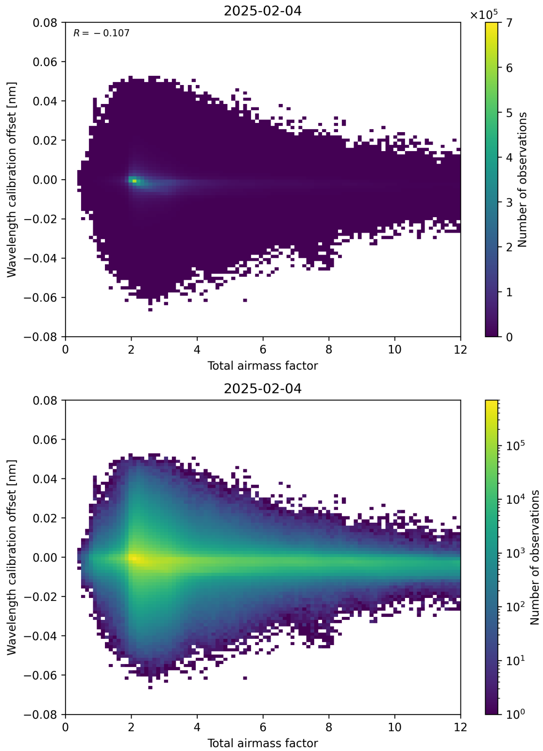
Figure 70: Scatter density plot of “Total airmass factor” against “Wavelength calibration offset” for 2025-02-04 to 2025-02-05.
