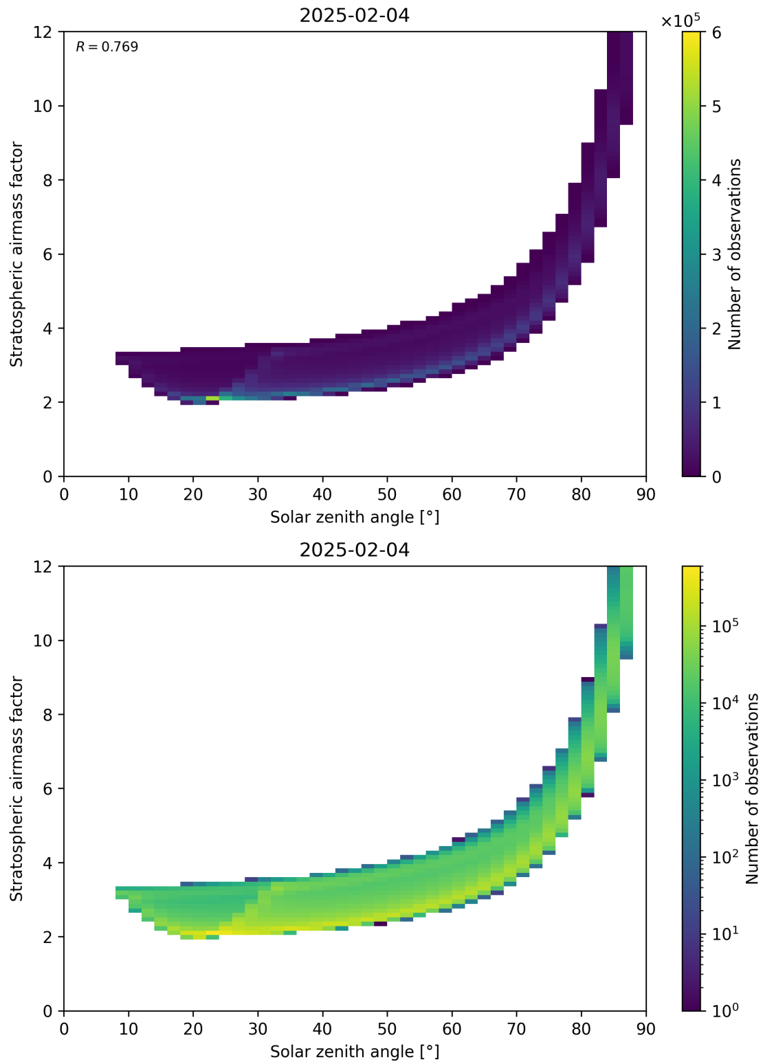
Figure 145: Scatter density plot of “Solar zenith angle” against “Stratospheric airmass factor” for 2025-02-04 to 2025-02-05.
