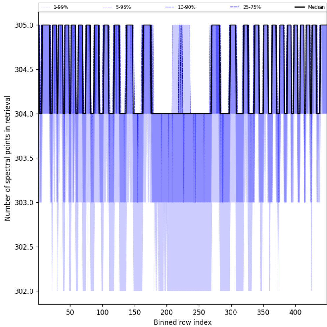
Figure 50: Along track statistics of “Number of spectral points in retrieval” for 2025-02-04 to 2025-02-05
