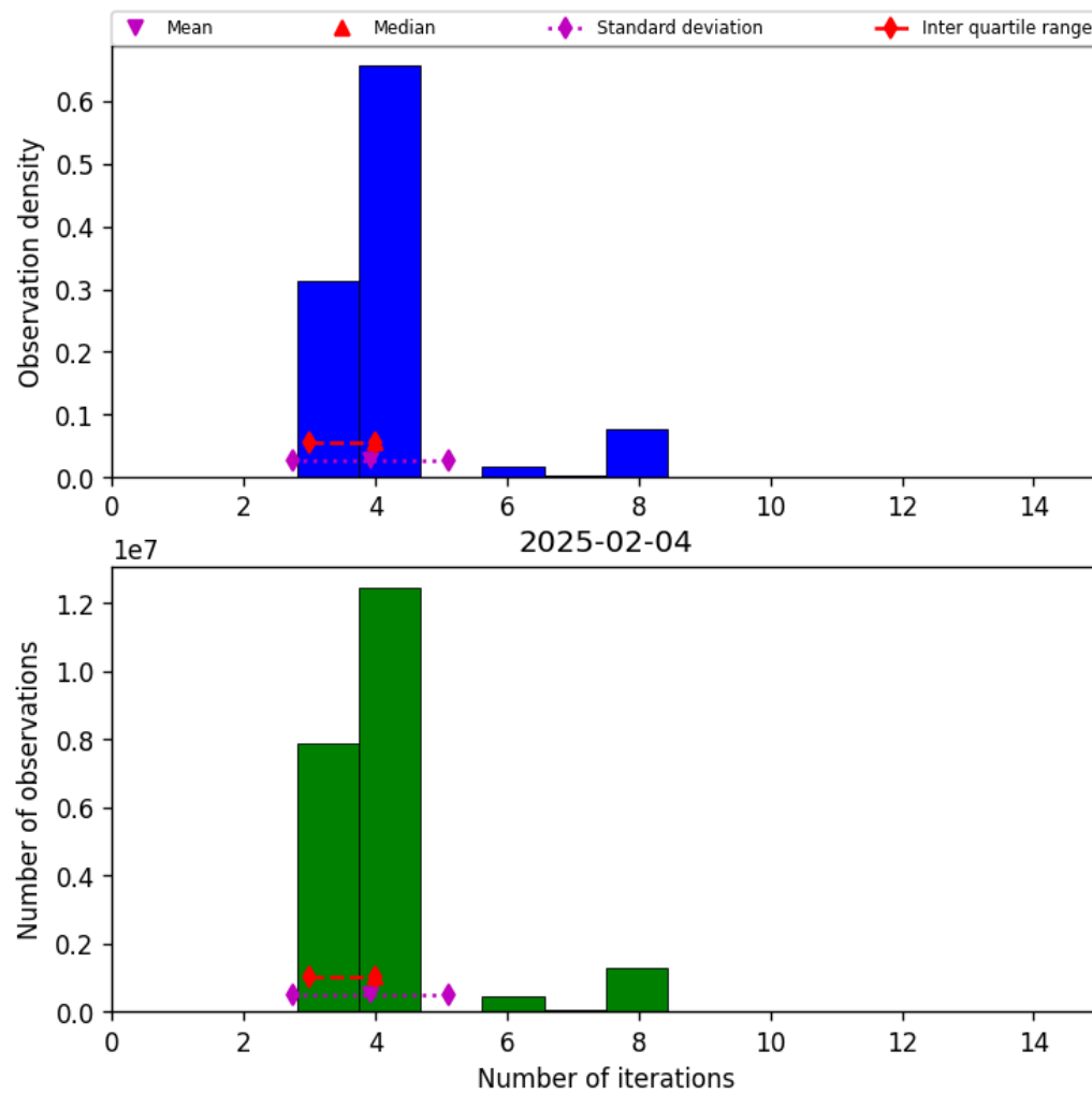
Figure 34: Histogram of “Number of iterations” for 2025-02-04 to 2025-02-05
