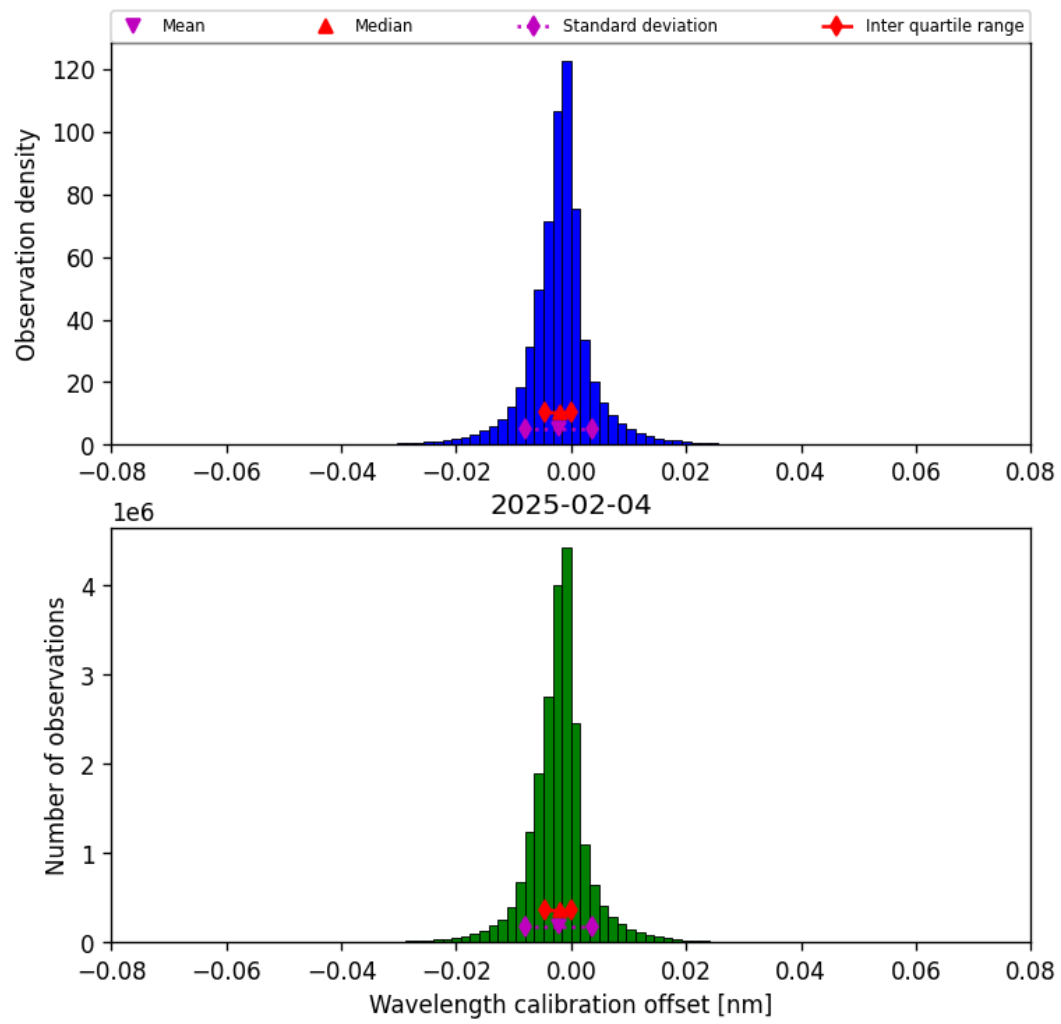
Figure 35: Histogram of “Wavelength calibration offset” for 2025-02-04 to 2025-02-05
