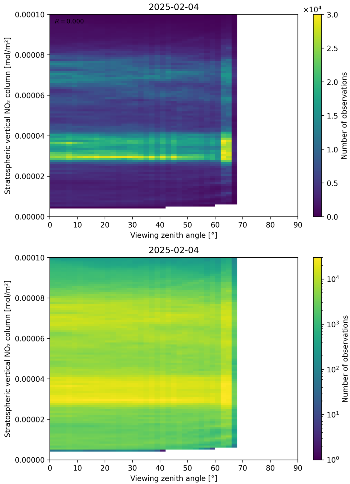
Figure 164: Scatter density plot of “Viewing zenith angle” against “Stratospheric vertical NO 2 column” for 2025-02-04 to 2025-02-05.
