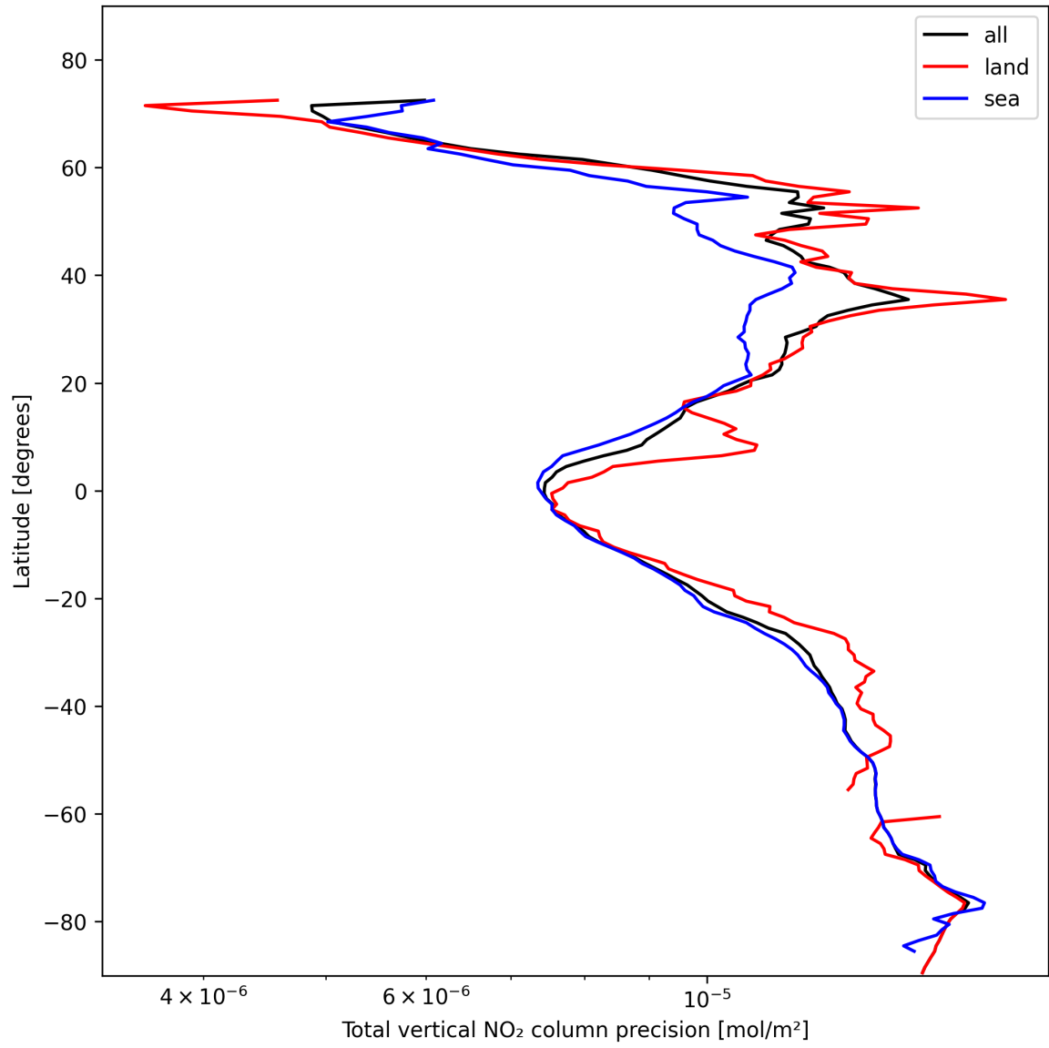
Figure 22: Zonal average of “Total vertical NO 2 column precision” for 2025-02-04 to 2025-02-05.
