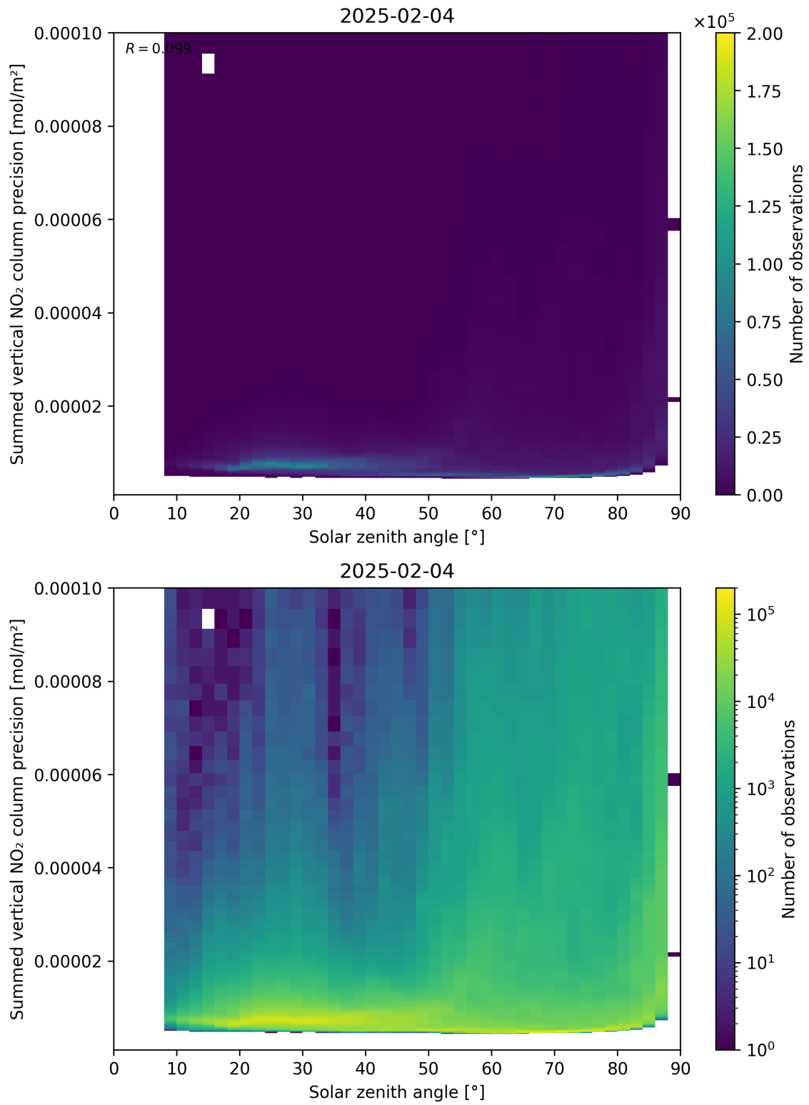
Figure 152: Scatter density plot of “Solar zenith angle” against “Summed vertical NO 2 column precision” for 2025-02-04 to 2025-02-05.
