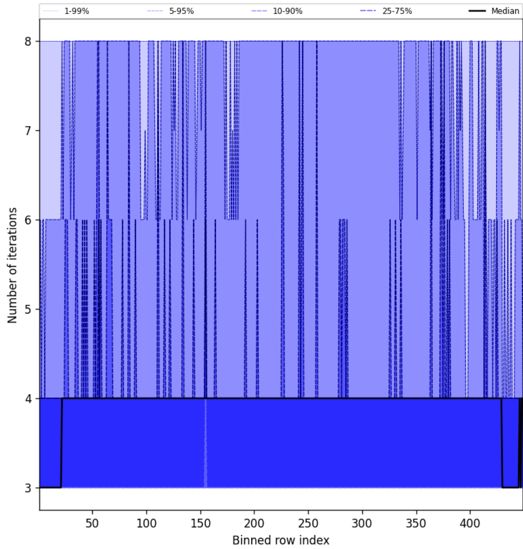
Figure 51: Along track statistics of “Number of iterations” for 2025-02-04 to 2025-02-05
