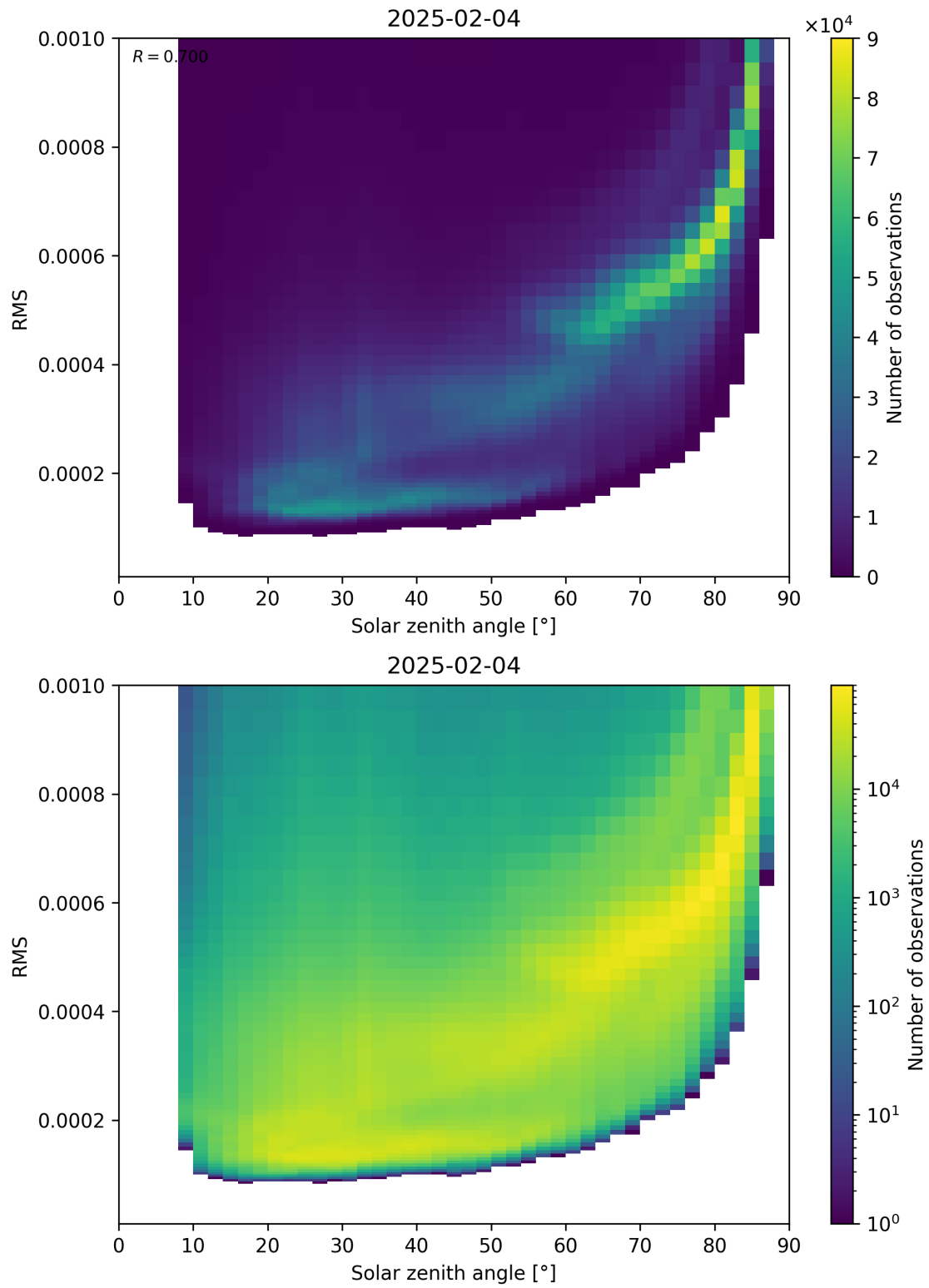
Figure 157: Scatter density plot of “Solar zenith angle” against “RMS” for 2025-02-04 to 2025-02-05.
