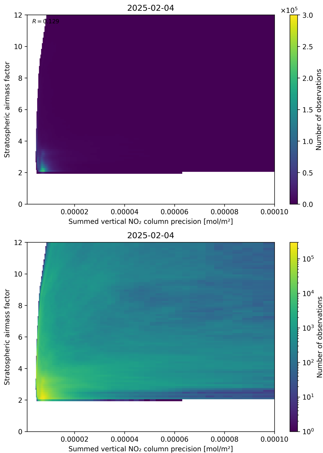
Figure 106: Scatter density plot of “Summed vertical NO 2 column precision” against “Stratospheric airmass factor” for 2025-02-04 to 2025-02-05.
