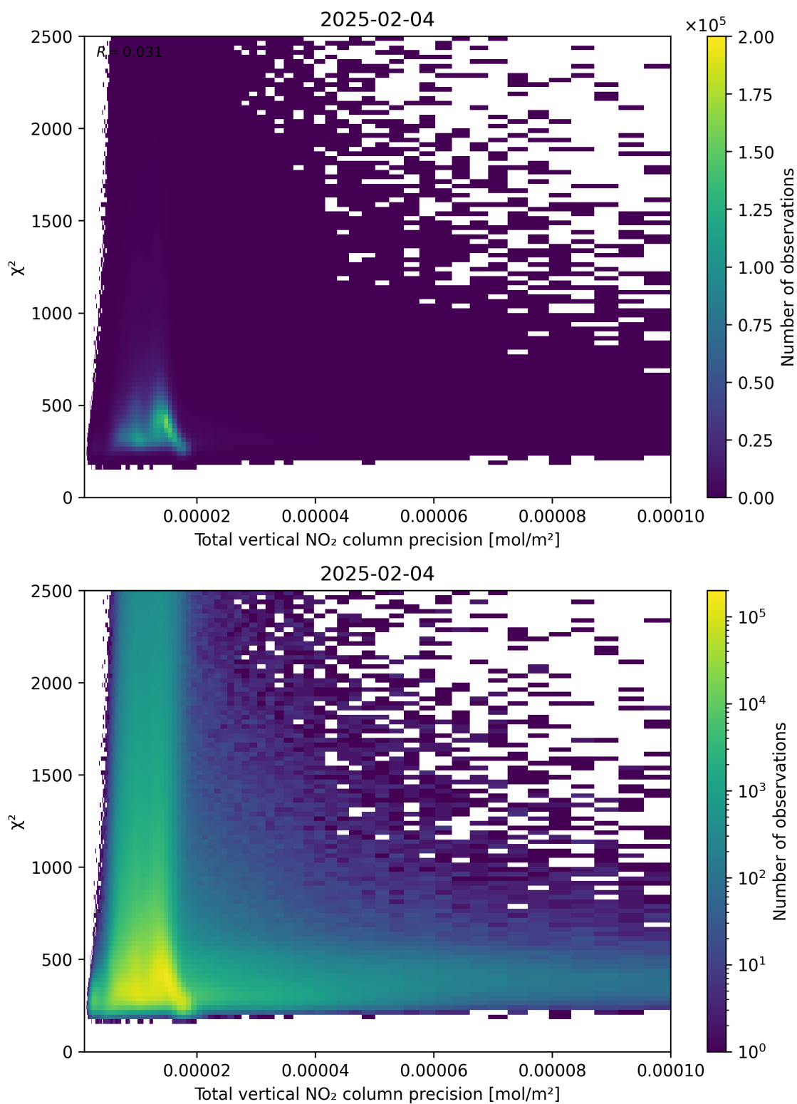
Figure 116: Scatter density plot of “Total vertical NO 2 column precision” against “ \chi^2 ” for 2025-02-04 to 2025-02-05.
