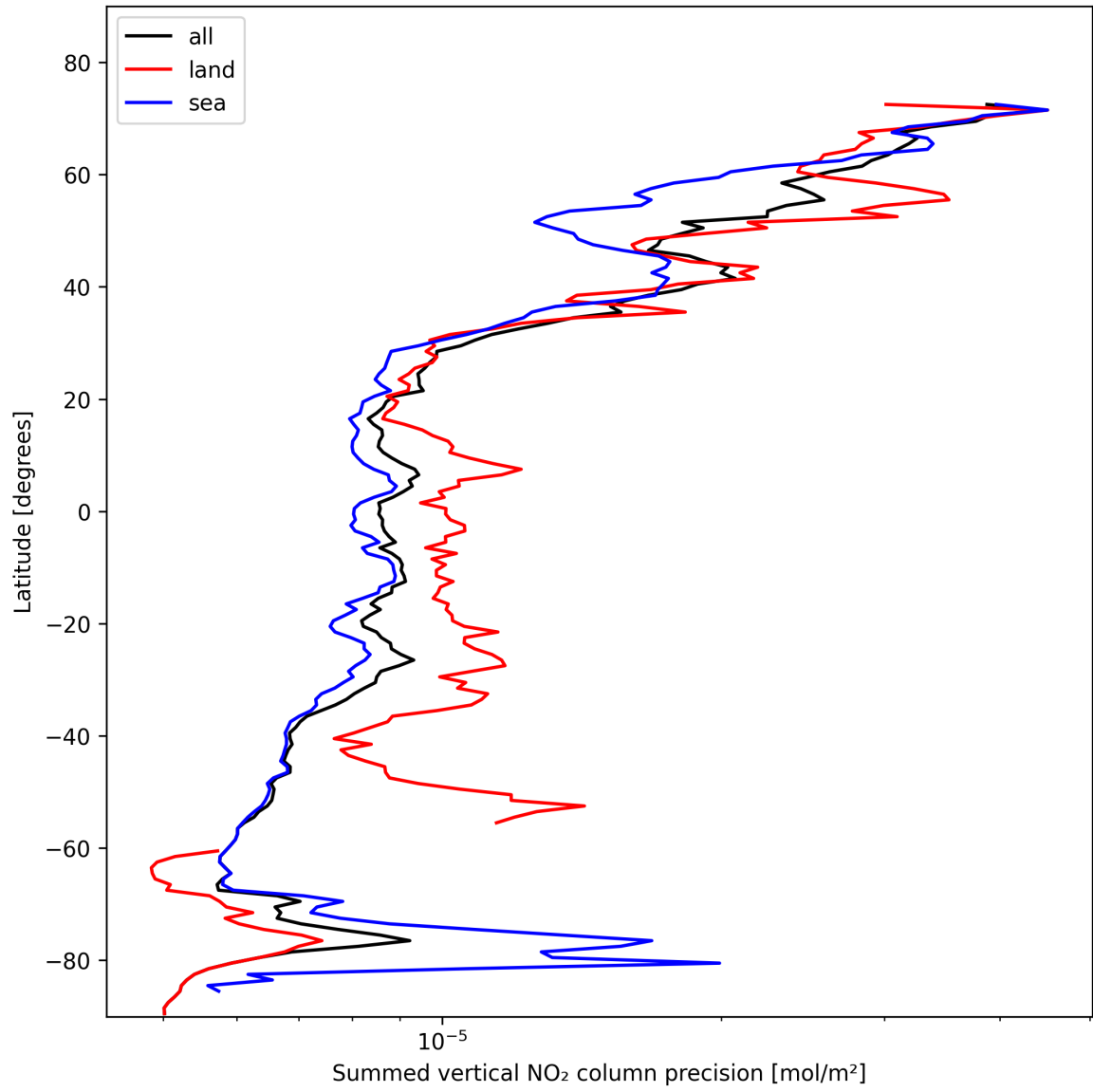
Figure 24: Zonal average of “Summed vertical NO 2 column precision” for 2025-02-04 to 2025-02-05.
