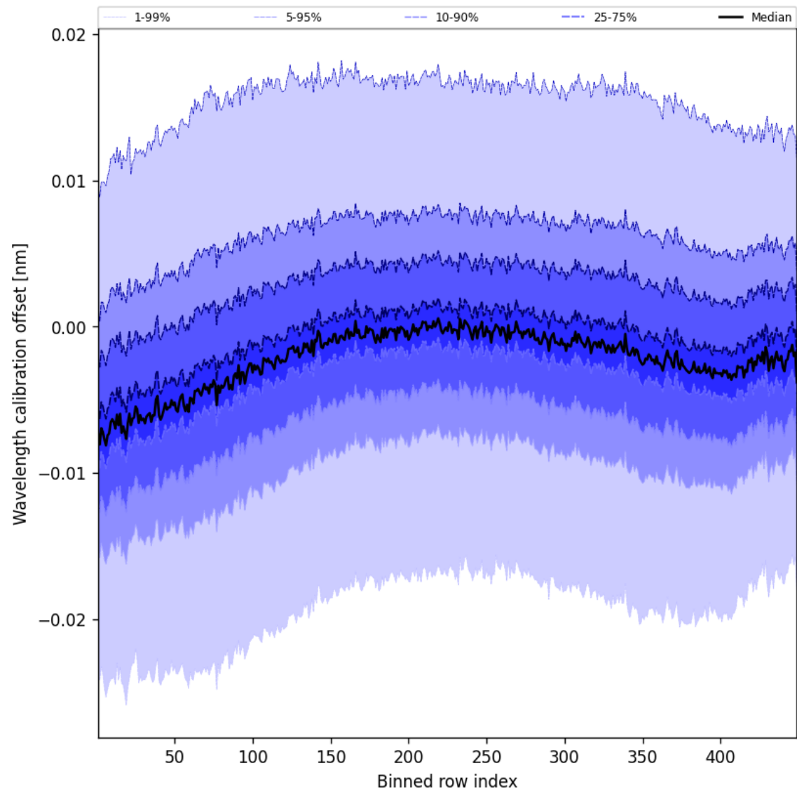
Figure 52: Along track statistics of “Wavelength calibration offset” for 2025-02-04 to 2025-02-05
