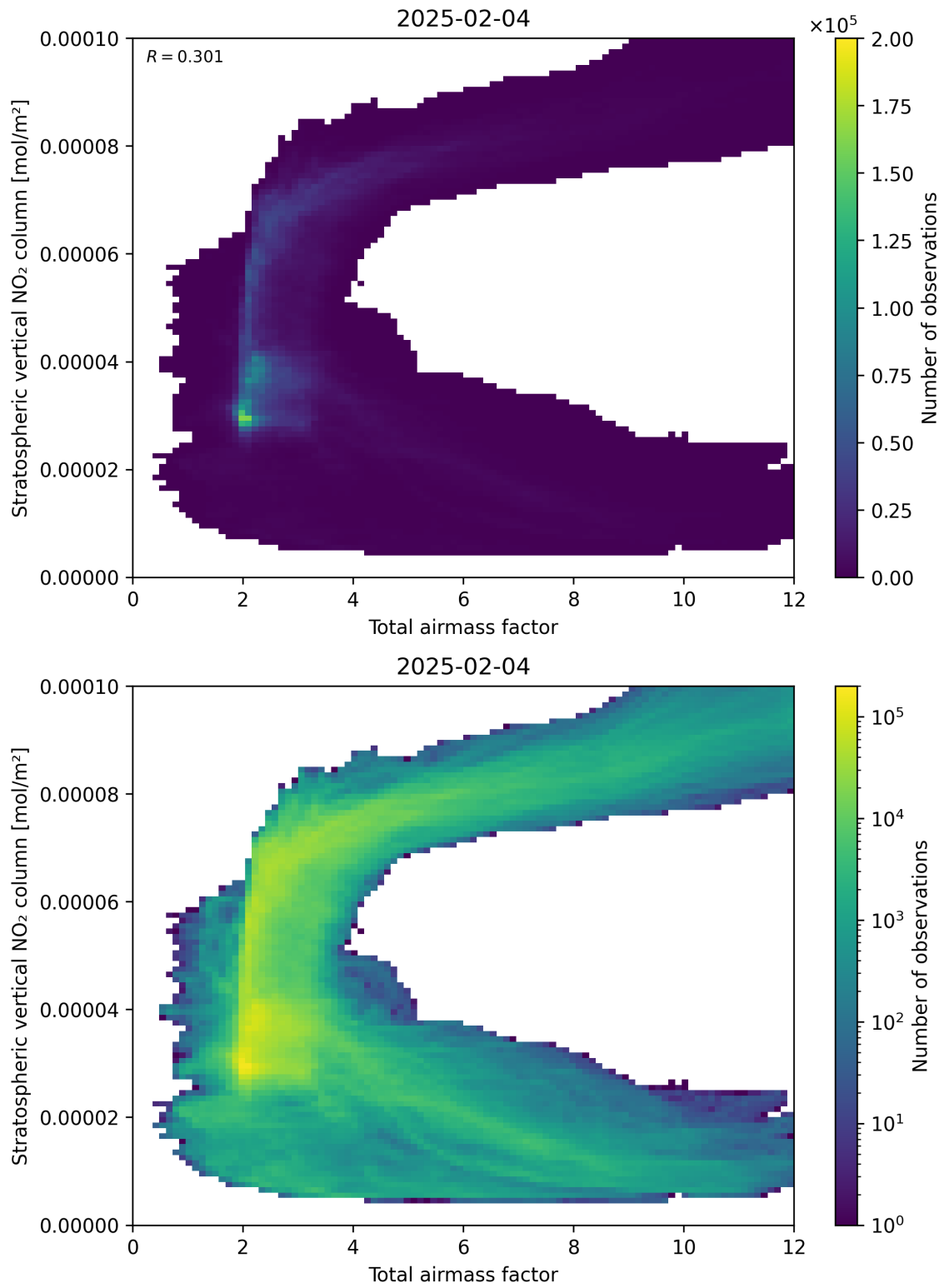
Figure 64: Scatter density plot of “Total airmass factor” against “Stratospheric vertical \text{NO}_2 column” for 2025-02-04 to 2025-02-05.
