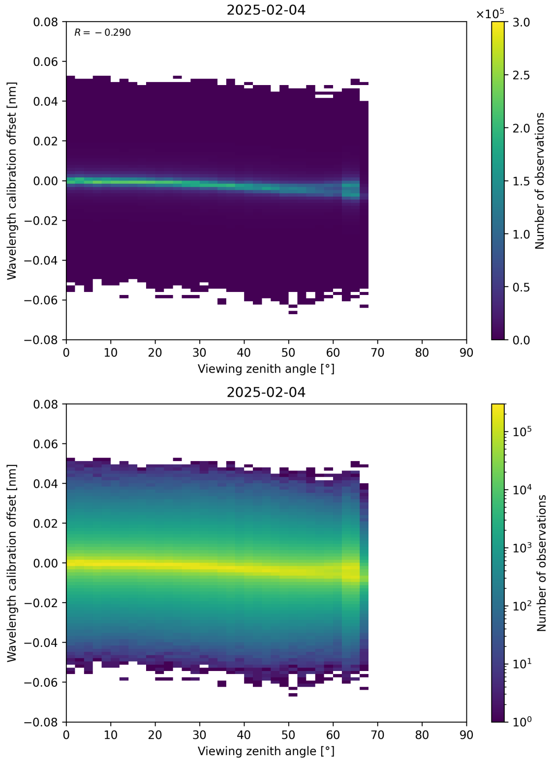
Figure 173: Scatter density plot of “Viewing zenith angle” against “Wavelength calibration offset” for 2025-02-04 to 2025-02-05.
