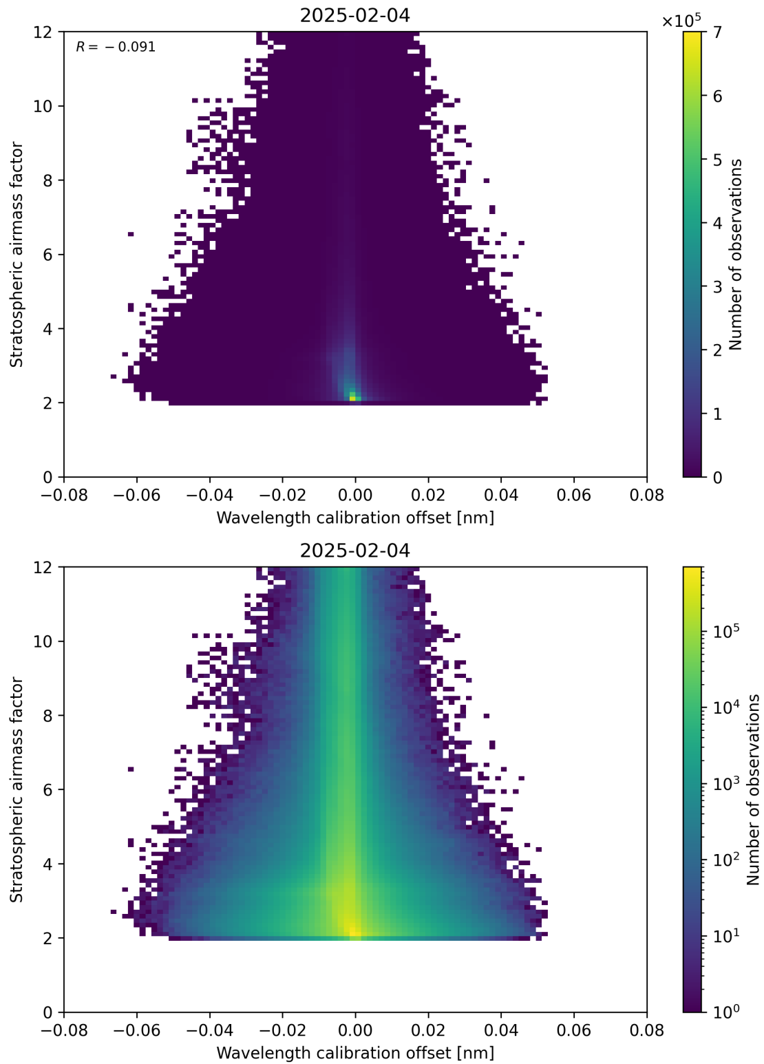
Figure 174: Scatter density plot of “Wavelength calibration offset” against “Stratospheric airmass factor” for 2025-02-04 to 2025-02-05.
