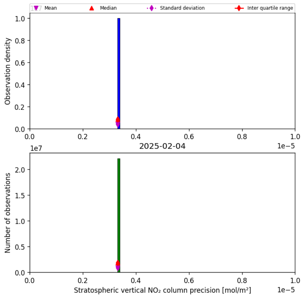
Figure 37: Histogram of “Stratospheric vertical NO 2 column precision” for 2025-02-04 to 2025-02-05
