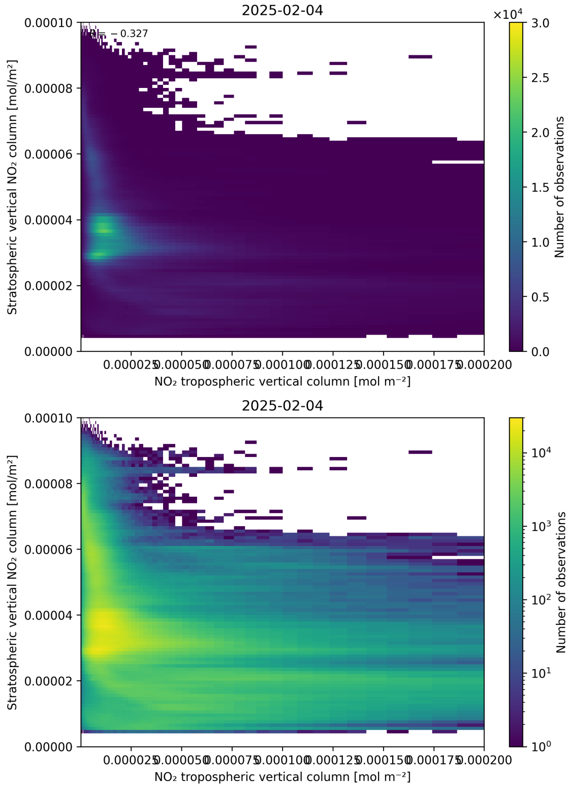
Figure 125: Scatter density plot of “NO 2 tropospheric vertical column” against “Stratospheric vertical NO 2 column” for 2025-02-04 to 2025-02-05.
