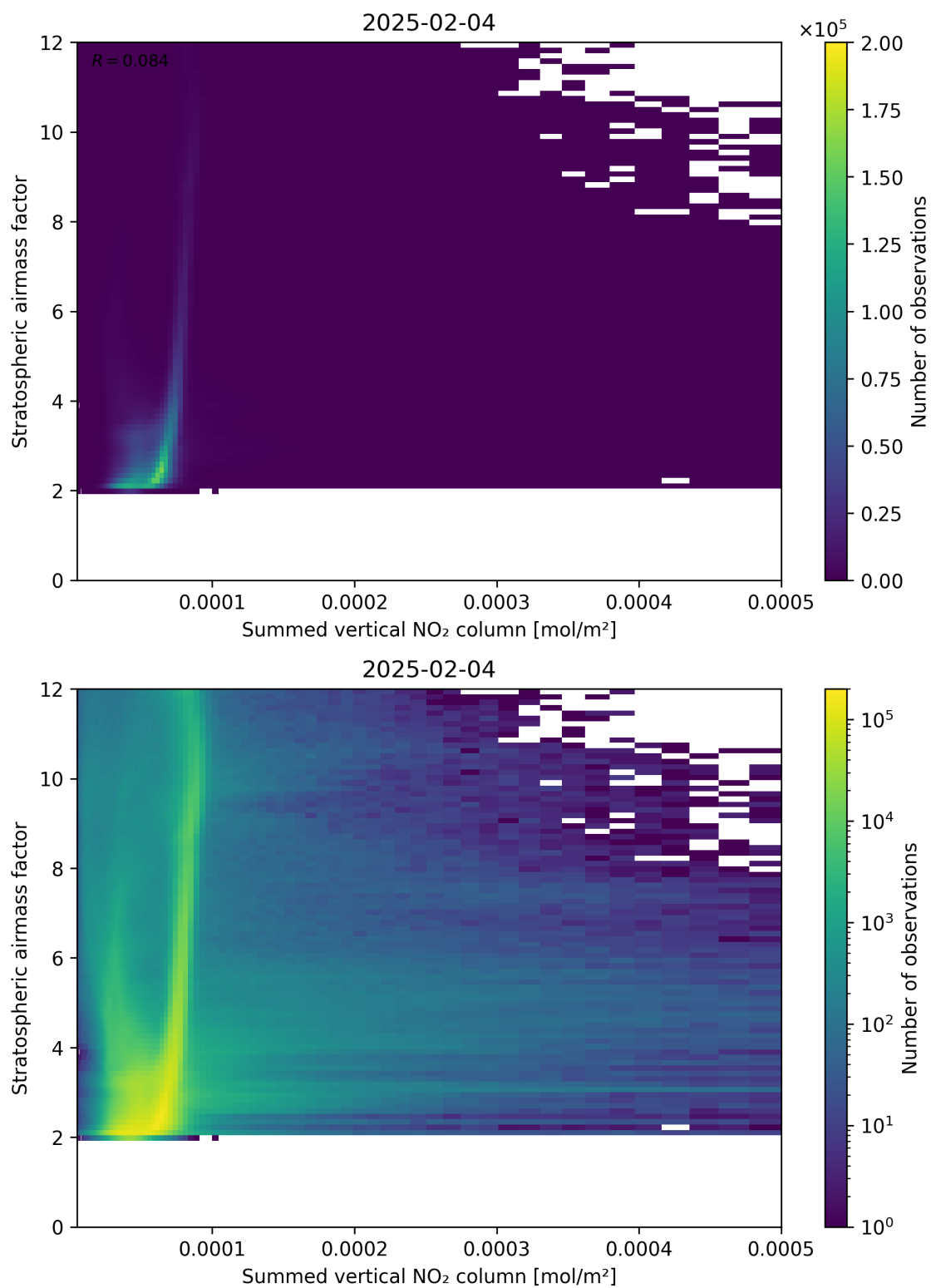
Figure 103: Scatter density plot of “Summed vertical NO 2 column” against “Stratospheric airmass factor” for 2025-02-04 to 2025-02-05.
