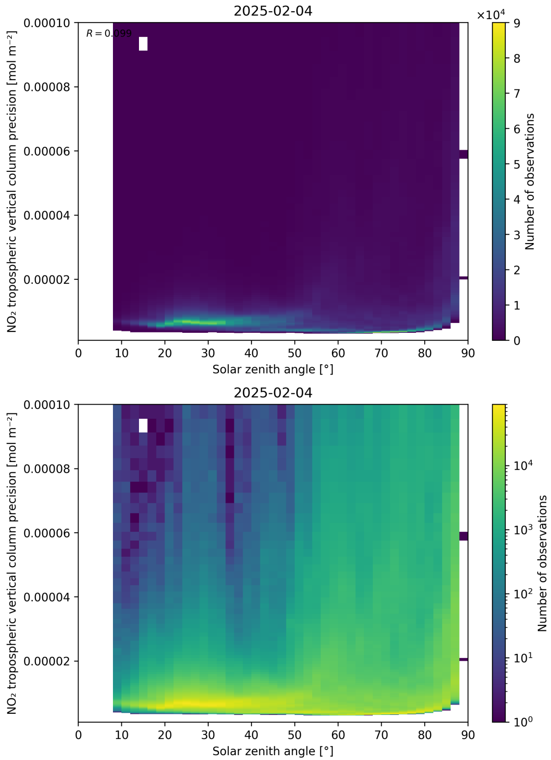
Figure 156: Scatter density plot of “Solar zenith angle” against “NO 2 tropospheric vertical column precision” for 2025-02-04 to 2025-02-05.
