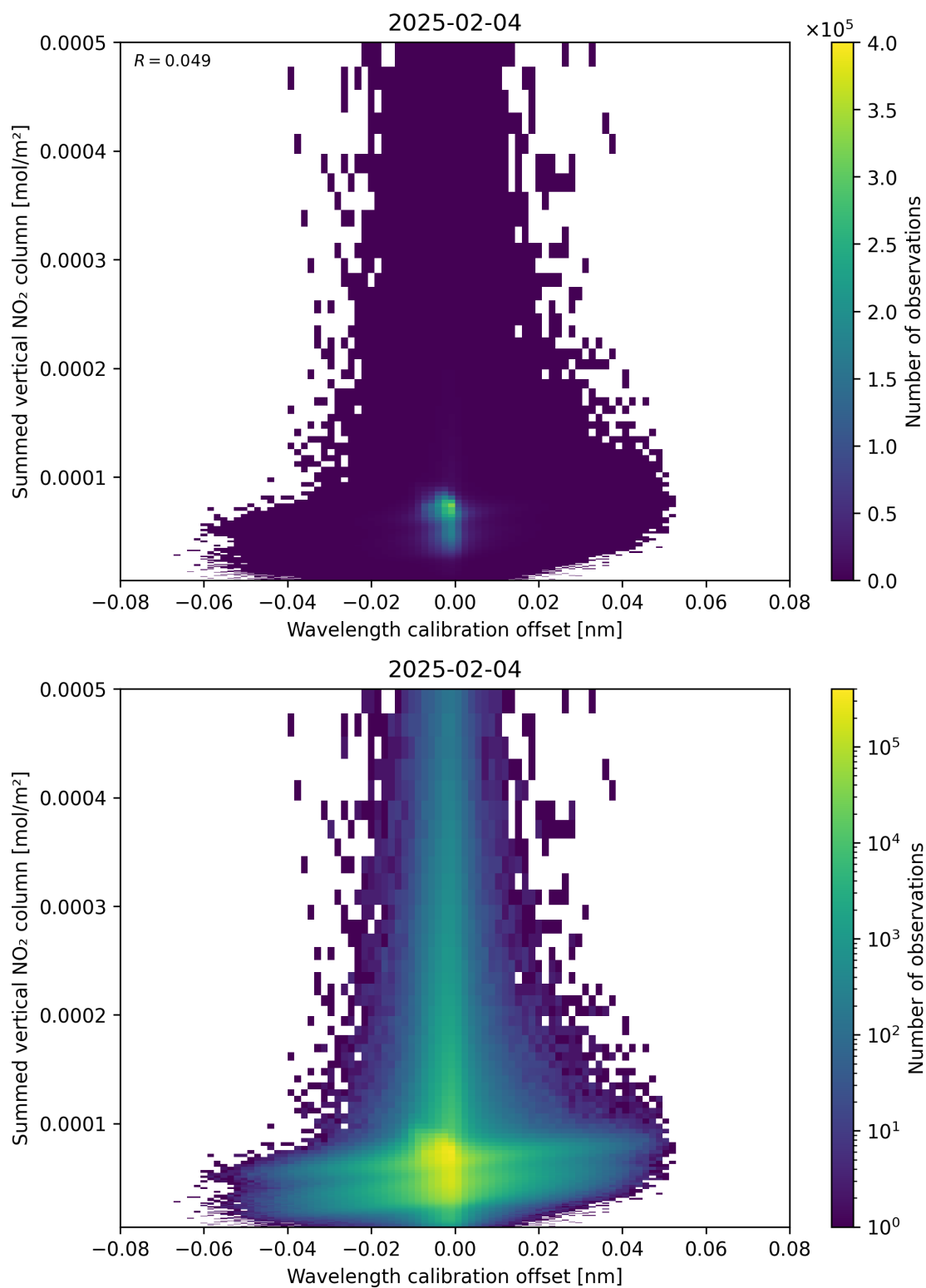
Figure 177: Scatter density plot of “Wavelength calibration offset” against “Summed vertical NO 2 column” for 2025-02-04 to 2025-02-05.
