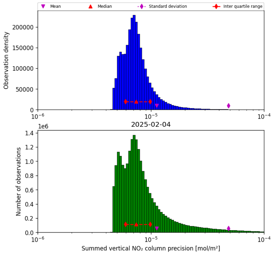
Figure 41: Histogram of “Summed vertical NO 2 column precision” for 2025-02-04 to 2025-02-05
