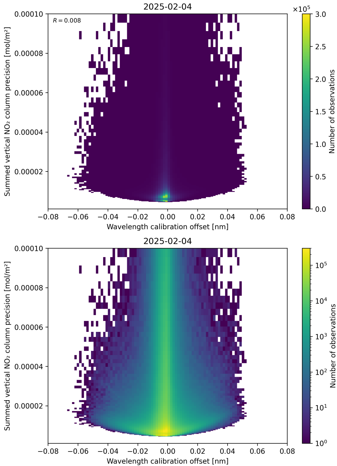
Figure 178: Scatter density plot of “Wavelength calibration offset” against “Summed vertical NO 2 column precision” for 2025-02-04 to 2025-02-05.
