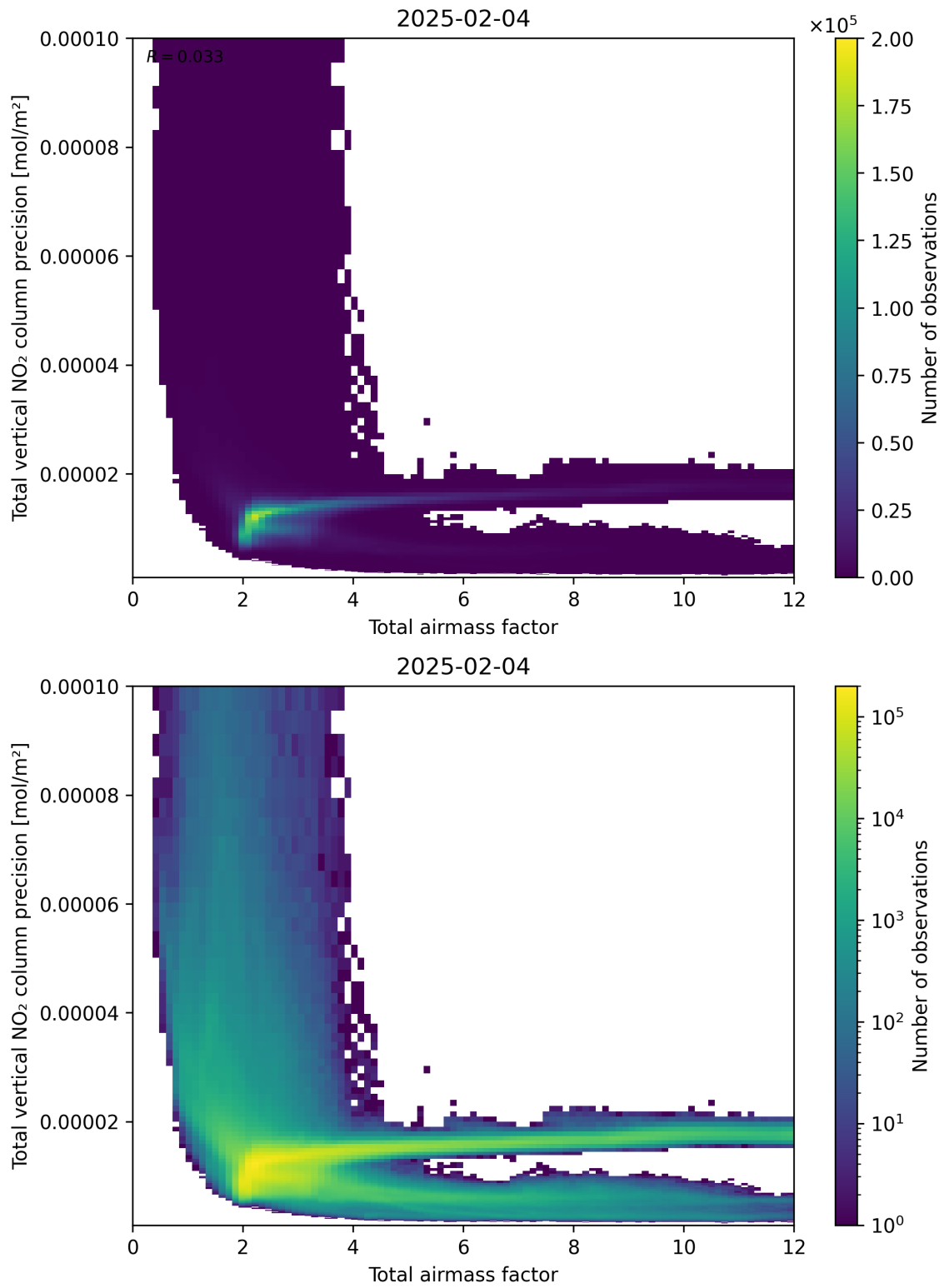
Figure 68: Scatter density plot of “Total airmass factor” against “Total vertical NO 2 column precision” for 2025-02-04 to 2025-02-05.
