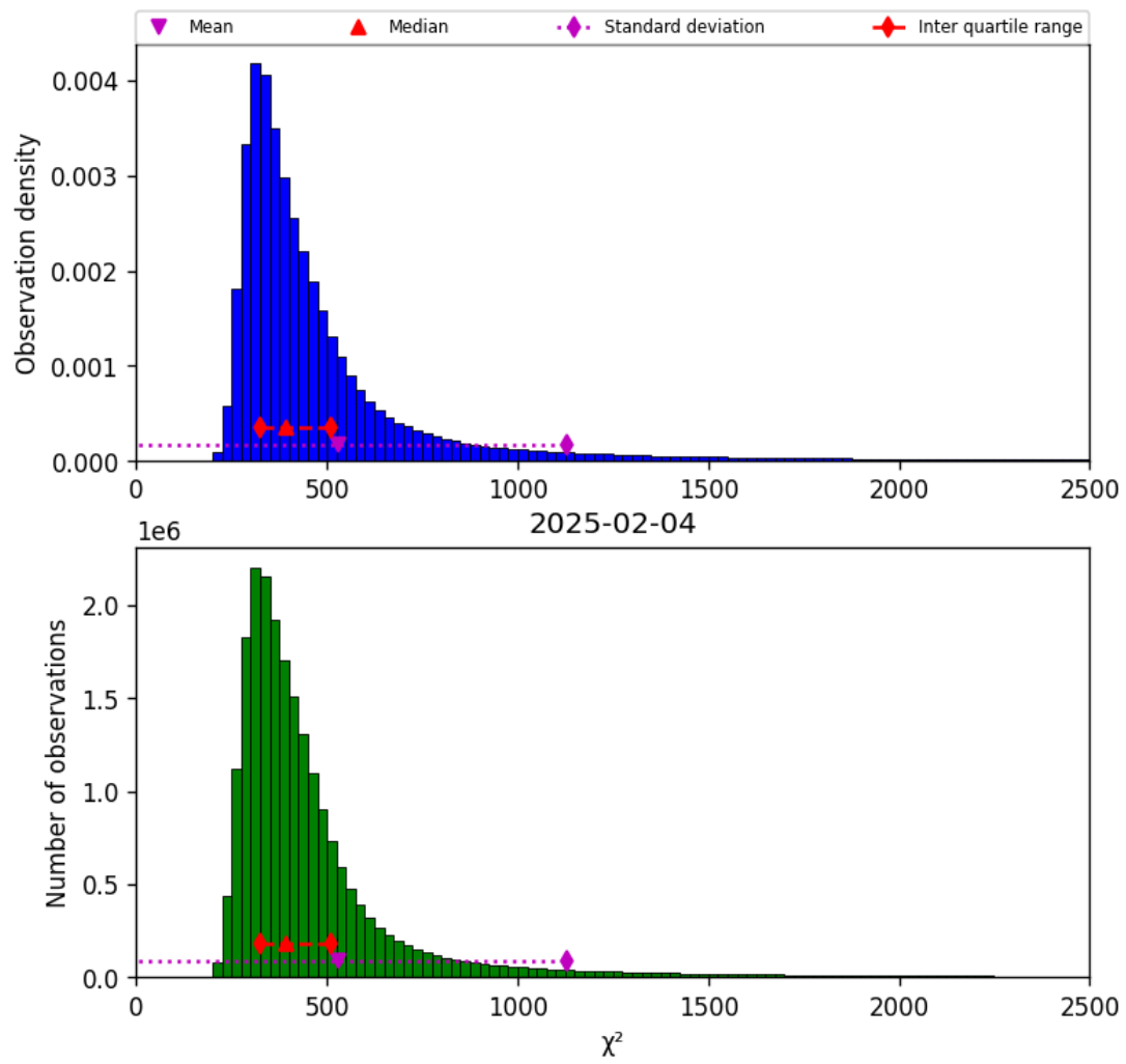
Figure 42: Histogram of “ \chi^2 ” for 2025-02-04 to 2025-02-05
