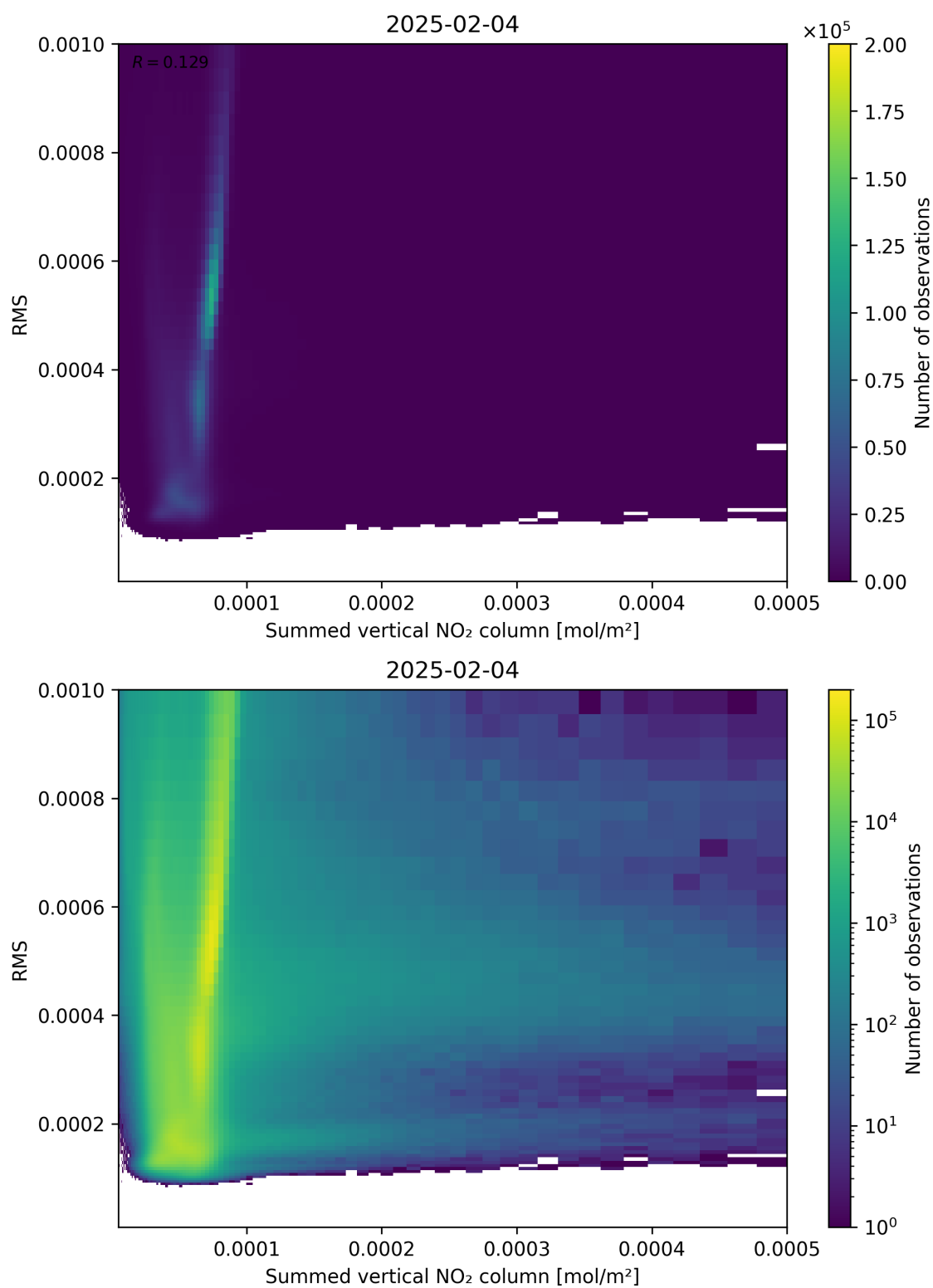
Figure 109: Scatter density plot of “Summed vertical NO 2 column” against “RMS” for 2025-02-04 to 2025-02-05.
