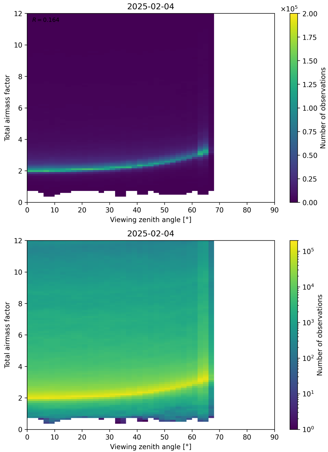
Figure 160: Scatter density plot of “Viewing zenith angle” against “Total airmass factor” for 2025-02-04 to 2025-02-05.
