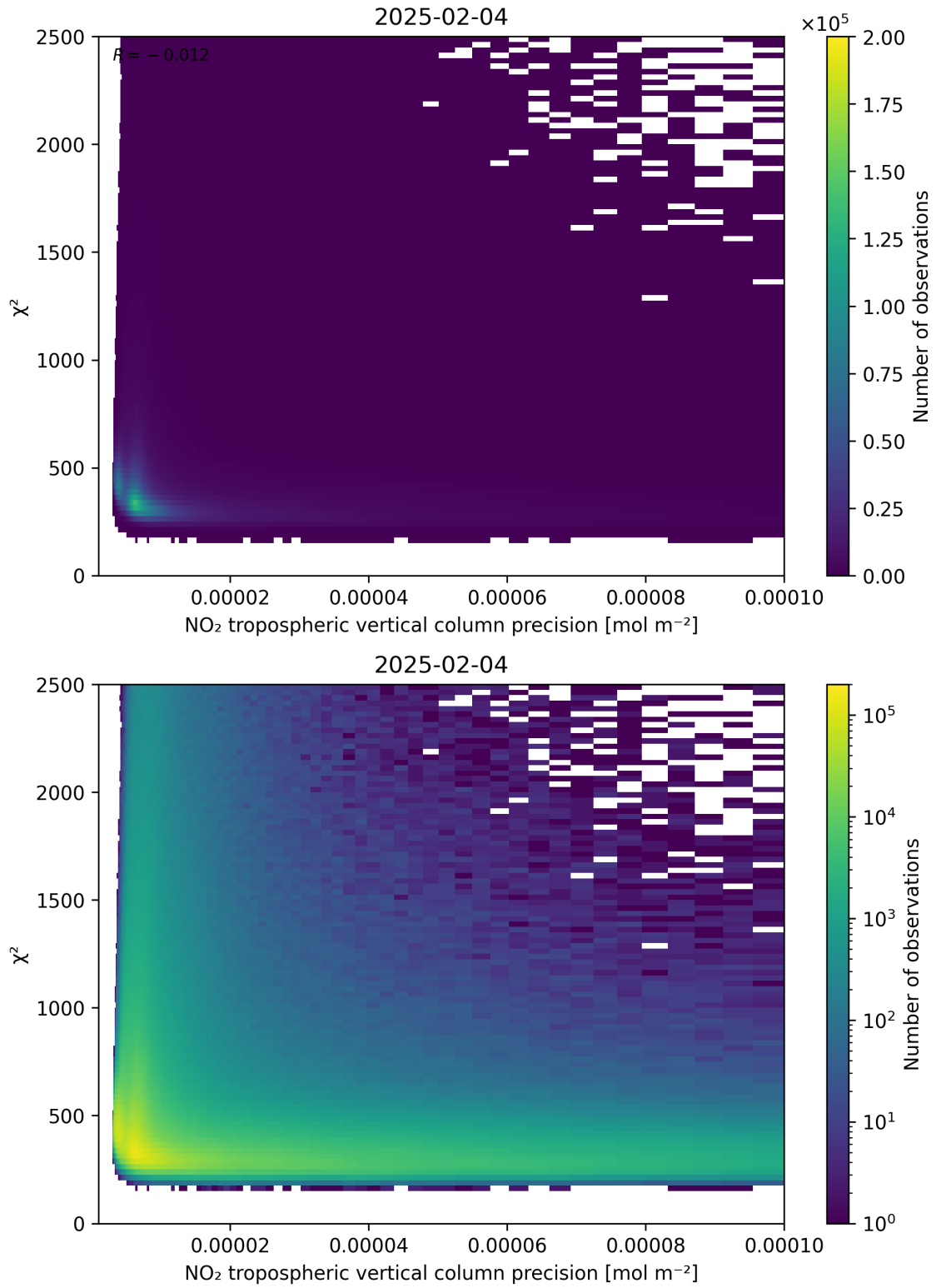
Figure 134: Scatter density plot of “NO 2 tropospheric vertical column precision” against “ \chi^2 ” for 2025-02-04 to 2025-02-05.
