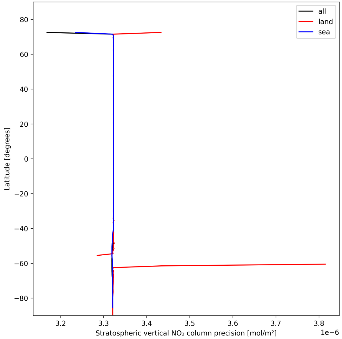
Figure 20: Zonal average of “Stratospheric vertical NO 2 column precision” for 2025-02-04 to 2025-02-05.
