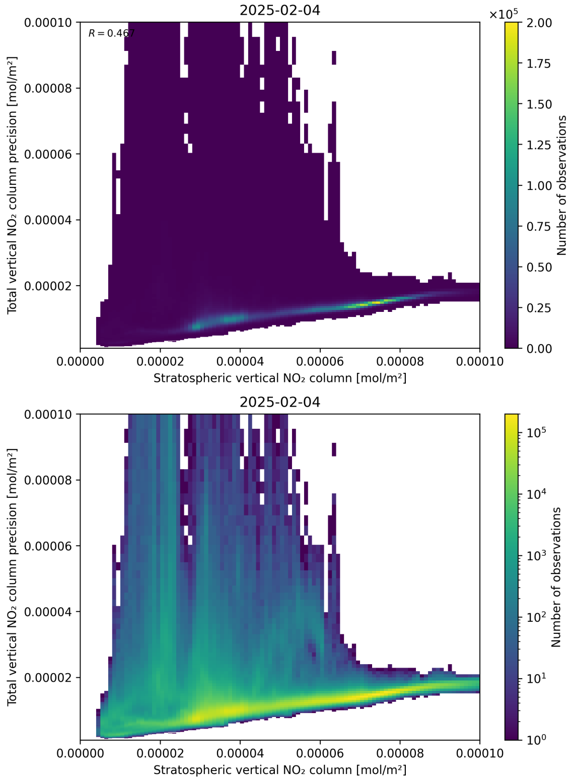
Figure 101: Scatter density plot of “Stratospheric vertical NO 2 column” against “Total vertical NO 2 column precision” for 2025-02-04 to 2025-02-05.
