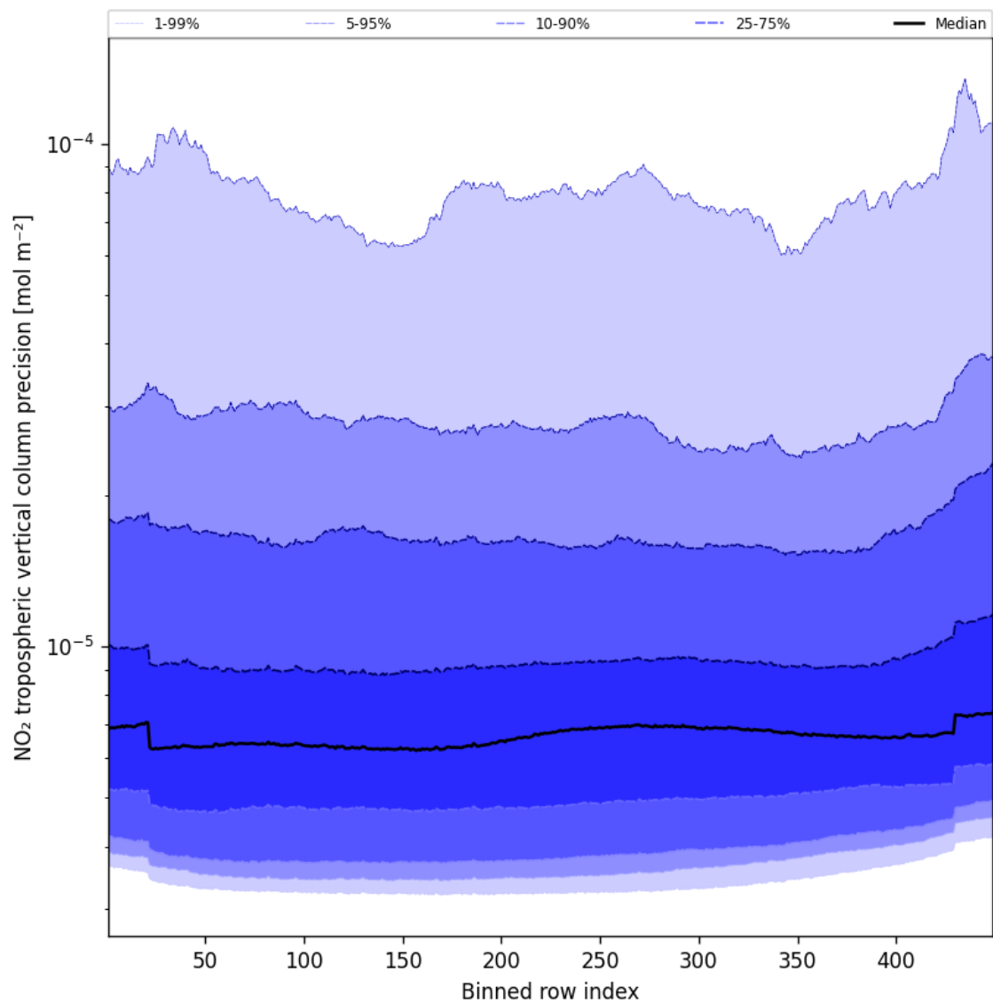
Figure 47: Along track statistics of “NO 2 tropospheric vertical column precision” for 2025-02-04 to 2025-02-05
