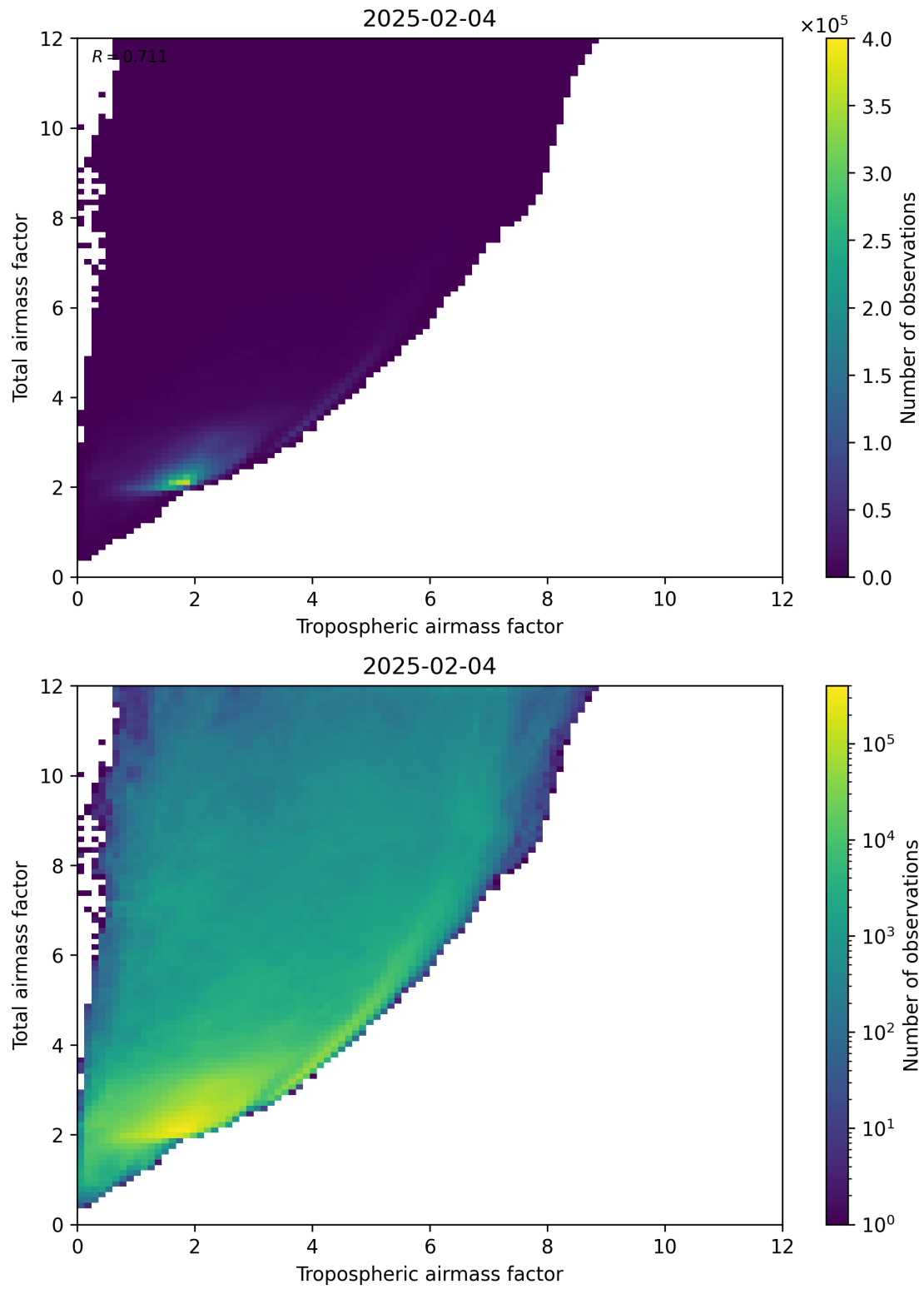
Figure 72: Scatter density plot of “Tropospheric airmass factor” against “Total airmass factor” for 2025-02-04 to 2025-02-05.
