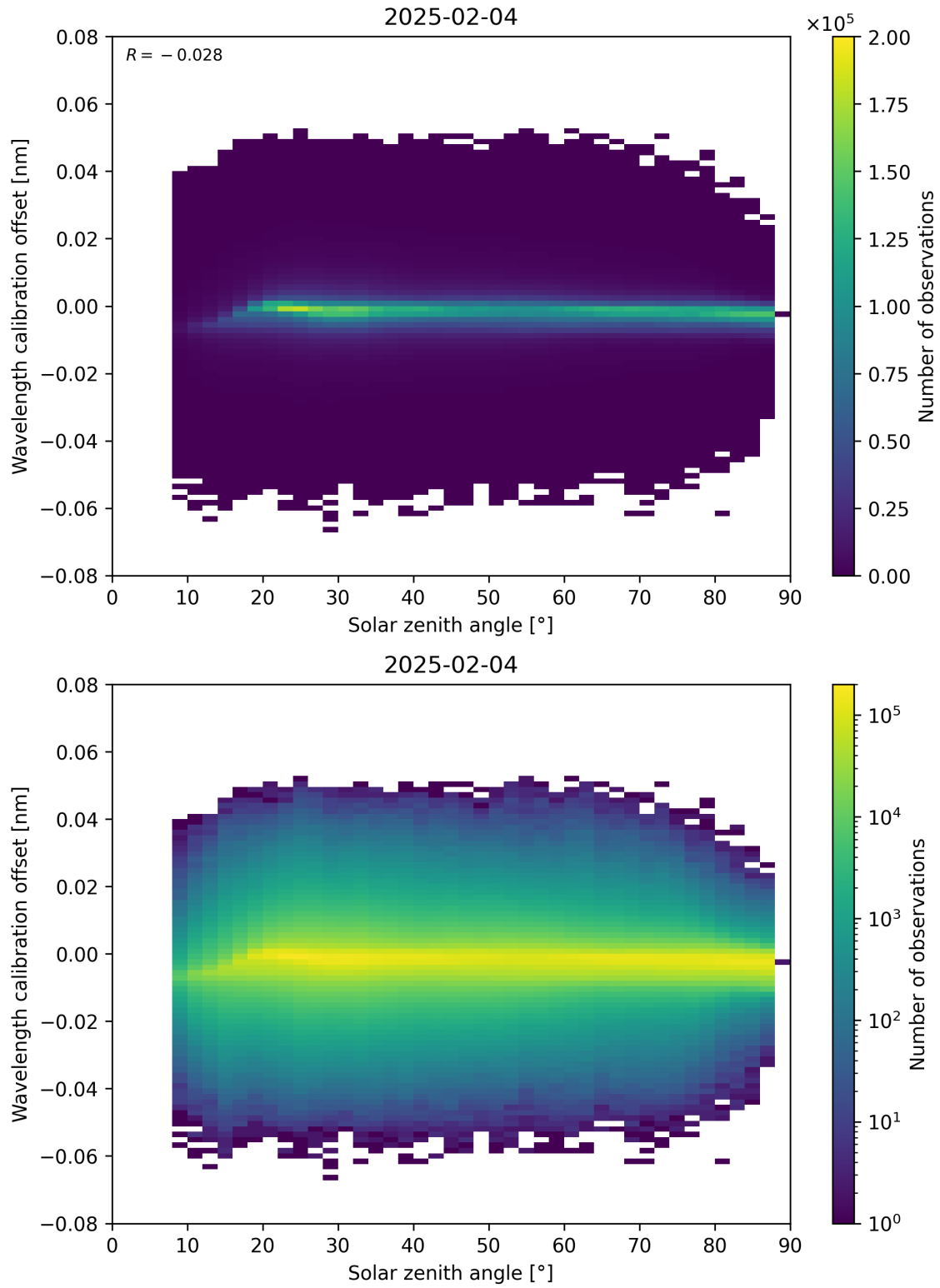
Figure 158: Scatter density plot of “Solar zenith angle” against “Wavelength calibration offset” for 2025-02-04 to 2025-02-05.
