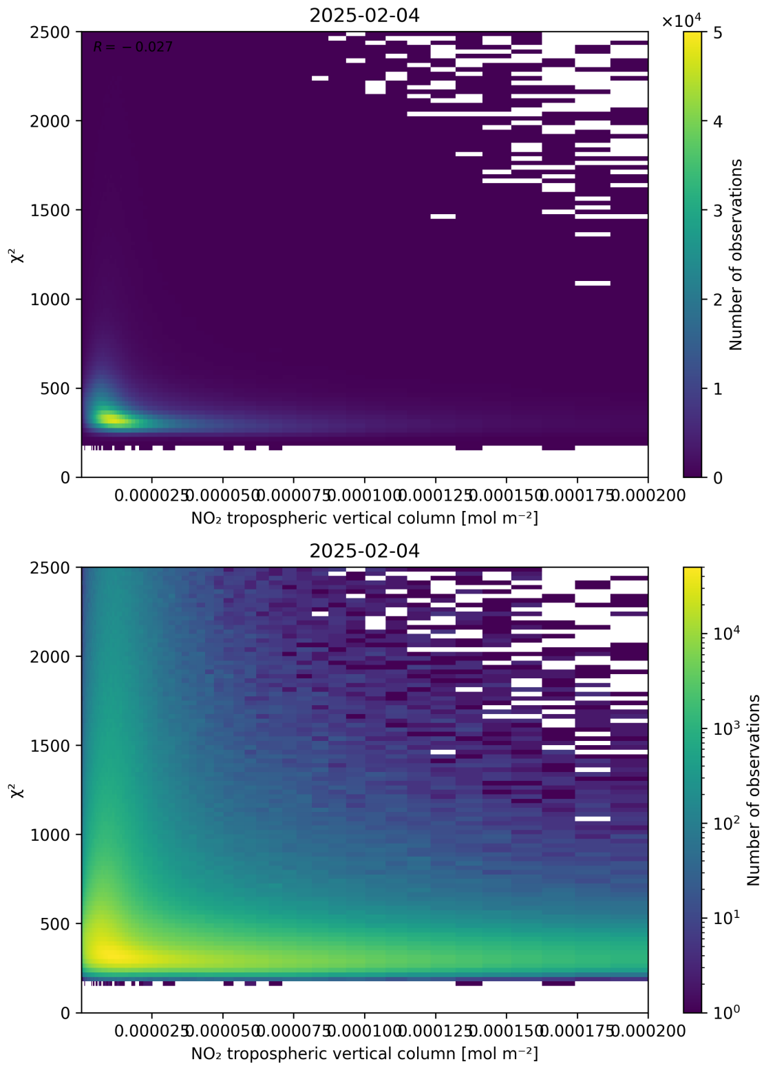
Figure 124: Scatter density plot of “NO 2 tropospheric vertical column” against “ \chi^2 ” for 2025-02-04 to 2025-02-05.
