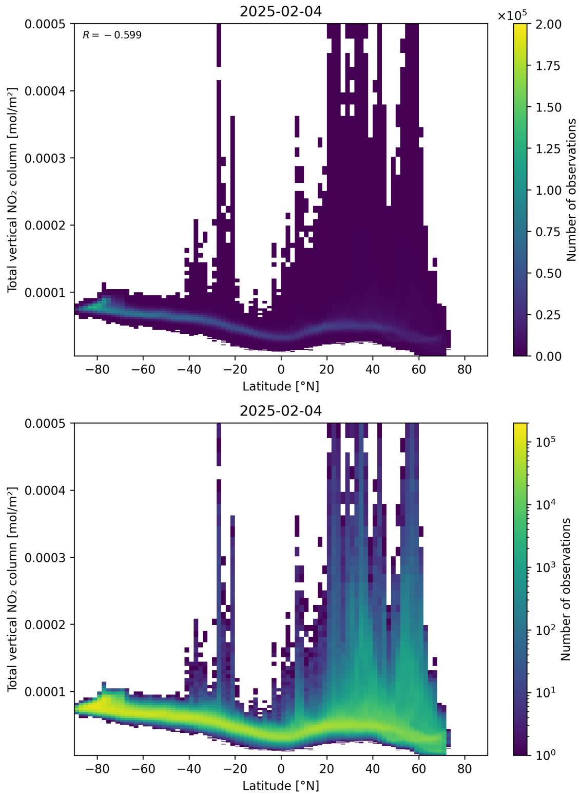
Figure 90: Scatter density plot of “Latitude” against “Total vertical NO 2 column” for 2025-02-04 to 2025-02-05.
