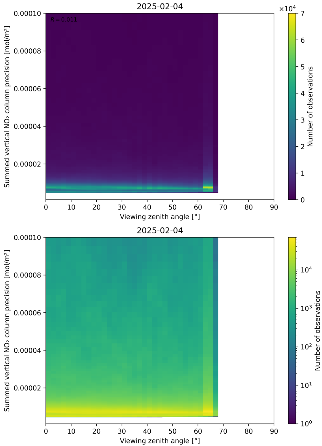
Figure 166: Scatter density plot of “Viewing zenith angle” against “Summed vertical NO 2 column precision” for 2025-02-04 to 2025-02-05.
