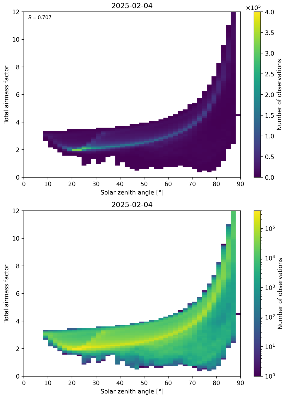
Figure 146: Scatter density plot of “Solar zenith angle” against “Total air mass factor” for 2025-02-04 to 2025-02-05.
