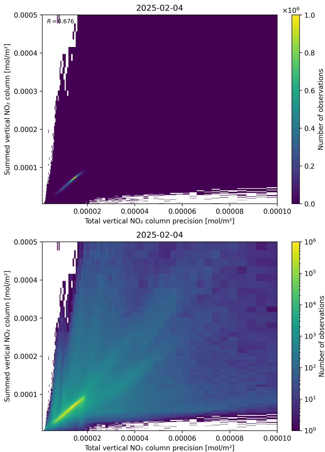
Figure 117: Scatter density plot of “Total vertical NO 2 column precision” against “Summed vertical NO 2 column” for 2025-02-04 to 2025-02-05.
