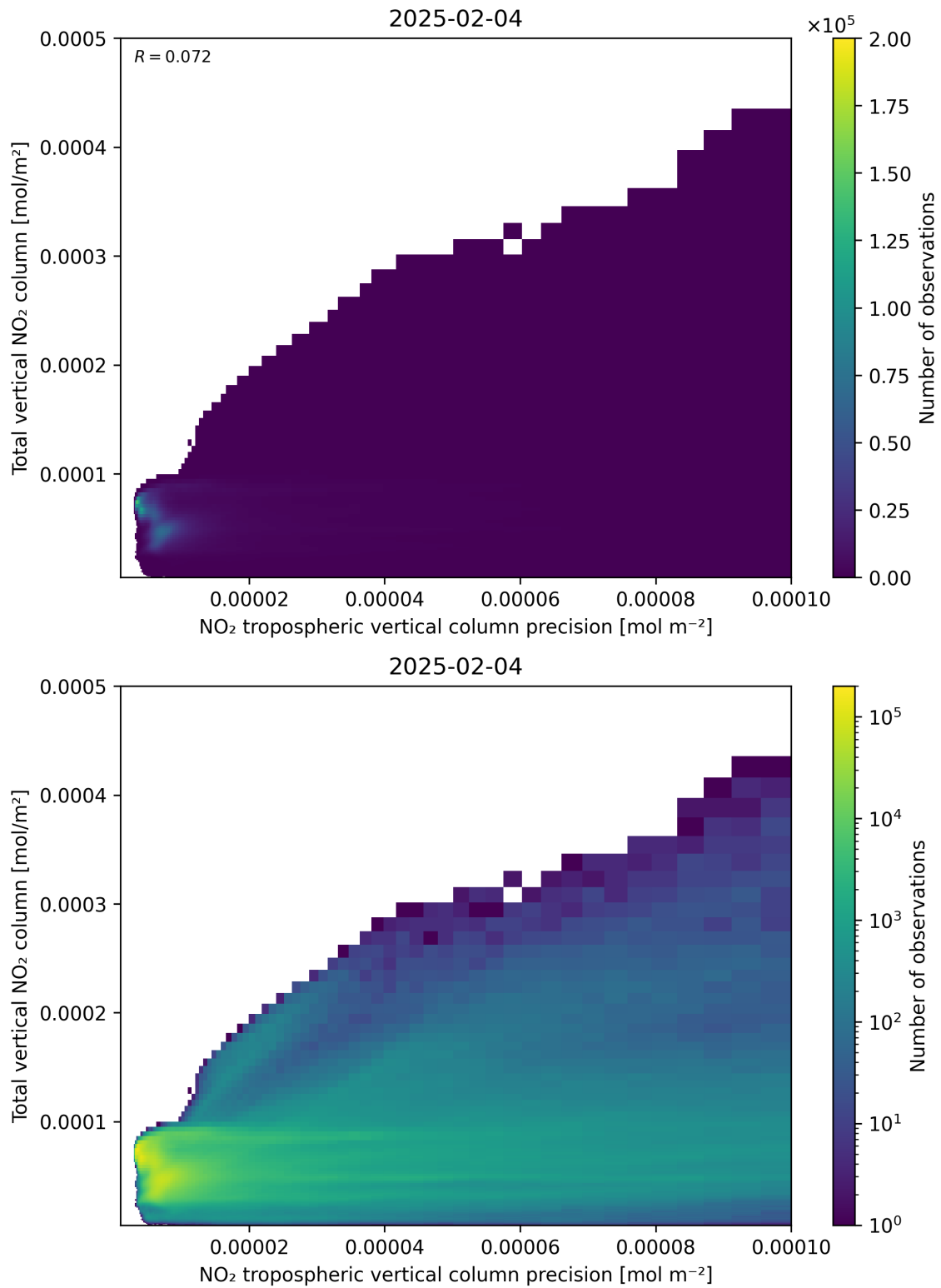
Figure 138: Scatter density plot of “NO 2 tropospheric vertical column precision” against “Total vertical NO 2 column” for 2025-02-04 to 2025-02-05.
