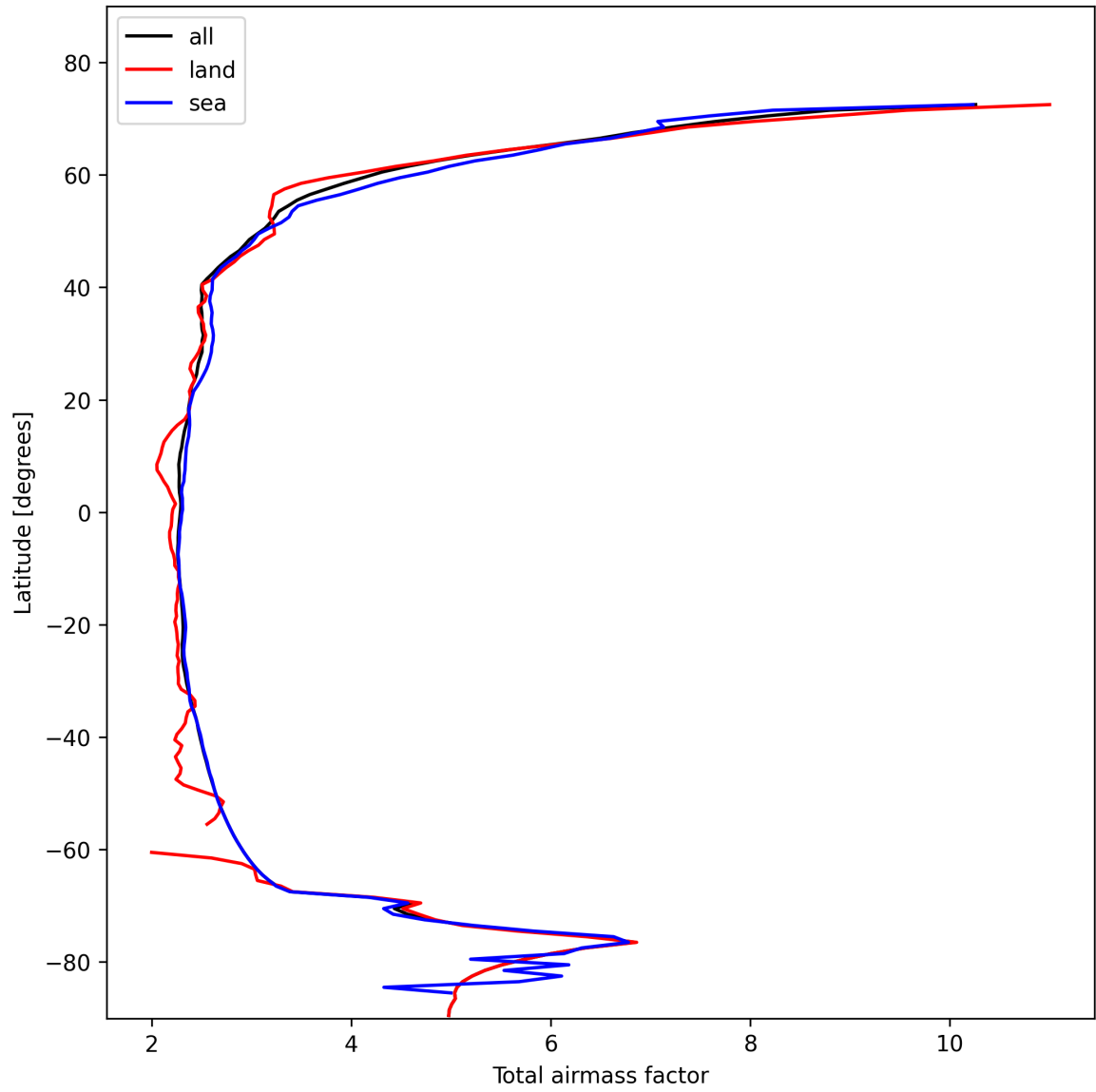
Figure 15: Zonal average of “Total airmass factor” for 2025-02-04 to 2025-02-05.
