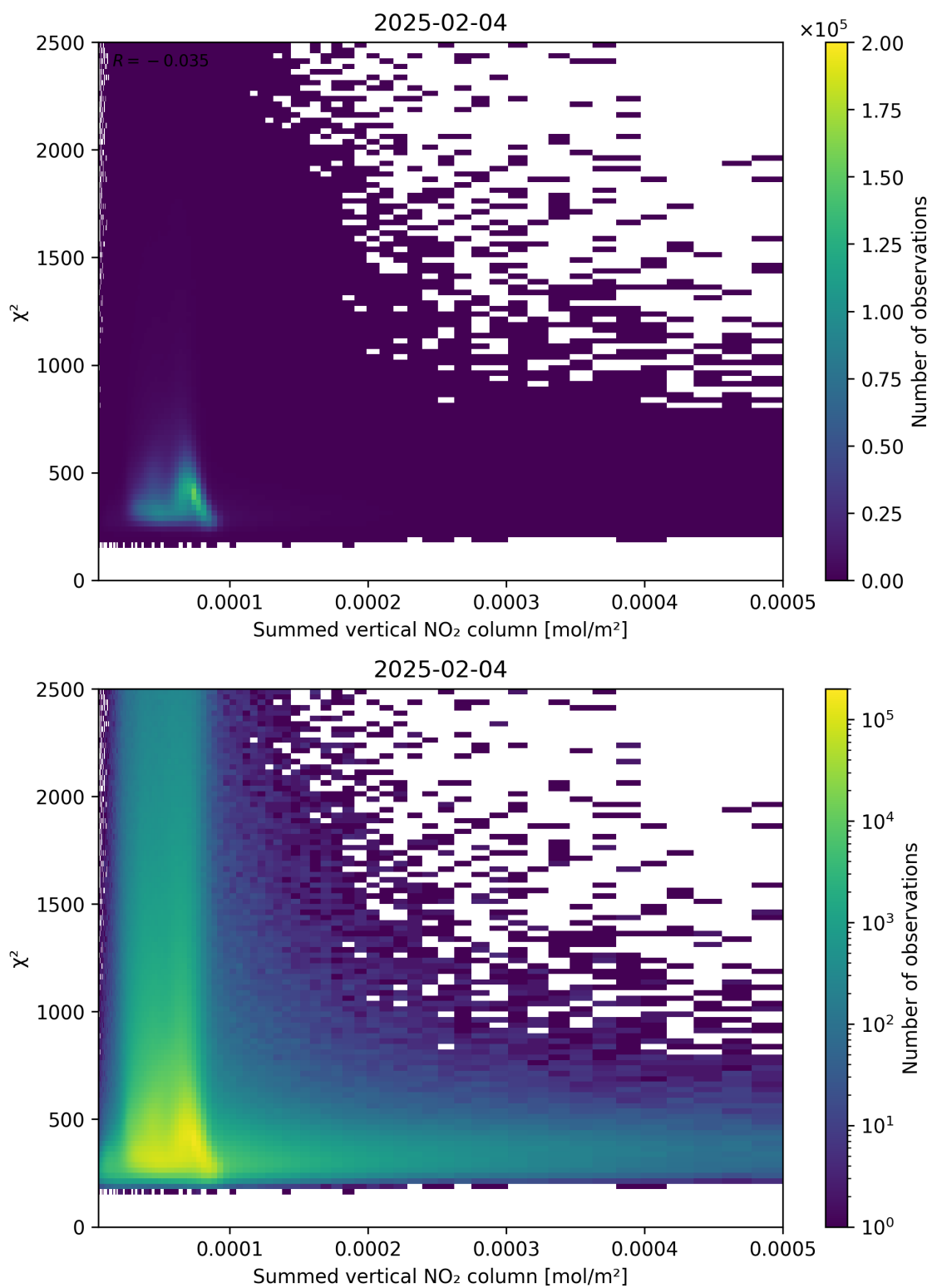
Figure 104: Scatter density plot of “Summed vertical NO 2 column” against “ \chi^2 ” for 2025-02-04 to 2025-02-05.
