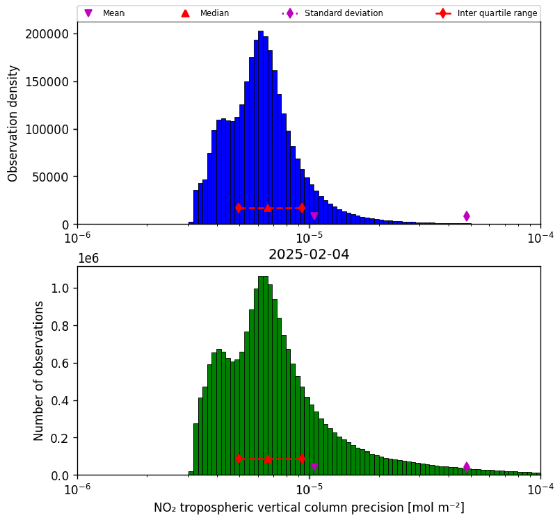
Figure 30: Histogram of “NO 2 tropospheric vertical column precision” for 2025-02-04 to 2025-02-05
