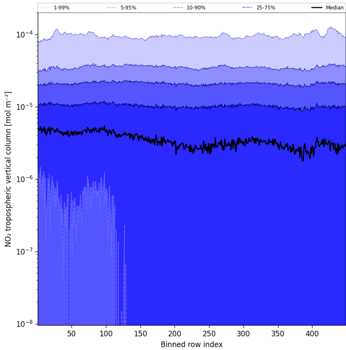
Figure 46: Along track statistics of “NO 2 tropospheric vertical column” for 2025-02-04 to 2025-02-05
