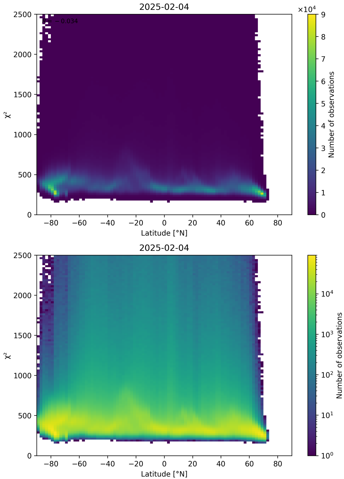
Figure 86: Scatter density plot of “Latitude” against “ \chi^2 ” for 2025-02-04 to 2025-02-05.
