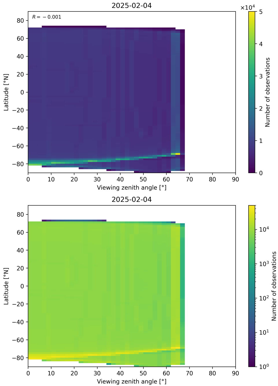
Figure 163: Scatter density plot of “Viewing zenith angle” against “Latitude” for 2025-02-04 to 2025-02-05.
