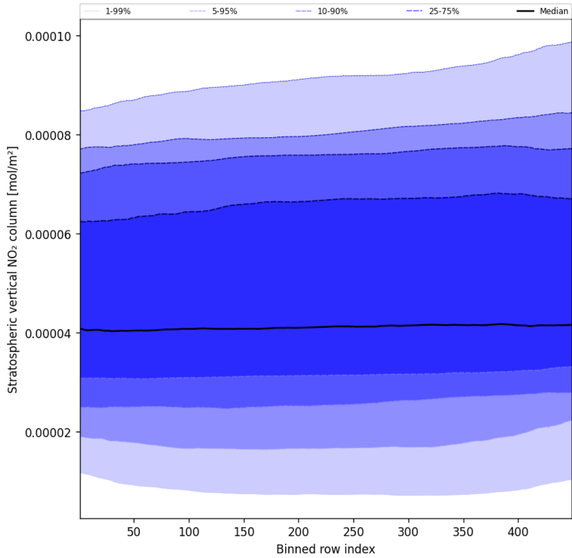
Figure 53: Along track statistics of “Stratospheric vertical NO 2 column” for 2025-02-04 to 2025-02-05
