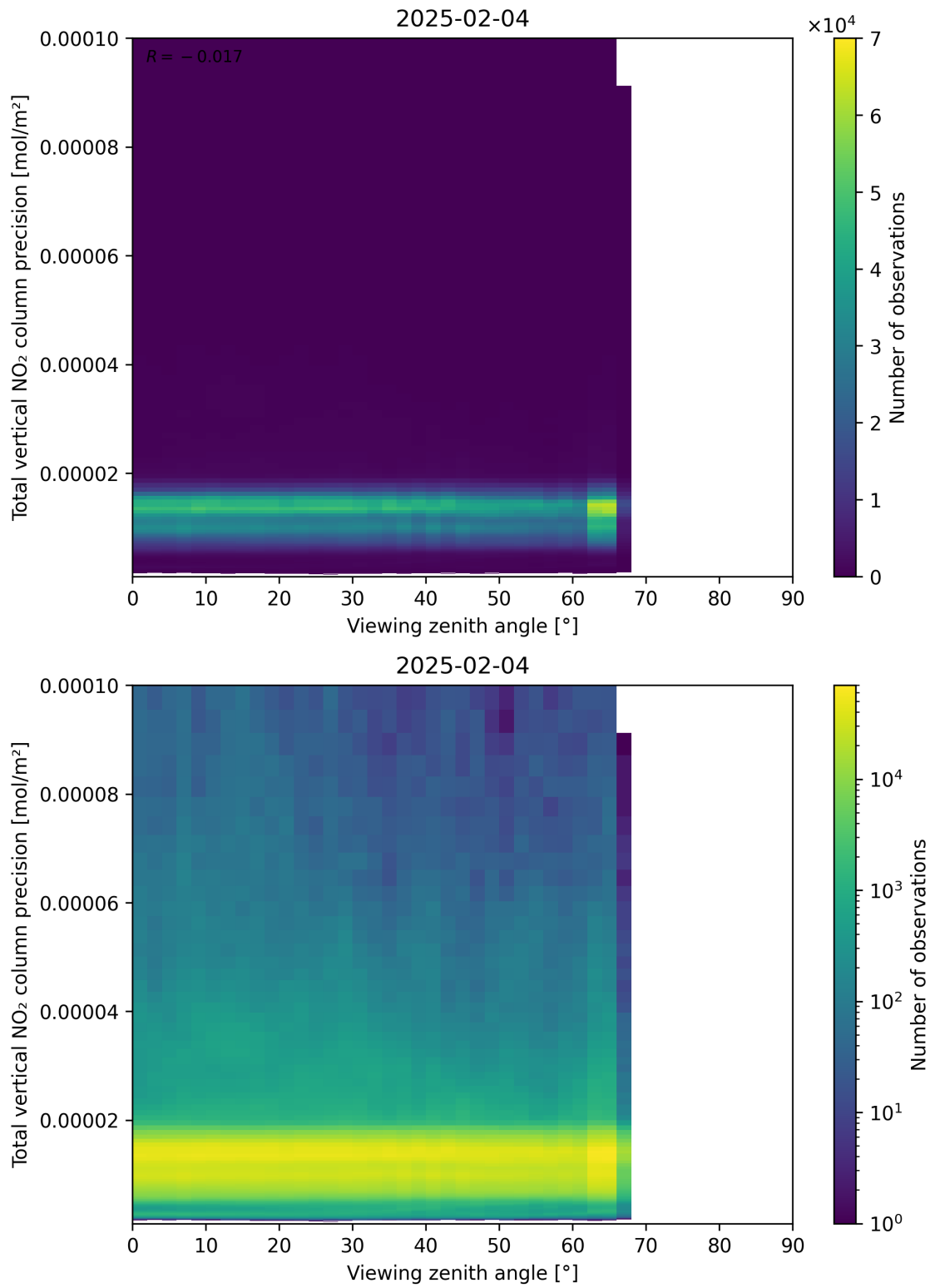
Figure 168: Scatter density plot of “Viewing zenith angle” against “Total vertical NO 2 column precision” for 2025-02-04 to 2025-02-05.
