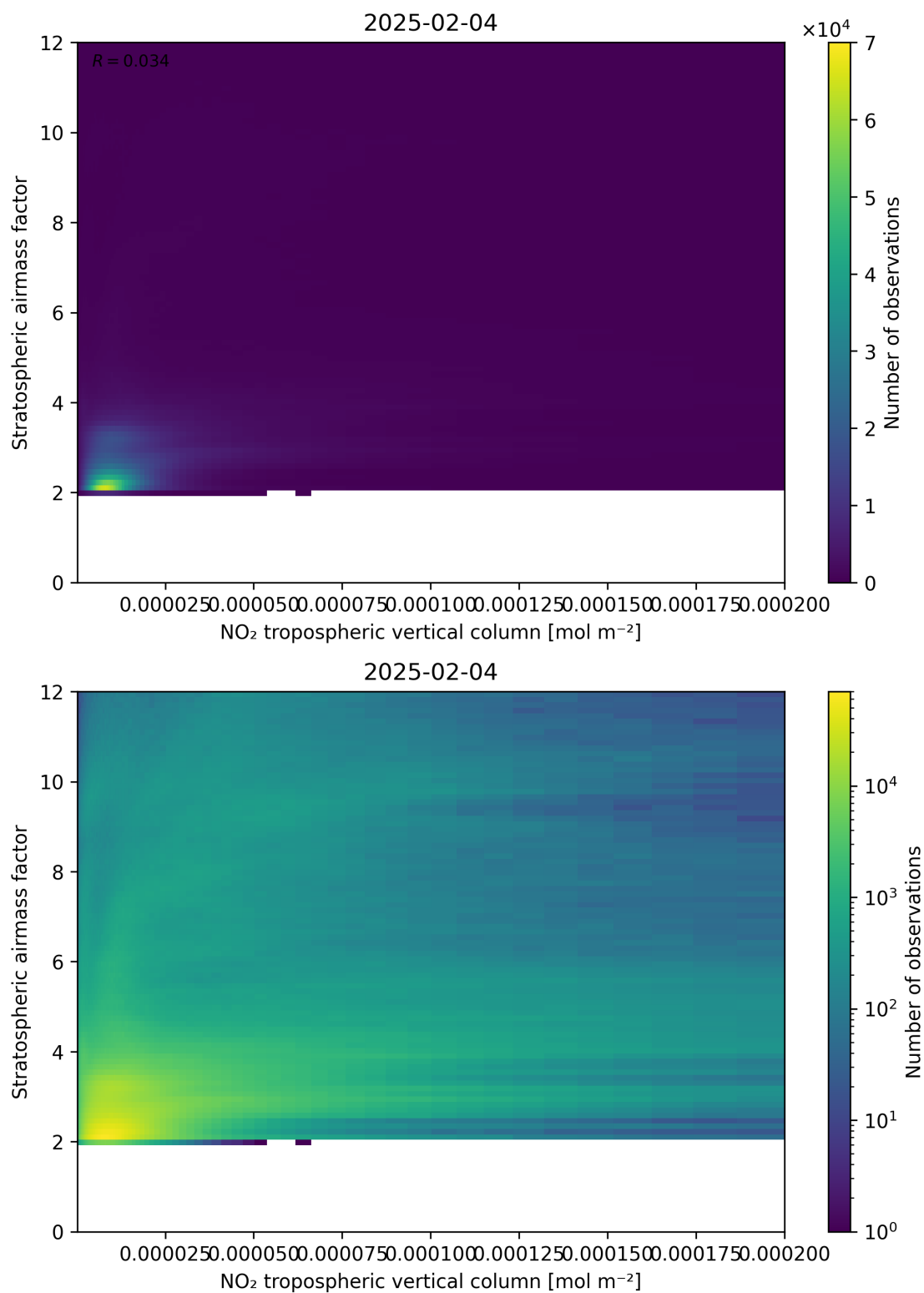
Figure 121: Scatter density plot of “NO 2 tropospheric vertical column” against “Stratospheric airmass factor” for 2025-02-04 to 2025-02-05.
