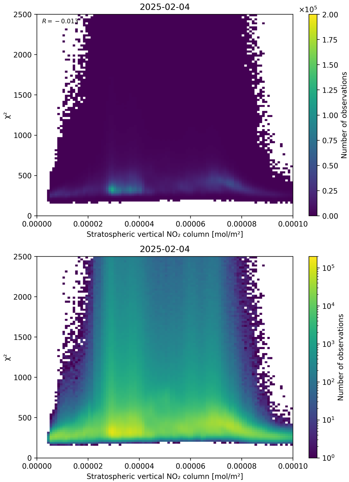
Figure 97: Scatter density plot of “Stratospheric vertical NO 2 column” against “ \chi^2 ” for 2025-02-04 to 2025-02-05.
