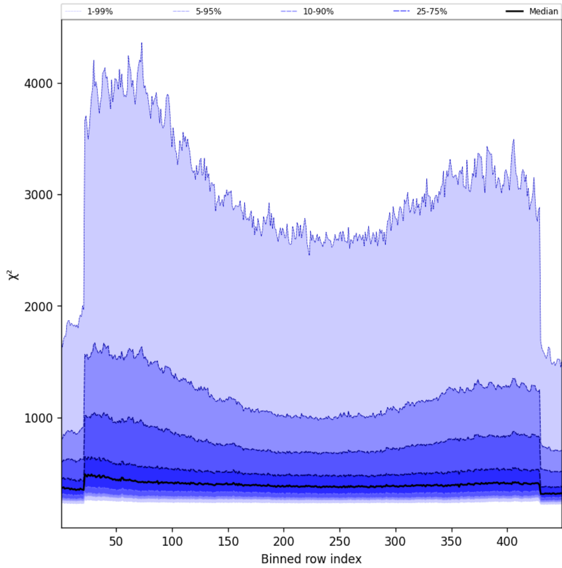
Figure 59: Along track statistics of “ \chi^2 ” for 2025-02-04 to 2025-02-05
