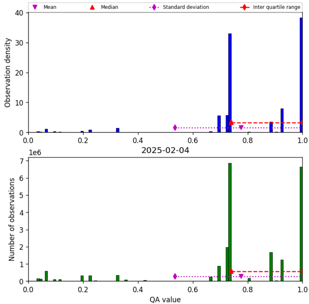
Figure 28: Histogram of “QA value” for 2025-02-04 to 2025-02-05
