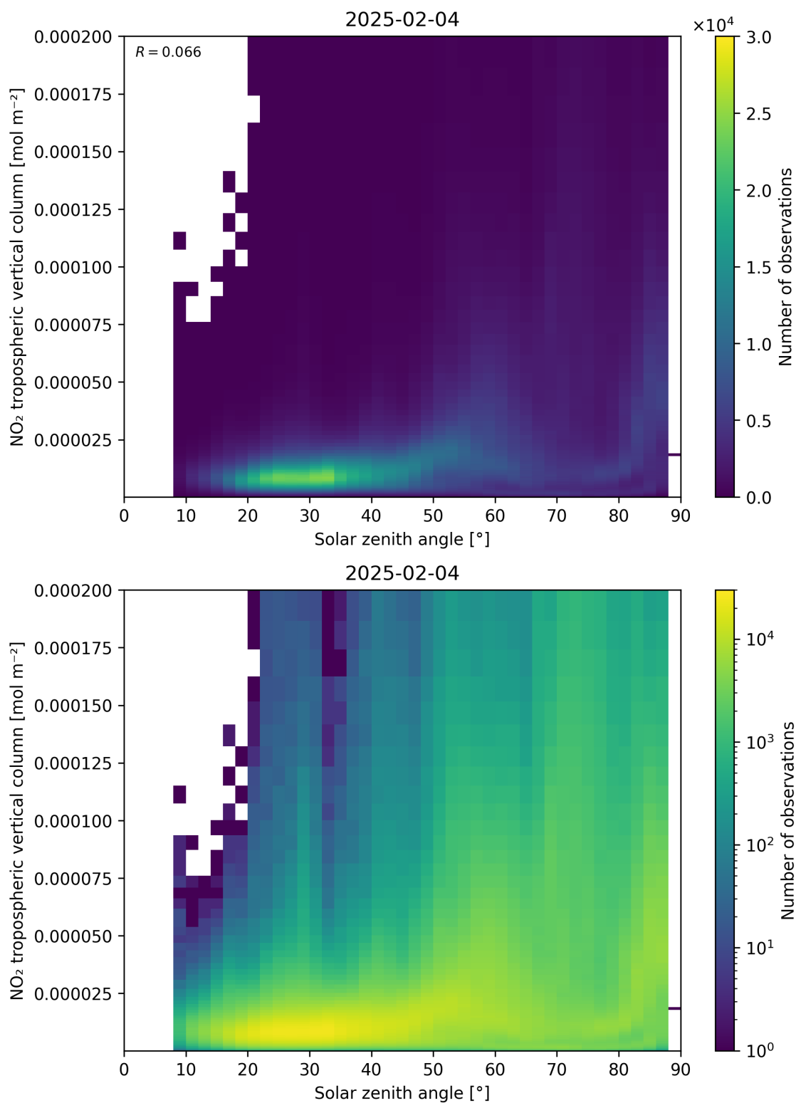
Figure 155: Scatter density plot of “Solar zenith angle” against “NO 2 tropospheric vertical column” for 2025-02-04 to 2025-02-05.
