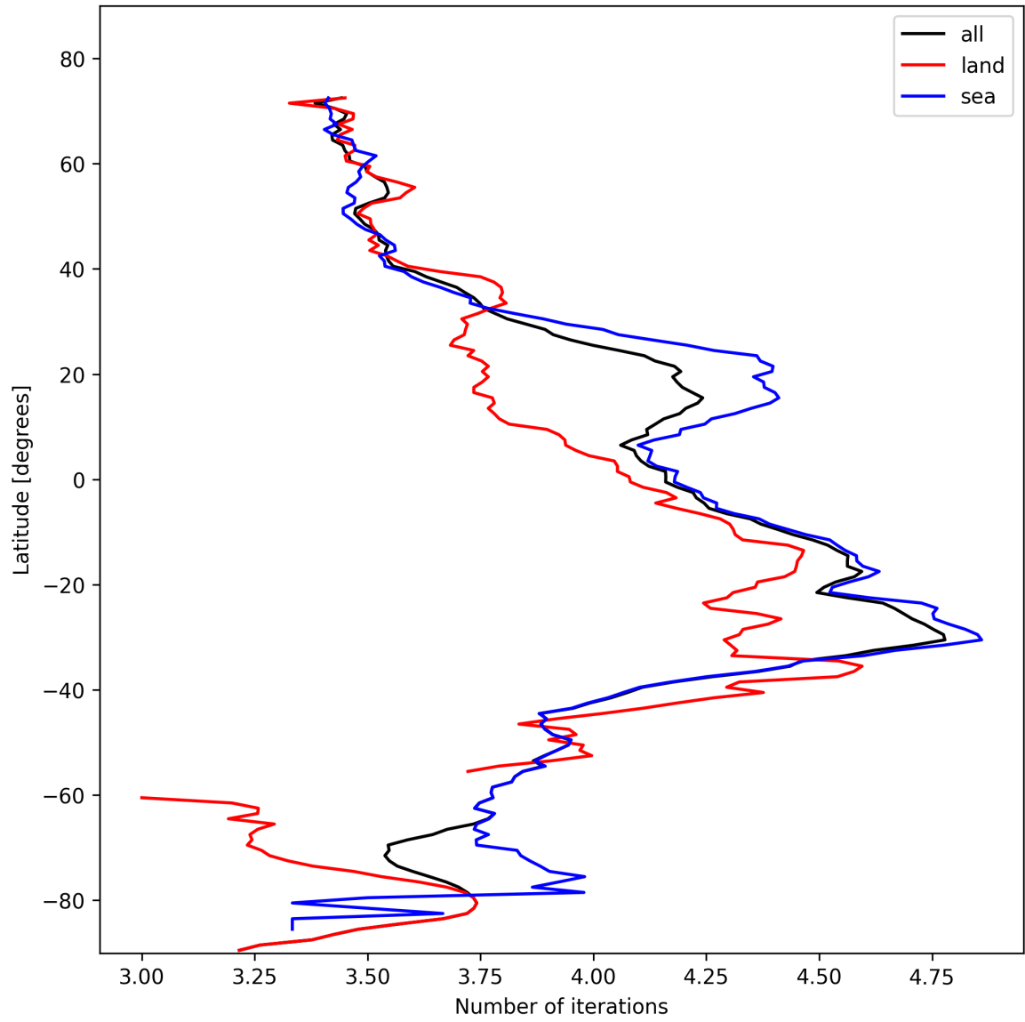
Figure 17: Zonal average of “Number of iterations” for 2025-02-04 to 2025-02-05.
