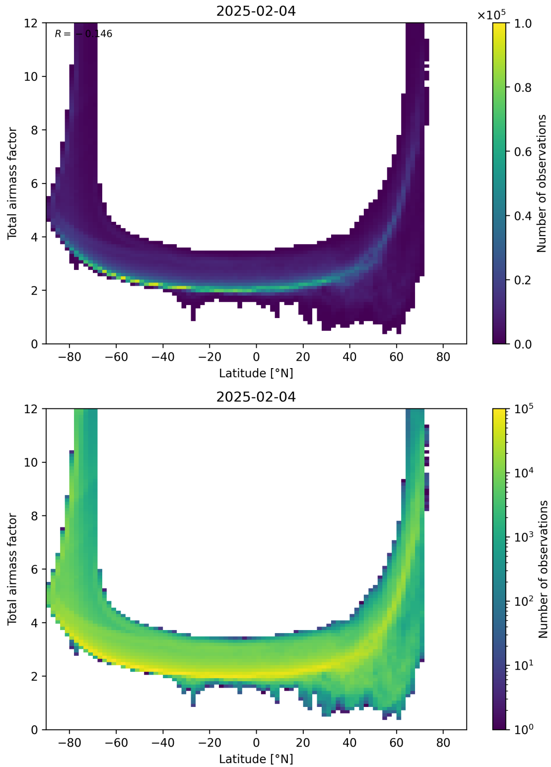
Figure 84: Scatter density plot of “Latitude” against “Total airmass factor” for 2025-02-04 to 2025-02-05.
