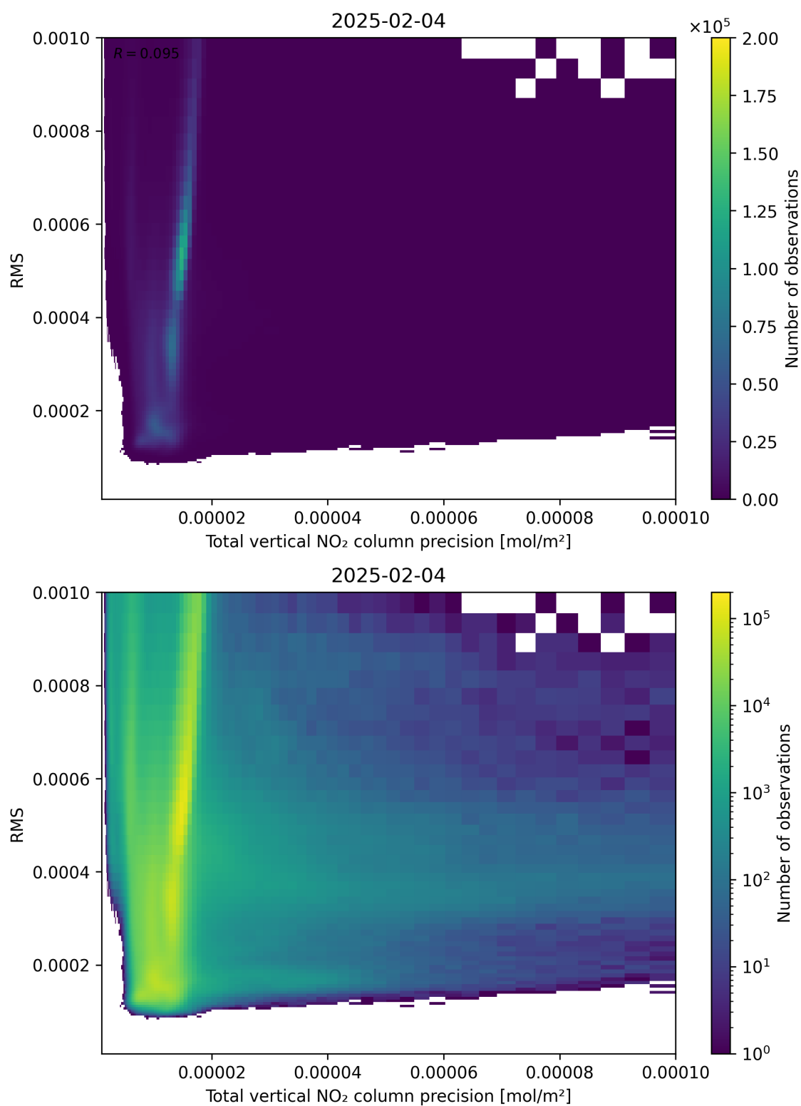
Figure 119: Scatter density plot of “Total vertical NO 2 column precision” against “RMS” for 2025-02-04 to 2025-02-05.
