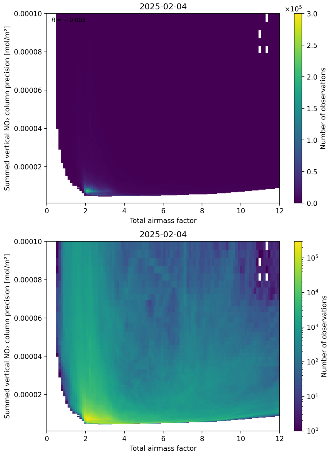
Figure 66: Scatter density plot of “Total airmass factor” against “Summed vertical NO 2 column precision” for 2025-02-04 to 2025-02-05.
