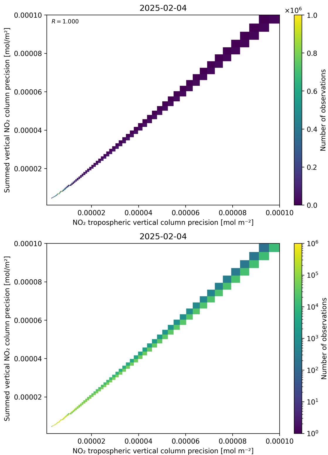
Figure 137: Scatter density plot of “NO 2 tropospheric vertical column precision” against “Summed vertical NO 2 column precision” for 2025-02-04 to 2025-02-05.
