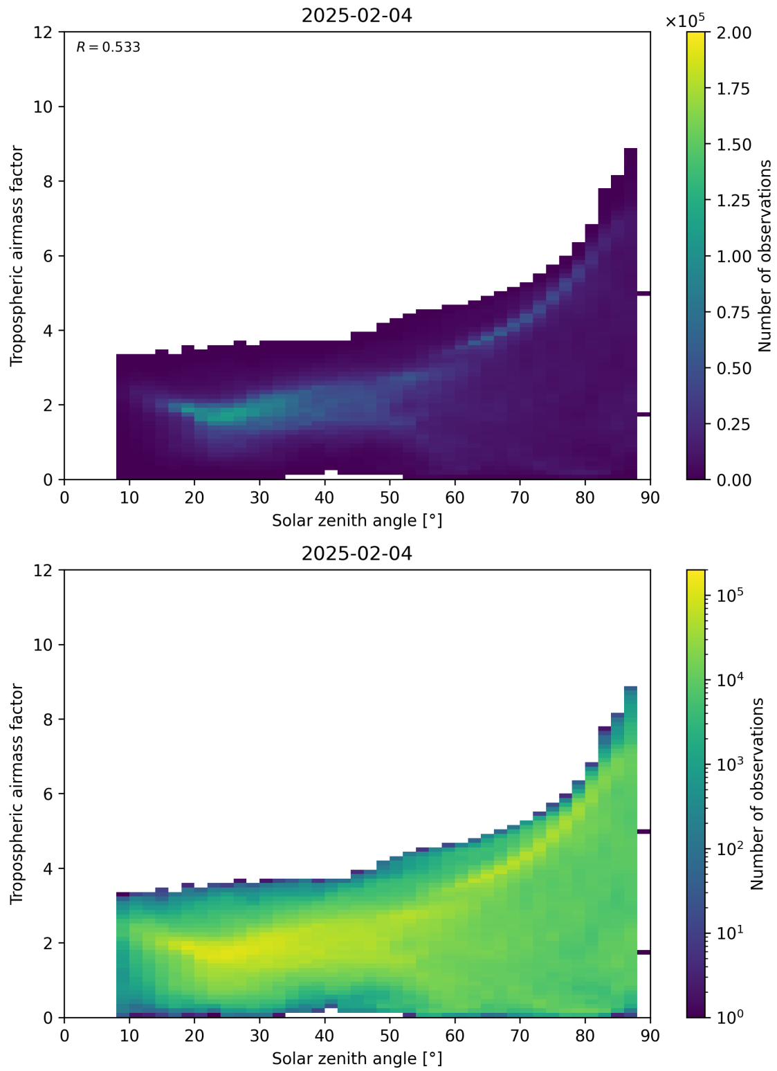
Figure 147: Scatter density plot of “Solar zenith angle” against “Tropospheric airmass factor” for 2025-02-04 to 2025-02-05.
