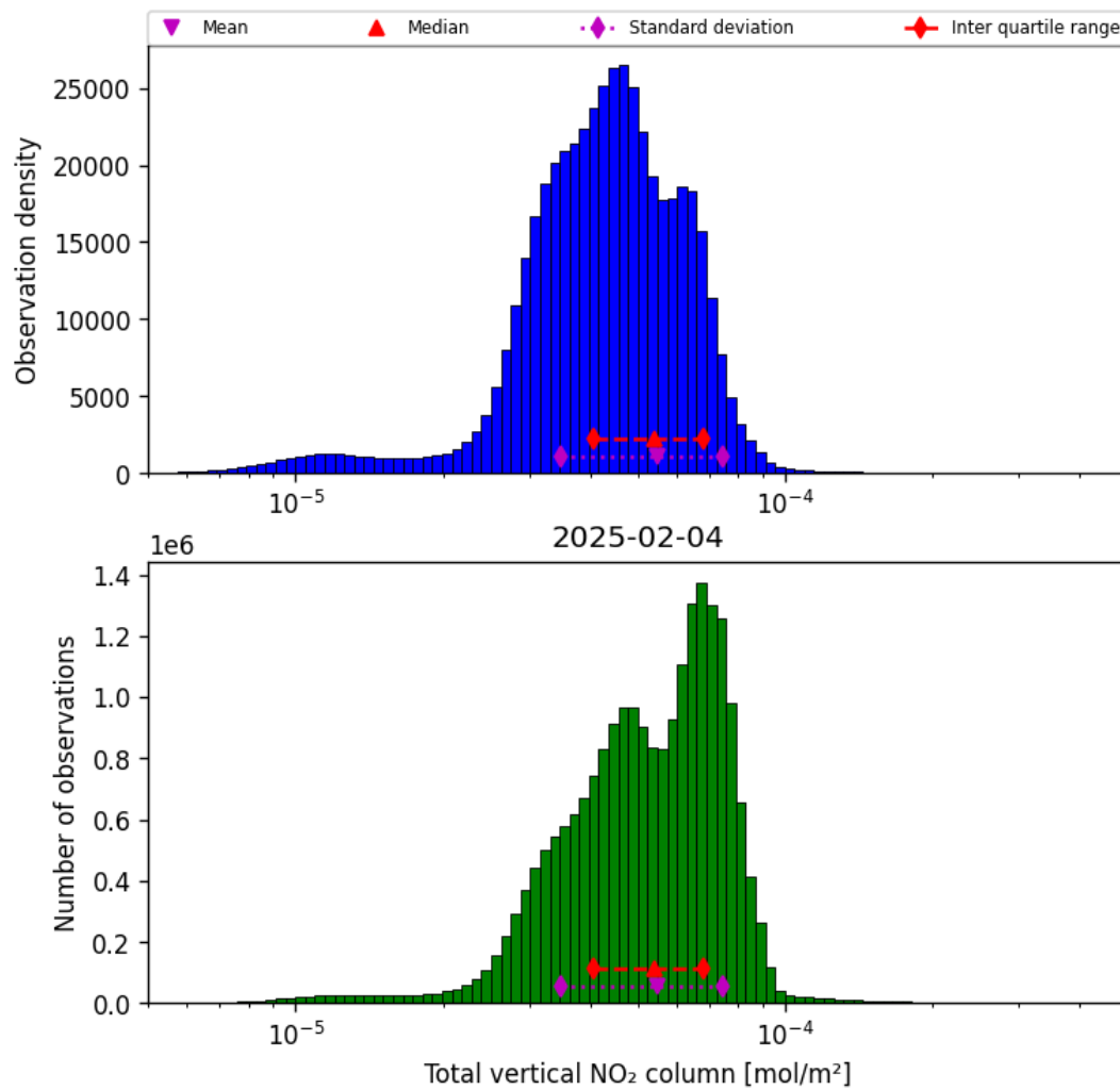
Figure 38: Histogram of “Total vertical NO 2 column” for 2025-02-04 to 2025-02-05
