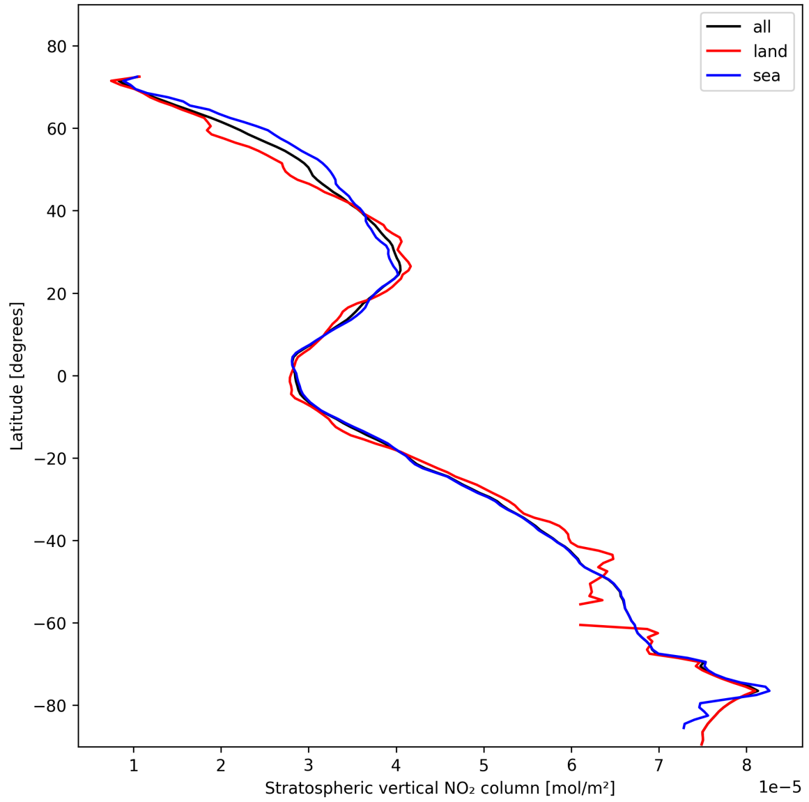
Figure 19: Zonal average of “Stratospheric vertical NO 2 column” for 2025-02-04 to 2025-02-05.
