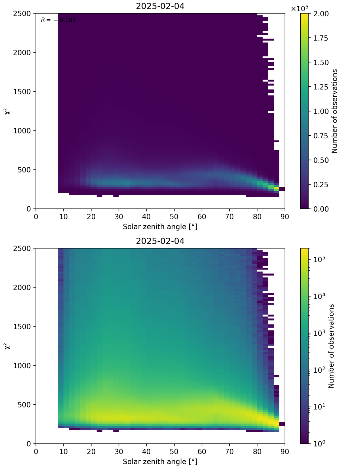
Figure 148: Scatter density plot of “Solar zenith angle” against “ \chi^2 ” for 2025-02-04 to 2025-02-05.
