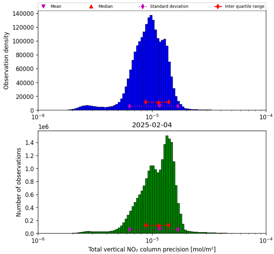
Figure 39: Histogram of “Total vertical NO 2 column precision” for 2025-02-04 to 2025-02-05
