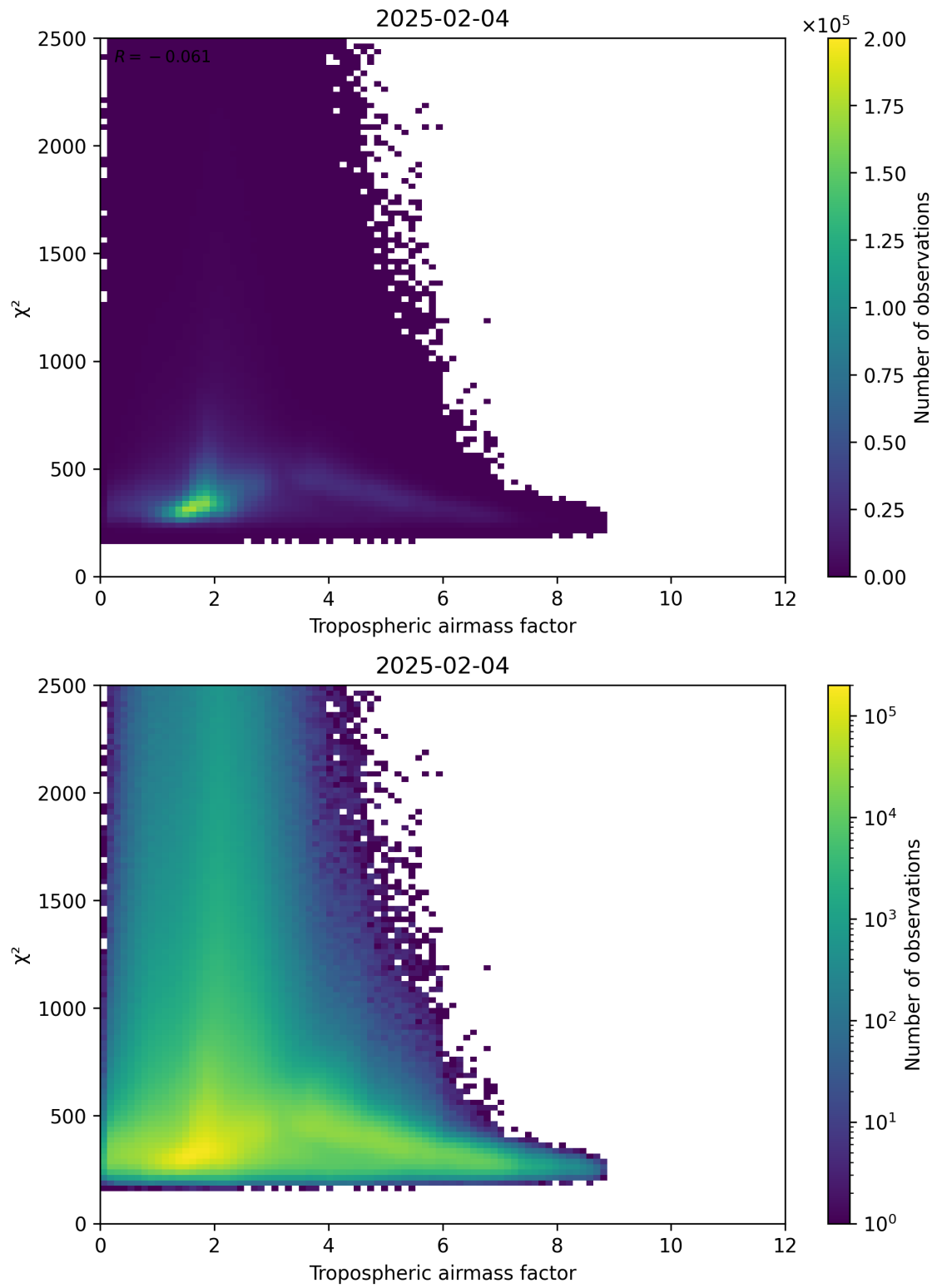
Figure 73: Scatter density plot of “Tropospheric airmass factor” against “ \chi^2 ” for 2025-02-04 to 2025-02-05.
