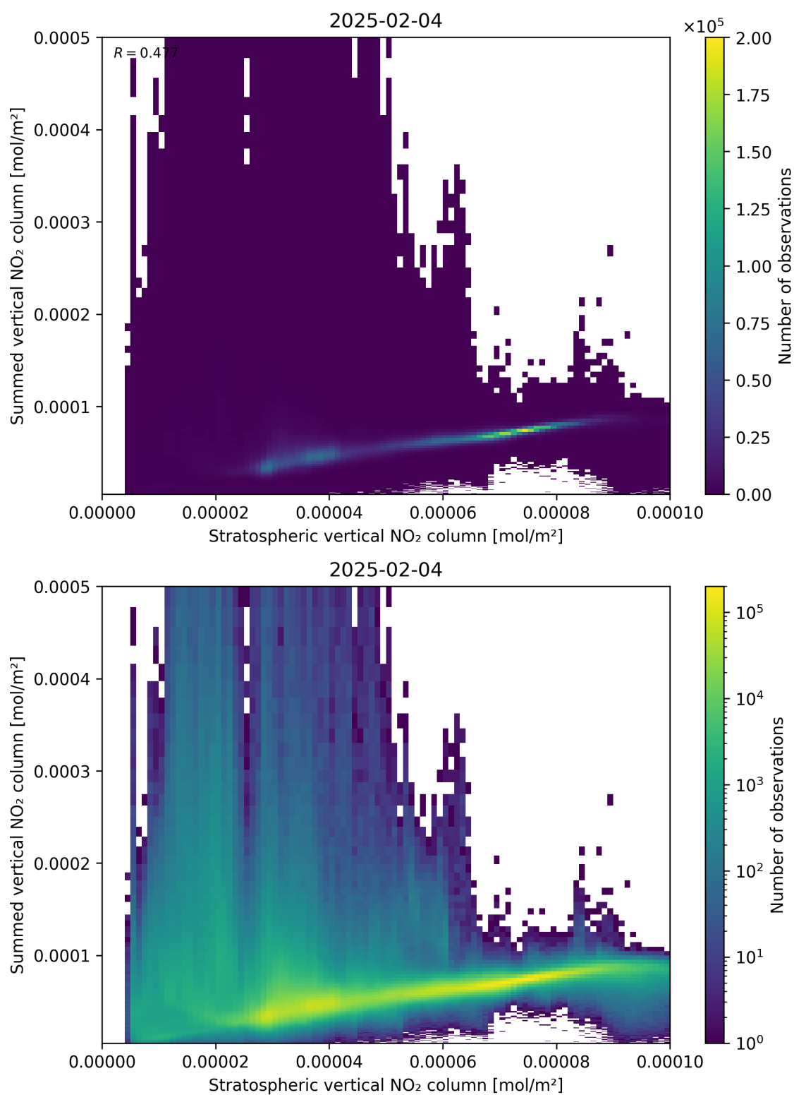
Figure 98: Scatter density plot of “Stratospheric vertical NO 2 column” against “Summed vertical NO 2 column” for 2025-02-04 to 2025-02-05.
