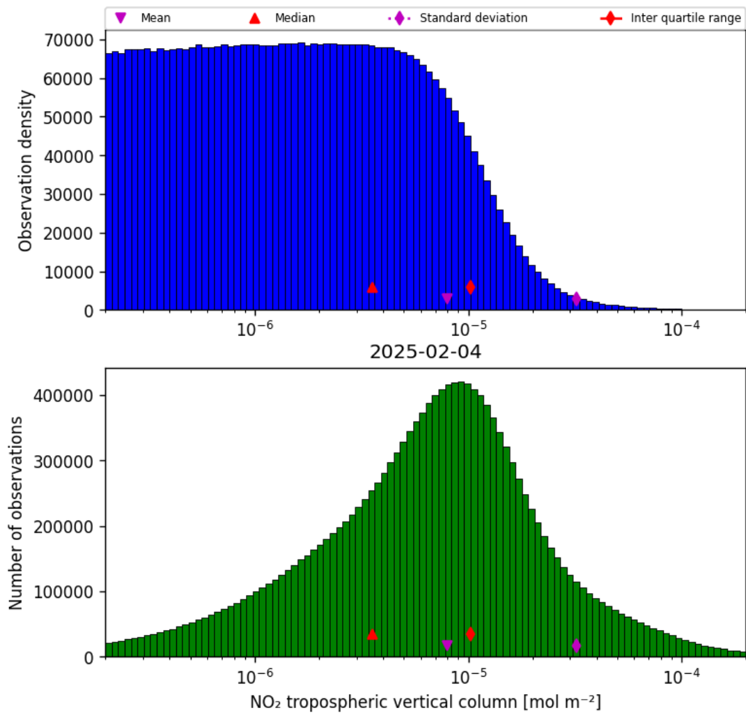
Figure 29: Histogram of “NO 2 tropospheric vertical column” for 2025-02-04 to 2025-02-05
