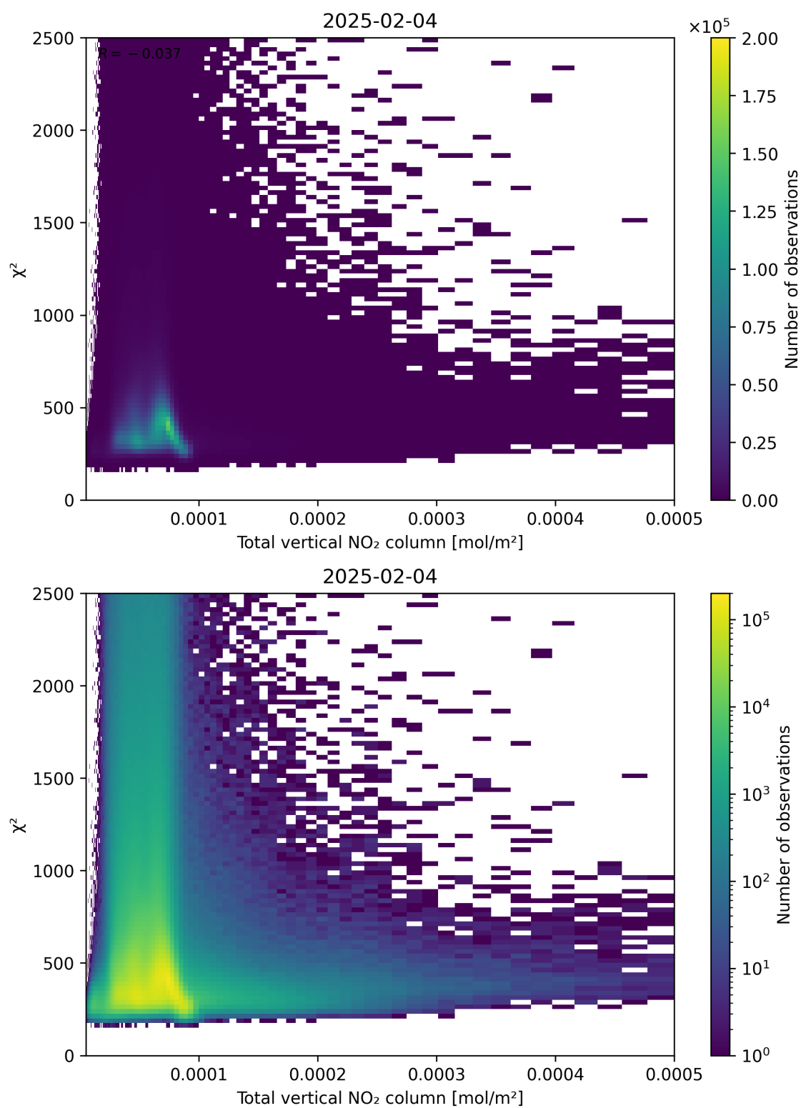
Figure 111: Scatter density plot of “Total vertical NO 2 column” against “ \chi^2 ” for 2025-02-04 to 2025-02-05.
