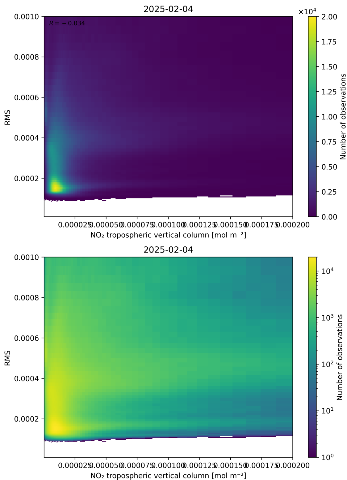
Figure 142: Scatter density plot of “NO 2 tropospheric vertical column” against “RMS” for 2025-02-04 to 2025-02-05.
