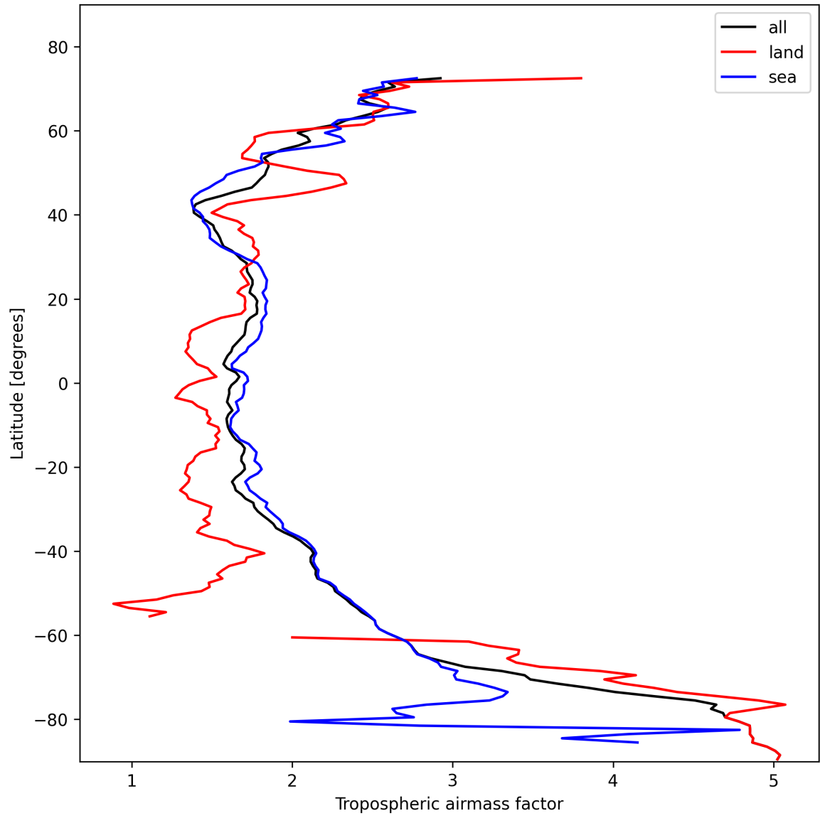
Figure 14: Zonal average of “Tropospheric airmass factor” for 2025-02-04 to 2025-02-05.
