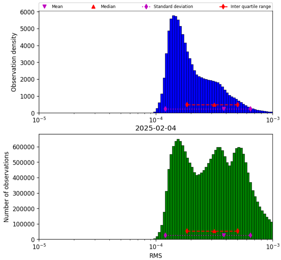
Figure 43: Histogram of “RMS” for 2025-02-04 to 2025-02-05
