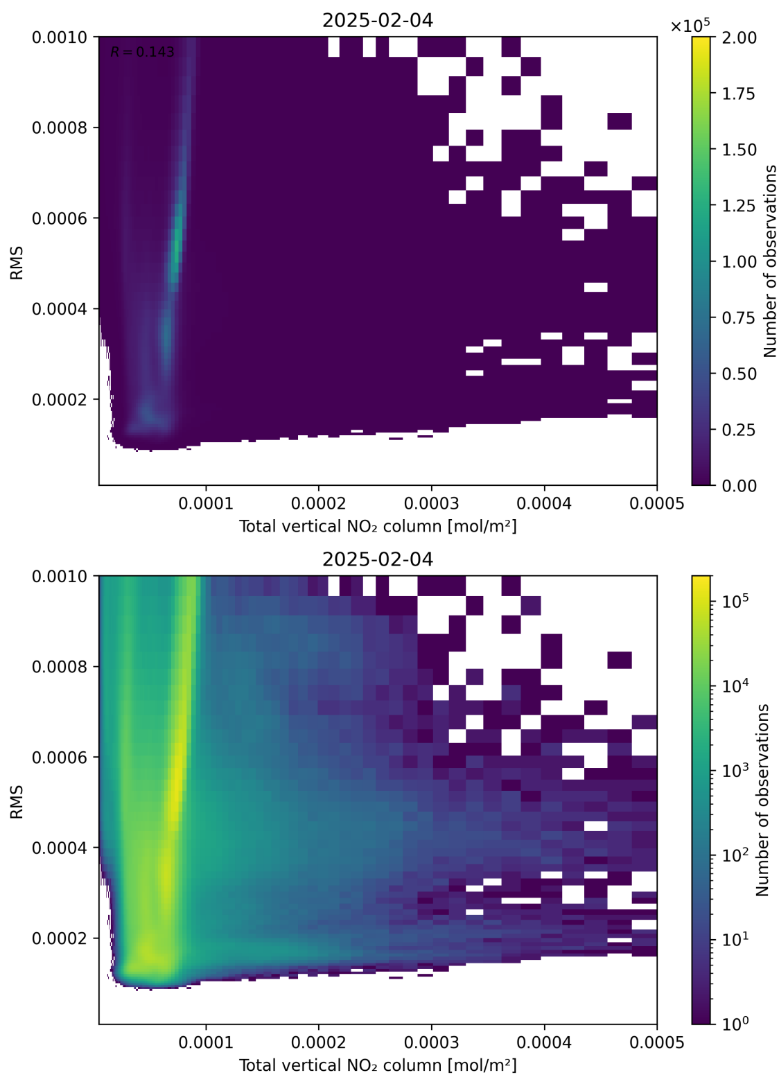
Figure 120: Scatter density plot of “Total vertical NO 2 column” against “RMS” for 2025-02-04 to 2025-02-05.
