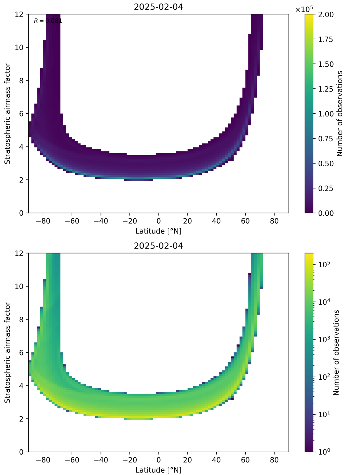
Figure 83: Scatter density plot of “Latitude” against “Stratospheric airmass factor” for 2025-02-04 to 2025-02-05.
