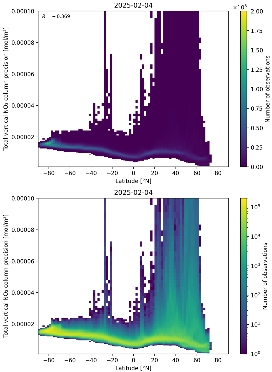
Figure 91: Scatter density plot of “Latitude” against “Total vertical NO 2 column precision” for 2025-02-04 to 2025-02-05.
