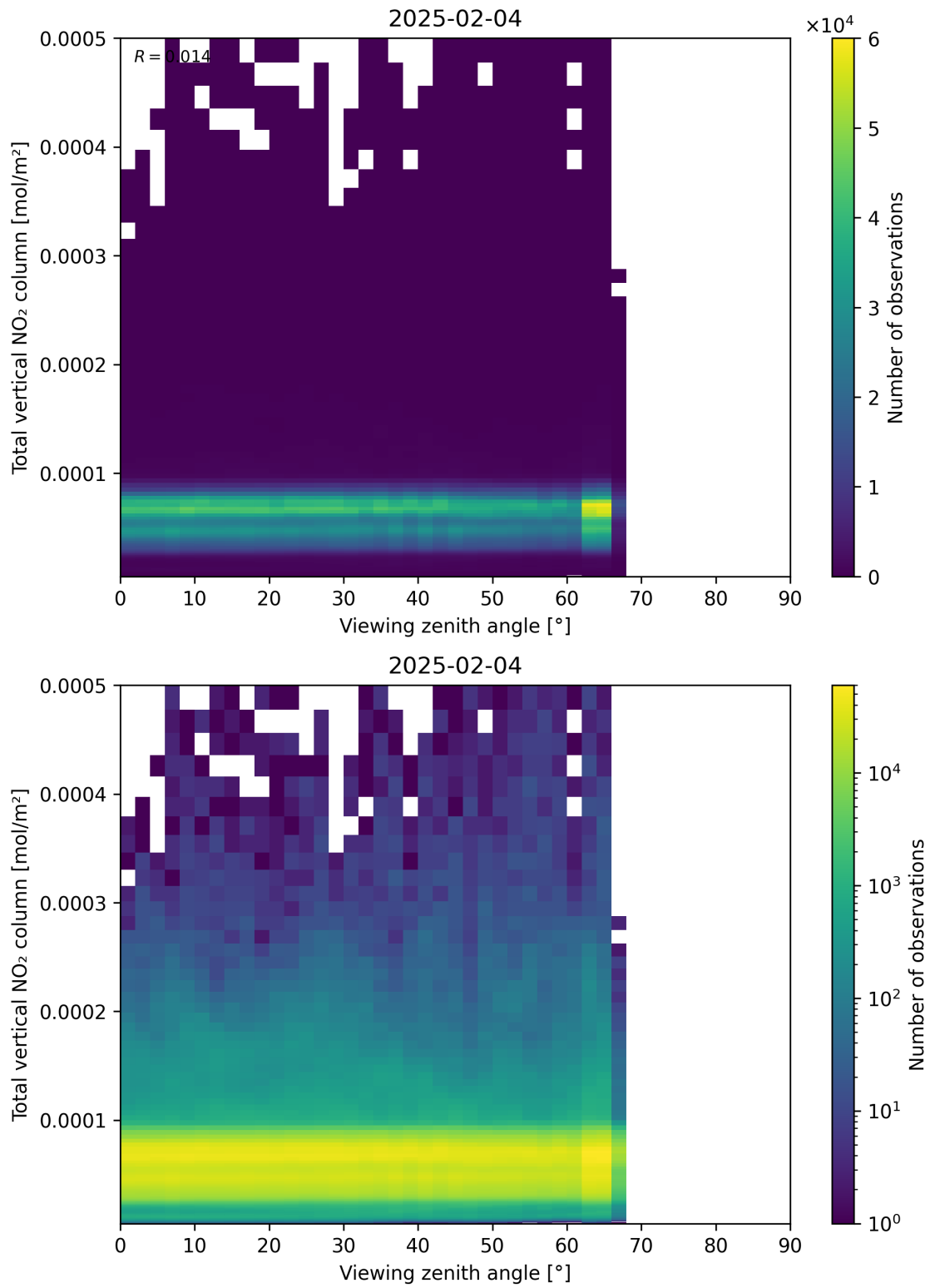
Figure 167: Scatter density plot of “Viewing zenith angle” against “Total vertical NO 2 column” for 2025-02-04 to 2025-02-05.
