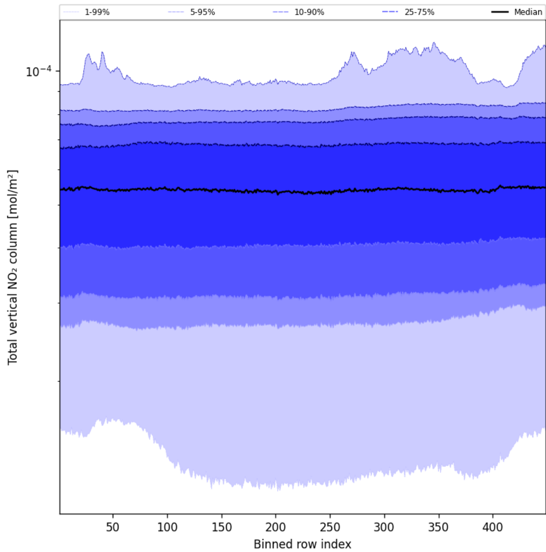
Figure 55: Along track statistics of “Total vertical NO 2 column” for 2025-02-04 to 2025-02-05
