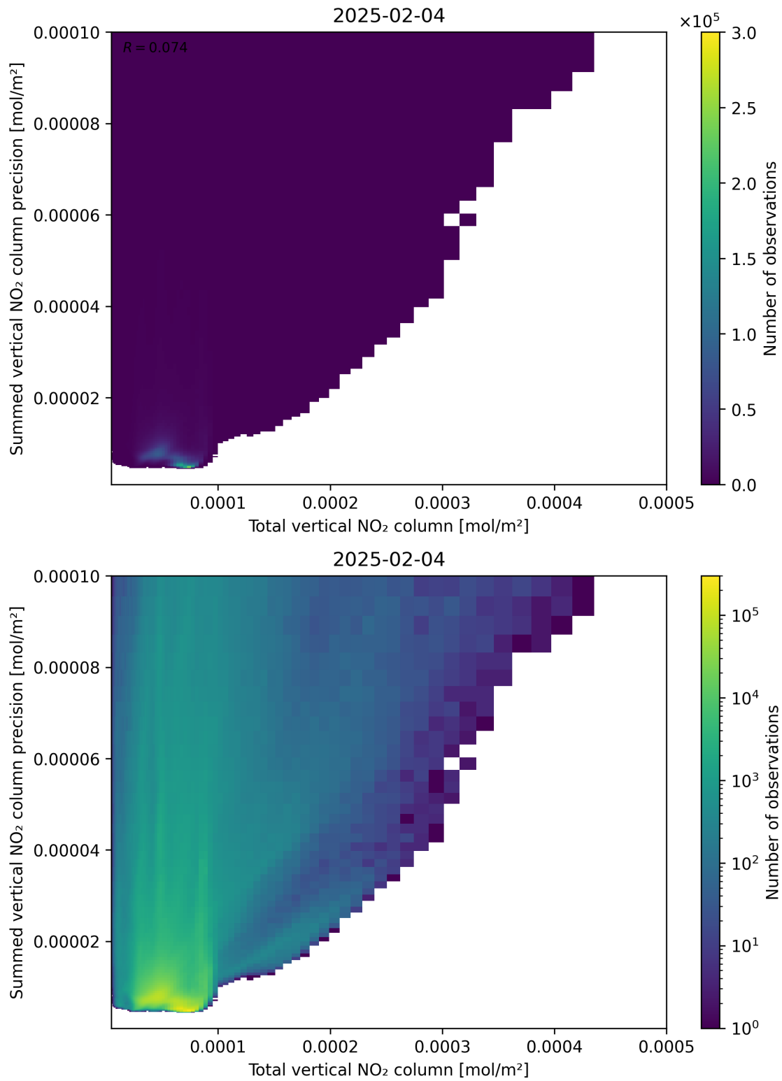
Figure 113: Scatter density plot of “Total vertical NO 2 column” against “Summed vertical NO 2 column precision” for 2025-02-04 to 2025-02-05.
