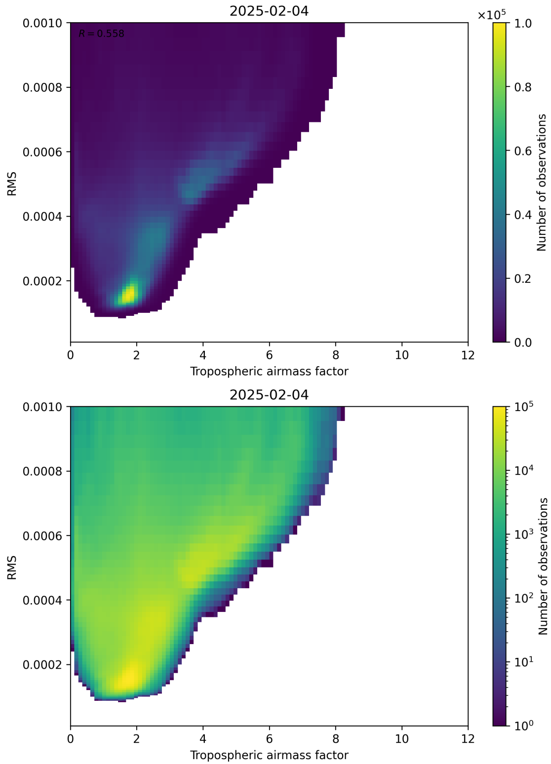
Figure 79: Scatter density plot of “Tropospheric airmass factor” against “RMS” for 2025-02-04 to 2025-02-05.
