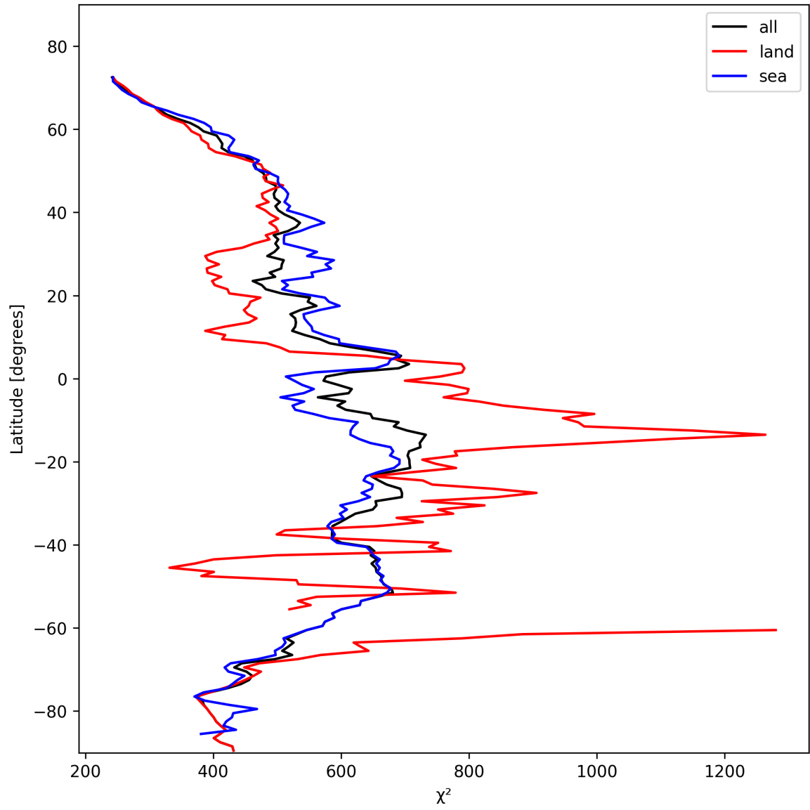
Figure 25: Zonal average of “ \chi^2 ” for 2025-02-04 to 2025-02-05.
