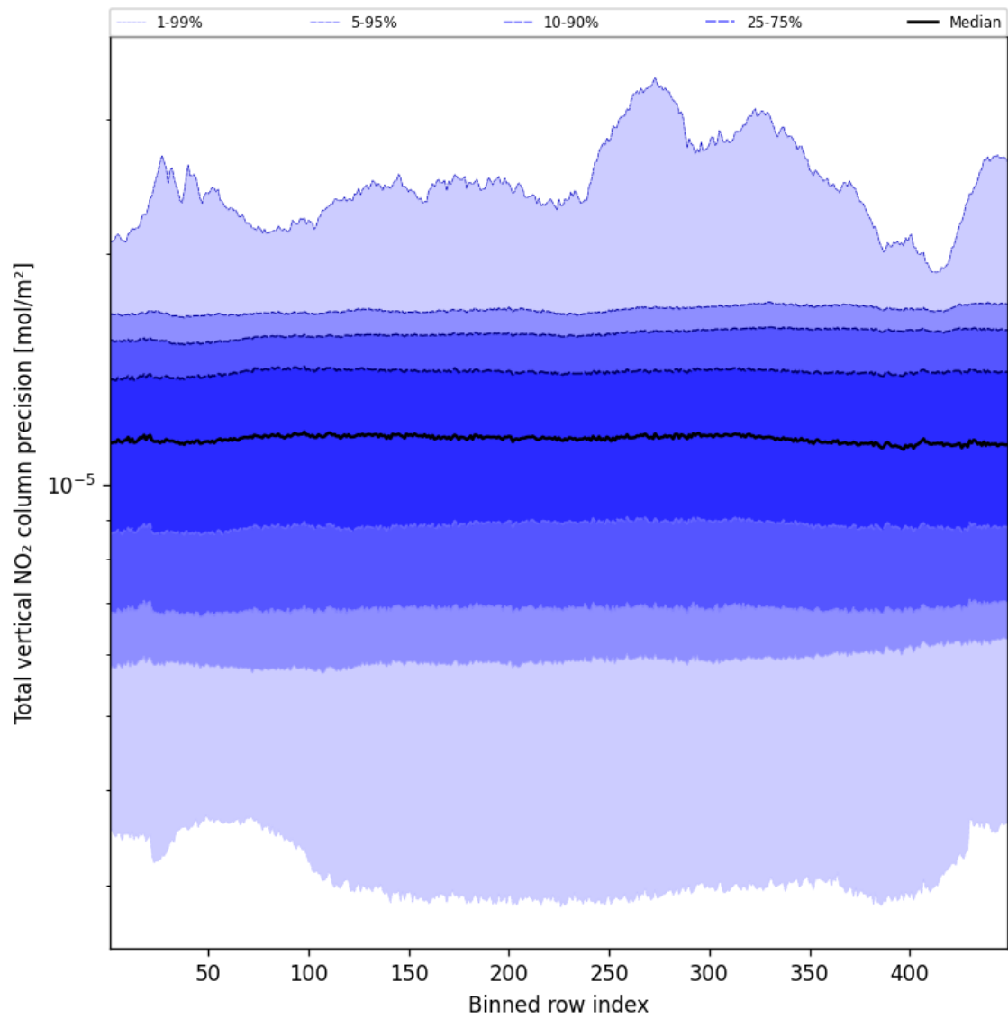
Figure 56: Along track statistics of “Total vertical NO 2 column precision” for 2025-02-04 to 2025-02-05
