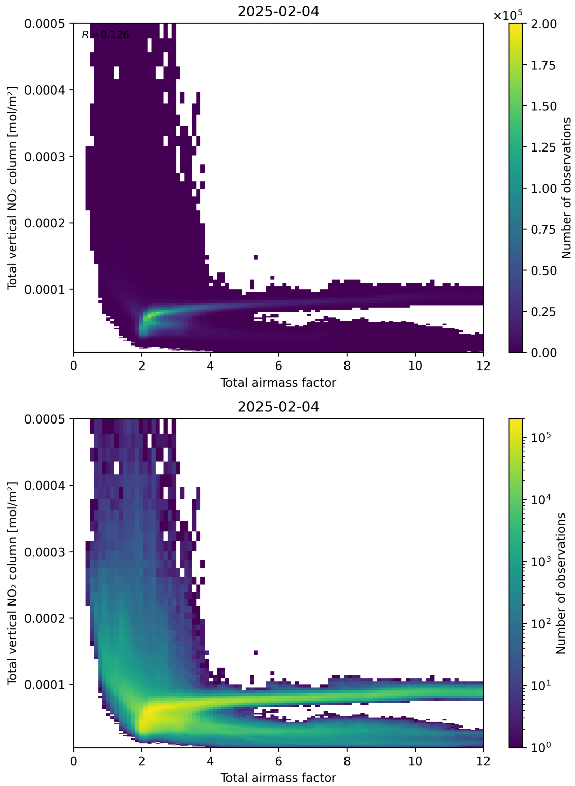
Figure 67: Scatter density plot of “Total airmass factor” against “Total vertical NO 2 column” for 2025-02-04 to 2025-02-05.
