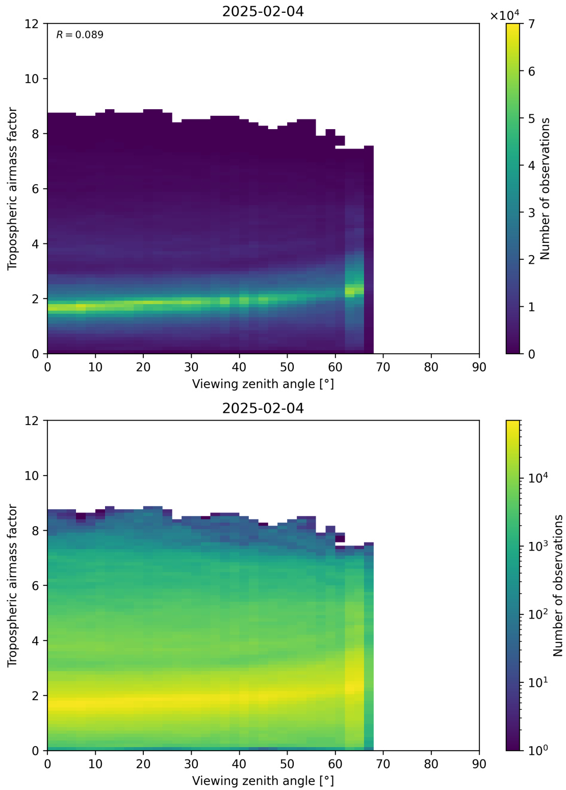
Figure 161: Scatter density plot of “Viewing zenith angle” against “Tropospheric airmass factor” for 2025-02-04 to 2025-02-05.
