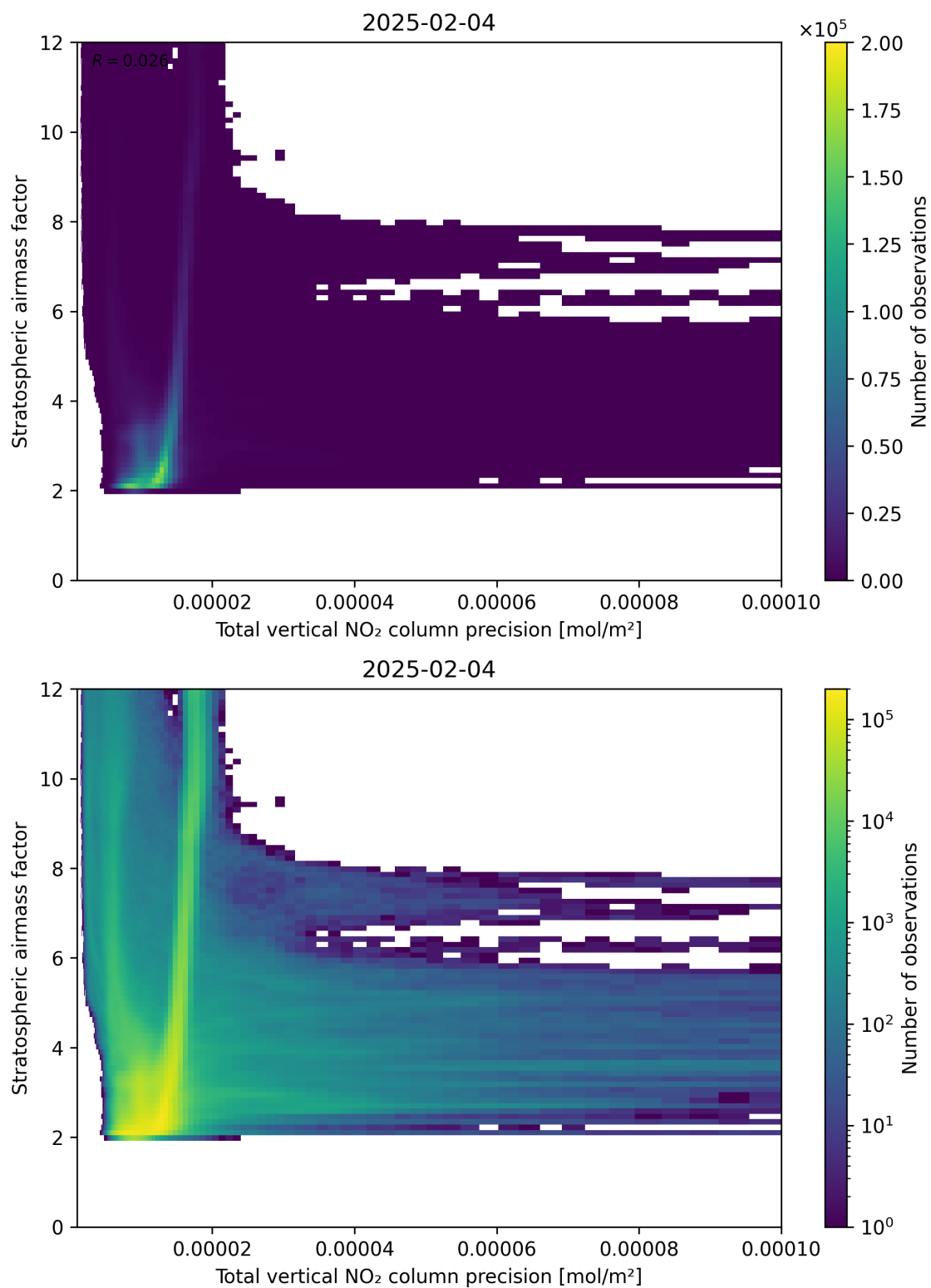
Figure 115: Scatter density plot of “Total vertical NO 2 column precision” against “Stratospheric air mass factor” for 2025-02-04 to 2025-02-05.
