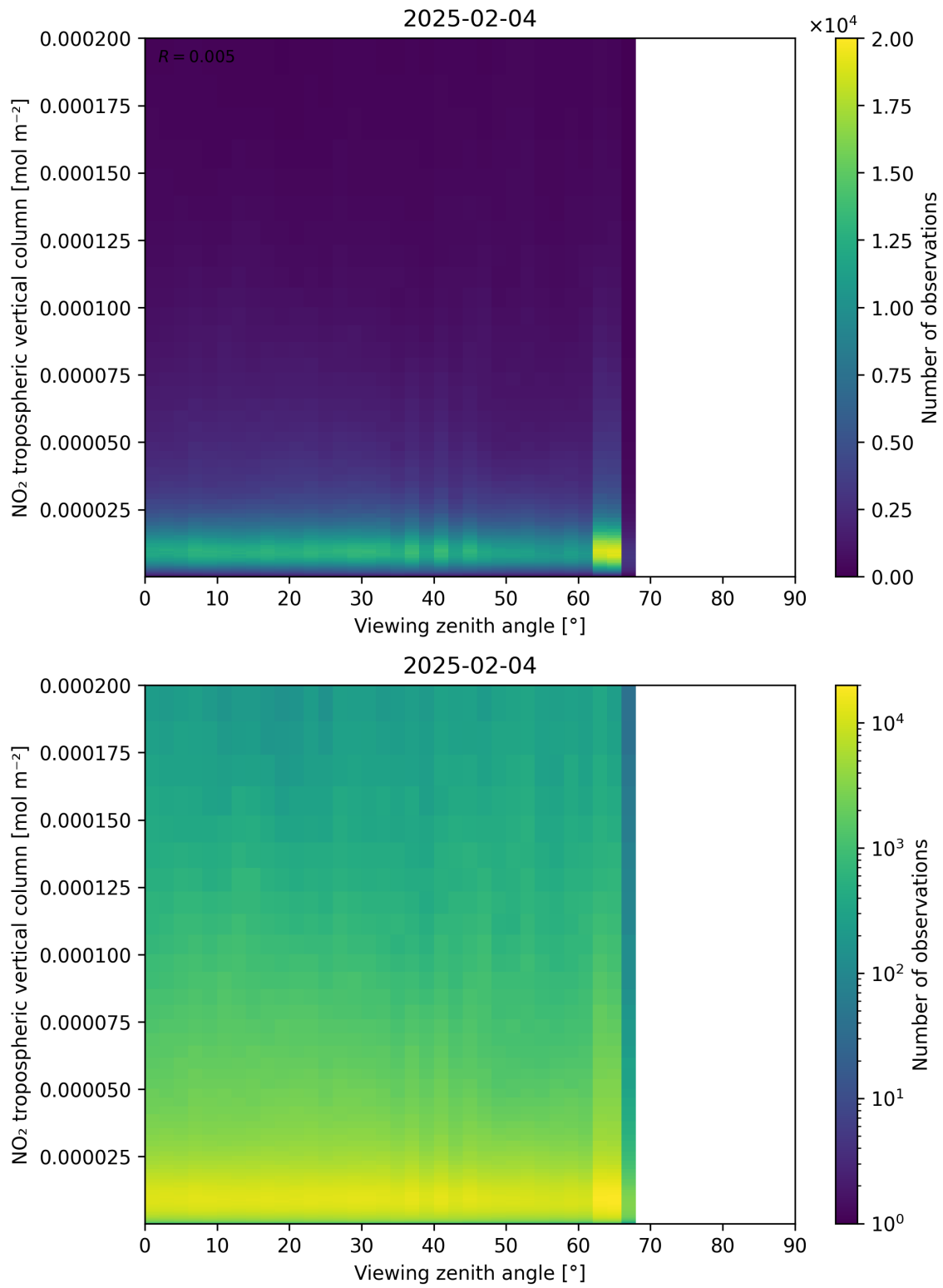
Figure 169: Scatter density plot of “Viewing zenith angle” against “NO 2 tropospheric vertical column” for 2025-02-04 to 2025-02-05.
