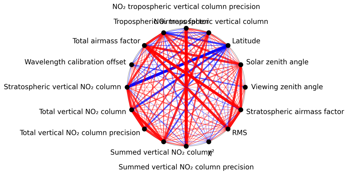
Figure 1: Map of correlation graph for 2025-02-04 to 2025-02-05.
