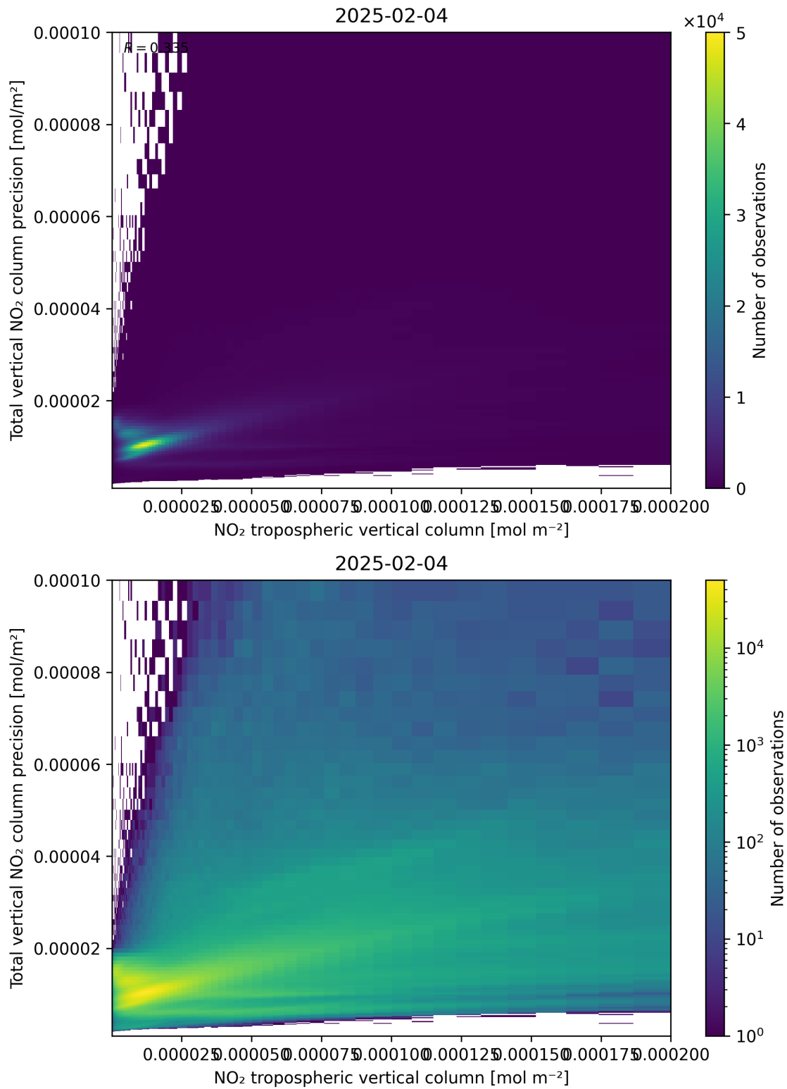
Figure 129: Scatter density plot of “NO 2 tropospheric vertical column” against “Total vertical NO 2 column precision” for 2025-02-04 to 2025-02-05.
