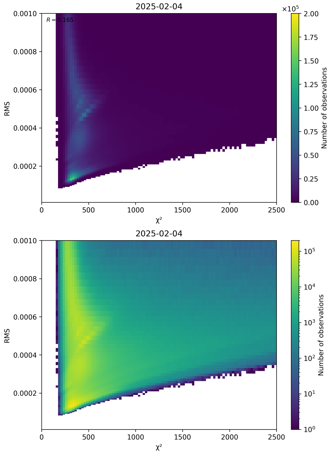
Figure 82: Scatter density plot of “ \chi^2 ” against “RMS” for 2025-02-04 to 2025-02-05.
