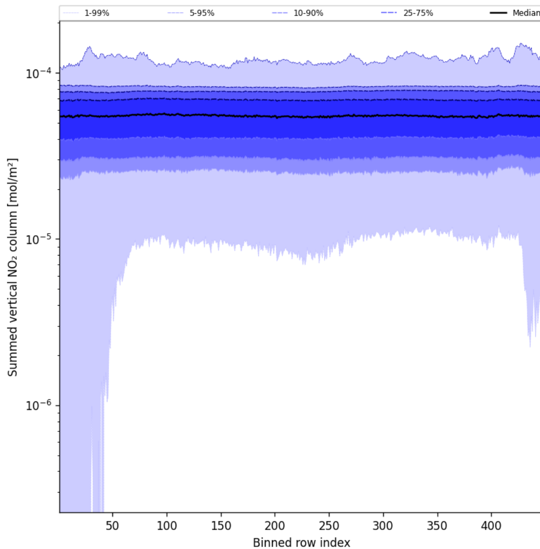
Figure 57: Along track statistics of “Summed vertical NO 2 column” for 2025-02-04 to 2025-02-05
