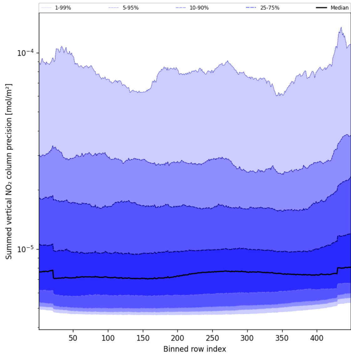
Figure 58: Along track statistics of “Summed vertical NO 2 column precision” for 2025-02-04 to 2025-02-05
