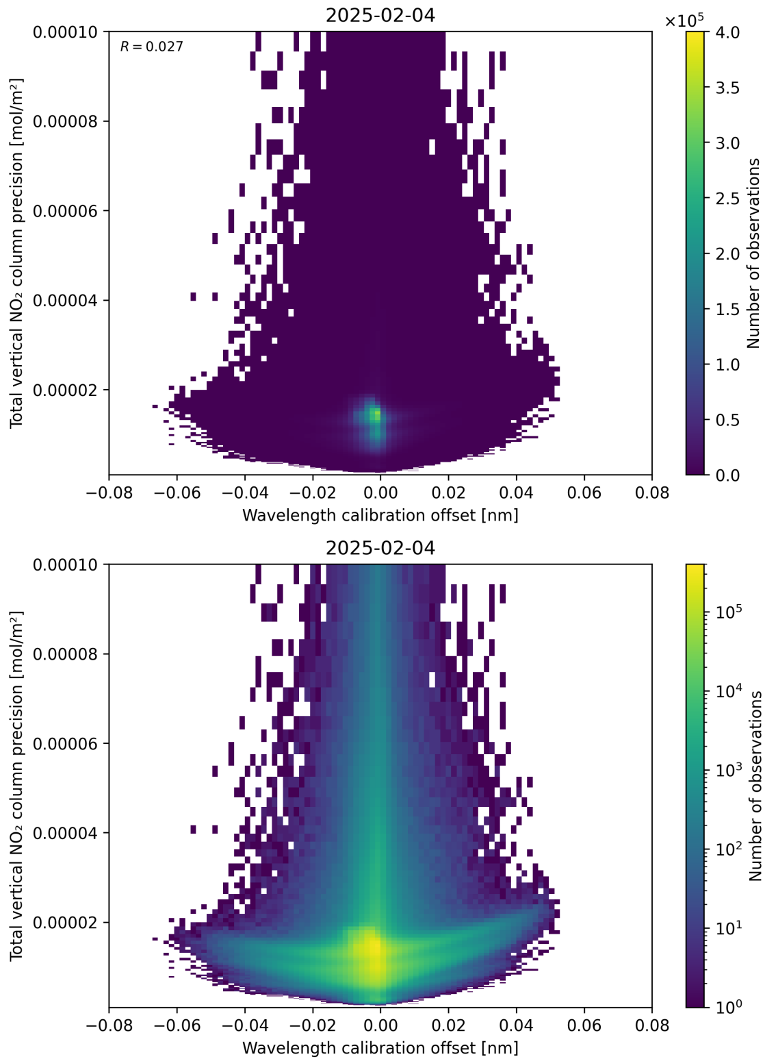
Figure 180: Scatter density plot of “Wavelength calibration offset” against “Total vertical NO 2 column precision” for 2025-02-04 to 2025-02-05.
