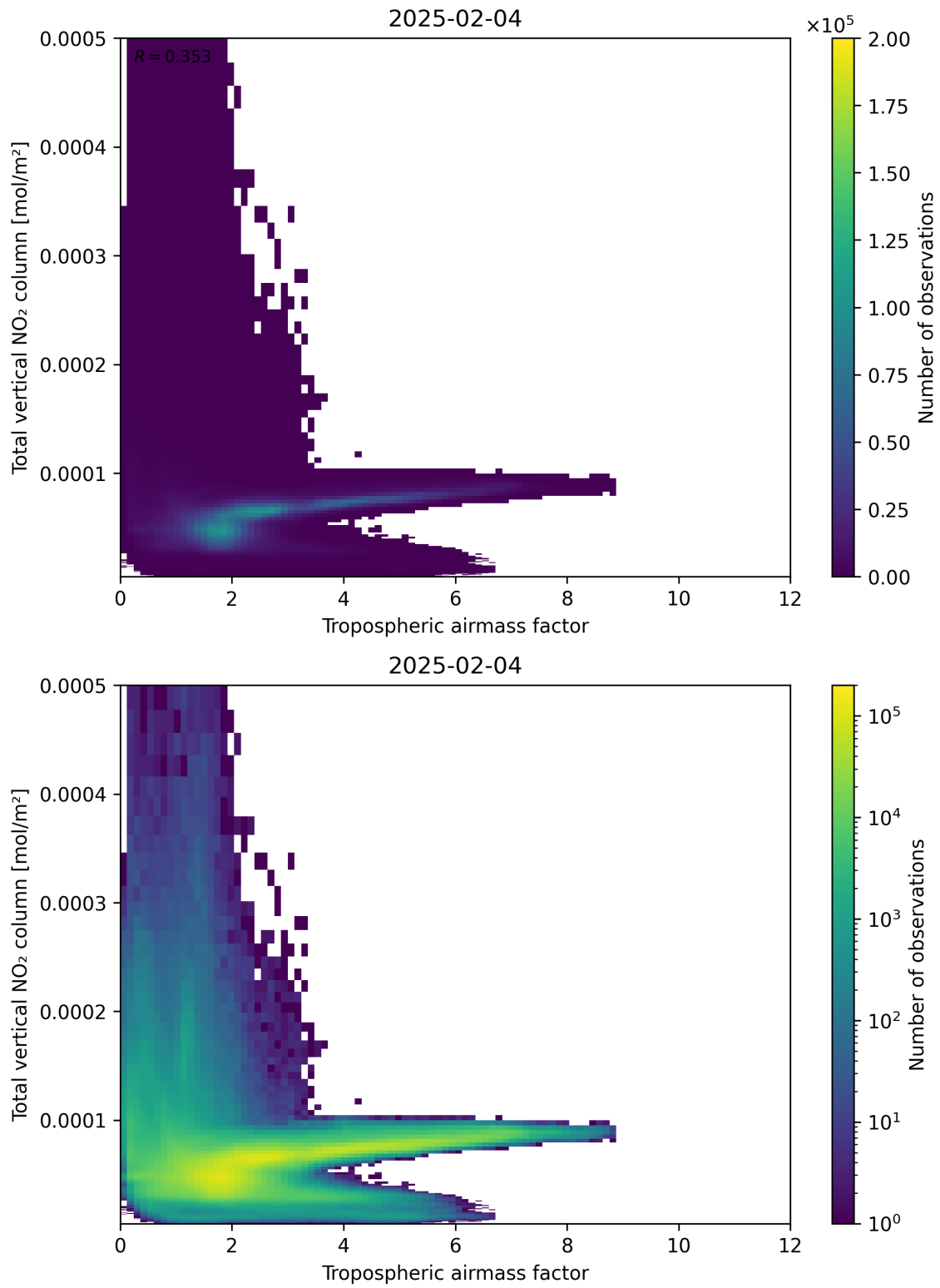
Figure 77: Scatter density plot of “Tropospheric airmass factor” against “Total vertical NO 2 column” for 2025-02-04 to 2025-02-05.
