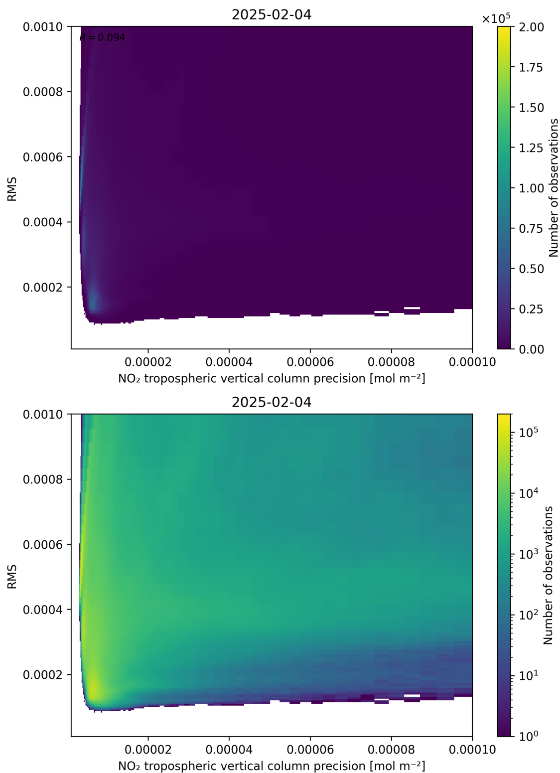
Figure 140: Scatter density plot of “NO 2 tropospheric vertical column precision” against “RMS” for 2025-02-04 to 2025-02-05.
