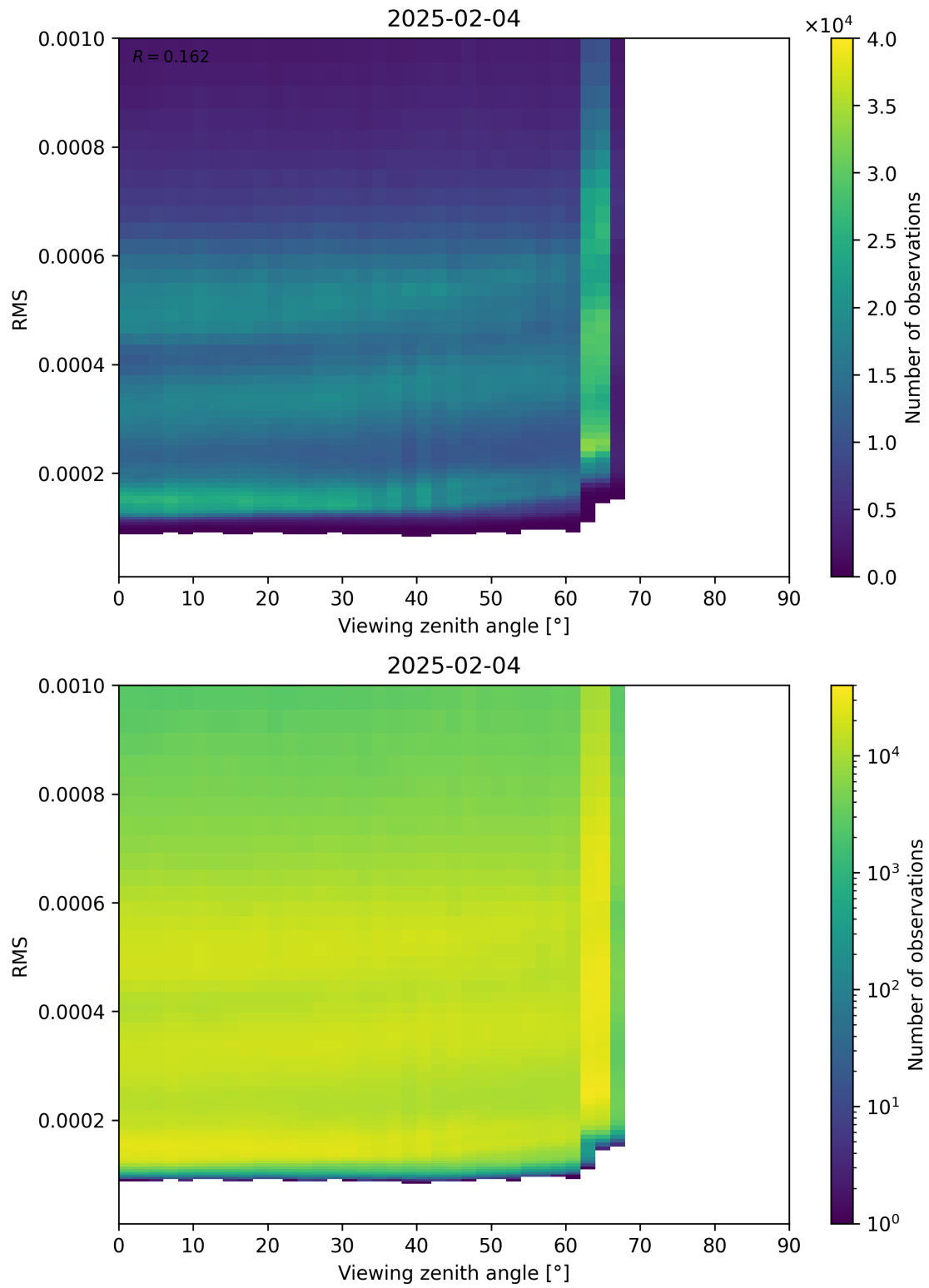
Figure 171: Scatter density plot of “Viewing zenith angle” against “RMS” for 2025-02-04 to 2025-02-05.
