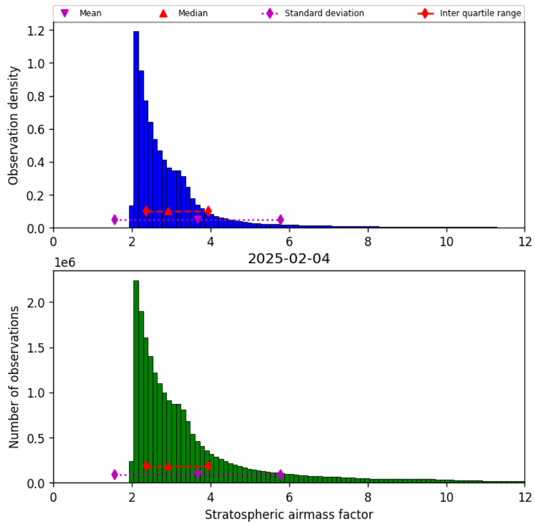
Figure 44: Histogram of “Stratospheric airmass factor” for 2025-02-04 to 2025-02-05
