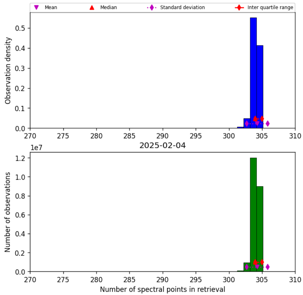
Figure 33: Histogram of “Number of spectral points in retrieval” for 2025-02-04 to 2025-02-05
