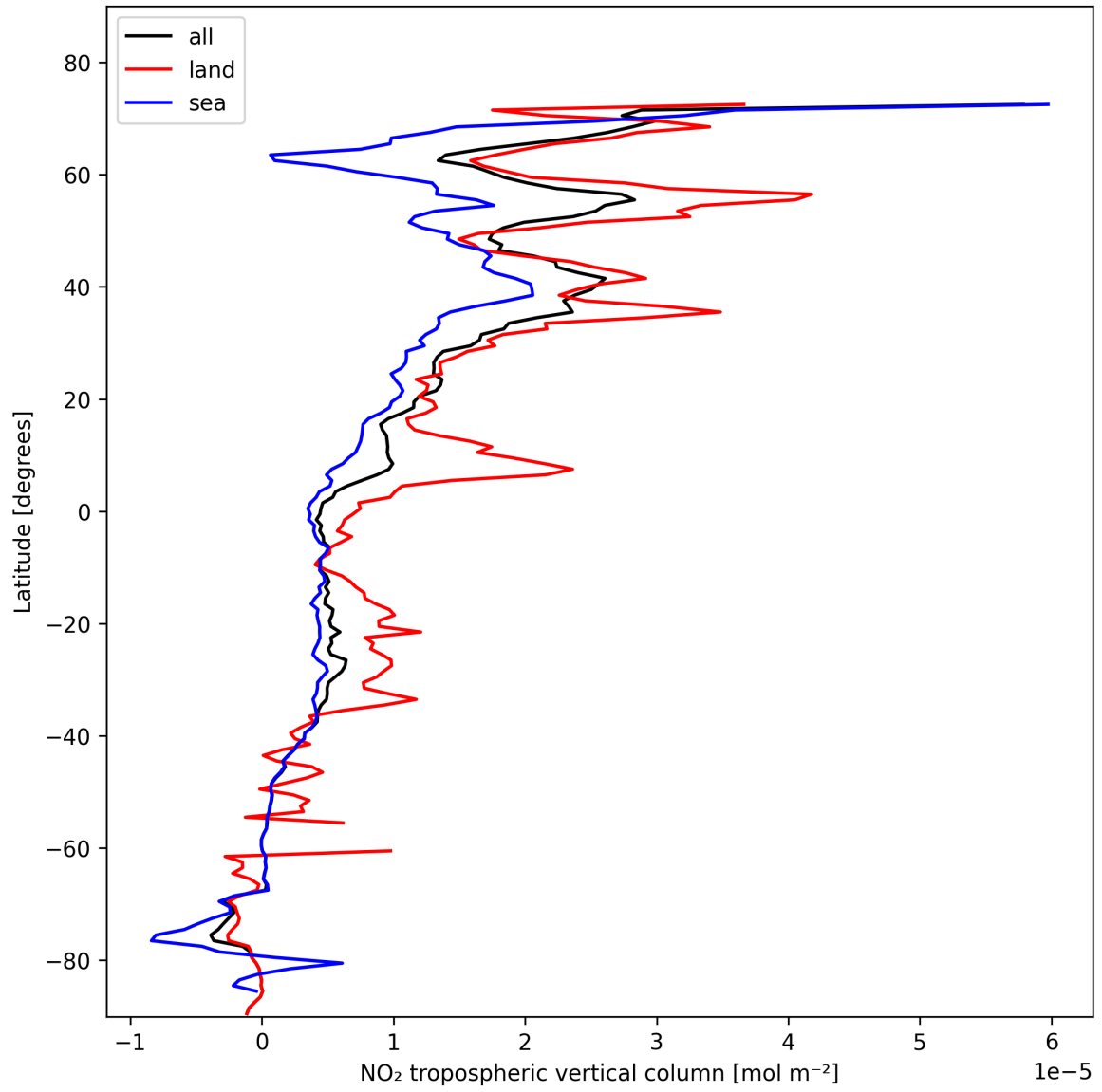
Figure 12: Zonal average of “NO 2 tropospheric vertical column” for 2025-02-04 to 2025-02-05.
