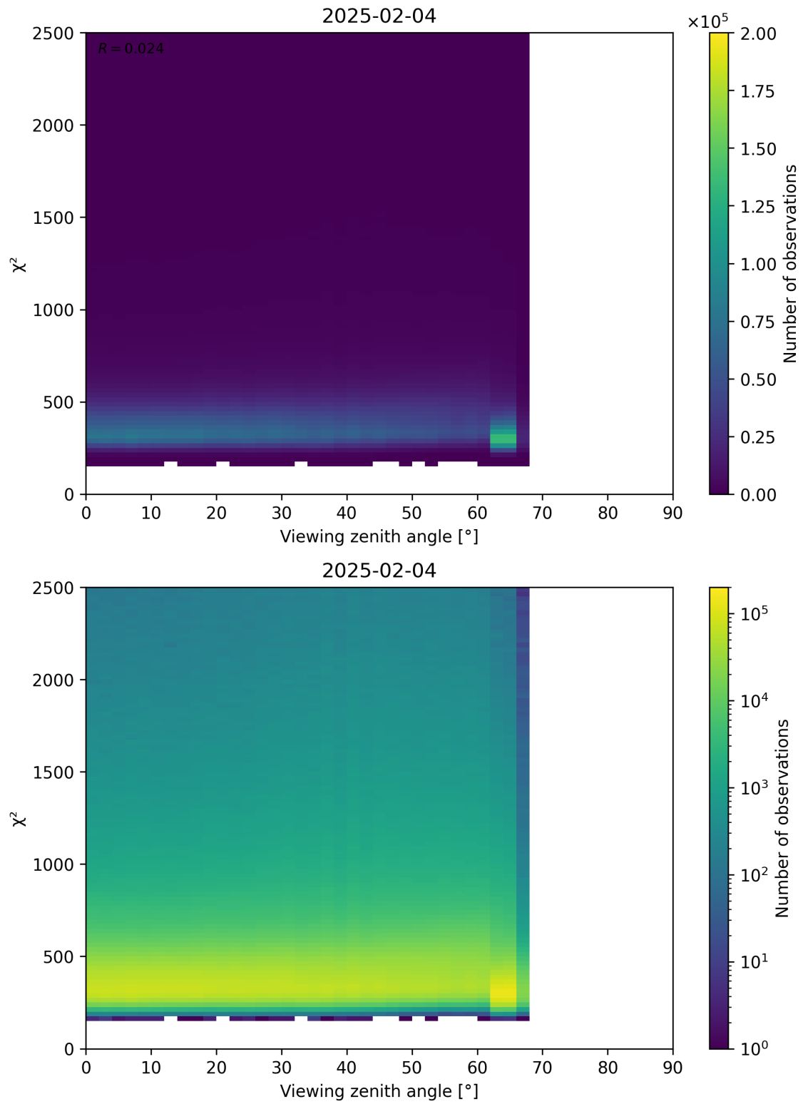
Figure 162: Scatter density plot of “Viewing zenith angle” against “ \chi^2 ” for 2025-02-04 to 2025-02-05.
