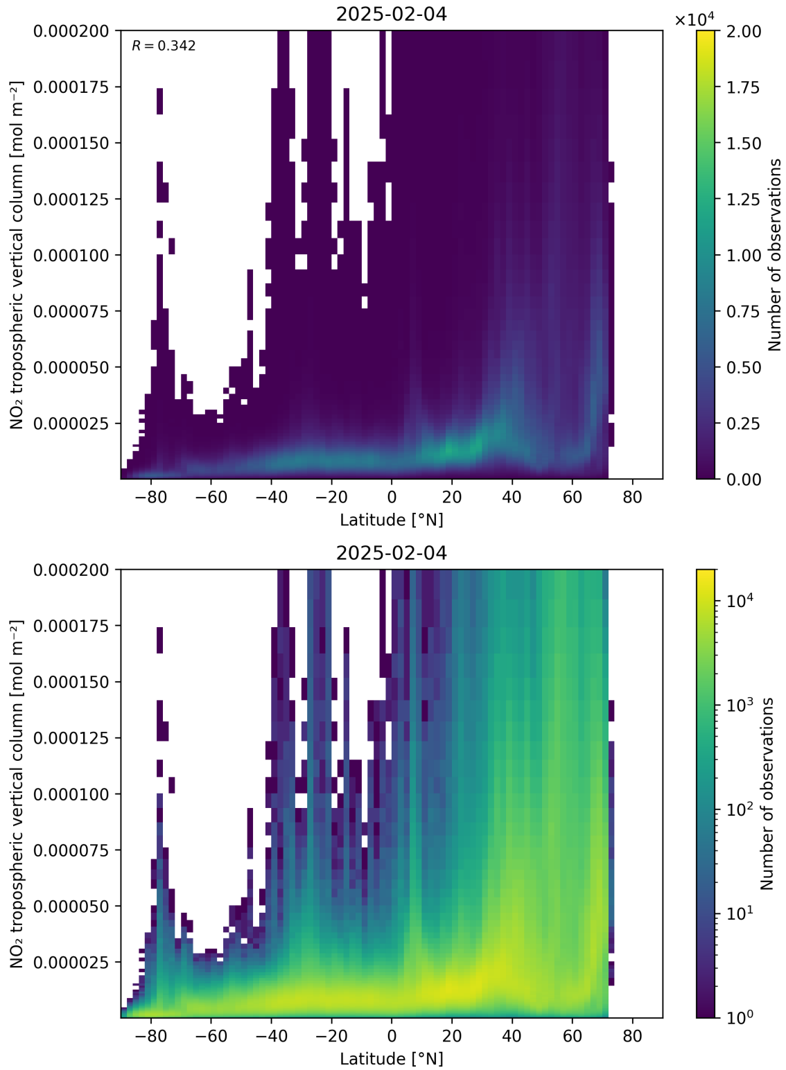
Figure 92: Scatter density plot of “Latitude” against “NO 2 tropospheric vertical column” for 2025-02-04 to 2025-02-05.
