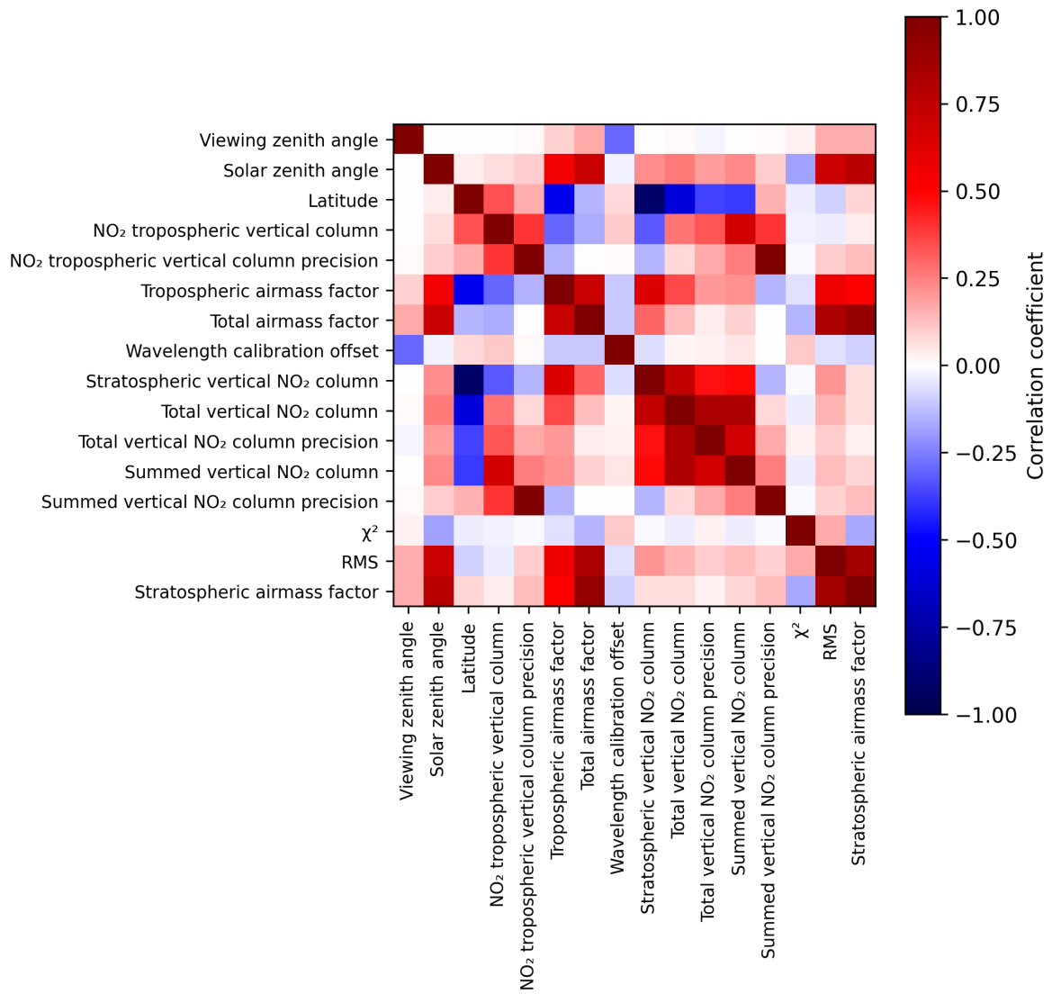
Figure 2: Map of correlation matrix for 2025-02-04 to 2025-02-05.
