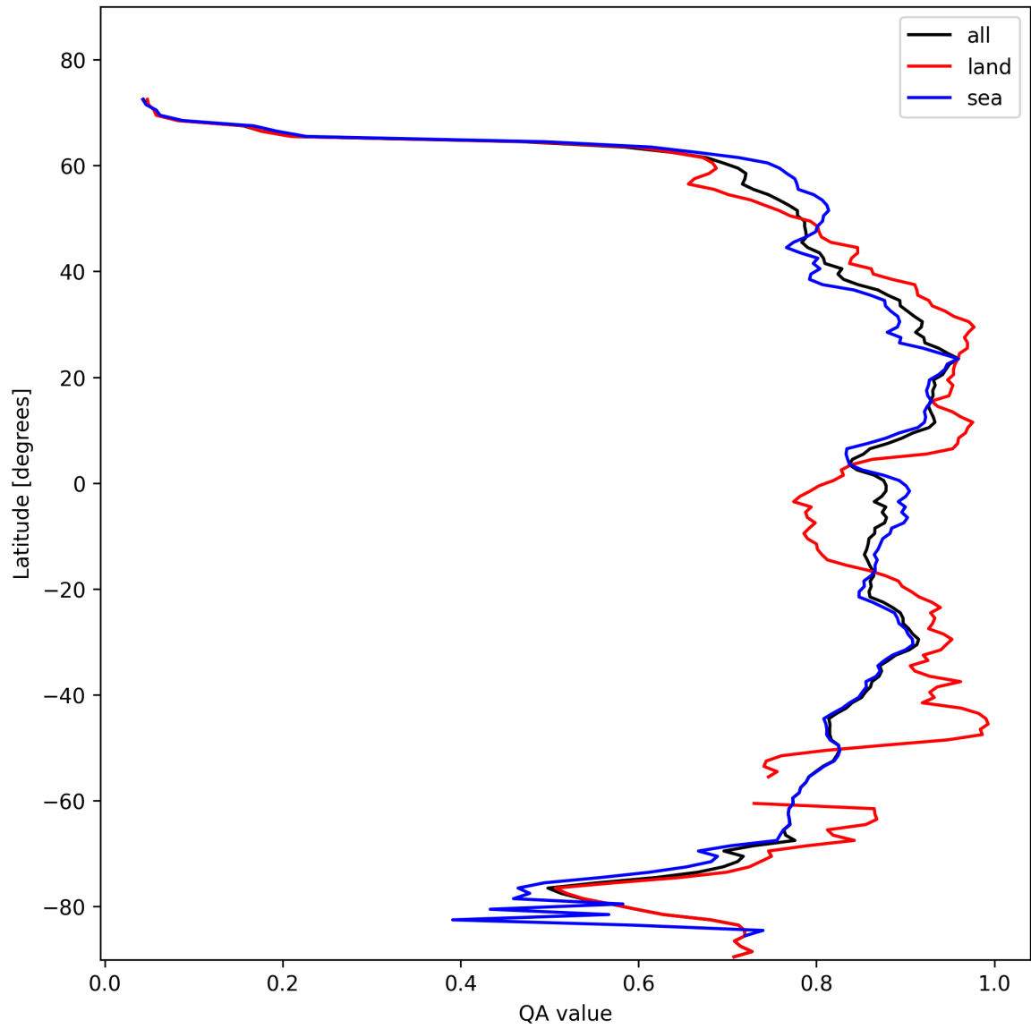
Figure 11: Zonal average of “QA value” for 2025-02-04 to 2025-02-05.
