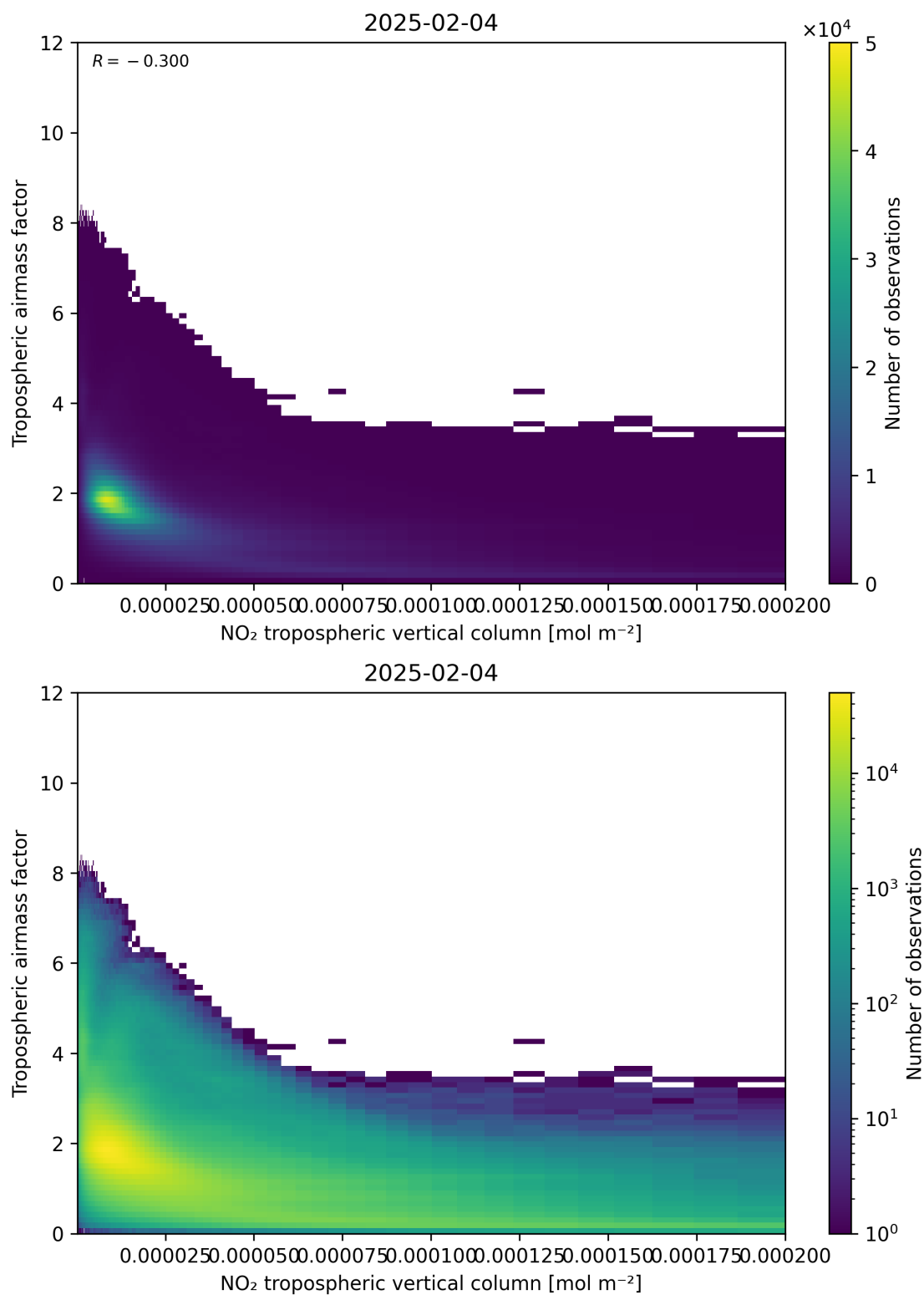
Figure 123: Scatter density plot of “NO 2 tropospheric vertical column” against “Tropospheric air mass factor” for 2025-02-04 to 2025-02-05.
