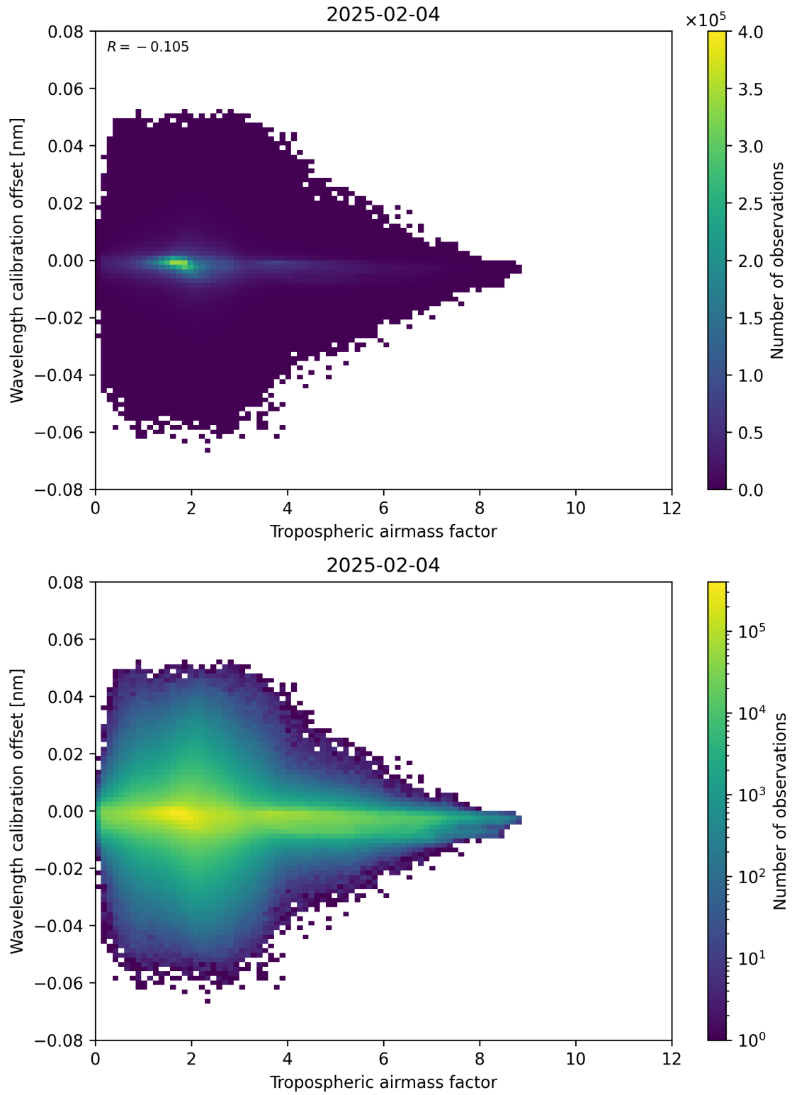
Figure 80: Scatter density plot of “Tropospheric airmass factor” against “Wavelength calibration offset” for 2025-02-04 to 2025-02-05.
