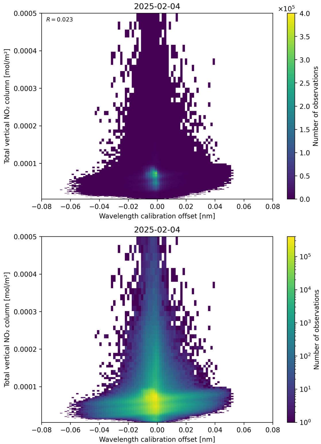
Figure 179: Scatter density plot of “Wavelength calibration offset” against “Total vertical NO 2 column” for 2025-02-04 to 2025-02-05.
