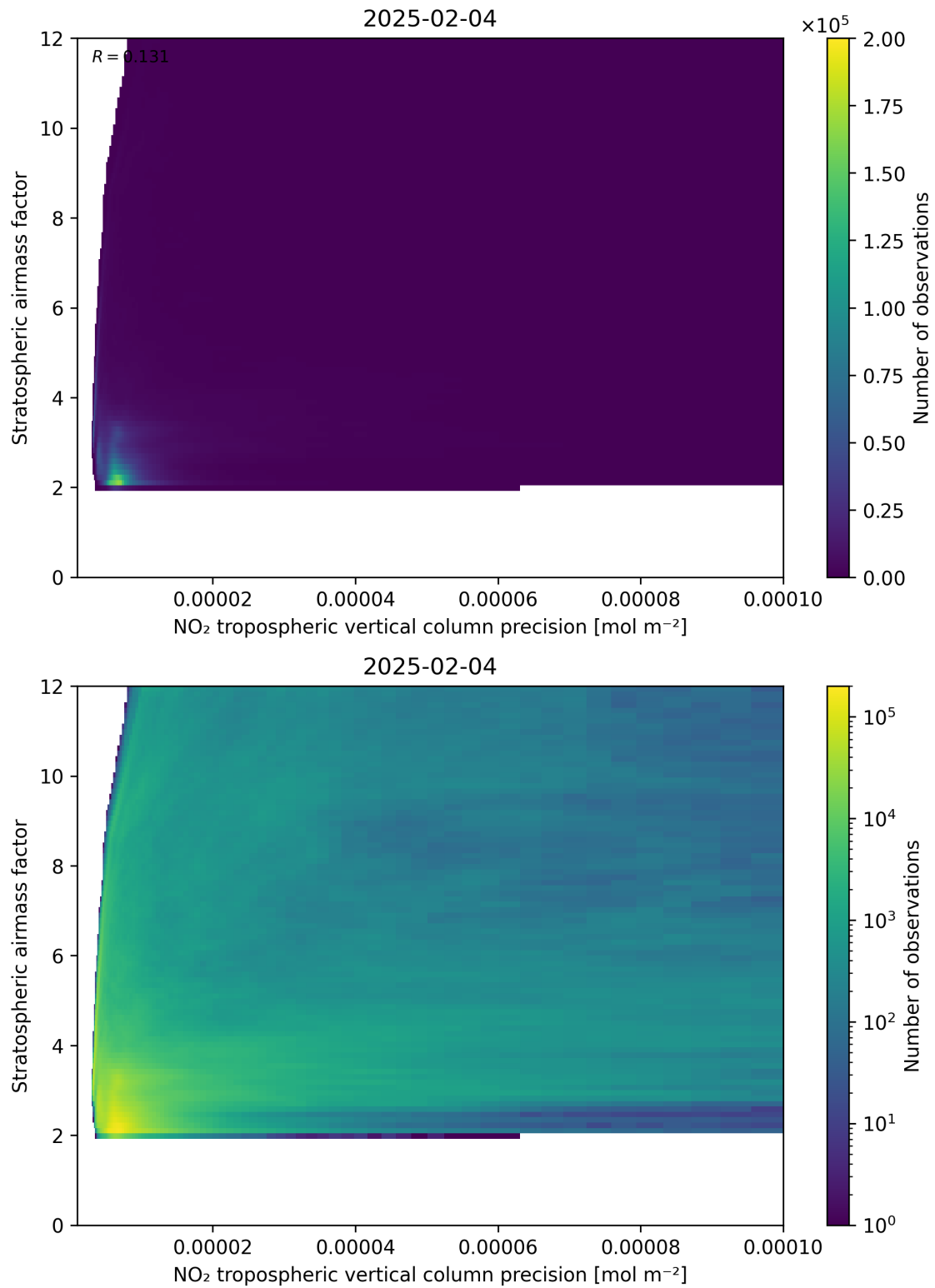
Figure 131: Scatter density plot of “NO 2 tropospheric vertical column precision” against “Stratospheric airmass factor” for 2025-02-04 to 2025-02-05.
