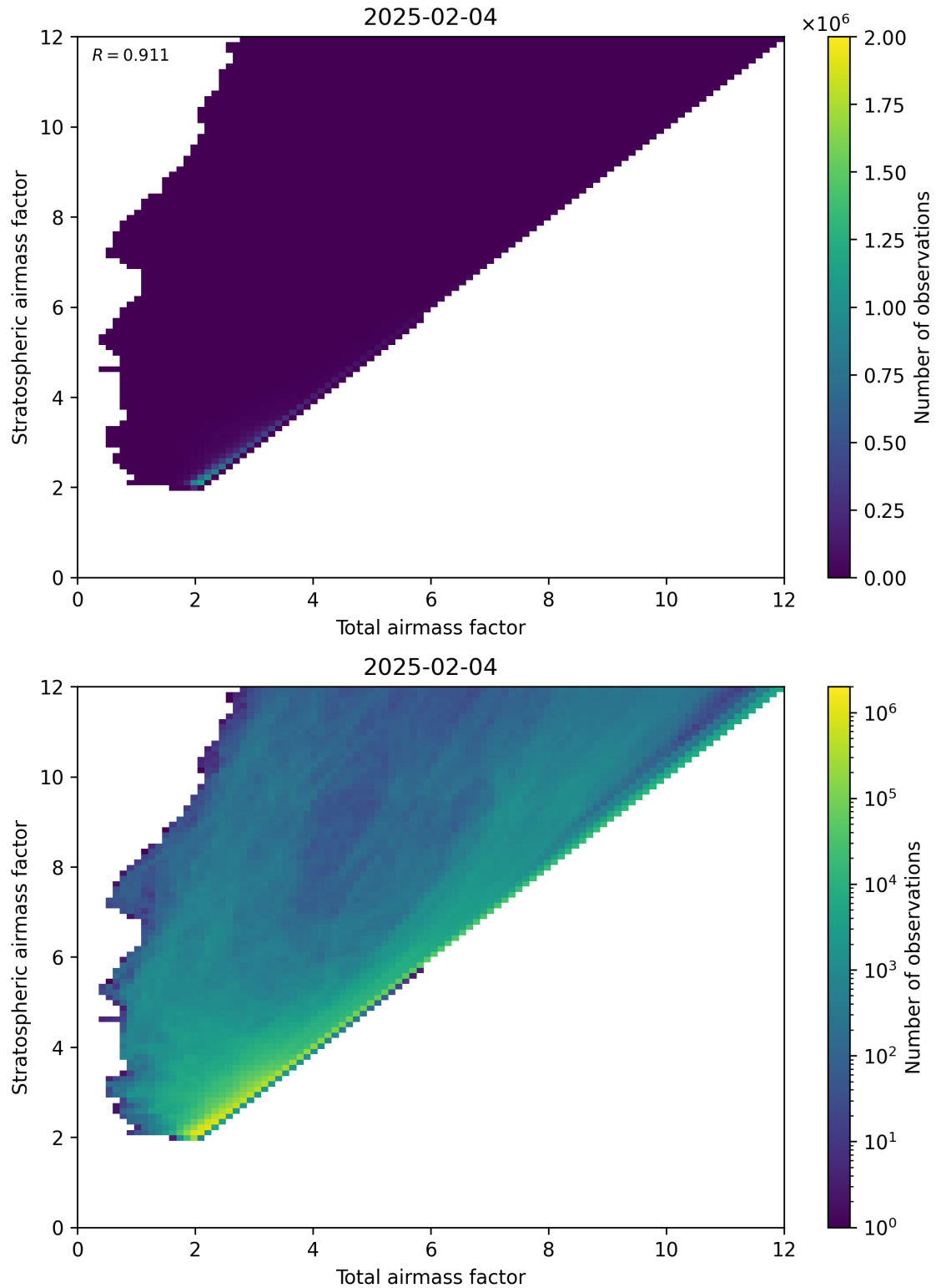
Figure 62: Scatter density plot of “Total airmass factor” against “Stratospheric airmass factor” for 2025-02-04 to 2025-02-05.
