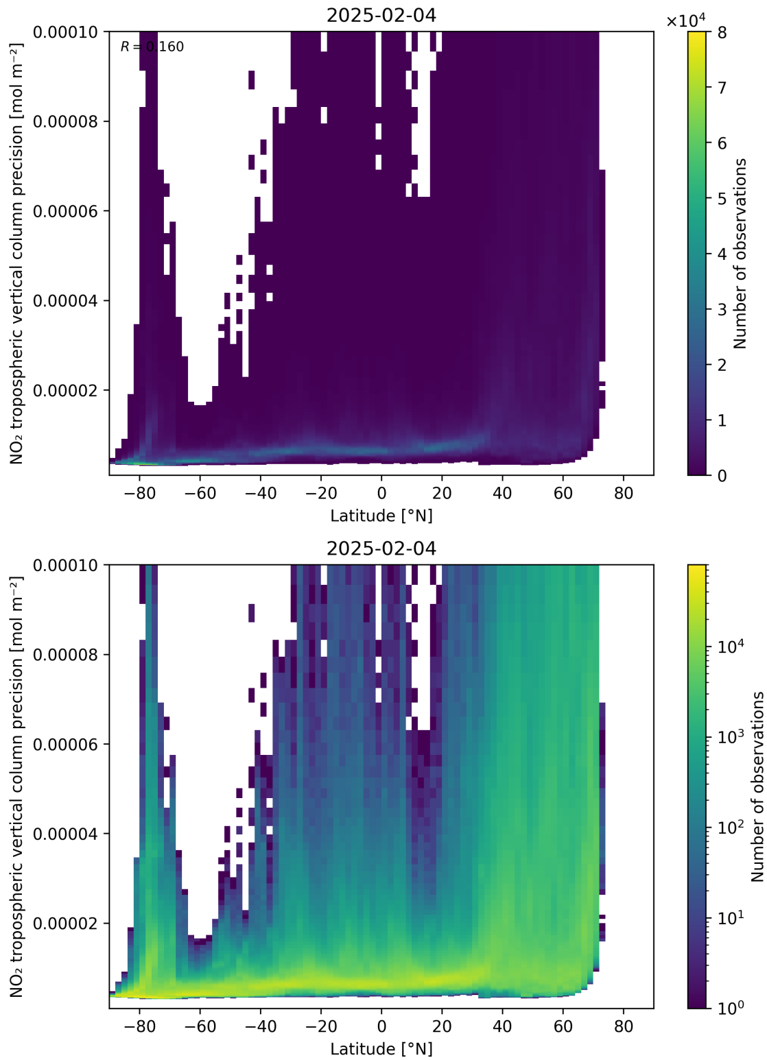
Figure 93: Scatter density plot of “Latitude” against “NO 2 tropospheric vertical column precision” for 2025-02-04 to 2025-02-05.
