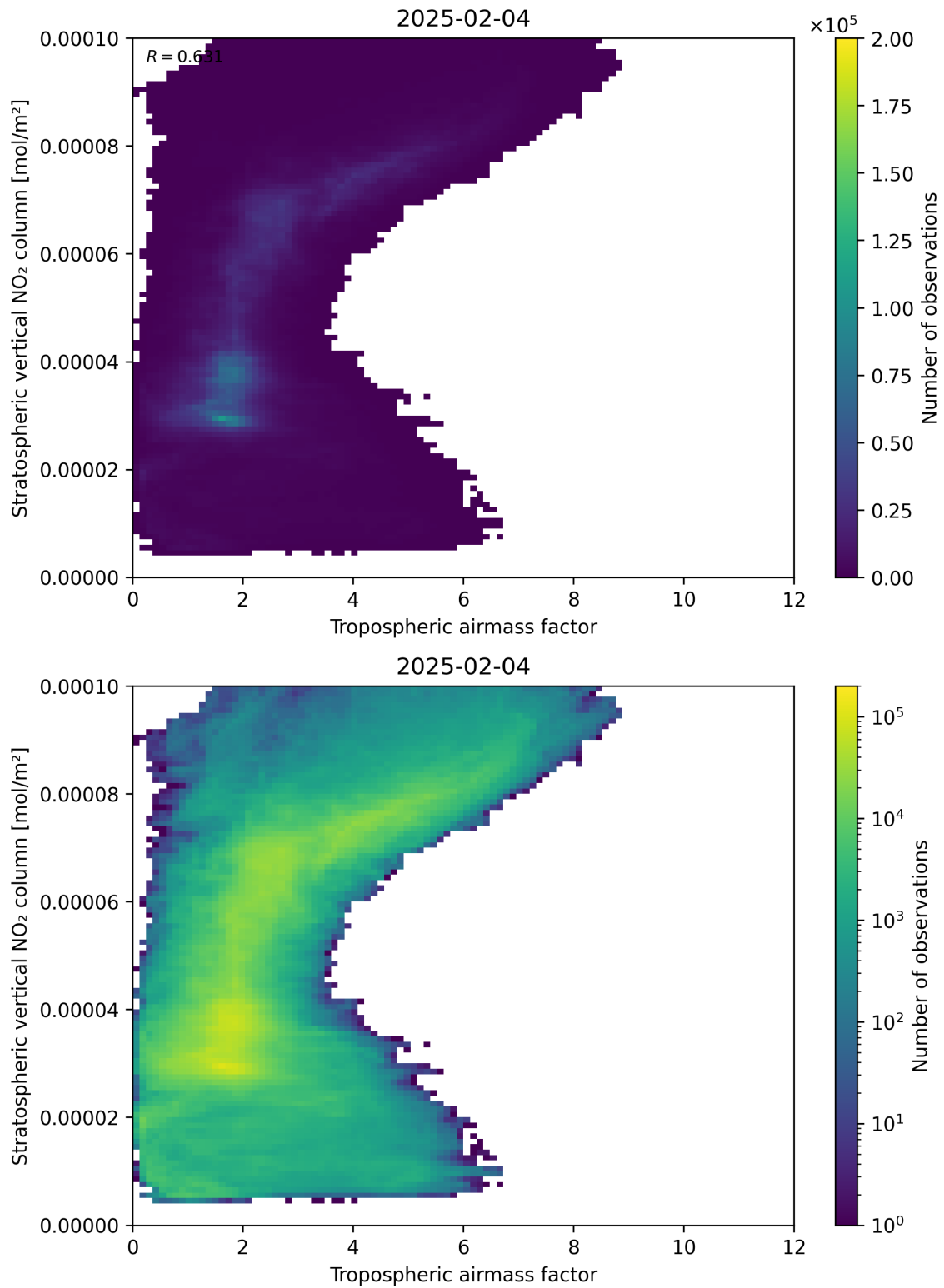
Figure 74: Scatter density plot of “Tropospheric air mass factor” against “Stratospheric vertical NO 2 column” for 2025-02-04 to 2025-02-05.
