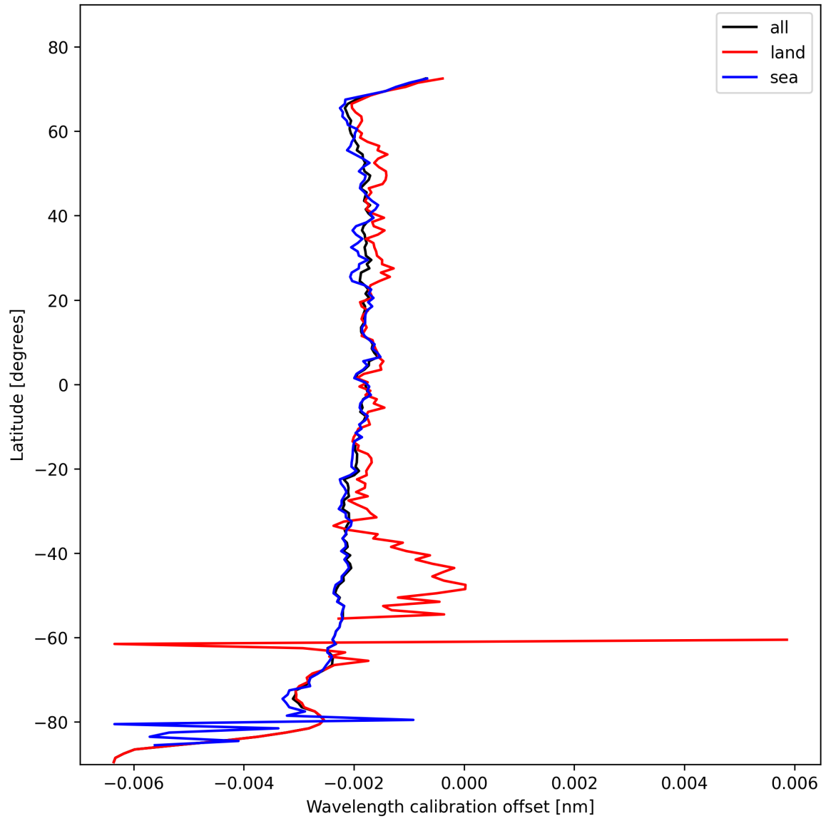
Figure 18: Zonal average of “Wavelength calibration offset” for 2025-02-04 to 2025-02-05.
