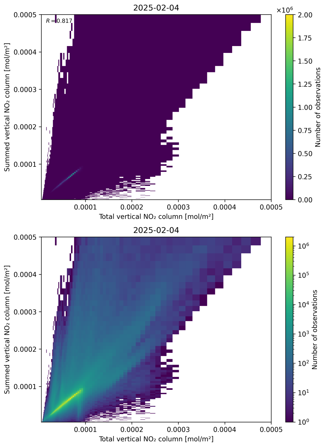
Figure 112: Scatter density plot of “Total vertical NO 2 column” against “Summed vertical NO 2 column” for 2025-02-04 to 2025-02-05.
