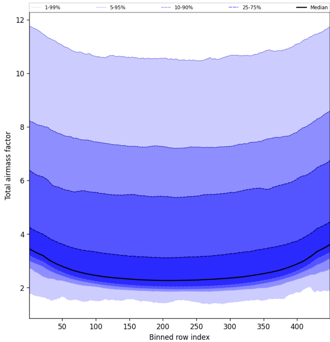
Figure 49: Along track statistics of “Total airmass factor” for 2025-02-04 to 2025-02-05
