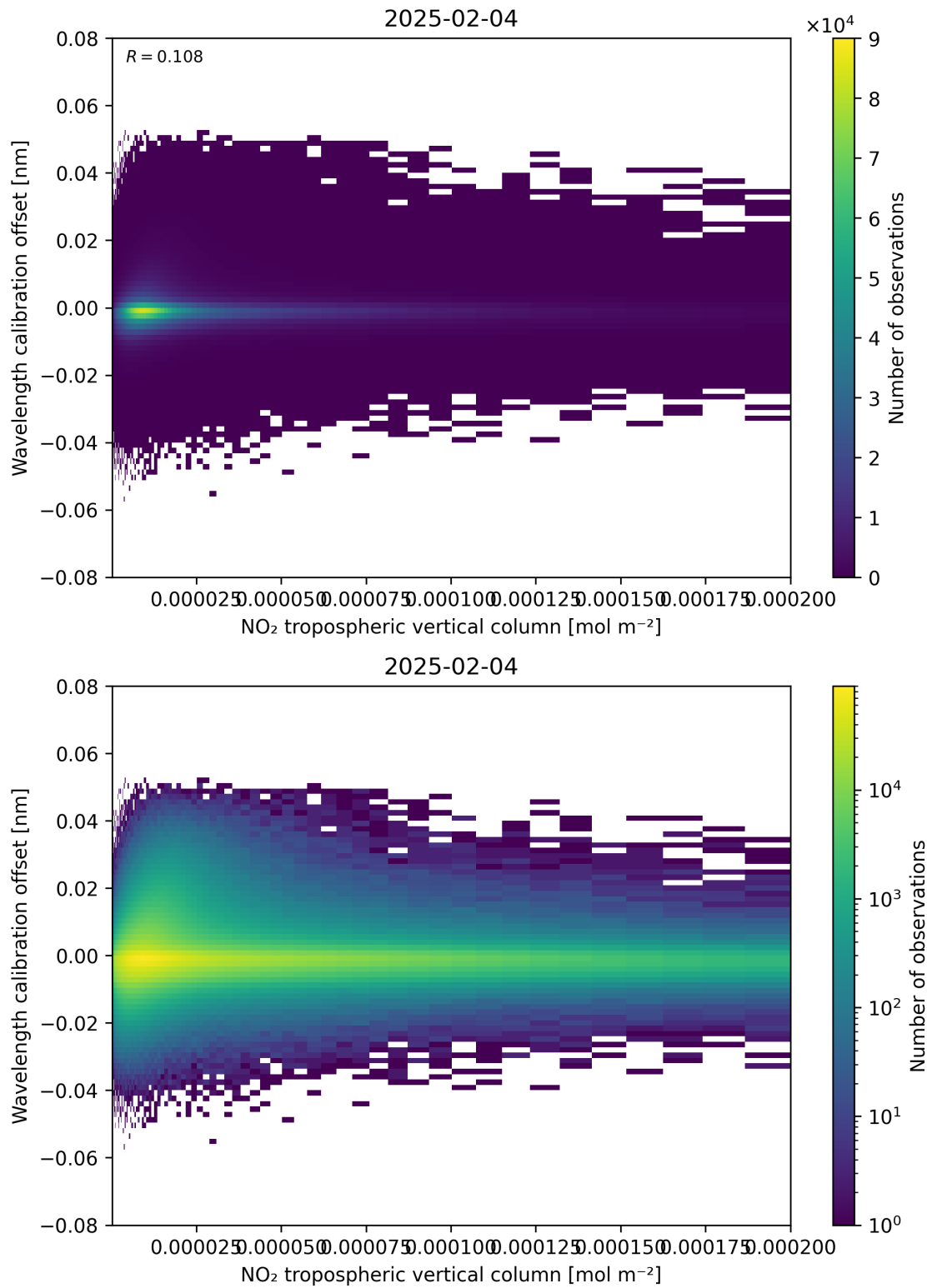
Figure 143: Scatter density plot of “NO 2 tropospheric vertical column” against “Wavelength calibration offset” for 2025-02-04 to 2025-02-05.
