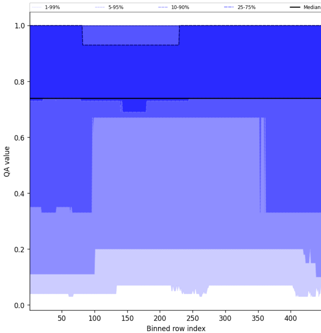
Figure 45: Along track statistics of “QA value” for 2025-02-04 to 2025-02-05
