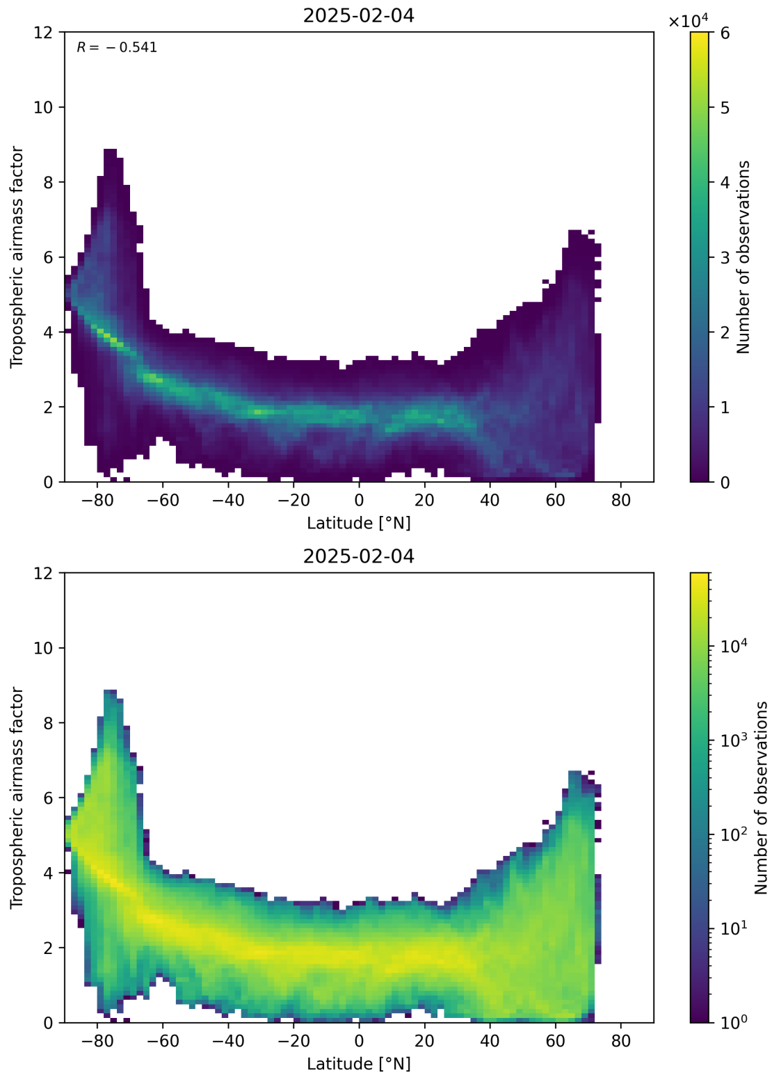
Figure 85: Scatter density plot of “Latitude” against “Tropospheric airmass factor” for 2025-02-04 to 2025-02-05.
