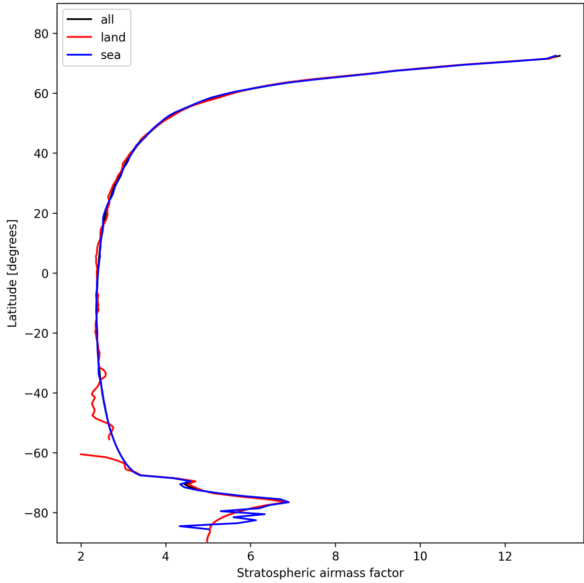
Figure 27: Zonal average of “Stratospheric airmass factor” for 2025-02-04 to 2025-02-05.
