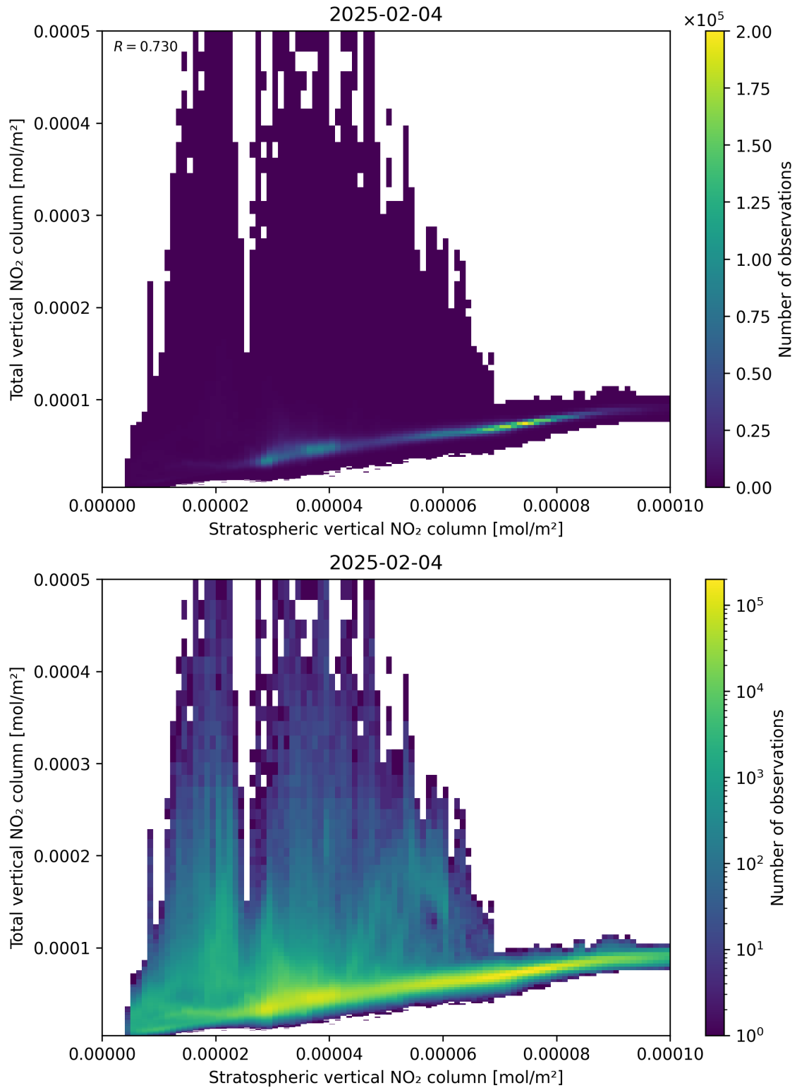
Figure 100: Scatter density plot of “Stratospheric vertical NO 2 column” against “Total vertical NO 2 column” for 2025-02-04 to 2025-02-05.
