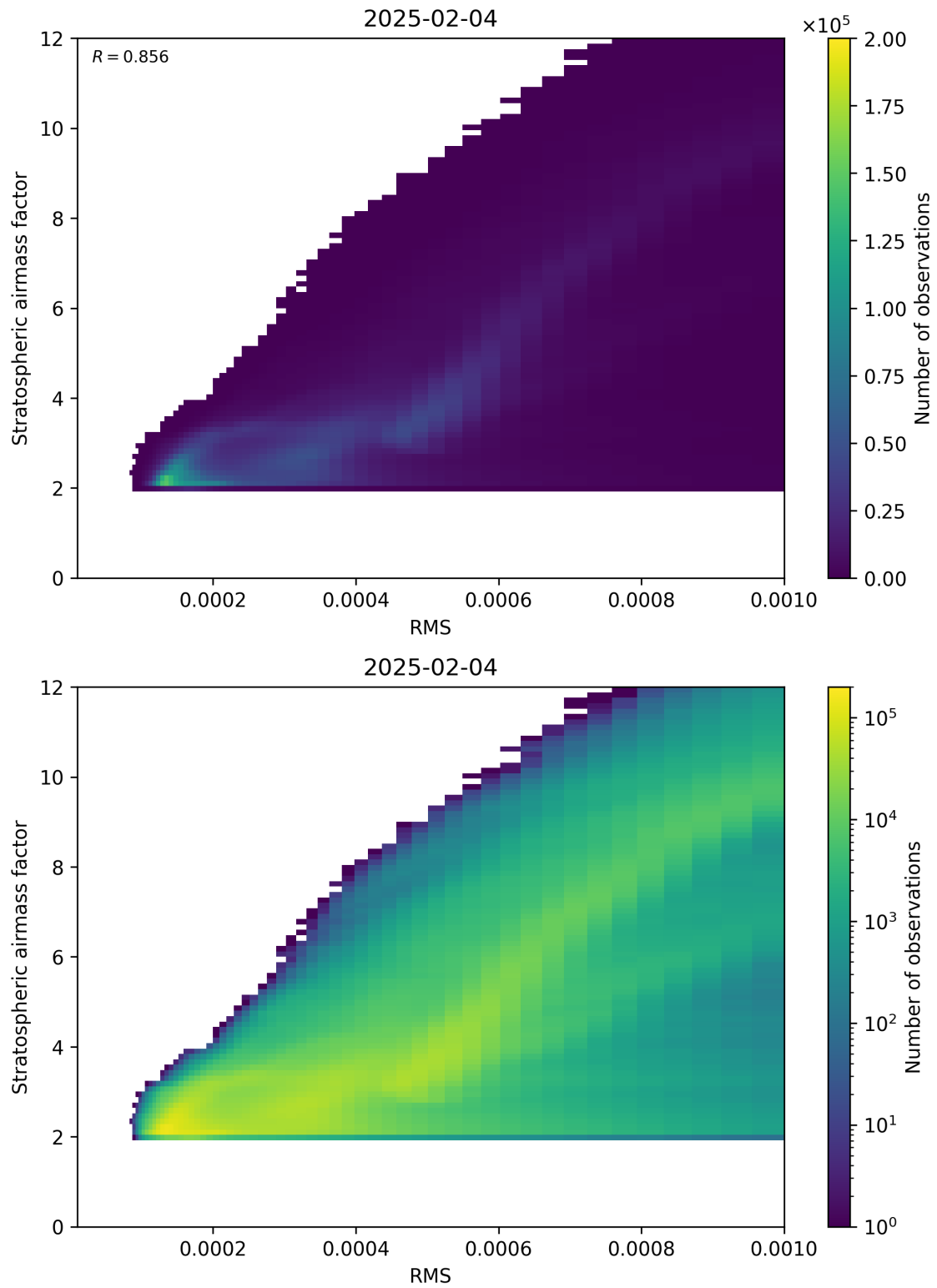
Figure 144: Scatter density plot of “RMS” against “Stratospheric airmass factor” for 2025-02-04 to 2025-02-05.
