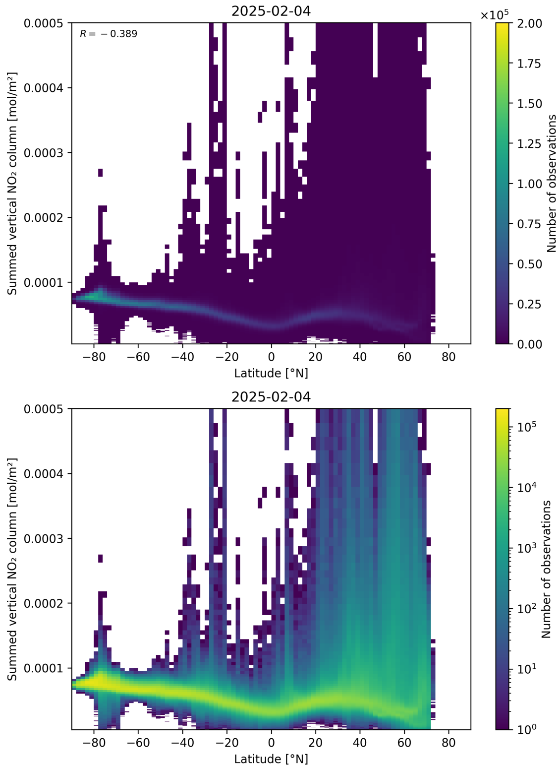
Figure 88: Scatter density plot of “Latitude” against “Summed vertical NO 2 column” for 2025-02-04 to 2025-02-05.
