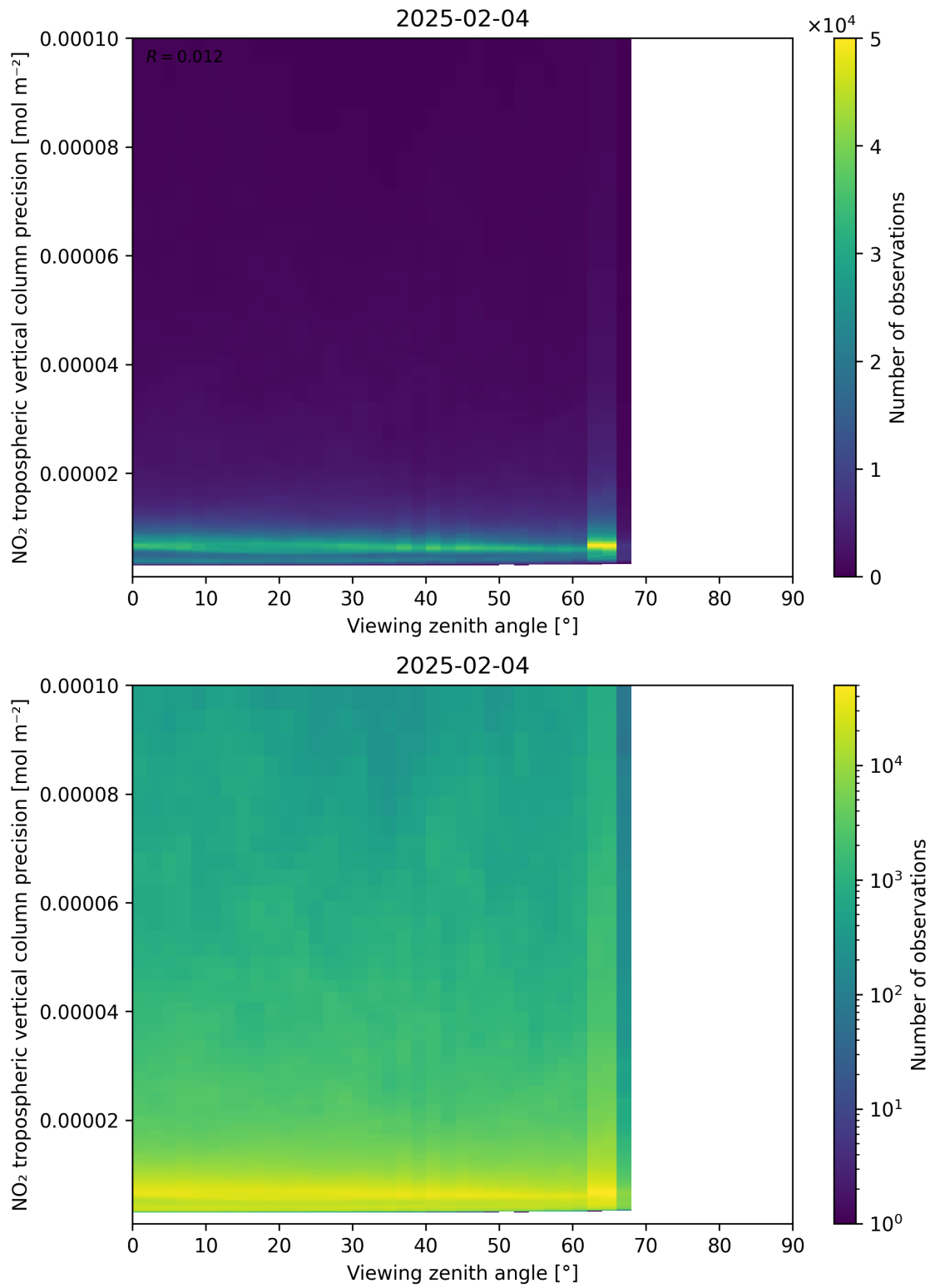
Figure 170: Scatter density plot of “Viewing zenith angle” against “NO 2 tropospheric vertical column precision” for 2025-02-04 to 2025-02-05.
