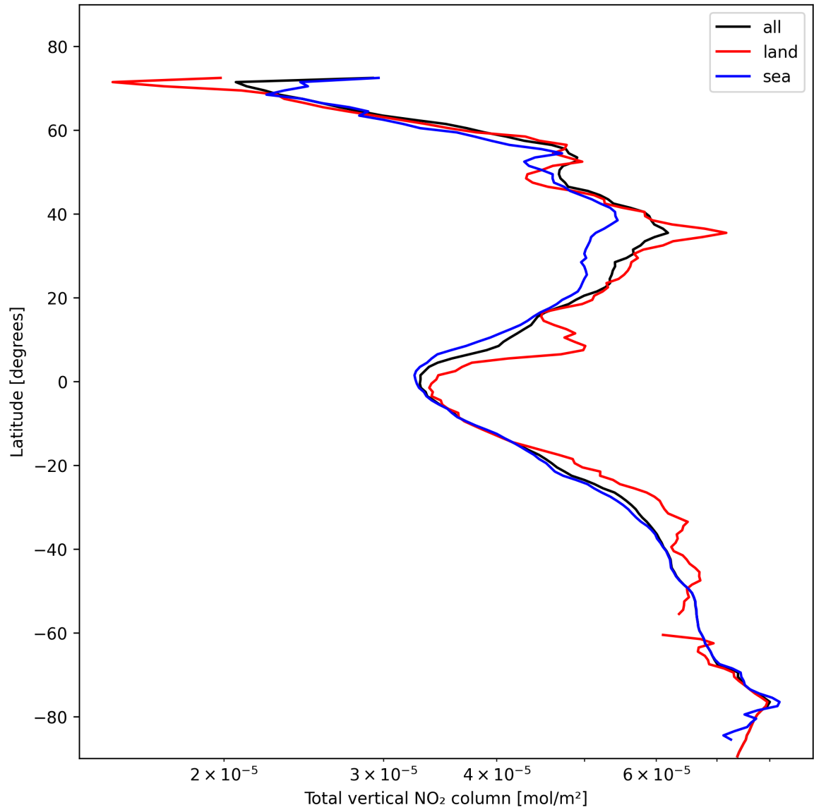
Figure 21: Zonal average of “Total vertical NO 2 column” for 2025-02-04 to 2025-02-05.
