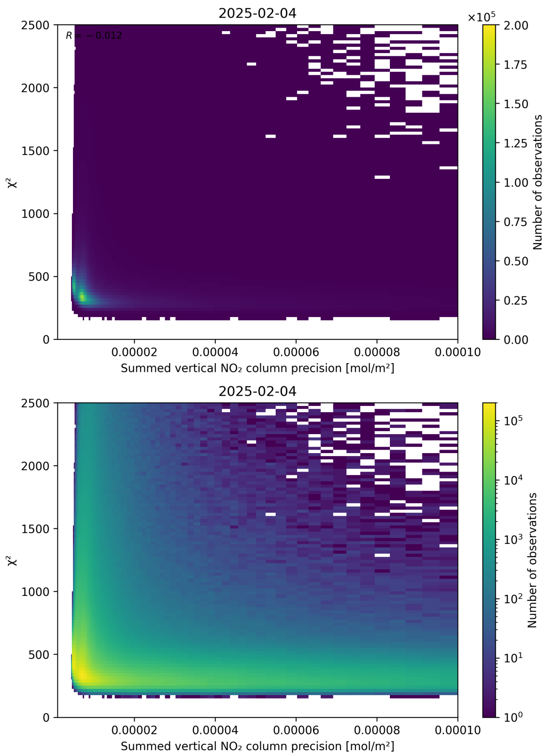
Figure 107: Scatter density plot of “Summed vertical NO 2 column precision” against “ \chi^2 ” for 2025-02-04 to 2025-02-05.
