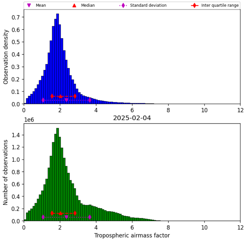
Figure 31: Histogram of “Tropospheric airmass factor” for 2025-02-04 to 2025-02-05
