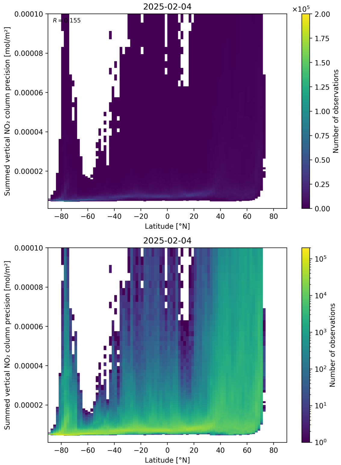
Figure 89: Scatter density plot of “Latitude” against “Summed vertical NO 2 column precision” for 2025-02-04 to 2025-02-05.
