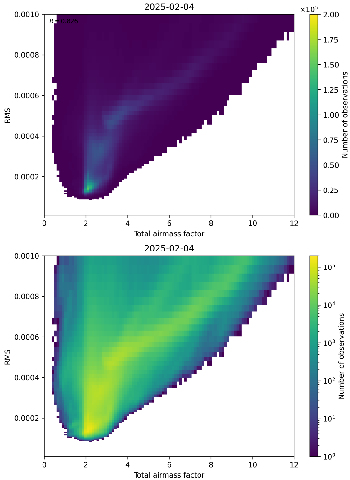
Figure 69: Scatter density plot of “Total airmass factor” against “RMS” for 2025-02-04 to 2025-02-05.
