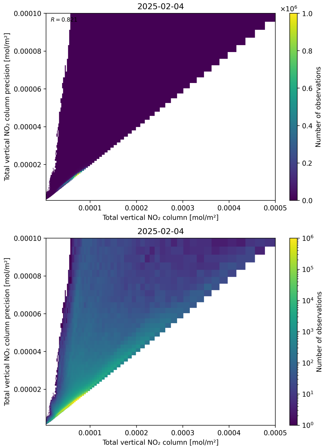
Figure 114: Scatter density plot of “Total vertical NO 2 column” against “Total vertical NO 2 column precision” for 2025-02-04 to 2025-02-05.
