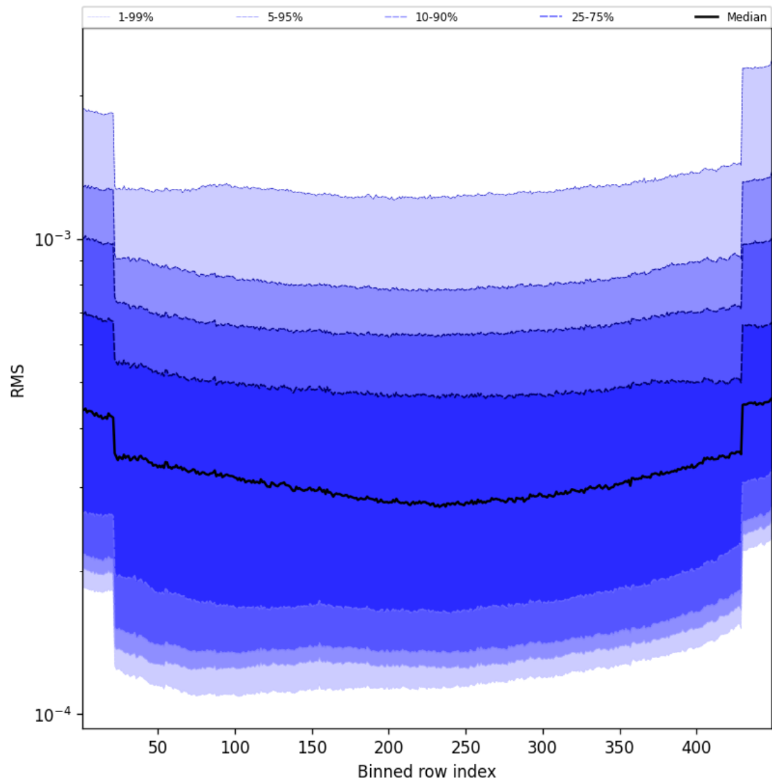
Figure 60: Along track statistics of “RMS” for 2025-02-04 to 2025-02-05
