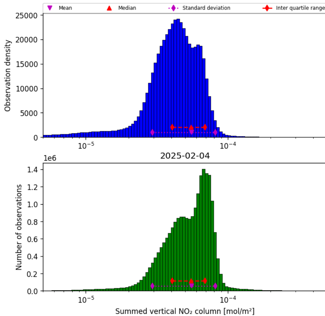
Figure 40: Histogram of “Summed vertical NO 2 column” for 2025-02-04 to 2025-02-05
