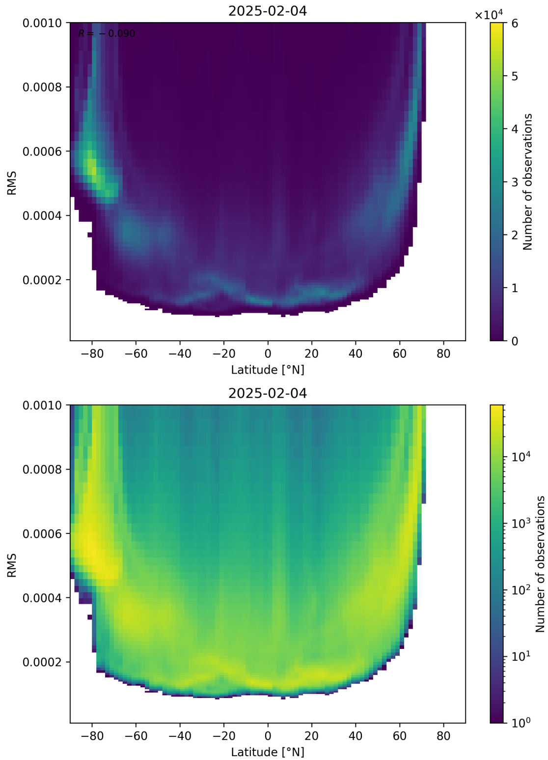
Figure 94: Scatter density plot of “Latitude” against “RMS” for 2025-02-04 to 2025-02-05.
