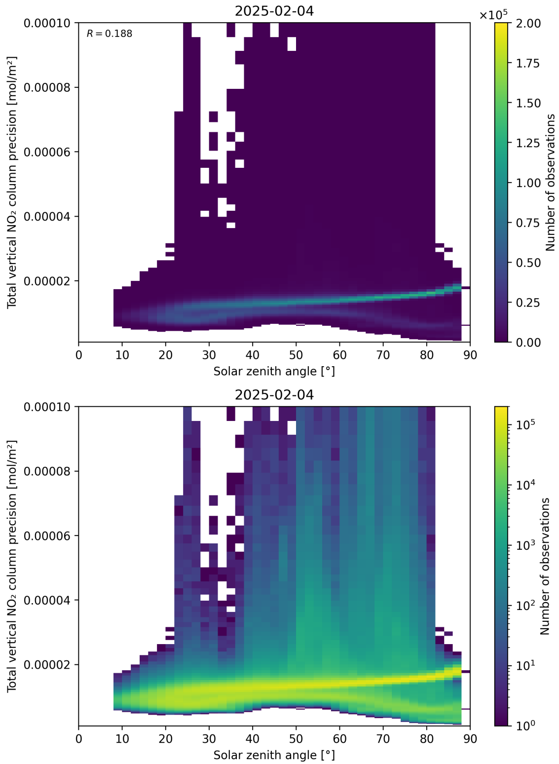
Figure 154: Scatter density plot of “Solar zenith angle” against “Total vertical NO 2 column precision” for 2025-02-04 to 2025-02-05.
