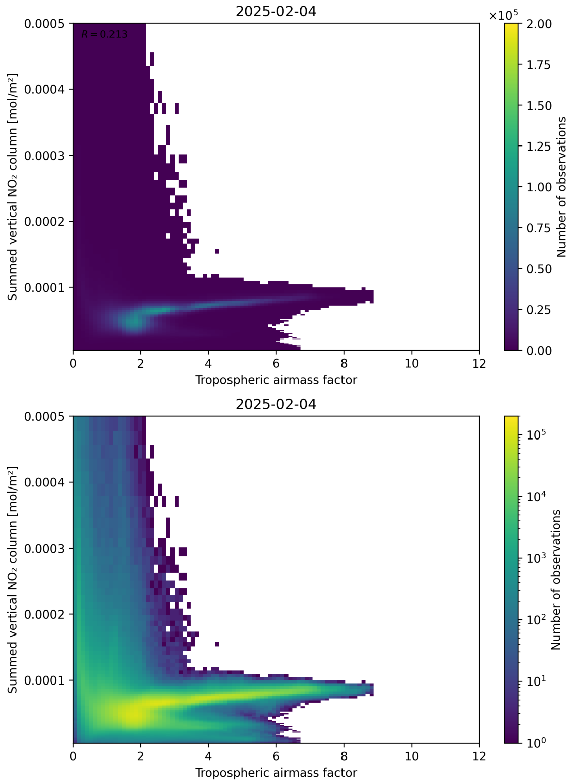
Figure 75: Scatter density plot of “Tropospheric air mass factor” against “Summed vertical NO 2 column” for 2025-02-04 to 2025-02-05.
