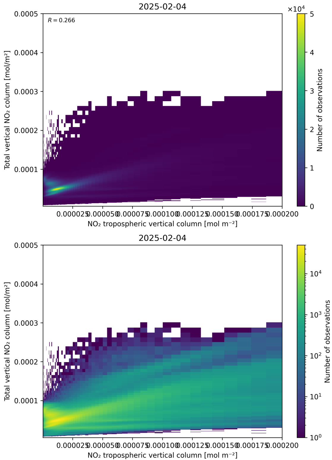
Figure 128: Scatter density plot of “NO 2 tropospheric vertical column” against “Total vertical NO 2 column” for 2025-02-04 to 2025-02-05.
