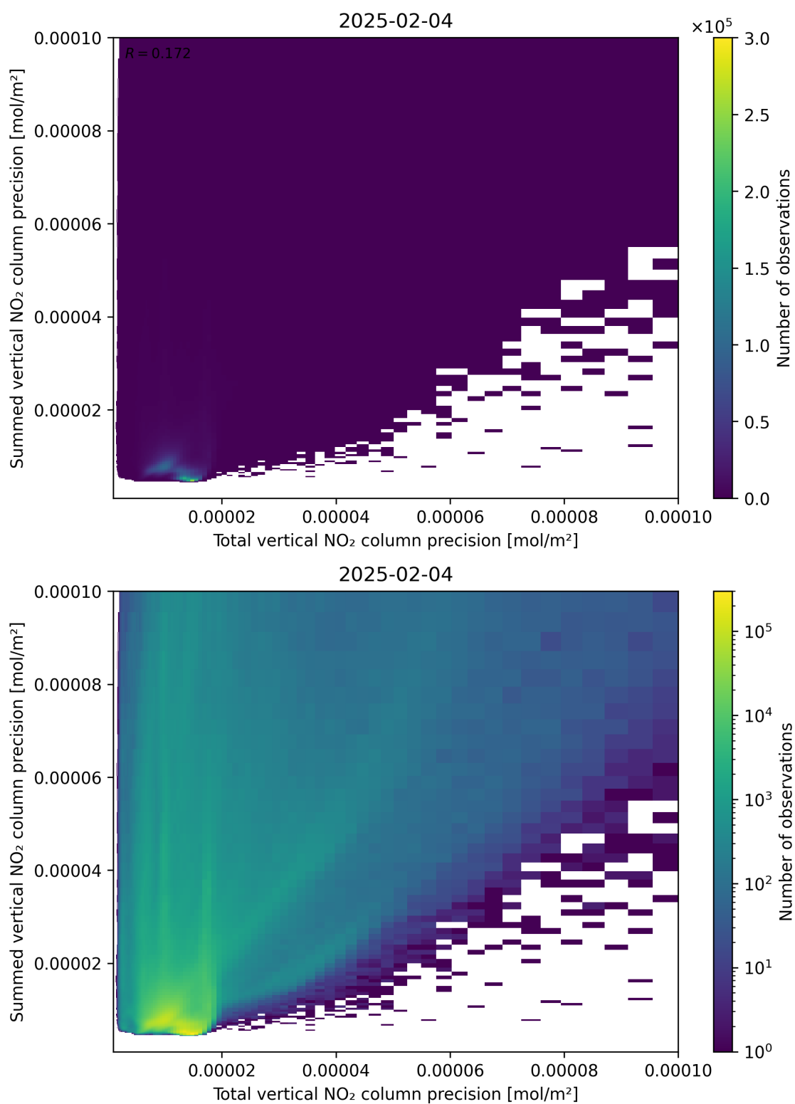
Figure 118: Scatter density plot of “Total vertical NO 2 column precision” against “Summed vertical NO 2 column precision” for 2025-02-04 to 2025-02-05.
