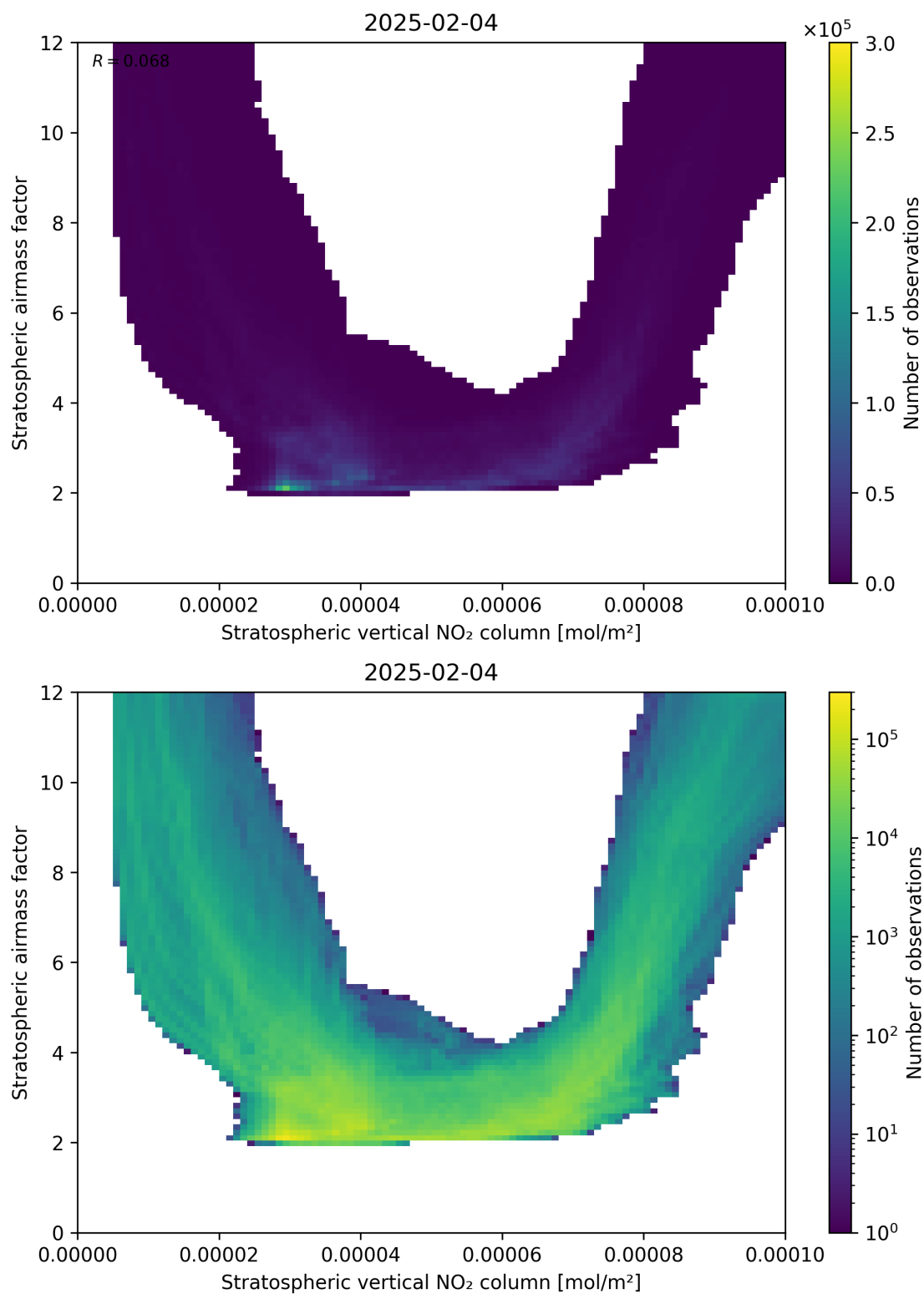
Figure 96: Scatter density plot of “Stratospheric vertical NO 2 column” against “Stratospheric airmass factor” for 2025-02-04 to 2025-02-05.
