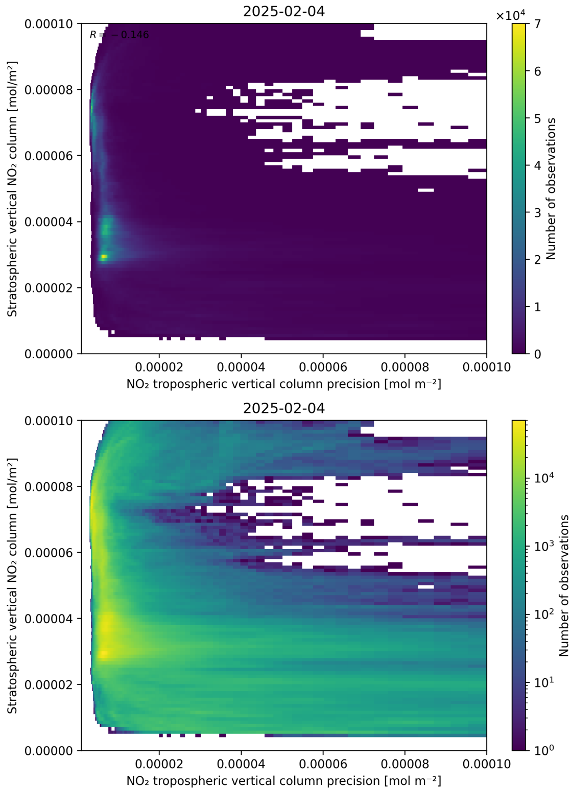
Figure 135: Scatter density plot of “NO 2 tropospheric vertical column precision” against “Stratospheric vertical NO 2 column” for 2025-02-04 to 2025-02-05.
