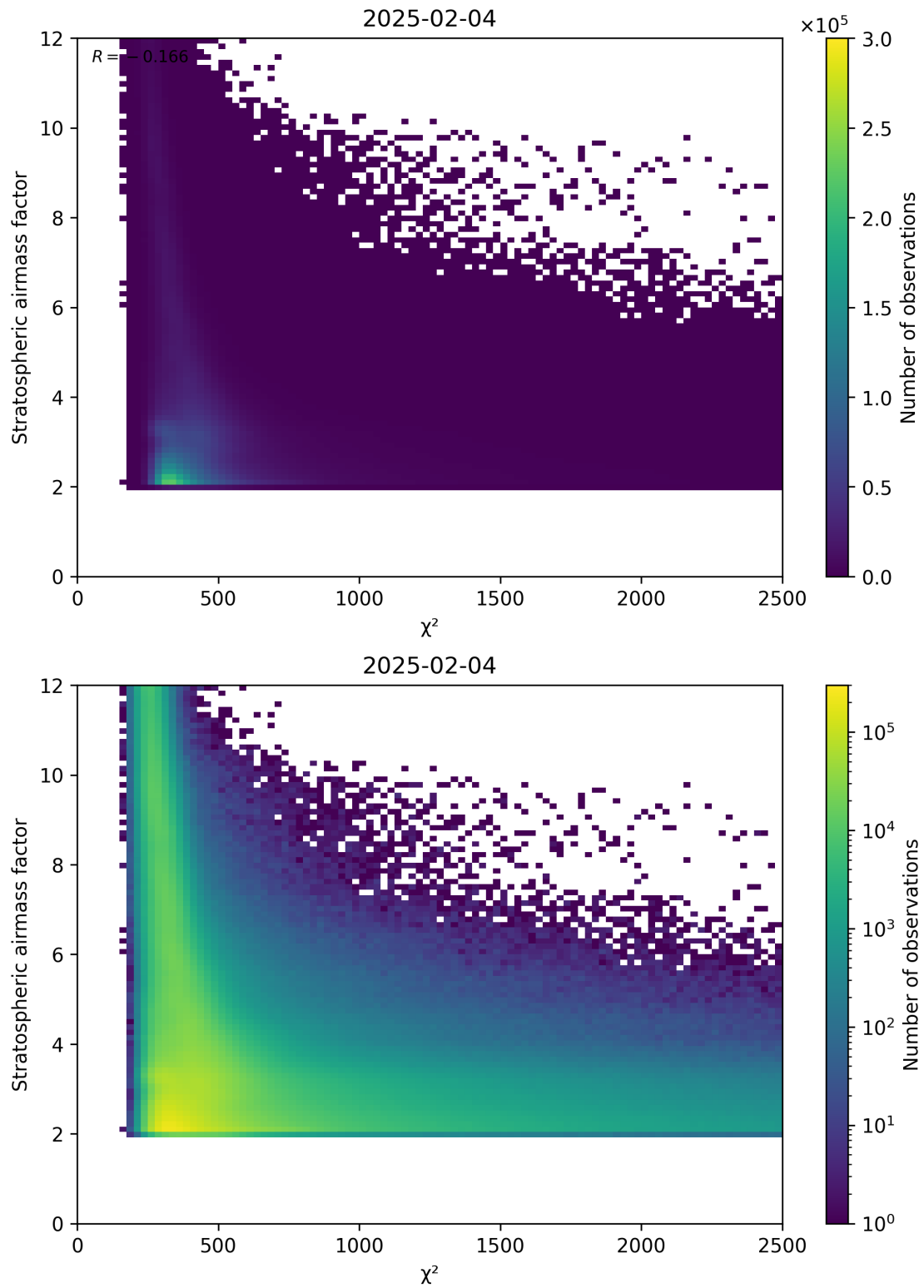
Figure 81: Scatter density plot of “ \chi^2 ” against “Stratospheric airmass factor” for 2025-02-04 to 2025-02-05.
