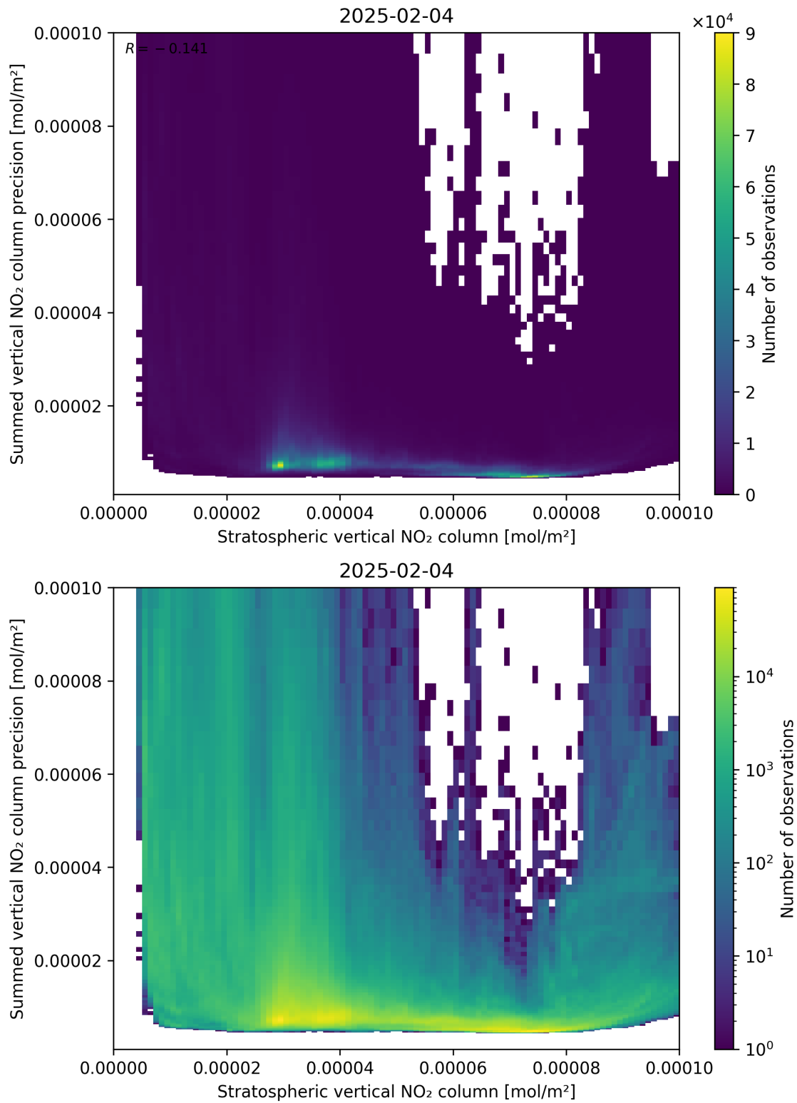
Figure 99: Scatter density plot of “Stratospheric vertical NO 2 column” against “Summed vertical NO 2 column precision” for 2025-02-04 to 2025-02-05.
