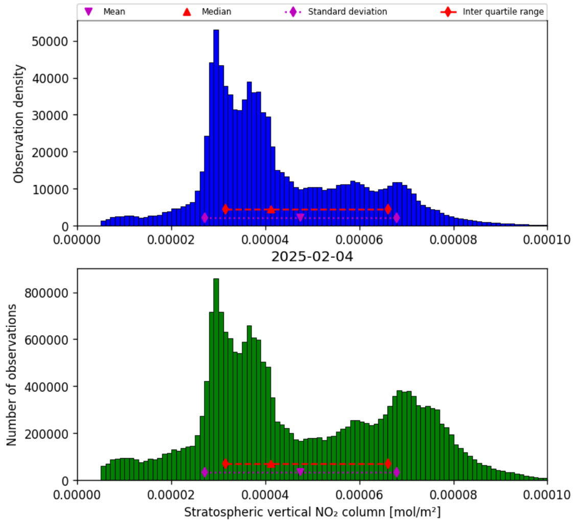
Figure 36: Histogram of “Stratospheric vertical NO 2 column” for 2025-02-04 to 2025-02-05
