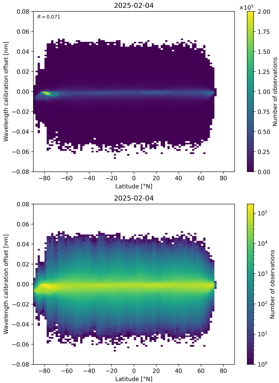
Figure 95: Scatter density plot of “Latitude” against “Wavelength calibration offset” for 2025-02-04 to 2025-02-05.
