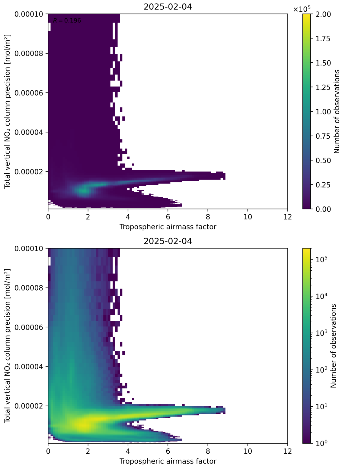
Figure 78: Scatter density plot of “Tropospheric air mass factor” against “Total vertical NO 2 column precision” for 2025-02-04 to 2025-02-05.
