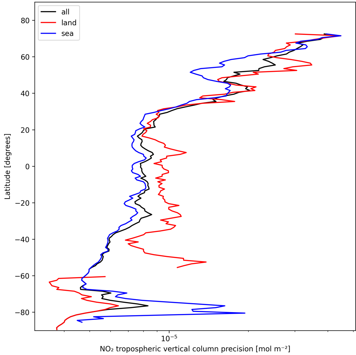
Figure 13: Zonal average of “NO 2 tropospheric vertical column precision” for 2025-02-04 to 2025-02-05.
