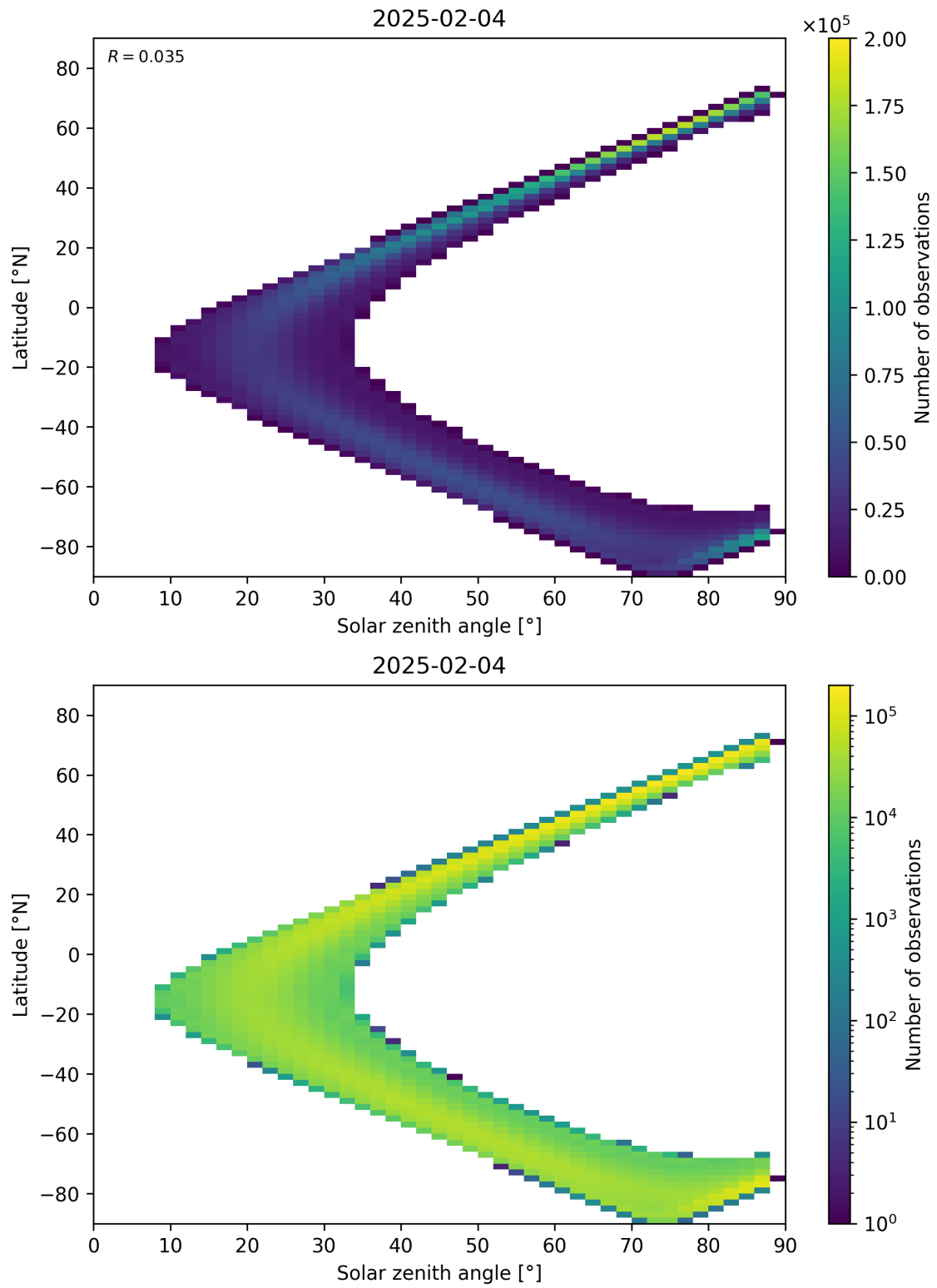
Figure 149: Scatter density plot of “Solar zenith angle” against “Latitude” for 2025-02-04 to 2025-02-05.
