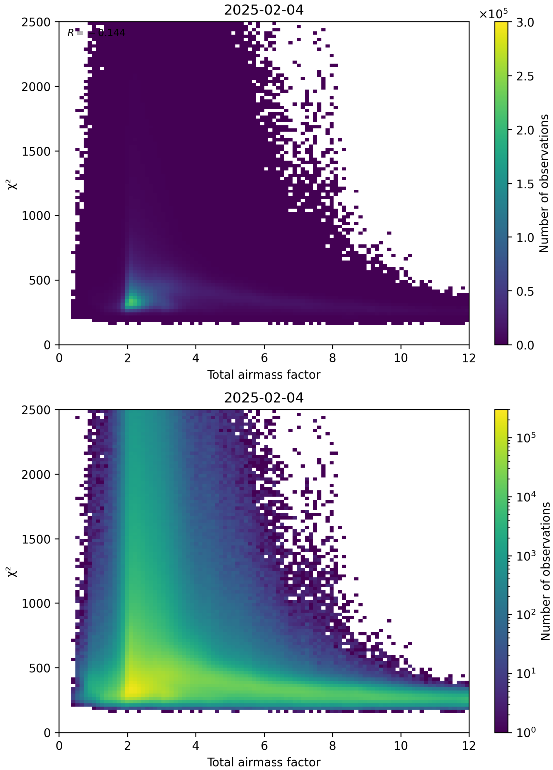
Figure 63: Scatter density plot of “Total airmass factor” against “ \chi^2 ” for 2025-02-04 to 2025-02-05.
