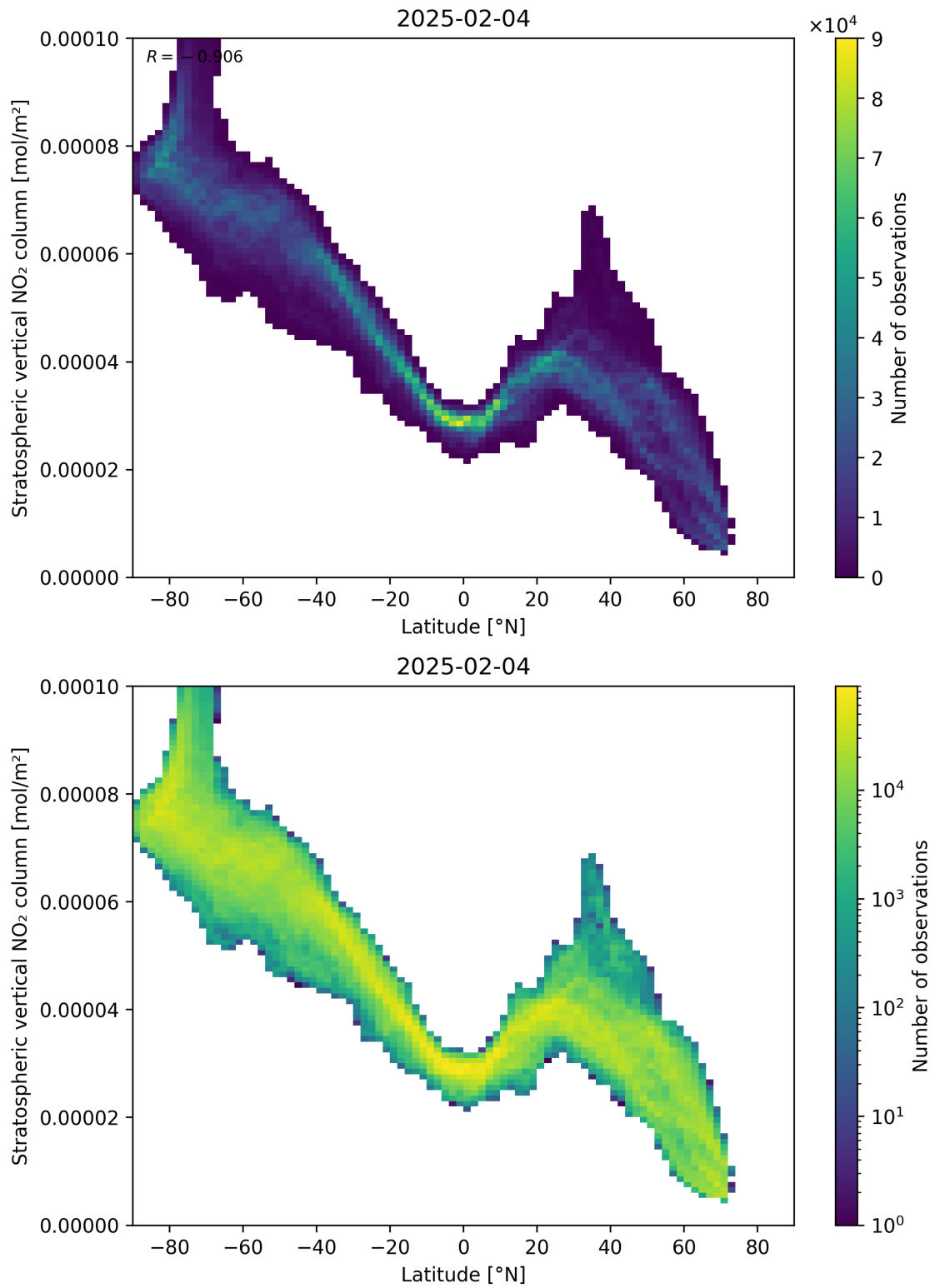
Figure 87: Scatter density plot of “Latitude” against “Stratospheric vertical NO 2 column” for 2025-02-04 to 2025-02-05.
