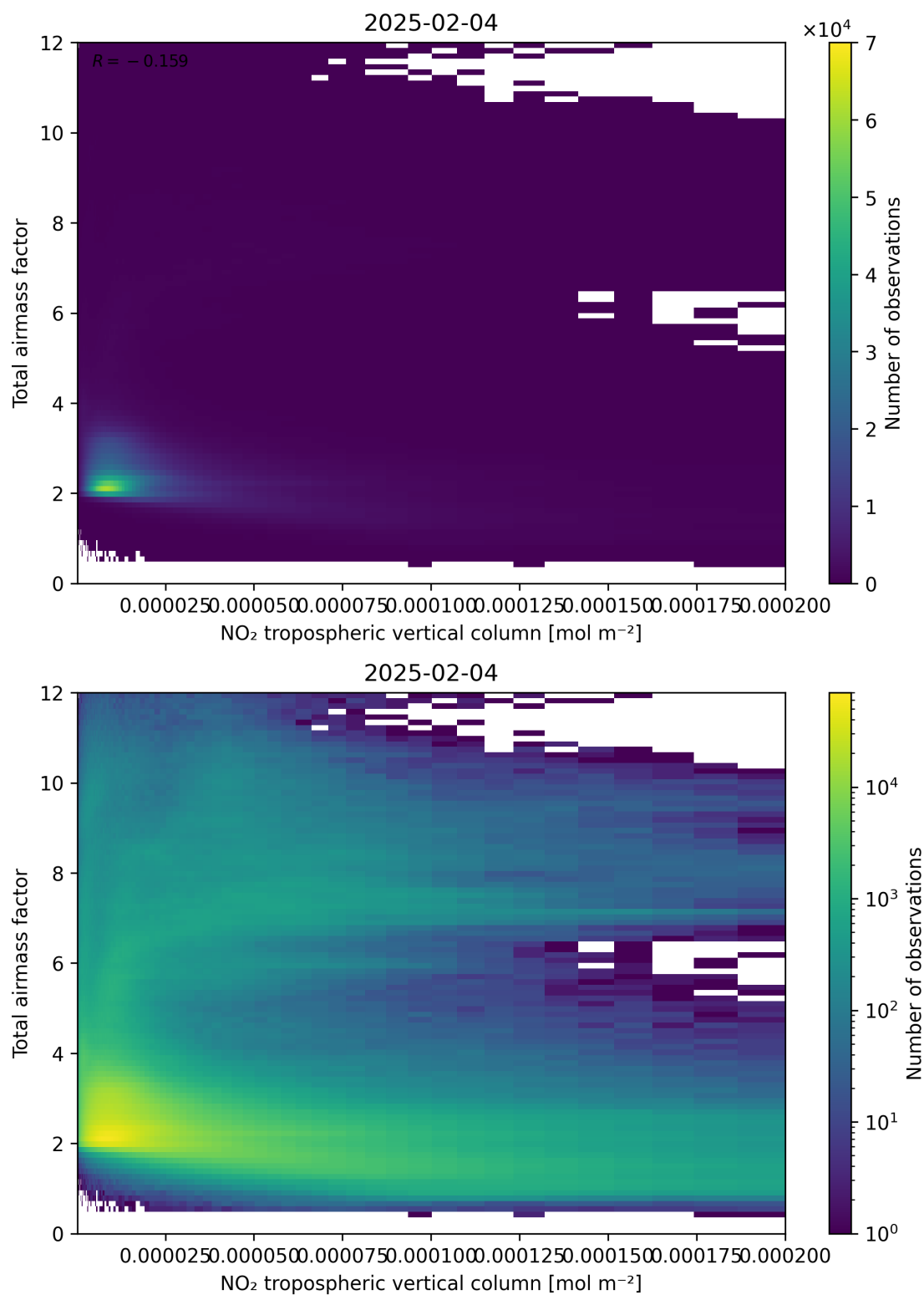
Figure 122: Scatter density plot of “NO 2 tropospheric vertical column” against “Total air mass factor” for 2025-02-04 to 2025-02-05.
