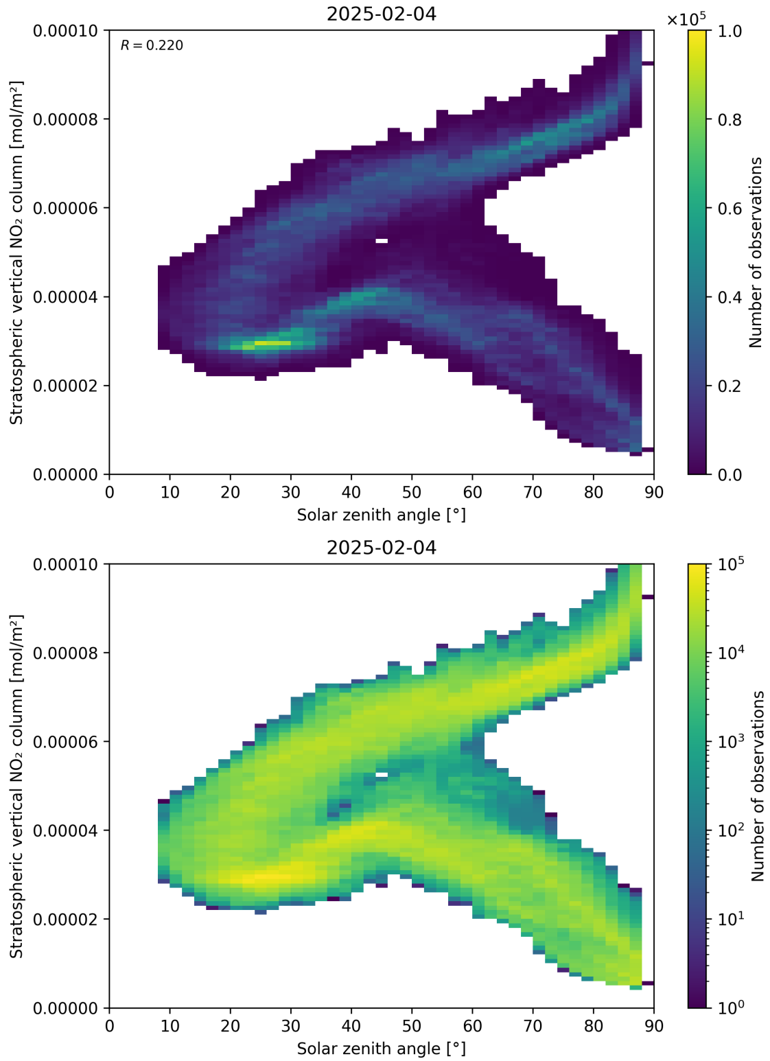
Figure 150: Scatter density plot of “Solar zenith angle” against “Stratospheric vertical NO 2 column” for 2025-02-04 to 2025-02-05.
