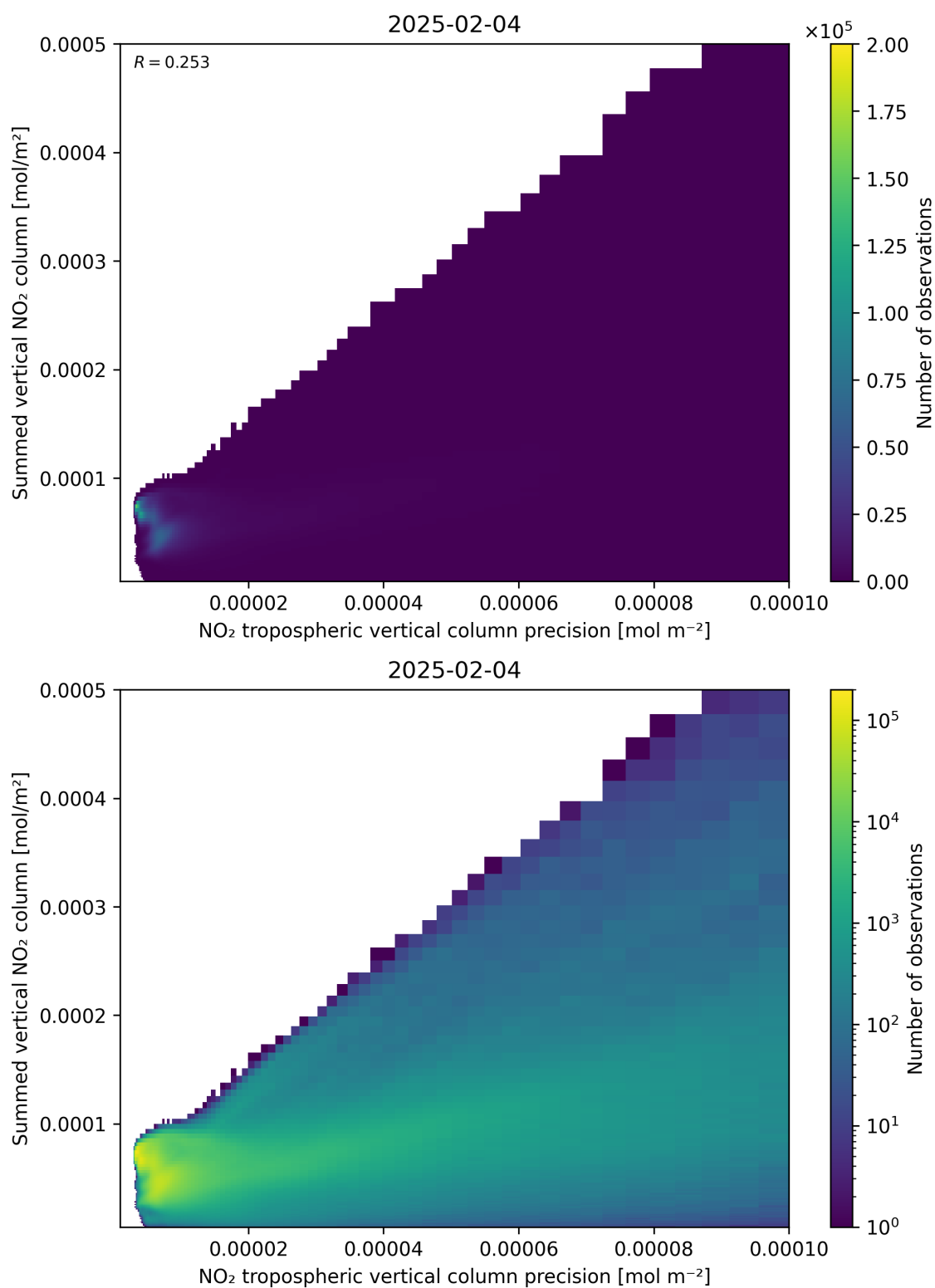
Figure 136: Scatter density plot of “NO 2 tropospheric vertical column precision” against “Summed vertical NO 2 column” for 2025-02-04 to 2025-02-05.
