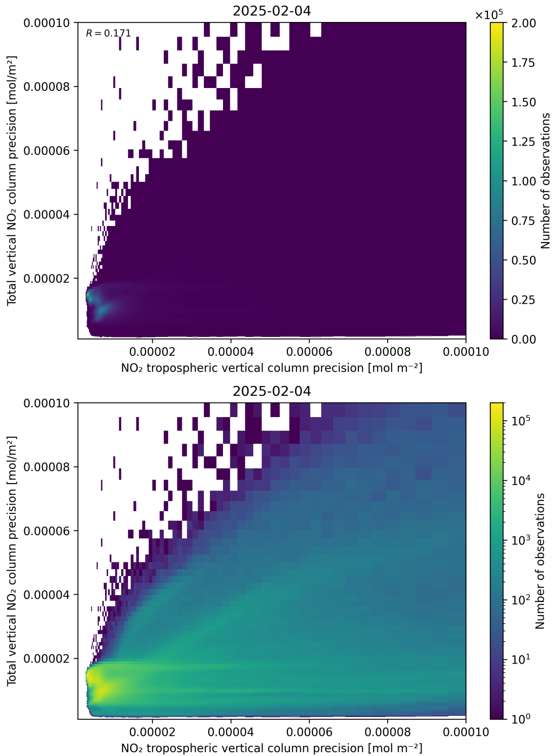
Figure 139: Scatter density plot of “NO 2 tropospheric vertical column precision” against “Total vertical NO 2 column precision” for 2025-02-04 to 2025-02-05.
