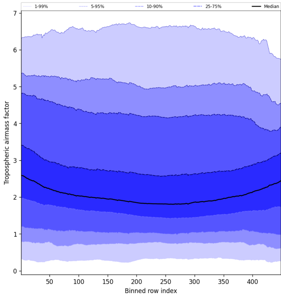
Figure 48: Along track statistics of “Tropospheric air mass factor” for 2025-02-04 to 2025-02-05
