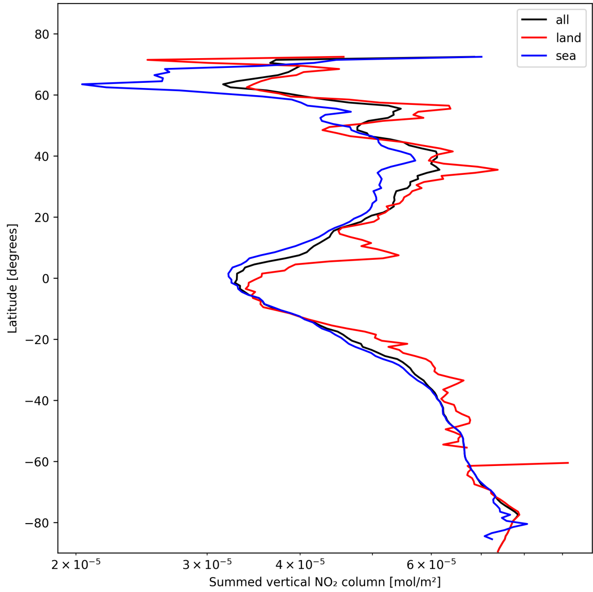
Figure 23: Zonal average of “Summed vertical NO 2 column” for 2025-02-04 to 2025-02-05.
