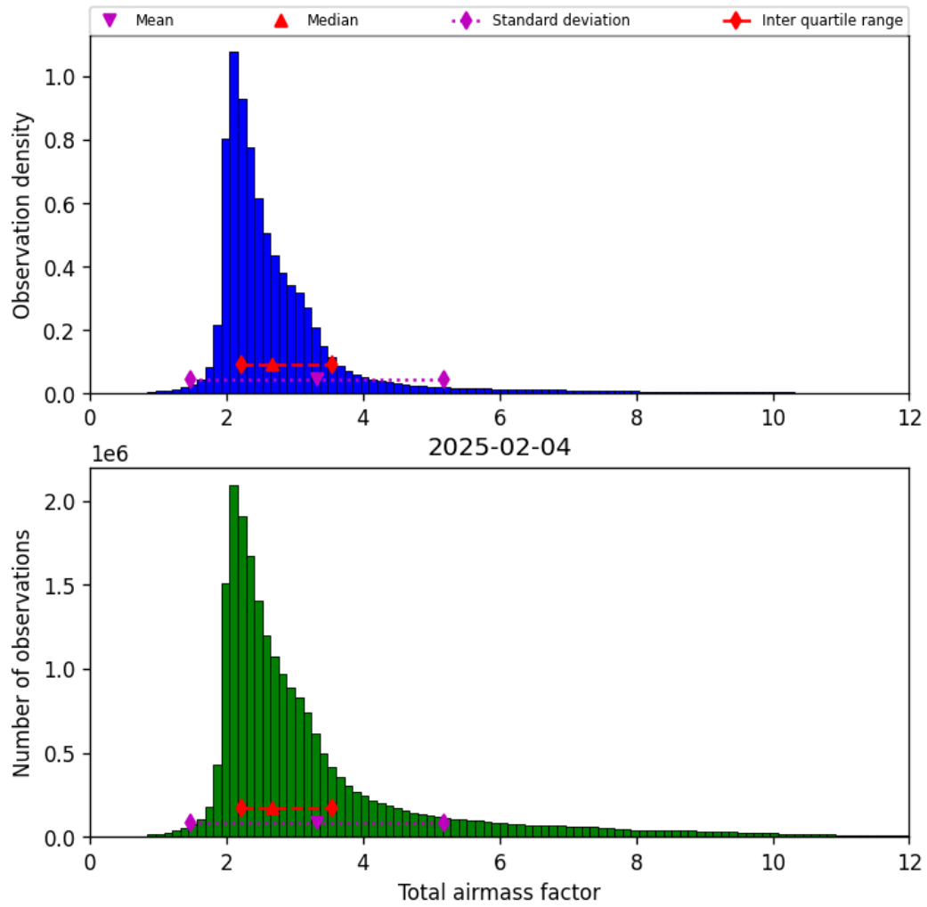
Figure 32: Histogram of “Total airmass factor” for 2025-02-04 to 2025-02-05
