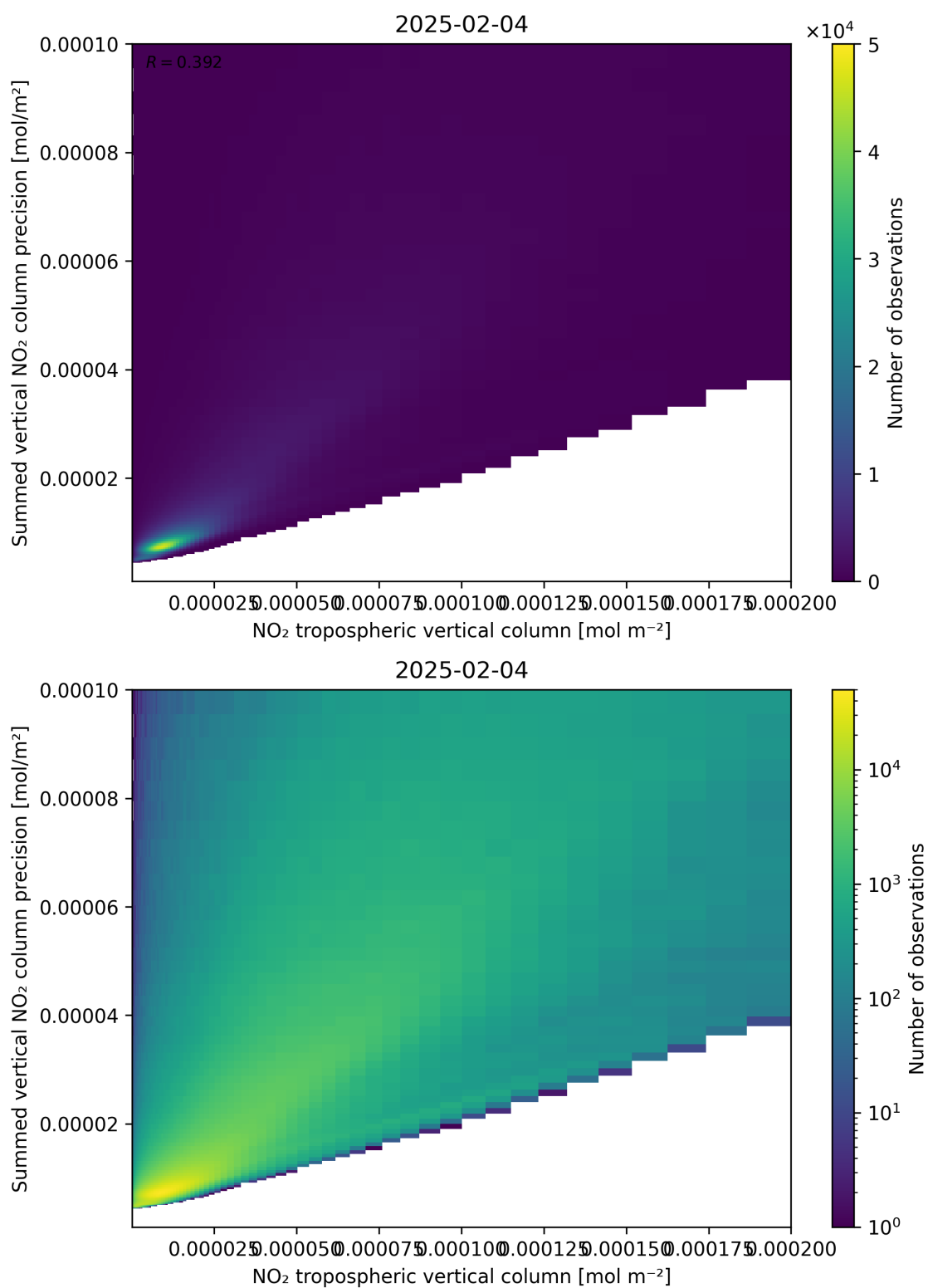
Figure 127: Scatter density plot of “NO 2 tropospheric vertical column” against “Summed vertical NO 2 column precision” for 2025-02-04 to 2025-02-05.
