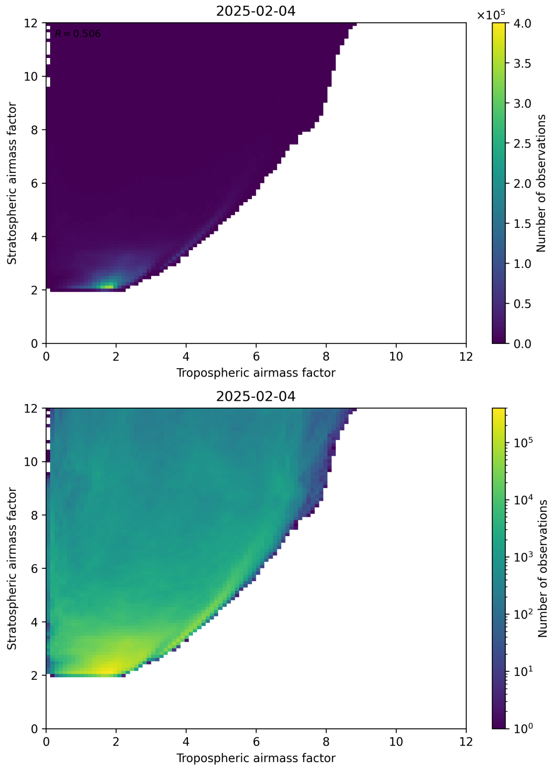
Figure 71: Scatter density plot of “Tropospheric airmass factor” against “Stratospheric airmass factor” for 2025-02-04 to 2025-02-05.
