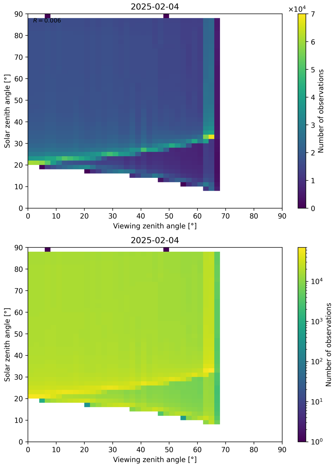
Figure 172: Scatter density plot of “Viewing zenith angle” against “Solar zenith angle” for 2025-02-04 to 2025-02-05.
