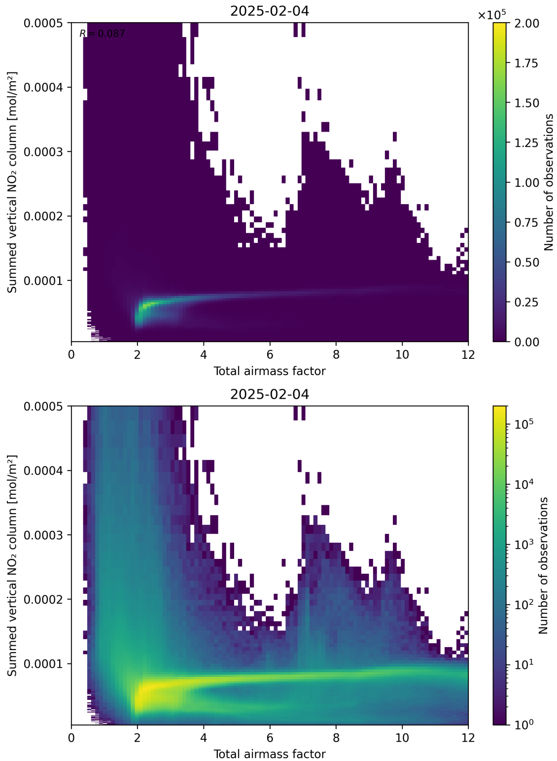
Figure 65: Scatter density plot of “Total airmass factor” against “Summed vertical NO 2 column” for 2025-02-04 to 2025-02-05.
