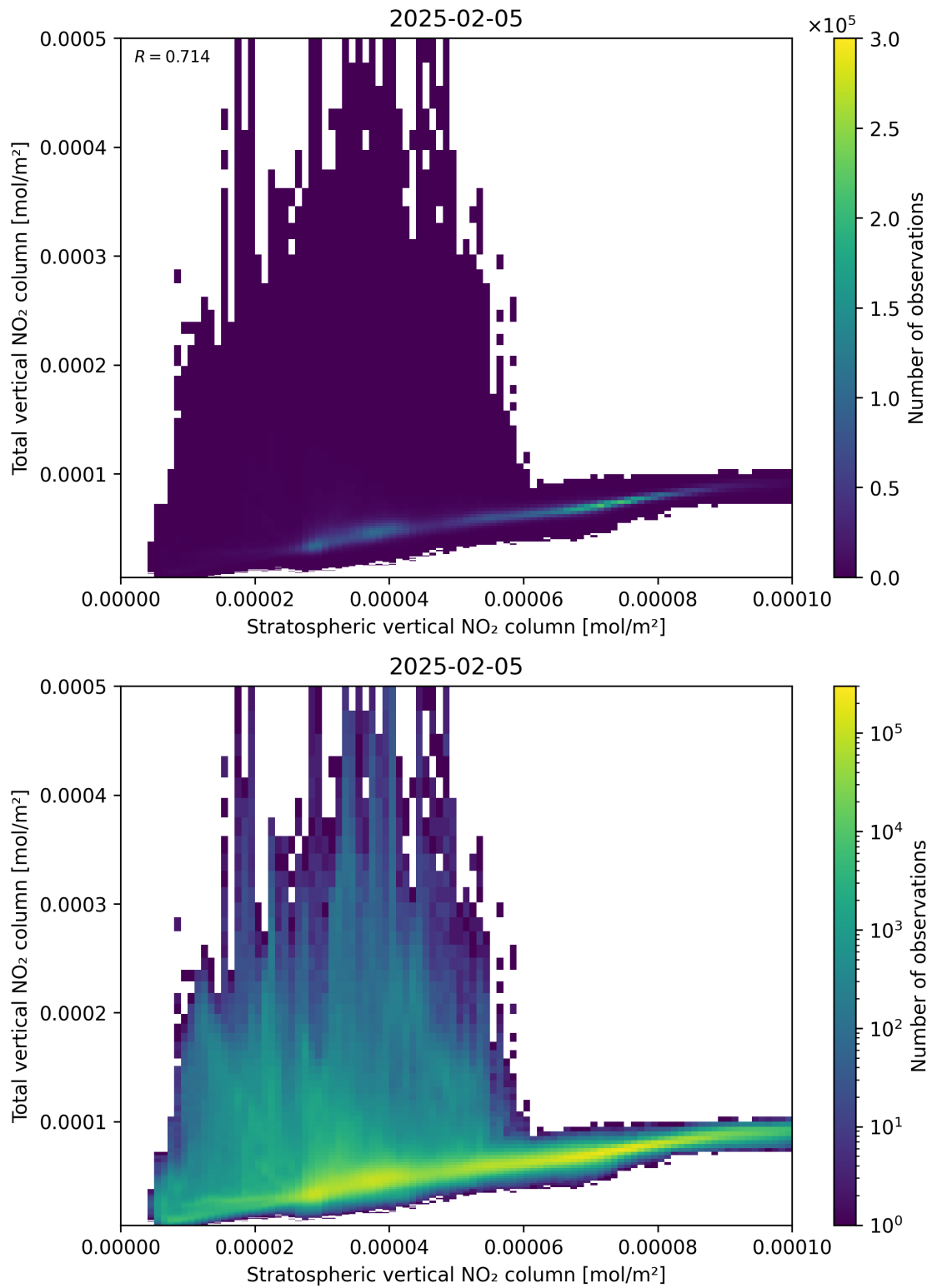
Figure 100: Scatter density plot of “Stratospheric vertical NO 2 column” against “Total vertical NO 2 column” for 2025-02-04 to 2025-02-06.
