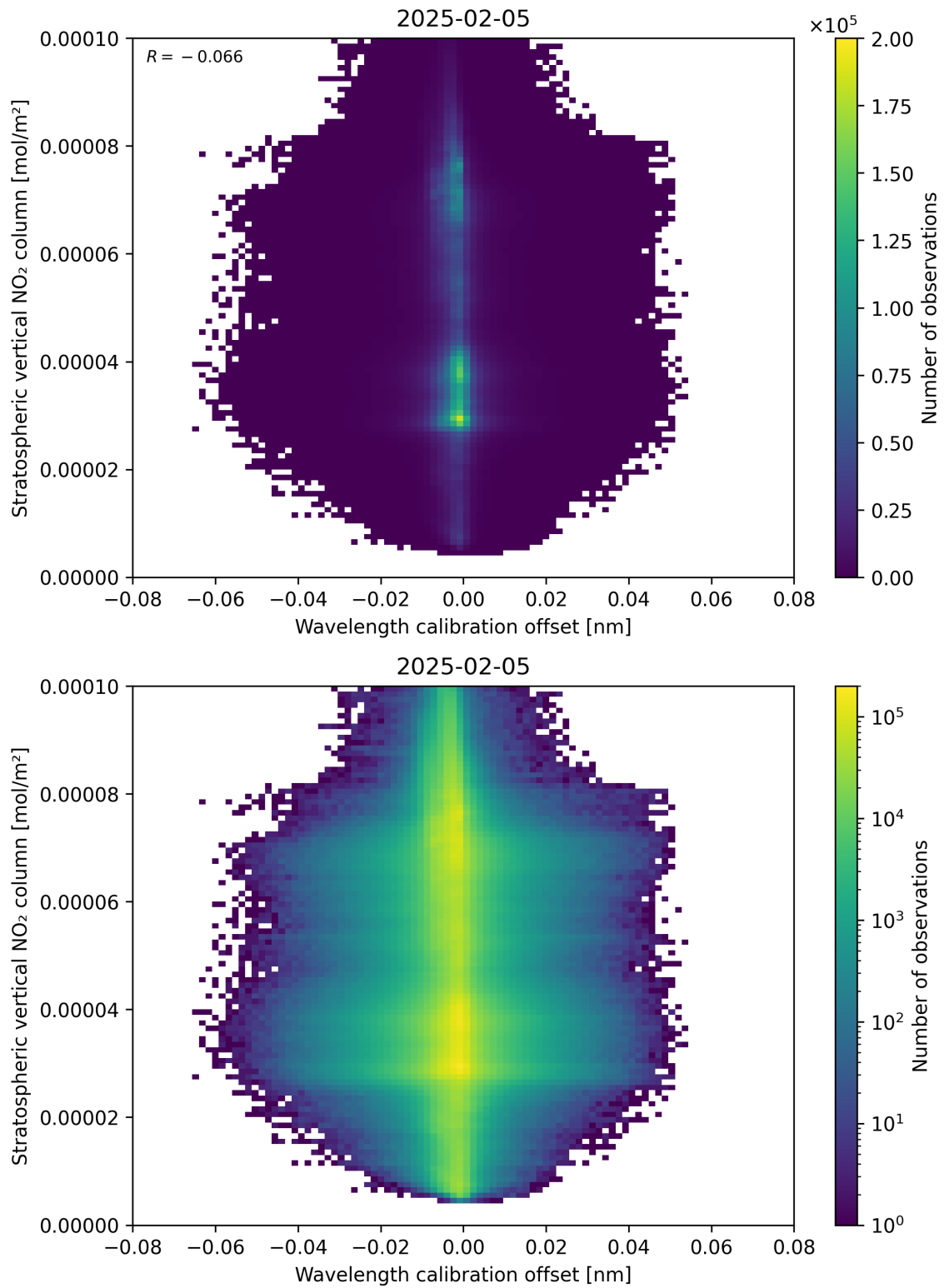
Figure 176: Scatter density plot of “Wavelength calibration offset” against “Stratospheric vertical NO 2 column” for 2025-02-04 to 2025-02-06.
