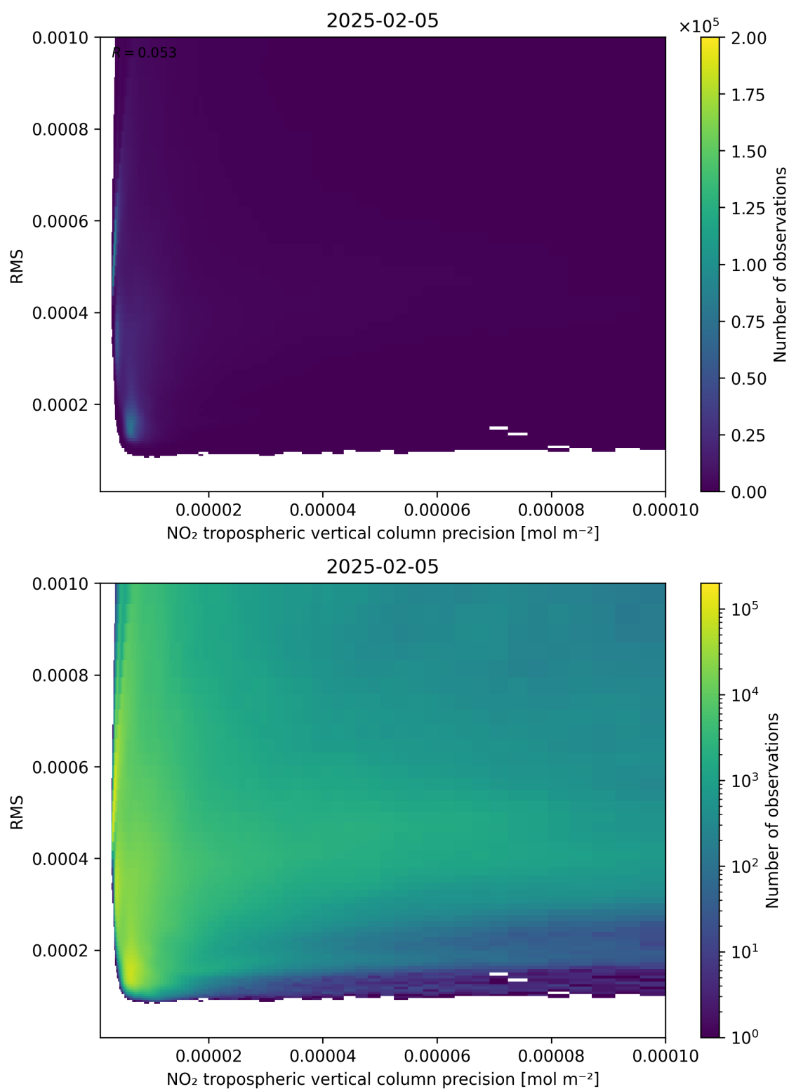
Figure 140: Scatter density plot of “NO 2 tropospheric vertical column precision” against “RMS” for 2025-02-04 to 2025-02-06.
