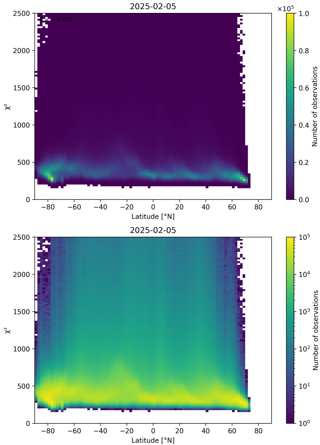
Figure 86: Scatter density plot of “Latitude” against “ \chi^2 ” for 2025-02-04 to 2025-02-06.
