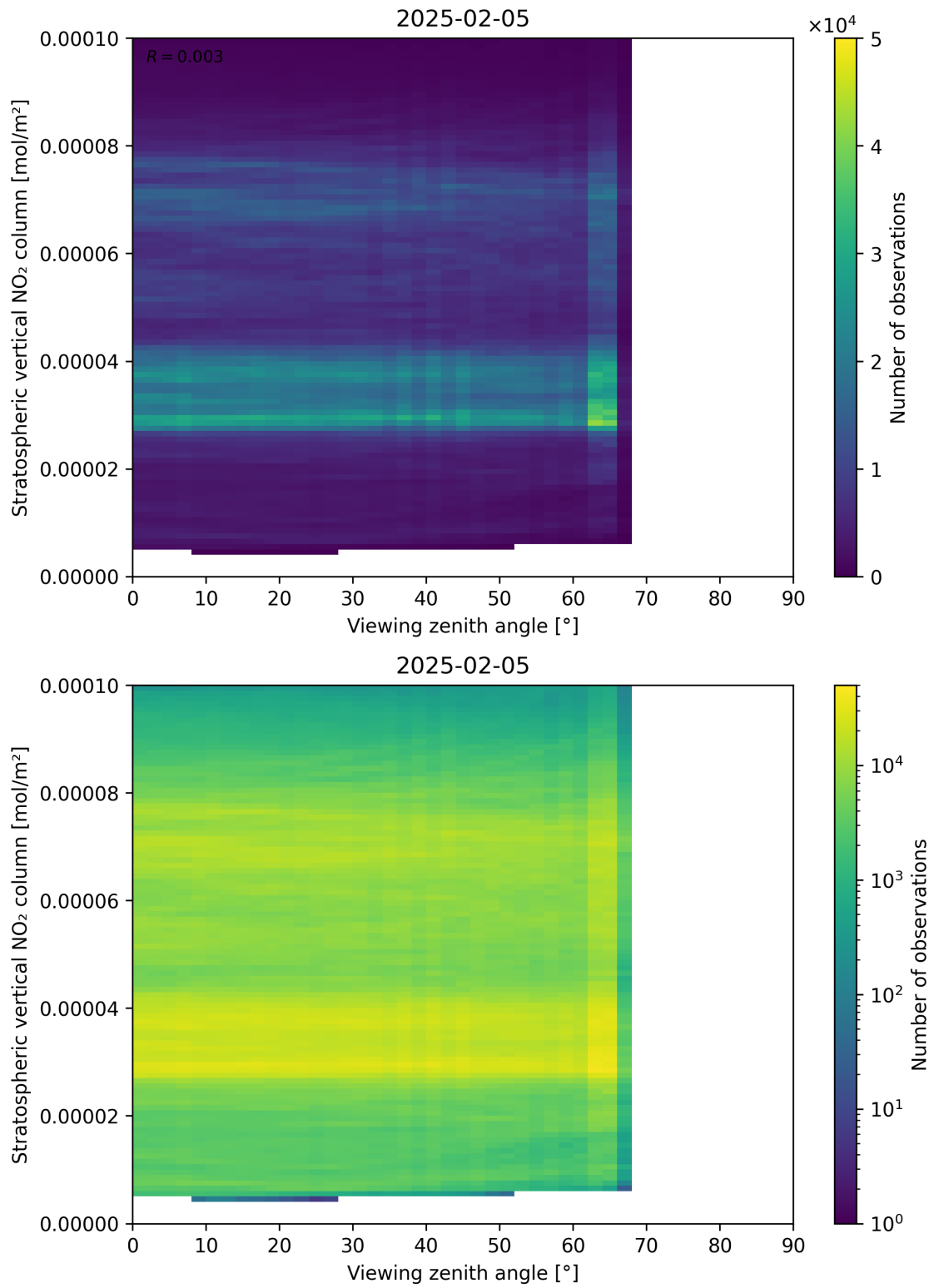
Figure 164: Scatter density plot of “Viewing zenith angle” against “Stratospheric vertical NO 2 column” for 2025-02-04 to 2025-02-06.
