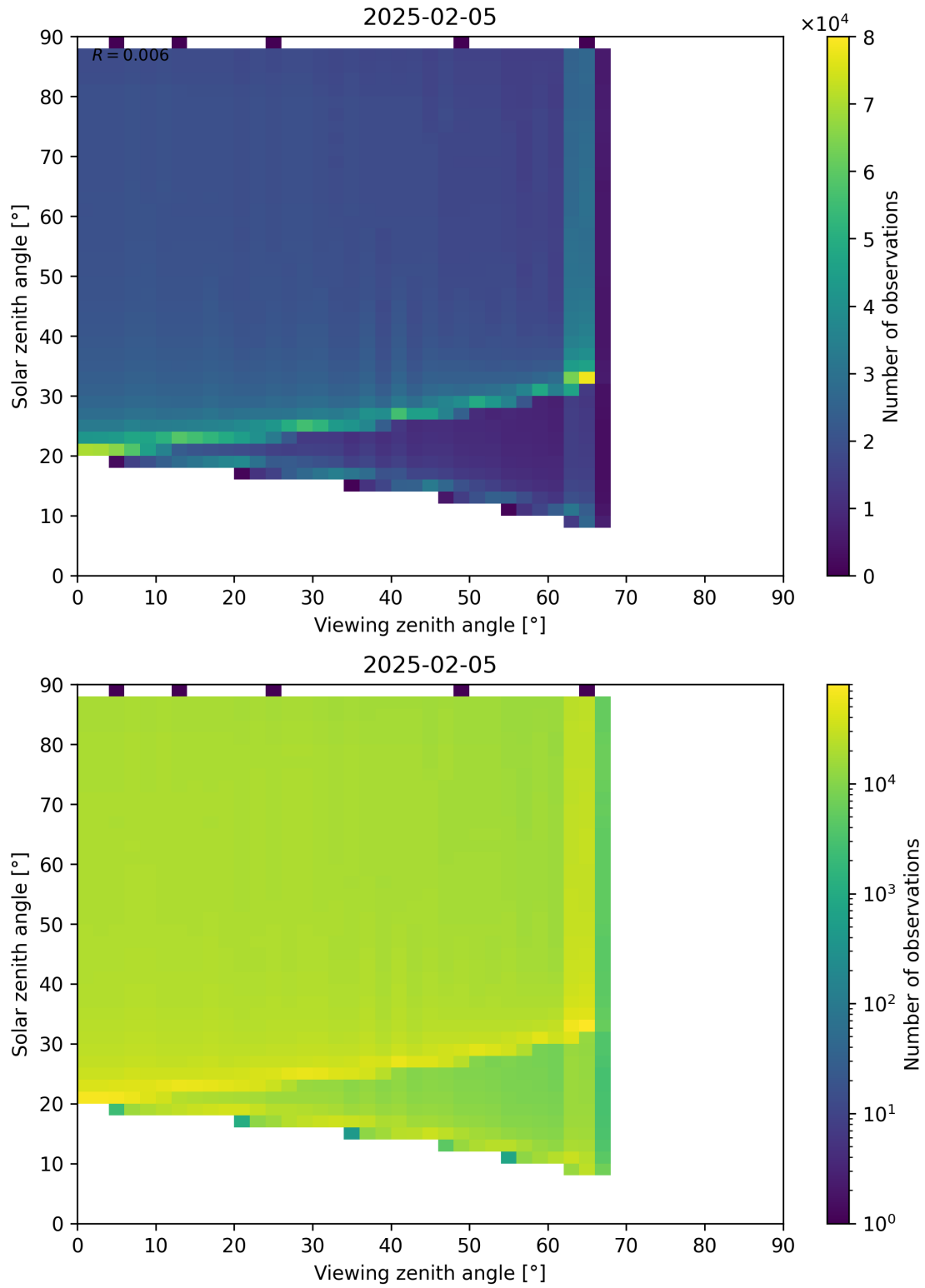
Figure 172: Scatter density plot of “Viewing zenith angle” against “Solar zenith angle” for 2025-02-04 to 2025-02-06.
