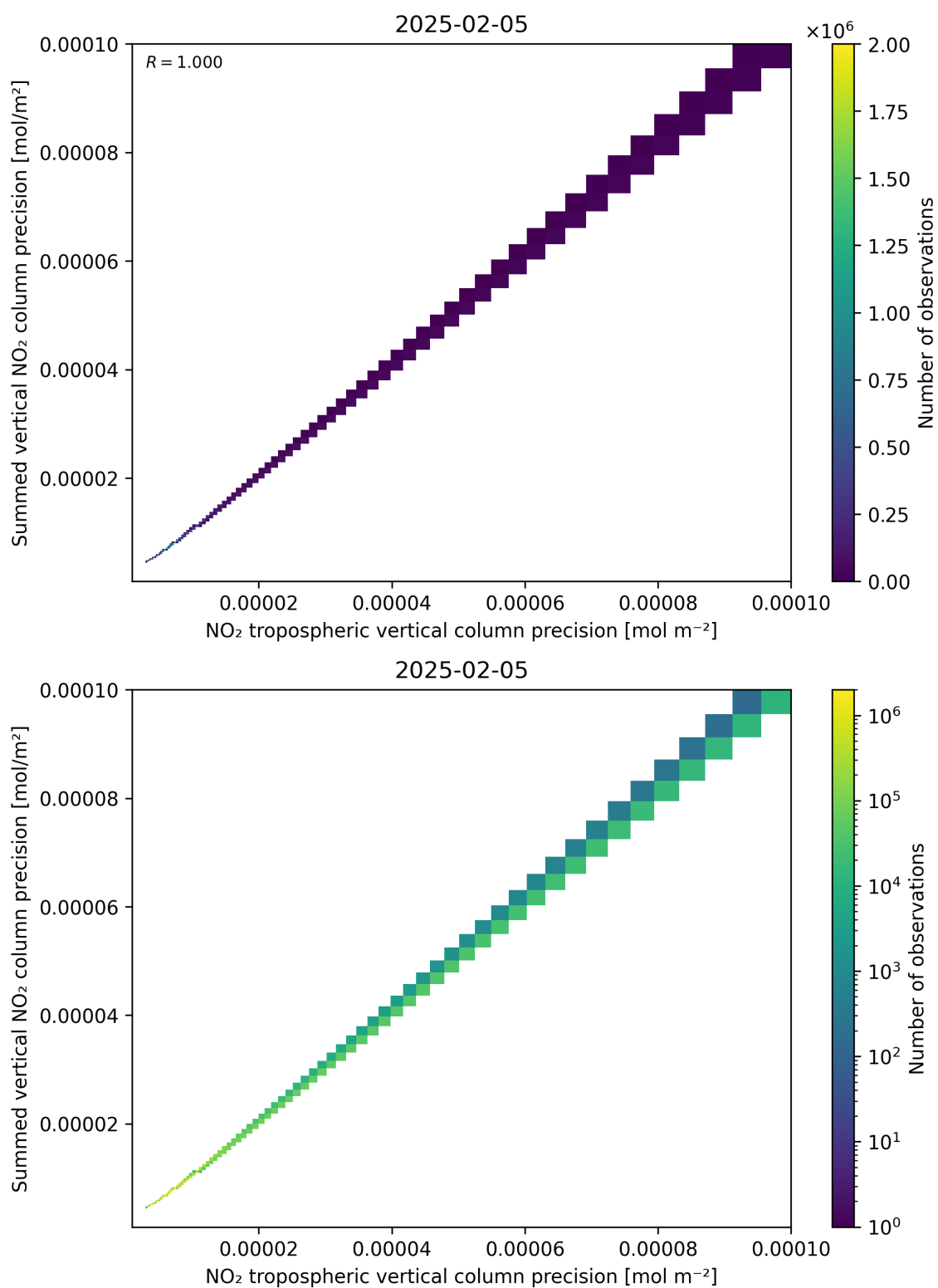
Figure 137: Scatter density plot of “NO 2 tropospheric vertical column precision” against “Summed vertical NO 2 column precision” for 2025-02-04 to 2025-02-06.
