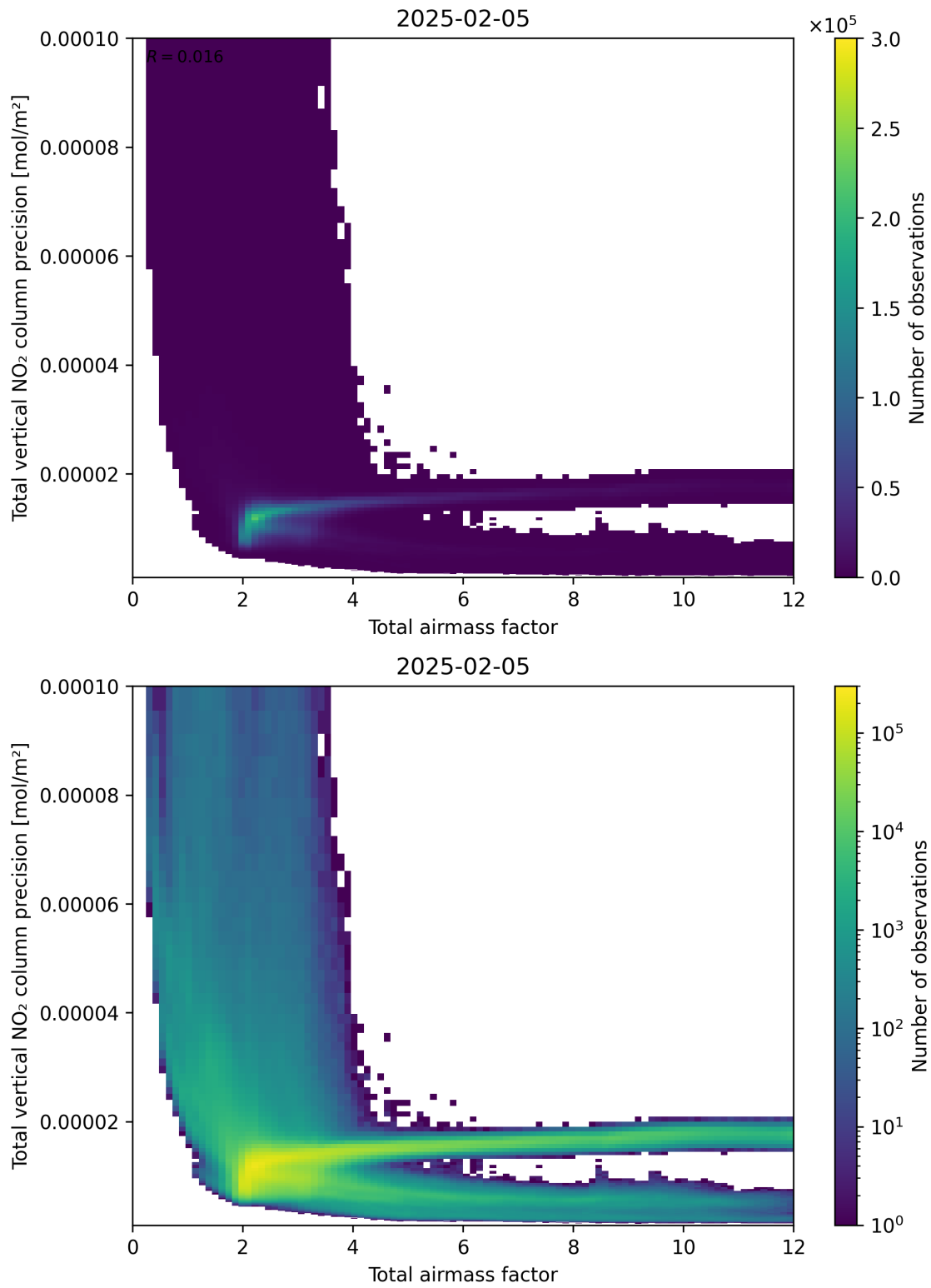
Figure 68: Scatter density plot of “Total airmass factor” against “Total vertical NO 2 column precision” for 2025-02-04 to 2025-02-06.
