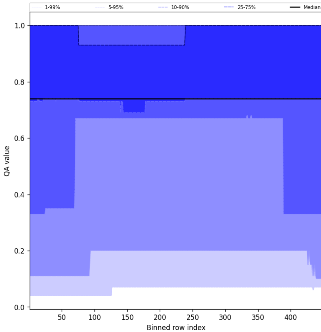
Figure 45: Along track statistics of “QA value” for 2025-02-04 to 2025-02-06
