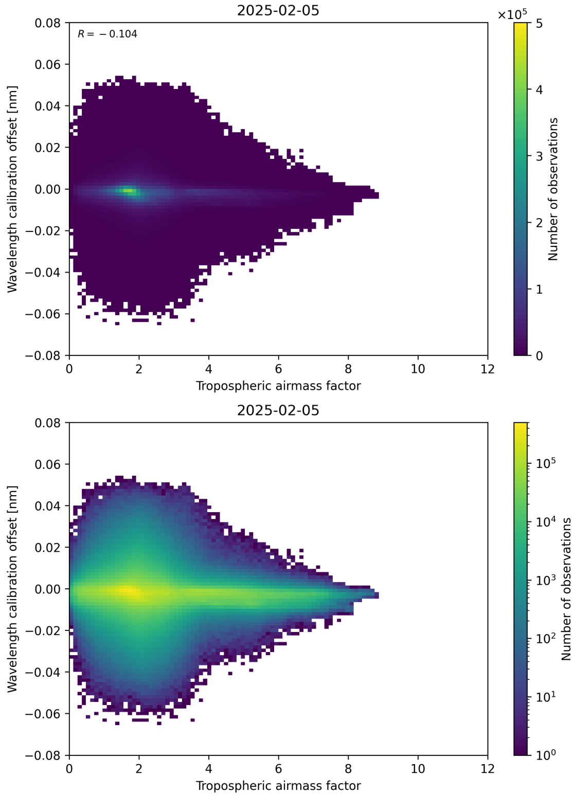
Figure 80: Scatter density plot of “Tropospheric airmass factor” against “Wavelength calibration offset” for 2025-02-04 to 2025-02-06.
