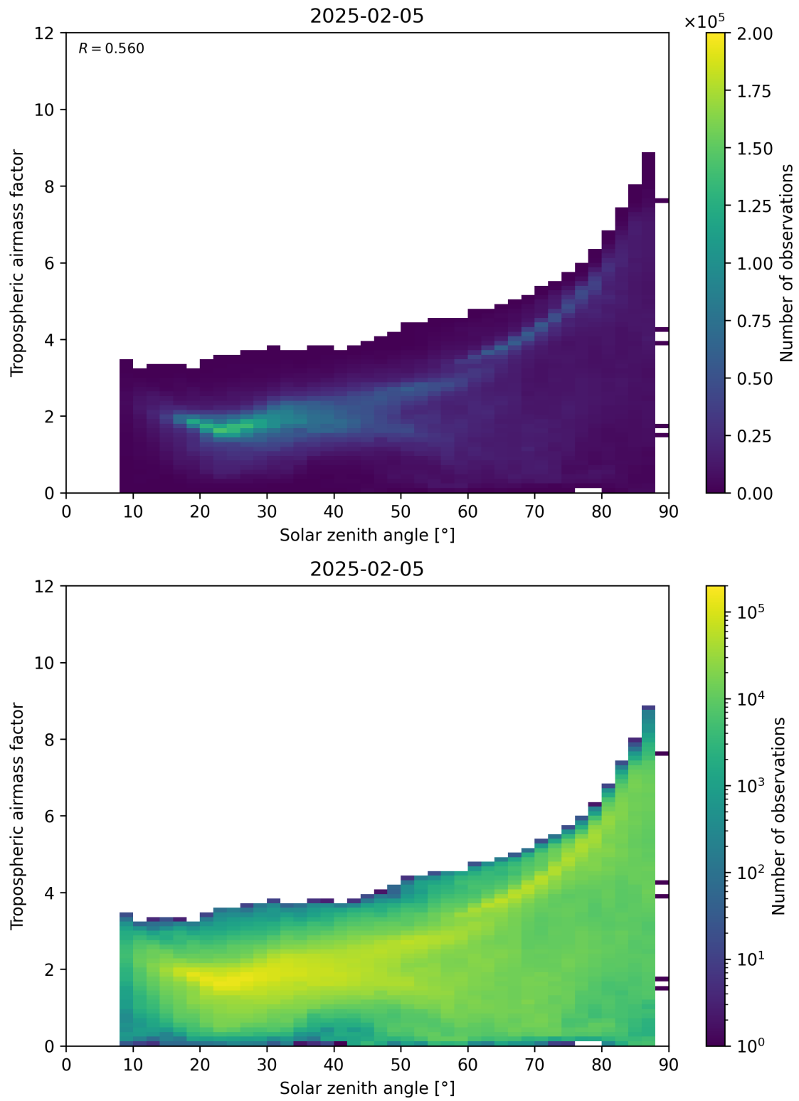
Figure 147: Scatter density plot of “Solar zenith angle” against “Tropospheric airmass factor” for 2025-02-04 to 2025-02-06.
