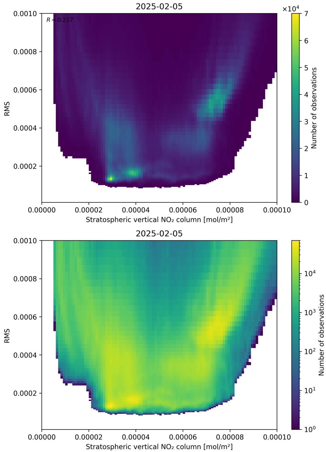
Figure 102: Scatter density plot of “Stratospheric vertical NO 2 column” against “RMS” for 2025-02-04 to 2025-02-06.
