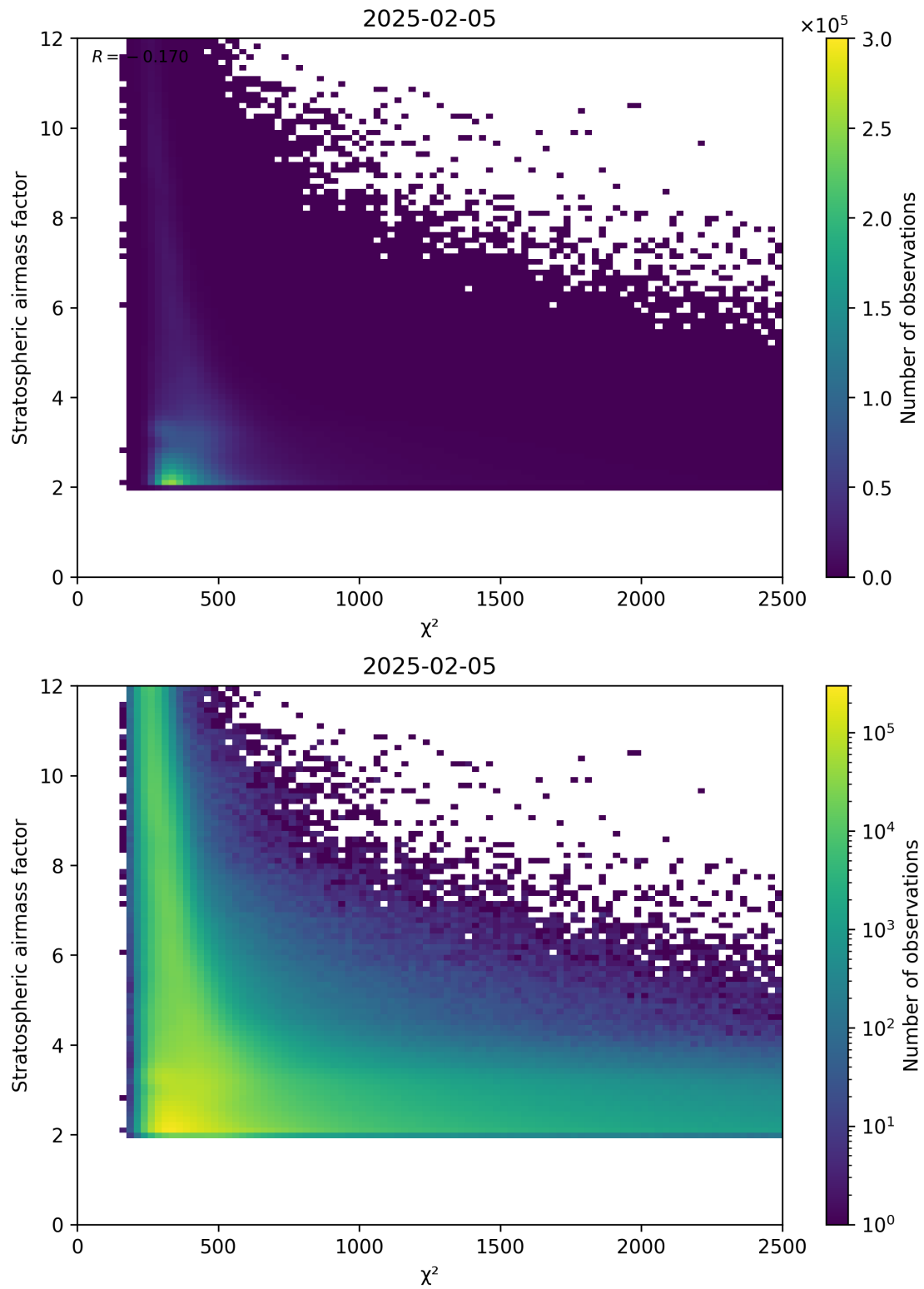
Figure 81: Scatter density plot of “ \chi^2 ” against “Stratospheric airmass factor” for 2025-02-04 to 2025-02-06.
