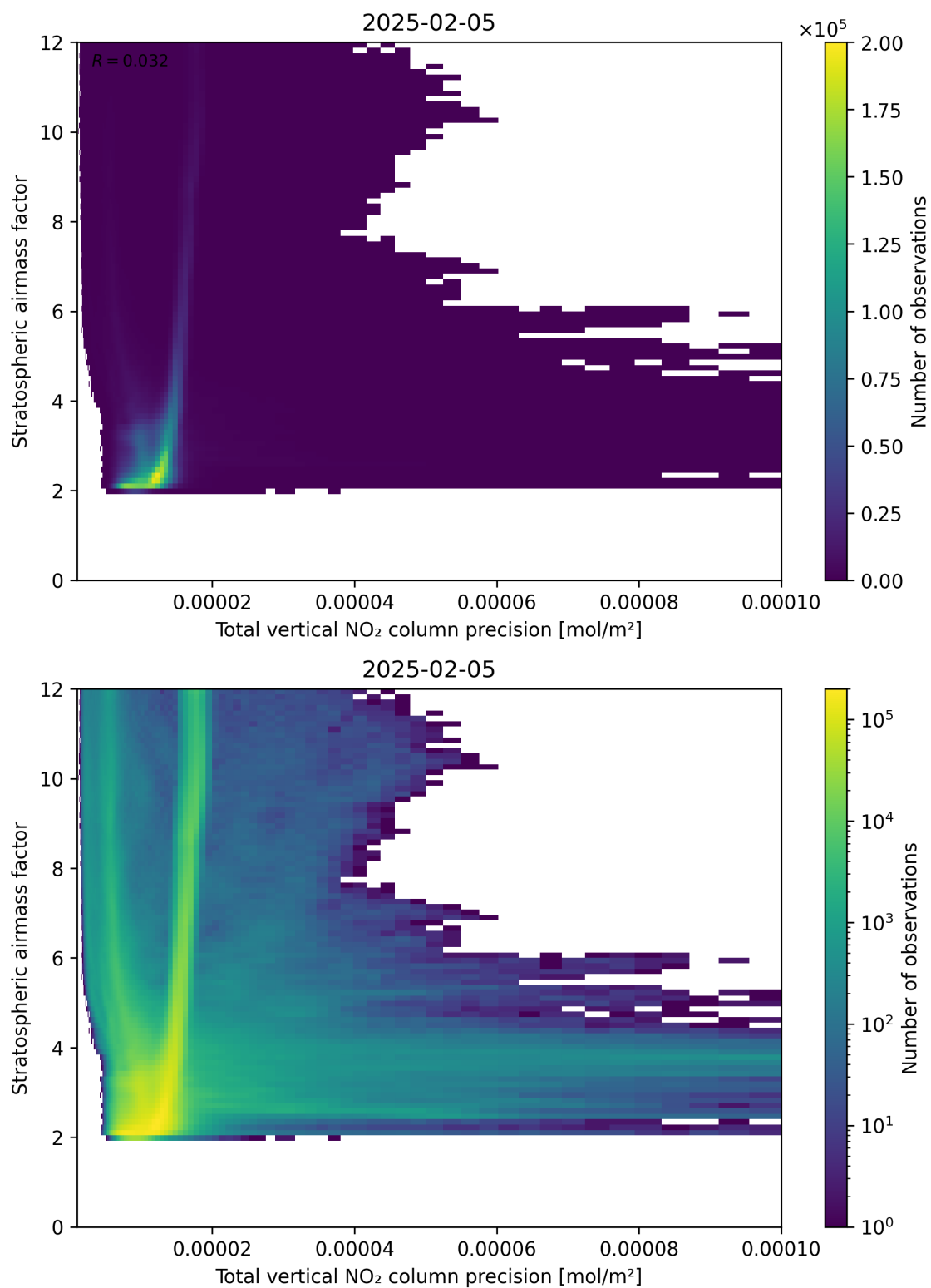
Figure 115: Scatter density plot of “Total vertical NO 2 column precision” against “Stratospheric air mass factor” for 2025-02-04 to 2025-02-06.
