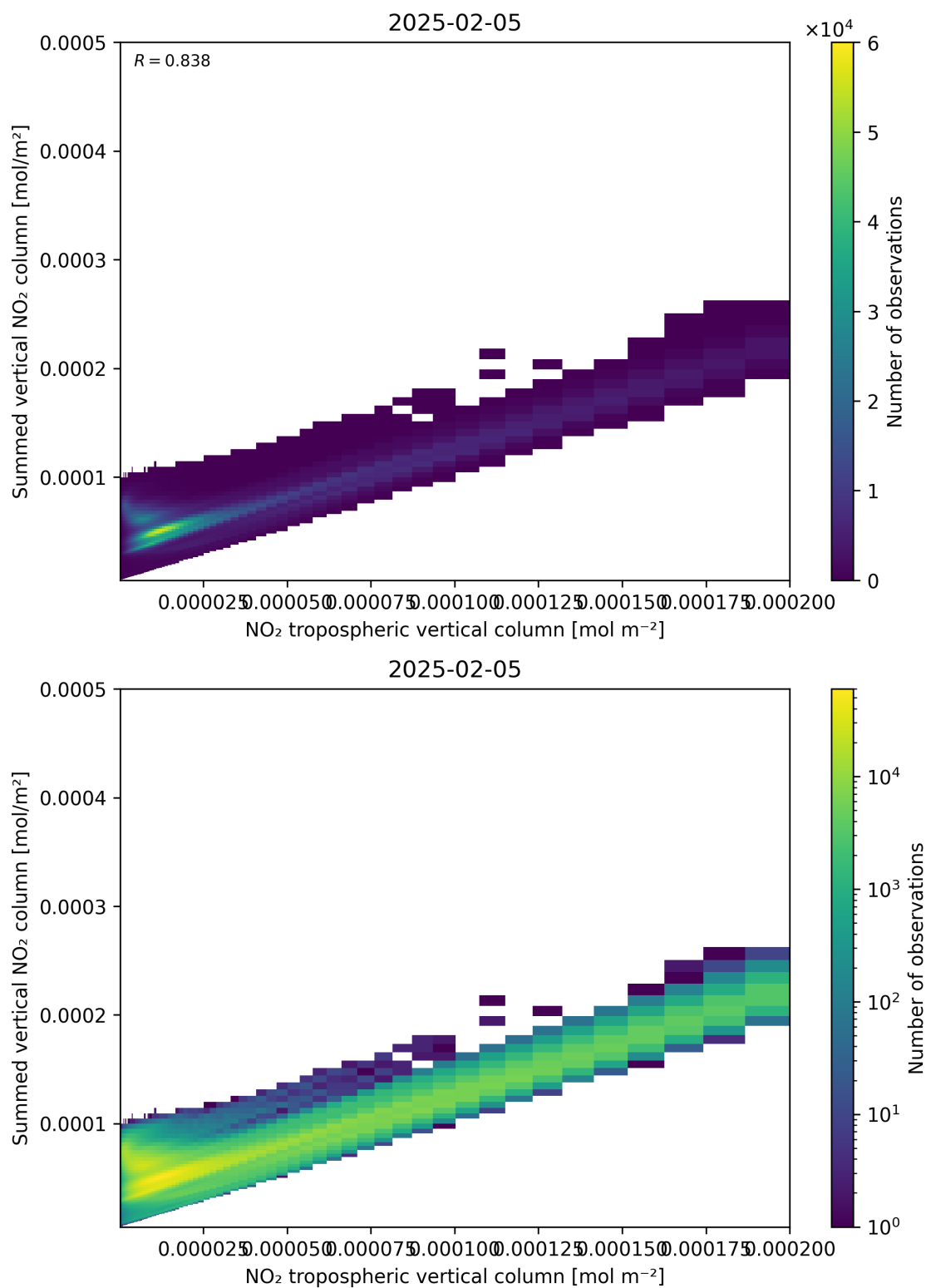
Figure 126: Scatter density plot of “NO 2 tropospheric vertical column” against “Summed vertical NO 2 column” for 2025-02-04 to 2025-02-06.
