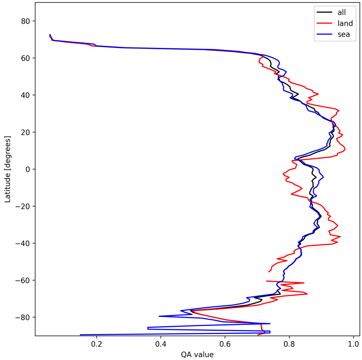
Figure 11: Zonal average of “QA value” for 2025-02-04 to 2025-02-06.
