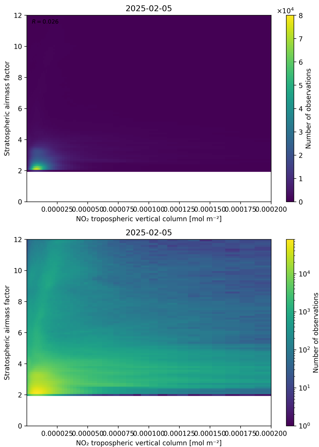
Figure 121: Scatter density plot of “NO 2 tropospheric vertical column” against “Stratospheric airmass factor” for 2025-02-04 to 2025-02-06.
