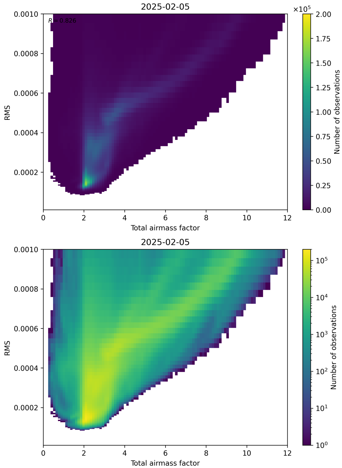
Figure 69: Scatter density plot of “Total airmass factor” against “RMS” for 2025-02-04 to 2025-02-06.
