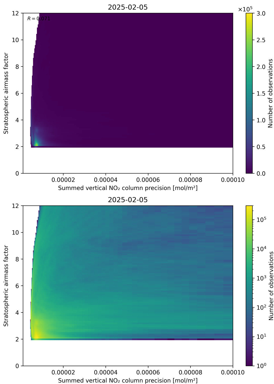
Figure 106: Scatter density plot of “Summed vertical NO 2 column precision” against “Stratospheric airmass factor” for 2025-02-04 to 2025-02-06.
