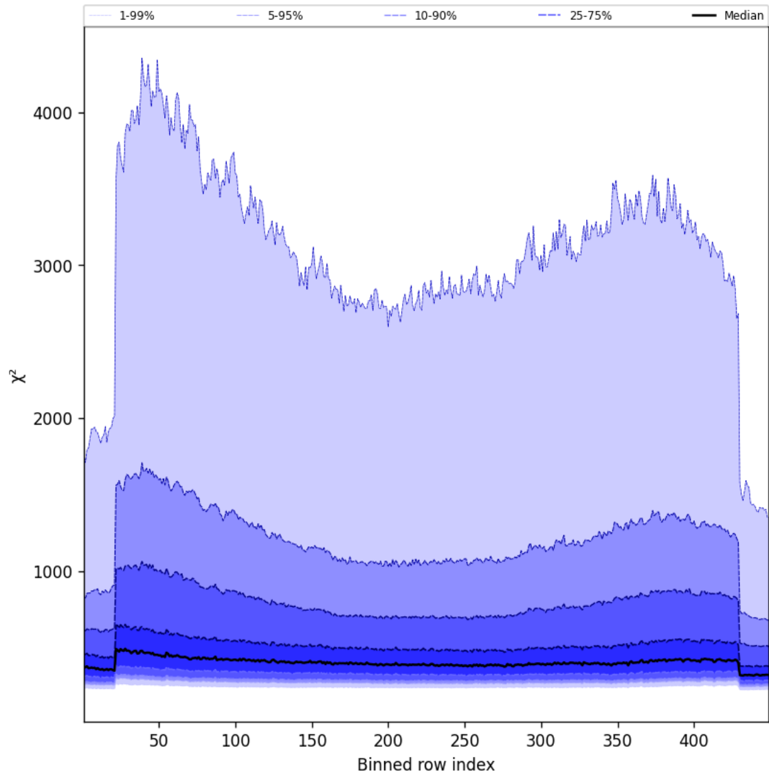
Figure 59: Along track statistics of “ \chi^2 ” for 2025-02-04 to 2025-02-06
