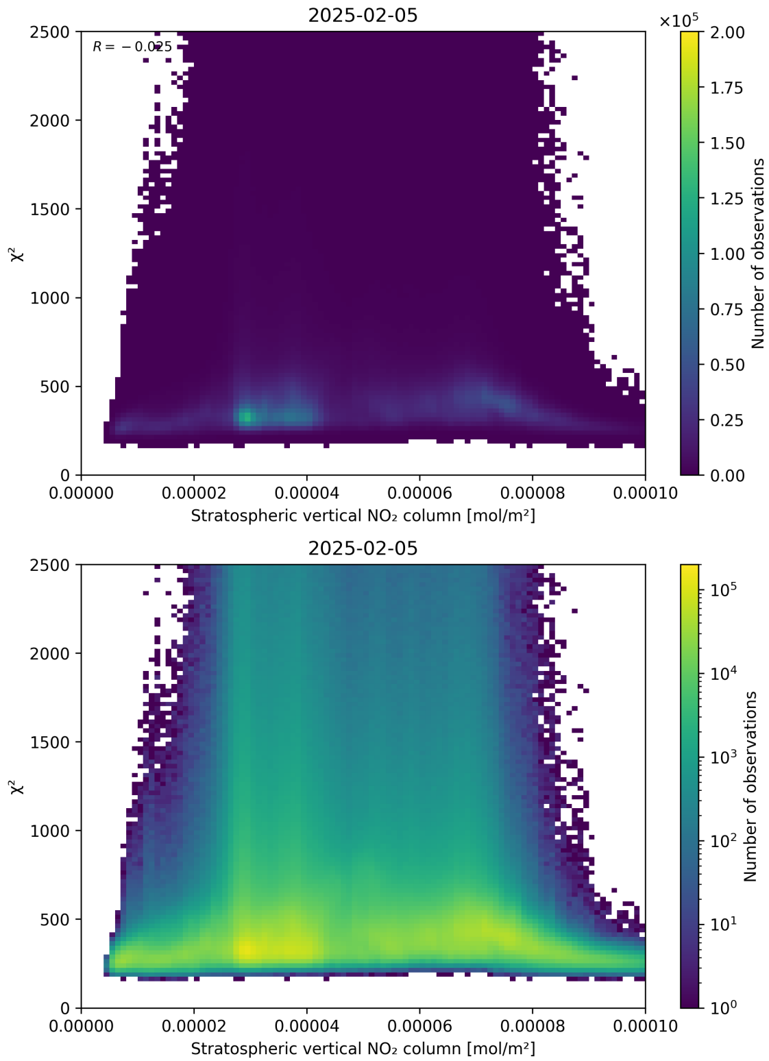
Figure 97: Scatter density plot of “Stratospheric vertical NO 2 column” against “ \chi^2 ” for 2025-02-04 to 2025-02-06.
