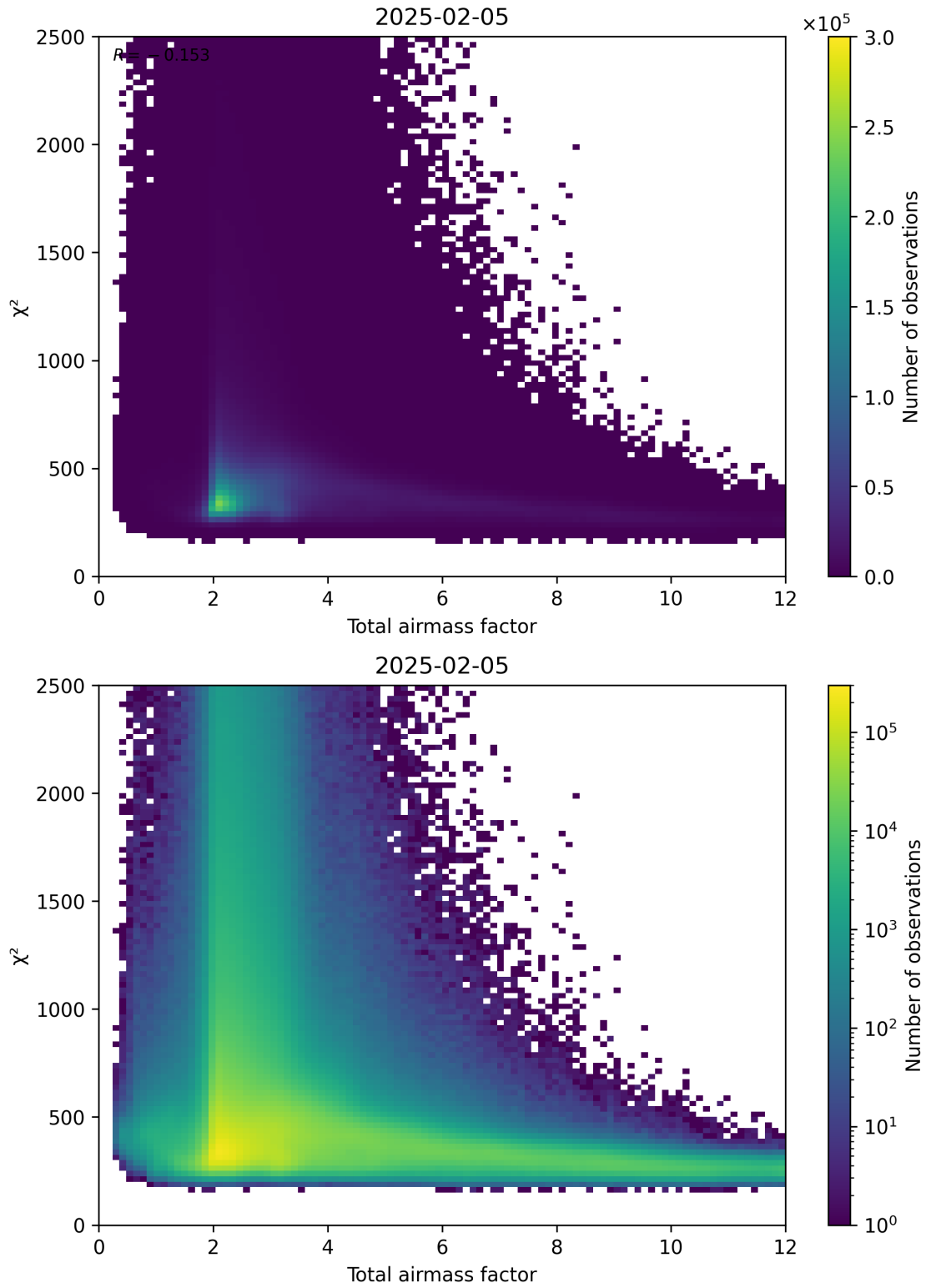
Figure 63: Scatter density plot of “Total airmass factor” against “ \chi^2 ” for 2025-02-04 to 2025-02-06.
