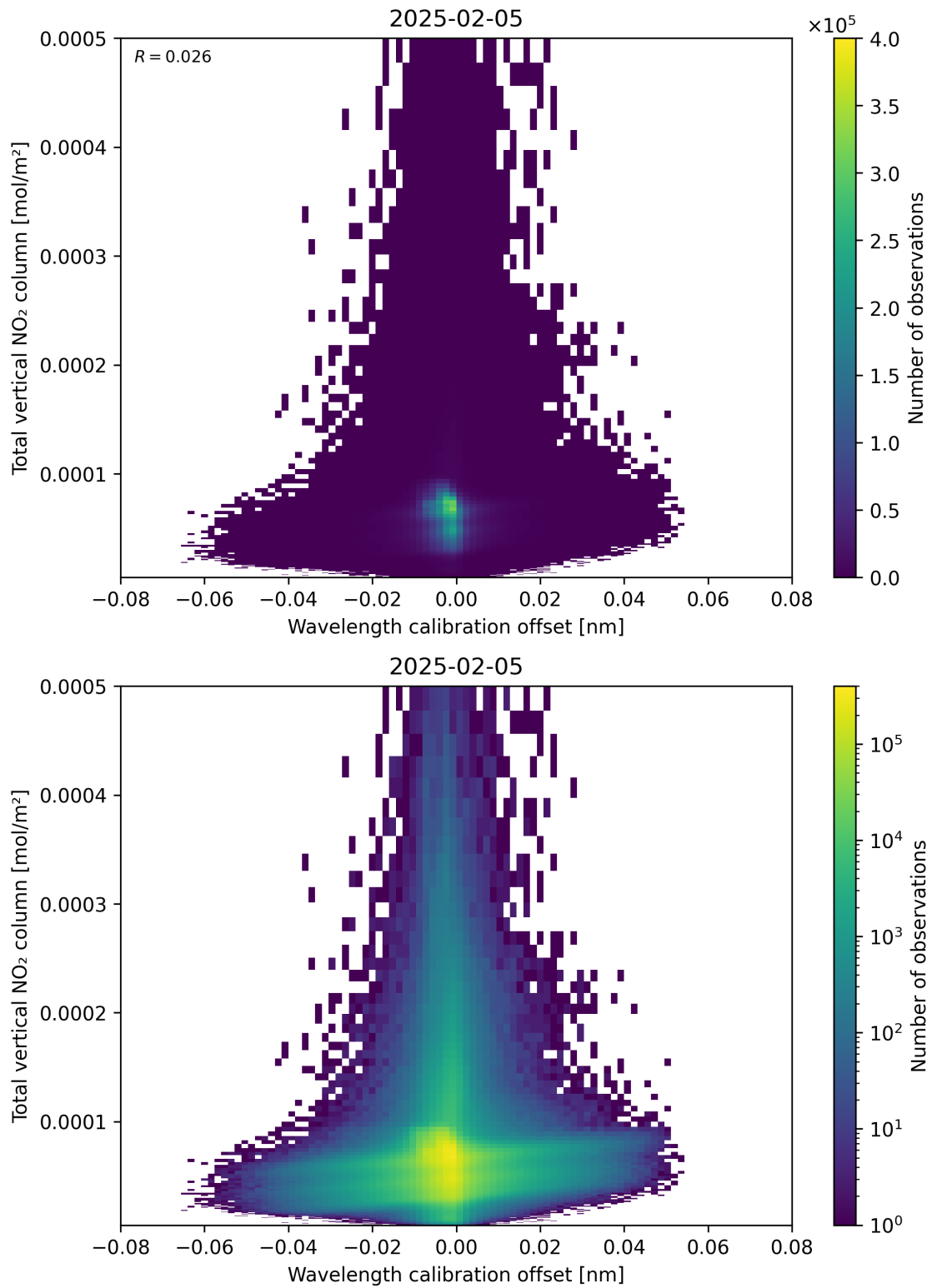
Figure 179: Scatter density plot of “Wavelength calibration offset” against “Total vertical NO 2 column” for 2025-02-04 to 2025-02-06.
