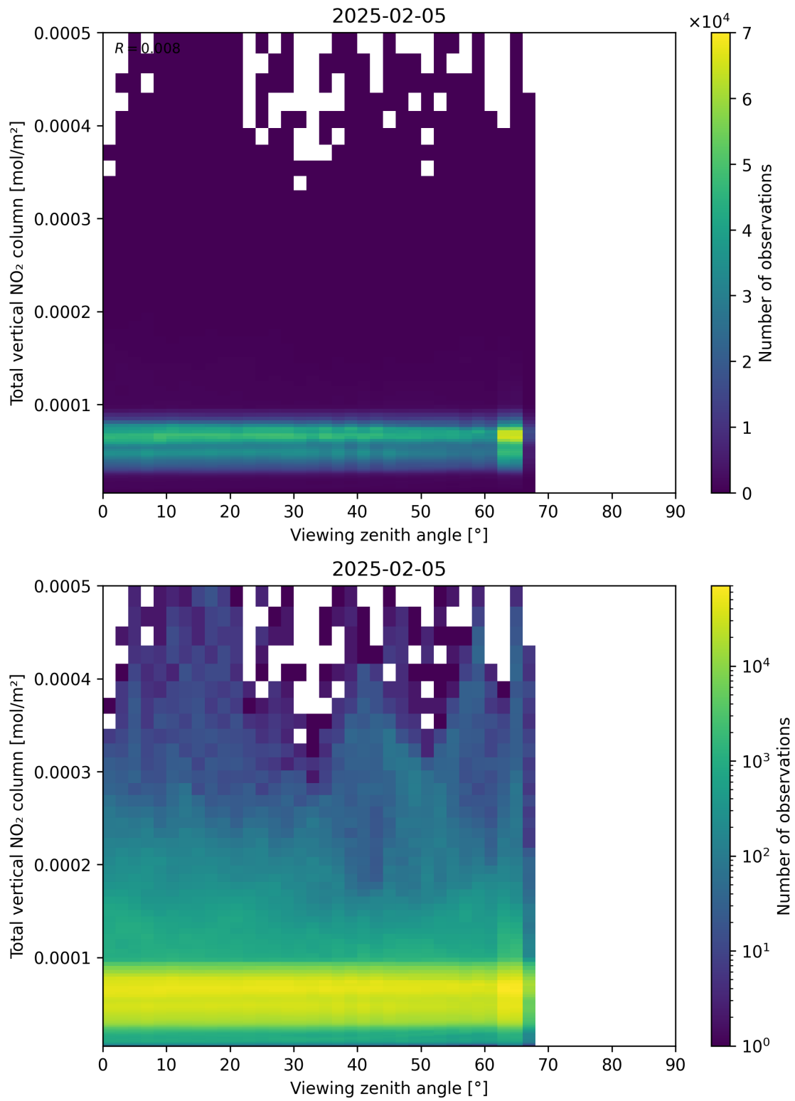
Figure 167: Scatter density plot of “Viewing zenith angle” against “Total vertical NO 2 column” for 2025-02-04 to 2025-02-06.
