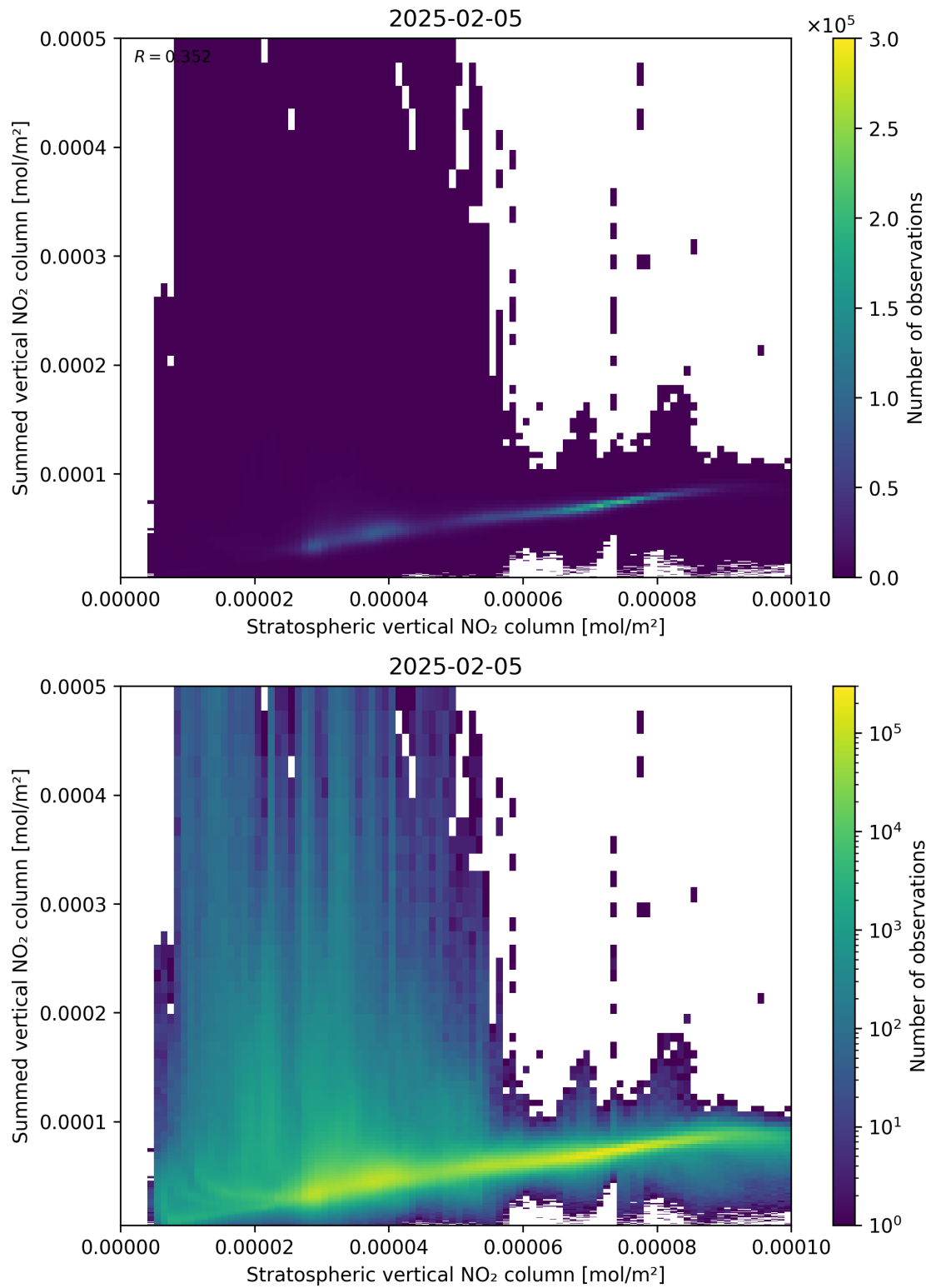
Figure 98: Scatter density plot of “Stratospheric vertical NO 2 column” against “Summed vertical NO 2 column” for 2025-02-04 to 2025-02-06.
