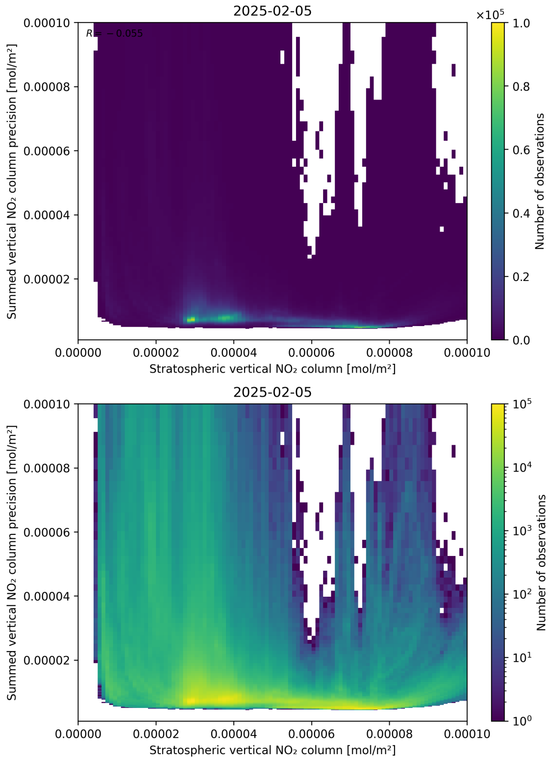
Figure 99: Scatter density plot of “Stratospheric vertical NO 2 column” against “Summed vertical NO 2 column precision” for 2025-02-04 to 2025-02-06.
