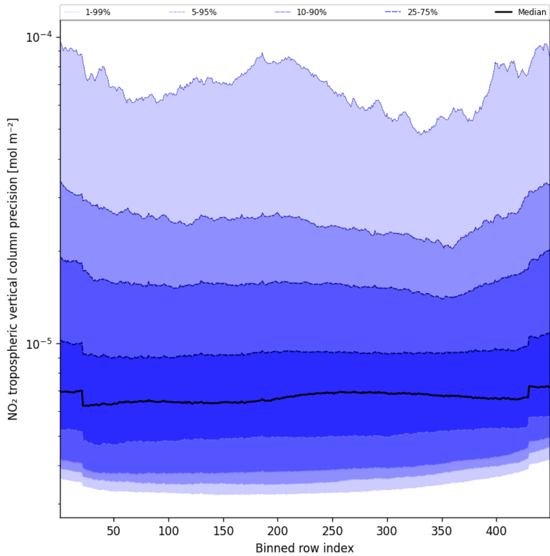
Figure 47: Along track statistics of “NO 2 tropospheric vertical column precision” for 2025-02-04 to 2025-02-06
