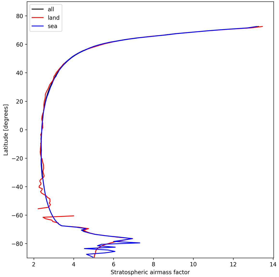
Figure 27: Zonal average of “Stratospheric airmass factor” for 2025-02-04 to 2025-02-06.
