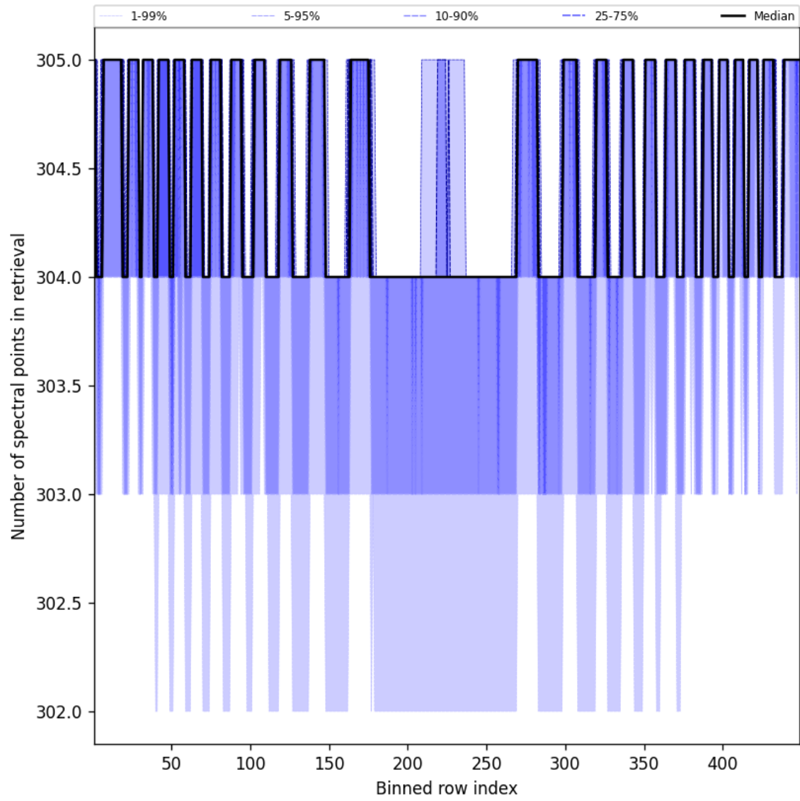
Figure 50: Along track statistics of “Number of spectral points in retrieval” for 2025-02-04 to 2025-02-06
