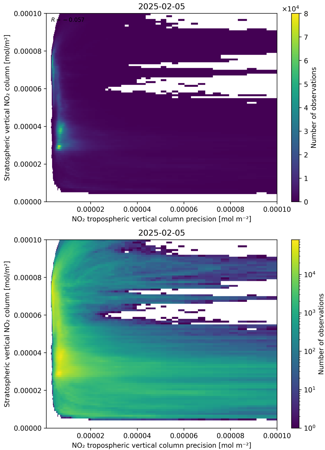
Figure 135: Scatter density plot of “NO 2 tropospheric vertical column precision” against “Stratospheric vertical NO 2 column” for 2025-02-04 to 2025-02-06.
