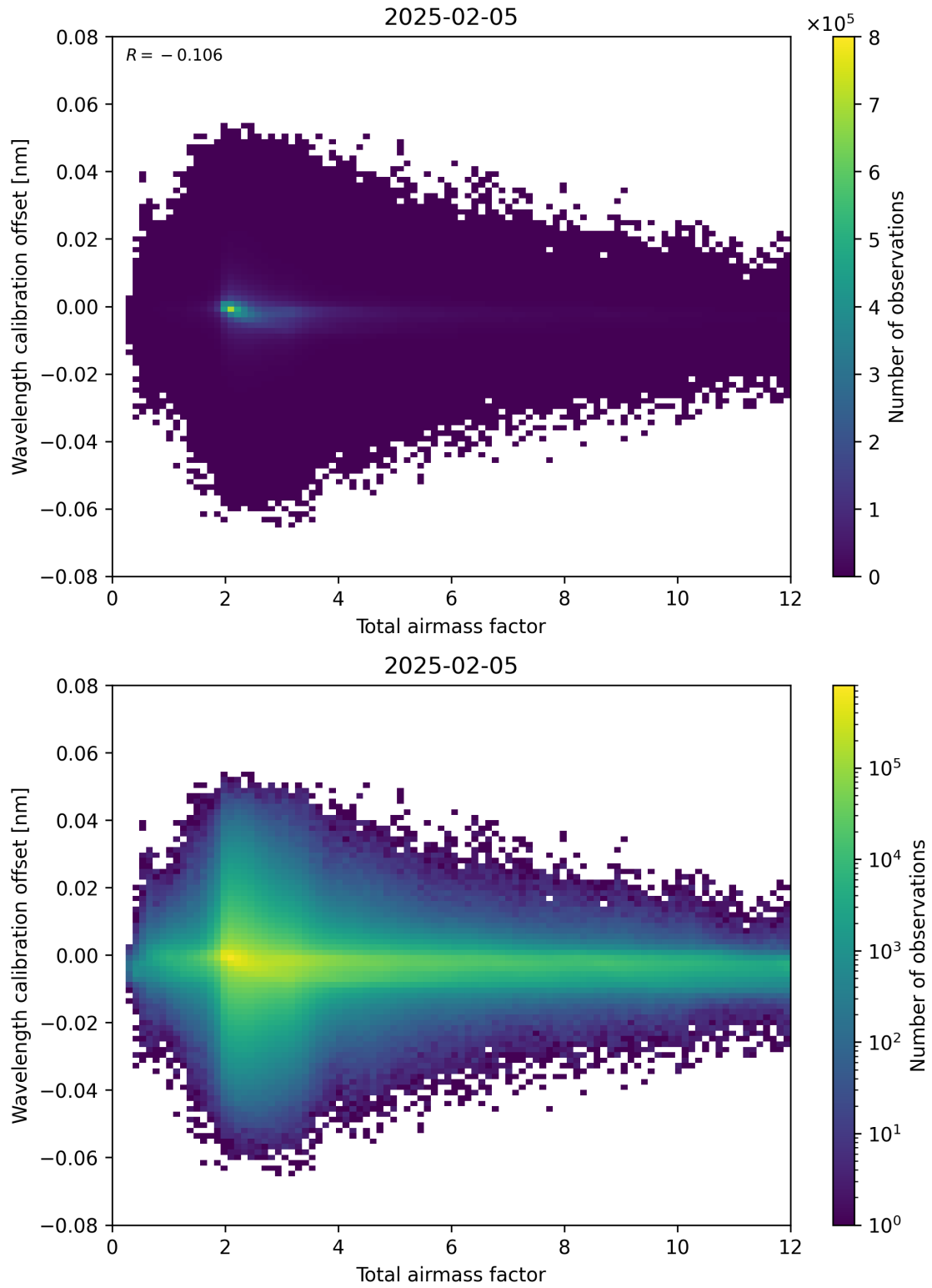
Figure 70: Scatter density plot of “Total airmass factor” against “Wavelength calibration offset” for 2025-02-04 to 2025-02-06.
