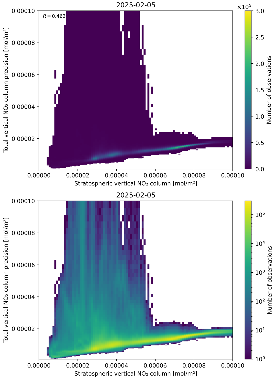
Figure 101: Scatter density plot of “Stratospheric vertical NO 2 column” against “Total vertical NO 2 column precision” for 2025-02-04 to 2025-02-06.
