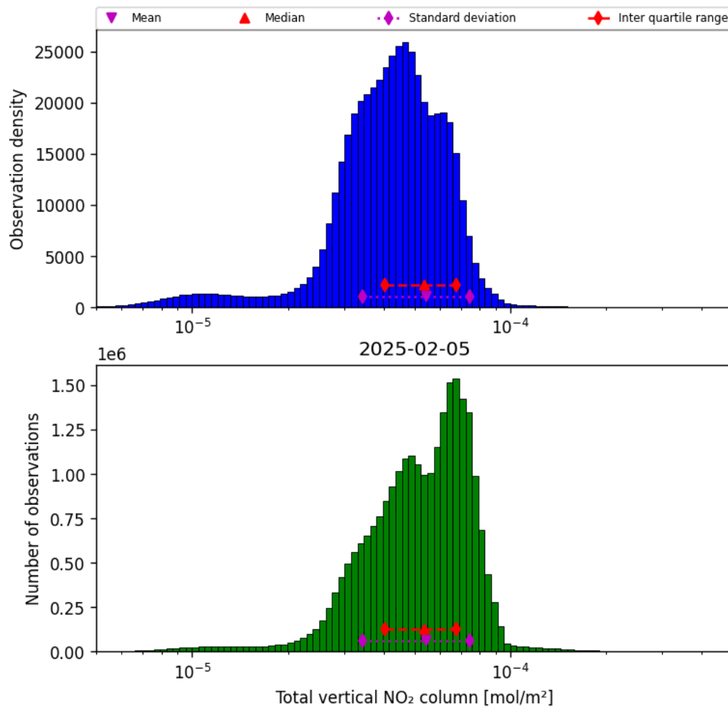
Figure 38: Histogram of “Total vertical NO 2 column” for 2025-02-04 to 2025-02-06
