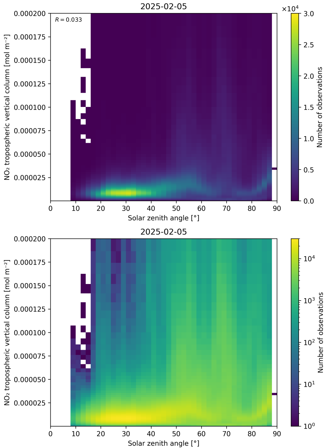
Figure 155: Scatter density plot of “Solar zenith angle” against “NO 2 tropospheric vertical column” for 2025-02-04 to 2025-02-06.
