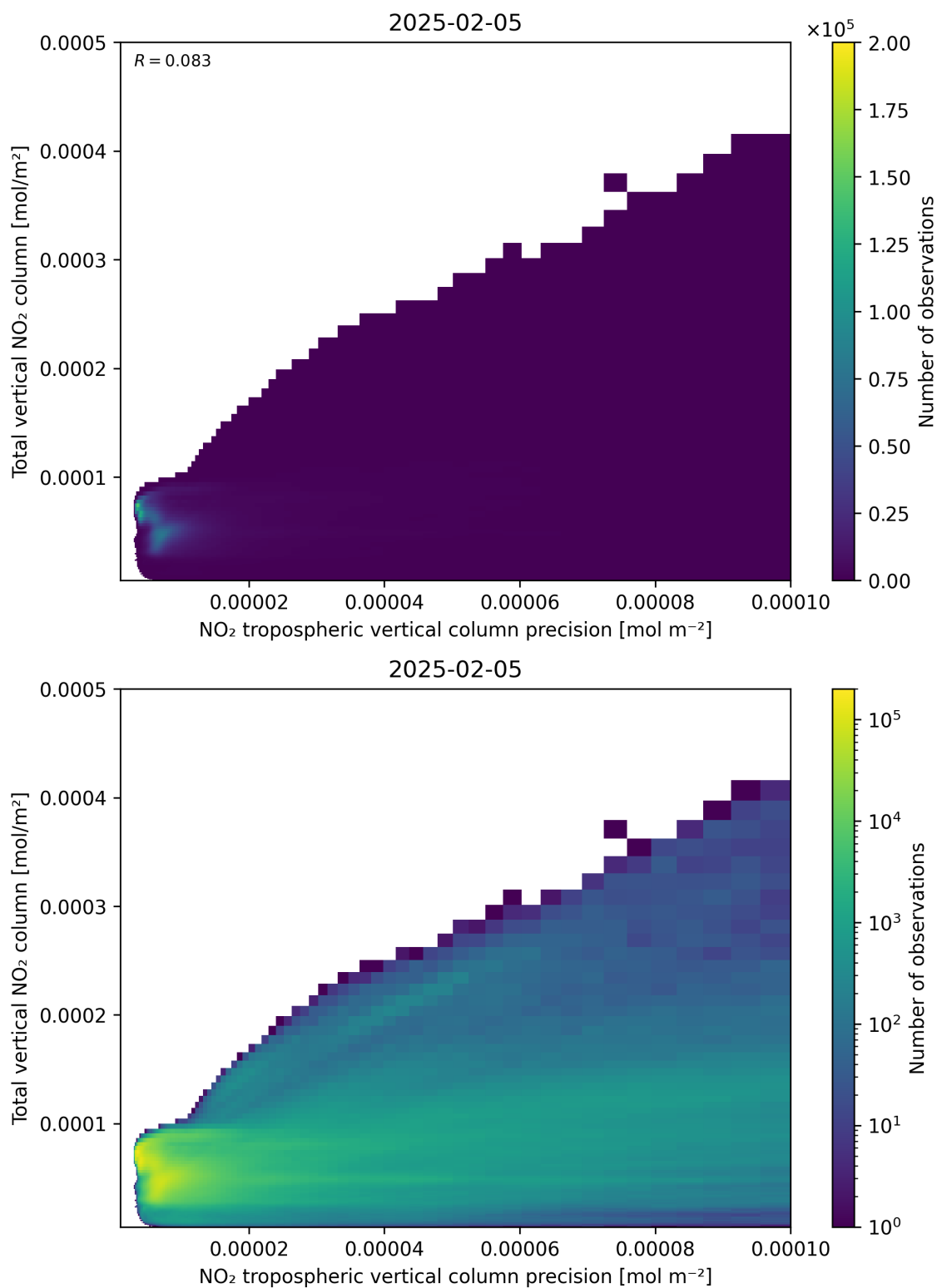
Figure 138: Scatter density plot of “NO 2 tropospheric vertical column precision” against “Total vertical NO 2 column” for 2025-02-04 to 2025-02-06.
