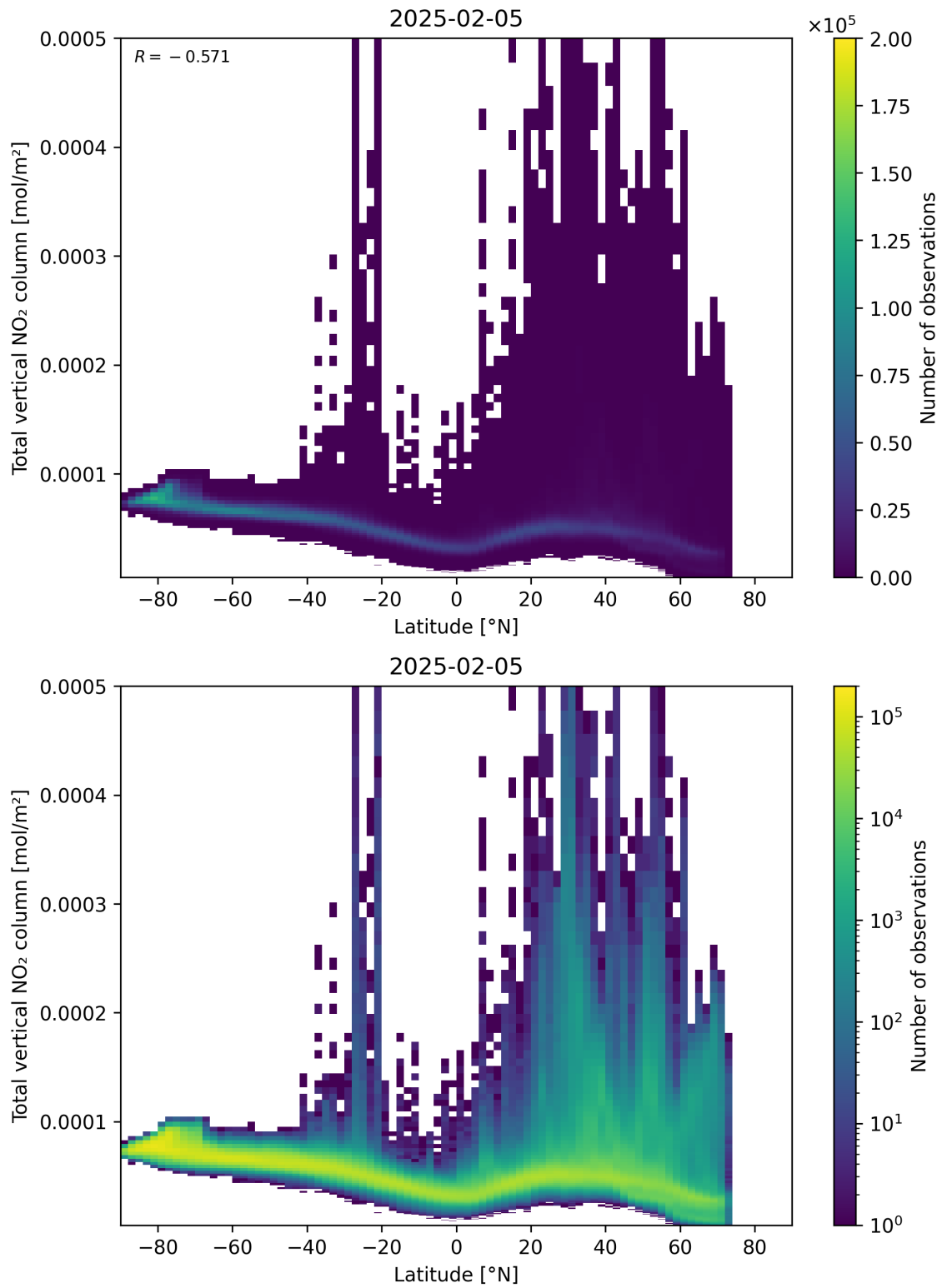
Figure 90: Scatter density plot of “Latitude” against “Total vertical NO 2 column” for 2025-02-04 to 2025-02-06.
