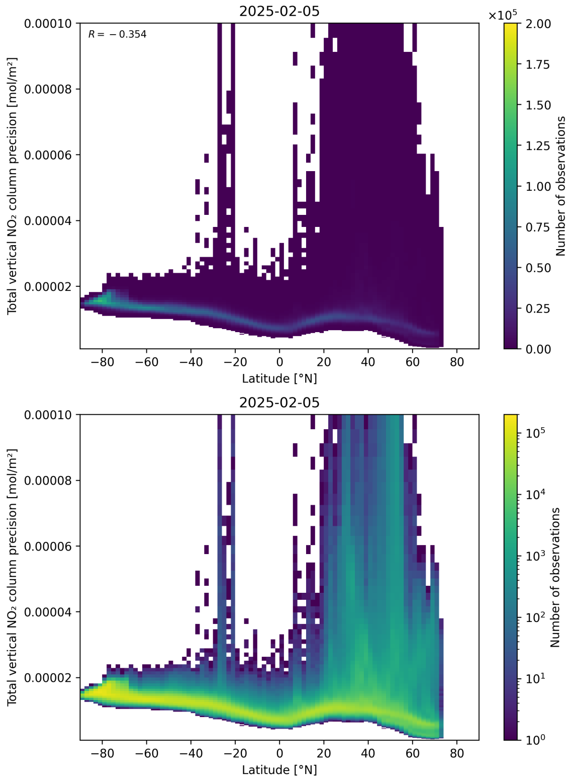
Figure 91: Scatter density plot of “Latitude” against “Total vertical NO 2 column precision” for 2025-02-04 to 2025-02-06.
