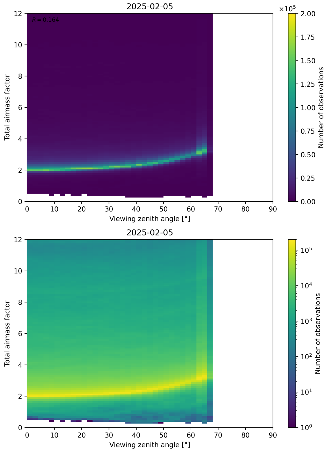
Figure 160: Scatter density plot of “Viewing zenith angle” against “Total airmass factor” for 2025-02-04 to 2025-02-06.
