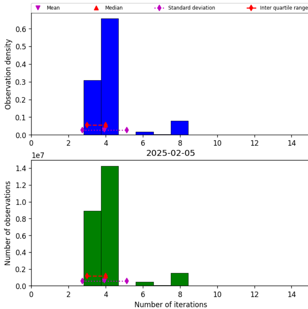
Figure 34: Histogram of “Number of iterations” for 2025-02-04 to 2025-02-06
