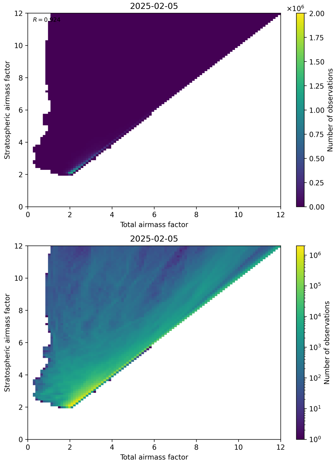
Figure 62: Scatter density plot of “Total airmass factor” against “Stratospheric airmass factor” for 2025-02-04 to 2025-02-06.
