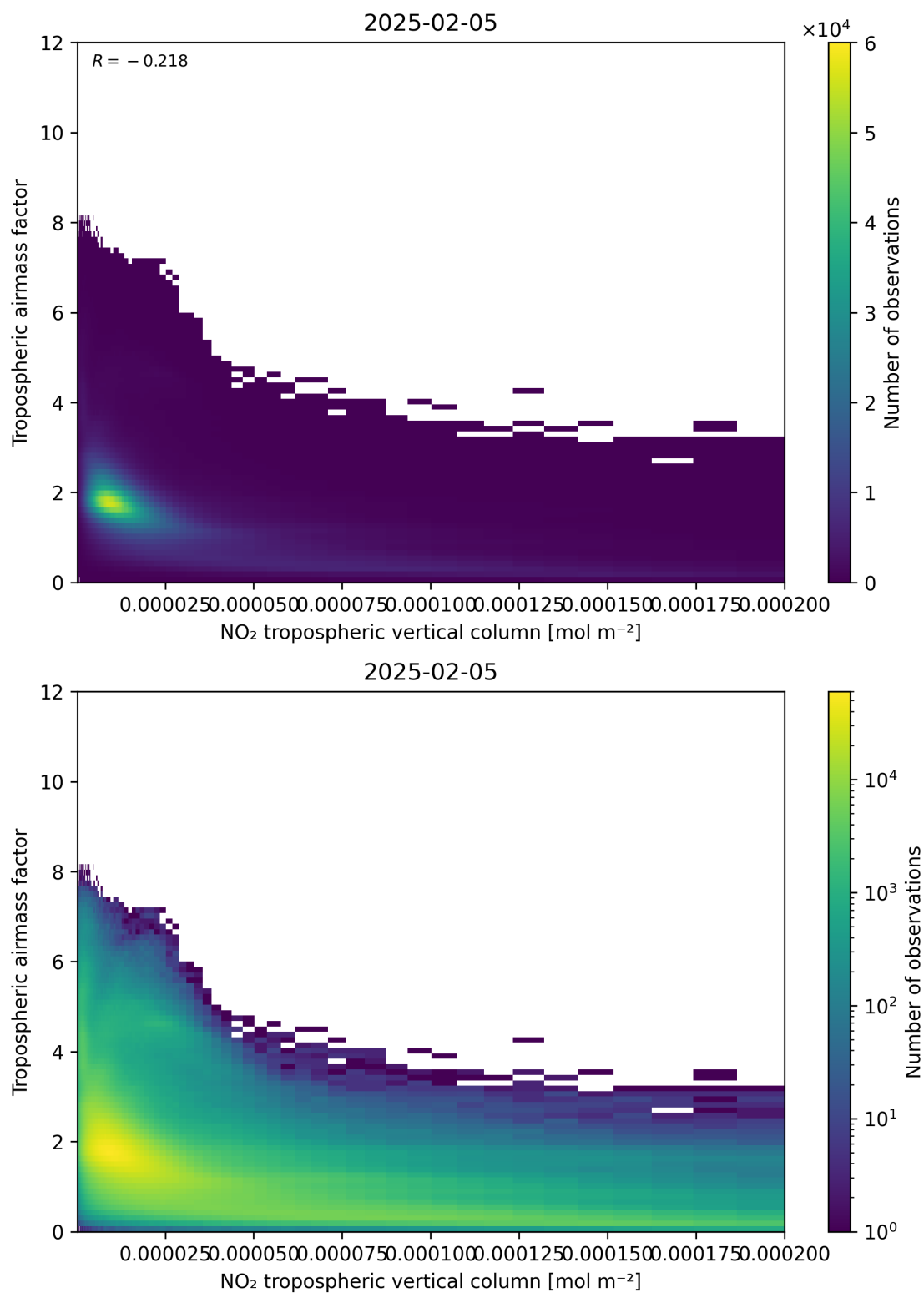
Figure 123: Scatter density plot of “NO 2 tropospheric vertical column” against “Tropospheric air mass factor” for 2025-02-04 to 2025-02-06.
