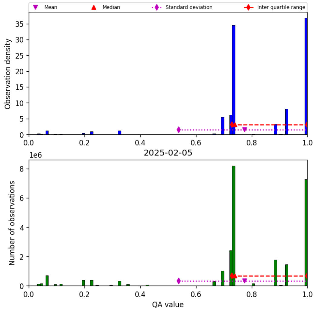
Figure 28: Histogram of “QA value” for 2025-02-04 to 2025-02-06
