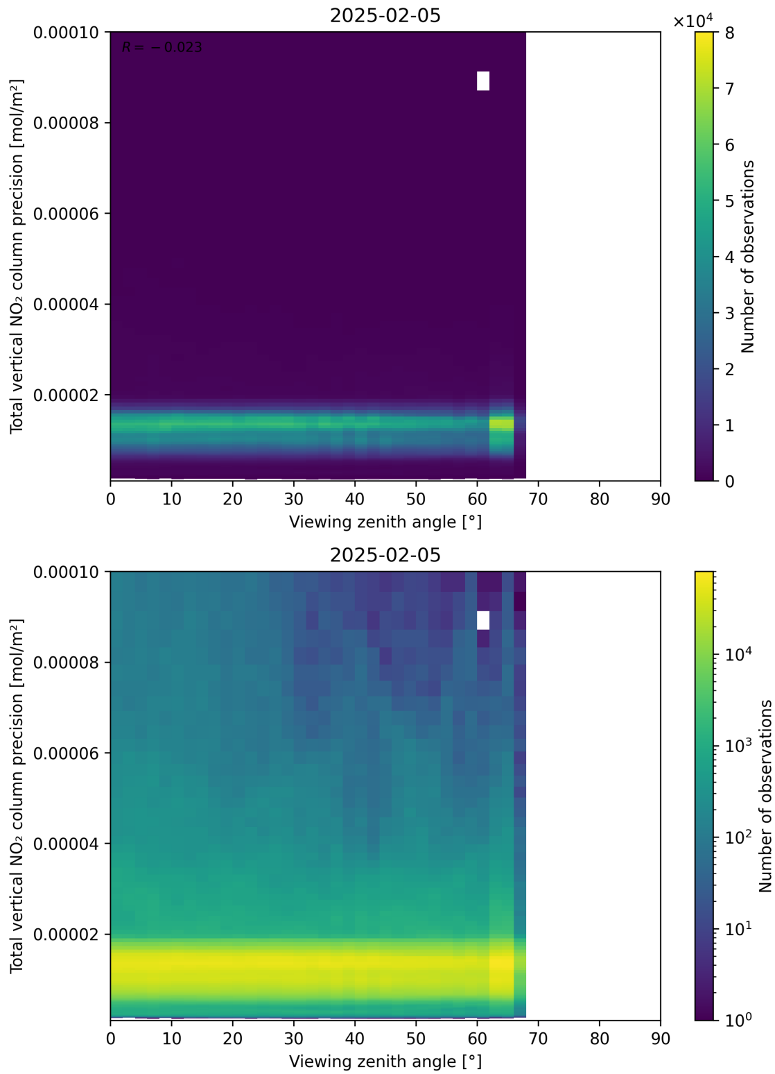
Figure 168: Scatter density plot of “Viewing zenith angle” against “Total vertical NO 2 column precision” for 2025-02-04 to 2025-02-06.
