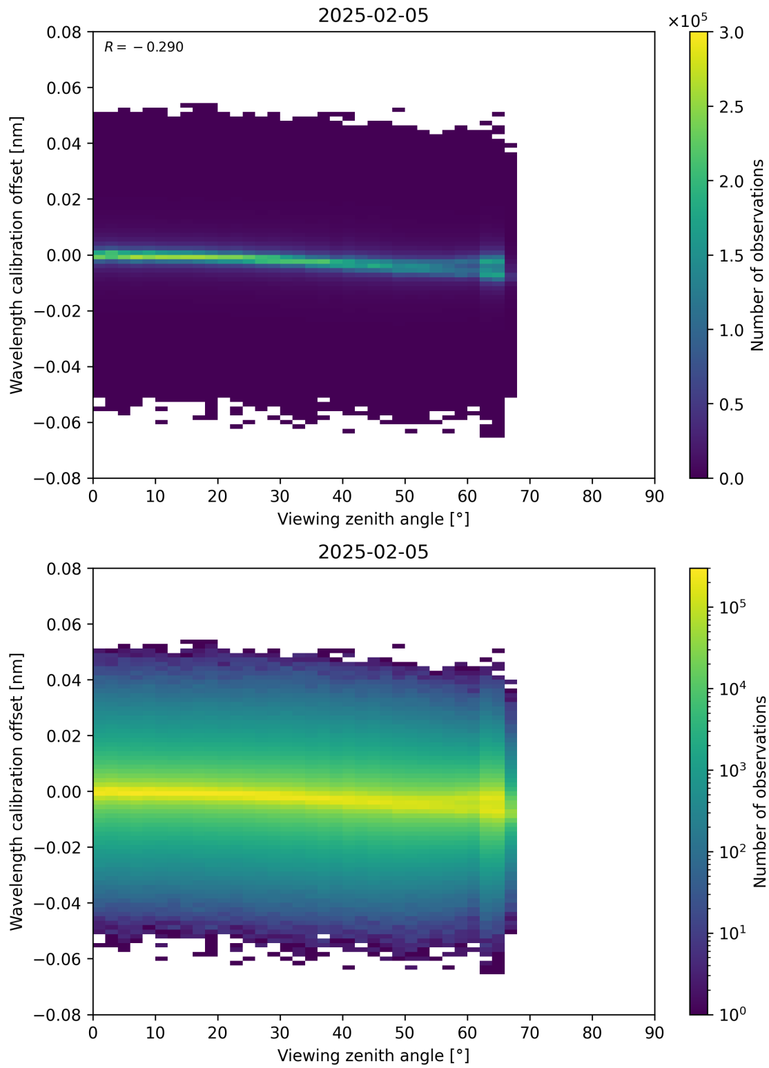
Figure 173: Scatter density plot of “Viewing zenith angle” against “Wavelength calibration offset” for 2025-02-04 to 2025-02-06.
