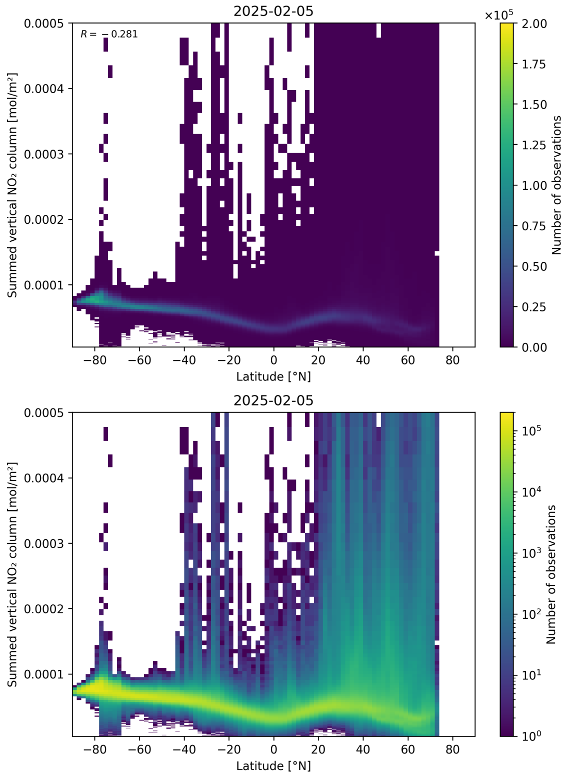
Figure 88: Scatter density plot of “Latitude” against “Summed vertical NO 2 column” for 2025-02-04 to 2025-02-06.
