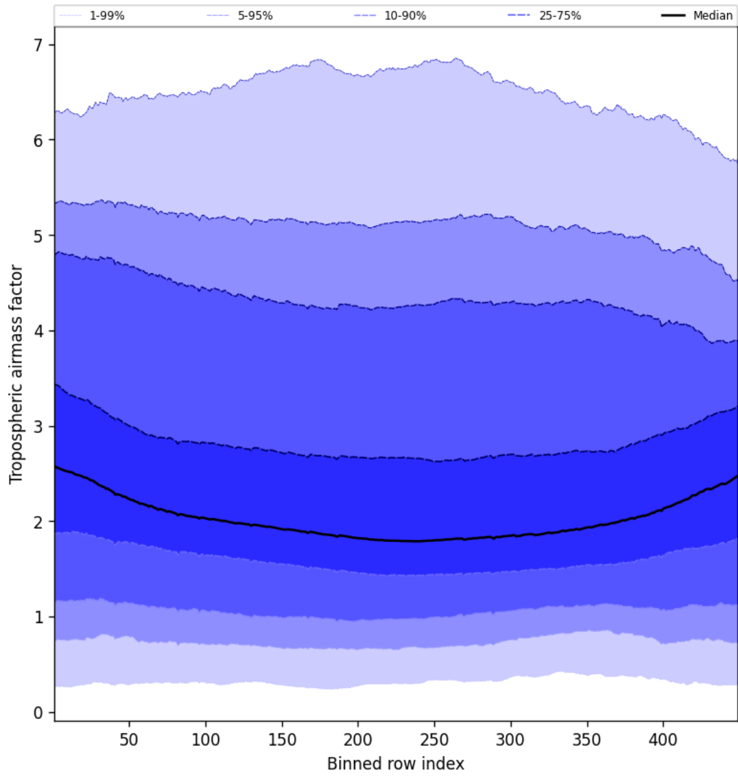
Figure 48: Along track statistics of “Tropospheric airmass factor” for 2025-02-04 to 2025-02-06
