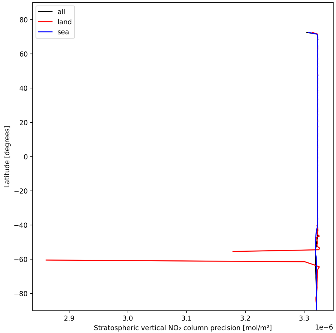
Figure 20: Zonal average of “Stratospheric vertical NO 2 column precision” for 2025-02-04 to 2025-02-06.
