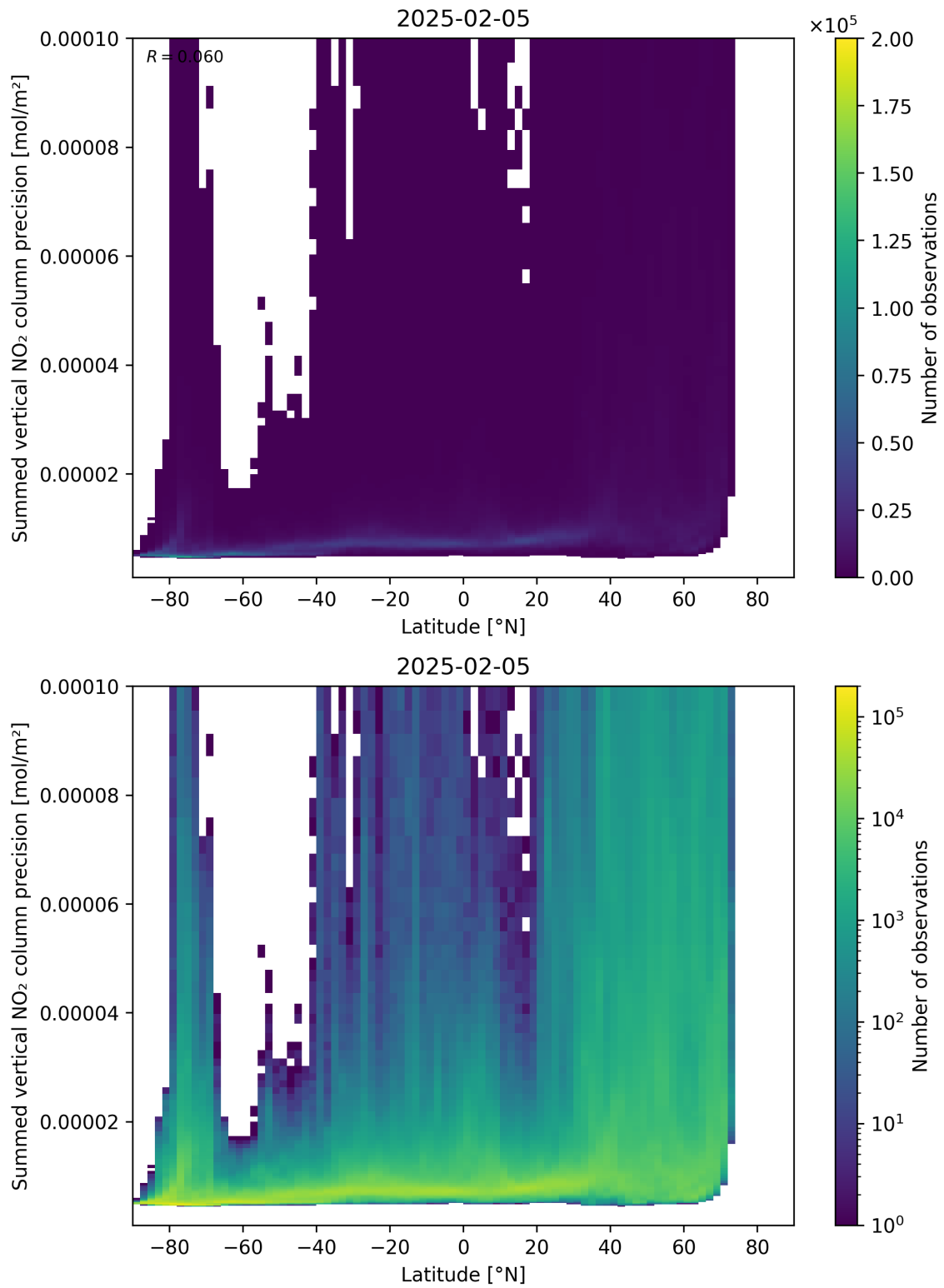
Figure 89: Scatter density plot of “Latitude” against “Summed vertical NO 2 column precision” for 2025-02-04 to 2025-02-06.
