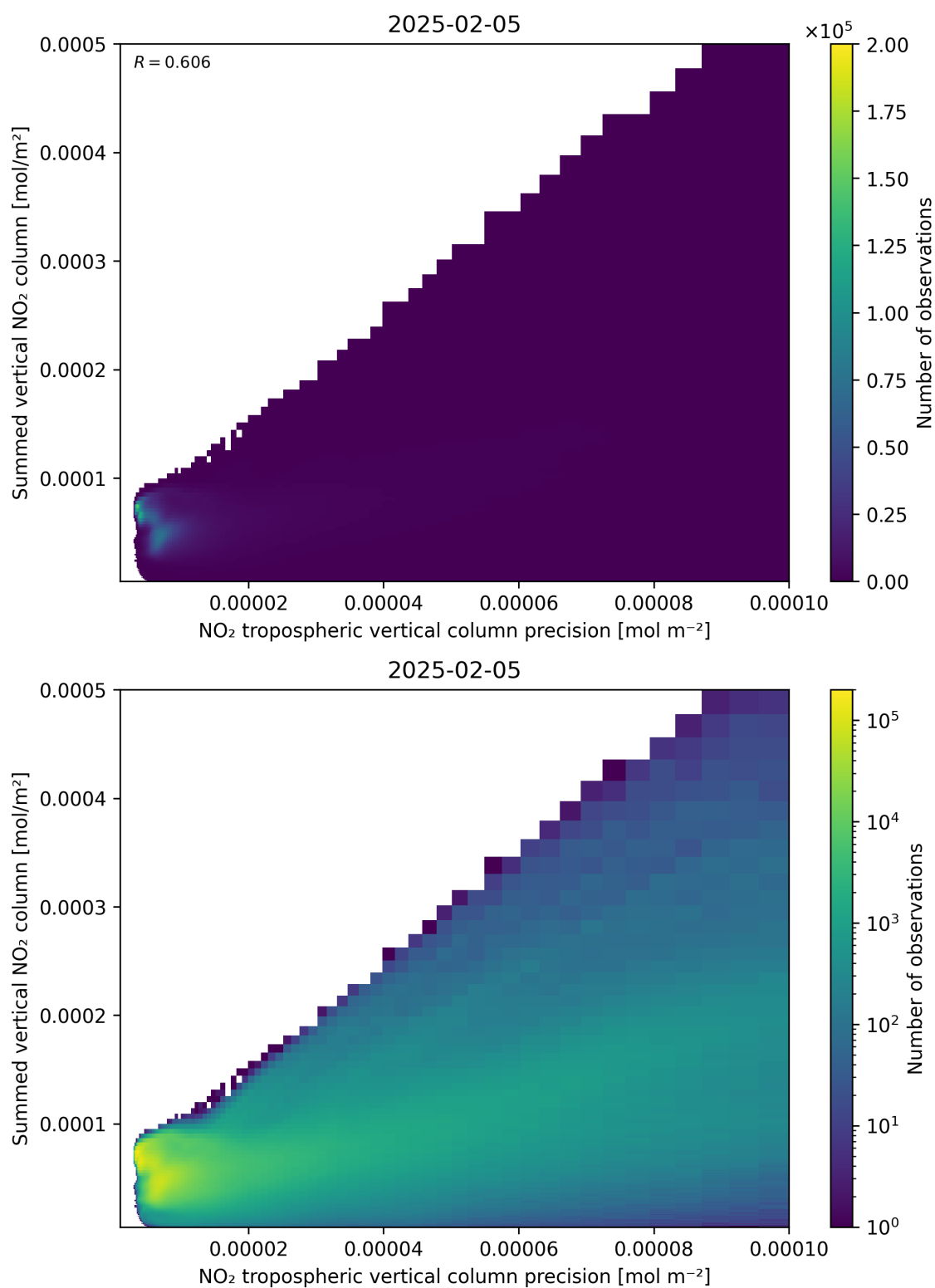
Figure 136: Scatter density plot of “NO 2 tropospheric vertical column precision” against “Summed vertical NO 2 column” for 2025-02-04 to 2025-02-06.
