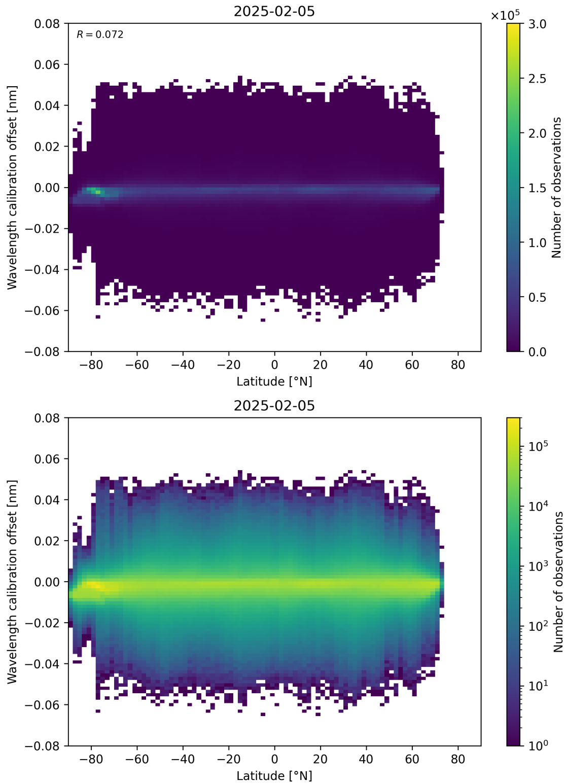
Figure 95: Scatter density plot of “Latitude” against “Wavelength calibration offset” for 2025-02-04 to 2025-02-06.
