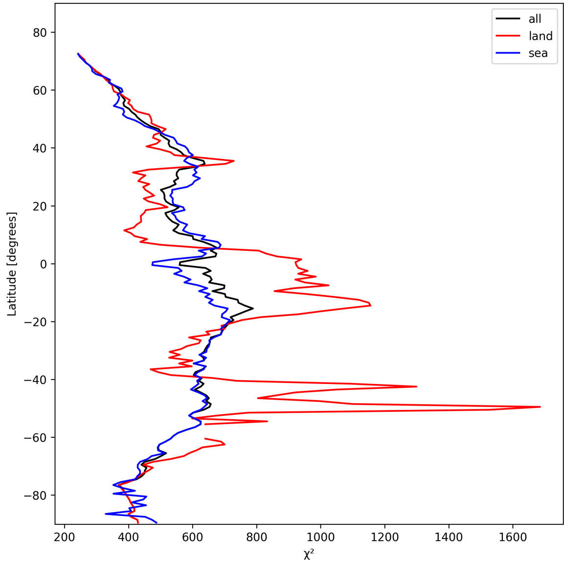
Figure 25: Zonal average of “ \chi^2 ” for 2025-02-04 to 2025-02-06.
