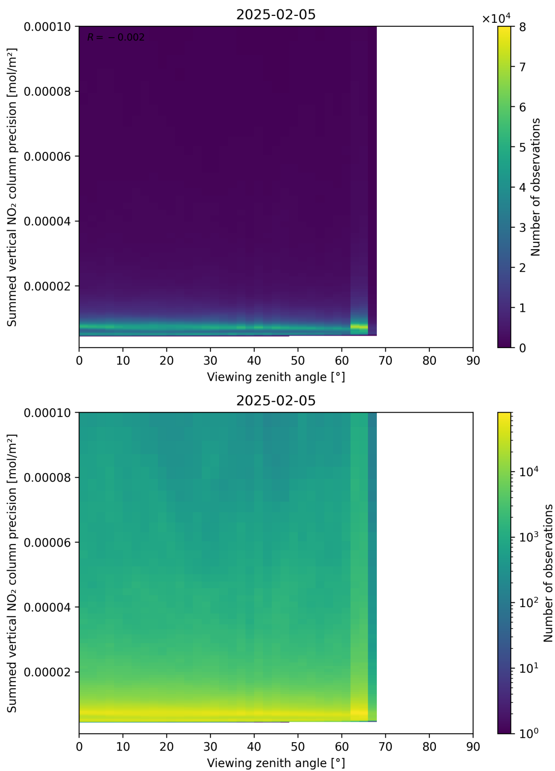
Figure 166: Scatter density plot of “Viewing zenith angle” against “Summed vertical NO 2 column precision” for 2025-02-04 to 2025-02-06.
