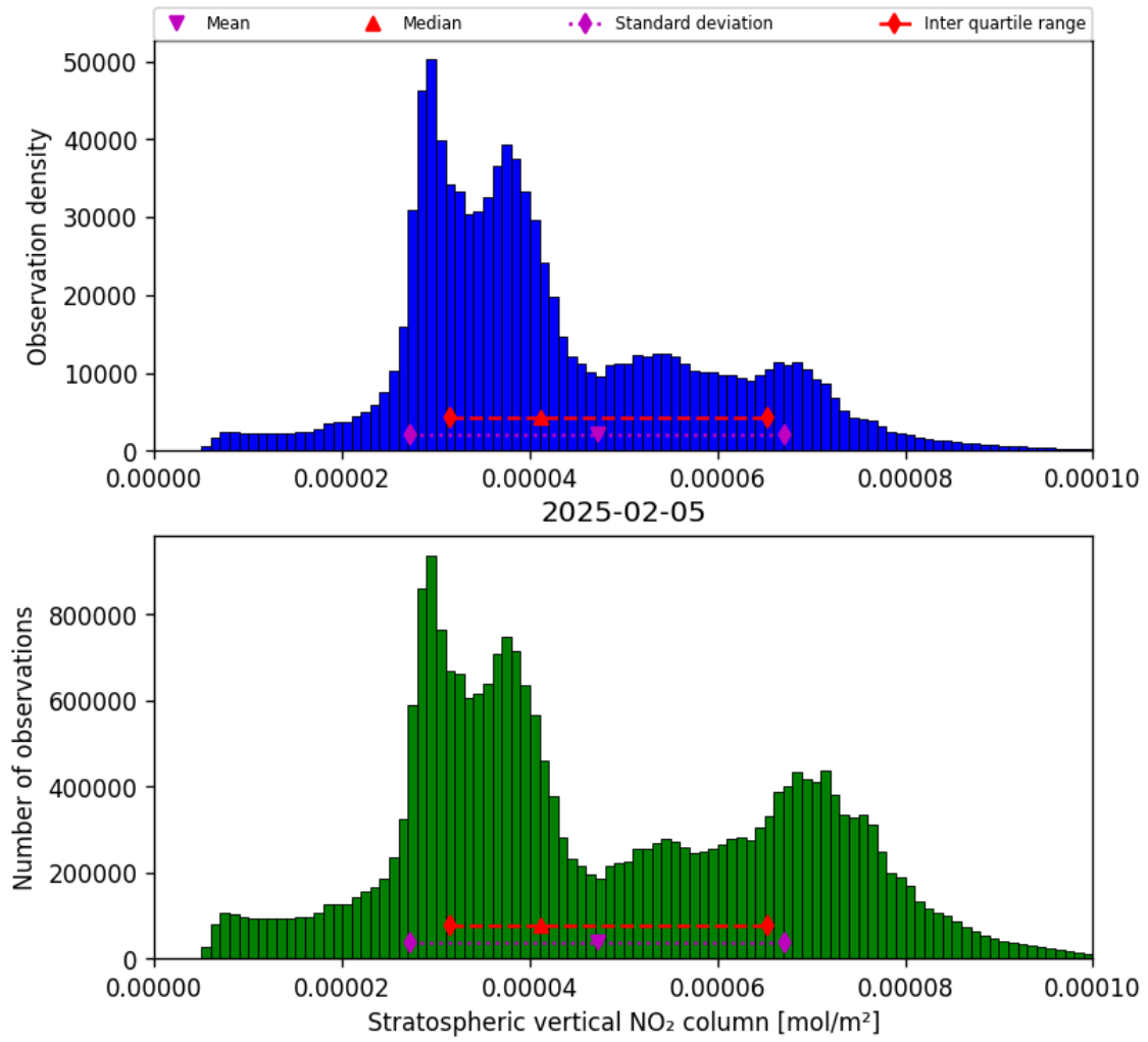
Figure 36: Histogram of “Stratospheric vertical NO 2 column” for 2025-02-04 to 2025-02-06
