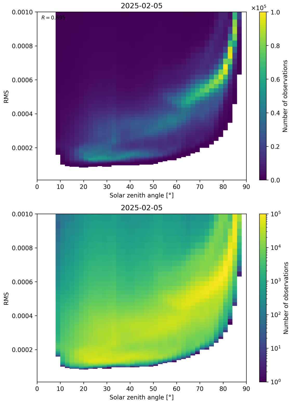
Figure 157: Scatter density plot of “Solar zenith angle” against “RMS” for 2025-02-04 to 2025-02-06.
