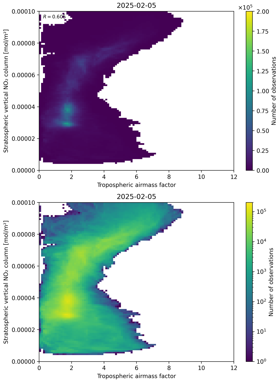
Figure 74: Scatter density plot of “Tropospheric air mass factor” against “Stratospheric vertical NO 2 column” for 2025-02-04 to 2025-02-06.
