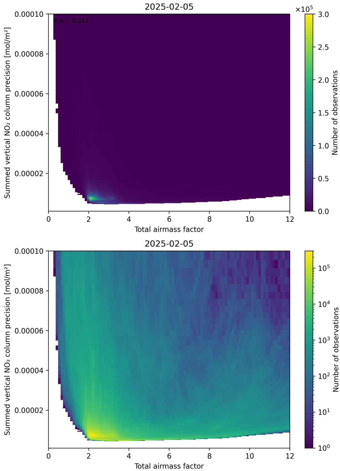
Figure 66: Scatter density plot of “Total airmass factor” against “Summed vertical NO 2 column precision” for 2025-02-04 to 2025-02-06.
