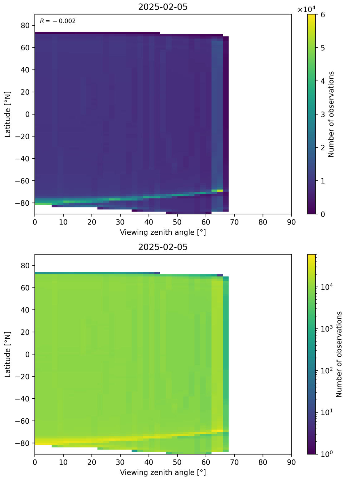
Figure 163: Scatter density plot of “Viewing zenith angle” against “Latitude” for 2025-02-04 to 2025-02-06.
