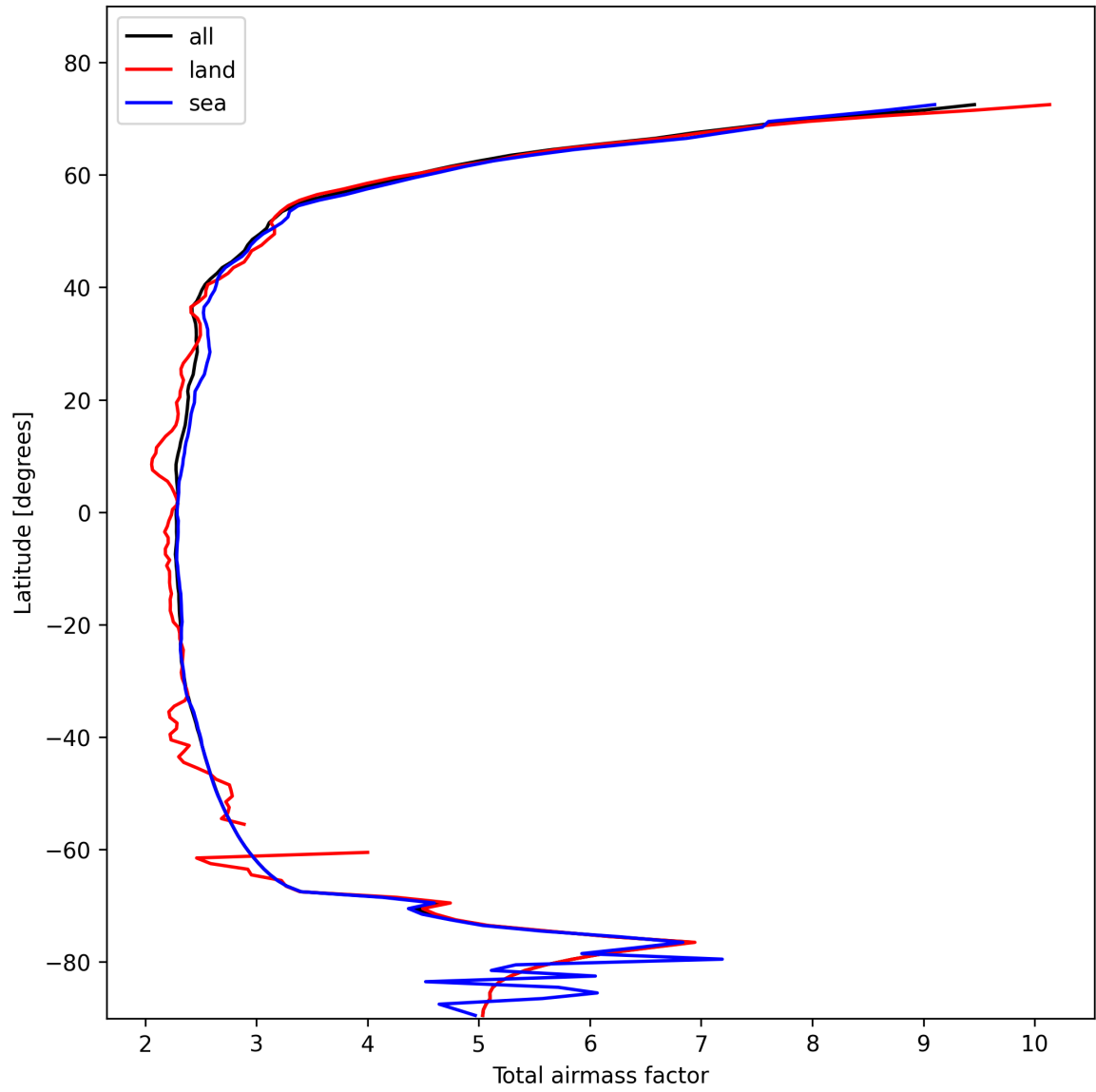
Figure 15: Zonal average of “Total airmass factor” for 2025-02-04 to 2025-02-06.
