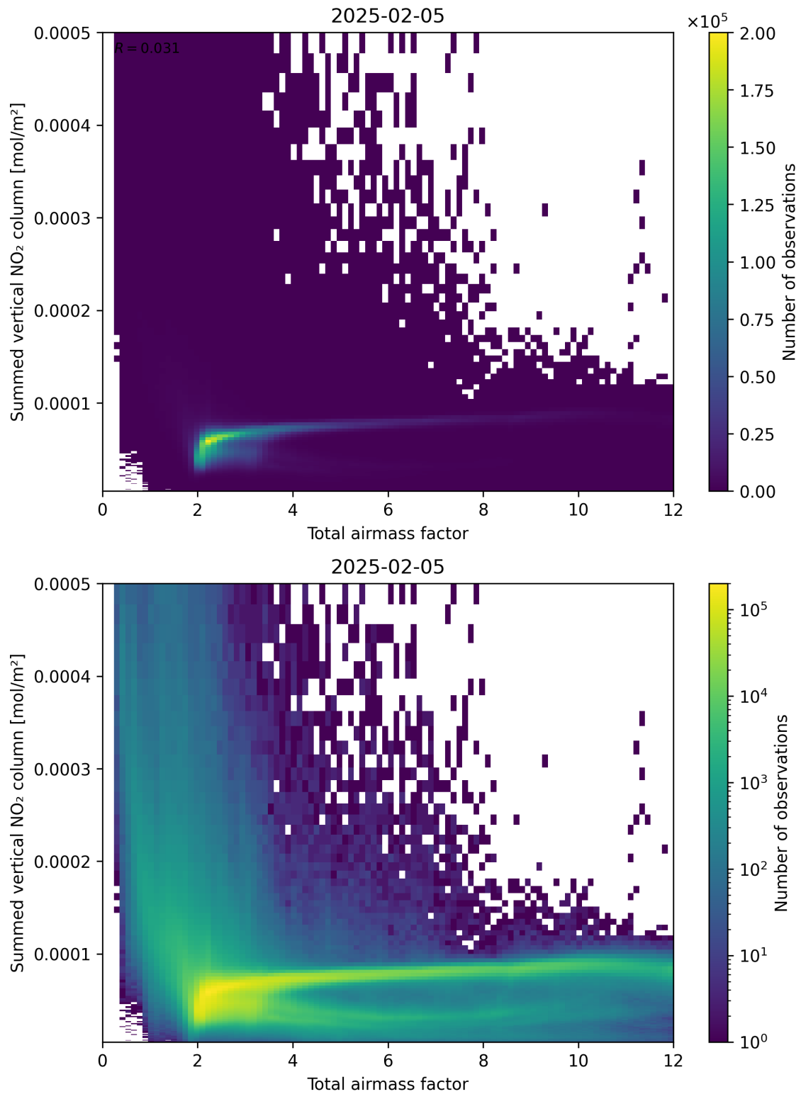
Figure 65: Scatter density plot of “Total airmass factor” against “Summed vertical NO 2 column” for 2025-02-04 to 2025-02-06.
