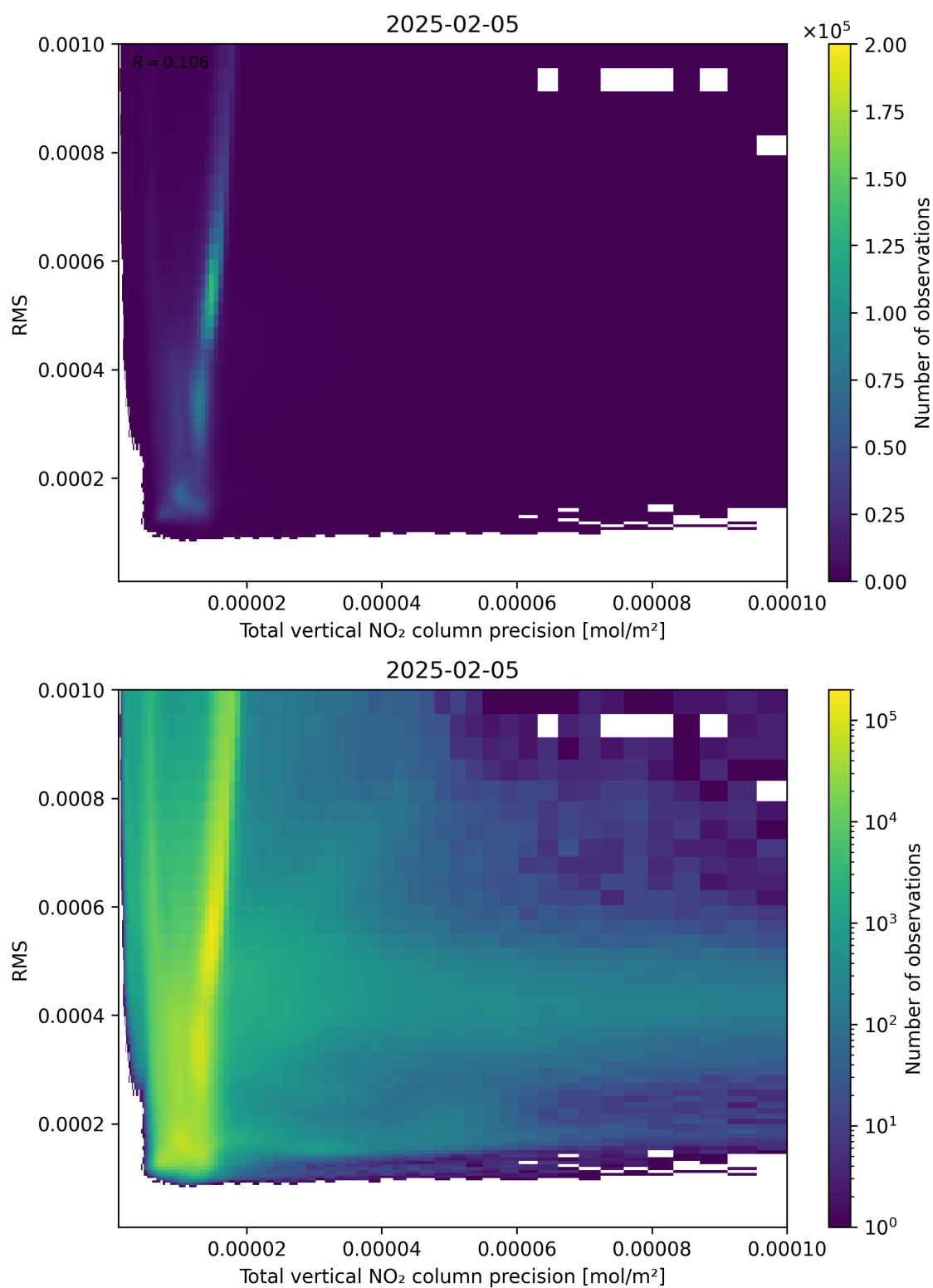
Figure 119: Scatter density plot of “Total vertical NO 2 column precision” against “RMS” for 2025-02-04 to 2025-02-06.
