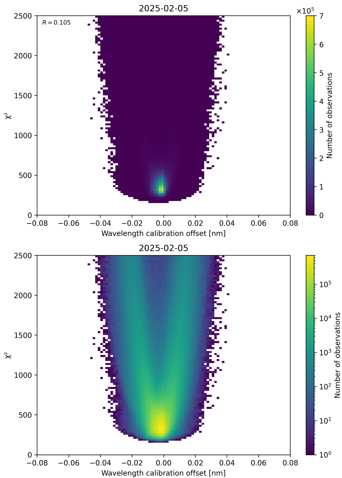
Figure 175: Scatter density plot of “Wavelength calibration offset” against “ \chi^2 ” for 2025-02-04 to 2025-02-06.
