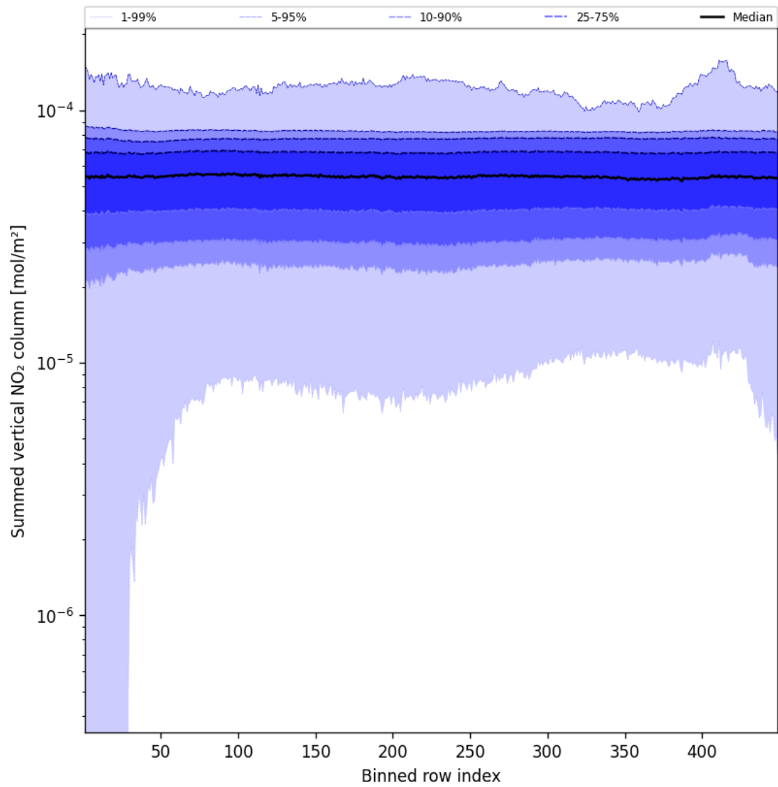
Figure 57: Along track statistics of “Summed vertical NO 2 column” for 2025-02-04 to 2025-02-06
