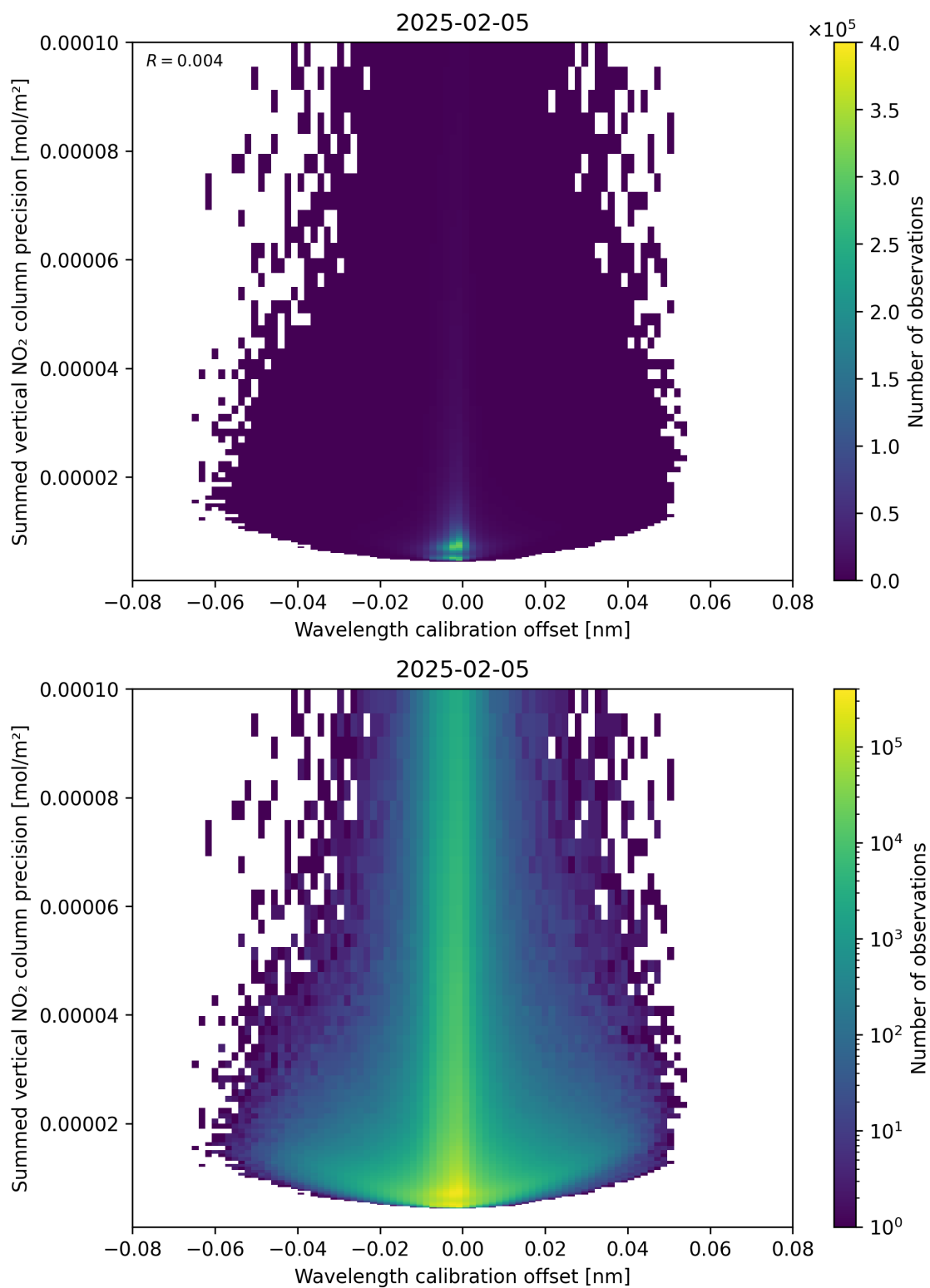
Figure 178: Scatter density plot of “Wavelength calibration offset” against “Summed vertical NO 2 column precision” for 2025-02-04 to 2025-02-06.
