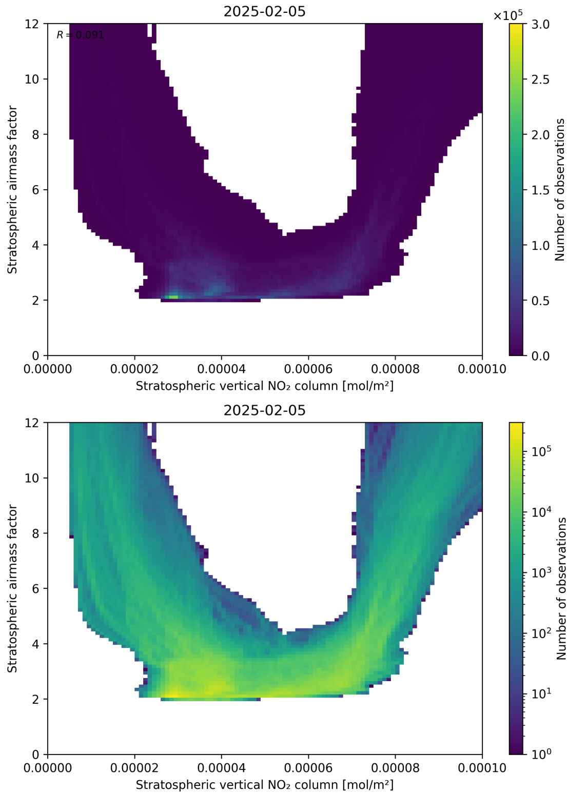
Figure 96: Scatter density plot of “Stratospheric vertical NO 2 column” against “Stratospheric airmass factor” for 2025-02-04 to 2025-02-06.
