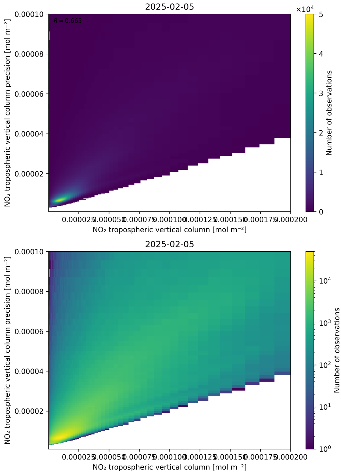
Figure 130: Scatter density plot of “NO 2 tropospheric vertical column” against “NO 2 tropospheric vertical column precision” for 2025-02-04 to 2025-02-06.
