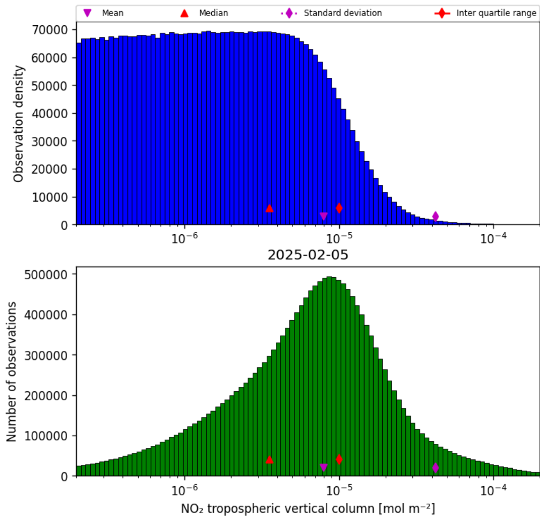
Figure 29: Histogram of “NO 2 tropospheric vertical column” for 2025-02-04 to 2025-02-06
