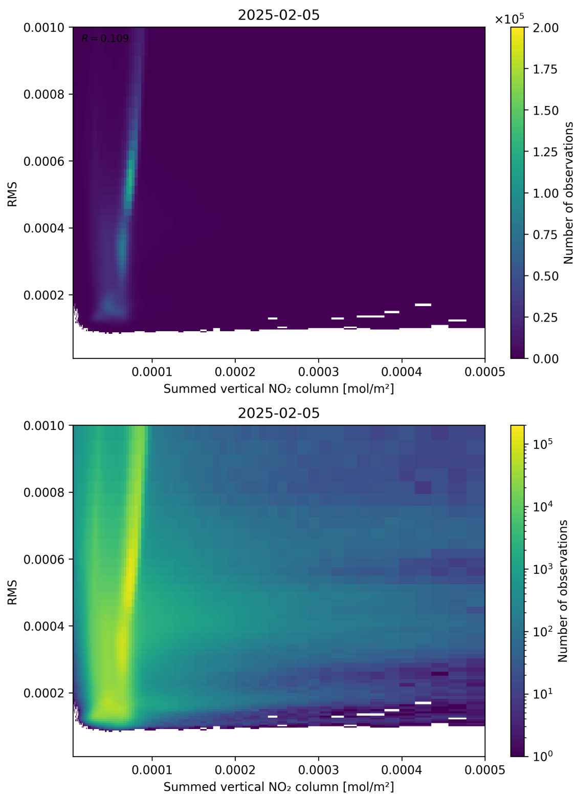
Figure 109: Scatter density plot of “Summed vertical NO 2 column” against “RMS” for 2025-02-04 to 2025-02-06.
