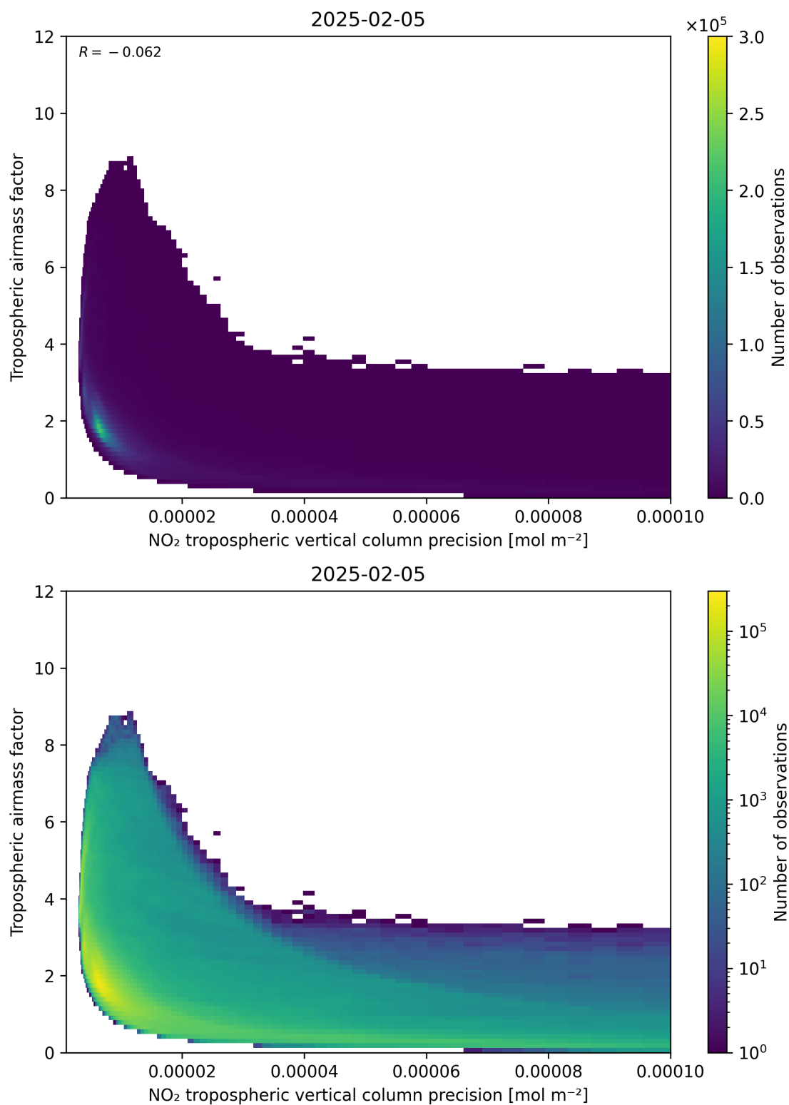
Figure 133: Scatter density plot of “NO 2 tropospheric vertical column precision” against “Tropospheric air mass factor” for 2025-02-04 to 2025-02-06.
