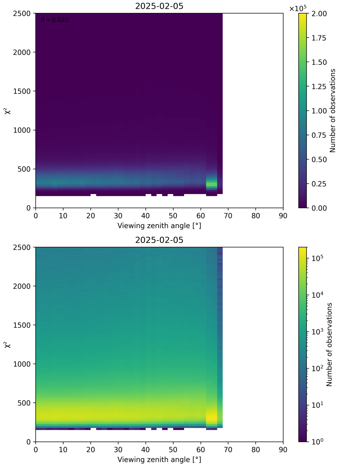
Figure 162: Scatter density plot of “Viewing zenith angle” against “ \chi^2 ” for 2025-02-04 to 2025-02-06.
