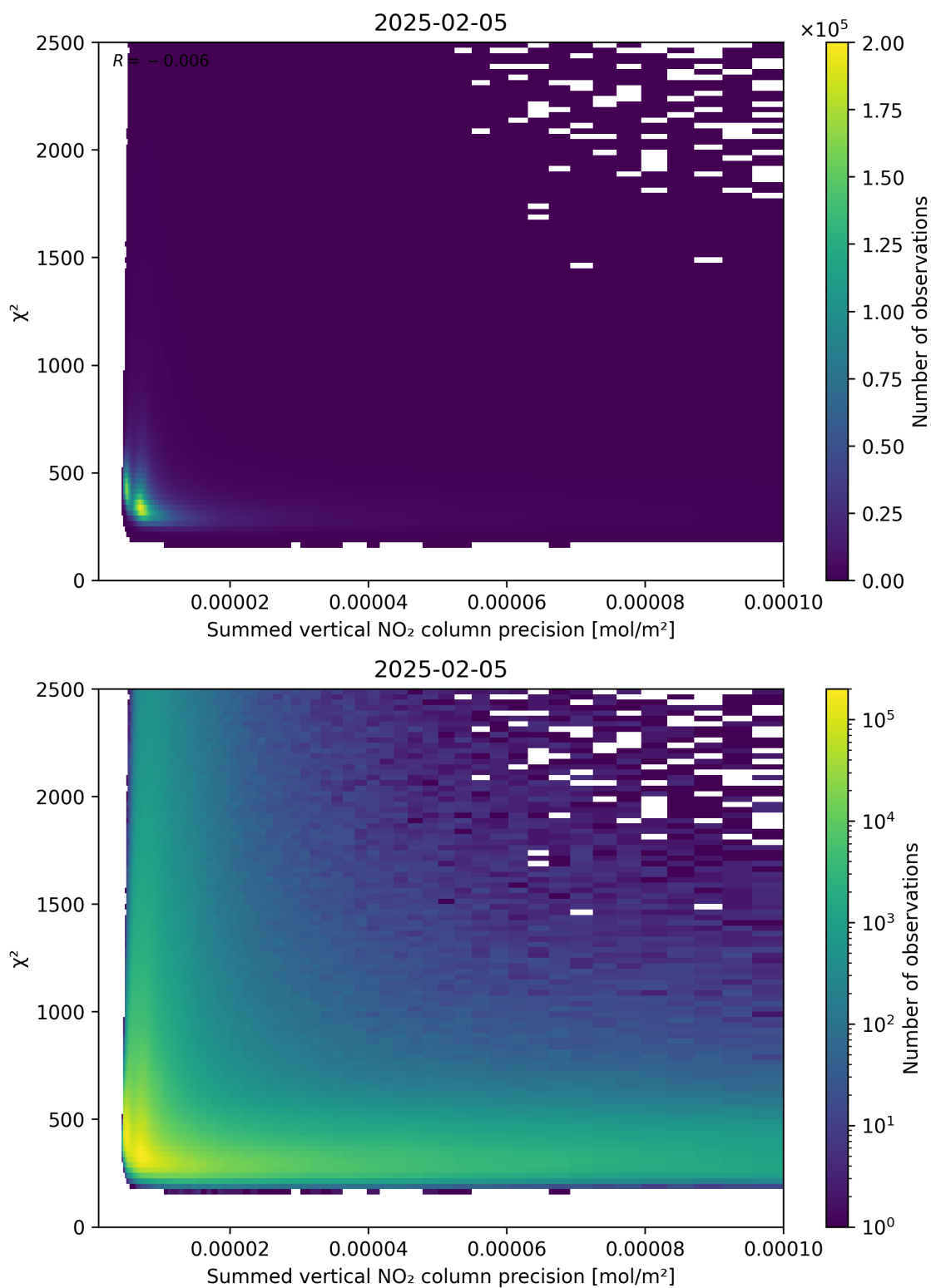
Figure 107: Scatter density plot of “Summed vertical NO 2 column precision” against “ \chi^2 ” for 2025-02-04 to 2025-02-06.
