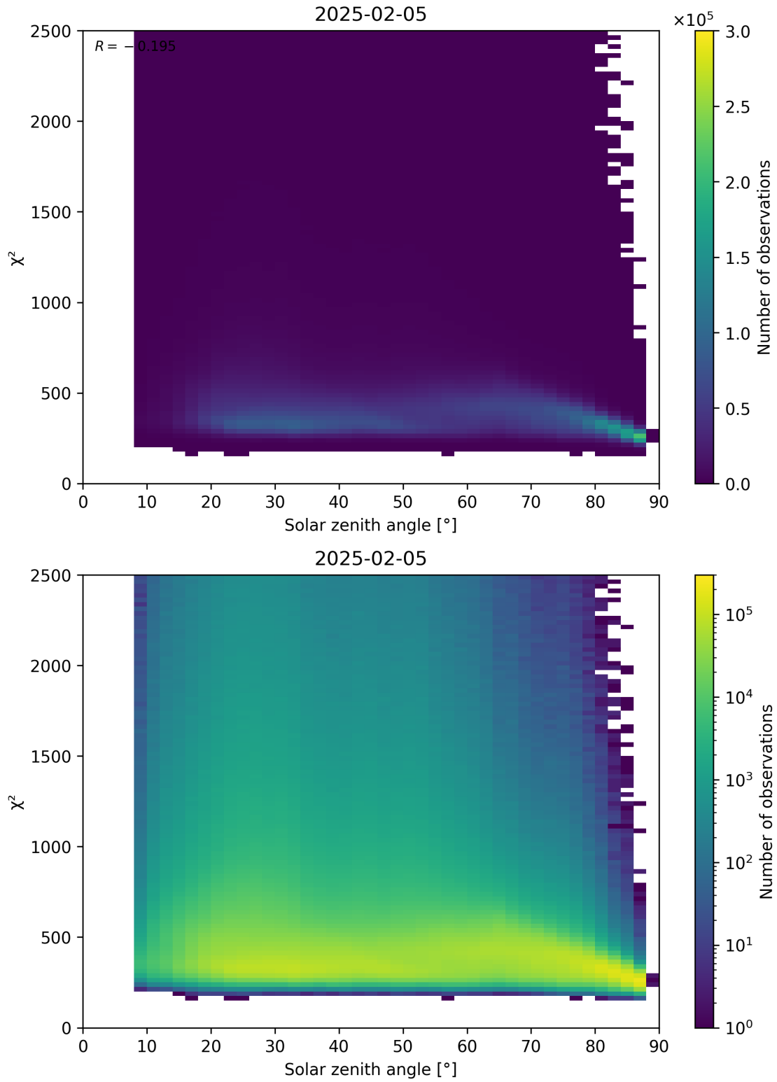
Figure 148: Scatter density plot of “Solar zenith angle” against “ \chi^2 ” for 2025-02-04 to 2025-02-06.
