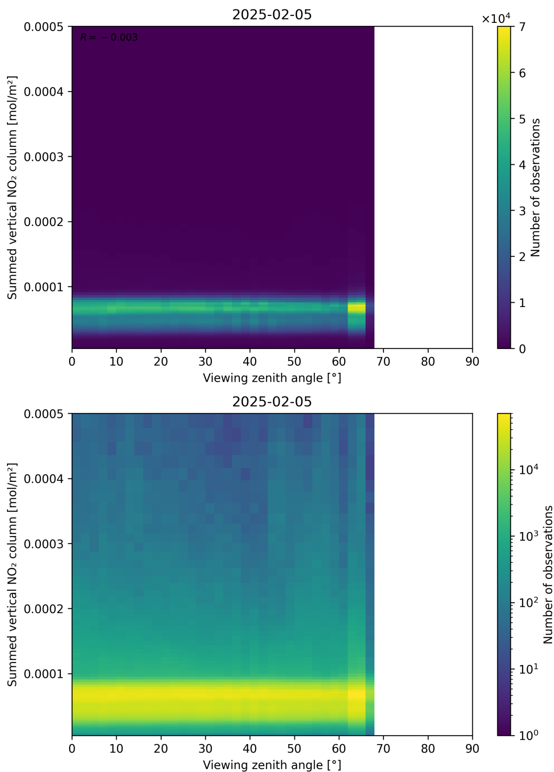
Figure 165: Scatter density plot of “Viewing zenith angle” against “Summed vertical NO 2 column” for 2025-02-04 to 2025-02-06.
