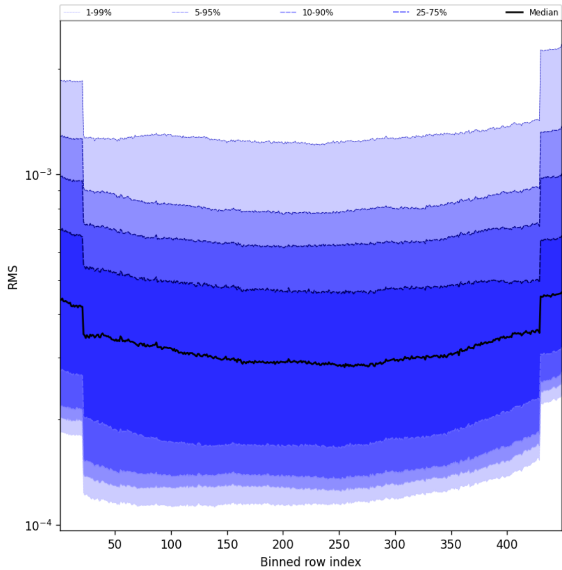
Figure 60: Along track statistics of “RMS” for 2025-02-04 to 2025-02-06
