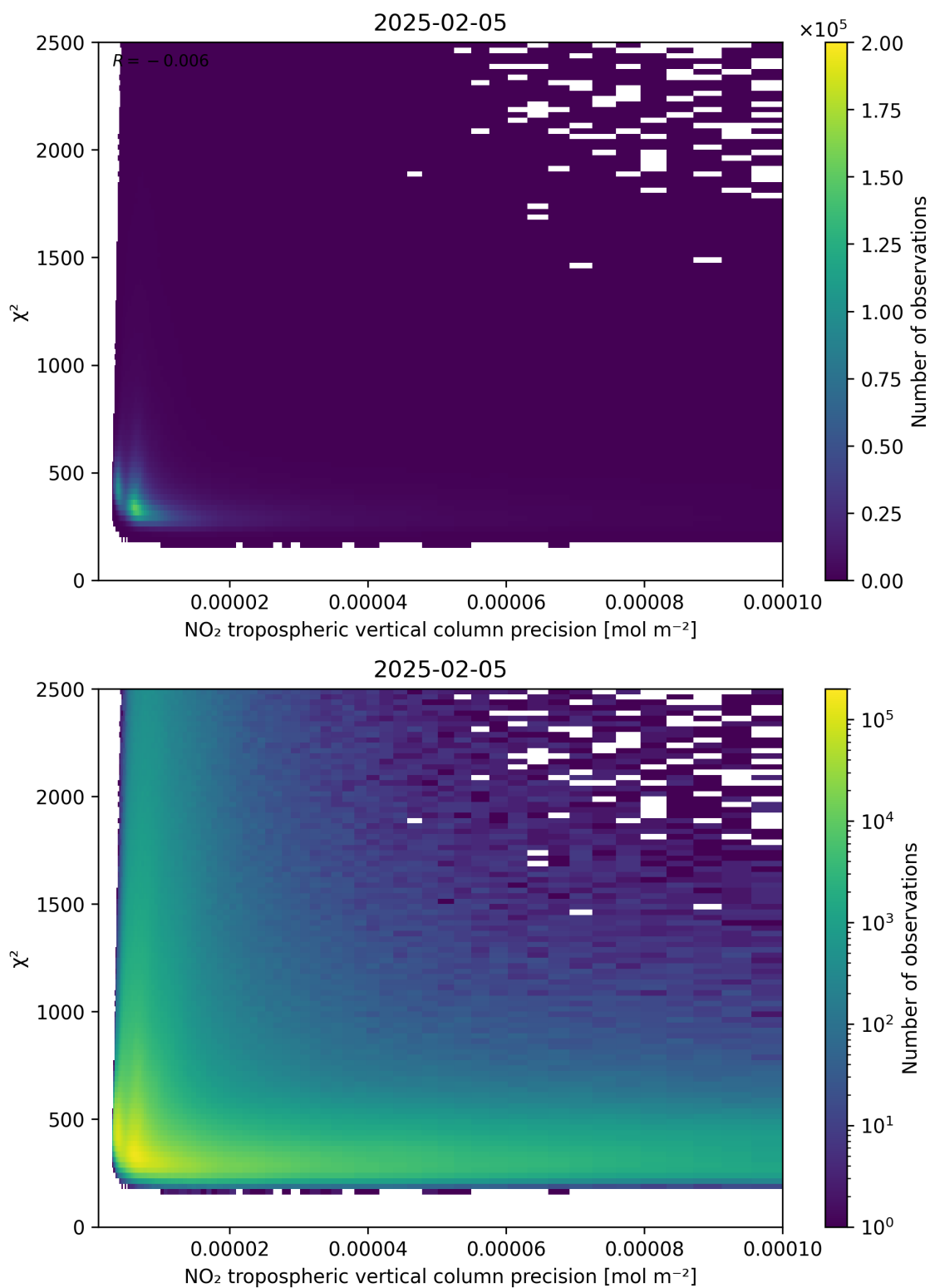
Figure 134: Scatter density plot of “NO 2 tropospheric vertical column precision” against “ \chi^2 ” for 2025-02-04 to 2025-02-06.
