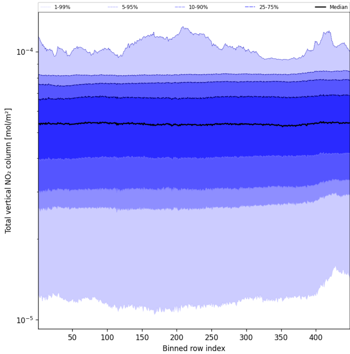
Figure 55: Along track statistics of “Total vertical NO 2 column” for 2025-02-04 to 2025-02-06
