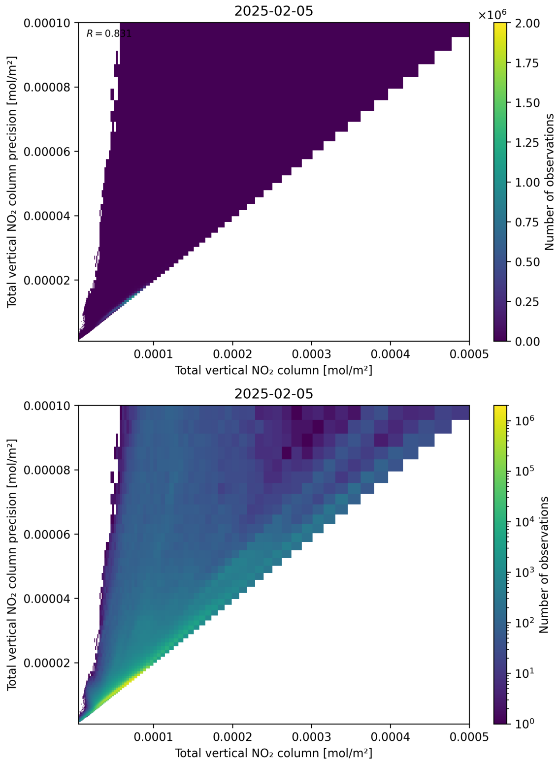
Figure 114: Scatter density plot of “Total vertical NO 2 column” against “Total vertical NO 2 column precision” for 2025-02-04 to 2025-02-06.
