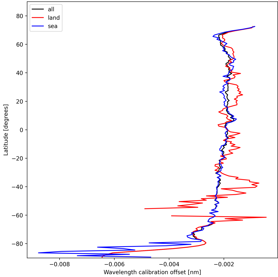
Figure 18: Zonal average of “Wavelength calibration offset” for 2025-02-04 to 2025-02-06.
