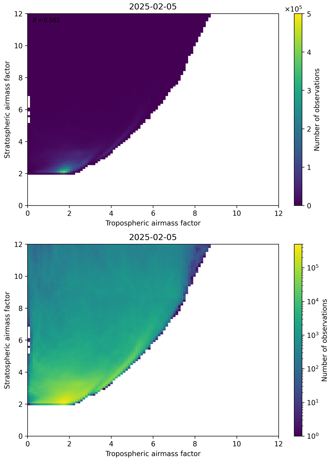
Figure 71: Scatter density plot of “Tropospheric airmass factor” against “Stratospheric airmass factor” for 2025-02-04 to 2025-02-06.
