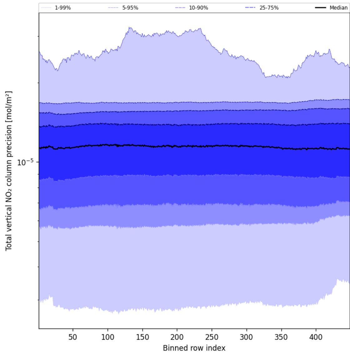
Figure 56: Along track statistics of “Total vertical NO 2 column precision” for 2025-02-04 to 2025-02-06
