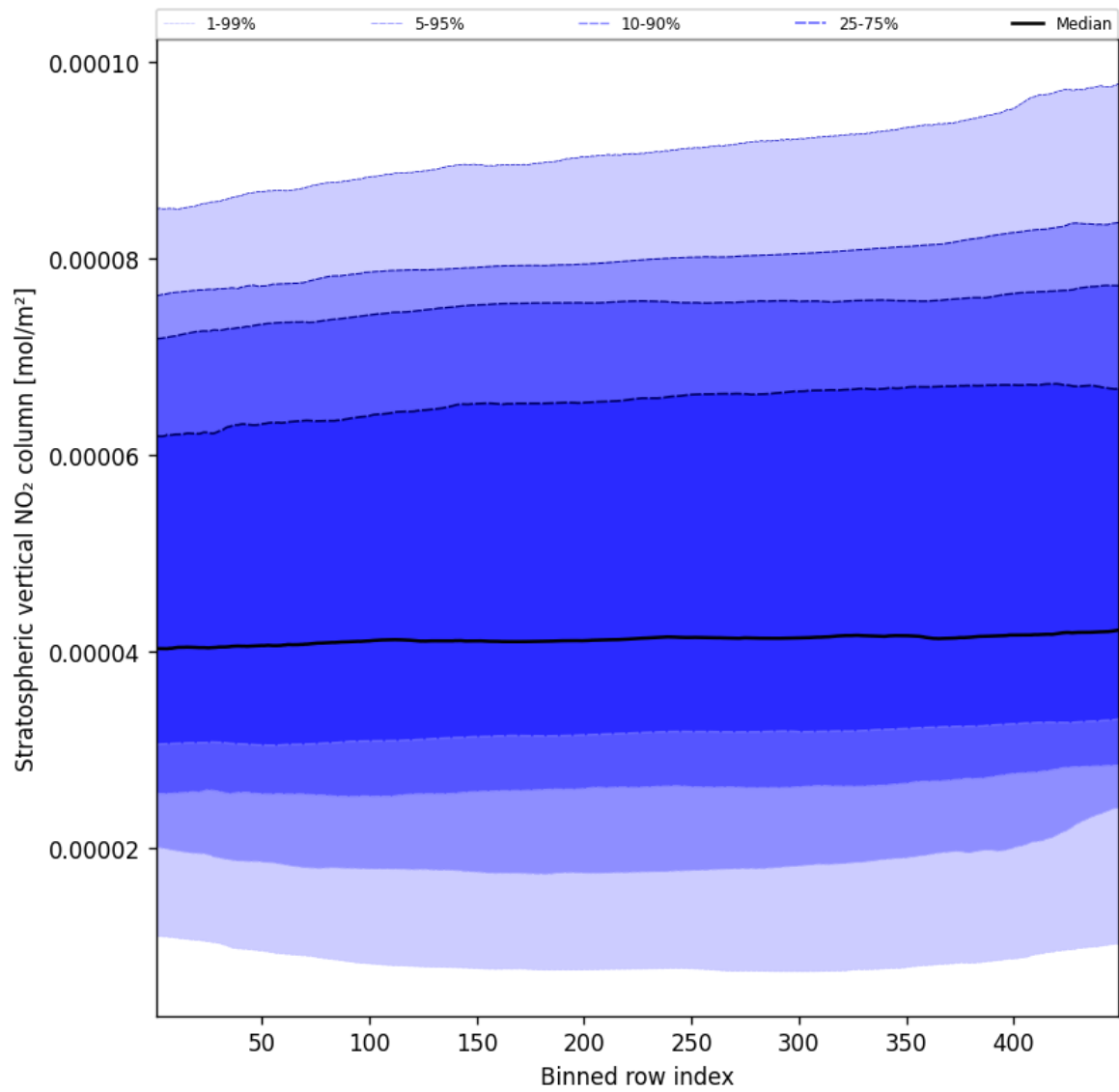
Figure 53: Along track statistics of “Stratospheric vertical NO 2 column” for 2025-02-04 to 2025-02-06
