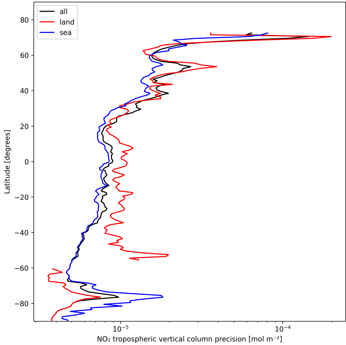
Figure 13: Zonal average of "NO 2 tropospheric vertical column precision" for 2025-02-04 to 2025-02-06.
