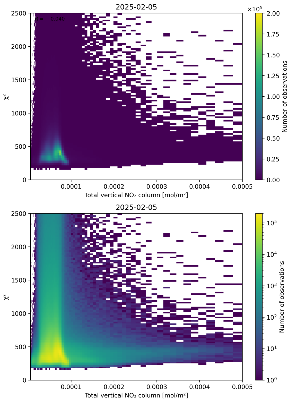
Figure 111: Scatter density plot of “Total vertical NO 2 column” against “ \chi^2 ” for 2025-02-04 to 2025-02-06.
