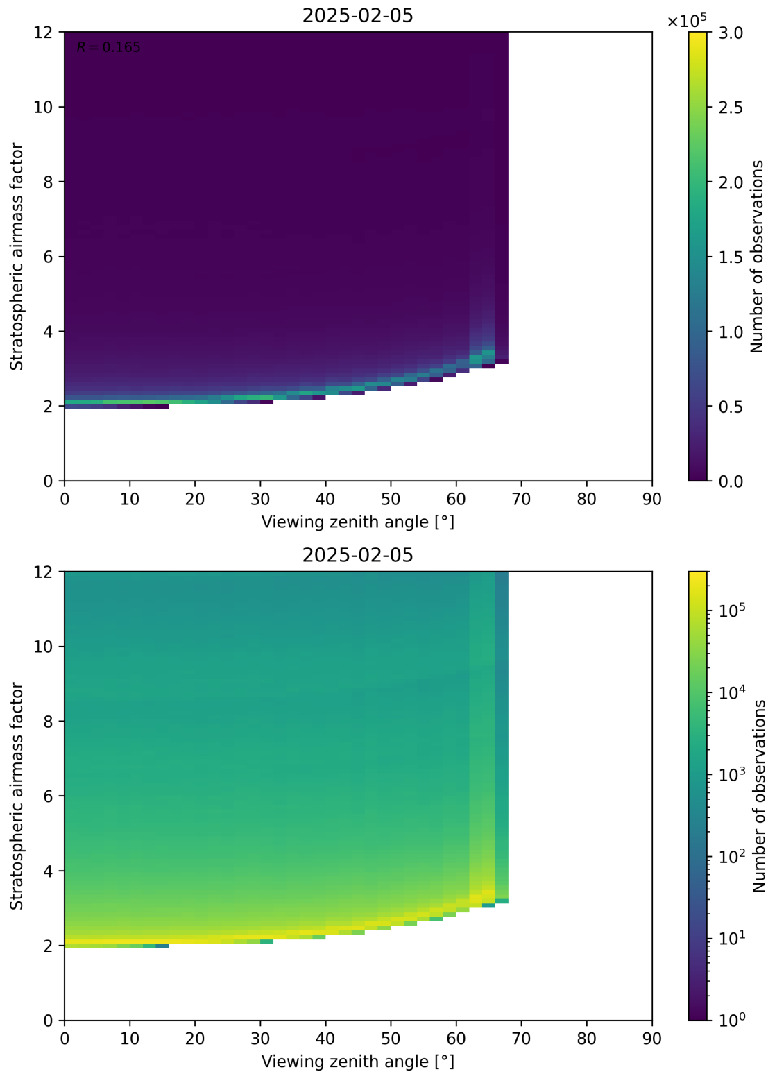
Figure 159: Scatter density plot of “Viewing zenith angle” against “Stratospheric airmass factor” for 2025-02-04 to 2025-02-06.
