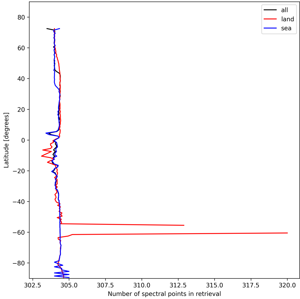
Figure 16: Zonal average of “Number of spectral points in retrieval” for 2025-02-04 to 2025-02-06.
