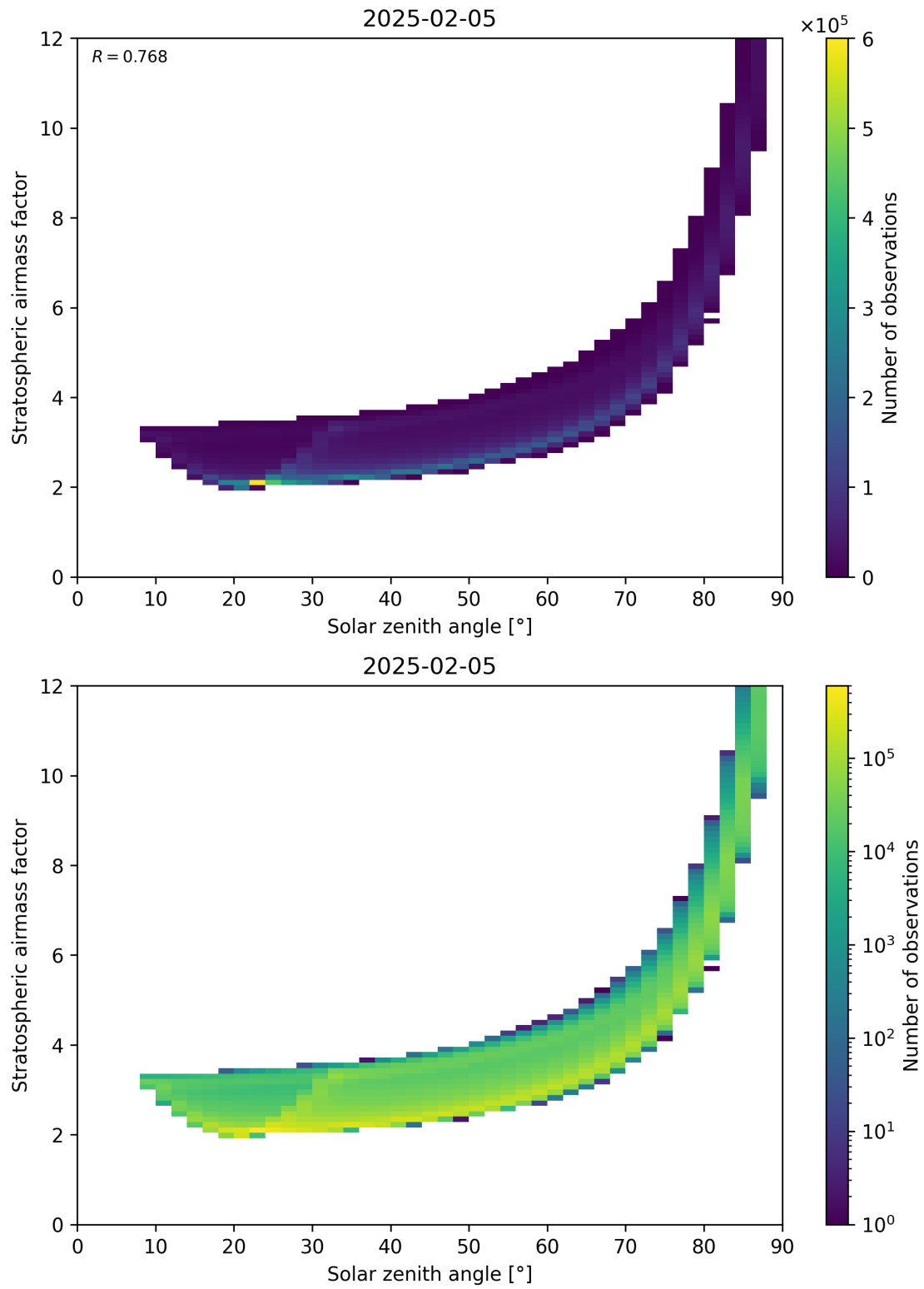
Figure 145: Scatter density plot of “Solar zenith angle” against “Stratospheric airmass factor” for 2025-02-04 to 2025-02-06.
