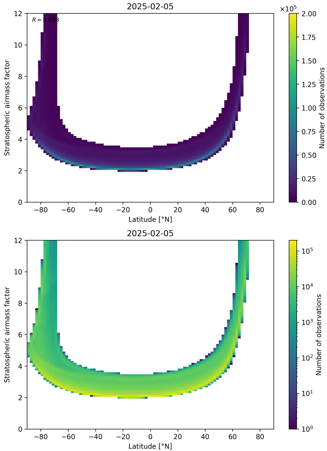
Figure 83: Scatter density plot of “Latitude” against “Stratospheric air mass factor” for 2025-02-04 to 2025-02-06.
