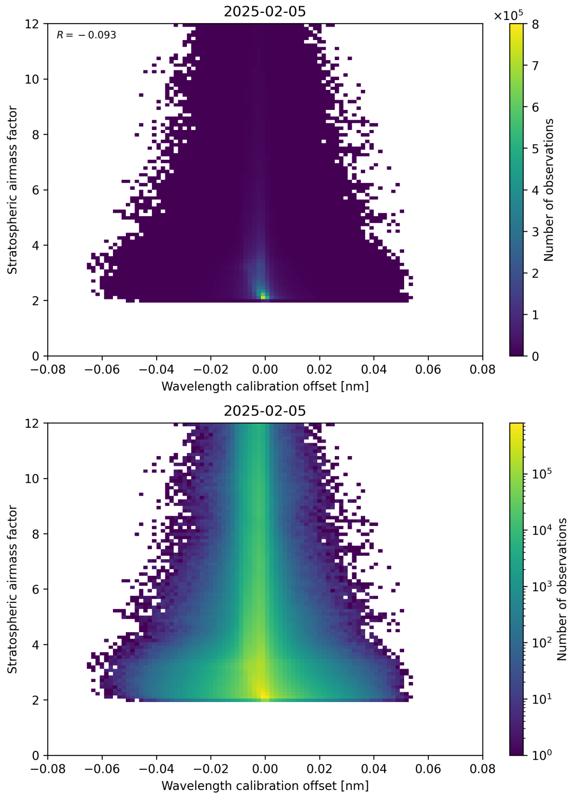
Figure 174: Scatter density plot of “Wavelength calibration offset” against “Stratospheric air mass factor” for 2025-02-04 to 2025-02-06.
