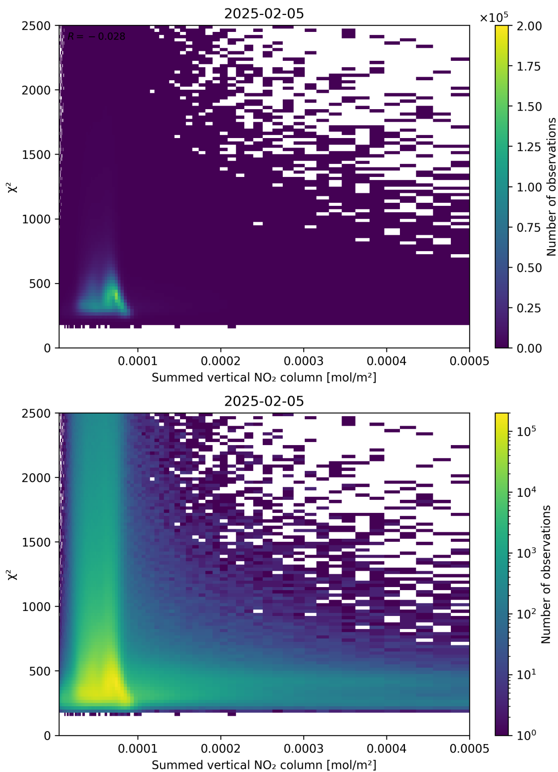
Figure 104: Scatter density plot of “Summed vertical NO 2 column” against “ \chi^2 ” for 2025-02-04 to 2025-02-06.
