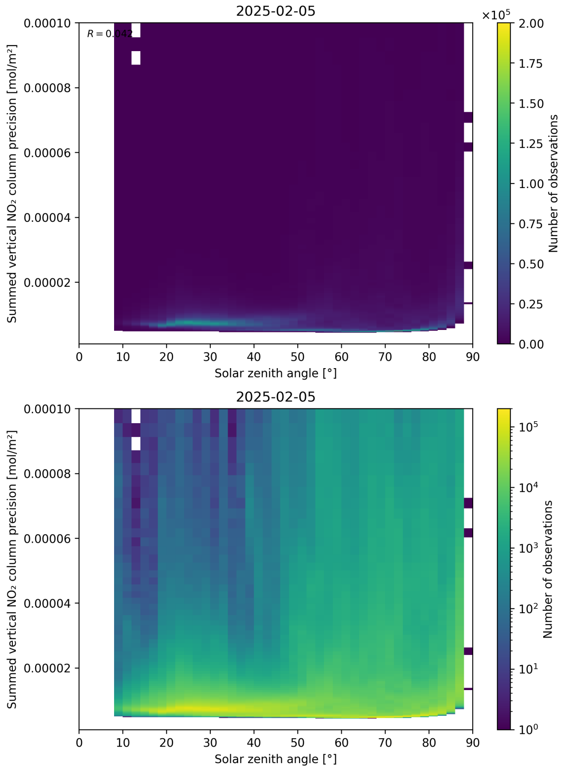
Figure 152: Scatter density plot of “Solar zenith angle” against “Summed vertical NO 2 column precision” for 2025-02-04 to 2025-02-06.
