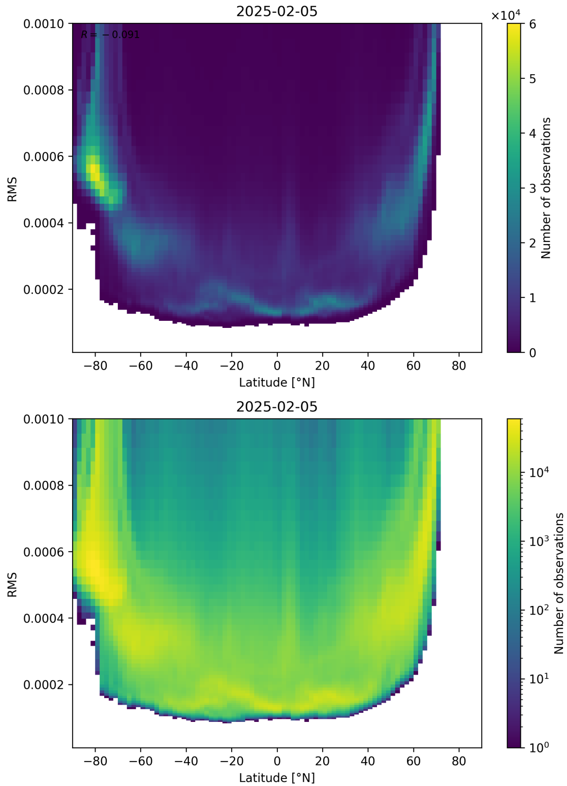
Figure 94: Scatter density plot of “Latitude” against “RMS” for 2025-02-04 to 2025-02-06.
