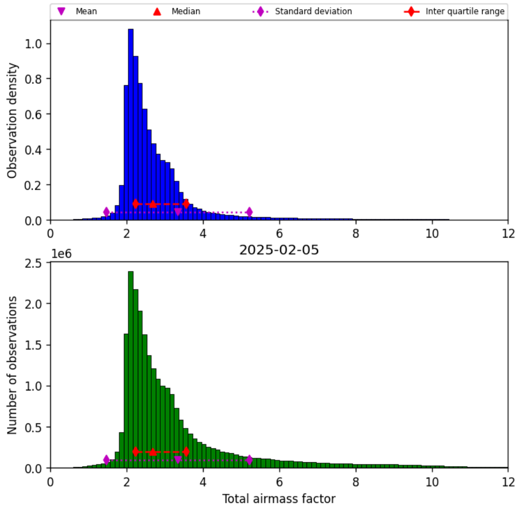
Figure 32: Histogram of “Total airmass factor” for 2025-02-04 to 2025-02-06
