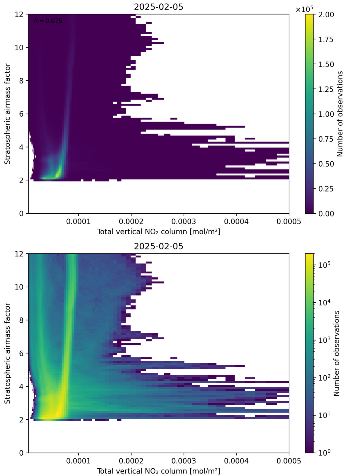
Figure 110: Scatter density plot of “Total vertical NO 2 column” against “Stratospheric airmass factor” for 2025-02-04 to 2025-02-06.
