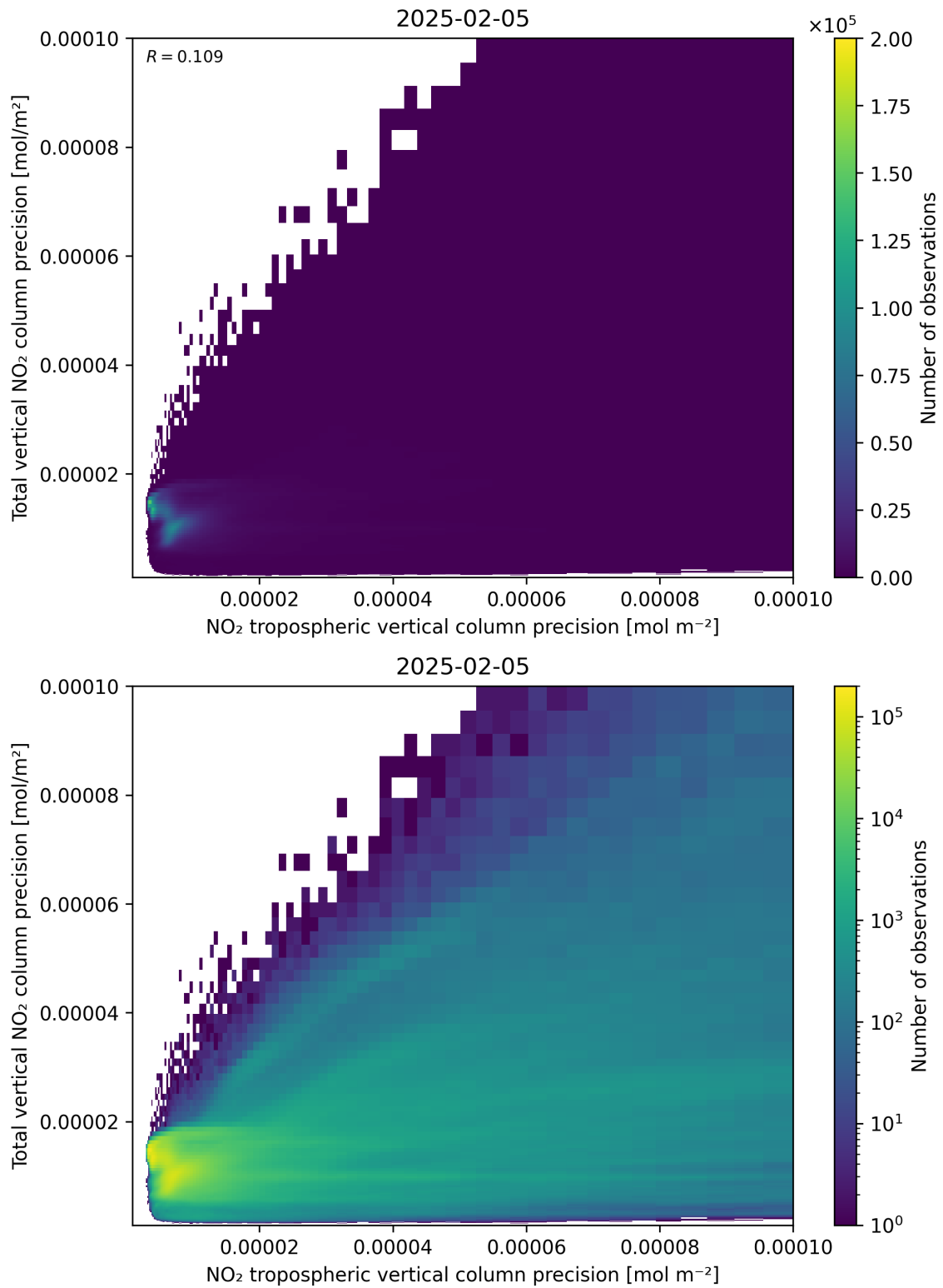
Figure 139: Scatter density plot of “NO 2 tropospheric vertical column precision” against “Total vertical NO 2 column precision” for 2025-02-04 to 2025-02-06.
