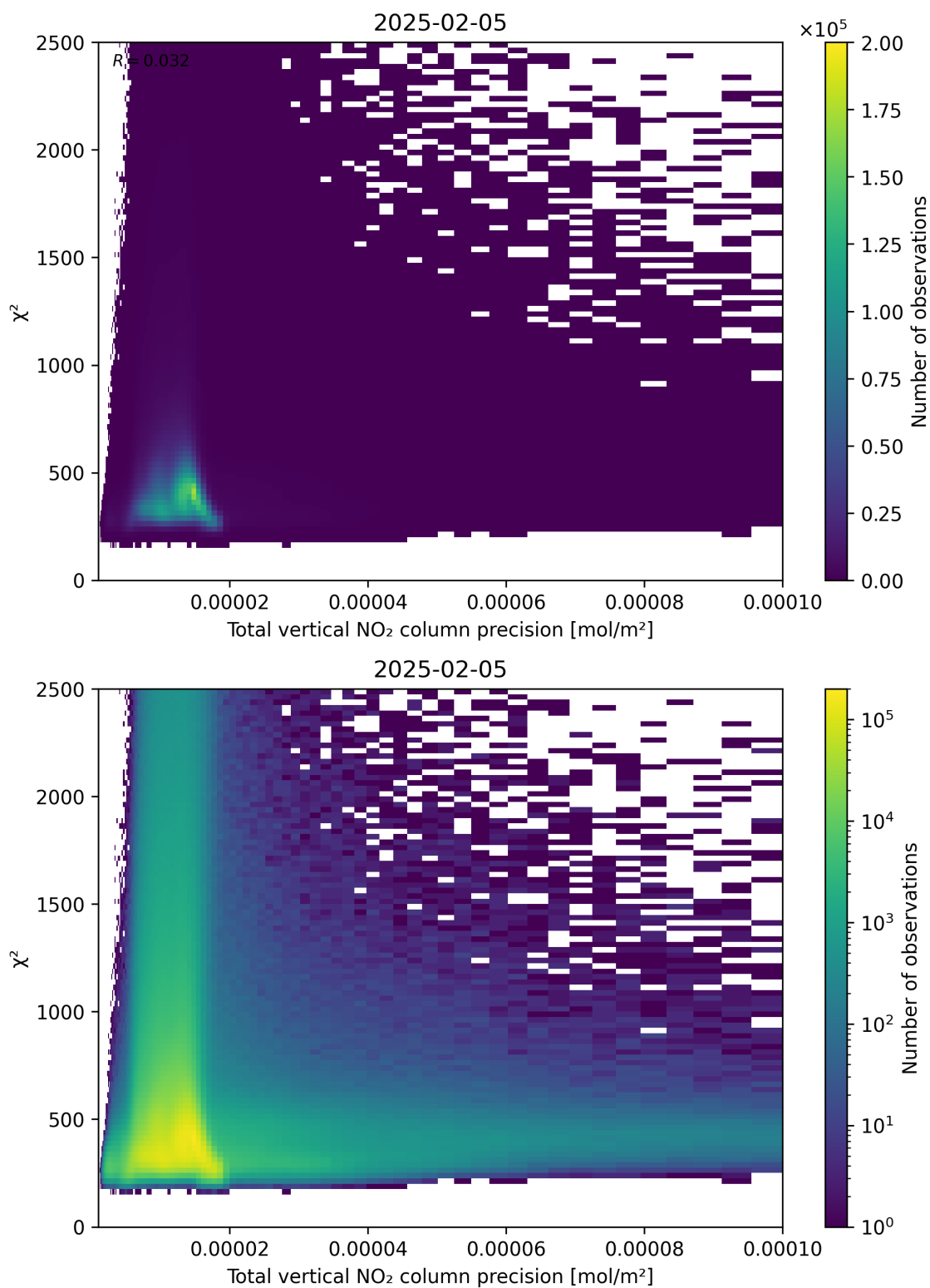
Figure 116: Scatter density plot of “Total vertical NO 2 column precision” against “ \chi^2 ” for 2025-02-04 to 2025-02-06.
