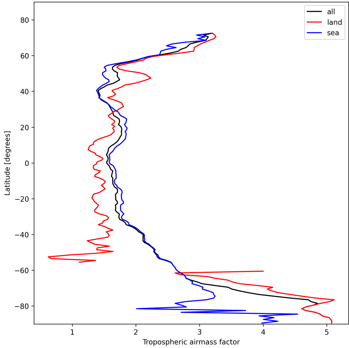
Figure 14: Zonal average of “Tropospheric airmass factor” for 2025-02-04 to 2025-02-06.
