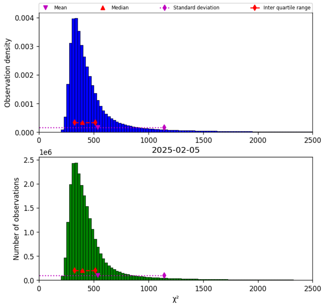
Figure 42: Histogram of “ \chi^2 ” for 2025-02-04 to 2025-02-06
