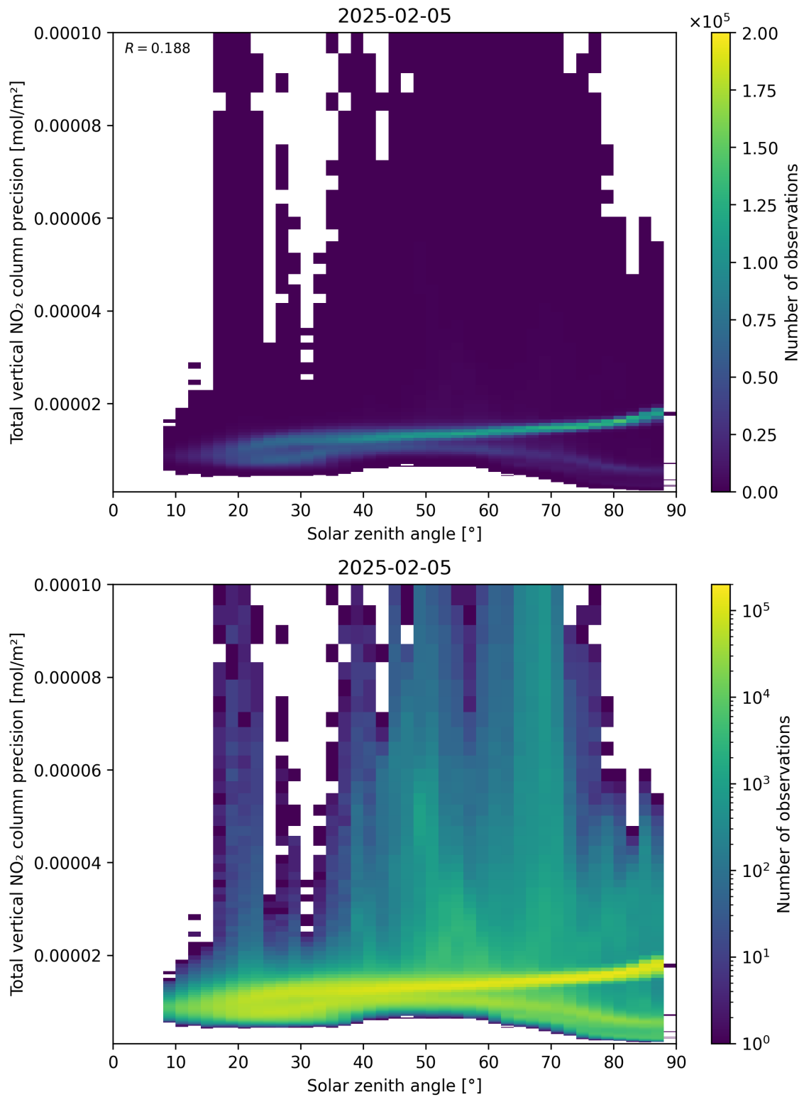
Figure 154: Scatter density plot of “Solar zenith angle” against “Total vertical NO 2 column precision” for 2025-02-04 to 2025-02-06.
