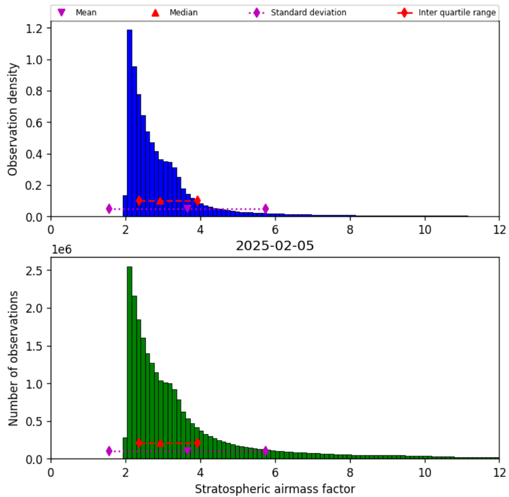
Figure 44: Histogram of “Stratospheric airmass factor” for 2025-02-04 to 2025-02-06
