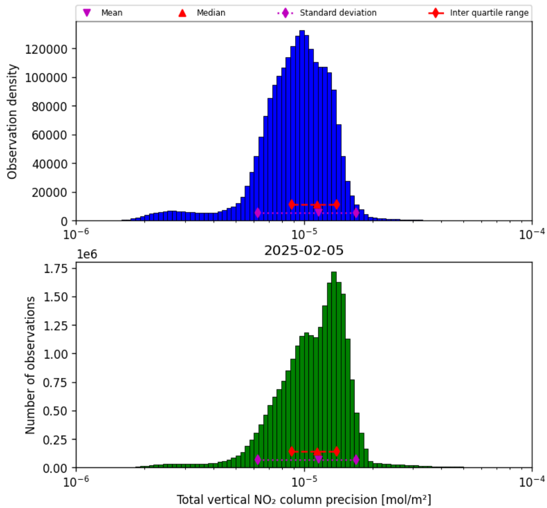
Figure 39: Histogram of “Total vertical NO 2 column precision” for 2025-02-04 to 2025-02-06
