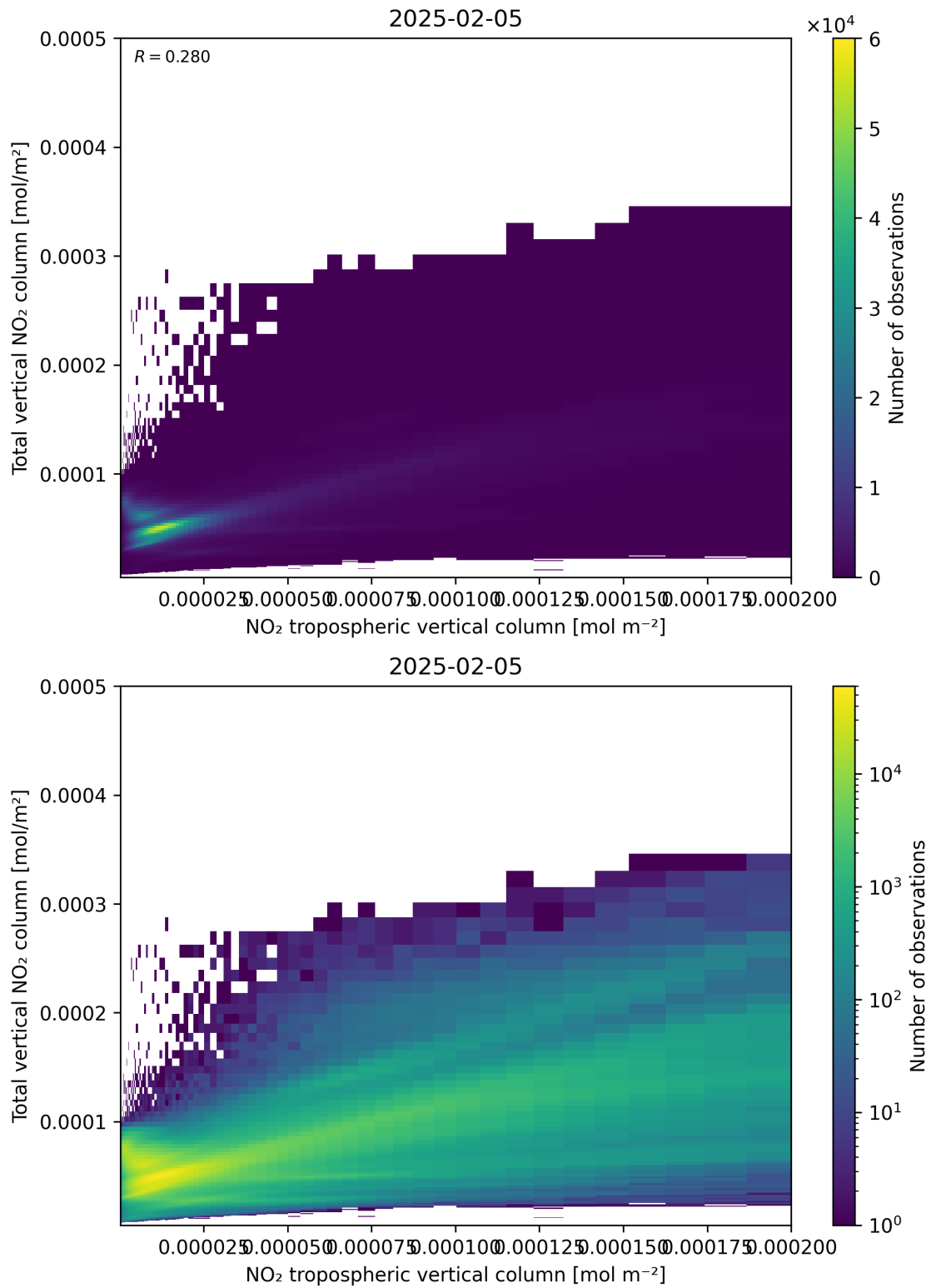
Figure 128: Scatter density plot of “NO 2 tropospheric vertical column” against “Total vertical NO 2 column” for 2025-02-04 to 2025-02-06.
