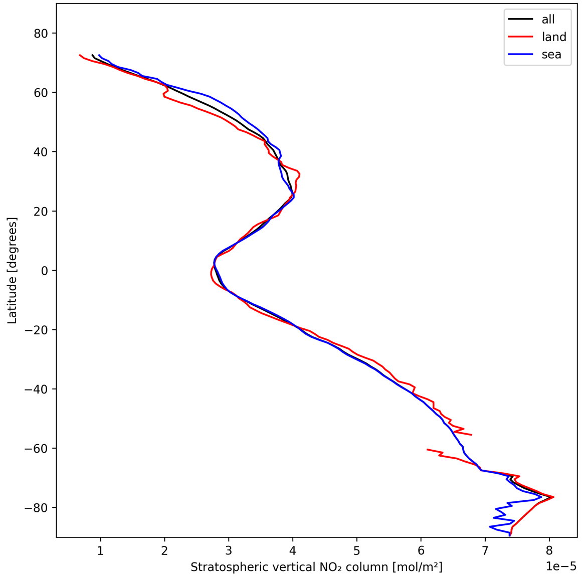
Figure 19: Zonal average of “Stratospheric vertical NO 2 column” for 2025-02-04 to 2025-02-06.
