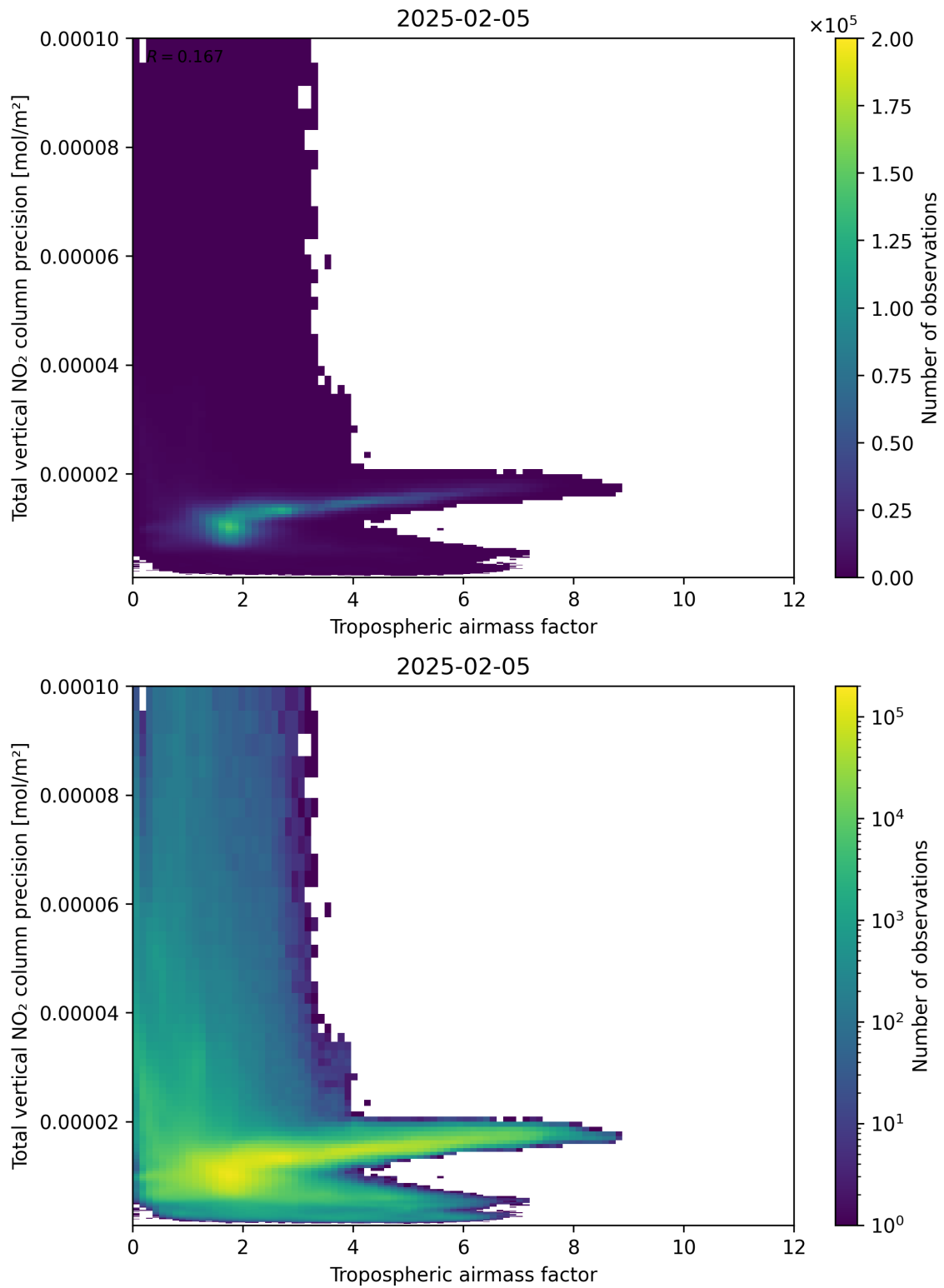
Figure 78: Scatter density plot of “Tropospheric air mass factor” against “Total vertical NO 2 column precision” for 2025-02-04 to 2025-02-06.
