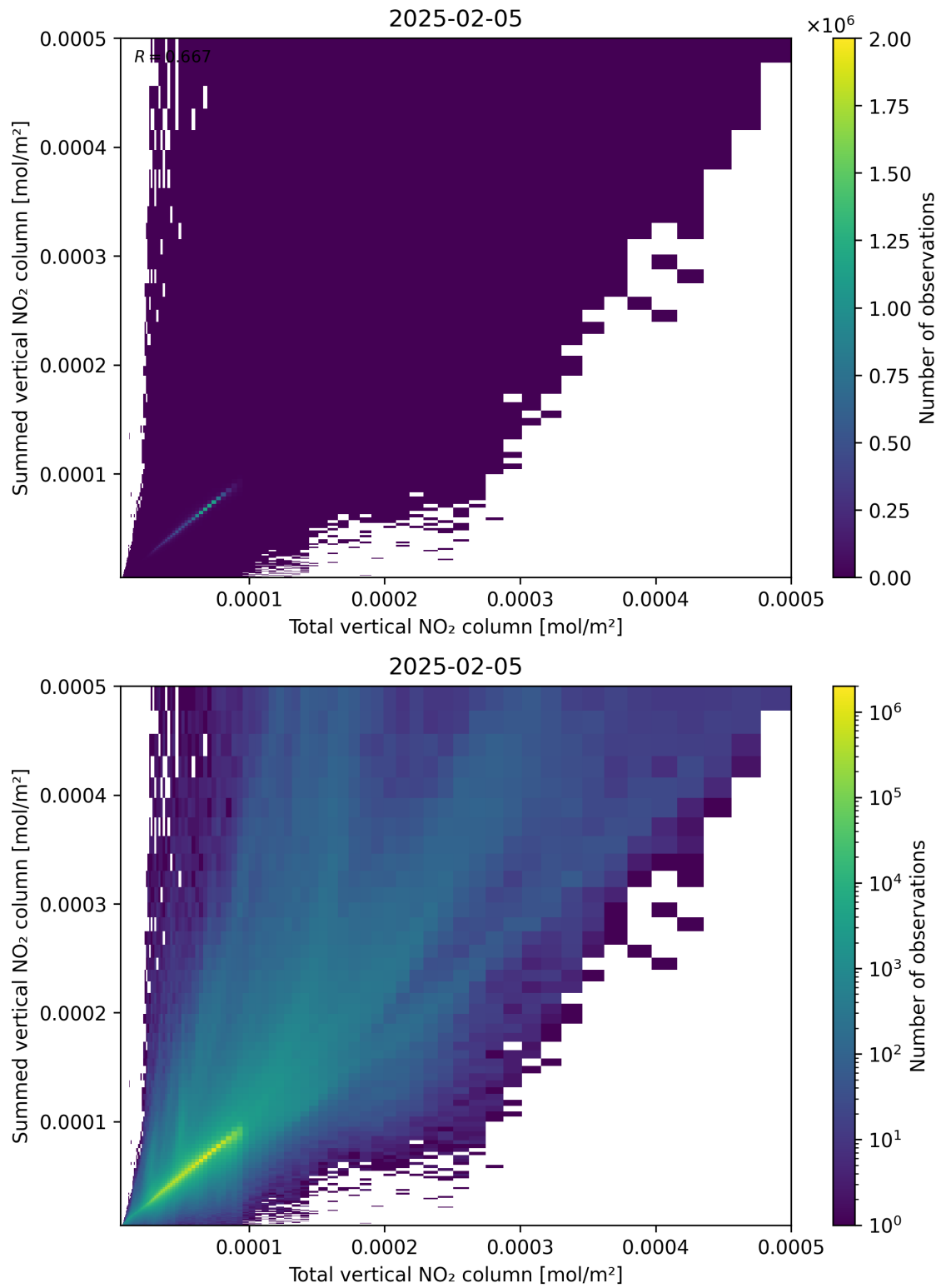
Figure 112: Scatter density plot of “Total vertical NO 2 column” against “Summed vertical NO 2 column” for 2025-02-04 to 2025-02-06.
