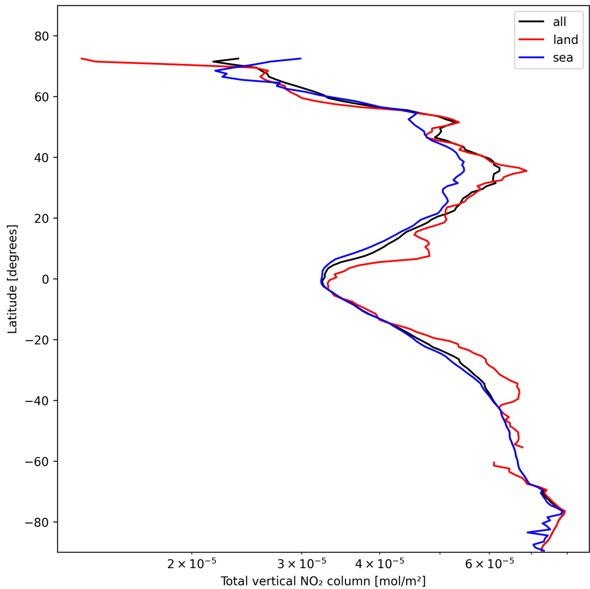
Figure 21: Zonal average of “Total vertical NO 2 column” for 2025-02-04 to 2025-02-06.
