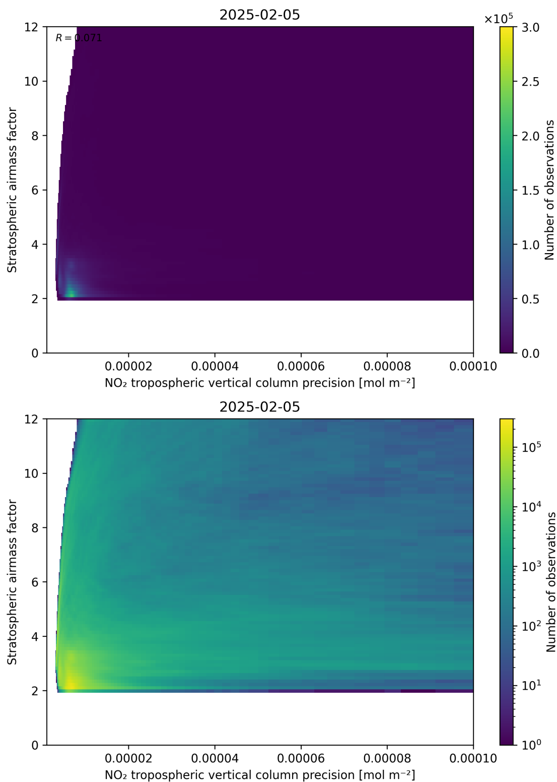
Figure 131: Scatter density plot of “NO 2 tropospheric vertical column precision” against “Stratospheric airmass factor” for 2025-02-04 to 2025-02-06.
