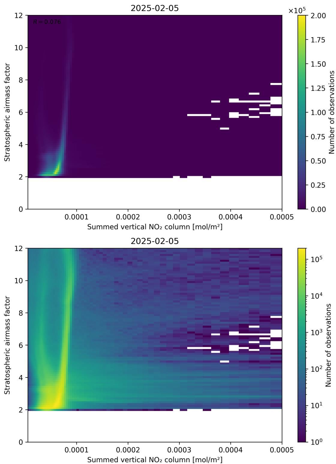
Figure 103: Scatter density plot of “Summed vertical NO 2 column” against “Stratospheric air mass factor” for 2025-02-04 to 2025-02-06.
