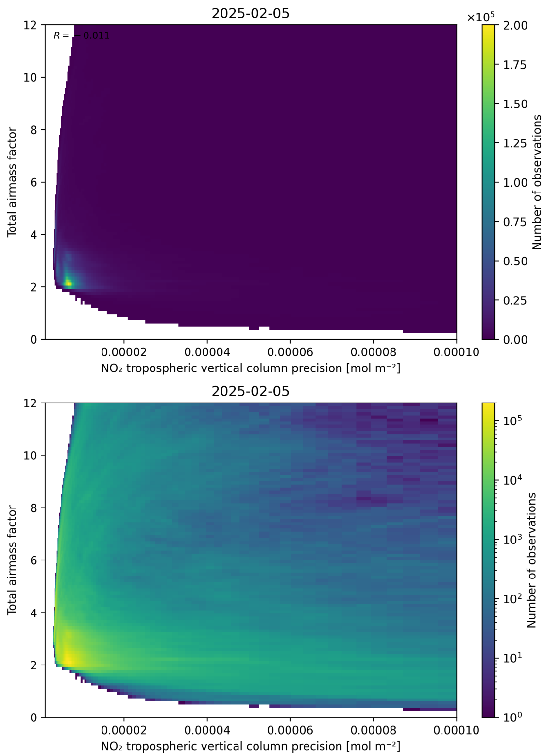
Figure 132: Scatter density plot of “NO 2 tropospheric vertical column precision” against “Total air mass factor” for 2025-02-04 to 2025-02-06.
