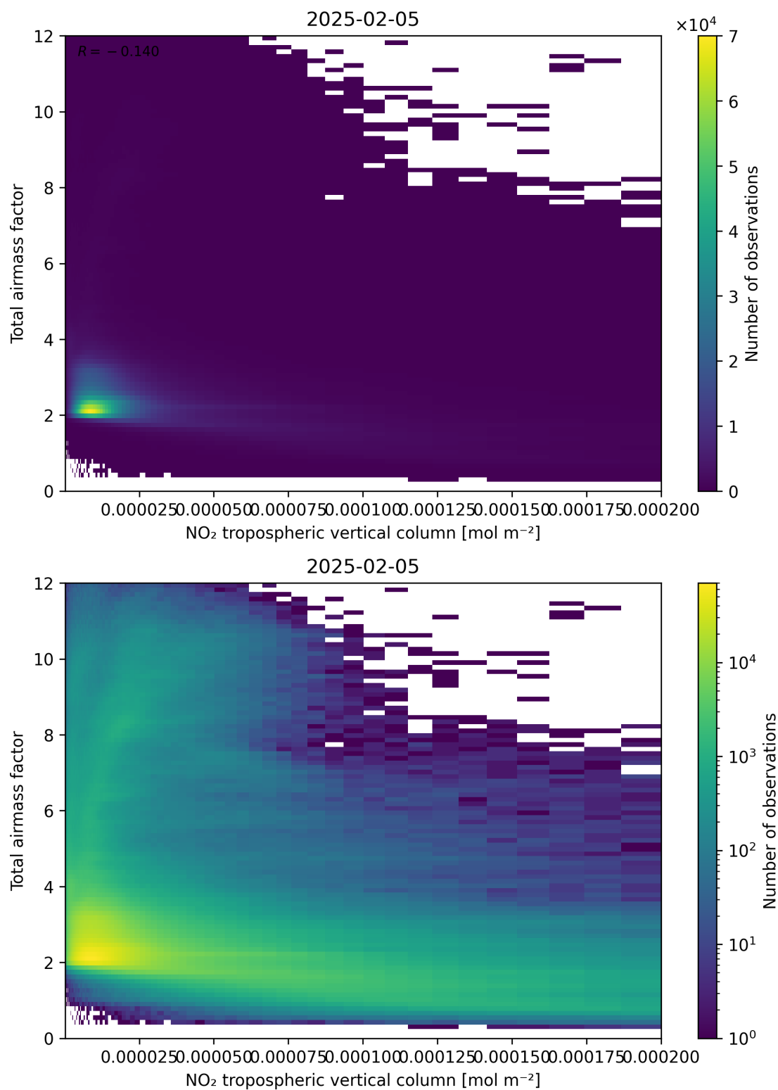
Figure 122: Scatter density plot of “NO 2 tropospheric vertical column” against “Total air mass factor” for 2025-02-04 to 2025-02-06.
