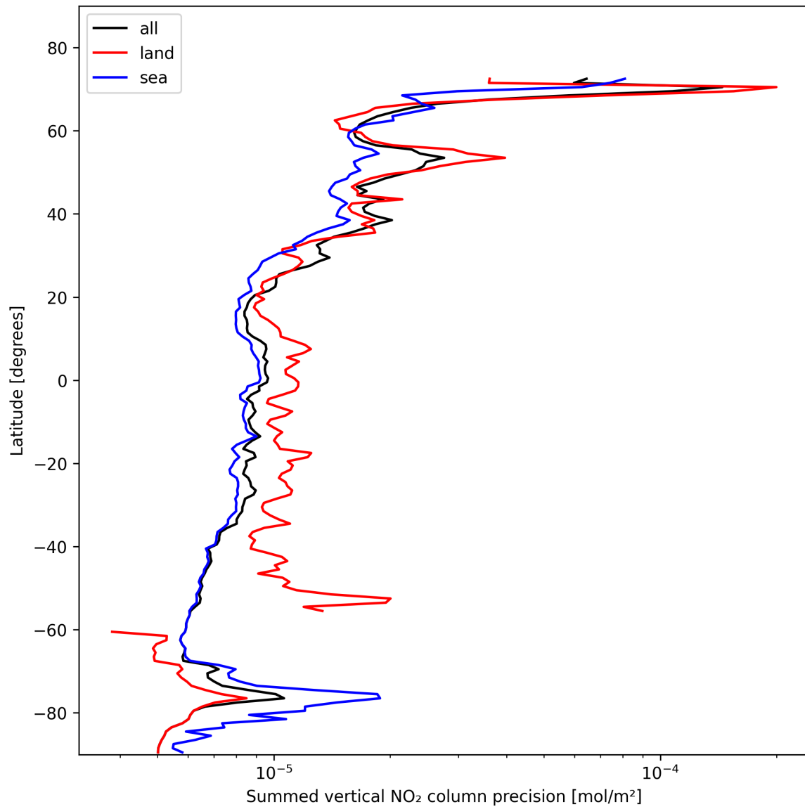
Figure 24: Zonal average of “Summed vertical NO 2 column precision” for 2025-02-04 to 2025-02-06.
