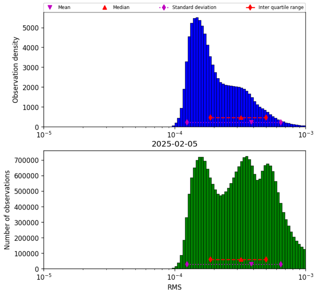
Figure 43: Histogram of “RMS” for 2025-02-04 to 2025-02-06
