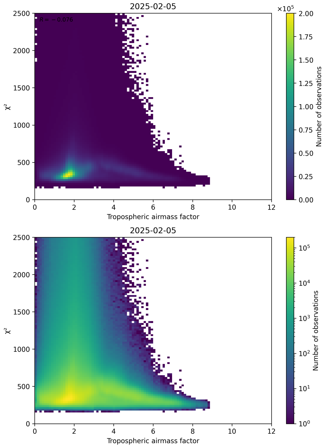
Figure 73: Scatter density plot of “Tropospheric airmass factor” against “ \chi^2 ” for 2025-02-04 to 2025-02-06.
