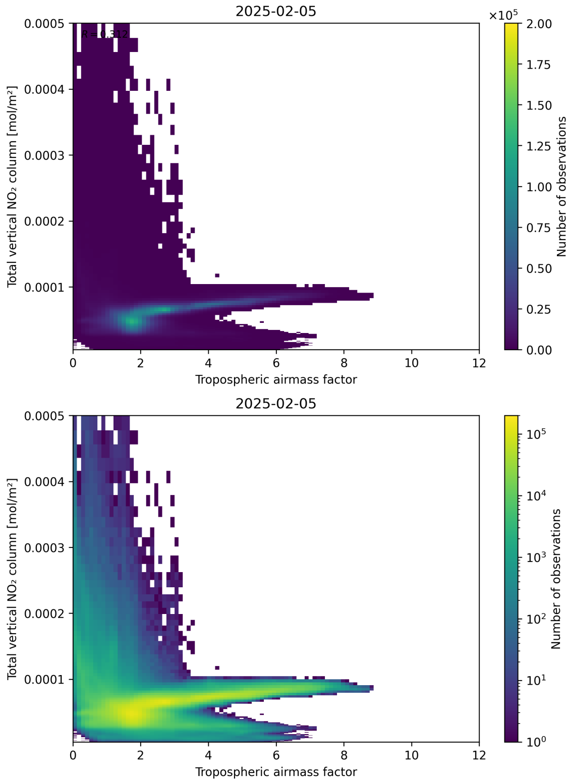
Figure 77: Scatter density plot of “Tropospheric airmass factor” against “Total vertical NO 2 column” for 2025-02-04 to 2025-02-06.
