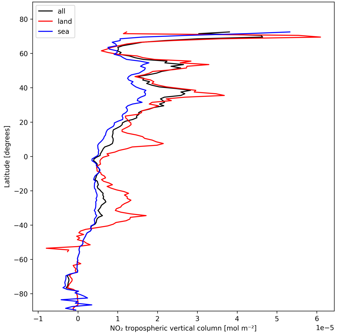
Figure 12: Zonal average of “NO 2 tropospheric vertical column” for 2025-02-04 to 2025-02-06.
