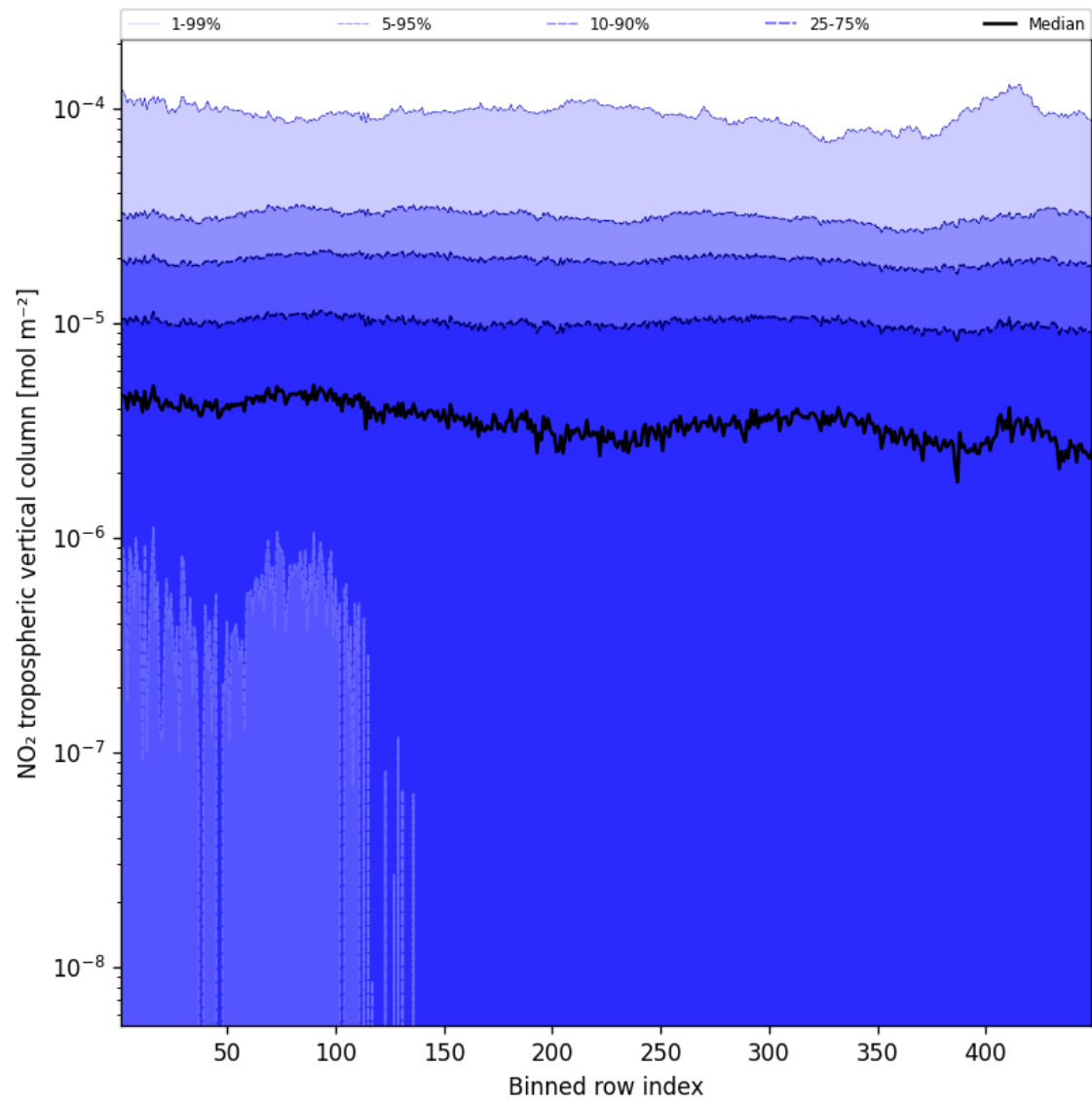
Figure 46: Along track statistics of “NO 2 tropospheric vertical column” for 2025-02-04 to 2025-02-06
