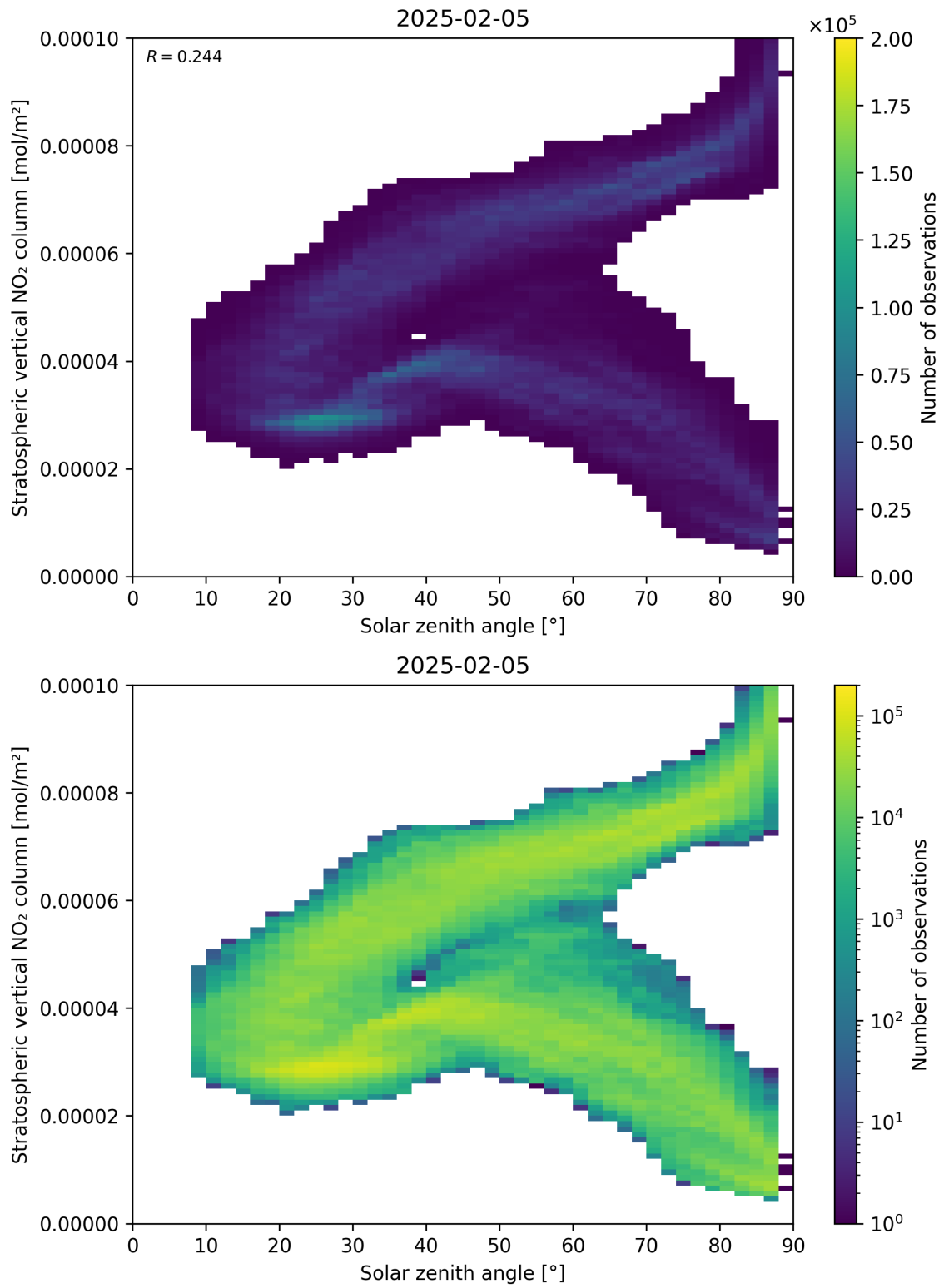
Figure 150: Scatter density plot of “Solar zenith angle” against “Stratospheric vertical NO 2 column” for 2025-02-04 to 2025-02-06.
