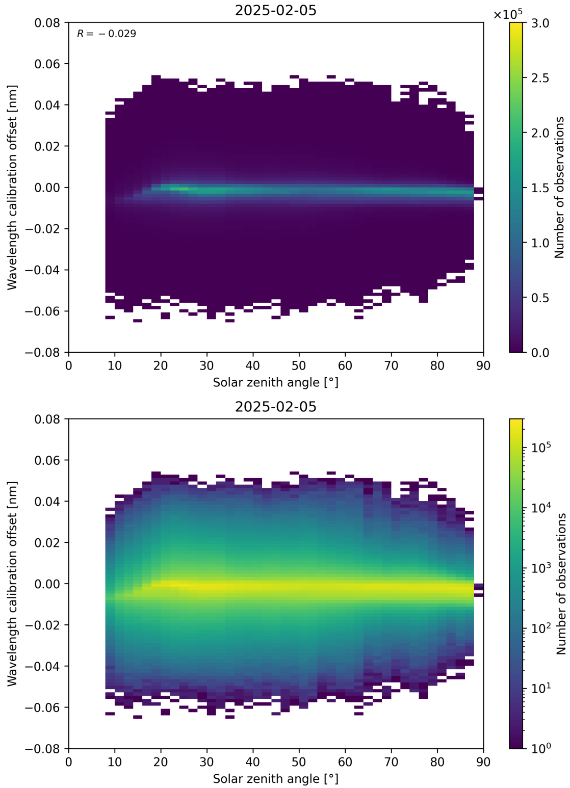
Figure 158: Scatter density plot of “Solar zenith angle” against “Wavelength calibration offset” for 2025-02-04 to 2025-02-06.
