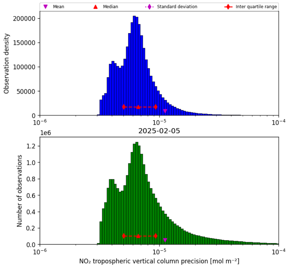
Figure 30: Histogram of “NO 2 tropospheric vertical column precision” for 2025-02-04 to 2025-02-06
