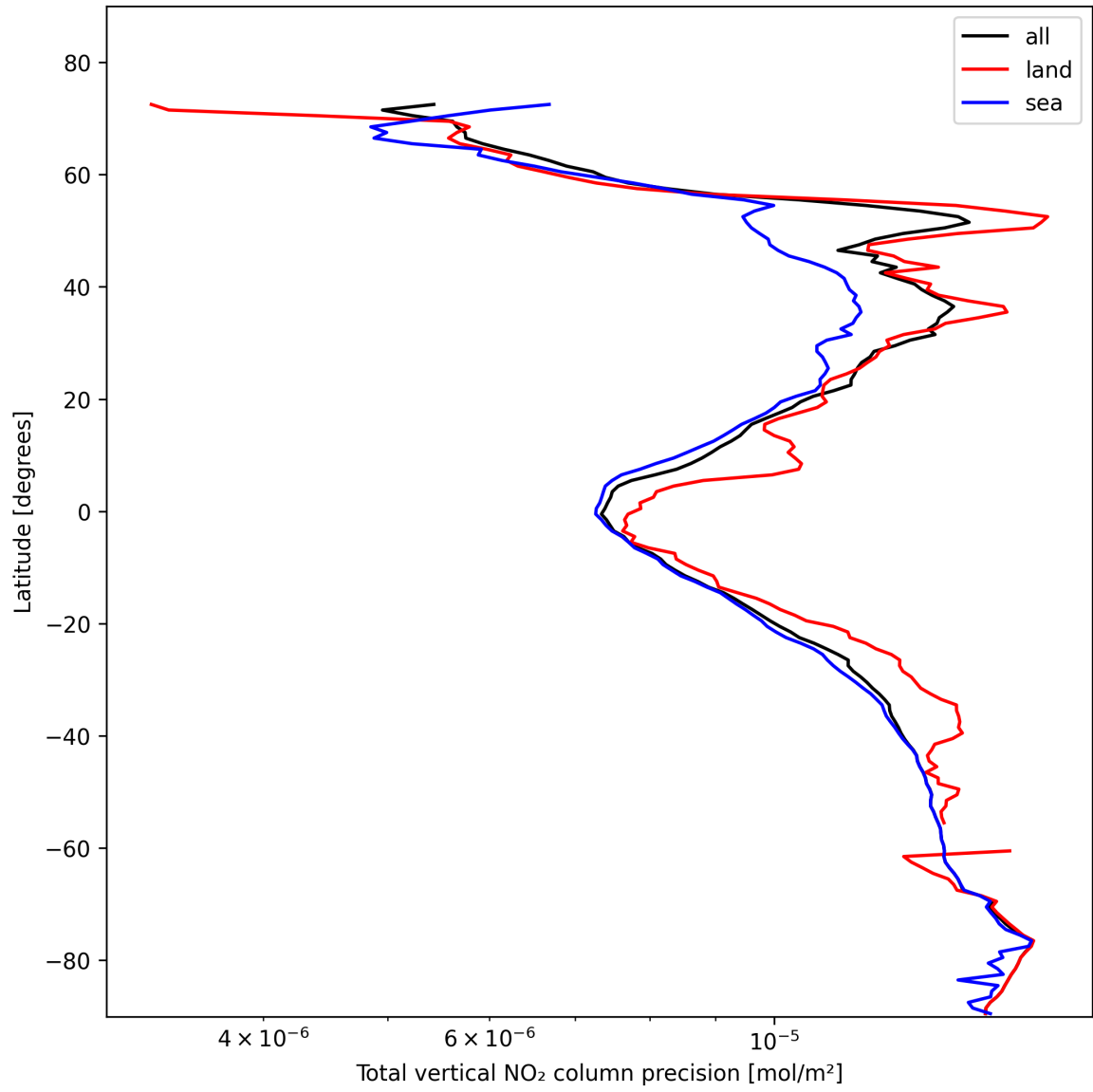
Figure 22: Zonal average of “Total vertical NO 2 column precision” for 2025-02-04 to 2025-02-06.
