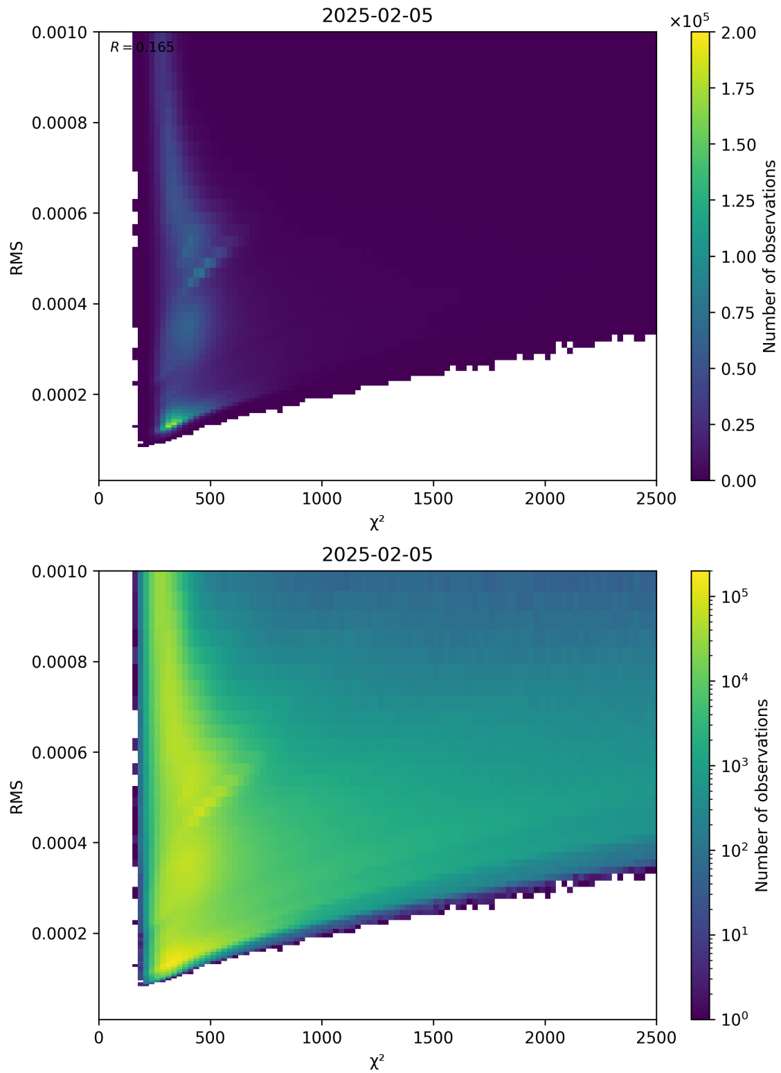
Figure 82: Scatter density plot of “ \chi^2 ” against “RMS” for 2025-02-04 to 2025-02-06.
