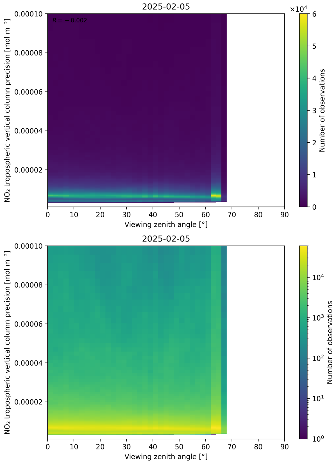
Figure 170: Scatter density plot of “Viewing zenith angle” against “NO 2 tropospheric vertical column precision” for 2025-02-04 to 2025-02-06.
