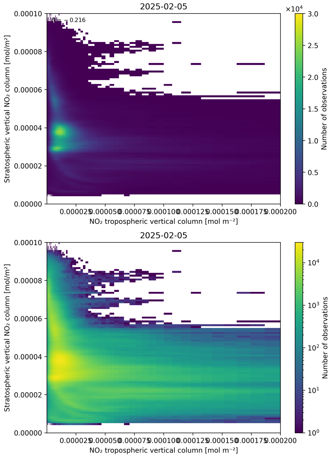
Figure 125: Scatter density plot of “NO 2 tropospheric vertical column” against “Stratospheric vertical NO 2 column” for 2025-02-04 to 2025-02-06.
