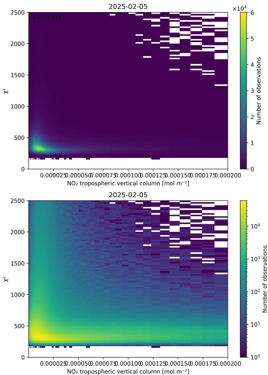
Figure 124: Scatter density plot of “NO 2 tropospheric vertical column” against “ \chi^2 ” for 2025-02-04 to 2025-02-06.
