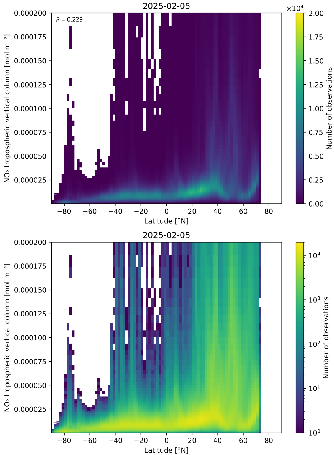
Figure 92: Scatter density plot of “Latitude” against “NO 2 tropospheric vertical column” for 2025-02-04 to 2025-02-06.
