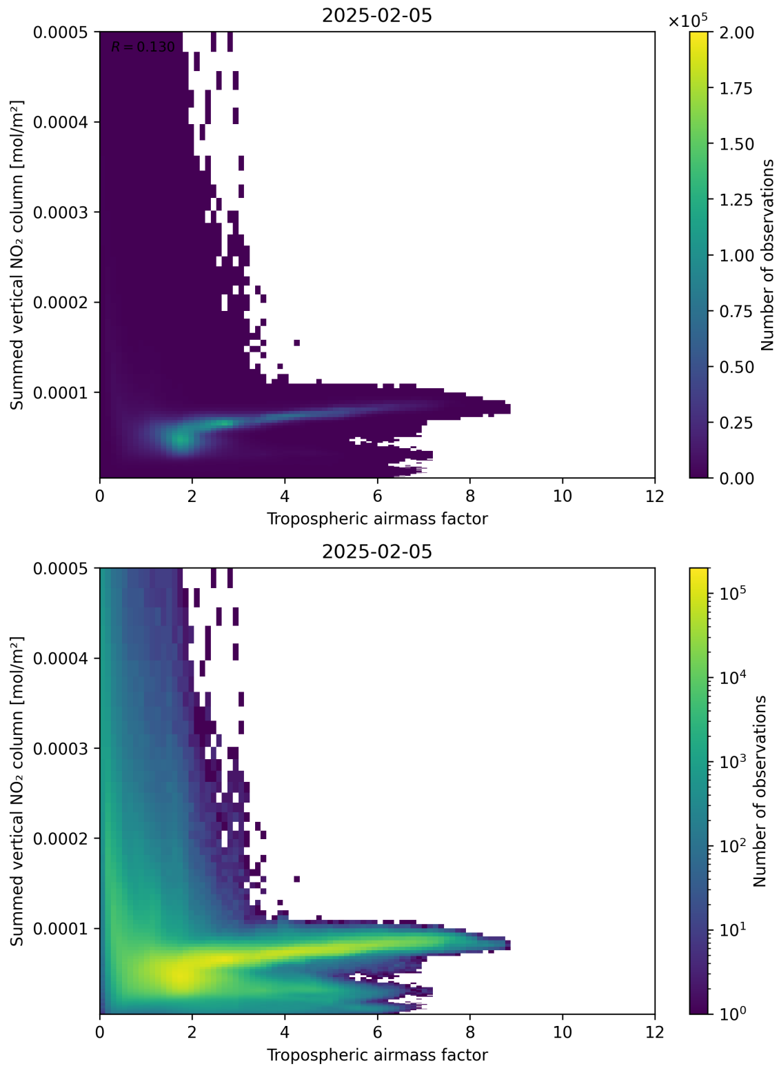
Figure 75: Scatter density plot of “Tropospheric air mass factor” against “Summed vertical NO 2 column” for 2025-02-04 to 2025-02-06.
