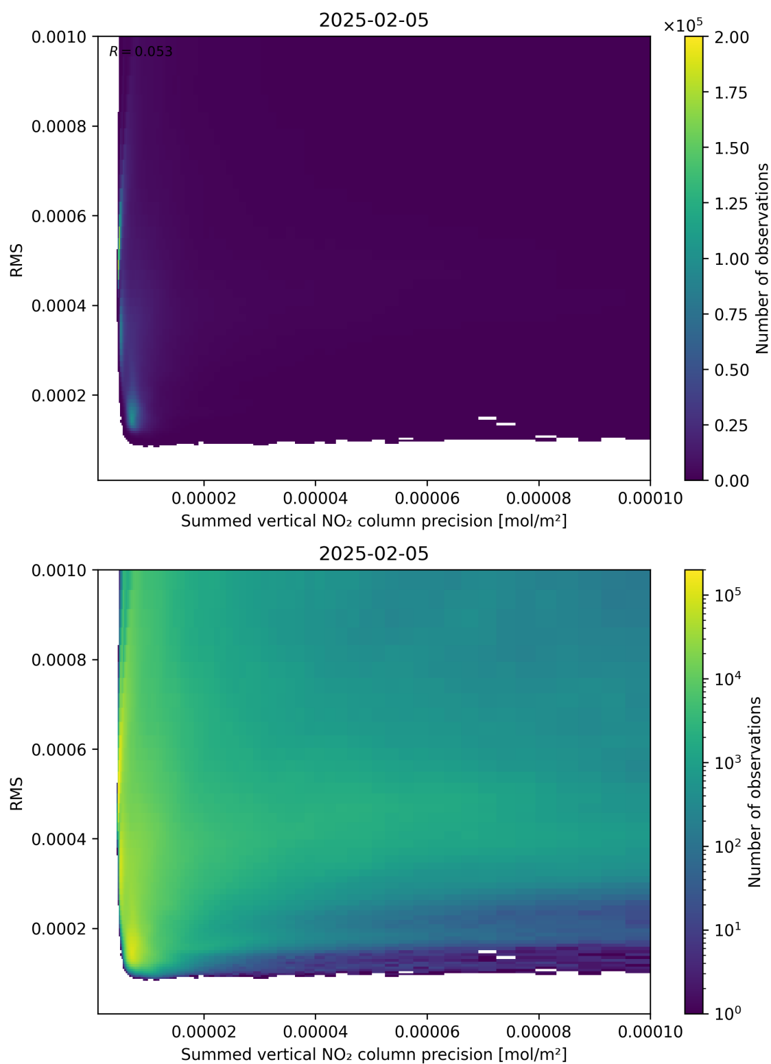
Figure 108: Scatter density plot of “Summed vertical NO 2 column precision” against “RMS” for 2025-02-04 to 2025-02-06.
