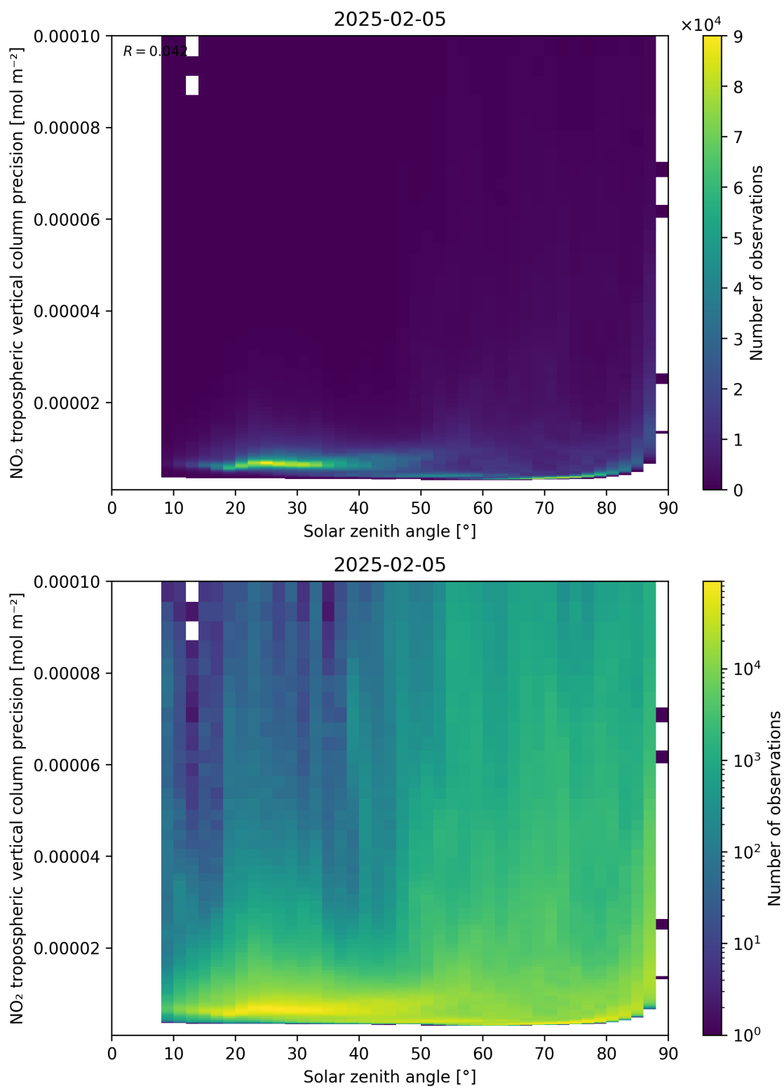
Figure 156: Scatter density plot of “Solar zenith angle” against “NO 2 tropospheric vertical column precision” for 2025-02-04 to 2025-02-06.
