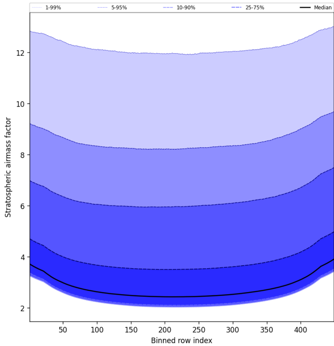
Figure 61: Along track statistics of “Stratospheric air mass factor” for 2025-02-04 to 2025-02-06
