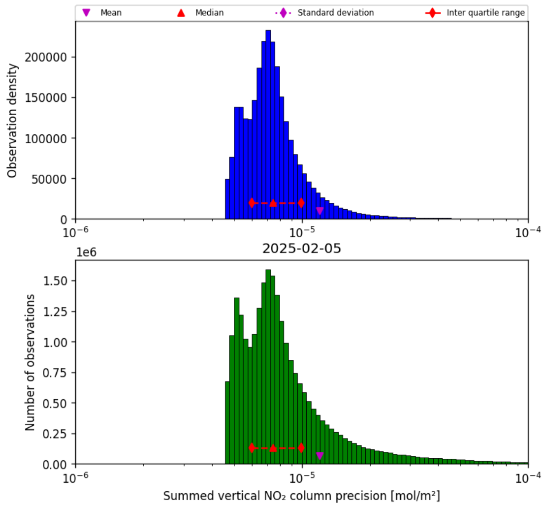
Figure 41: Histogram of “Summed vertical NO 2 column precision” for 2025-02-04 to 2025-02-06
