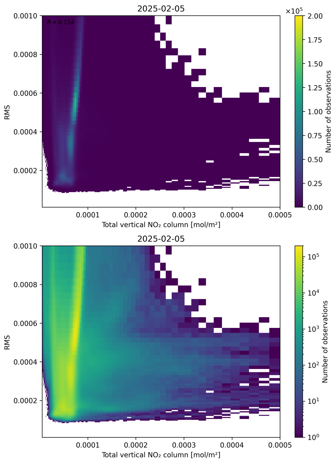
Figure 120: Scatter density plot of “Total vertical NO 2 column” against “RMS” for 2025-02-04 to 2025-02-06.
