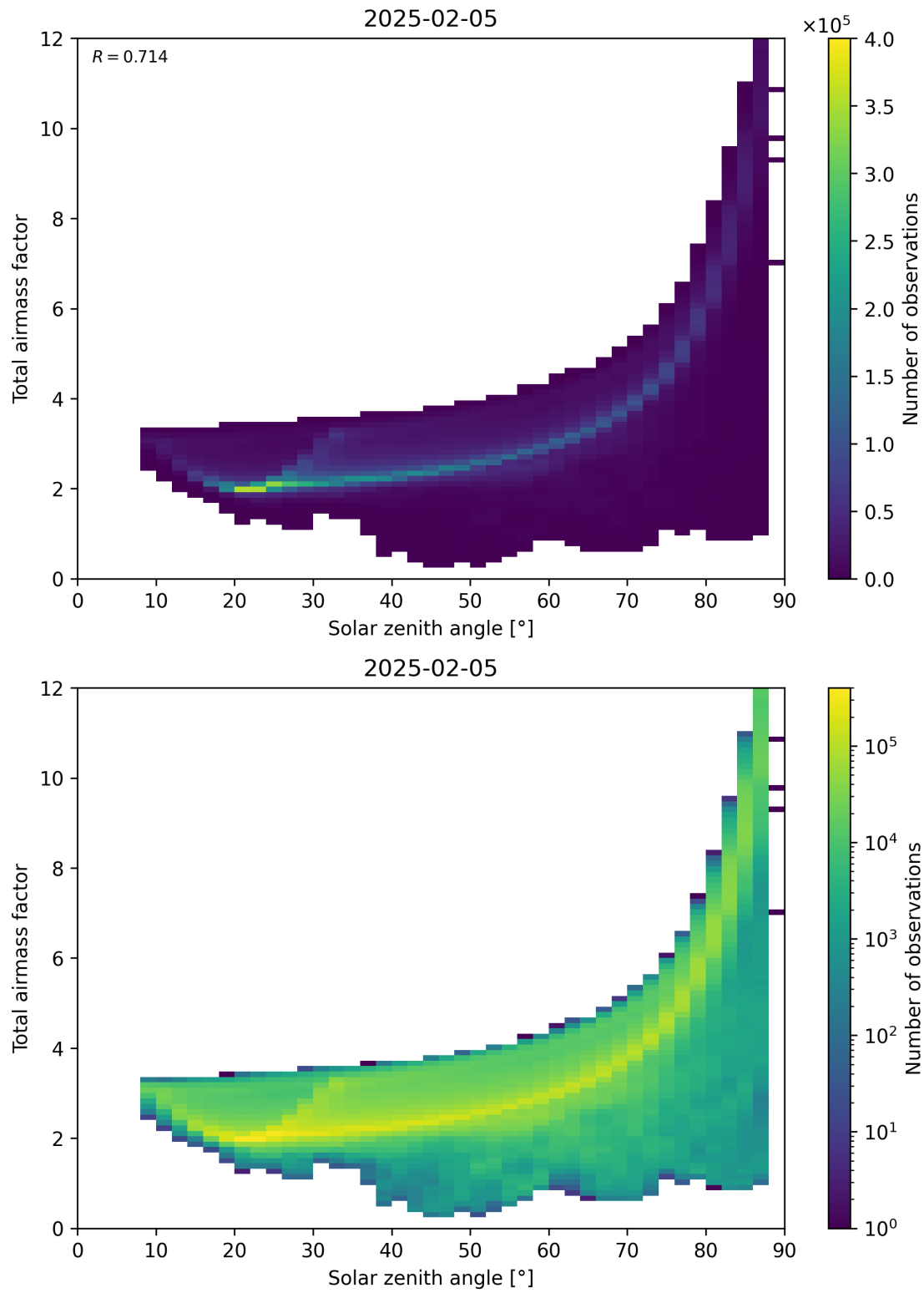
Figure 146: Scatter density plot of “Solar zenith angle” against “Total air mass factor” for 2025-02-04 to 2025-02-06.
