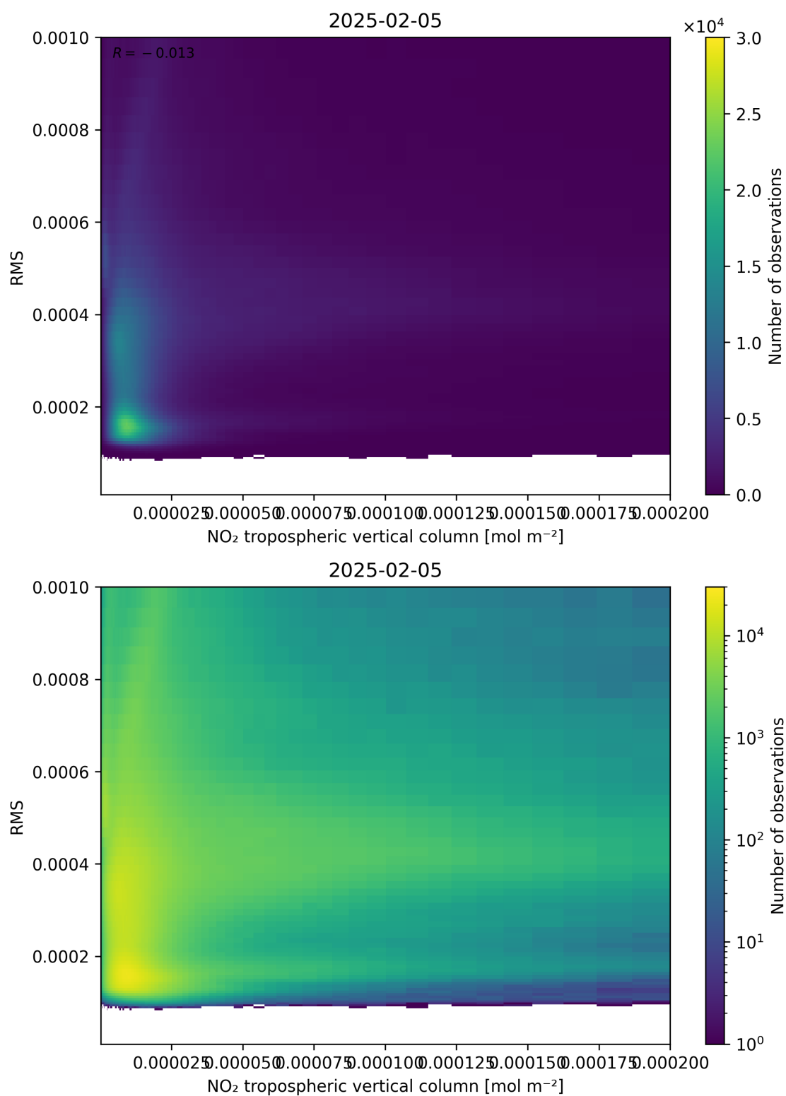
Figure 142: Scatter density plot of “NO 2 tropospheric vertical column” against “RMS” for 2025-02-04 to 2025-02-06.
