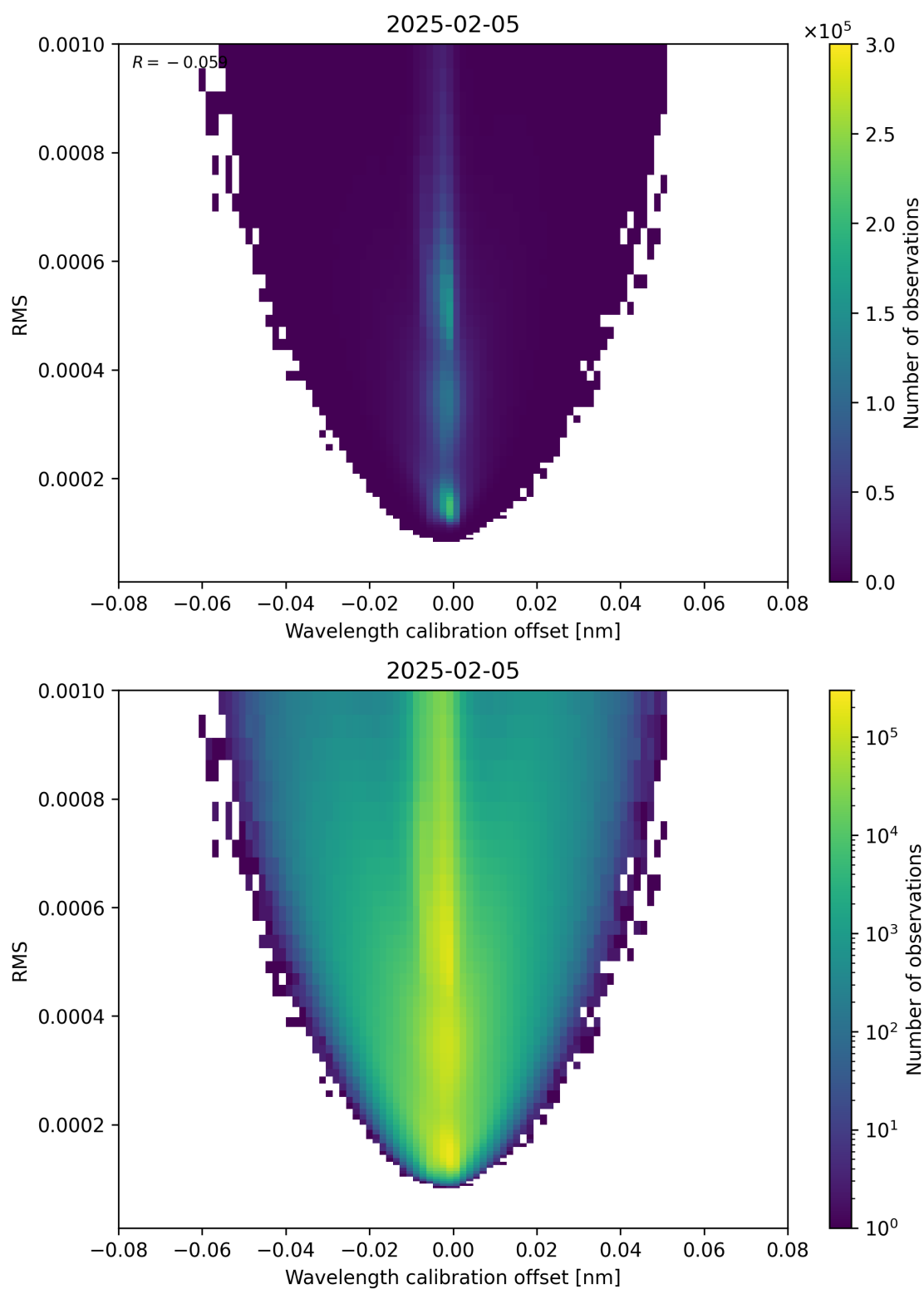
Figure 181: Scatter density plot of “Wavelength calibration offset” against “RMS” for 2025-02-04 to 2025-02-06.
