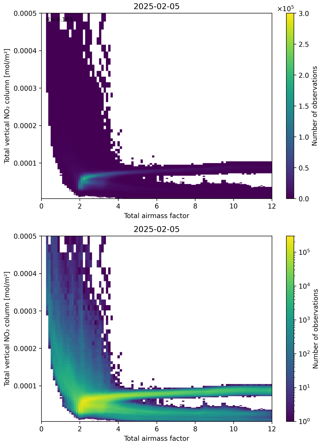
Figure 67: Scatter density plot of “Total airmass factor” against “Total vertical NO 2 column” for 2025-02-04 to 2025-02-06.
