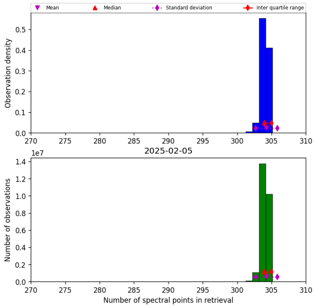
Figure 33: Histogram of “Number of spectral points in retrieval” for 2025-02-04 to 2025-02-06
