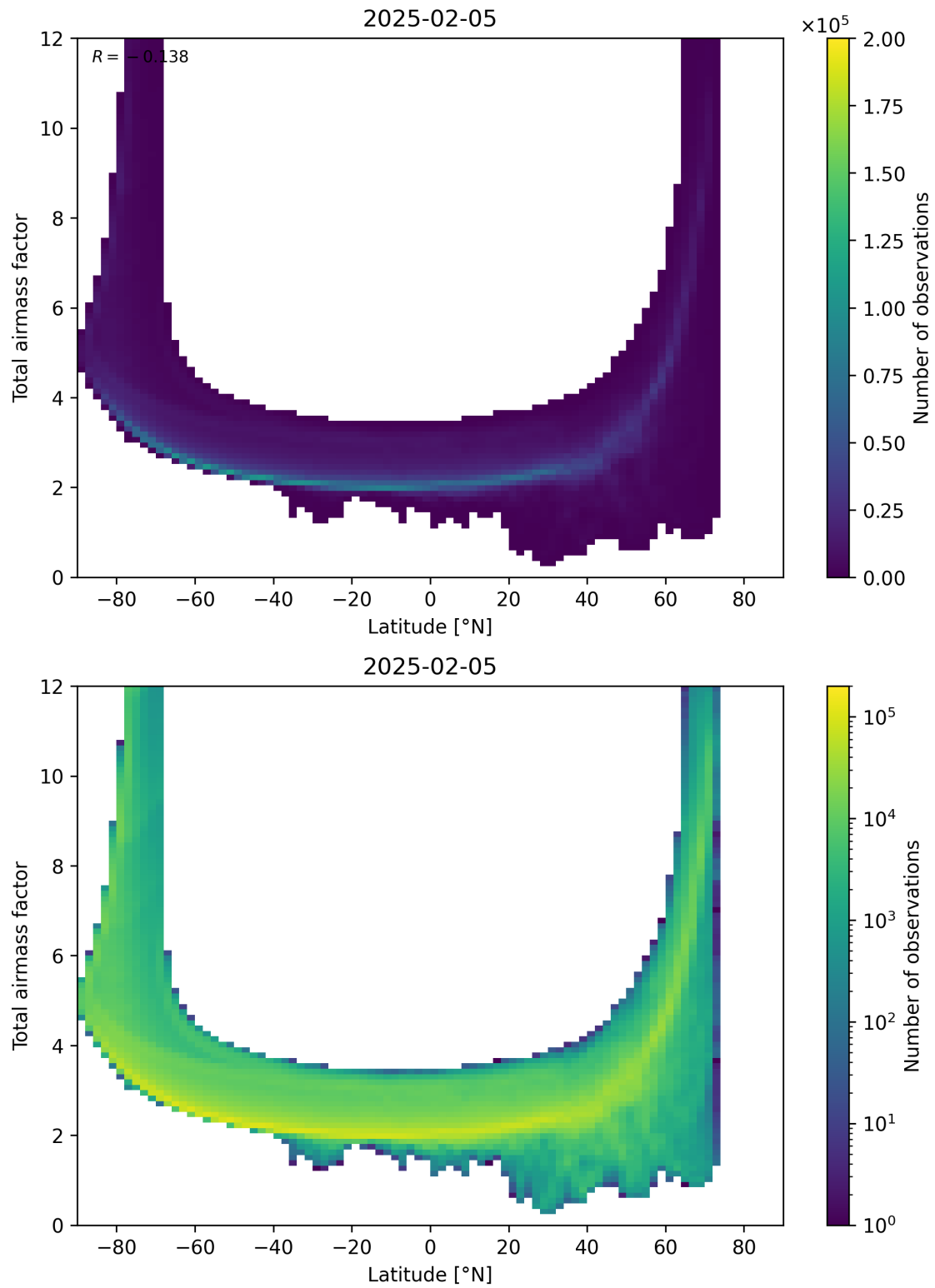
Figure 84: Scatter density plot of “Latitude” against “Total airmass factor” for 2025-02-04 to 2025-02-06.
