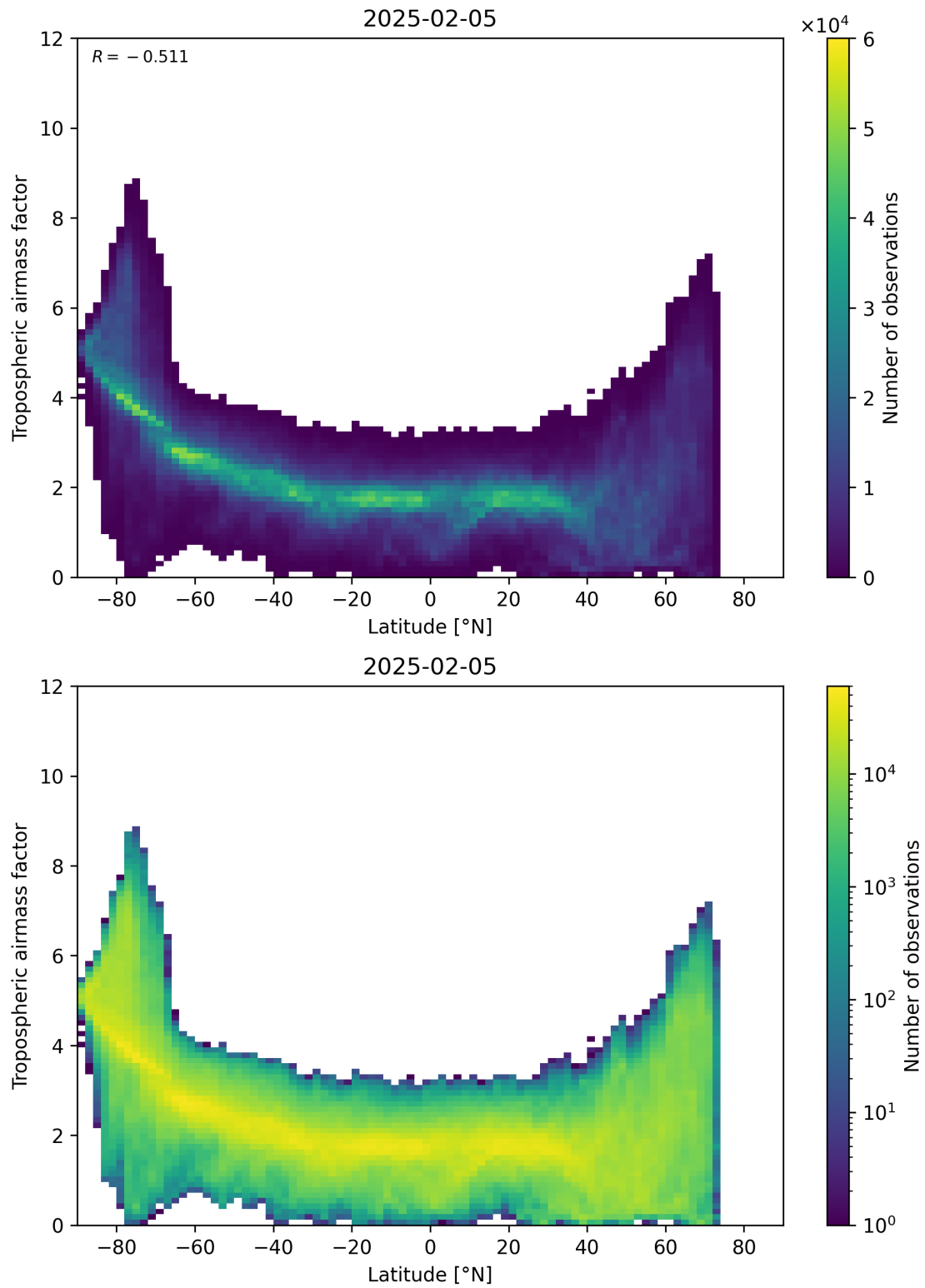
Figure 85: Scatter density plot of “Latitude” against “Tropospheric airmass factor” for 2025-02-04 to 2025-02-06.
