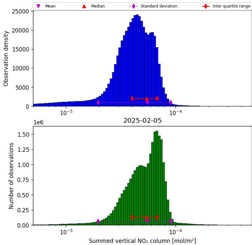
Figure 40: Histogram of “Summed vertical NO 2 column” for 2025-02-04 to 2025-02-06
