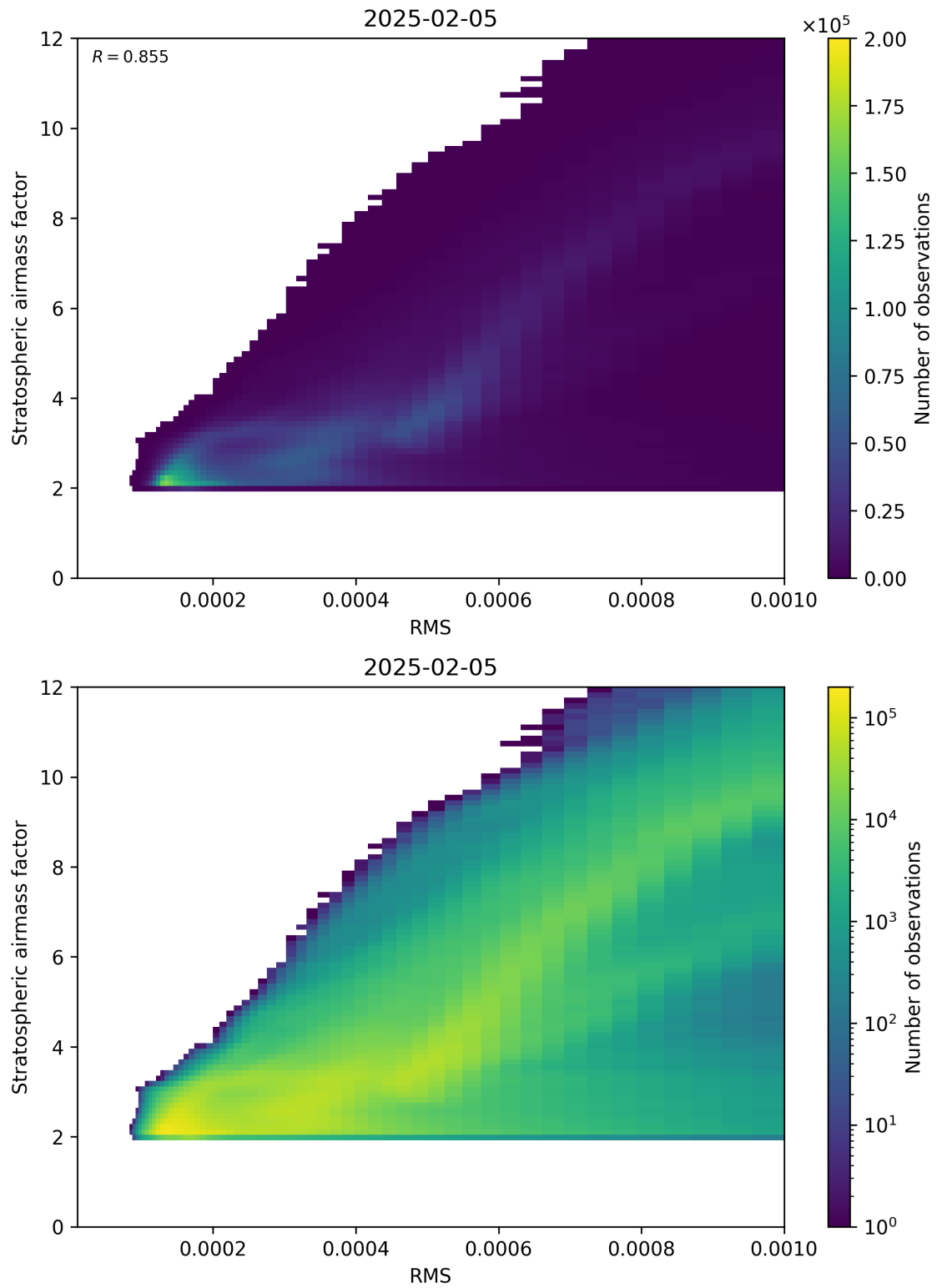
Figure 144: Scatter density plot of “RMS” against “Stratospheric airmass factor” for 2025-02-04 to 2025-02-06.
