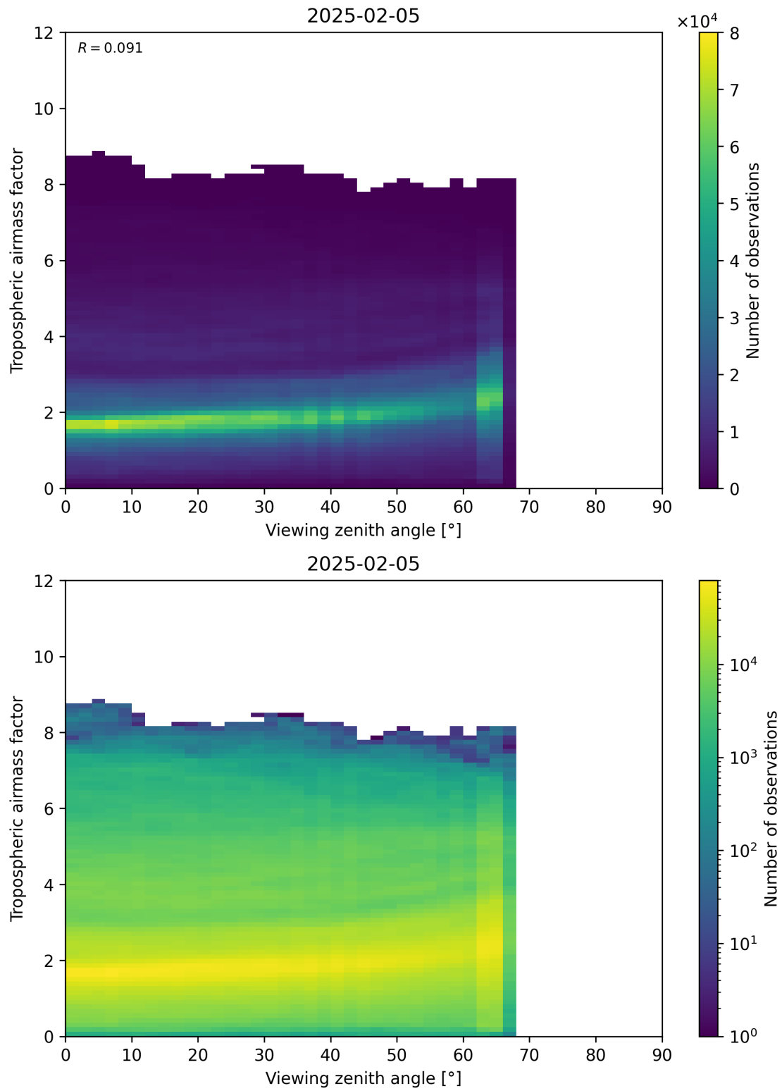
Figure 161: Scatter density plot of “Viewing zenith angle” against “Tropospheric airmass factor” for 2025-02-04 to 2025-02-06.
