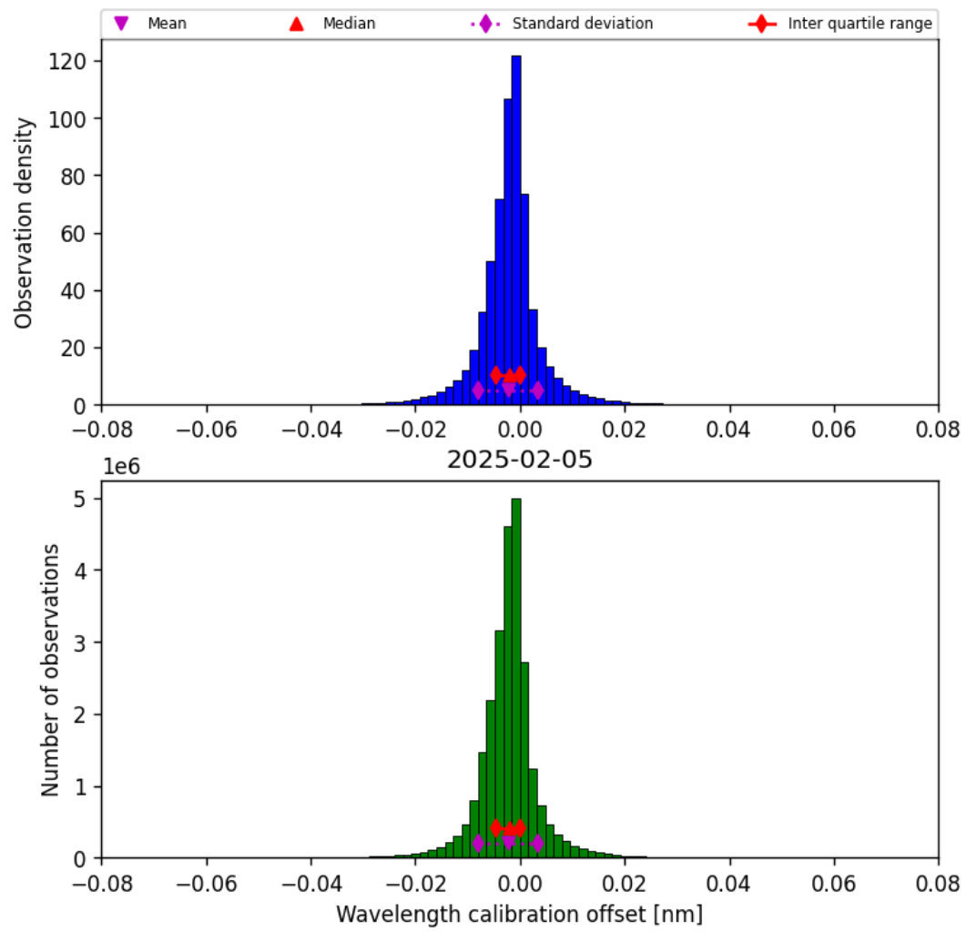
Figure 35: Histogram of “Wavelength calibration offset” for 2025-02-04 to 2025-02-06
