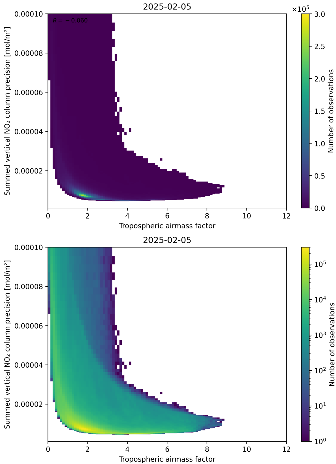
Figure 76: Scatter density plot of “Tropospheric air mass factor” against “Summed vertical NO 2 column precision” for 2025-02-04 to 2025-02-06.
