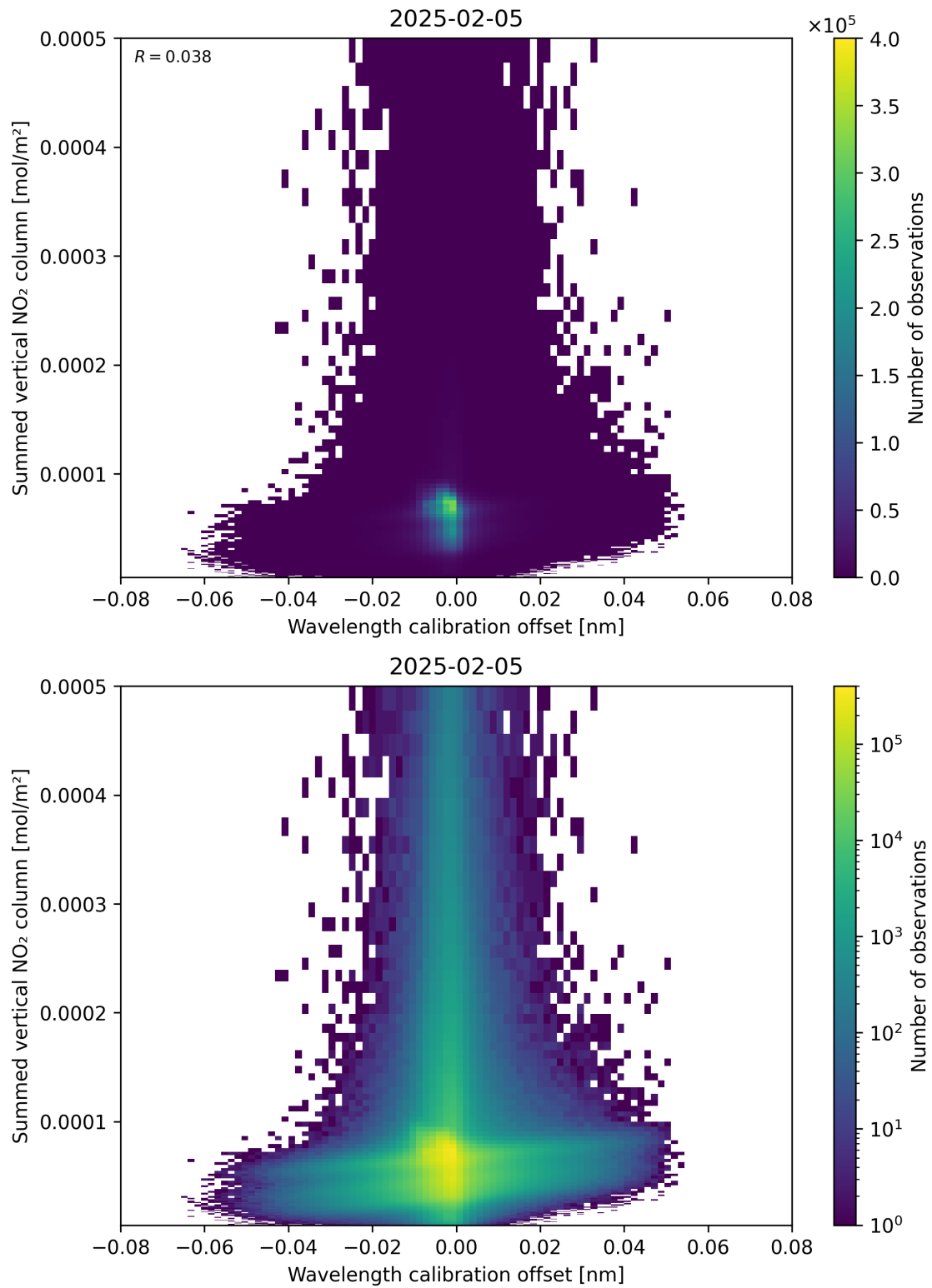
Figure 177: Scatter density plot of “Wavelength calibration offset” against “Summed vertical NO 2 column” for 2025-02-04 to 2025-02-06.
