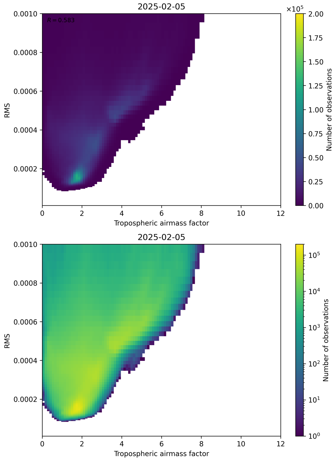
Figure 79: Scatter density plot of “Tropospheric airmass factor” against “RMS” for 2025-02-04 to 2025-02-06.
