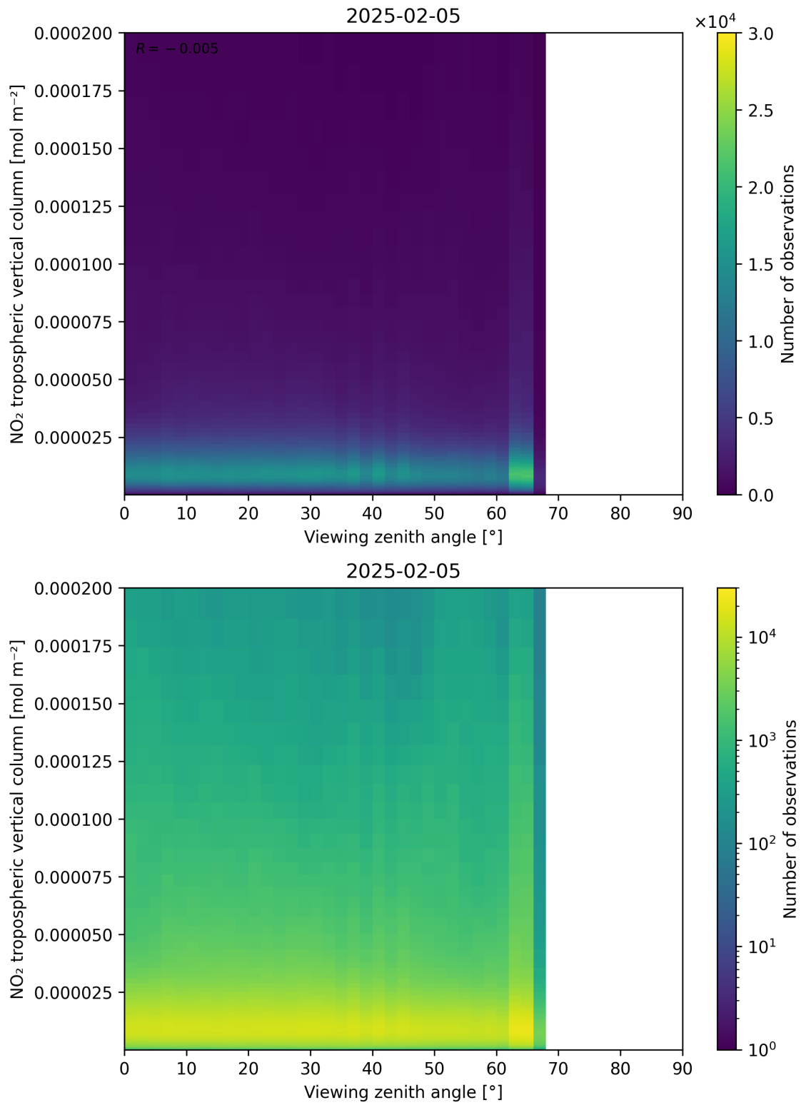
Figure 169: Scatter density plot of “Viewing zenith angle” against “NO 2 tropospheric vertical column” for 2025-02-04 to 2025-02-06.
