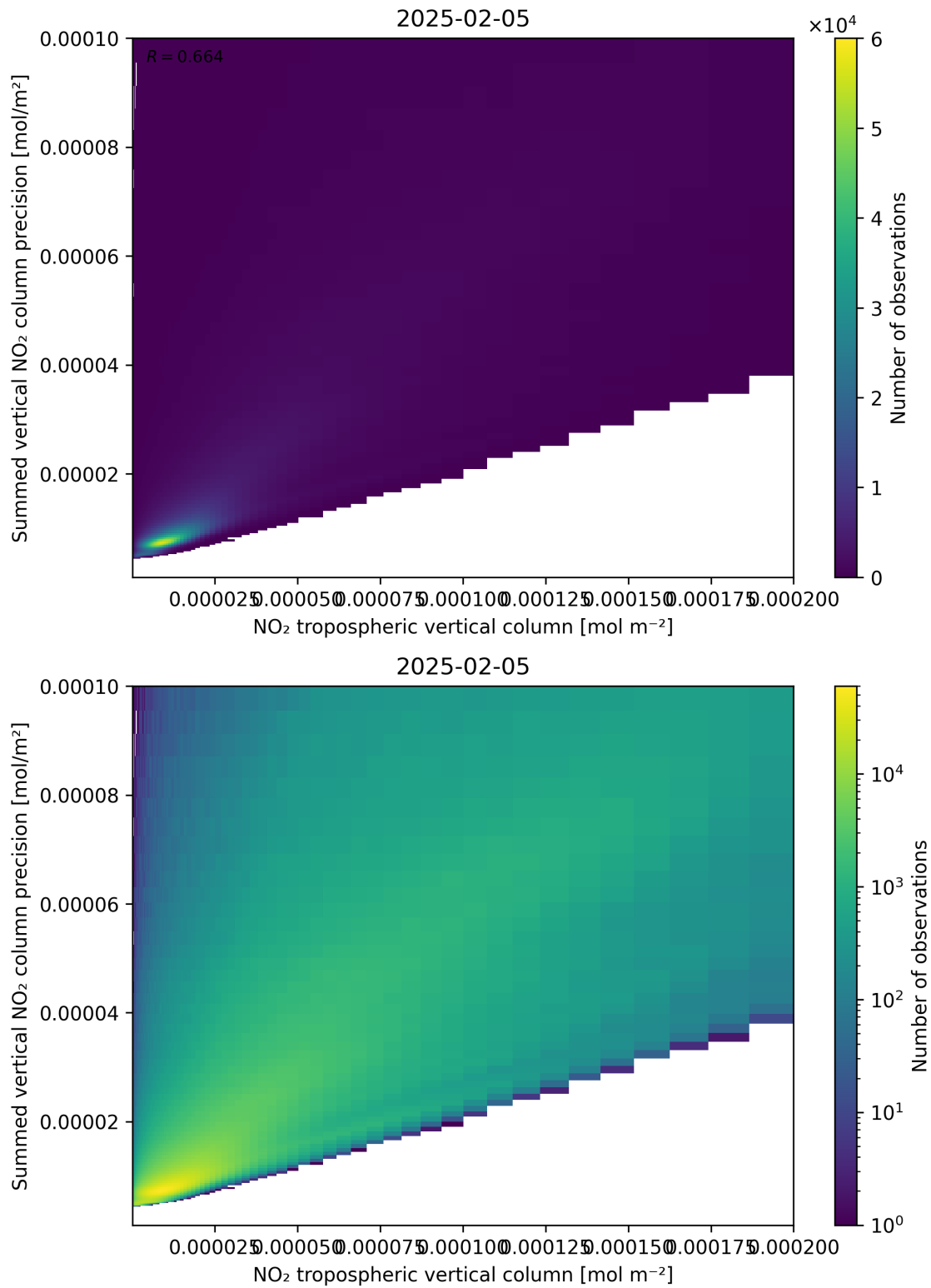
Figure 127: Scatter density plot of “NO 2 tropospheric vertical column” against “Summed vertical NO 2 column precision” for 2025-02-04 to 2025-02-06.
