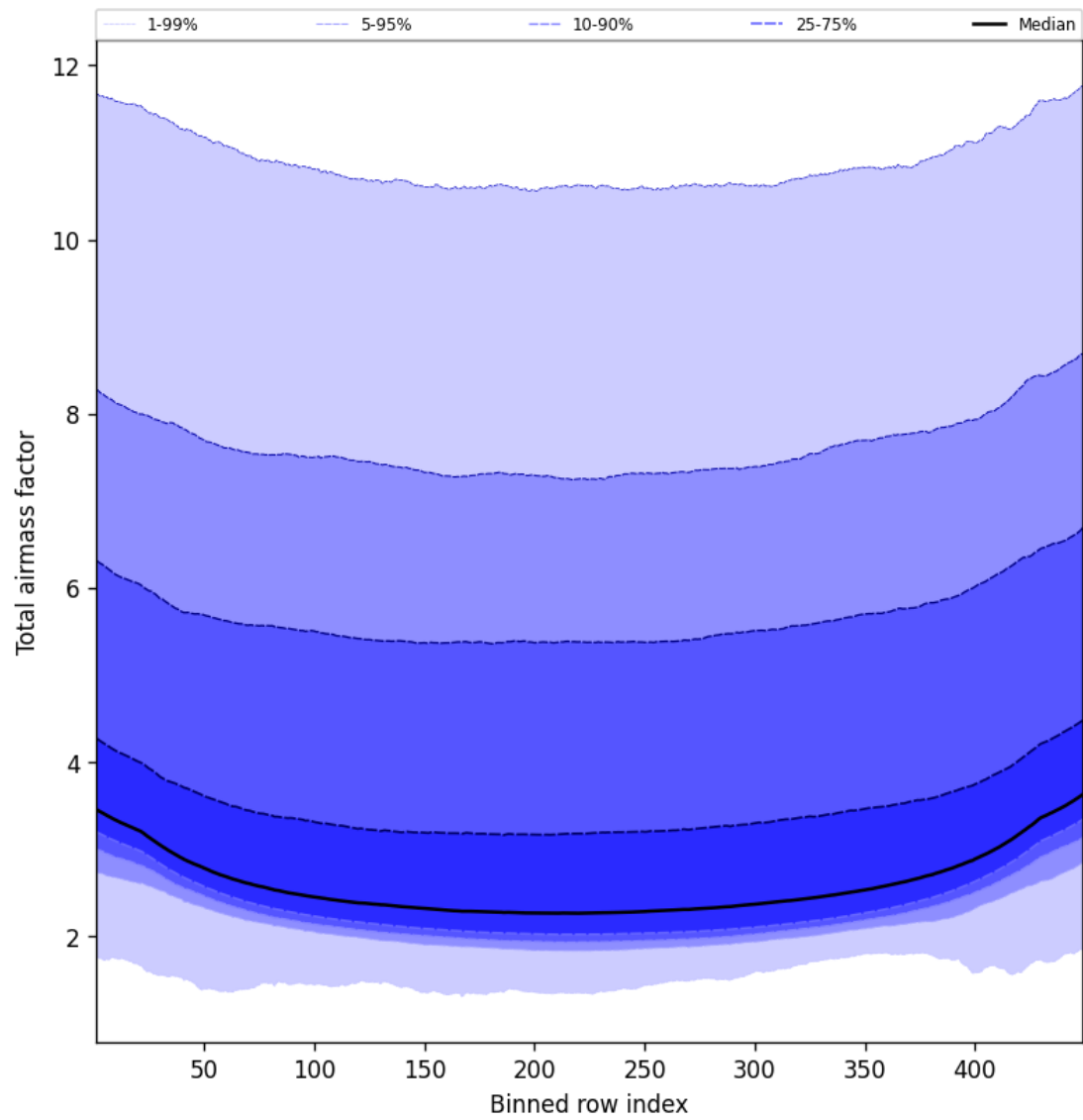
Figure 49: Along track statistics of “Total airmass factor” for 2025-02-04 to 2025-02-06
