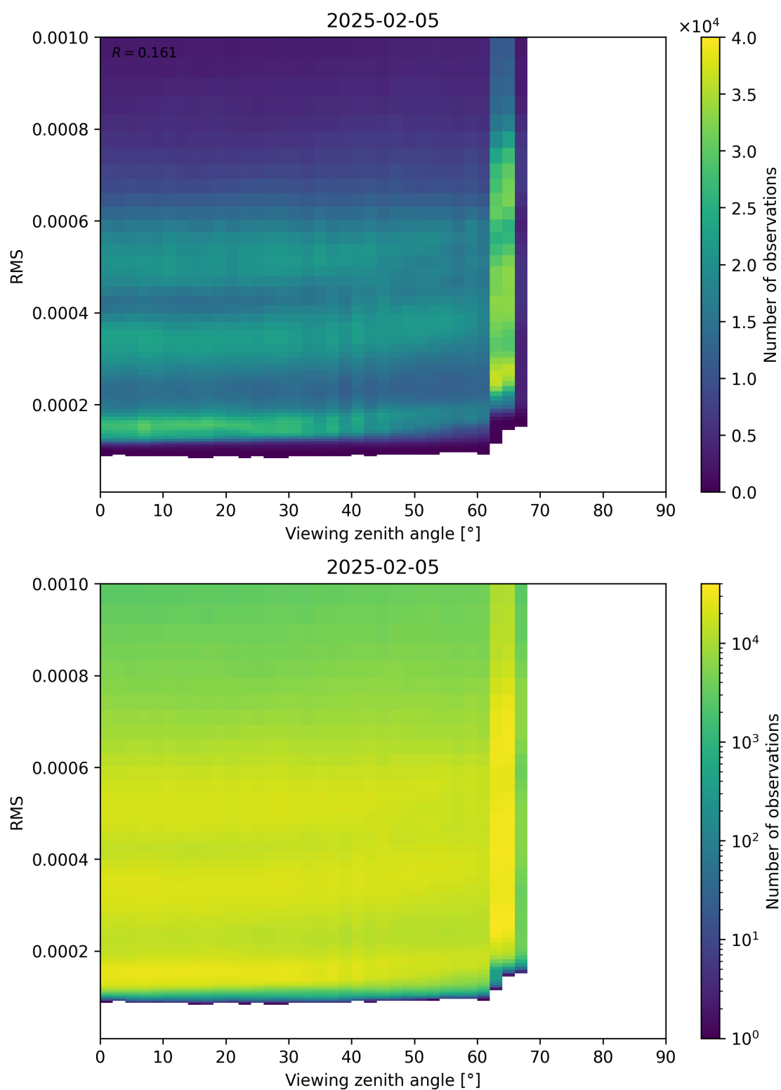
Figure 171: Scatter density plot of “Viewing zenith angle” against “RMS” for 2025-02-04 to 2025-02-06.
