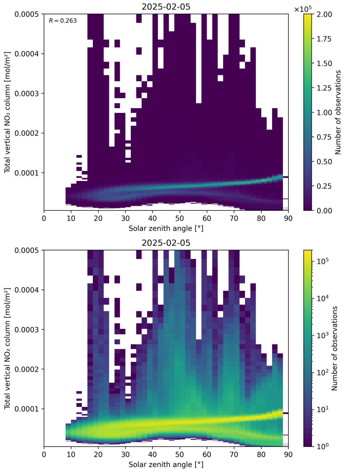
Figure 153: Scatter density plot of “Solar zenith angle” against “Total vertical NO 2 column” for 2025-02-04 to 2025-02-06.
