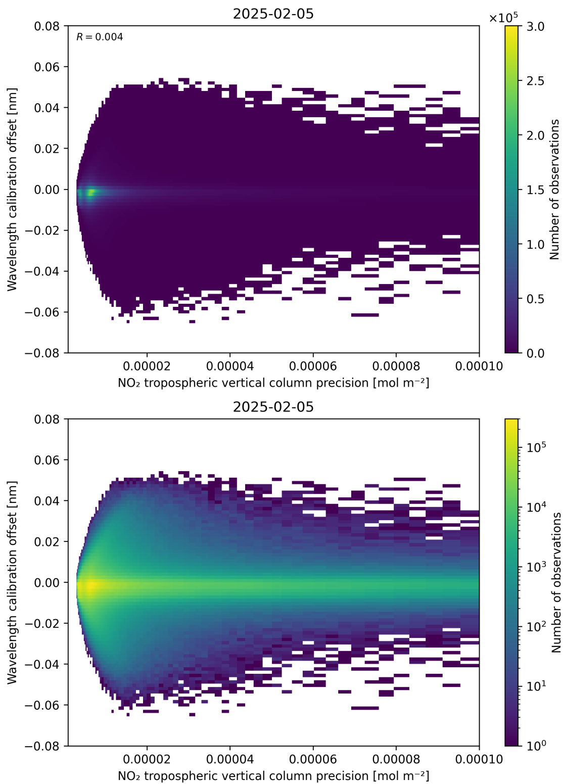
Figure 141: Scatter density plot of “NO 2 tropospheric vertical column precision” against “Wavelength calibration offset” for 2025-02-04 to 2025-02-06.
