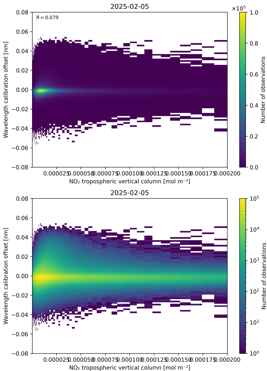
Figure 143: Scatter density plot of “NO 2 tropospheric vertical column” against “Wavelength calibration offset” for 2025-02-04 to 2025-02-06.
