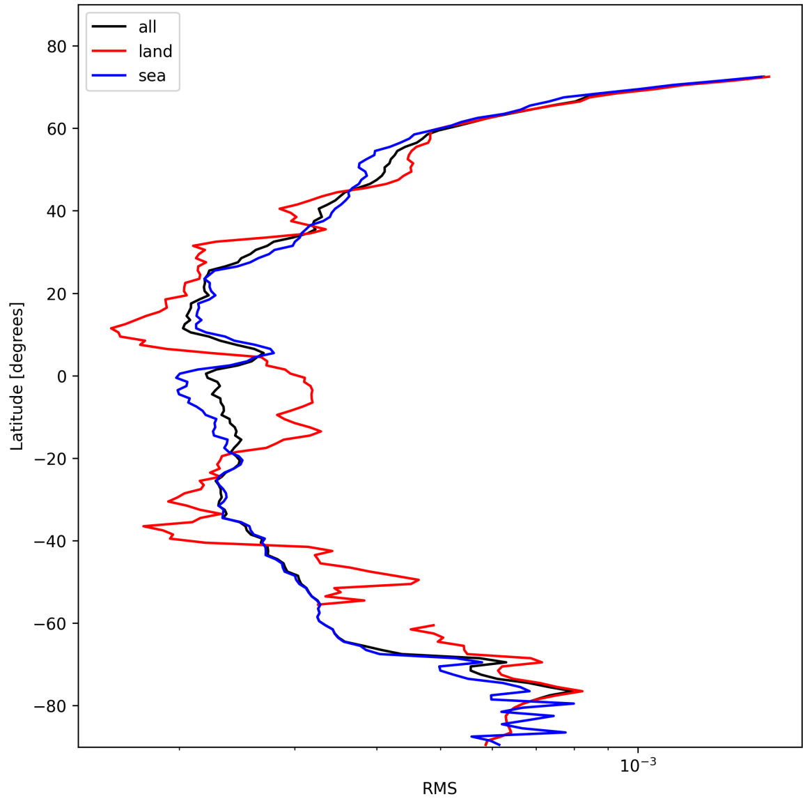
Figure 26: Zonal average of “RMS” for 2025-02-04 to 2025-02-06.
