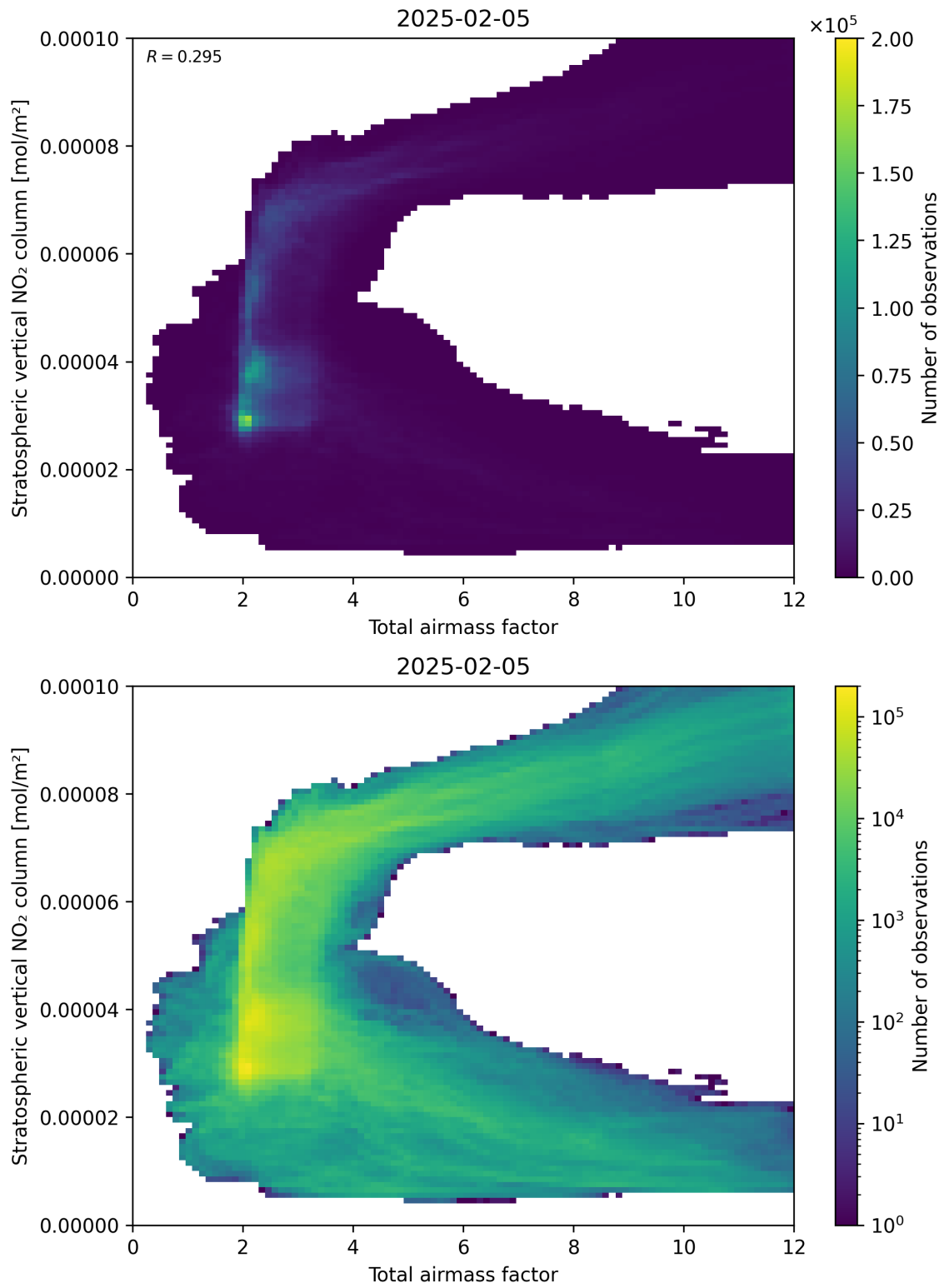
Figure 64: Scatter density plot of “Total airmass factor” against “Stratospheric vertical NO 2 column” for 2025-02-04 to 2025-02-06.
