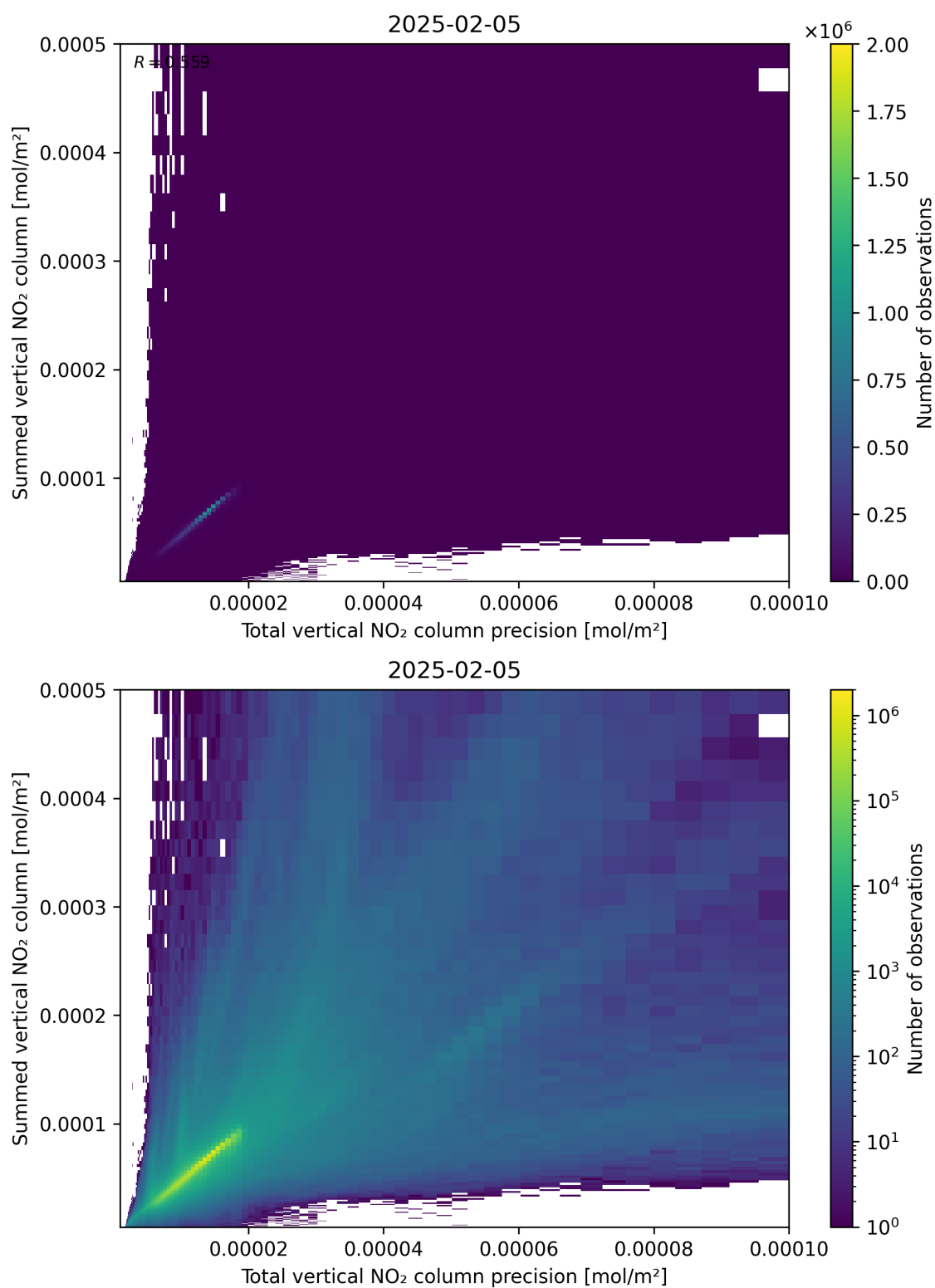
Figure 117: Scatter density plot of “Total vertical NO 2 column precision” against “Summed vertical NO 2 column” for 2025-02-04 to 2025-02-06.
