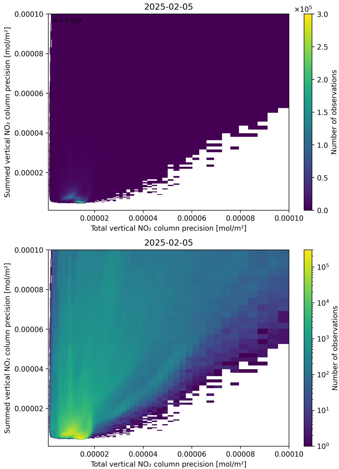
Figure 118: Scatter density plot of “Total vertical NO 2 column precision” against “Summed vertical NO 2 column precision” for 2025-02-04 to 2025-02-06.
