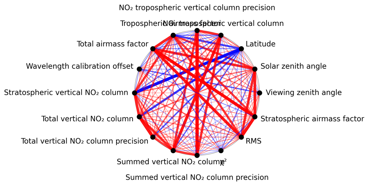
Figure 1: Map of correlation graph for 2025-02-04 to 2025-02-06.
