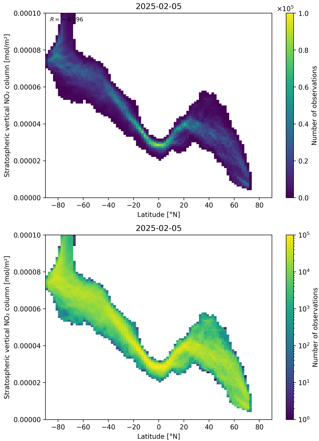
Figure 87: Scatter density plot of “Latitude” against “Stratospheric vertical NO 2 column” for 2025-02-04 to 2025-02-06.
