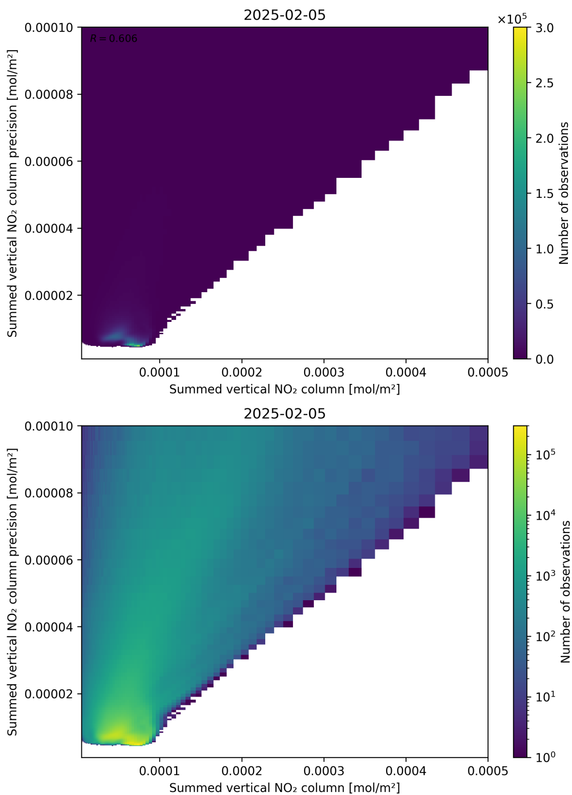
Figure 105: Scatter density plot of “Summed vertical NO 2 column” against “Summed vertical NO 2 column precision” for 2025-02-04 to 2025-02-06.
