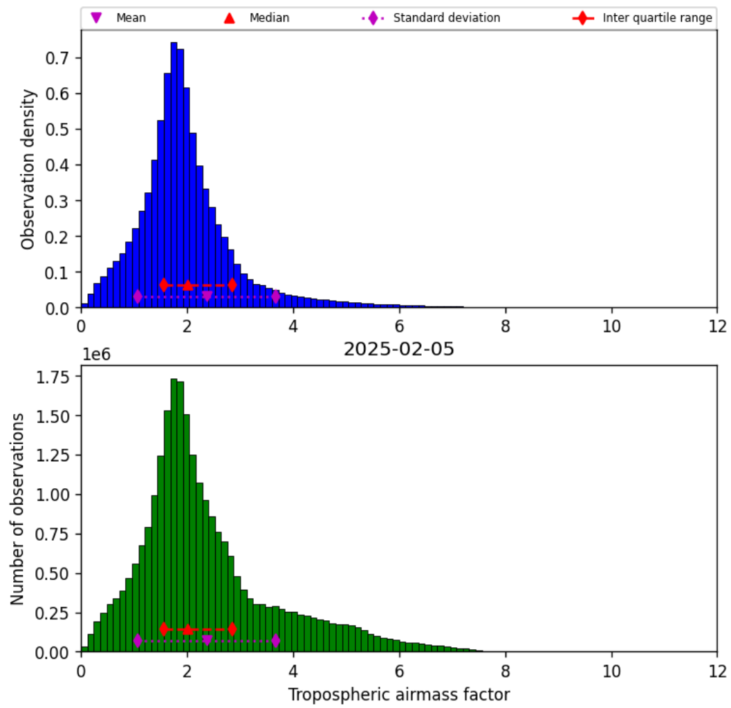
Figure 31: Histogram of “Tropospheric airmass factor” for 2025-02-04 to 2025-02-06
