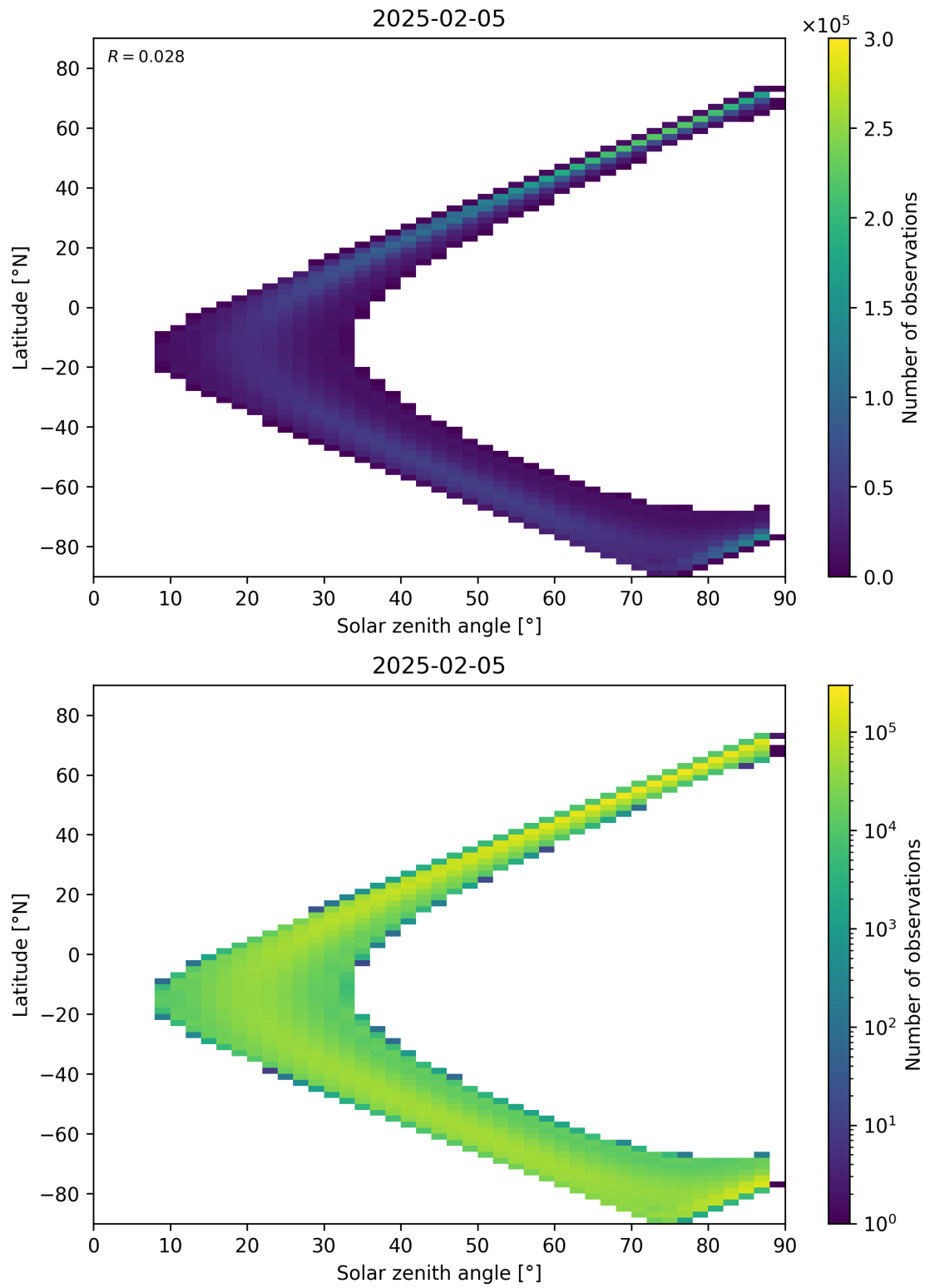
Figure 149: Scatter density plot of “Solar zenith angle” against “Latitude” for 2025-02-04 to 2025-02-06.
