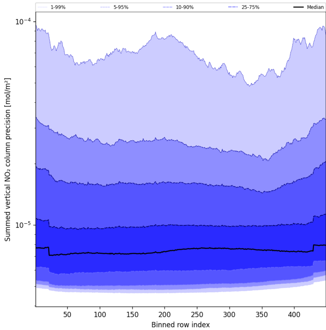
Figure 58: Along track statistics of “Summed vertical NO 2 column precision” for 2025-02-04 to 2025-02-06
