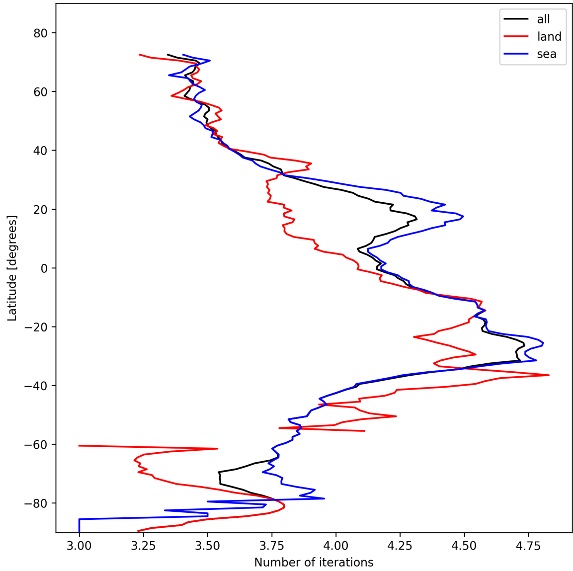
Figure 17: Zonal average of “Number of iterations” for 2025-02-04 to 2025-02-06.
