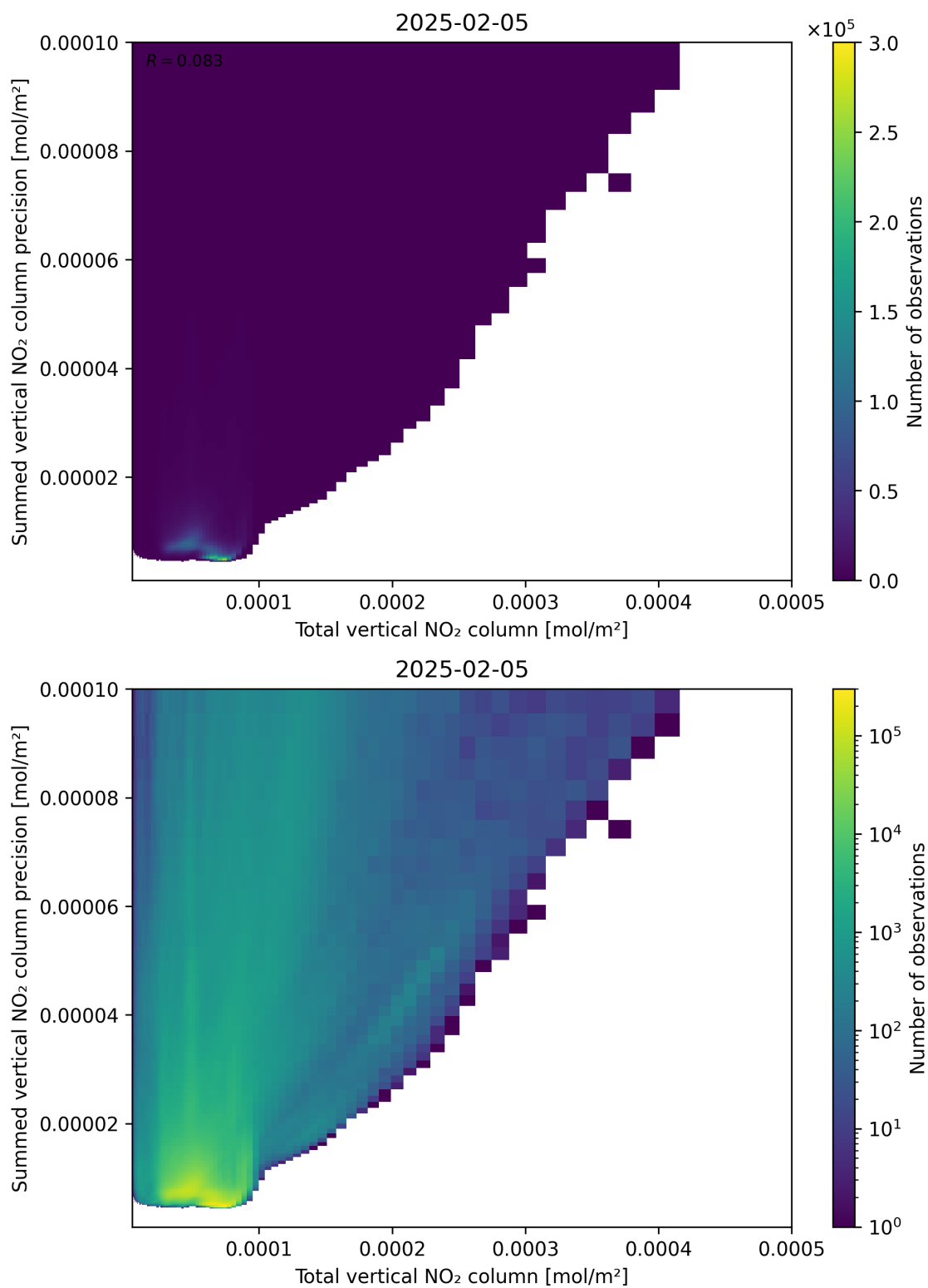
Figure 113: Scatter density plot of “Total vertical NO 2 column” against “Summed vertical NO 2 column precision” for 2025-02-04 to 2025-02-06.
