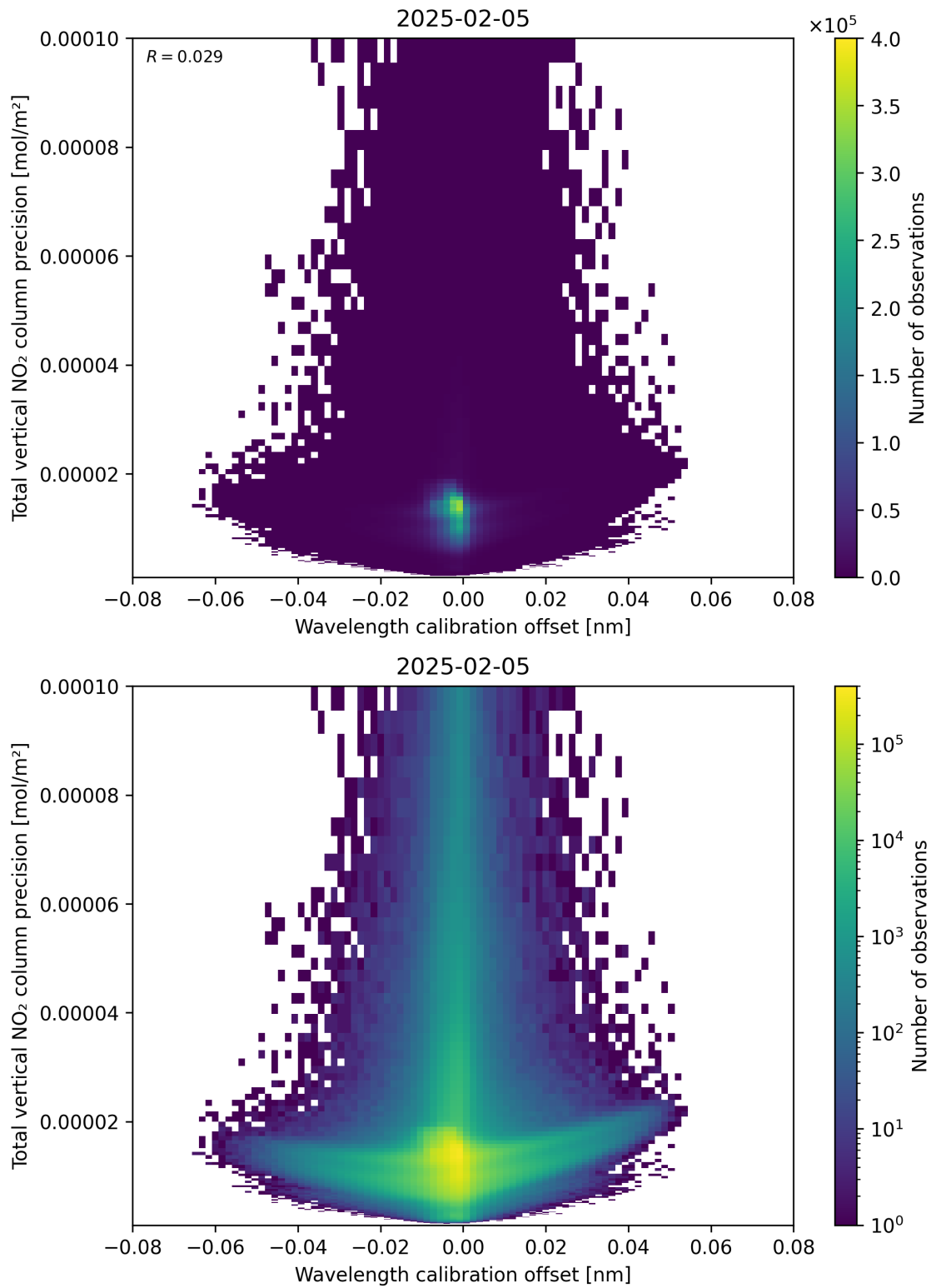
Figure 180: Scatter density plot of “Wavelength calibration offset” against “Total vertical NO 2 column precision” for 2025-02-04 to 2025-02-06.
