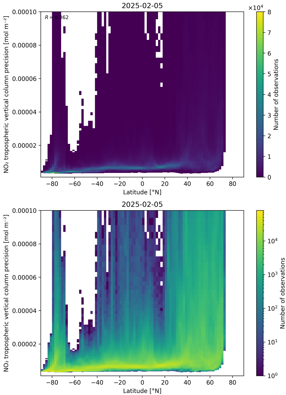
Figure 93: Scatter density plot of “Latitude” against “NO 2 tropospheric vertical column precision” for 2025-02-04 to 2025-02-06.
