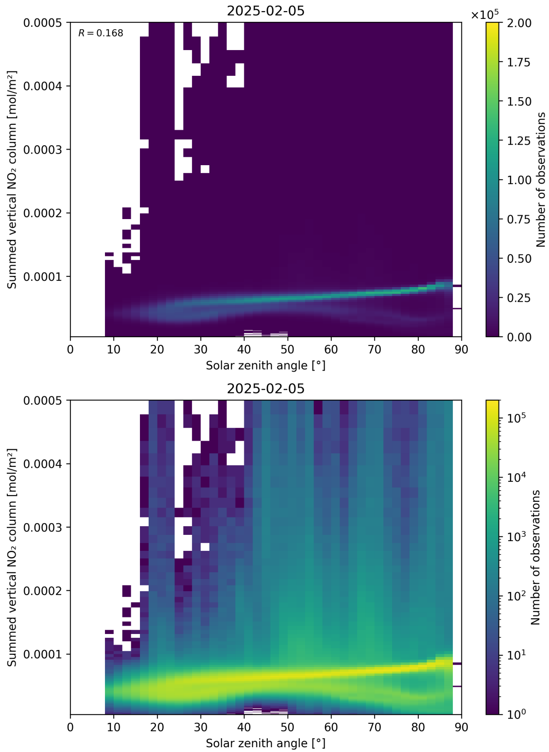
Figure 151: Scatter density plot of “Solar zenith angle” against “Summed vertical NO 2 column” for 2025-02-04 to 2025-02-06.
