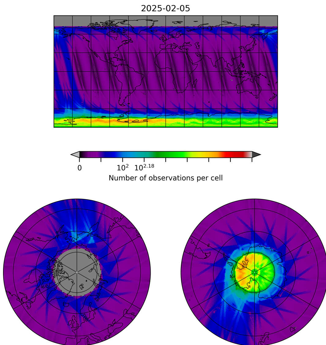
Figure 10: Map of the number of observations for 2025-02-04 to 2025-02-06
