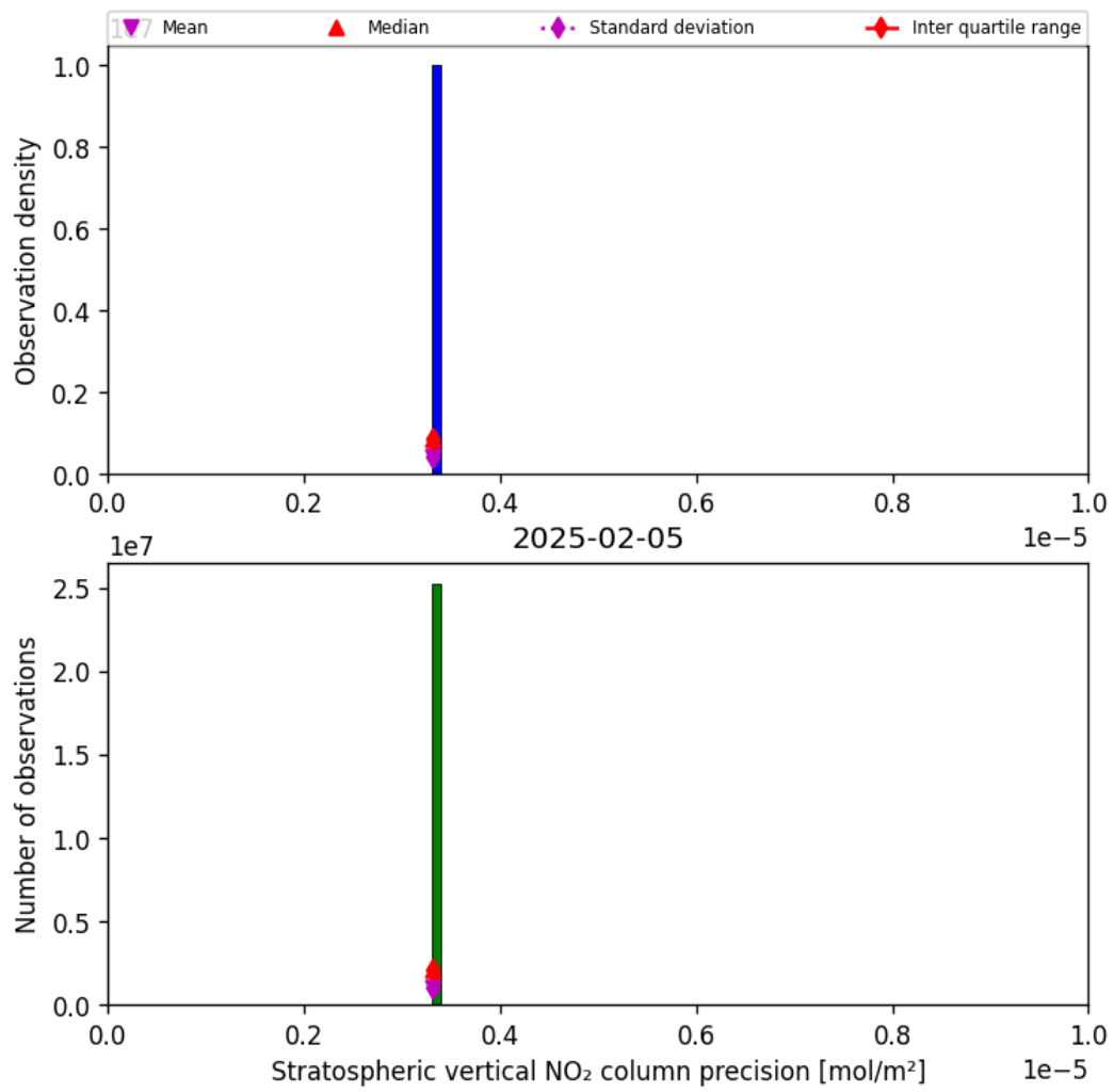
Figure 37: Histogram of “Stratospheric vertical NO 2 column precision” for 2025-02-04 to 2025-02-06
