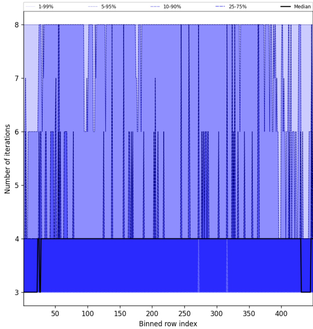
Figure 51: Along track statistics of “Number of iterations” for 2025-02-04 to 2025-02-06
