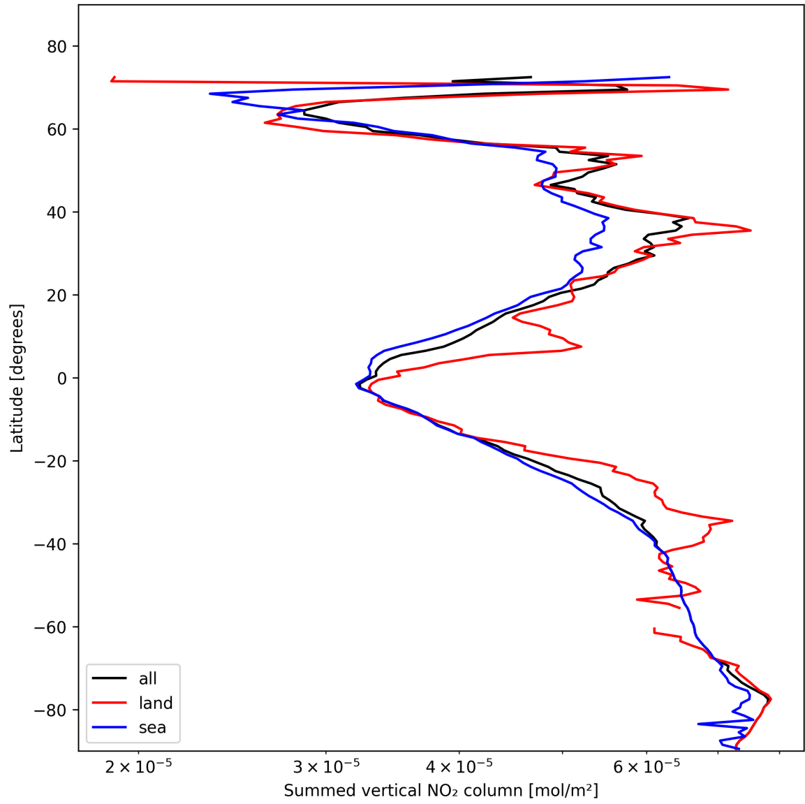
Figure 23: Zonal average of “Summed vertical NO 2 column” for 2025-02-04 to 2025-02-06.
