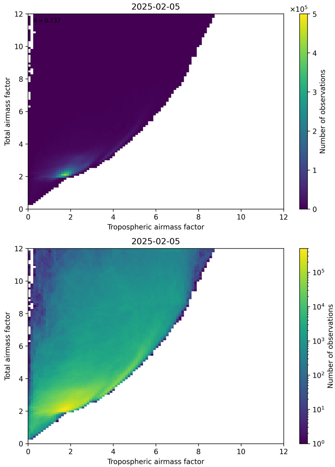
Figure 72: Scatter density plot of “Tropospheric airmass factor” against “Total airmass factor” for 2025-02-04 to 2025-02-06.
