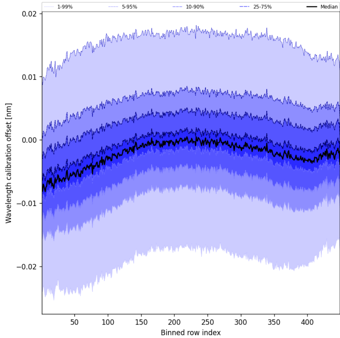
Figure 52: Along track statistics of “Wavelength calibration offset” for 2025-02-04 to 2025-02-06
