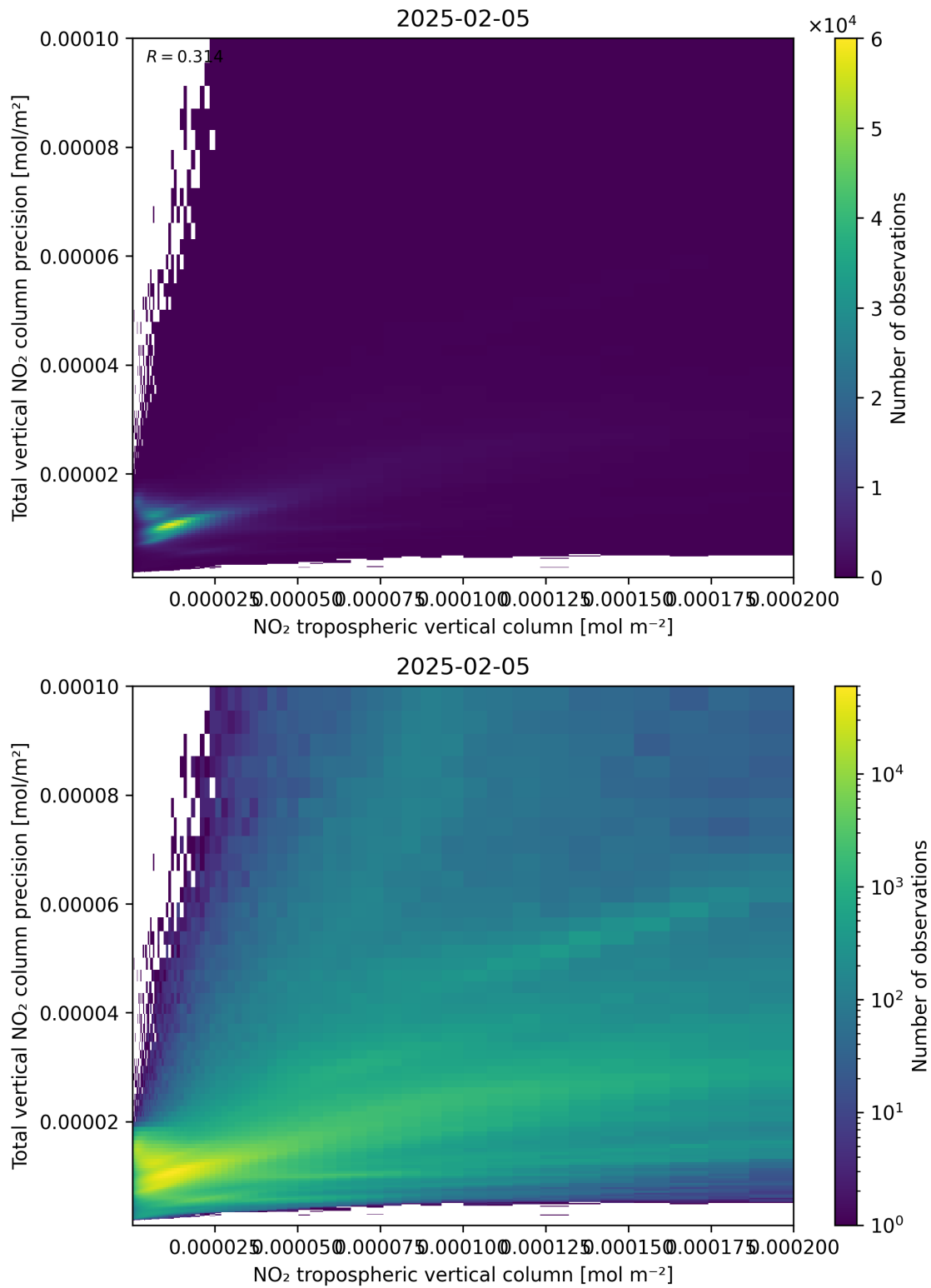
Figure 129: Scatter density plot of “NO 2 tropospheric vertical column” against “Total vertical NO 2 column precision” for 2025-02-04 to 2025-02-06.
