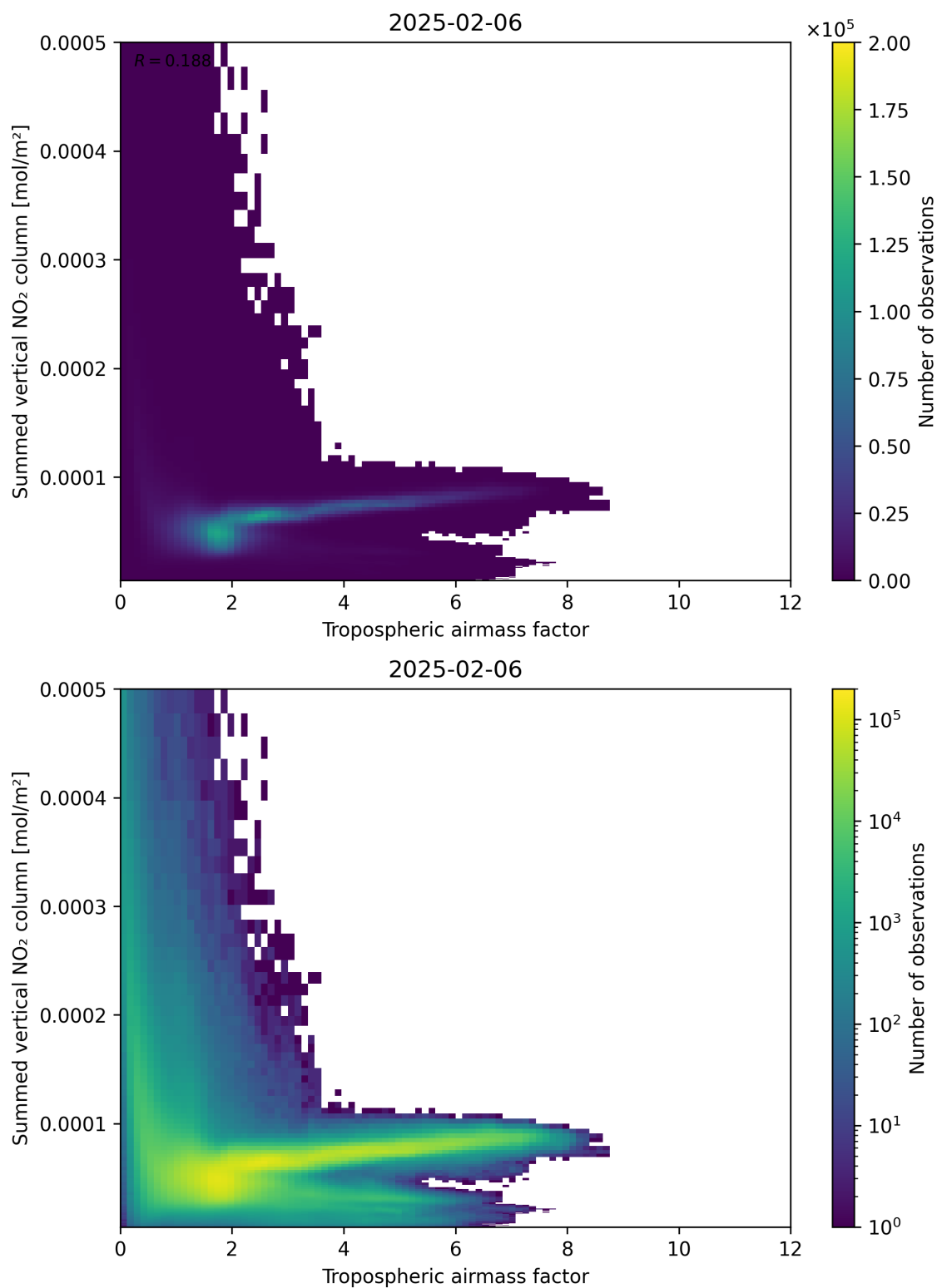
Figure 75: Scatter density plot of “Tropospheric airmass factor” against “Summed vertical NO 2 column” for 2025-02-05 to 2025-02-07.
