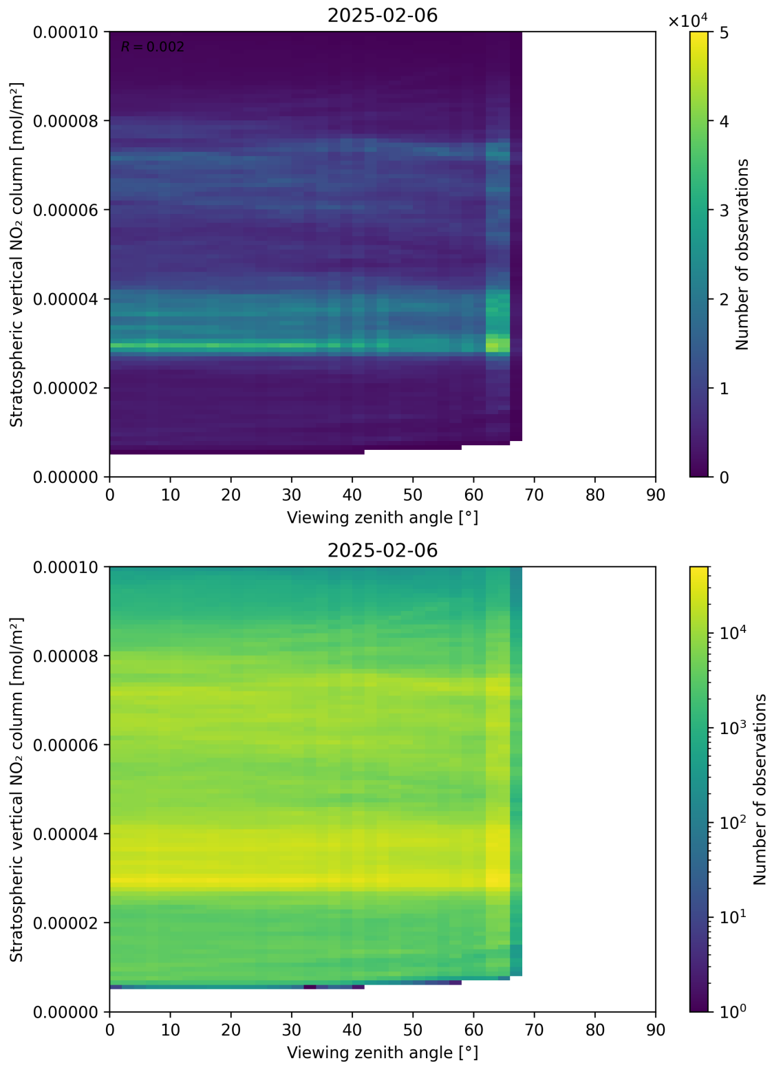
Figure 164: Scatter density plot of “Viewing zenith angle” against “Stratospheric vertical NO 2 column” for 2025-02-05 to 2025-02-07.
