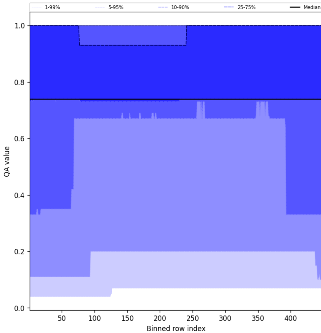
Figure 45: Along track statistics of “QA value” for 2025-02-05 to 2025-02-07
