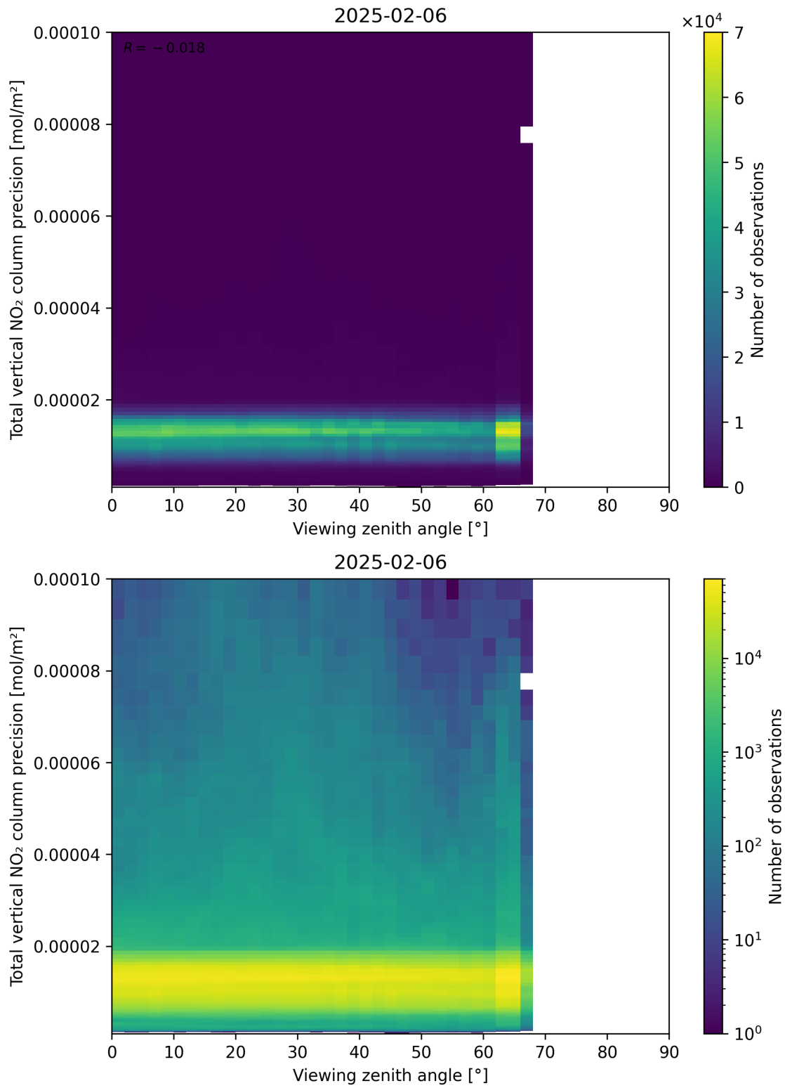
Figure 168: Scatter density plot of “Viewing zenith angle” against “Total vertical NO 2 column precision” for 2025-02-05 to 2025-02-07.
