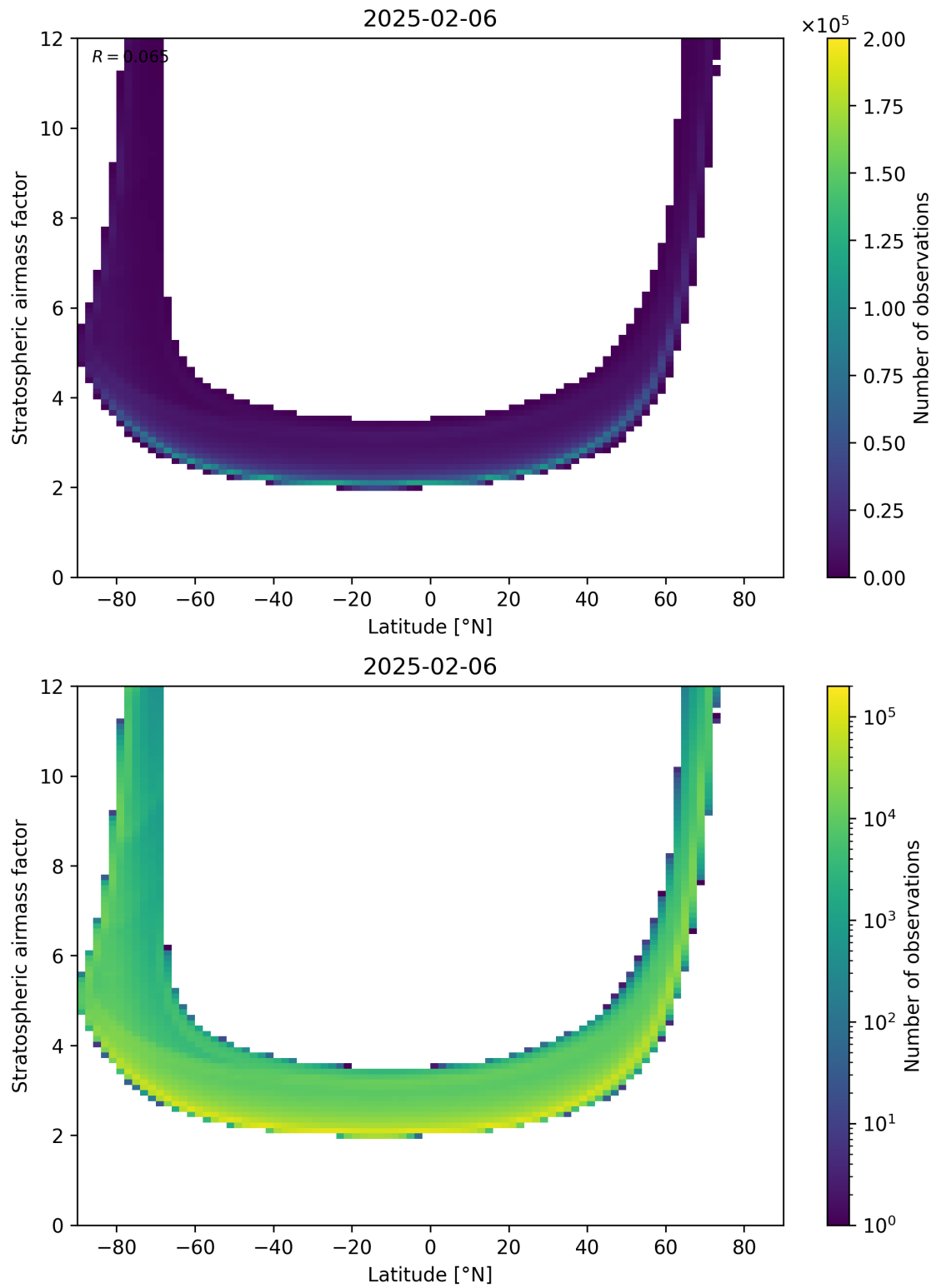
Figure 83: Scatter density plot of “Latitude” against “Stratospheric airmass factor” for 2025-02-05 to 2025-02-07.
