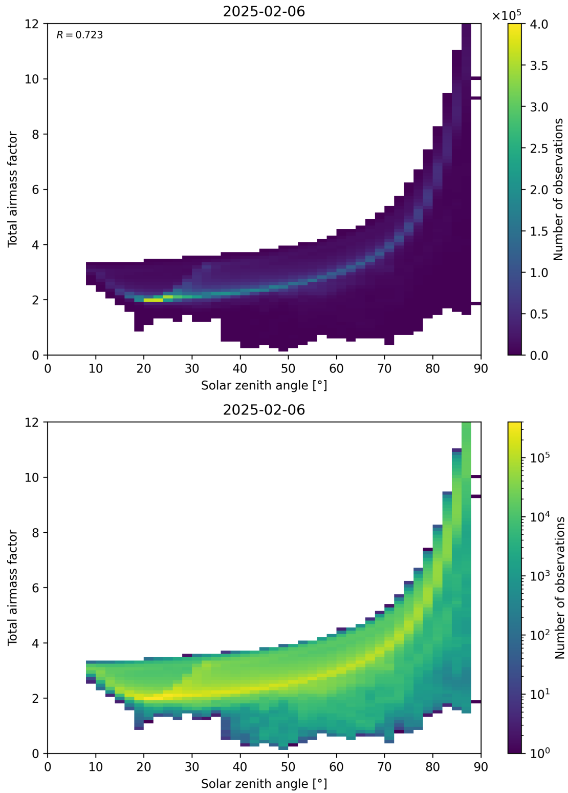
Figure 146: Scatter density plot of “Solar zenith angle” against “Total air mass factor” for 2025-02-05 to 2025-02-07.
