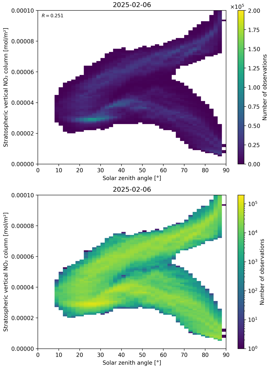
Figure 150: Scatter density plot of “Solar zenith angle” against “Stratospheric vertical NO 2 column” for 2025-02-05 to 2025-02-07.
