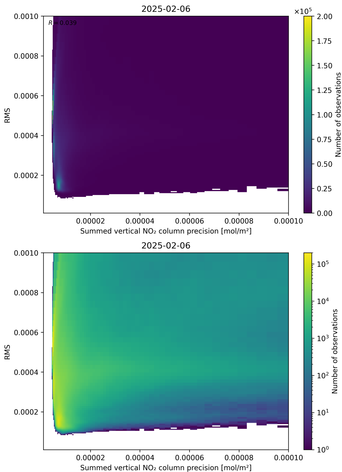
Figure 108: Scatter density plot of “Summed vertical NO 2 column precision” against “RMS” for 2025-02-05 to 2025-02-07.
