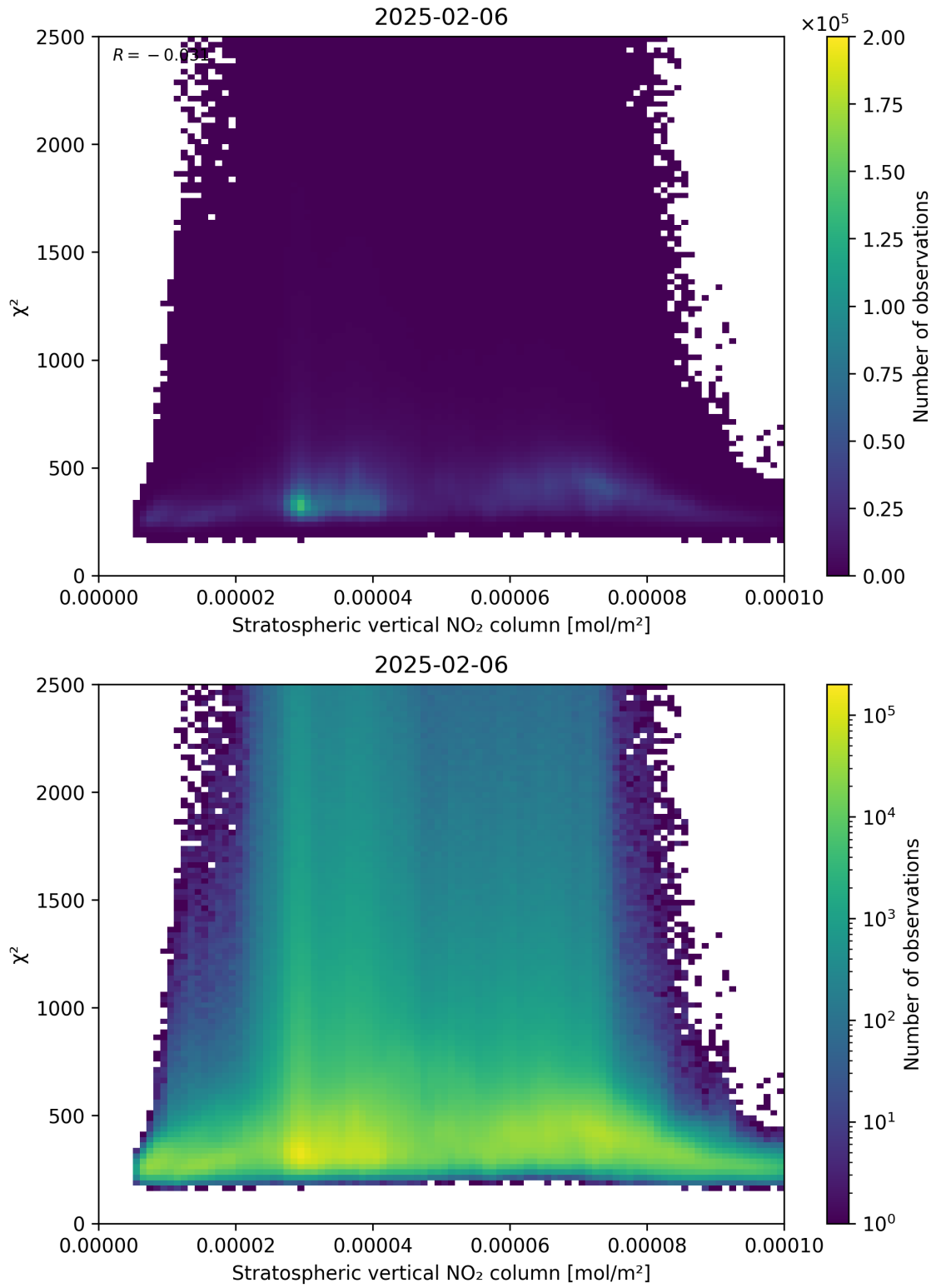
Figure 97: Scatter density plot of “Stratospheric vertical NO 2 column” against “ \chi^2 ” for 2025-02-05 to 2025-02-07.
