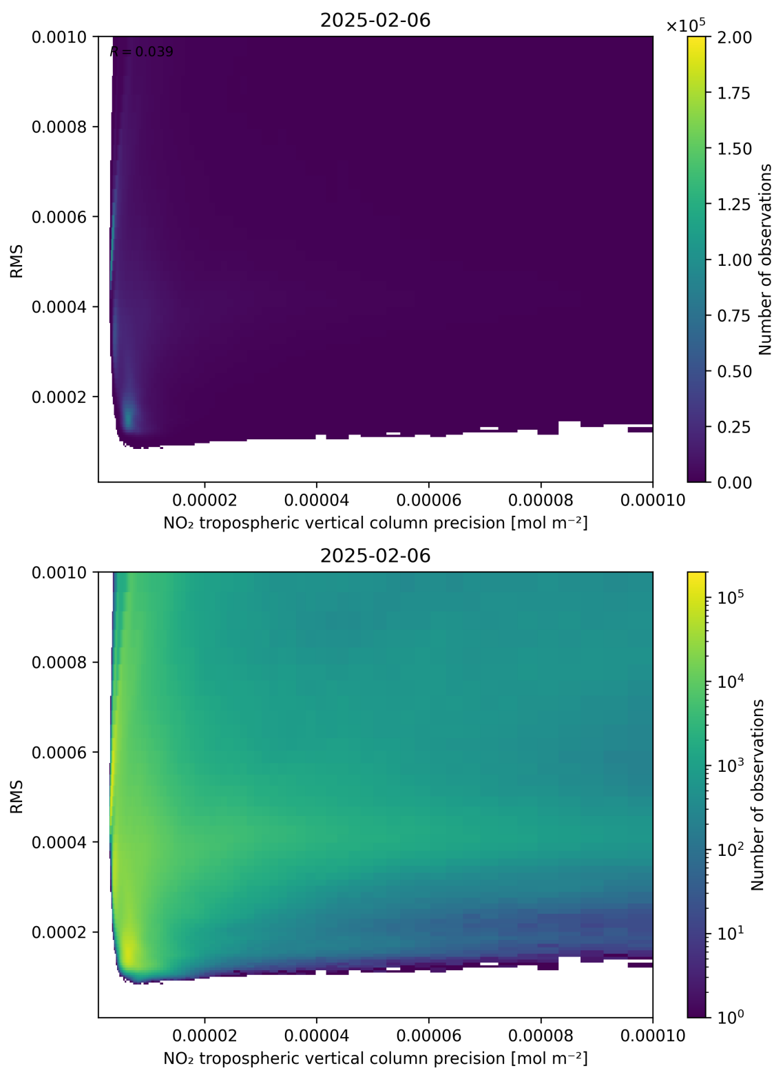
Figure 140: Scatter density plot of “NO 2 tropospheric vertical column precision” against “RMS” for 2025-02-05 to 2025-02-07.
