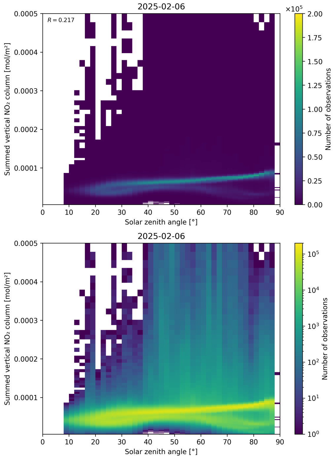
Figure 151: Scatter density plot of “Solar zenith angle” against “Summed vertical NO 2 column” for 2025-02-05 to 2025-02-07.
