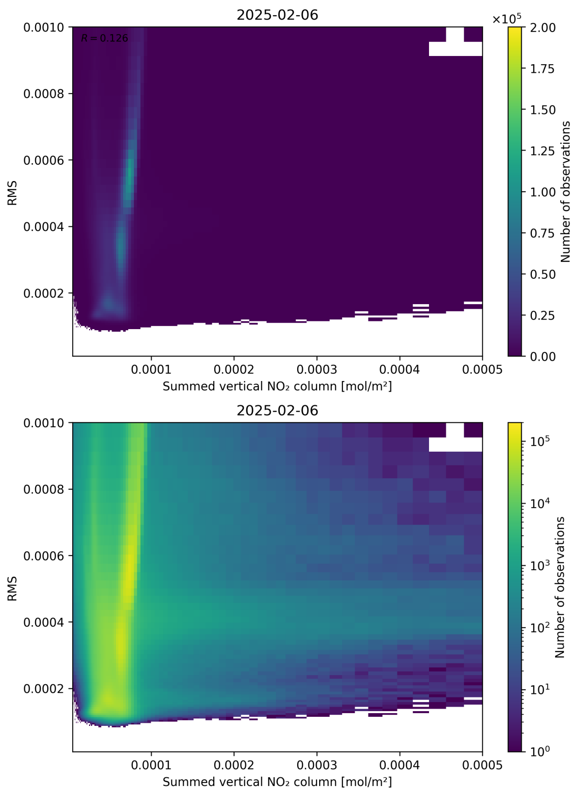
Figure 109: Scatter density plot of “Summed vertical NO 2 column” against “RMS” for 2025-02-05 to 2025-02-07.
