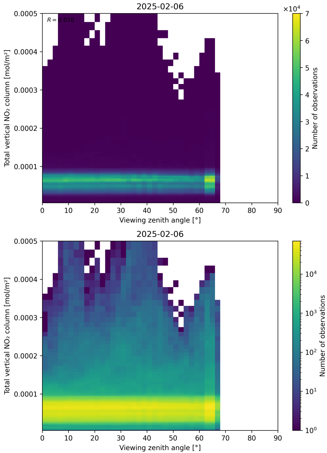
Figure 167: Scatter density plot of “Viewing zenith angle” against “Total vertical NO 2 column” for 2025-02-05 to 2025-02-07.
