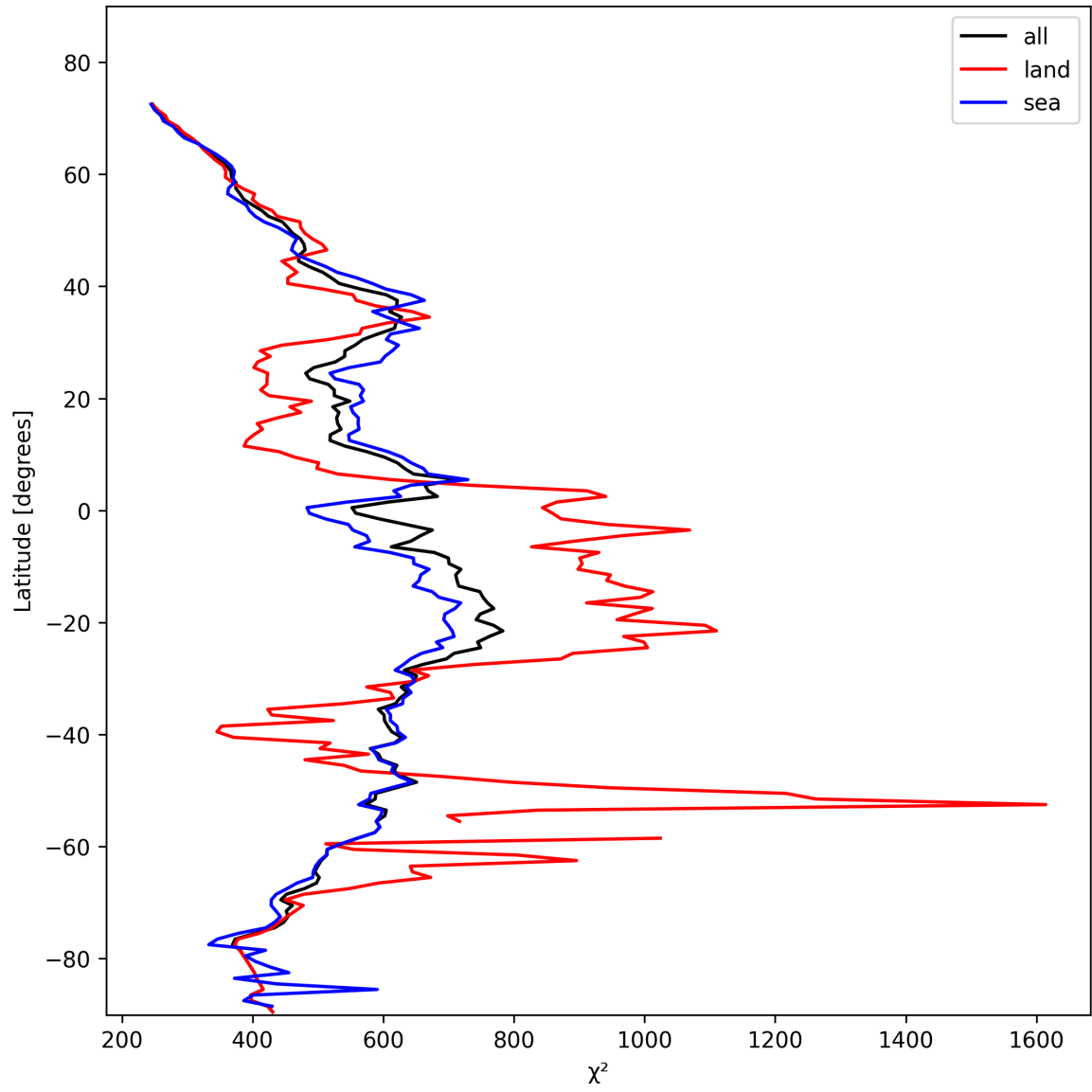
Figure 25: Zonal average of “ \chi^2 ” for 2025-02-05 to 2025-02-07.
