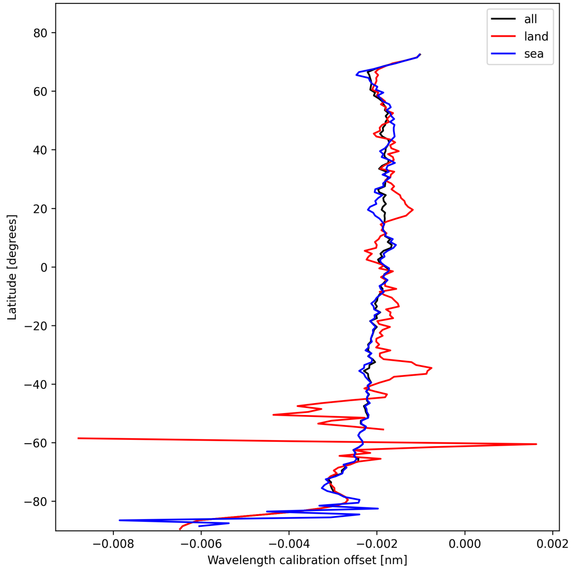
Figure 18: Zonal average of “Wavelength calibration offset” for 2025-02-05 to 2025-02-07.
