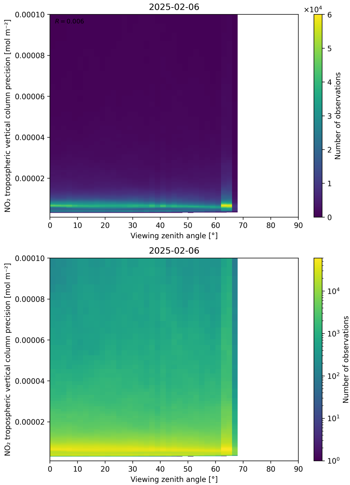
Figure 170: Scatter density plot of “Viewing zenith angle” against “NO 2 tropospheric vertical column precision” for 2025-02-05 to 2025-02-07.
