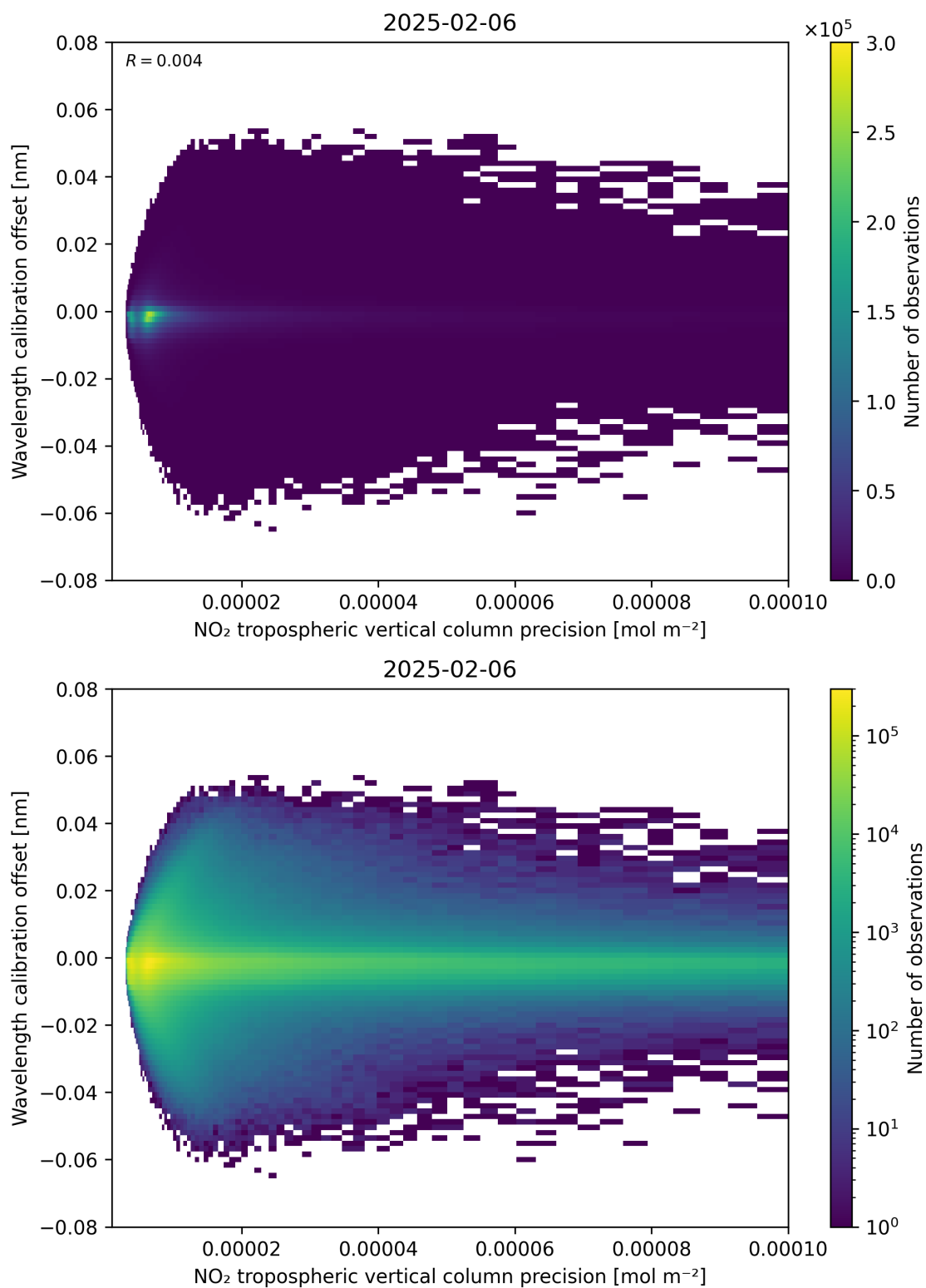
Figure 141: Scatter density plot of “NO 2 tropospheric vertical column precision” against “Wavelength calibration offset” for 2025-02-05 to 2025-02-07.
