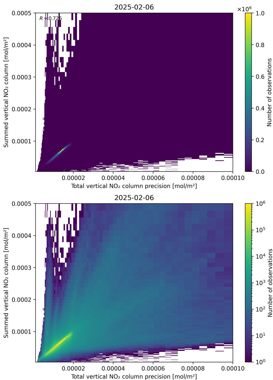
Figure 117: Scatter density plot of “Total vertical NO 2 column precision” against “Summed vertical NO 2 column” for 2025-02-05 to 2025-02-07.
