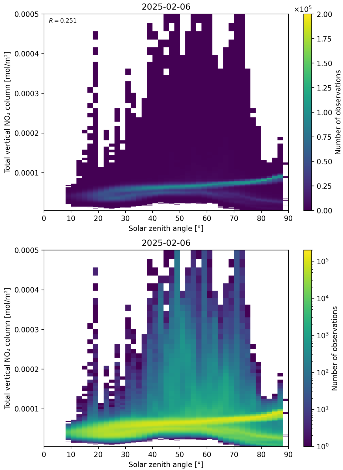
Figure 153: Scatter density plot of “Solar zenith angle” against “Total vertical NO 2 column” for 2025-02-05 to 2025-02-07.
