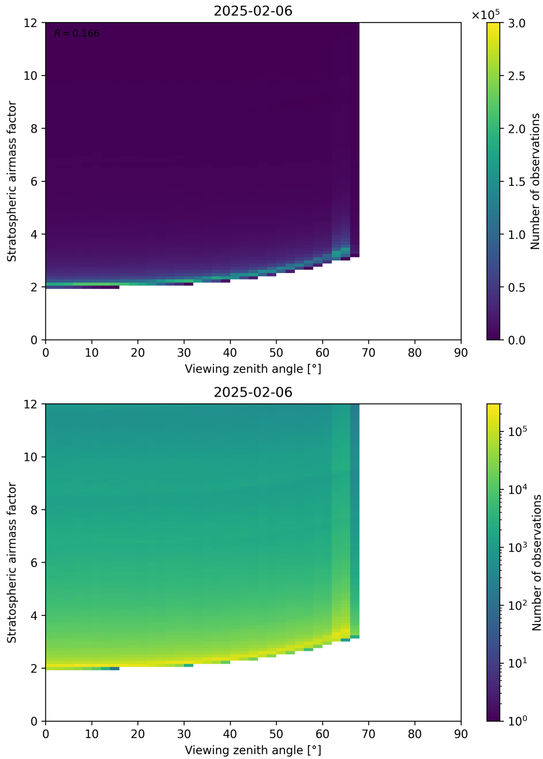
Figure 159: Scatter density plot of “Viewing zenith angle” against “Stratospheric airmass factor” for 2025-02-05 to 2025-02-07.
