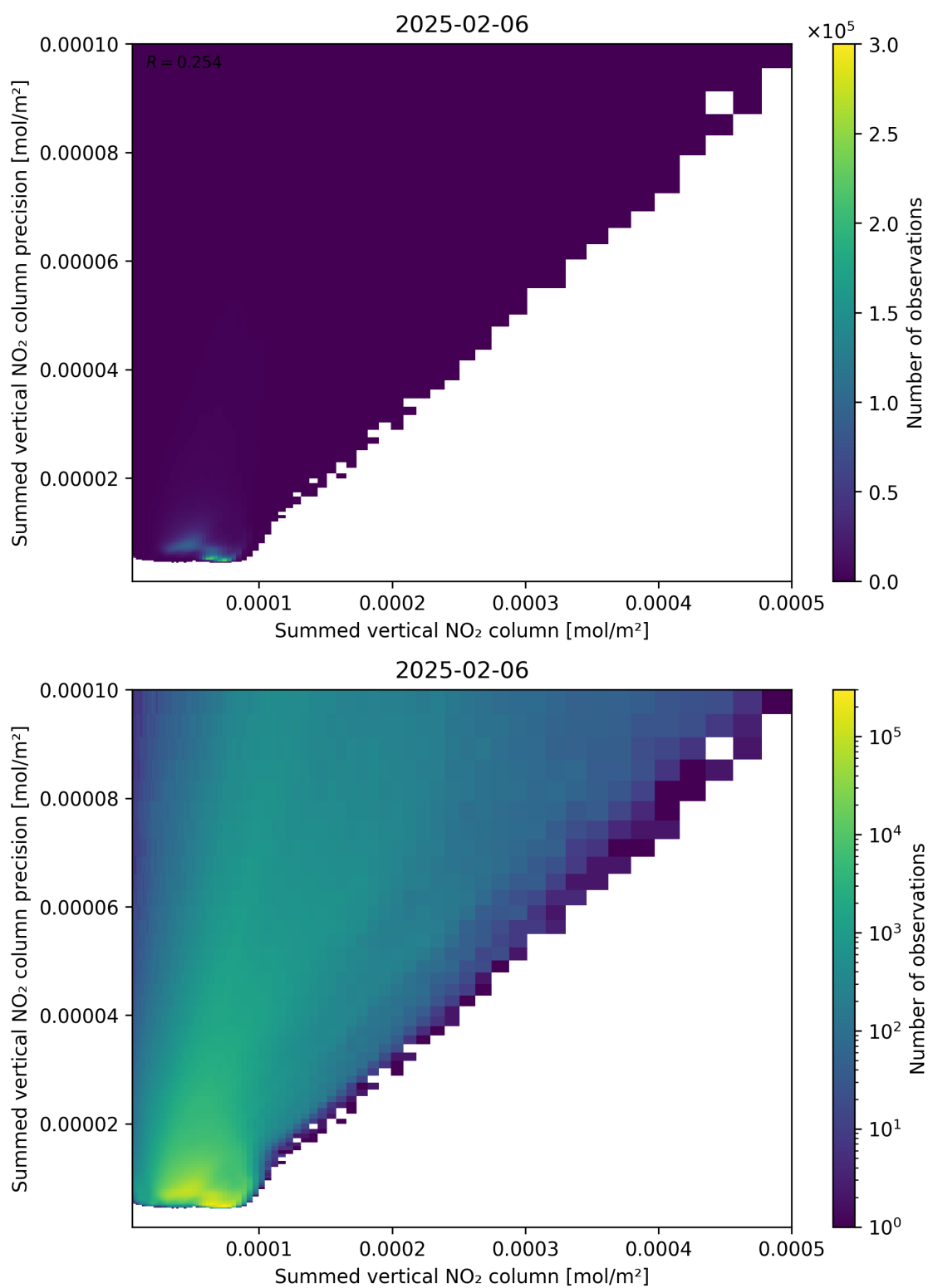
Figure 105: Scatter density plot of “Summed vertical NO 2 column” against “Summed vertical NO 2 column precision” for 2025-02-05 to 2025-02-07.
