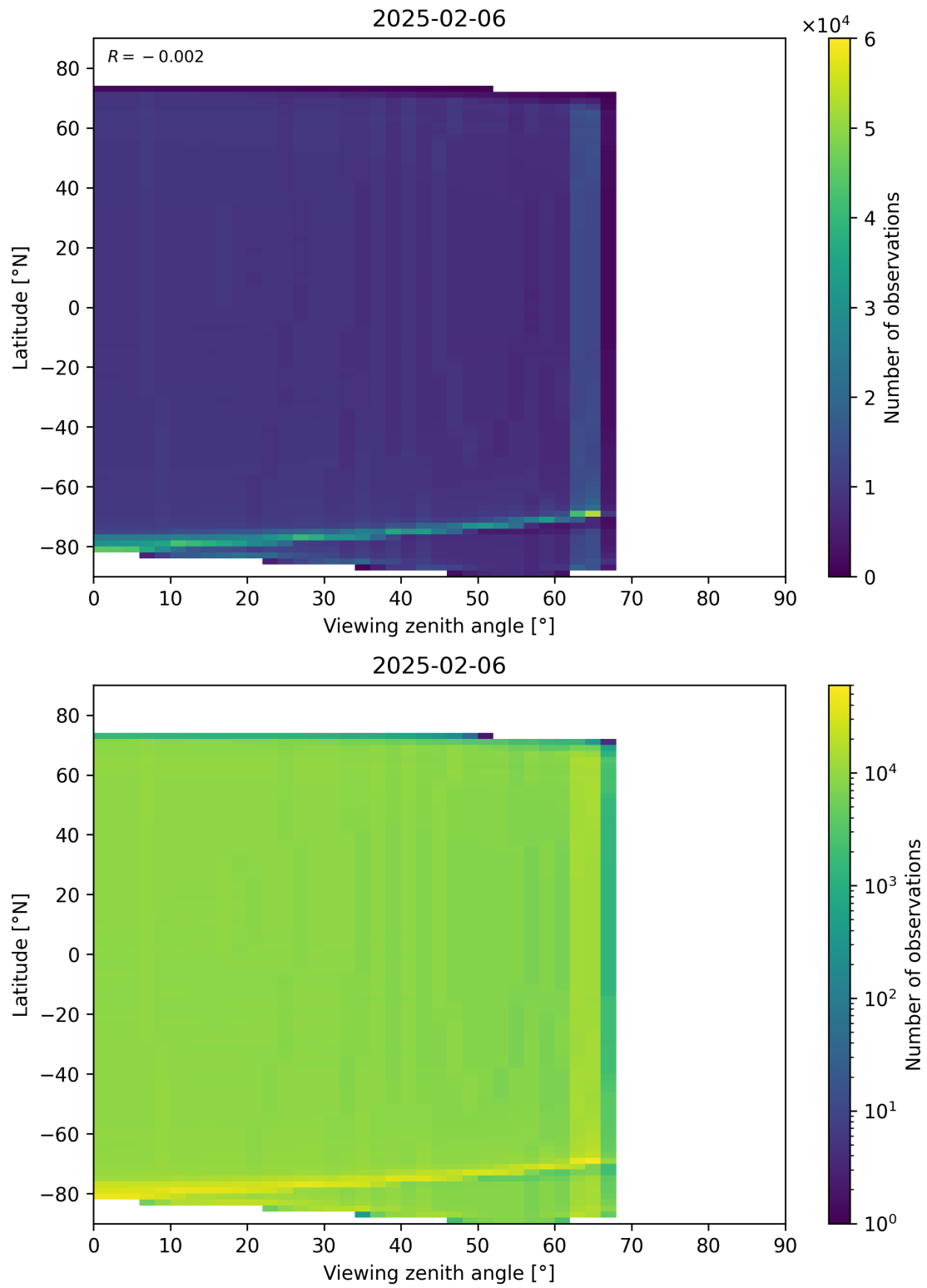
Figure 163: Scatter density plot of “Viewing zenith angle” against “Latitude” for 2025-02-05 to 2025-02-07.
