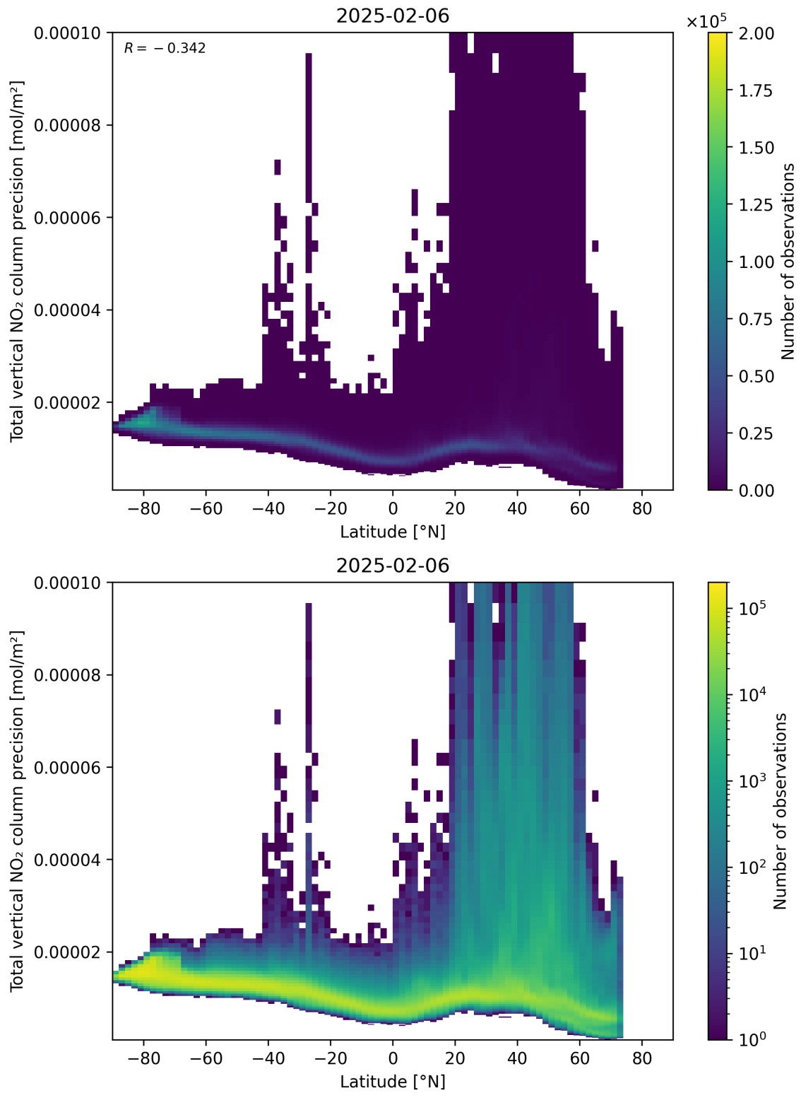
Figure 91: Scatter density plot of “Latitude” against “Total vertical NO 2 column precision” for 2025-02-05 to 2025-02-07.
