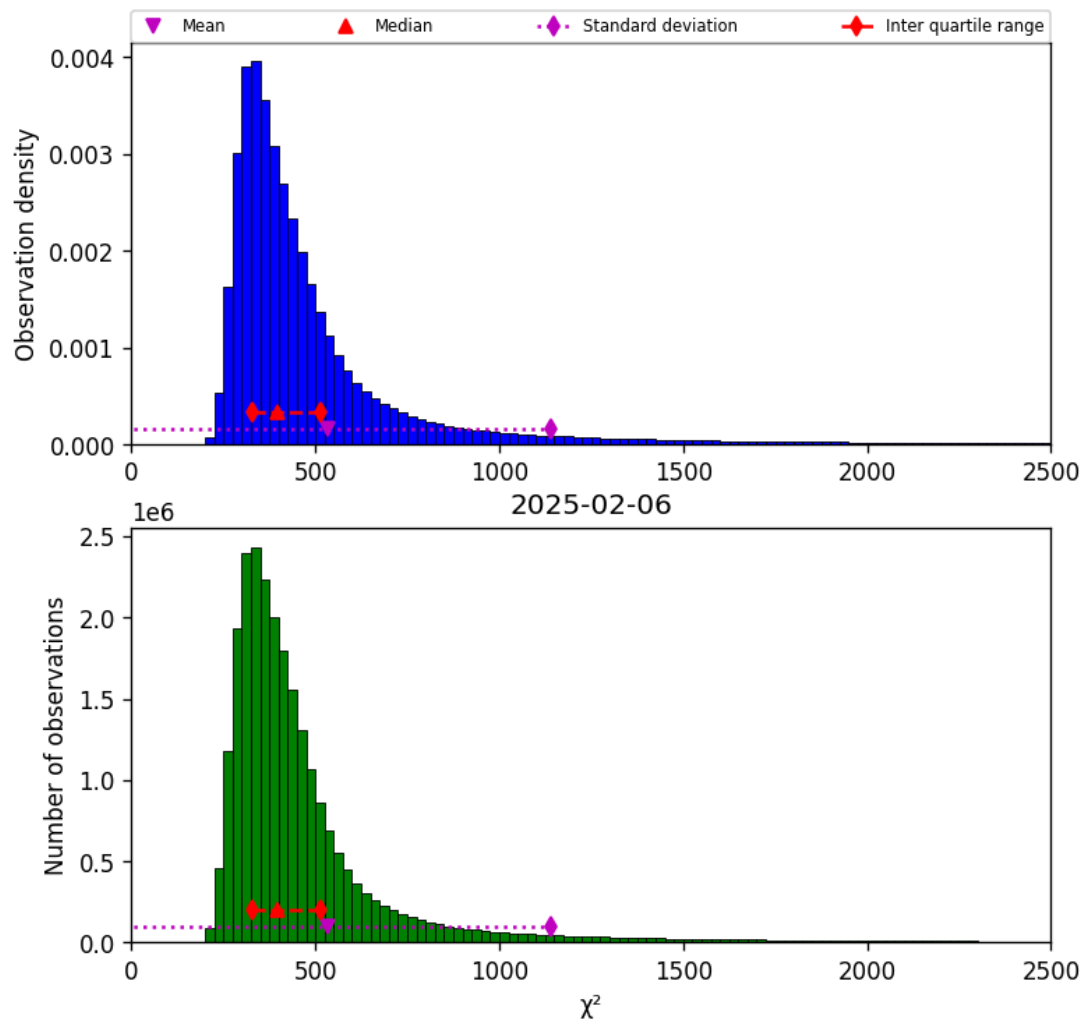
Figure 42: Histogram of “ \chi^2 ” for 2025-02-05 to 2025-02-07
