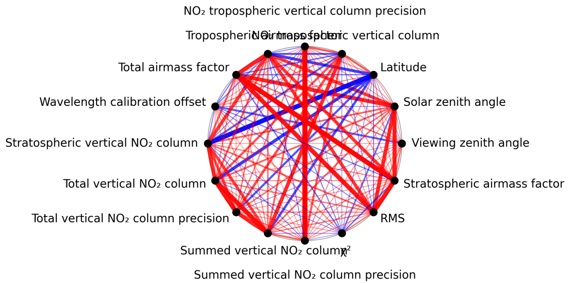
Figure 1: Map of correlation graph for 2025-02-05 to 2025-02-07.
