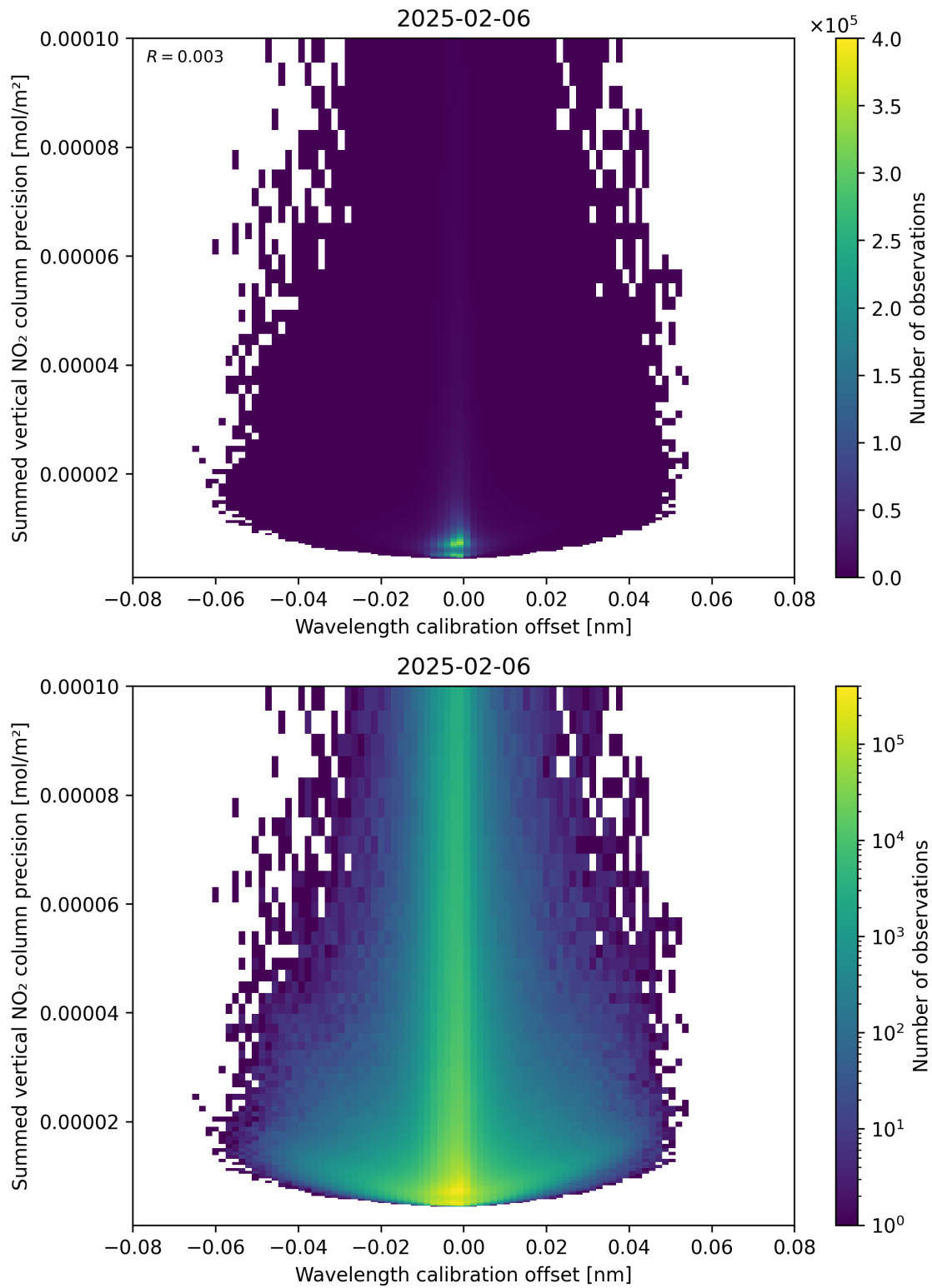
Figure 178: Scatter density plot of “Wavelength calibration offset” against “Summed vertical NO 2 column precision” for 2025-02-05 to 2025-02-07.
