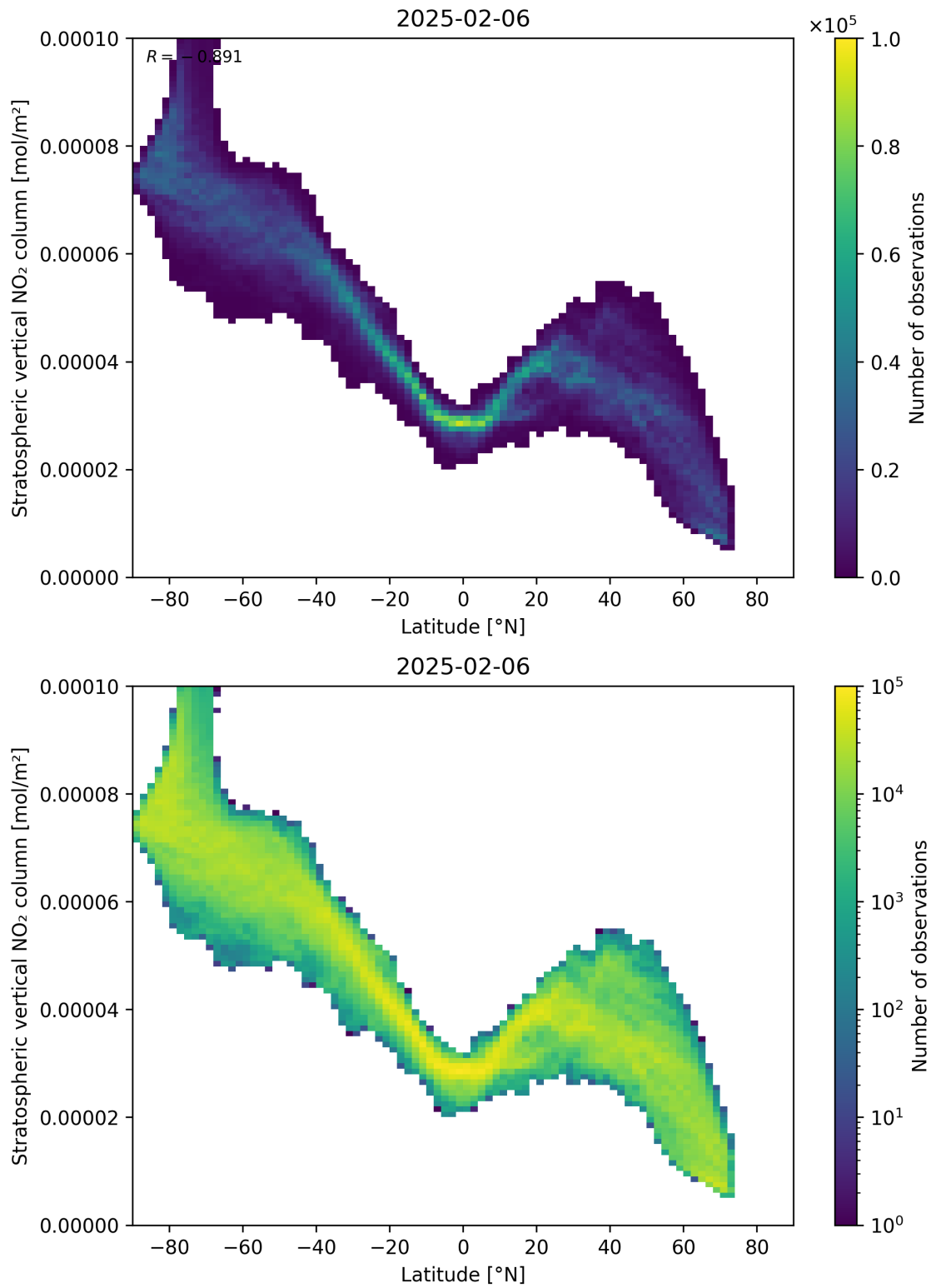
Figure 87: Scatter density plot of “Latitude” against “Stratospheric vertical NO 2 column” for 2025-02-05 to 2025-02-07.
