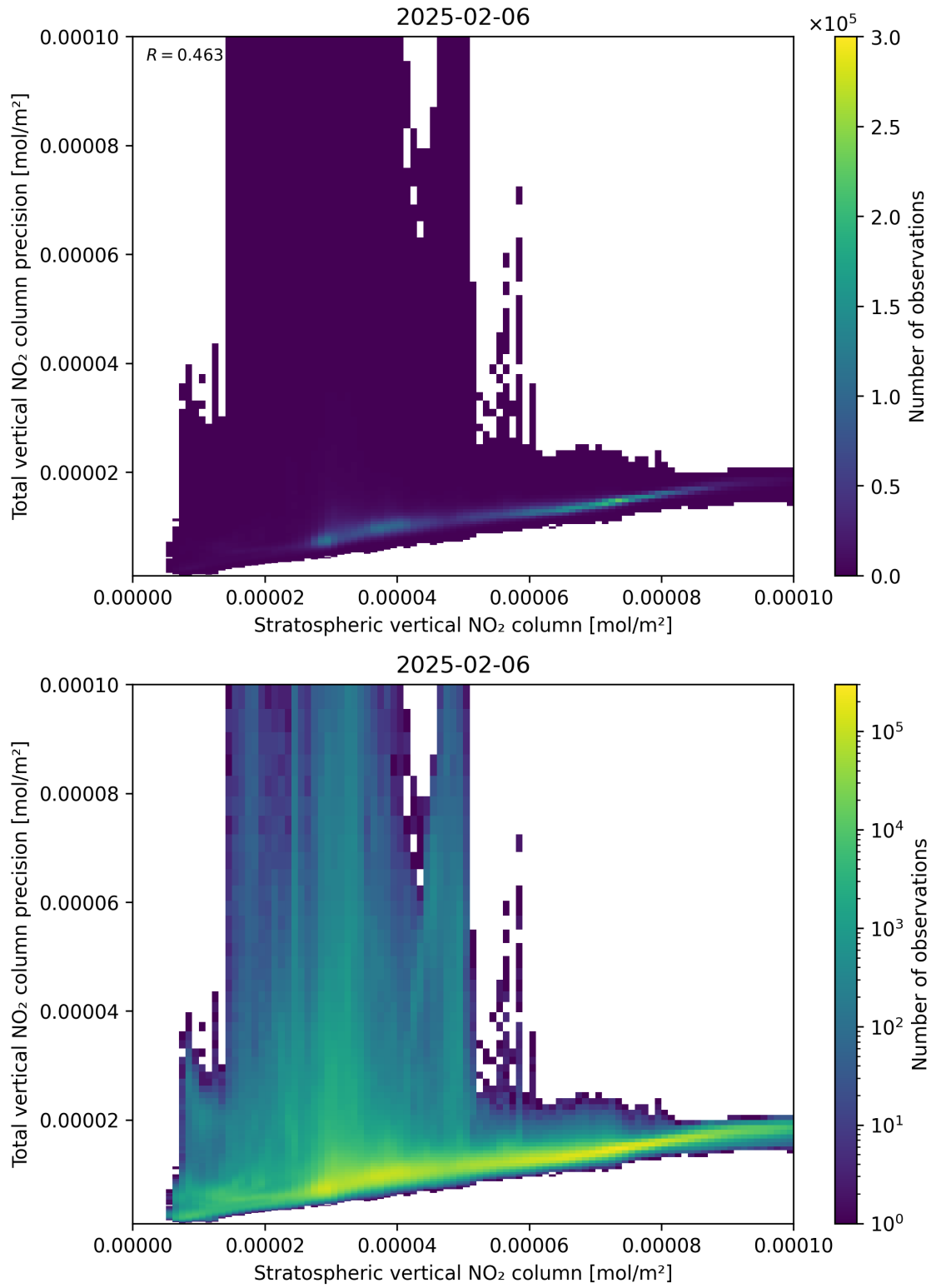
Figure 101: Scatter density plot of “Stratospheric vertical NO 2 column” against “Total vertical NO 2 column precision” for 2025-02-05 to 2025-02-07.
