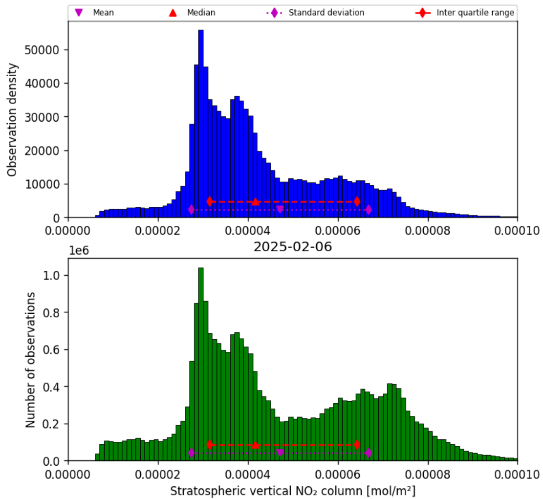
Figure 36: Histogram of “Stratospheric vertical NO 2 column” for 2025-02-05 to 2025-02-07
