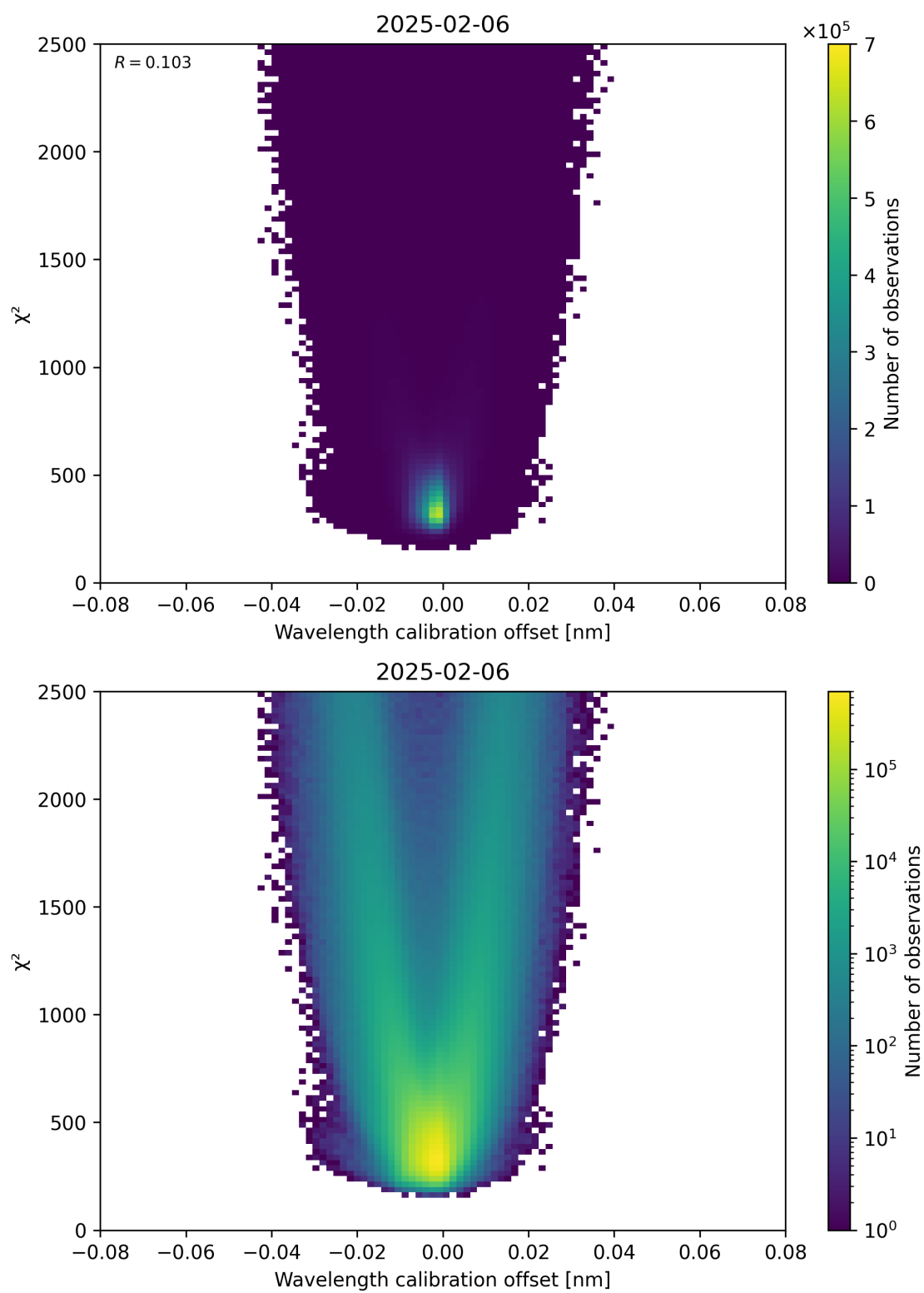
Figure 175: Scatter density plot of “Wavelength calibration offset” against “ \chi^2 ” for 2025-02-05 to 2025-02-07.
