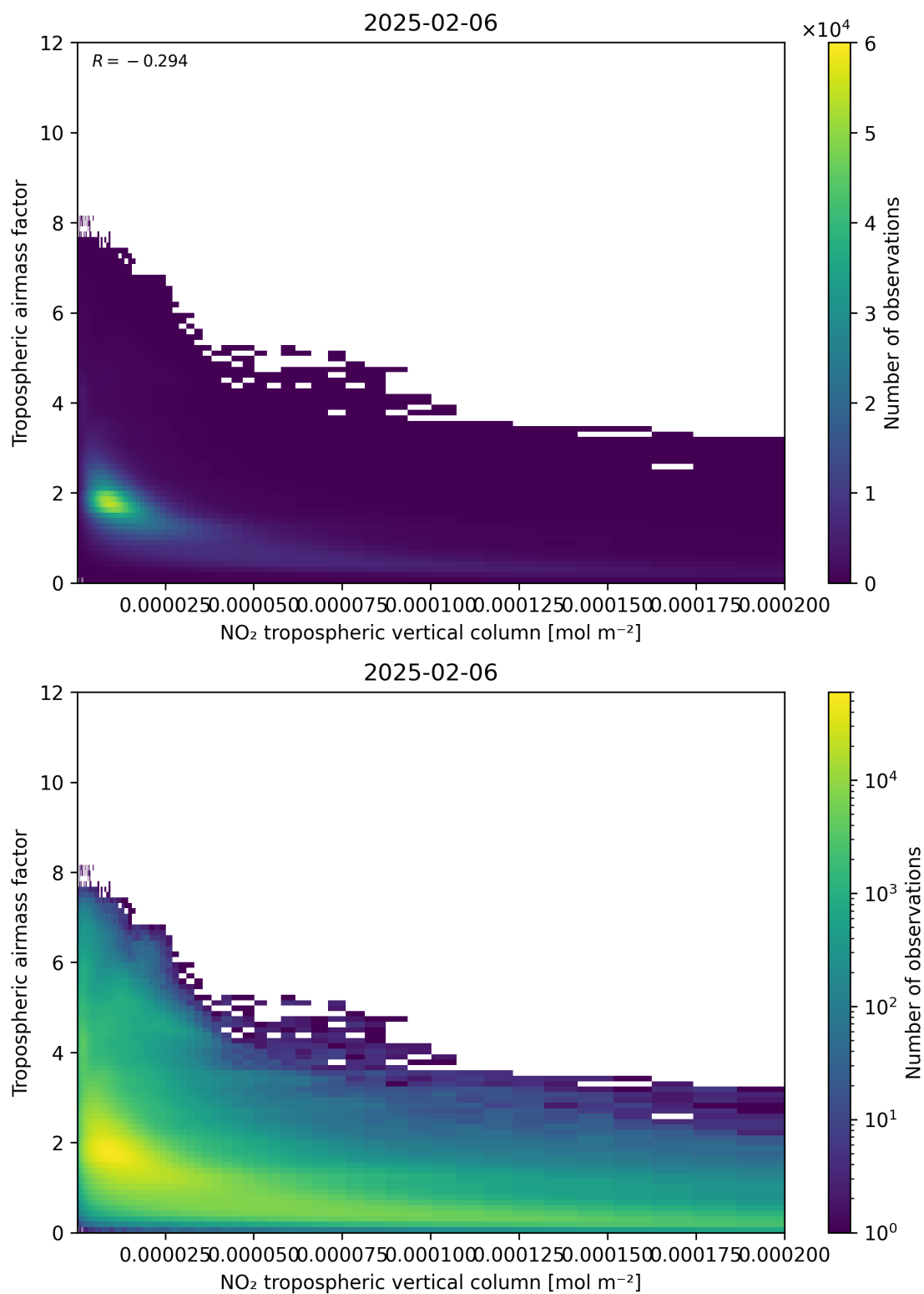
Figure 123: Scatter density plot of “NO 2 tropospheric vertical column” against “Tropospheric air mass factor” for 2025-02-05 to 2025-02-07.
