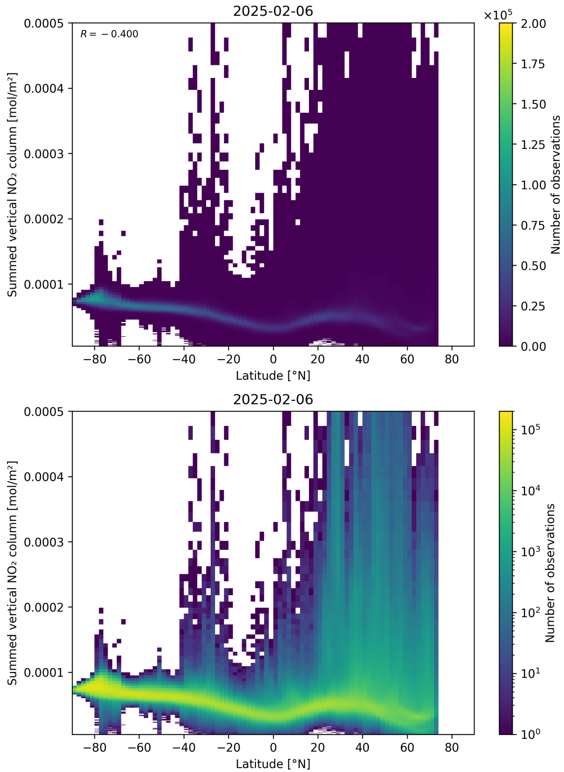
Figure 88: Scatter density plot of “Latitude” against “Summed vertical NO 2 column” for 2025-02-05 to 2025-02-07.
