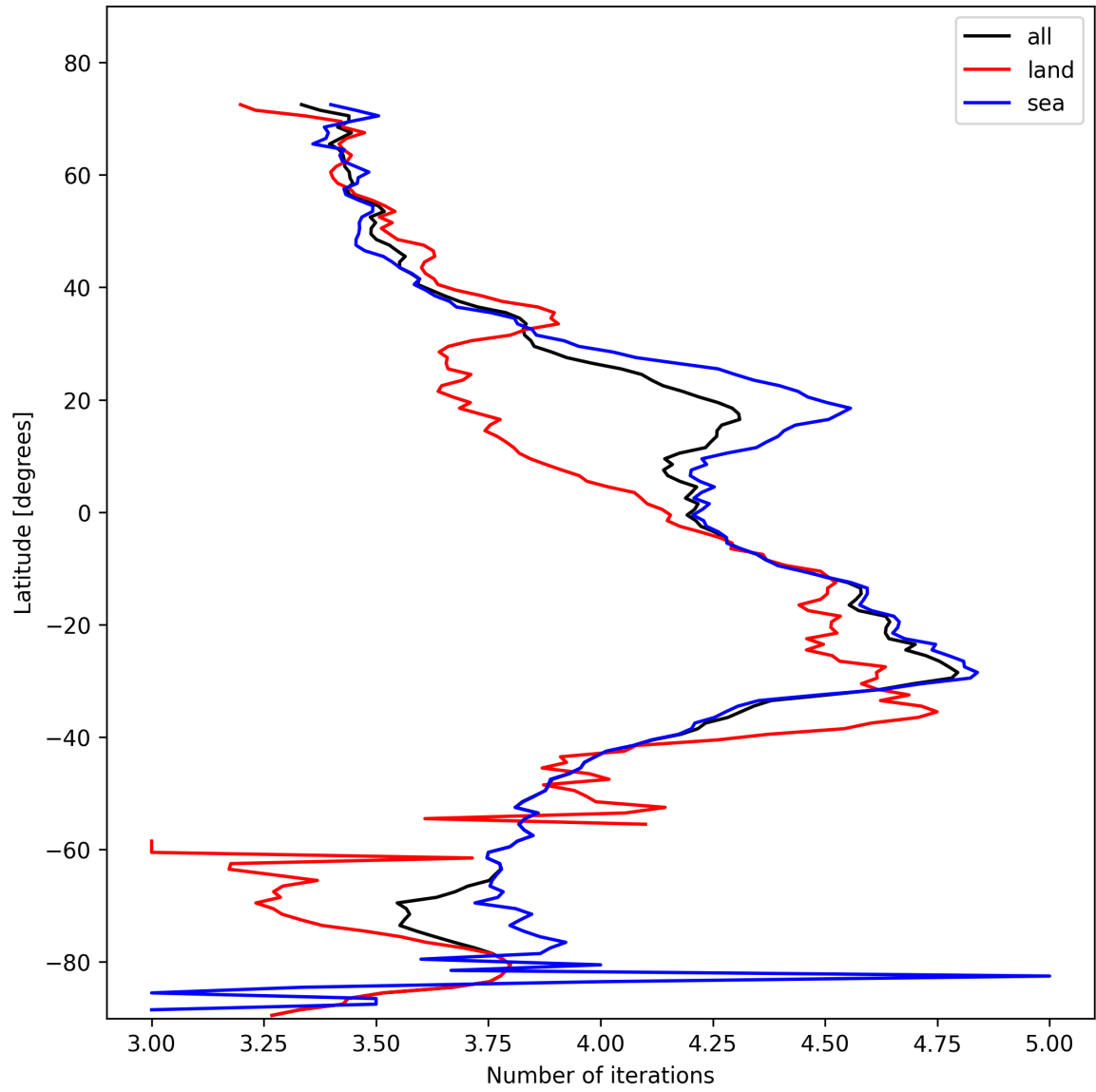
Figure 17: Zonal average of “Number of iterations” for 2025-02-05 to 2025-02-07.
