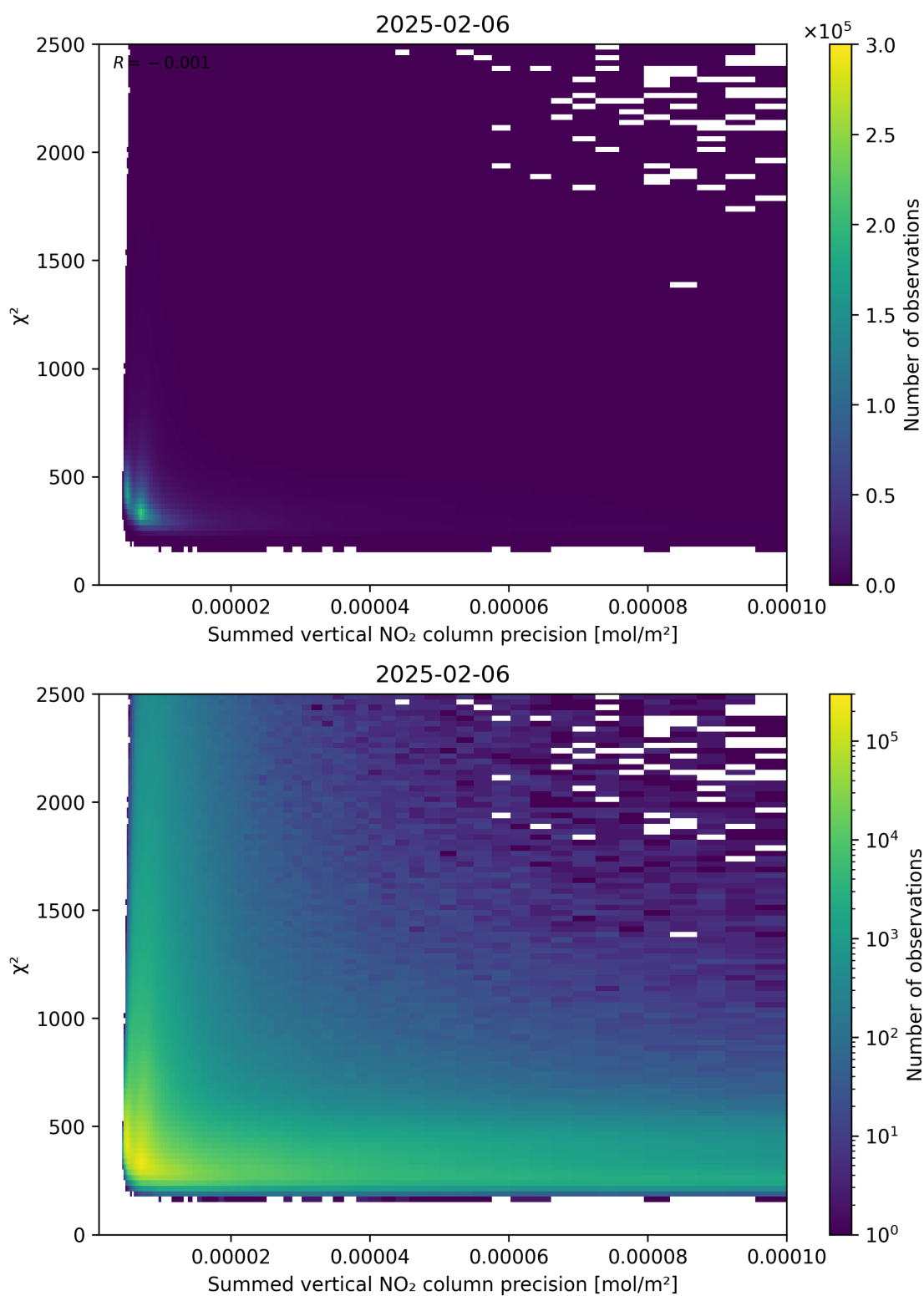
Figure 107: Scatter density plot of “Summed vertical NO 2 column precision” against “ \chi^2 ” for 2025-02-05 to 2025-02-07.
