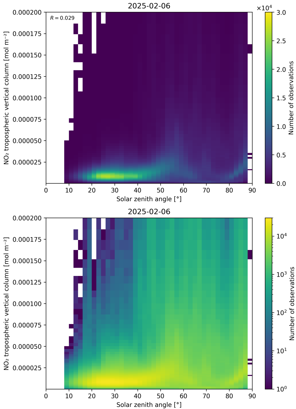
Figure 155: Scatter density plot of “Solar zenith angle” against “NO 2 tropospheric vertical column” for 2025-02-05 to 2025-02-07.
