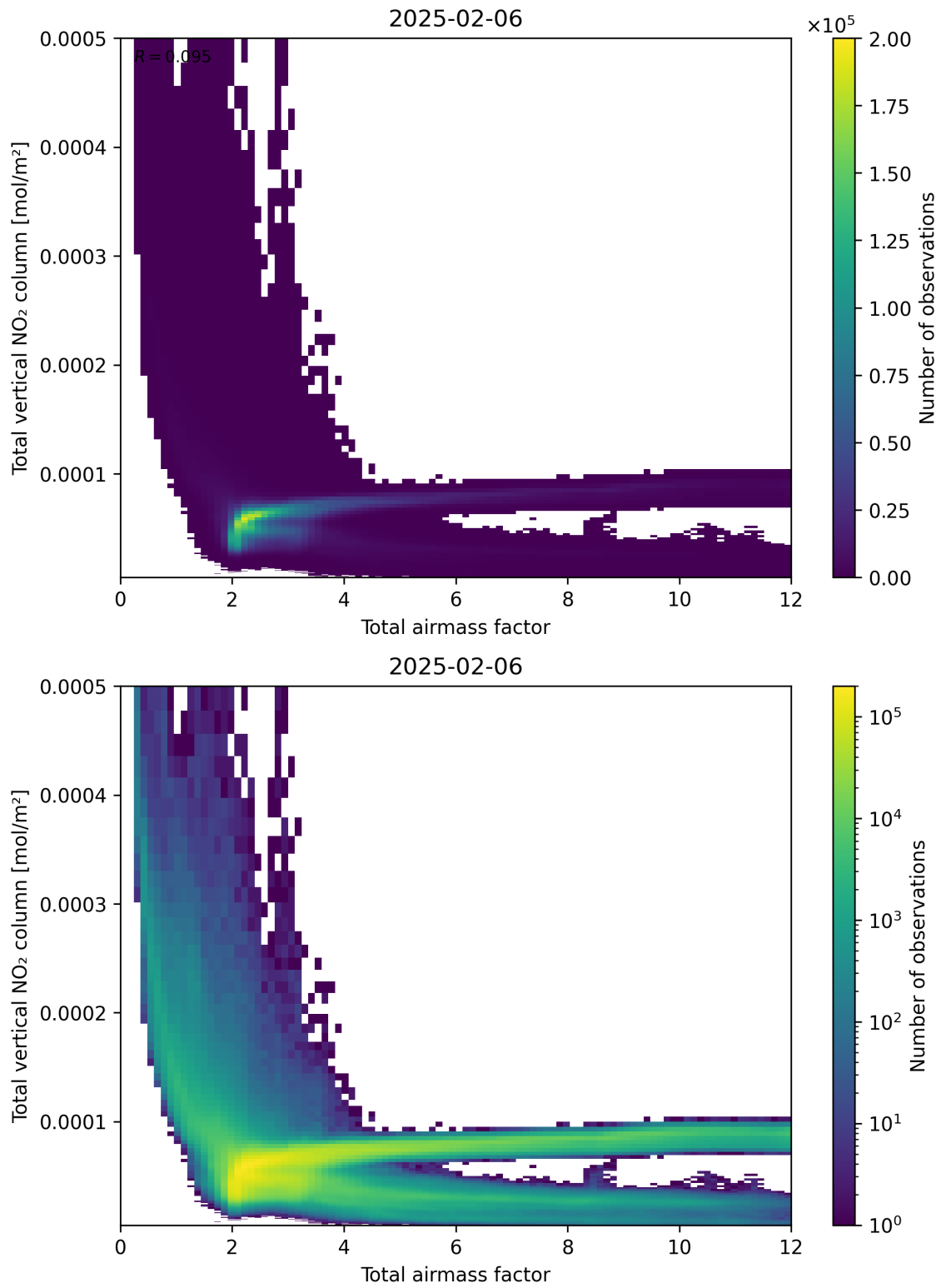
Figure 67: Scatter density plot of “Total airmass factor” against “Total vertical NO 2 column” for 2025-02-05 to 2025-02-07.
