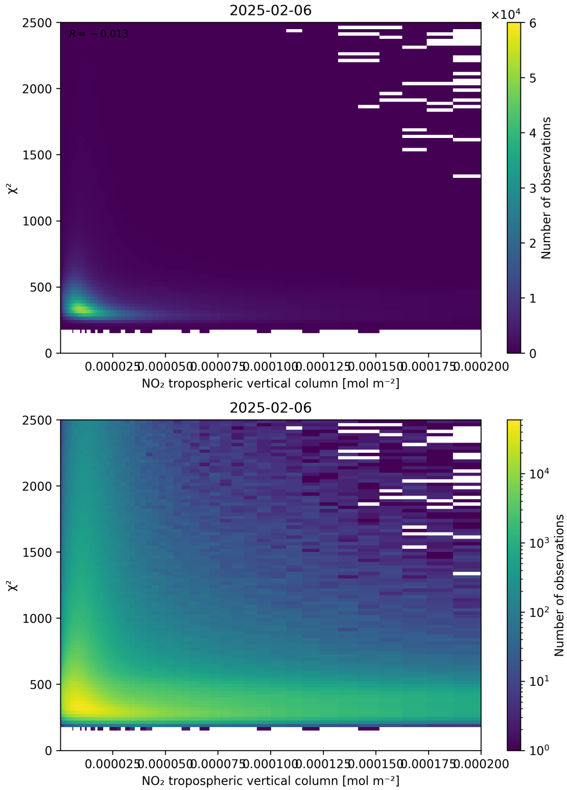
Figure 124: Scatter density plot of “NO 2 tropospheric vertical column” against “ \chi^2 ” for 2025-02-05 to 2025-02-07.
