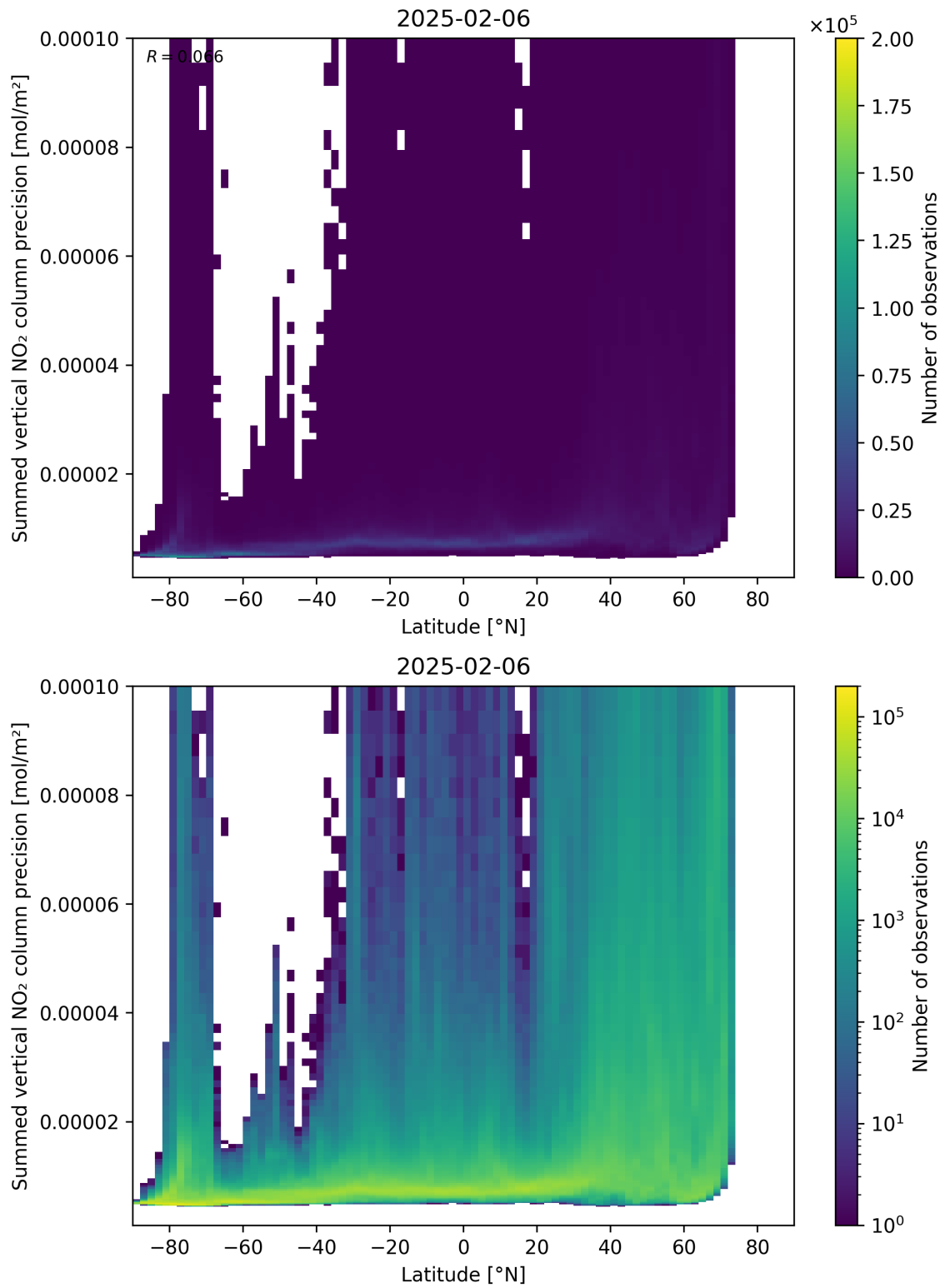
Figure 89: Scatter density plot of “Latitude” against “Summed vertical NO 2 column precision” for 2025-02-05 to 2025-02-07.
