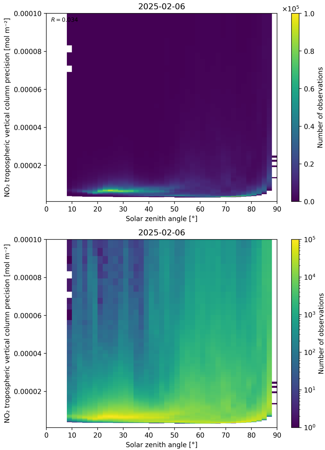
Figure 156: Scatter density plot of “Solar zenith angle” against “NO 2 tropospheric vertical column precision” for 2025-02-05 to 2025-02-07.
