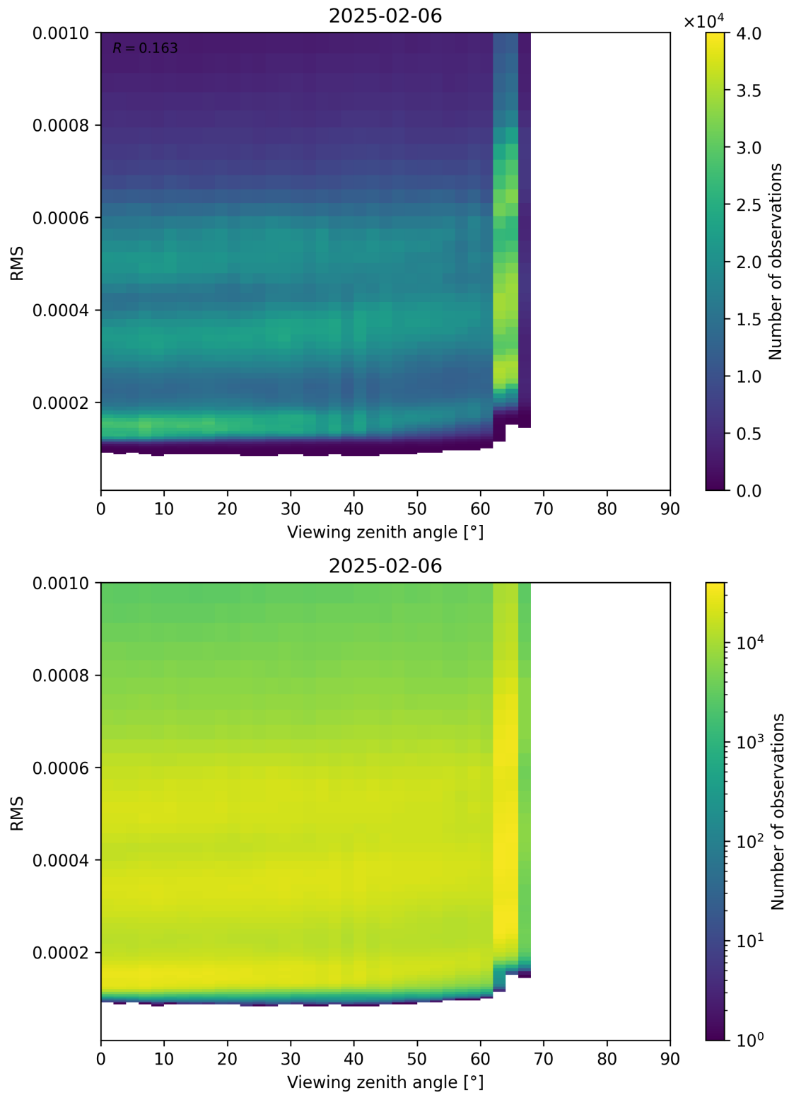
Figure 171: Scatter density plot of “Viewing zenith angle” against “RMS” for 2025-02-05 to 2025-02-07.
