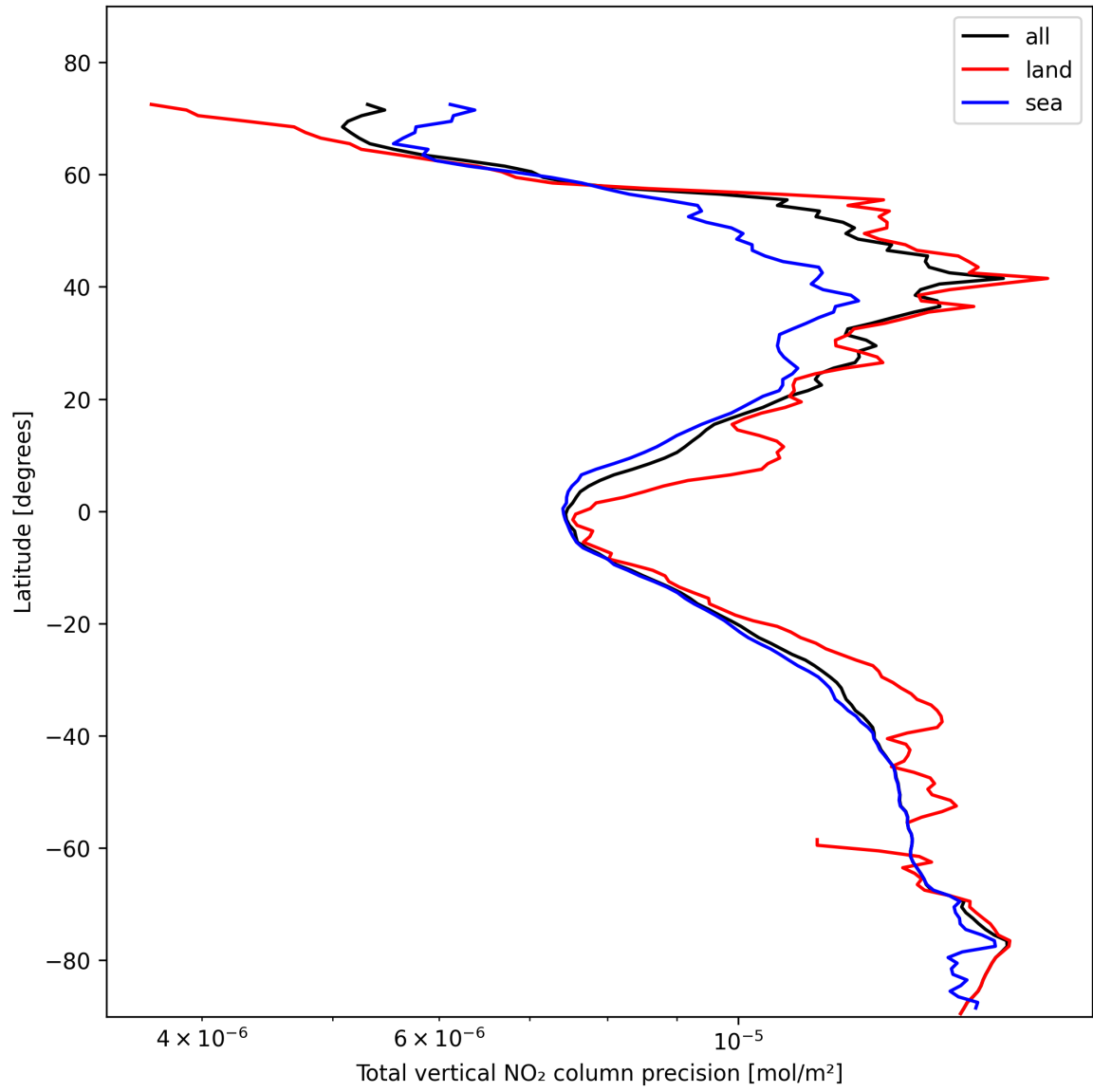
Figure 22: Zonal average of “Total vertical NO 2 column precision” for 2025-02-05 to 2025-02-07.
