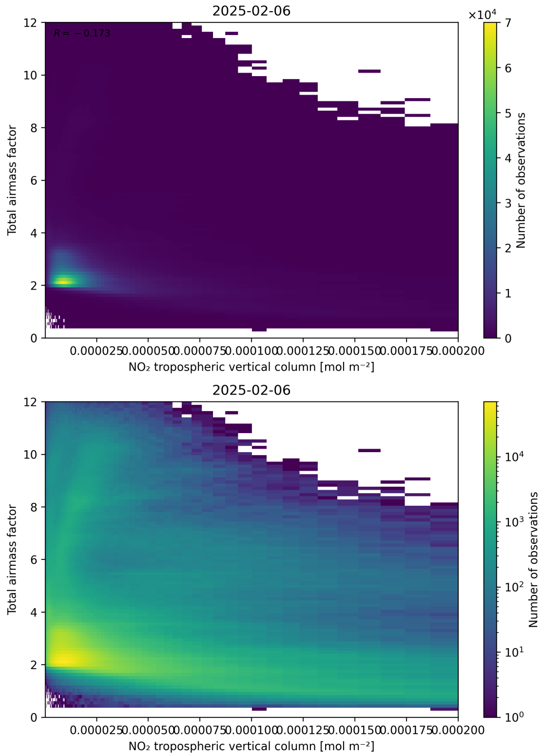
Figure 122: Scatter density plot of “NO 2 tropospheric vertical column” against “Total air mass factor” for 2025-02-05 to 2025-02-07.
