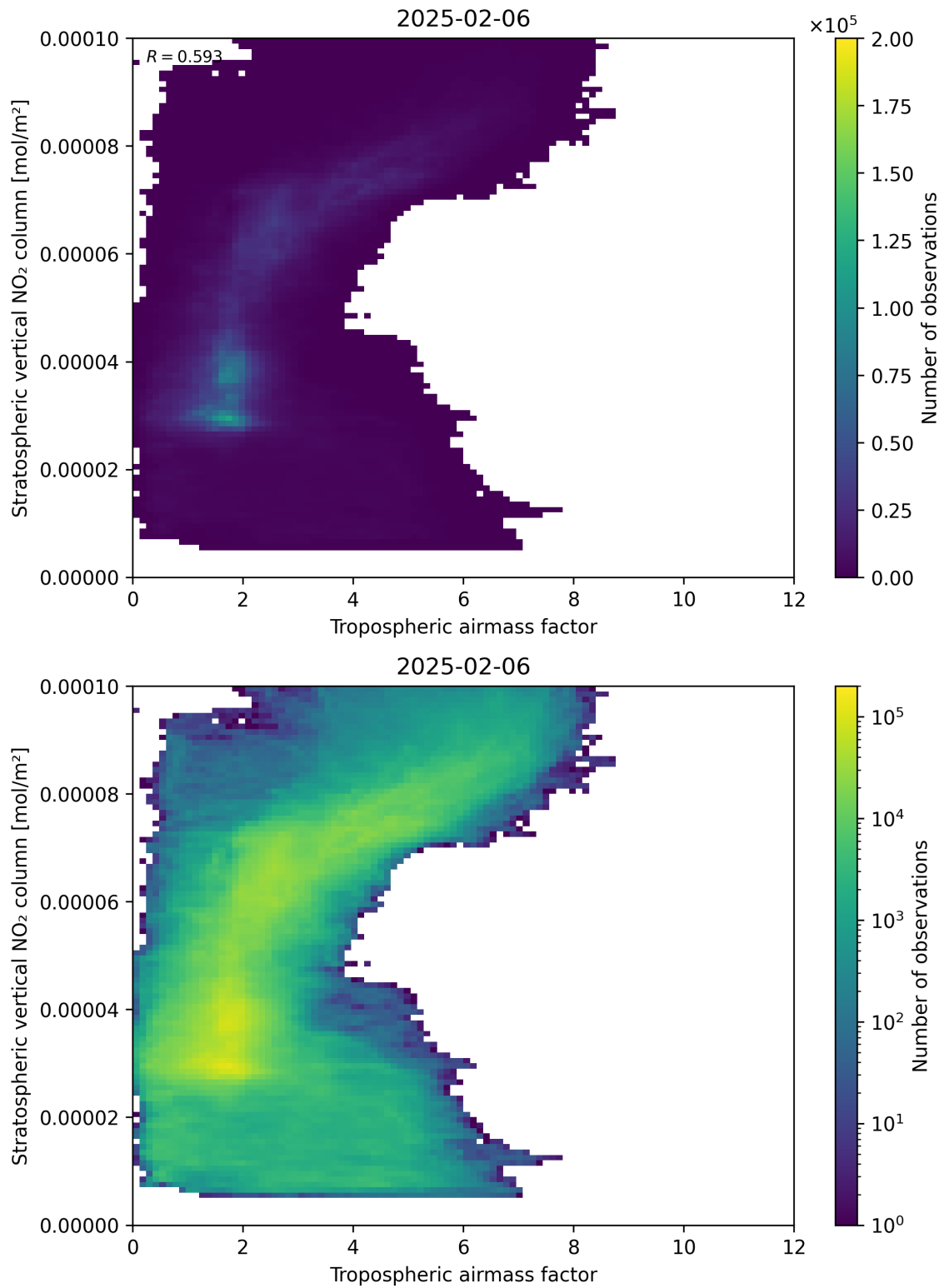
Figure 74: Scatter density plot of “Tropospheric air mass factor” against “Stratospheric vertical NO 2 column” for 2025-02-05 to 2025-02-07.
