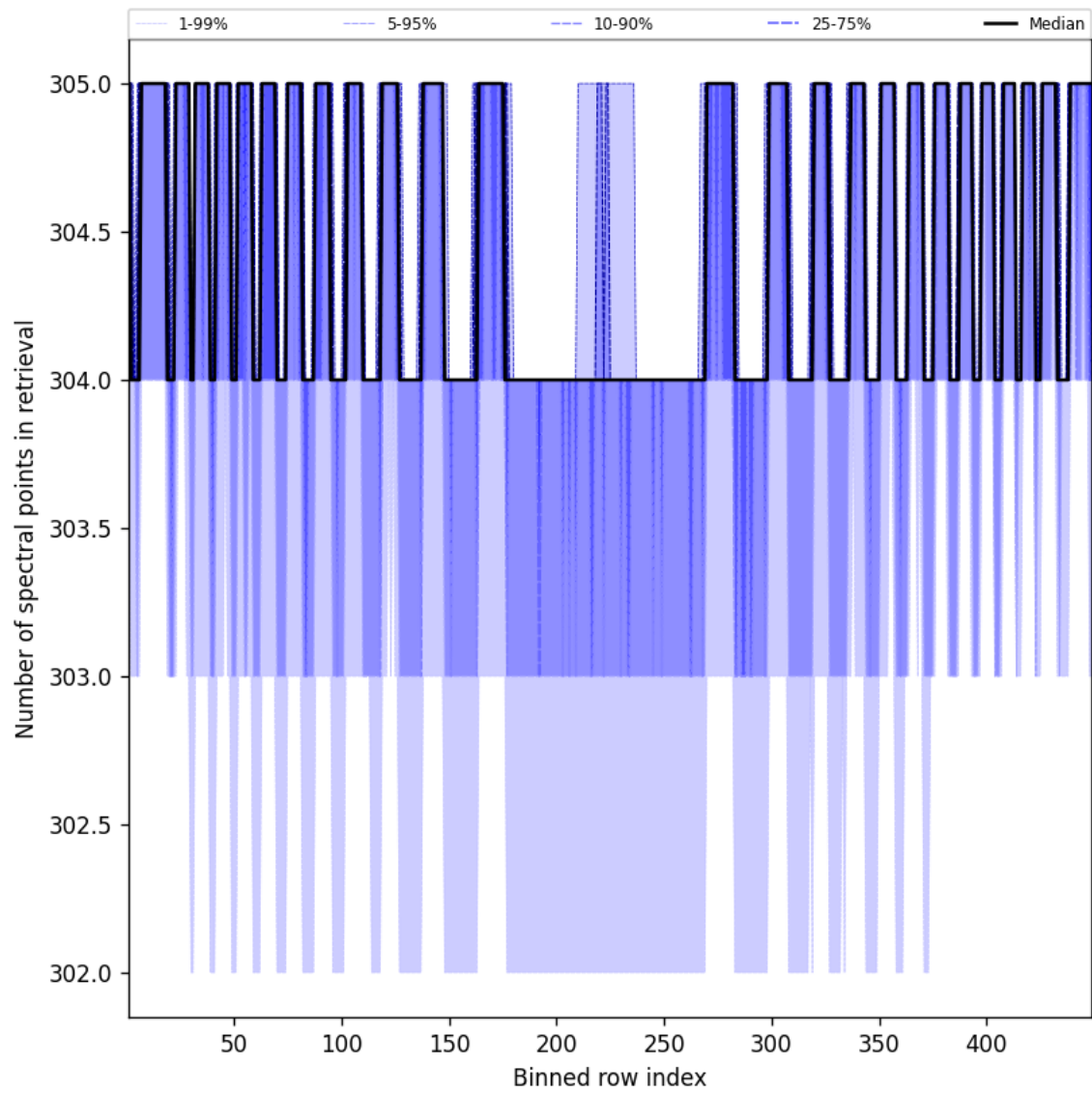
Figure 50: Along track statistics of “Number of spectral points in retrieval” for 2025-02-05 to 2025-02-07
