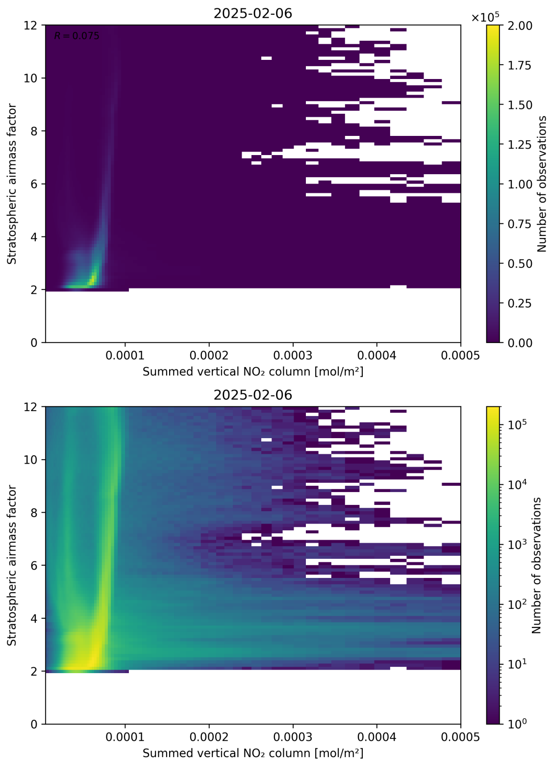
Figure 103: Scatter density plot of “Summed vertical NO 2 column” against “Stratospheric air mass factor” for 2025-02-05 to 2025-02-07.
