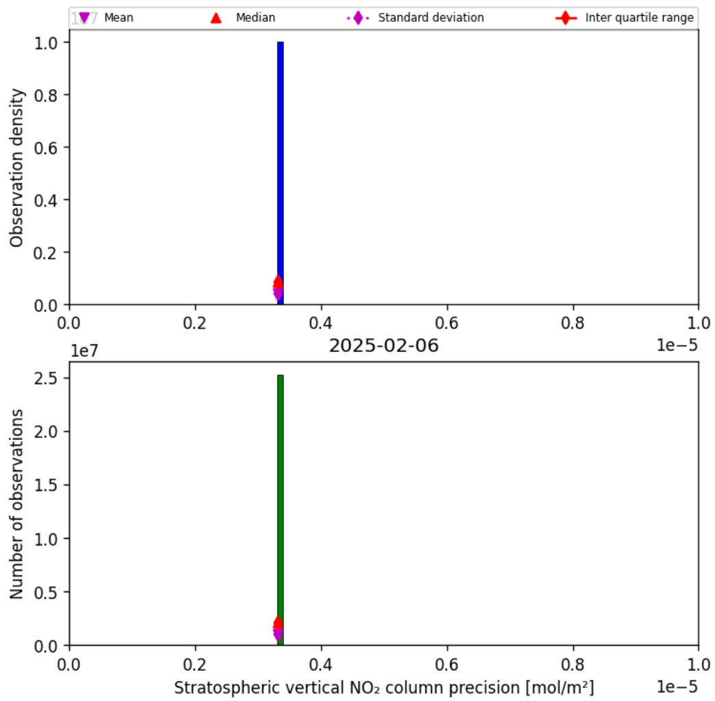
Figure 37: Histogram of “Stratospheric vertical NO 2 column precision” for 2025-02-05 to 2025-02-07
