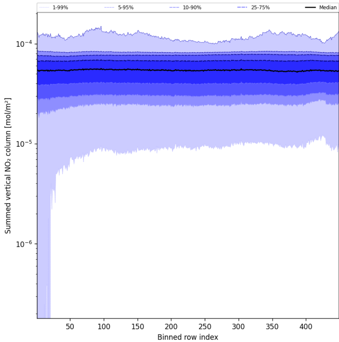
Figure 57: Along track statistics of “Summed vertical NO 2 column” for 2025-02-05 to 2025-02-07
