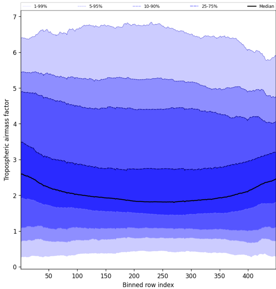
Figure 48: Along track statistics of "Tropospheric airmass factor" for 2025-02-05 to 2025-02-07
