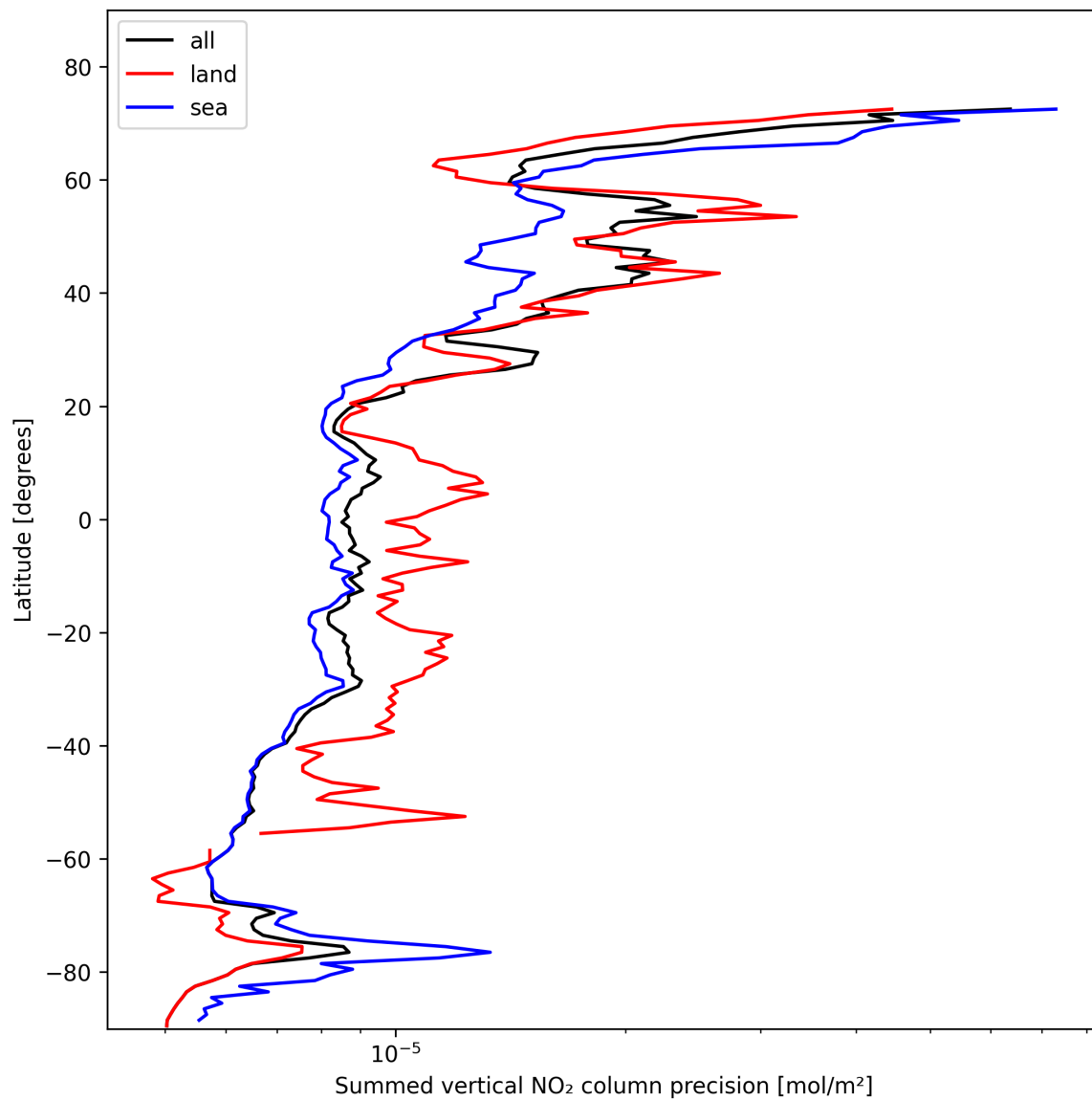
Figure 24: Zonal average of “Summed vertical NO 2 column precision” for 2025-02-05 to 2025-02-07.
