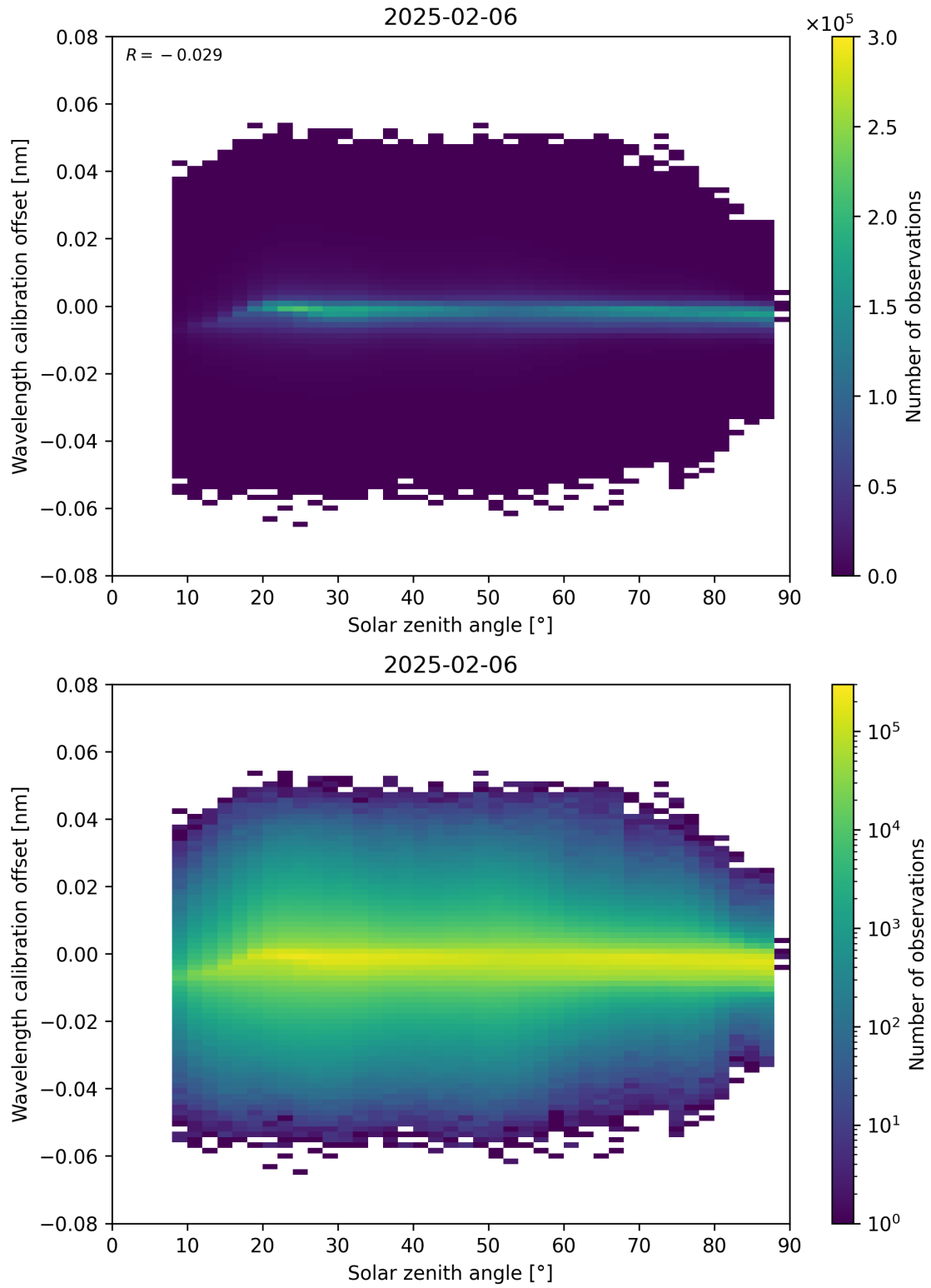
Figure 158: Scatter density plot of “Solar zenith angle” against “Wavelength calibration offset” for 2025-02-05 to 2025-02-07.
