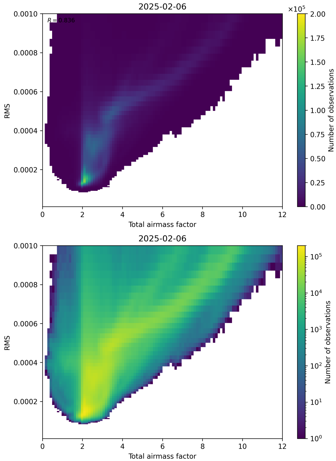
Figure 69: Scatter density plot of “Total airmass factor” against “RMS” for 2025-02-05 to 2025-02-07.
