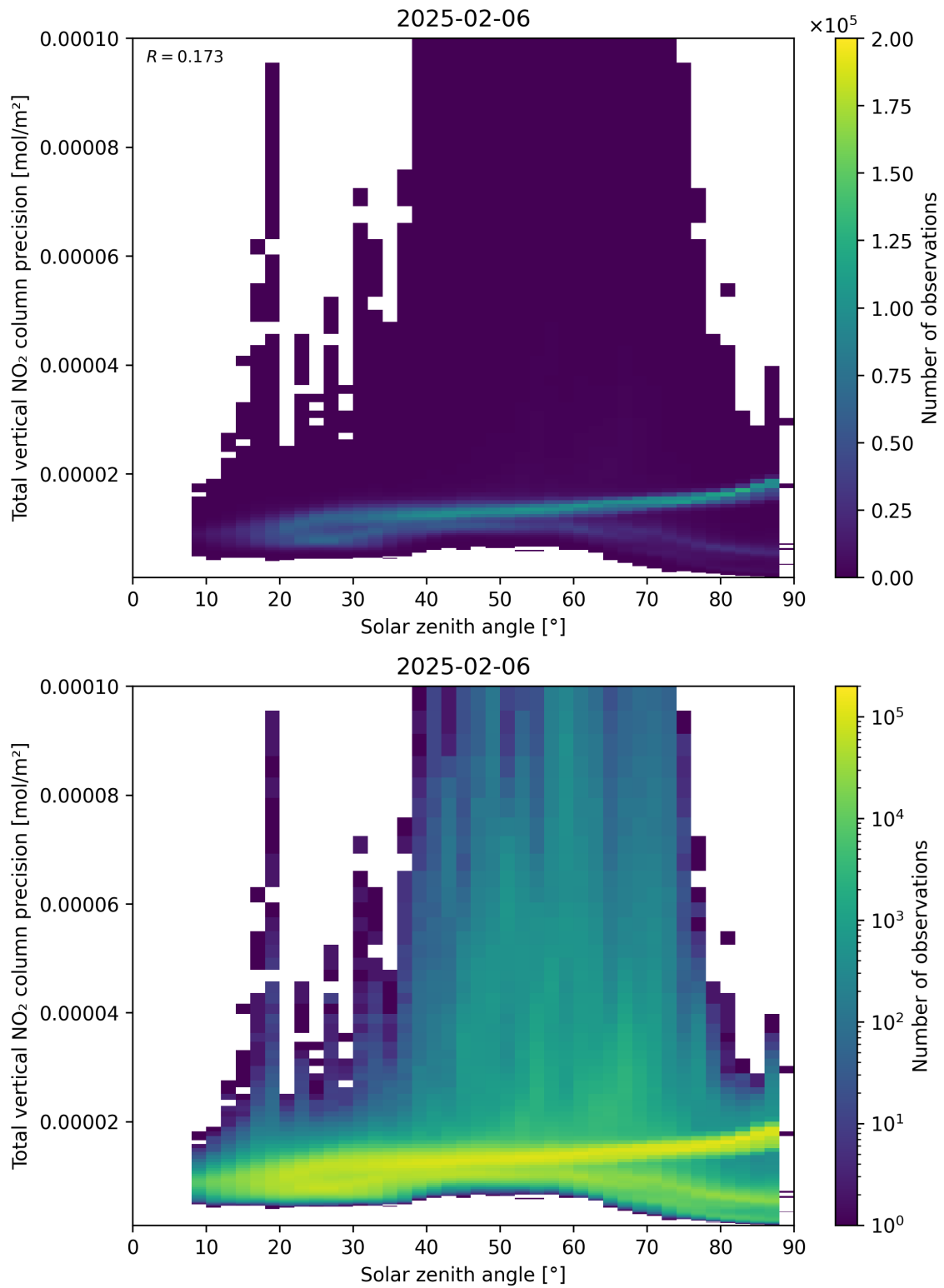
Figure 154: Scatter density plot of “Solar zenith angle” against “Total vertical NO 2 column precision” for 2025-02-05 to 2025-02-07.
