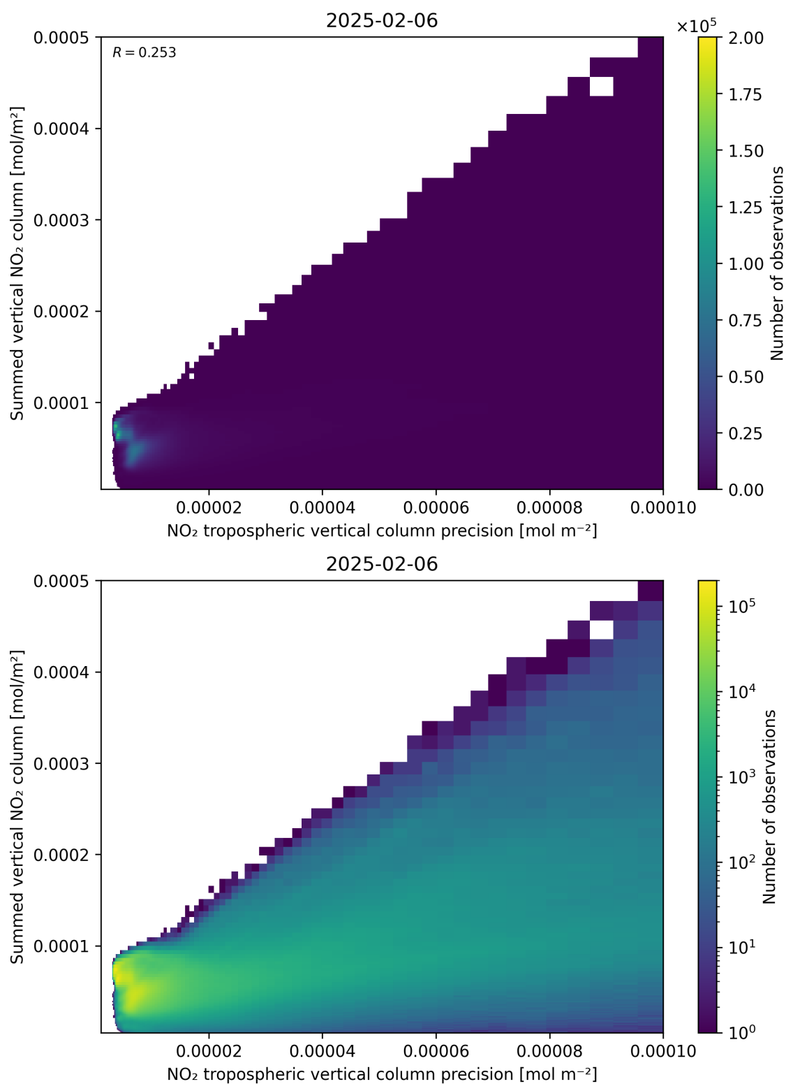
Figure 136: Scatter density plot of “NO 2 tropospheric vertical column precision” against “Summed vertical NO 2 column” for 2025-02-05 to 2025-02-07.
