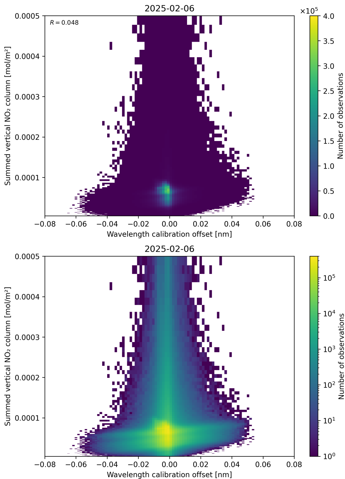
Figure 177: Scatter density plot of “Wavelength calibration offset” against “Summed vertical NO 2 column” for 2025-02-05 to 2025-02-07.
