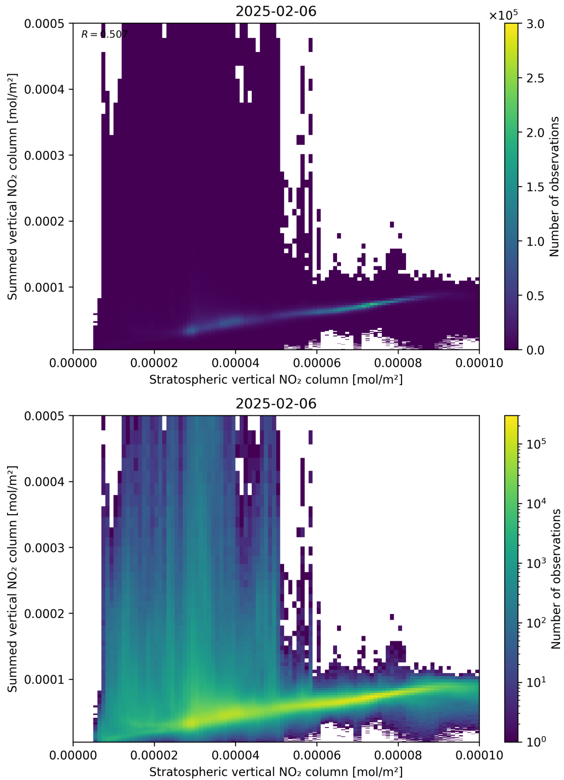
Figure 98: Scatter density plot of “Stratospheric vertical NO 2 column” against “Summed vertical NO 2 column” for 2025-02-05 to 2025-02-07.
