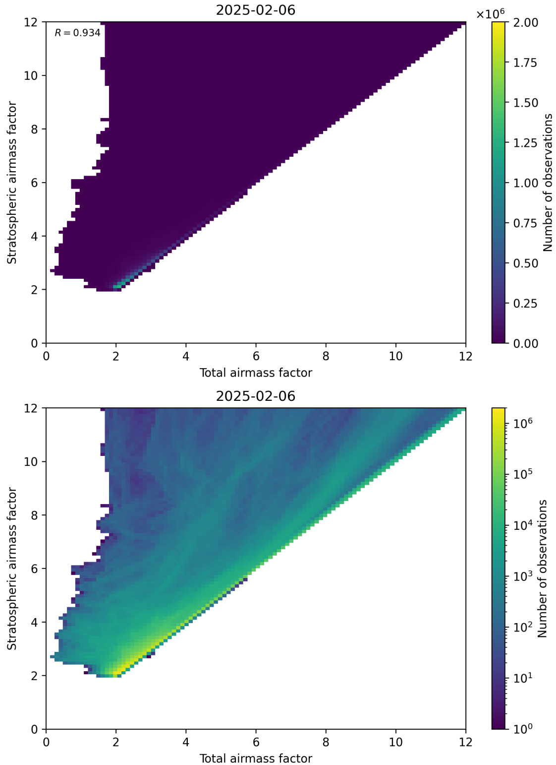
Figure 62: Scatter density plot of “Total airmass factor” against “Stratospheric airmass factor” for 2025-02-05 to 2025-02-07.
