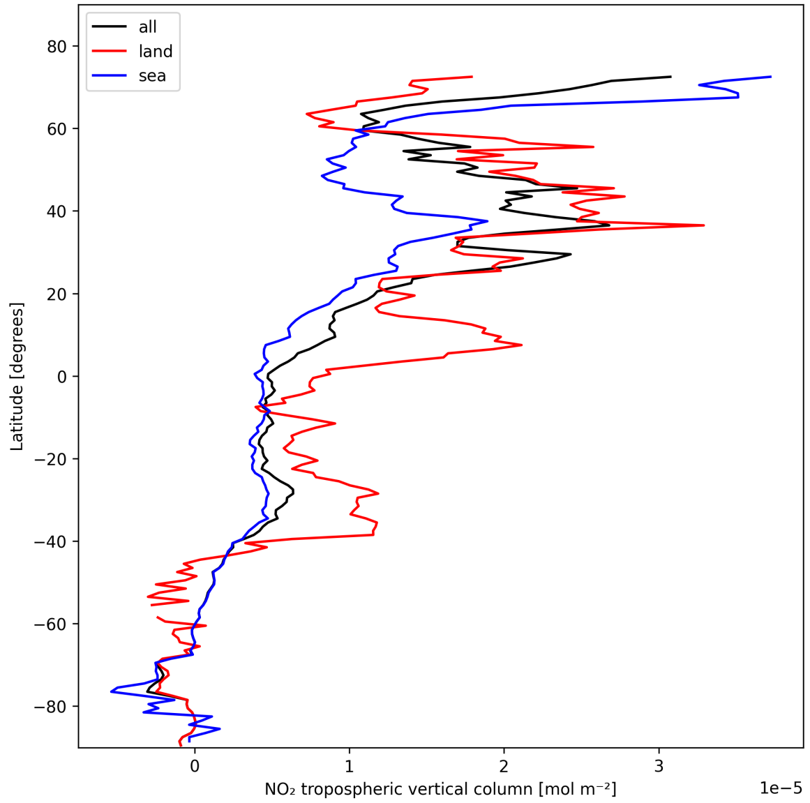
Figure 12: Zonal average of “NO 2 tropospheric vertical column” for 2025-02-05 to 2025-02-07.
