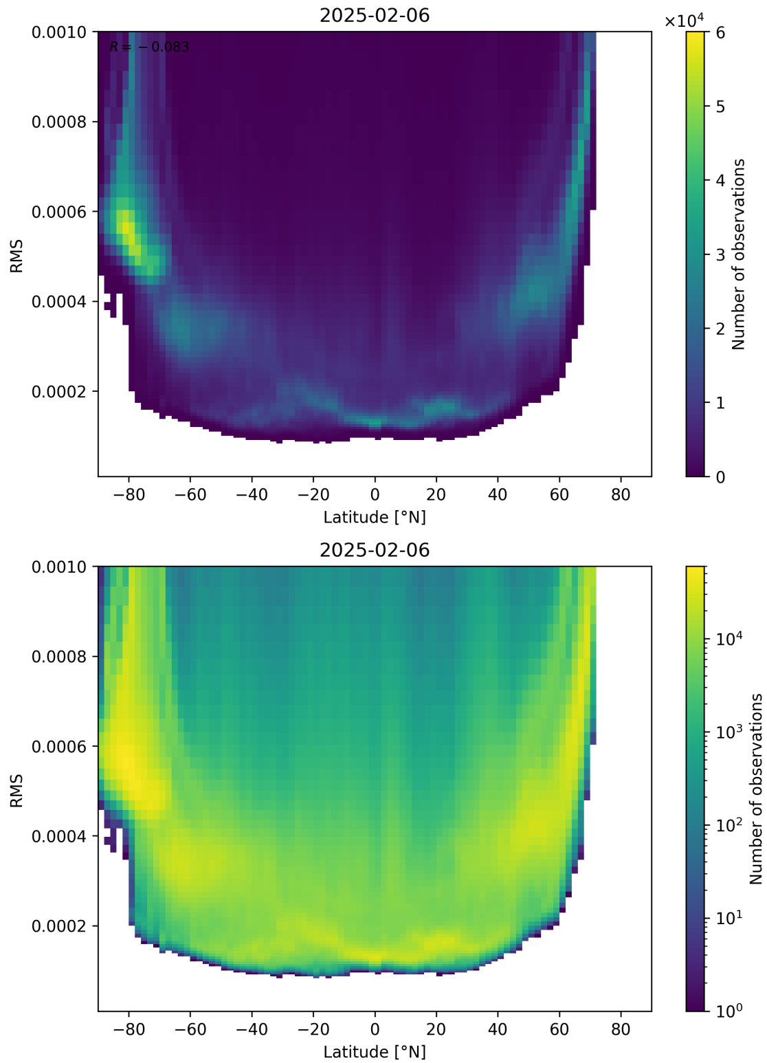
Figure 94: Scatter density plot of “Latitude” against “RMS” for 2025-02-05 to 2025-02-07.
