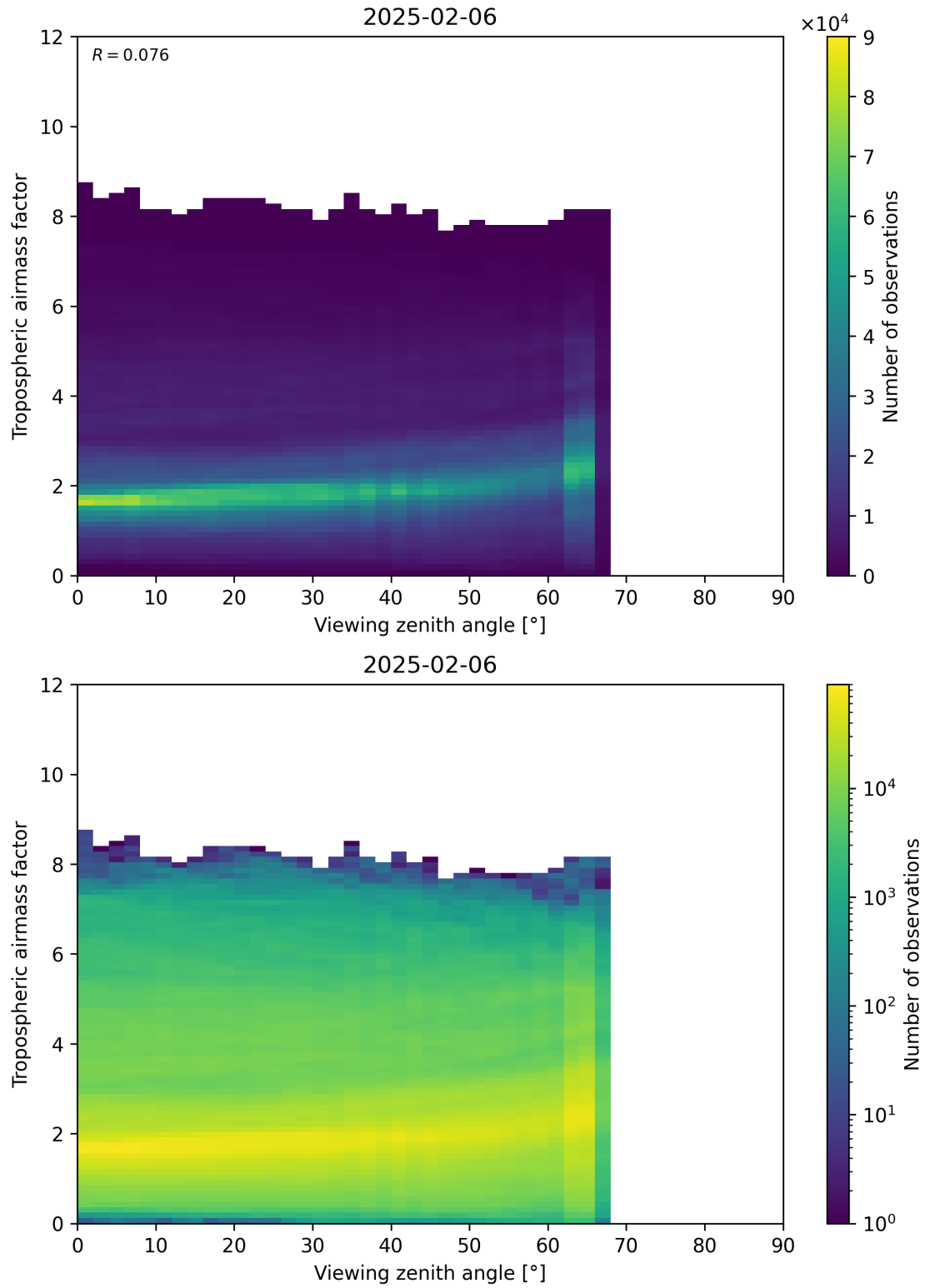
Figure 161: Scatter density plot of “Viewing zenith angle” against “Tropospheric airmass factor” for 2025-02-05 to 2025-02-07.
