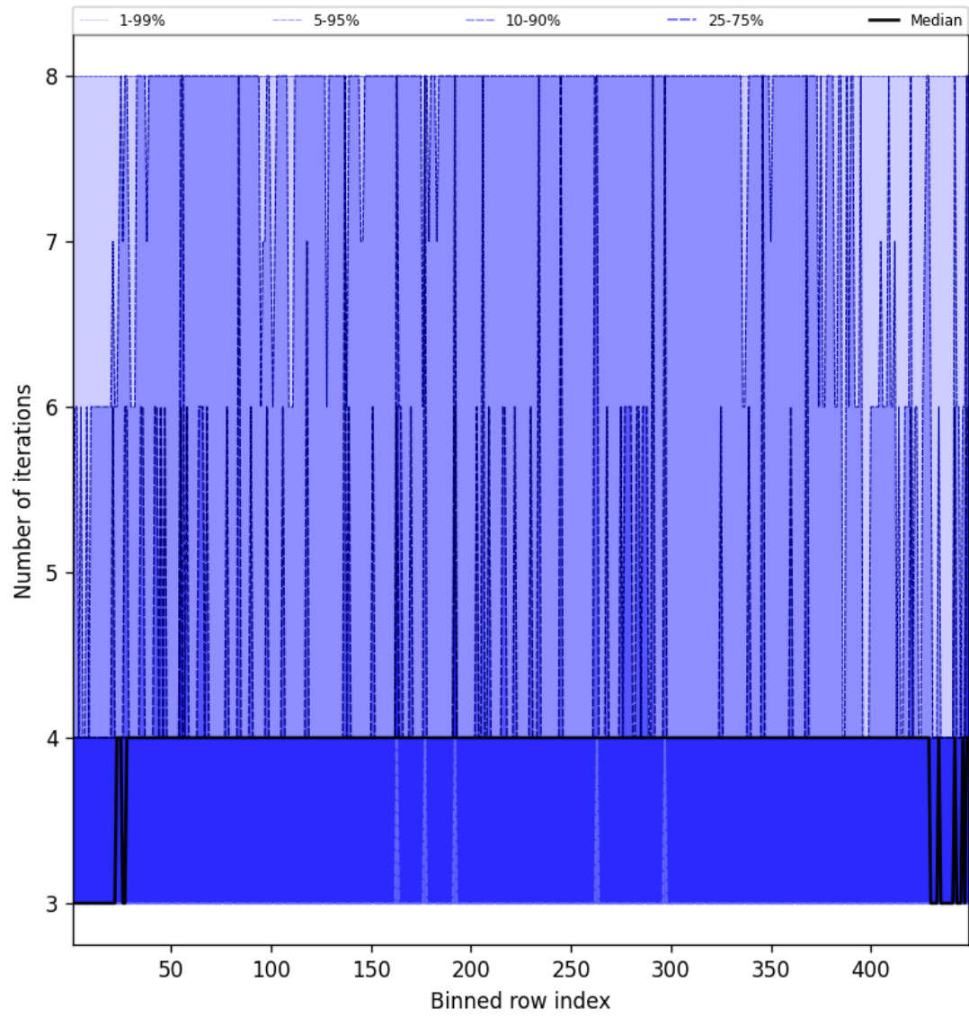
Figure 51: Along track statistics of “Number of iterations” for 2025-02-05 to 2025-02-07
