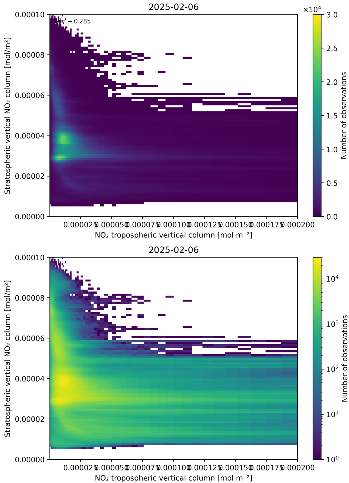
Figure 125: Scatter density plot of “NO 2 tropospheric vertical column” against “Stratospheric vertical NO 2 column” for 2025-02-05 to 2025-02-07.
