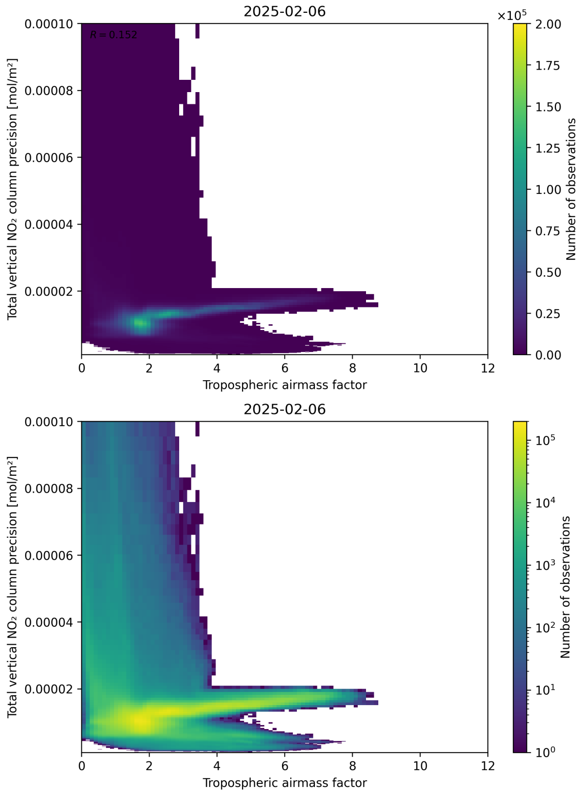
Figure 78: Scatter density plot of “Tropospheric air mass factor” against “Total vertical NO 2 column precision” for 2025-02-05 to 2025-02-07.
