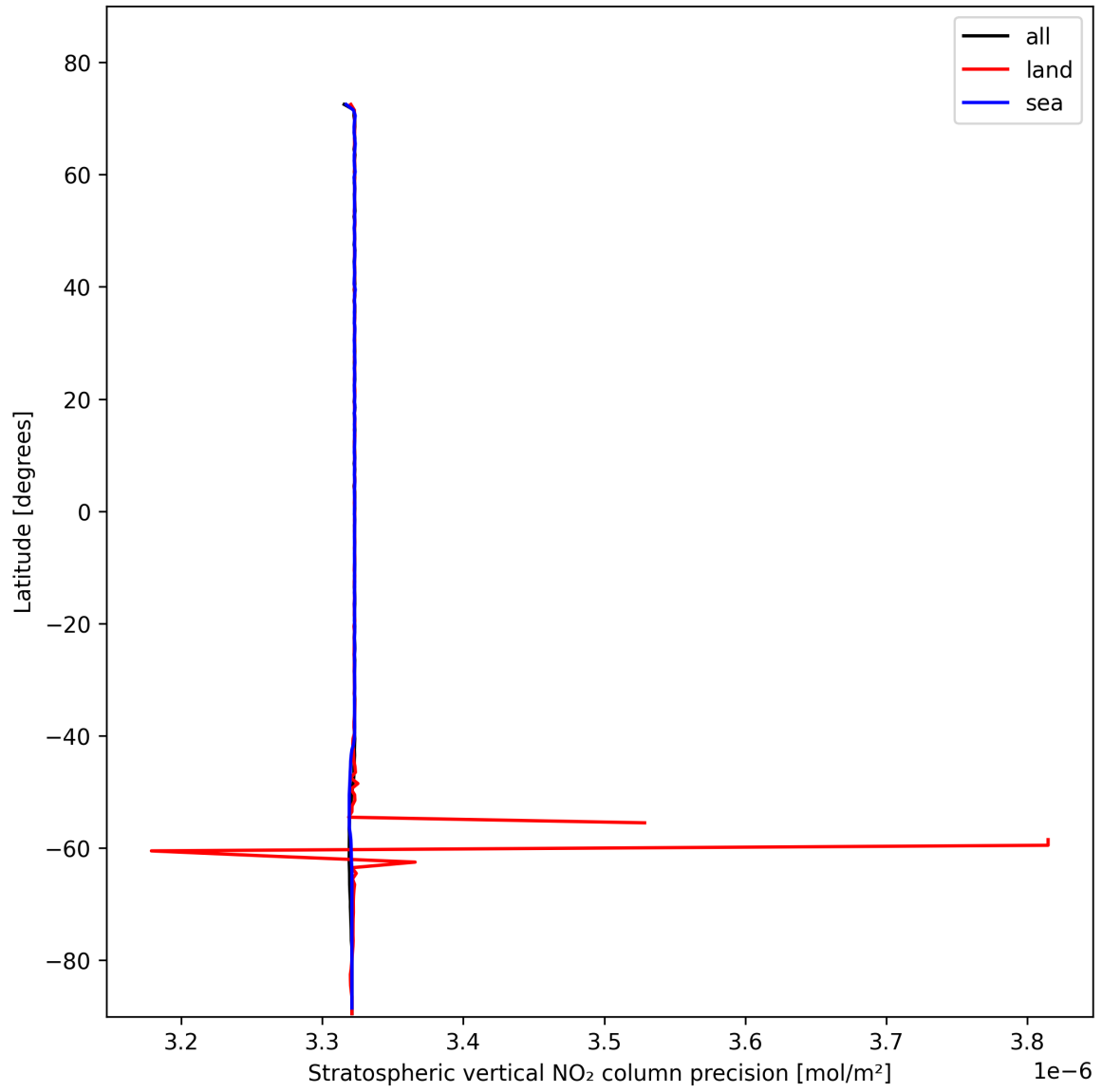
Figure 20: Zonal average of “Stratospheric vertical NO 2 column precision” for 2025-02-05 to 2025-02-07.
