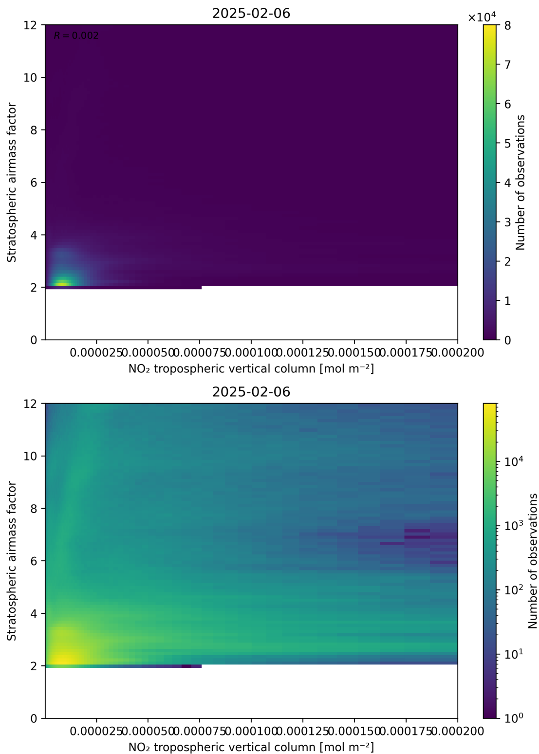
Figure 121: Scatter density plot of “NO 2 tropospheric vertical column” against “Stratospheric airmass factor” for 2025-02-05 to 2025-02-07.
