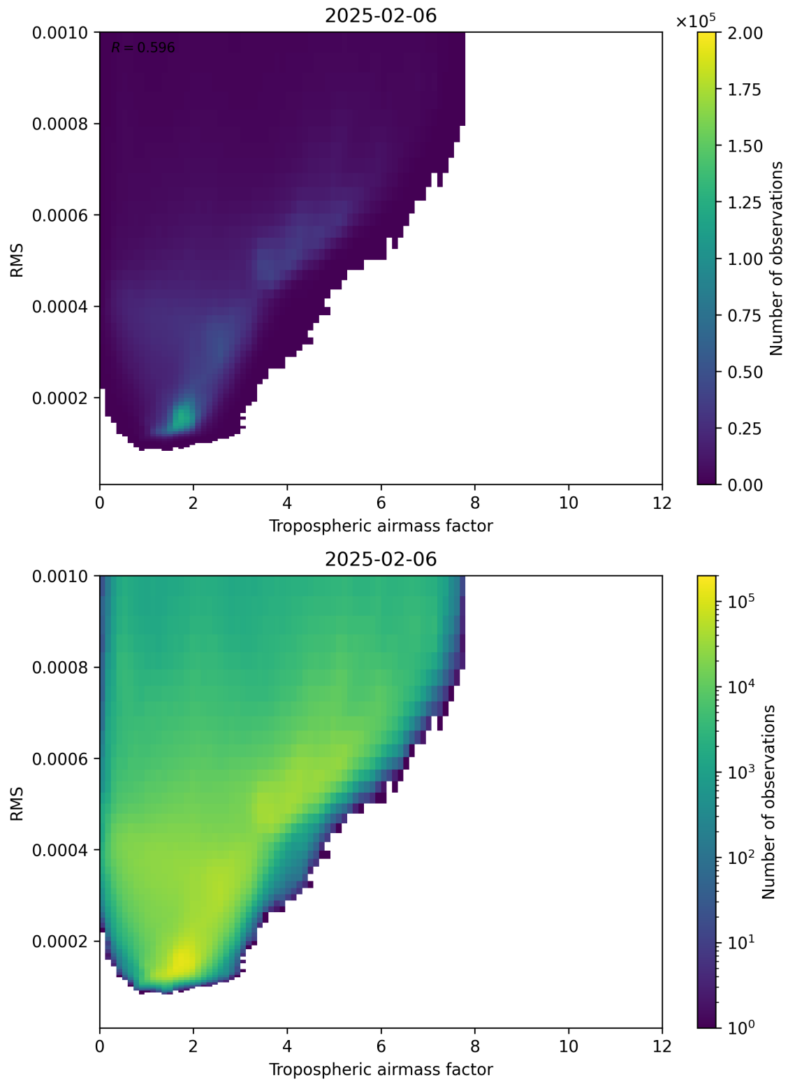
Figure 79: Scatter density plot of “Tropospheric airmass factor” against “RMS” for 2025-02-05 to 2025-02-07.
