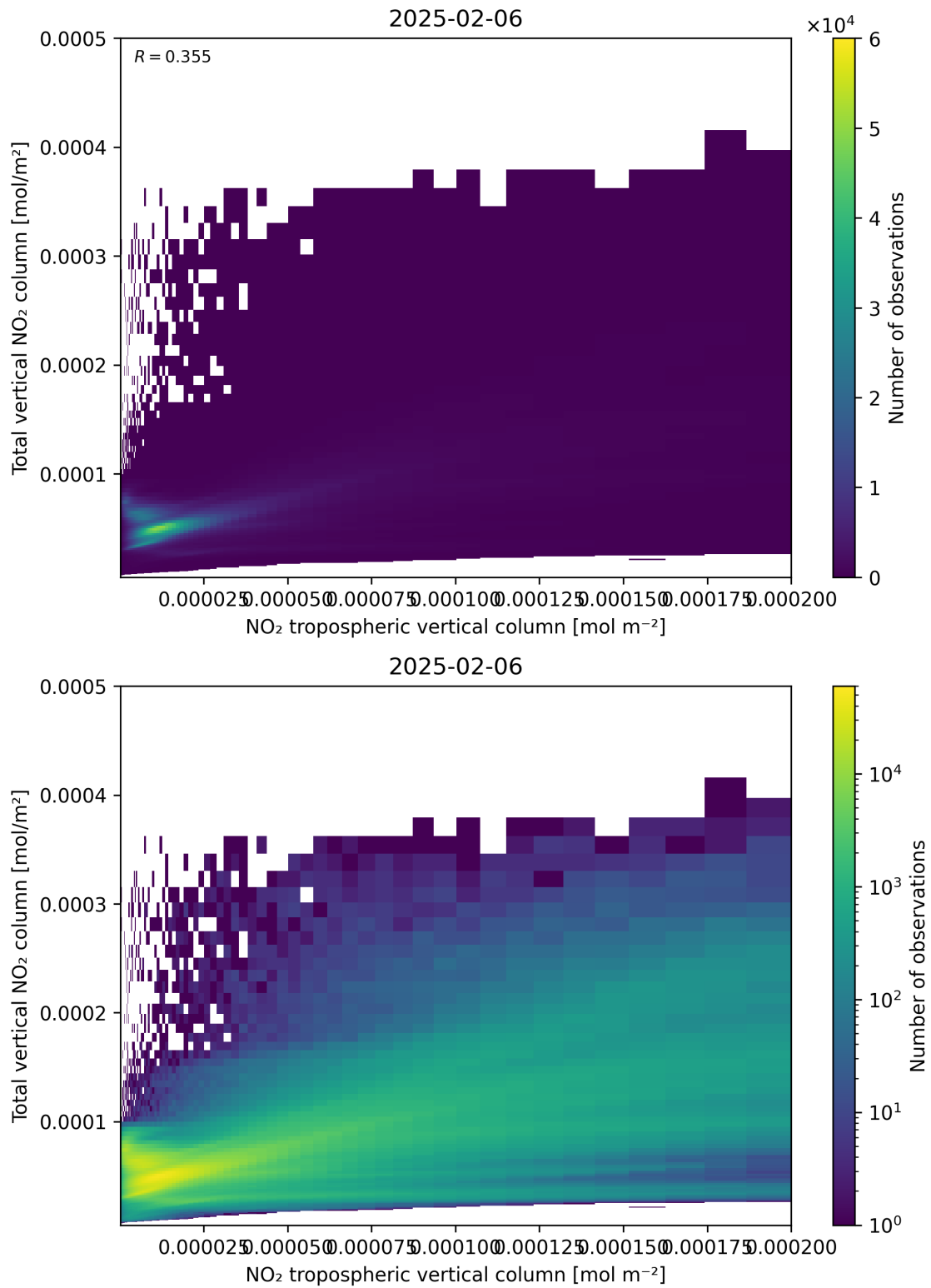
Figure 128: Scatter density plot of “NO 2 tropospheric vertical column” against “Total vertical NO 2 column” for 2025-02-05 to 2025-02-07.
