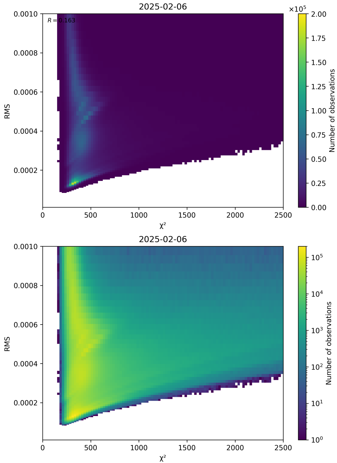
Figure 82: Scatter density plot of “ \chi^2 ” against “RMS” for 2025-02-05 to 2025-02-07.
