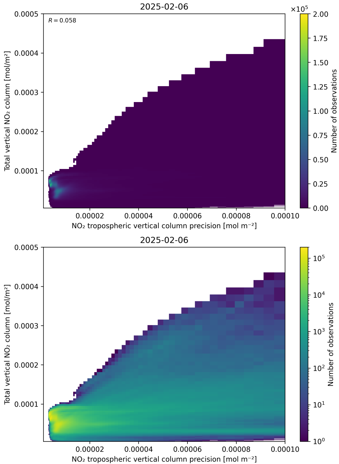
Figure 138: Scatter density plot of “NO 2 tropospheric vertical column precision” against “Total vertical NO 2 column” for 2025-02-05 to 2025-02-07.
