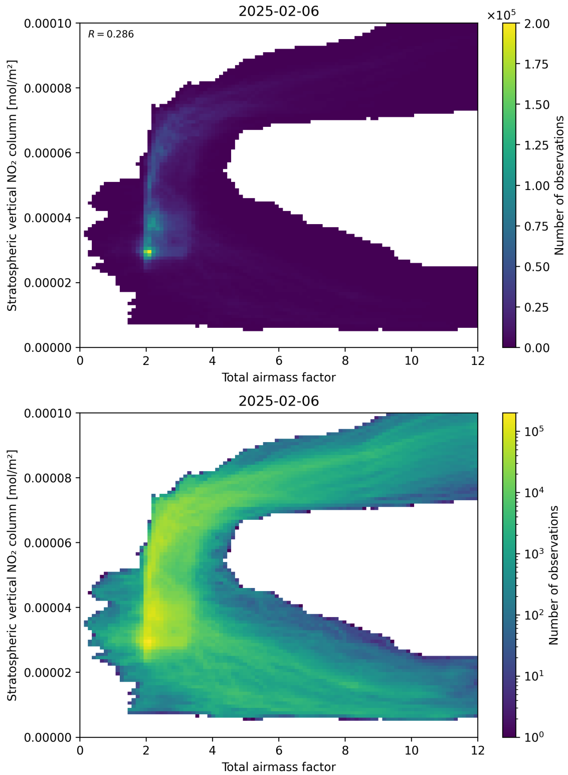
Figure 64: Scatter density plot of “Total airmass factor” against “Stratospheric vertical NO 2 column” for 2025-02-05 to 2025-02-07.
