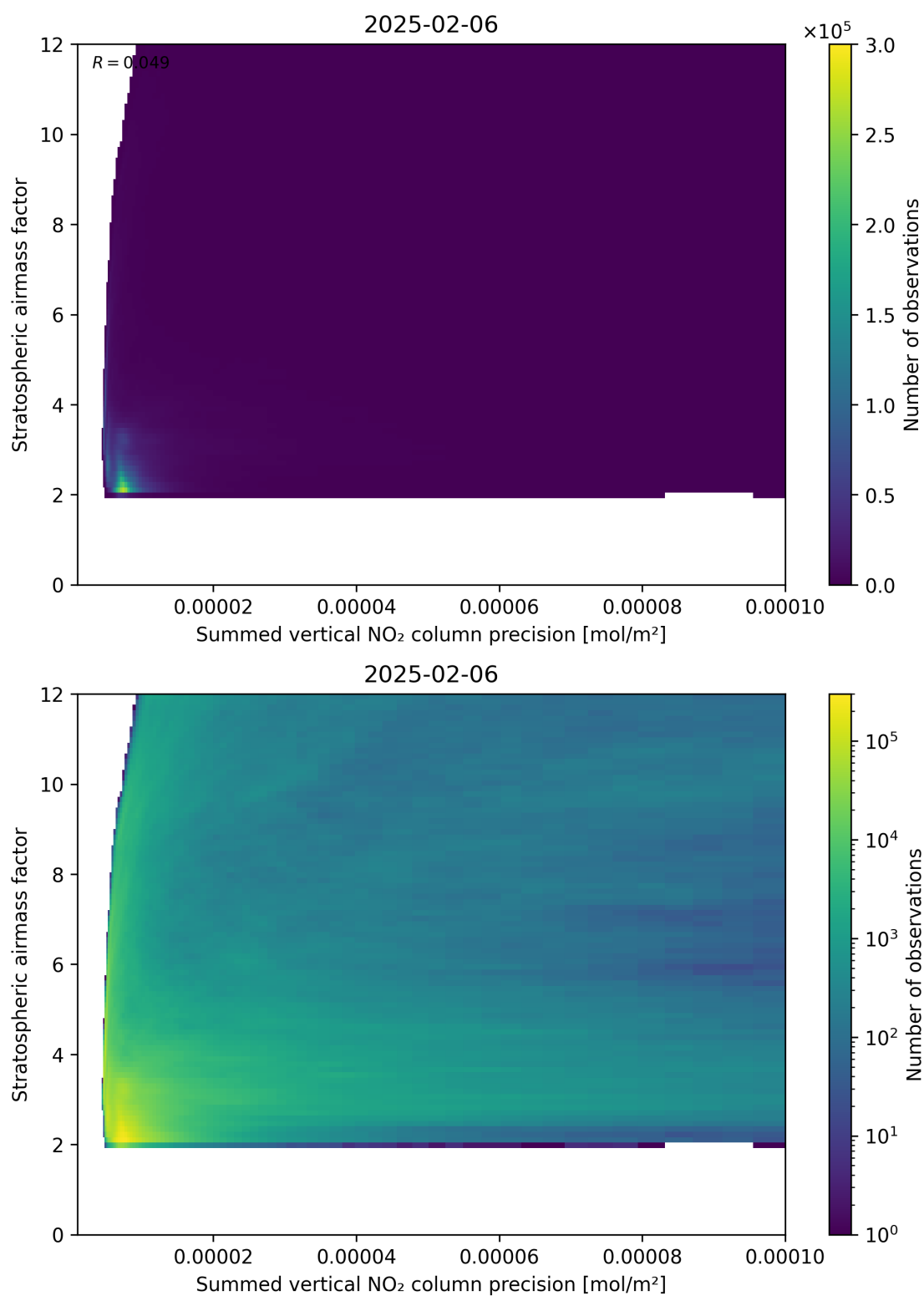
Figure 106: Scatter density plot of “Summed vertical NO 2 column precision” against “Stratospheric airmass factor” for 2025-02-05 to 2025-02-07.
