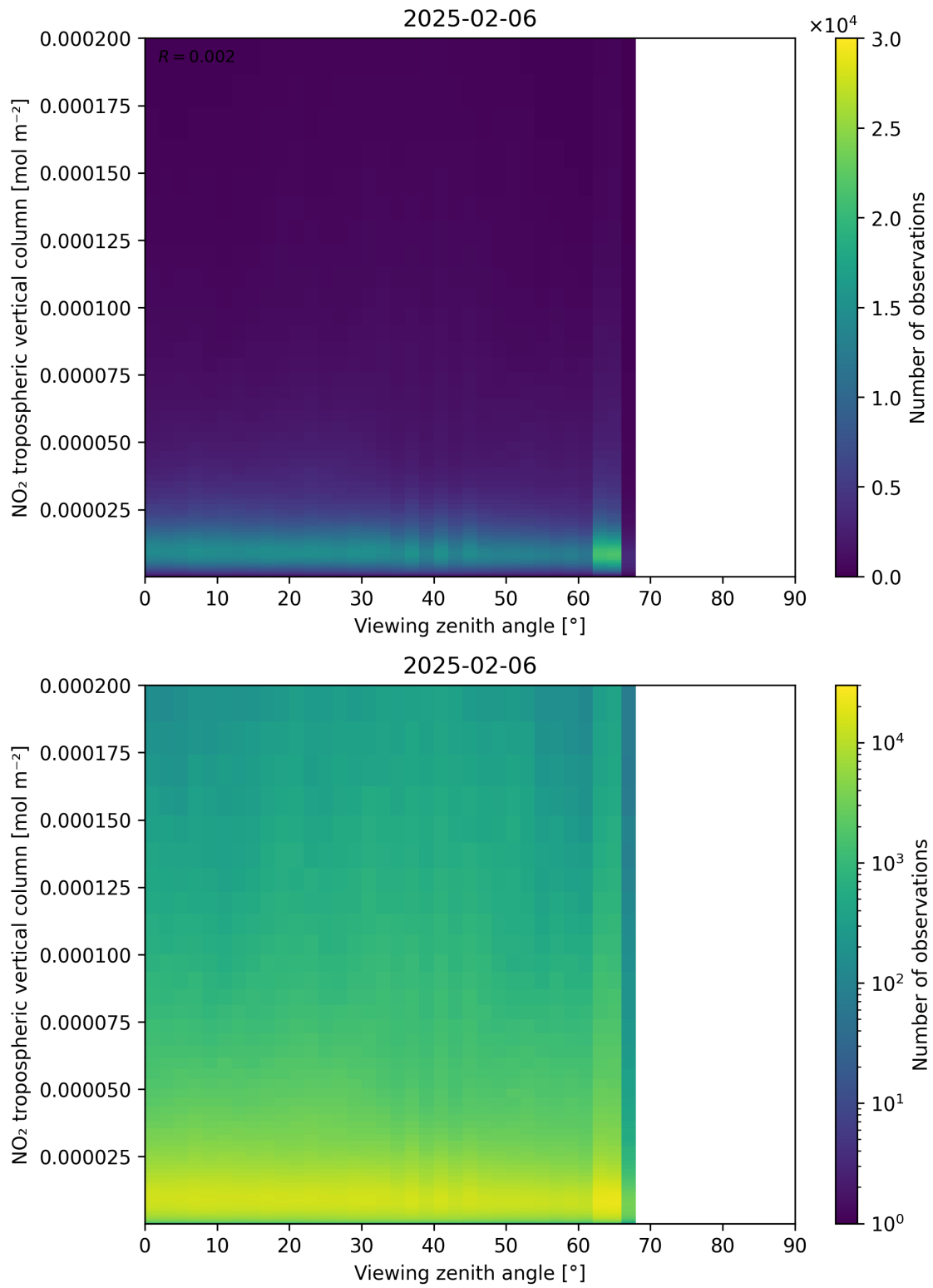
Figure 169: Scatter density plot of “Viewing zenith angle” against “NO 2 tropospheric vertical column” for 2025-02-05 to 2025-02-07.
