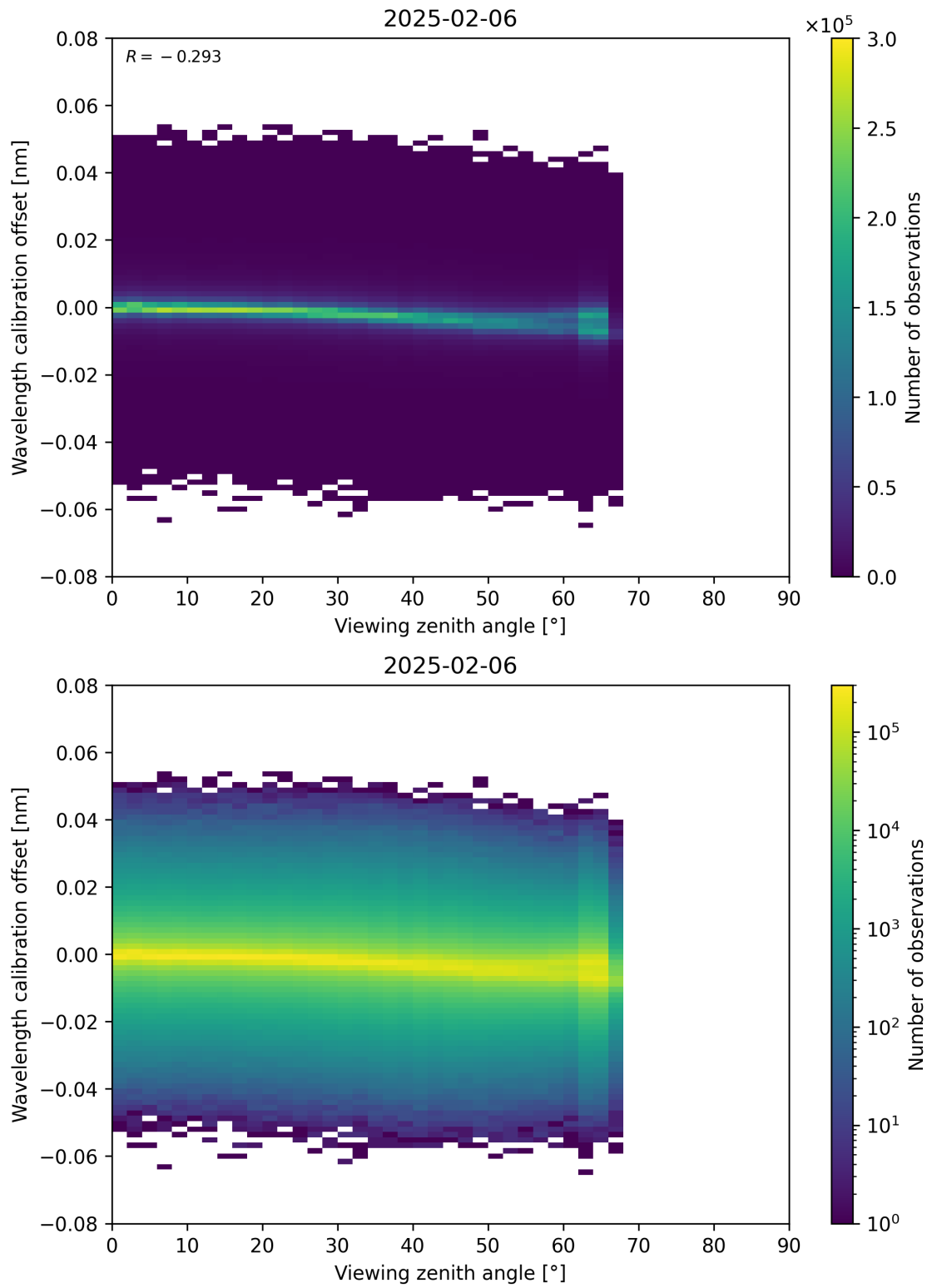
Figure 173: Scatter density plot of “Viewing zenith angle” against “Wavelength calibration offset” for 2025-02-05 to 2025-02-07.
