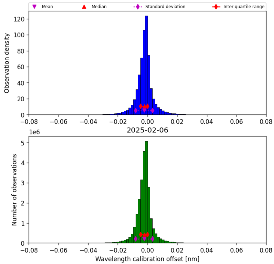
Figure 35: Histogram of “Wavelength calibration offset” for 2025-02-05 to 2025-02-07
