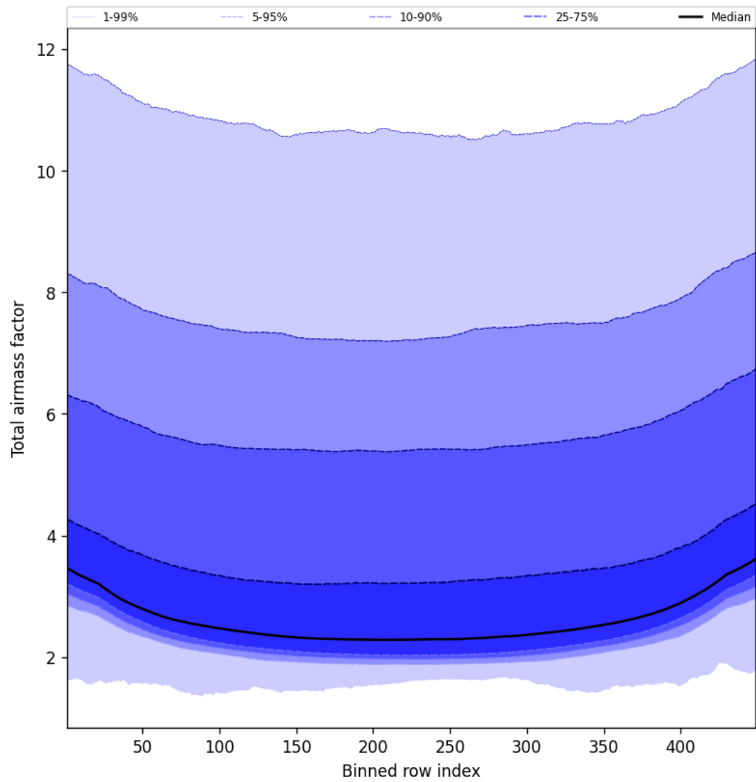
Figure 49: Along track statistics of “Total airmass factor” for 2025-02-05 to 2025-02-07
