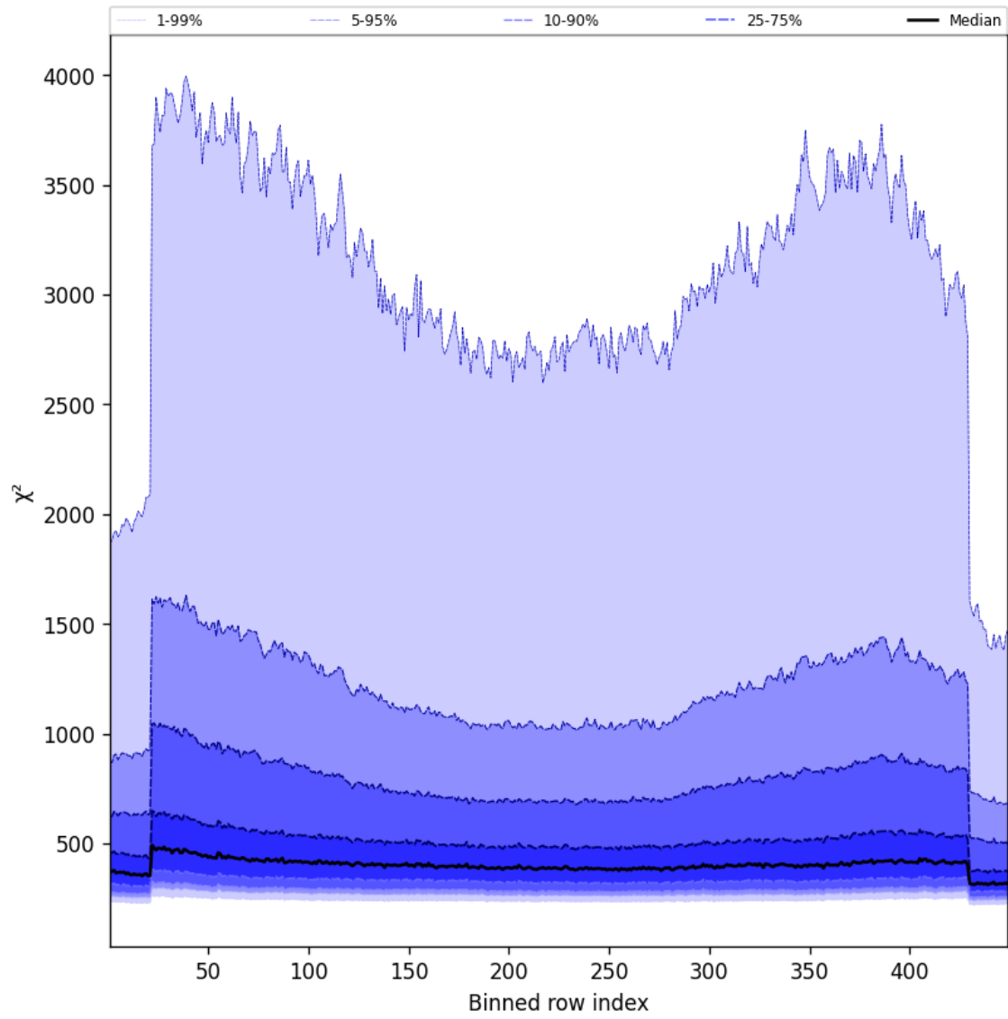
Figure 59: Along track statistics of “ \chi^2 ” for 2025-02-05 to 2025-02-07
