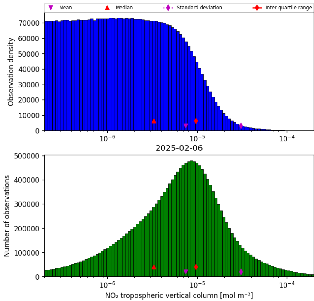
Figure 29: Histogram of “NO 2 tropospheric vertical column” for 2025-02-05 to 2025-02-07
