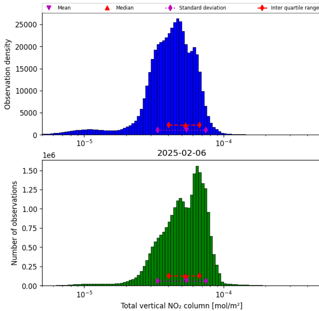
Figure 38: Histogram of “Total vertical NO 2 column” for 2025-02-05 to 2025-02-07
