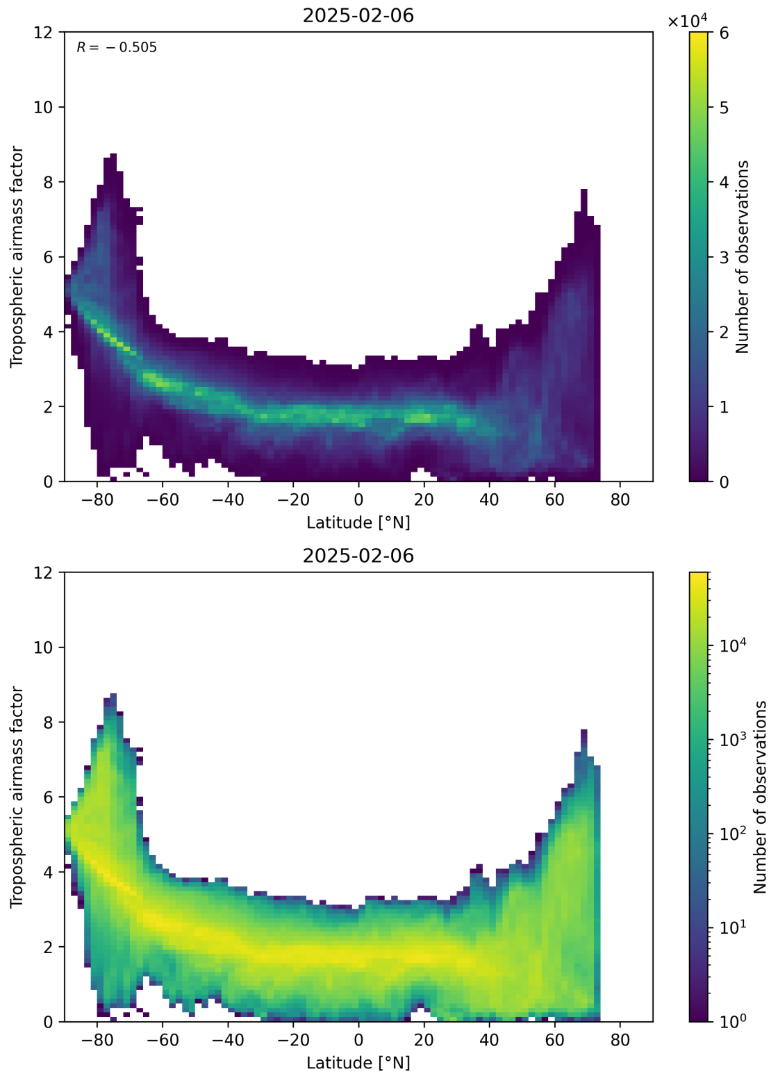
Figure 85: Scatter density plot of “Latitude” against “Tropospheric air mass factor” for 2025-02-05 to 2025-02-07.
