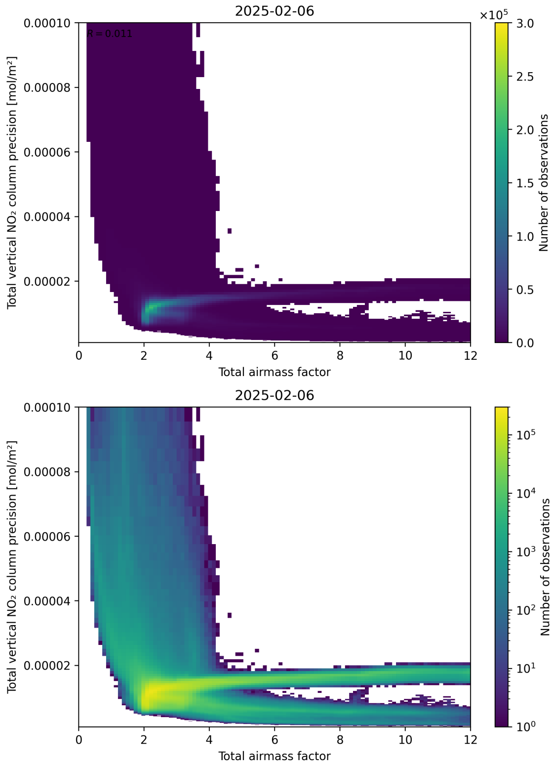
Figure 68: Scatter density plot of “Total airmass factor” against “Total vertical NO 2 column precision” for 2025-02-05 to 2025-02-07.
