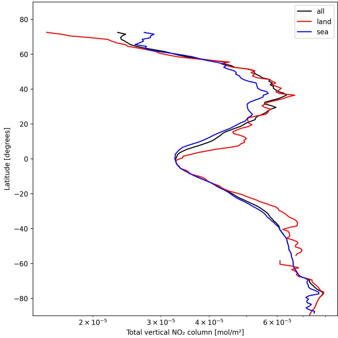
Figure 21: Zonal average of “Total vertical NO 2 column” for 2025-02-05 to 2025-02-07.
