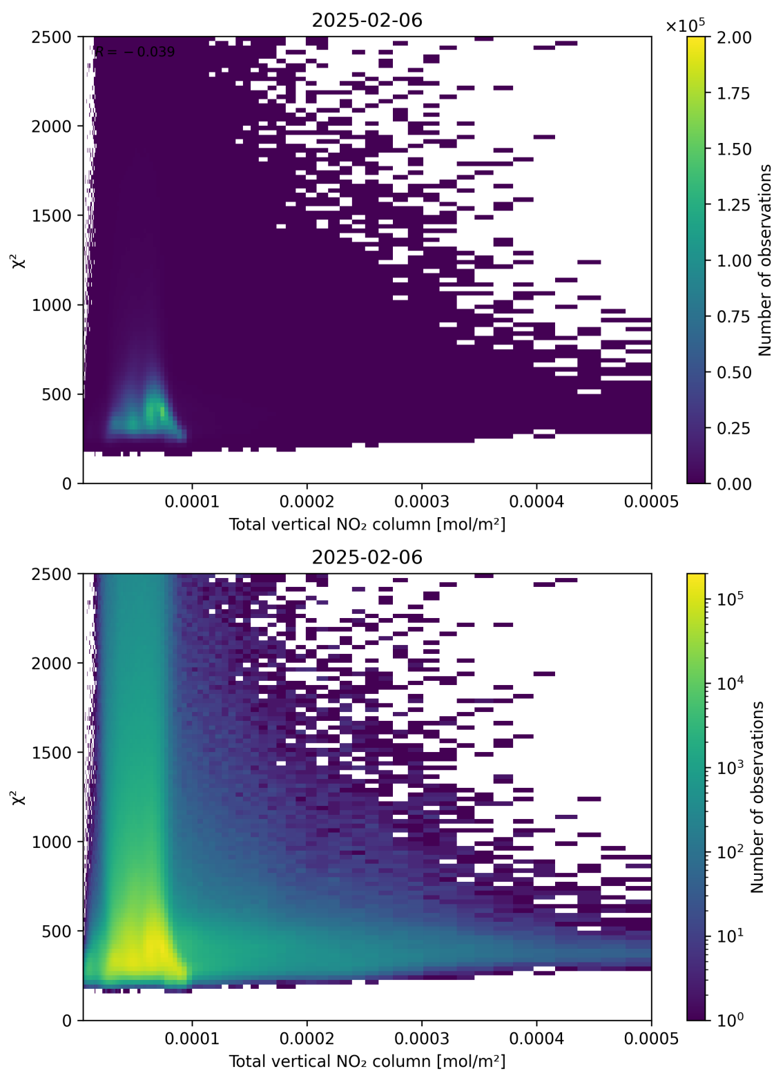
Figure 111: Scatter density plot of “Total vertical NO 2 column” against “ \chi^2 ” for 2025-02-05 to 2025-02-07.
