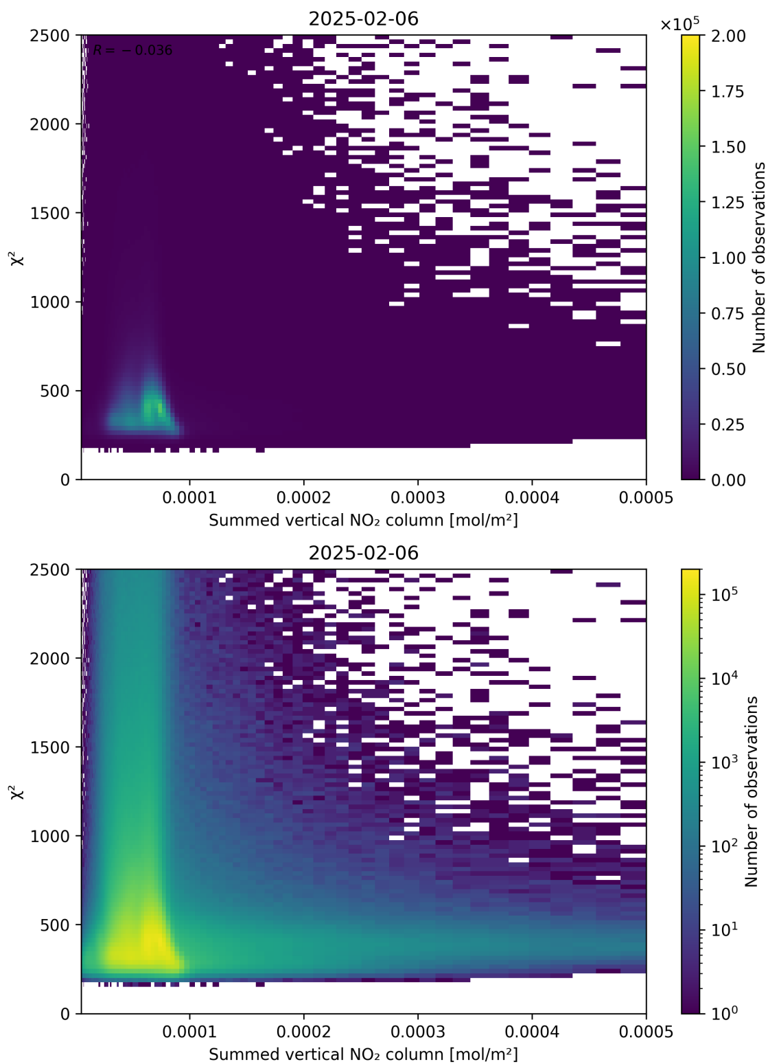
Figure 104: Scatter density plot of “Summed vertical NO 2 column” against “ \chi^2 ” for 2025-02-05 to 2025-02-07.
