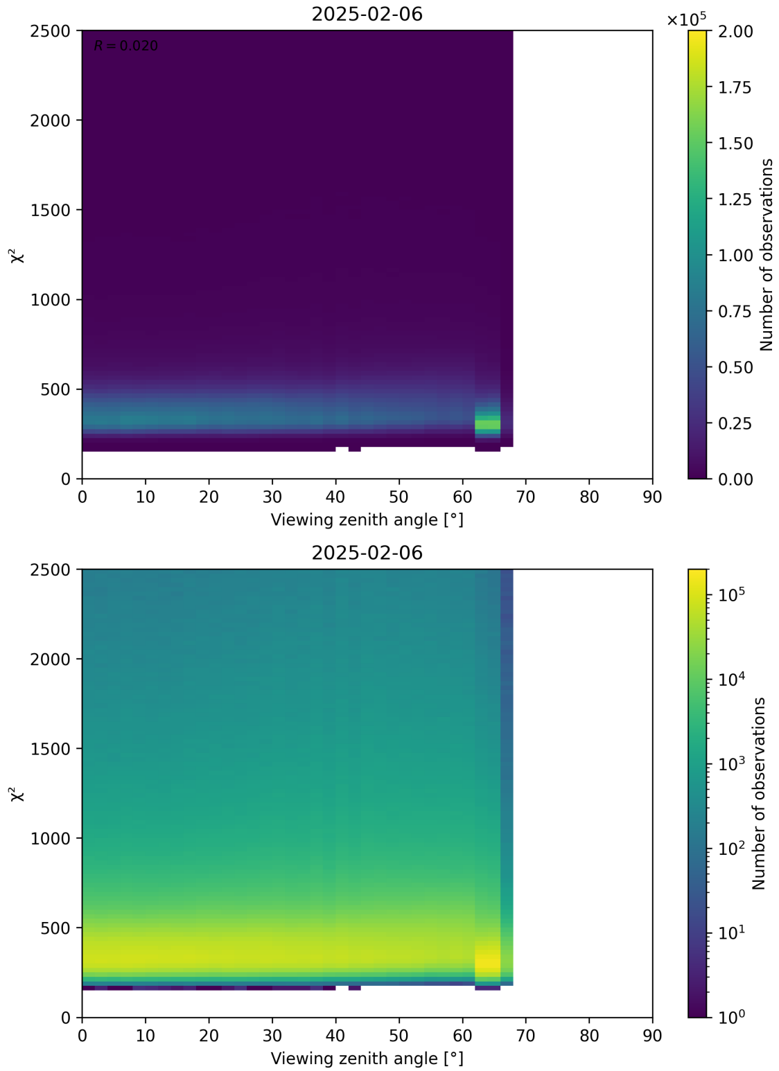
Figure 162: Scatter density plot of “Viewing zenith angle” against “ \chi^2 ” for 2025-02-05 to 2025-02-07.
