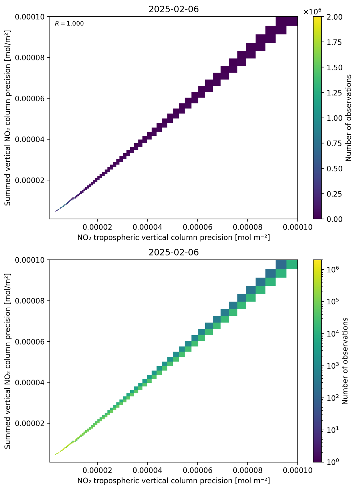
Figure 137: Scatter density plot of “NO 2 tropospheric vertical column precision” against “Summed vertical NO 2 column precision” for 2025-02-05 to 2025-02-07.
