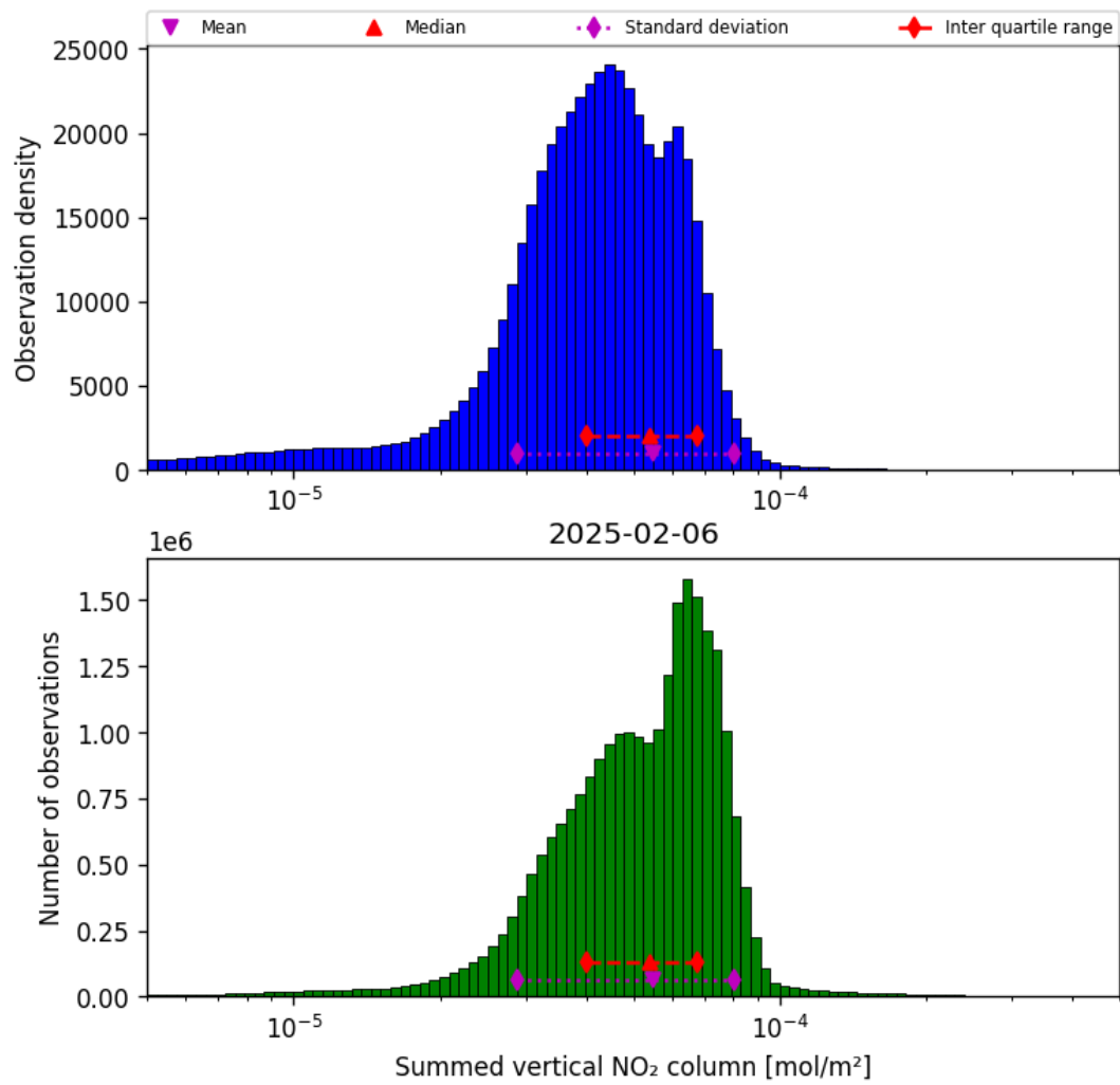
Figure 40: Histogram of “Summed vertical NO 2 column” for 2025-02-05 to 2025-02-07
