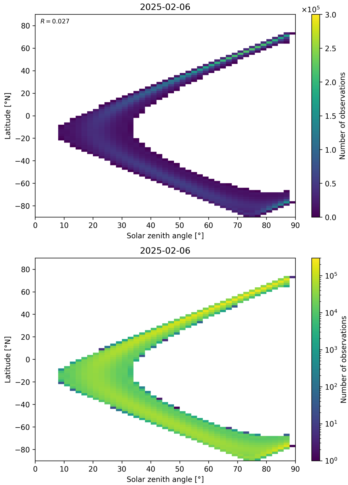
Figure 149: Scatter density plot of “Solar zenith angle” against “Latitude” for 2025-02-05 to 2025-02-07.
