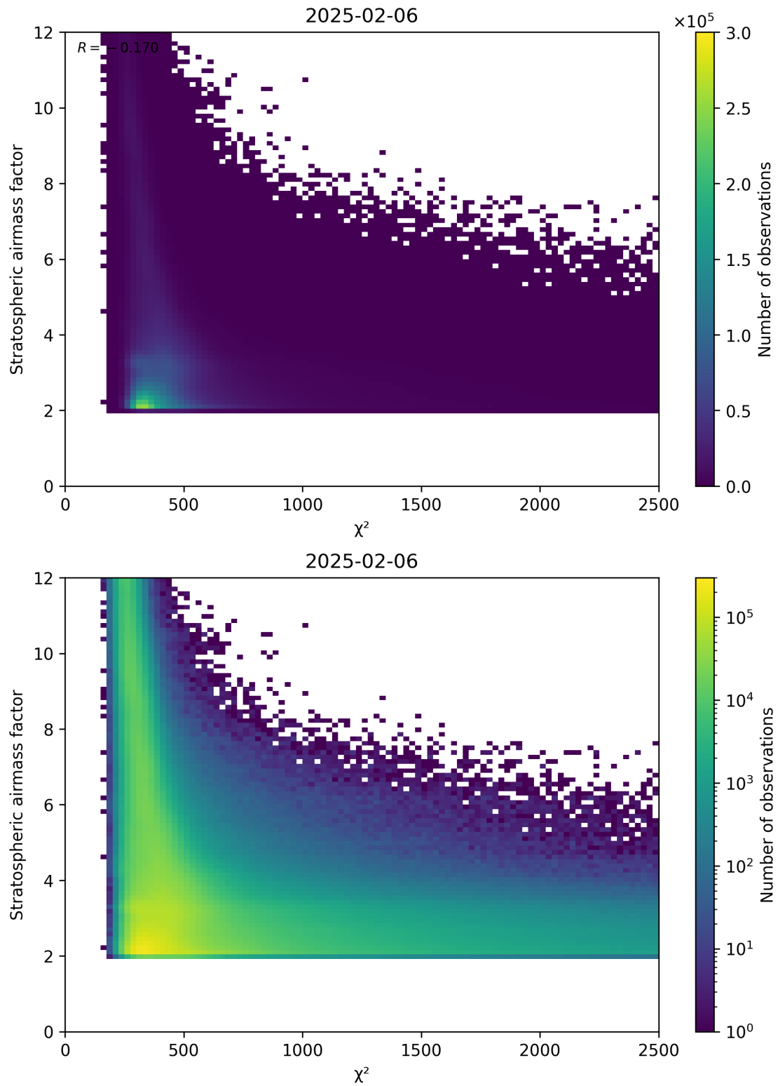
Figure 81: Scatter density plot of “ \chi^2 ” against “Stratospheric airmass factor” for 2025-02-05 to 2025-02-07.
