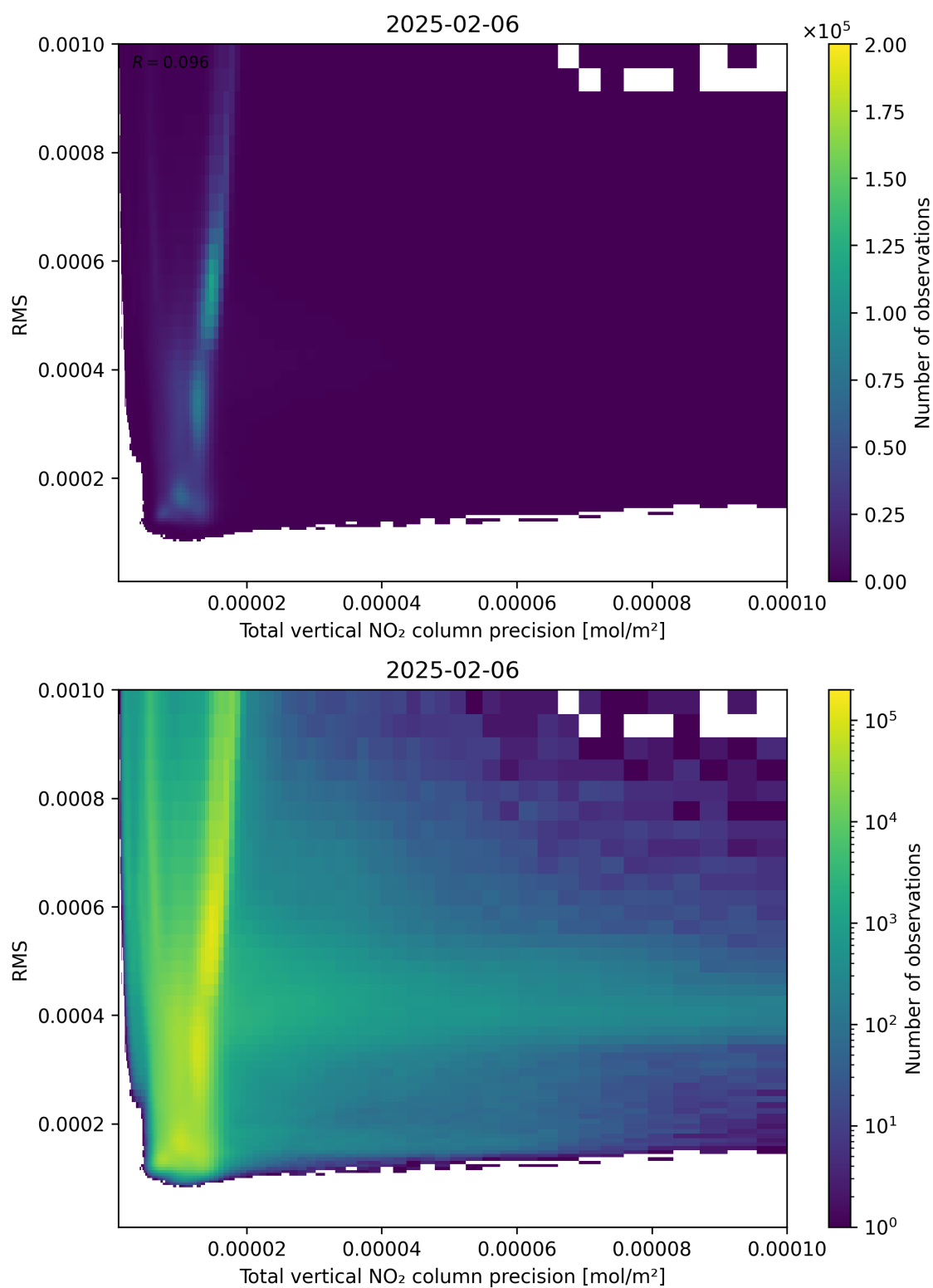
Figure 119: Scatter density plot of “Total vertical NO 2 column precision” against “RMS” for 2025-02-05 to 2025-02-07.
