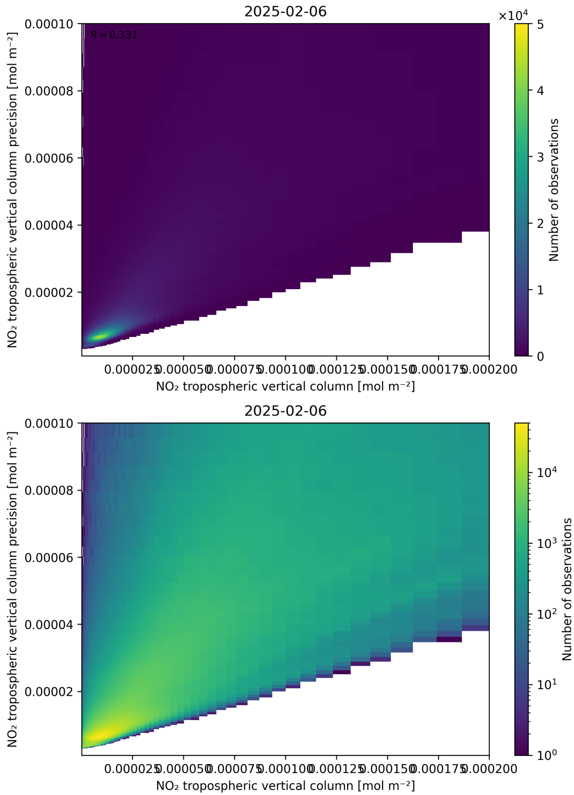
Figure 130: Scatter density plot of “NO 2 tropospheric vertical column” against “NO 2 tropospheric vertical column precision” for 2025-02-05 to 2025-02-07.
