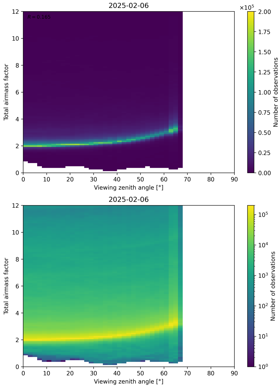
Figure 160: Scatter density plot of “Viewing zenith angle” against “Total airmass factor” for 2025-02-05 to 2025-02-07.
