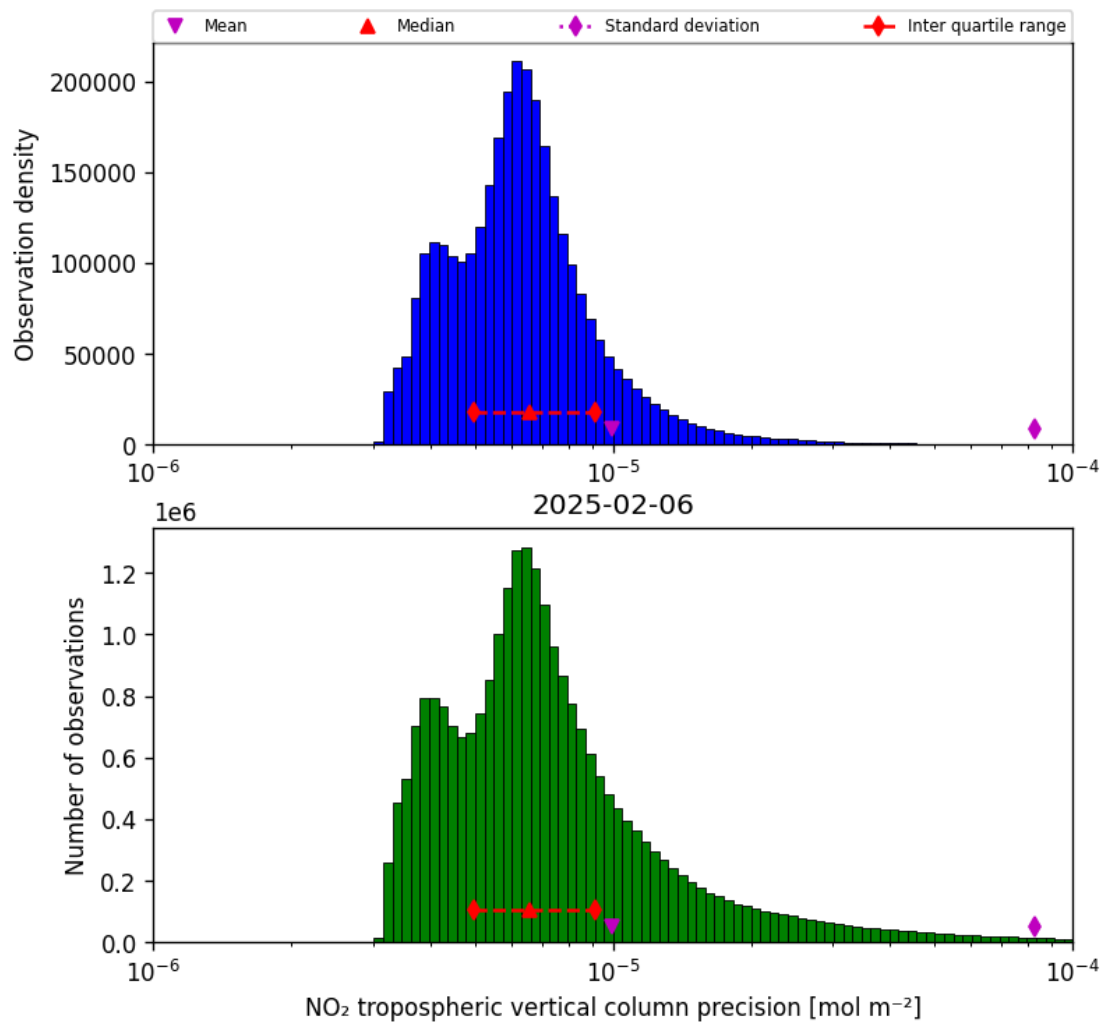
Figure 30: Histogram of “NO 2 tropospheric vertical column precision” for 2025-02-05 to 2025-02-07
