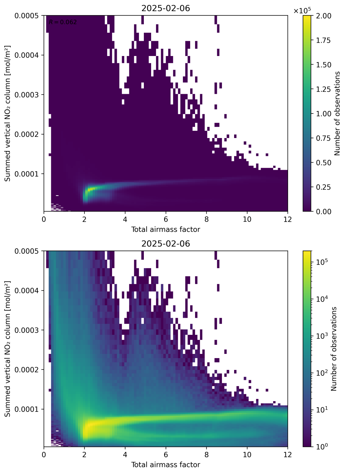
Figure 65: Scatter density plot of “Total airmass factor” against “Summed vertical NO 2 column” for 2025-02-05 to 2025-02-07.
