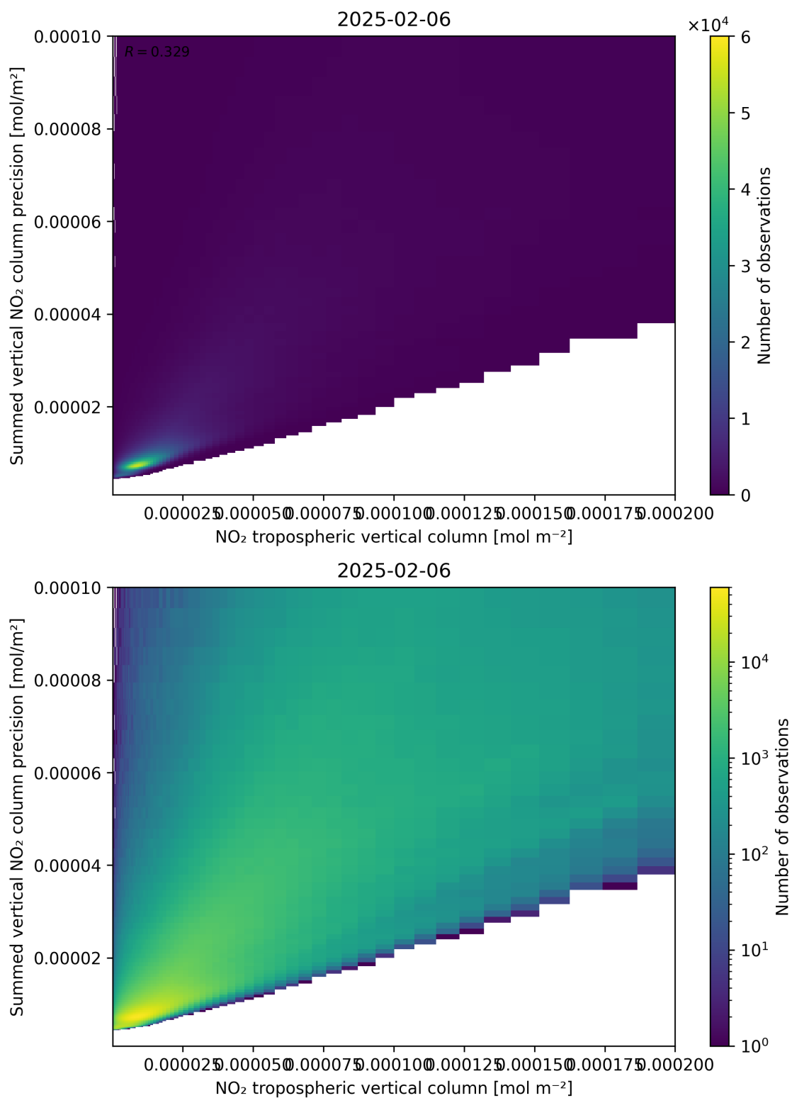
Figure 127: Scatter density plot of “NO 2 tropospheric vertical column” against “Summed vertical NO 2 column precision” for 2025-02-05 to 2025-02-07.
