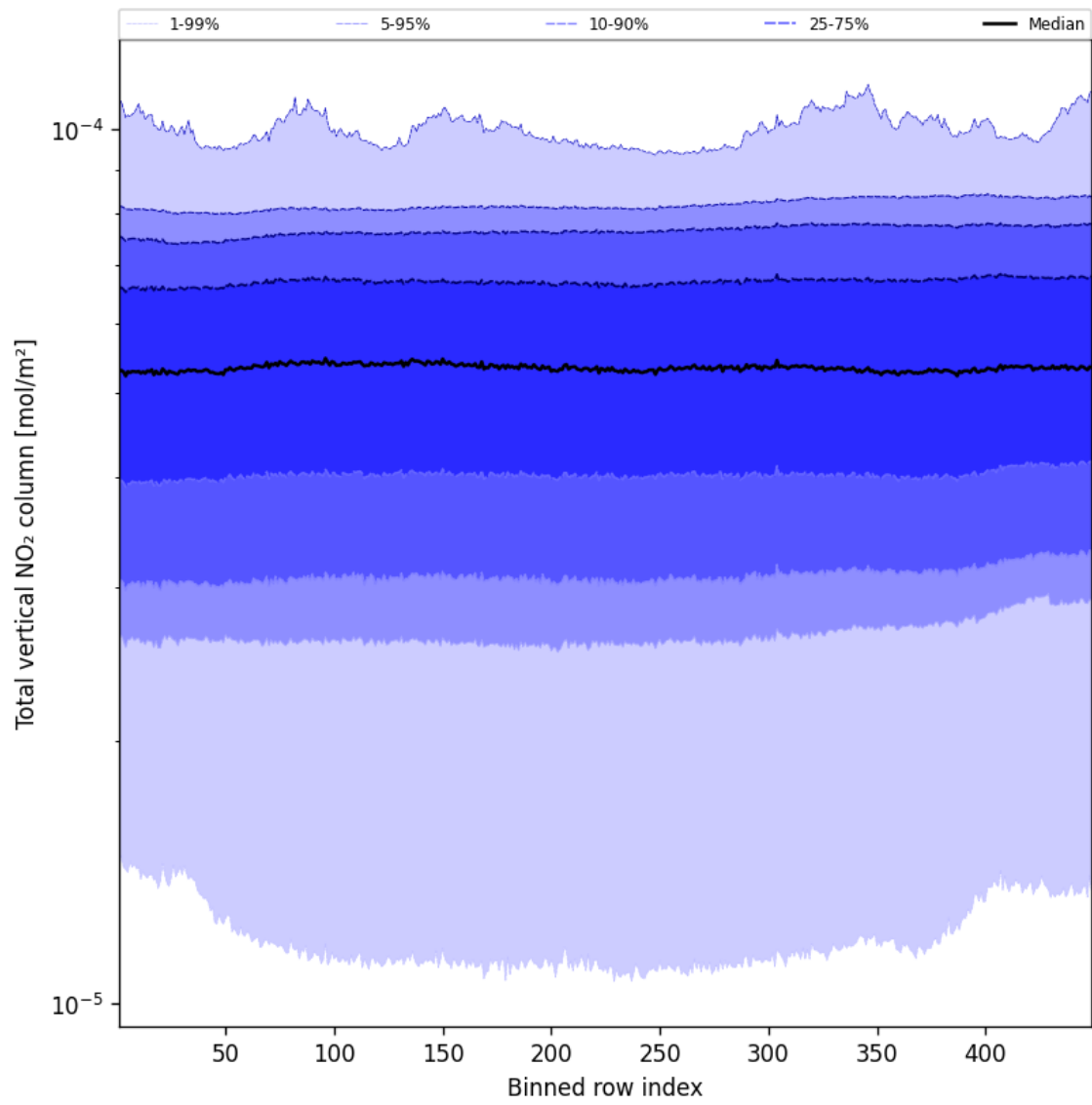
Figure 55: Along track statistics of “Total vertical NO 2 column” for 2025-02-05 to 2025-02-07
