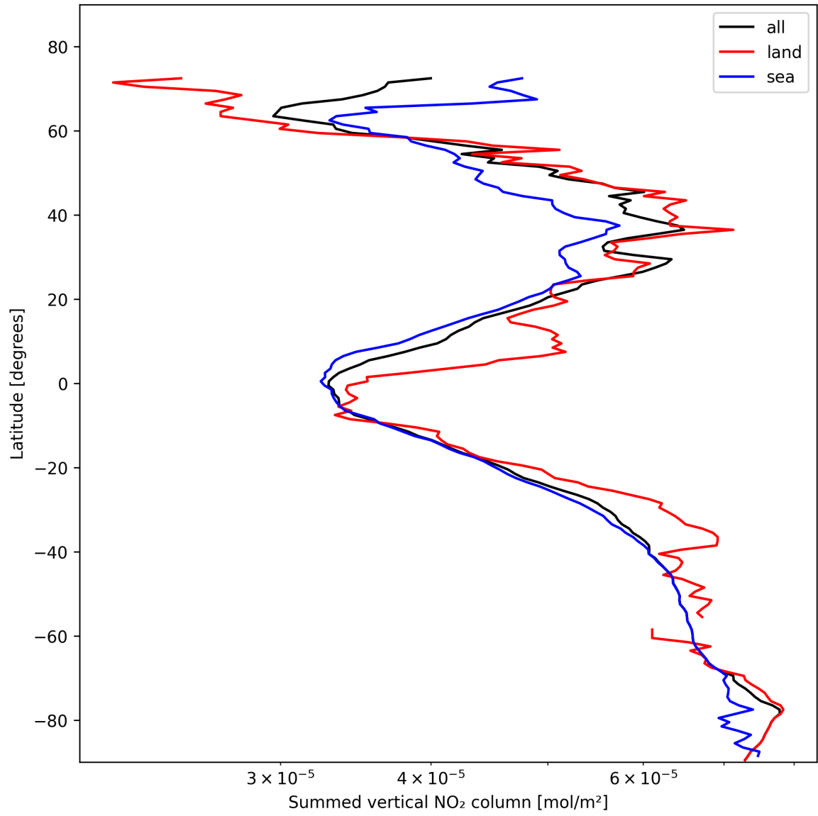
Figure 23: Zonal average of “Summed vertical NO 2 column” for 2025-02-05 to 2025-02-07.
