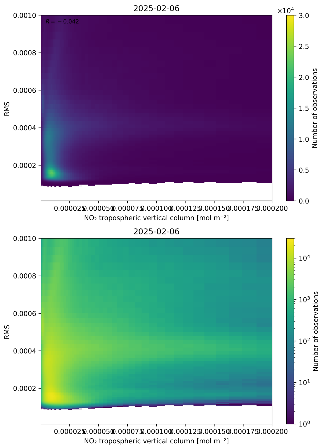
Figure 142: Scatter density plot of “NO 2 tropospheric vertical column” against “RMS” for 2025-02-05 to 2025-02-07.
