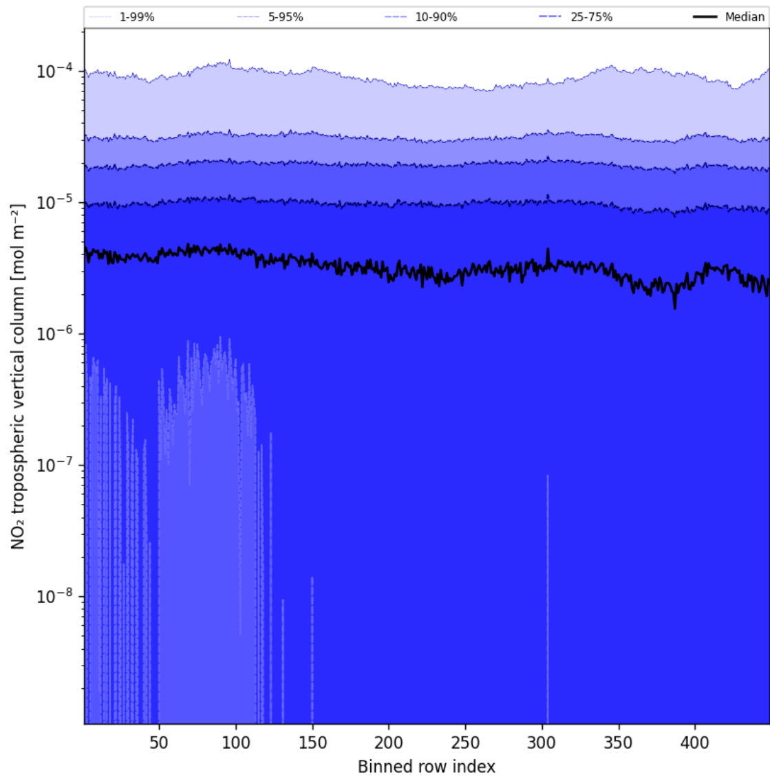
Figure 46: Along track statistics of “NO 2 tropospheric vertical column” for 2025-02-05 to 2025-02-07
