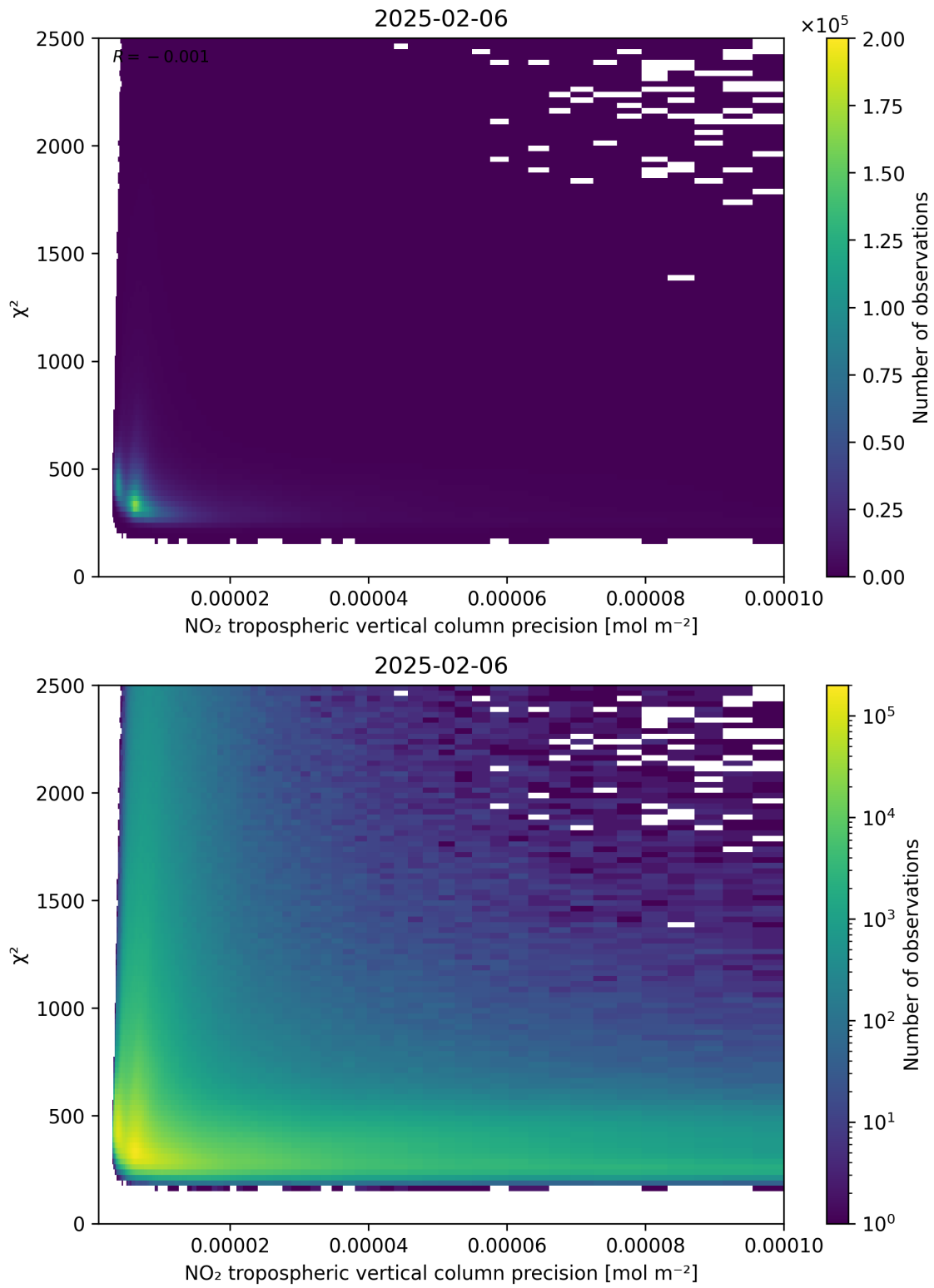
Figure 134: Scatter density plot of “NO 2 tropospheric vertical column precision” against “ \chi^2 ” for 2025-02-05 to 2025-02-07.
