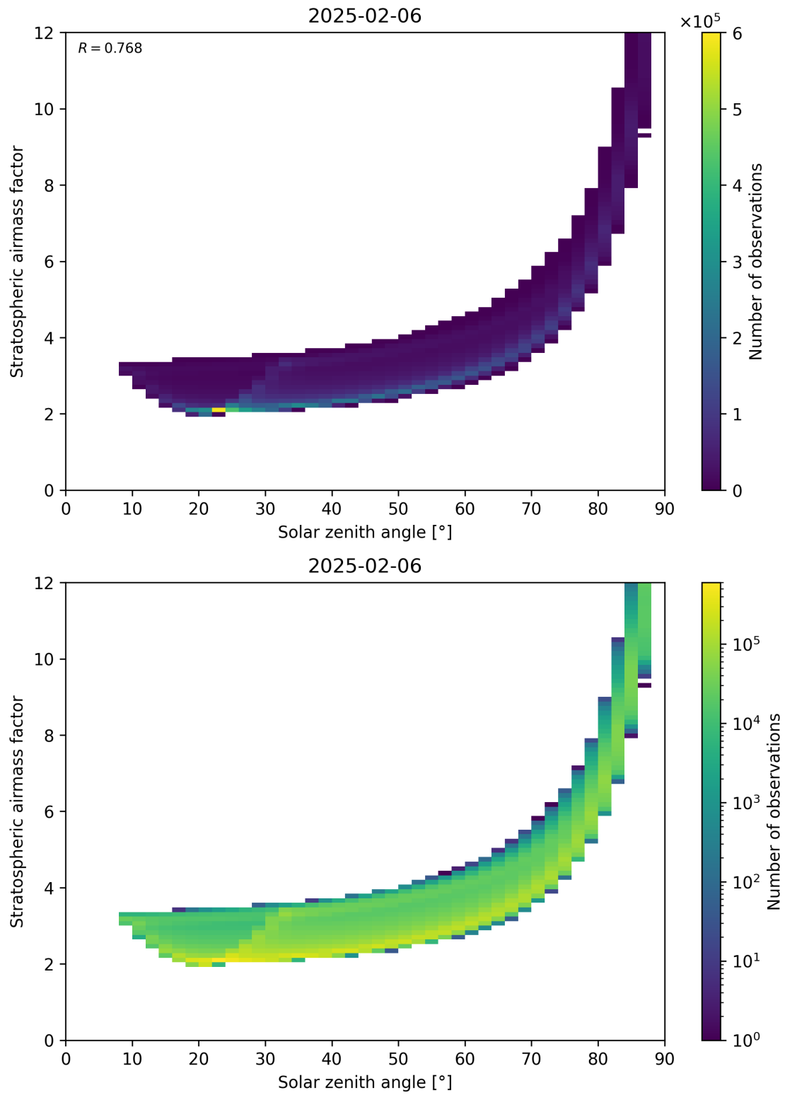
Figure 145: Scatter density plot of “Solar zenith angle” against “Stratospheric airmass factor” for 2025-02-05 to 2025-02-07.
