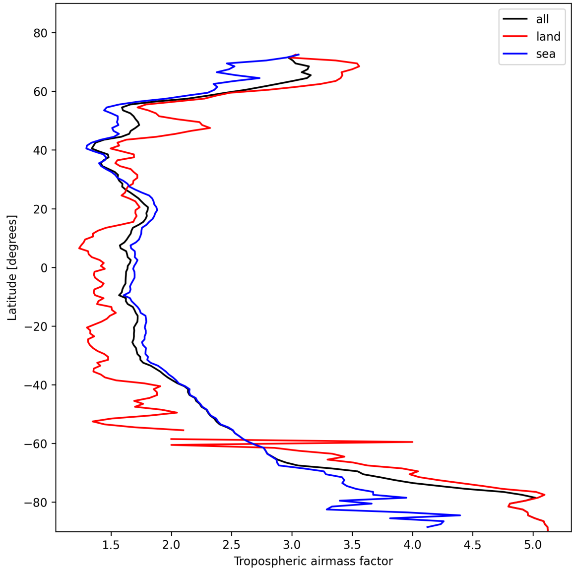
Figure 14: Zonal average of “Tropospheric airmass factor” for 2025-02-05 to 2025-02-07.
