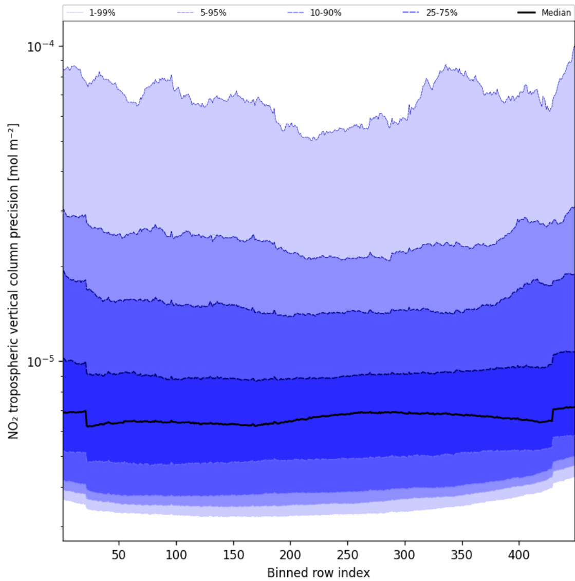
Figure 47: Along track statistics of “NO 2 tropospheric vertical column precision” for 2025-02-05 to 2025-02-07
