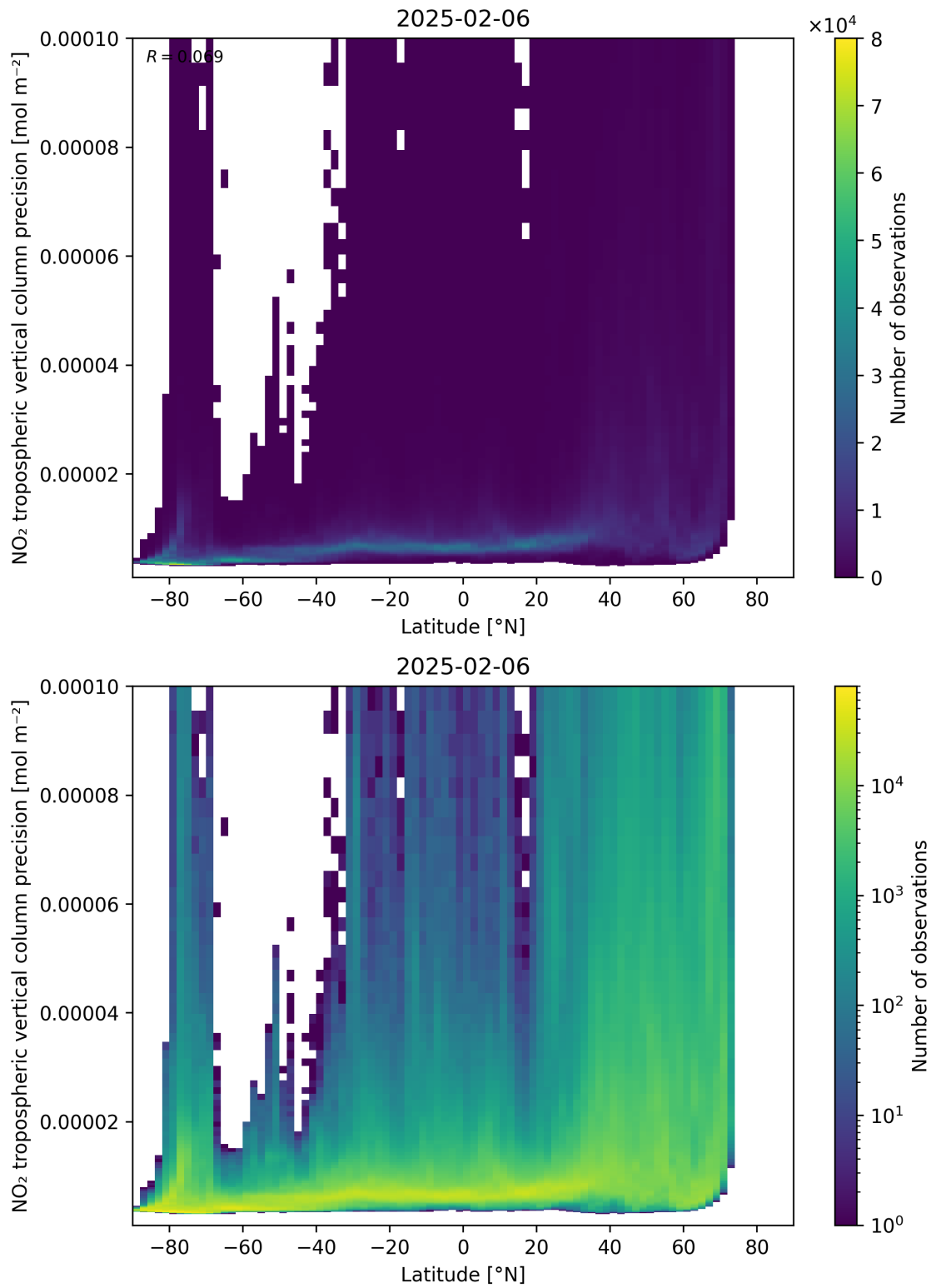
Figure 93: Scatter density plot of “Latitude” against “NO 2 tropospheric vertical column precision” for 2025-02-05 to 2025-02-07.
