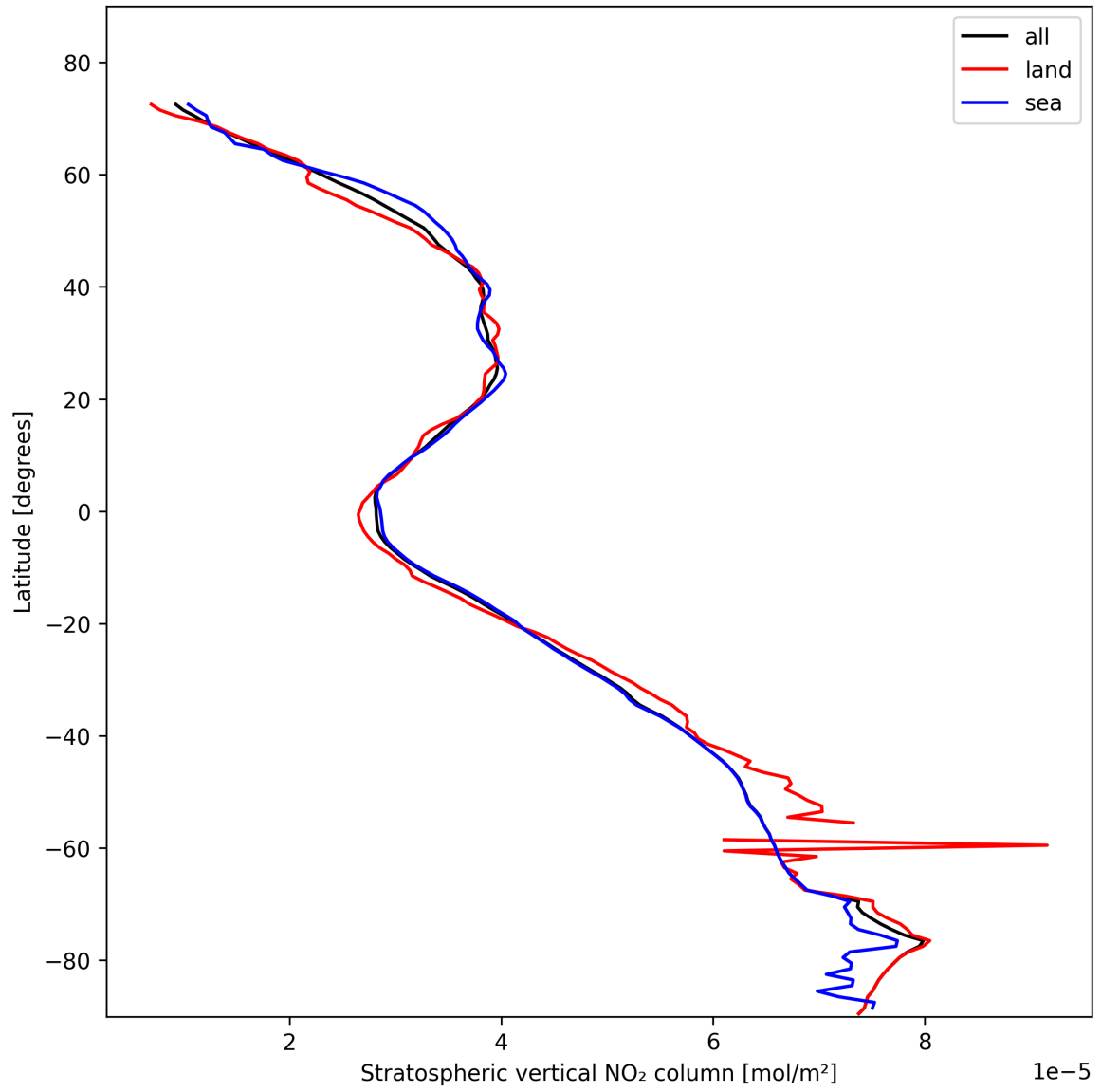
Figure 19: Zonal average of “Stratospheric vertical NO 2 column” for 2025-02-05 to 2025-02-07.
