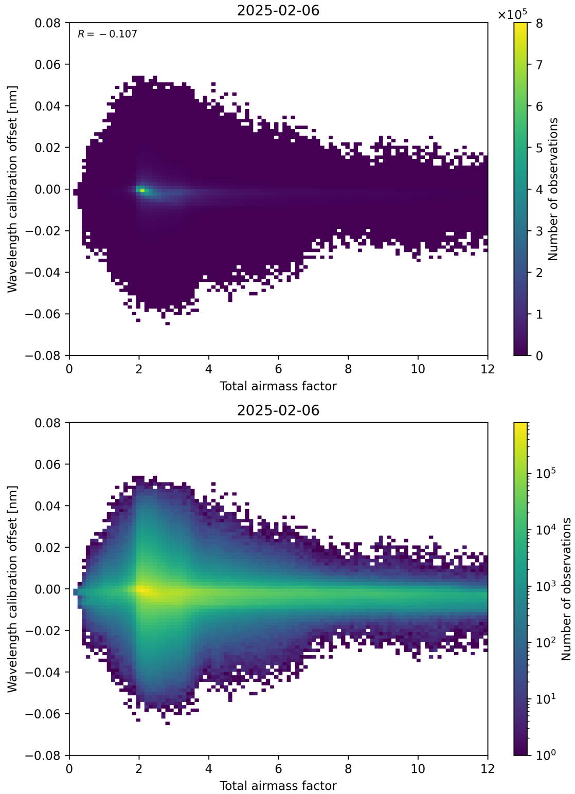
Figure 70: Scatter density plot of “Total airmass factor” against “Wavelength calibration offset” for 2025-02-05 to 2025-02-07.
