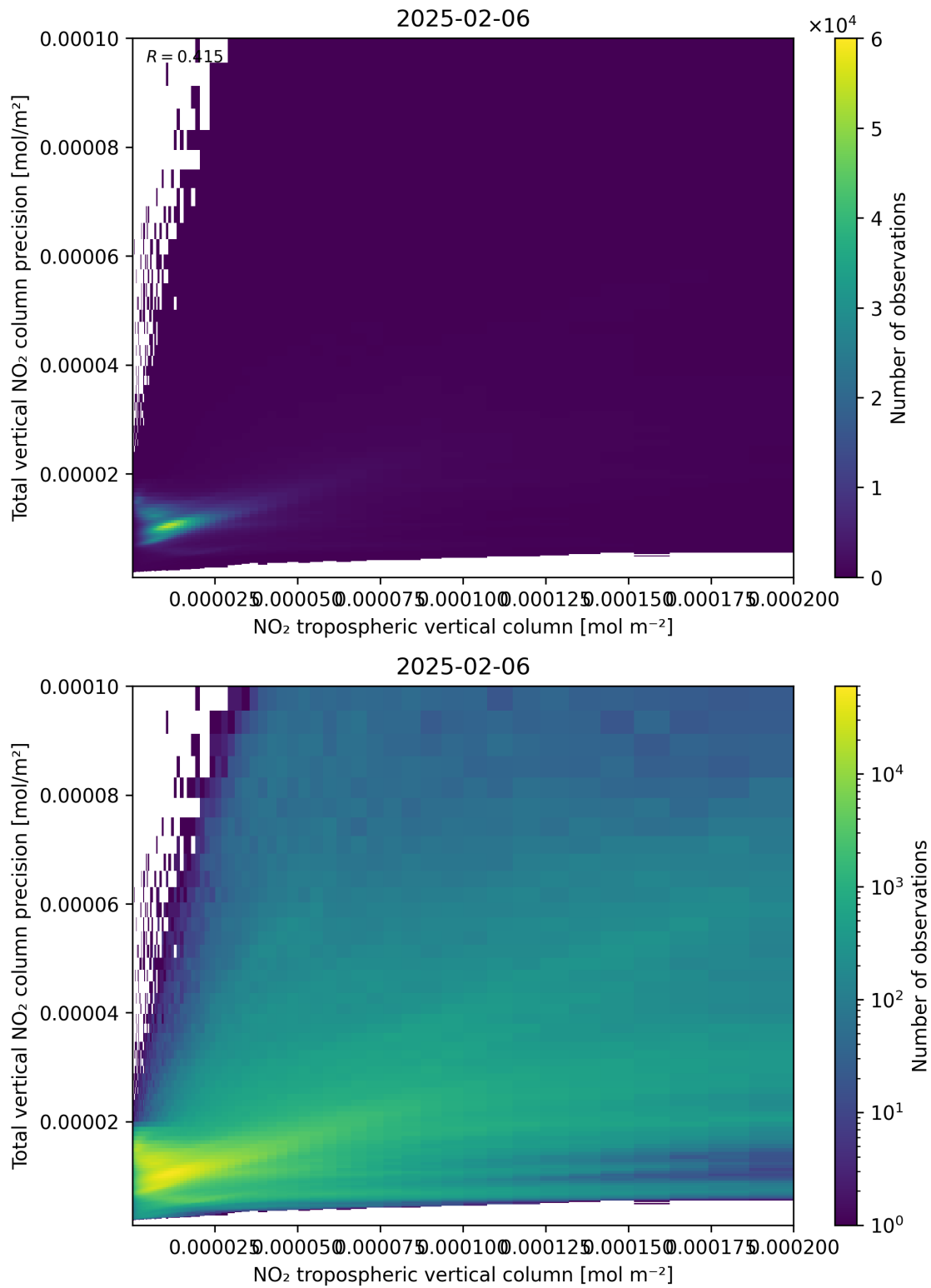
Figure 129: Scatter density plot of “NO 2 tropospheric vertical column” against “Total vertical NO 2 column precision” for 2025-02-05 to 2025-02-07.
