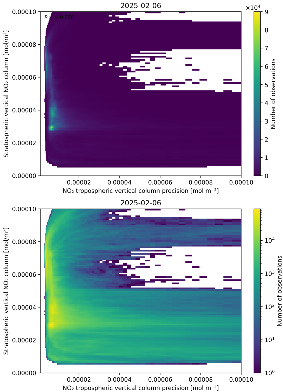
Figure 135: Scatter density plot of “NO 2 tropospheric vertical column precision” against “Stratospheric vertical NO 2 column” for 2025-02-05 to 2025-02-07.
