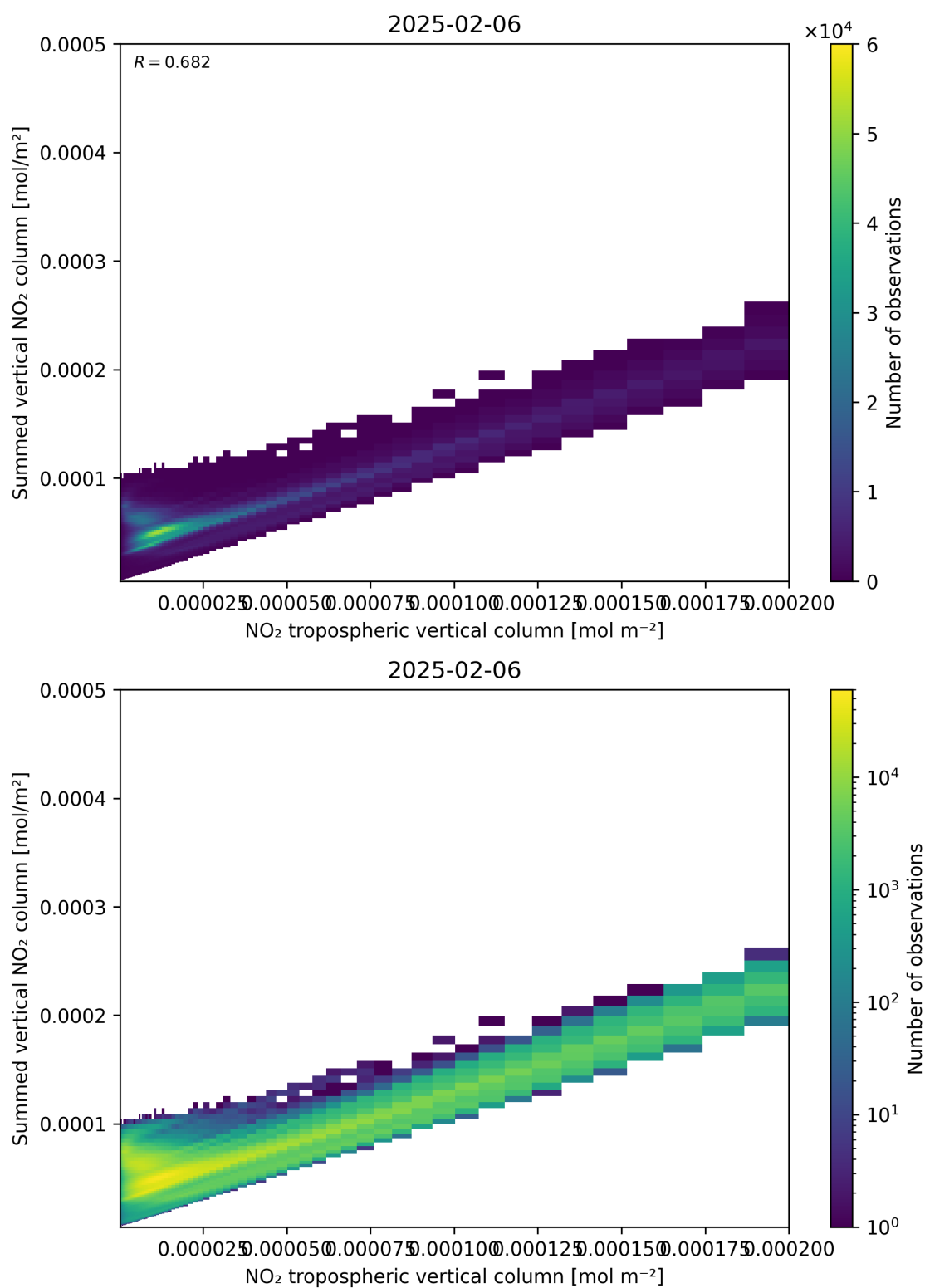
Figure 126: Scatter density plot of “NO 2 tropospheric vertical column” against “Summed vertical NO 2 column” for 2025-02-05 to 2025-02-07.
