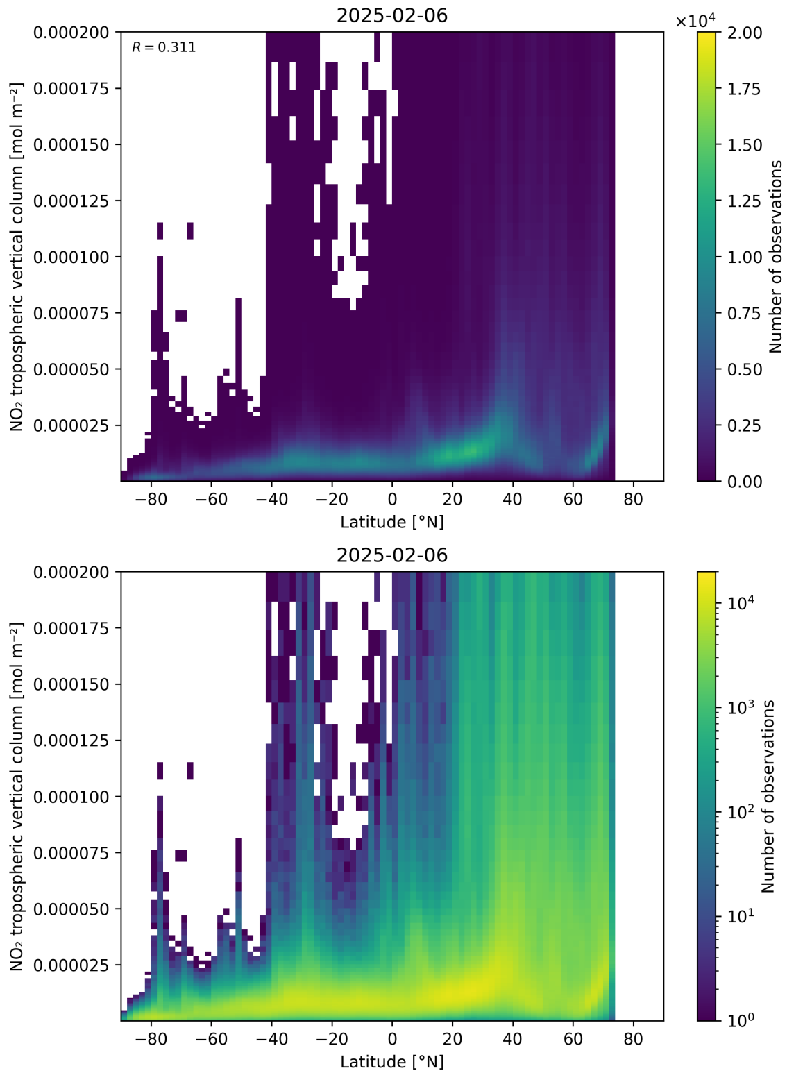
Figure 92: Scatter density plot of “Latitude” against “NO 2 tropospheric vertical column” for 2025-02-05 to 2025-02-07.
