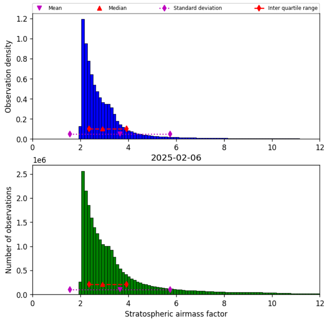
Figure 44: Histogram of “Stratospheric airmass factor” for 2025-02-05 to 2025-02-07
