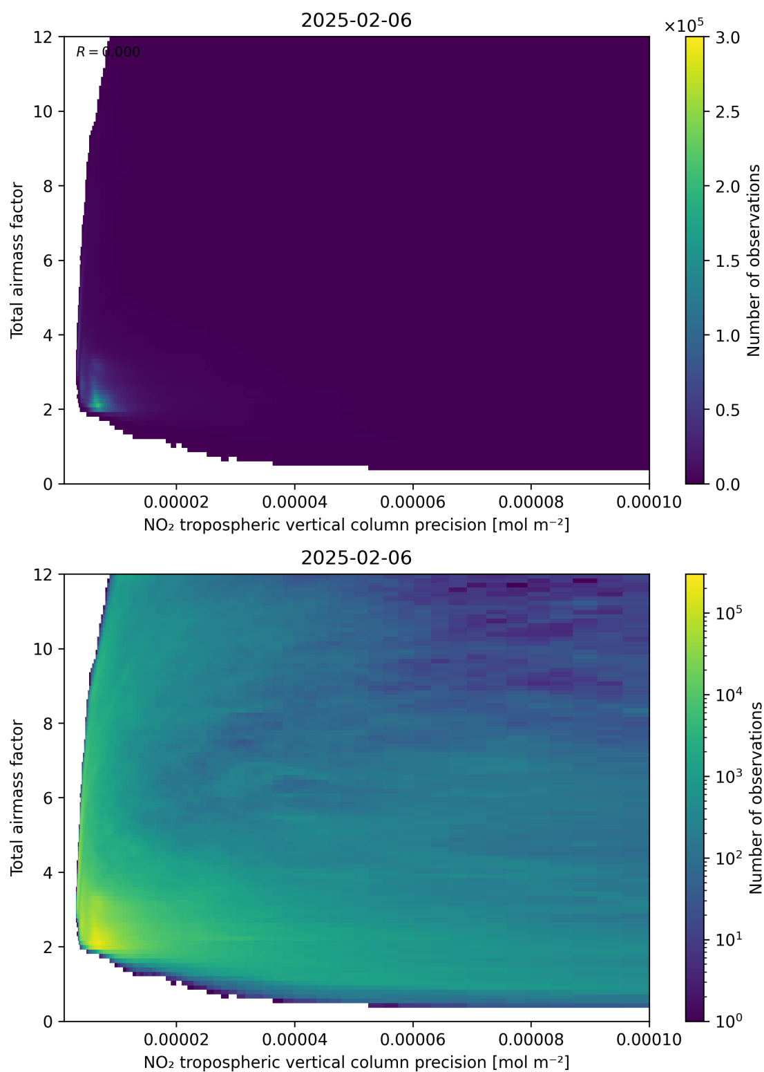
Figure 132: Scatter density plot of “NO 2 tropospheric vertical column precision” against “Total air mass factor” for 2025-02-05 to 2025-02-07.
