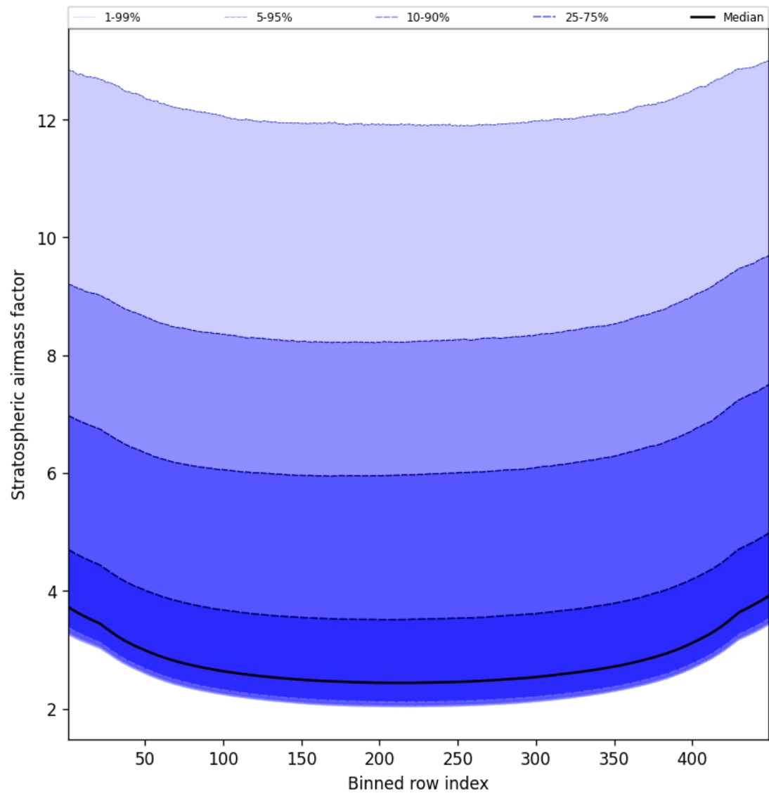
Figure 61: Along track statistics of “Stratospheric airmass factor” for 2025-02-05 to 2025-02-07
