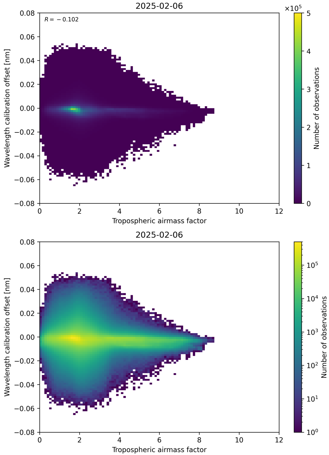
Figure 80: Scatter density plot of “Tropospheric airmass factor” against “Wavelength calibration offset” for 2025-02-05 to 2025-02-07.
