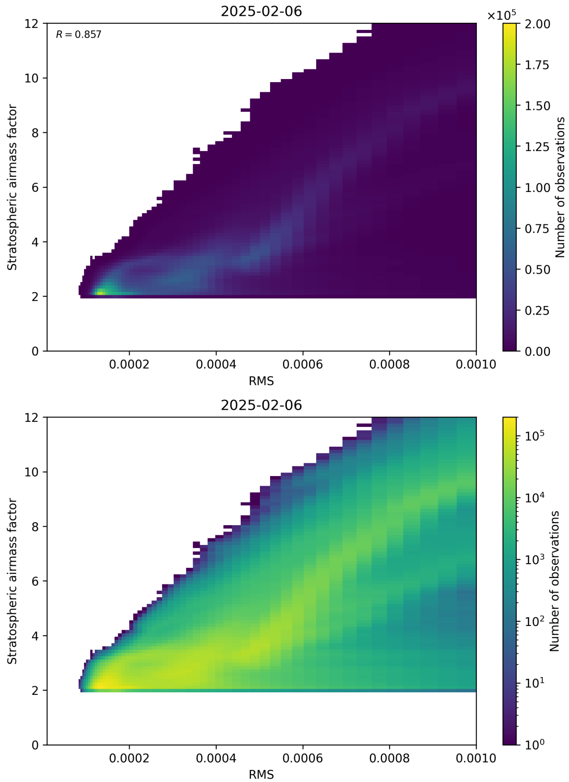
Figure 144: Scatter density plot of “RMS” against “Stratospheric airmass factor” for 2025-02-05 to 2025-02-07.
