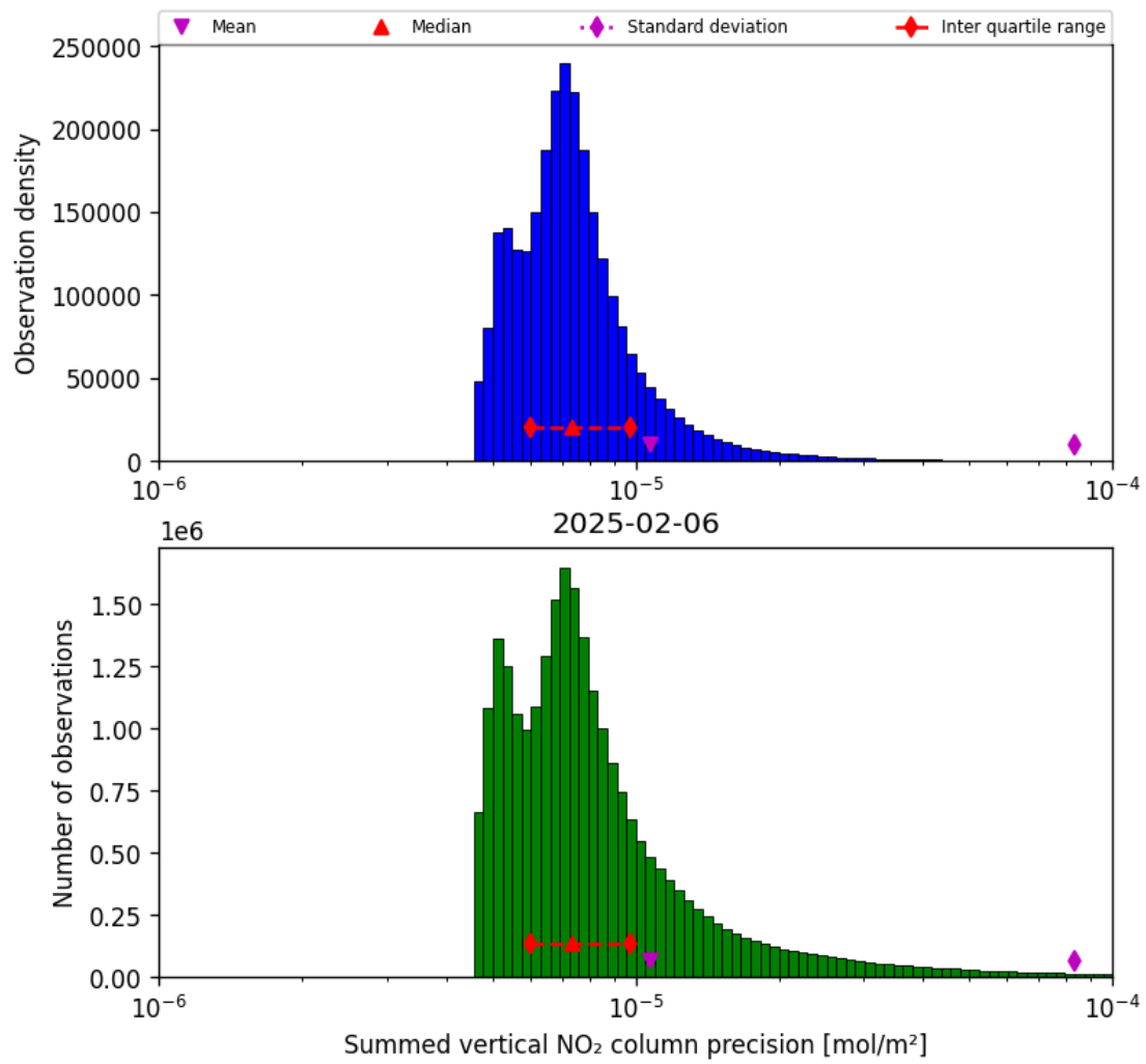
Figure 41: Histogram of "Summed vertical NO 2 column precision" for 2025-02-05 to 2025-02-07
