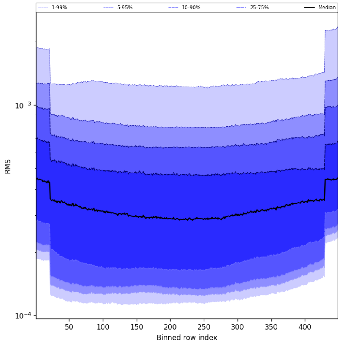
Figure 60: Along track statistics of “RMS” for 2025-02-05 to 2025-02-07
