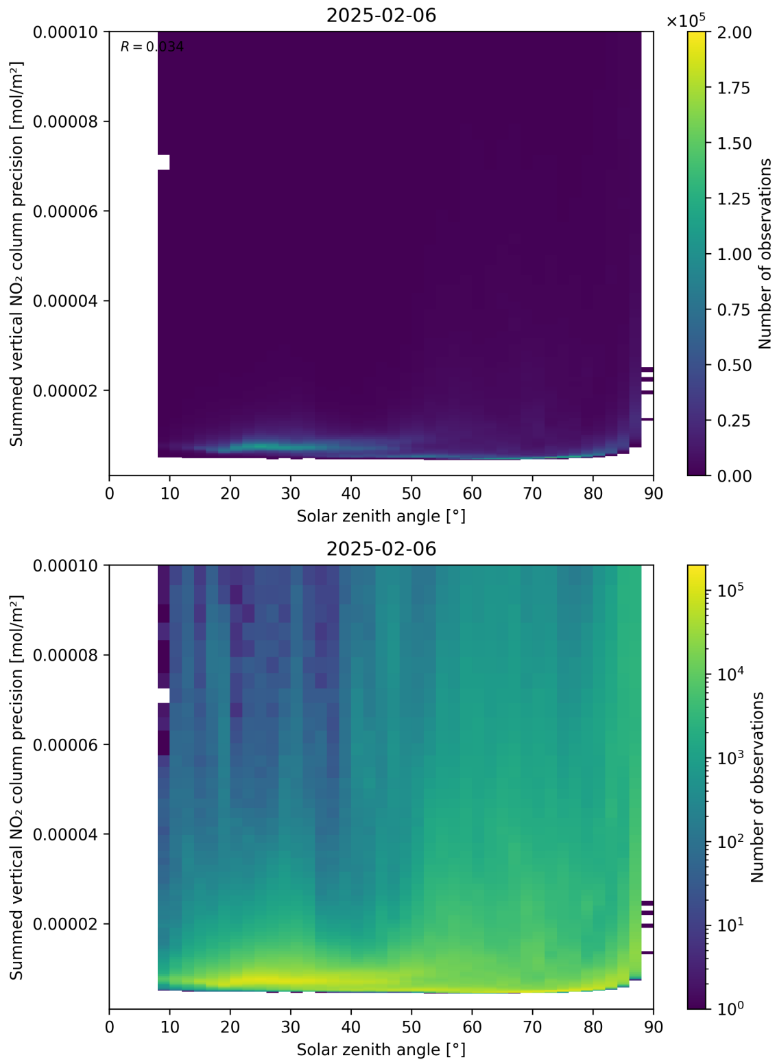
Figure 152: Scatter density plot of “Solar zenith angle” against “Summed vertical NO 2 column precision” for 2025-02-05 to 2025-02-07.
