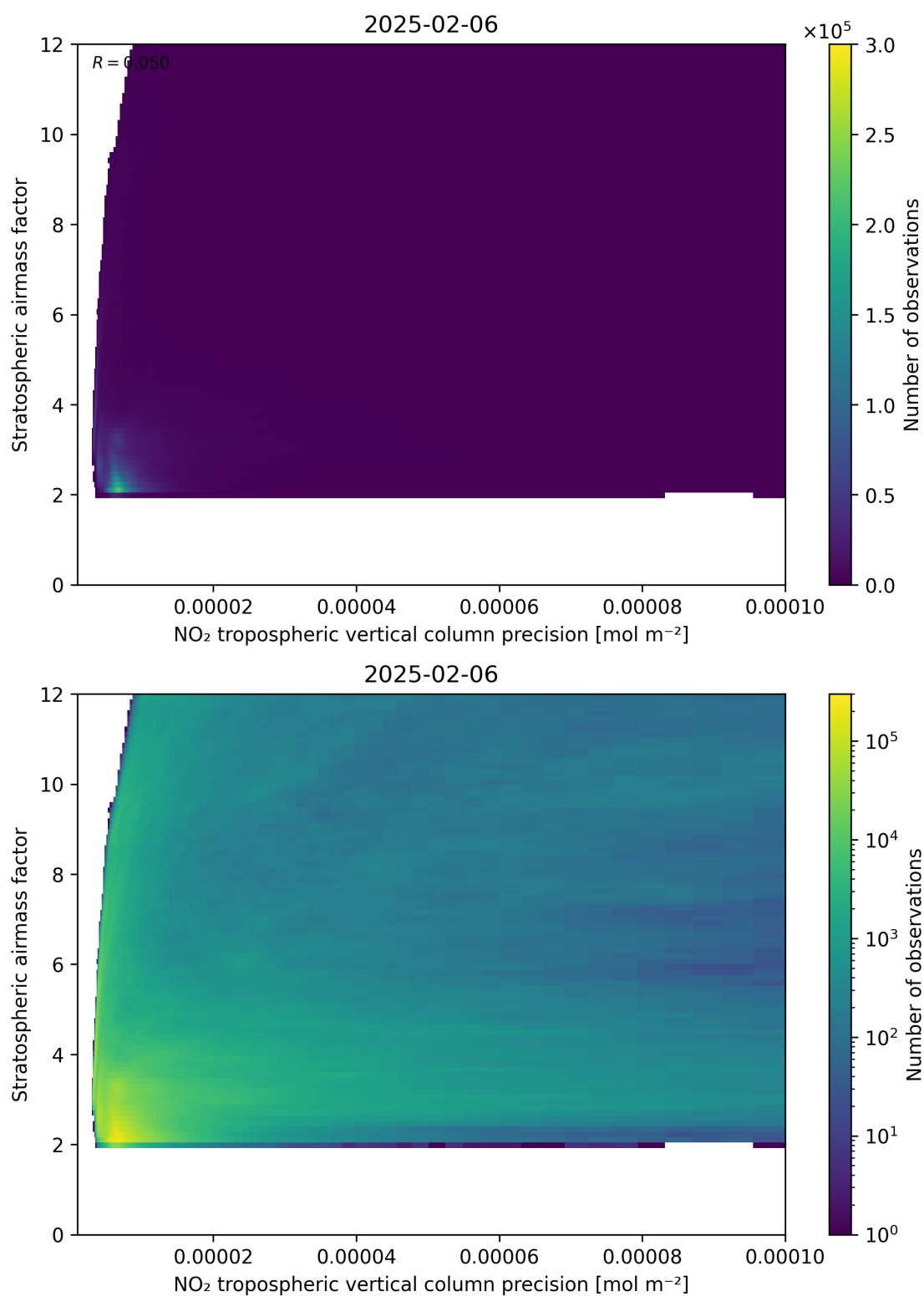
Figure 131: Scatter density plot of “NO 2 tropospheric vertical column precision” against “Stratospheric airmass factor” for 2025-02-05 to 2025-02-07.
