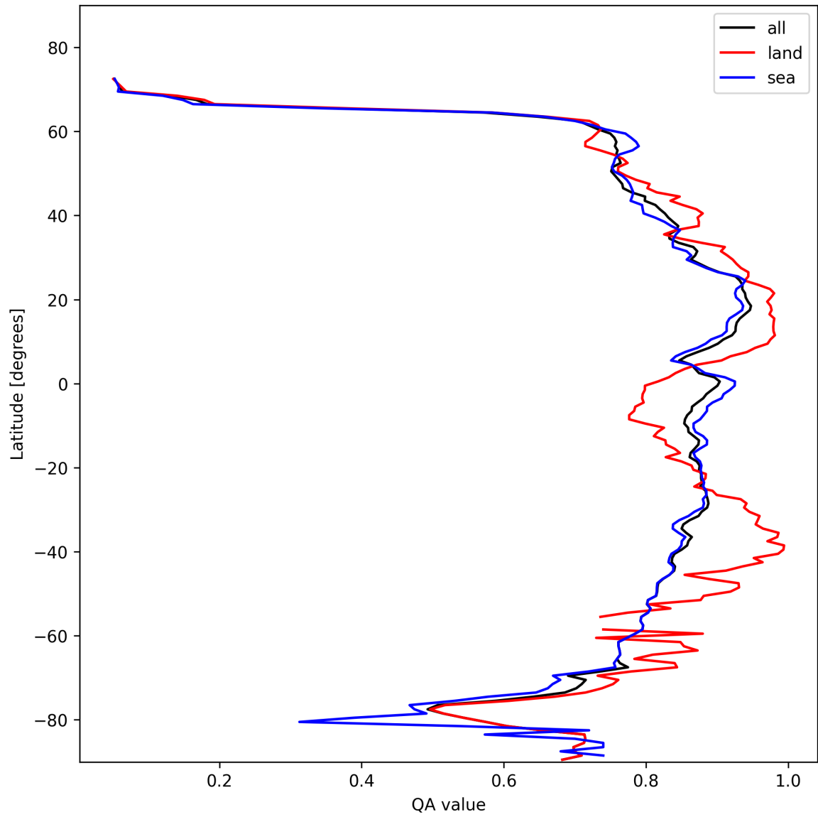
Figure 11: Zonal average of “QA value” for 2025-02-05 to 2025-02-07.
