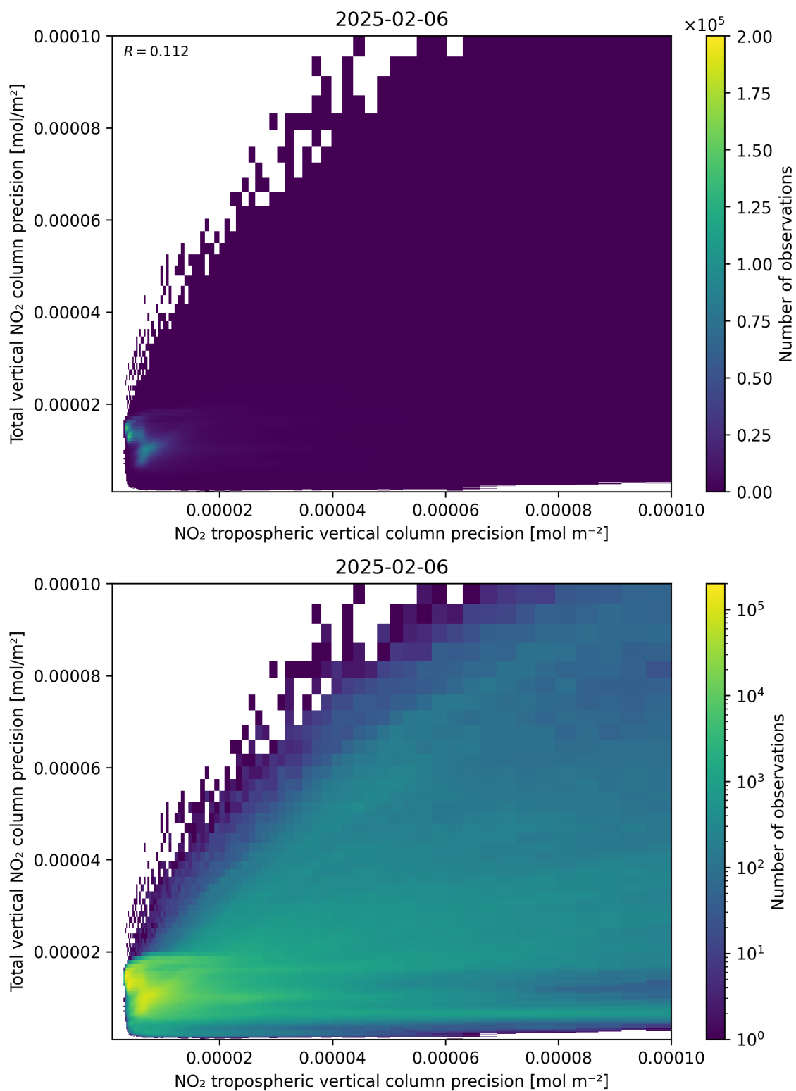
Figure 139: Scatter density plot of “NO 2 tropospheric vertical column precision” against “Total vertical NO 2 column precision” for 2025-02-05 to 2025-02-07.
