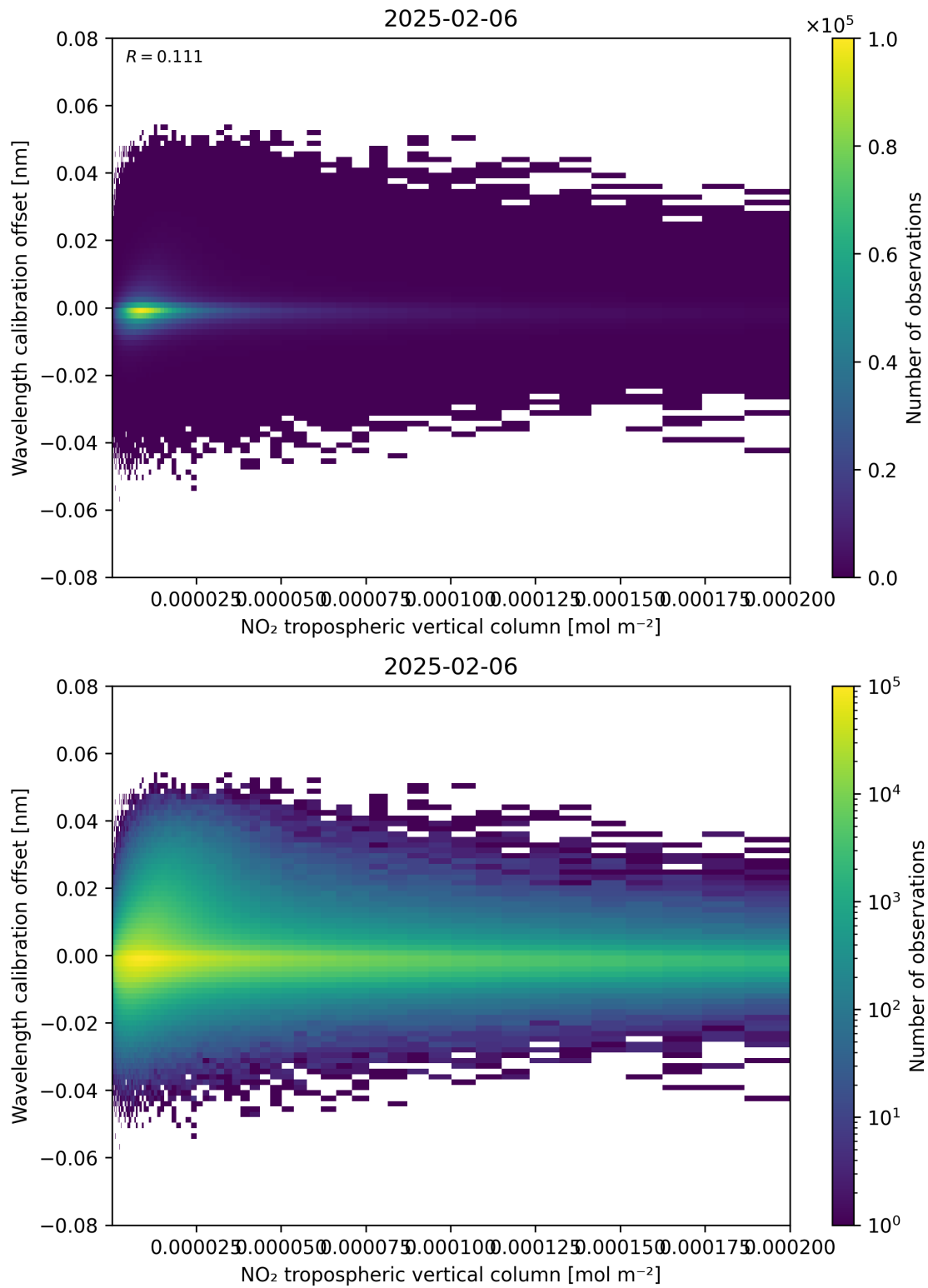
Figure 143: Scatter density plot of “NO 2 tropospheric vertical column” against “Wavelength calibration offset” for 2025-02-05 to 2025-02-07.
