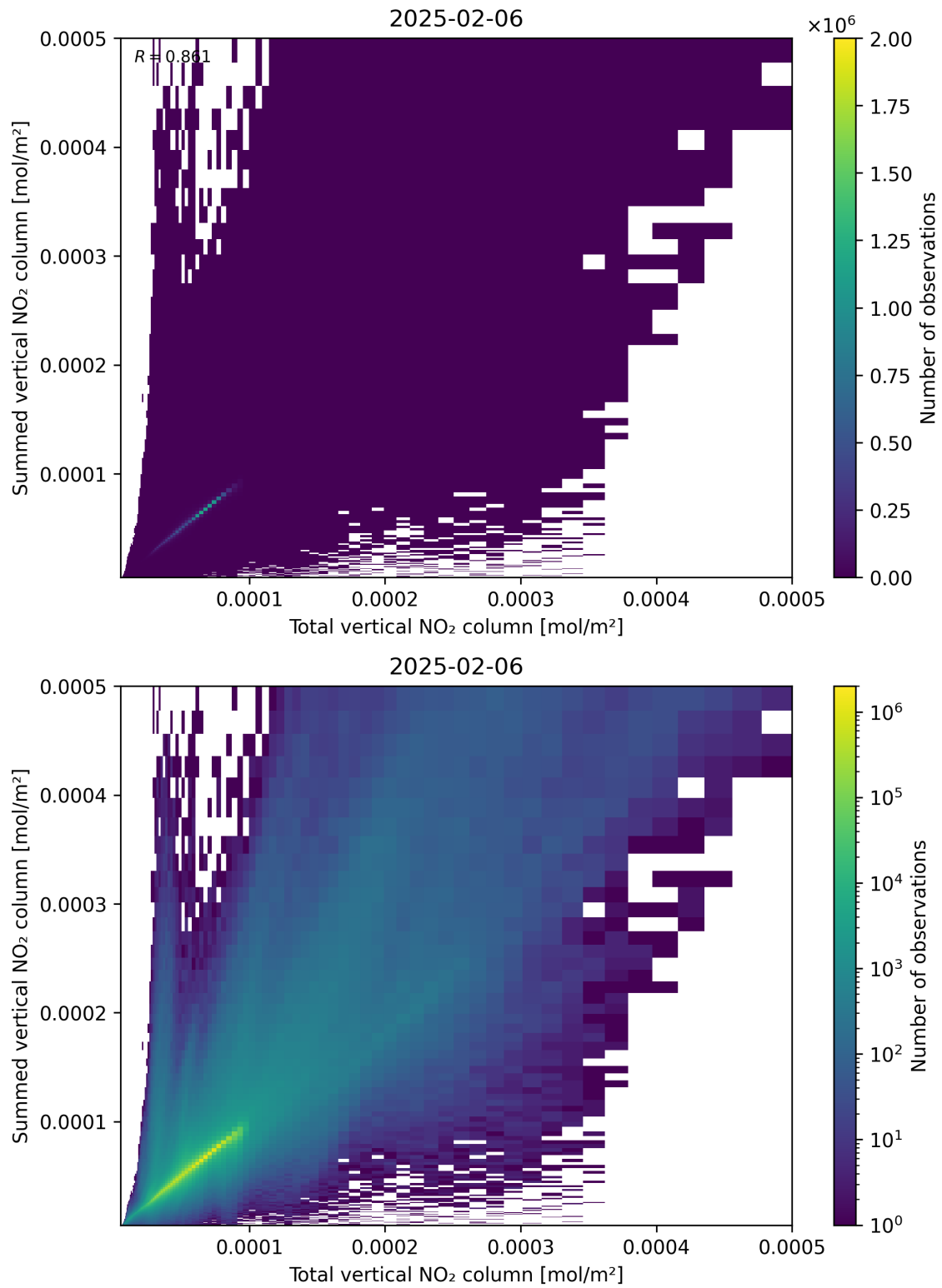
Figure 112: Scatter density plot of “Total vertical NO 2 column” against “Summed vertical NO 2 column” for 2025-02-05 to 2025-02-07.
