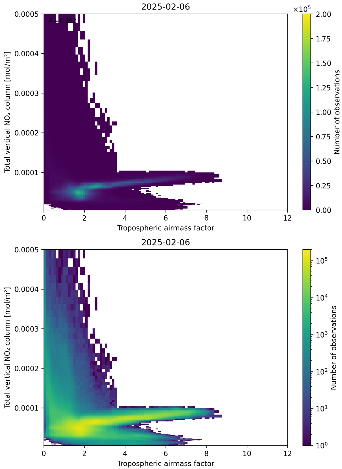
Figure 77: Scatter density plot of “Tropospheric airmass factor” against “Total vertical NO 2 column” for 2025-02-05 to 2025-02-07.
