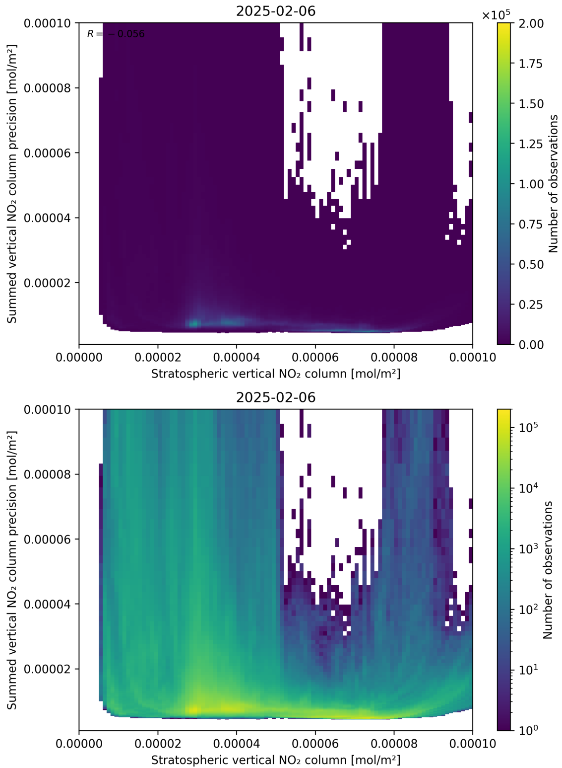
Figure 99: Scatter density plot of “Stratospheric vertical NO 2 column” against “Summed vertical NO 2 column precision” for 2025-02-05 to 2025-02-07.
