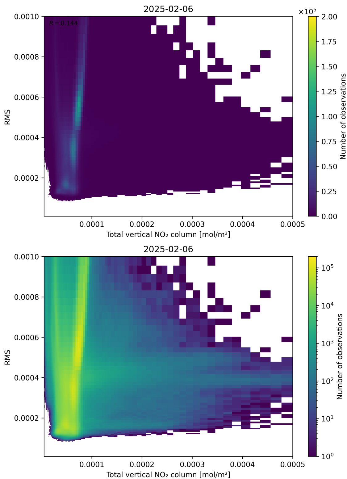
Figure 120: Scatter density plot of “Total vertical NO 2 column” against “RMS” for 2025-02-05 to 2025-02-07.
