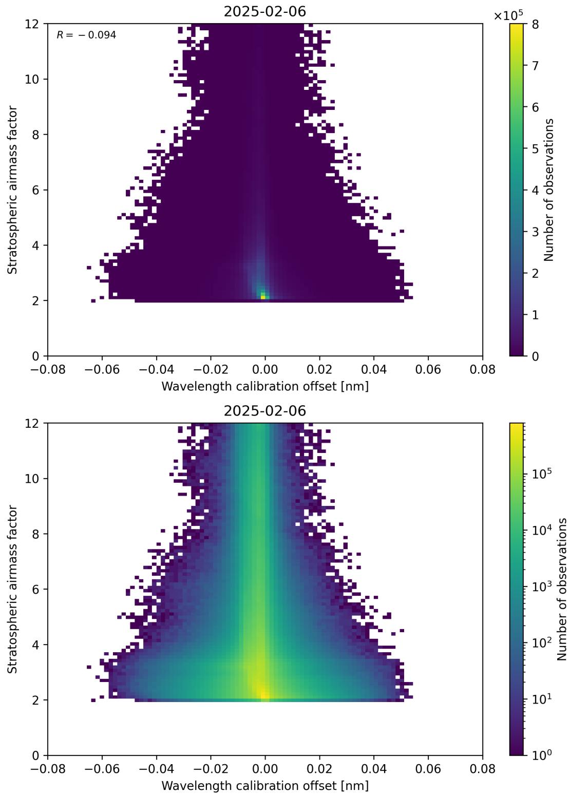
Figure 174: Scatter density plot of “Wavelength calibration offset” against “Stratospheric airmass factor” for 2025-02-05 to 2025-02-07.
