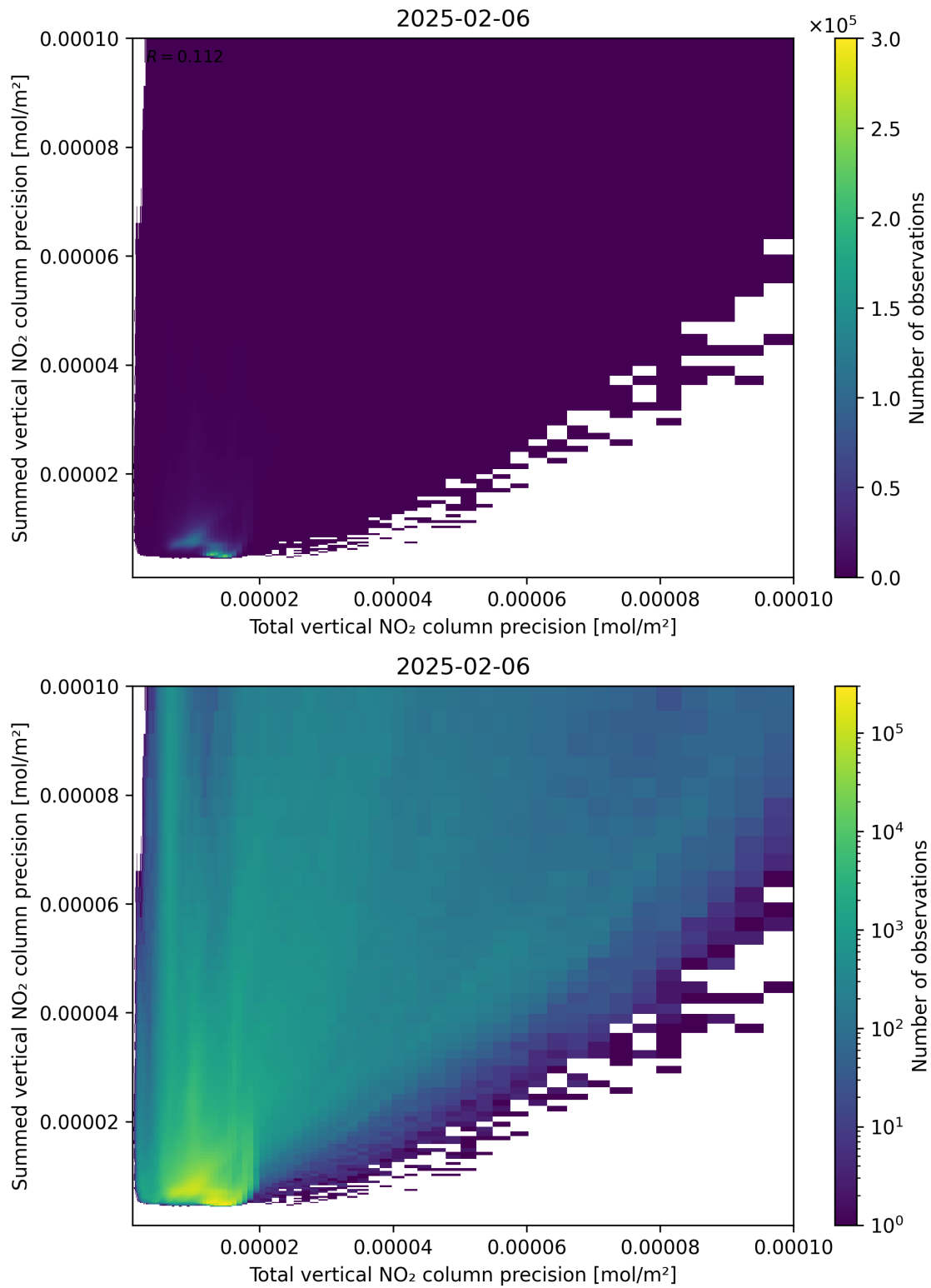
Figure 118: Scatter density plot of “Total vertical NO 2 column precision” against “Summed vertical NO 2 column precision” for 2025-02-05 to 2025-02-07.
