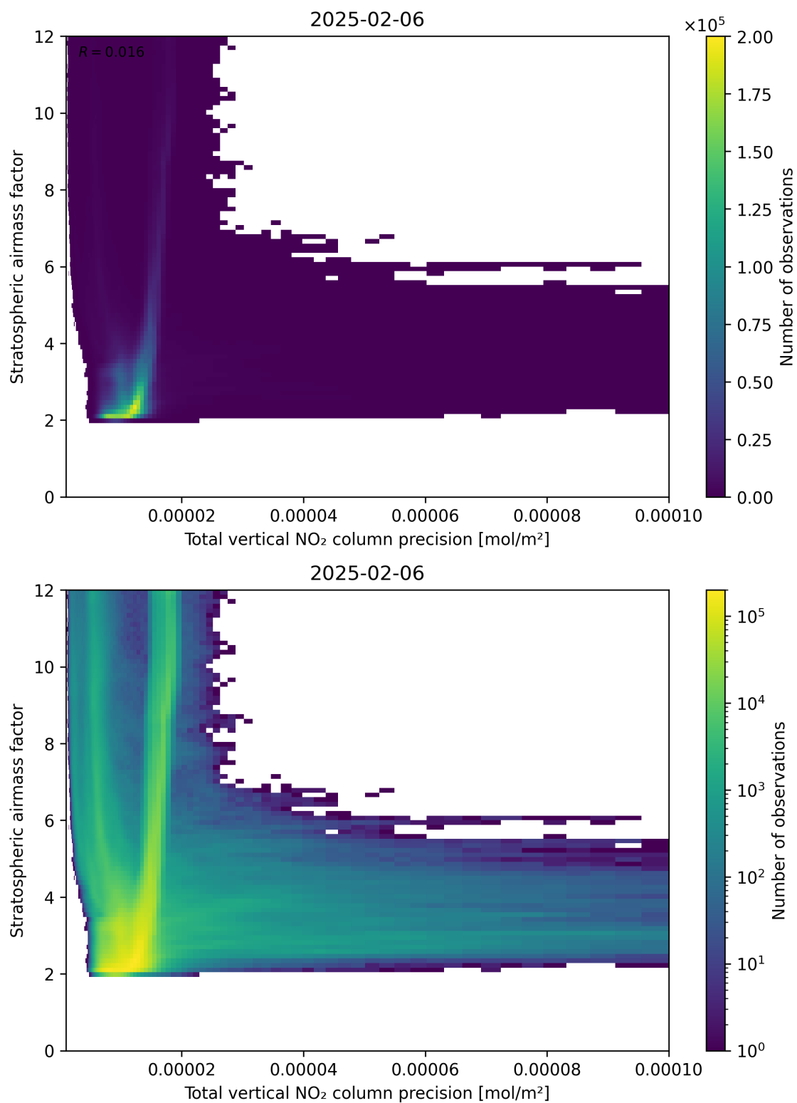
Figure 115: Scatter density plot of “Total vertical NO 2 column precision” against “Stratospheric airmass factor” for 2025-02-05 to 2025-02-07.
