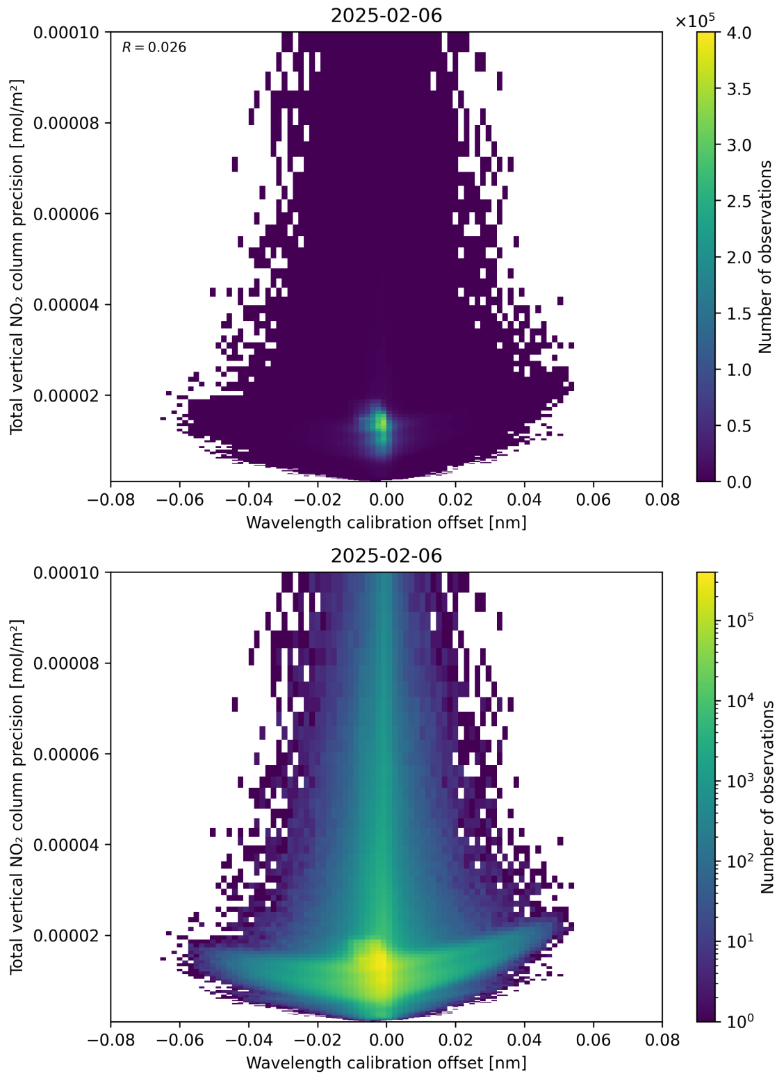
Figure 180: Scatter density plot of “Wavelength calibration offset” against “Total vertical NO 2 column precision” for 2025-02-05 to 2025-02-07.
