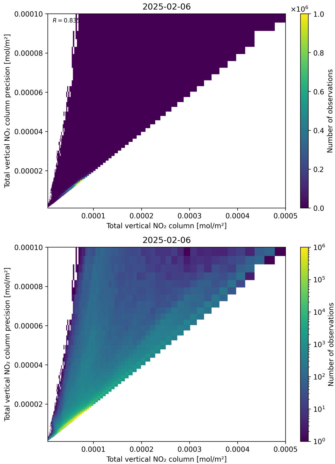
Figure 114: Scatter density plot of “Total vertical NO 2 column” against “Total vertical NO 2 column precision” for 2025-02-05 to 2025-02-07.
