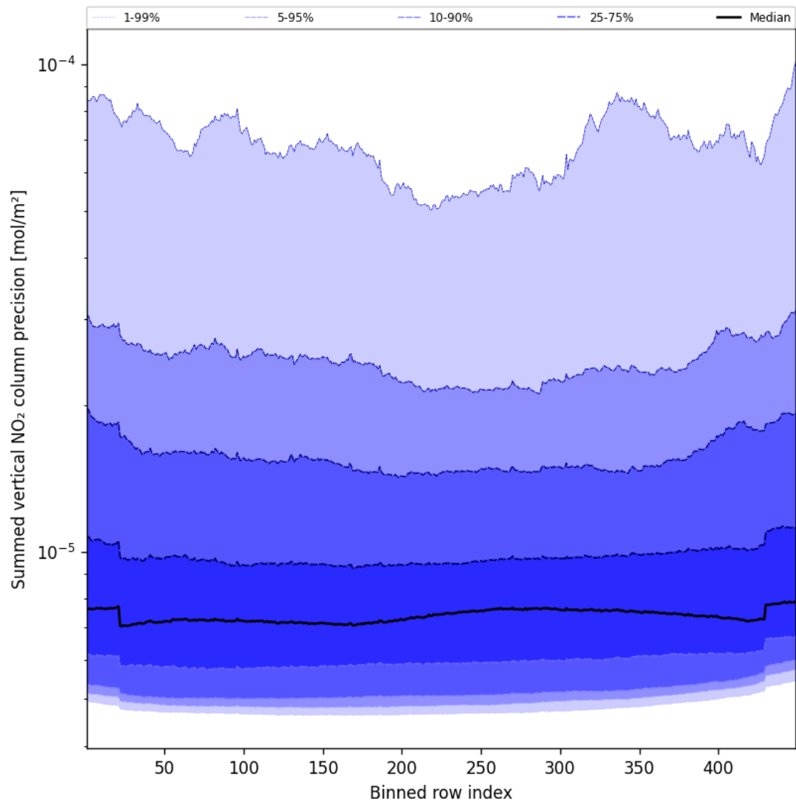
Figure 58: Along track statistics of “Summed vertical NO 2 column precision” for 2025-02-05 to 2025-02-07
