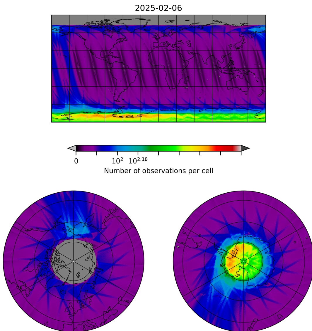
Figure 10: Map of the number of observations for 2025-02-05 to 2025-02-07
