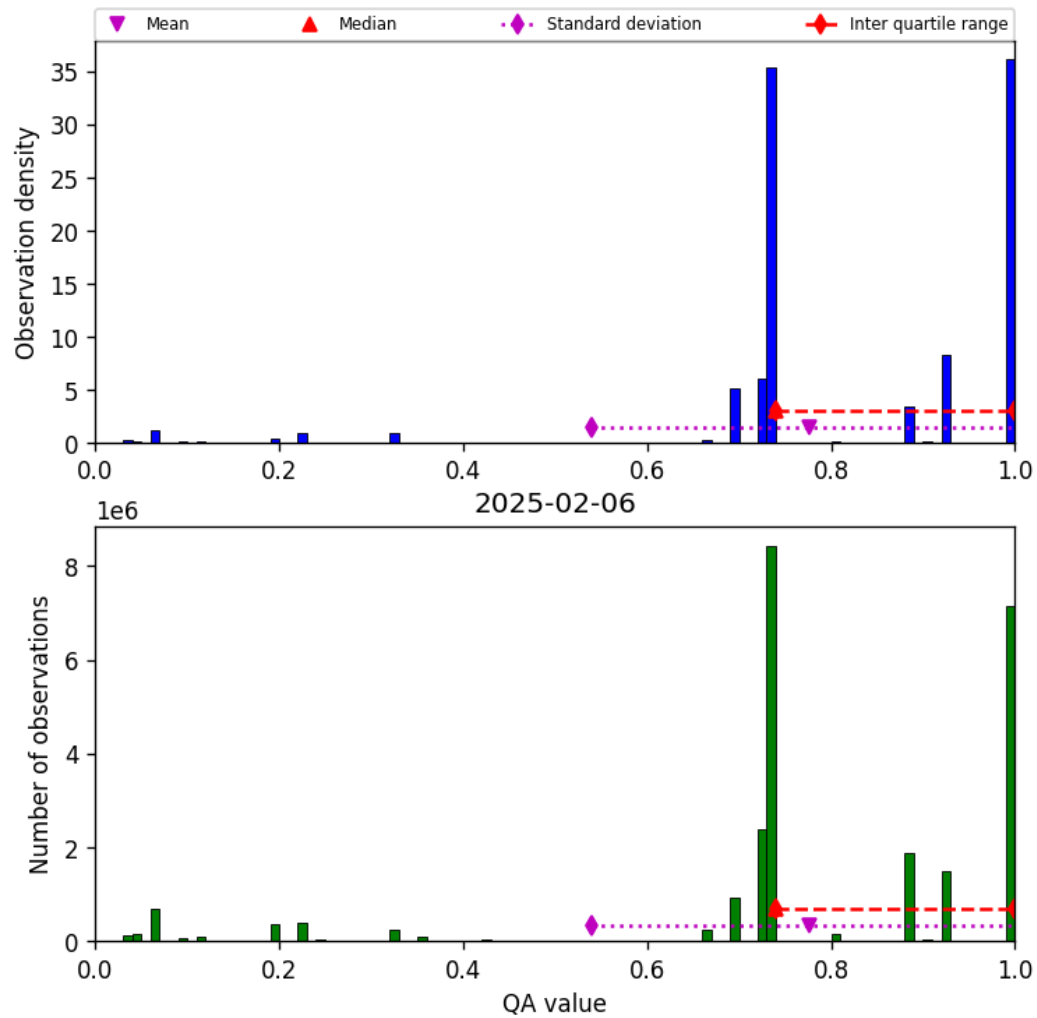
Figure 28: Histogram of “QA value” for 2025-02-05 to 2025-02-07
