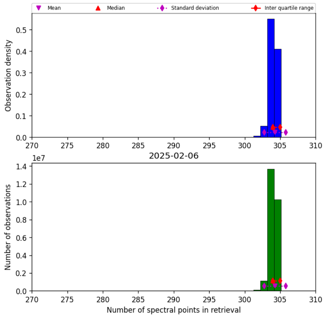
Figure 33: Histogram of “Number of spectral points in retrieval” for 2025-02-05 to 2025-02-07
