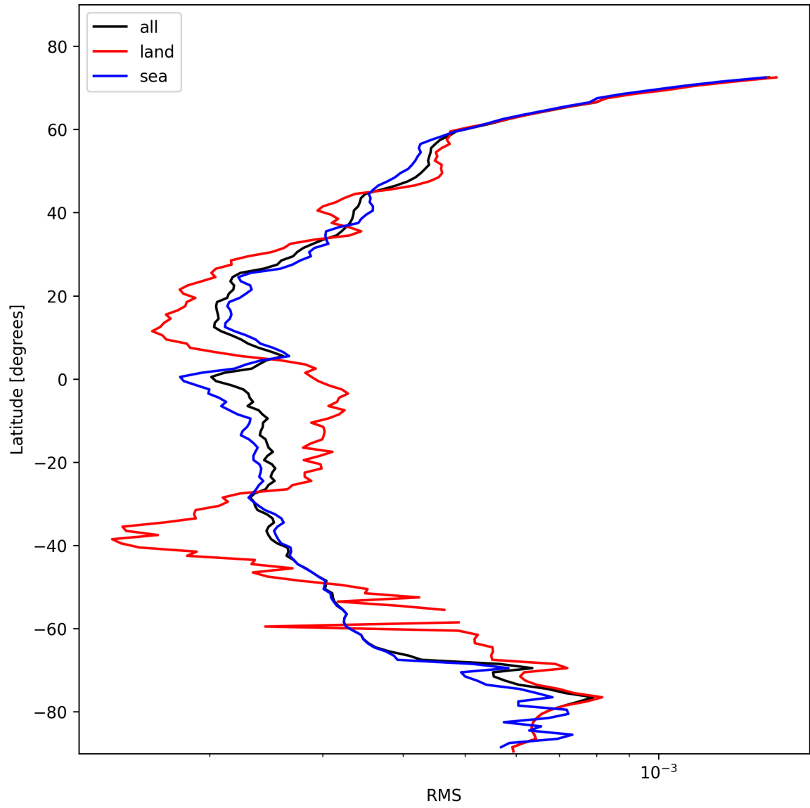
Figure 26: Zonal average of “RMS” for 2025-02-05 to 2025-02-07.
