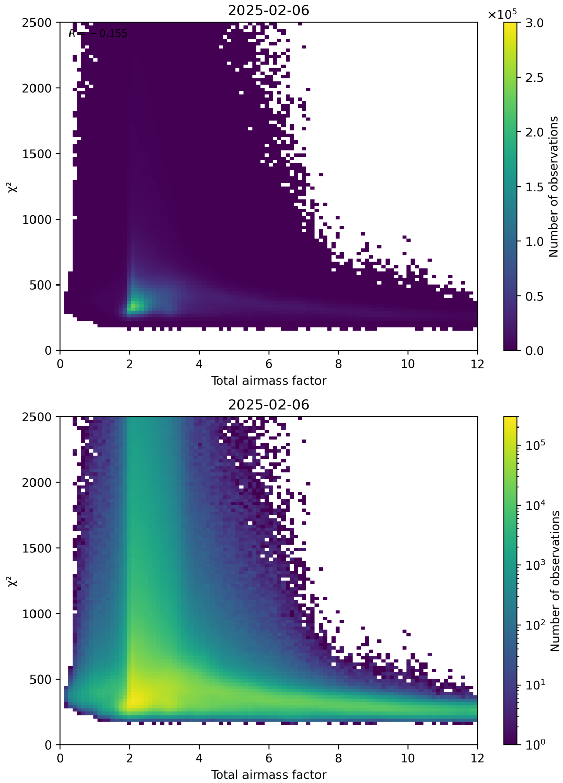
Figure 63: Scatter density plot of “Total airmass factor” against “ \chi^2 ” for 2025-02-05 to 2025-02-07.
