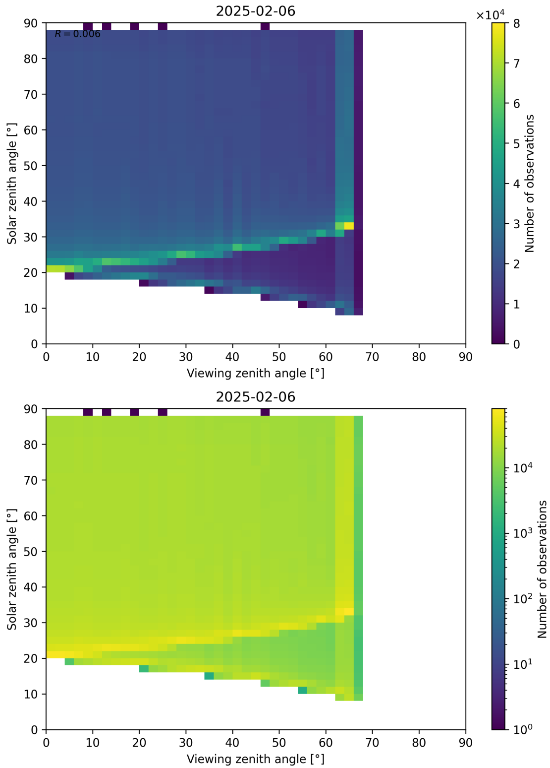
Figure 172: Scatter density plot of “Viewing zenith angle” against “Solar zenith angle” for 2025-02-05 to 2025-02-07.
