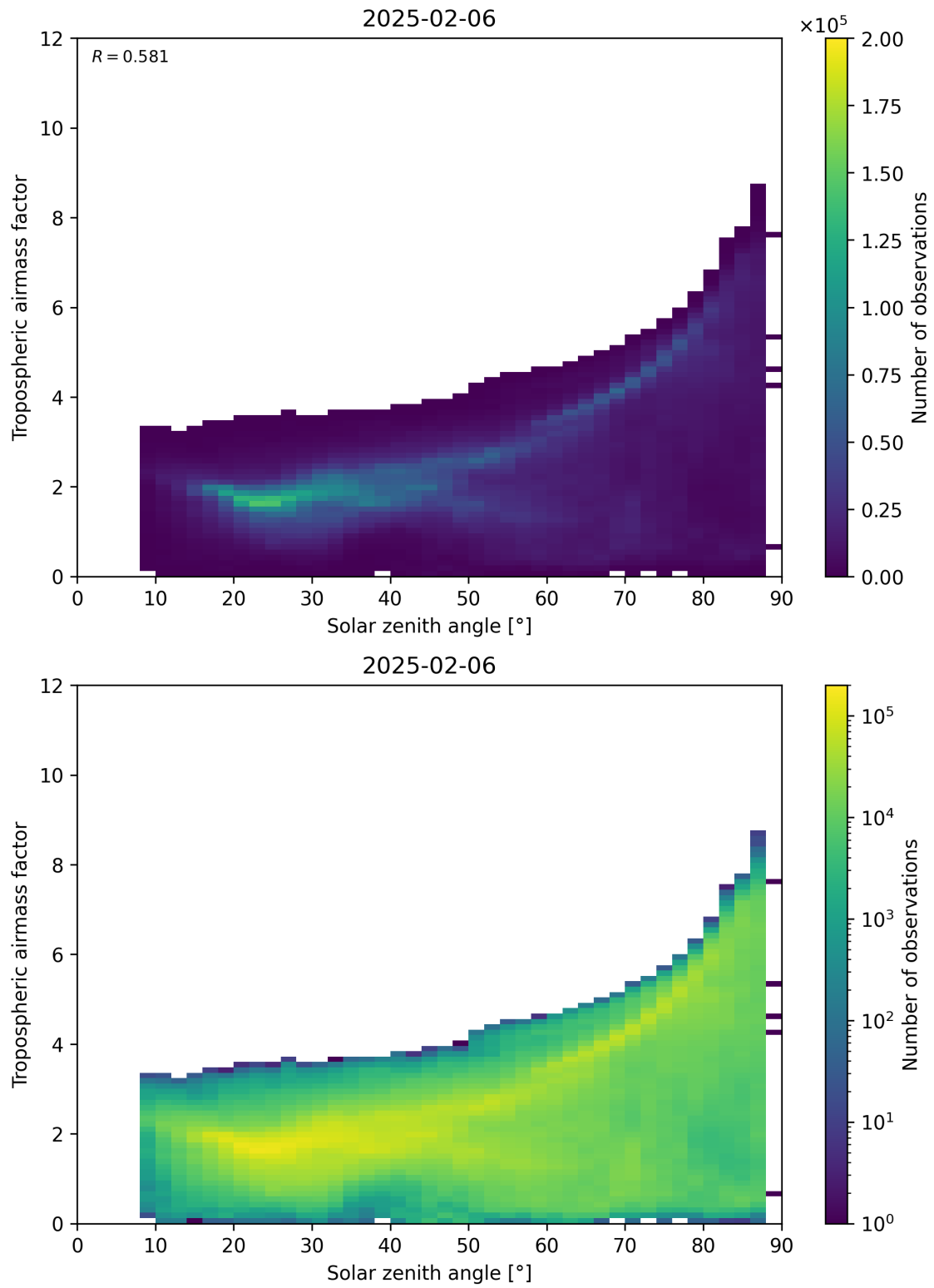
Figure 147: Scatter density plot of “Solar zenith angle” against “Tropospheric airmass factor” for 2025-02-05 to 2025-02-07.
