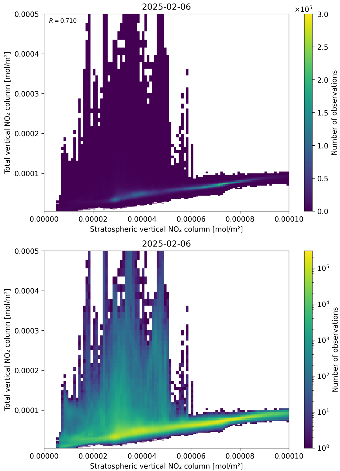
Figure 100: Scatter density plot of “Stratospheric vertical NO 2 column” against “Total vertical NO 2 column” for 2025-02-05 to 2025-02-07.
