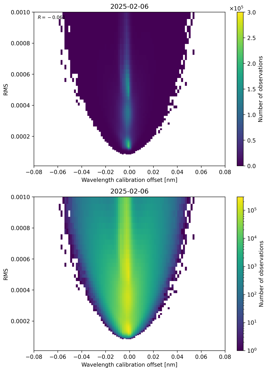
Figure 181: Scatter density plot of “Wavelength calibration offset” against “RMS” for 2025-02-05 to 2025-02-07.
