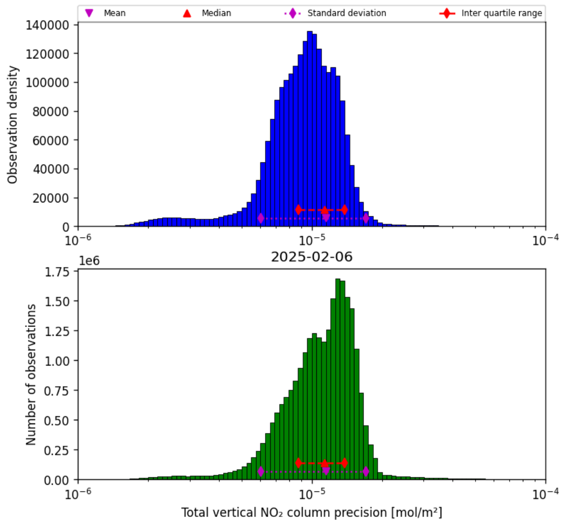
Figure 39: Histogram of “Total vertical NO 2 column precision” for 2025-02-05 to 2025-02-07
