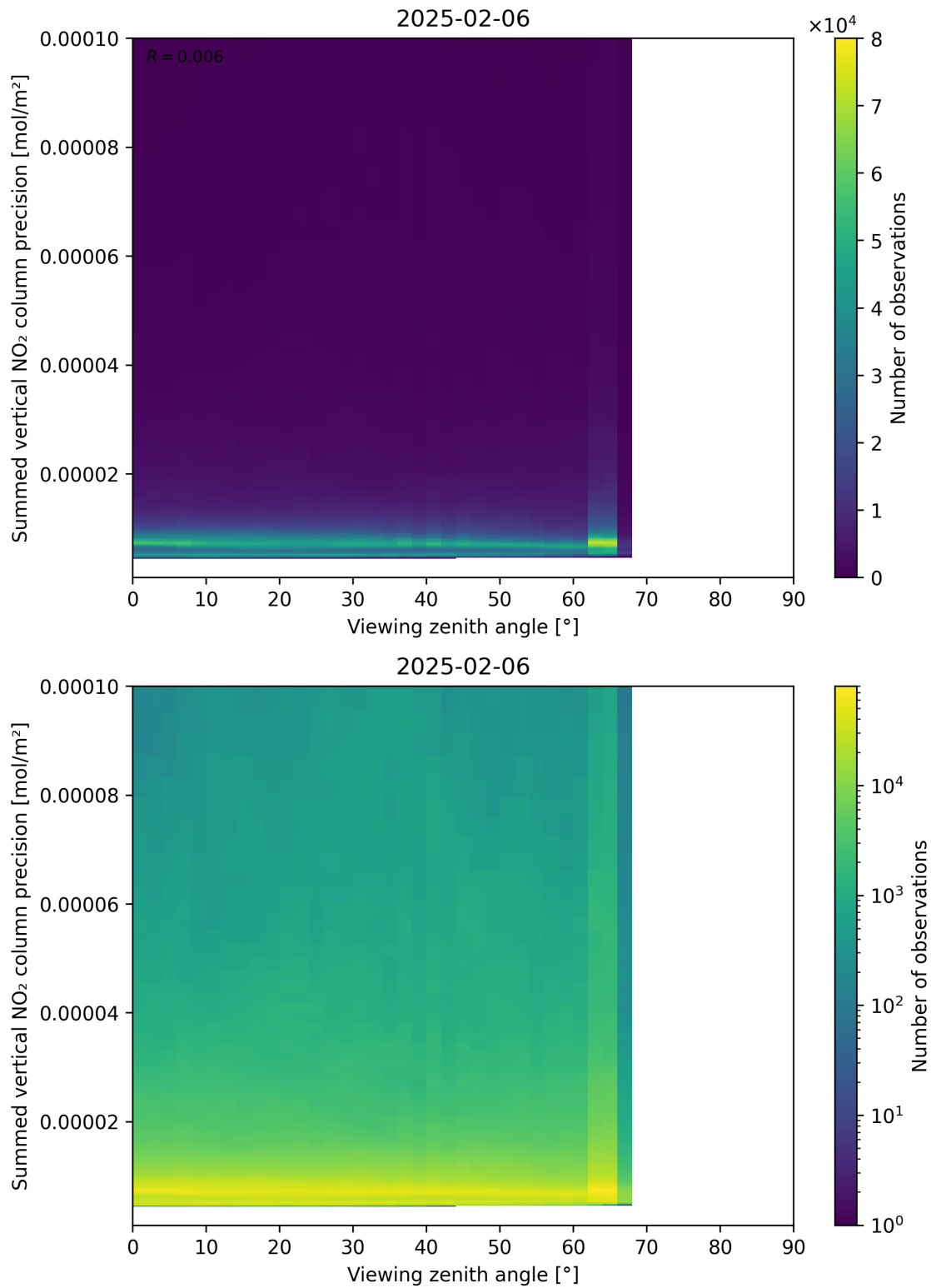
Figure 166: Scatter density plot of “Viewing zenith angle” against “Summed vertical NO 2 column precision” for 2025-02-05 to 2025-02-07.
