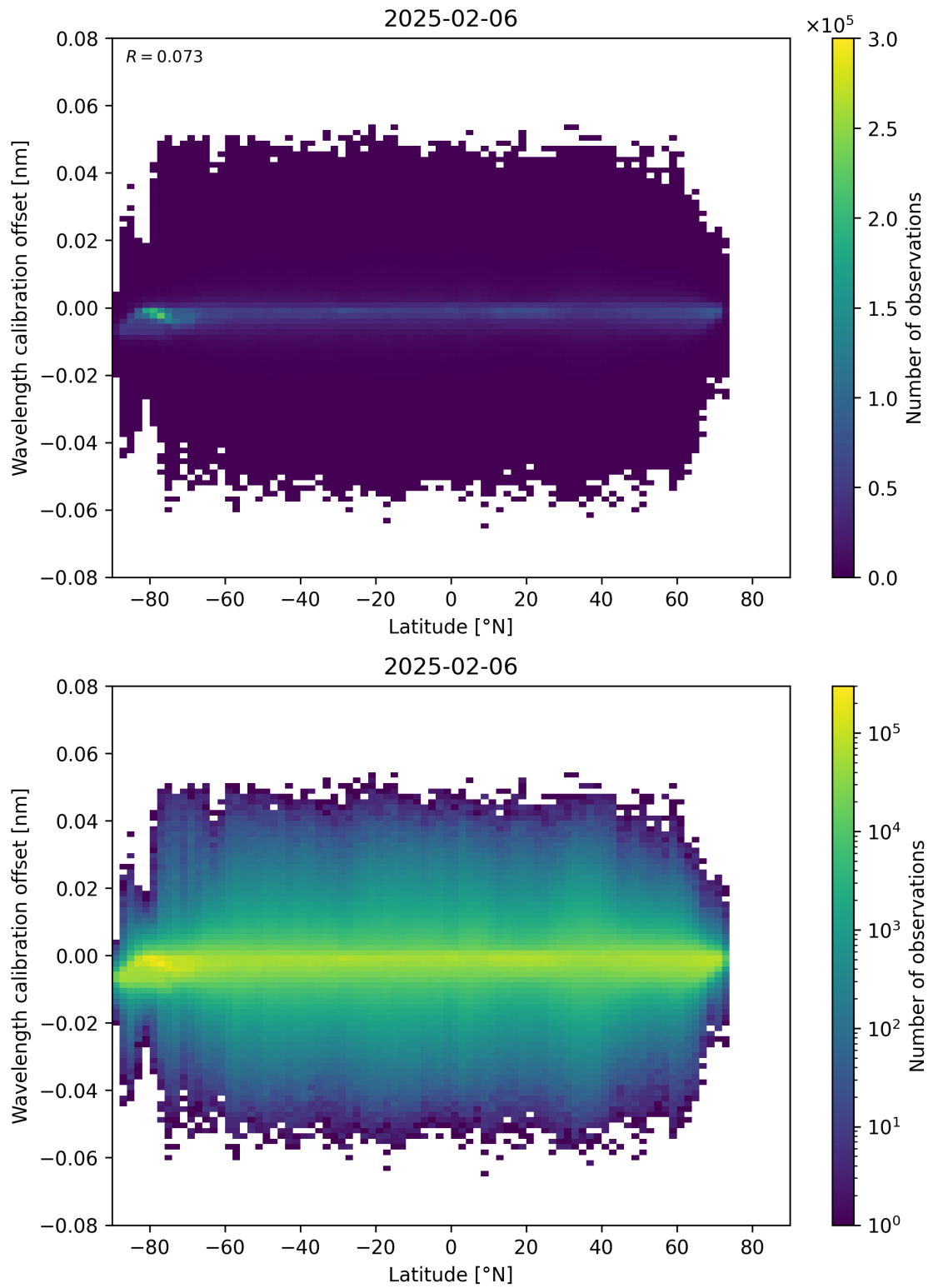
Figure 95: Scatter density plot of “Latitude” against “Wavelength calibration offset” for 2025-02-05 to 2025-02-07.
