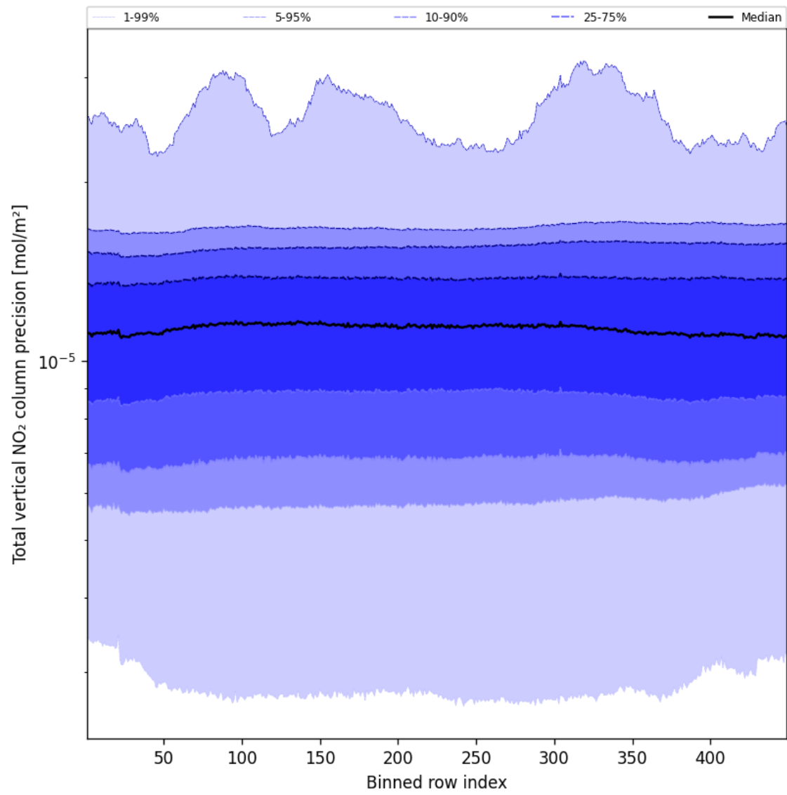
Figure 56: Along track statistics of “Total vertical NO 2 column precision” for 2025-02-05 to 2025-02-07
