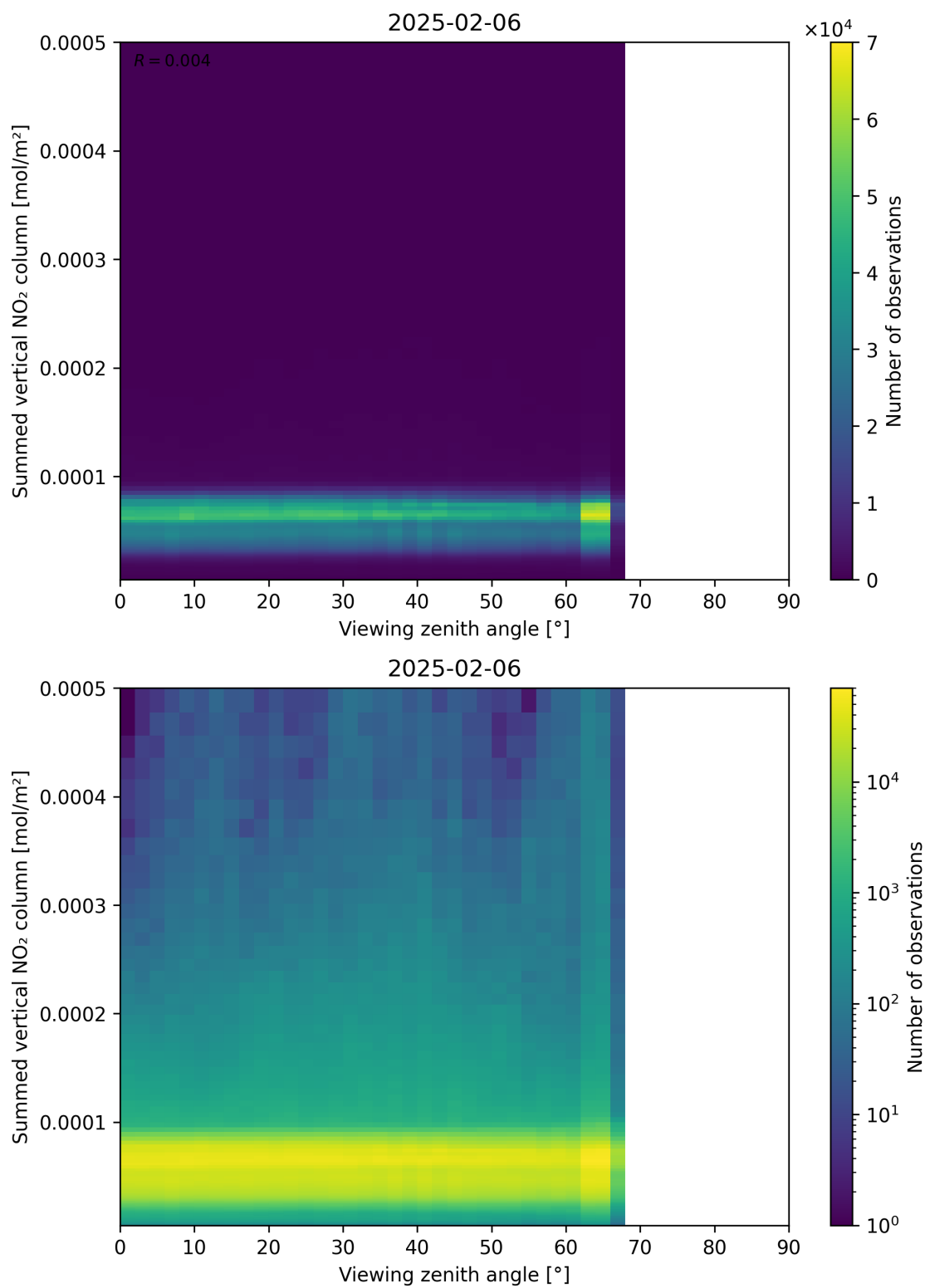
Figure 165: Scatter density plot of “Viewing zenith angle” against “Summed vertical NO 2 column” for 2025-02-05 to 2025-02-07.
