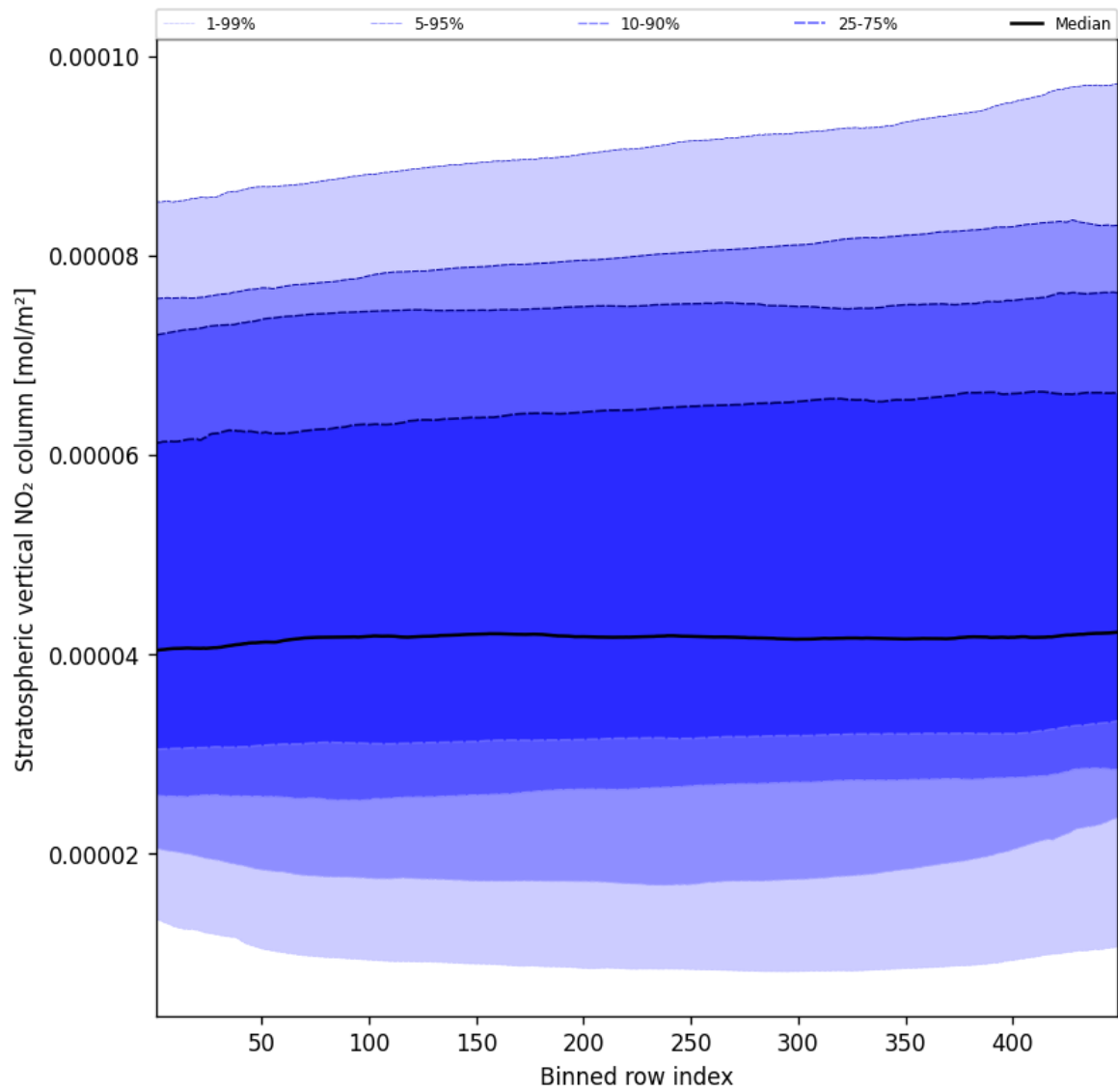
Figure 53: Along track statistics of “Stratospheric vertical NO 2 column” for 2025-02-05 to 2025-02-07
