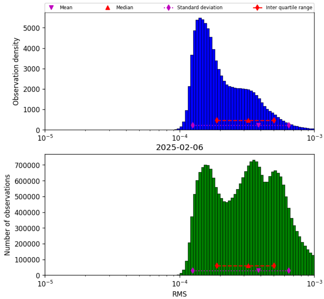
Figure 43: Histogram of “RMS” for 2025-02-05 to 2025-02-07
