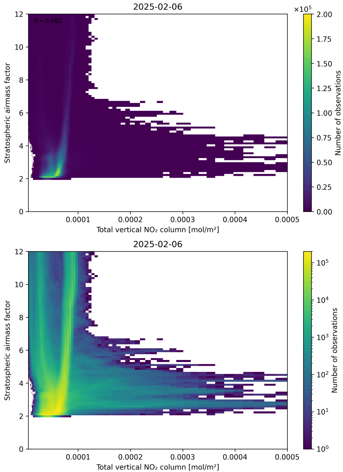
Figure 110: Scatter density plot of “Total vertical NO 2 column” against “Stratospheric airmass factor” for 2025-02-05 to 2025-02-07.
