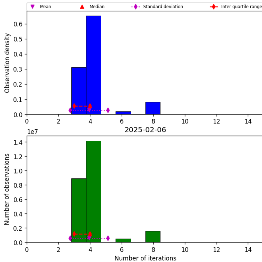
Figure 34: Histogram of “Number of iterations” for 2025-02-05 to 2025-02-07
