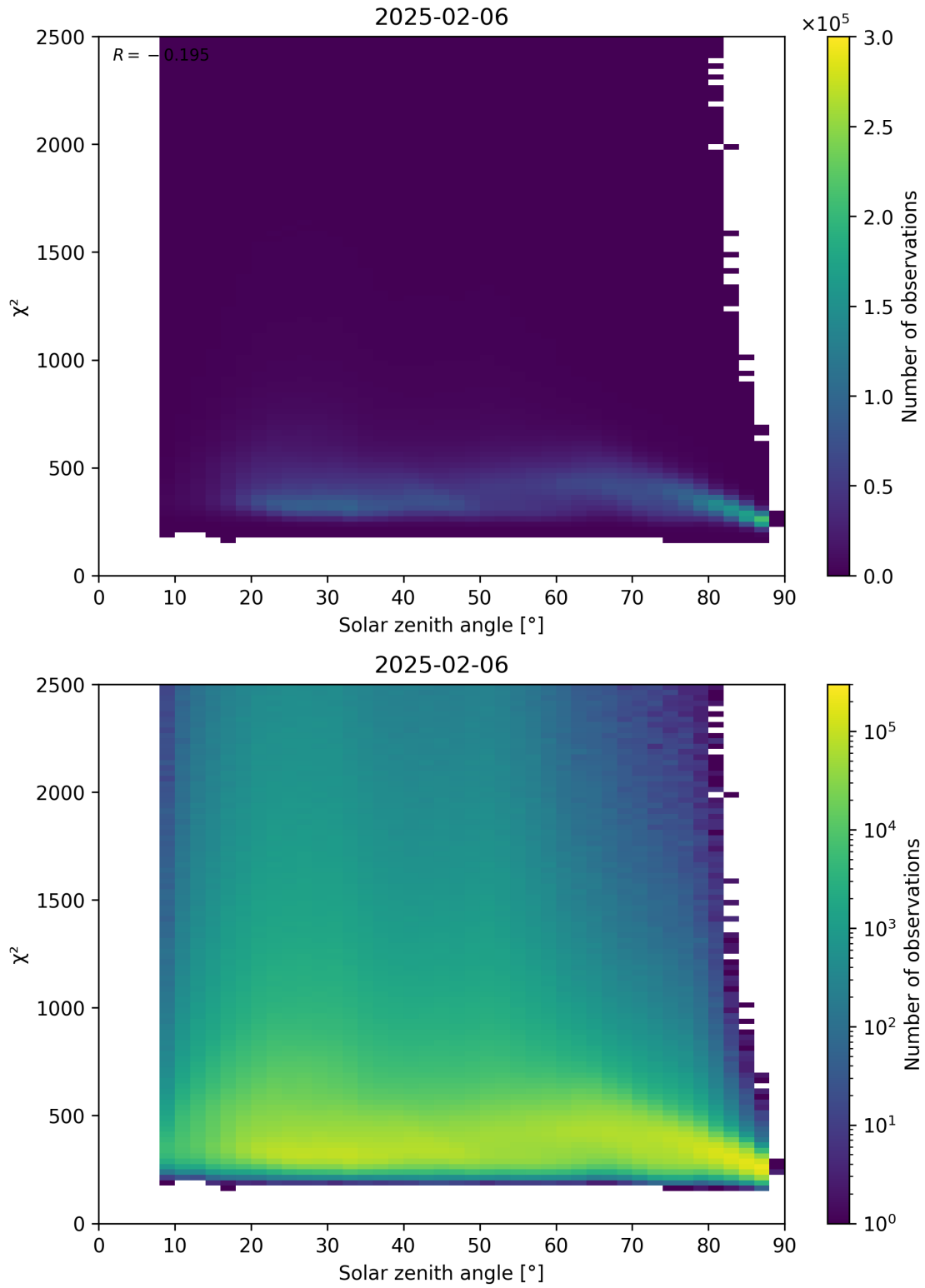
Figure 148: Scatter density plot of “Solar zenith angle” against “ \chi^2 ” for 2025-02-05 to 2025-02-07.
