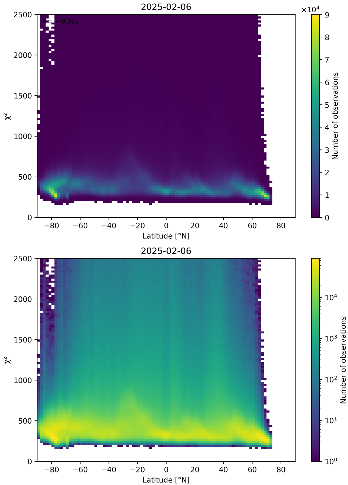
Figure 86: Scatter density plot of “Latitude” against “ \chi^2 ” for 2025-02-05 to 2025-02-07.
