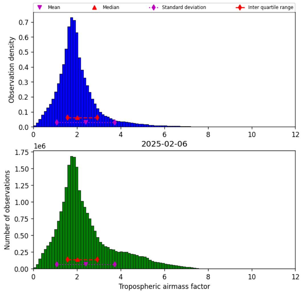
Figure 31: Histogram of “Tropospheric airmass factor” for 2025-02-05 to 2025-02-07
