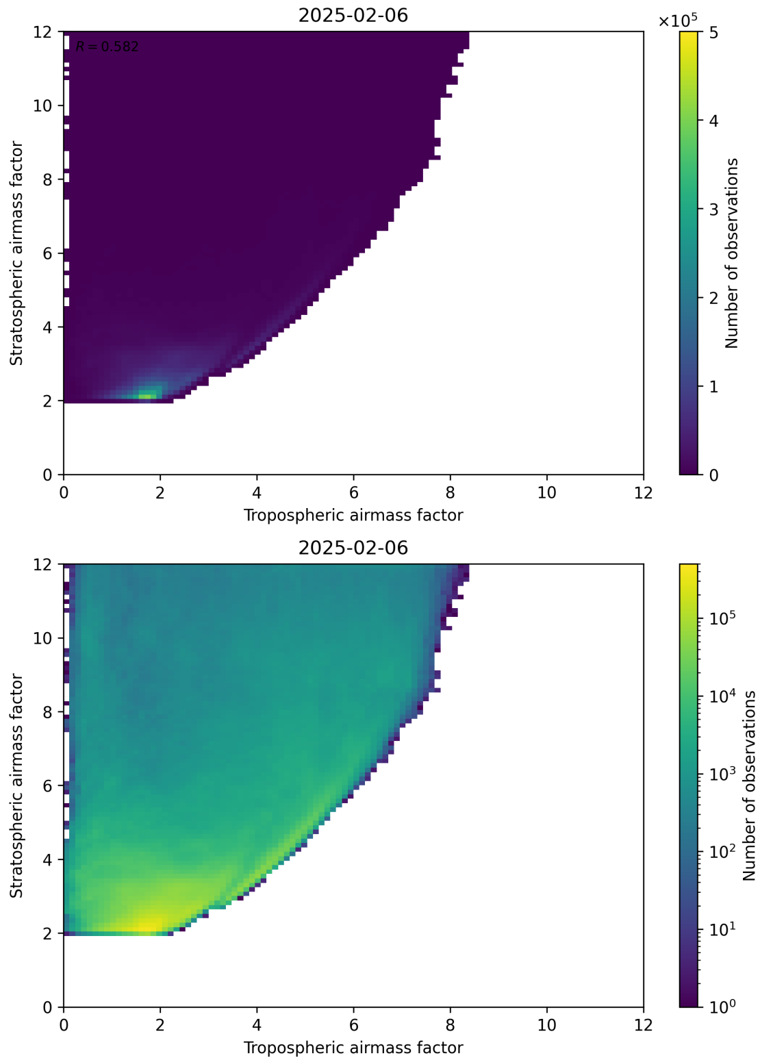
Figure 71: Scatter density plot of “Tropospheric airmass factor” against “Stratospheric airmass factor” for 2025-02-05 to 2025-02-07.
