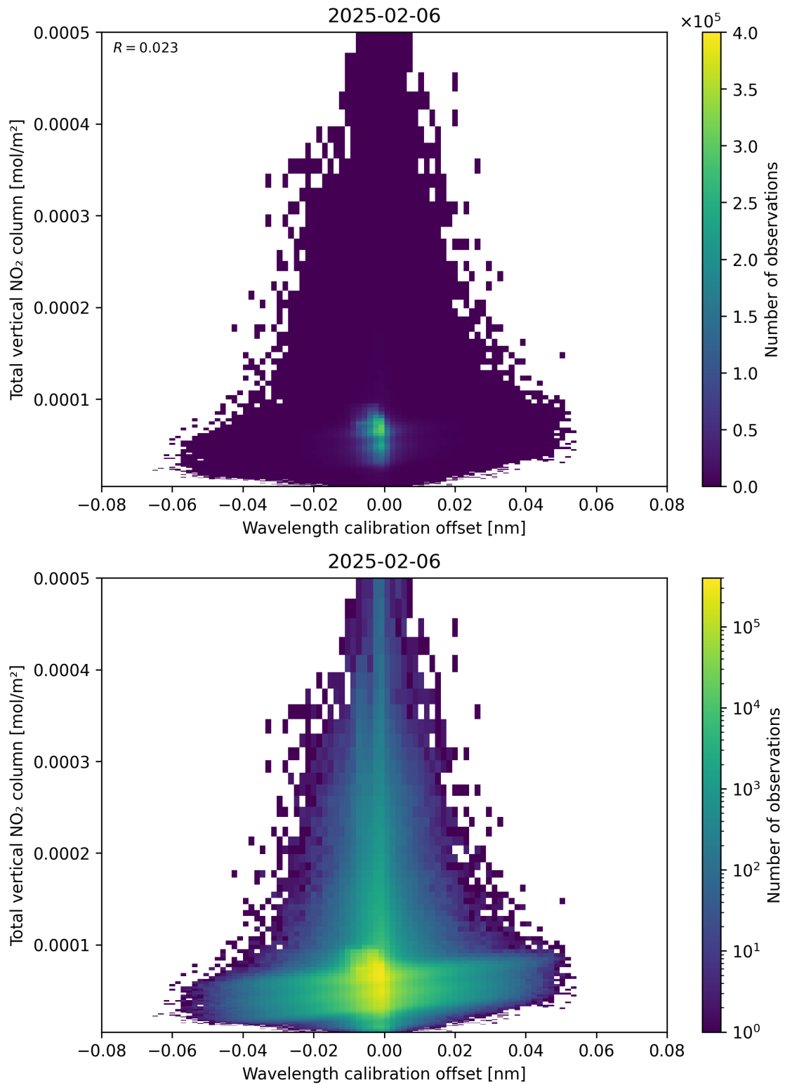
Figure 179: Scatter density plot of “Wavelength calibration offset” against “Total vertical NO 2 column” for 2025-02-05 to 2025-02-07.
