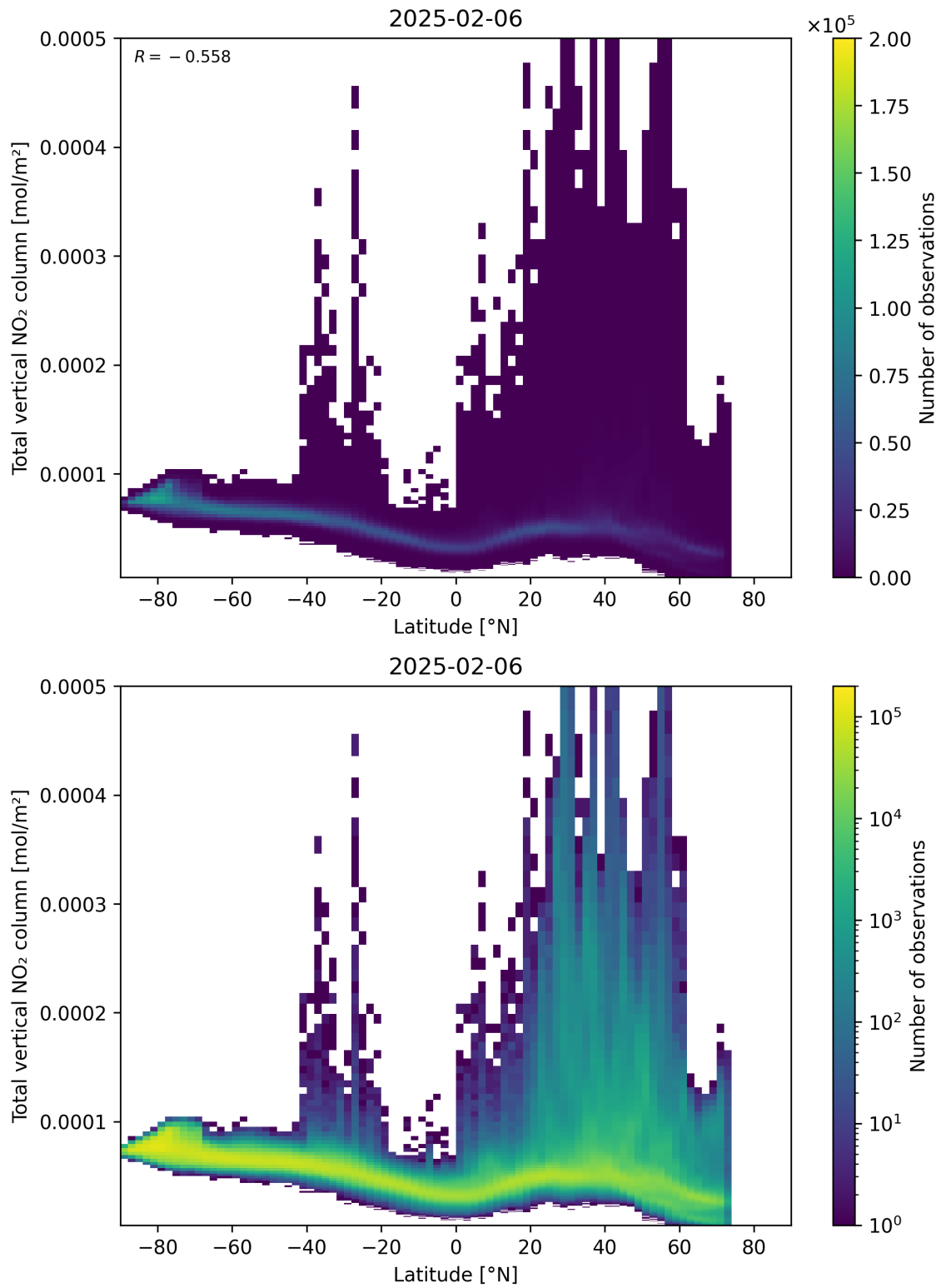
Figure 90: Scatter density plot of “Latitude” against “Total vertical NO 2 column” for 2025-02-05 to 2025-02-07.
