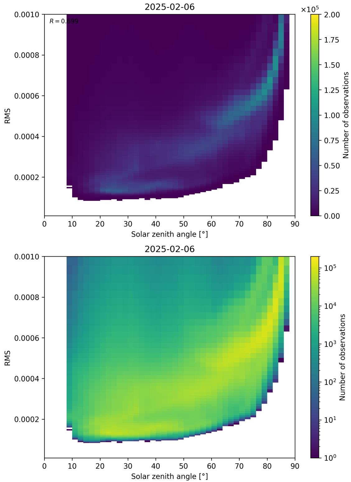
Figure 157: Scatter density plot of “Solar zenith angle” against “RMS” for 2025-02-05 to 2025-02-07.
