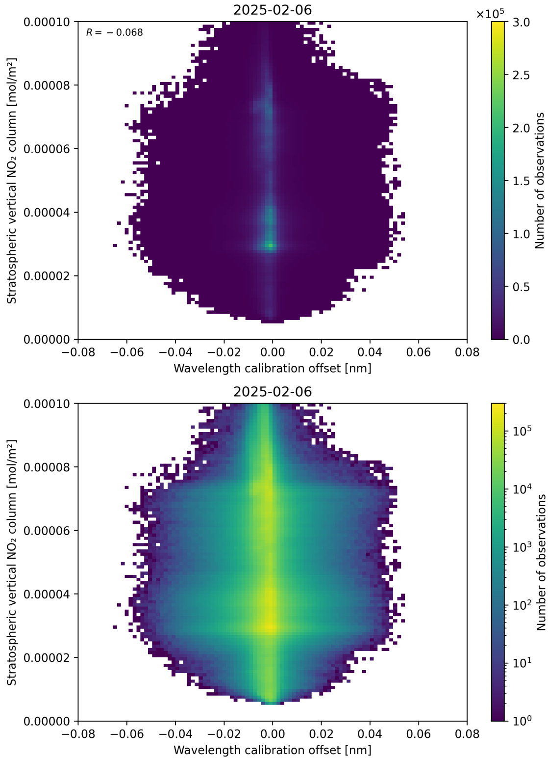
Figure 176: Scatter density plot of “Wavelength calibration offset” against “Stratospheric vertical NO 2 column” for 2025-02-05 to 2025-02-07.
