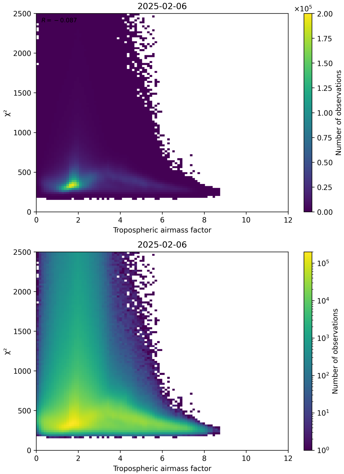
Figure 73: Scatter density plot of “Tropospheric airmass factor” against “ \chi^2 ” for 2025-02-05 to 2025-02-07.
