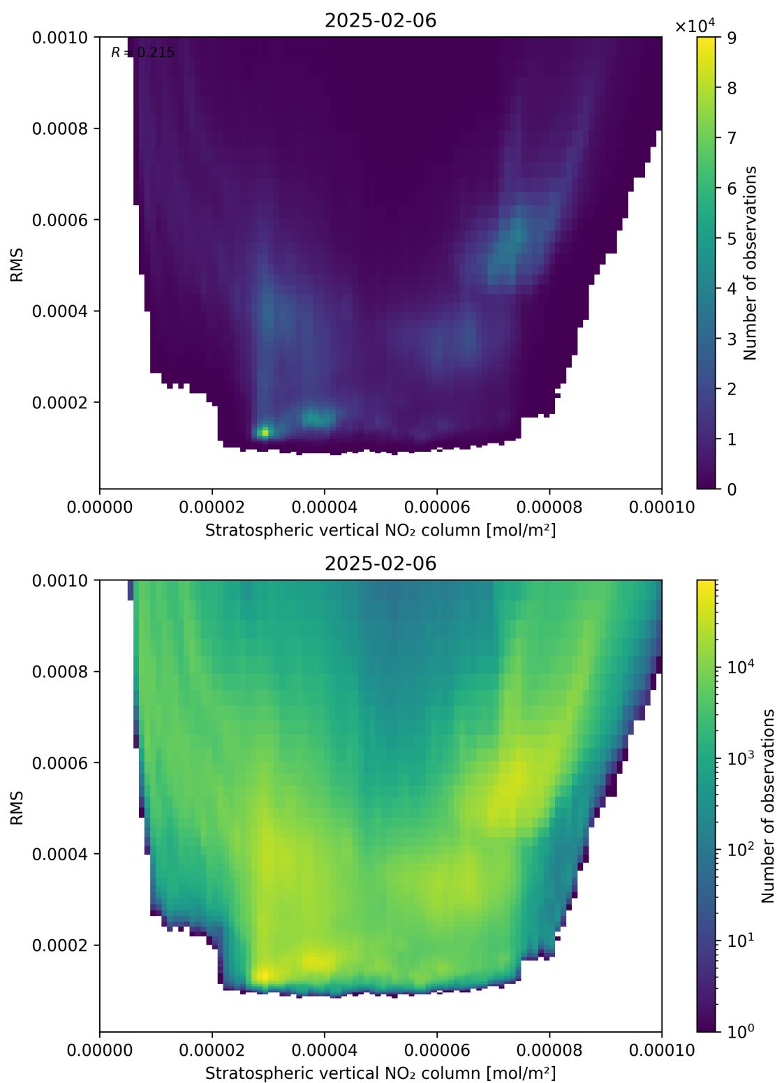
Figure 102: Scatter density plot of “Stratospheric vertical NO 2 column” against “RMS” for 2025-02-05 to 2025-02-07.
