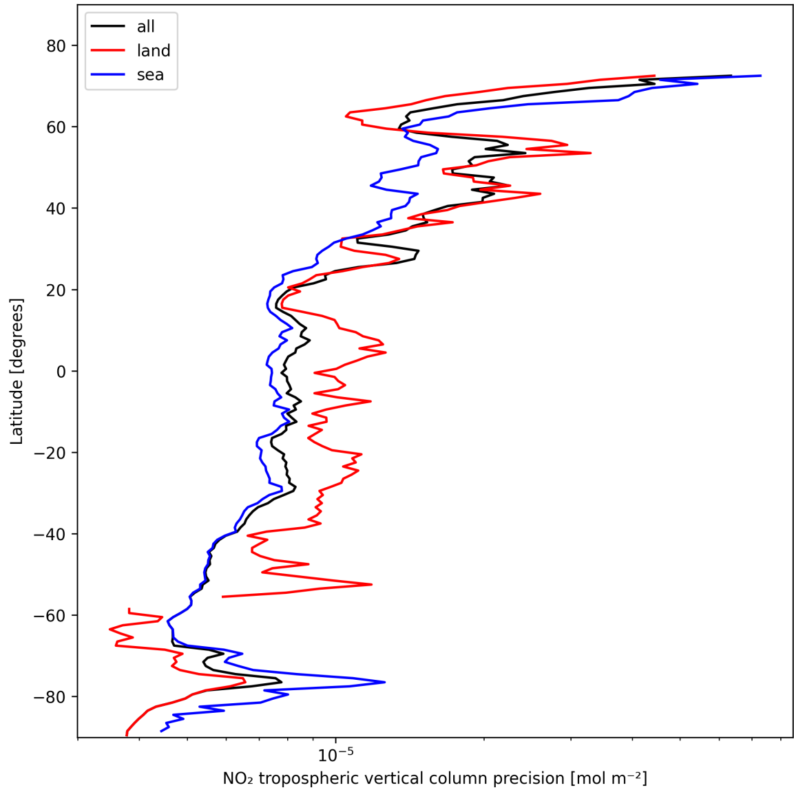
Figure 13: Zonal average of “NO 2 tropospheric vertical column precision” for 2025-02-05 to 2025-02-07.
