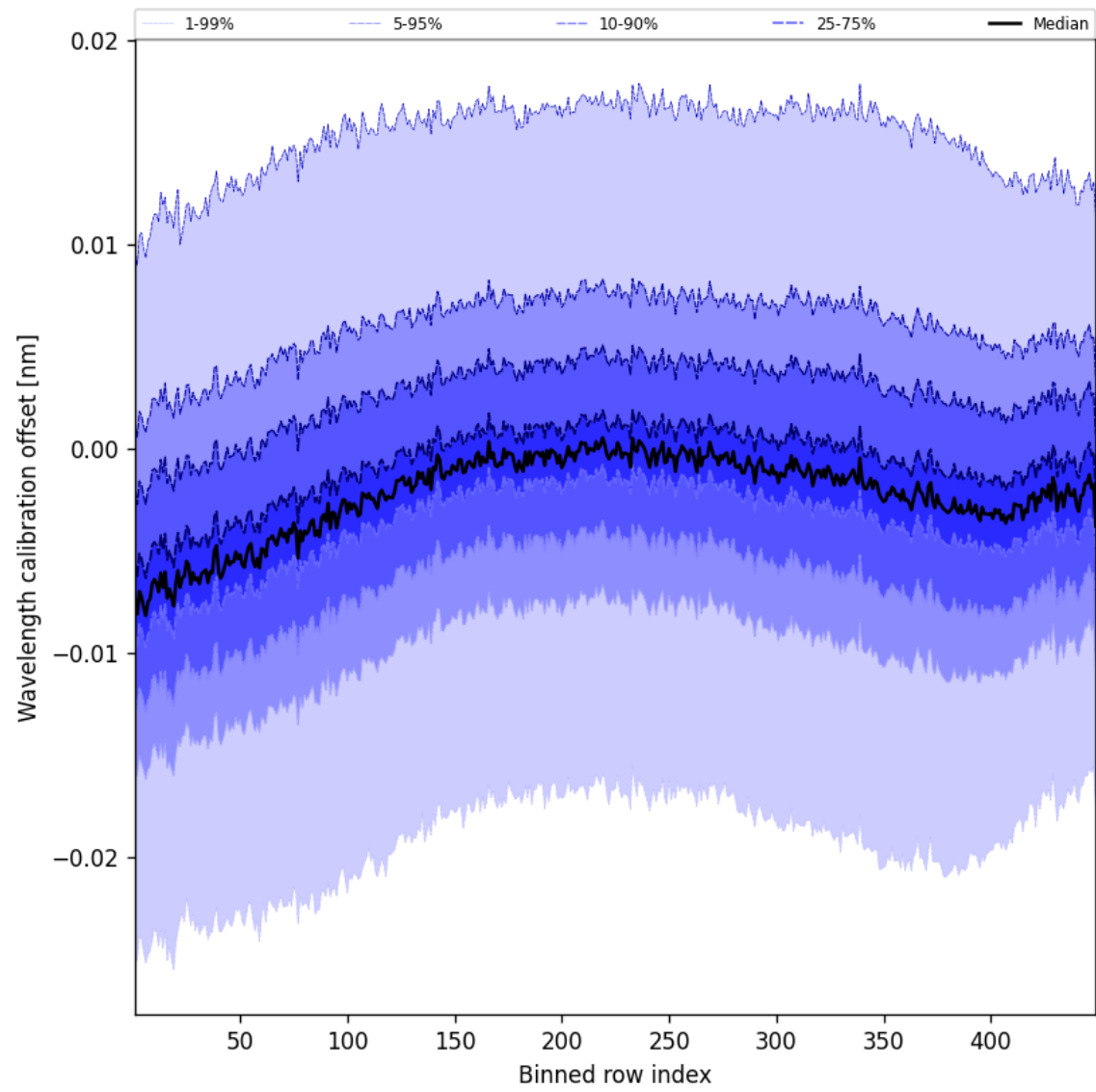
Figure 52: Along track statistics of “Wavelength calibration offset” for 2025-02-05 to 2025-02-07
