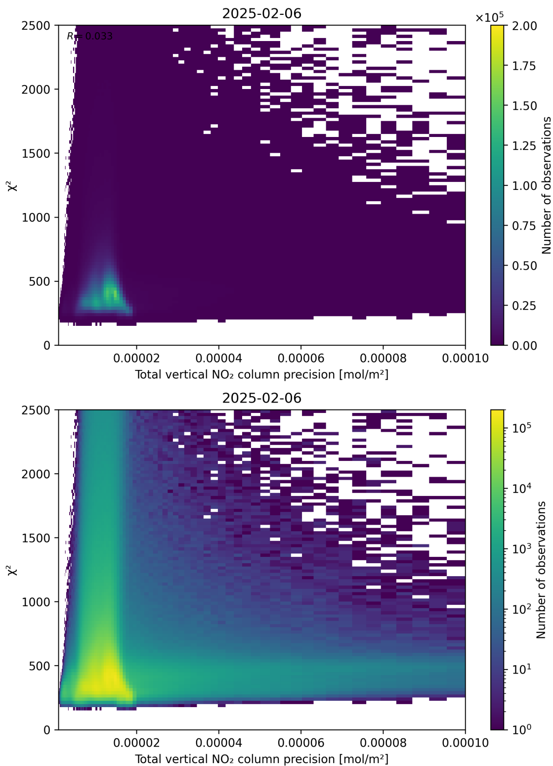
Figure 116: Scatter density plot of “Total vertical NO 2 column precision” against “ \chi^2 ” for 2025-02-05 to 2025-02-07.
