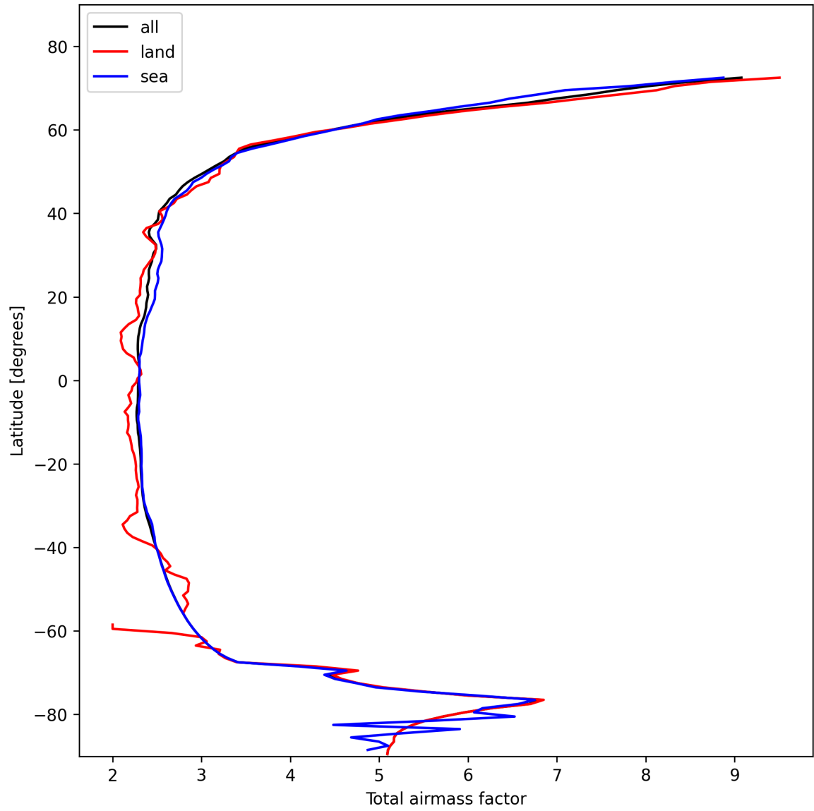
Figure 15: Zonal average of “Total airmass factor” for 2025-02-05 to 2025-02-07.
