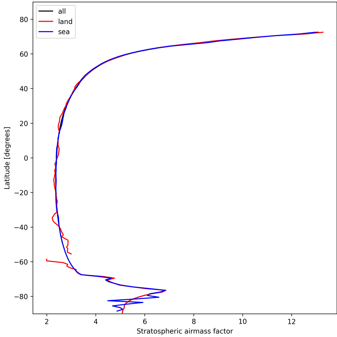
Figure 27: Zonal average of “Stratospheric airmass factor” for 2025-02-05 to 2025-02-07.
