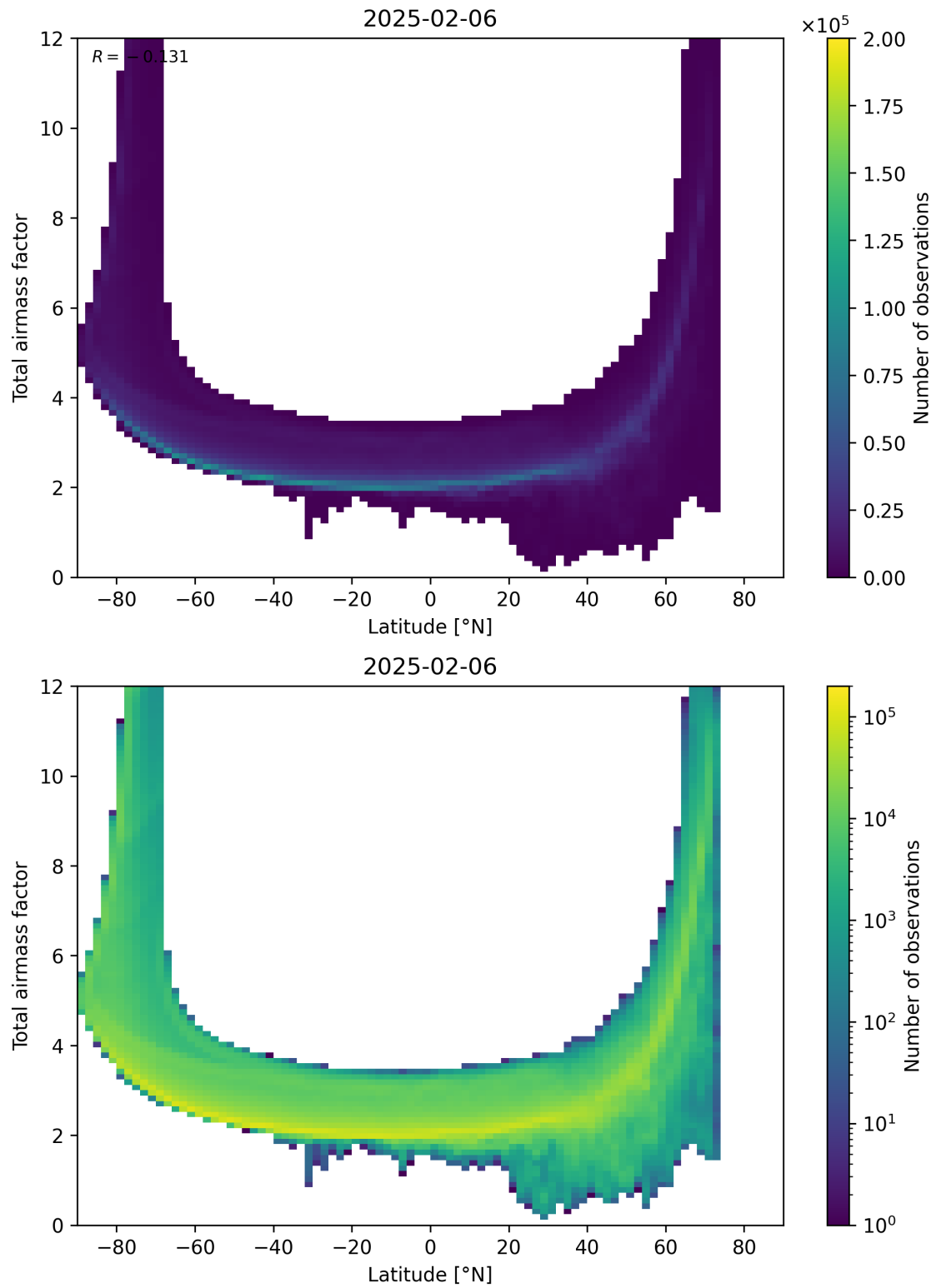
Figure 84: Scatter density plot of “Latitude” against “Total airmass factor” for 2025-02-05 to 2025-02-07.
