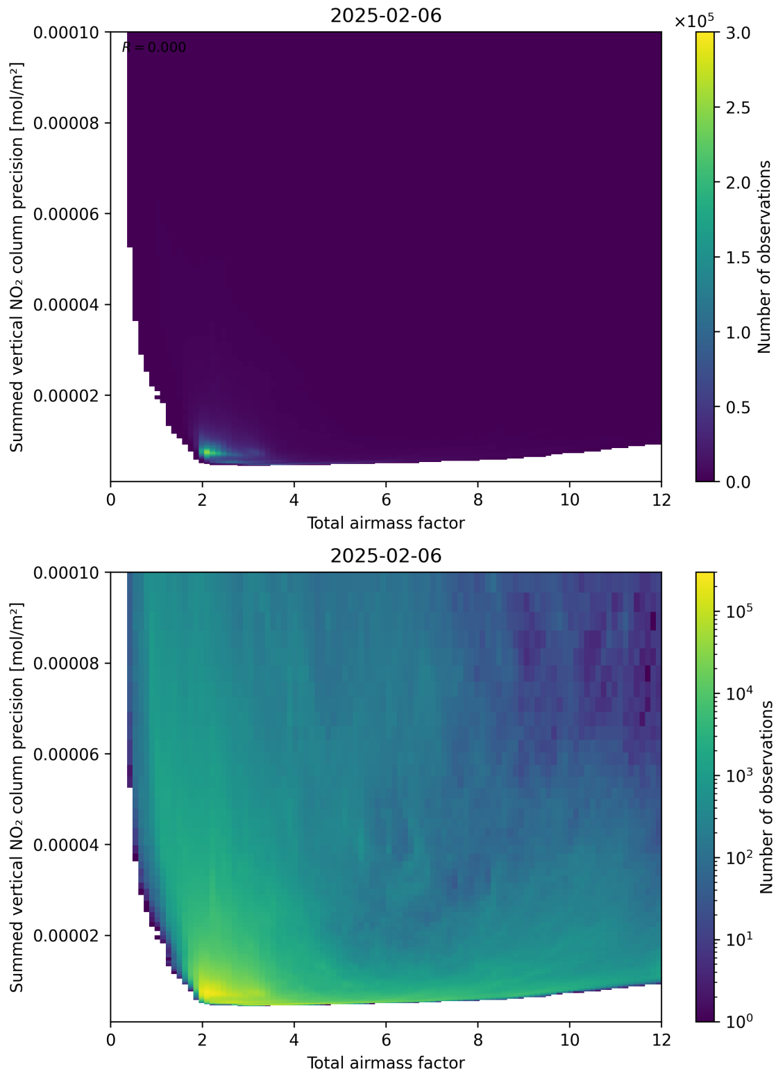
Figure 66: Scatter density plot of “Total airmass factor” against “Summed vertical NO 2 column precision” for 2025-02-05 to 2025-02-07.
