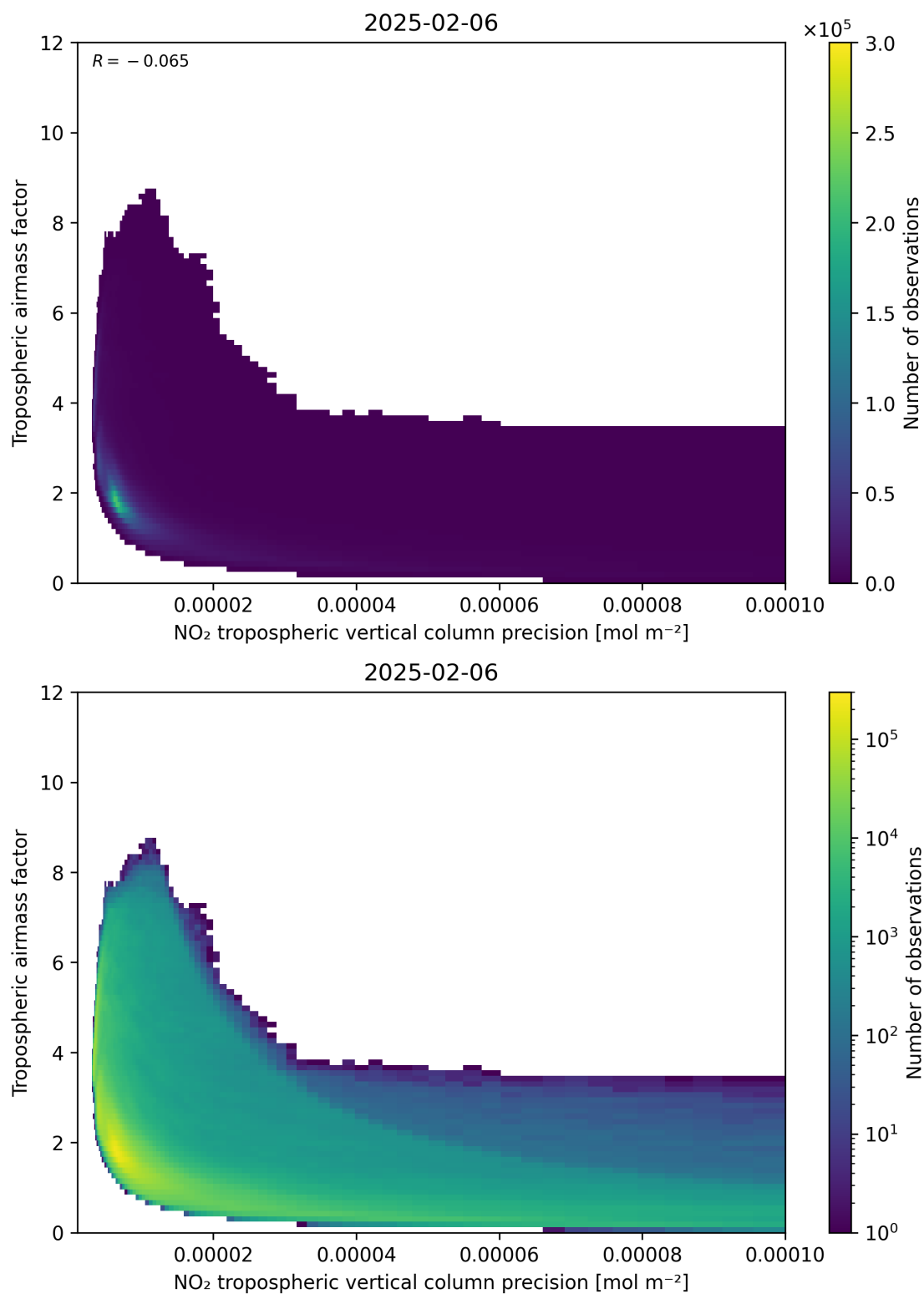
Figure 133: Scatter density plot of “NO 2 tropospheric vertical column precision” against “Tropospheric air mass factor” for 2025-02-05 to 2025-02-07.
