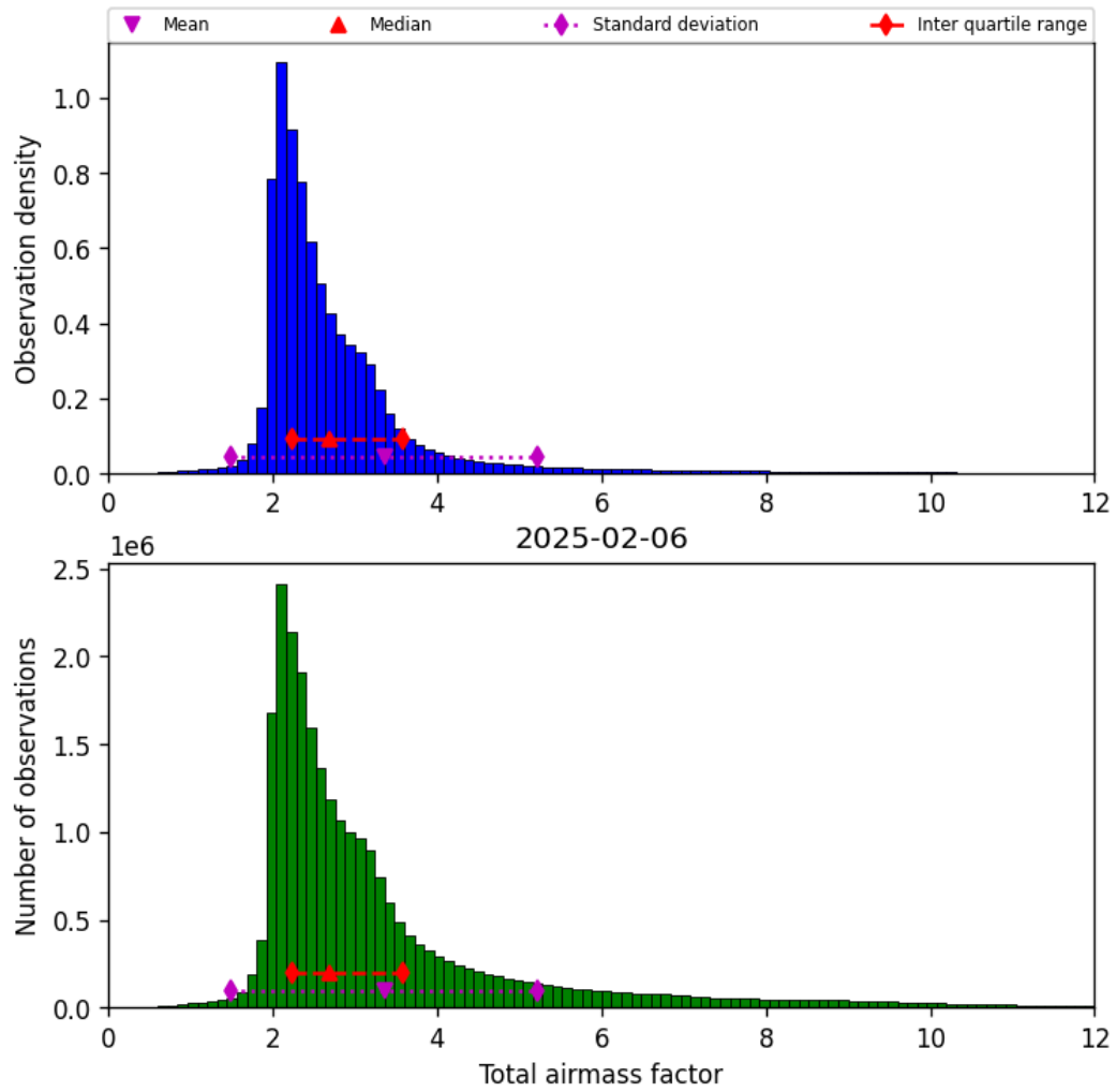
Figure 32: Histogram of “Total airmass factor” for 2025-02-05 to 2025-02-07
