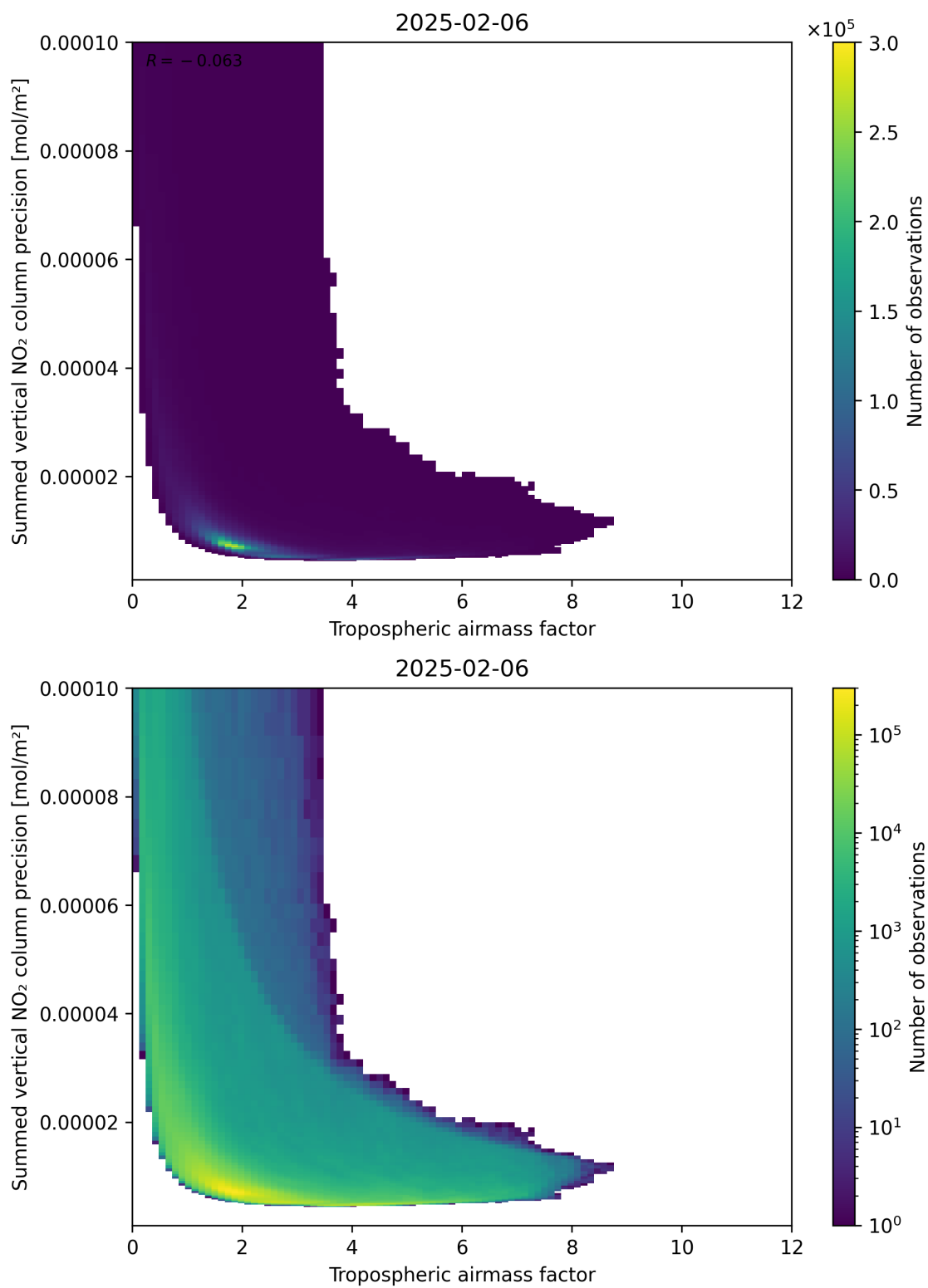
Figure 76: Scatter density plot of “Tropospheric air mass factor” against “Summed vertical NO 2 column precision” for 2025-02-05 to 2025-02-07.
