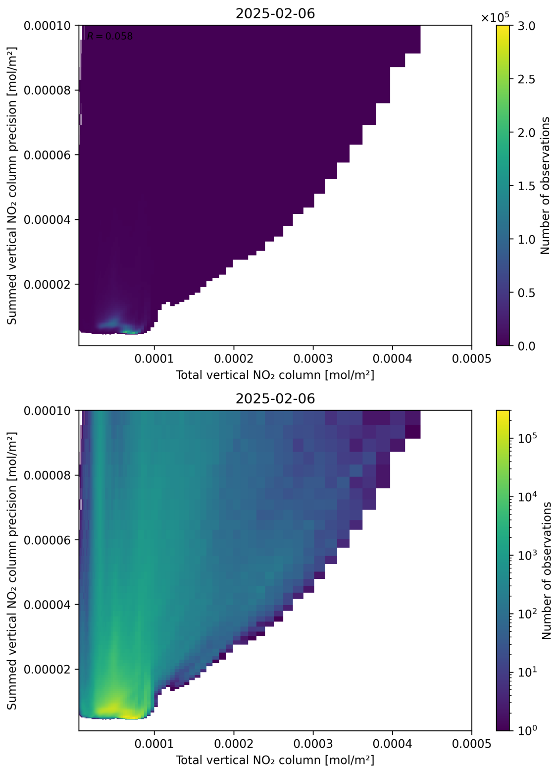
Figure 113: Scatter density plot of “Total vertical NO 2 column” against “Summed vertical NO 2 column precision” for 2025-02-05 to 2025-02-07.
