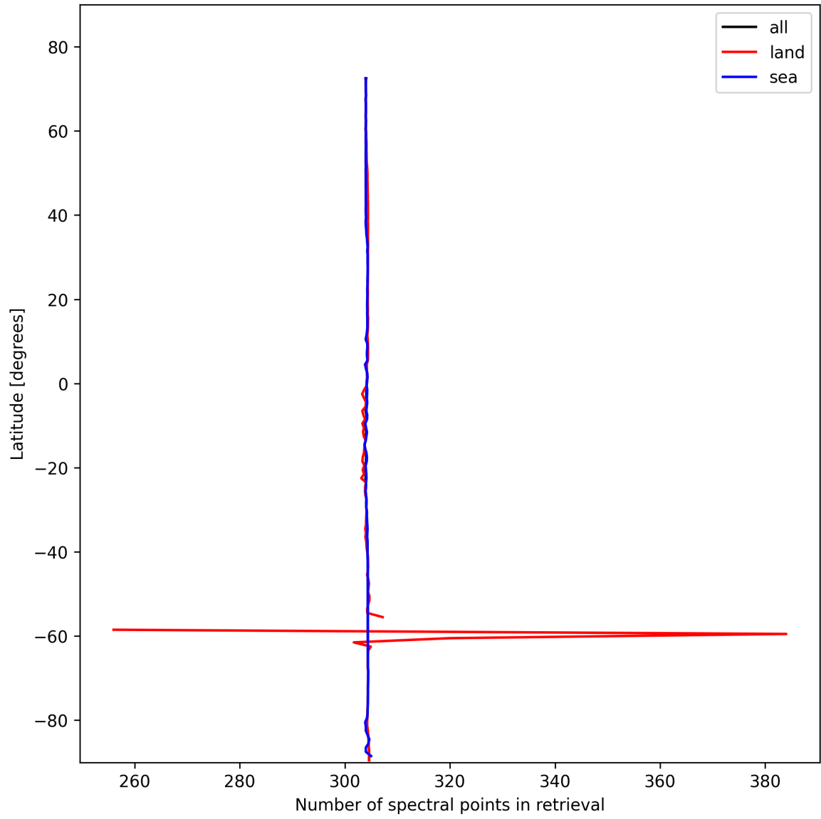
Figure 16: Zonal average of “Number of spectral points in retrieval” for 2025-02-05 to 2025-02-07.
