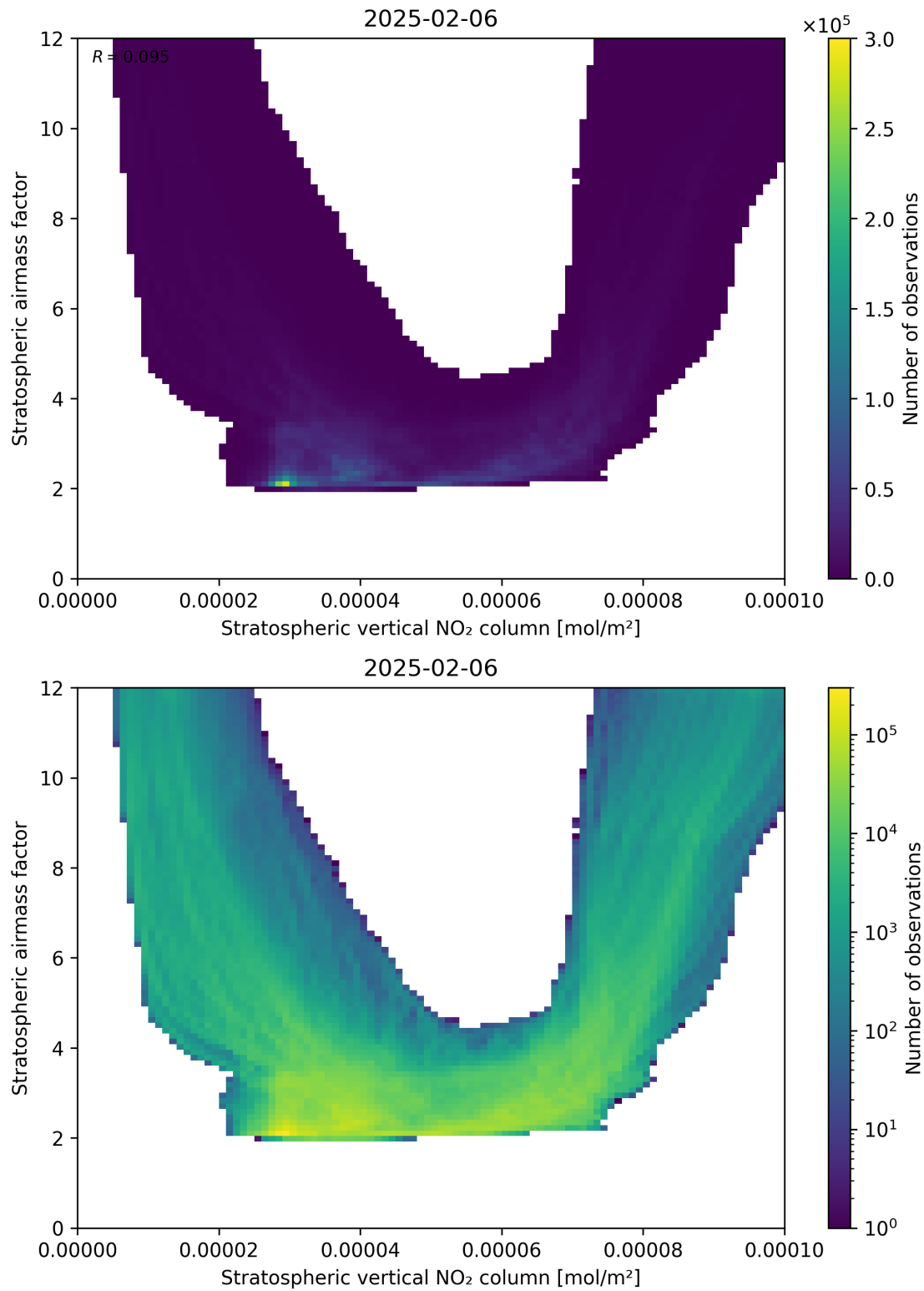
Figure 96: Scatter density plot of “Stratospheric vertical NO 2 column” against “Stratospheric airmass factor” for 2025-02-05 to 2025-02-07.
