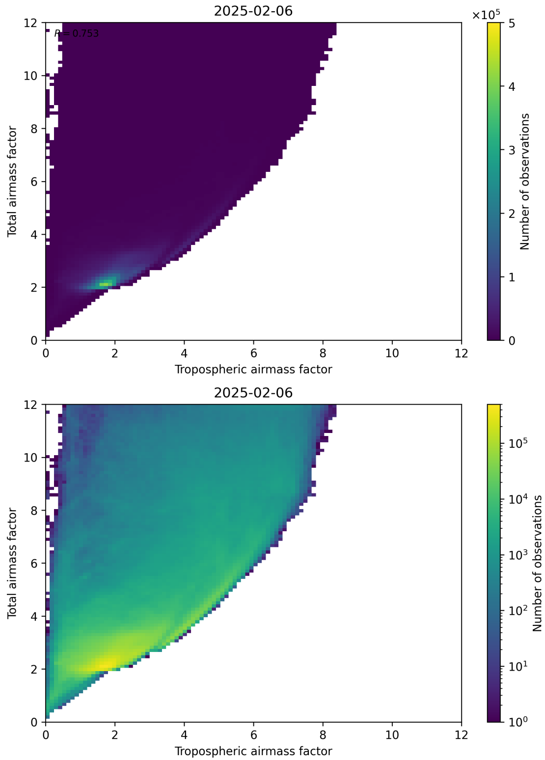
Figure 72: Scatter density plot of “Tropospheric airmass factor” against “Total airmass factor” for 2025-02-05 to 2025-02-07.
