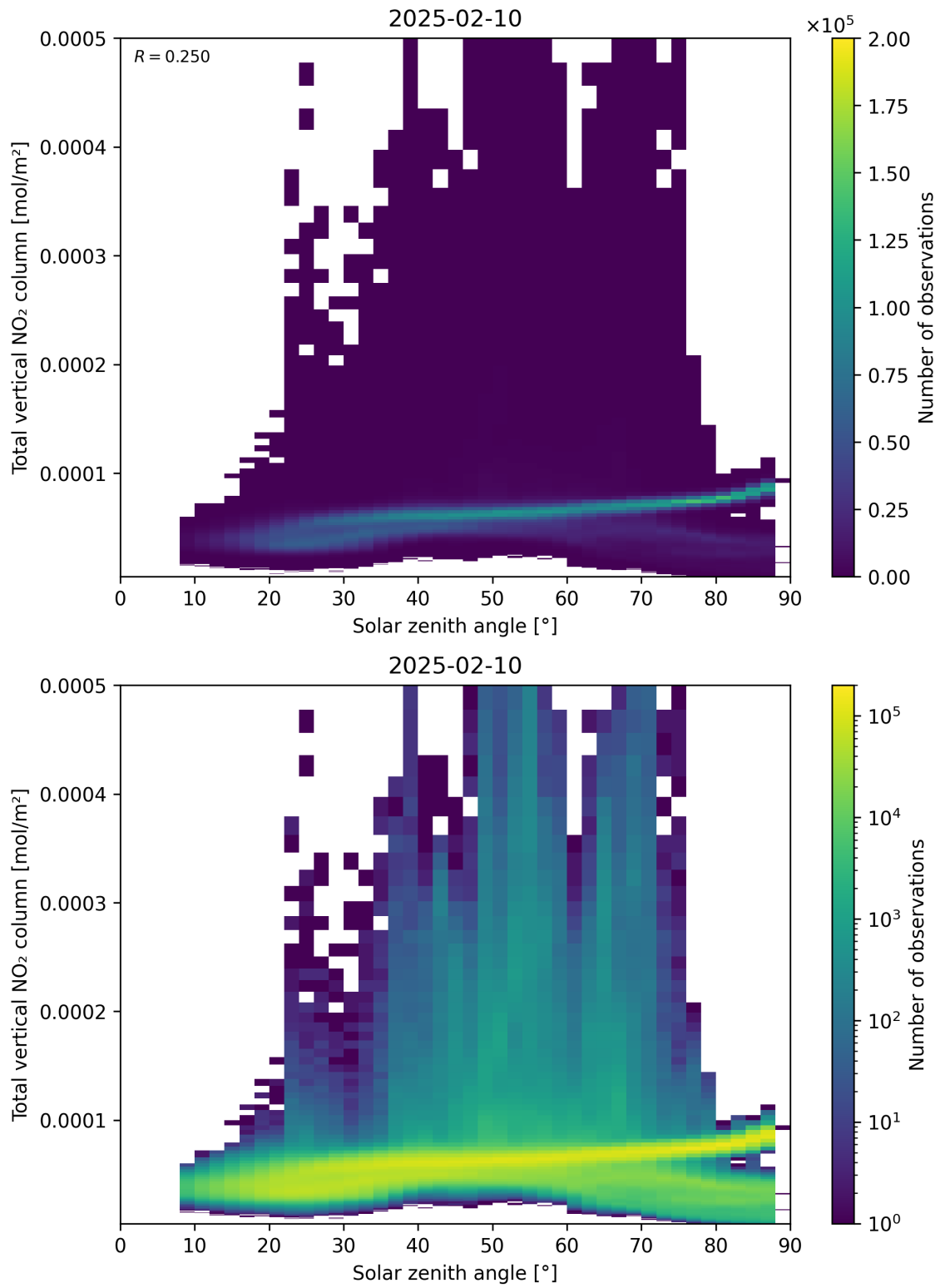
Figure 153: Scatter density plot of “Solar zenith angle” against “Total vertical NO 2 column” for 2025-02-09 to 2025-02-11.
