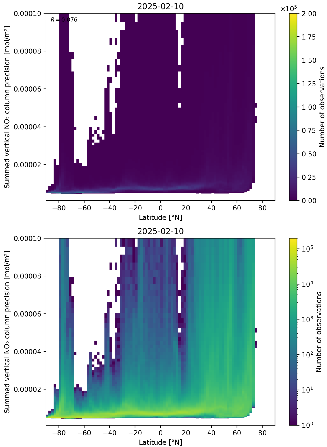
Figure 89: Scatter density plot of “Latitude” against “Summed vertical NO 2 column precision” for 2025-02-09 to 2025-02-11.
