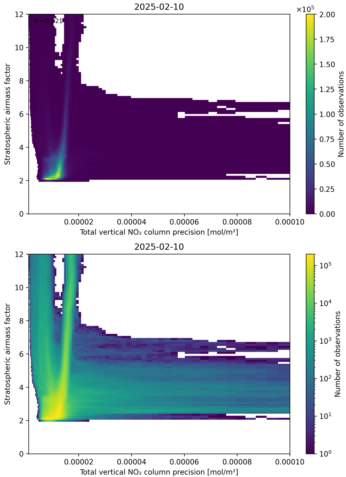
Figure 115: Scatter density plot of “Total vertical NO 2 column precision” against “Stratospheric air mass factor” for 2025-02-09 to 2025-02-11.
