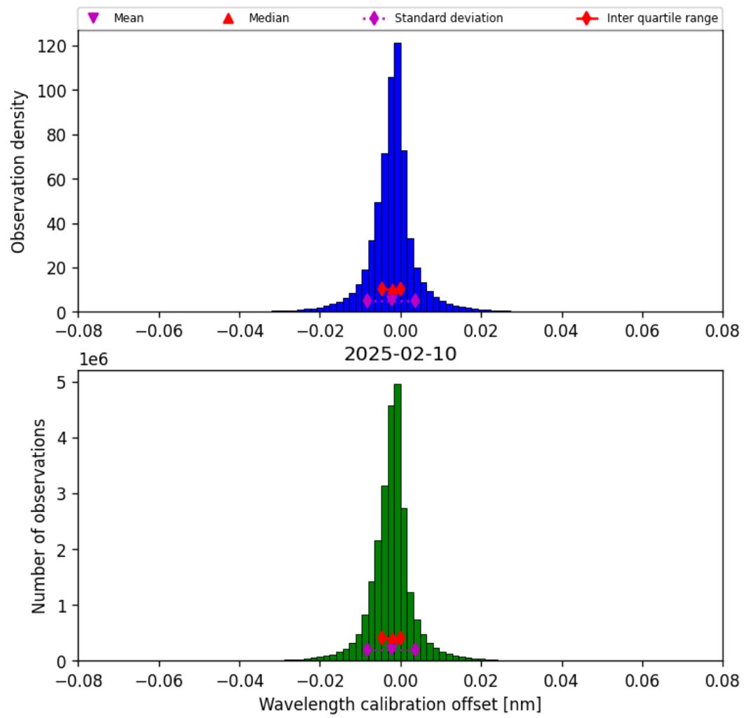
Figure 35: Histogram of “Wavelength calibration offset” for 2025-02-09 to 2025-02-11
