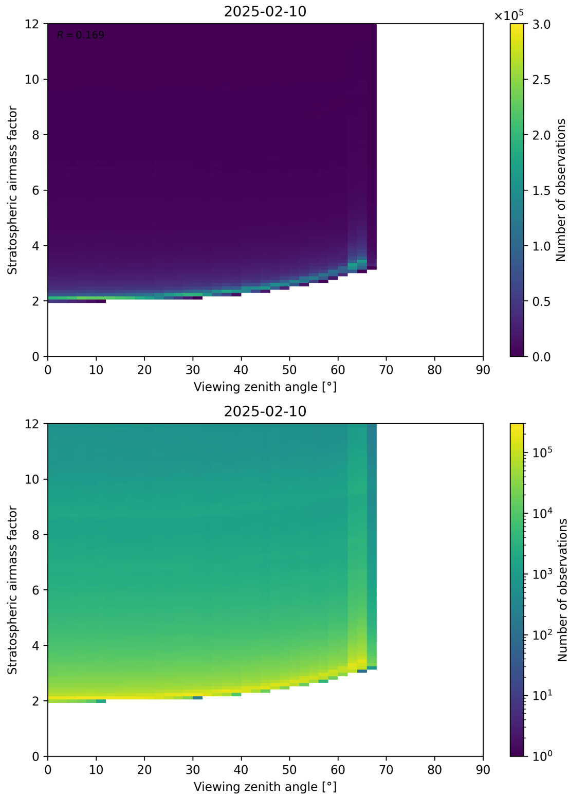
Figure 159: Scatter density plot of “Viewing zenith angle” against “Stratospheric airmass factor” for 2025-02-09 to 2025-02-11.
