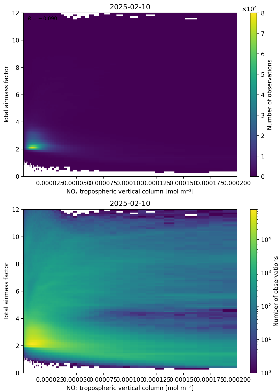
Figure 122: Scatter density plot of “NO 2 tropospheric vertical column” against “Total air mass factor” for 2025-02-09 to 2025-02-11.
