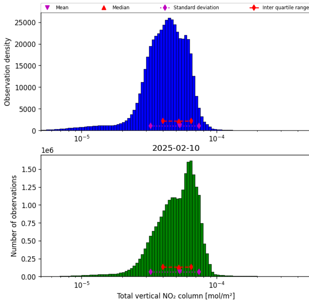
Figure 38: Histogram of “Total vertical NO 2 column” for 2025-02-09 to 2025-02-11
