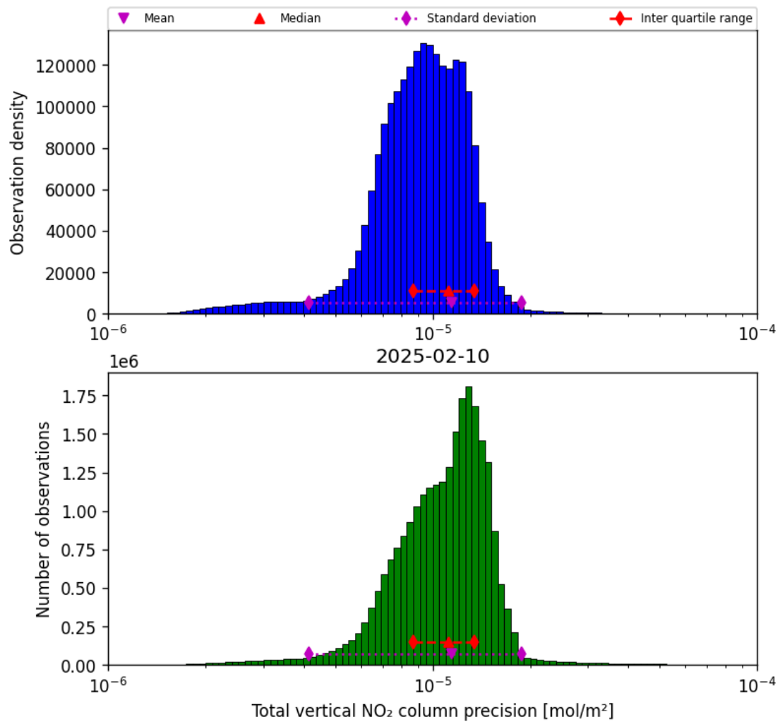
Figure 39: Histogram of “Total vertical NO 2 column precision” for 2025-02-09 to 2025-02-11
