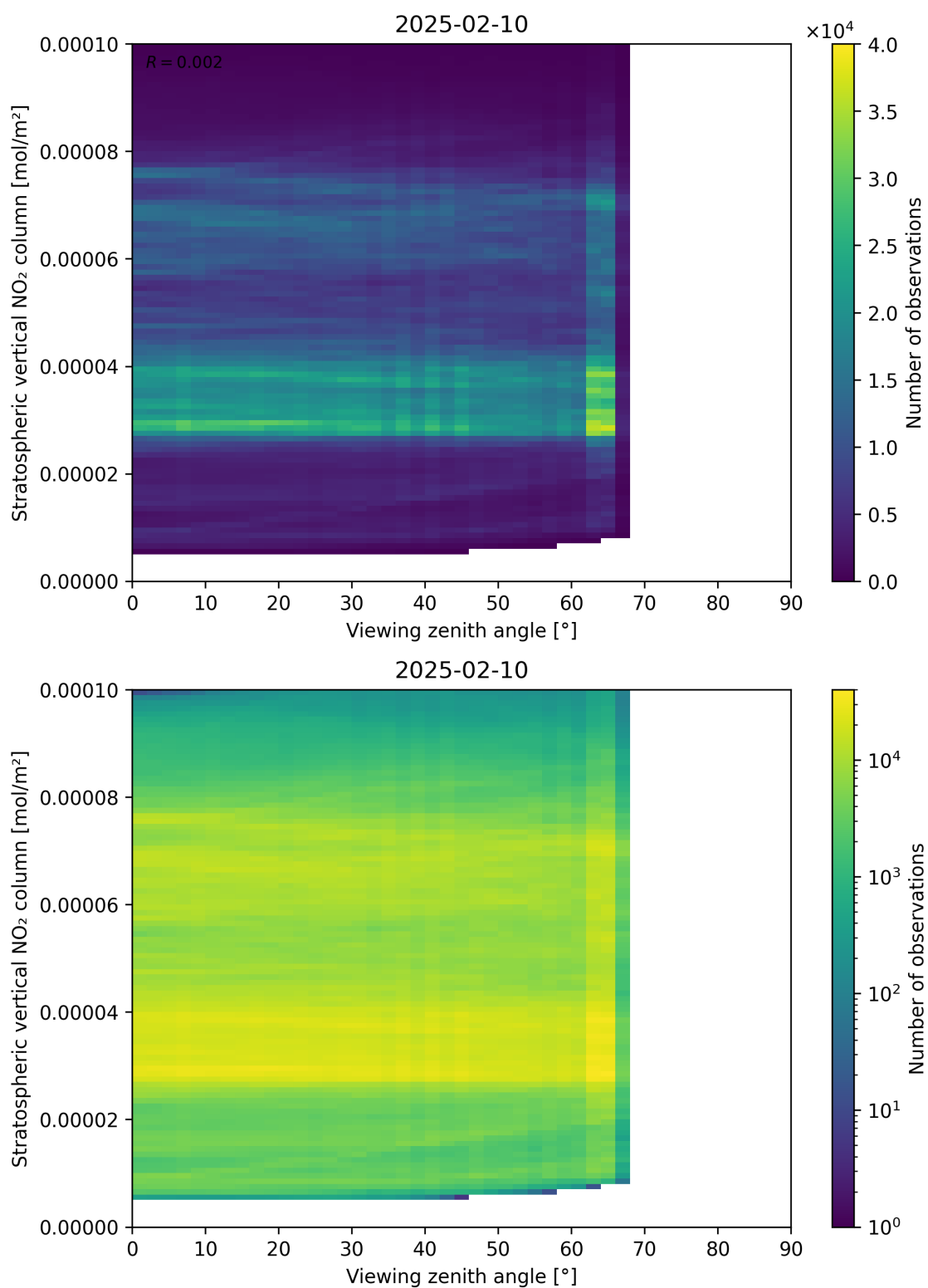
Figure 164: Scatter density plot of “Viewing zenith angle” against “Stratospheric vertical NO 2 column” for 2025-02-09 to 2025-02-11.
