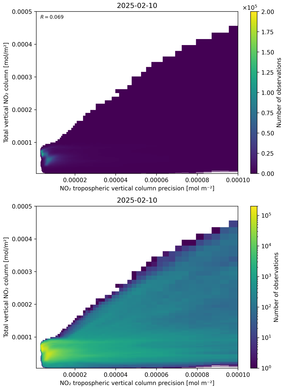
Figure 138: Scatter density plot of “NO 2 tropospheric vertical column precision” against “Total vertical NO 2 column” for 2025-02-09 to 2025-02-11.
