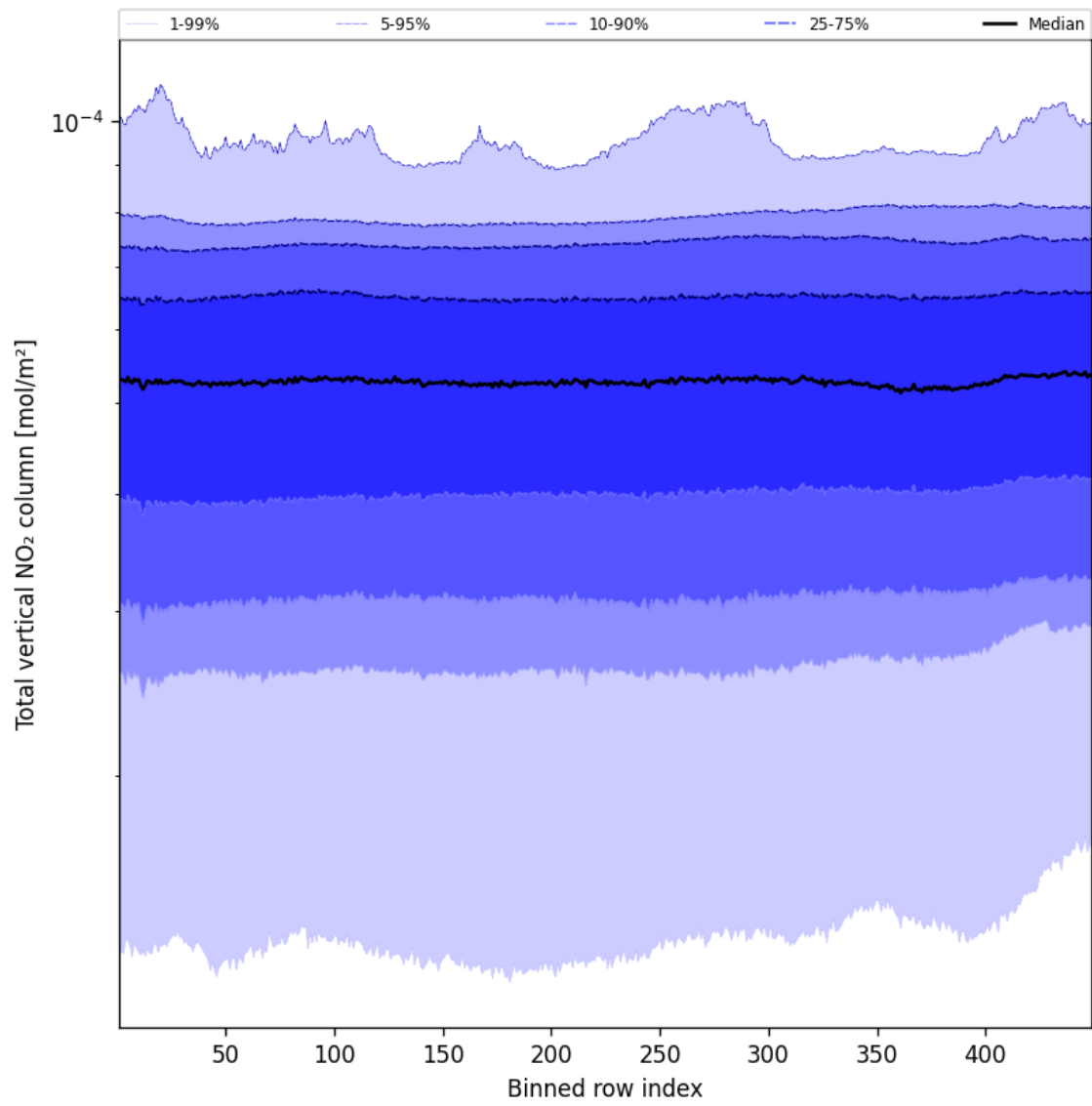
Figure 55: Along track statistics of “Total vertical NO 2 column” for 2025-02-09 to 2025-02-11
