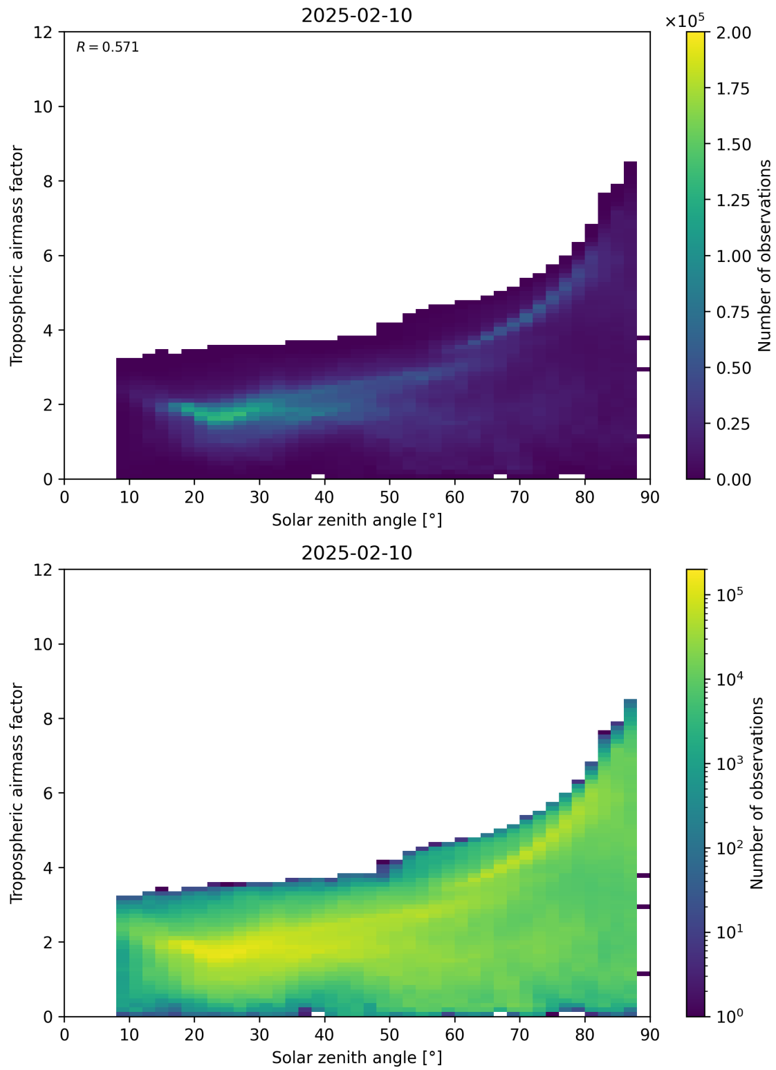
Figure 147: Scatter density plot of “Solar zenith angle” against “Tropospheric airmass factor” for 2025-02-09 to 2025-02-11.
