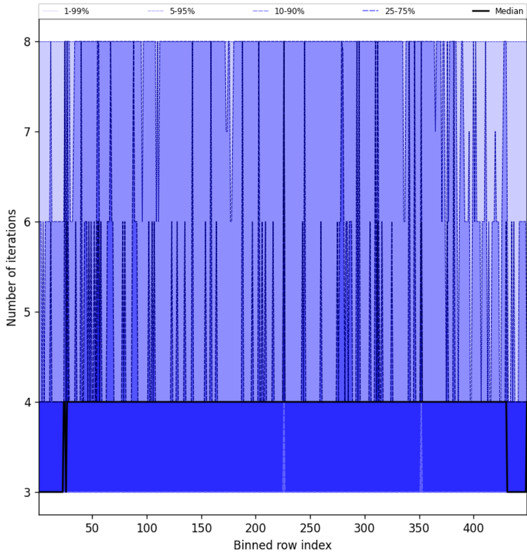
Figure 51: Along track statistics of “Number of iterations” for 2025-02-09 to 2025-02-11
