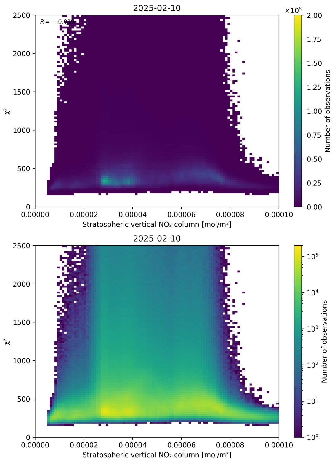
Figure 97: Scatter density plot of “Stratospheric vertical NO 2 column” against “ \chi^2 ” for 2025-02-09 to 2025-02-11.
