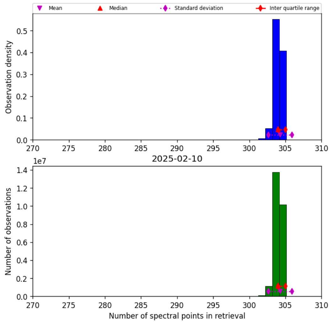
Figure 33: Histogram of “Number of spectral points in retrieval” for 2025-02-09 to 2025-02-11
