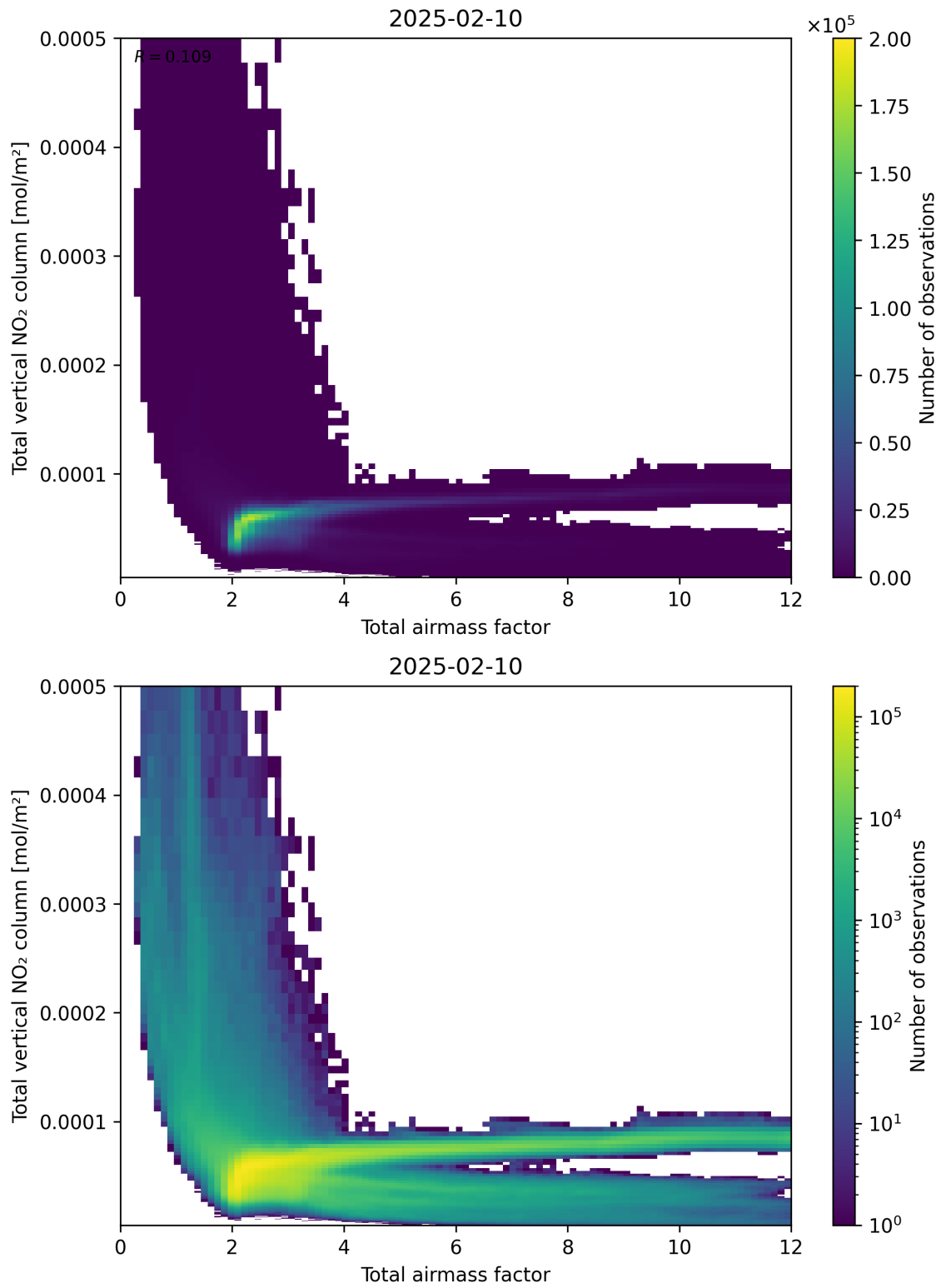
Figure 67: Scatter density plot of “Total airmass factor” against “Total vertical NO 2 column” for 2025-02-09 to 2025-02-11.
