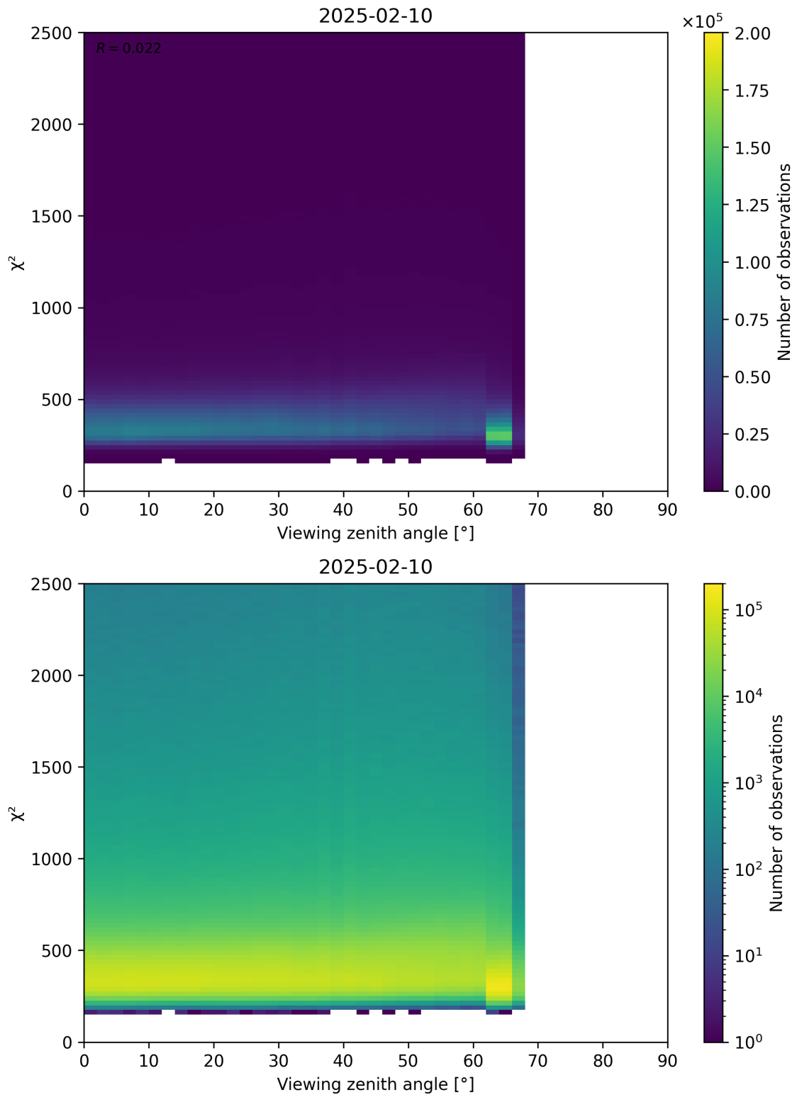
Figure 162: Scatter density plot of “Viewing zenith angle” against “ \chi^2 ” for 2025-02-09 to 2025-02-11.
