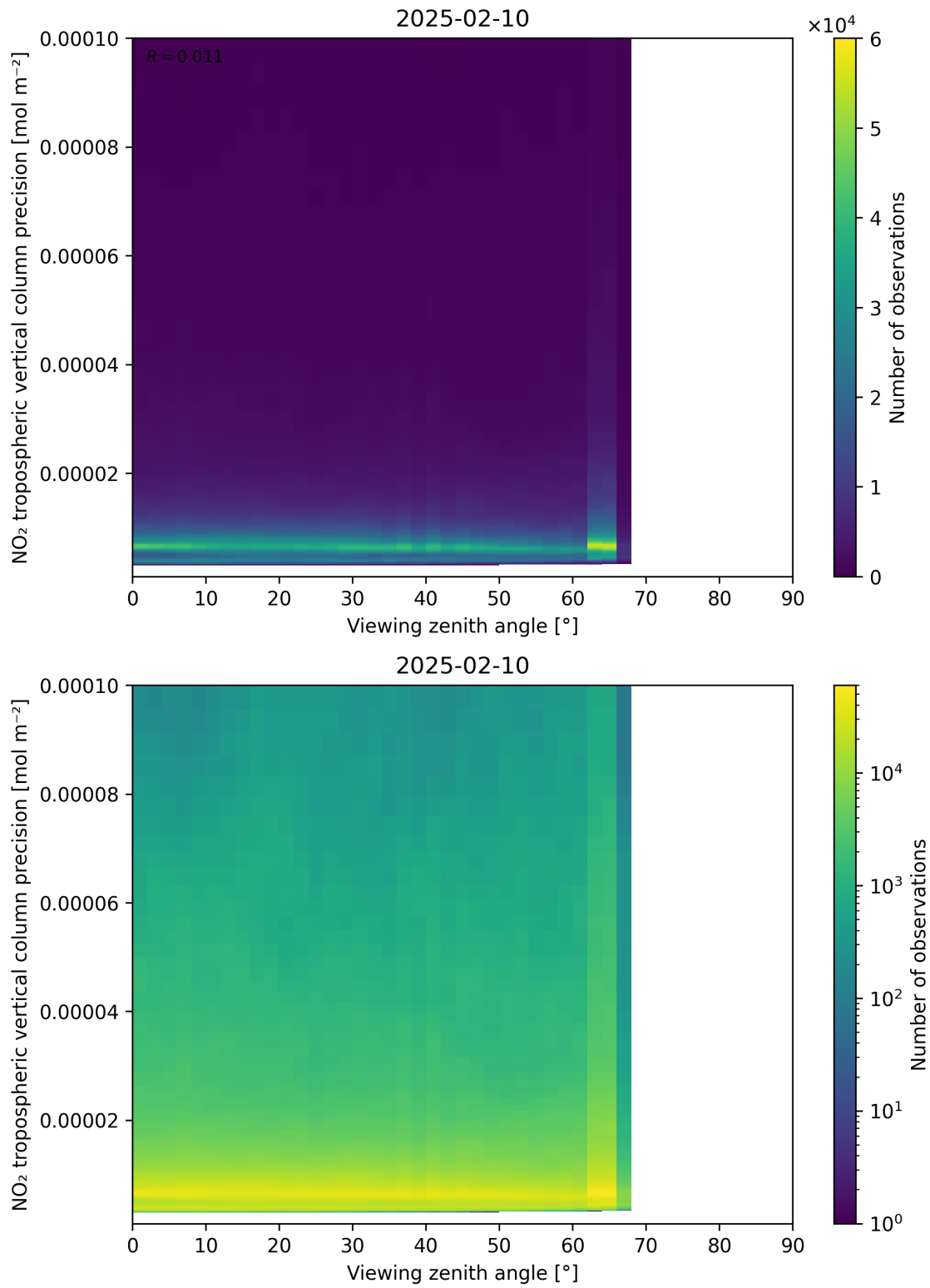
Figure 170: Scatter density plot of “Viewing zenith angle” against “NO 2 tropospheric vertical column precision” for 2025-02-09 to 2025-02-11.
