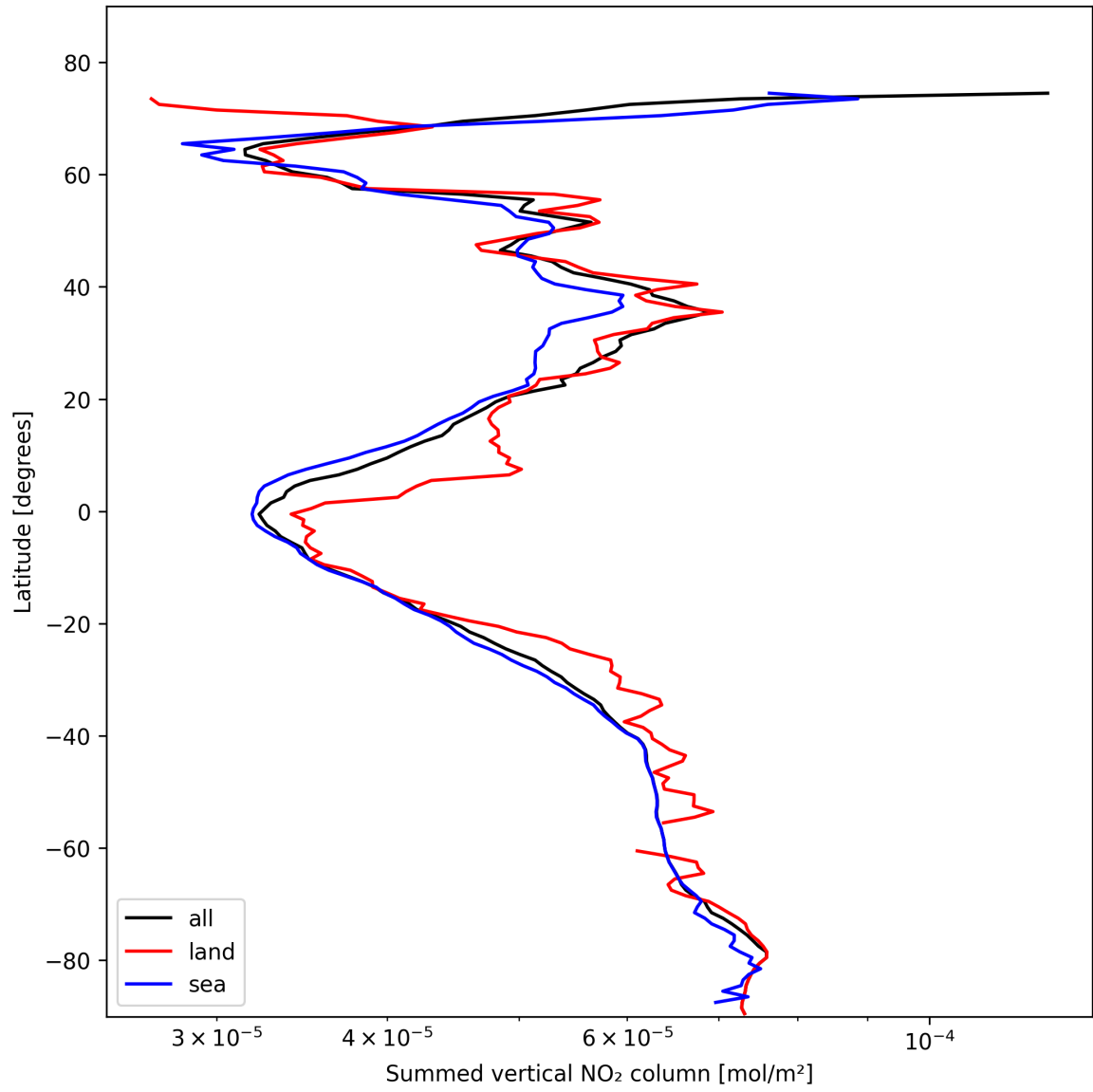
Figure 23: Zonal average of “Summed vertical NO 2 column” for 2025-02-09 to 2025-02-11.
