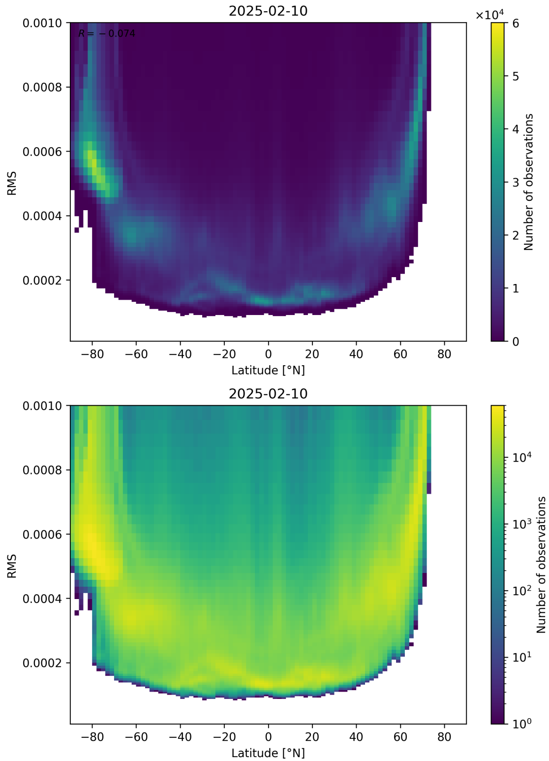
Figure 94: Scatter density plot of “Latitude” against “RMS” for 2025-02-09 to 2025-02-11.
