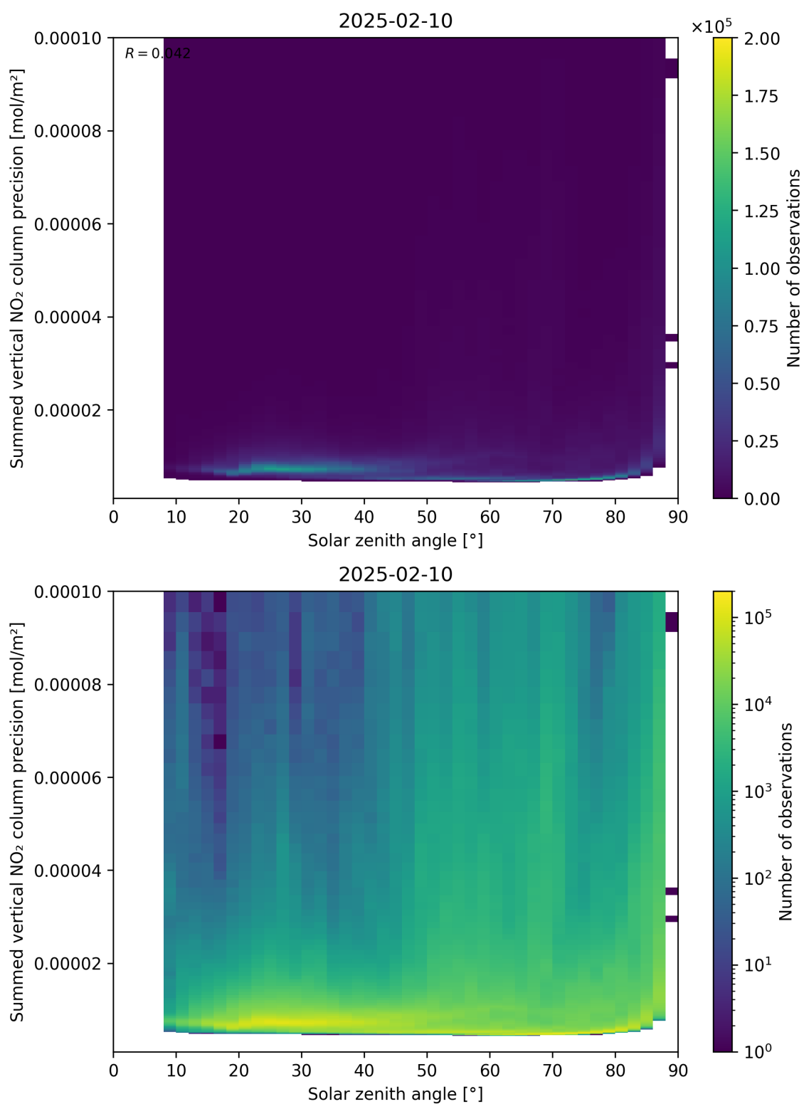
Figure 152: Scatter density plot of “Solar zenith angle” against “Summed vertical NO 2 column precision” for 2025-02-09 to 2025-02-11.
