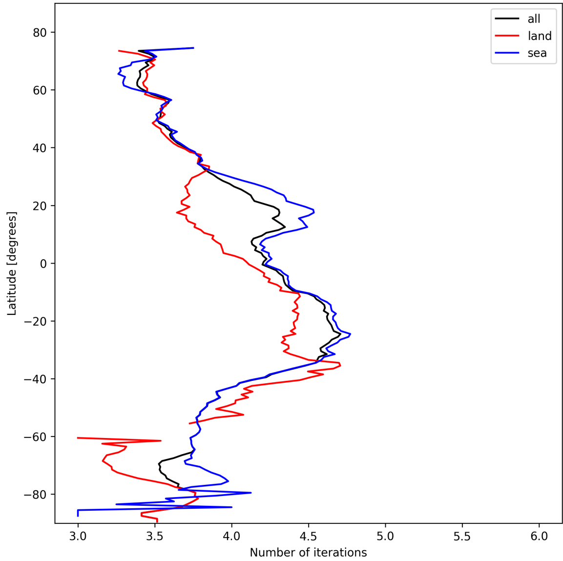
Figure 17: Zonal average of “Number of iterations” for 2025-02-09 to 2025-02-11.
