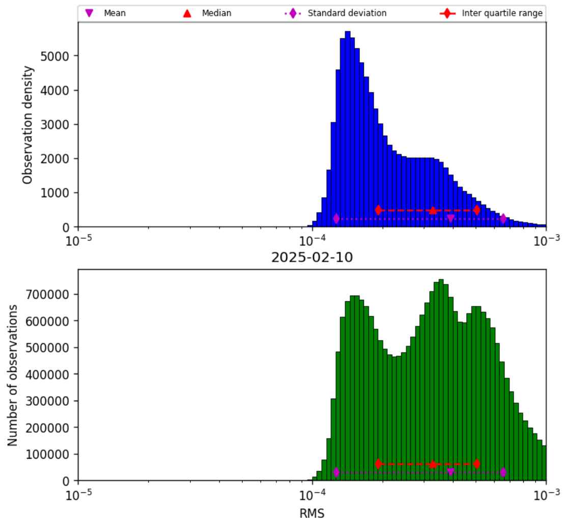
Figure 43: Histogram of “RMS” for 2025-02-09 to 2025-02-11
