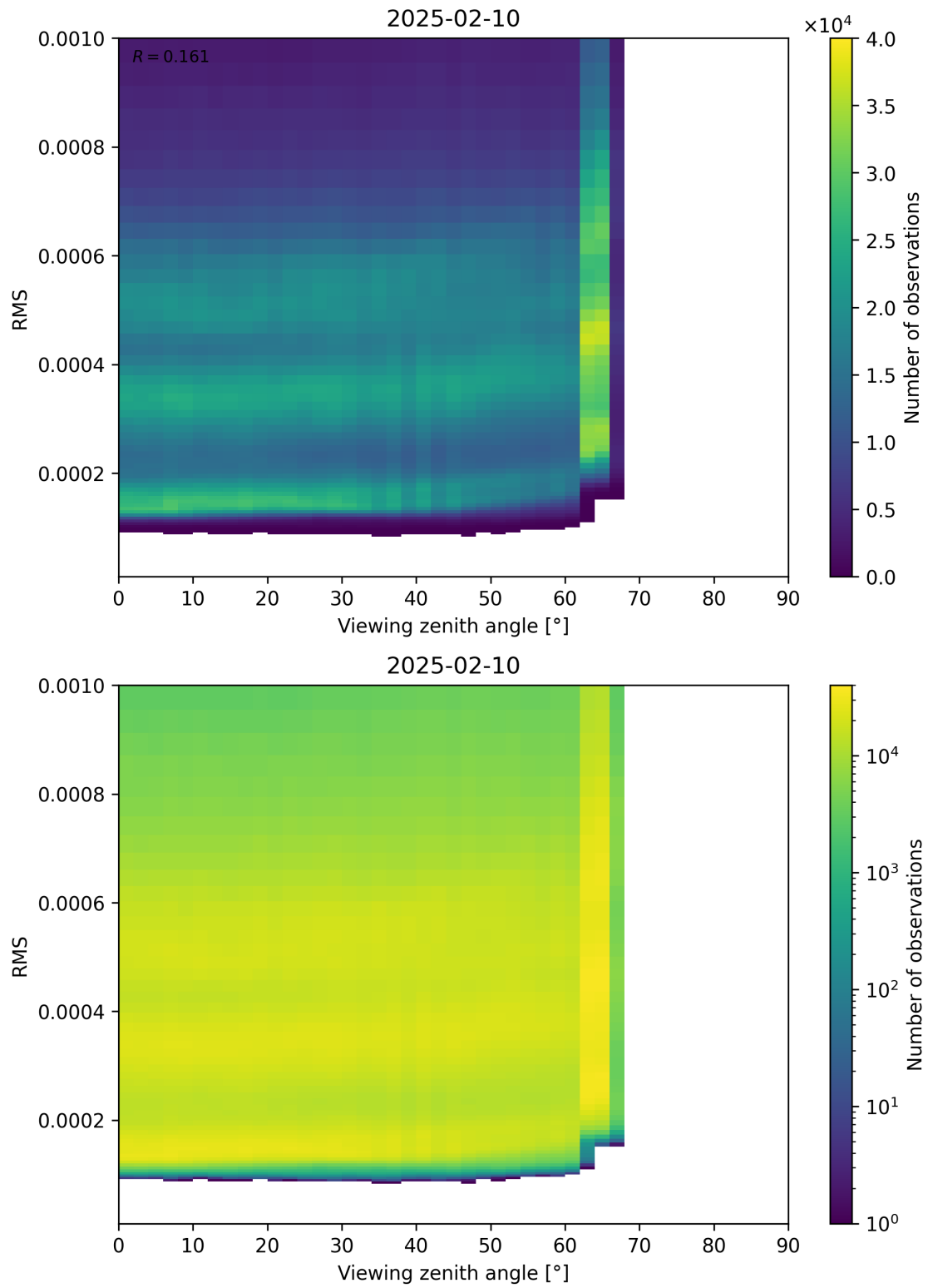
Figure 171: Scatter density plot of “Viewing zenith angle” against “RMS” for 2025-02-09 to 2025-02-11.
