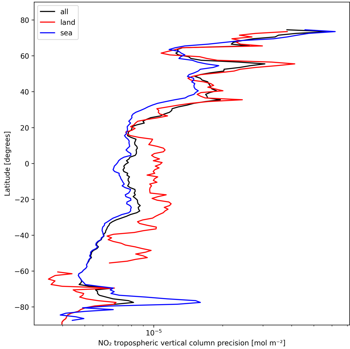
Figure 13: Zonal average of “NO 2 tropospheric vertical column precision” for 2025-02-09 to 2025-02-11.
