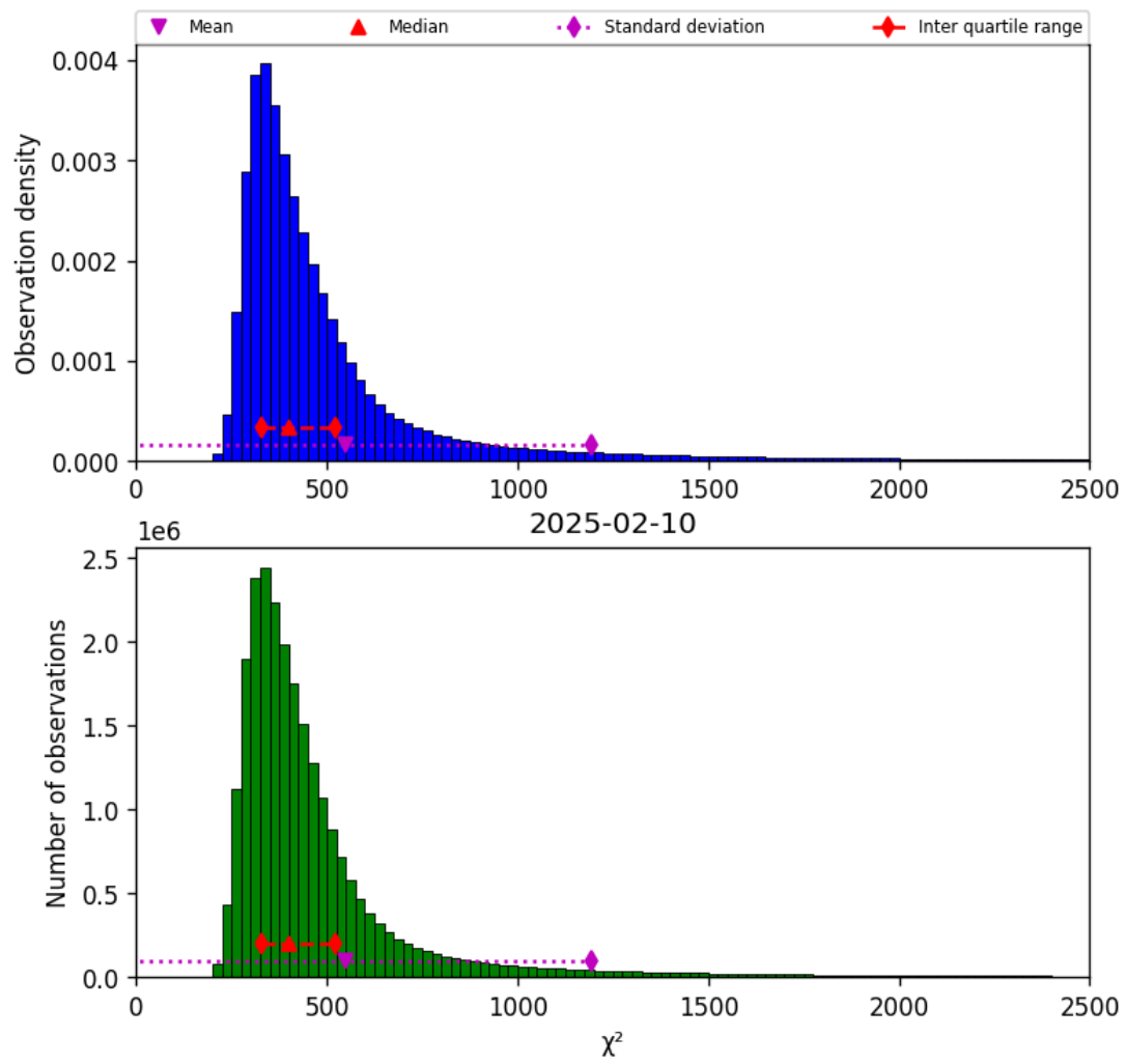
Figure 42: Histogram of “ \chi^2 ” for 2025-02-09 to 2025-02-11
