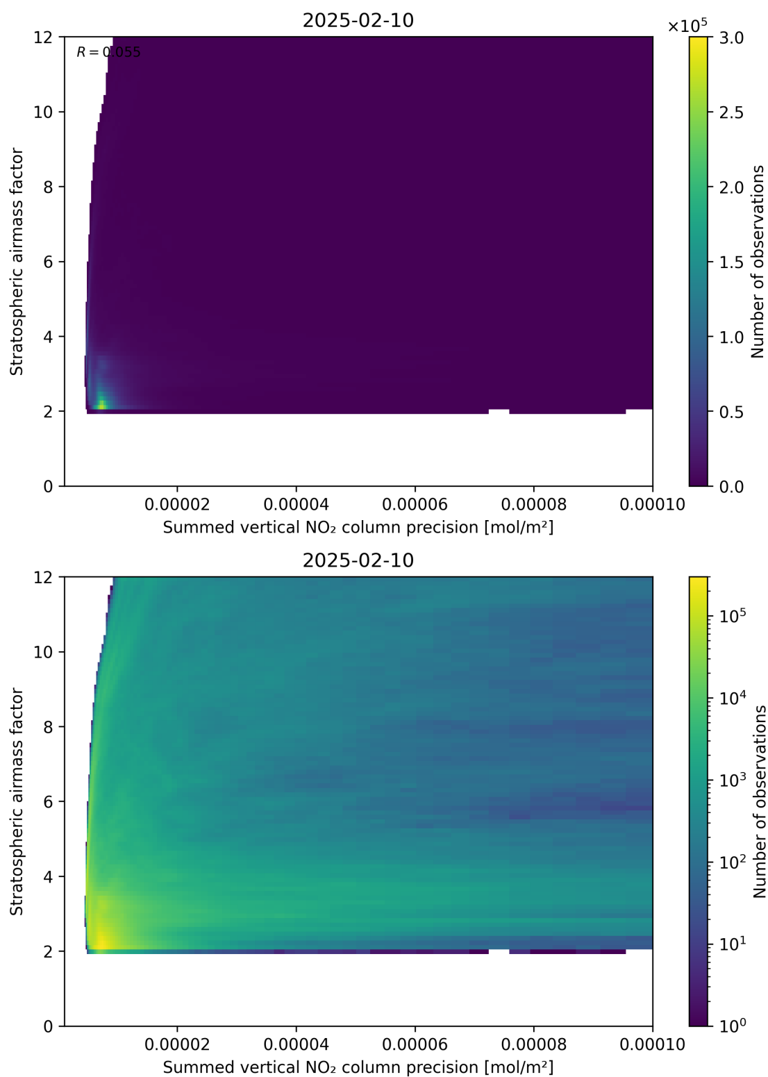
Figure 106: Scatter density plot of “Summed vertical NO 2 column precision” against “Stratospheric airmass factor” for 2025-02-09 to 2025-02-11.
