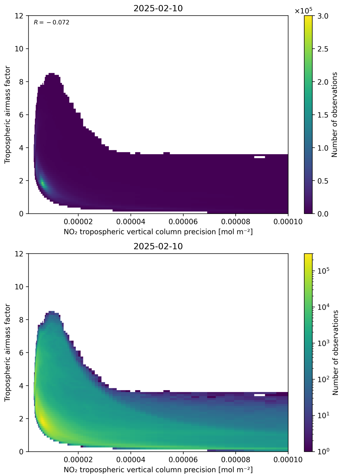
Figure 133: Scatter density plot of “NO 2 tropospheric vertical column precision” against “Tropospheric air mass factor” for 2025-02-09 to 2025-02-11.
