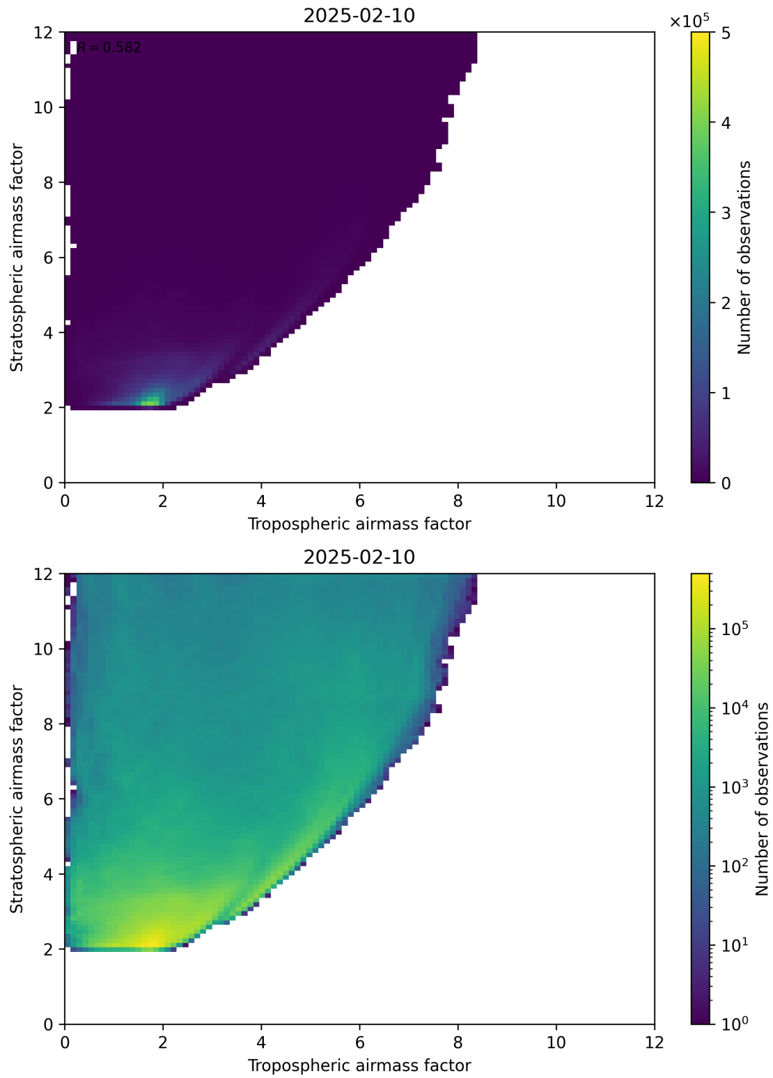
Figure 71: Scatter density plot of “Tropospheric airmass factor” against “Stratospheric airmass factor” for 2025-02-09 to 2025-02-11.
