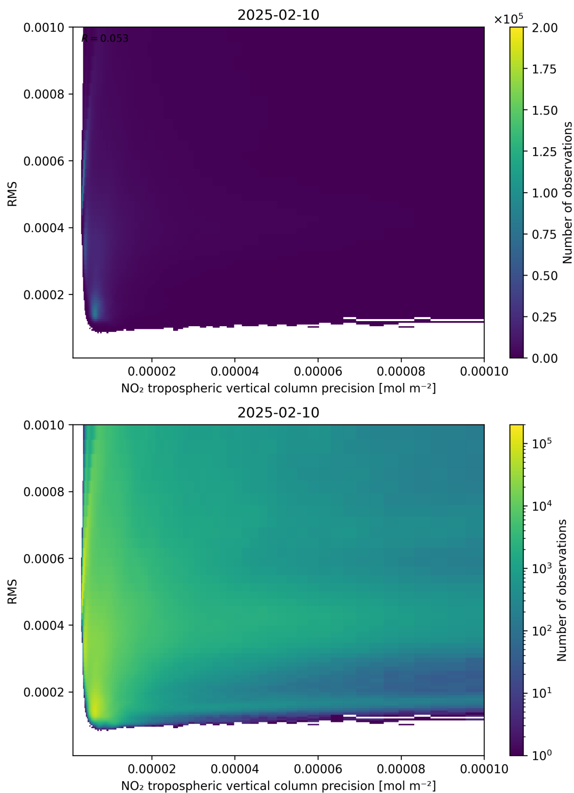
Figure 140: Scatter density plot of “NO 2 tropospheric vertical column precision” against “RMS” for 2025-02-09 to 2025-02-11.
