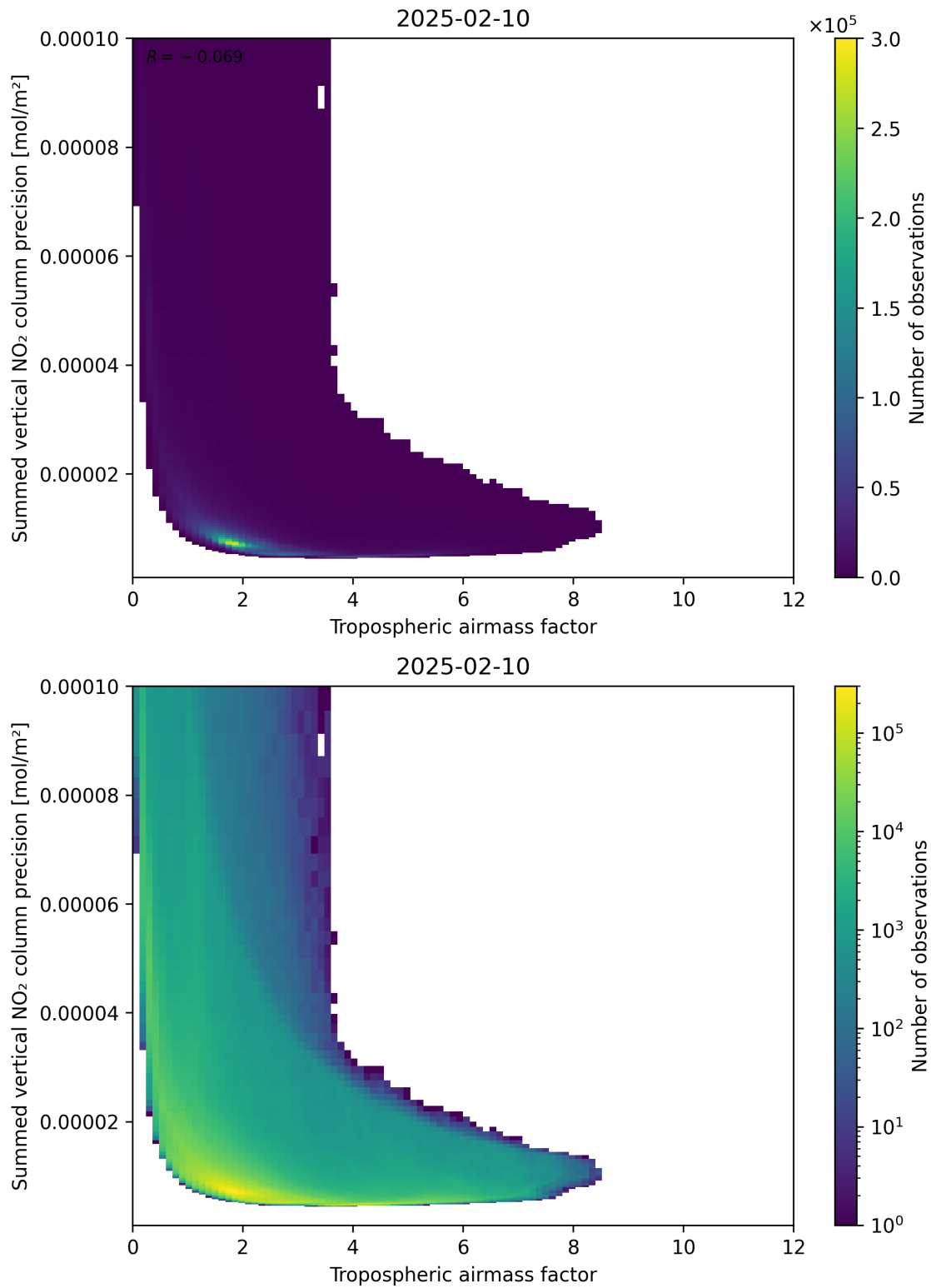
Figure 76: Scatter density plot of “Tropospheric air mass factor” against “Summed vertical NO 2 column precision” for 2025-02-09 to 2025-02-11.
