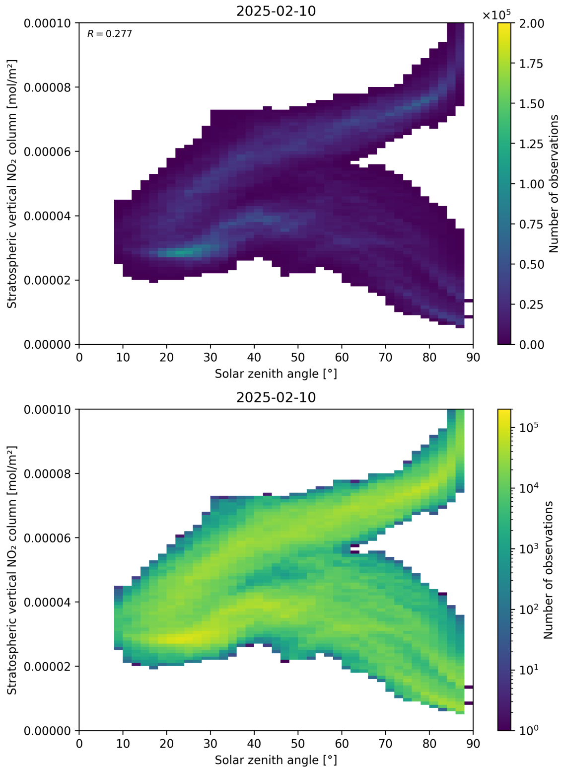
Figure 150: Scatter density plot of “Solar zenith angle” against “Stratospheric vertical NO 2 column” for 2025-02-09 to 2025-02-11.
