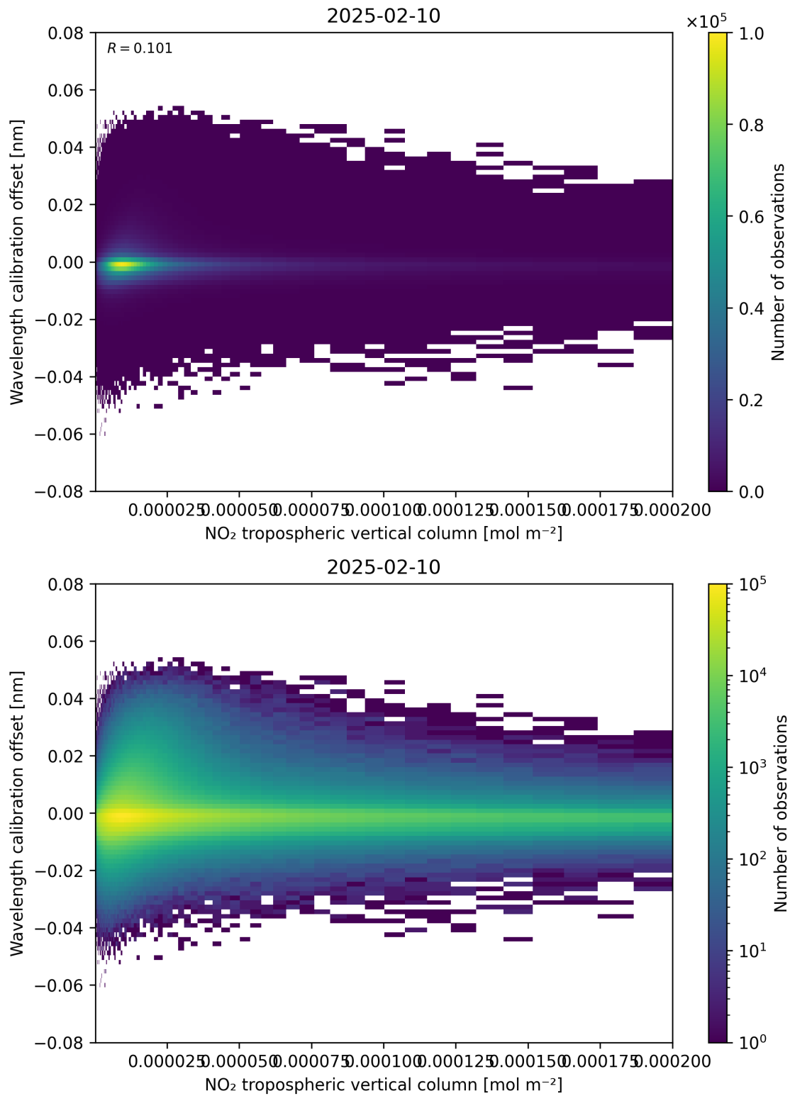
Figure 143: Scatter density plot of “NO 2 tropospheric vertical column” against “Wavelength calibration offset” for 2025-02-09 to 2025-02-11.
