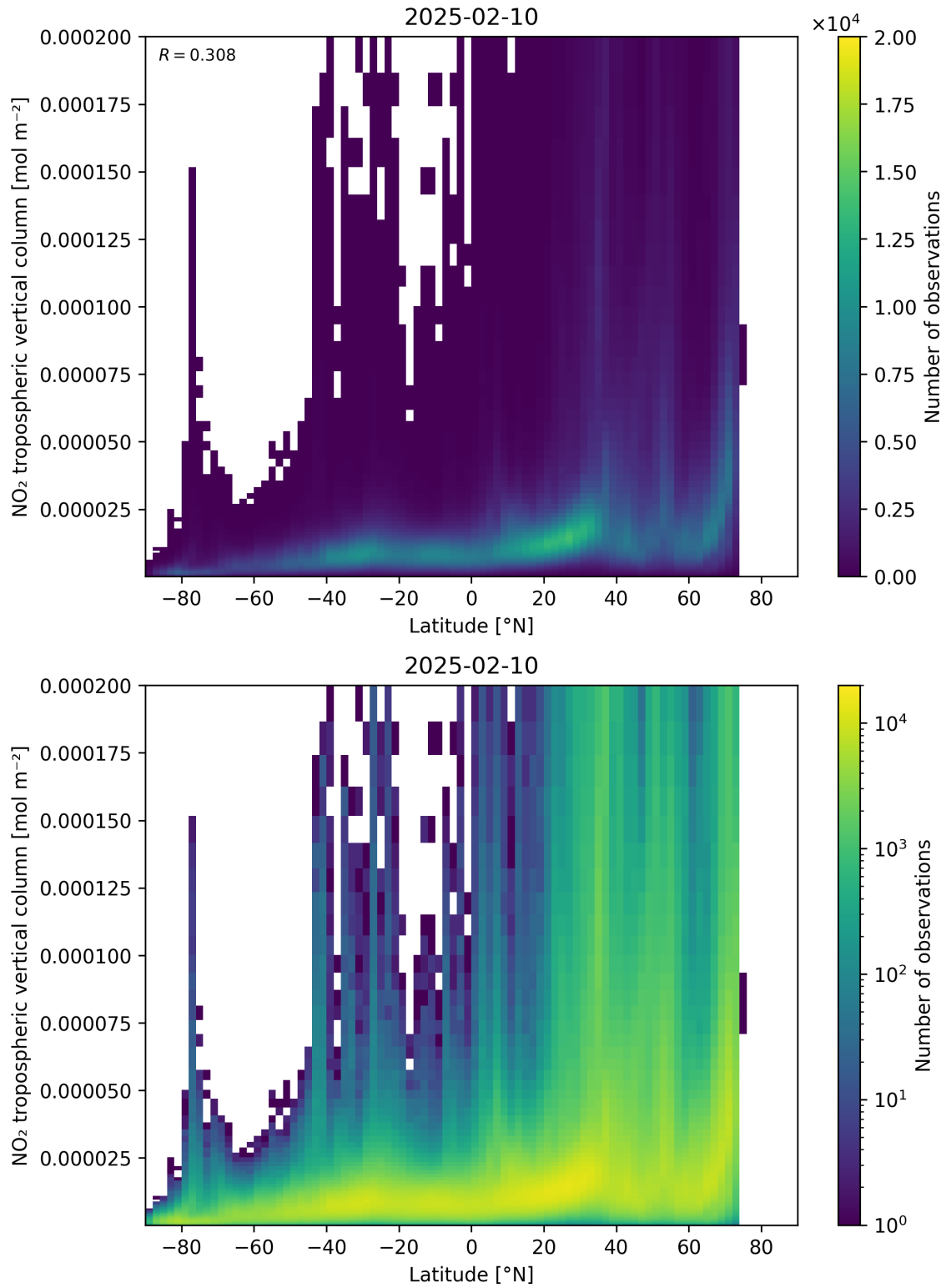
Figure 92: Scatter density plot of “Latitude” against “NO 2 tropospheric vertical column” for 2025-02-09 to 2025-02-11.
