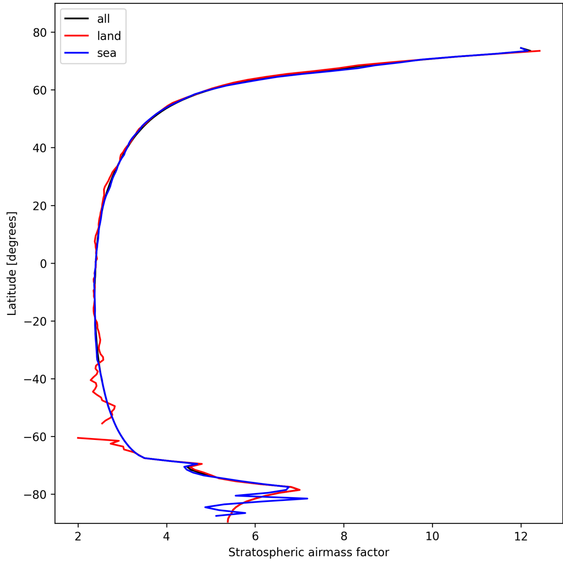
Figure 27: Zonal average of “Stratospheric airmass factor” for 2025-02-09 to 2025-02-11.
