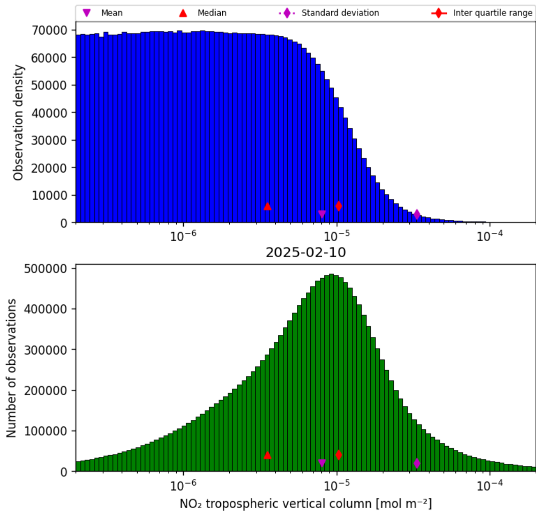
Figure 29: Histogram of “NO 2 tropospheric vertical column” for 2025-02-09 to 2025-02-11
