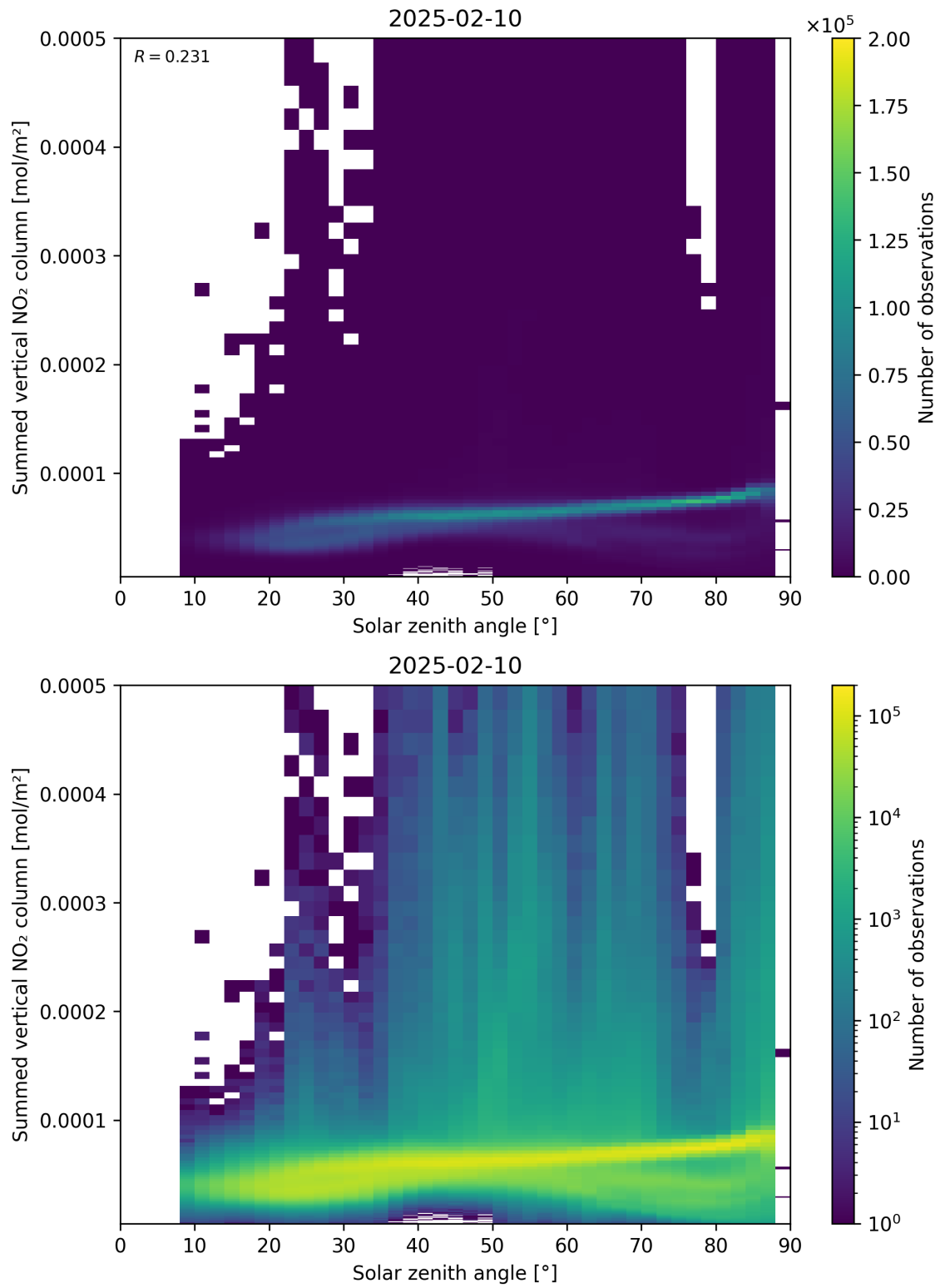
Figure 151: Scatter density plot of “Solar zenith angle” against “Summed vertical NO 2 column” for 2025-02-09 to 2025-02-11.
