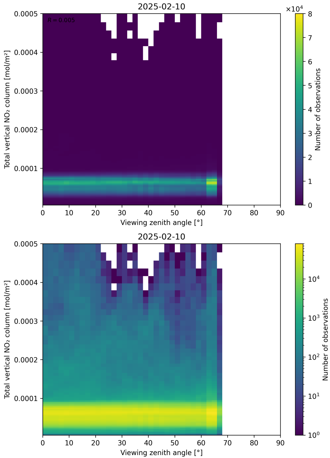
Figure 167: Scatter density plot of “Viewing zenith angle” against “Total vertical NO 2 column” for 2025-02-09 to 2025-02-11.
