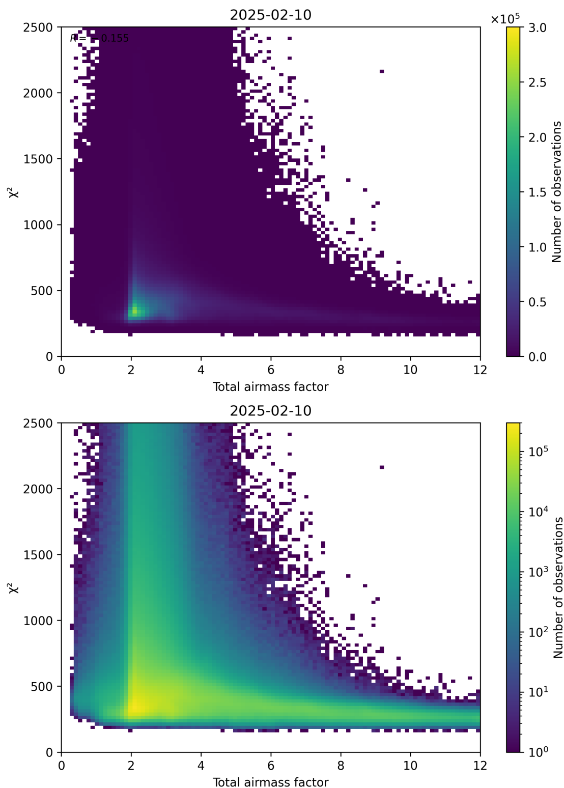
Figure 63: Scatter density plot of “Total airmass factor” against “ \chi^2 ” for 2025-02-09 to 2025-02-11.
