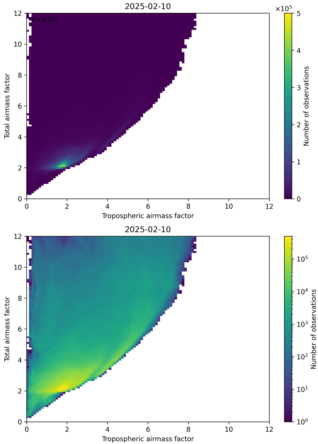
Figure 72: Scatter density plot of “Tropospheric airmass factor” against “Total airmass factor” for 2025-02-09 to 2025-02-11.
