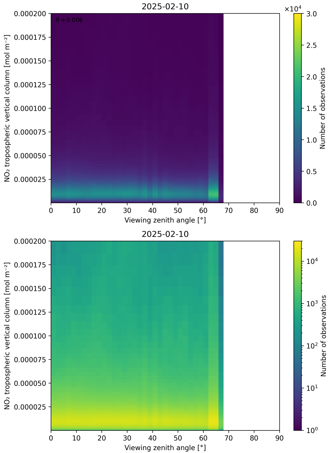
Figure 169: Scatter density plot of “Viewing zenith angle” against “NO 2 tropospheric vertical column” for 2025-02-09 to 2025-02-11.
