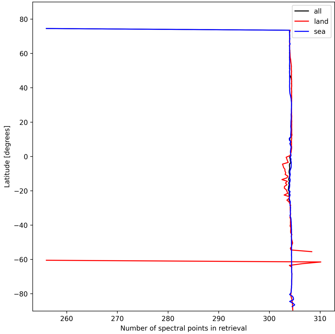
Figure 16: Zonal average of “Number of spectral points in retrieval” for 2025-02-09 to 2025-02-11.
