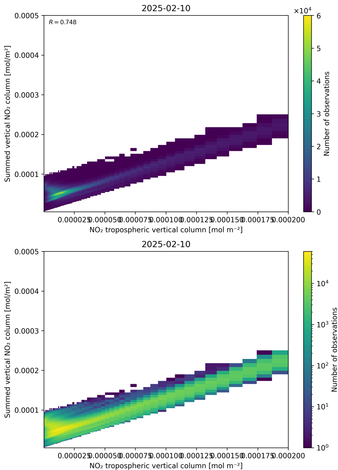
Figure 126: Scatter density plot of “NO 2 tropospheric vertical column” against “Summed vertical NO 2 column” for 2025-02-09 to 2025-02-11.
