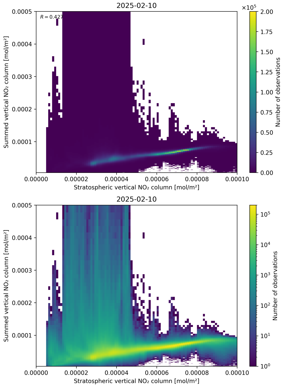
Figure 98: Scatter density plot of “Stratospheric vertical NO 2 column” against “Summed vertical NO 2 column” for 2025-02-09 to 2025-02-11.
