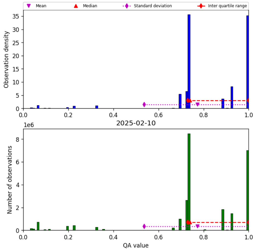
Figure 28: Histogram of “QA value” for 2025-02-09 to 2025-02-11
