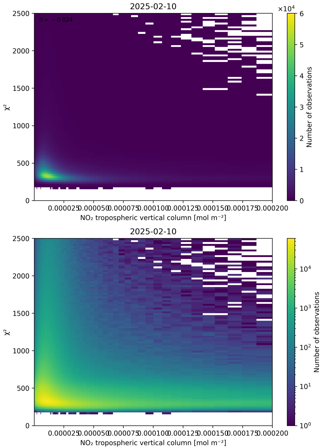
Figure 124: Scatter density plot of “NO 2 tropospheric vertical column” against “ \chi^2 ” for 2025-02-09 to 2025-02-11.
