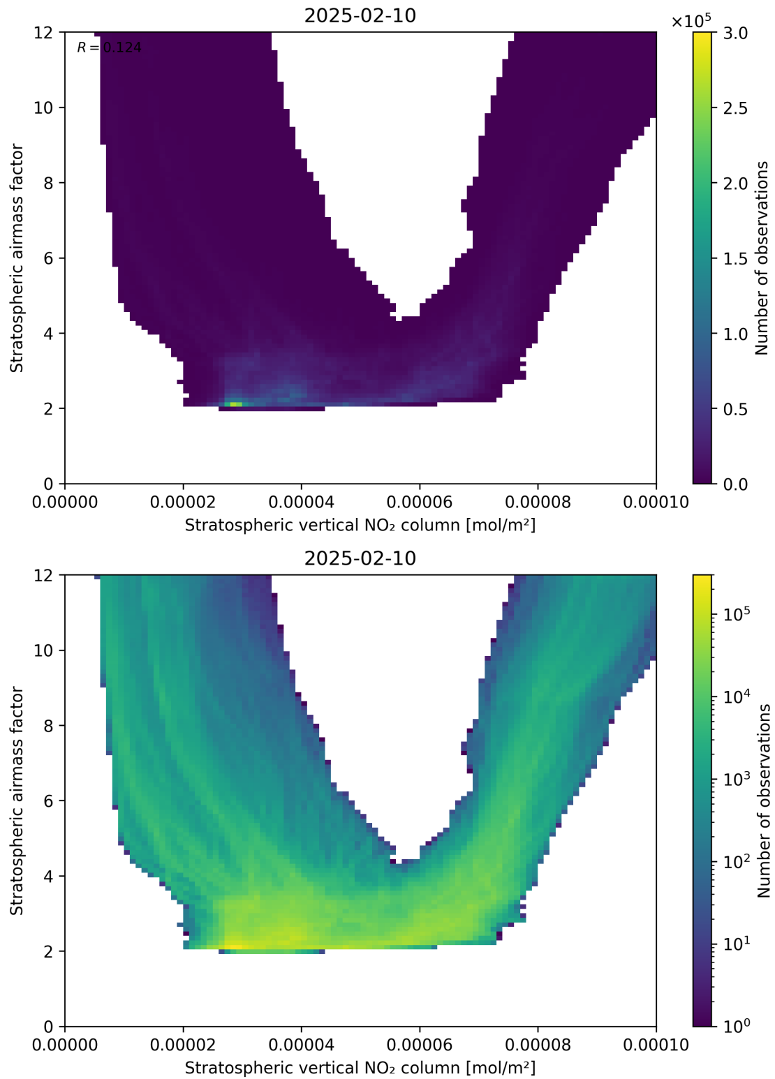
Figure 96: Scatter density plot of “Stratospheric vertical NO 2 column” against “Stratospheric airmass factor” for 2025-02-09 to 2025-02-11.
