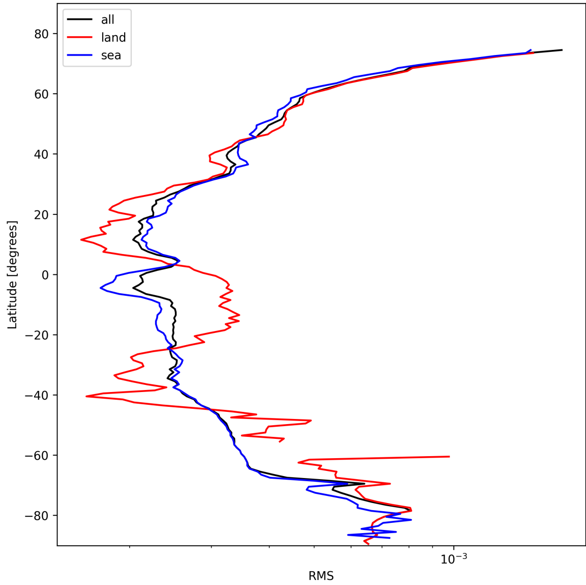
Figure 26: Zonal average of “RMS” for 2025-02-09 to 2025-02-11.
