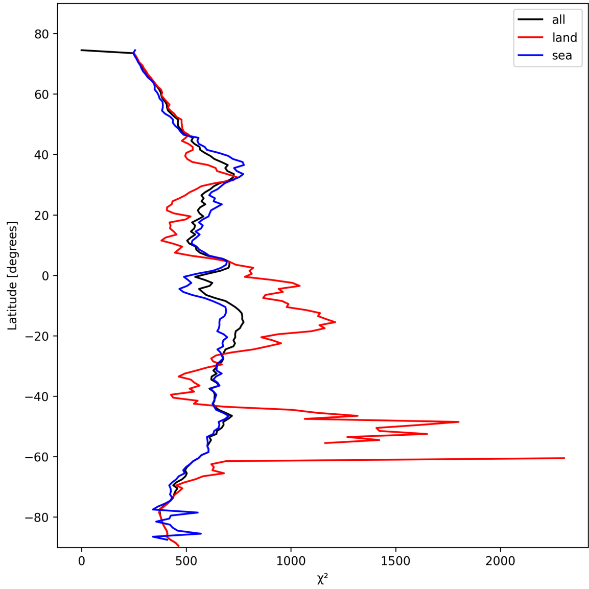
Figure 25: Zonal average of “ \chi^2 ” for 2025-02-09 to 2025-02-11.
