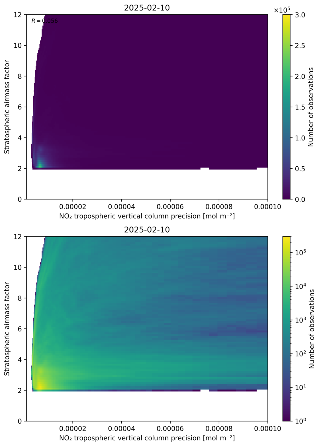
Figure 131: Scatter density plot of “NO 2 tropospheric vertical column precision” against “Stratospheric airmass factor” for 2025-02-09 to 2025-02-11.
