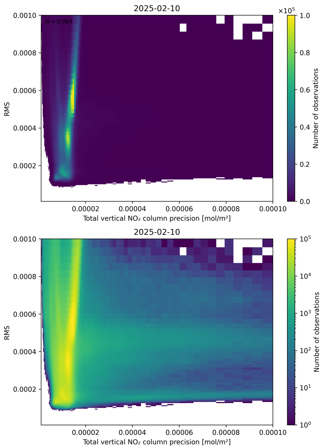
Figure 119: Scatter density plot of “Total vertical NO 2 column precision” against “RMS” for 2025-02-09 to 2025-02-11.
