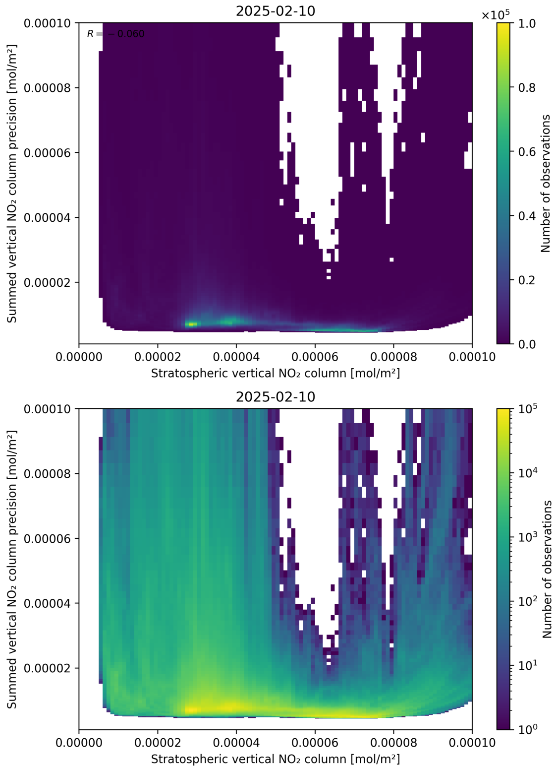
Figure 99: Scatter density plot of “Stratospheric vertical NO 2 column” against “Summed vertical NO 2 column precision” for 2025-02-09 to 2025-02-11.
