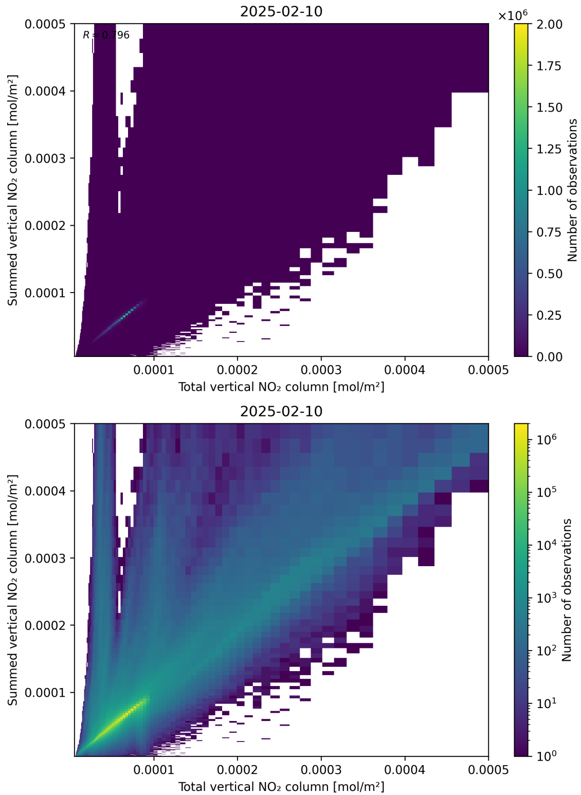
Figure 112: Scatter density plot of “Total vertical NO 2 column” against “Summed vertical NO 2 column” for 2025-02-09 to 2025-02-11.
