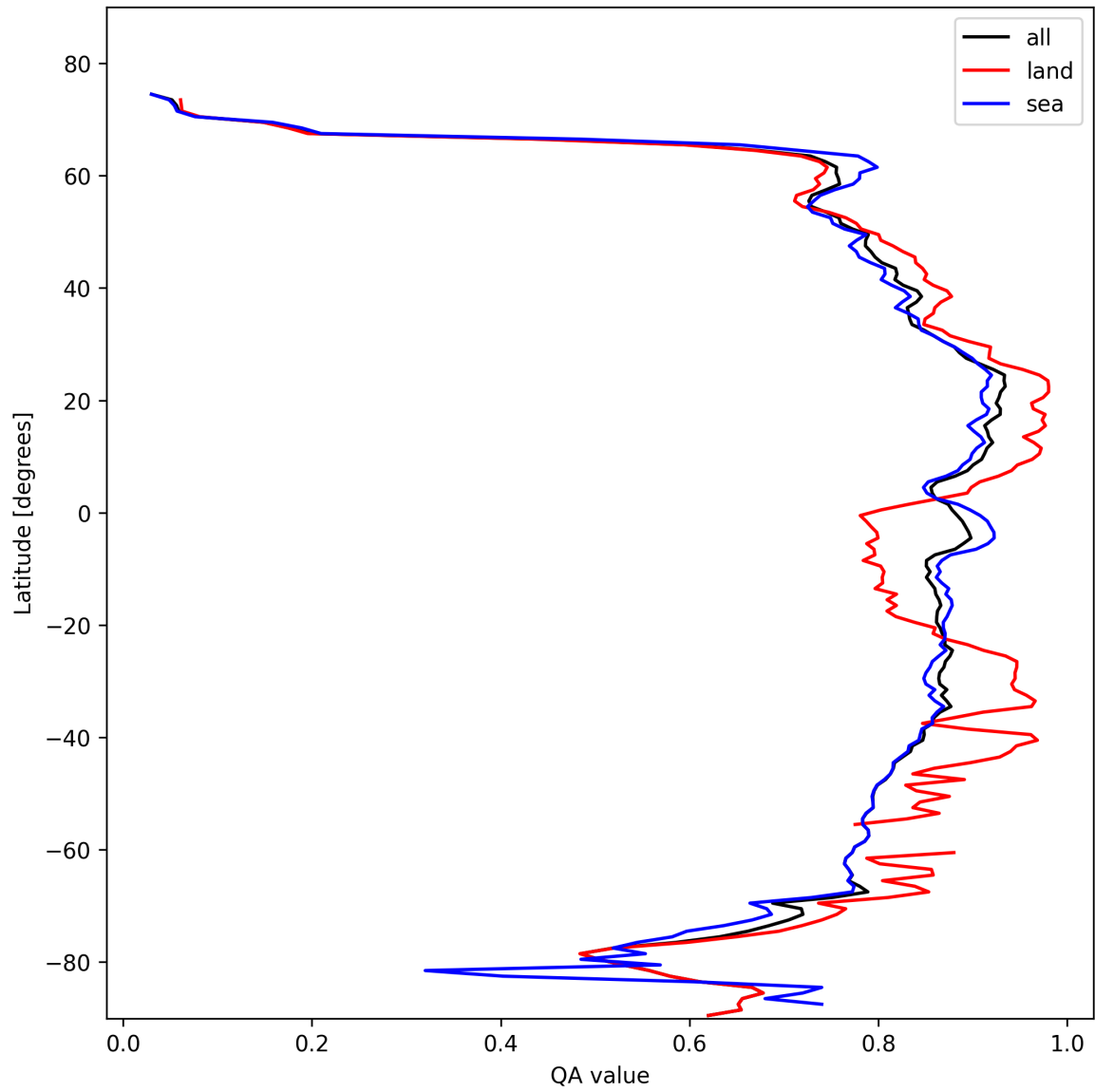
Figure 11: Zonal average of “QA value” for 2025-02-09 to 2025-02-11.
