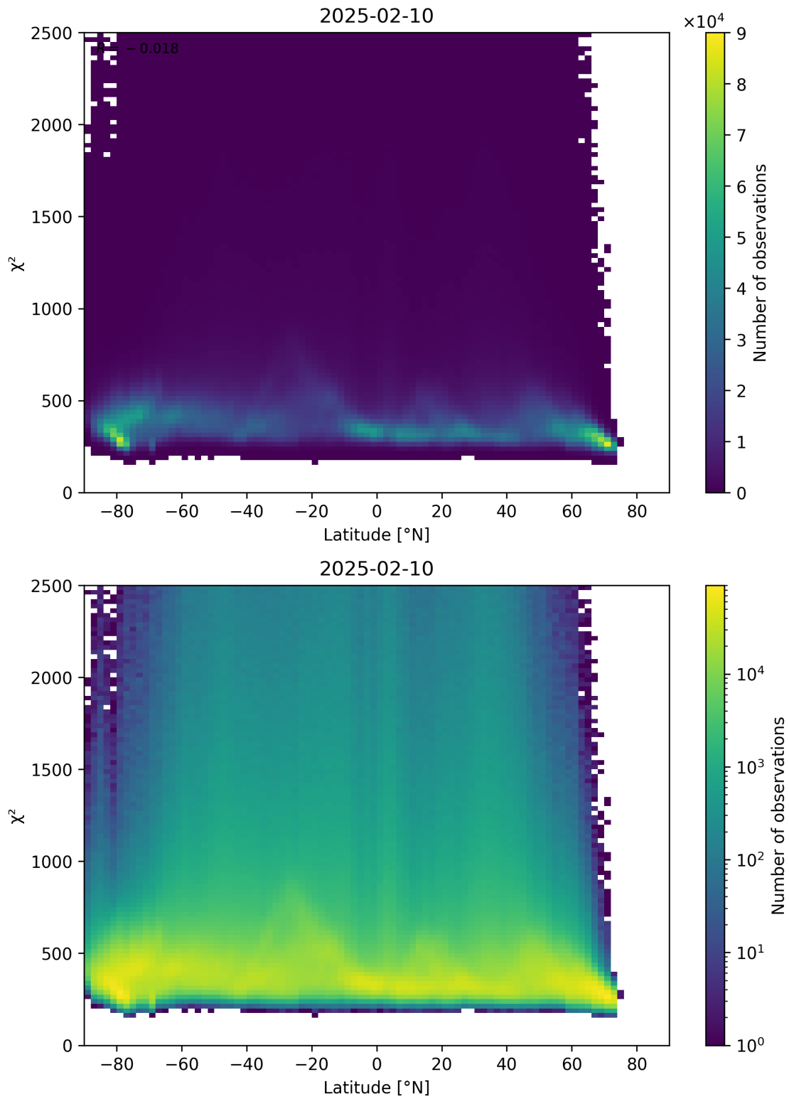
Figure 86: Scatter density plot of “Latitude” against “ \chi^2 ” for 2025-02-09 to 2025-02-11.
