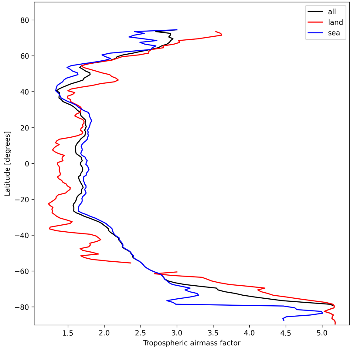
Figure 14: Zonal average of “Tropospheric airmass factor” for 2025-02-09 to 2025-02-11.
