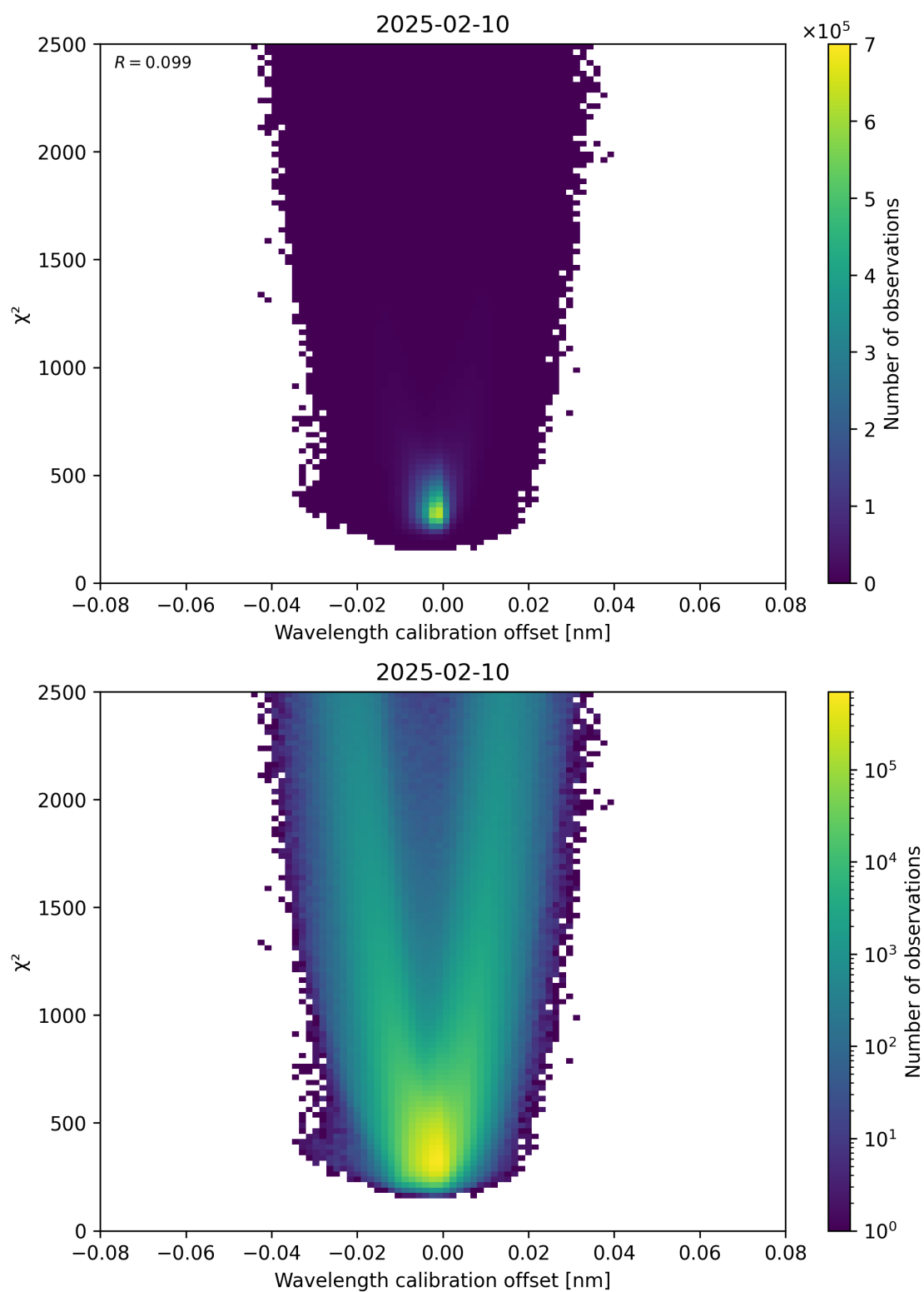
Figure 175: Scatter density plot of “Wavelength calibration offset” against “ \chi^2 ” for 2025-02-09 to 2025-02-11.
