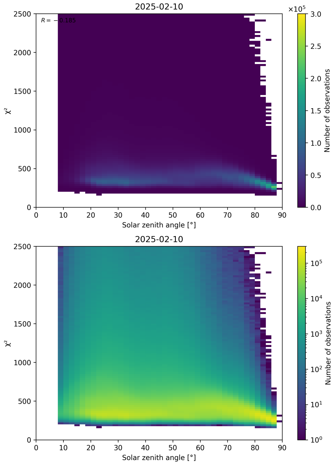
Figure 148: Scatter density plot of “Solar zenith angle” against “ \chi^2 ” for 2025-02-09 to 2025-02-11.
