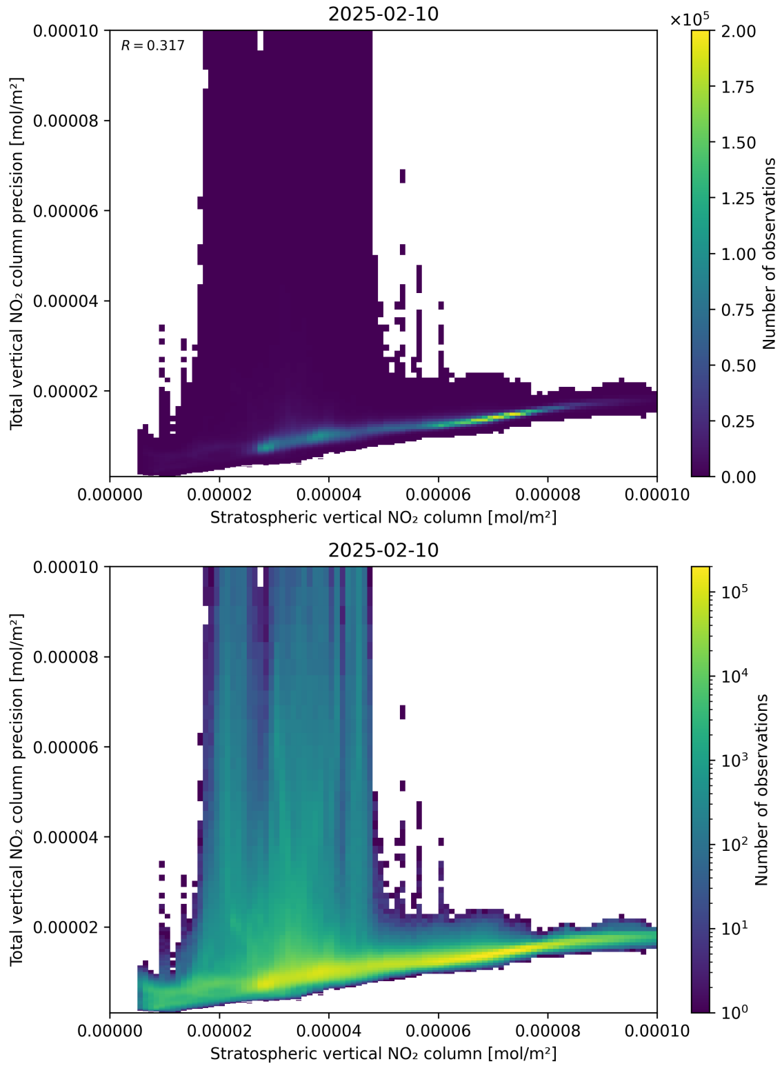
Figure 101: Scatter density plot of “Stratospheric vertical NO 2 column” against “Total vertical NO 2 column precision” for 2025-02-09 to 2025-02-11.
