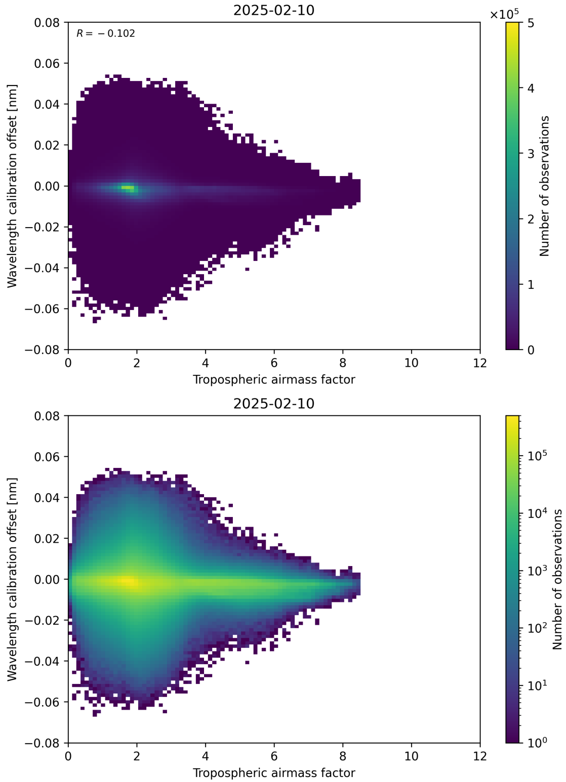
Figure 80: Scatter density plot of “Tropospheric airmass factor” against “Wavelength calibration offset” for 2025-02-09 to 2025-02-11.
