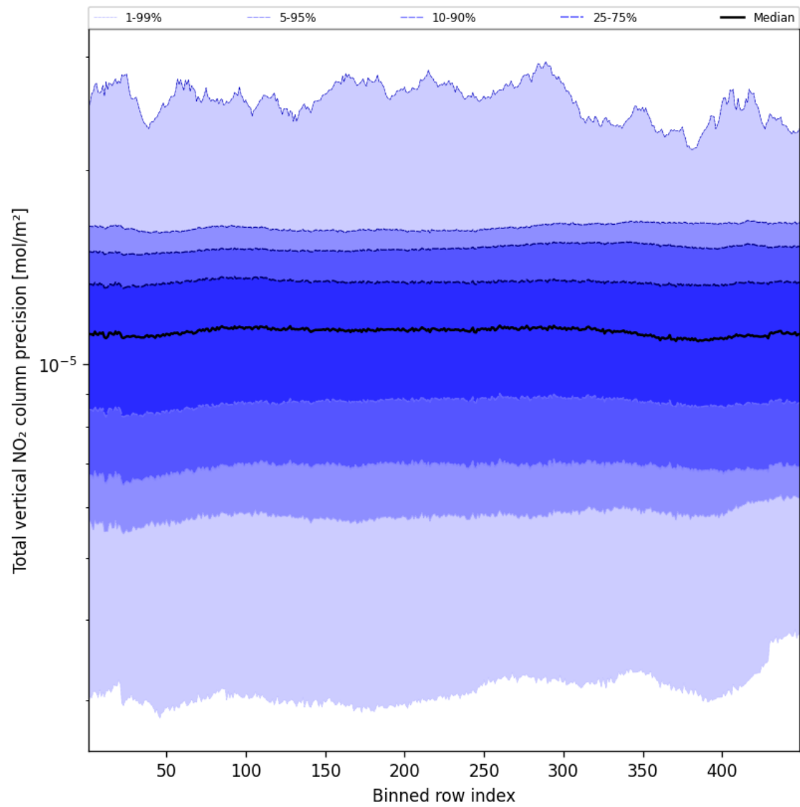
Figure 56: Along track statistics of “Total vertical NO 2 column precision” for 2025-02-09 to 2025-02-11
