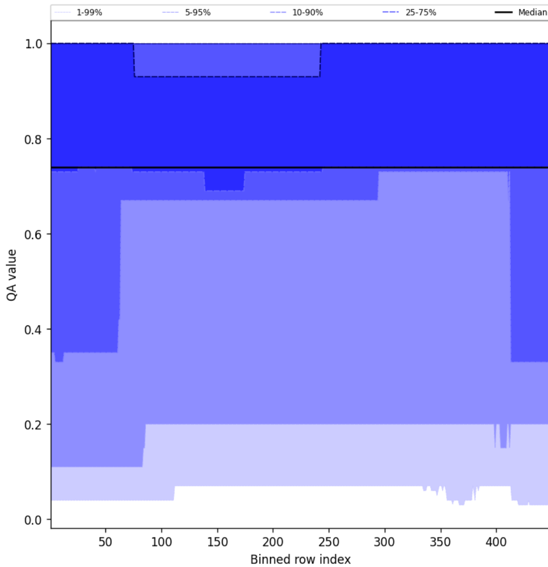
Figure 45: Along track statistics of “QA value” for 2025-02-09 to 2025-02-11
