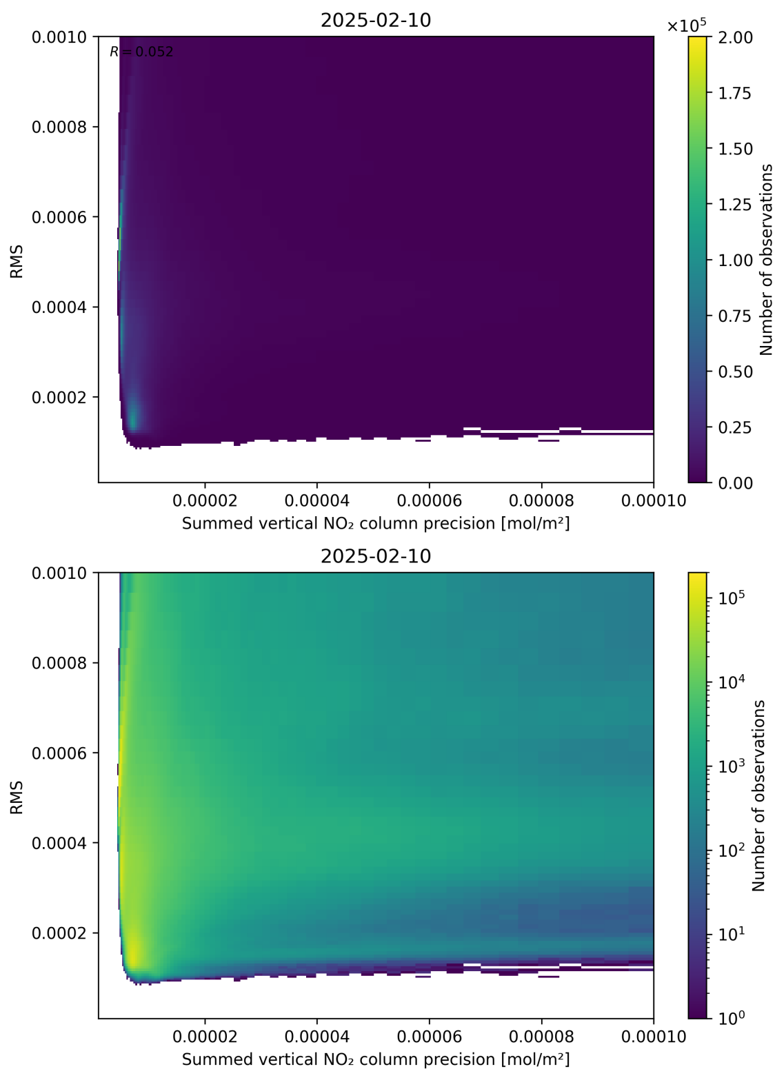
Figure 108: Scatter density plot of “Summed vertical NO 2 column precision” against “RMS” for 2025-02-09 to 2025-02-11.
