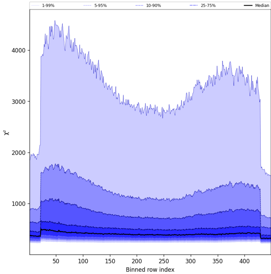
Figure 59: Along track statistics of “ \chi^2 ” for 2025-02-09 to 2025-02-11
