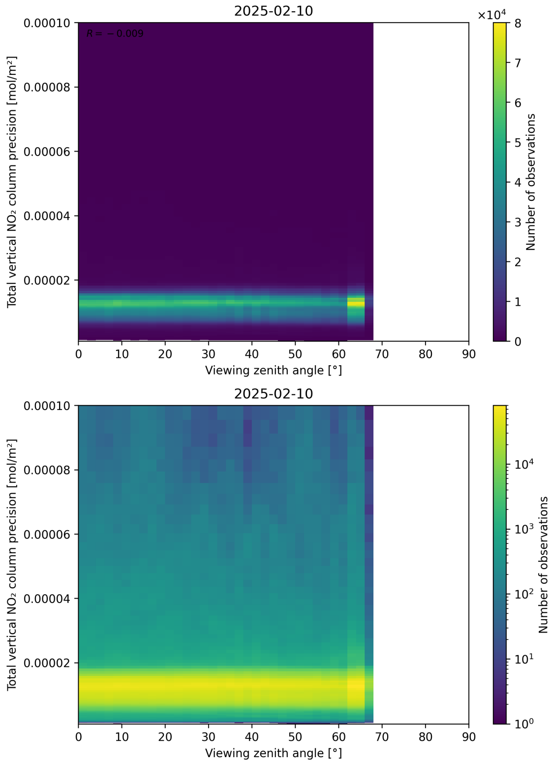
Figure 168: Scatter density plot of “Viewing zenith angle” against “Total vertical NO 2 column precision” for 2025-02-09 to 2025-02-11.
