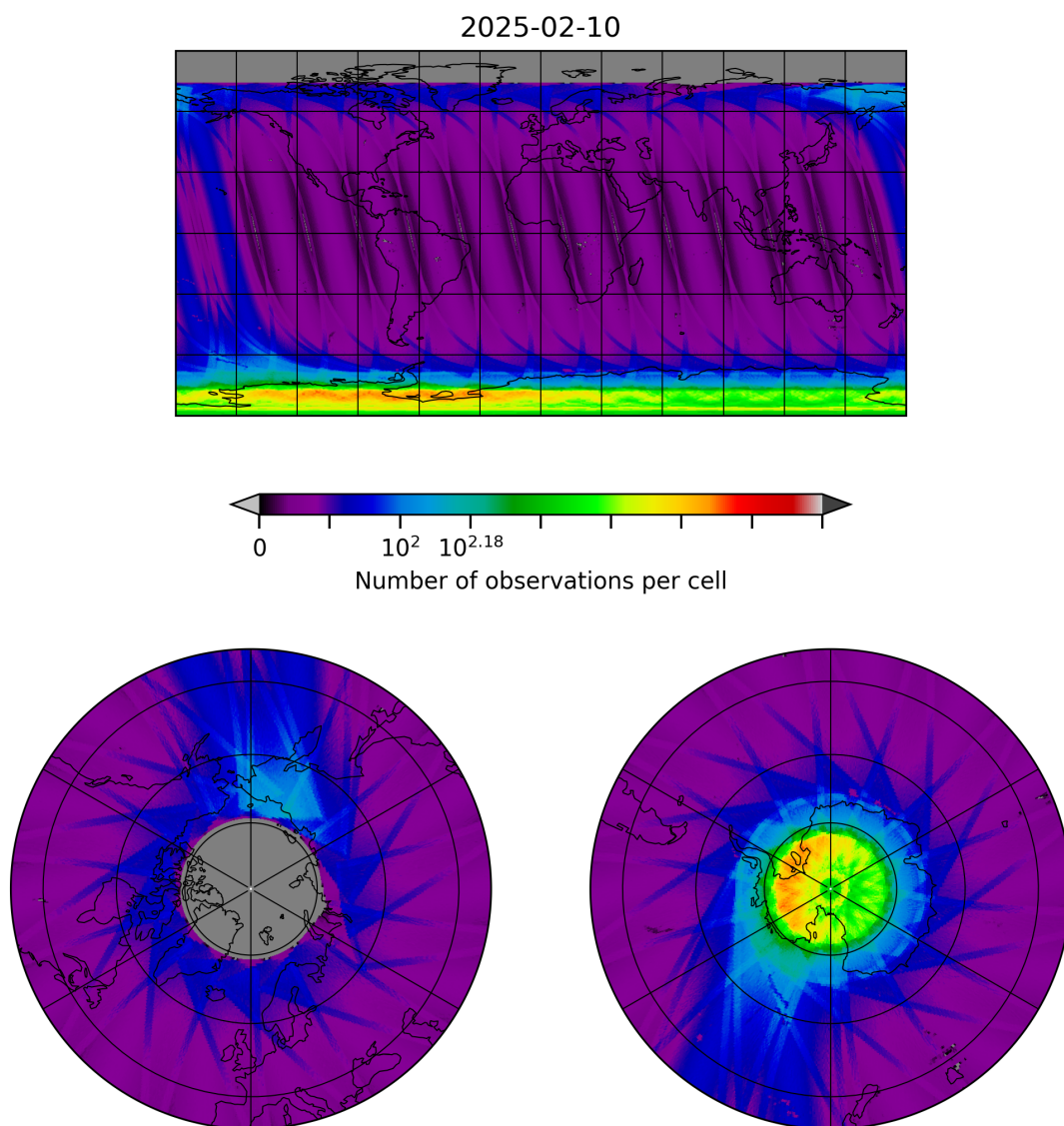
Figure 10: Map of the number of observations for 2025-02-09 to 2025-02-11
