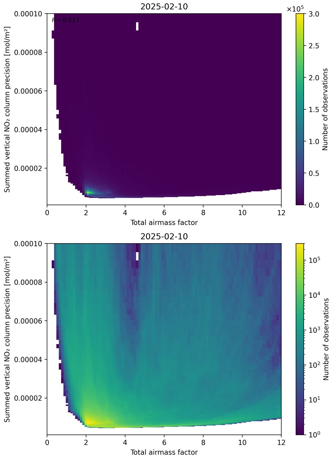
Figure 66: Scatter density plot of “Total airmass factor” against “Summed vertical NO 2 column precision” for 2025-02-09 to 2025-02-11.
