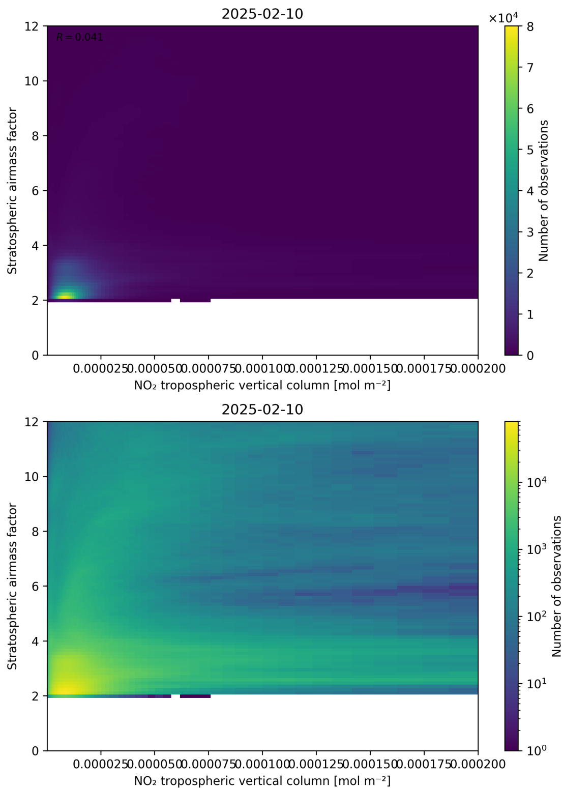
Figure 121: Scatter density plot of “NO 2 tropospheric vertical column” against “Stratospheric airmass factor” for 2025-02-09 to 2025-02-11.
