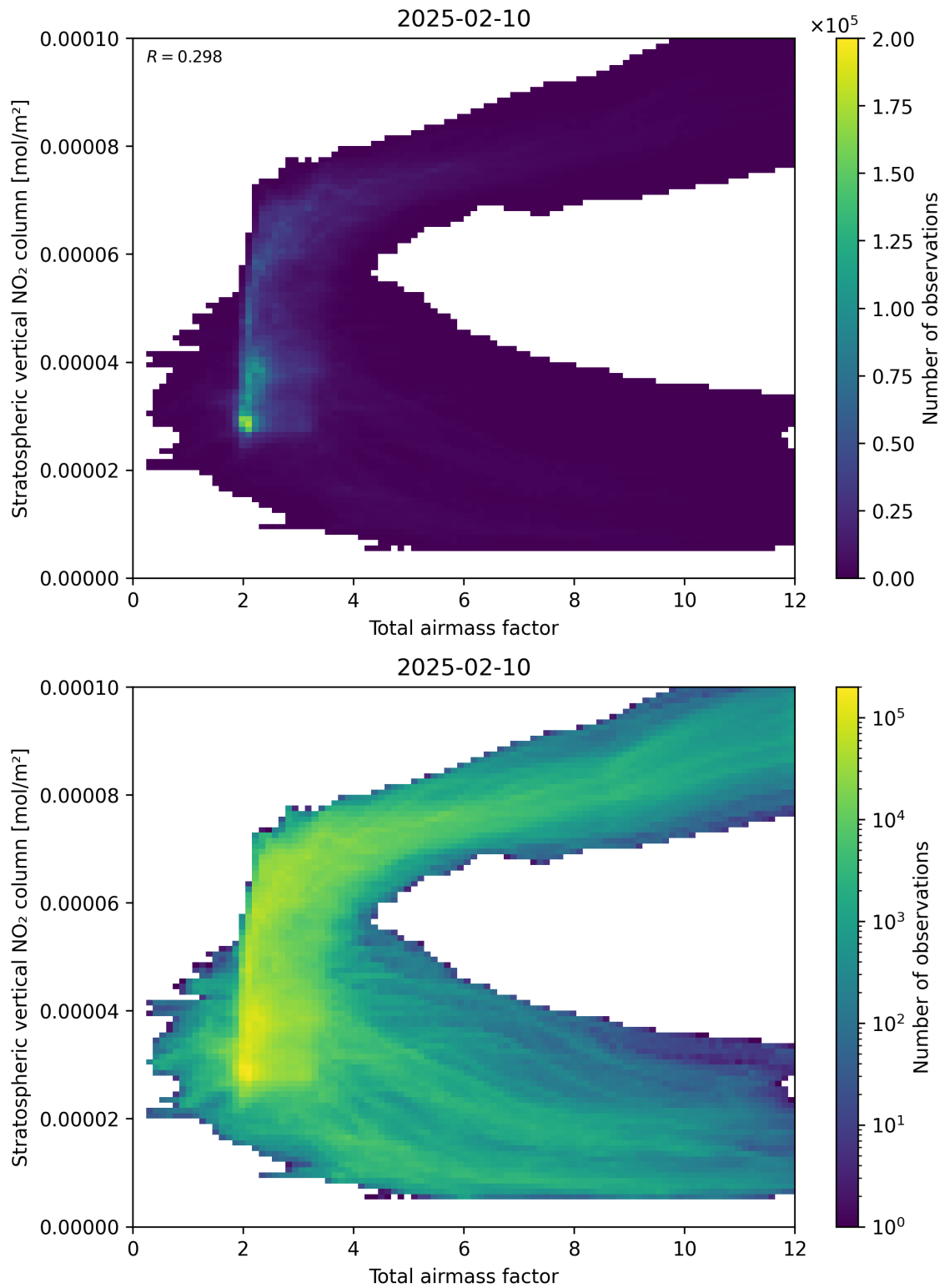
Figure 64: Scatter density plot of “Total airmass factor” against “Stratospheric vertical NO 2 column” for 2025-02-09 to 2025-02-11.
