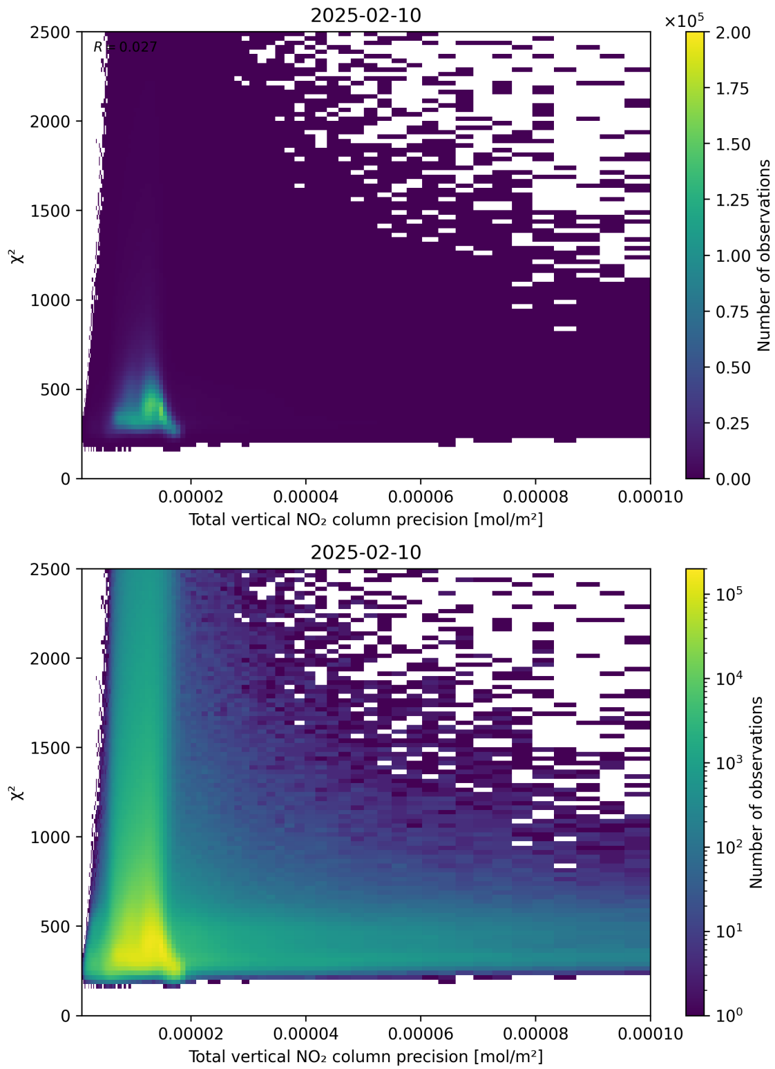
Figure 116: Scatter density plot of “Total vertical NO 2 column precision” against “ \chi^2 ” for 2025-02-09 to 2025-02-11.
