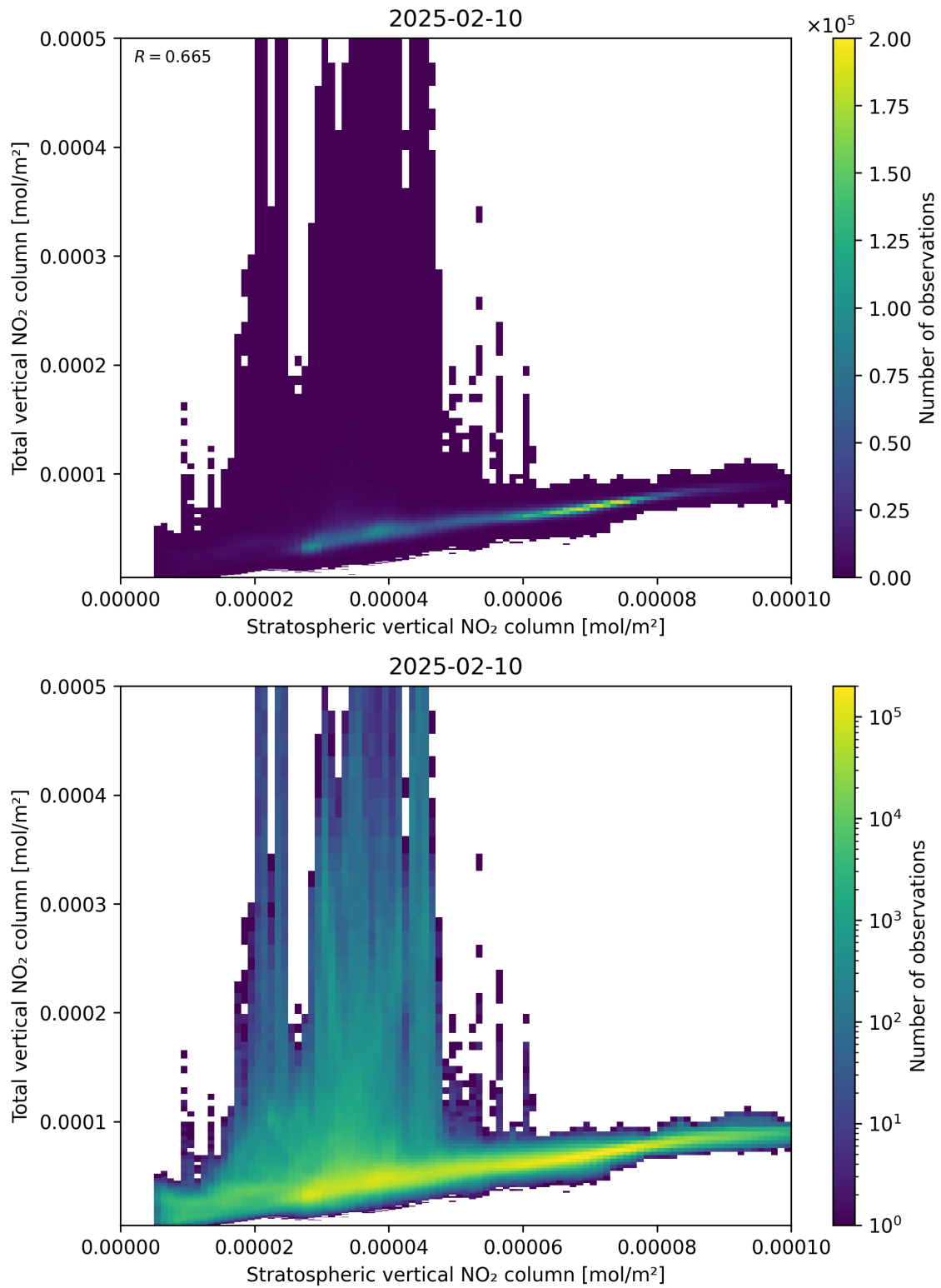
Figure 100: Scatter density plot of “Stratospheric vertical NO 2 column” against “Total vertical NO 2 column” for 2025-02-09 to 2025-02-11.
