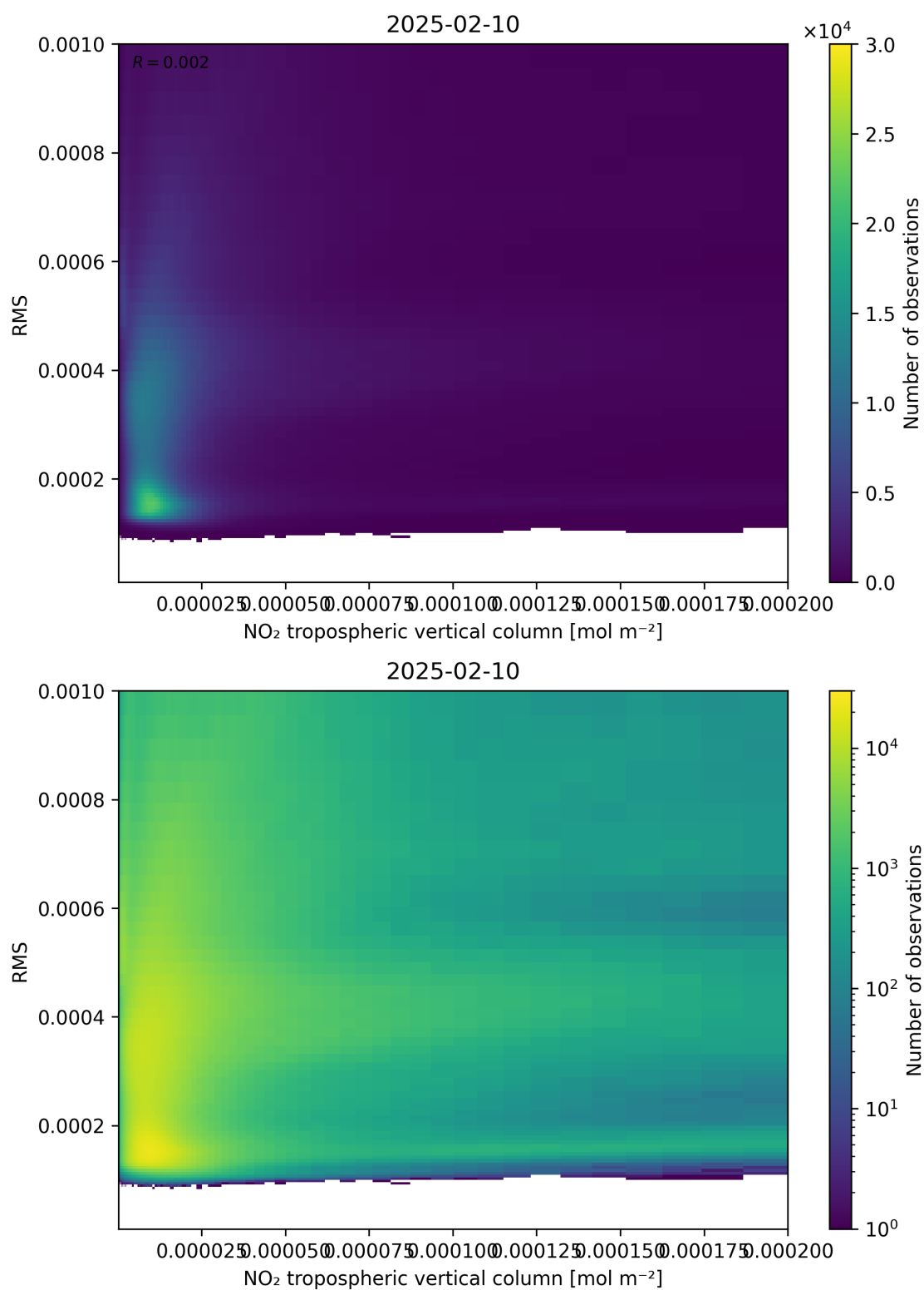
Figure 142: Scatter density plot of “NO 2 tropospheric vertical column” against “RMS” for 2025-02-09 to 2025-02-11.
