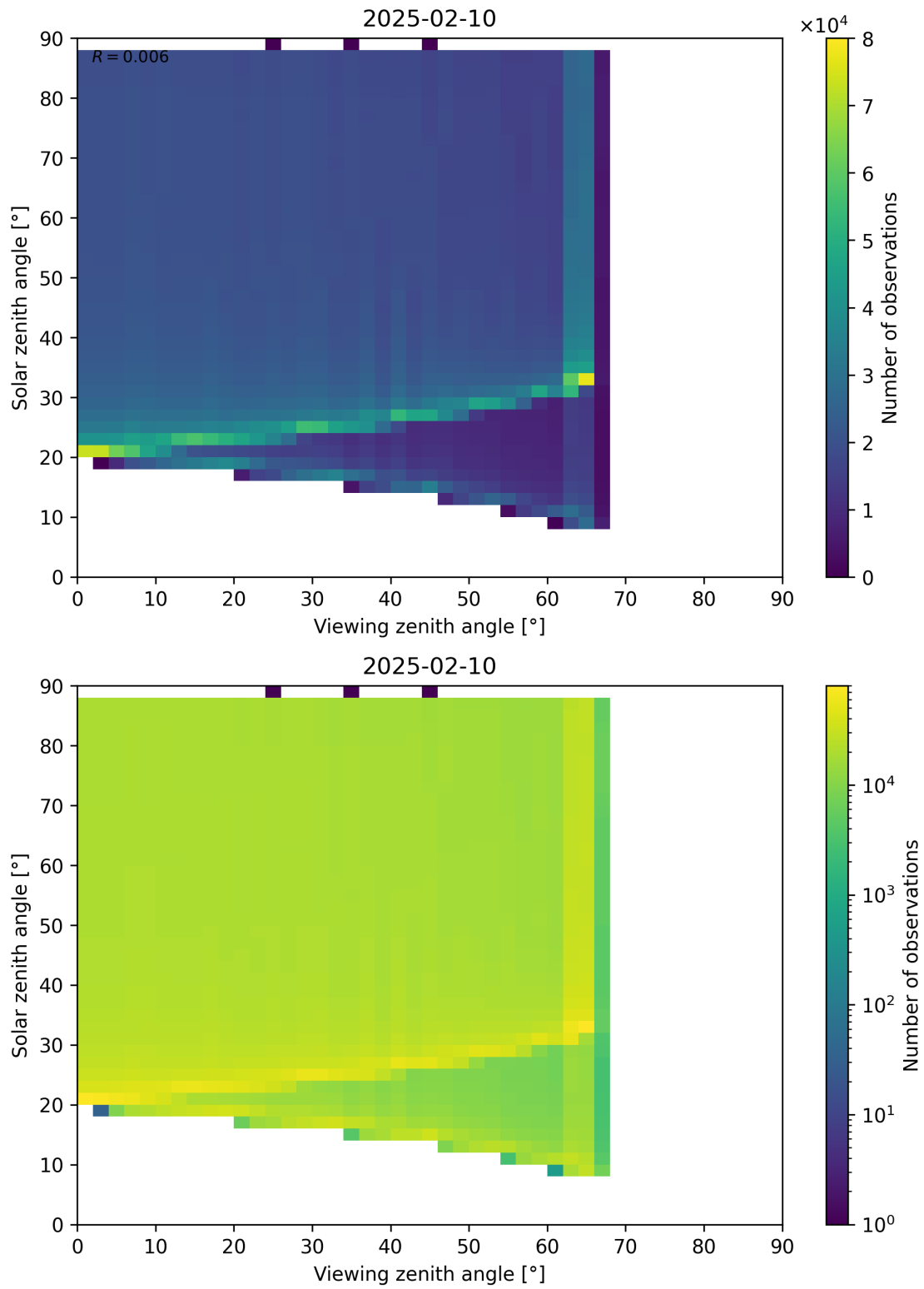
Figure 172: Scatter density plot of “Viewing zenith angle” against “Solar zenith angle” for 2025-02-09 to 2025-02-11.
