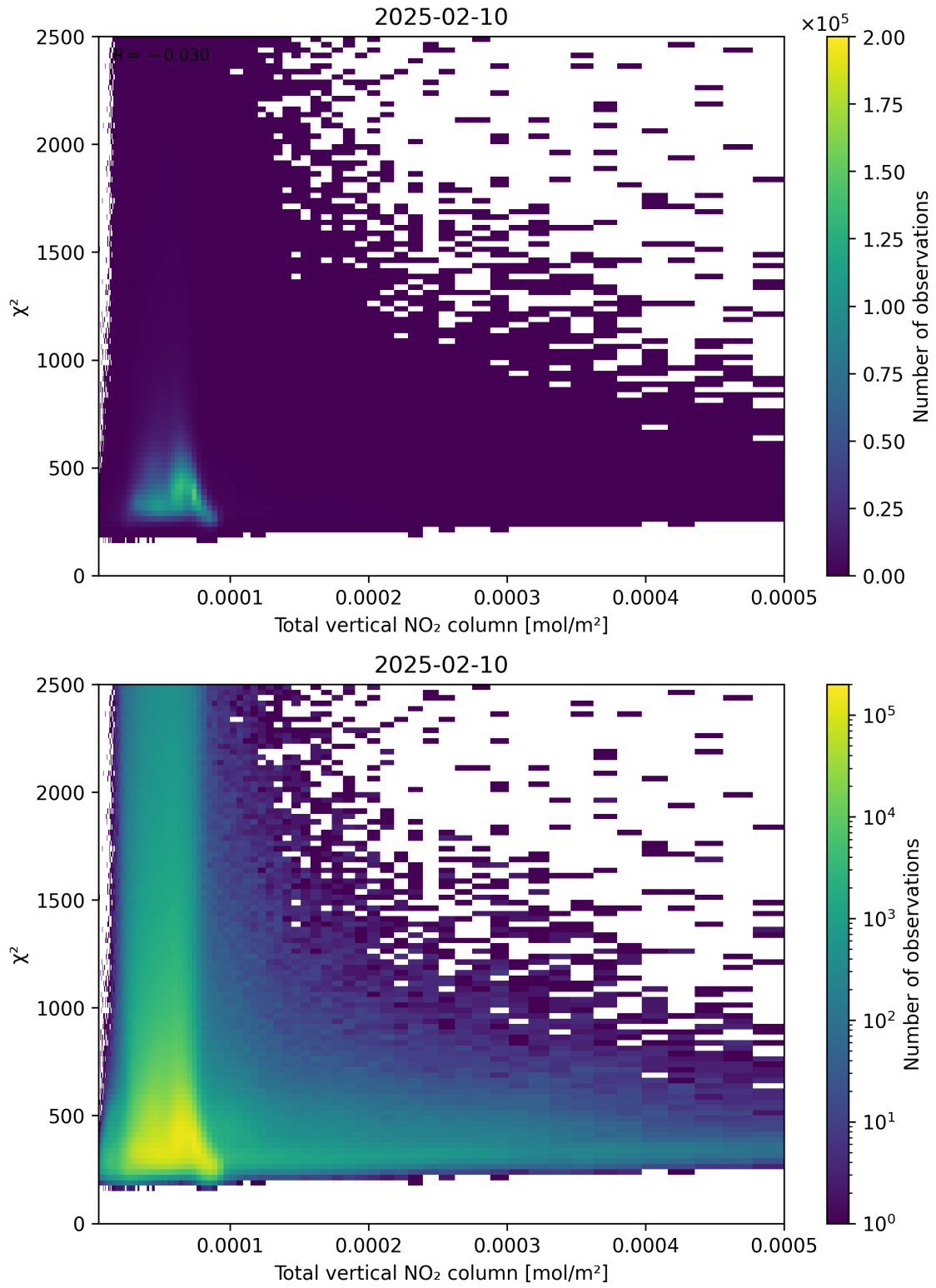
Figure 111: Scatter density plot of “Total vertical NO 2 column” against “ \chi^2 ” for 2025-02-09 to 2025-02-11.
