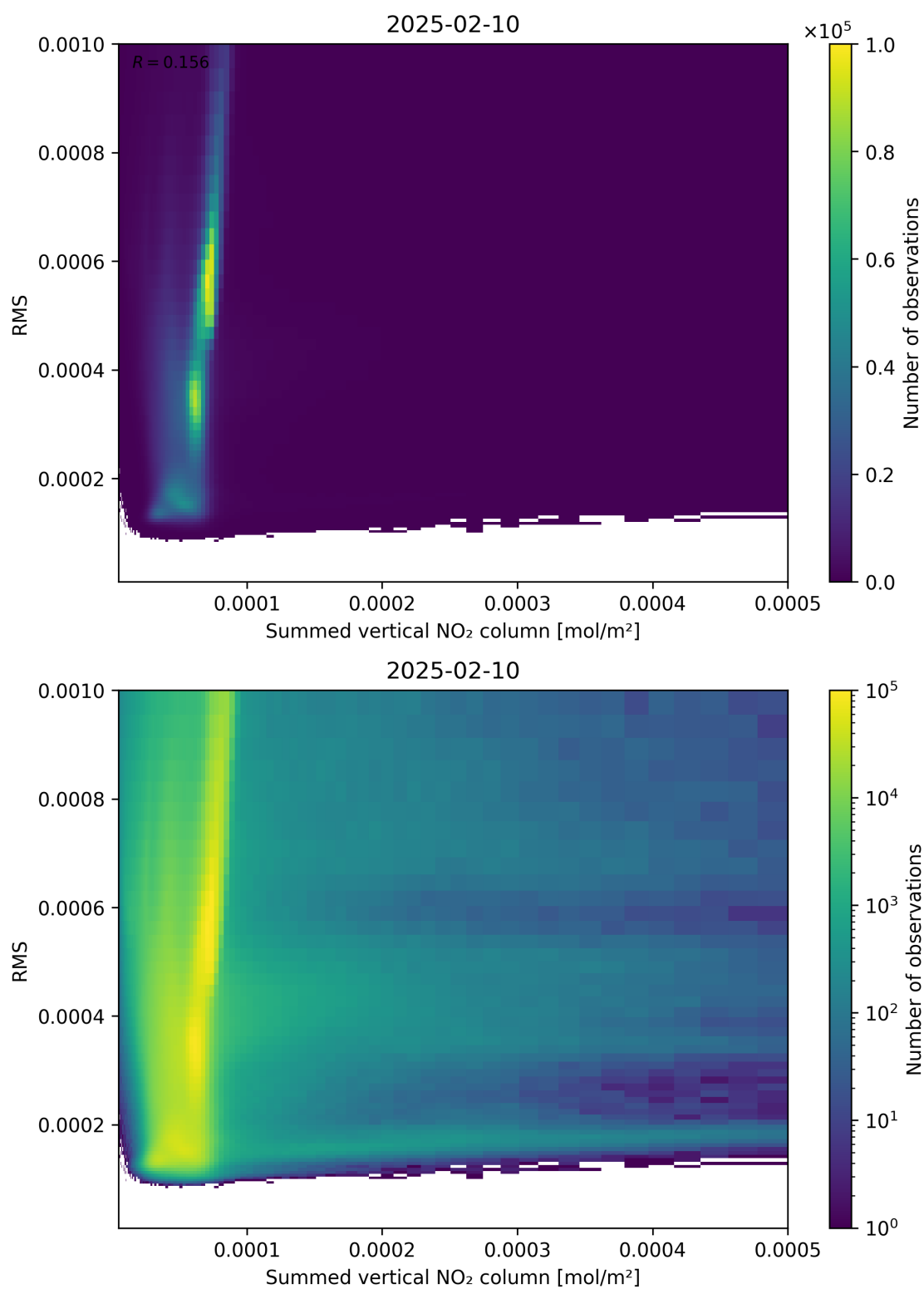
Figure 109: Scatter density plot of “Summed vertical NO 2 column” against “RMS” for 2025-02-09 to 2025-02-11.
