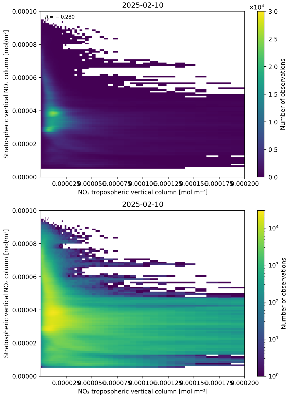
Figure 125: Scatter density plot of “NO 2 tropospheric vertical column” against “Stratospheric vertical NO 2 column” for 2025-02-09 to 2025-02-11.
