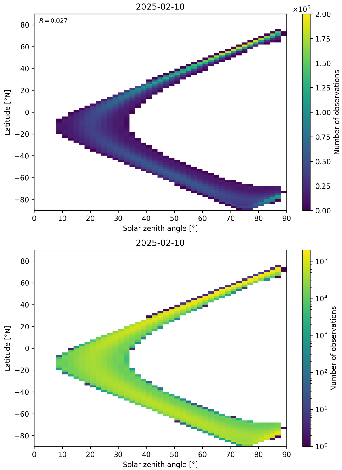
Figure 149: Scatter density plot of “Solar zenith angle” against “Latitude” for 2025-02-09 to 2025-02-11.
