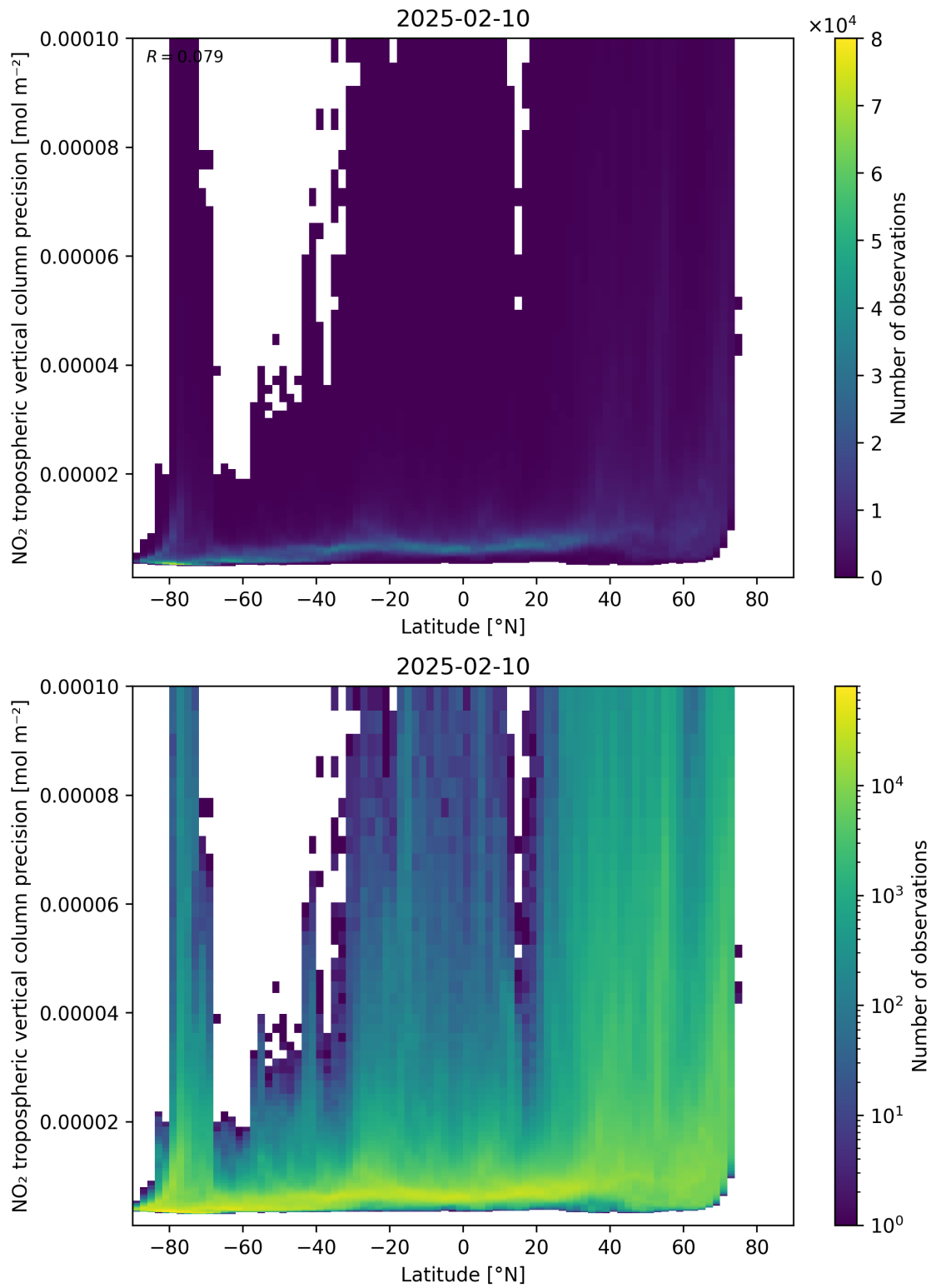
Figure 93: Scatter density plot of “Latitude” against “NO 2 tropospheric vertical column precision” for 2025-02-09 to 2025-02-11.
