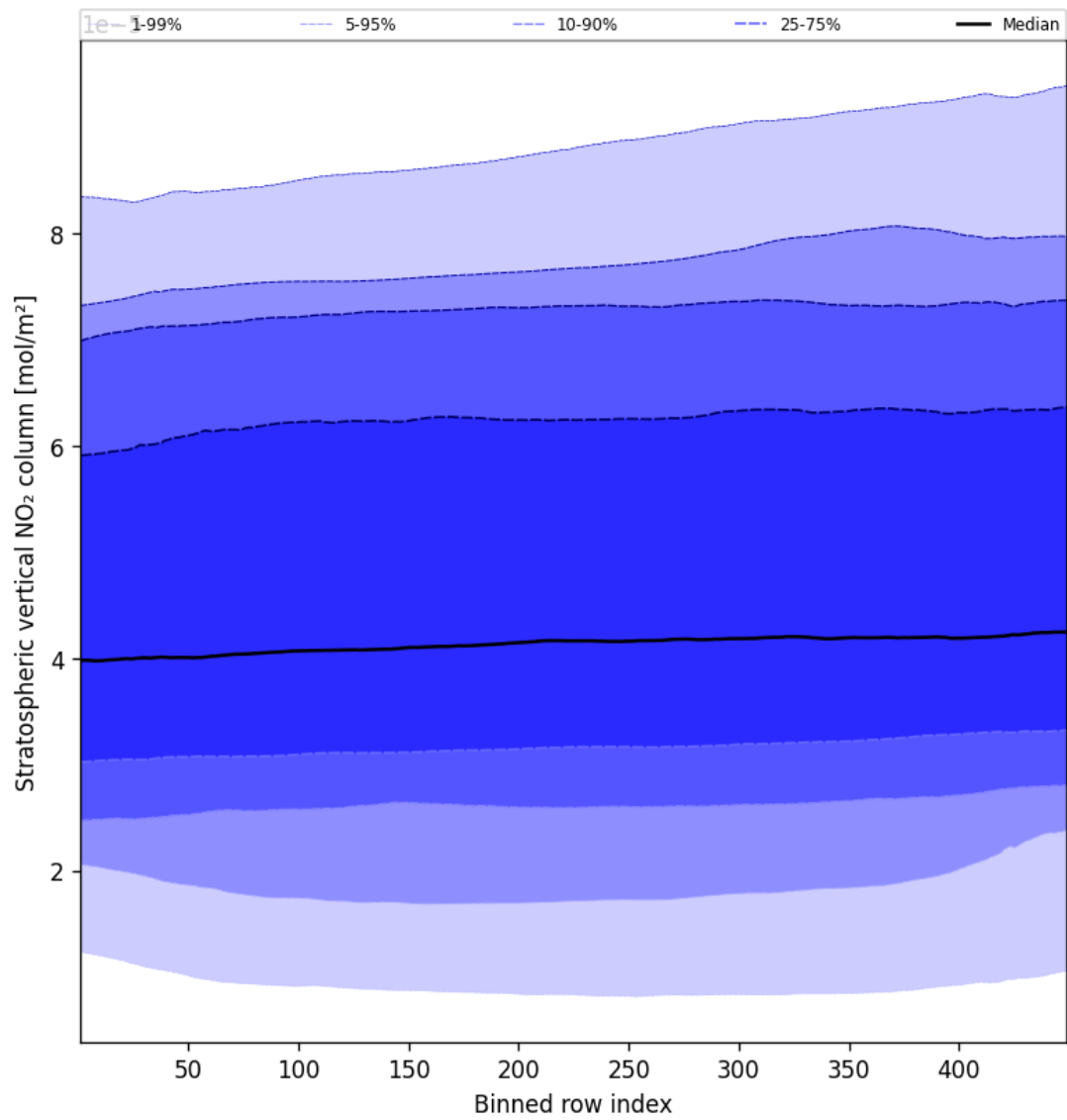
Figure 53: Along track statistics of “Stratospheric vertical NO 2 column” for 2025-02-09 to 2025-02-11
