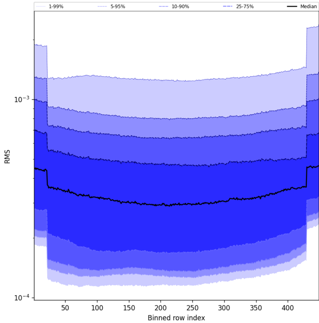
Figure 60: Along track statistics of “RMS” for 2025-02-09 to 2025-02-11
