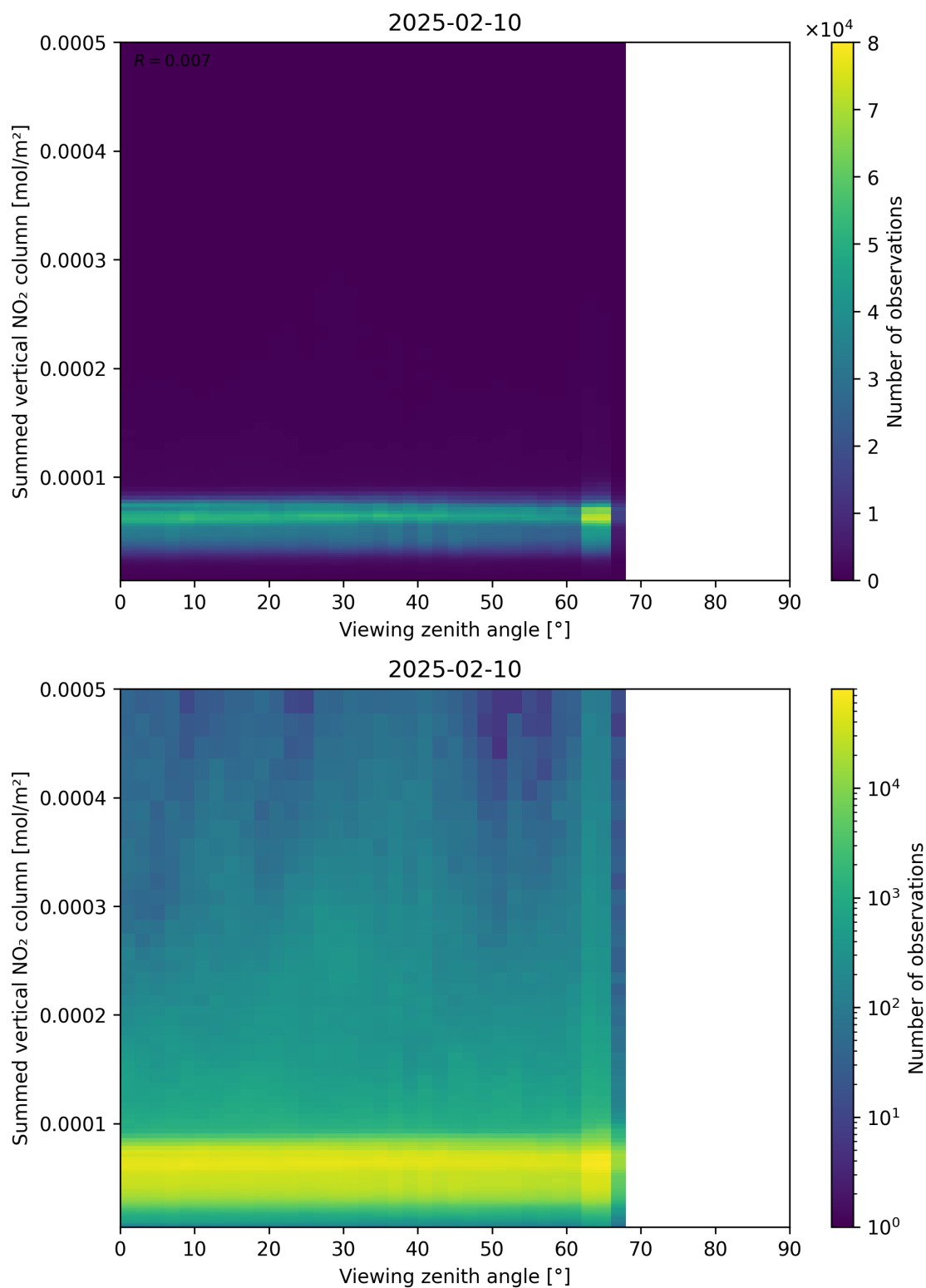
Figure 165: Scatter density plot of “Viewing zenith angle” against “Summed vertical NO 2 column” for 2025-02-09 to 2025-02-11.
