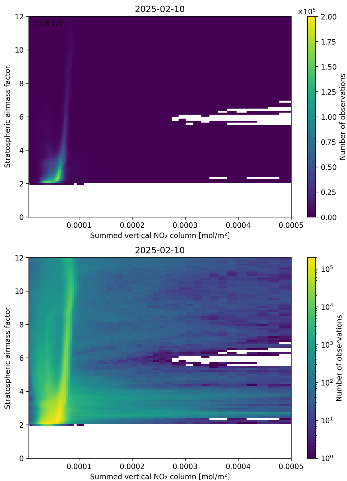
Figure 103: Scatter density plot of “Summed vertical NO 2 column” against “Stratospheric air mass factor” for 2025-02-09 to 2025-02-11.
