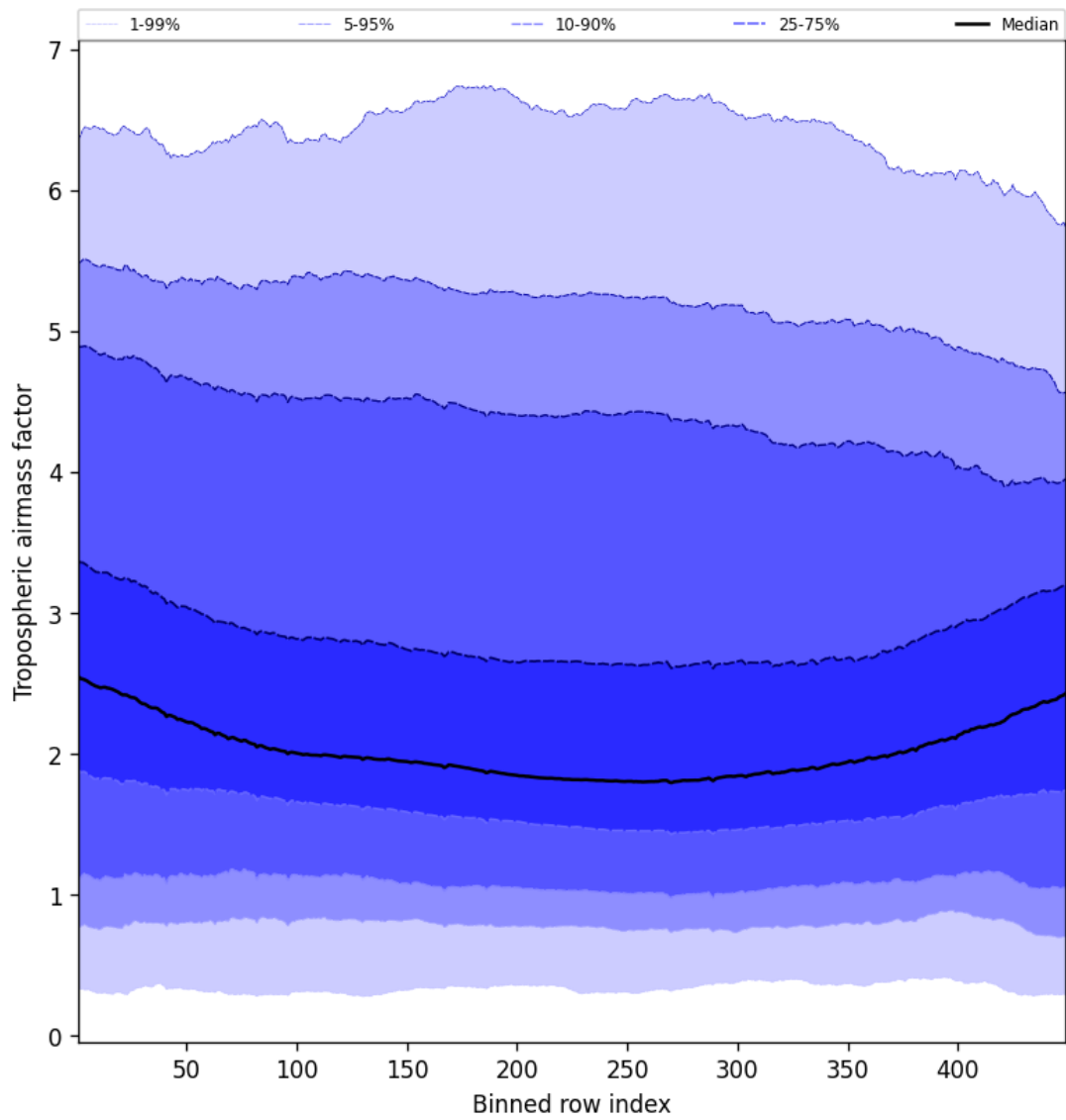
Figure 48: Along track statistics of “Tropospheric air mass factor” for 2025-02-09 to 2025-02-11
