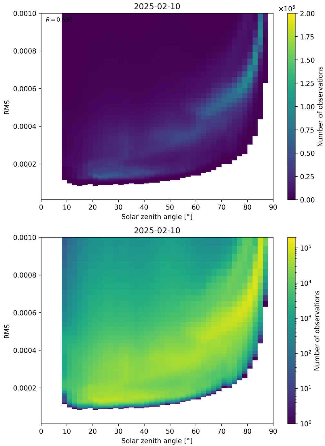
Figure 157: Scatter density plot of “Solar zenith angle” against “RMS” for 2025-02-09 to 2025-02-11.
