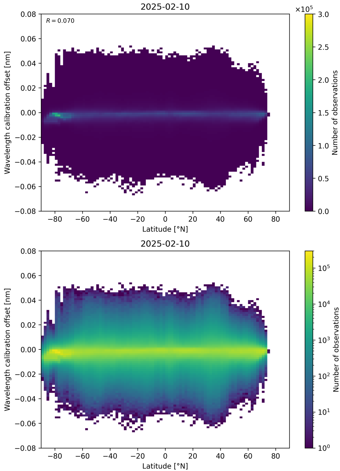
Figure 95: Scatter density plot of “Latitude” against “Wavelength calibration offset” for 2025-02-09 to 2025-02-11.
