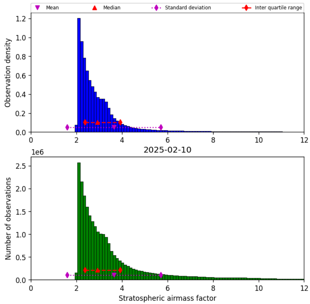
Figure 44: Histogram of “Stratospheric airmass factor” for 2025-02-09 to 2025-02-11
