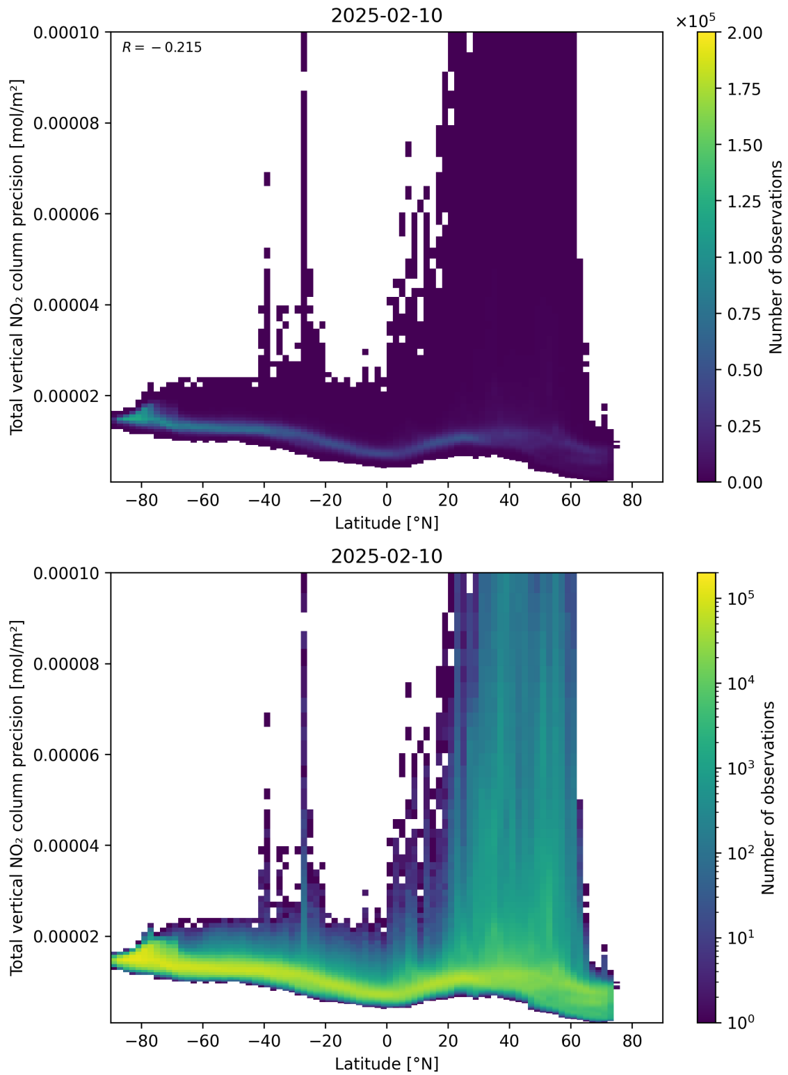
Figure 91: Scatter density plot of “Latitude” against “Total vertical NO 2 column precision” for 2025-02-09 to 2025-02-11.
