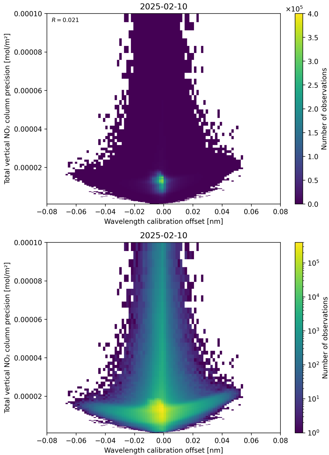
Figure 180: Scatter density plot of “Wavelength calibration offset” against “Total vertical NO 2 column precision” for 2025-02-09 to 2025-02-11.
