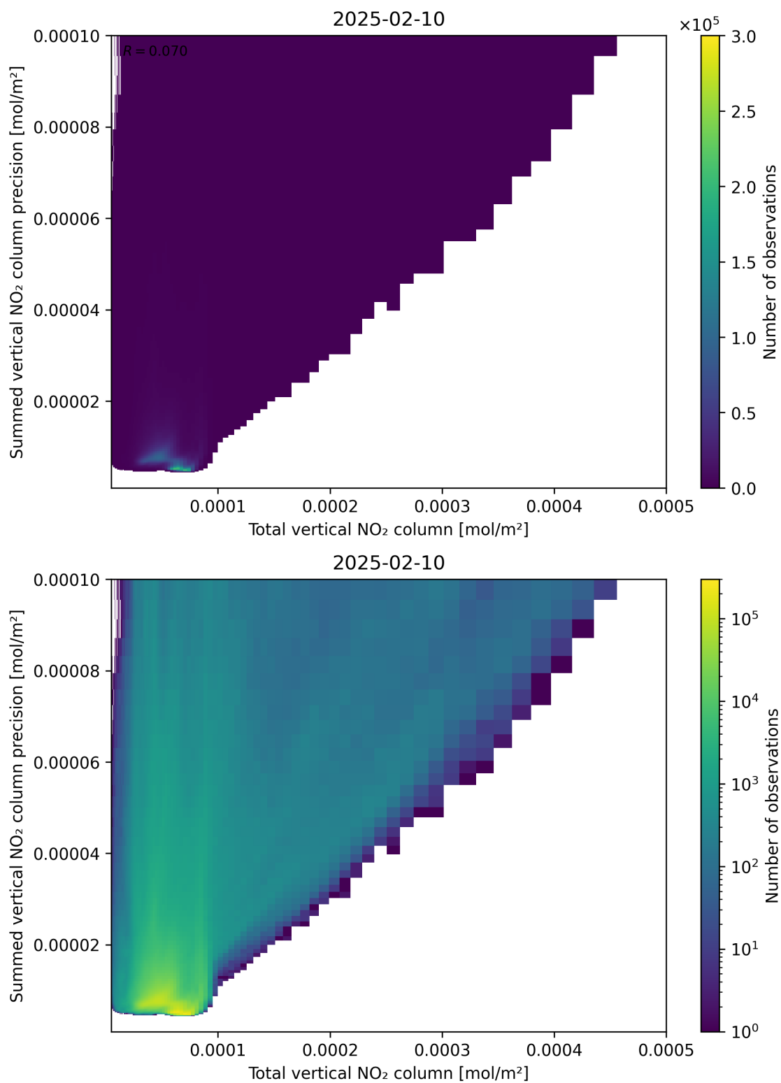
Figure 113: Scatter density plot of “Total vertical NO 2 column” against “Summed vertical NO 2 column precision” for 2025-02-09 to 2025-02-11.
