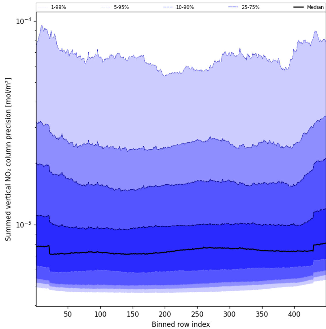
Figure 58: Along track statistics of “Summed vertical NO 2 column precision” for 2025-02-09 to 2025-02-11
