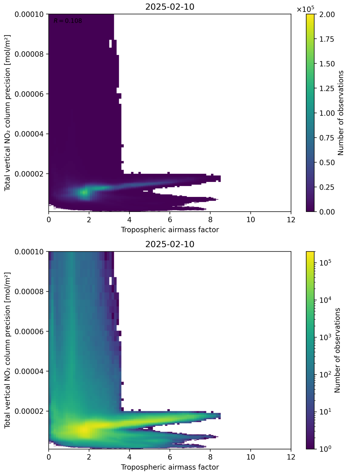
Figure 78: Scatter density plot of “Tropospheric airmass factor” against “Total vertical NO 2 column precision” for 2025-02-09 to 2025-02-11.
