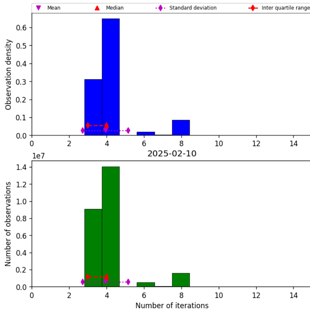
Figure 34: Histogram of “Number of iterations” for 2025-02-09 to 2025-02-11
