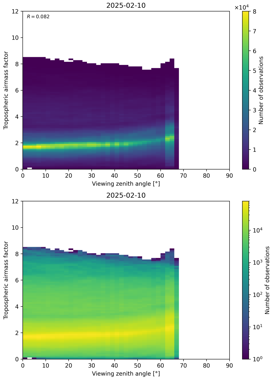
Figure 161: Scatter density plot of “Viewing zenith angle” against “Tropospheric airmass factor” for 2025-02-09 to 2025-02-11.
