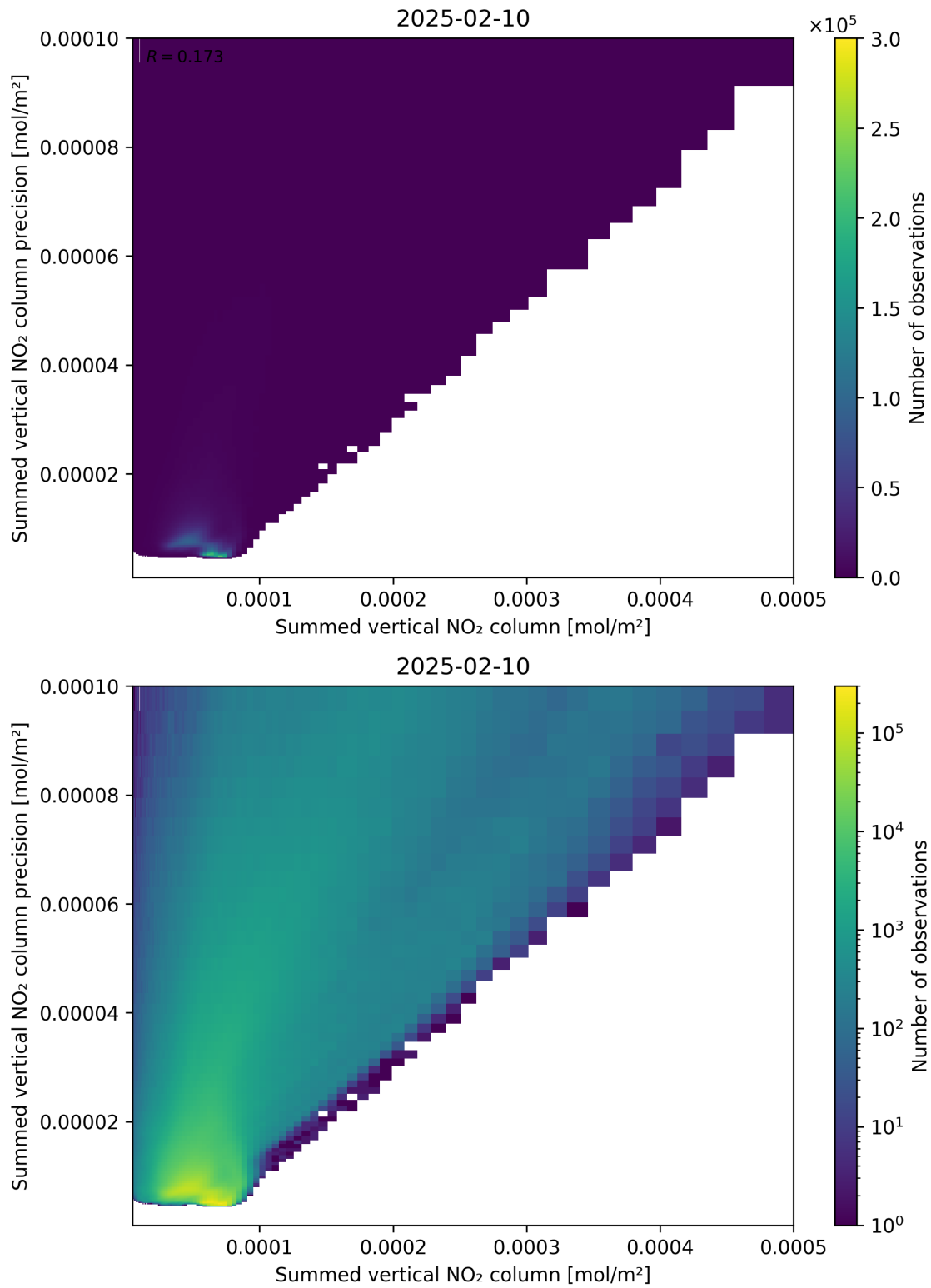
Figure 105: Scatter density plot of “Summed vertical NO 2 column” against “Summed vertical NO 2 column precision” for 2025-02-09 to 2025-02-11.
