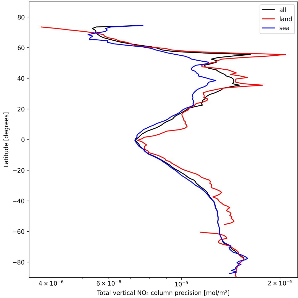
Figure 22: Zonal average of “Total vertical NO 2 column precision” for 2025-02-09 to 2025-02-11.
