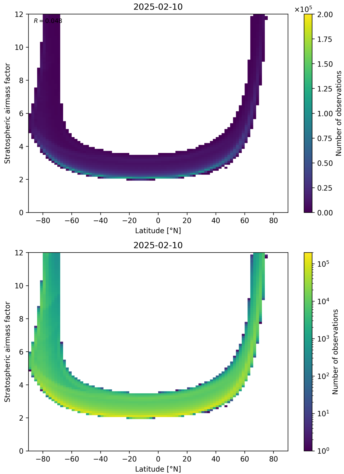
Figure 83: Scatter density plot of “Latitude” against “Stratospheric airmass factor” for 2025-02-09 to 2025-02-11.
