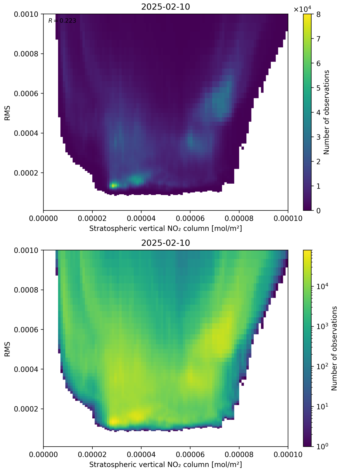
Figure 102: Scatter density plot of “Stratospheric vertical NO 2 column” against “RMS” for 2025-02-09 to 2025-02-11.
