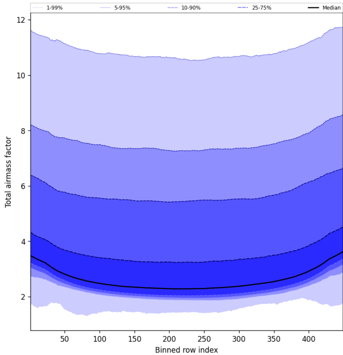
Figure 49: Along track statistics of “Total airmass factor” for 2025-02-09 to 2025-02-11
