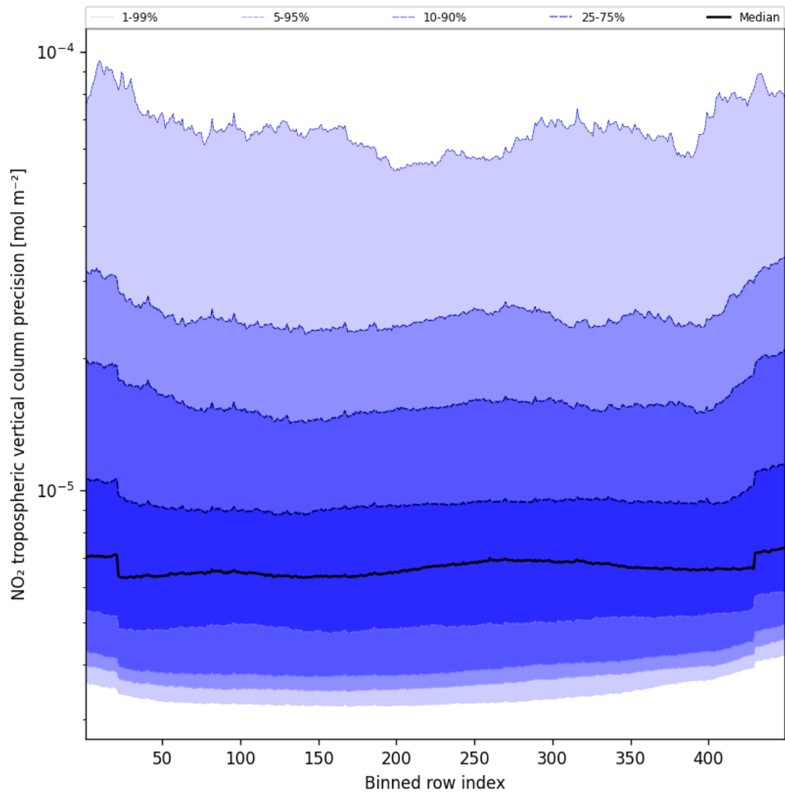
Figure 47: Along track statistics of “NO 2 tropospheric vertical column precision” for 2025-02-09 to 2025-02-11
