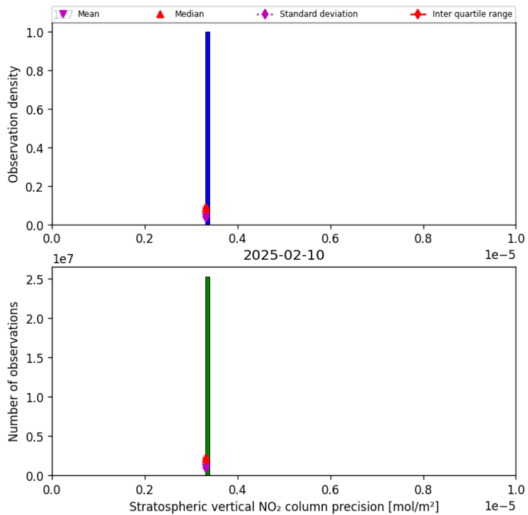
Figure 37: Histogram of “Stratospheric vertical NO 2 column precision” for 2025-02-09 to 2025-02-11
