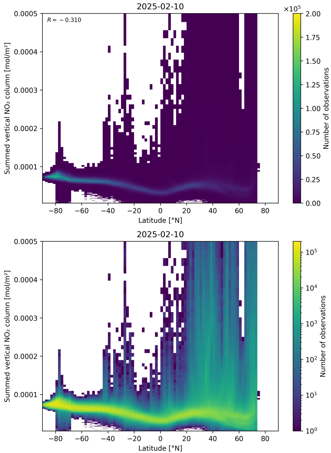
Figure 88: Scatter density plot of “Latitude” against “Summed vertical NO 2 column” for 2025-02-09 to 2025-02-11.
