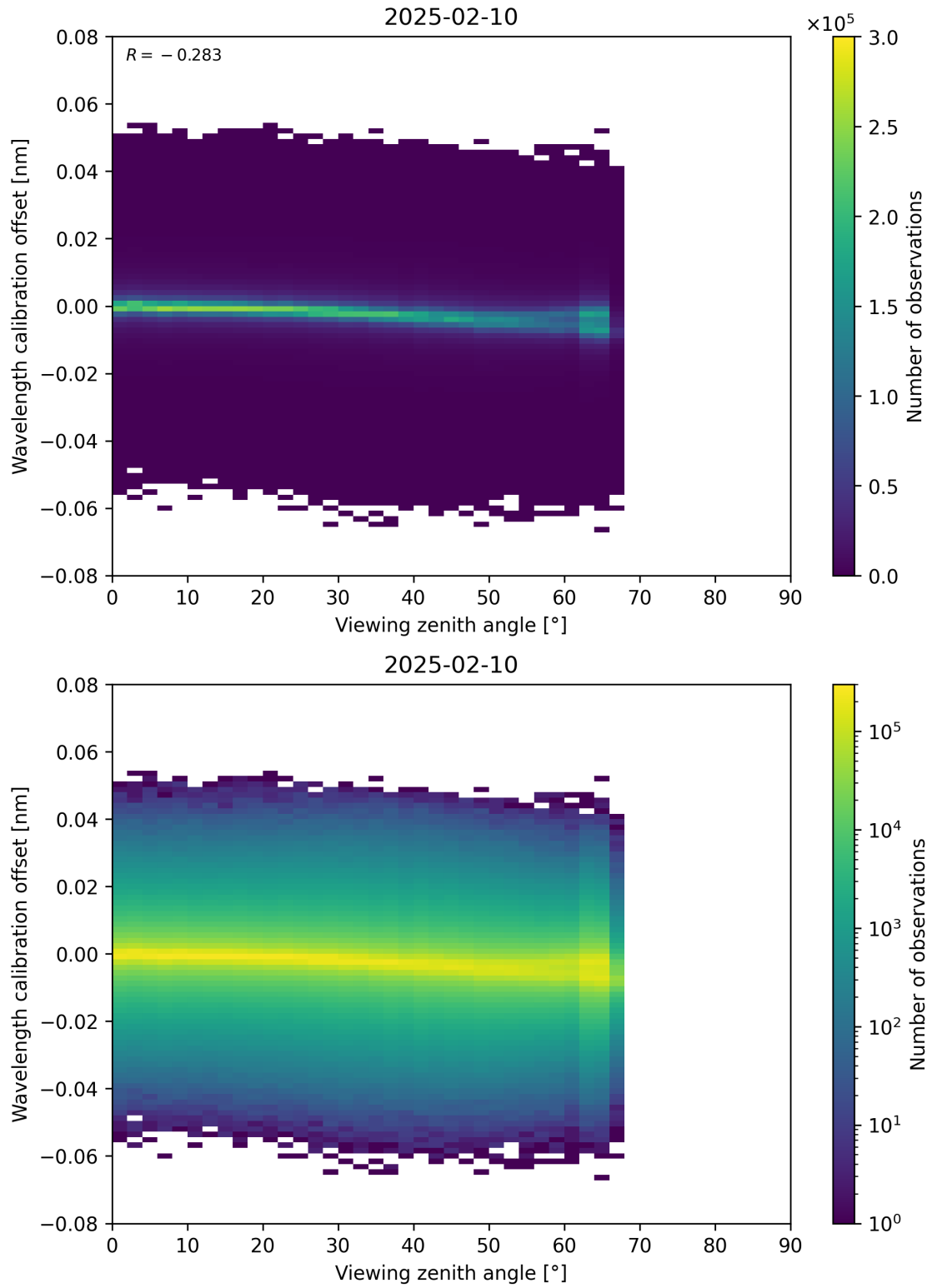
Figure 173: Scatter density plot of “Viewing zenith angle” against “Wavelength calibration offset” for 2025-02-09 to 2025-02-11.
