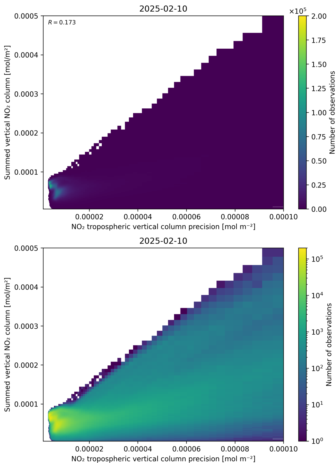
Figure 136: Scatter density plot of “NO 2 tropospheric vertical column precision” against “Summed vertical NO 2 column” for 2025-02-09 to 2025-02-11.
