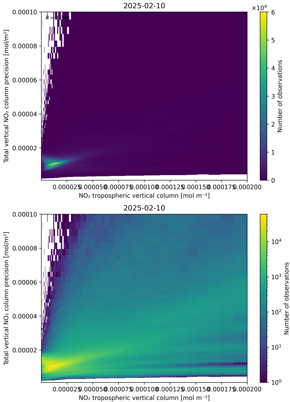
Figure 129: Scatter density plot of “NO 2 tropospheric vertical column” against “Total vertical NO 2 column precision” for 2025-02-09 to 2025-02-11.
