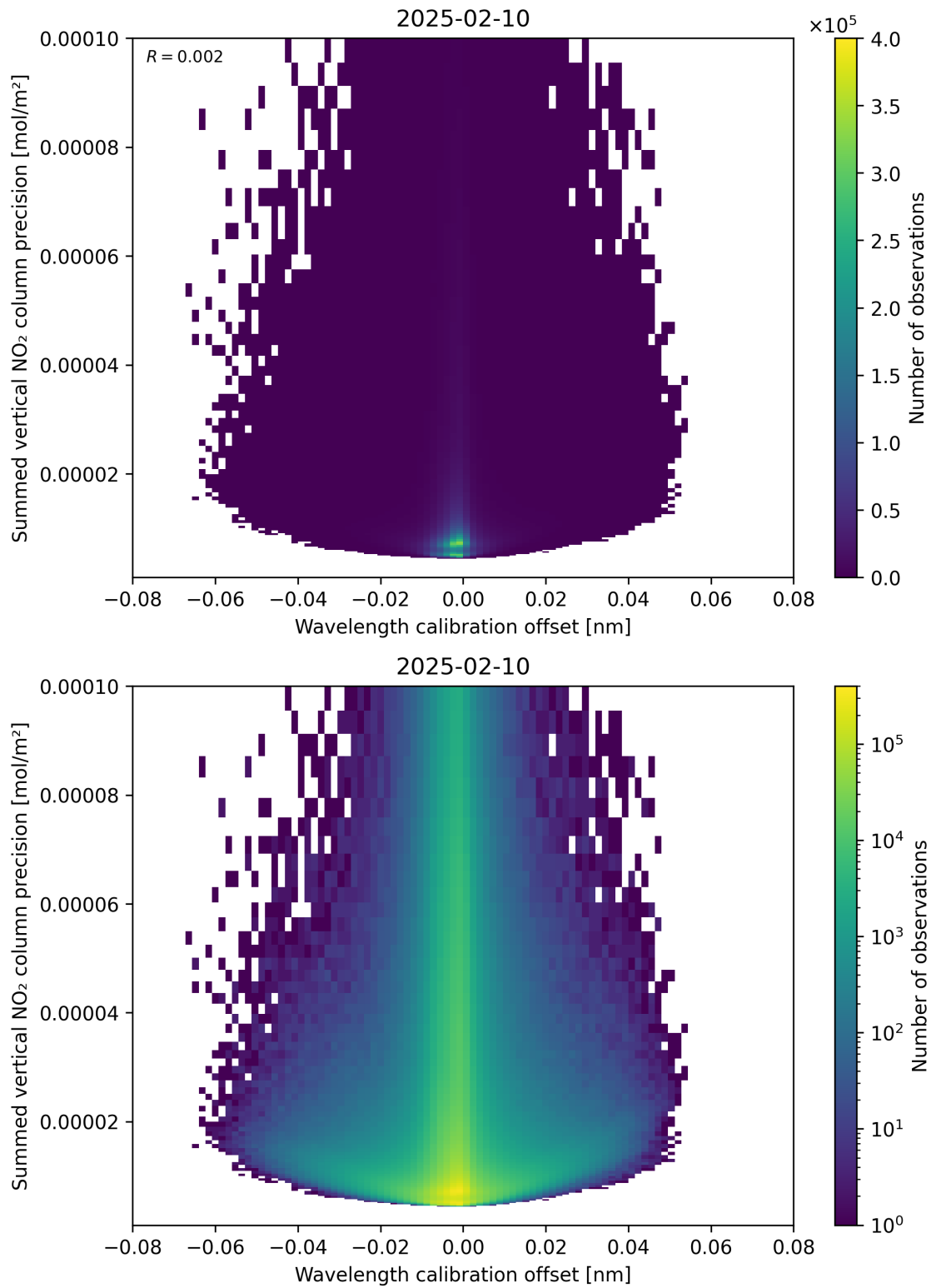
Figure 178: Scatter density plot of “Wavelength calibration offset” against “Summed vertical NO 2 column precision” for 2025-02-09 to 2025-02-11.
