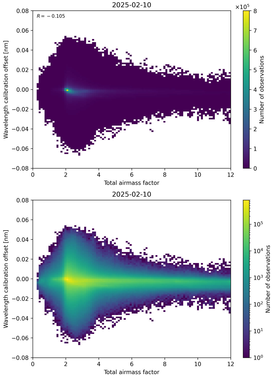
Figure 70: Scatter density plot of “Total airmass factor” against “Wavelength calibration offset” for 2025-02-09 to 2025-02-11.
