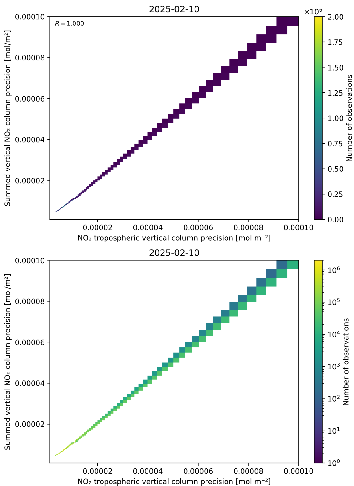
Figure 137: Scatter density plot of “NO 2 tropospheric vertical column precision” against “Summed vertical NO 2 column precision” for 2025-02-09 to 2025-02-11.
