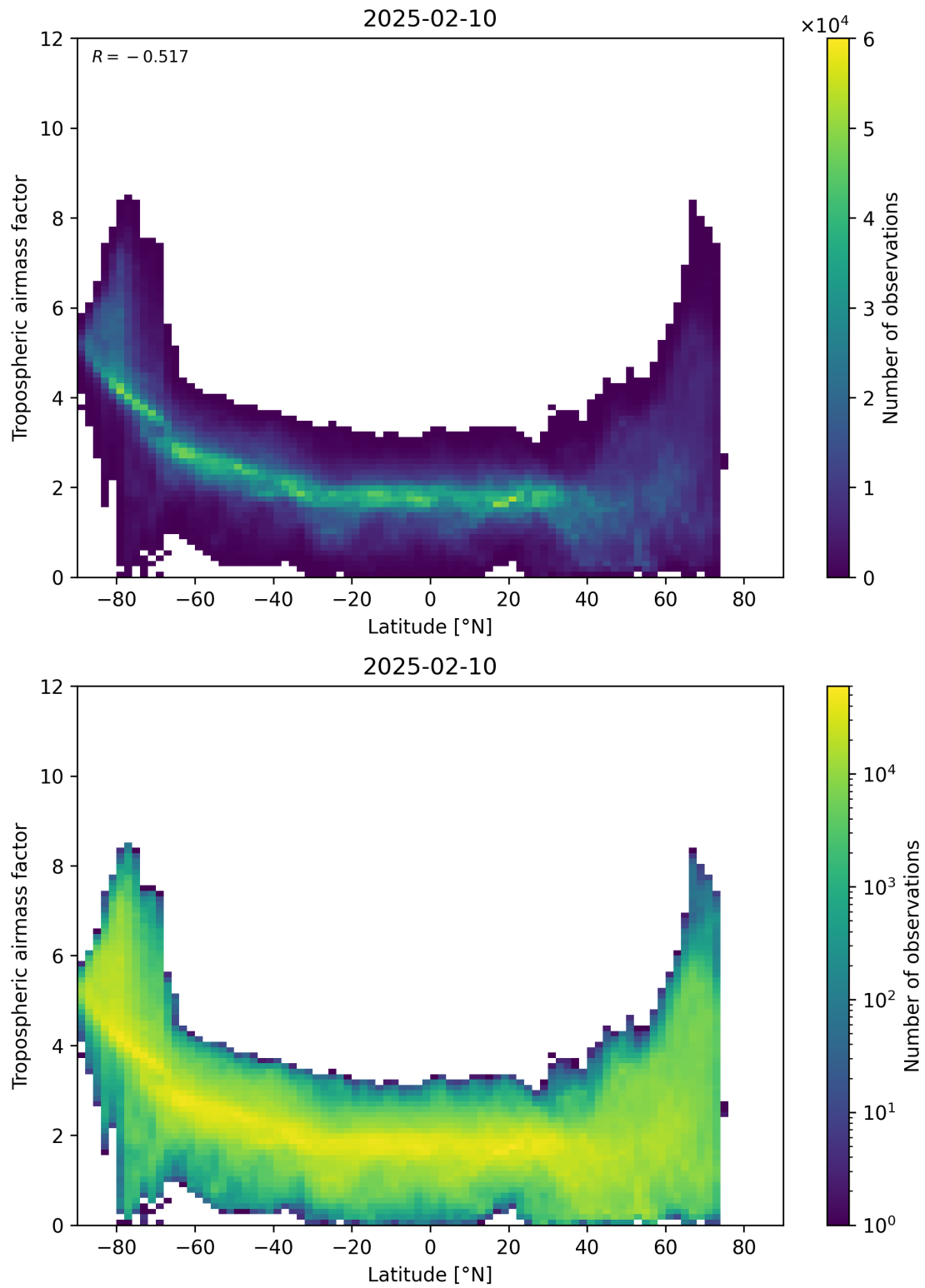
Figure 85: Scatter density plot of “Latitude” against “Tropospheric airmass factor” for 2025-02-09 to 2025-02-11.
