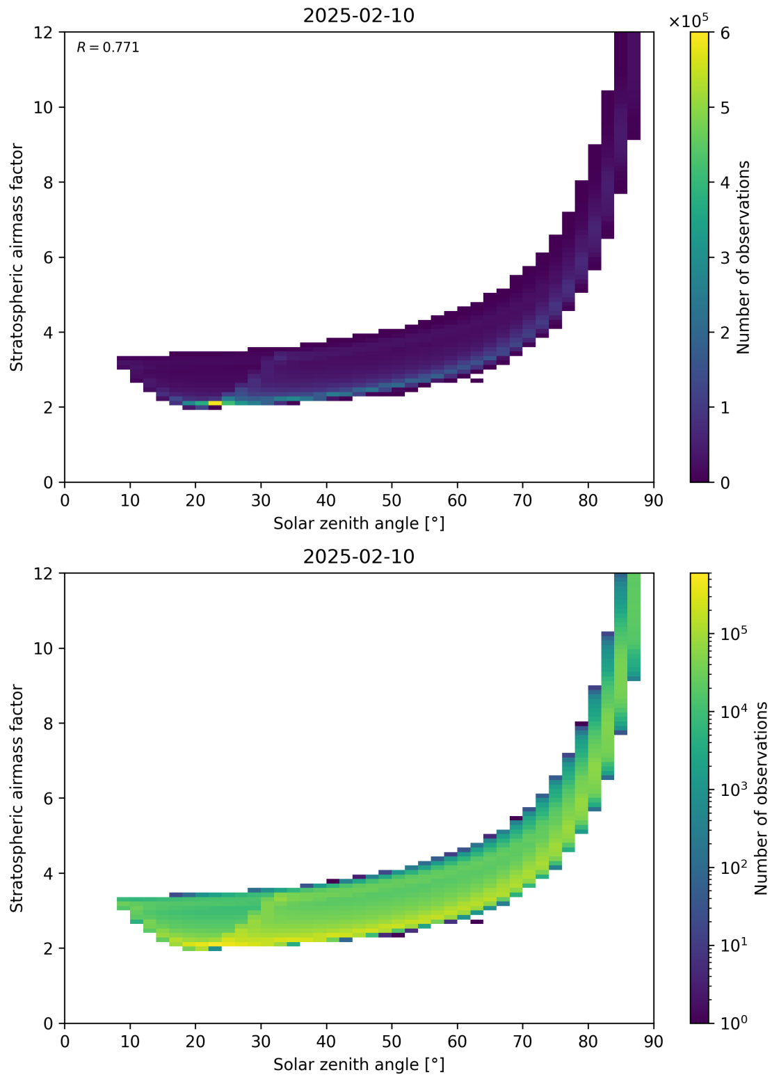
Figure 145: Scatter density plot of “Solar zenith angle” against “Stratospheric airmass factor” for 2025-02-09 to 2025-02-11.
