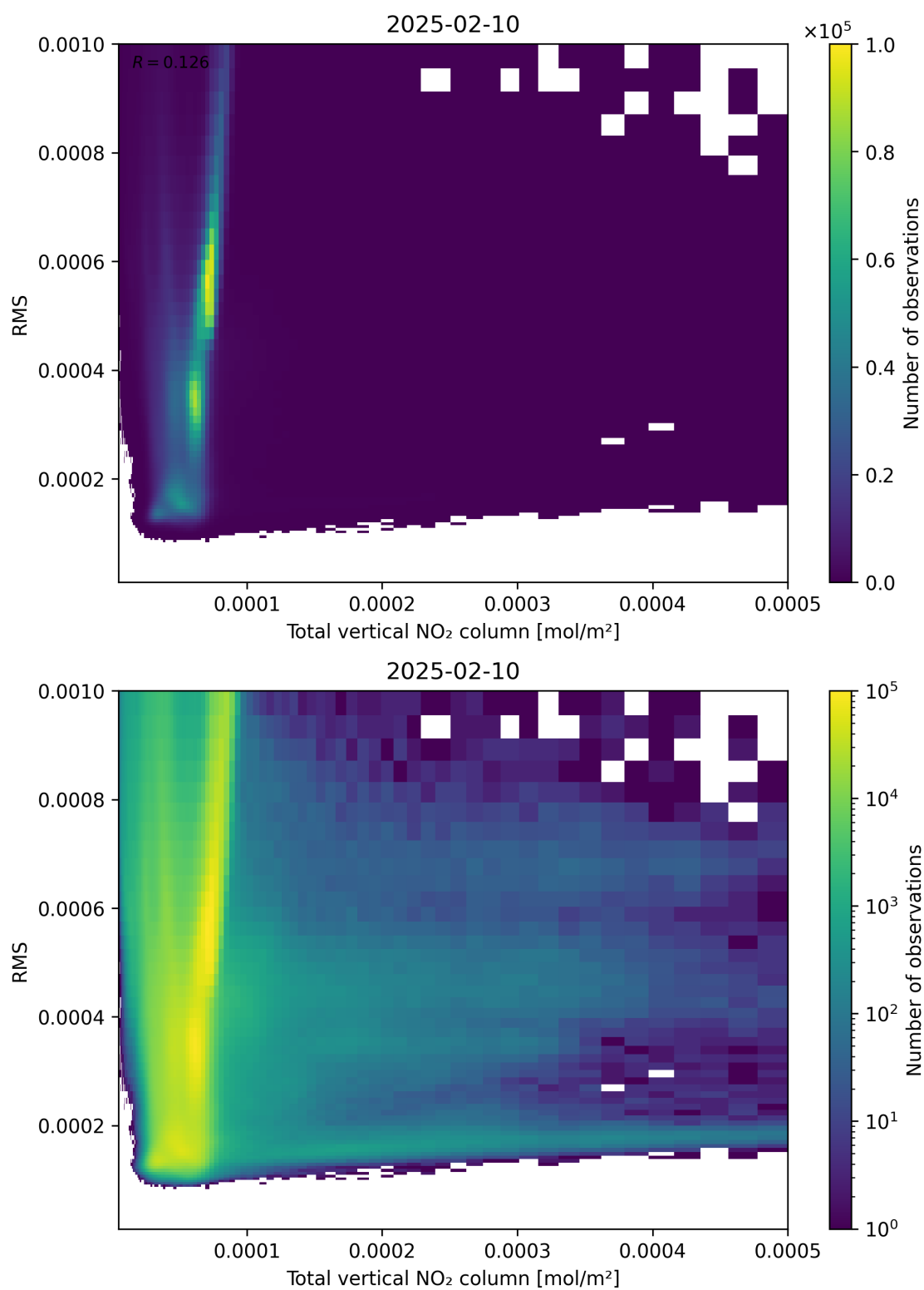
Figure 120: Scatter density plot of “Total vertical NO 2 column” against “RMS” for 2025-02-09 to 2025-02-11.
