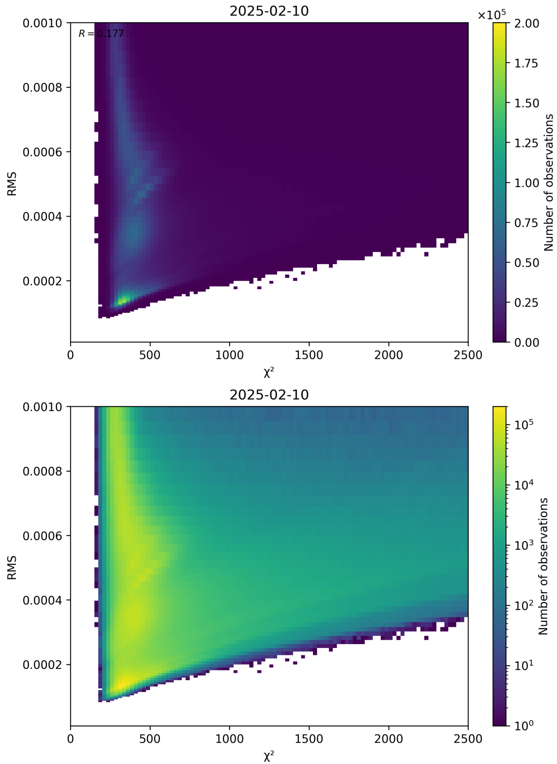
Figure 82: Scatter density plot of “ \chi^2 ” against “RMS” for 2025-02-09 to 2025-02-11.
