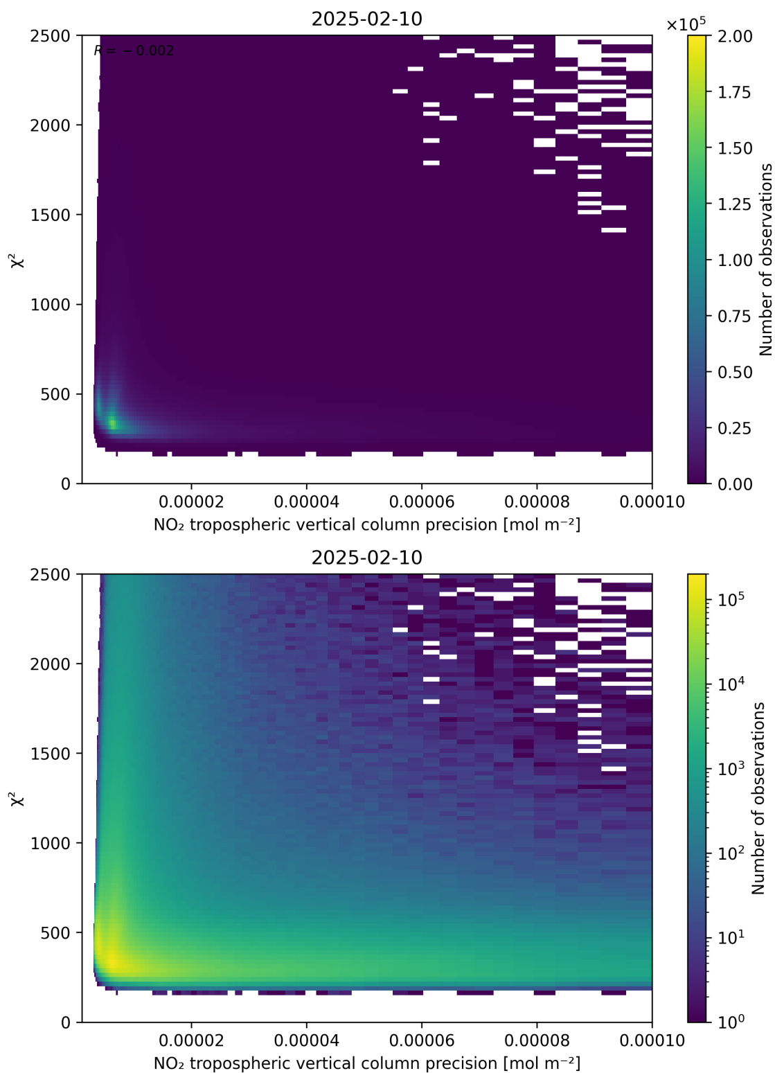
Figure 134: Scatter density plot of “NO 2 tropospheric vertical column precision” against “ \chi^2 ” for 2025-02-09 to 2025-02-11.
