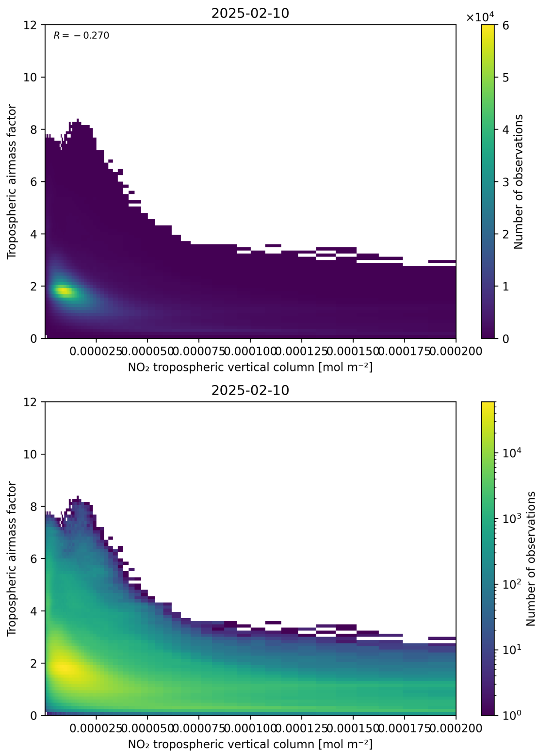
Figure 123: Scatter density plot of “NO 2 tropospheric vertical column” against “Tropospheric air mass factor” for 2025-02-09 to 2025-02-11.
