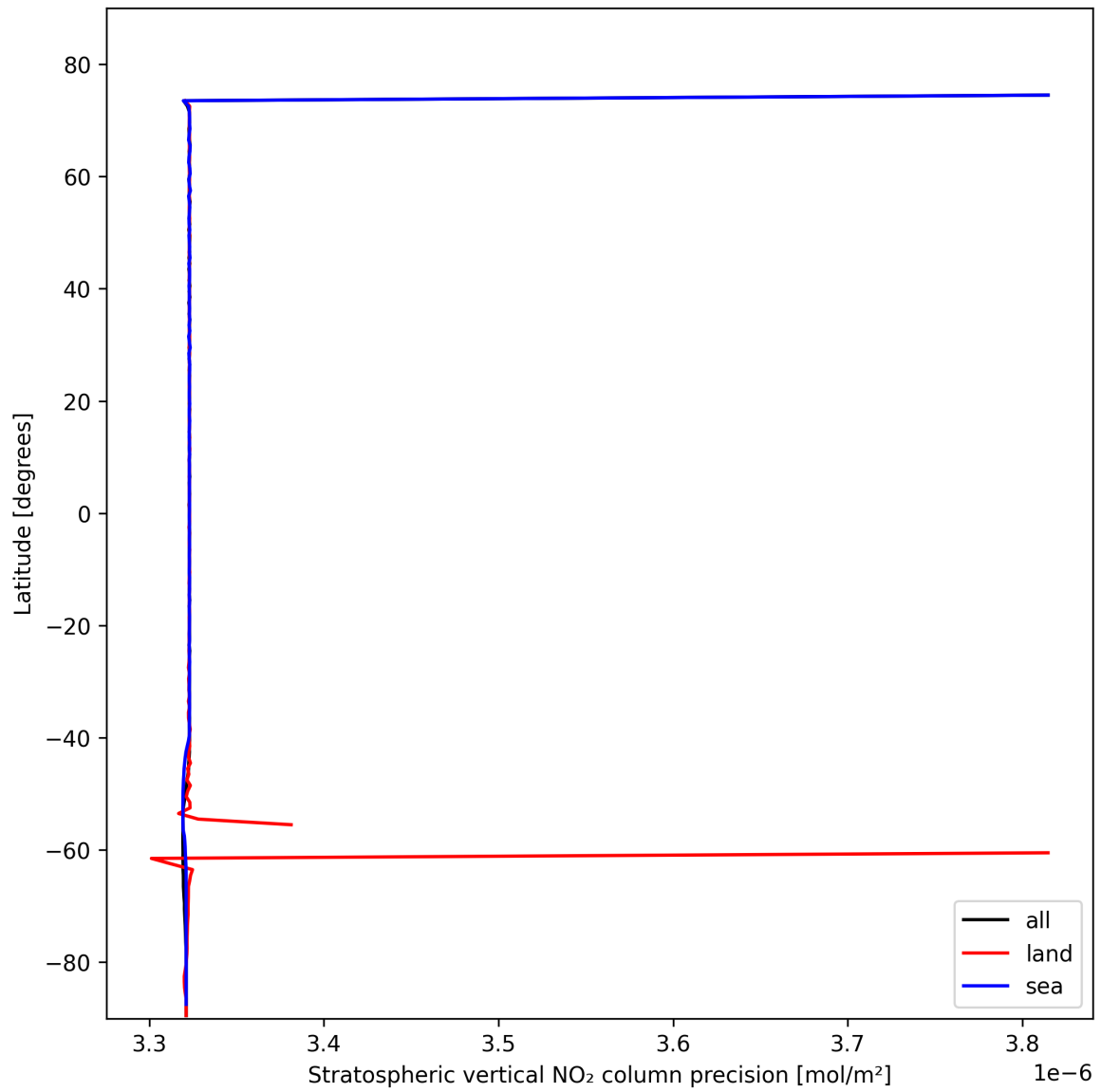
Figure 20: Zonal average of “Stratospheric vertical NO 2 column precision” for 2025-02-09 to 2025-02-11.
