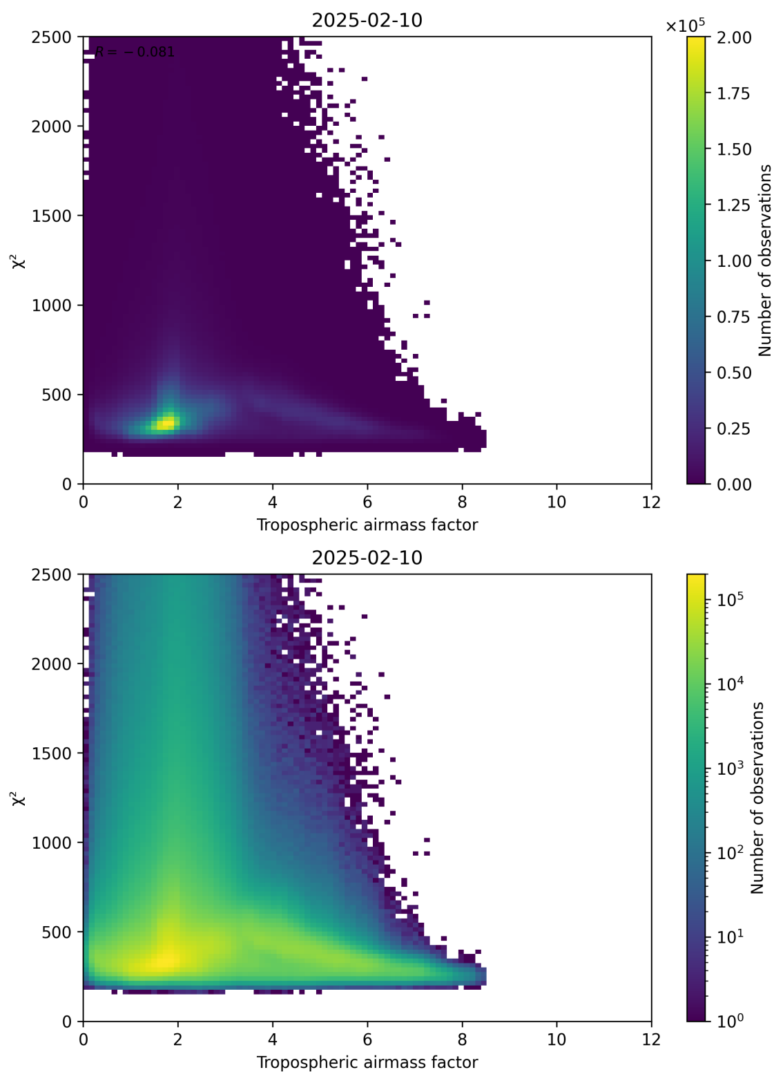
Figure 73: Scatter density plot of “Tropospheric airmass factor” against “ \chi^2 ” for 2025-02-09 to 2025-02-11.
