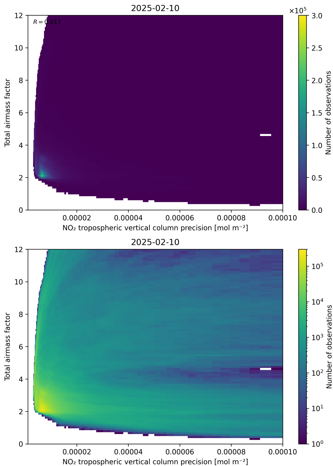
Figure 132: Scatter density plot of “NO 2 tropospheric vertical column precision” against “Total air mass factor” for 2025-02-09 to 2025-02-11.
