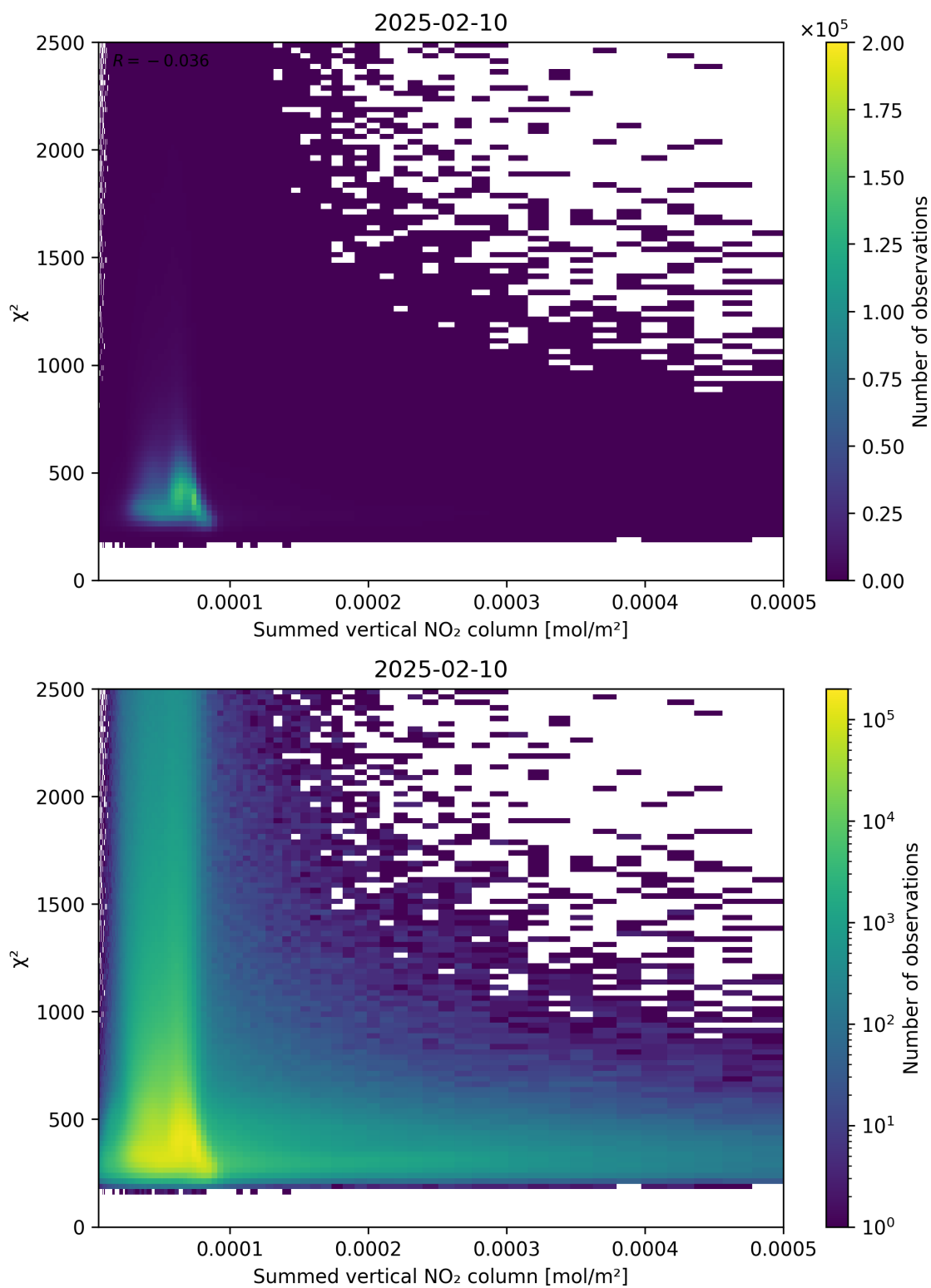
Figure 104: Scatter density plot of “Summed vertical NO 2 column” against “ \chi^2 ” for 2025-02-09 to 2025-02-11.
