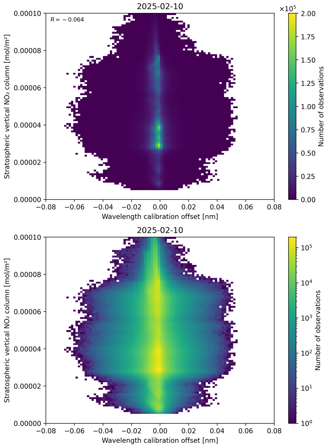
Figure 176: Scatter density plot of “Wavelength calibration offset” against “Stratospheric vertical NO 2 column” for 2025-02-09 to 2025-02-11.
