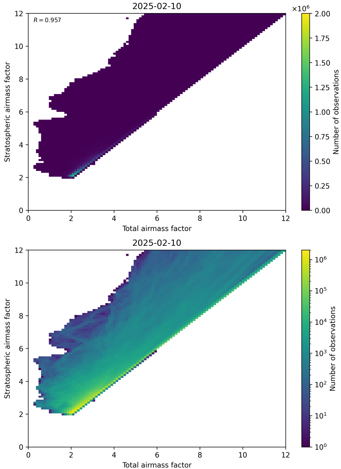
Figure 62: Scatter density plot of “Total airmass factor” against “Stratospheric airmass factor” for 2025-02-09 to 2025-02-11.
