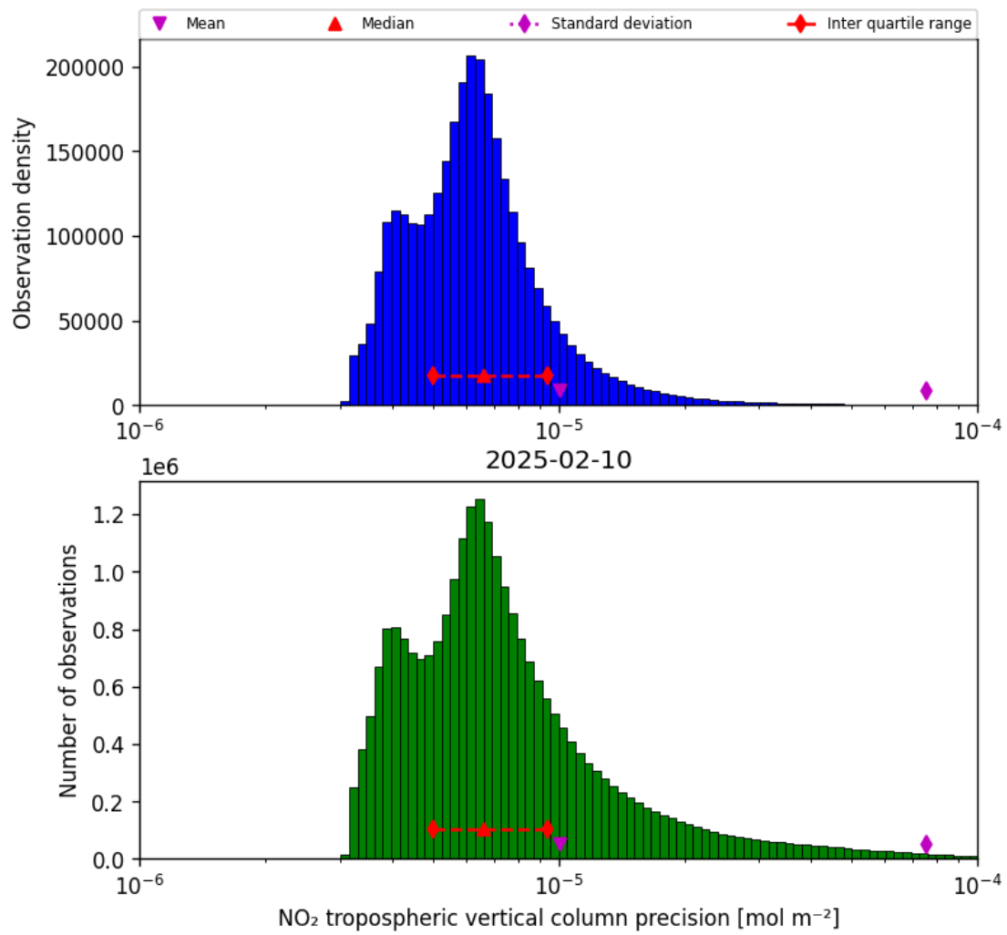
Figure 30: Histogram of “NO 2 tropospheric vertical column precision” for 2025-02-09 to 2025-02-11
