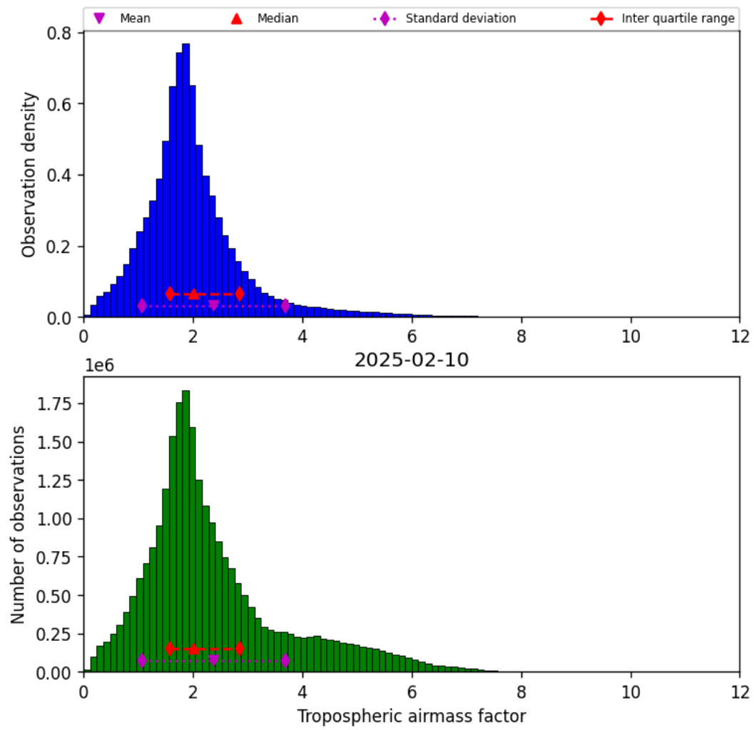
Figure 31: Histogram of “Tropospheric airmass factor” for 2025-02-09 to 2025-02-11
