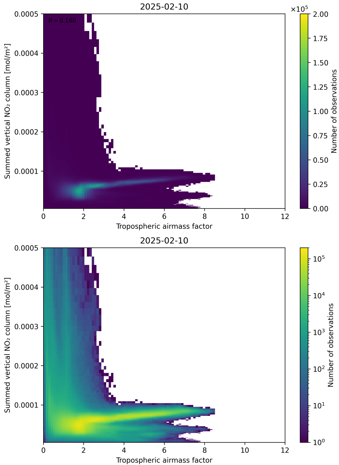
Figure 75: Scatter density plot of “Tropospheric airmass factor” against “Summed vertical NO 2 column” for 2025-02-09 to 2025-02-11.
