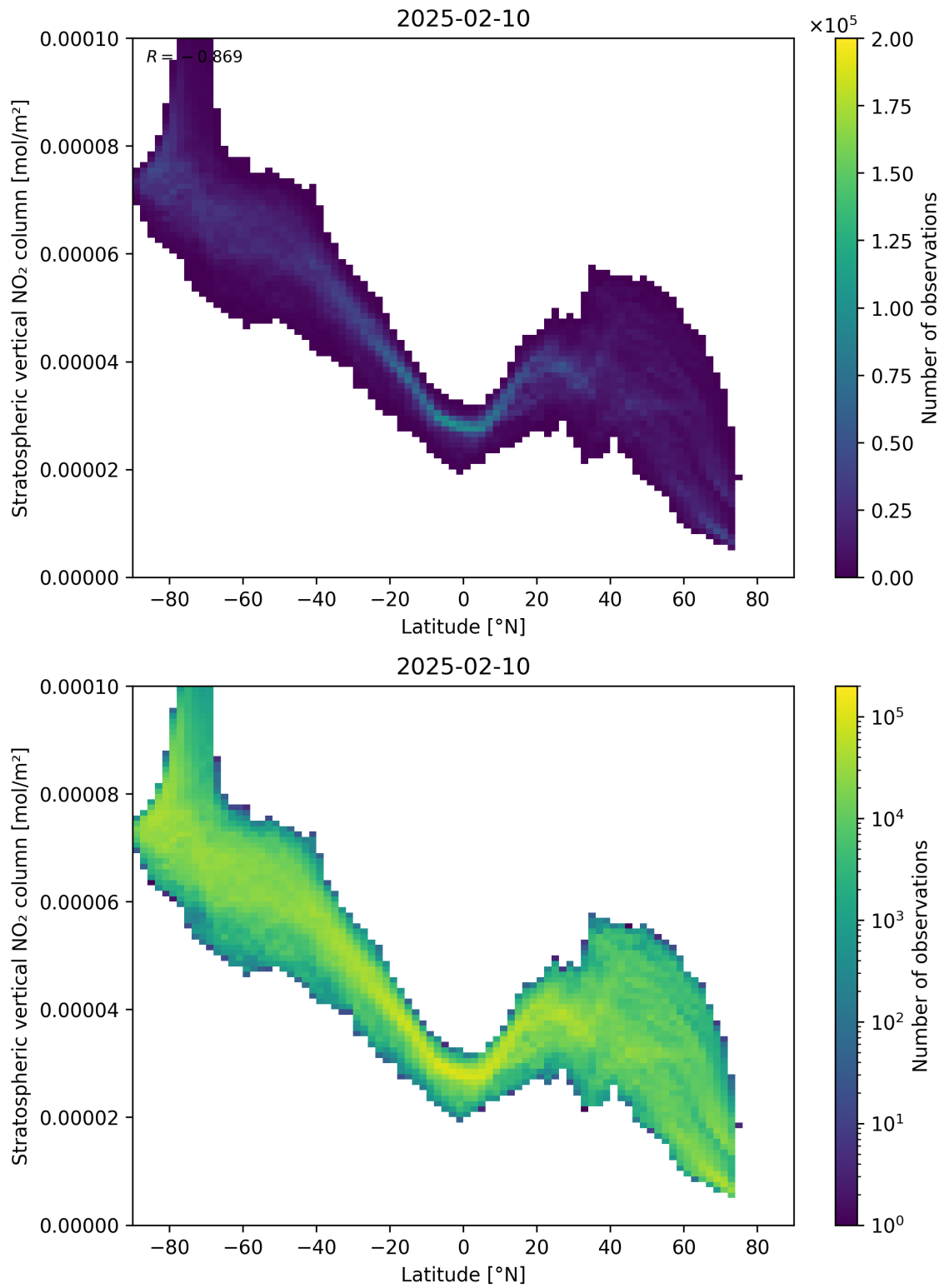
Figure 87: Scatter density plot of “Latitude” against “Stratospheric vertical NO 2 column” for 2025-02-09 to 2025-02-11.
