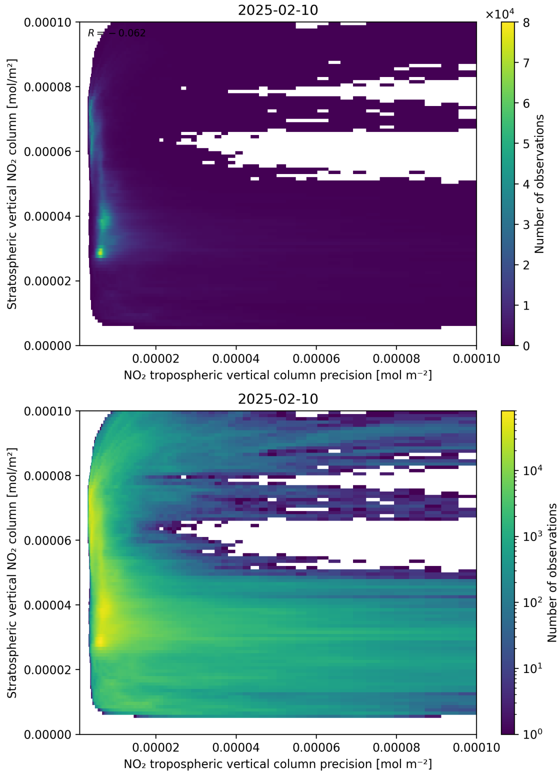
Figure 135: Scatter density plot of “NO 2 tropospheric vertical column precision” against “Stratospheric vertical NO 2 column” for 2025-02-09 to 2025-02-11.
