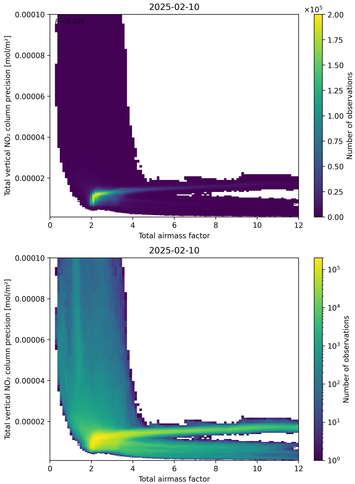
Figure 68: Scatter density plot of “Total airmass factor” against “Total vertical NO 2 column precision” for 2025-02-09 to 2025-02-11.
