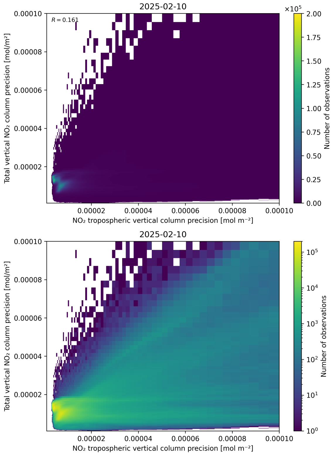
Figure 139: Scatter density plot of “NO 2 tropospheric vertical column precision” against “Total vertical NO 2 column precision” for 2025-02-09 to 2025-02-11.
