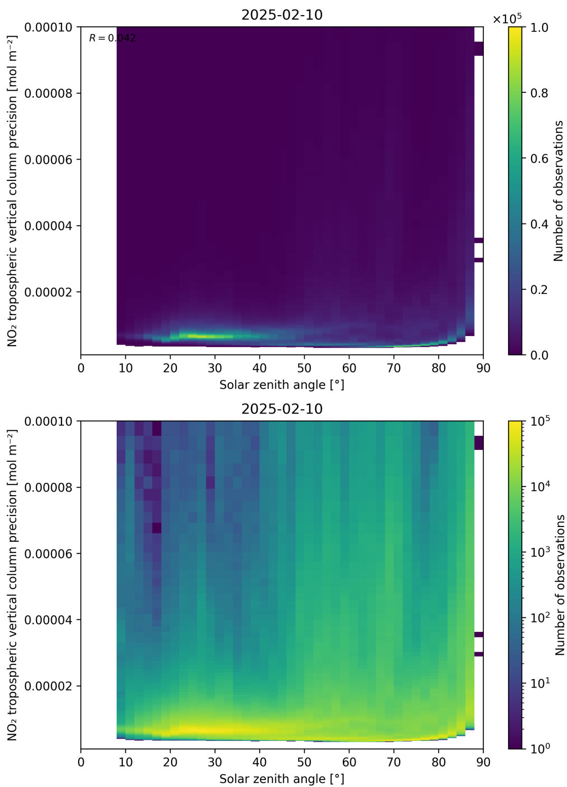
Figure 156: Scatter density plot of “Solar zenith angle” against “NO 2 tropospheric vertical column precision” for 2025-02-09 to 2025-02-11.
