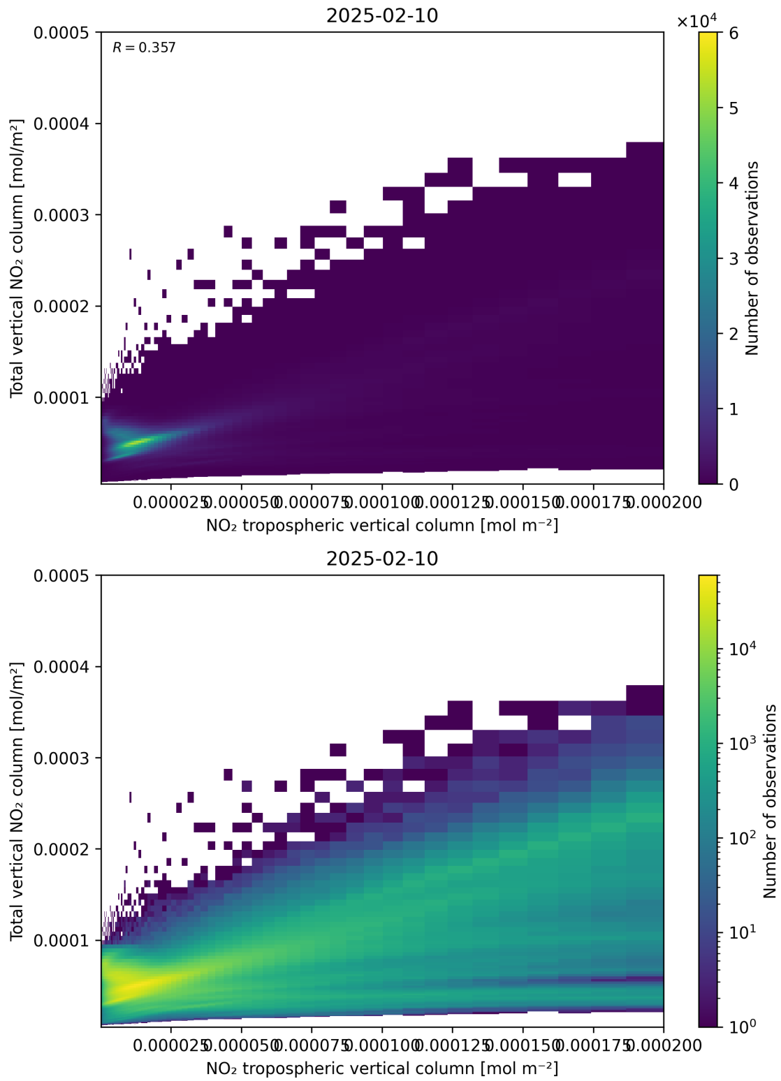
Figure 128: Scatter density plot of “NO 2 tropospheric vertical column” against “Total vertical NO 2 column” for 2025-02-09 to 2025-02-11.
