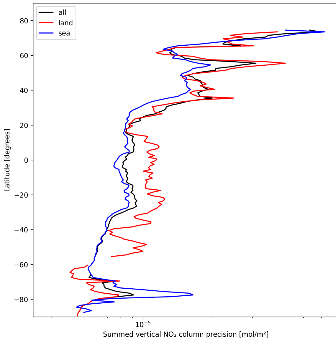
Figure 24: Zonal average of “Summed vertical NO 2 column precision” for 2025-02-09 to 2025-02-11.
