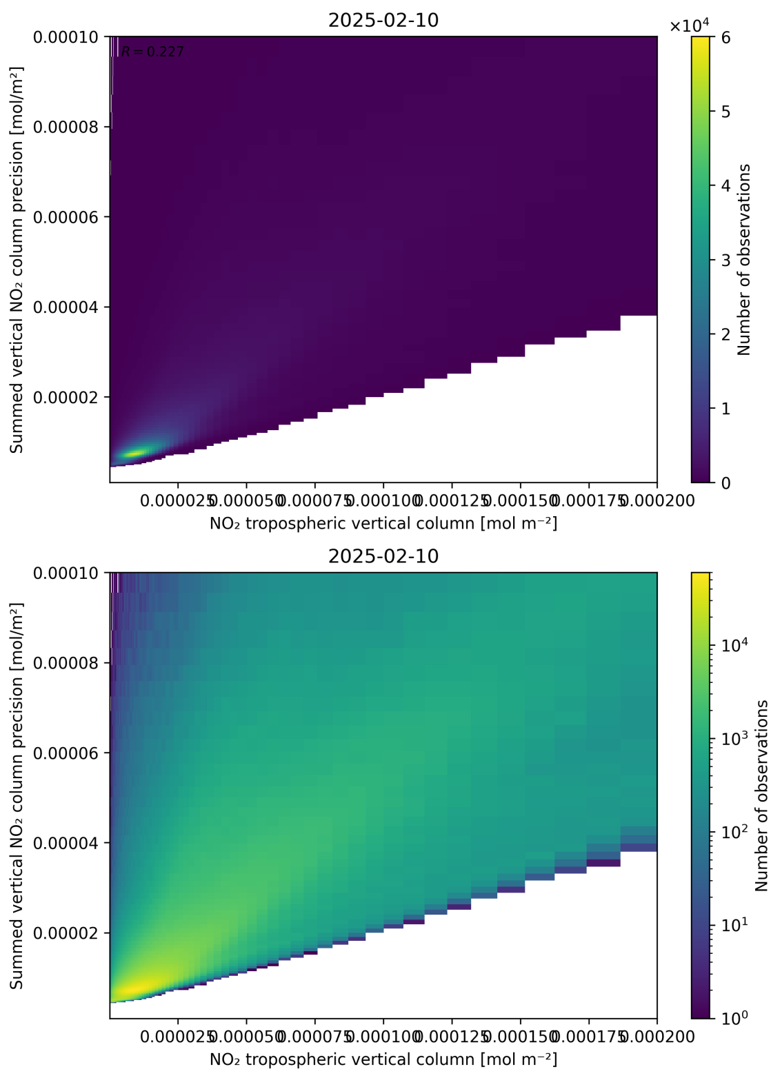
Figure 127: Scatter density plot of “NO 2 tropospheric vertical column” against “Summed vertical NO 2 column precision” for 2025-02-09 to 2025-02-11.
