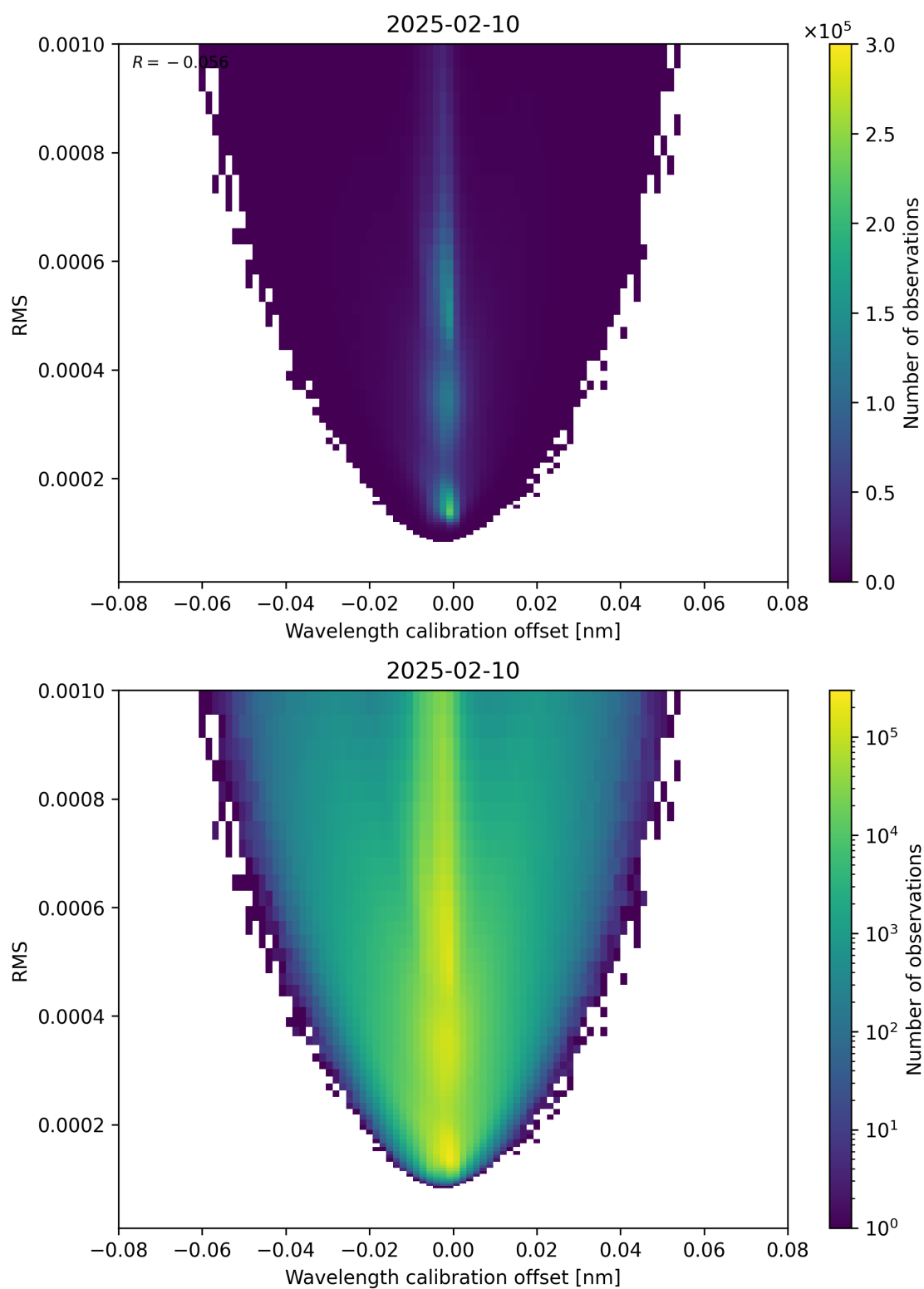
Figure 181: Scatter density plot of “Wavelength calibration offset” against “RMS” for 2025-02-09 to 2025-02-11.
