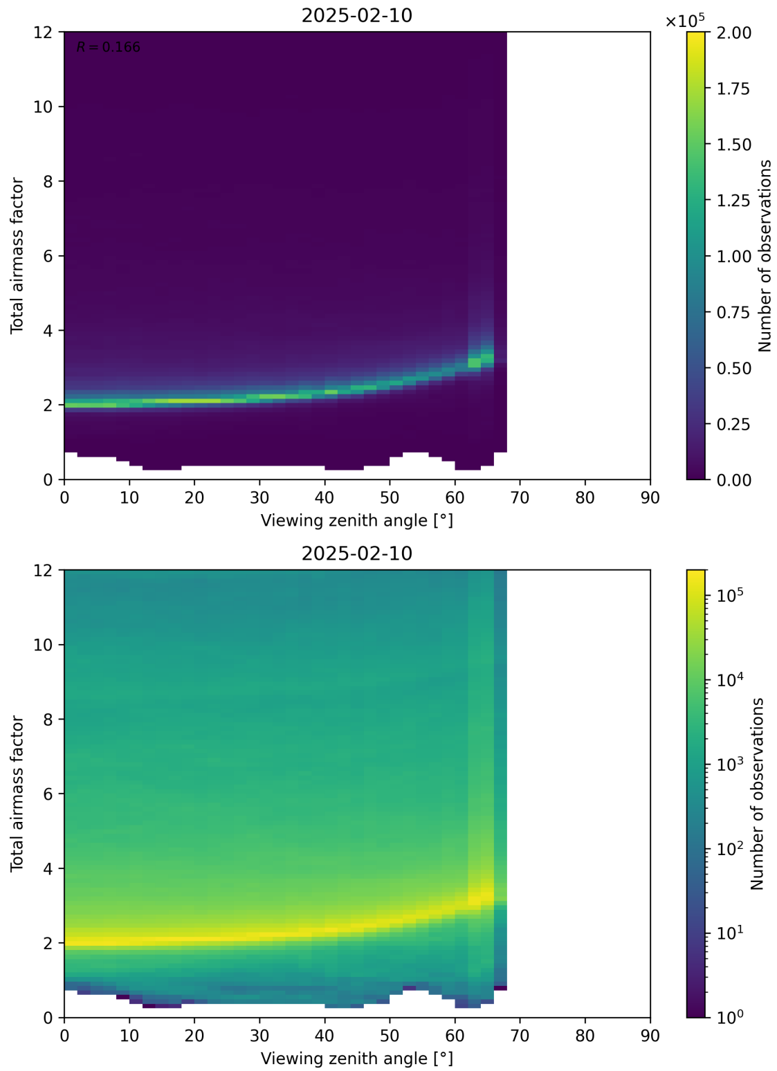
Figure 160: Scatter density plot of “Viewing zenith angle” against “Total airmass factor” for 2025-02-09 to 2025-02-11.
