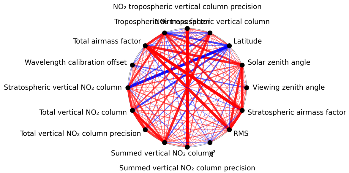
Figure 1: Map of correlation graph for 2025-02-09 to 2025-02-11.
