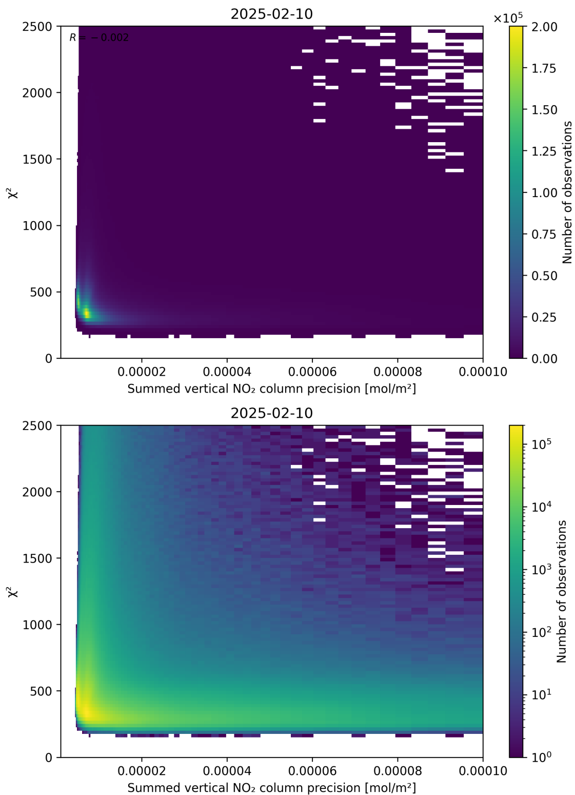
Figure 107: Scatter density plot of “Summed vertical NO 2 column precision” against “ \chi^2 ” for 2025-02-09 to 2025-02-11.
