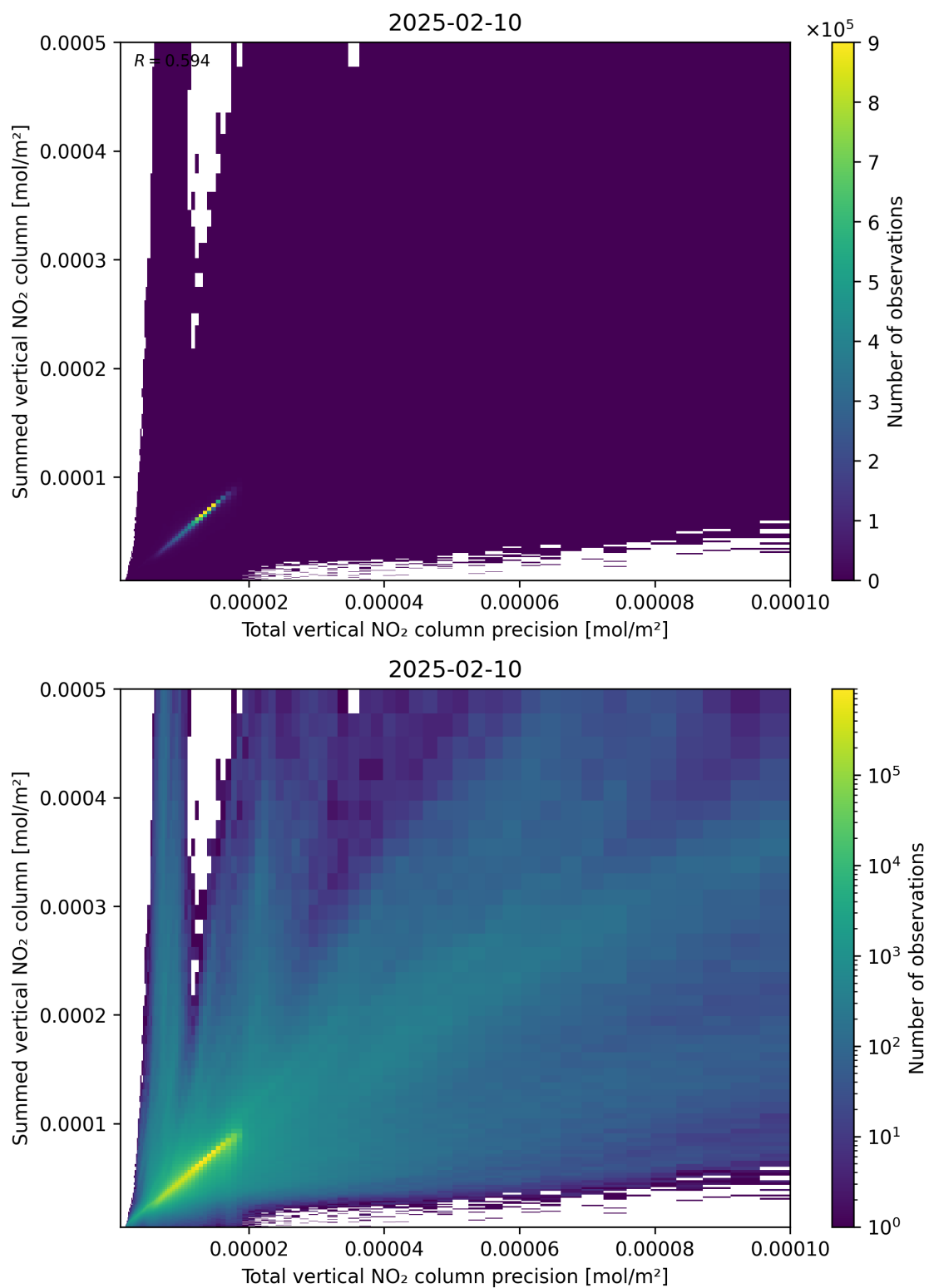
Figure 117: Scatter density plot of “Total vertical NO 2 column precision” against “Summed vertical NO 2 column” for 2025-02-09 to 2025-02-11.
