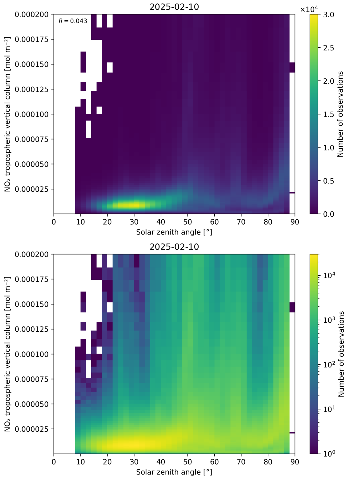
Figure 155: Scatter density plot of “Solar zenith angle” against “NO 2 tropospheric vertical column” for 2025-02-09 to 2025-02-11.
