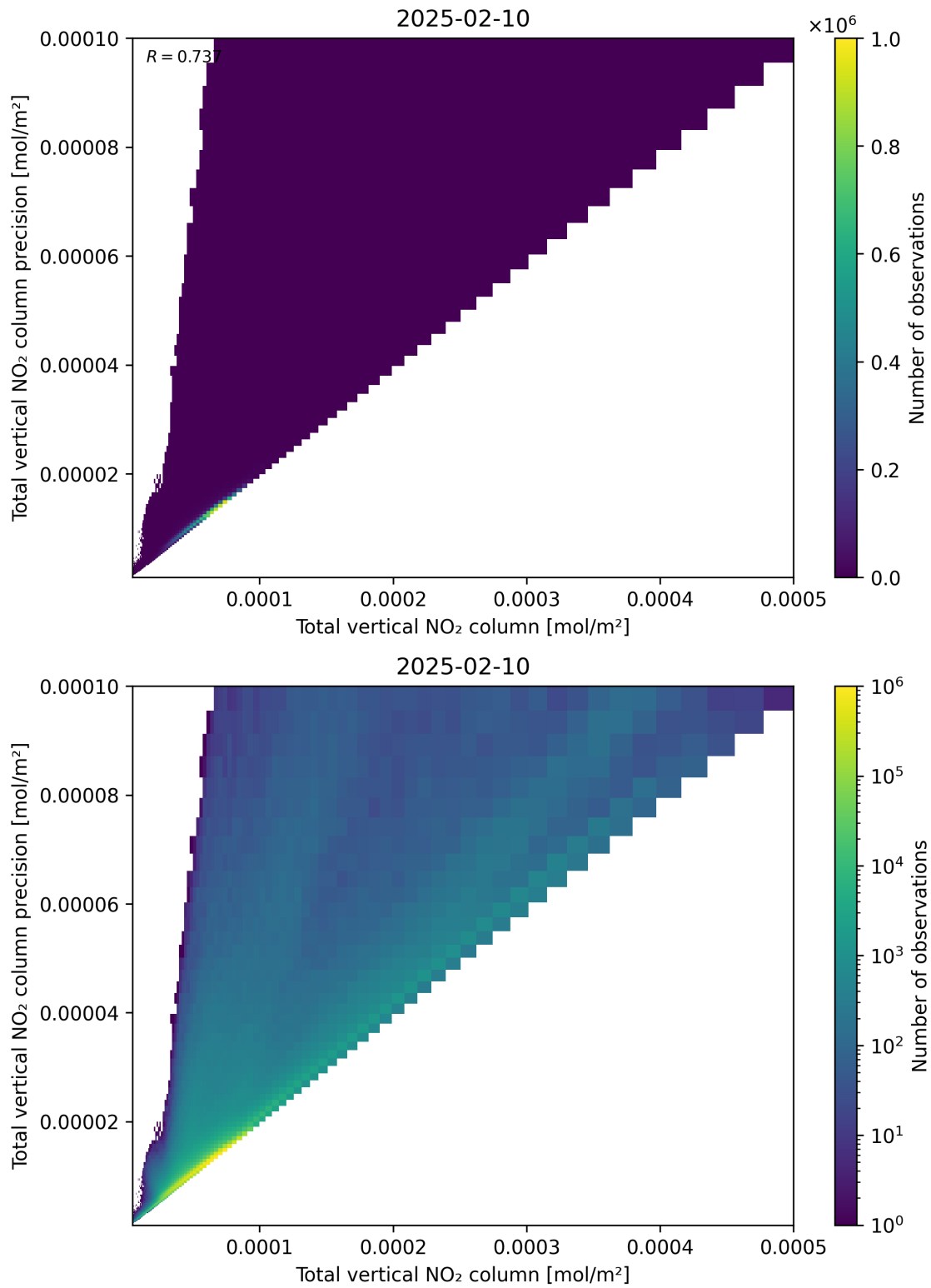
Figure 114: Scatter density plot of “Total vertical NO 2 column” against “Total vertical NO 2 column precision” for 2025-02-09 to 2025-02-11.
