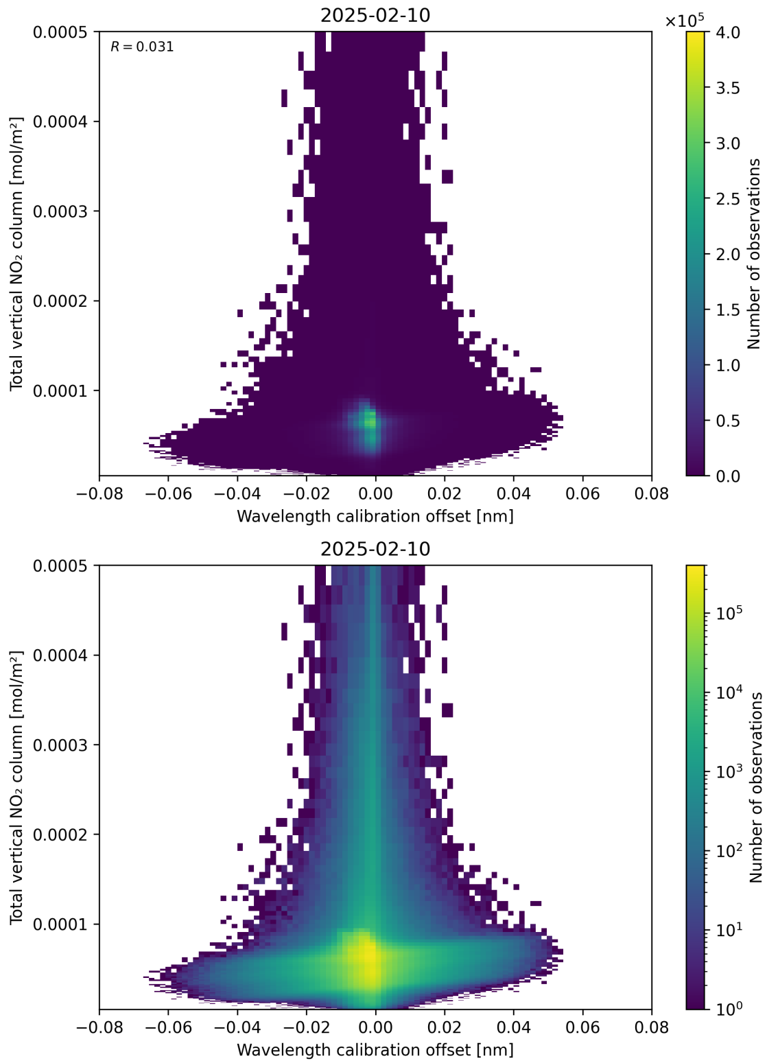
Figure 179: Scatter density plot of “Wavelength calibration offset” against “Total vertical NO 2 column” for 2025-02-09 to 2025-02-11.
