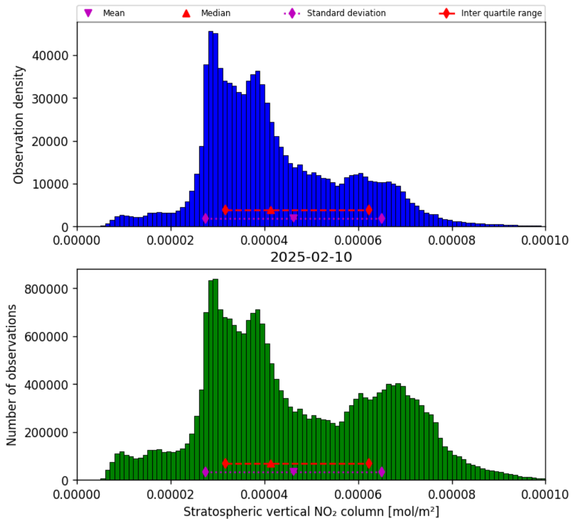
Figure 36: Histogram of “Stratospheric vertical NO 2 column” for 2025-02-09 to 2025-02-11
