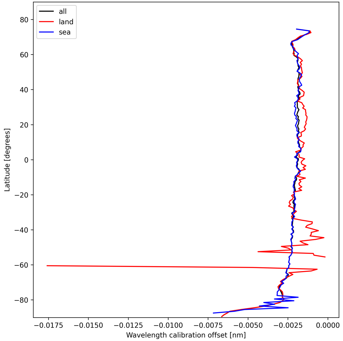
Figure 18: Zonal average of “Wavelength calibration offset” for 2025-02-09 to 2025-02-11.
