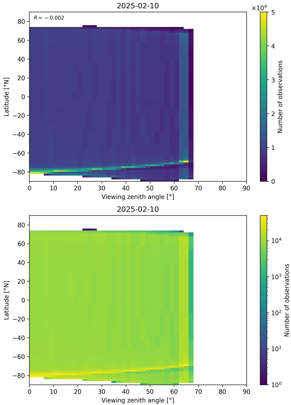
Figure 163: Scatter density plot of “Viewing zenith angle” against “Latitude” for 2025-02-09 to 2025-02-11.
