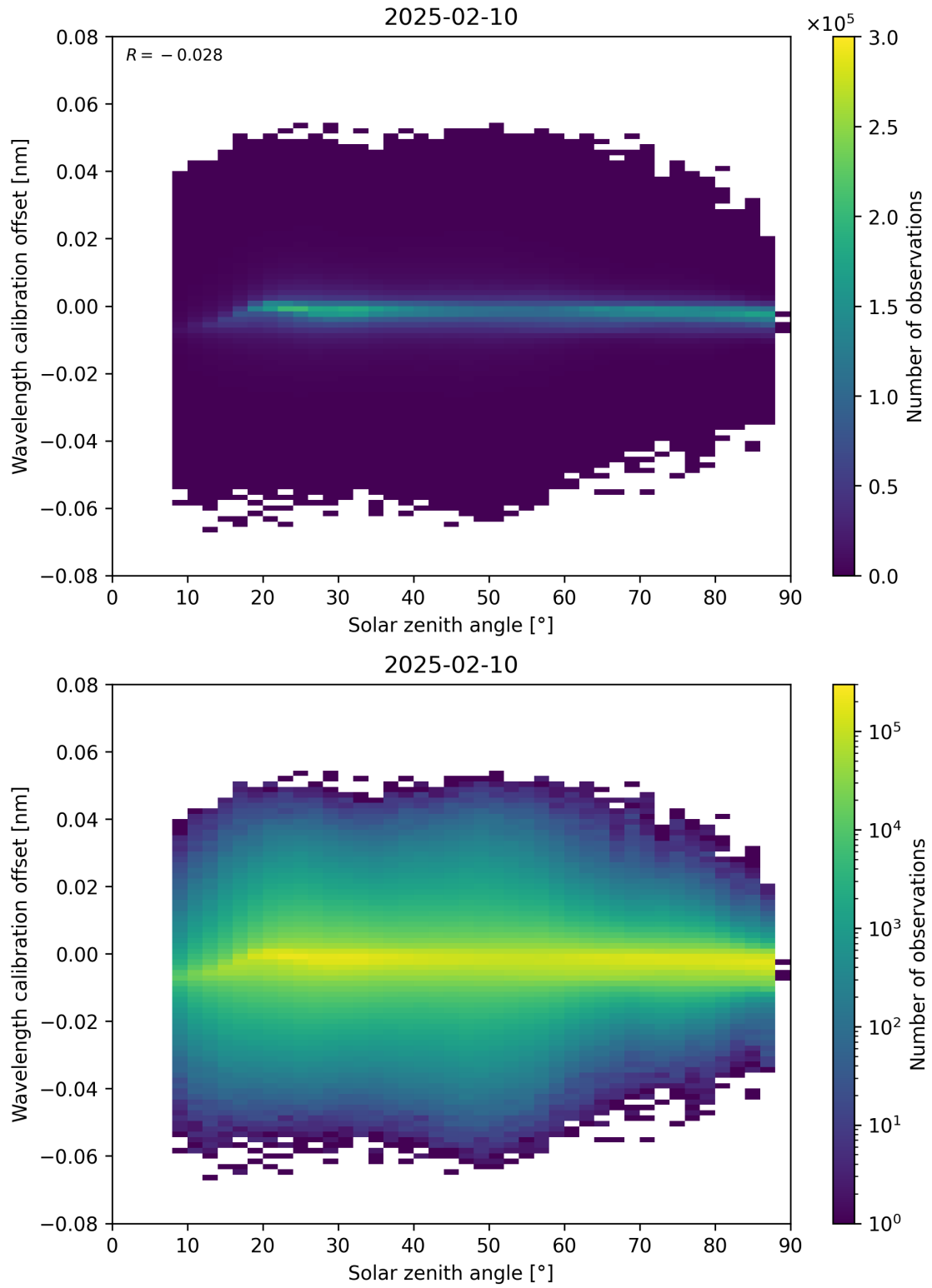
Figure 158: Scatter density plot of “Solar zenith angle” against “Wavelength calibration offset” for 2025-02-09 to 2025-02-11.
