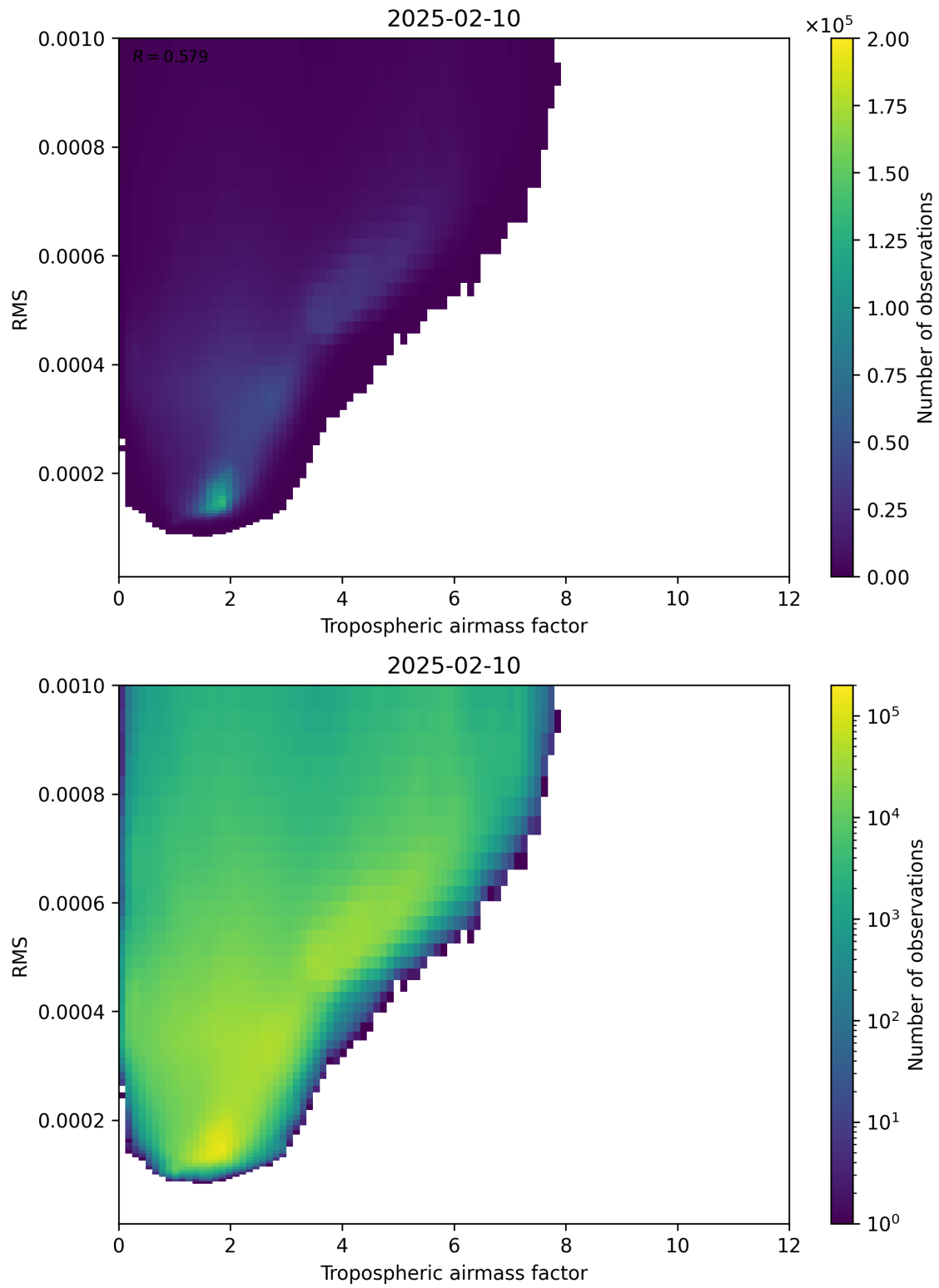
Figure 79: Scatter density plot of “Tropospheric airmass factor” against “RMS” for 2025-02-09 to 2025-02-11.
