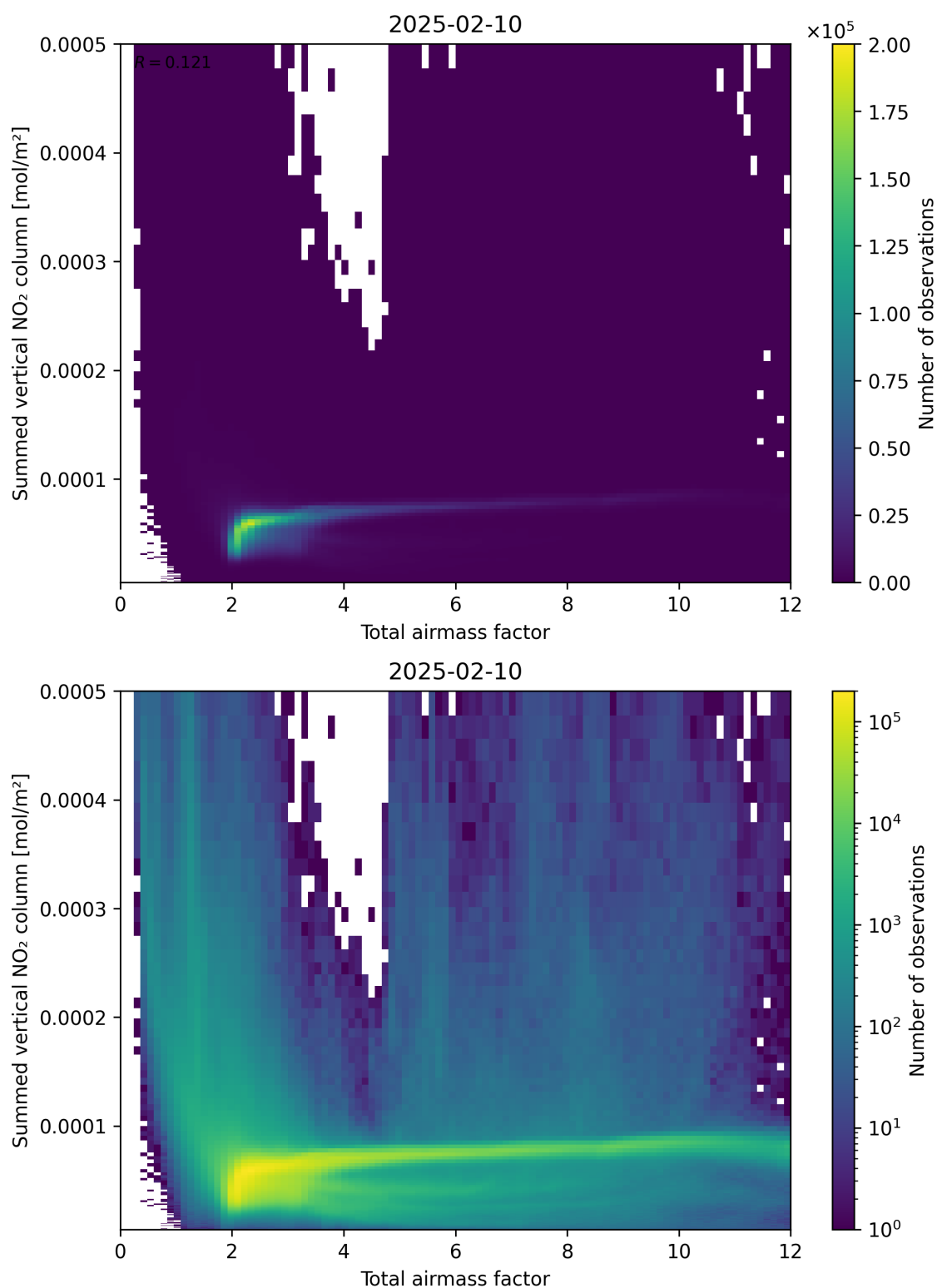
Figure 65: Scatter density plot of “Total airmass factor” against “Summed vertical NO 2 column” for 2025-02-09 to 2025-02-11.
