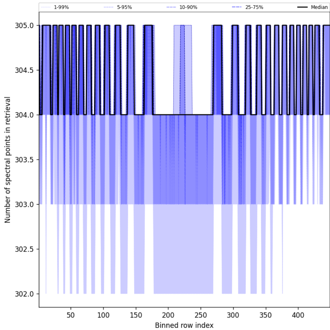
Figure 50: Along track statistics of “Number of spectral points in retrieval” for 2025-02-09 to 2025-02-11
