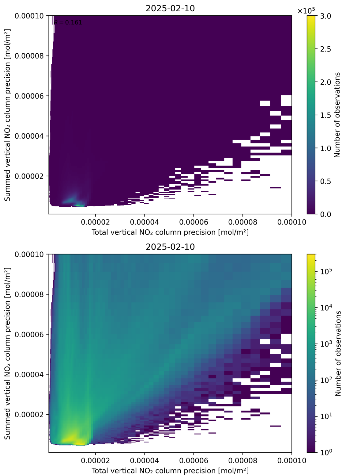
Figure 118: Scatter density plot of “Total vertical NO 2 column precision” against “Summed vertical NO 2 column precision” for 2025-02-09 to 2025-02-11.
