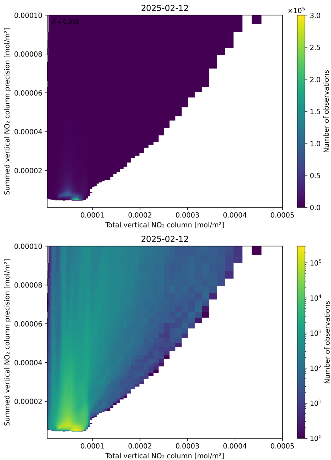
Figure 113: Scatter density plot of “Total vertical NO 2 column” against “Summed vertical NO 2 column precision” for 2025-02-11 to 2025-02-13.
