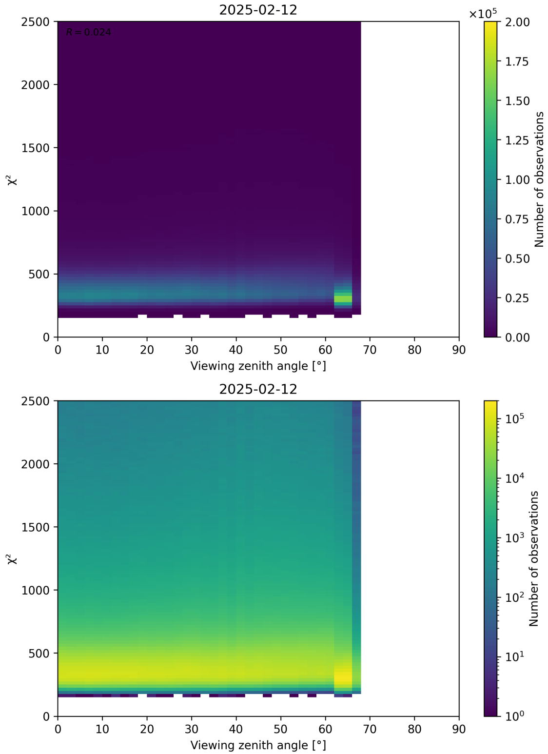
Figure 162: Scatter density plot of “Viewing zenith angle” against “ \chi^2 ” for 2025-02-11 to 2025-02-13.
