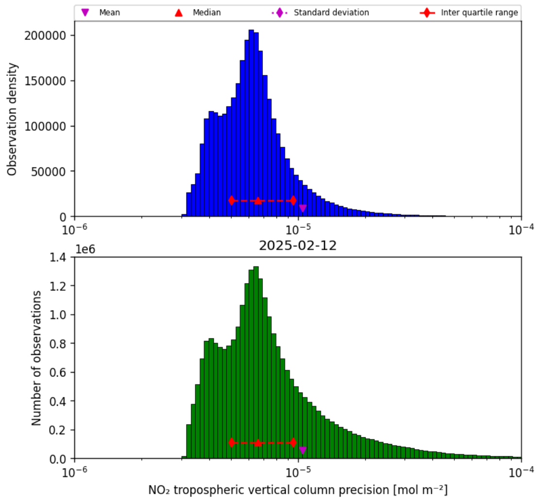
Figure 30: Histogram of “NO 2 tropospheric vertical column precision” for 2025-02-11 to 2025-02-13
