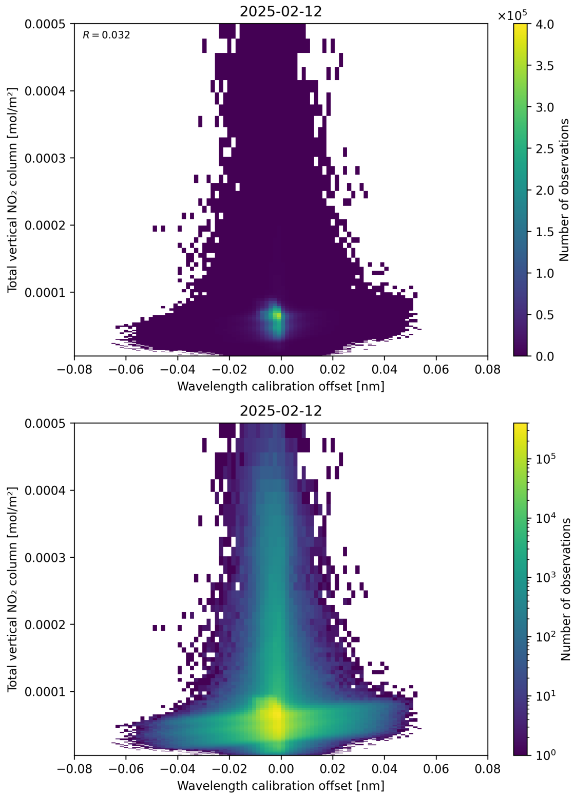
Figure 179: Scatter density plot of “Wavelength calibration offset” against “Total vertical NO 2 column” for 2025-02-11 to 2025-02-13.
