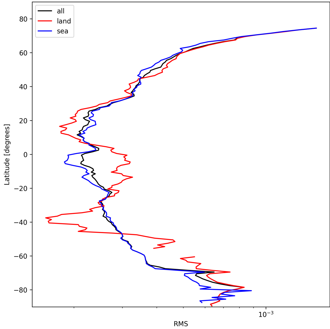
Figure 26: Zonal average of “RMS” for 2025-02-11 to 2025-02-13.
