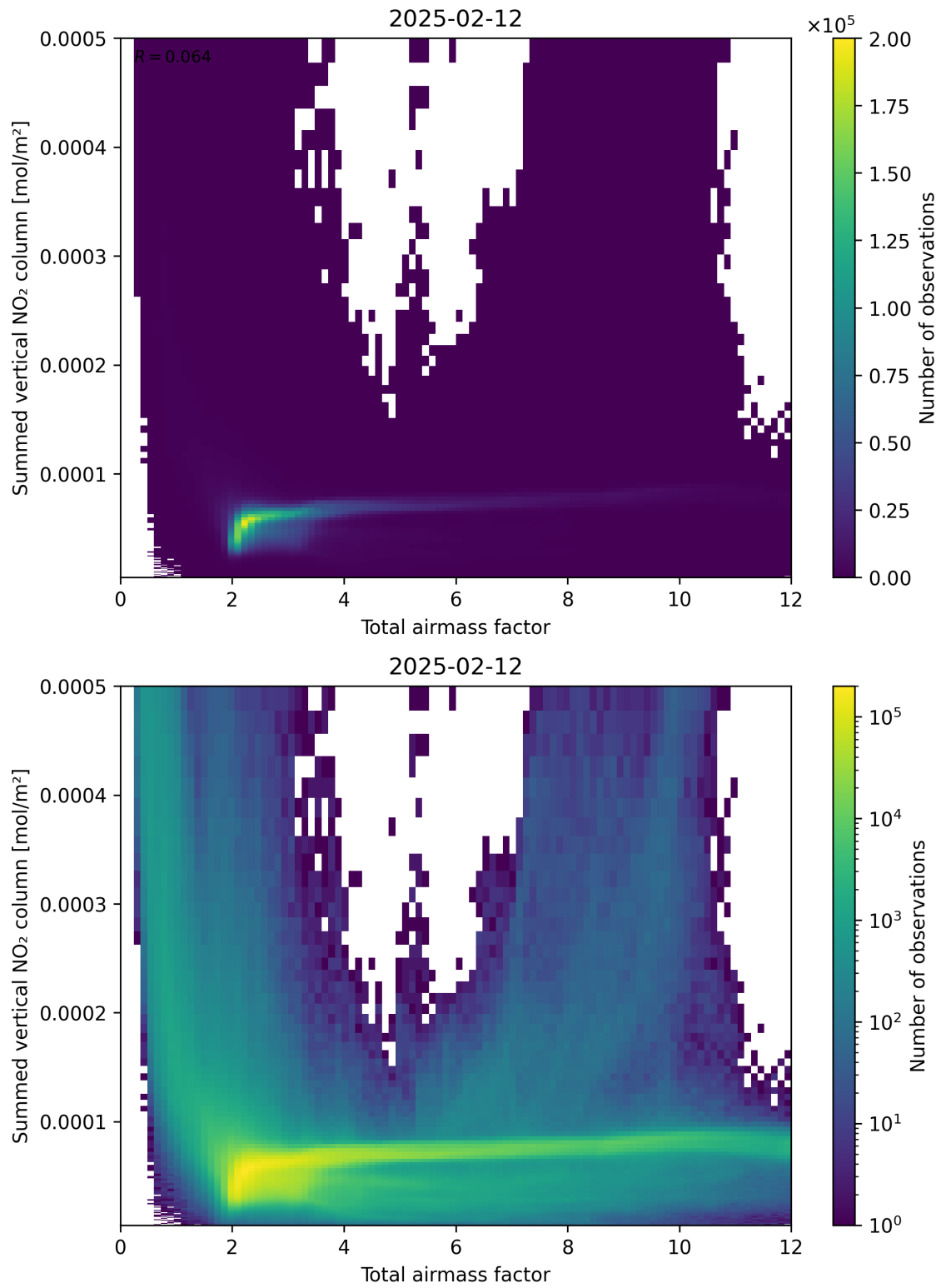
Figure 65: Scatter density plot of “Total airmass factor” against “Summed vertical NO 2 column” for 2025-02-11 to 2025-02-13.
