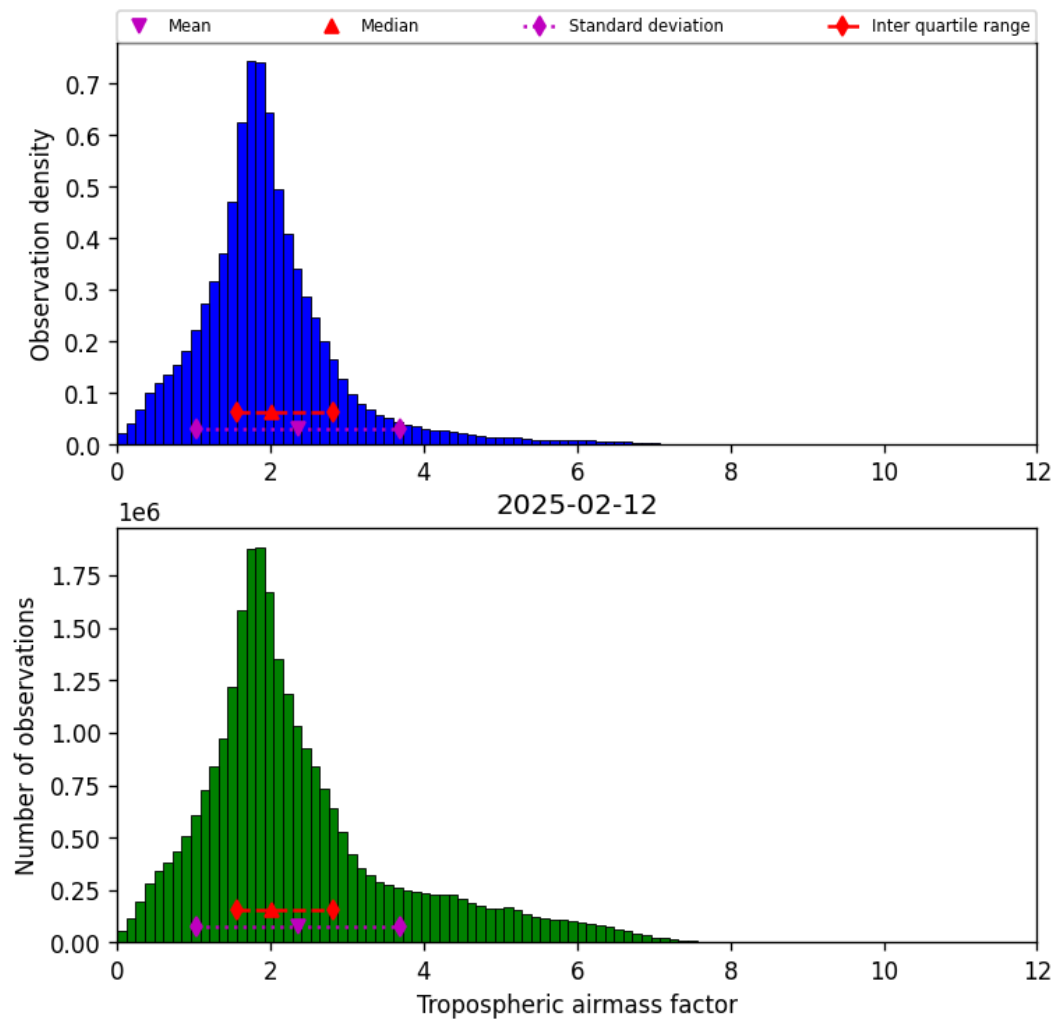
Figure 31: Histogram of “Tropospheric airmass factor” for 2025-02-11 to 2025-02-13
