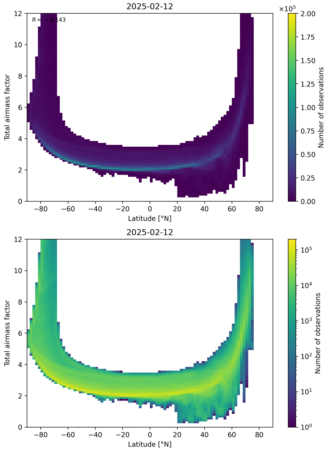
Figure 84: Scatter density plot of “Latitude” against “Total airmass factor” for 2025-02-11 to 2025-02-13.
