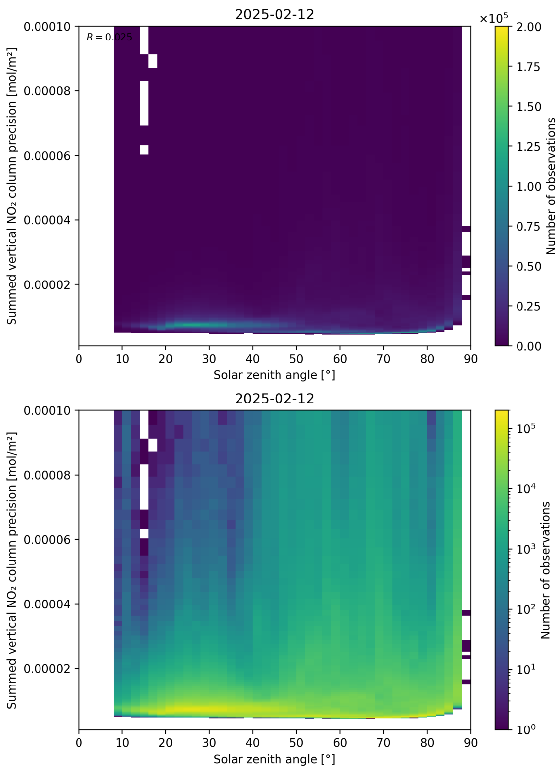
Figure 152: Scatter density plot of “Solar zenith angle” against “Summed vertical NO 2 column precision” for 2025-02-11 to 2025-02-13.
