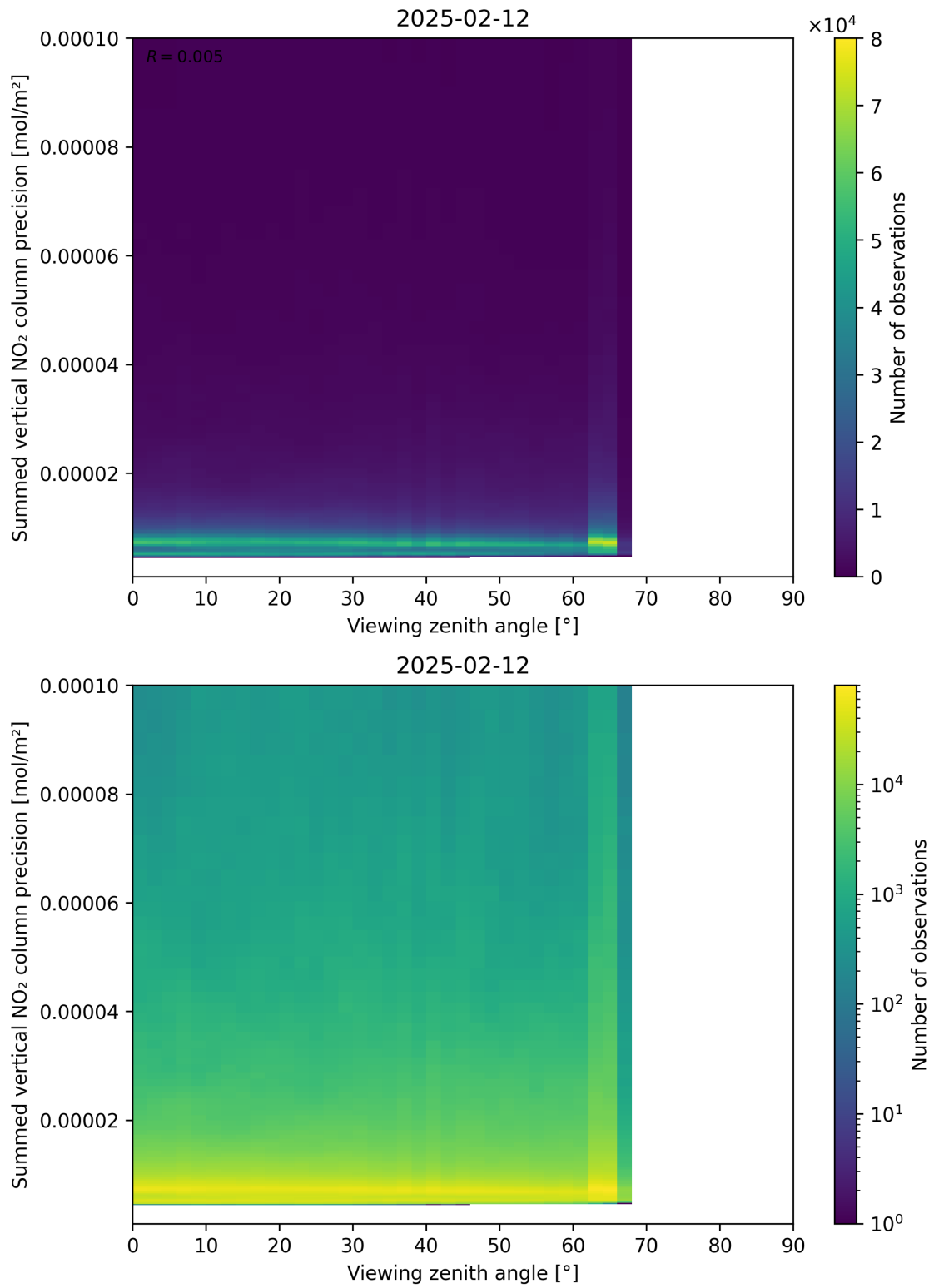
Figure 166: Scatter density plot of “Viewing zenith angle” against “Summed vertical NO 2 column precision” for 2025-02-11 to 2025-02-13.
