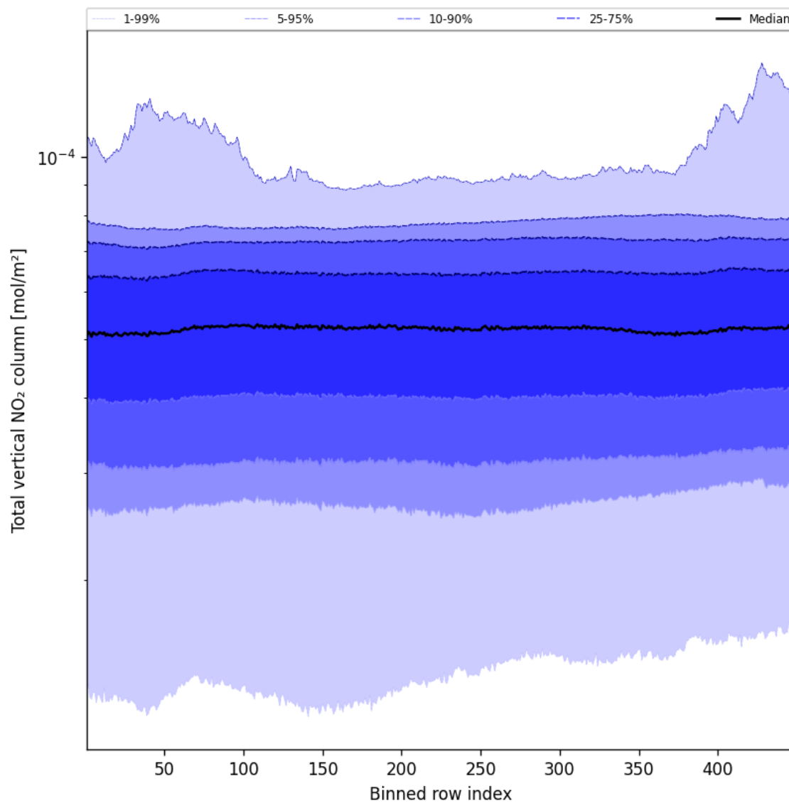
Figure 55: Along track statistics of “Total vertical NO 2 column” for 2025-02-11 to 2025-02-13
