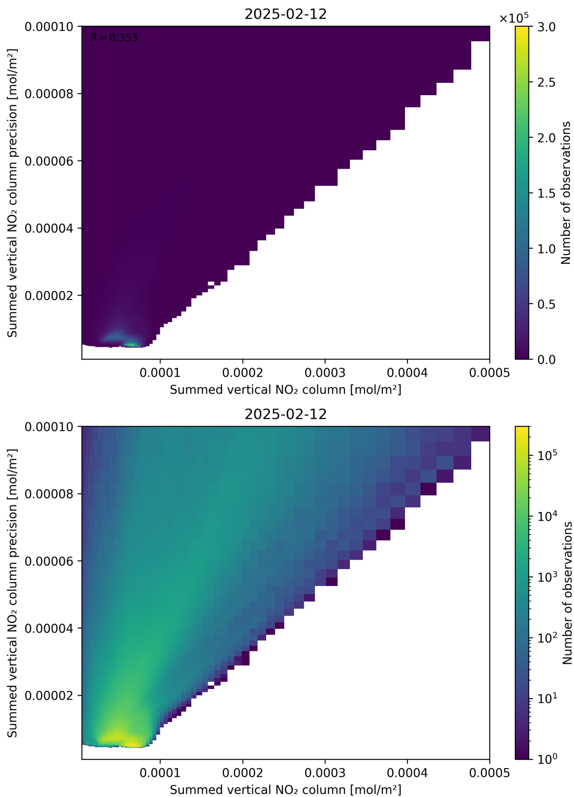
Figure 105: Scatter density plot of “Summed vertical NO 2 column” against “Summed vertical NO 2 column precision” for 2025-02-11 to 2025-02-13.
