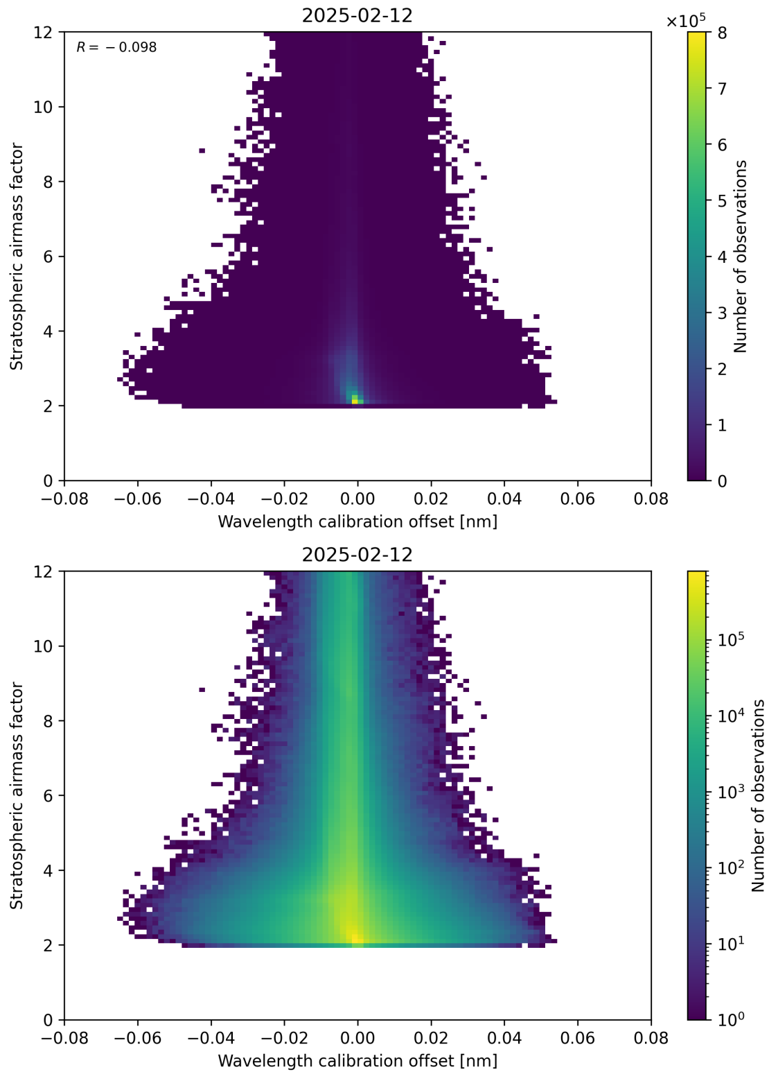
Figure 174: Scatter density plot of “Wavelength calibration offset” against “Stratospheric airmass factor” for 2025-02-11 to 2025-02-13.
