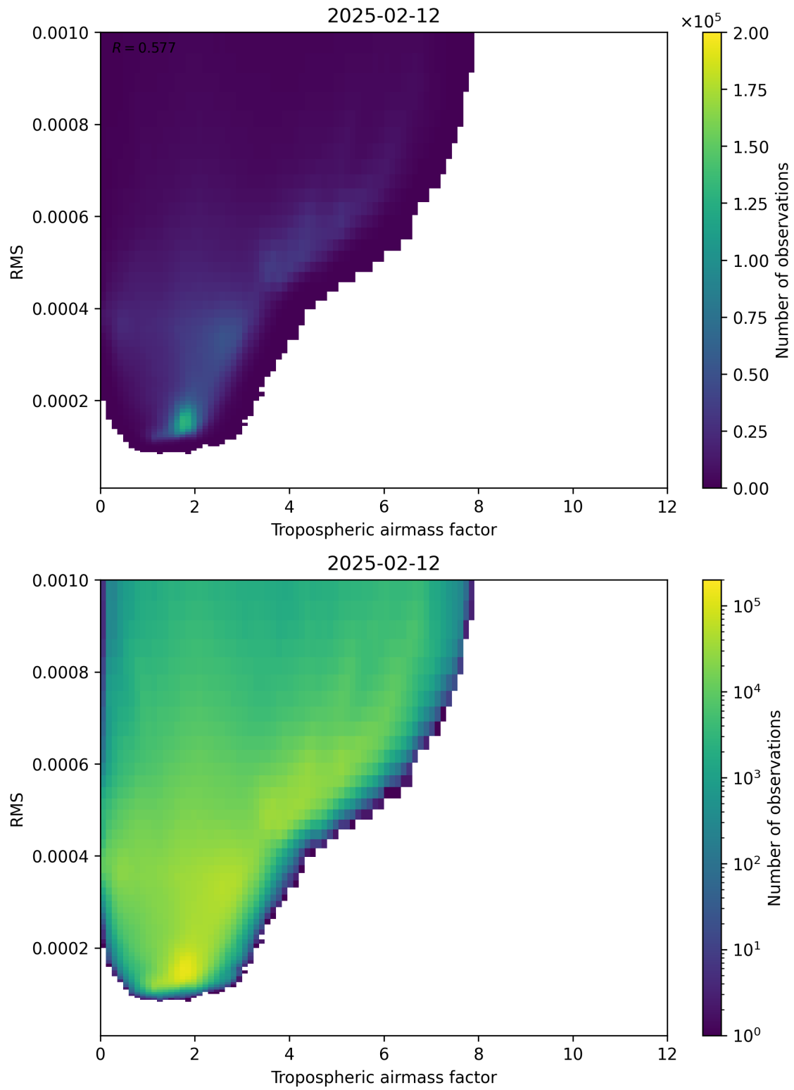
Figure 79: Scatter density plot of “Tropospheric airmass factor” against “RMS” for 2025-02-11 to 2025-02-13.
