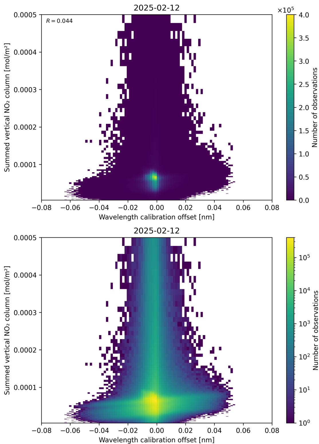
Figure 177: Scatter density plot of “Wavelength calibration offset” against “Summed vertical NO 2 column” for 2025-02-11 to 2025-02-13.
