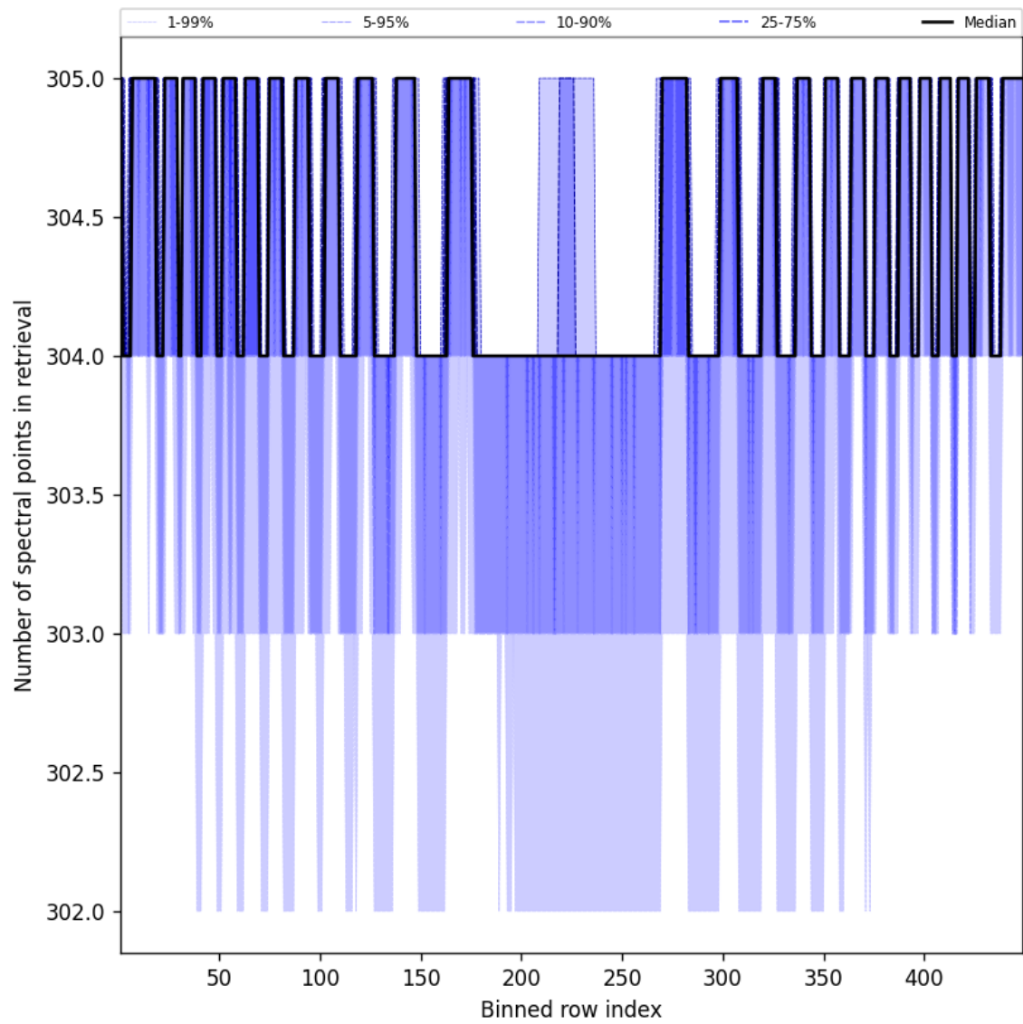
Figure 50: Along track statistics of “Number of spectral points in retrieval” for 2025-02-11 to 2025-02-13
