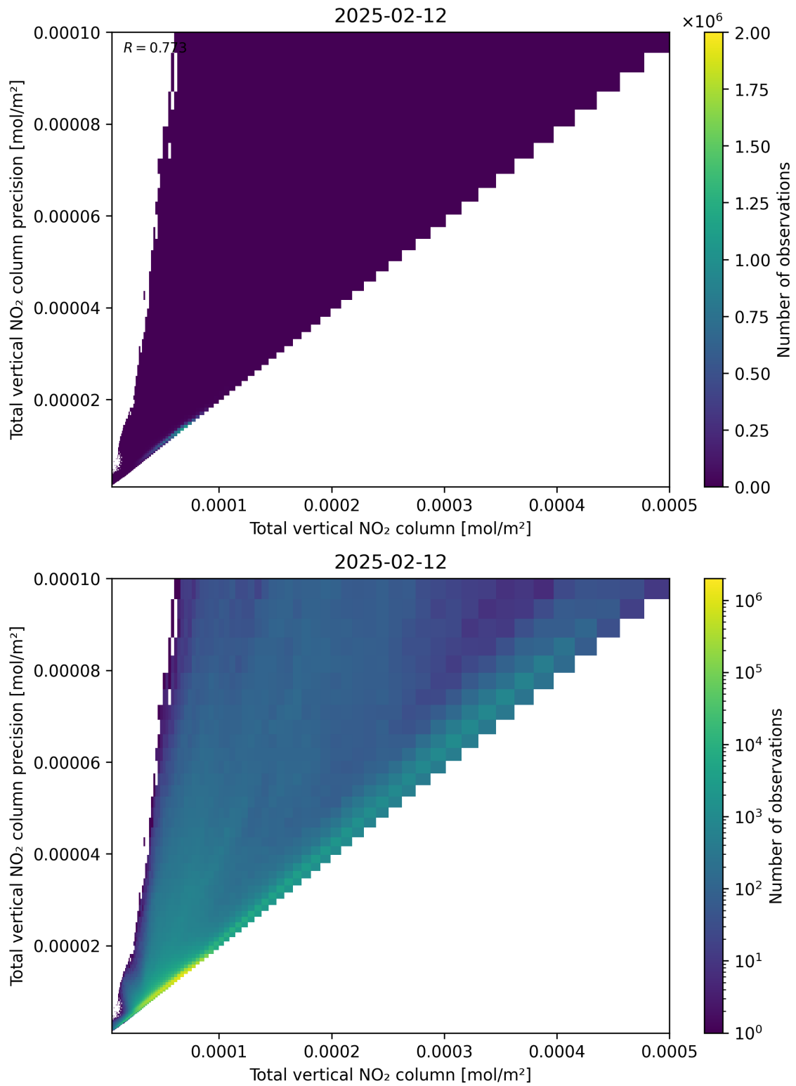
Figure 114: Scatter density plot of “Total vertical NO 2 column” against “Total vertical NO 2 column precision” for 2025-02-11 to 2025-02-13.
