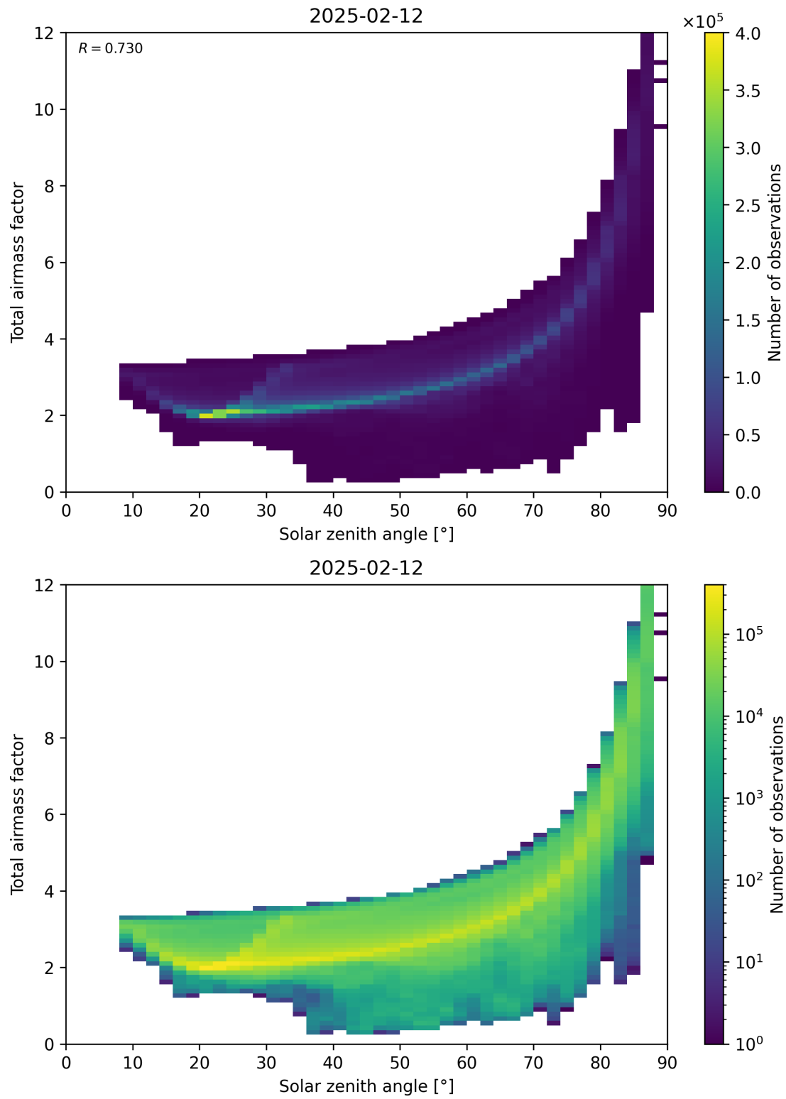
Figure 146: Scatter density plot of “Solar zenith angle” against “Total air mass factor” for 2025-02-11 to 2025-02-13.
