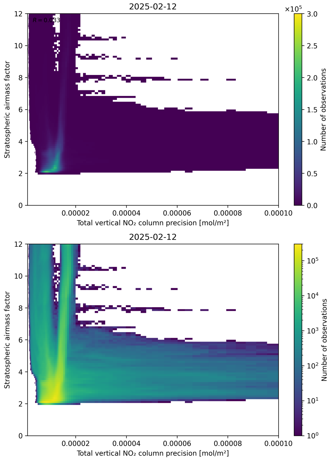
Figure 115: Scatter density plot of “Total vertical NO 2 column precision” against “Stratospheric air mass factor” for 2025-02-11 to 2025-02-13.
