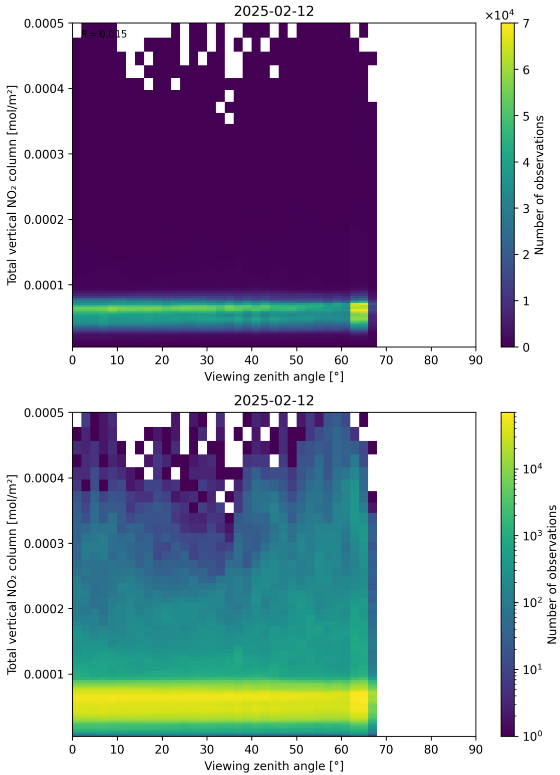
Figure 167: Scatter density plot of “Viewing zenith angle” against “Total vertical NO 2 column” for 2025-02-11 to 2025-02-13.
