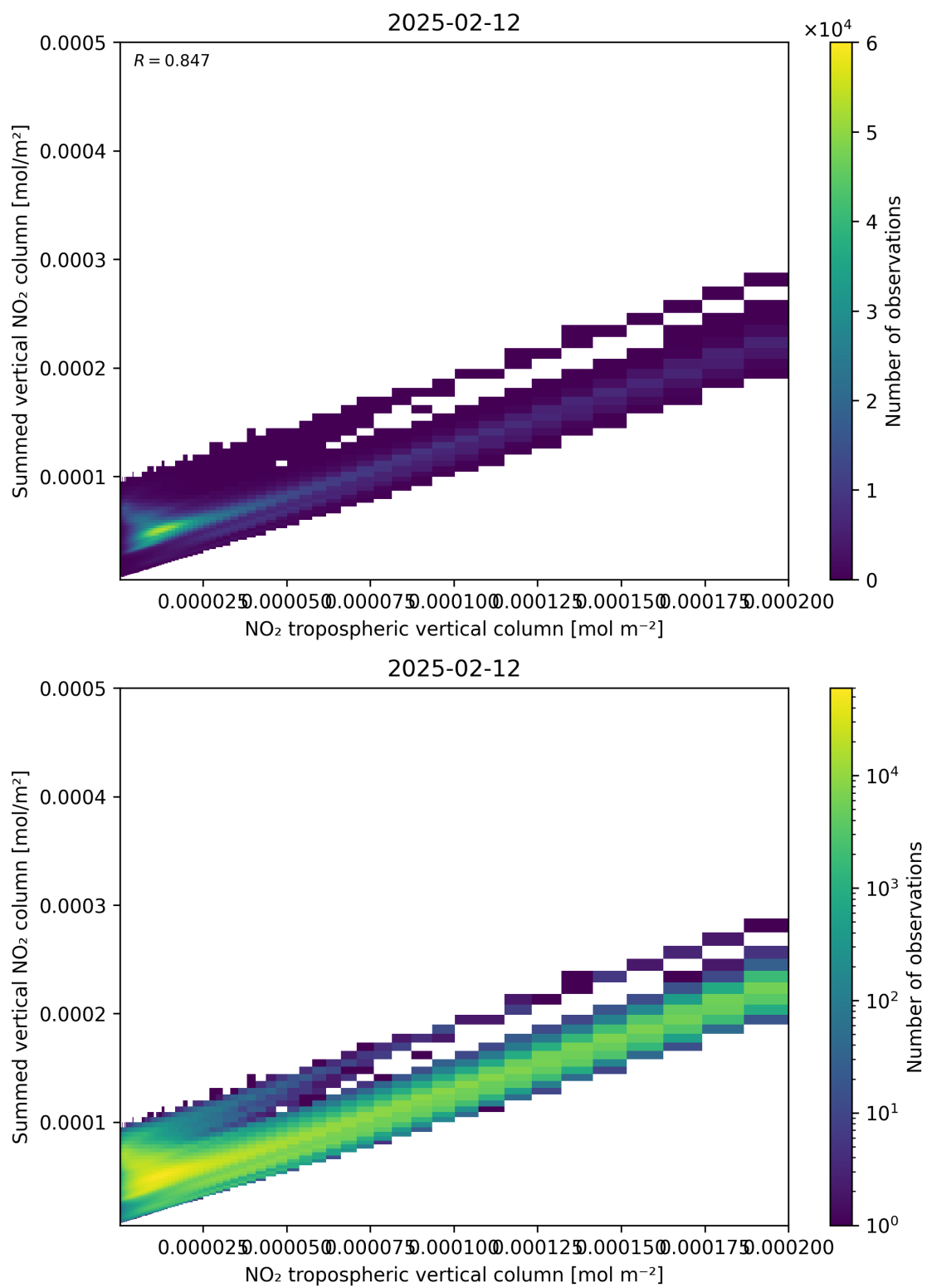
Figure 126: Scatter density plot of “NO 2 tropospheric vertical column” against “Summed vertical NO 2 column” for 2025-02-11 to 2025-02-13.
