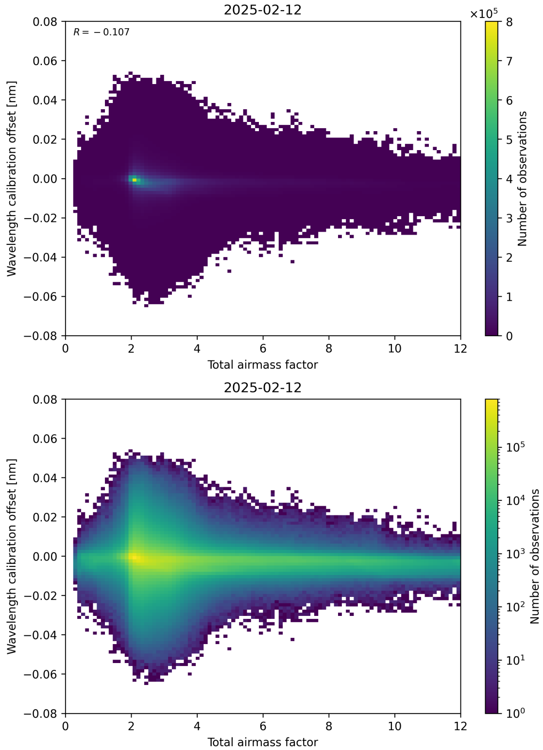
Figure 70: Scatter density plot of “Total airmass factor” against “Wavelength calibration offset” for 2025-02-11 to 2025-02-13.
