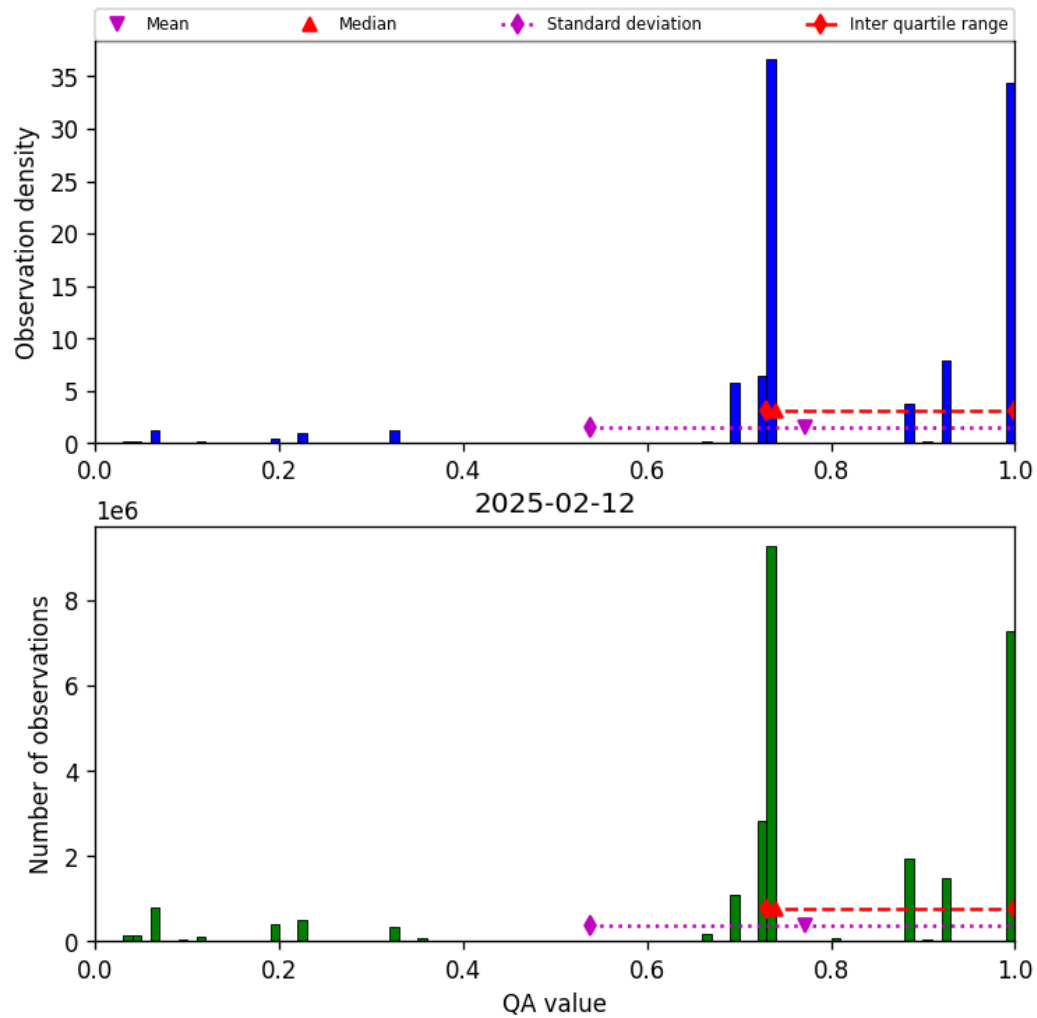
Figure 28: Histogram of “QA value” for 2025-02-11 to 2025-02-13
