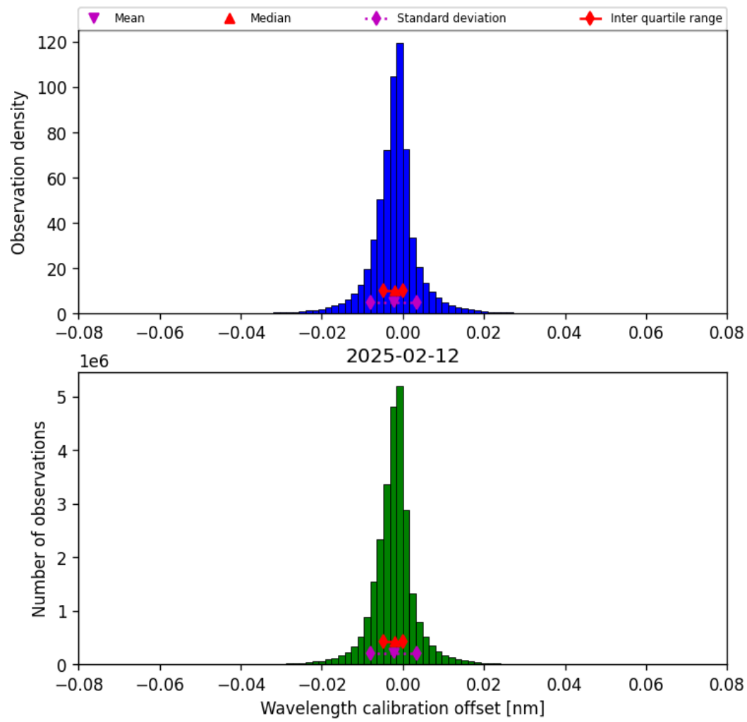
Figure 35: Histogram of “Wavelength calibration offset” for 2025-02-11 to 2025-02-13
