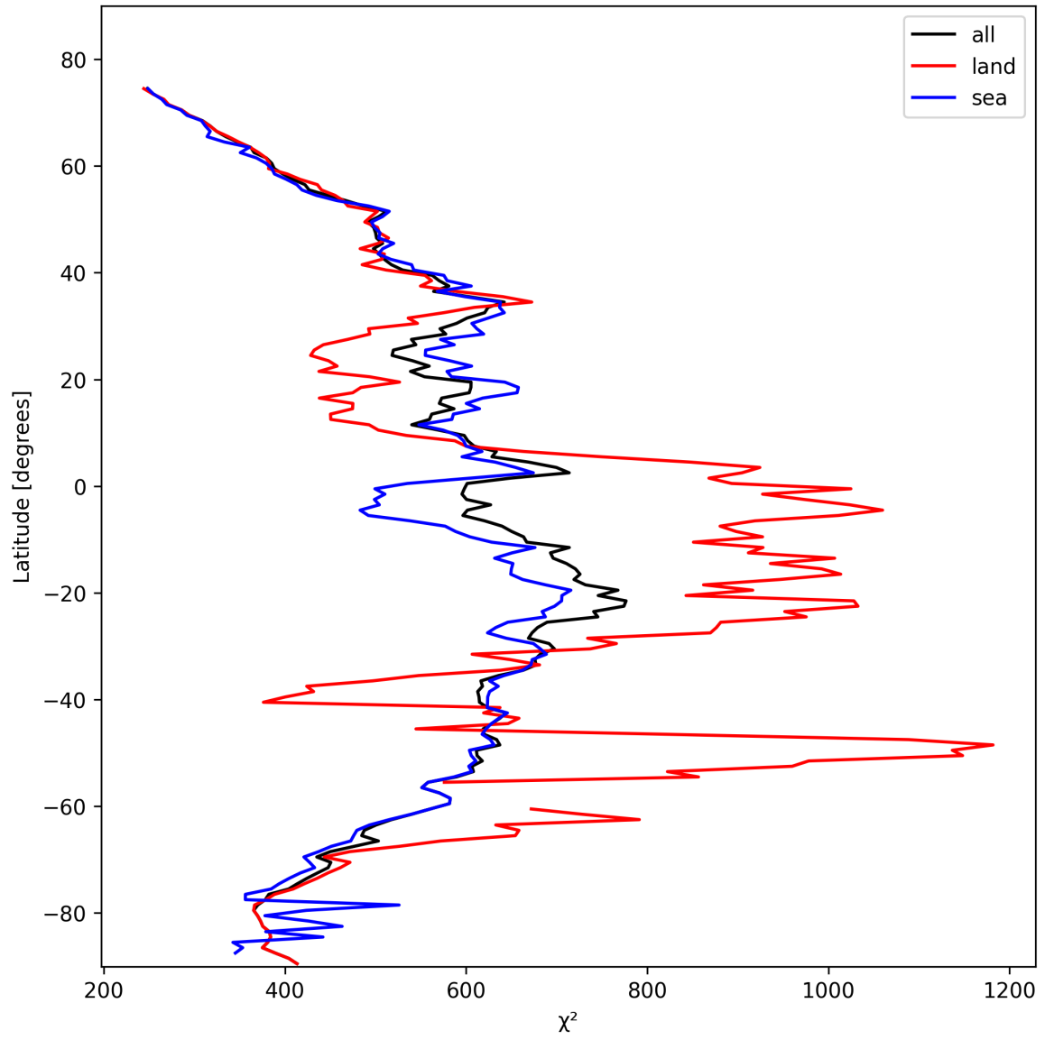
Figure 25: Zonal average of “ \chi^2 ” for 2025-02-11 to 2025-02-13.
