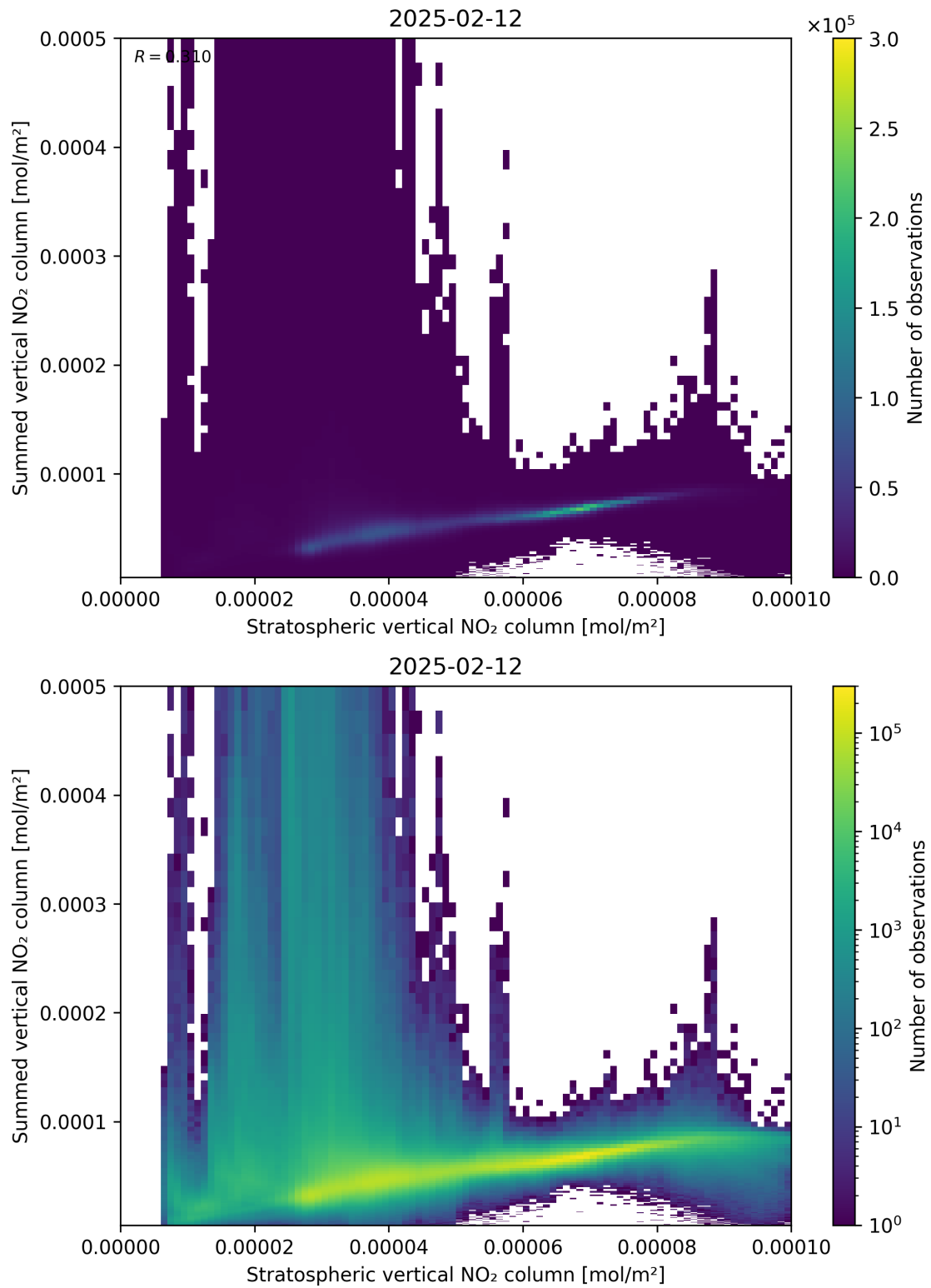
Figure 98: Scatter density plot of “Stratospheric vertical NO 2 column” against “Summed vertical NO 2 column” for 2025-02-11 to 2025-02-13.
