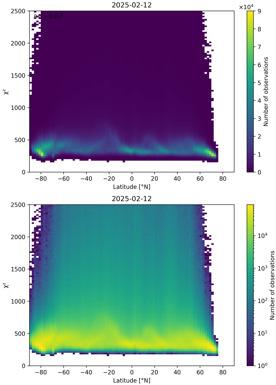
Figure 86: Scatter density plot of “Latitude” against “ \chi^2 ” for 2025-02-11 to 2025-02-13.
