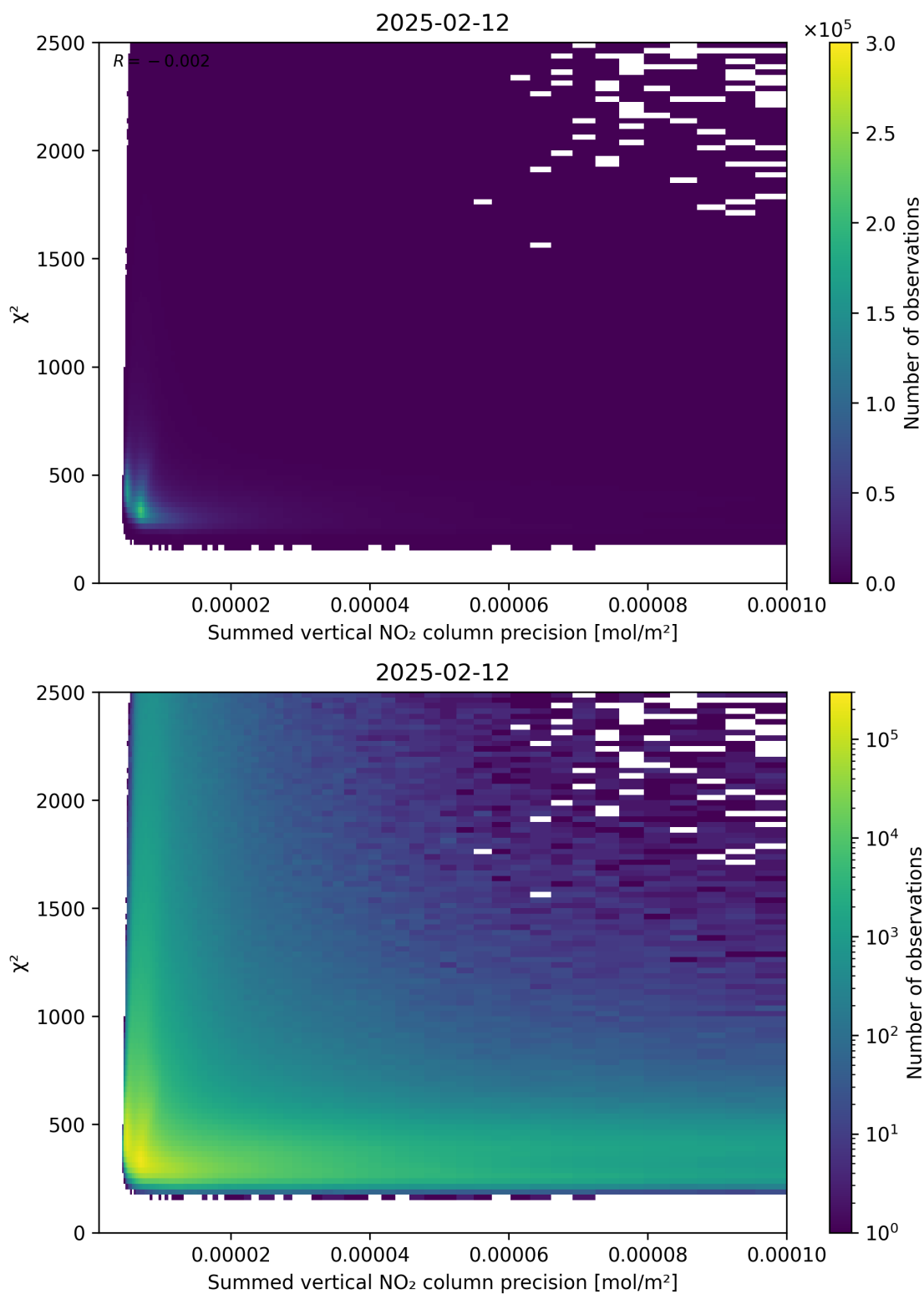
Figure 107: Scatter density plot of “Summed vertical NO 2 column precision” against “ \chi^2 ” for 2025-02-11 to 2025-02-13.
