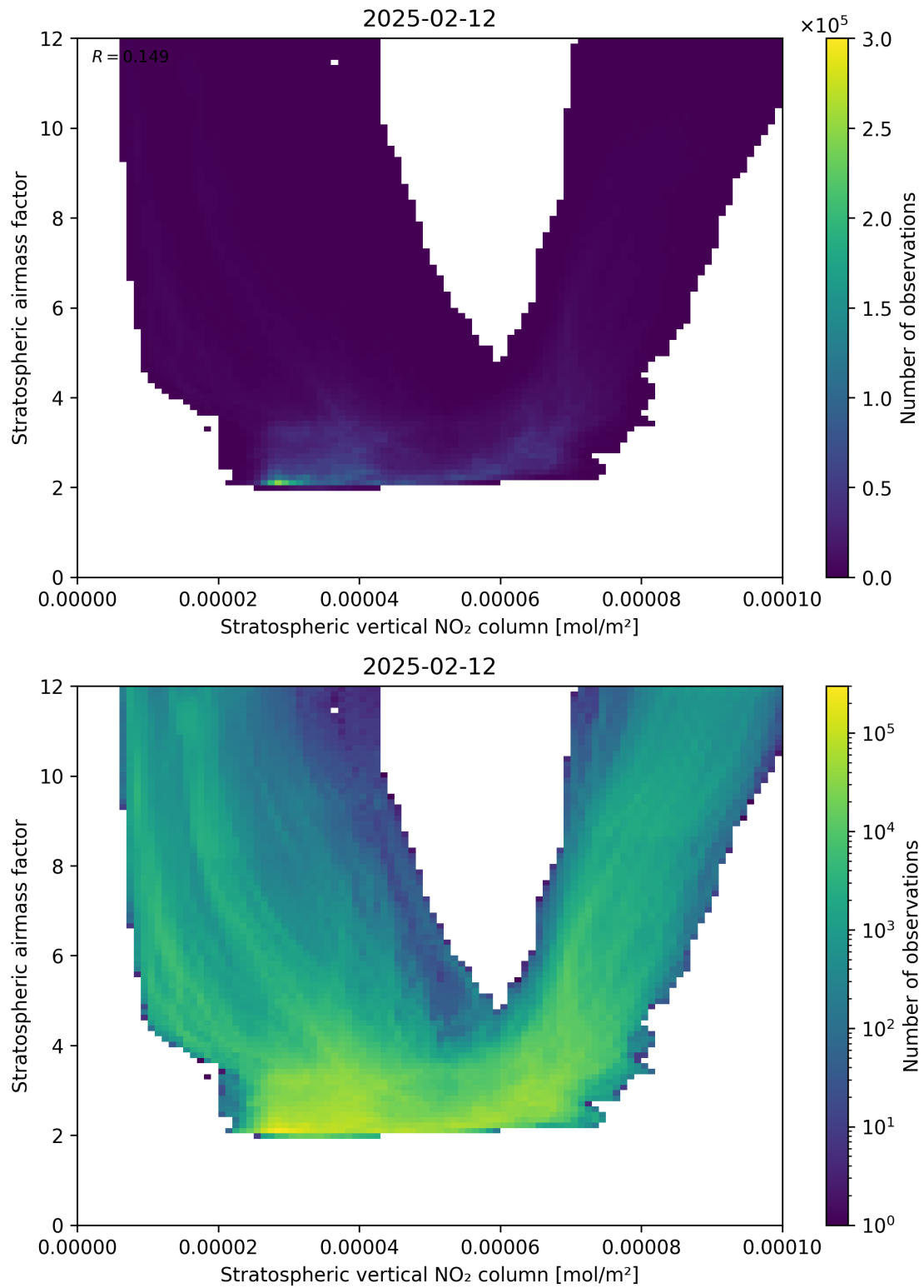
Figure 96: Scatter density plot of “Stratospheric vertical NO 2 column” against “Stratospheric airmass factor” for 2025-02-11 to 2025-02-13.
