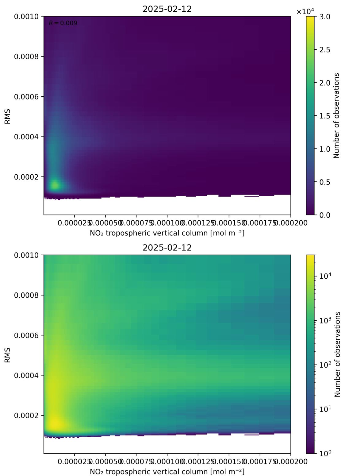
Figure 142: Scatter density plot of “NO 2 tropospheric vertical column” against “RMS” for 2025-02-11 to 2025-02-13.
