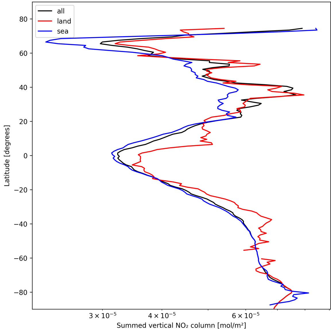
Figure 23: Zonal average of “Summed vertical NO 2 column” for 2025-02-11 to 2025-02-13.
