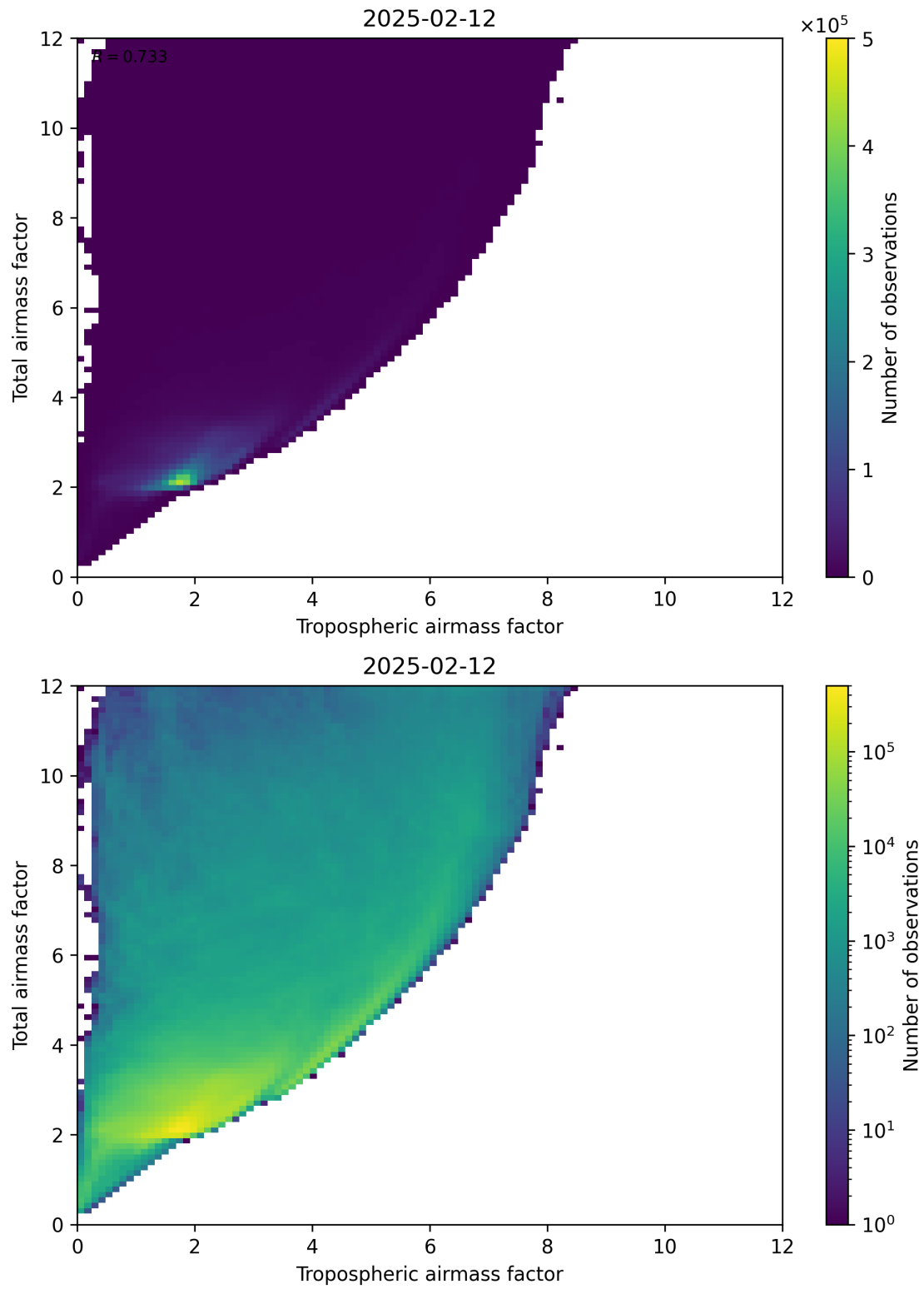
Figure 72: Scatter density plot of “Tropospheric airmass factor” against “Total airmass factor” for 2025-02-11 to 2025-02-13.
