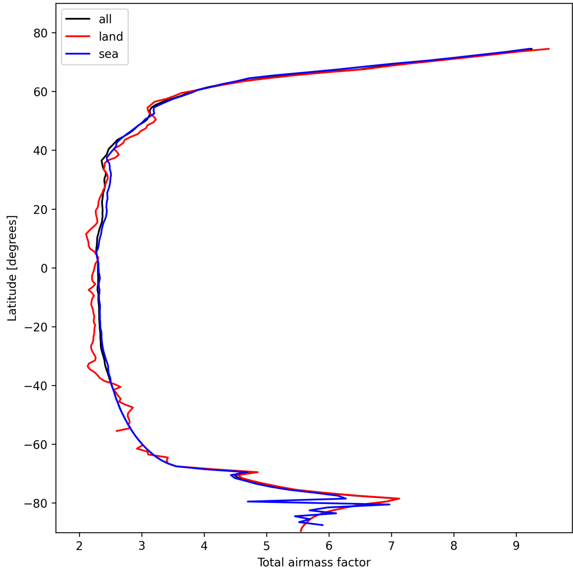
Figure 15: Zonal average of “Total airmass factor” for 2025-02-11 to 2025-02-13.
