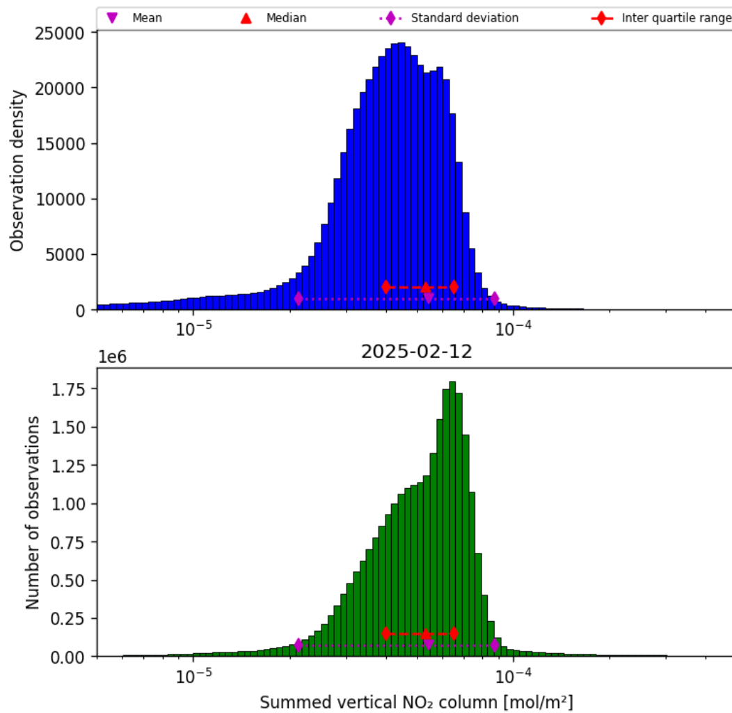
Figure 40: Histogram of “Summed vertical NO 2 column” for 2025-02-11 to 2025-02-13
