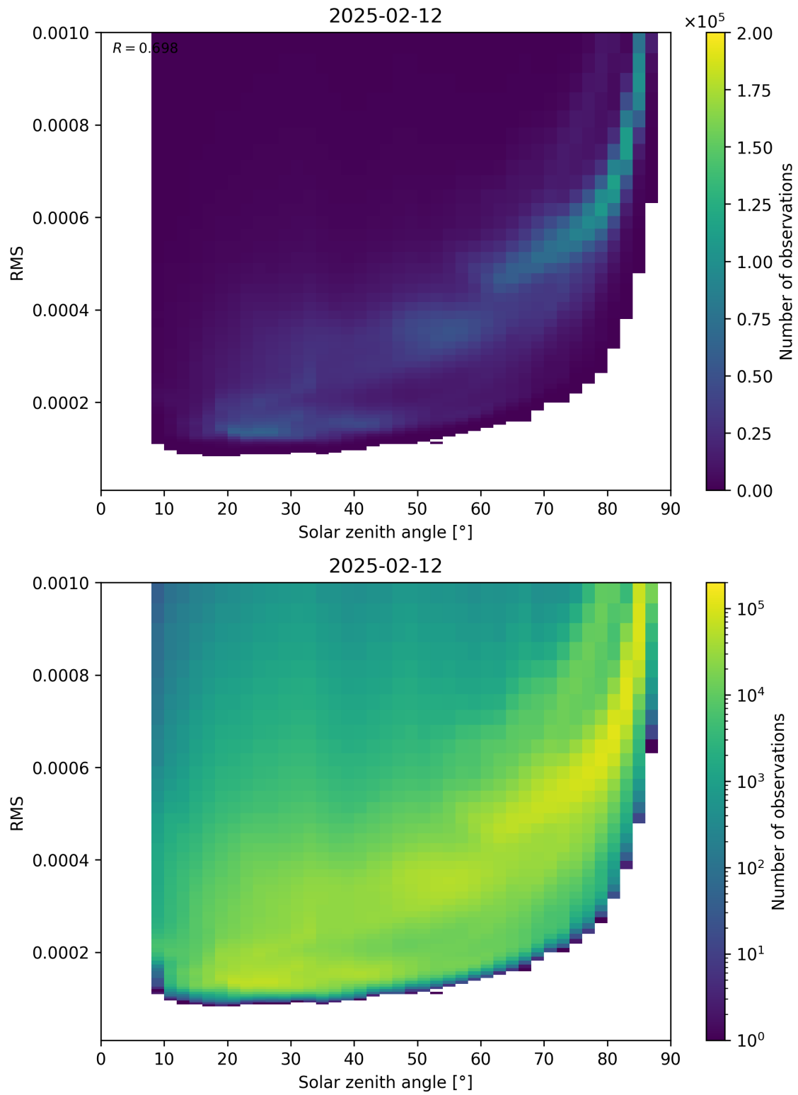
Figure 157: Scatter density plot of “Solar zenith angle” against “RMS” for 2025-02-11 to 2025-02-13.
