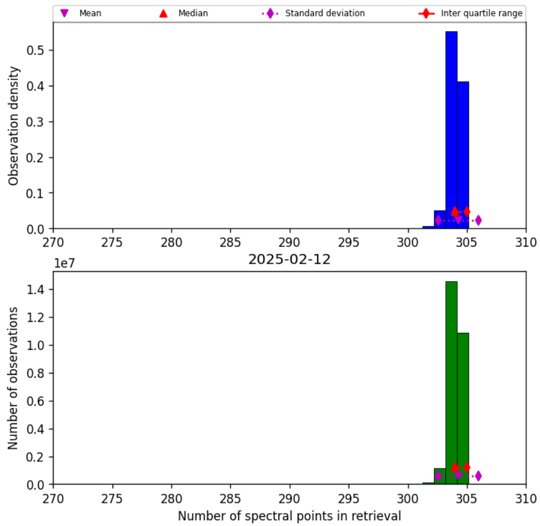
Figure 33: Histogram of “Number of spectral points in retrieval” for 2025-02-11 to 2025-02-13
