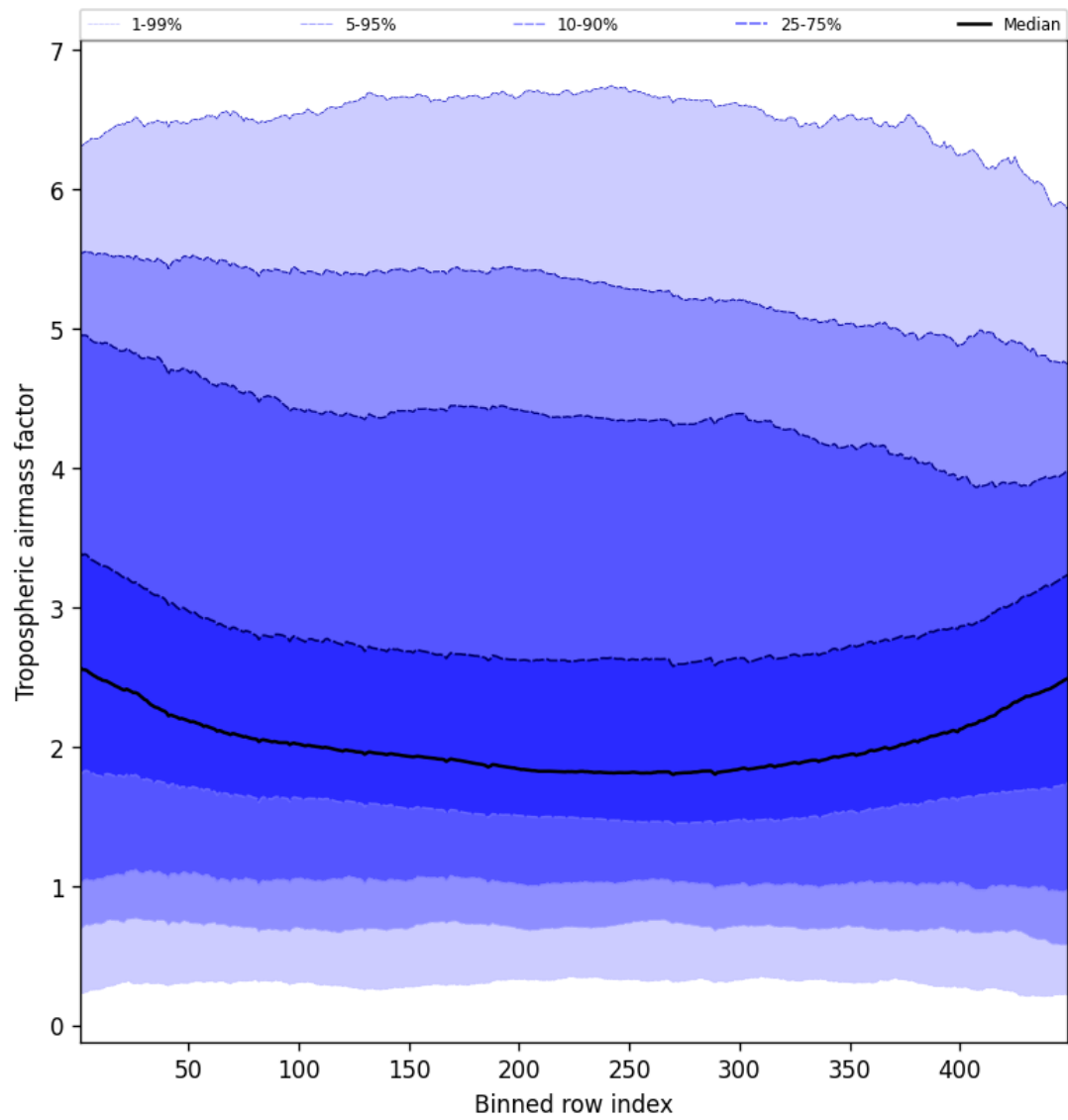
Figure 48: Along track statistics of “Tropospheric airmass factor” for 2025-02-11 to 2025-02-13
