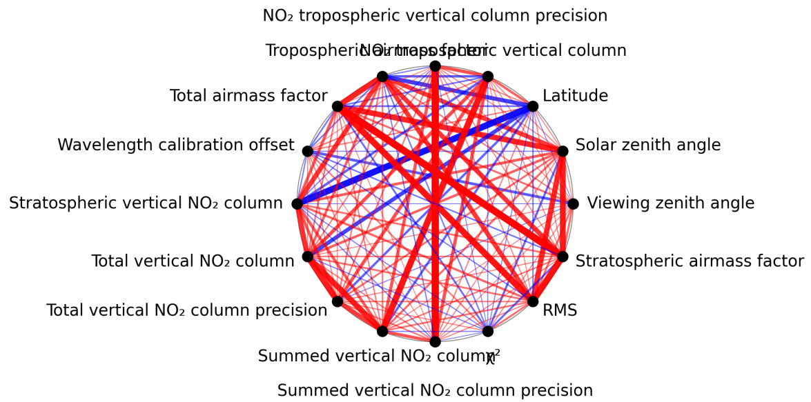
Figure 1: Map of correlation graph for 2025-02-11 to 2025-02-13.
