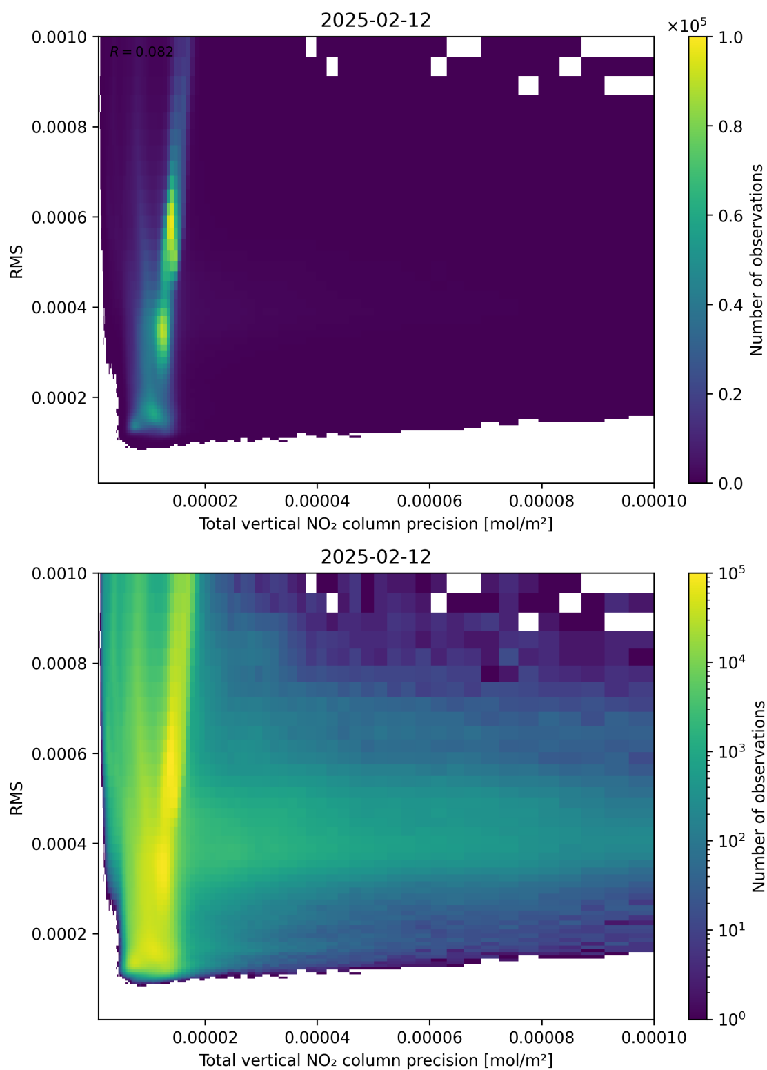
Figure 119: Scatter density plot of “Total vertical NO 2 column precision” against “RMS” for 2025-02-11 to 2025-02-13.
