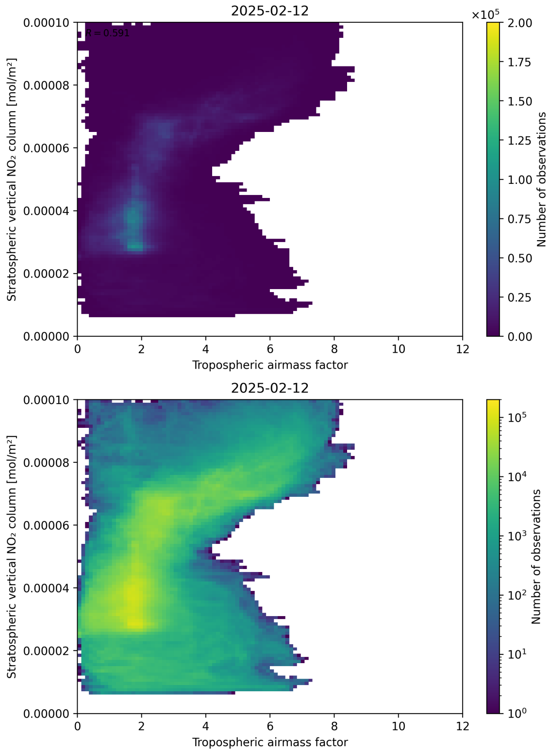
Figure 74: Scatter density plot of “Tropospheric airmass factor” against “Stratospheric vertical NO 2 column” for 2025-02-11 to 2025-02-13.
