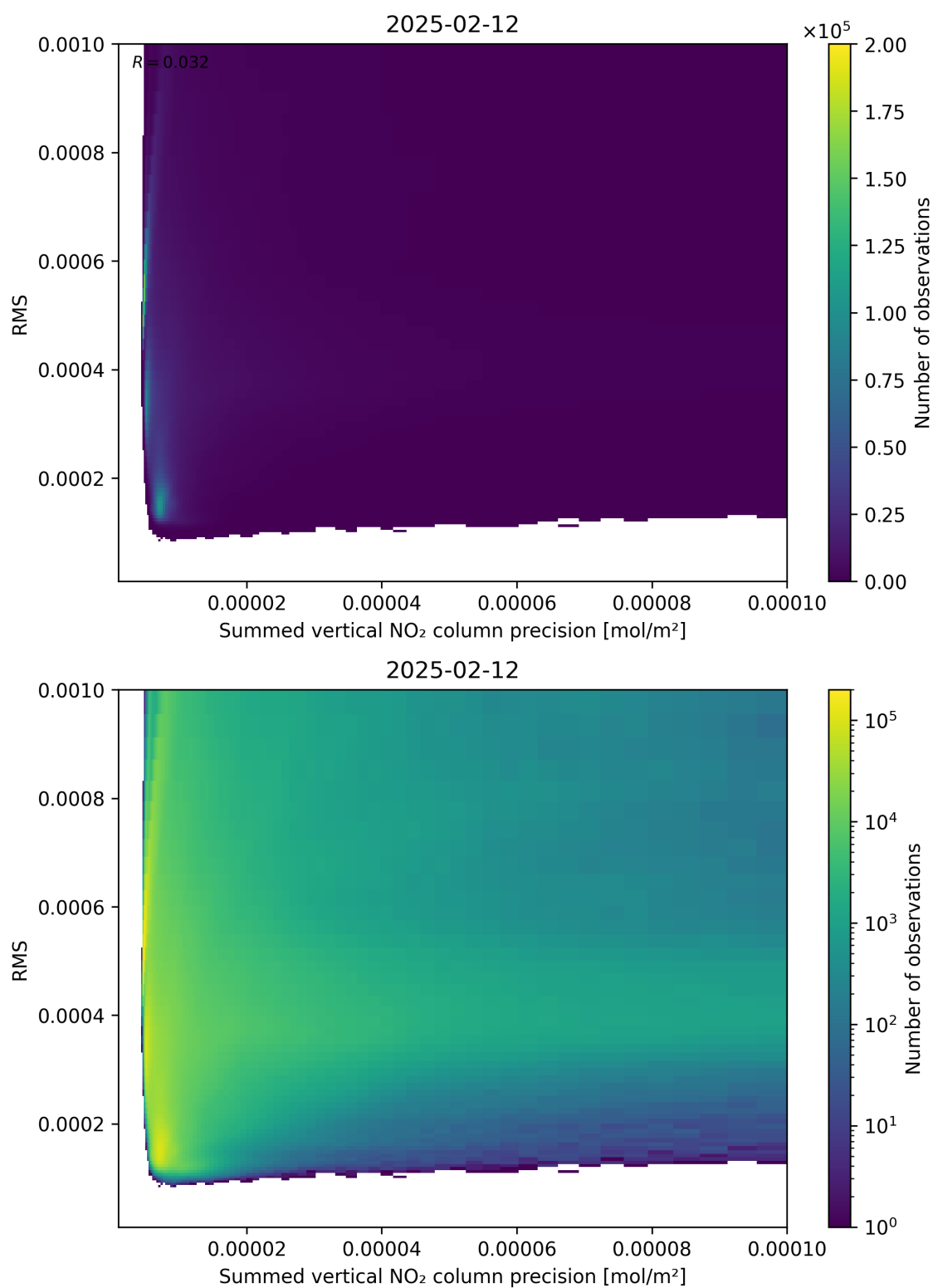
Figure 108: Scatter density plot of “Summed vertical NO 2 column precision” against “RMS” for 2025-02-11 to 2025-02-13.
