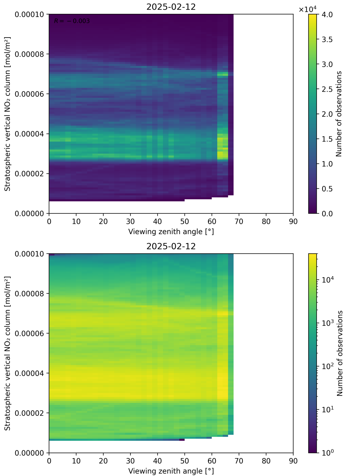
Figure 164: Scatter density plot of “Viewing zenith angle” against “Stratospheric vertical NO 2 column” for 2025-02-11 to 2025-02-13.
