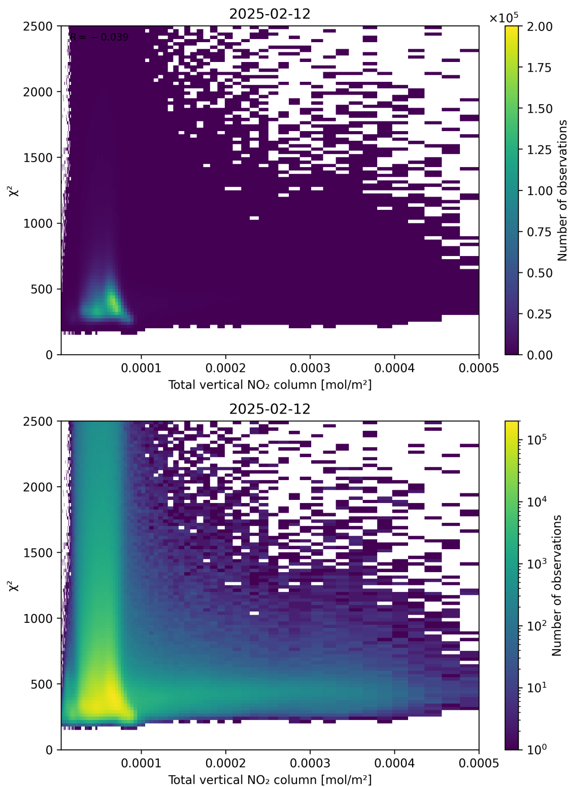
Figure 111: Scatter density plot of “Total vertical NO 2 column” against “ \chi^2 ” for 2025-02-11 to 2025-02-13.
