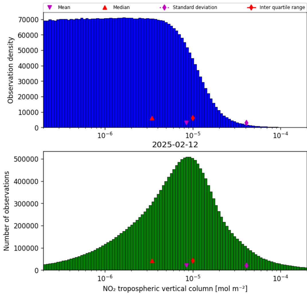
Figure 29: Histogram of “NO 2 tropospheric vertical column” for 2025-02-11 to 2025-02-13
