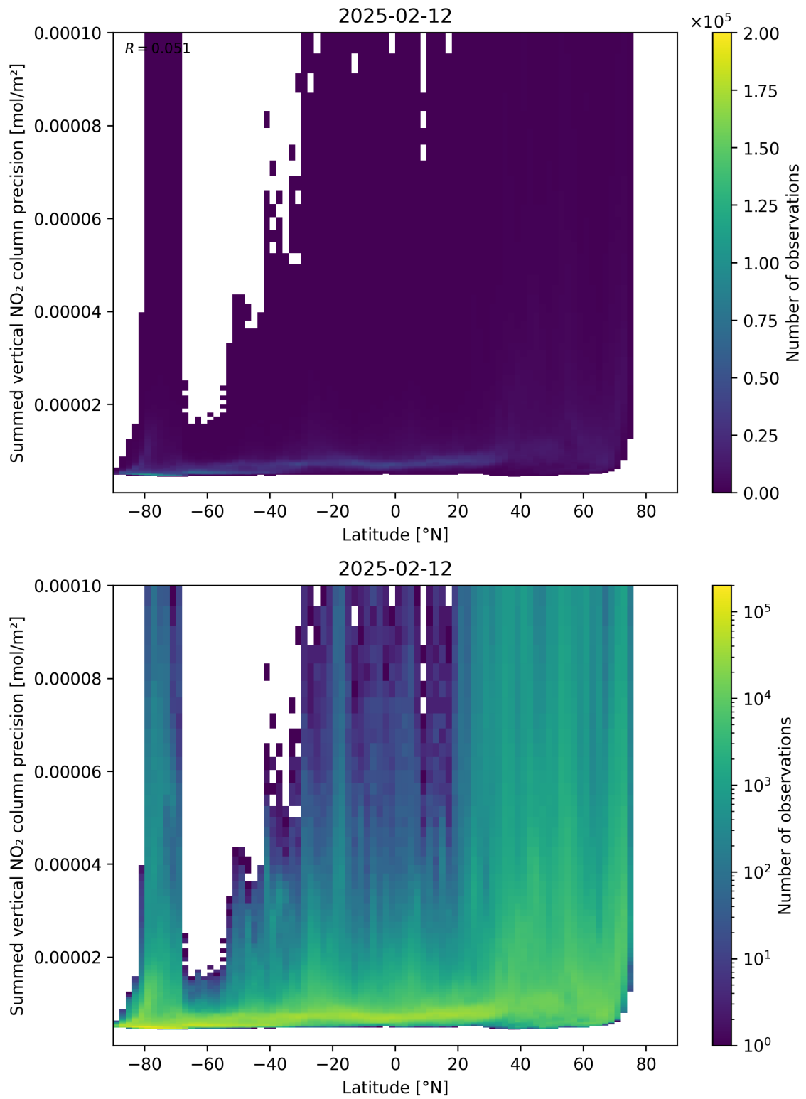
Figure 89: Scatter density plot of “Latitude” against “Summed vertical NO 2 column precision” for 2025-02-11 to 2025-02-13.
