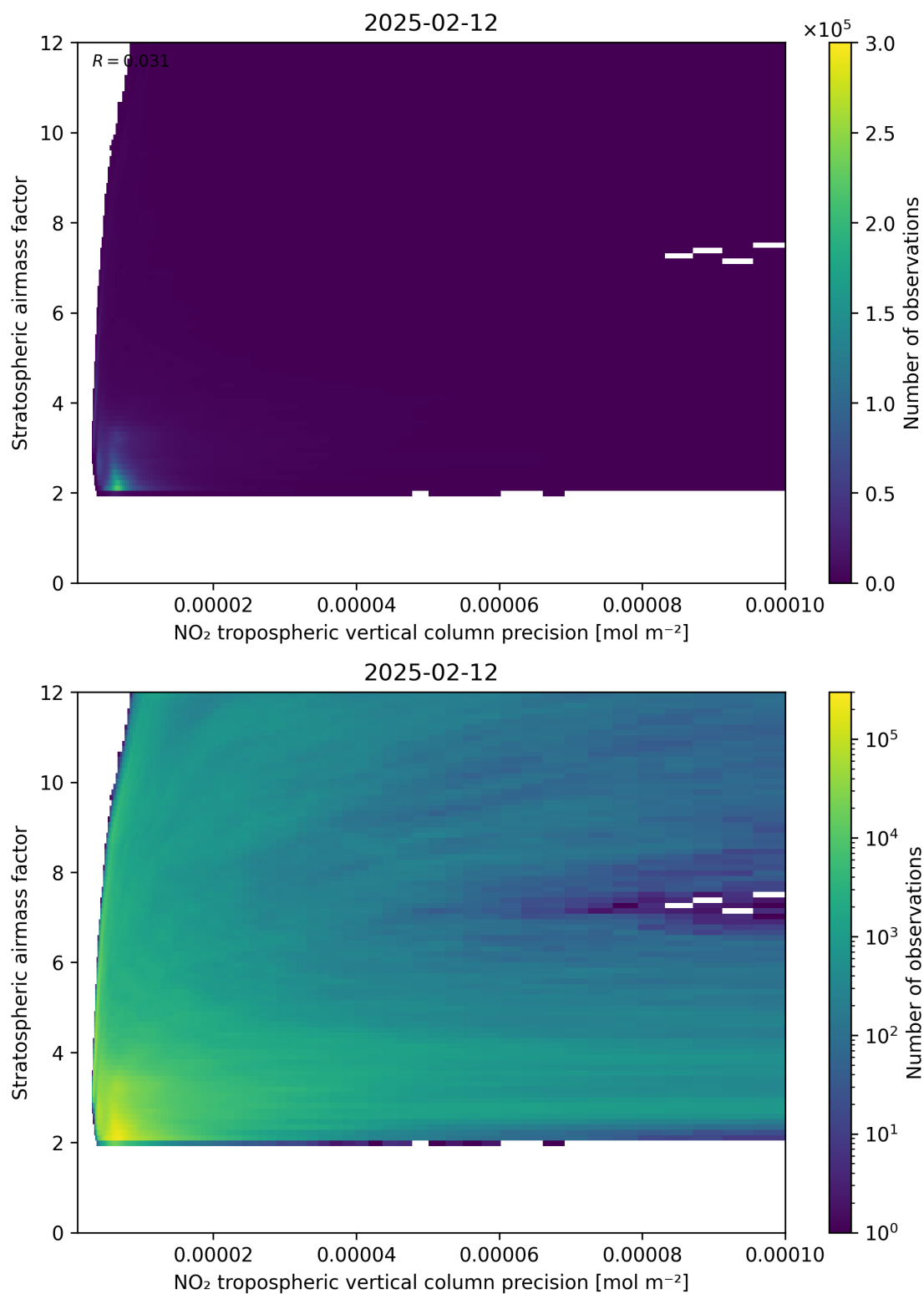
Figure 131: Scatter density plot of “NO 2 tropospheric vertical column precision” against “Stratospheric airmass factor” for 2025-02-11 to 2025-02-13.
