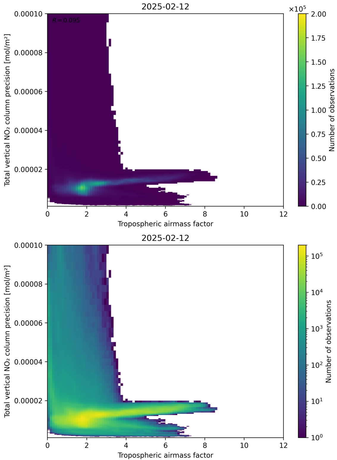
Figure 78: Scatter density plot of “Tropospheric airmass factor” against “Total vertical NO 2 column precision” for 2025-02-11 to 2025-02-13.
