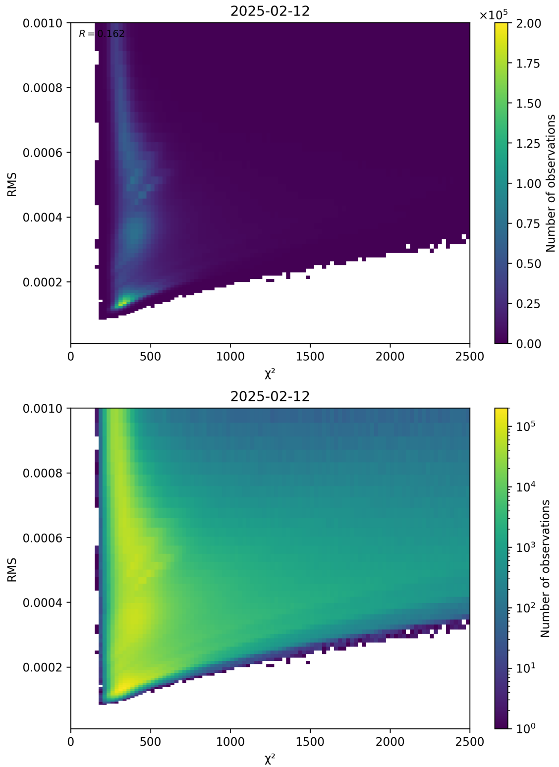
Figure 82: Scatter density plot of “ \chi^2 ” against “RMS” for 2025-02-11 to 2025-02-13.
