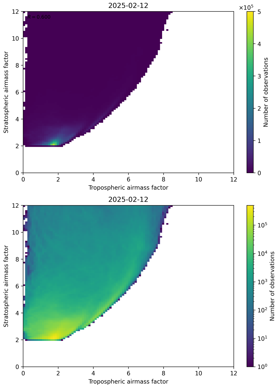
Figure 71: Scatter density plot of “Tropospheric airmass factor” against “Stratospheric airmass factor” for 2025-02-11 to 2025-02-13.
