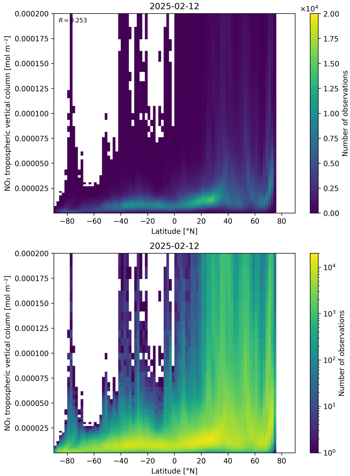
Figure 92: Scatter density plot of “Latitude” against “NO 2 tropospheric vertical column” for 2025-02-11 to 2025-02-13.
