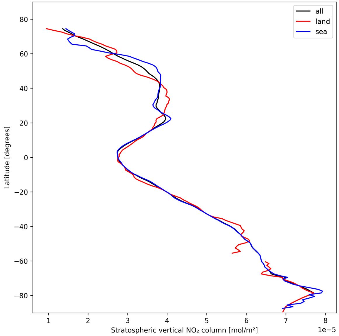
Figure 19: Zonal average of “Stratospheric vertical NO 2 column” for 2025-02-11 to 2025-02-13.
