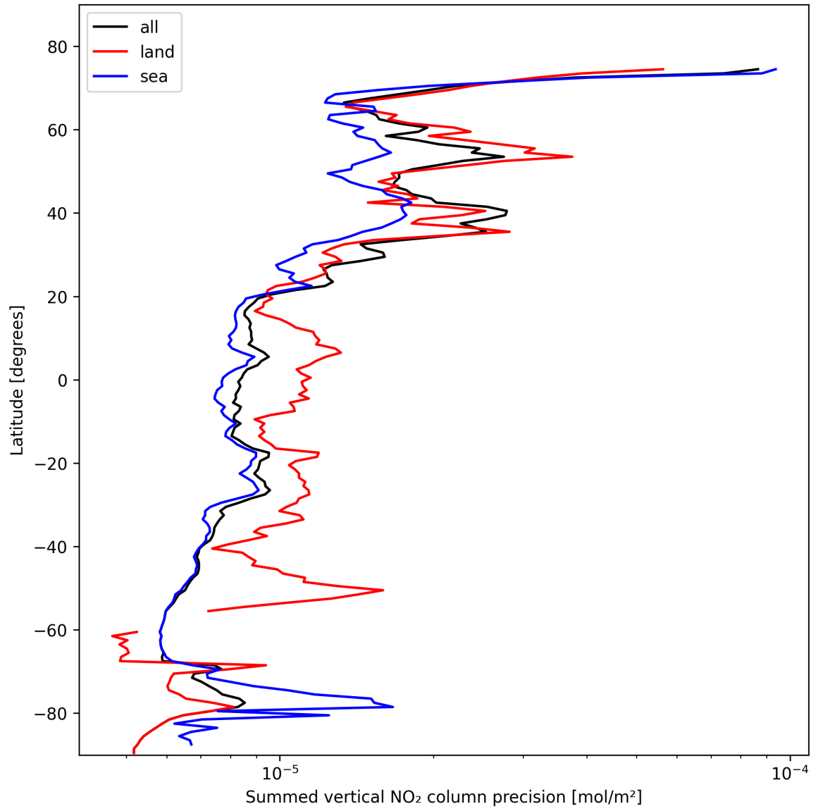
Figure 24: Zonal average of “Summed vertical NO 2 column precision” for 2025-02-11 to 2025-02-13.
