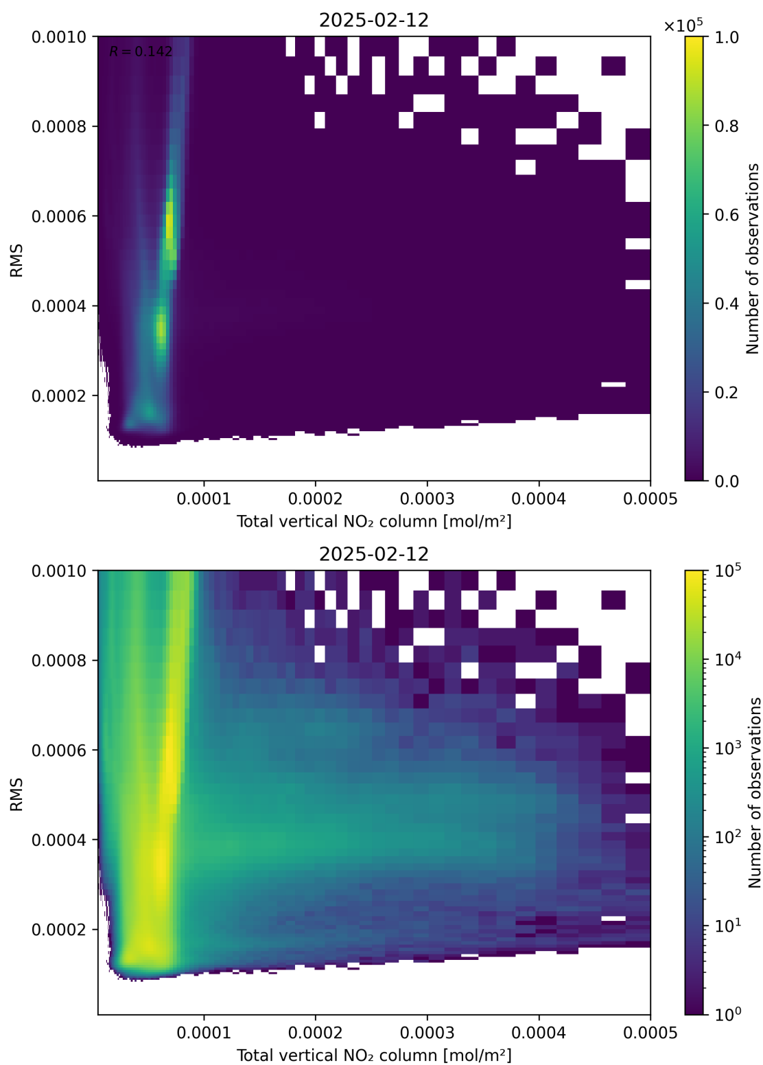
Figure 120: Scatter density plot of “Total vertical NO 2 column” against “RMS” for 2025-02-11 to 2025-02-13.
