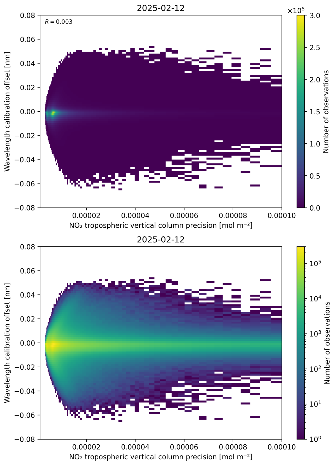
Figure 141: Scatter density plot of “NO 2 tropospheric vertical column precision” against “Wavelength calibration offset” for 2025-02-11 to 2025-02-13.
