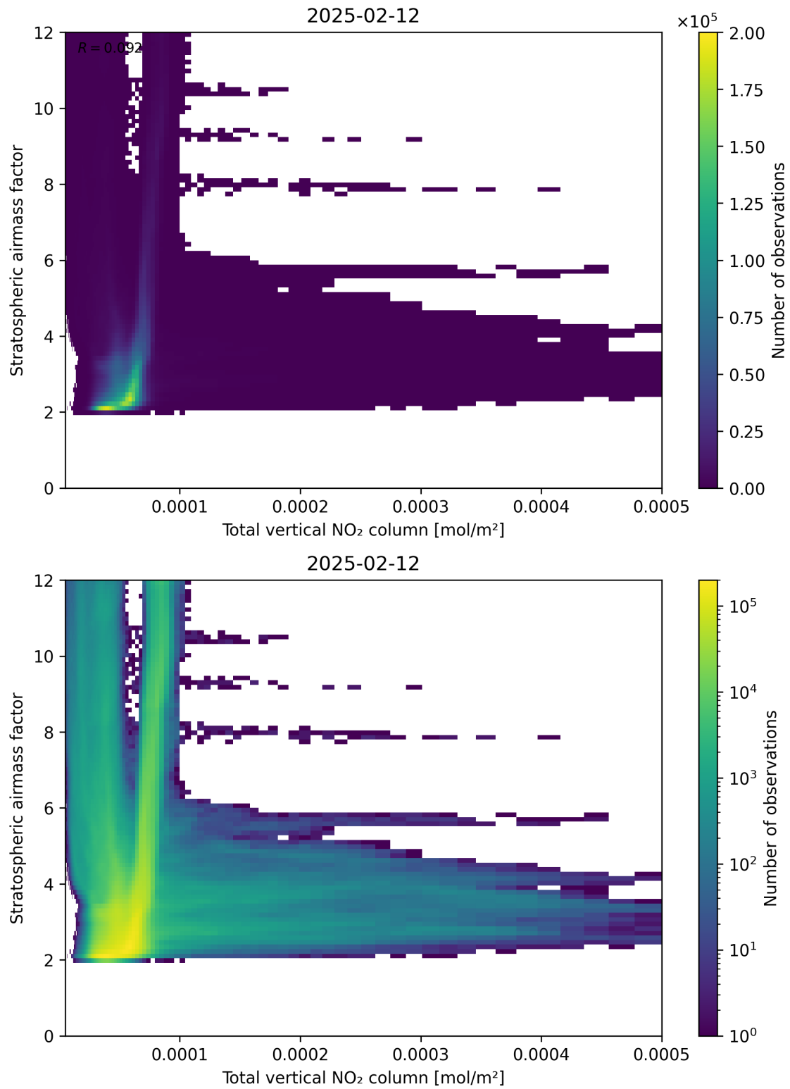
Figure 110: Scatter density plot of “Total vertical NO 2 column” against “Stratospheric airmass factor” for 2025-02-11 to 2025-02-13.
