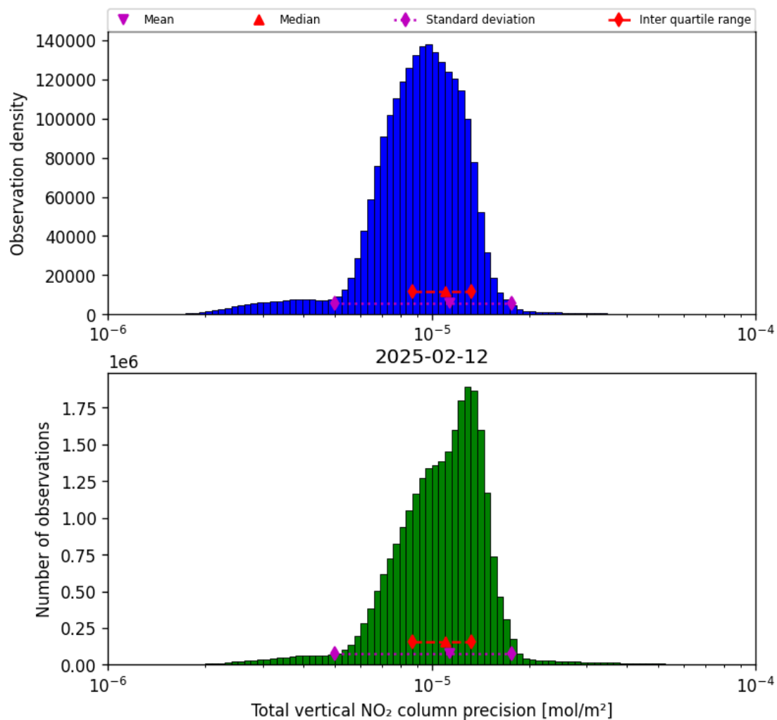
Figure 39: Histogram of “Total vertical NO 2 column precision” for 2025-02-11 to 2025-02-13
