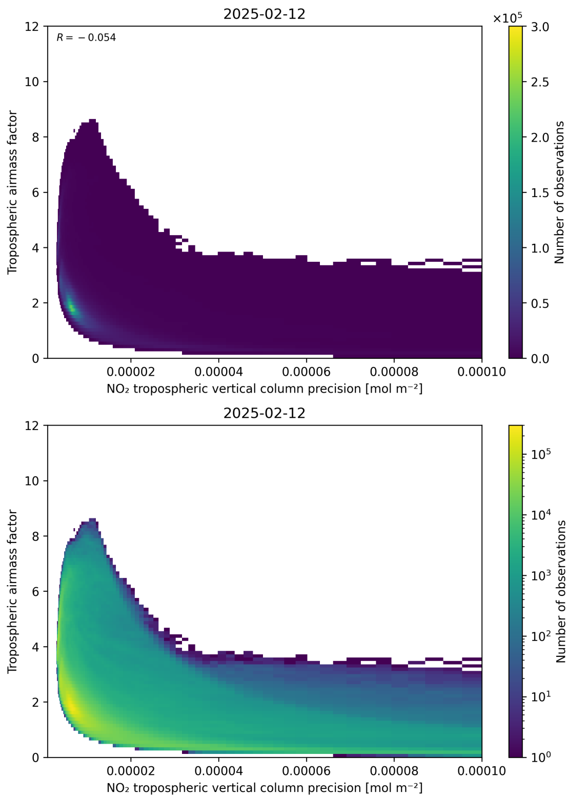
Figure 133: Scatter density plot of “NO 2 tropospheric vertical column precision” against “Tropospheric airmass factor” for 2025-02-11 to 2025-02-13.
