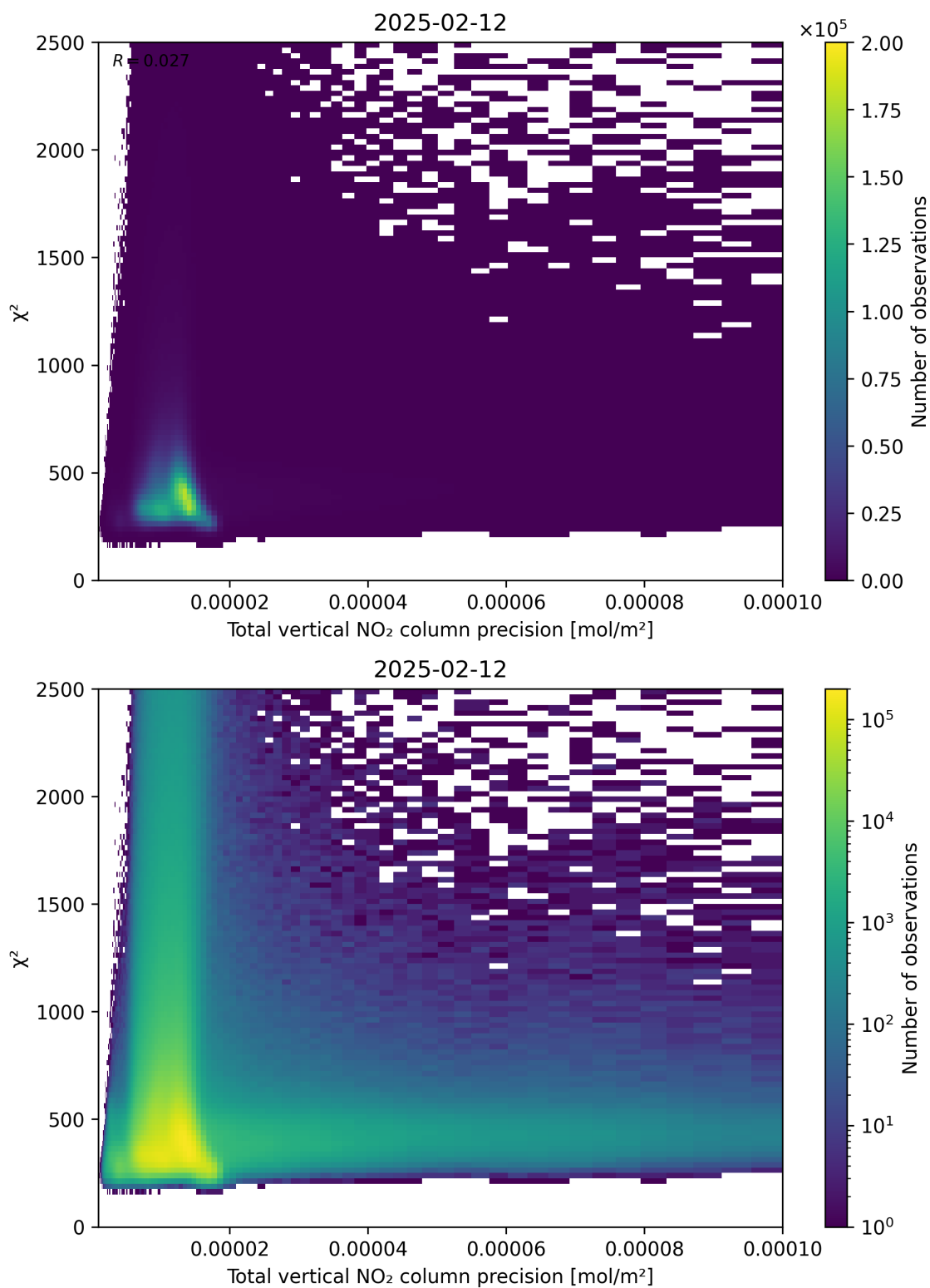
Figure 116: Scatter density plot of “Total vertical NO 2 column precision” against “ \chi^2 ” for 2025-02-11 to 2025-02-13.
