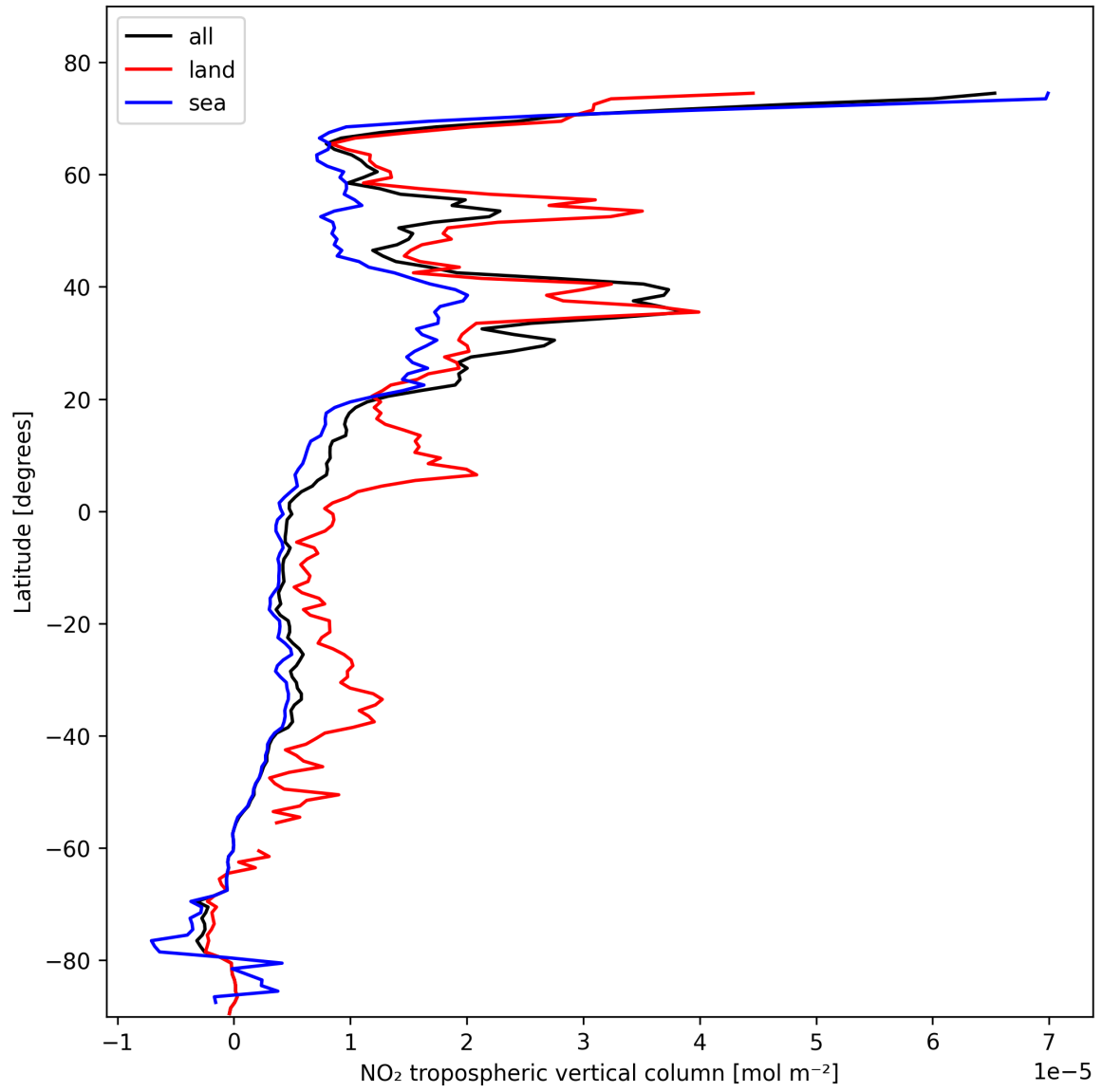
Figure 12: Zonal average of “NO 2 tropospheric vertical column” for 2025-02-11 to 2025-02-13.
