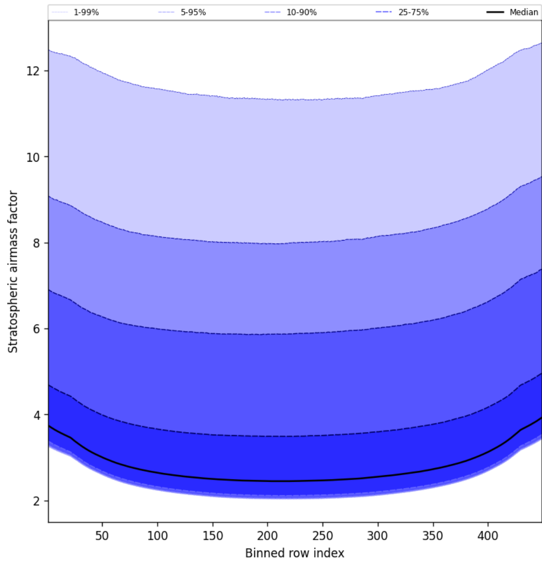
Figure 61: Along track statistics of “Stratospheric airmass factor” for 2025-02-11 to 2025-02-13
