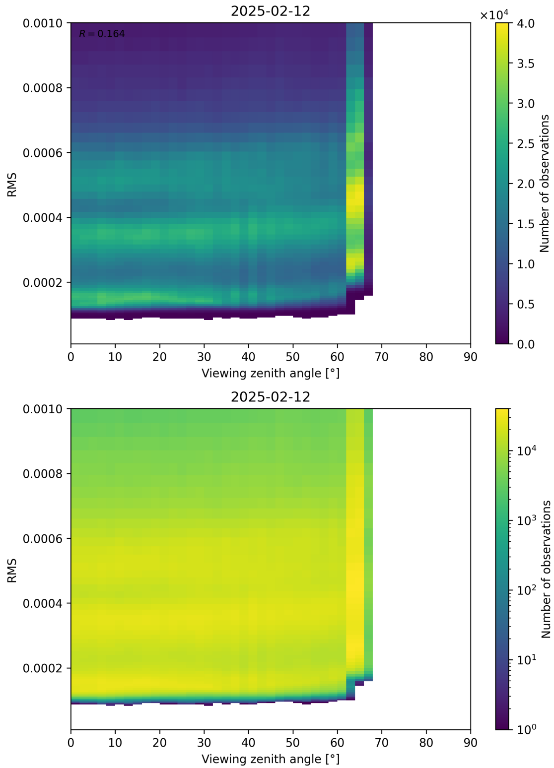
Figure 171: Scatter density plot of “Viewing zenith angle” against “RMS” for 2025-02-11 to 2025-02-13.
