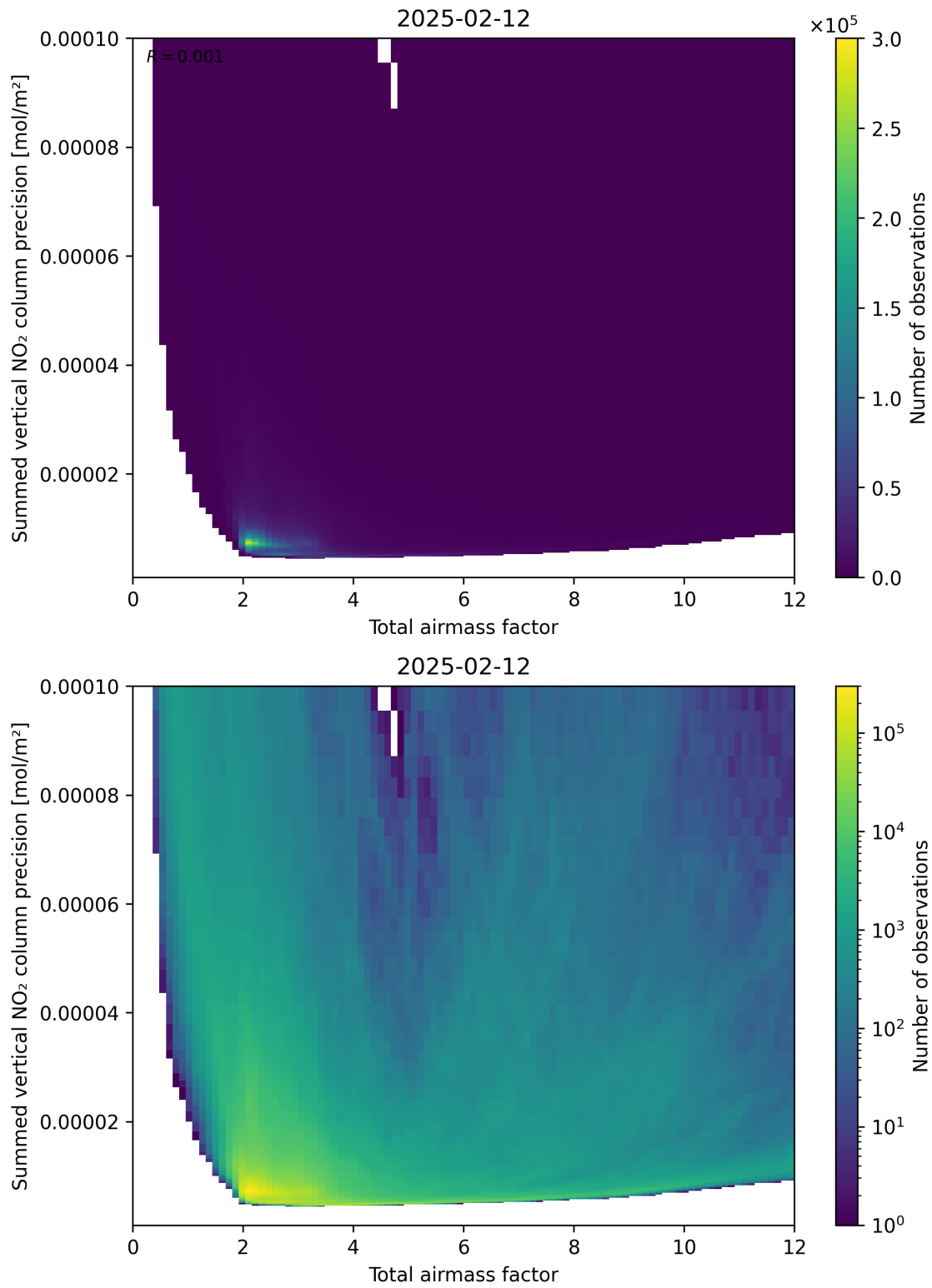
Figure 66: Scatter density plot of “Total airmass factor” against “Summed vertical NO 2 column precision” for 2025-02-11 to 2025-02-13.
