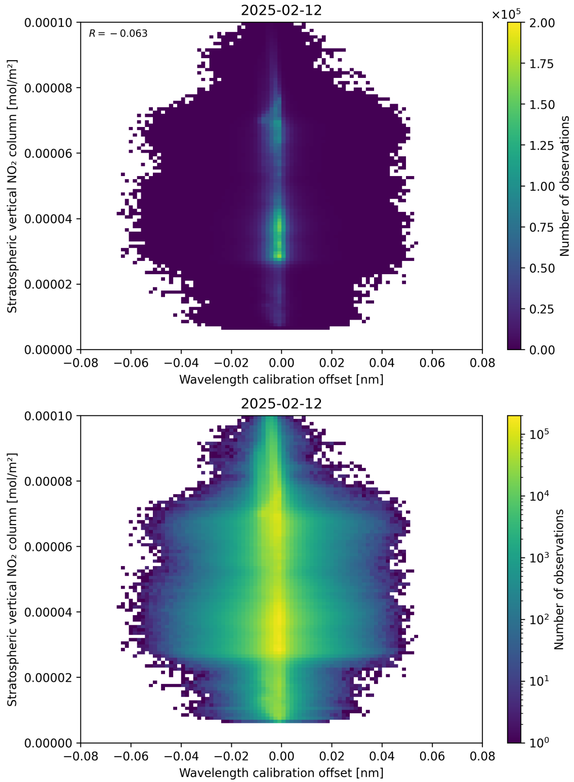
Figure 176: Scatter density plot of “Wavelength calibration offset” against “Stratospheric vertical NO 2 column” for 2025-02-11 to 2025-02-13.
