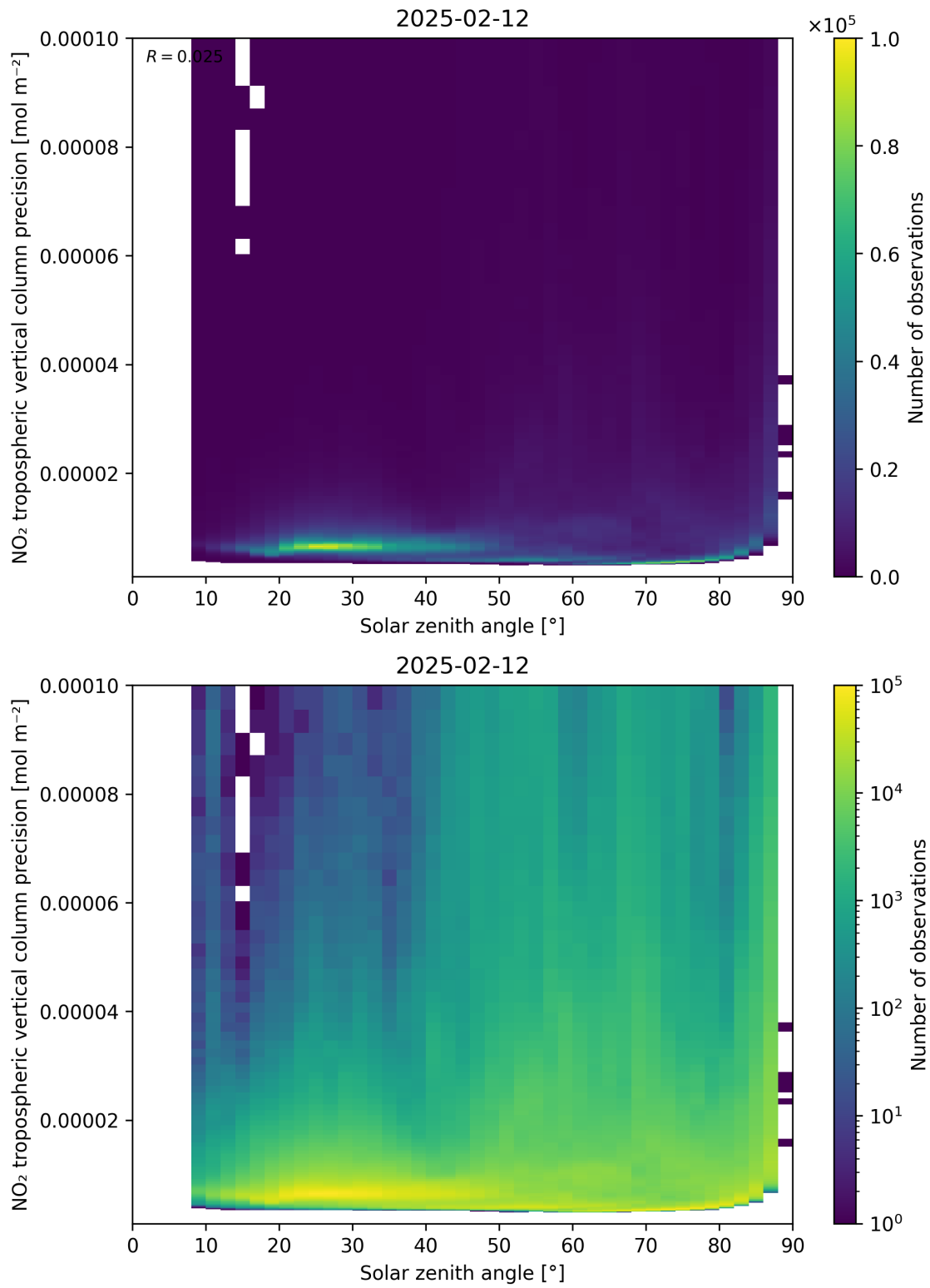
Figure 156: Scatter density plot of “Solar zenith angle” against “NO 2 tropospheric vertical column precision” for 2025-02-11 to 2025-02-13.
