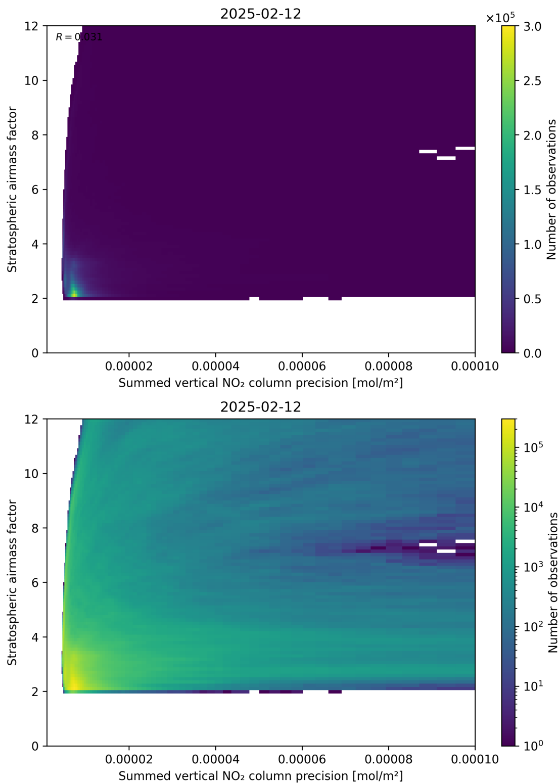
Figure 106: Scatter density plot of “Summed vertical NO 2 column precision” against “Stratospheric airmass factor” for 2025-02-11 to 2025-02-13.
