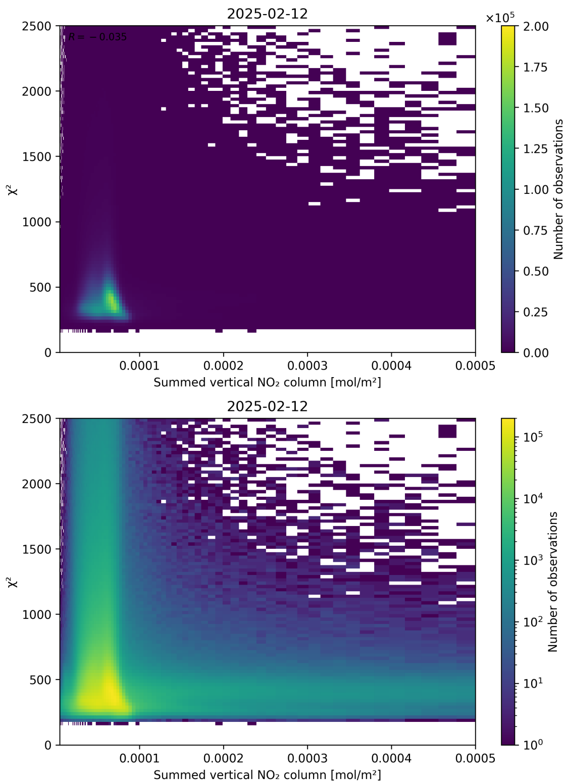
Figure 104: Scatter density plot of “Summed vertical NO 2 column” against “ \chi^2 ” for 2025-02-11 to 2025-02-13.
