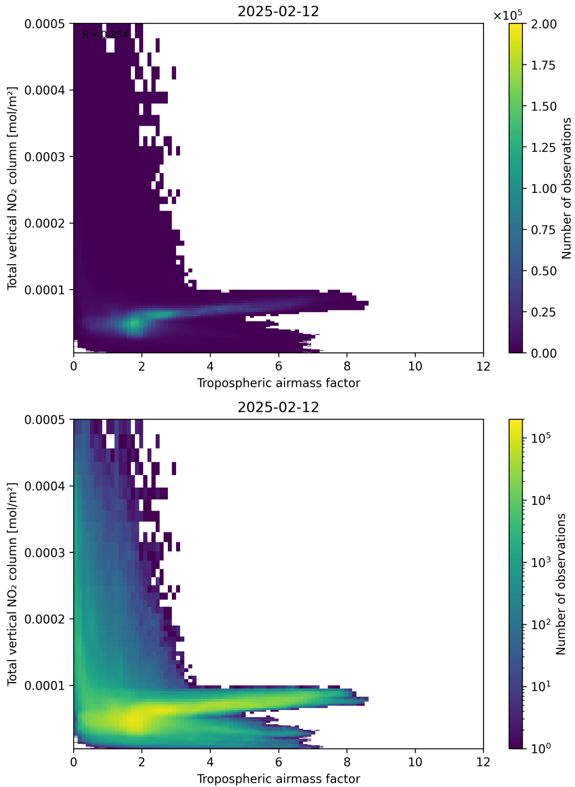
Figure 77: Scatter density plot of “Tropospheric airmass factor” against “Total vertical NO 2 column” for 2025-02-11 to 2025-02-13.
