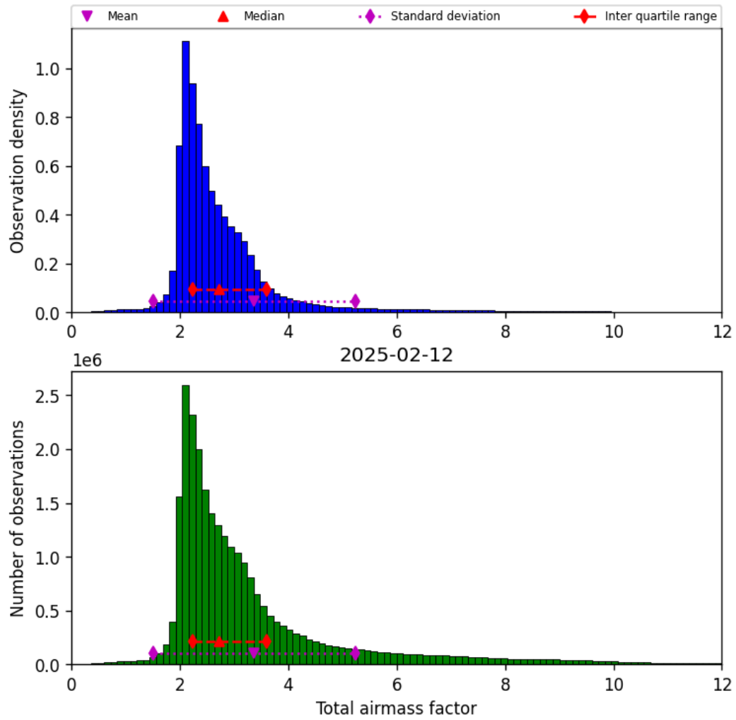
Figure 32: Histogram of “Total airmass factor” for 2025-02-11 to 2025-02-13
