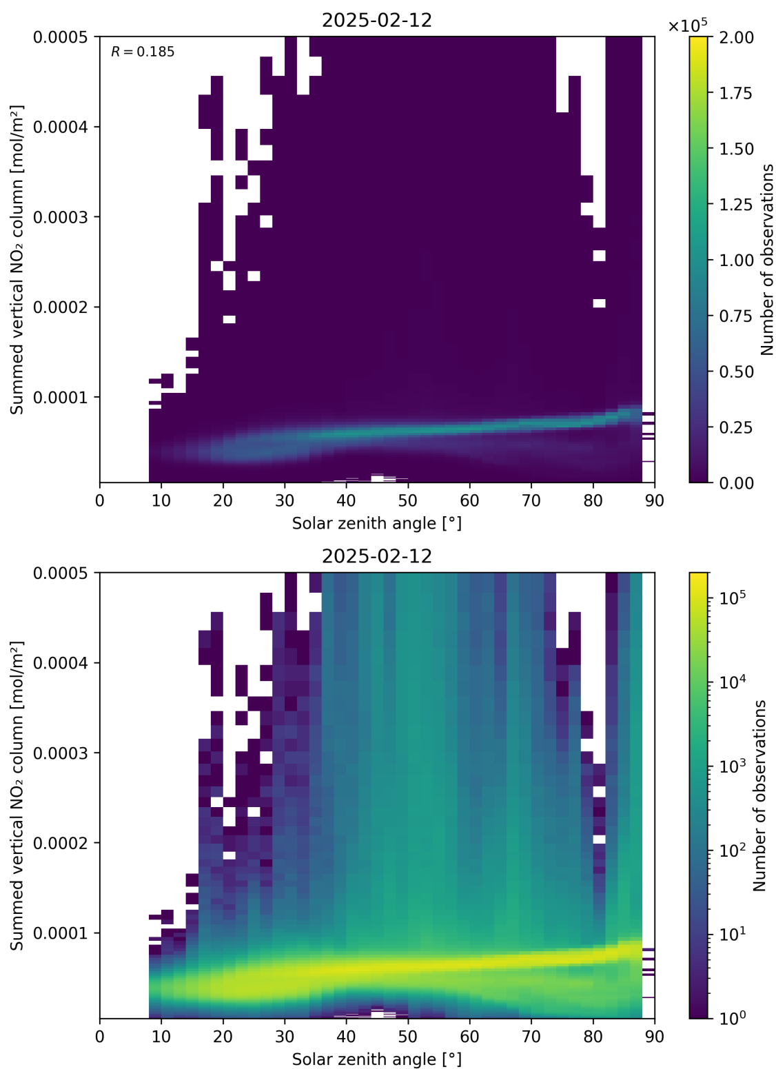
Figure 151: Scatter density plot of “Solar zenith angle” against “Summed vertical NO 2 column” for 2025-02-11 to 2025-02-13.
