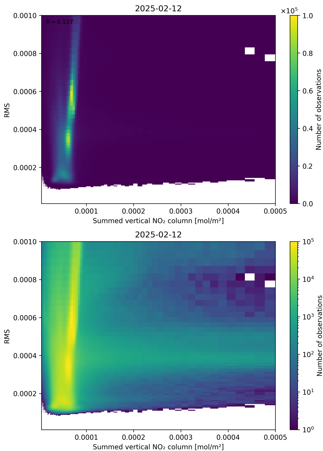
Figure 109: Scatter density plot of “Summed vertical NO 2 column” against “RMS” for 2025-02-11 to 2025-02-13.
