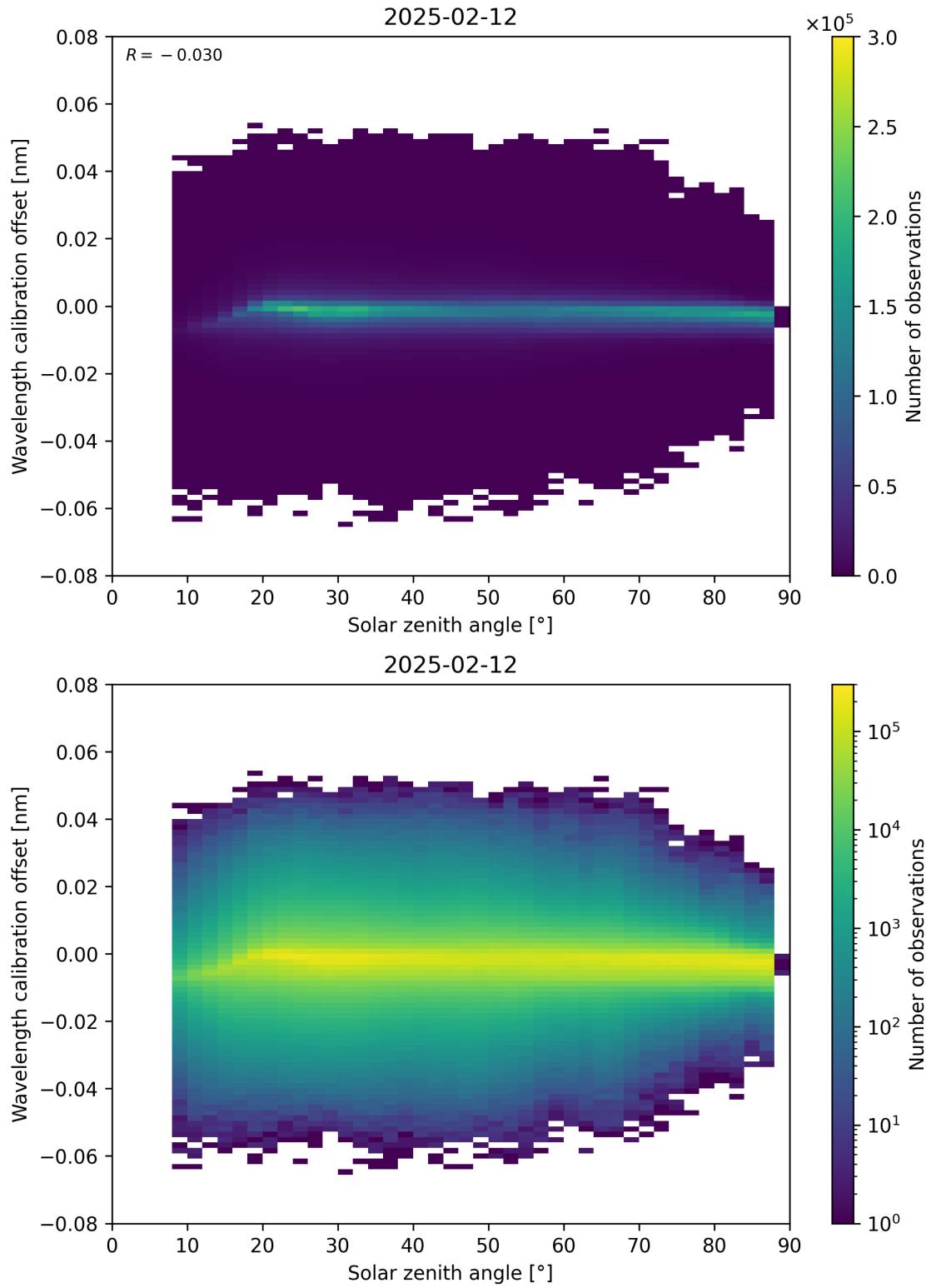
Figure 158: Scatter density plot of “Solar zenith angle” against “Wavelength calibration offset” for 2025-02-11 to 2025-02-13.
