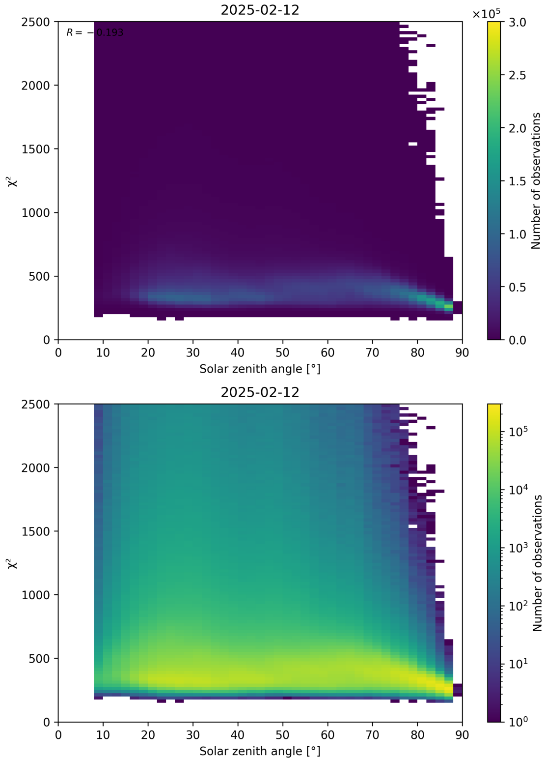
Figure 148: Scatter density plot of “Solar zenith angle” against “ \chi^2 ” for 2025-02-11 to 2025-02-13.
