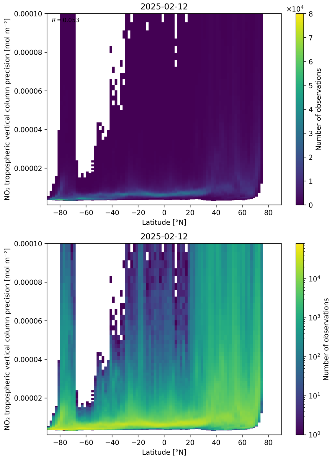
Figure 93: Scatter density plot of “Latitude” against “NO 2 tropospheric vertical column precision” for 2025-02-11 to 2025-02-13.
