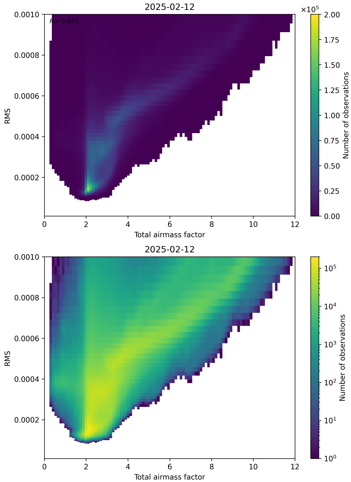
Figure 69: Scatter density plot of “Total airmass factor” against “RMS” for 2025-02-11 to 2025-02-13.
