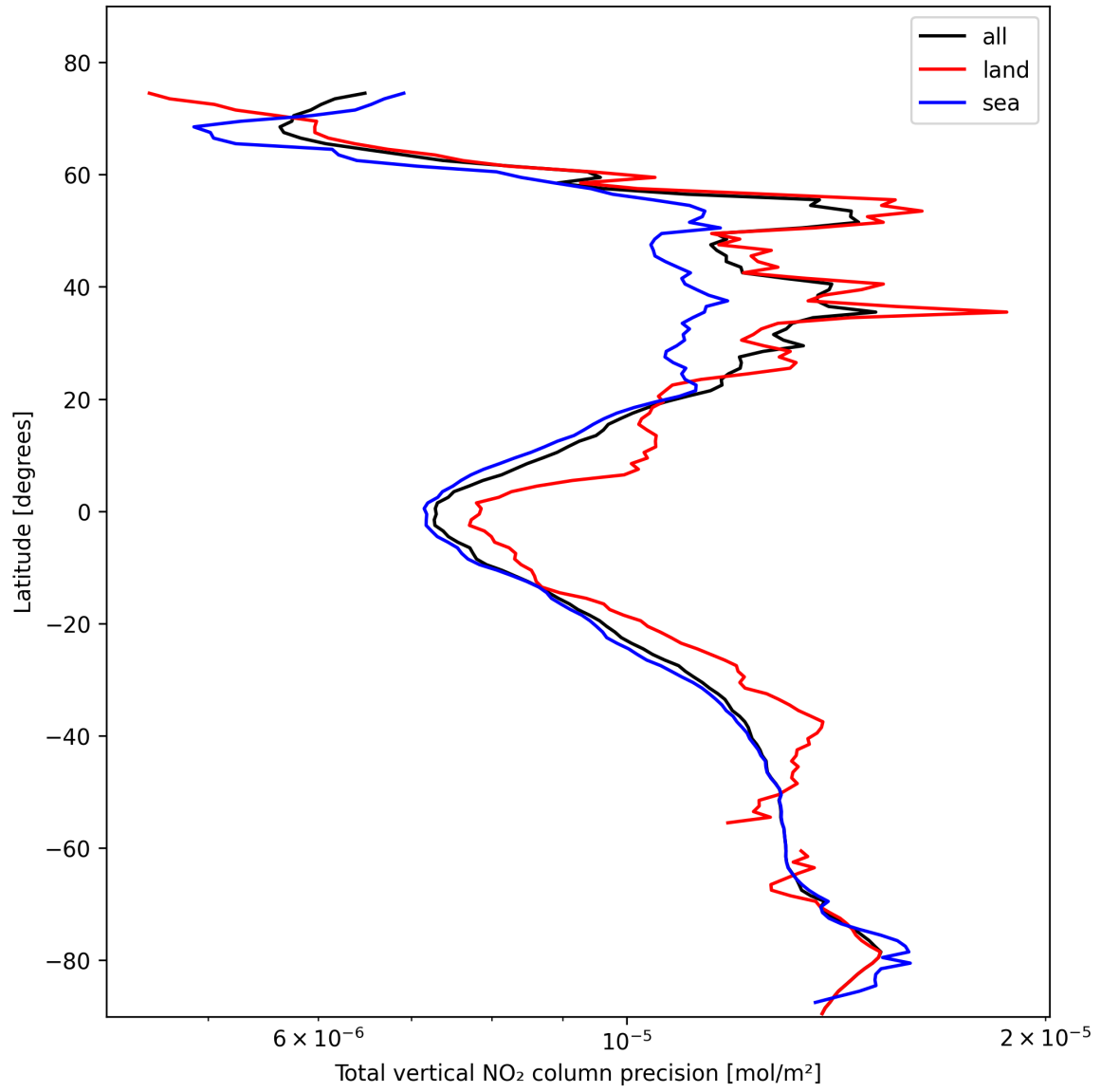
Figure 22: Zonal average of “Total vertical NO 2 column precision” for 2025-02-11 to 2025-02-13.
