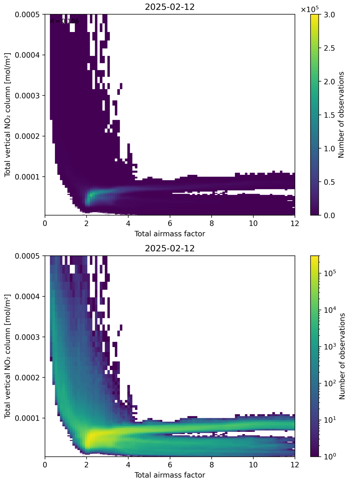
Figure 67: Scatter density plot of “Total airmass factor” against “Total vertical NO 2 column” for 2025-02-11 to 2025-02-13.
