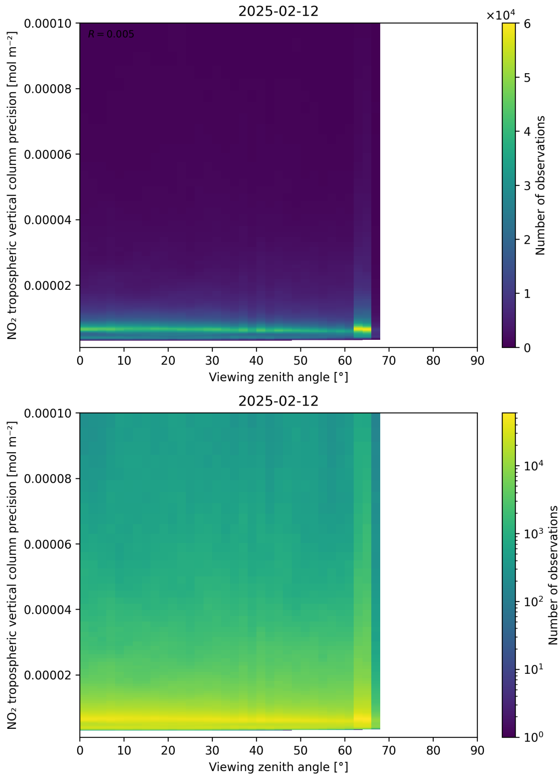
Figure 170: Scatter density plot of “Viewing zenith angle” against “NO 2 tropospheric vertical column precision” for 2025-02-11 to 2025-02-13.
