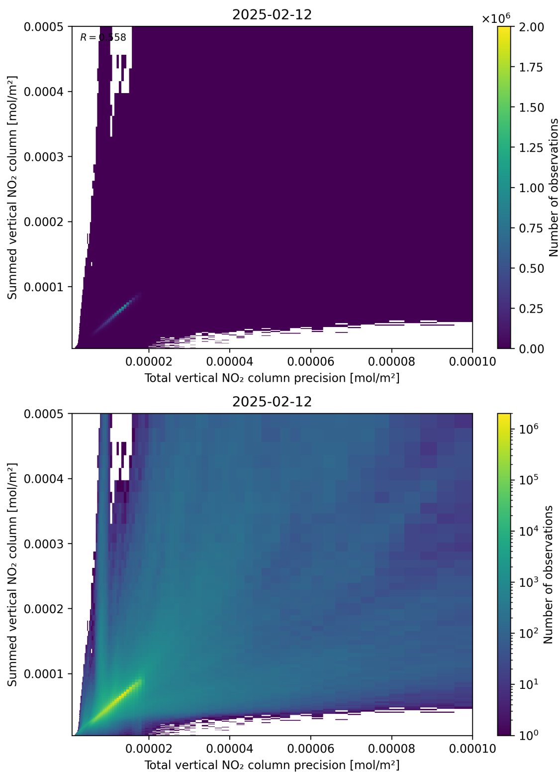
Figure 117: Scatter density plot of “Total vertical NO 2 column precision” against “Summed vertical NO 2 column” for 2025-02-11 to 2025-02-13.
