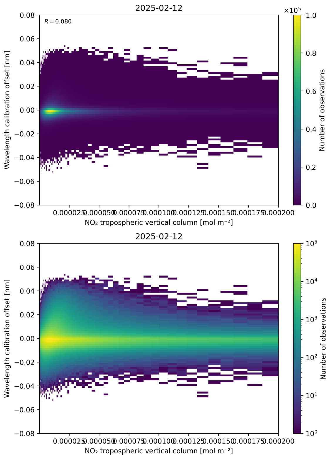
Figure 143: Scatter density plot of “NO 2 tropospheric vertical column” against “Wavelength calibration offset” for 2025-02-11 to 2025-02-13.
