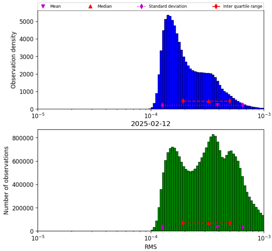
Figure 43: Histogram of “RMS” for 2025-02-11 to 2025-02-13
