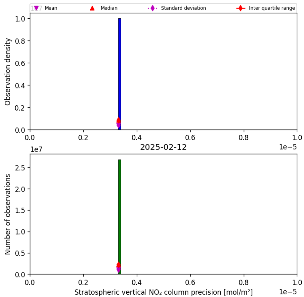
Figure 37: Histogram of “Stratospheric vertical NO 2 column precision” for 2025-02-11 to 2025-02-13
