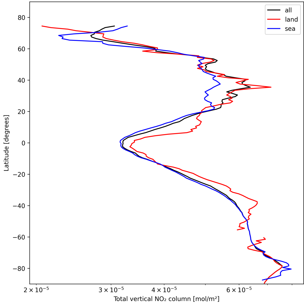
Figure 21: Zonal average of “Total vertical NO 2 column” for 2025-02-11 to 2025-02-13.
