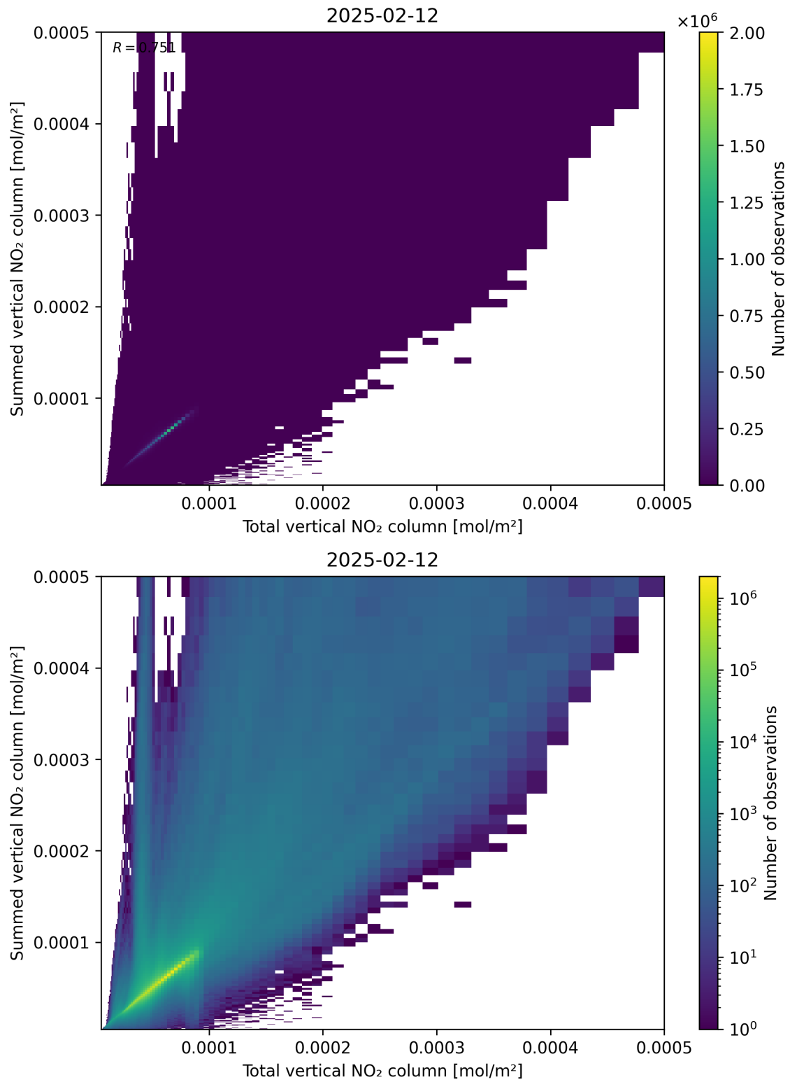
Figure 112: Scatter density plot of “Total vertical NO 2 column” against “Summed vertical NO 2 column” for 2025-02-11 to 2025-02-13.
