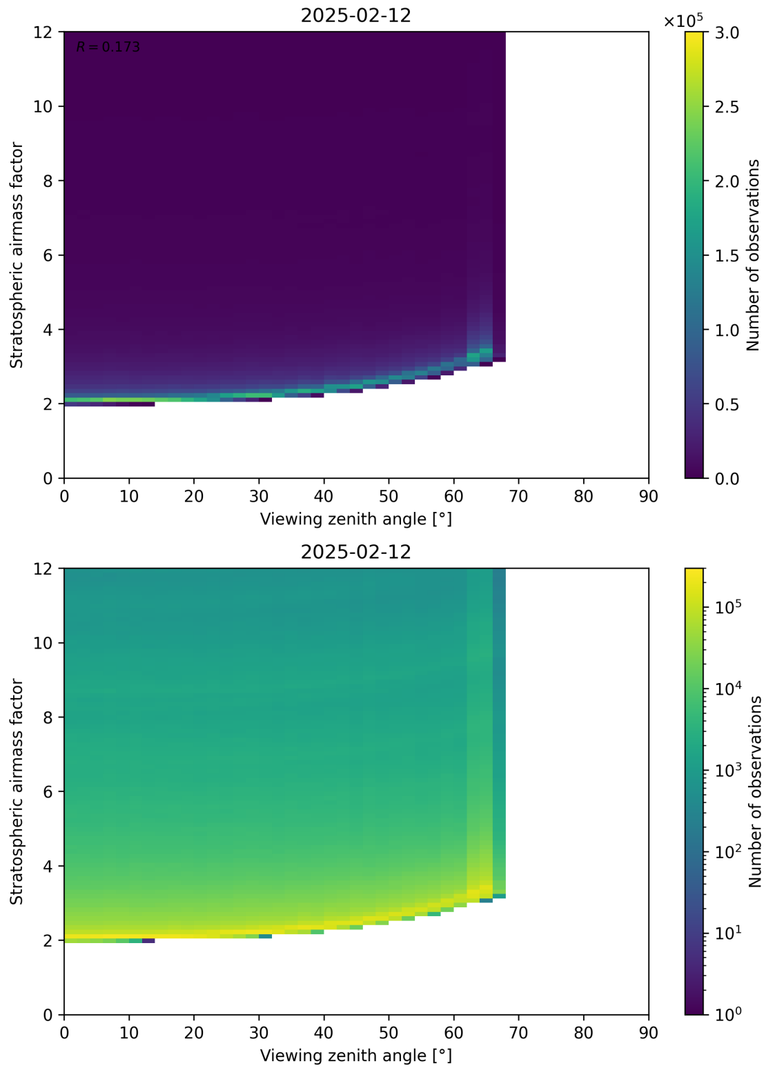
Figure 159: Scatter density plot of “Viewing zenith angle” against “Stratospheric airmass factor” for 2025-02-11 to 2025-02-13.
