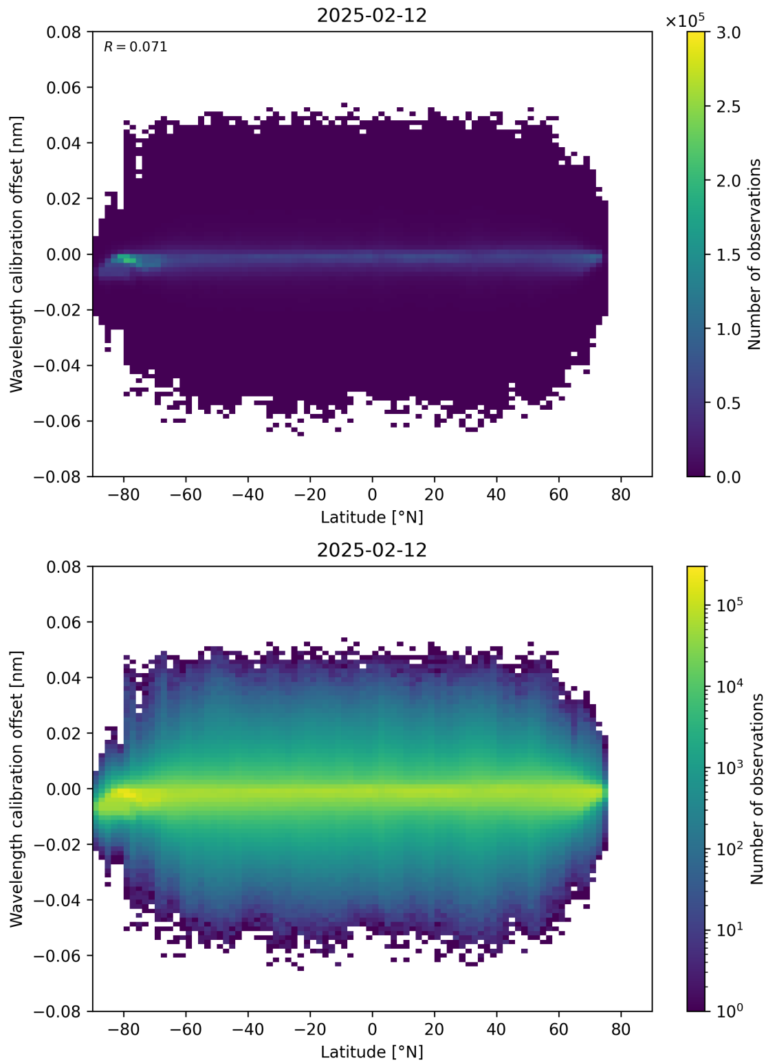
Figure 95: Scatter density plot of “Latitude” against “Wavelength calibration offset” for 2025-02-11 to 2025-02-13.
