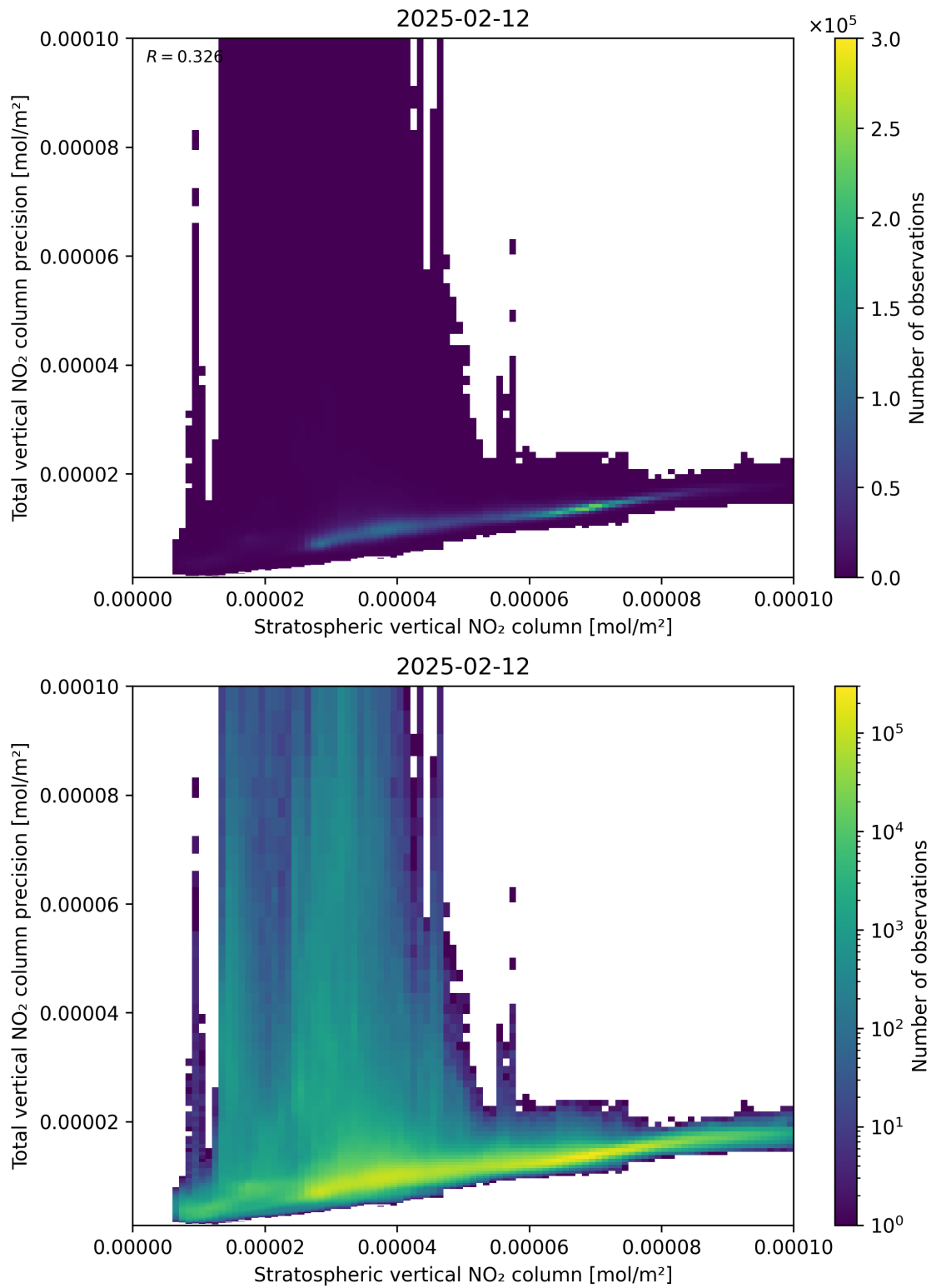
Figure 101: Scatter density plot of “Stratospheric vertical NO 2 column” against “Total vertical NO 2 column precision” for 2025-02-11 to 2025-02-13.
