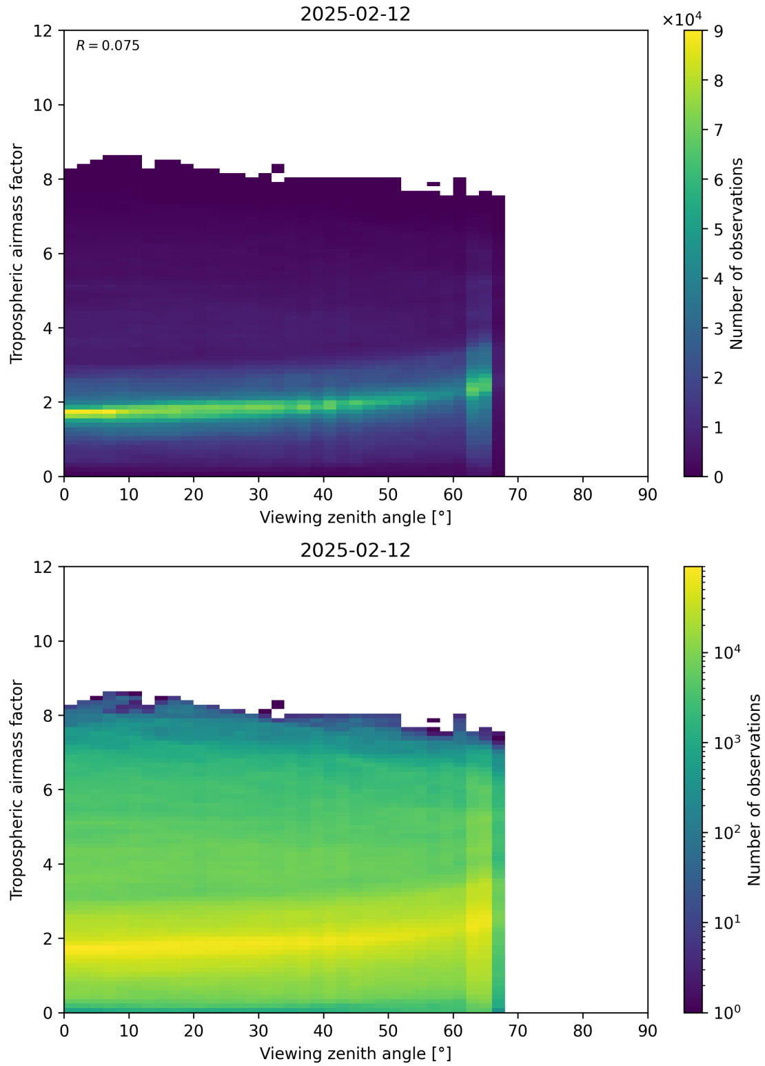
Figure 161: Scatter density plot of “Viewing zenith angle” against “Tropospheric airmass factor” for 2025-02-11 to 2025-02-13.
