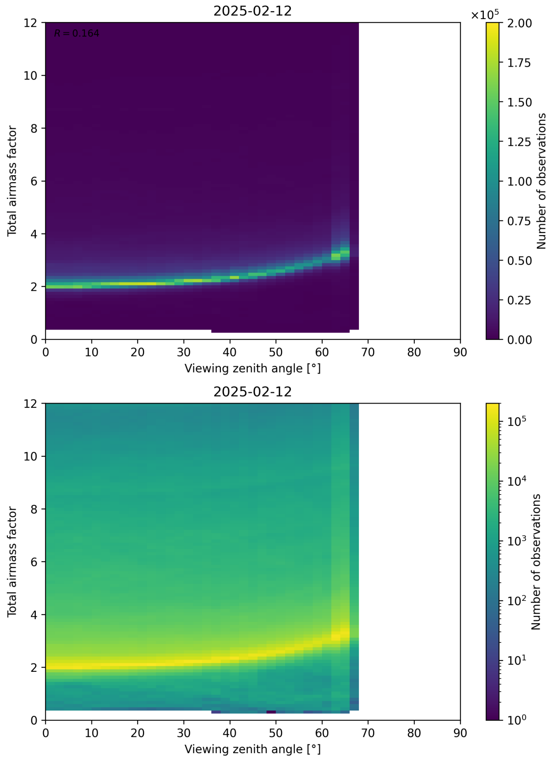
Figure 160: Scatter density plot of “Viewing zenith angle” against “Total airmass factor” for 2025-02-11 to 2025-02-13.
