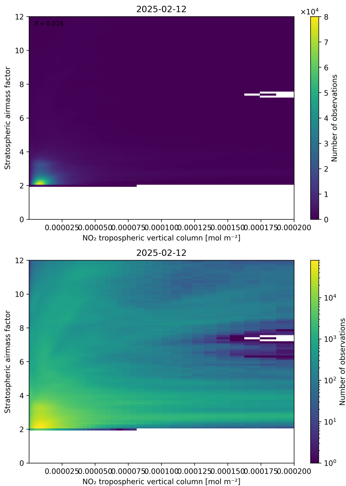
Figure 121: Scatter density plot of “NO 2 tropospheric vertical column” against “Stratospheric airmass factor” for 2025-02-11 to 2025-02-13.
