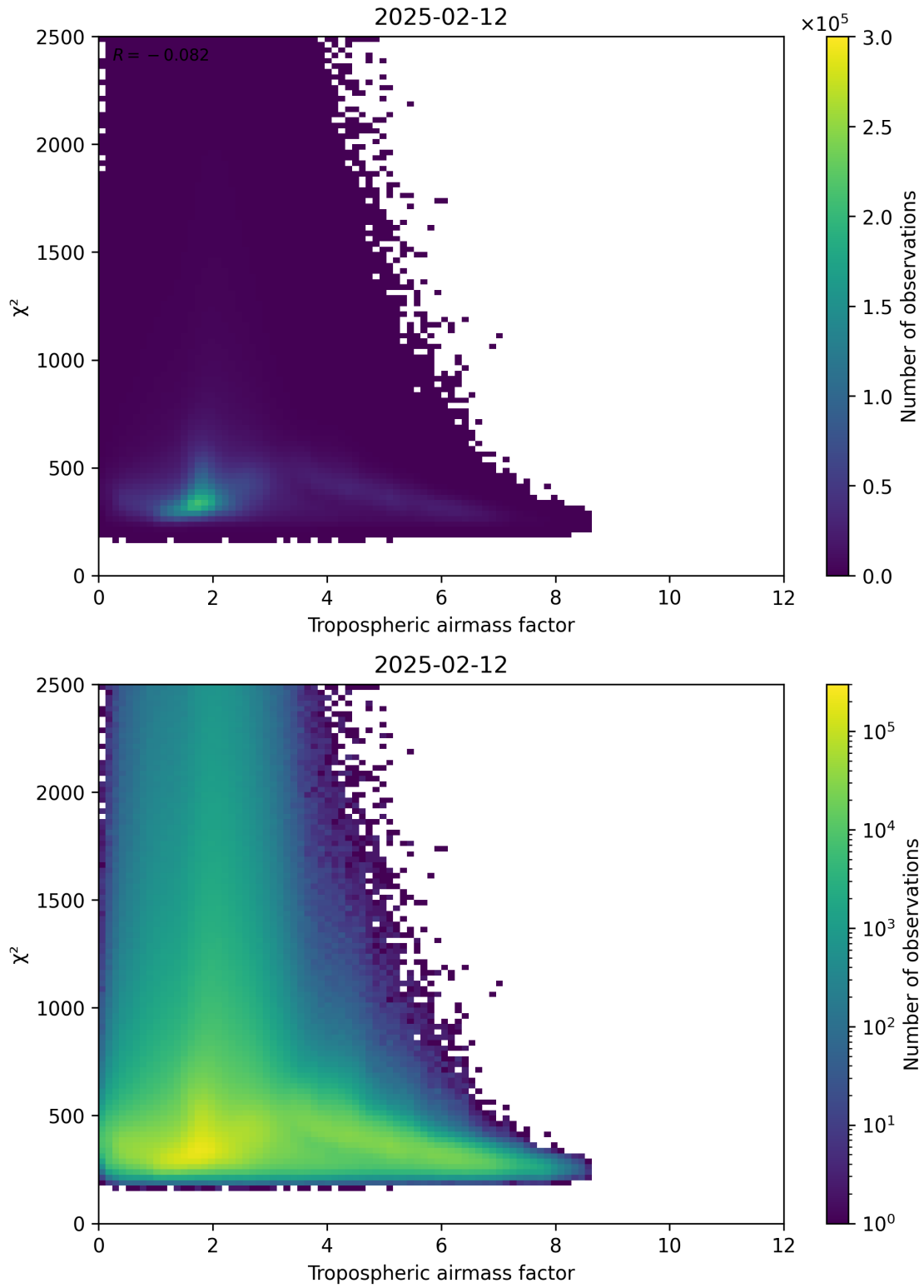
Figure 73: Scatter density plot of “Tropospheric airmass factor” against “ \chi^2 ” for 2025-02-11 to 2025-02-13.
