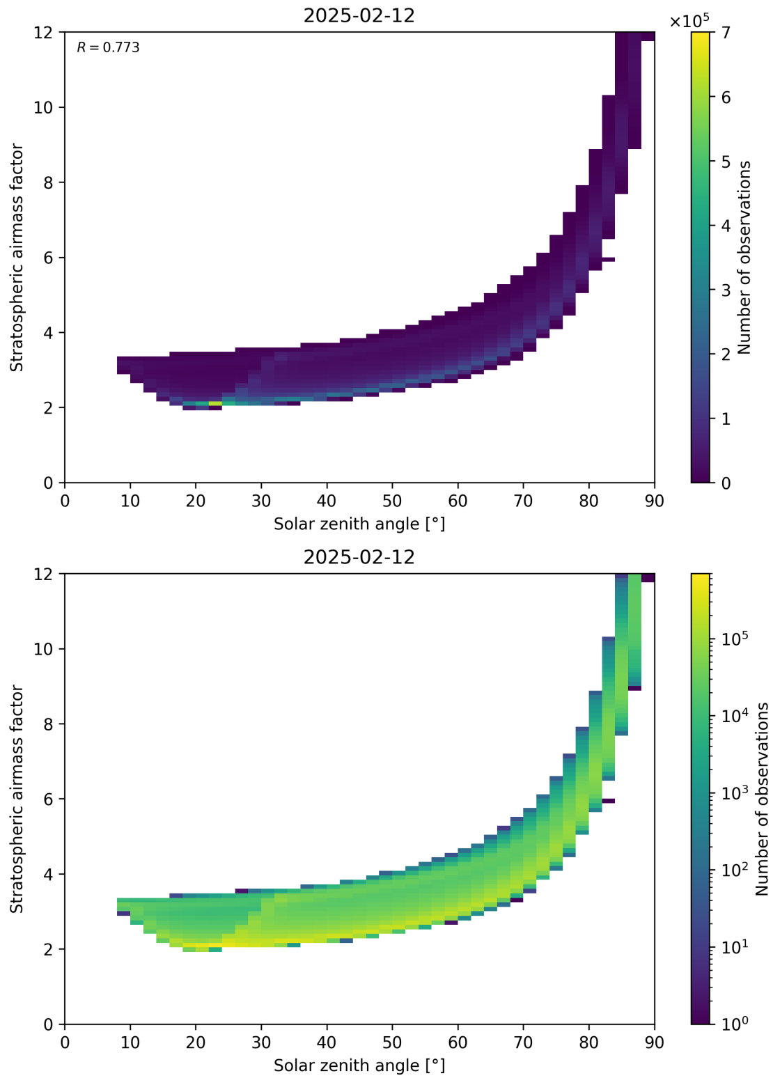
Figure 145: Scatter density plot of “Solar zenith angle” against “Stratospheric airmass factor” for 2025-02-11 to 2025-02-13.
