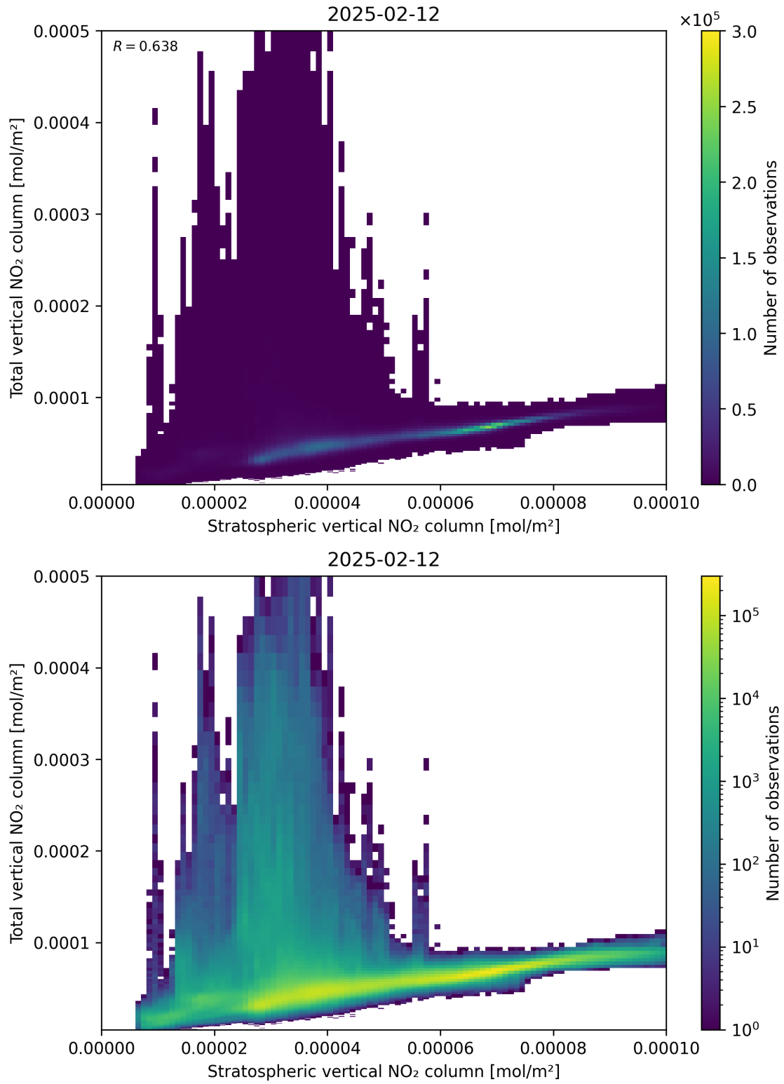
Figure 100: Scatter density plot of “Stratospheric vertical NO 2 column” against “Total vertical NO 2 column” for 2025-02-11 to 2025-02-13.
