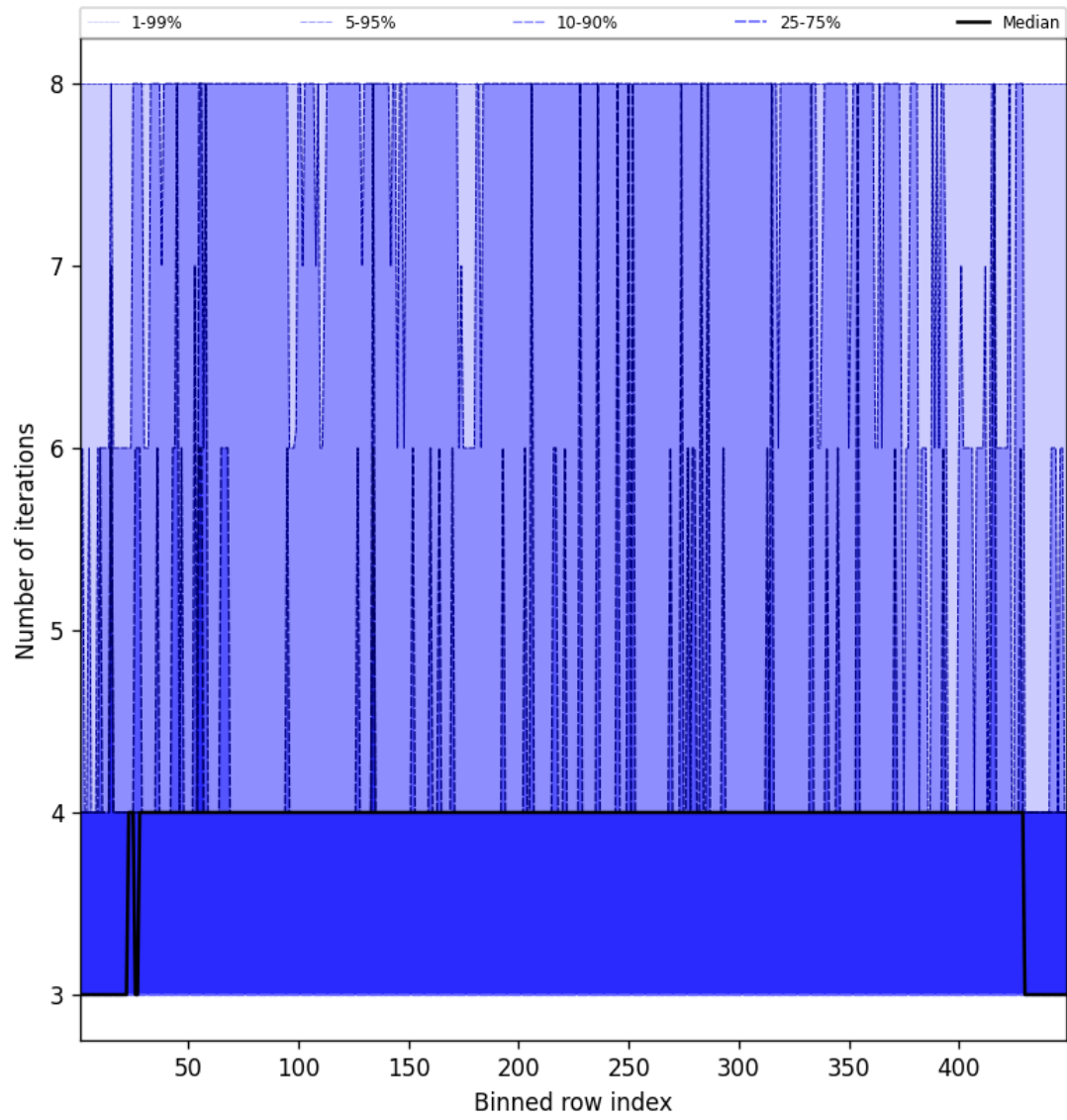
Figure 51: Along track statistics of “Number of iterations” for 2025-02-11 to 2025-02-13
