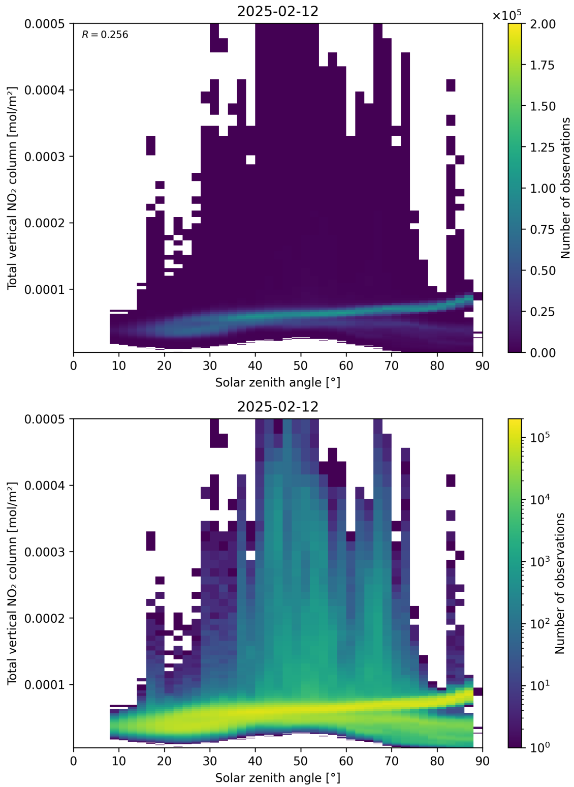
Figure 153: Scatter density plot of “Solar zenith angle” against “Total vertical \text{NO}_2 column” for 2025-02-11 to 2025-02-13.
