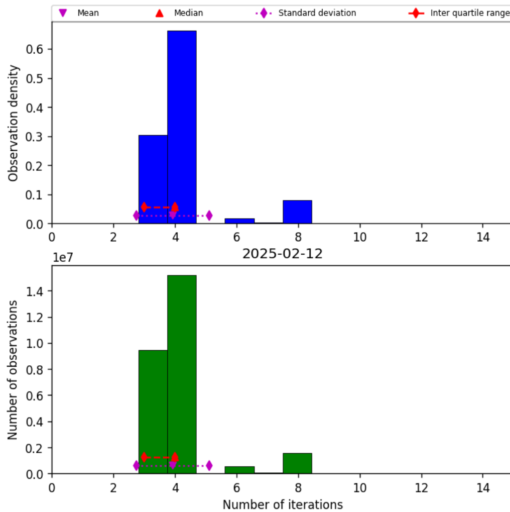
Figure 34: Histogram of “Number of iterations” for 2025-02-11 to 2025-02-13
