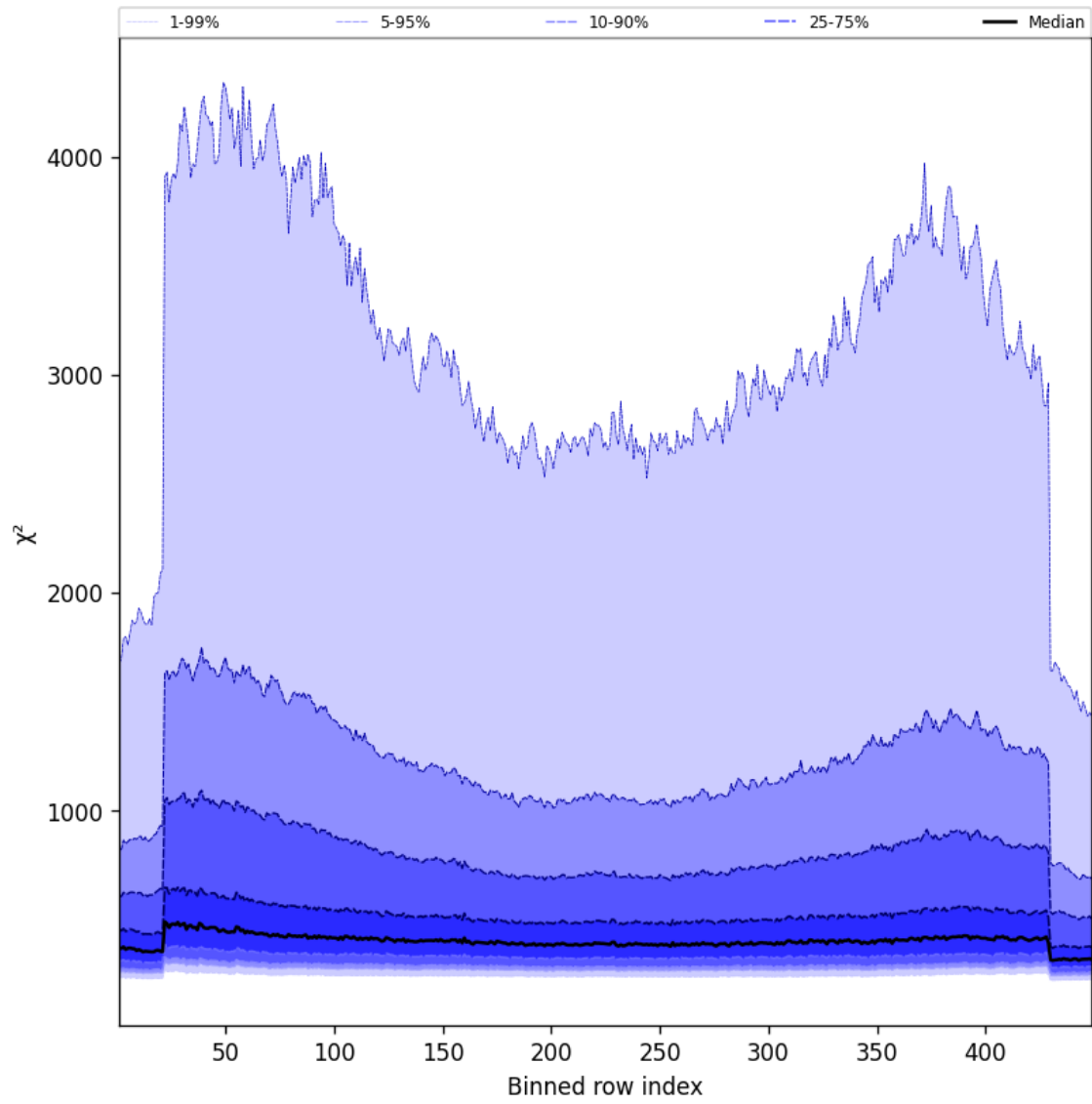
Figure 59: Along track statistics of “ \chi^2 ” for 2025-02-11 to 2025-02-13
