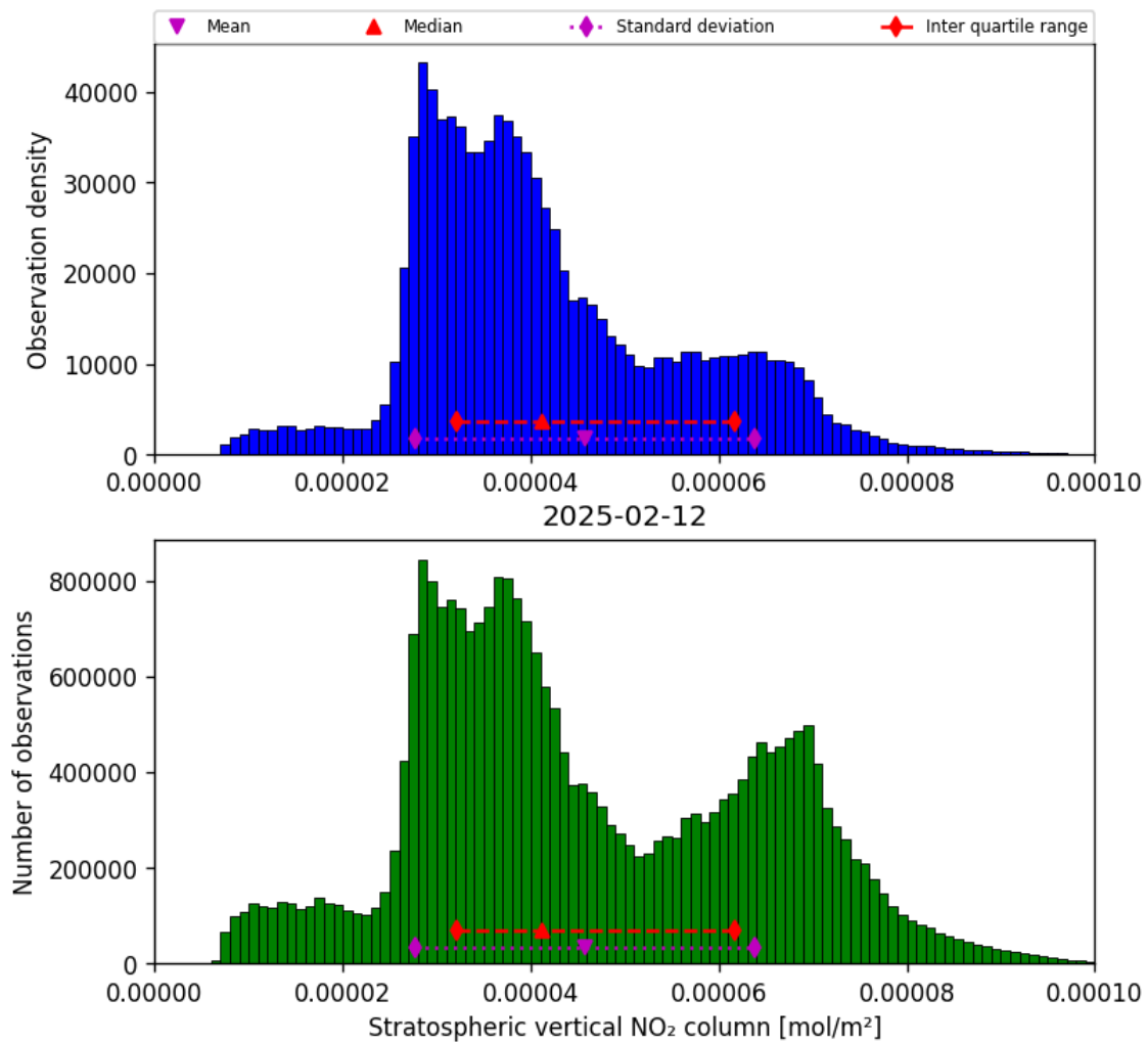
Figure 36: Histogram of “Stratospheric vertical NO 2 column” for 2025-02-11 to 2025-02-13
