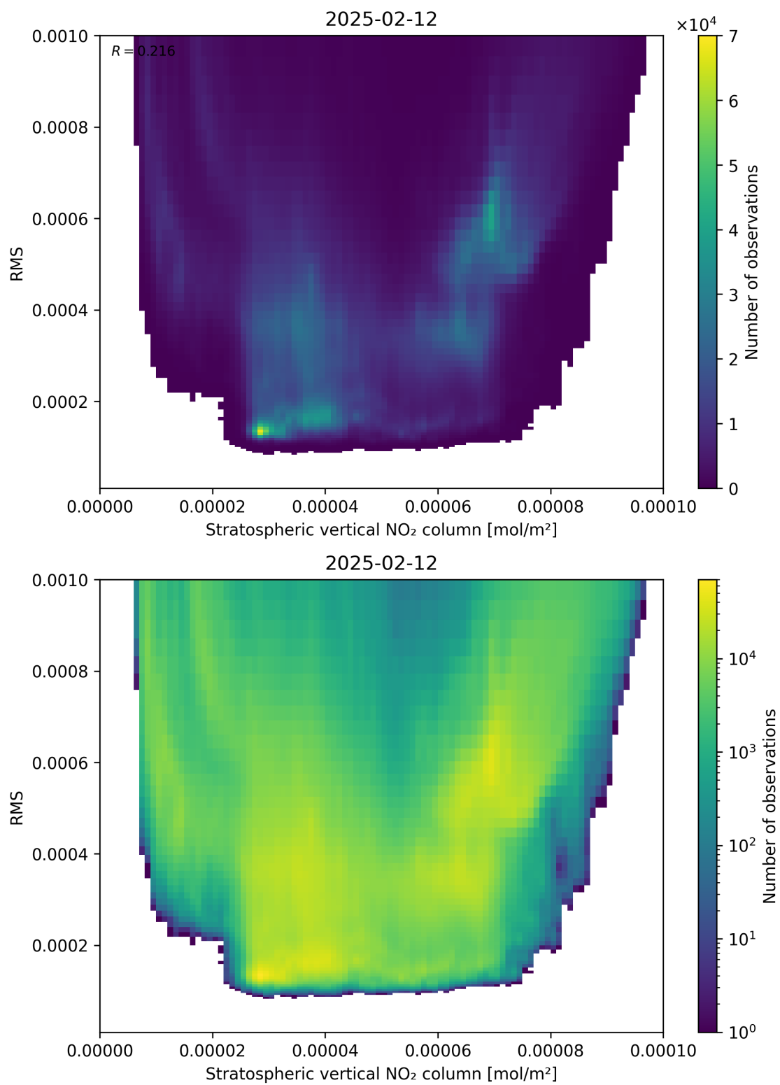
Figure 102: Scatter density plot of “Stratospheric vertical NO 2 column” against “RMS” for 2025-02-11 to 2025-02-13.
