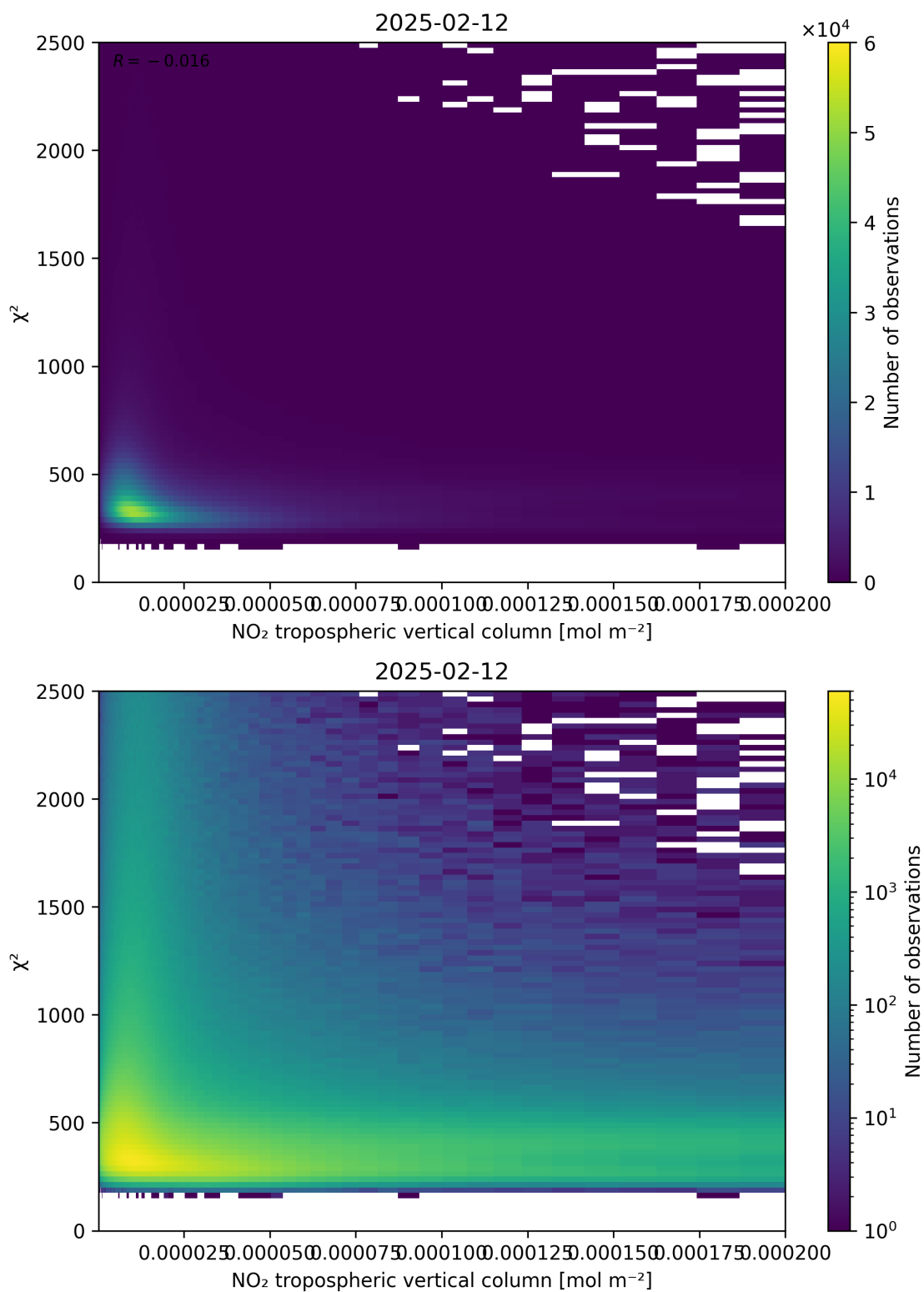
Figure 124: Scatter density plot of “NO 2 tropospheric vertical column” against “ \chi^2 ” for 2025-02-11 to 2025-02-13.
