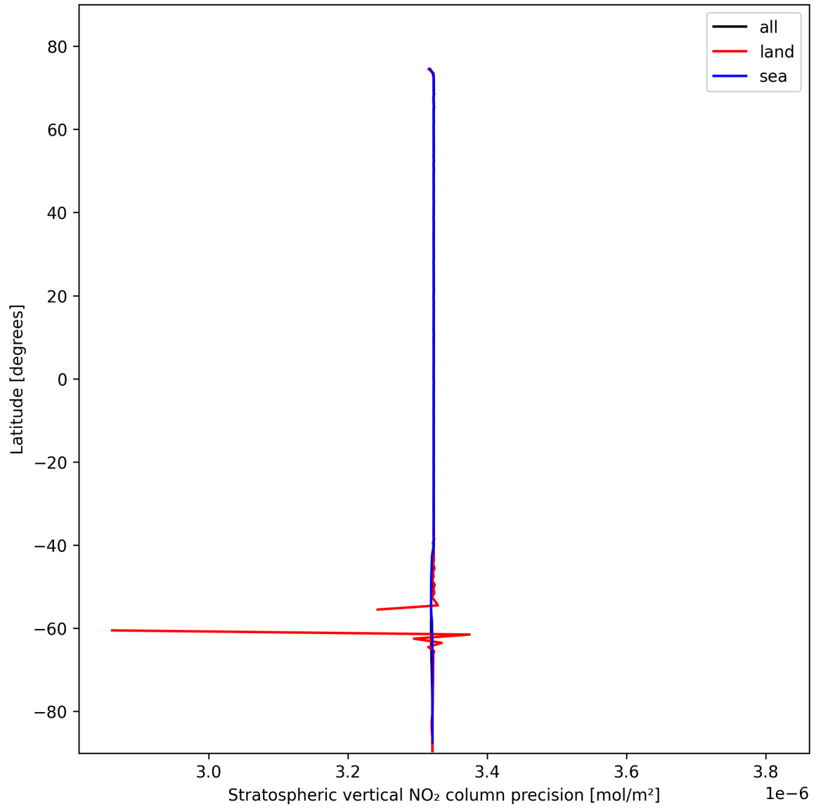
Figure 20: Zonal average of “Stratospheric vertical NO 2 column precision” for 2025-02-11 to 2025-02-13.
