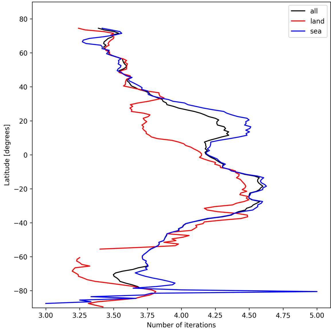
Figure 17: Zonal average of “Number of iterations” for 2025-02-11 to 2025-02-13.
