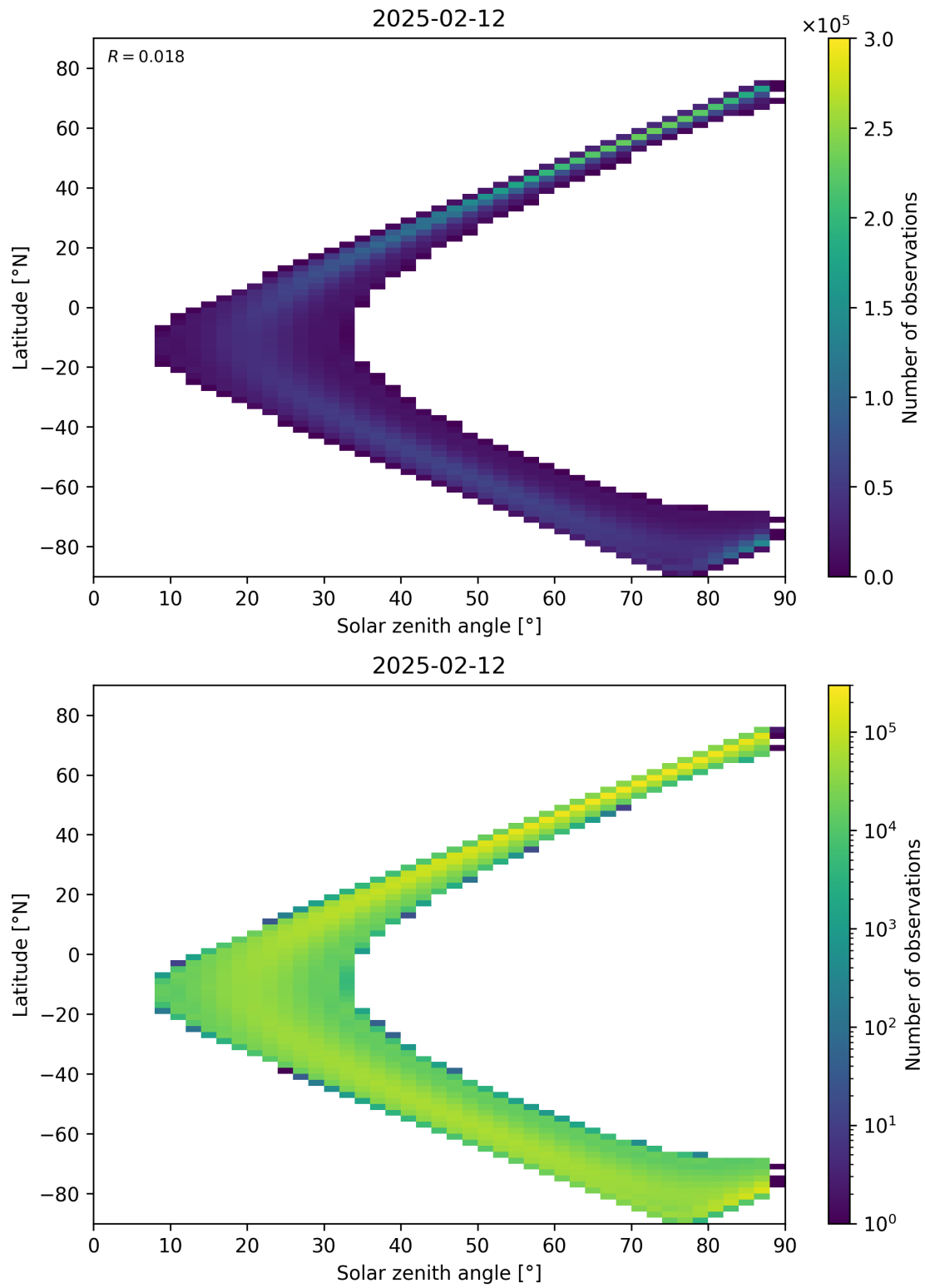
Figure 149: Scatter density plot of “Solar zenith angle” against “Latitude” for 2025-02-11 to 2025-02-13.
