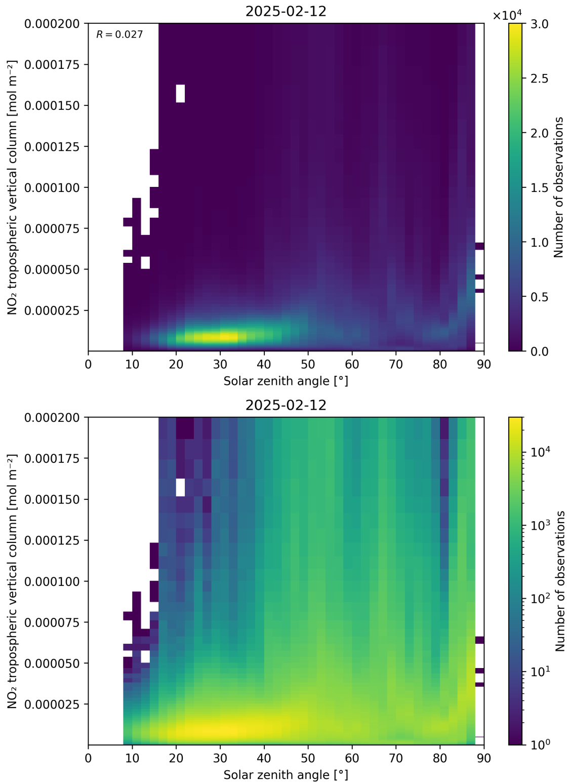
Figure 155: Scatter density plot of “Solar zenith angle” against “NO 2 tropospheric vertical column” for 2025-02-11 to 2025-02-13.
