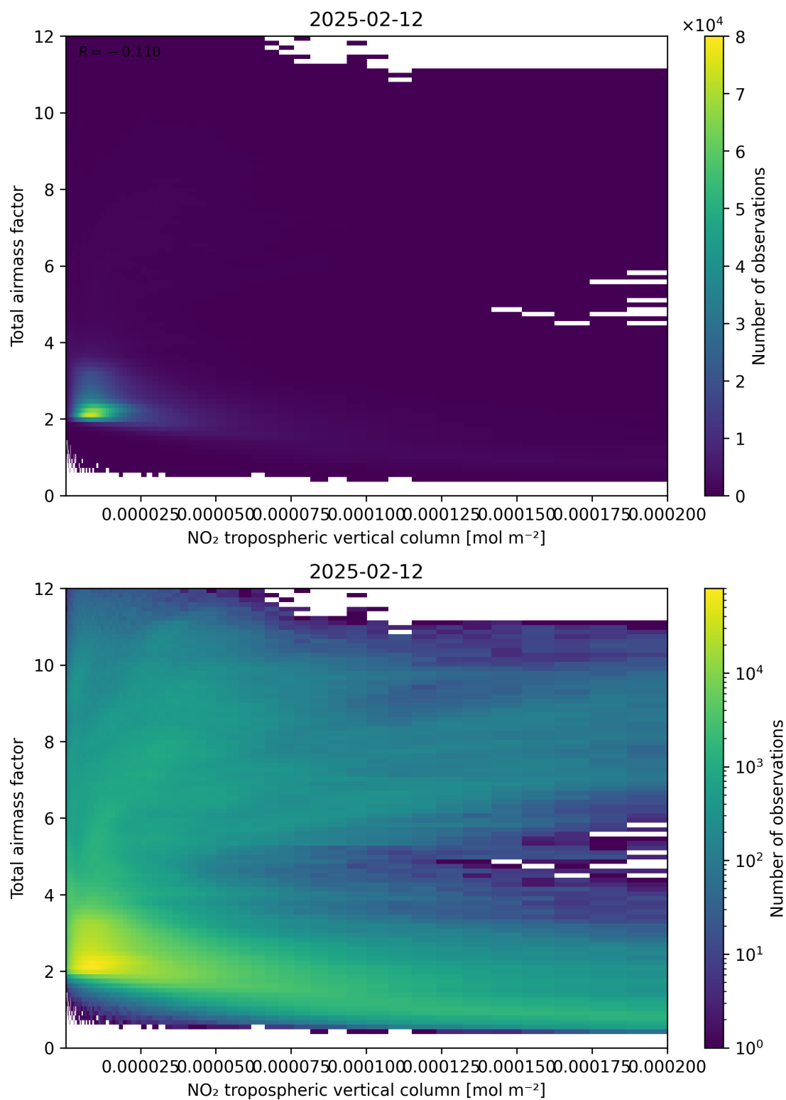
Figure 122: Scatter density plot of “NO 2 tropospheric vertical column” against “Total air mass factor” for 2025-02-11 to 2025-02-13.
