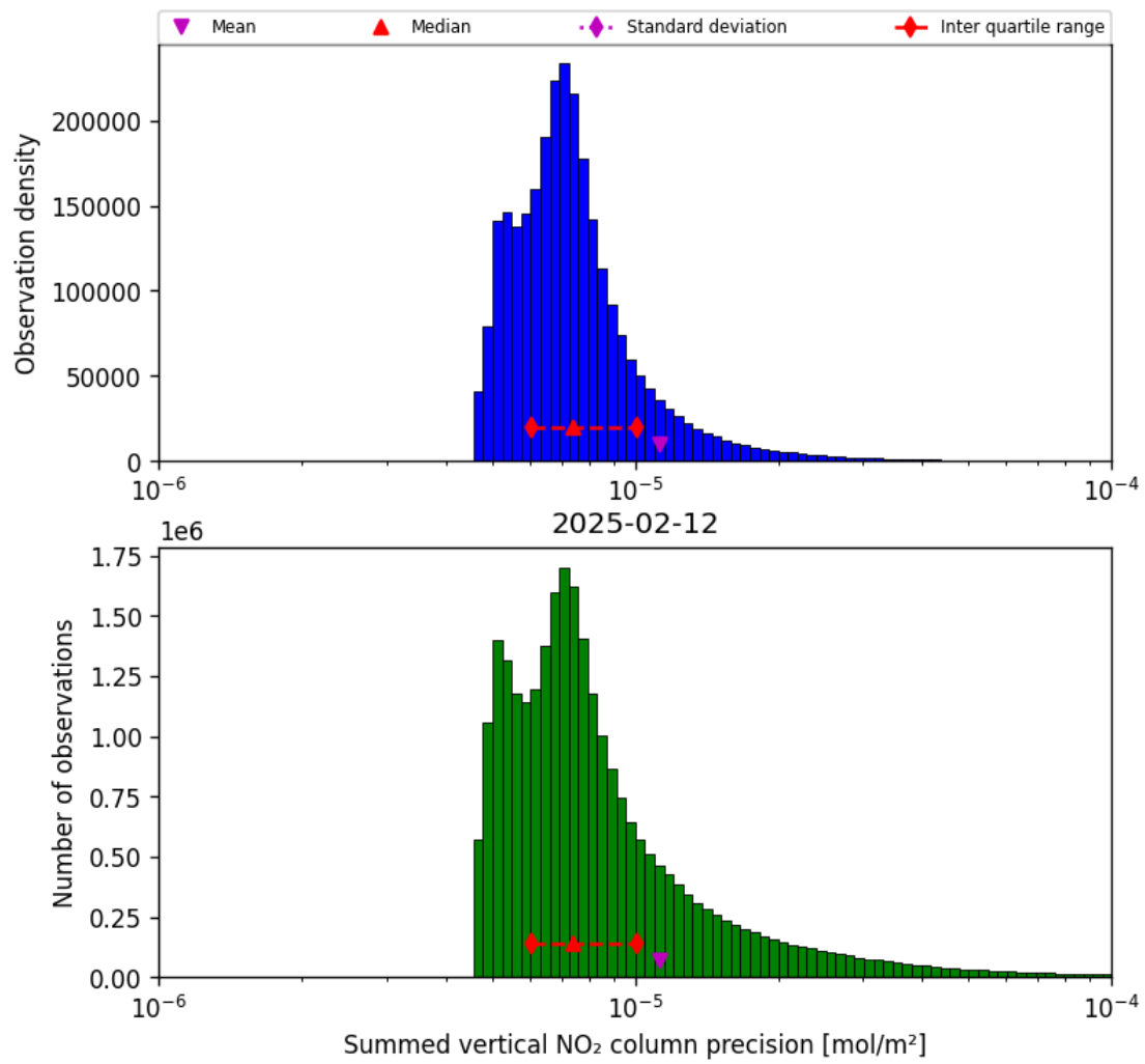
Figure 41: Histogram of “Summed vertical NO 2 column precision” for 2025-02-11 to 2025-02-13
