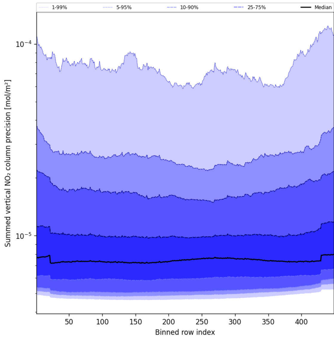
Figure 58: Along track statistics of “Summed vertical NO 2 column precision” for 2025-02-11 to 2025-02-13
