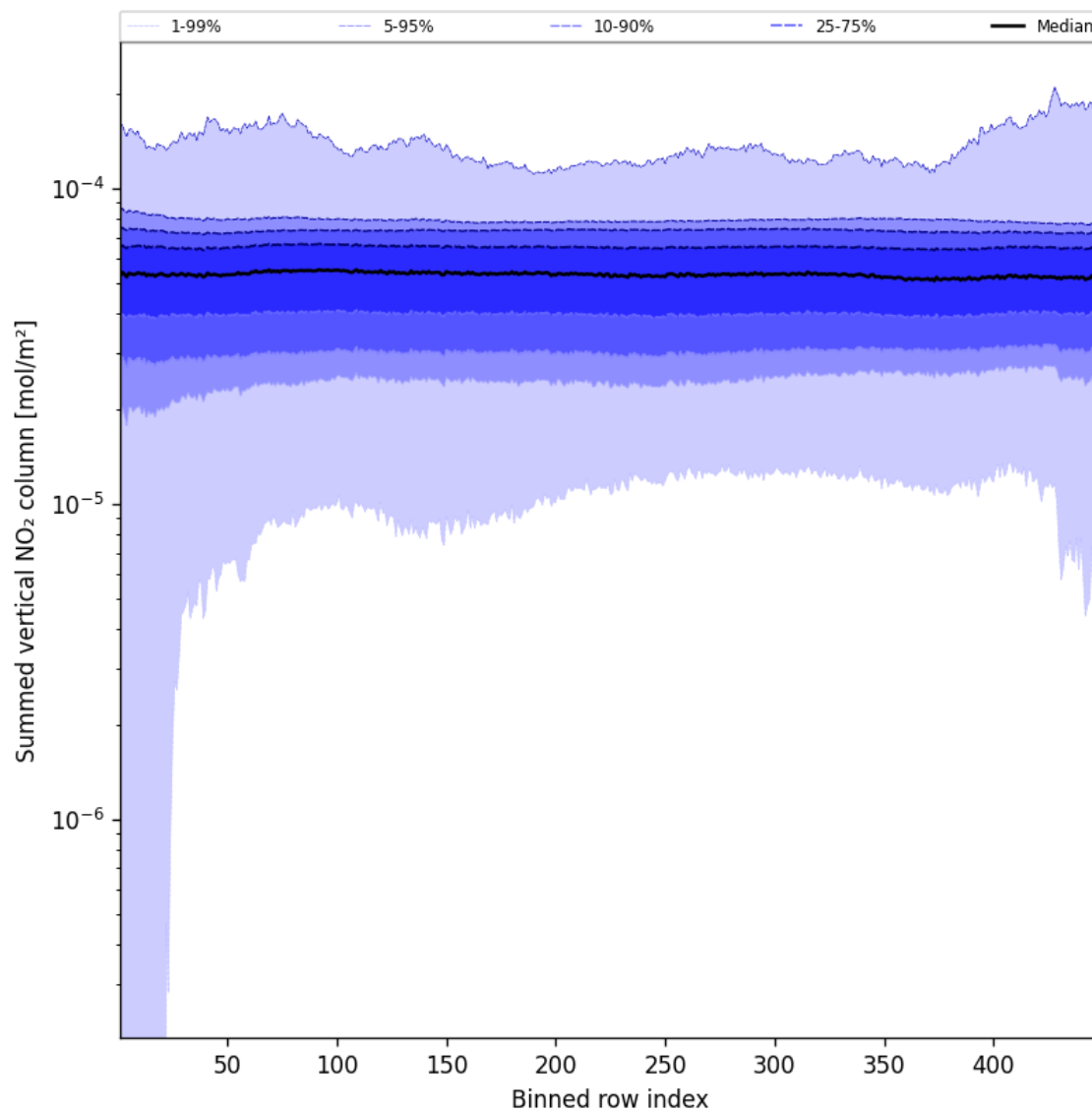
Figure 57: Along track statistics of “Summed vertical NO 2 column” for 2025-02-11 to 2025-02-13
