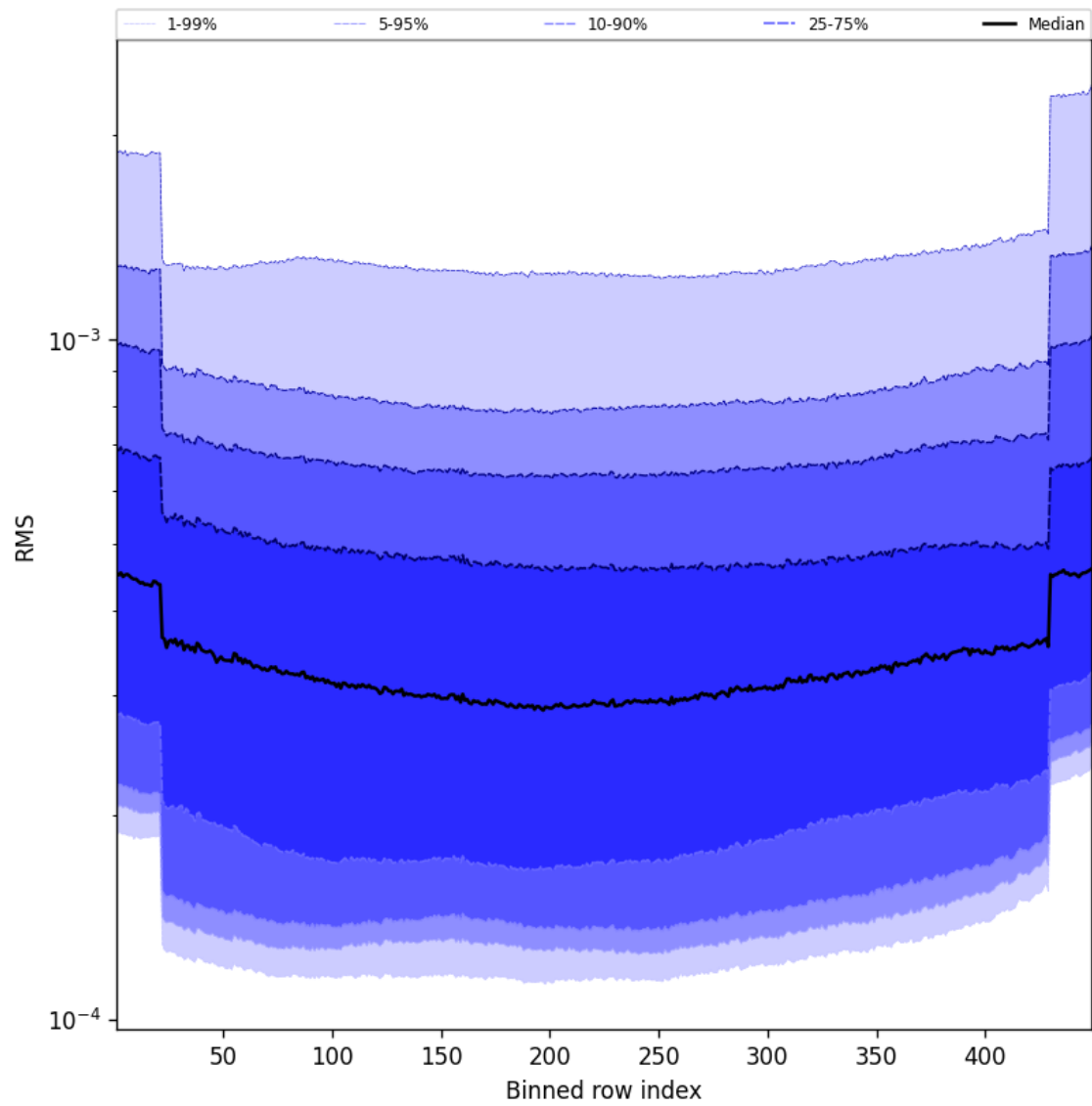
Figure 60: Along track statistics of “RMS” for 2025-02-11 to 2025-02-13
