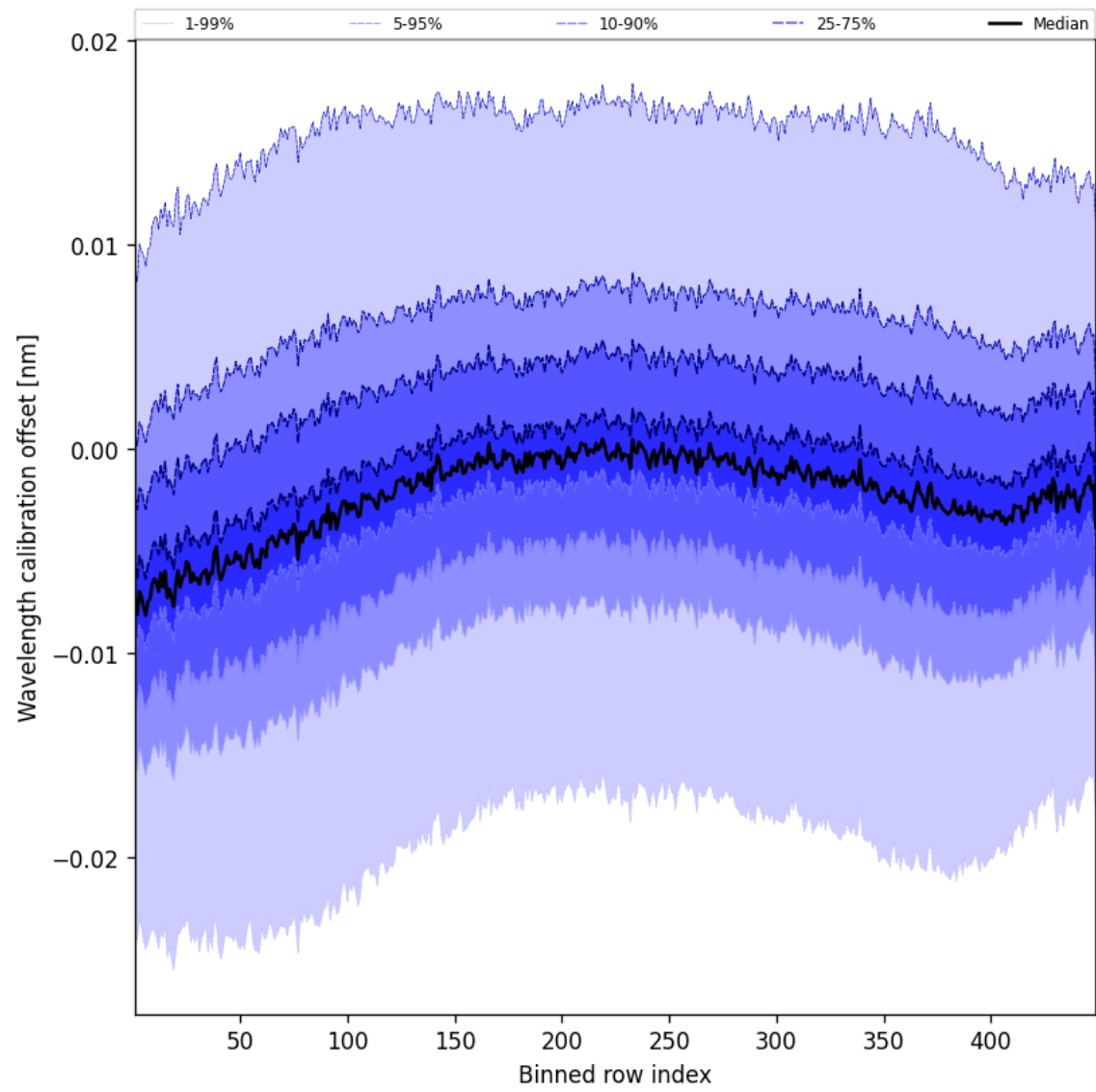
Figure 52: Along track statistics of “Wavelength calibration offset” for 2025-02-11 to 2025-02-13
