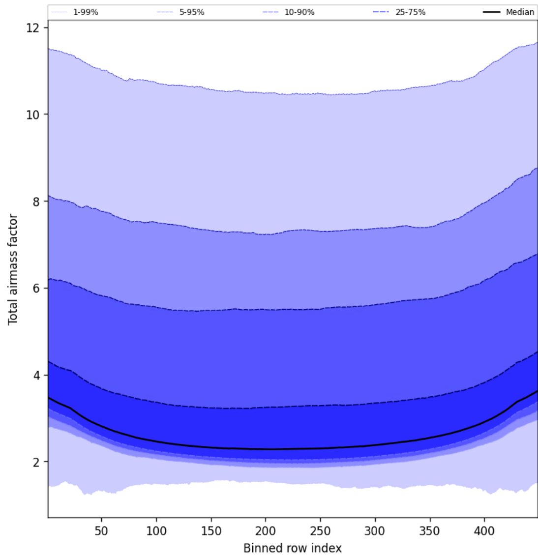
Figure 49: Along track statistics of “Total airmass factor” for 2025-02-11 to 2025-02-13
