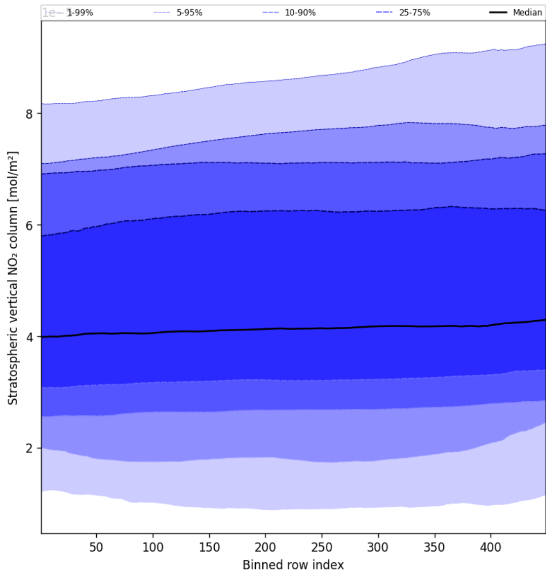
Figure 53: Along track statistics of “Stratospheric vertical NO 2 column” for 2025-02-11 to 2025-02-13
