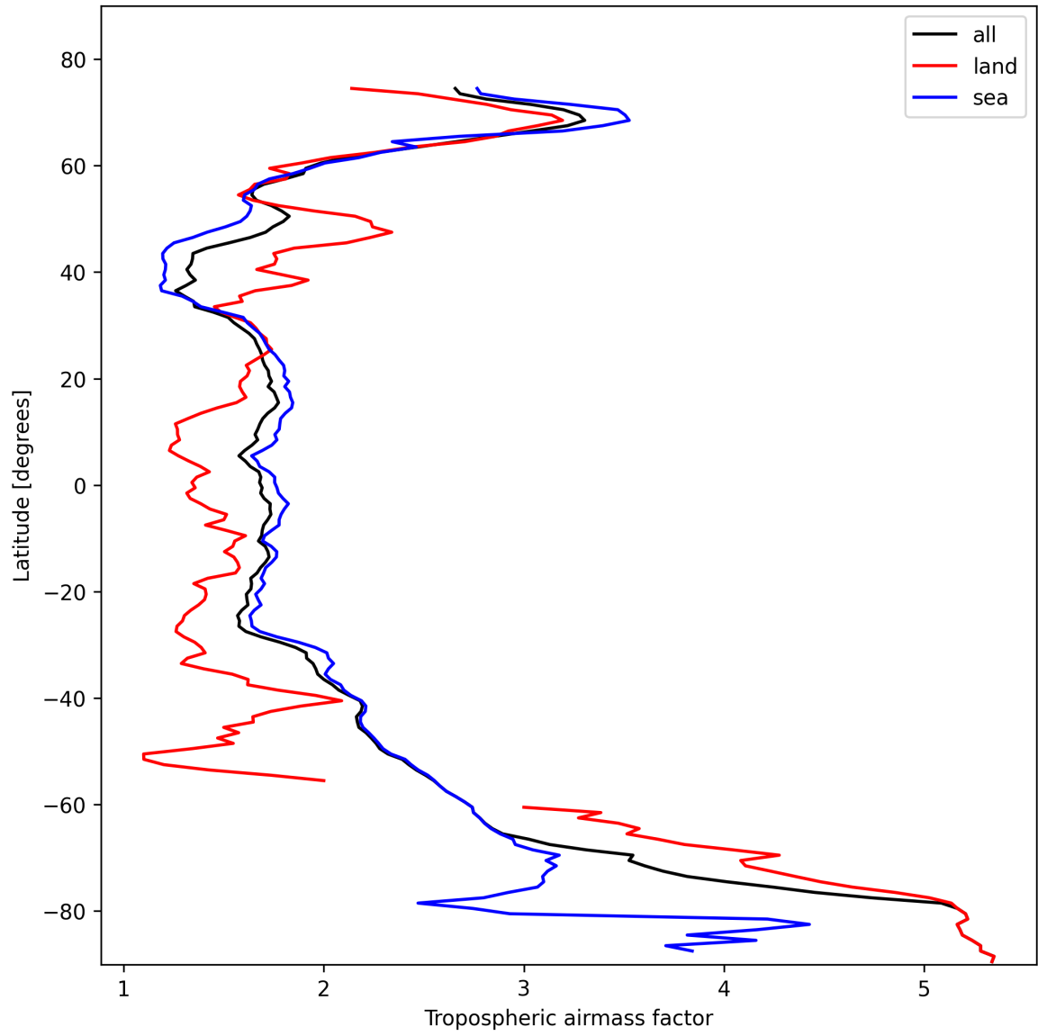
Figure 14: Zonal average of “Tropospheric airmass factor” for 2025-02-11 to 2025-02-13.
