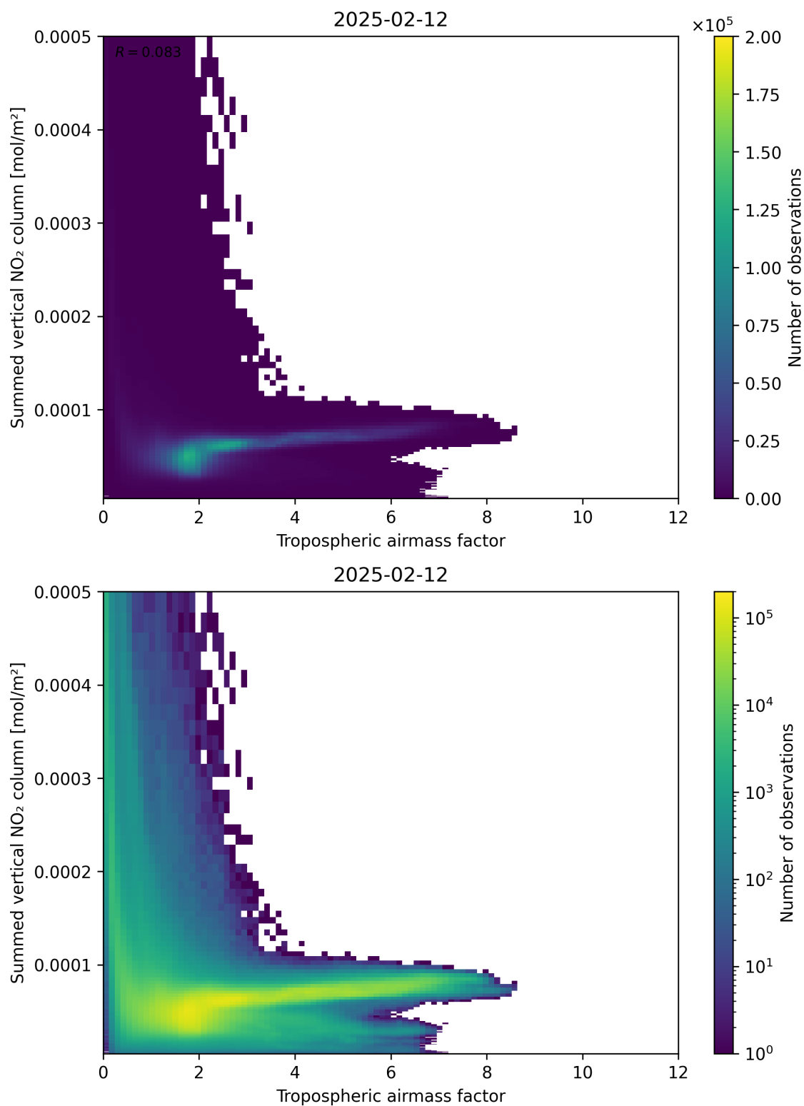
Figure 75: Scatter density plot of “Tropospheric air mass factor” against “Summed vertical NO 2 column” for 2025-02-11 to 2025-02-13.
