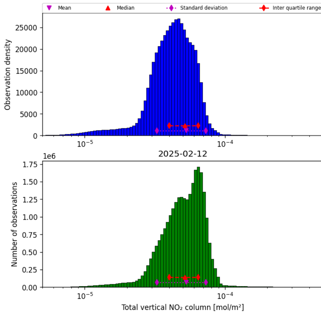
Figure 38: Histogram of “Total vertical NO 2 column” for 2025-02-11 to 2025-02-13
