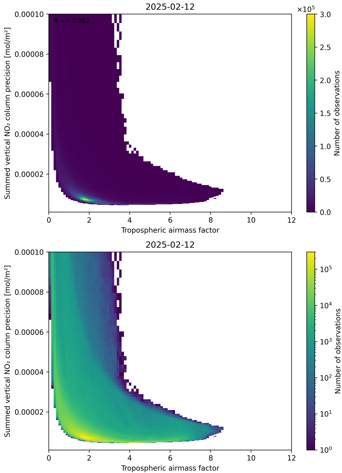
Figure 76: Scatter density plot of “Tropospheric air mass factor” against “Summed vertical NO 2 column precision” for 2025-02-11 to 2025-02-13.
