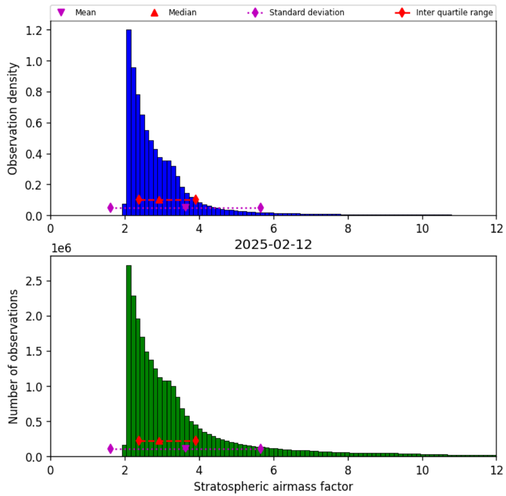
Figure 44: Histogram of “Stratospheric airmass factor” for 2025-02-11 to 2025-02-13
