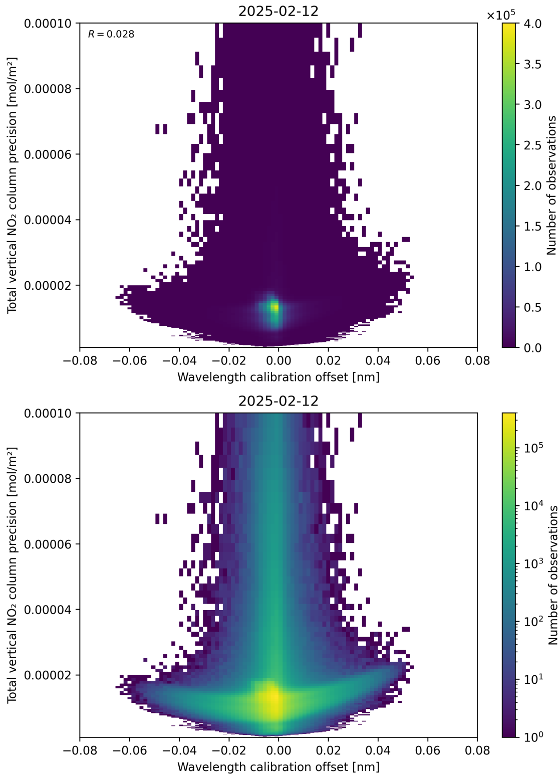
Figure 180: Scatter density plot of “Wavelength calibration offset” against “Total vertical NO 2 column precision” for 2025-02-11 to 2025-02-13.
