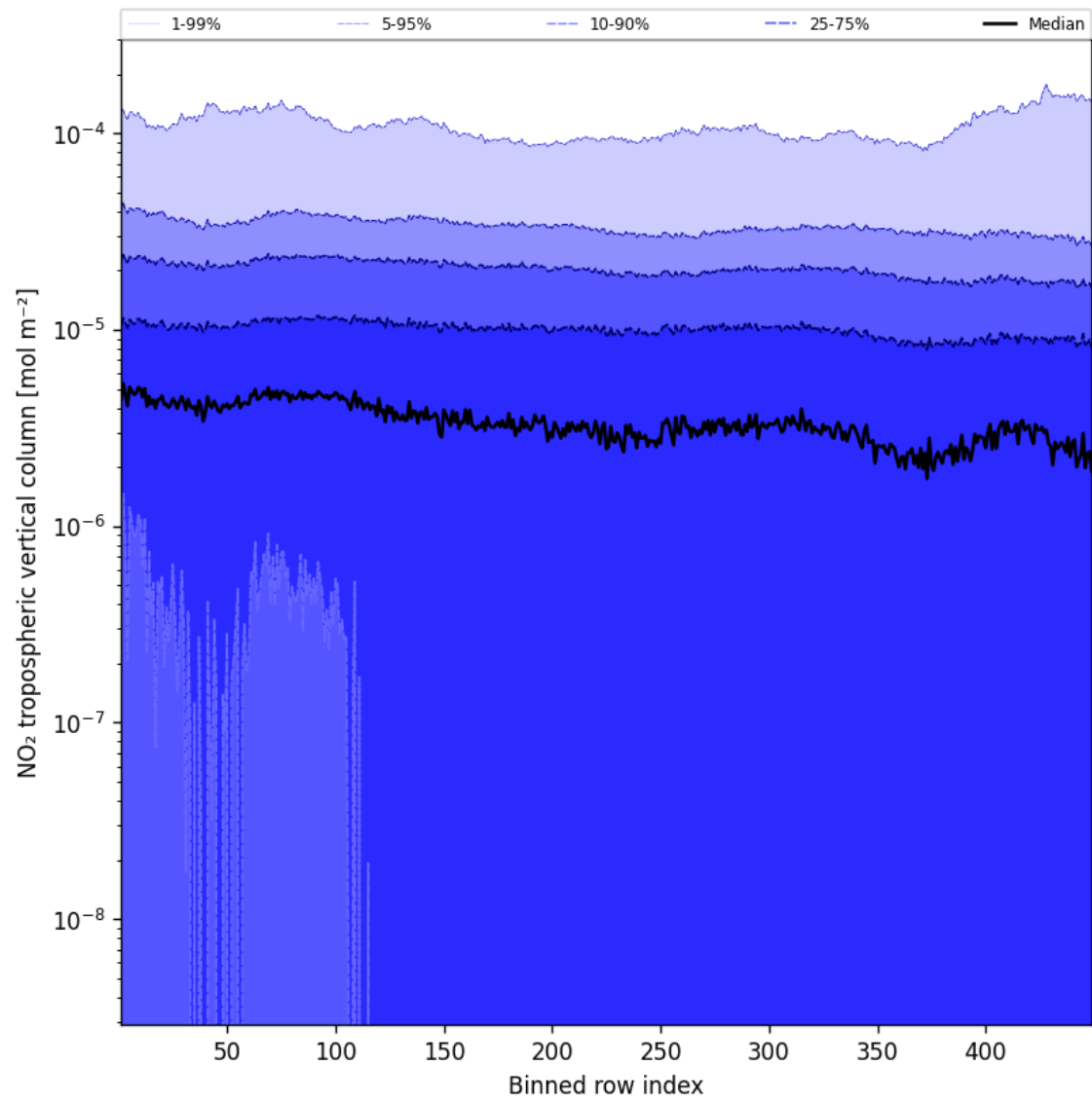
Figure 46: Along track statistics of “NO 2 tropospheric vertical column” for 2025-02-11 to 2025-02-13
