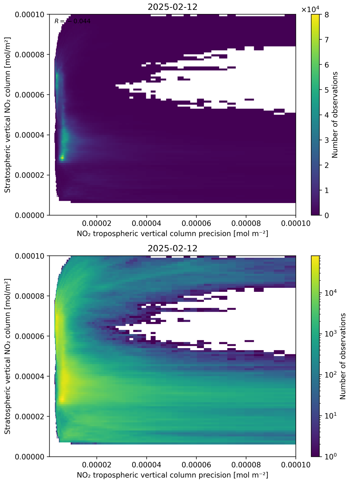
Figure 135: Scatter density plot of “NO 2 tropospheric vertical column precision” against “Stratospheric vertical NO 2 column” for 2025-02-11 to 2025-02-13.
