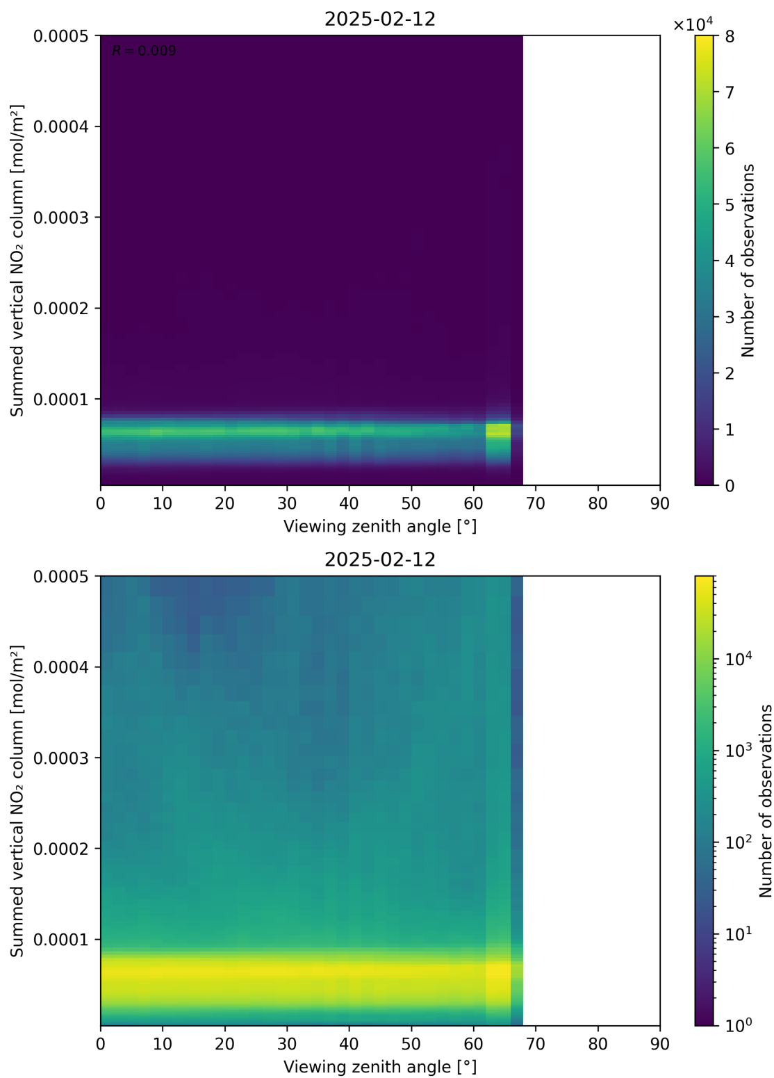
Figure 165: Scatter density plot of “Viewing zenith angle” against “Summed vertical NO 2 column” for 2025-02-11 to 2025-02-13.
