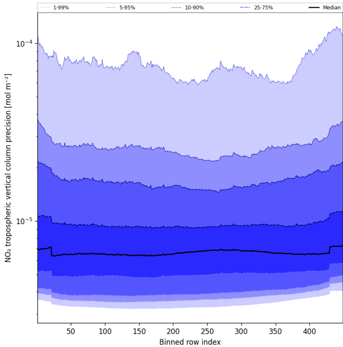
Figure 47: Along track statistics of “NO 2 tropospheric vertical column precision” for 2025-02-11 to 2025-02-13
