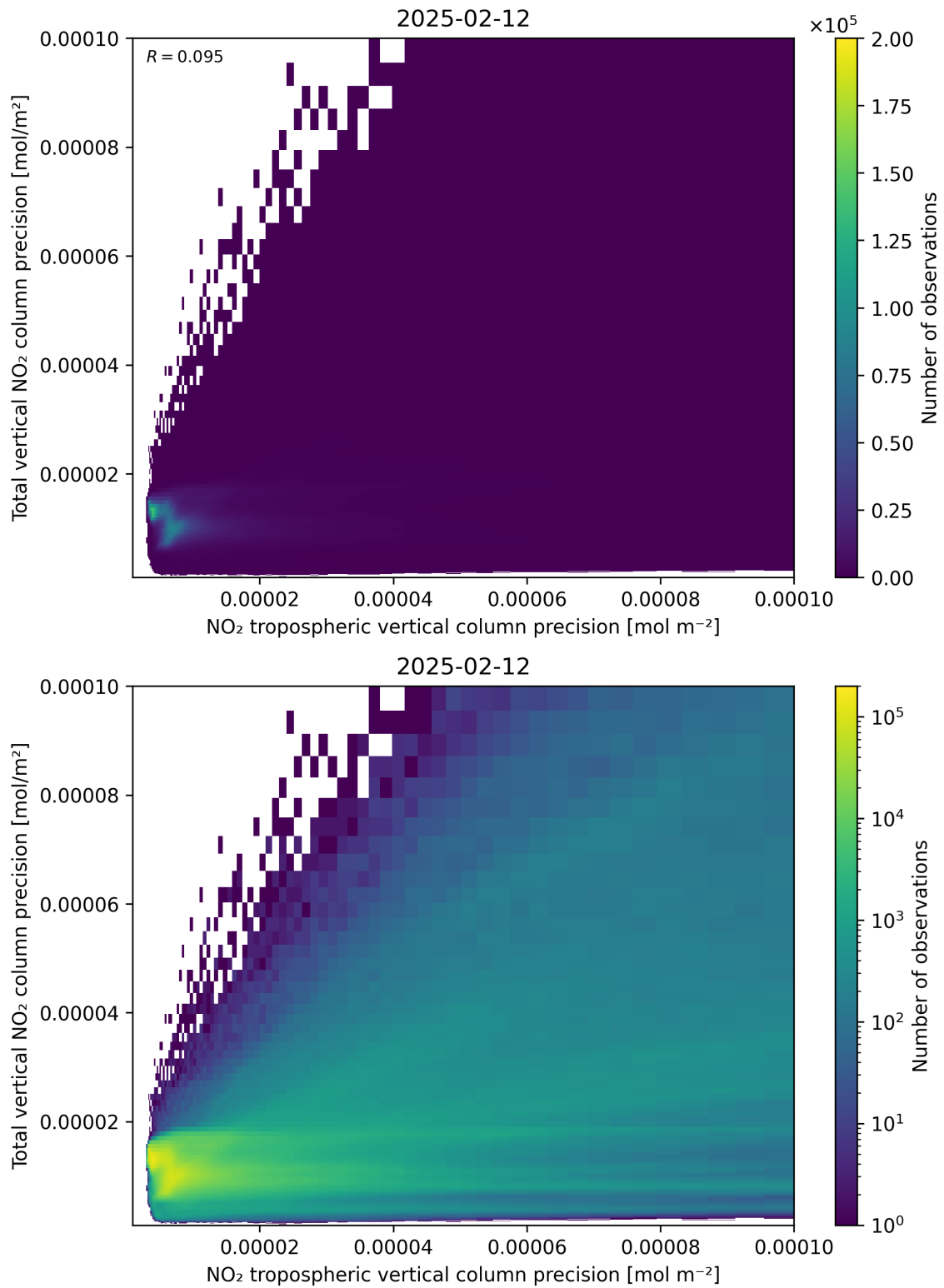
Figure 139: Scatter density plot of “NO 2 tropospheric vertical column precision” against “Total vertical NO 2 column precision” for 2025-02-11 to 2025-02-13.
