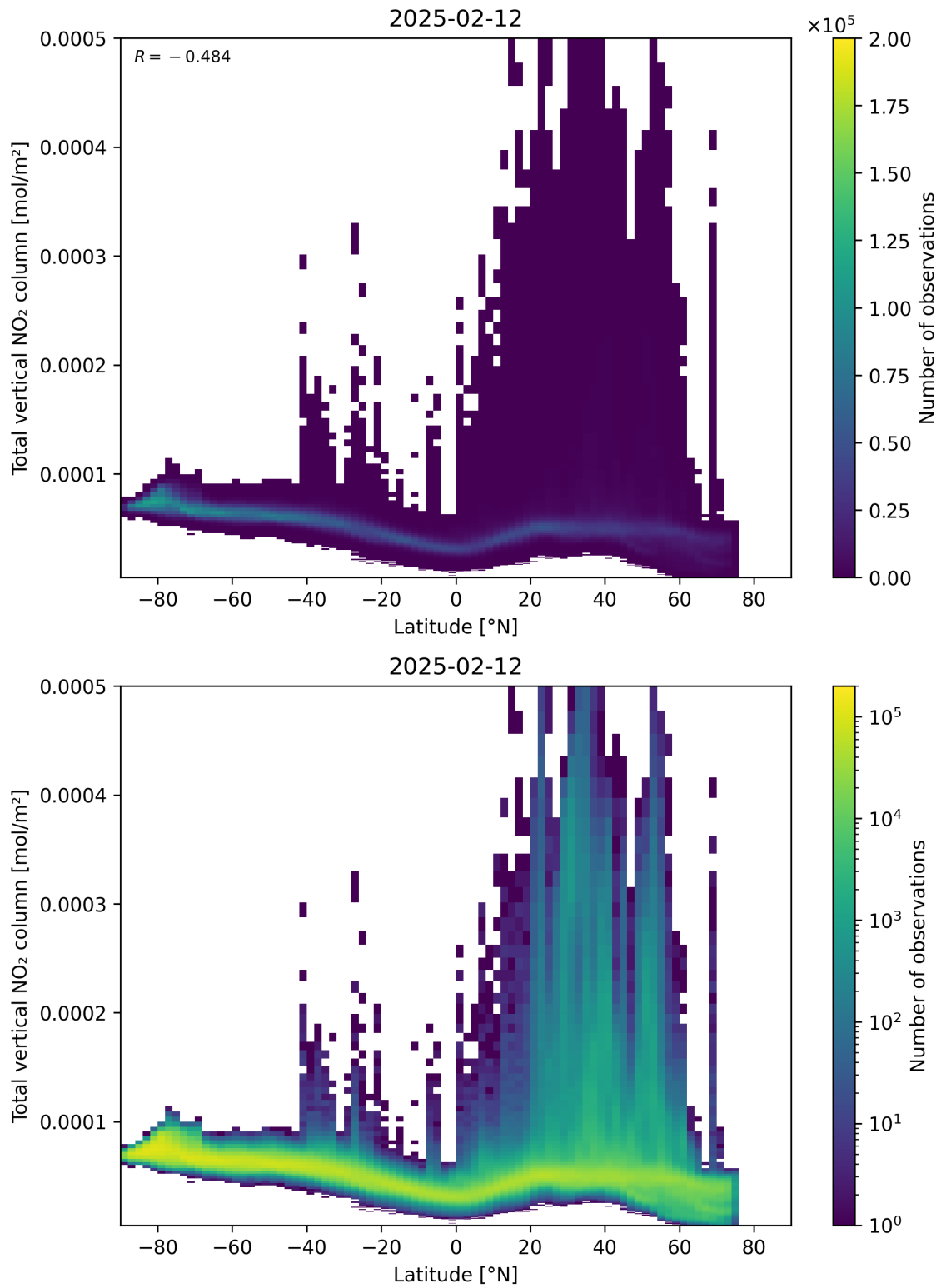
Figure 90: Scatter density plot of “Latitude” against “Total vertical NO 2 column” for 2025-02-11 to 2025-02-13.
