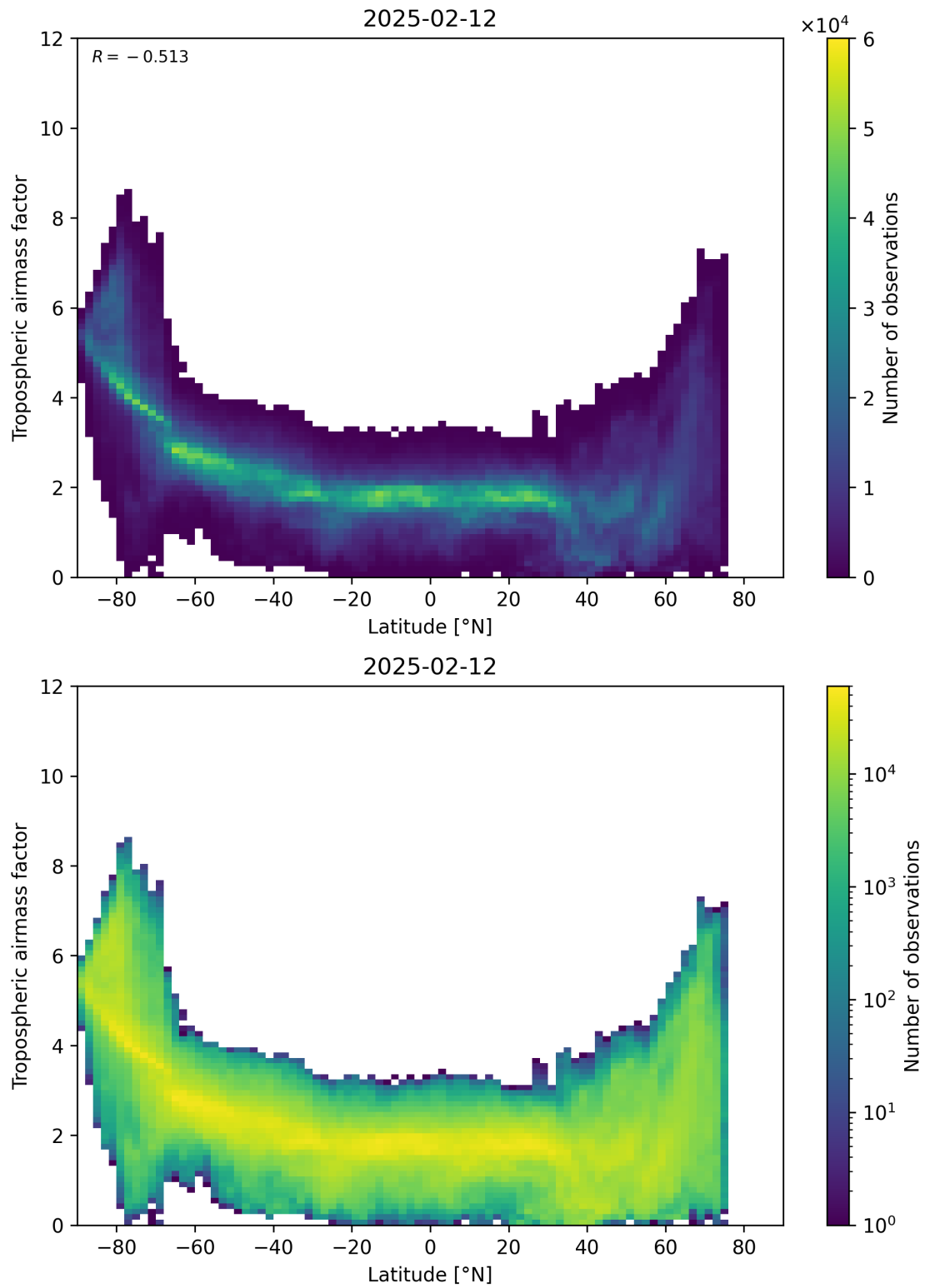
Figure 85: Scatter density plot of “Latitude” against “Tropospheric airmass factor” for 2025-02-11 to 2025-02-13.
