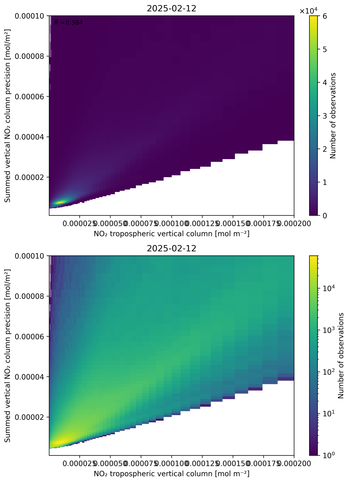
Figure 127: Scatter density plot of “NO 2 tropospheric vertical column” against “Summed vertical NO 2 column precision” for 2025-02-11 to 2025-02-13.
