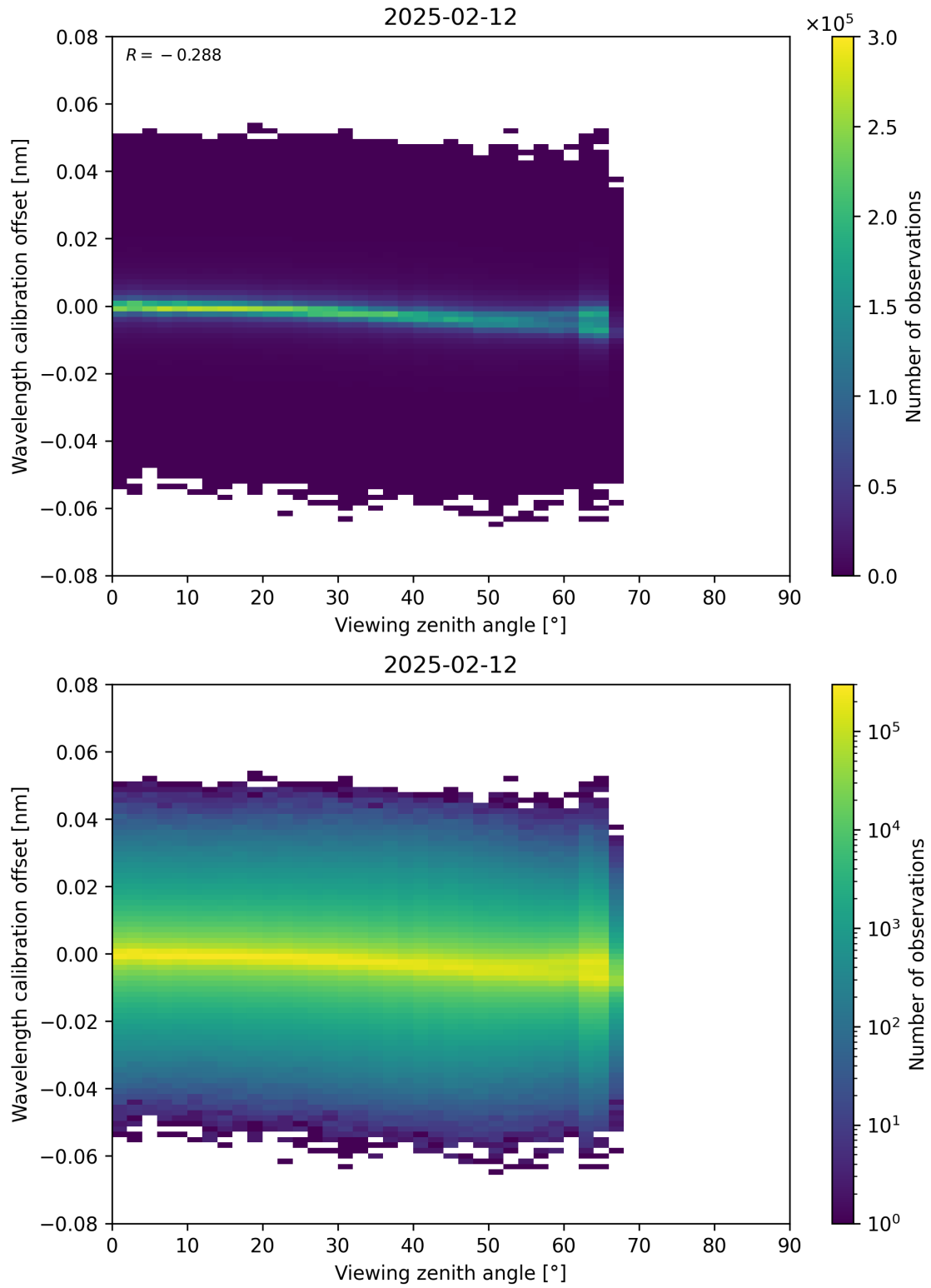
Figure 173: Scatter density plot of “Viewing zenith angle” against “Wavelength calibration offset” for 2025-02-11 to 2025-02-13.
