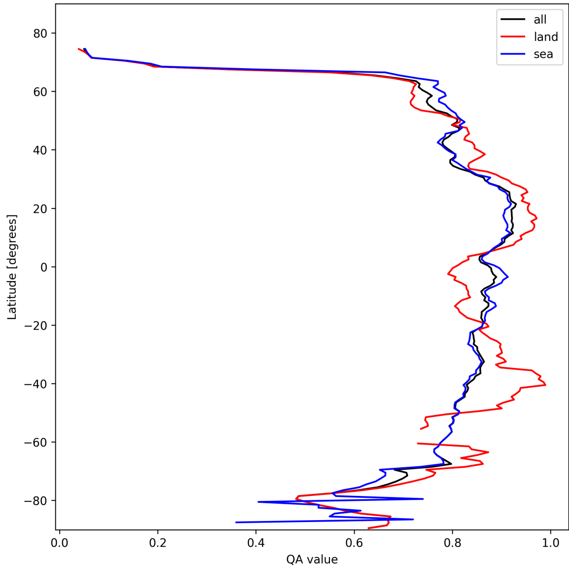
Figure 11: Zonal average of “QA value” for 2025-02-11 to 2025-02-13.
