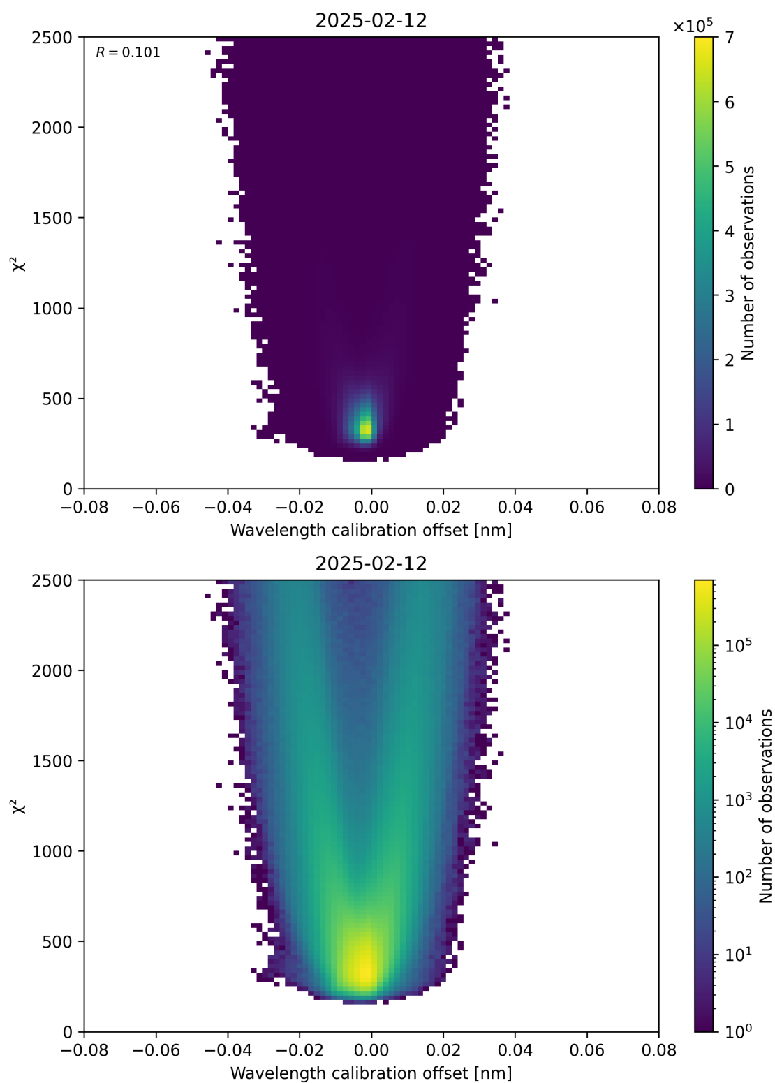
Figure 175: Scatter density plot of “Wavelength calibration offset” against “ \chi^2 ” for 2025-02-11 to 2025-02-13.
