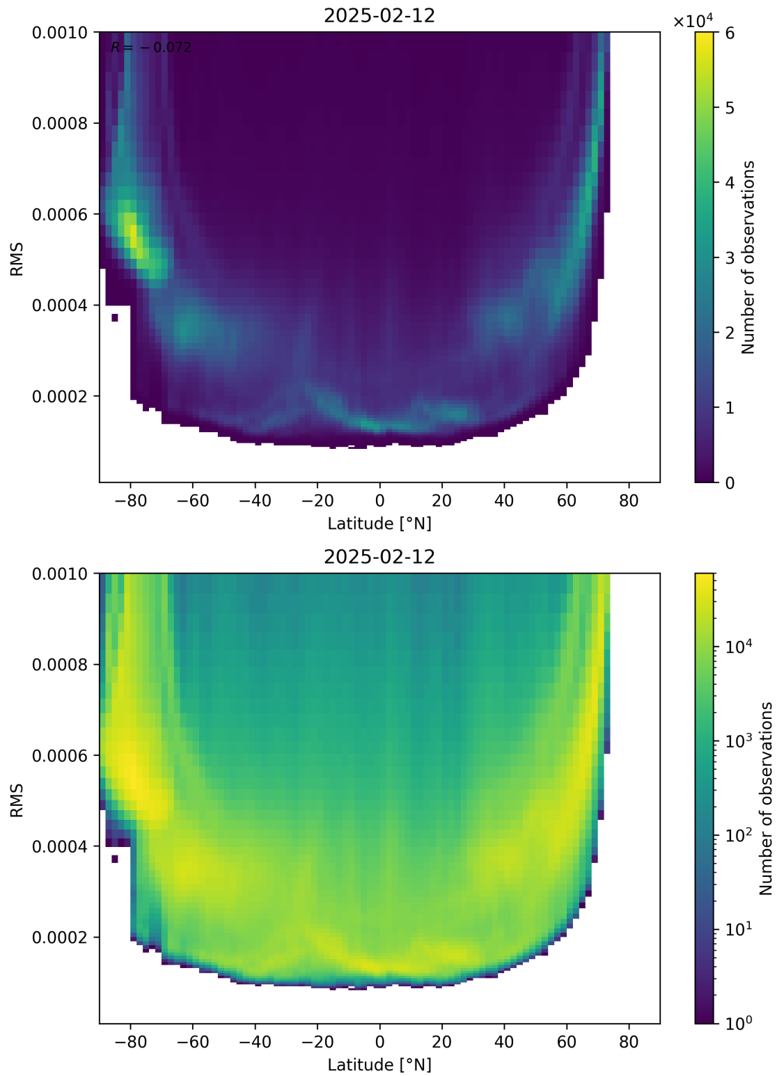
Figure 94: Scatter density plot of “Latitude” against “RMS” for 2025-02-11 to 2025-02-13.
