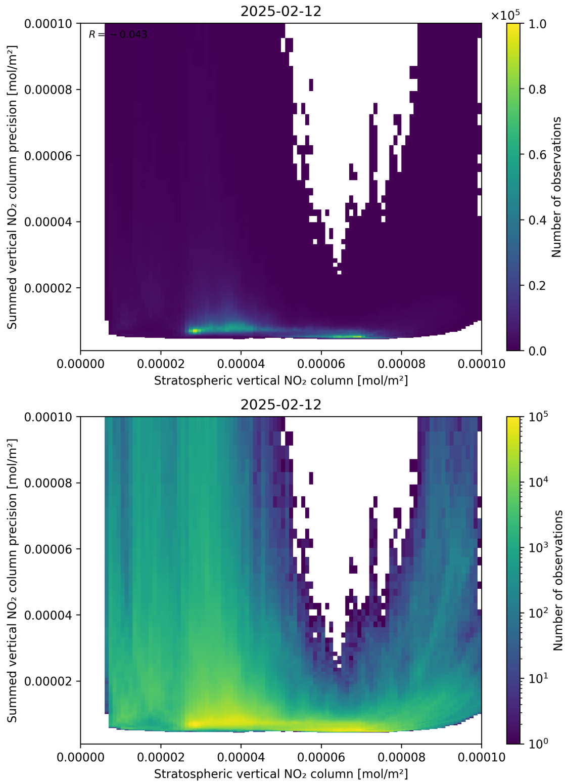
Figure 99: Scatter density plot of “Stratospheric vertical NO 2 column” against “Summed vertical NO 2 column precision” for 2025-02-11 to 2025-02-13.
