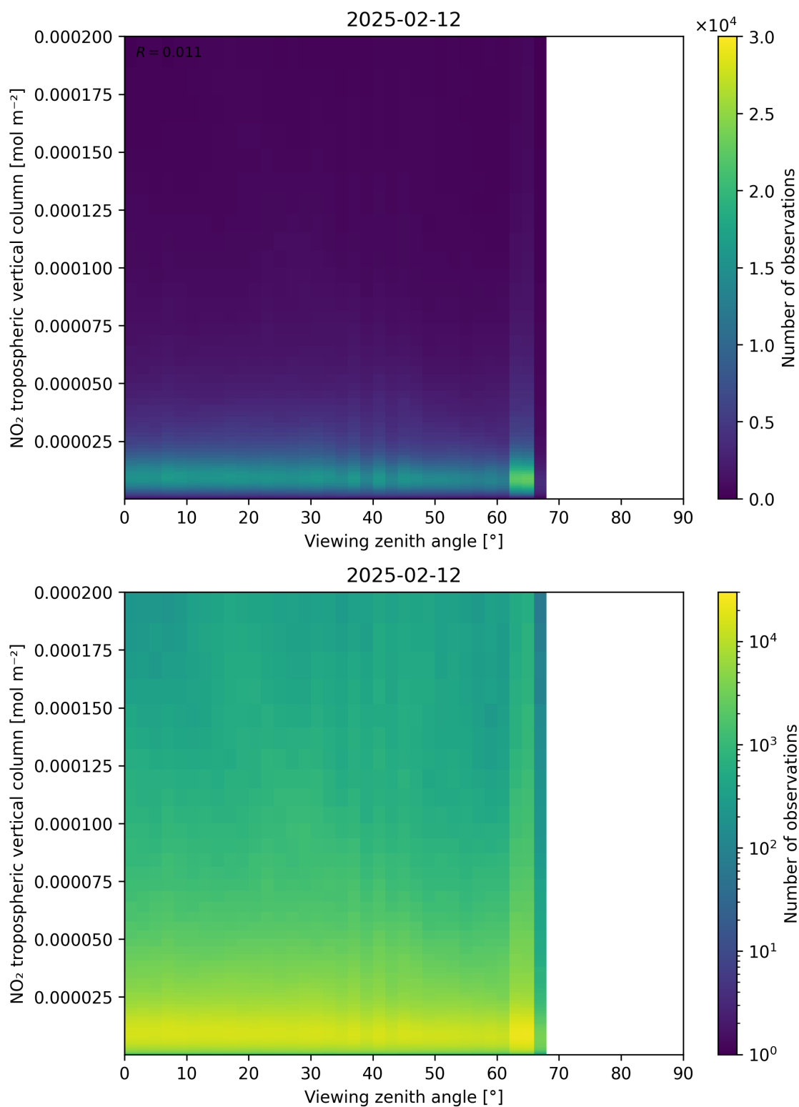
Figure 169: Scatter density plot of “Viewing zenith angle” against “NO 2 tropospheric vertical column” for 2025-02-11 to 2025-02-13.
