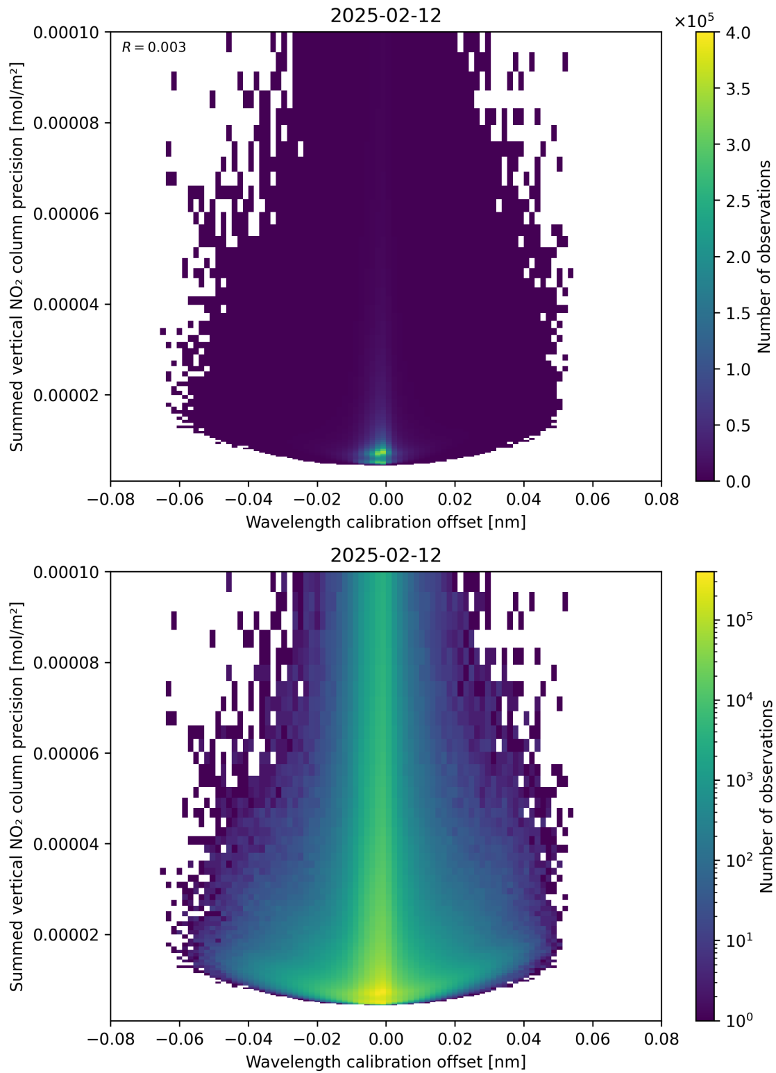
Figure 178: Scatter density plot of “Wavelength calibration offset” against “Summed vertical NO 2 column precision” for 2025-02-11 to 2025-02-13.
