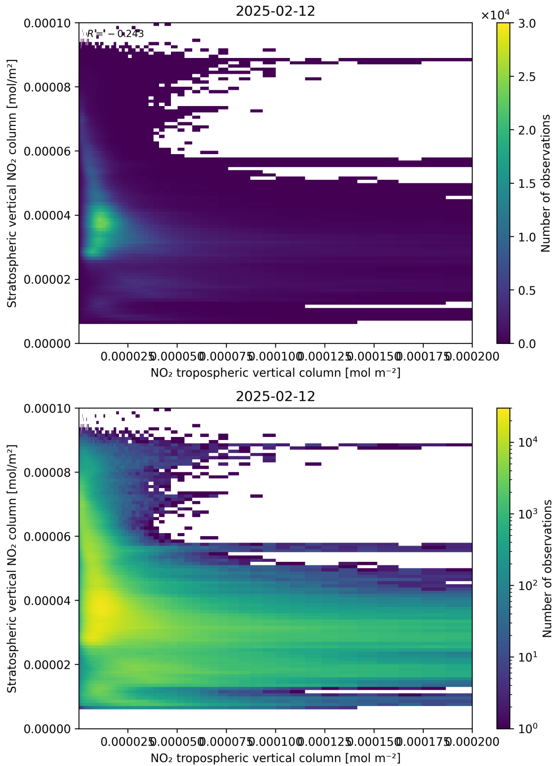
Figure 125: Scatter density plot of “NO 2 tropospheric vertical column” against “Stratospheric vertical NO 2 column” for 2025-02-11 to 2025-02-13.
