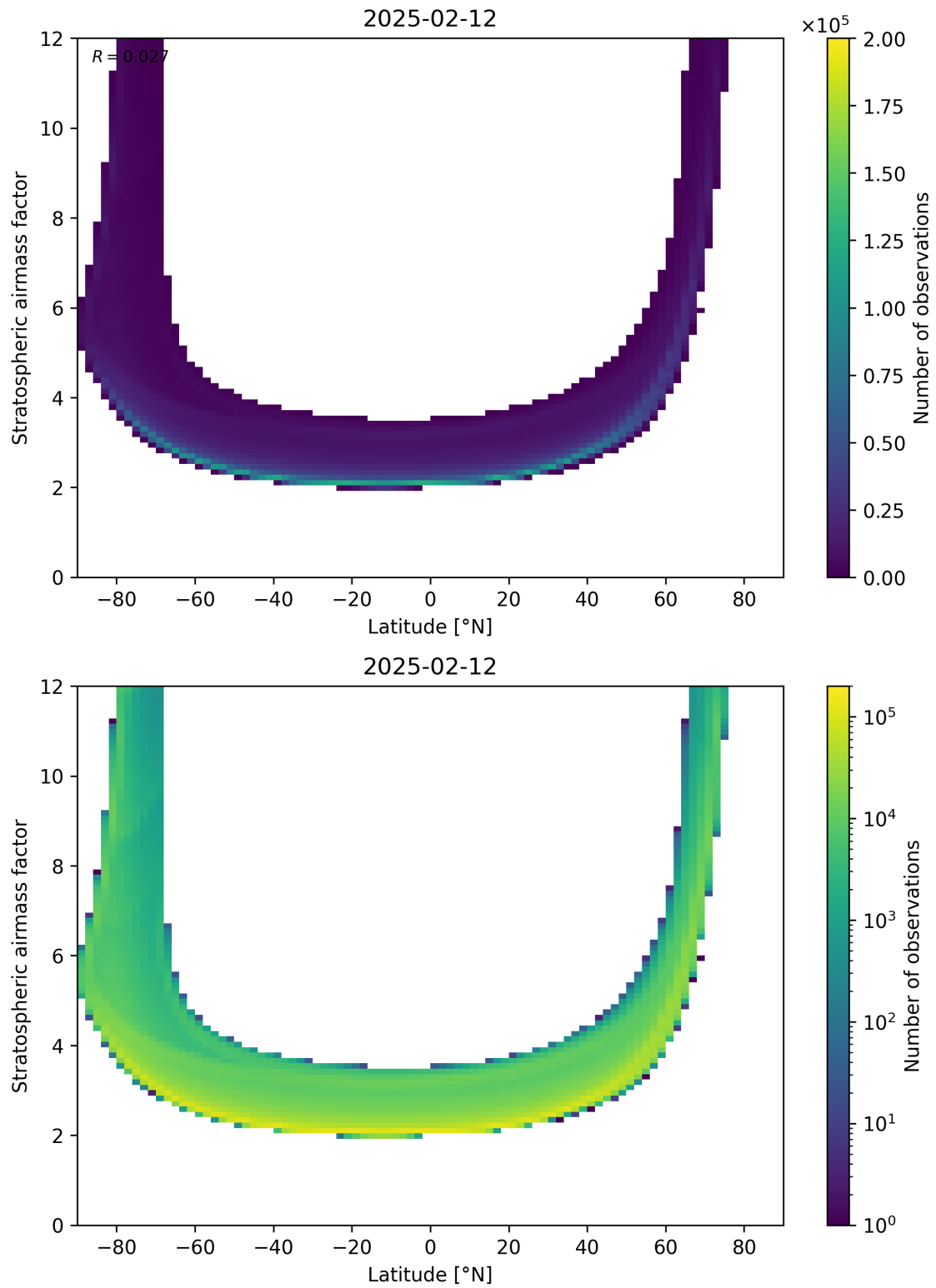
Figure 83: Scatter density plot of “Latitude” against “Stratospheric airmass factor” for 2025-02-11 to 2025-02-13.
