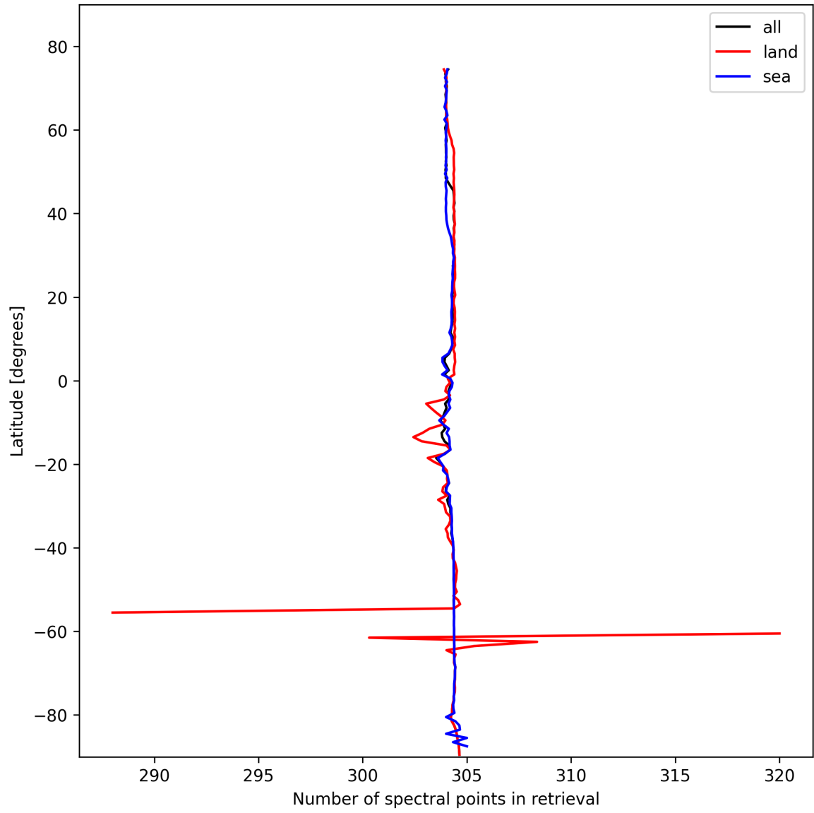
Figure 16: Zonal average of “Number of spectral points in retrieval” for 2025-02-11 to 2025-02-13.
