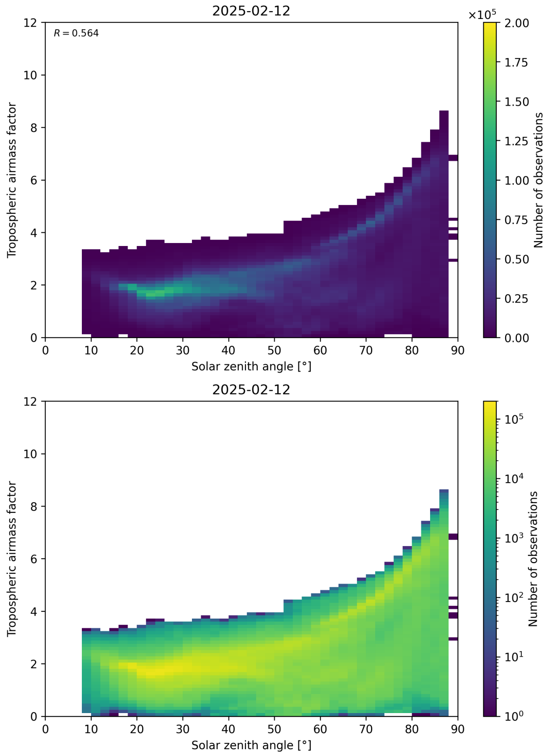
Figure 147: Scatter density plot of “Solar zenith angle” against “Tropospheric airmass factor” for 2025-02-11 to 2025-02-13.
