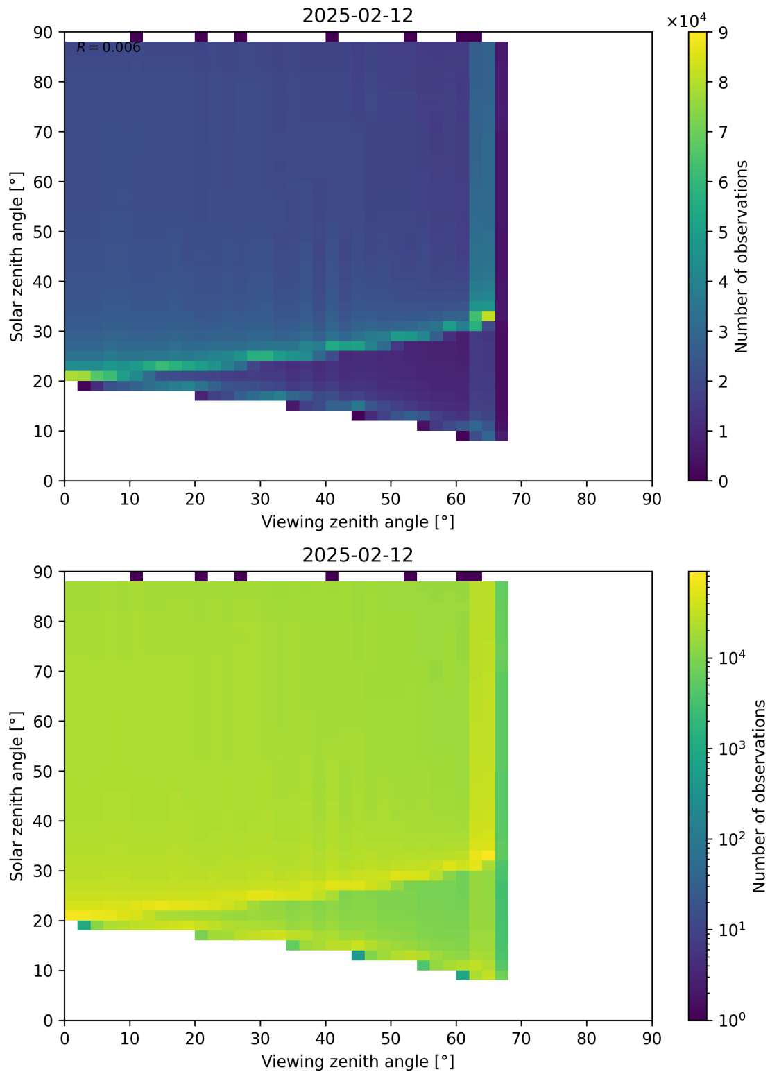
Figure 172: Scatter density plot of “Viewing zenith angle” against “Solar zenith angle” for 2025-02-11 to 2025-02-13.
