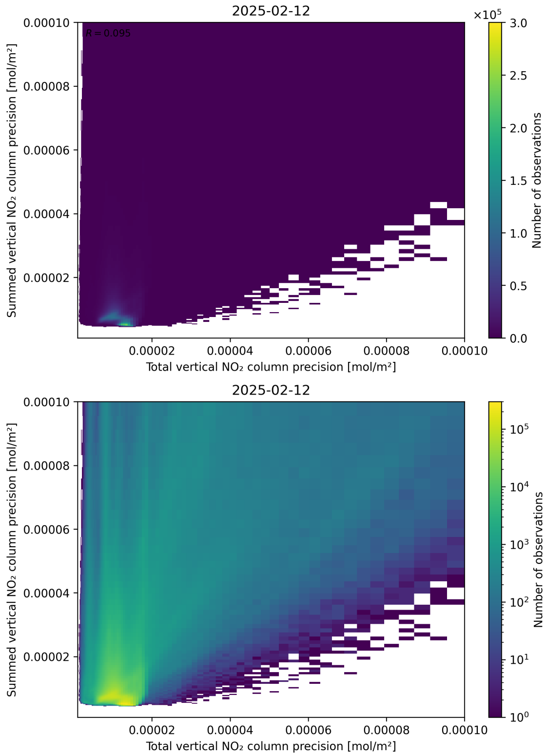
Figure 118: Scatter density plot of “Total vertical NO 2 column precision” against “Summed vertical NO 2 column precision” for 2025-02-11 to 2025-02-13.
