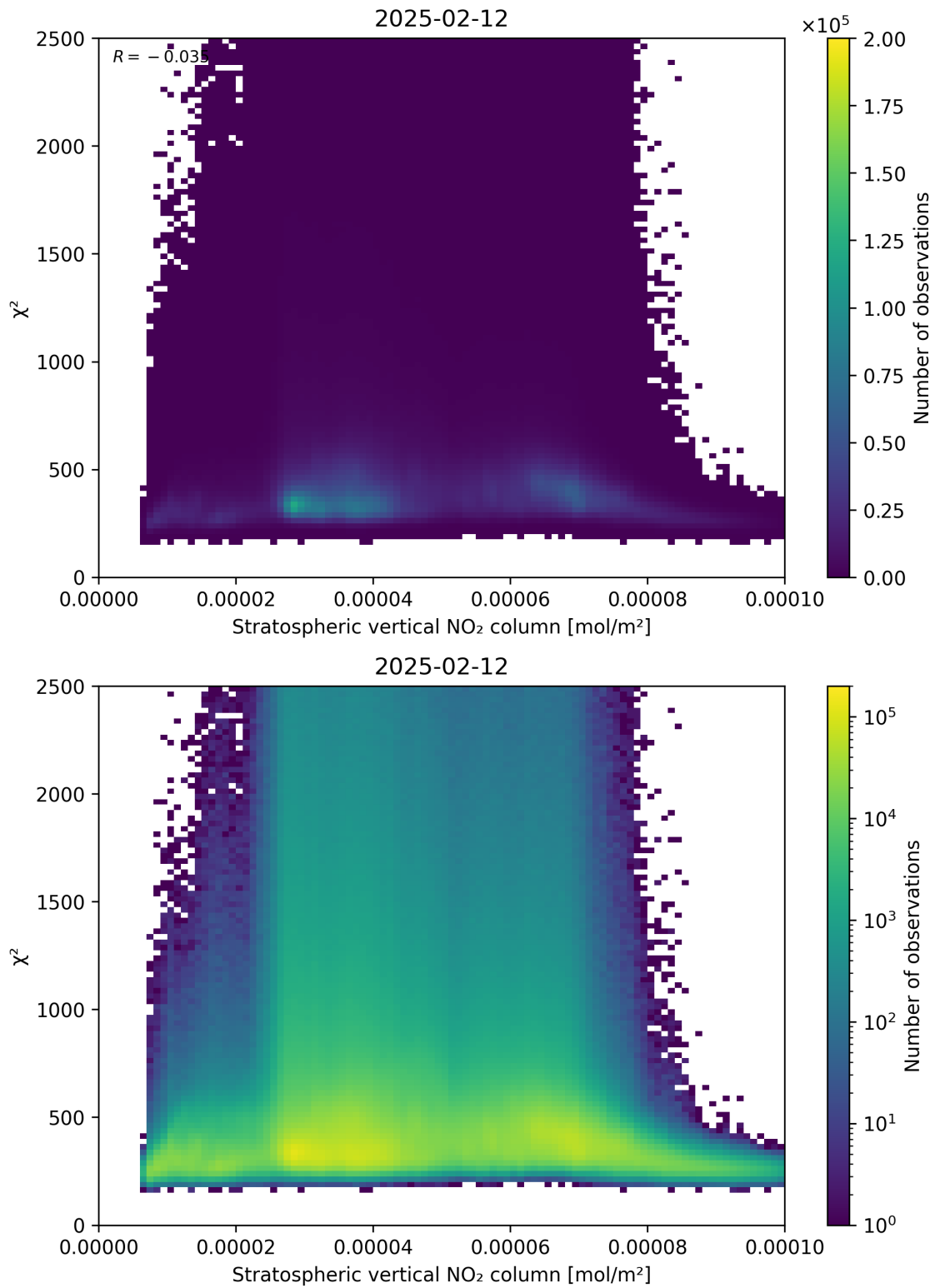
Figure 97: Scatter density plot of “Stratospheric vertical NO 2 column” against “ \chi^2 ” for 2025-02-11 to 2025-02-13.
