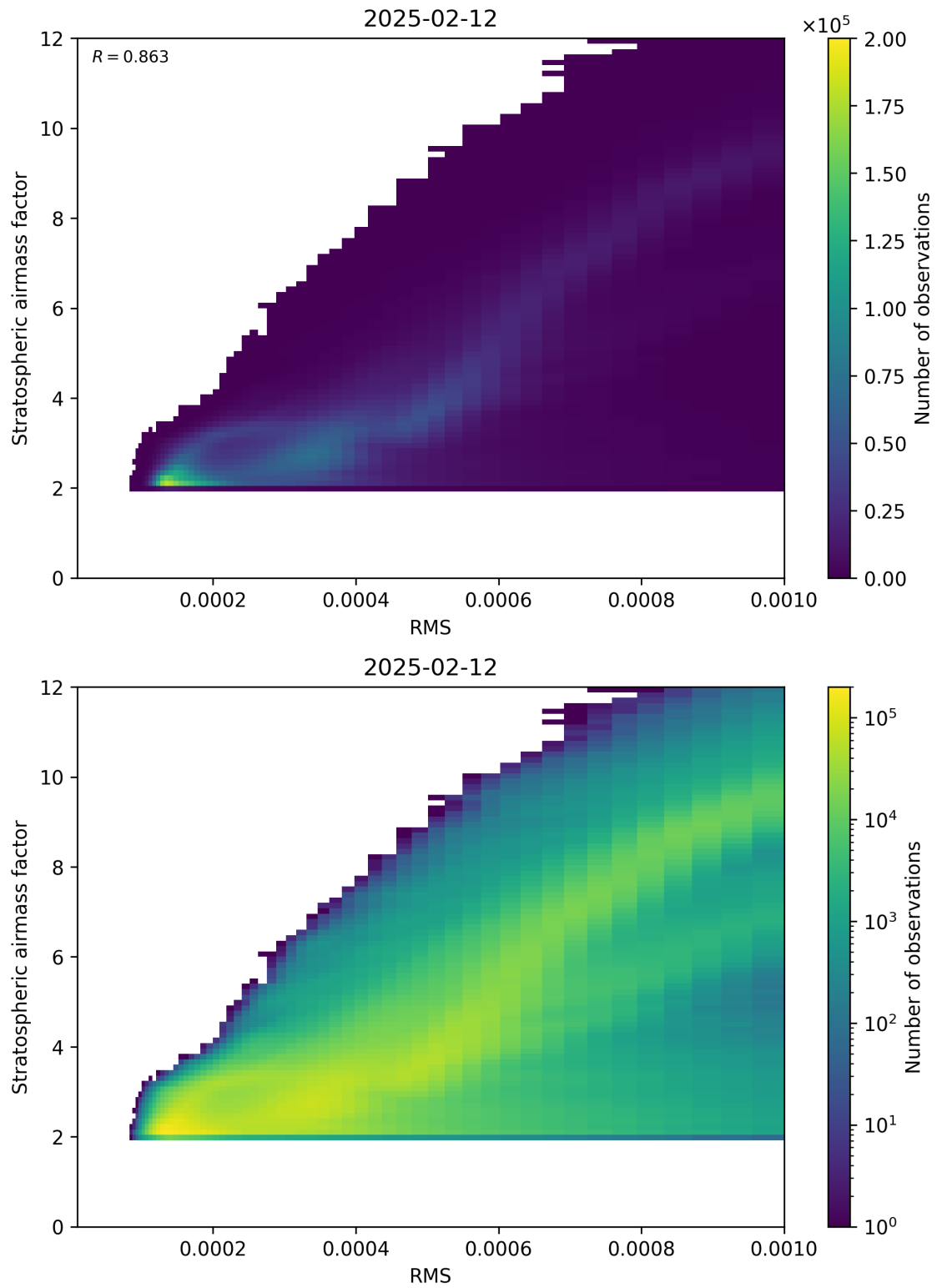
Figure 144: Scatter density plot of “RMS” against “Stratospheric airmass factor” for 2025-02-11 to 2025-02-13.
