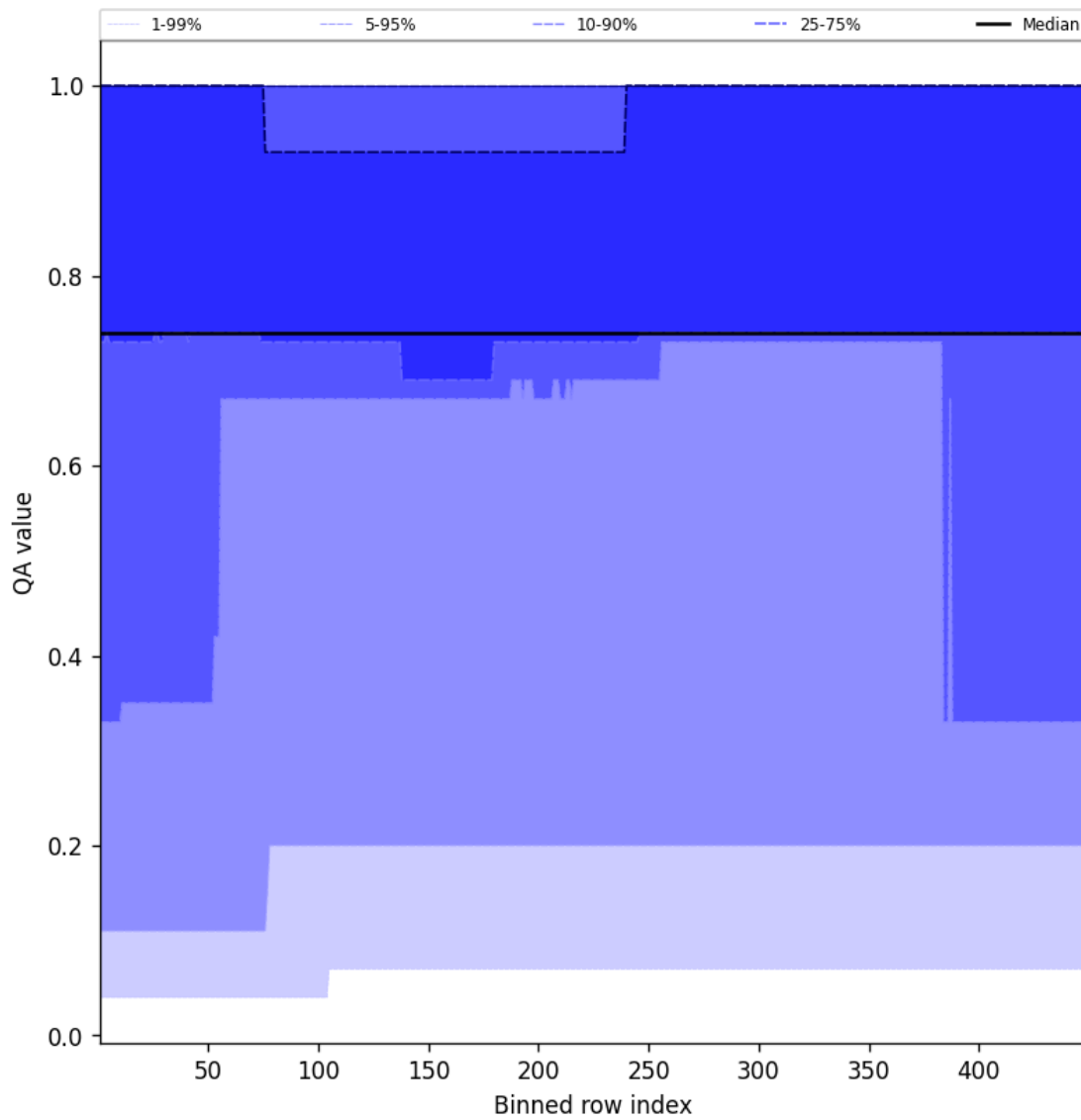
Figure 45: Along track statistics of “QA value” for 2025-02-11 to 2025-02-13
