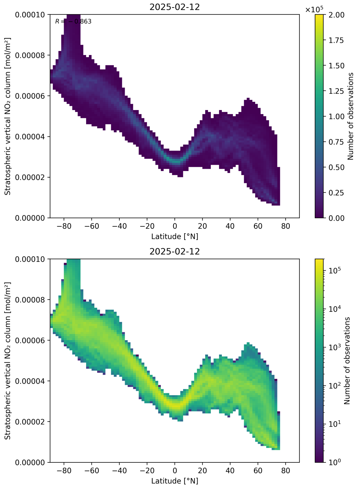
Figure 87: Scatter density plot of “Latitude” against “Stratospheric vertical NO 2 column” for 2025-02-11 to 2025-02-13.
