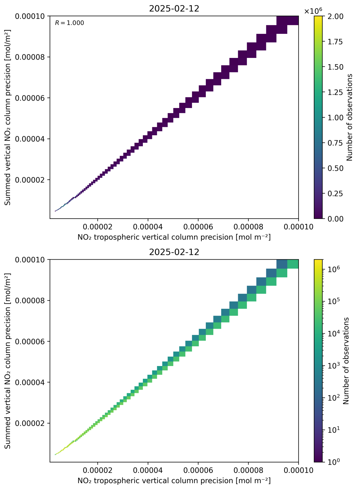
Figure 137: Scatter density plot of “NO 2 tropospheric vertical column precision” against “Summed vertical NO 2 column precision” for 2025-02-11 to 2025-02-13.
