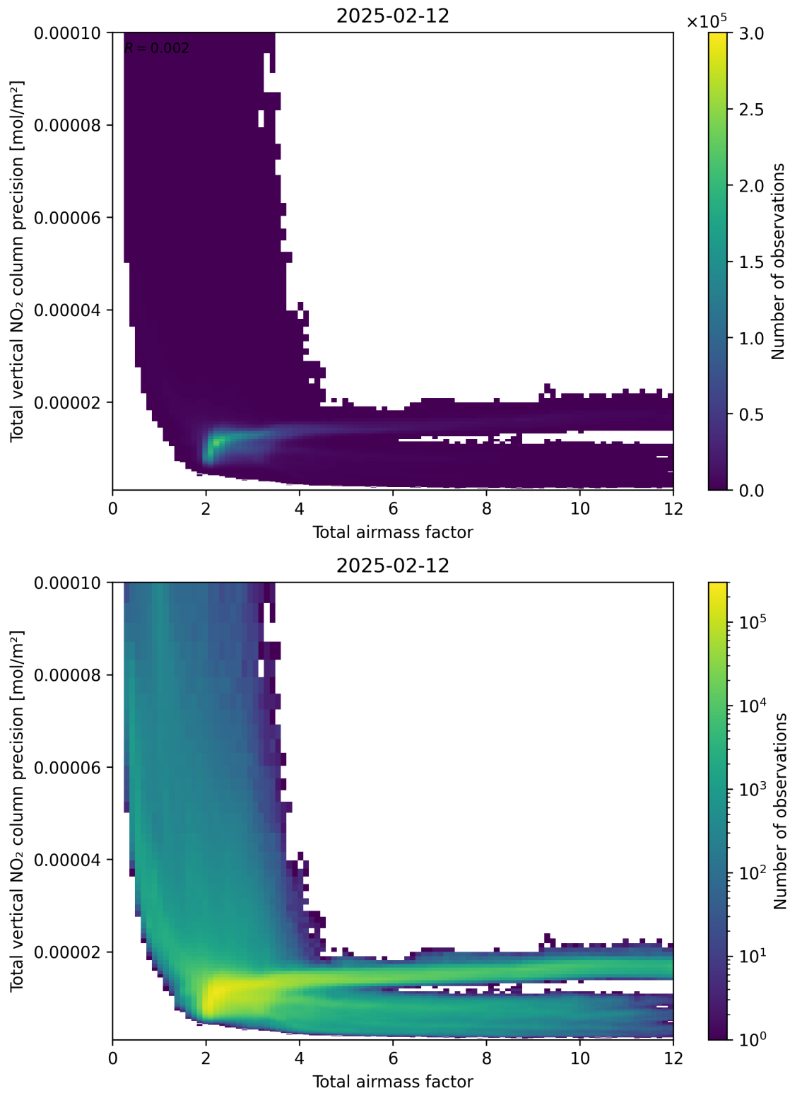
Figure 68: Scatter density plot of “Total airmass factor” against “Total vertical NO 2 column precision” for 2025-02-11 to 2025-02-13.
