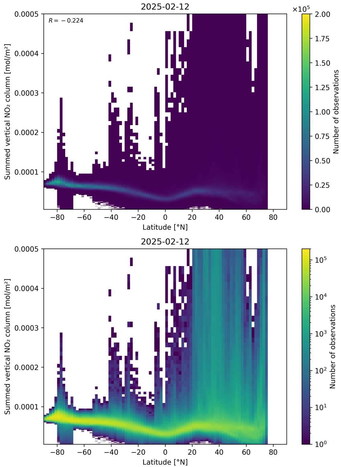
Figure 88: Scatter density plot of “Latitude” against “Summed vertical NO 2 column” for 2025-02-11 to 2025-02-13.
