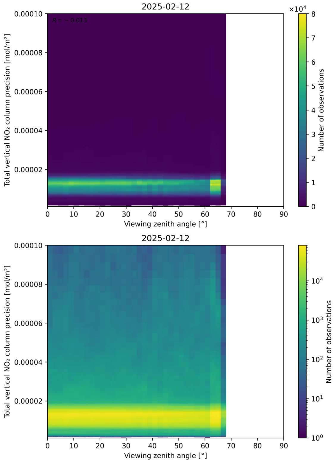
Figure 168: Scatter density plot of “Viewing zenith angle” against “Total vertical NO 2 column precision” for 2025-02-11 to 2025-02-13.
