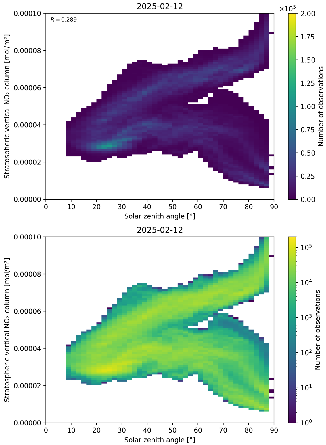
Figure 150: Scatter density plot of “Solar zenith angle” against “Stratospheric vertical NO 2 column” for 2025-02-11 to 2025-02-13.
