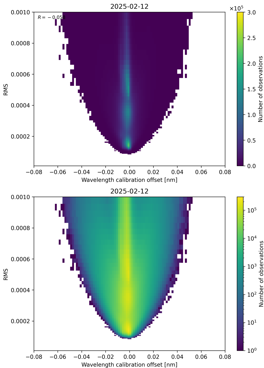
Figure 181: Scatter density plot of “Wavelength calibration offset” against “RMS” for 2025-02-11 to 2025-02-13.
