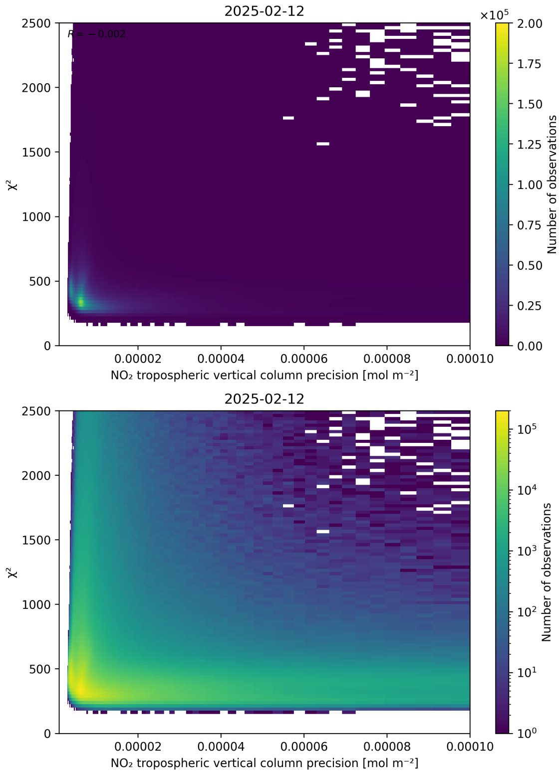
Figure 134: Scatter density plot of “NO 2 tropospheric vertical column precision” against “ \chi^2 ” for 2025-02-11 to 2025-02-13.
