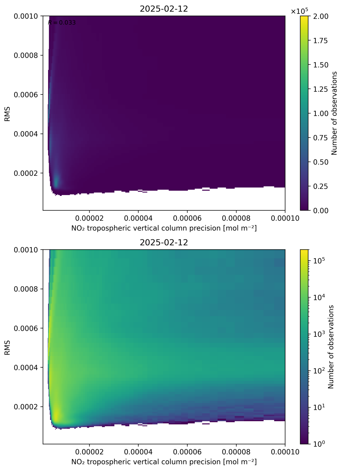
Figure 140: Scatter density plot of “NO 2 tropospheric vertical column precision” against “RMS” for 2025-02-11 to 2025-02-13.
