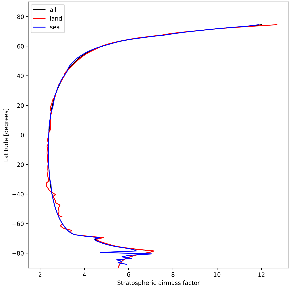
Figure 27: Zonal average of “Stratospheric air mass factor” for 2025-02-11 to 2025-02-13.
