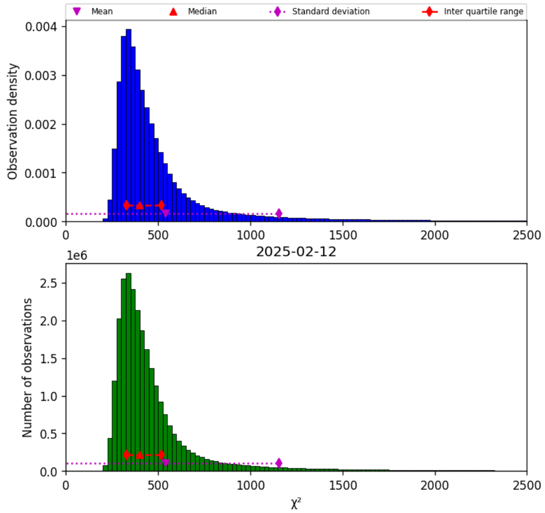
Figure 42: Histogram of “ \chi^2 ” for 2025-02-11 to 2025-02-13
