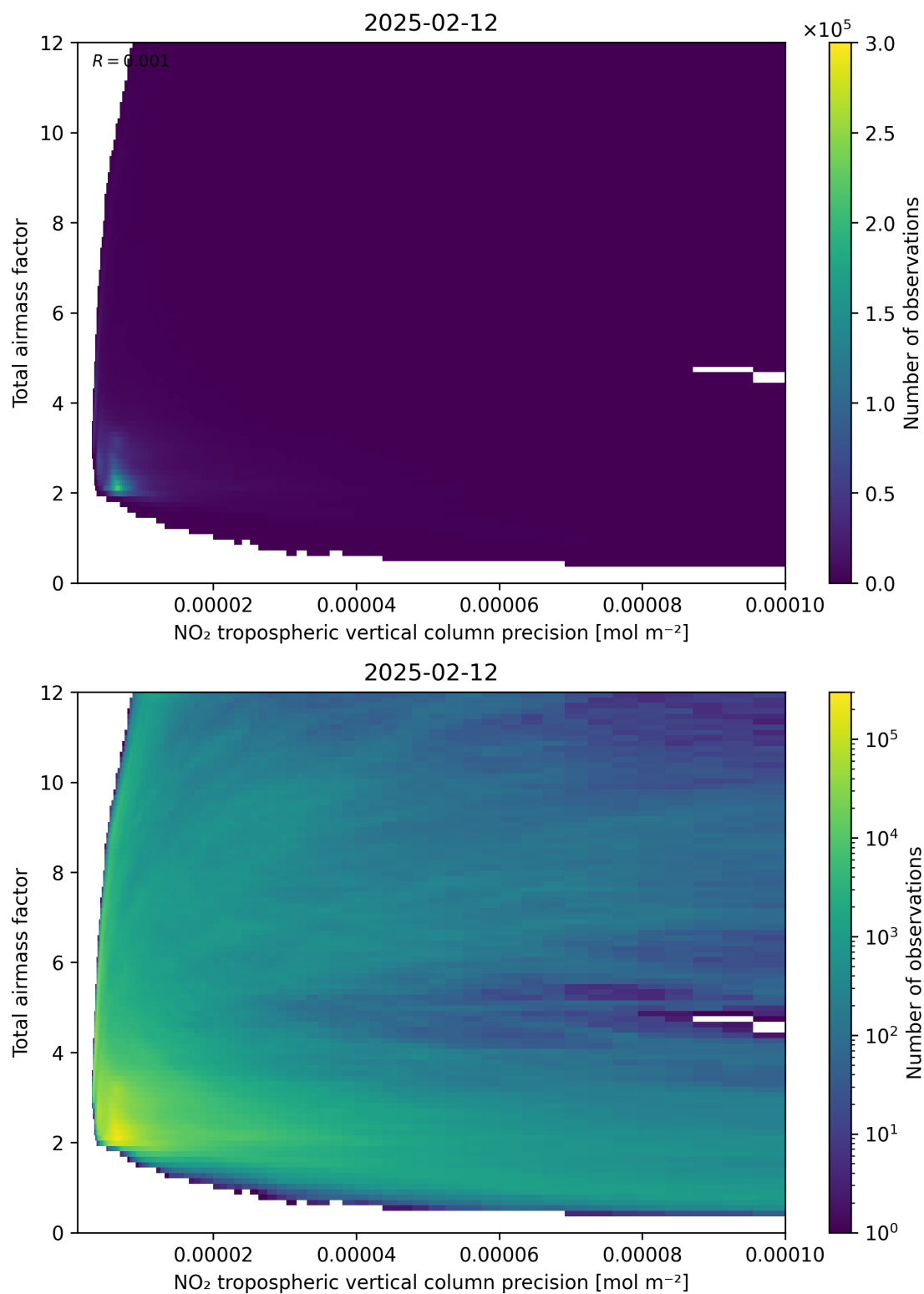
Figure 132: Scatter density plot of “NO 2 tropospheric vertical column precision” against “Total air mass factor” for 2025-02-11 to 2025-02-13.
