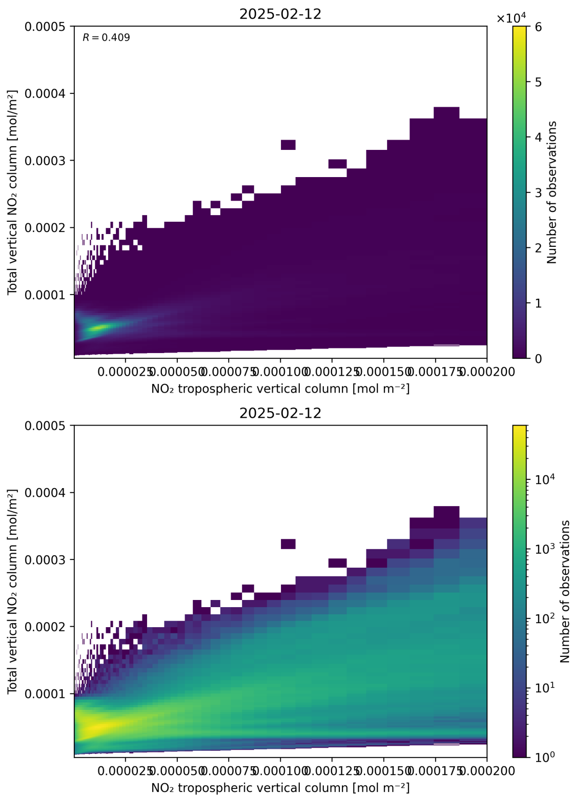
Figure 128: Scatter density plot of “NO 2 tropospheric vertical column” against “Total vertical NO 2 column” for 2025-02-11 to 2025-02-13.
