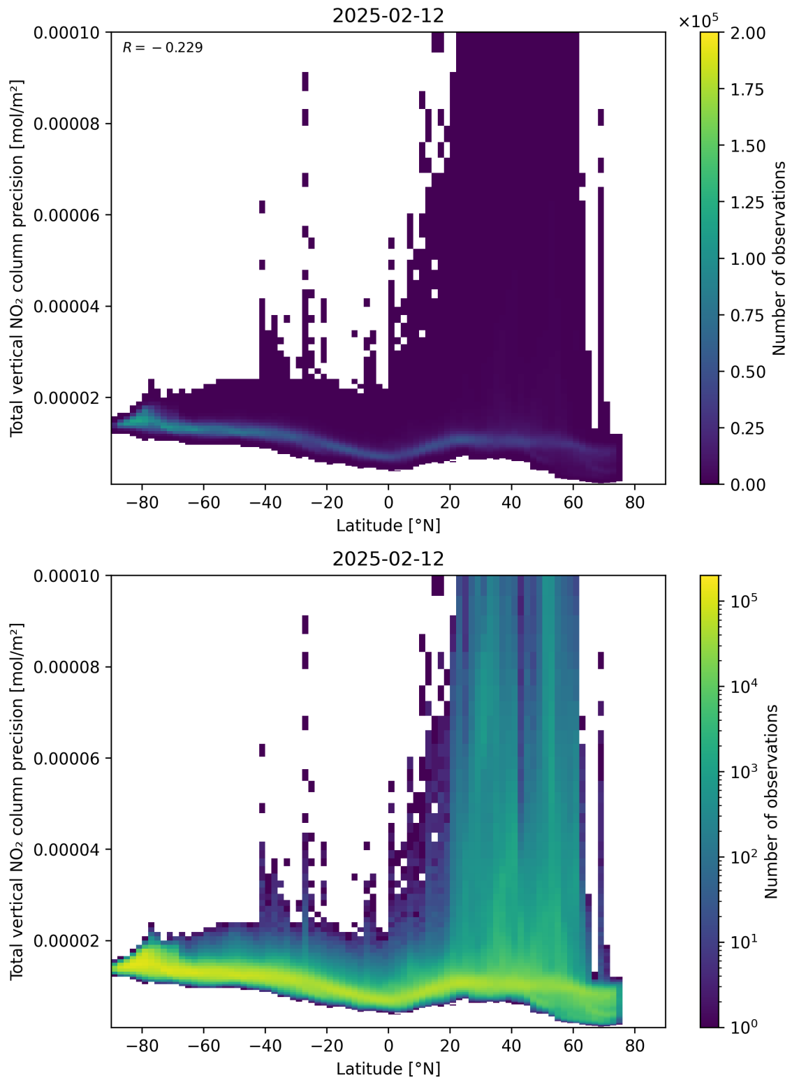
Figure 91: Scatter density plot of “Latitude” against “Total vertical NO 2 column precision” for 2025-02-11 to 2025-02-13.
