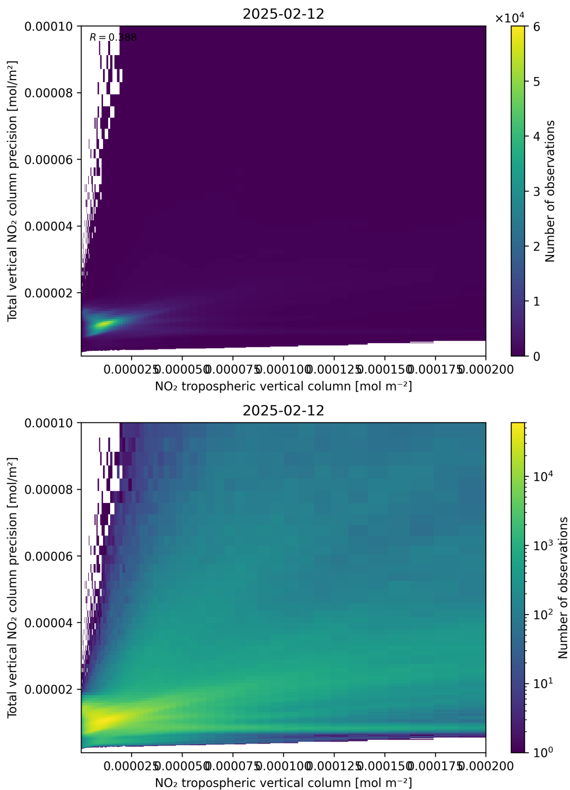
Figure 129: Scatter density plot of “NO 2 tropospheric vertical column” against “Total vertical NO 2 column precision” for 2025-02-11 to 2025-02-13.
