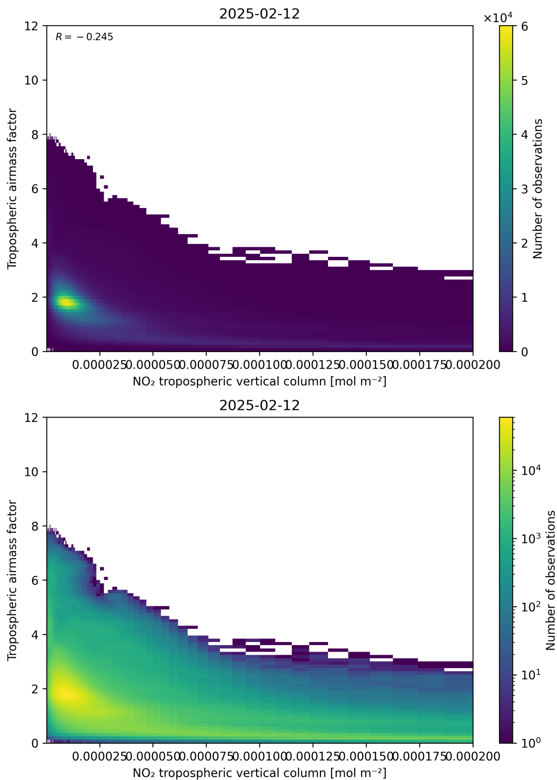
Figure 123: Scatter density plot of “NO 2 tropospheric vertical column” against “Tropospheric air mass factor” for 2025-02-11 to 2025-02-13.
