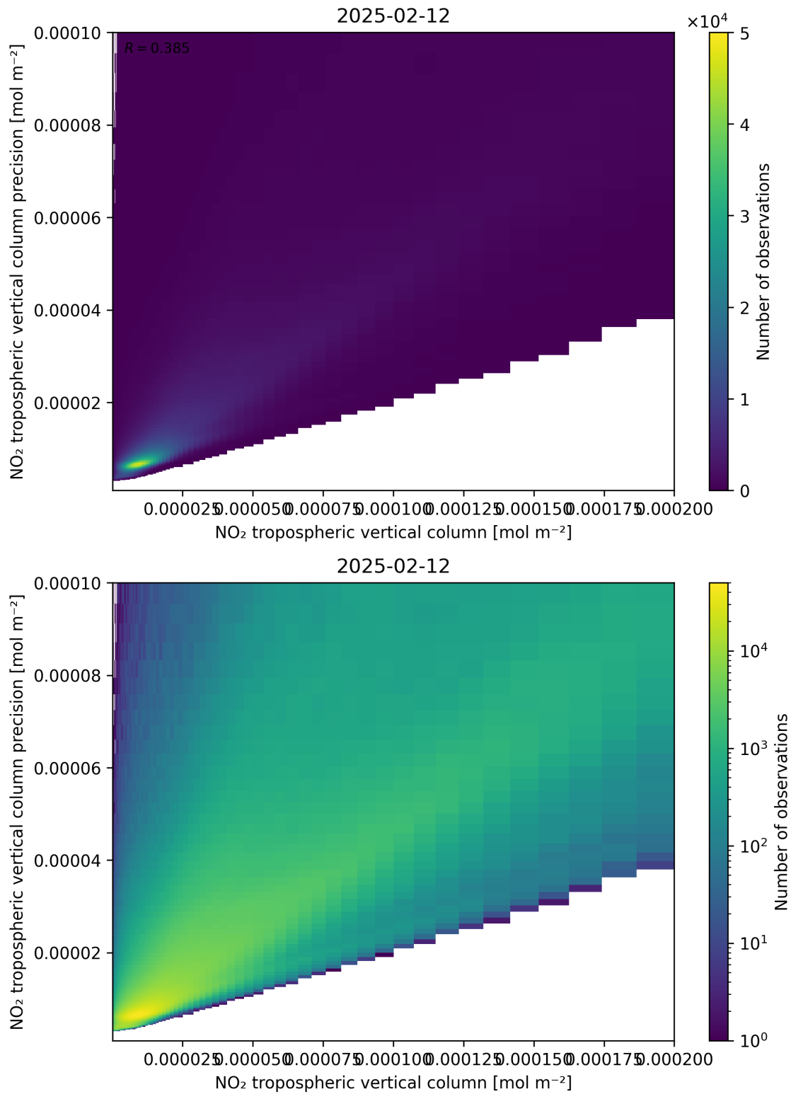
Figure 130: Scatter density plot of “NO 2 tropospheric vertical column” against “NO 2 tropospheric vertical column precision” for 2025-02-11 to 2025-02-13.
