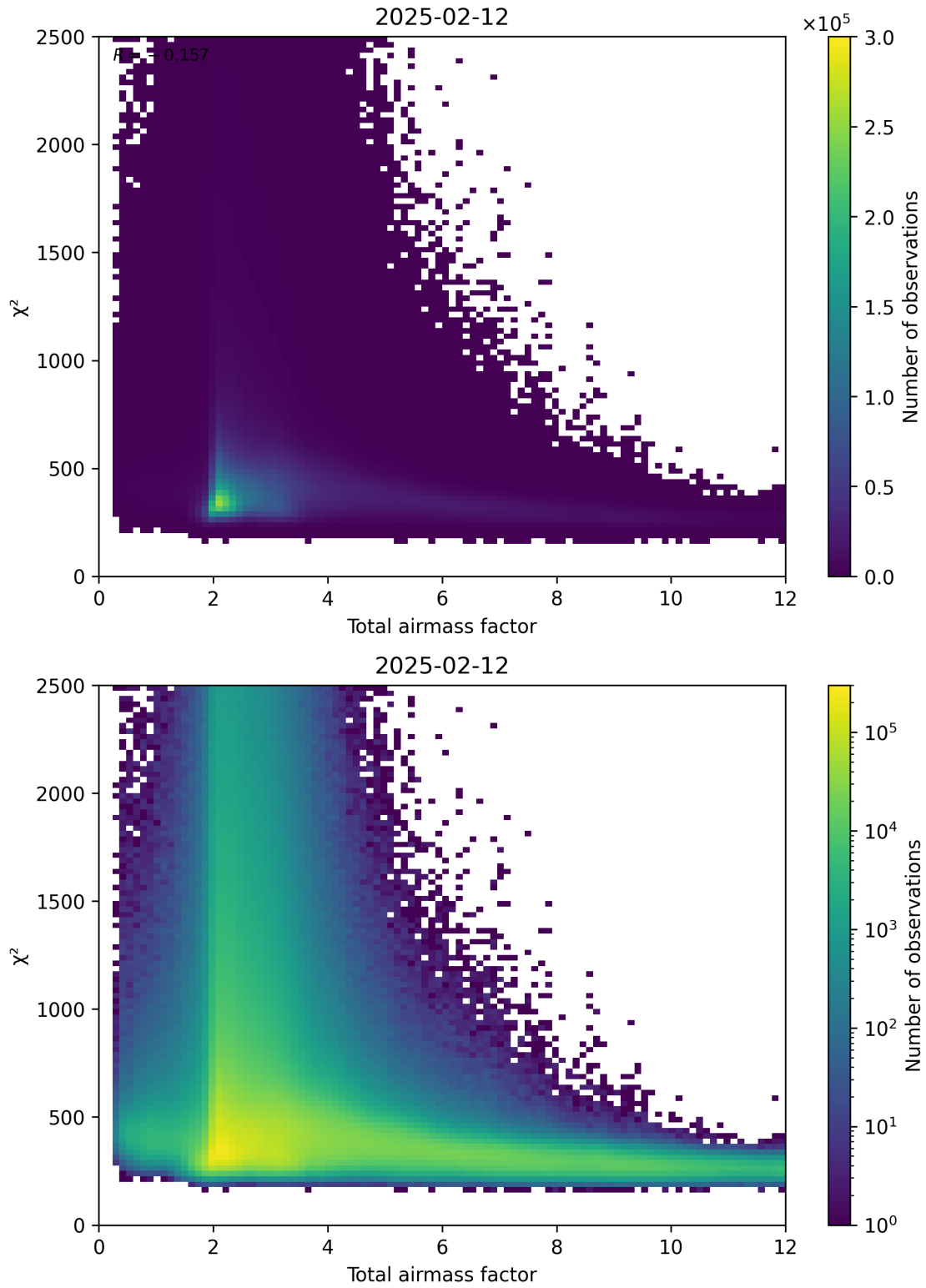
Figure 63: Scatter density plot of “Total airmass factor” against “ \chi^2 ” for 2025-02-11 to 2025-02-13.
