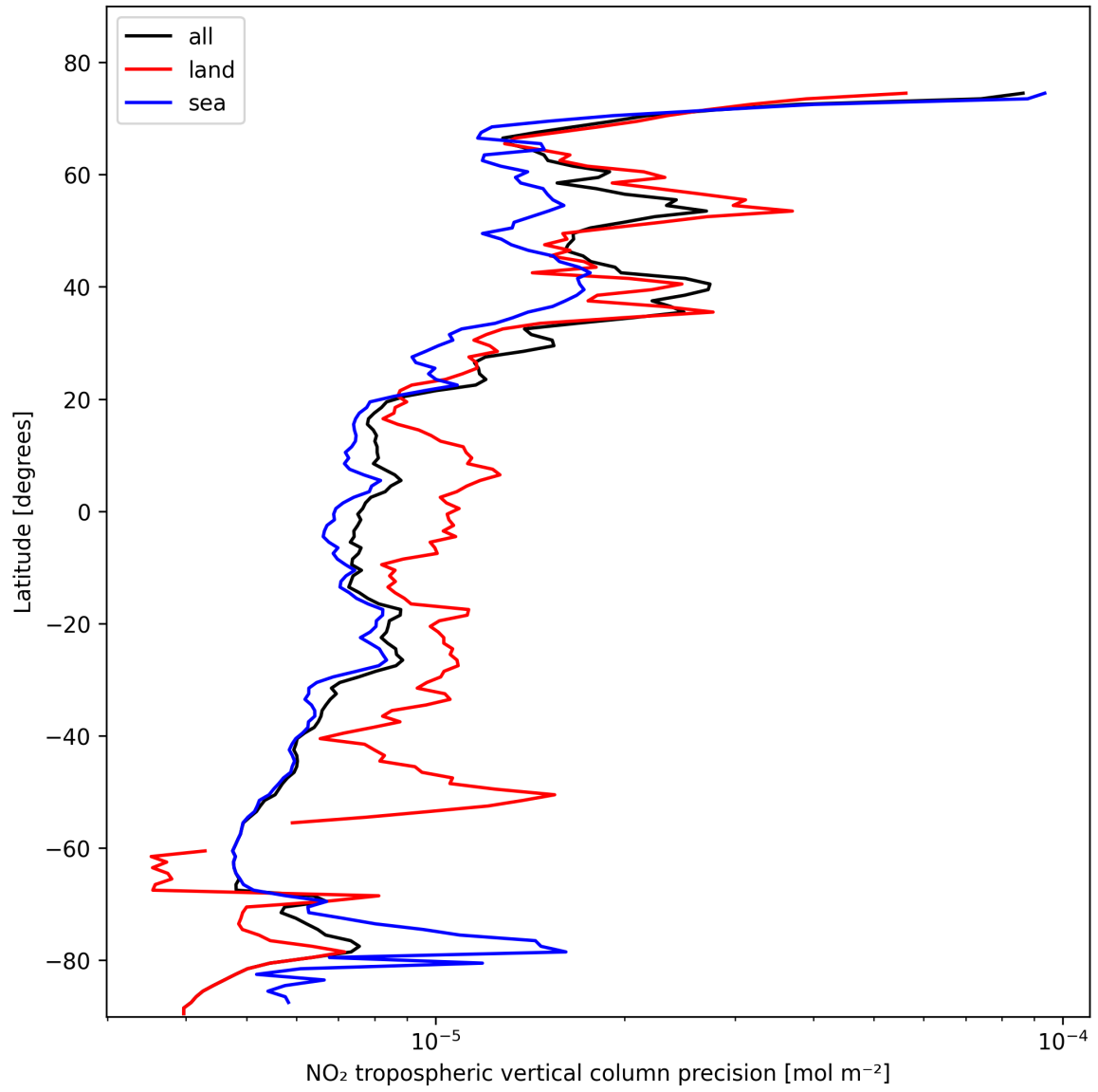
Figure 13: Zonal average of “NO 2 tropospheric vertical column precision” for 2025-02-11 to 2025-02-13.
