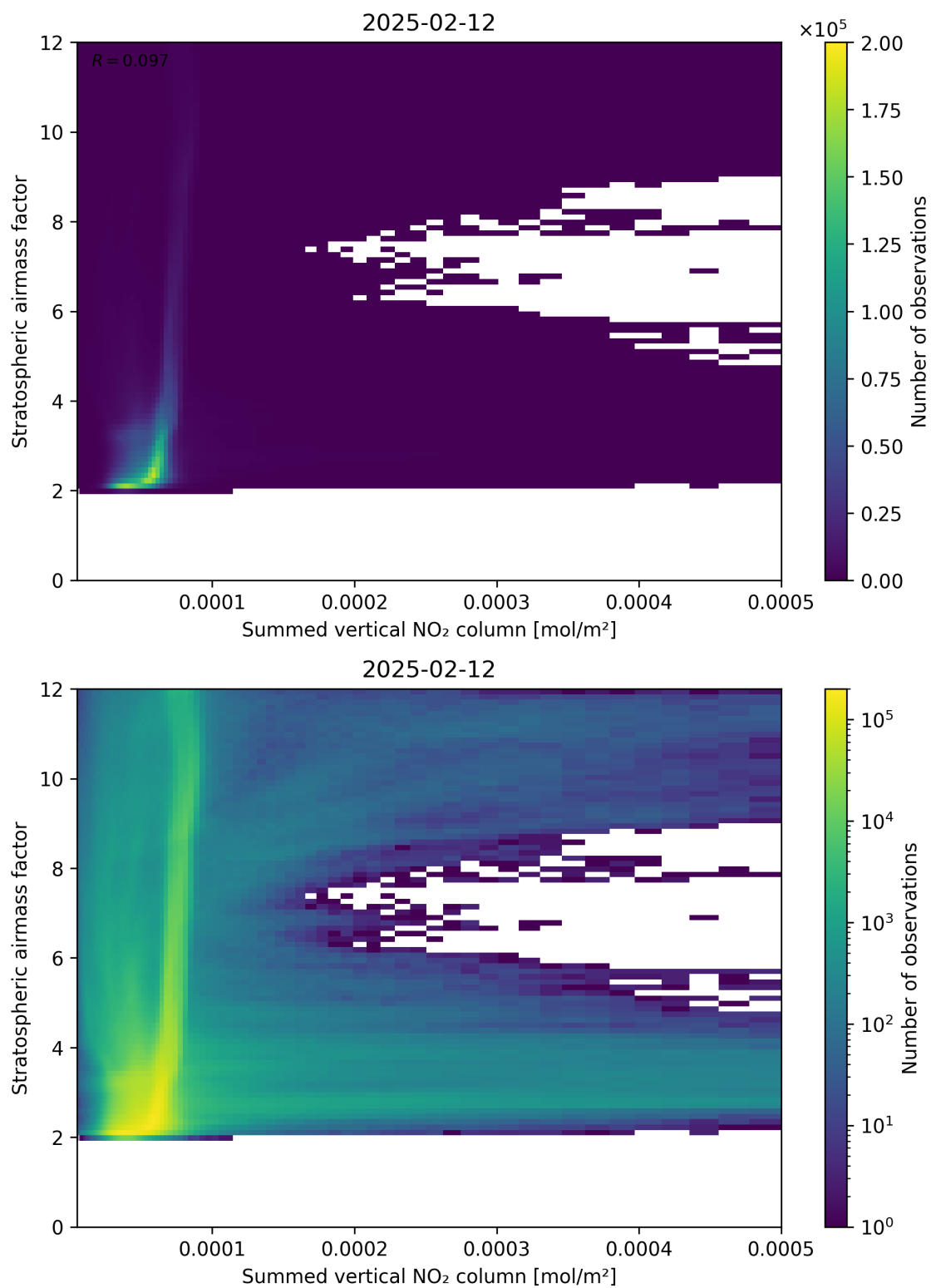
Figure 103: Scatter density plot of “Summed vertical NO 2 column” against “Stratospheric air mass factor” for 2025-02-11 to 2025-02-13.
