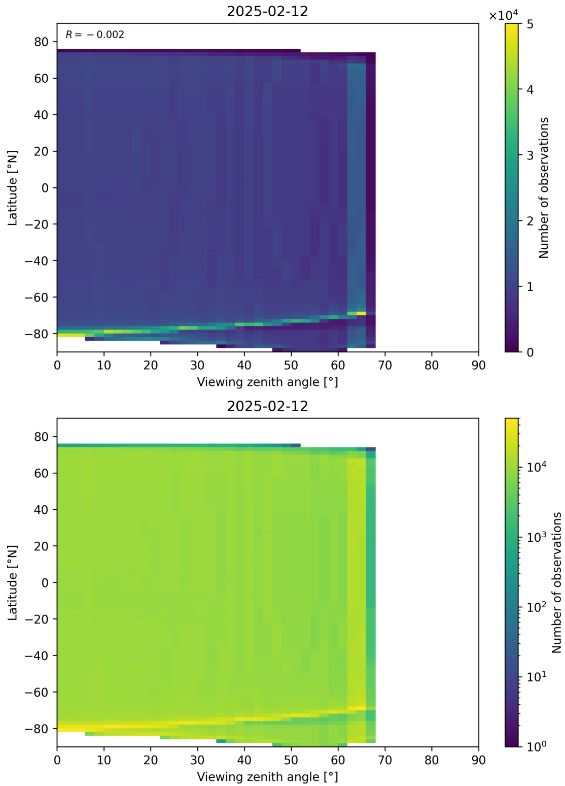
Figure 163: Scatter density plot of “Viewing zenith angle” against “Latitude” for 2025-02-11 to 2025-02-13.
