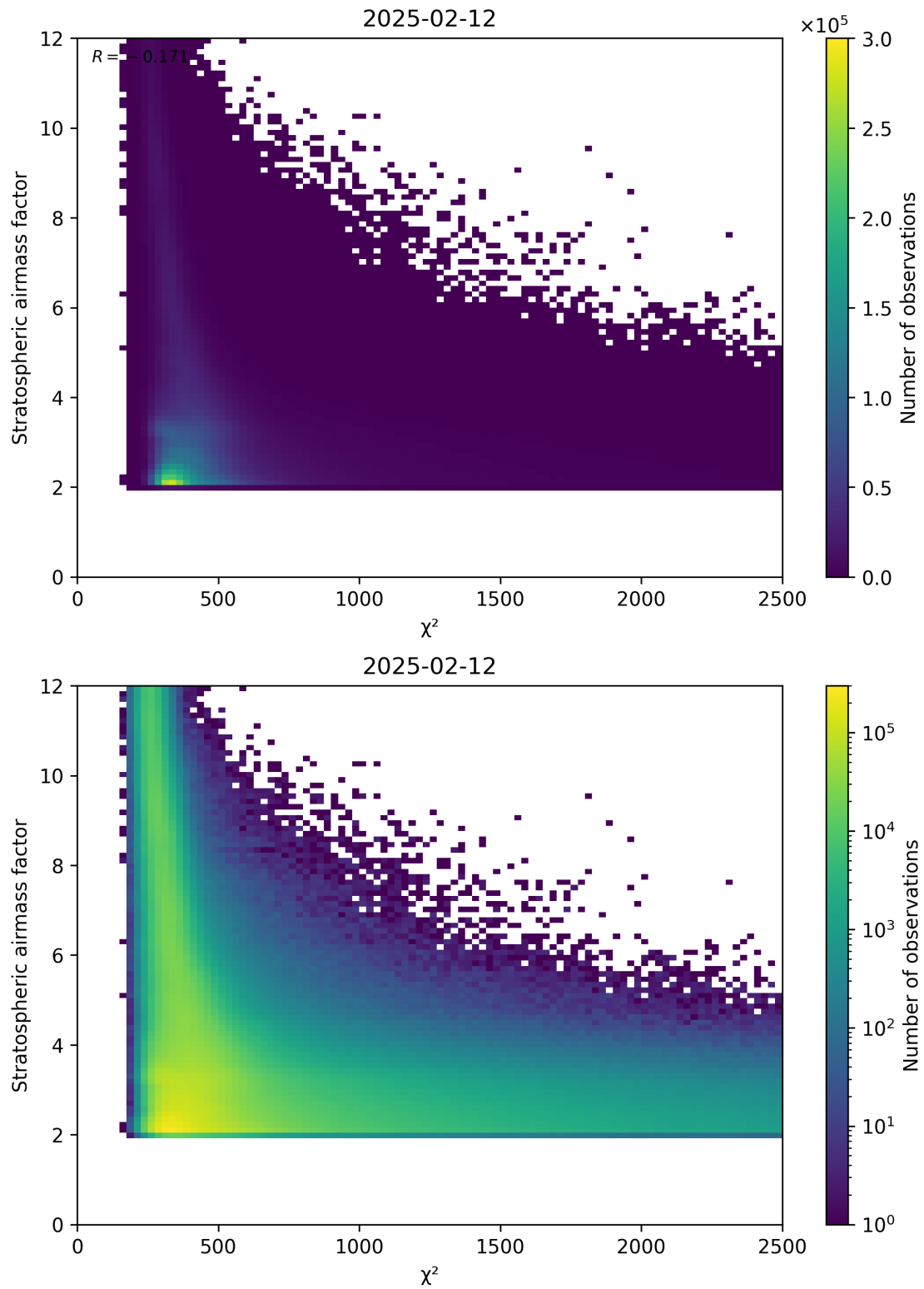
Figure 81: Scatter density plot of “ \chi^2 ” against “Stratospheric airmass factor” for 2025-02-11 to 2025-02-13.
