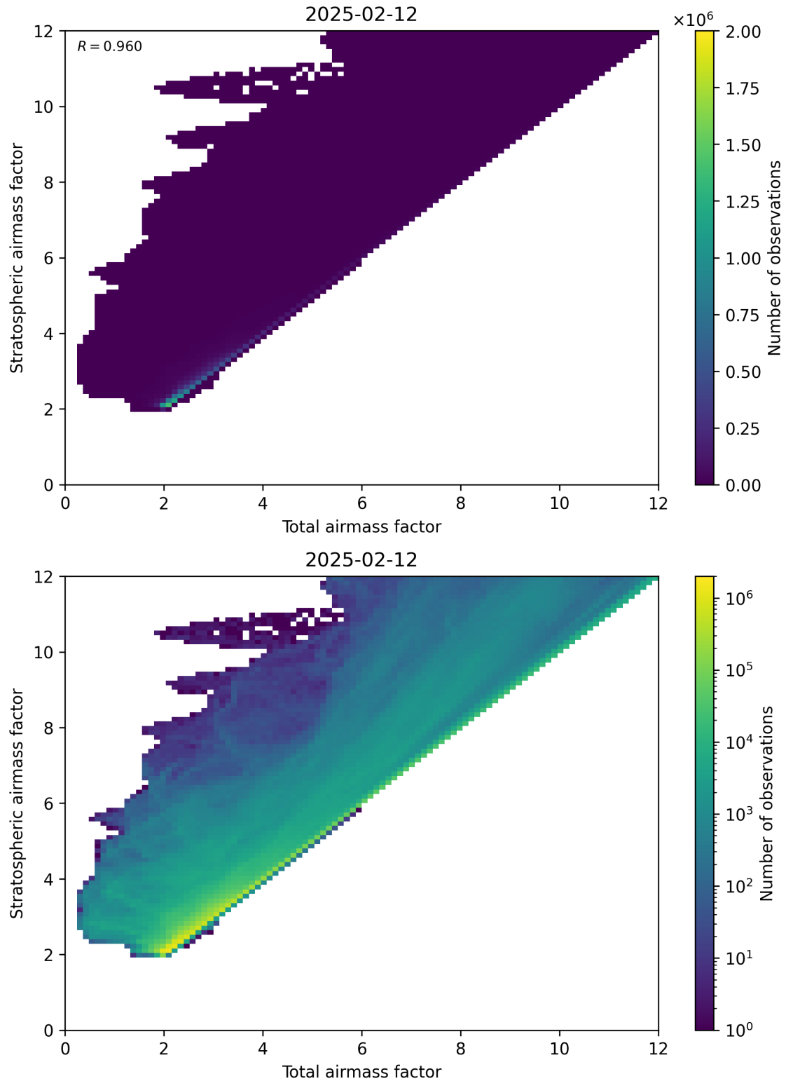
Figure 62: Scatter density plot of “Total airmass factor” against “Stratospheric airmass factor” for 2025-02-11 to 2025-02-13.
