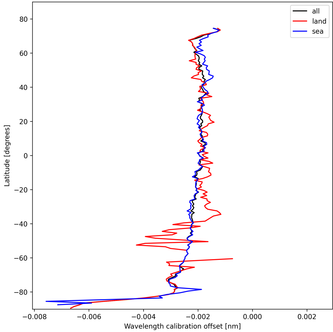
Figure 18: Zonal average of “Wavelength calibration offset” for 2025-02-11 to 2025-02-13.
