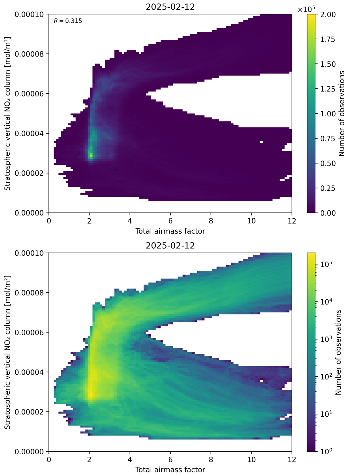
Figure 64: Scatter density plot of “Total airmass factor” against “Stratospheric vertical NO 2 column” for 2025-02-11 to 2025-02-13.
