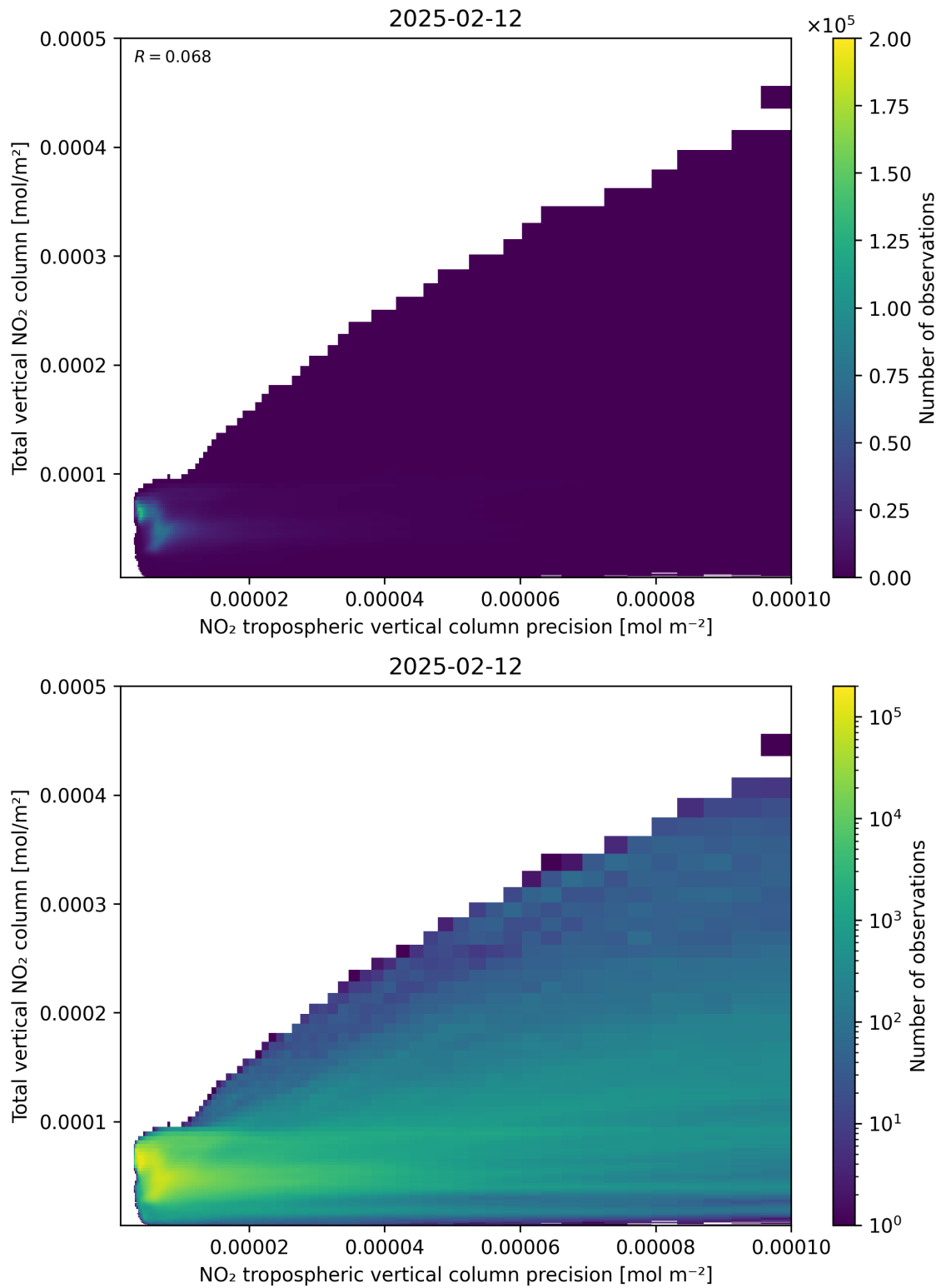
Figure 138: Scatter density plot of “NO 2 tropospheric vertical column precision” against “Total vertical NO 2 column” for 2025-02-11 to 2025-02-13.
