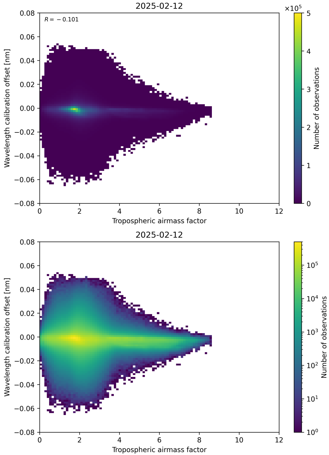
Figure 80: Scatter density plot of “Tropospheric airmass factor” against “Wavelength calibration offset” for 2025-02-11 to 2025-02-13.
