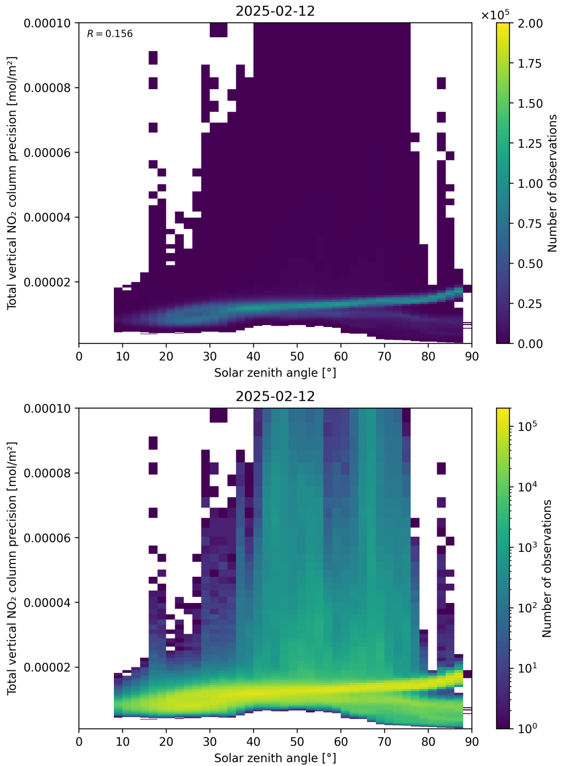
Figure 154: Scatter density plot of “Solar zenith angle” against “Total vertical NO 2 column precision” for 2025-02-11 to 2025-02-13.
