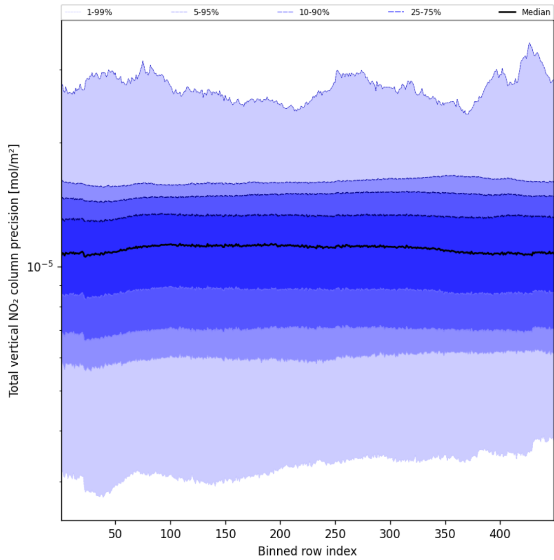
Figure 56: Along track statistics of “Total vertical NO 2 column precision” for 2025-02-11 to 2025-02-13
