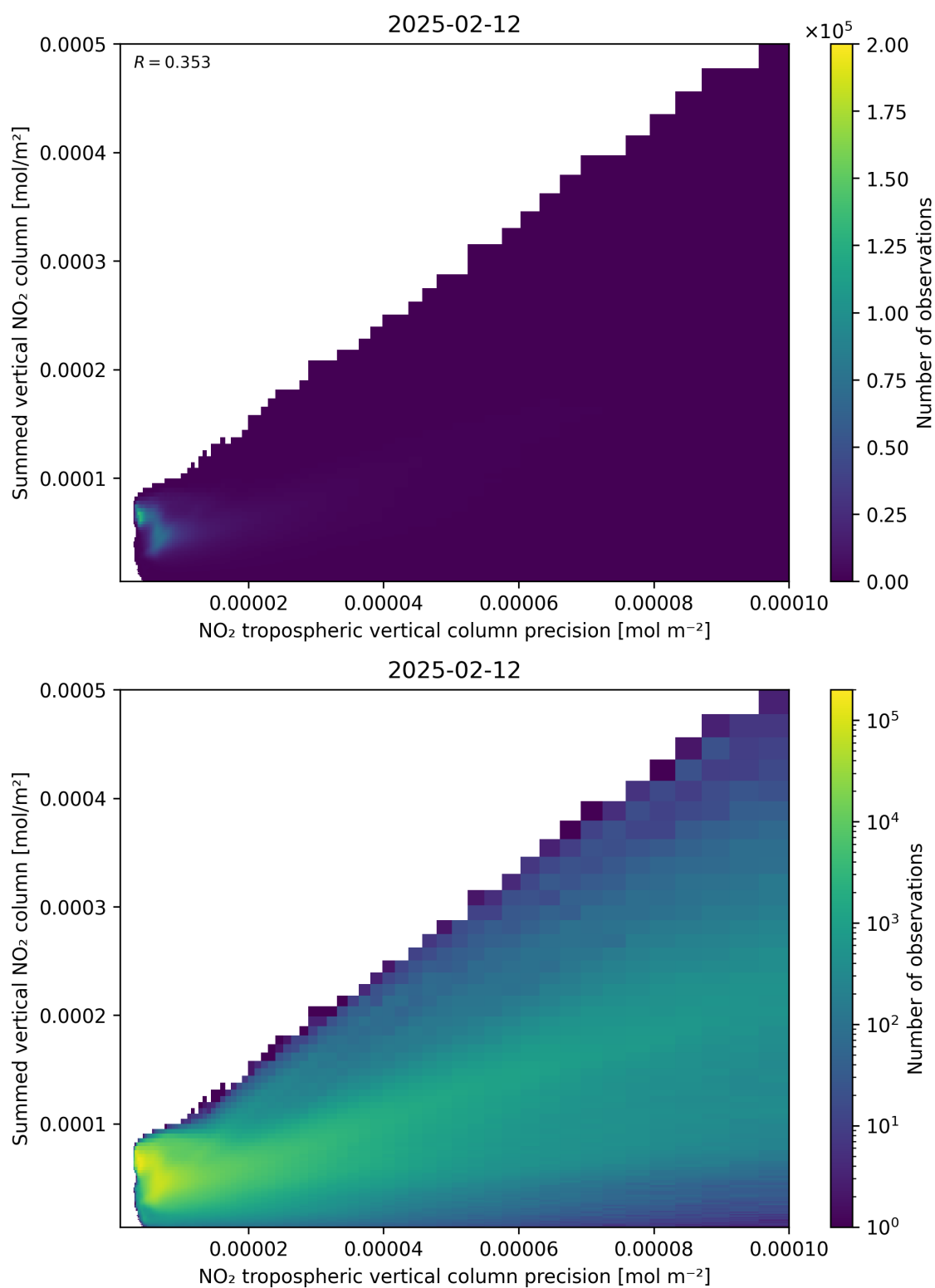
Figure 136: Scatter density plot of “NO 2 tropospheric vertical column precision” against “Summed vertical NO 2 column” for 2025-02-11 to 2025-02-13.
