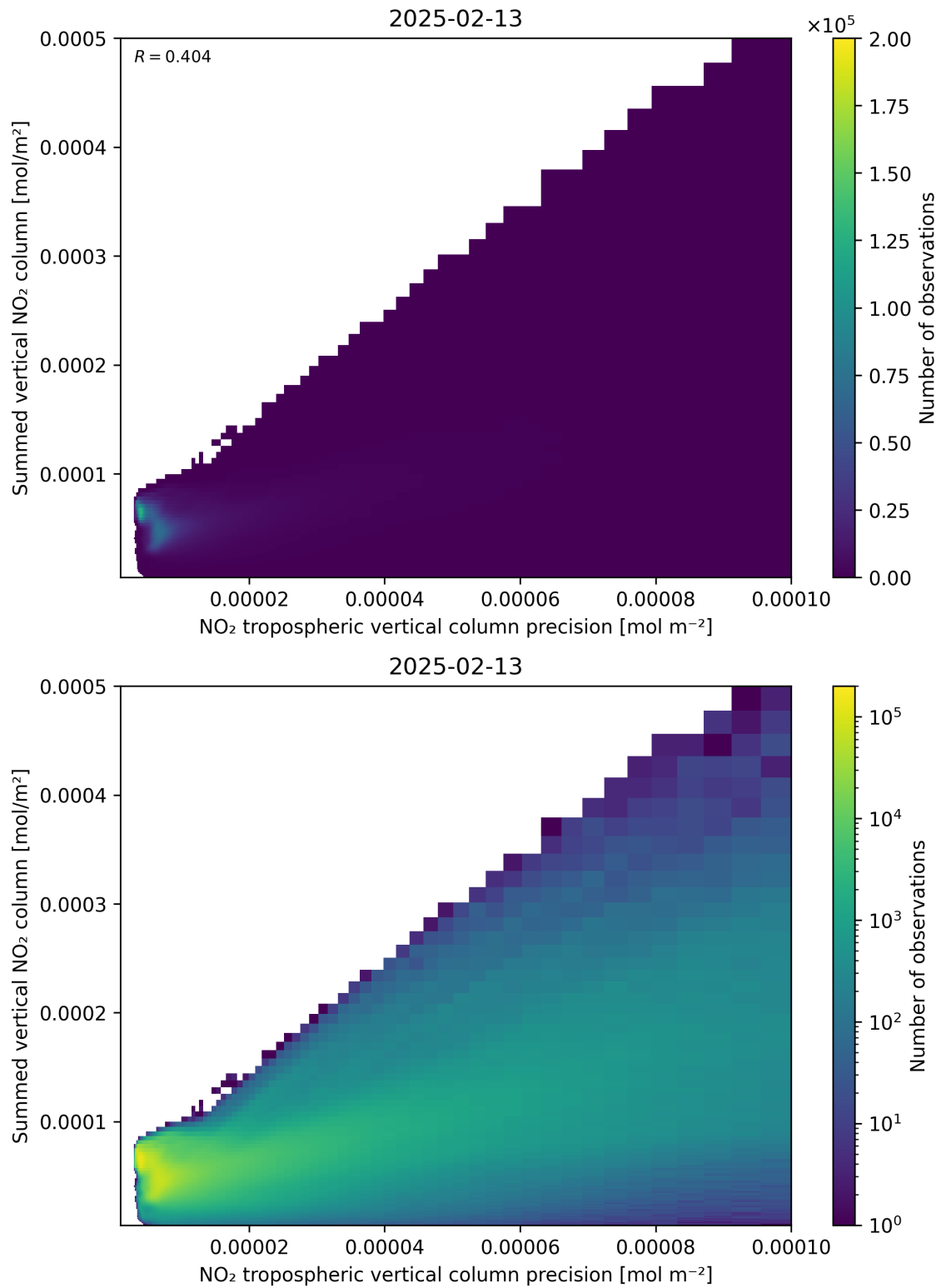
Figure 136: Scatter density plot of “NO 2 tropospheric vertical column precision” against “Summed vertical NO 2 column” for 2025-02-13 to 2025-02-14.
