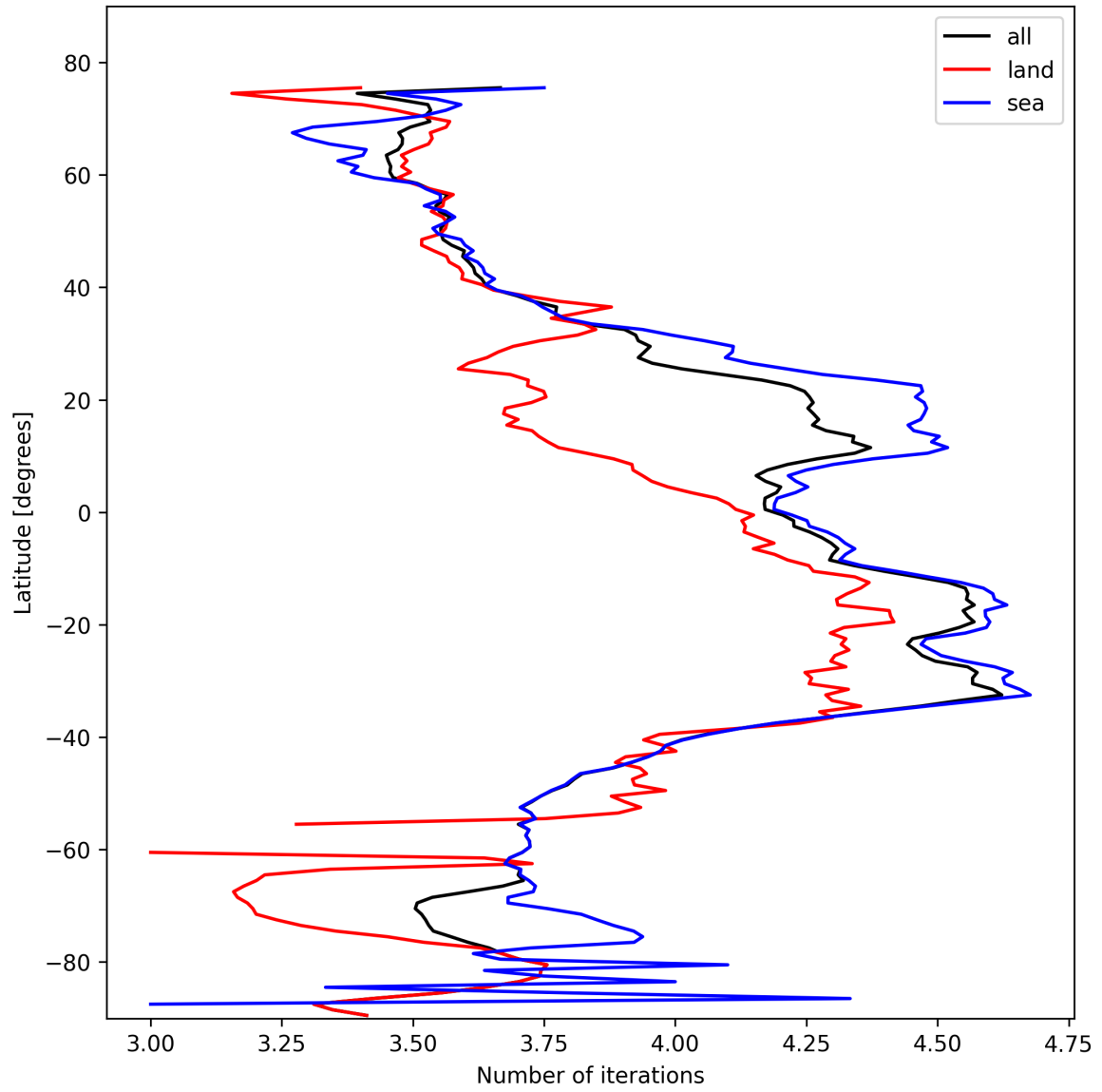
Figure 17: Zonal average of “Number of iterations” for 2025-02-13 to 2025-02-14.
