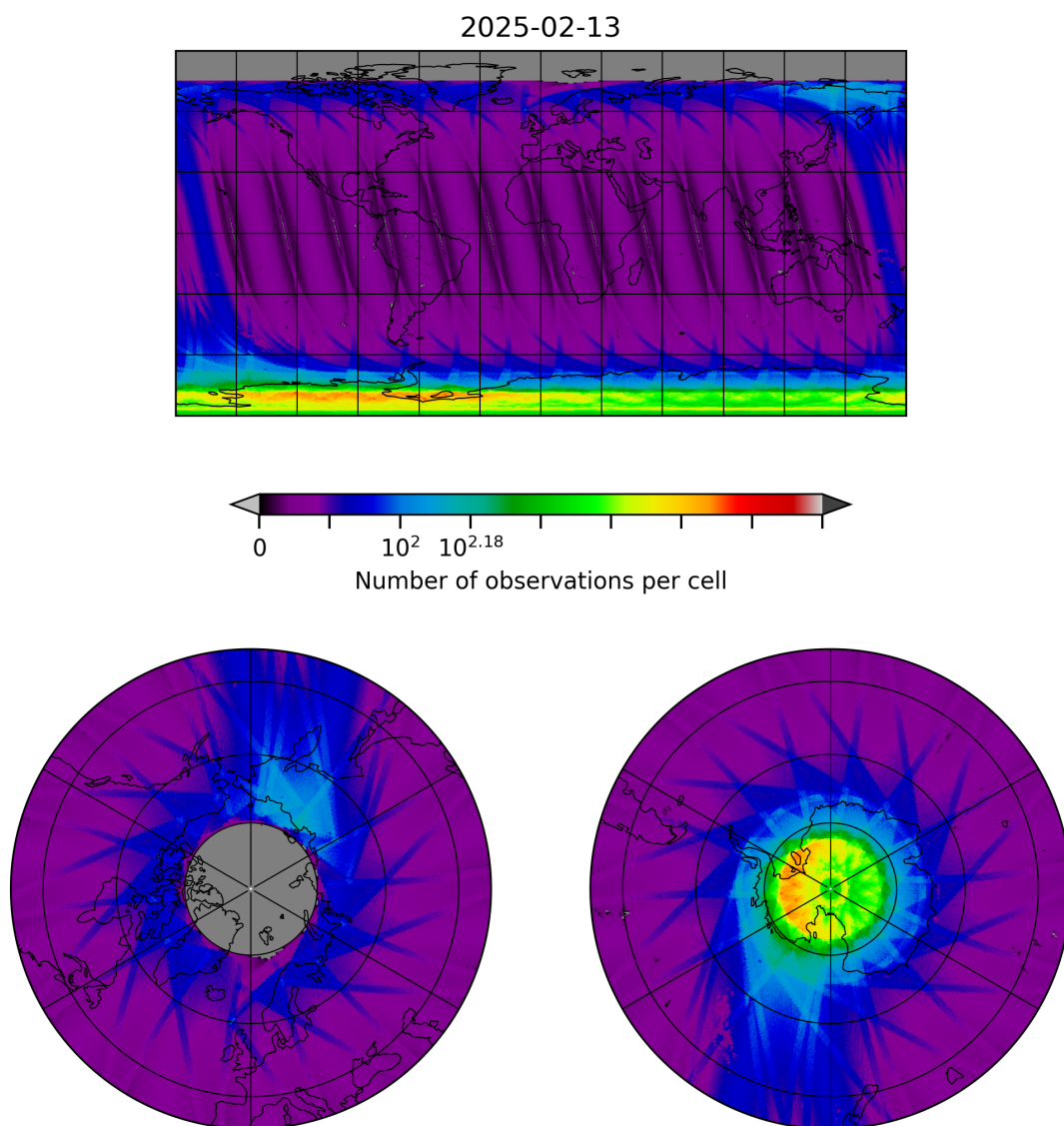
Figure 10: Map of the number of observations for 2025-02-13 to 2025-02-14
