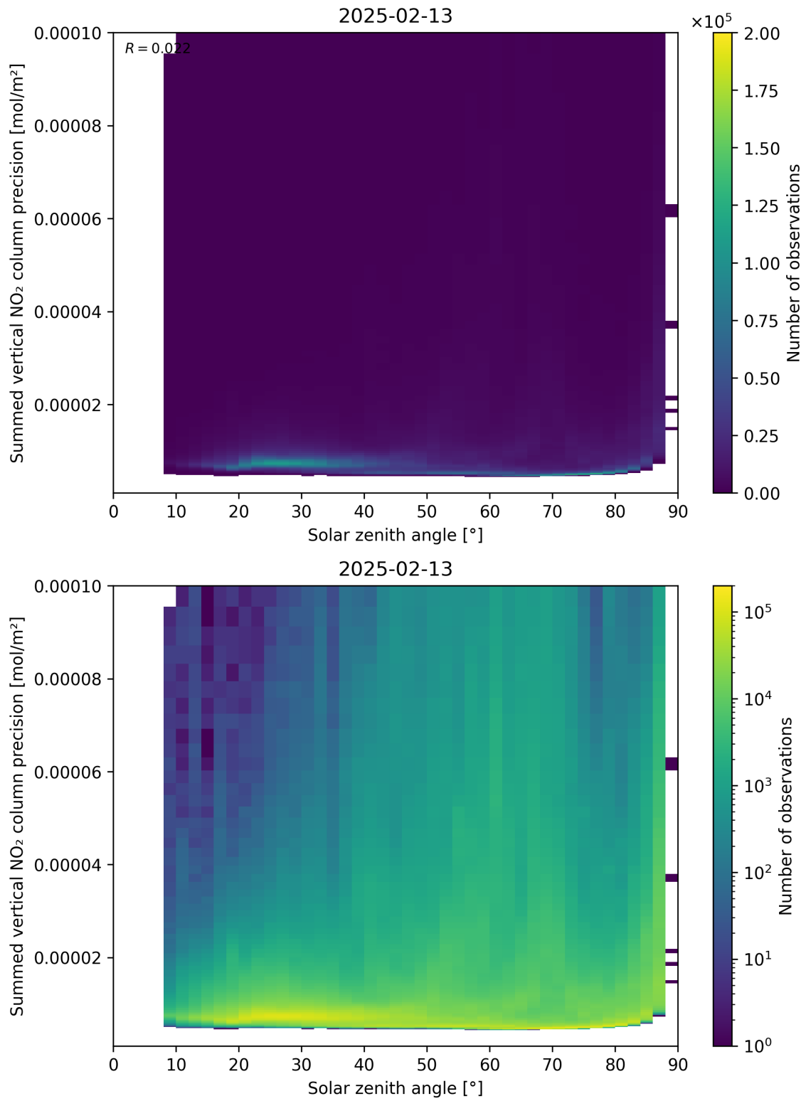
Figure 152: Scatter density plot of “Solar zenith angle” against “Summed vertical NO 2 column precision” for 2025-02-13 to 2025-02-14.
