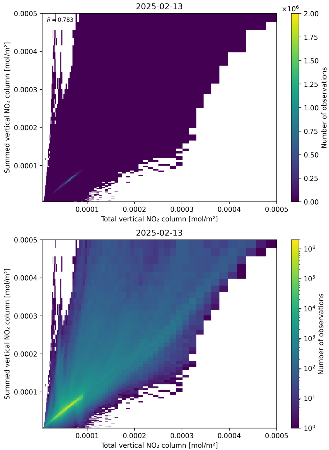
Figure 112: Scatter density plot of “Total vertical NO 2 column” against “Summed vertical NO 2 column” for 2025-02-13 to 2025-02-14.
