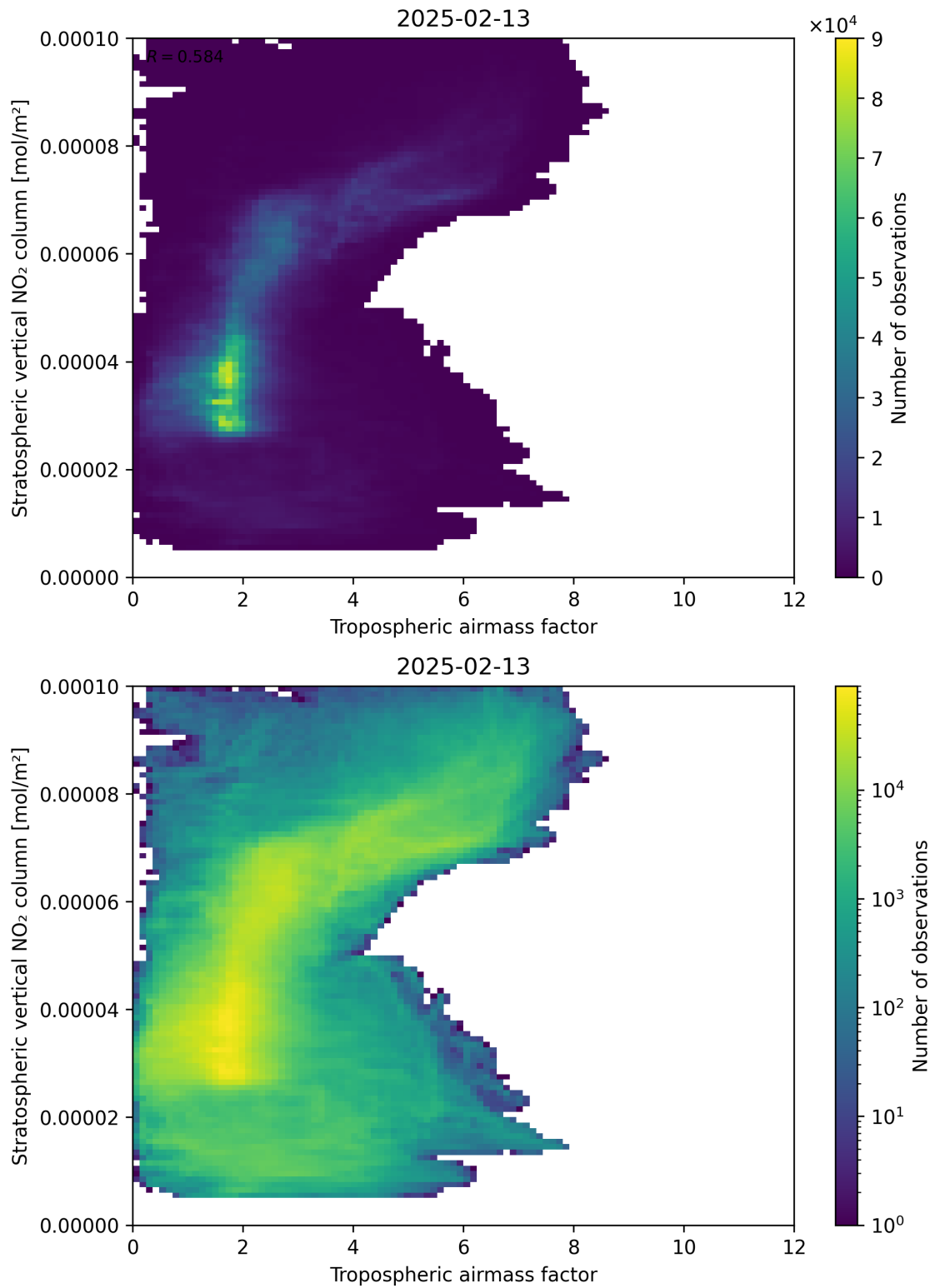
Figure 74: Scatter density plot of “Tropospheric airmass factor” against “Stratospheric vertical NO 2 column” for 2025-02-13 to 2025-02-14.
