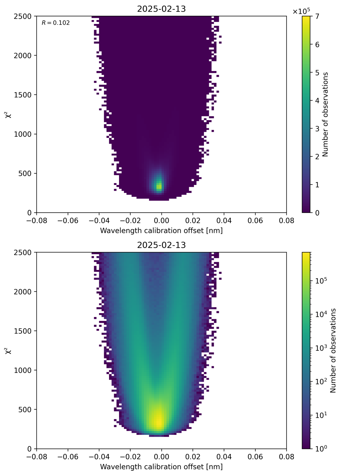
Figure 175: Scatter density plot of “Wavelength calibration offset” against “ \chi^2 ” for 2025-02-13 to 2025-02-14.
