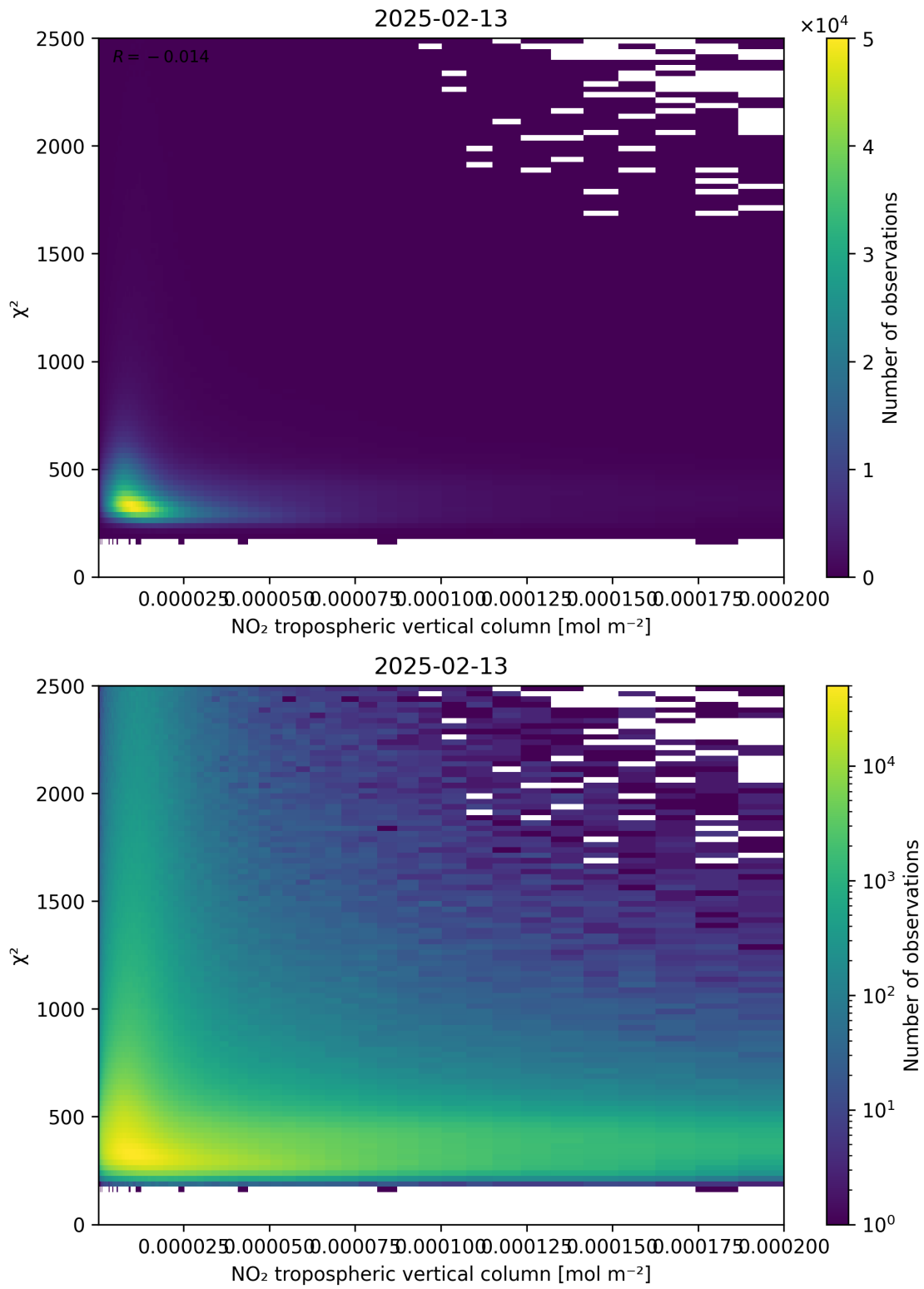
Figure 124: Scatter density plot of “NO 2 tropospheric vertical column” against “ \chi^2 ” for 2025-02-13 to 2025-02-14.
