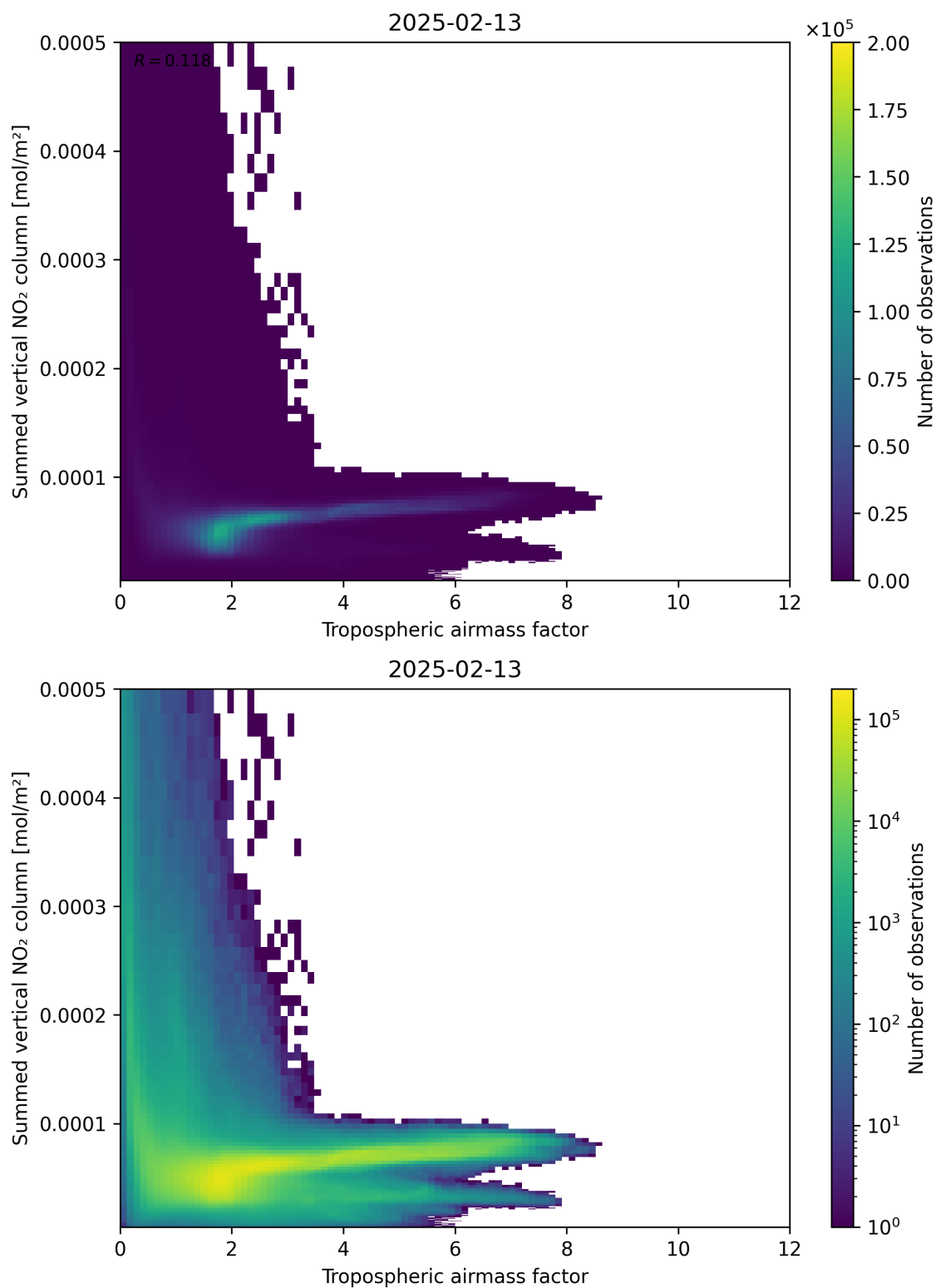
Figure 75: Scatter density plot of “Tropospheric airmass factor” against “Summed vertical NO 2 column” for 2025-02-13 to 2025-02-14.
