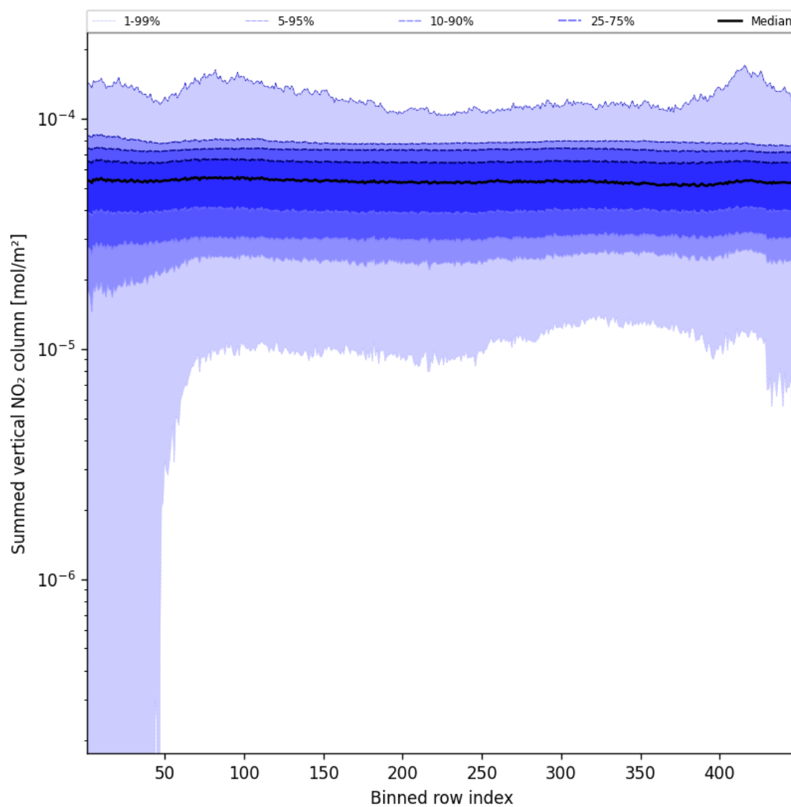
Figure 57: Along track statistics of “Summed vertical NO 2 column” for 2025-02-13 to 2025-02-14
