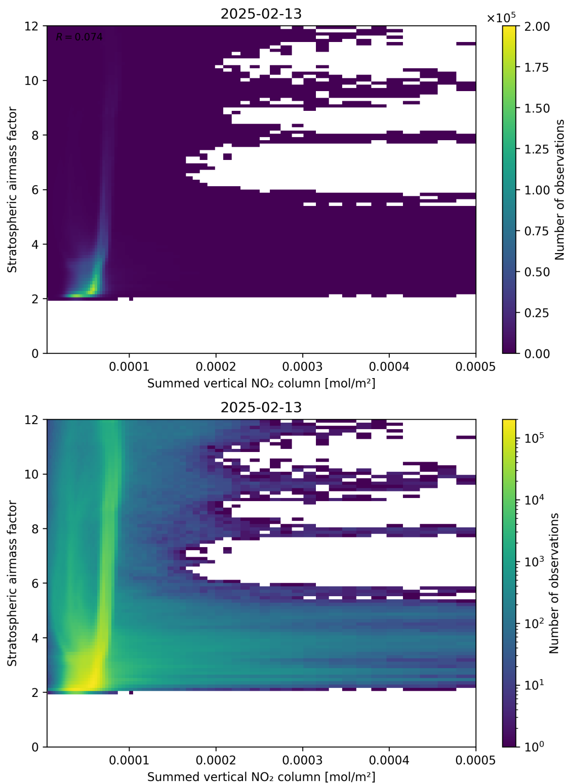
Figure 103: Scatter density plot of “Summed vertical NO 2 column” against “Stratospheric air mass factor” for 2025-02-13 to 2025-02-14.
