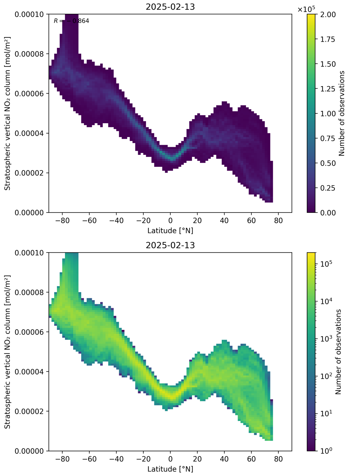
Figure 87: Scatter density plot of “Latitude” against “Stratospheric vertical NO 2 column” for 2025-02-13 to 2025-02-14.
