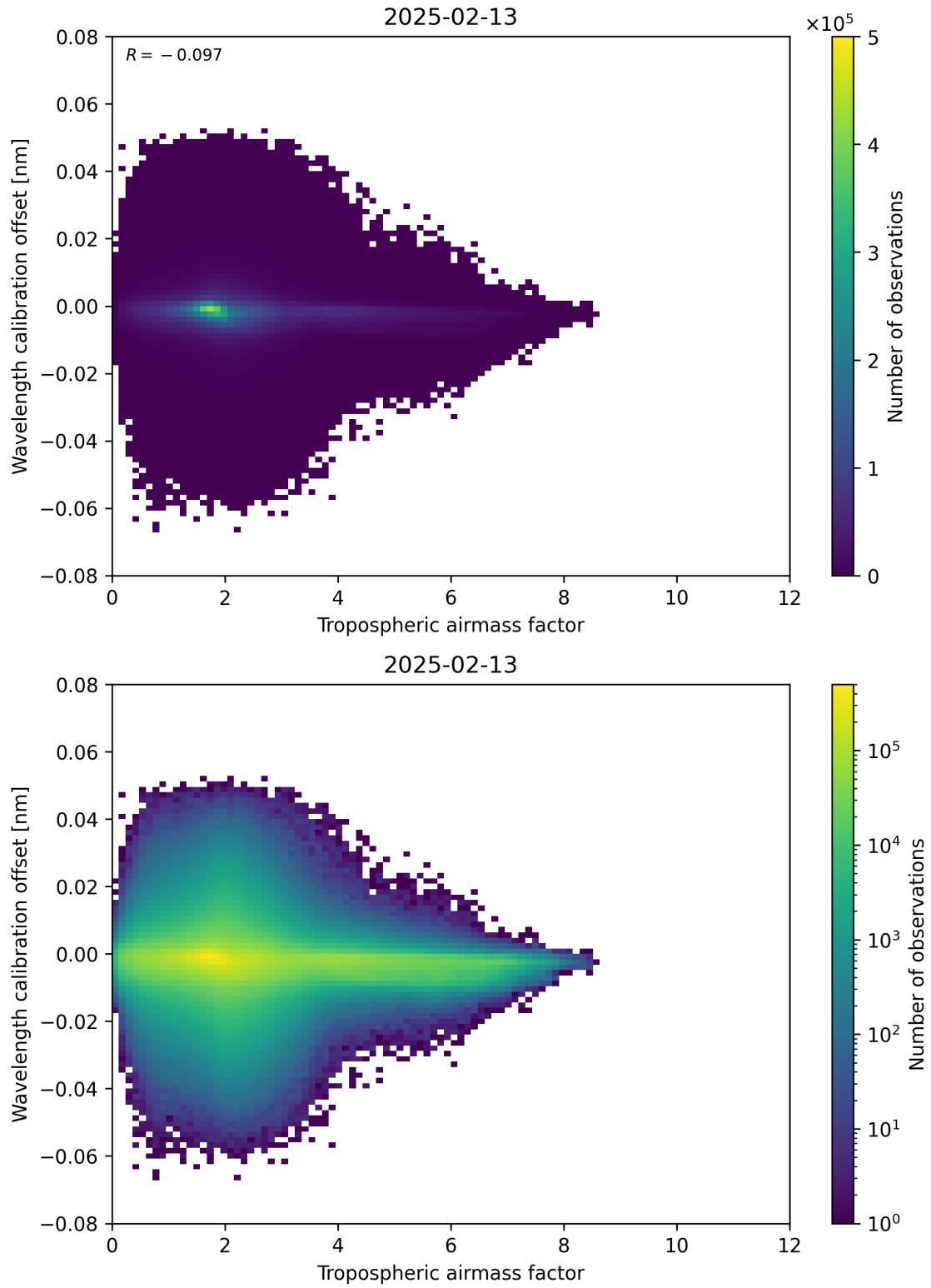
Figure 80: Scatter density plot of “Tropospheric airmass factor” against “Wavelength calibration offset” for 2025-02-13 to 2025-02-14.
