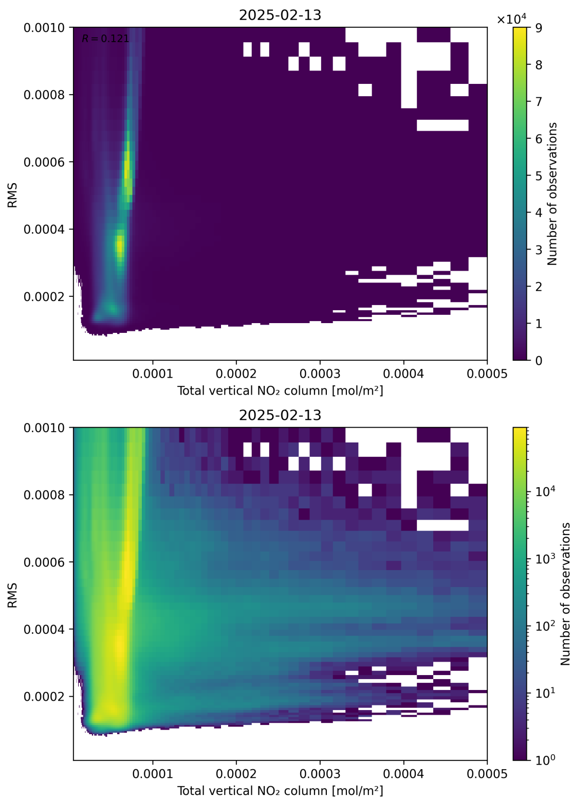
Figure 120: Scatter density plot of “Total vertical NO 2 column” against “RMS” for 2025-02-13 to 2025-02-14.
