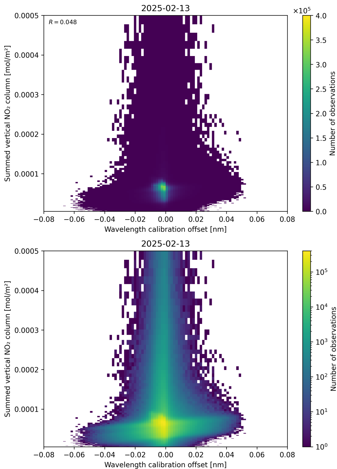
Figure 177: Scatter density plot of “Wavelength calibration offset” against “Summed vertical NO 2 column” for 2025-02-13 to 2025-02-14.
