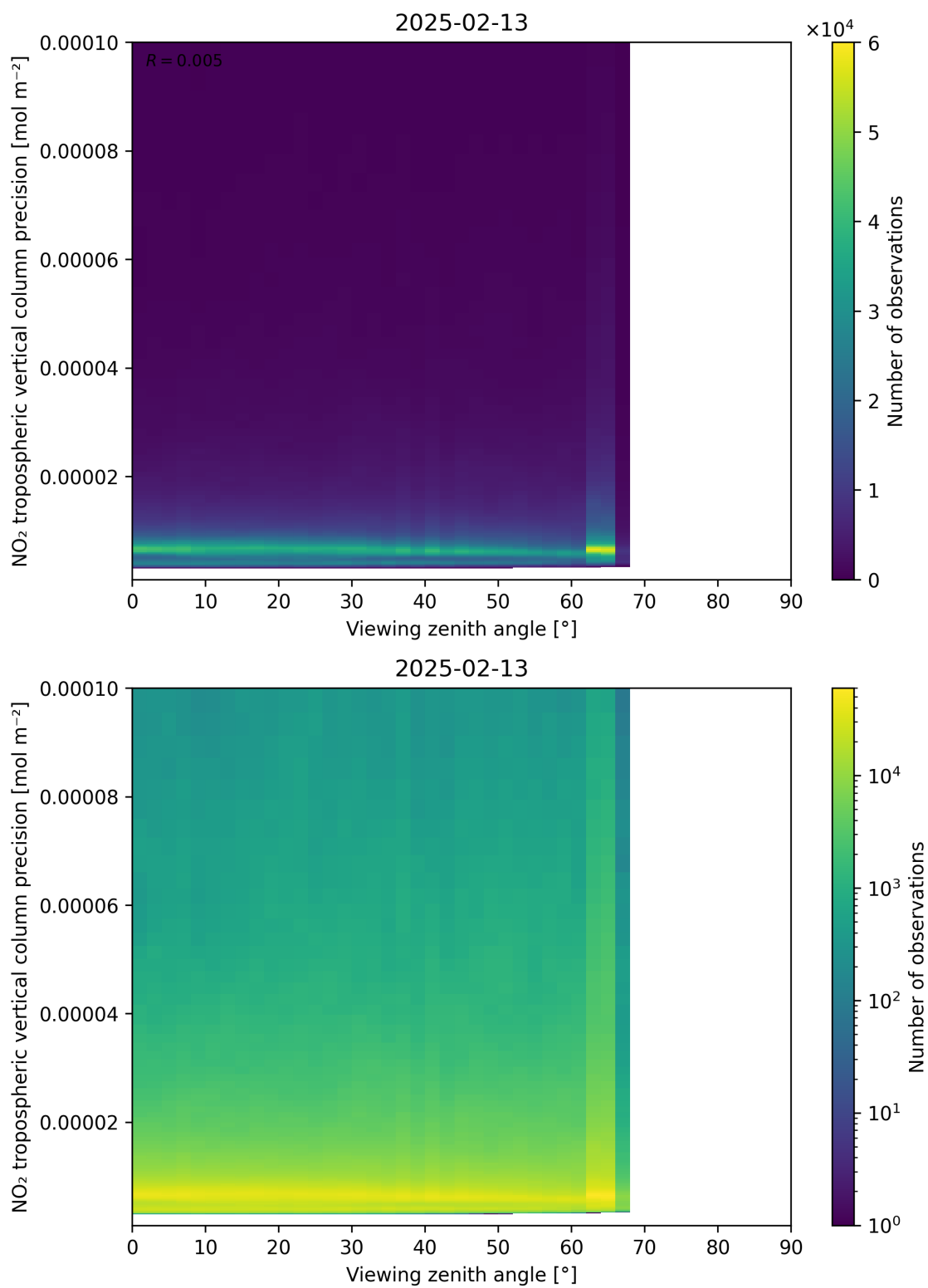
Figure 170: Scatter density plot of “Viewing zenith angle” against “NO 2 tropospheric vertical column precision” for 2025-02-13 to 2025-02-14.
