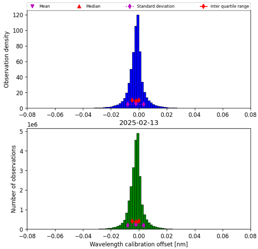
Figure 35: Histogram of “Wavelength calibration offset” for 2025-02-13 to 2025-02-14
