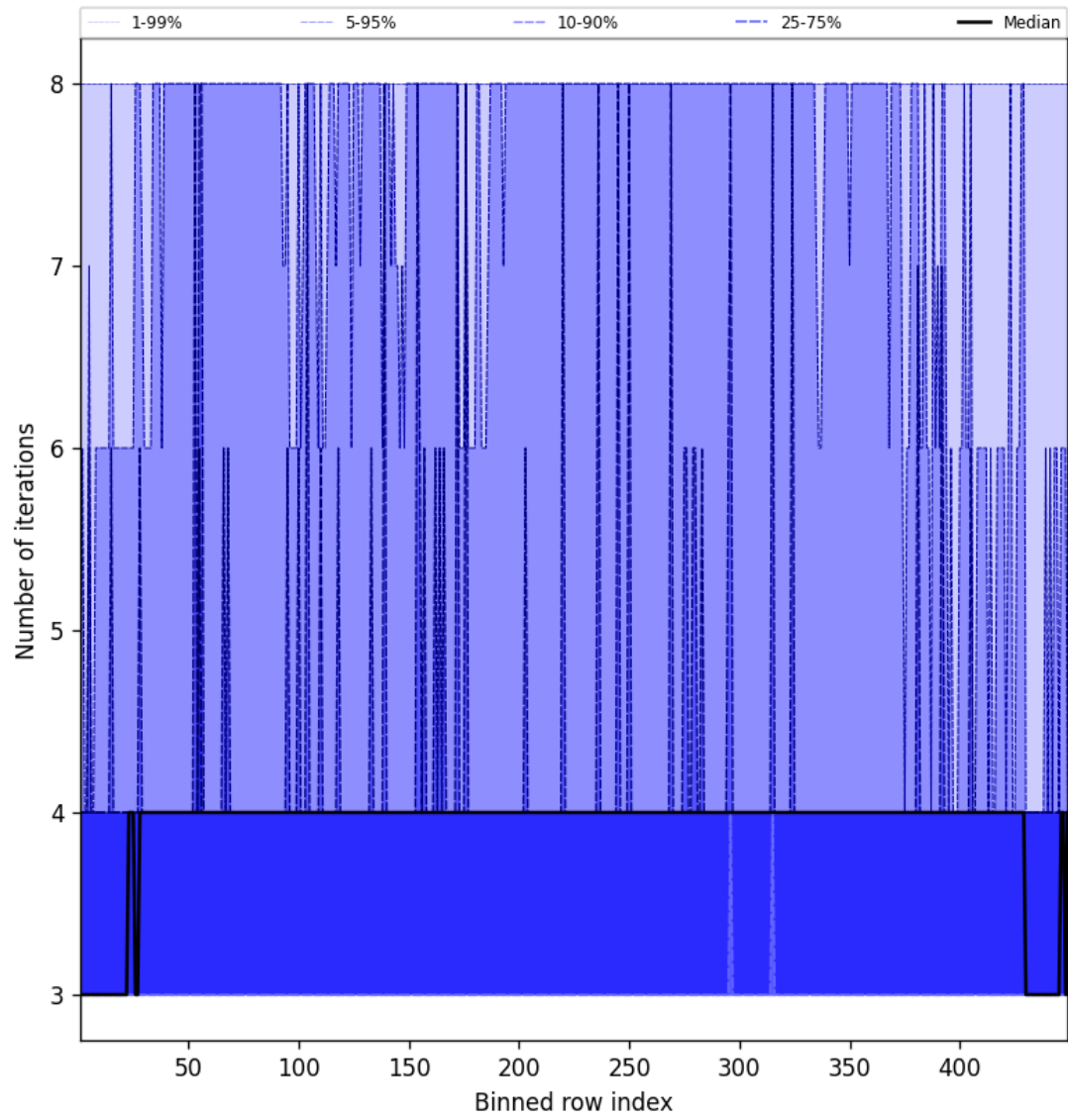
Figure 51: Along track statistics of “Number of iterations” for 2025-02-13 to 2025-02-14
