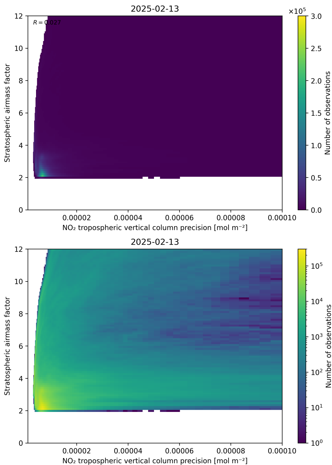
Figure 131: Scatter density plot of “NO 2 tropospheric vertical column precision” against “Stratospheric airmass factor” for 2025-02-13 to 2025-02-14.
