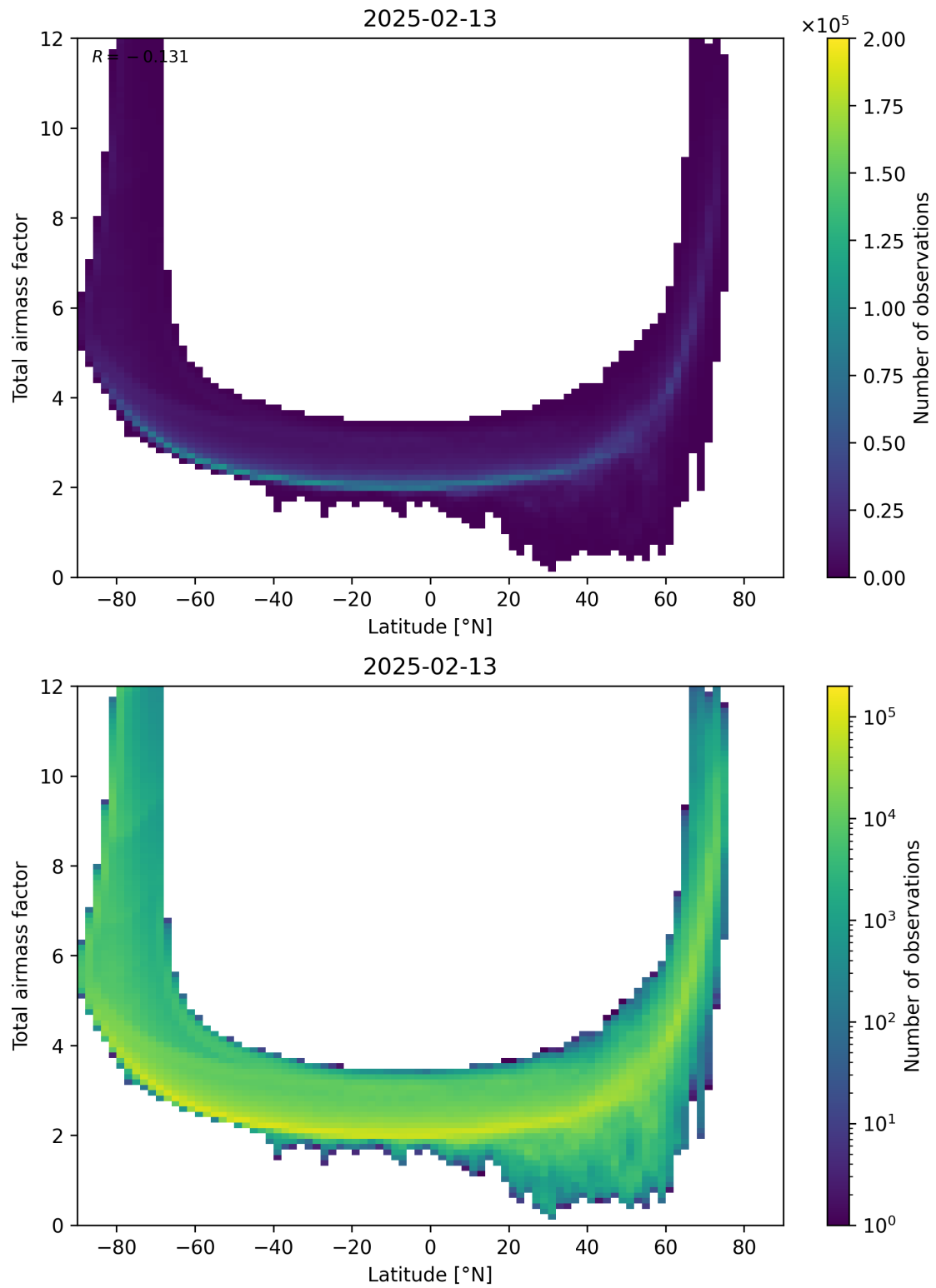
Figure 84: Scatter density plot of “Latitude” against “Total airmass factor” for 2025-02-13 to 2025-02-14.
