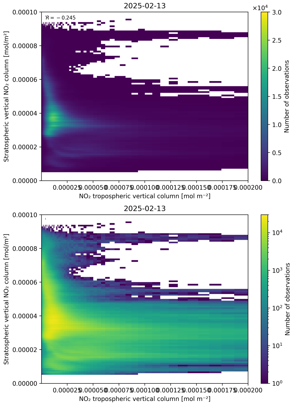
Figure 125: Scatter density plot of “NO 2 tropospheric vertical column” against “Stratospheric vertical NO 2 column” for 2025-02-13 to 2025-02-14.
