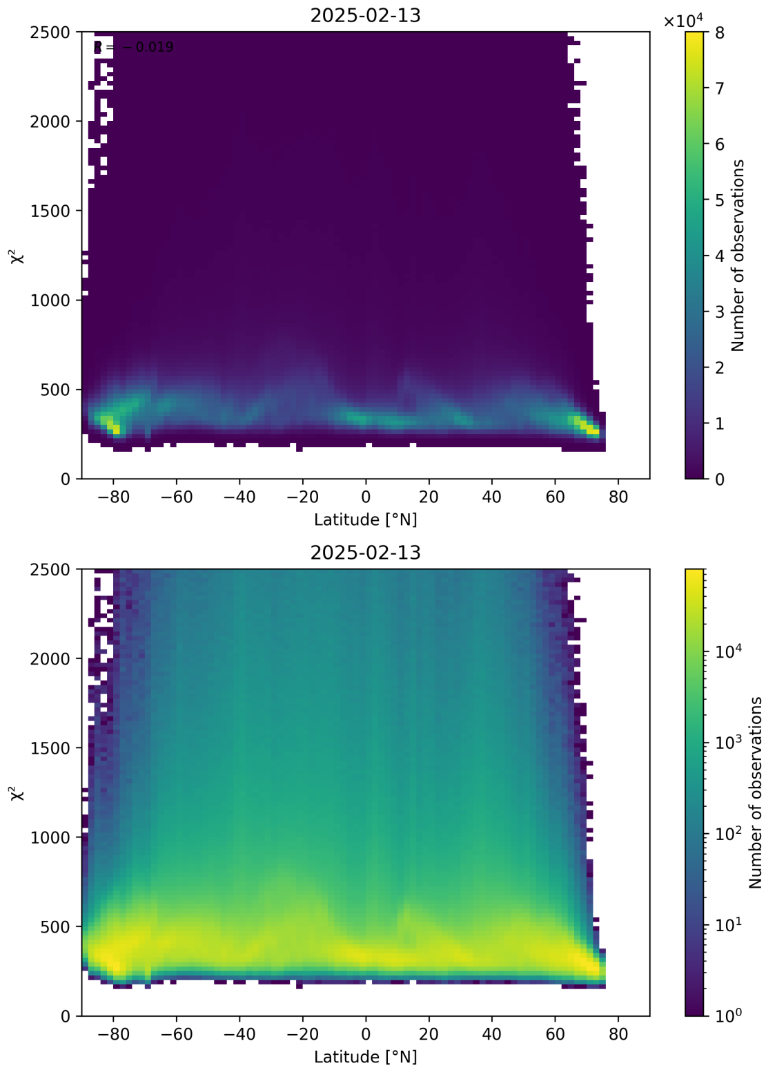
Figure 86: Scatter density plot of “Latitude” against “ \chi^2 ” for 2025-02-13 to 2025-02-14.
