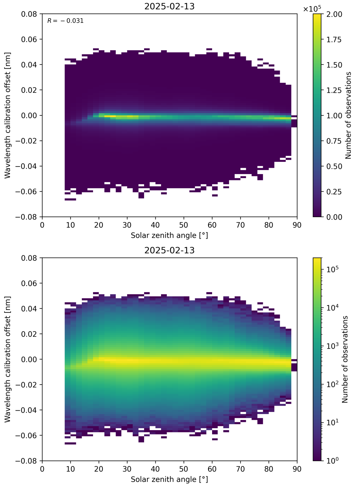
Figure 158: Scatter density plot of “Solar zenith angle” against “Wavelength calibration offset” for 2025-02-13 to 2025-02-14.
