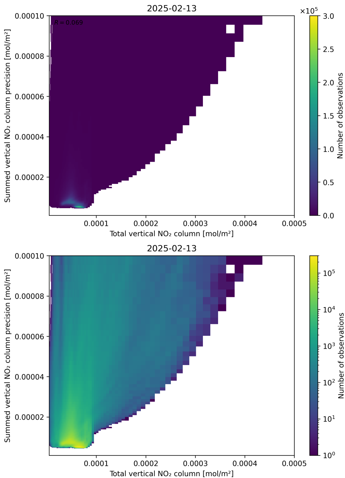
Figure 113: Scatter density plot of “Total vertical NO 2 column” against “Summed vertical NO 2 column precision” for 2025-02-13 to 2025-02-14.
