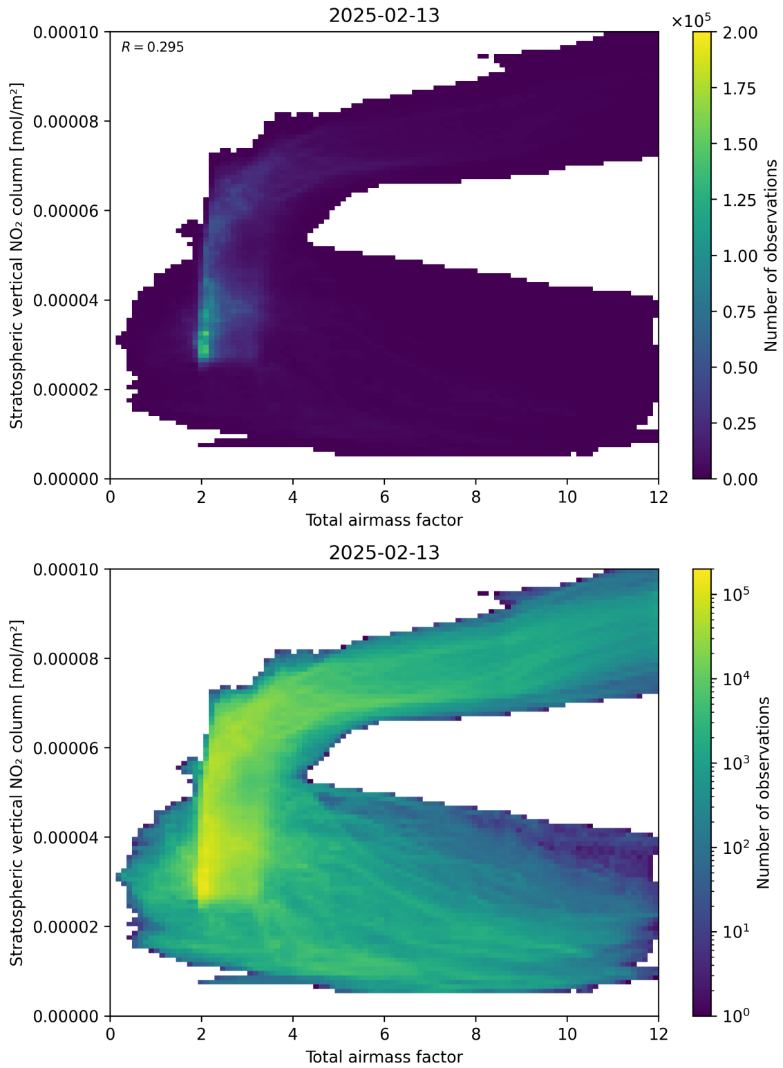
Figure 64: Scatter density plot of “Total airmass factor” against “Stratospheric vertical NO 2 column” for 2025-02-13 to 2025-02-14.
