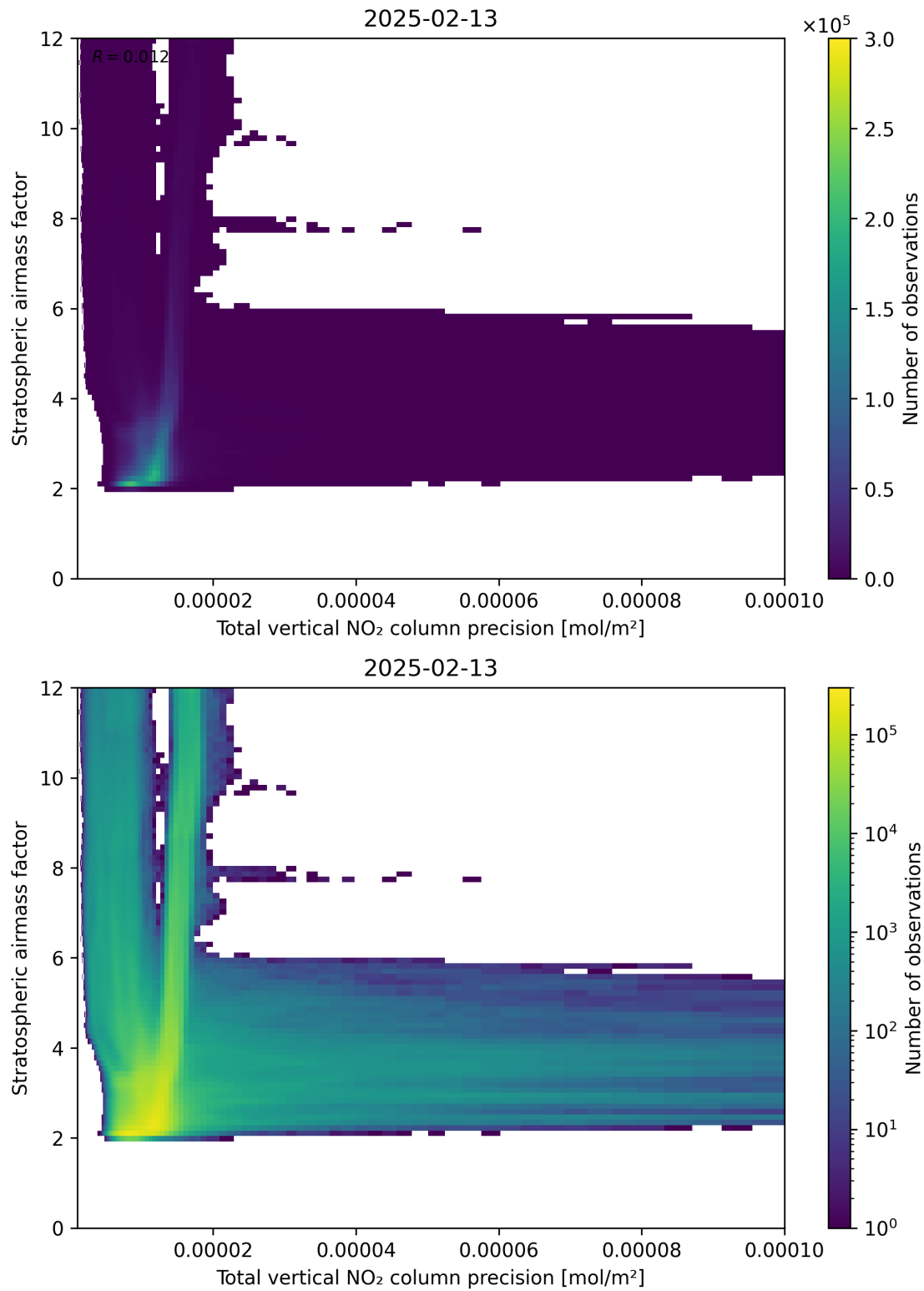
Figure 115: Scatter density plot of “Total vertical NO 2 column precision” against “Stratospheric air mass factor” for 2025-02-13 to 2025-02-14.
