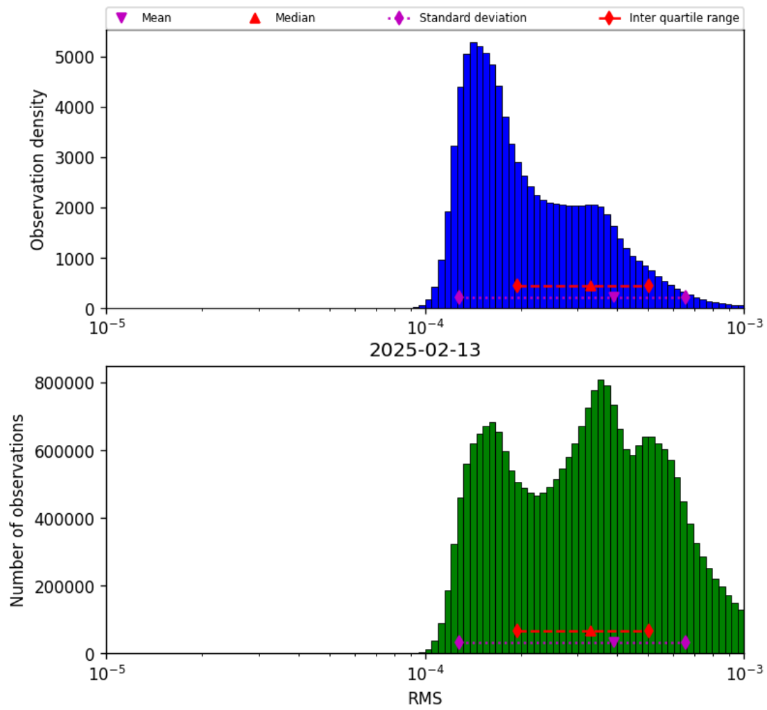
Figure 43: Histogram of “RMS” for 2025-02-13 to 2025-02-14
