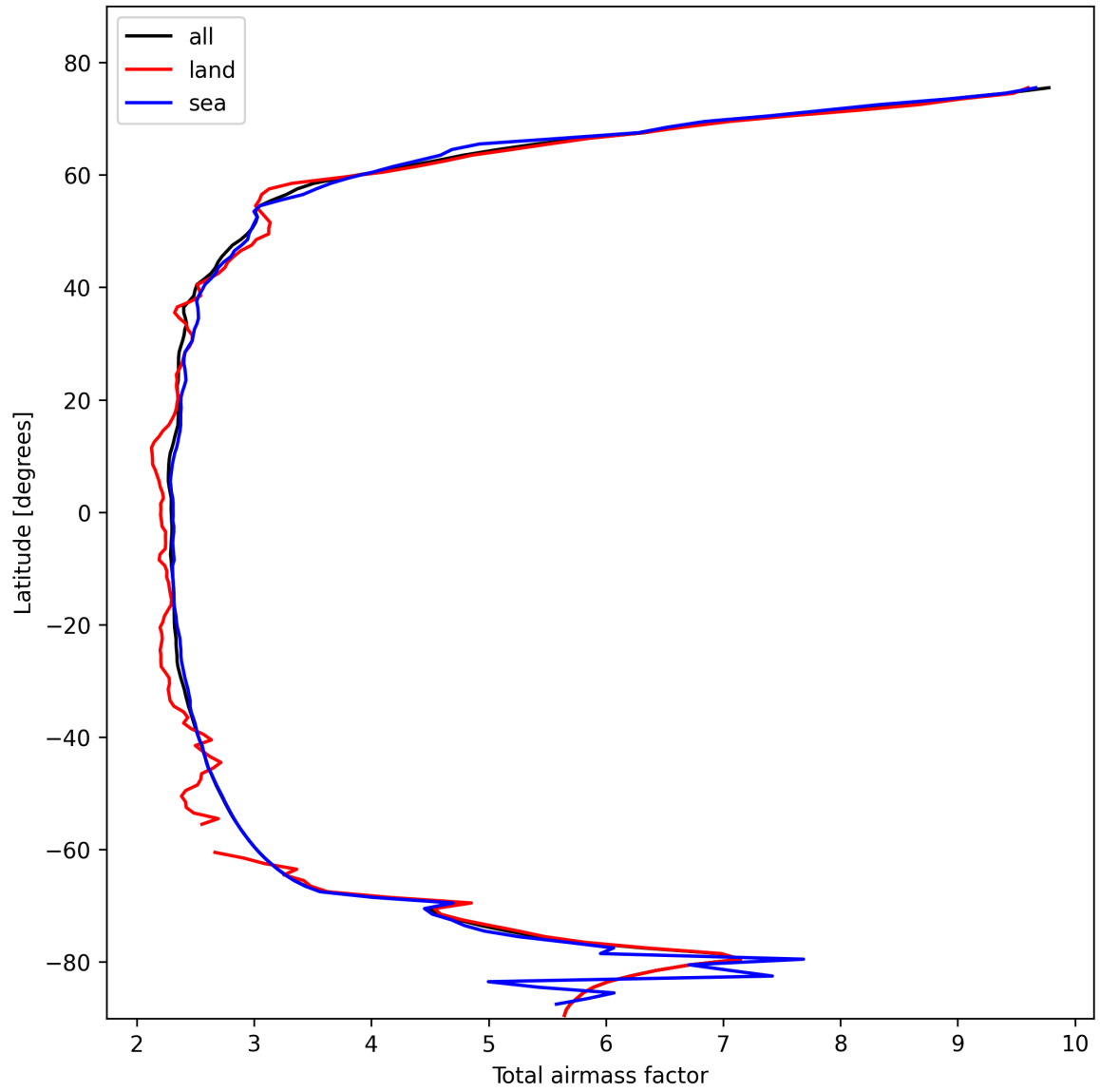
Figure 15: Zonal average of “Total airmass factor” for 2025-02-13 to 2025-02-14.
