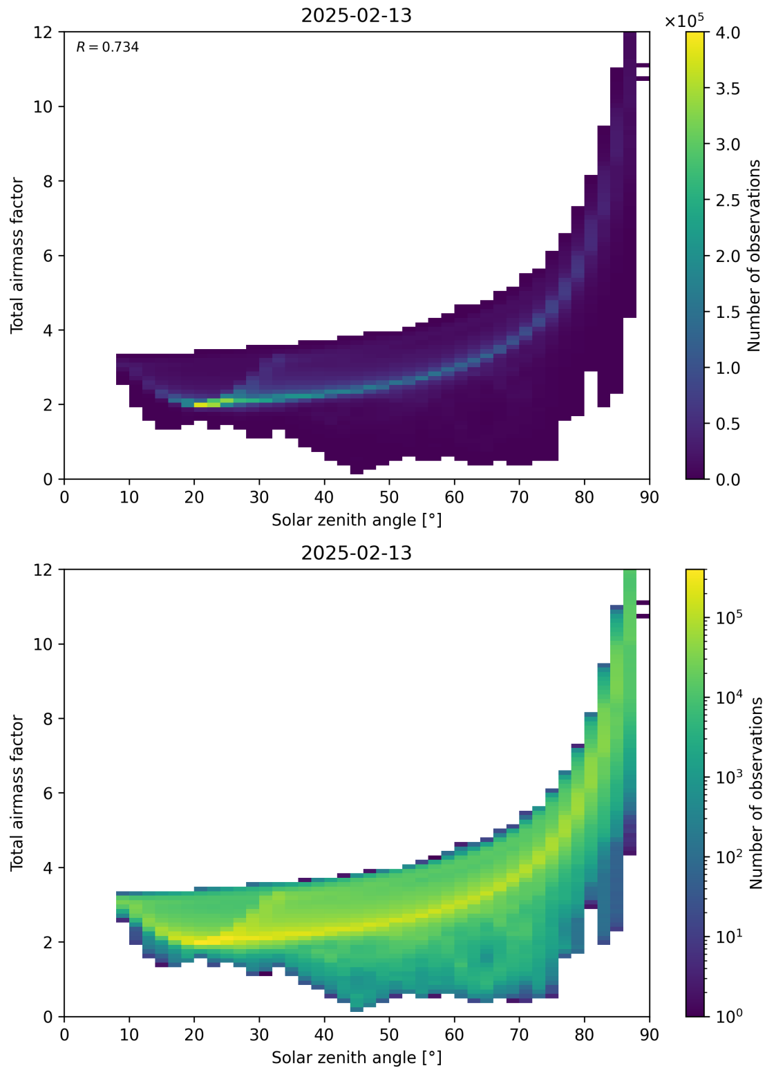
Figure 146: Scatter density plot of “Solar zenith angle” against “Total air mass factor” for 2025-02-13 to 2025-02-14.
