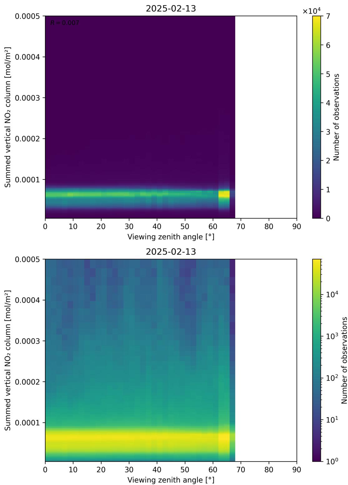
Figure 165: Scatter density plot of “Viewing zenith angle” against “Summed vertical NO 2 column” for 2025-02-13 to 2025-02-14.
