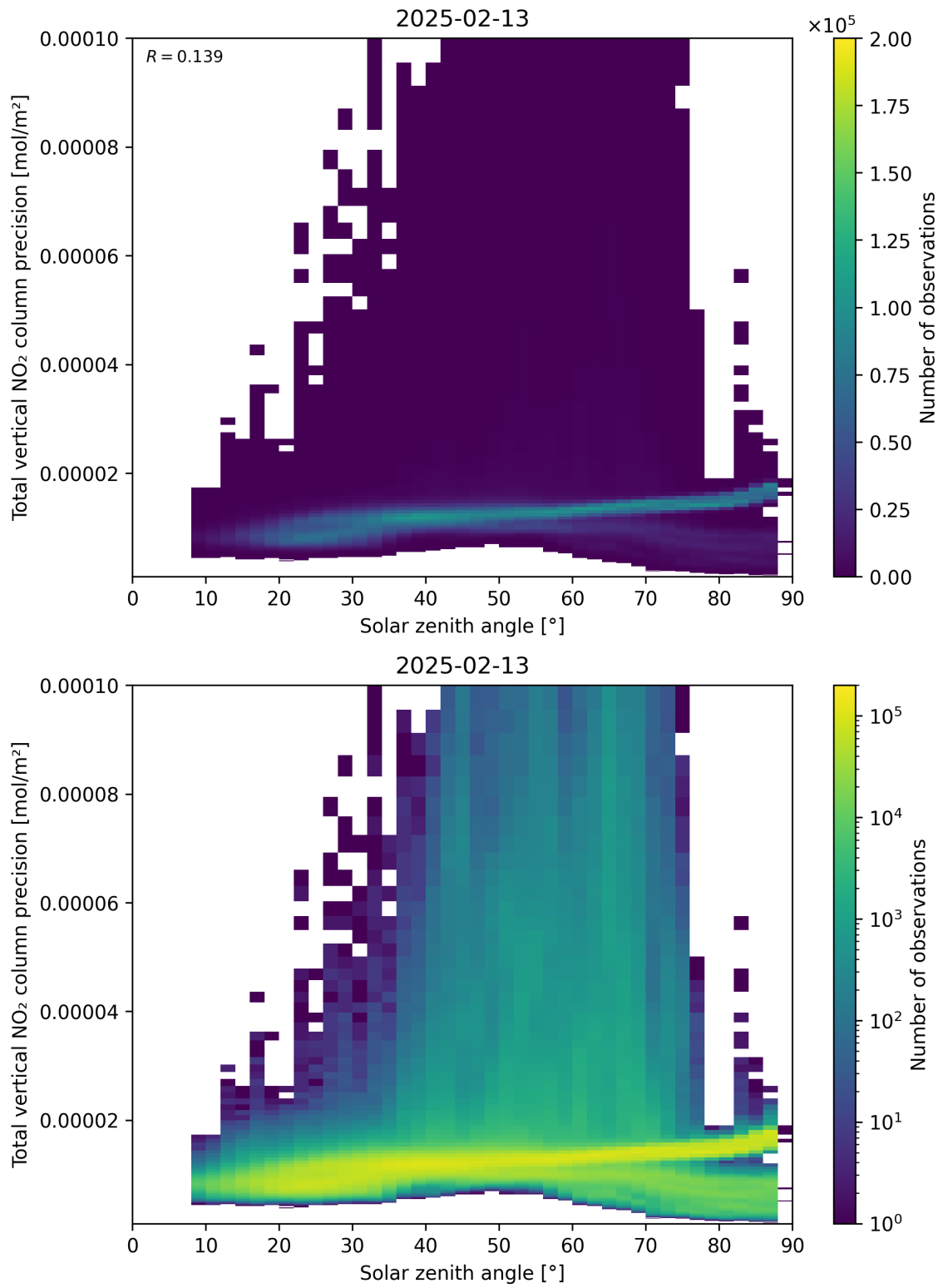
Figure 154: Scatter density plot of “Solar zenith angle” against “Total vertical NO 2 column precision” for 2025-02-13 to 2025-02-14.
