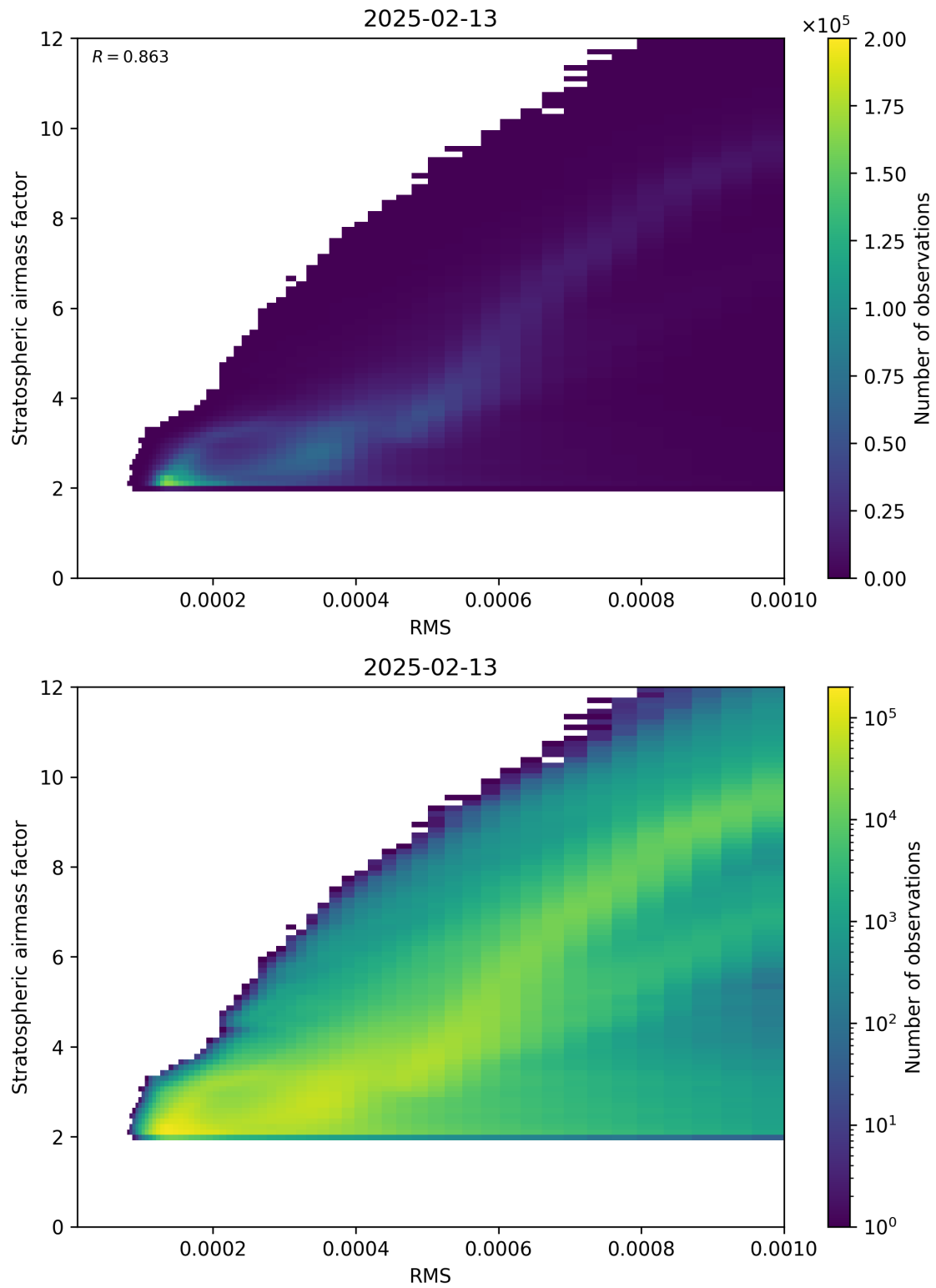
Figure 144: Scatter density plot of “RMS” against “Stratospheric airmass factor” for 2025-02-13 to 2025-02-14.
