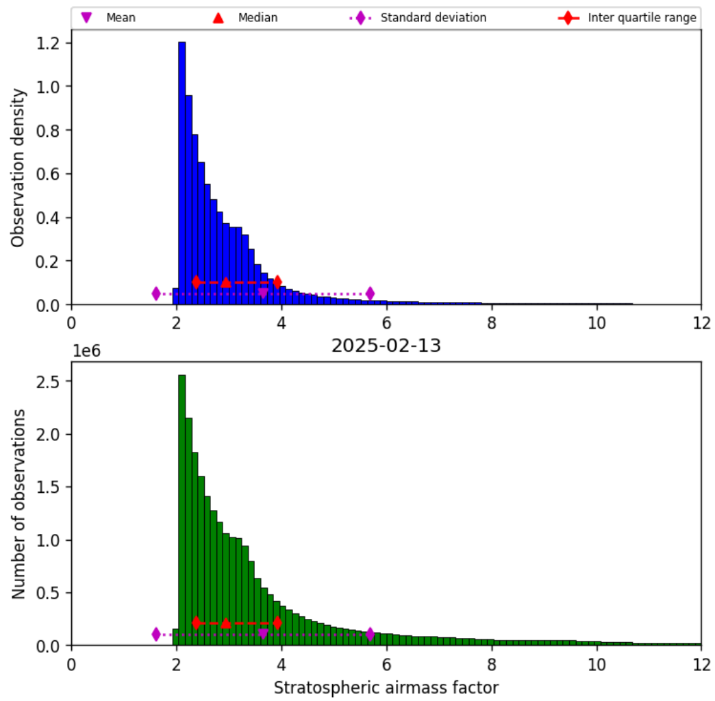
Figure 44: Histogram of “Stratospheric airmass factor” for 2025-02-13 to 2025-02-14
