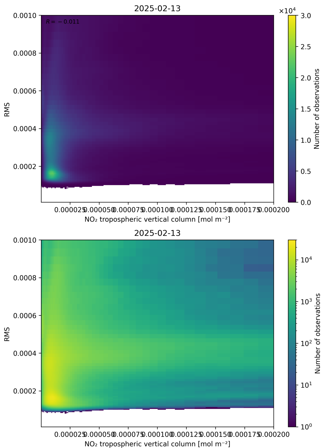
Figure 142: Scatter density plot of “NO 2 tropospheric vertical column” against “RMS” for 2025-02-13 to 2025-02-14.
