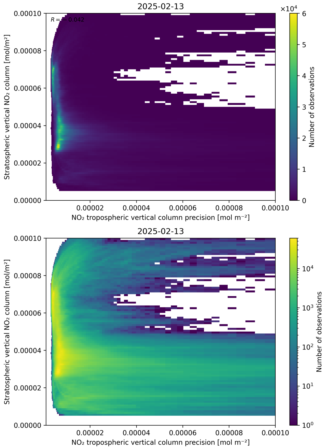
Figure 135: Scatter density plot of “NO 2 tropospheric vertical column precision” against “Stratospheric vertical NO 2 column” for 2025-02-13 to 2025-02-14.
