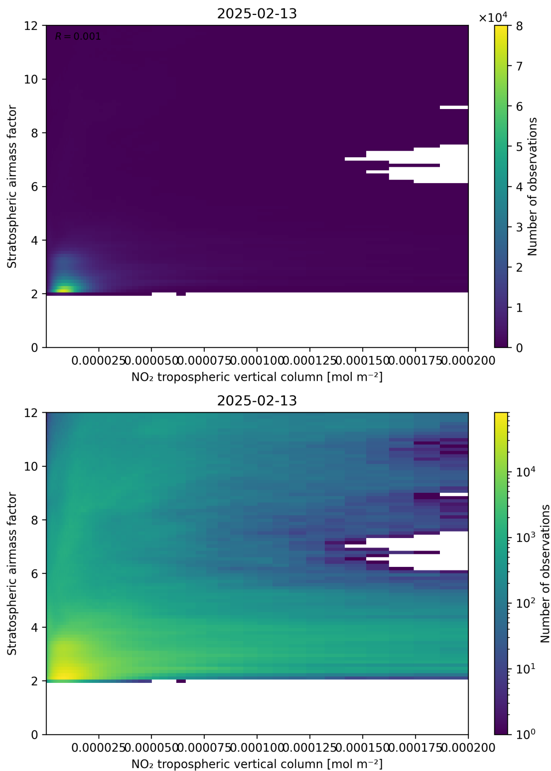
Figure 121: Scatter density plot of “NO 2 tropospheric vertical column” against “Stratospheric air mass factor” for 2025-02-13 to 2025-02-14.
