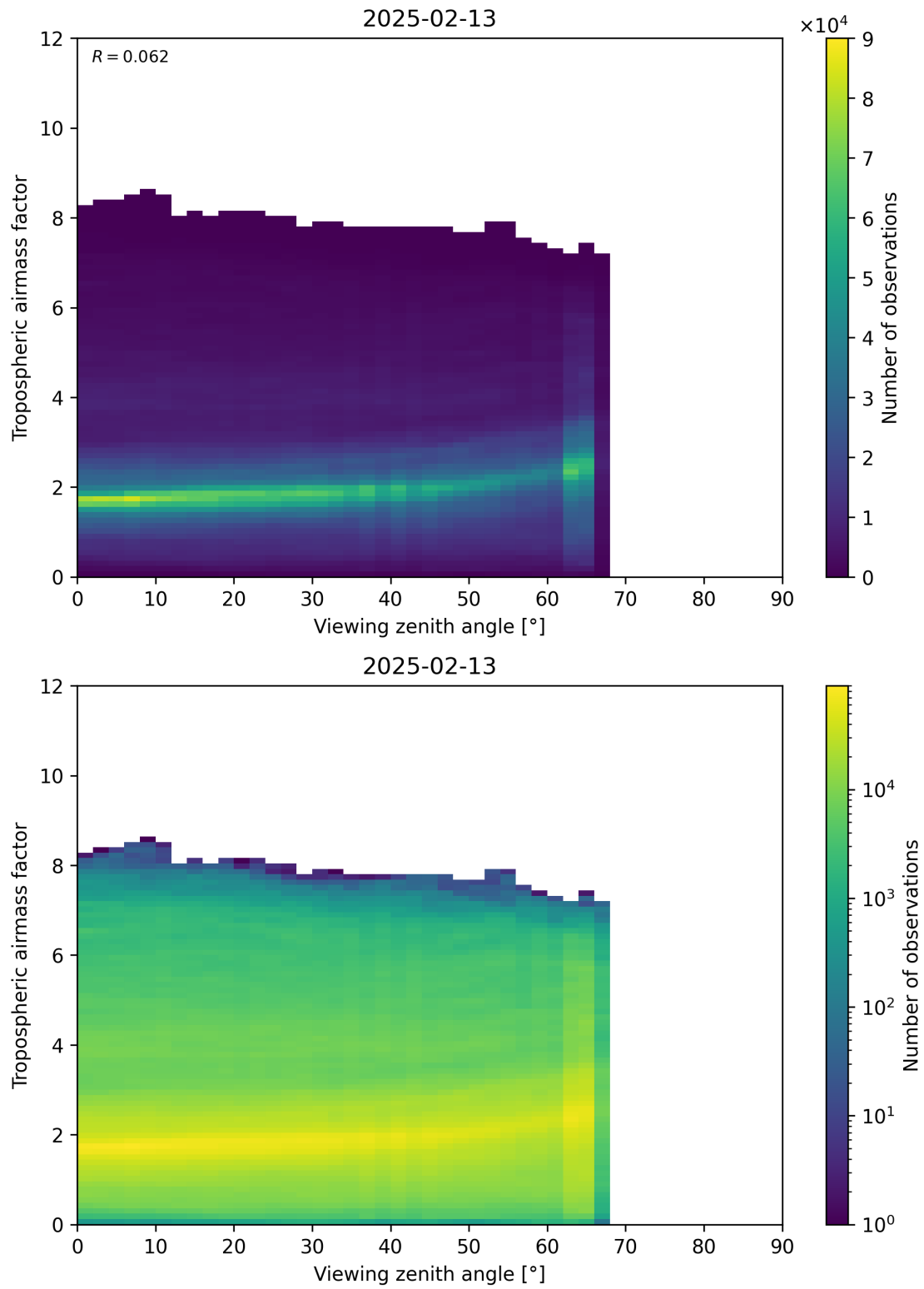
Figure 161: Scatter density plot of “Viewing zenith angle” against “Tropospheric airmass factor” for 2025-02-13 to 2025-02-14.
