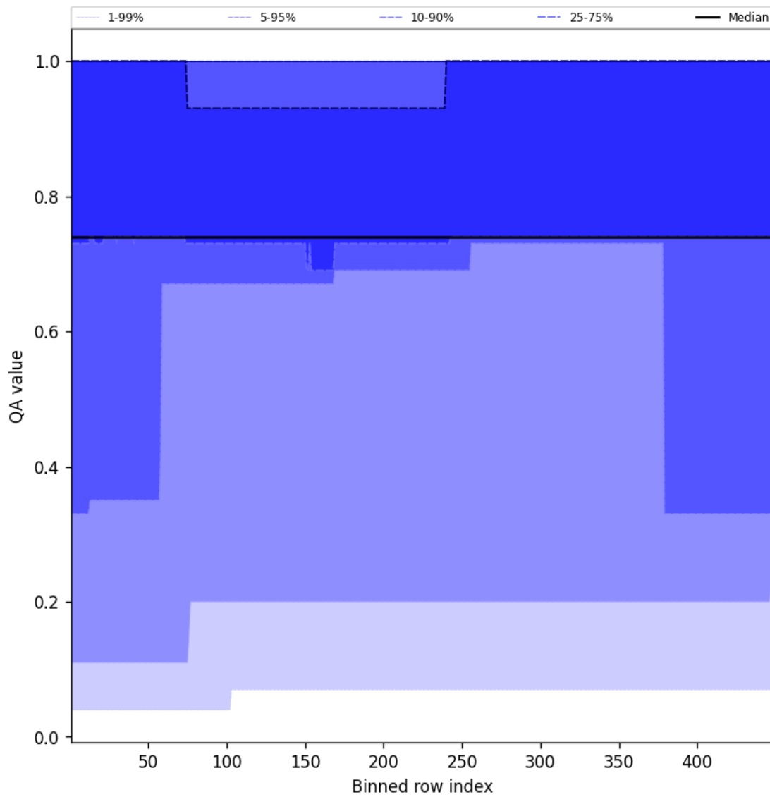
Figure 45: Along track statistics of “QA value” for 2025-02-13 to 2025-02-14
