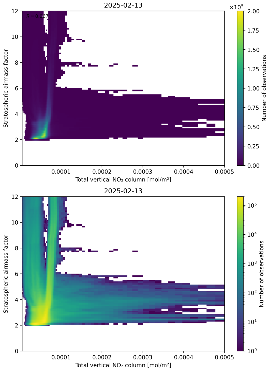
Figure 110: Scatter density plot of “Total vertical NO 2 column” against “Stratospheric airmass factor” for 2025-02-13 to 2025-02-14.
