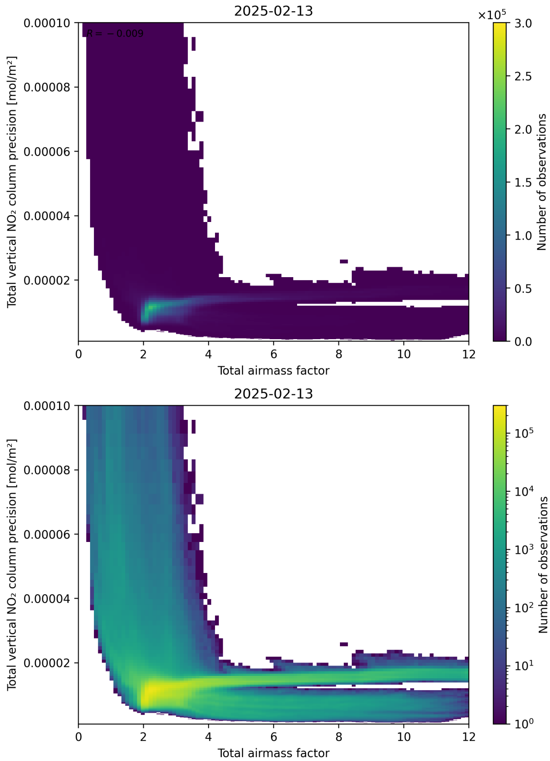
Figure 68: Scatter density plot of “Total airmass factor” against “Total vertical NO 2 column precision” for 2025-02-13 to 2025-02-14.
