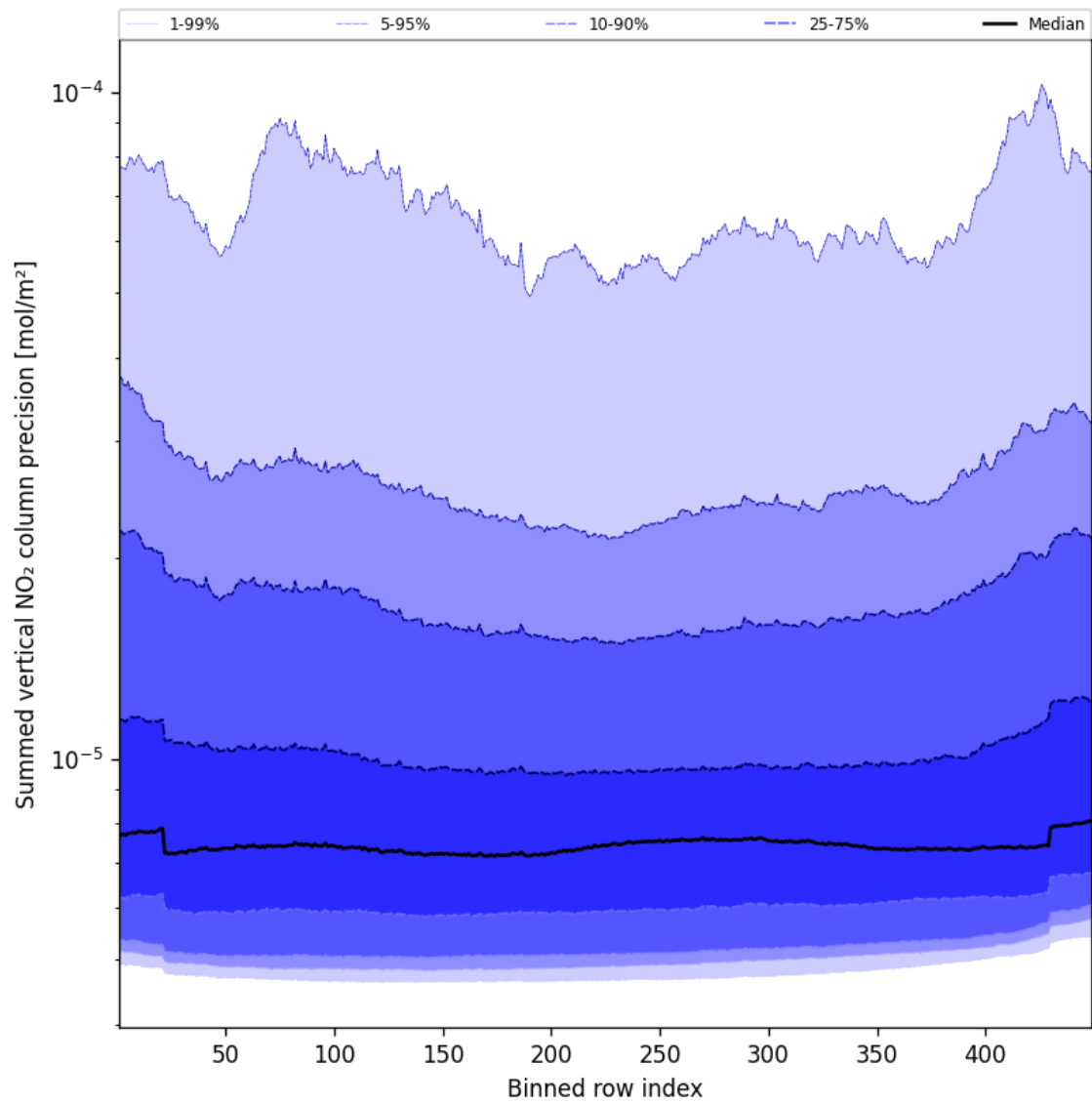
Figure 58: Along track statistics of “Summed vertical NO 2 column precision” for 2025-02-13 to 2025-02-14
