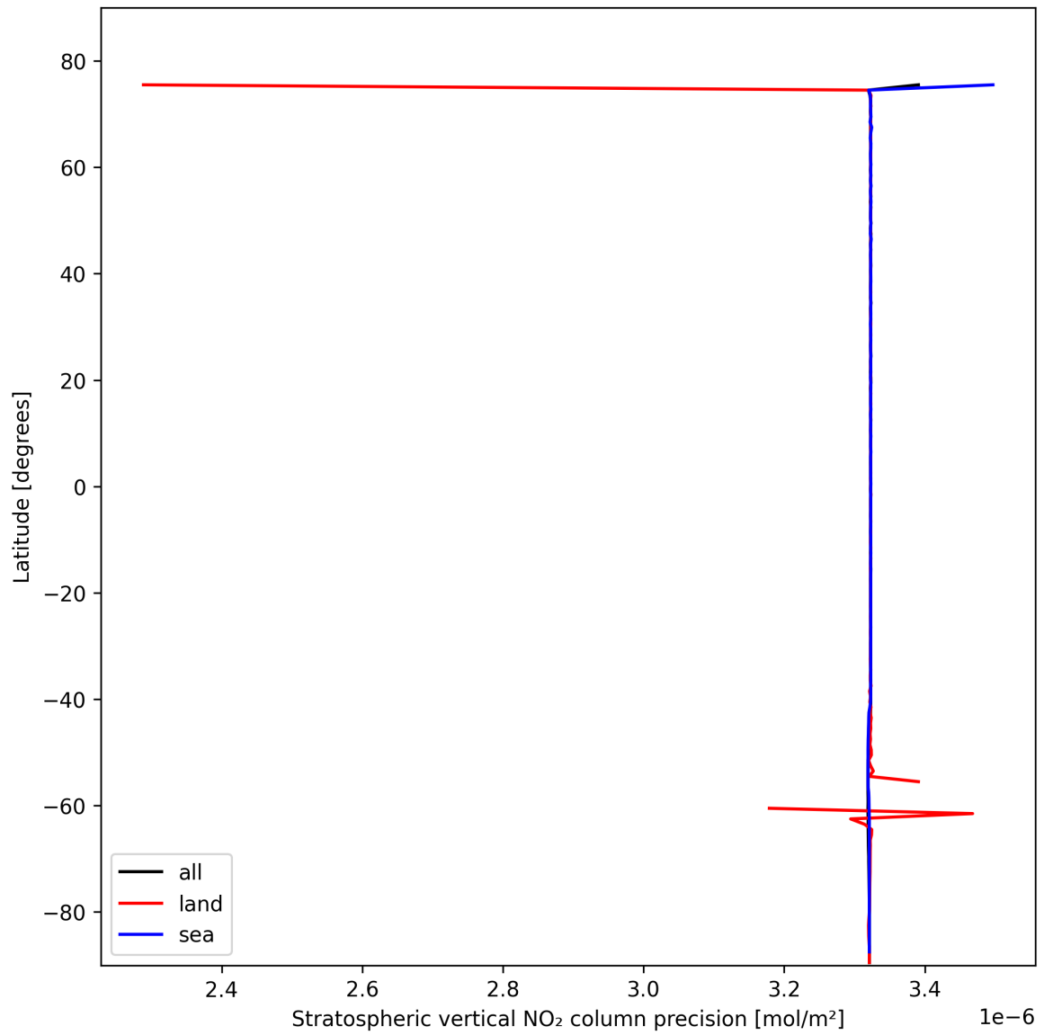
Figure 20: Zonal average of “Stratospheric vertical NO 2 column precision” for 2025-02-13 to 2025-02-14.
