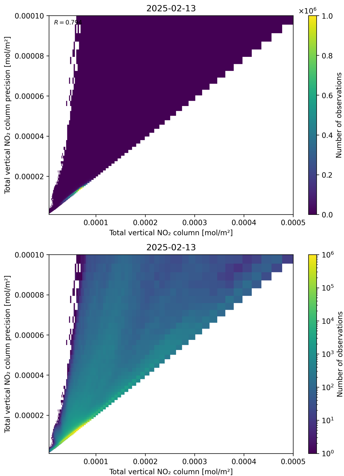
Figure 114: Scatter density plot of “Total vertical NO 2 column” against “Total vertical NO 2 column precision” for 2025-02-13 to 2025-02-14.
