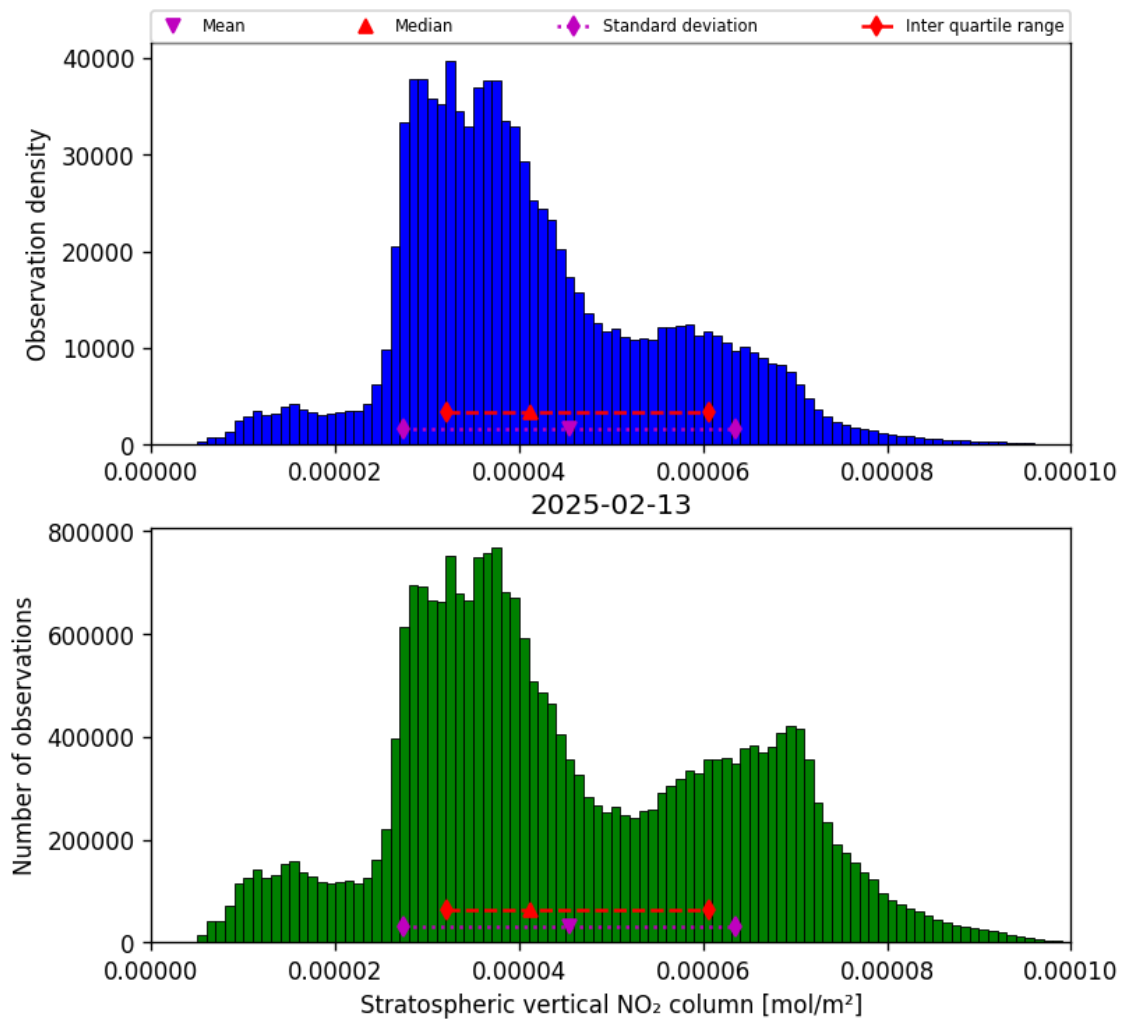
Figure 36: Histogram of “Stratospheric vertical NO 2 column” for 2025-02-13 to 2025-02-14
