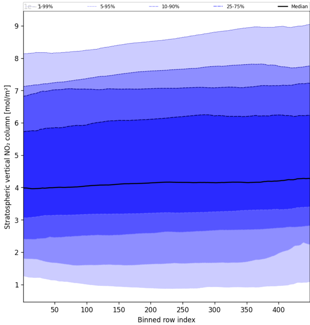
Figure 53: Along track statistics of “Stratospheric vertical NO 2 column” for 2025-02-13 to 2025-02-14
