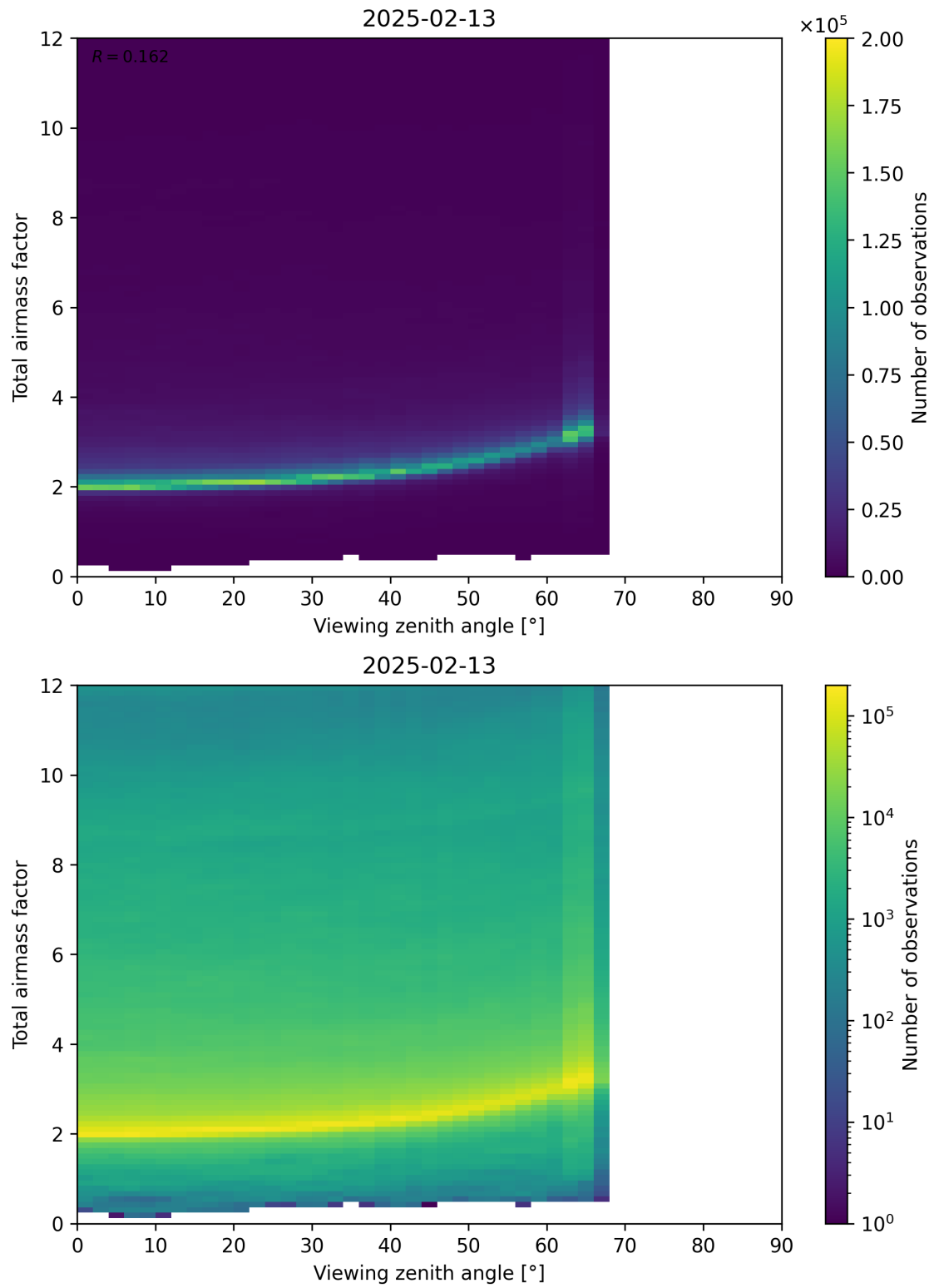
Figure 160: Scatter density plot of “Viewing zenith angle” against “Total airmass factor” for 2025-02-13 to 2025-02-14.
