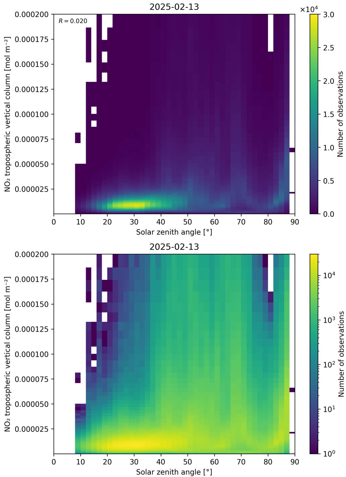
Figure 155: Scatter density plot of “Solar zenith angle” against “NO 2 tropospheric vertical column” for 2025-02-13 to 2025-02-14.
