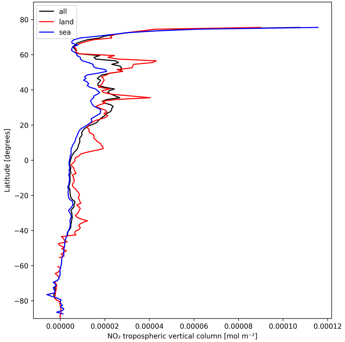
Figure 12: Zonal average of “NO 2 tropospheric vertical column” for 2025-02-13 to 2025-02-14.
