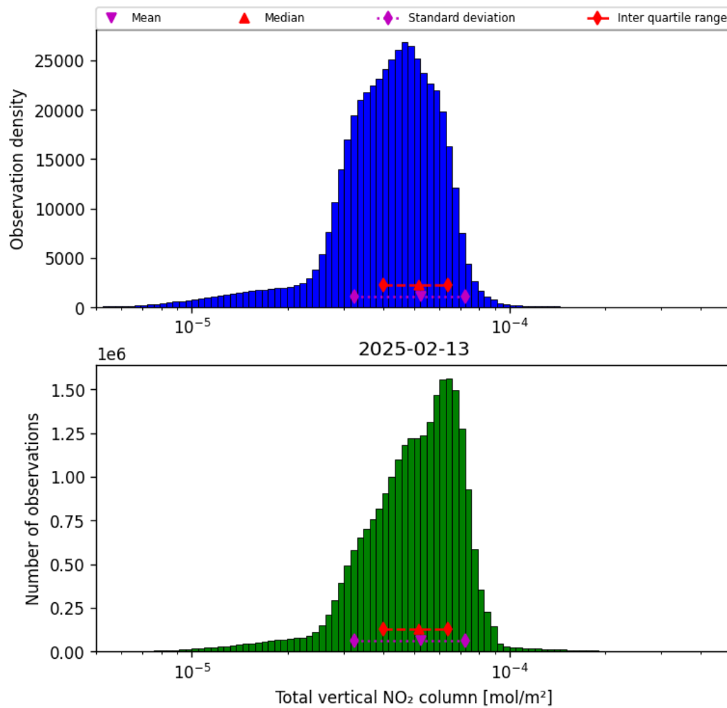
Figure 38: Histogram of “Total vertical NO 2 column” for 2025-02-13 to 2025-02-14
