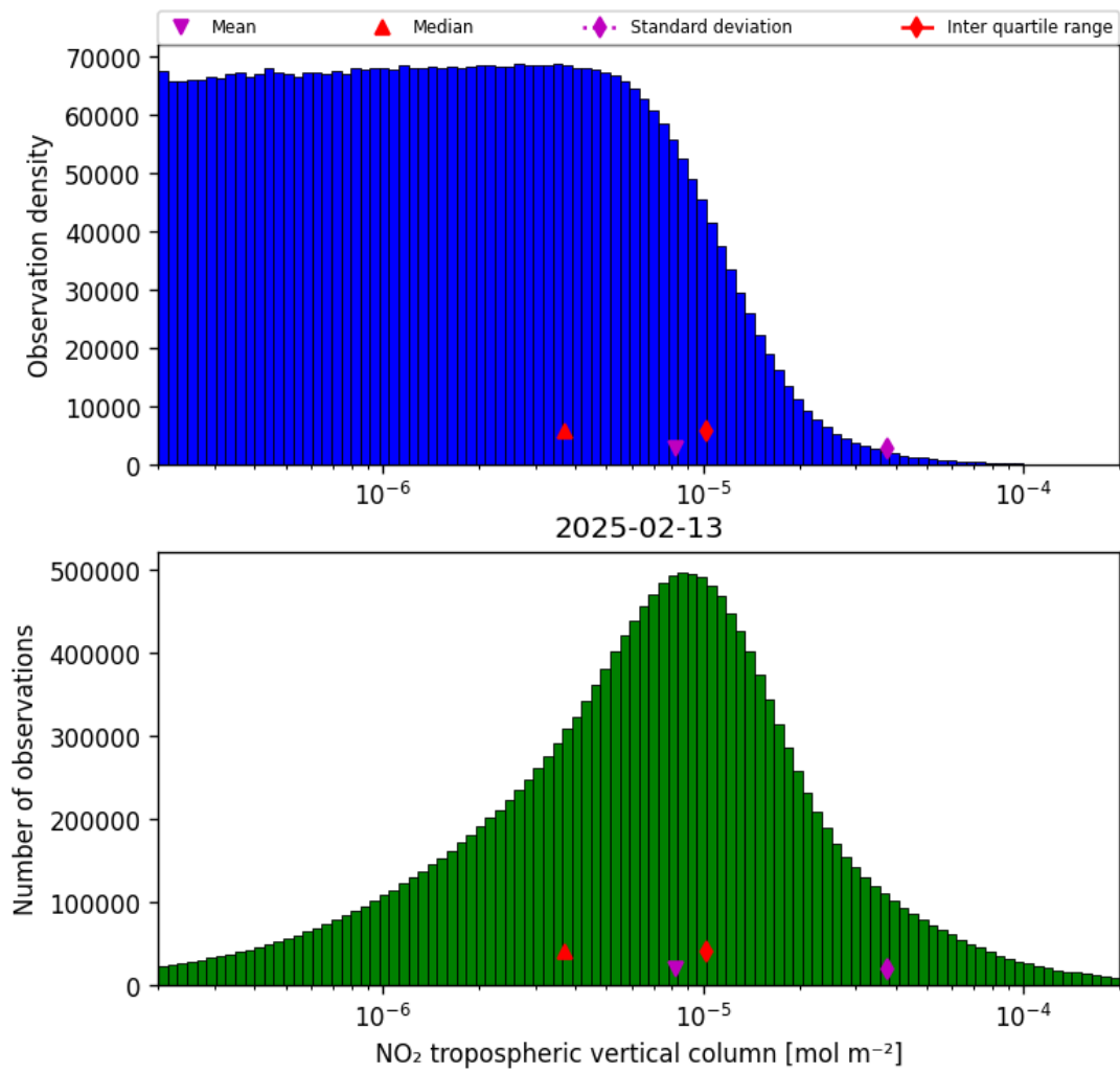
Figure 29: Histogram of “NO 2 tropospheric vertical column” for 2025-02-13 to 2025-02-14
