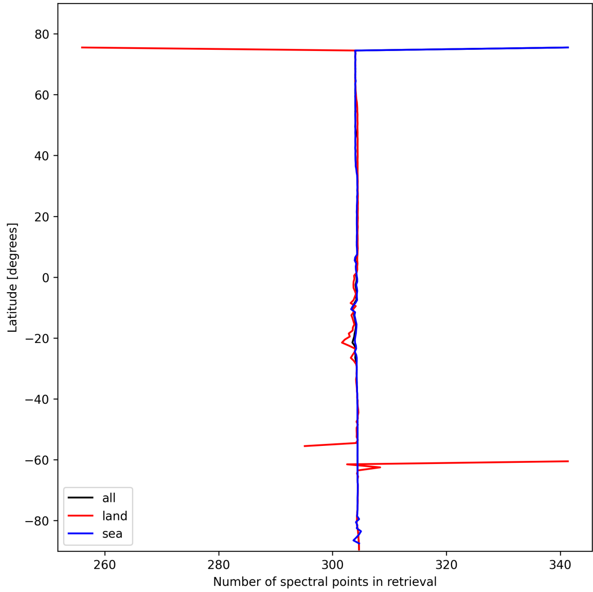
Figure 16: Zonal average of “Number of spectral points in retrieval” for 2025-02-13 to 2025-02-14.
