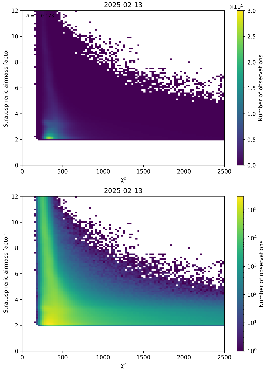
Figure 81: Scatter density plot of “ \chi^2 ” against “Stratospheric airmass factor” for 2025-02-13 to 2025-02-14.
