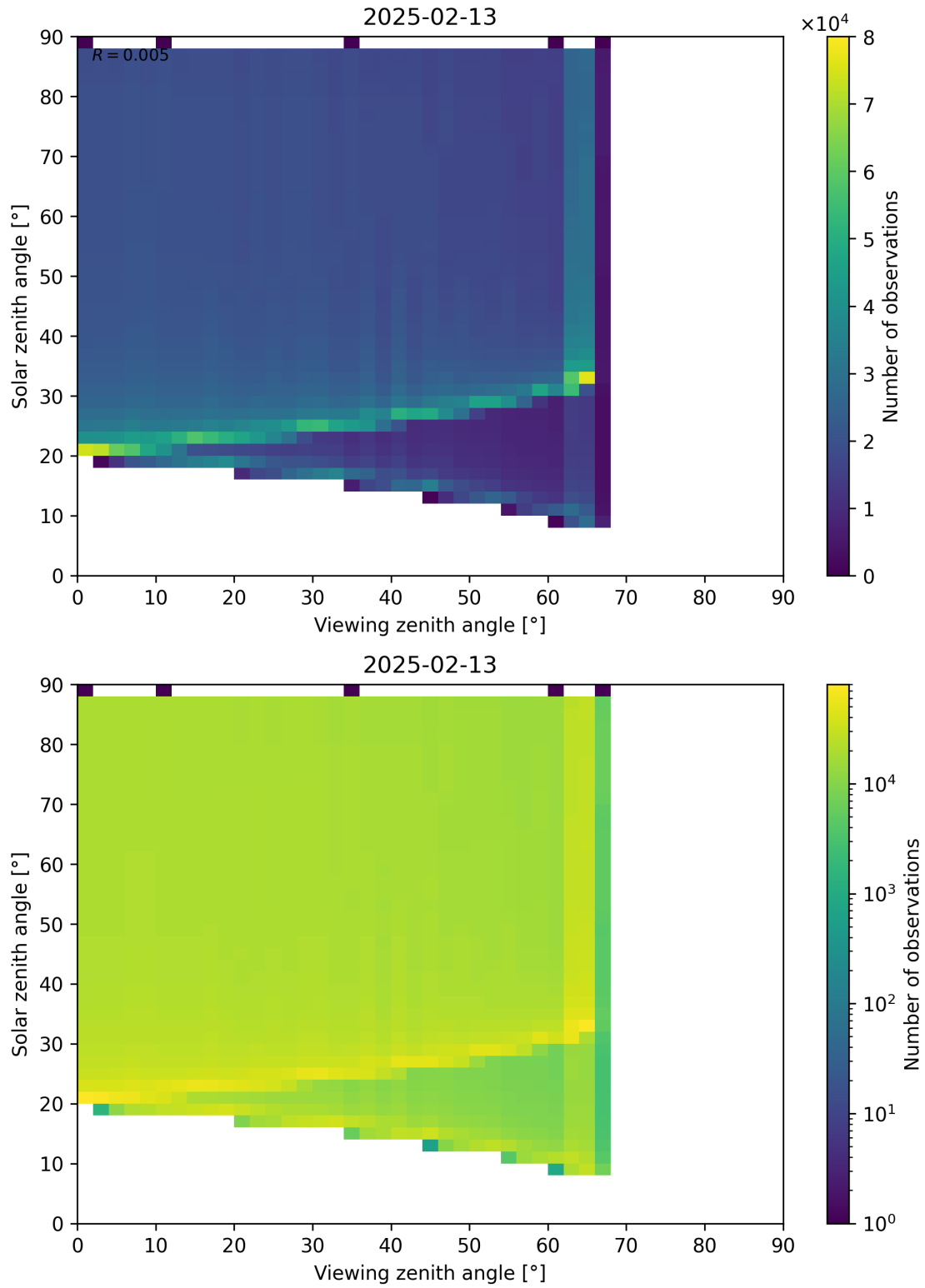
Figure 172: Scatter density plot of “Viewing zenith angle” against “Solar zenith angle” for 2025-02-13 to 2025-02-14.
