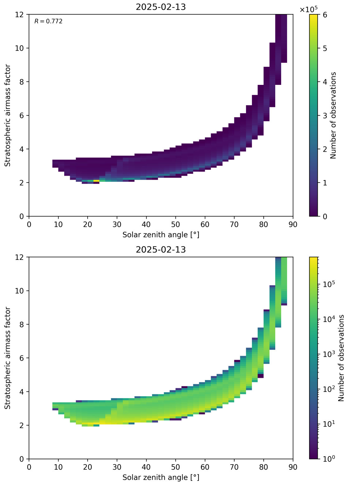
Figure 145: Scatter density plot of “Solar zenith angle” against “Stratospheric airmass factor” for 2025-02-13 to 2025-02-14.
