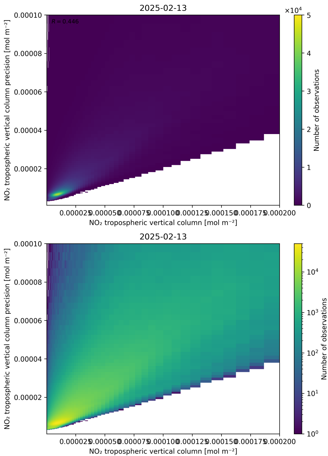
Figure 130: Scatter density plot of “NO 2 tropospheric vertical column” against “NO 2 tropospheric vertical column precision” for 2025-02-13 to 2025-02-14.
