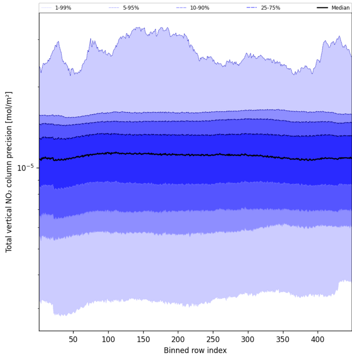
Figure 56: Along track statistics of “Total vertical NO 2 column precision” for 2025-02-13 to 2025-02-14
