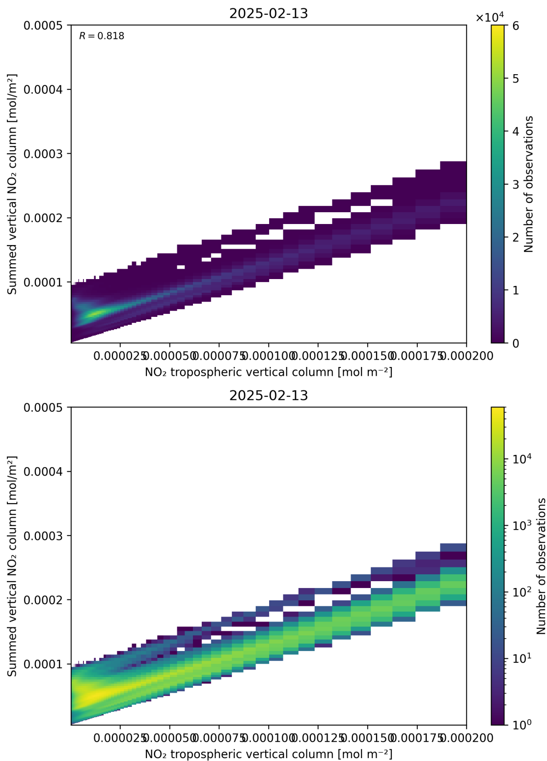
Figure 126: Scatter density plot of “NO 2 tropospheric vertical column” against “Summed vertical NO 2 column” for 2025-02-13 to 2025-02-14.
