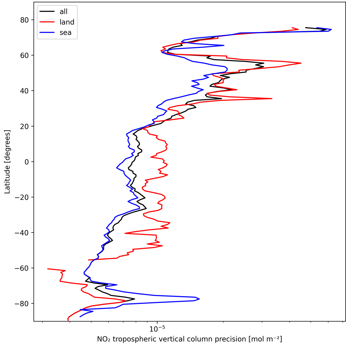
Figure 13: Zonal average of “NO 2 tropospheric vertical column precision” for 2025-02-13 to 2025-02-14.
