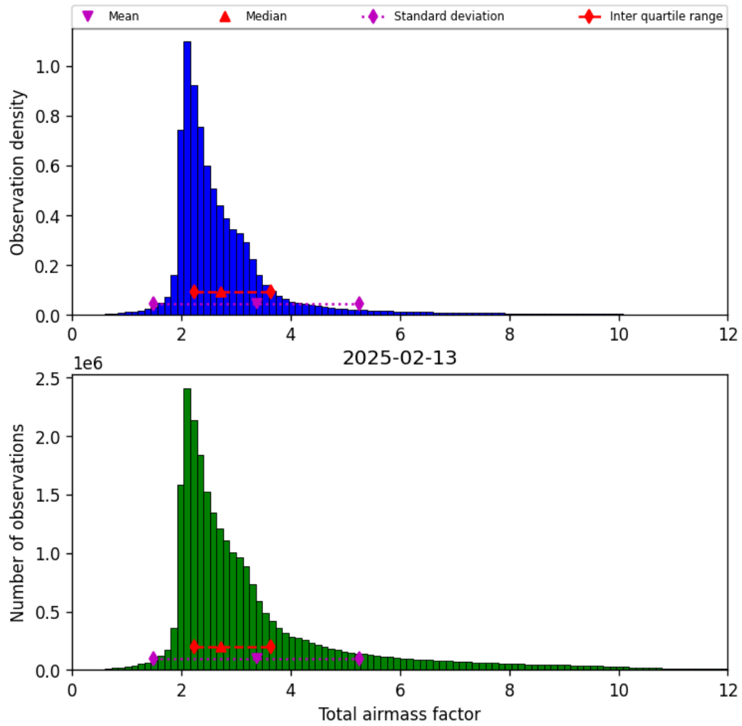
Figure 32: Histogram of “Total airmass factor” for 2025-02-13 to 2025-02-14
