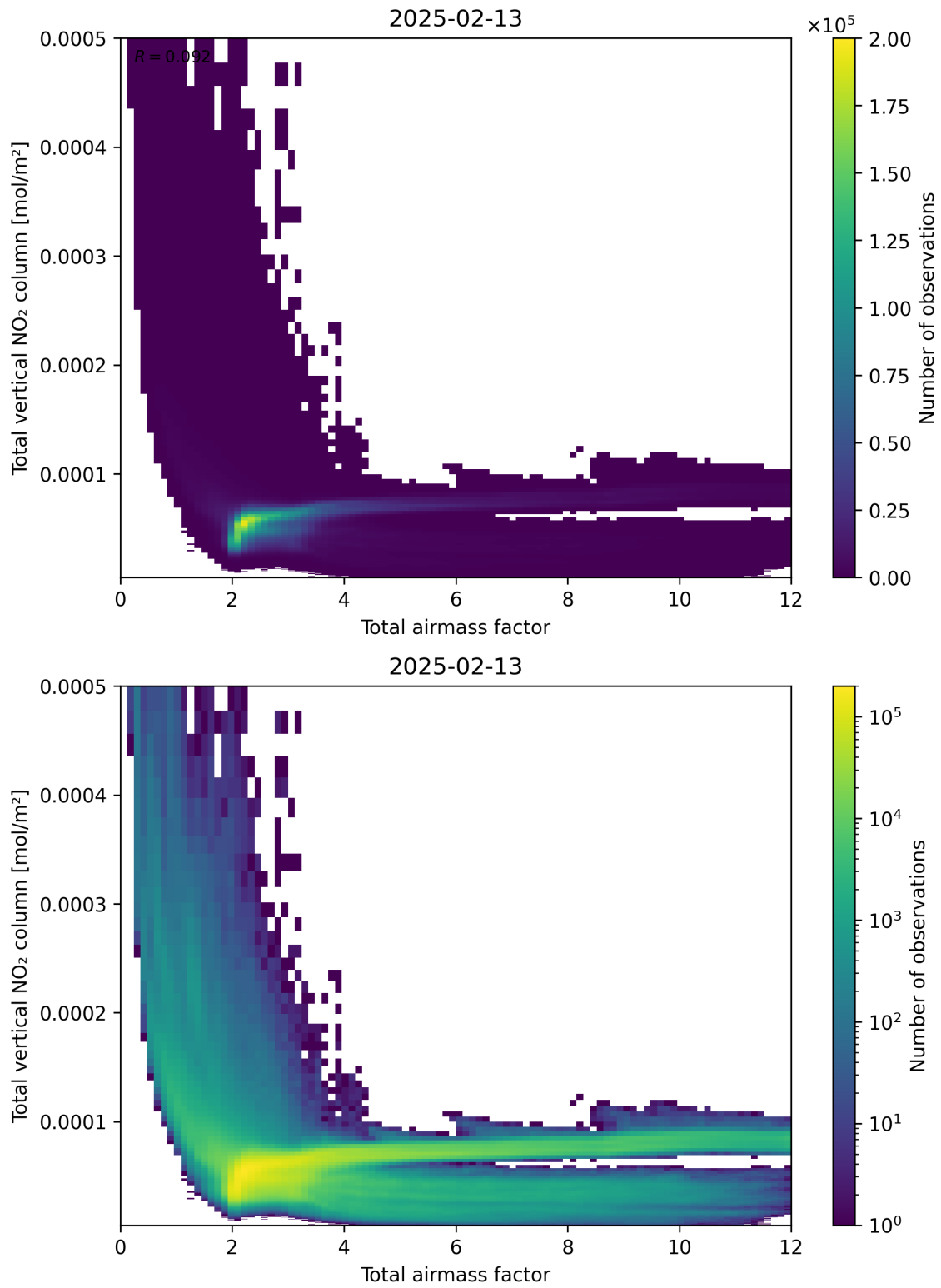
Figure 67: Scatter density plot of “Total airmass factor” against “Total vertical NO 2 column” for 2025-02-13 to 2025-02-14.
