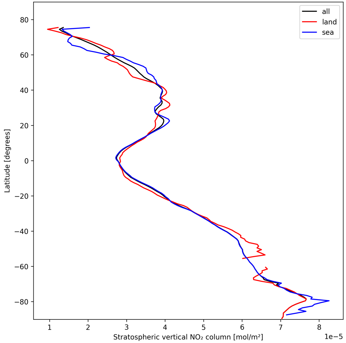
Figure 19: Zonal average of “Stratospheric vertical NO 2 column” for 2025-02-13 to 2025-02-14.
