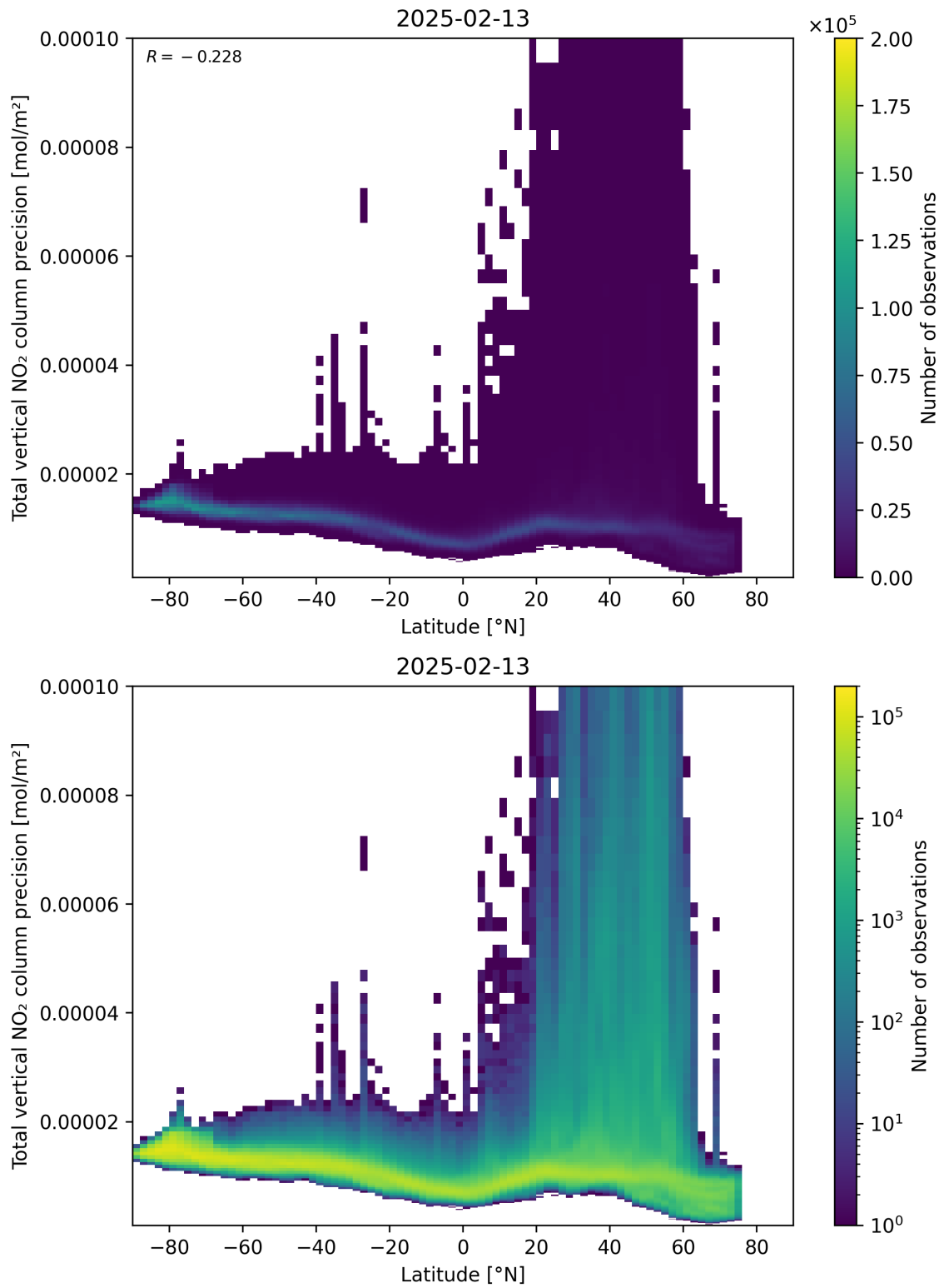
Figure 91: Scatter density plot of “Latitude” against “Total vertical NO 2 column precision” for 2025-02-13 to 2025-02-14.
