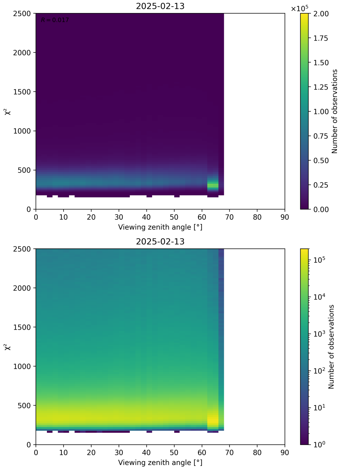
Figure 162: Scatter density plot of “Viewing zenith angle” against “ \chi^2 ” for 2025-02-13 to 2025-02-14.
