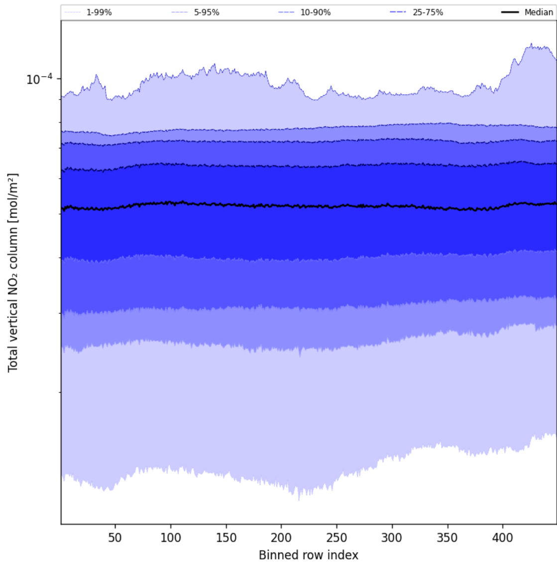
Figure 55: Along track statistics of “Total vertical NO 2 column” for 2025-02-13 to 2025-02-14
