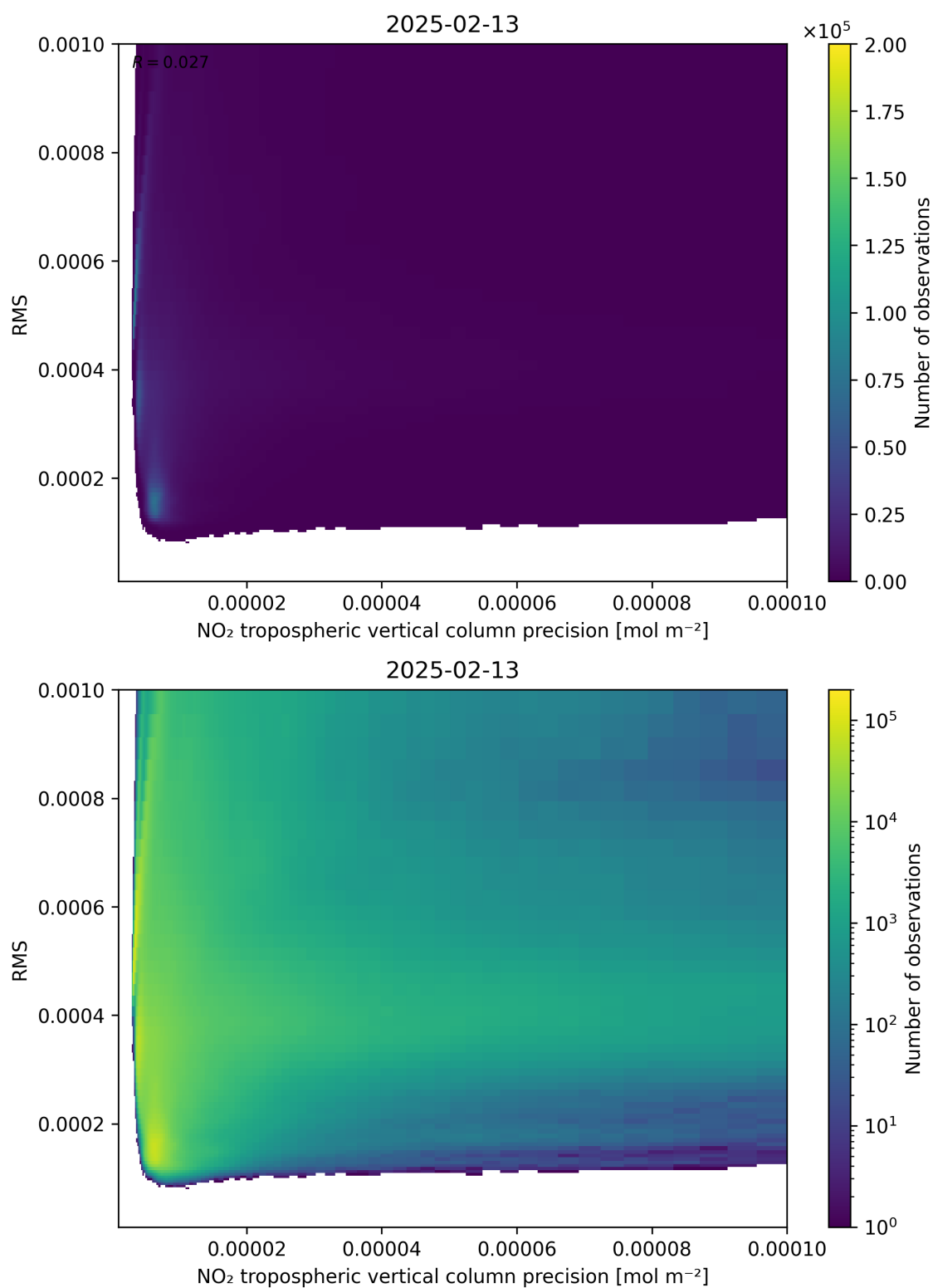
Figure 140: Scatter density plot of “NO 2 tropospheric vertical column precision” against “RMS” for 2025-02-13 to 2025-02-14.
