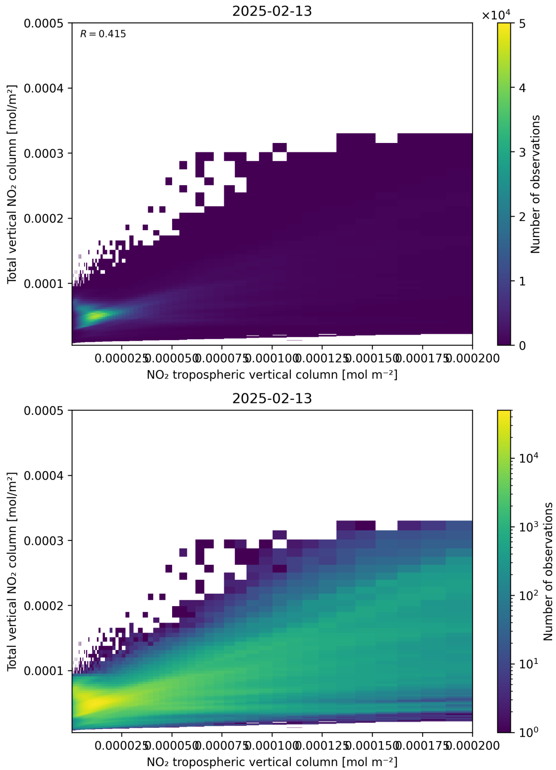
Figure 128: Scatter density plot of “NO 2 tropospheric vertical column” against “Total vertical NO 2 column” for 2025-02-13 to 2025-02-14.
