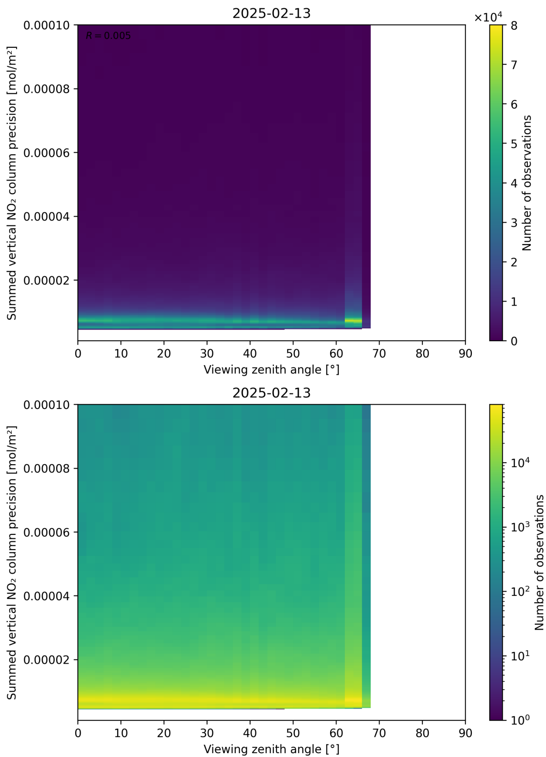
Figure 166: Scatter density plot of “Viewing zenith angle” against “Summed vertical NO 2 column precision” for 2025-02-13 to 2025-02-14.
