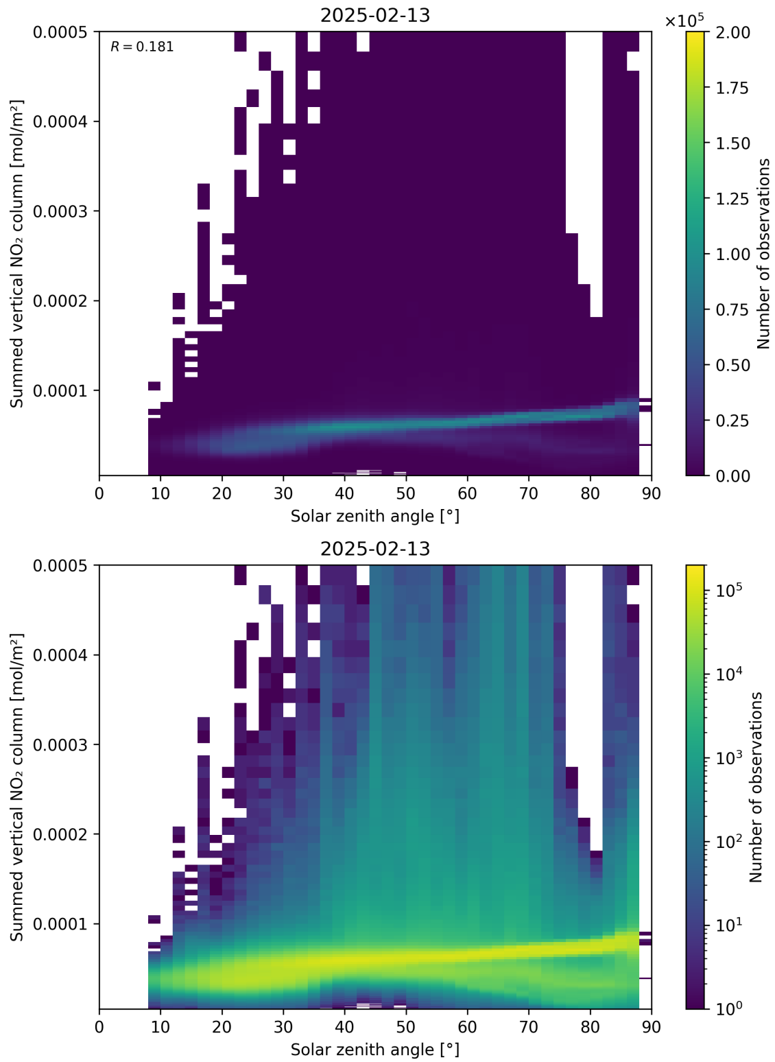
Figure 151: Scatter density plot of “Solar zenith angle” against “Summed vertical NO 2 column” for 2025-02-13 to 2025-02-14.
