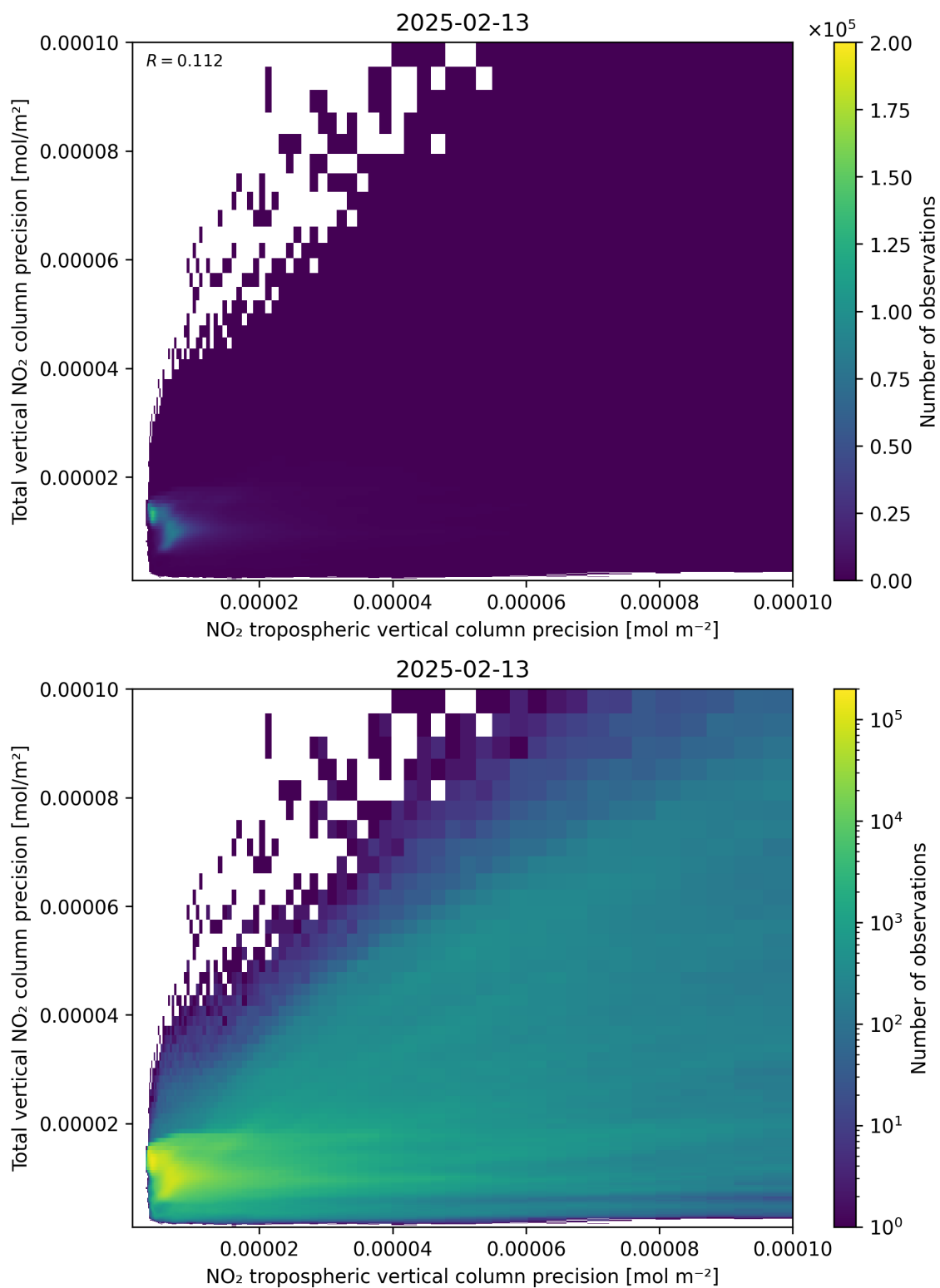
Figure 139: Scatter density plot of “NO 2 tropospheric vertical column precision” against “Total vertical NO 2 column precision” for 2025-02-13 to 2025-02-14.
