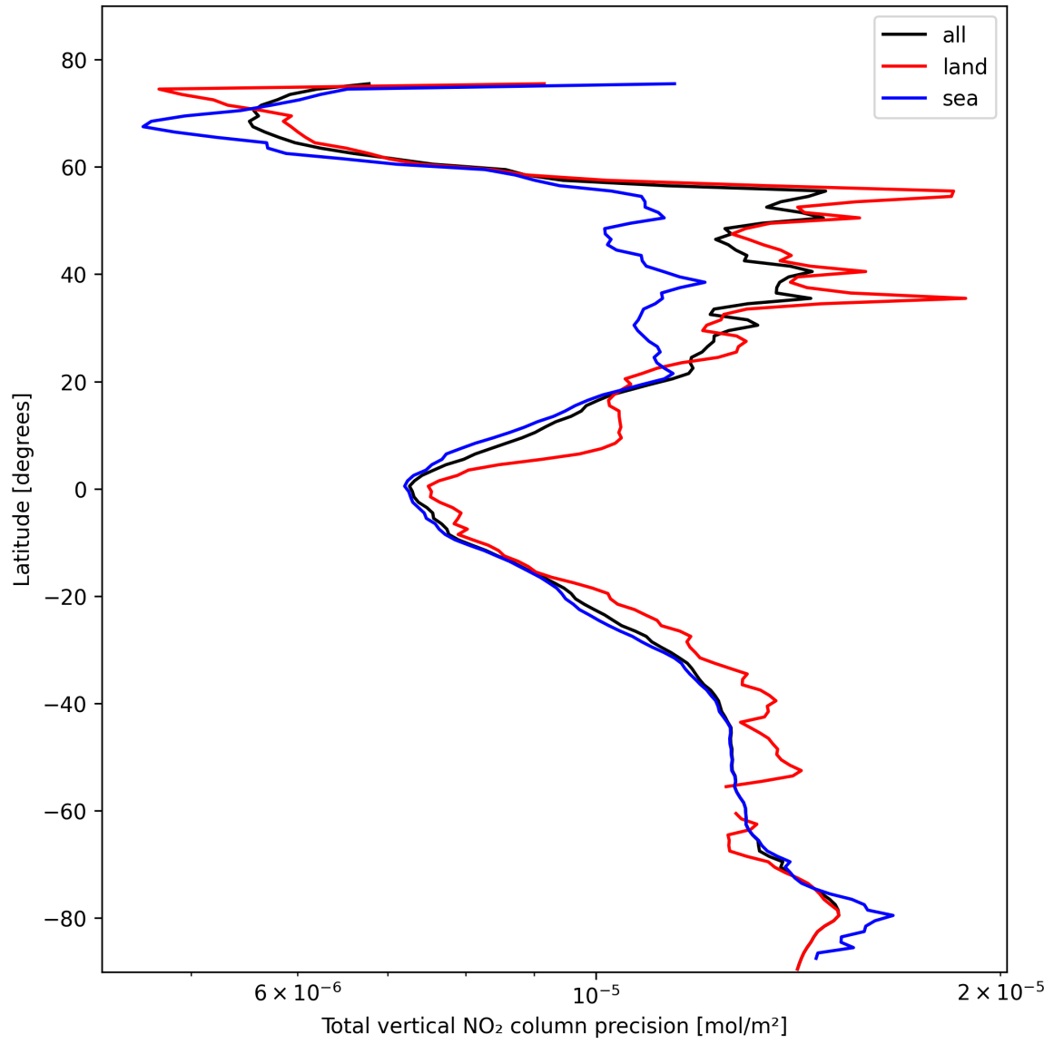
Figure 22: Zonal average of “Total vertical NO 2 column precision” for 2025-02-13 to 2025-02-14.
