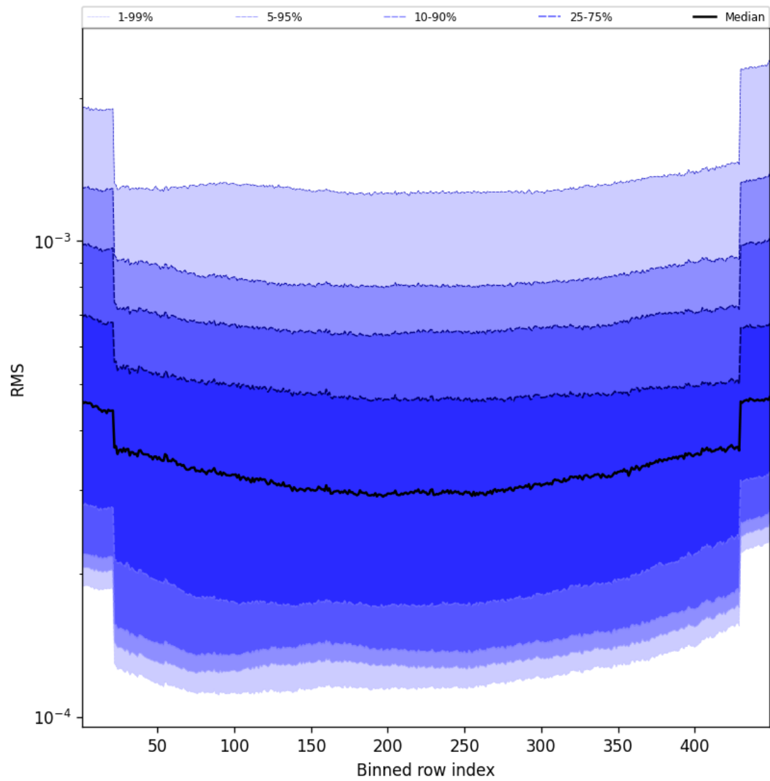
Figure 60: Along track statistics of “RMS” for 2025-02-13 to 2025-02-14
