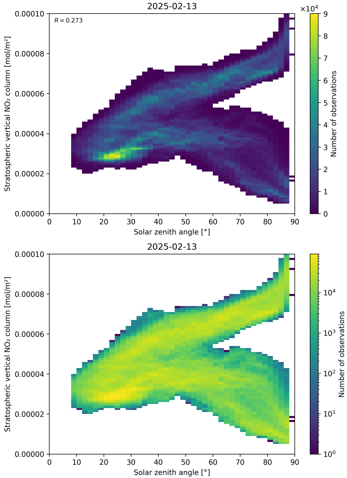
Figure 150: Scatter density plot of “Solar zenith angle” against “Stratospheric vertical NO 2 column” for 2025-02-13 to 2025-02-14.
