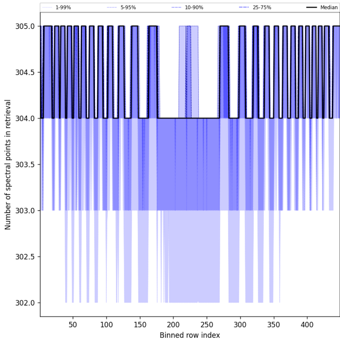
Figure 50: Along track statistics of “Number of spectral points in retrieval” for 2025-02-13 to 2025-02-14
