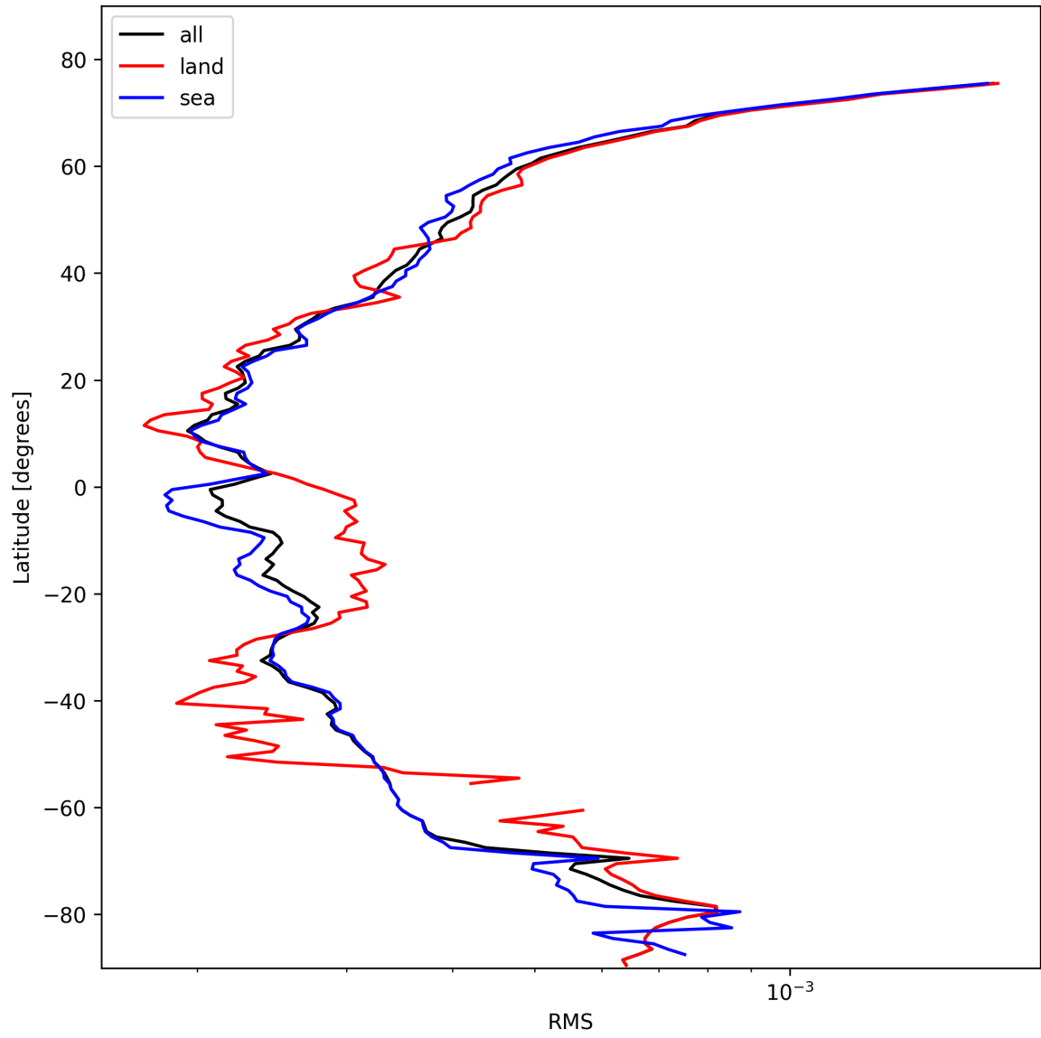
Figure 26: Zonal average of “RMS” for 2025-02-13 to 2025-02-14.
