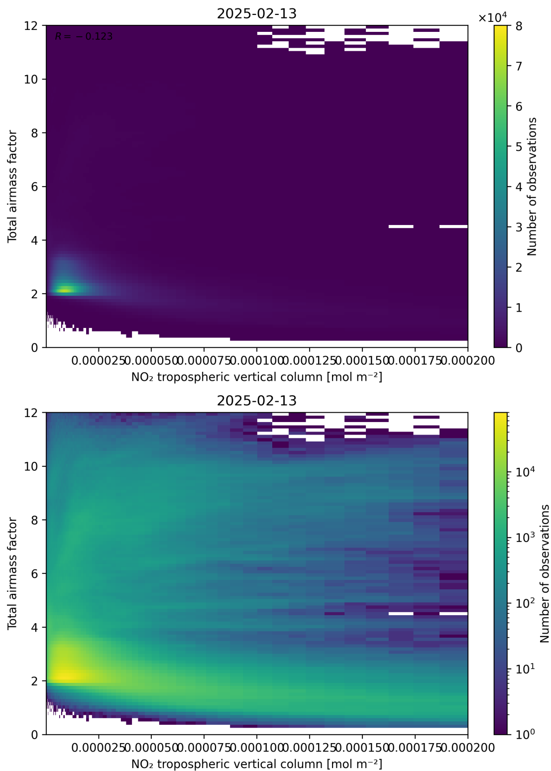
Figure 122: Scatter density plot of “NO 2 tropospheric vertical column” against “Total air mass factor” for 2025-02-13 to 2025-02-14.
