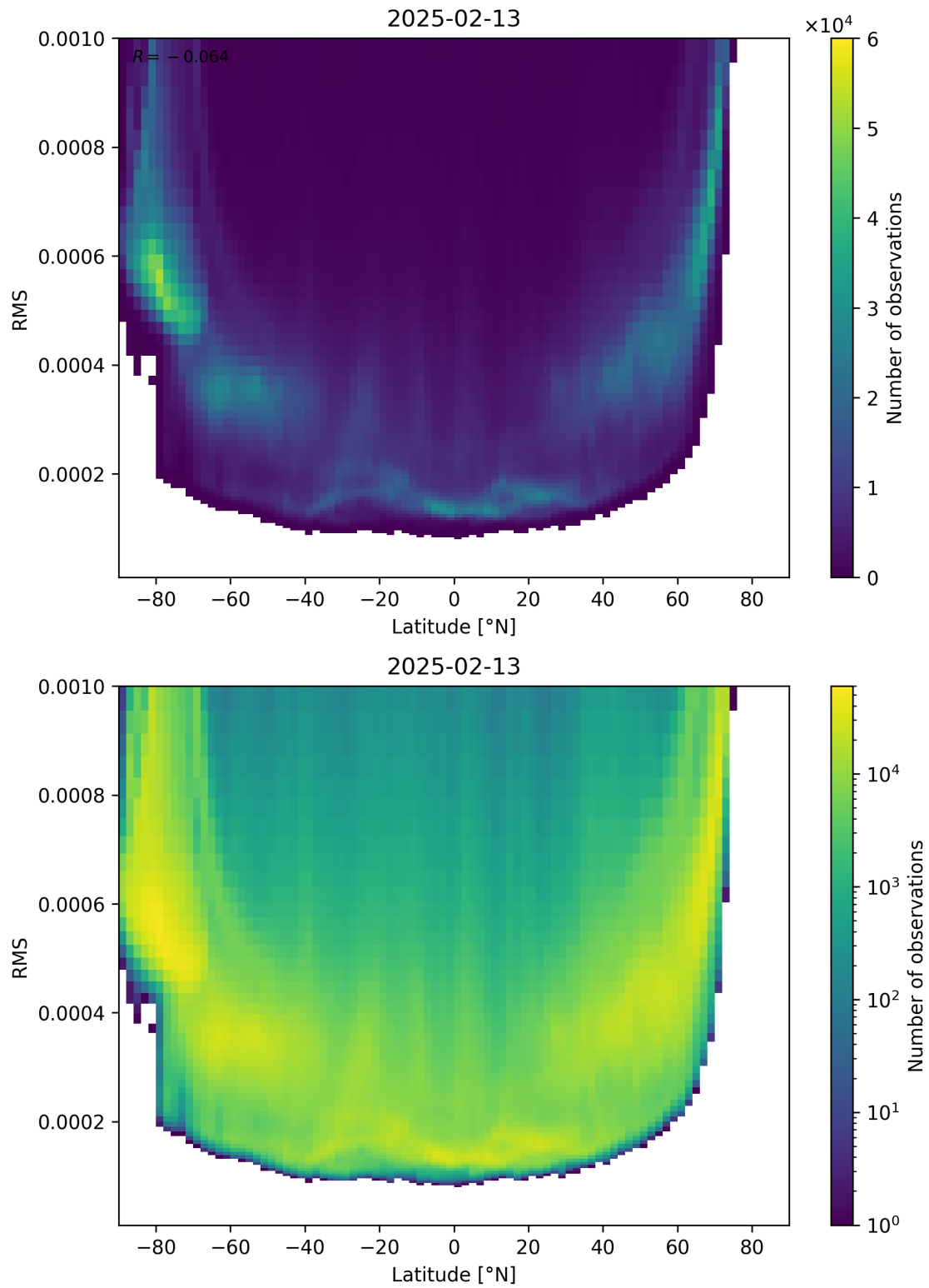
Figure 94: Scatter density plot of “Latitude” against “RMS” for 2025-02-13 to 2025-02-14.
