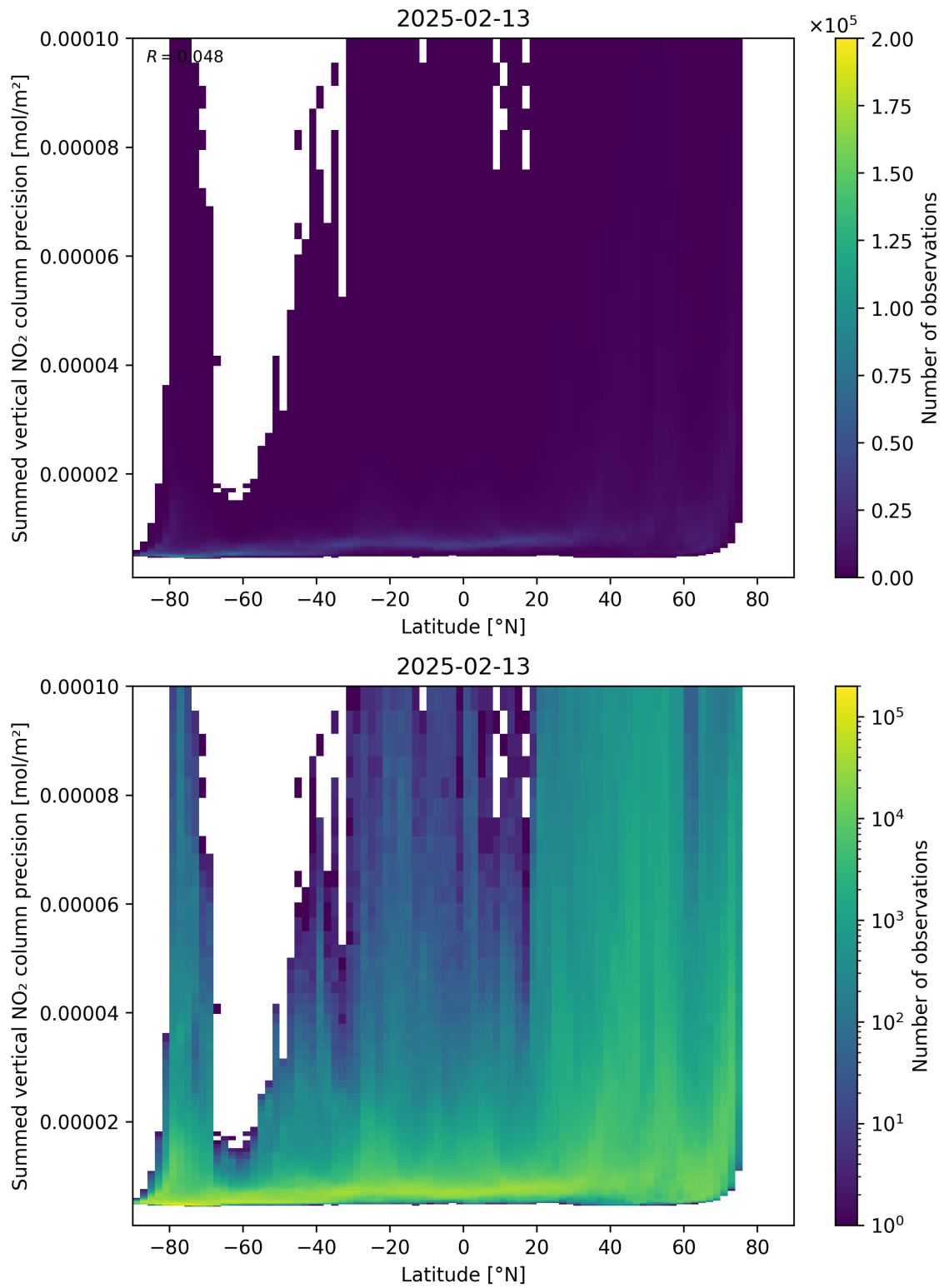
Figure 89: Scatter density plot of “Latitude” against “Summed vertical NO 2 column precision” for 2025-02-13 to 2025-02-14.
