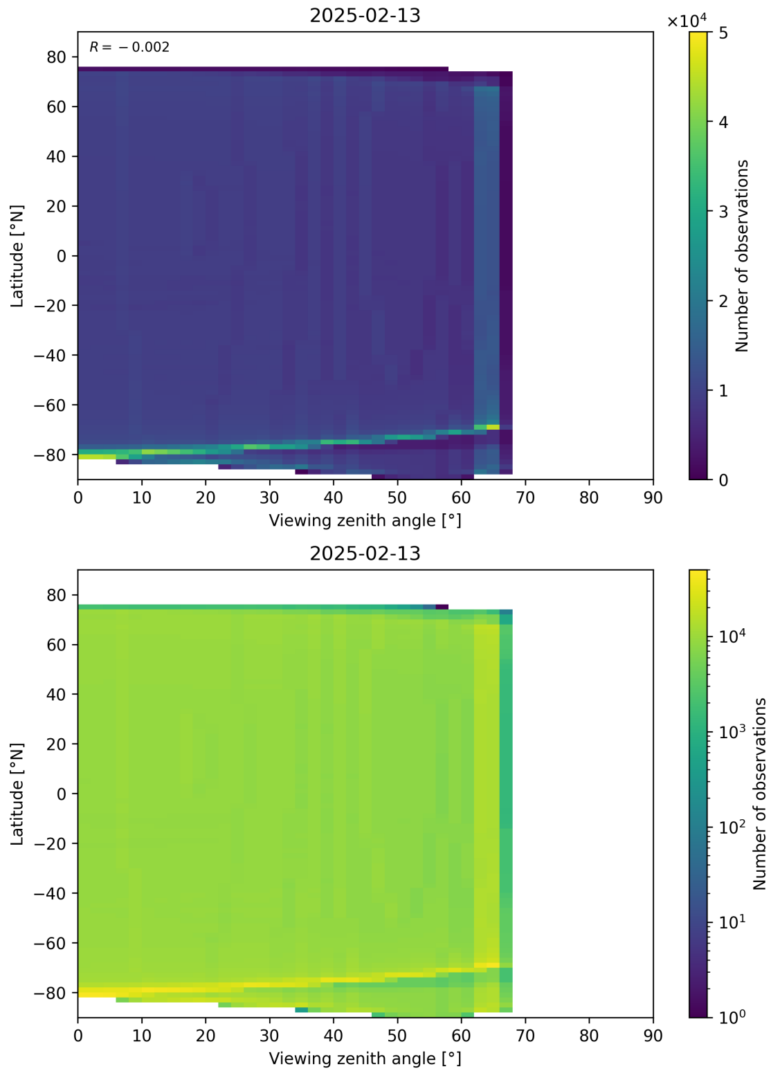
Figure 163: Scatter density plot of “Viewing zenith angle” against “Latitude” for 2025-02-13 to 2025-02-14.
