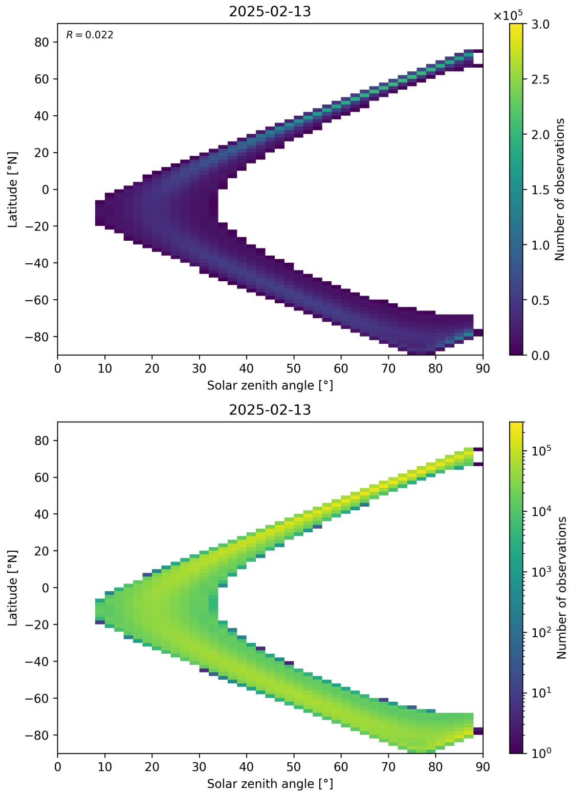
Figure 149: Scatter density plot of “Solar zenith angle” against “Latitude” for 2025-02-13 to 2025-02-14.
