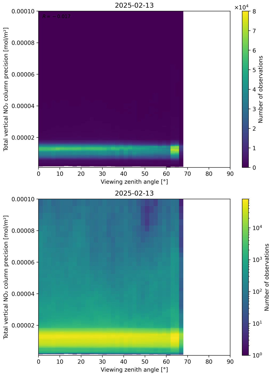
Figure 168: Scatter density plot of “Viewing zenith angle” against “Total vertical NO 2 column precision” for 2025-02-13 to 2025-02-14.
