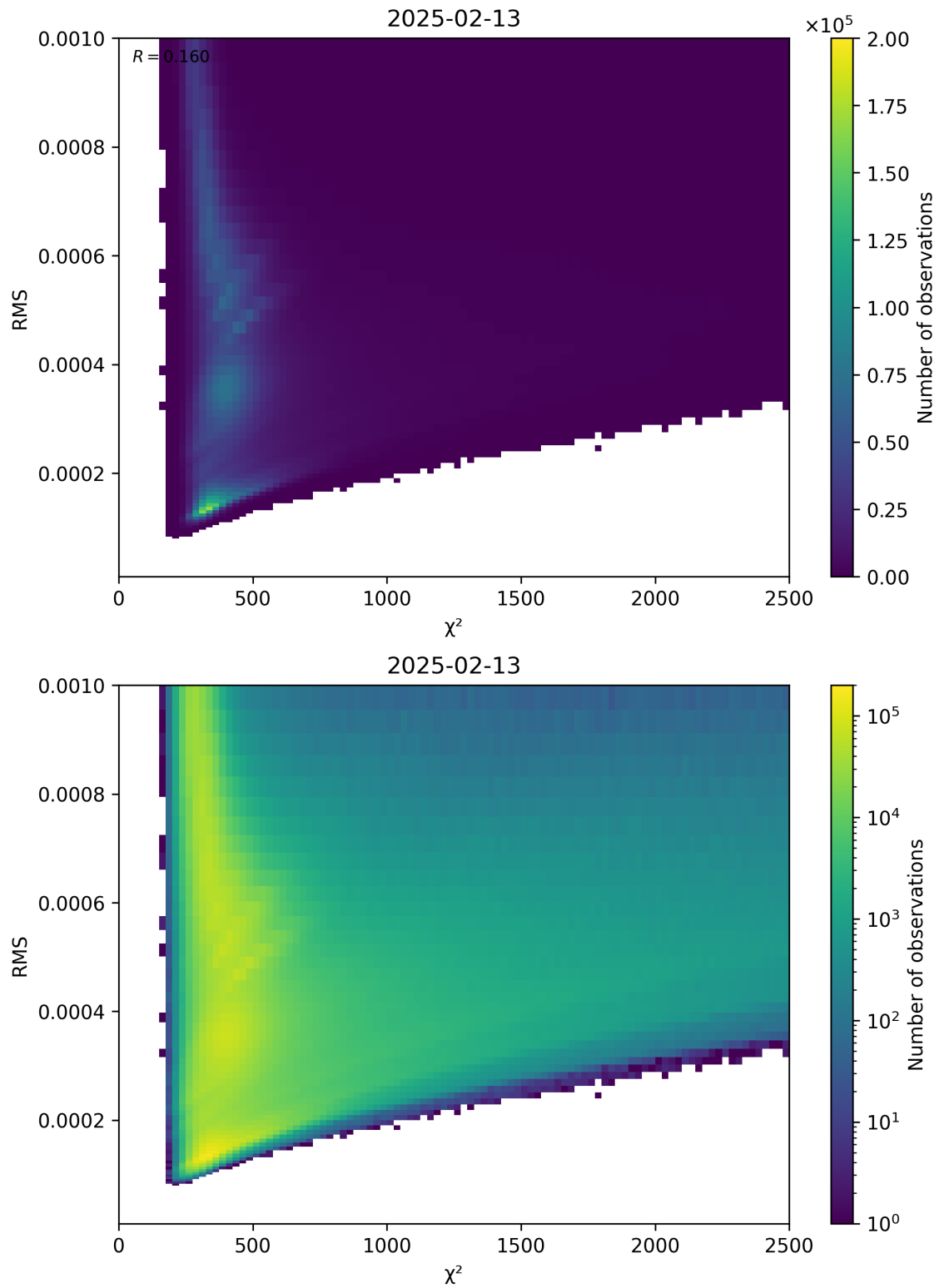
Figure 82: Scatter density plot of “ \chi^2 ” against “RMS” for 2025-02-13 to 2025-02-14.
