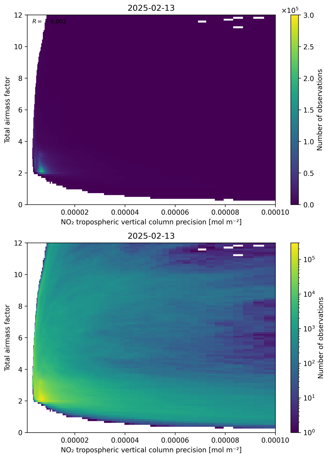
Figure 132: Scatter density plot of “NO 2 tropospheric vertical column precision” against “Total air mass factor” for 2025-02-13 to 2025-02-14.
