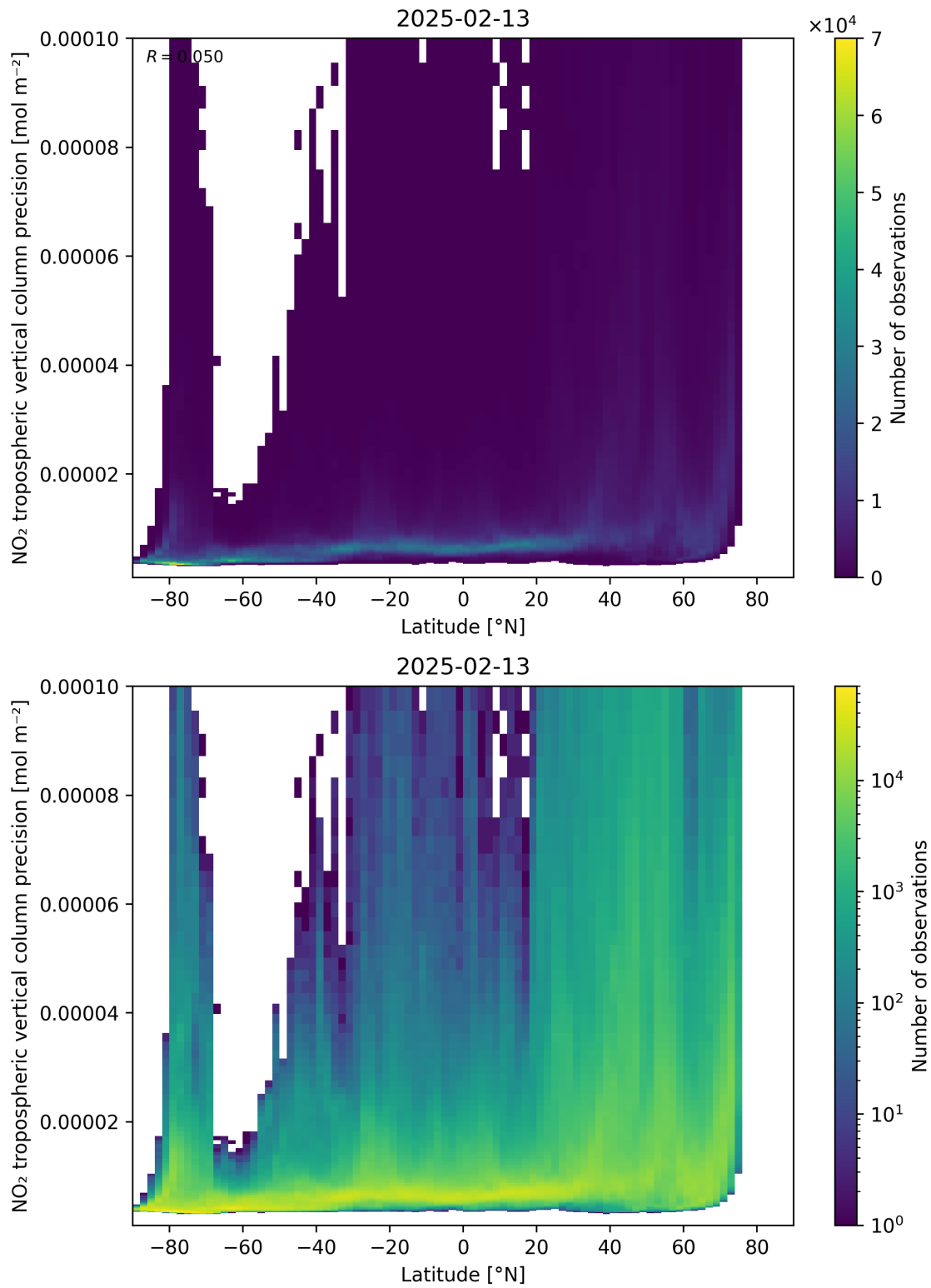
Figure 93: Scatter density plot of “Latitude” against “NO 2 tropospheric vertical column precision” for 2025-02-13 to 2025-02-14.
