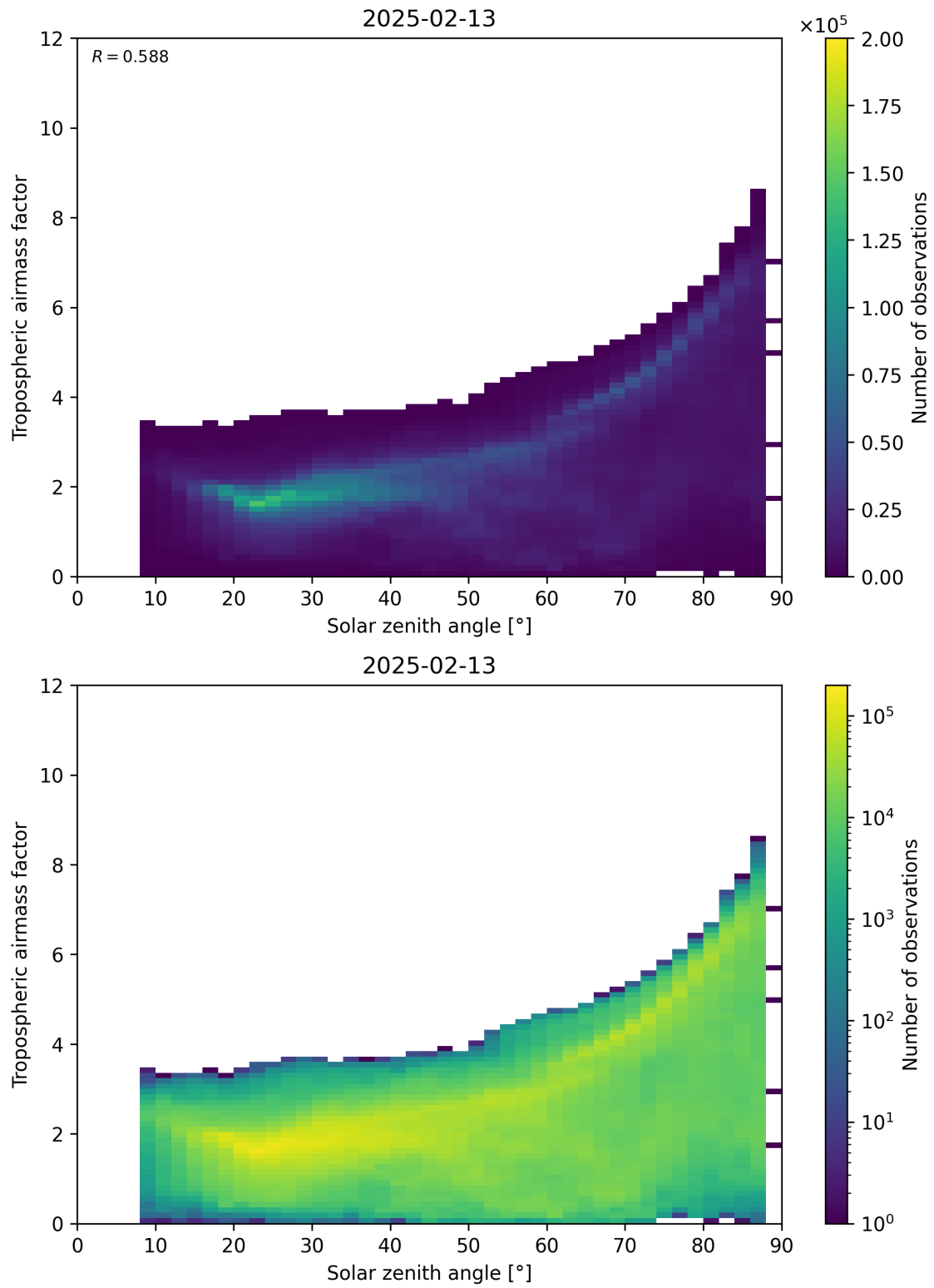
Figure 147: Scatter density plot of “Solar zenith angle” against “Tropospheric airmass factor” for 2025-02-13 to 2025-02-14.
