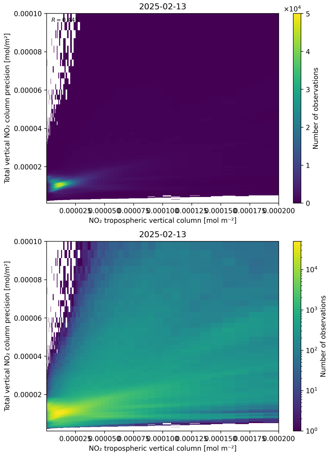
Figure 129: Scatter density plot of “NO 2 tropospheric vertical column” against “Total vertical NO 2 column precision” for 2025-02-13 to 2025-02-14.
