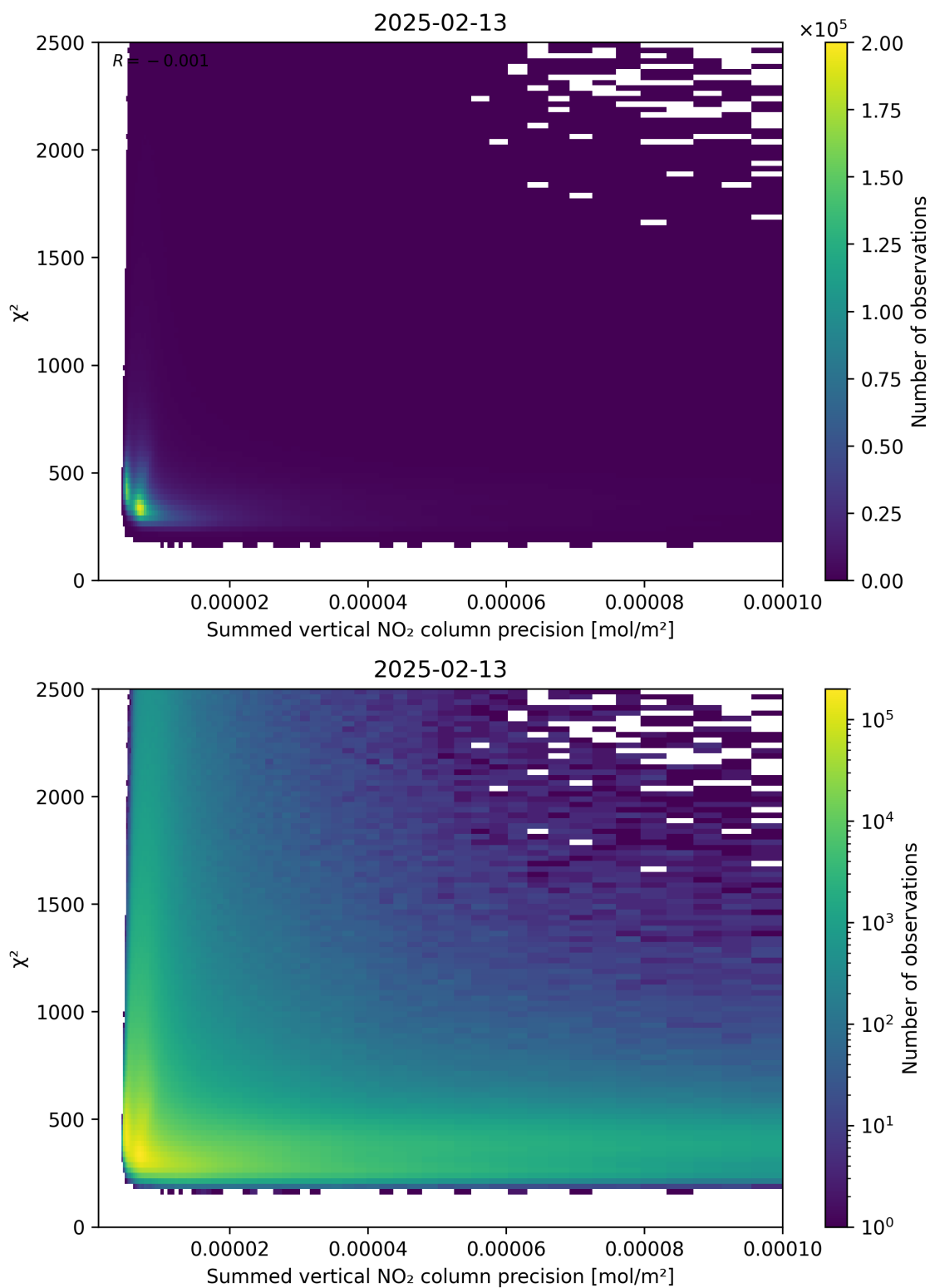
Figure 107: Scatter density plot of “Summed vertical NO 2 column precision” against “ \chi^2 ” for 2025-02-13 to 2025-02-14.
