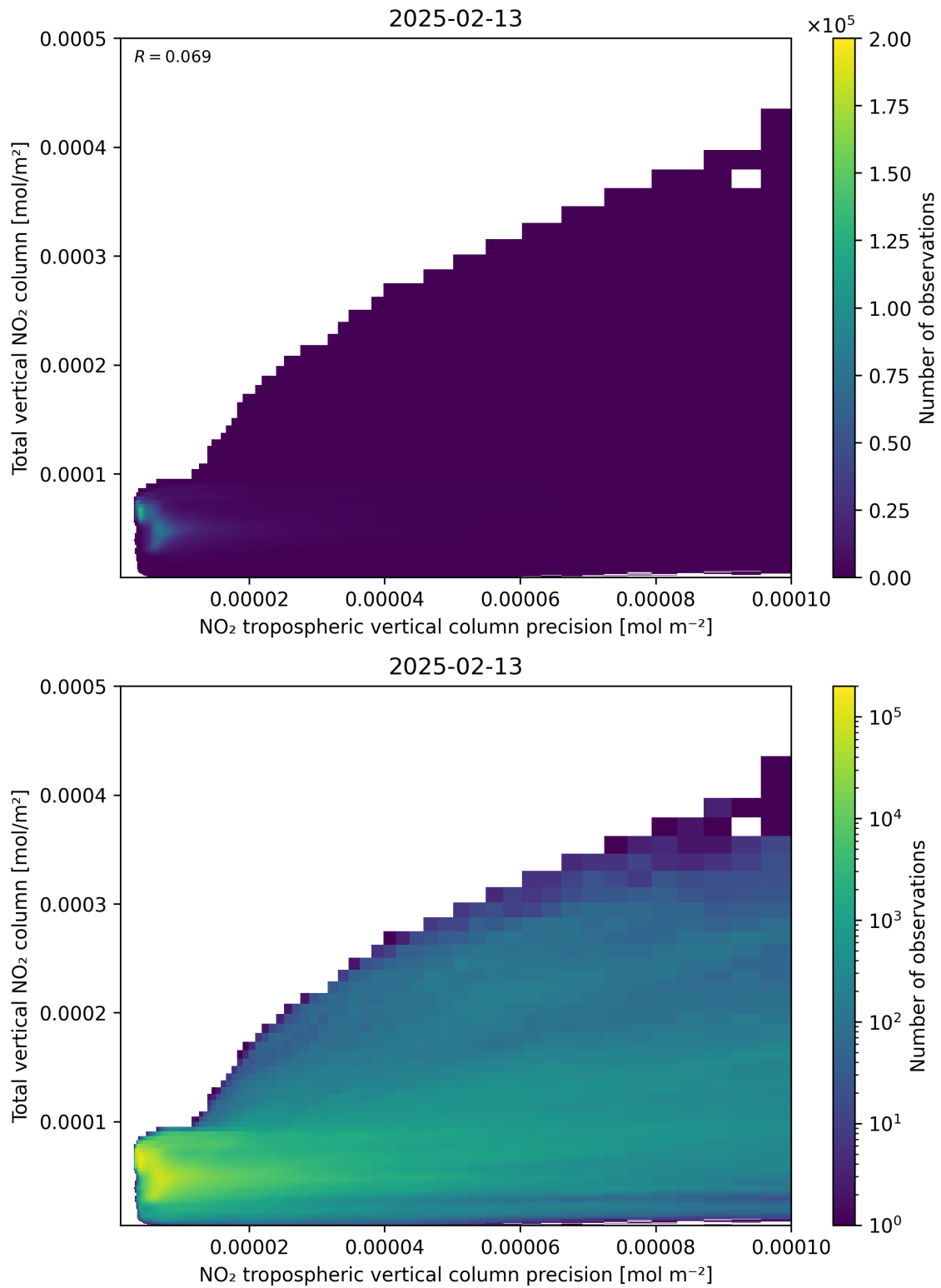
Figure 138: Scatter density plot of “NO 2 tropospheric vertical column precision” against “Total vertical NO 2 column” for 2025-02-13 to 2025-02-14.
