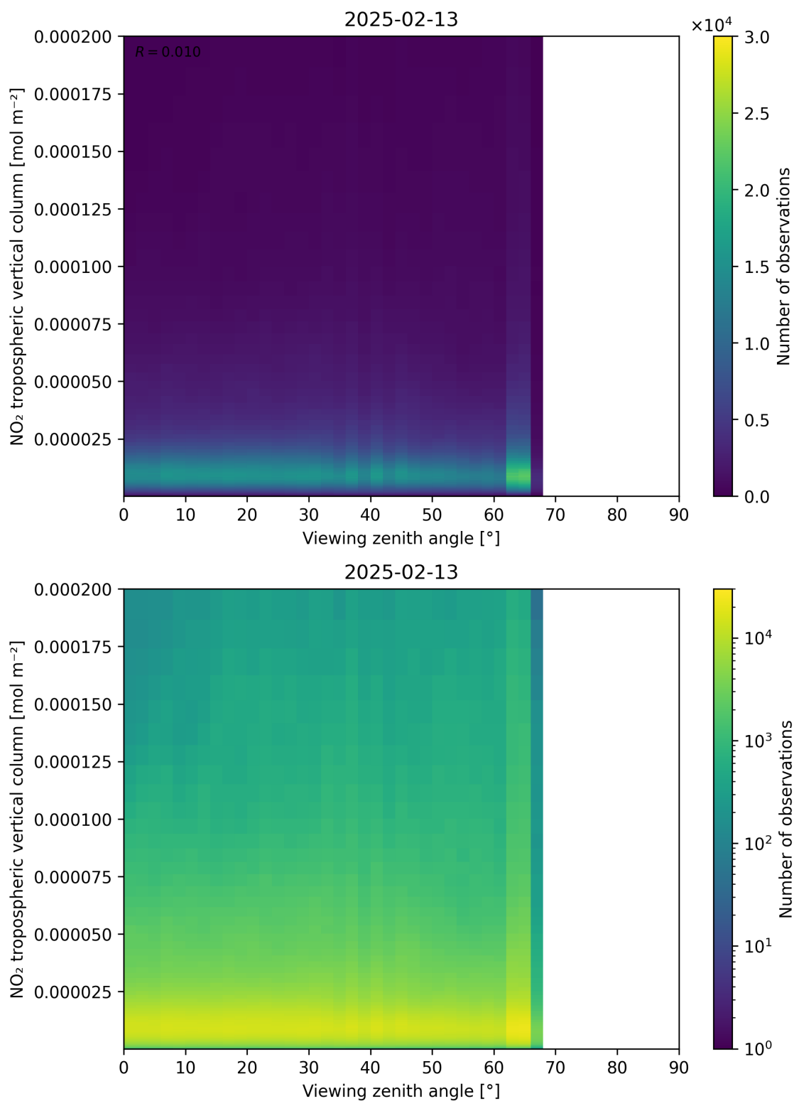
Figure 169: Scatter density plot of “Viewing zenith angle” against “NO 2 tropospheric vertical column” for 2025-02-13 to 2025-02-14.
