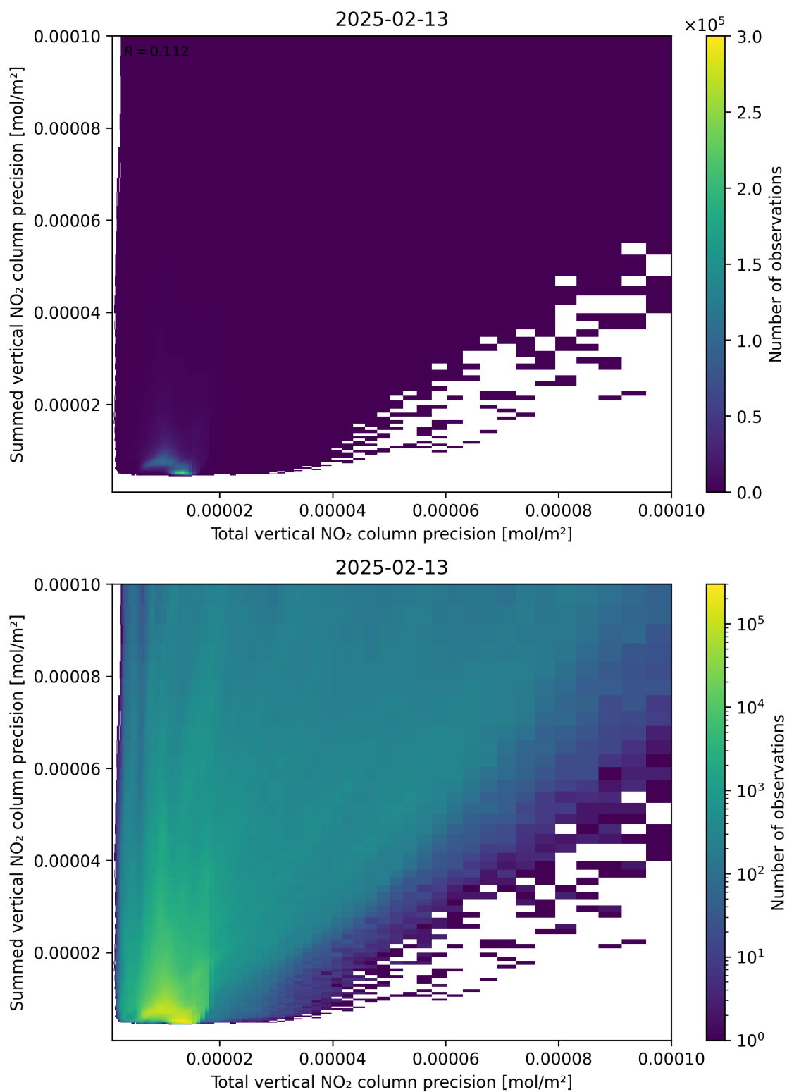
Figure 118: Scatter density plot of “Total vertical NO 2 column precision” against “Summed vertical NO 2 column precision” for 2025-02-13 to 2025-02-14.
