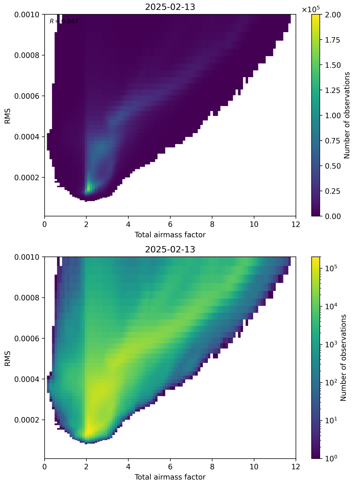
Figure 69: Scatter density plot of “Total airmass factor” against “RMS” for 2025-02-13 to 2025-02-14.
