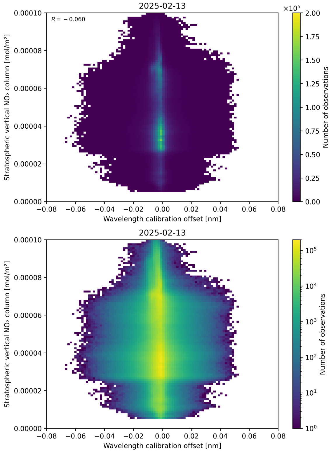
Figure 176: Scatter density plot of “Wavelength calibration offset” against “Stratospheric vertical NO 2 column” for 2025-02-13 to 2025-02-14.
