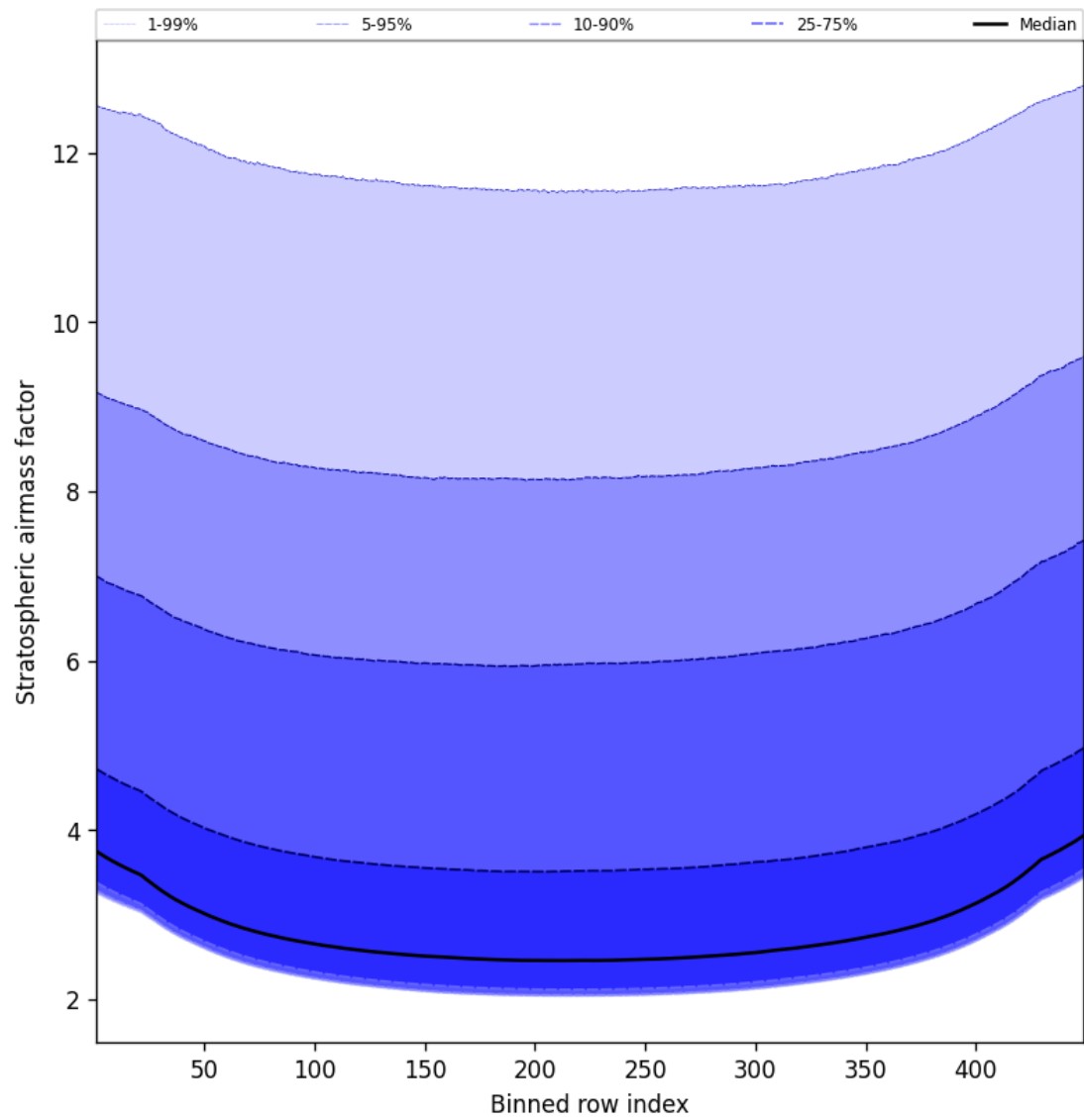
Figure 61: Along track statistics of “Stratospheric airmass factor” for 2025-02-13 to 2025-02-14
