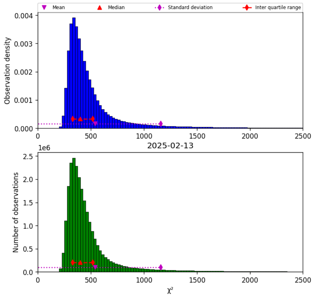
Figure 42: Histogram of “ \chi^2 ” for 2025-02-13 to 2025-02-14
