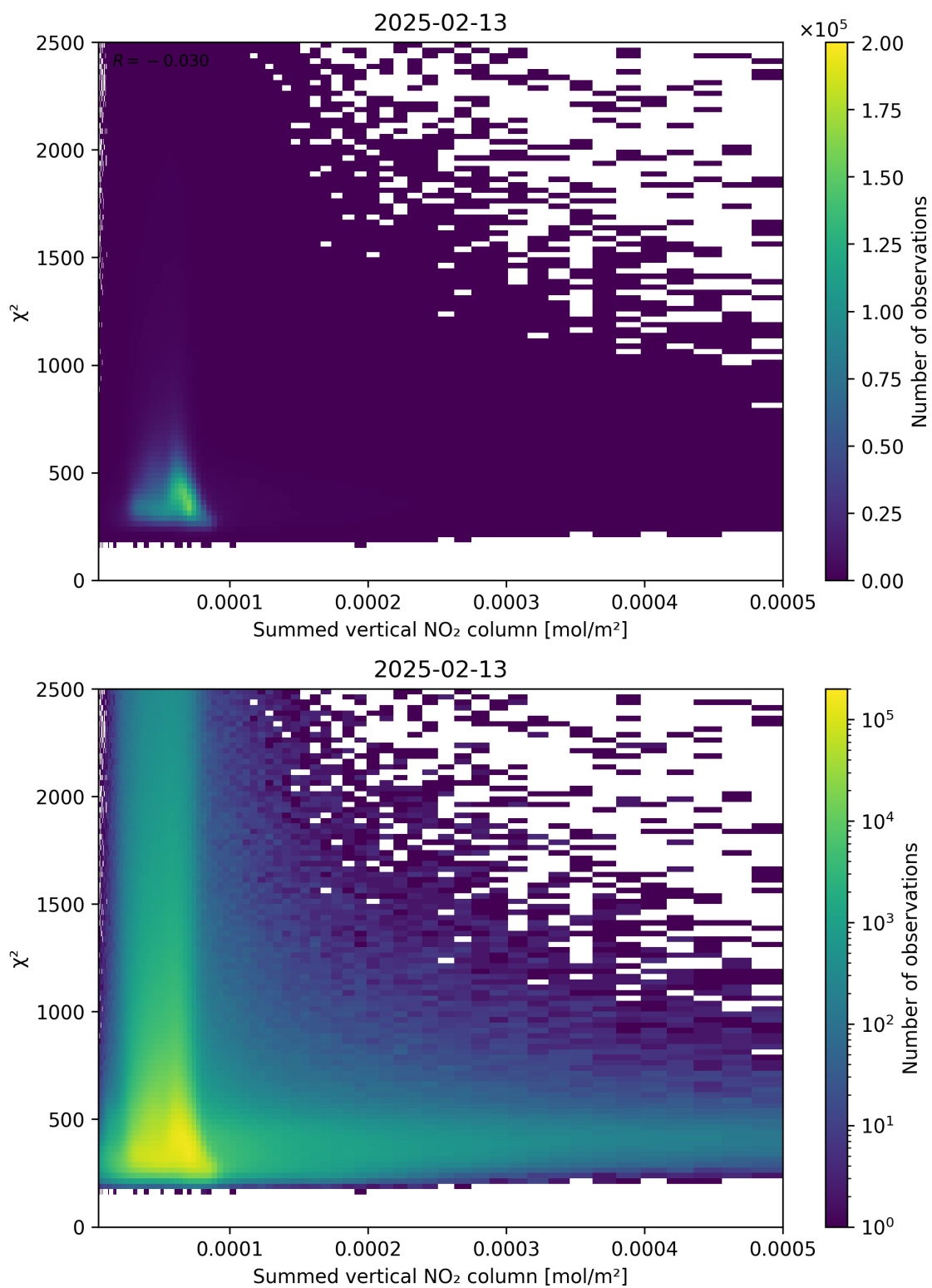
Figure 104: Scatter density plot of “Summed vertical NO 2 column” against “ \chi^2 ” for 2025-02-13 to 2025-02-14.
