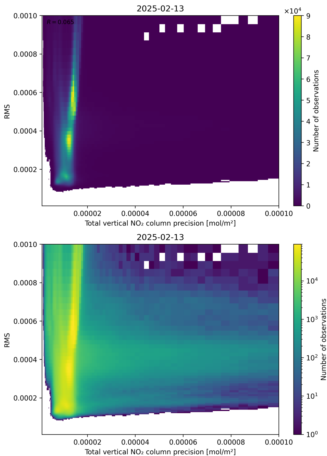
Figure 119: Scatter density plot of “Total vertical NO 2 column precision” against “RMS” for 2025-02-13 to 2025-02-14.
