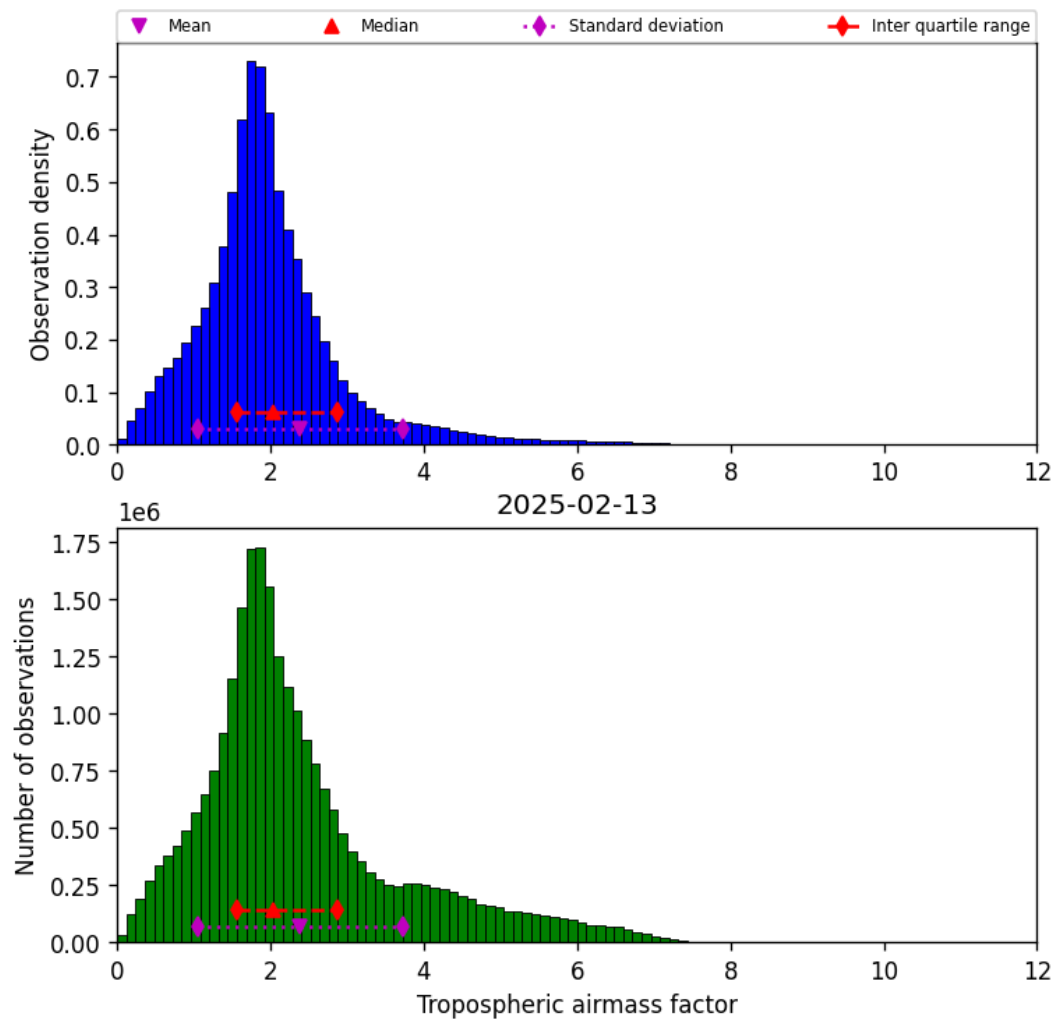
Figure 31: Histogram of “Tropospheric airmass factor” for 2025-02-13 to 2025-02-14
