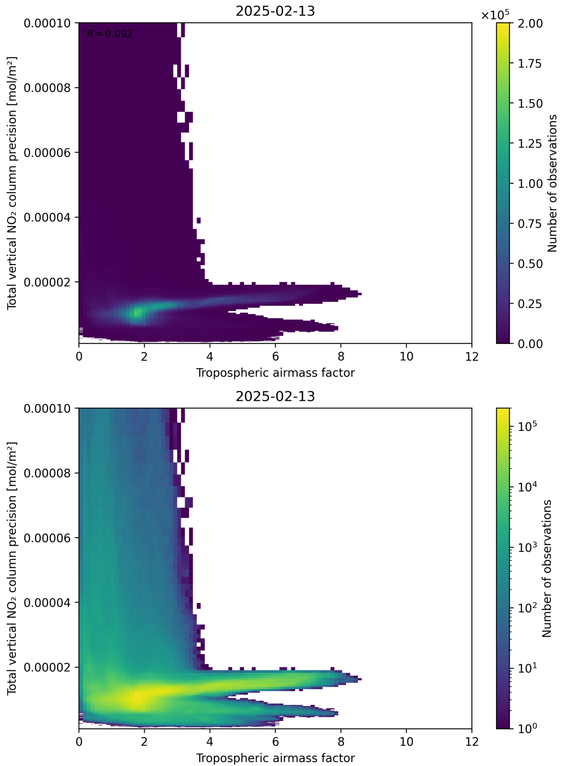
Figure 78: Scatter density plot of “Tropospheric air mass factor” against “Total vertical NO 2 column precision” for 2025-02-13 to 2025-02-14.
