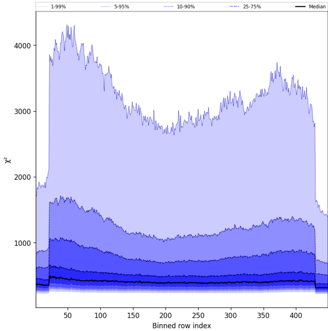
Figure 59: Along track statistics of “ \chi^2 ” for 2025-02-13 to 2025-02-14
