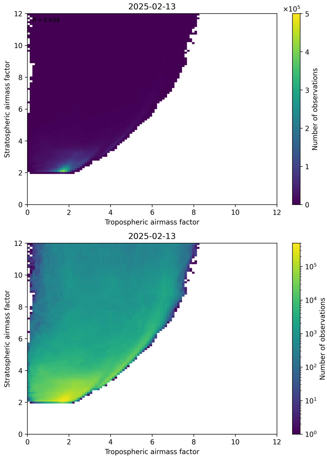
Figure 71: Scatter density plot of “Tropospheric airmass factor” against “Stratospheric airmass factor” for 2025-02-13 to 2025-02-14.
