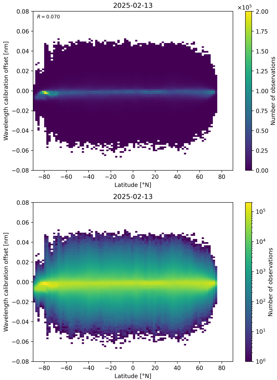
Figure 95: Scatter density plot of “Latitude” against “Wavelength calibration offset” for 2025-02-13 to 2025-02-14.
