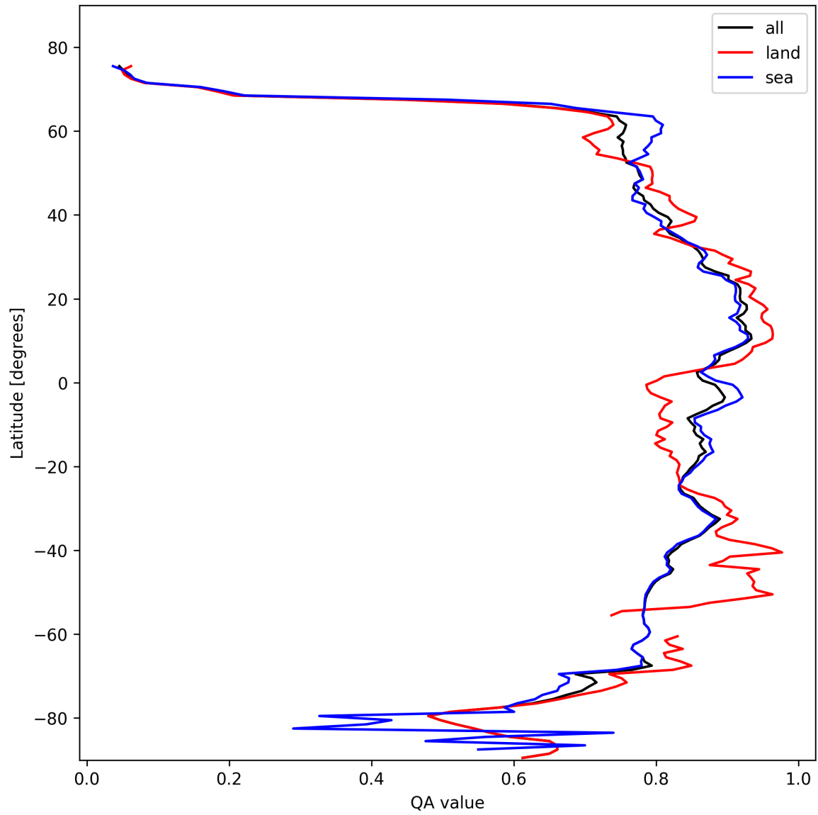
Figure 11: Zonal average of “QA value” for 2025-02-13 to 2025-02-14.
