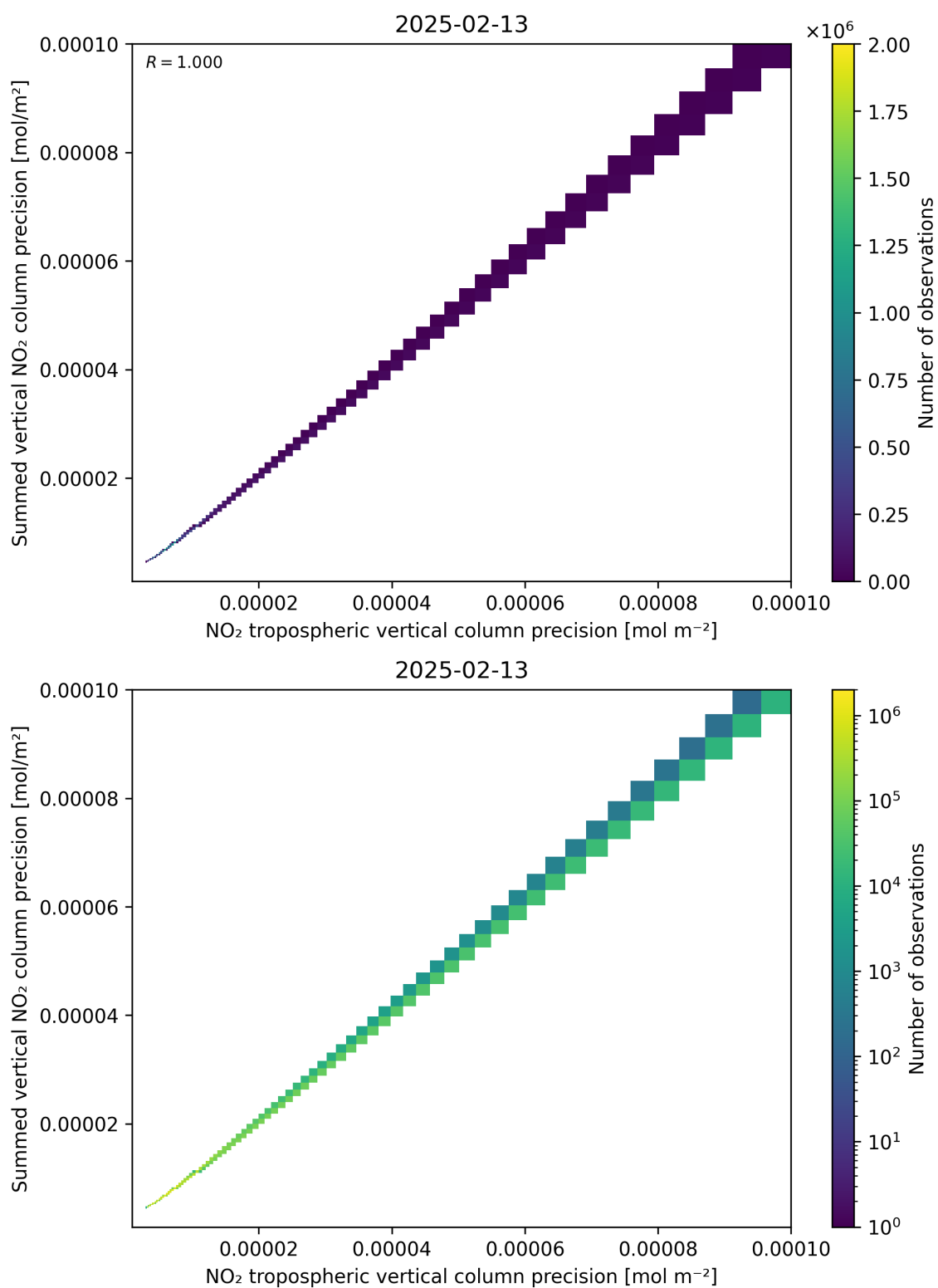
Figure 137: Scatter density plot of “NO 2 tropospheric vertical column precision” against “Summed vertical NO 2 column precision” for 2025-02-13 to 2025-02-14.
