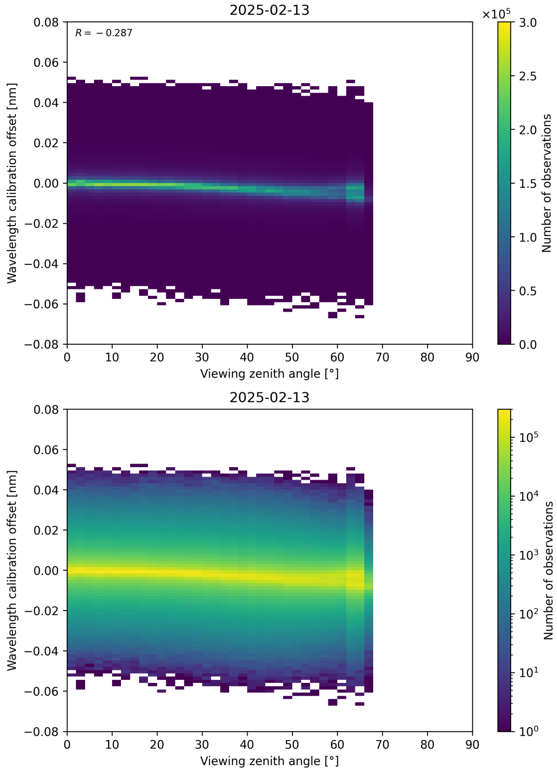
Figure 173: Scatter density plot of “Viewing zenith angle” against “Wavelength calibration offset” for 2025-02-13 to 2025-02-14.
