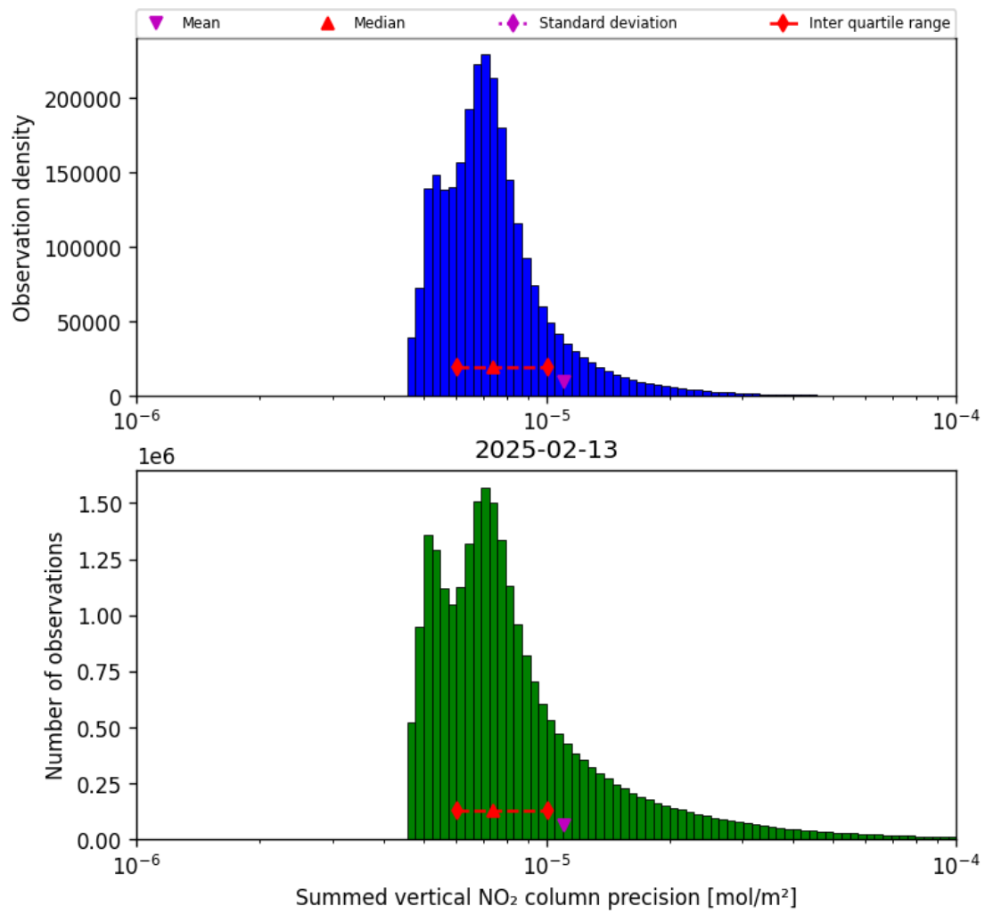
Figure 41: Histogram of “Summed vertical NO 2 column precision” for 2025-02-13 to 2025-02-14
