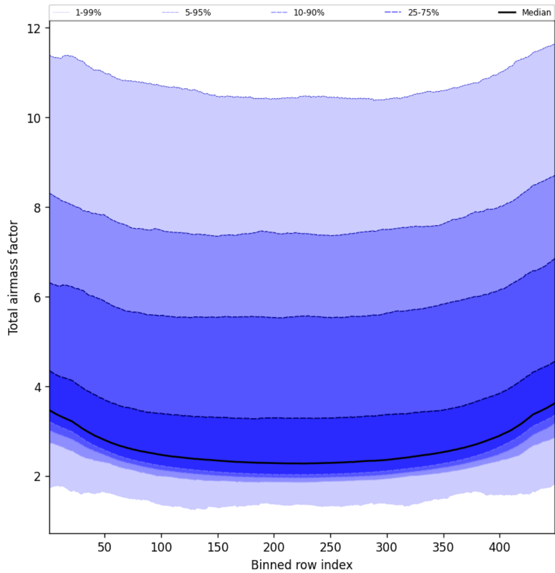
Figure 49: Along track statistics of “Total airmass factor” for 2025-02-13 to 2025-02-14
