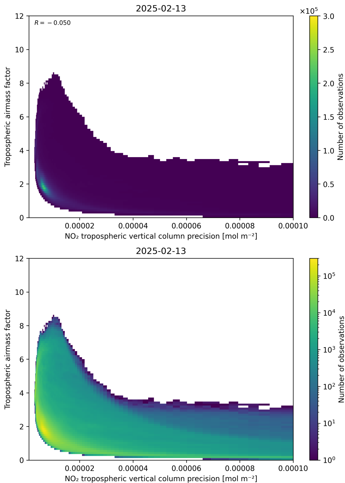
Figure 133: Scatter density plot of “NO 2 tropospheric vertical column precision” against “Tropospheric airmass factor” for 2025-02-13 to 2025-02-14.
