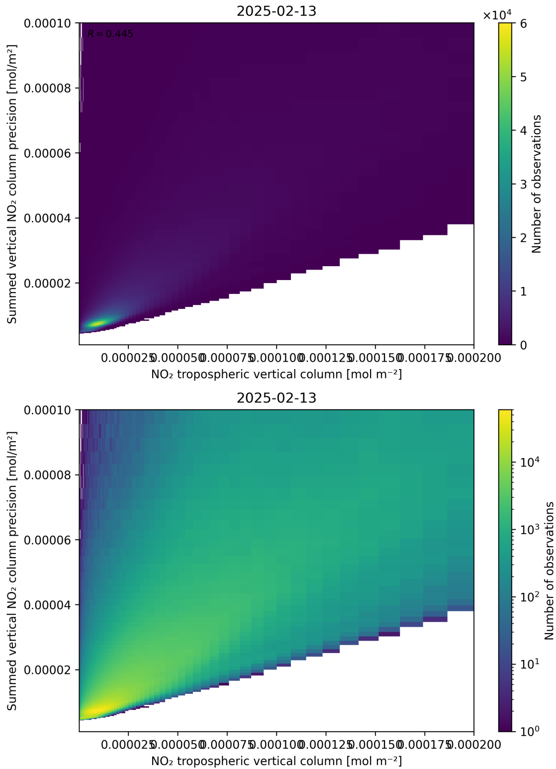
Figure 127: Scatter density plot of “NO 2 tropospheric vertical column” against “Summed vertical NO 2 column precision” for 2025-02-13 to 2025-02-14.
