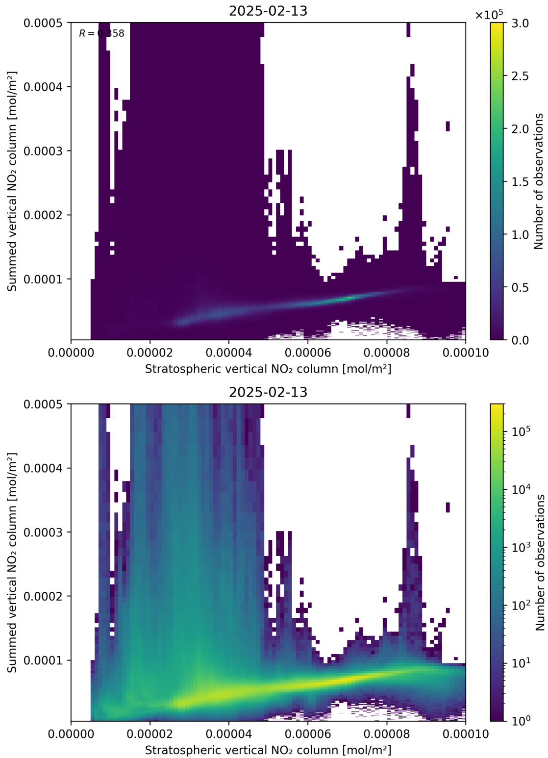
Figure 98: Scatter density plot of “Stratospheric vertical NO 2 column” against “Summed vertical NO 2 column” for 2025-02-13 to 2025-02-14.
