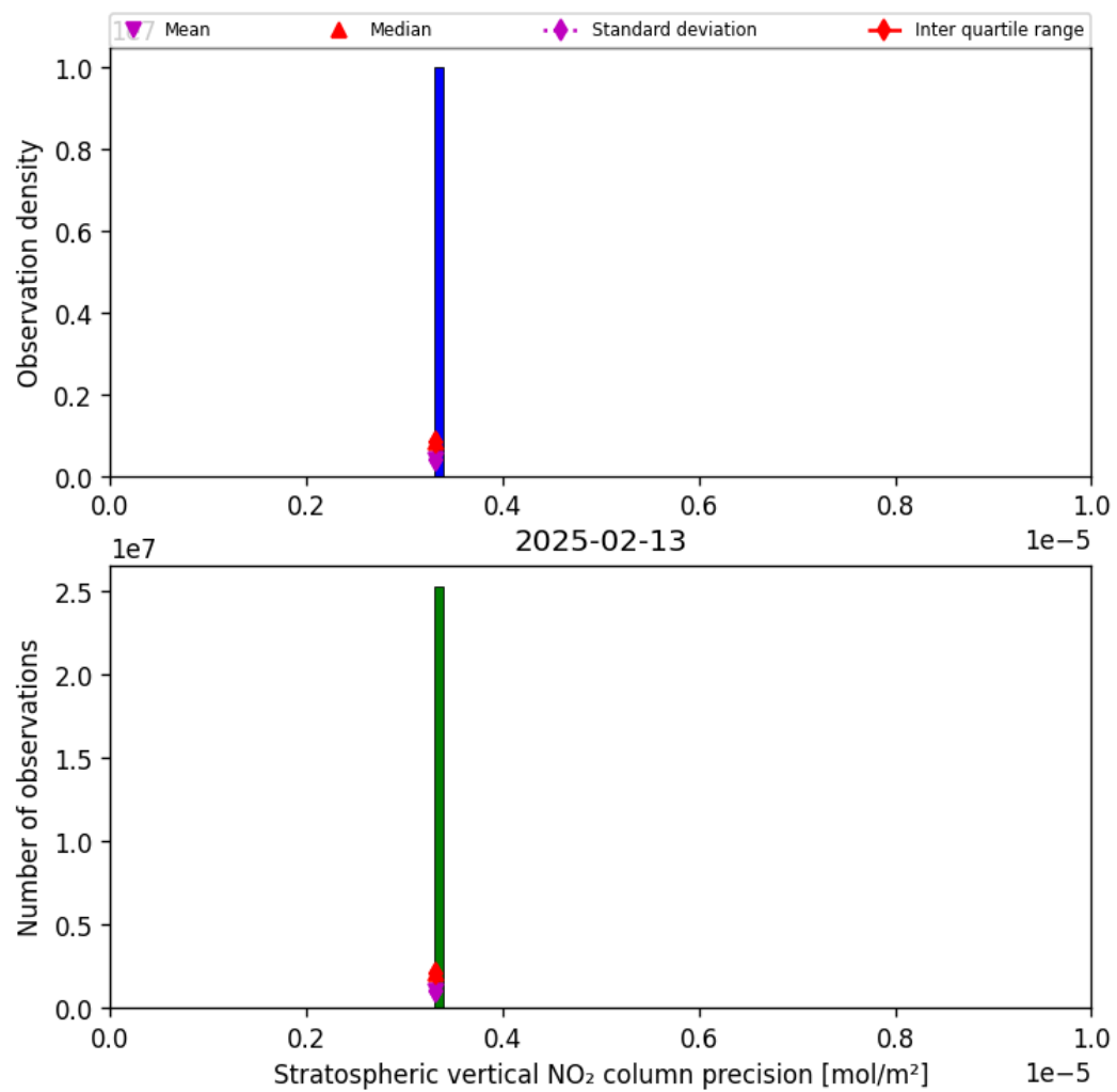
Figure 37: Histogram of “Stratospheric vertical NO 2 column precision” for 2025-02-13 to 2025-02-14
