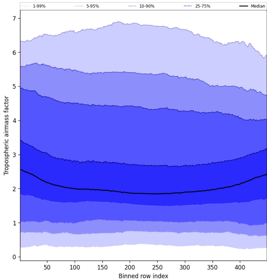
Figure 48: Along track statistics of “Tropospheric air mass factor” for 2025-02-13 to 2025-02-14
