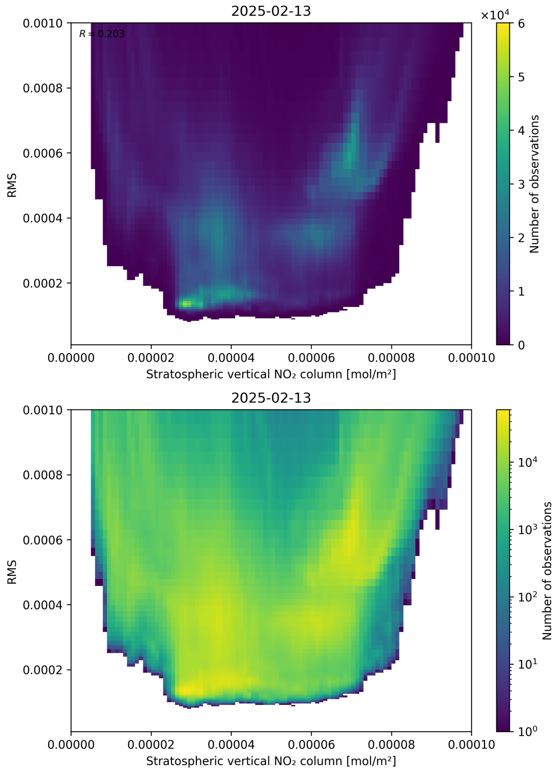
Figure 102: Scatter density plot of “Stratospheric vertical NO 2 column” against “RMS” for 2025-02-13 to 2025-02-14.
