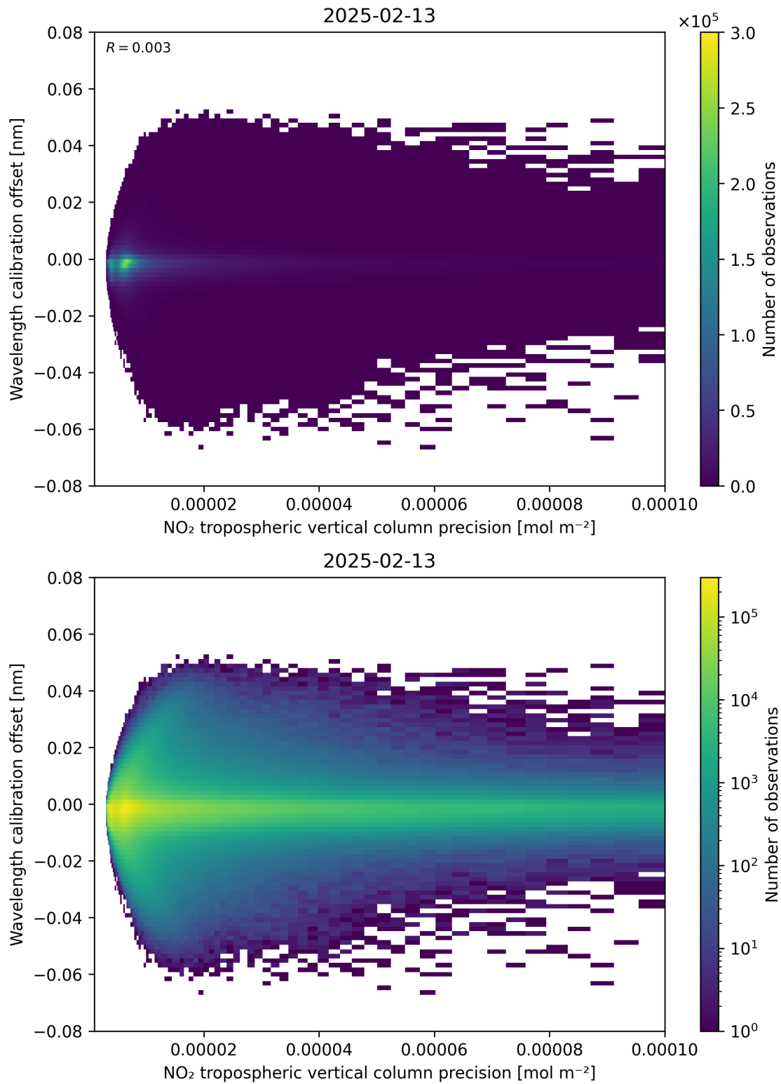
Figure 141: Scatter density plot of “NO 2 tropospheric vertical column precision” against “Wavelength calibration offset” for 2025-02-13 to 2025-02-14.
