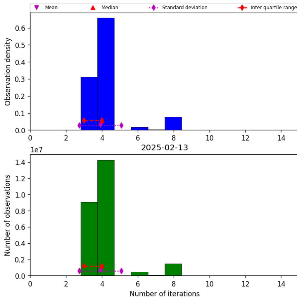
Figure 34: Histogram of “Number of iterations” for 2025-02-13 to 2025-02-14
