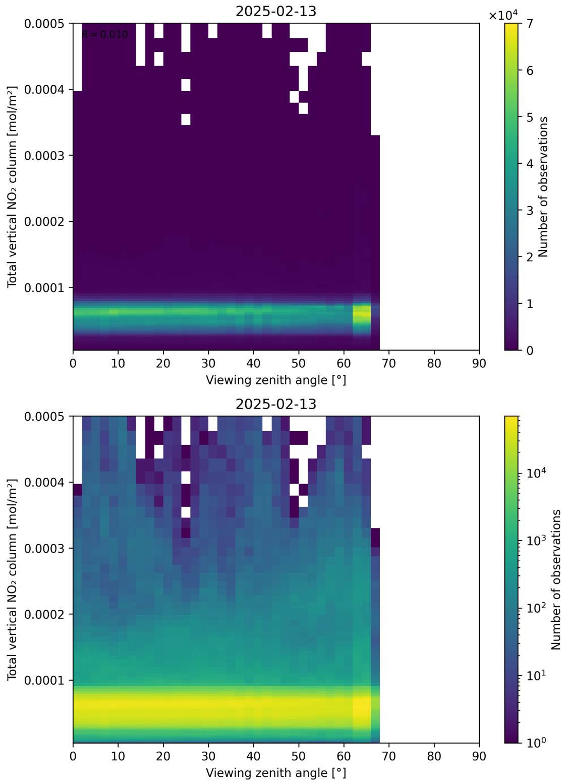
Figure 167: Scatter density plot of “Viewing zenith angle” against “Total vertical NO 2 column” for 2025-02-13 to 2025-02-14.
