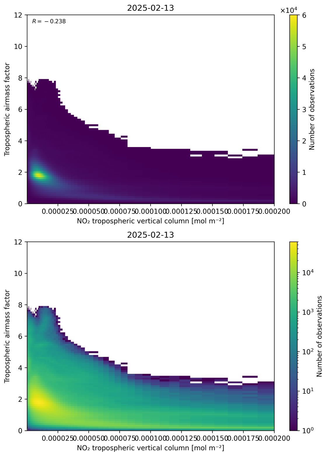
Figure 123: Scatter density plot of “NO 2 tropospheric vertical column” against “Tropospheric air mass factor” for 2025-02-13 to 2025-02-14.
