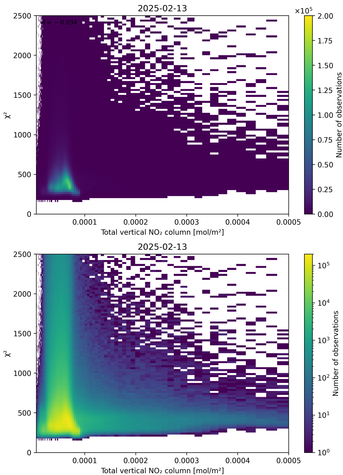
Figure 111: Scatter density plot of “Total vertical NO 2 column” against “ \chi^2 ” for 2025-02-13 to 2025-02-14.
