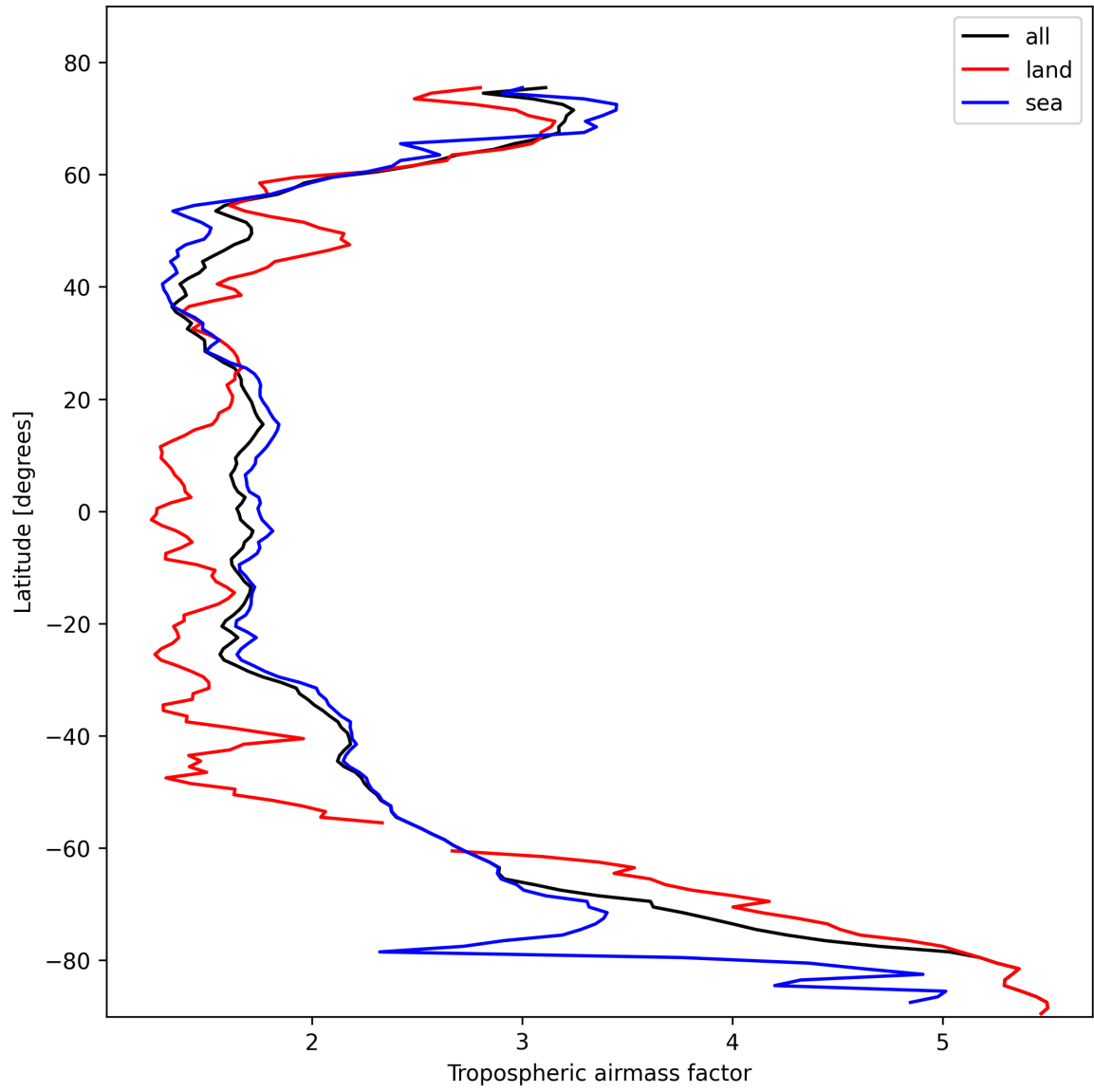
Figure 14: Zonal average of “Tropospheric airmass factor” for 2025-02-13 to 2025-02-14.
