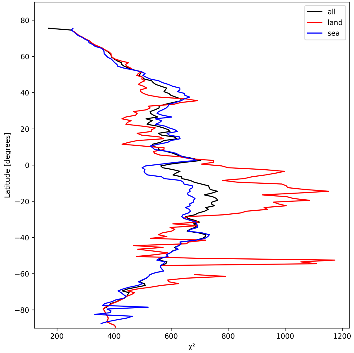
Figure 25: Zonal average of “ \chi^2 ” for 2025-02-13 to 2025-02-14.
