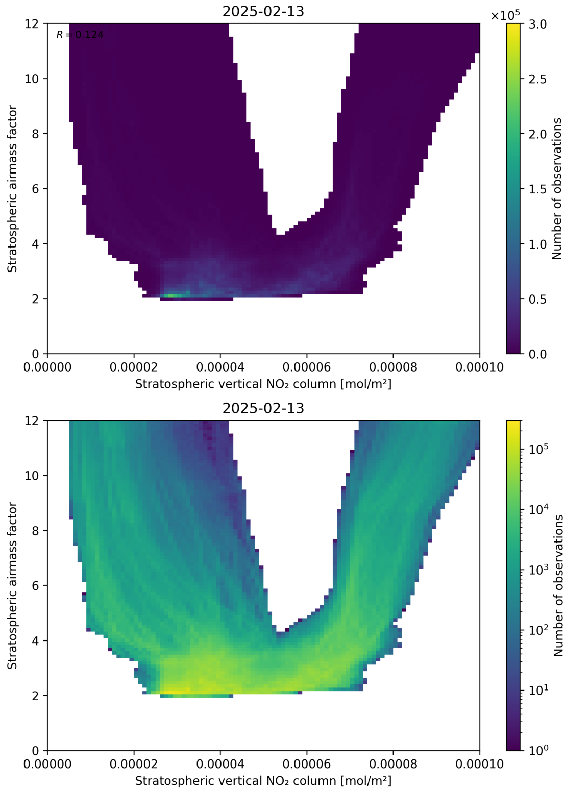
Figure 96: Scatter density plot of “Stratospheric vertical NO 2 column” against “Stratospheric airmass factor” for 2025-02-13 to 2025-02-14.
