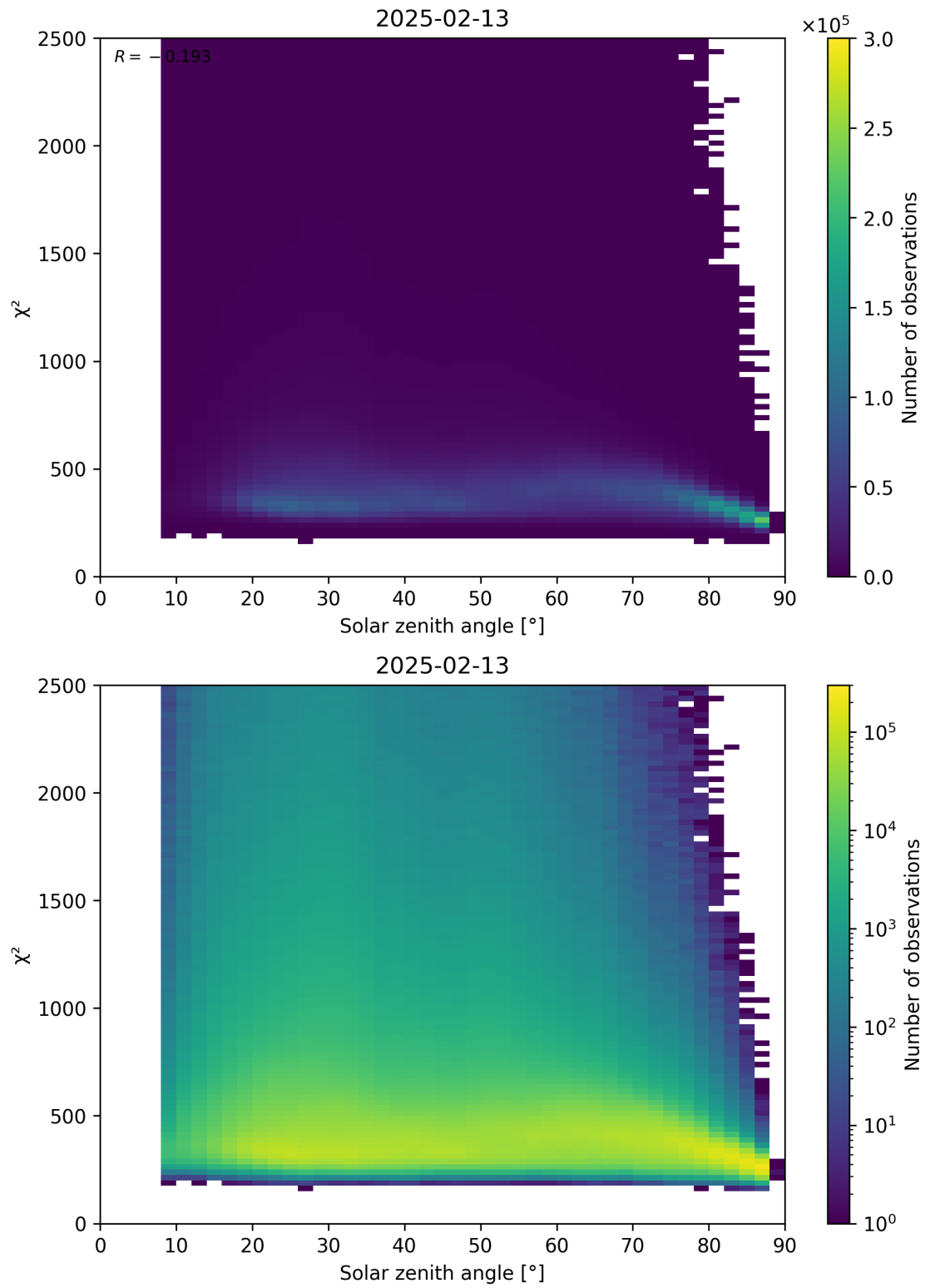
Figure 148: Scatter density plot of “Solar zenith angle” against “ \chi^2 ” for 2025-02-13 to 2025-02-14.
