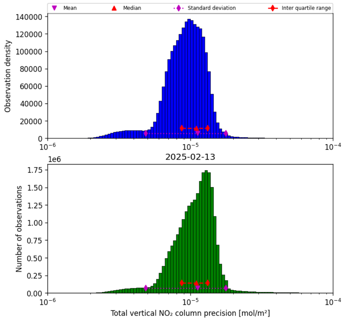
Figure 39: Histogram of “Total vertical NO 2 column precision” for 2025-02-13 to 2025-02-14
