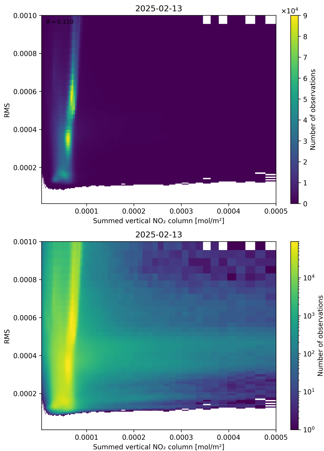
Figure 109: Scatter density plot of “Summed vertical NO 2 column” against “RMS” for 2025-02-13 to 2025-02-14.
