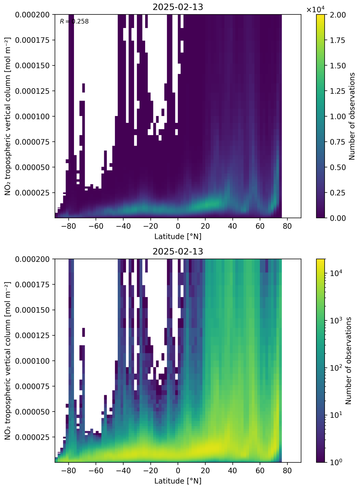
Figure 92: Scatter density plot of “Latitude” against “NO 2 tropospheric vertical column” for 2025-02-13 to 2025-02-14.
