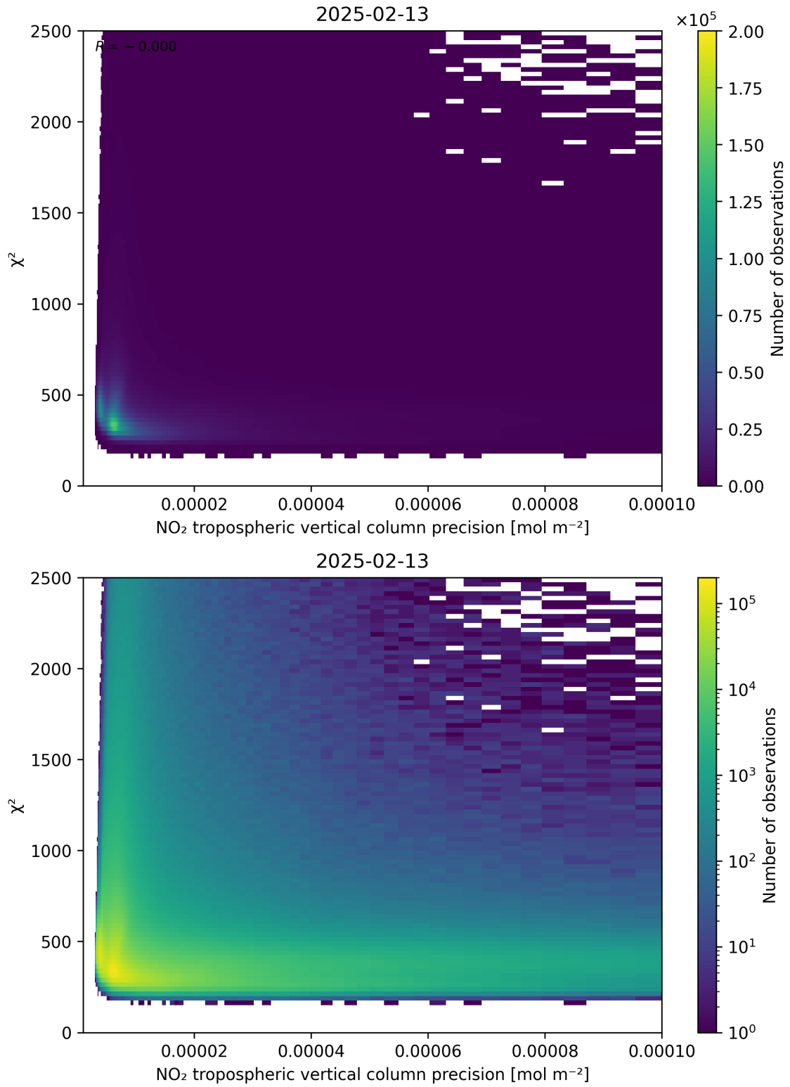
Figure 134: Scatter density plot of “NO 2 tropospheric vertical column precision” against “ \chi^2 ” for 2025-02-13 to 2025-02-14.
