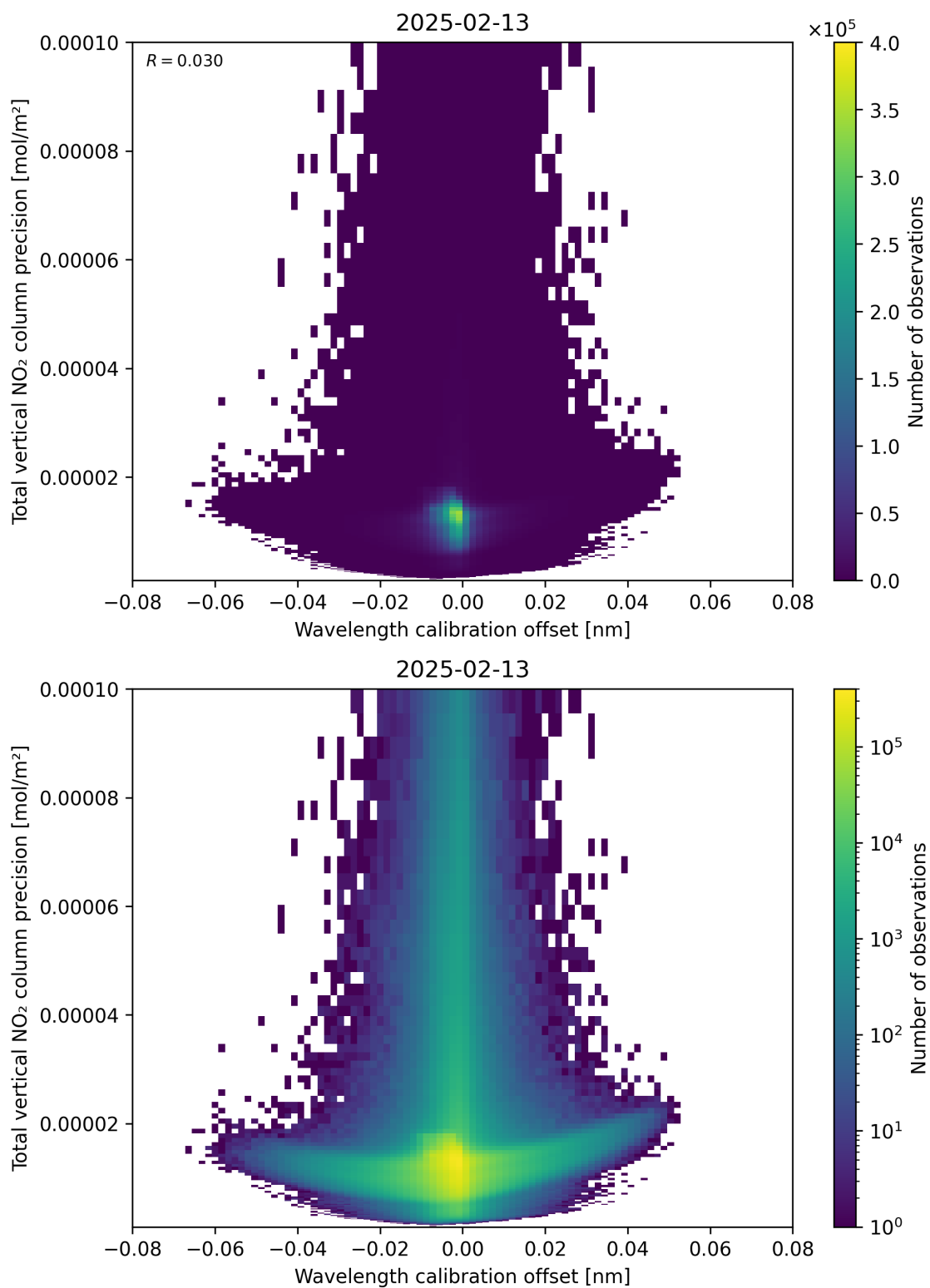
Figure 180: Scatter density plot of “Wavelength calibration offset” against “Total vertical NO 2 column precision” for 2025-02-13 to 2025-02-14.
