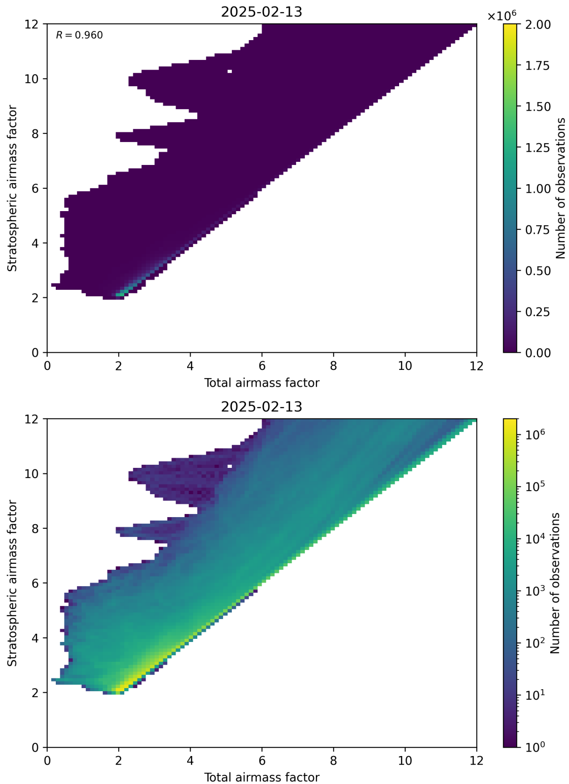
Figure 62: Scatter density plot of “Total airmass factor” against “Stratospheric airmass factor” for 2025-02-13 to 2025-02-14.
