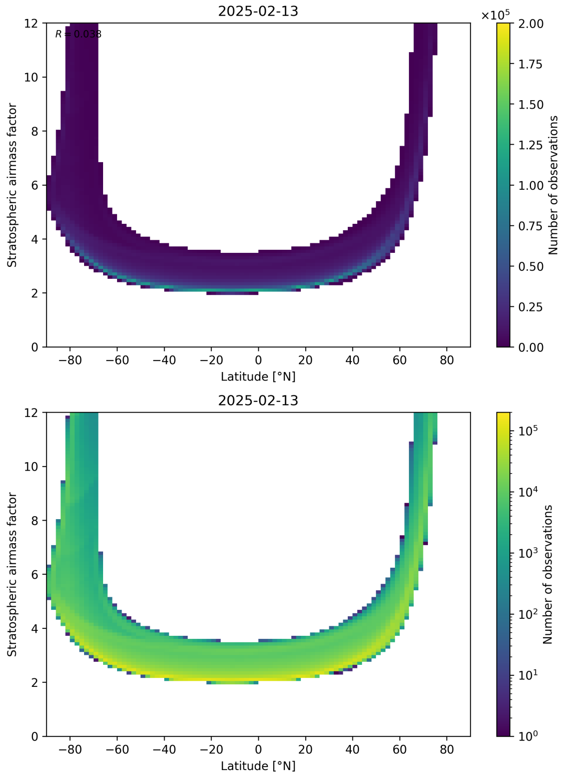
Figure 83: Scatter density plot of “Latitude” against “Stratospheric air mass factor” for 2025-02-13 to 2025-02-14.
