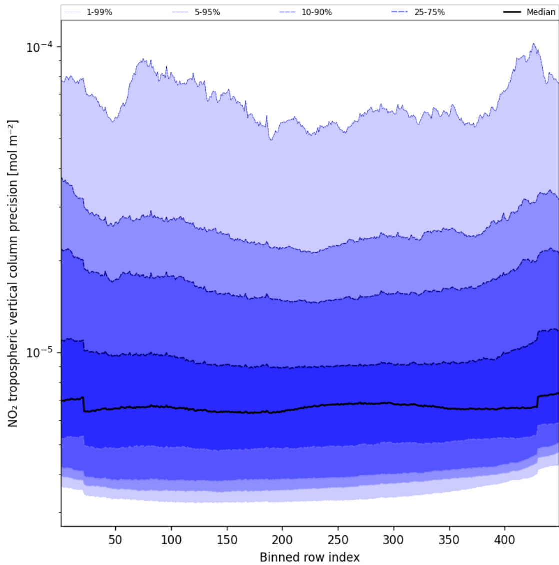
Figure 47: Along track statistics of “NO 2 tropospheric vertical column precision” for 2025-02-13 to 2025-02-14
