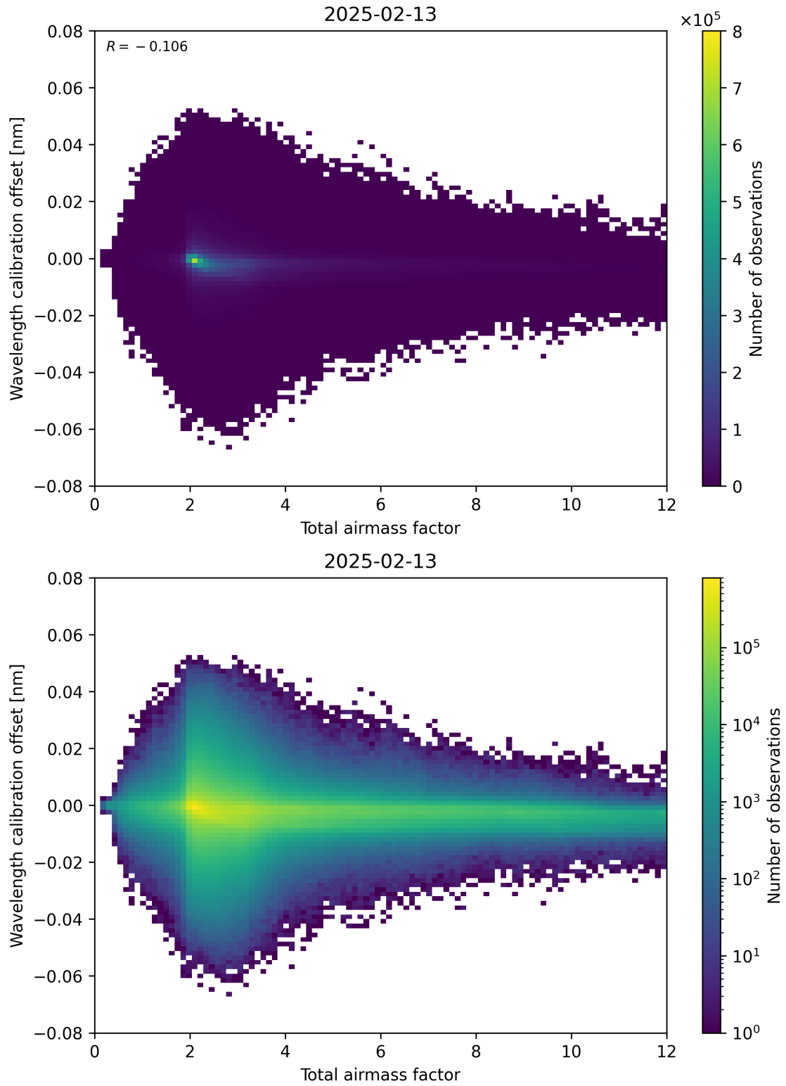
Figure 70: Scatter density plot of “Total airmass factor” against “Wavelength calibration offset” for 2025-02-13 to 2025-02-14.
