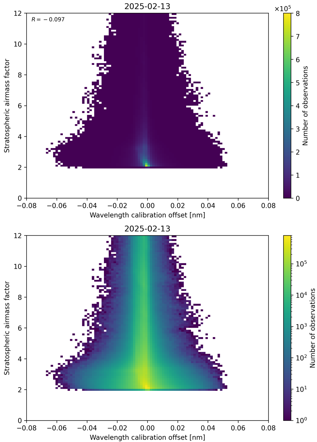
Figure 174: Scatter density plot of “Wavelength calibration offset” against “Stratospheric airmass factor” for 2025-02-13 to 2025-02-14.
