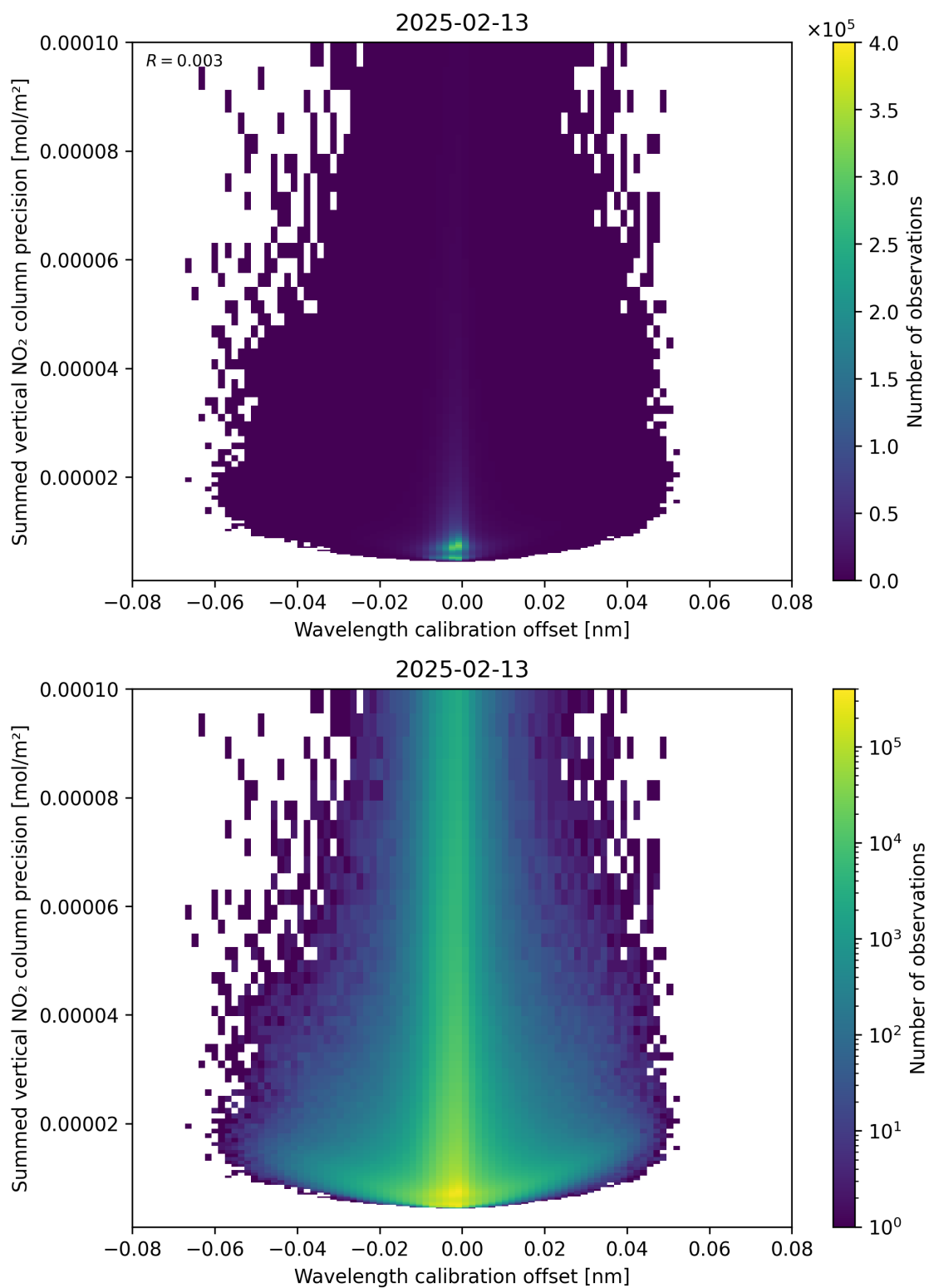
Figure 178: Scatter density plot of “Wavelength calibration offset” against “Summed vertical NO 2 column precision” for 2025-02-13 to 2025-02-14.
