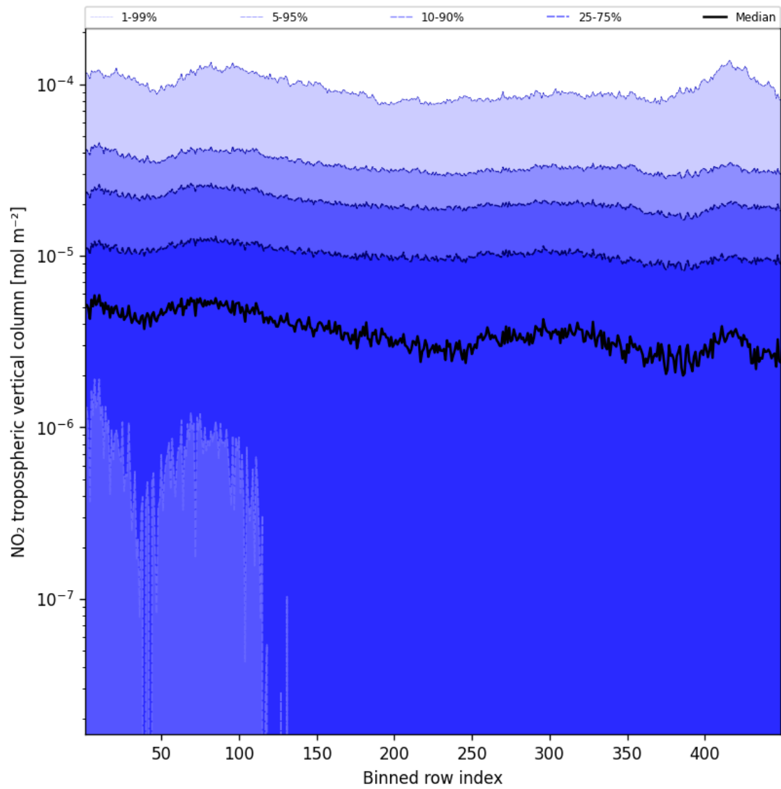
Figure 46: Along track statistics of “NO 2 tropospheric vertical column” for 2025-02-13 to 2025-02-14
