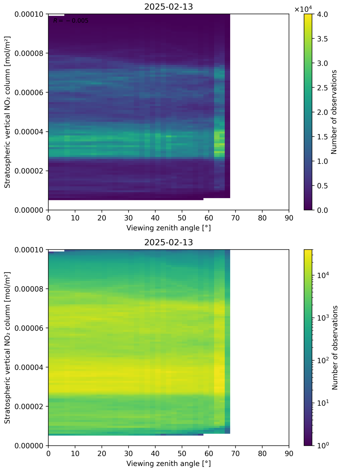
Figure 164: Scatter density plot of “Viewing zenith angle” against “Stratospheric vertical NO 2 column” for 2025-02-13 to 2025-02-14.
