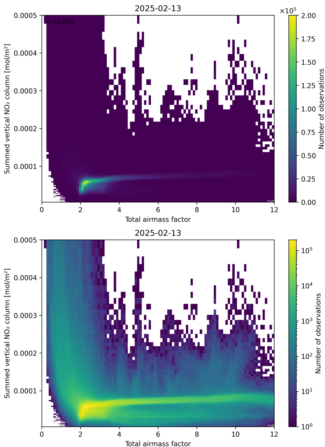
Figure 65: Scatter density plot of “Total airmass factor” against “Summed vertical NO 2 column” for 2025-02-13 to 2025-02-14.
