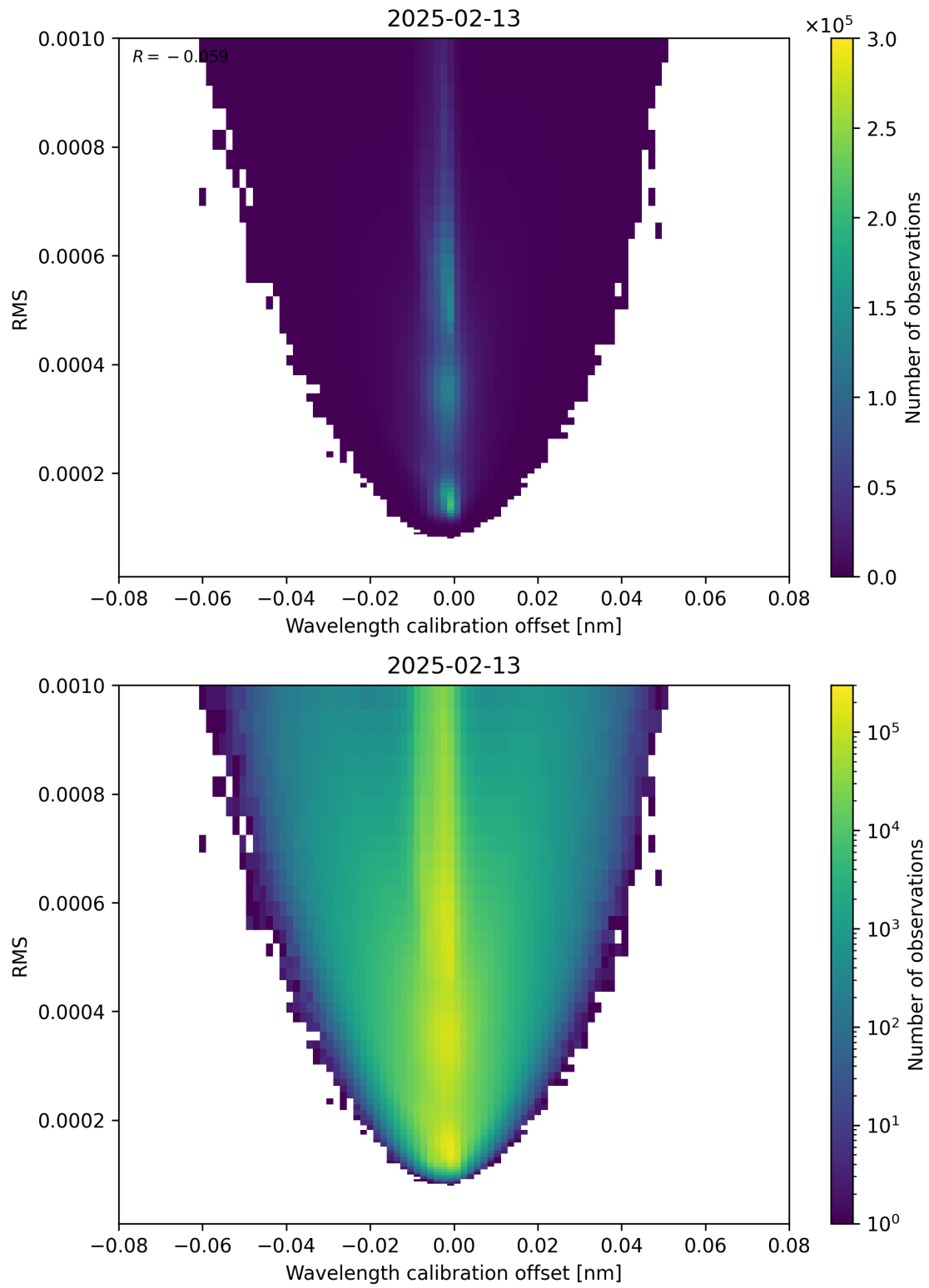
Figure 181: Scatter density plot of “Wavelength calibration offset” against “RMS” for 2025-02-13 to 2025-02-14.
