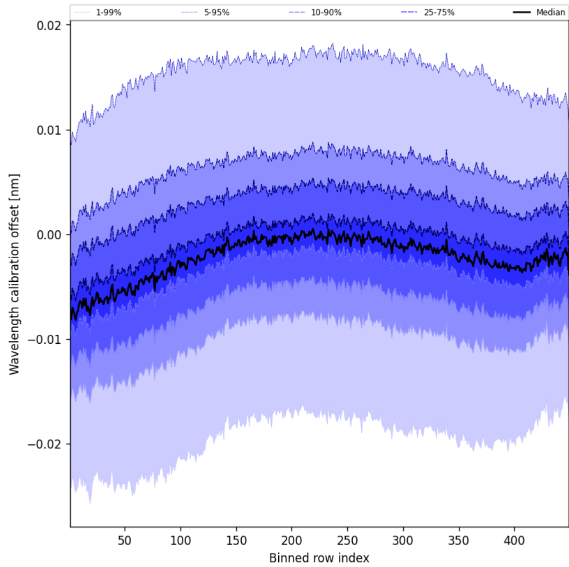
Figure 52: Along track statistics of “Wavelength calibration offset” for 2025-02-13 to 2025-02-14
