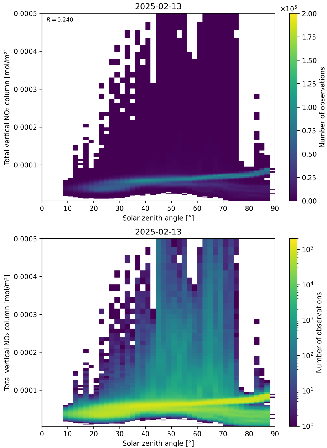
Figure 153: Scatter density plot of “Solar zenith angle” against “Total vertical NO 2 column” for 2025-02-13 to 2025-02-14.
