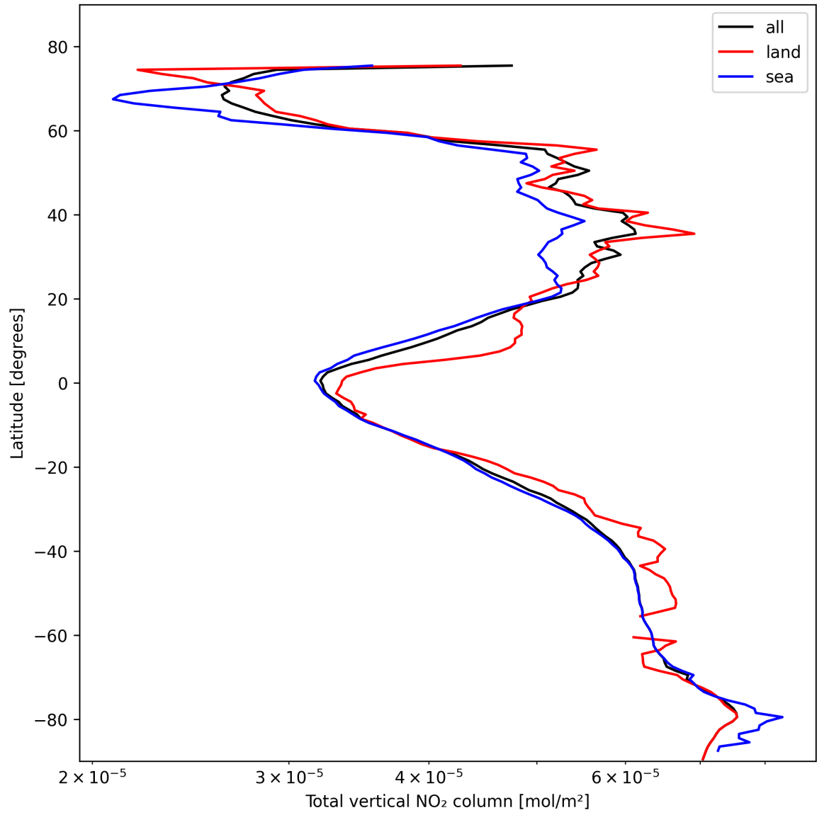
Figure 21: Zonal average of “Total vertical NO 2 column” for 2025-02-13 to 2025-02-14.
