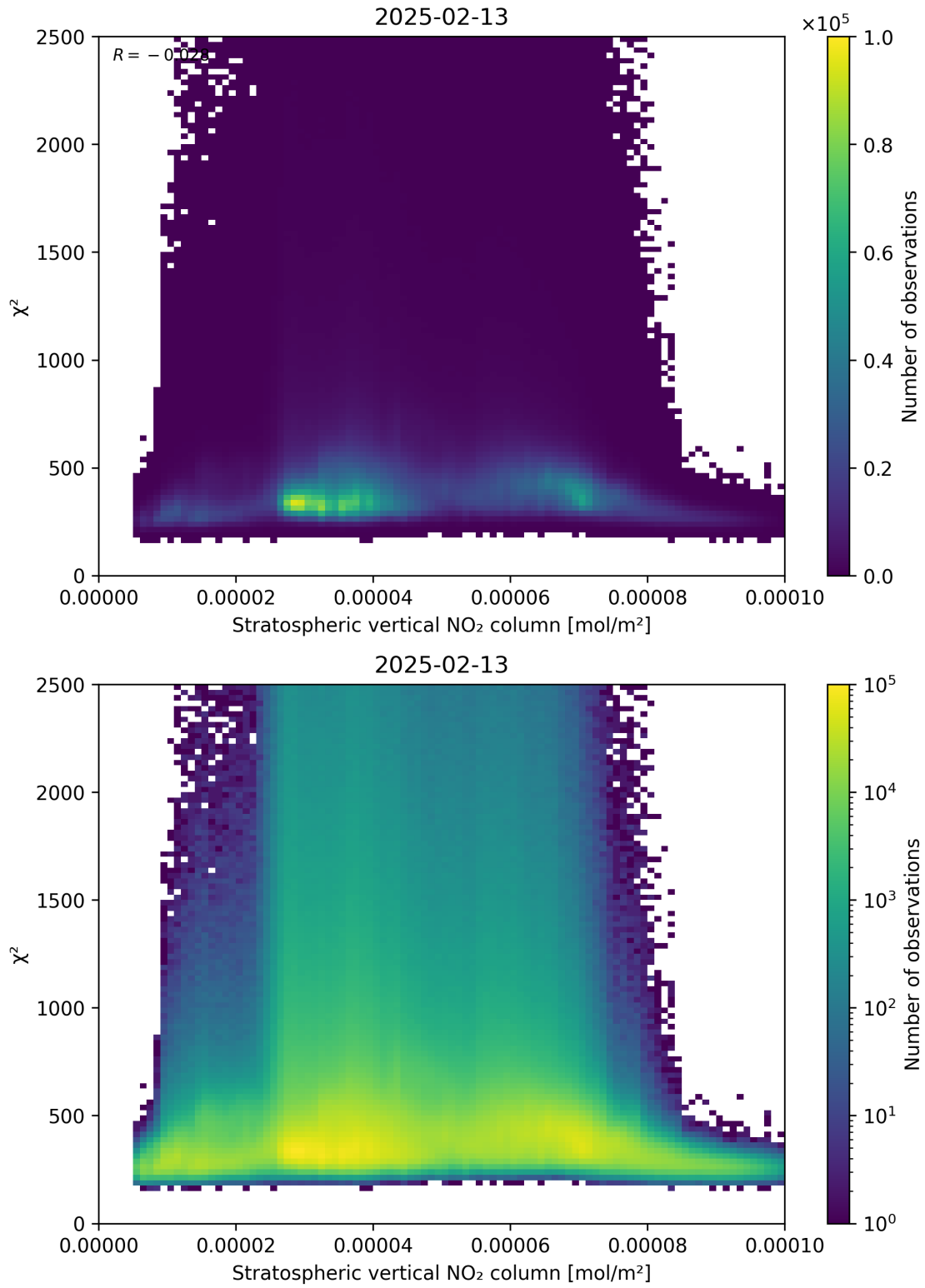
Figure 97: Scatter density plot of “Stratospheric vertical NO 2 column” against “ \chi^2 ” for 2025-02-13 to 2025-02-14.
