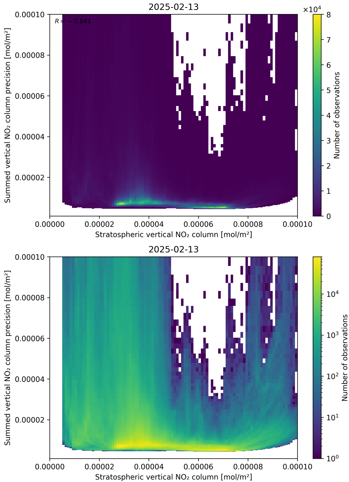
Figure 99: Scatter density plot of “Stratospheric vertical NO 2 column” against “Summed vertical NO 2 column precision” for 2025-02-13 to 2025-02-14.
