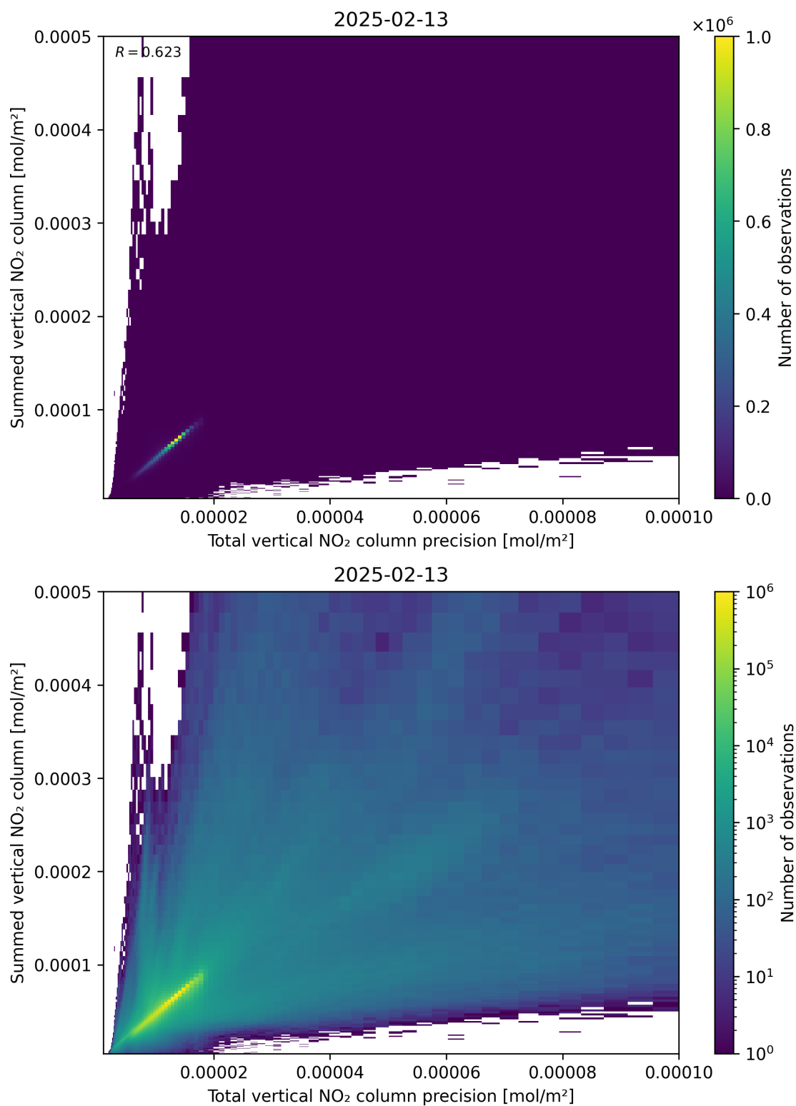
Figure 117: Scatter density plot of “Total vertical NO 2 column precision” against “Summed vertical NO 2 column” for 2025-02-13 to 2025-02-14.
