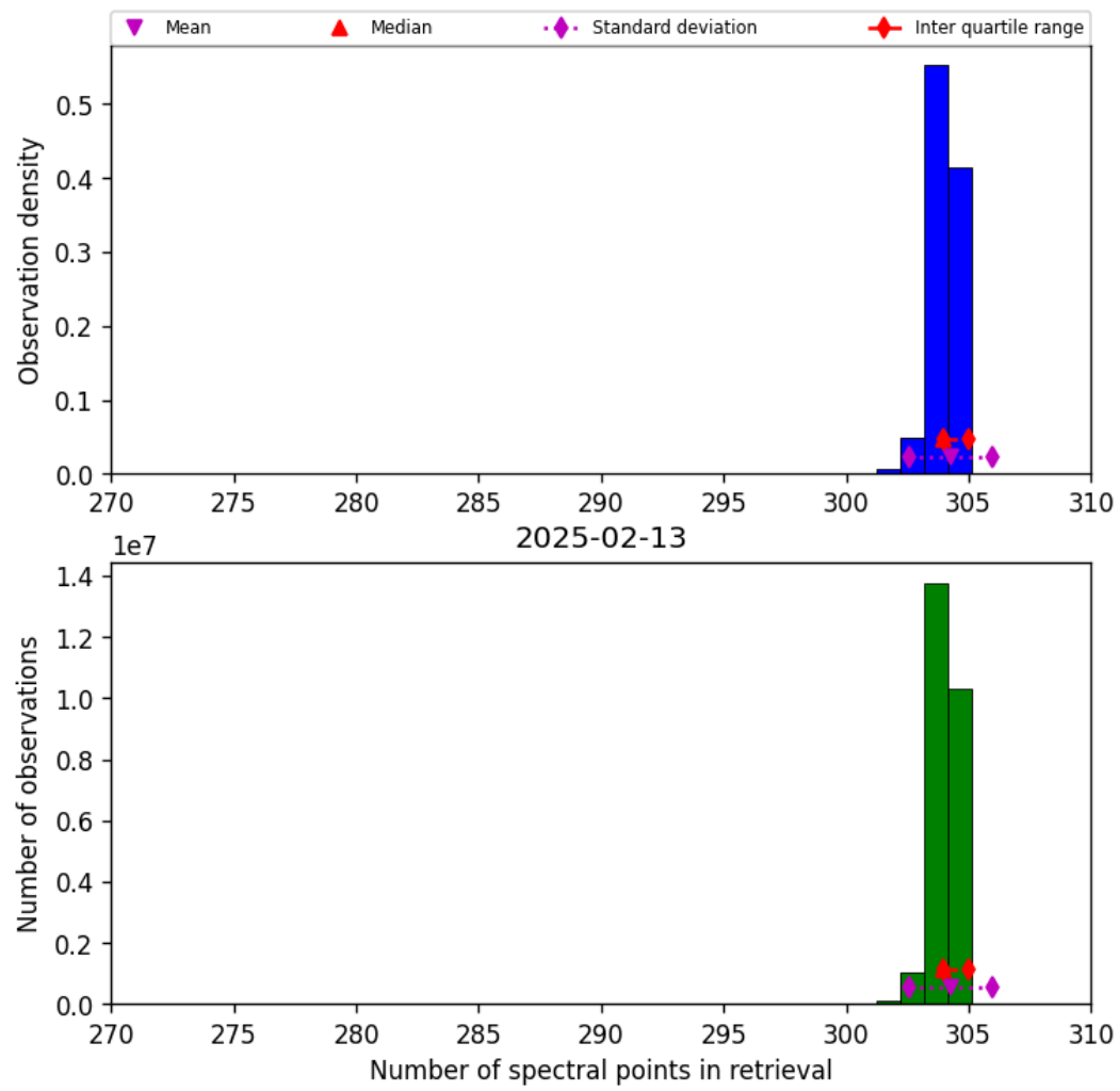
Figure 33: Histogram of “Number of spectral points in retrieval” for 2025-02-13 to 2025-02-14
