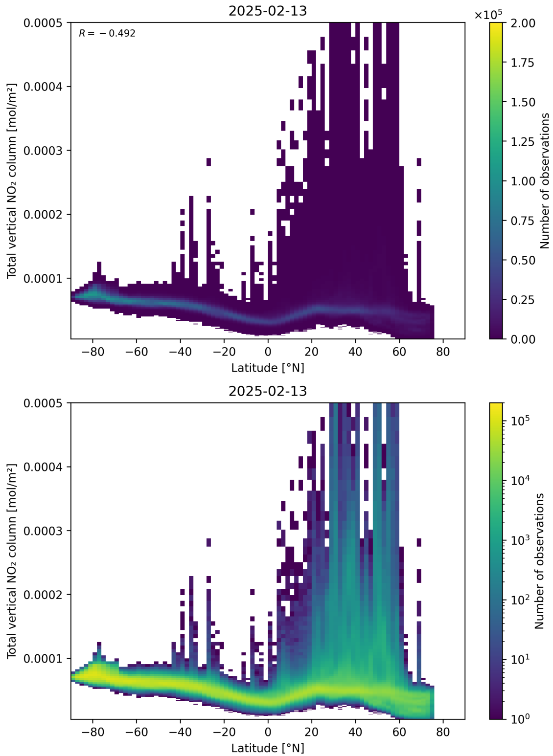
Figure 90: Scatter density plot of “Latitude” against “Total vertical NO 2 column” for 2025-02-13 to 2025-02-14.
