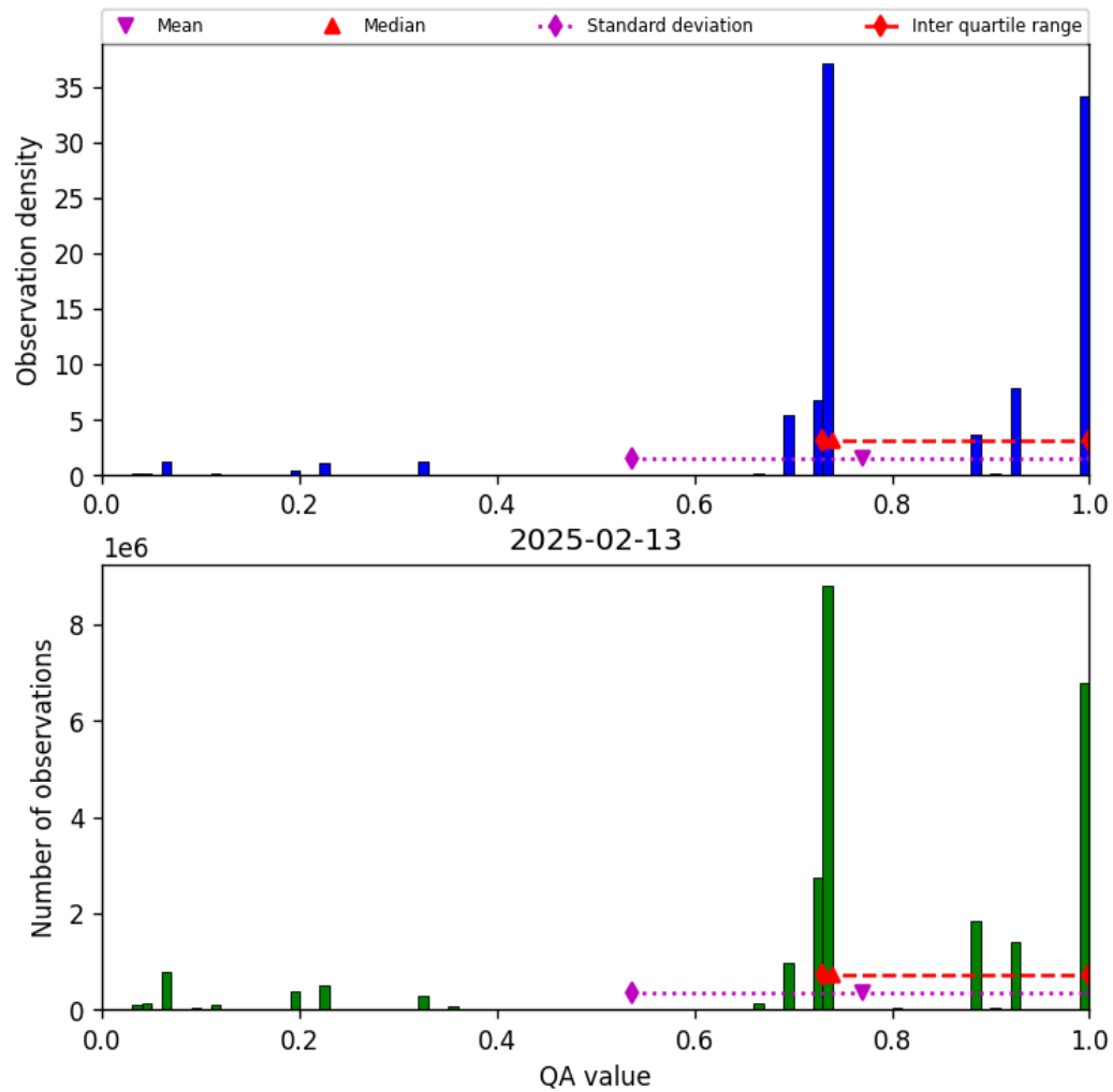
Figure 28: Histogram of “QA value” for 2025-02-13 to 2025-02-14
