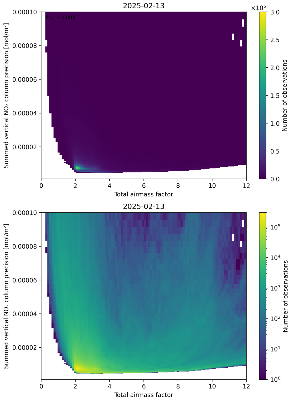
Figure 66: Scatter density plot of “Total airmass factor” against “Summed vertical NO 2 column precision” for 2025-02-13 to 2025-02-14.
