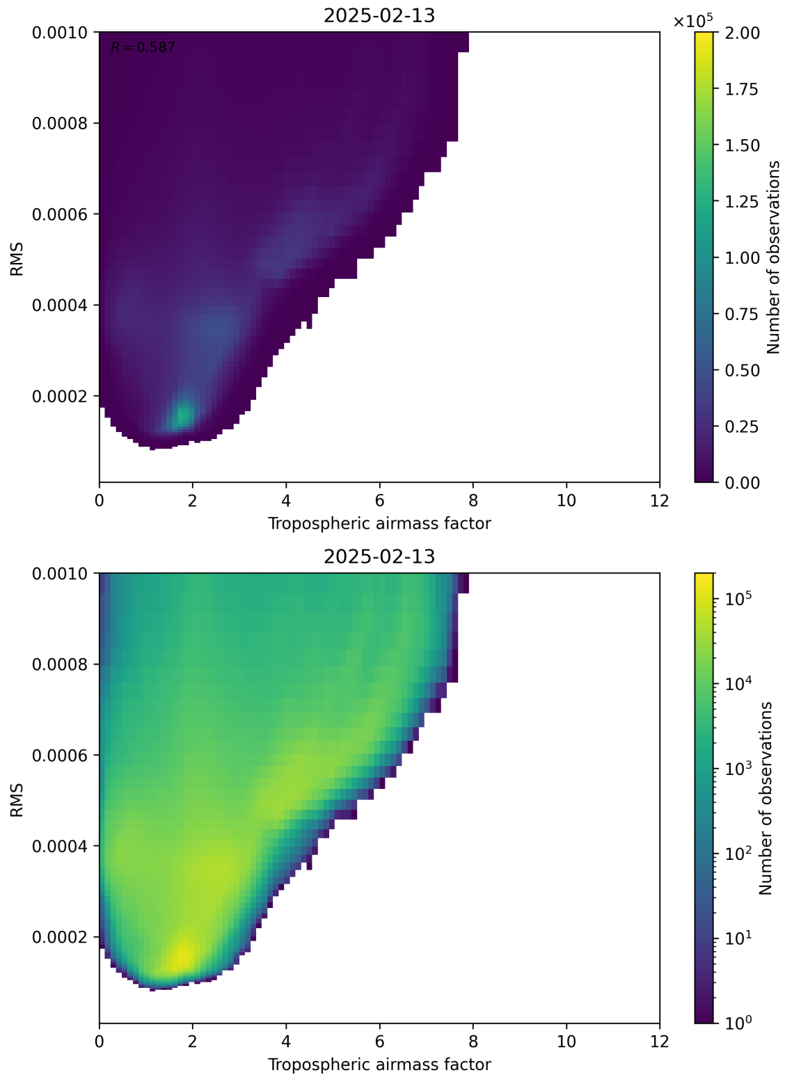
Figure 79: Scatter density plot of “Tropospheric airmass factor” against “RMS” for 2025-02-13 to 2025-02-14.
