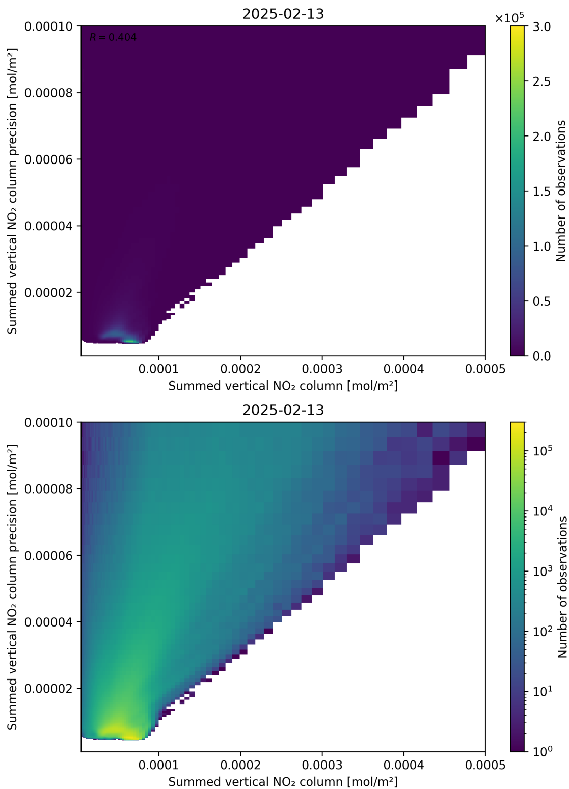
Figure 105: Scatter density plot of “Summed vertical NO 2 column” against “Summed vertical NO 2 column precision” for 2025-02-13 to 2025-02-14.
