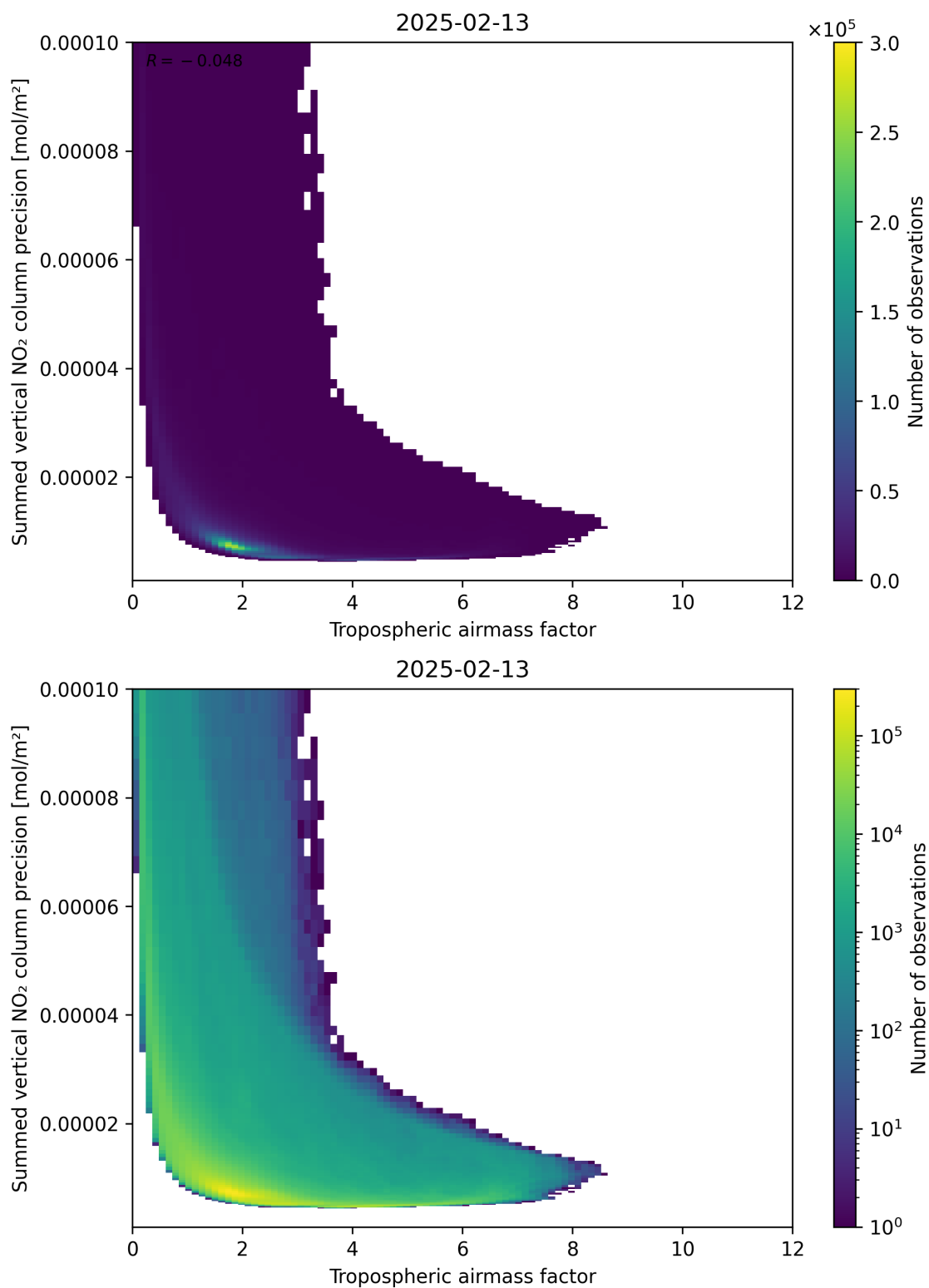
Figure 76: Scatter density plot of “Tropospheric airmass factor” against “Summed vertical NO 2 column precision” for 2025-02-13 to 2025-02-14.
