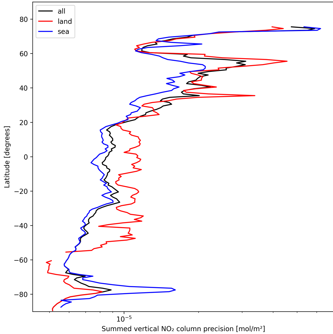
Figure 24: Zonal average of “Summed vertical NO 2 column precision” for 2025-02-13 to 2025-02-14.
