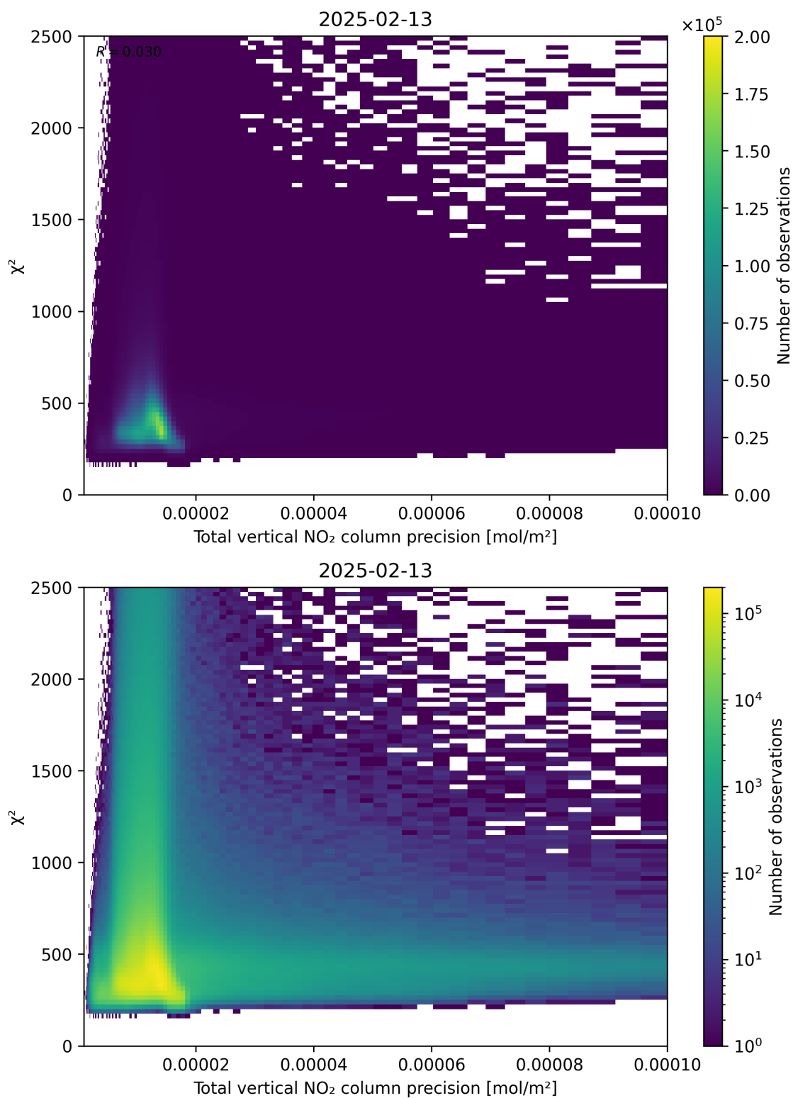
Figure 116: Scatter density plot of “Total vertical NO 2 column precision” against “ \chi^2 ” for 2025-02-13 to 2025-02-14.
