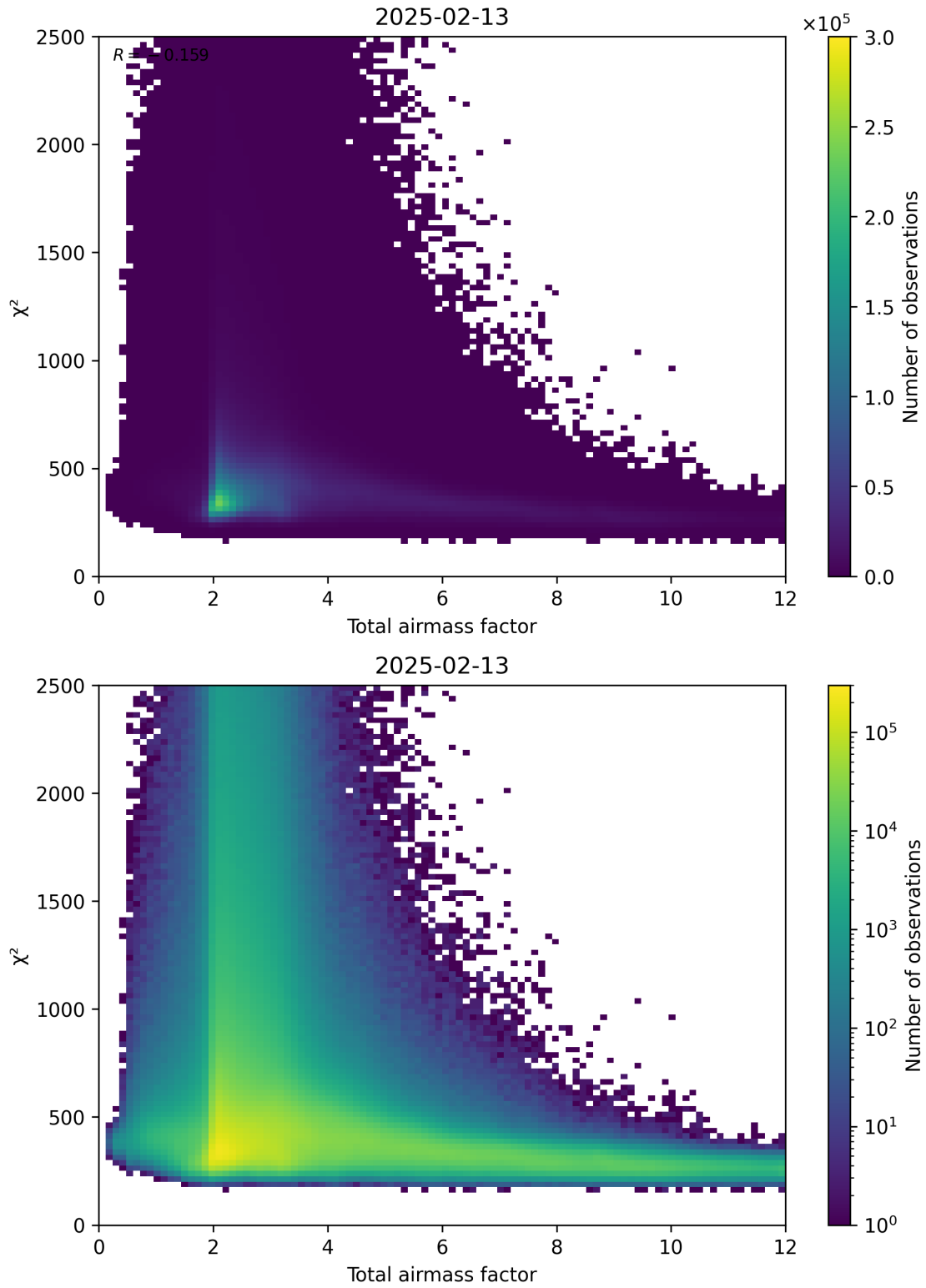
Figure 63: Scatter density plot of “Total airmass factor” against “ \chi^2 ” for 2025-02-13 to 2025-02-14.
