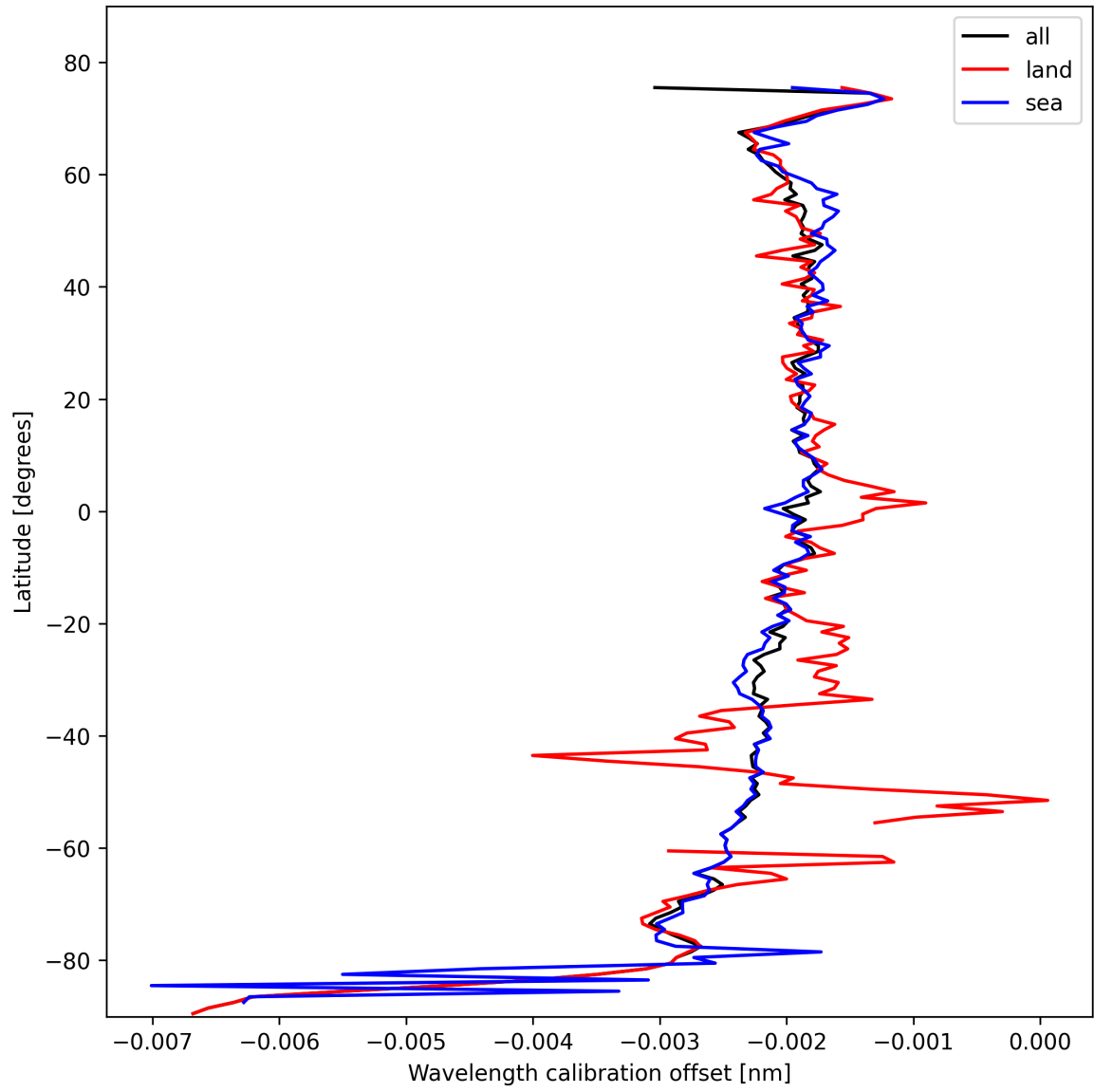
Figure 18: Zonal average of “Wavelength calibration offset” for 2025-02-13 to 2025-02-14.
