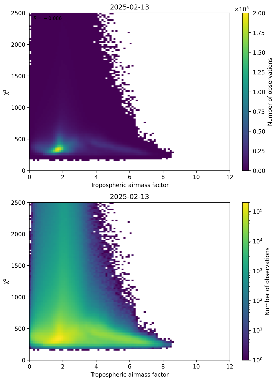
Figure 73: Scatter density plot of “Tropospheric airmass factor” against “ \chi^2 ” for 2025-02-13 to 2025-02-14.
