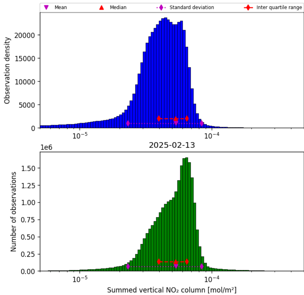
Figure 40: Histogram of “Summed vertical NO 2 column” for 2025-02-13 to 2025-02-14
