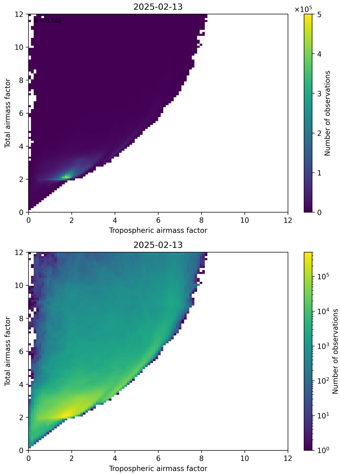
Figure 72: Scatter density plot of “Tropospheric airmass factor” against “Total airmass factor” for 2025-02-13 to 2025-02-14.
