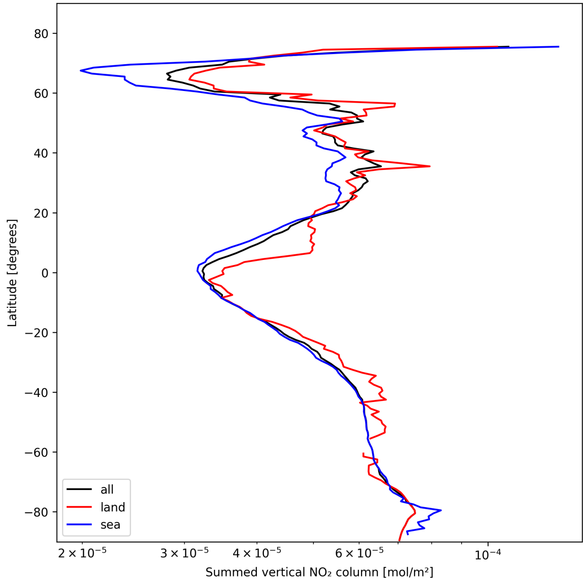
Figure 23: Zonal average of “Summed vertical NO 2 column” for 2025-02-13 to 2025-02-14.
