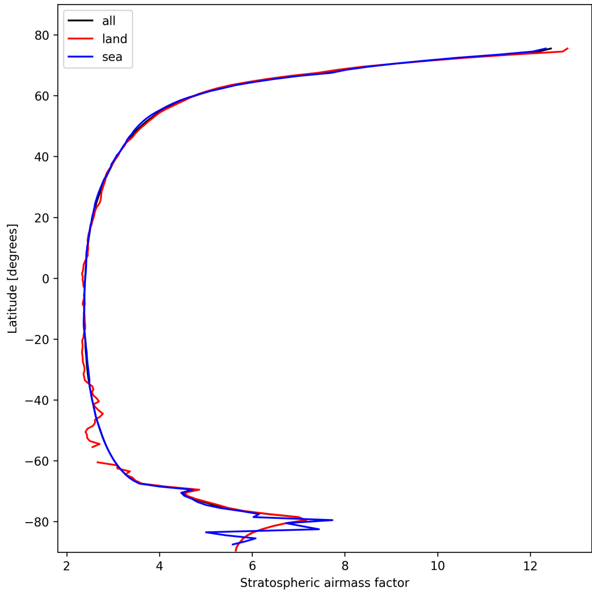
Figure 27: Zonal average of “Stratospheric airmass factor” for 2025-02-13 to 2025-02-14.
