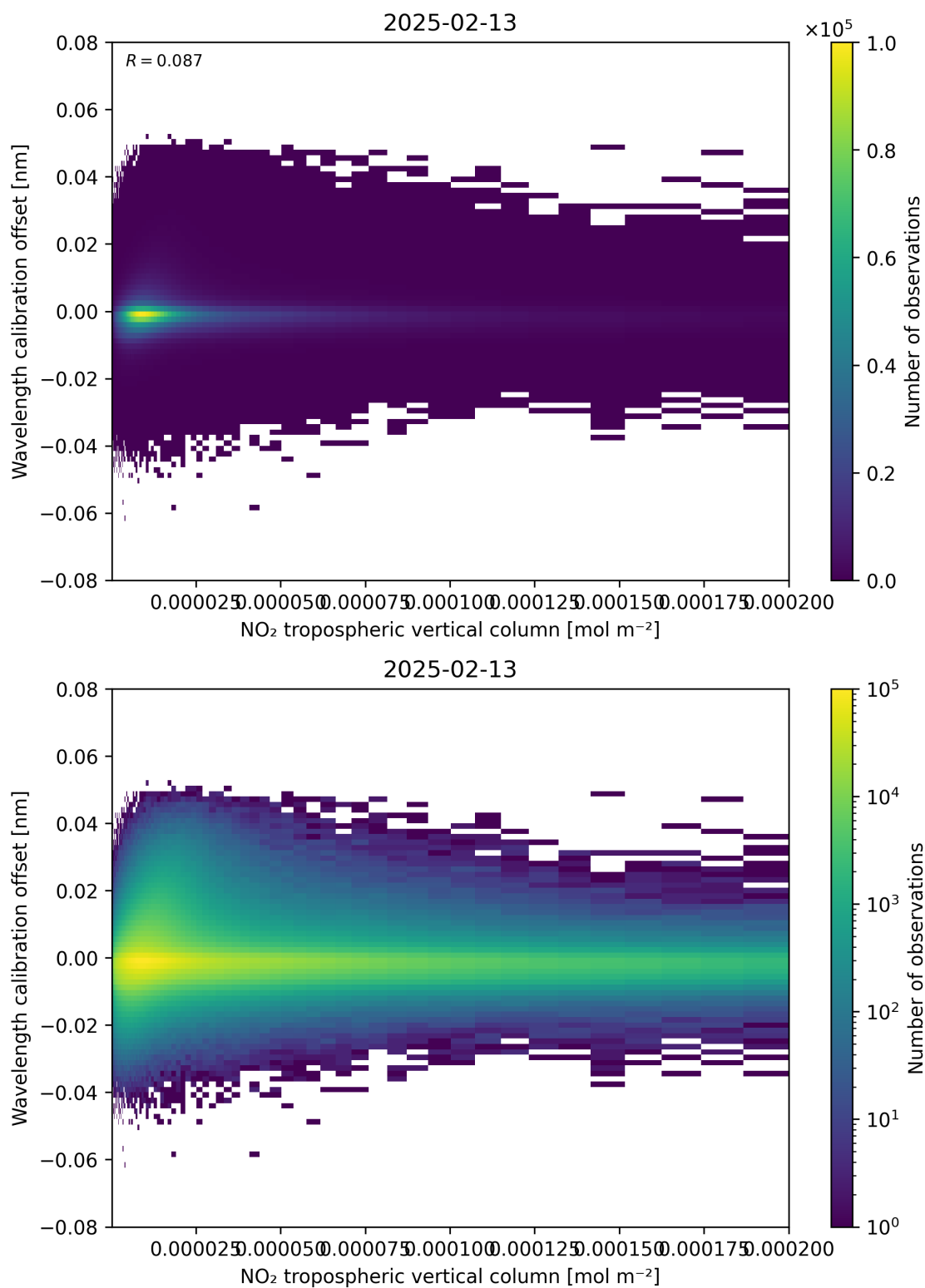
Figure 143: Scatter density plot of “NO 2 tropospheric vertical column” against “Wavelength calibration offset” for 2025-02-13 to 2025-02-14.
