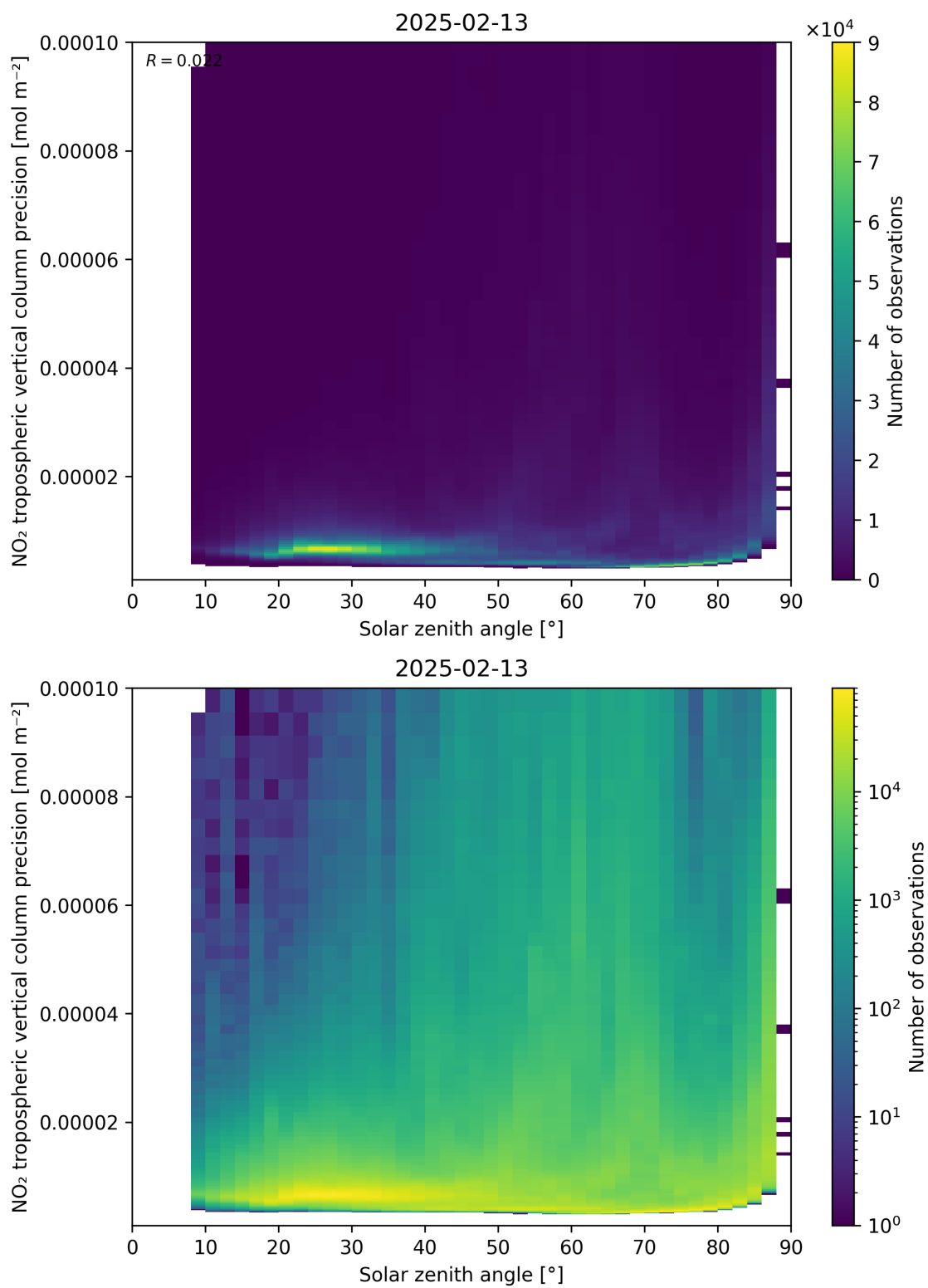
Figure 156: Scatter density plot of “Solar zenith angle” against “NO 2 tropospheric vertical column precision” for 2025-02-13 to 2025-02-14.
