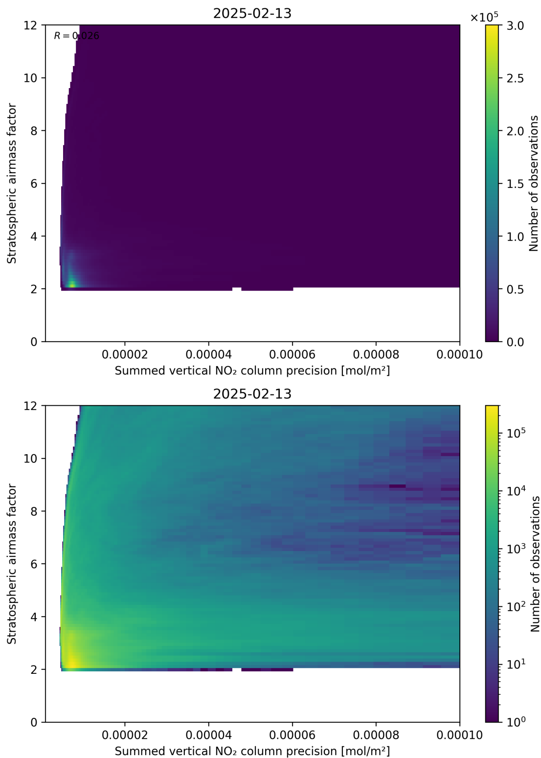
Figure 106: Scatter density plot of “Summed vertical NO 2 column precision” against “Stratospheric airmass factor” for 2025-02-13 to 2025-02-14.
