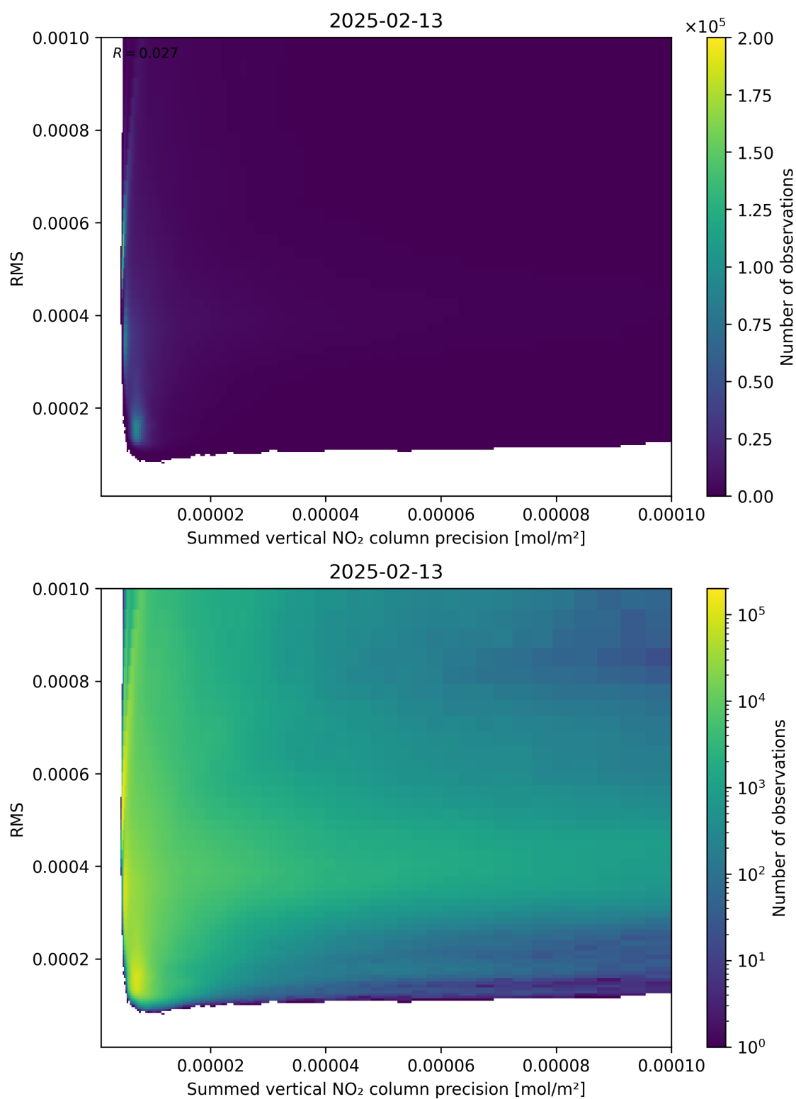
Figure 108: Scatter density plot of “Summed vertical NO 2 column precision” against “RMS” for 2025-02-13 to 2025-02-14.
