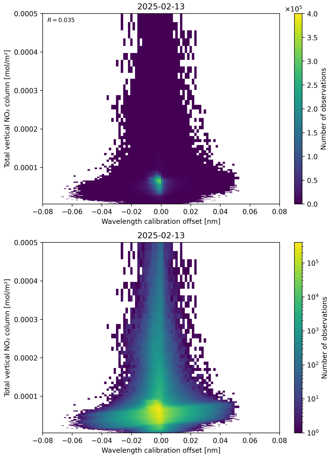
Figure 179: Scatter density plot of “Wavelength calibration offset” against “Total vertical NO 2 column” for 2025-02-13 to 2025-02-14.
