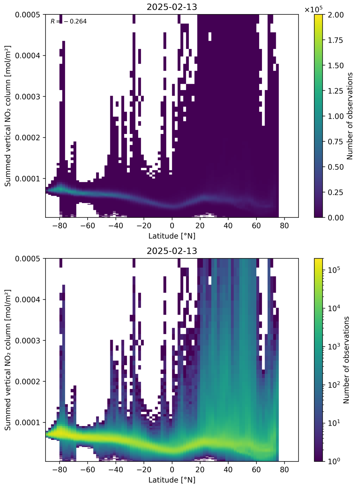
Figure 88: Scatter density plot of “Latitude” against “Summed vertical NO 2 column” for 2025-02-13 to 2025-02-14.
