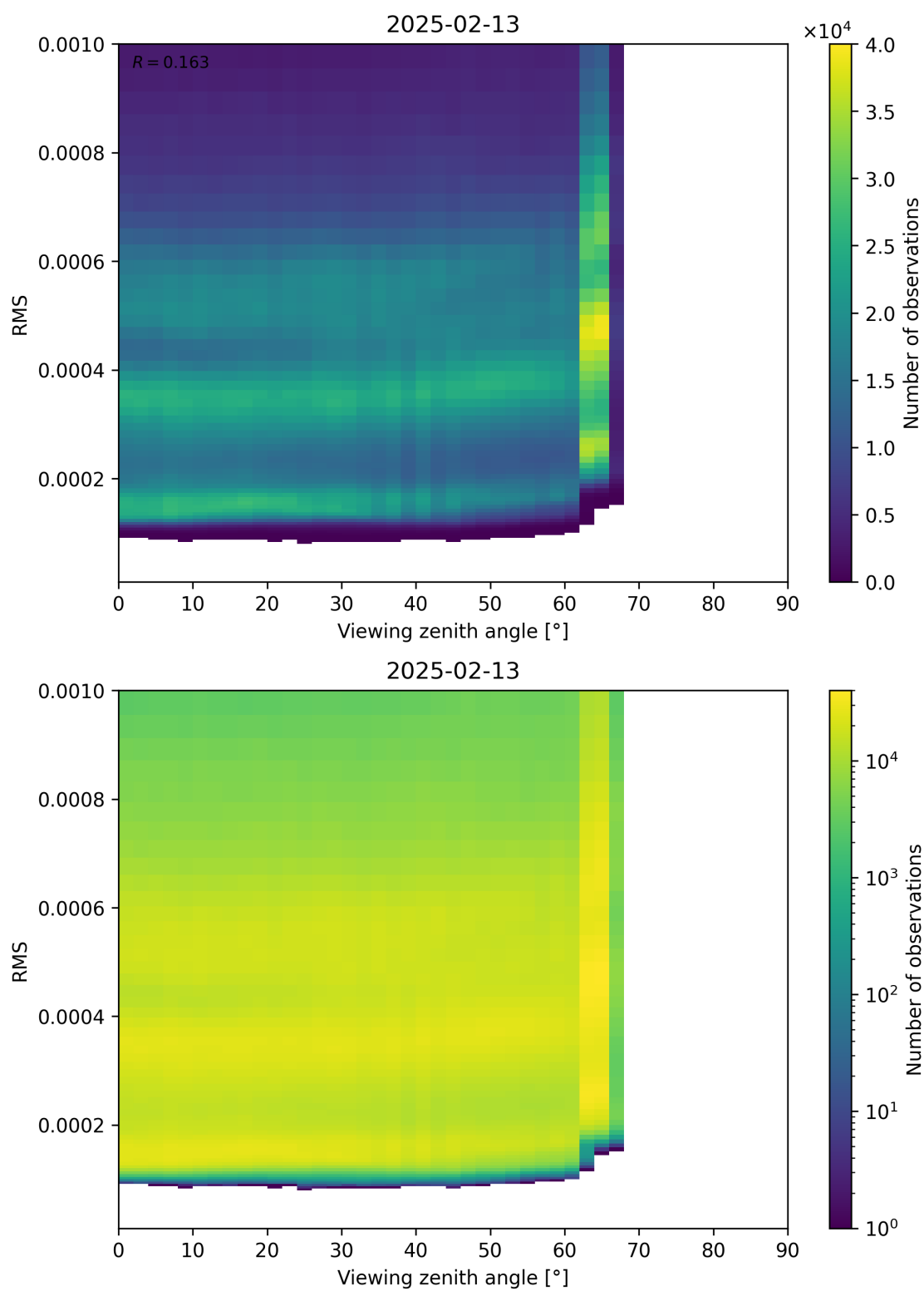
Figure 171: Scatter density plot of “Viewing zenith angle” against “RMS” for 2025-02-13 to 2025-02-14.
