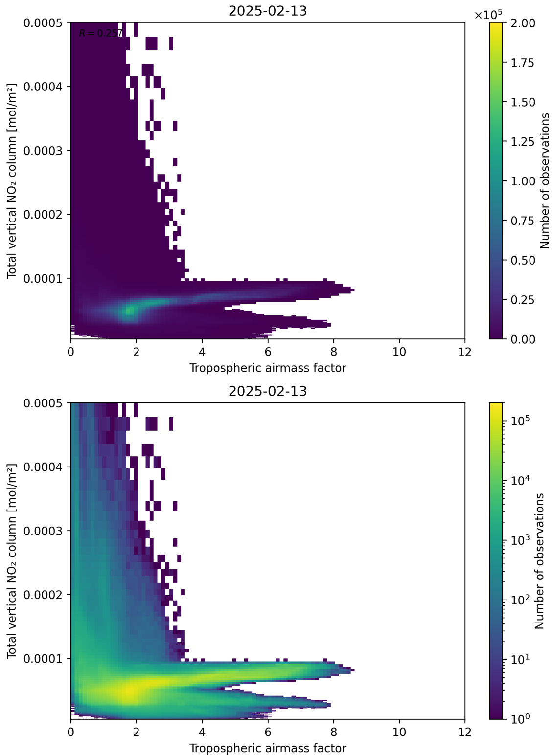
Figure 77: Scatter density plot of “Tropospheric airmass factor” against “Total vertical NO 2 column” for 2025-02-13 to 2025-02-14.
