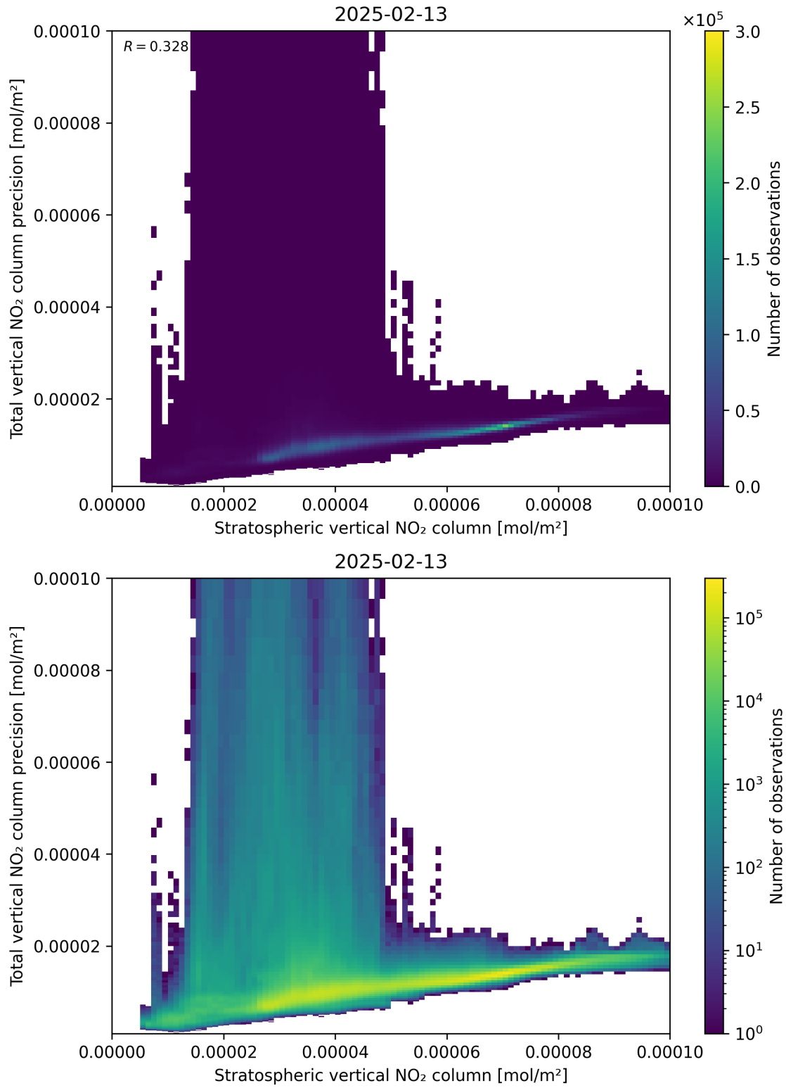
Figure 101: Scatter density plot of “Stratospheric vertical NO 2 column” against “Total vertical NO 2 column precision” for 2025-02-13 to 2025-02-14.
