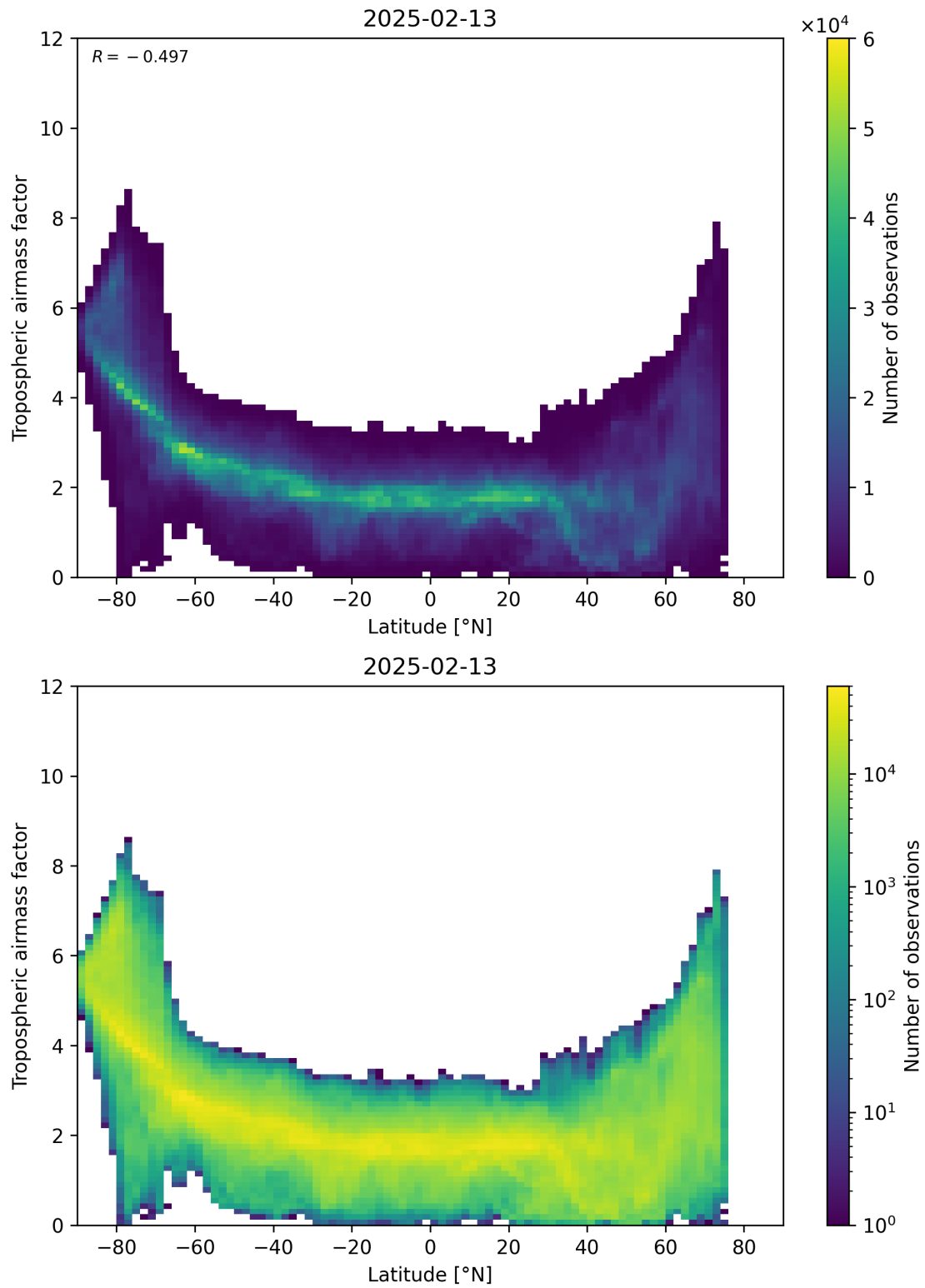
Figure 85: Scatter density plot of “Latitude” against “Tropospheric airmass factor” for 2025-02-13 to 2025-02-14.
