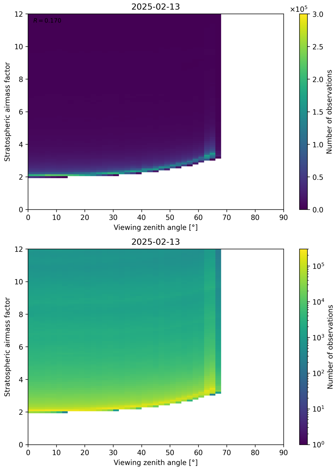
Figure 159: Scatter density plot of “Viewing zenith angle” against “Stratospheric airmass factor” for 2025-02-13 to 2025-02-14.
