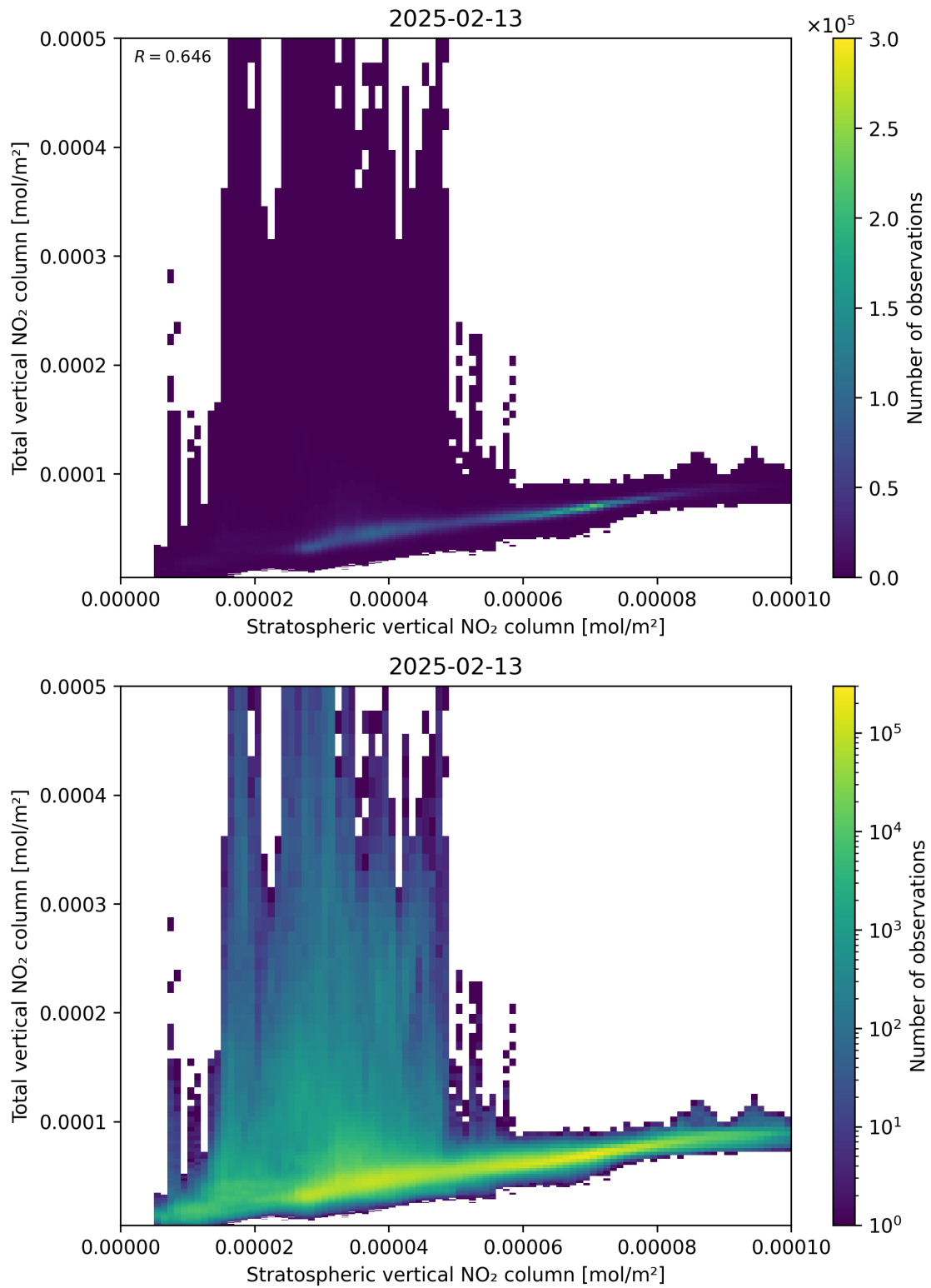
Figure 100: Scatter density plot of “Stratospheric vertical NO 2 column” against “Total vertical NO 2 column” for 2025-02-13 to 2025-02-14.
