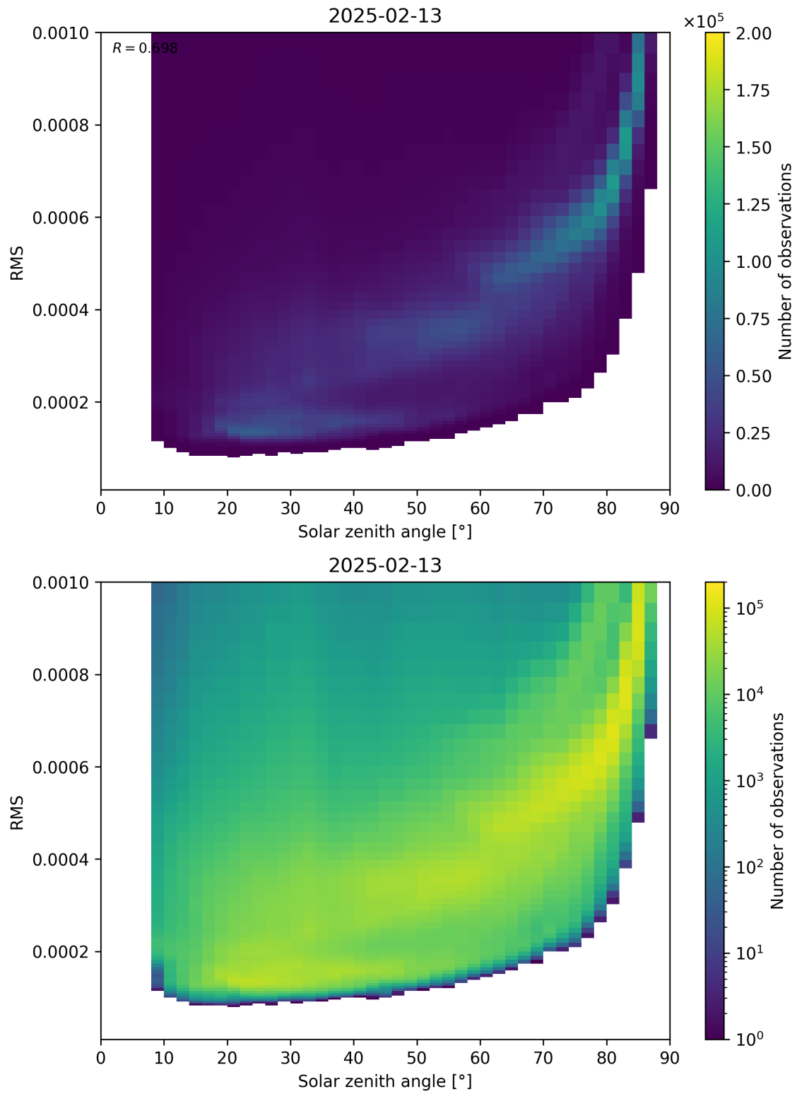
Figure 157: Scatter density plot of “Solar zenith angle” against “RMS” for 2025-02-13 to 2025-02-14.
