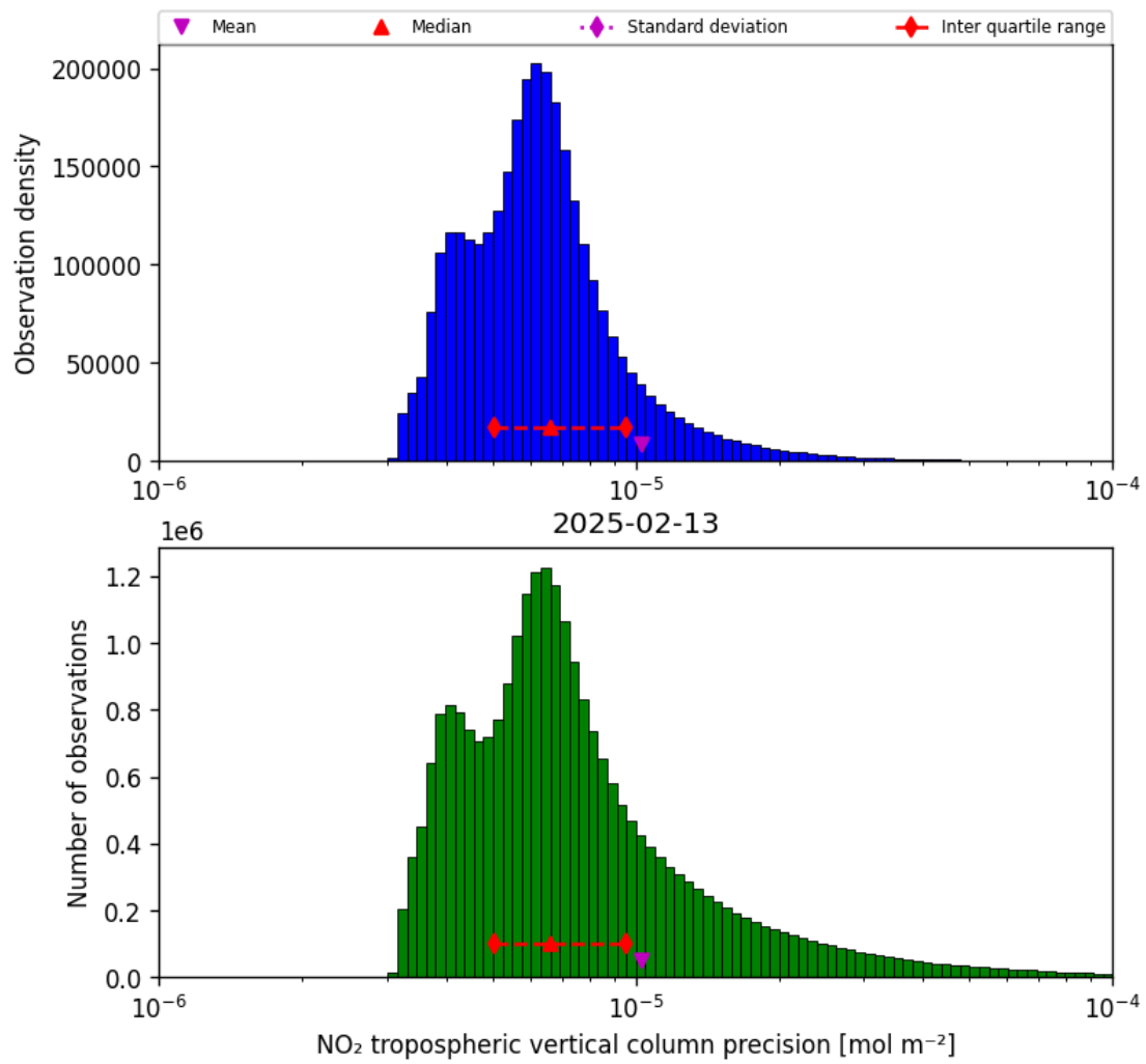
Figure 30: Histogram of “NO 2 tropospheric vertical column precision” for 2025-02-13 to 2025-02-14
