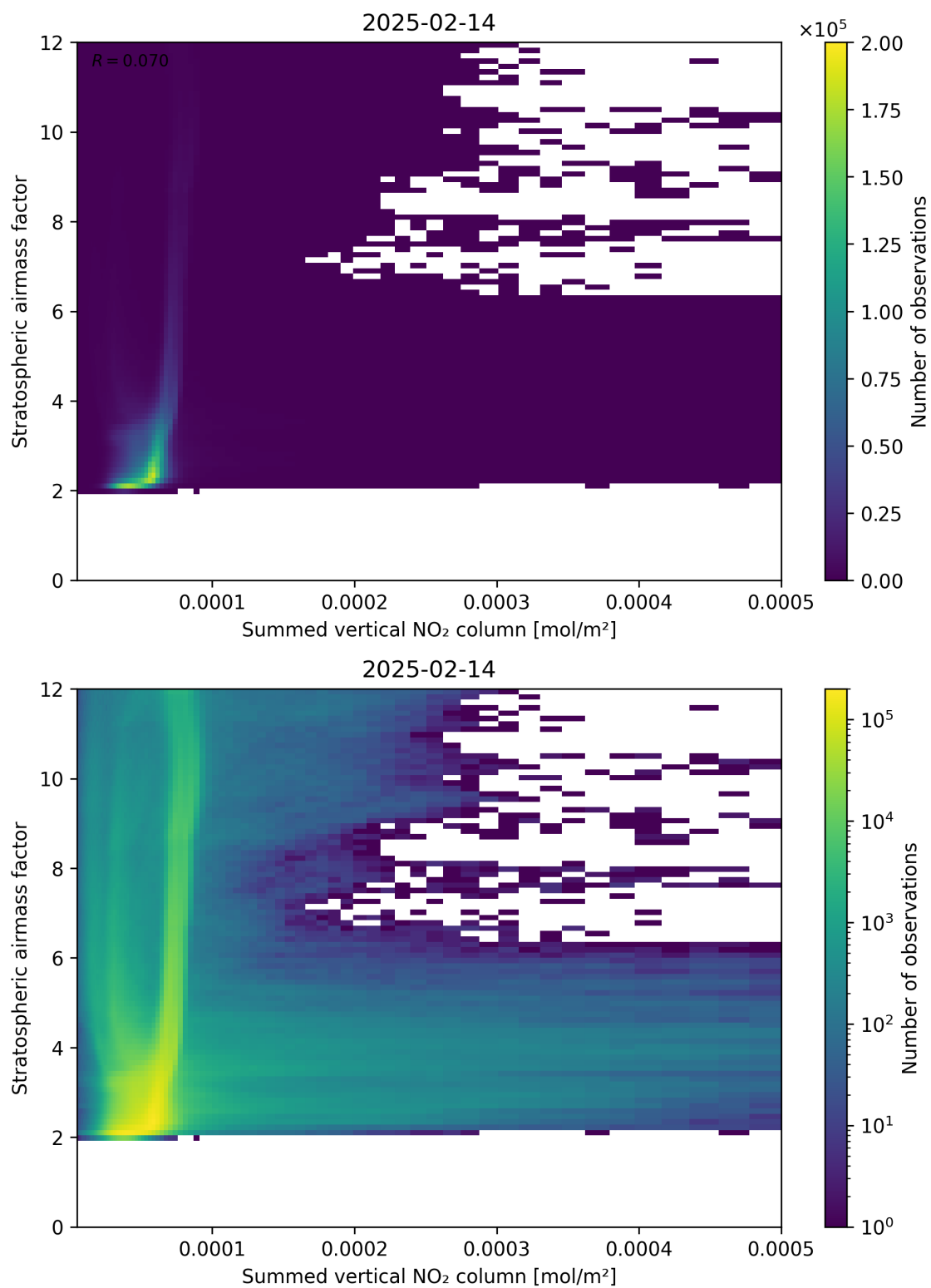
Figure 103: Scatter density plot of “Summed vertical NO 2 column” against “Stratospheric air mass factor” for 2025-02-13 to 2025-02-15.
