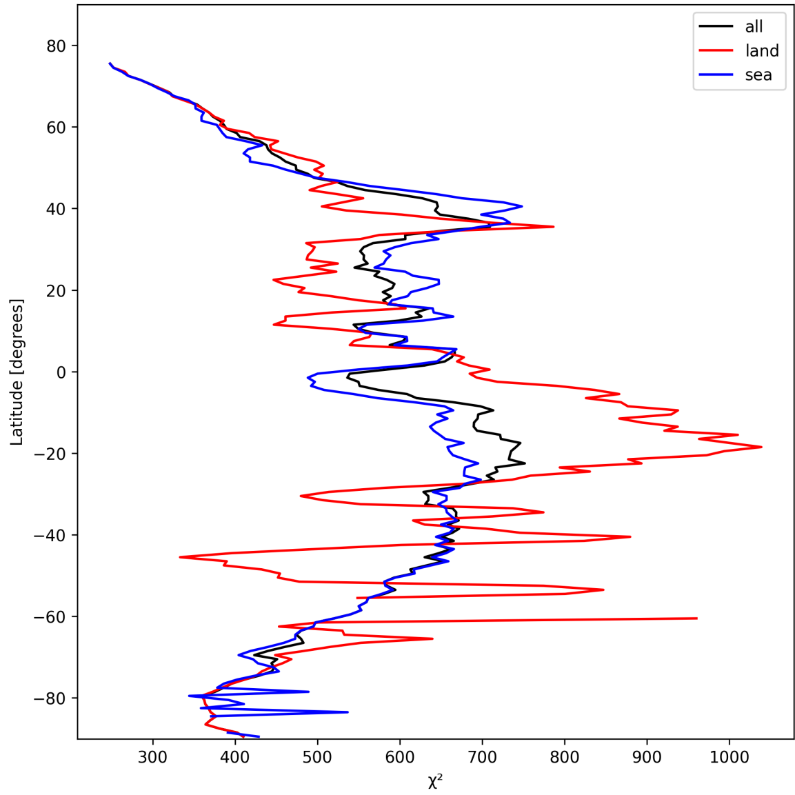
Figure 25: Zonal average of “ \chi^2 ” for 2025-02-13 to 2025-02-15.
