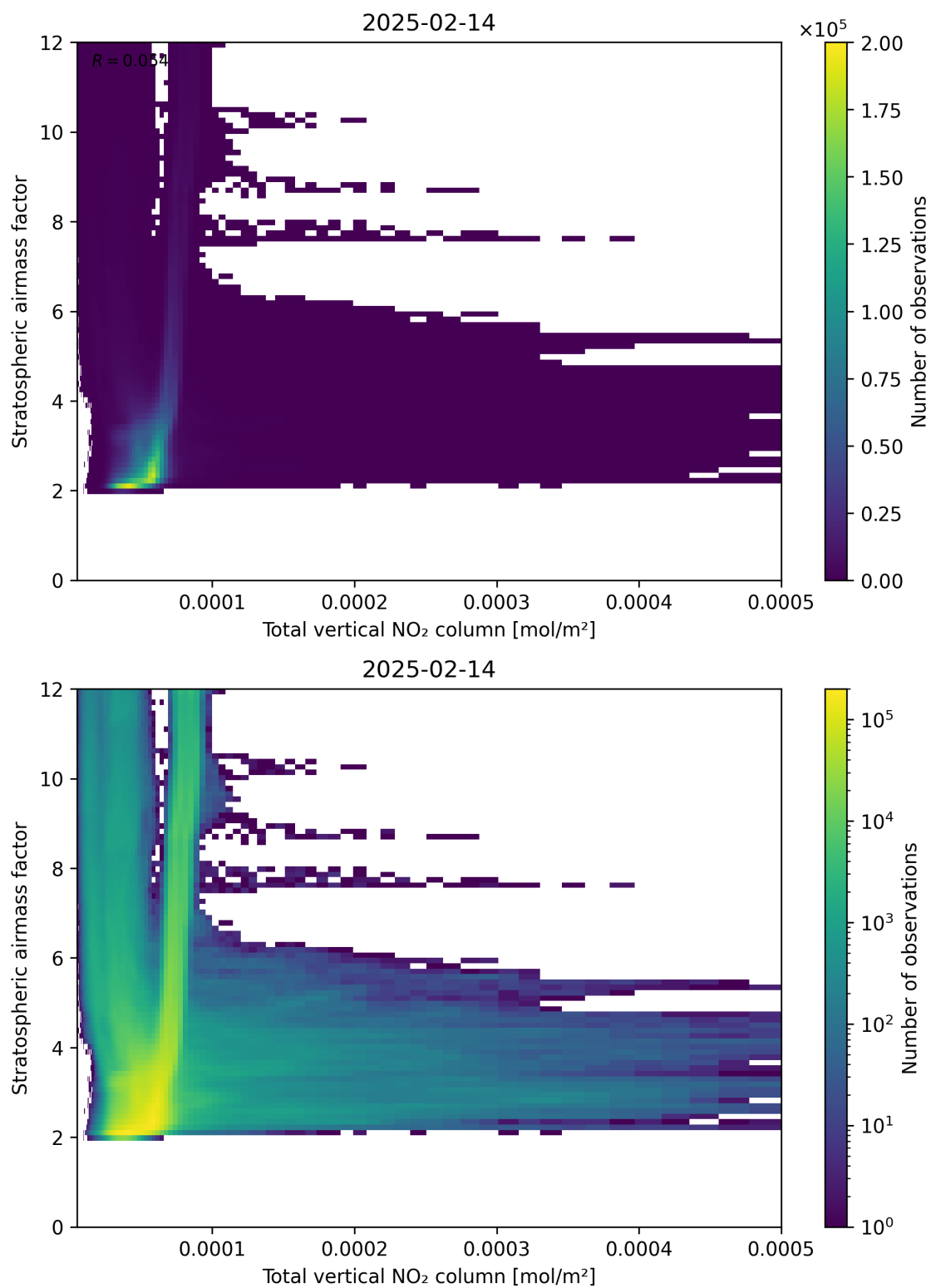
Figure 110: Scatter density plot of “Total vertical NO 2 column” against “Stratospheric airmass factor” for 2025-02-13 to 2025-02-15.
