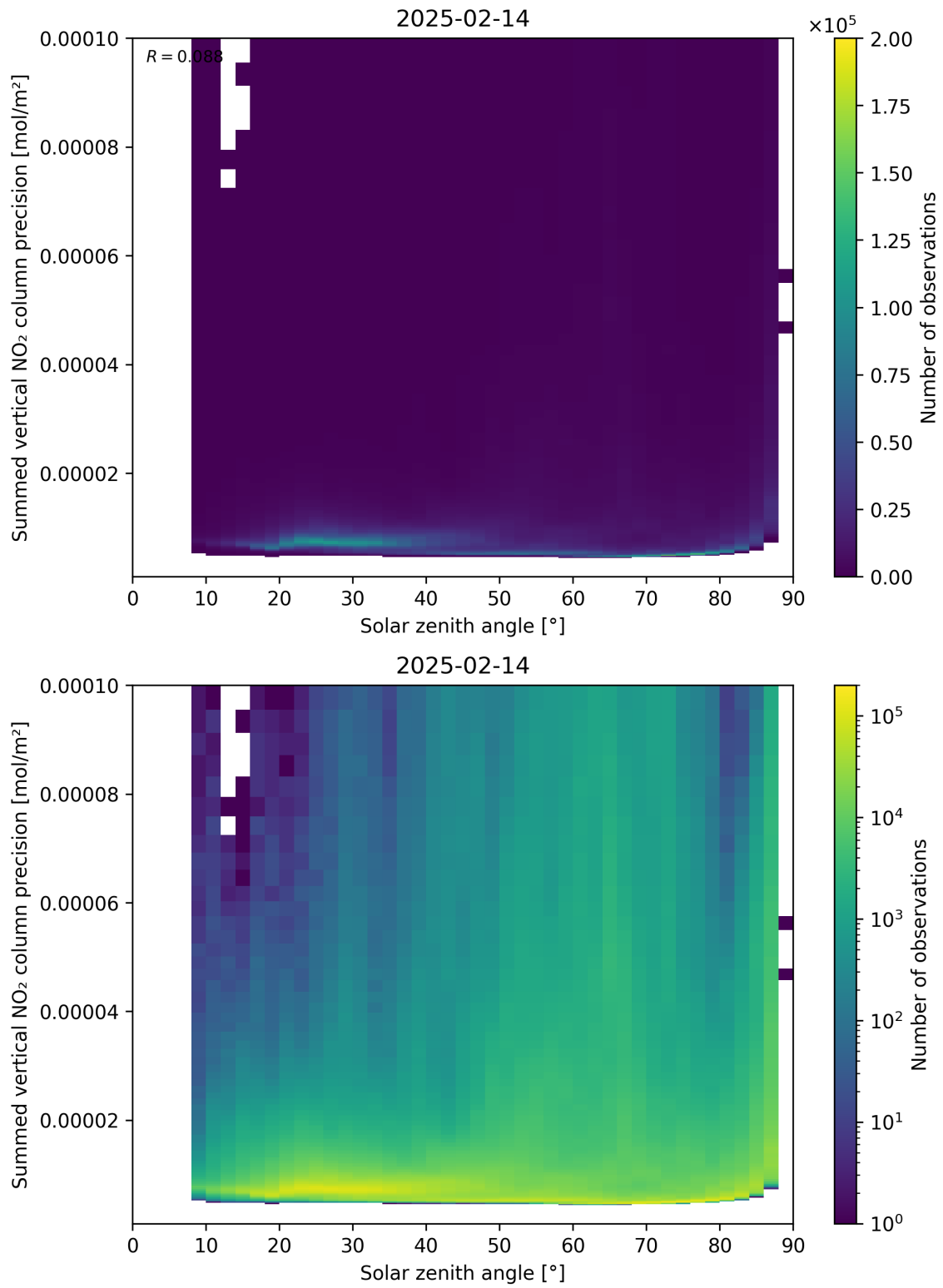
Figure 152: Scatter density plot of “Solar zenith angle” against “Summed vertical NO 2 column precision” for 2025-02-13 to 2025-02-15.
