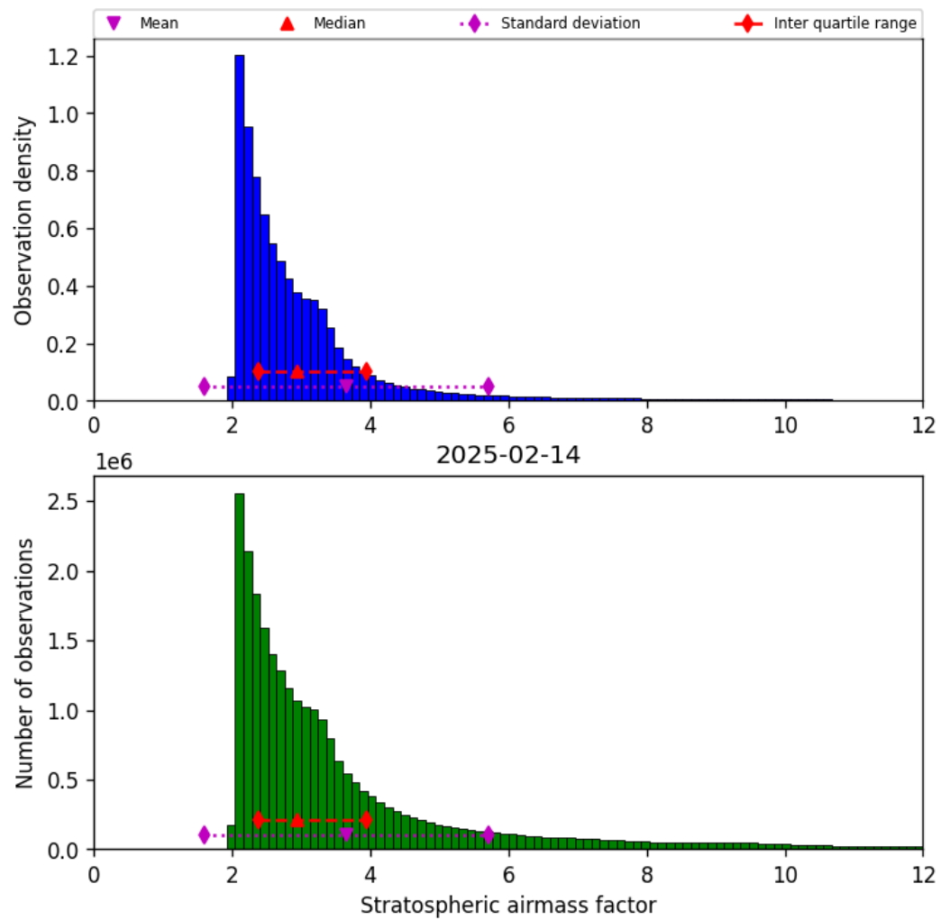
Figure 44: Histogram of “Stratospheric airmass factor” for 2025-02-13 to 2025-02-15
