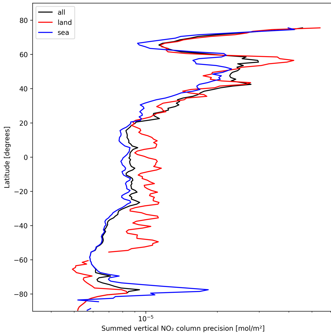
Figure 24: Zonal average of “Summed vertical NO 2 column precision” for 2025-02-13 to 2025-02-15.
