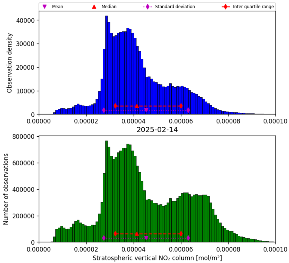
Figure 36: Histogram of “Stratospheric vertical NO 2 column” for 2025-02-13 to 2025-02-15
