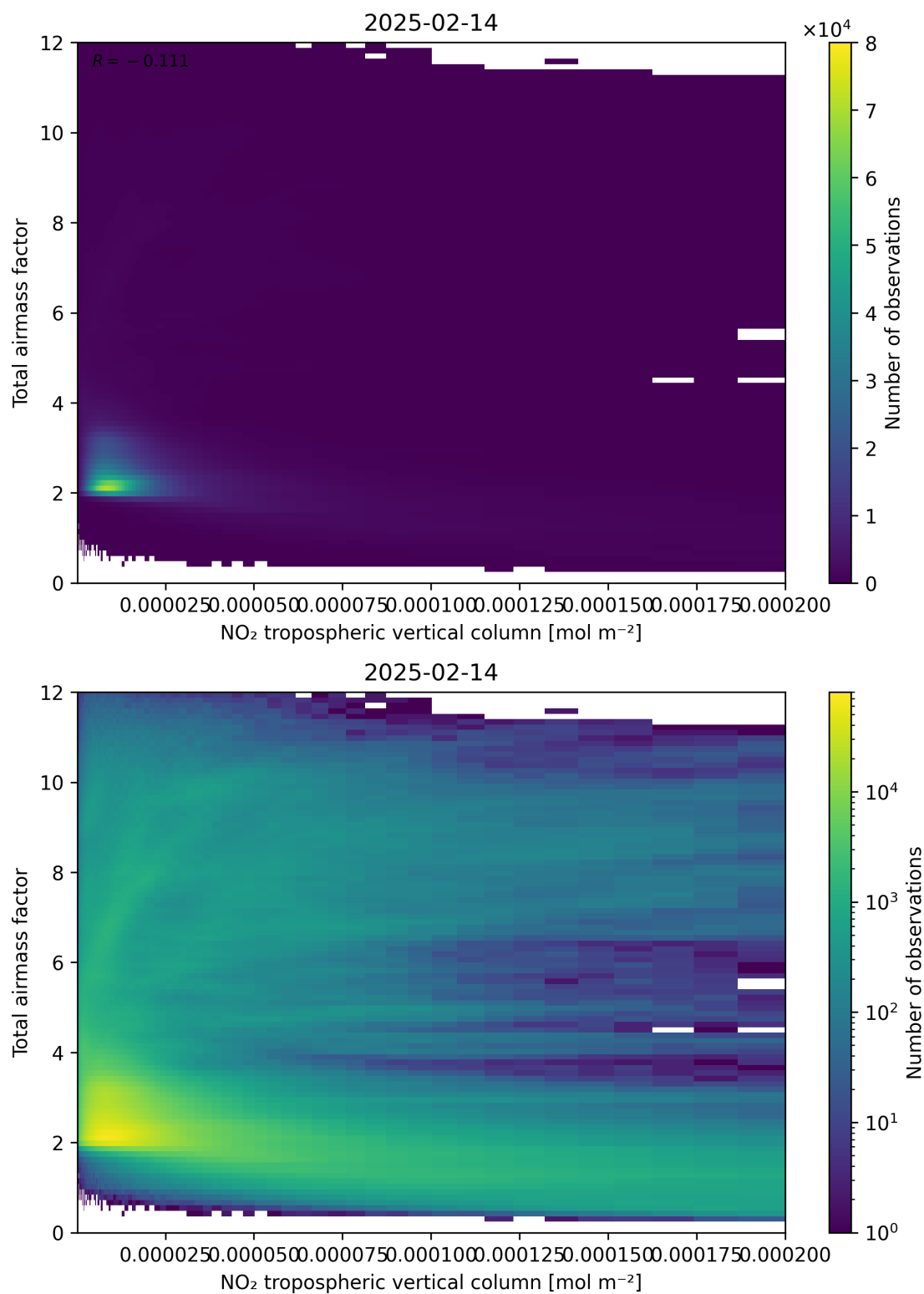
Figure 122: Scatter density plot of “NO 2 tropospheric vertical column” against “Total air mass factor” for 2025-02-13 to 2025-02-15.
