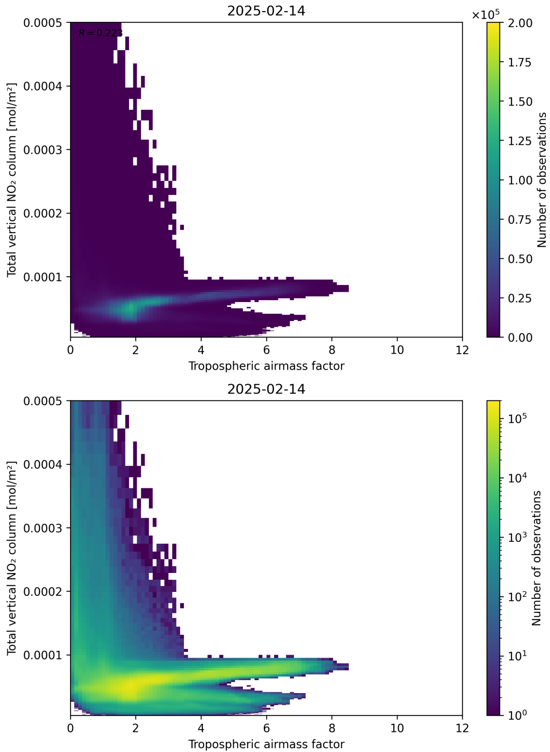
Figure 77: Scatter density plot of “Tropospheric airmass factor” against “Total vertical NO 2 column” for 2025-02-13 to 2025-02-15.
