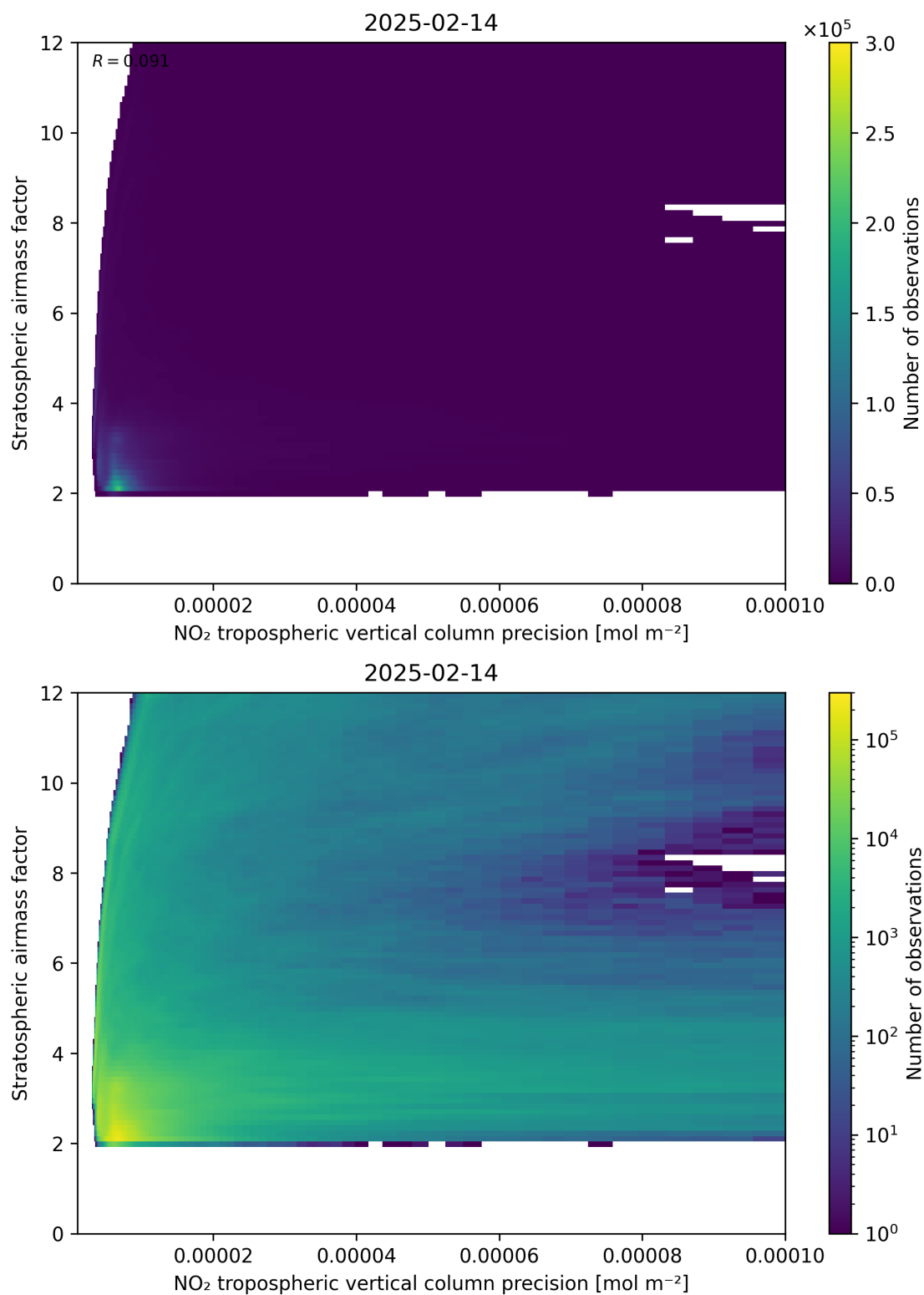
Figure 131: Scatter density plot of “NO 2 tropospheric vertical column precision” against “Stratospheric airmass factor” for 2025-02-13 to 2025-02-15.
