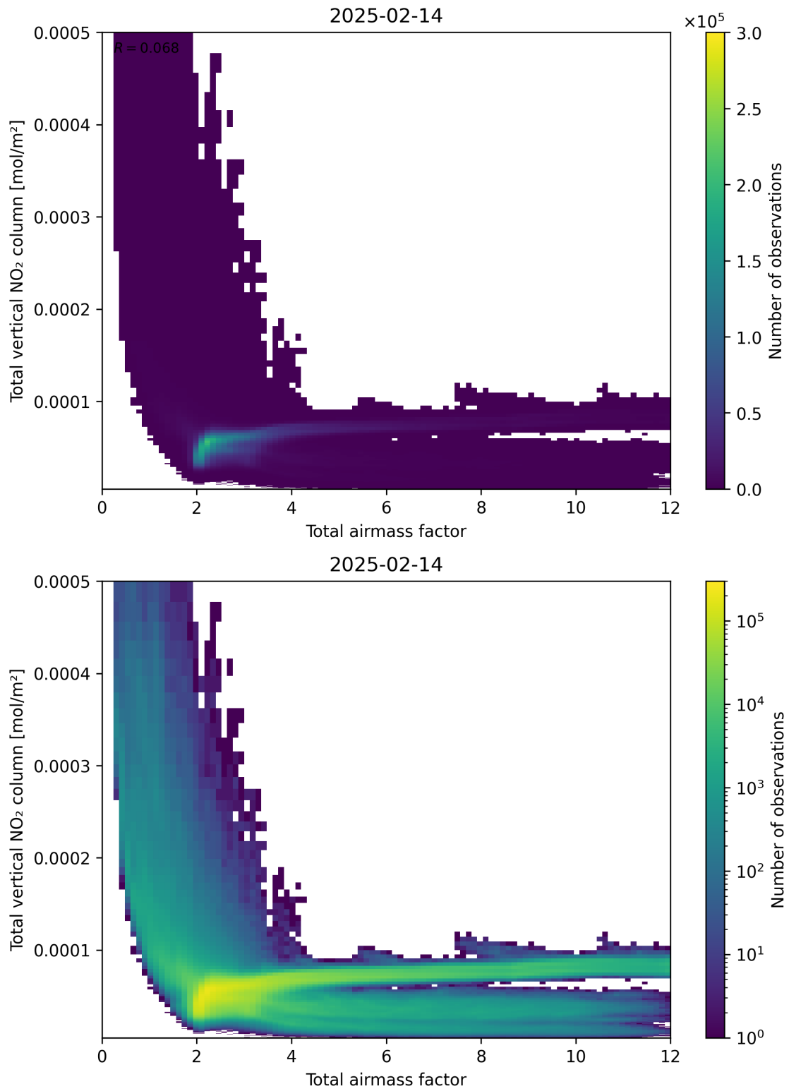
Figure 67: Scatter density plot of “Total airmass factor” against “Total vertical NO 2 column” for 2025-02-13 to 2025-02-15.
