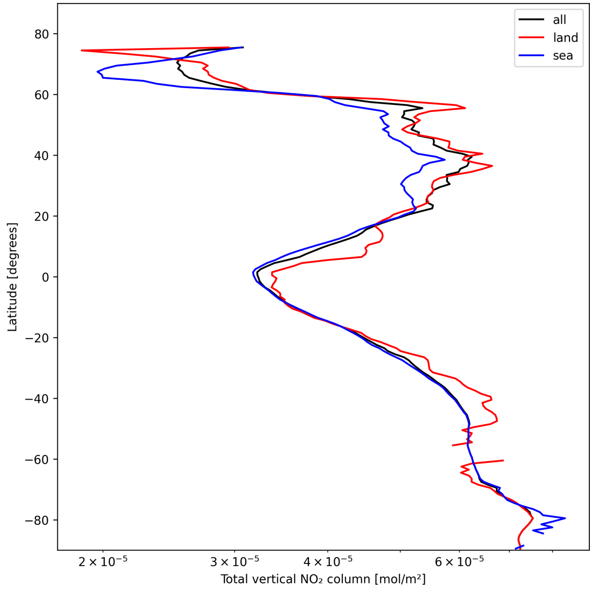
Figure 21: Zonal average of “Total vertical NO 2 column” for 2025-02-13 to 2025-02-15.
