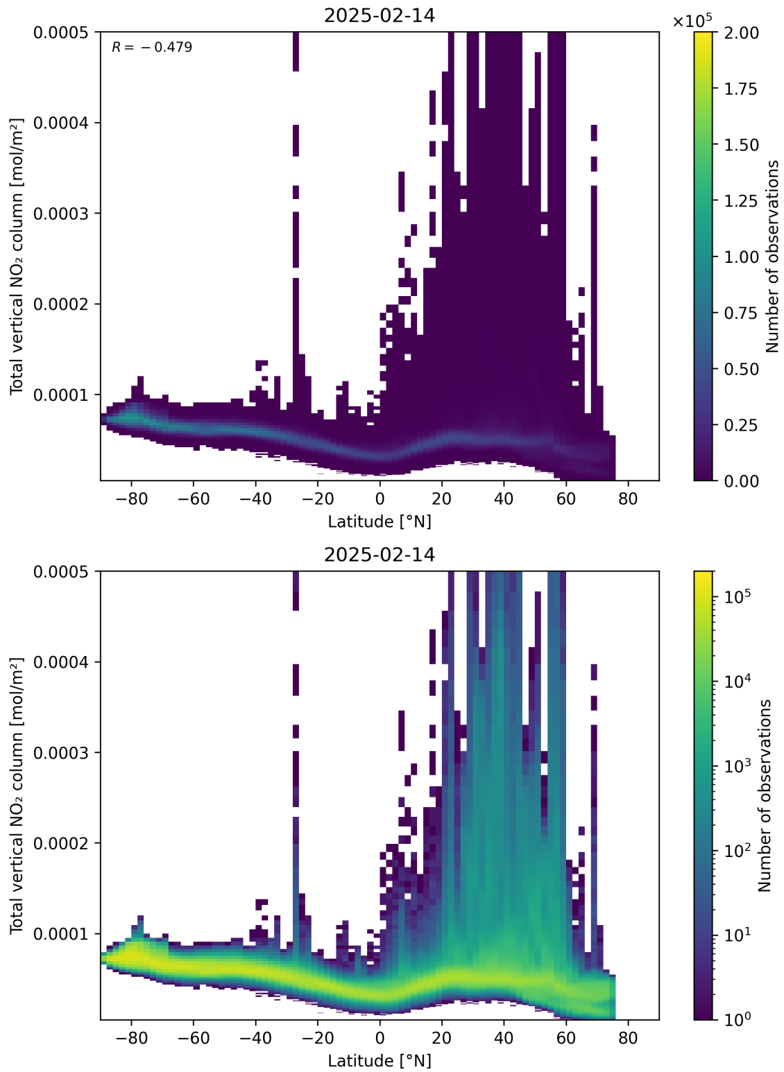
Figure 90: Scatter density plot of “Latitude” against “Total vertical NO 2 column” for 2025-02-13 to 2025-02-15.
