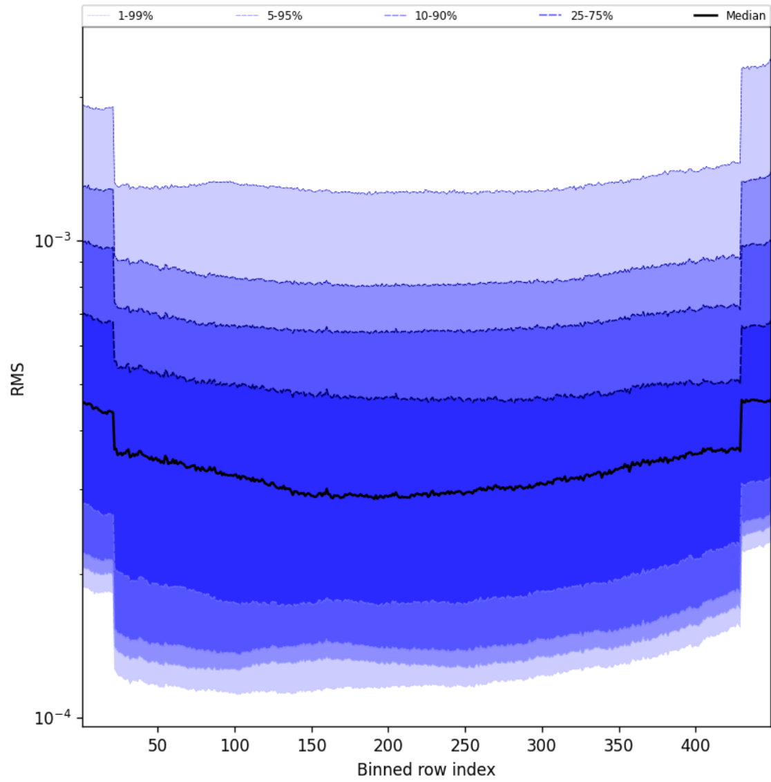
Figure 60: Along track statistics of “RMS” for 2025-02-13 to 2025-02-15
