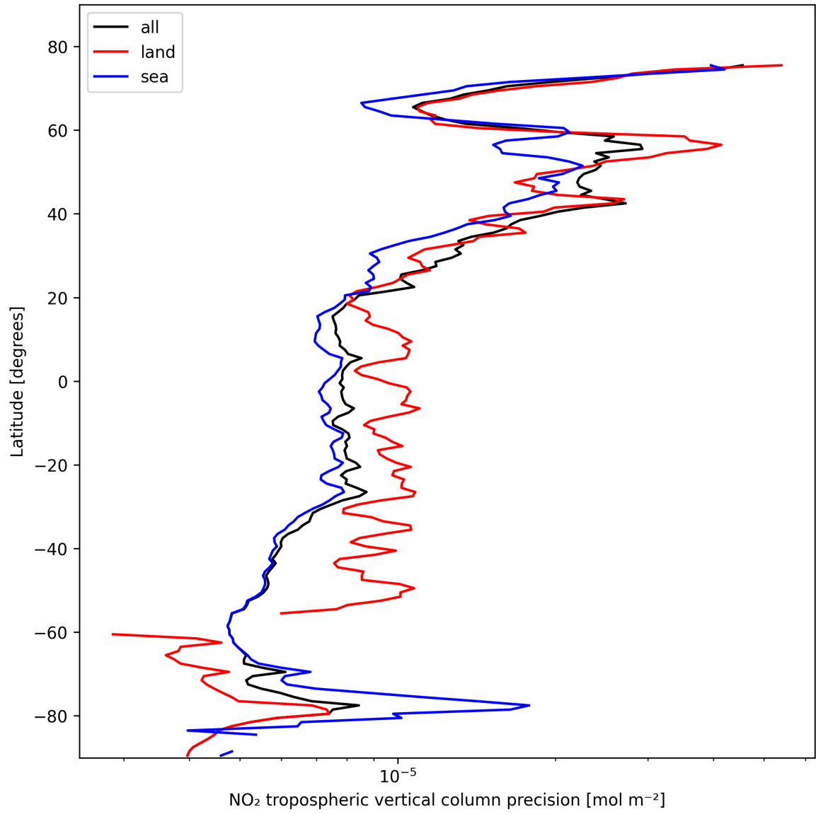
Figure 13: Zonal average of “NO 2 tropospheric vertical column precision” for 2025-02-13 to 2025-02-15.
