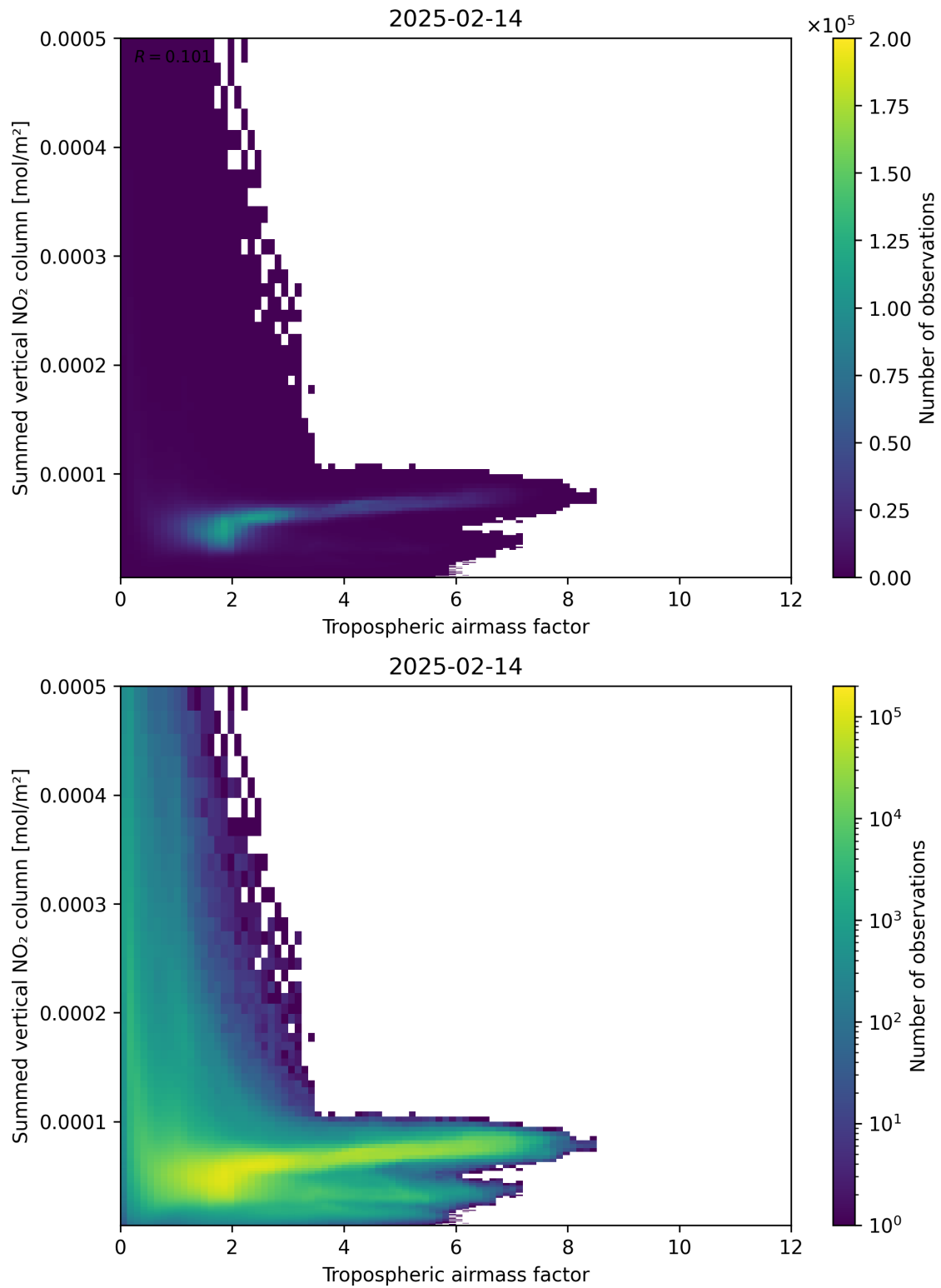
Figure 75: Scatter density plot of “Tropospheric air mass factor” against “Summed vertical NO 2 column” for 2025-02-13 to 2025-02-15.
