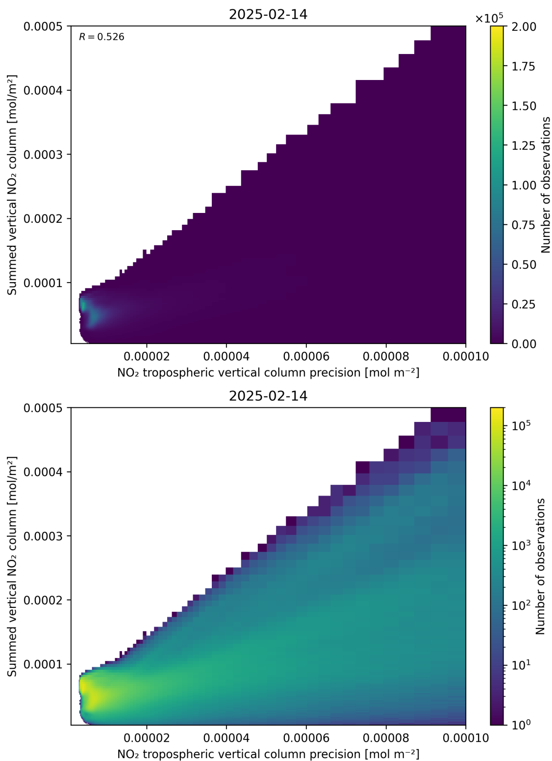
Figure 136: Scatter density plot of “NO 2 tropospheric vertical column precision” against “Summed vertical NO 2 column” for 2025-02-13 to 2025-02-15.
