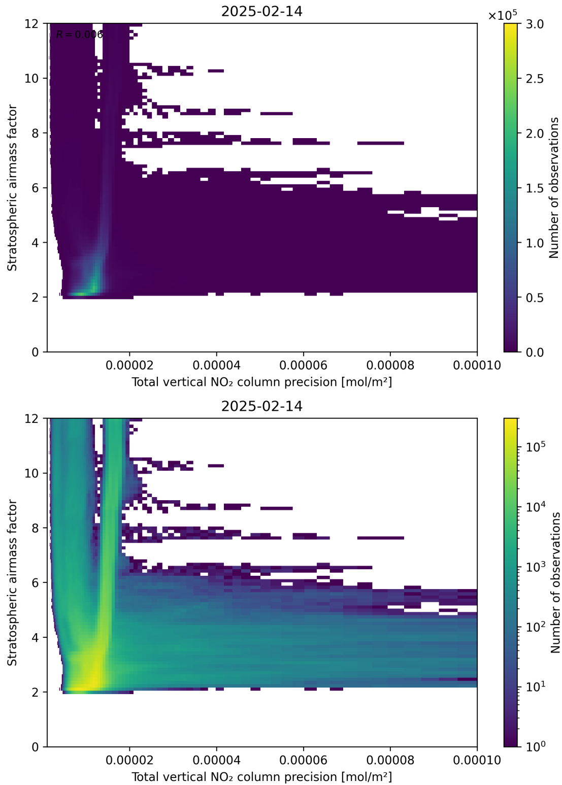
Figure 115: Scatter density plot of “Total vertical NO 2 column precision” against “Stratospheric air mass factor” for 2025-02-13 to 2025-02-15.
