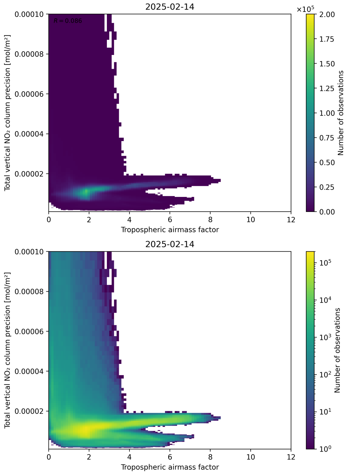
Figure 78: Scatter density plot of “Tropospheric airmass factor” against “Total vertical NO 2 column precision” for 2025-02-13 to 2025-02-15.
