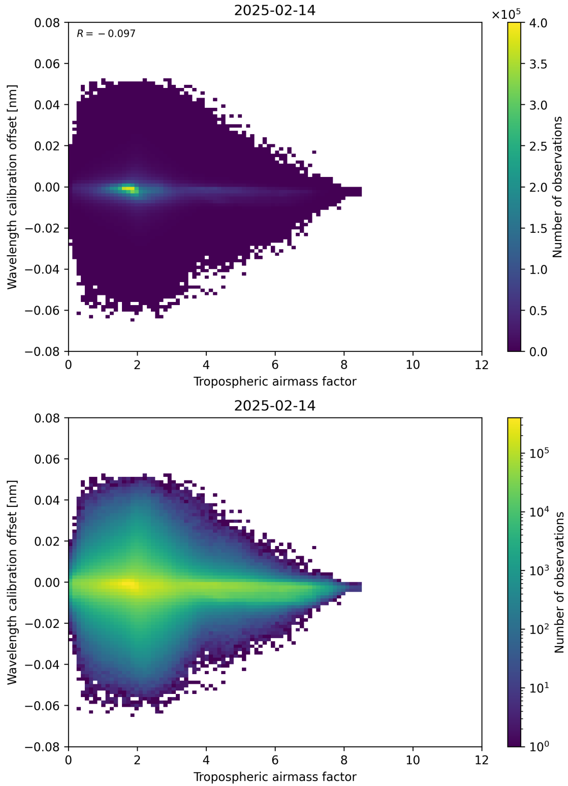
Figure 80: Scatter density plot of “Tropospheric airmass factor” against “Wavelength calibration offset” for 2025-02-13 to 2025-02-15.
