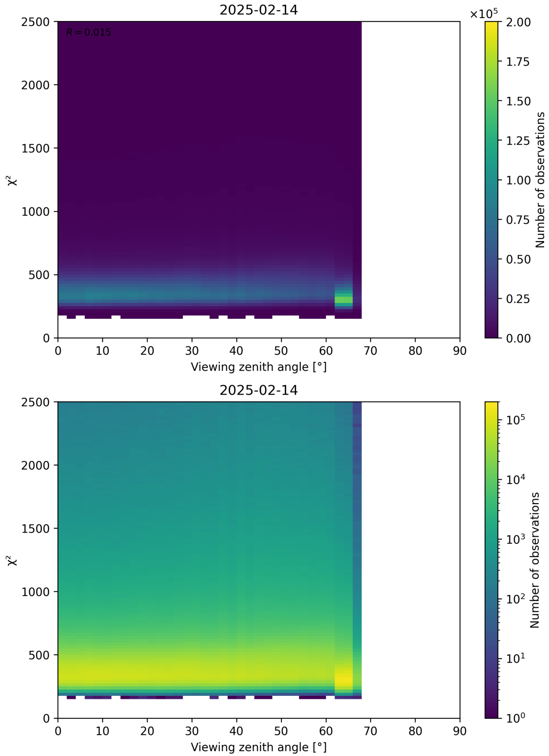
Figure 162: Scatter density plot of “Viewing zenith angle” against “ \chi^2 ” for 2025-02-13 to 2025-02-15.
