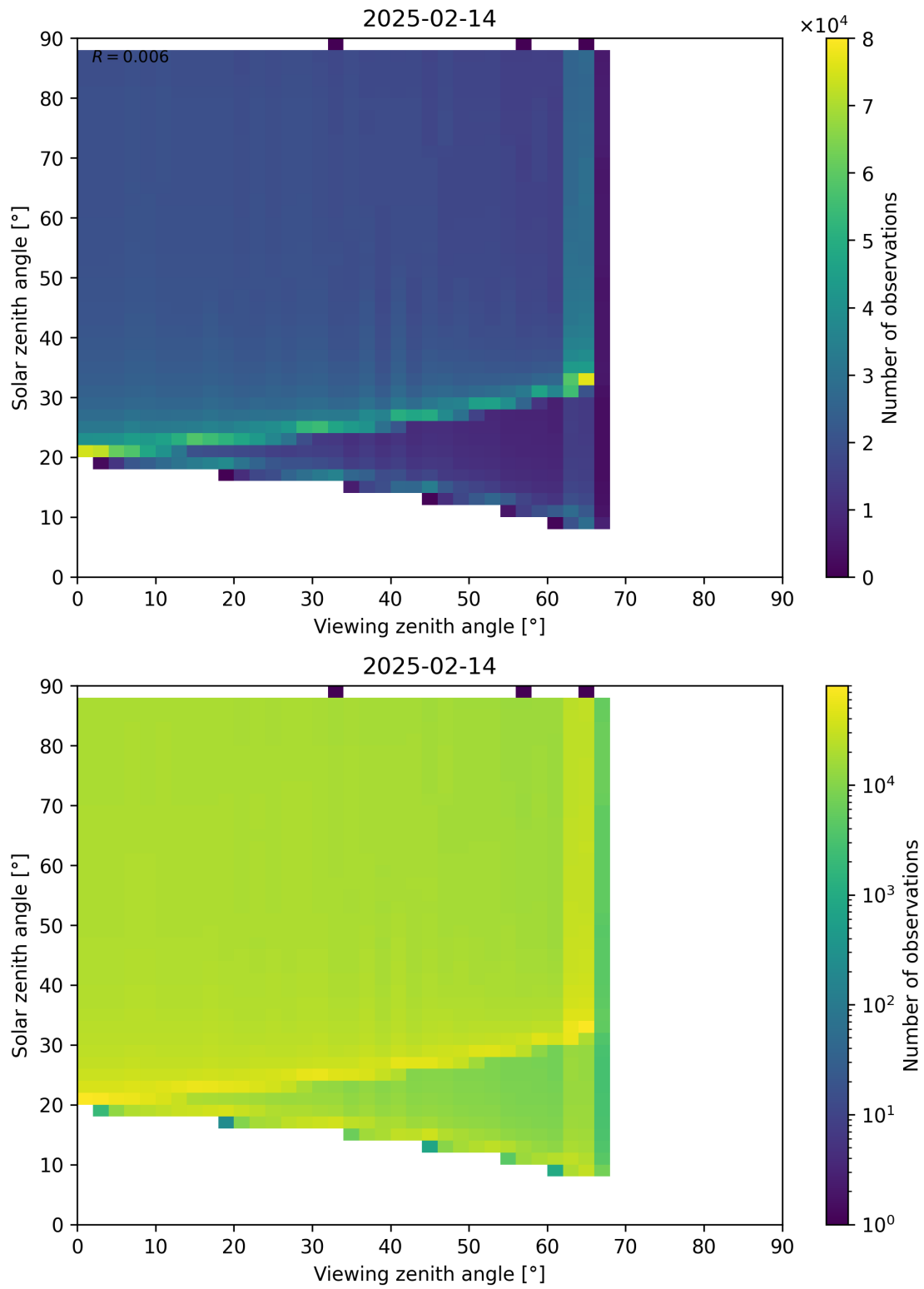
Figure 172: Scatter density plot of “Viewing zenith angle” against “Solar zenith angle” for 2025-02-13 to 2025-02-15.
