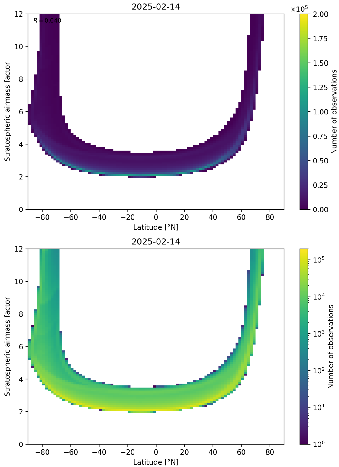
Figure 83: Scatter density plot of “Latitude” against “Stratospheric airmass factor” for 2025-02-13 to 2025-02-15.
