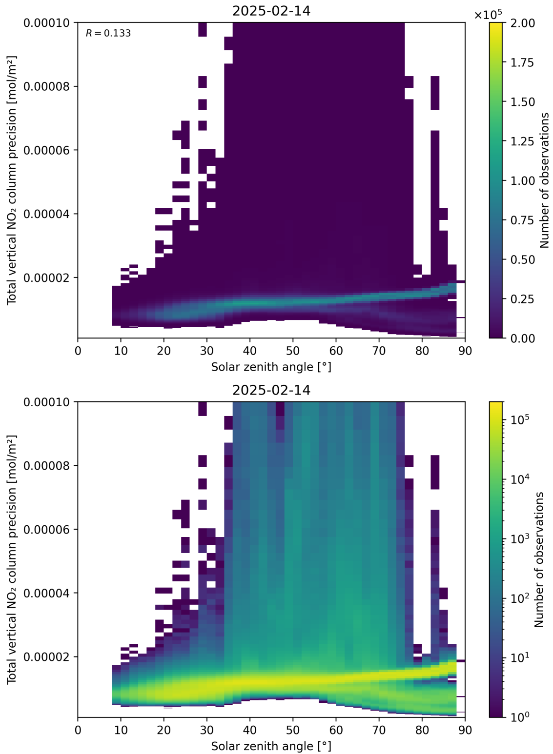
Figure 154: Scatter density plot of “Solar zenith angle” against “Total vertical NO 2 column precision” for 2025-02-13 to 2025-02-15.
