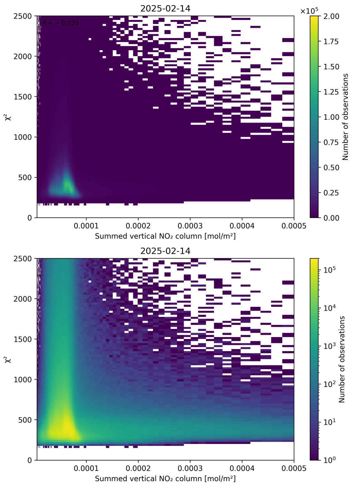
Figure 104: Scatter density plot of “Summed vertical NO 2 column” against “ \chi^2 ” for 2025-02-13 to 2025-02-15.
