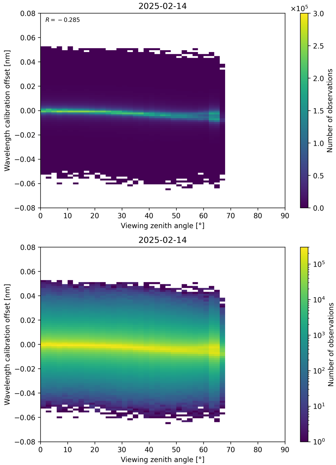
Figure 173: Scatter density plot of “Viewing zenith angle” against “Wavelength calibration offset” for 2025-02-13 to 2025-02-15.
