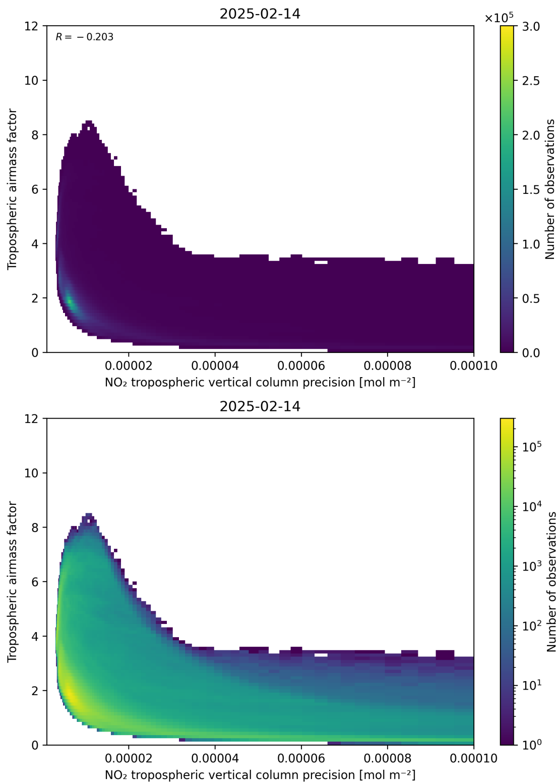
Figure 133: Scatter density plot of “NO 2 tropospheric vertical column precision” against “Tropospheric air mass factor” for 2025-02-13 to 2025-02-15.
