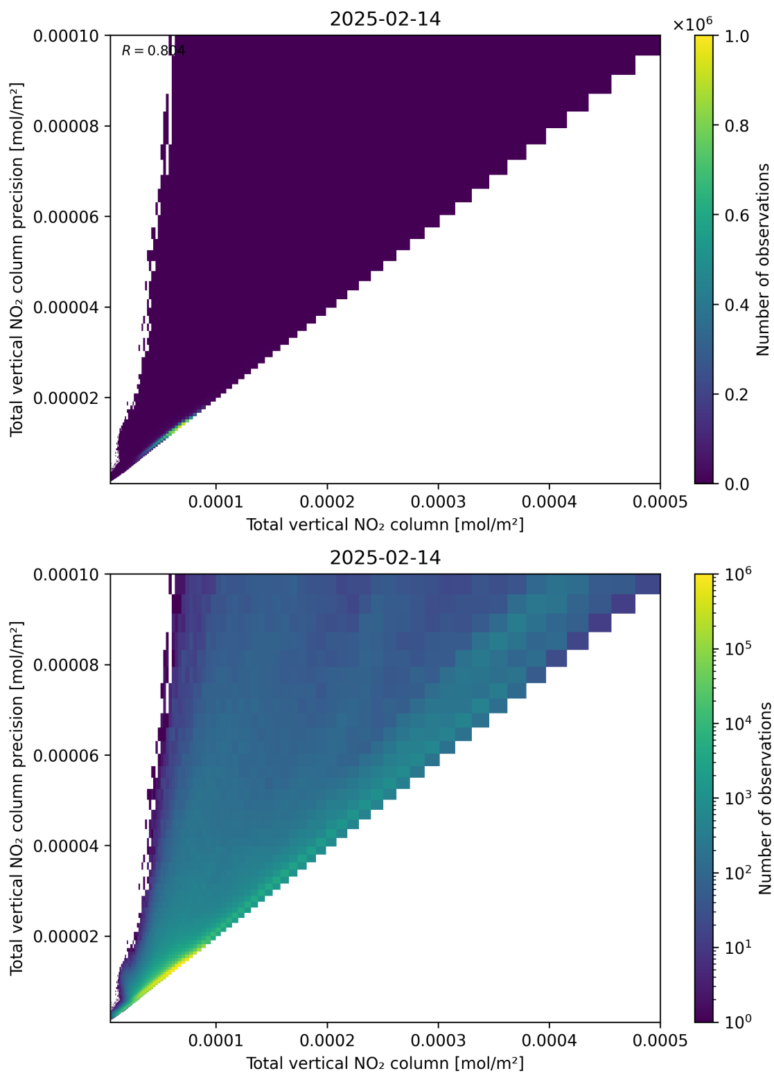
Figure 114: Scatter density plot of “Total vertical NO 2 column” against “Total vertical NO 2 column precision” for 2025-02-13 to 2025-02-15.
