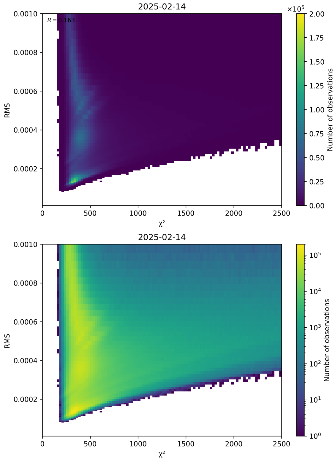
Figure 82: Scatter density plot of “ \chi^2 ” against “RMS” for 2025-02-13 to 2025-02-15.
