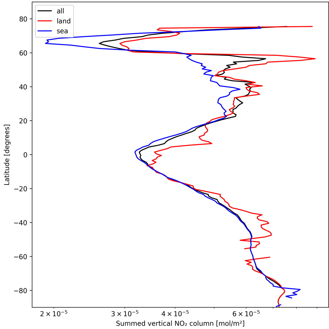
Figure 23: Zonal average of “Summed vertical NO 2 column” for 2025-02-13 to 2025-02-15.
