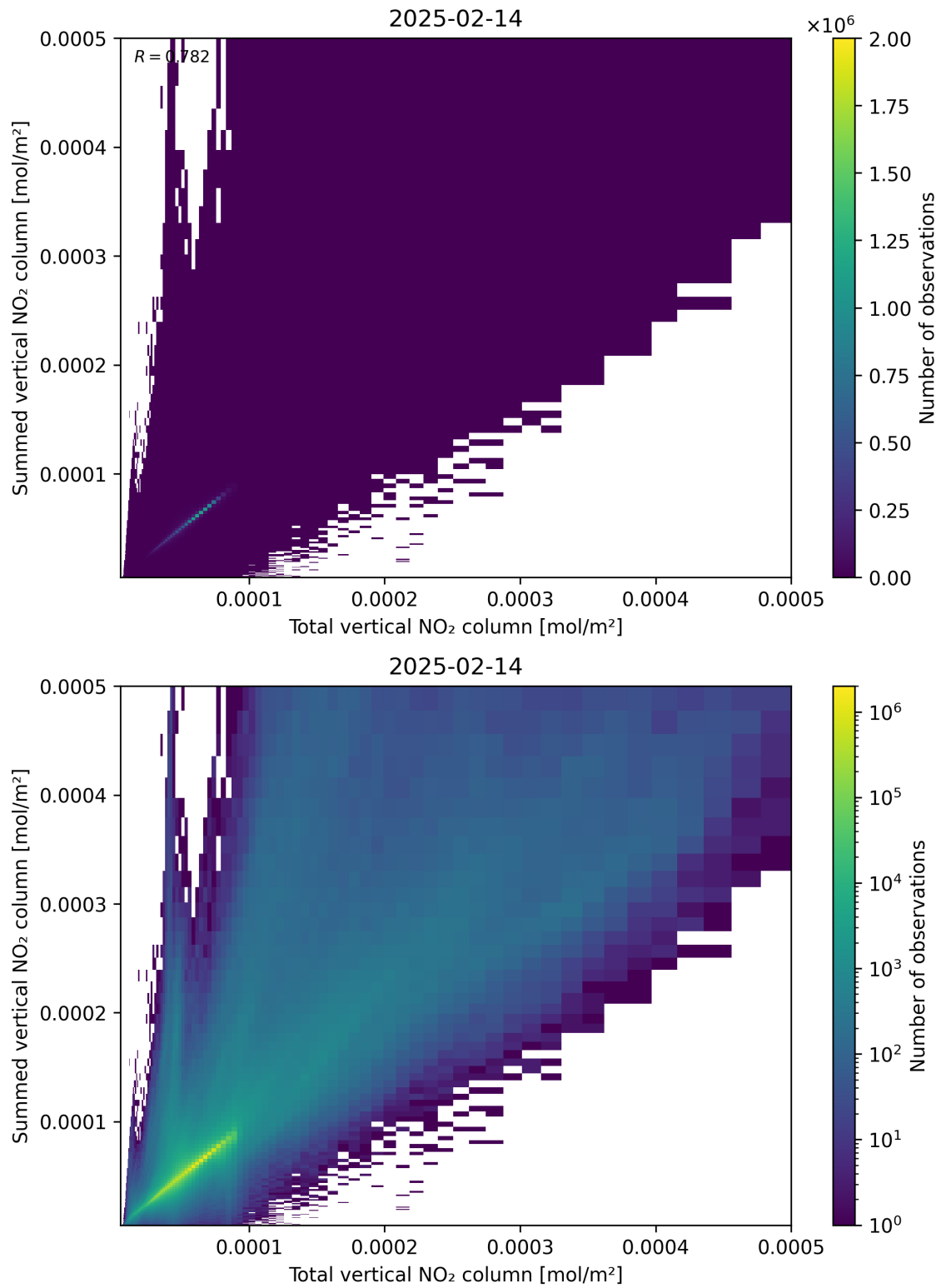
Figure 112: Scatter density plot of “Total vertical NO 2 column” against “Summed vertical NO 2 column” for 2025-02-13 to 2025-02-15.
