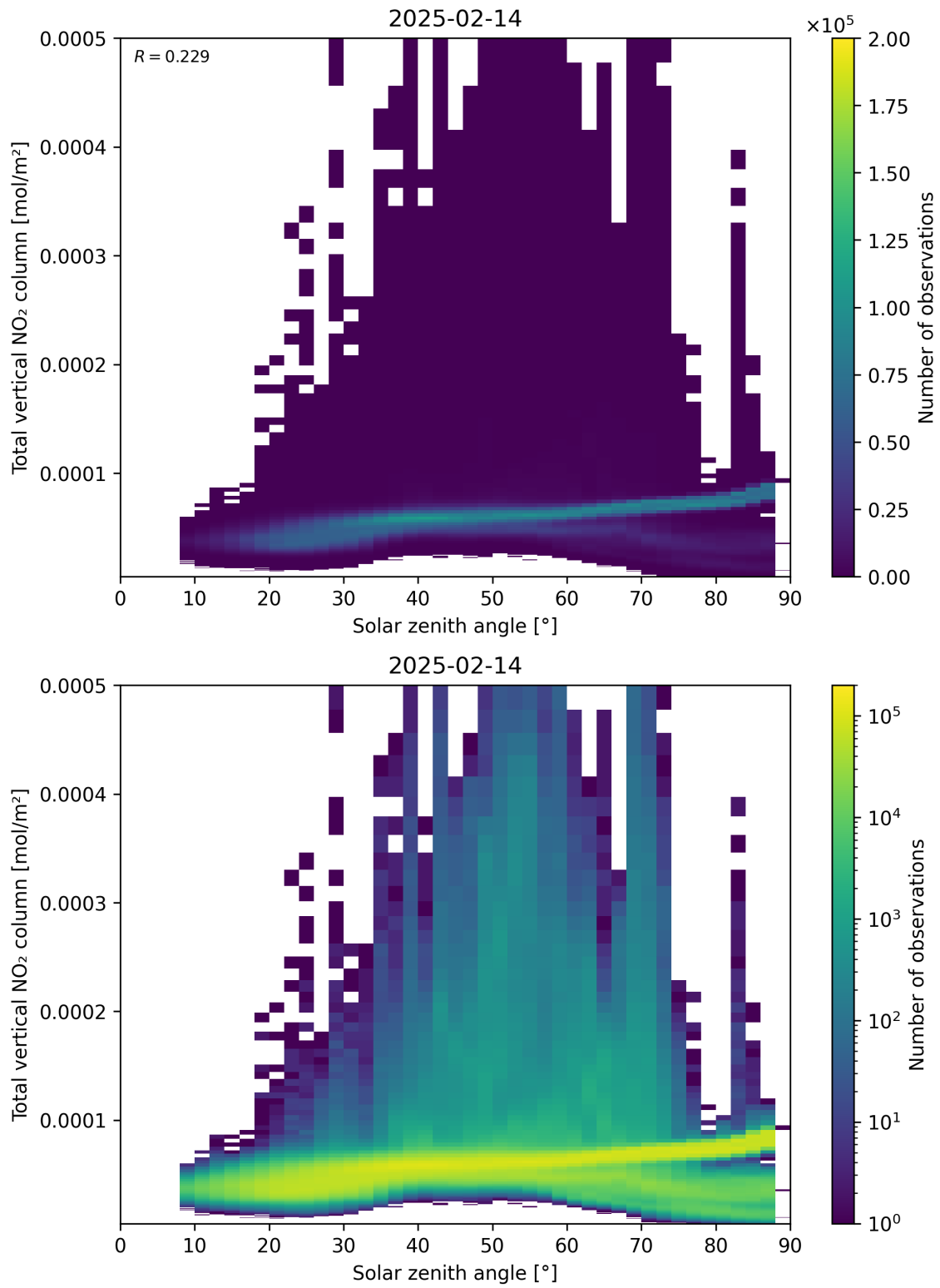
Figure 153: Scatter density plot of “Solar zenith angle” against “Total vertical NO 2 column” for 2025-02-13 to 2025-02-15.
