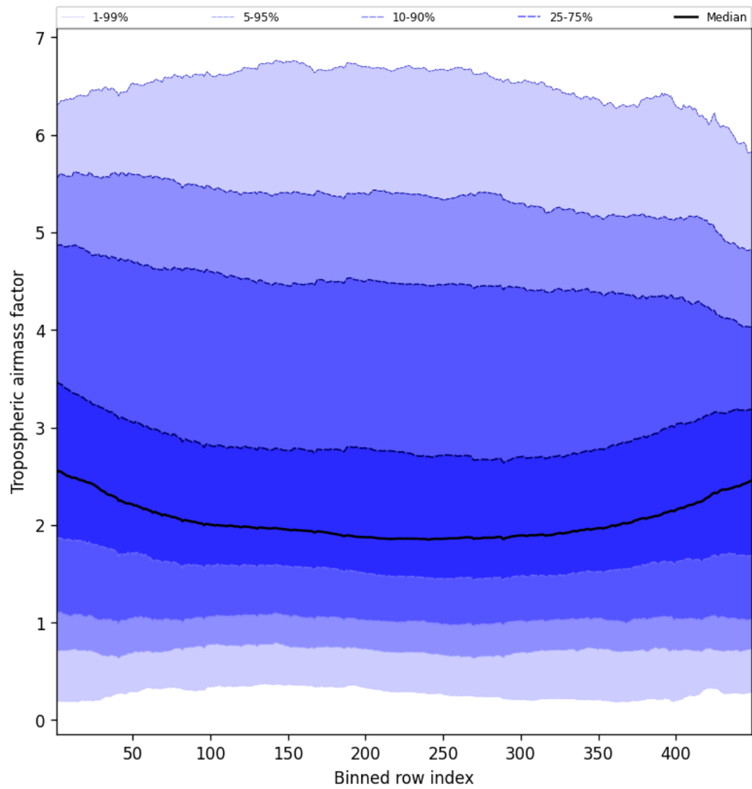
Figure 48: Along track statistics of “Tropospheric airmass factor” for 2025-02-13 to 2025-02-15
