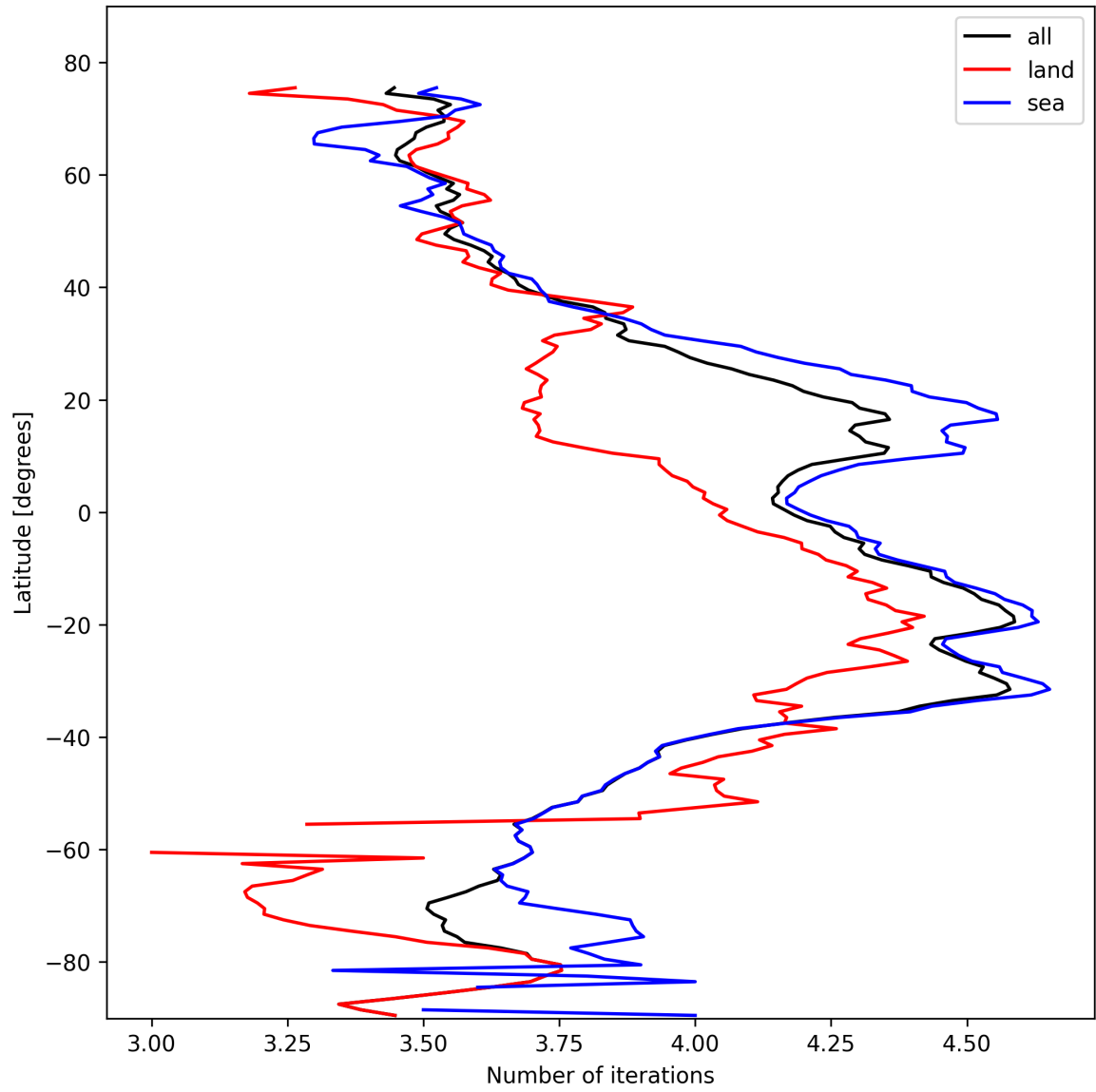
Figure 17: Zonal average of “Number of iterations” for 2025-02-13 to 2025-02-15.
