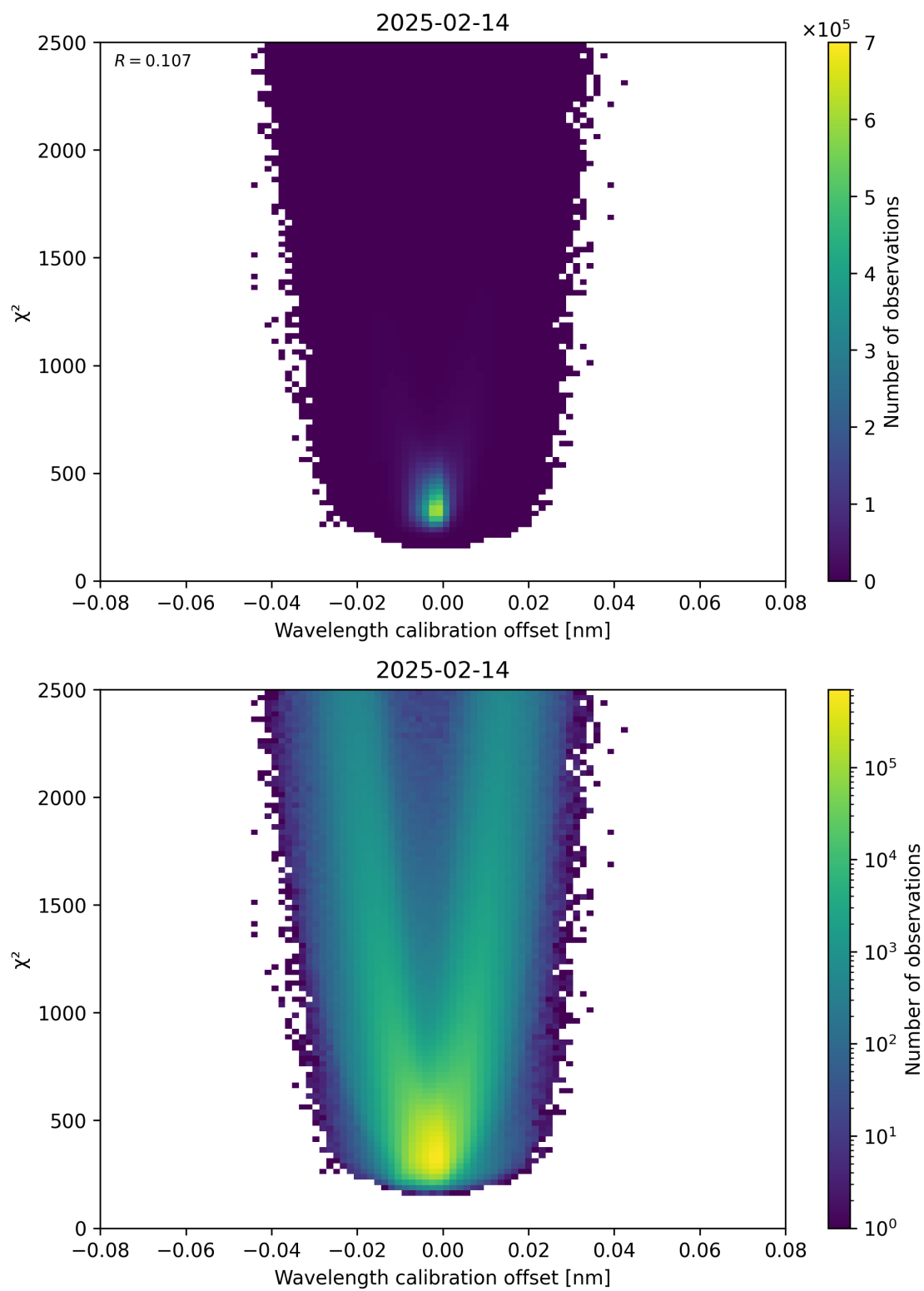
Figure 175: Scatter density plot of “Wavelength calibration offset” against “ \chi^2 ” for 2025-02-13 to 2025-02-15.
