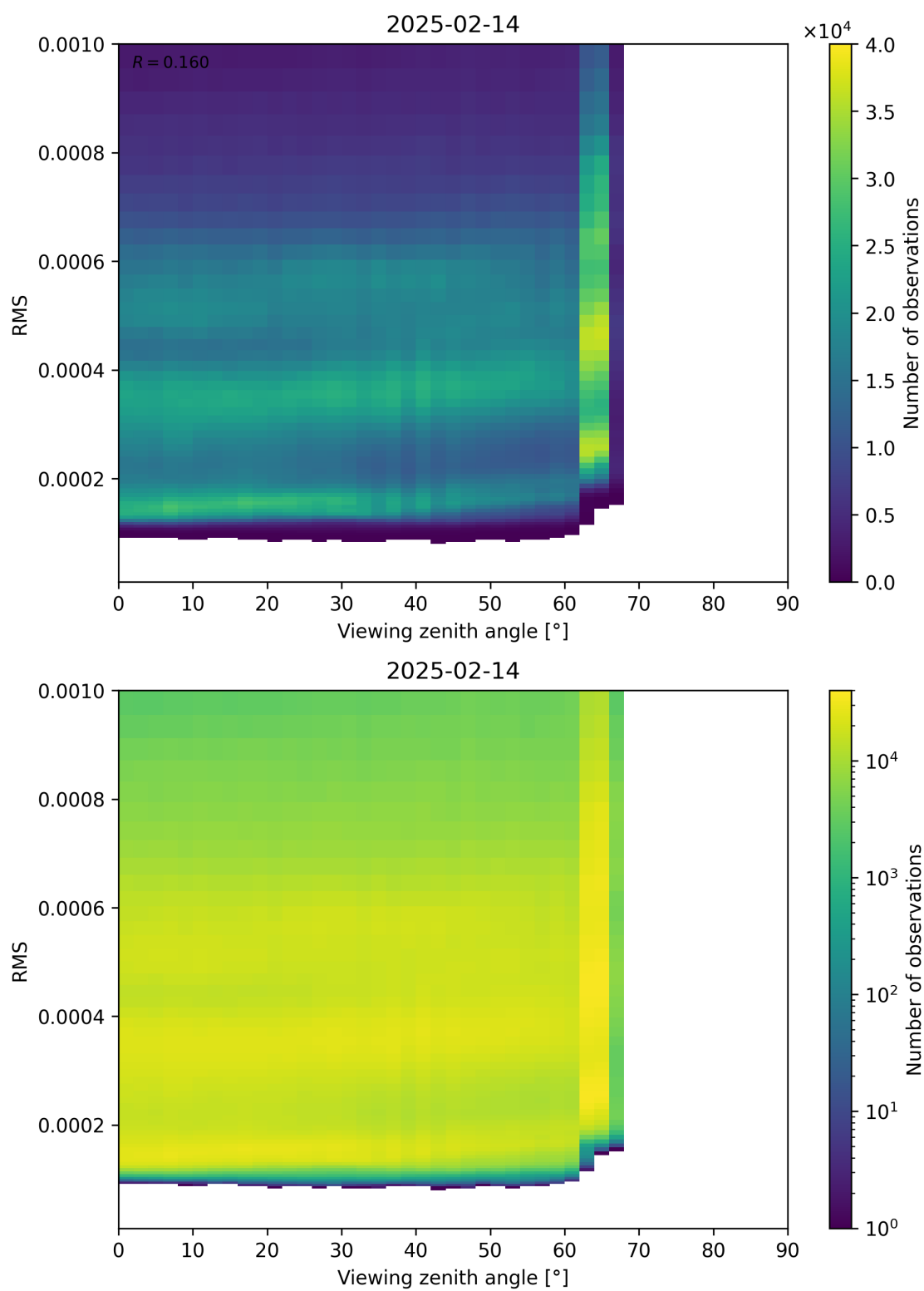
Figure 171: Scatter density plot of “Viewing zenith angle” against “RMS” for 2025-02-13 to 2025-02-15.
