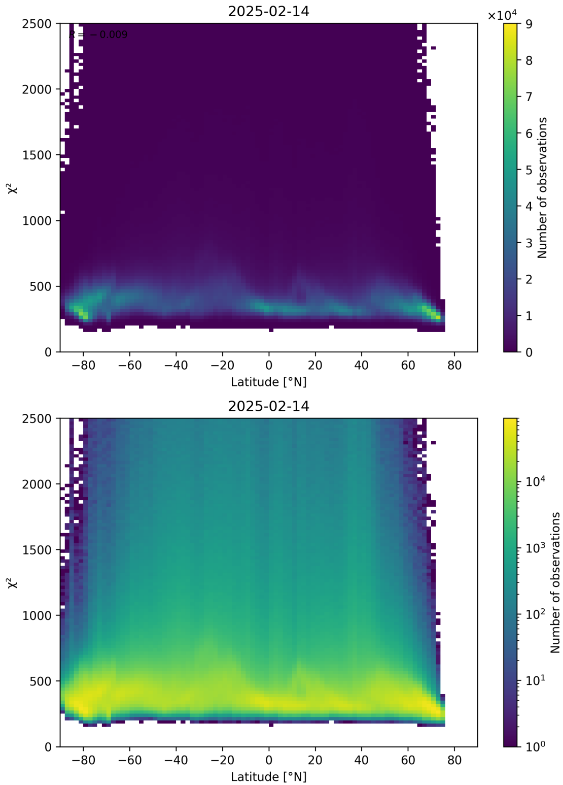
Figure 86: Scatter density plot of “Latitude” against “ \chi^2 ” for 2025-02-13 to 2025-02-15.
