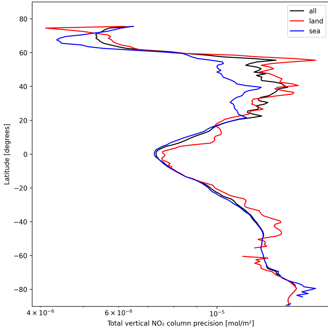
Figure 22: Zonal average of “Total vertical NO 2 column precision” for 2025-02-13 to 2025-02-15.
