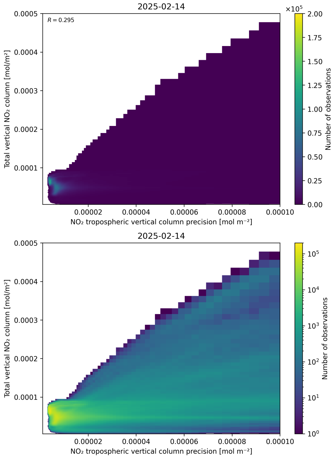
Figure 138: Scatter density plot of “NO 2 tropospheric vertical column precision” against “Total vertical NO 2 column” for 2025-02-13 to 2025-02-15.
