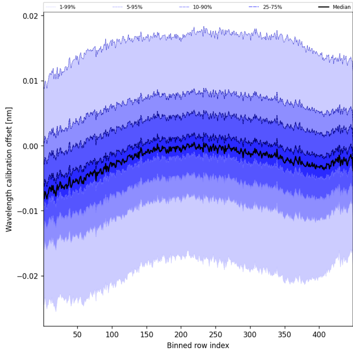
Figure 52: Along track statistics of “Wavelength calibration offset” for 2025-02-13 to 2025-02-15
