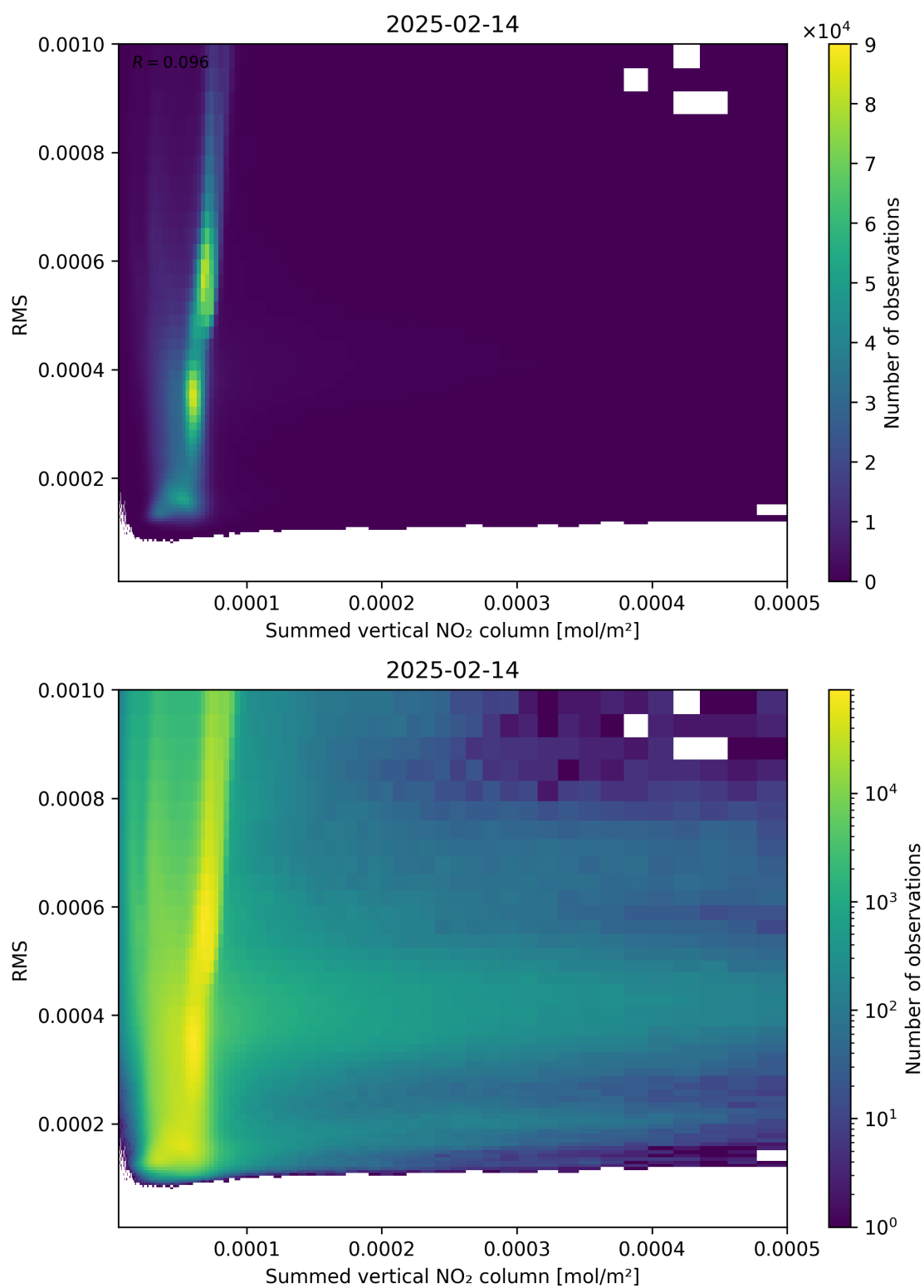
Figure 109: Scatter density plot of “Summed vertical NO 2 column” against “RMS” for 2025-02-13 to 2025-02-15.
