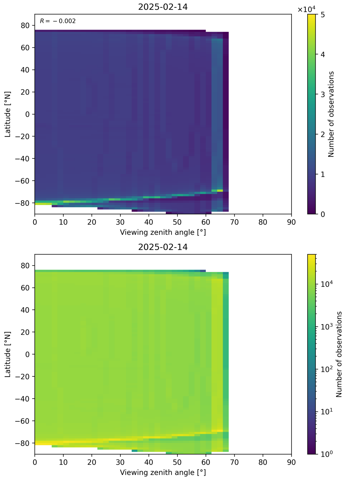
Figure 163: Scatter density plot of “Viewing zenith angle” against “Latitude” for 2025-02-13 to 2025-02-15.
