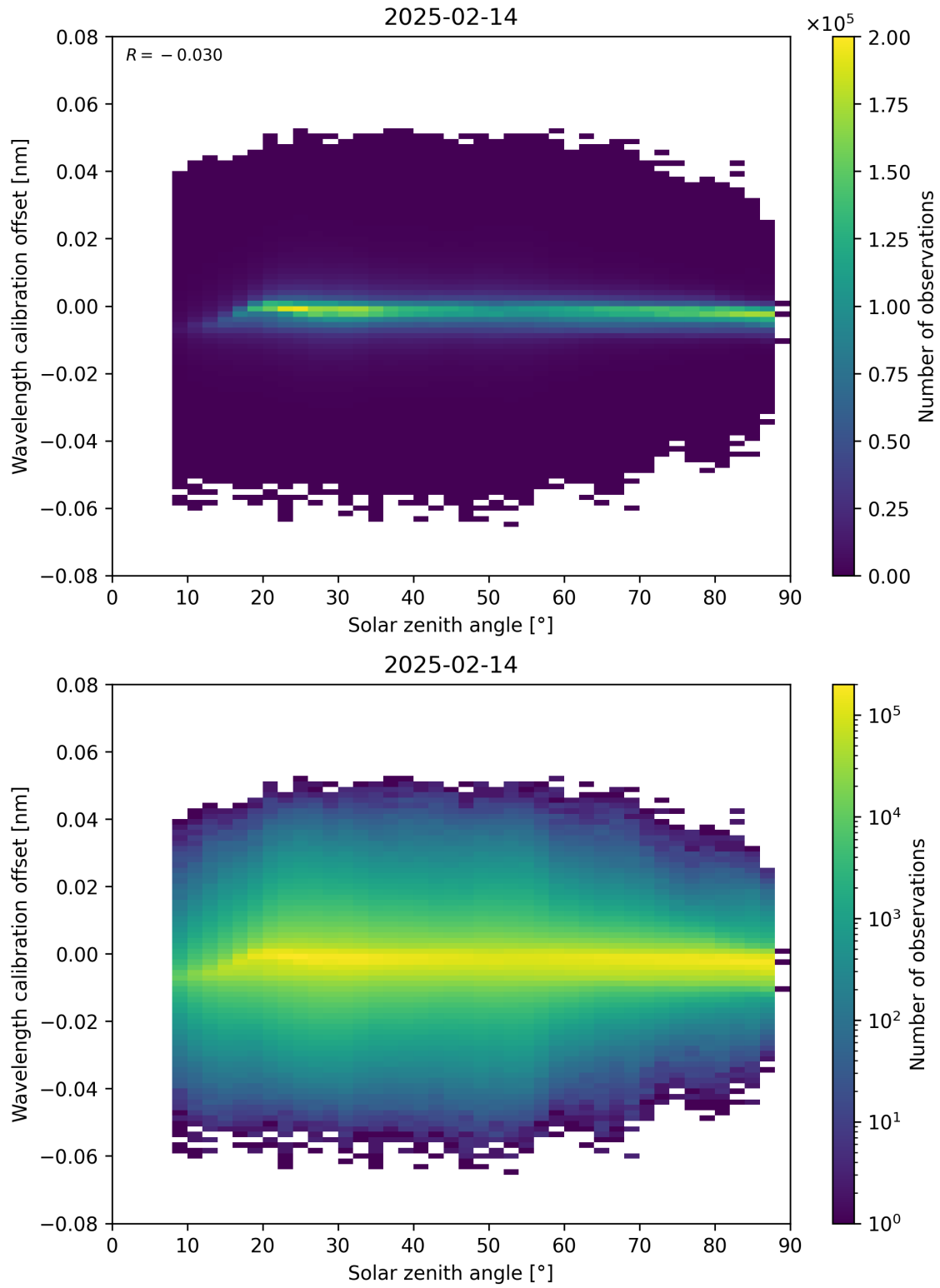
Figure 158: Scatter density plot of “Solar zenith angle” against “Wavelength calibration offset” for 2025-02-13 to 2025-02-15.
