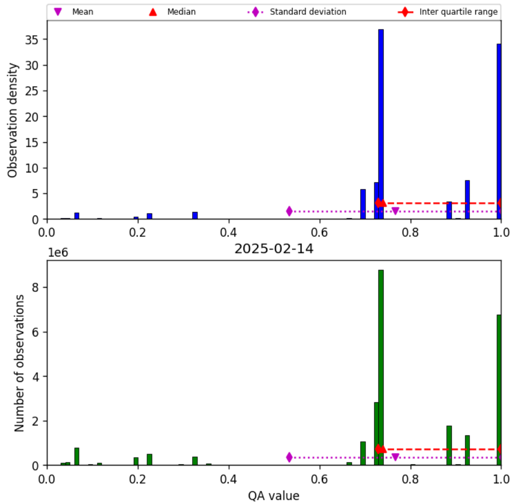
Figure 28: Histogram of “QA value” for 2025-02-13 to 2025-02-15
