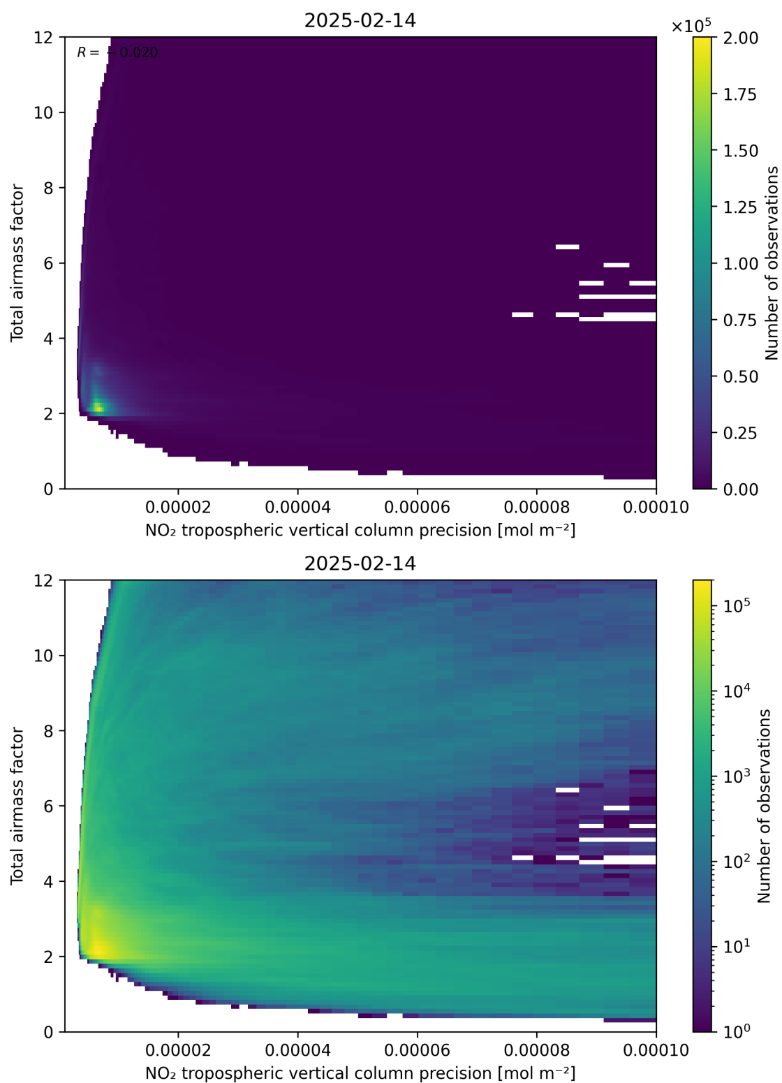
Figure 132: Scatter density plot of “NO 2 tropospheric vertical column precision” against “Total airmass factor” for 2025-02-13 to 2025-02-15.
