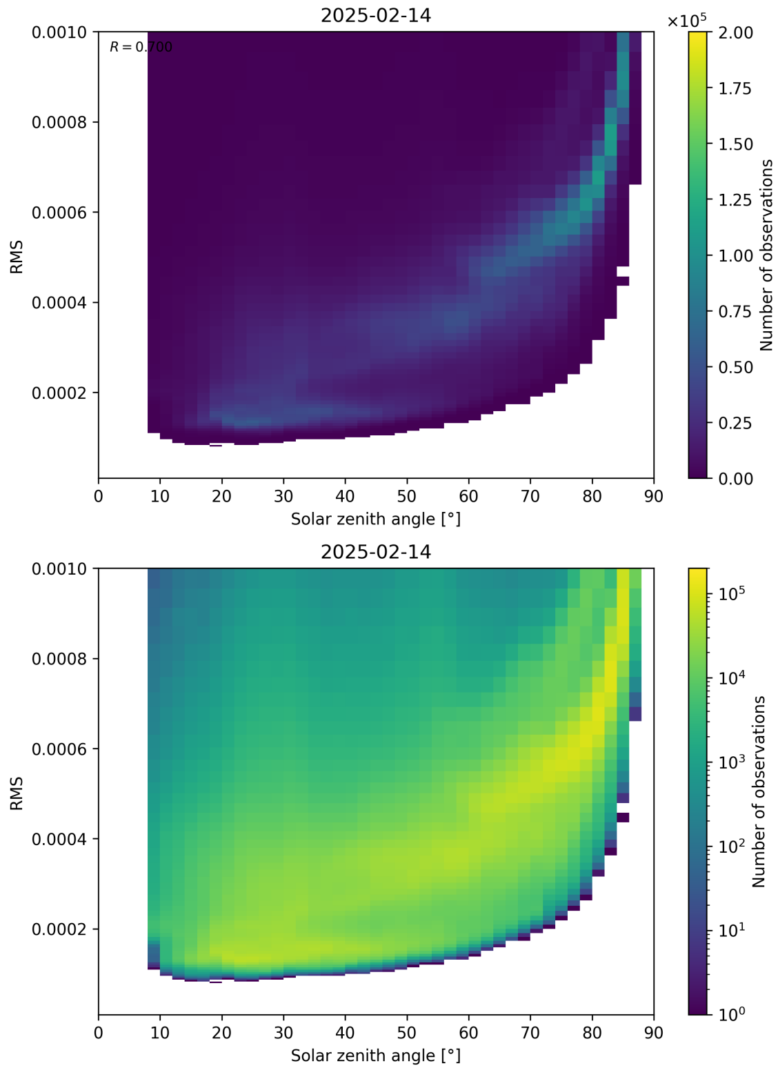
Figure 157: Scatter density plot of “Solar zenith angle” against “RMS” for 2025-02-13 to 2025-02-15.
