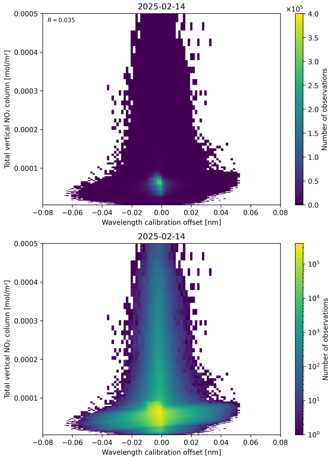
Figure 179: Scatter density plot of “Wavelength calibration offset” against “Total vertical NO 2 column” for 2025-02-13 to 2025-02-15.
