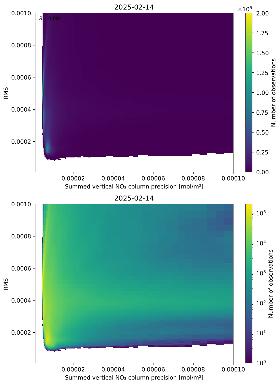
Figure 108: Scatter density plot of “Summed vertical NO 2 column precision” against “RMS” for 2025-02-13 to 2025-02-15.
