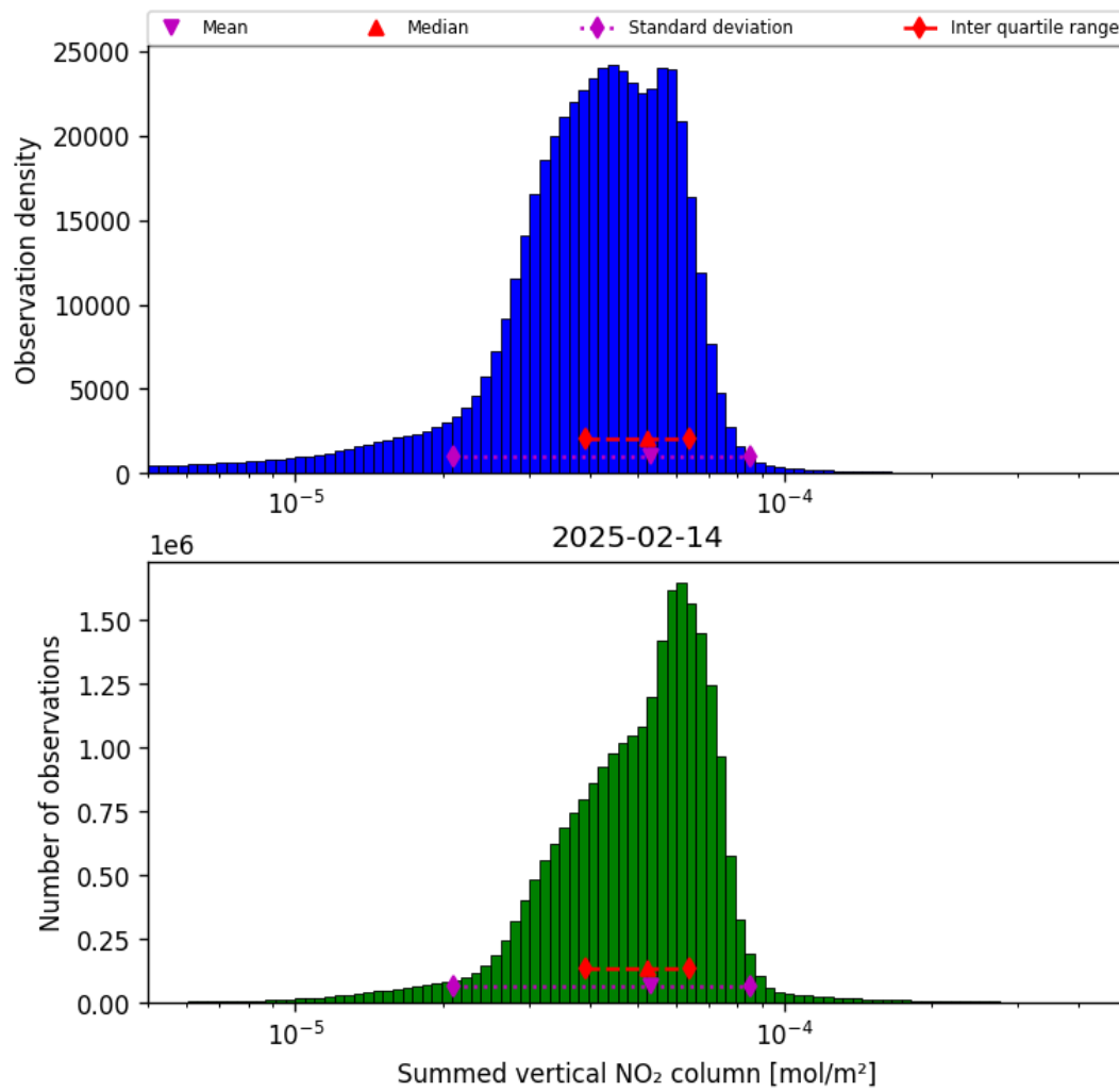
Figure 40: Histogram of “Summed vertical NO 2 column” for 2025-02-13 to 2025-02-15
