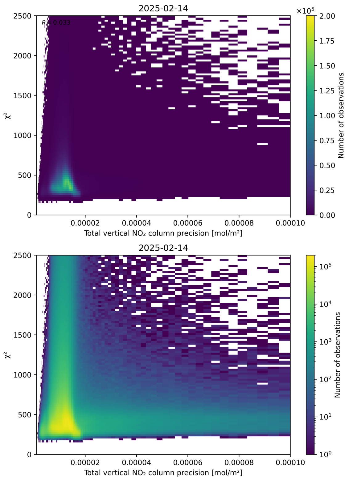
Figure 116: Scatter density plot of “Total vertical NO 2 column precision” against “ \chi^2 ” for 2025-02-13 to 2025-02-15.
