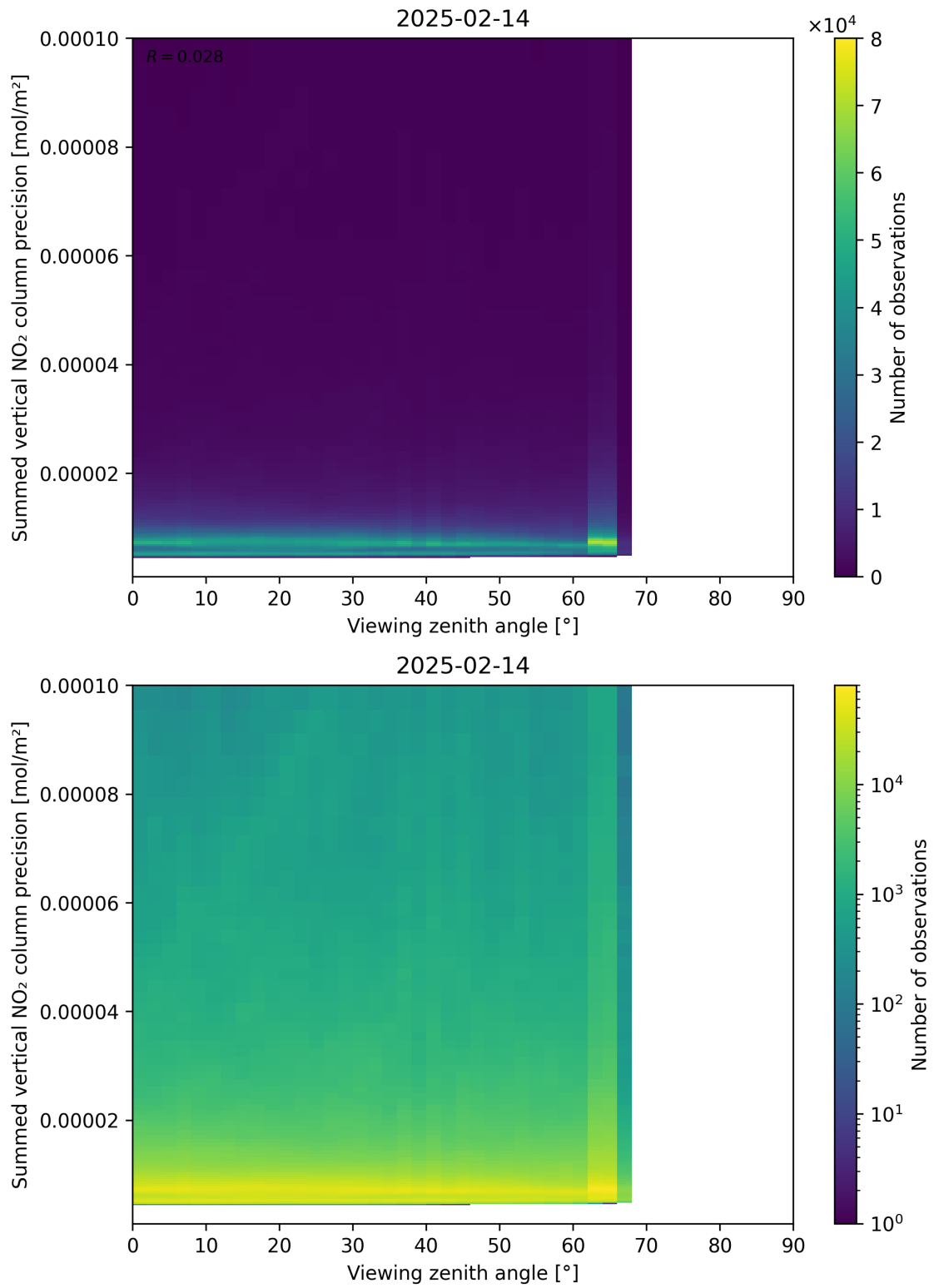
Figure 166: Scatter density plot of “Viewing zenith angle” against “Summed vertical NO 2 column precision” for 2025-02-13 to 2025-02-15.
