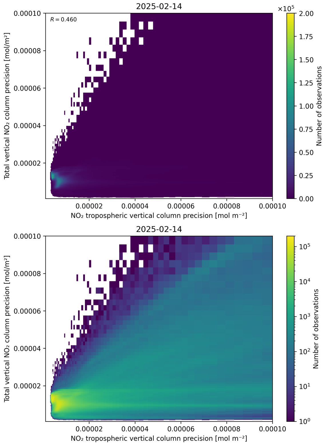
Figure 139: Scatter density plot of “NO 2 tropospheric vertical column precision” against “Total vertical NO 2 column precision” for 2025-02-13 to 2025-02-15.
