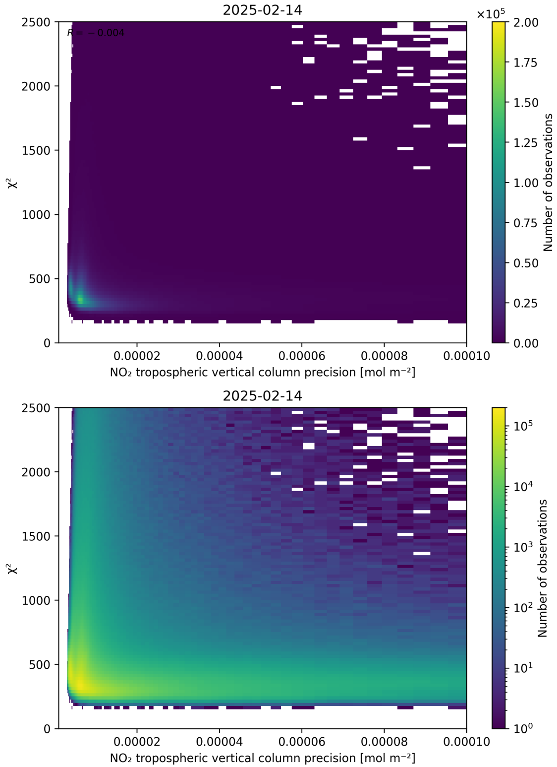
Figure 134: Scatter density plot of “NO 2 tropospheric vertical column precision” against “ \chi^2 ” for 2025-02-13 to 2025-02-15.
