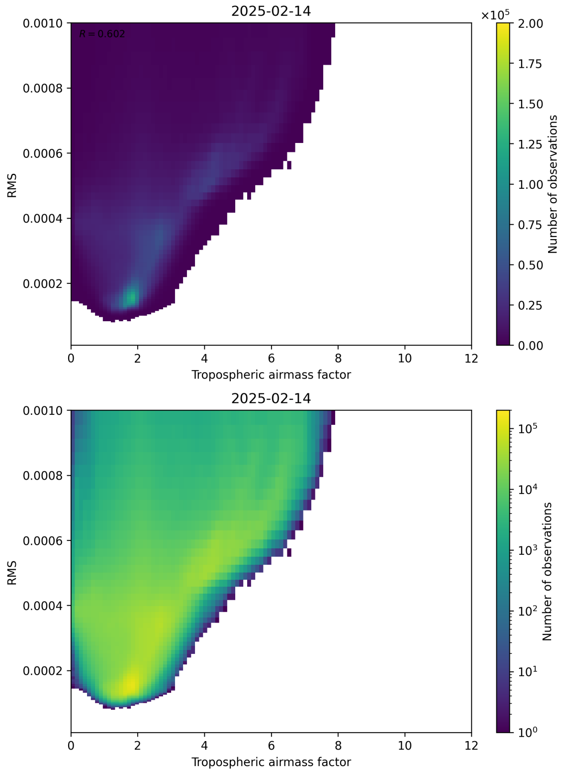
Figure 79: Scatter density plot of “Tropospheric airmass factor” against “RMS” for 2025-02-13 to 2025-02-15.
