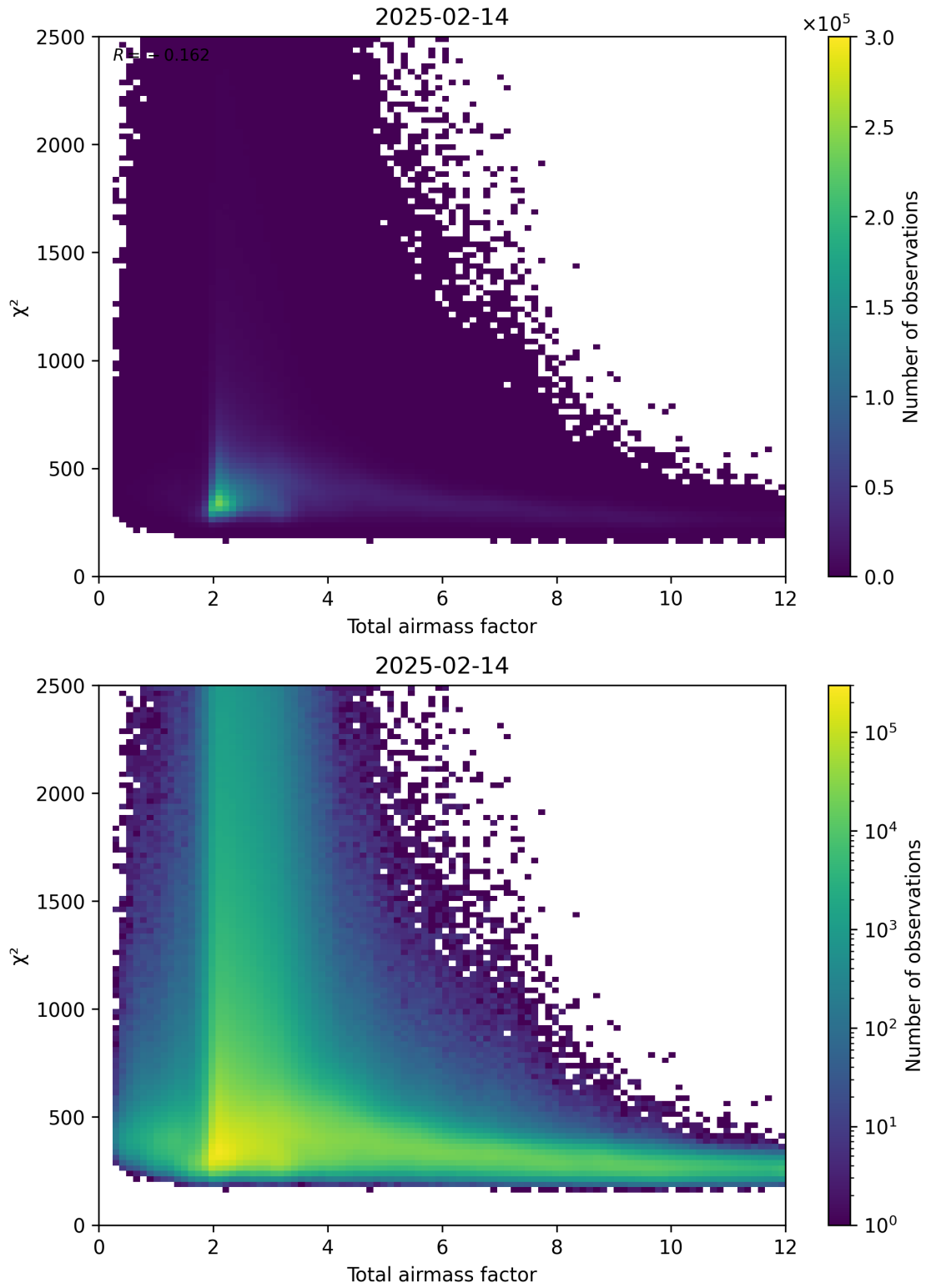
Figure 63: Scatter density plot of “Total airmass factor” against “ \chi^2 ” for 2025-02-13 to 2025-02-15.
