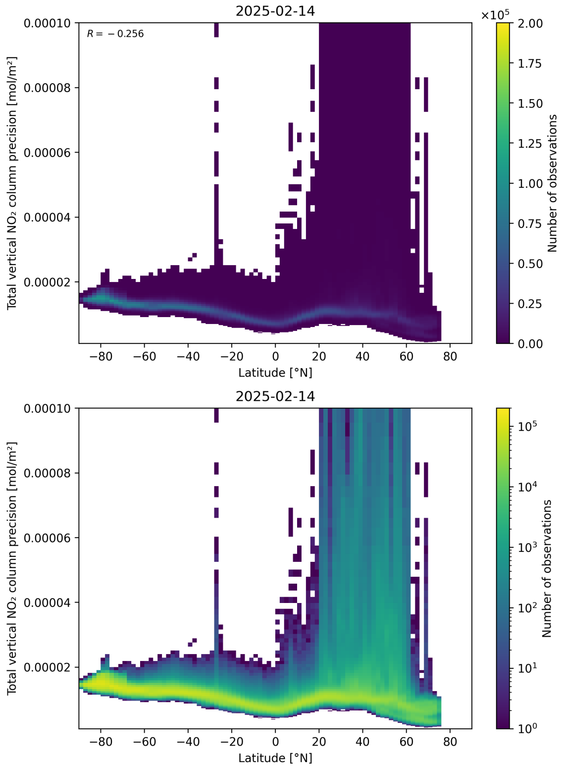
Figure 91: Scatter density plot of “Latitude” against “Total vertical NO 2 column precision” for 2025-02-13 to 2025-02-15.
