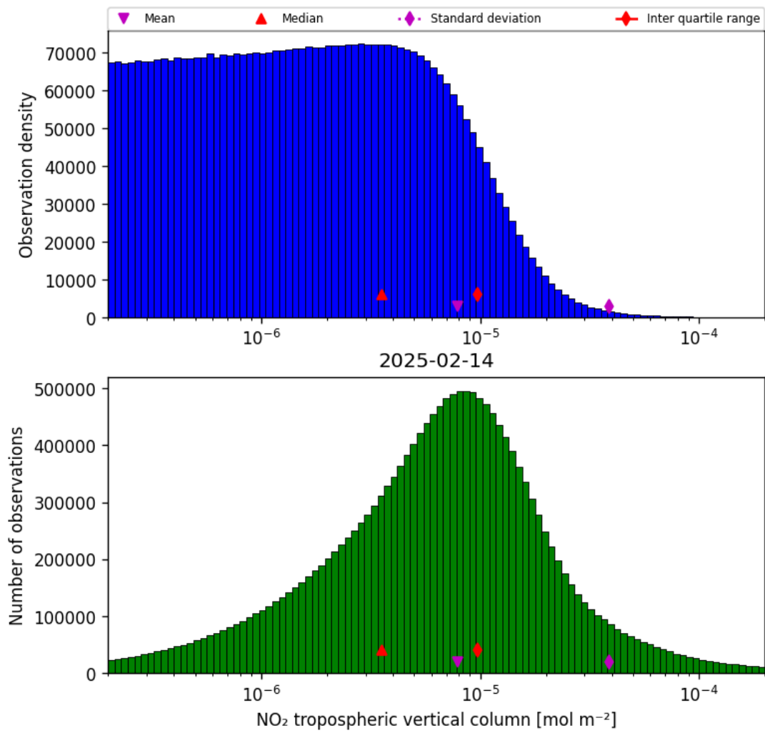
Figure 29: Histogram of “NO 2 tropospheric vertical column” for 2025-02-13 to 2025-02-15
