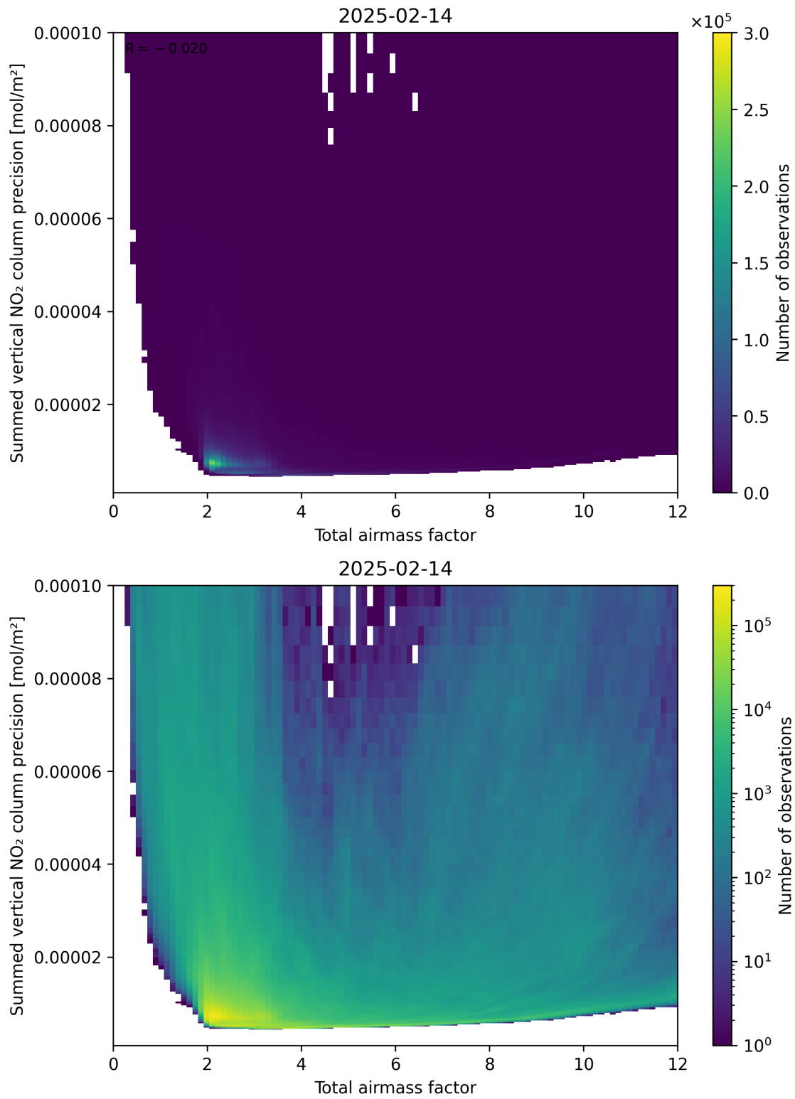
Figure 66: Scatter density plot of “Total airmass factor” against “Summed vertical NO 2 column precision” for 2025-02-13 to 2025-02-15.
