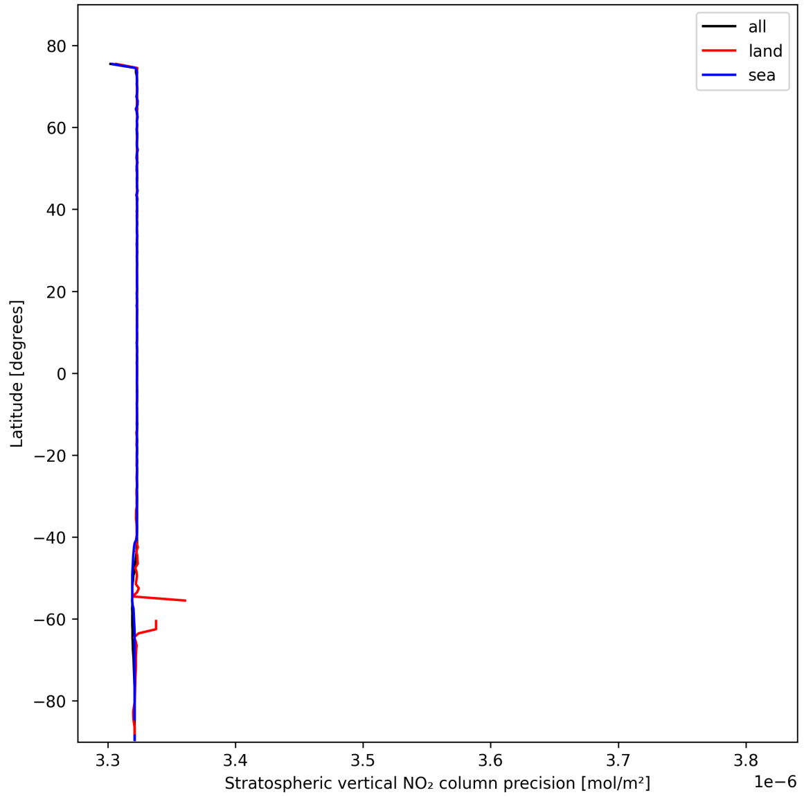
Figure 20: Zonal average of “Stratospheric vertical NO 2 column precision” for 2025-02-13 to 2025-02-15.
