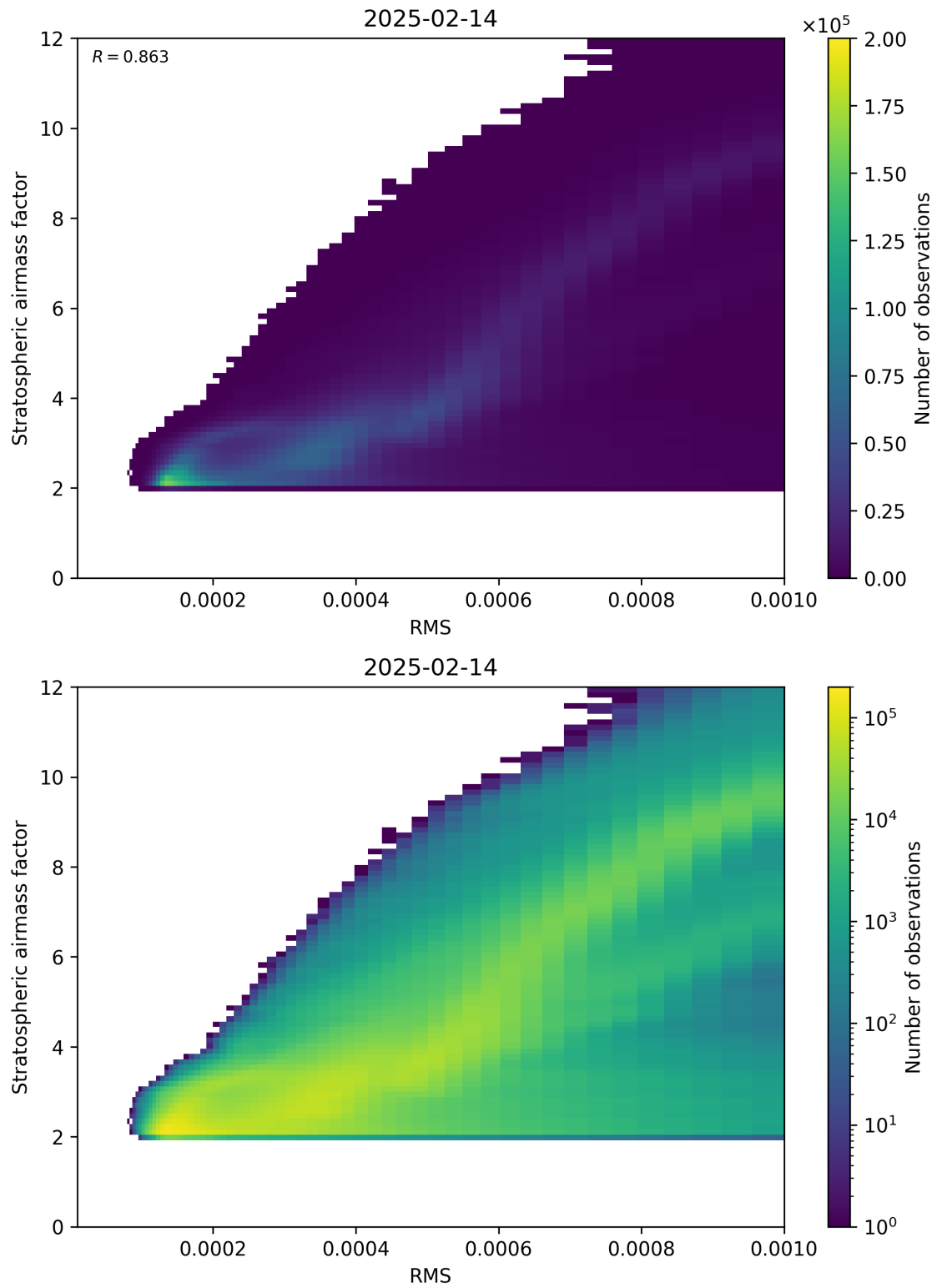
Figure 144: Scatter density plot of “RMS” against “Stratospheric airmass factor” for 2025-02-13 to 2025-02-15.
