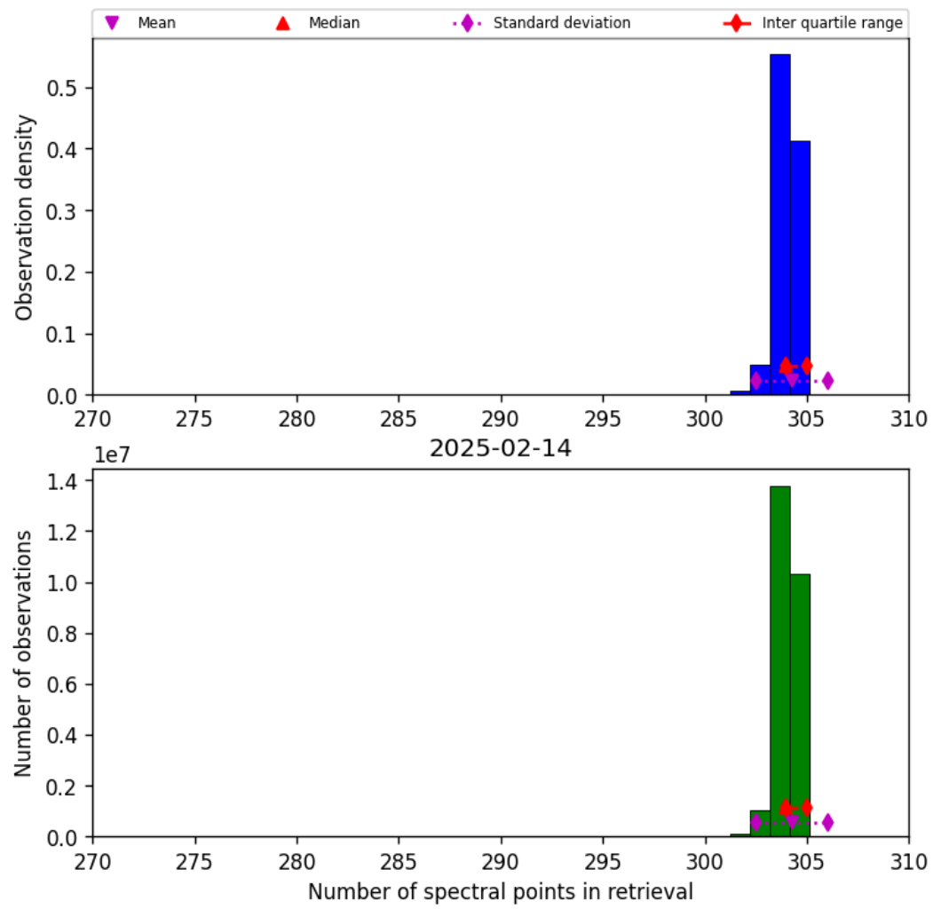
Figure 33: Histogram of “Number of spectral points in retrieval” for 2025-02-13 to 2025-02-15
