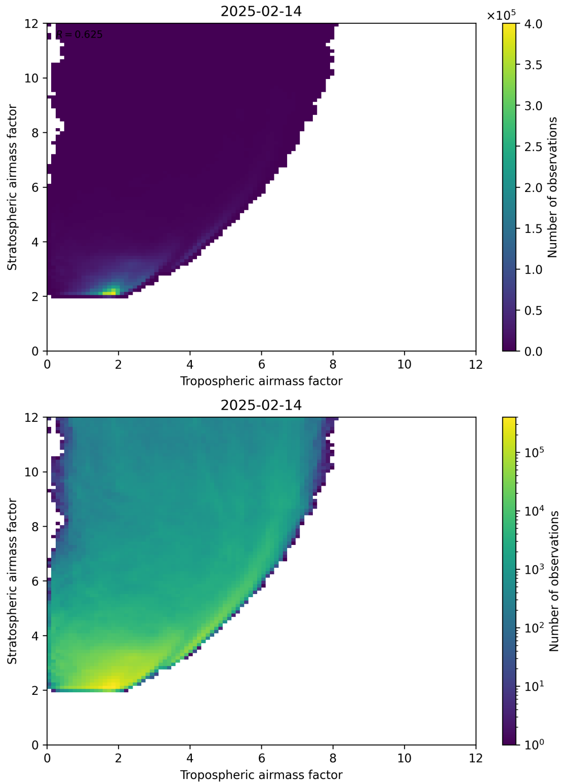
Figure 71: Scatter density plot of “Tropospheric airmass factor” against “Stratospheric airmass factor” for 2025-02-13 to 2025-02-15.
