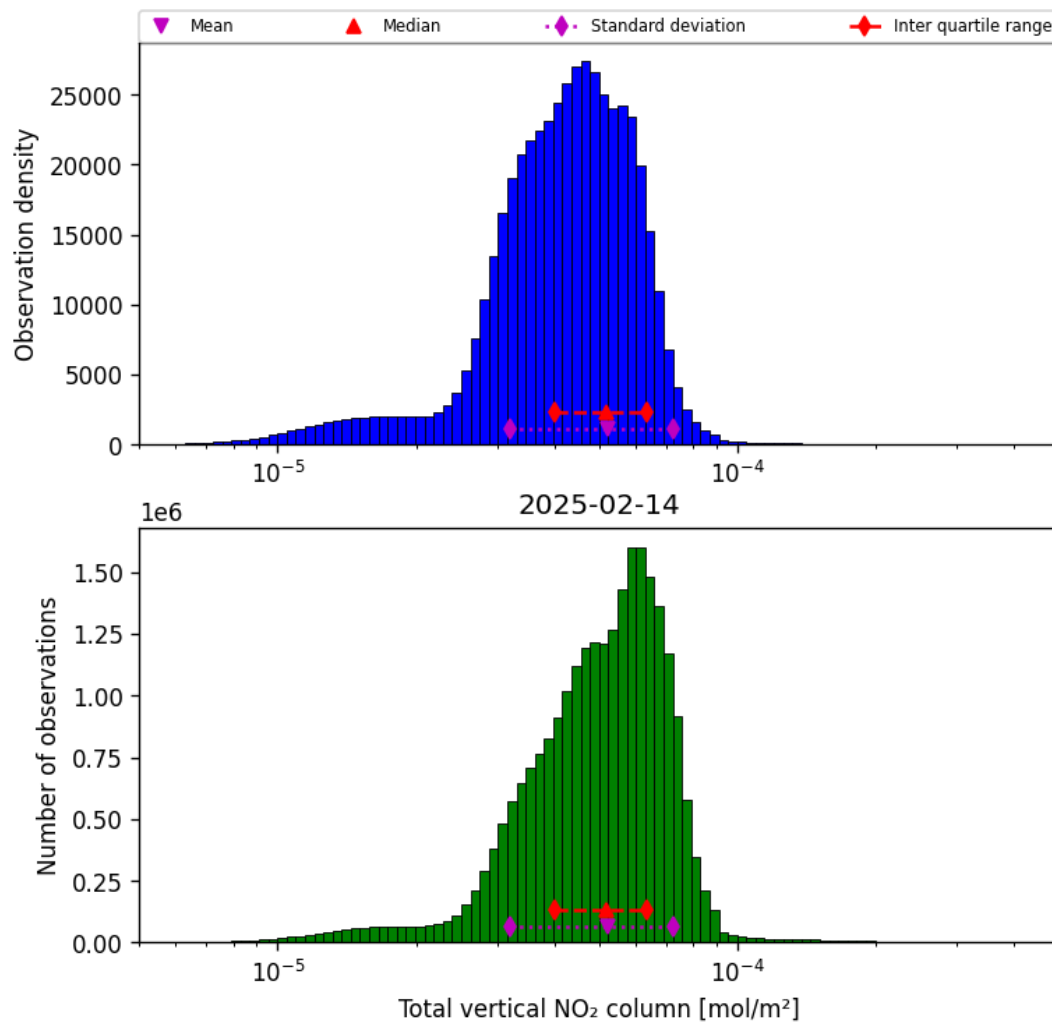
Figure 38: Histogram of “Total vertical NO 2 column” for 2025-02-13 to 2025-02-15
