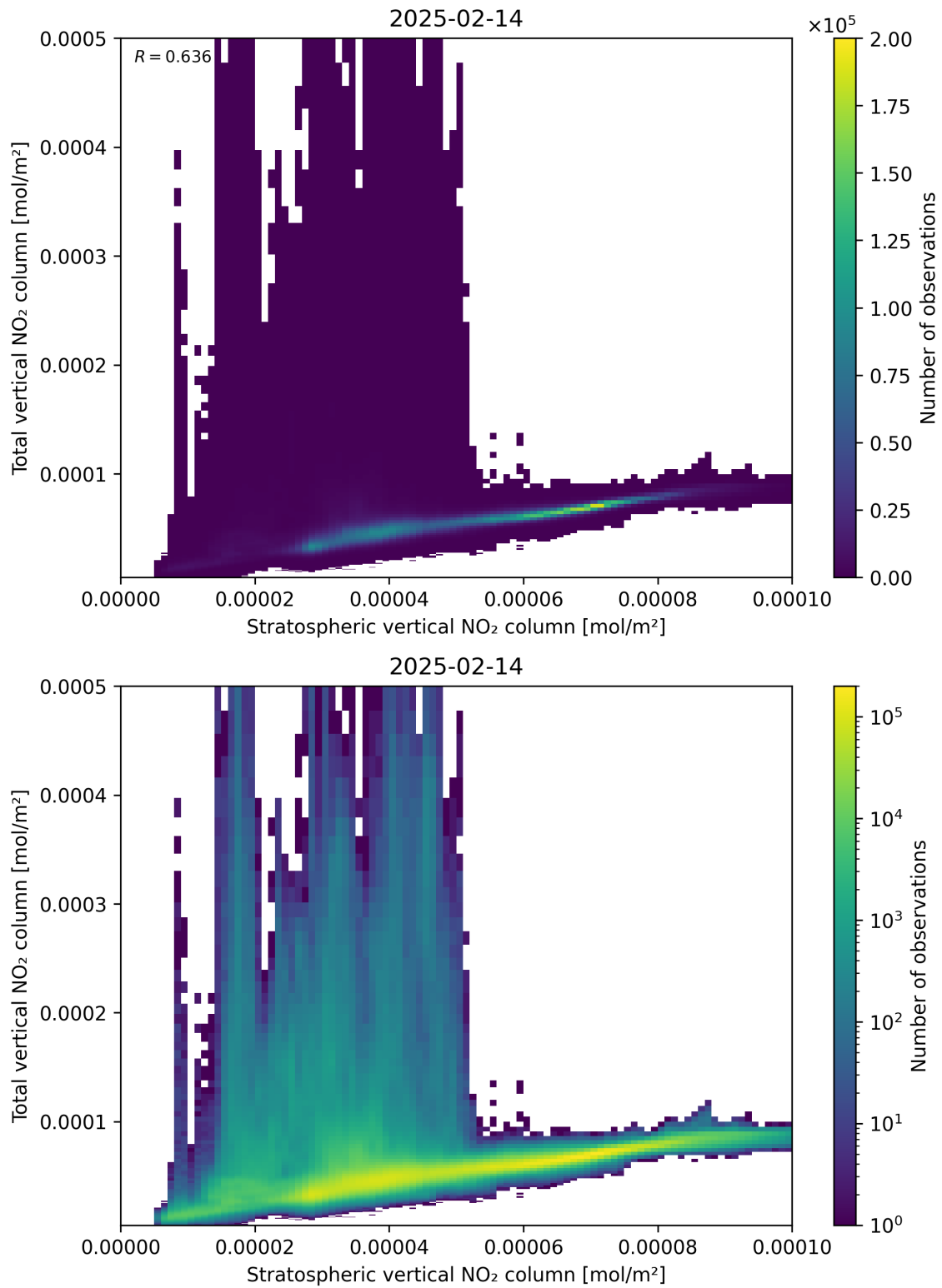
Figure 100: Scatter density plot of “Stratospheric vertical NO 2 column” against “Total vertical NO 2 column” for 2025-02-13 to 2025-02-15.
