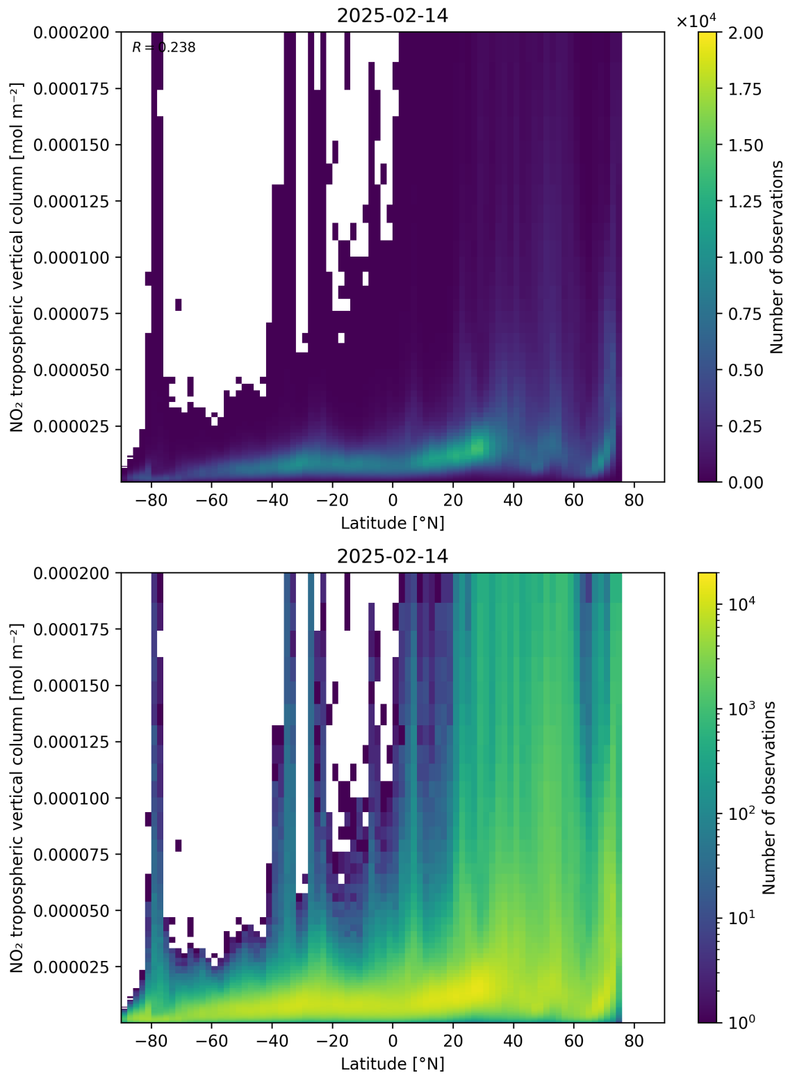
Figure 92: Scatter density plot of “Latitude” against “NO 2 tropospheric vertical column” for 2025-02-13 to 2025-02-15.
