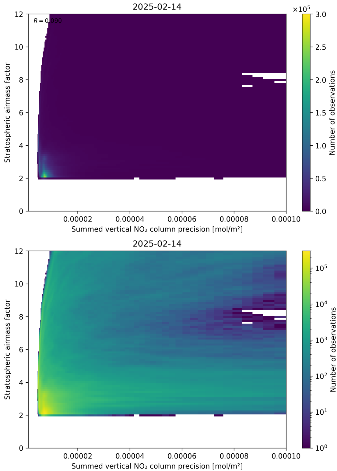
Figure 106: Scatter density plot of “Summed vertical NO 2 column precision” against “Stratospheric airmass factor” for 2025-02-13 to 2025-02-15.
