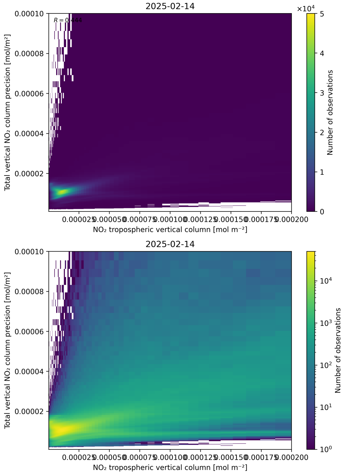
Figure 129: Scatter density plot of “NO 2 tropospheric vertical column” against “Total vertical NO 2 column precision” for 2025-02-13 to 2025-02-15.
