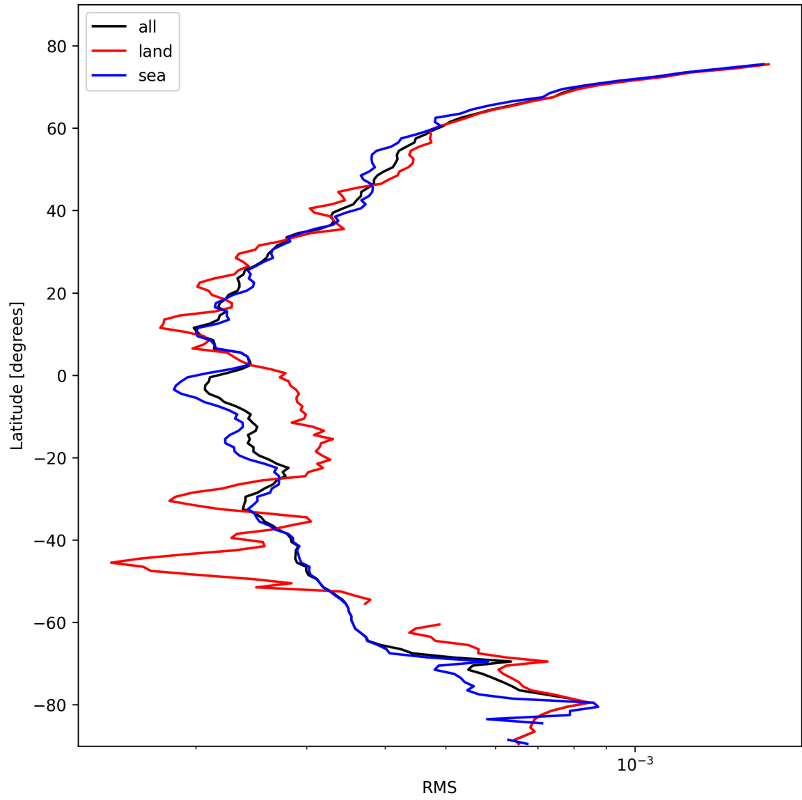
Figure 26: Zonal average of “RMS” for 2025-02-13 to 2025-02-15.
