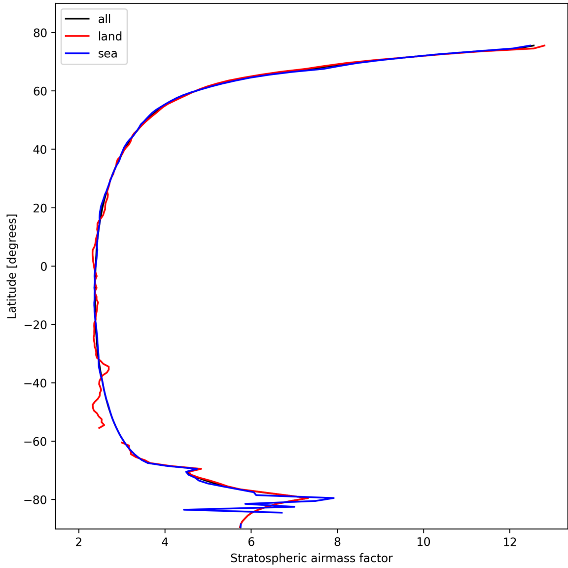
Figure 27: Zonal average of “Stratospheric airmass factor” for 2025-02-13 to 2025-02-15.
