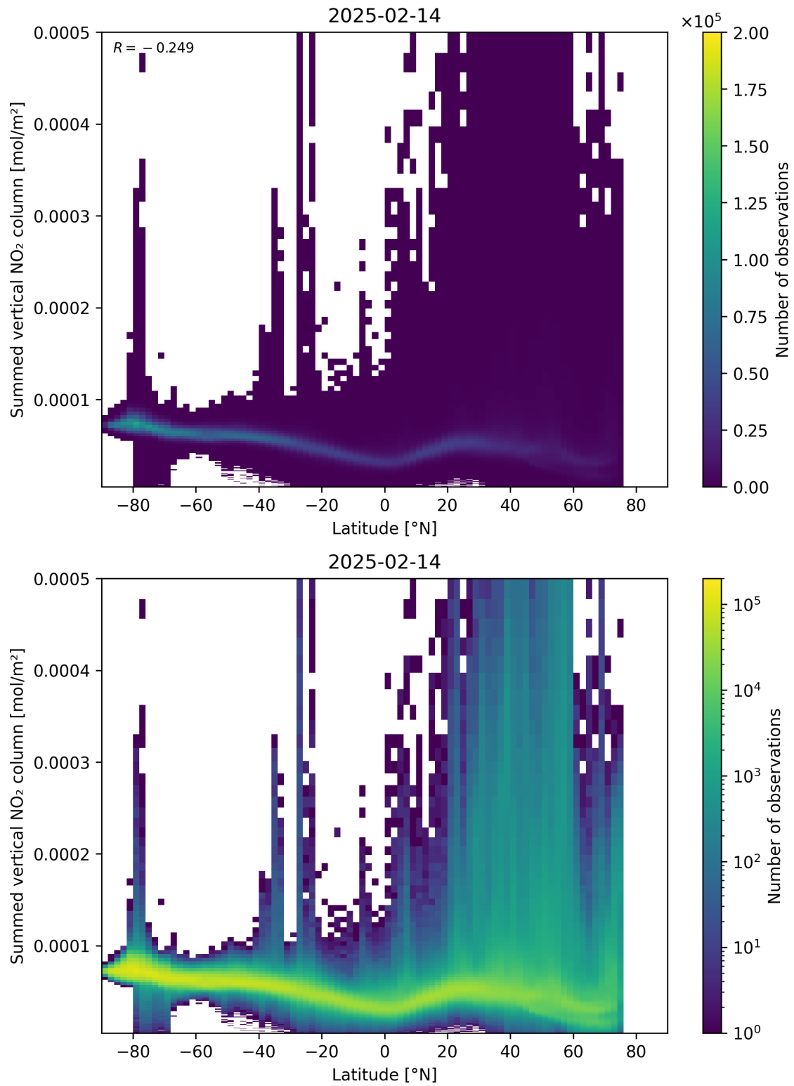
Figure 88: Scatter density plot of “Latitude” against “Summed vertical NO 2 column” for 2025-02-13 to 2025-02-15.
