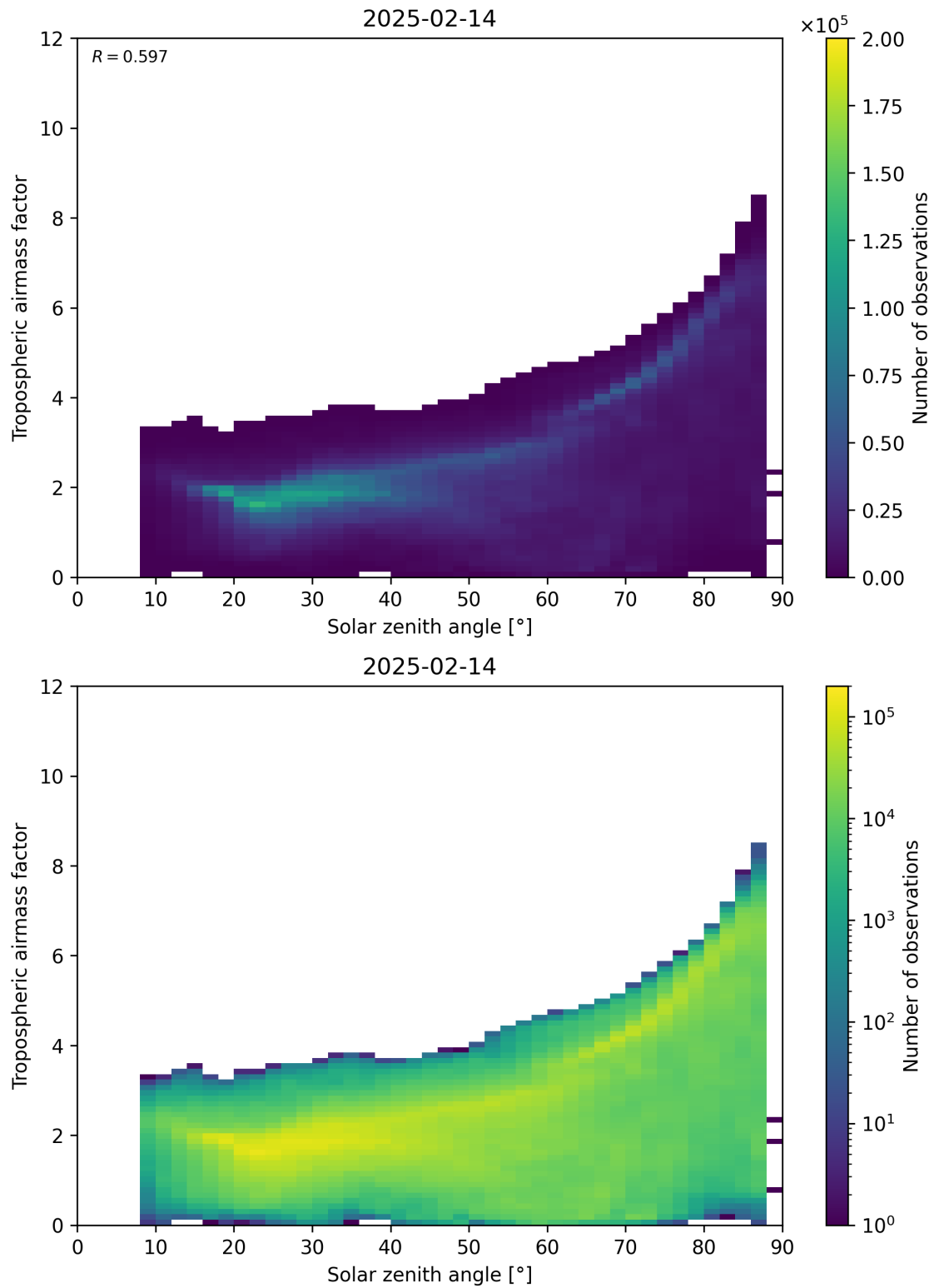
Figure 147: Scatter density plot of “Solar zenith angle” against “Tropospheric airmass factor” for 2025-02-13 to 2025-02-15.
