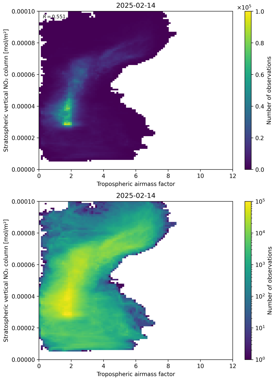
Figure 74: Scatter density plot of “Tropospheric air mass factor” against “Stratospheric vertical NO 2 column” for 2025-02-13 to 2025-02-15.
