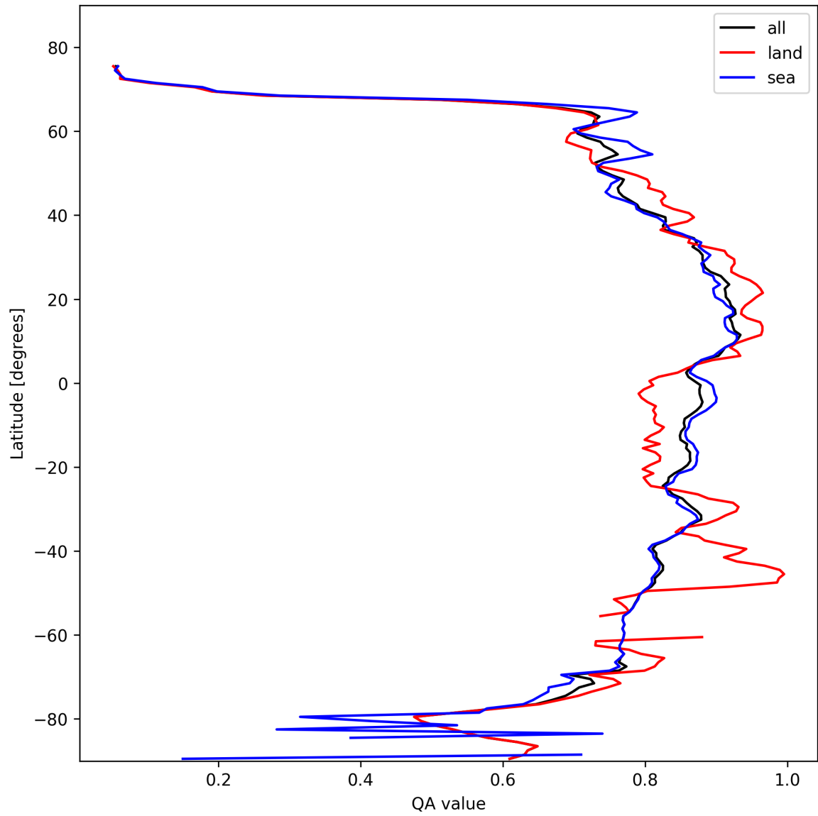
Figure 11: Zonal average of “QA value” for 2025-02-13 to 2025-02-15.
