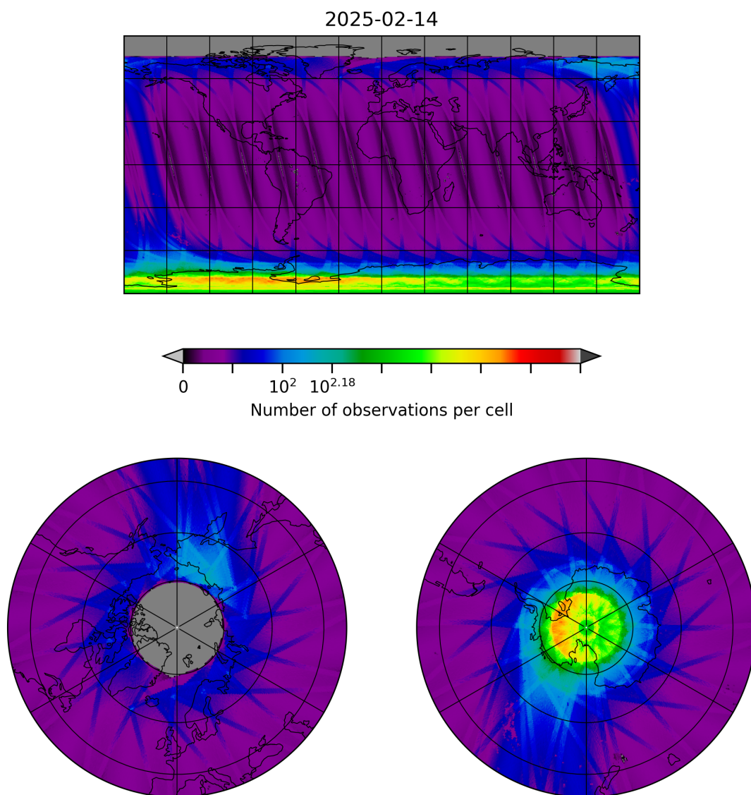
Figure 10: Map of the number of observations for 2025-02-13 to 2025-02-15
