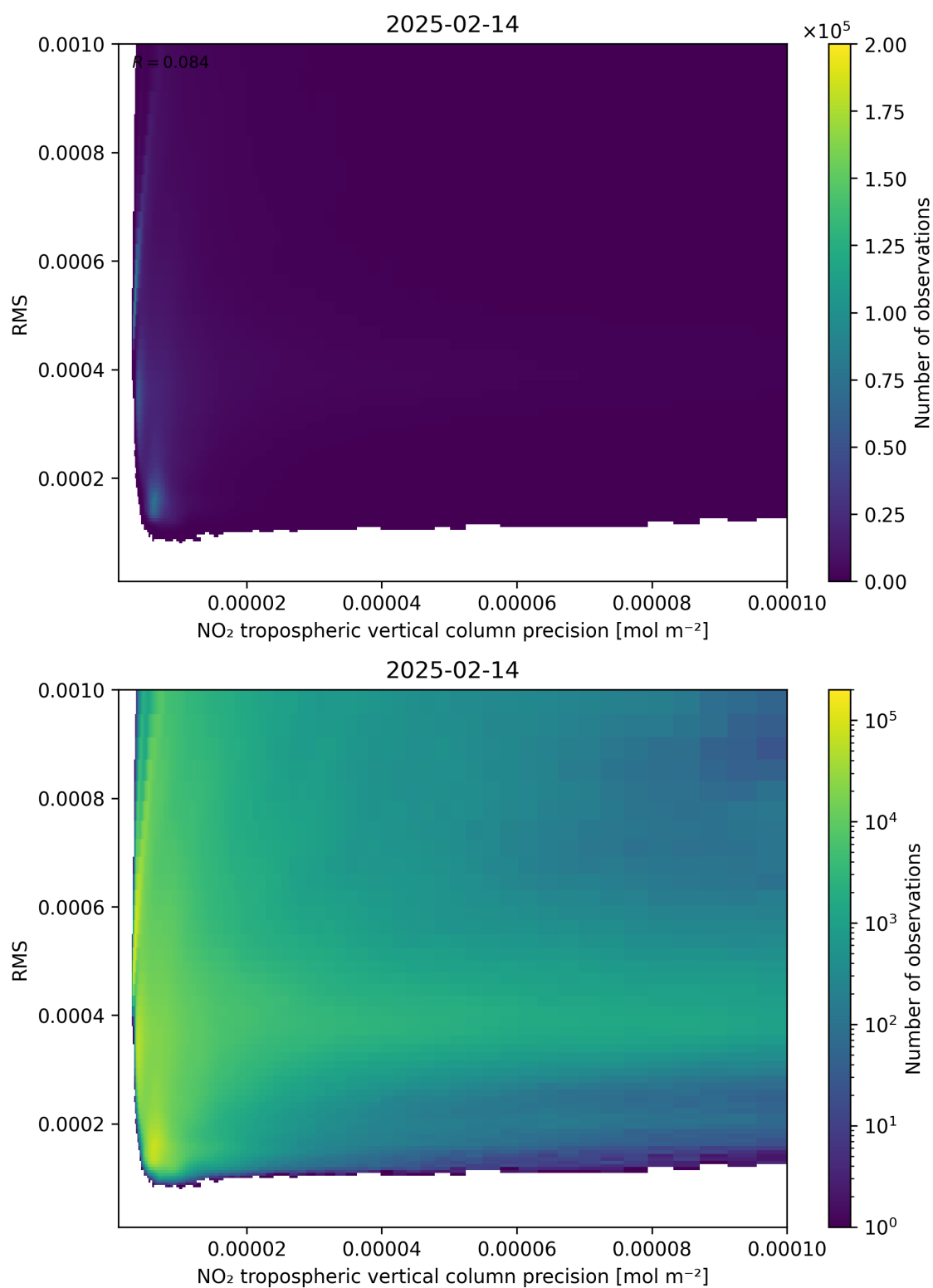
Figure 140: Scatter density plot of “NO 2 tropospheric vertical column precision” against “RMS” for 2025-02-13 to 2025-02-15.
