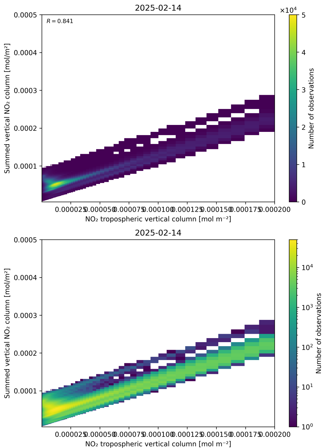
Figure 126: Scatter density plot of “NO 2 tropospheric vertical column” against “Summed vertical NO 2 column” for 2025-02-13 to 2025-02-15.
