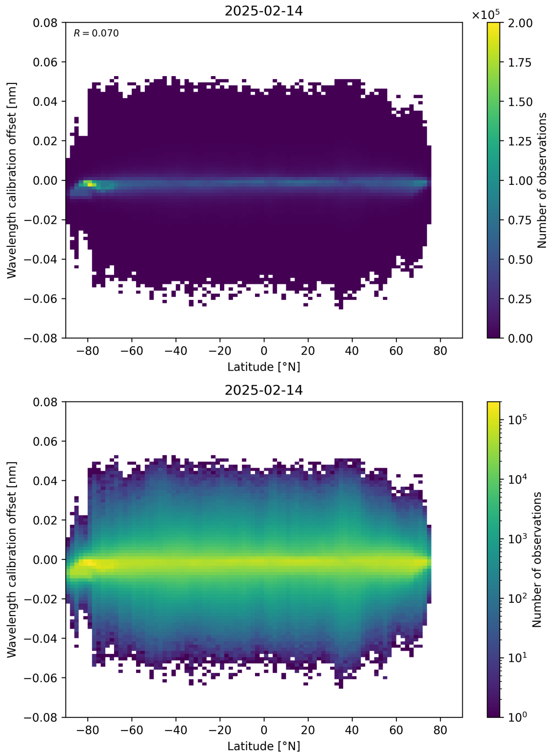
Figure 95: Scatter density plot of “Latitude” against “Wavelength calibration offset” for 2025-02-13 to 2025-02-15.
