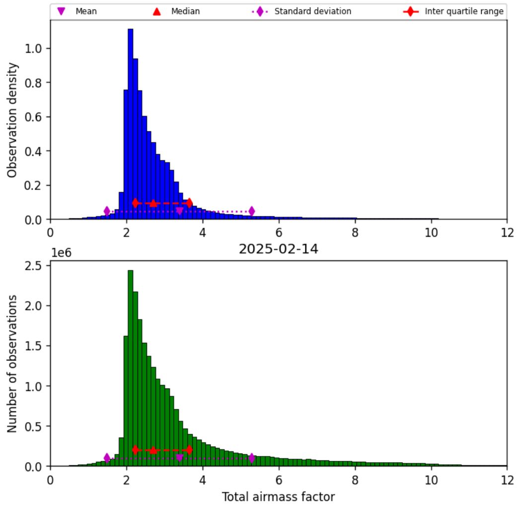
Figure 32: Histogram of “Total airmass factor” for 2025-02-13 to 2025-02-15
