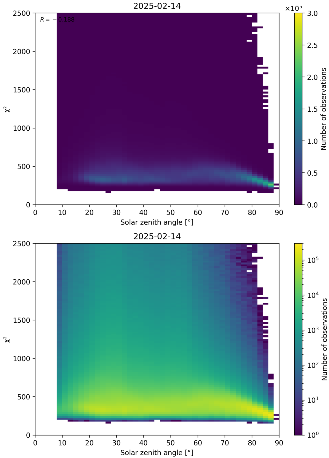
Figure 148: Scatter density plot of “Solar zenith angle” against “ \chi^2 ” for 2025-02-13 to 2025-02-15.
