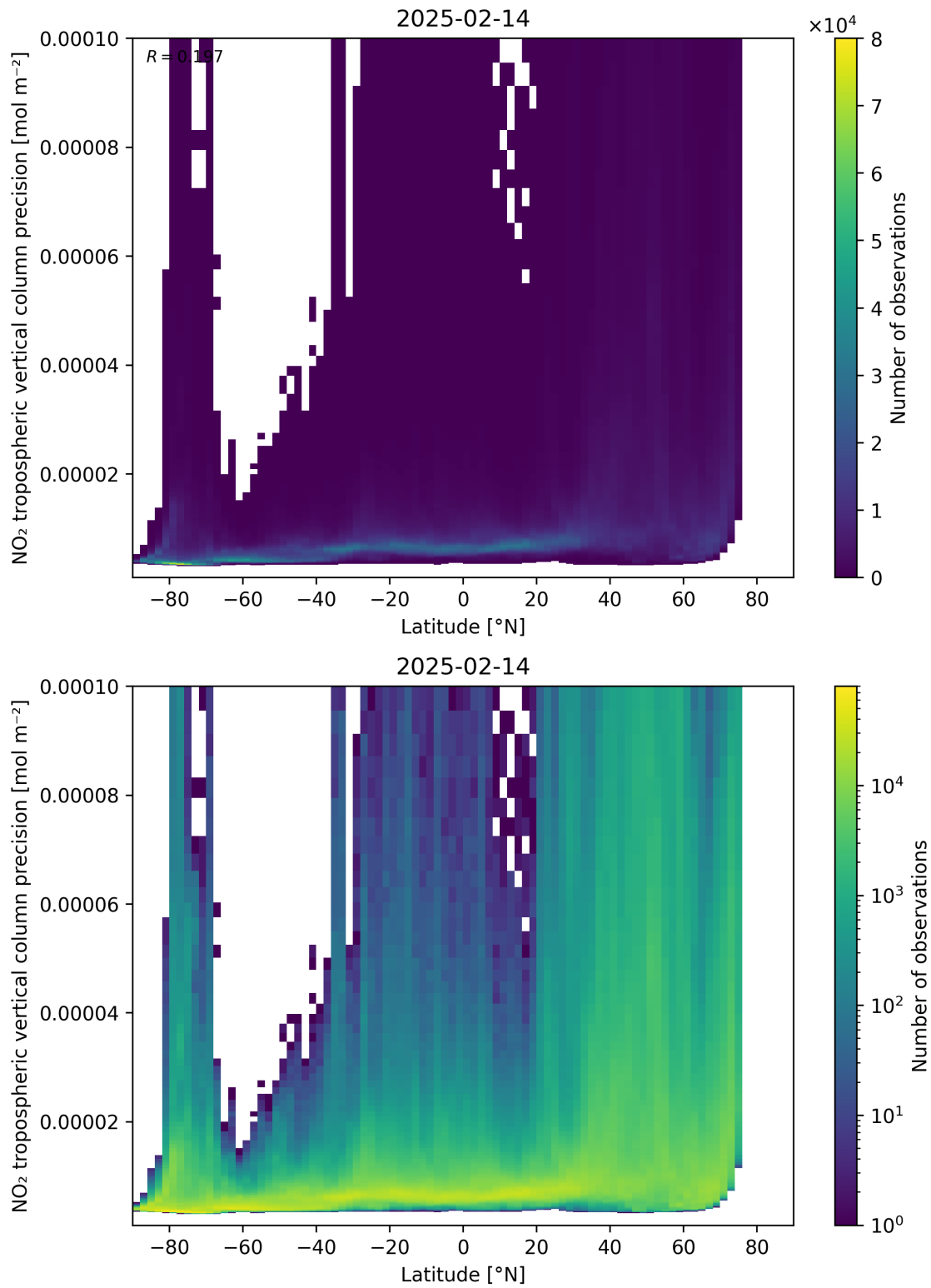
Figure 93: Scatter density plot of “Latitude” against “NO 2 tropospheric vertical column precision” for 2025-02-13 to 2025-02-15.
