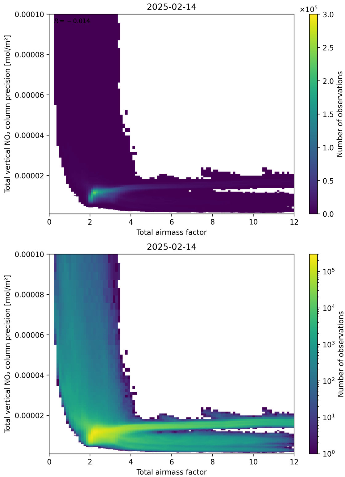
Figure 68: Scatter density plot of “Total airmass factor” against “Total vertical NO 2 column precision” for 2025-02-13 to 2025-02-15.
