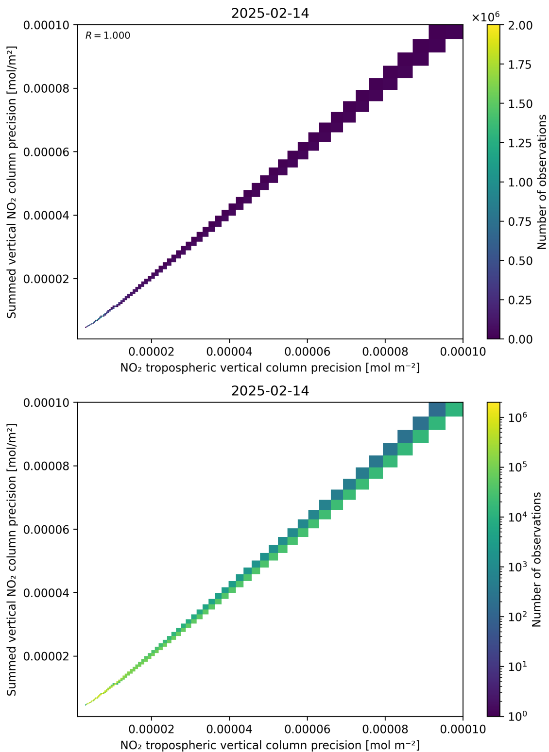
Figure 137: Scatter density plot of “NO 2 tropospheric vertical column precision” against “Summed vertical NO 2 column precision” for 2025-02-13 to 2025-02-15.
