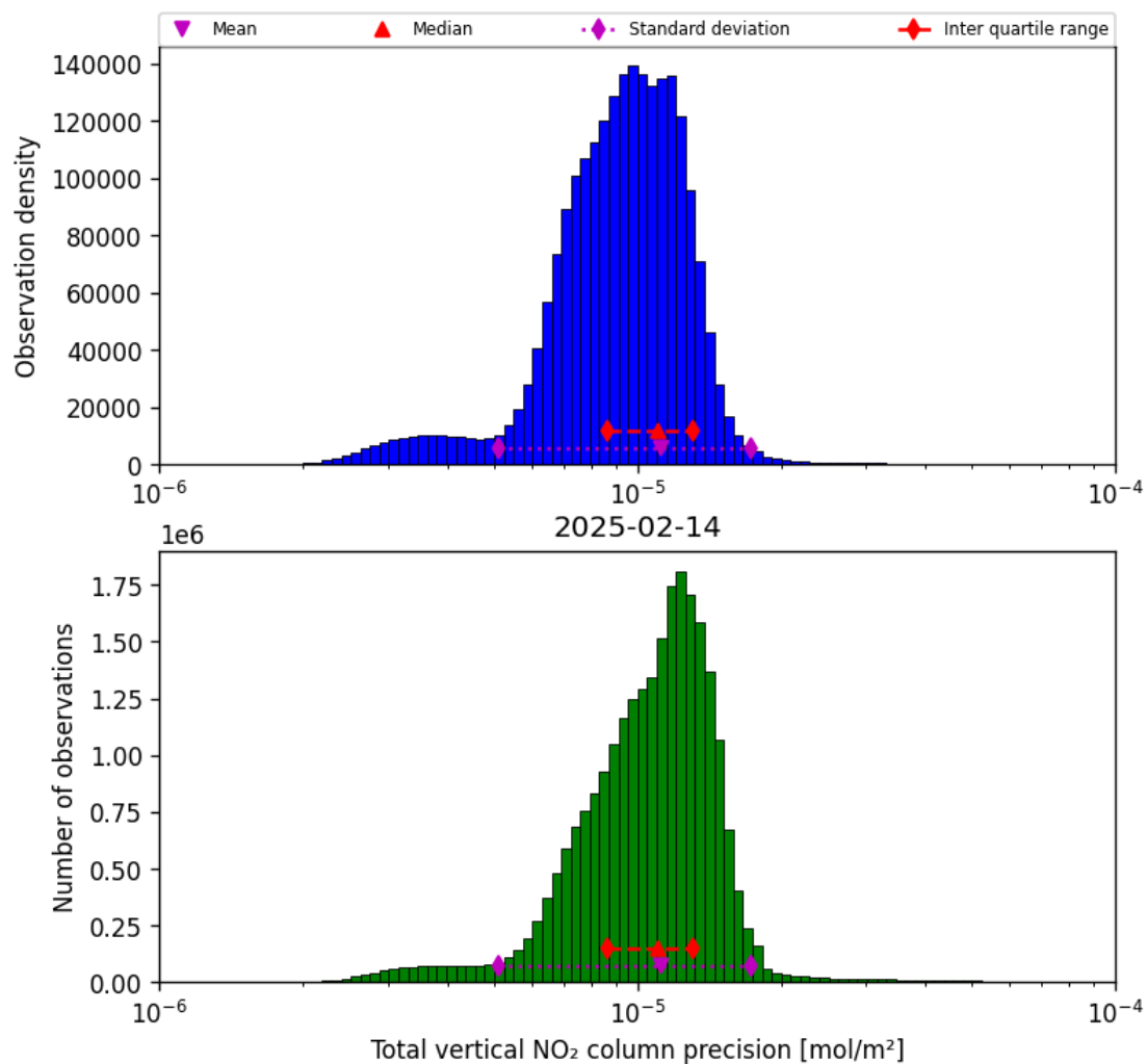
Figure 39: Histogram of “Total vertical NO 2 column precision” for 2025-02-13 to 2025-02-15
