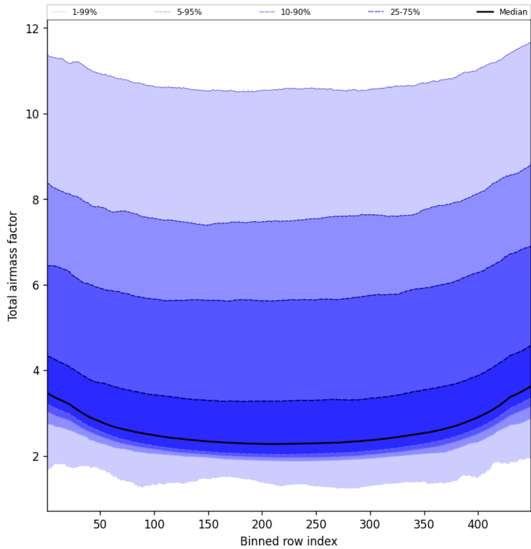
Figure 49: Along track statistics of “Total airmass factor” for 2025-02-13 to 2025-02-15
