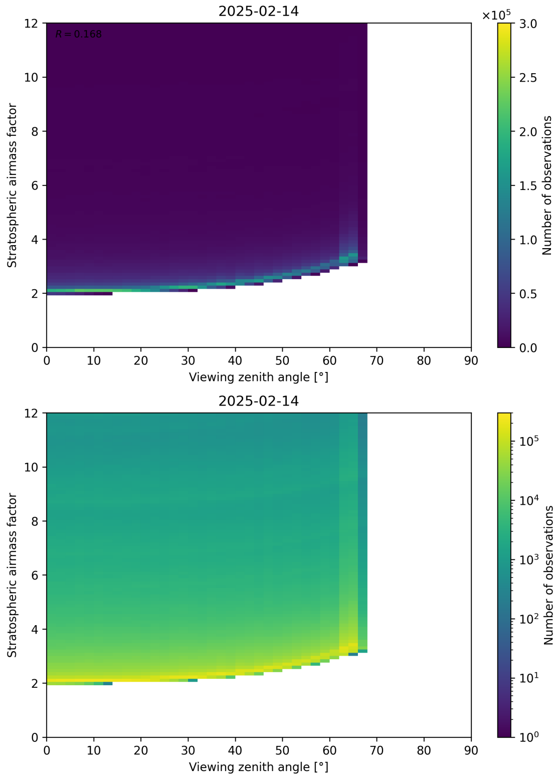
Figure 159: Scatter density plot of “Viewing zenith angle” against “Stratospheric airmass factor” for 2025-02-13 to 2025-02-15.
