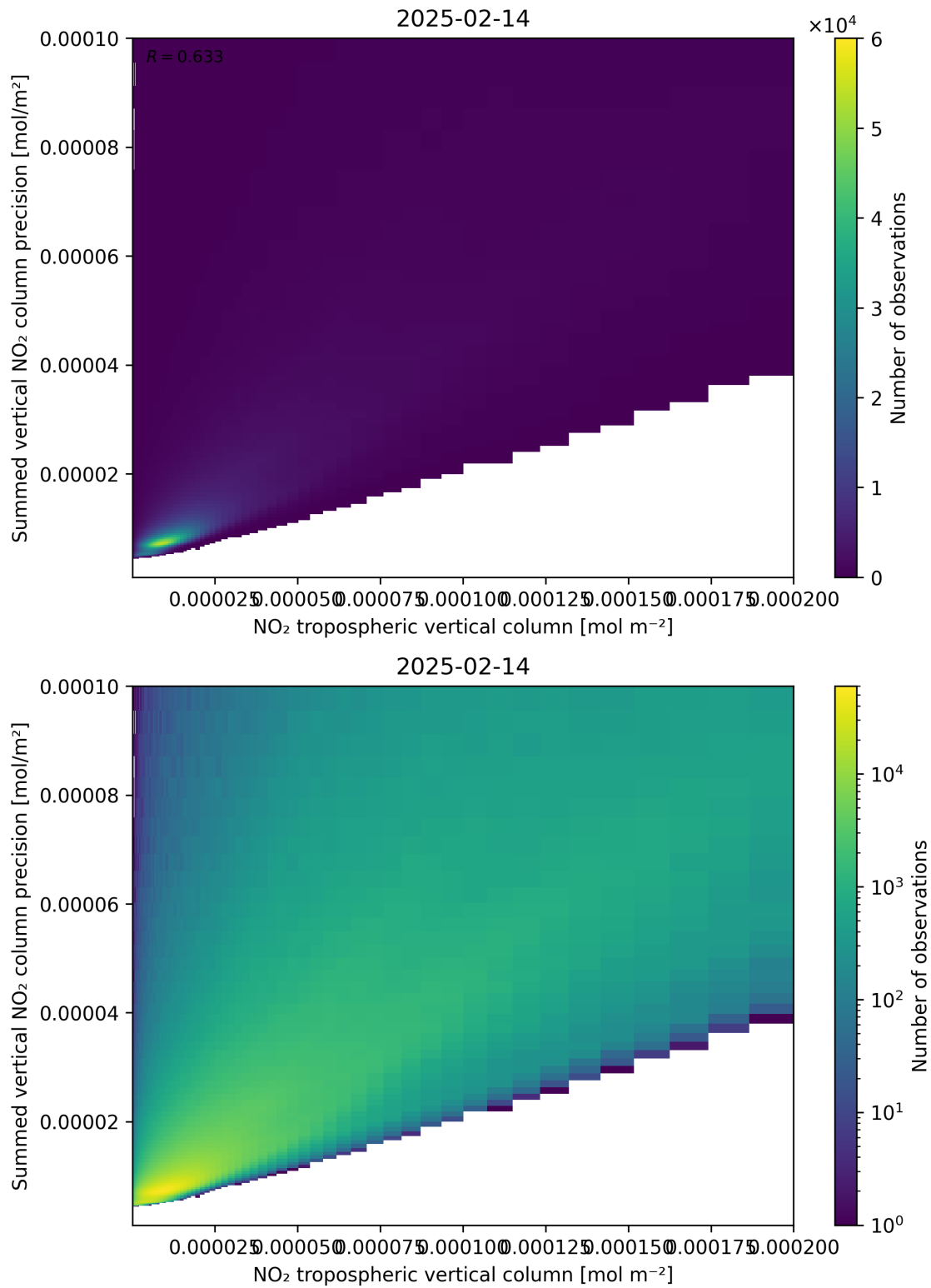
Figure 127: Scatter density plot of “NO 2 tropospheric vertical column” against “Summed vertical NO 2 column precision” for 2025-02-13 to 2025-02-15.
