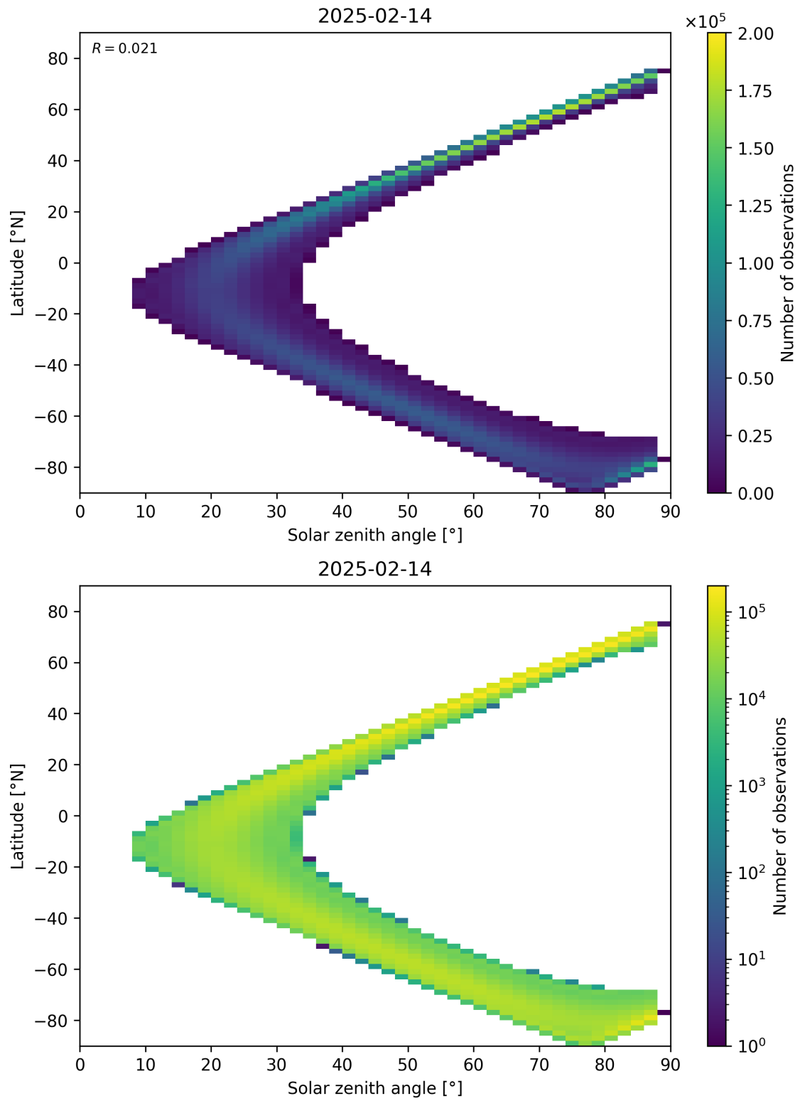
Figure 149: Scatter density plot of “Solar zenith angle” against “Latitude” for 2025-02-13 to 2025-02-15.
