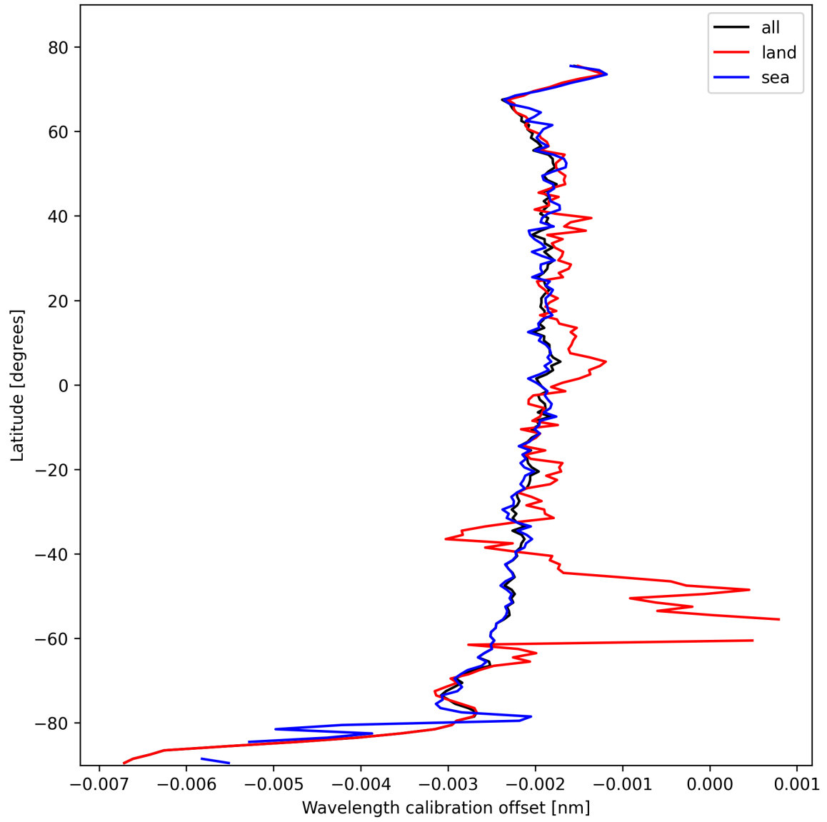
Figure 18: Zonal average of “Wavelength calibration offset” for 2025-02-13 to 2025-02-15.
