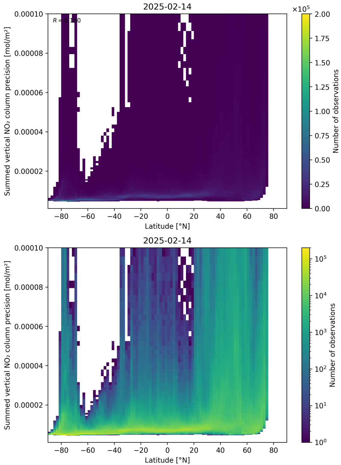
Figure 89: Scatter density plot of “Latitude” against “Summed vertical NO 2 column precision” for 2025-02-13 to 2025-02-15.
