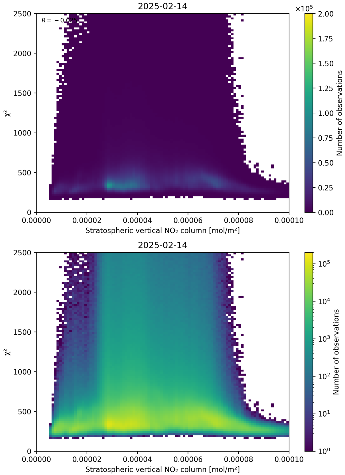
Figure 97: Scatter density plot of “Stratospheric vertical NO 2 column” against “ \chi^2 ” for 2025-02-13 to 2025-02-15.
