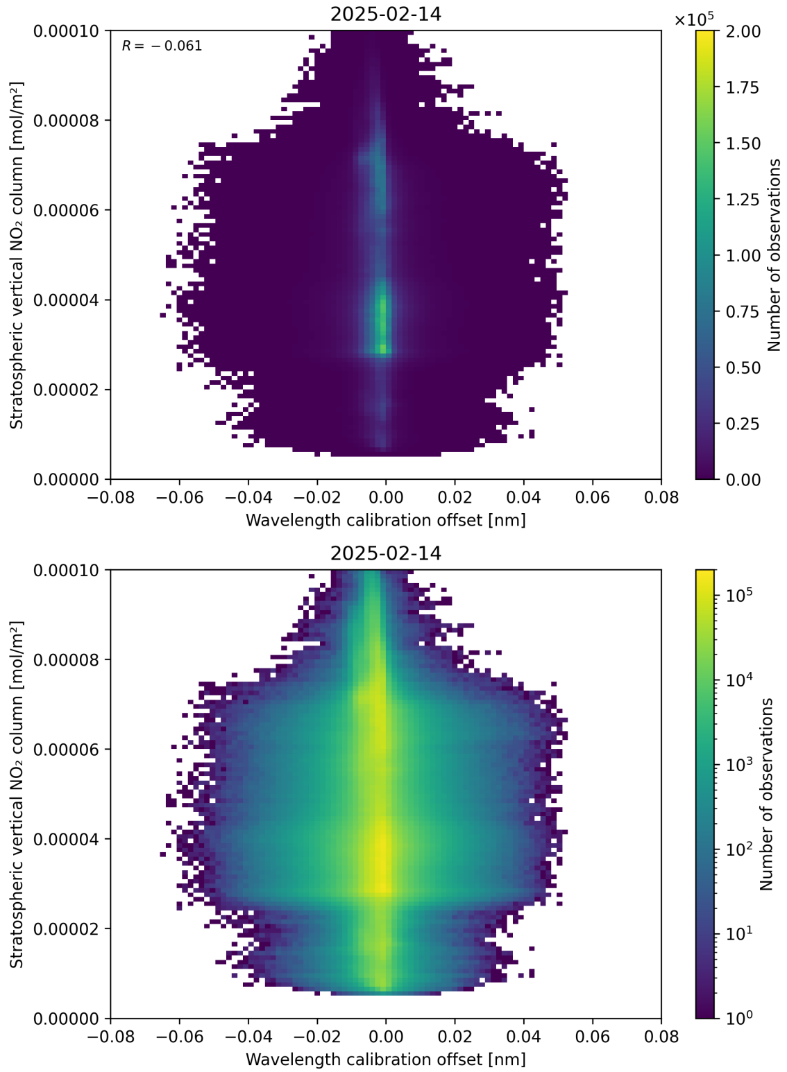
Figure 176: Scatter density plot of “Wavelength calibration offset” against “Stratospheric vertical NO 2 column” for 2025-02-13 to 2025-02-15.
