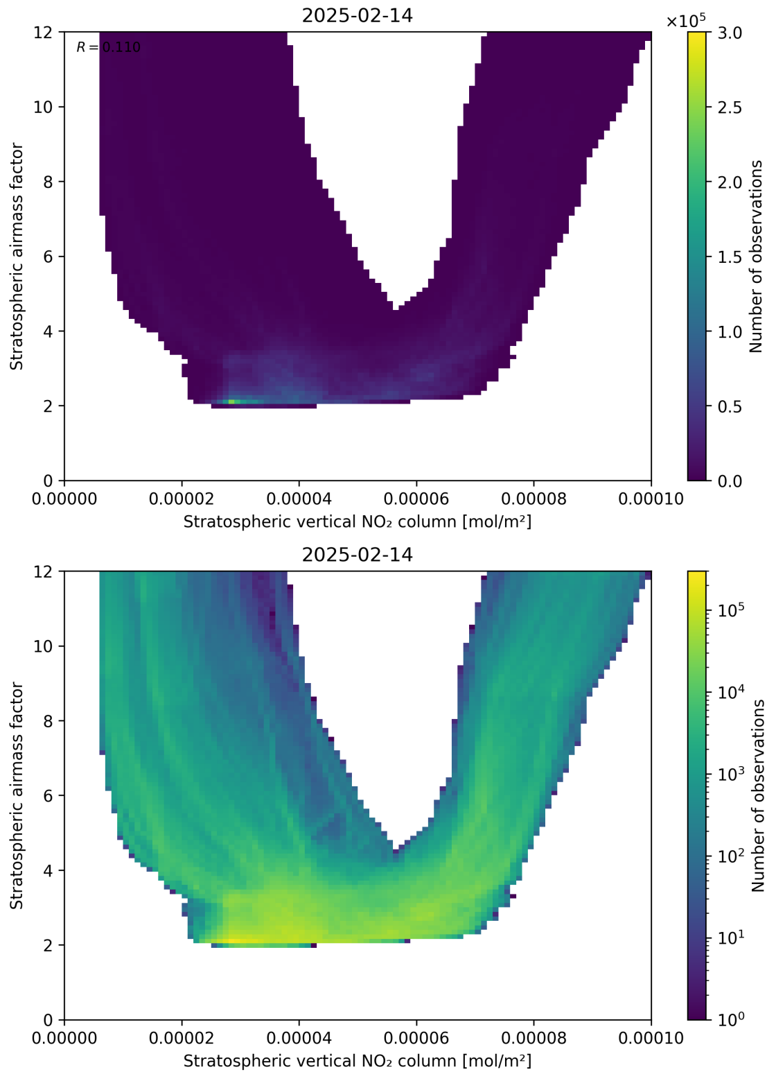
Figure 96: Scatter density plot of “Stratospheric vertical NO 2 column” against “Stratospheric airmass factor” for 2025-02-13 to 2025-02-15.
