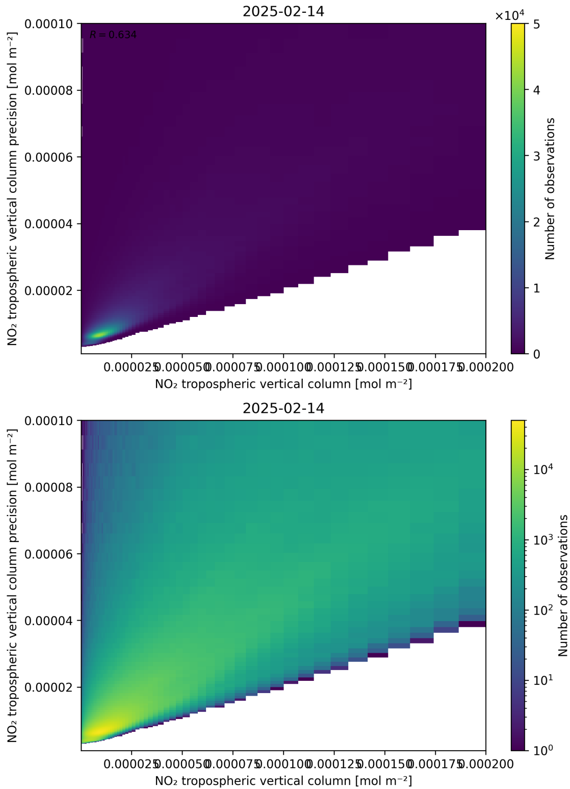
Figure 130: Scatter density plot of “NO 2 tropospheric vertical column” against “NO 2 tropospheric vertical column precision” for 2025-02-13 to 2025-02-15.
