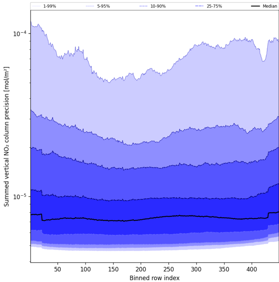
Figure 58: Along track statistics of “Summed vertical NO 2 column precision” for 2025-02-13 to 2025-02-15
