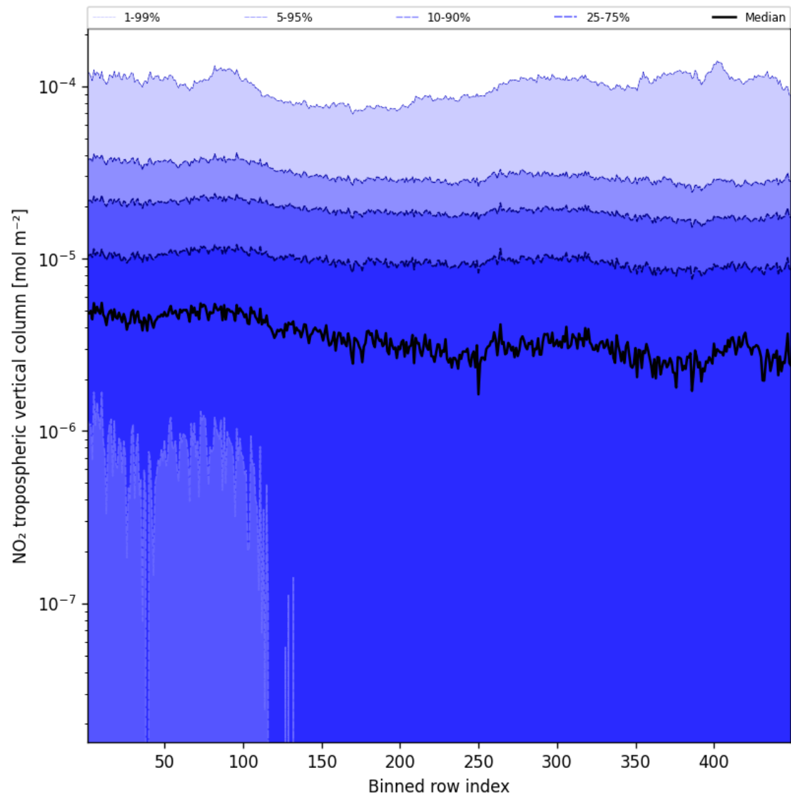
Figure 46: Along track statistics of “NO 2 tropospheric vertical column” for 2025-02-13 to 2025-02-15
