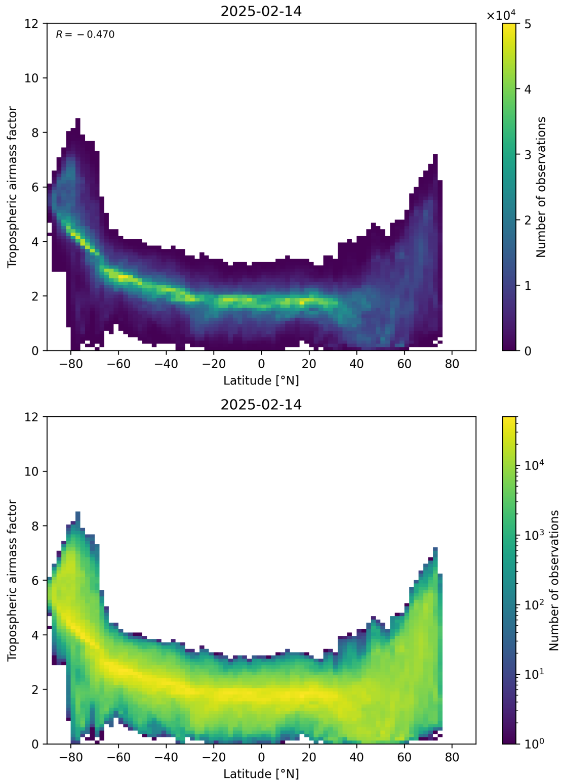
Figure 85: Scatter density plot of “Latitude” against “Tropospheric airmass factor” for 2025-02-13 to 2025-02-15.
