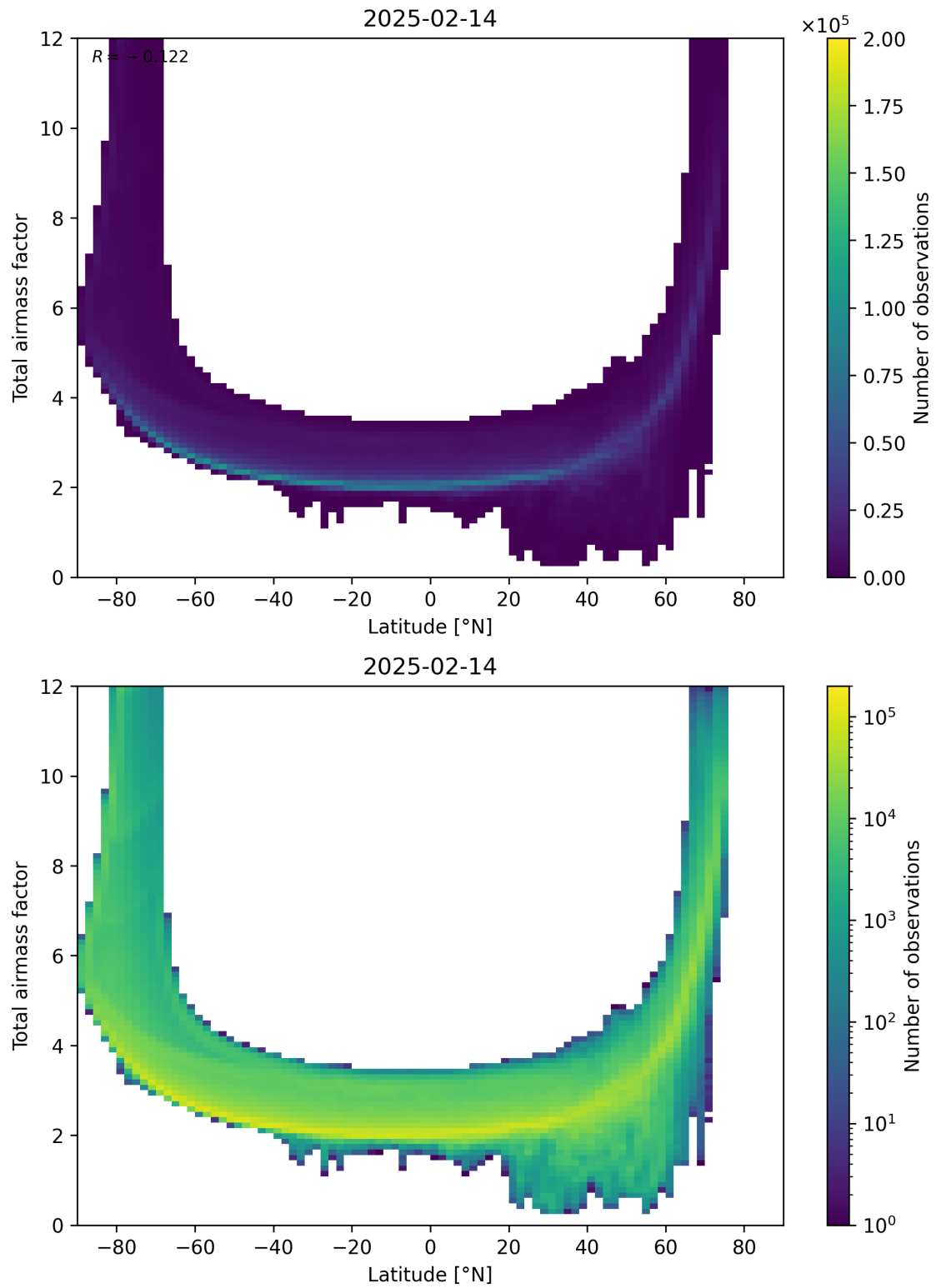
Figure 84: Scatter density plot of “Latitude” against “Total airmass factor” for 2025-02-13 to 2025-02-15.
