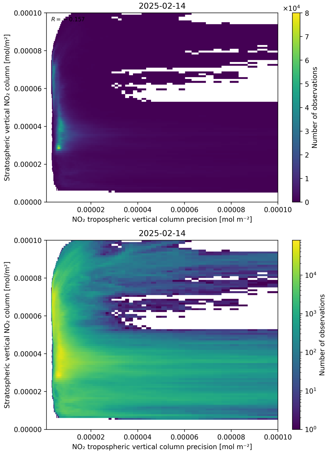
Figure 135: Scatter density plot of “NO 2 tropospheric vertical column precision” against “Stratospheric vertical NO 2 column” for 2025-02-13 to 2025-02-15.
