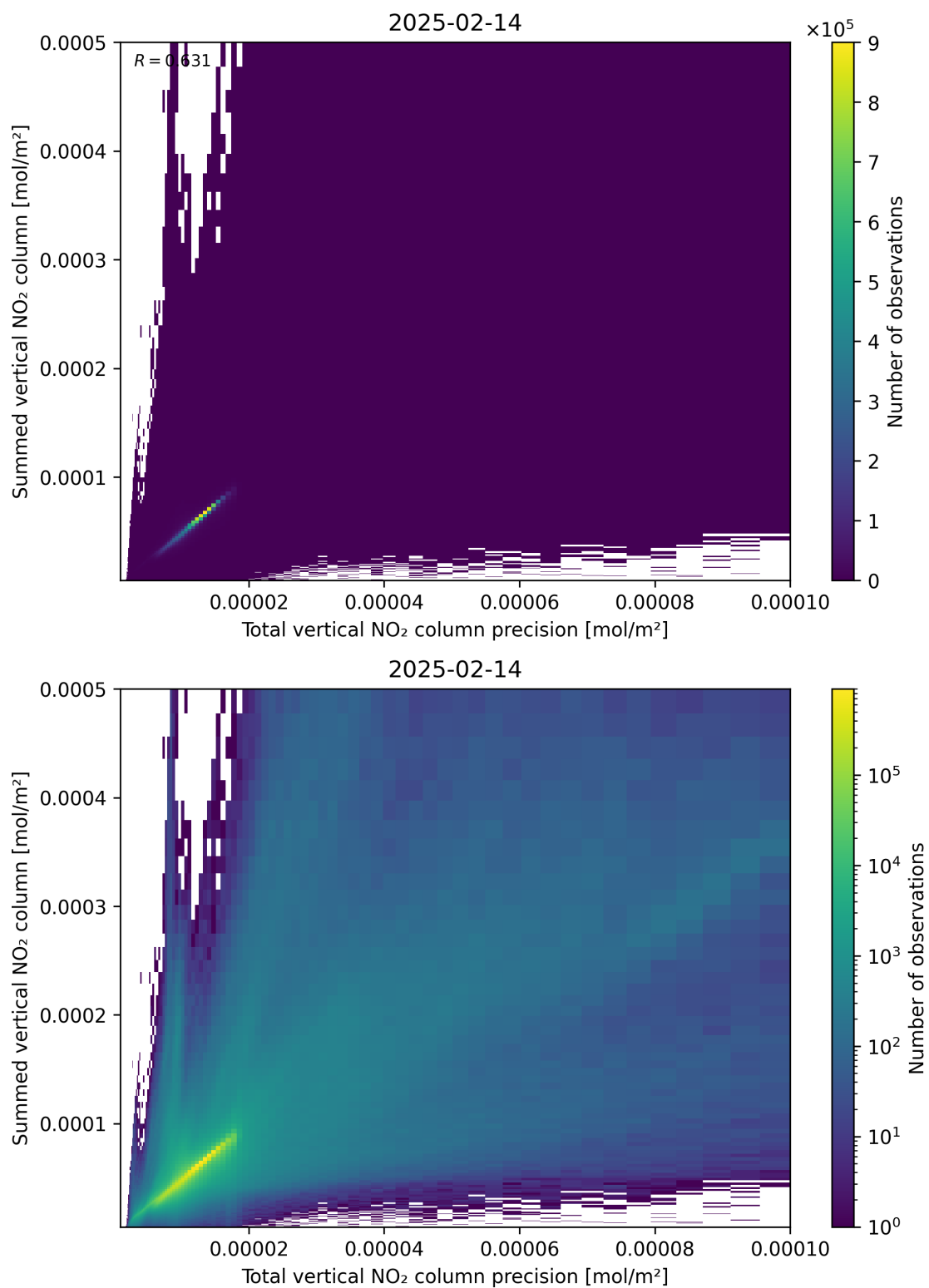
Figure 117: Scatter density plot of “Total vertical NO 2 column precision” against “Summed vertical NO 2 column” for 2025-02-13 to 2025-02-15.
