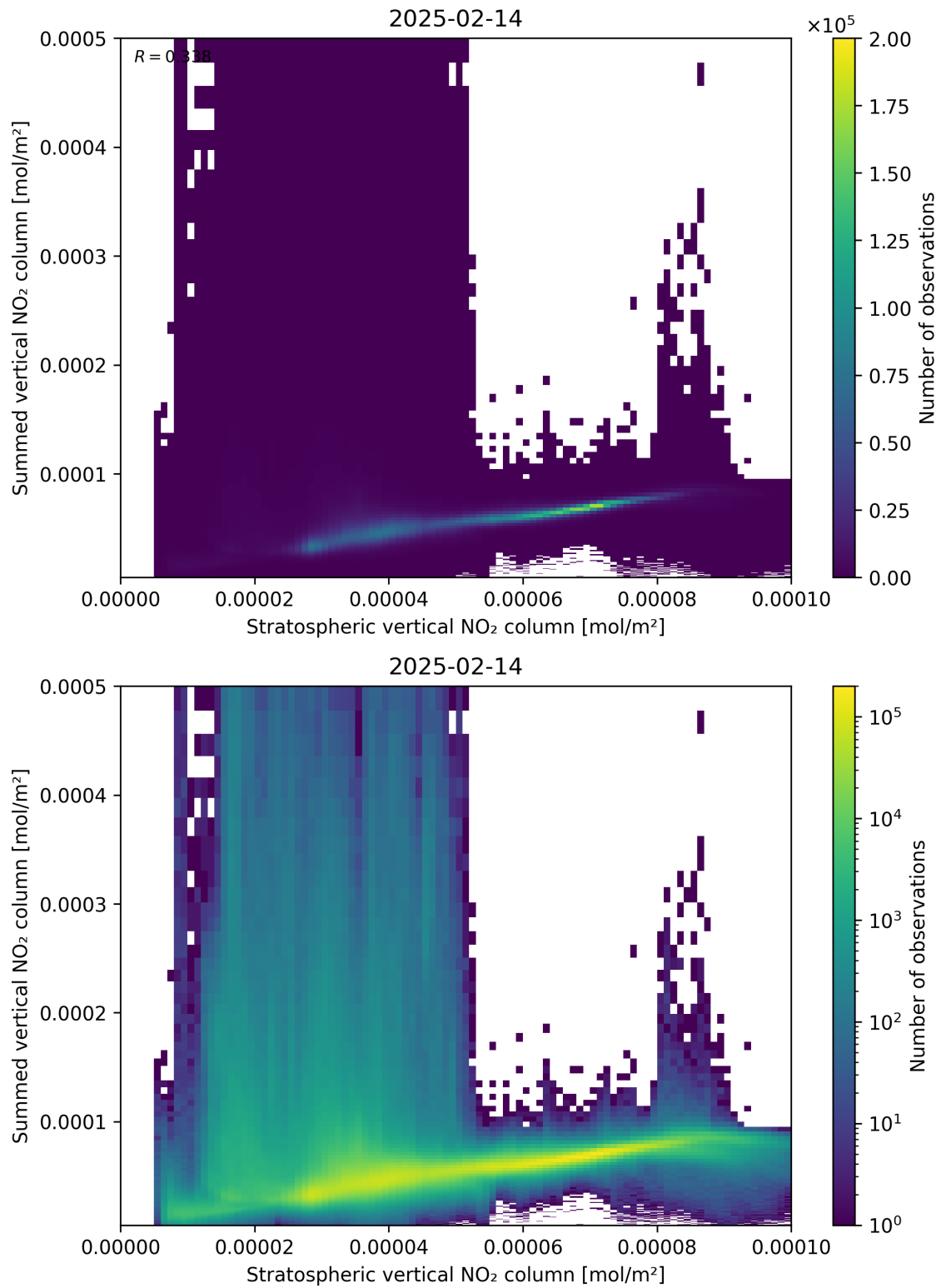
Figure 98: Scatter density plot of “Stratospheric vertical NO 2 column” against “Summed vertical NO 2 column” for 2025-02-13 to 2025-02-15.
