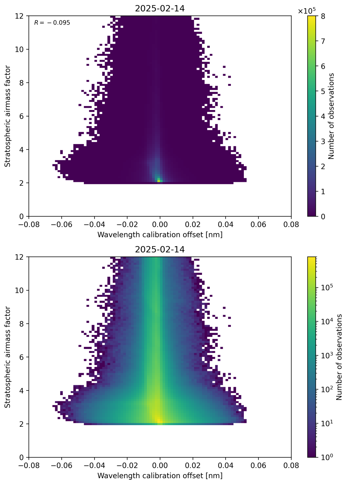
Figure 174: Scatter density plot of “Wavelength calibration offset” against “Stratospheric airmass factor” for 2025-02-13 to 2025-02-15.
