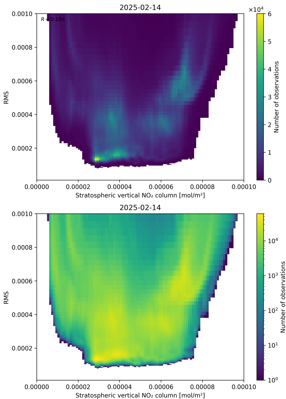
Figure 102: Scatter density plot of “Stratospheric vertical NO 2 column” against “RMS” for 2025-02-13 to 2025-02-15.
