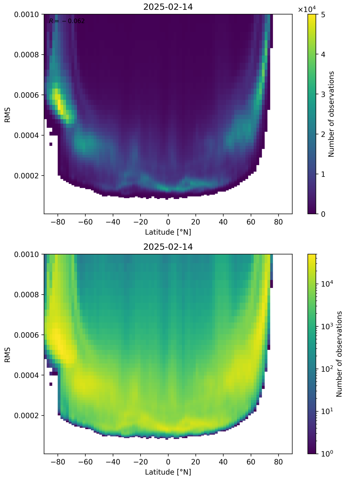
Figure 94: Scatter density plot of “Latitude” against “RMS” for 2025-02-13 to 2025-02-15.
