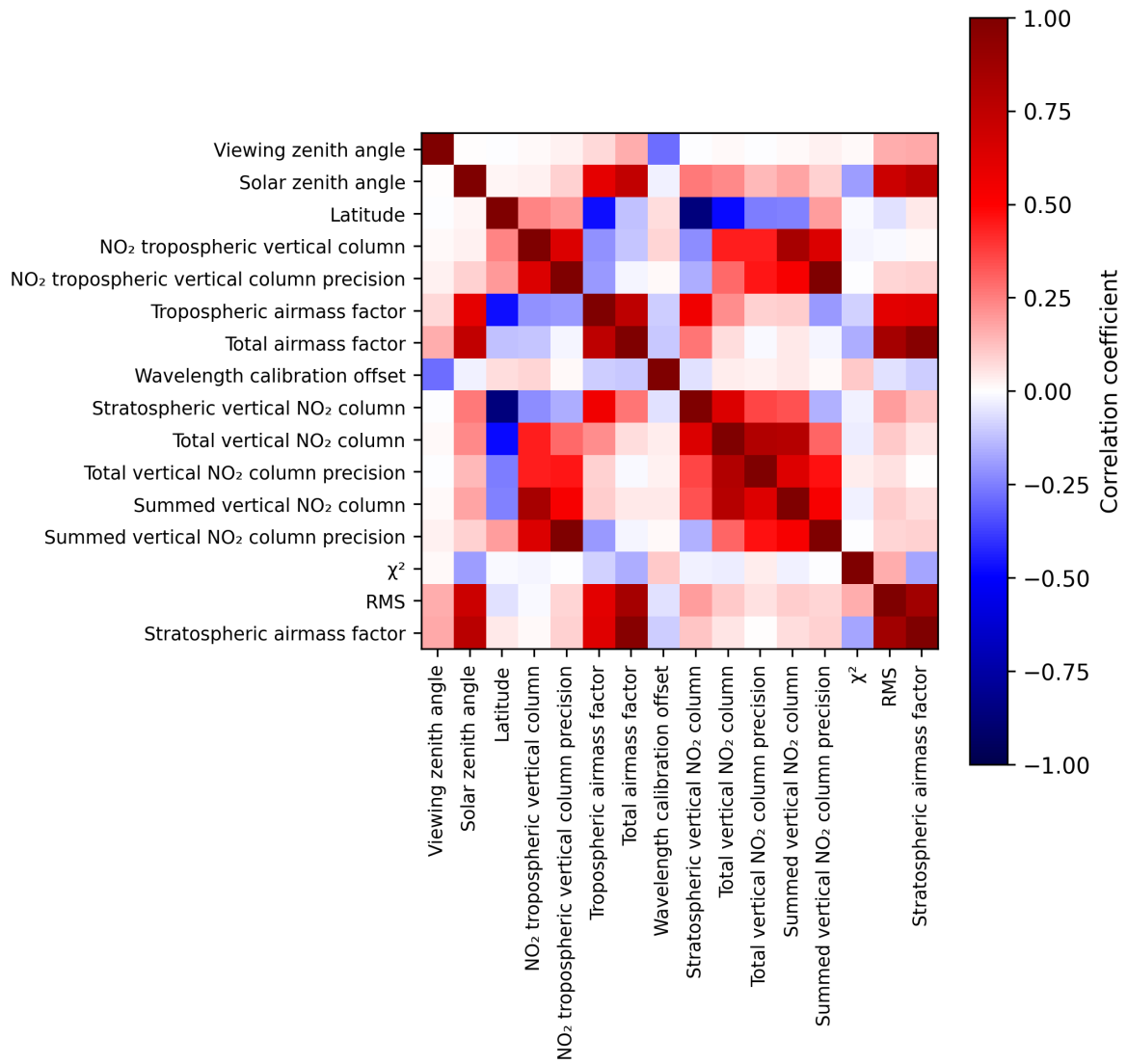
Figure 2: Map of correlation matrix for 2025-02-13 to 2025-02-15.
