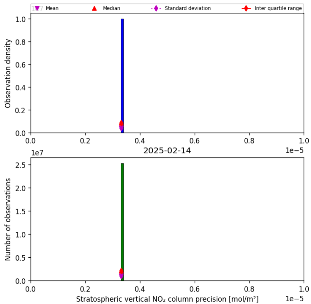
Figure 37: Histogram of “Stratospheric vertical NO 2 column precision” for 2025-02-13 to 2025-02-15
