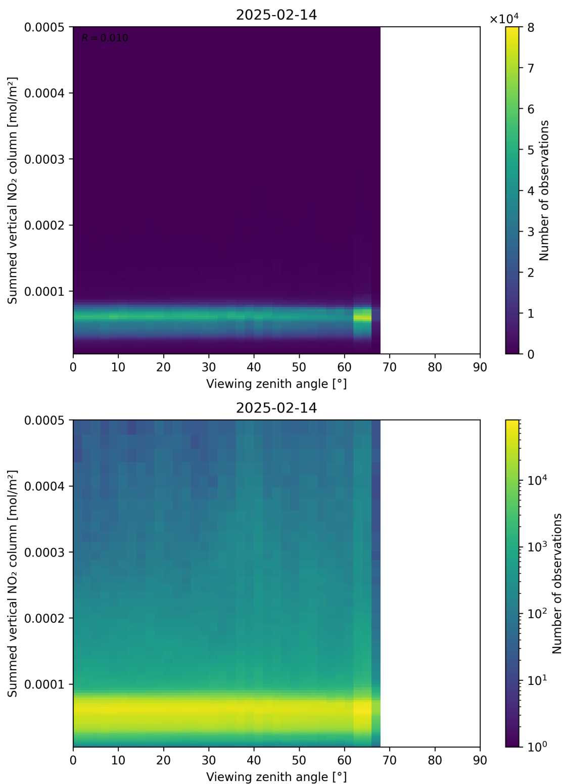
Figure 165: Scatter density plot of “Viewing zenith angle” against “Summed vertical NO 2 column” for 2025-02-13 to 2025-02-15.
