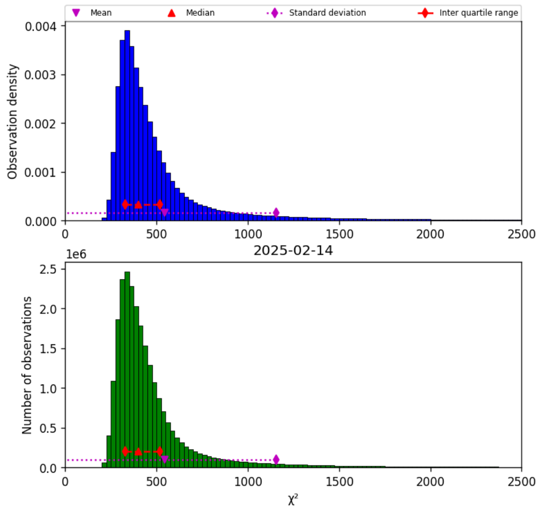
Figure 42: Histogram of " \chi^2 " for 2025-02-13 to 2025-02-15
