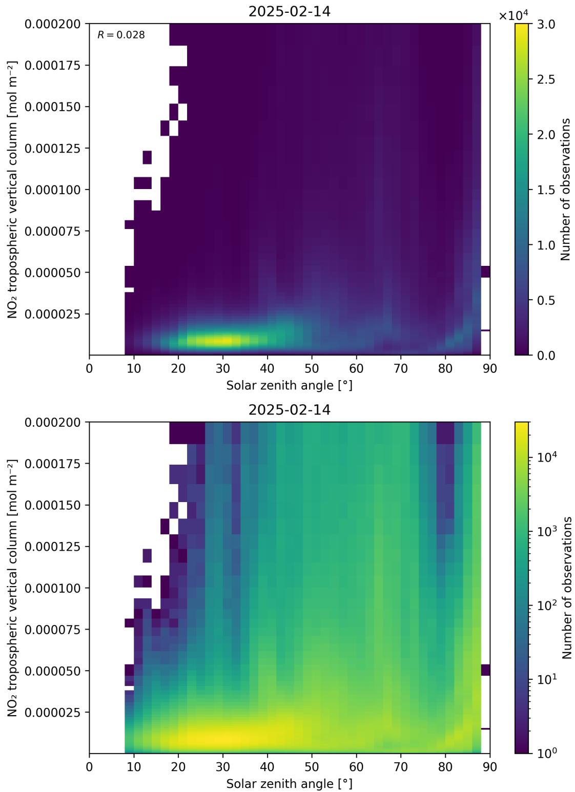
Figure 155: Scatter density plot of “Solar zenith angle” against “NO 2 tropospheric vertical column” for 2025-02-13 to 2025-02-15.
