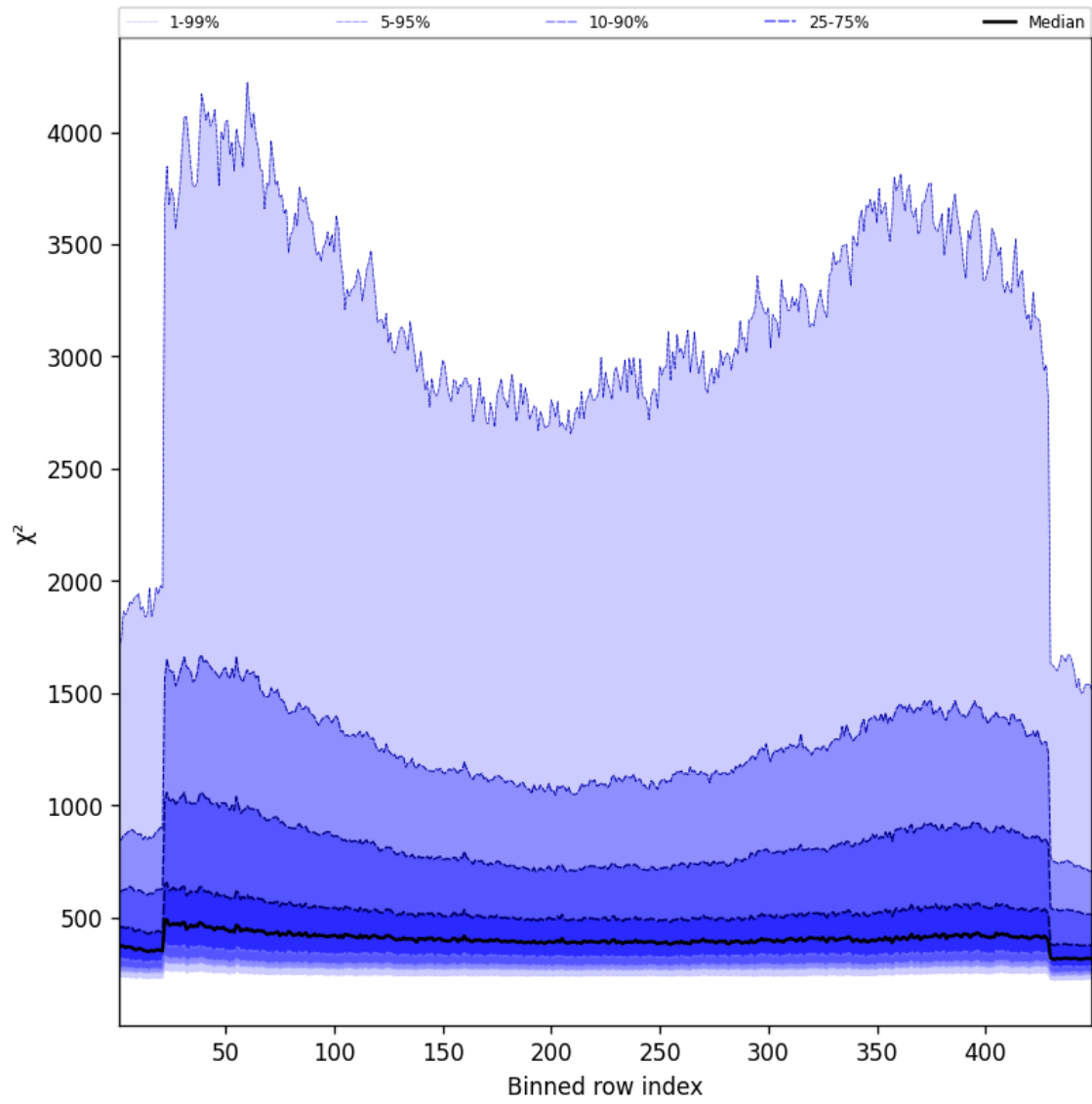
Figure 59: Along track statistics of “ \chi^2 ” for 2025-02-13 to 2025-02-15
