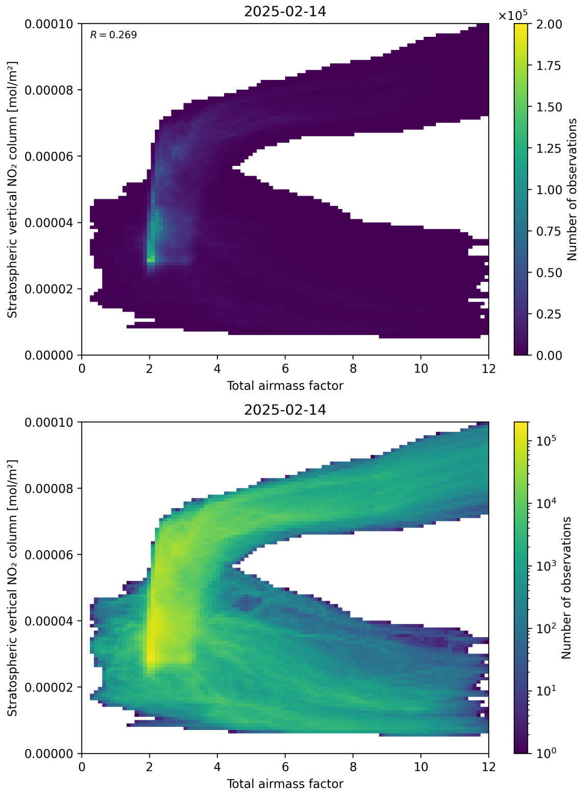
Figure 64: Scatter density plot of “Total airmass factor” against “Stratospheric vertical NO 2 column” for 2025-02-13 to 2025-02-15.
