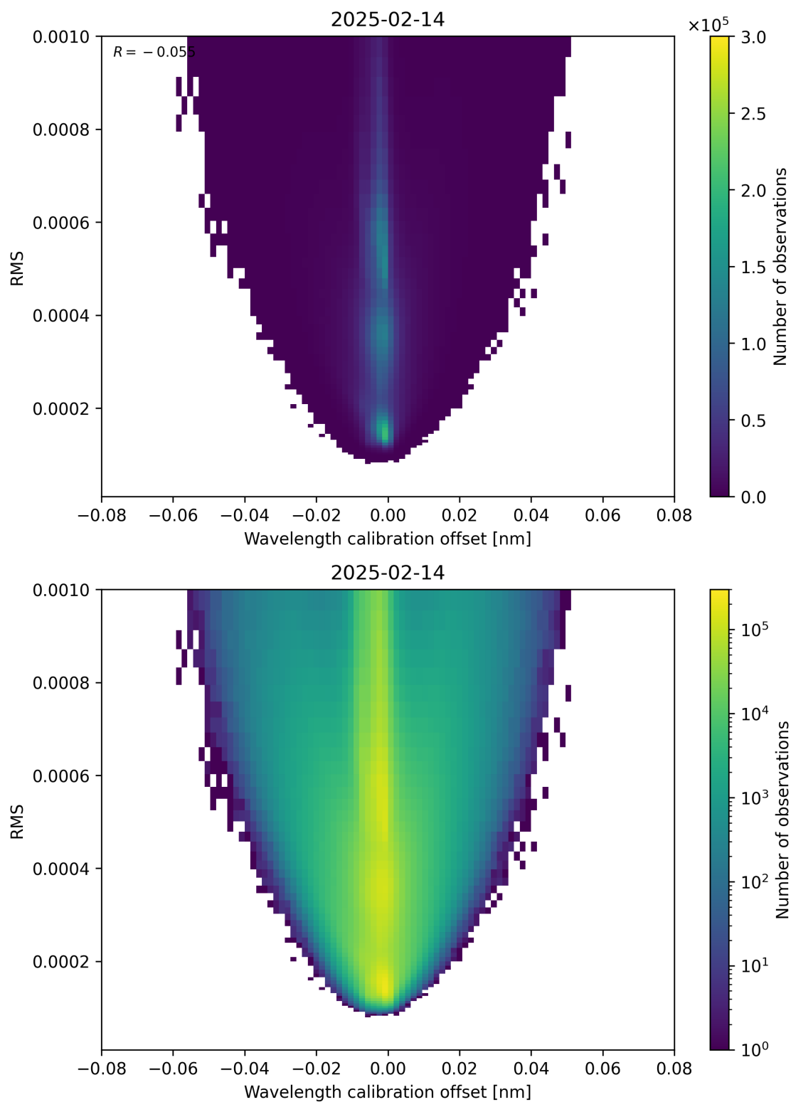
Figure 181: Scatter density plot of “Wavelength calibration offset” against “RMS” for 2025-02-13 to 2025-02-15.
