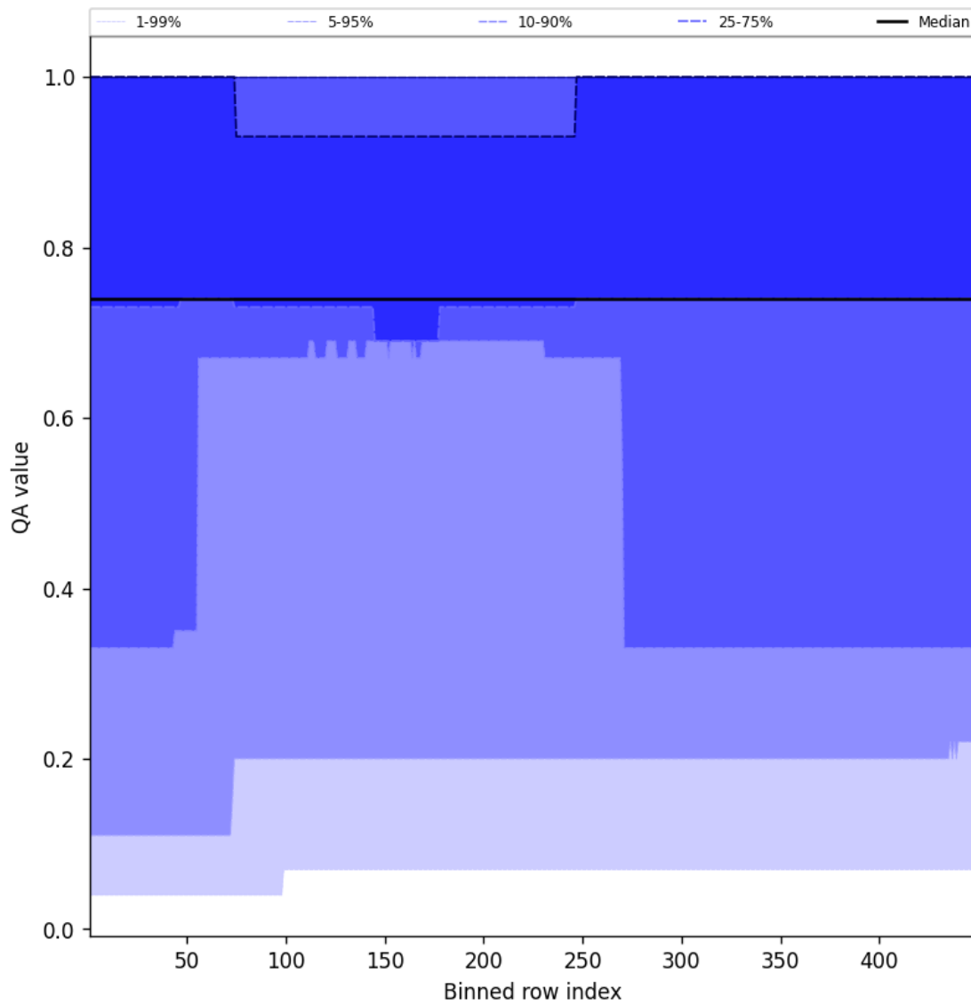
Figure 45: Along track statistics of “QA value” for 2025-02-13 to 2025-02-15
