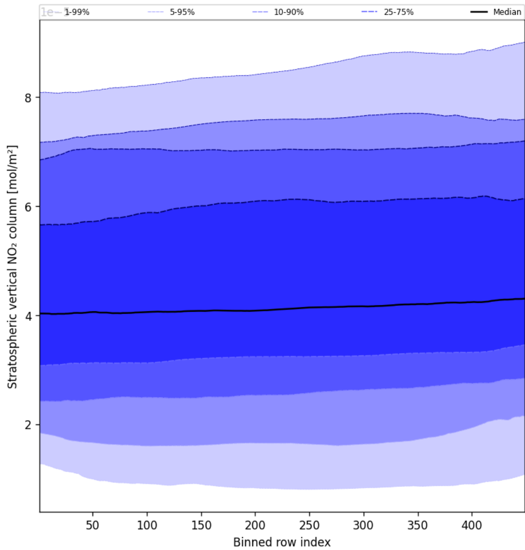
Figure 53: Along track statistics of “Stratospheric vertical NO 2 column” for 2025-02-13 to 2025-02-15
