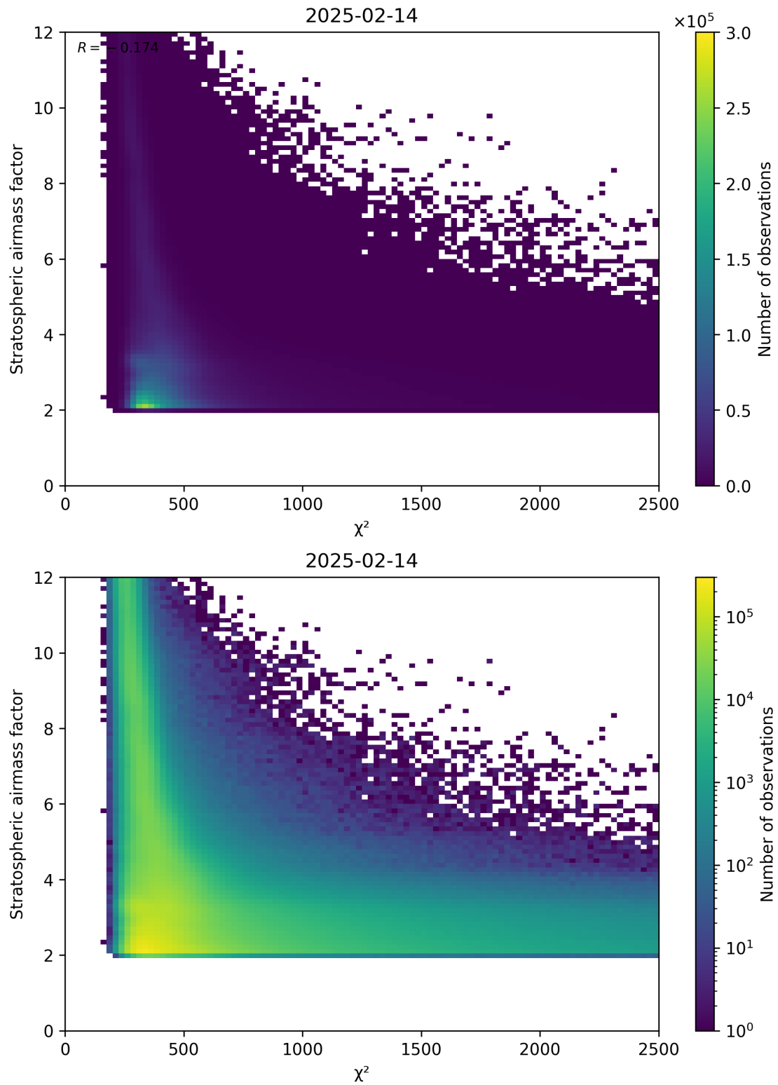
Figure 81: Scatter density plot of “ \chi^2 ” against “Stratospheric airmass factor” for 2025-02-13 to 2025-02-15.
