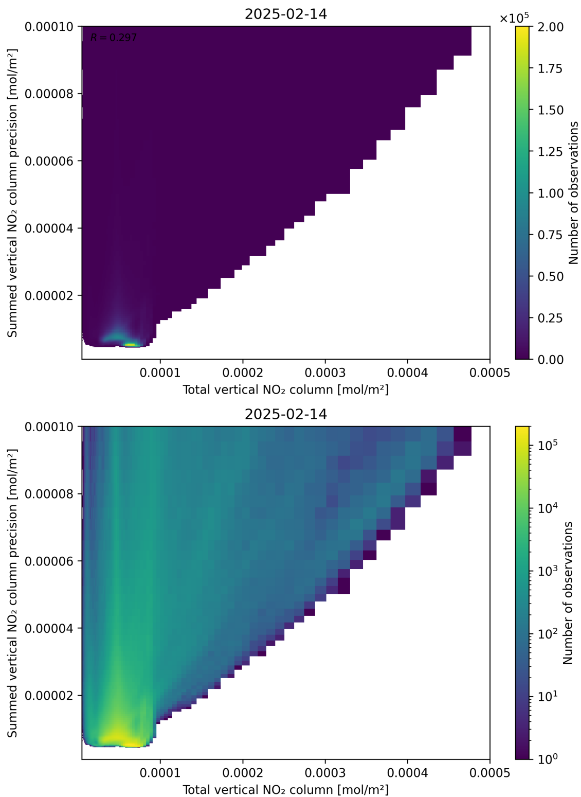
Figure 113: Scatter density plot of “Total vertical NO 2 column” against “Summed vertical NO 2 column precision” for 2025-02-13 to 2025-02-15.
