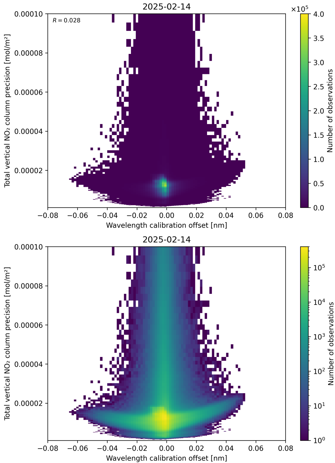
Figure 180: Scatter density plot of “Wavelength calibration offset” against “Total vertical NO 2 column precision” for 2025-02-13 to 2025-02-15.
