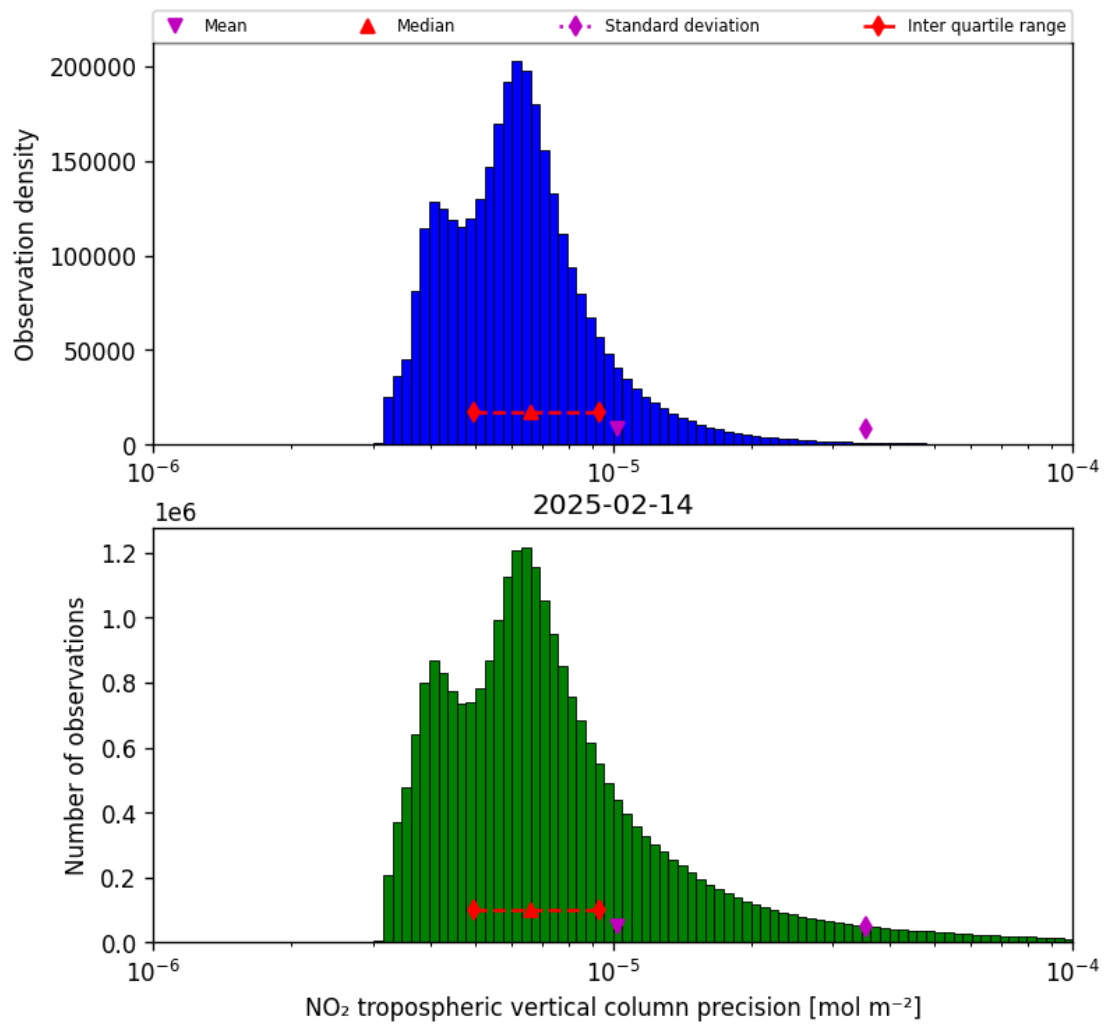
Figure 30: Histogram of “NO 2 tropospheric vertical column precision” for 2025-02-13 to 2025-02-15
