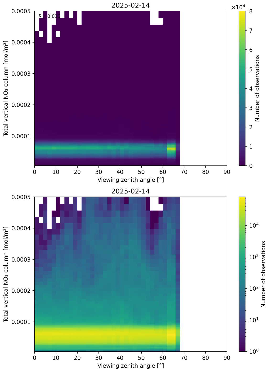
Figure 167: Scatter density plot of “Viewing zenith angle” against “Total vertical NO 2 column” for 2025-02-13 to 2025-02-15.
