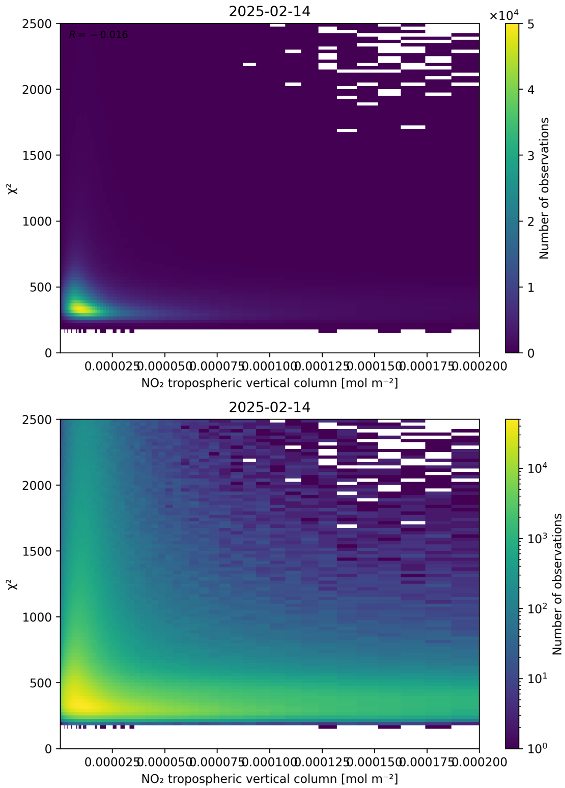
Figure 124: Scatter density plot of “NO 2 tropospheric vertical column” against “ \chi^2 ” for 2025-02-13 to 2025-02-15.
