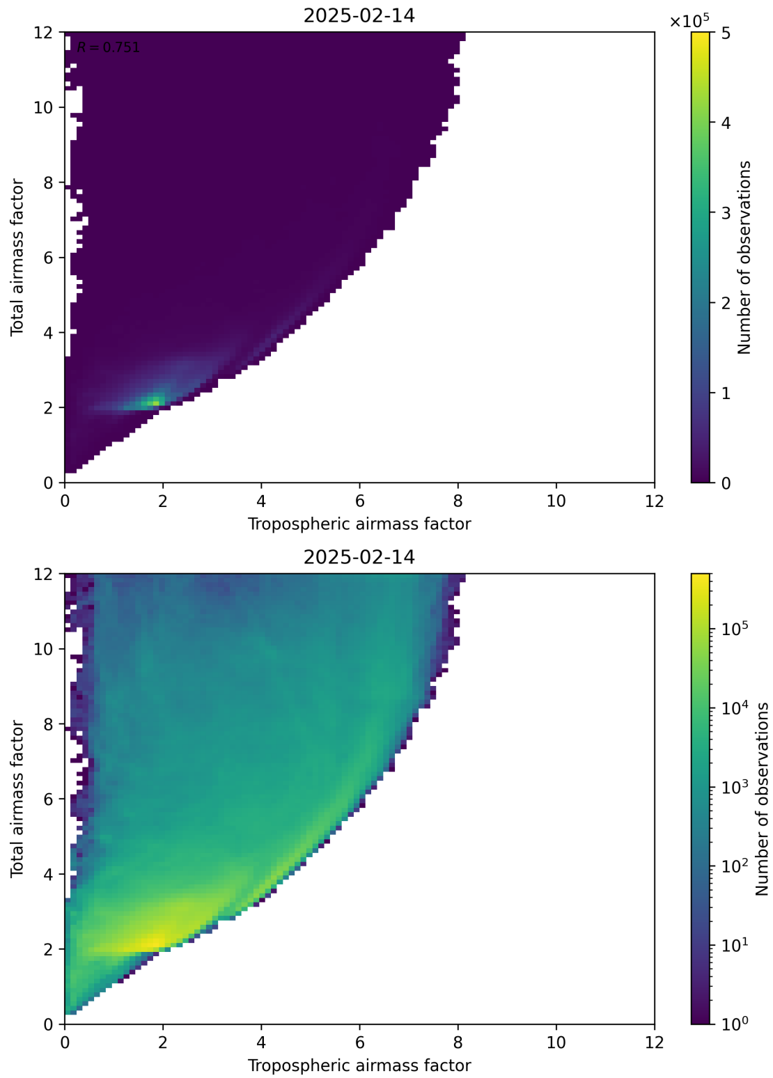
Figure 72: Scatter density plot of “Tropospheric airmass factor” against “Total airmass factor” for 2025-02-13 to 2025-02-15.
