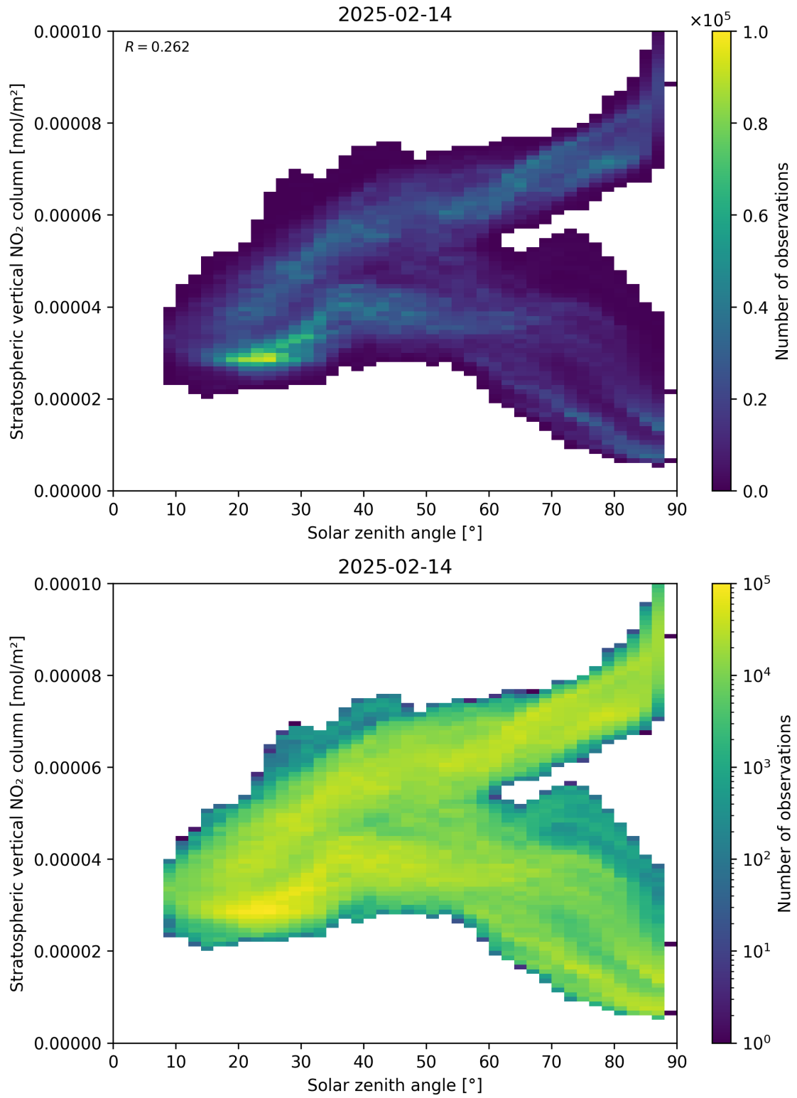
Figure 150: Scatter density plot of “Solar zenith angle” against “Stratospheric vertical NO 2 column” for 2025-02-13 to 2025-02-15.
