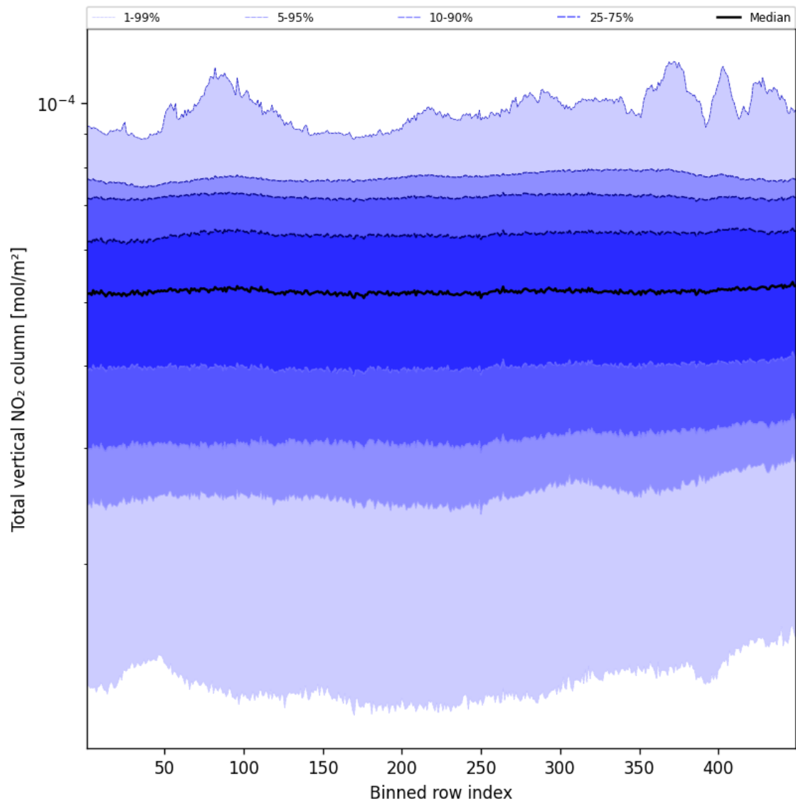
Figure 55: Along track statistics of “Total vertical NO 2 column” for 2025-02-13 to 2025-02-15
