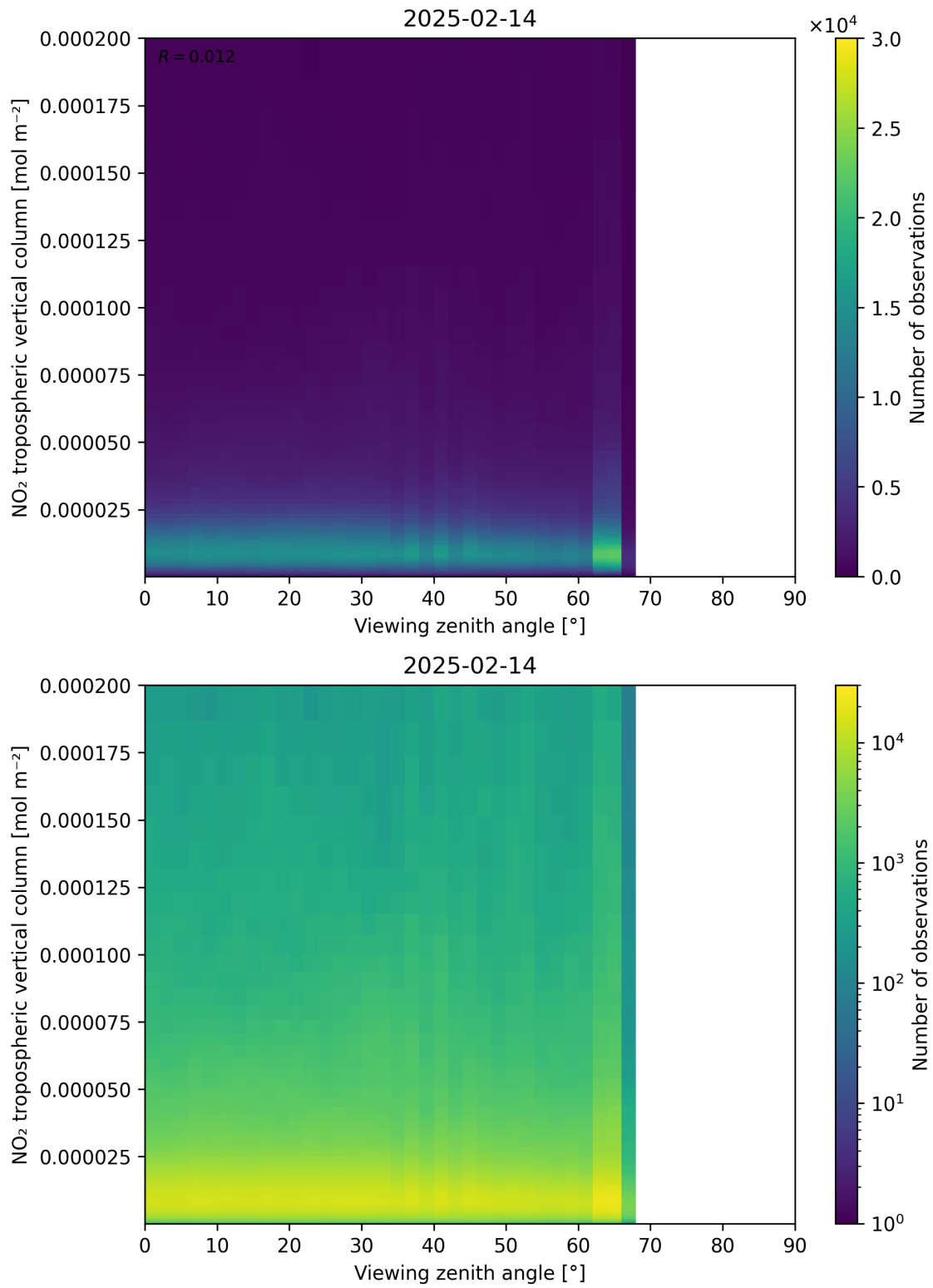
Figure 169: Scatter density plot of “Viewing zenith angle” against “NO 2 tropospheric vertical column” for 2025-02-13 to 2025-02-15.
