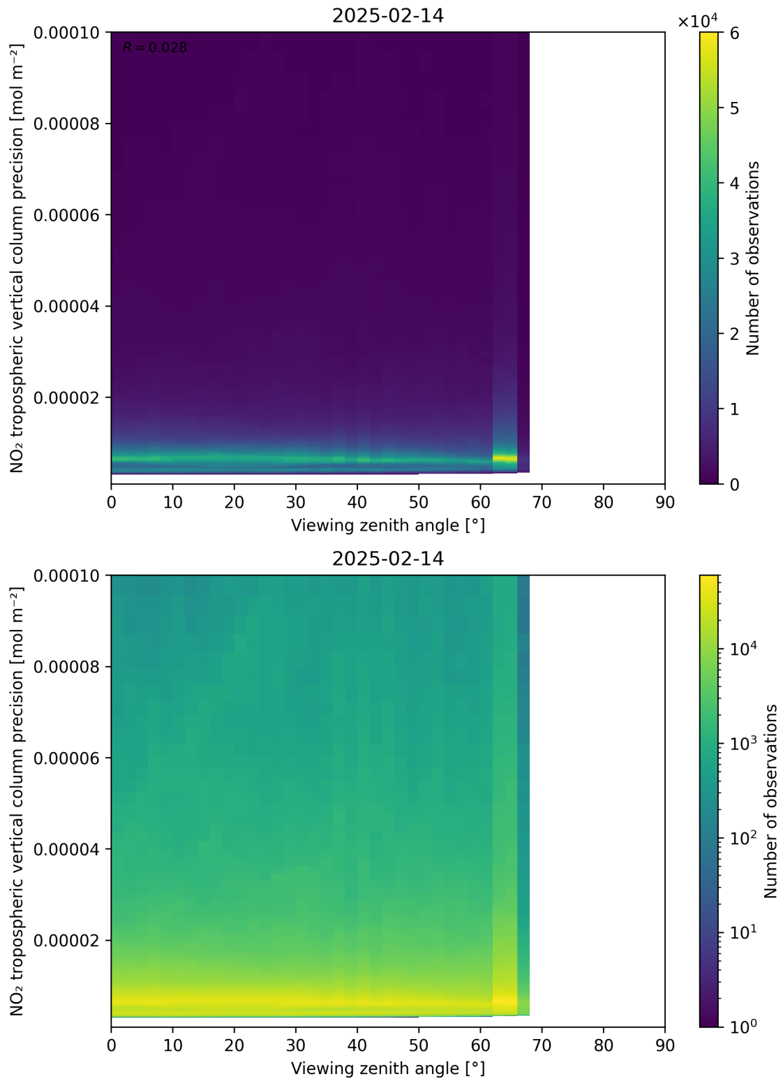
Figure 170: Scatter density plot of “Viewing zenith angle” against “NO 2 tropospheric vertical column precision” for 2025-02-13 to 2025-02-15.
