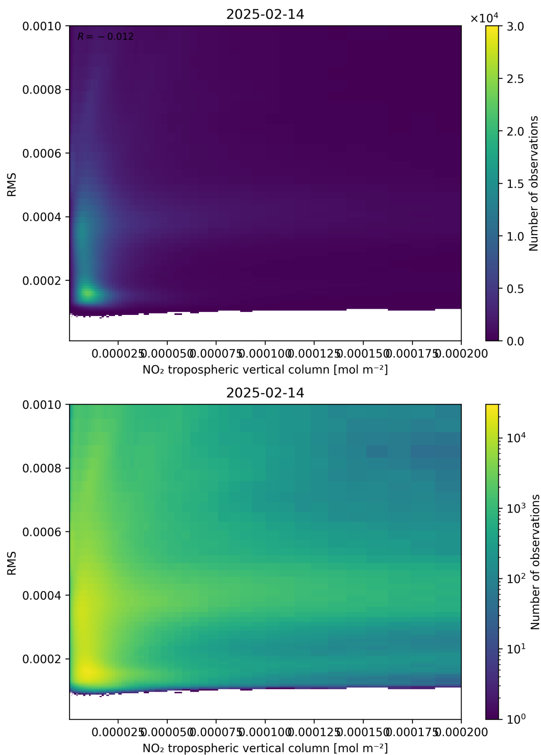
Figure 142: Scatter density plot of “NO 2 tropospheric vertical column” against “RMS” for 2025-02-13 to 2025-02-15.
