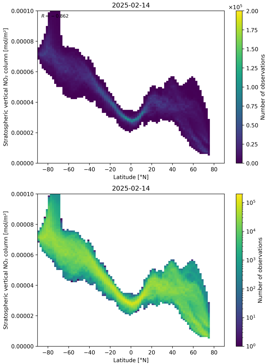
Figure 87: Scatter density plot of “Latitude” against “Stratospheric vertical NO 2 column” for 2025-02-13 to 2025-02-15.
