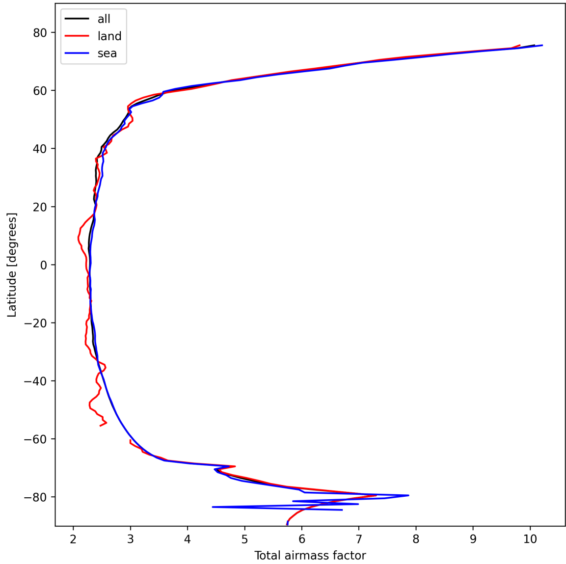
Figure 15: Zonal average of “Total airmass factor” for 2025-02-13 to 2025-02-15.
