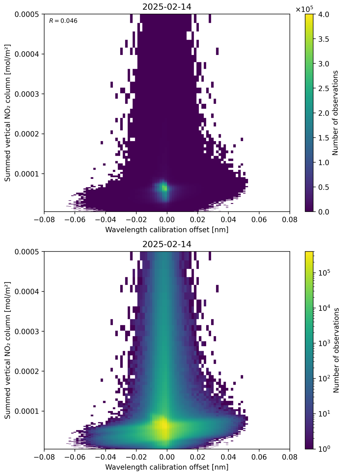
Figure 177: Scatter density plot of “Wavelength calibration offset” against “Summed vertical NO 2 column” for 2025-02-13 to 2025-02-15.
