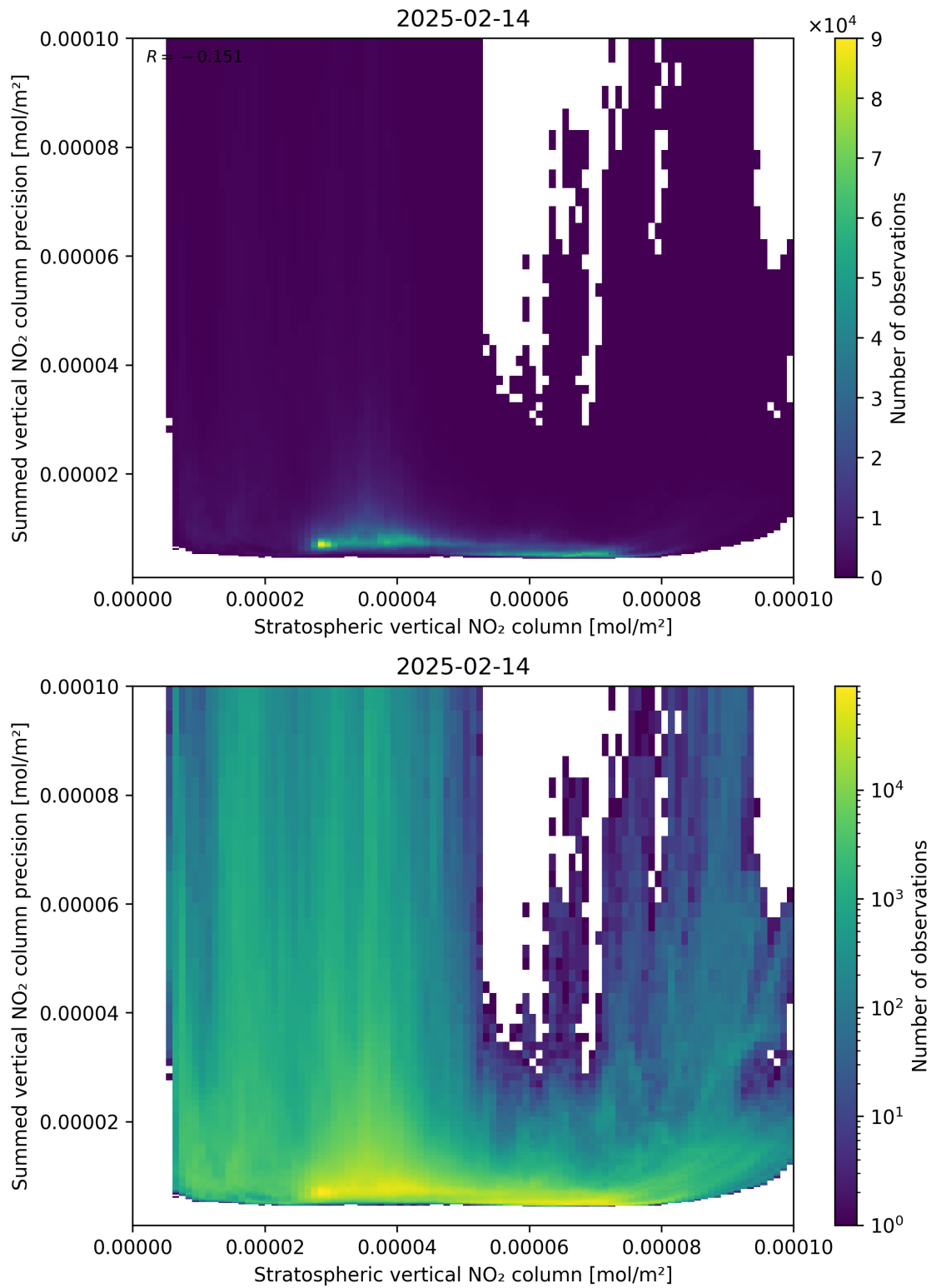
Figure 99: Scatter density plot of “Stratospheric vertical NO 2 column” against “Summed vertical NO 2 column precision” for 2025-02-13 to 2025-02-15.
