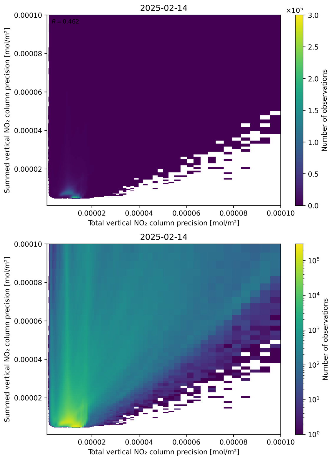
Figure 118: Scatter density plot of “Total vertical NO 2 column precision” against “Summed vertical NO 2 column precision” for 2025-02-13 to 2025-02-15.
