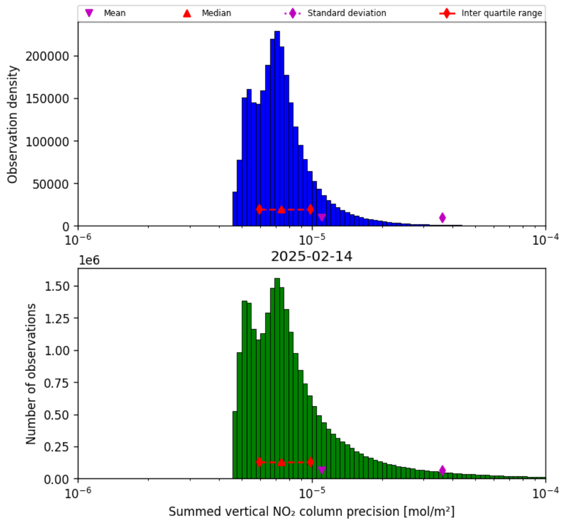
Figure 41: Histogram of "Summed vertical NO 2 column precision" for 2025-02-13 to 2025-02-15
