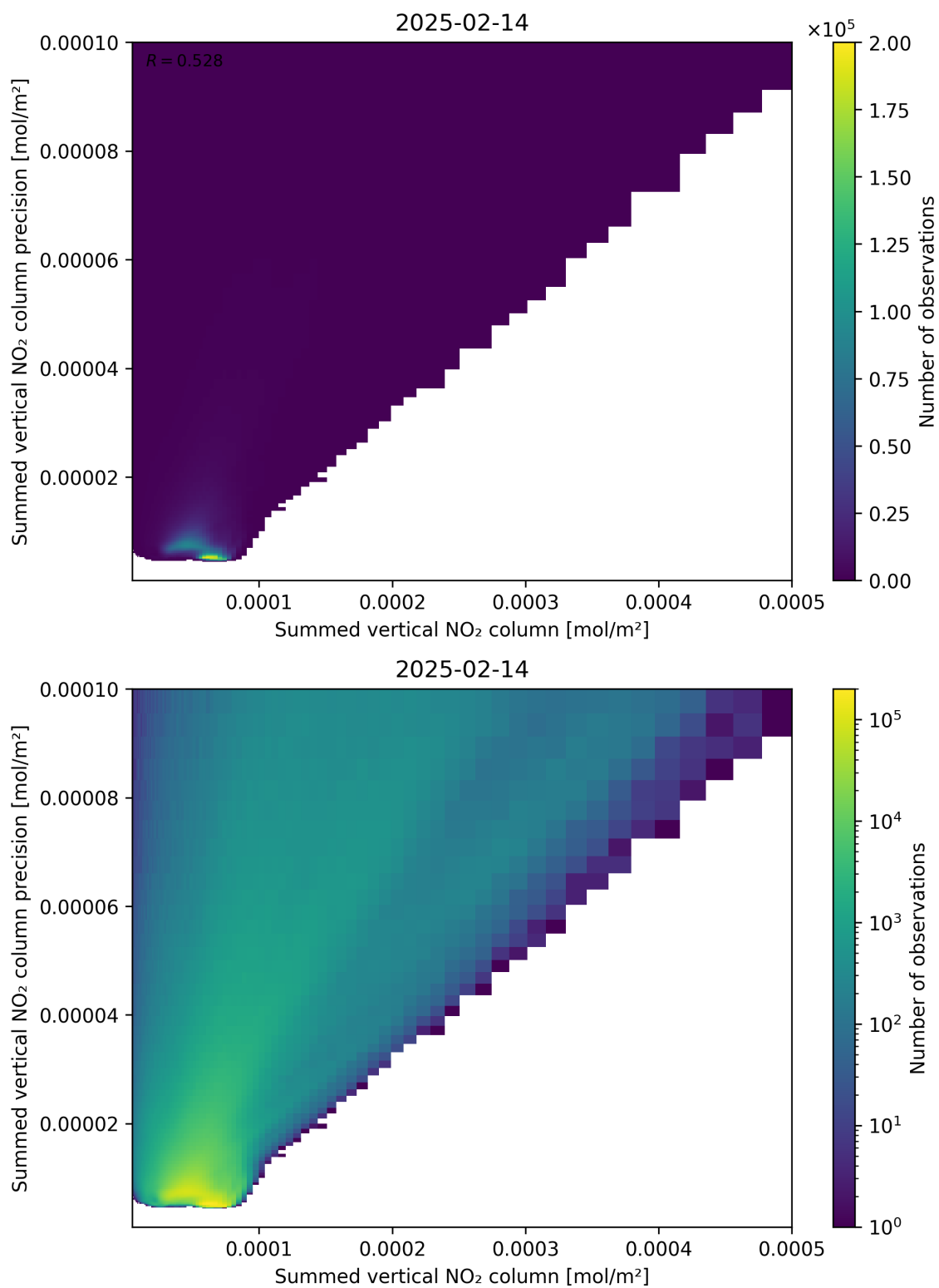
Figure 105: Scatter density plot of “Summed vertical NO 2 column” against “Summed vertical NO 2 column precision” for 2025-02-13 to 2025-02-15.
