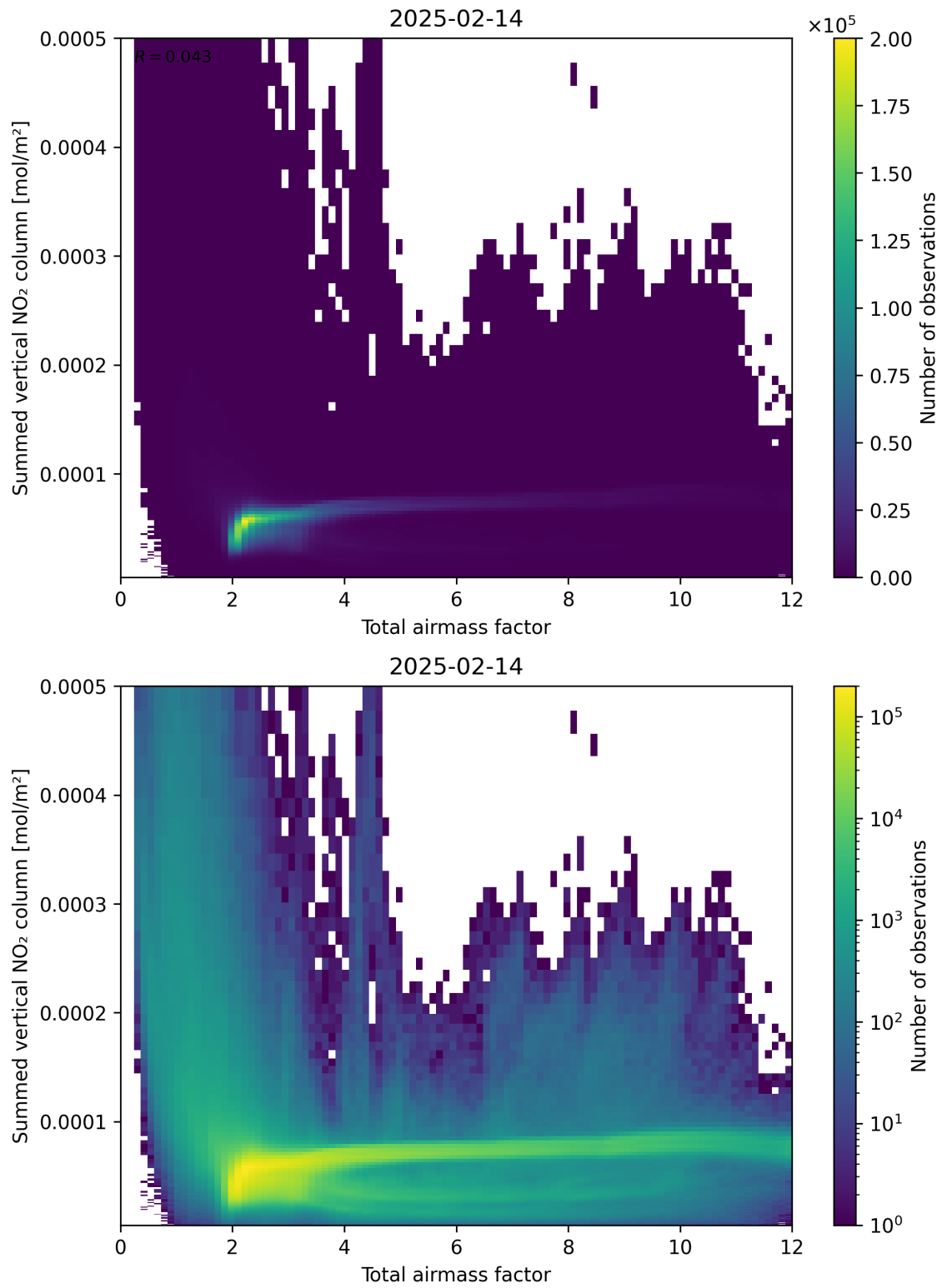
Figure 65: Scatter density plot of “Total airmass factor” against “Summed vertical NO 2 column” for 2025-02-13 to 2025-02-15.
