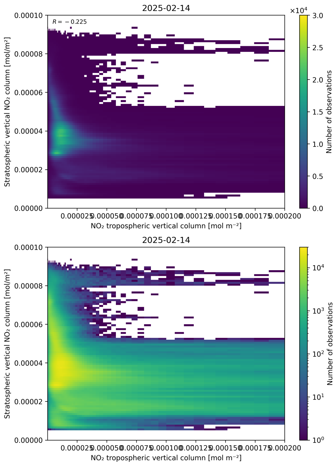
Figure 125: Scatter density plot of “NO 2 tropospheric vertical column” against “Stratospheric vertical NO 2 column” for 2025-02-13 to 2025-02-15.
