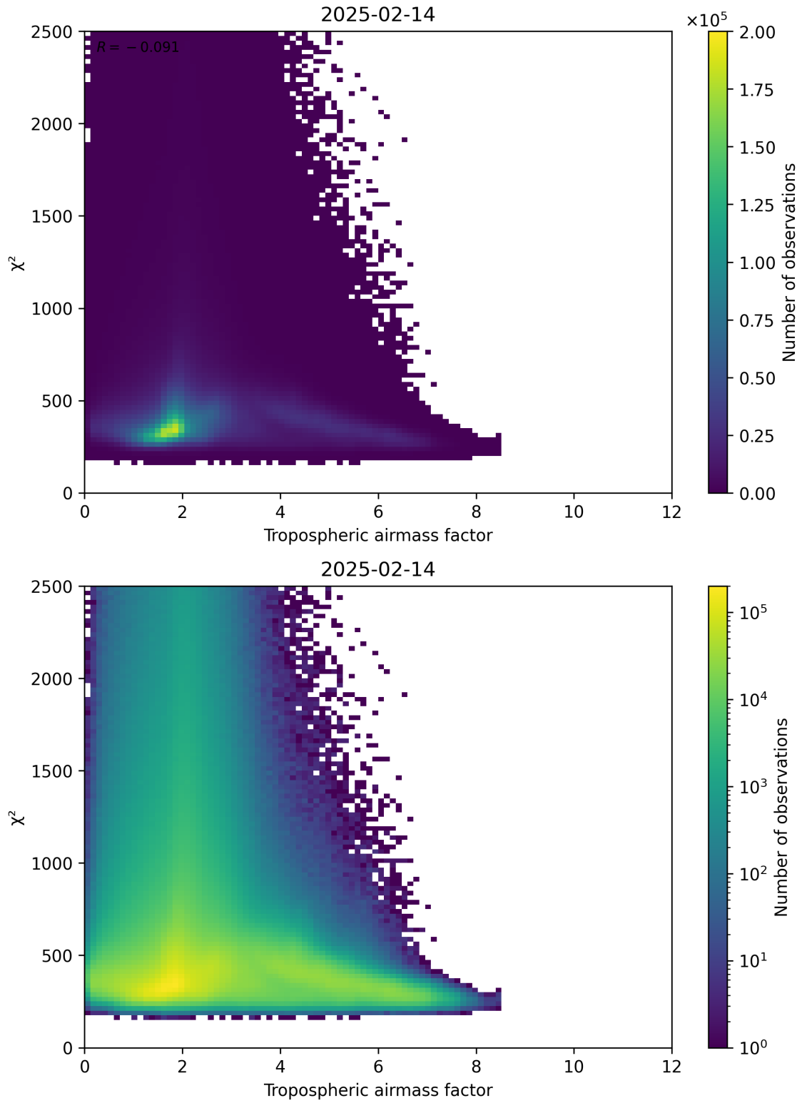
Figure 73: Scatter density plot of “Tropospheric airmass factor” against “ \chi^2 ” for 2025-02-13 to 2025-02-15.
