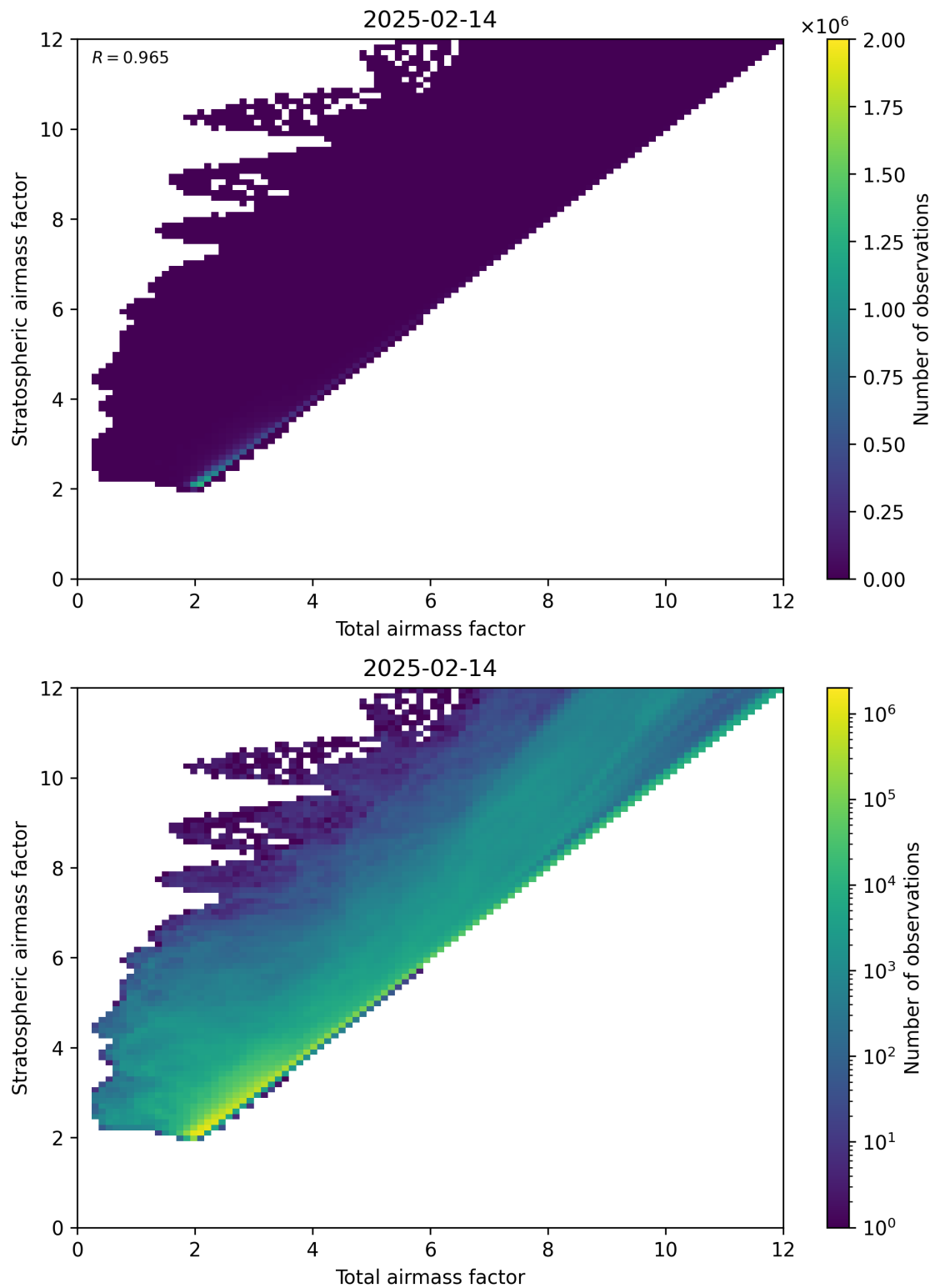
Figure 62: Scatter density plot of “Total airmass factor” against “Stratospheric airmass factor” for 2025-02-13 to 2025-02-15.
