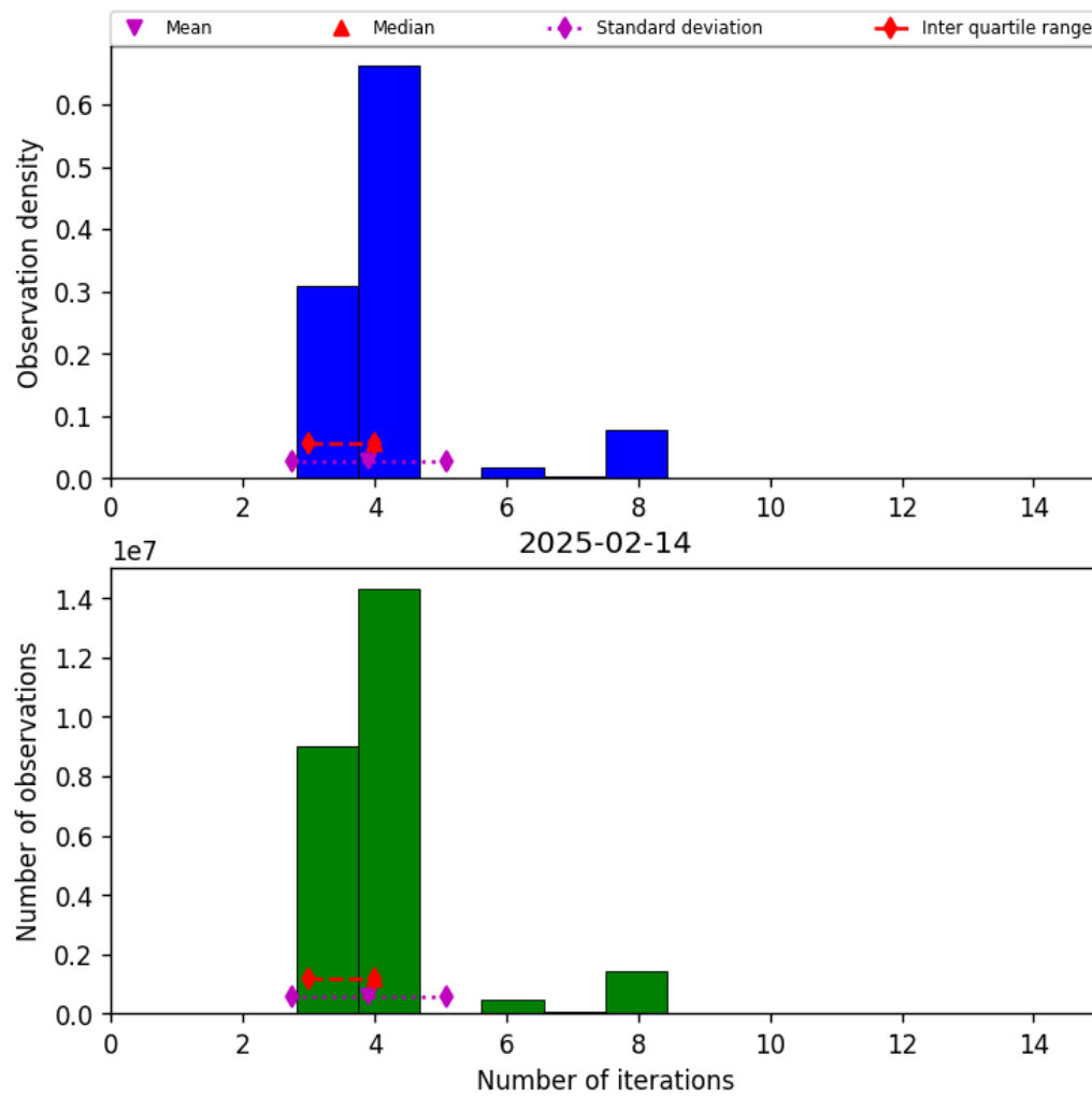
Figure 34: Histogram of “Number of iterations” for 2025-02-13 to 2025-02-15
