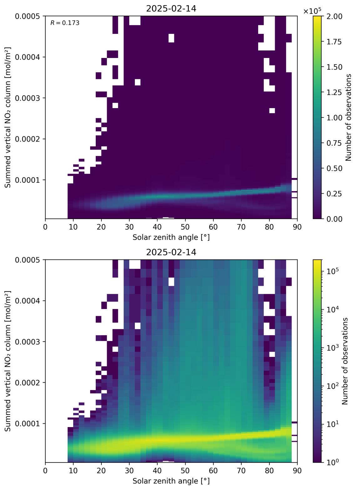
Figure 151: Scatter density plot of “Solar zenith angle” against “Summed vertical NO 2 column” for 2025-02-13 to 2025-02-15.
