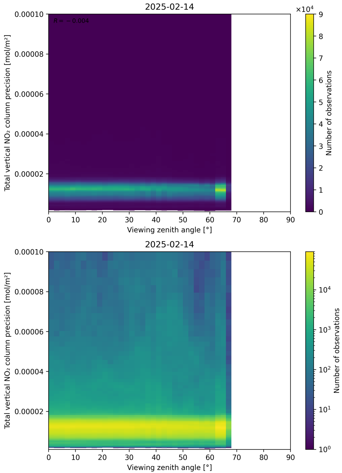
Figure 168: Scatter density plot of “Viewing zenith angle” against “Total vertical NO 2 column precision” for 2025-02-13 to 2025-02-15.
