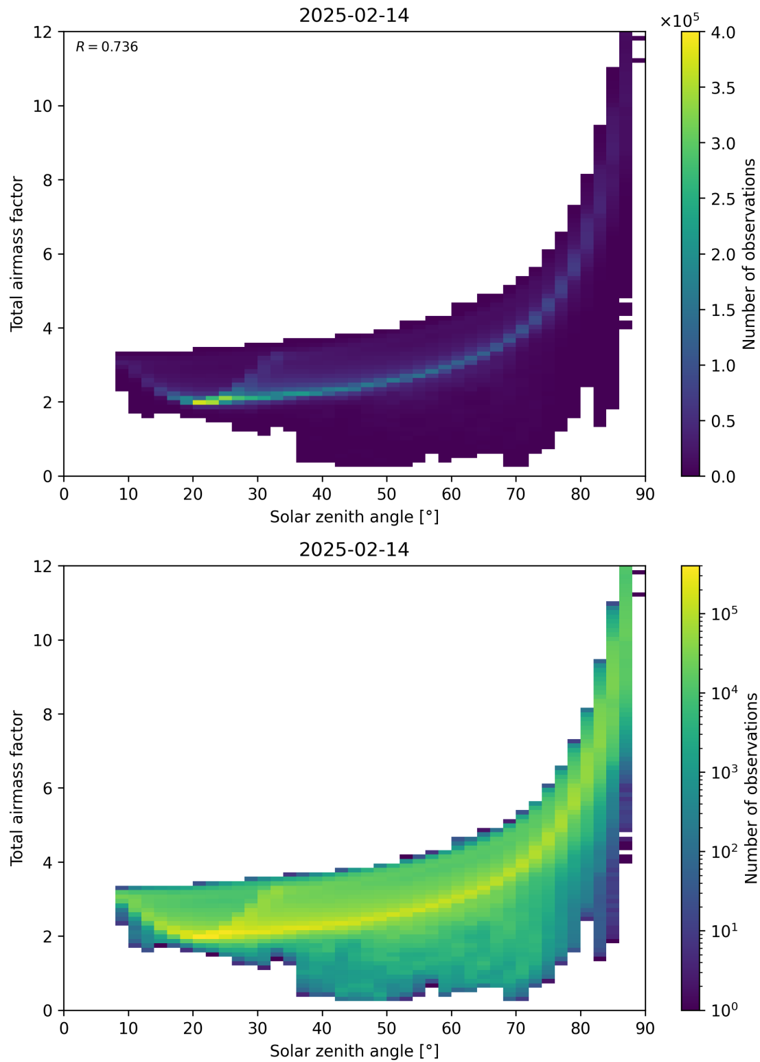
Figure 146: Scatter density plot of “Solar zenith angle” against “Total air mass factor” for 2025-02-13 to 2025-02-15.
