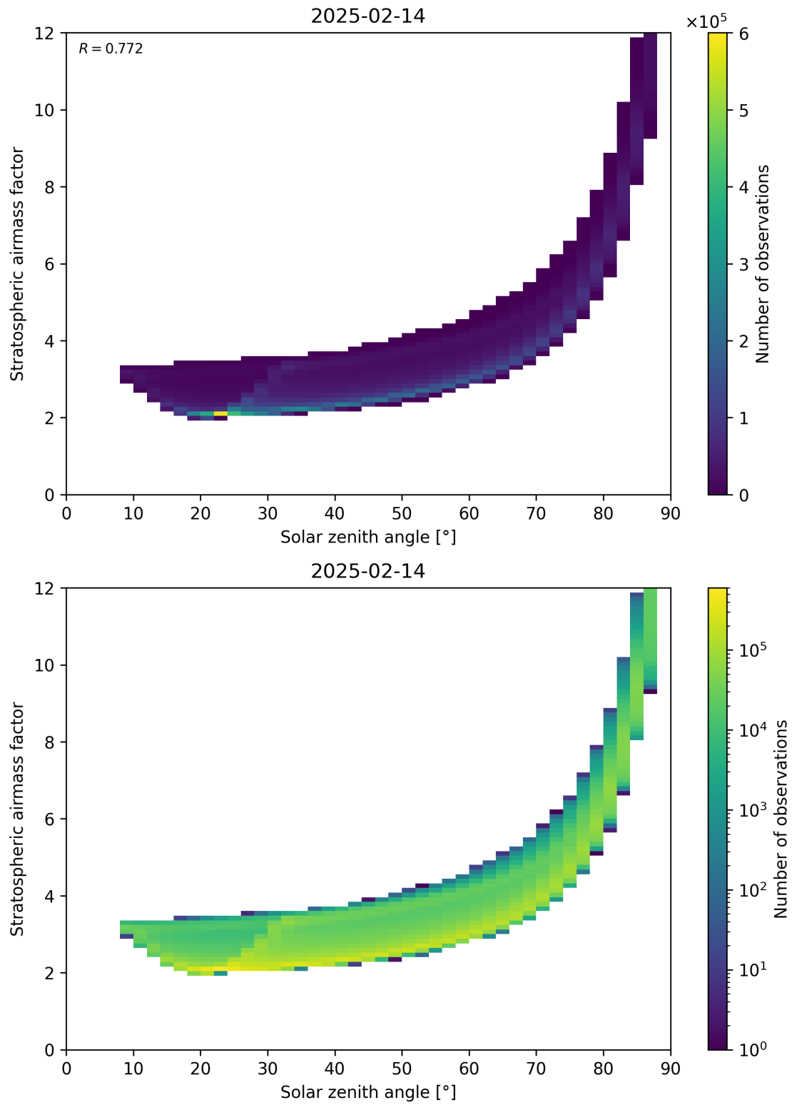
Figure 145: Scatter density plot of “Solar zenith angle” against “Stratospheric airmass factor” for 2025-02-13 to 2025-02-15.
