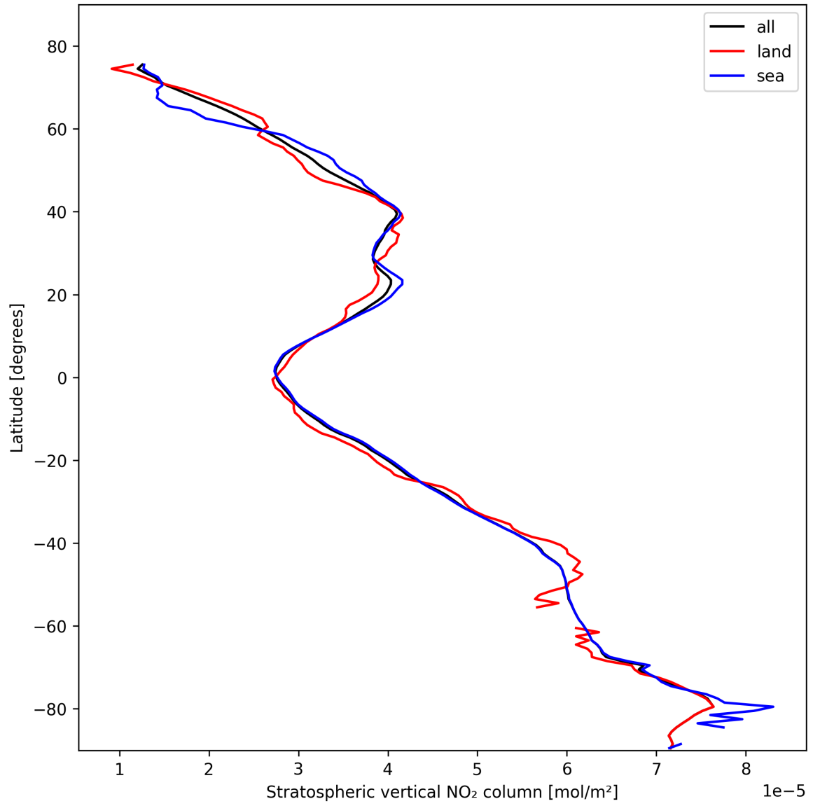
Figure 19: Zonal average of “Stratospheric vertical NO 2 column” for 2025-02-13 to 2025-02-15.
