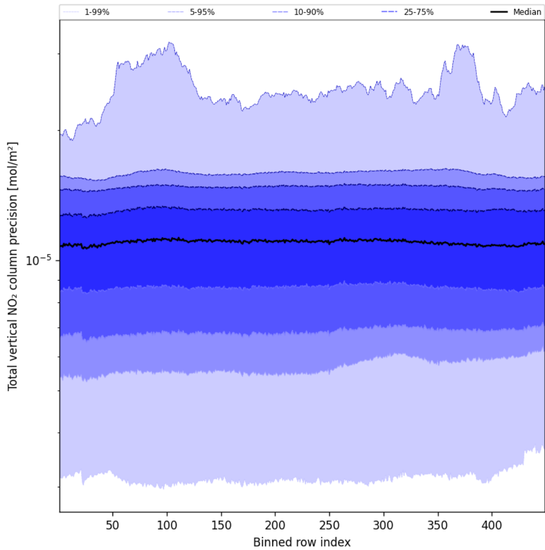
Figure 56: Along track statistics of “Total vertical NO 2 column precision” for 2025-02-13 to 2025-02-15
