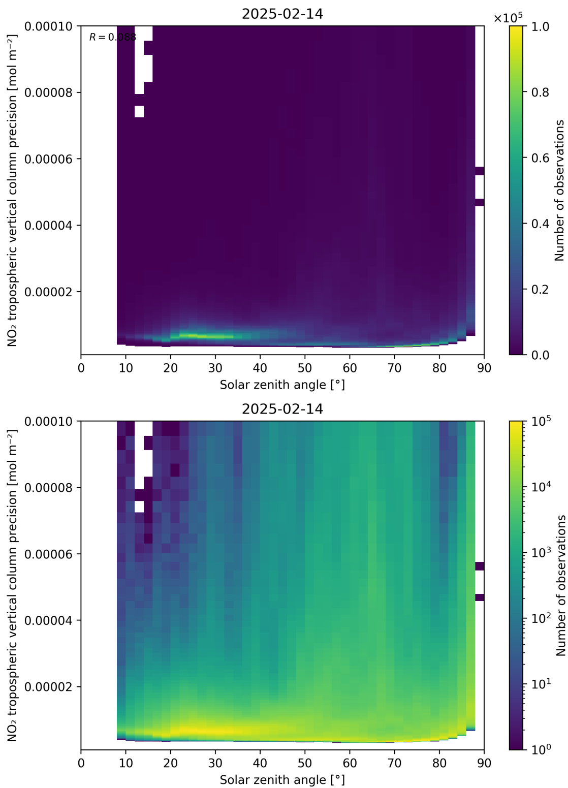
Figure 156: Scatter density plot of “Solar zenith angle” against “NO 2 tropospheric vertical column precision” for 2025-02-13 to 2025-02-15.
