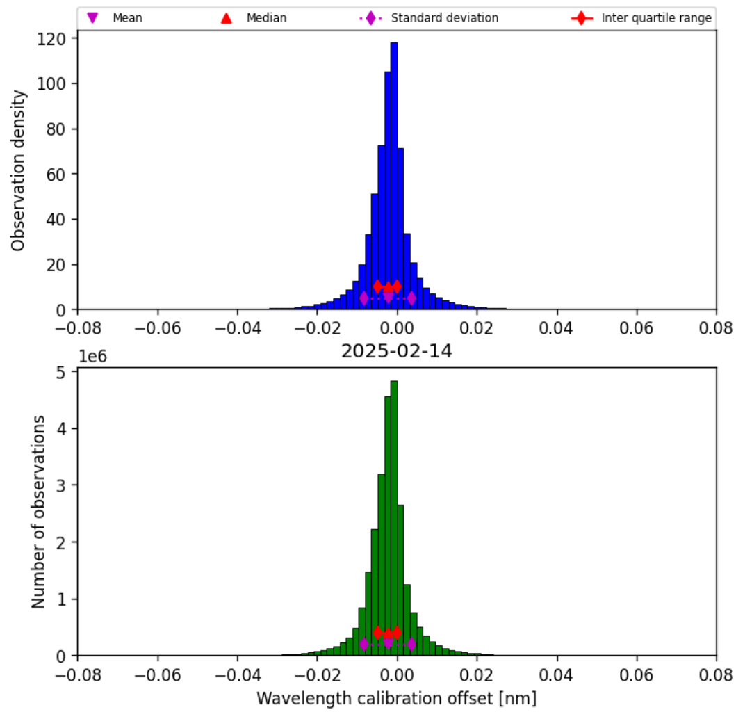
Figure 35: Histogram of “Wavelength calibration offset” for 2025-02-13 to 2025-02-15
