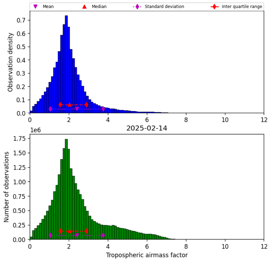
Figure 31: Histogram of “Tropospheric airmass factor” for 2025-02-13 to 2025-02-15
