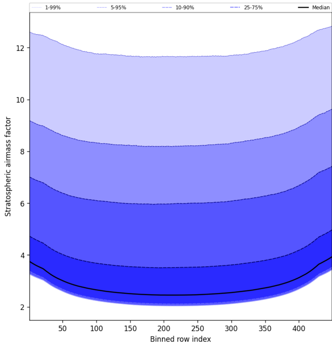
Figure 61: Along track statistics of “Stratospheric airmass factor” for 2025-02-13 to 2025-02-15
