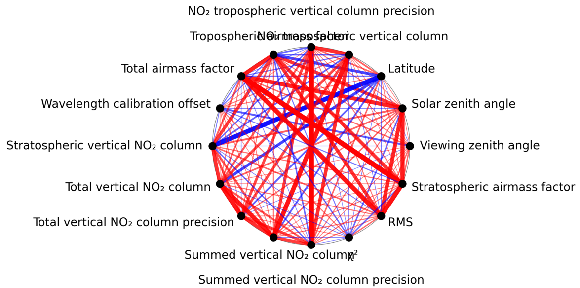
Figure 1: Map of correlation graph for 2025-02-13 to 2025-02-15.
