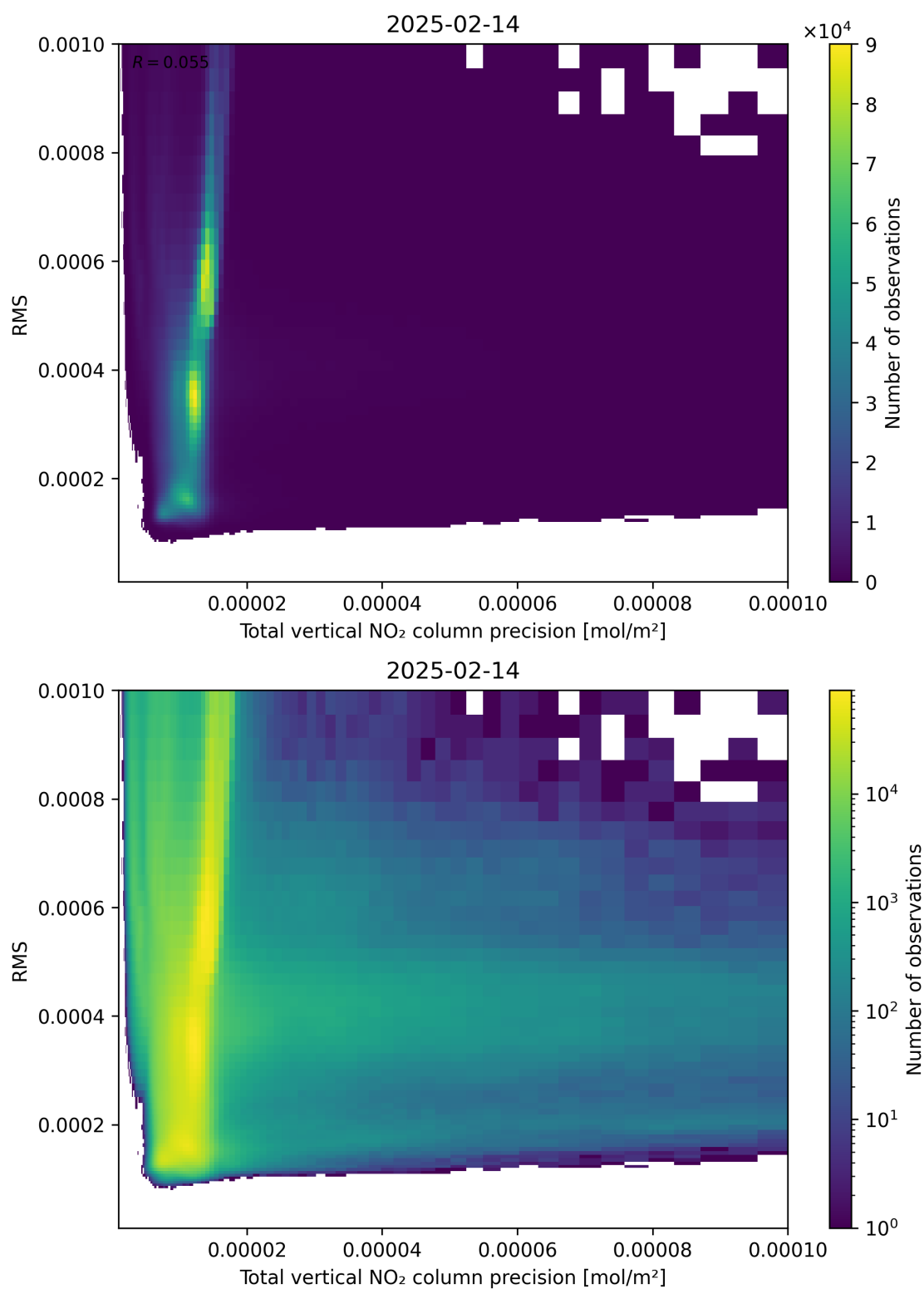
Figure 119: Scatter density plot of “Total vertical NO 2 column precision” against “RMS” for 2025-02-13 to 2025-02-15.
