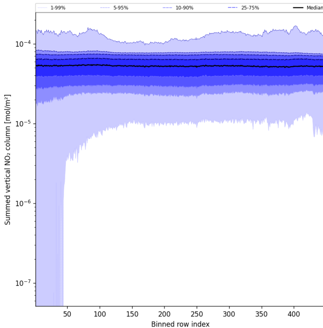
Figure 57: Along track statistics of “Summed vertical NO 2 column” for 2025-02-13 to 2025-02-15
