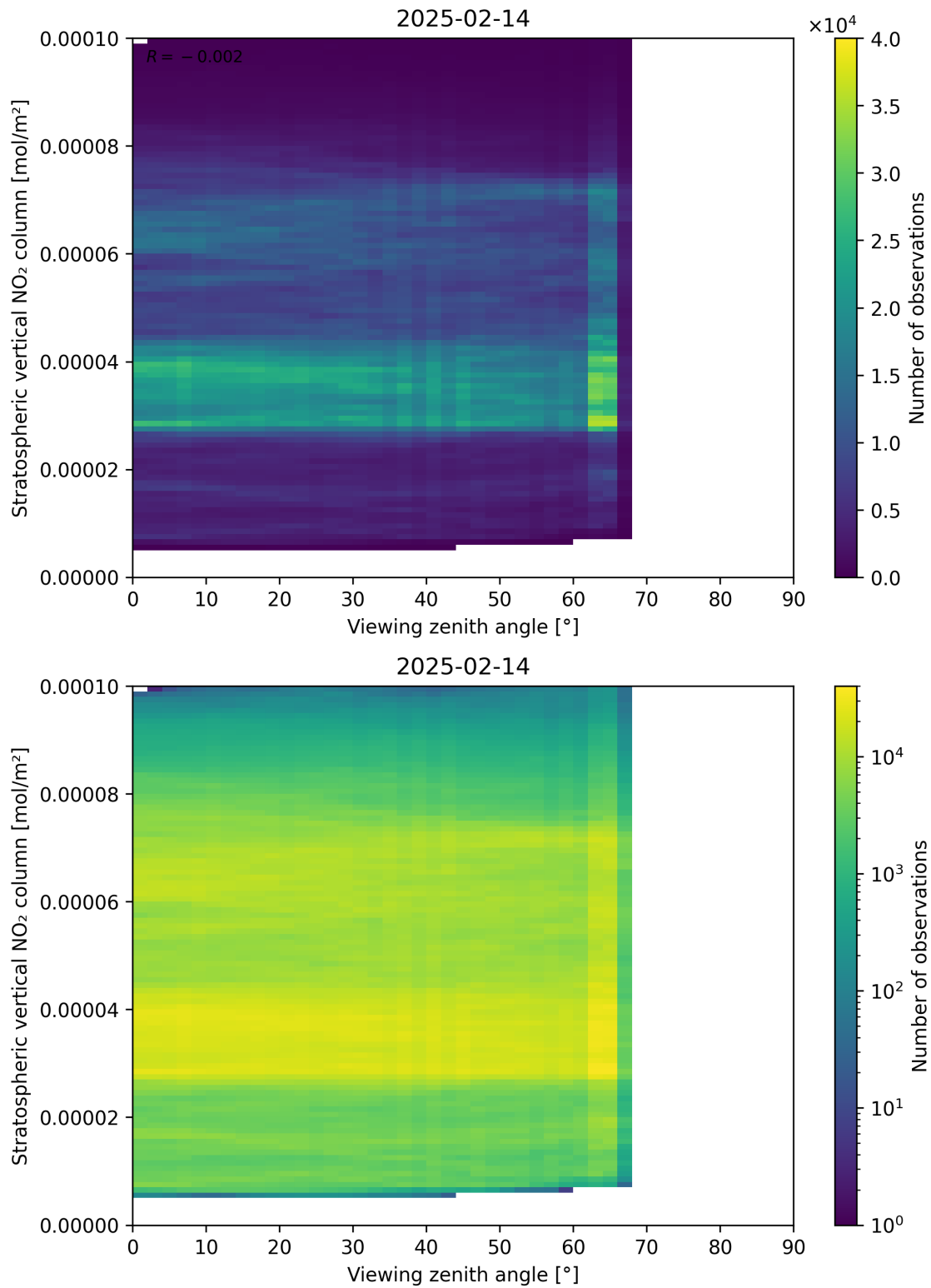
Figure 164: Scatter density plot of “Viewing zenith angle” against “Stratospheric vertical NO 2 column” for 2025-02-13 to 2025-02-15.
