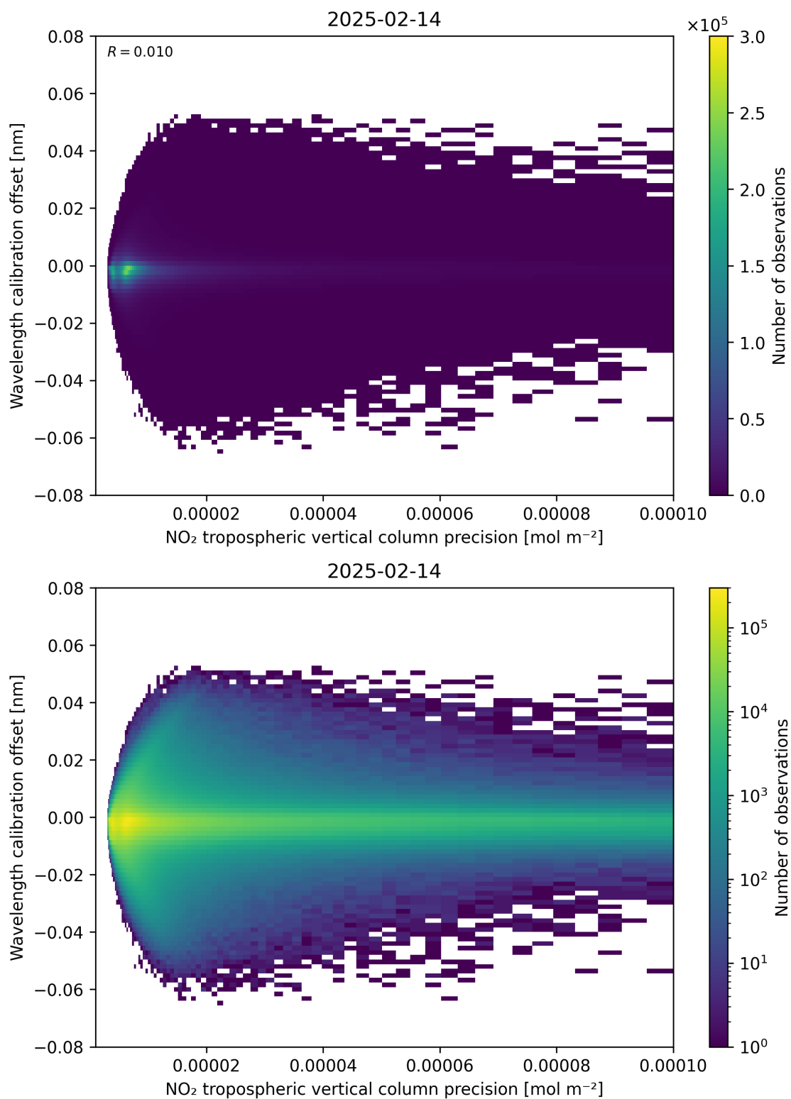
Figure 141: Scatter density plot of “NO 2 tropospheric vertical column precision” against “Wavelength calibration offset” for 2025-02-13 to 2025-02-15.
