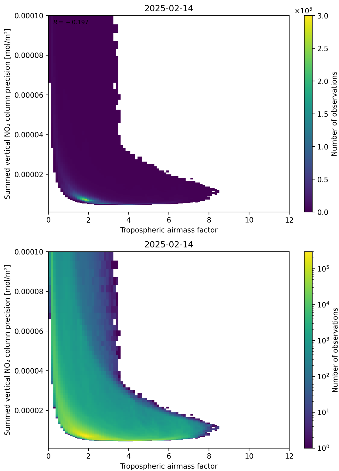
Figure 76: Scatter density plot of “Tropospheric air mass factor” against “Summed vertical NO 2 column precision” for 2025-02-13 to 2025-02-15.
