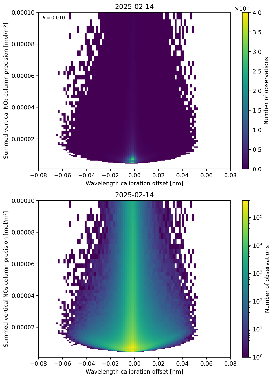
Figure 178: Scatter density plot of “Wavelength calibration offset” against “Summed vertical NO 2 column precision” for 2025-02-13 to 2025-02-15.
