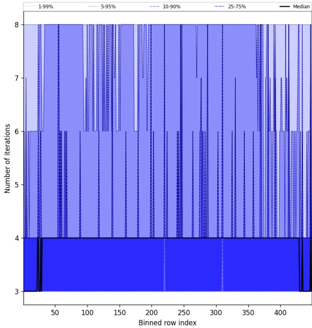
Figure 51: Along track statistics of “Number of iterations” for 2025-02-13 to 2025-02-15
