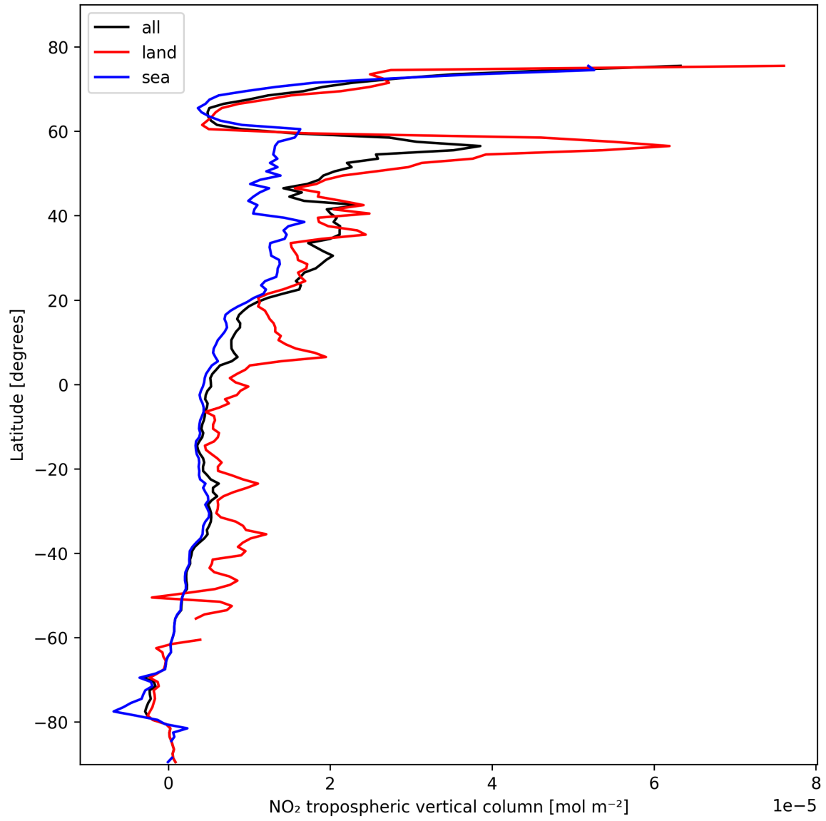
Figure 12: Zonal average of “NO 2 tropospheric vertical column” for 2025-02-13 to 2025-02-15.
