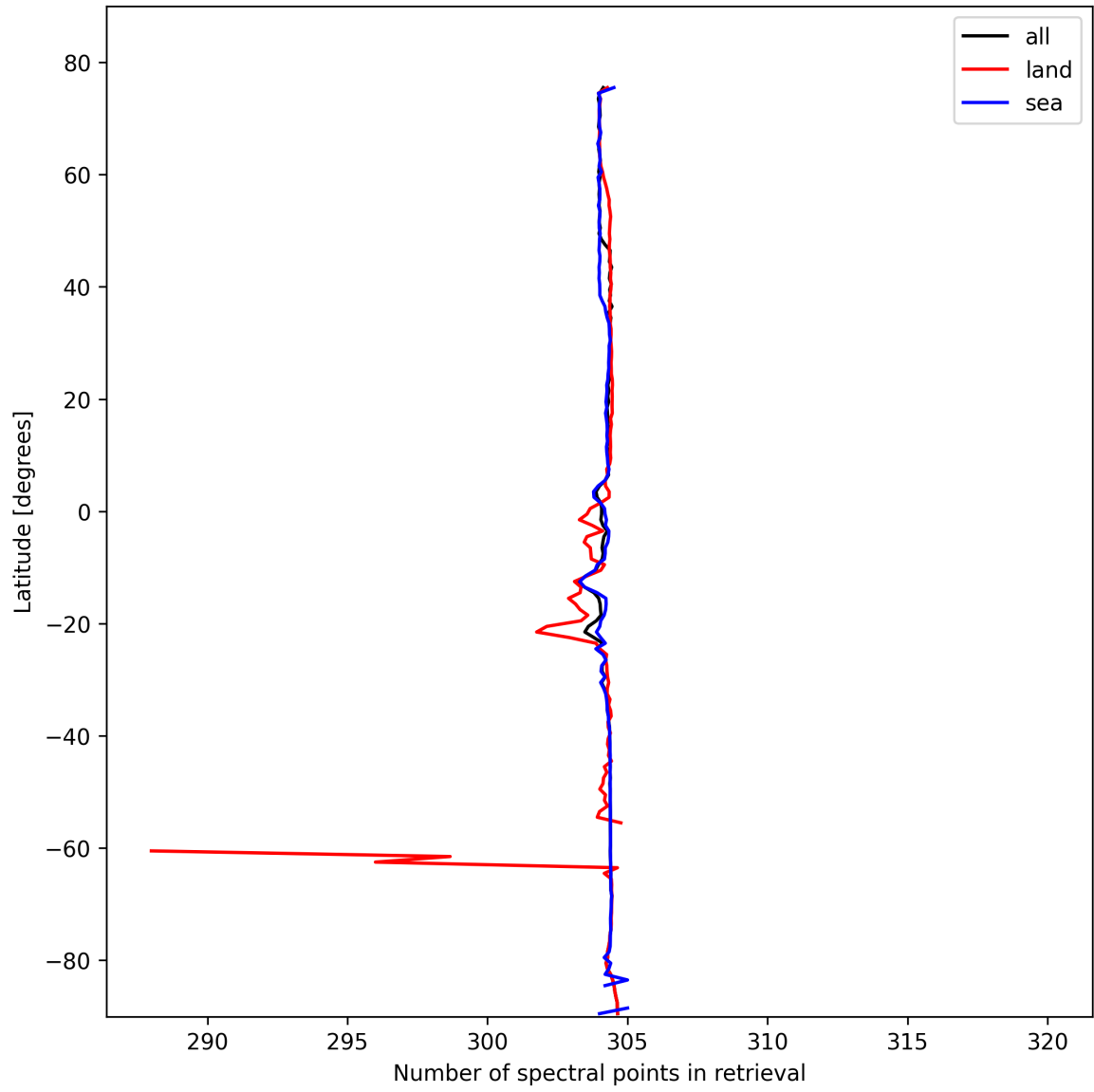
Figure 16: Zonal average of “Number of spectral points in retrieval” for 2025-02-13 to 2025-02-15.
