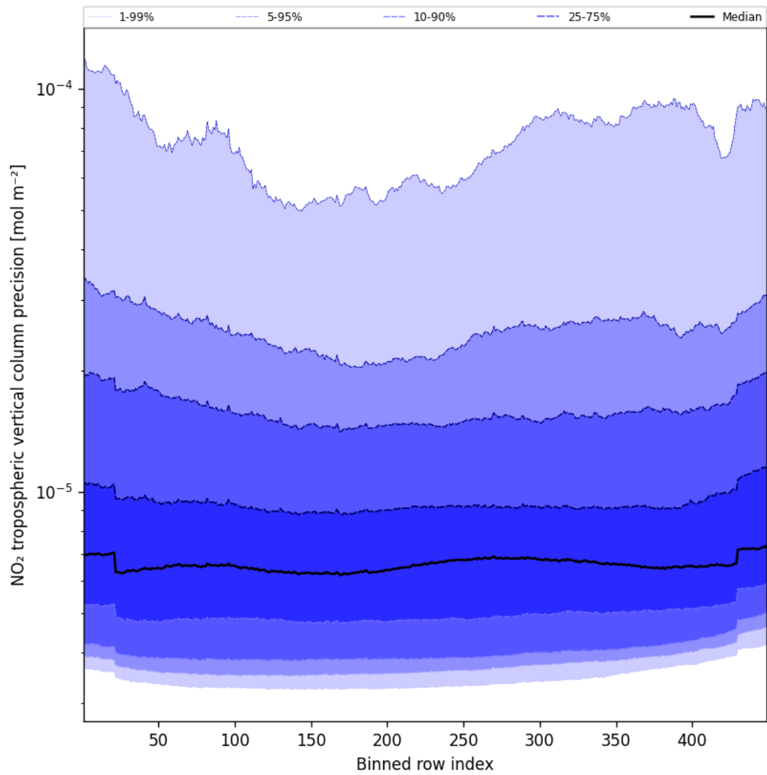
Figure 47: Along track statistics of “NO 2 tropospheric vertical column precision” for 2025-02-13 to 2025-02-15
