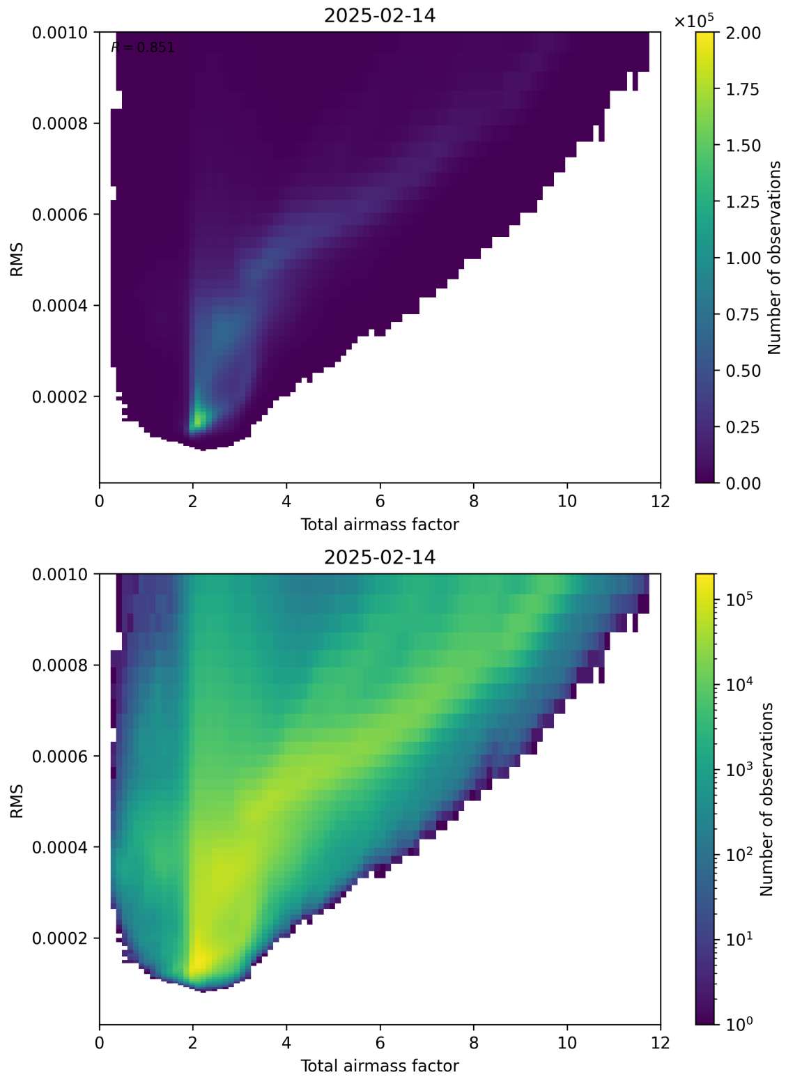
Figure 69: Scatter density plot of “Total airmass factor” against “RMS” for 2025-02-13 to 2025-02-15.
