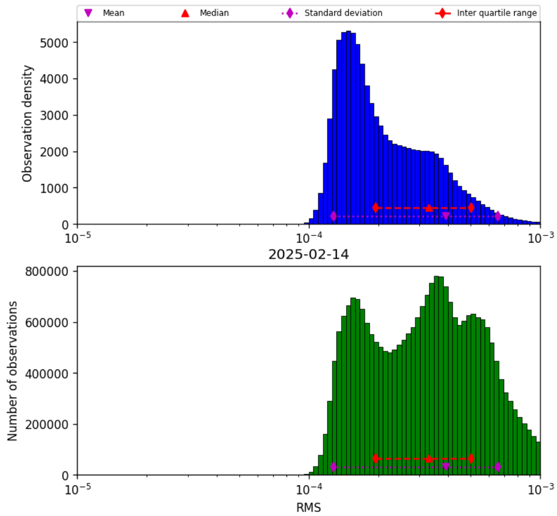
Figure 43: Histogram of “RMS” for 2025-02-13 to 2025-02-15
