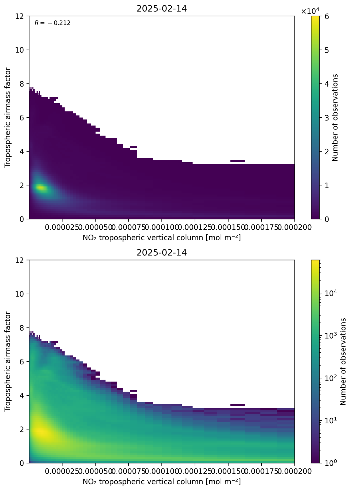
Figure 123: Scatter density plot of “NO 2 tropospheric vertical column” against “Tropospheric air mass factor” for 2025-02-13 to 2025-02-15.
