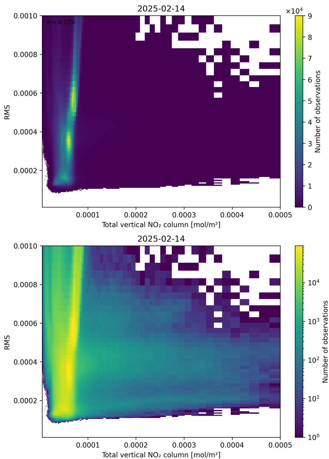
Figure 120: Scatter density plot of “Total vertical NO 2 column” against “RMS” for 2025-02-13 to 2025-02-15.
