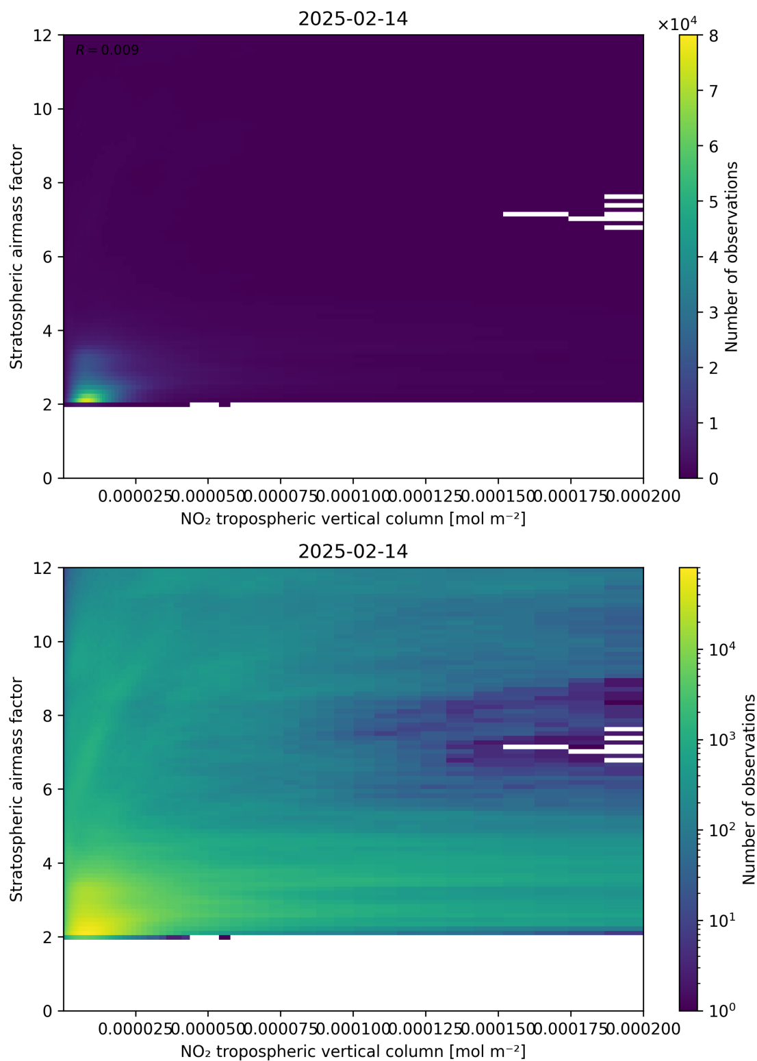
Figure 121: Scatter density plot of “NO 2 tropospheric vertical column” against “Stratospheric airmass factor” for 2025-02-13 to 2025-02-15.
