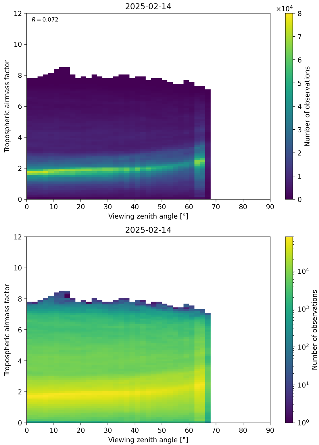
Figure 161: Scatter density plot of “Viewing zenith angle” against “Tropospheric airmass factor” for 2025-02-13 to 2025-02-15.
