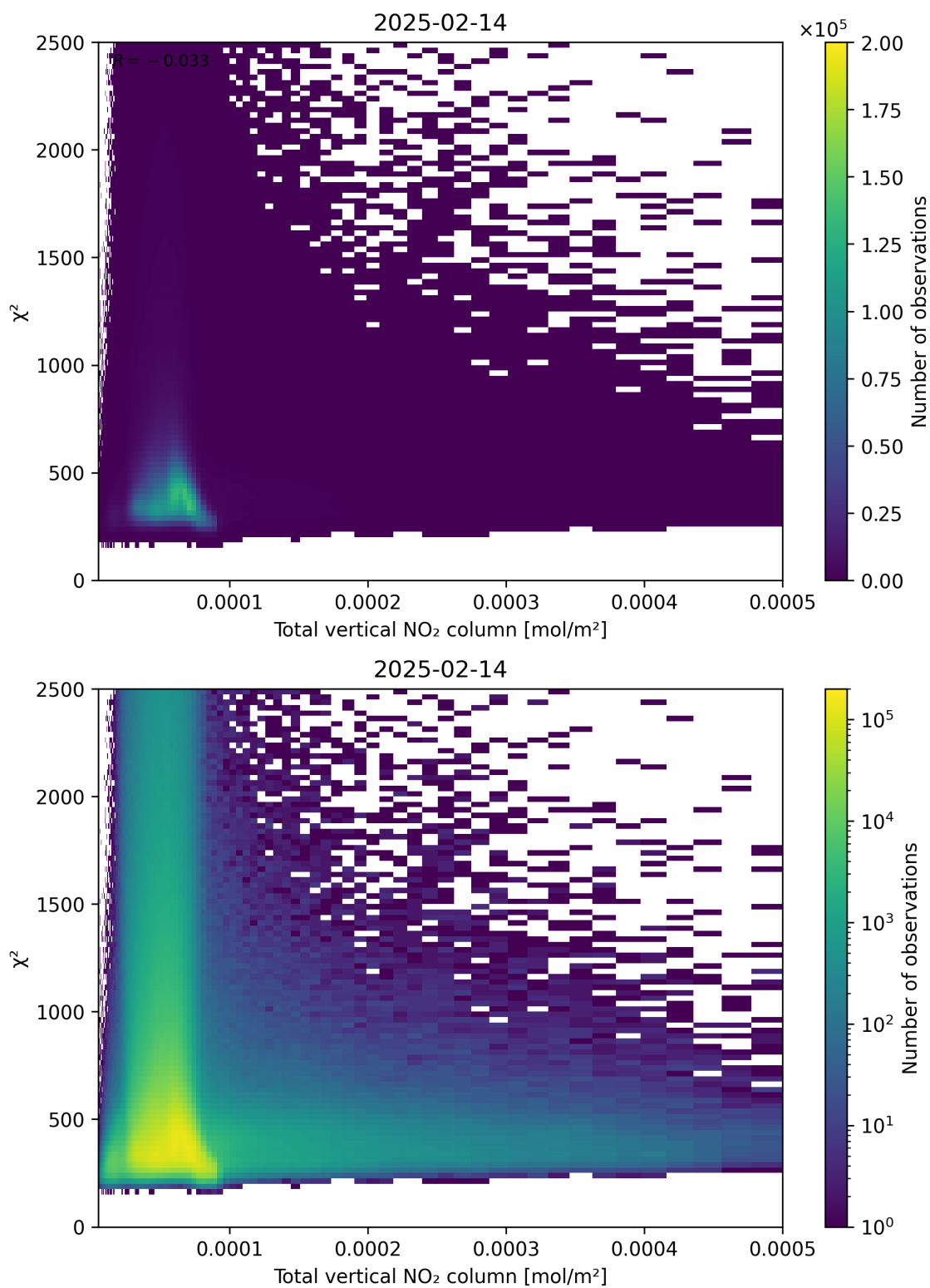
Figure 111: Scatter density plot of “Total vertical NO 2 column” against “ \chi^2 ” for 2025-02-13 to 2025-02-15.
