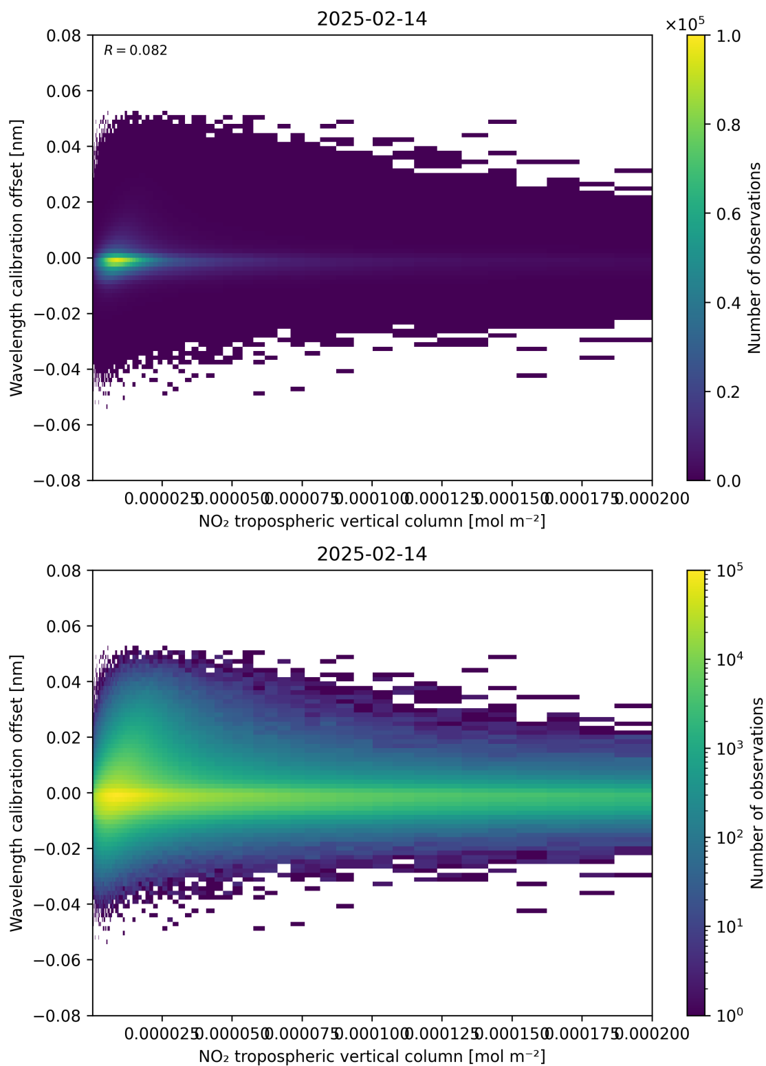
Figure 143: Scatter density plot of “NO 2 tropospheric vertical column” against “Wavelength calibration offset” for 2025-02-13 to 2025-02-15.
