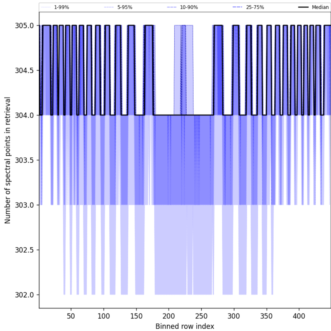
Figure 50: Along track statistics of “Number of spectral points in retrieval” for 2025-02-13 to 2025-02-15
