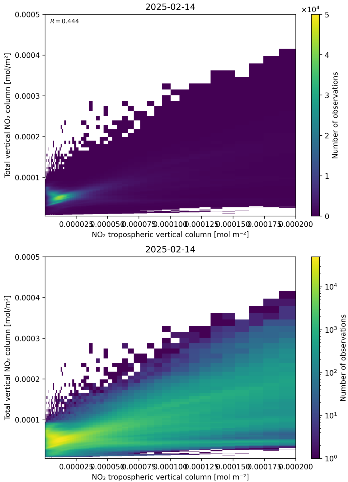
Figure 128: Scatter density plot of “NO 2 tropospheric vertical column” against “Total vertical NO 2 column” for 2025-02-13 to 2025-02-15.
