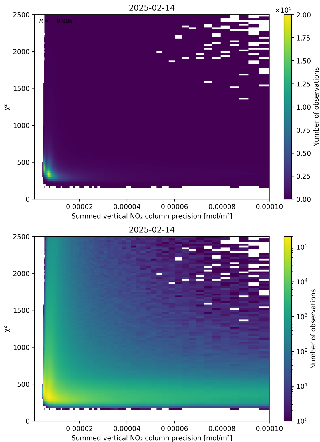
Figure 107: Scatter density plot of “Summed vertical NO 2 column precision” against “ \chi^2 ” for 2025-02-13 to 2025-02-15.
