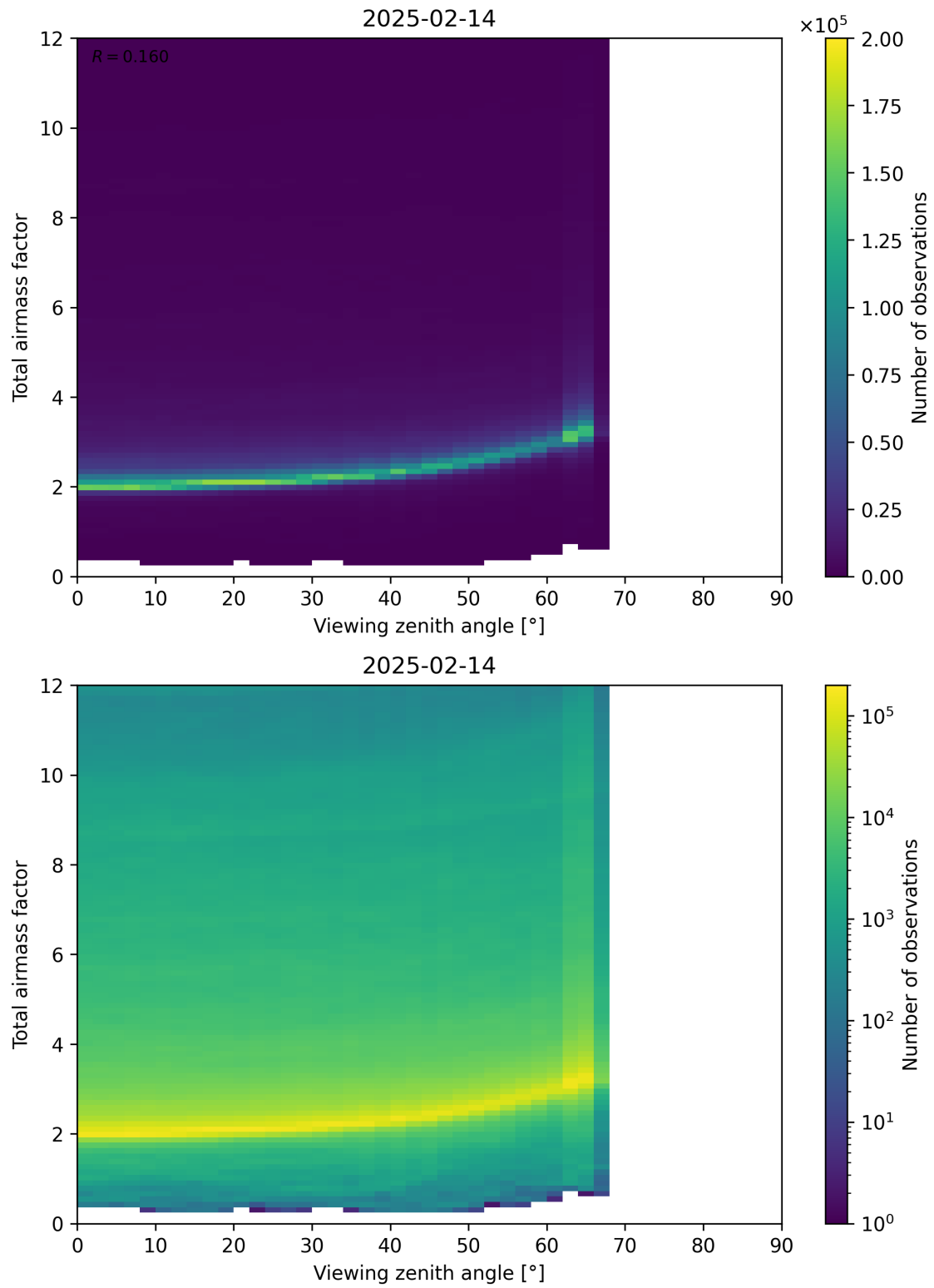
Figure 160: Scatter density plot of “Viewing zenith angle” against “Total airmass factor” for 2025-02-13 to 2025-02-15.
