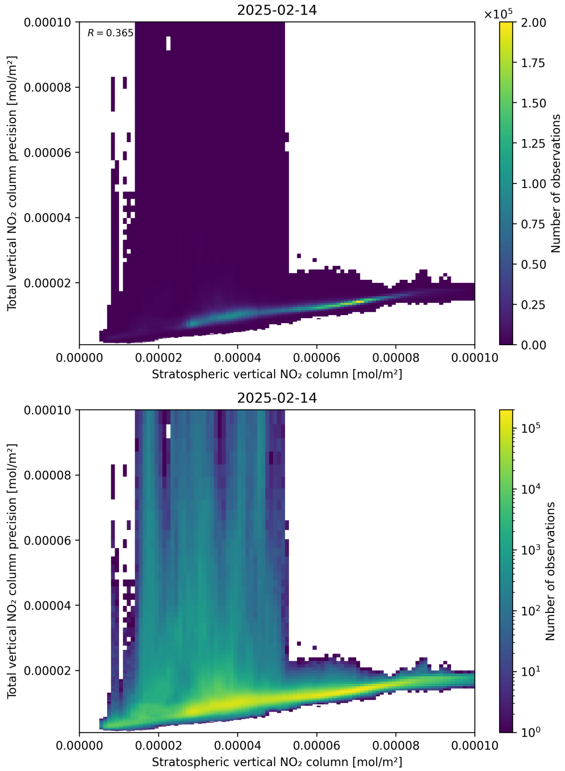
Figure 101: Scatter density plot of “Stratospheric vertical NO 2 column” against “Total vertical NO 2 column precision” for 2025-02-13 to 2025-02-15.
