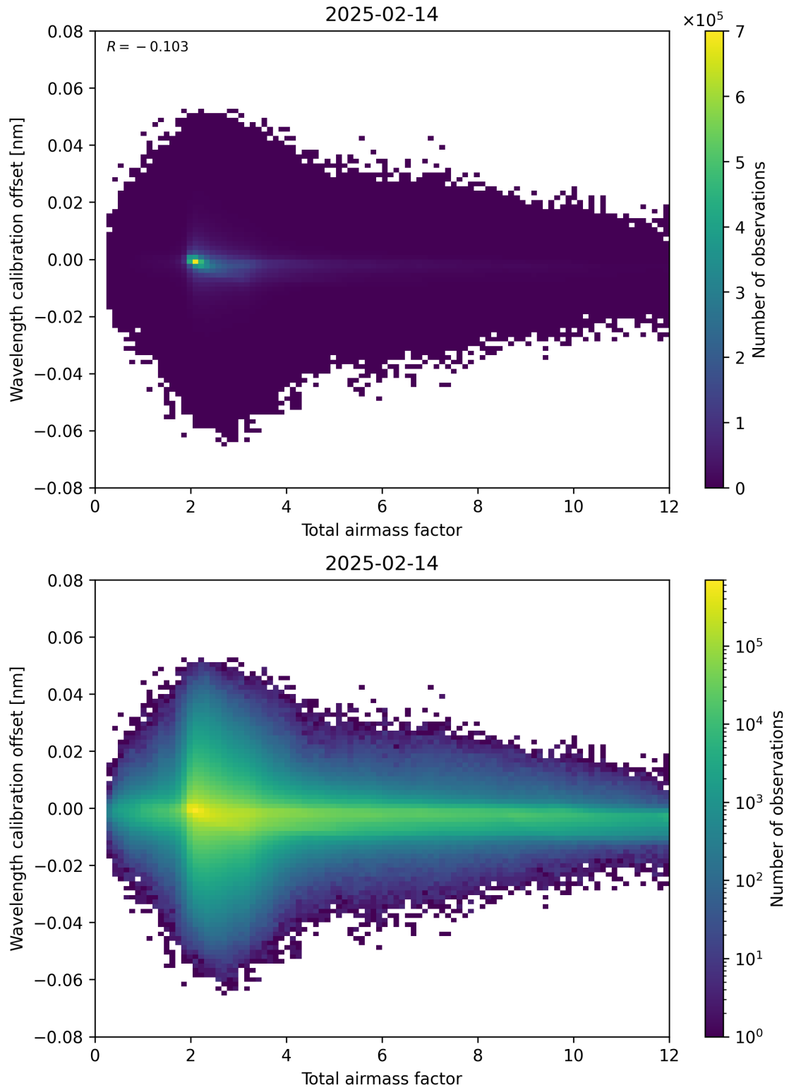
Figure 70: Scatter density plot of “Total airmass factor” against “Wavelength calibration offset” for 2025-02-13 to 2025-02-15.
