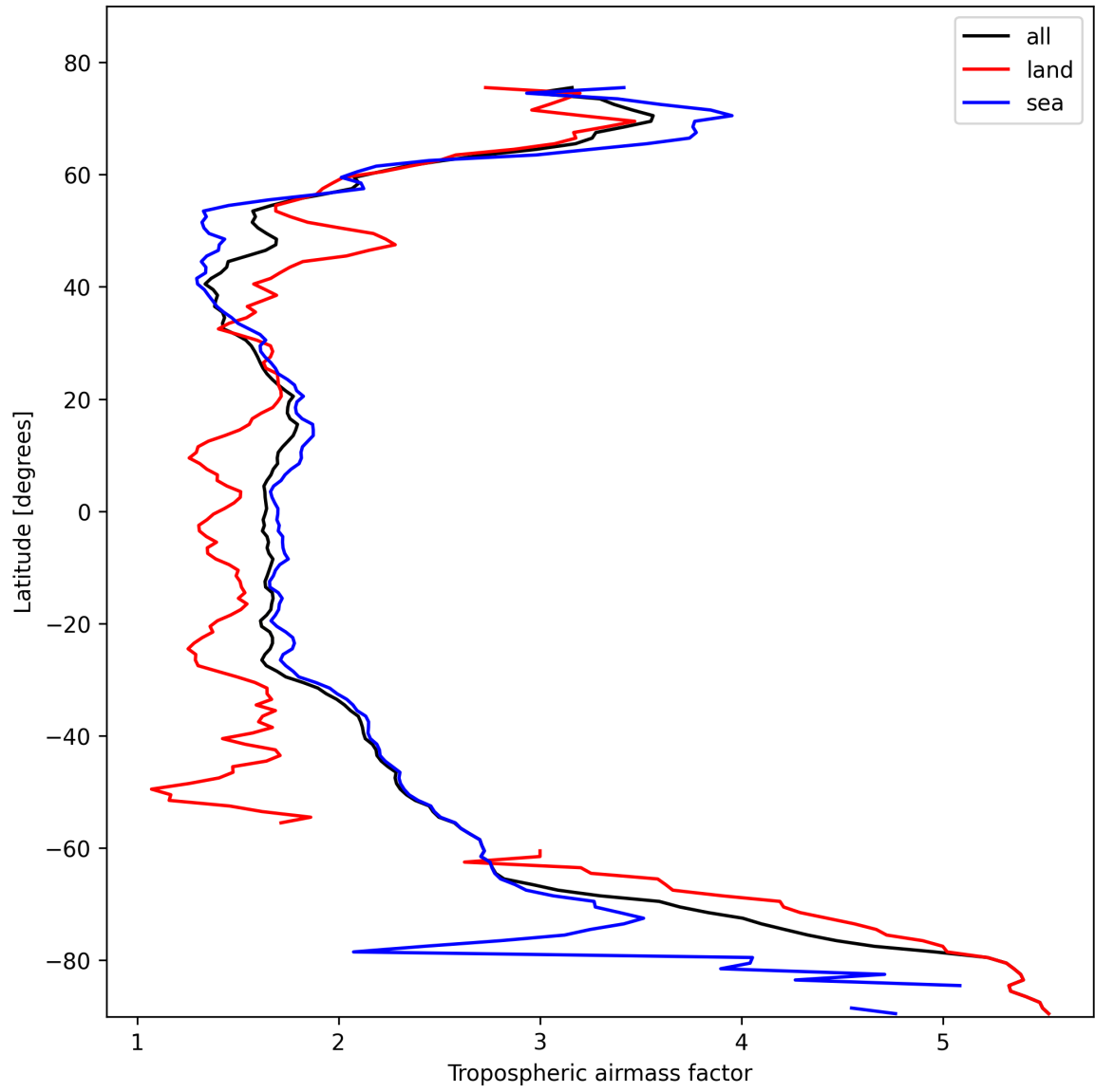
Figure 14: Zonal average of “Tropospheric airmass factor” for 2025-02-13 to 2025-02-15.
