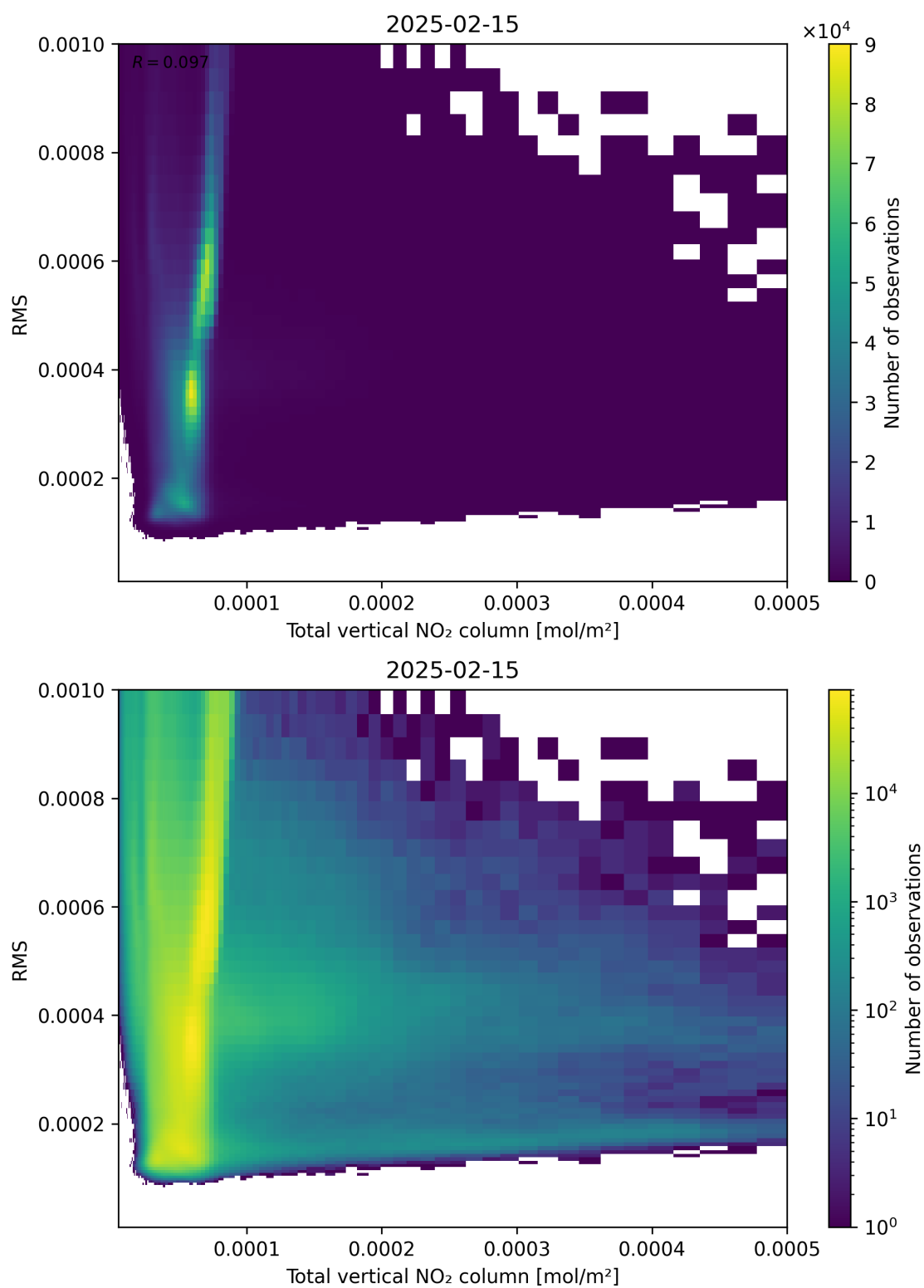
Figure 120: Scatter density plot of “Total vertical NO 2 column” against “RMS” for 2025-02-14 to 2025-02-16.
