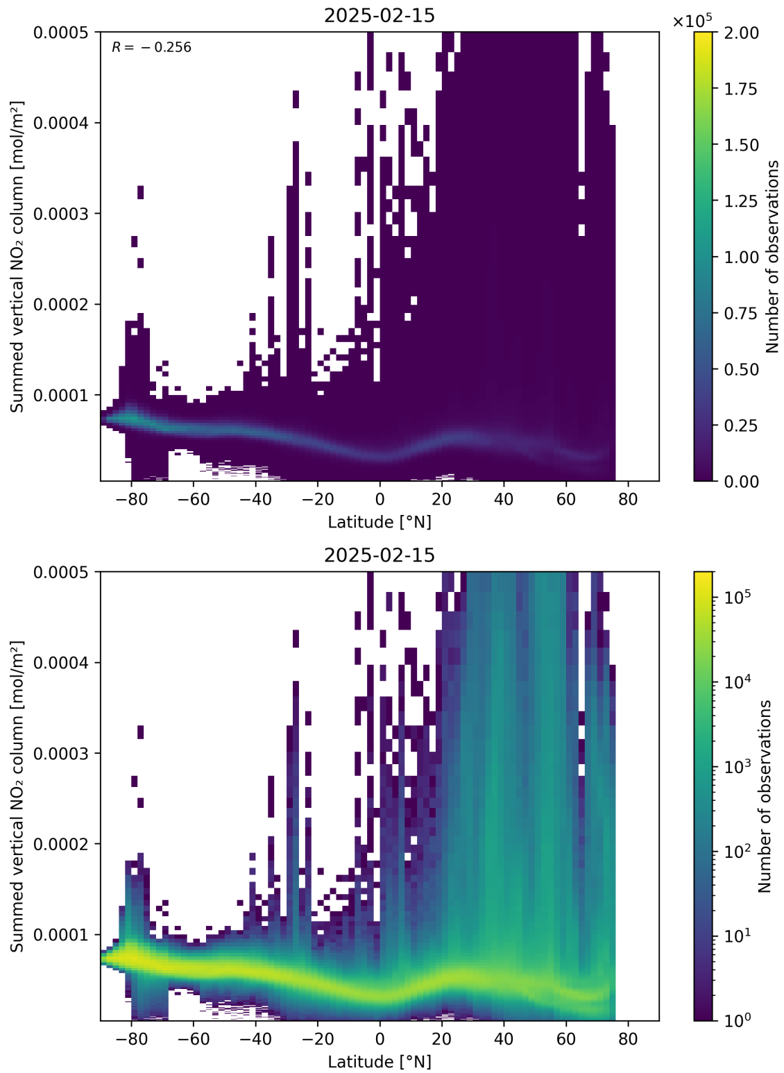
Figure 88: Scatter density plot of “Latitude” against “Summed vertical NO 2 column” for 2025-02-14 to 2025-02-16.
