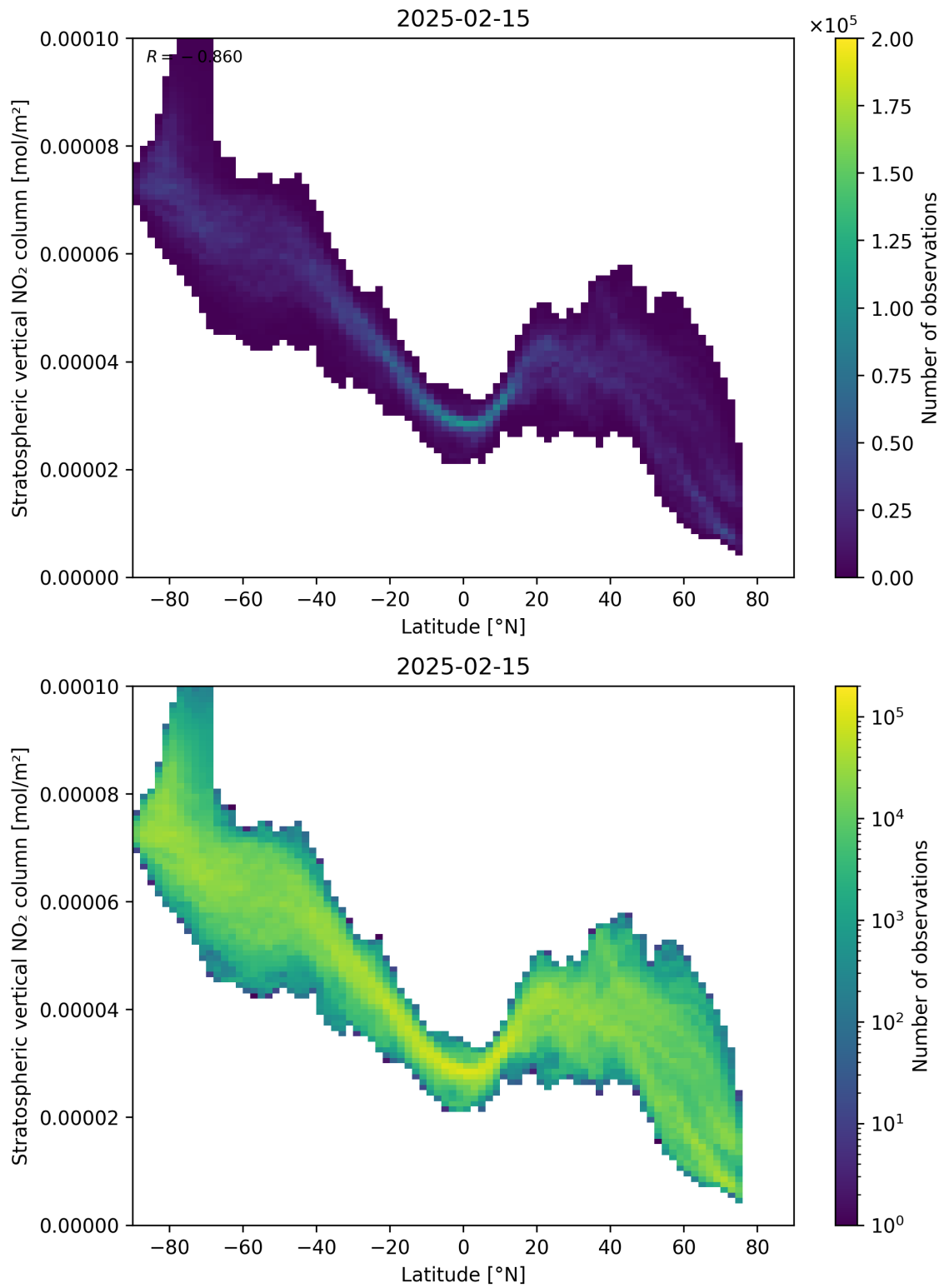
Figure 87: Scatter density plot of “Latitude” against “Stratospheric vertical NO 2 column” for 2025-02-14 to 2025-02-16.
