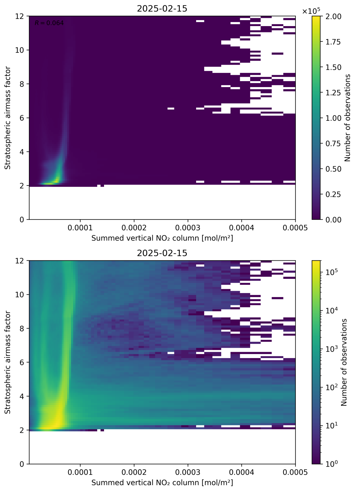
Figure 103: Scatter density plot of “Summed vertical NO 2 column” against “Stratospheric air mass factor” for 2025-02-14 to 2025-02-16.
