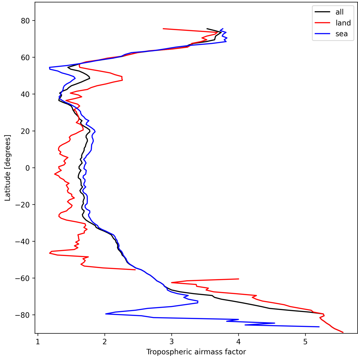
Figure 14: Zonal average of “Tropospheric airmass factor” for 2025-02-14 to 2025-02-16.
