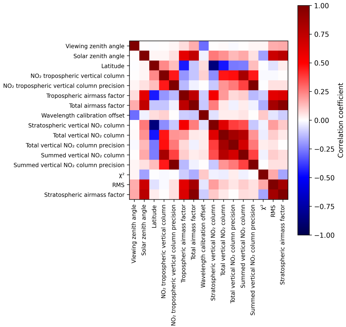
Figure 2: Map of correlation matrix for 2025-02-14 to 2025-02-16.
