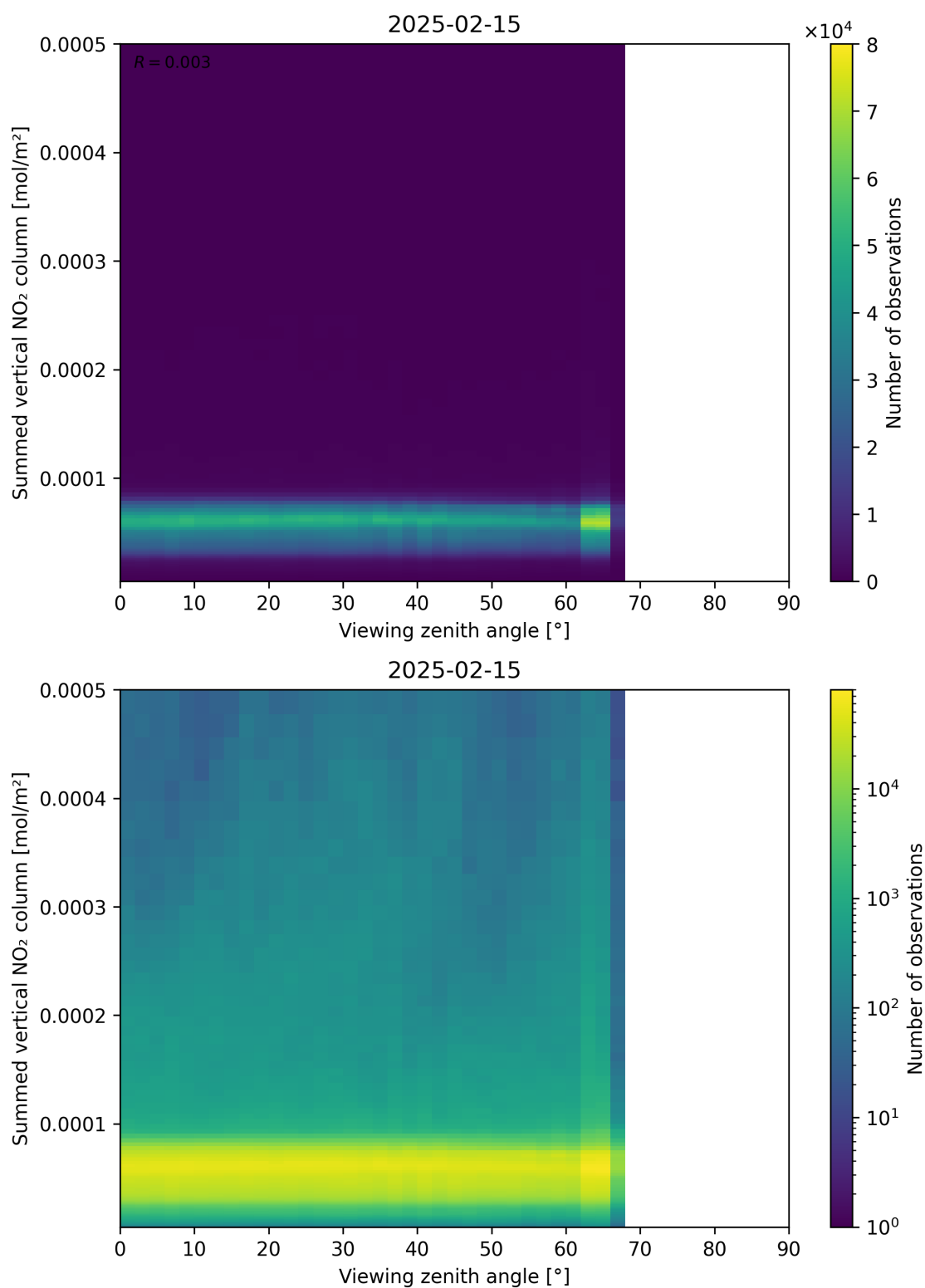
Figure 165: Scatter density plot of “Viewing zenith angle” against “Summed vertical NO 2 column” for 2025-02-14 to 2025-02-16.
