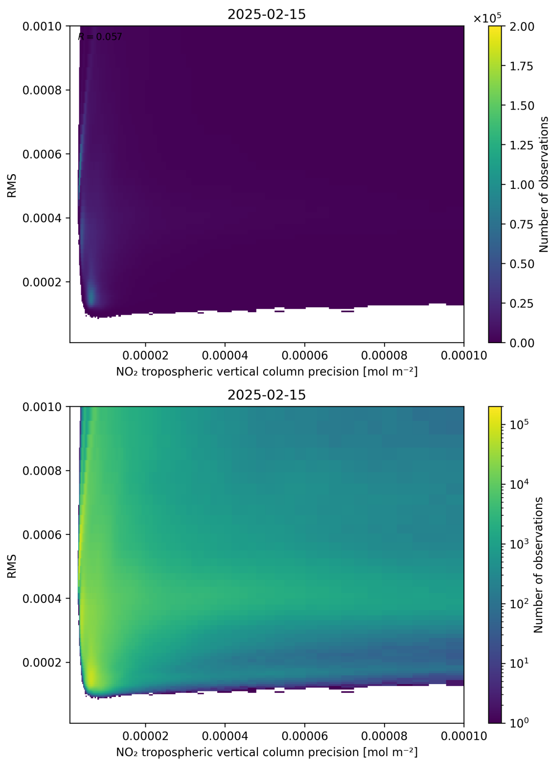
Figure 140: Scatter density plot of “NO 2 tropospheric vertical column precision” against “RMS” for 2025-02-14 to 2025-02-16.
