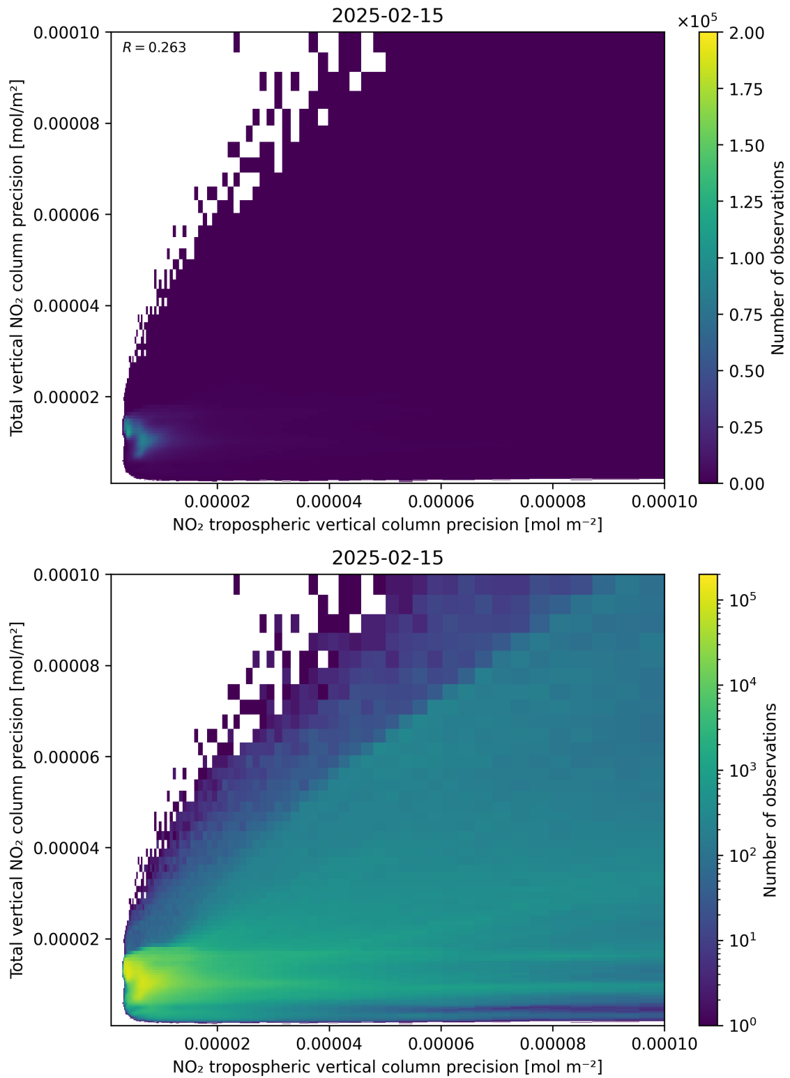
Figure 139: Scatter density plot of “NO 2 tropospheric vertical column precision” against “Total vertical NO 2 column precision” for 2025-02-14 to 2025-02-16.
