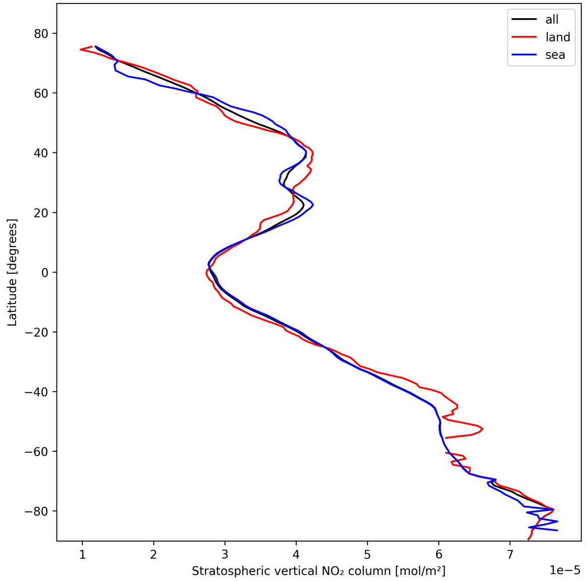
Figure 19: Zonal average of “Stratospheric vertical NO 2 column” for 2025-02-14 to 2025-02-16.
