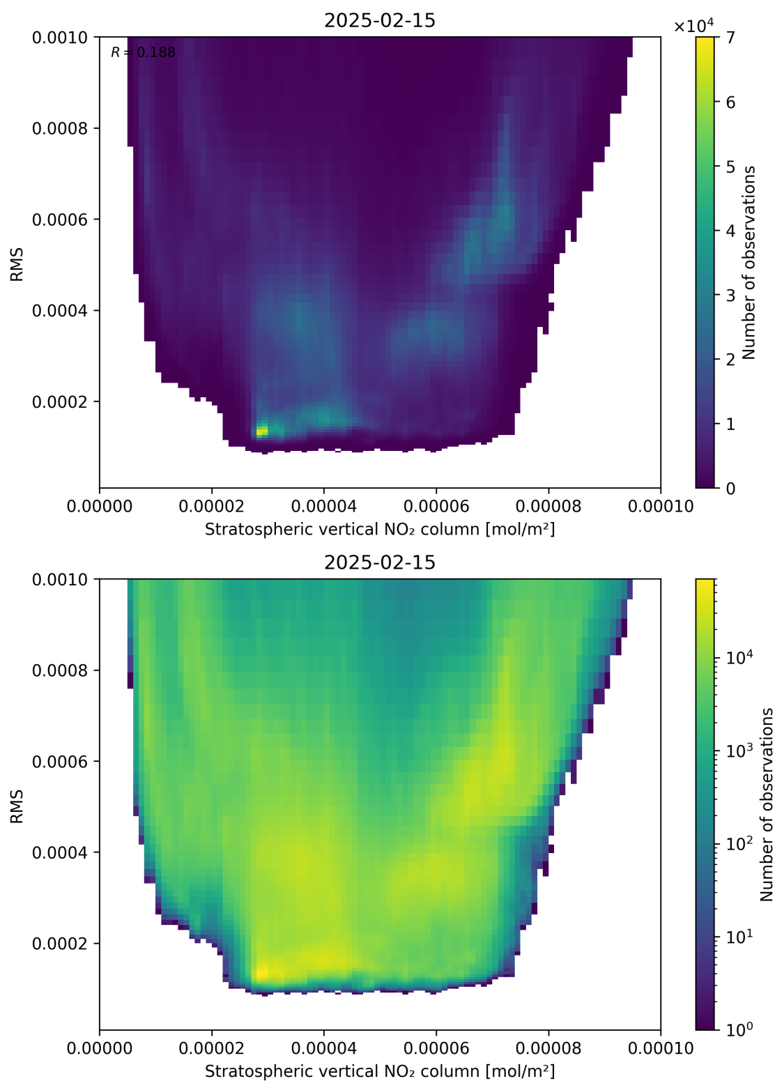
Figure 102: Scatter density plot of “Stratospheric vertical NO 2 column” against “RMS” for 2025-02-14 to 2025-02-16.
