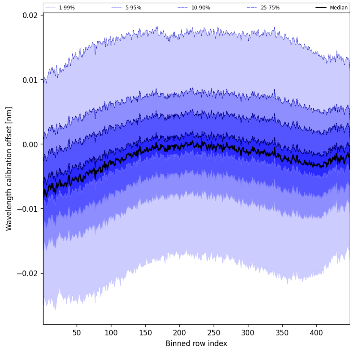
Figure 52: Along track statistics of “Wavelength calibration offset” for 2025-02-14 to 2025-02-16
