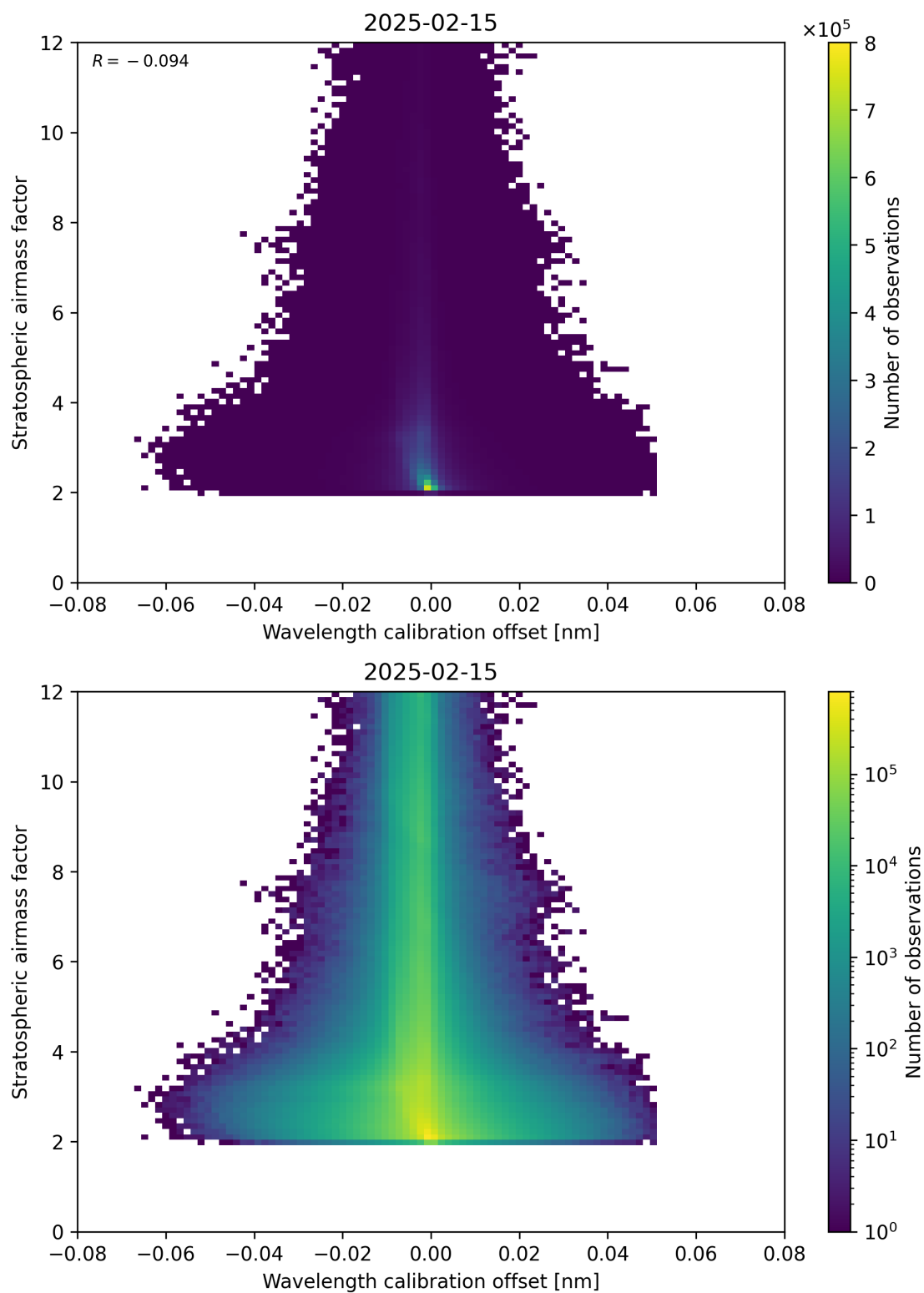
Figure 174: Scatter density plot of “Wavelength calibration offset” against “Stratospheric airmass factor” for 2025-02-14 to 2025-02-16.
