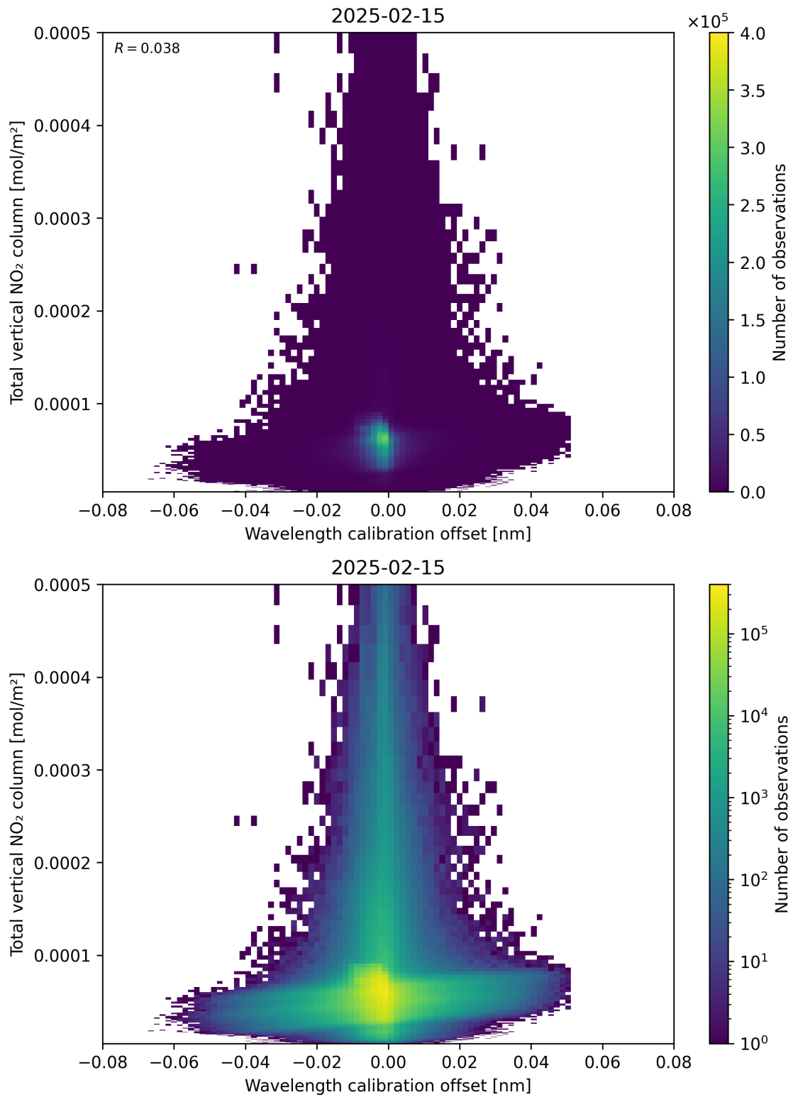
Figure 179: Scatter density plot of “Wavelength calibration offset” against “Total vertical NO 2 column” for 2025-02-14 to 2025-02-16.
