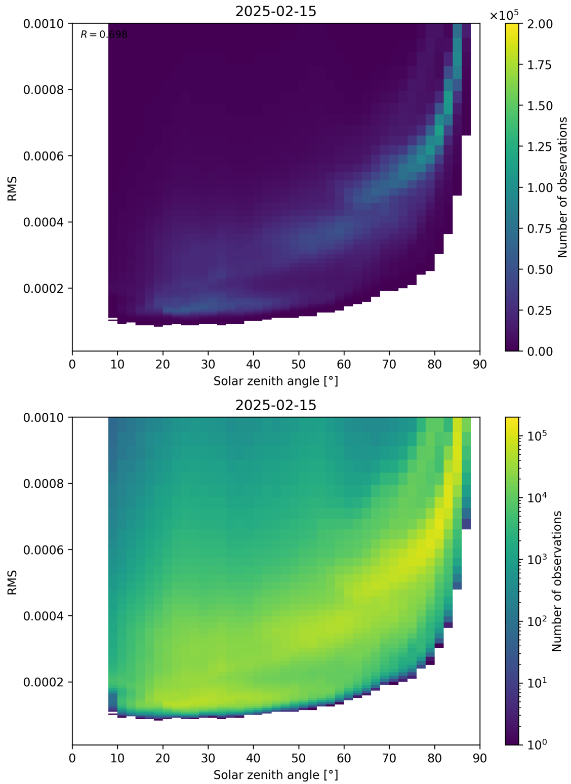
Figure 157: Scatter density plot of “Solar zenith angle” against “RMS” for 2025-02-14 to 2025-02-16.
