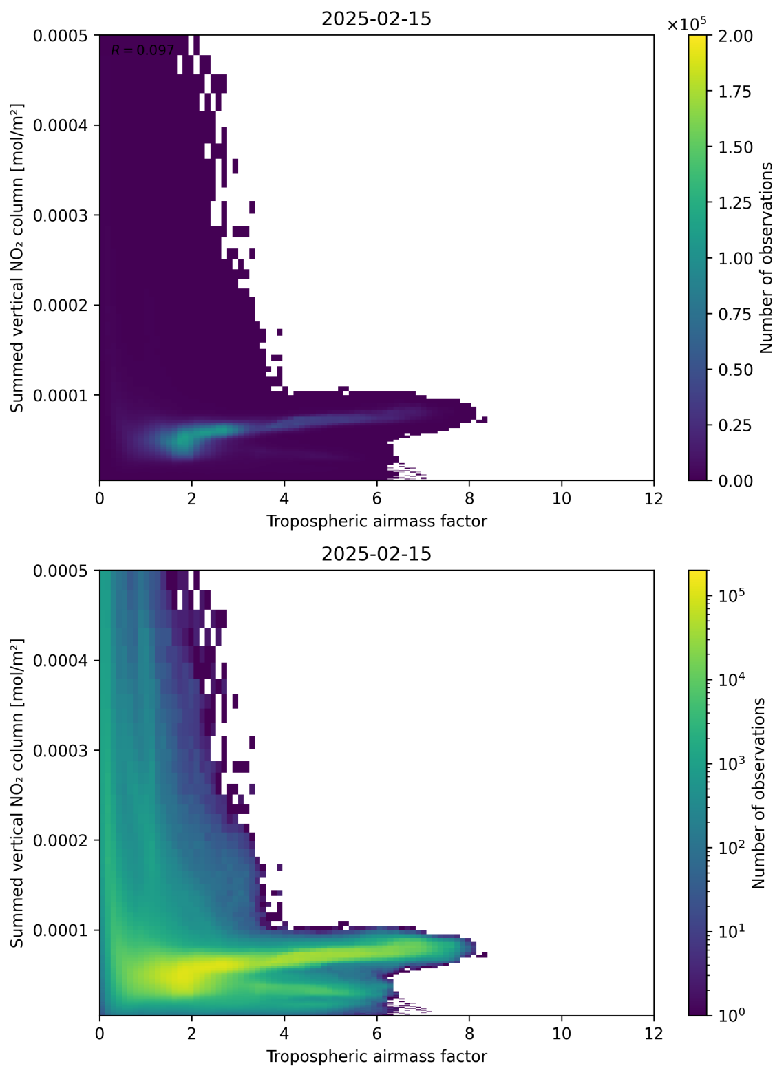
Figure 75: Scatter density plot of “Tropospheric air mass factor” against “Summed vertical NO 2 column” for 2025-02-14 to 2025-02-16.
