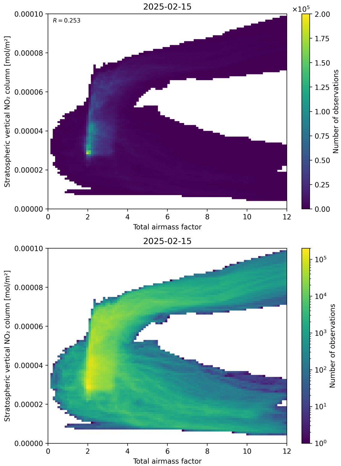
Figure 64: Scatter density plot of “Total airmass factor” against “Stratospheric vertical NO 2 column” for 2025-02-14 to 2025-02-16.
