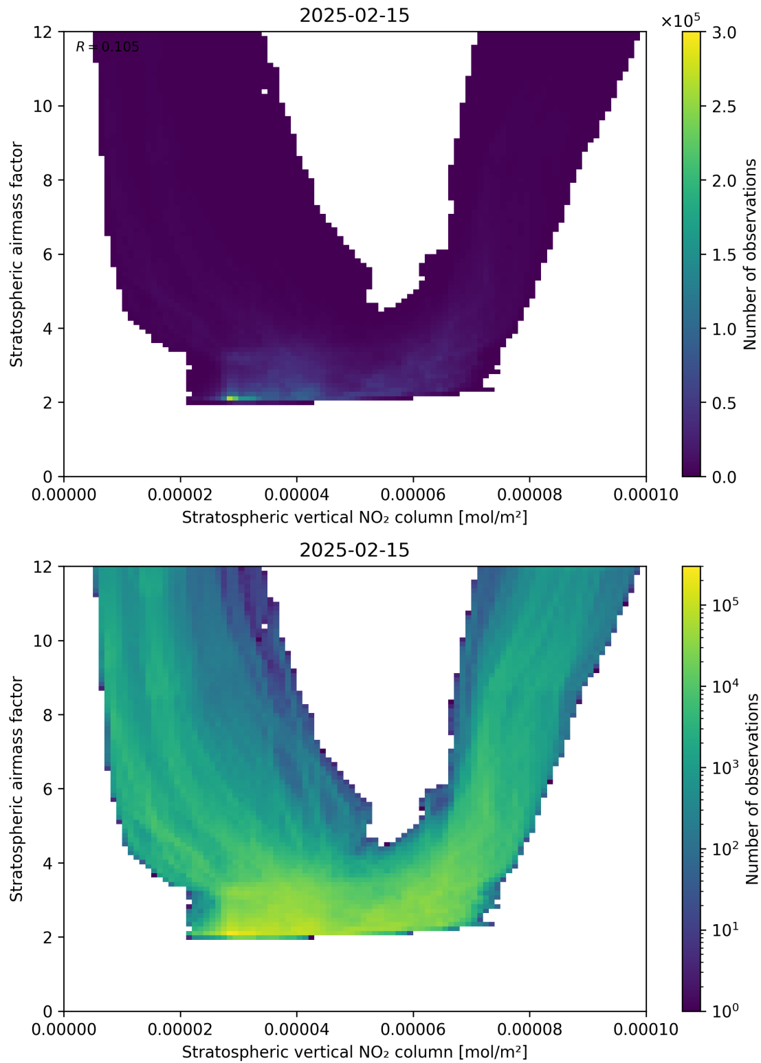
Figure 96: Scatter density plot of “Stratospheric vertical NO 2 column” against “Stratospheric airmass factor” for 2025-02-14 to 2025-02-16.
