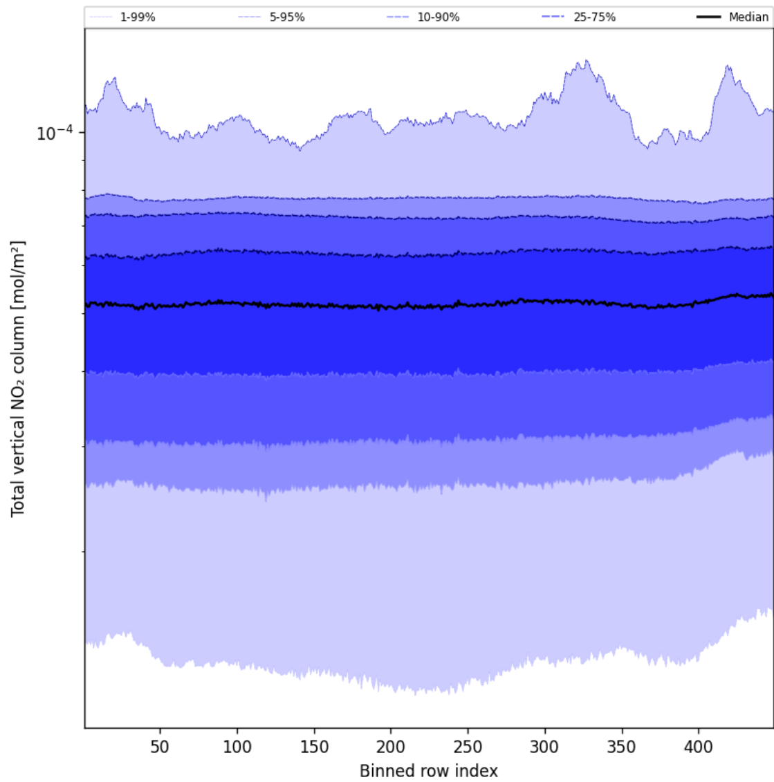
Figure 55: Along track statistics of “Total vertical NO 2 column” for 2025-02-14 to 2025-02-16
