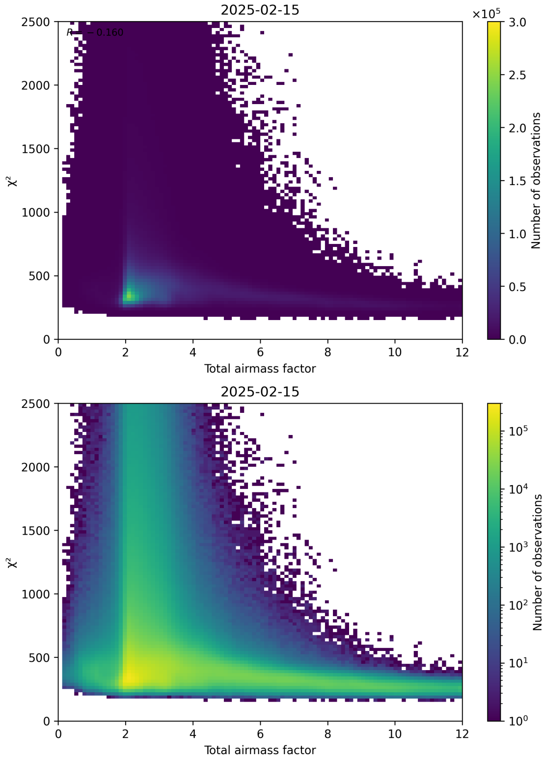
Figure 63: Scatter density plot of “Total airmass factor” against “ \chi^2 ” for 2025-02-14 to 2025-02-16.
