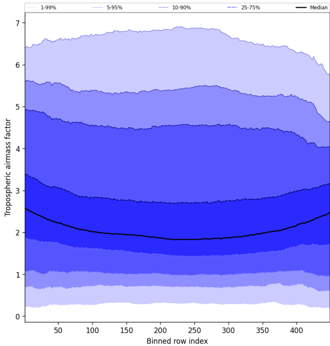
Figure 48: Along track statistics of “Tropospheric airmass factor” for 2025-02-14 to 2025-02-16
