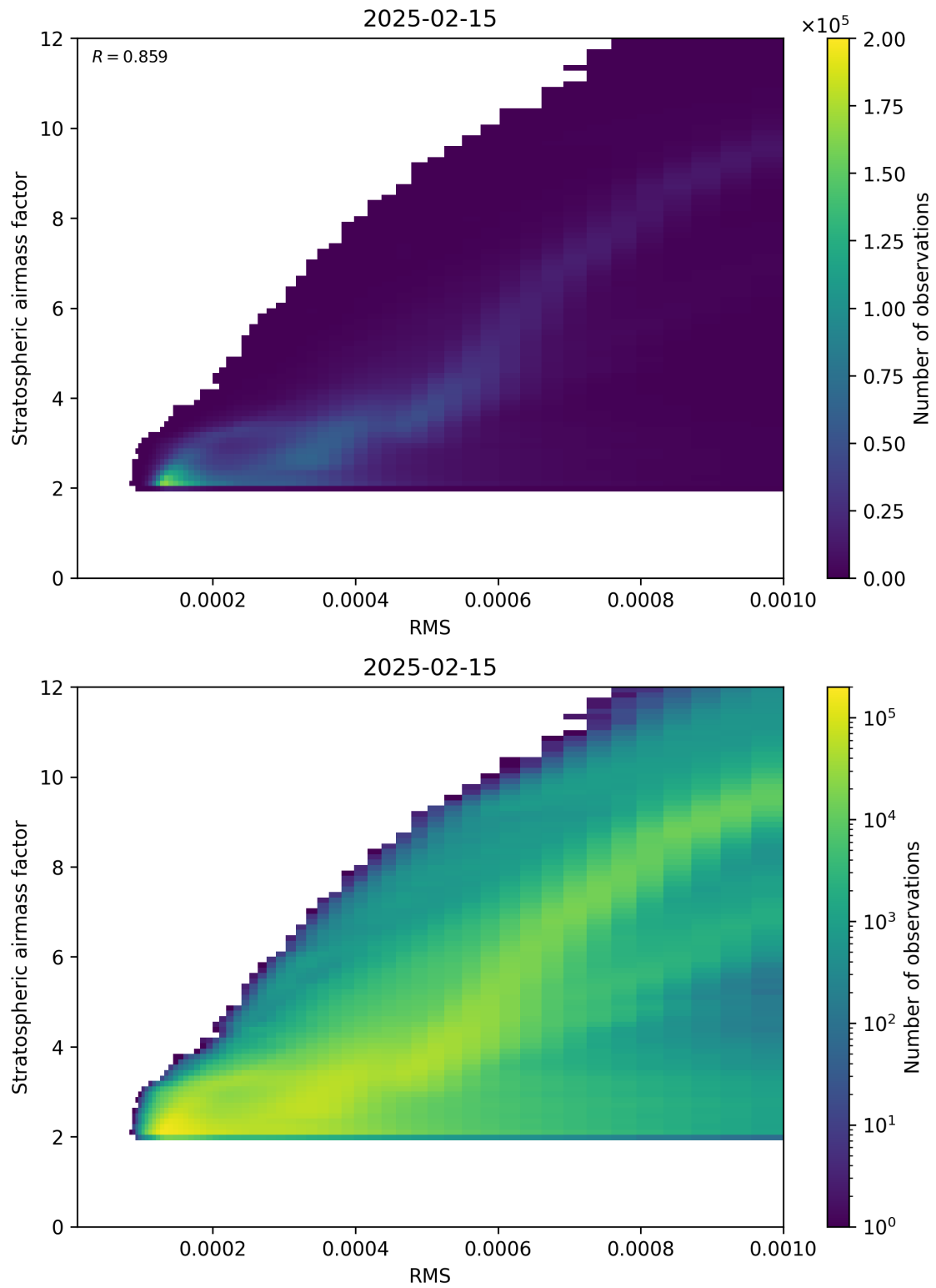
Figure 144: Scatter density plot of “RMS” against “Stratospheric airmass factor” for 2025-02-14 to 2025-02-16.
