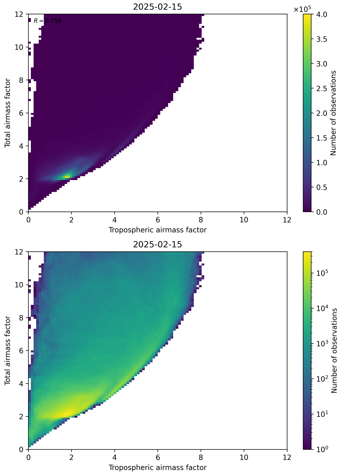
Figure 72: Scatter density plot of “Tropospheric airmass factor” against “Total airmass factor” for 2025-02-14 to 2025-02-16.
