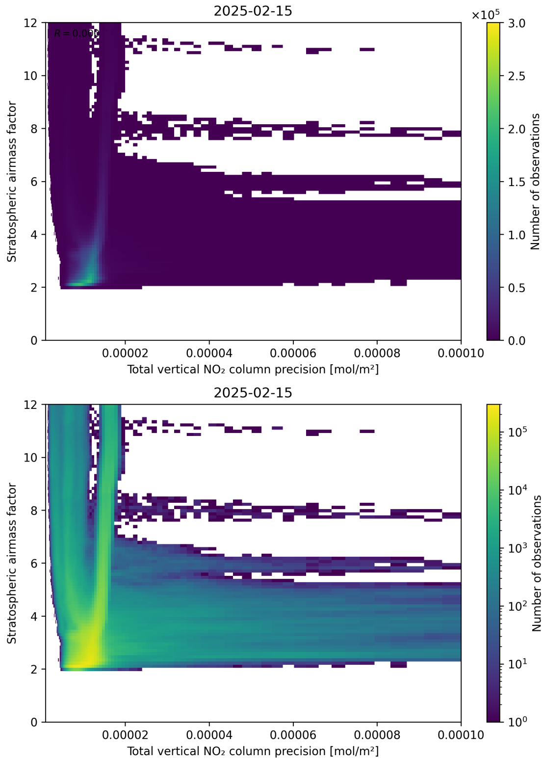
Figure 115: Scatter density plot of “Total vertical NO 2 column precision” against “Stratospheric air mass factor” for 2025-02-14 to 2025-02-16.
