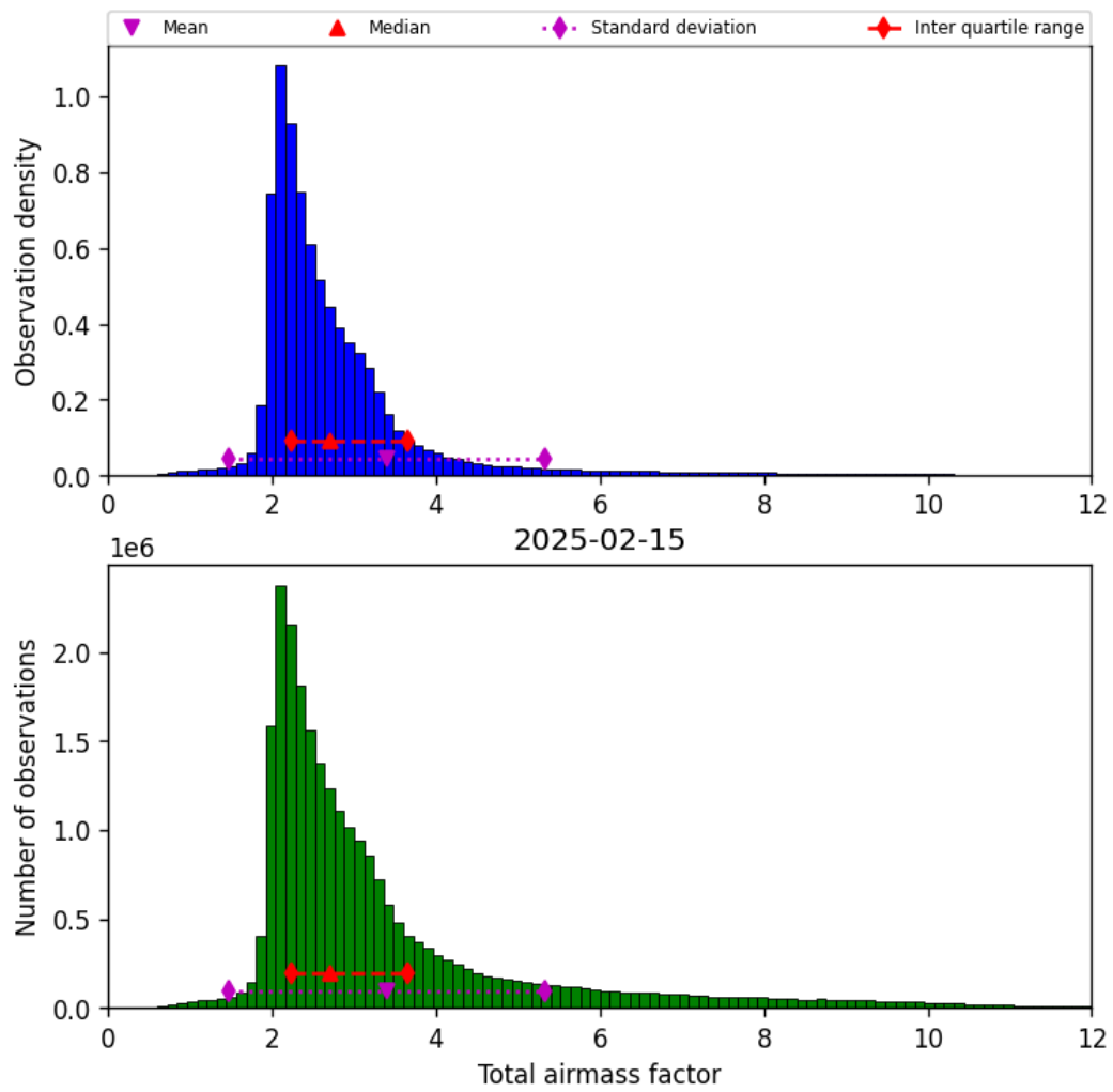
Figure 32: Histogram of “Total airmass factor” for 2025-02-14 to 2025-02-16
