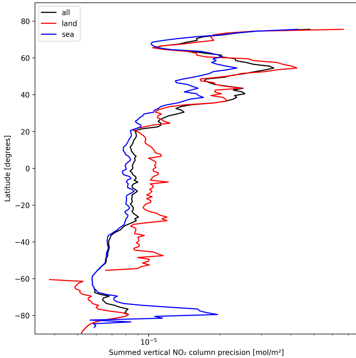
Figure 24: Zonal average of “Summed vertical NO 2 column precision” for 2025-02-14 to 2025-02-16.
