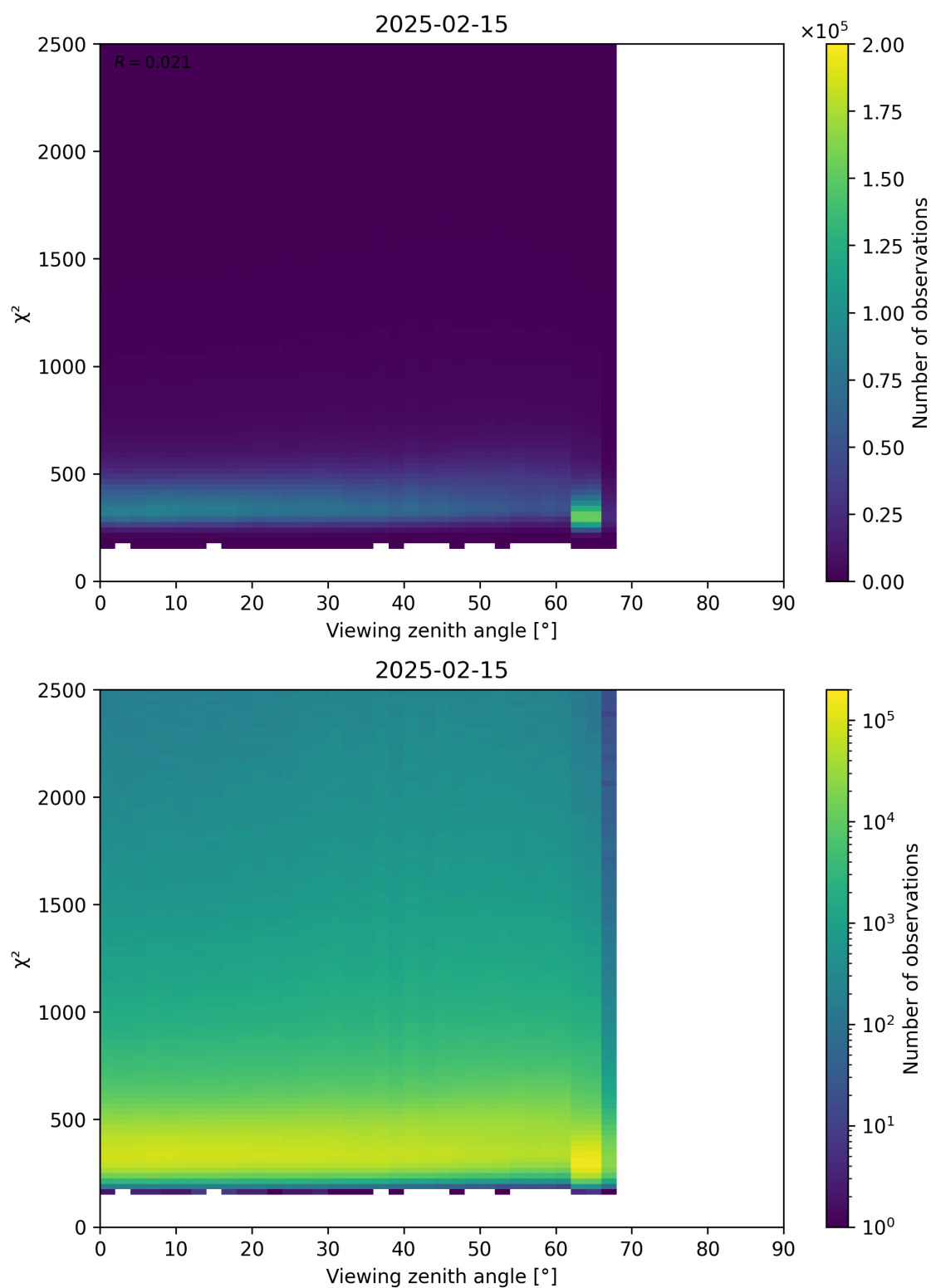
Figure 162: Scatter density plot of “Viewing zenith angle” against “ \chi^2 ” for 2025-02-14 to 2025-02-16.
