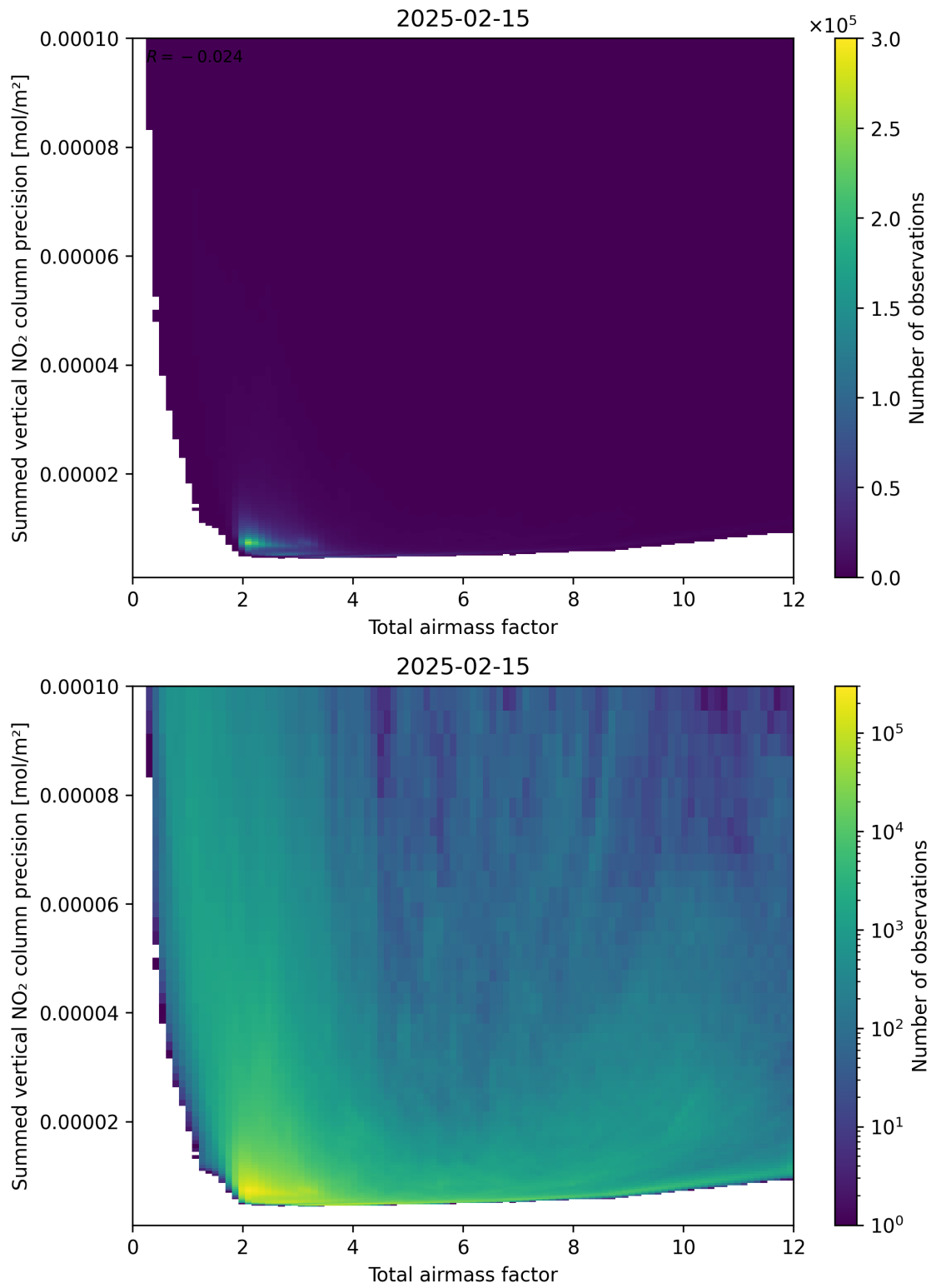
Figure 66: Scatter density plot of “Total airmass factor” against “Summed vertical NO 2 column precision” for 2025-02-14 to 2025-02-16.
