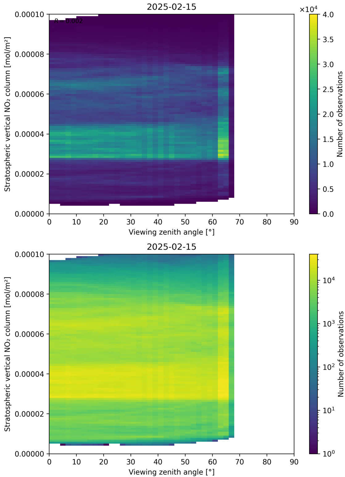
Figure 164: Scatter density plot of “Viewing zenith angle” against “Stratospheric vertical NO 2 column” for 2025-02-14 to 2025-02-16.
