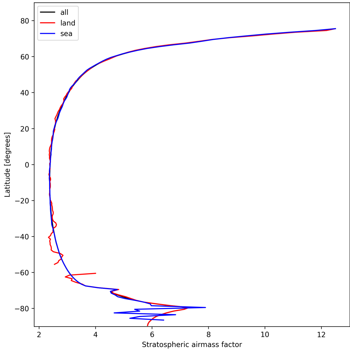
Figure 27: Zonal average of “Stratospheric airmass factor” for 2025-02-14 to 2025-02-16.
