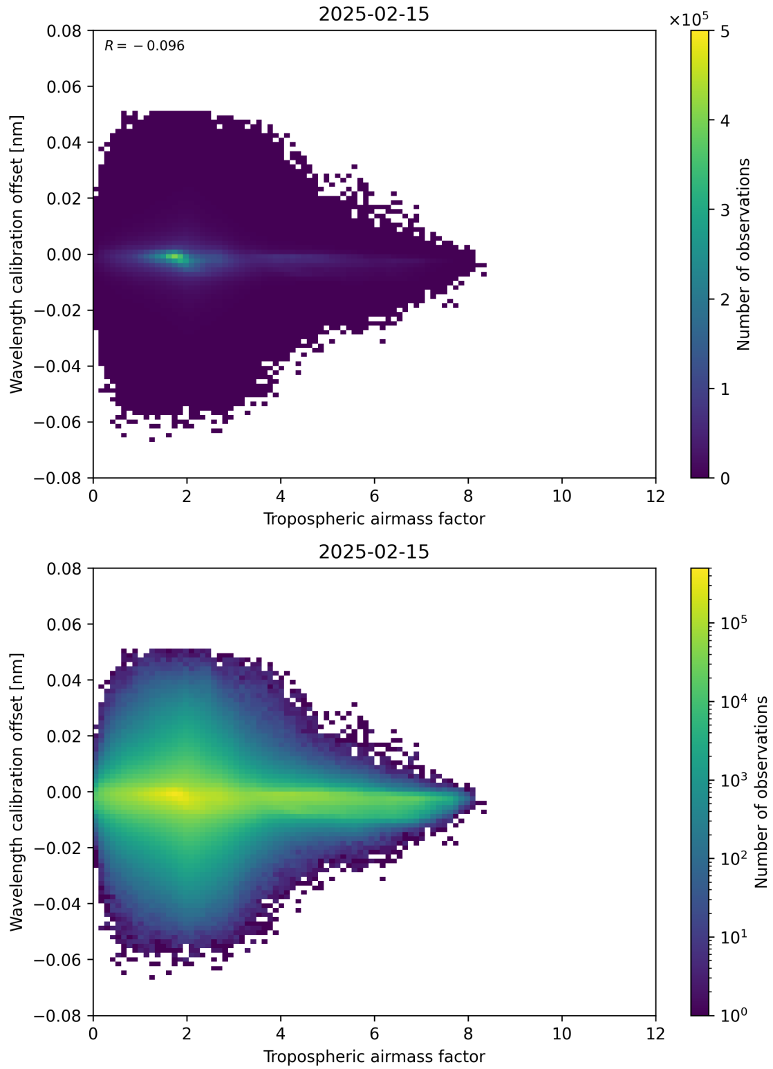
Figure 80: Scatter density plot of “Tropospheric airmass factor” against “Wavelength calibration offset” for 2025-02-14 to 2025-02-16.
