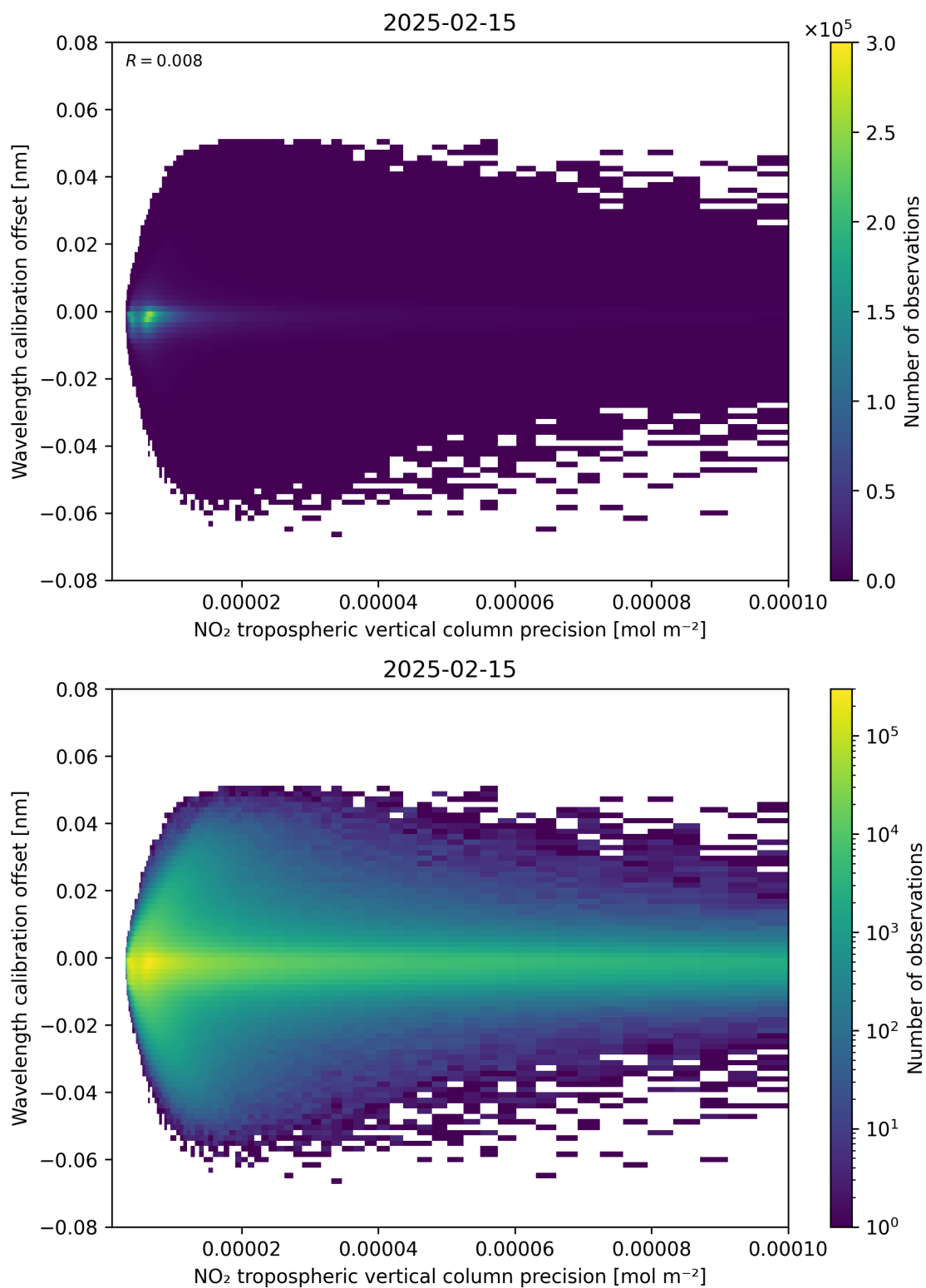
Figure 141: Scatter density plot of “NO 2 tropospheric vertical column precision” against “Wavelength calibration offset” for 2025-02-14 to 2025-02-16.
