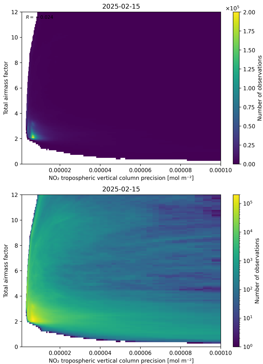
Figure 132: Scatter density plot of “NO 2 tropospheric vertical column precision” against “Total air mass factor” for 2025-02-14 to 2025-02-16.
