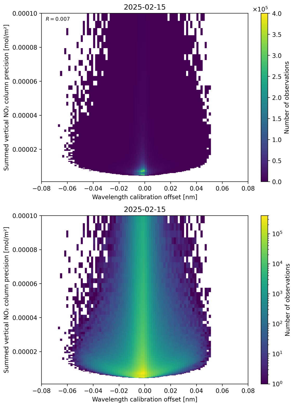
Figure 178: Scatter density plot of “Wavelength calibration offset” against “Summed vertical NO 2 column precision” for 2025-02-14 to 2025-02-16.
