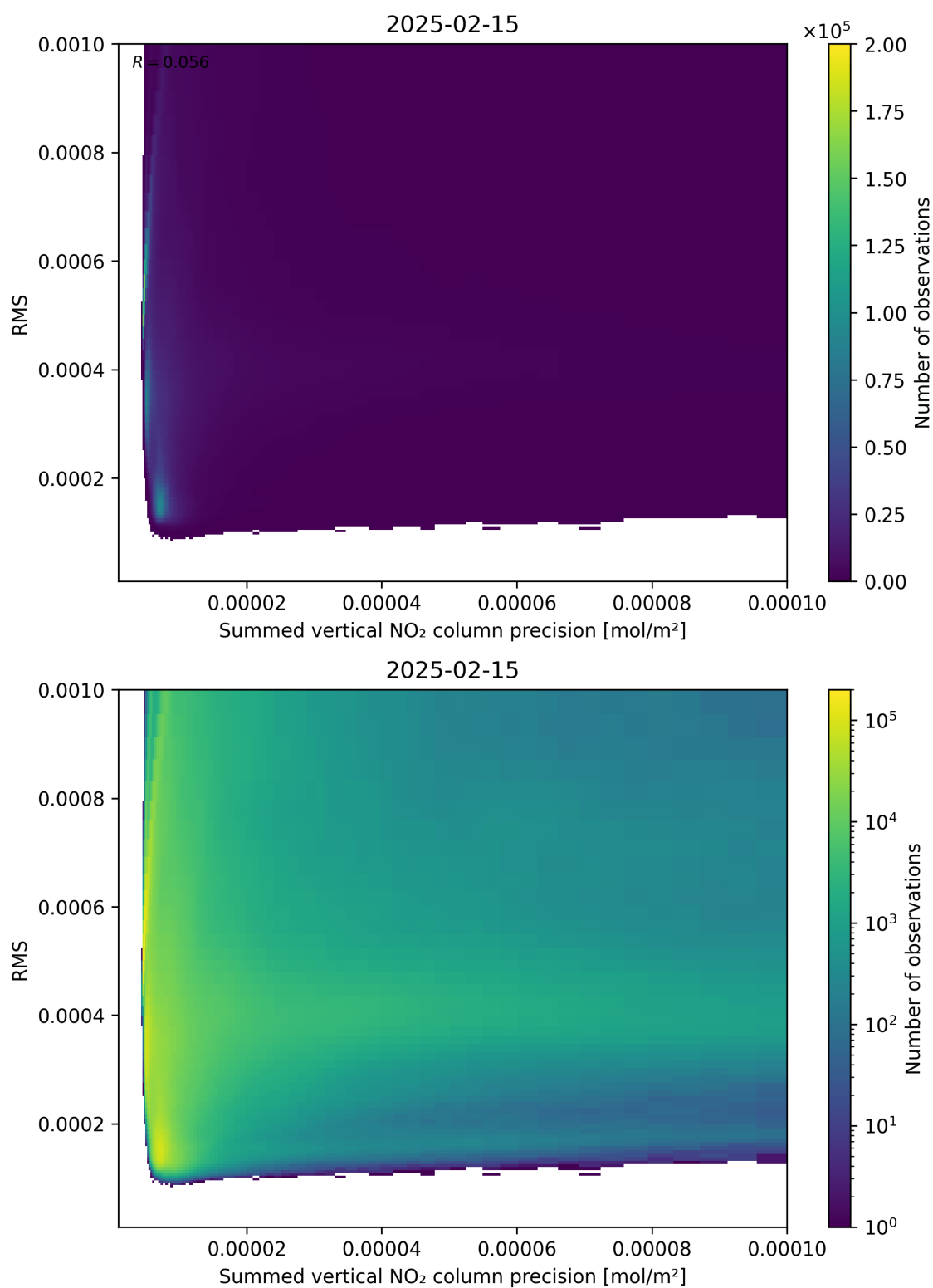
Figure 108: Scatter density plot of “Summed vertical NO 2 column precision” against “RMS” for 2025-02-14 to 2025-02-16.
