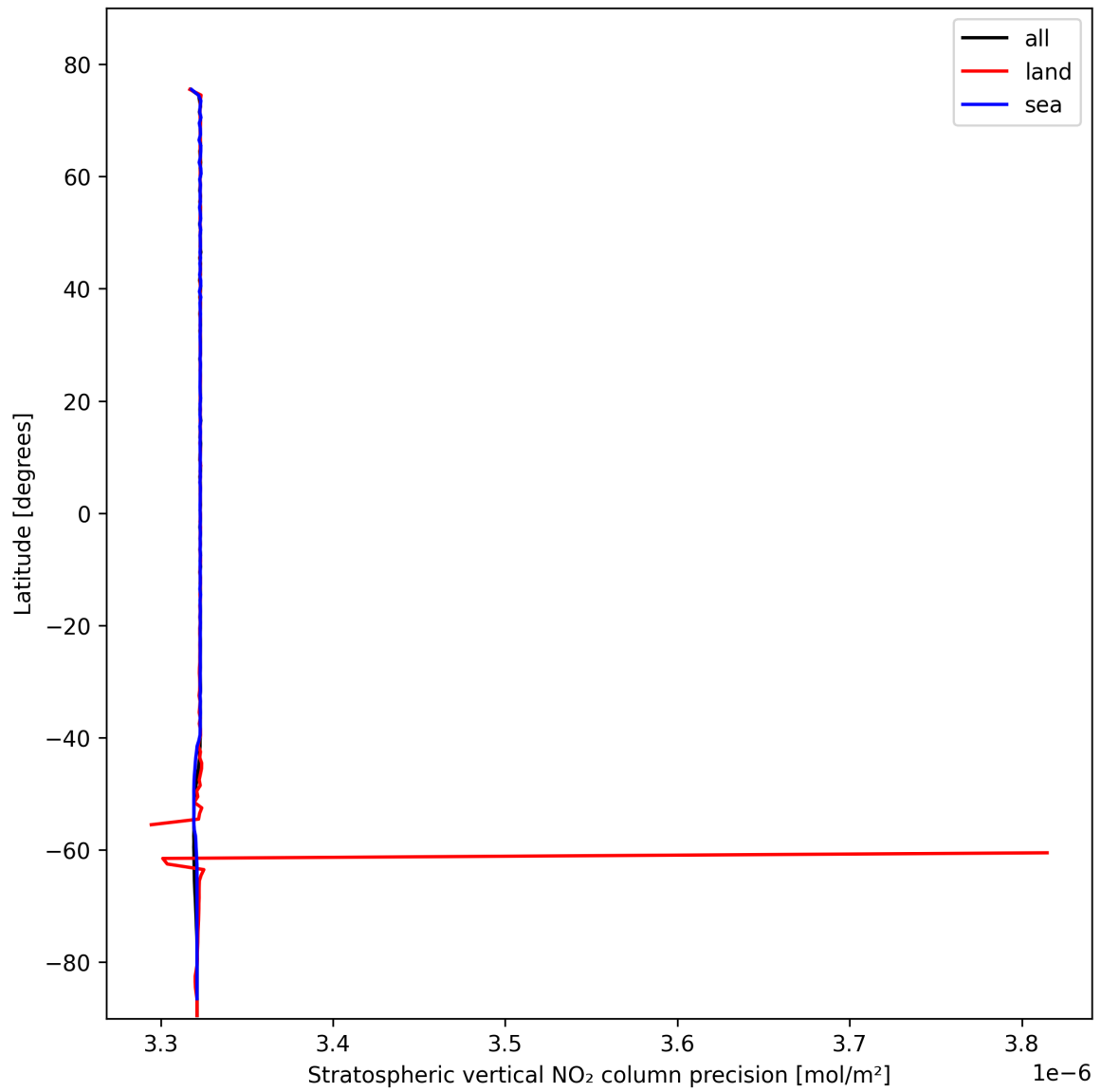
Figure 20: Zonal average of "Stratospheric vertical NO 2 column precision" for 2025-02-14 to 2025-02-16.
