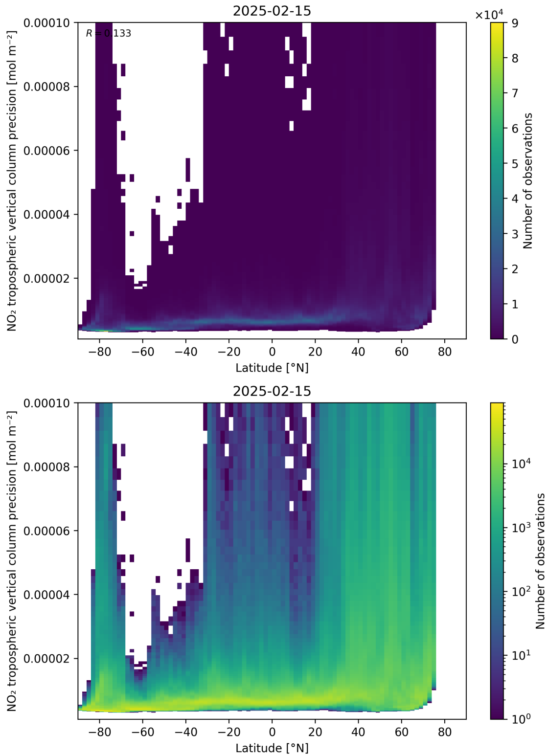
Figure 93: Scatter density plot of “Latitude” against “NO 2 tropospheric vertical column precision” for 2025-02-14 to 2025-02-16.
