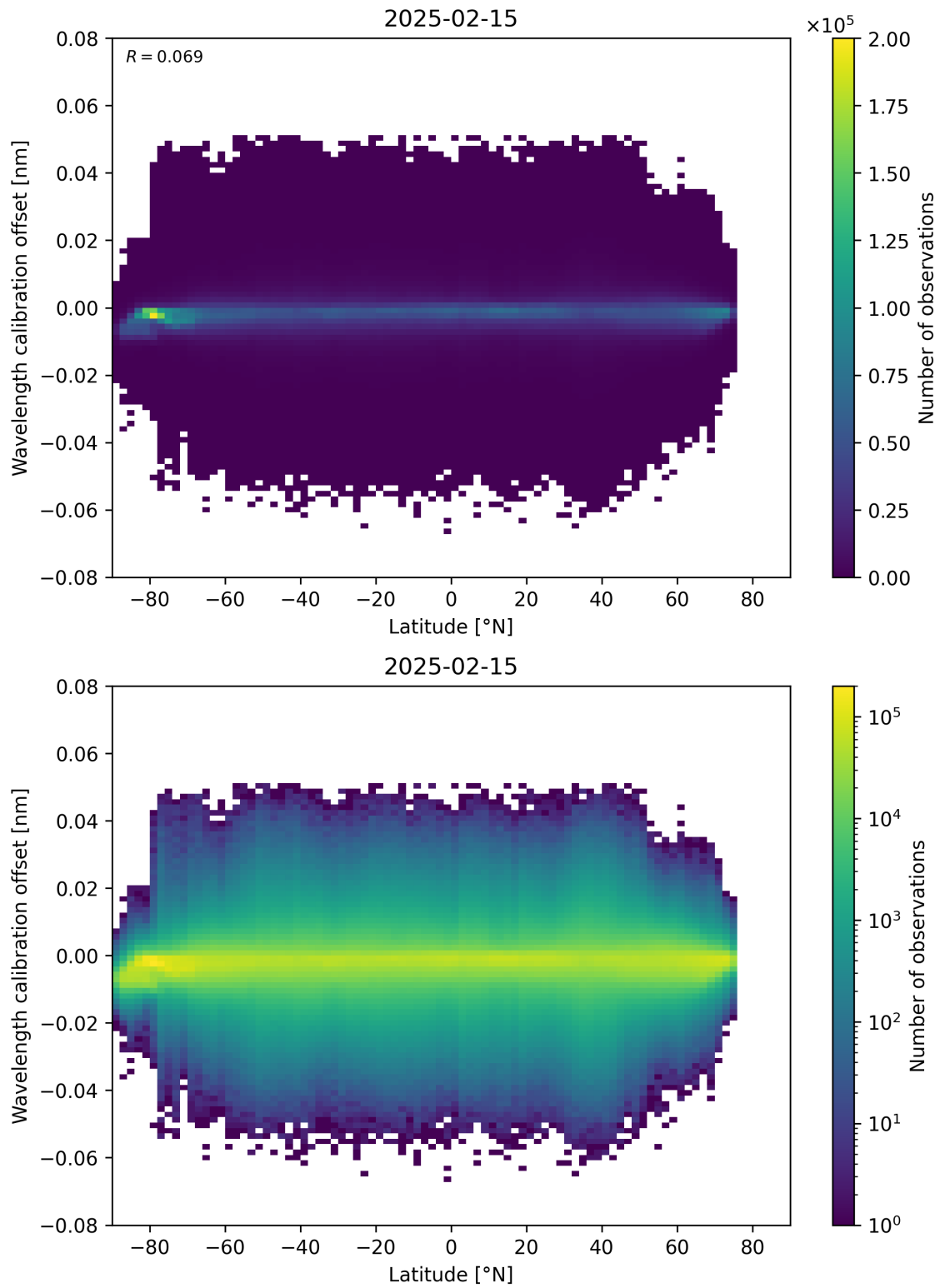
Figure 95: Scatter density plot of “Latitude” against “Wavelength calibration offset” for 2025-02-14 to 2025-02-16.
