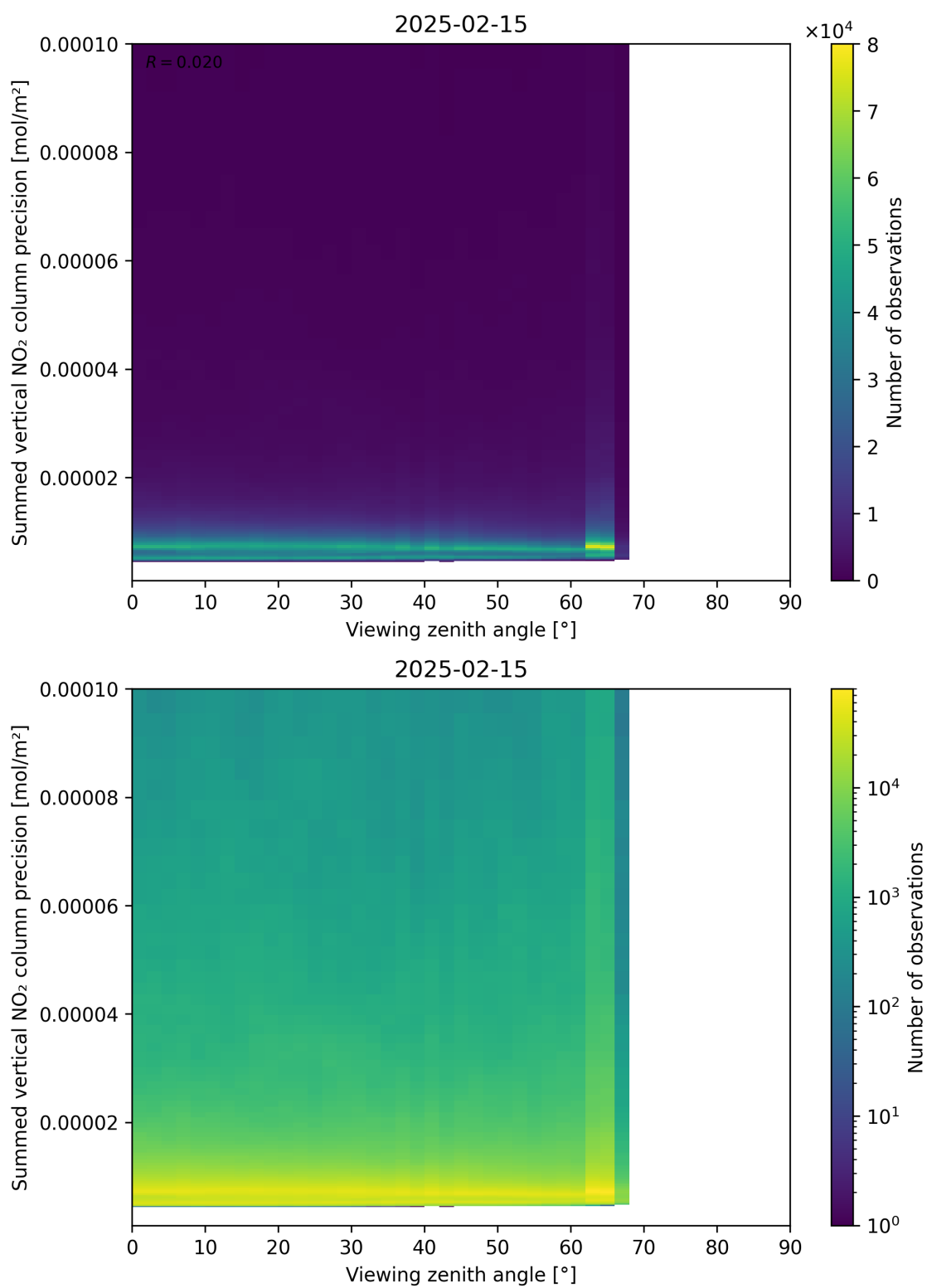
Figure 166: Scatter density plot of “Viewing zenith angle” against “Summed vertical NO 2 column precision” for 2025-02-14 to 2025-02-16.
