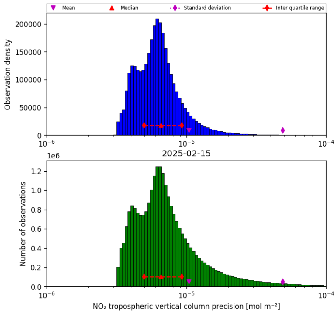
Figure 30: Histogram of “NO 2 tropospheric vertical column precision” for 2025-02-14 to 2025-02-16
