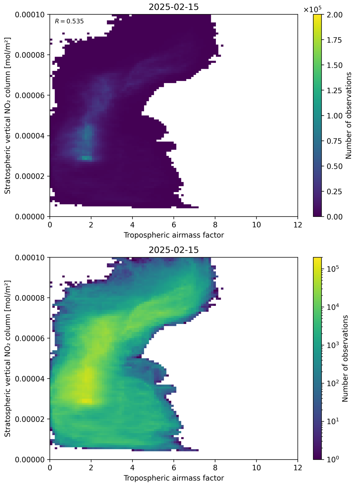
Figure 74: Scatter density plot of “Tropospheric airmass factor” against “Stratospheric vertical NO 2 column” for 2025-02-14 to 2025-02-16.
