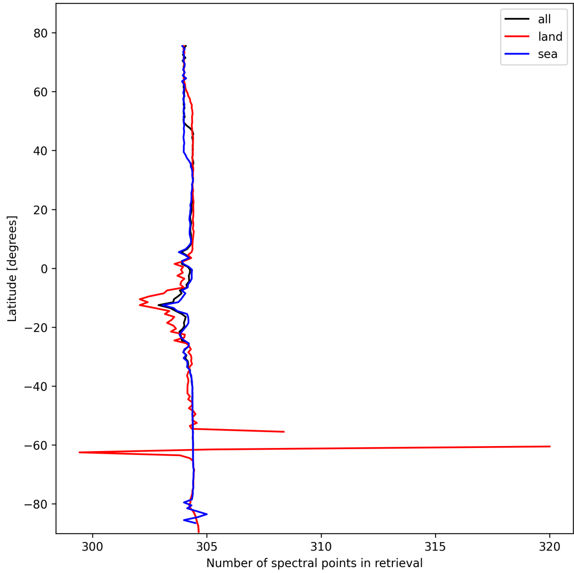
Figure 16: Zonal average of “Number of spectral points in retrieval” for 2025-02-14 to 2025-02-16.
