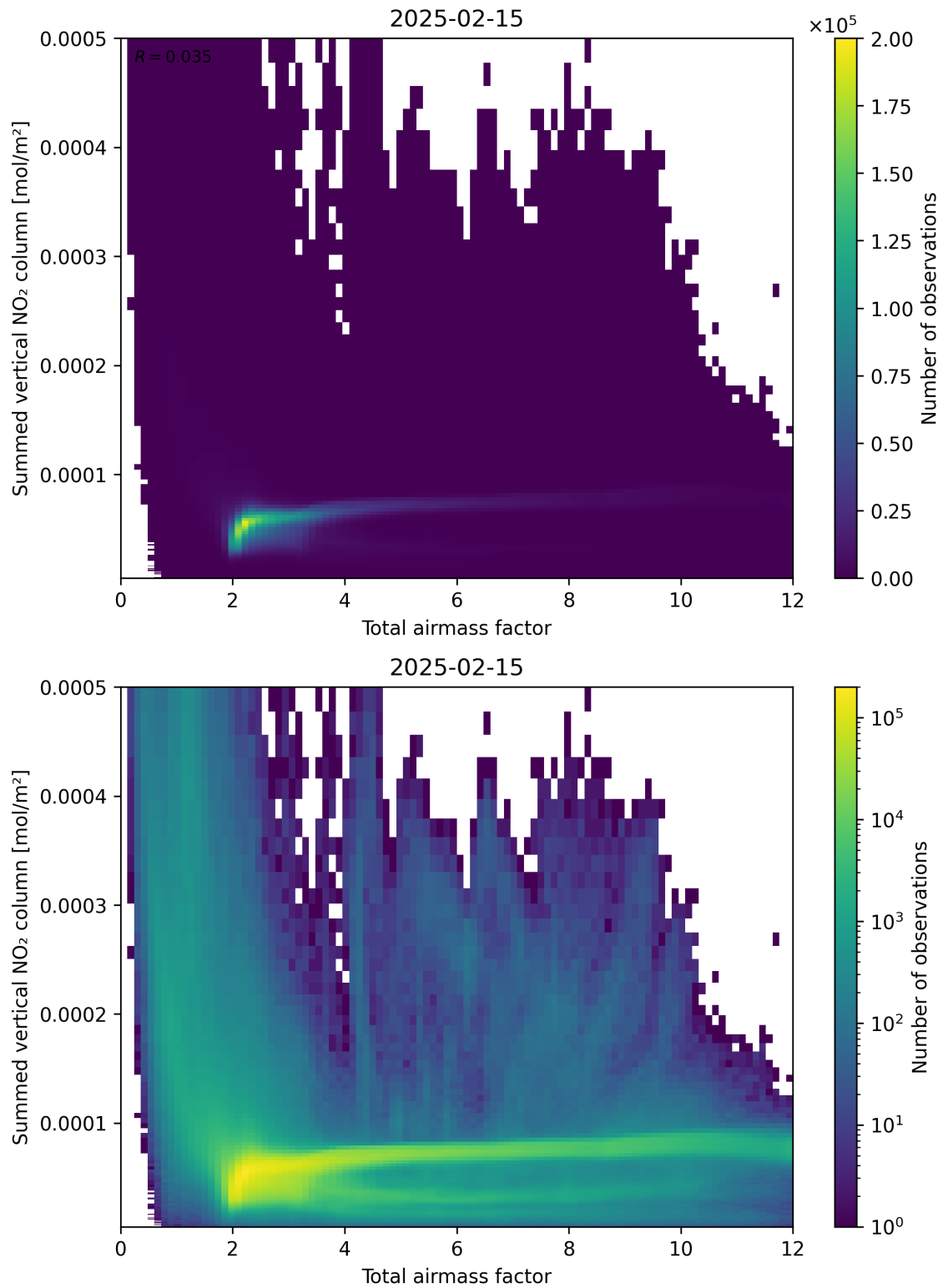
Figure 65: Scatter density plot of “Total airmass factor” against “Summed vertical NO 2 column” for 2025-02-14 to 2025-02-16.
