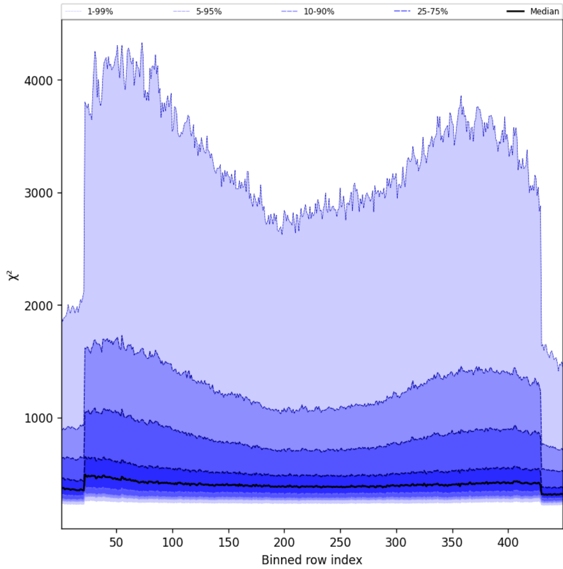
Figure 59: Along track statistics of “ \chi^2 ” for 2025-02-14 to 2025-02-16
