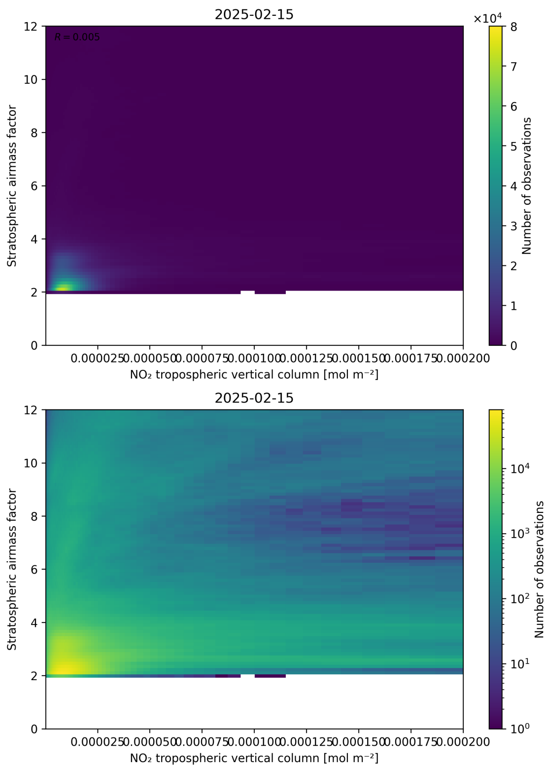
Figure 121: Scatter density plot of “NO 2 tropospheric vertical column” against “Stratospheric airmass factor” for 2025-02-14 to 2025-02-16.
