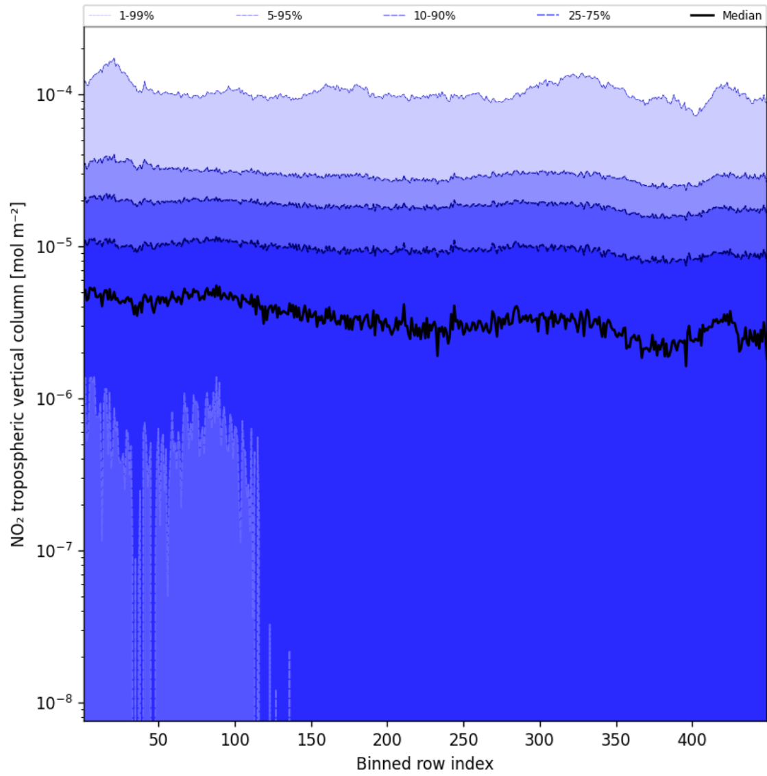
Figure 46: Along track statistics of “NO 2 tropospheric vertical column” for 2025-02-14 to 2025-02-16
