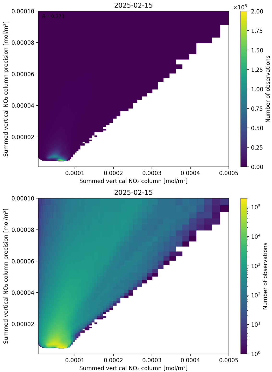
Figure 105: Scatter density plot of “Summed vertical NO 2 column” against “Summed vertical NO 2 column precision” for 2025-02-14 to 2025-02-16.
