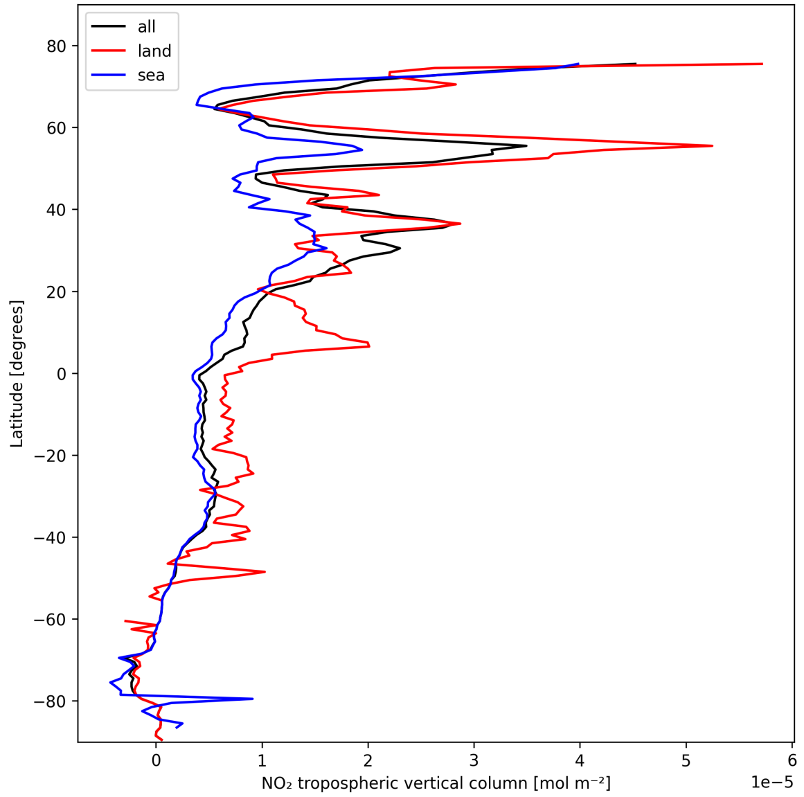
Figure 12: Zonal average of “NO 2 tropospheric vertical column” for 2025-02-14 to 2025-02-16.
