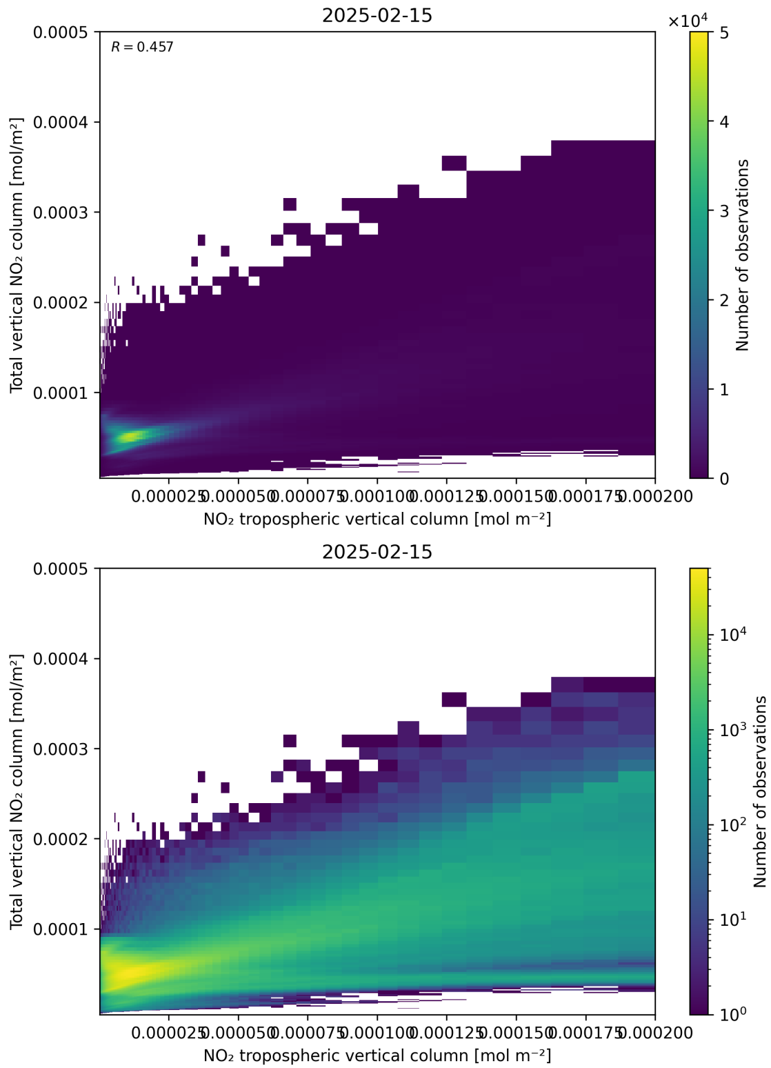
Figure 128: Scatter density plot of “NO 2 tropospheric vertical column” against “Total vertical NO 2 column” for 2025-02-14 to 2025-02-16.
