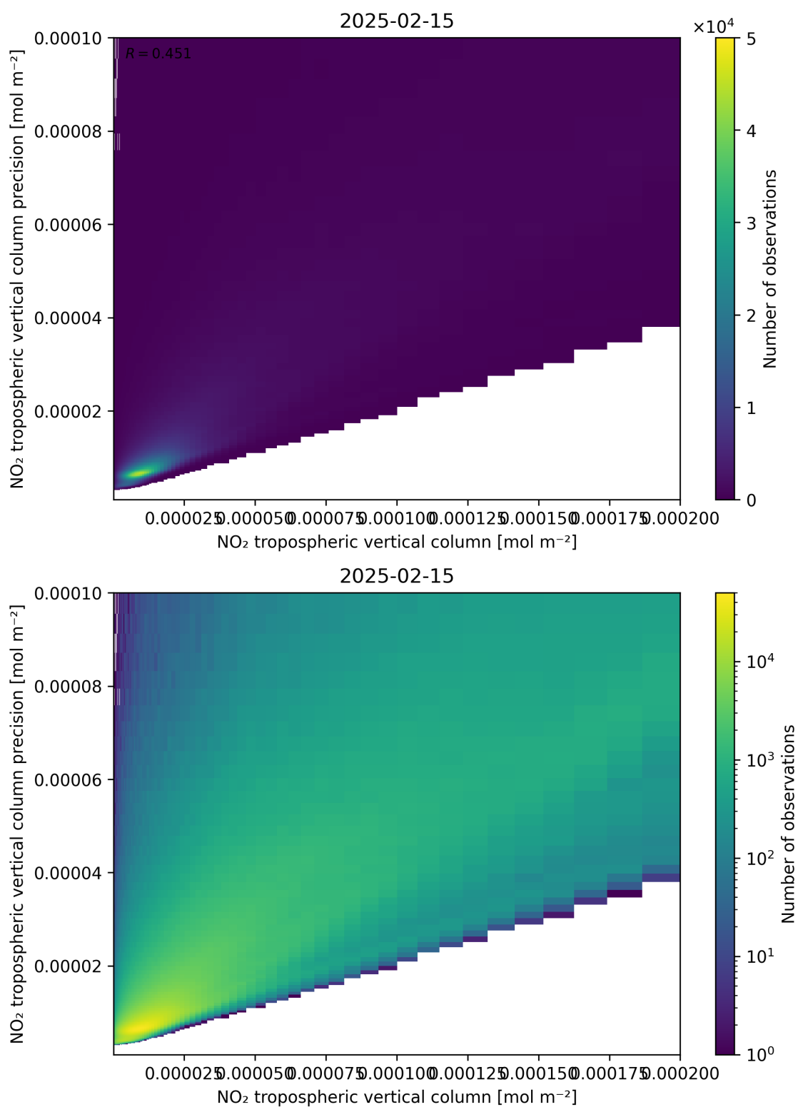
Figure 130: Scatter density plot of “NO 2 tropospheric vertical column” against “NO 2 tropospheric vertical column precision” for 2025-02-14 to 2025-02-16.
