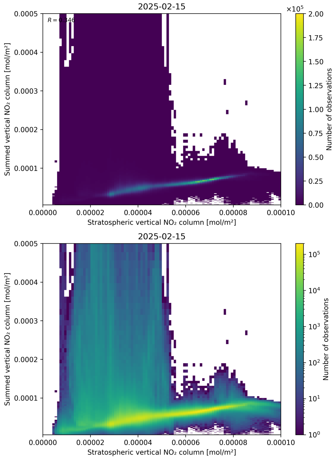
Figure 98: Scatter density plot of “Stratospheric vertical NO 2 column” against “Summed vertical NO 2 column” for 2025-02-14 to 2025-02-16.
