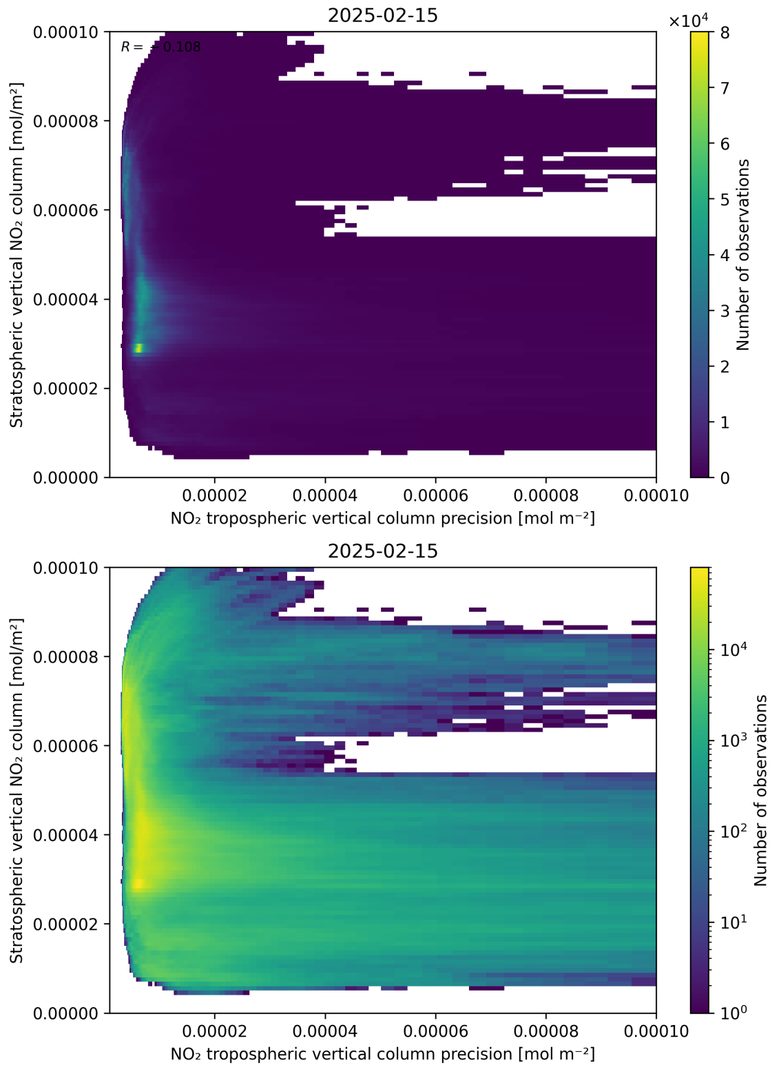
Figure 135: Scatter density plot of “NO 2 tropospheric vertical column precision” against “Stratospheric vertical NO 2 column” for 2025-02-14 to 2025-02-16.
