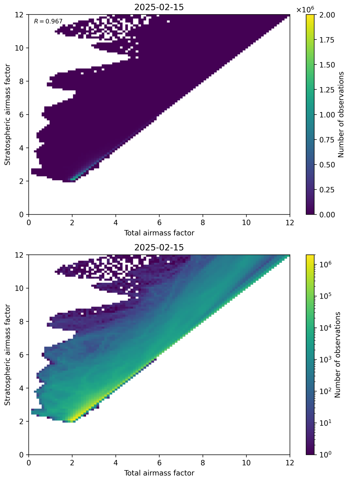
Figure 62: Scatter density plot of “Total airmass factor” against “Stratospheric airmass factor” for 2025-02-14 to 2025-02-16.
