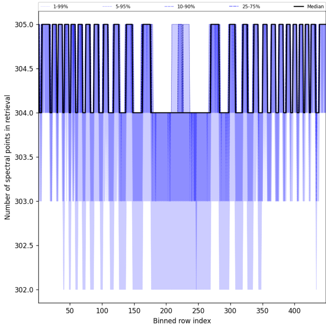
Figure 50: Along track statistics of “Number of spectral points in retrieval” for 2025-02-14 to 2025-02-16
