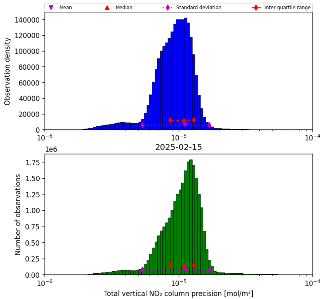
Figure 39: Histogram of “Total vertical NO 2 column precision” for 2025-02-14 to 2025-02-16
