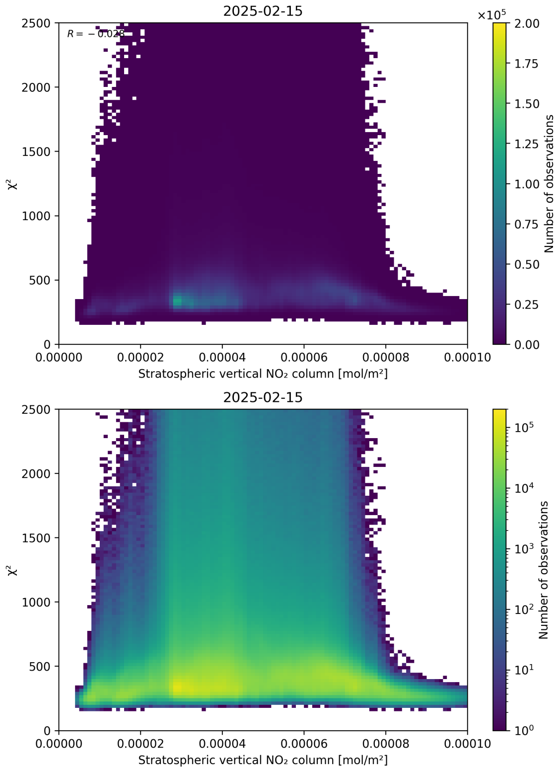
Figure 97: Scatter density plot of “Stratospheric vertical NO 2 column” against “ \chi^2 ” for 2025-02-14 to 2025-02-16.
