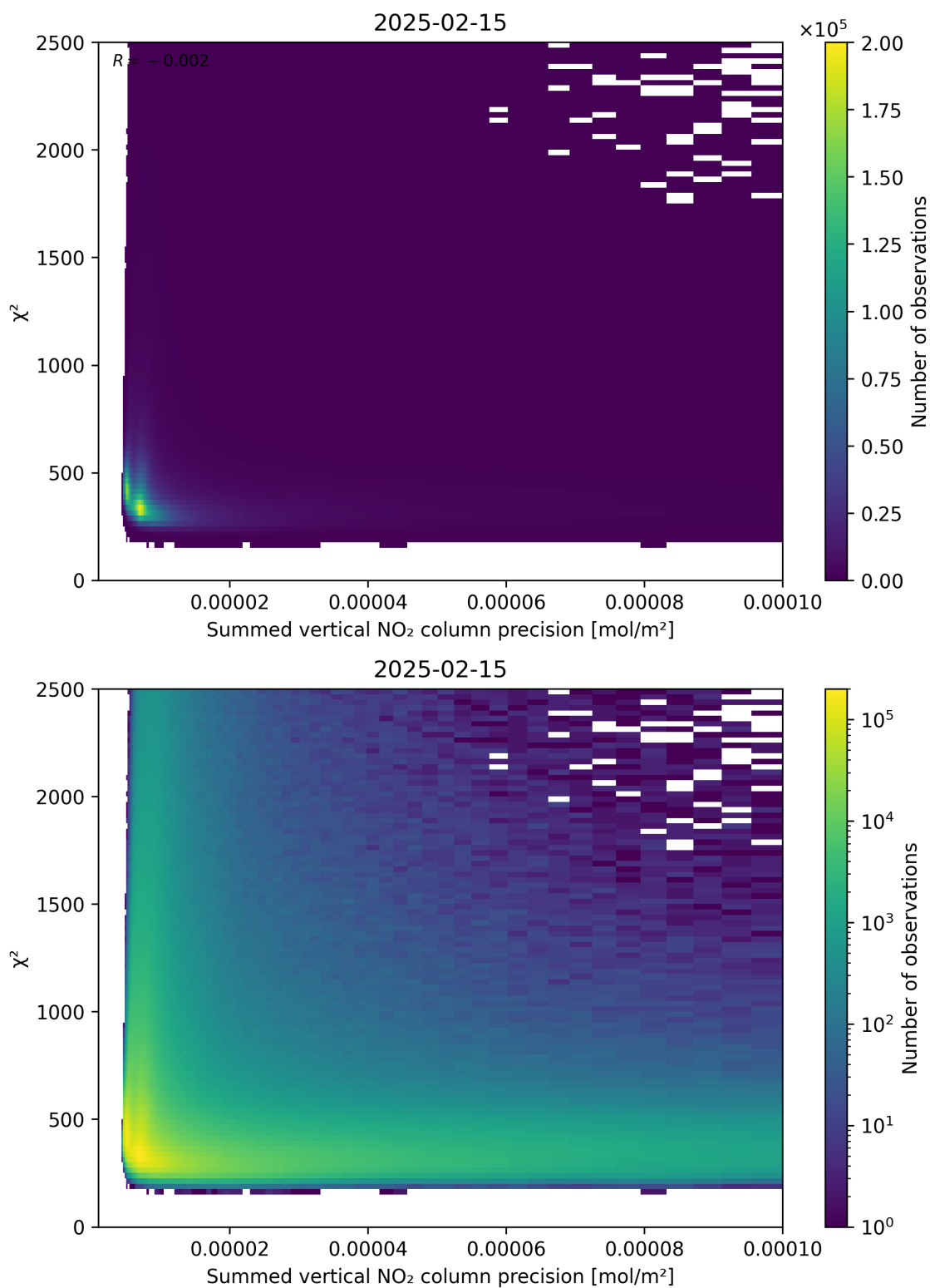
Figure 107: Scatter density plot of “Summed vertical NO 2 column precision” against “ \chi^2 ” for 2025-02-14 to 2025-02-16.
