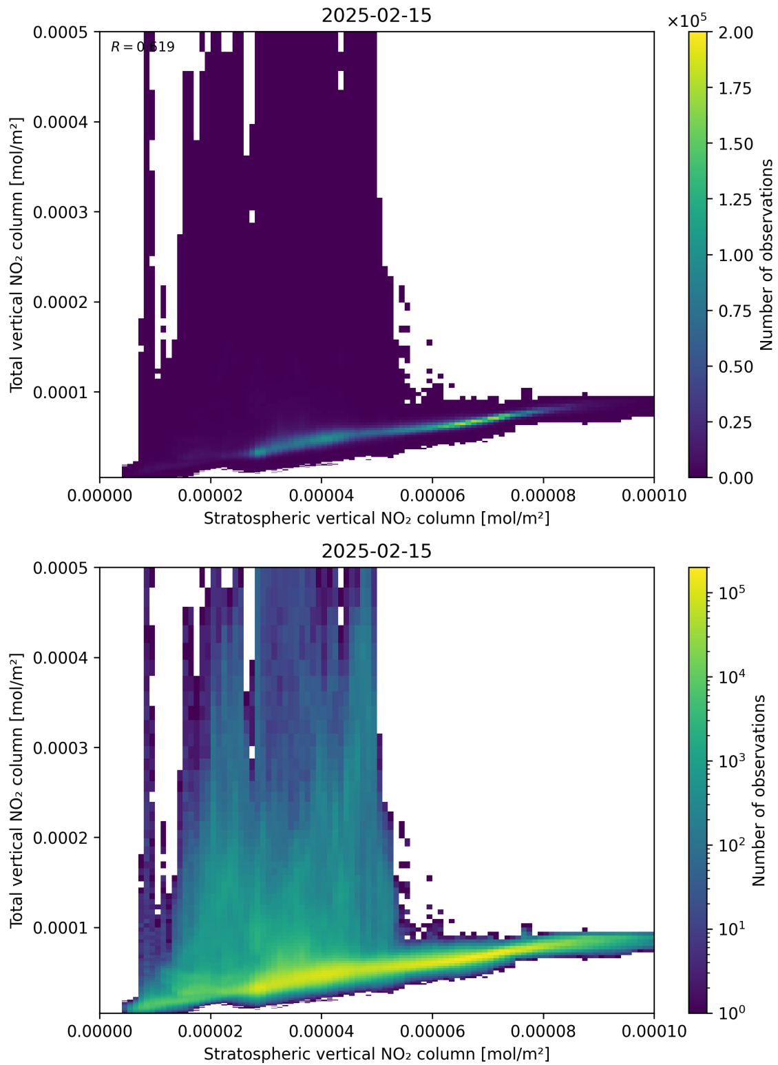
Figure 100: Scatter density plot of “Stratospheric vertical NO 2 column” against “Total vertical NO 2 column” for 2025-02-14 to 2025-02-16.
