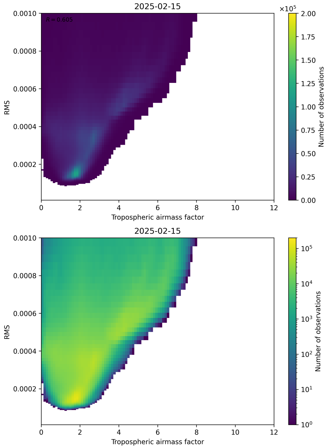
Figure 79: Scatter density plot of “Tropospheric airmass factor” against “RMS” for 2025-02-14 to 2025-02-16.
