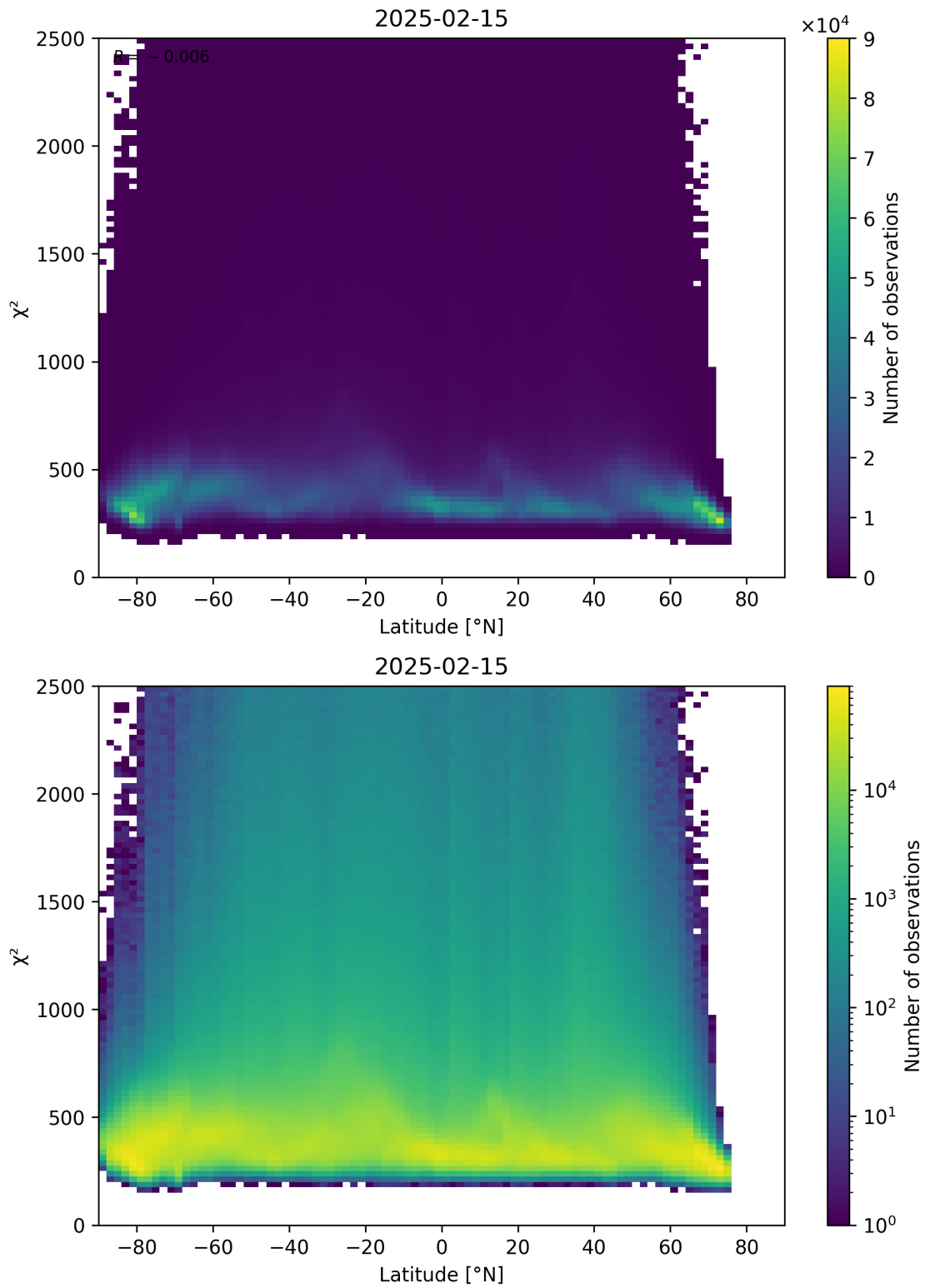
Figure 86: Scatter density plot of “Latitude” against “ \chi^2 ” for 2025-02-14 to 2025-02-16.
