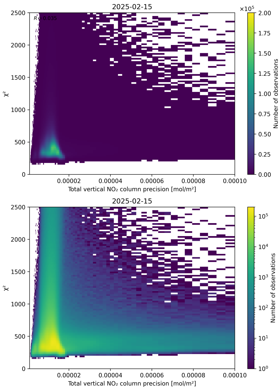
Figure 116: Scatter density plot of “Total vertical NO 2 column precision” against “ \chi^2 ” for 2025-02-14 to 2025-02-16.
