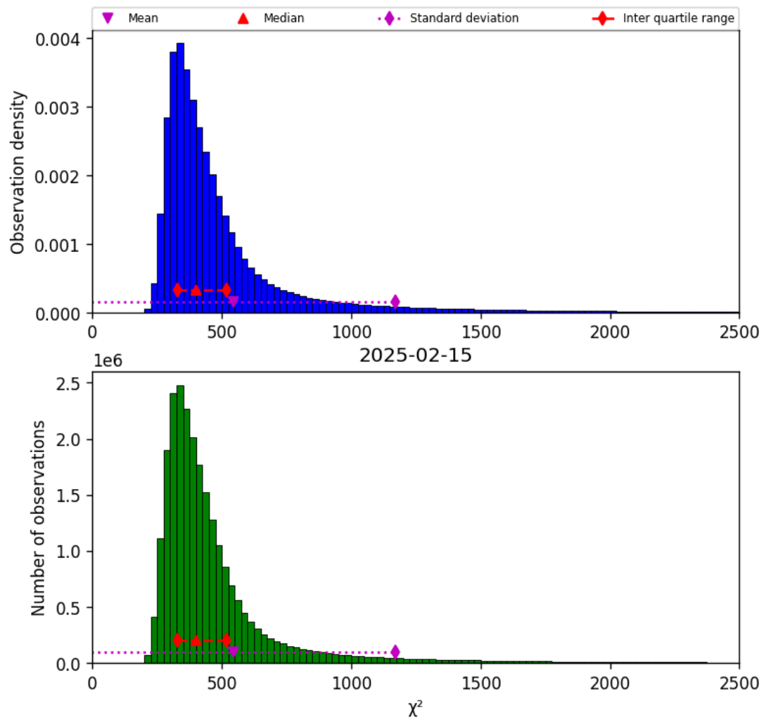
Figure 42: Histogram of " \chi^2 " for 2025-02-14 to 2025-02-16
