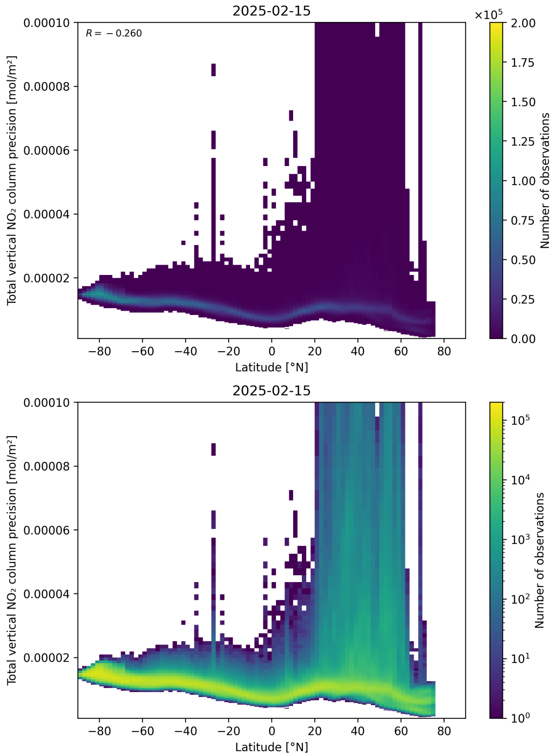
Figure 91: Scatter density plot of “Latitude” against “Total vertical NO 2 column precision” for 2025-02-14 to 2025-02-16.
