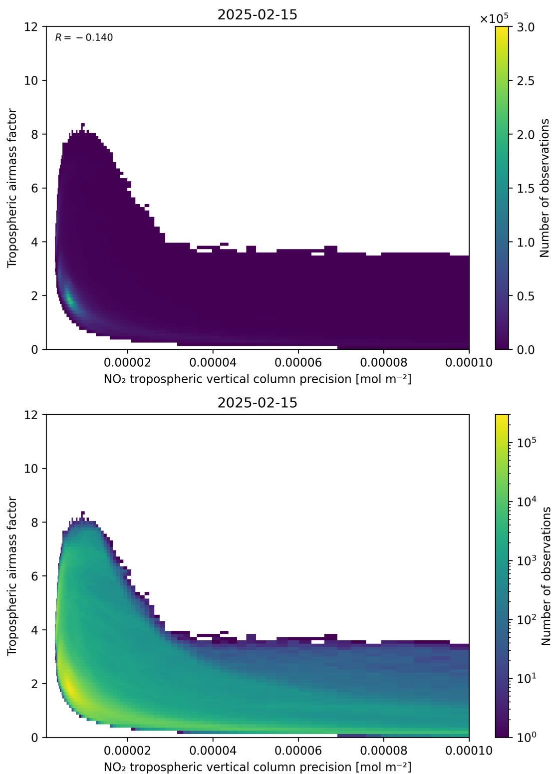
Figure 133: Scatter density plot of “NO 2 tropospheric vertical column precision” against “Tropospheric air mass factor” for 2025-02-14 to 2025-02-16.
