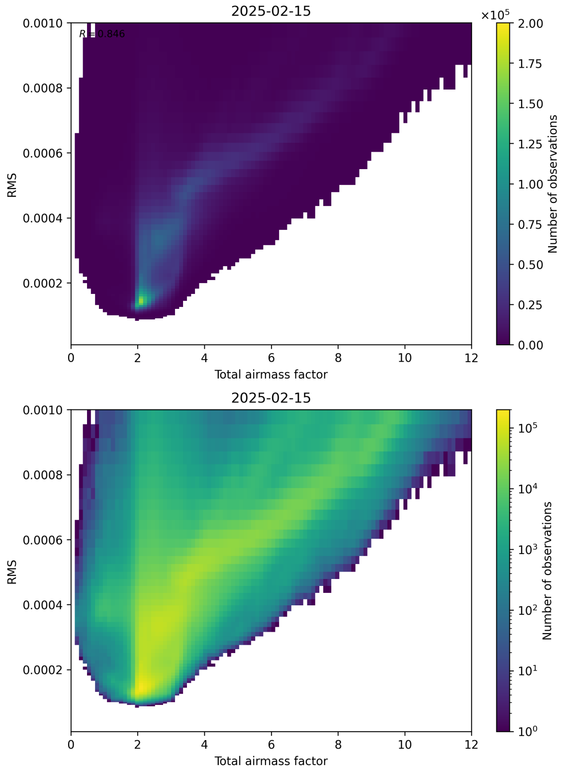
Figure 69: Scatter density plot of “Total airmass factor” against “RMS” for 2025-02-14 to 2025-02-16.
