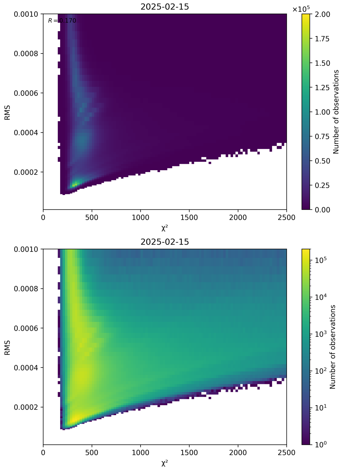
Figure 82: Scatter density plot of “ \chi^2 ” against “RMS” for 2025-02-14 to 2025-02-16.
