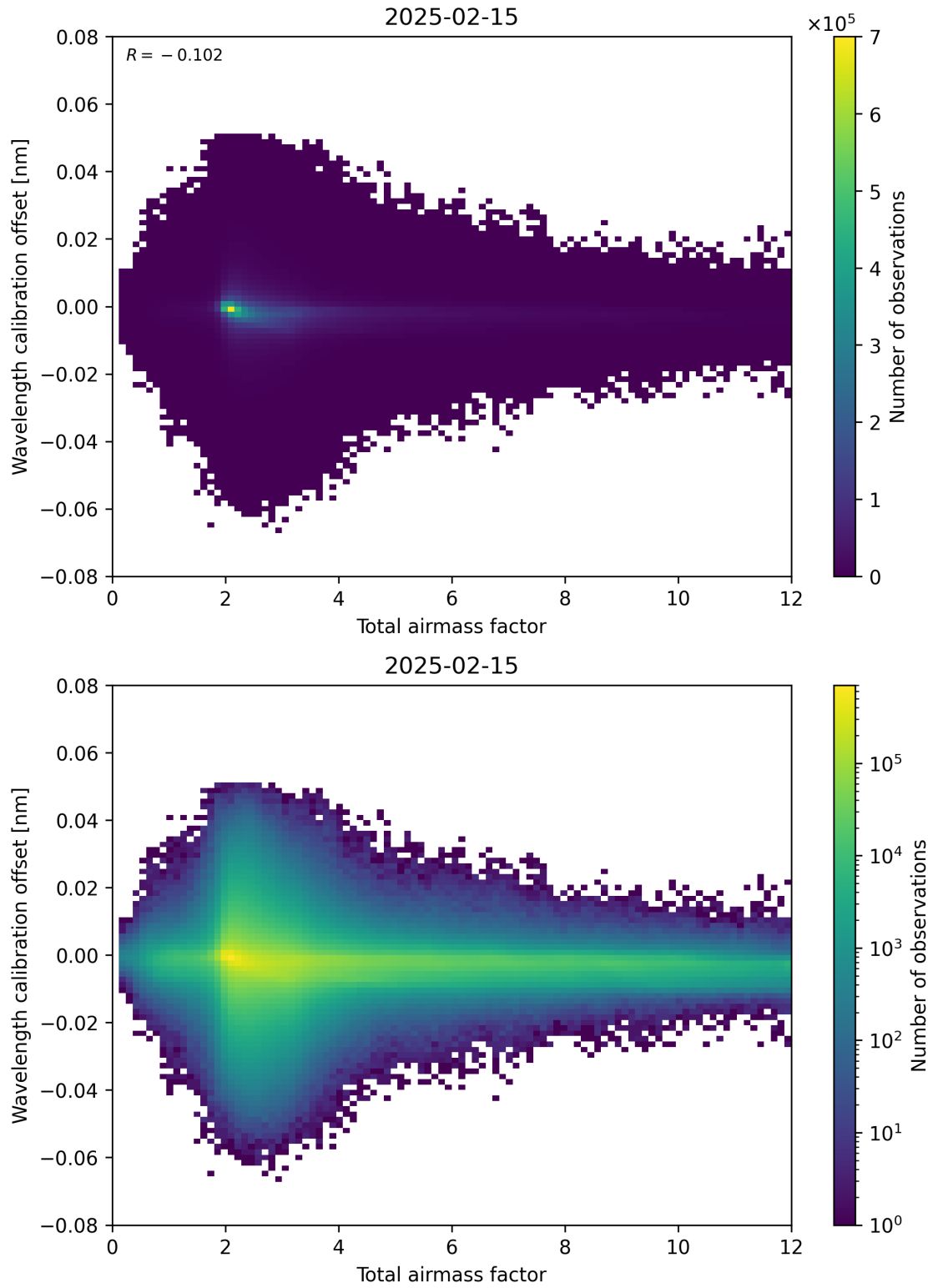
Figure 70: Scatter density plot of “Total airmass factor” against “Wavelength calibration offset” for 2025-02-14 to 2025-02-16.
