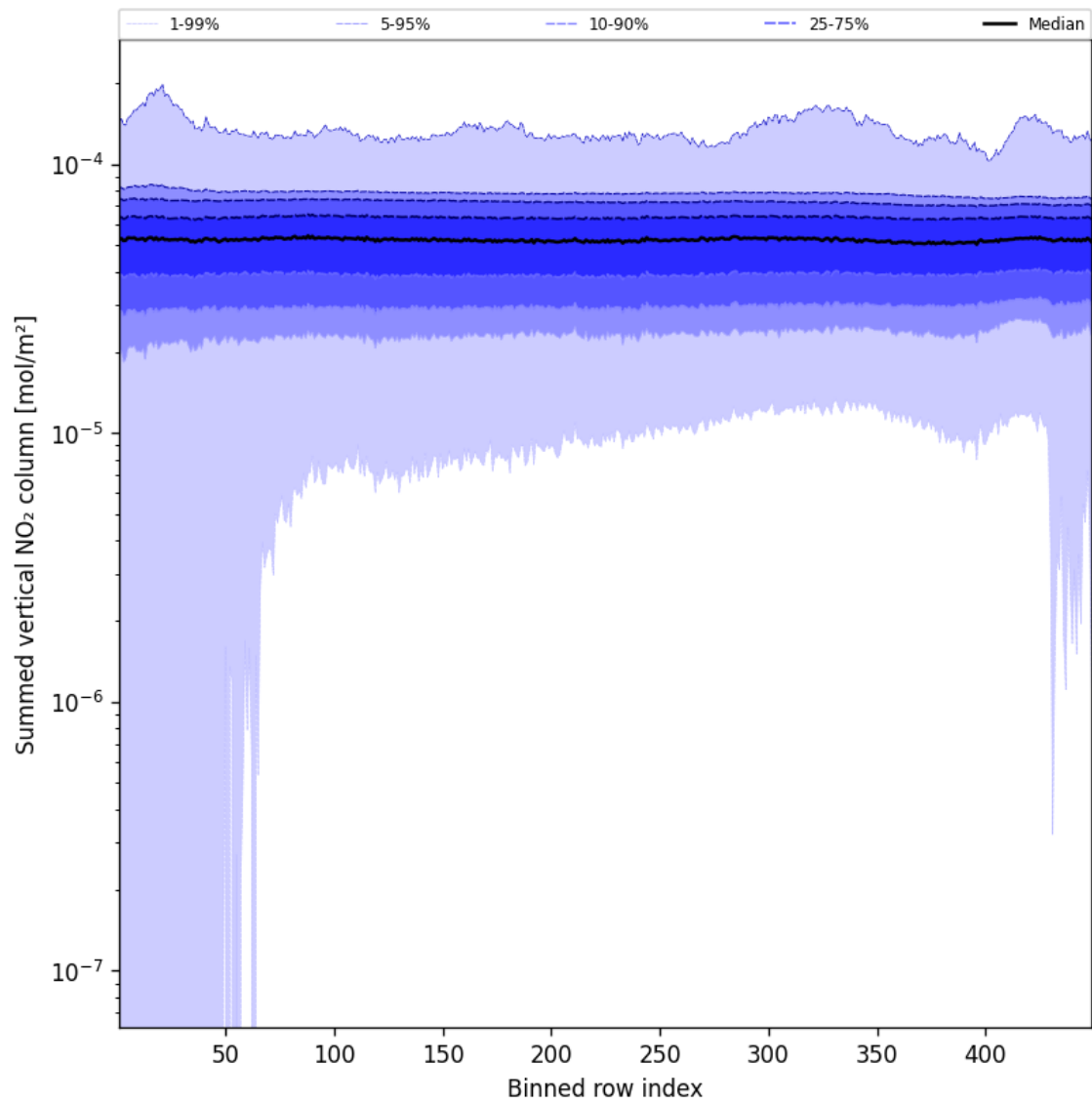
Figure 57: Along track statistics of “Summed vertical NO 2 column” for 2025-02-14 to 2025-02-16
