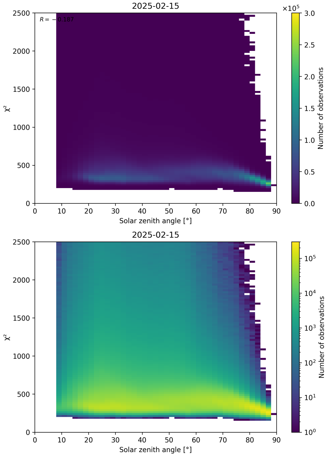
Figure 148: Scatter density plot of “Solar zenith angle” against “ \chi^2 ” for 2025-02-14 to 2025-02-16.
