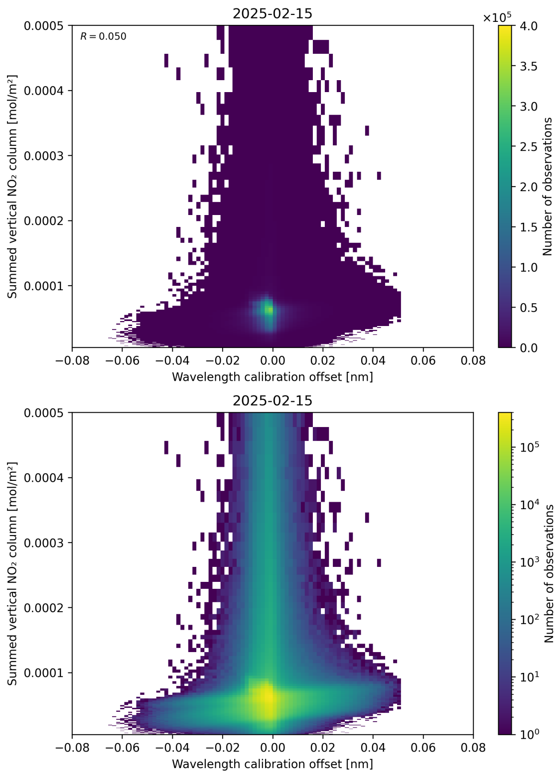
Figure 177: Scatter density plot of “Wavelength calibration offset” against “Summed vertical NO 2 column” for 2025-02-14 to 2025-02-16.
