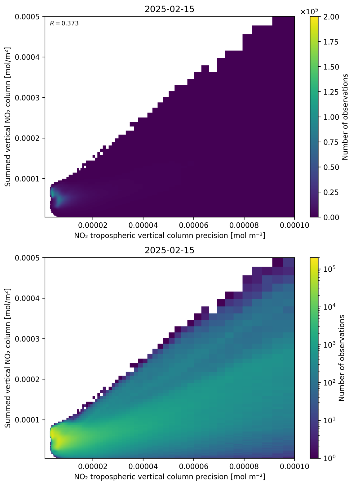
Figure 136: Scatter density plot of “NO 2 tropospheric vertical column precision” against “Summed vertical NO 2 column” for 2025-02-14 to 2025-02-16.
