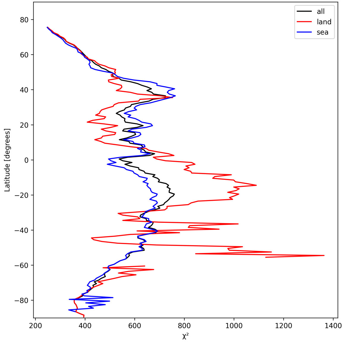
Figure 25: Zonal average of “ \chi^2 ” for 2025-02-14 to 2025-02-16.
