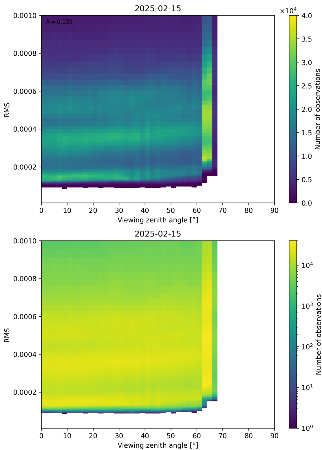
Figure 171: Scatter density plot of “Viewing zenith angle” against “RMS” for 2025-02-14 to 2025-02-16.
