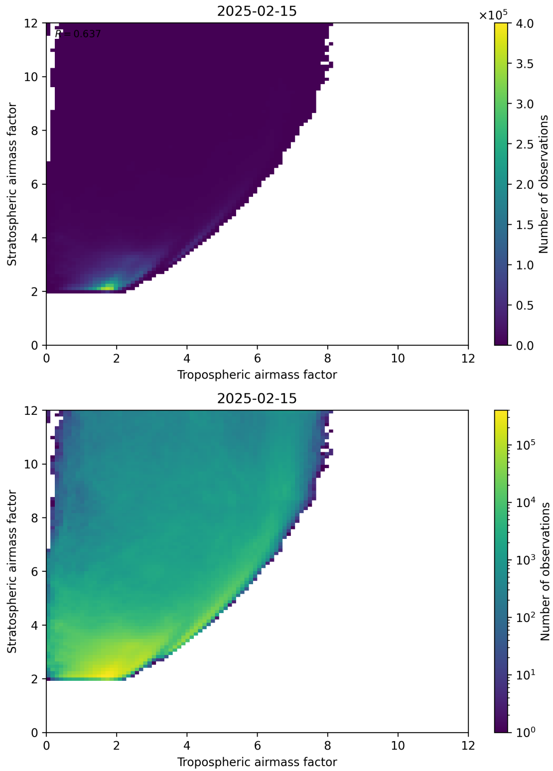
Figure 71: Scatter density plot of “Tropospheric airmass factor” against “Stratospheric airmass factor” for 2025-02-14 to 2025-02-16.
