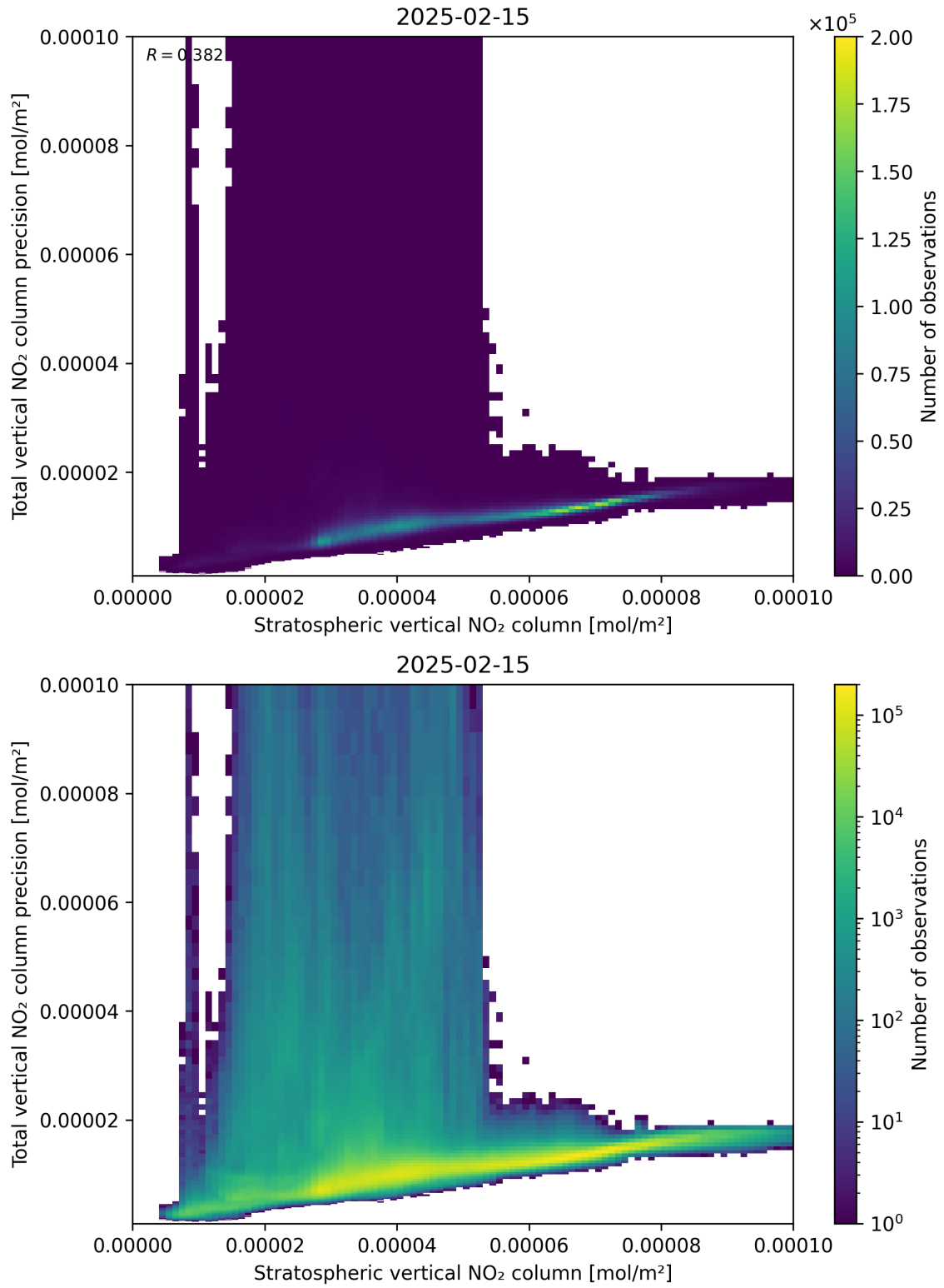
Figure 101: Scatter density plot of “Stratospheric vertical NO 2 column” against “Total vertical NO 2 column precision” for 2025-02-14 to 2025-02-16.
