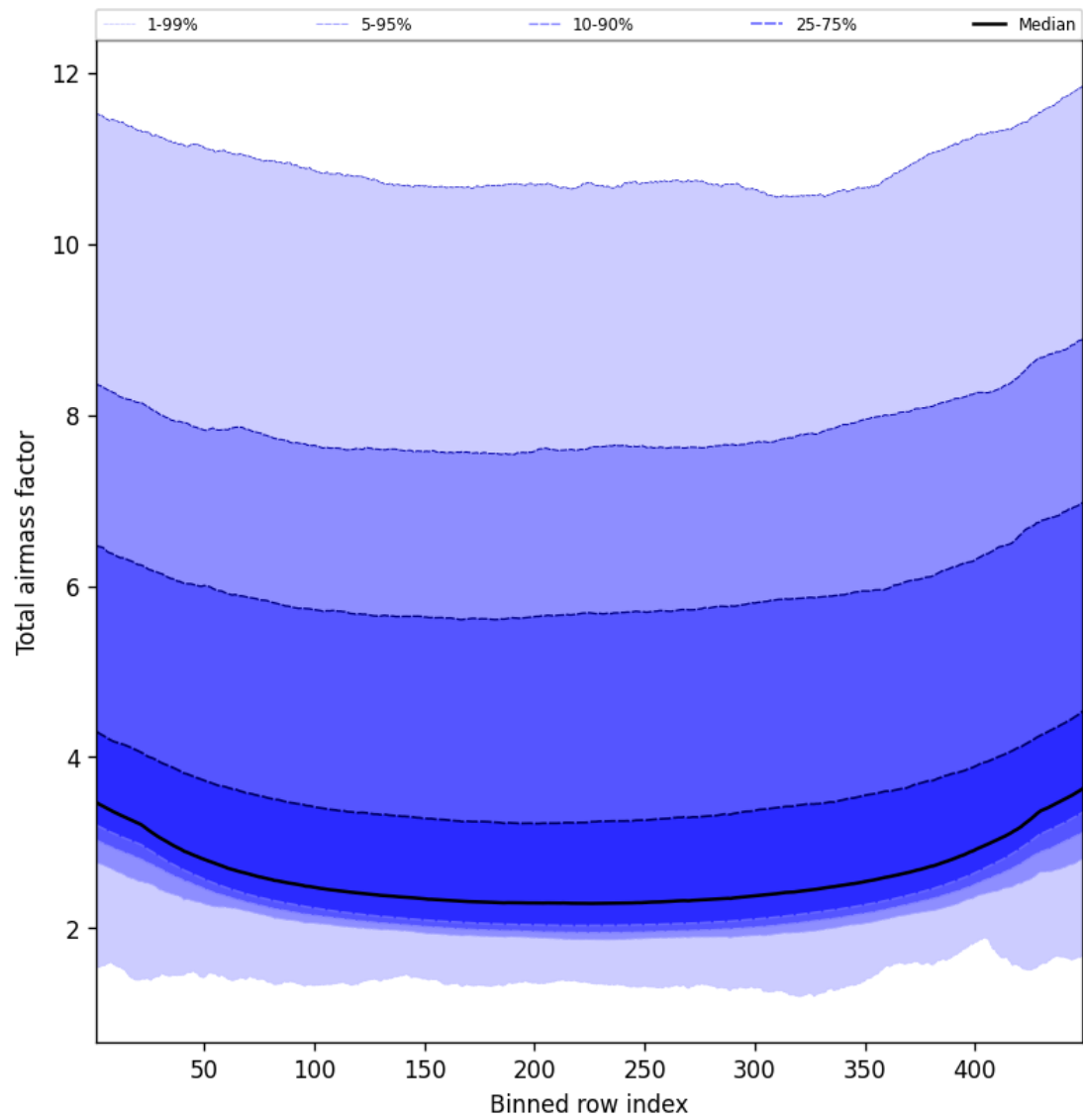
Figure 49: Along track statistics of “Total airmass factor” for 2025-02-14 to 2025-02-16
