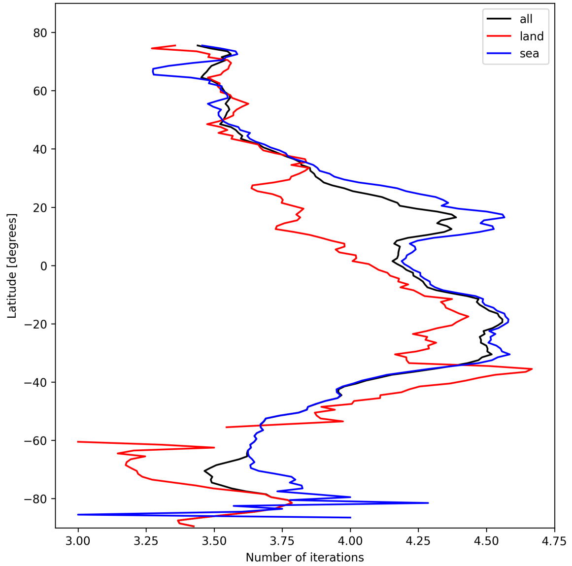
Figure 17: Zonal average of “Number of iterations” for 2025-02-14 to 2025-02-16.
