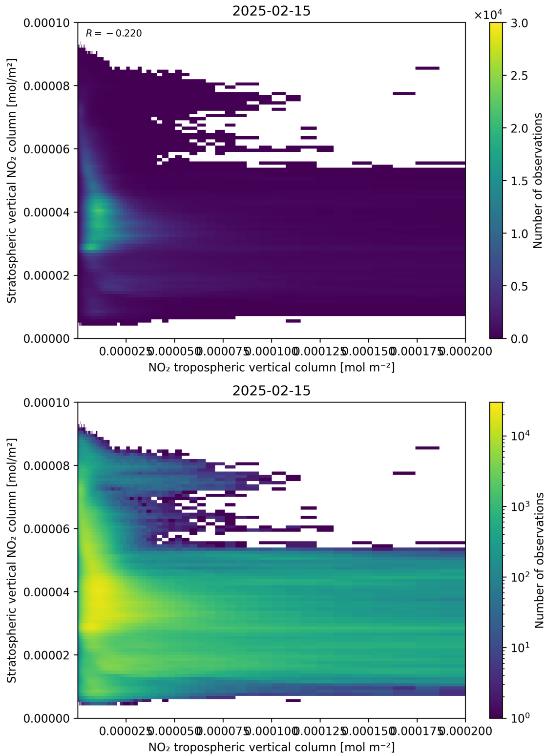
Figure 125: Scatter density plot of “NO 2 tropospheric vertical column” against “Stratospheric vertical NO 2 column” for 2025-02-14 to 2025-02-16.
