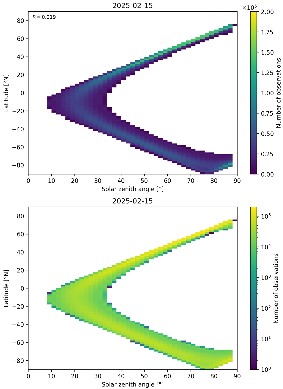
Figure 149: Scatter density plot of “Solar zenith angle” against “Latitude” for 2025-02-14 to 2025-02-16.
