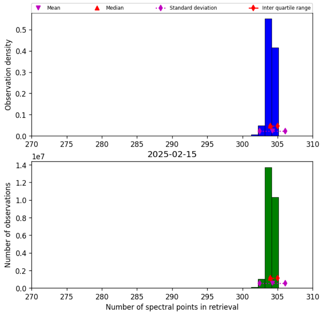
Figure 33: Histogram of “Number of spectral points in retrieval” for 2025-02-14 to 2025-02-16
