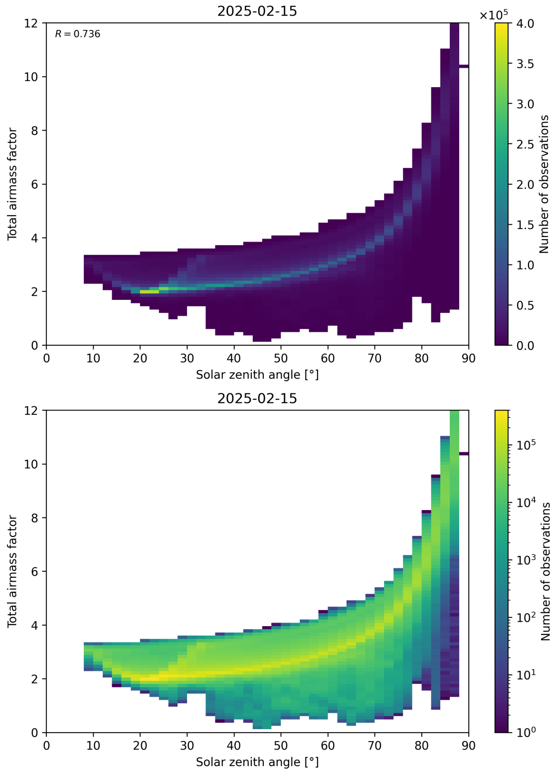
Figure 146: Scatter density plot of “Solar zenith angle” against “Total air mass factor” for 2025-02-14 to 2025-02-16.
