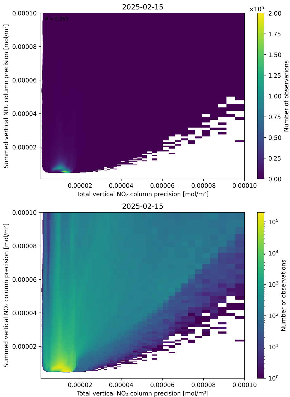
Figure 118: Scatter density plot of “Total vertical NO 2 column precision” against “Summed vertical NO 2 column precision” for 2025-02-14 to 2025-02-16.
