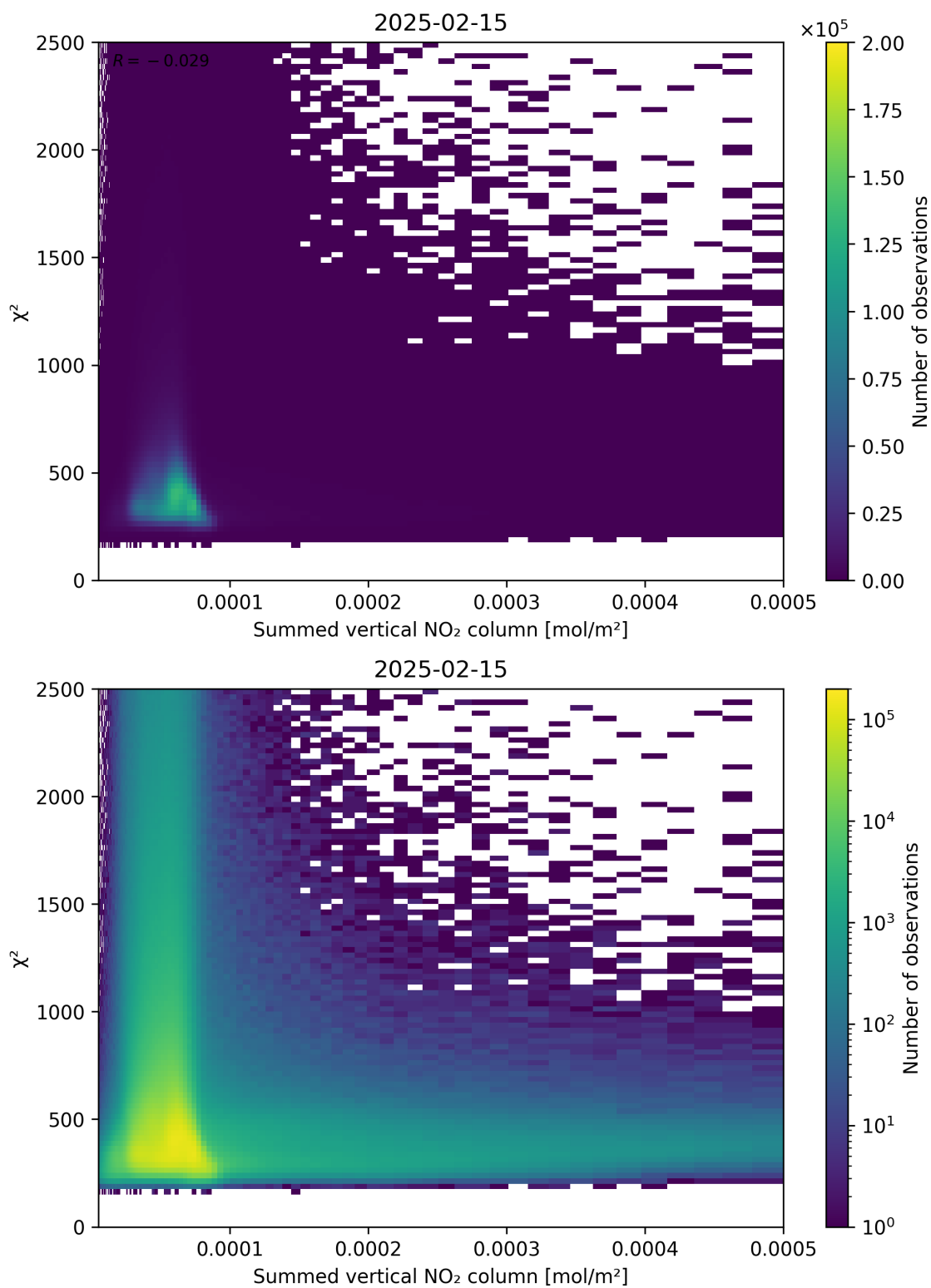
Figure 104: Scatter density plot of “Summed vertical NO 2 column” against “ \chi^2 ” for 2025-02-14 to 2025-02-16.
