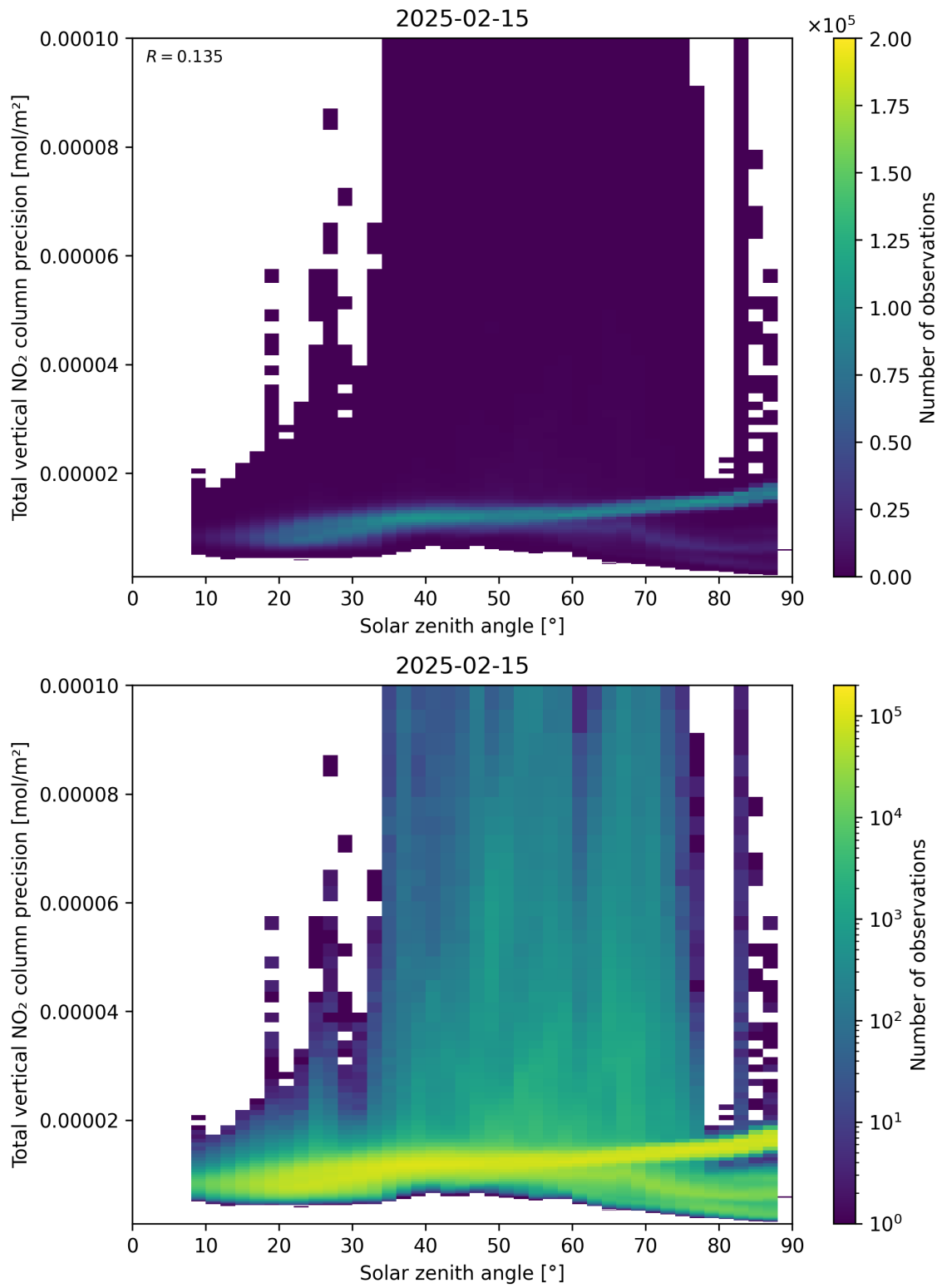
Figure 154: Scatter density plot of “Solar zenith angle” against “Total vertical NO 2 column precision” for 2025-02-14 to 2025-02-16.
