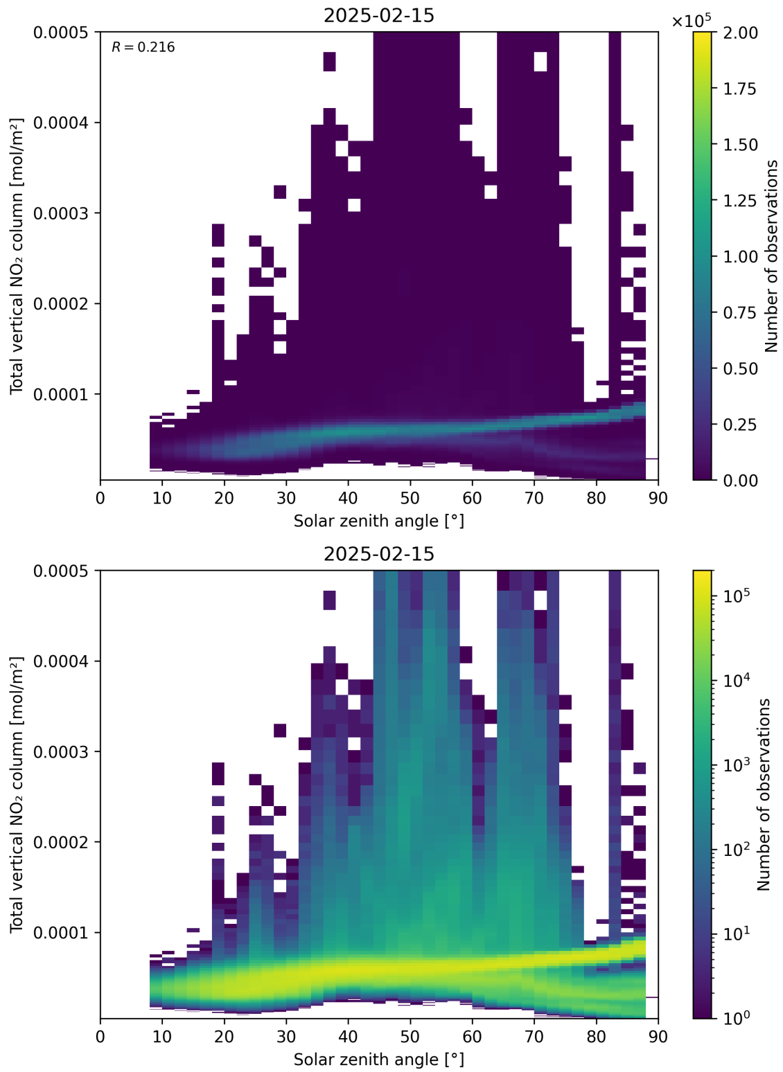
Figure 153: Scatter density plot of “Solar zenith angle” against “Total vertical NO 2 column” for 2025-02-14 to 2025-02-16.
