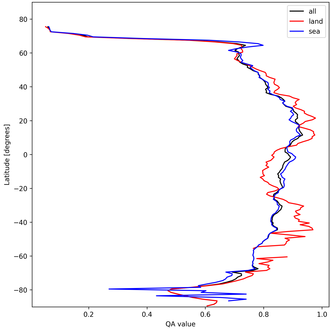
Figure 11: Zonal average of “QA value” for 2025-02-14 to 2025-02-16.
