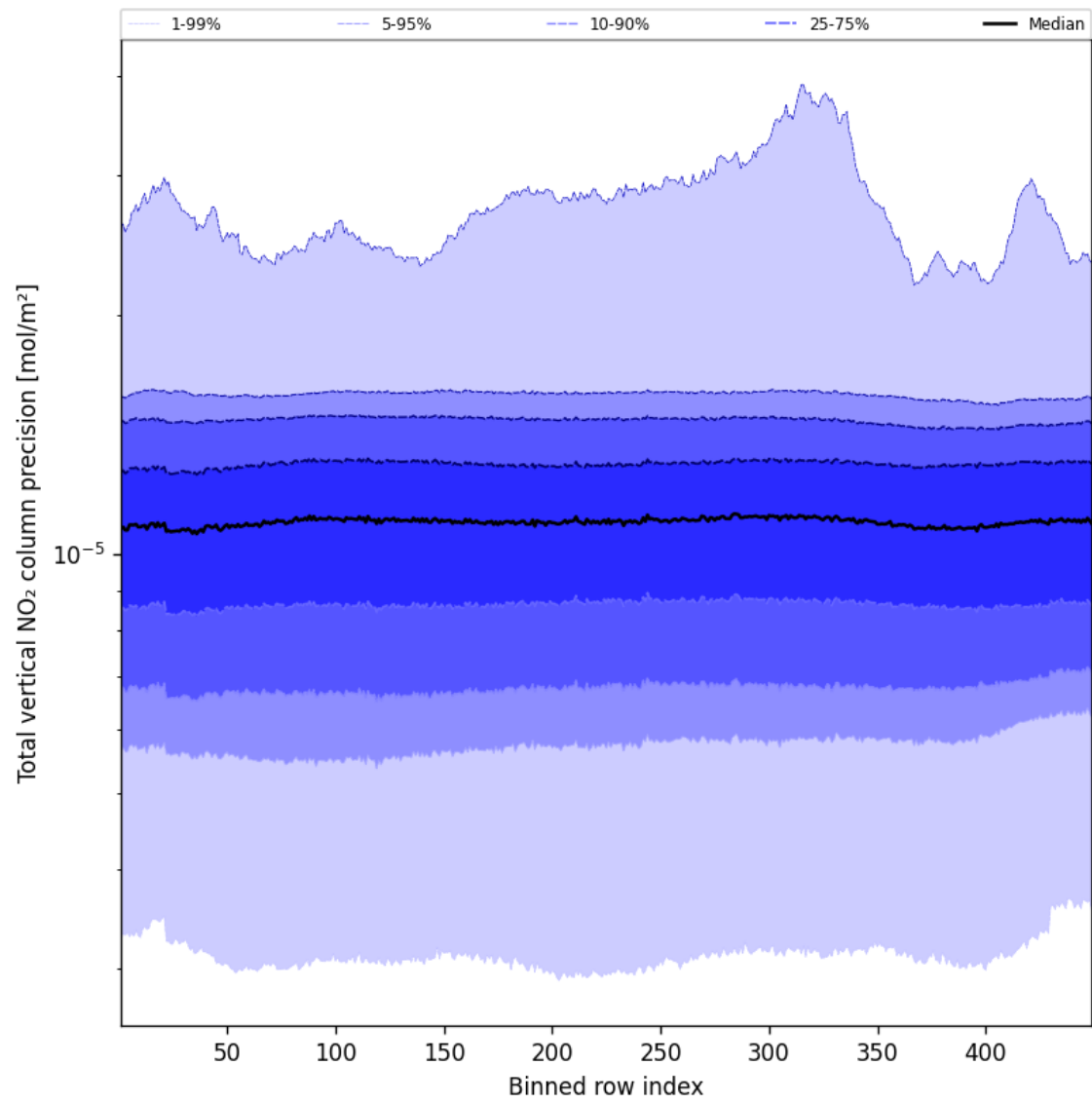
Figure 56: Along track statistics of “Total vertical NO 2 column precision” for 2025-02-14 to 2025-02-16
