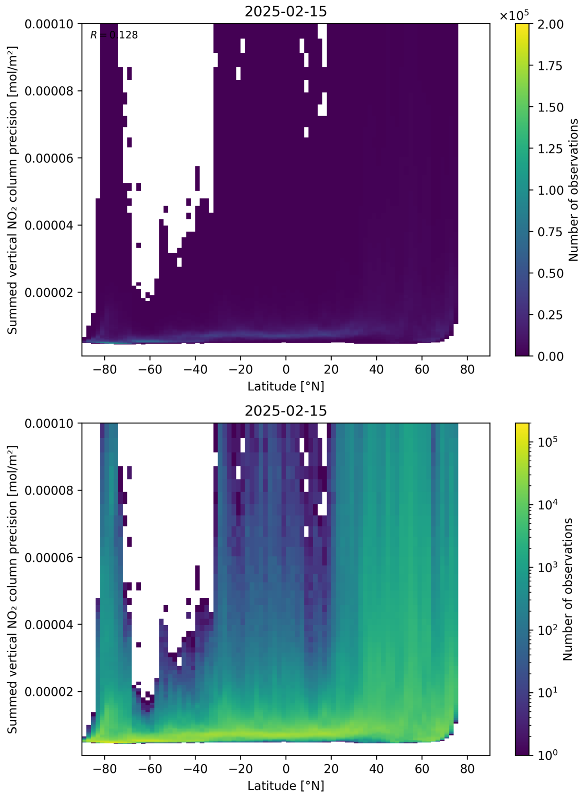
Figure 89: Scatter density plot of “Latitude” against “Summed vertical NO 2 column precision” for 2025-02-14 to 2025-02-16.
