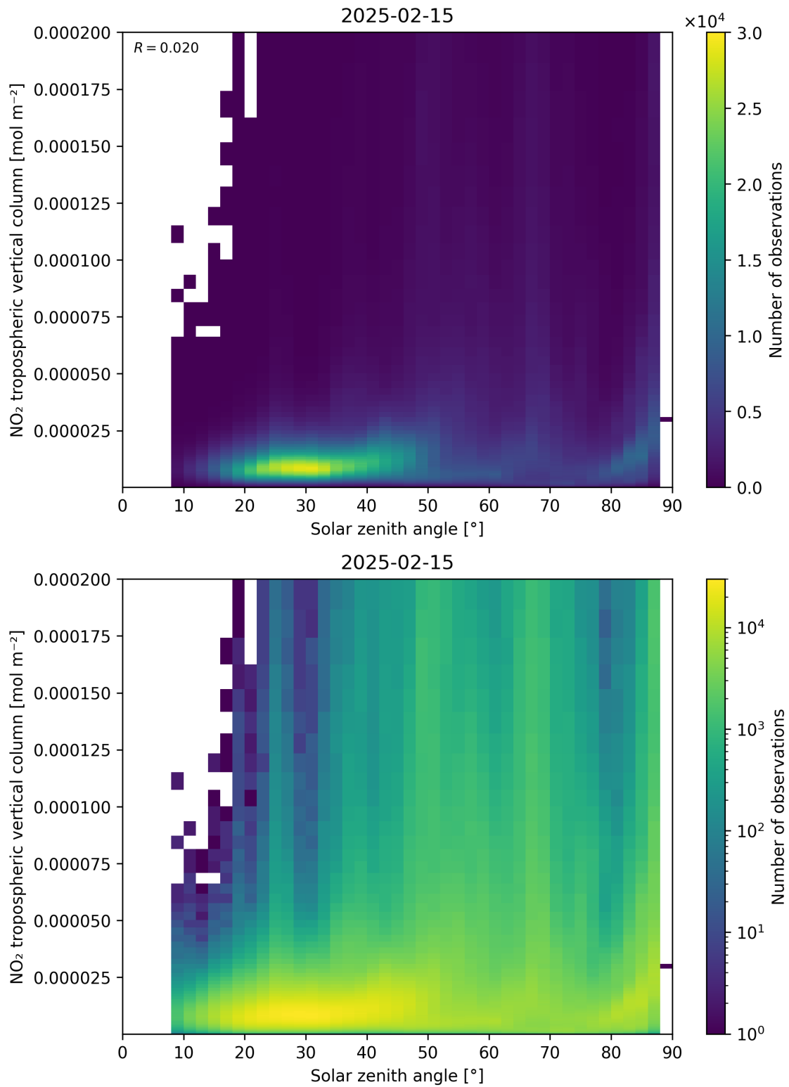
Figure 155: Scatter density plot of “Solar zenith angle” against “NO 2 tropospheric vertical column” for 2025-02-14 to 2025-02-16.
