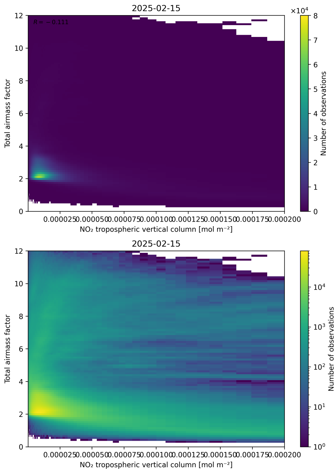
Figure 122: Scatter density plot of “NO 2 tropospheric vertical column” against “Total air mass factor” for 2025-02-14 to 2025-02-16.
