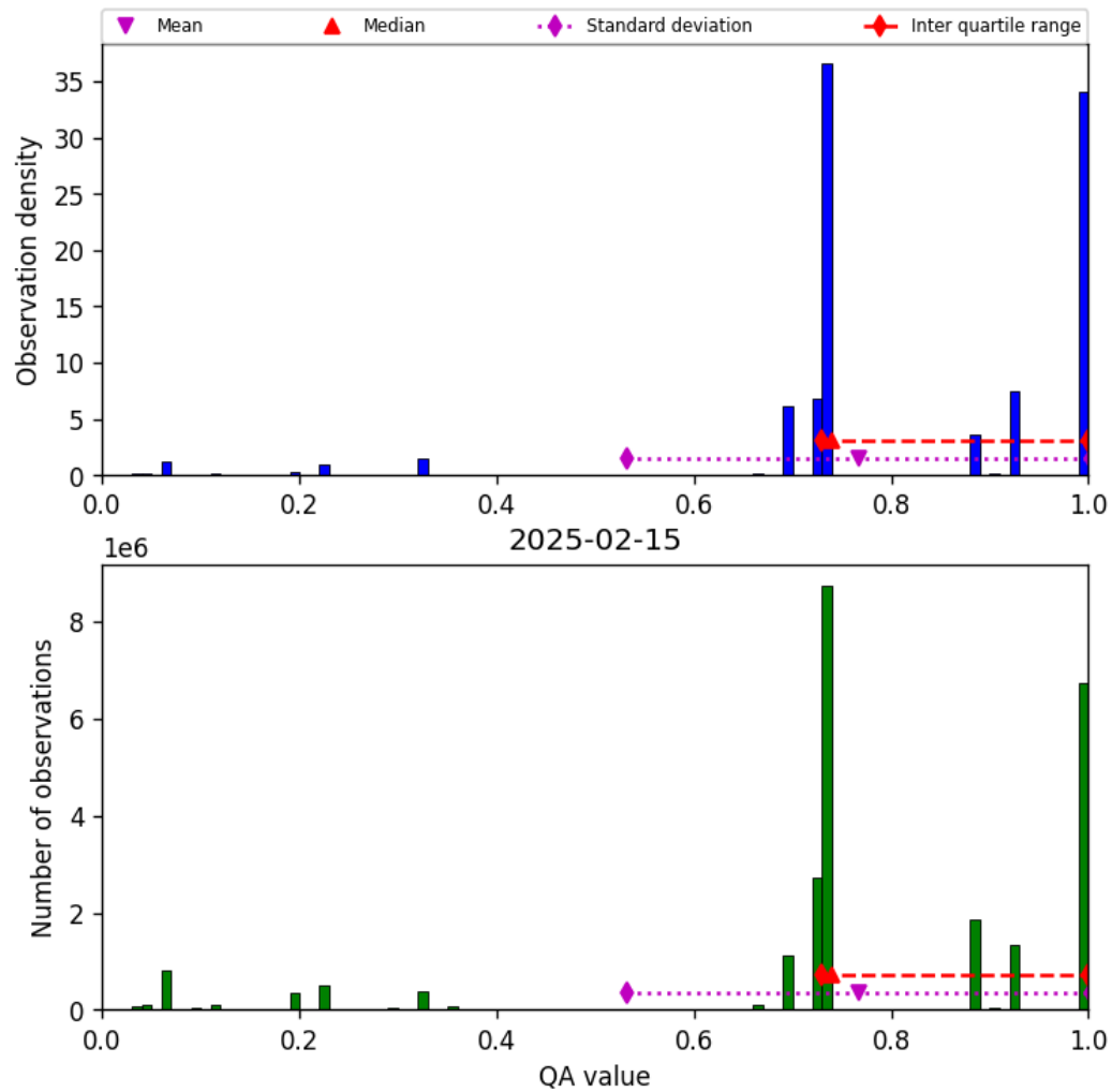
Figure 28: Histogram of “QA value” for 2025-02-14 to 2025-02-16
