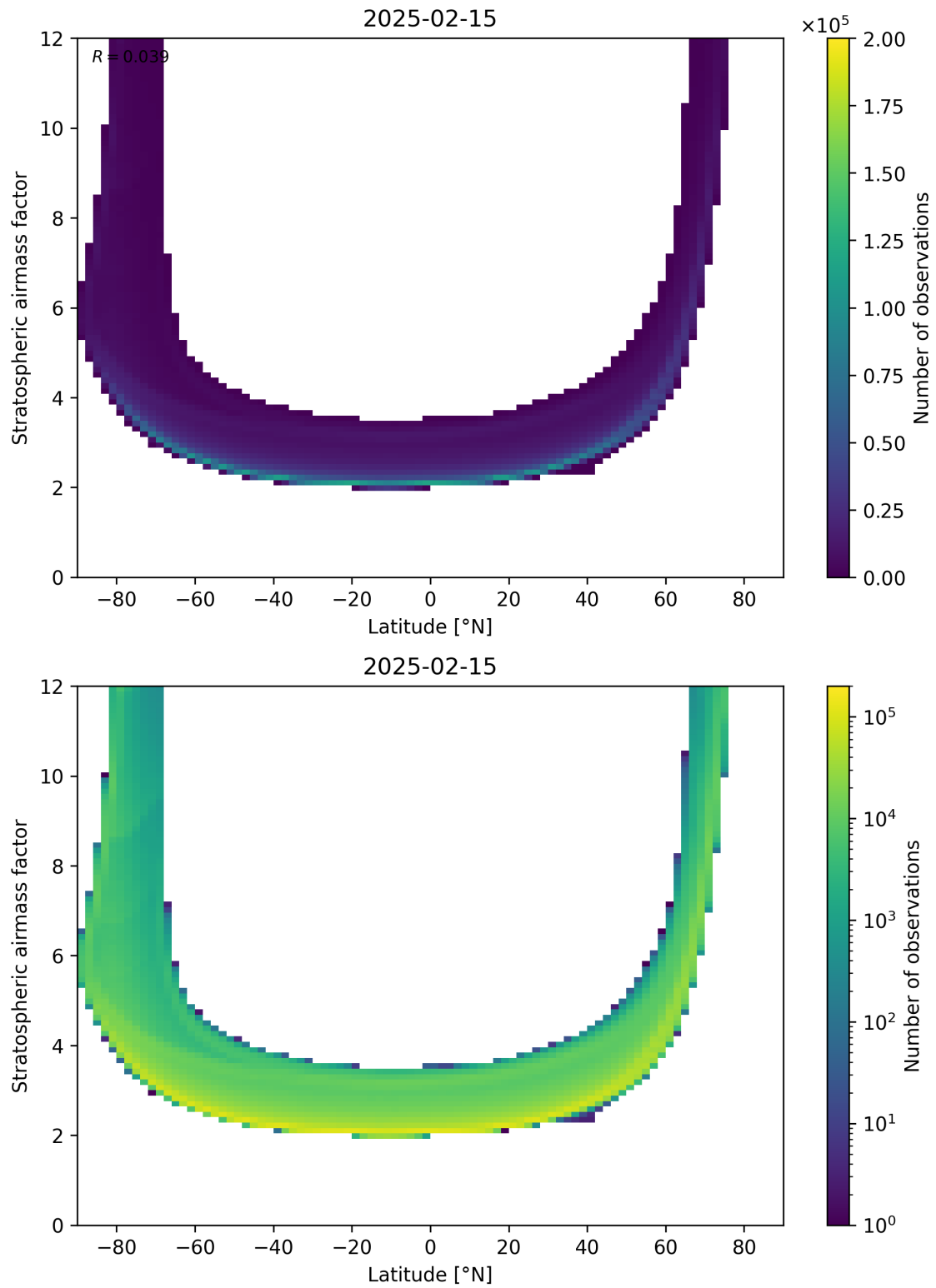
Figure 83: Scatter density plot of “Latitude” against “Stratospheric air mass factor” for 2025-02-14 to 2025-02-16.
