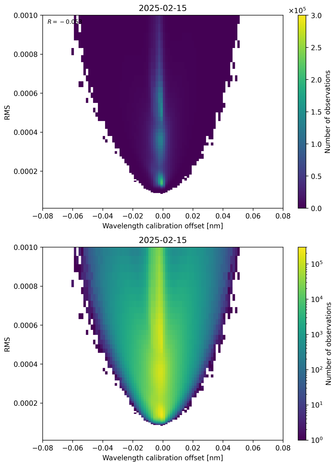
Figure 181: Scatter density plot of “Wavelength calibration offset” against “RMS” for 2025-02-14 to 2025-02-16.
