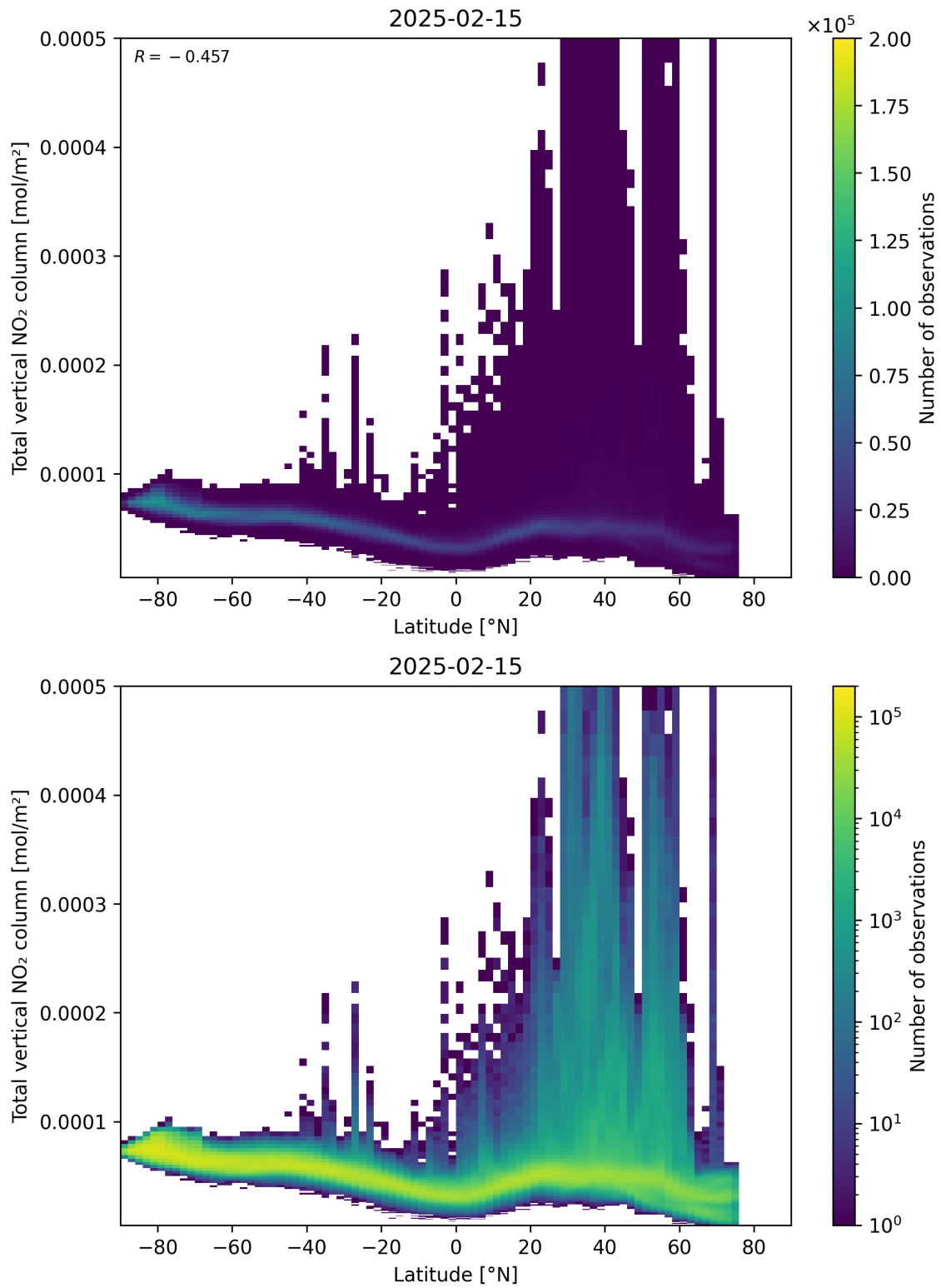
Figure 90: Scatter density plot of “Latitude” against “Total vertical NO 2 column” for 2025-02-14 to 2025-02-16.
