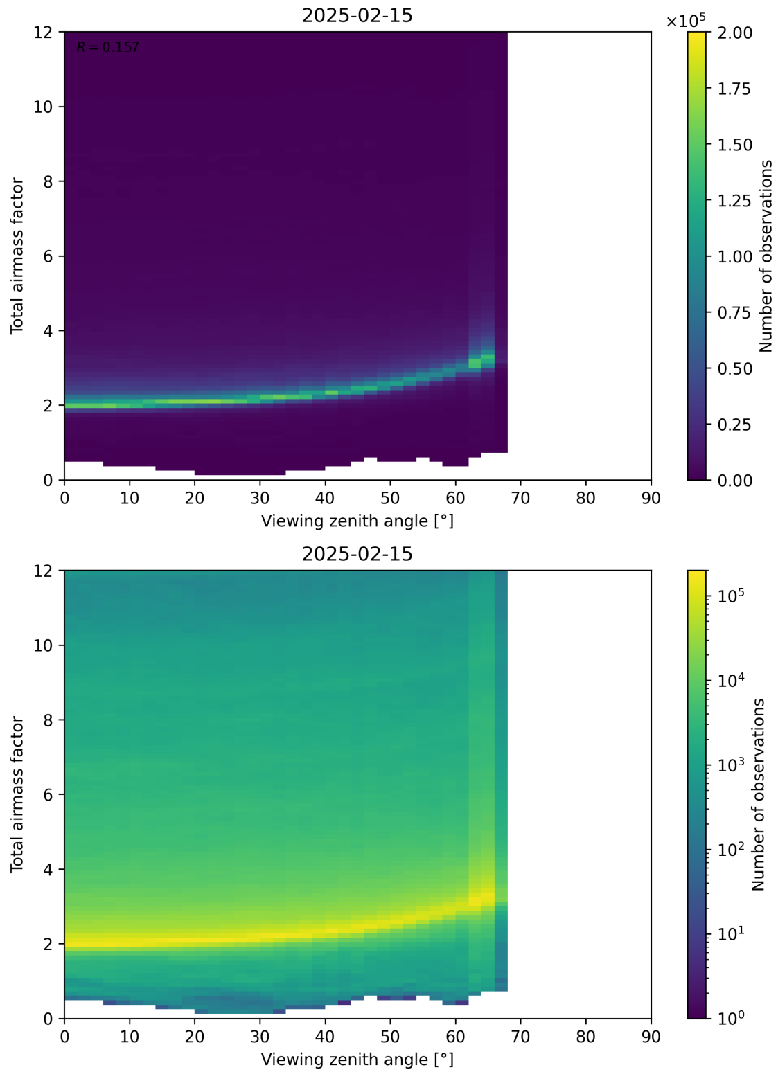
Figure 160: Scatter density plot of “Viewing zenith angle” against “Total airmass factor” for 2025-02-14 to 2025-02-16.
