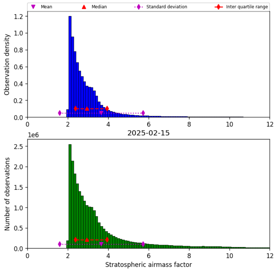
Figure 44: Histogram of “Stratospheric airmass factor” for 2025-02-14 to 2025-02-16
