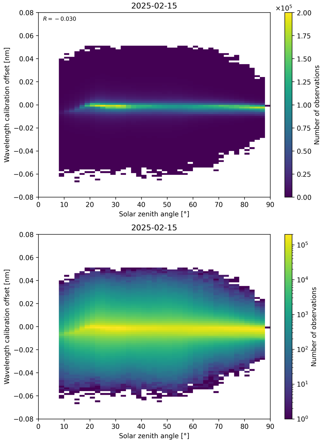
Figure 158: Scatter density plot of “Solar zenith angle” against “Wavelength calibration offset” for 2025-02-14 to 2025-02-16.
