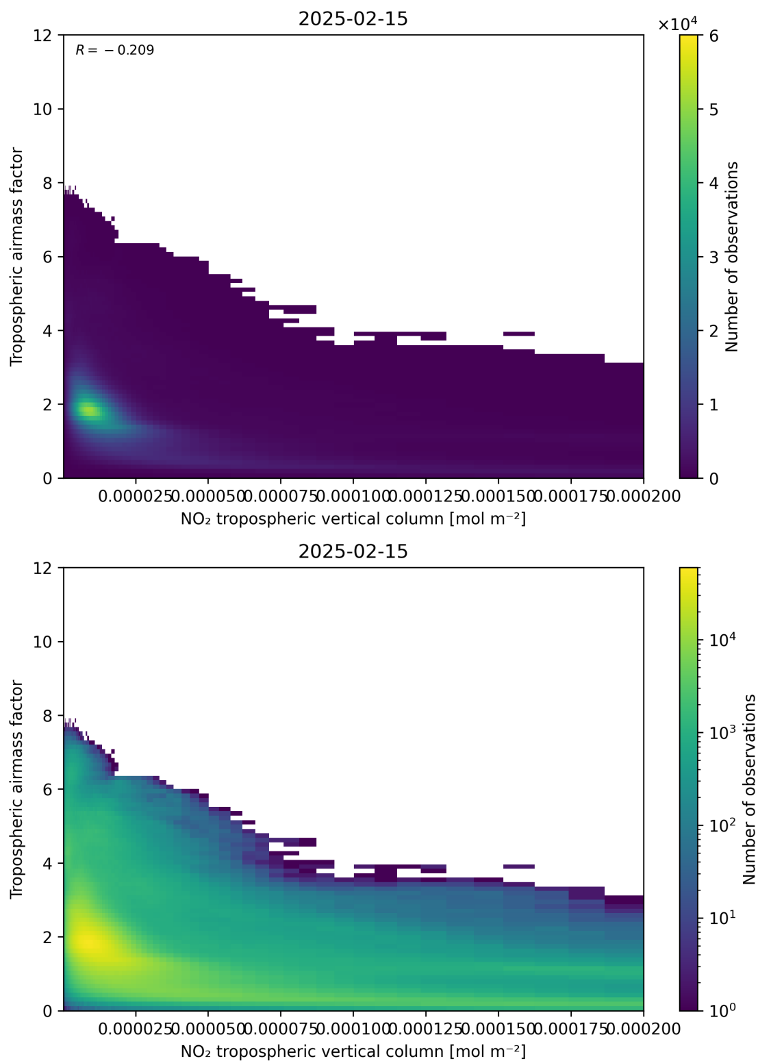
Figure 123: Scatter density plot of “NO 2 tropospheric vertical column” against “Tropospheric air mass factor” for 2025-02-14 to 2025-02-16.
