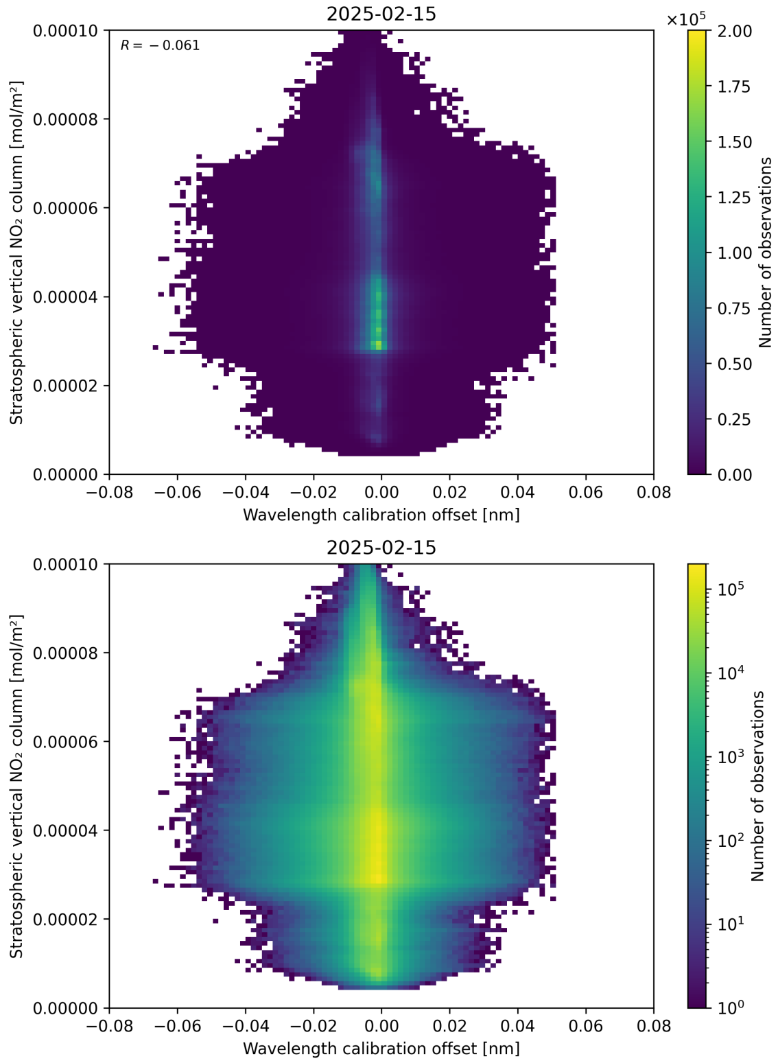
Figure 176: Scatter density plot of “Wavelength calibration offset” against “Stratospheric vertical NO 2 column” for 2025-02-14 to 2025-02-16.
