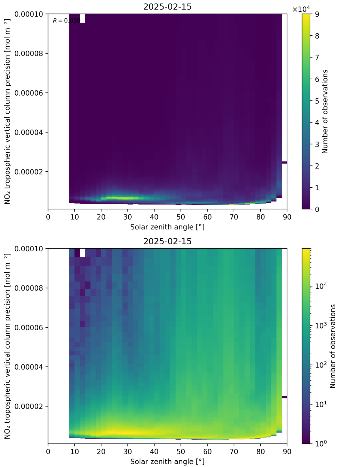
Figure 156: Scatter density plot of “Solar zenith angle” against “NO 2 tropospheric vertical column precision” for 2025-02-14 to 2025-02-16.
