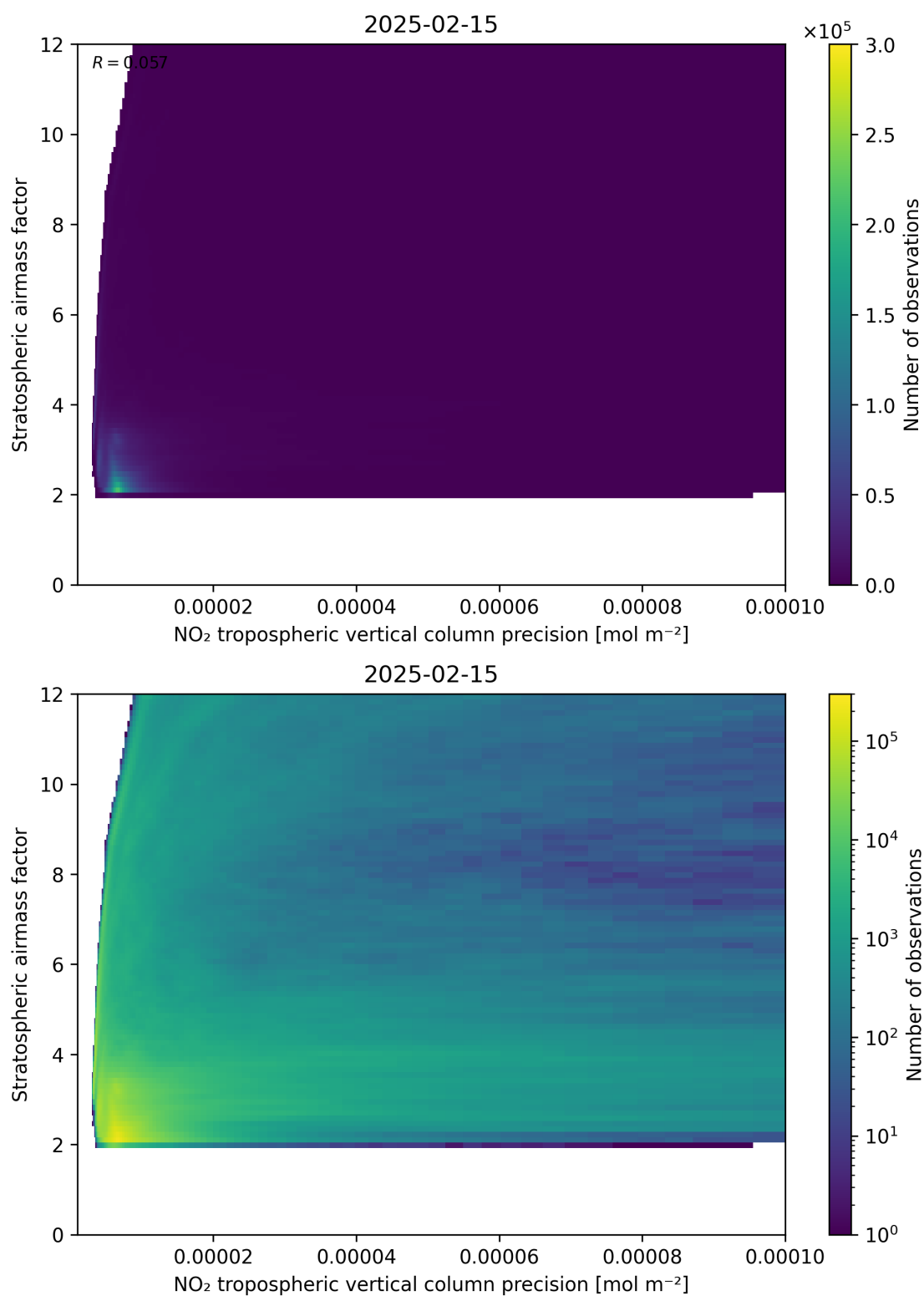
Figure 131: Scatter density plot of “NO 2 tropospheric vertical column precision” against “Stratospheric airmass factor” for 2025-02-14 to 2025-02-16.
