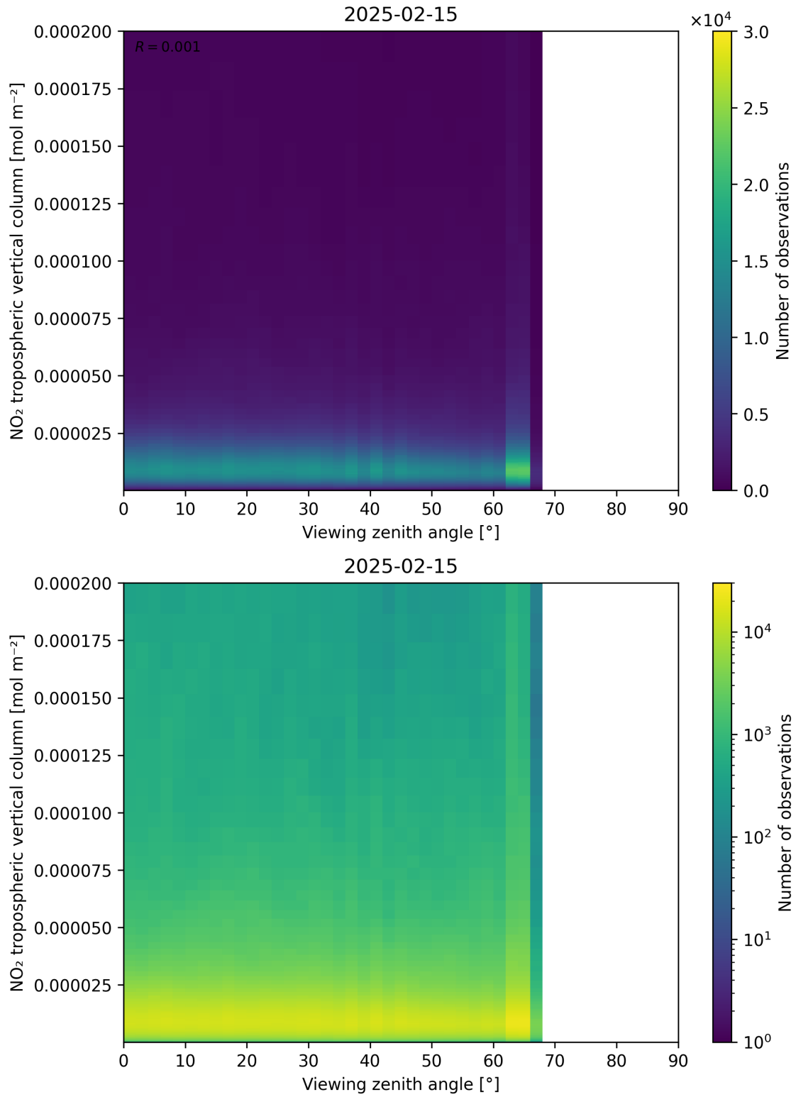
Figure 169: Scatter density plot of “Viewing zenith angle” against “NO 2 tropospheric vertical column” for 2025-02-14 to 2025-02-16.
