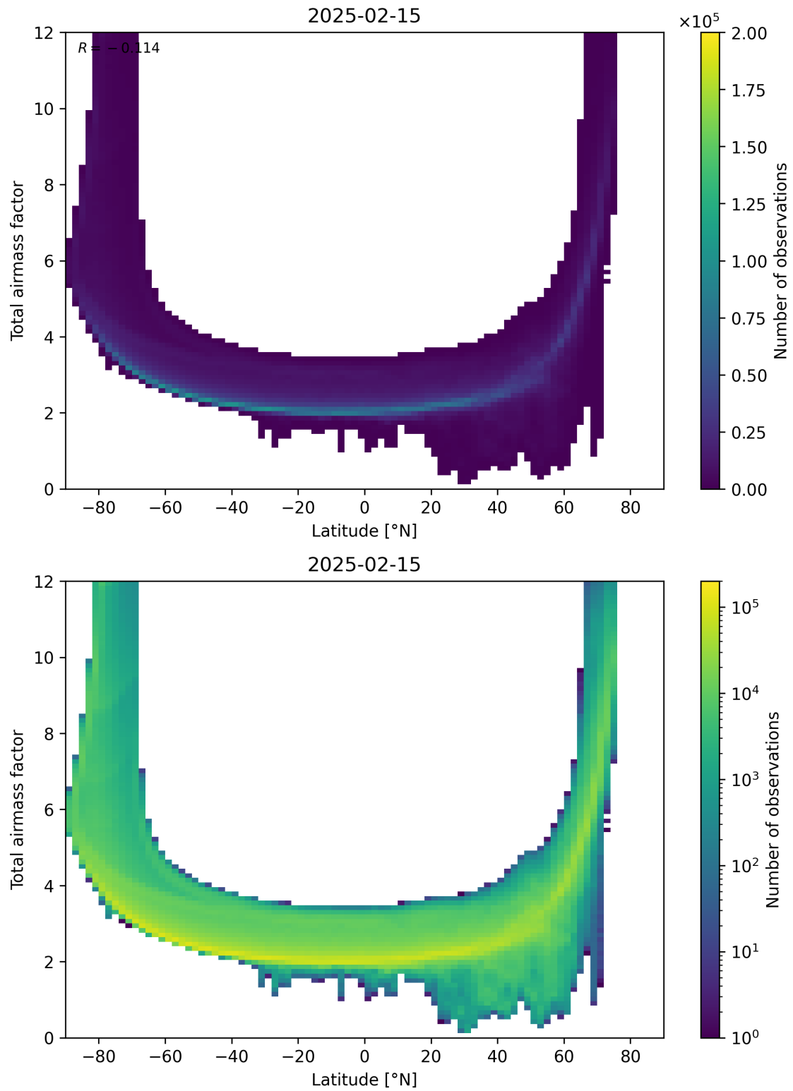
Figure 84: Scatter density plot of “Latitude” against “Total airmass factor” for 2025-02-14 to 2025-02-16.
