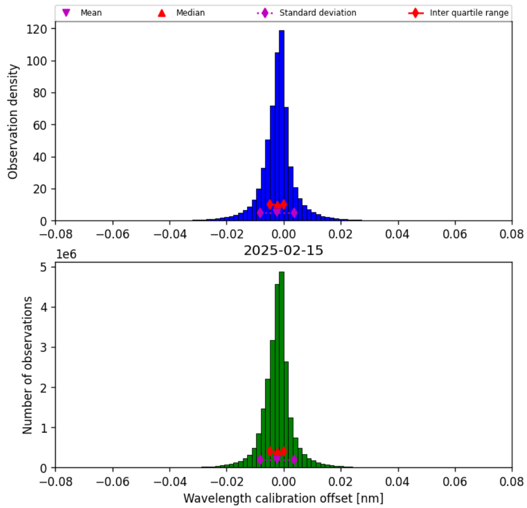
Figure 35: Histogram of “Wavelength calibration offset” for 2025-02-14 to 2025-02-16
