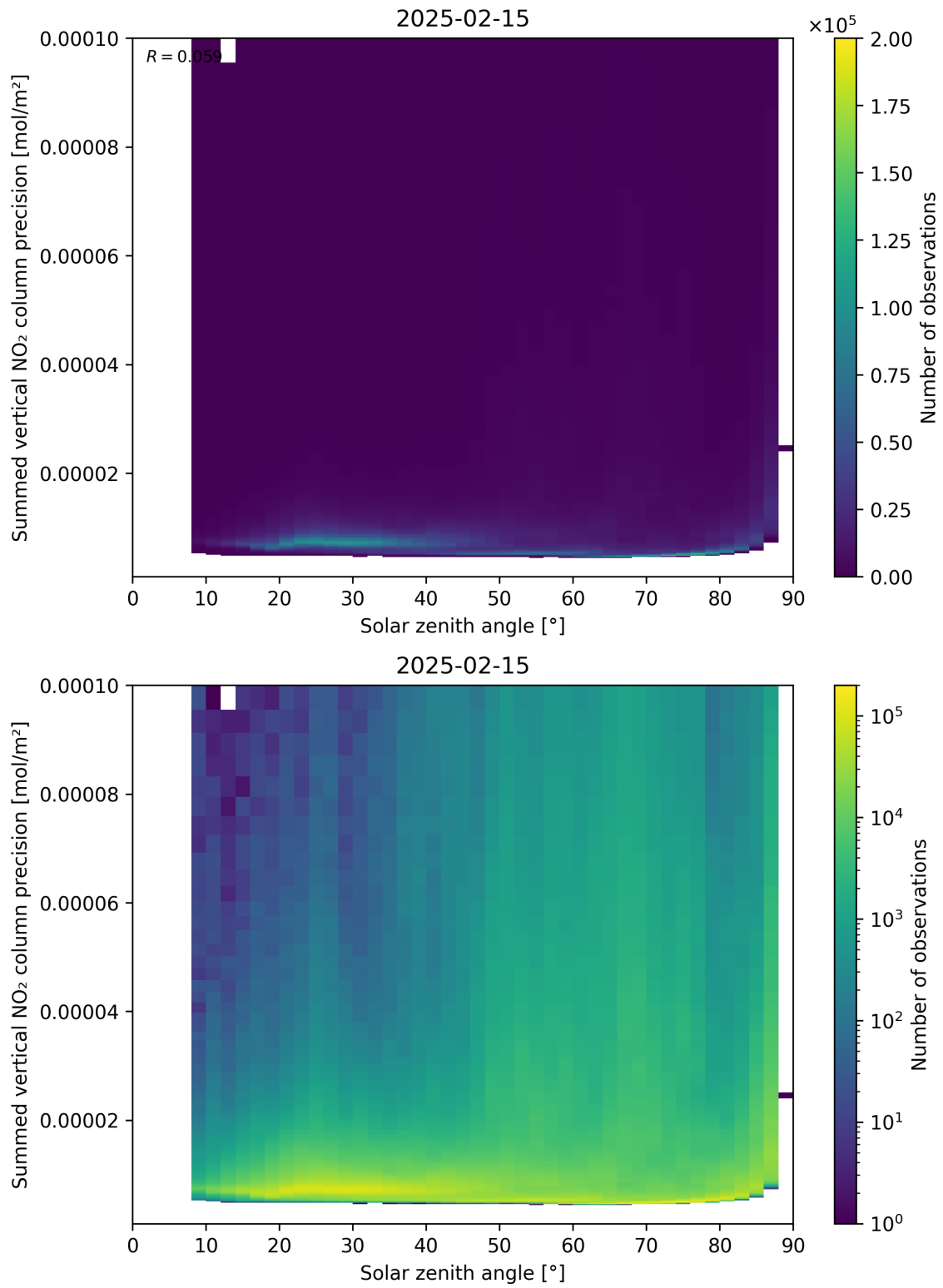
Figure 152: Scatter density plot of “Solar zenith angle” against “Summed vertical NO 2 column precision” for 2025-02-14 to 2025-02-16.
