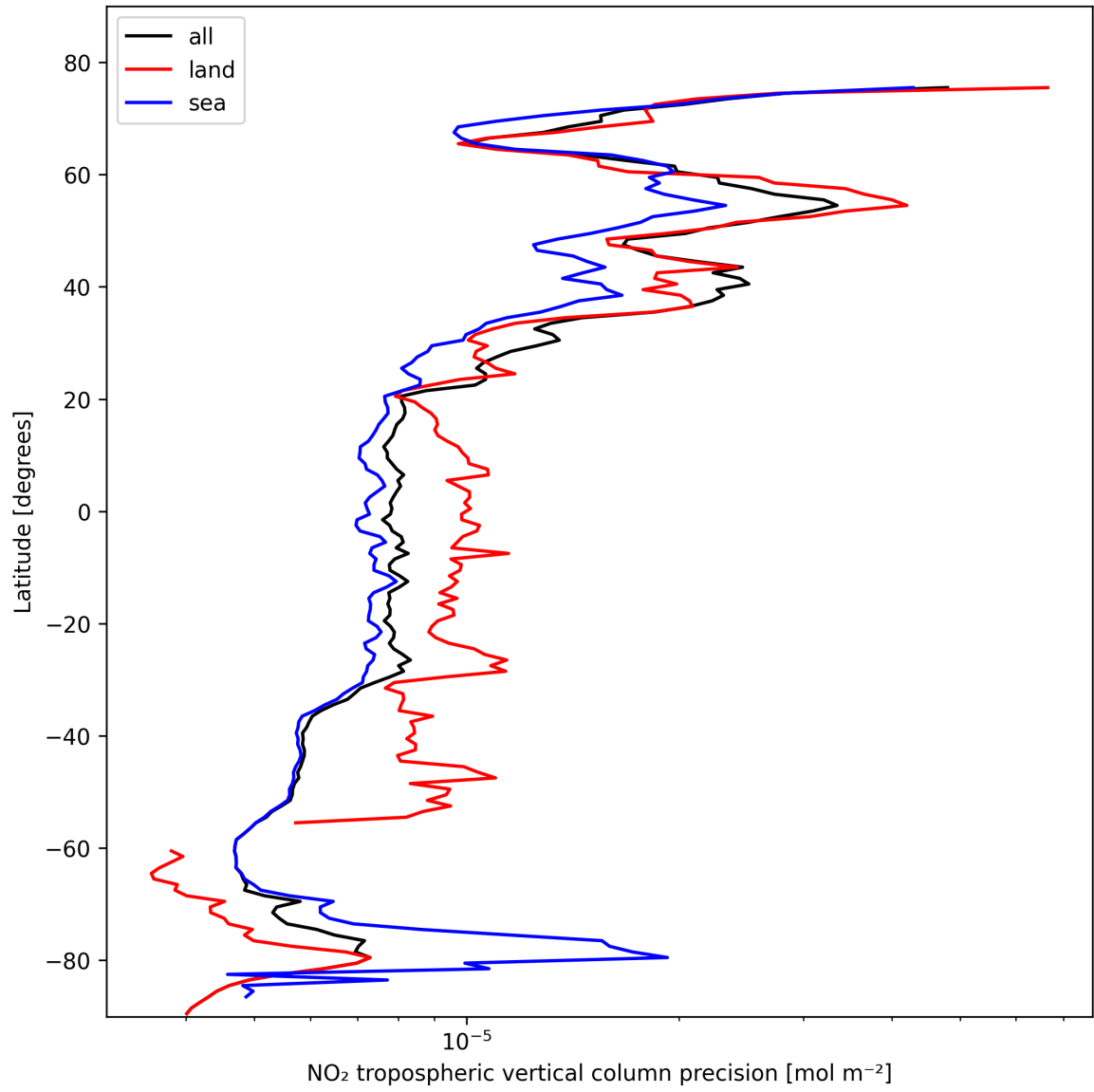
Figure 13: Zonal average of “NO 2 tropospheric vertical column precision” for 2025-02-14 to 2025-02-16.
