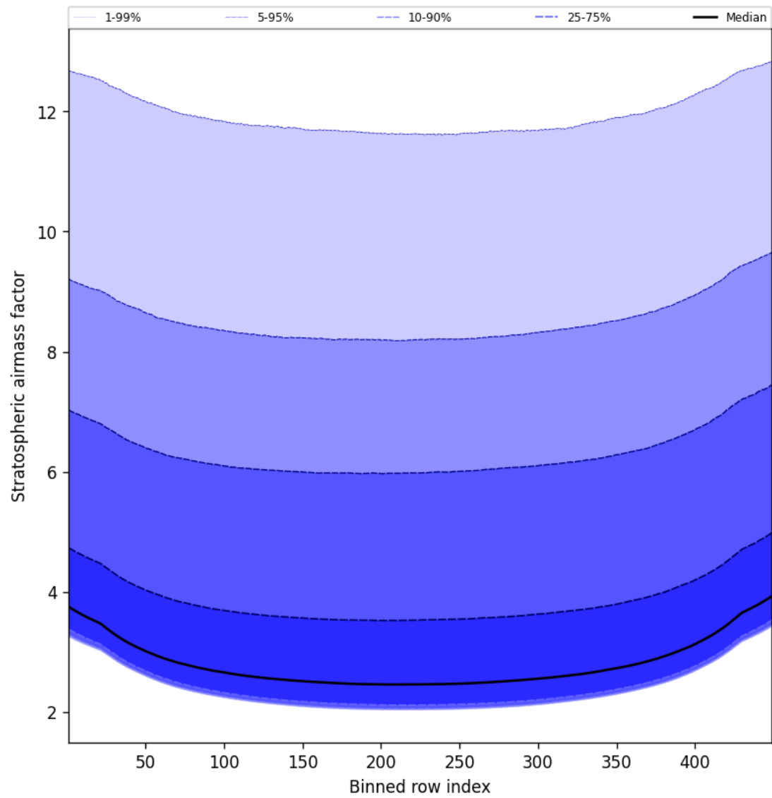
Figure 61: Along track statistics of “Stratospheric airmass factor” for 2025-02-14 to 2025-02-16
