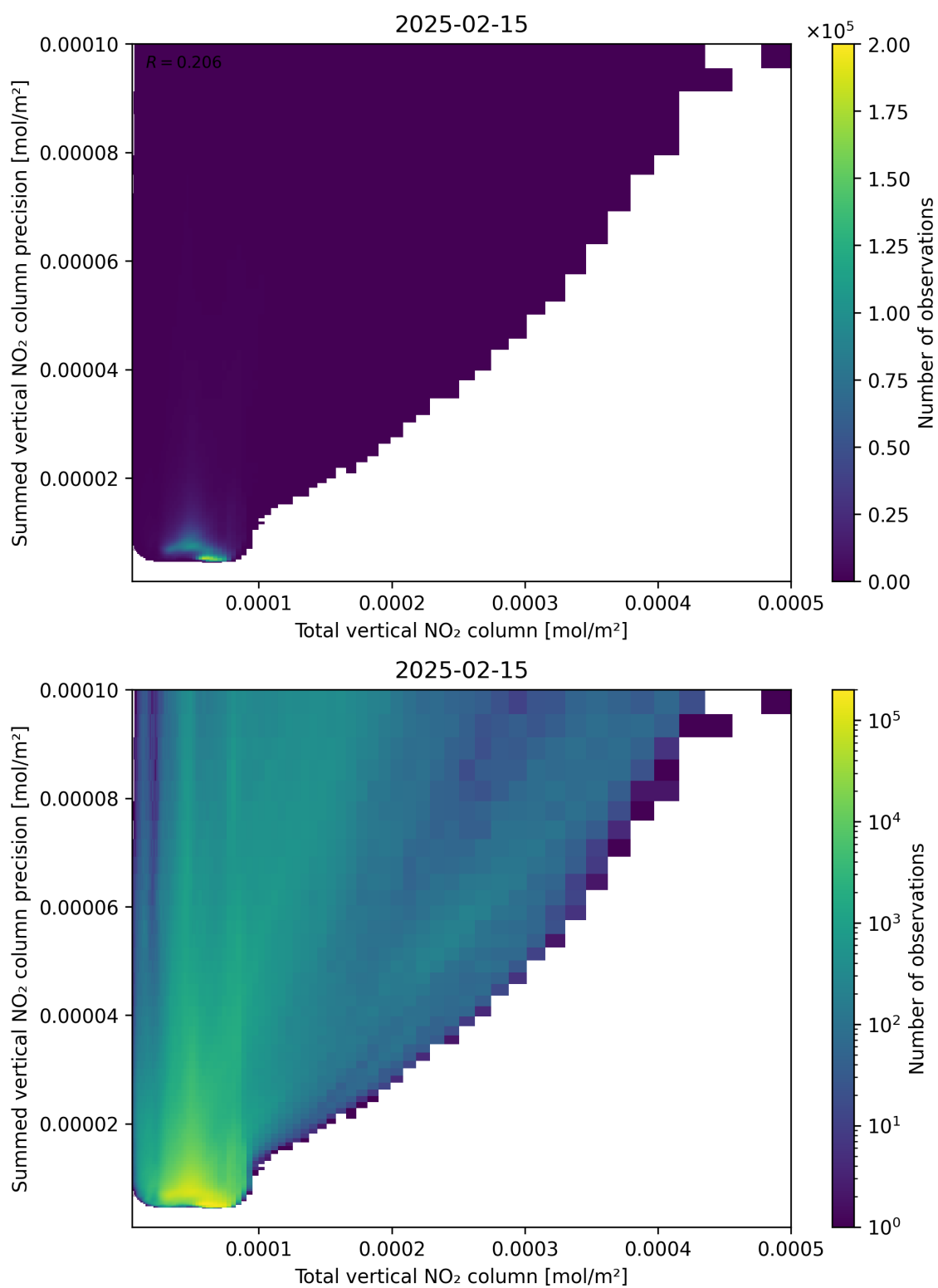
Figure 113: Scatter density plot of “Total vertical NO 2 column” against “Summed vertical NO 2 column precision” for 2025-02-14 to 2025-02-16.
