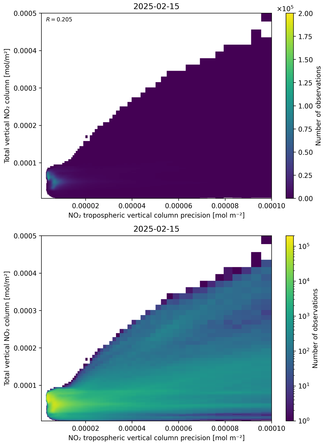
Figure 138: Scatter density plot of “NO 2 tropospheric vertical column precision” against “Total vertical NO 2 column” for 2025-02-14 to 2025-02-16.
