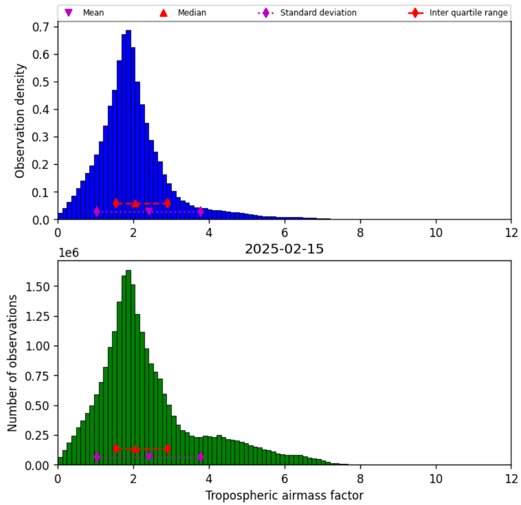
Figure 31: Histogram of “Tropospheric airmass factor” for 2025-02-14 to 2025-02-16
