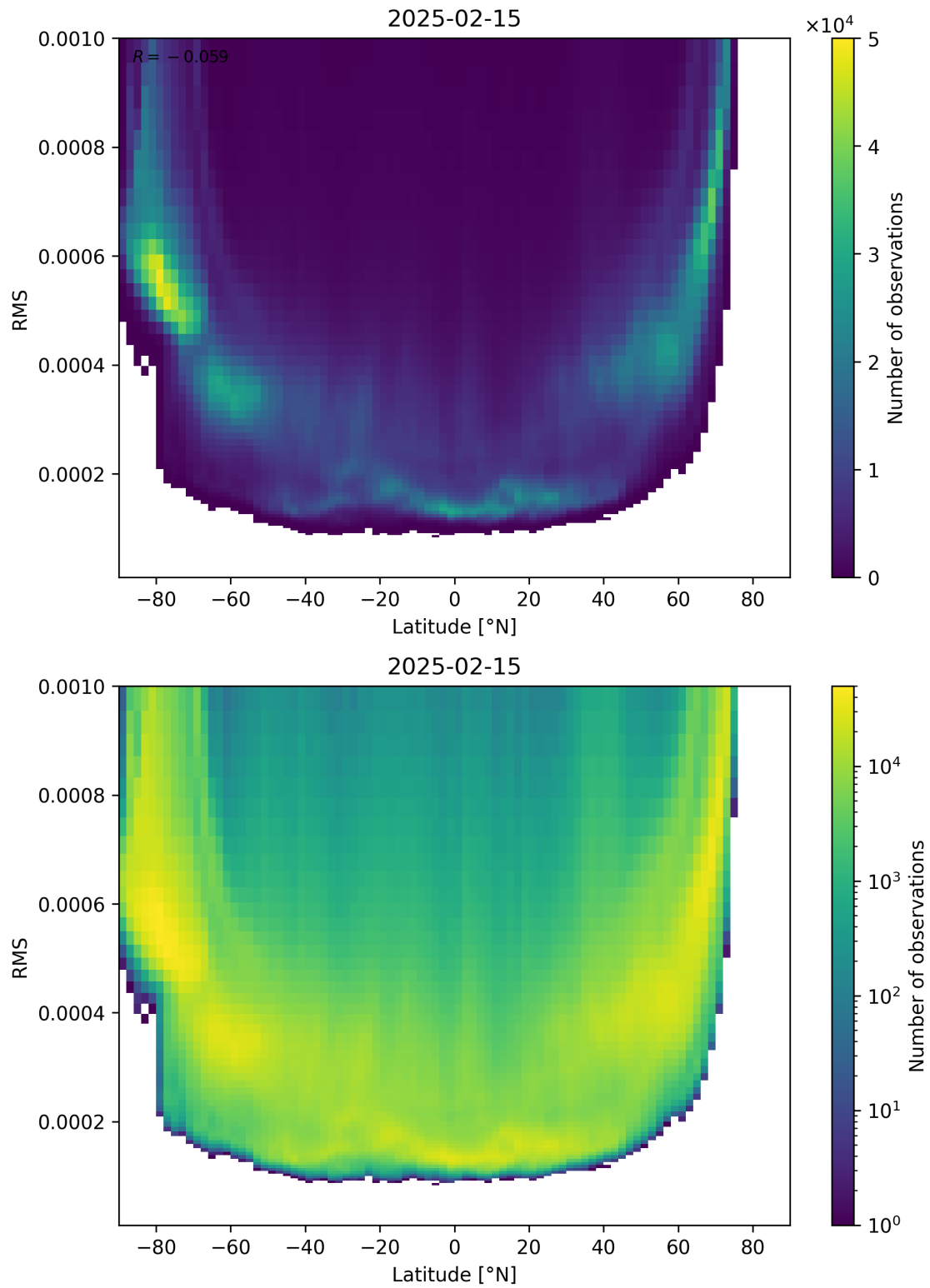
Figure 94: Scatter density plot of “Latitude” against “RMS” for 2025-02-14 to 2025-02-16.
