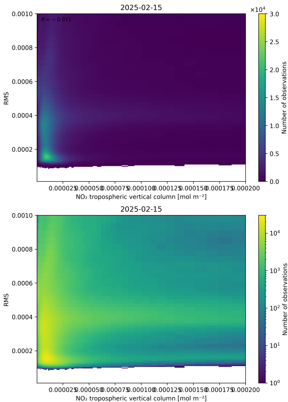
Figure 142: Scatter density plot of “NO 2 tropospheric vertical column” against “RMS” for 2025-02-14 to 2025-02-16.
