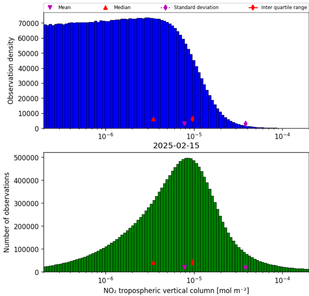
Figure 29: Histogram of “NO 2 tropospheric vertical column” for 2025-02-14 to 2025-02-16
