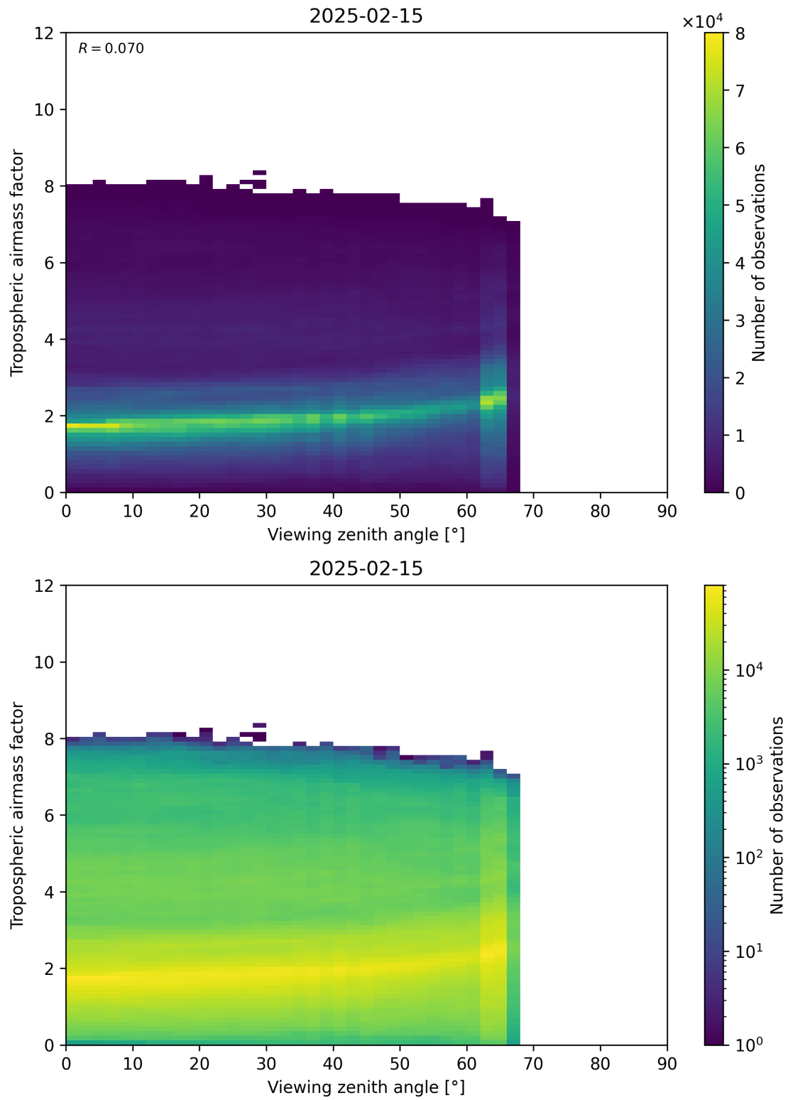
Figure 161: Scatter density plot of “Viewing zenith angle” against “Tropospheric airmass factor” for 2025-02-14 to 2025-02-16.
