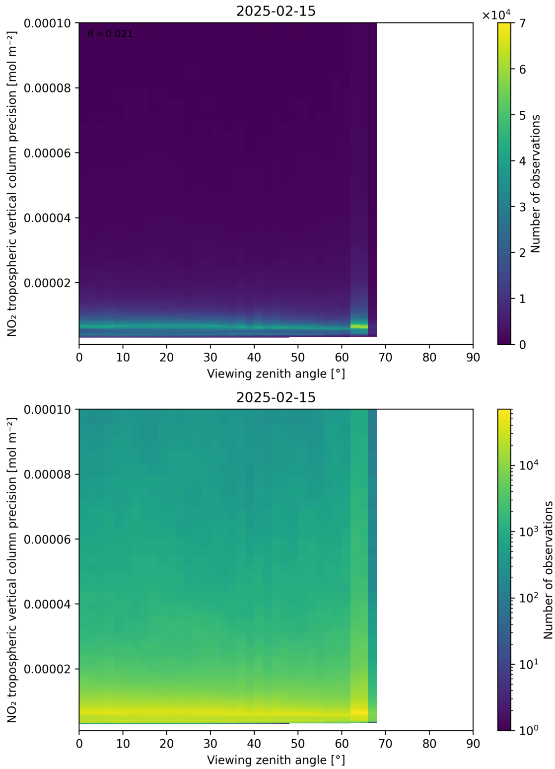
Figure 170: Scatter density plot of “Viewing zenith angle” against “NO 2 tropospheric vertical column precision” for 2025-02-14 to 2025-02-16.
