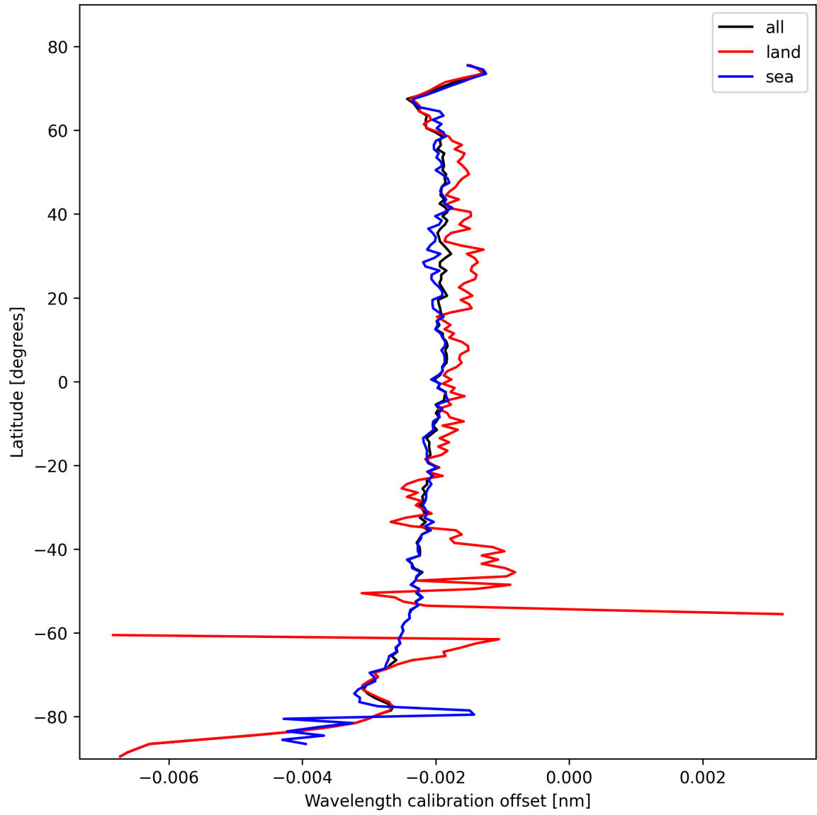
Figure 18: Zonal average of “Wavelength calibration offset” for 2025-02-14 to 2025-02-16.
