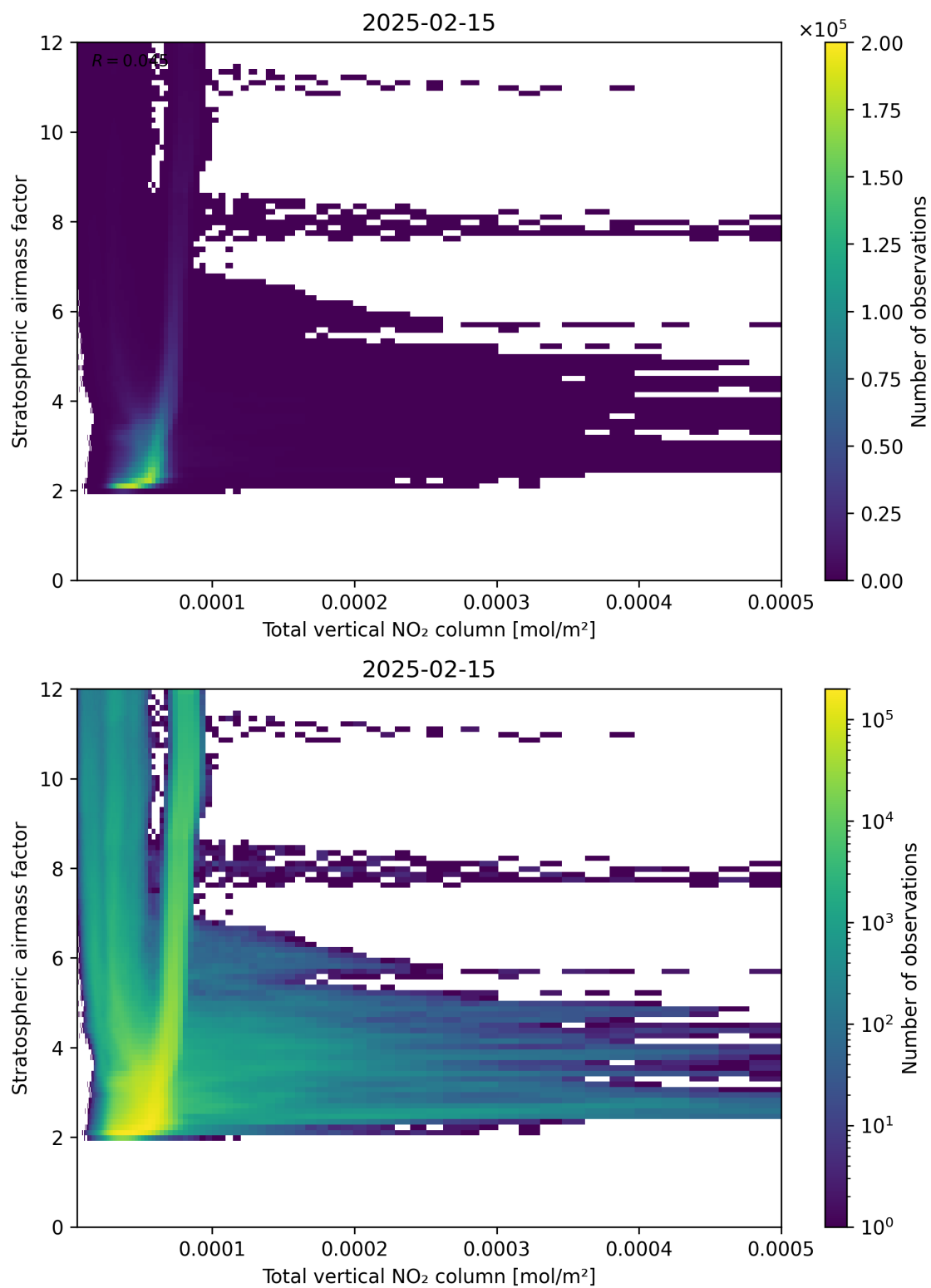
Figure 110: Scatter density plot of “Total vertical NO 2 column” against “Stratospheric air mass factor” for 2025-02-14 to 2025-02-16.
