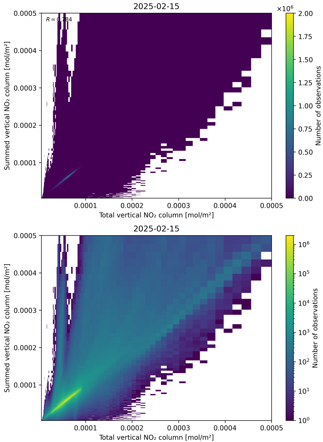
Figure 112: Scatter density plot of “Total vertical NO 2 column” against “Summed vertical NO 2 column” for 2025-02-14 to 2025-02-16.
