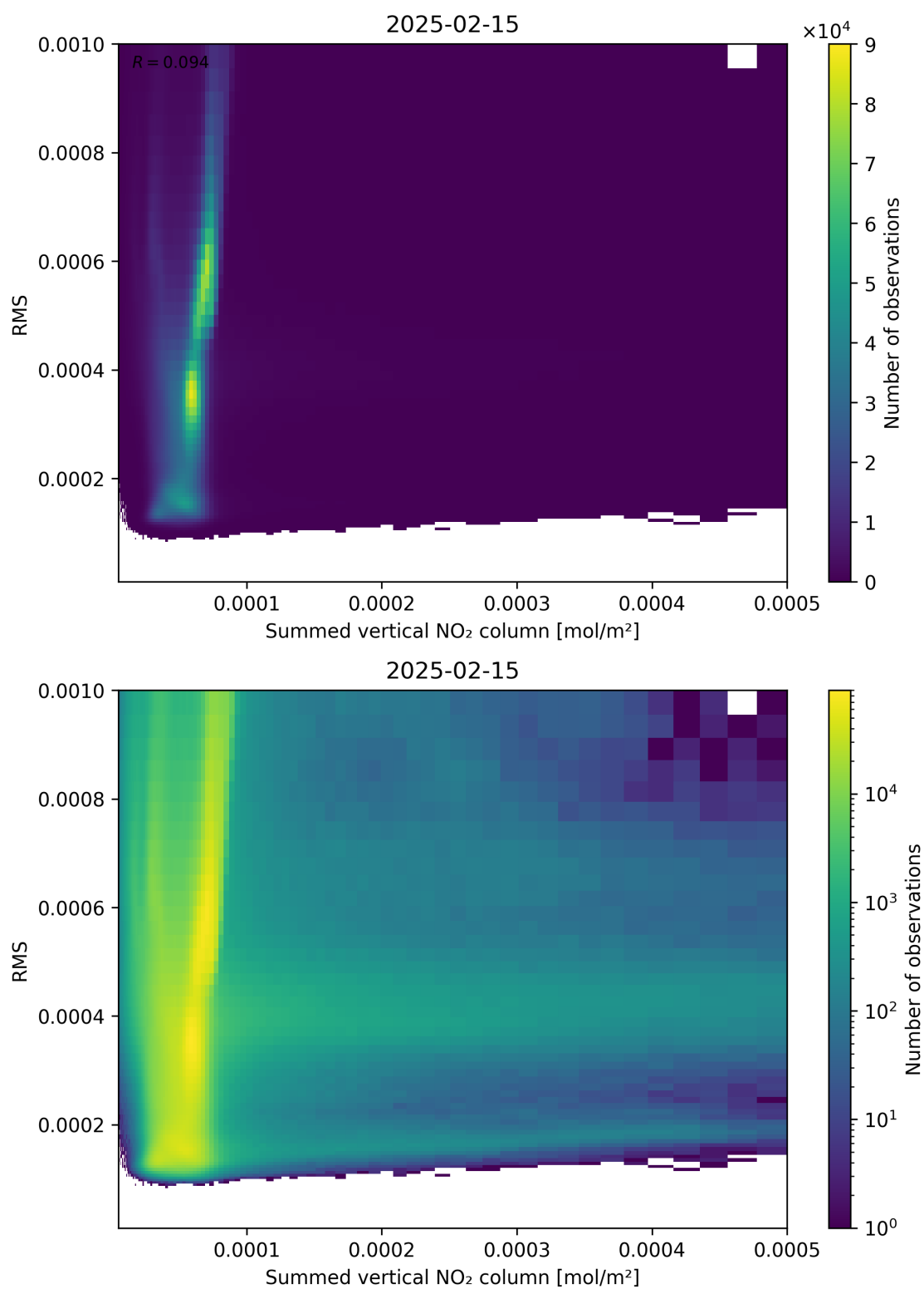
Figure 109: Scatter density plot of “Summed vertical NO 2 column” against “RMS” for 2025-02-14 to 2025-02-16.
