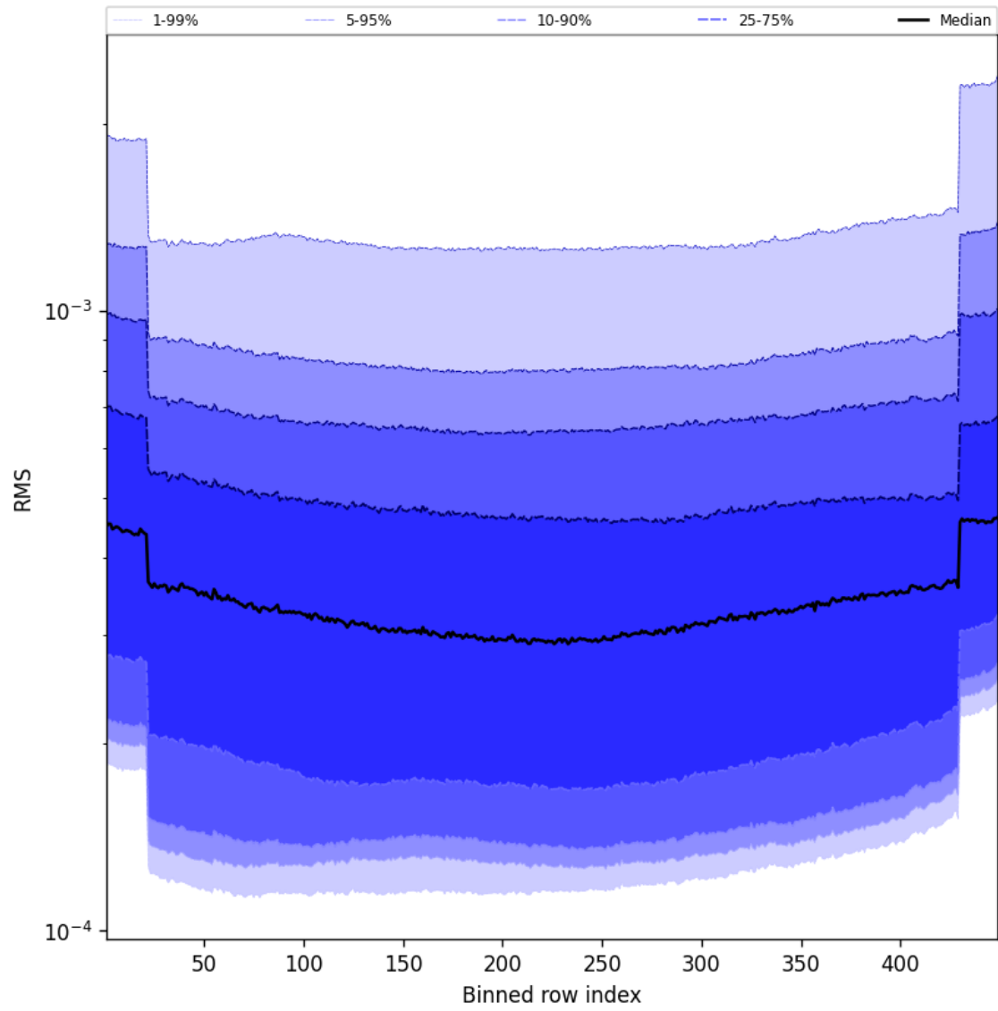
Figure 60: Along track statistics of “RMS” for 2025-02-14 to 2025-02-16
