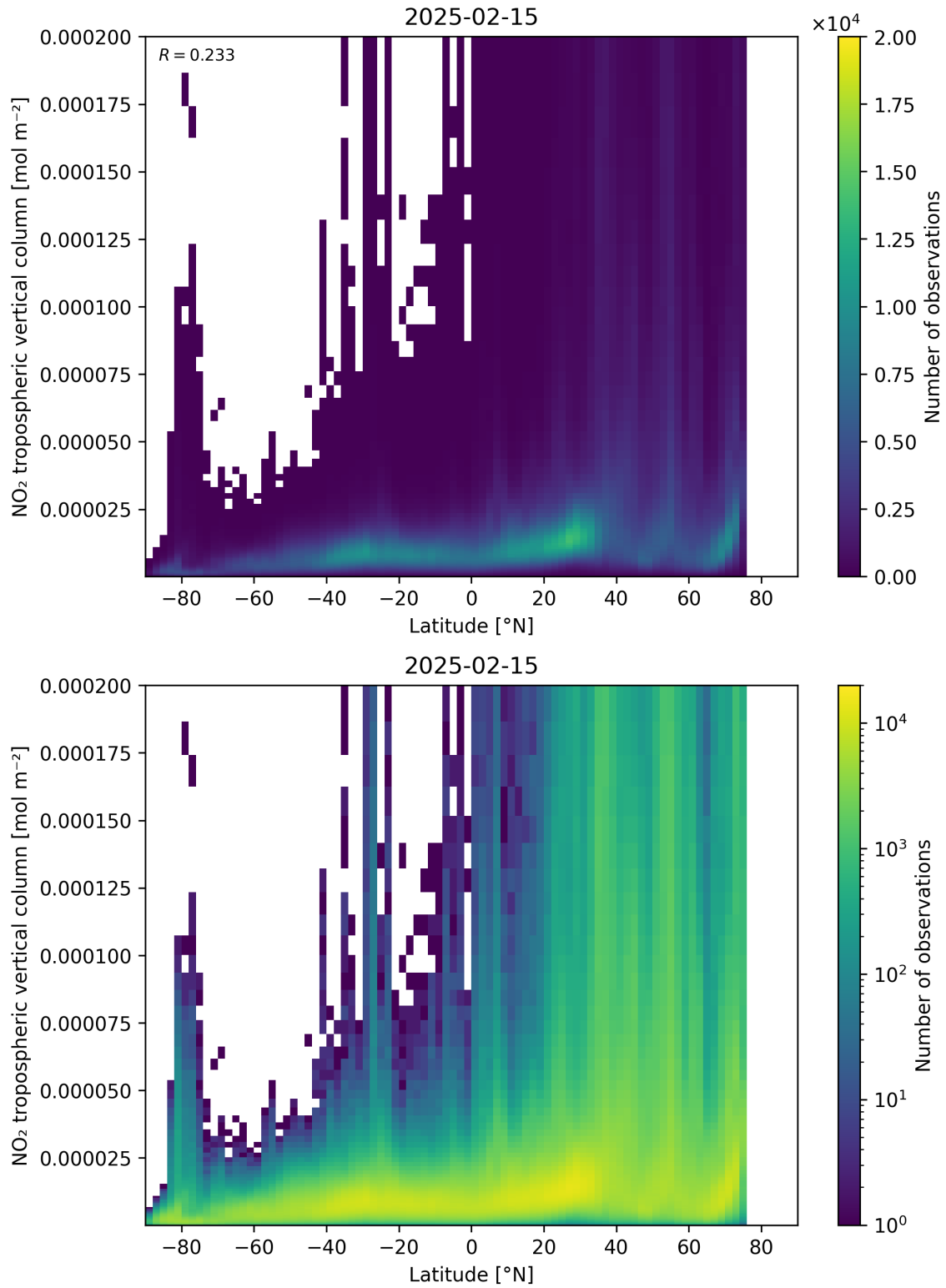
Figure 92: Scatter density plot of “Latitude” against “NO 2 tropospheric vertical column” for 2025-02-14 to 2025-02-16.
