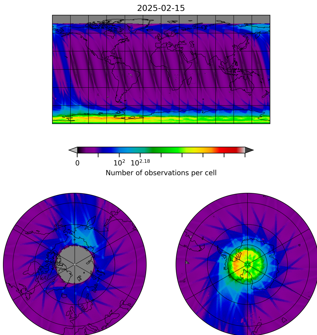
Figure 10: Map of the number of observations for 2025-02-14 to 2025-02-16
