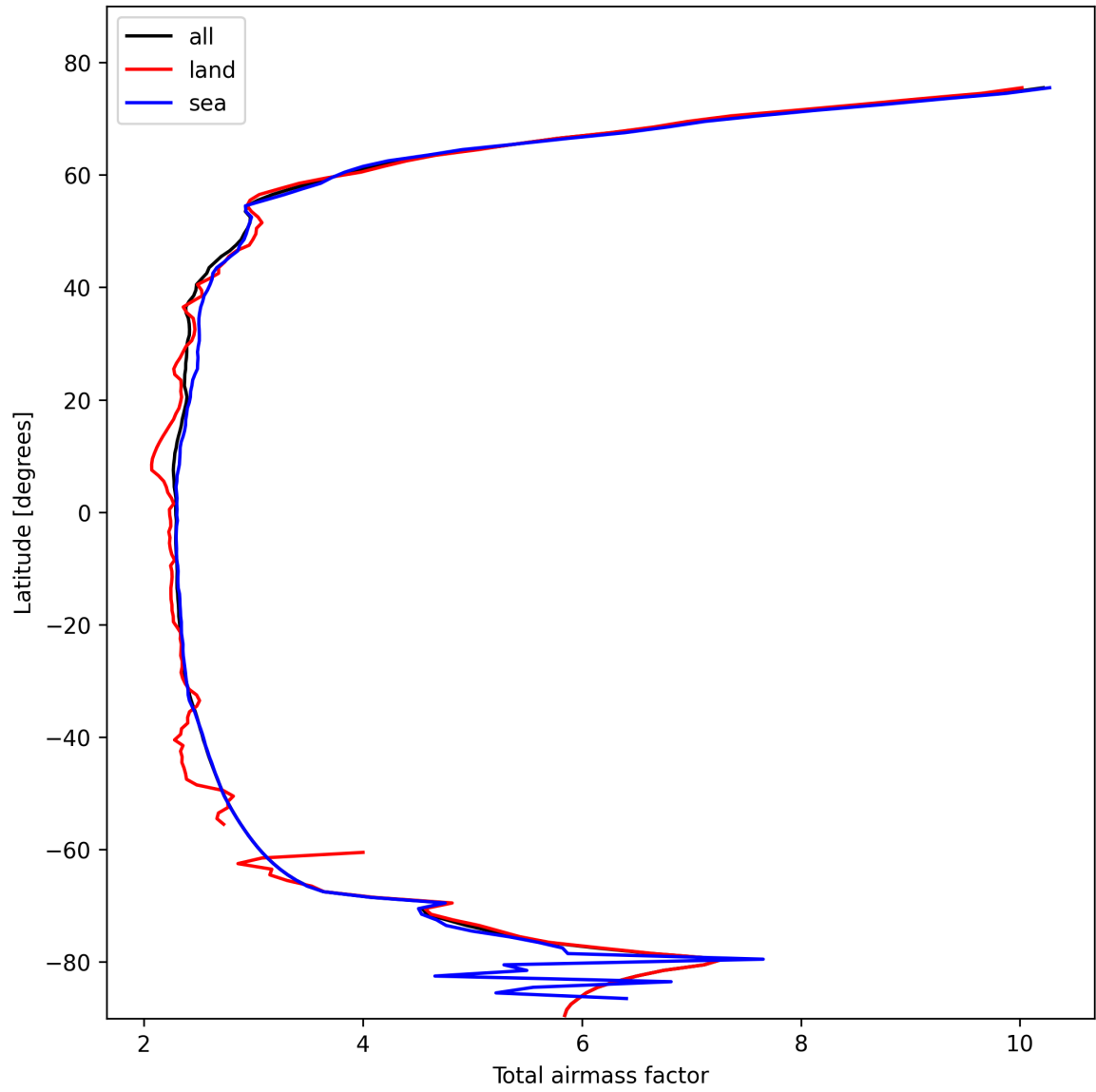
Figure 15: Zonal average of “Total airmass factor” for 2025-02-14 to 2025-02-16.
