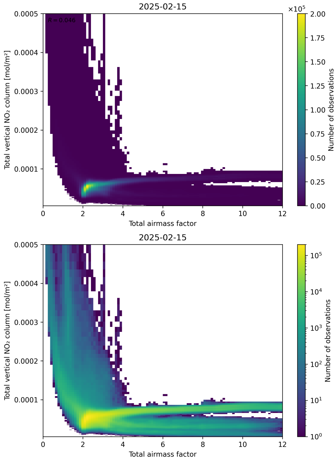
Figure 67: Scatter density plot of “Total airmass factor” against “Total vertical NO 2 column” for 2025-02-14 to 2025-02-16.
