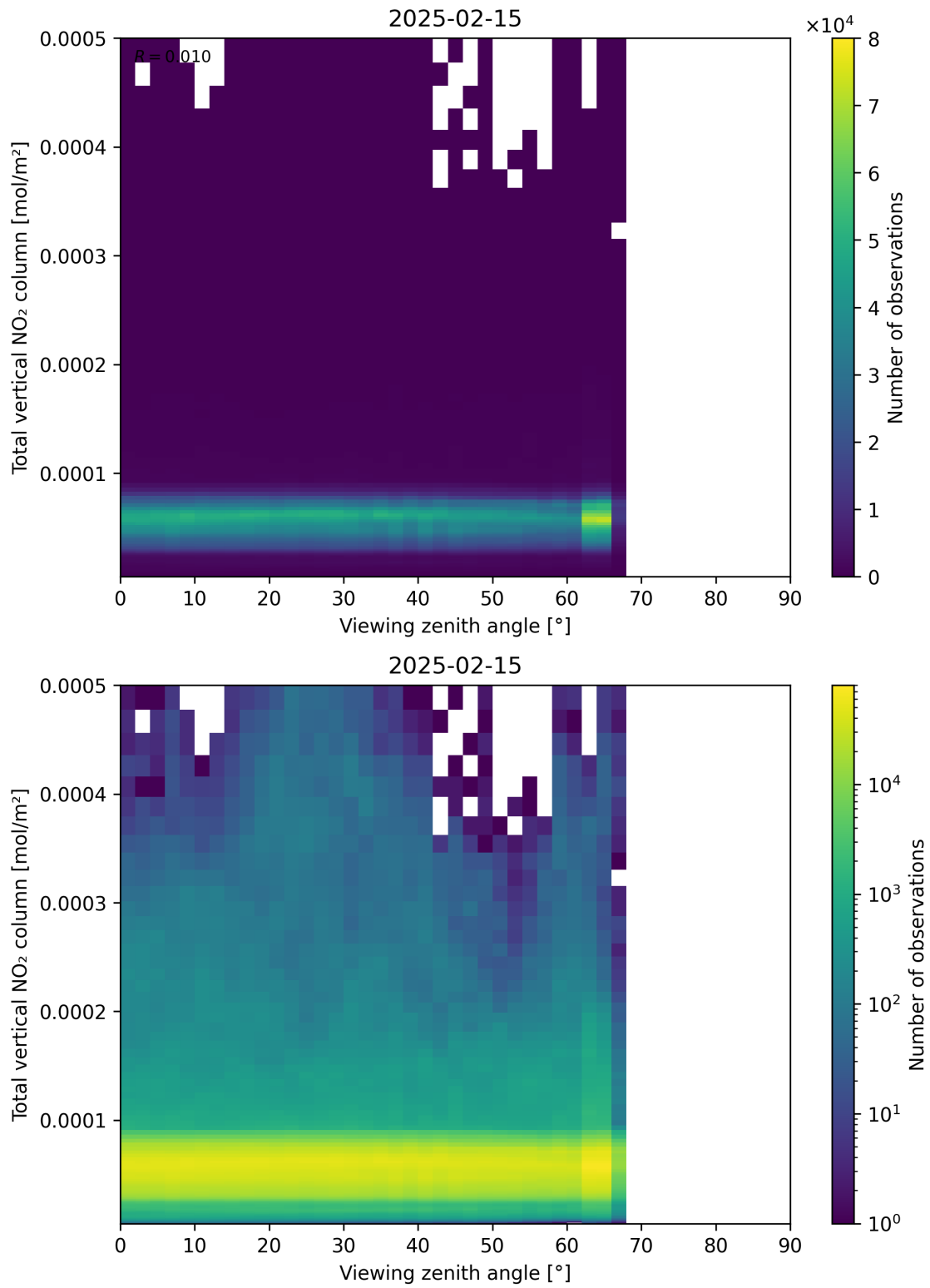
Figure 167: Scatter density plot of “Viewing zenith angle” against “Total vertical NO 2 column” for 2025-02-14 to 2025-02-16.
