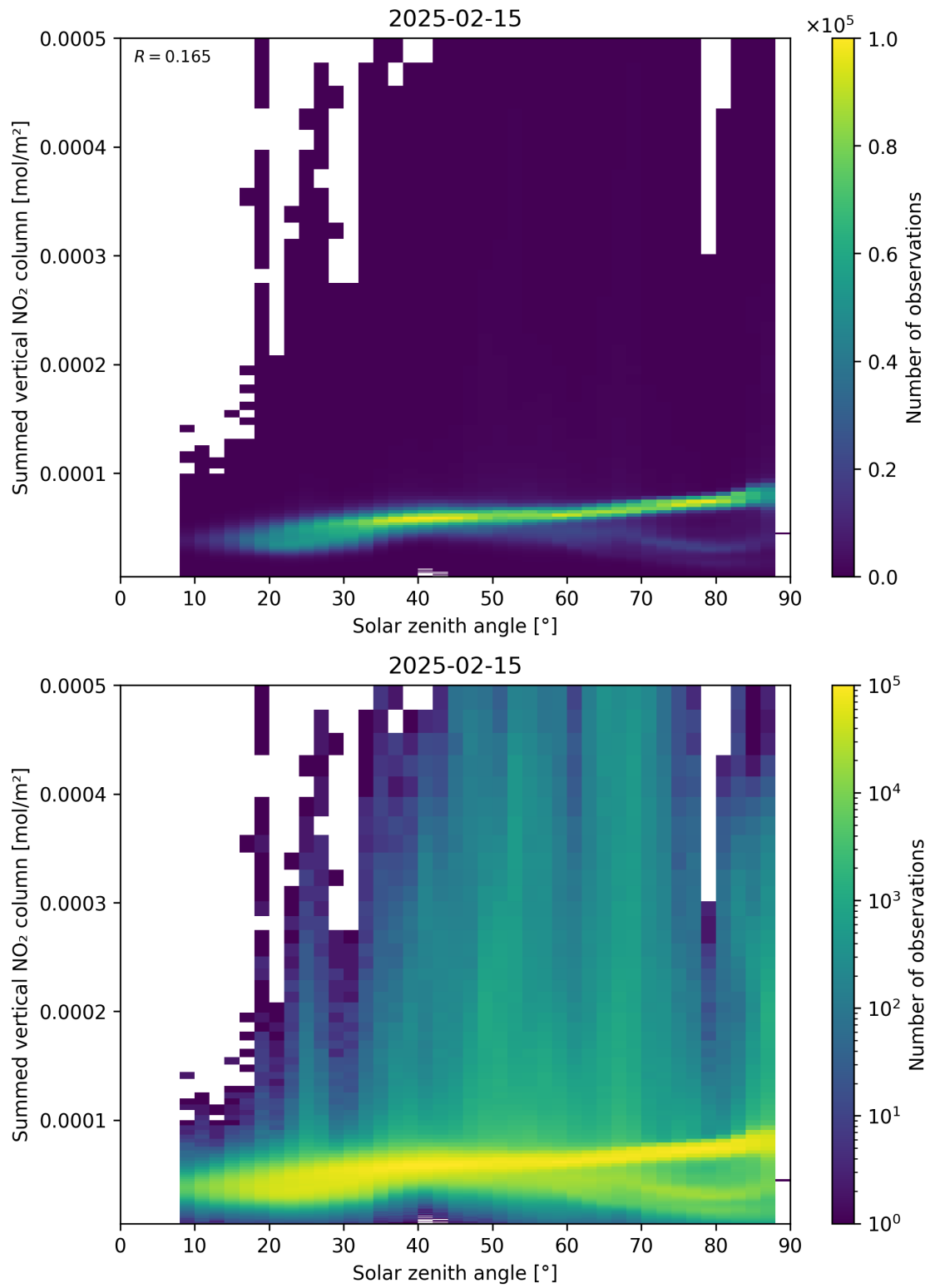
Figure 151: Scatter density plot of “Solar zenith angle” against “Summed vertical NO 2 column” for 2025-02-14 to 2025-02-16.
