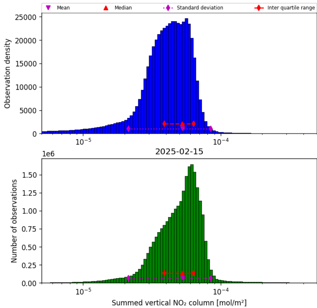
Figure 40: Histogram of “Summed vertical NO 2 column” for 2025-02-14 to 2025-02-16
