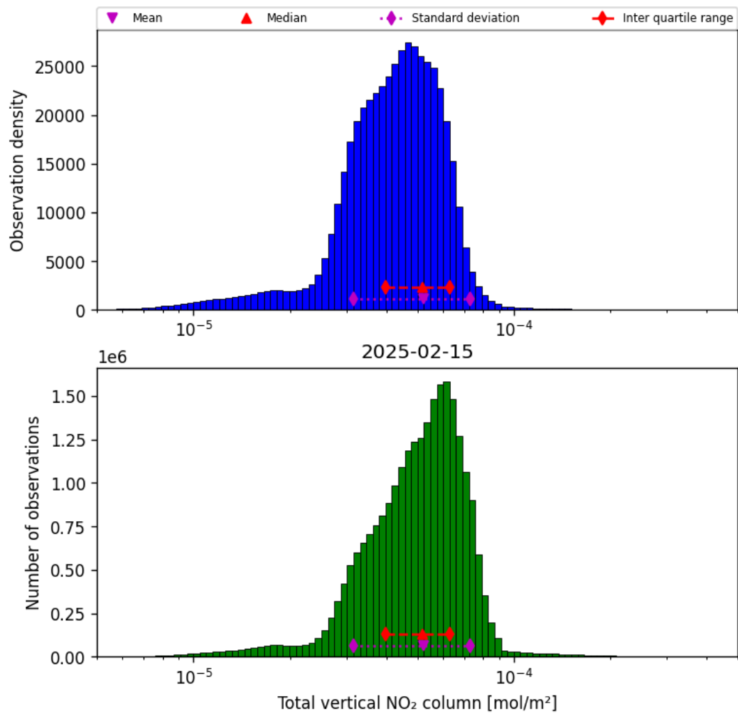
Figure 38: Histogram of “Total vertical NO 2 column” for 2025-02-14 to 2025-02-16
