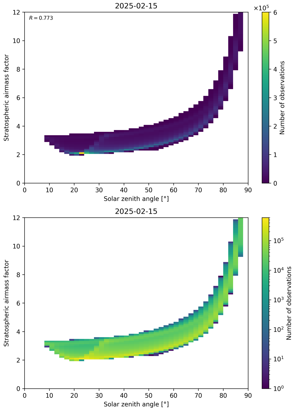
Figure 145: Scatter density plot of “Solar zenith angle” against “Stratospheric airmass factor” for 2025-02-14 to 2025-02-16.
