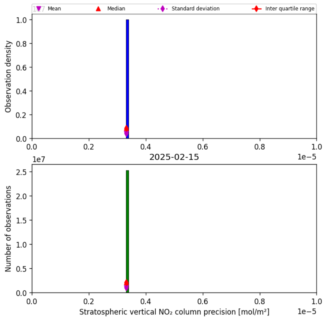
Figure 37: Histogram of “Stratospheric vertical NO 2 column precision” for 2025-02-14 to 2025-02-16
