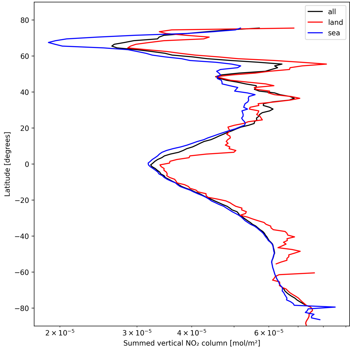
Figure 23: Zonal average of “Summed vertical NO 2 column” for 2025-02-14 to 2025-02-16.
