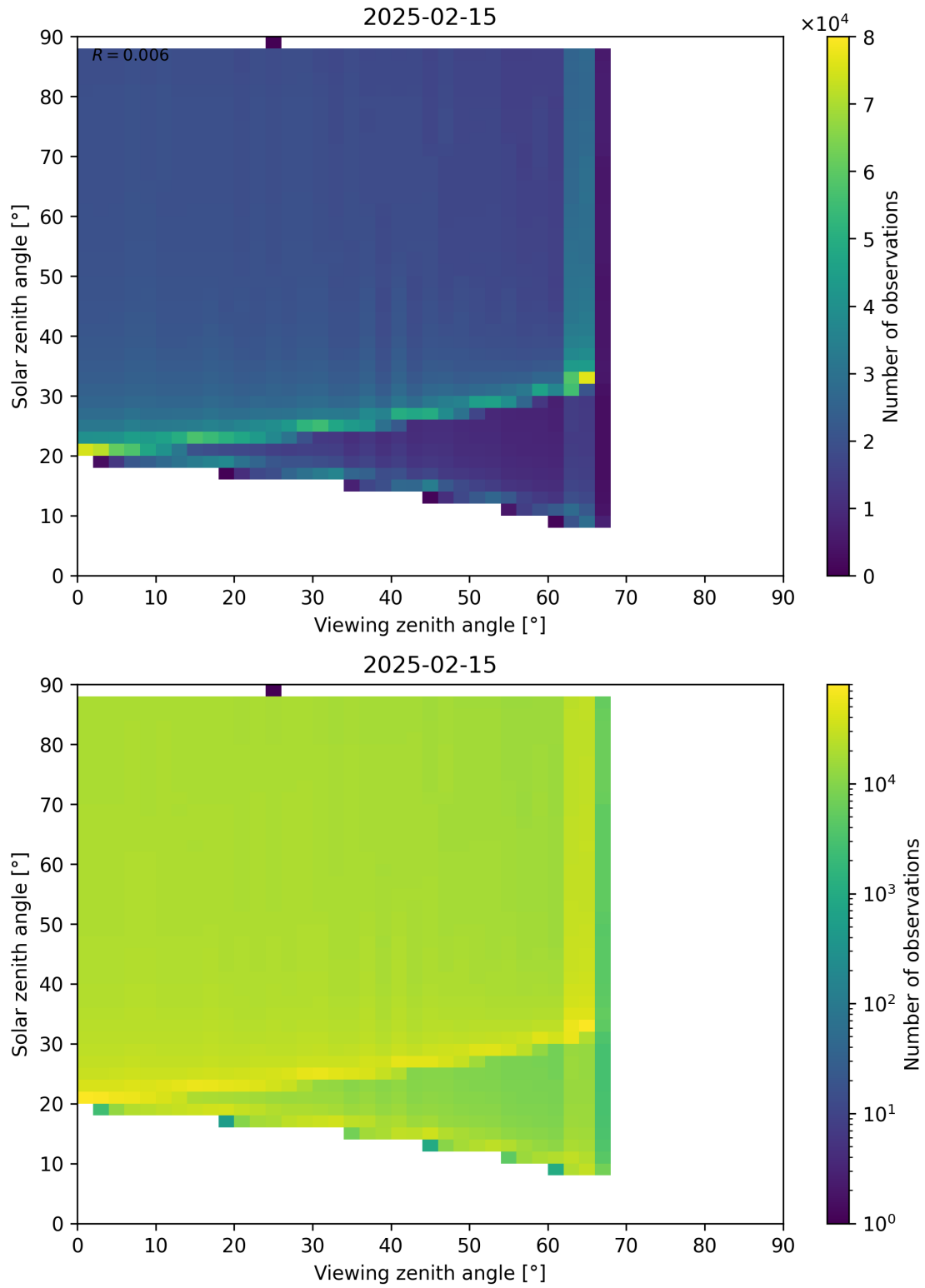
Figure 172: Scatter density plot of “Viewing zenith angle” against “Solar zenith angle” for 2025-02-14 to 2025-02-16.
