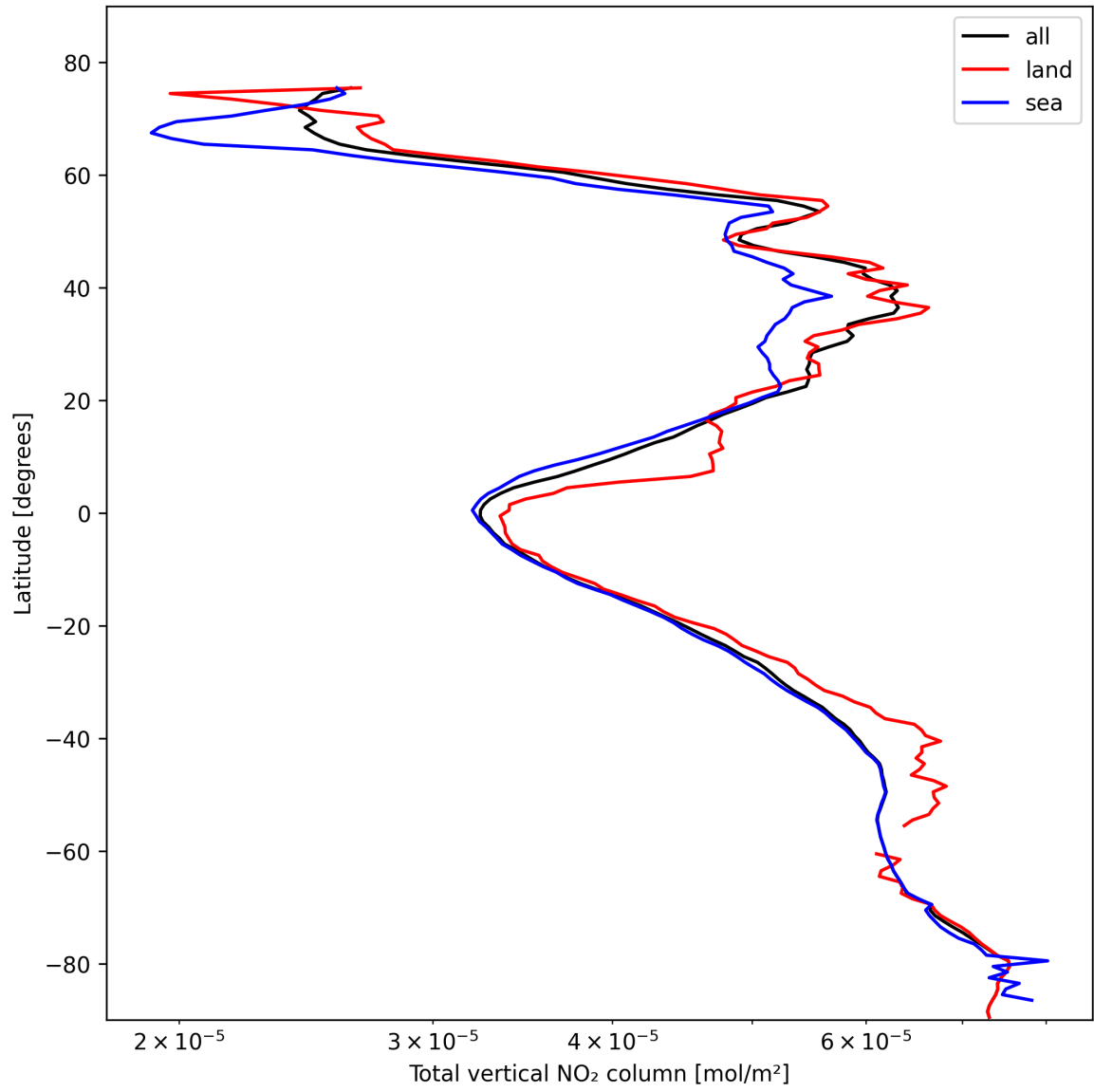
Figure 21: Zonal average of “Total vertical NO 2 column” for 2025-02-14 to 2025-02-16.
