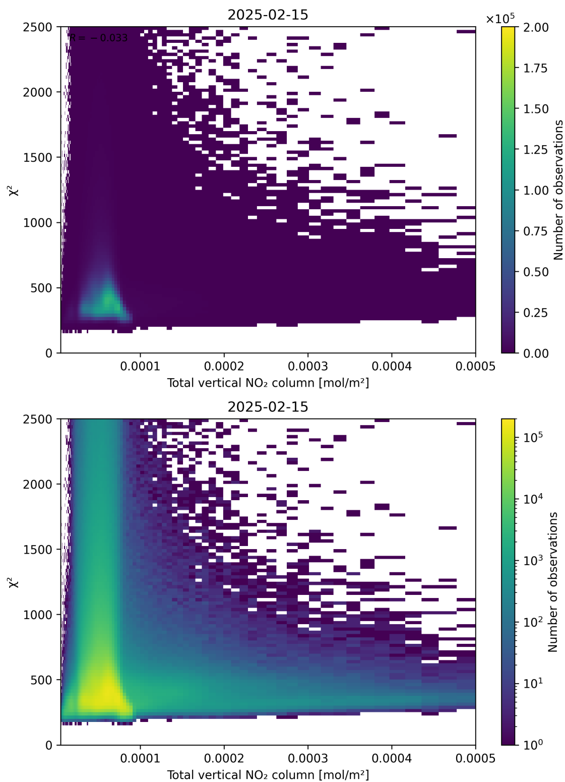
Figure 111: Scatter density plot of “Total vertical NO 2 column” against “ \chi^2 ” for 2025-02-14 to 2025-02-16.
