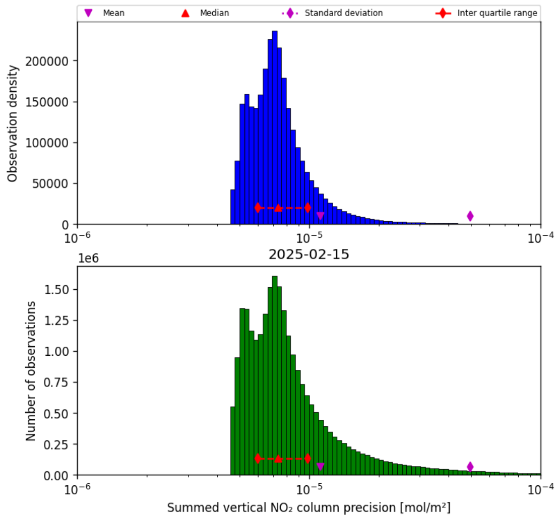
Figure 41: Histogram of “Summed vertical NO 2 column precision” for 2025-02-14 to 2025-02-16
