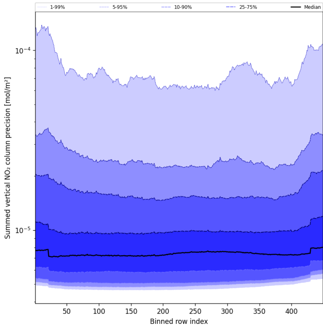
Figure 58: Along track statistics of “Summed vertical NO 2 column precision” for 2025-02-14 to 2025-02-16
