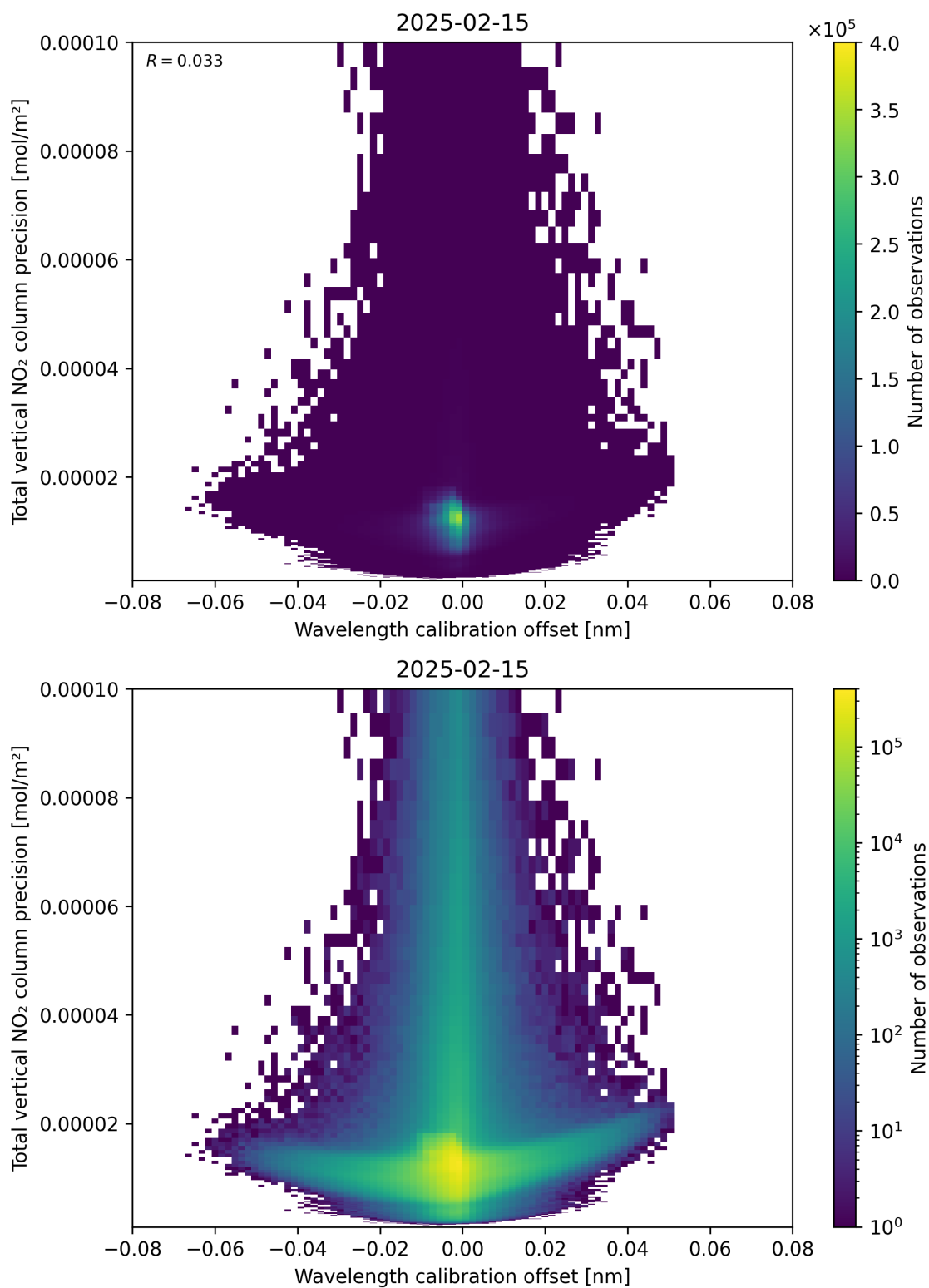
Figure 180: Scatter density plot of “Wavelength calibration offset” against “Total vertical NO 2 column precision” for 2025-02-14 to 2025-02-16.
