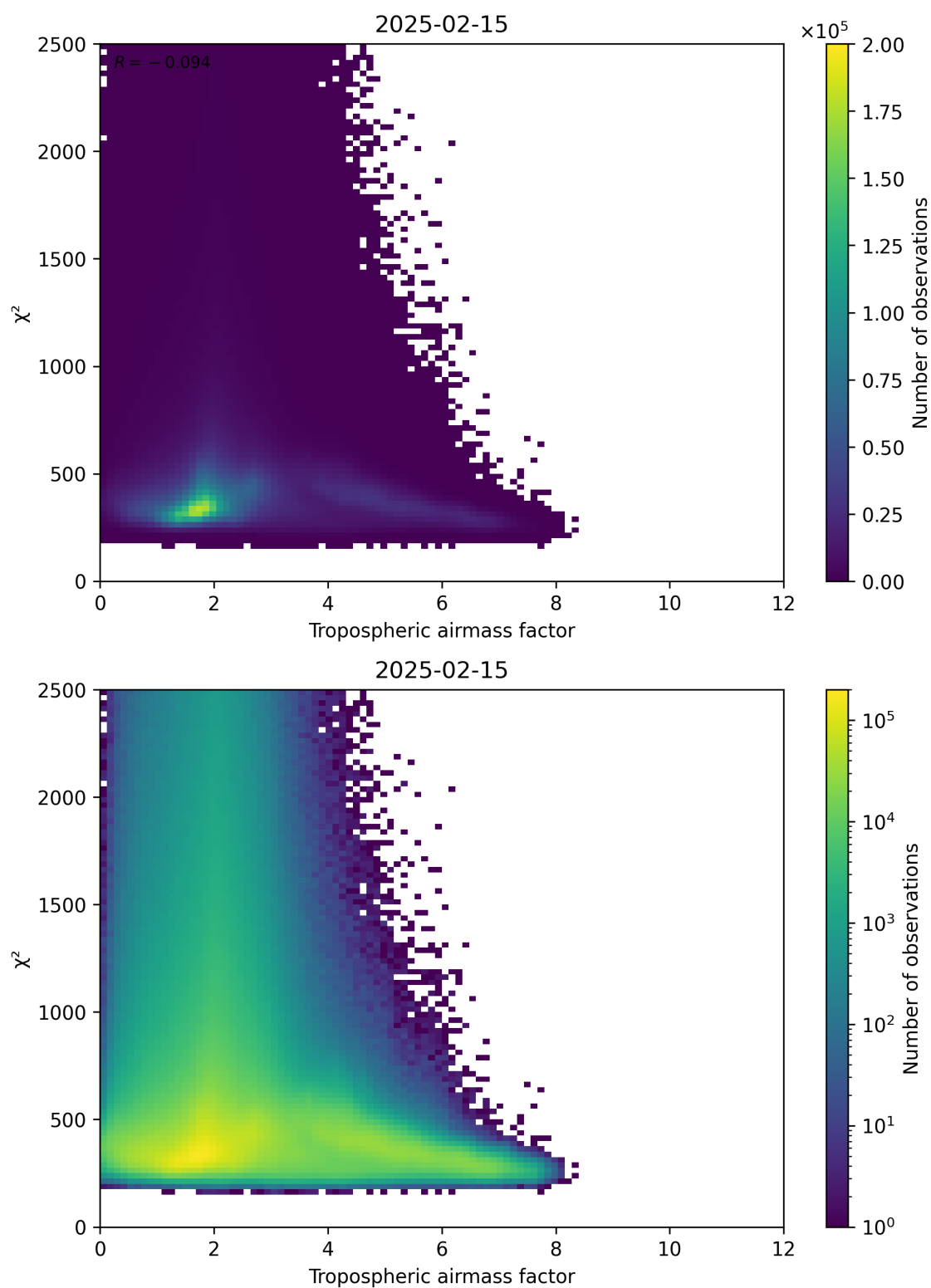
Figure 73: Scatter density plot of “Tropospheric airmass factor” against “ \chi^2 ” for 2025-02-14 to 2025-02-16.
