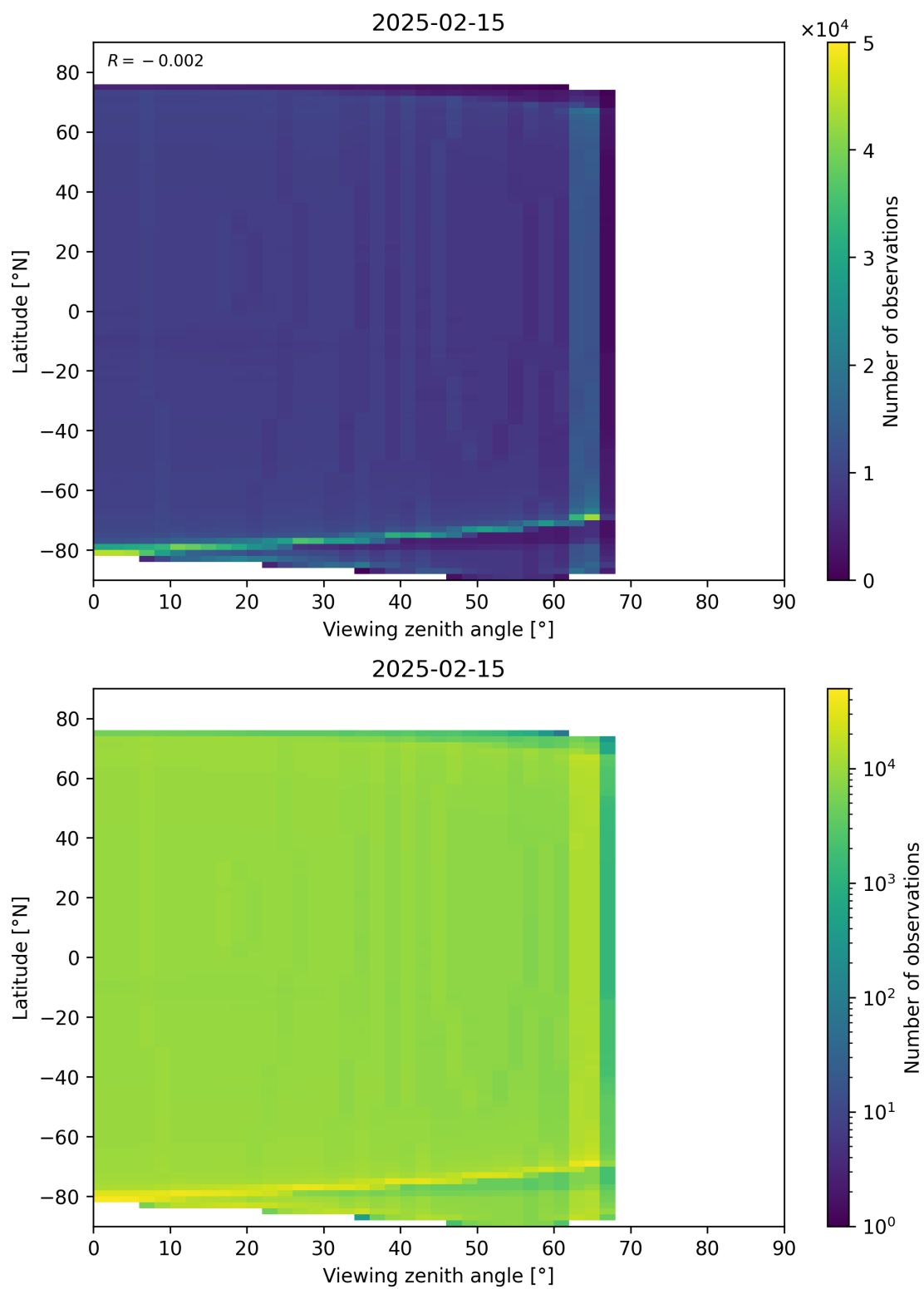
Figure 163: Scatter density plot of “Viewing zenith angle” against “Latitude” for 2025-02-14 to 2025-02-16.
