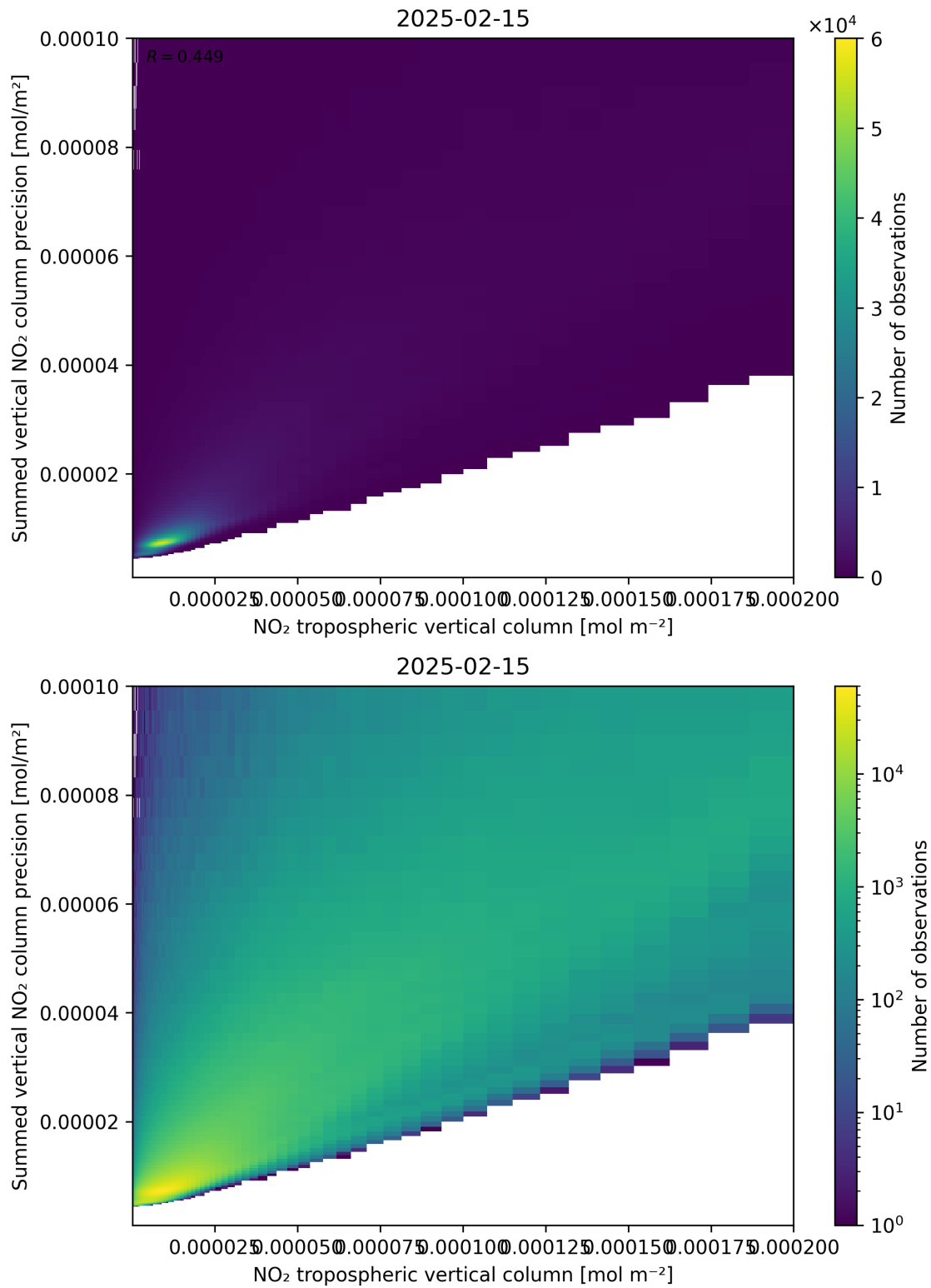
Figure 127: Scatter density plot of “NO 2 tropospheric vertical column” against “Summed vertical NO 2 column precision” for 2025-02-14 to 2025-02-16.
