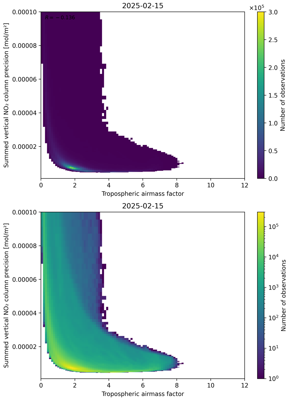
Figure 76: Scatter density plot of “Tropospheric air mass factor” against “Summed vertical NO 2 column precision” for 2025-02-14 to 2025-02-16.
