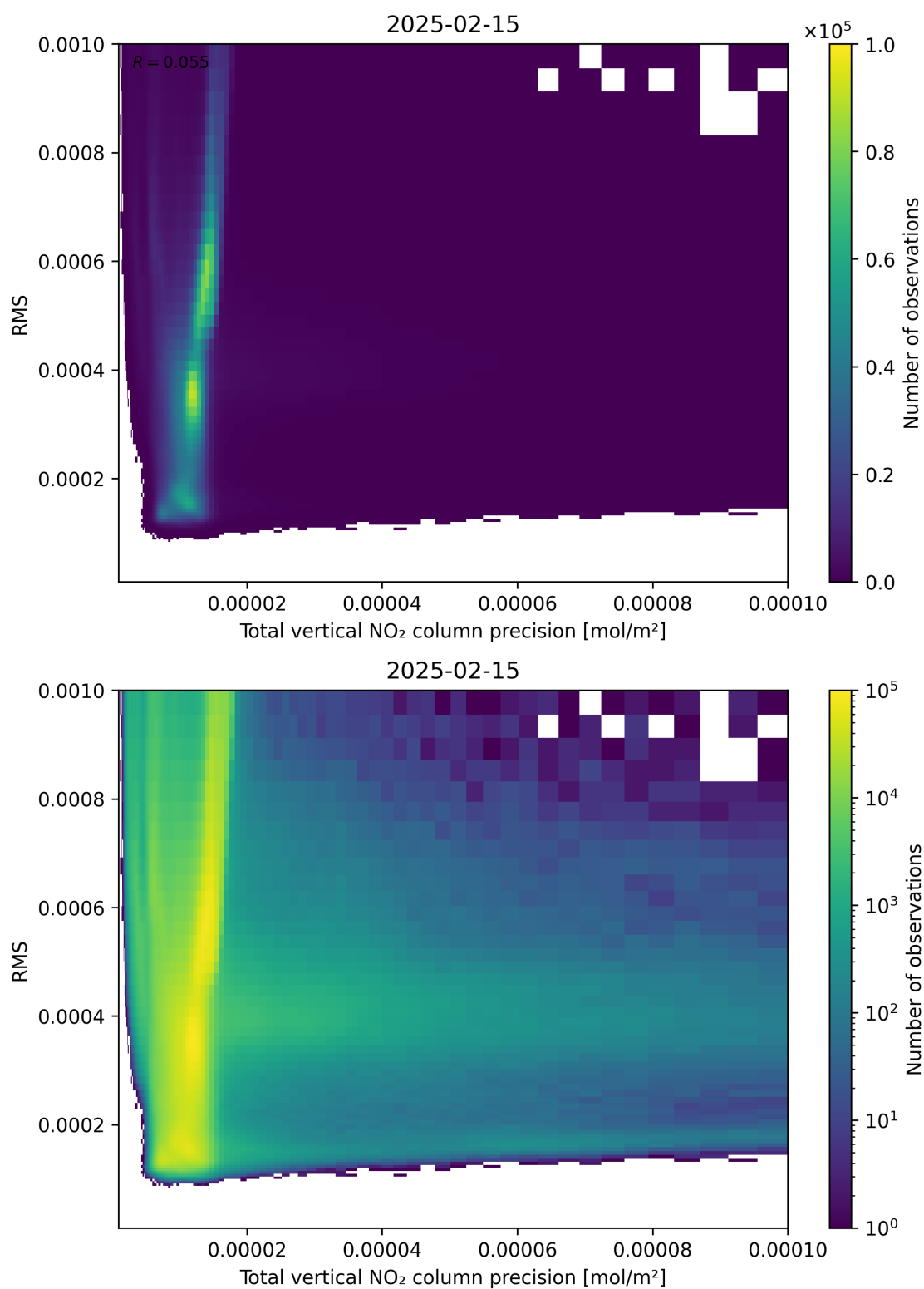
Figure 119: Scatter density plot of “Total vertical NO 2 column precision” against “RMS” for 2025-02-14 to 2025-02-16.
