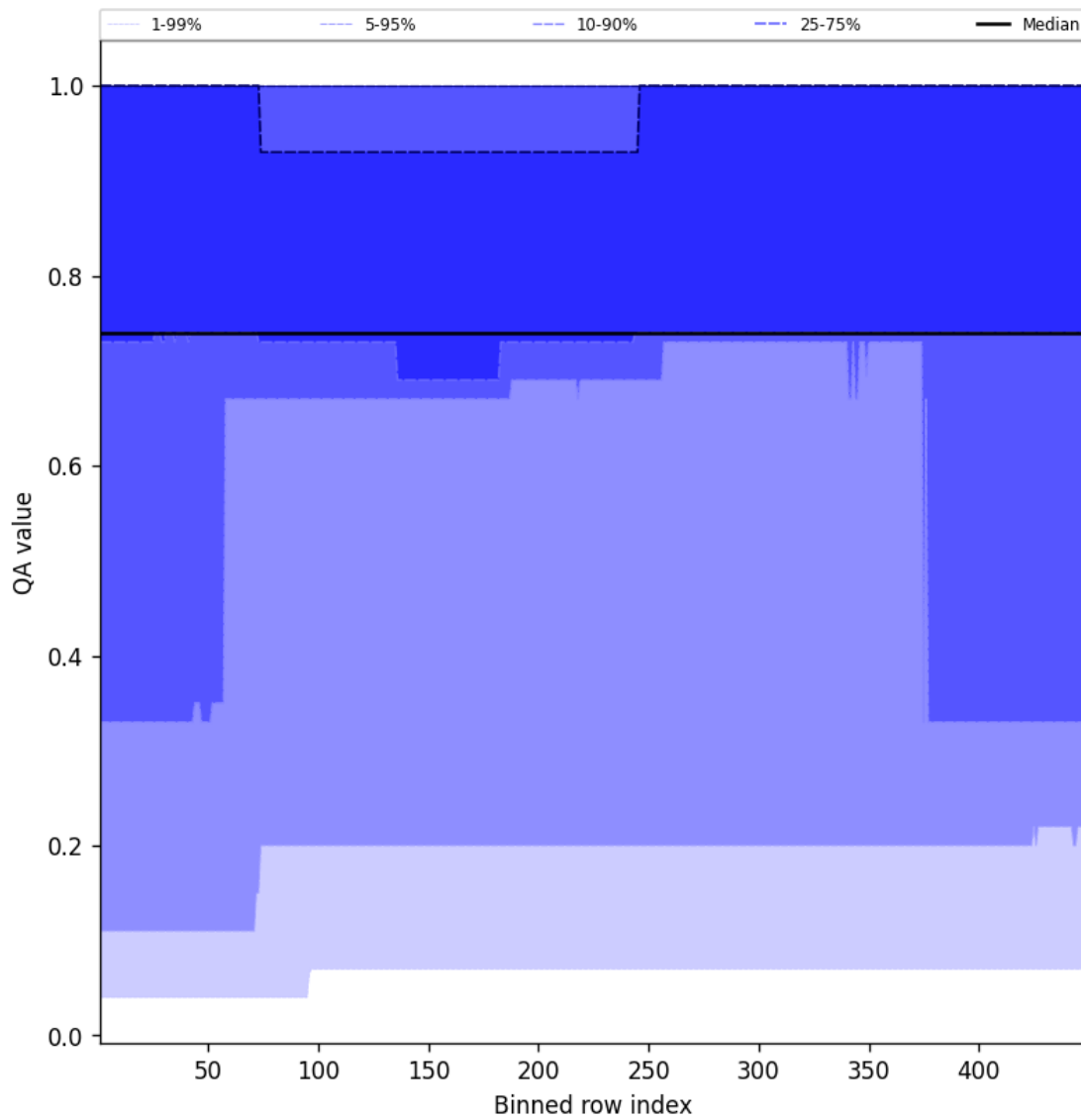
Figure 45: Along track statistics of “QA value” for 2025-02-14 to 2025-02-16
