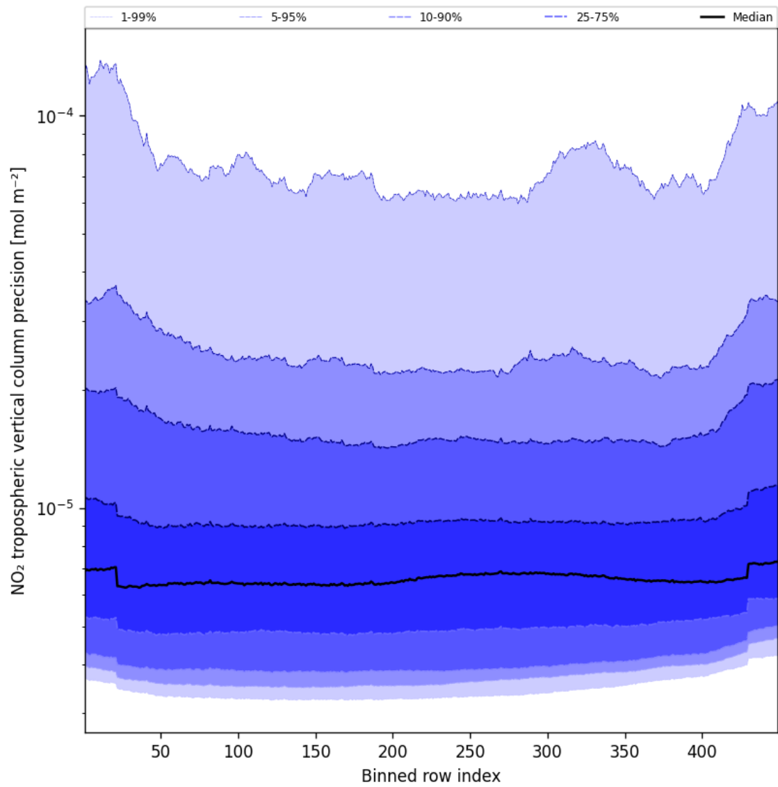
Figure 47: Along track statistics of “NO 2 tropospheric vertical column precision” for 2025-02-14 to 2025-02-16
