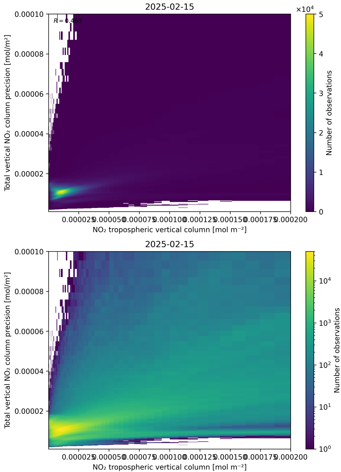
Figure 129: Scatter density plot of “NO 2 tropospheric vertical column” against “Total vertical NO 2 column precision” for 2025-02-14 to 2025-02-16.
