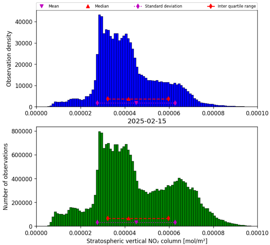
Figure 36: Histogram of “Stratospheric vertical NO 2 column” for 2025-02-14 to 2025-02-16
