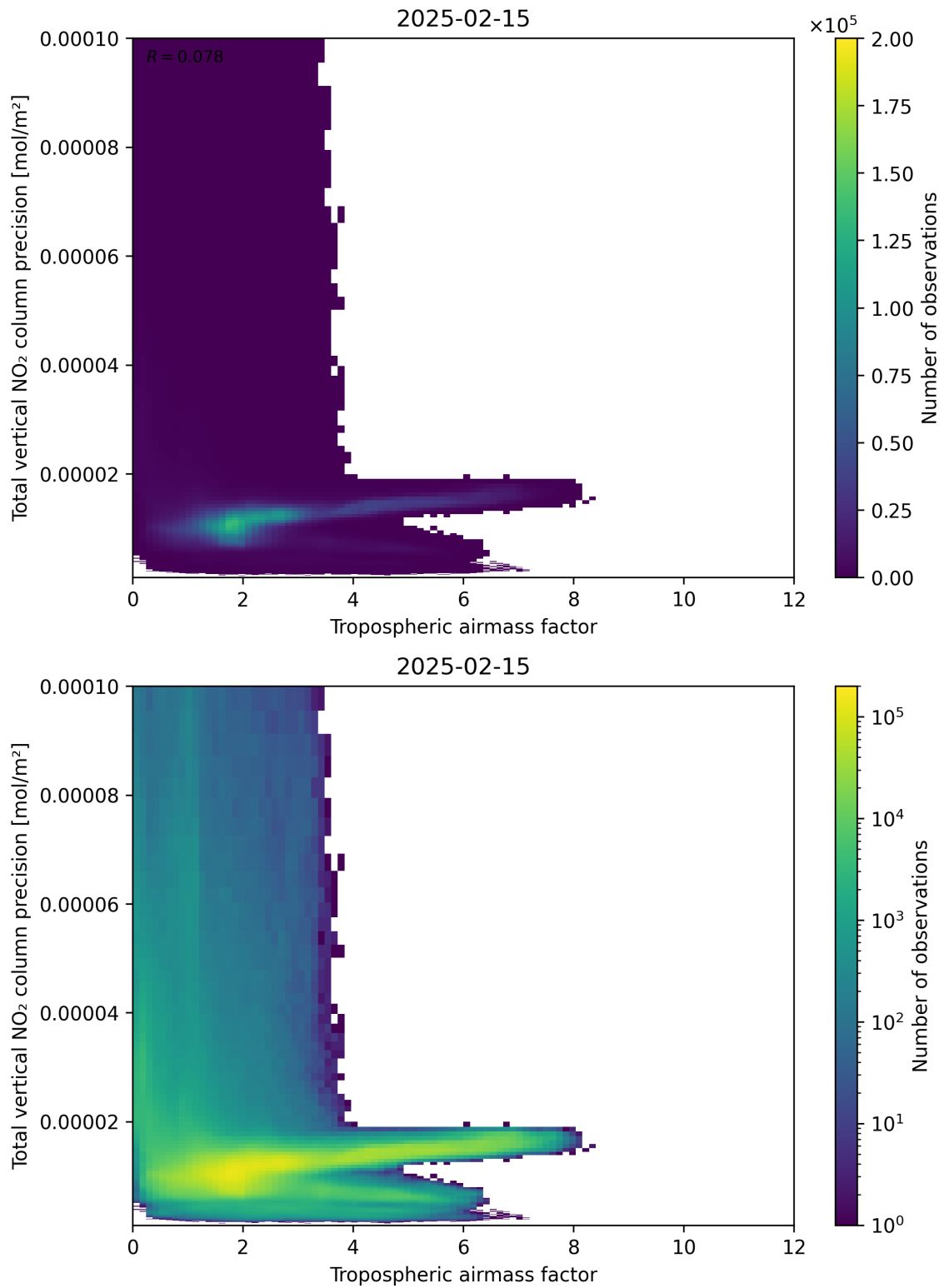
Figure 78: Scatter density plot of “Tropospheric air mass factor” against “Total vertical NO 2 column precision” for 2025-02-14 to 2025-02-16.
