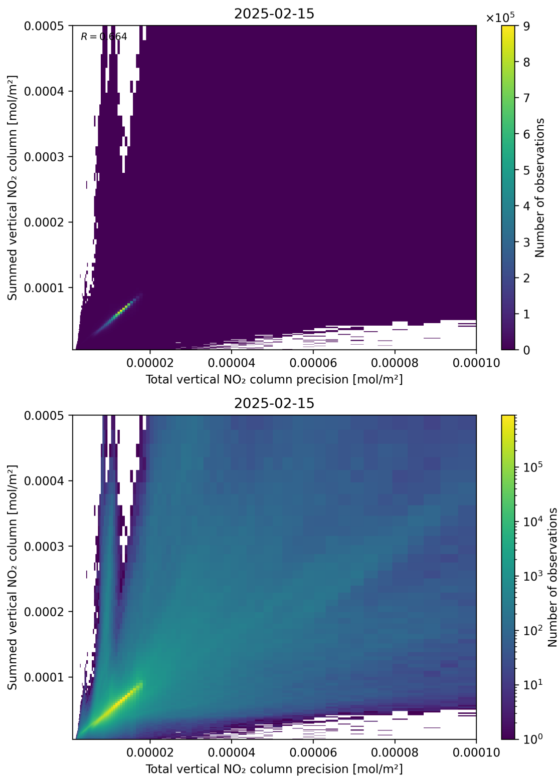
Figure 117: Scatter density plot of “Total vertical NO 2 column precision” against “Summed vertical NO 2 column” for 2025-02-14 to 2025-02-16.
