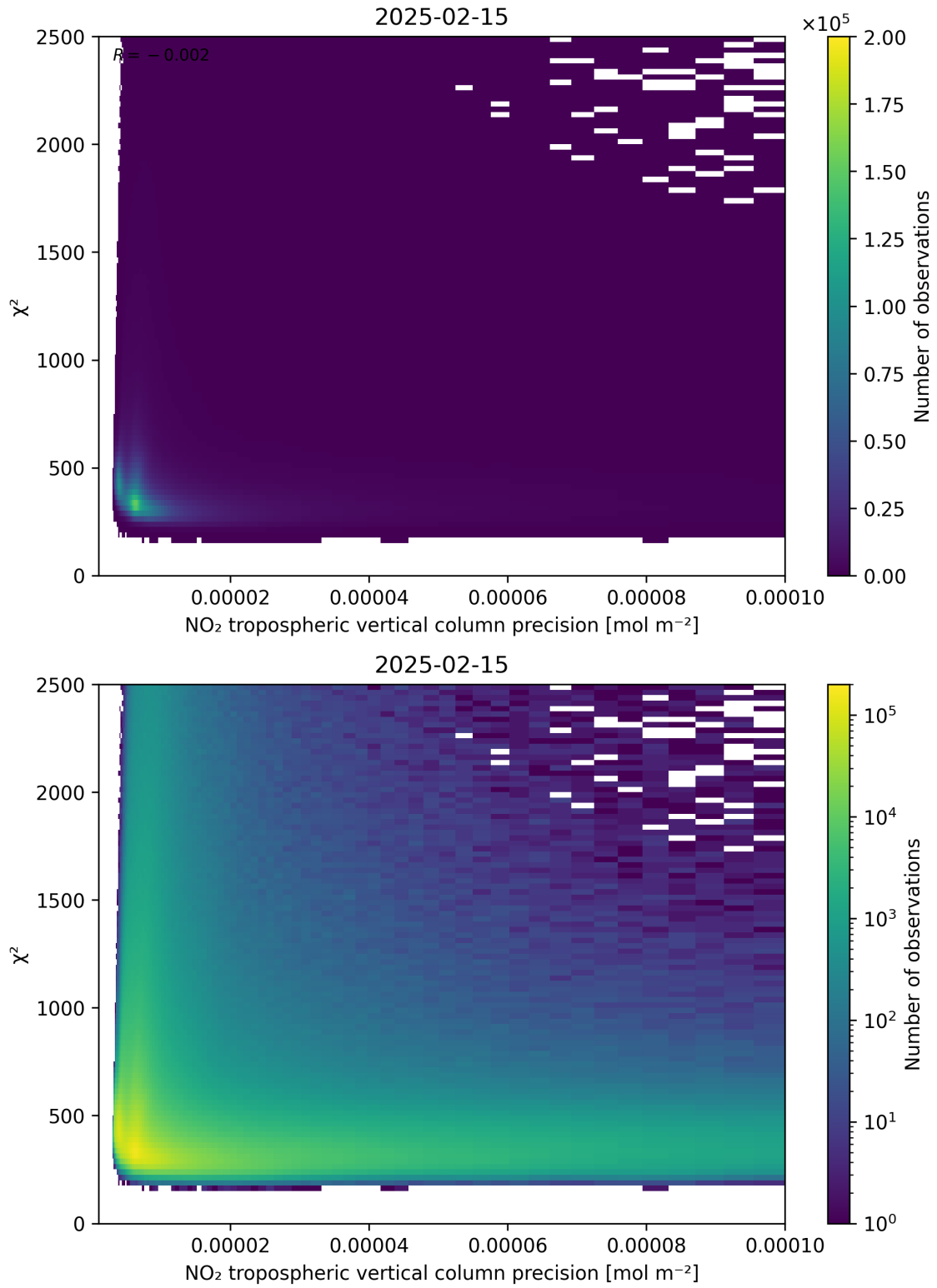
Figure 134: Scatter density plot of “NO 2 tropospheric vertical column precision” against “ \chi^2 ” for 2025-02-14 to 2025-02-16.
