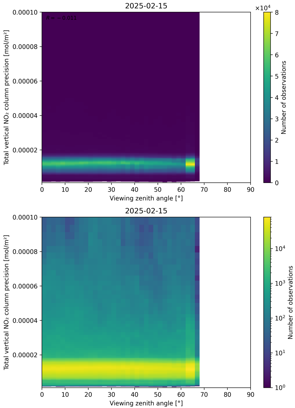
Figure 168: Scatter density plot of “Viewing zenith angle” against “Total vertical NO 2 column precision” for 2025-02-14 to 2025-02-16.
