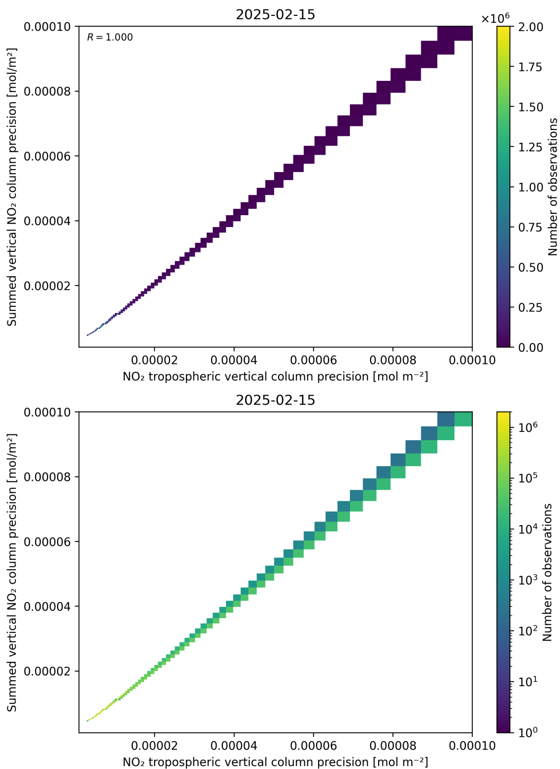
Figure 137: Scatter density plot of “NO 2 tropospheric vertical column precision” against “Summed vertical NO 2 column precision” for 2025-02-14 to 2025-02-16.
