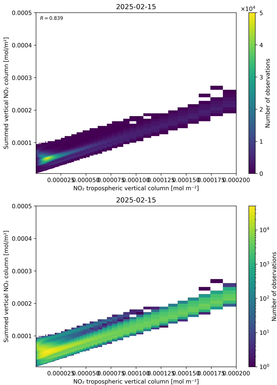
Figure 126: Scatter density plot of “NO 2 tropospheric vertical column” against “Summed vertical NO 2 column” for 2025-02-14 to 2025-02-16.
