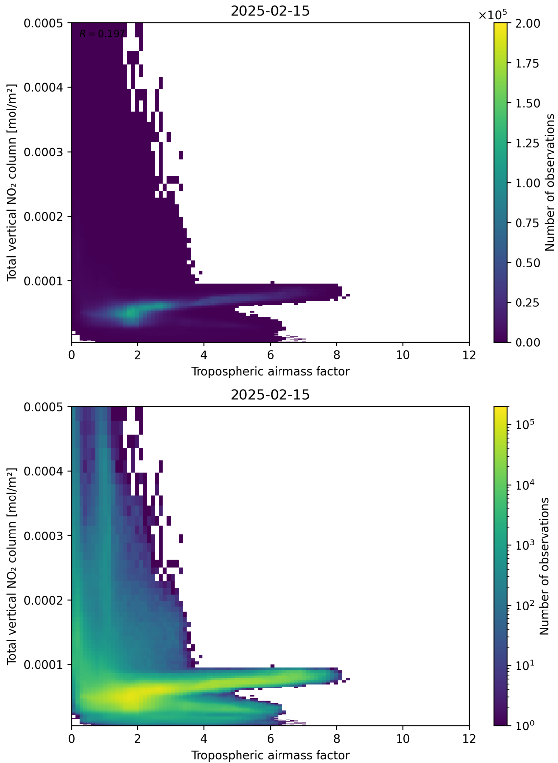
Figure 77: Scatter density plot of “Tropospheric airmass factor” against “Total vertical NO 2 column” for 2025-02-14 to 2025-02-16.
