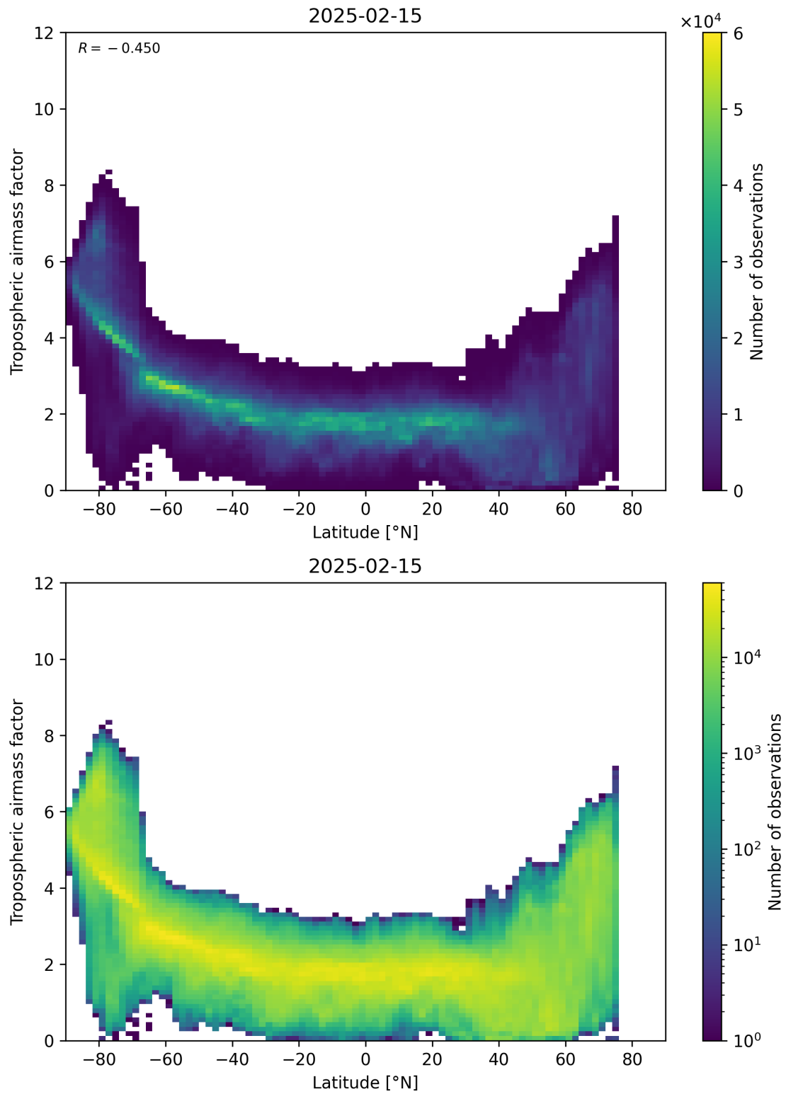
Figure 85: Scatter density plot of “Latitude” against “Tropospheric airmass factor” for 2025-02-14 to 2025-02-16.
