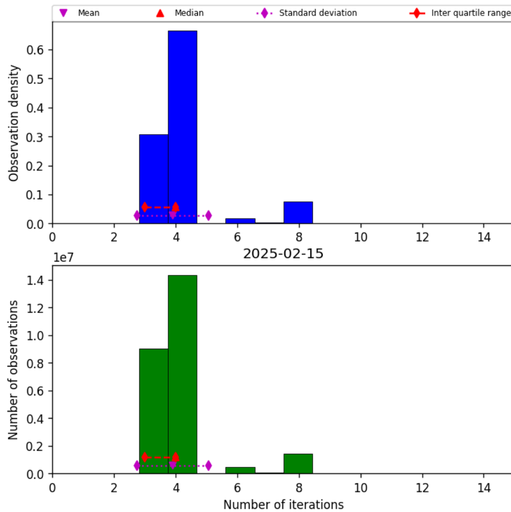
Figure 34: Histogram of “Number of iterations” for 2025-02-14 to 2025-02-16
