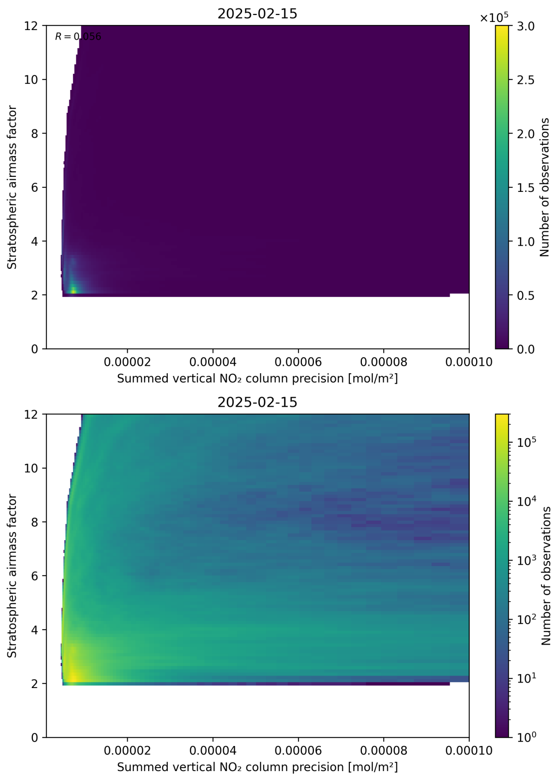
Figure 106: Scatter density plot of “Summed vertical NO 2 column precision” against “Stratospheric airmass factor” for 2025-02-14 to 2025-02-16.
