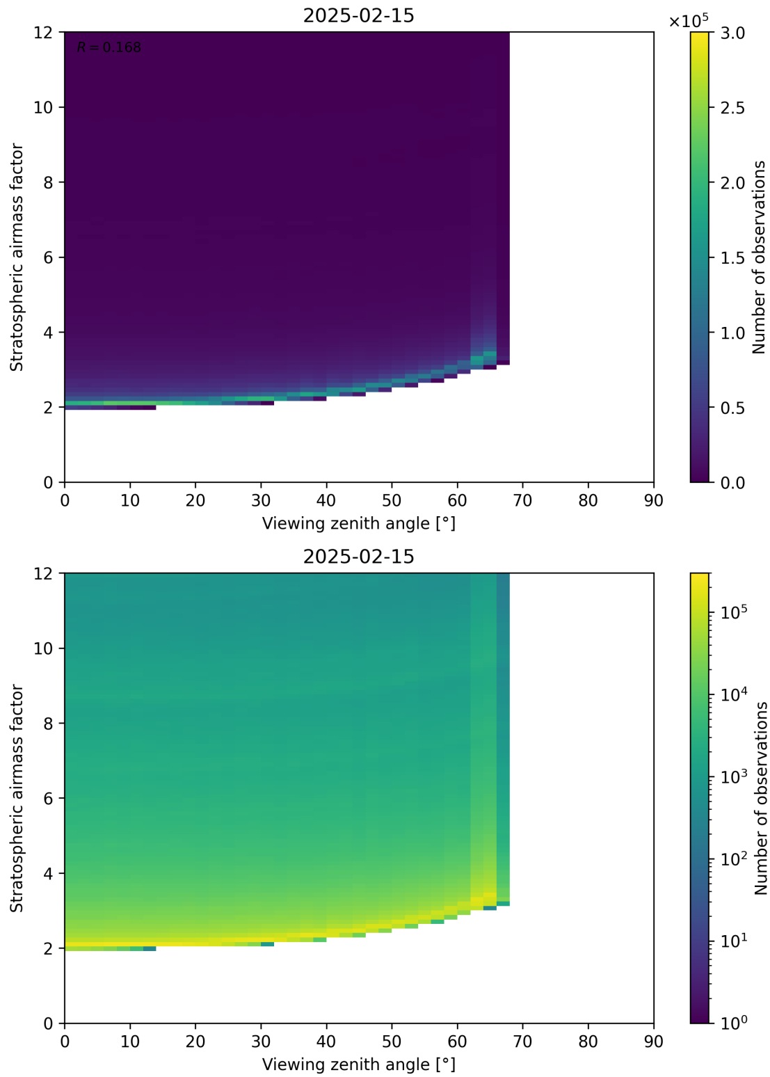
Figure 159: Scatter density plot of “Viewing zenith angle” against “Stratospheric airmass factor” for 2025-02-14 to 2025-02-16.
