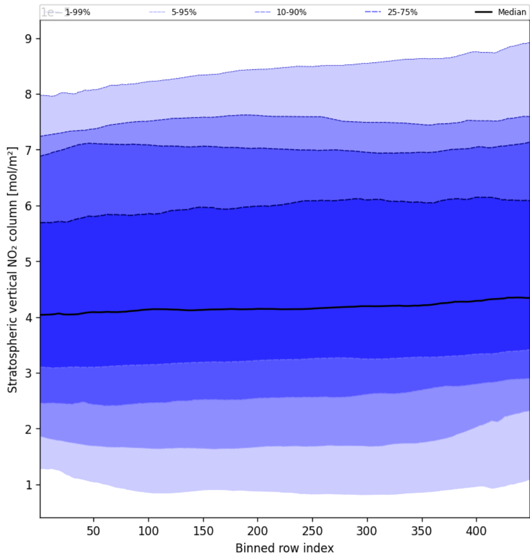
Figure 53: Along track statistics of “Stratospheric vertical NO 2 column” for 2025-02-14 to 2025-02-16
