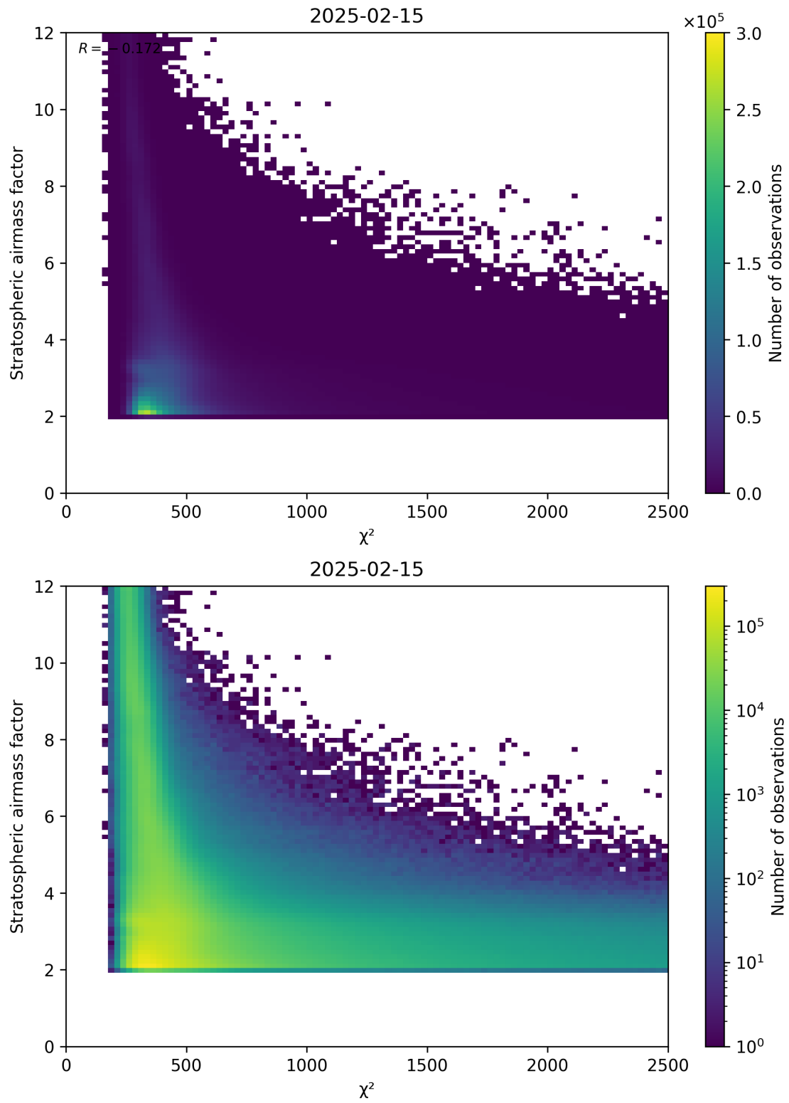
Figure 81: Scatter density plot of “ \chi^2 ” against “Stratospheric airmass factor” for 2025-02-14 to 2025-02-16.
