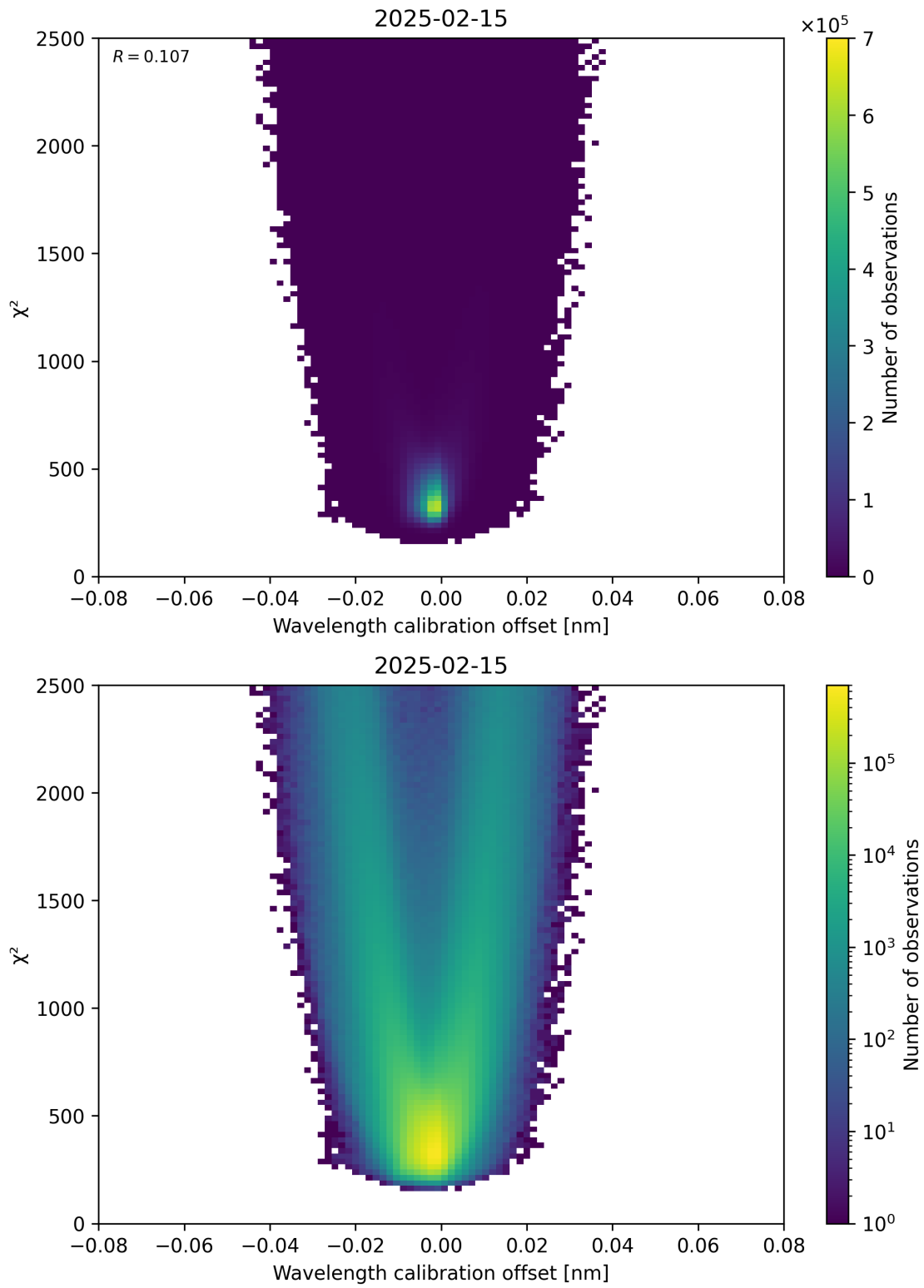
Figure 175: Scatter density plot of “Wavelength calibration offset” against “ \chi^2 ” for 2025-02-14 to 2025-02-16.
