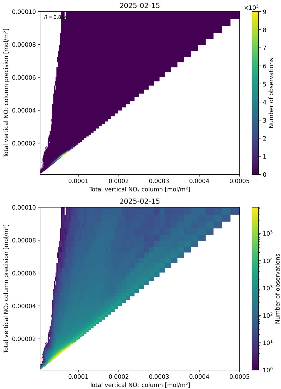
Figure 114: Scatter density plot of “Total vertical NO 2 column” against “Total vertical NO 2 column precision” for 2025-02-14 to 2025-02-16.
