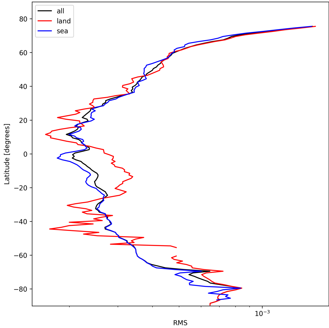
Figure 26: Zonal average of “RMS” for 2025-02-14 to 2025-02-16.
