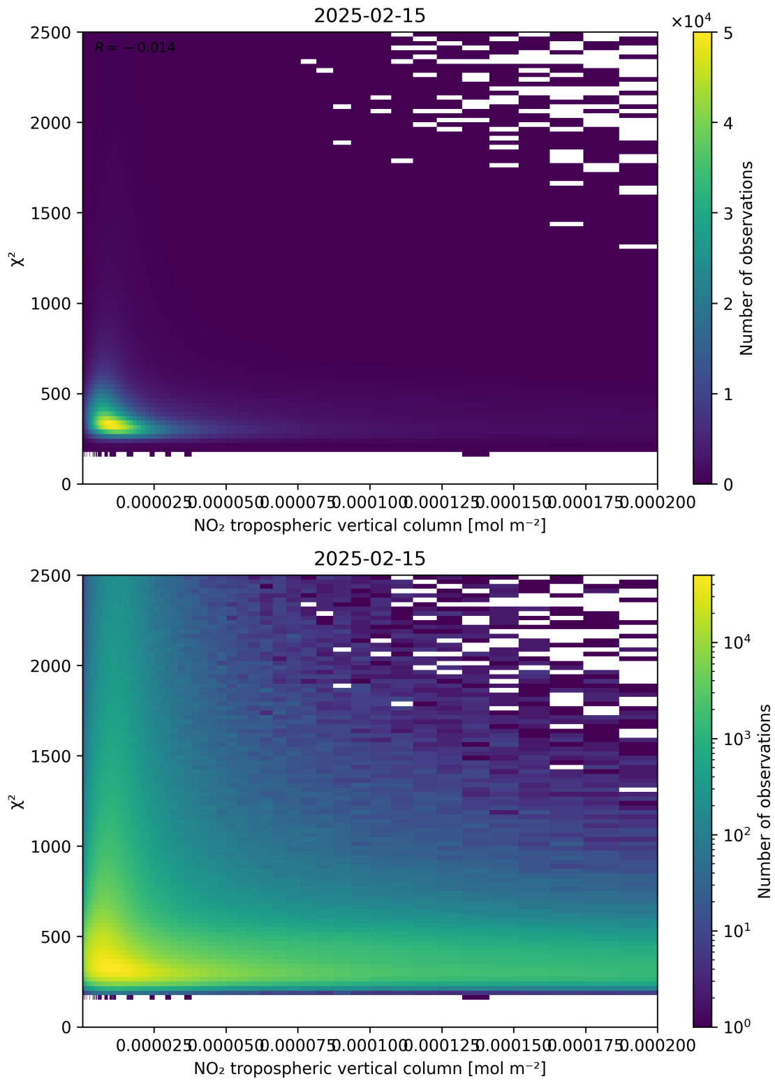
Figure 124: Scatter density plot of “NO 2 tropospheric vertical column” against “ \chi^2 ” for 2025-02-14 to 2025-02-16.
