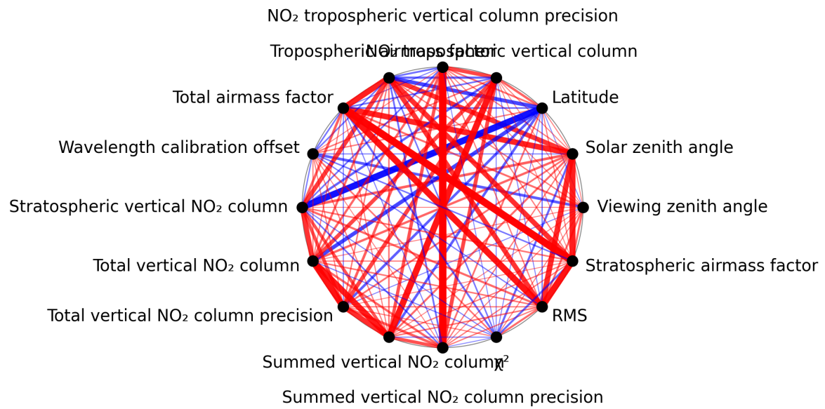
Figure 1: Map of correlation graph for 2025-02-14 to 2025-02-16.
