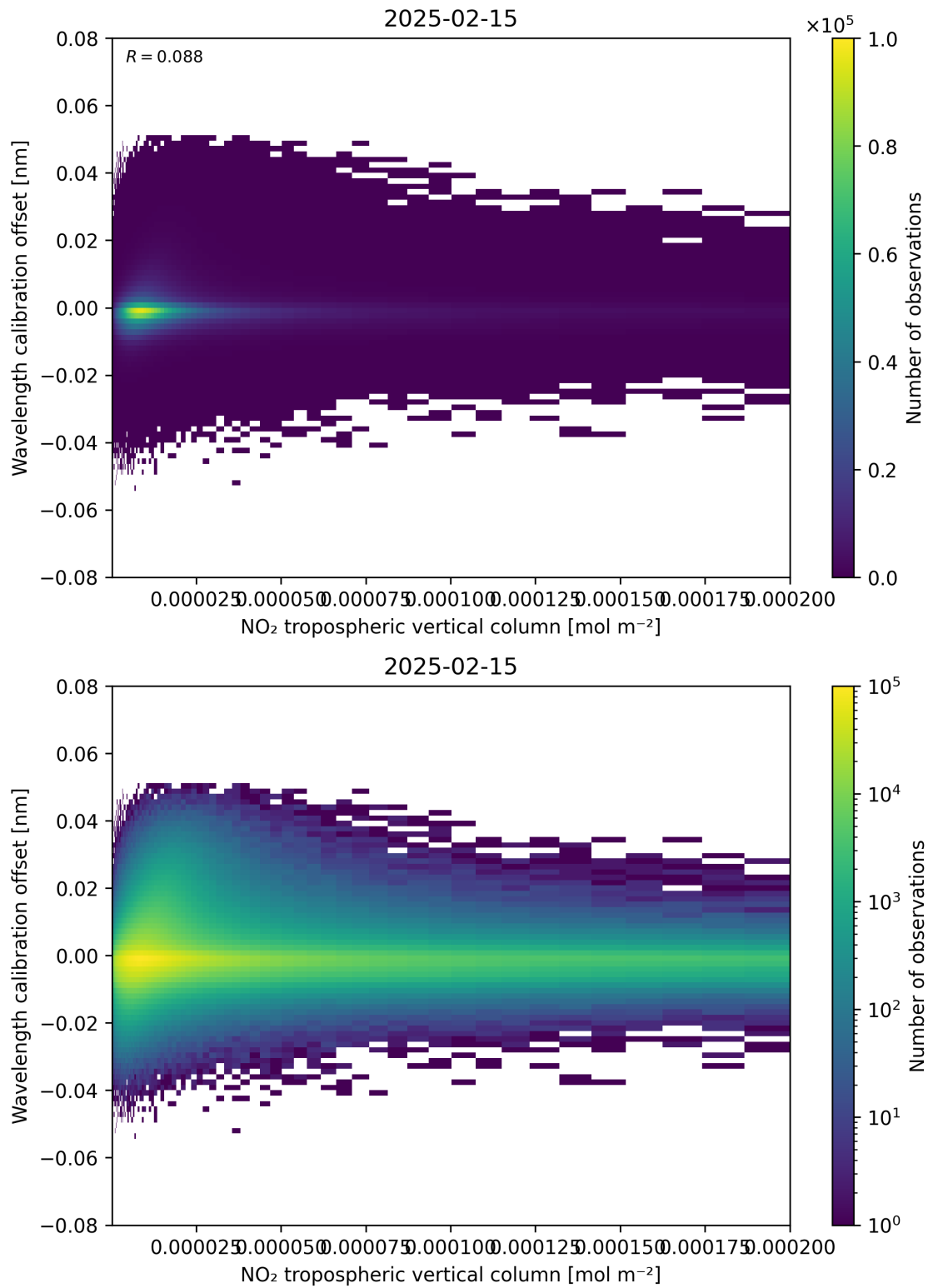
Figure 143: Scatter density plot of “NO 2 tropospheric vertical column” against “Wavelength calibration offset” for 2025-02-14 to 2025-02-16.
