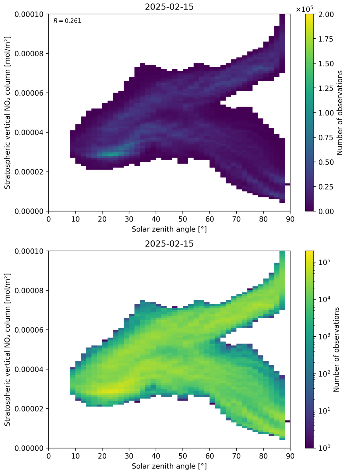
Figure 150: Scatter density plot of “Solar zenith angle” against “Stratospheric vertical NO 2 column” for 2025-02-14 to 2025-02-16.
