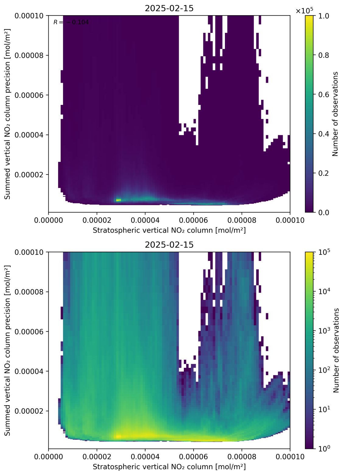
Figure 99: Scatter density plot of “Stratospheric vertical NO 2 column” against “Summed vertical NO 2 column precision” for 2025-02-14 to 2025-02-16.
