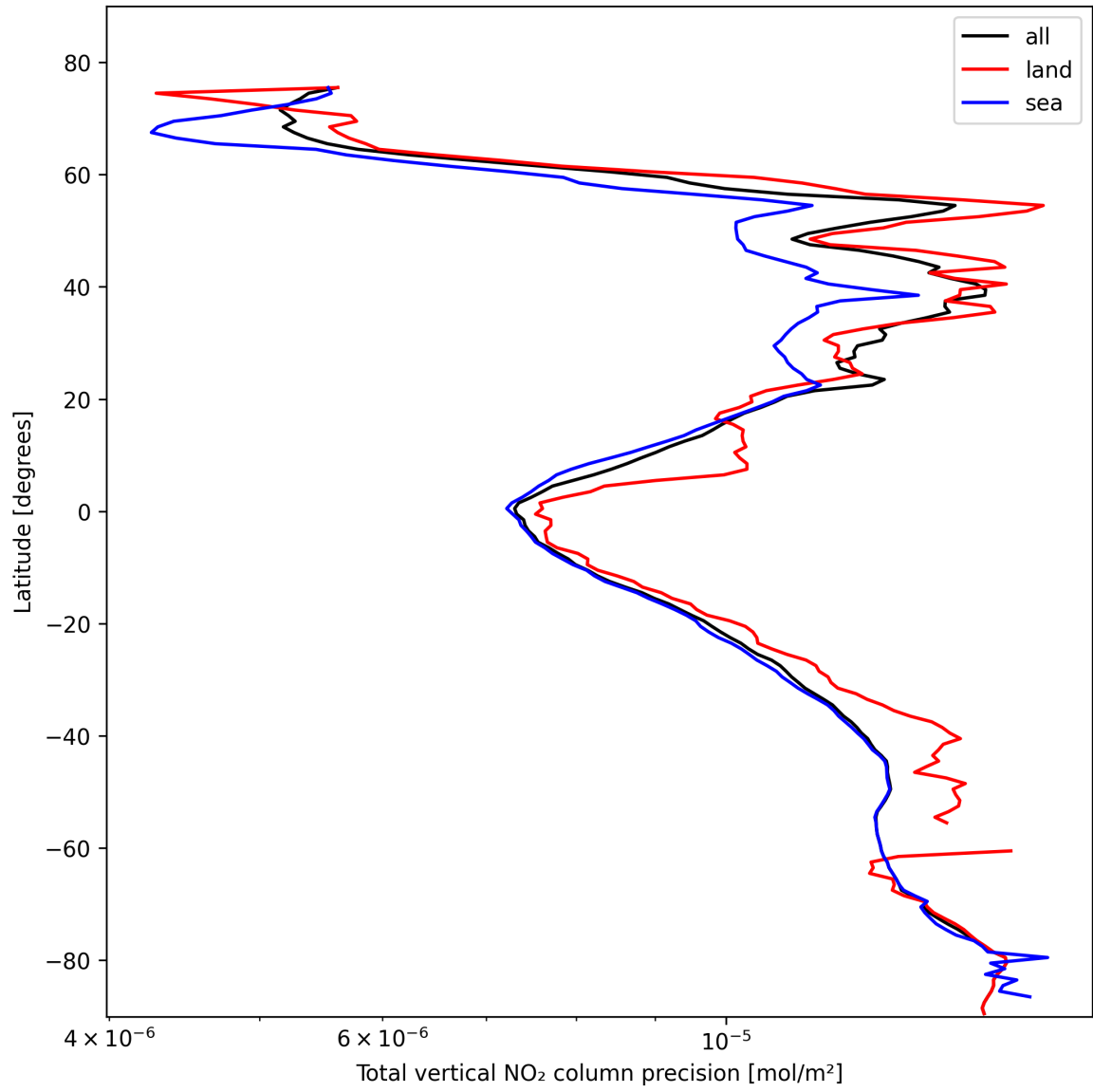
Figure 22: Zonal average of “Total vertical NO 2 column precision” for 2025-02-14 to 2025-02-16.
