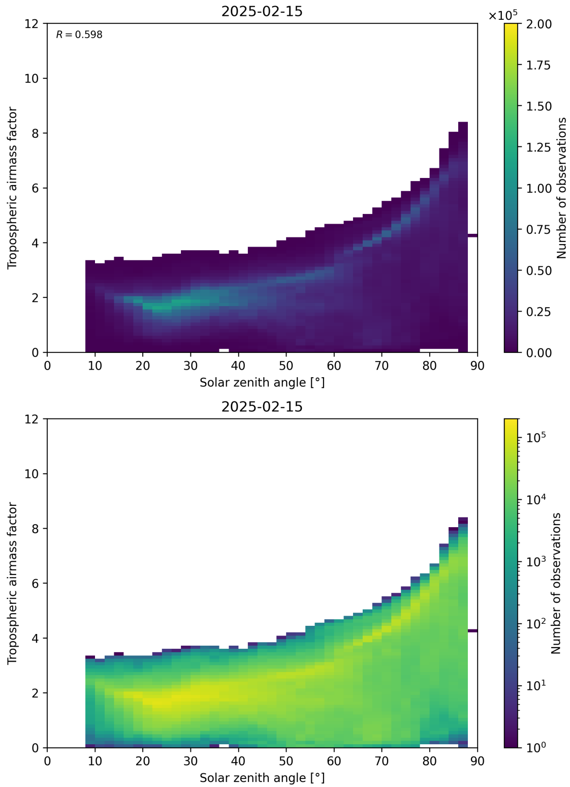
Figure 147: Scatter density plot of “Solar zenith angle” against “Tropospheric airmass factor” for 2025-02-14 to 2025-02-16.
