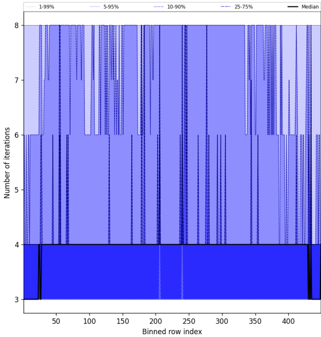
Figure 51: Along track statistics of “Number of iterations” for 2025-02-14 to 2025-02-16
