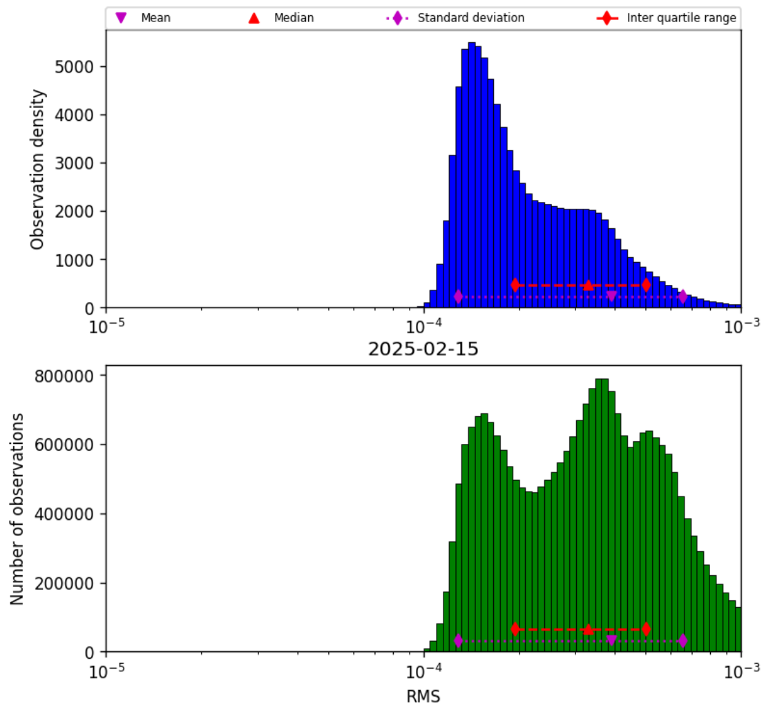
Figure 43: Histogram of “RMS” for 2025-02-14 to 2025-02-16
