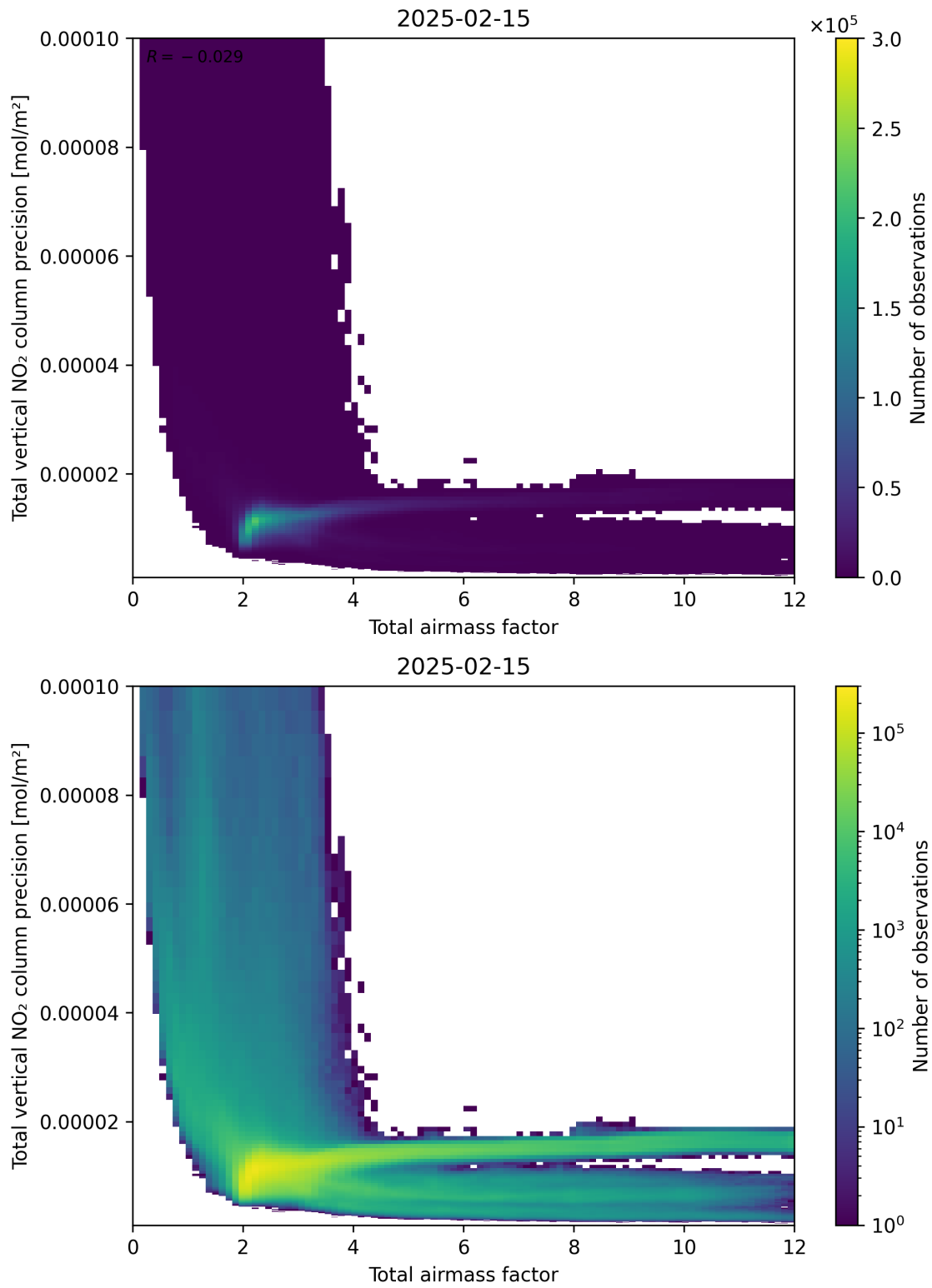
Figure 68: Scatter density plot of “Total airmass factor” against “Total vertical NO 2 column precision” for 2025-02-14 to 2025-02-16.
