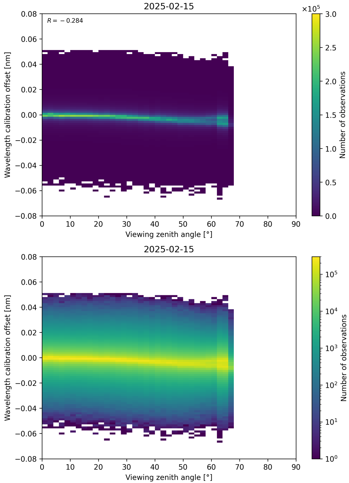
Figure 173: Scatter density plot of “Viewing zenith angle” against “Wavelength calibration offset” for 2025-02-14 to 2025-02-16.
