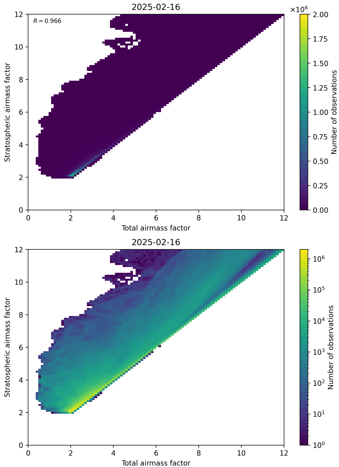
Figure 62: Scatter density plot of “Total airmass factor” against “Stratospheric airmass factor” for 2025-02-15 to 2025-02-17.
