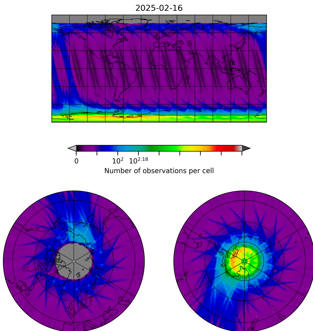
Figure 10: Map of the number of observations for 2025-02-15 to 2025-02-17
