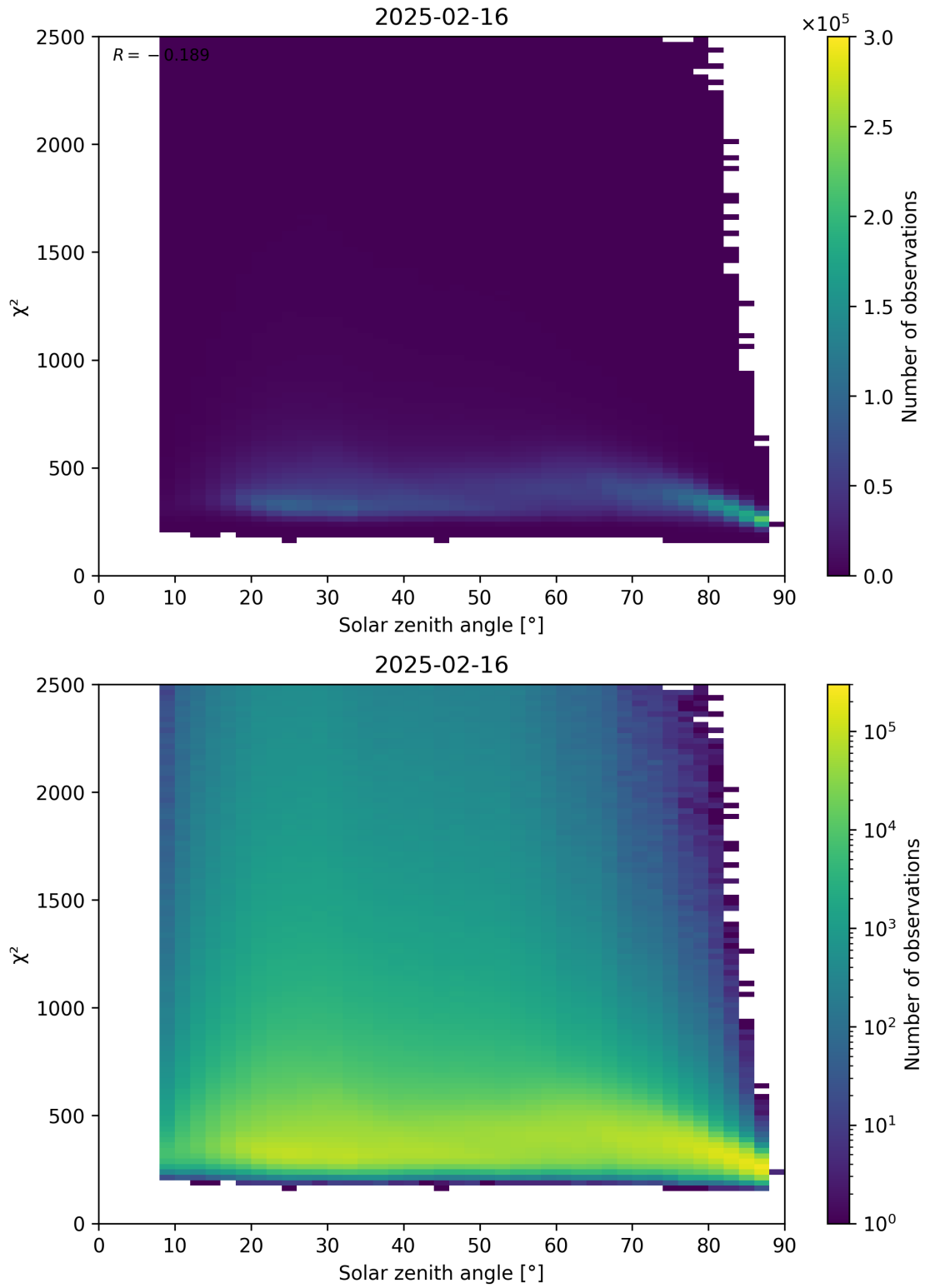
Figure 148: Scatter density plot of “Solar zenith angle” against “ \chi^2 ” for 2025-02-15 to 2025-02-17.
