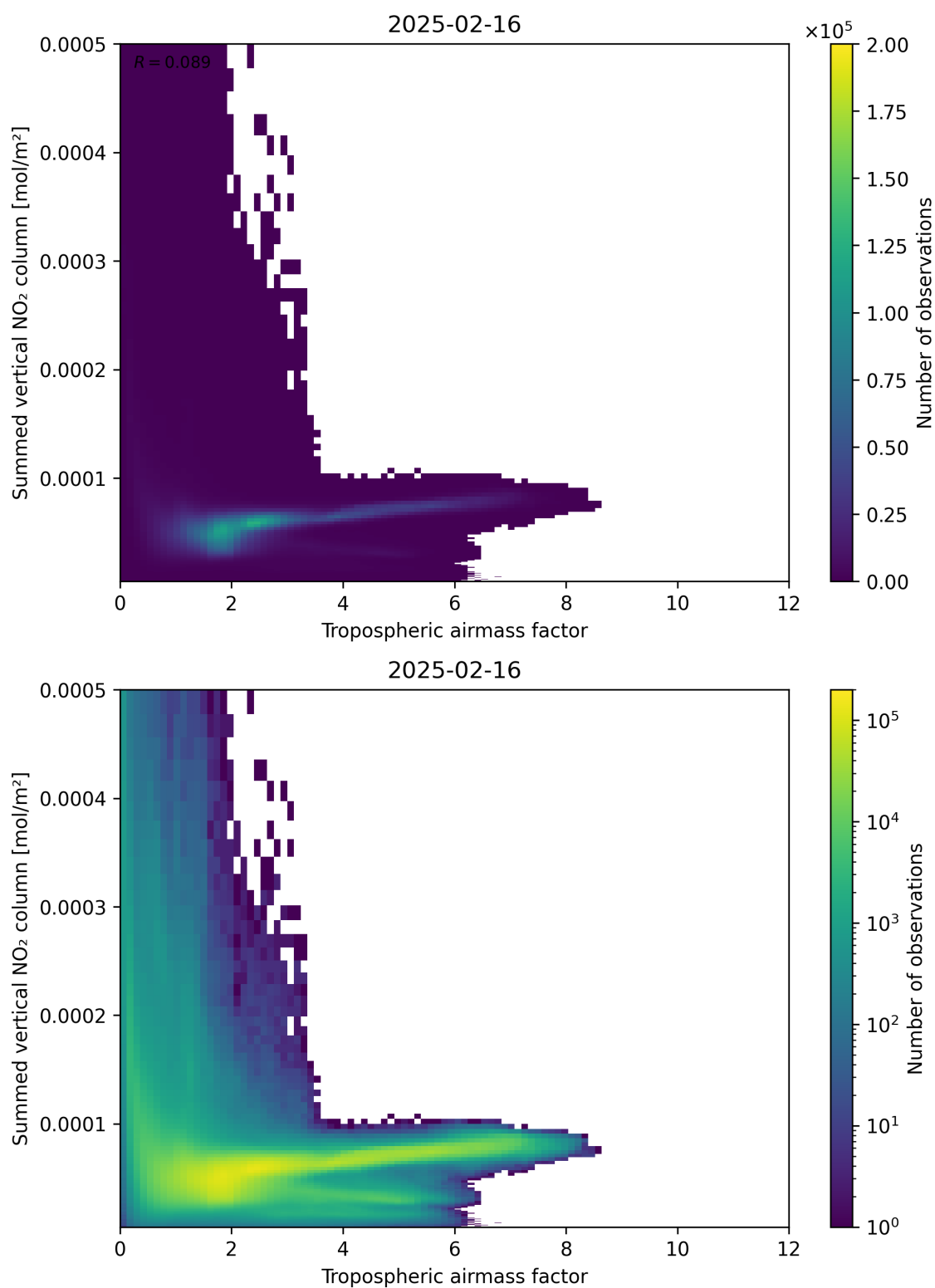
Figure 75: Scatter density plot of “Tropospheric air mass factor” against “Summed vertical NO 2 column” for 2025-02-15 to 2025-02-17.
