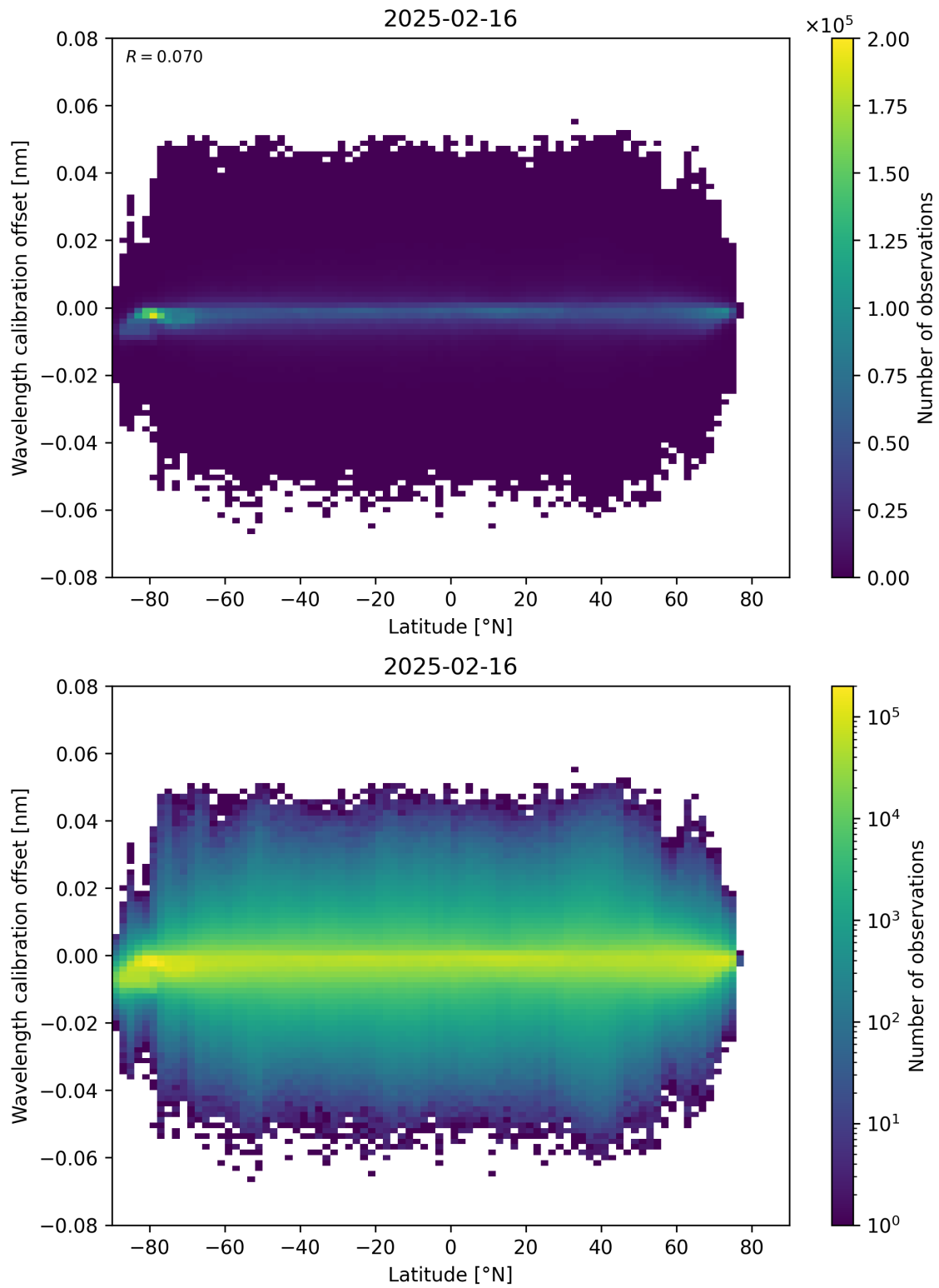
Figure 95: Scatter density plot of “Latitude” against “Wavelength calibration offset” for 2025-02-15 to 2025-02-17.
