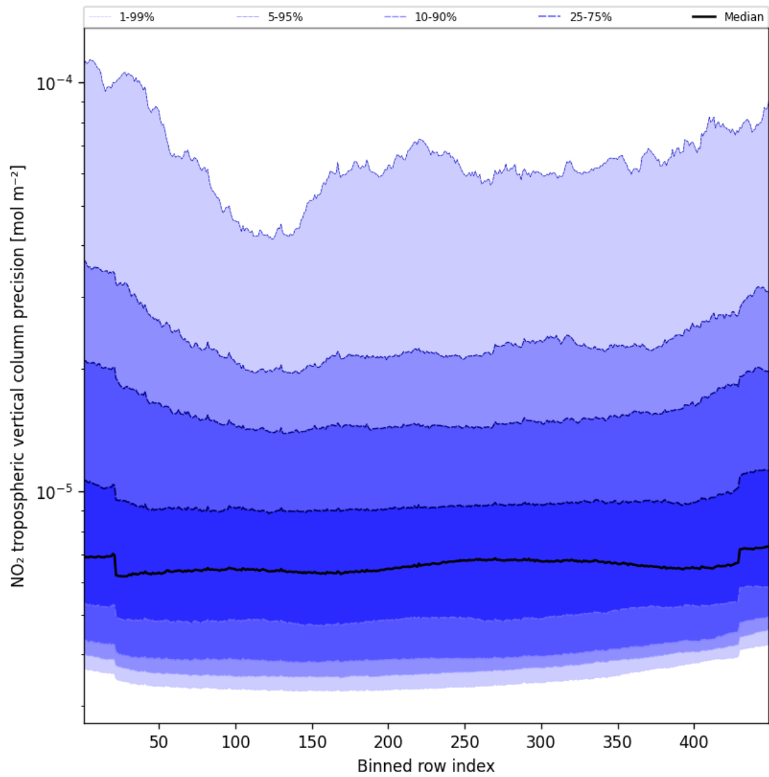
Figure 47: Along track statistics of “NO 2 tropospheric vertical column precision” for 2025-02-15 to 2025-02-17
