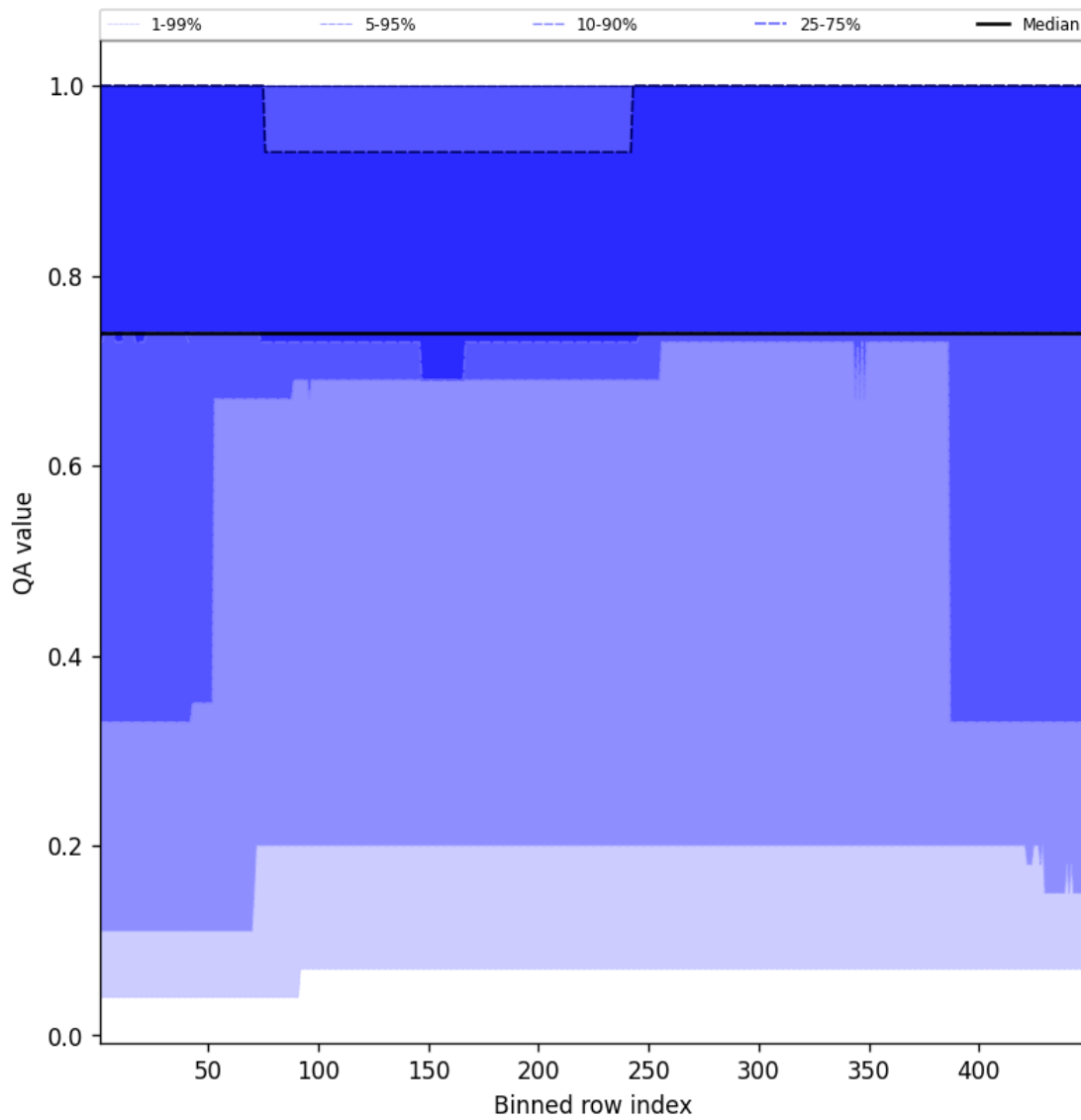
Figure 45: Along track statistics of “QA value” for 2025-02-15 to 2025-02-17
