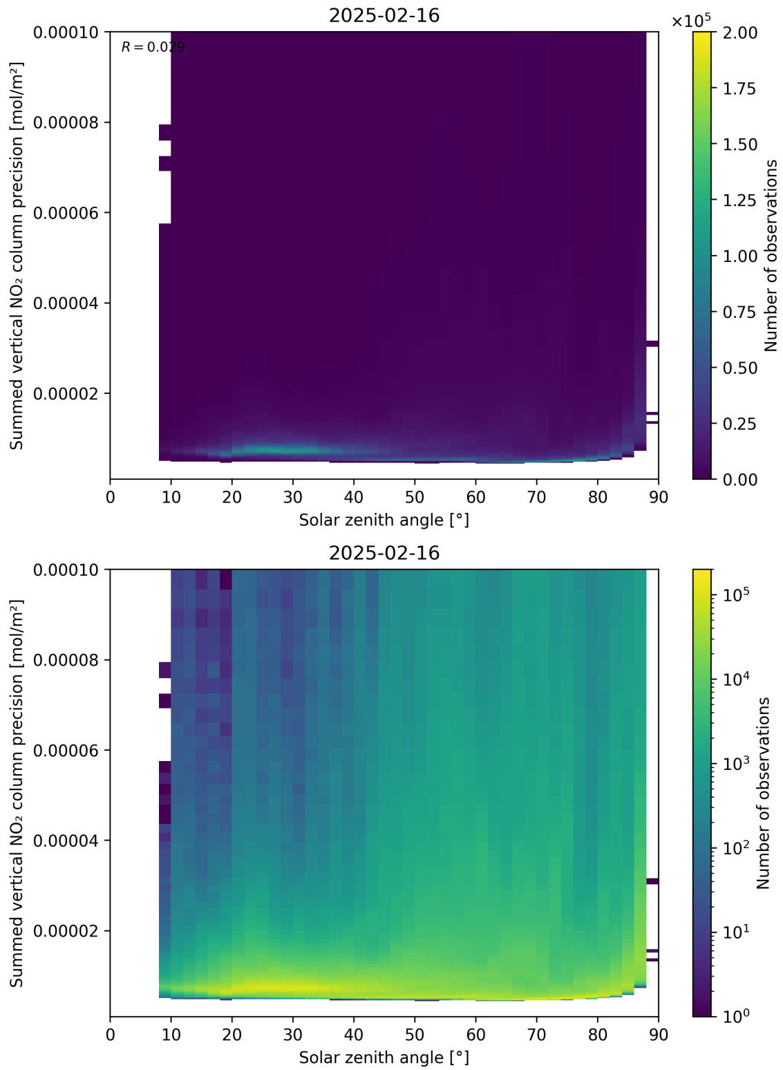
Figure 152: Scatter density plot of “Solar zenith angle” against “Summed vertical NO 2 column precision” for 2025-02-15 to 2025-02-17.
