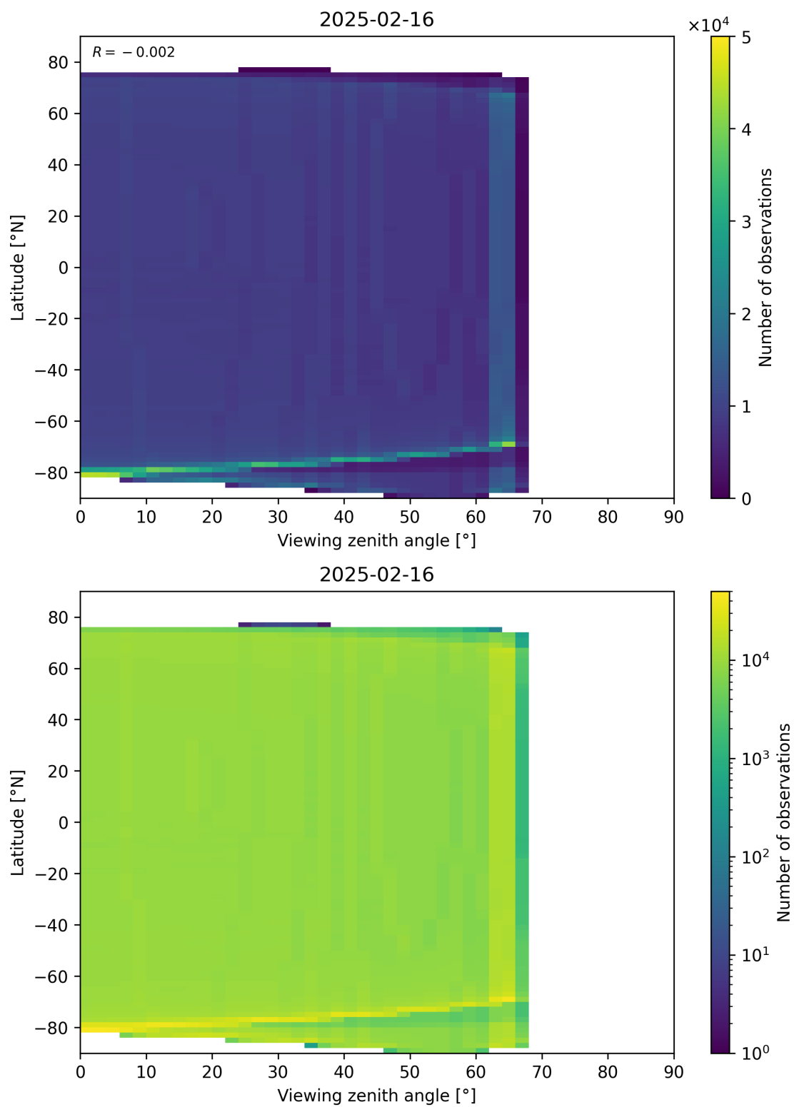
Figure 163: Scatter density plot of “Viewing zenith angle” against “Latitude” for 2025-02-15 to 2025-02-17.
