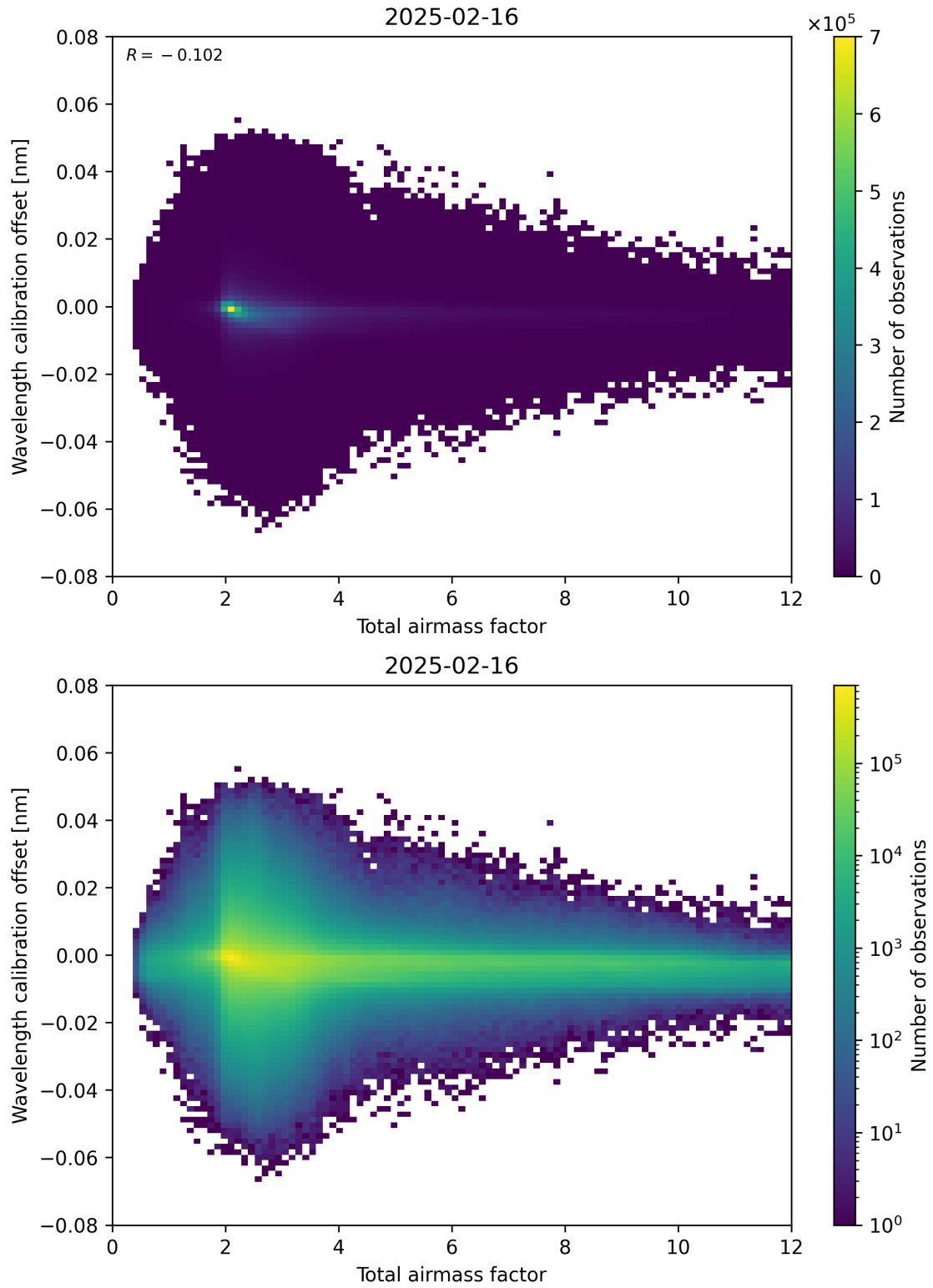
Figure 70: Scatter density plot of “Total airmass factor” against “Wavelength calibration offset” for 2025-02-15 to 2025-02-17.
