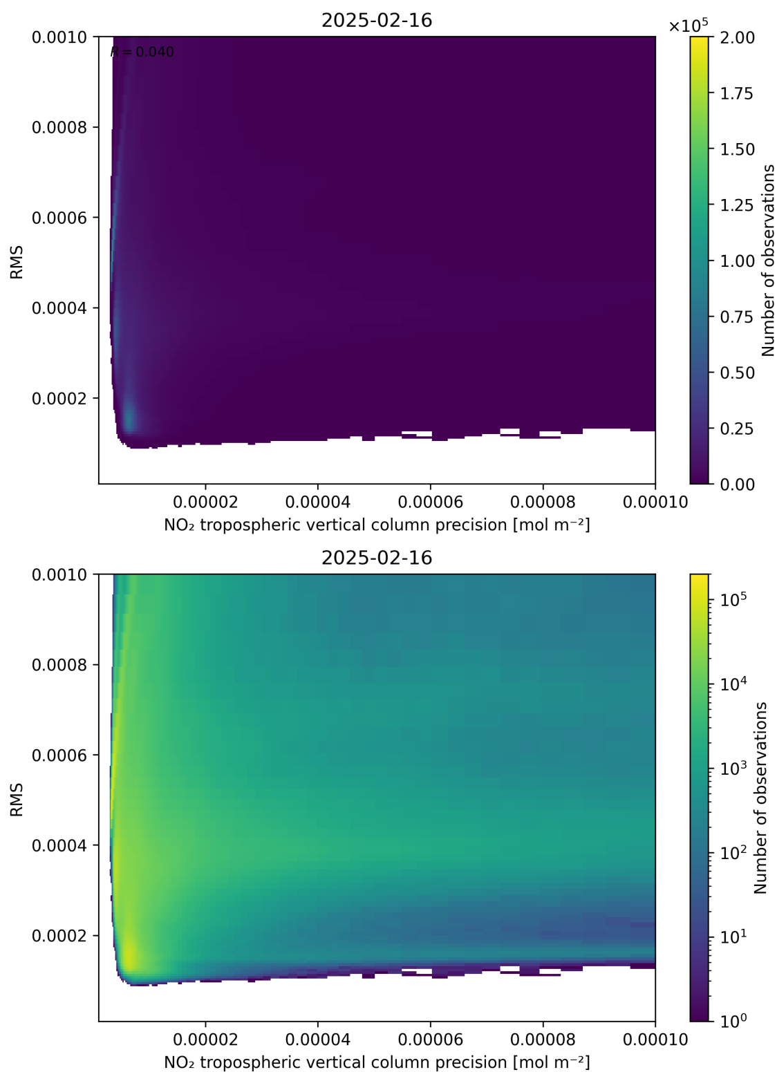
Figure 140: Scatter density plot of “NO 2 tropospheric vertical column precision” against “RMS” for 2025-02-15 to 2025-02-17.
