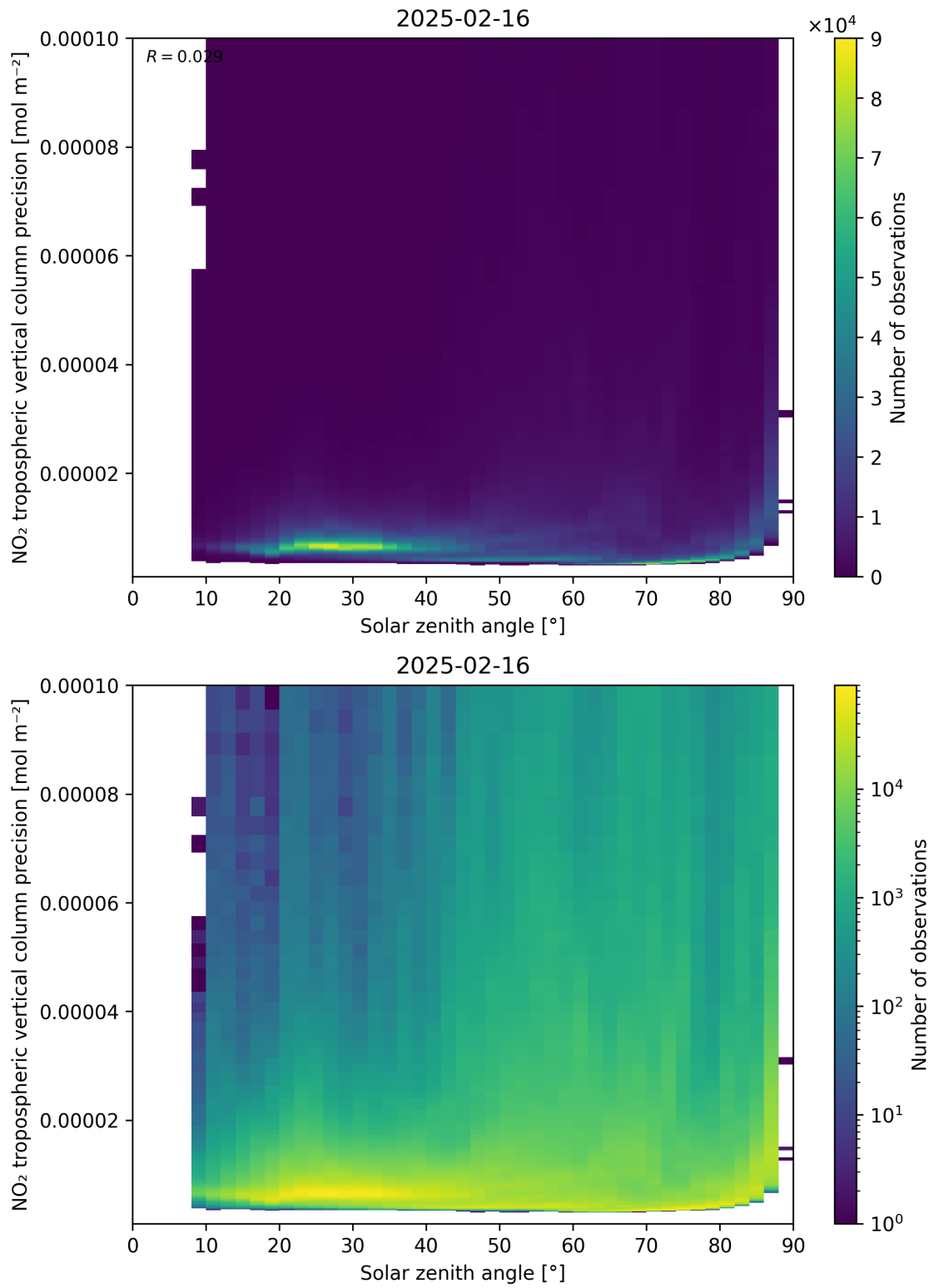
Figure 156: Scatter density plot of “Solar zenith angle” against “NO 2 tropospheric vertical column precision” for 2025-02-15 to 2025-02-17.
