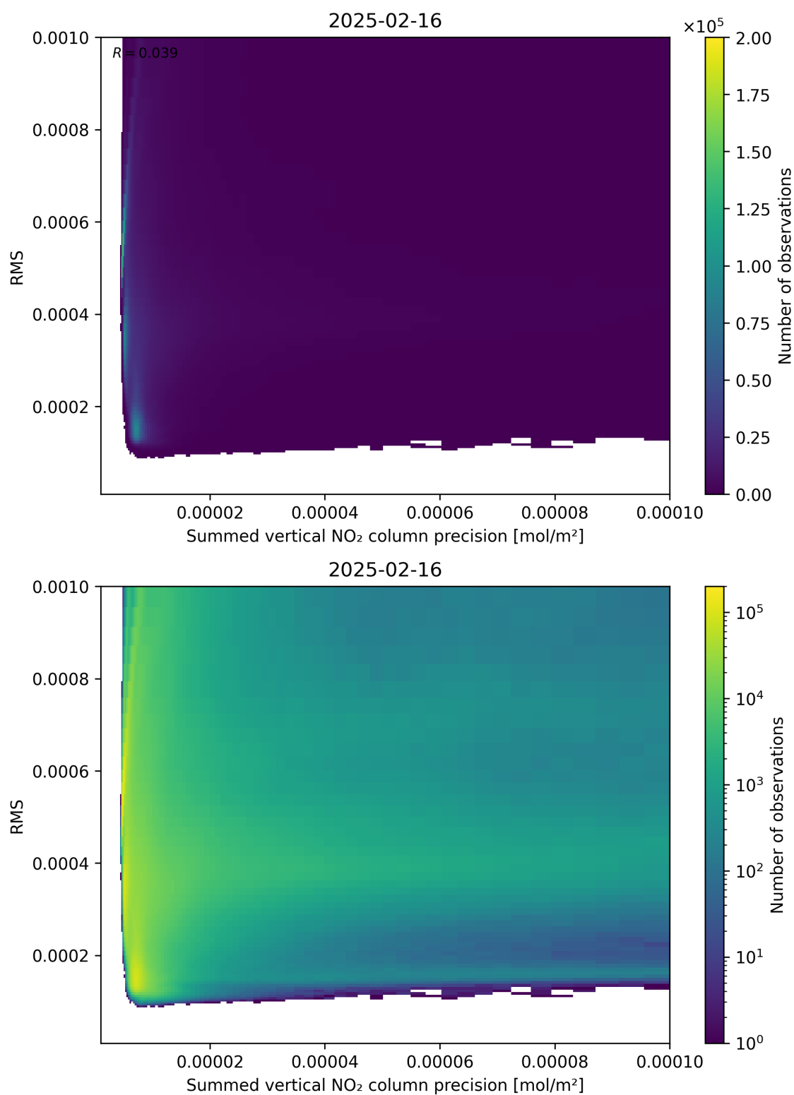
Figure 108: Scatter density plot of “Summed vertical NO 2 column precision” against “RMS” for 2025-02-15 to 2025-02-17.
