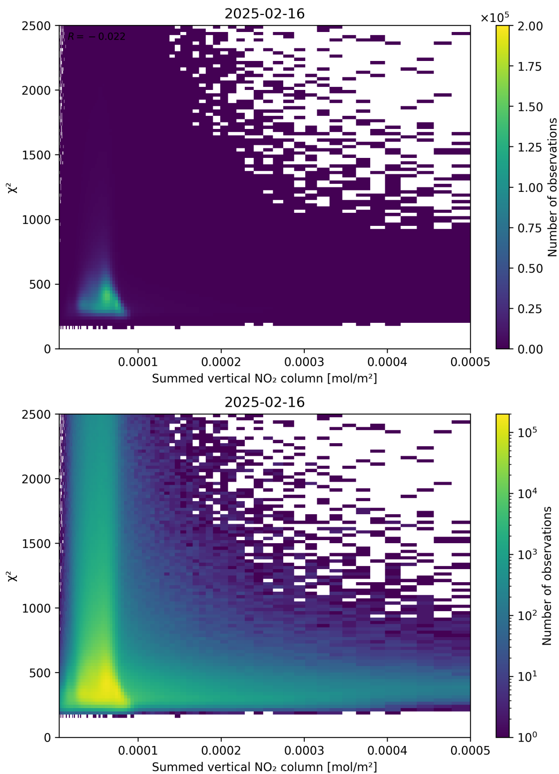
Figure 104: Scatter density plot of “Summed vertical NO 2 column” against “ \chi^2 ” for 2025-02-15 to 2025-02-17.
