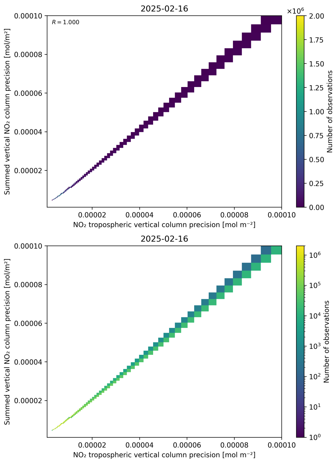
Figure 137: Scatter density plot of “NO 2 tropospheric vertical column precision” against “Summed vertical NO 2 column precision” for 2025-02-15 to 2025-02-17.
