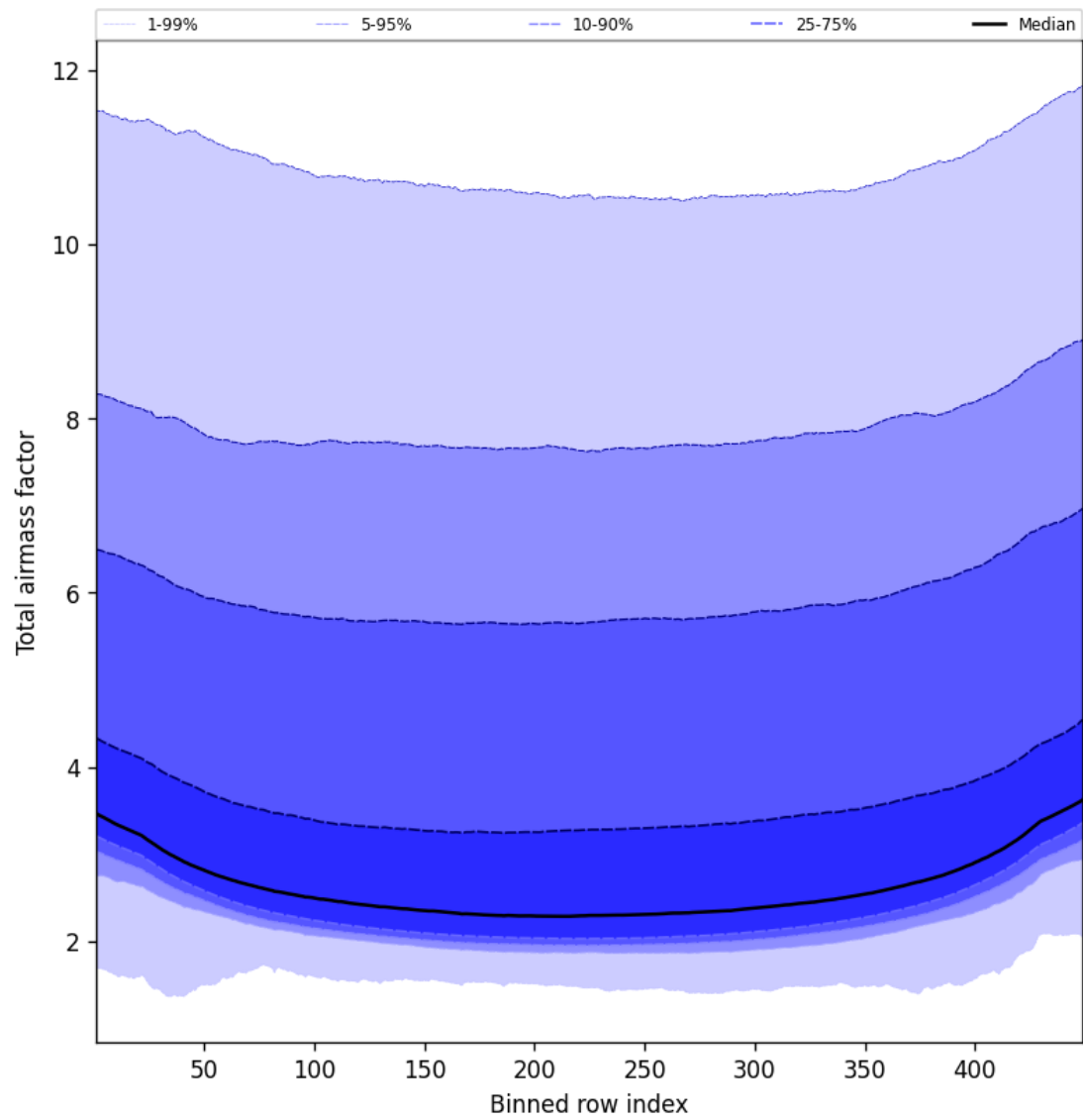
Figure 49: Along track statistics of “Total airmass factor” for 2025-02-15 to 2025-02-17
