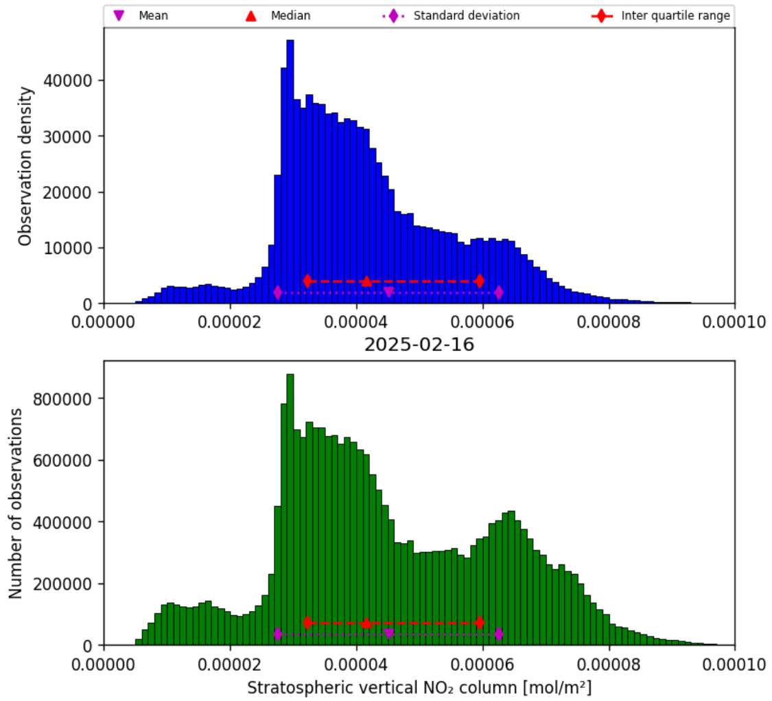
Figure 36: Histogram of “Stratospheric vertical NO 2 column” for 2025-02-15 to 2025-02-17
