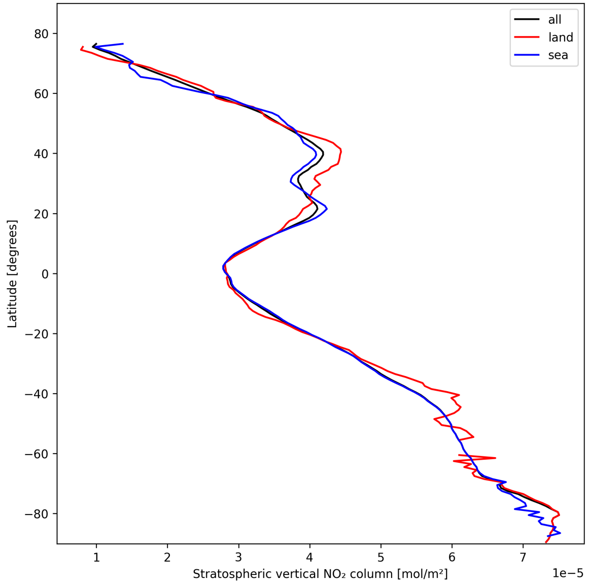
Figure 19: Zonal average of “Stratospheric vertical NO 2 column” for 2025-02-15 to 2025-02-17.
