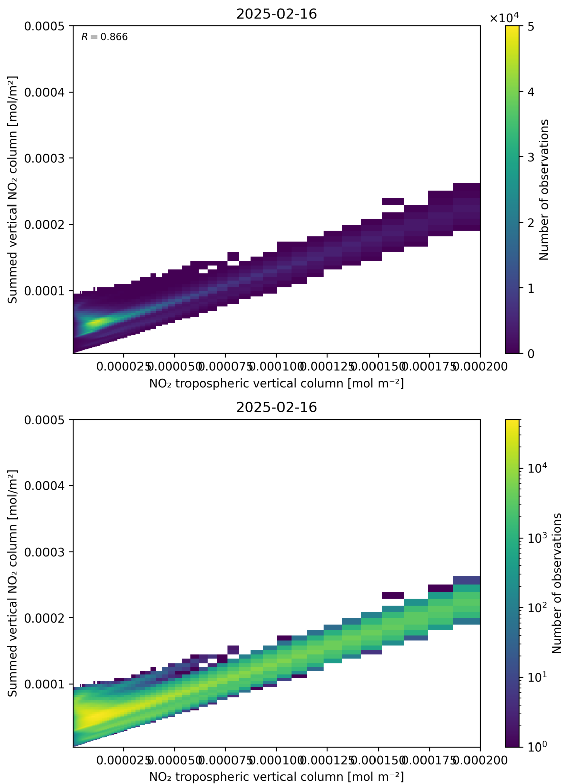
Figure 126: Scatter density plot of “NO 2 tropospheric vertical column” against “Summed vertical NO 2 column” for 2025-02-15 to 2025-02-17.
