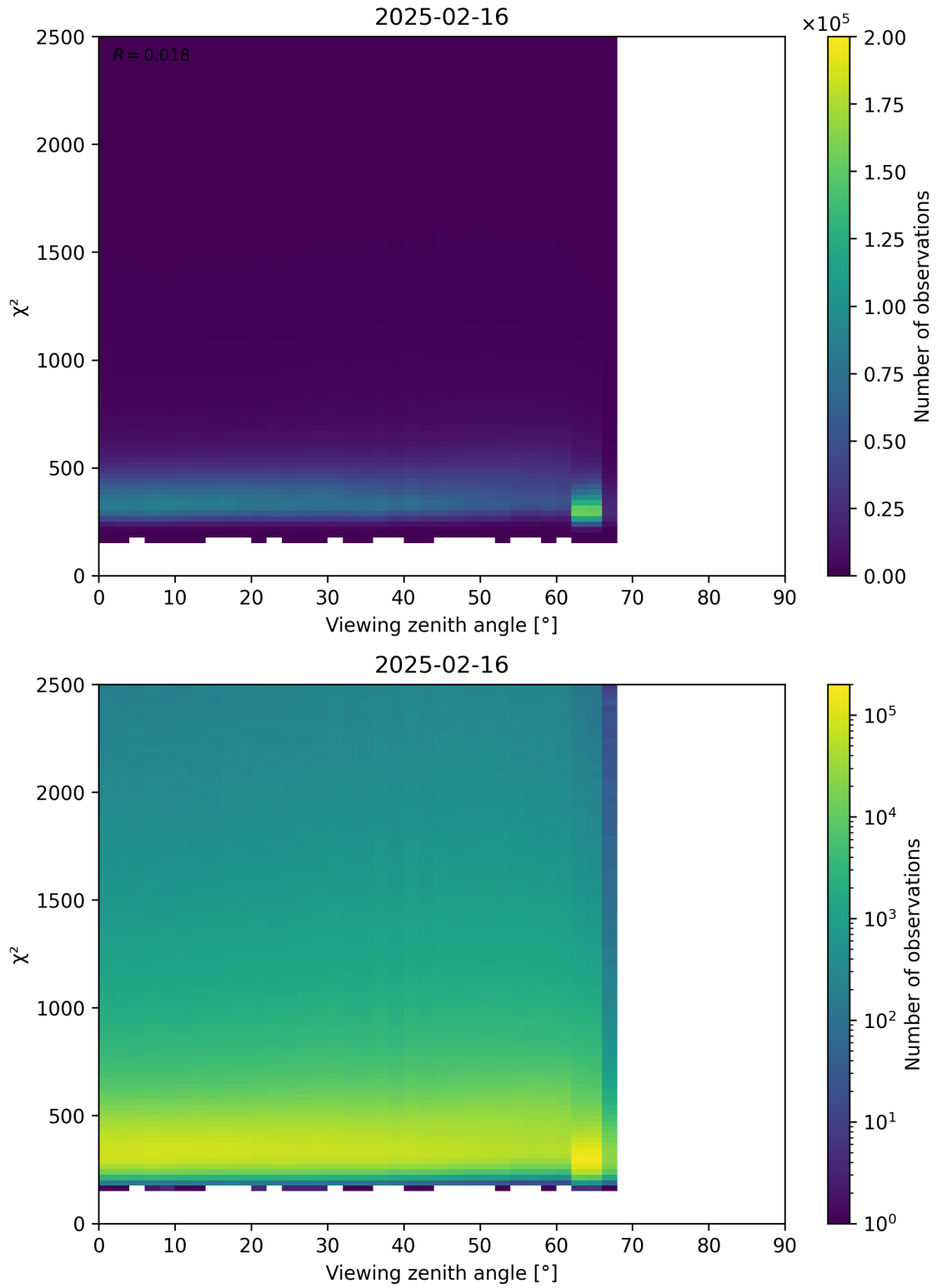
Figure 162: Scatter density plot of “Viewing zenith angle” against “ \chi^2 ” for 2025-02-15 to 2025-02-17.
