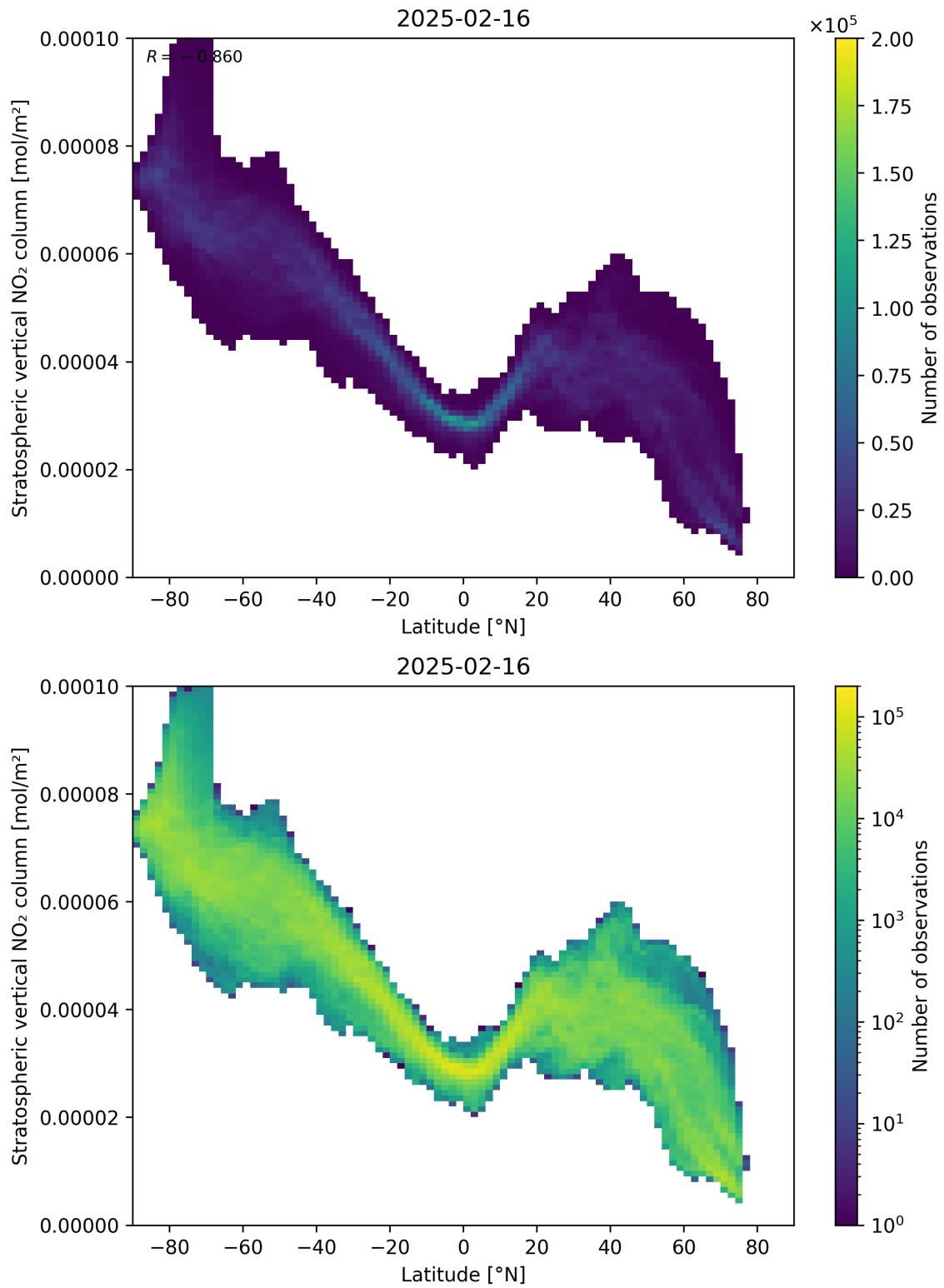
Figure 87: Scatter density plot of “Latitude” against “Stratospheric vertical NO 2 column” for 2025-02-15 to 2025-02-17.
