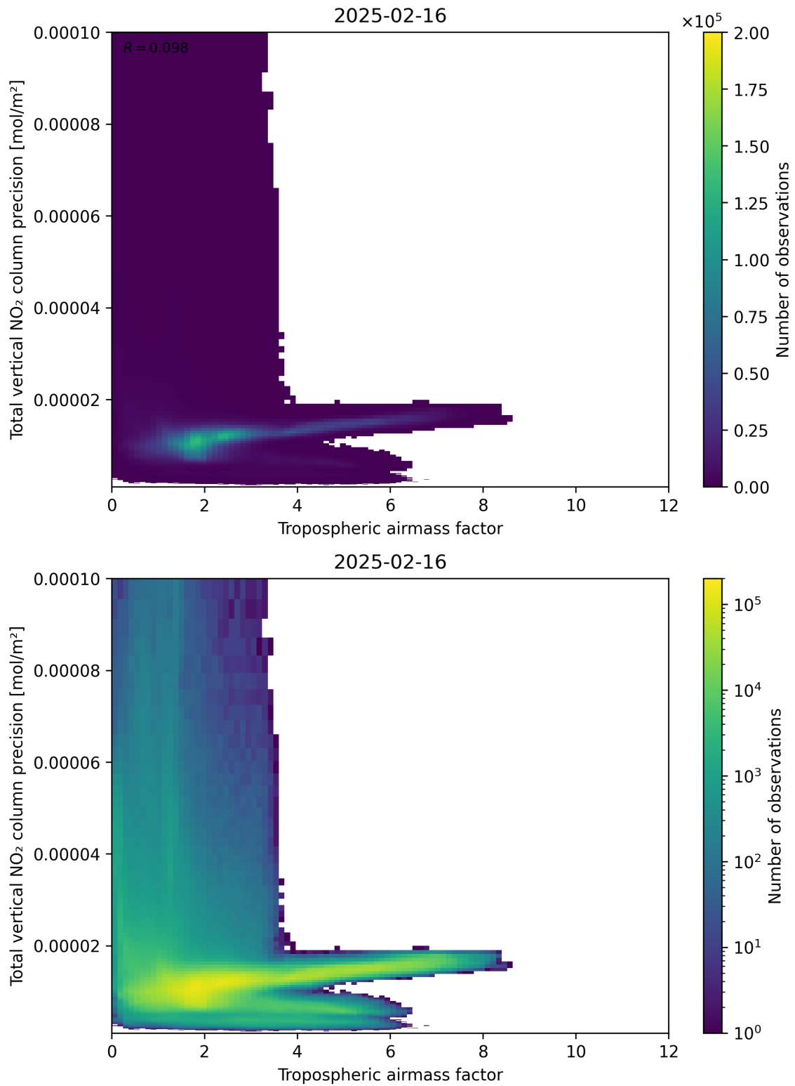
Figure 78: Scatter density plot of “Tropospheric air mass factor” against “Total vertical NO 2 column precision” for 2025-02-15 to 2025-02-17.
