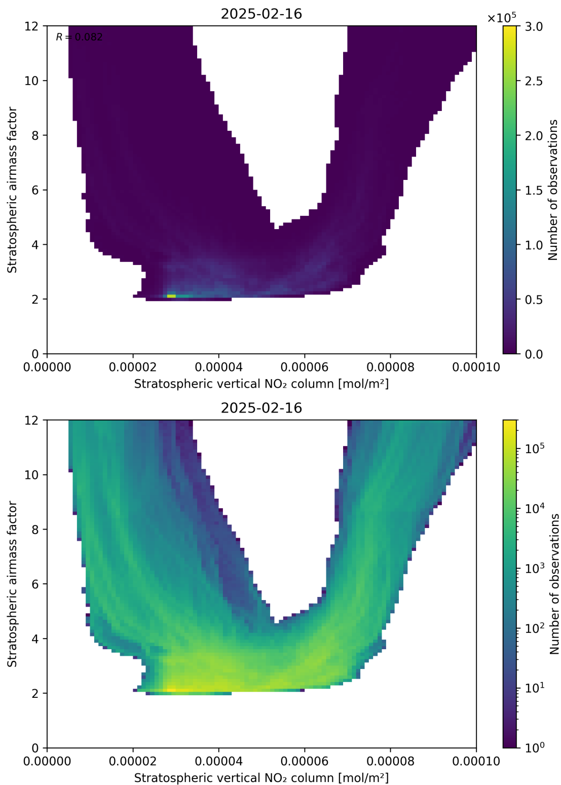
Figure 96: Scatter density plot of “Stratospheric vertical NO 2 column” against “Stratospheric airmass factor” for 2025-02-15 to 2025-02-17.
