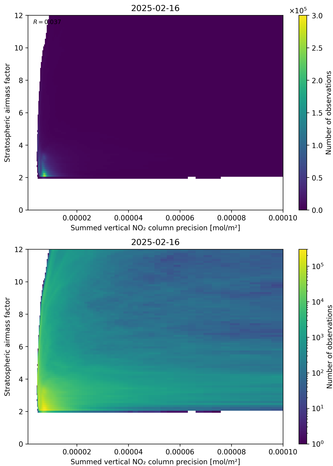
Figure 106: Scatter density plot of “Summed vertical NO 2 column precision” against “Stratospheric airmass factor” for 2025-02-15 to 2025-02-17.
