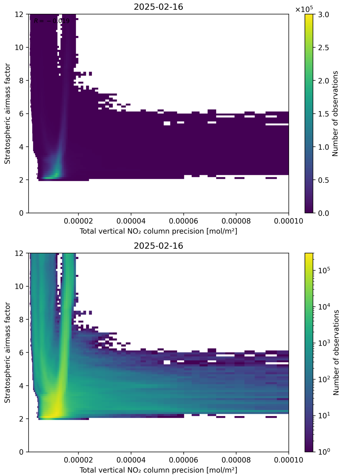
Figure 115: Scatter density plot of “Total vertical NO 2 column precision” against “Stratospheric air mass factor” for 2025-02-15 to 2025-02-17.
