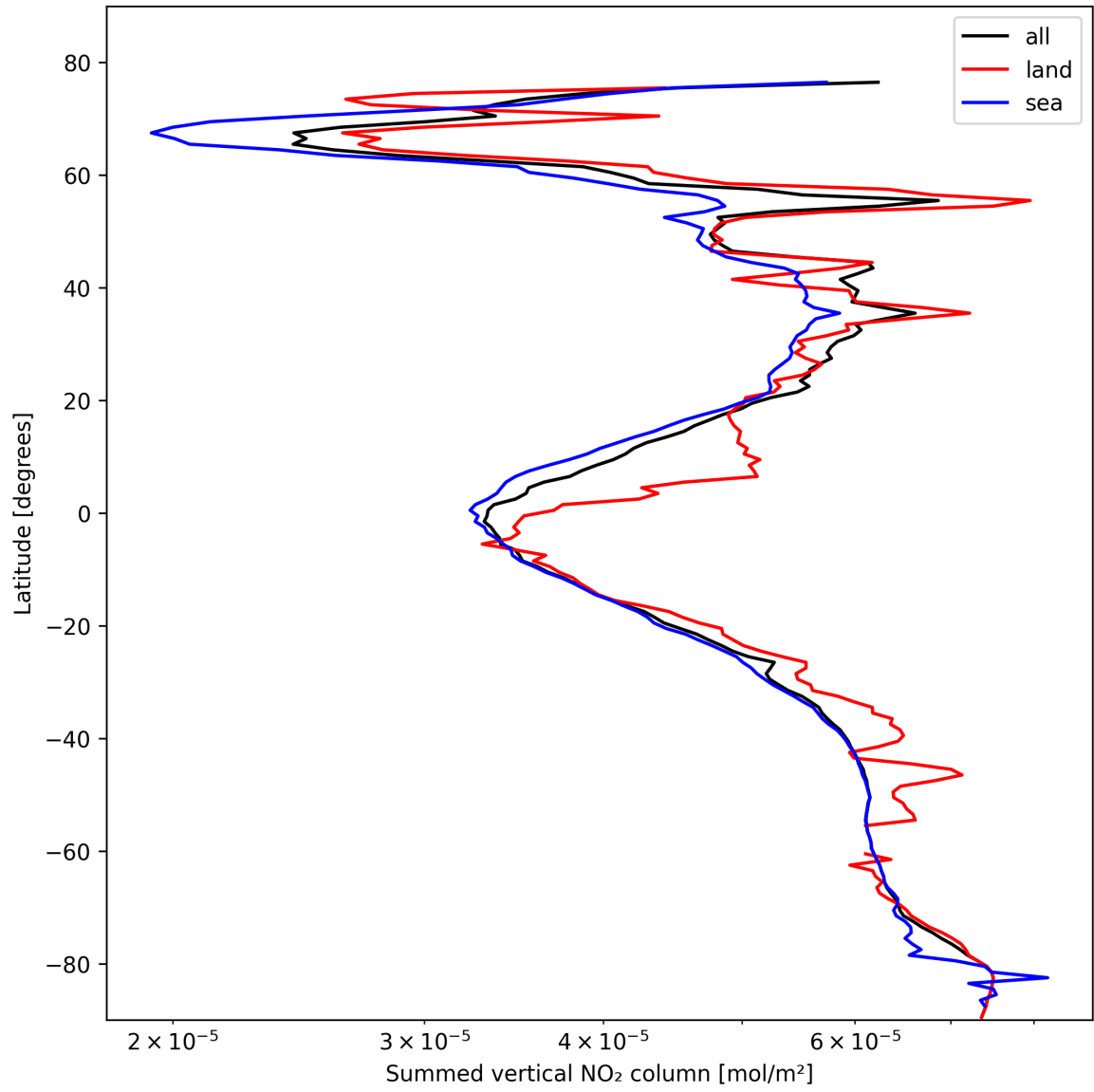
Figure 23: Zonal average of “Summed vertical NO 2 column” for 2025-02-15 to 2025-02-17.
