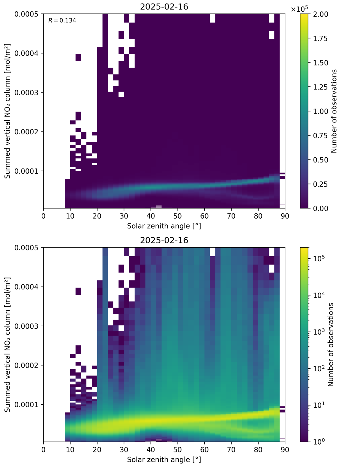
Figure 151: Scatter density plot of “Solar zenith angle” against “Summed vertical NO 2 column” for 2025-02-15 to 2025-02-17.
