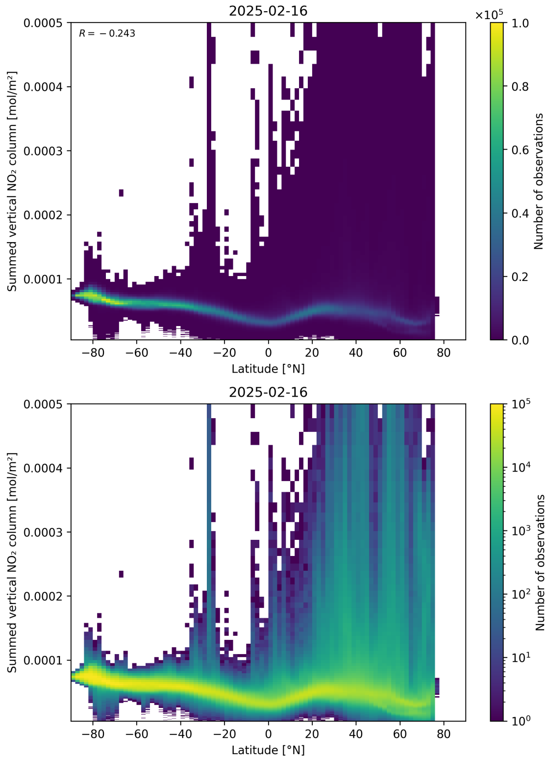
Figure 88: Scatter density plot of “Latitude” against “Summed vertical NO 2 column” for 2025-02-15 to 2025-02-17.
