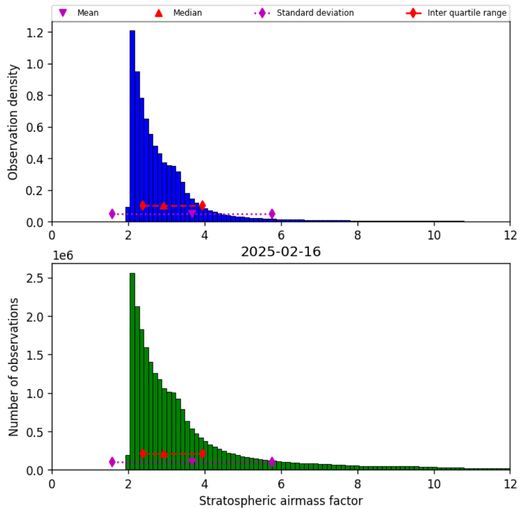
Figure 44: Histogram of “Stratospheric airmass factor” for 2025-02-15 to 2025-02-17
