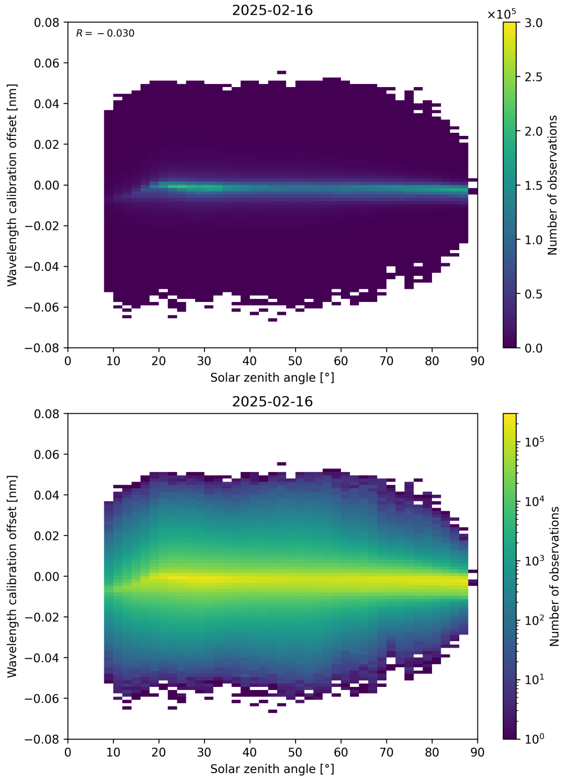
Figure 158: Scatter density plot of “Solar zenith angle” against “Wavelength calibration offset” for 2025-02-15 to 2025-02-17.
