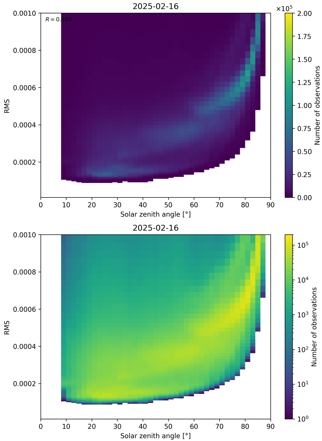
Figure 157: Scatter density plot of “Solar zenith angle” against “RMS” for 2025-02-15 to 2025-02-17.
