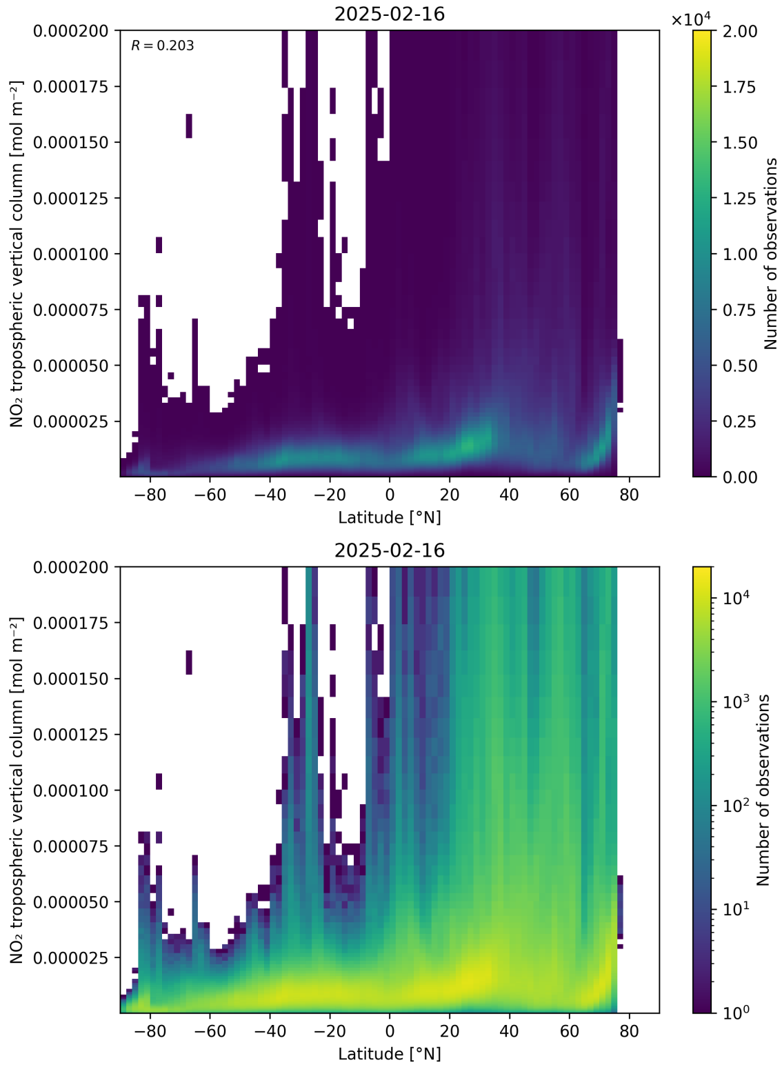
Figure 92: Scatter density plot of “Latitude” against “NO 2 tropospheric vertical column” for 2025-02-15 to 2025-02-17.
