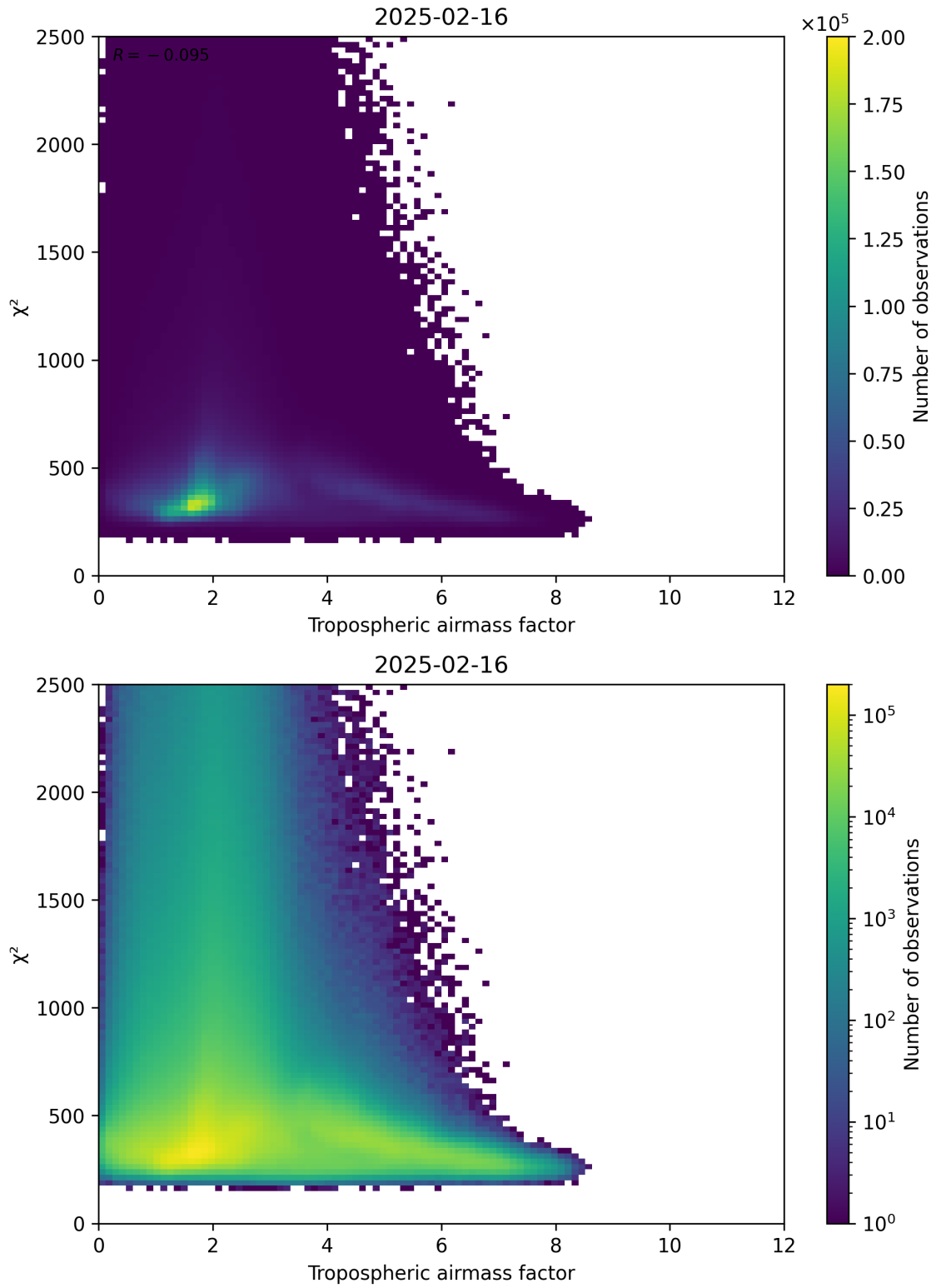
Figure 73: Scatter density plot of “Tropospheric airmass factor” against “ \chi^2 ” for 2025-02-15 to 2025-02-17.
