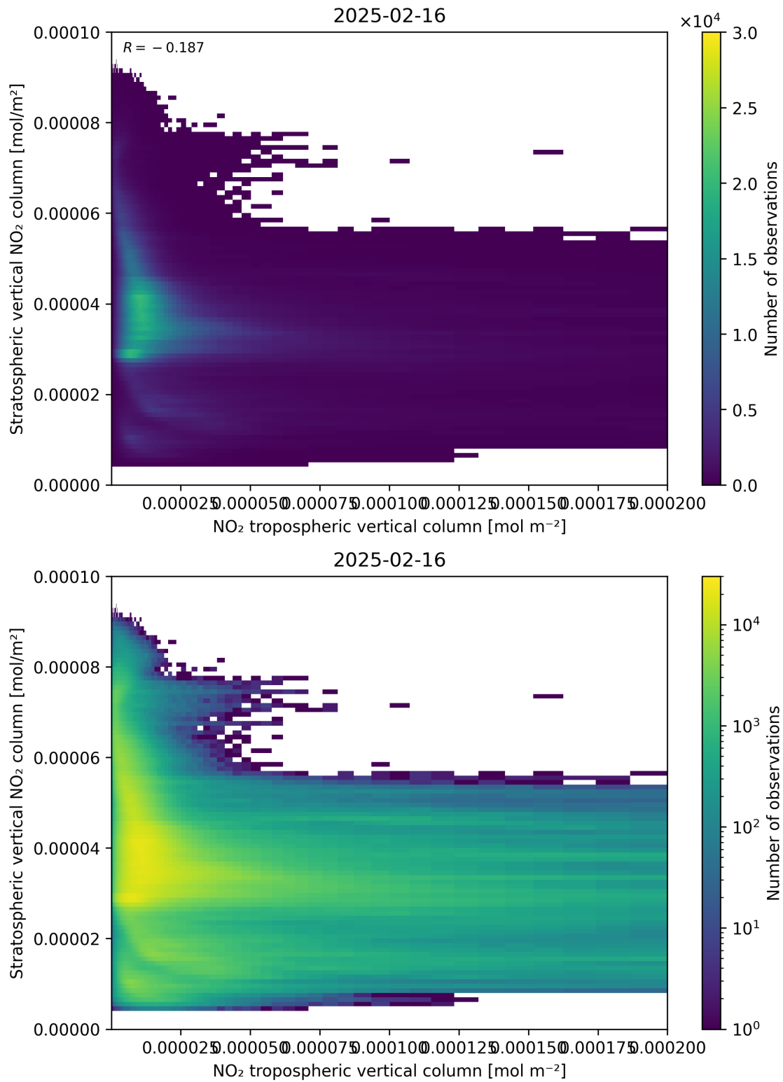
Figure 125: Scatter density plot of “NO 2 tropospheric vertical column” against “Stratospheric vertical NO 2 column” for 2025-02-15 to 2025-02-17.
