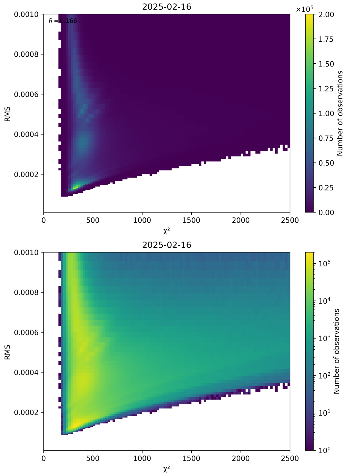
Figure 82: Scatter density plot of “ \chi^2 ” against “RMS” for 2025-02-15 to 2025-02-17.
