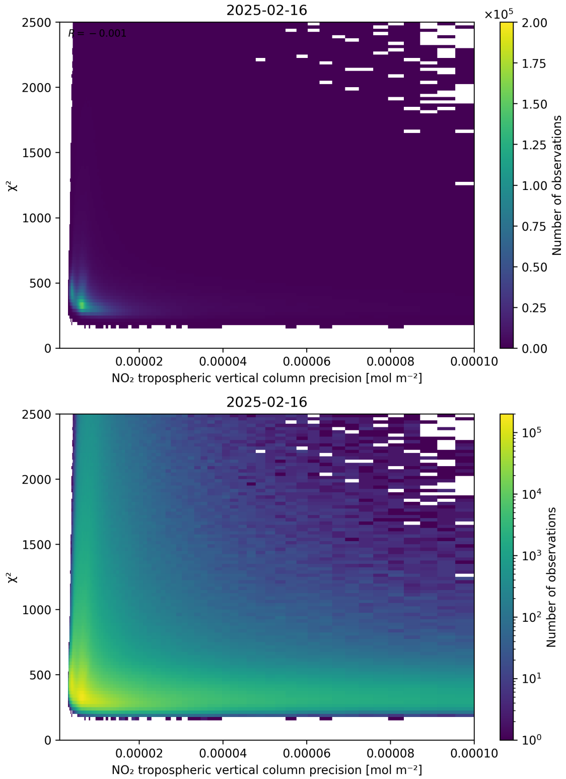
Figure 134: Scatter density plot of “NO 2 tropospheric vertical column precision” against “ \chi^2 ” for 2025-02-15 to 2025-02-17.
