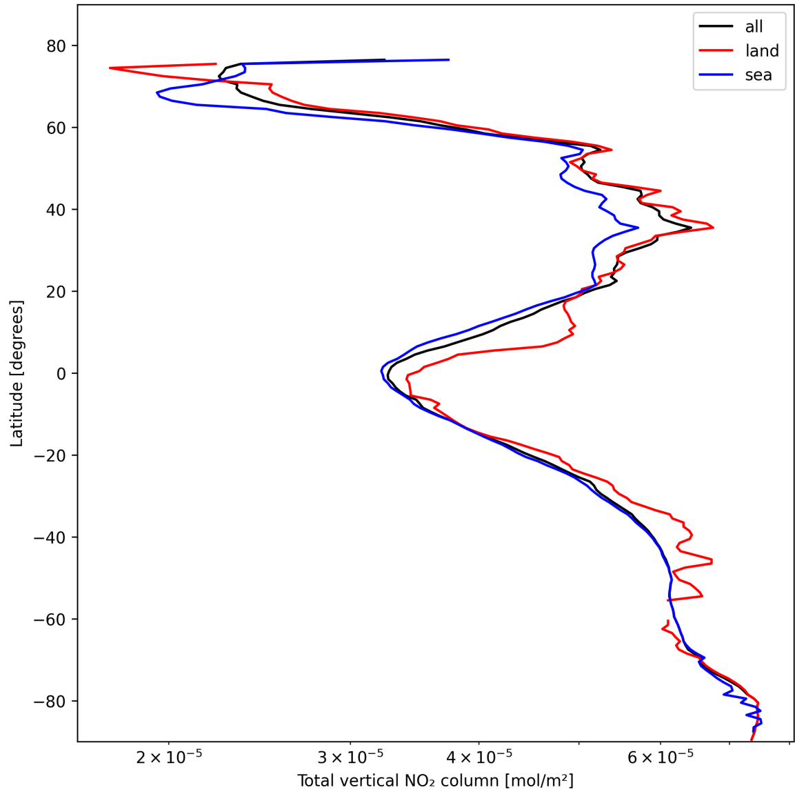
Figure 21: Zonal average of “Total vertical NO 2 column” for 2025-02-15 to 2025-02-17.
