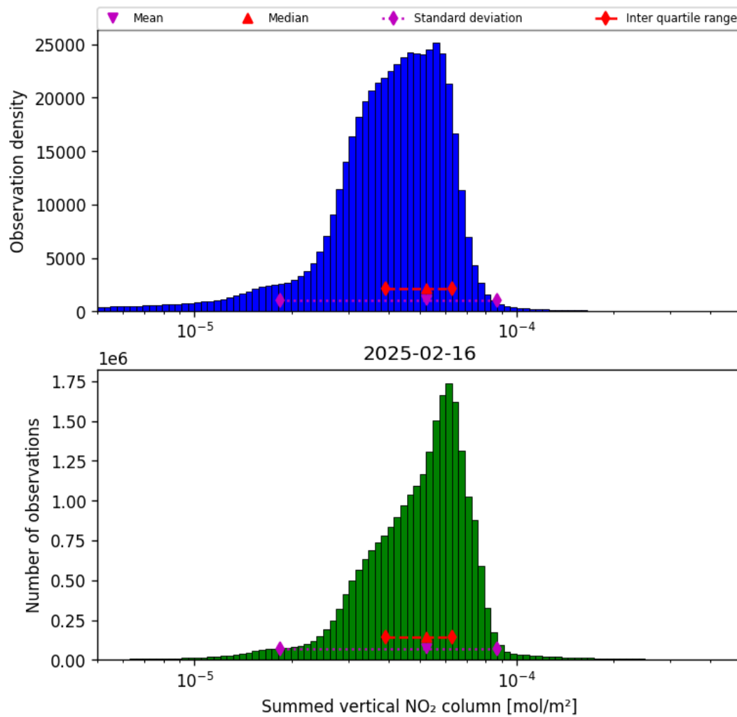
Figure 40: Histogram of “Summed vertical NO 2 column” for 2025-02-15 to 2025-02-17
