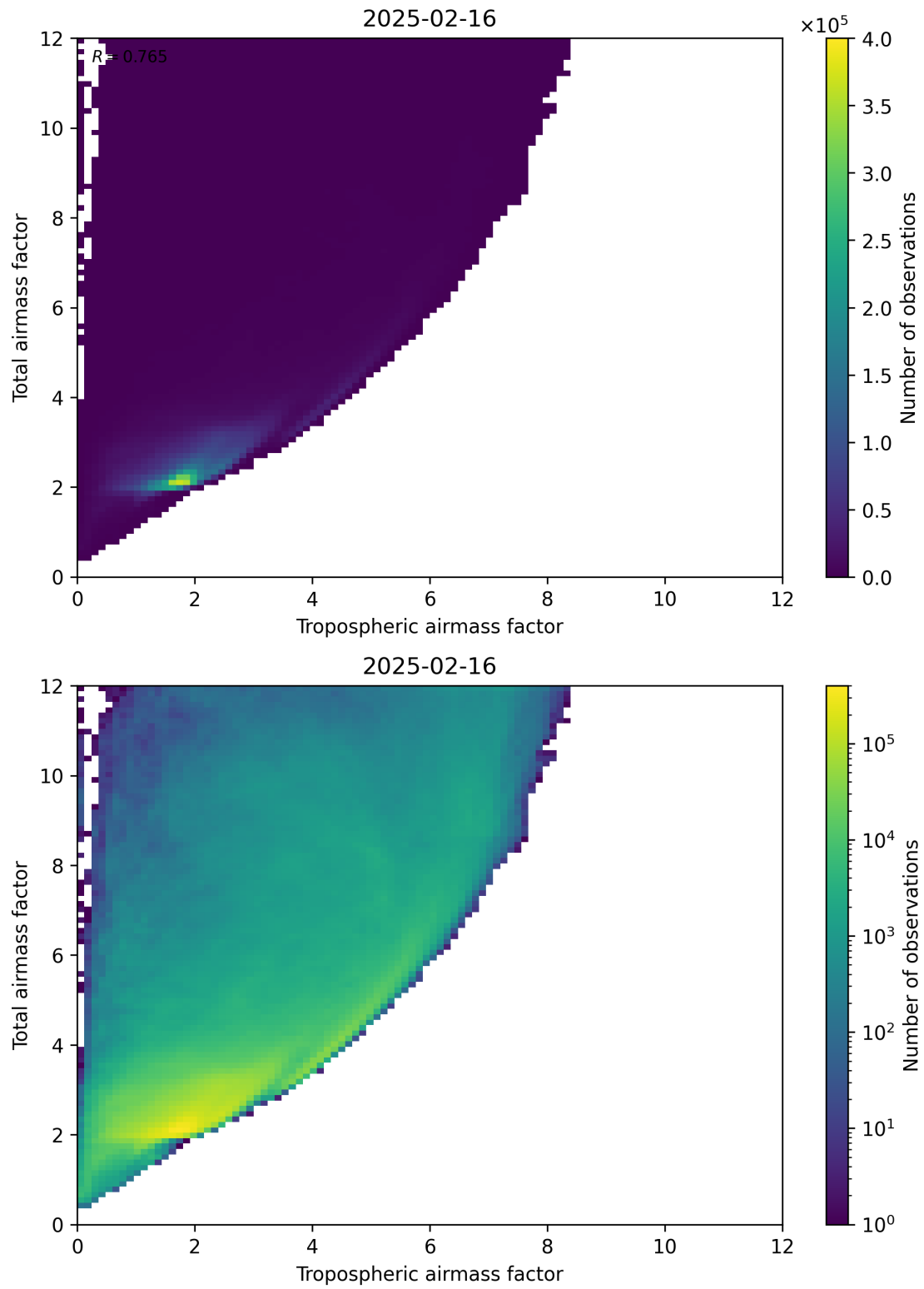
Figure 72: Scatter density plot of “Tropospheric airmass factor” against “Total airmass factor” for 2025-02-15 to 2025-02-17.
