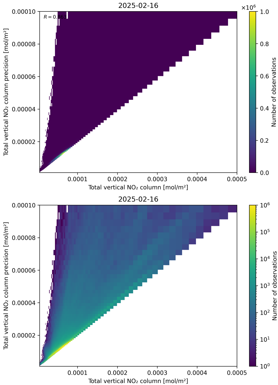
Figure 114: Scatter density plot of “Total vertical NO 2 column” against “Total vertical NO 2 column precision” for 2025-02-15 to 2025-02-17.
