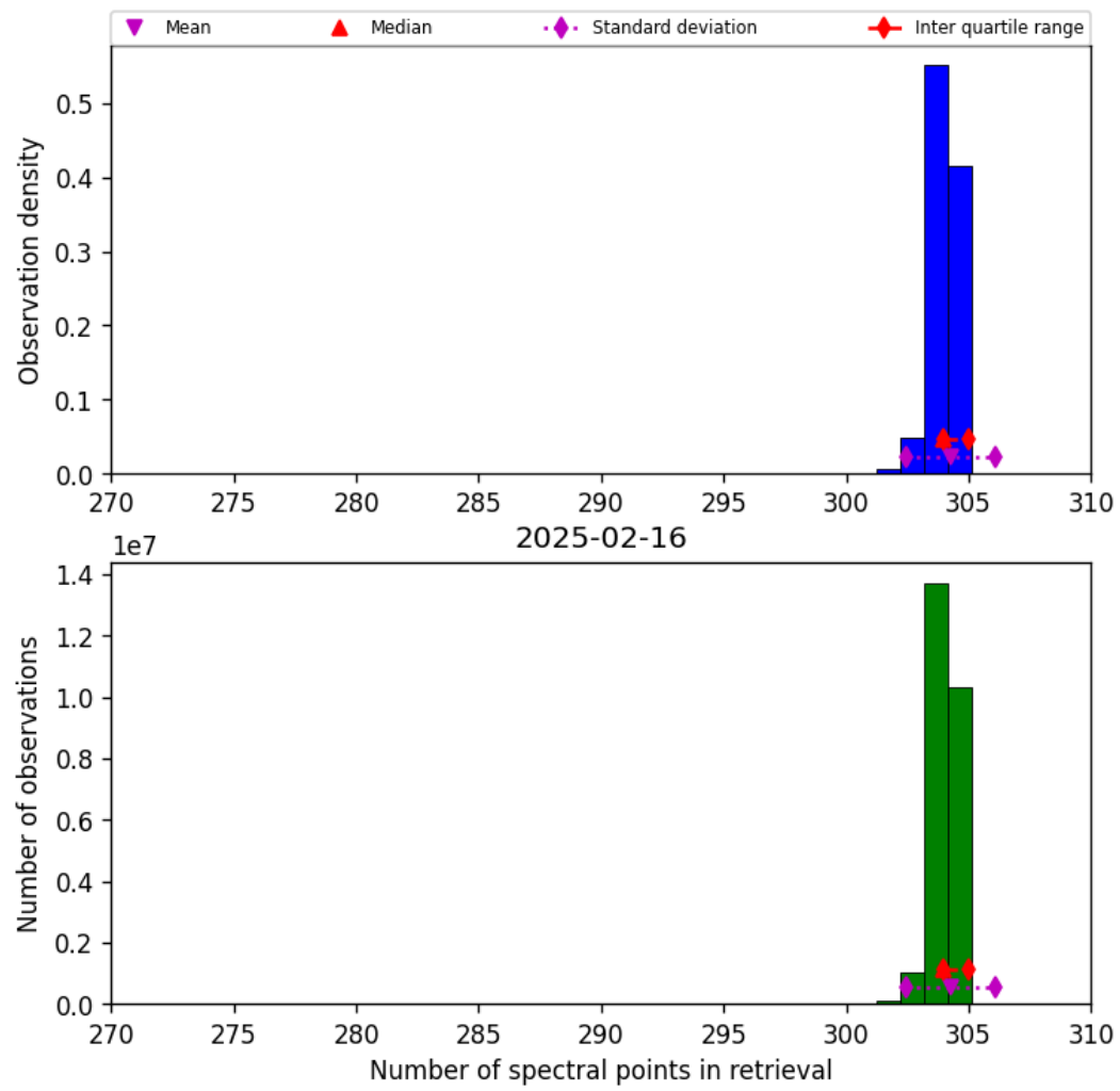
Figure 33: Histogram of “Number of spectral points in retrieval” for 2025-02-15 to 2025-02-17
