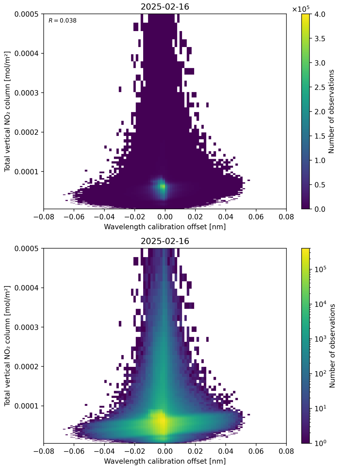
Figure 179: Scatter density plot of “Wavelength calibration offset” against “Total vertical NO 2 column” for 2025-02-15 to 2025-02-17.
