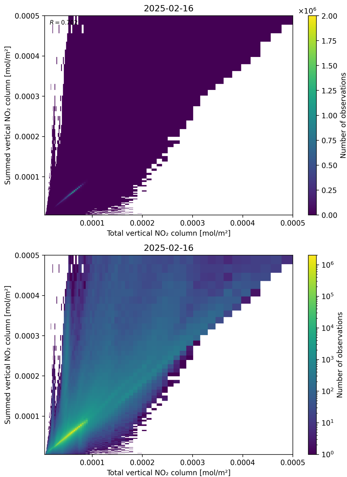
Figure 112: Scatter density plot of “Total vertical NO 2 column” against “Summed vertical NO 2 column” for 2025-02-15 to 2025-02-17.
