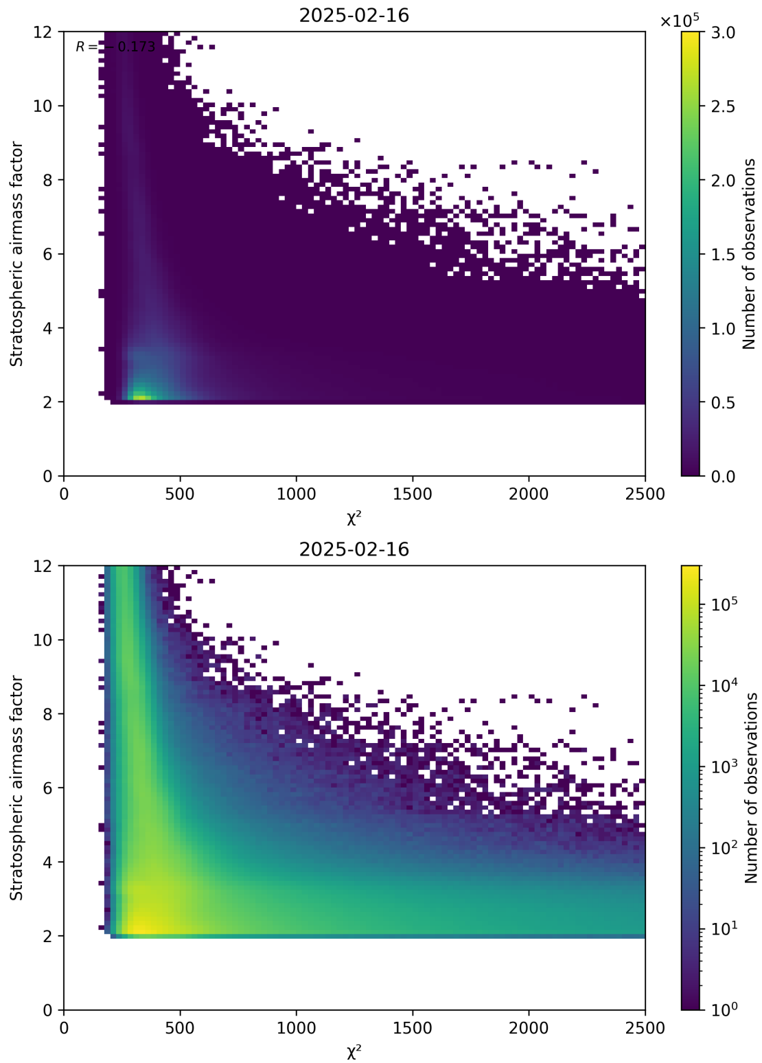
Figure 81: Scatter density plot of “ \chi^2 ” against “Stratospheric airmass factor” for 2025-02-15 to 2025-02-17.
