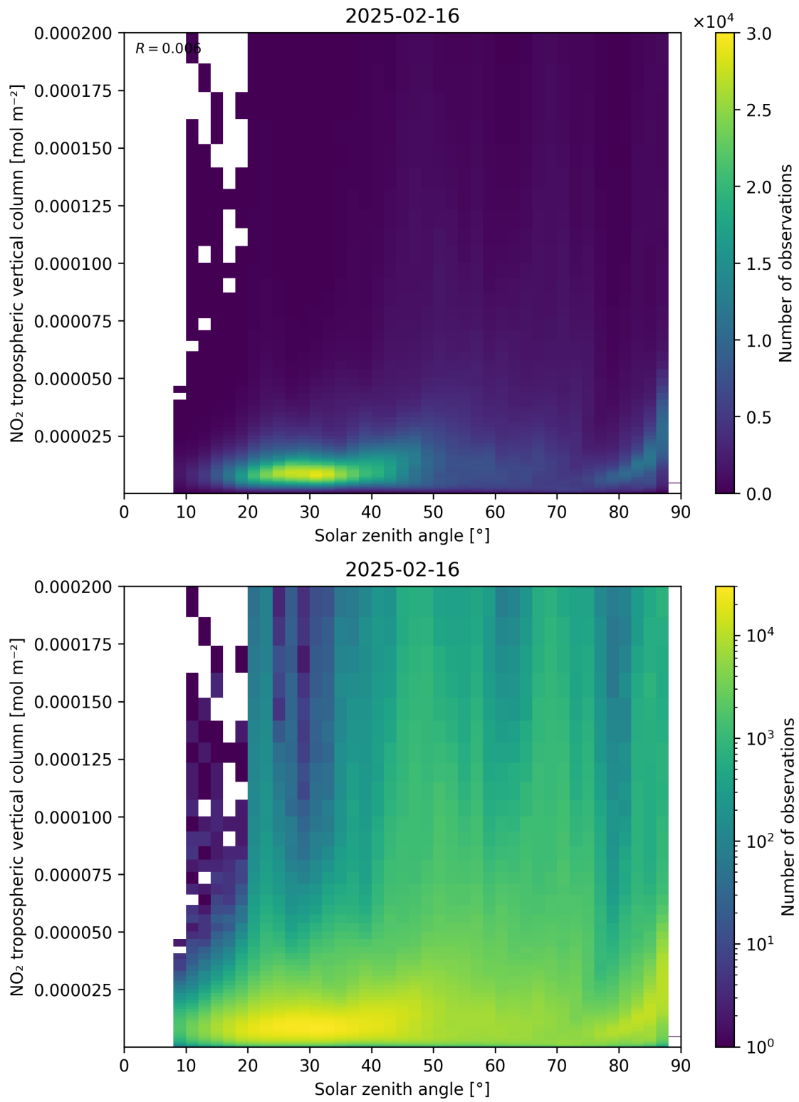
Figure 155: Scatter density plot of “Solar zenith angle” against “NO 2 tropospheric vertical column” for 2025-02-15 to 2025-02-17.
