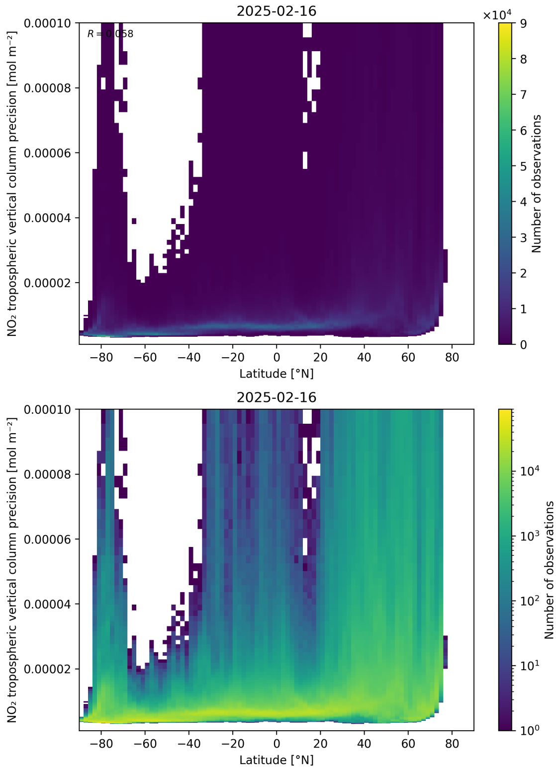
Figure 93: Scatter density plot of “Latitude” against “NO 2 tropospheric vertical column precision” for 2025-02-15 to 2025-02-17.
