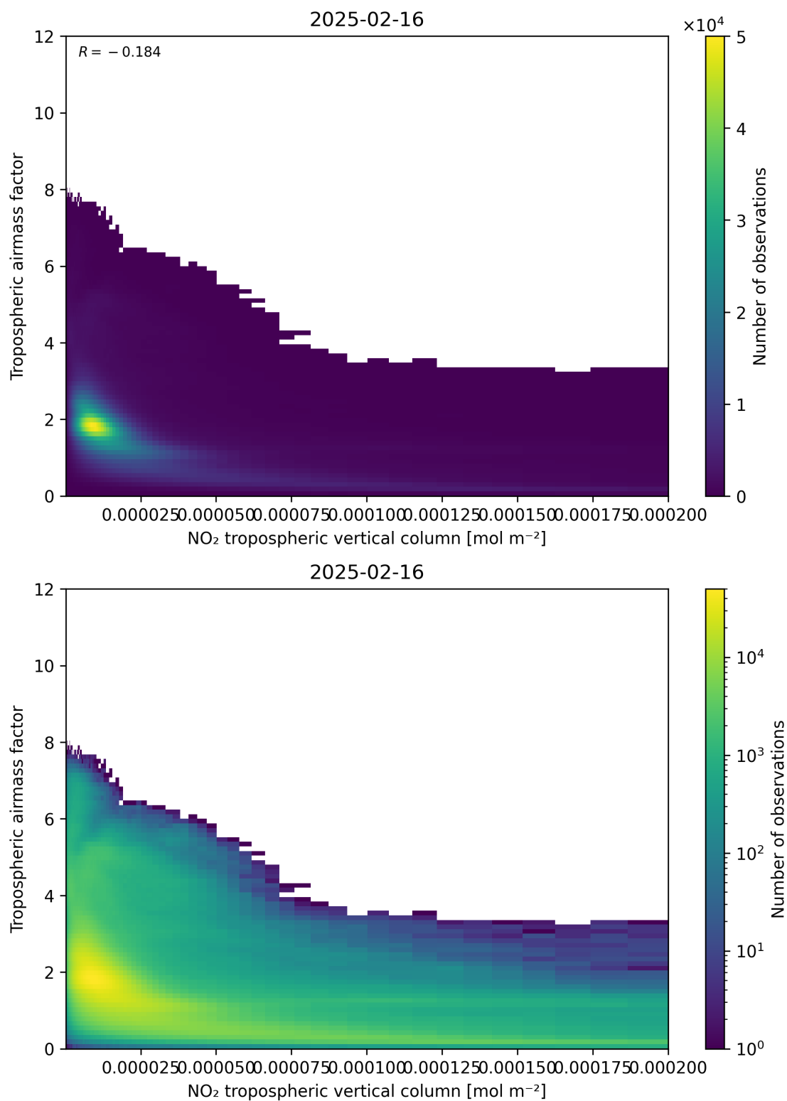
Figure 123: Scatter density plot of “NO 2 tropospheric vertical column” against “Tropospheric air mass factor” for 2025-02-15 to 2025-02-17.
