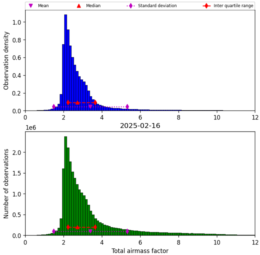
Figure 32: Histogram of “Total airmass factor” for 2025-02-15 to 2025-02-17
