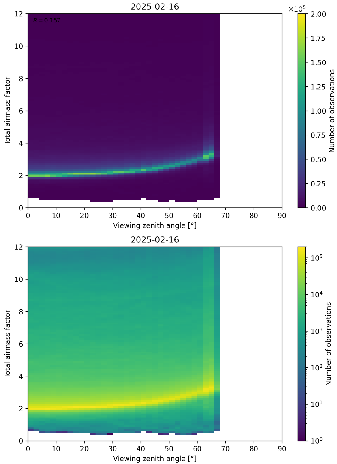
Figure 160: Scatter density plot of “Viewing zenith angle” against “Total airmass factor” for 2025-02-15 to 2025-02-17.
