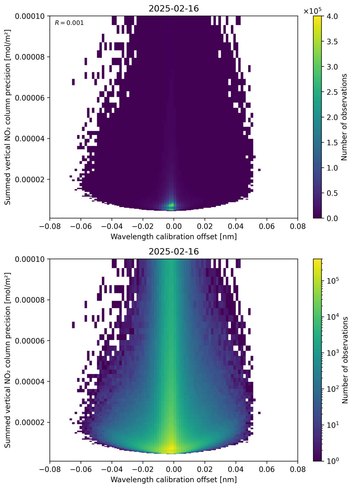
Figure 178: Scatter density plot of “Wavelength calibration offset” against “Summed vertical NO 2 column precision” for 2025-02-15 to 2025-02-17.
