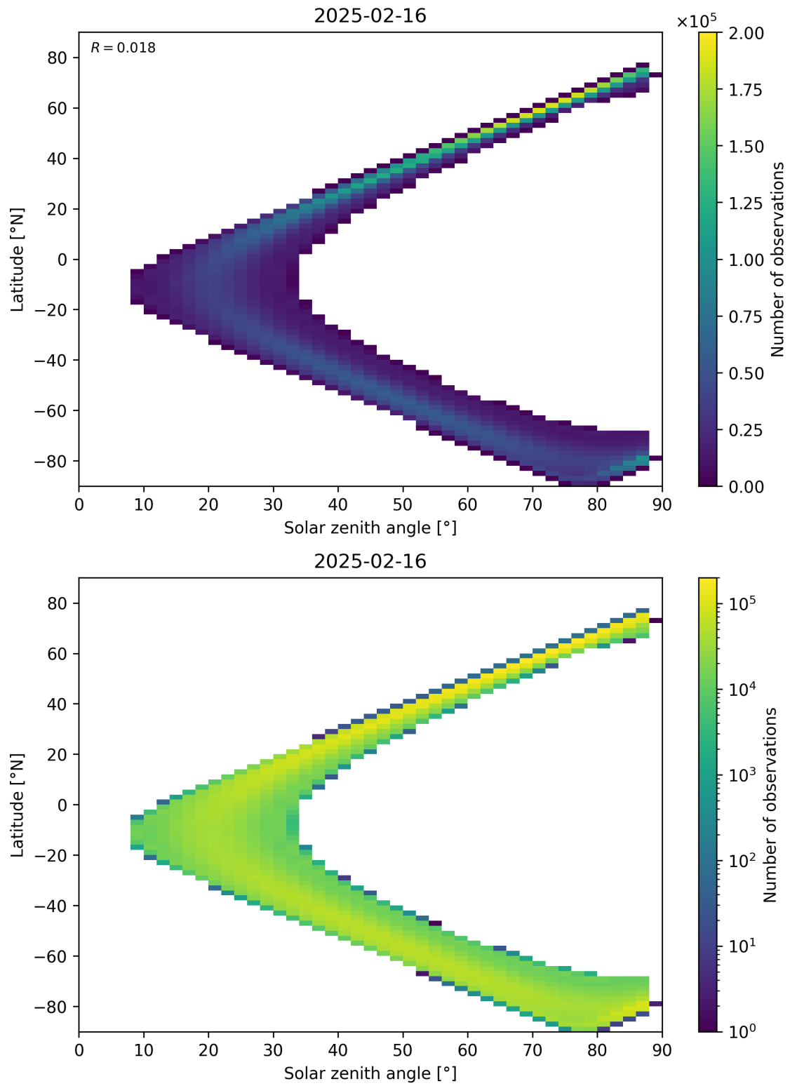
Figure 149: Scatter density plot of “Solar zenith angle” against “Latitude” for 2025-02-15 to 2025-02-17.
