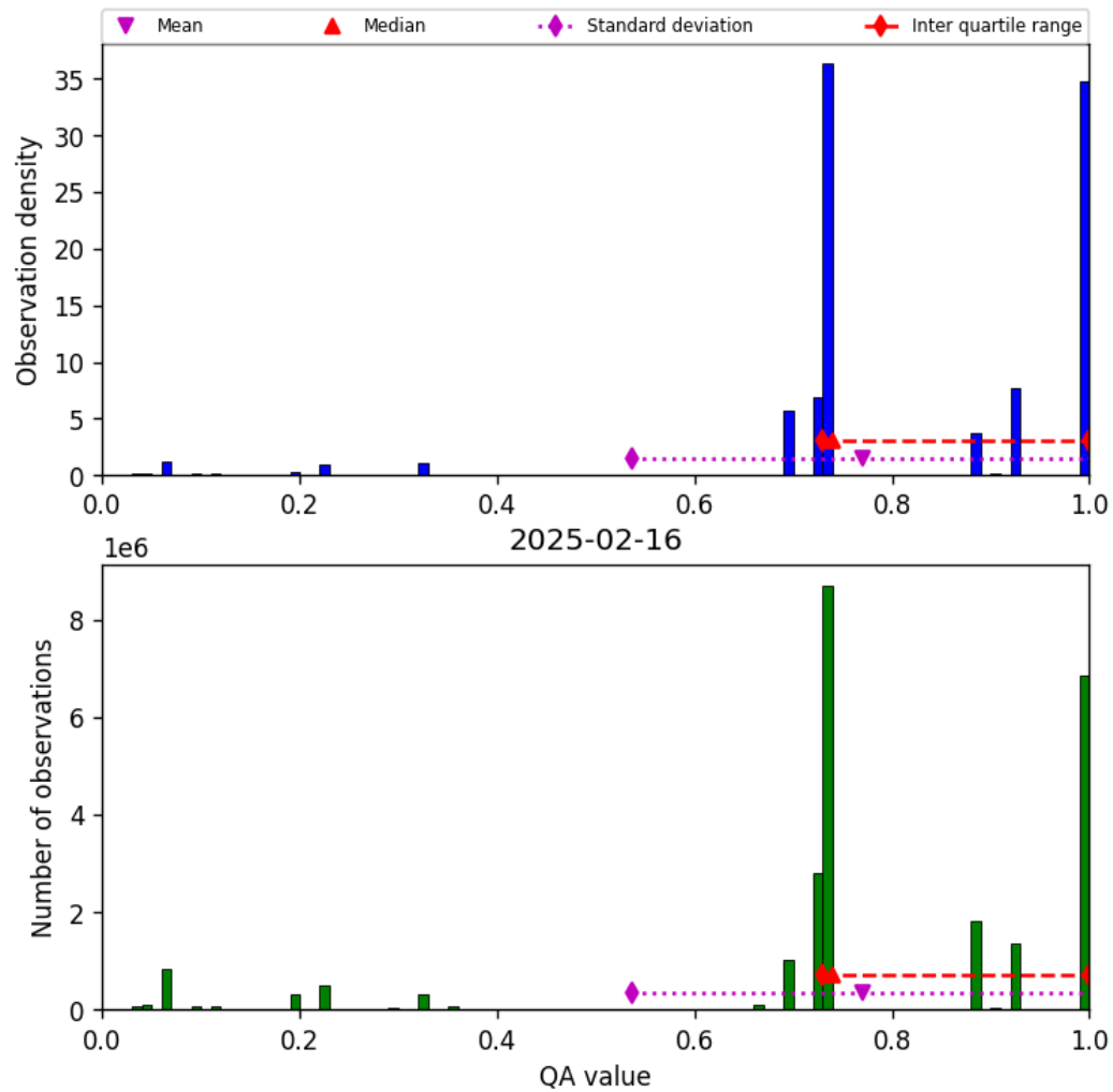
Figure 28: Histogram of “QA value” for 2025-02-15 to 2025-02-17
