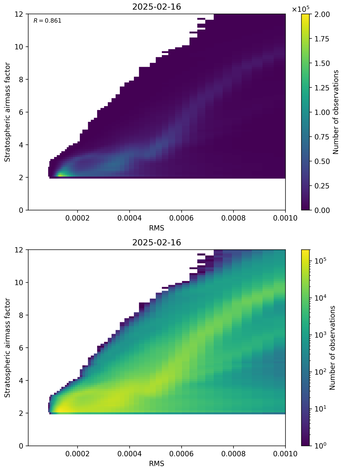
Figure 144: Scatter density plot of “RMS” against “Stratospheric airmass factor” for 2025-02-15 to 2025-02-17.
