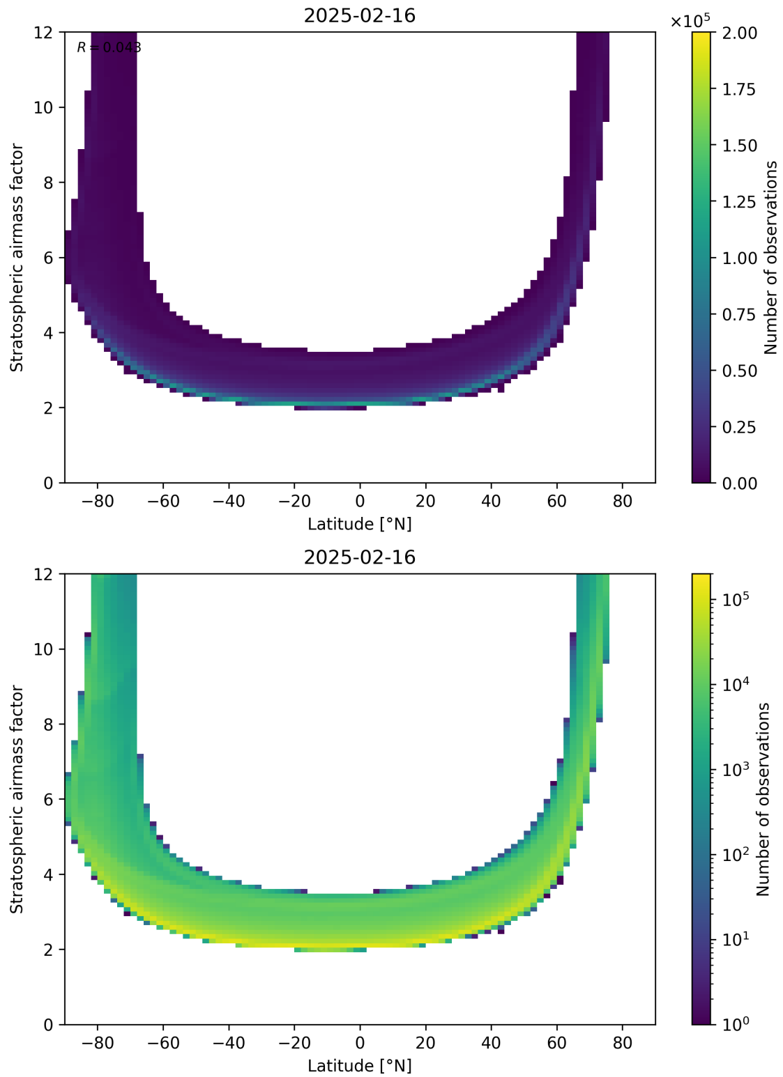
Figure 83: Scatter density plot of “Latitude” against “Stratospheric airmass factor” for 2025-02-15 to 2025-02-17.
