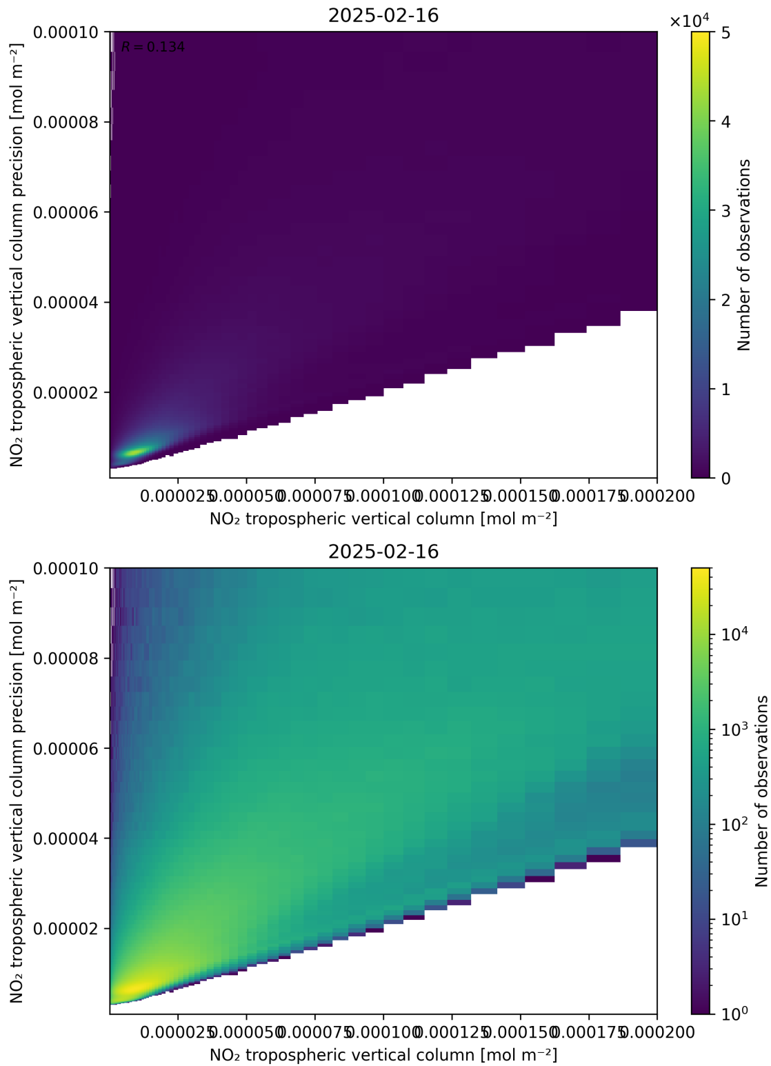
Figure 130: Scatter density plot of “NO 2 tropospheric vertical column” against “NO 2 tropospheric vertical column precision” for 2025-02-15 to 2025-02-17.
