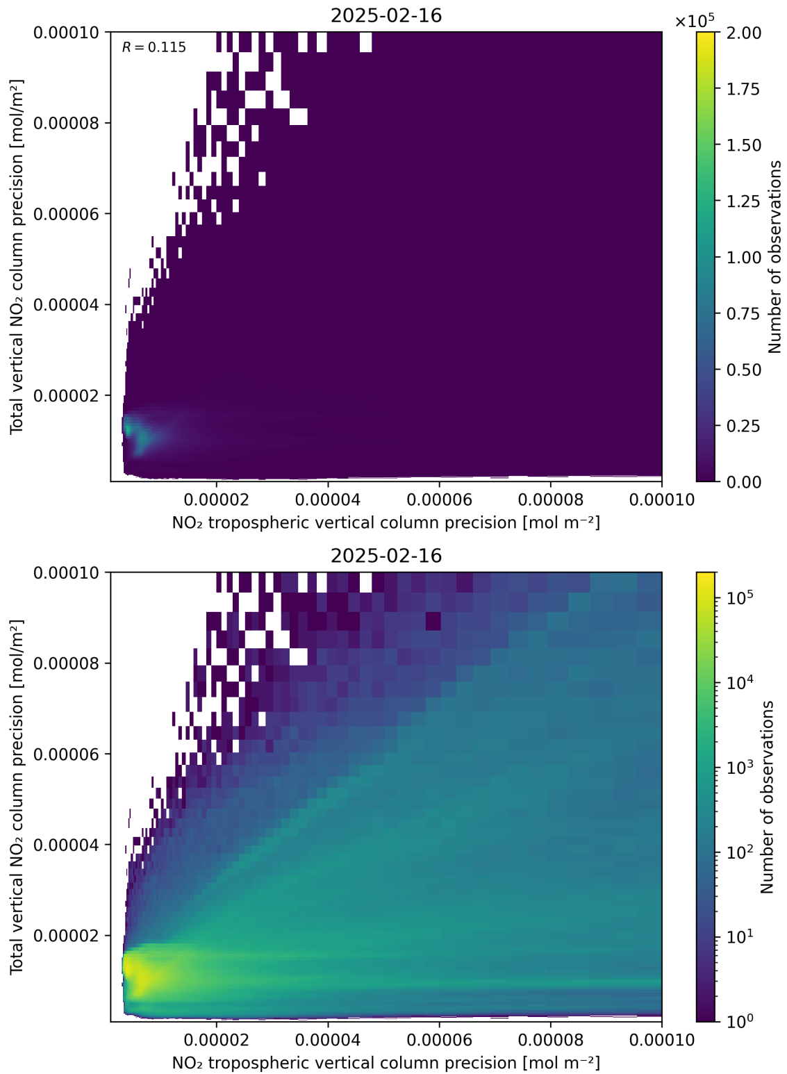
Figure 139: Scatter density plot of “NO 2 tropospheric vertical column precision” against “Total vertical NO 2 column precision” for 2025-02-15 to 2025-02-17.
