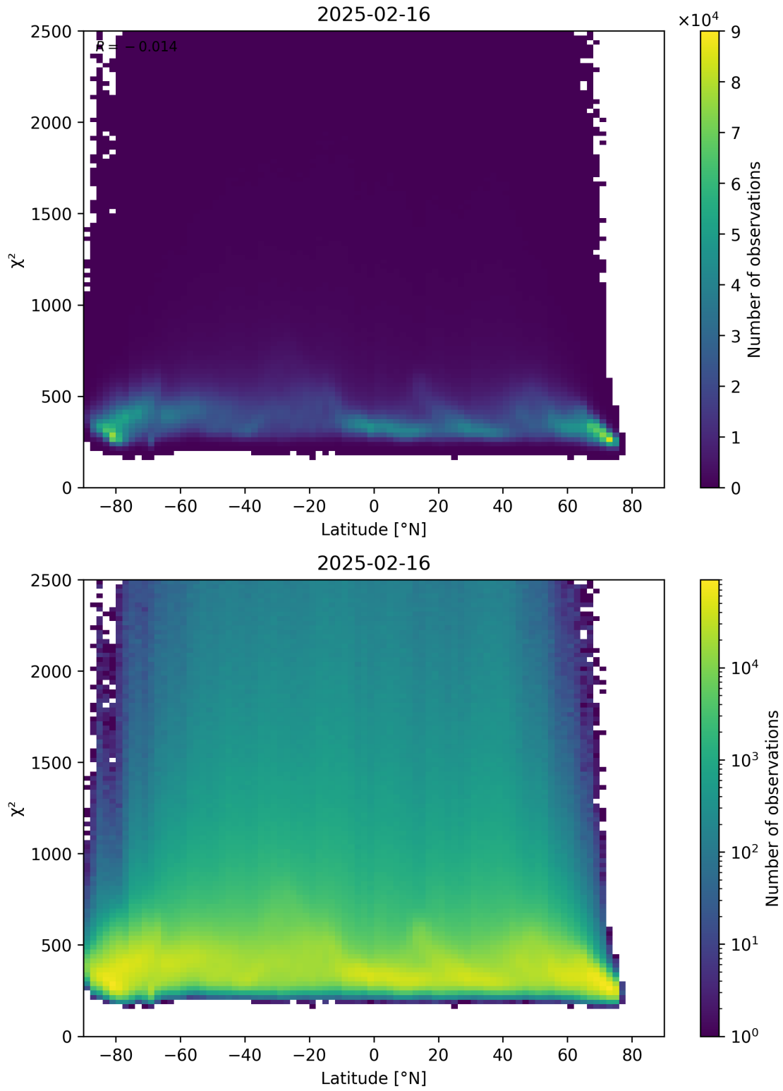
Figure 86: Scatter density plot of “Latitude” against “ \chi^2 ” for 2025-02-15 to 2025-02-17.
