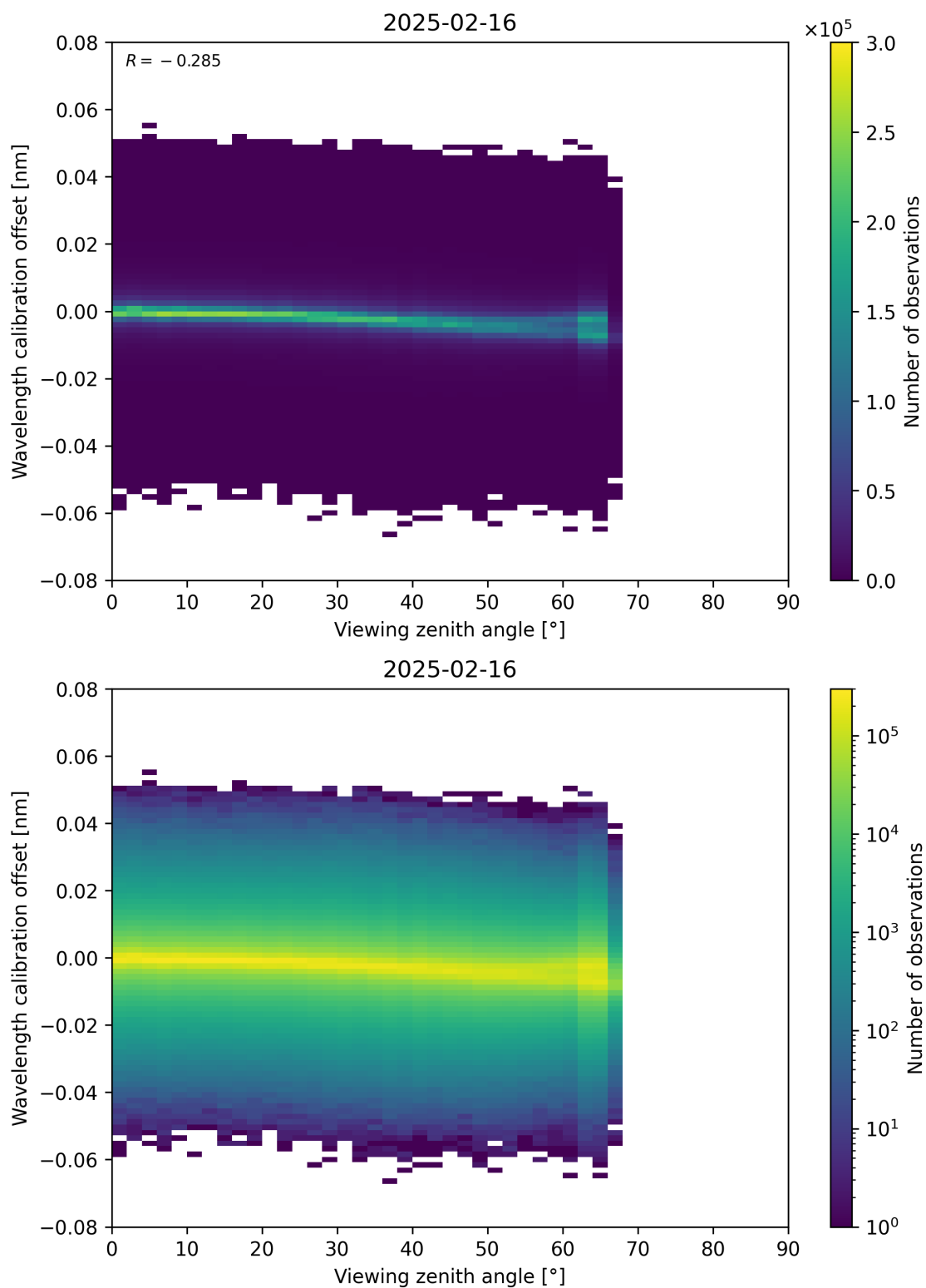
Figure 173: Scatter density plot of “Viewing zenith angle” against “Wavelength calibration offset” for 2025-02-15 to 2025-02-17.
