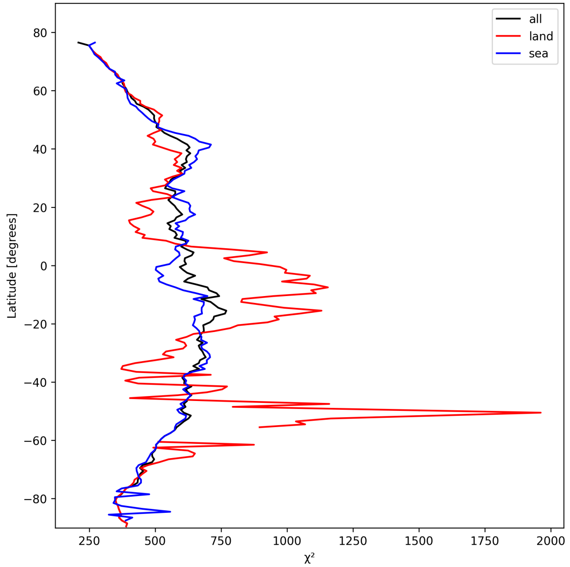
Figure 25: Zonal average of “ \chi^2 ” for 2025-02-15 to 2025-02-17.
