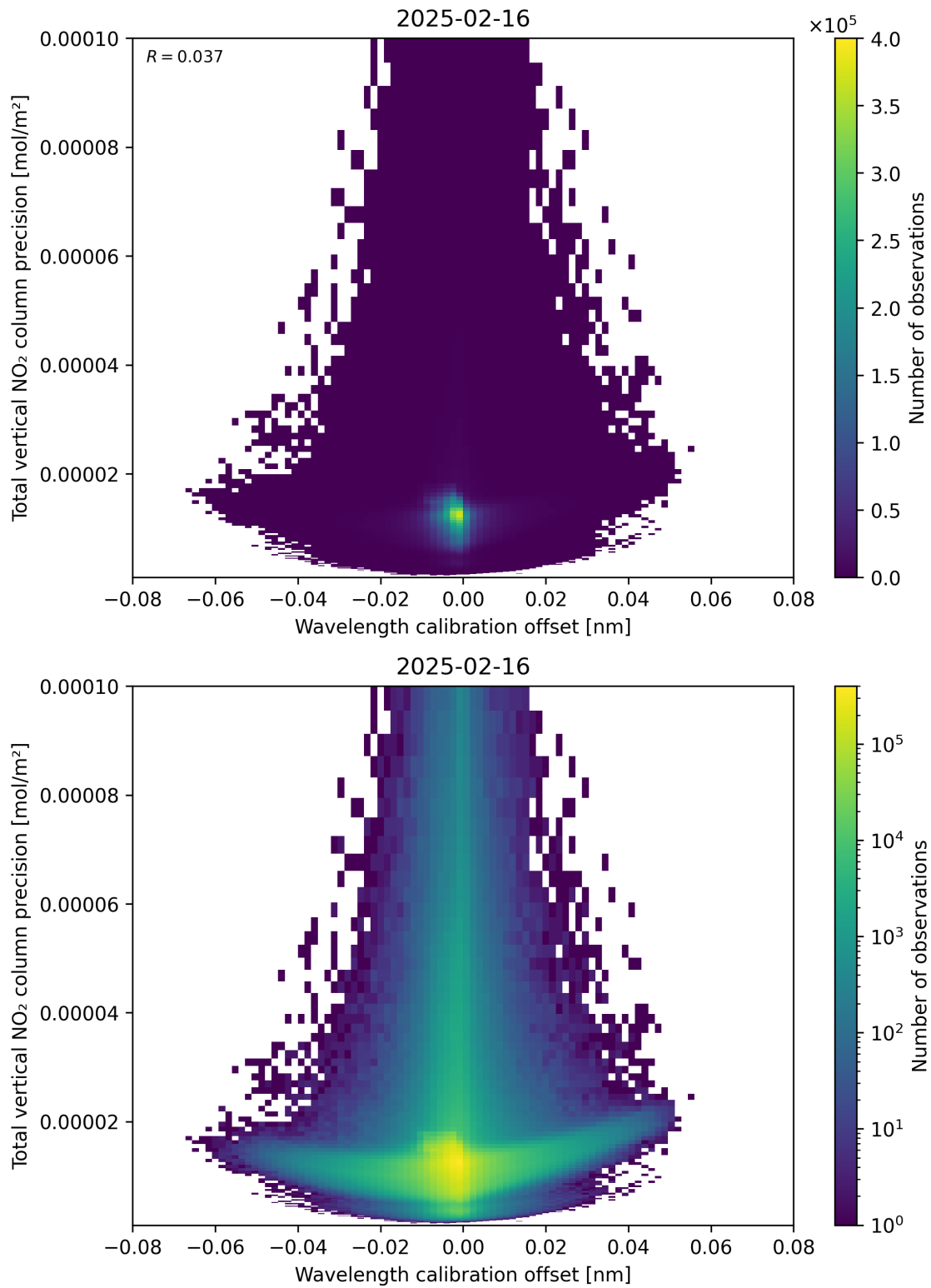
Figure 180: Scatter density plot of “Wavelength calibration offset” against “Total vertical NO 2 column precision” for 2025-02-15 to 2025-02-17.
