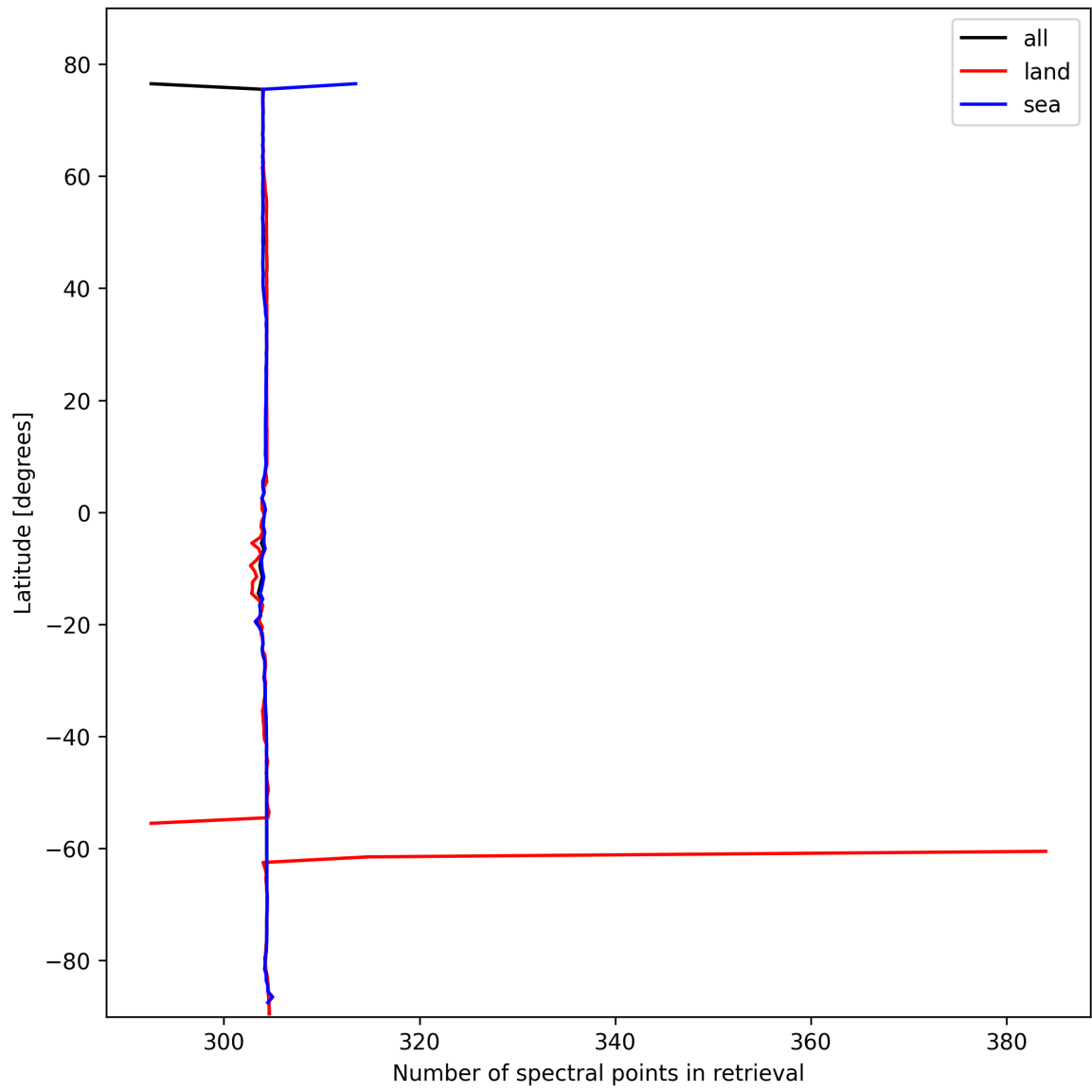
Figure 16: Zonal average of “Number of spectral points in retrieval” for 2025-02-15 to 2025-02-17.
