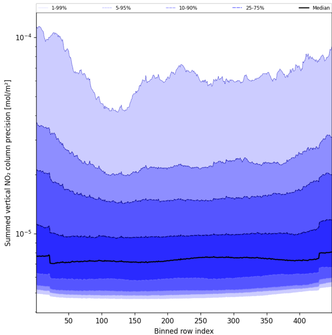
Figure 58: Along track statistics of “Summed vertical NO 2 column precision” for 2025-02-15 to 2025-02-17
