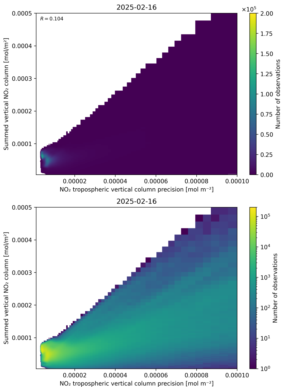
Figure 136: Scatter density plot of “NO 2 tropospheric vertical column precision” against “Summed vertical NO 2 column” for 2025-02-15 to 2025-02-17.
