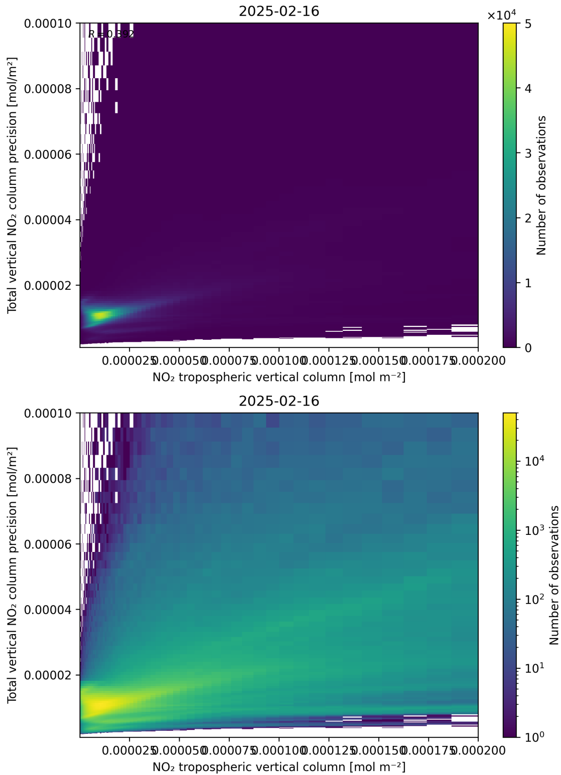
Figure 129: Scatter density plot of “NO 2 tropospheric vertical column” against “Total vertical NO 2 column precision” for 2025-02-15 to 2025-02-17.
