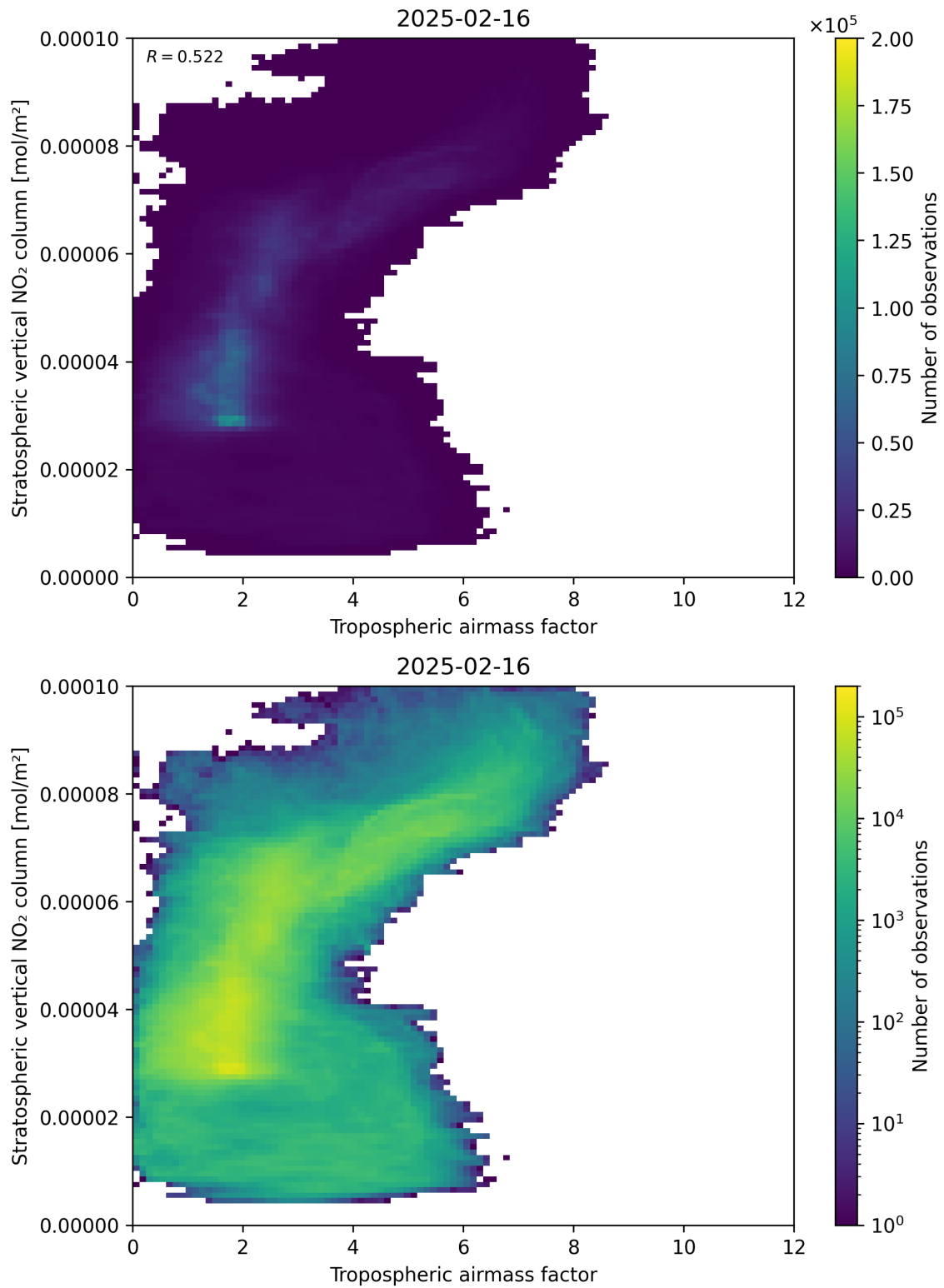
Figure 74: Scatter density plot of “Tropospheric air mass factor” against “Stratospheric vertical \text{NO}_2 column” for 2025-02-15 to 2025-02-17.
