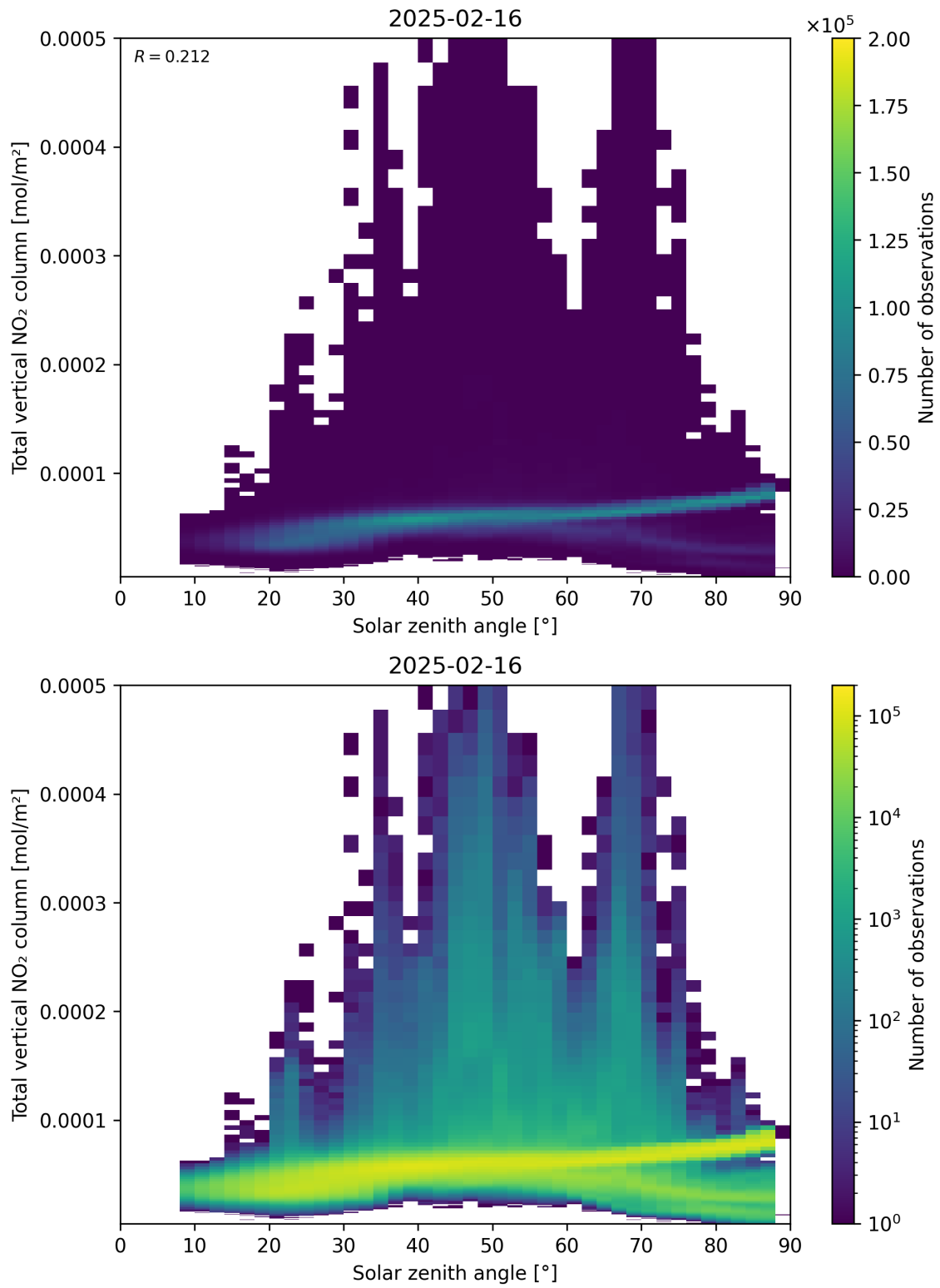
Figure 153: Scatter density plot of “Solar zenith angle” against “Total vertical NO 2 column” for 2025-02-15 to 2025-02-17.
