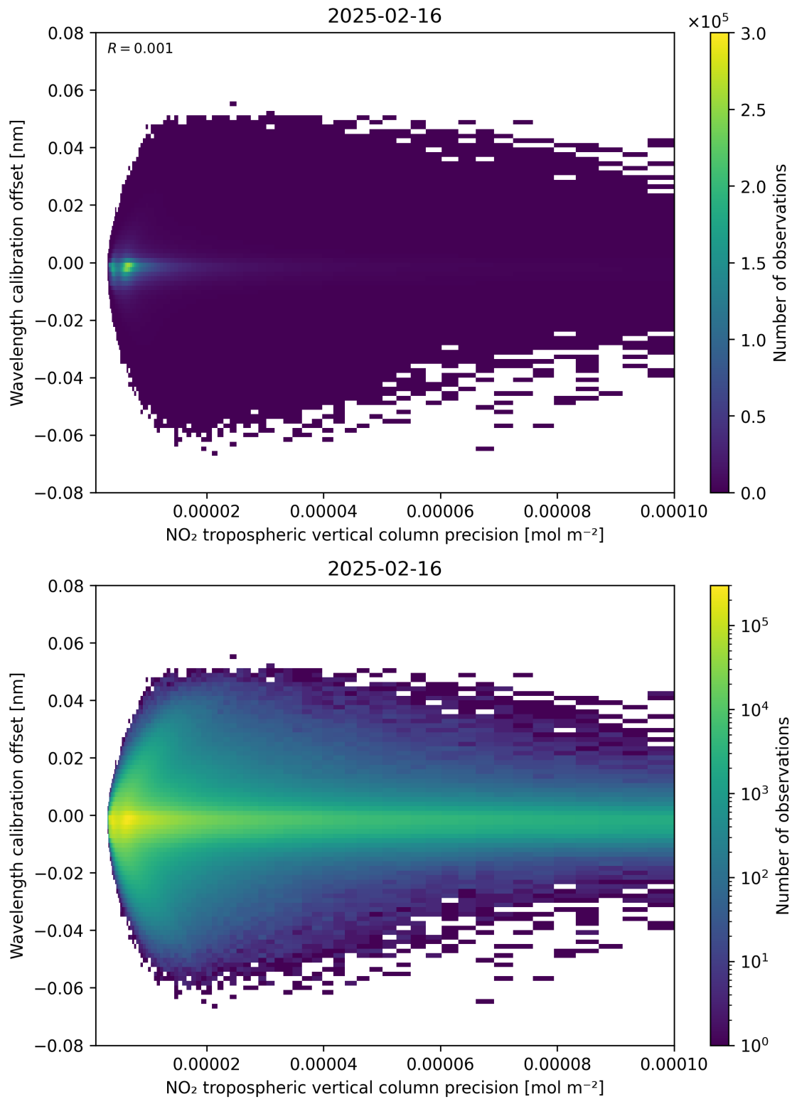
Figure 141: Scatter density plot of “NO 2 tropospheric vertical column precision” against “Wavelength calibration offset” for 2025-02-15 to 2025-02-17.
