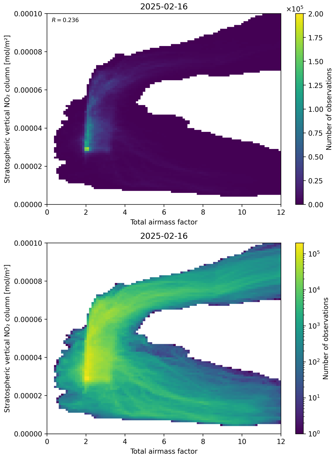
Figure 64: Scatter density plot of “Total airmass factor” against “Stratospheric vertical \text{NO}_2 column” for 2025-02-15 to 2025-02-17.
