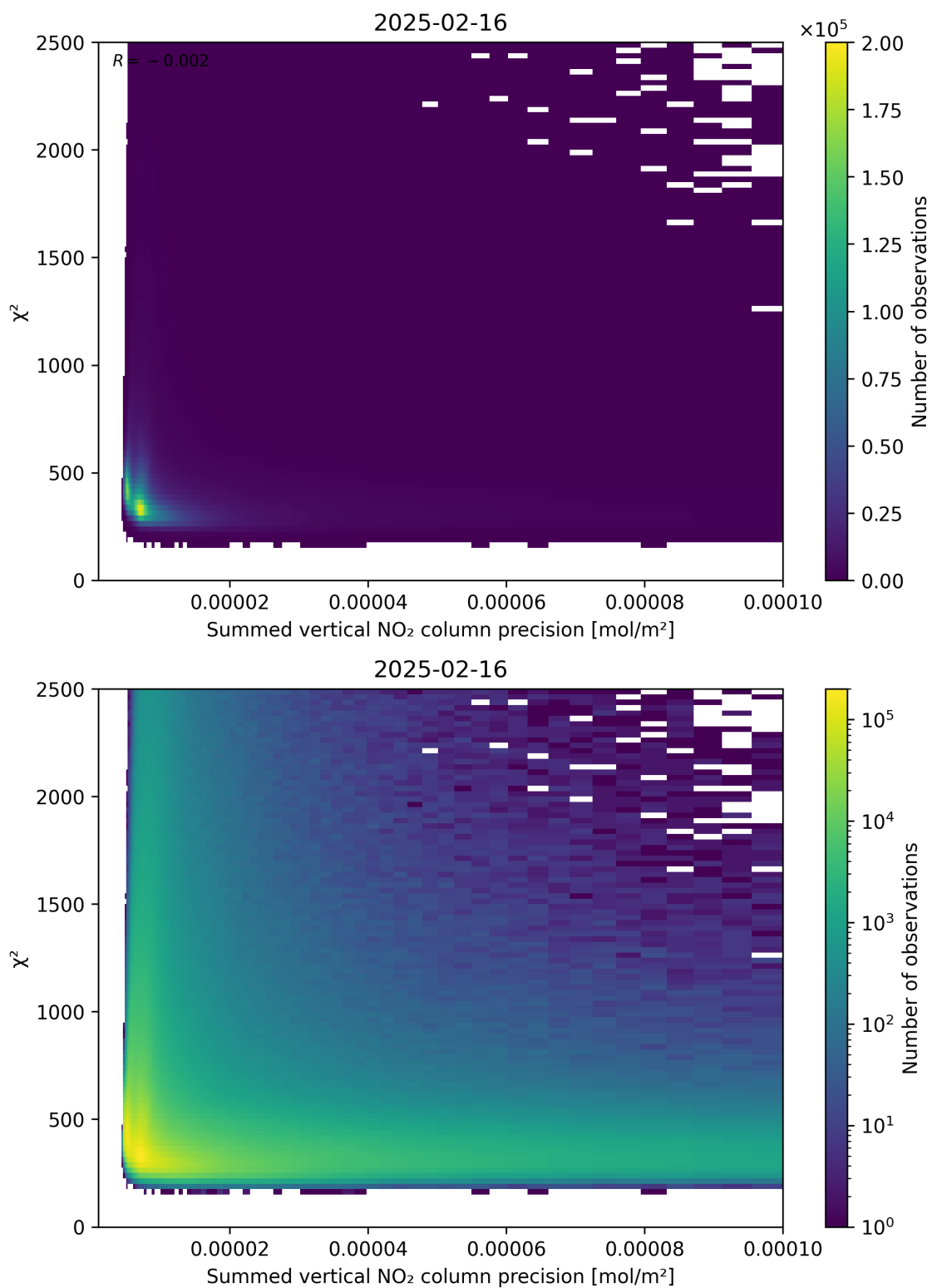
Figure 107: Scatter density plot of “Summed vertical NO 2 column precision” against “ \chi^2 ” for 2025-02-15 to 2025-02-17.
