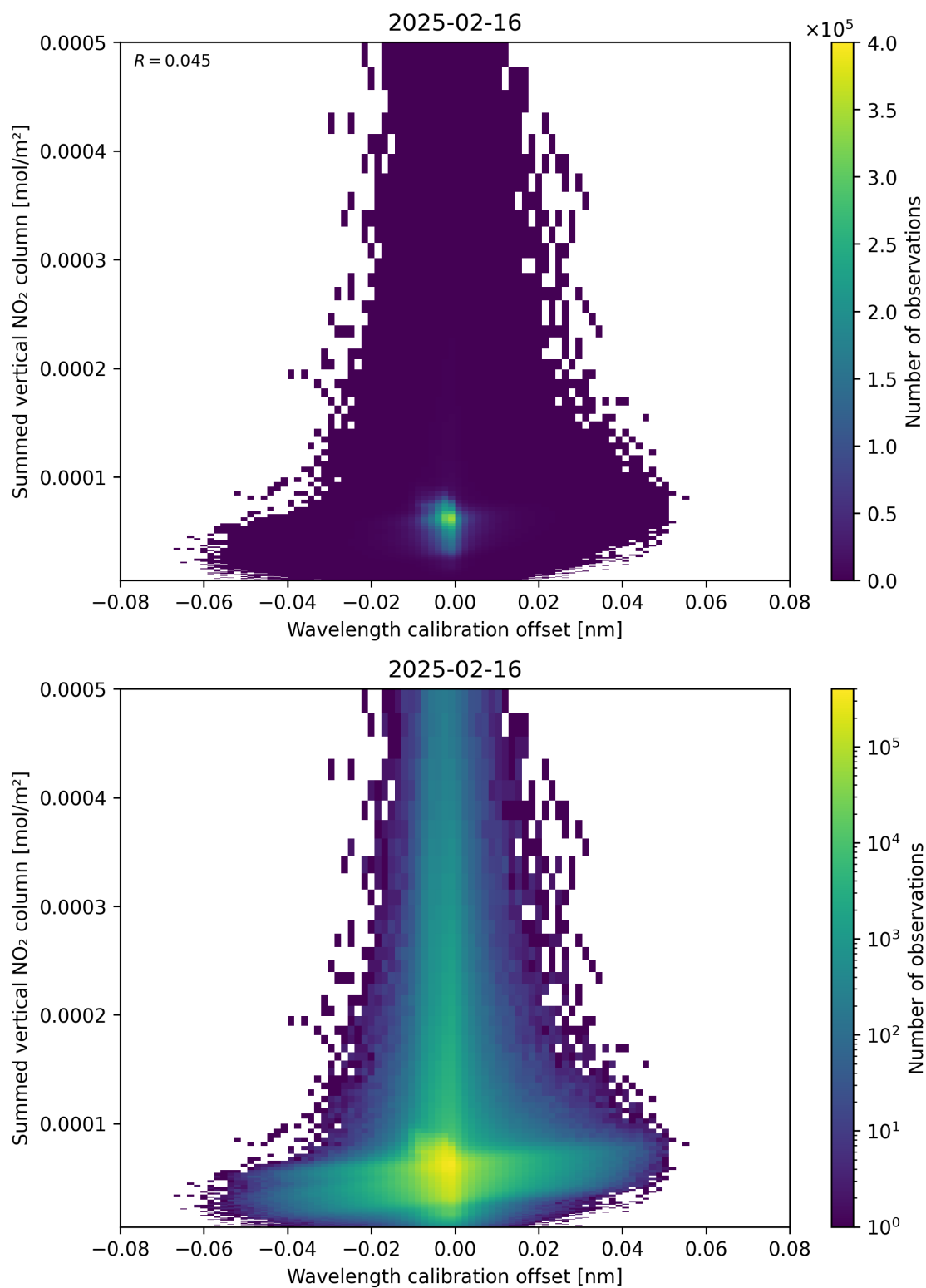
Figure 177: Scatter density plot of “Wavelength calibration offset” against “Summed vertical NO 2 column” for 2025-02-15 to 2025-02-17.
