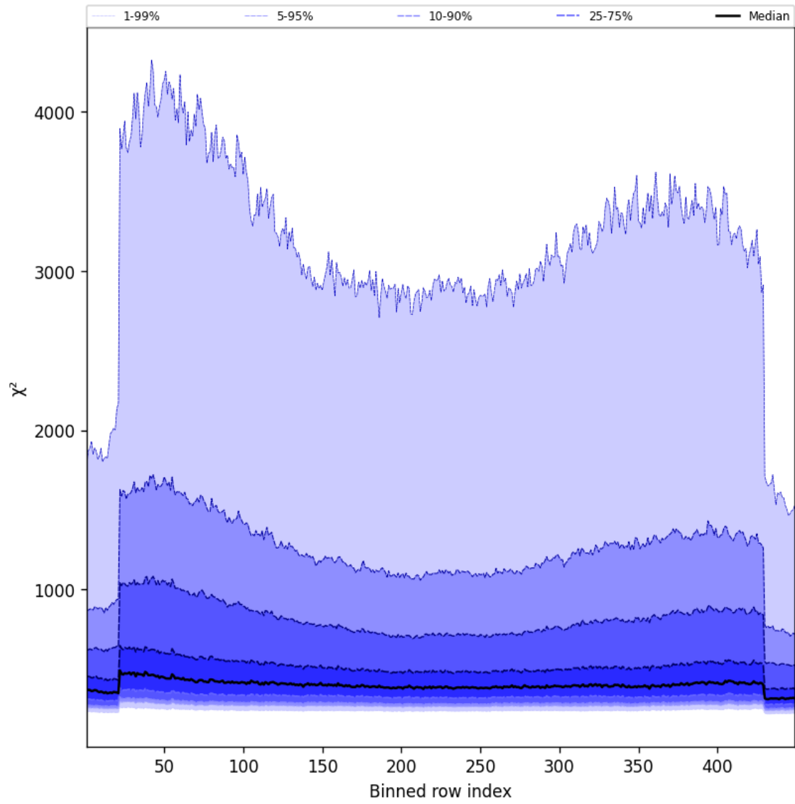
Figure 59: Along track statistics of “ \chi^2 ” for 2025-02-15 to 2025-02-17
