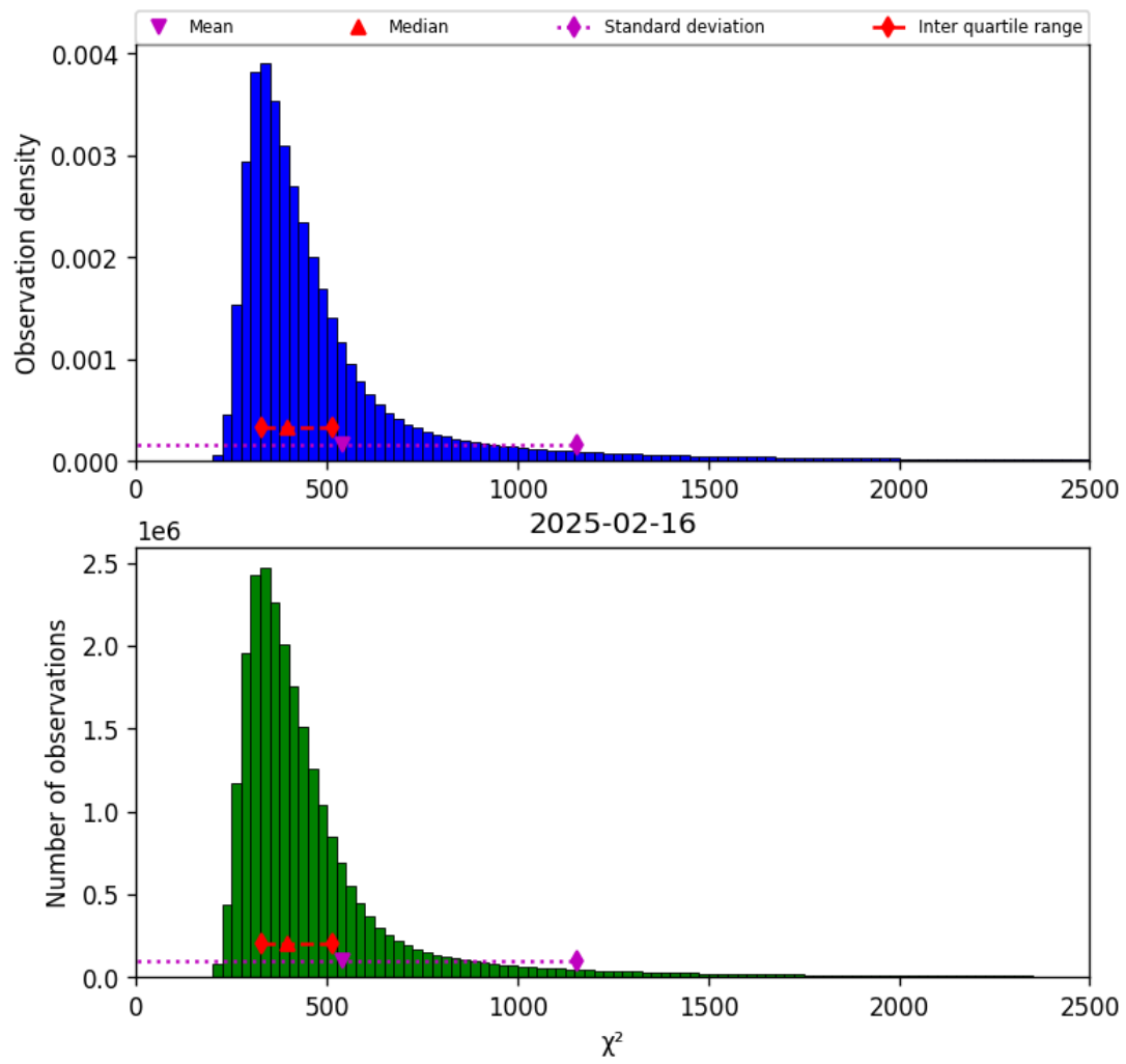
Figure 42: Histogram of “ \chi^2 ” for 2025-02-15 to 2025-02-17
