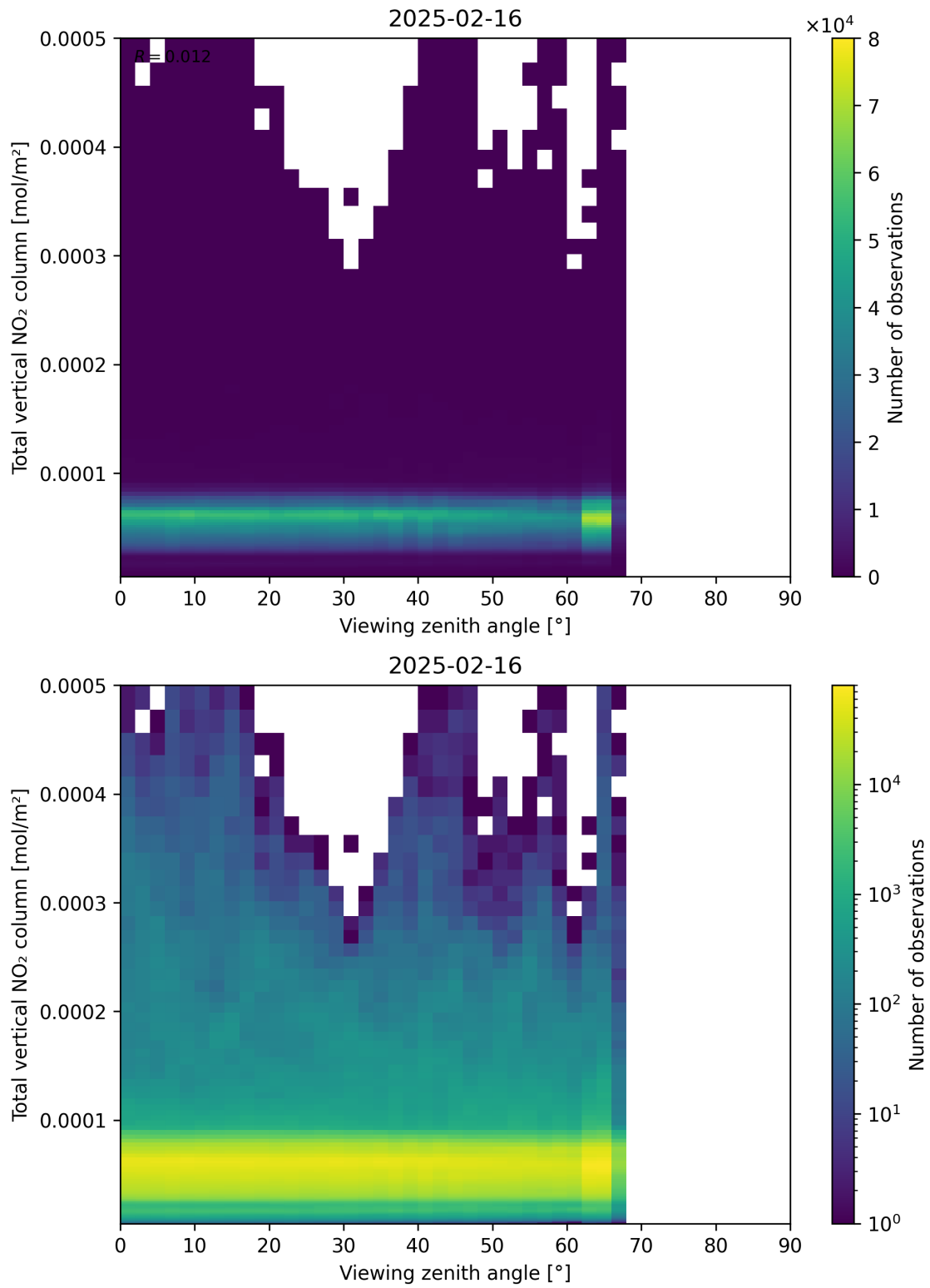
Figure 167: Scatter density plot of “Viewing zenith angle” against “Total vertical NO 2 column” for 2025-02-15 to 2025-02-17.
