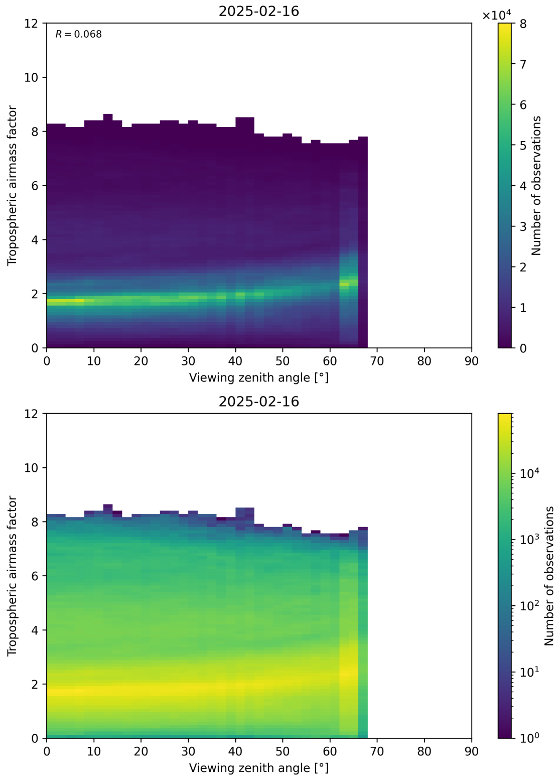
Figure 161: Scatter density plot of “Viewing zenith angle” against “Tropospheric airmass factor” for 2025-02-15 to 2025-02-17.
