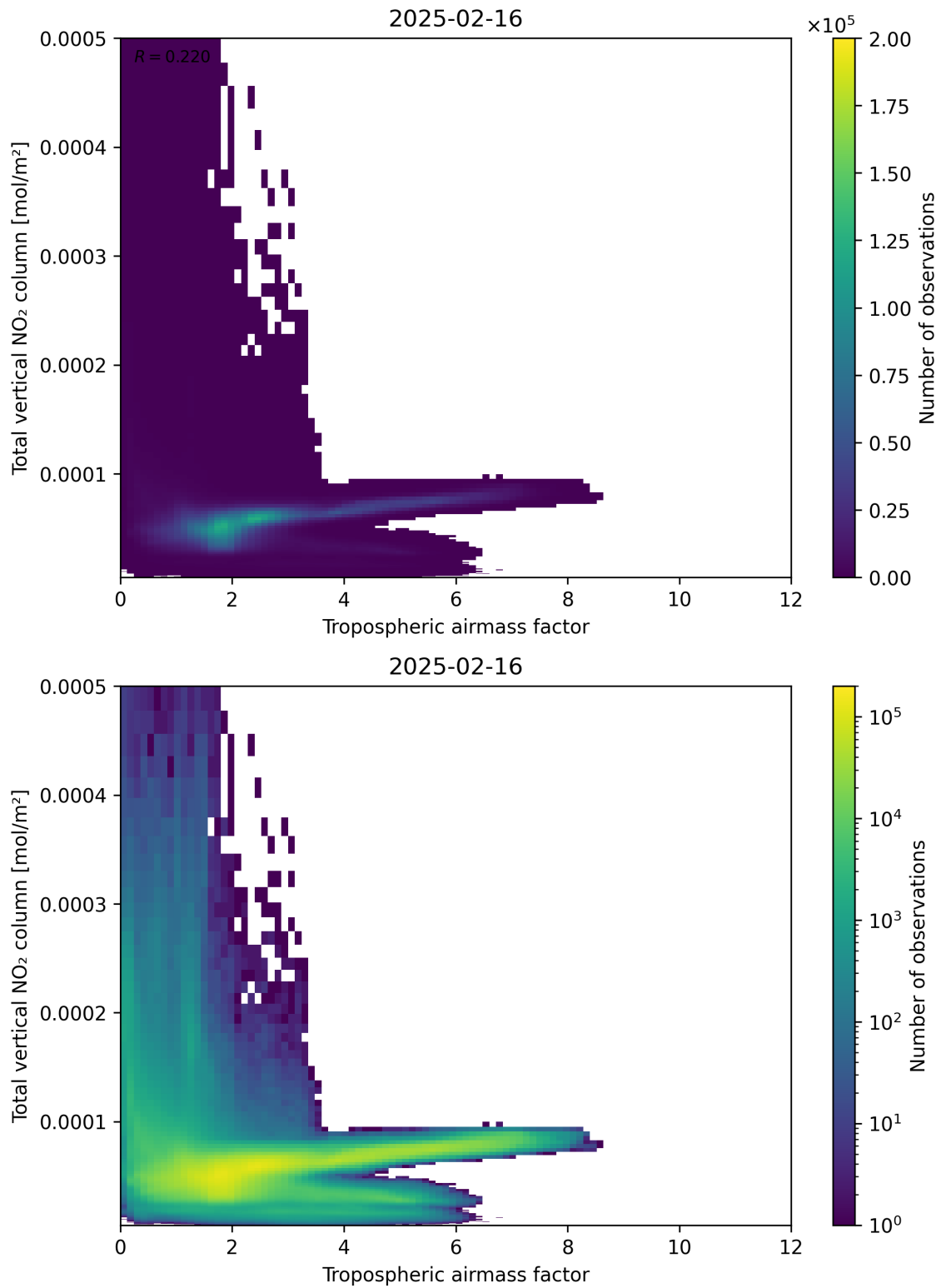
Figure 77: Scatter density plot of “Tropospheric airmass factor” against “Total vertical NO 2 column” for 2025-02-15 to 2025-02-17.
