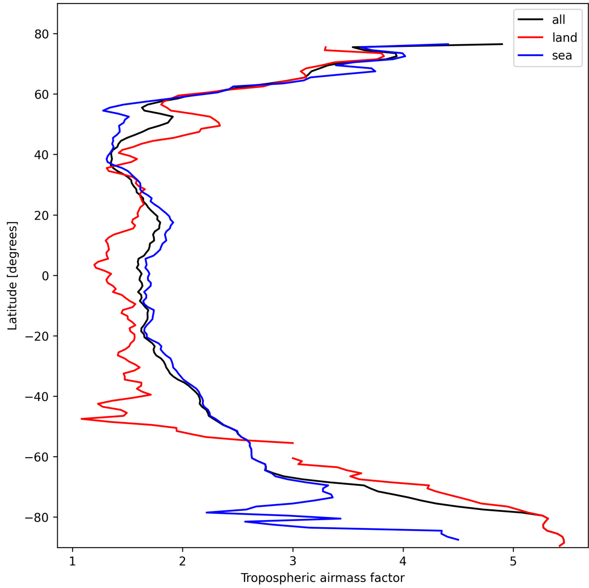
Figure 14: Zonal average of “Tropospheric airmass factor” for 2025-02-15 to 2025-02-17.
