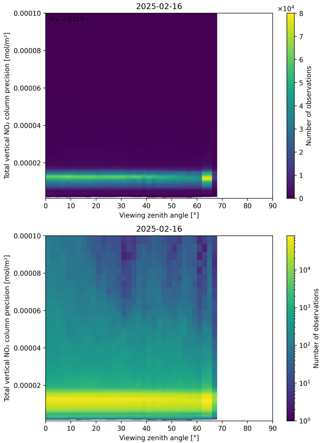
Figure 168: Scatter density plot of “Viewing zenith angle” against “Total vertical NO 2 column precision” for 2025-02-15 to 2025-02-17.
