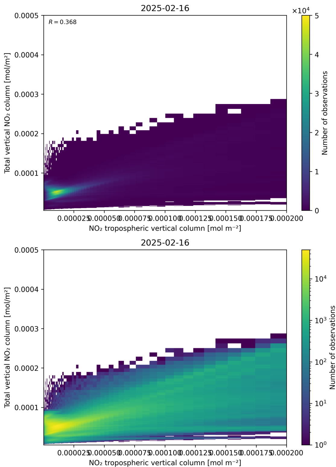
Figure 128: Scatter density plot of “NO 2 tropospheric vertical column” against “Total vertical NO 2 column” for 2025-02-15 to 2025-02-17.
