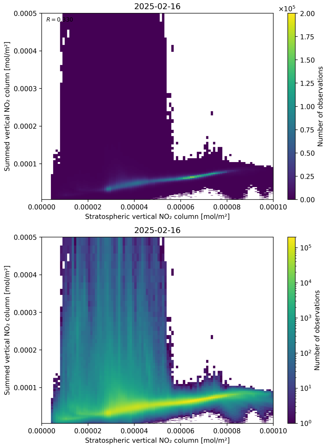
Figure 98: Scatter density plot of “Stratospheric vertical NO 2 column” against “Summed vertical NO 2 column” for 2025-02-15 to 2025-02-17.
