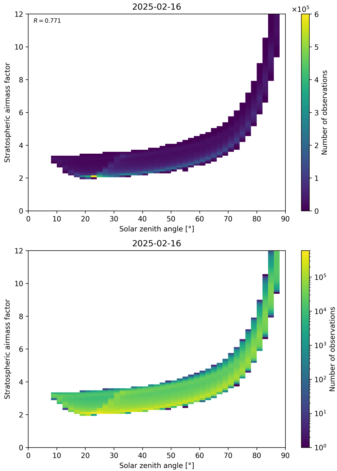
Figure 145: Scatter density plot of “Solar zenith angle” against “Stratospheric airmass factor” for 2025-02-15 to 2025-02-17.
