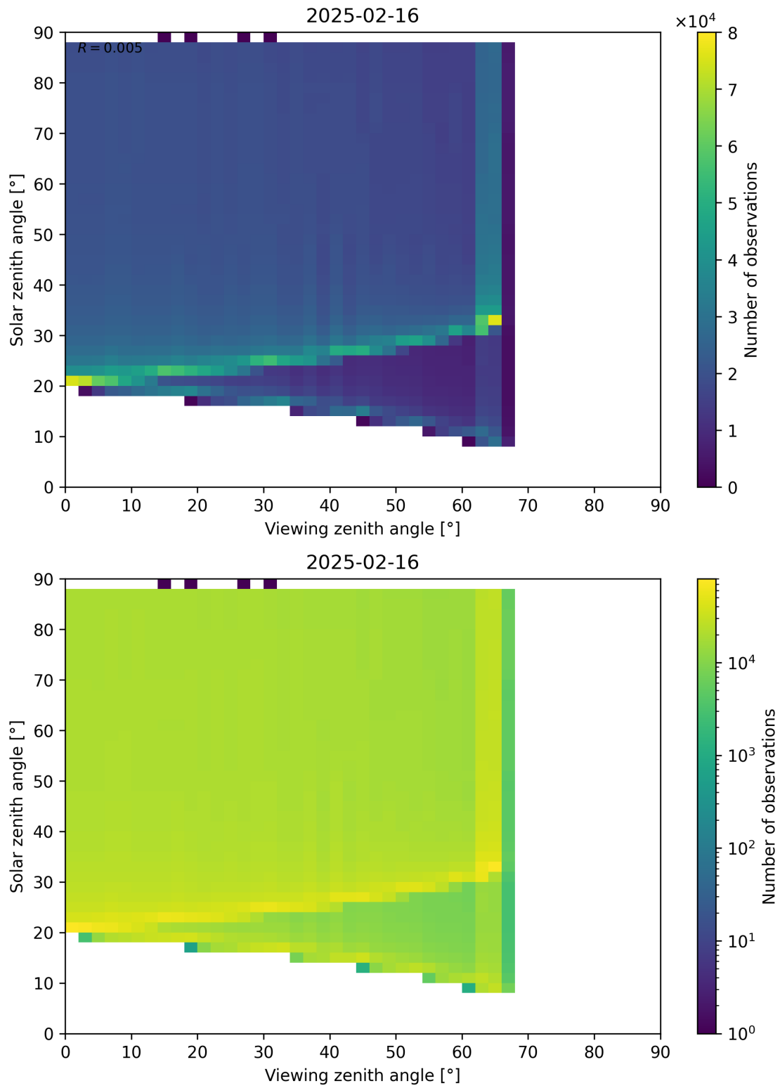
Figure 172: Scatter density plot of “Viewing zenith angle” against “Solar zenith angle” for 2025-02-15 to 2025-02-17.
