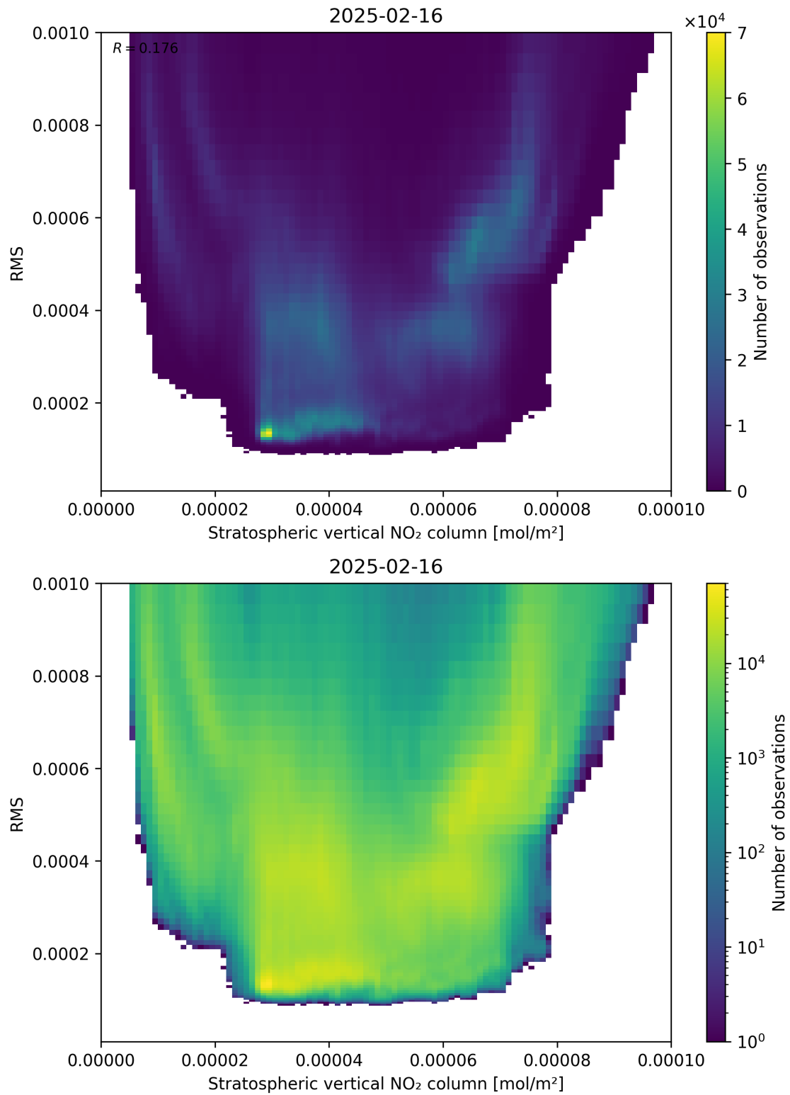
Figure 102: Scatter density plot of “Stratospheric vertical NO 2 column” against “RMS” for 2025-02-15 to 2025-02-17.
