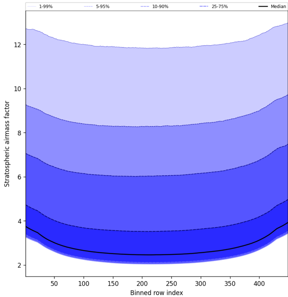
Figure 61: Along track statistics of “Stratospheric air mass factor” for 2025-02-15 to 2025-02-17
