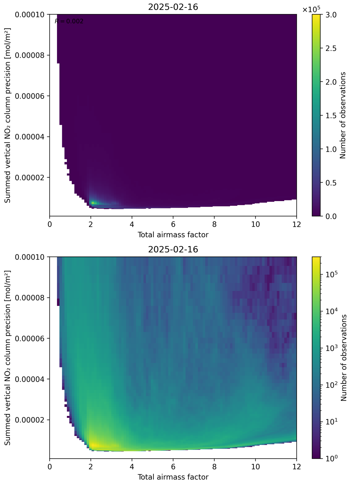
Figure 66: Scatter density plot of “Total airmass factor” against “Summed vertical NO 2 column precision” for 2025-02-15 to 2025-02-17.
