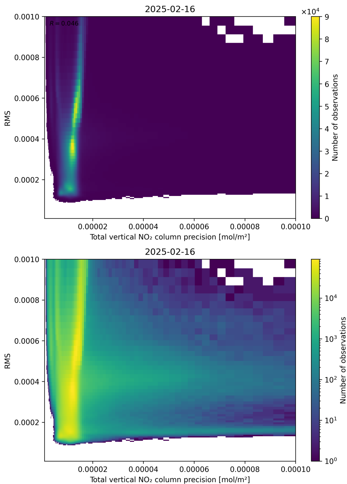
Figure 119: Scatter density plot of “Total vertical NO 2 column precision” against “RMS” for 2025-02-15 to 2025-02-17.
