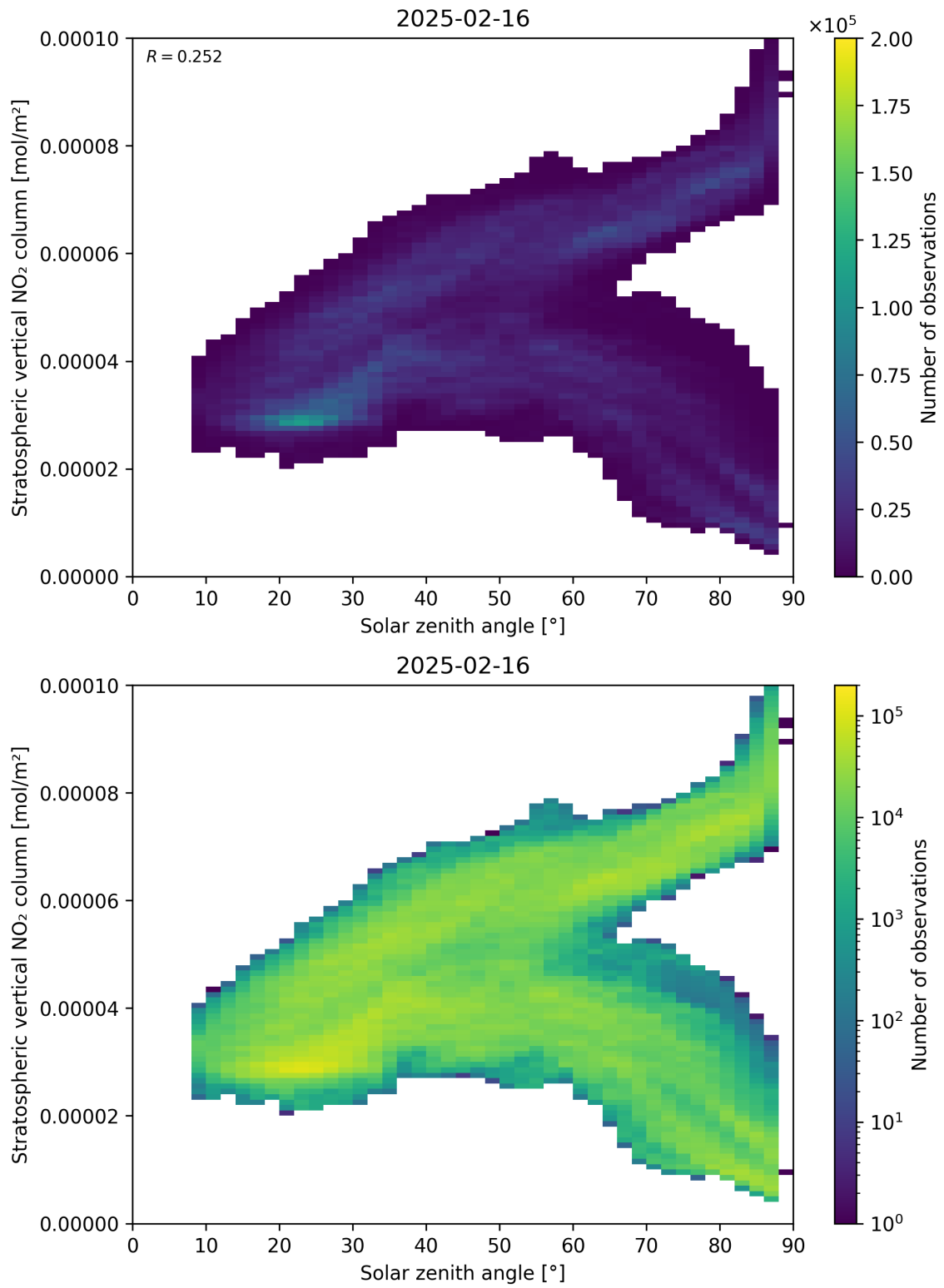
Figure 150: Scatter density plot of “Solar zenith angle” against “Stratospheric vertical NO 2 column” for 2025-02-15 to 2025-02-17.
