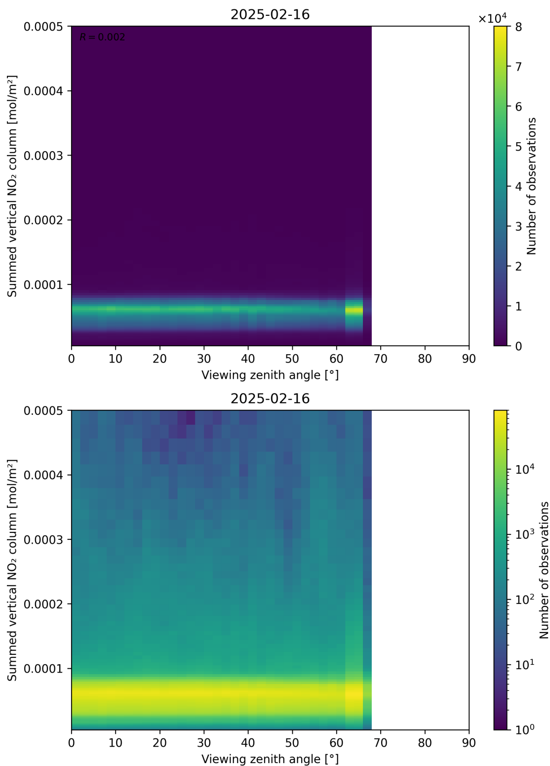
Figure 165: Scatter density plot of “Viewing zenith angle” against “Summed vertical NO 2 column” for 2025-02-15 to 2025-02-17.
