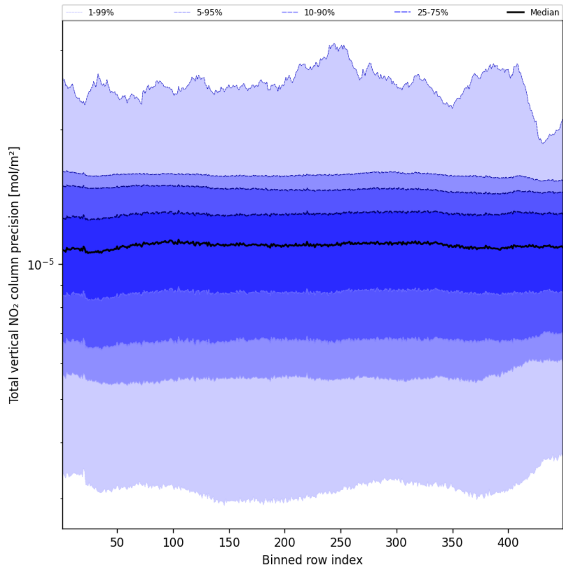
Figure 56: Along track statistics of “Total vertical NO 2 column precision” for 2025-02-15 to 2025-02-17
