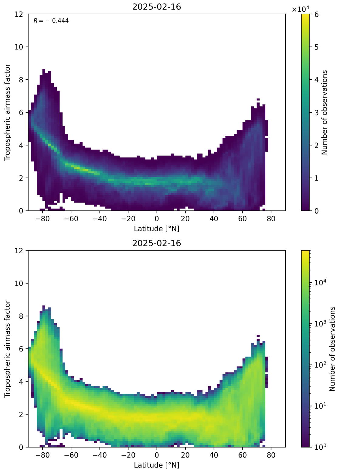
Figure 85: Scatter density plot of “Latitude” against “Tropospheric airmass factor” for 2025-02-15 to 2025-02-17.
