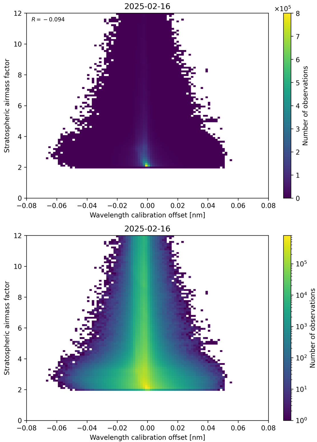
Figure 174: Scatter density plot of “Wavelength calibration offset” against “Stratospheric airmass factor” for 2025-02-15 to 2025-02-17.
