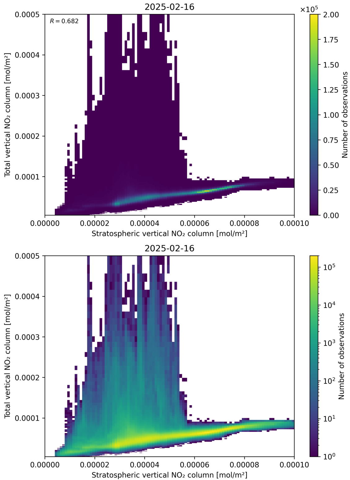
Figure 100: Scatter density plot of “Stratospheric vertical NO 2 column” against “Total vertical NO 2 column” for 2025-02-15 to 2025-02-17.
