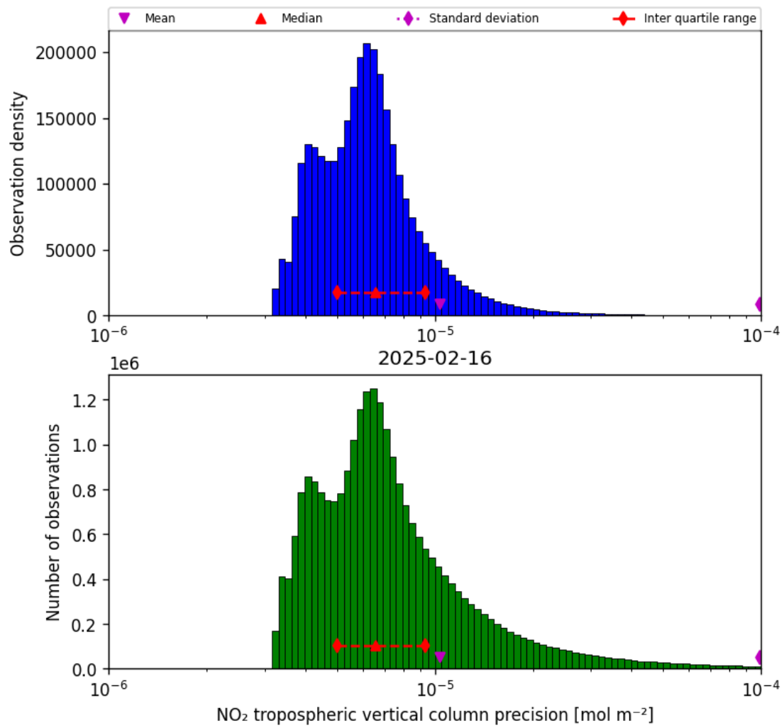
Figure 30: Histogram of “NO 2 tropospheric vertical column precision” for 2025-02-15 to 2025-02-17
