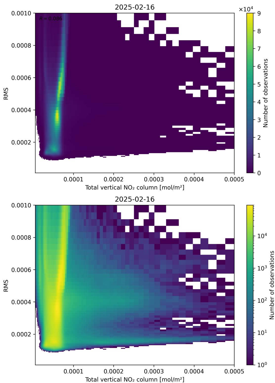
Figure 120: Scatter density plot of “Total vertical NO 2 column” against “RMS” for 2025-02-15 to 2025-02-17.
