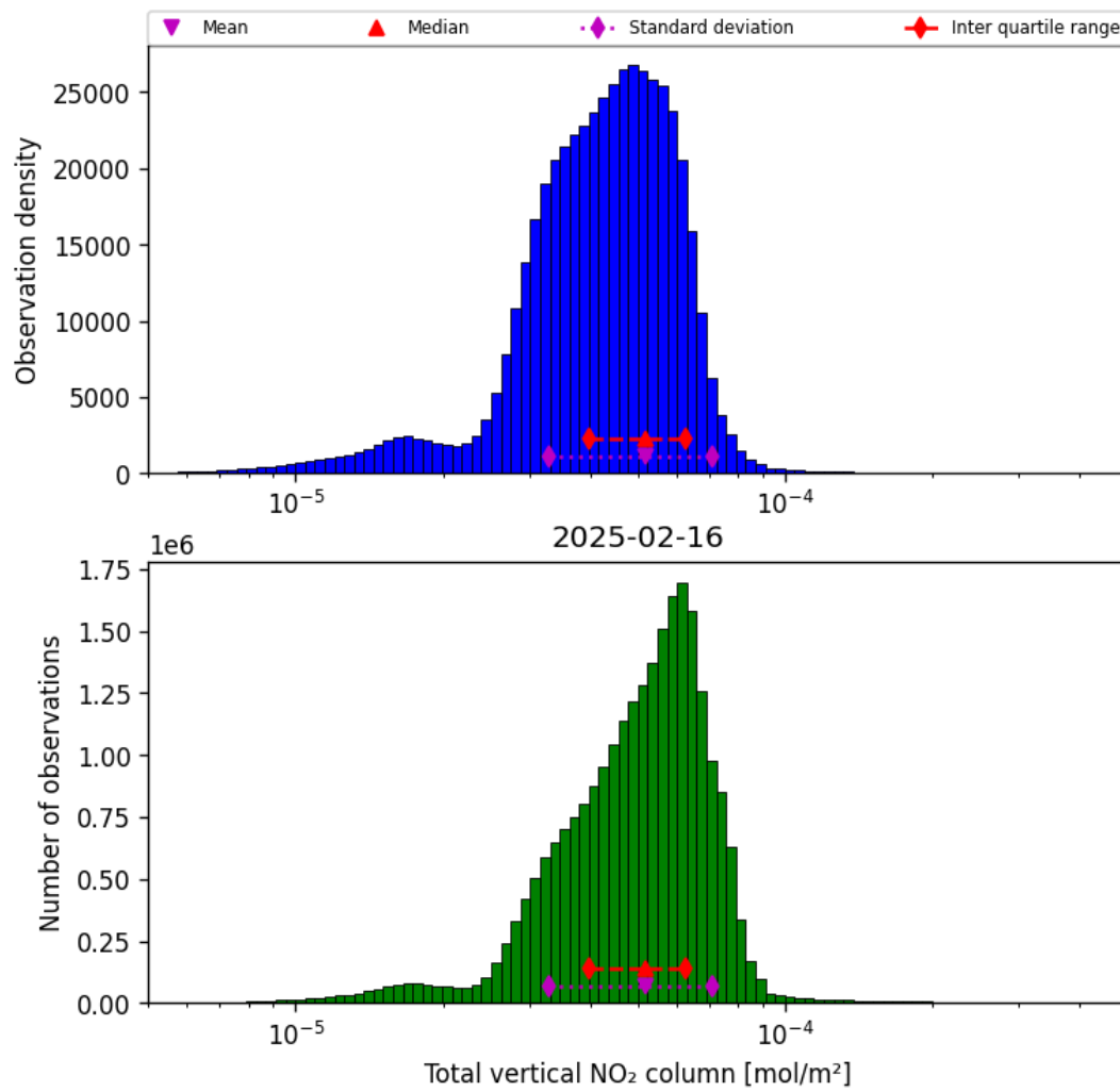
Figure 38: Histogram of “Total vertical NO 2 column” for 2025-02-15 to 2025-02-17
