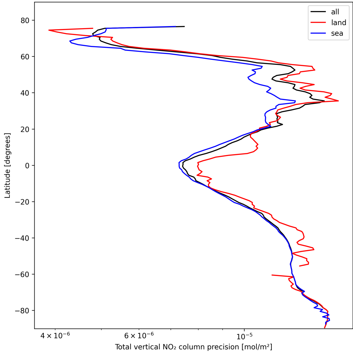
Figure 22: Zonal average of “Total vertical NO 2 column precision” for 2025-02-15 to 2025-02-17.
