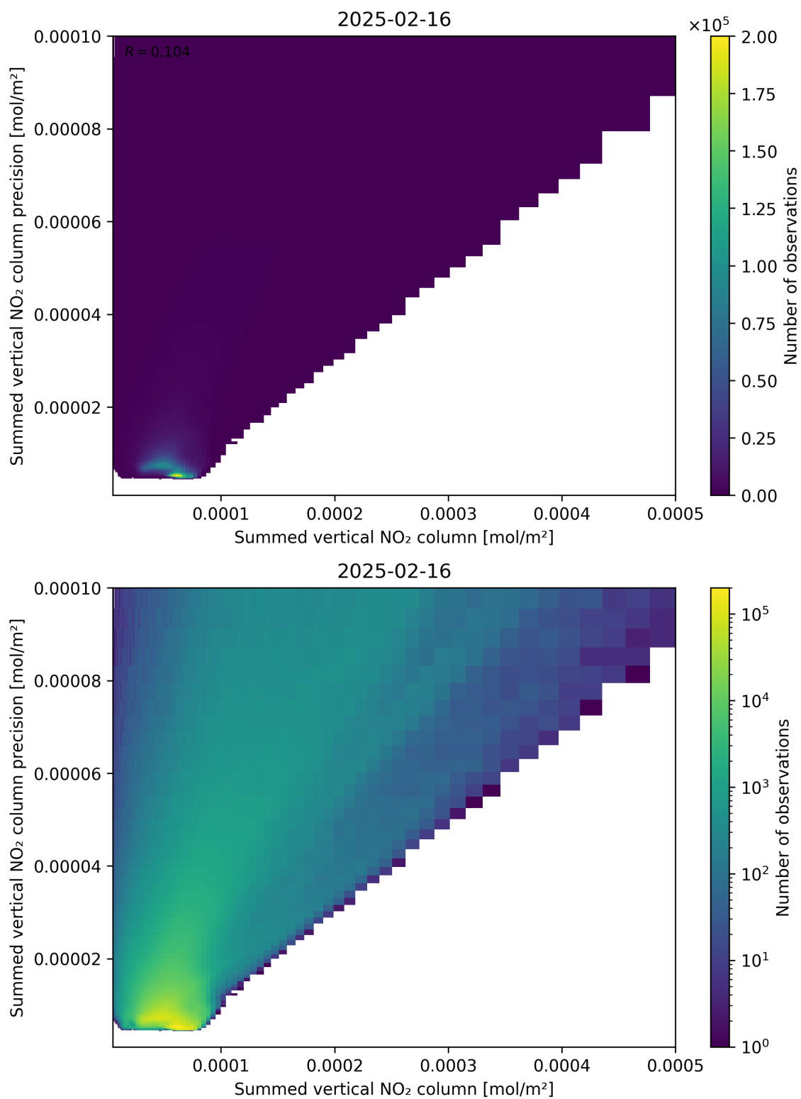
Figure 105: Scatter density plot of “Summed vertical NO 2 column” against “Summed vertical NO 2 column precision” for 2025-02-15 to 2025-02-17.
