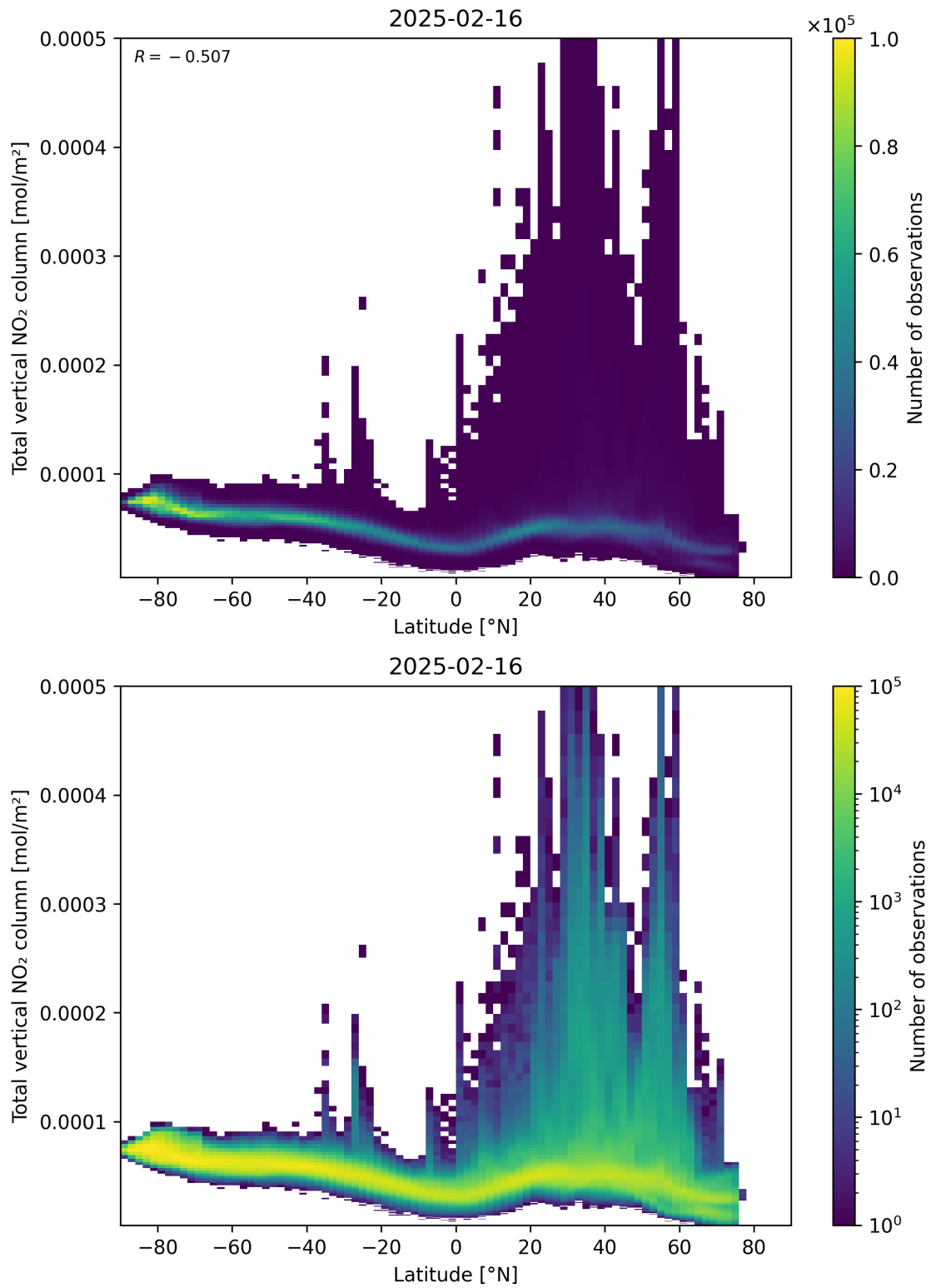
Figure 90: Scatter density plot of “Latitude” against “Total vertical NO 2 column” for 2025-02-15 to 2025-02-17.
