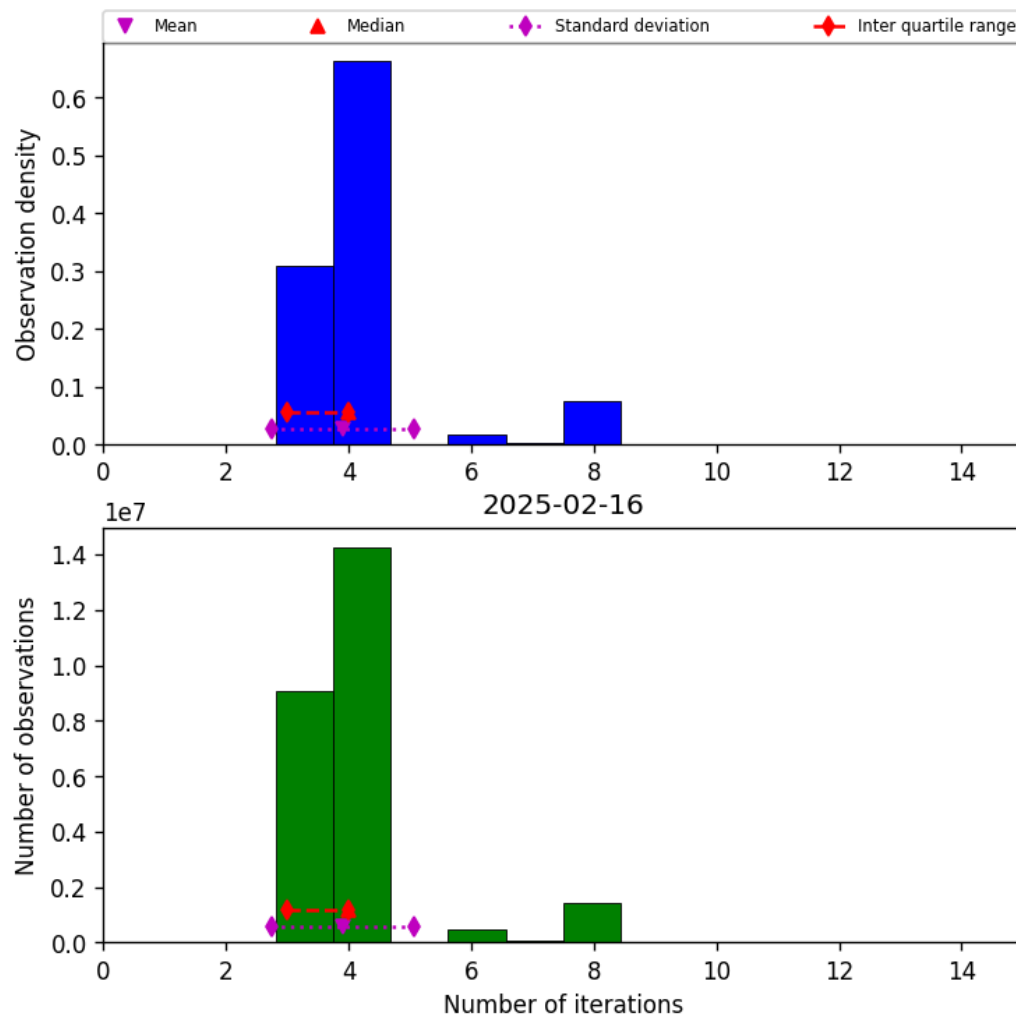
Figure 34: Histogram of “Number of iterations” for 2025-02-15 to 2025-02-17
