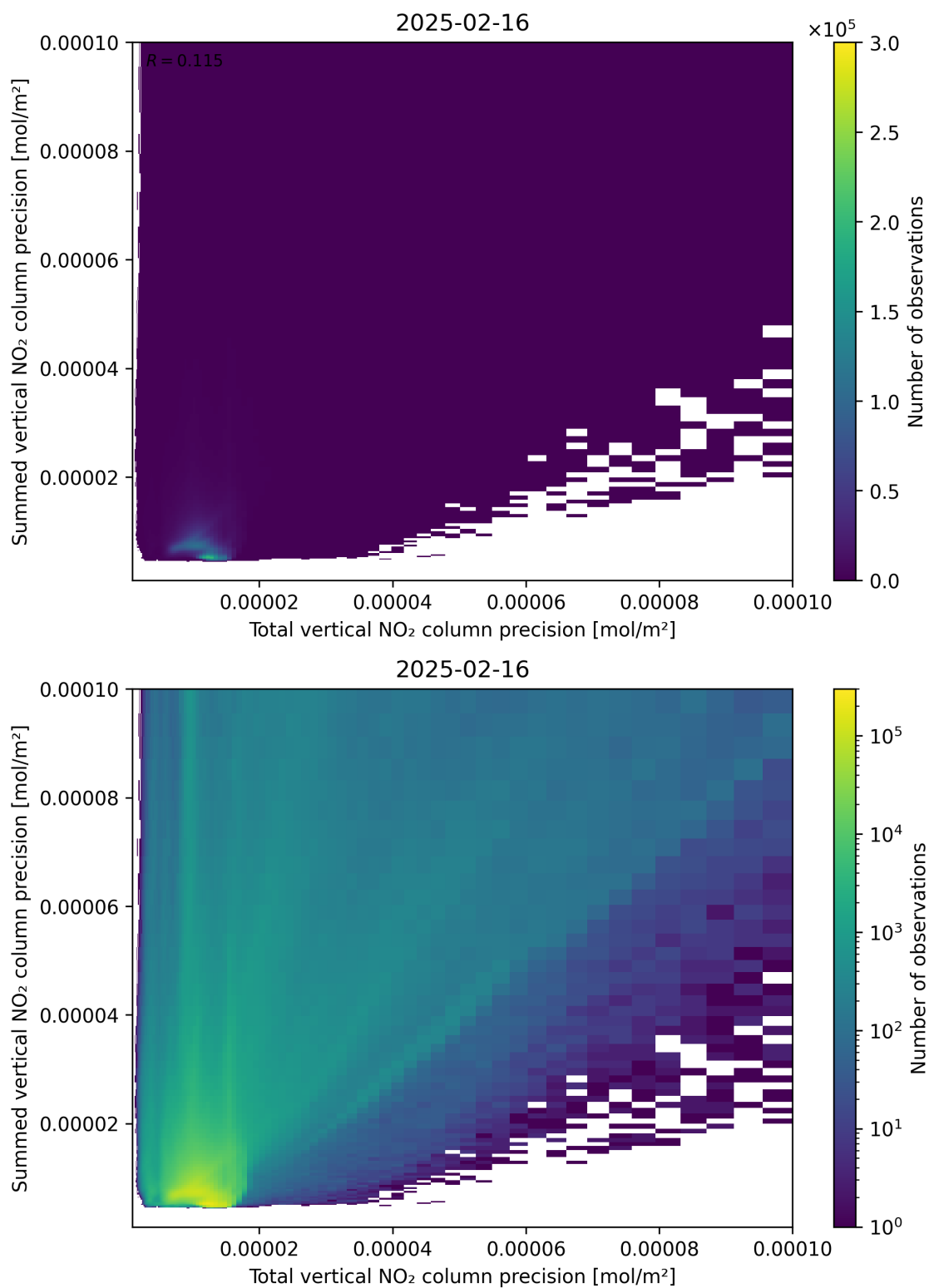
Figure 118: Scatter density plot of “Total vertical NO 2 column precision” against “Summed vertical NO 2 column precision” for 2025-02-15 to 2025-02-17.
