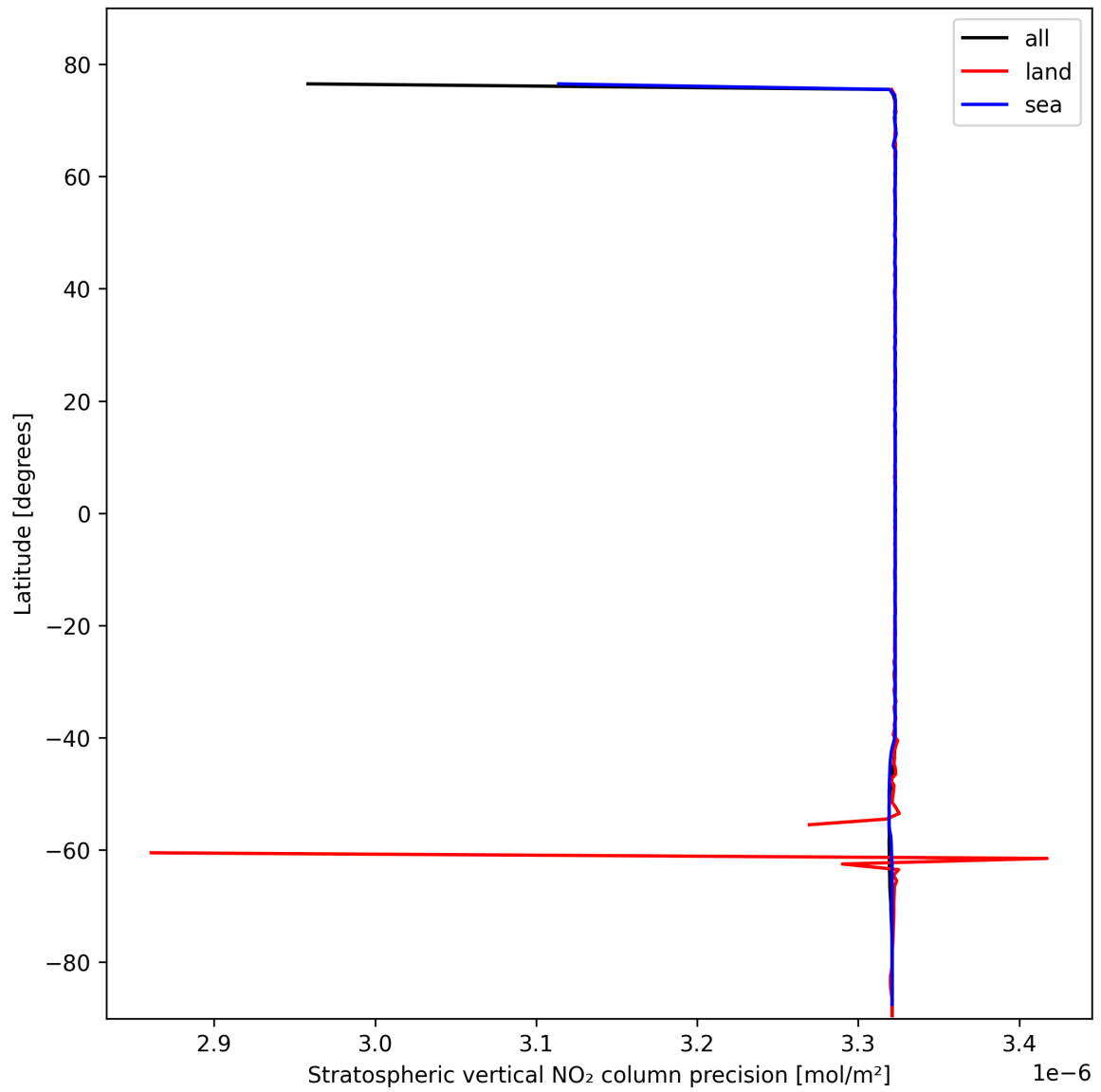
Figure 20: Zonal average of “Stratospheric vertical NO 2 column precision” for 2025-02-15 to 2025-02-17.
