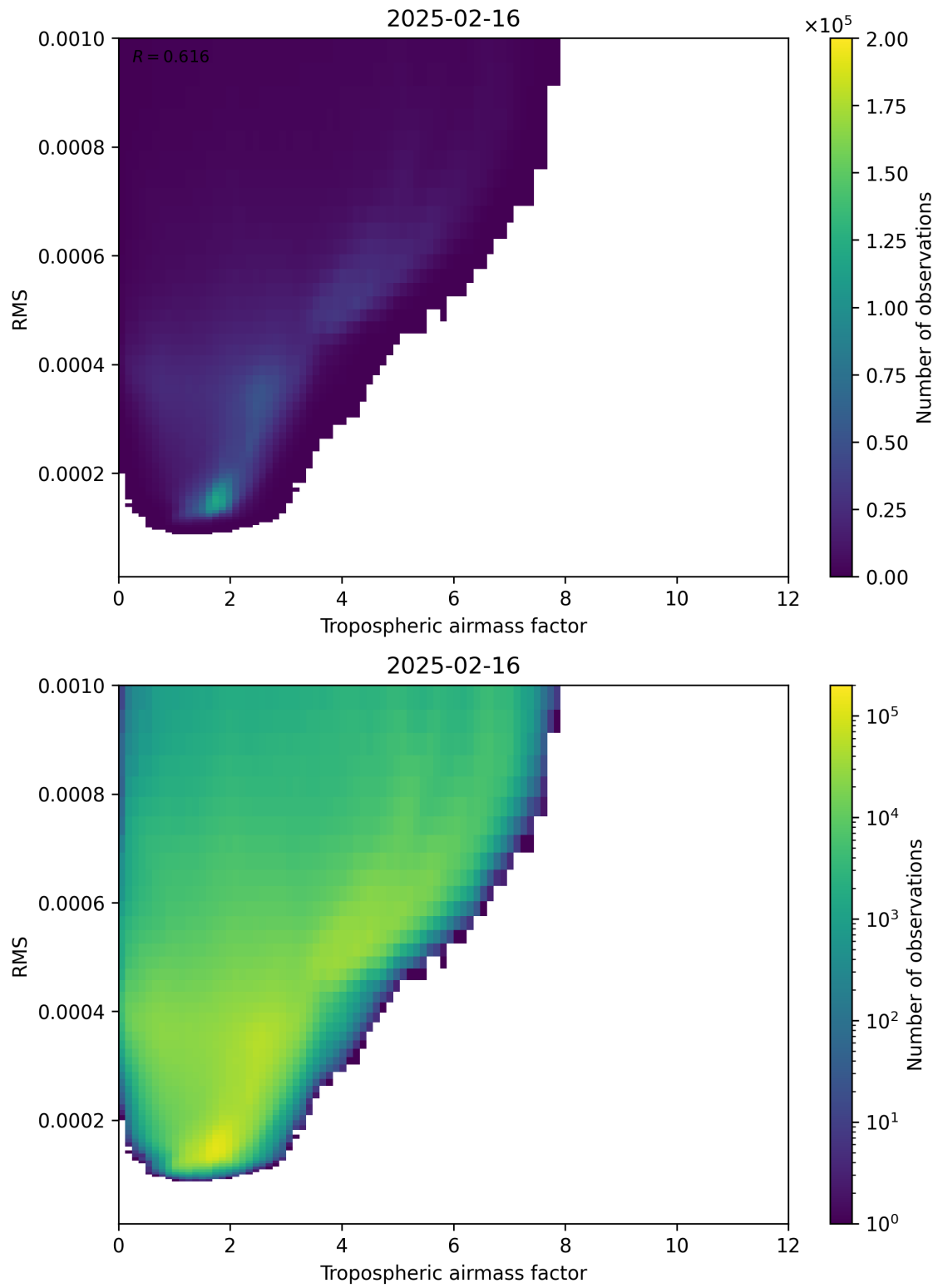
Figure 79: Scatter density plot of “Tropospheric airmass factor” against “RMS” for 2025-02-15 to 2025-02-17.
