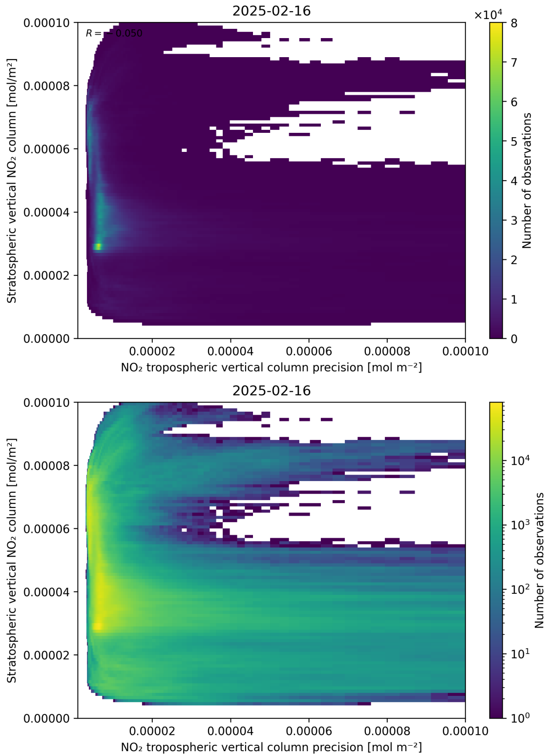
Figure 135: Scatter density plot of “NO 2 tropospheric vertical column precision” against “Stratospheric vertical NO 2 column” for 2025-02-15 to 2025-02-17.
