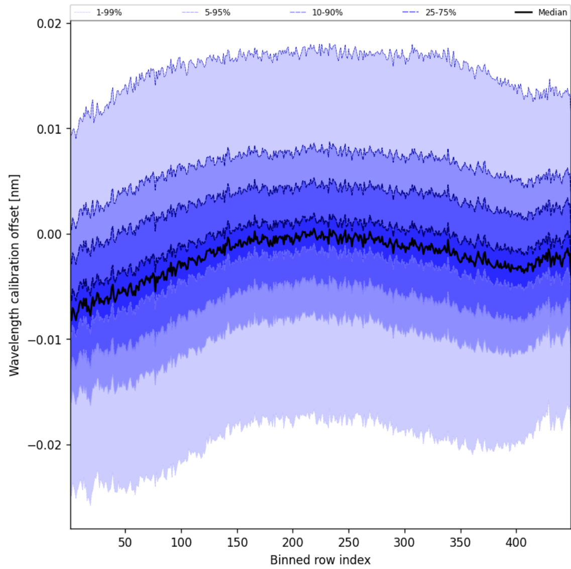
Figure 52: Along track statistics of “Wavelength calibration offset” for 2025-02-15 to 2025-02-17
