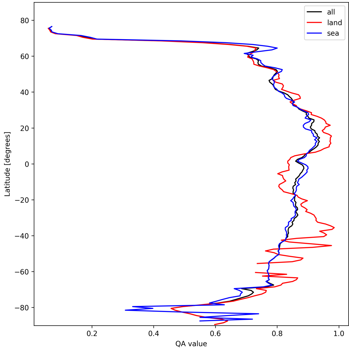
Figure 11: Zonal average of “QA value” for 2025-02-15 to 2025-02-17.
