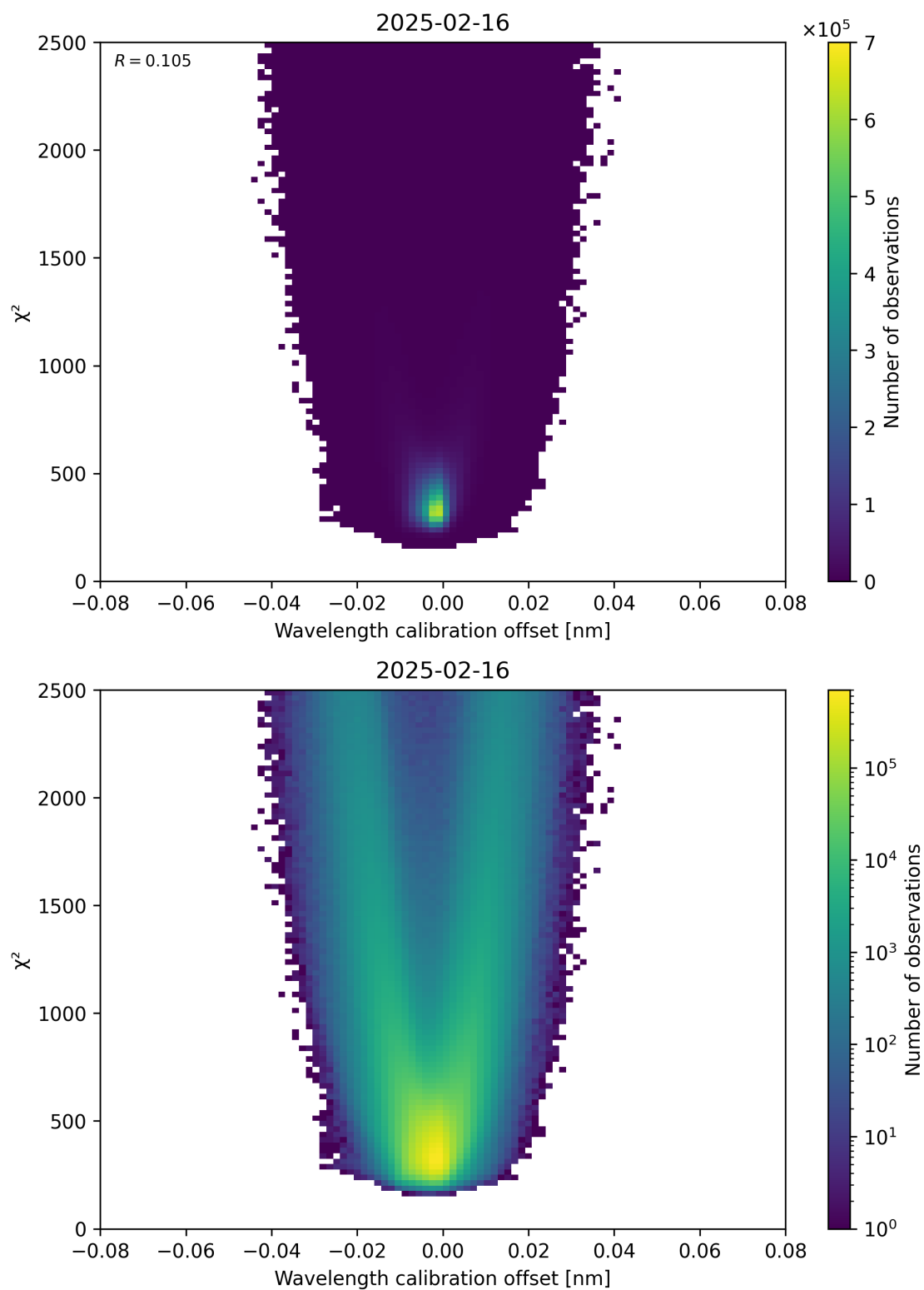
Figure 175: Scatter density plot of “Wavelength calibration offset” against “ \chi^2 ” for 2025-02-15 to 2025-02-17.
