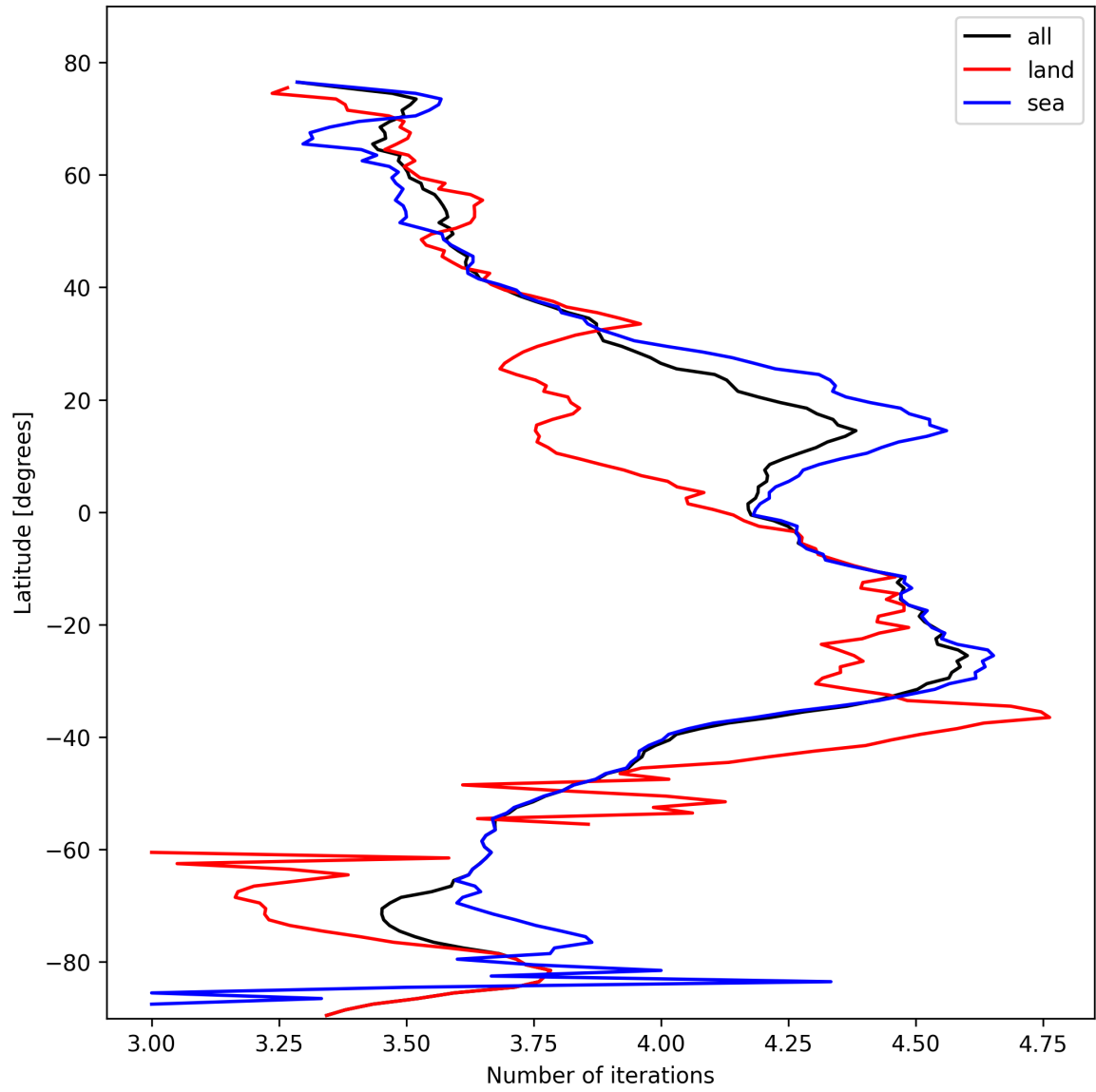
Figure 17: Zonal average of “Number of iterations” for 2025-02-15 to 2025-02-17.
