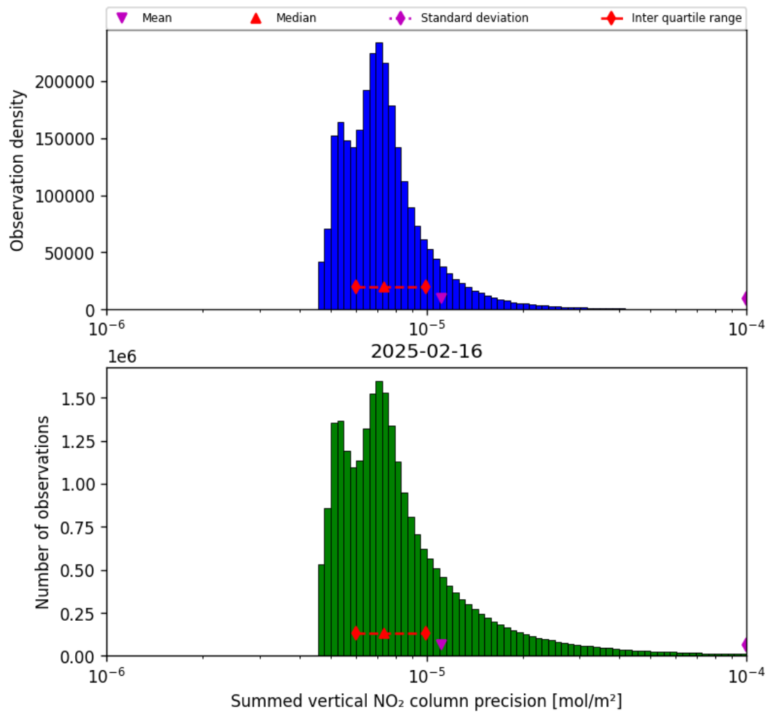
Figure 41: Histogram of “Summed vertical NO 2 column precision” for 2025-02-15 to 2025-02-17
