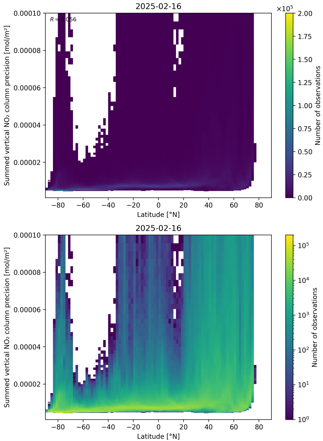
Figure 89: Scatter density plot of “Latitude” against “Summed vertical NO 2 column precision” for 2025-02-15 to 2025-02-17.
