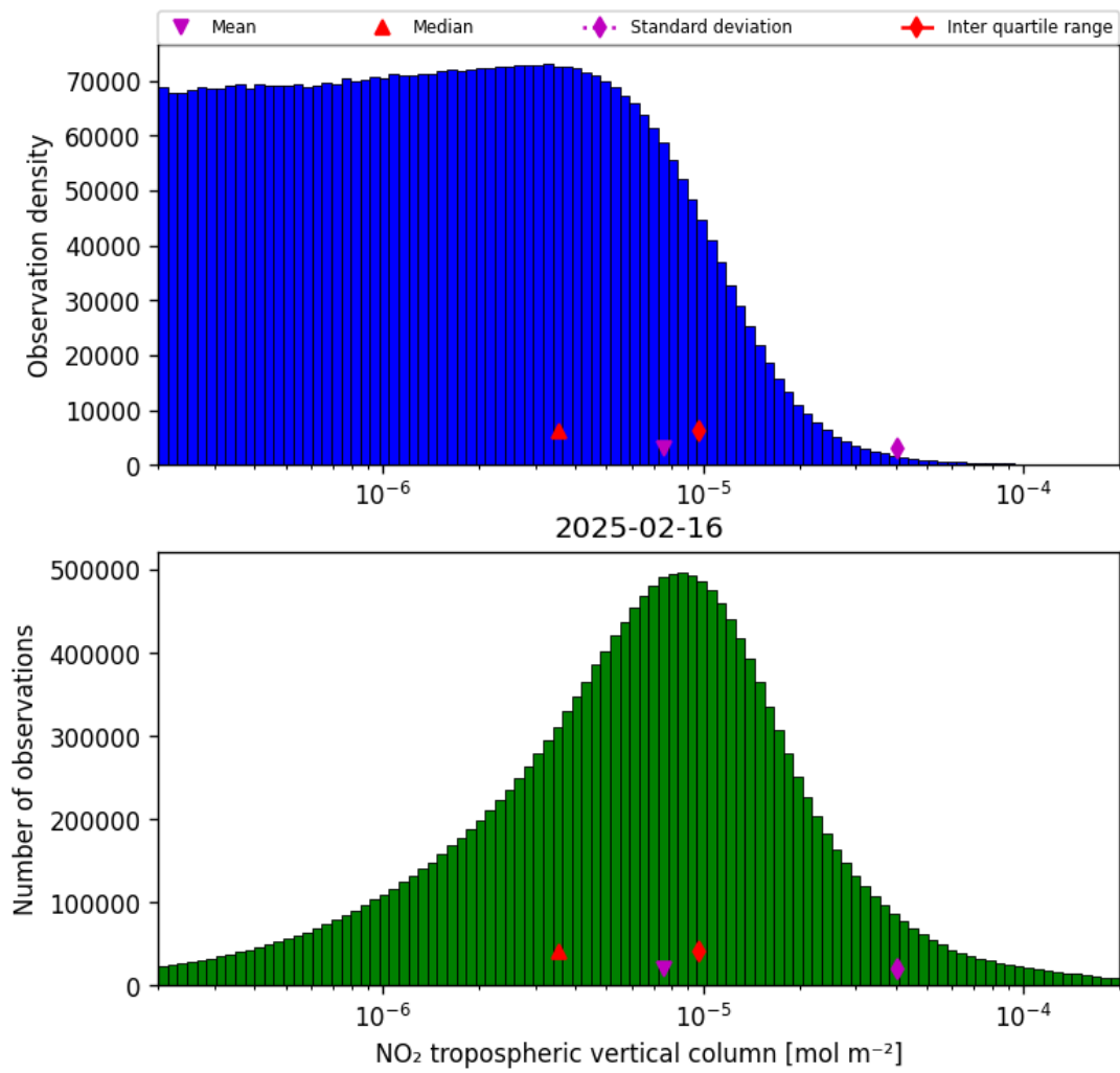
Figure 29: Histogram of “NO 2 tropospheric vertical column” for 2025-02-15 to 2025-02-17
