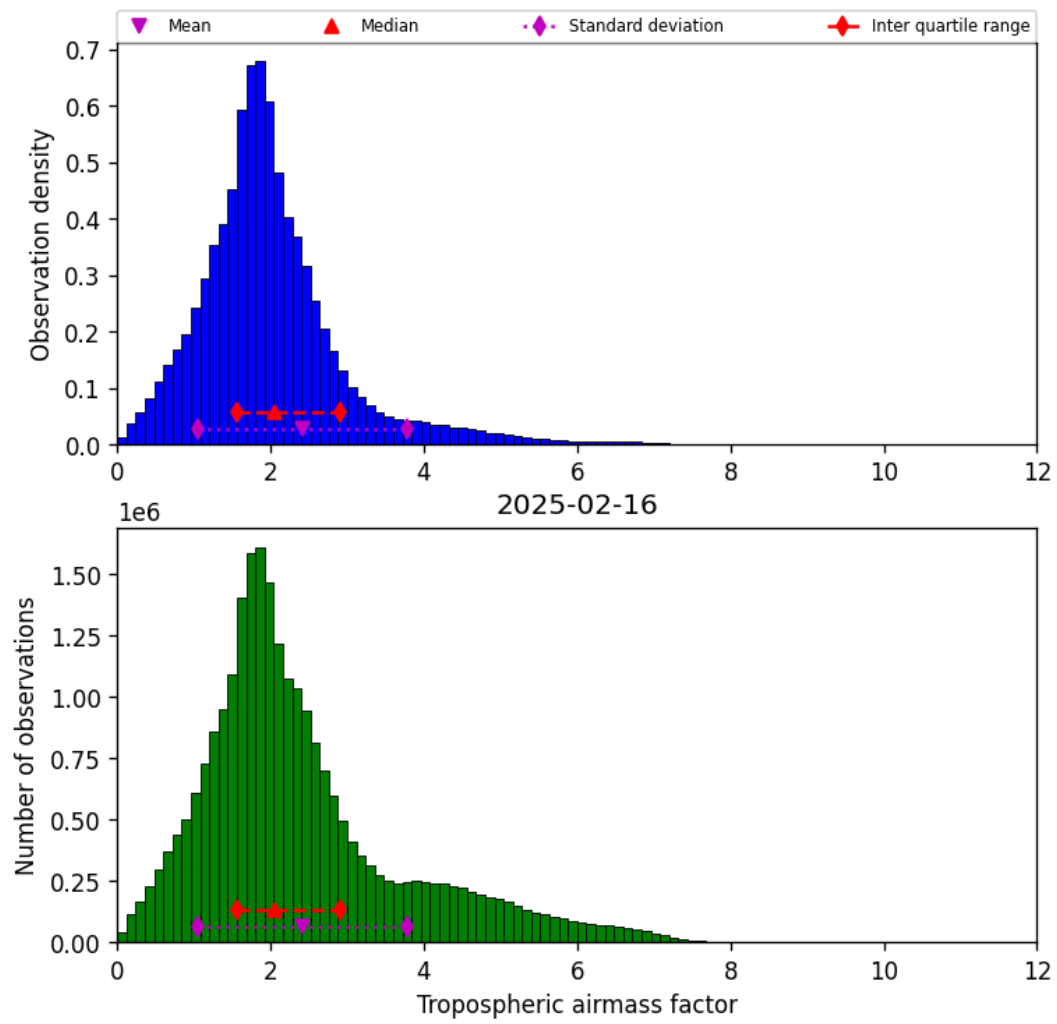
Figure 31: Histogram of “Tropospheric airmass factor” for 2025-02-15 to 2025-02-17
