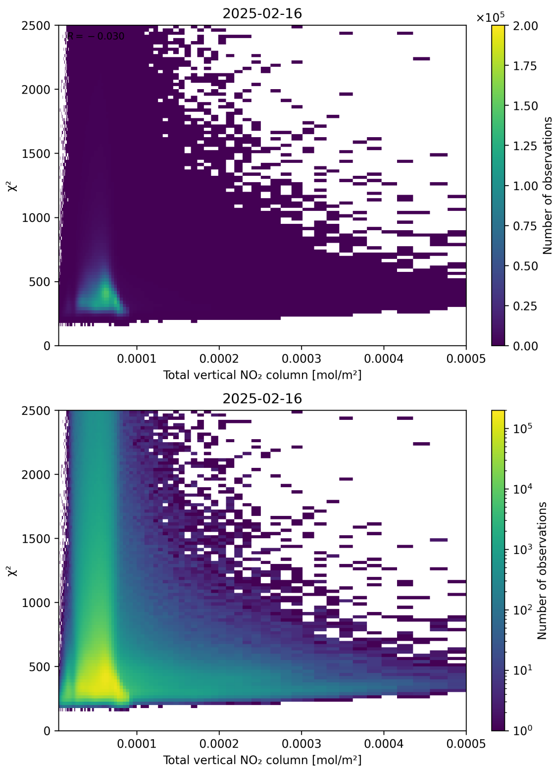
Figure 111: Scatter density plot of “Total vertical NO 2 column” against “ \chi^2 ” for 2025-02-15 to 2025-02-17.
