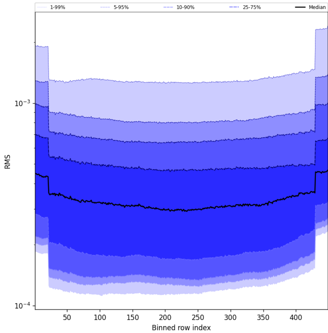
Figure 60: Along track statistics of “RMS” for 2025-02-15 to 2025-02-17
