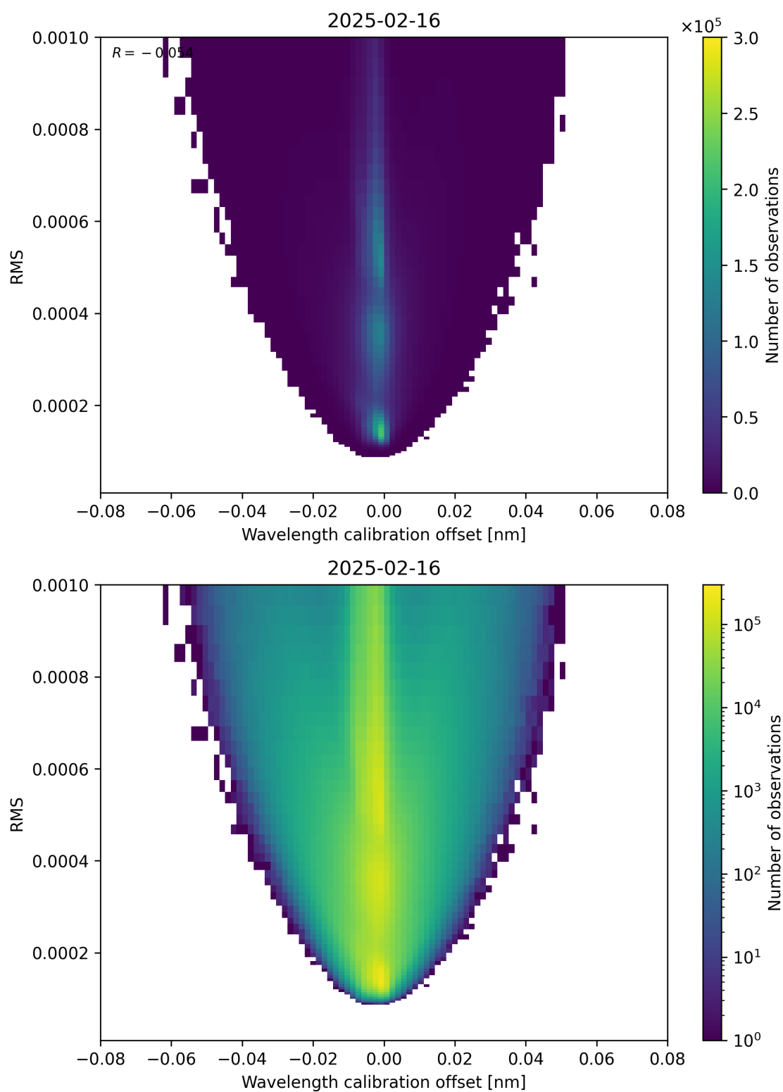
Figure 181: Scatter density plot of “Wavelength calibration offset” against “RMS” for 2025-02-15 to 2025-02-17.
