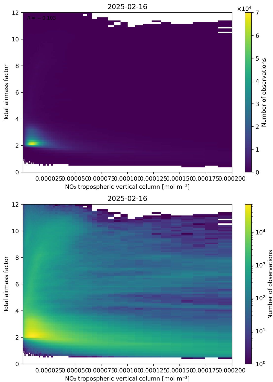
Figure 122: Scatter density plot of “NO 2 tropospheric vertical column” against “Total air mass factor” for 2025-02-15 to 2025-02-17.
