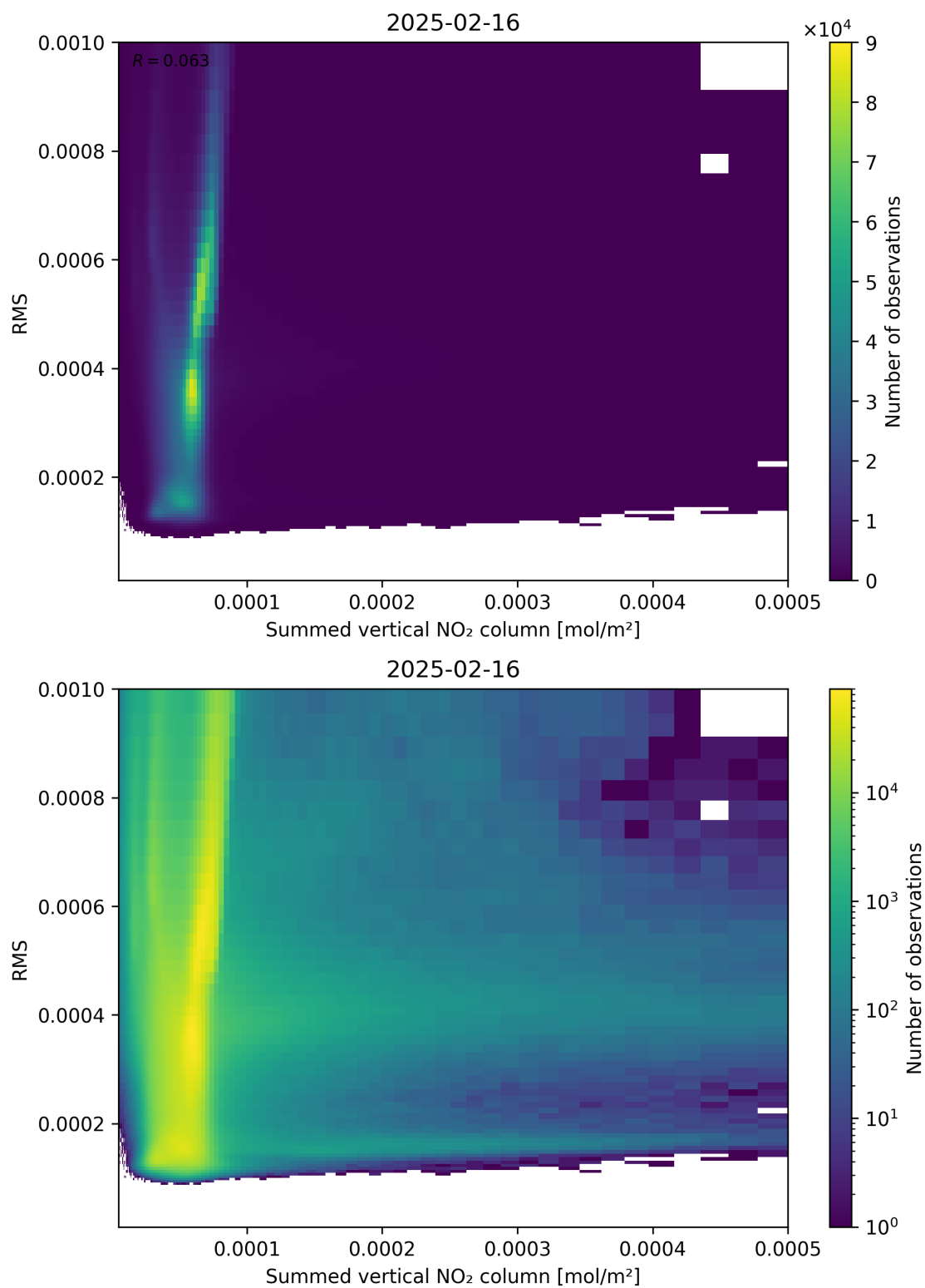
Figure 109: Scatter density plot of “Summed vertical NO 2 column” against “RMS” for 2025-02-15 to 2025-02-17.
