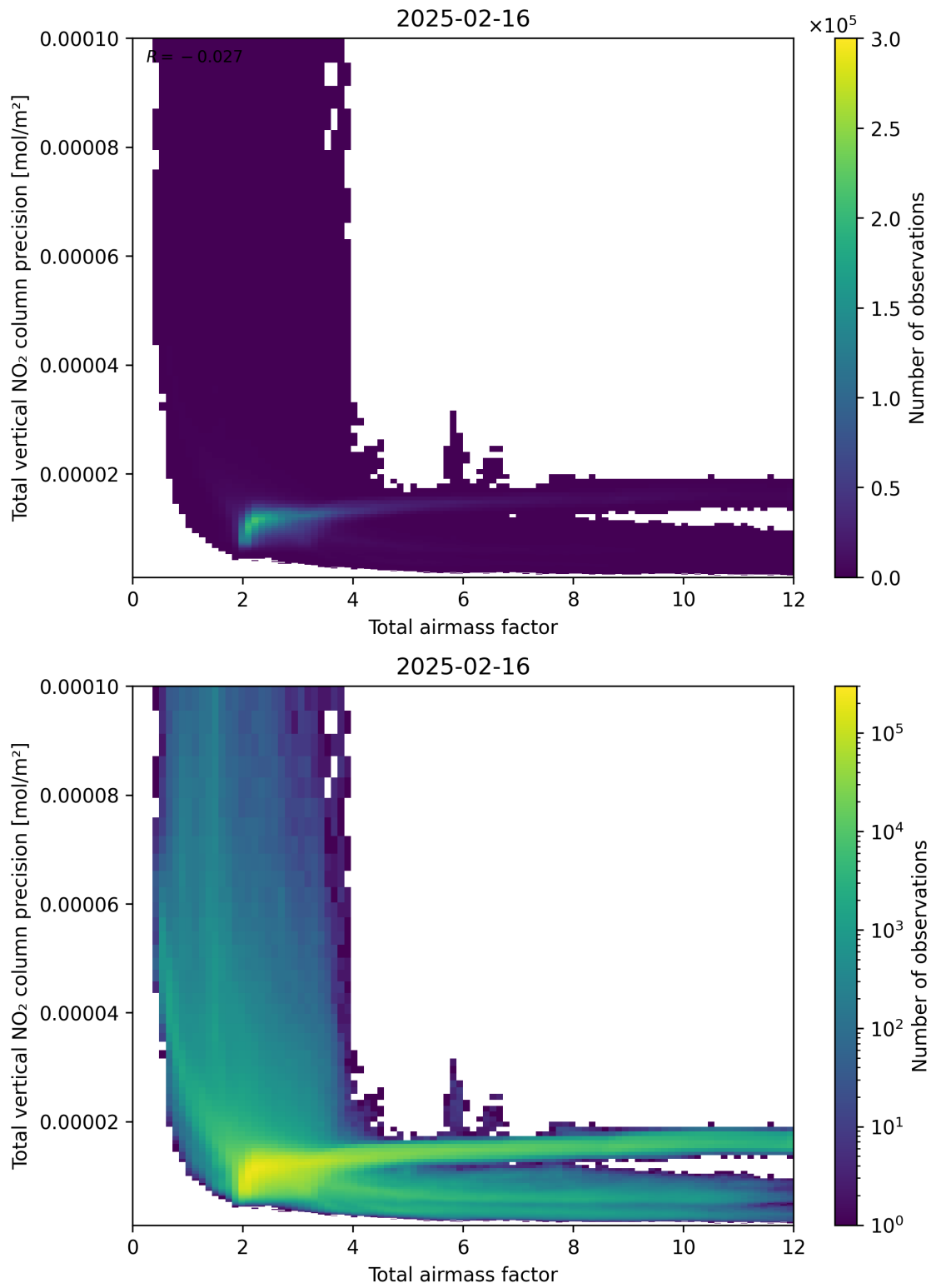
Figure 68: Scatter density plot of “Total airmass factor” against “Total vertical NO 2 column precision” for 2025-02-15 to 2025-02-17.
