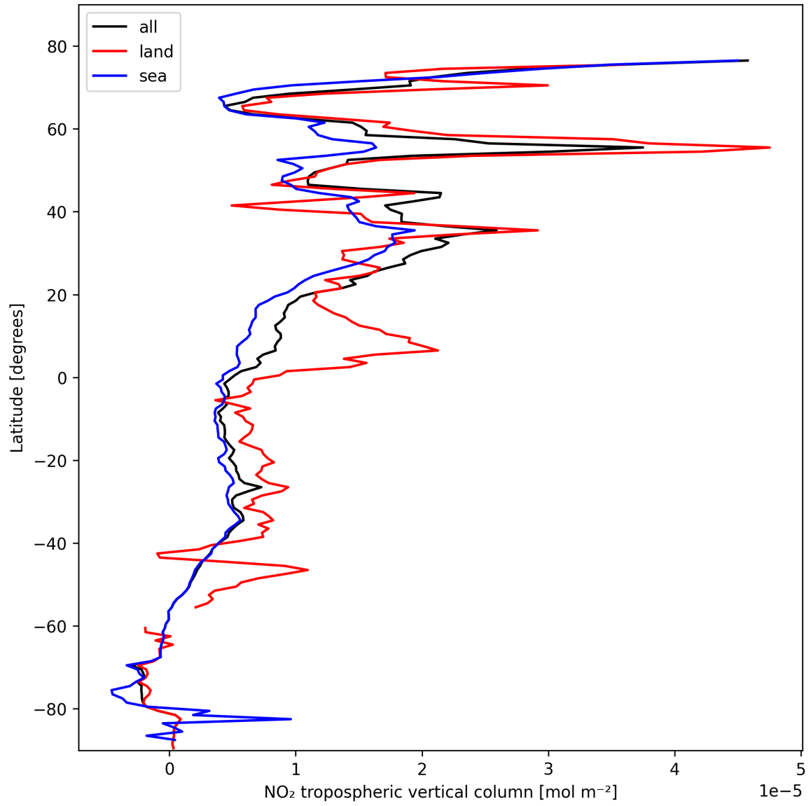
Figure 12: Zonal average of “NO 2 tropospheric vertical column” for 2025-02-15 to 2025-02-17.
