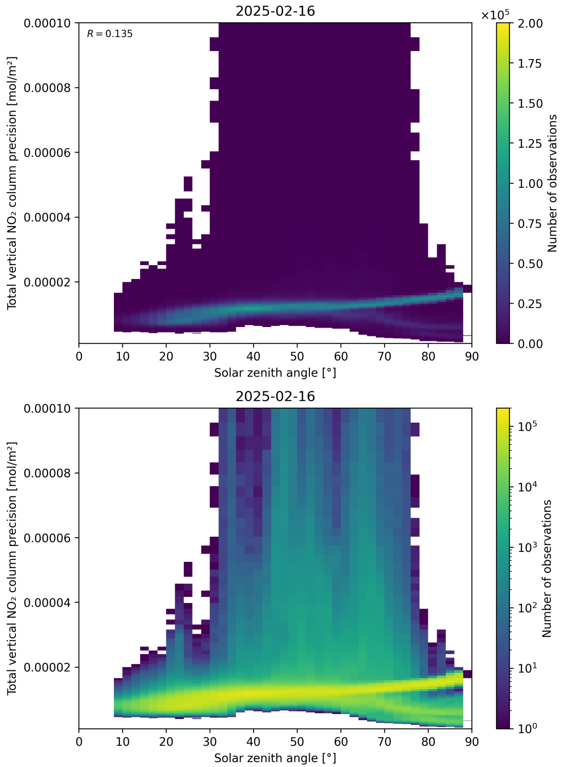
Figure 154: Scatter density plot of “Solar zenith angle” against “Total vertical NO 2 column precision” for 2025-02-15 to 2025-02-17.
