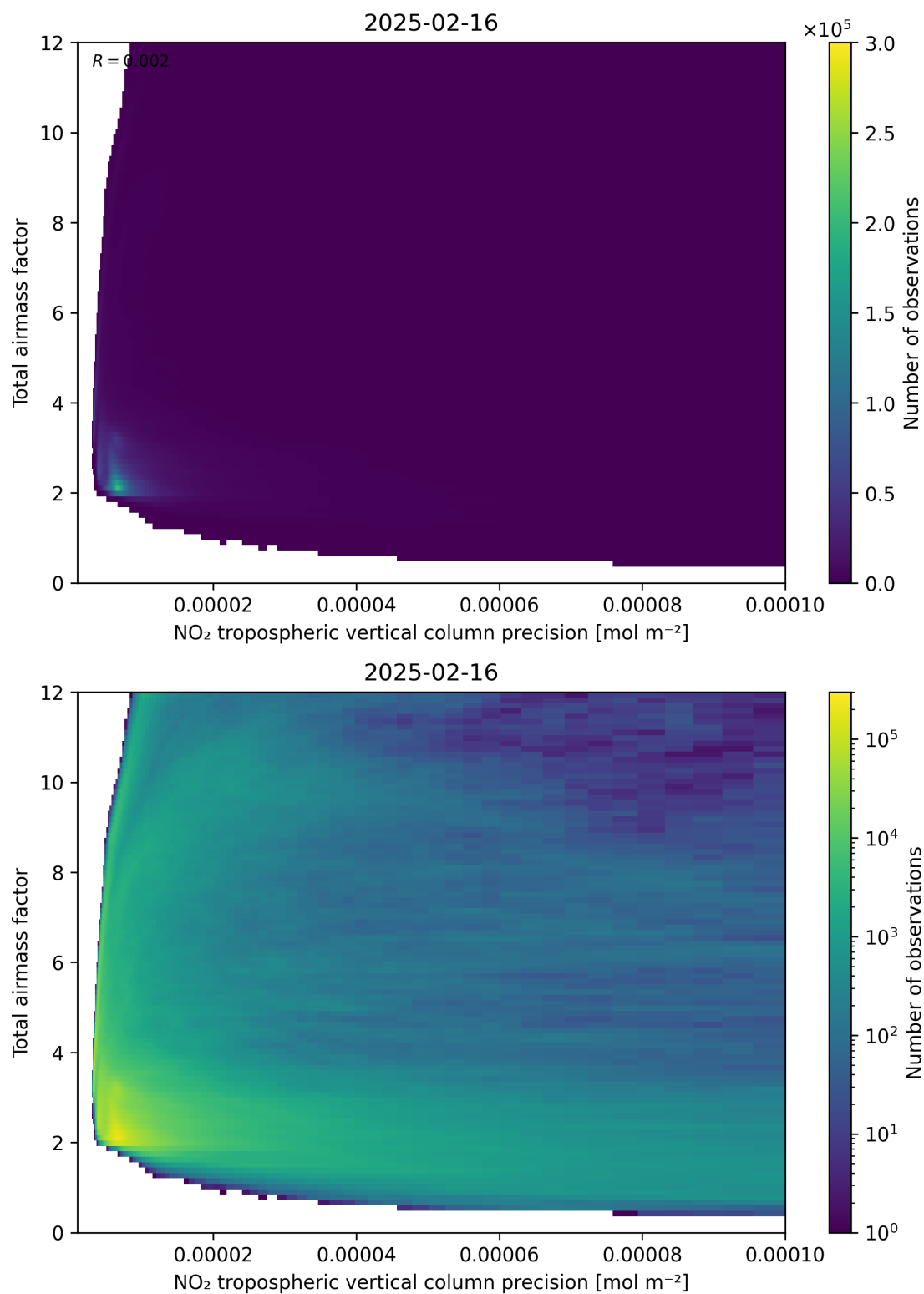
Figure 132: Scatter density plot of “NO 2 tropospheric vertical column precision” against “Total air mass factor” for 2025-02-15 to 2025-02-17.
