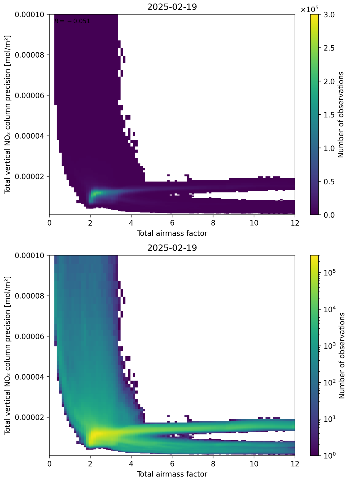
Figure 68: Scatter density plot of “Total airmass factor” against “Total vertical NO 2 column precision” for 2025-02-19 to 2025-02-20.
