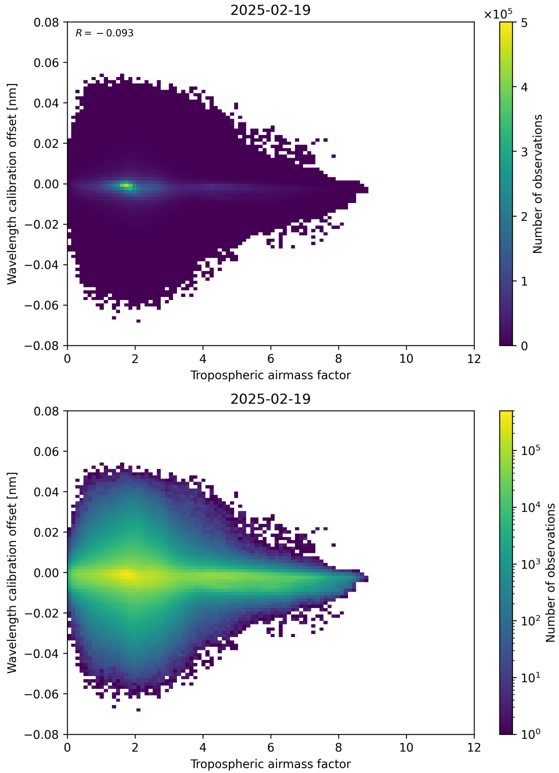
Figure 80: Scatter density plot of “Tropospheric airmass factor” against “Wavelength calibration offset” for 2025-02-19 to 2025-02-20.
