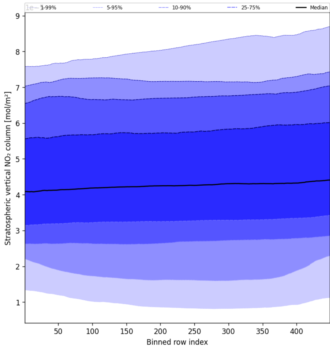
Figure 53: Along track statistics of “Stratospheric vertical NO 2 column” for 2025-02-19 to 2025-02-20
