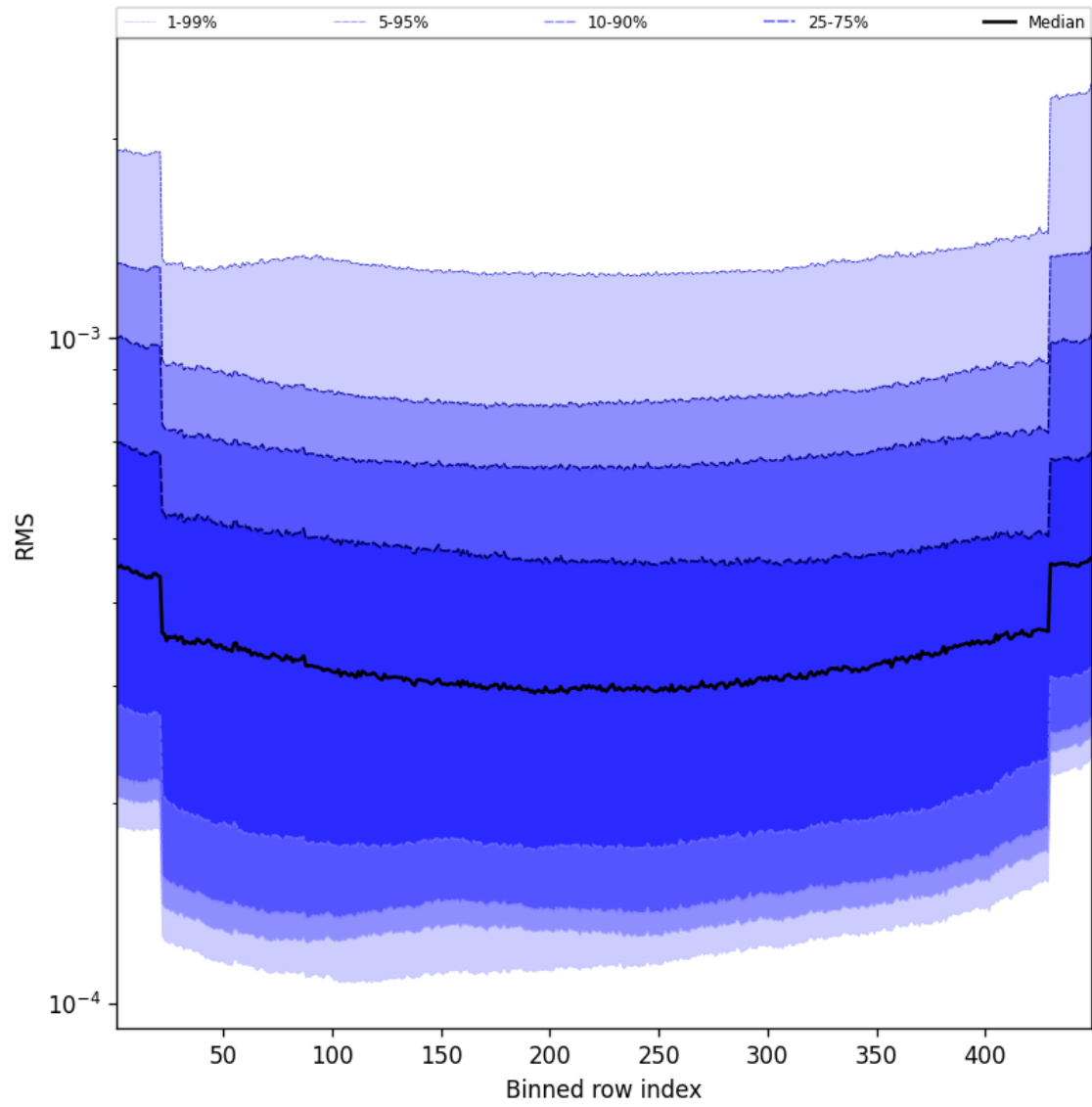
Figure 60: Along track statistics of “RMS” for 2025-02-19 to 2025-02-20
