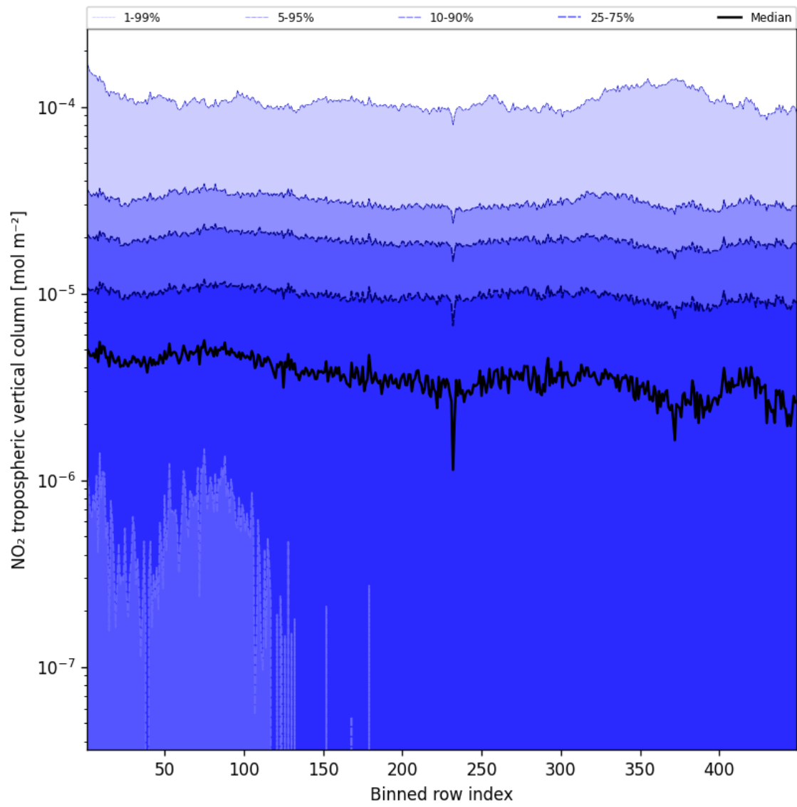
Figure 46: Along track statistics of “NO 2 tropospheric vertical column” for 2025-02-19 to 2025-02-20
