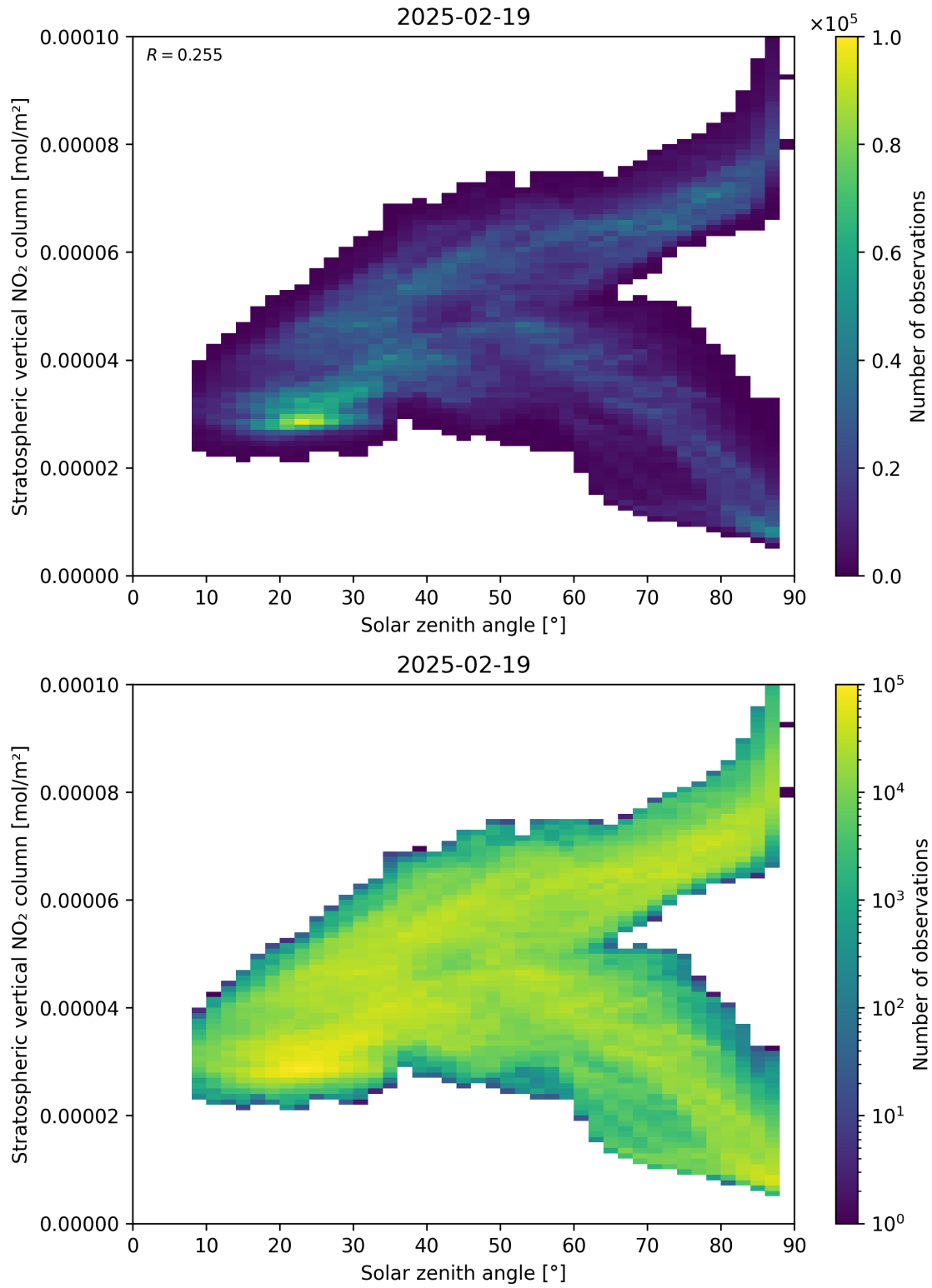
Figure 150: Scatter density plot of “Solar zenith angle” against “Stratospheric vertical NO 2 column” for 2025-02-19 to 2025-02-20.
