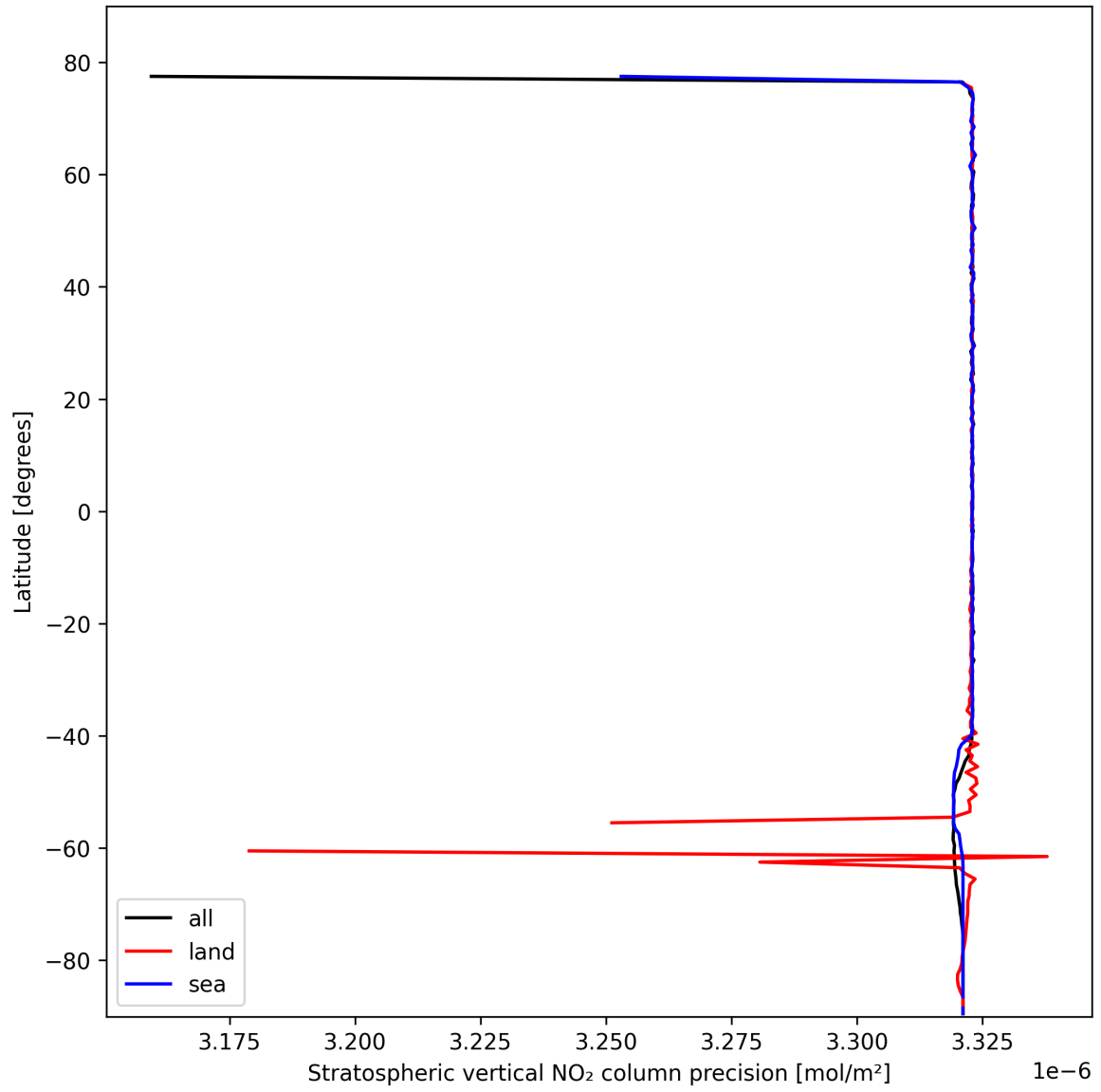
Figure 20: Zonal average of “Stratospheric vertical NO 2 column precision” for 2025-02-19 to 2025-02-20.
