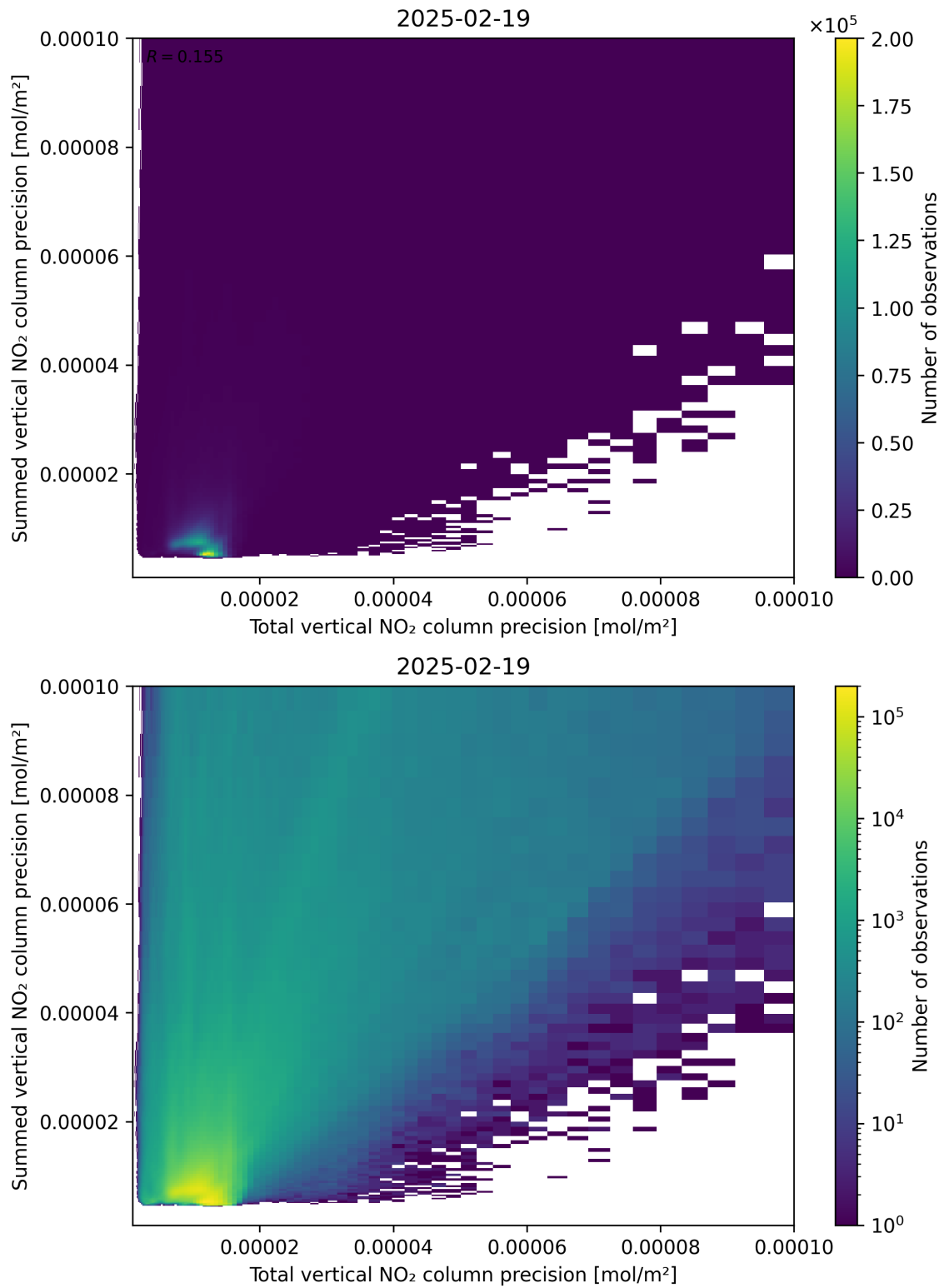
Figure 118: Scatter density plot of “Total vertical NO 2 column precision” against “Summed vertical NO 2 column precision” for 2025-02-19 to 2025-02-20.
