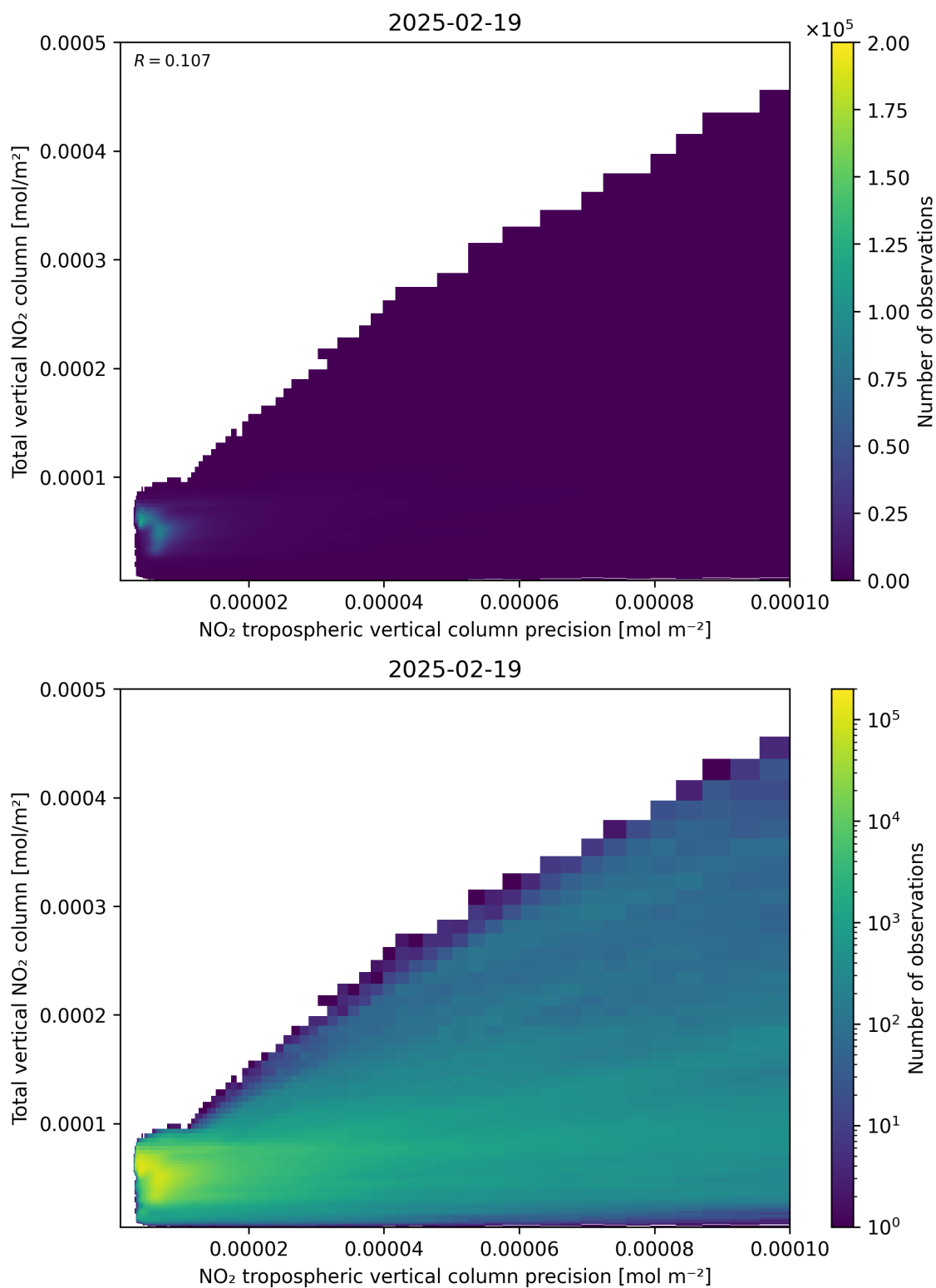
Figure 138: Scatter density plot of “NO 2 tropospheric vertical column precision” against “Total vertical NO 2 column” for 2025-02-19 to 2025-02-20.
