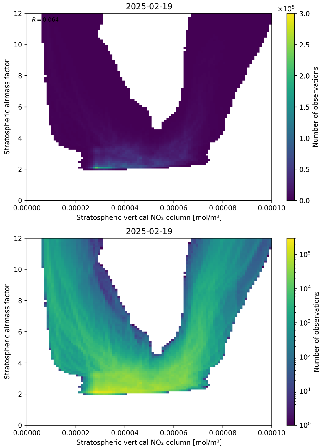
Figure 96: Scatter density plot of “Stratospheric vertical NO 2 column” against “Stratospheric airmass factor” for 2025-02-19 to 2025-02-20.
