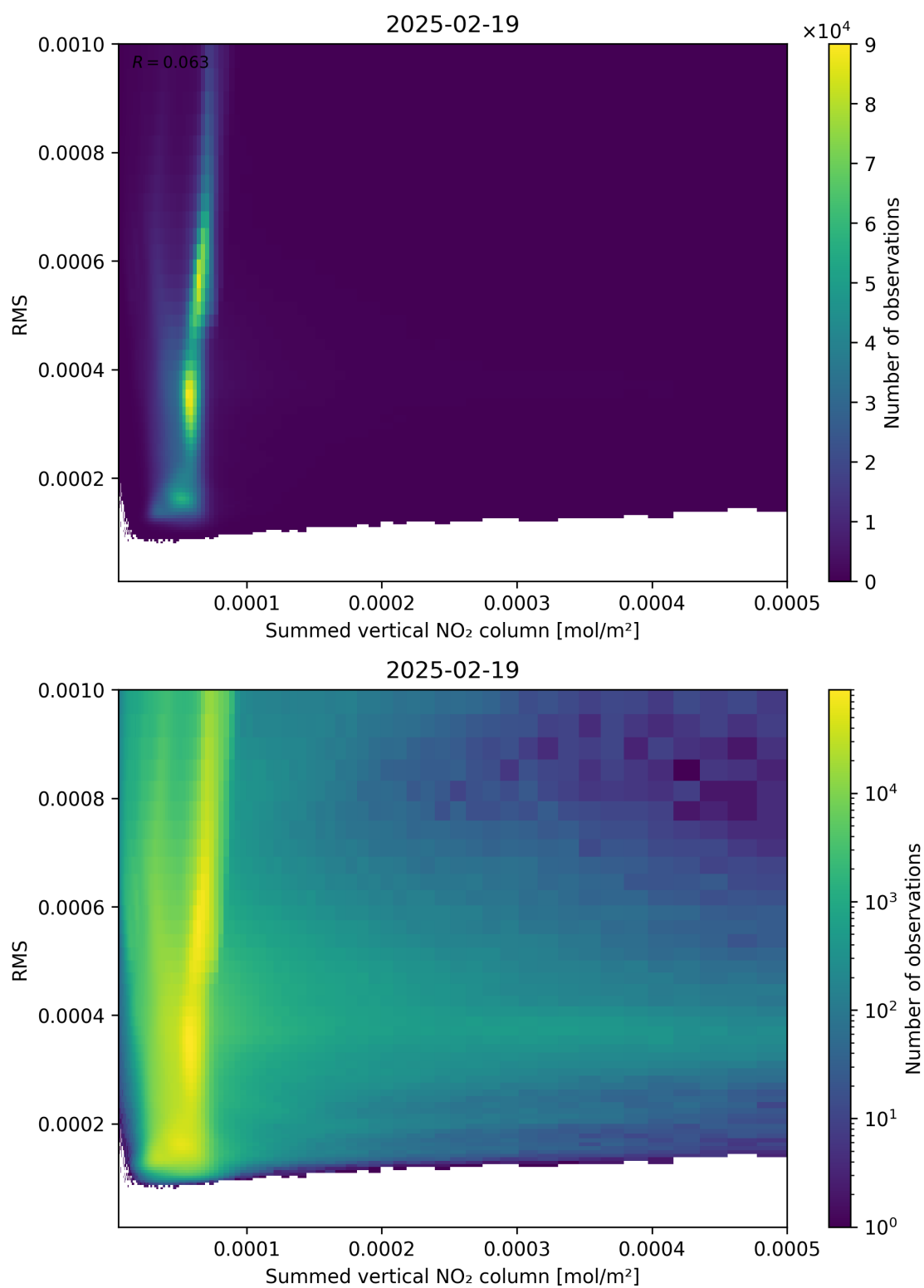
Figure 109: Scatter density plot of “Summed vertical NO 2 column” against “RMS” for 2025-02-19 to 2025-02-20.
