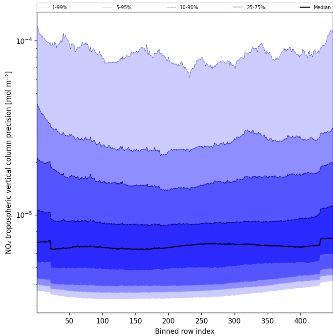
Figure 47: Along track statistics of “NO 2 tropospheric vertical column precision” for 2025-02-19 to 2025-02-20
