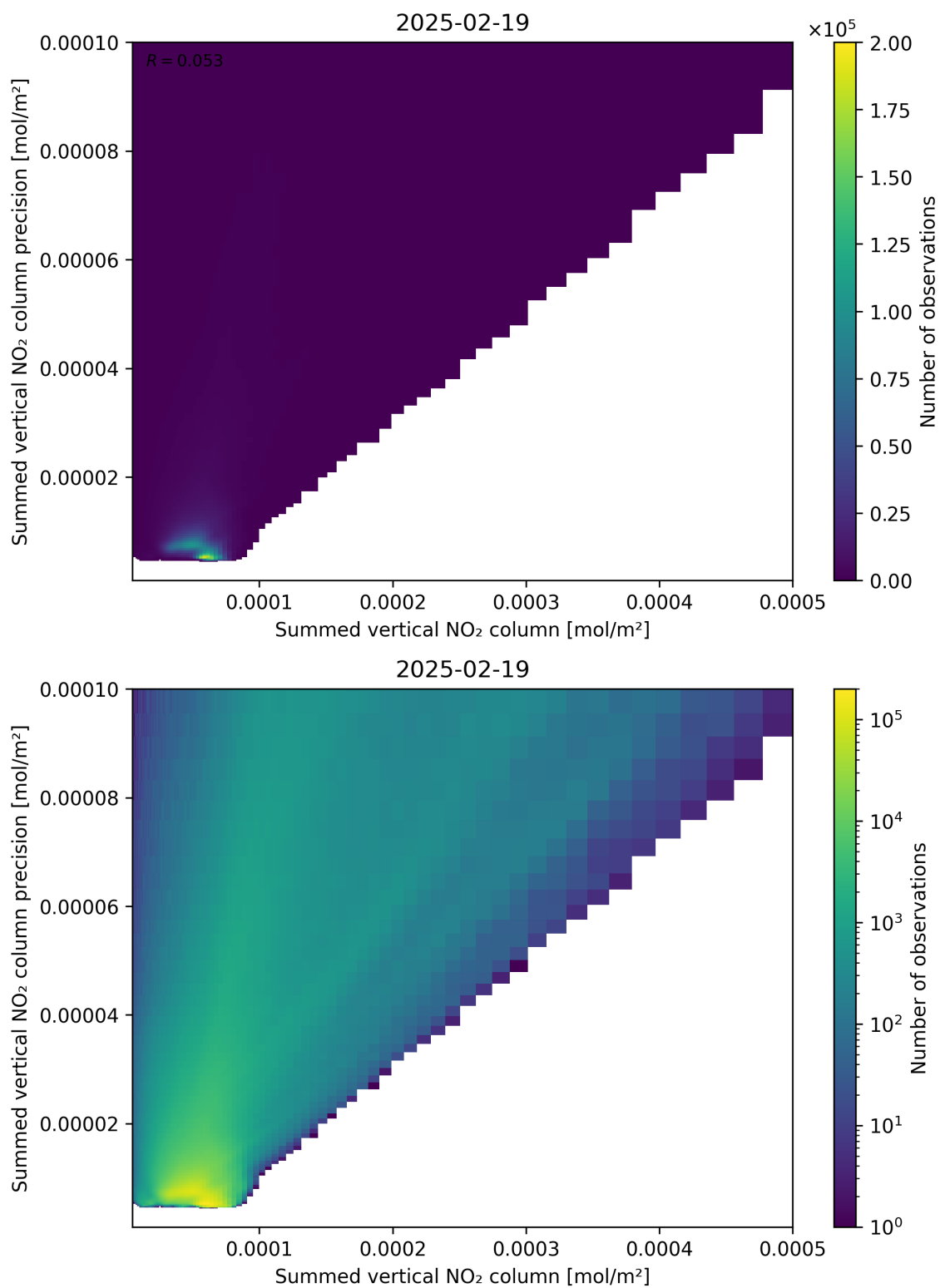
Figure 105: Scatter density plot of “Summed vertical NO 2 column” against “Summed vertical NO 2 column precision” for 2025-02-19 to 2025-02-20.
