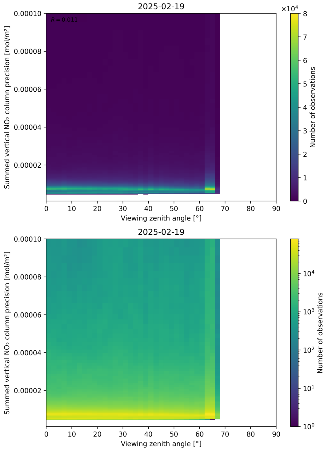
Figure 166: Scatter density plot of “Viewing zenith angle” against “Summed vertical NO 2 column precision” for 2025-02-19 to 2025-02-20.
