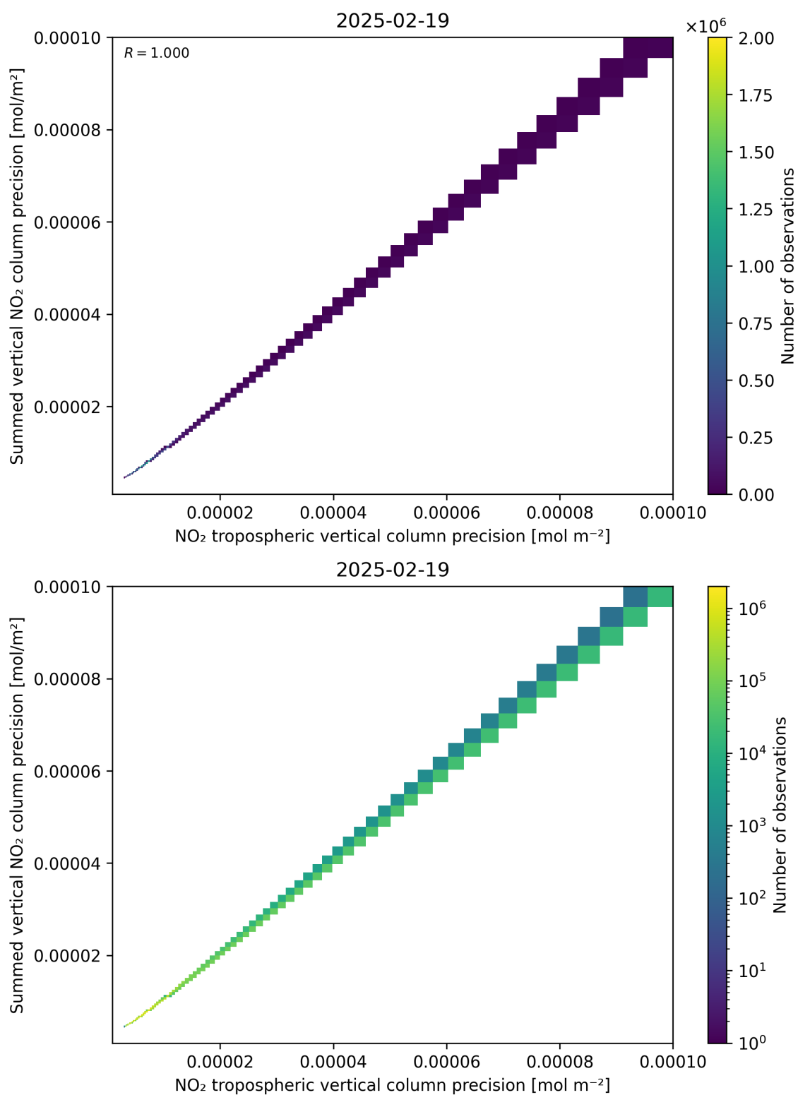
Figure 137: Scatter density plot of “NO 2 tropospheric vertical column precision” against “Summed vertical NO 2 column precision” for 2025-02-19 to 2025-02-20.
