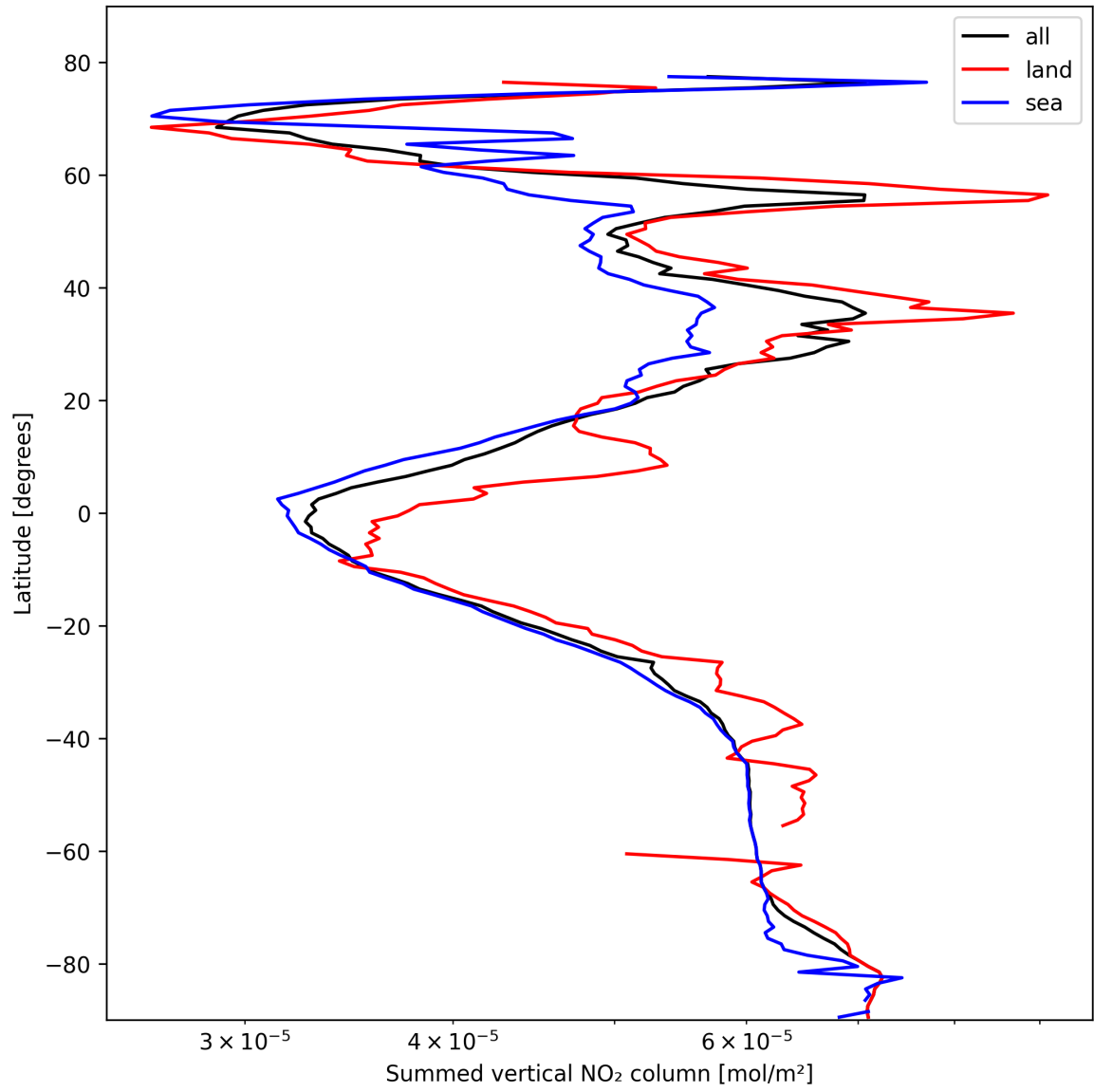
Figure 23: Zonal average of “Summed vertical NO 2 column” for 2025-02-19 to 2025-02-20.
