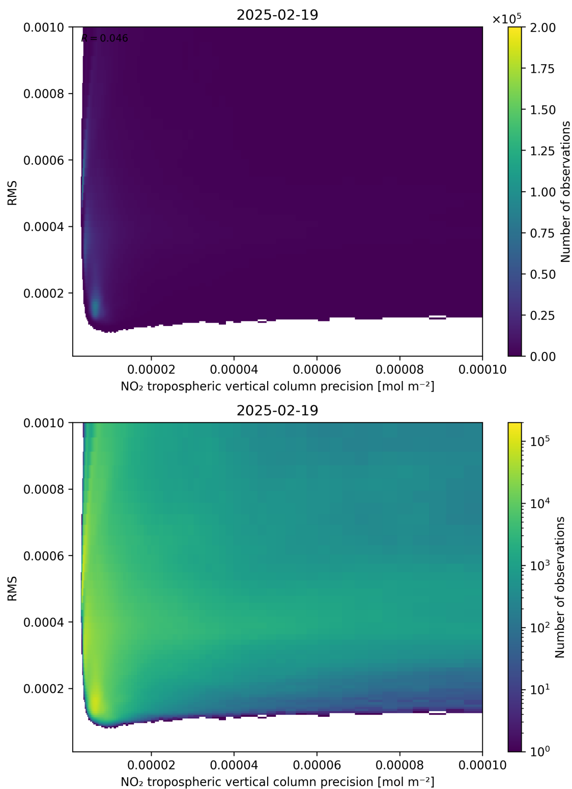
Figure 140: Scatter density plot of “NO 2 tropospheric vertical column precision” against “RMS” for 2025-02-19 to 2025-02-20.
