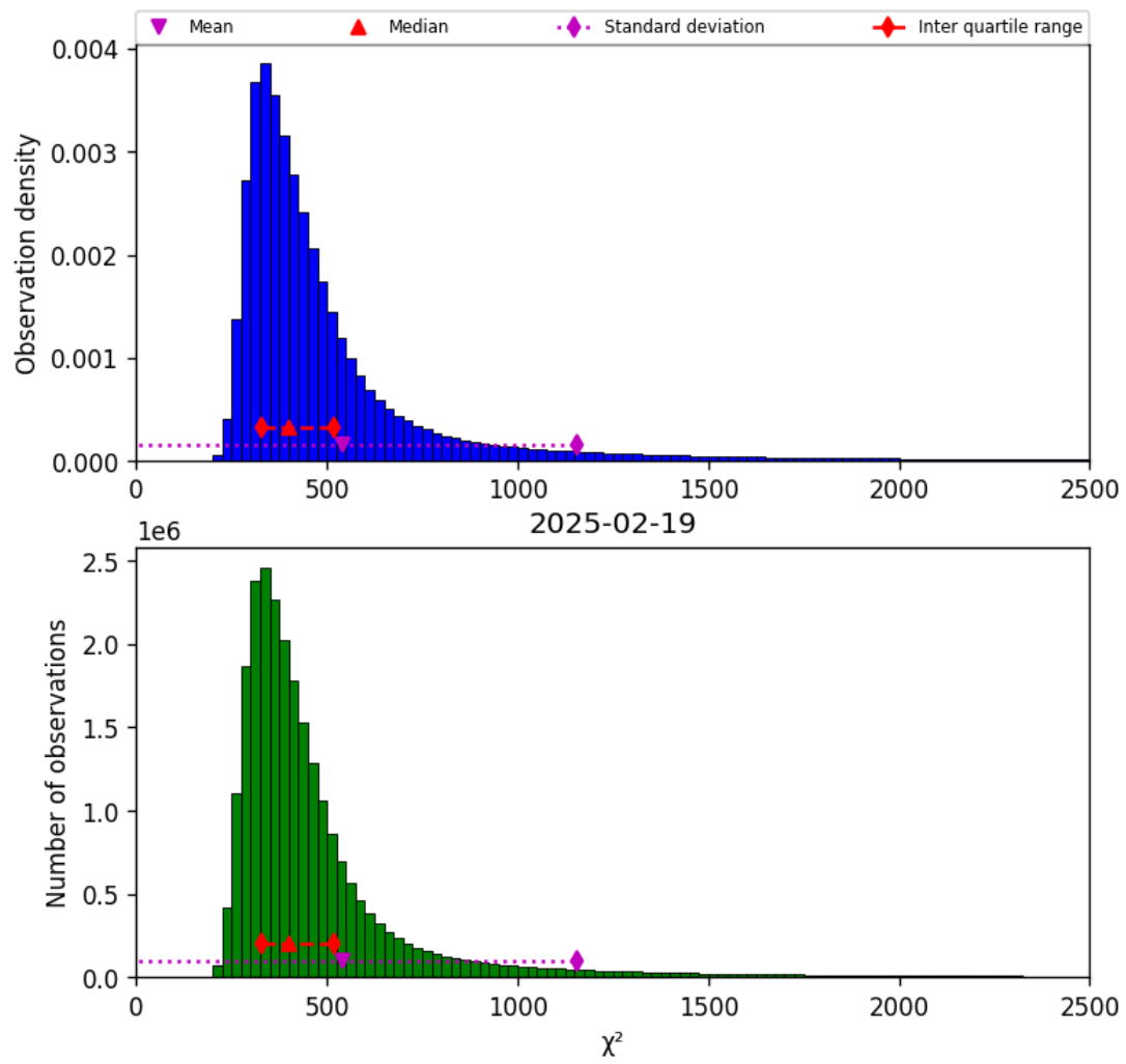
Figure 42: Histogram of “ \chi^2 ” for 2025-02-19 to 2025-02-20
