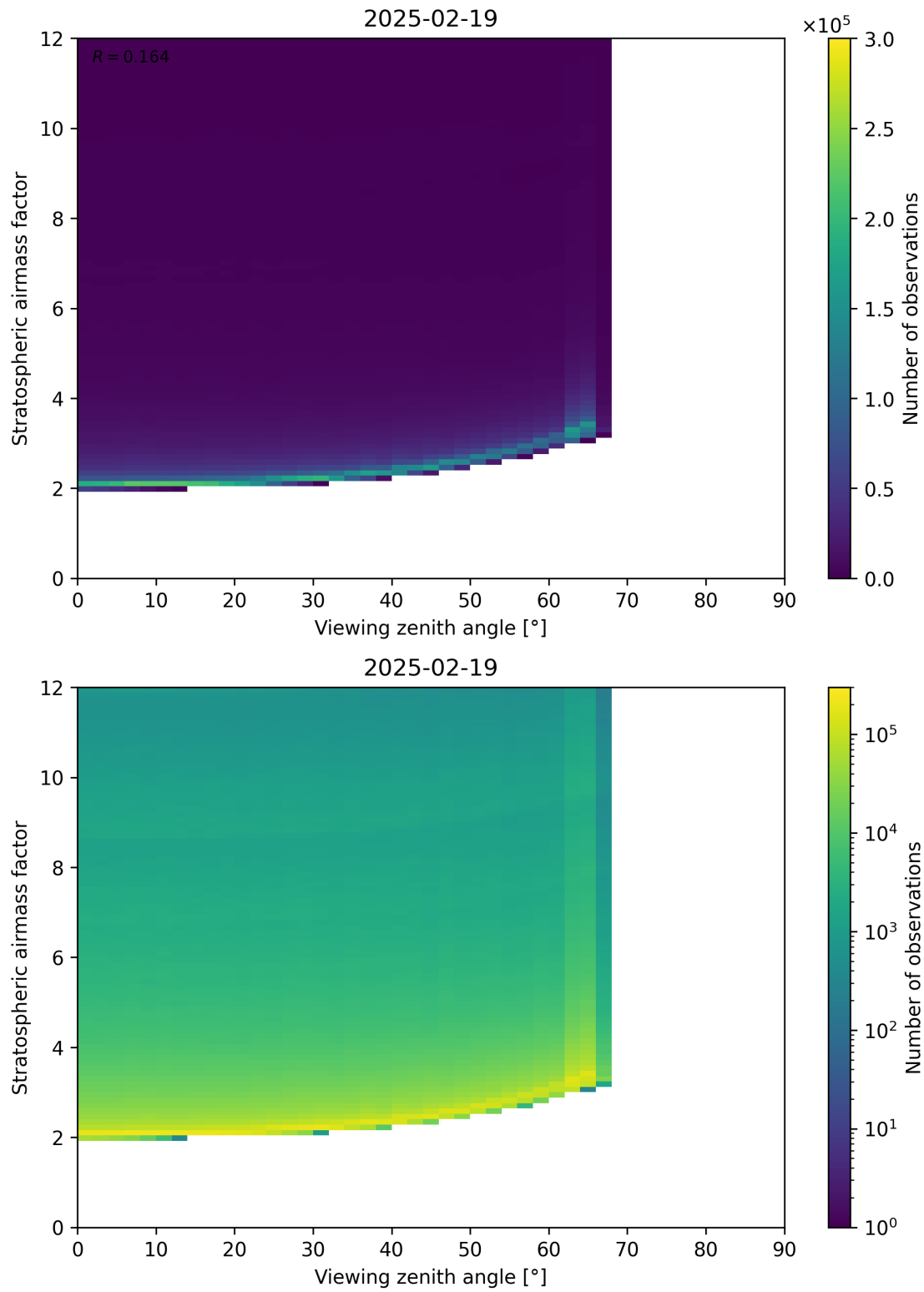
Figure 159: Scatter density plot of “Viewing zenith angle” against “Stratospheric airmass factor” for 2025-02-19 to 2025-02-20.
