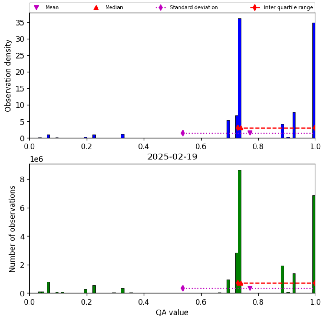
Figure 28: Histogram of “QA value” for 2025-02-19 to 2025-02-20
