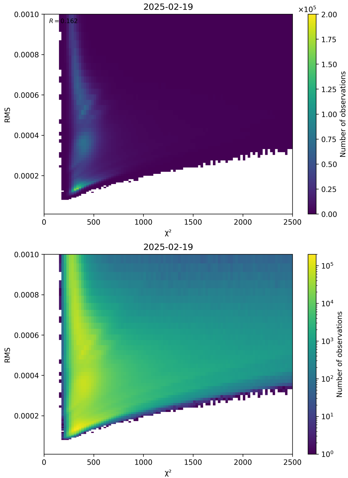
Figure 82: Scatter density plot of “ \chi^2 ” against “RMS” for 2025-02-19 to 2025-02-20.
