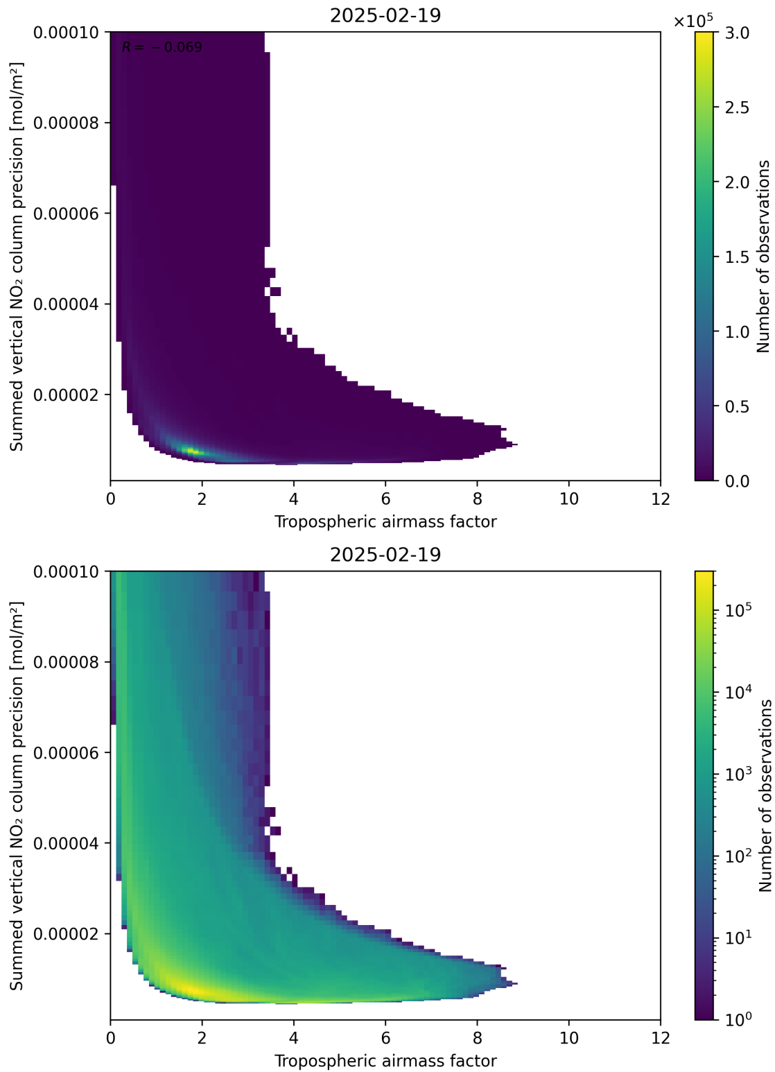
Figure 76: Scatter density plot of “Tropospheric air mass factor” against “Summed vertical NO 2 column precision” for 2025-02-19 to 2025-02-20.
