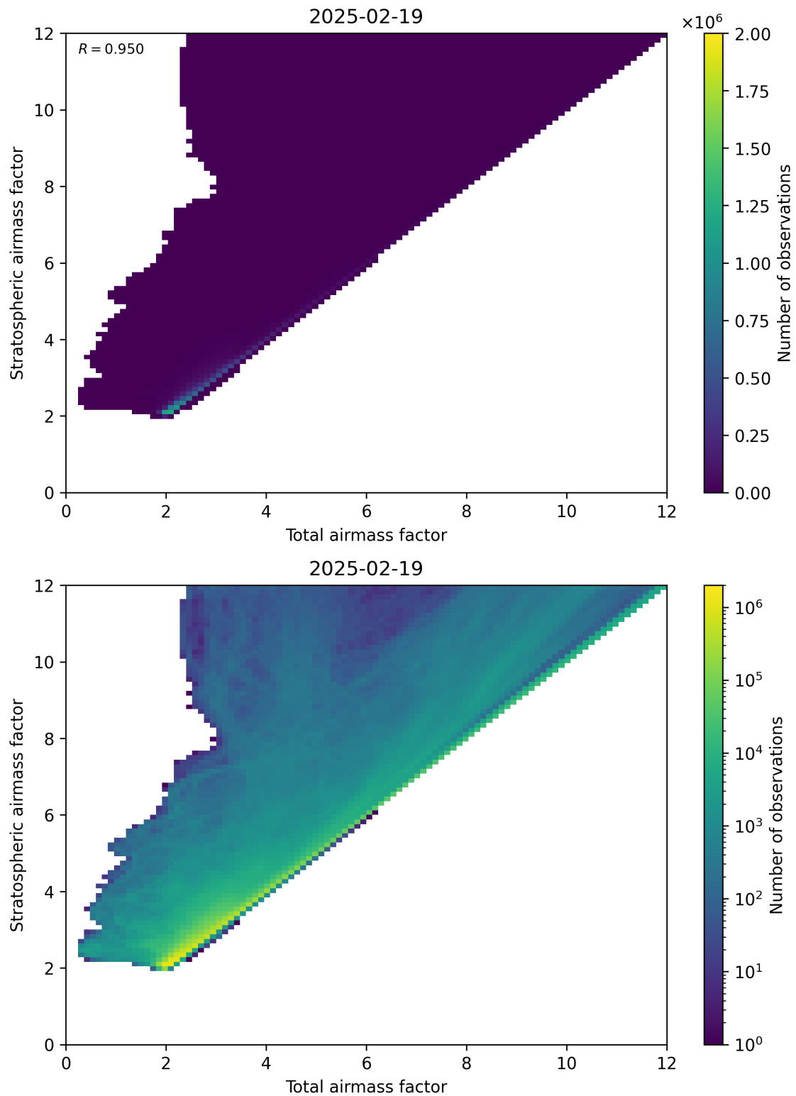
Figure 62: Scatter density plot of “Total air mass factor” against “Stratospheric air mass factor” for 2025-02-19 to 2025-02-20.
