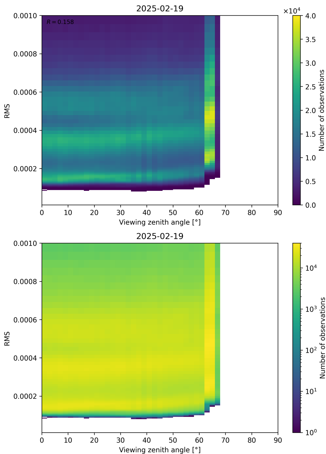
Figure 171: Scatter density plot of “Viewing zenith angle” against “RMS” for 2025-02-19 to 2025-02-20.
