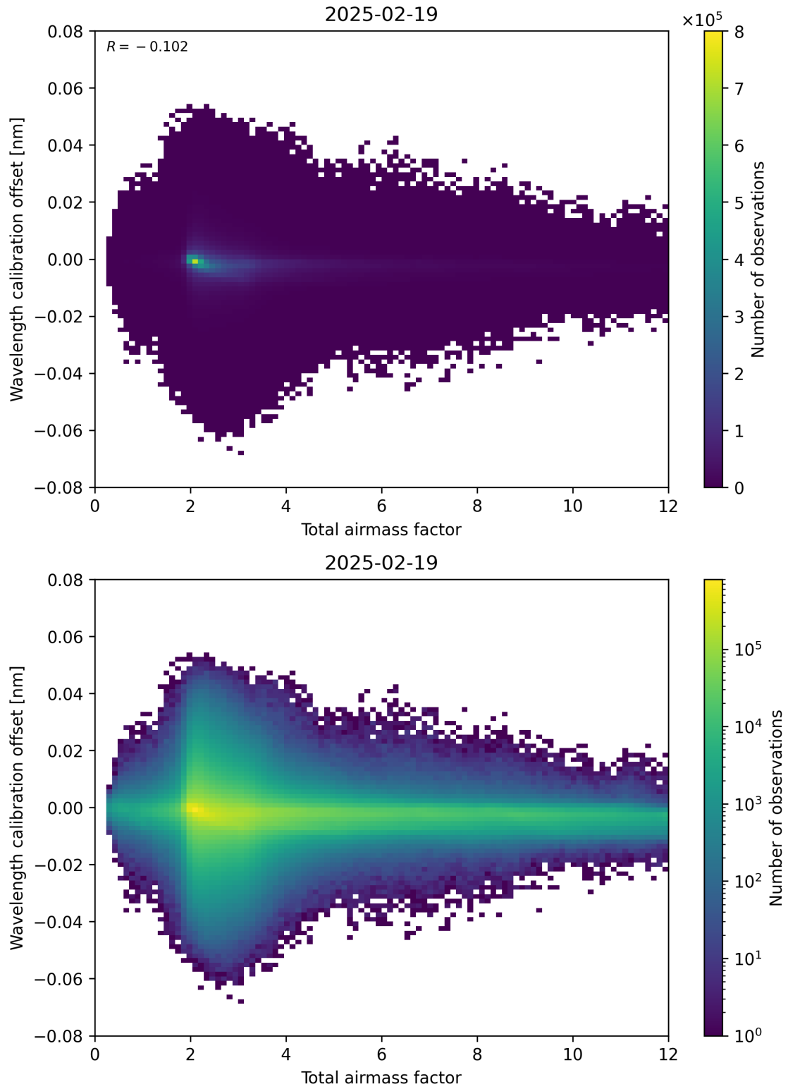
Figure 70: Scatter density plot of “Total airmass factor” against “Wavelength calibration offset” for 2025-02-19 to 2025-02-20.
