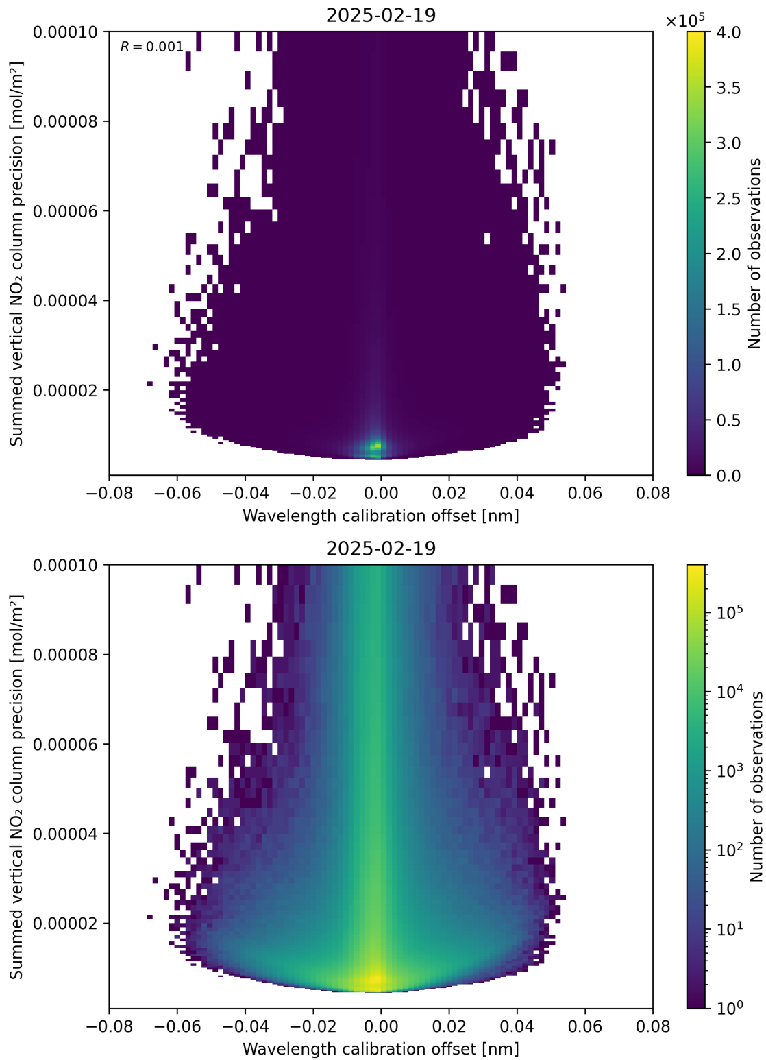
Figure 178: Scatter density plot of “Wavelength calibration offset” against “Summed vertical NO 2 column precision” for 2025-02-19 to 2025-02-20.
