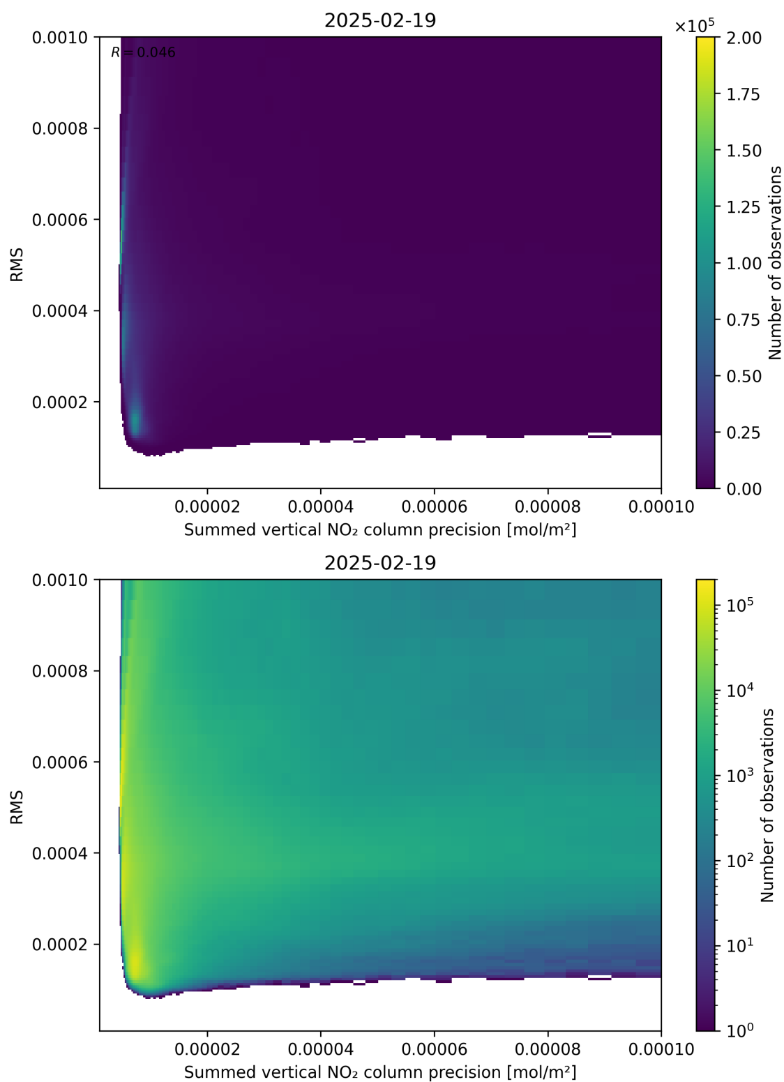
Figure 108: Scatter density plot of “Summed vertical NO 2 column precision” against “RMS” for 2025-02-19 to 2025-02-20.
