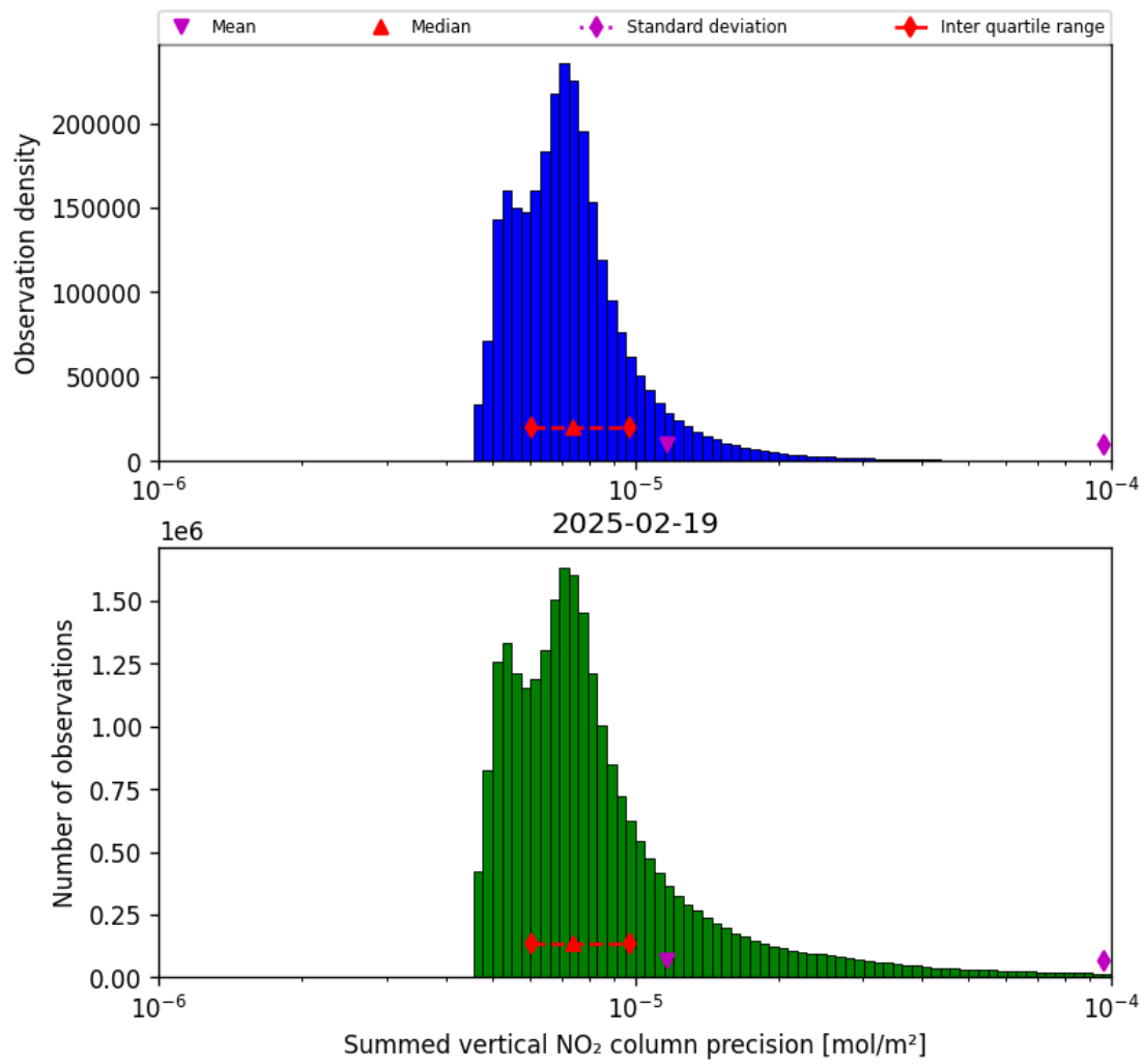
Figure 41: Histogram of "Summed vertical NO 2 column precision" for 2025-02-19 to 2025-02-20
