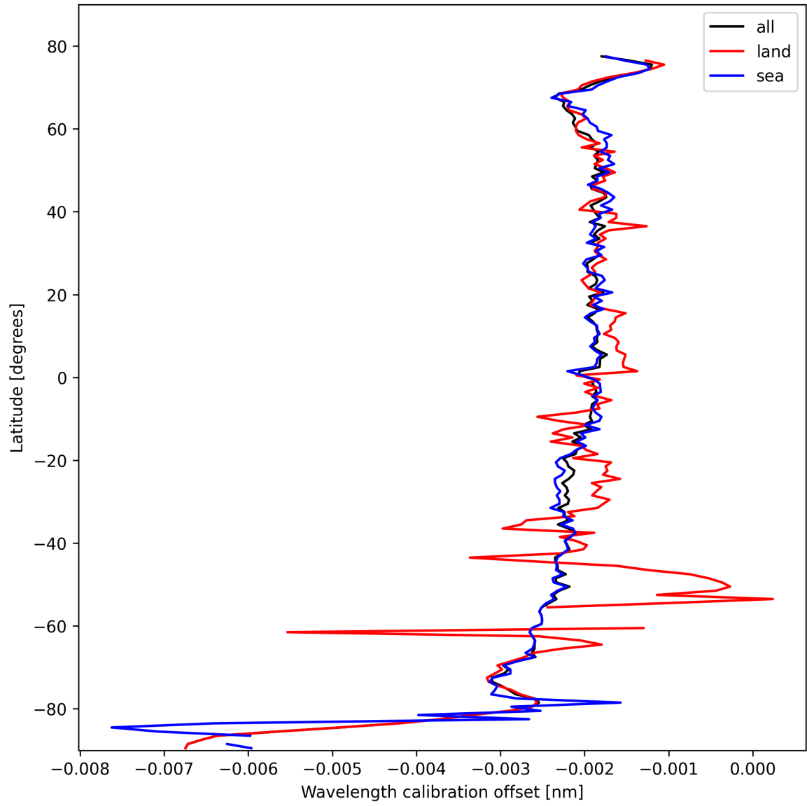
Figure 18: Zonal average of “Wavelength calibration offset” for 2025-02-19 to 2025-02-20.
