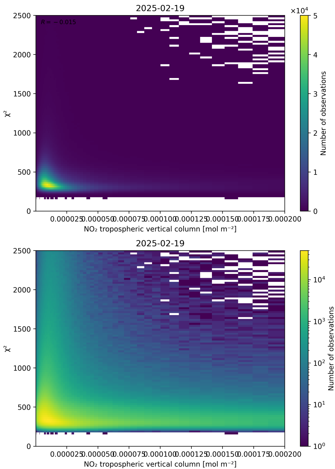
Figure 124: Scatter density plot of “NO 2 tropospheric vertical column” against “ \chi^2 ” for 2025-02-19 to 2025-02-20.
