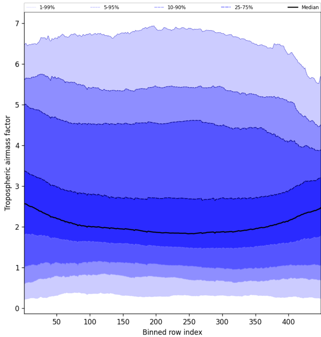
Figure 48: Along track statistics of “Tropospheric airmass factor” for 2025-02-19 to 2025-02-20
