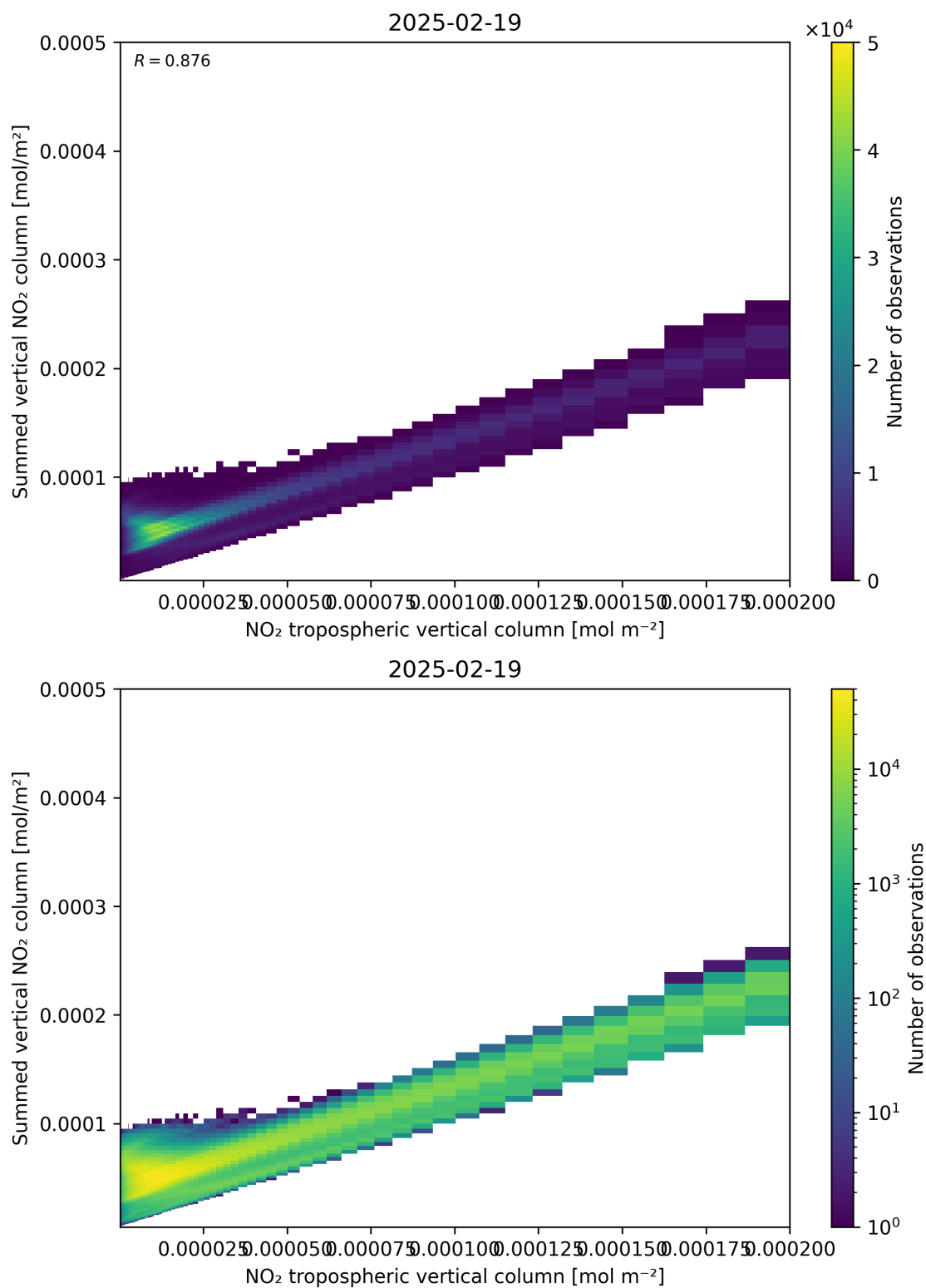
Figure 126: Scatter density plot of “NO 2 tropospheric vertical column” against “Summed vertical NO 2 column” for 2025-02-19 to 2025-02-20.
