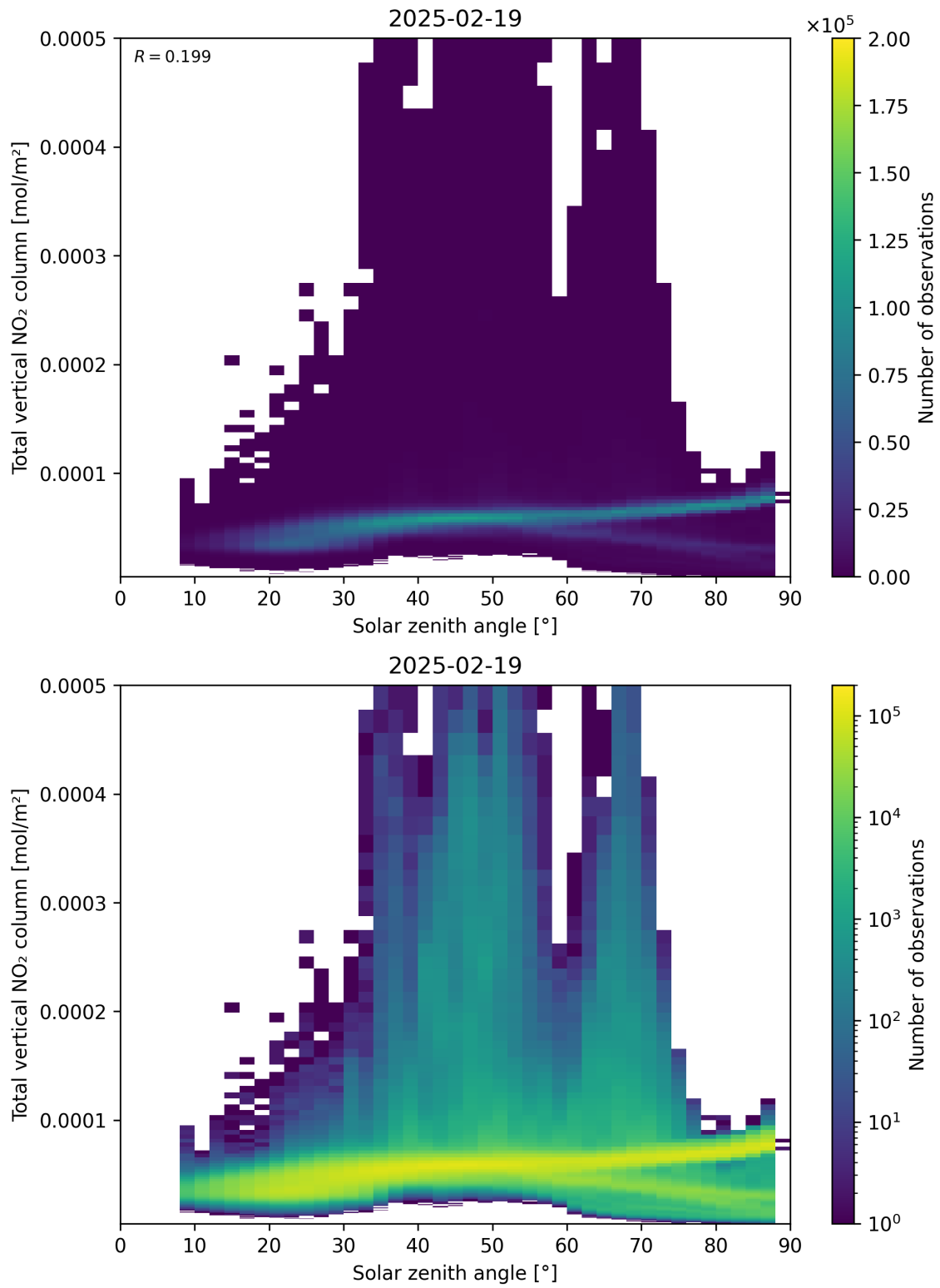
Figure 153: Scatter density plot of “Solar zenith angle” against “Total vertical NO 2 column” for 2025-02-19 to 2025-02-20.
