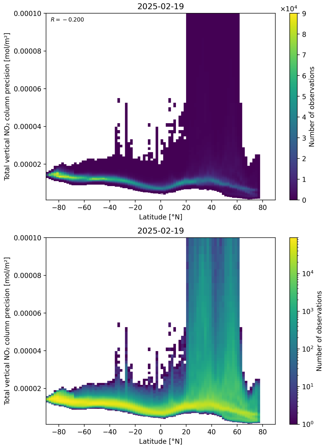
Figure 91: Scatter density plot of “Latitude” against “Total vertical NO 2 column precision” for 2025-02-19 to 2025-02-20.
