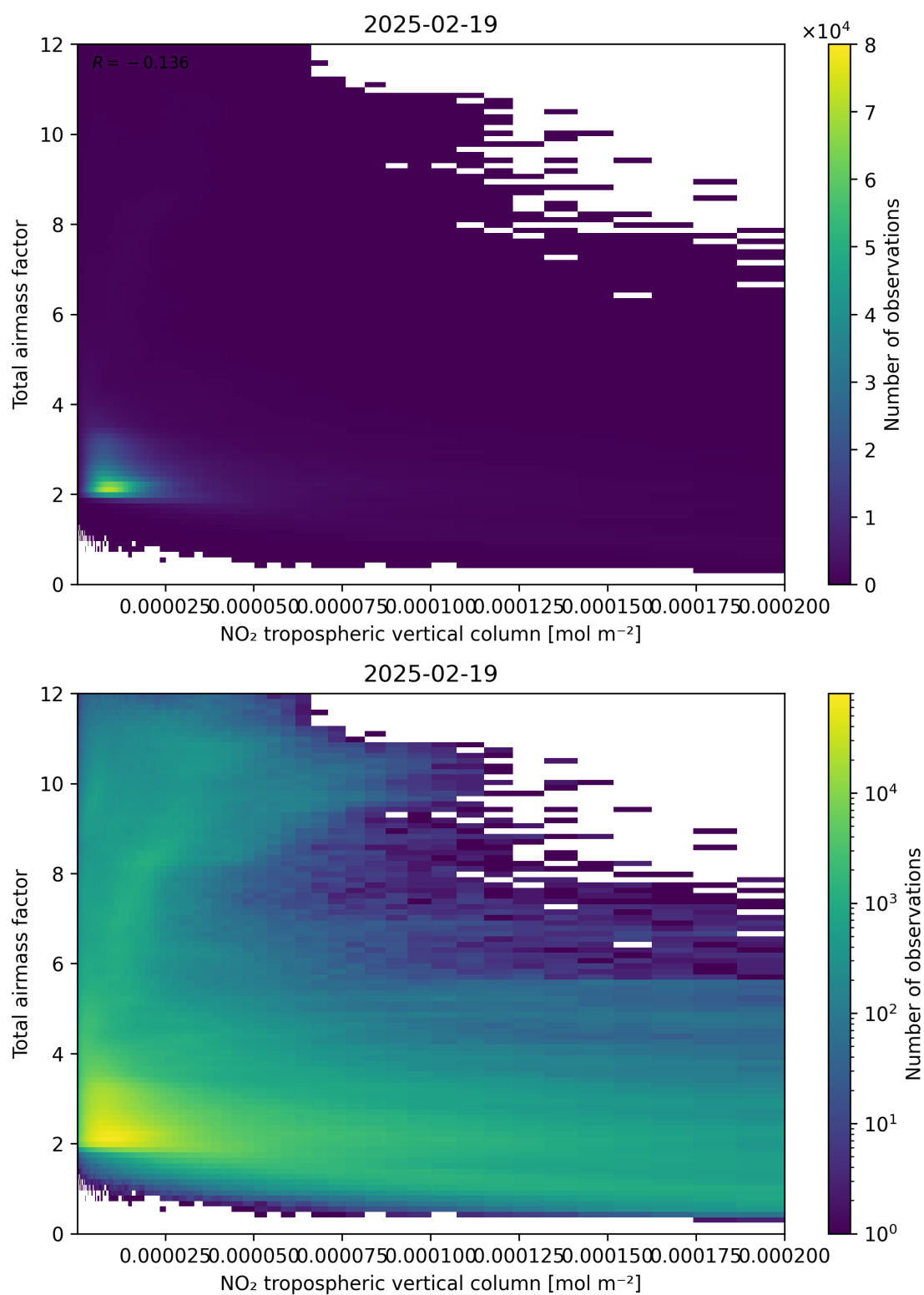
Figure 122: Scatter density plot of “NO 2 tropospheric vertical column” against “Total air mass factor” for 2025-02-19 to 2025-02-20.
