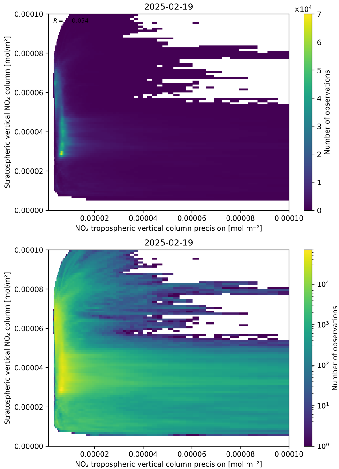
Figure 135: Scatter density plot of “NO 2 tropospheric vertical column precision” against “Stratospheric vertical NO 2 column” for 2025-02-19 to 2025-02-20.
