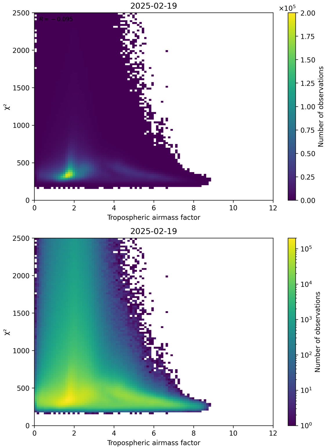
Figure 73: Scatter density plot of “Tropospheric airmass factor” against “ \chi^2 ” for 2025-02-19 to 2025-02-20.
