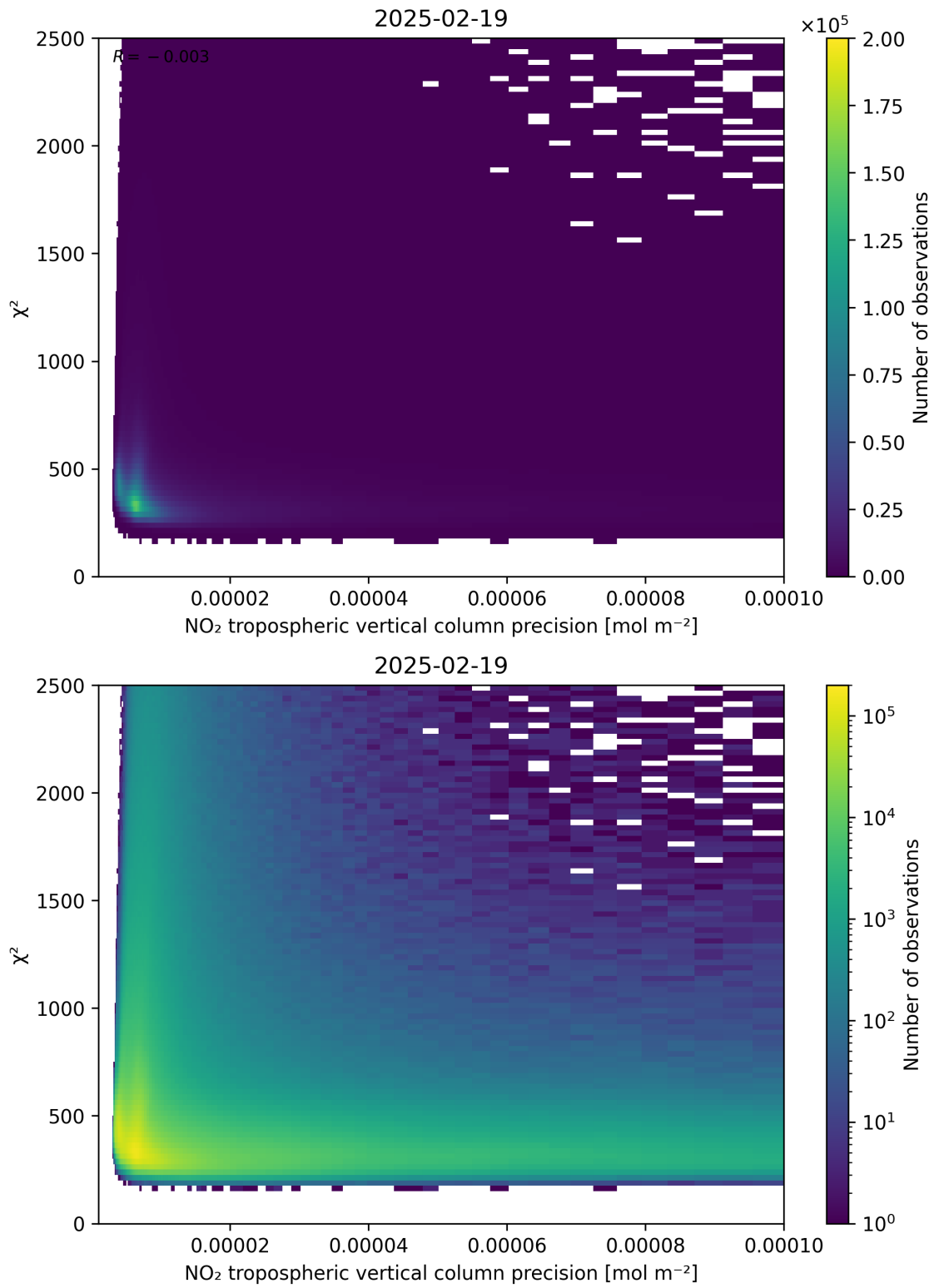
Figure 134: Scatter density plot of “NO 2 tropospheric vertical column precision” against “ \chi^2 ” for 2025-02-19 to 2025-02-20.
