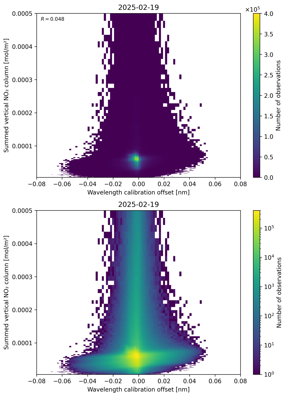
Figure 177: Scatter density plot of “Wavelength calibration offset” against “Summed vertical NO 2 column” for 2025-02-19 to 2025-02-20.
