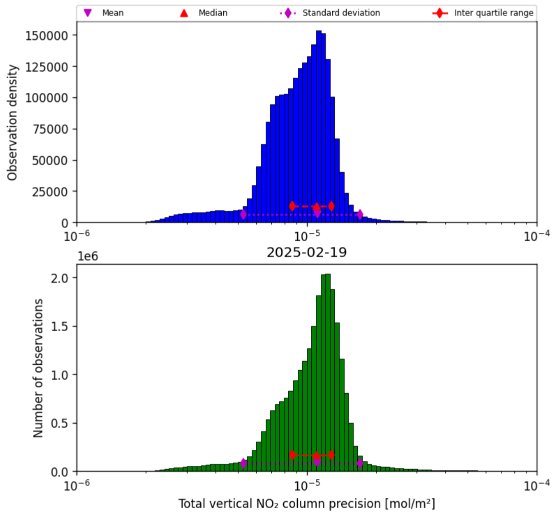
Figure 39: Histogram of “Total vertical NO 2 column precision” for 2025-02-19 to 2025-02-20
