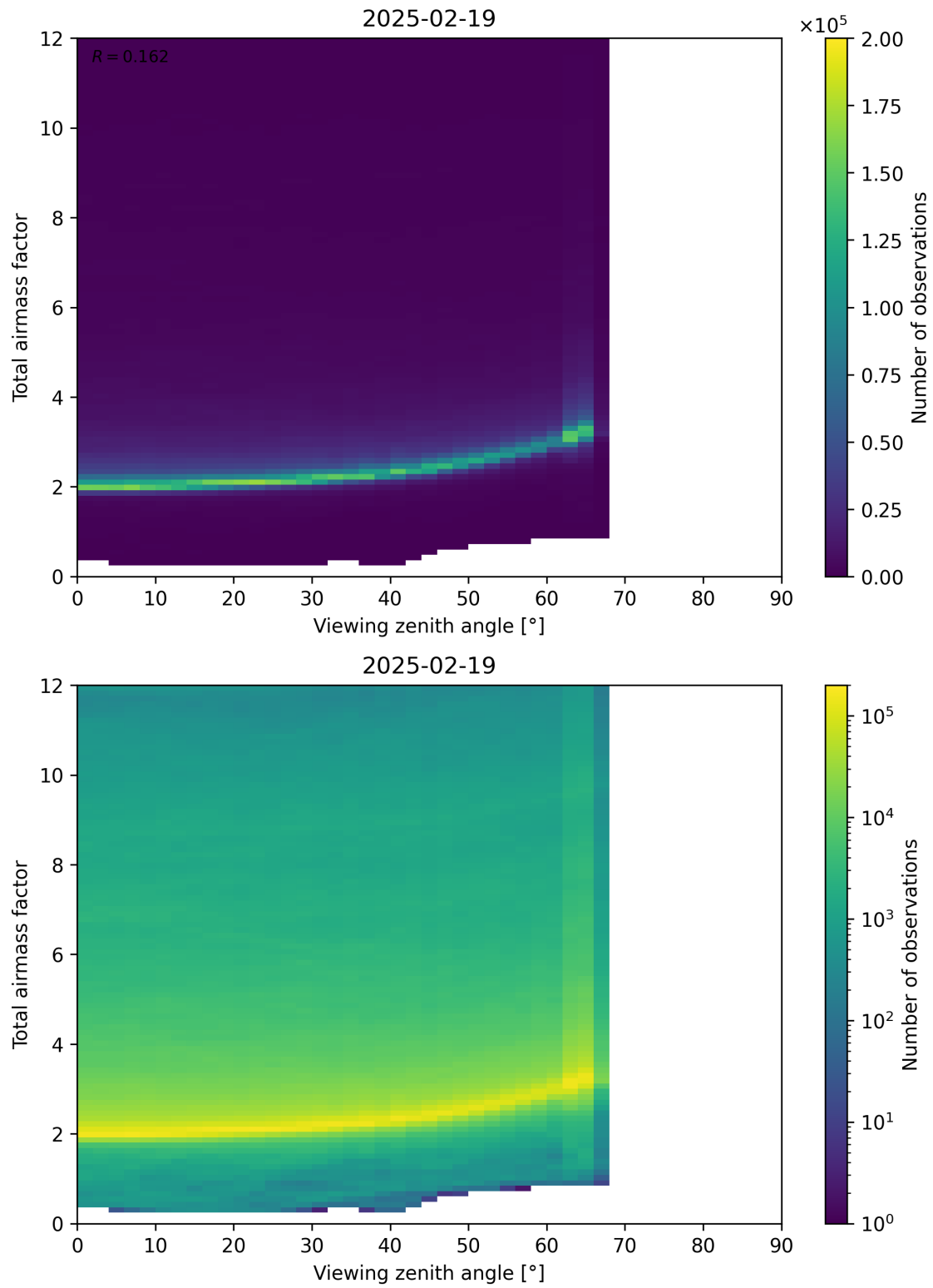
Figure 160: Scatter density plot of “Viewing zenith angle” against “Total airmass factor” for 2025-02-19 to 2025-02-20.
