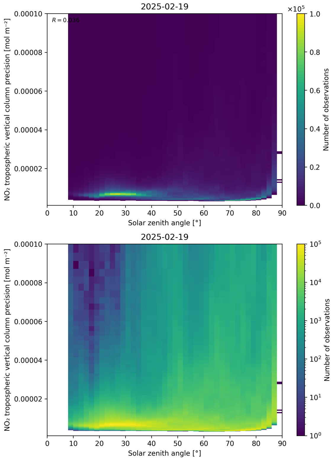
Figure 156: Scatter density plot of “Solar zenith angle” against “NO 2 tropospheric vertical column precision” for 2025-02-19 to 2025-02-20.
