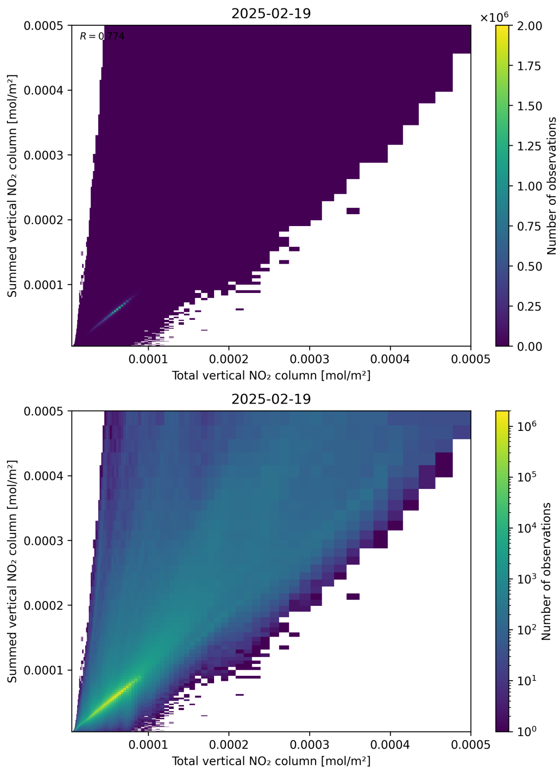
Figure 112: Scatter density plot of “Total vertical NO 2 column” against “Summed vertical NO 2 column” for 2025-02-19 to 2025-02-20.
