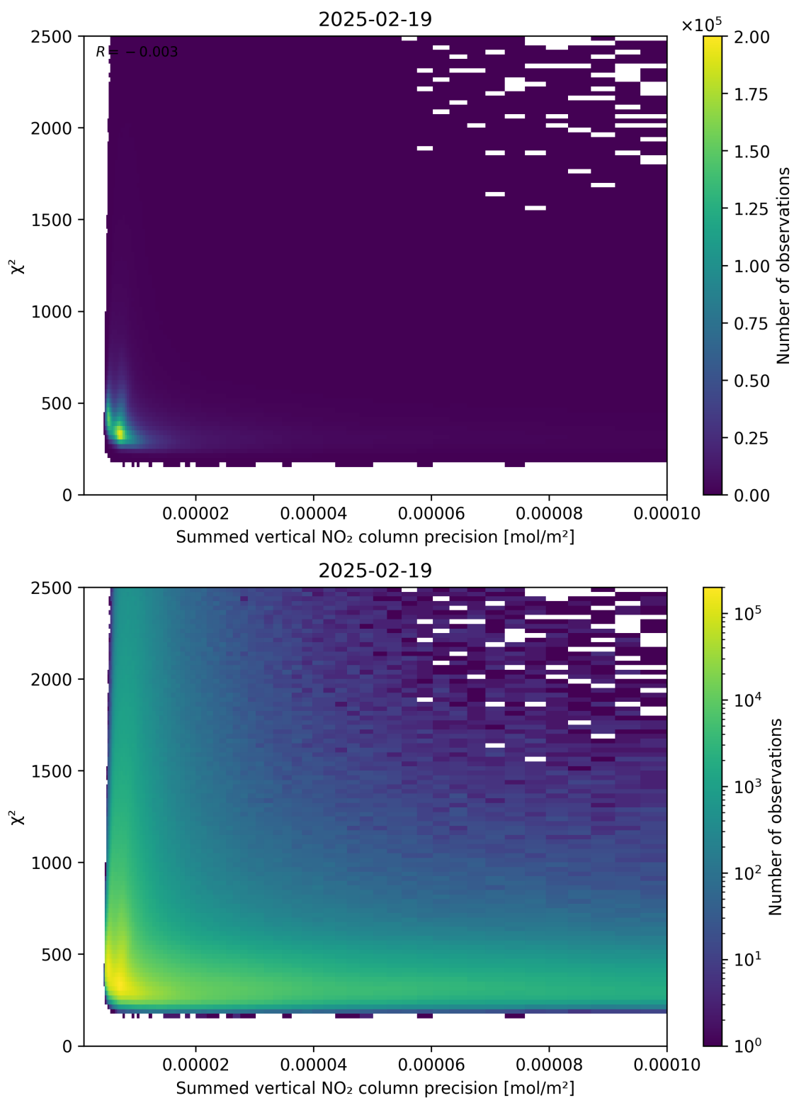
Figure 107: Scatter density plot of “Summed vertical NO 2 column precision” against “ \chi^2 ” for 2025-02-19 to 2025-02-20.
