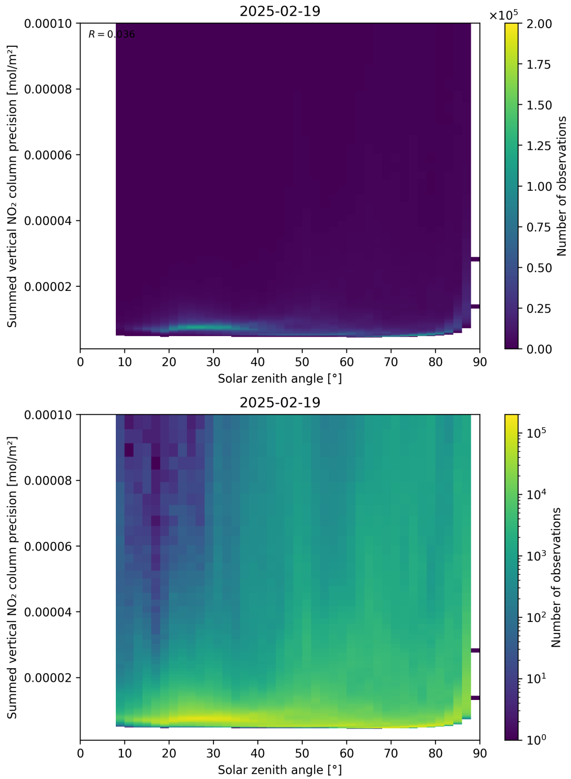
Figure 152: Scatter density plot of “Solar zenith angle” against “Summed vertical NO 2 column precision” for 2025-02-19 to 2025-02-20.
