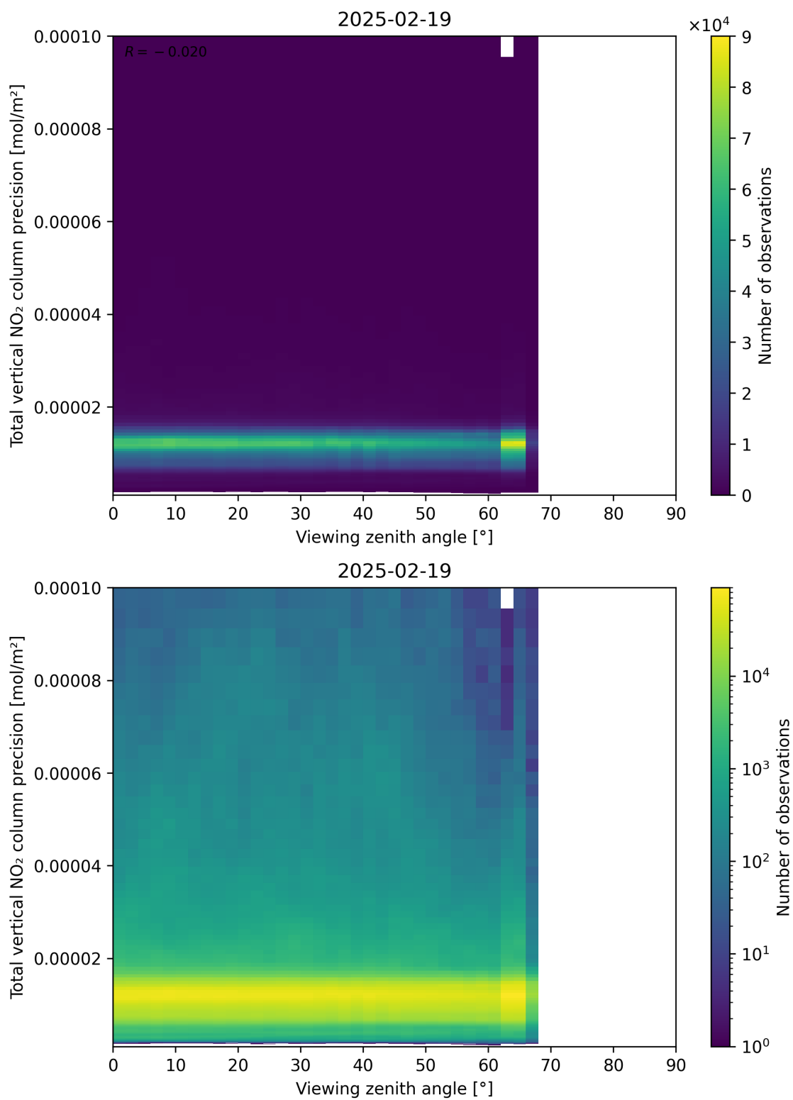
Figure 168: Scatter density plot of “Viewing zenith angle” against “Total vertical NO 2 column precision” for 2025-02-19 to 2025-02-20.
