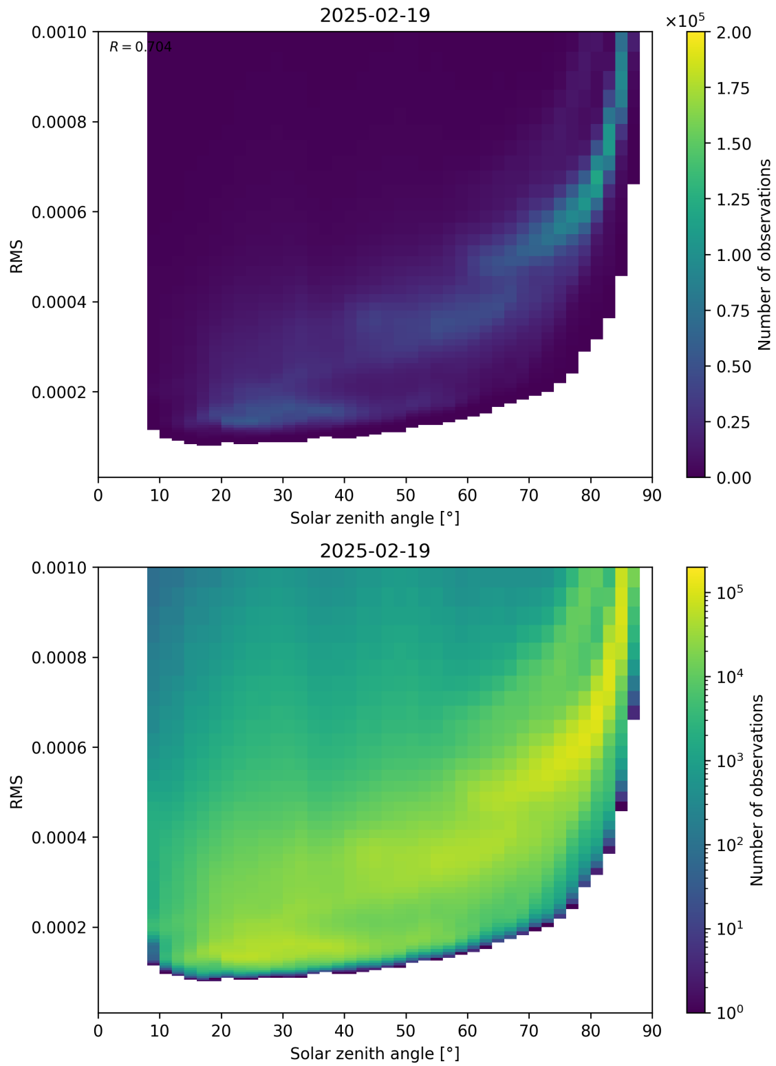
Figure 157: Scatter density plot of “Solar zenith angle” against “RMS” for 2025-02-19 to 2025-02-20.
