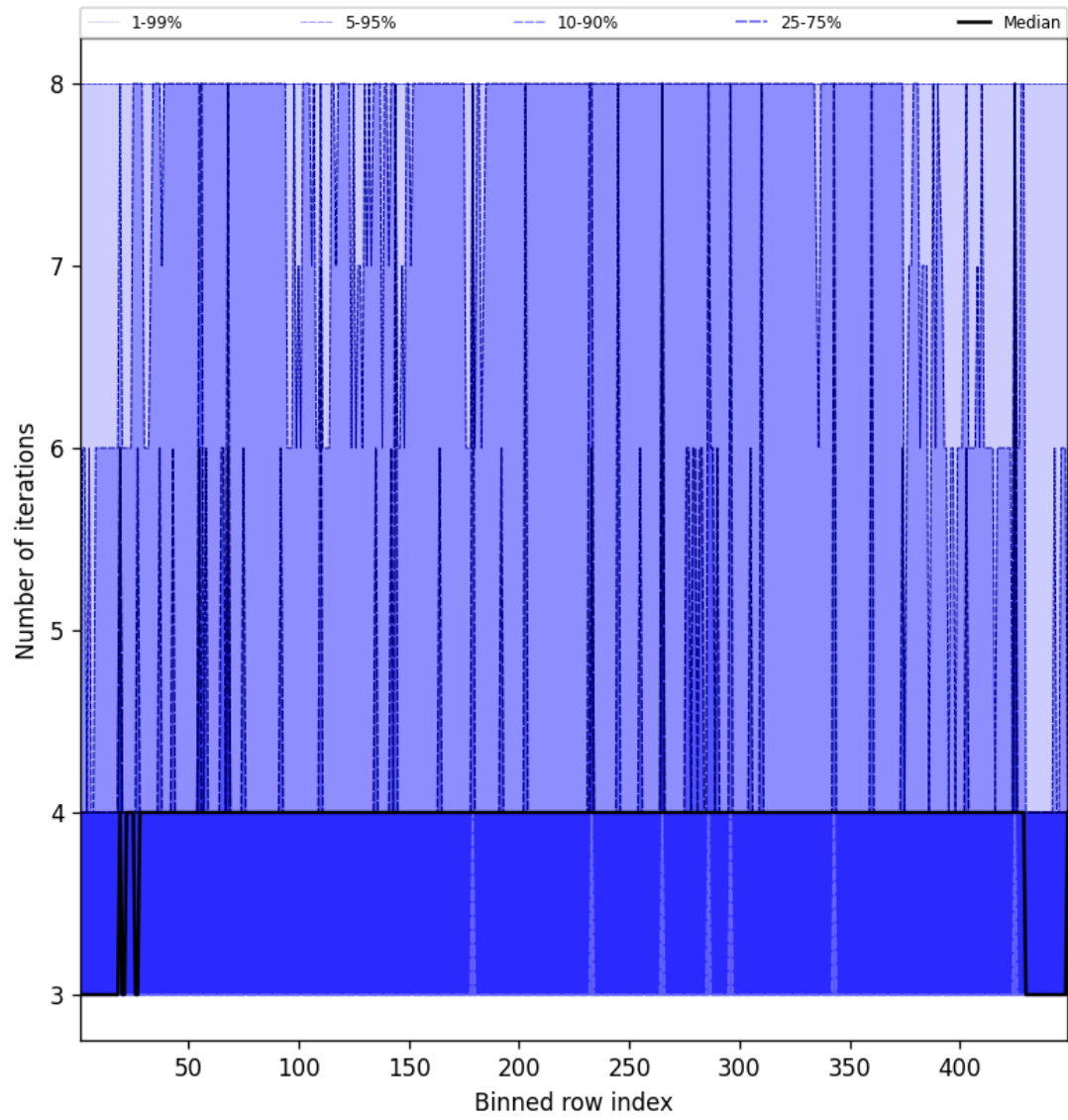
Figure 51: Along track statistics of “Number of iterations” for 2025-02-19 to 2025-02-20
