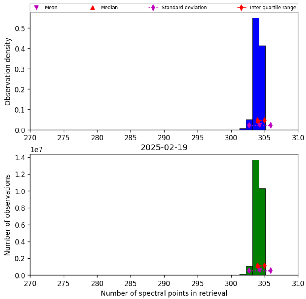
Figure 33: Histogram of “Number of spectral points in retrieval” for 2025-02-19 to 2025-02-20
