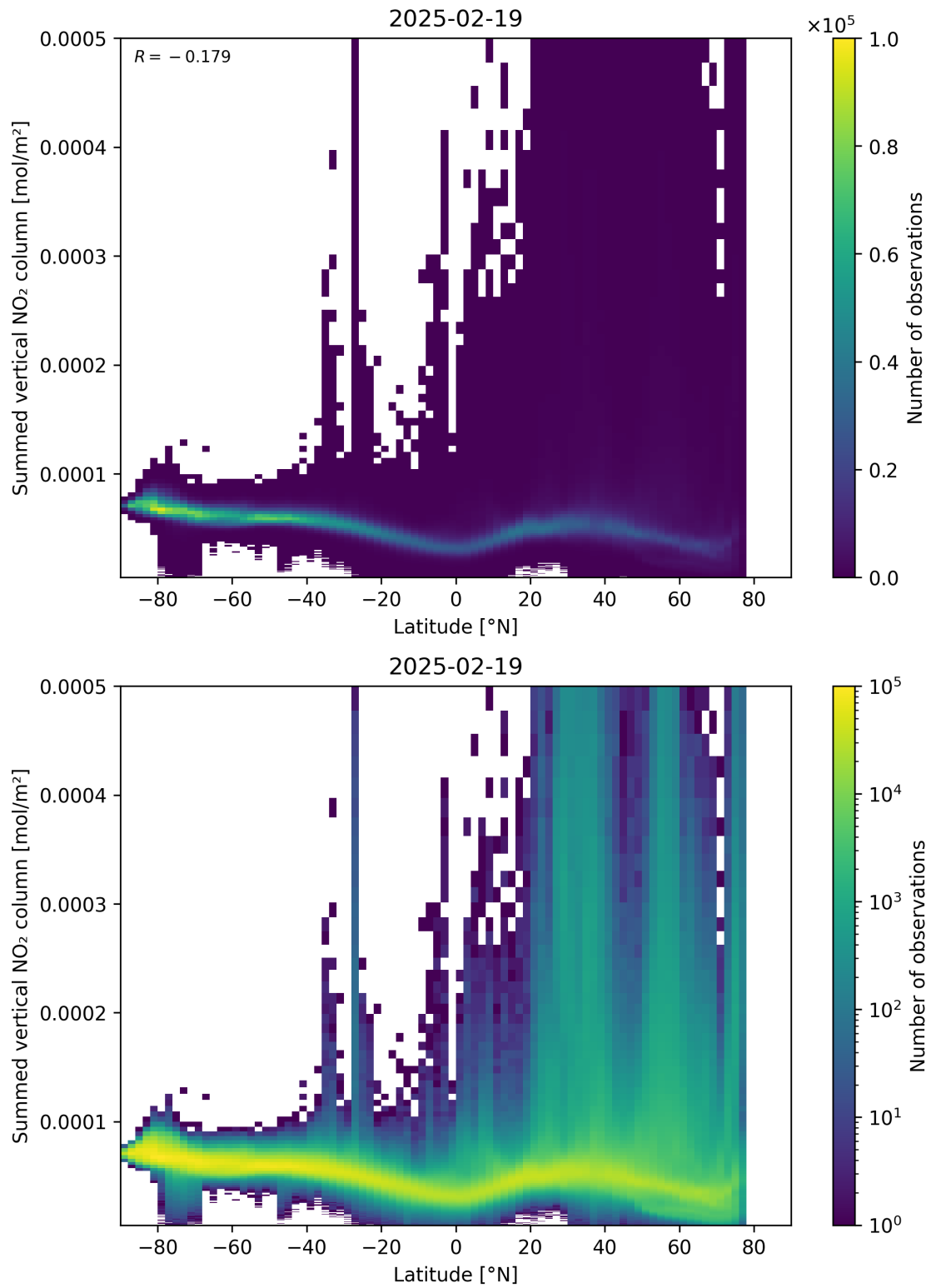
Figure 88: Scatter density plot of “Latitude” against “Summed vertical NO 2 column” for 2025-02-19 to 2025-02-20.
