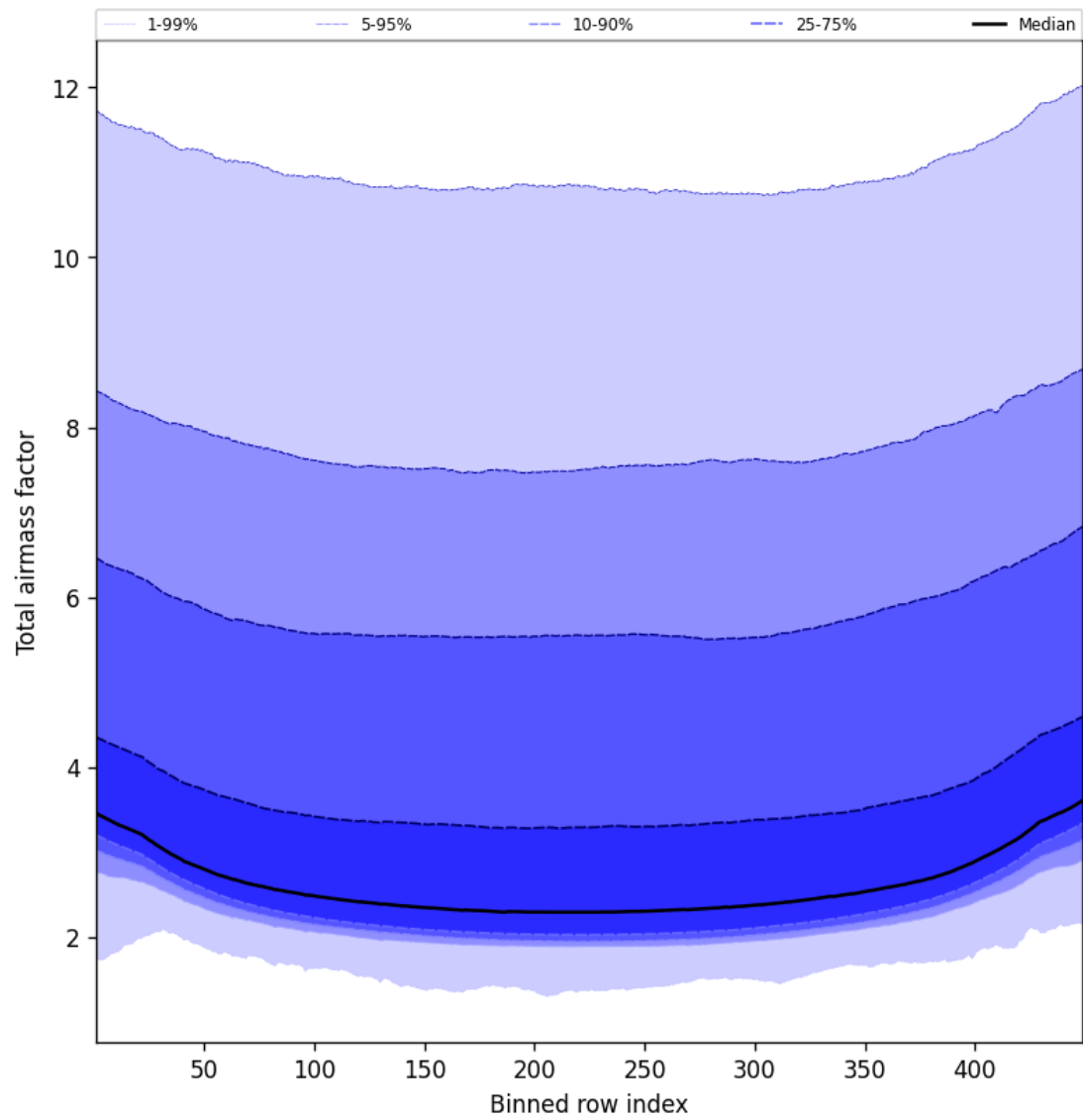
Figure 49: Along track statistics of “Total airmass factor” for 2025-02-19 to 2025-02-20
