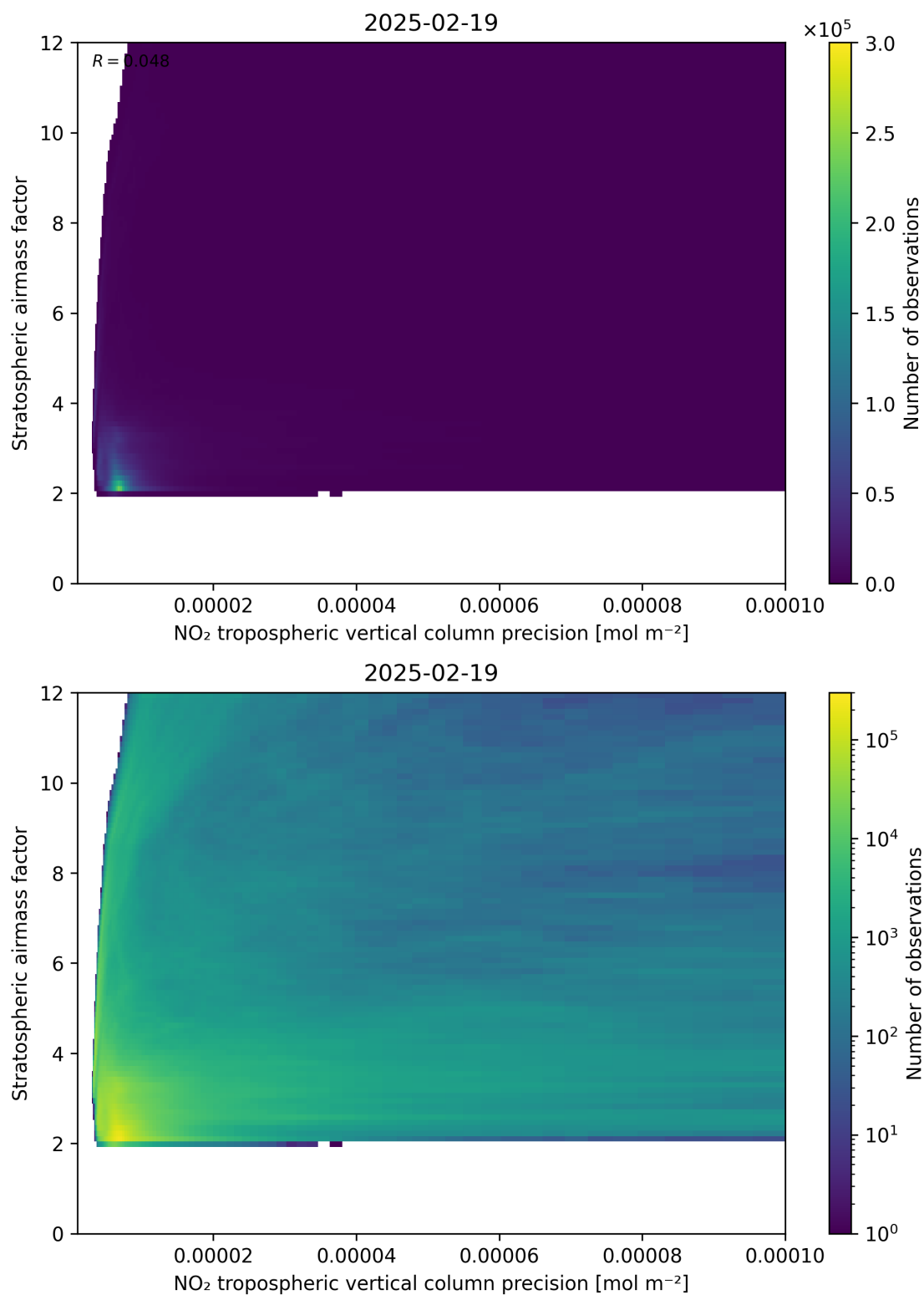
Figure 131: Scatter density plot of “NO 2 tropospheric vertical column precision” against “Stratospheric airmass factor” for 2025-02-19 to 2025-02-20.
