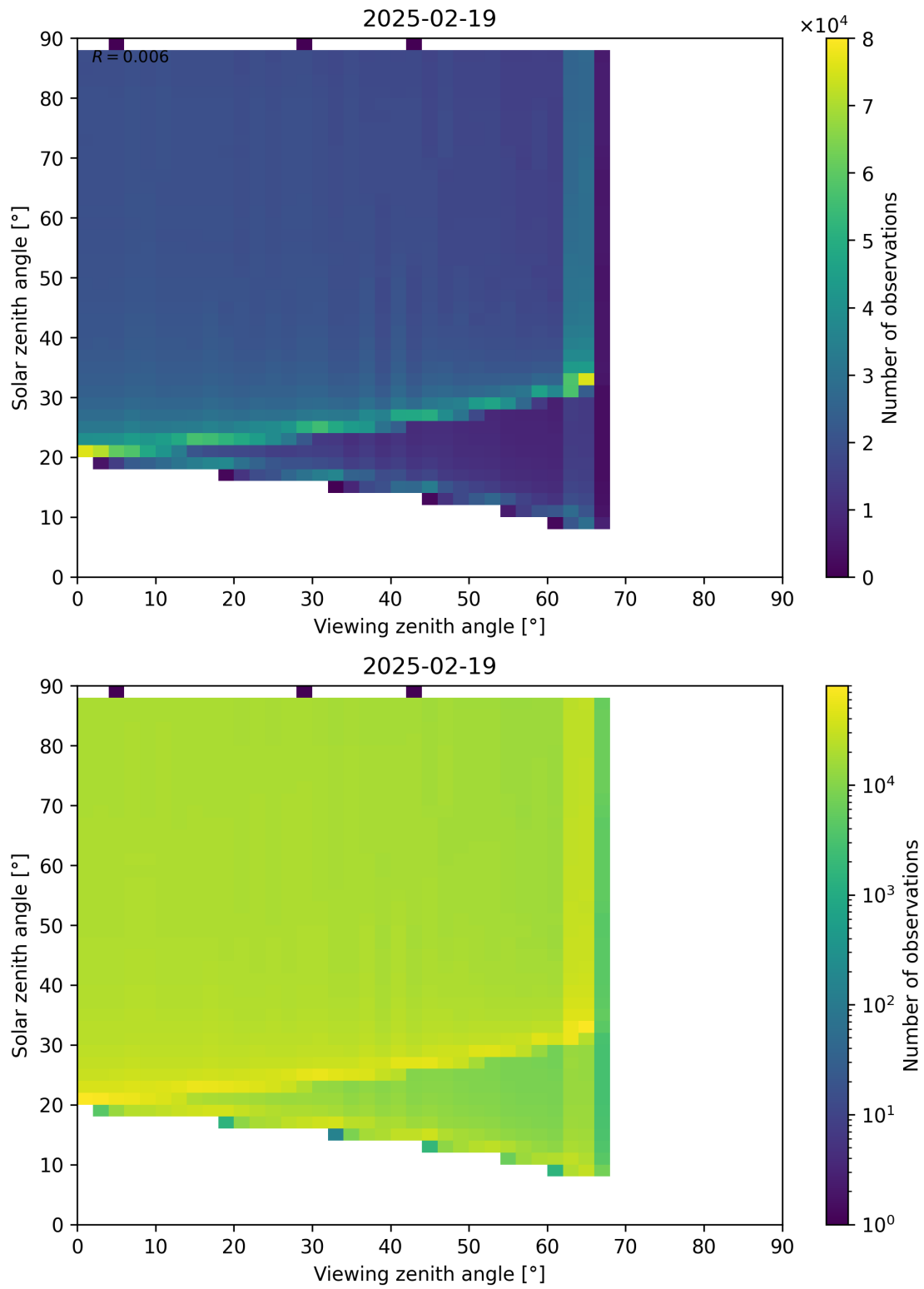
Figure 172: Scatter density plot of “Viewing zenith angle” against “Solar zenith angle” for 2025-02-19 to 2025-02-20.
