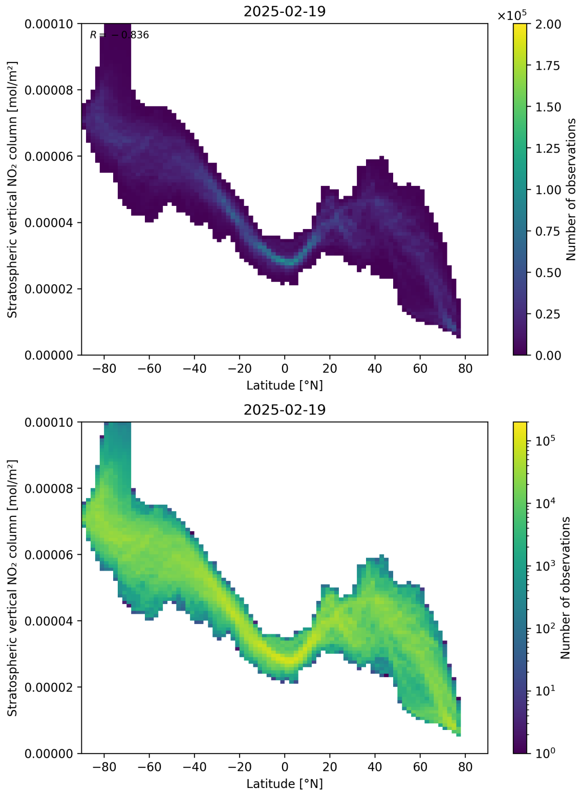
Figure 87: Scatter density plot of “Latitude” against “Stratospheric vertical NO 2 column” for 2025-02-19 to 2025-02-20.
