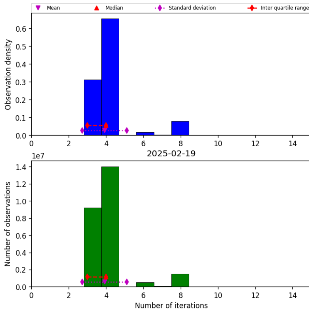
Figure 34: Histogram of “Number of iterations” for 2025-02-19 to 2025-02-20
