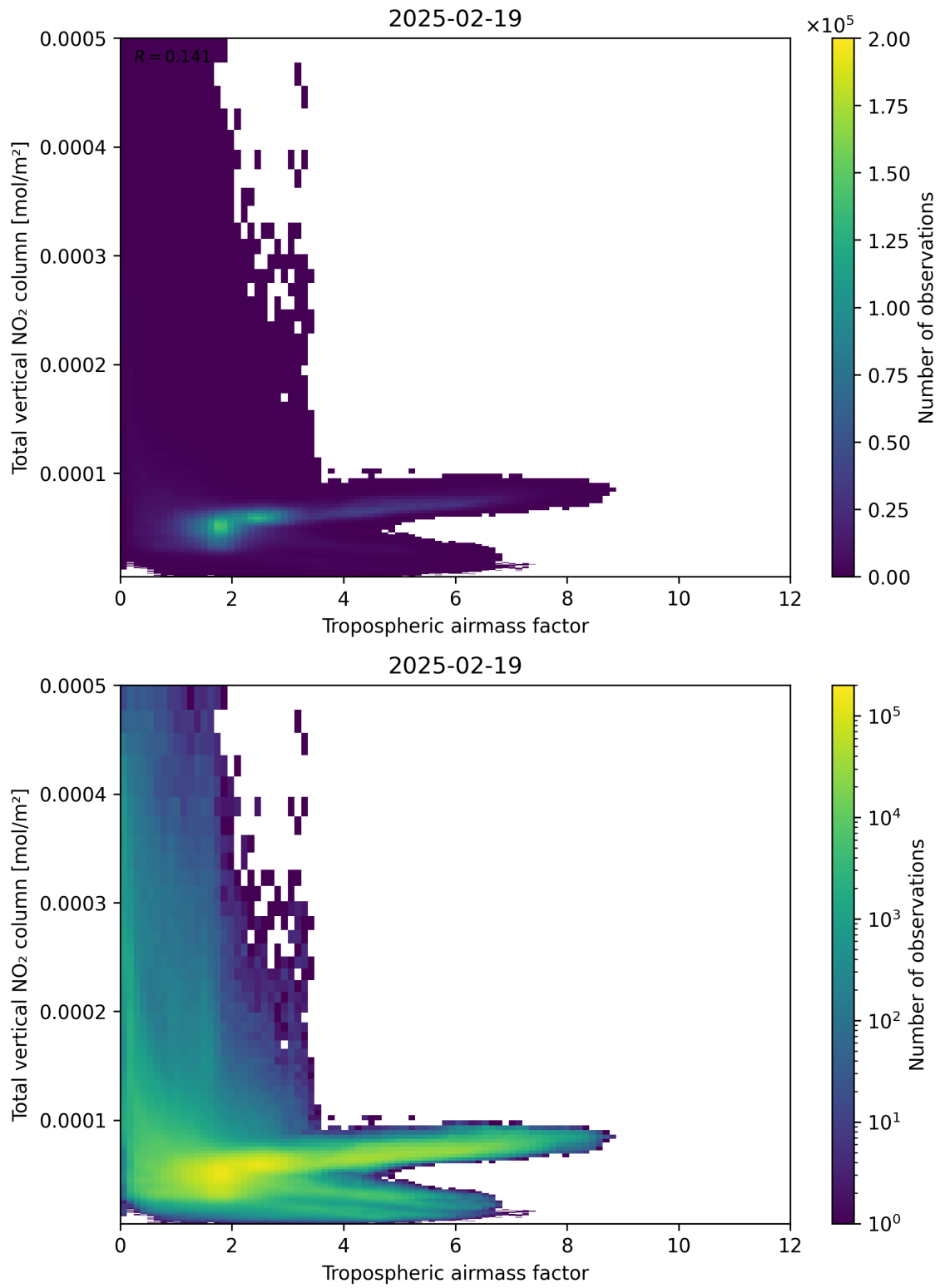
Figure 77: Scatter density plot of “Tropospheric airmass factor” against “Total vertical NO 2 column” for 2025-02-19 to 2025-02-20.
