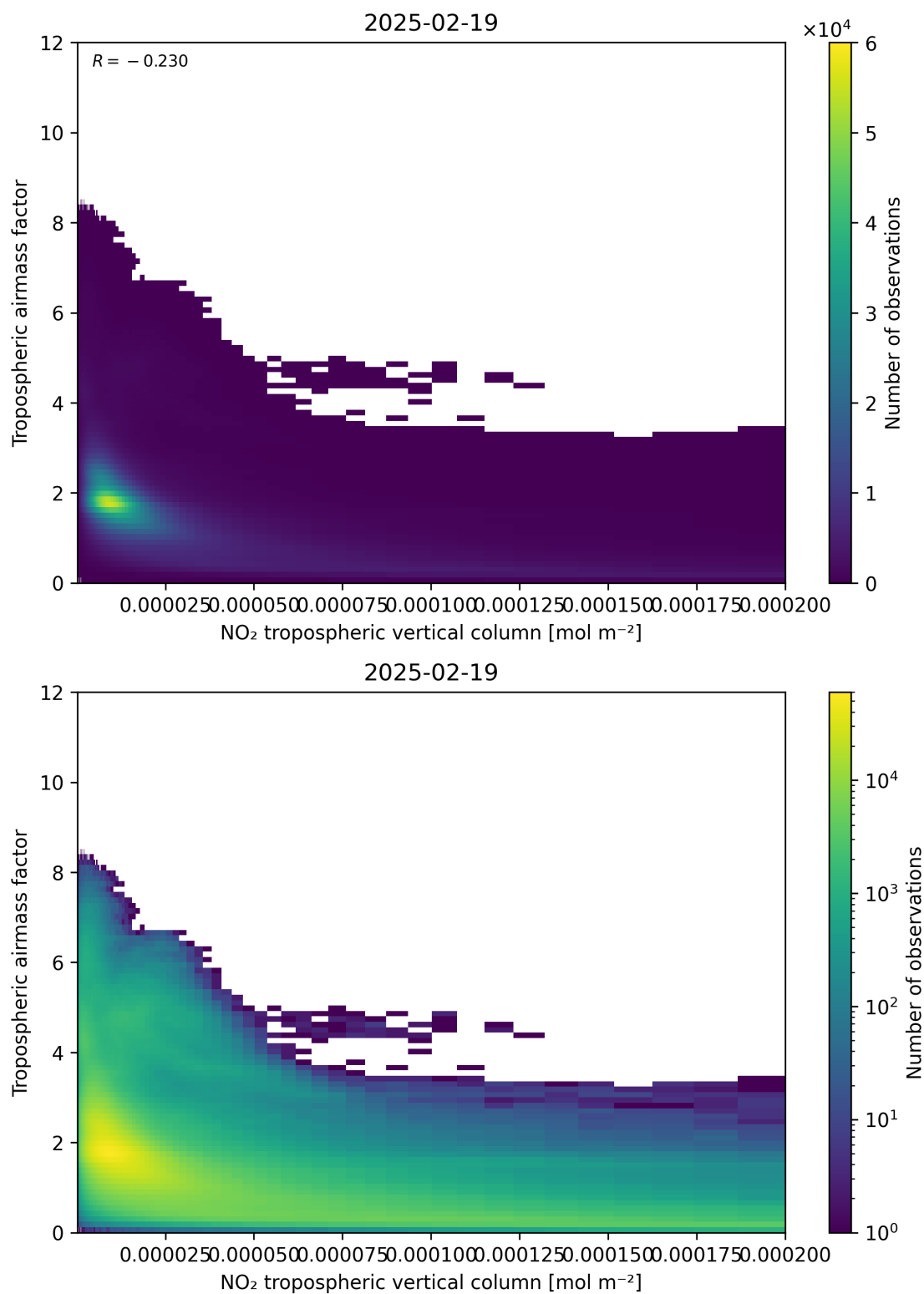
Figure 123: Scatter density plot of “NO 2 tropospheric vertical column” against “Tropospheric air mass factor” for 2025-02-19 to 2025-02-20.
