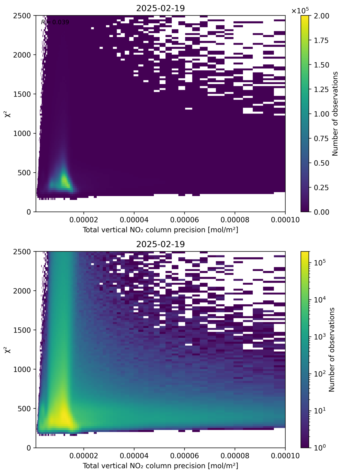
Figure 116: Scatter density plot of “Total vertical NO 2 column precision” against “ \chi^2 ” for 2025-02-19 to 2025-02-20.
