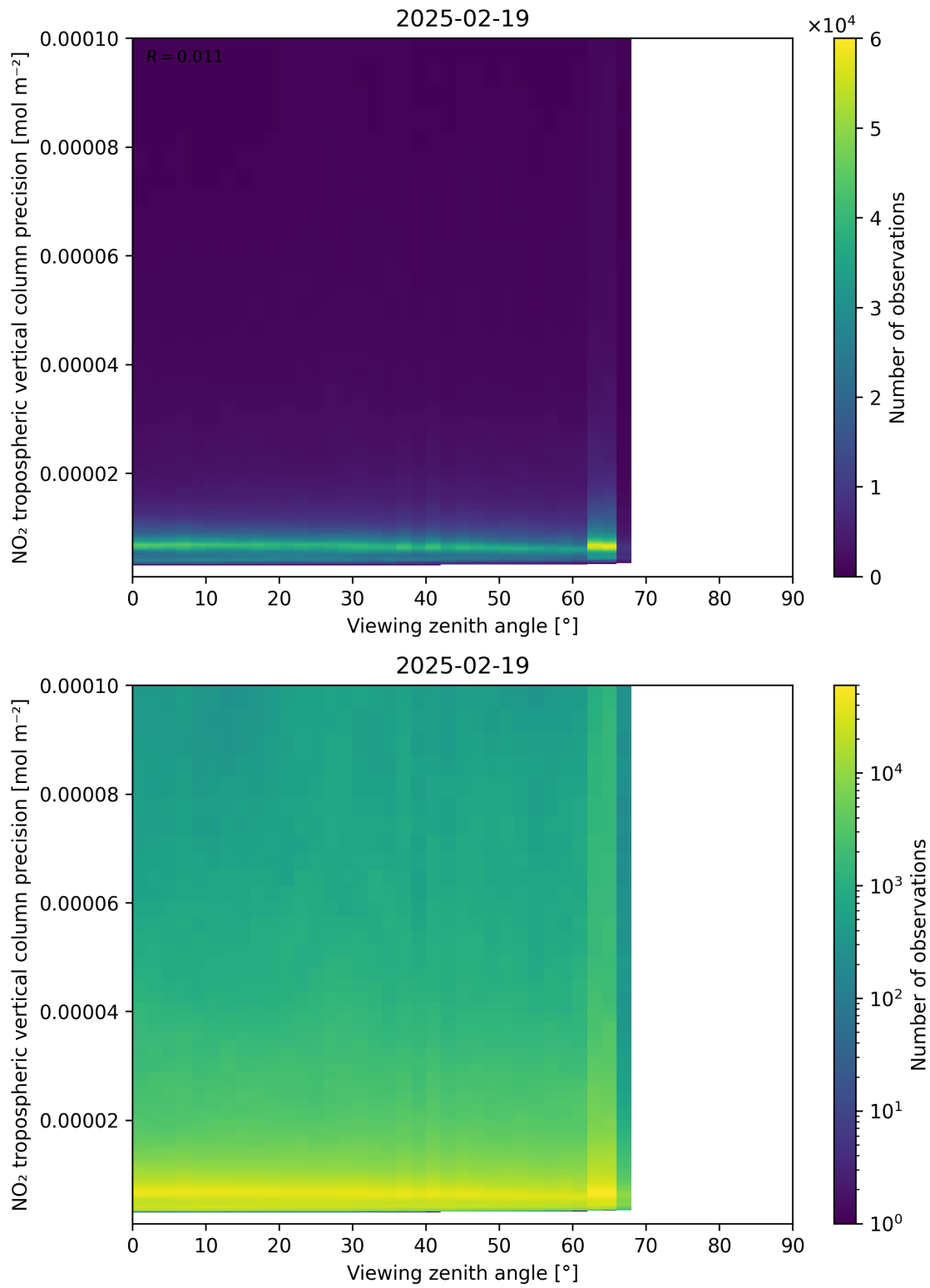
Figure 170: Scatter density plot of “Viewing zenith angle” against “NO 2 tropospheric vertical column precision” for 2025-02-19 to 2025-02-20.
