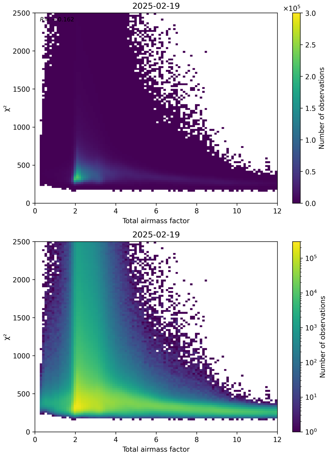
Figure 63: Scatter density plot of “Total airmass factor” against “ \chi^2 ” for 2025-02-19 to 2025-02-20.
