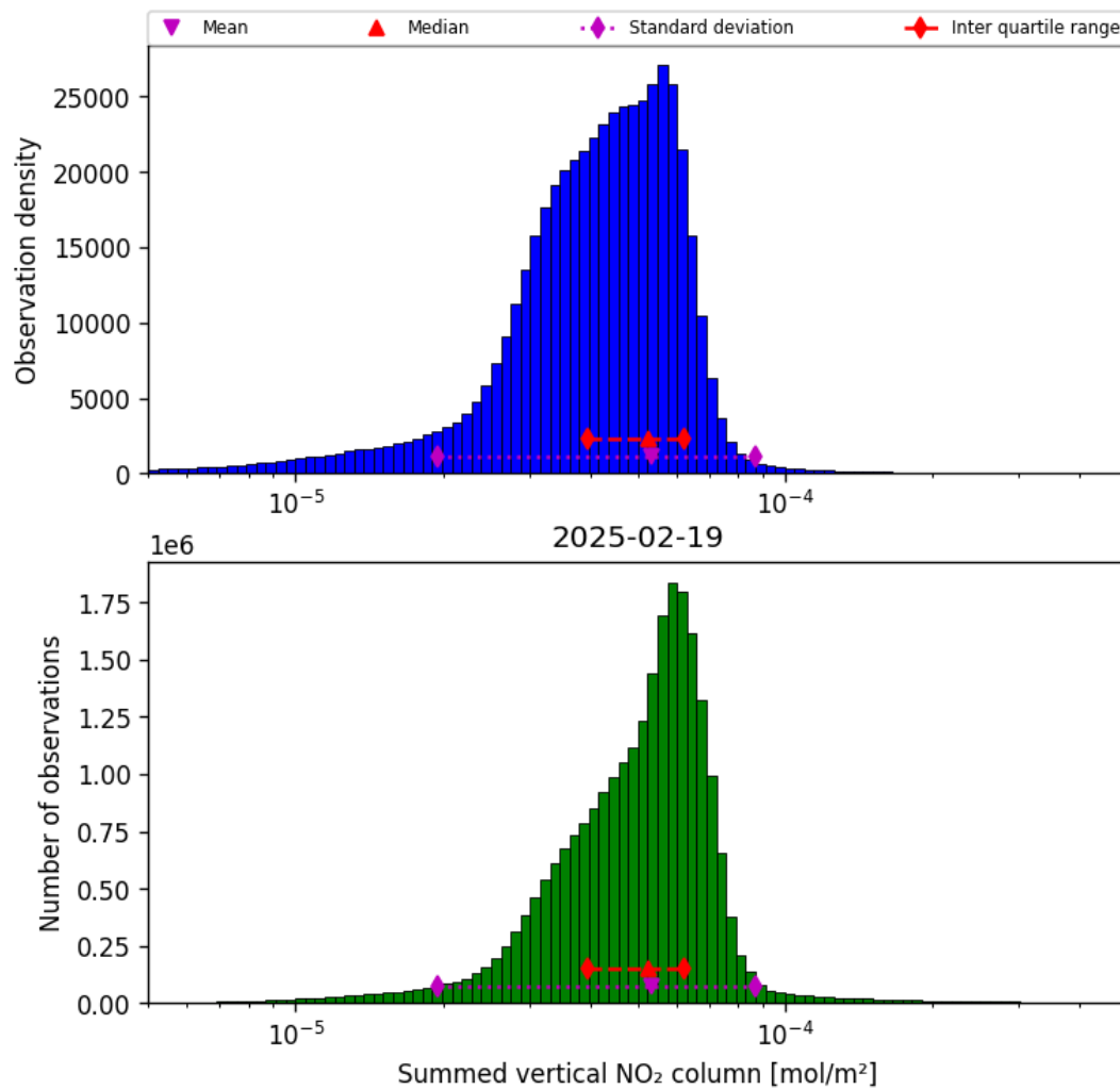
Figure 40: Histogram of “Summed vertical NO 2 column” for 2025-02-19 to 2025-02-20
