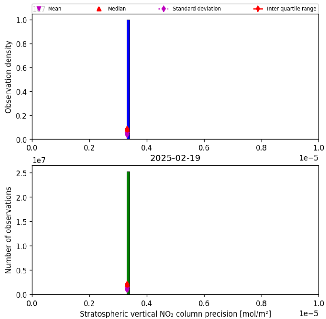
Figure 37: Histogram of “Stratospheric vertical NO 2 column precision” for 2025-02-19 to 2025-02-20
