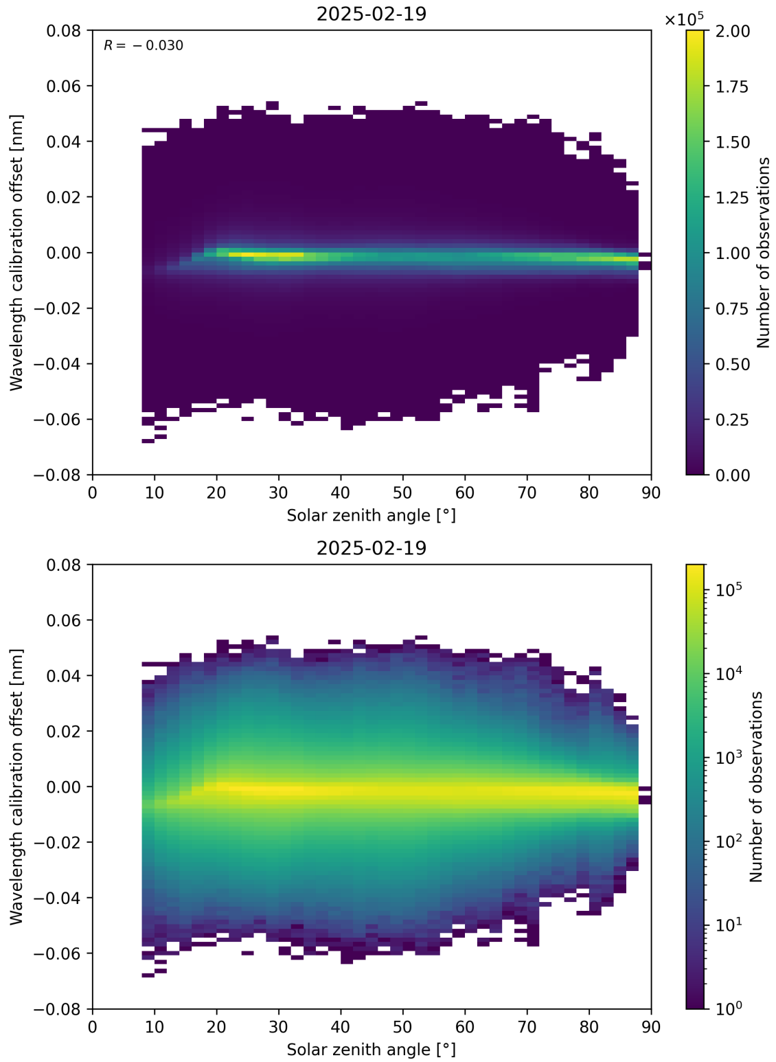
Figure 158: Scatter density plot of “Solar zenith angle” against “Wavelength calibration offset” for 2025-02-19 to 2025-02-20.
