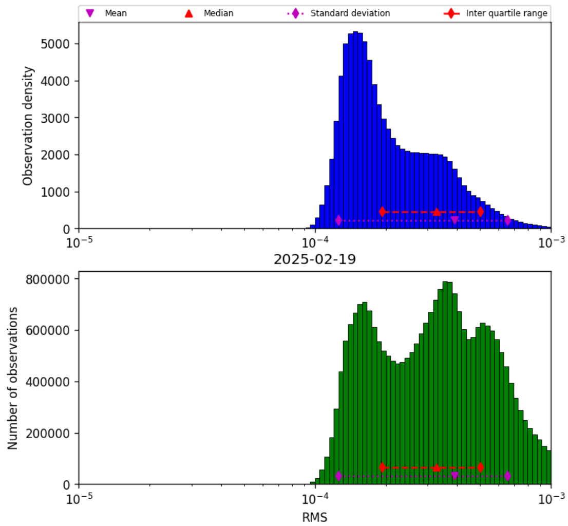
Figure 43: Histogram of “RMS” for 2025-02-19 to 2025-02-20
