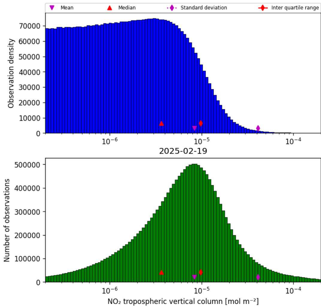
Figure 29: Histogram of “NO 2 tropospheric vertical column” for 2025-02-19 to 2025-02-20
