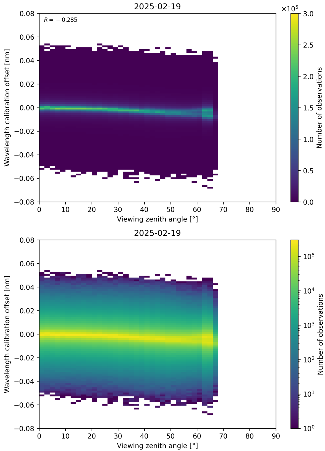
Figure 173: Scatter density plot of “Viewing zenith angle” against “Wavelength calibration offset” for 2025-02-19 to 2025-02-20.
