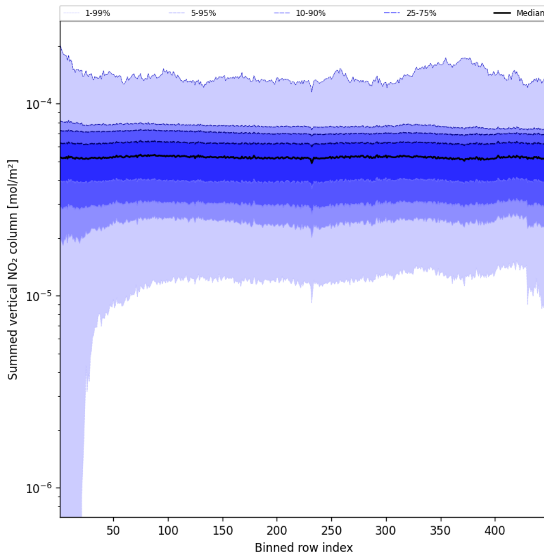
Figure 57: Along track statistics of “Summed vertical NO 2 column” for 2025-02-19 to 2025-02-20
