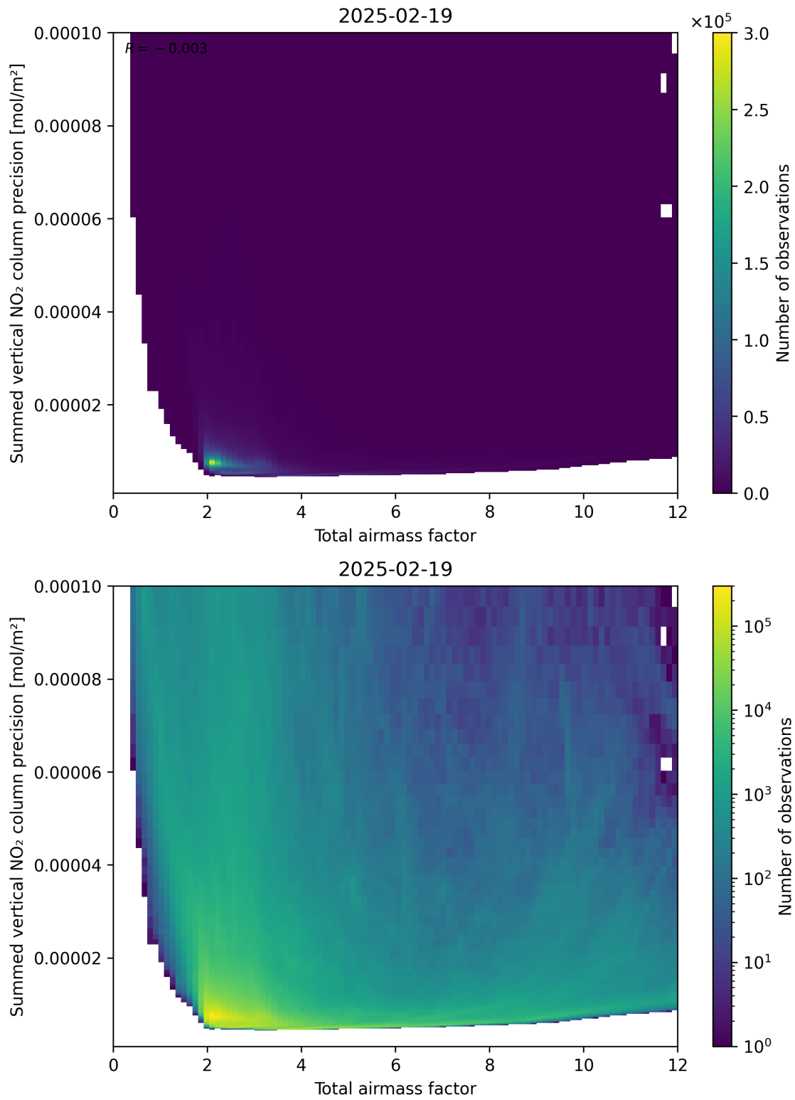
Figure 66: Scatter density plot of “Total airmass factor” against “Summed vertical NO 2 column precision” for 2025-02-19 to 2025-02-20.
