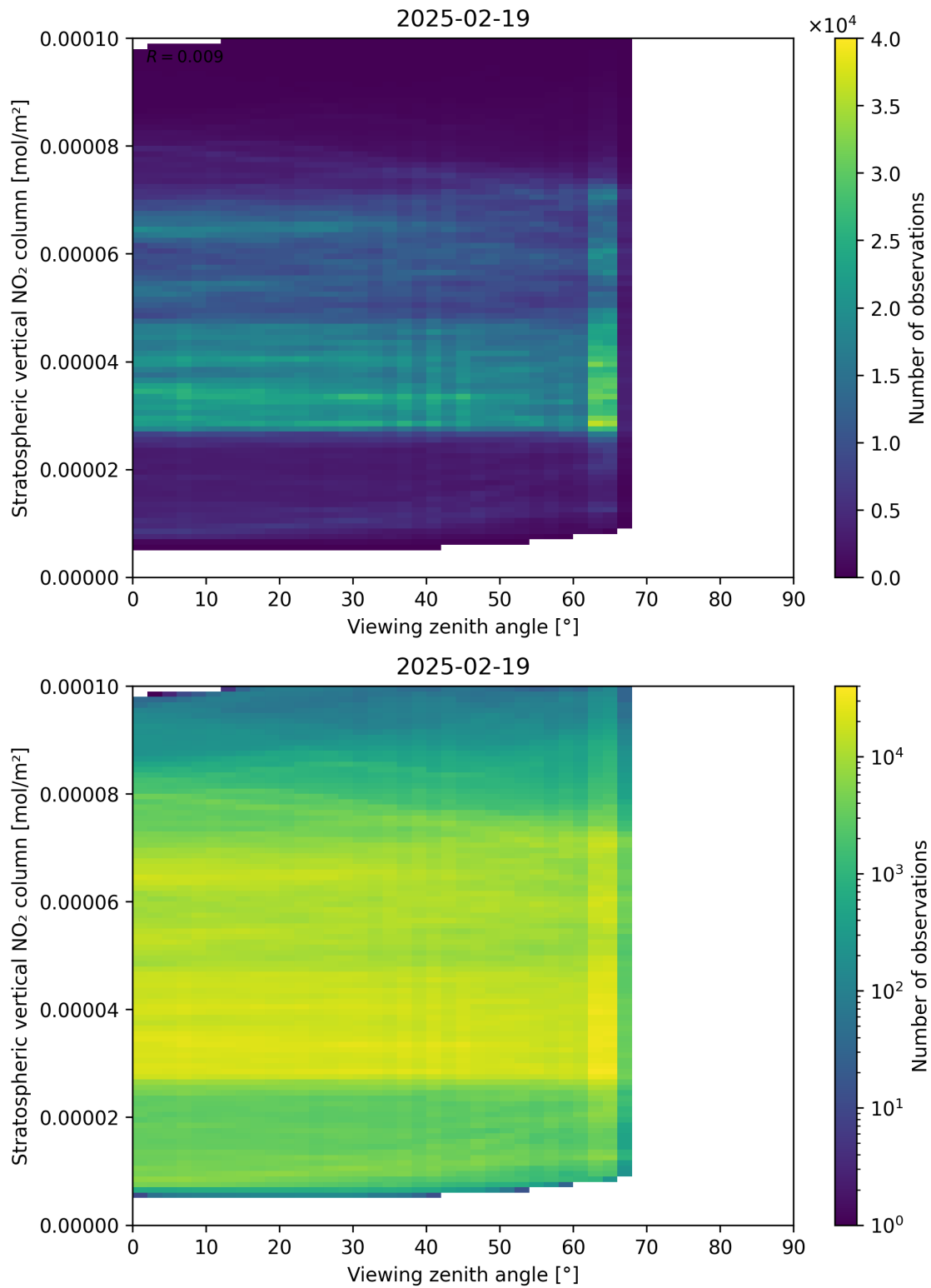
Figure 164: Scatter density plot of “Viewing zenith angle” against “Stratospheric vertical NO 2 column” for 2025-02-19 to 2025-02-20.
