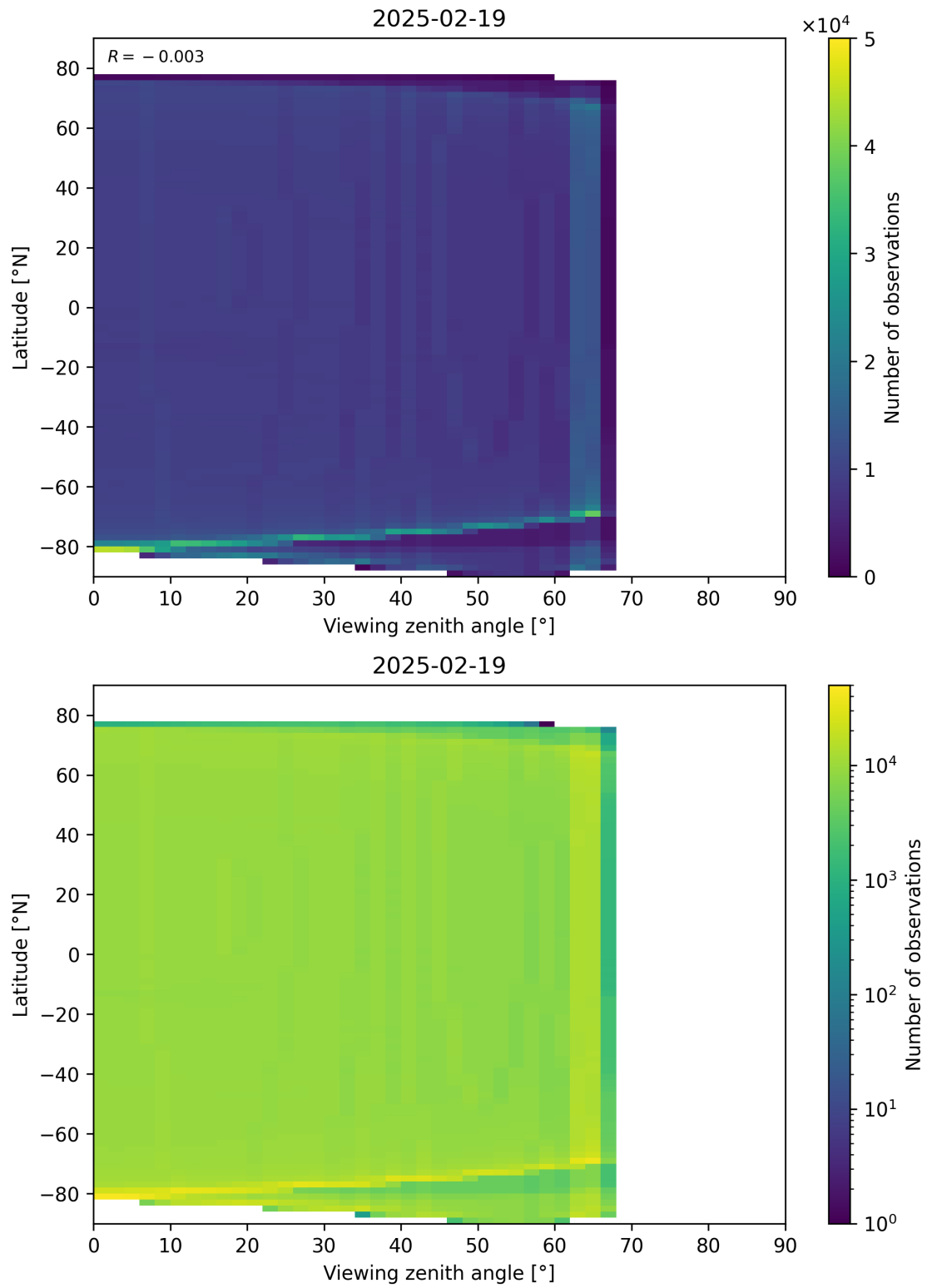
Figure 163: Scatter density plot of “Viewing zenith angle” against “Latitude” for 2025-02-19 to 2025-02-20.
