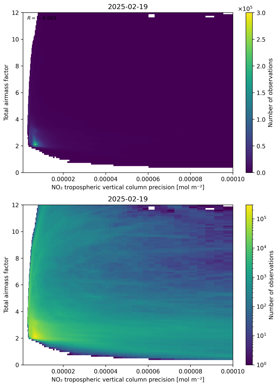
Figure 132: Scatter density plot of “NO 2 tropospheric vertical column precision” against “Total airmass factor” for 2025-02-19 to 2025-02-20.
