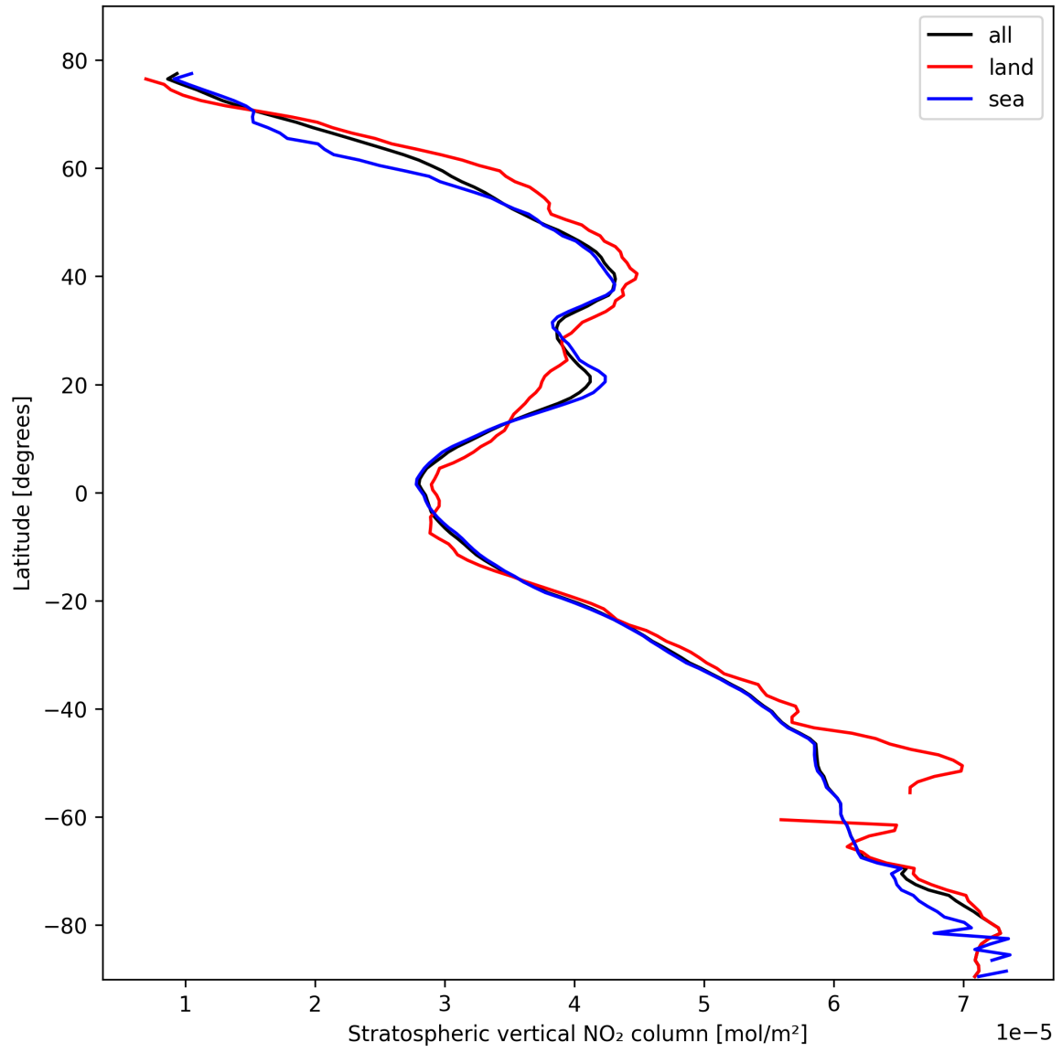
Figure 19: Zonal average of “Stratospheric vertical NO 2 column” for 2025-02-19 to 2025-02-20.
