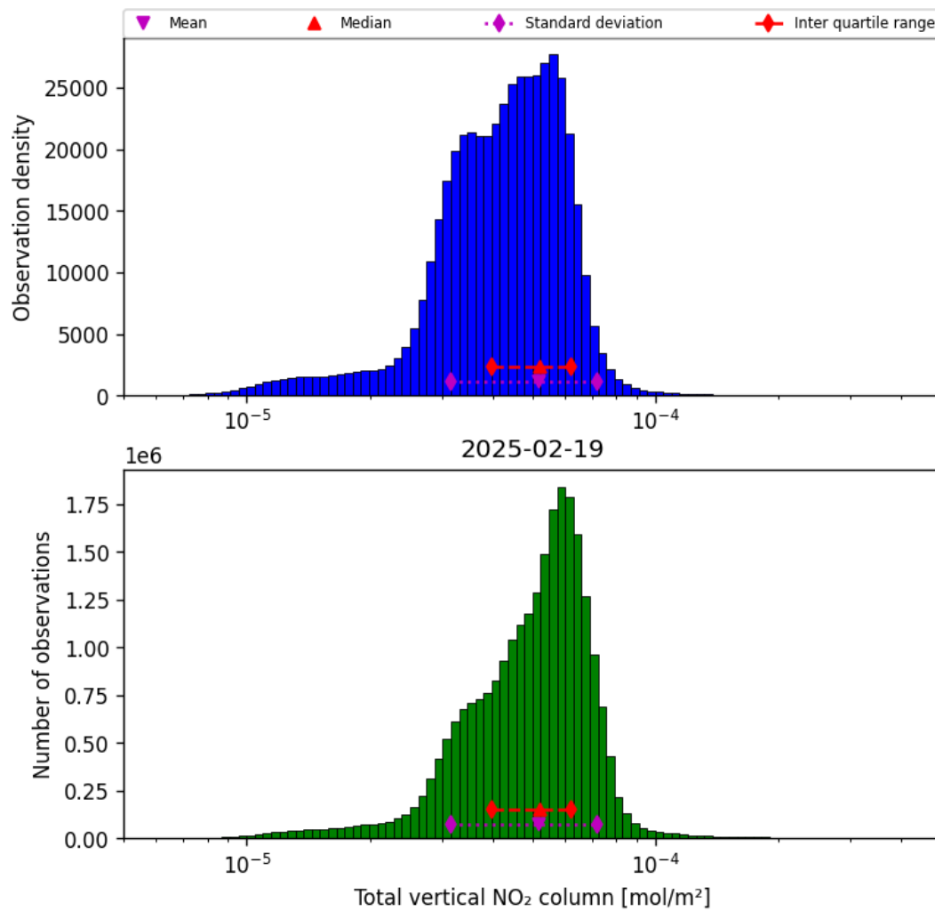
Figure 38: Histogram of “Total vertical NO 2 column” for 2025-02-19 to 2025-02-20
