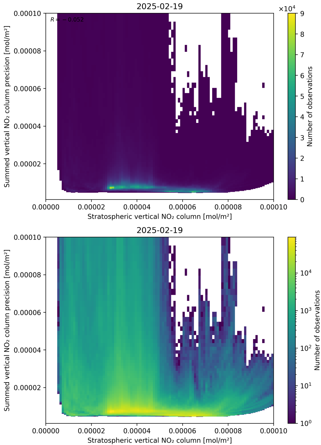
Figure 99: Scatter density plot of “Stratospheric vertical NO 2 column” against “Summed vertical NO 2 column precision” for 2025-02-19 to 2025-02-20.
