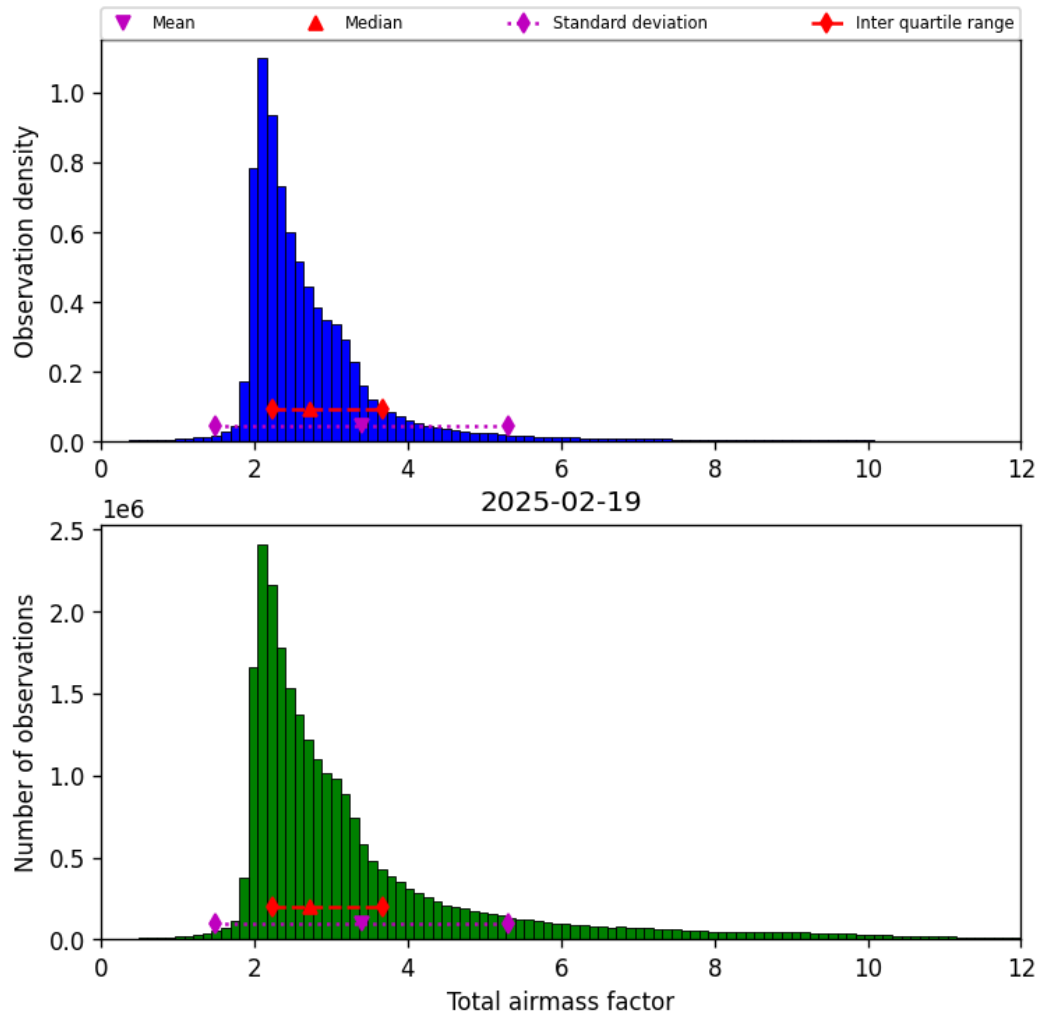
Figure 32: Histogram of “Total airmass factor” for 2025-02-19 to 2025-02-20
