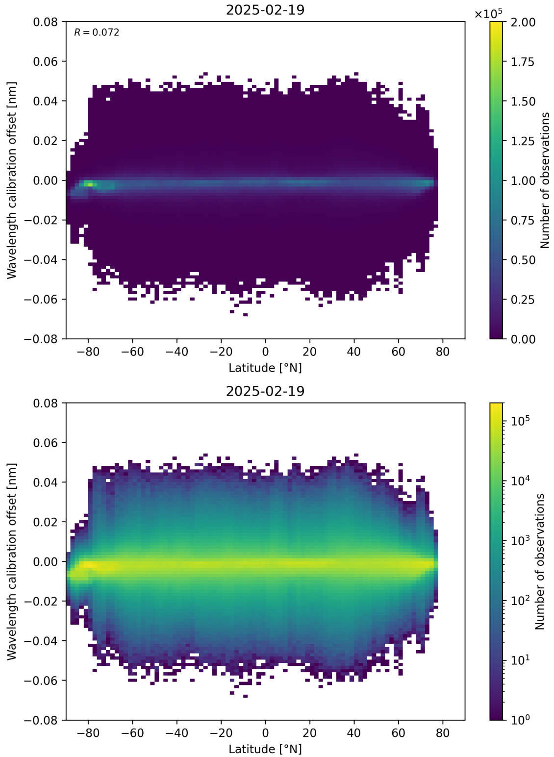
Figure 95: Scatter density plot of “Latitude” against “Wavelength calibration offset” for 2025-02-19 to 2025-02-20.
