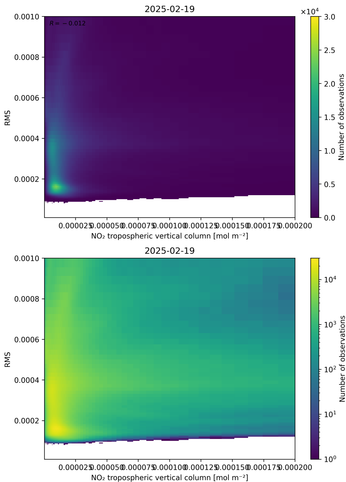
Figure 142: Scatter density plot of “NO 2 tropospheric vertical column” against “RMS” for 2025-02-19 to 2025-02-20.
