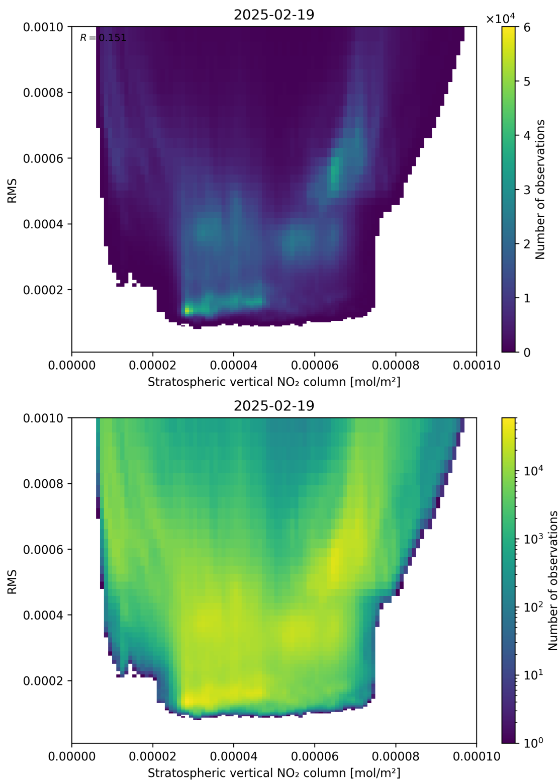
Figure 102: Scatter density plot of “Stratospheric vertical NO 2 column” against “RMS” for 2025-02-19 to 2025-02-20.
