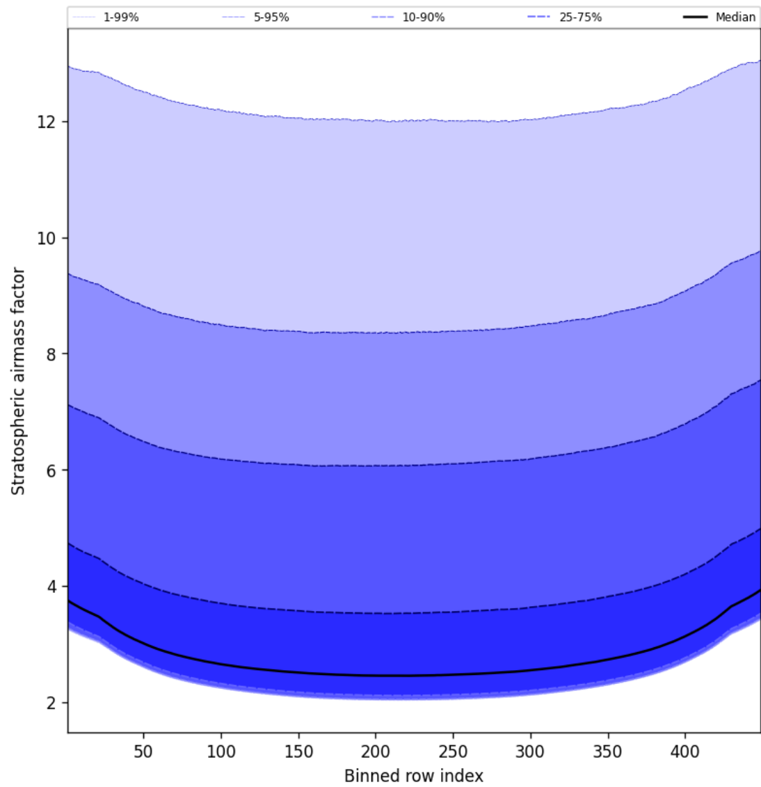
Figure 61: Along track statistics of “Stratospheric airmass factor” for 2025-02-19 to 2025-02-20
