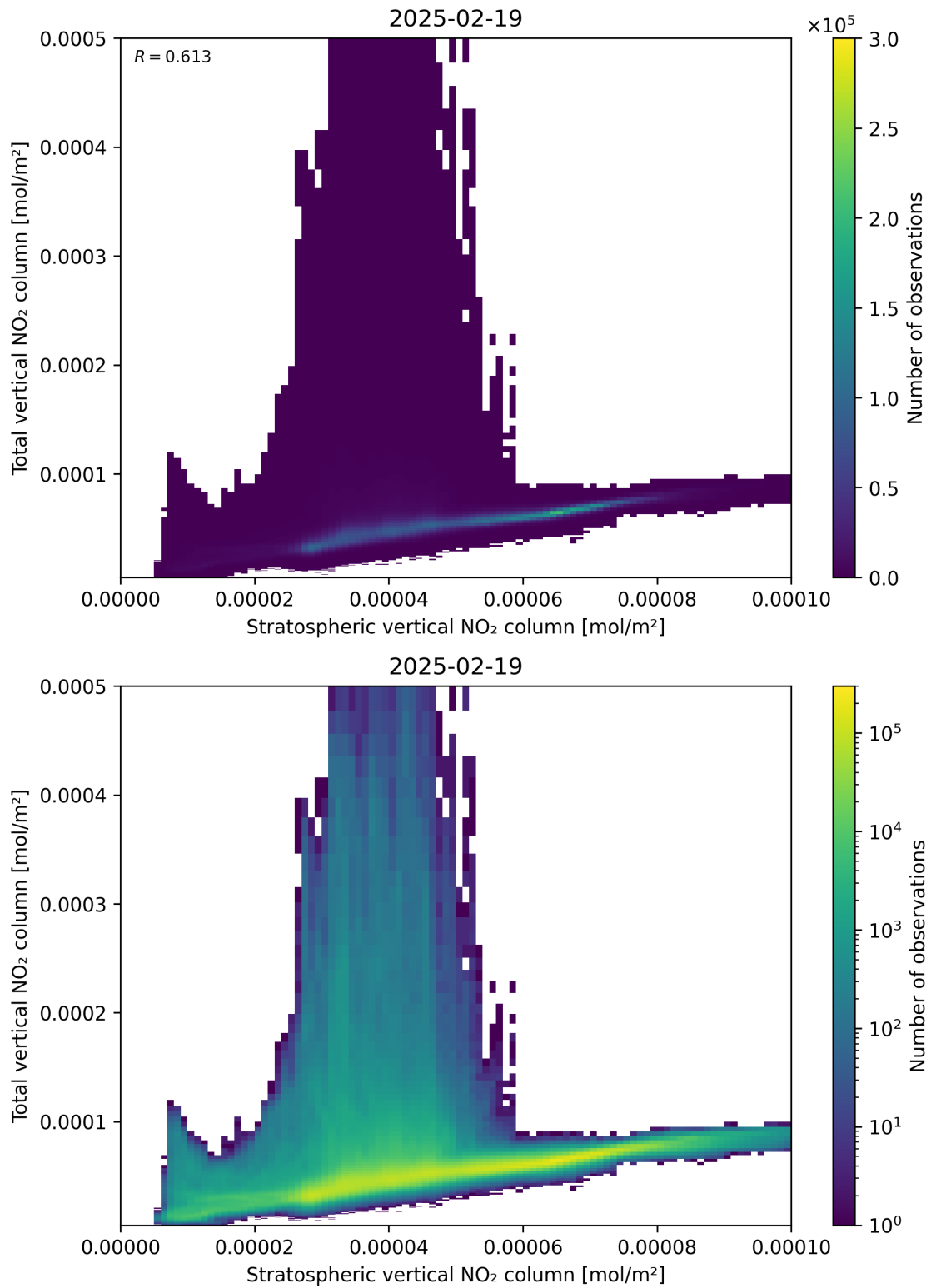
Figure 100: Scatter density plot of “Stratospheric vertical NO 2 column” against “Total vertical NO 2 column” for 2025-02-19 to 2025-02-20.
