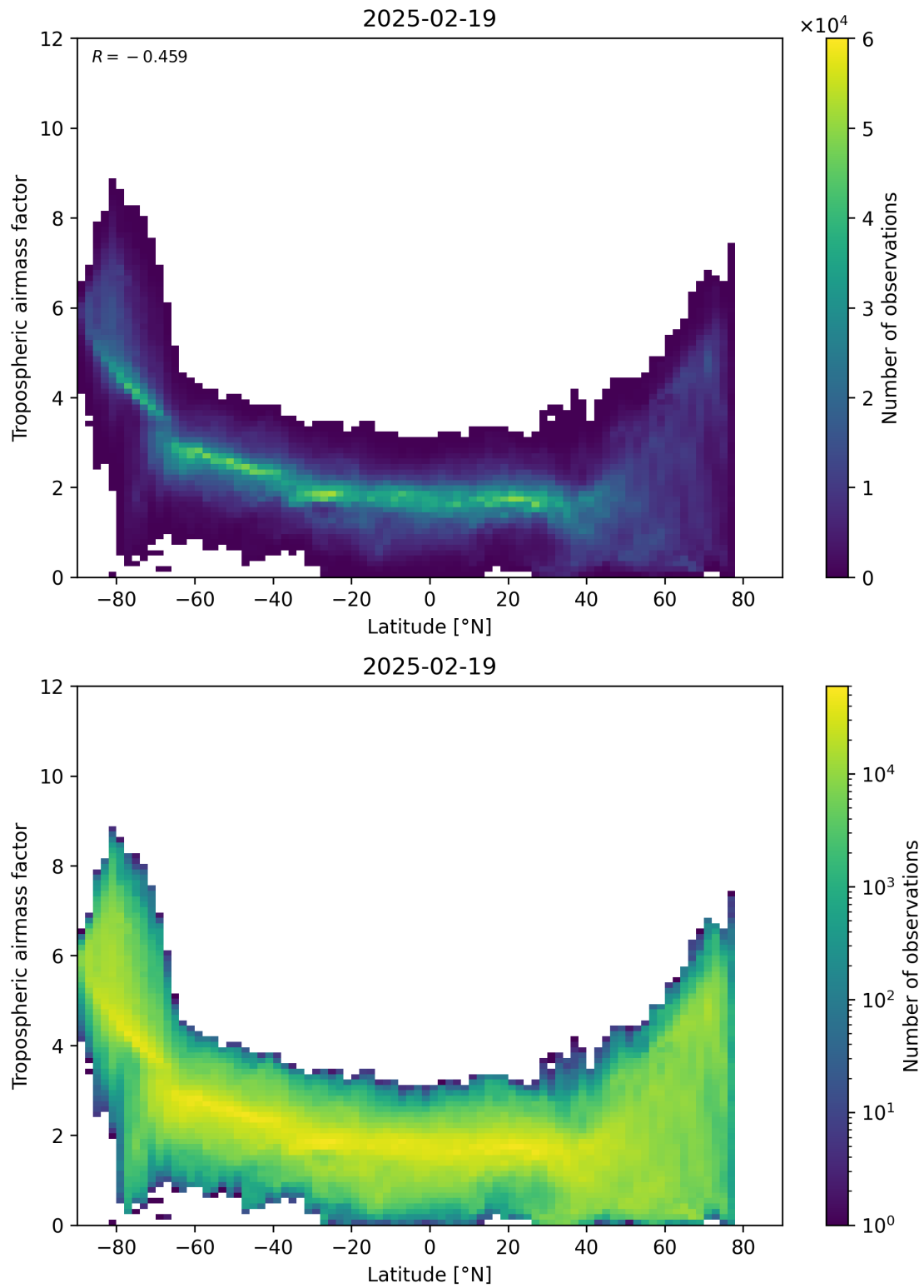
Figure 85: Scatter density plot of “Latitude” against “Tropospheric airmass factor” for 2025-02-19 to 2025-02-20.
