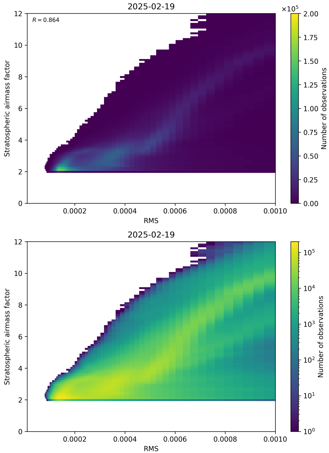
Figure 144: Scatter density plot of “RMS” against “Stratospheric airmass factor” for 2025-02-19 to 2025-02-20.
