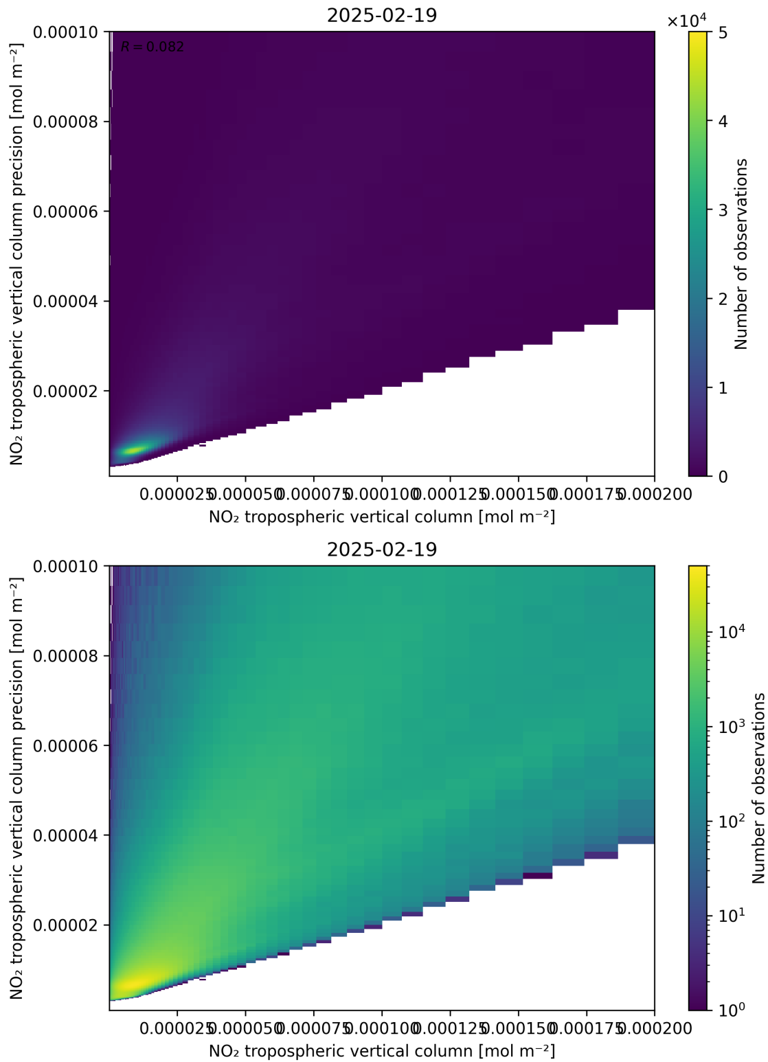
Figure 130: Scatter density plot of “NO 2 tropospheric vertical column” against “NO 2 tropospheric vertical column precision” for 2025-02-19 to 2025-02-20.
