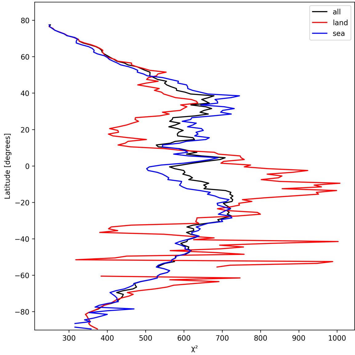
Figure 25: Zonal average of “ \chi^2 ” for 2025-02-19 to 2025-02-20.
