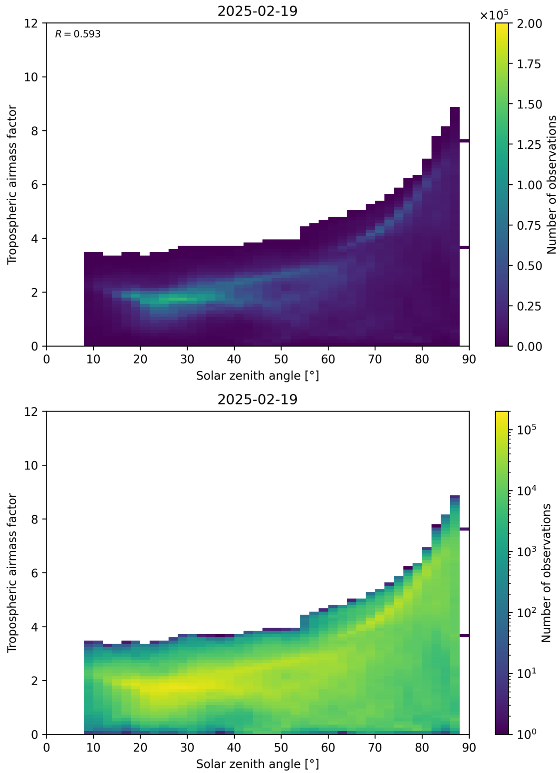
Figure 147: Scatter density plot of “Solar zenith angle” against “Tropospheric airmass factor” for 2025-02-19 to 2025-02-20.
