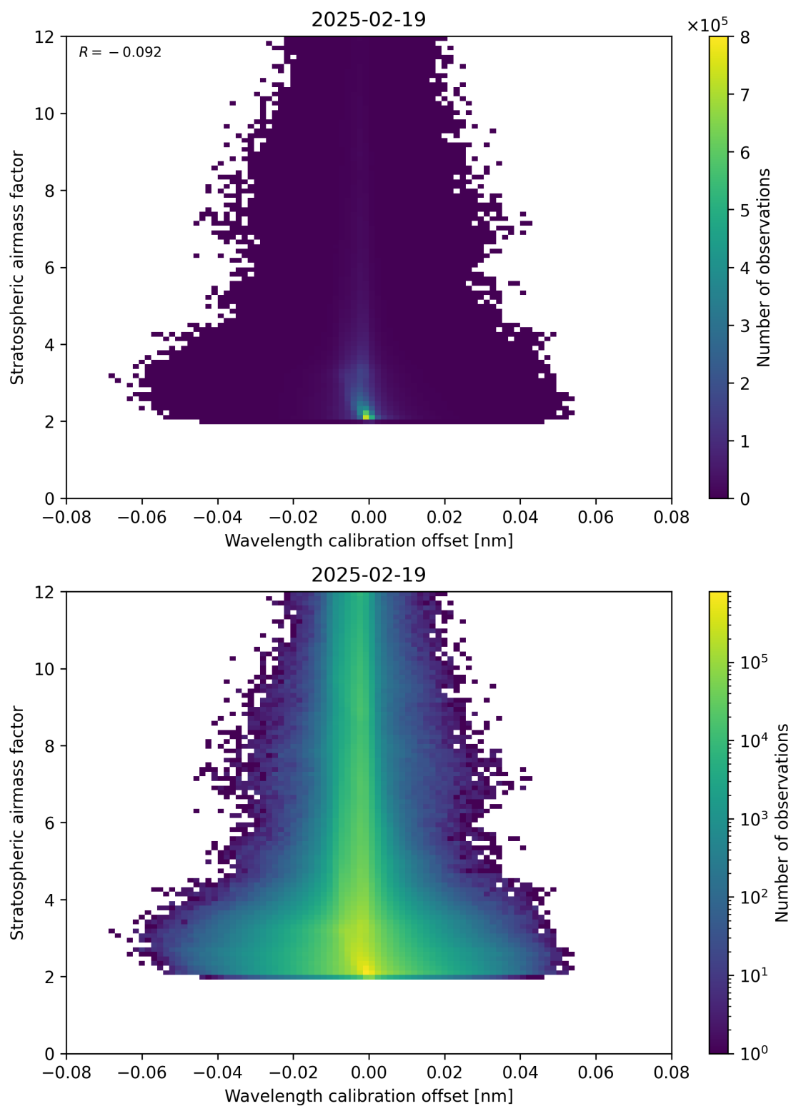
Figure 174: Scatter density plot of “Wavelength calibration offset” against “Stratospheric airmass factor” for 2025-02-19 to 2025-02-20.
