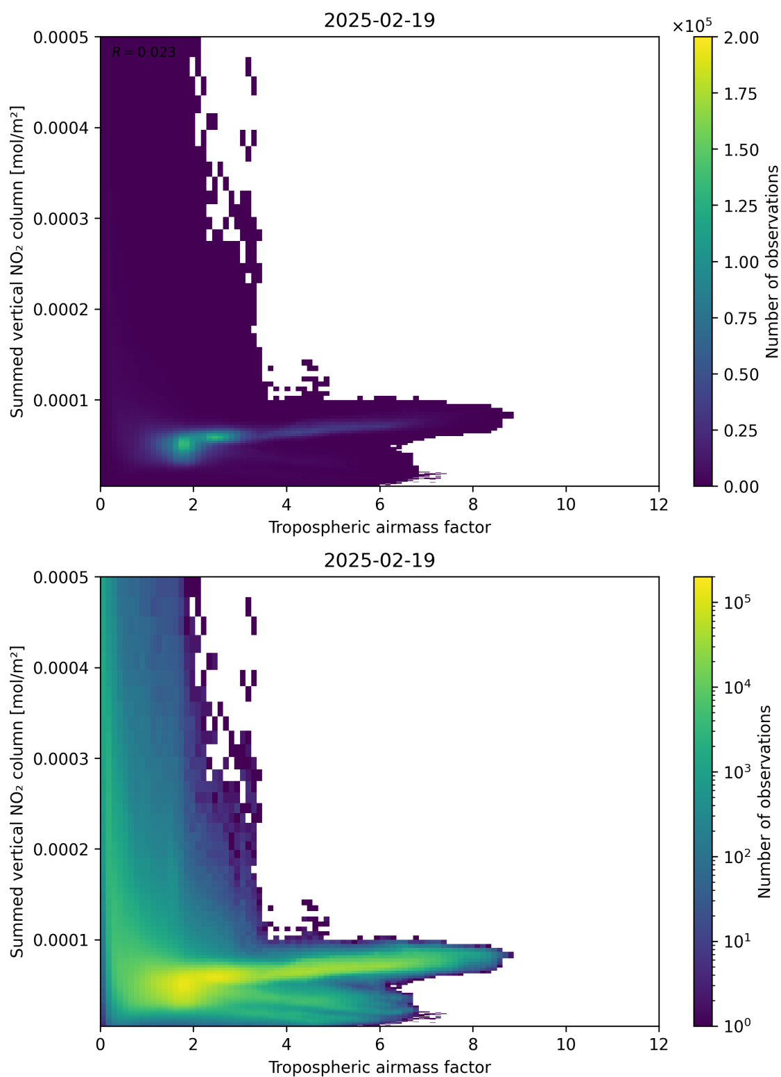
Figure 75: Scatter density plot of “Tropospheric air mass factor” against “Summed vertical NO 2 column” for 2025-02-19 to 2025-02-20.
