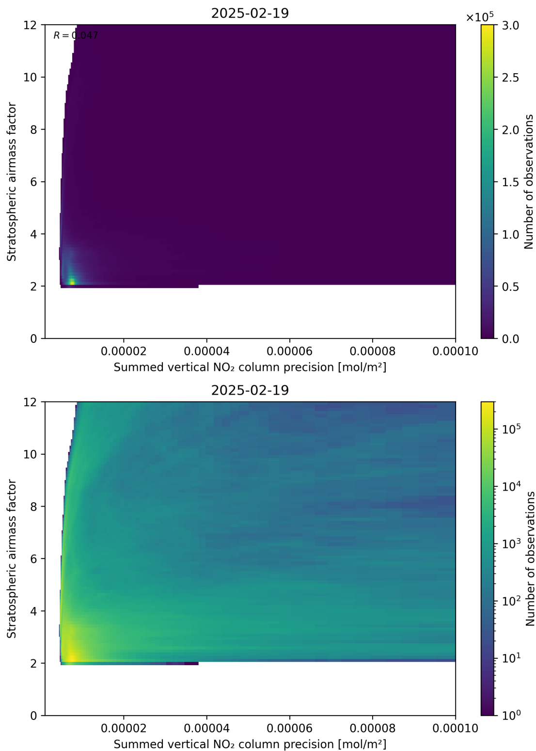
Figure 106: Scatter density plot of “Summed vertical NO 2 column precision” against “Stratospheric airmass factor” for 2025-02-19 to 2025-02-20.
