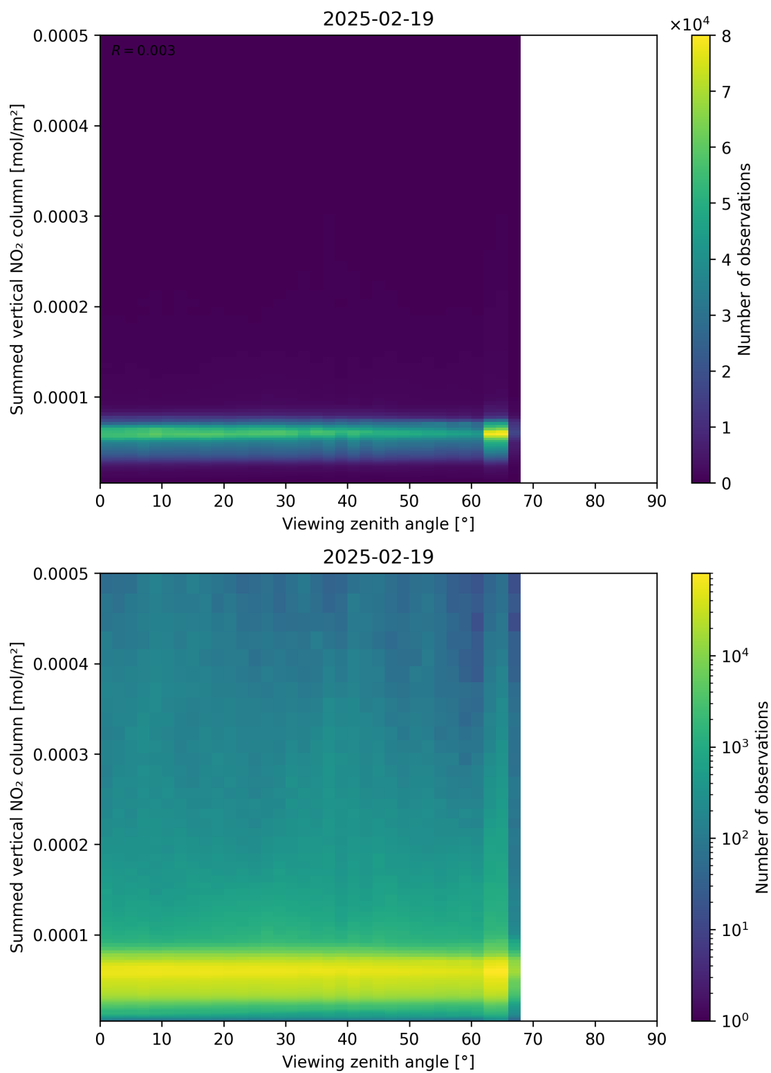
Figure 165: Scatter density plot of “Viewing zenith angle” against “Summed vertical NO 2 column” for 2025-02-19 to 2025-02-20.
