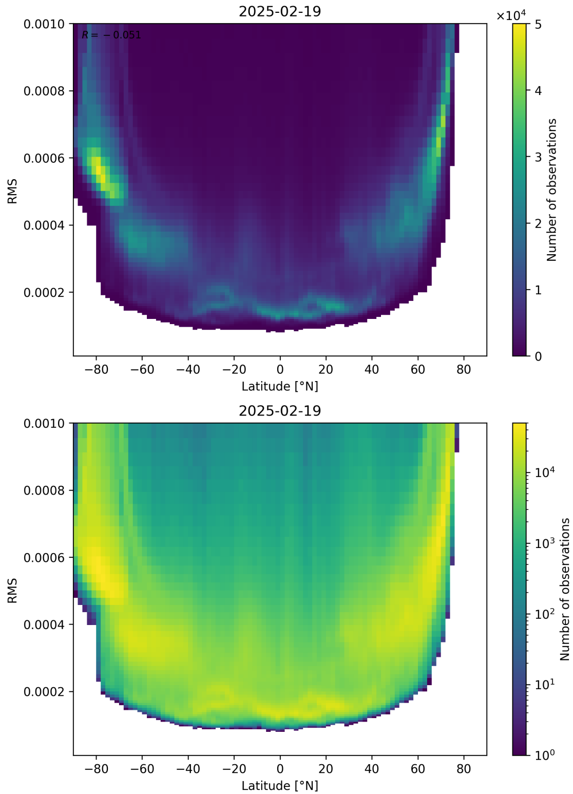
Figure 94: Scatter density plot of “Latitude” against “RMS” for 2025-02-19 to 2025-02-20.
