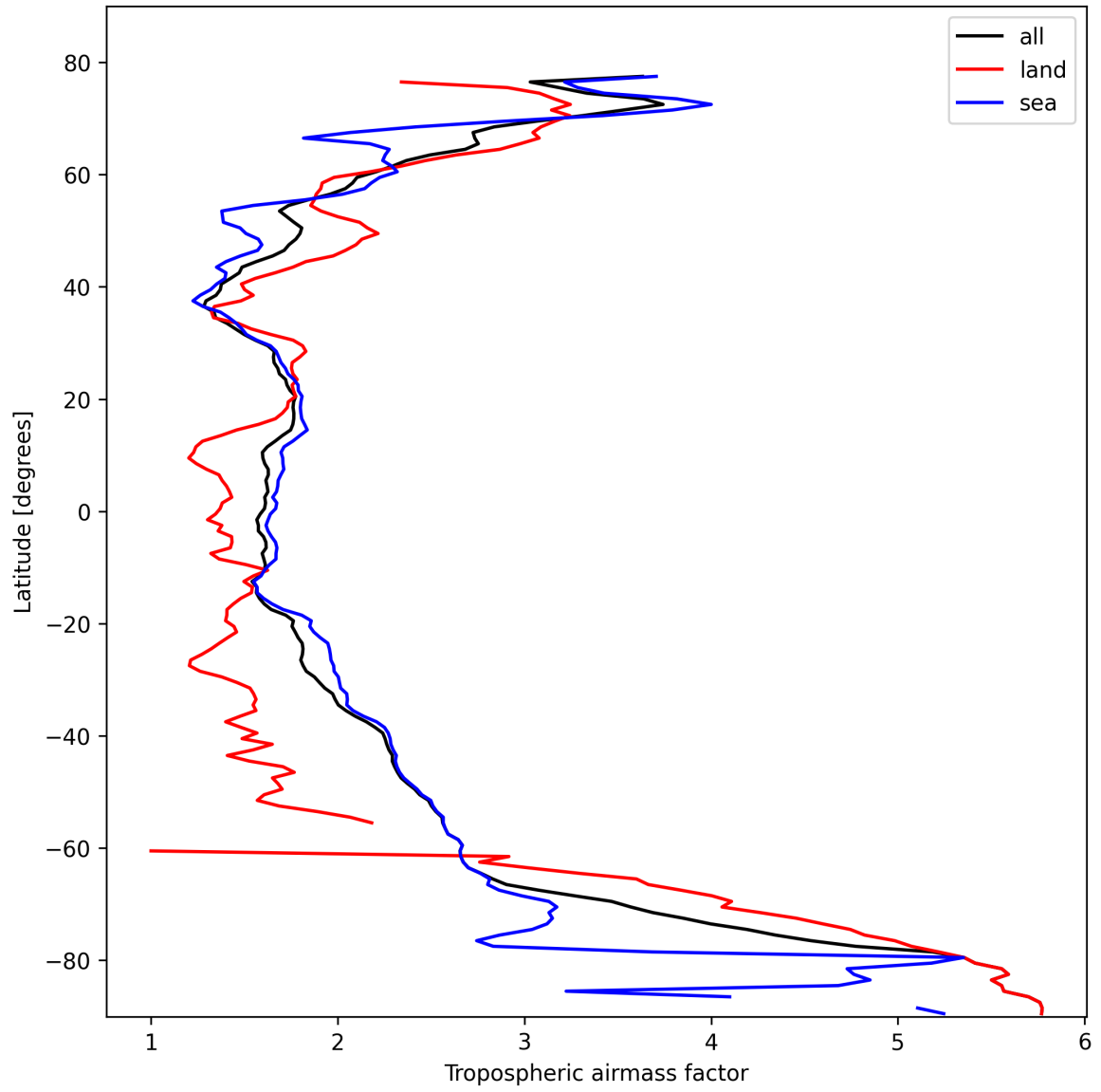
Figure 14: Zonal average of “Tropospheric airmass factor” for 2025-02-19 to 2025-02-20.
