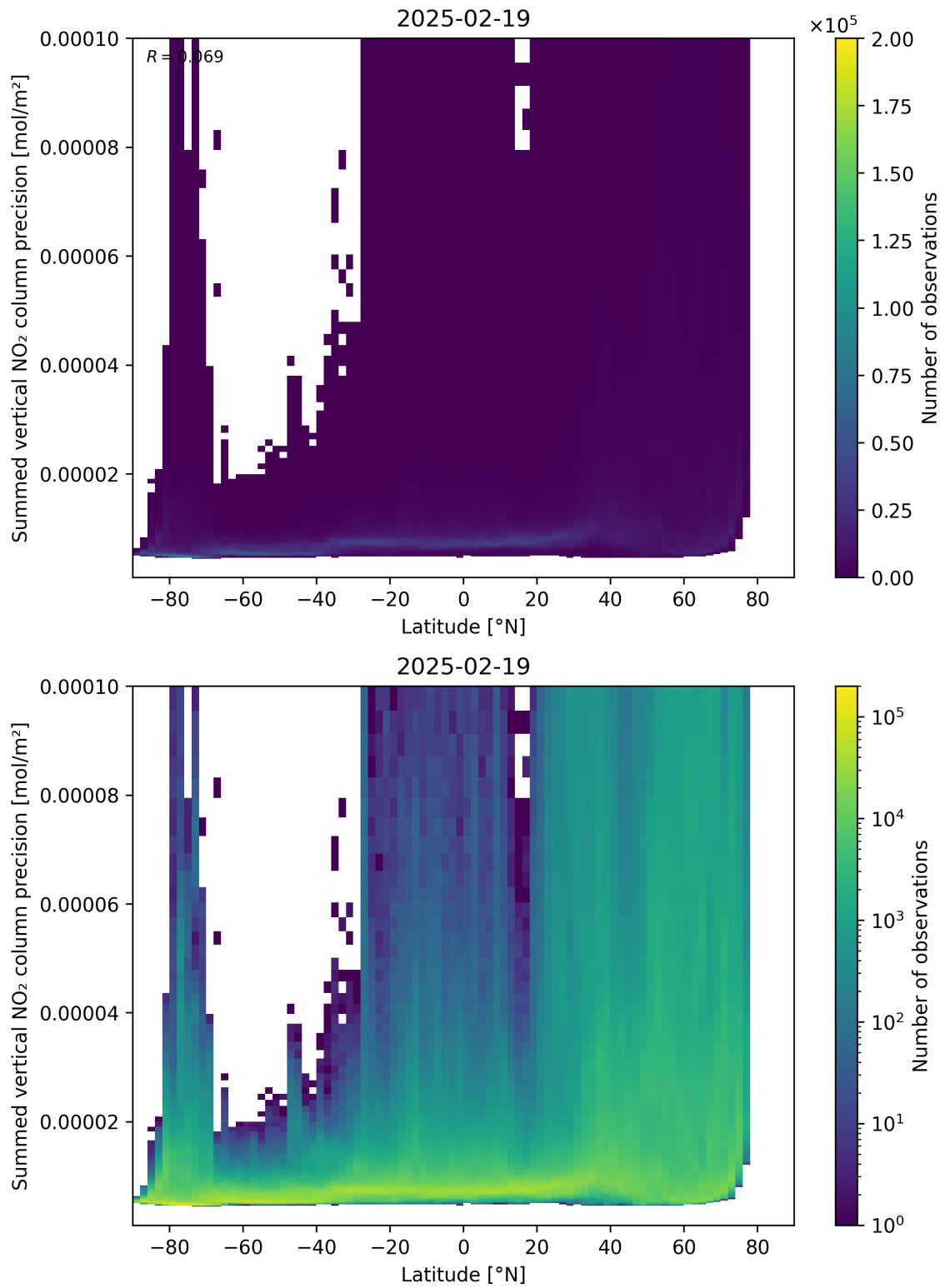
Figure 89: Scatter density plot of “Latitude” against “Summed vertical NO 2 column precision” for 2025-02-19 to 2025-02-20.
