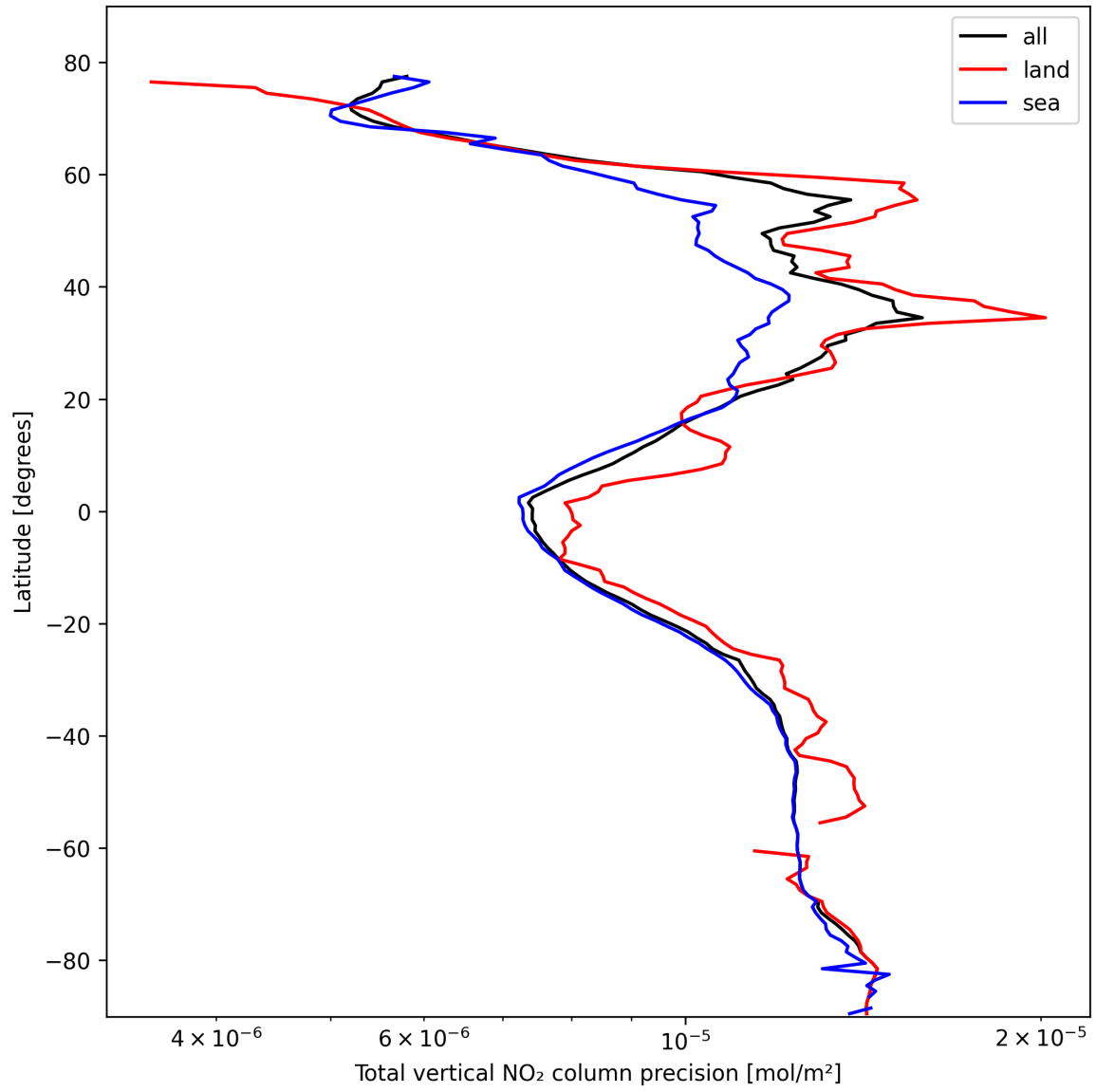
Figure 22: Zonal average of “Total vertical NO 2 column precision” for 2025-02-19 to 2025-02-20.
