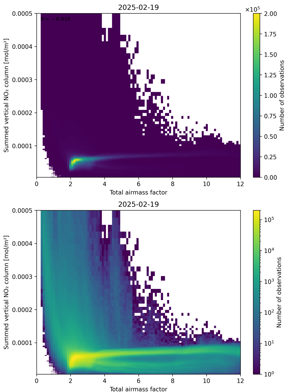
Figure 65: Scatter density plot of “Total airmass factor” against “Summed vertical NO 2 column” for 2025-02-19 to 2025-02-20.
