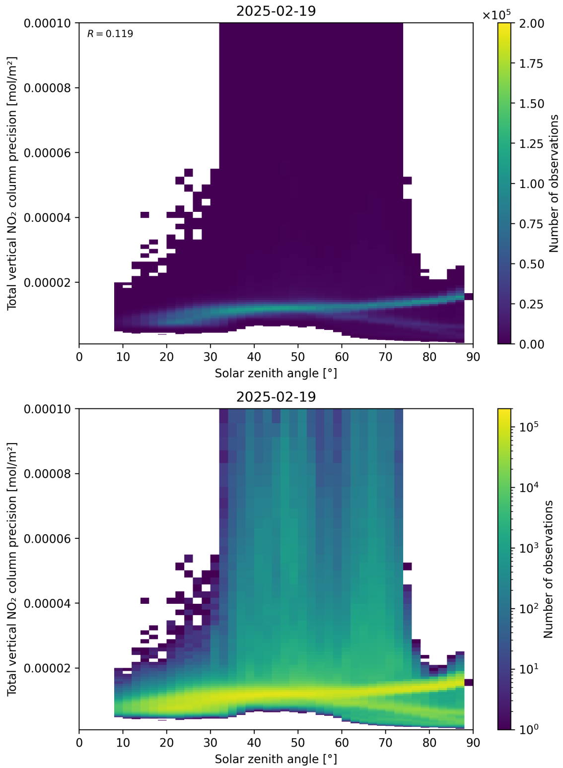
Figure 154: Scatter density plot of “Solar zenith angle” against “Total vertical NO 2 column precision” for 2025-02-19 to 2025-02-20.
