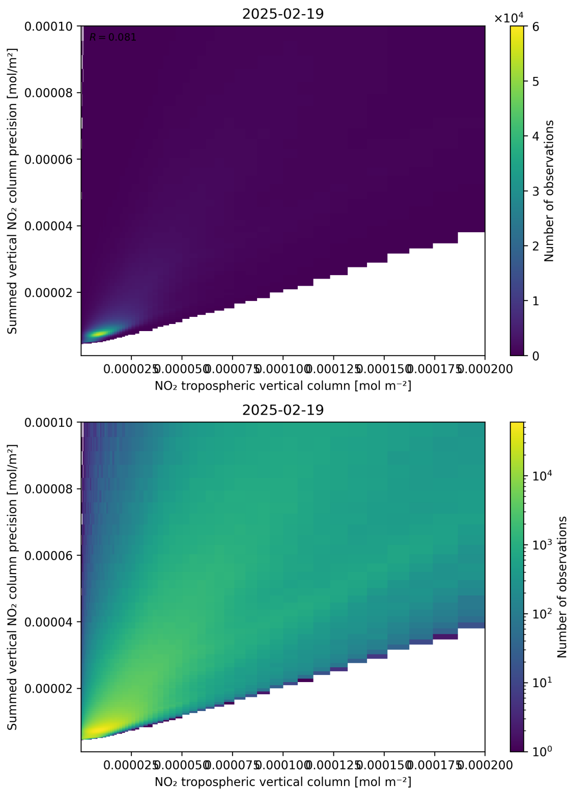
Figure 127: Scatter density plot of “NO 2 tropospheric vertical column” against “Summed vertical NO 2 column precision” for 2025-02-19 to 2025-02-20.
