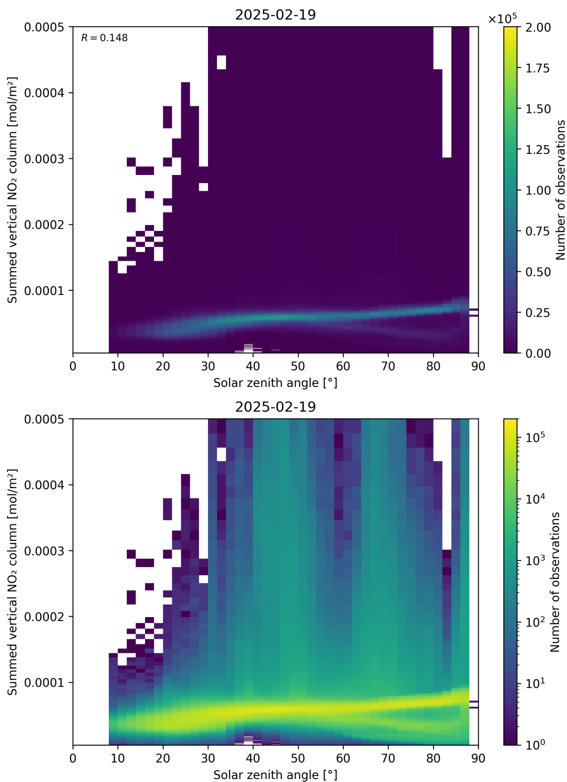
Figure 151: Scatter density plot of “Solar zenith angle” against “Summed vertical NO 2 column” for 2025-02-19 to 2025-02-20.
