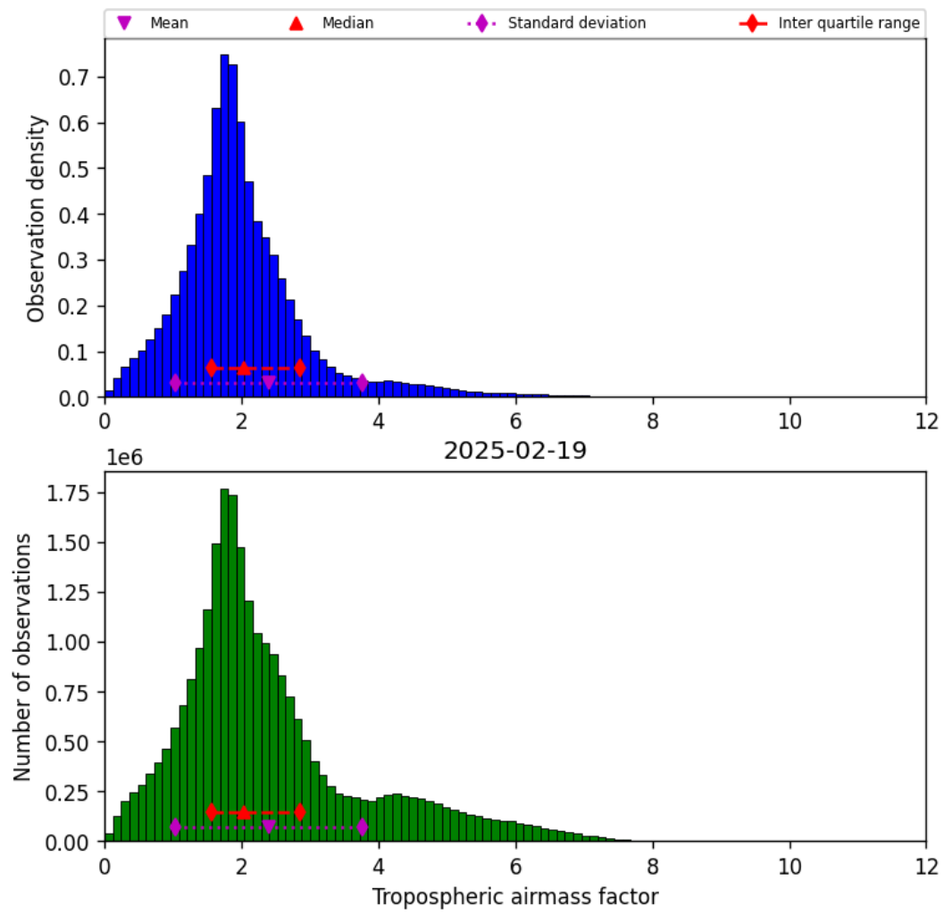
Figure 31: Histogram of “Tropospheric airmass factor” for 2025-02-19 to 2025-02-20
