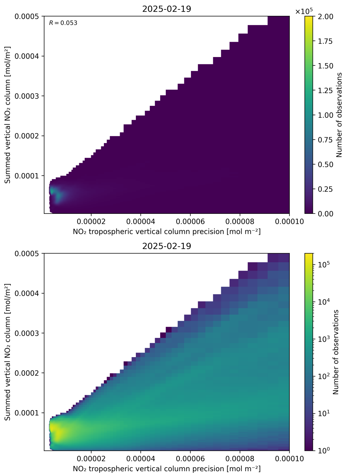
Figure 136: Scatter density plot of “NO 2 tropospheric vertical column precision” against “Summed vertical NO 2 column” for 2025-02-19 to 2025-02-20.
