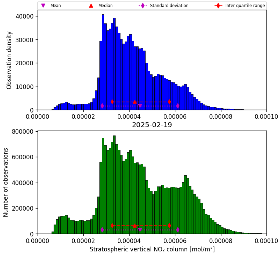
Figure 36: Histogram of “Stratospheric vertical NO 2 column” for 2025-02-19 to 2025-02-20
