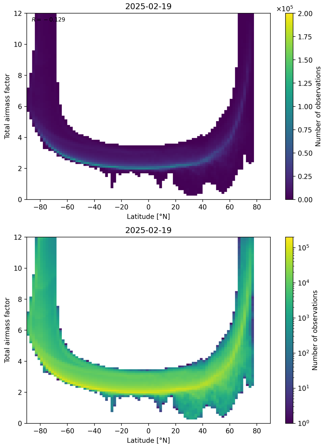
Figure 84: Scatter density plot of “Latitude” against “Total airmass factor” for 2025-02-19 to 2025-02-20.
