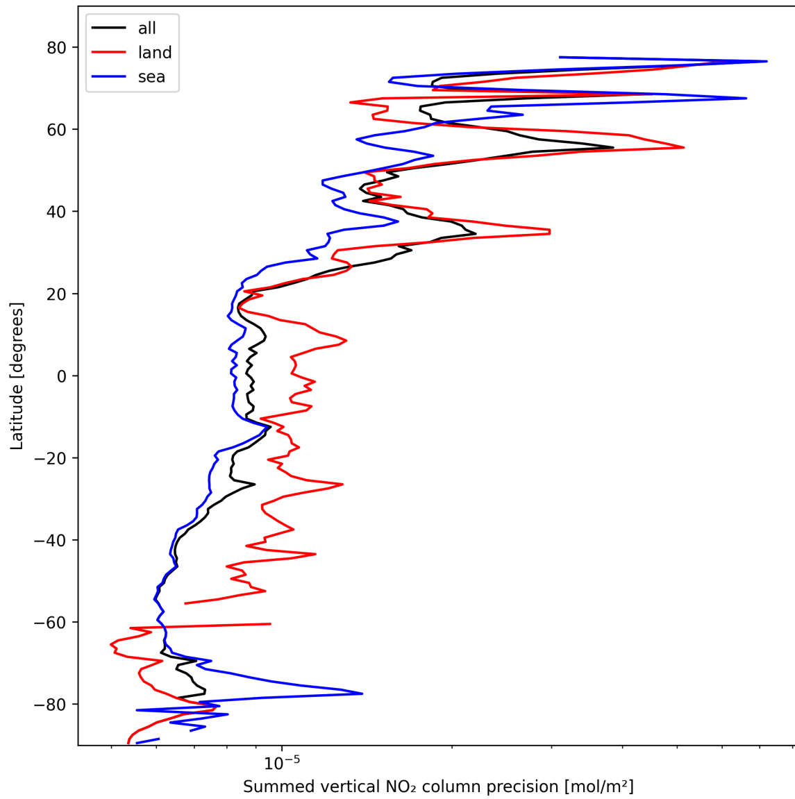
Figure 24: Zonal average of “Summed vertical NO 2 column precision” for 2025-02-19 to 2025-02-20.
