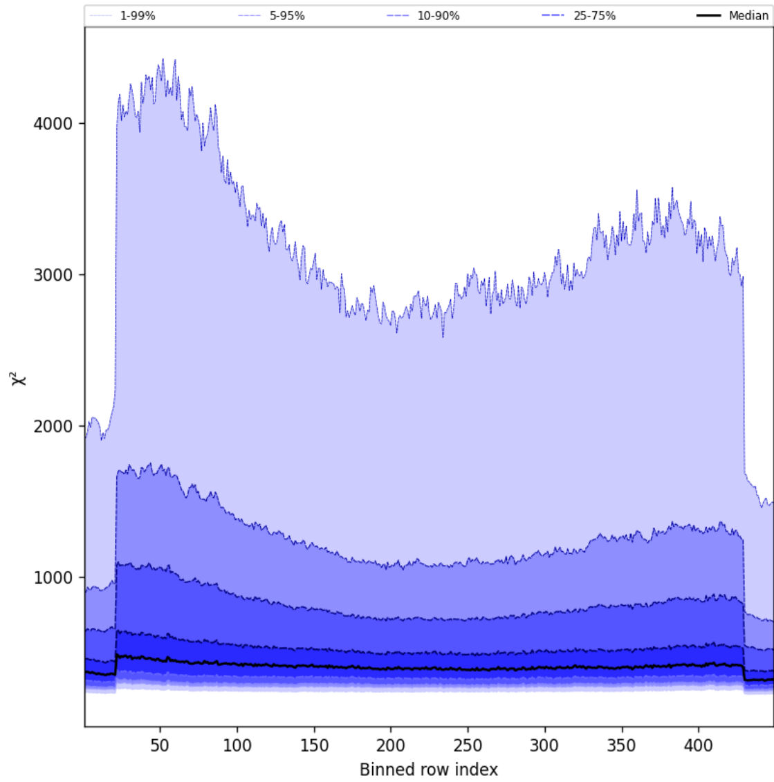
Figure 59: Along track statistics of “ \chi^2 ” for 2025-02-19 to 2025-02-20
