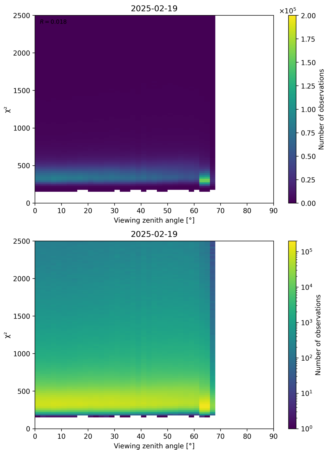
Figure 162: Scatter density plot of “Viewing zenith angle” against “ \chi^2 ” for 2025-02-19 to 2025-02-20.
