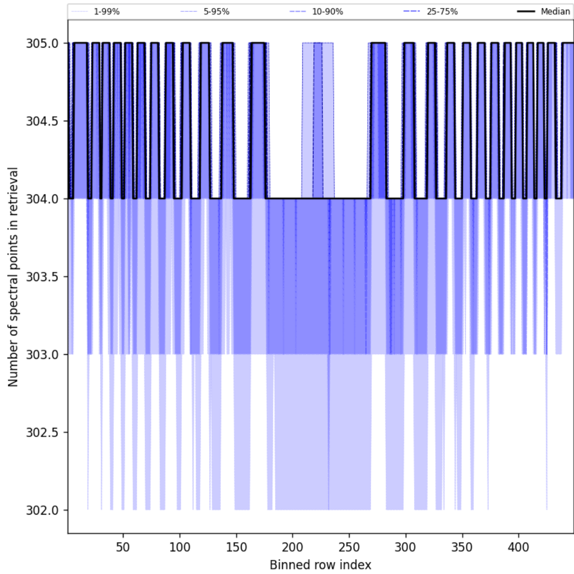
Figure 50: Along track statistics of “Number of spectral points in retrieval” for 2025-02-19 to 2025-02-20
