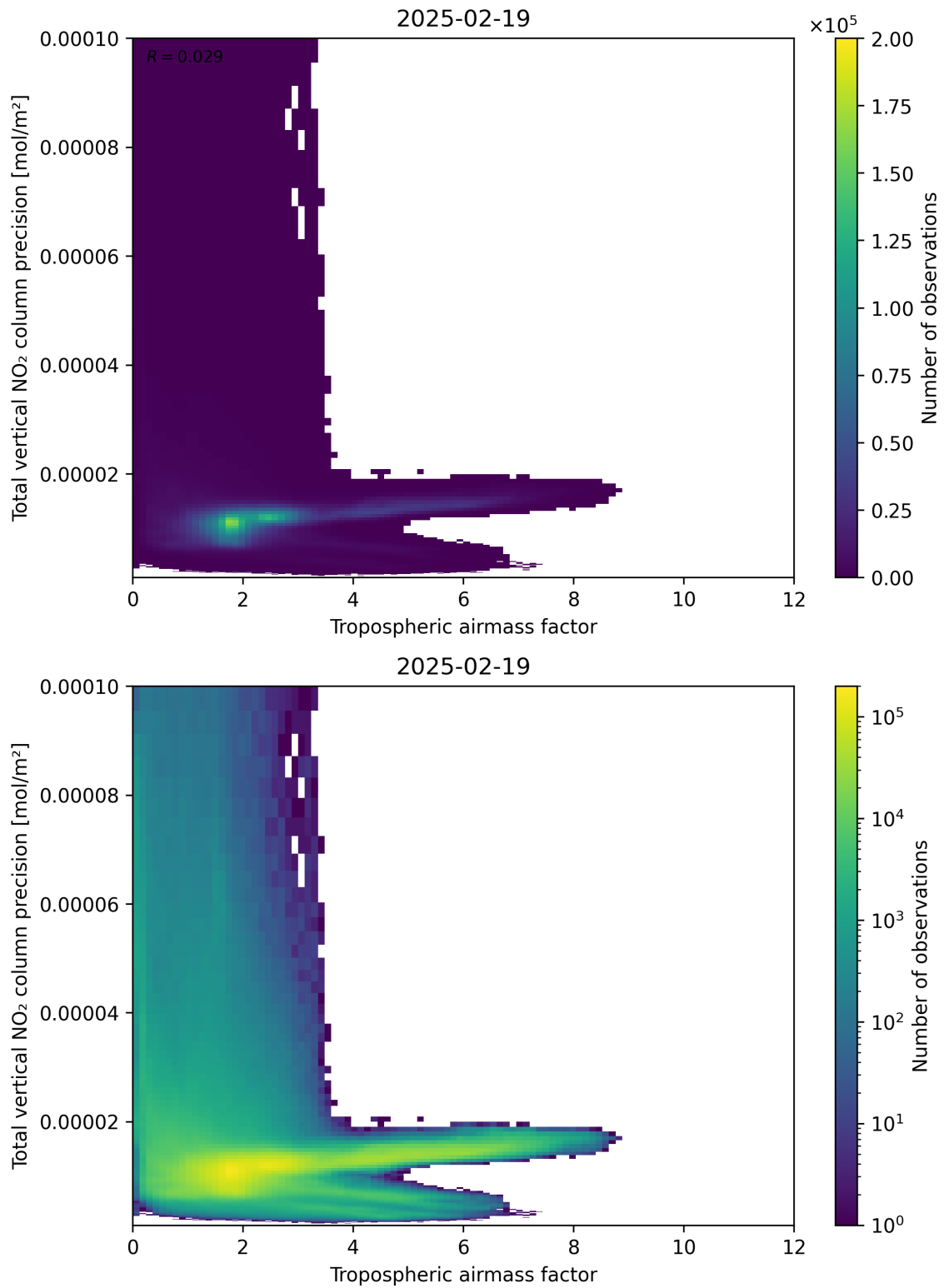
Figure 78: Scatter density plot of “Tropospheric air mass factor” against “Total vertical NO 2 column precision” for 2025-02-19 to 2025-02-20.
