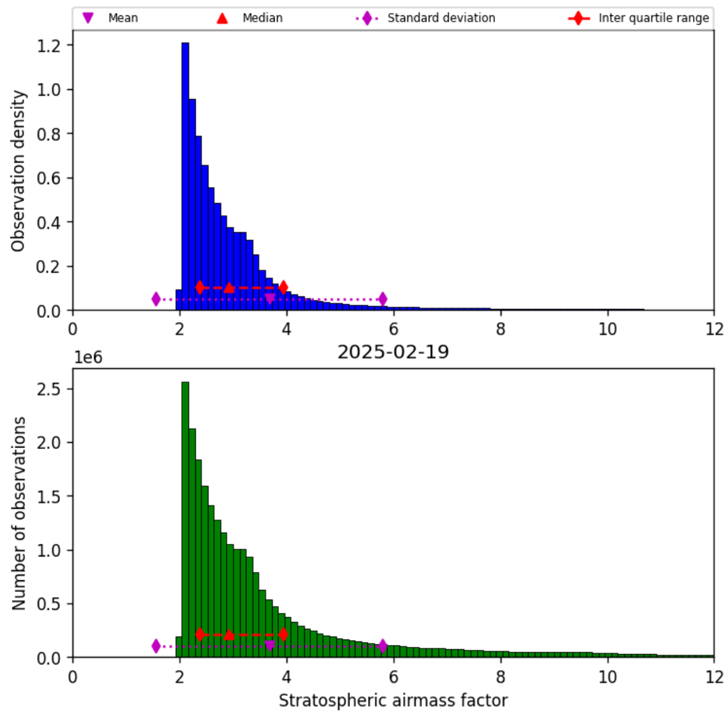
Figure 44: Histogram of “Stratospheric airmass factor” for 2025-02-19 to 2025-02-20
