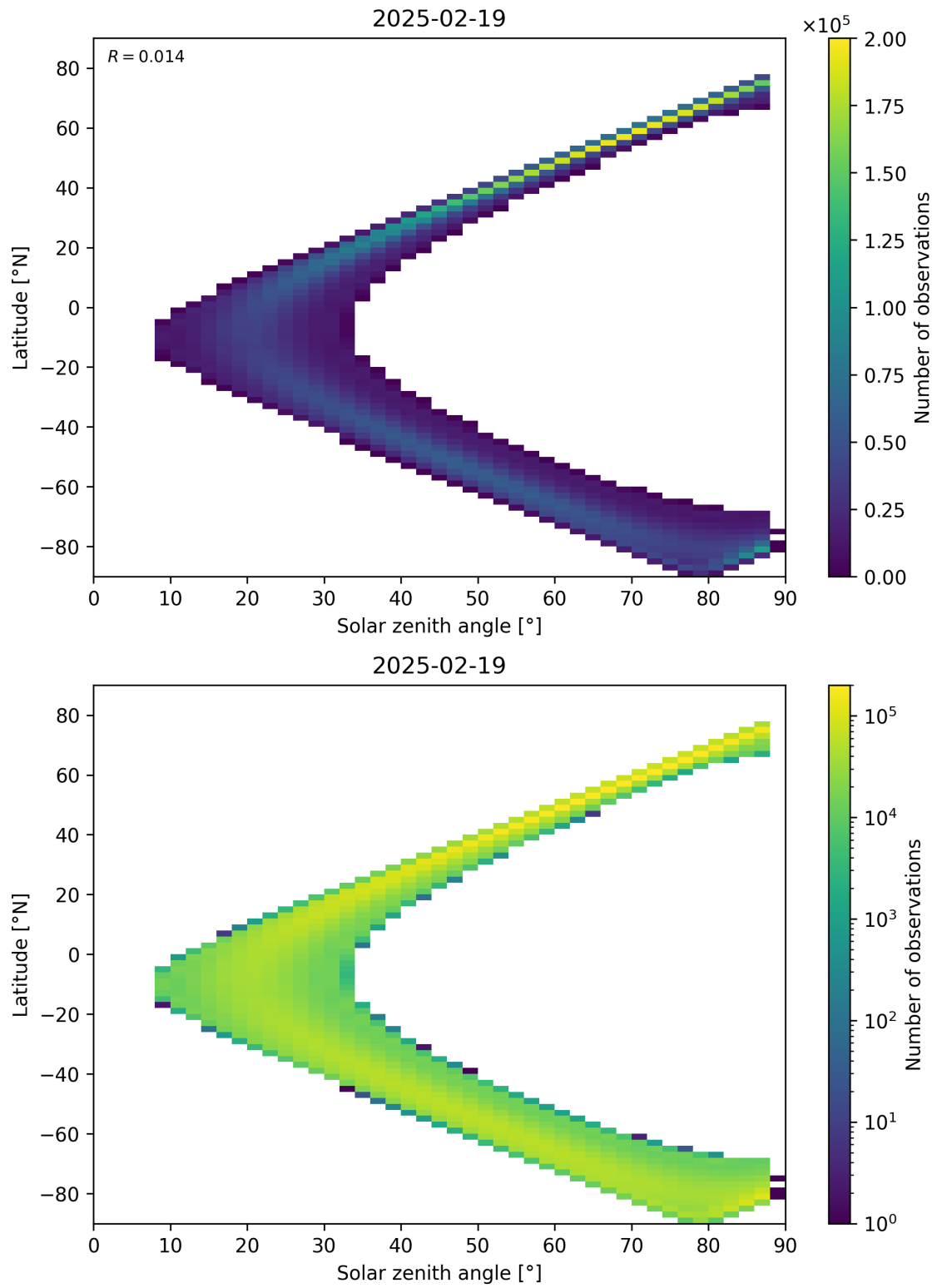
Figure 149: Scatter density plot of “Solar zenith angle” against “Latitude” for 2025-02-19 to 2025-02-20.
