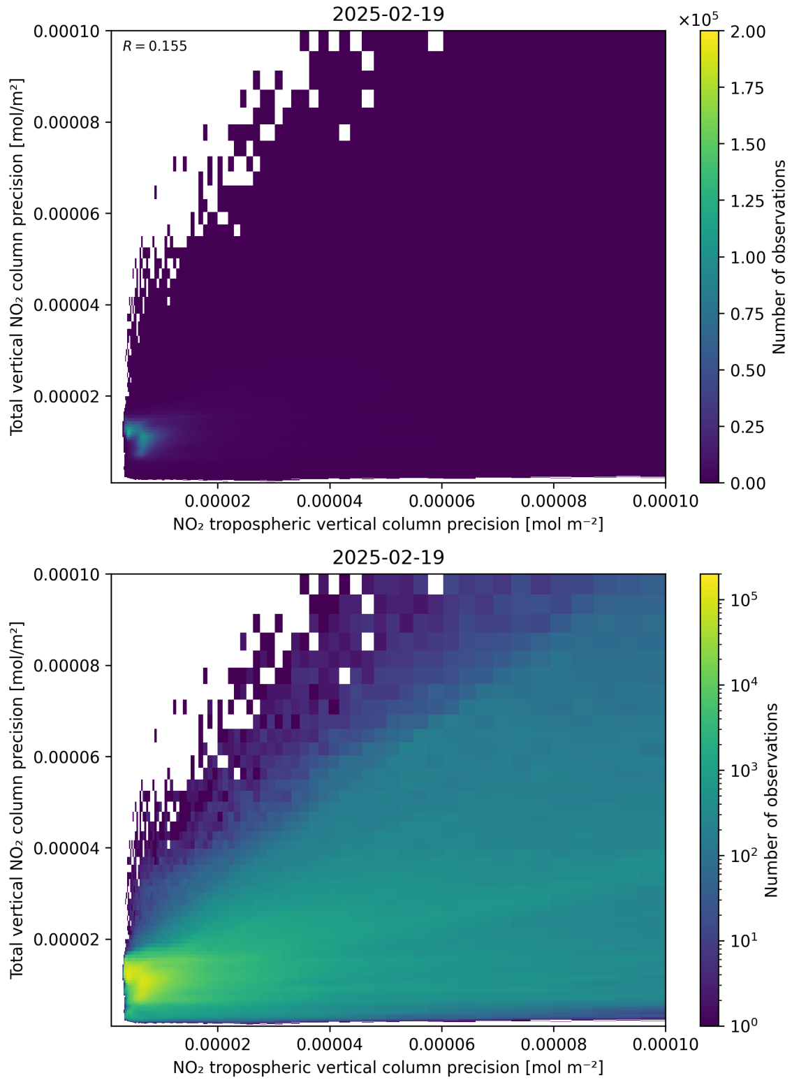
Figure 139: Scatter density plot of “NO 2 tropospheric vertical column precision” against “Total vertical NO 2 column precision” for 2025-02-19 to 2025-02-20.
