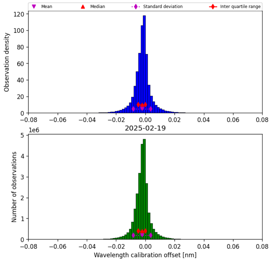
Figure 35: Histogram of “Wavelength calibration offset” for 2025-02-19 to 2025-02-20
