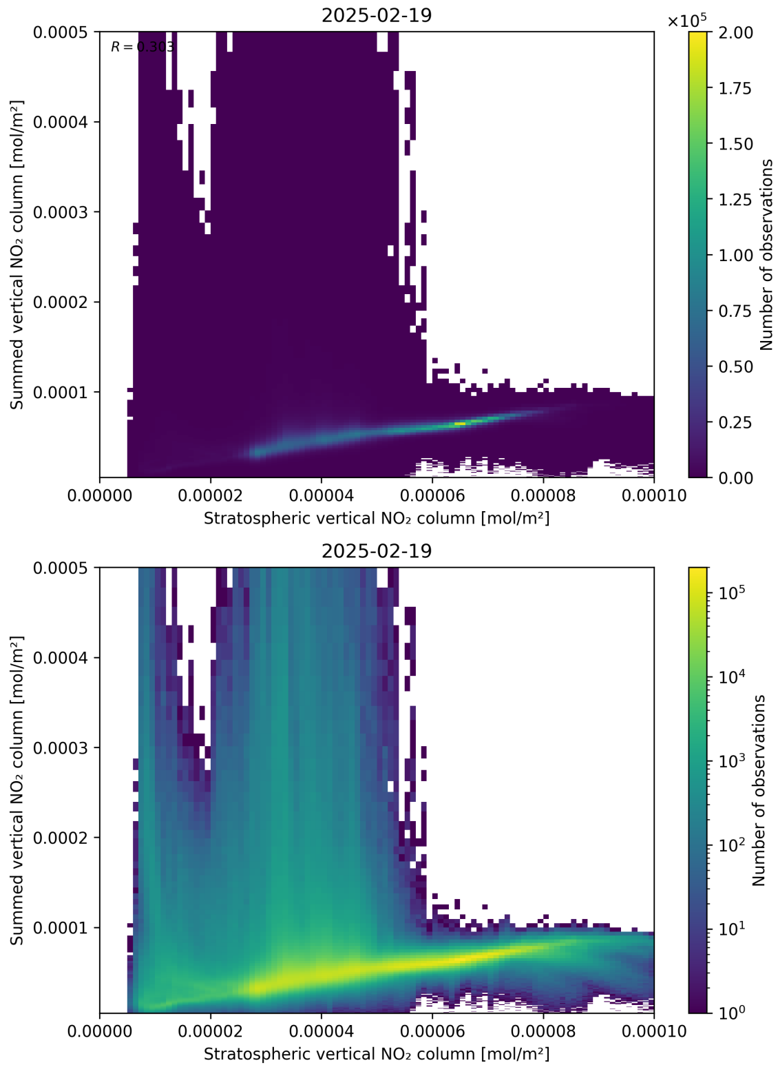
Figure 98: Scatter density plot of “Stratospheric vertical NO 2 column” against “Summed vertical NO 2 column” for 2025-02-19 to 2025-02-20.
