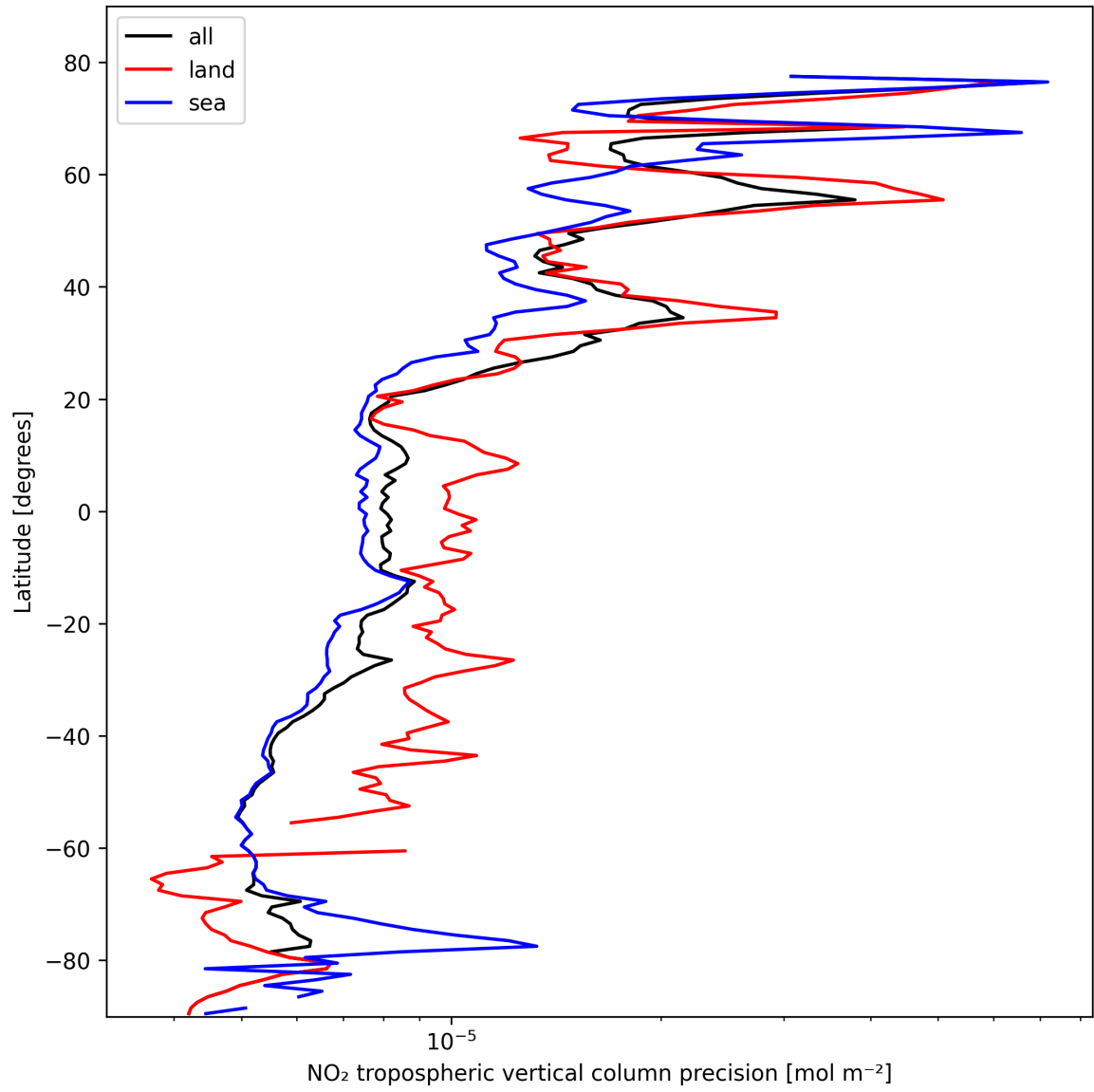
Figure 13: Zonal average of "NO 2 tropospheric vertical column precision" for 2025-02-19 to 2025-02-20.
