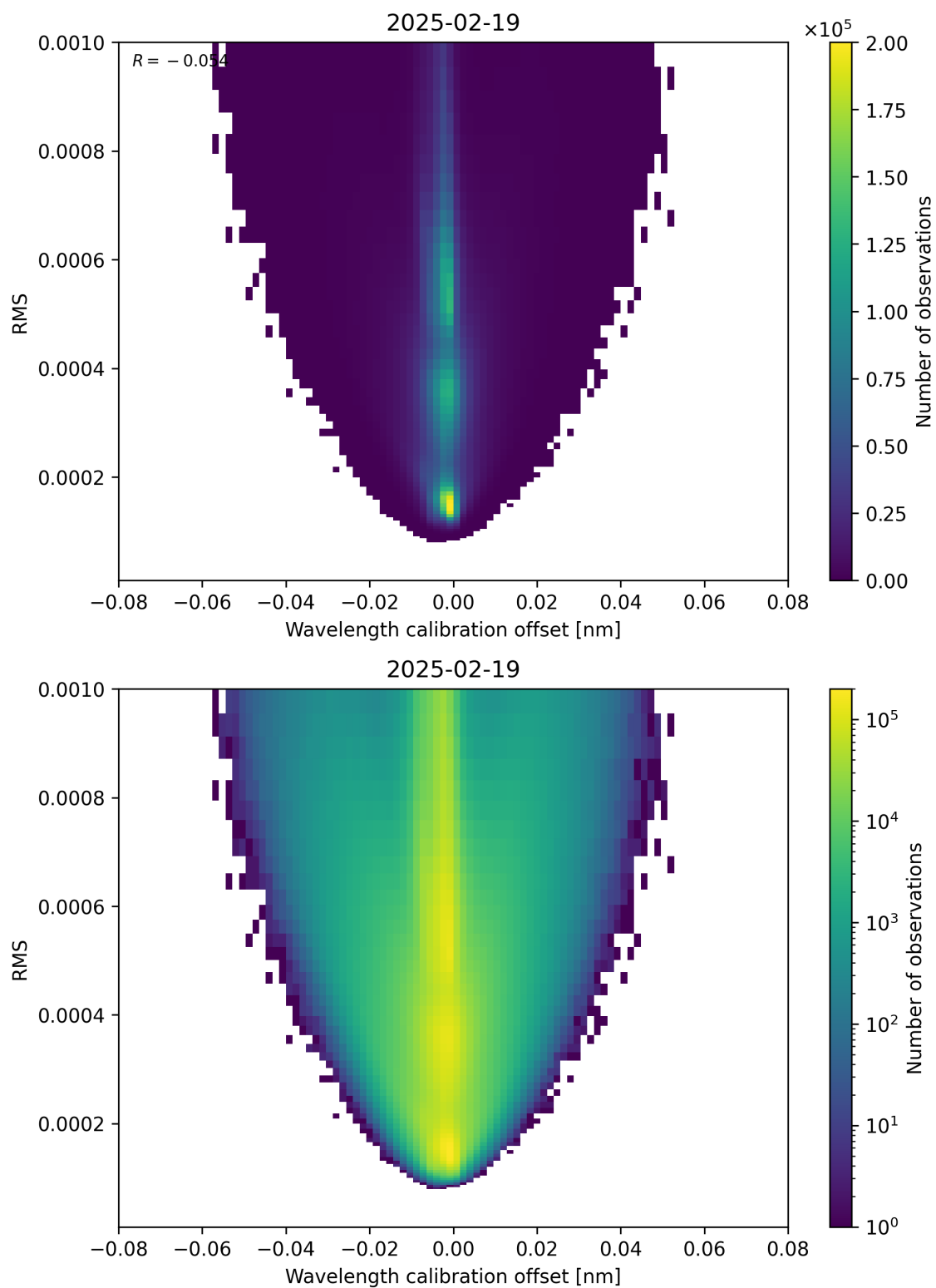
Figure 181: Scatter density plot of “Wavelength calibration offset” against “RMS” for 2025-02-19 to 2025-02-20.
