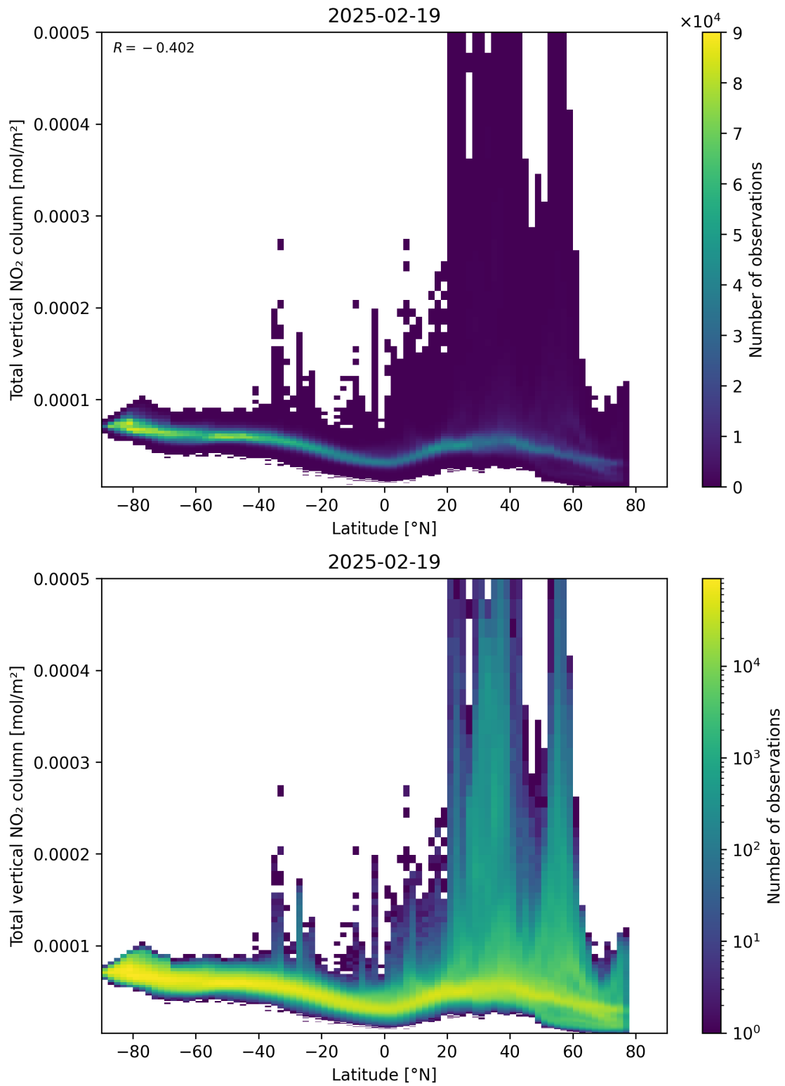
Figure 90: Scatter density plot of “Latitude” against “Total vertical NO 2 column” for 2025-02-19 to 2025-02-20.
