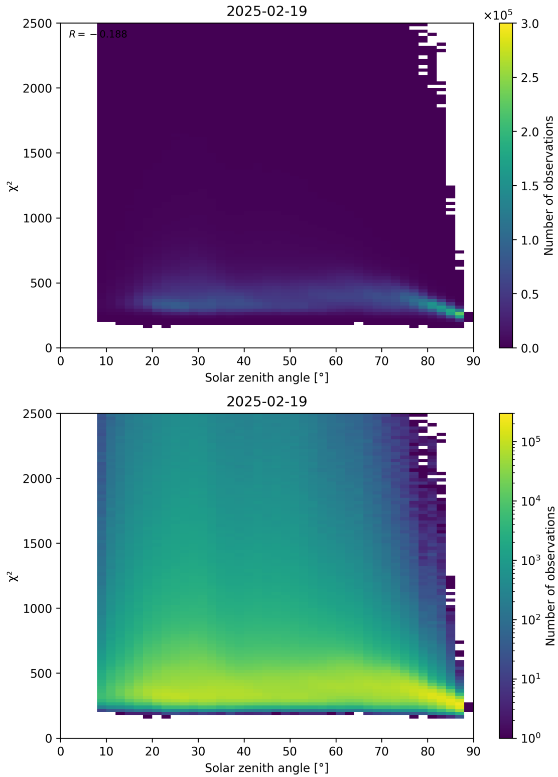
Figure 148: Scatter density plot of “Solar zenith angle” against “ \chi^2 ” for 2025-02-19 to 2025-02-20.
