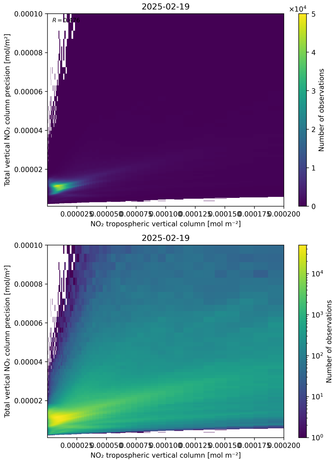
Figure 129: Scatter density plot of “NO 2 tropospheric vertical column” against “Total vertical NO 2 column precision” for 2025-02-19 to 2025-02-20.
