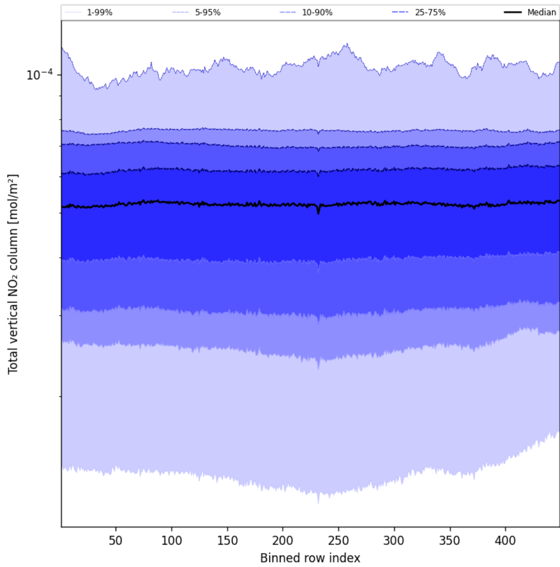
Figure 55: Along track statistics of “Total vertical NO 2 column” for 2025-02-19 to 2025-02-20
