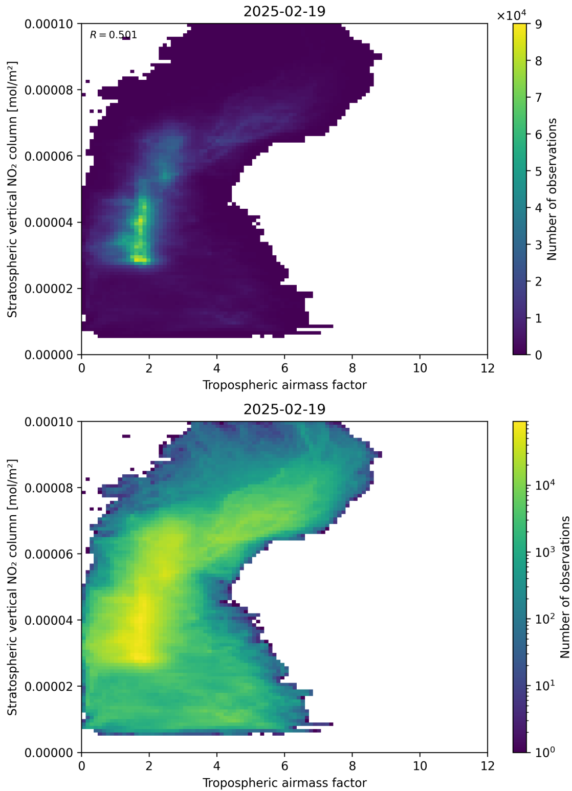
Figure 74: Scatter density plot of “Tropospheric air mass factor” against “Stratospheric vertical NO 2 column” for 2025-02-19 to 2025-02-20.
