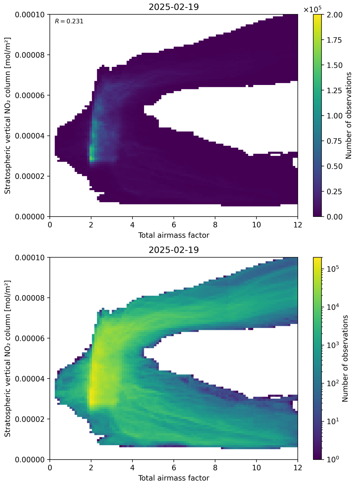
Figure 64: Scatter density plot of “Total airmass factor” against “Stratospheric vertical NO 2 column” for 2025-02-19 to 2025-02-20.
