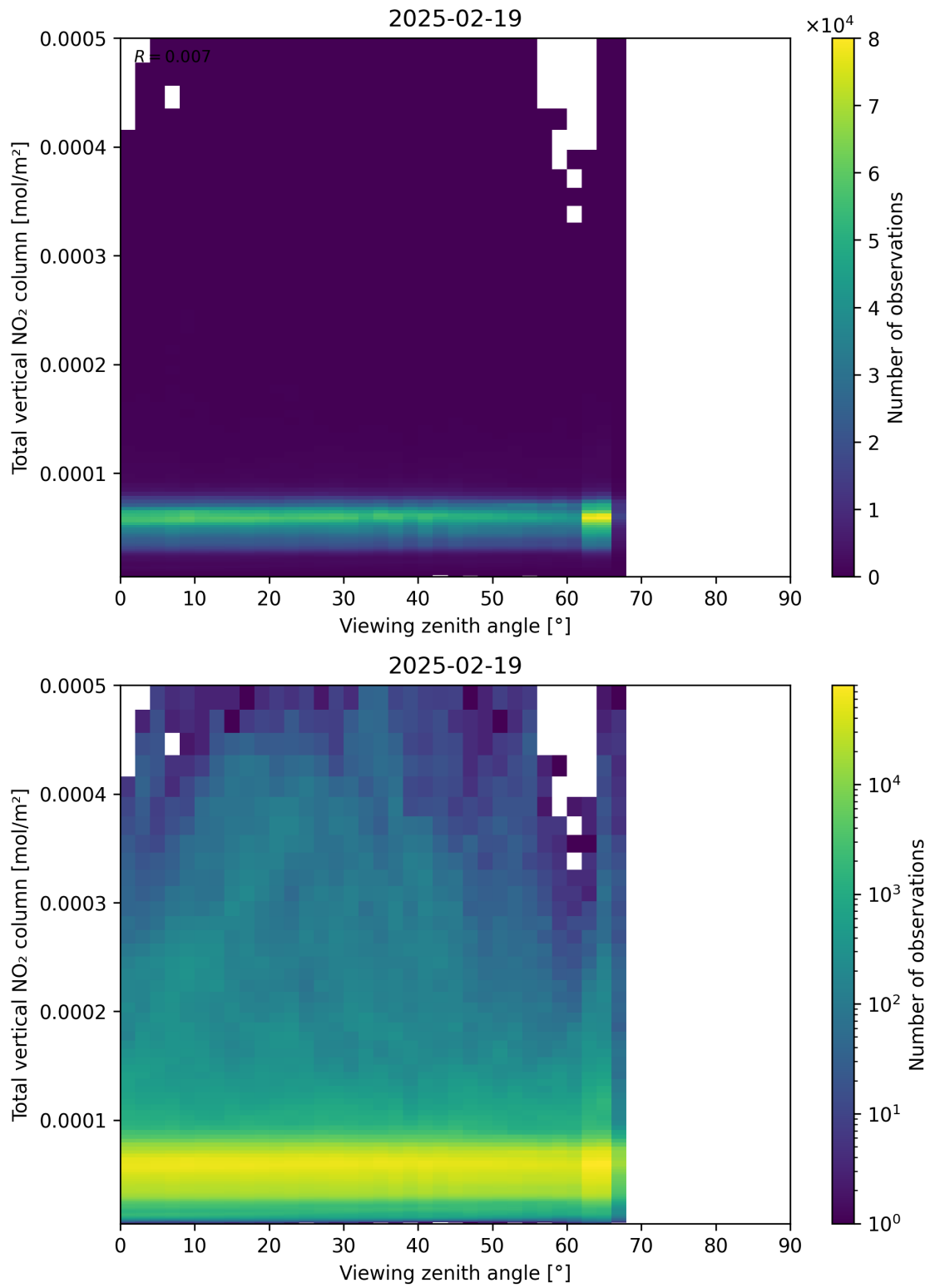
Figure 167: Scatter density plot of “Viewing zenith angle” against “Total vertical NO 2 column” for 2025-02-19 to 2025-02-20.
