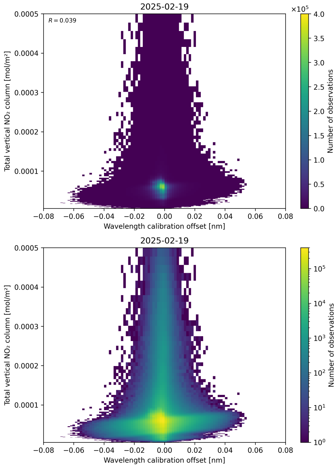
Figure 179: Scatter density plot of “Wavelength calibration offset” against “Total vertical NO 2 column” for 2025-02-19 to 2025-02-20.
