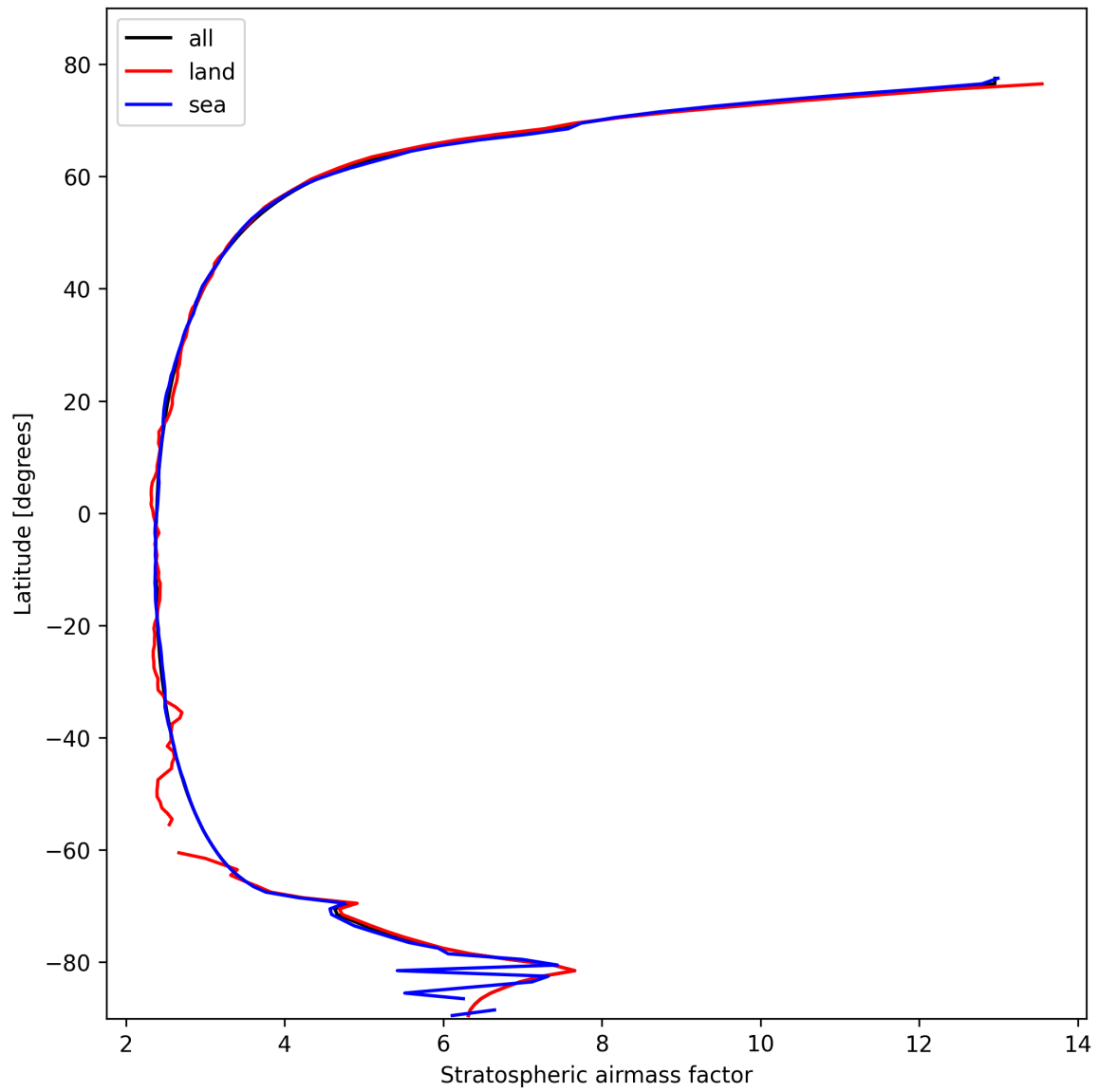
Figure 27: Zonal average of “Stratospheric air mass factor” for 2025-02-19 to 2025-02-20.
