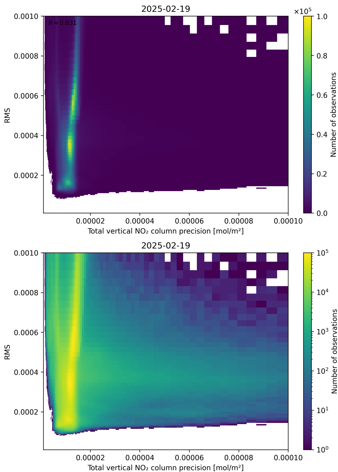
Figure 119: Scatter density plot of “Total vertical NO 2 column precision” against “RMS” for 2025-02-19 to 2025-02-20.
