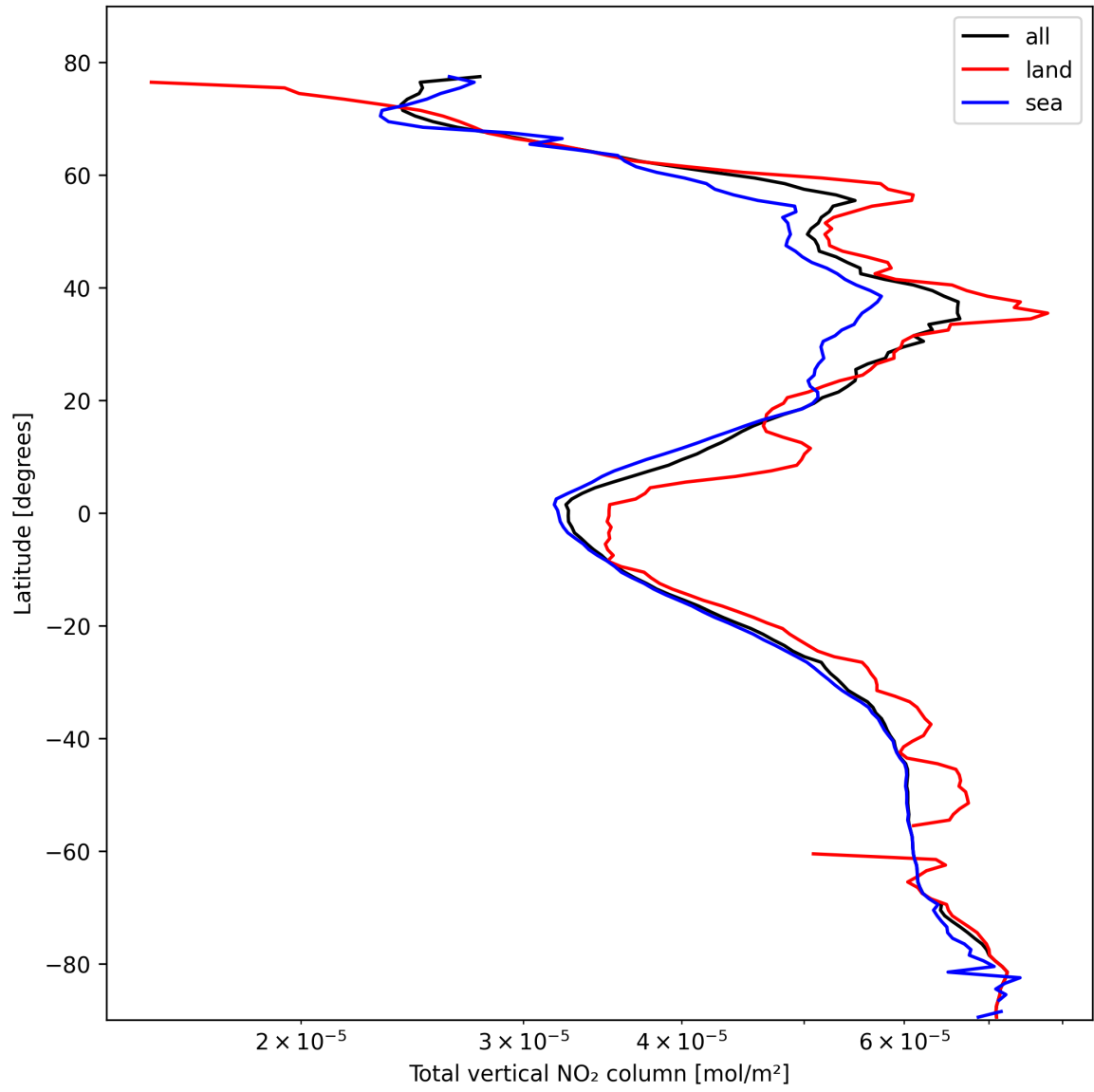
Figure 21: Zonal average of “Total vertical NO 2 column” for 2025-02-19 to 2025-02-20.
