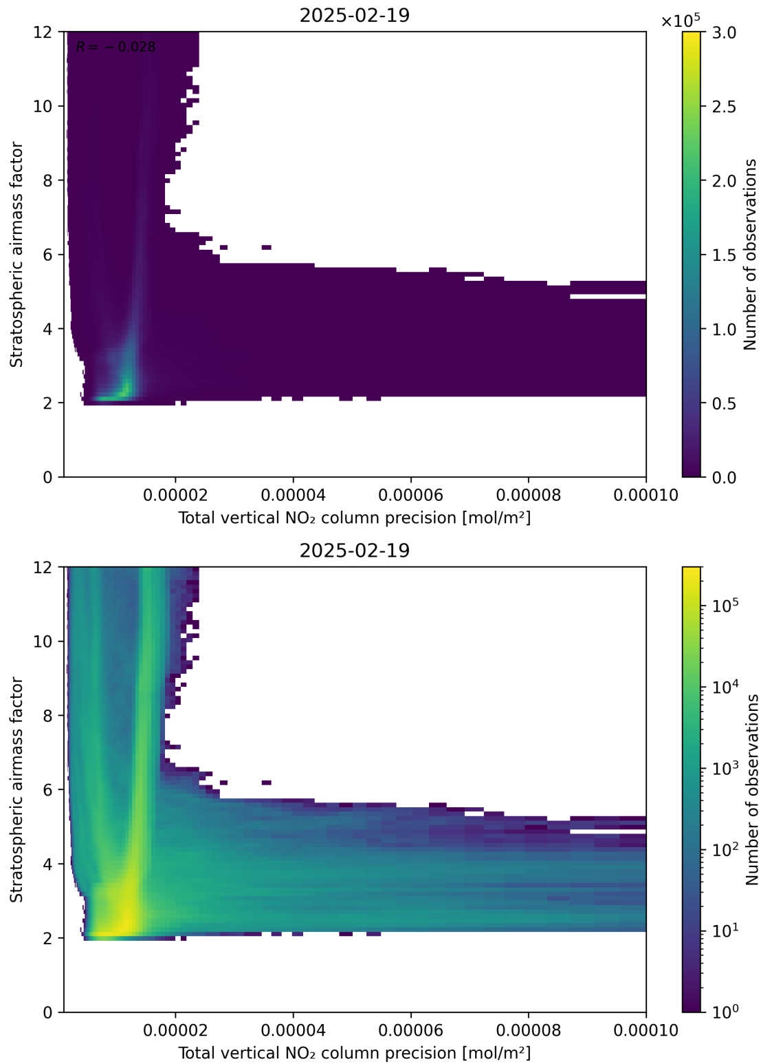
Figure 115: Scatter density plot of “Total vertical NO 2 column precision” against “Stratospheric air mass factor” for 2025-02-19 to 2025-02-20.
