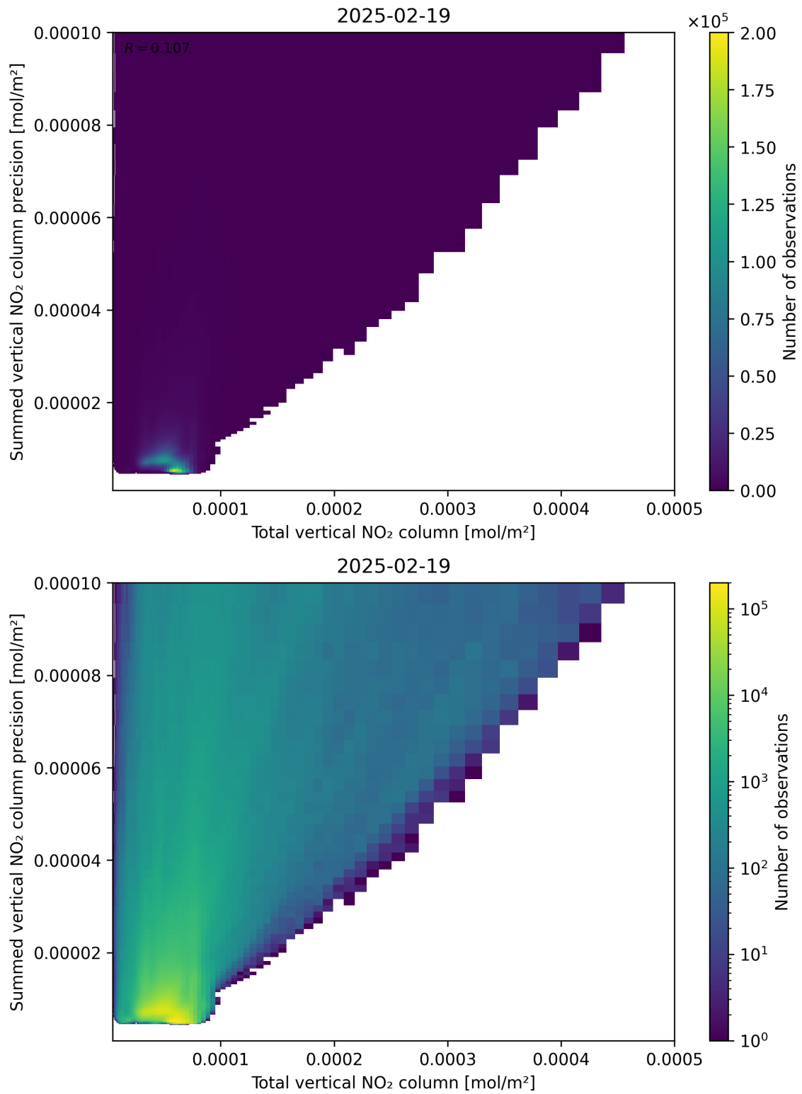
Figure 113: Scatter density plot of “Total vertical NO 2 column” against “Summed vertical NO 2 column precision” for 2025-02-19 to 2025-02-20.
