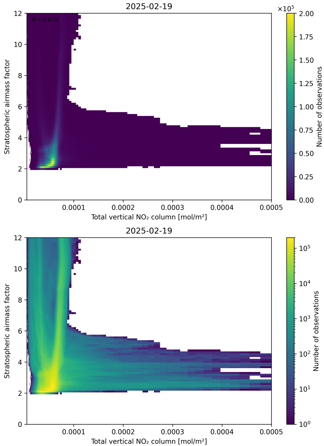
Figure 110: Scatter density plot of “Total vertical NO 2 column” against “Stratospheric airmass factor” for 2025-02-19 to 2025-02-20.
