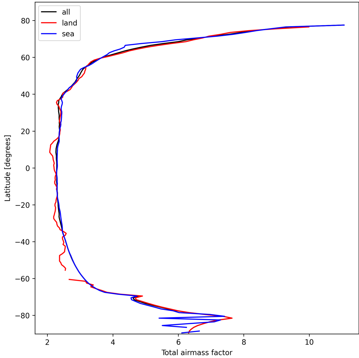
Figure 15: Zonal average of “Total airmass factor” for 2025-02-19 to 2025-02-20.
