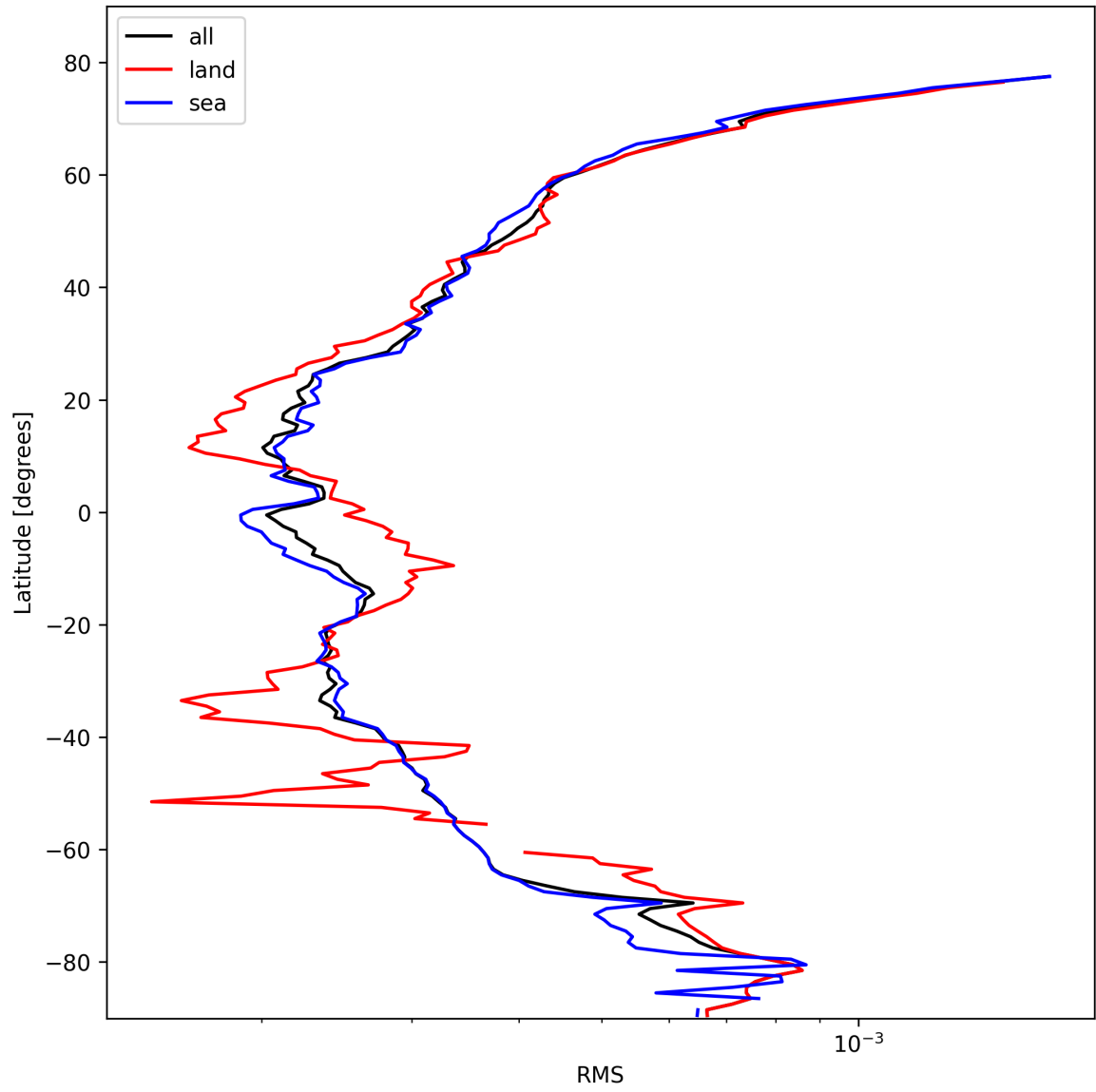
Figure 26: Zonal average of “RMS” for 2025-02-19 to 2025-02-20.
