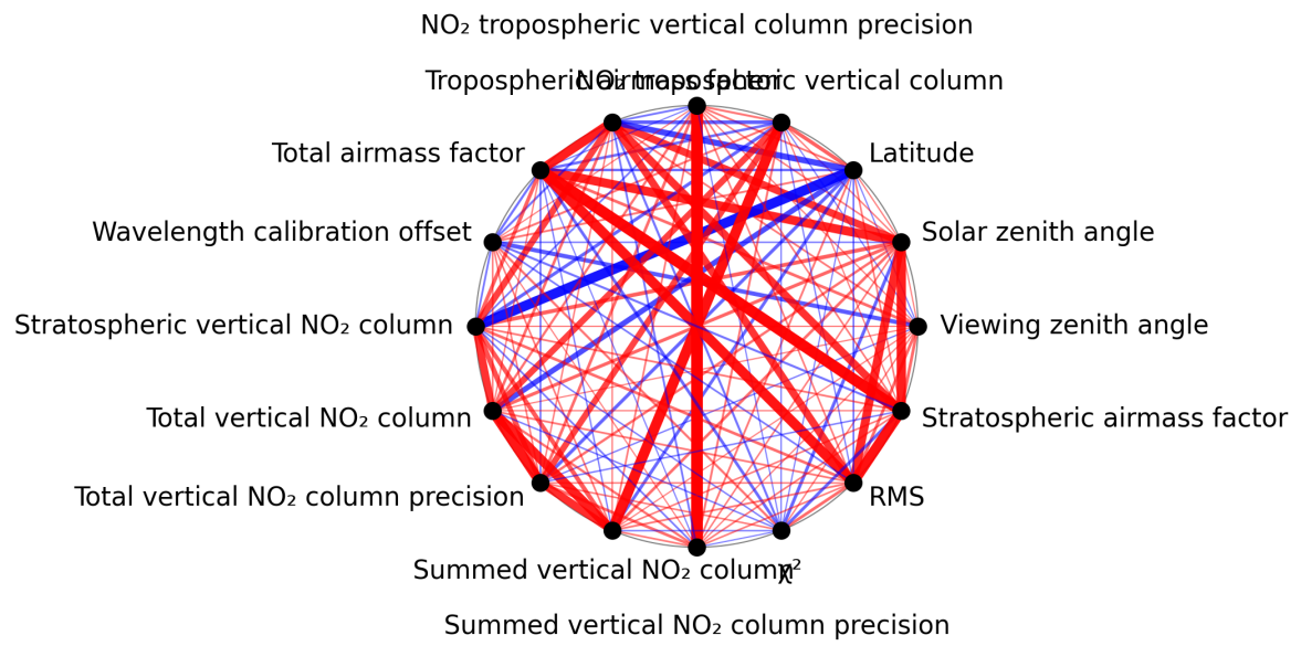
Figure 1: Map of correlation graph for 2025-02-19 to 2025-02-20.
