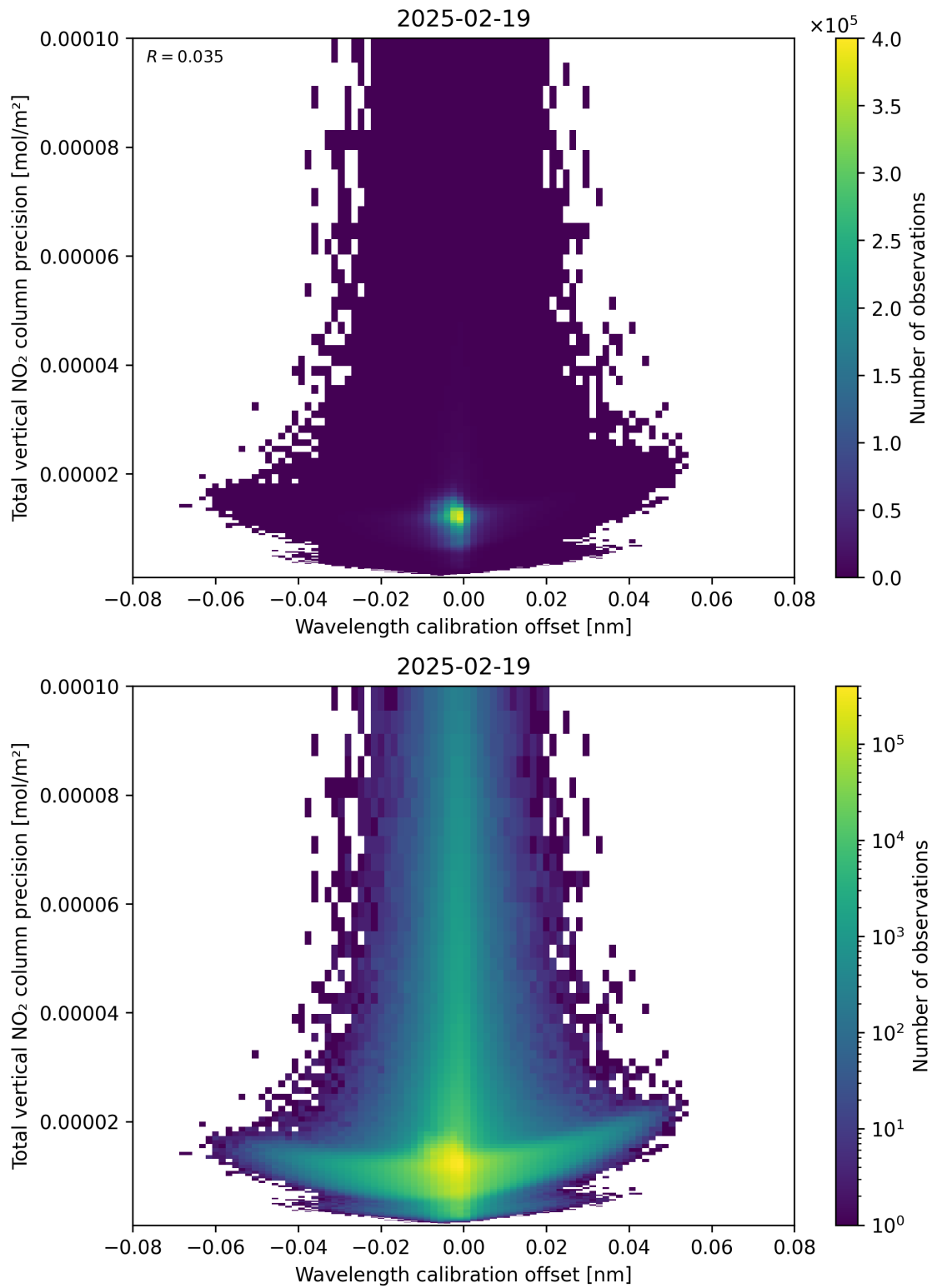
Figure 180: Scatter density plot of “Wavelength calibration offset” against “Total vertical NO 2 column precision” for 2025-02-19 to 2025-02-20.
