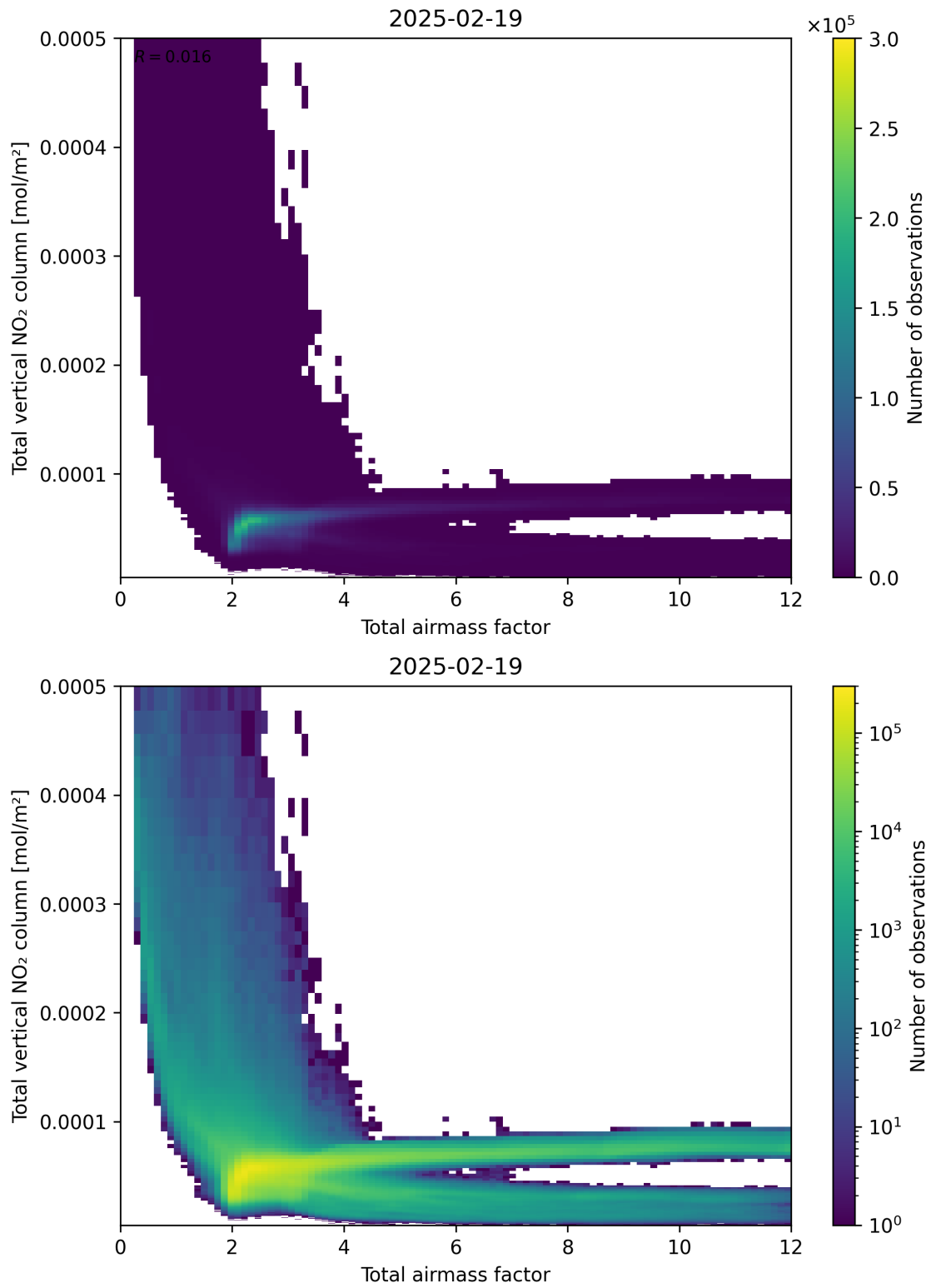
Figure 67: Scatter density plot of “Total airmass factor” against “Total vertical NO 2 column” for 2025-02-19 to 2025-02-20.
