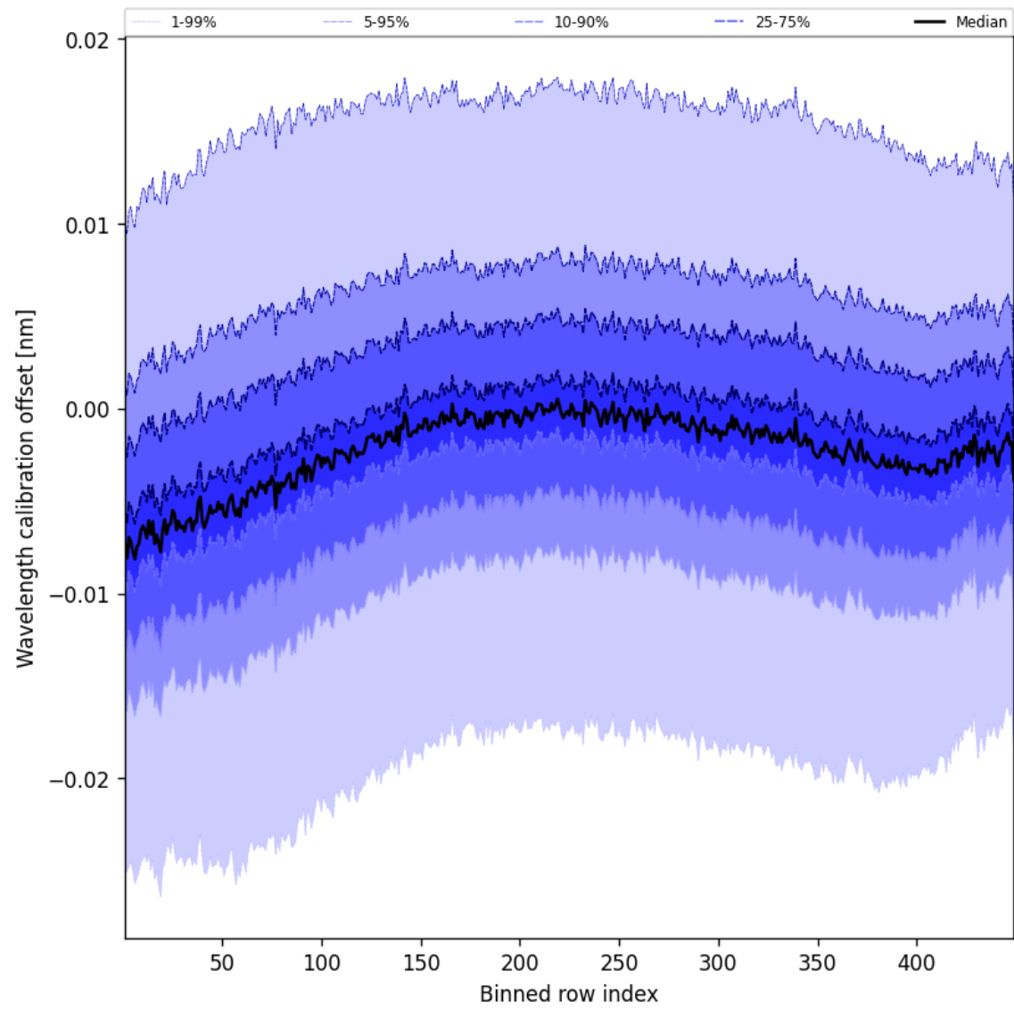
Figure 52: Along track statistics of “Wavelength calibration offset” for 2025-02-19 to 2025-02-20
