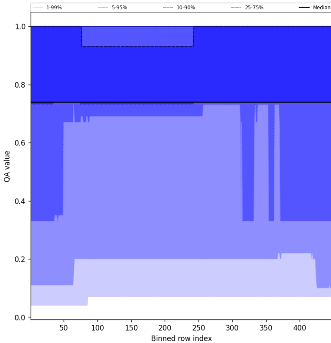
Figure 45: Along track statistics of “QA value” for 2025-02-19 to 2025-02-20
