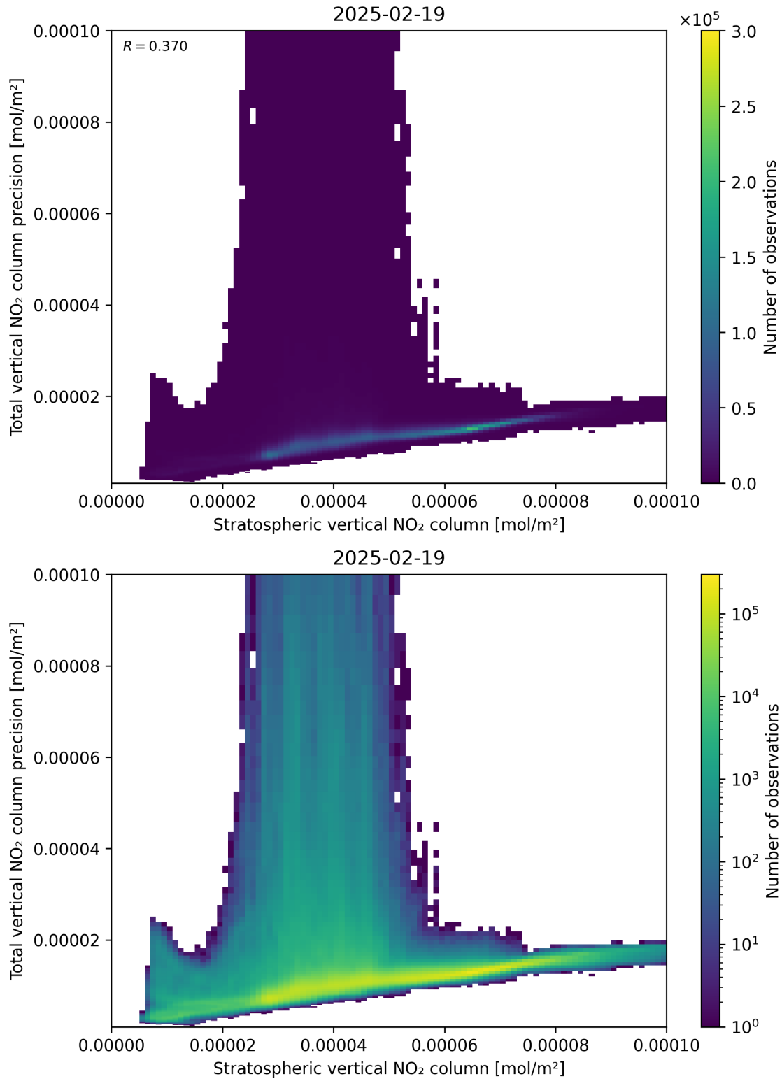
Figure 101: Scatter density plot of “Stratospheric vertical NO 2 column” against “Total vertical NO 2 column precision” for 2025-02-19 to 2025-02-20.
