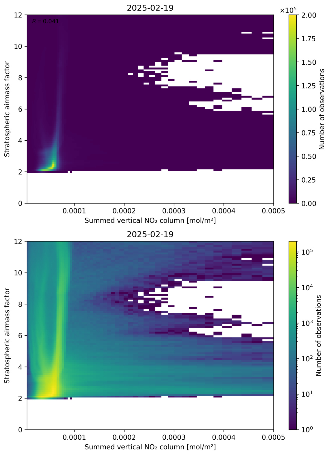
Figure 103: Scatter density plot of “Summed vertical NO 2 column” against “Stratospheric airmass factor” for 2025-02-19 to 2025-02-20.
