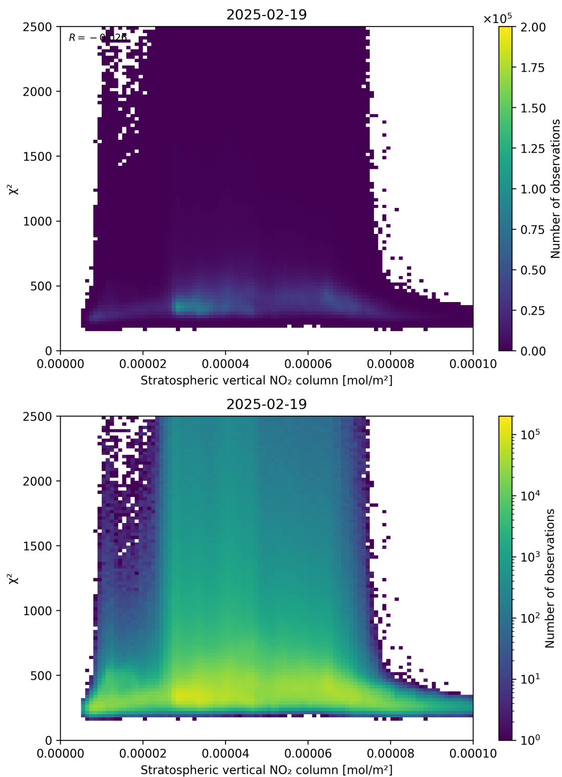
Figure 97: Scatter density plot of “Stratospheric vertical NO 2 column” against “ \chi^2 ” for 2025-02-19 to 2025-02-20.
