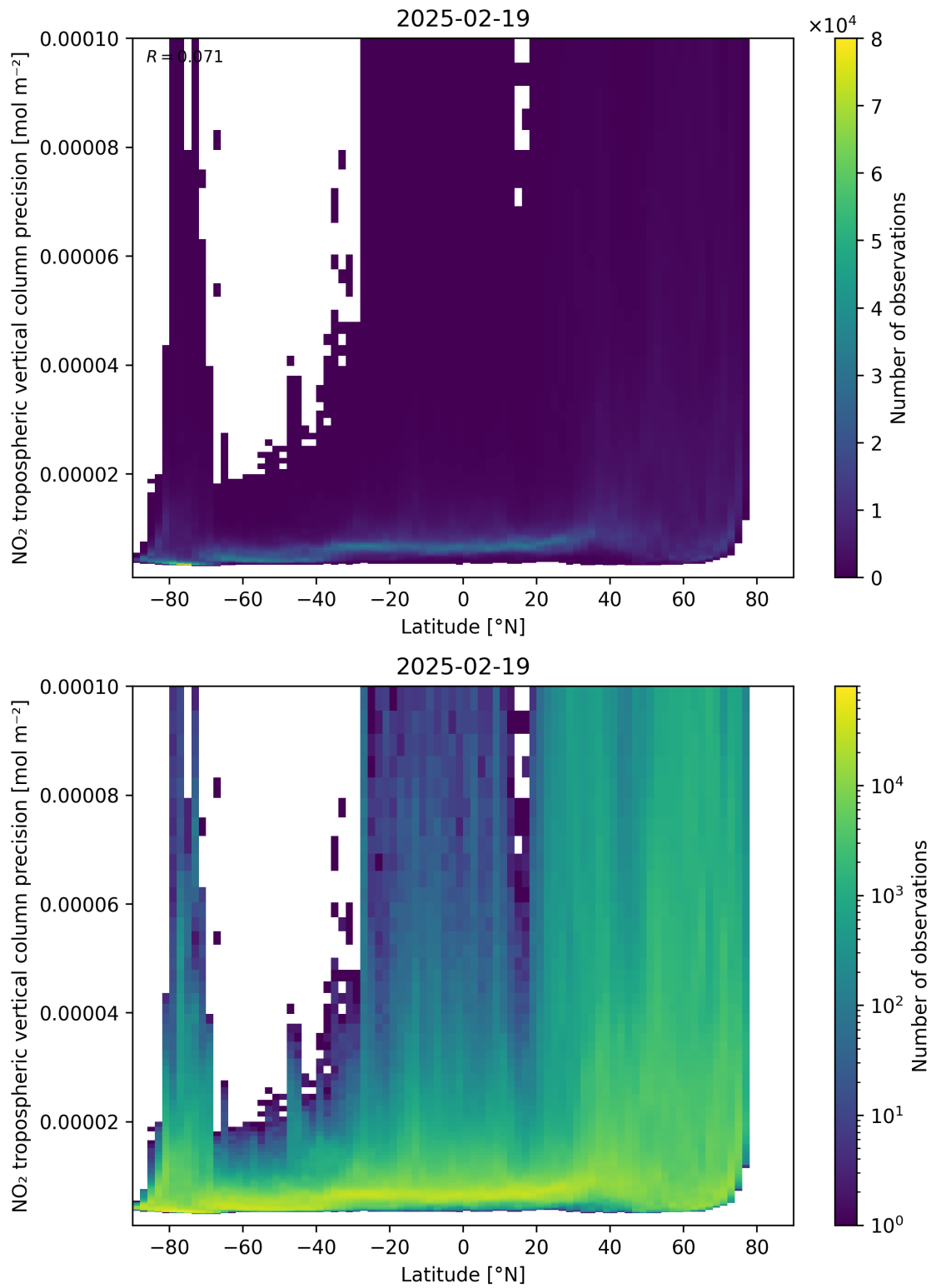
Figure 93: Scatter density plot of “Latitude” against “NO 2 tropospheric vertical column precision” for 2025-02-19 to 2025-02-20.
