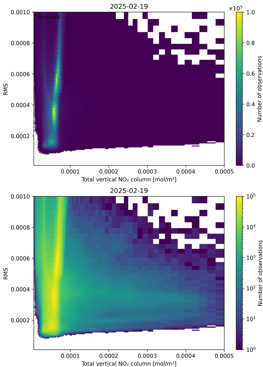
Figure 120: Scatter density plot of “Total vertical NO 2 column” against “RMS” for 2025-02-19 to 2025-02-20.
