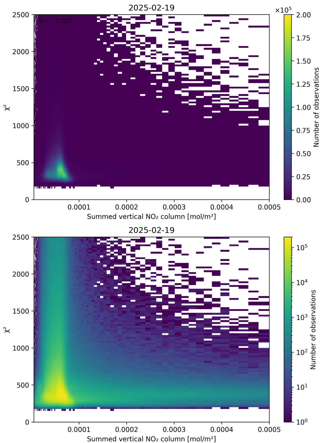
Figure 104: Scatter density plot of “Summed vertical NO 2 column” against “ \chi^2 ” for 2025-02-19 to 2025-02-20.
