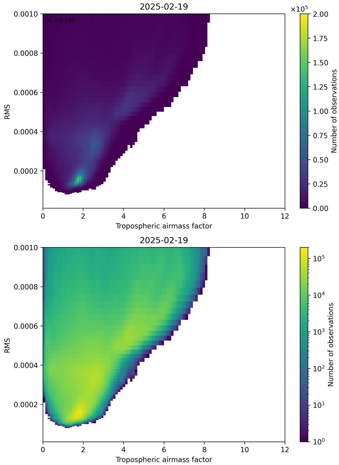
Figure 79: Scatter density plot of “Tropospheric airmass factor” against “RMS” for 2025-02-19 to 2025-02-20.
