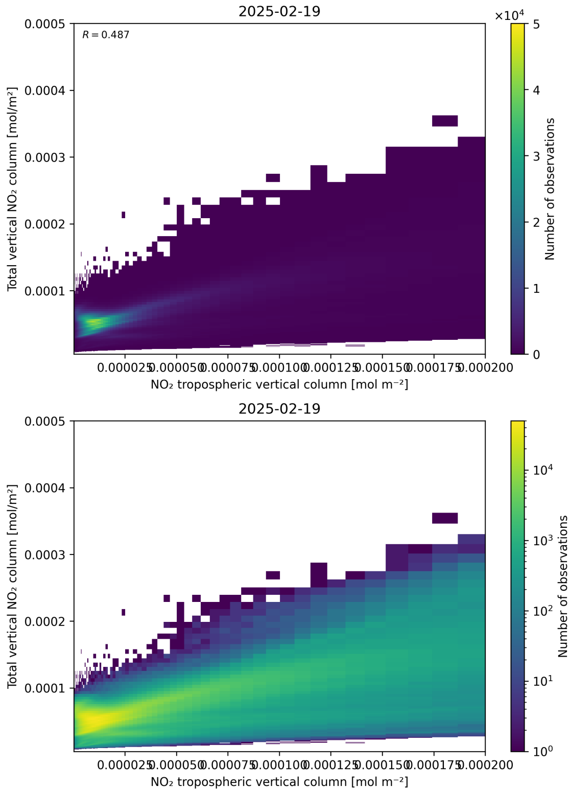
Figure 128: Scatter density plot of “NO 2 tropospheric vertical column” against “Total vertical NO 2 column” for 2025-02-19 to 2025-02-20.
