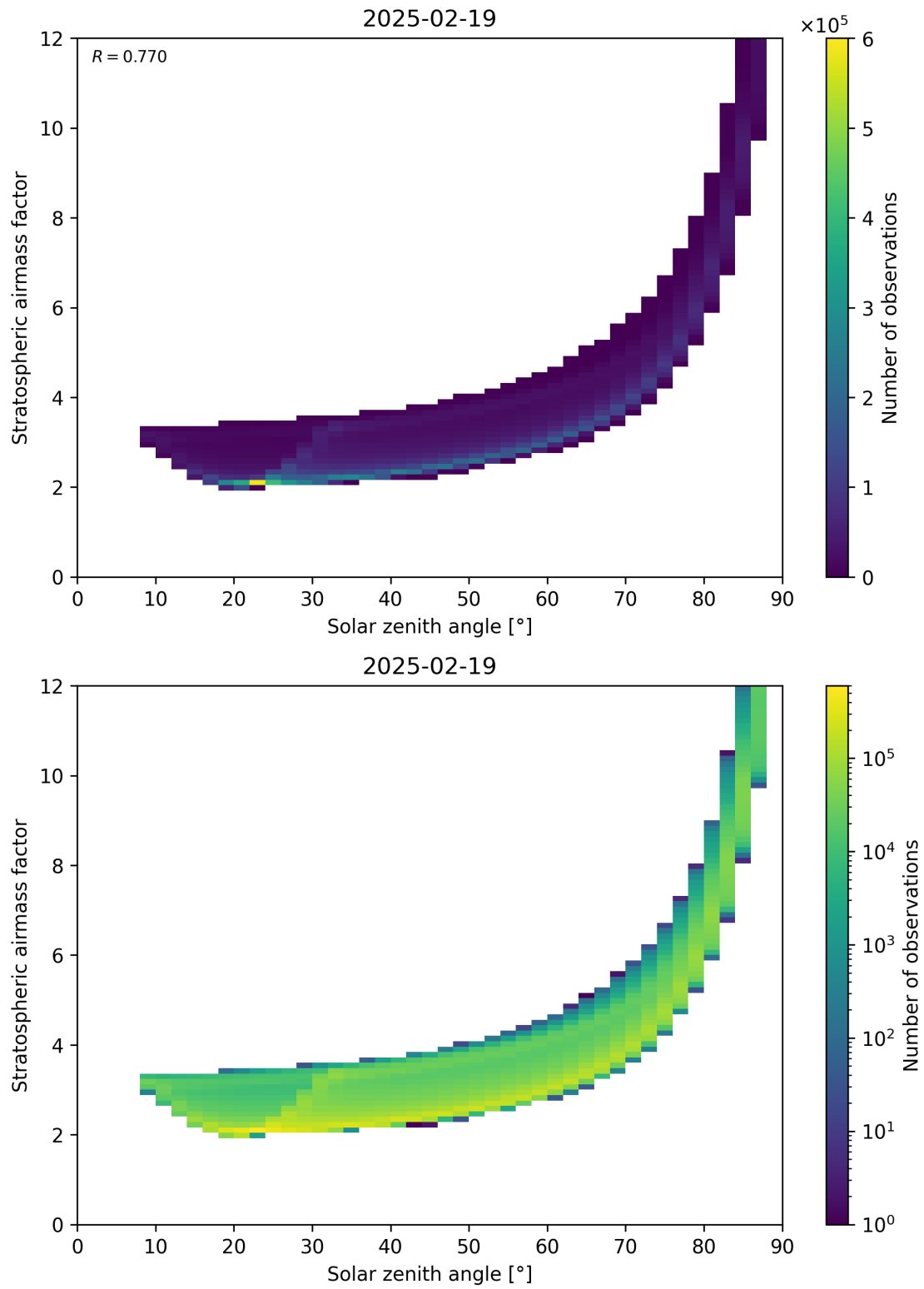
Figure 145: Scatter density plot of “Solar zenith angle” against “Stratospheric airmass factor” for 2025-02-19 to 2025-02-20.
