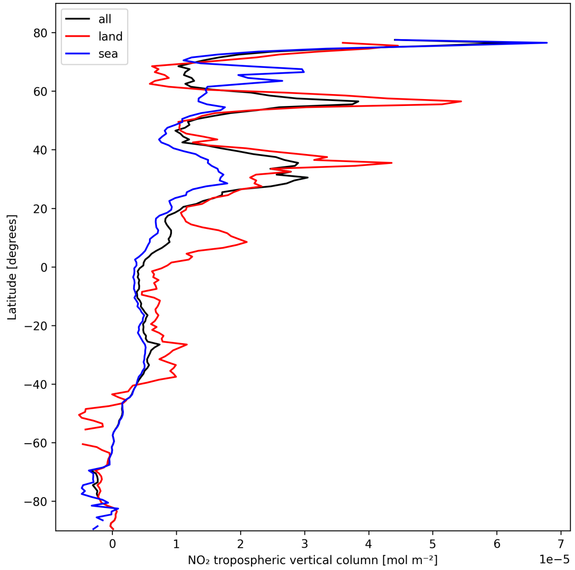
Figure 12: Zonal average of “NO 2 tropospheric vertical column” for 2025-02-19 to 2025-02-20.
