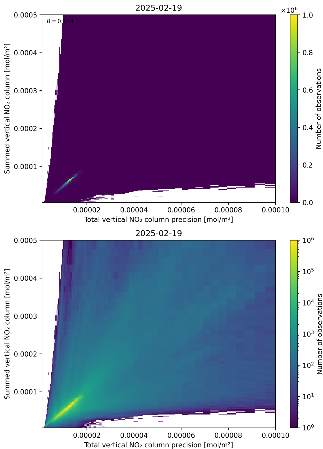
Figure 117: Scatter density plot of “Total vertical NO 2 column precision” against “Summed vertical NO 2 column” for 2025-02-19 to 2025-02-20.
