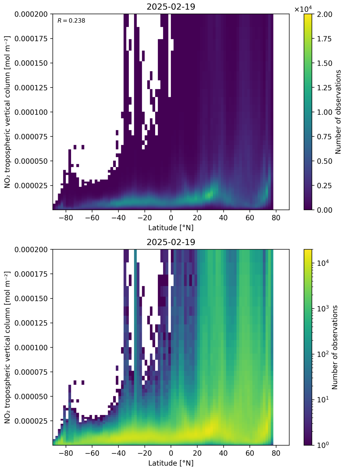
Figure 92: Scatter density plot of “Latitude” against “NO 2 tropospheric vertical column” for 2025-02-19 to 2025-02-20.
