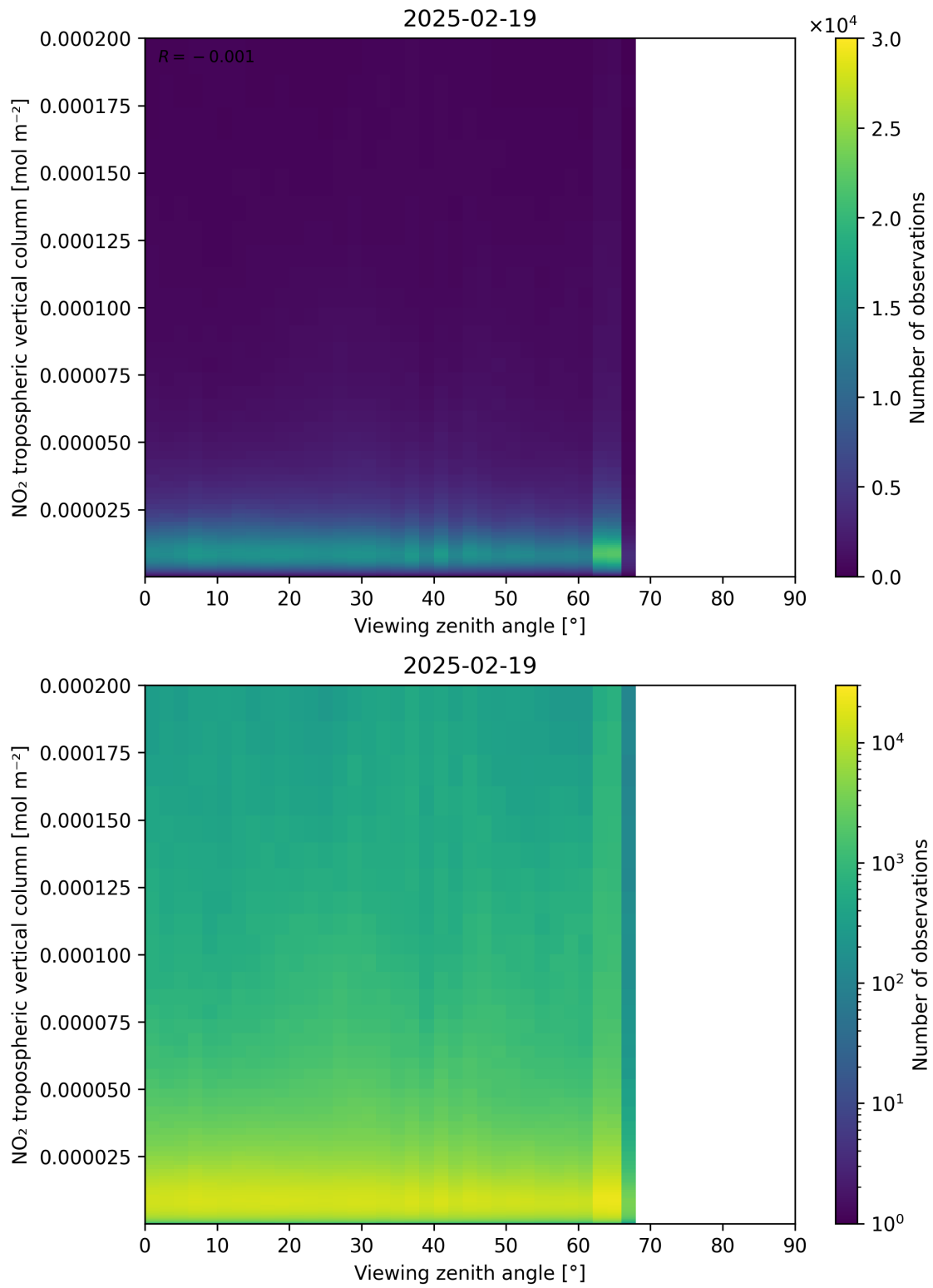
Figure 169: Scatter density plot of “Viewing zenith angle” against “NO 2 tropospheric vertical column” for 2025-02-19 to 2025-02-20.
