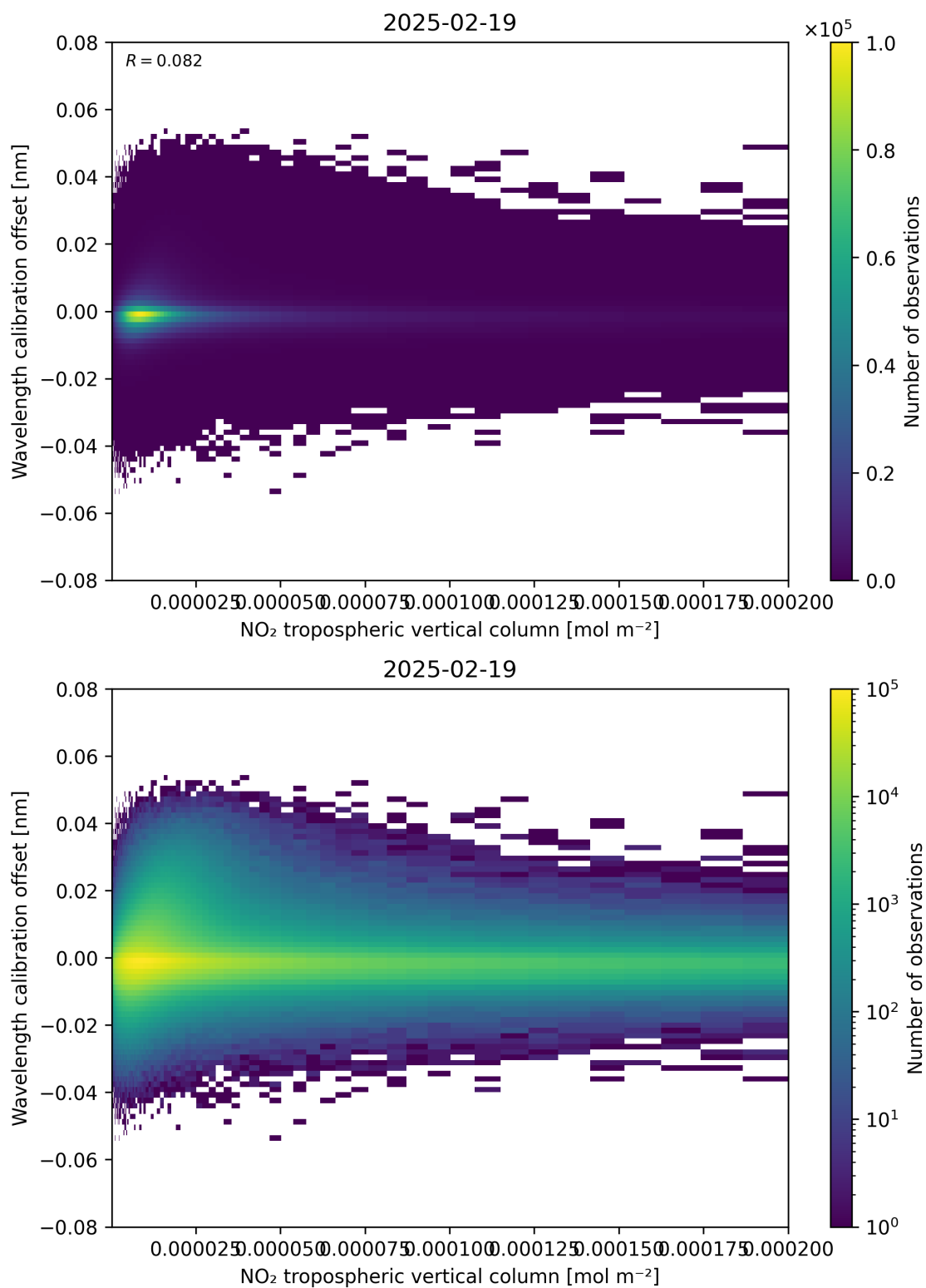
Figure 143: Scatter density plot of “NO 2 tropospheric vertical column” against “Wavelength calibration offset” for 2025-02-19 to 2025-02-20.
