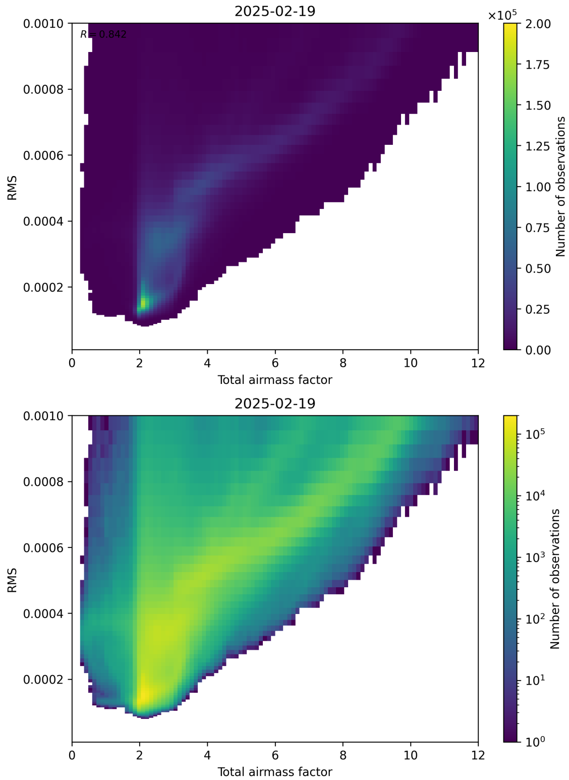
Figure 69: Scatter density plot of “Total airmass factor” against “RMS” for 2025-02-19 to 2025-02-20.
