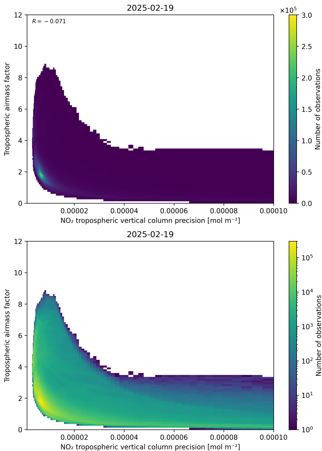
Figure 133: Scatter density plot of “NO 2 tropospheric vertical column precision” against “Tropospheric air mass factor” for 2025-02-19 to 2025-02-20.
