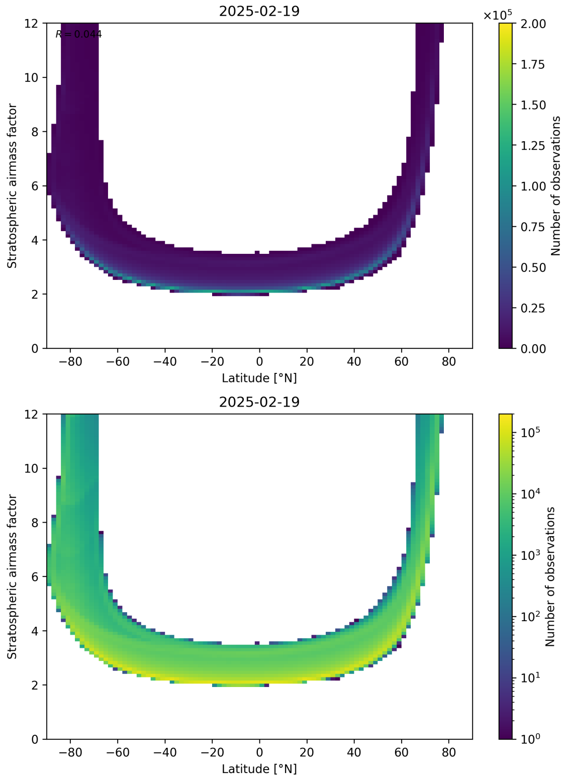
Figure 83: Scatter density plot of “Latitude” against “Stratospheric airmass factor” for 2025-02-19 to 2025-02-20.
