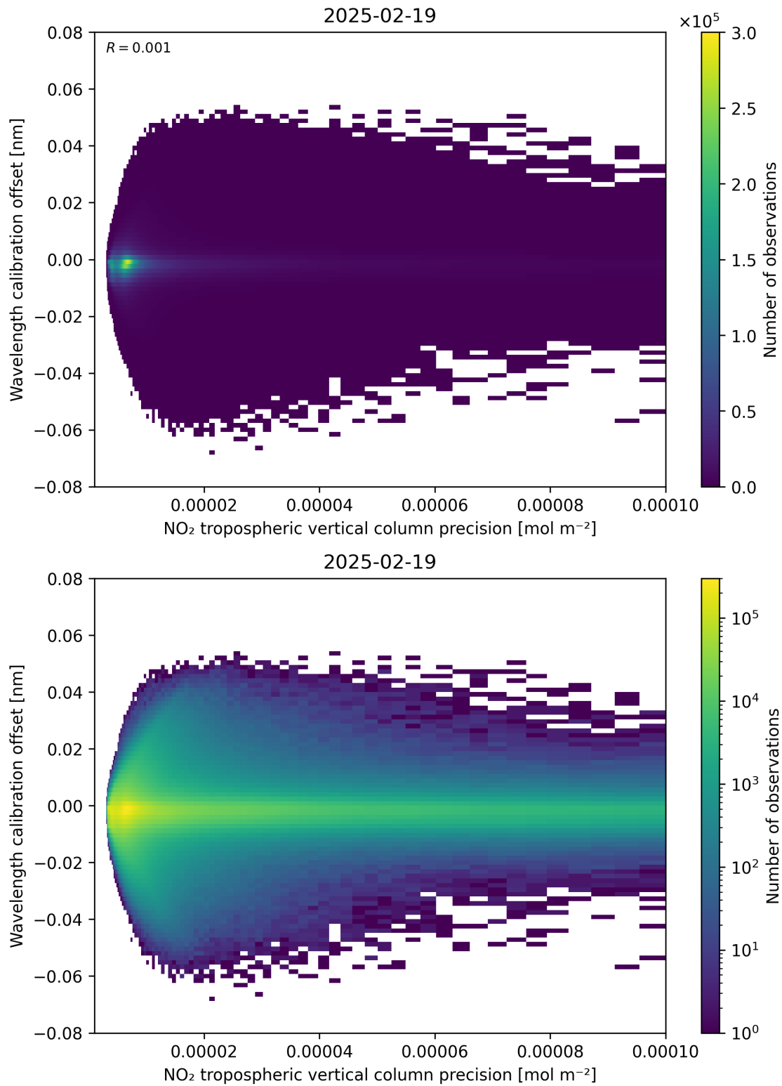
Figure 141: Scatter density plot of “NO 2 tropospheric vertical column precision” against “Wavelength calibration offset” for 2025-02-19 to 2025-02-20.
