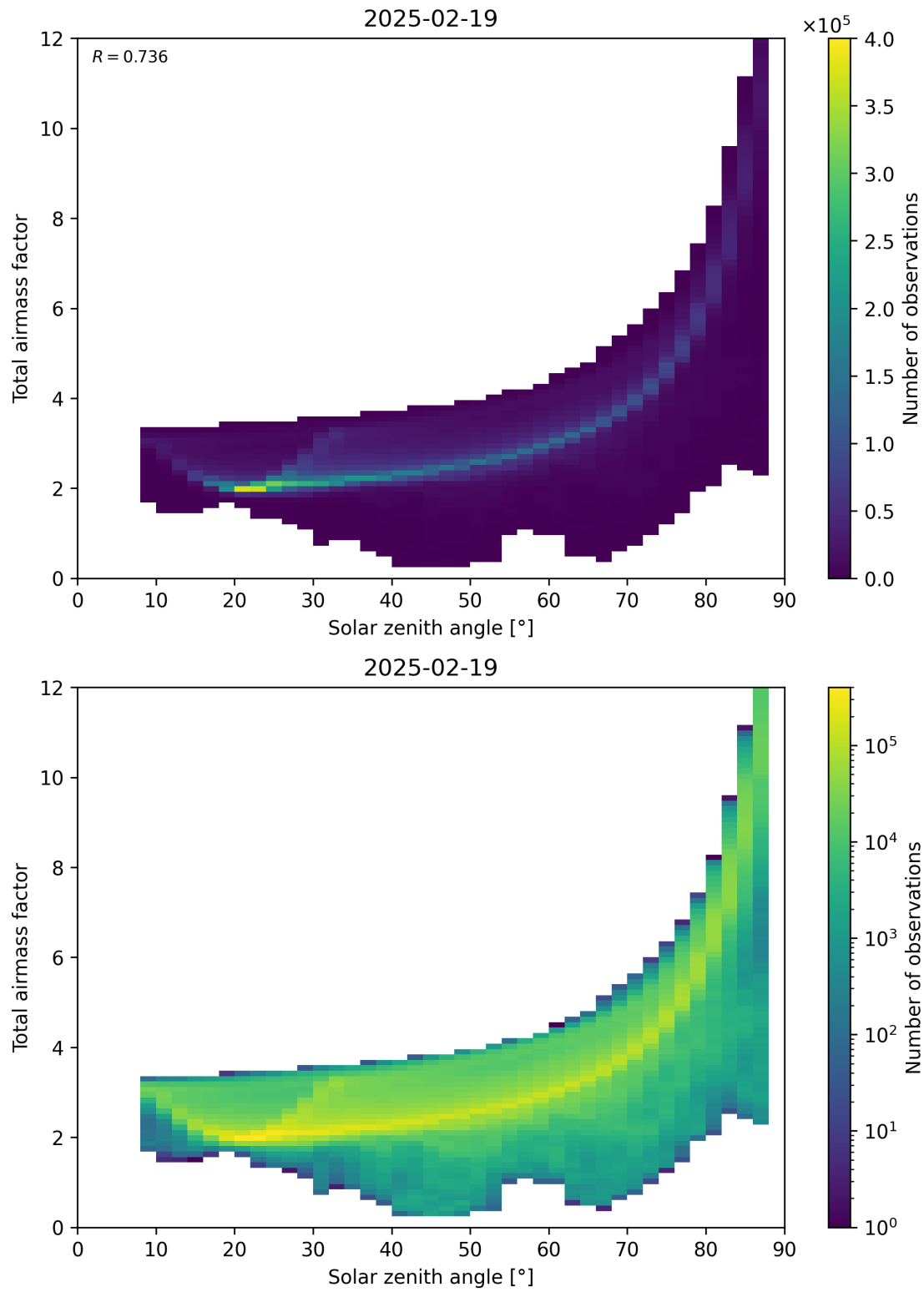
Figure 146: Scatter density plot of “Solar zenith angle” against “Total air mass factor” for 2025-02-19 to 2025-02-20.
