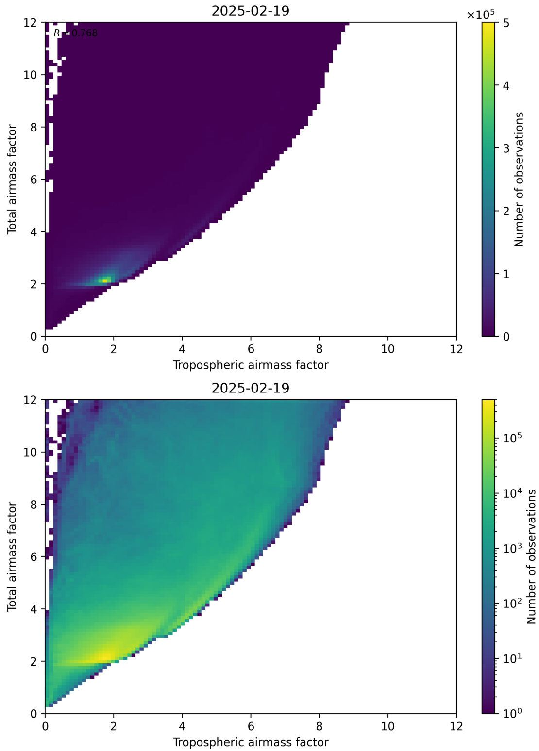
Figure 72: Scatter density plot of “Tropospheric airmass factor” against “Total airmass factor” for 2025-02-19 to 2025-02-20.
