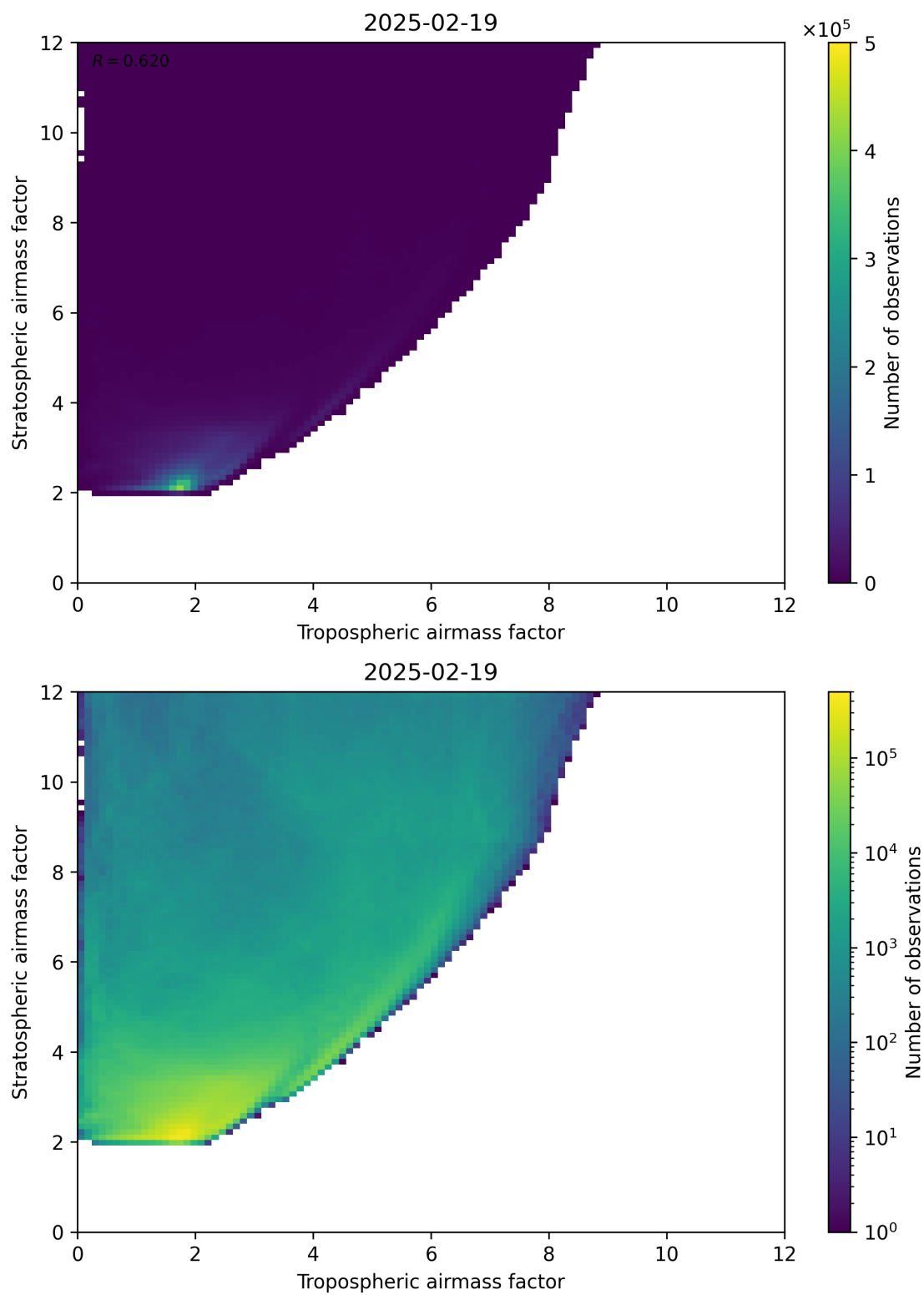
Figure 71: Scatter density plot of “Tropospheric airmass factor” against “Stratospheric airmass factor” for 2025-02-19 to 2025-02-20.
