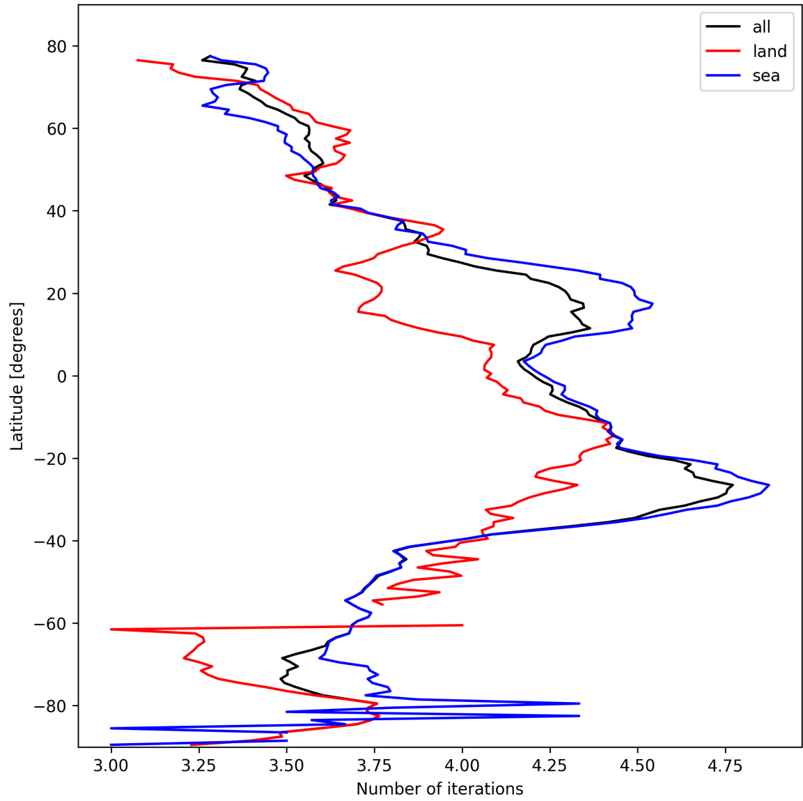
Figure 17: Zonal average of “Number of iterations” for 2025-02-19 to 2025-02-20.
