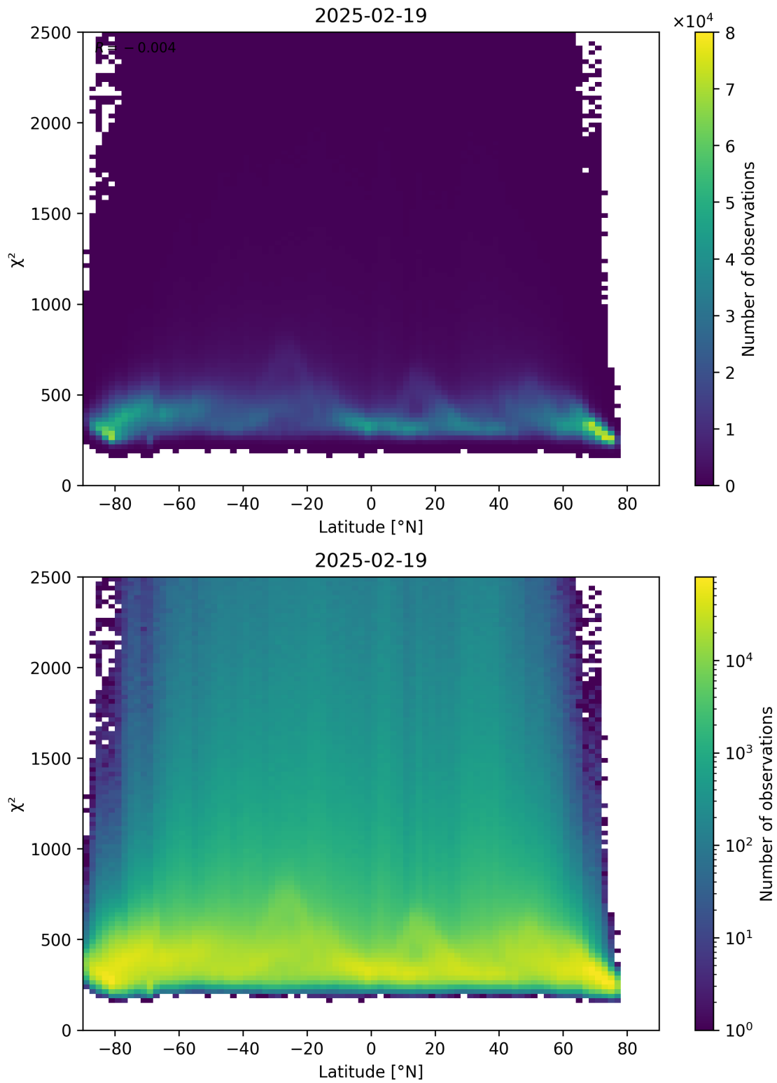
Figure 86: Scatter density plot of “Latitude” against “ \chi^2 ” for 2025-02-19 to 2025-02-20.
