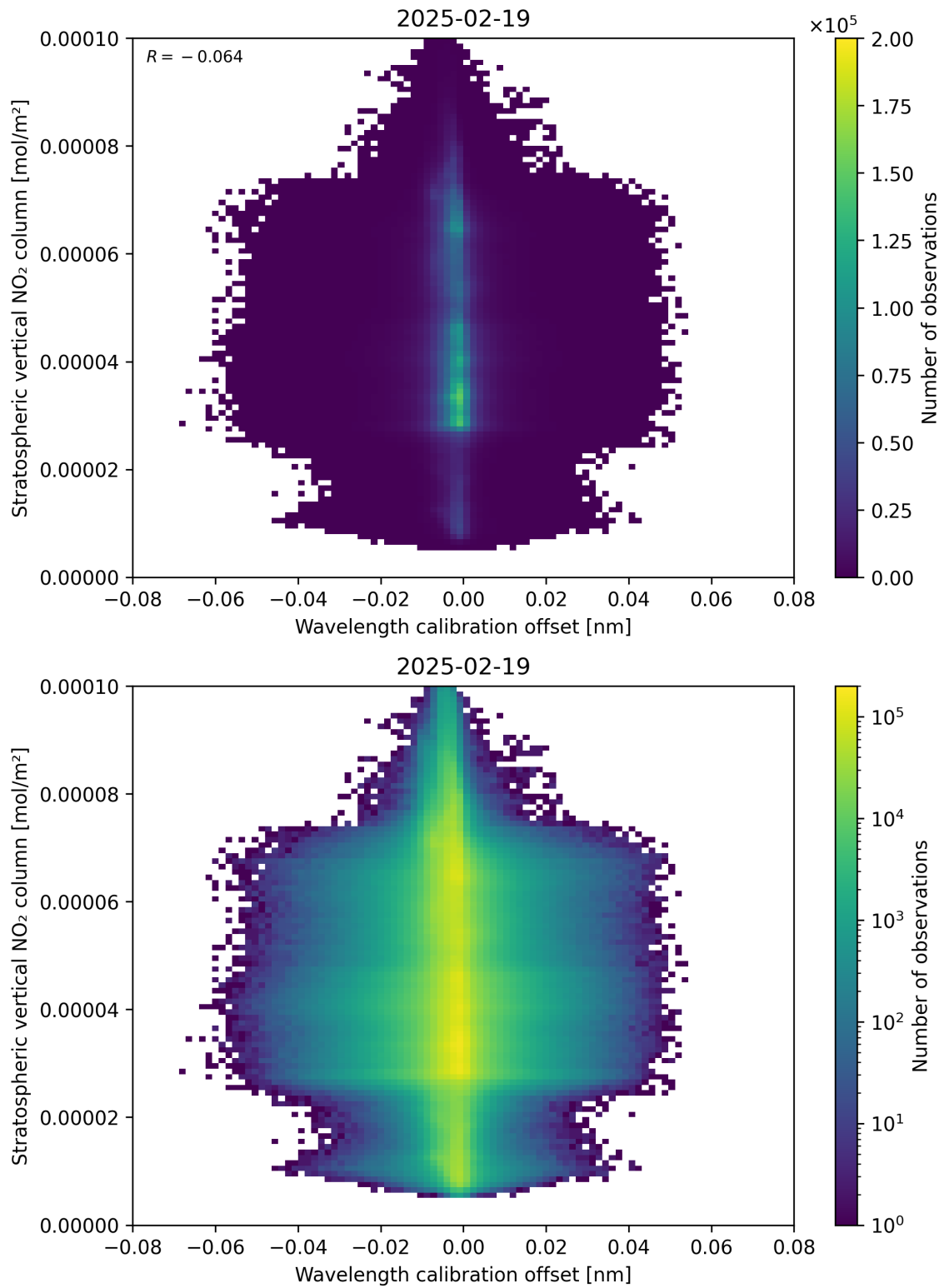
Figure 176: Scatter density plot of “Wavelength calibration offset” against “Stratospheric vertical NO 2 column” for 2025-02-19 to 2025-02-20.
