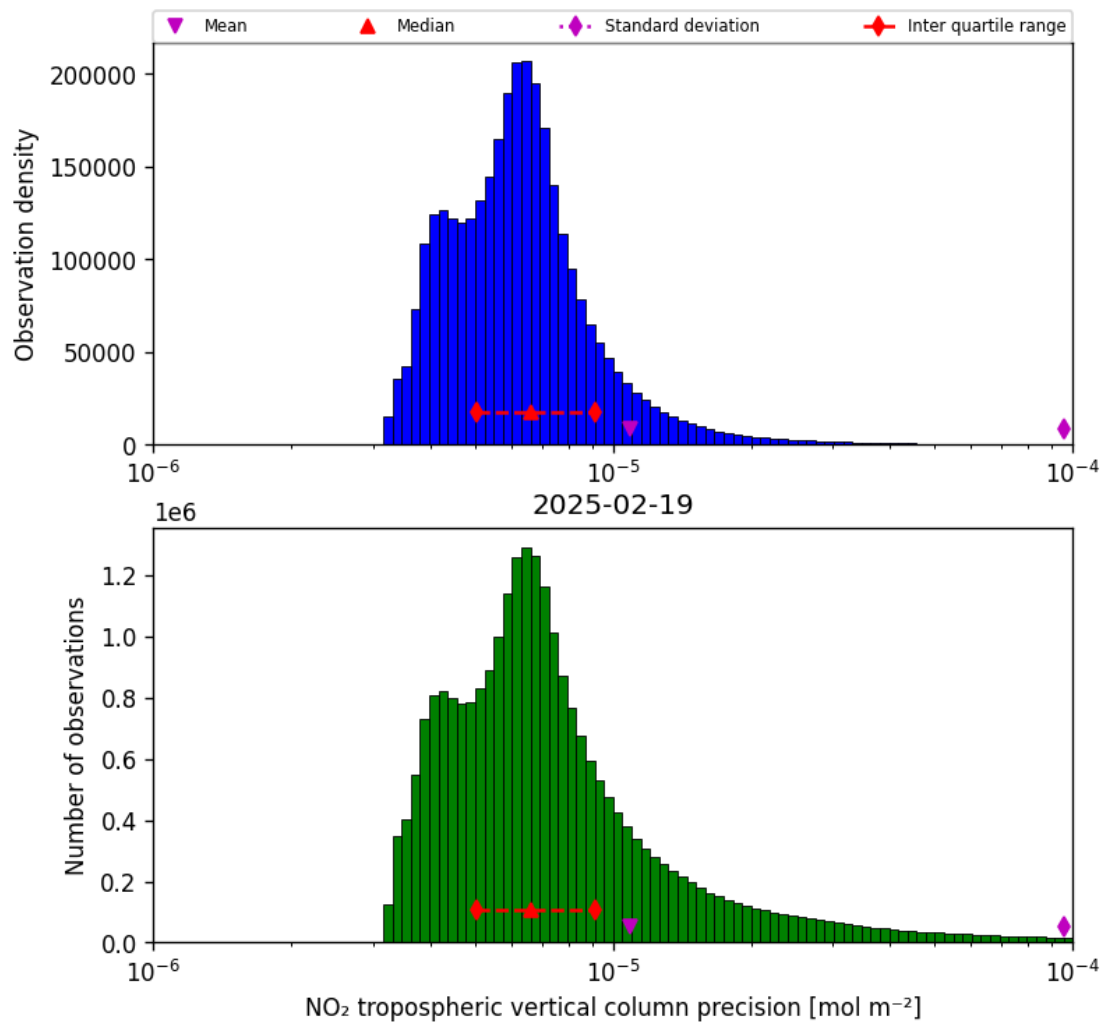
Figure 30: Histogram of “NO 2 tropospheric vertical column precision” for 2025-02-19 to 2025-02-20
