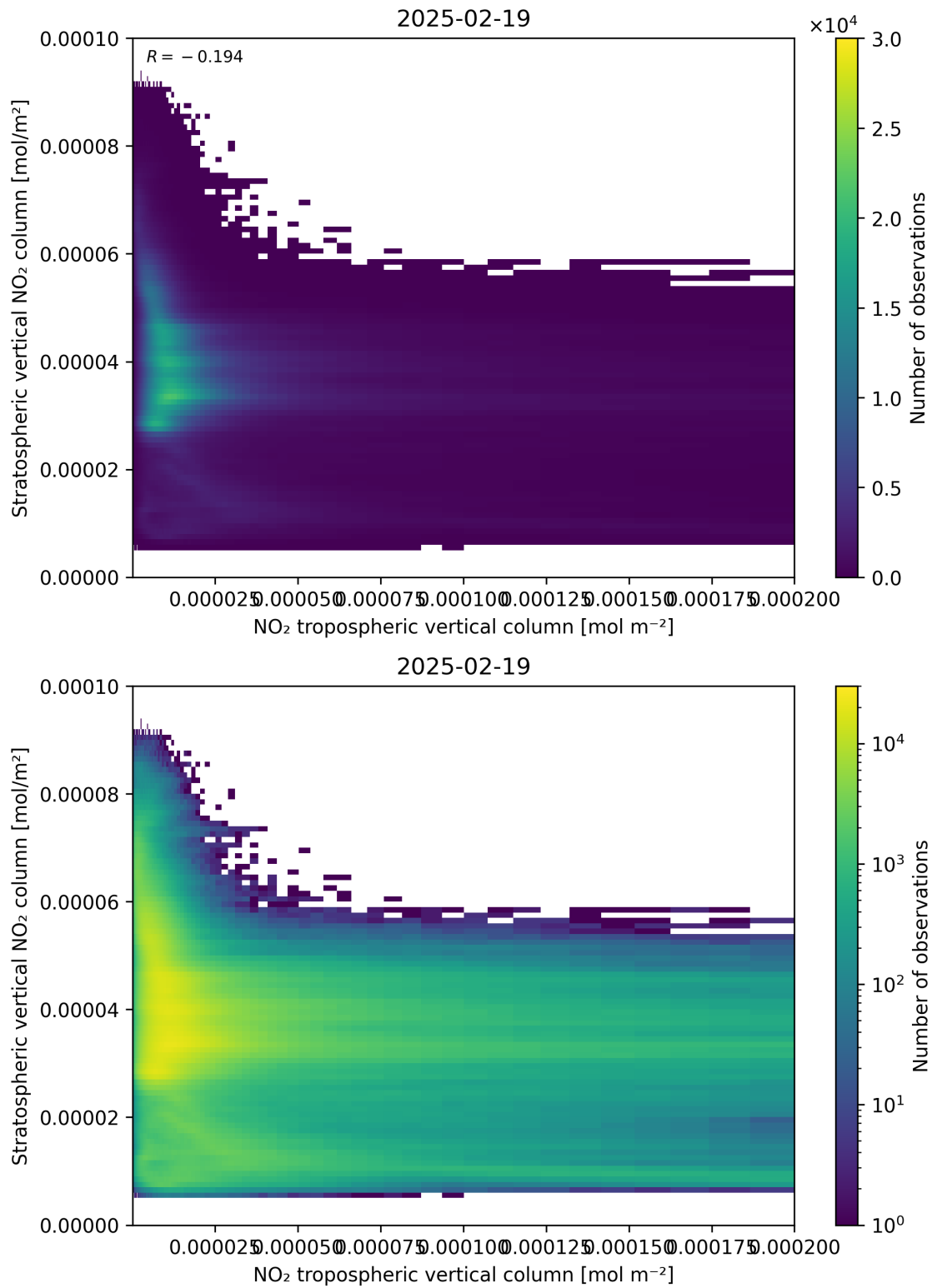
Figure 125: Scatter density plot of “NO 2 tropospheric vertical column” against “Stratospheric vertical NO 2 column” for 2025-02-19 to 2025-02-20.
