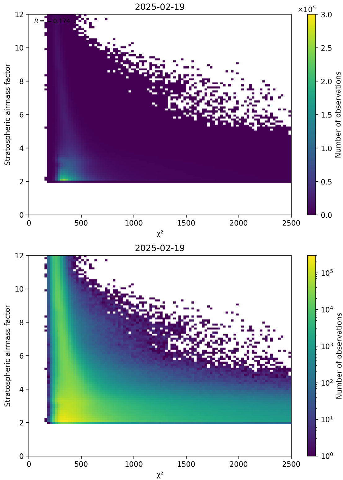
Figure 81: Scatter density plot of “ \chi^2 ” against “Stratospheric airmass factor” for 2025-02-19 to 2025-02-20.
