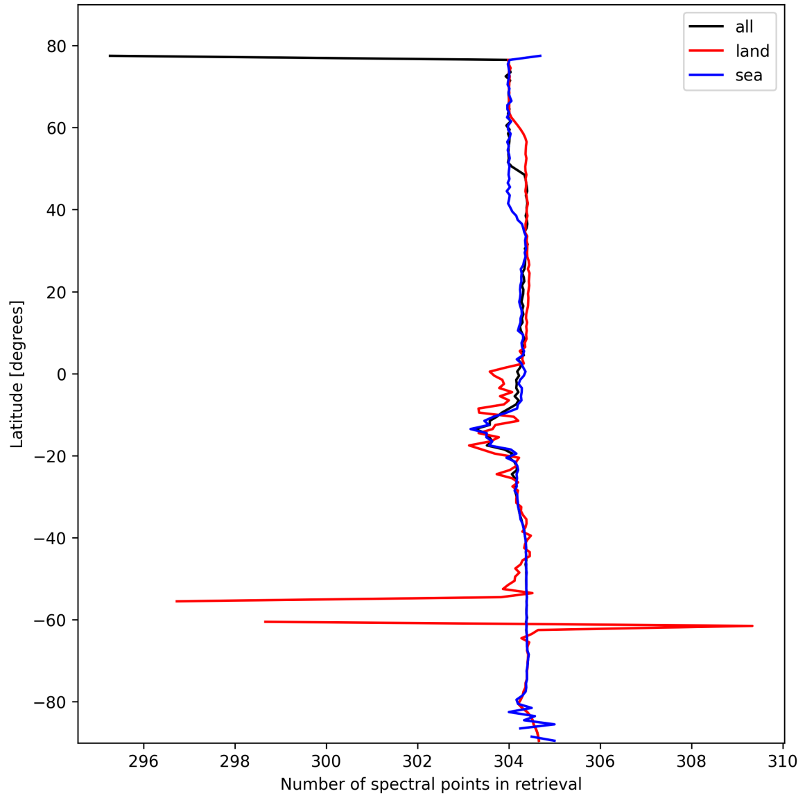
Figure 16: Zonal average of “Number of spectral points in retrieval” for 2025-02-19 to 2025-02-20.
