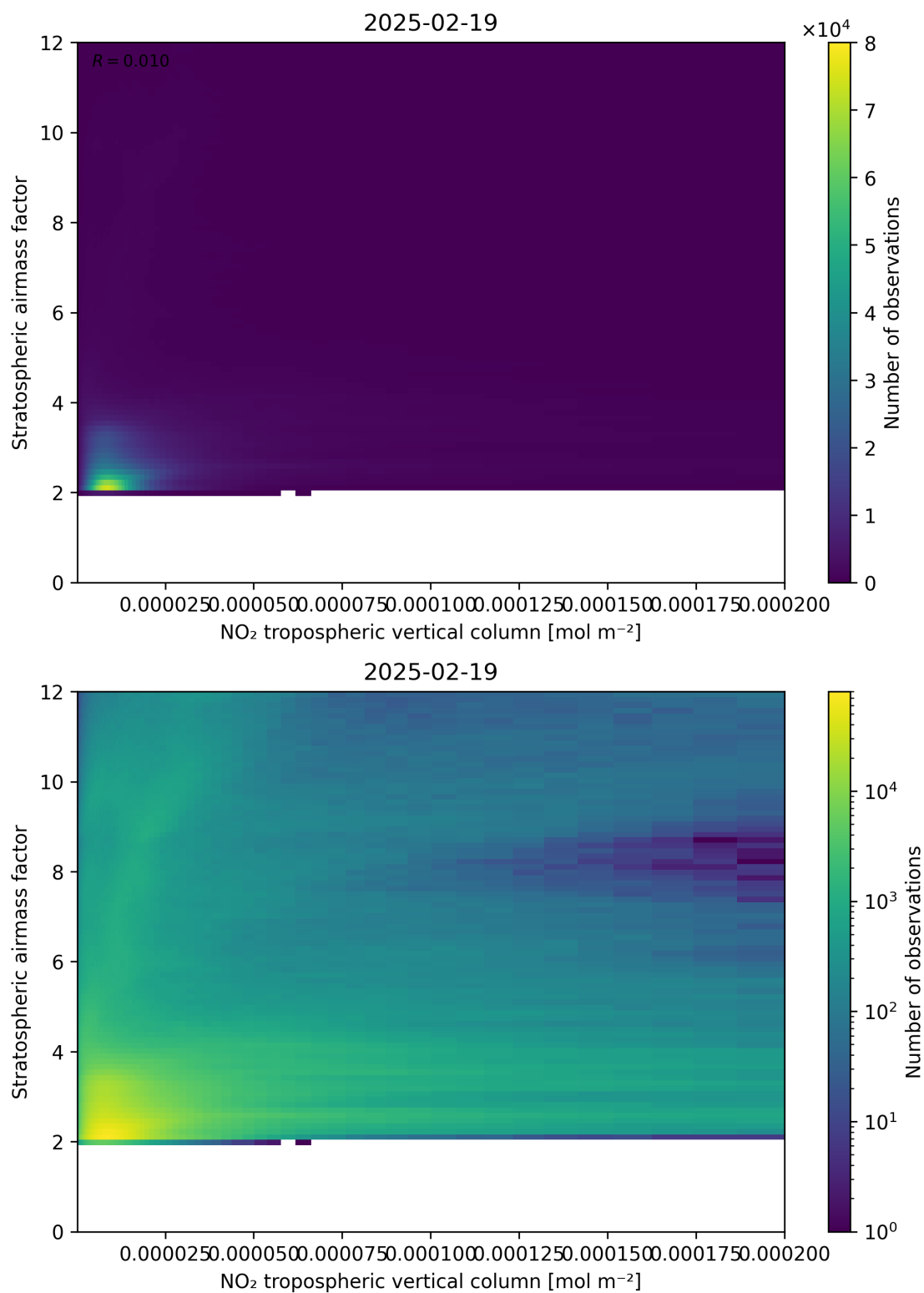
Figure 121: Scatter density plot of “NO 2 tropospheric vertical column” against “Stratospheric airmass factor” for 2025-02-19 to 2025-02-20.
