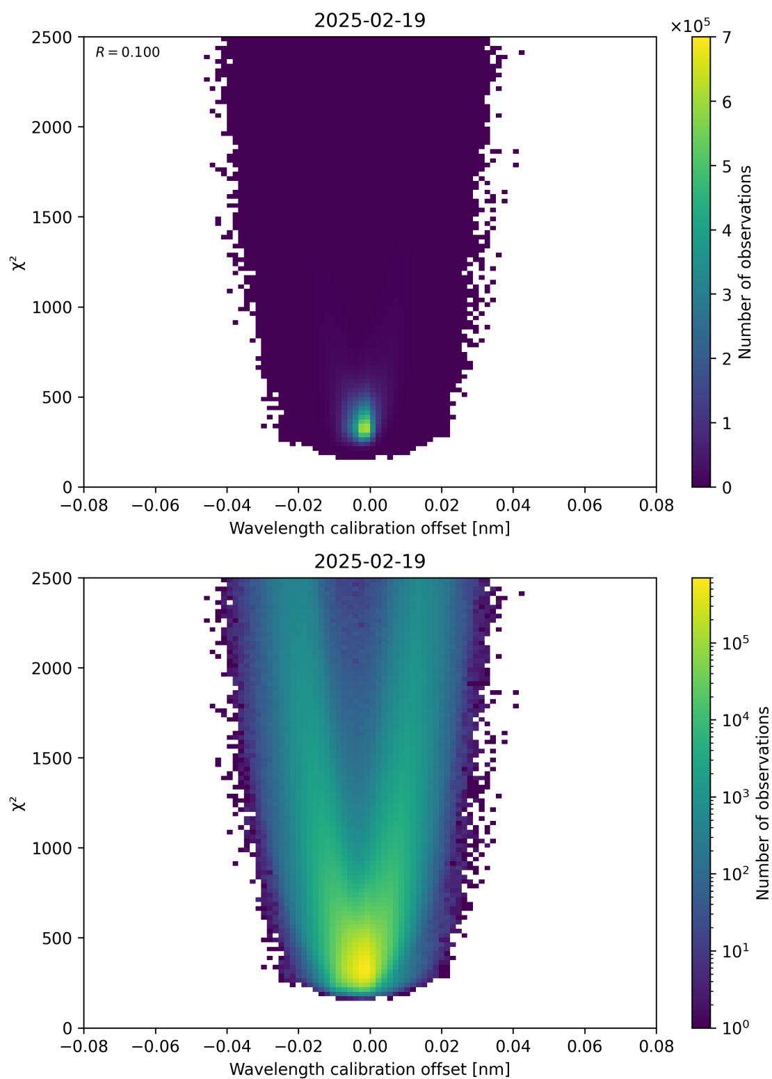
Figure 175: Scatter density plot of “Wavelength calibration offset” against “ \chi^2 ” for 2025-02-19 to 2025-02-20.
