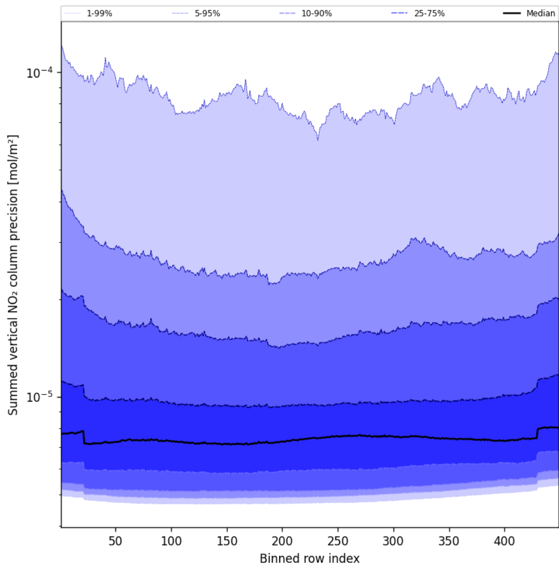
Figure 58: Along track statistics of “Summed vertical NO 2 column precision” for 2025-02-19 to 2025-02-20
