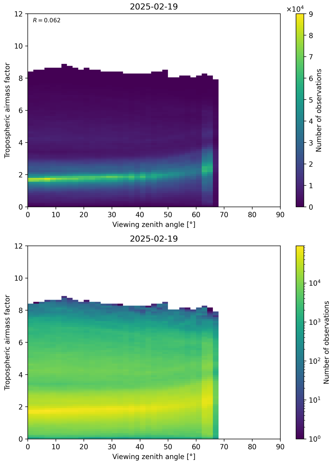
Figure 161: Scatter density plot of “Viewing zenith angle” against “Tropospheric airmass factor” for 2025-02-19 to 2025-02-20.
