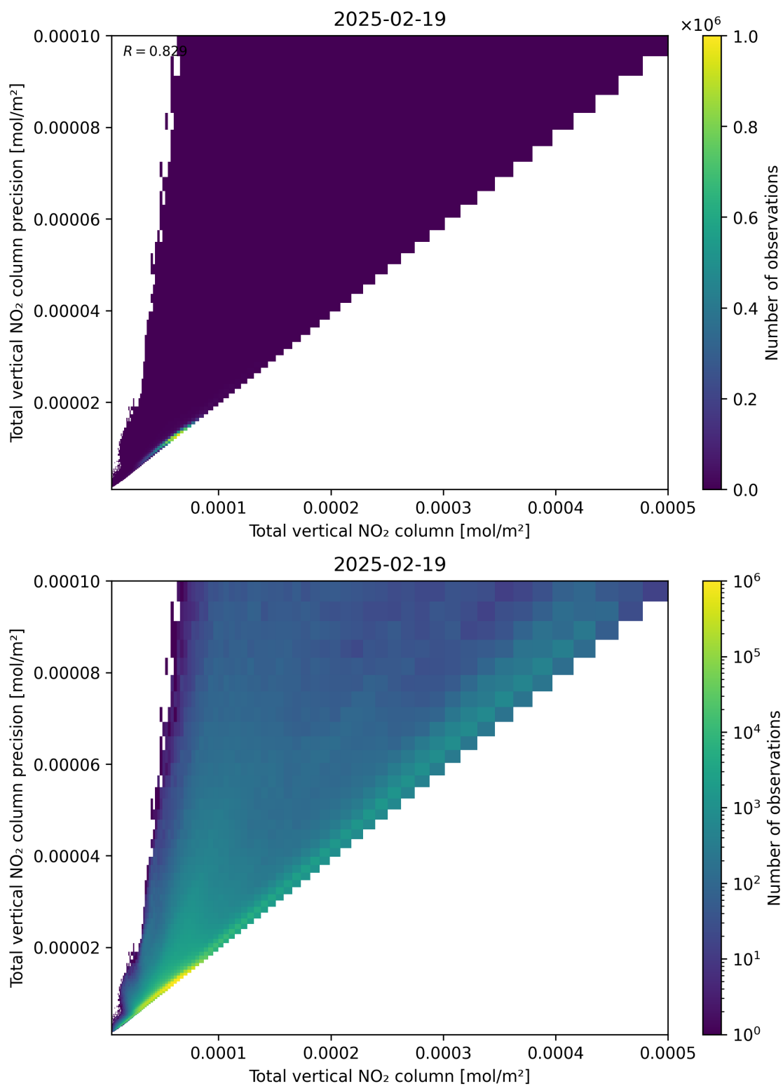
Figure 114: Scatter density plot of “Total vertical NO 2 column” against “Total vertical NO 2 column precision” for 2025-02-19 to 2025-02-20.
