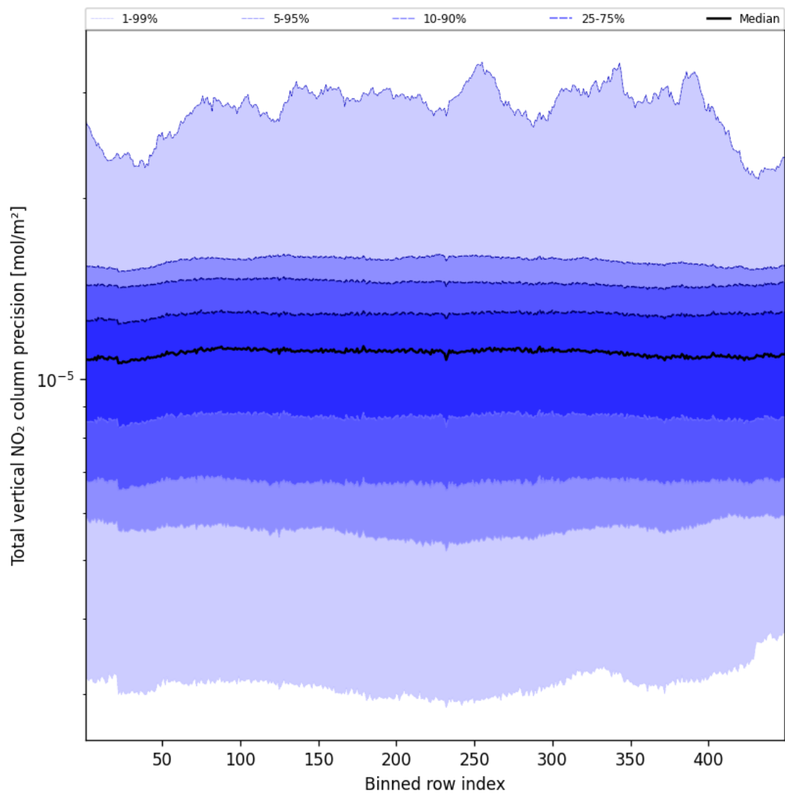
Figure 56: Along track statistics of “Total vertical NO 2 column precision” for 2025-02-19 to 2025-02-20
