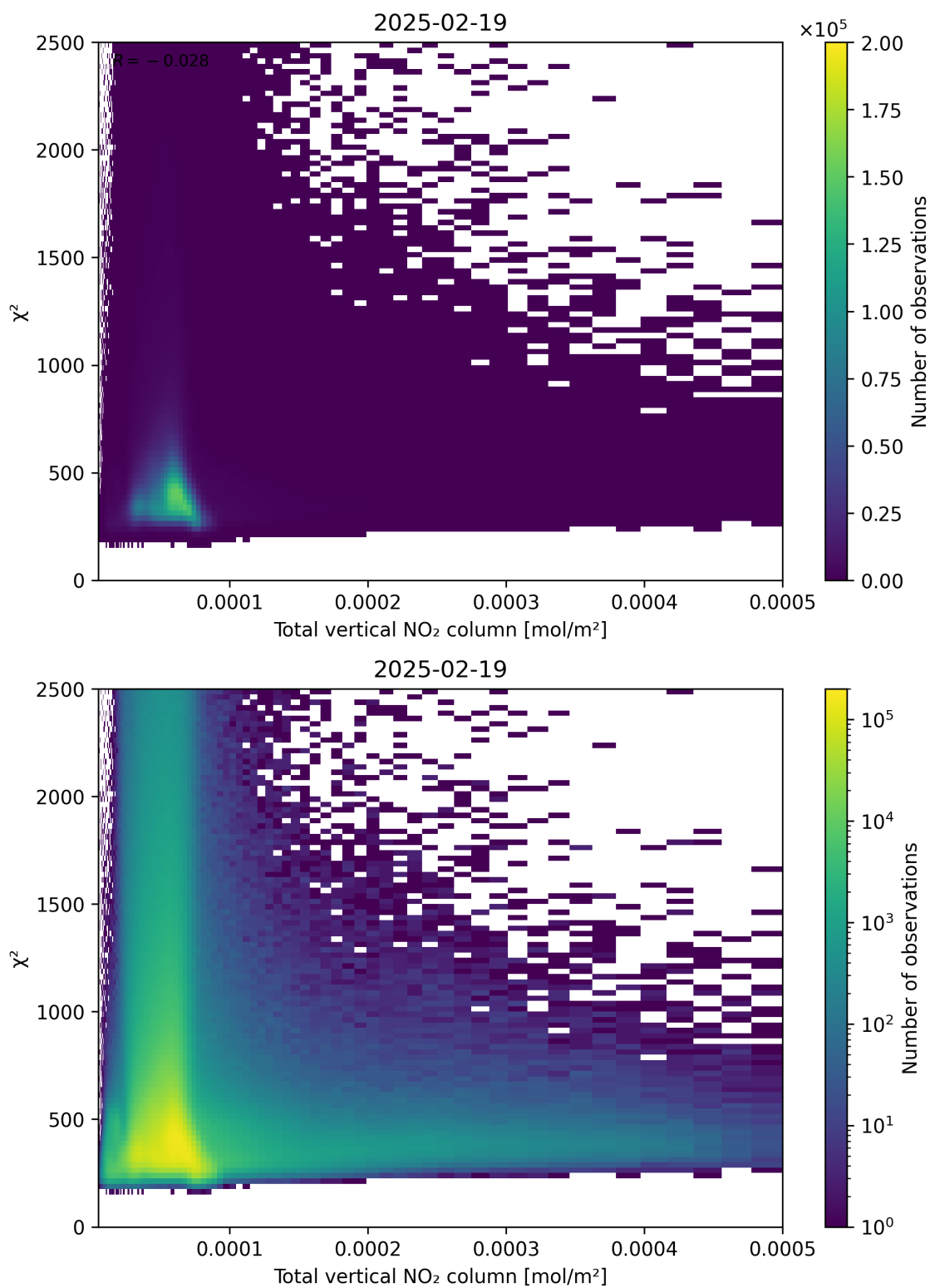
Figure 111: Scatter density plot of “Total vertical NO 2 column” against “ \chi^2 ” for 2025-02-19 to 2025-02-20.
