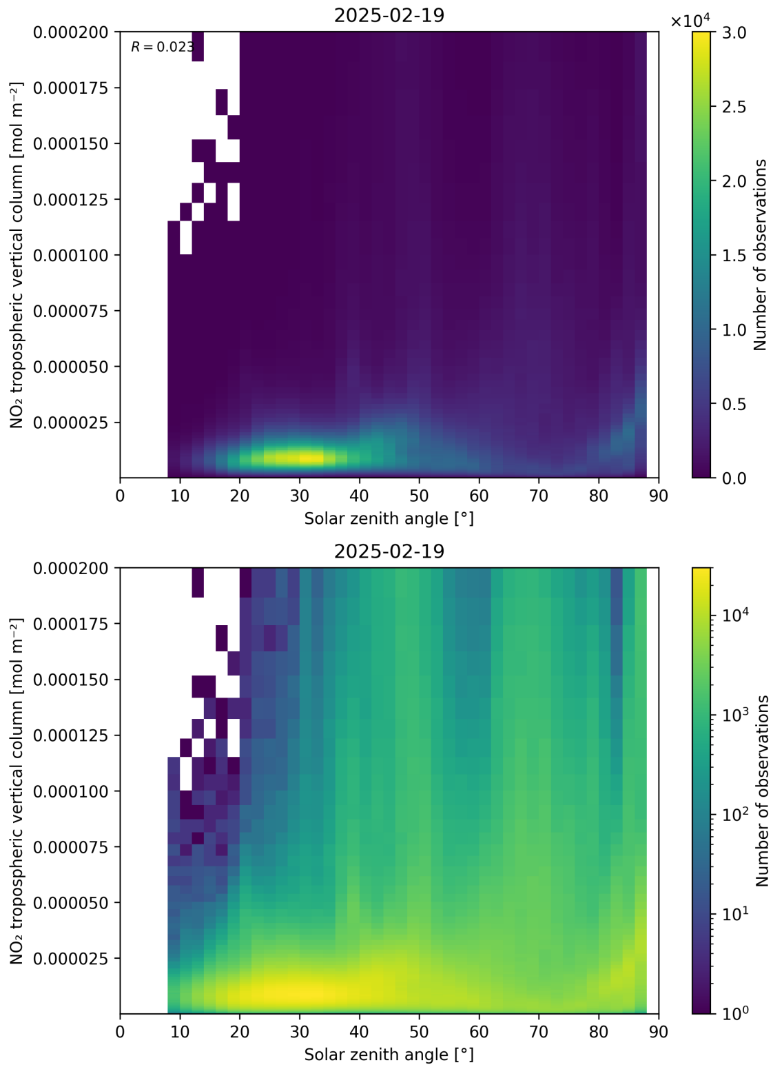
Figure 155: Scatter density plot of “Solar zenith angle” against “NO 2 tropospheric vertical column” for 2025-02-19 to 2025-02-20.
