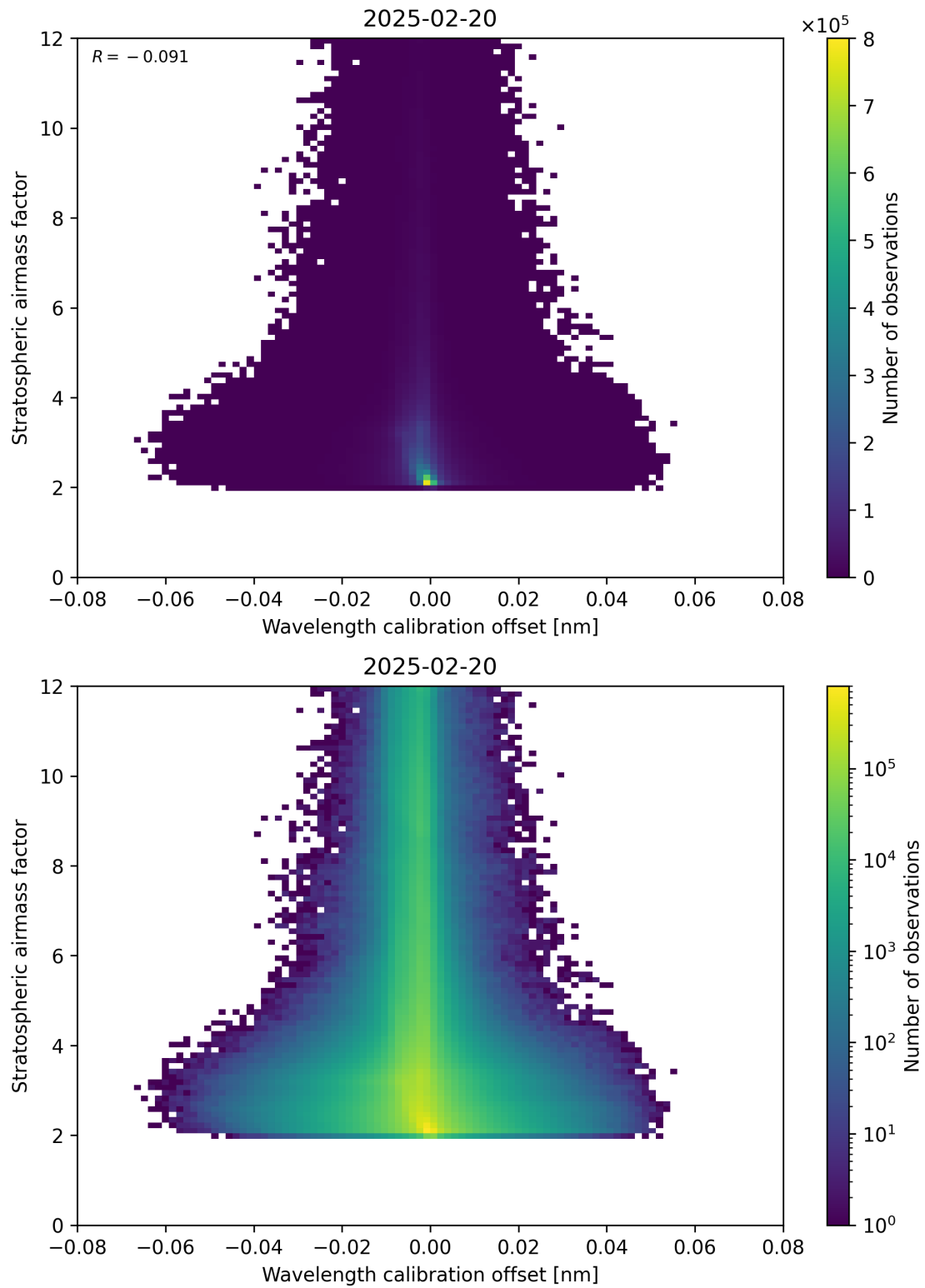
Figure 174: Scatter density plot of “Wavelength calibration offset” against “Stratospheric airmass factor” for 2025-02-19 to 2025-02-21.
