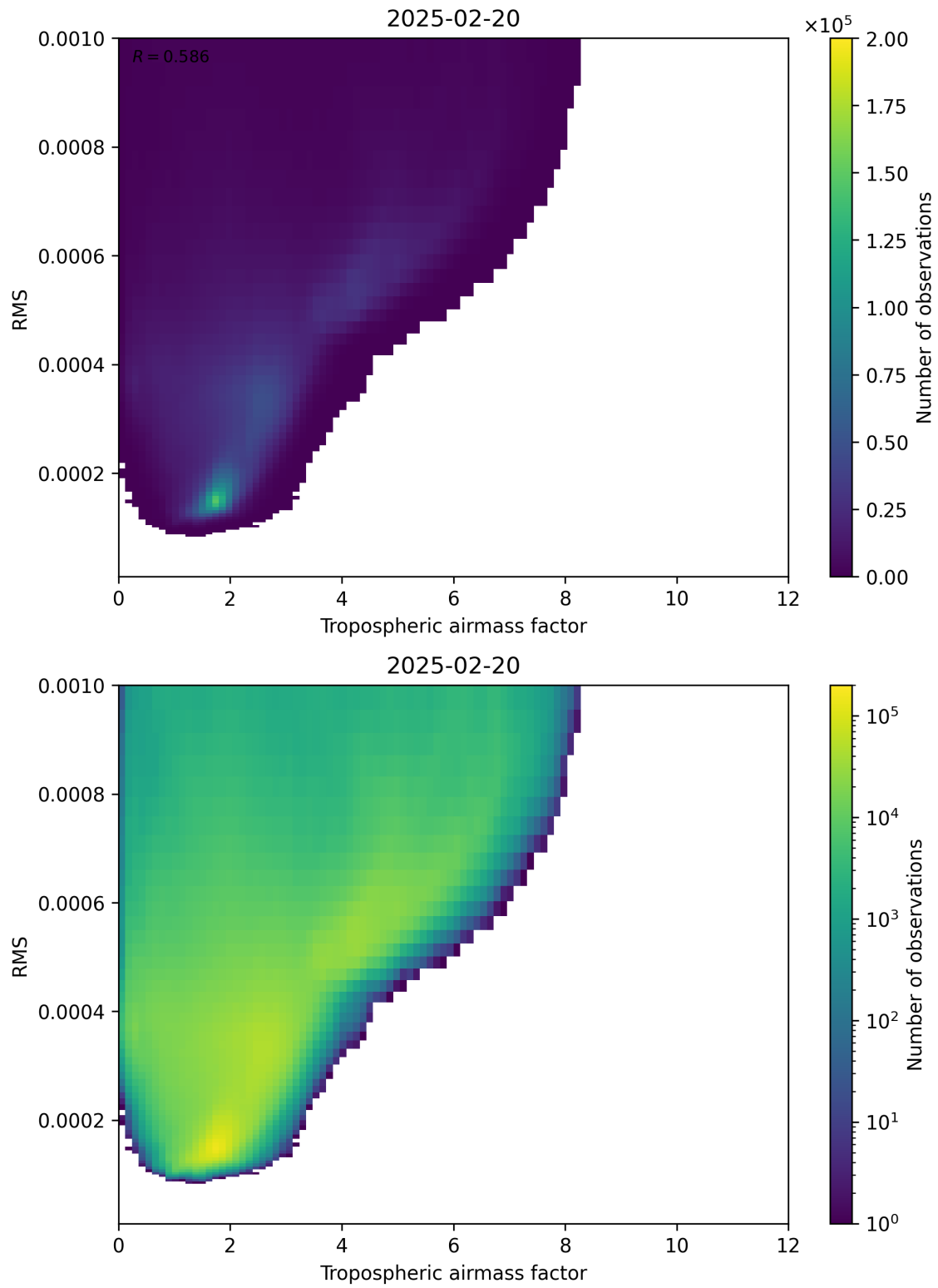
Figure 79: Scatter density plot of “Tropospheric airmass factor” against “RMS” for 2025-02-19 to 2025-02-21.
