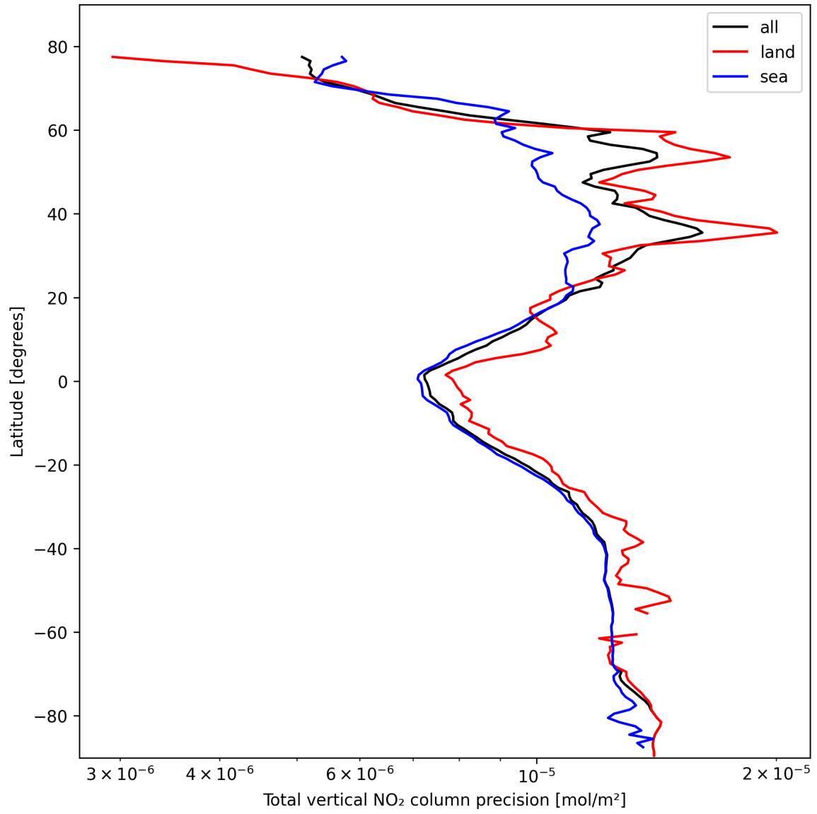
Figure 22: Zonal average of “Total vertical NO 2 column precision” for 2025-02-19 to 2025-02-21.
