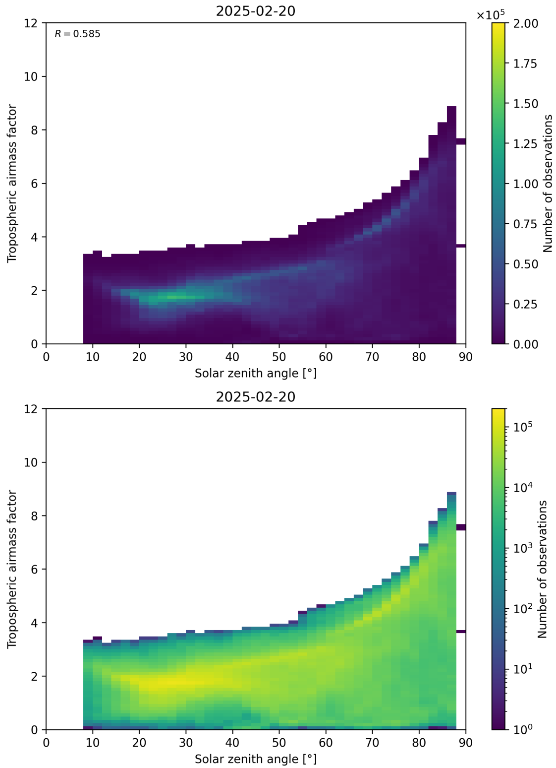
Figure 147: Scatter density plot of “Solar zenith angle” against “Tropospheric airmass factor” for 2025-02-19 to 2025-02-21.
