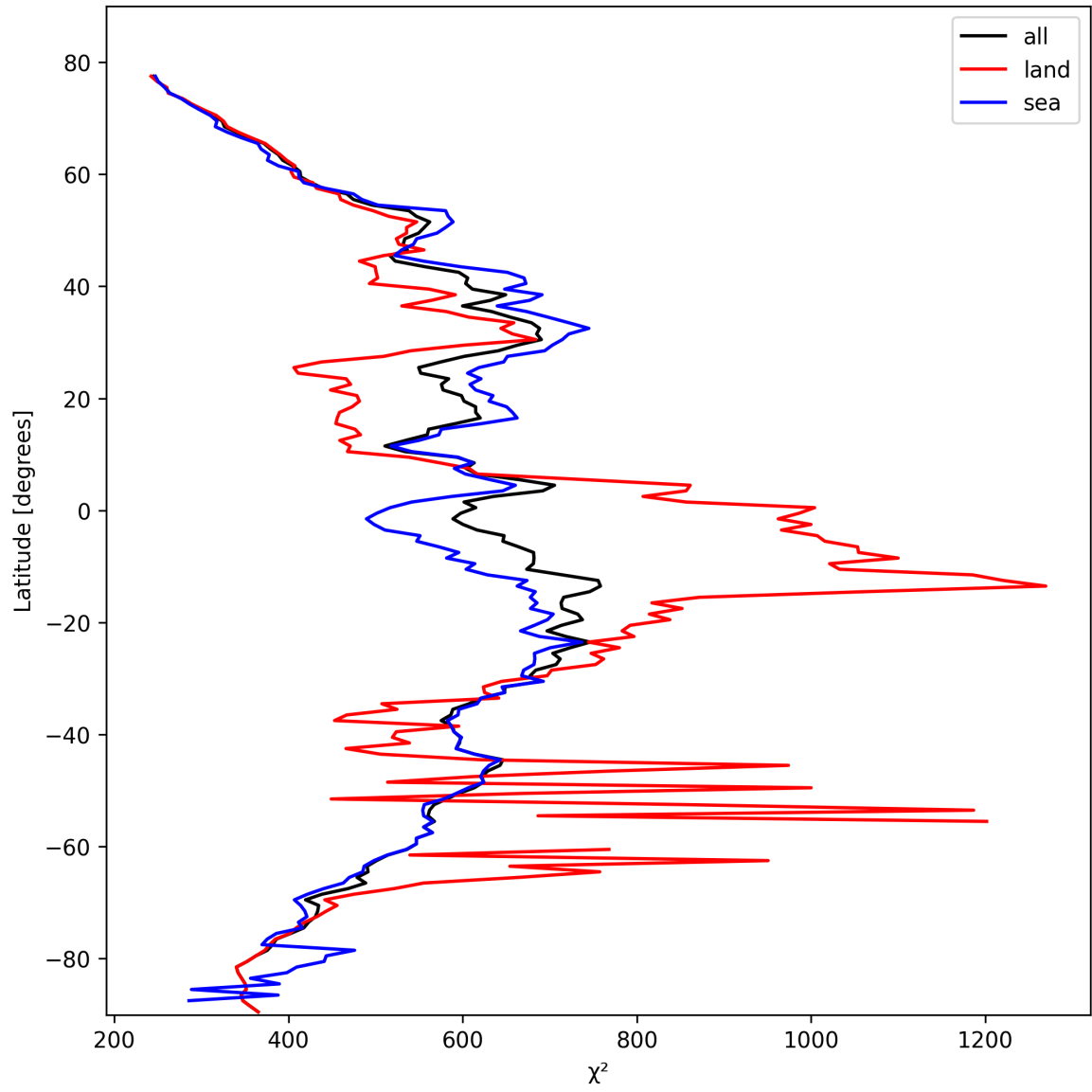
Figure 25: Zonal average of “ \chi^2 ” for 2025-02-19 to 2025-02-21.
