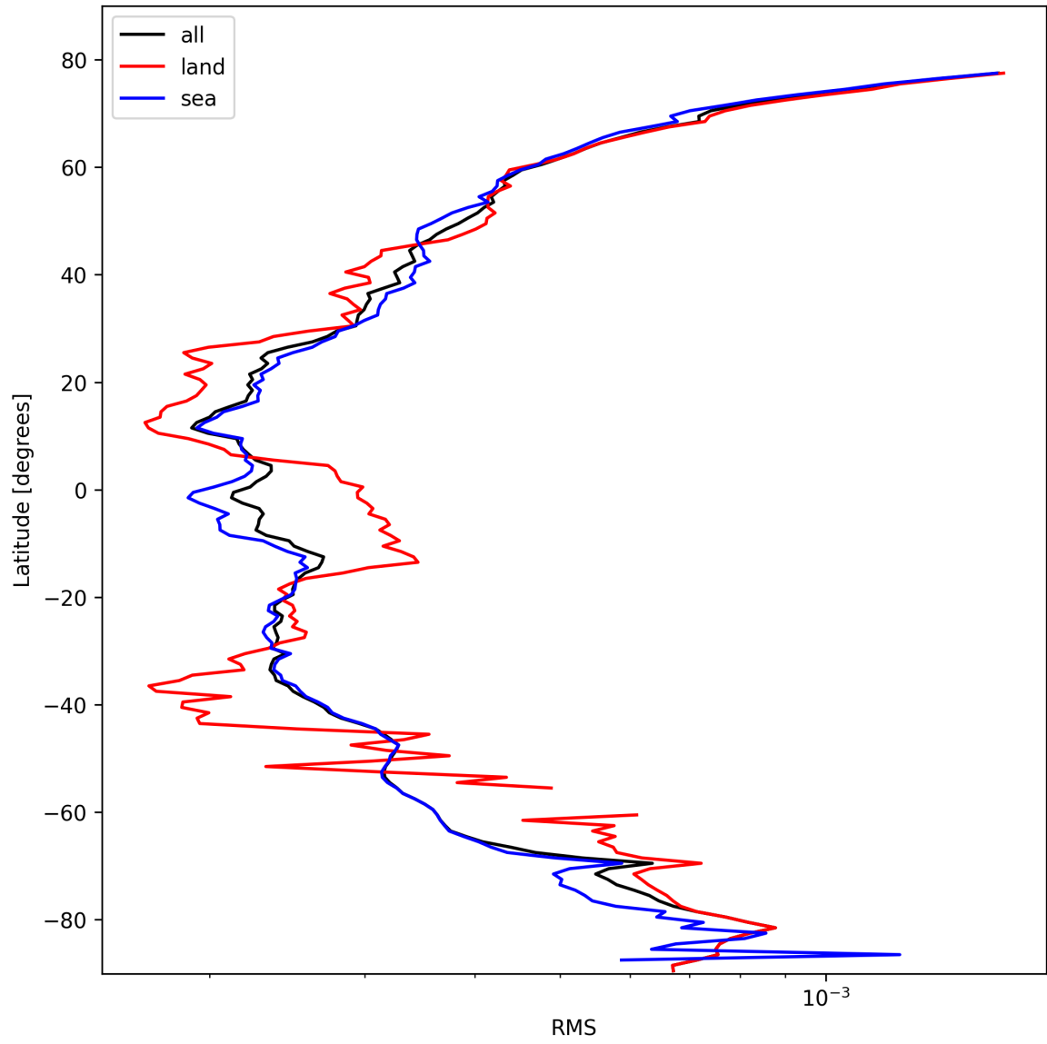
Figure 26: Zonal average of “RMS” for 2025-02-19 to 2025-02-21.
