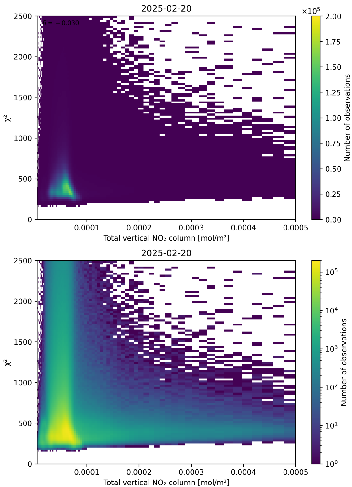
Figure 111: Scatter density plot of “Total vertical NO 2 column” against “ \chi^2 ” for 2025-02-19 to 2025-02-21.
