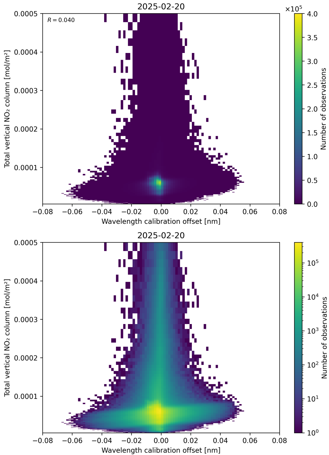
Figure 179: Scatter density plot of “Wavelength calibration offset” against “Total vertical NO 2 column” for 2025-02-19 to 2025-02-21.
