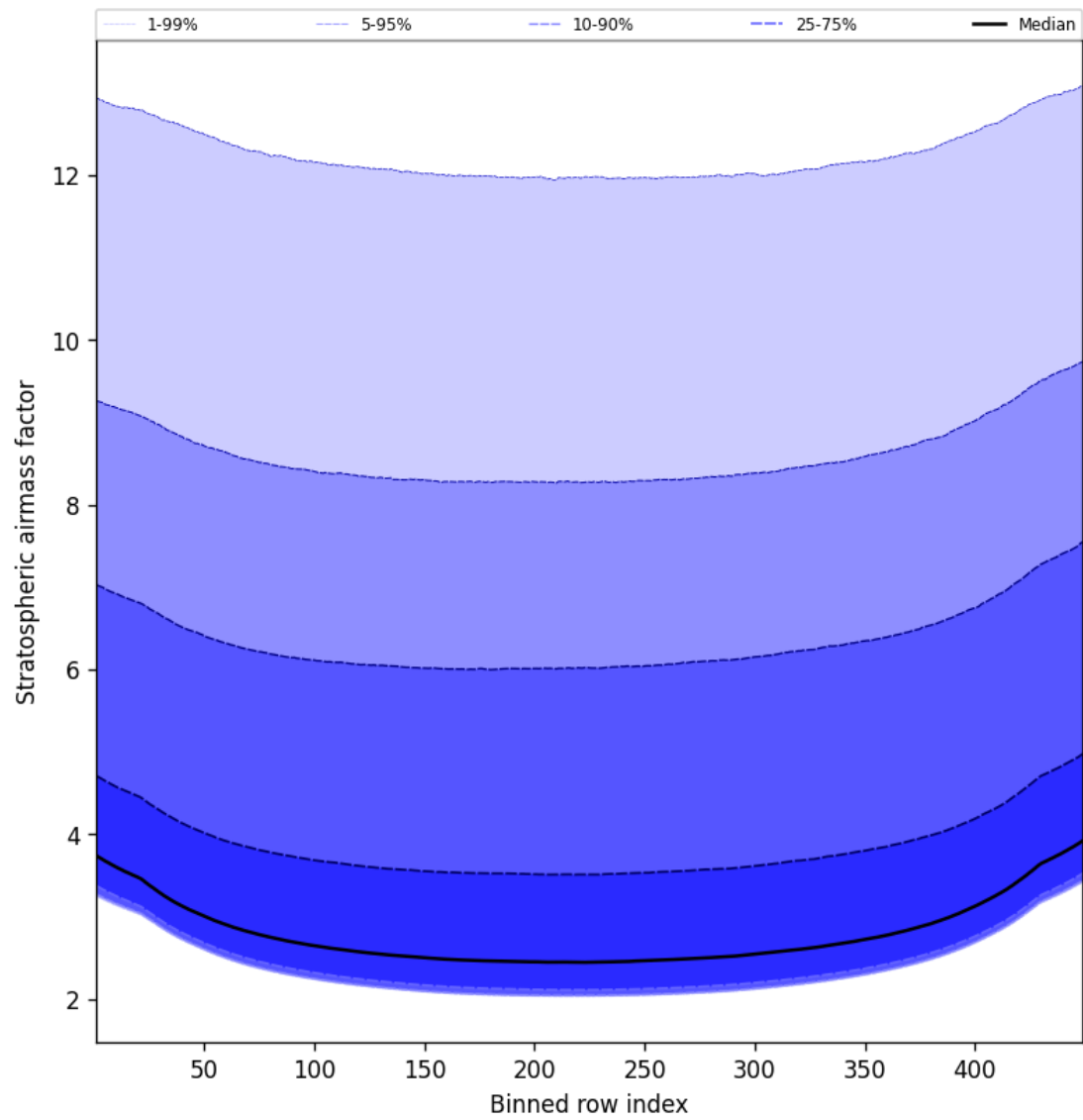
Figure 61: Along track statistics of “Stratospheric airmass factor” for 2025-02-19 to 2025-02-21
