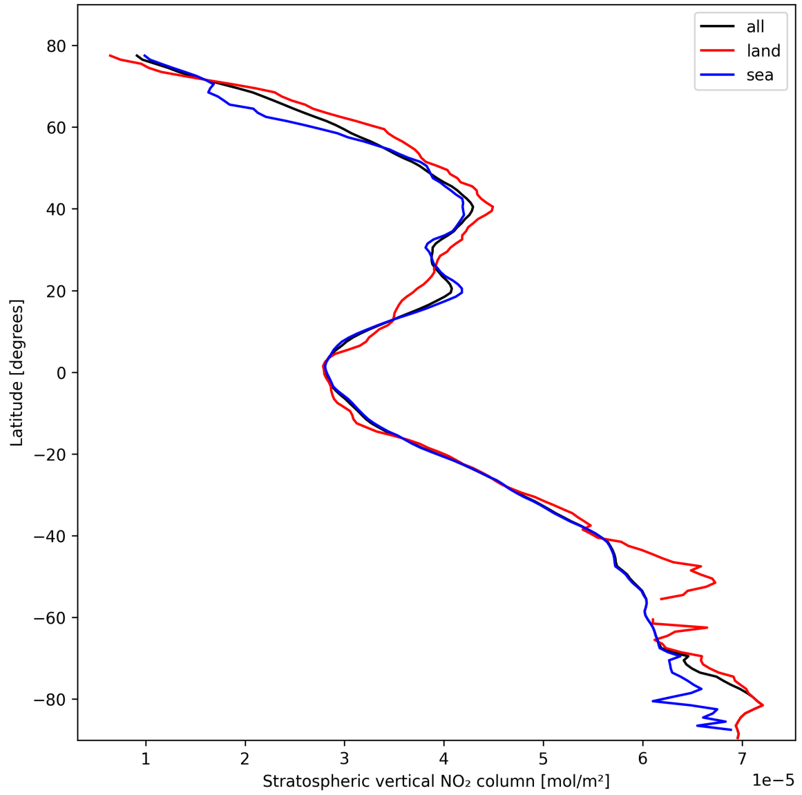
Figure 19: Zonal average of “Stratospheric vertical NO 2 column” for 2025-02-19 to 2025-02-21.
