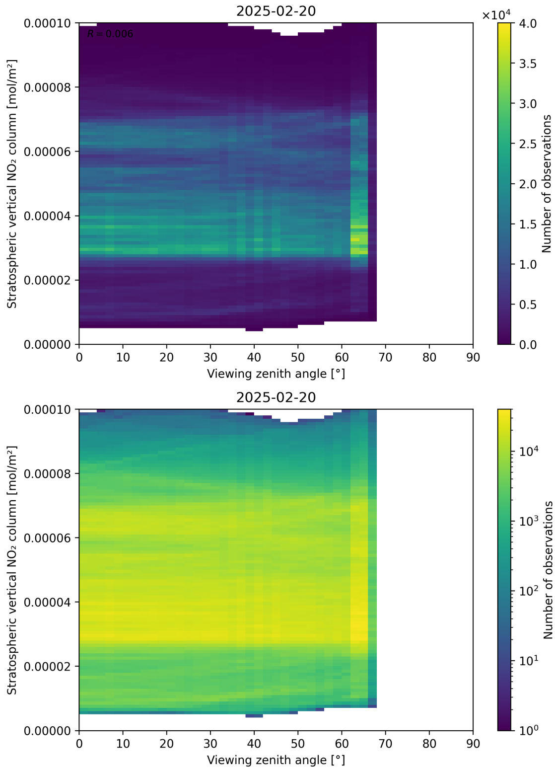
Figure 164: Scatter density plot of “Viewing zenith angle” against “Stratospheric vertical NO 2 column” for 2025-02-19 to 2025-02-21.
