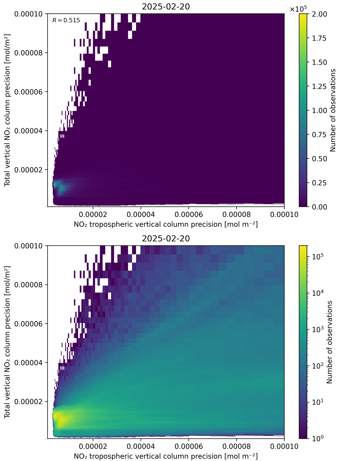
Figure 139: Scatter density plot of “NO 2 tropospheric vertical column precision” against “Total vertical NO 2 column precision” for 2025-02-19 to 2025-02-21.
