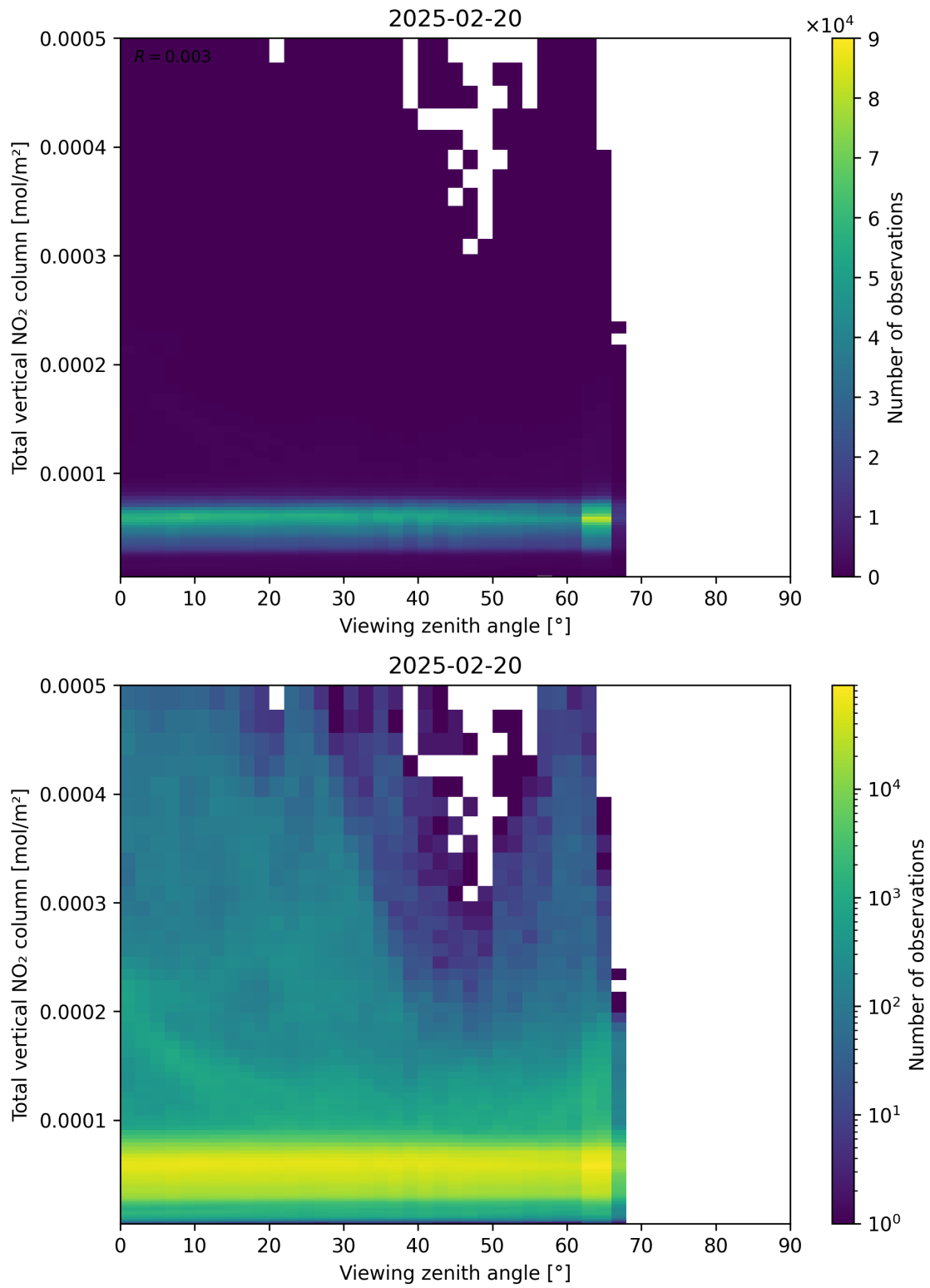
Figure 167: Scatter density plot of “Viewing zenith angle” against “Total vertical NO 2 column” for 2025-02-19 to 2025-02-21.
