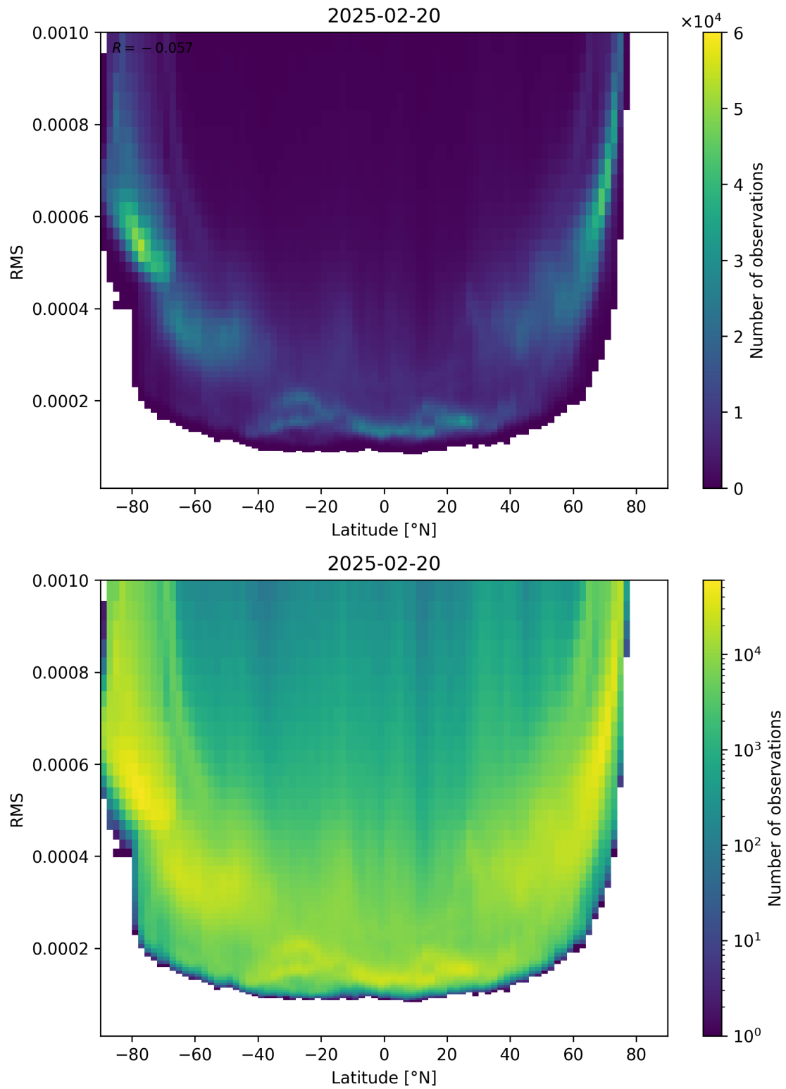
Figure 94: Scatter density plot of “Latitude” against “RMS” for 2025-02-19 to 2025-02-21.
