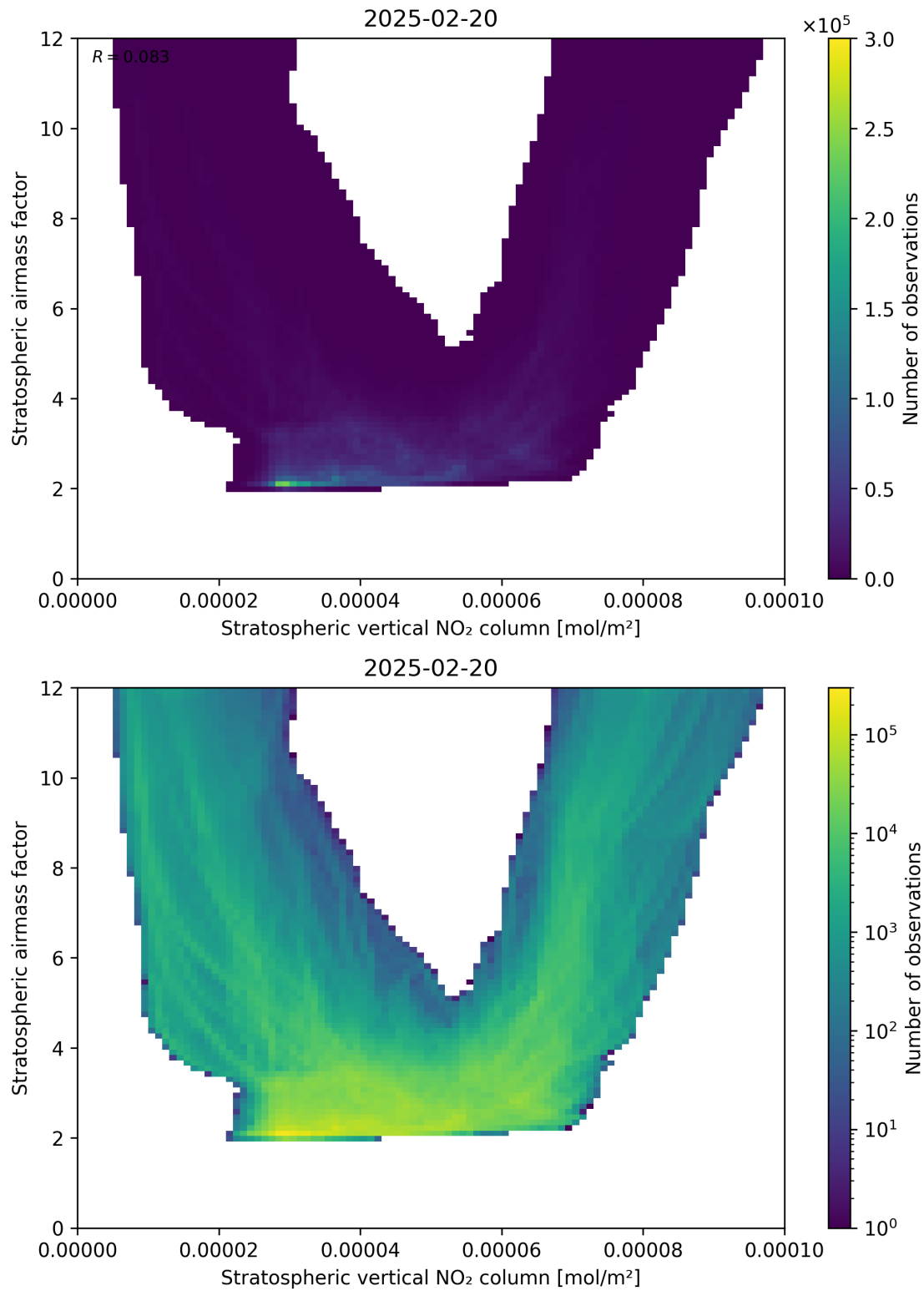
Figure 96: Scatter density plot of “Stratospheric vertical NO 2 column” against “Stratospheric airmass factor” for 2025-02-19 to 2025-02-21.
