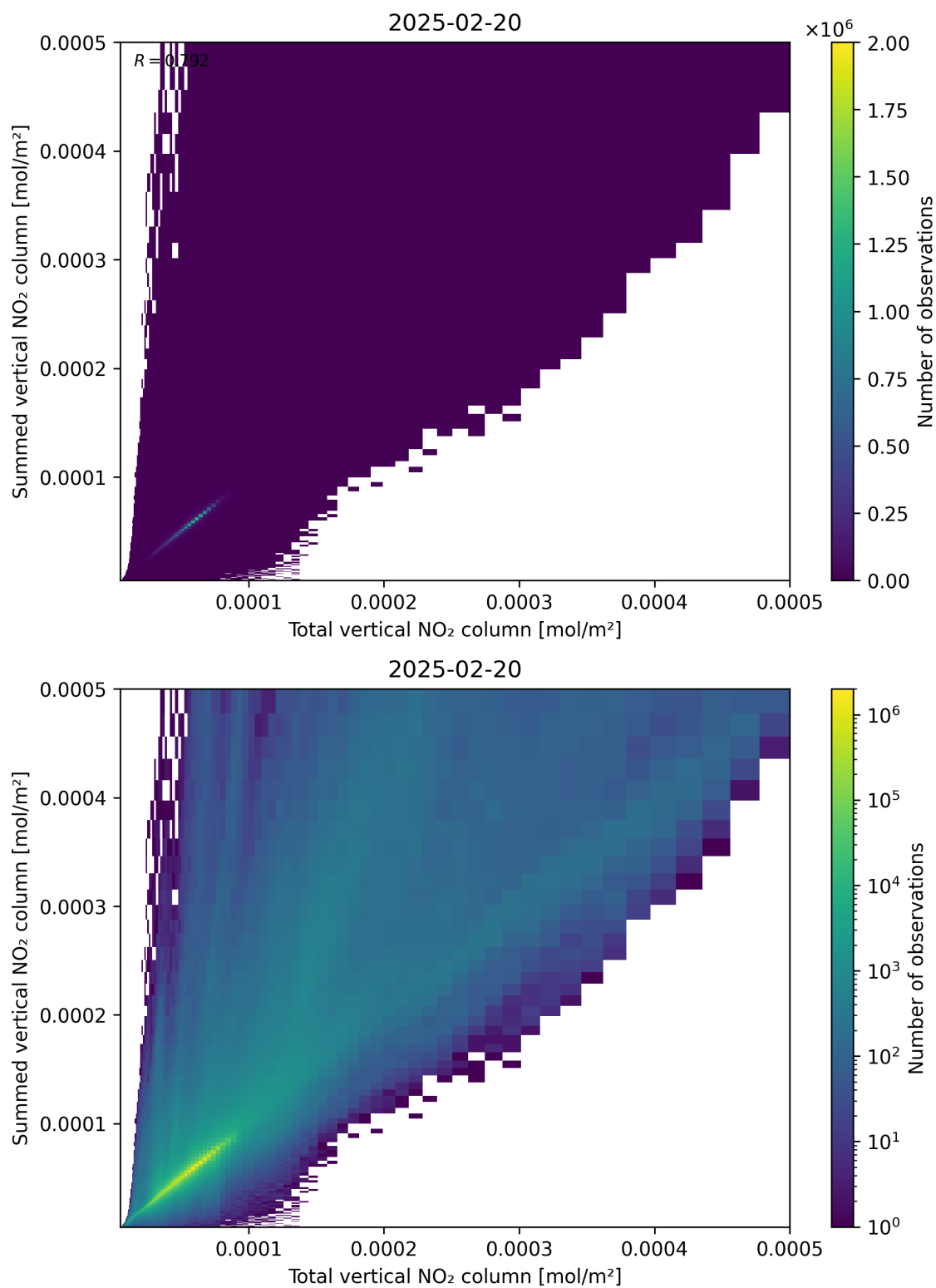
Figure 112: Scatter density plot of “Total vertical NO 2 column” against “Summed vertical NO 2 column” for 2025-02-19 to 2025-02-21.
