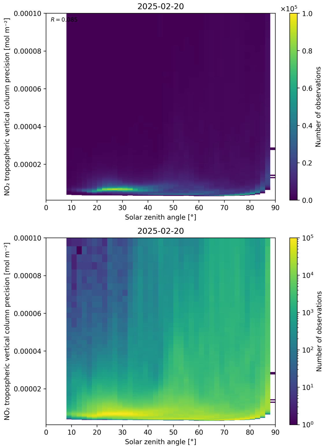
Figure 156: Scatter density plot of “Solar zenith angle” against “NO 2 tropospheric vertical column precision” for 2025-02-19 to 2025-02-21.
