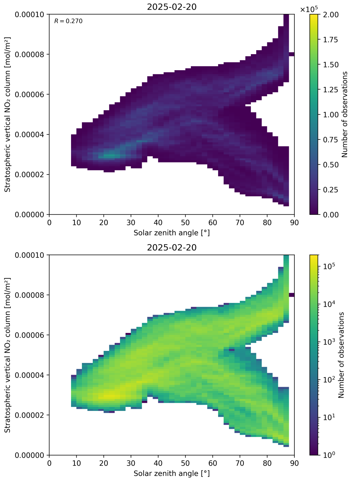
Figure 150: Scatter density plot of “Solar zenith angle” against “Stratospheric vertical NO 2 column” for 2025-02-19 to 2025-02-21.
