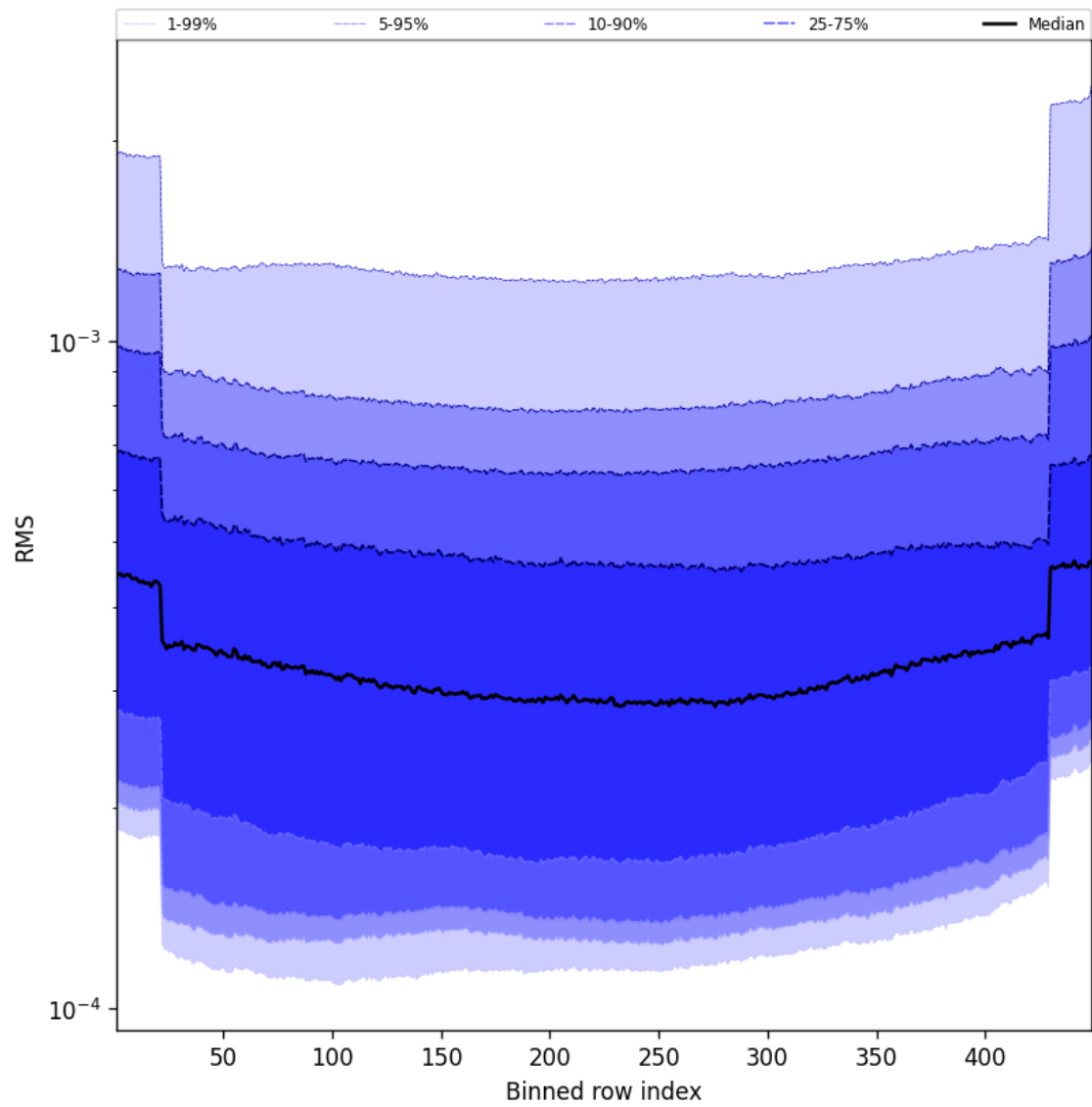
Figure 60: Along track statistics of “RMS” for 2025-02-19 to 2025-02-21
