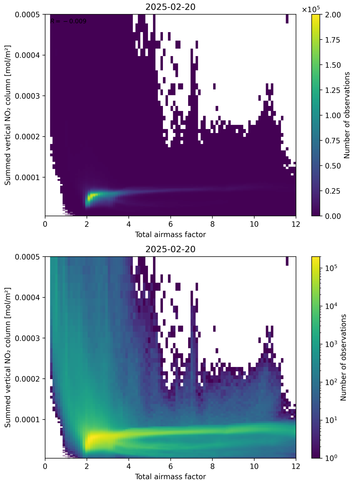
Figure 65: Scatter density plot of “Total airmass factor” against “Summed vertical NO 2 column” for 2025-02-19 to 2025-02-21.
