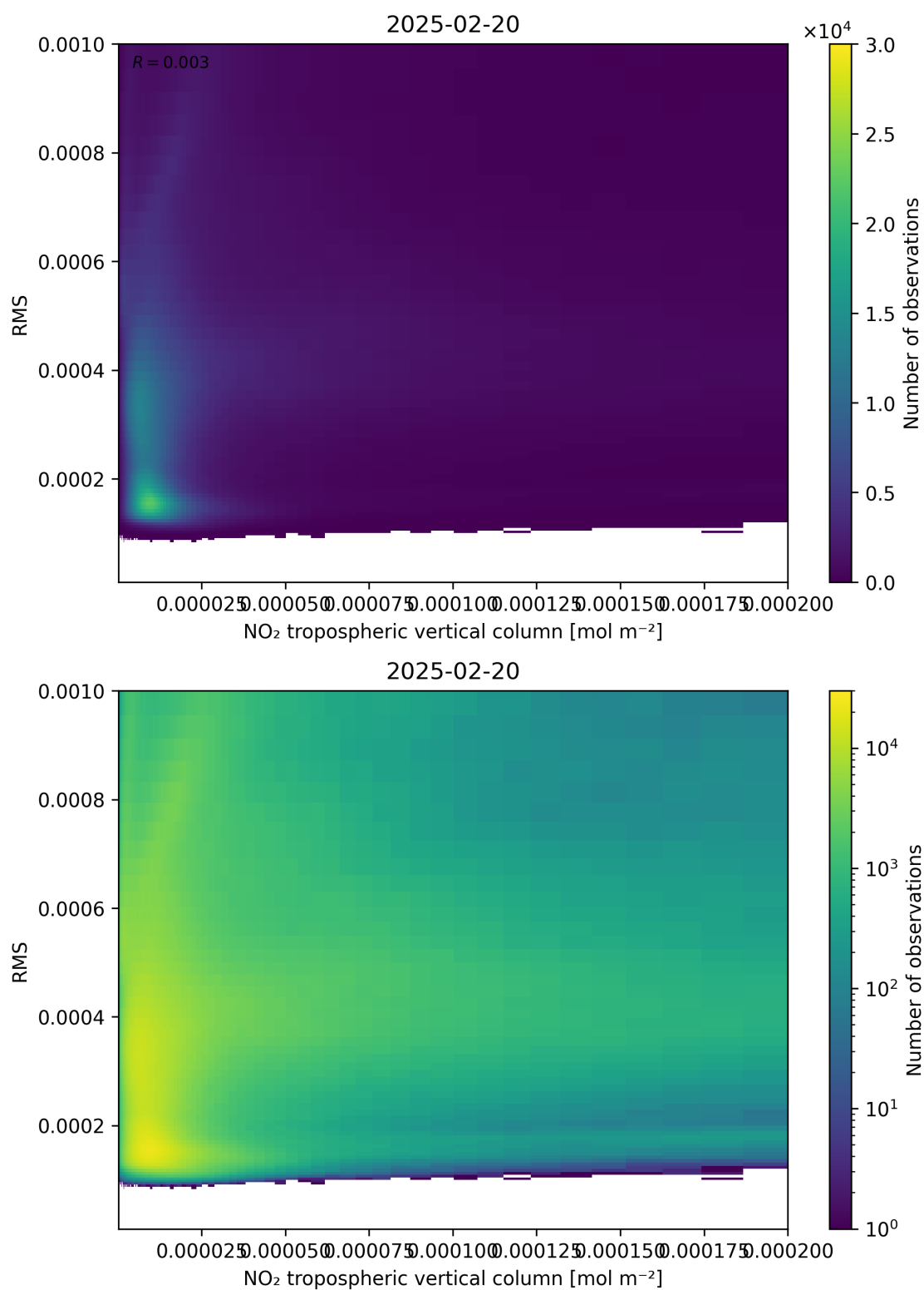
Figure 142: Scatter density plot of “NO 2 tropospheric vertical column” against “RMS” for 2025-02-19 to 2025-02-21.
