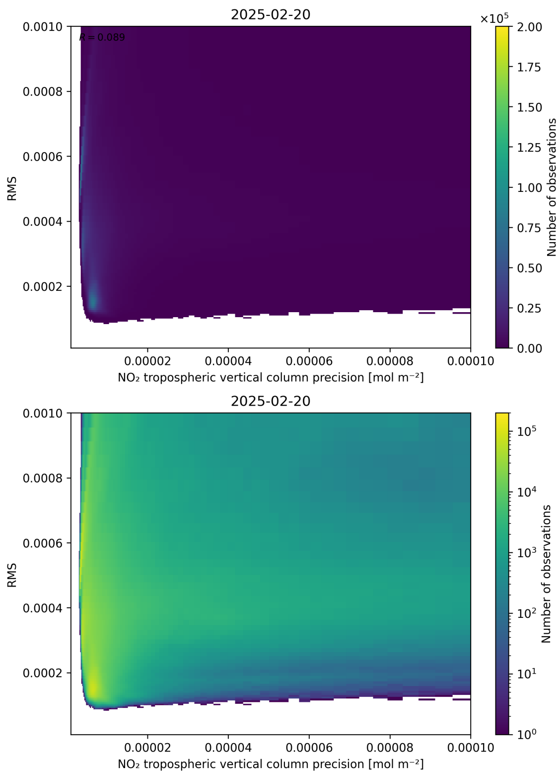
Figure 140: Scatter density plot of “NO 2 tropospheric vertical column precision” against “RMS” for 2025-02-19 to 2025-02-21.
