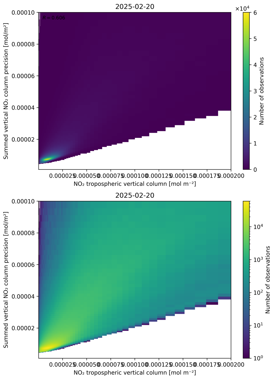
Figure 127: Scatter density plot of “NO 2 tropospheric vertical column” against “Summed vertical NO 2 column precision” for 2025-02-19 to 2025-02-21.
