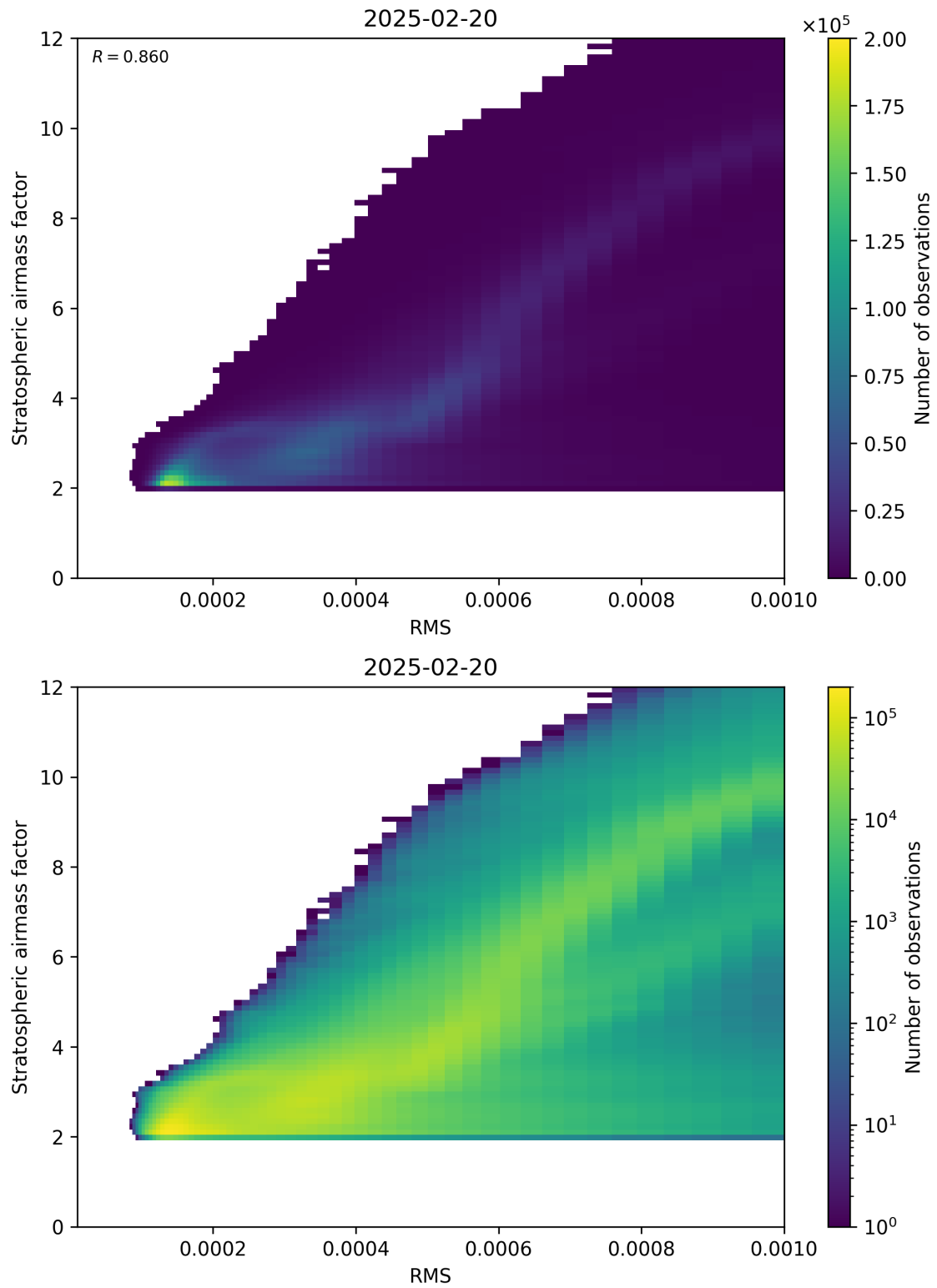
Figure 144: Scatter density plot of “RMS” against “Stratospheric airmass factor” for 2025-02-19 to 2025-02-21.
