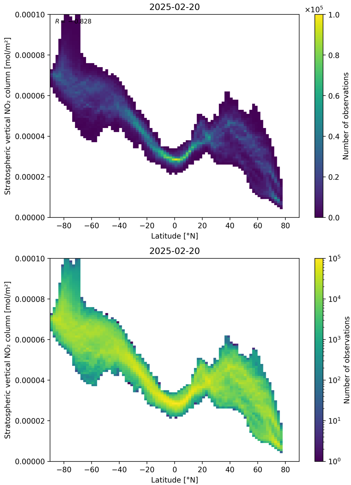
Figure 87: Scatter density plot of “Latitude” against “Stratospheric vertical NO 2 column” for 2025-02-19 to 2025-02-21.
