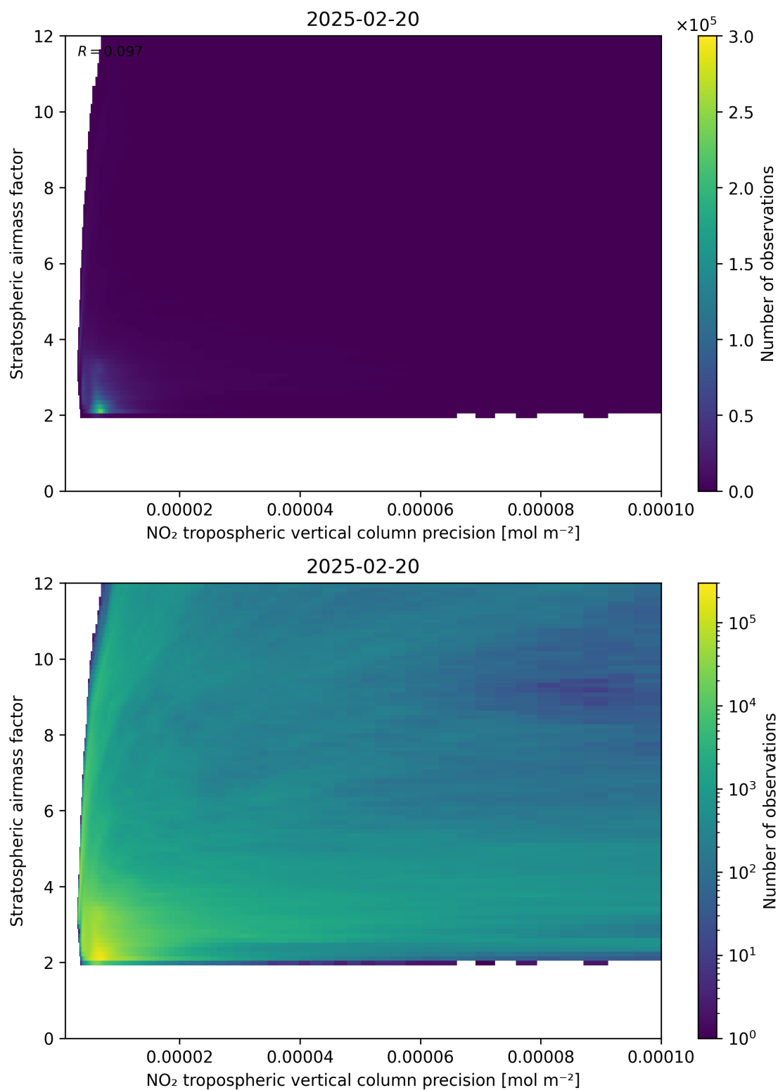
Figure 131: Scatter density plot of “NO 2 tropospheric vertical column precision” against “Stratospheric airmass factor” for 2025-02-19 to 2025-02-21.
