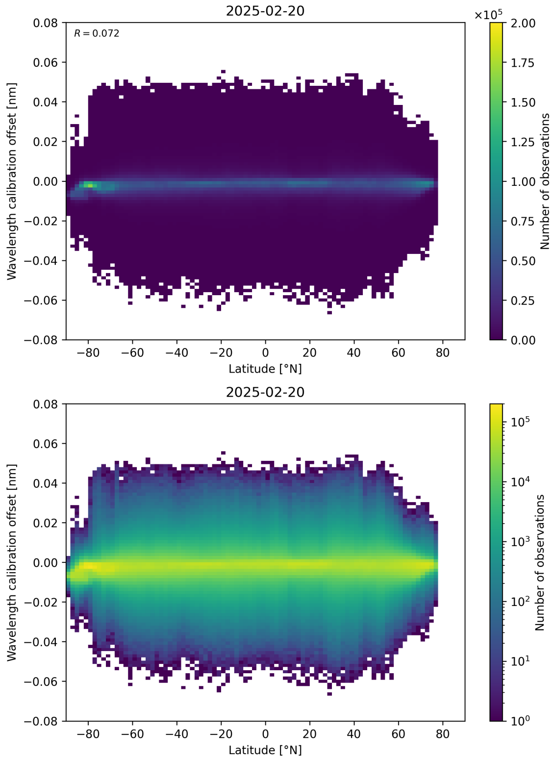
Figure 95: Scatter density plot of “Latitude” against “Wavelength calibration offset” for 2025-02-19 to 2025-02-21.
