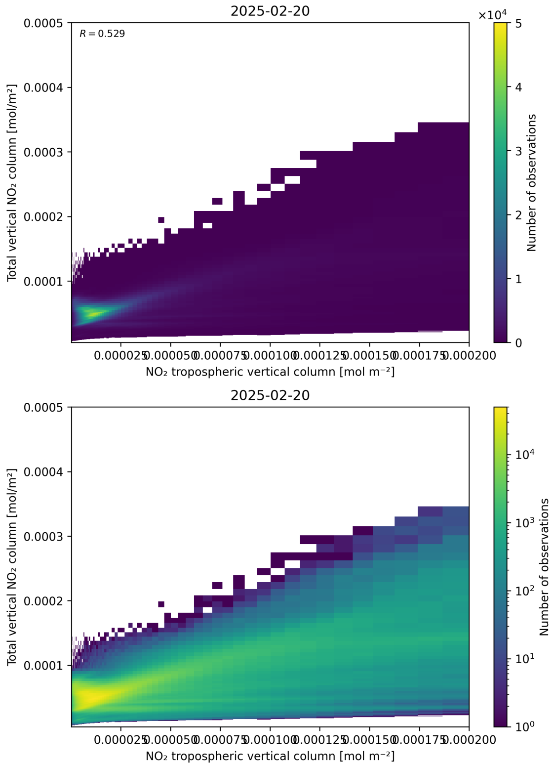
Figure 128: Scatter density plot of “NO 2 tropospheric vertical column” against “Total vertical NO 2 column” for 2025-02-19 to 2025-02-21.
