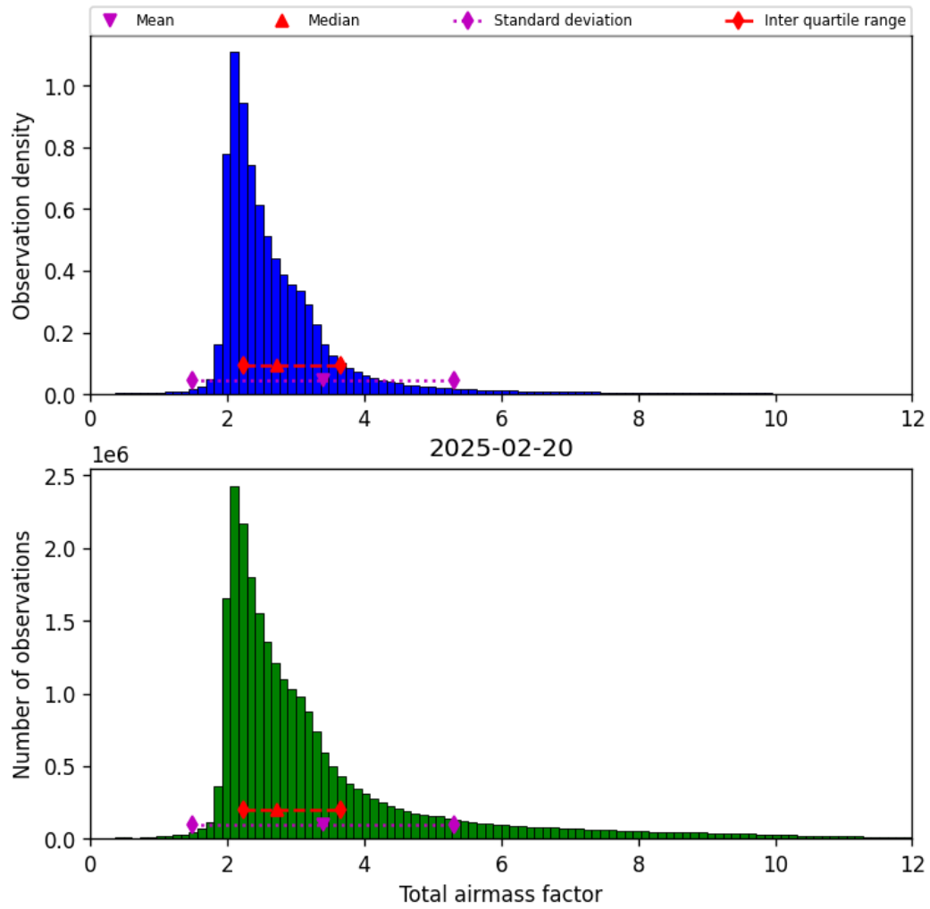
Figure 32: Histogram of “Total airmass factor” for 2025-02-19 to 2025-02-21
