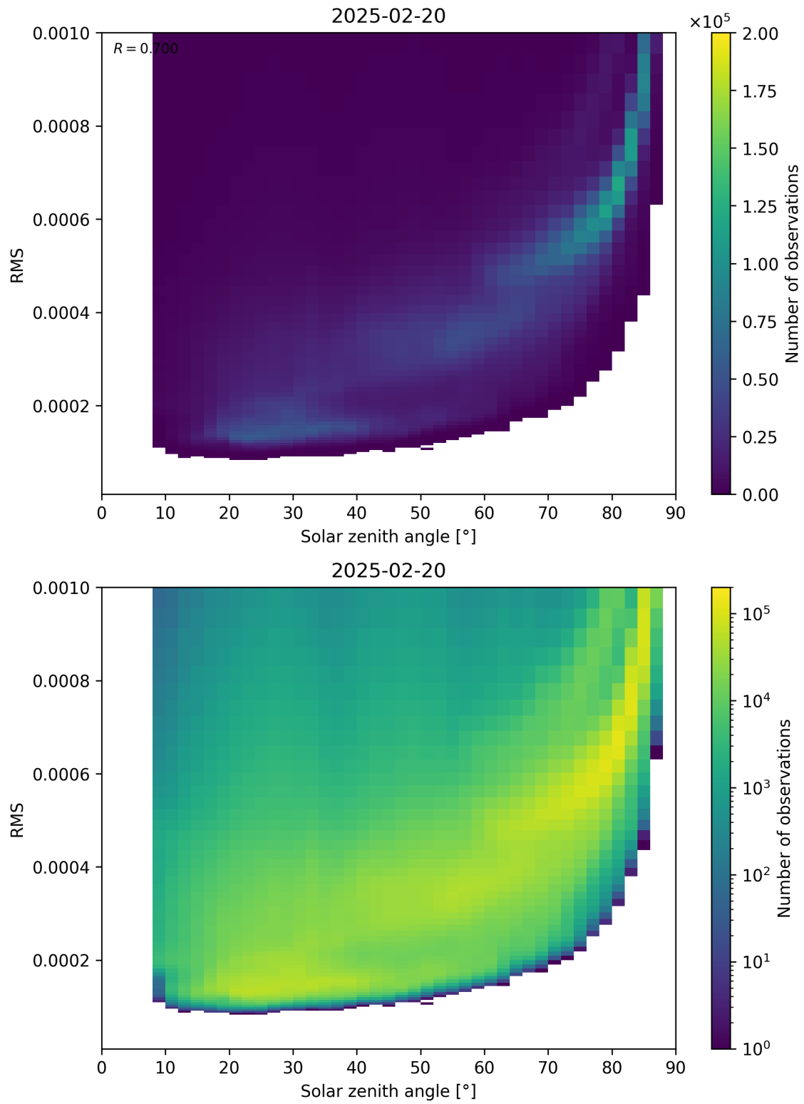
Figure 157: Scatter density plot of “Solar zenith angle” against “RMS” for 2025-02-19 to 2025-02-21.
