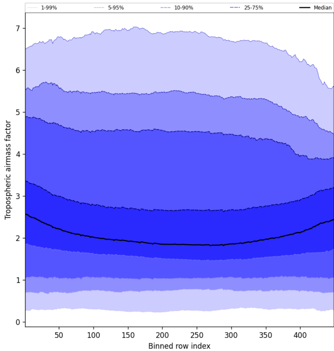
Figure 48: Along track statistics of “Tropospheric airmass factor” for 2025-02-19 to 2025-02-21
