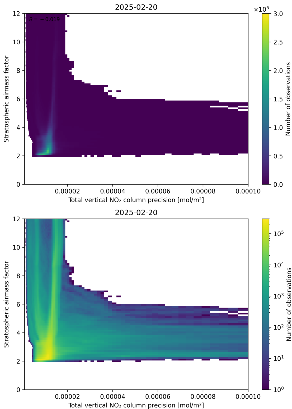
Figure 115: Scatter density plot of “Total vertical NO 2 column precision” against “Stratospheric air mass factor” for 2025-02-19 to 2025-02-21.
