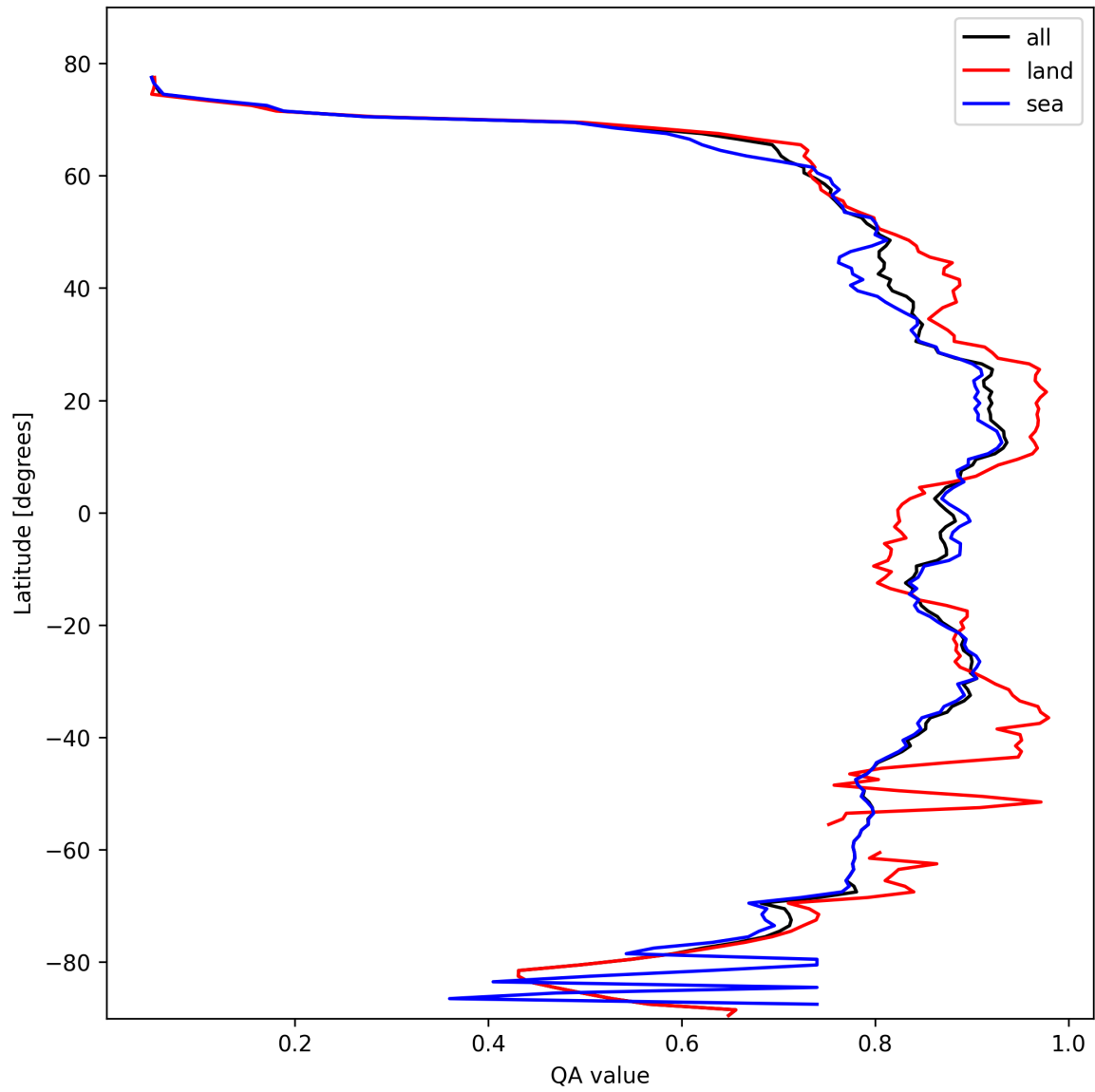
Figure 11: Zonal average of “QA value” for 2025-02-19 to 2025-02-21.
