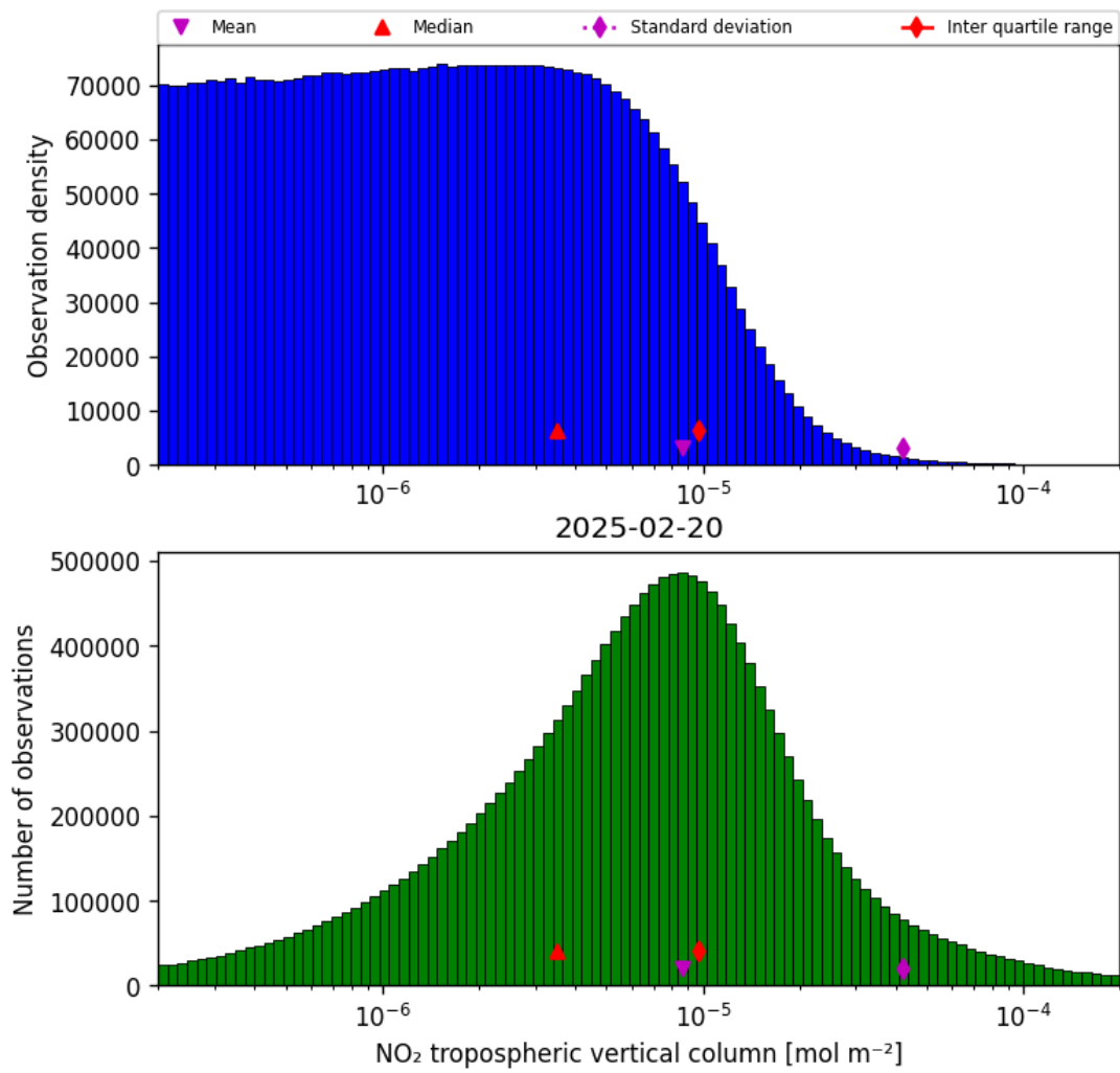
Figure 29: Histogram of “NO 2 tropospheric vertical column” for 2025-02-19 to 2025-02-21
