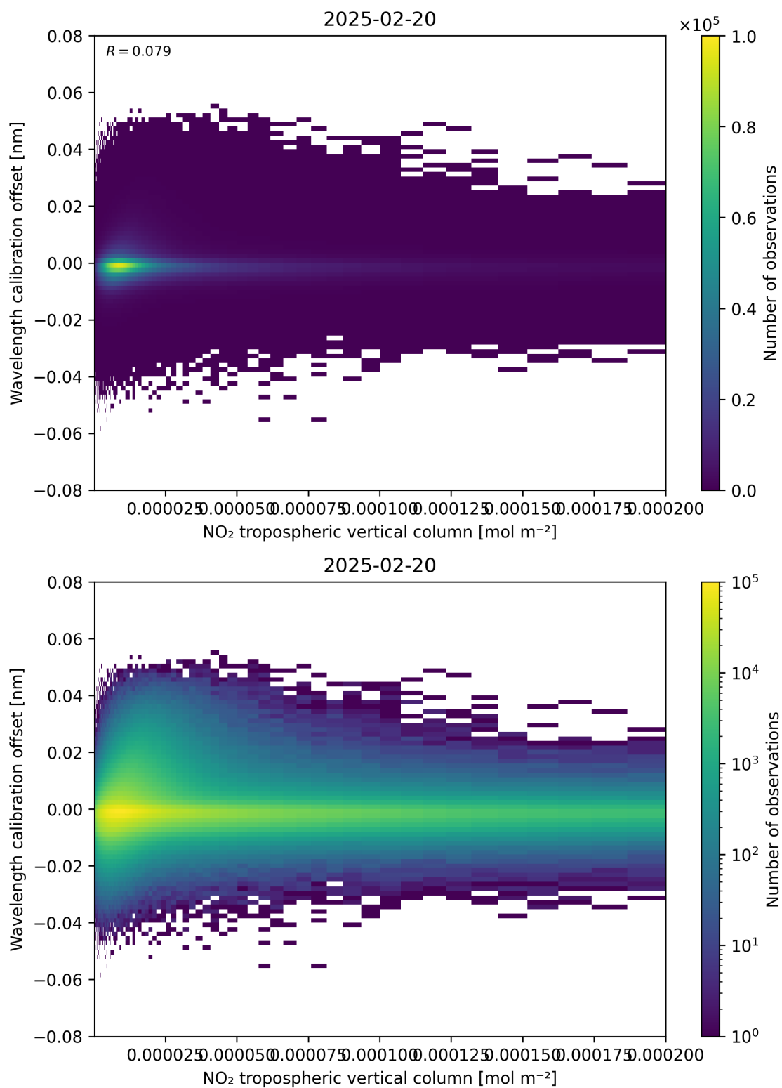
Figure 143: Scatter density plot of “NO 2 tropospheric vertical column” against “Wavelength calibration offset” for 2025-02-19 to 2025-02-21.
