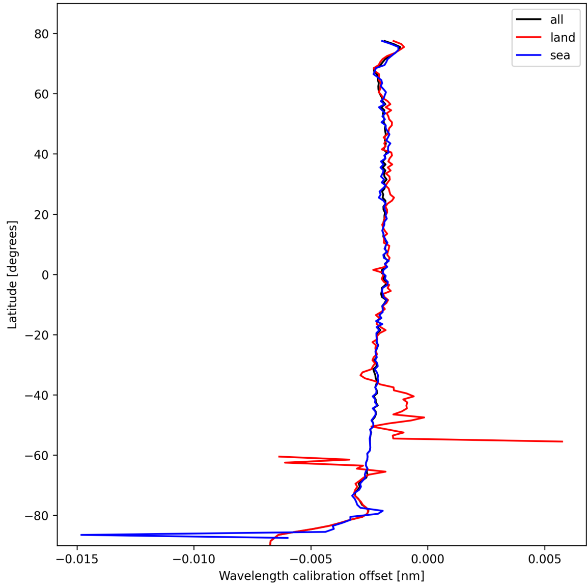
Figure 18: Zonal average of “Wavelength calibration offset” for 2025-02-19 to 2025-02-21.
