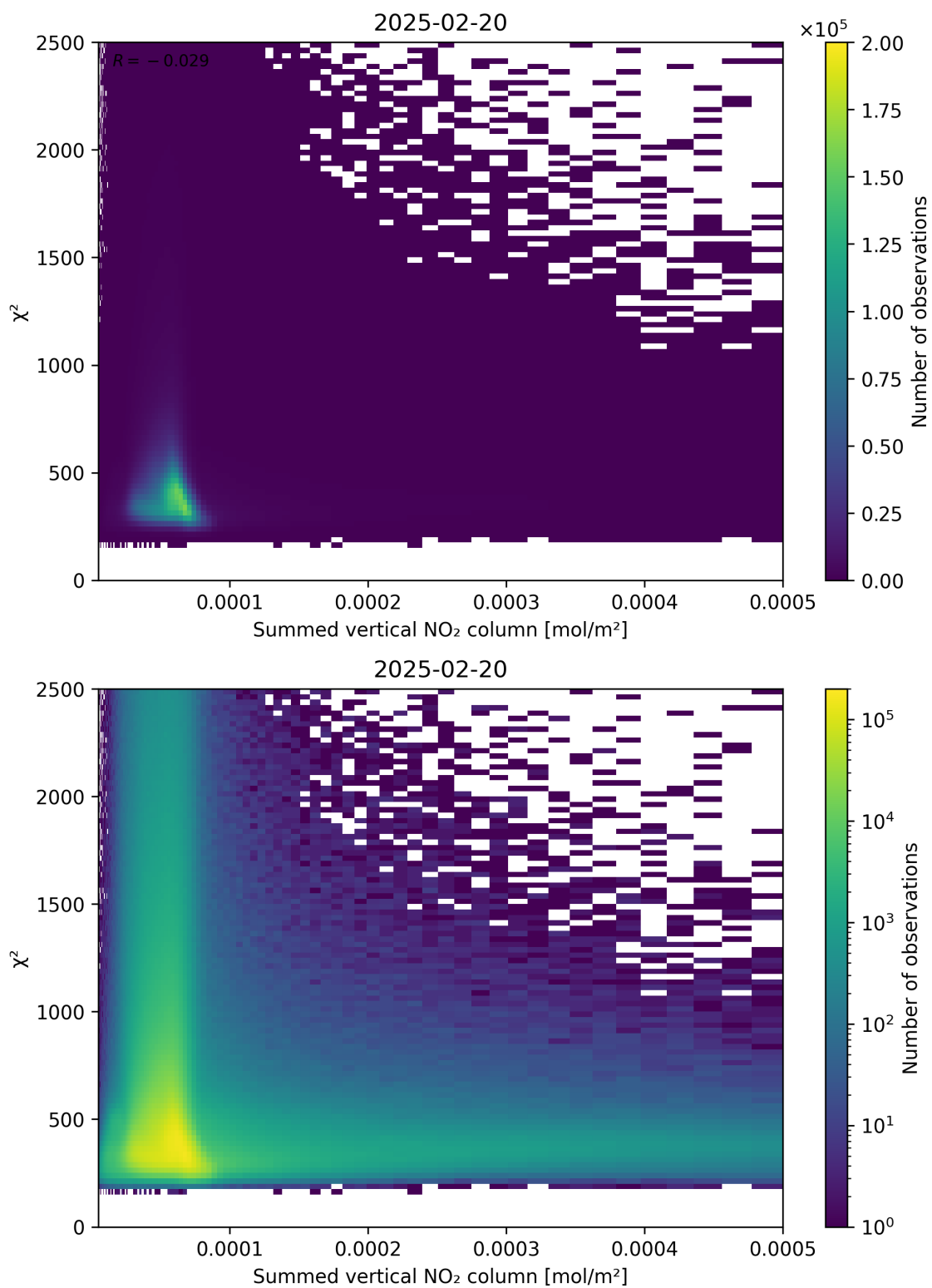
Figure 104: Scatter density plot of “Summed vertical NO 2 column” against “ \chi^2 ” for 2025-02-19 to 2025-02-21.
