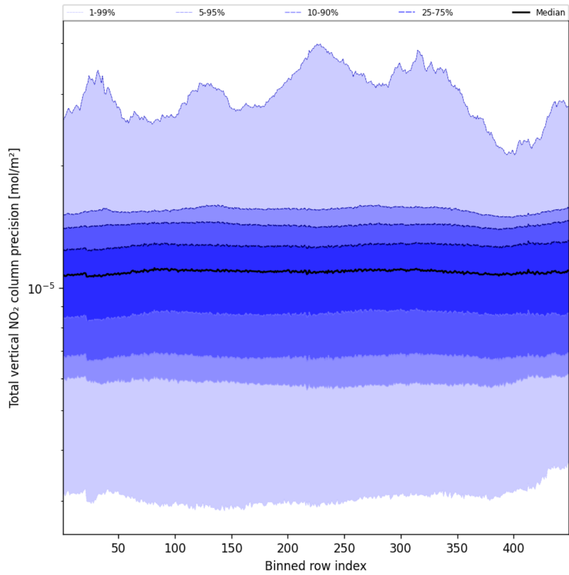
Figure 56: Along track statistics of “Total vertical NO 2 column precision” for 2025-02-19 to 2025-02-21
