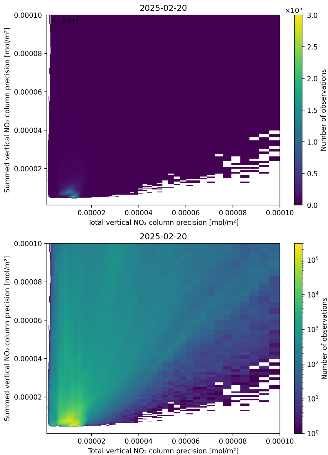
Figure 118: Scatter density plot of “Total vertical NO 2 column precision” against “Summed vertical NO 2 column precision” for 2025-02-19 to 2025-02-21.
