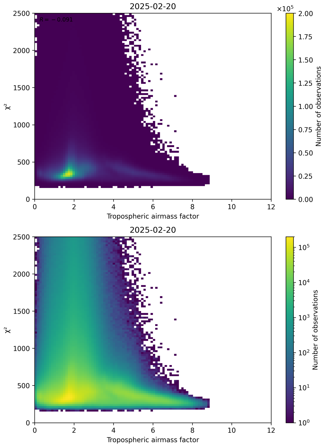
Figure 73: Scatter density plot of “Tropospheric airmass factor” against “ \chi^2 ” for 2025-02-19 to 2025-02-21.
