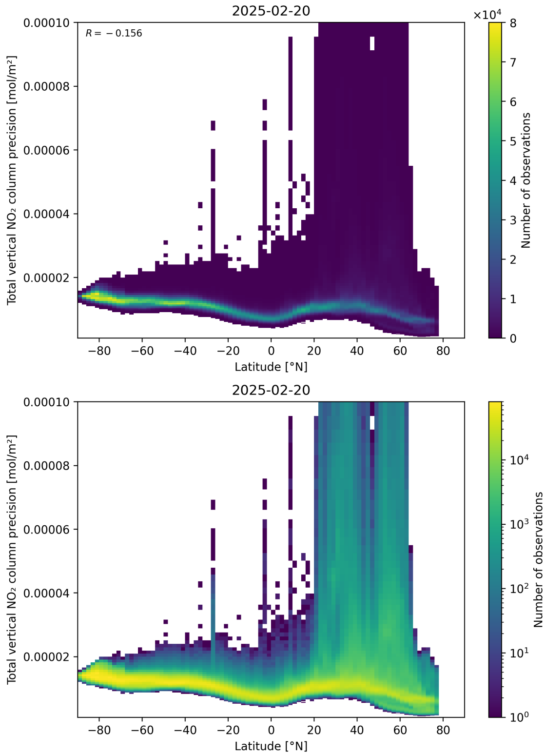
Figure 91: Scatter density plot of “Latitude” against “Total vertical NO 2 column precision” for 2025-02-19 to 2025-02-21.
