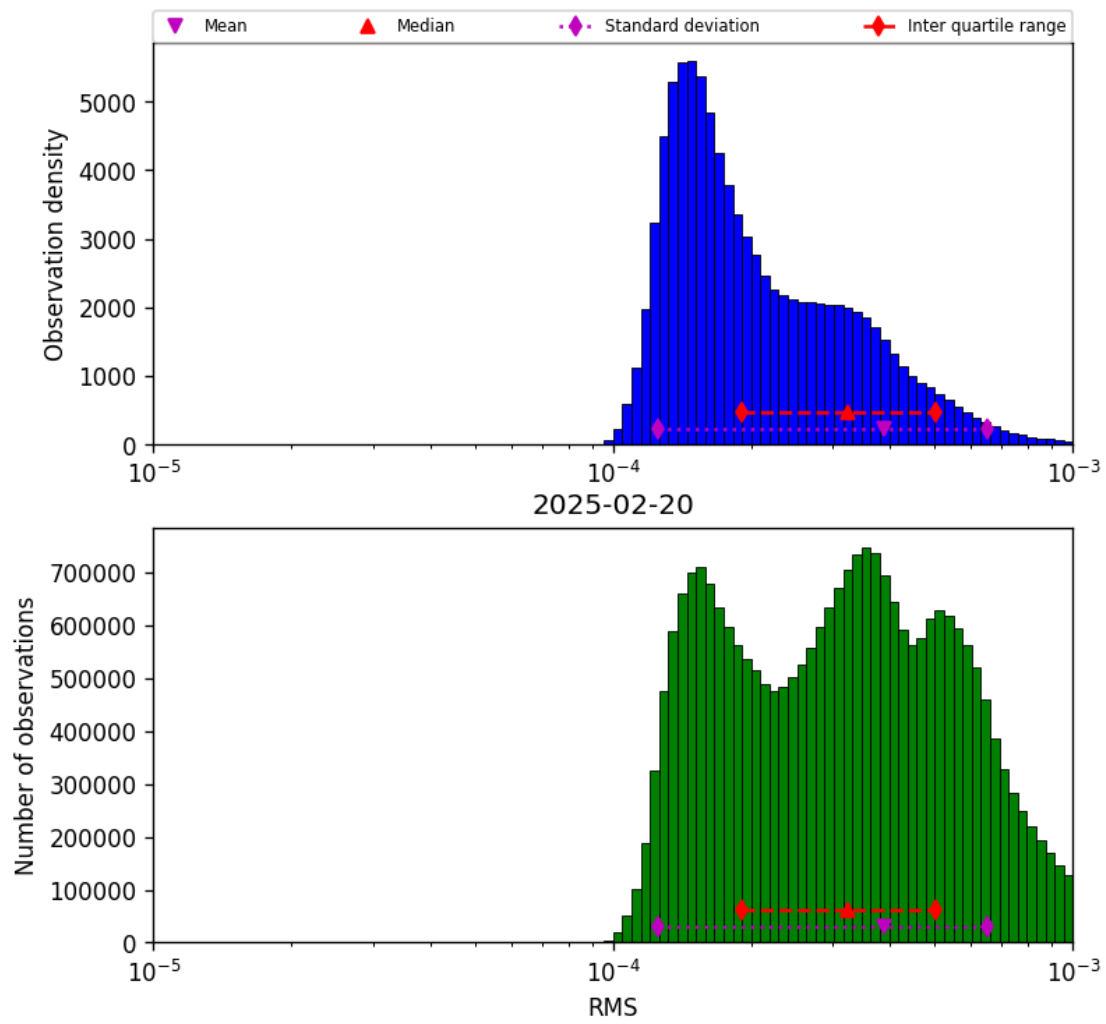
Figure 43: Histogram of “RMS” for 2025-02-19 to 2025-02-21
