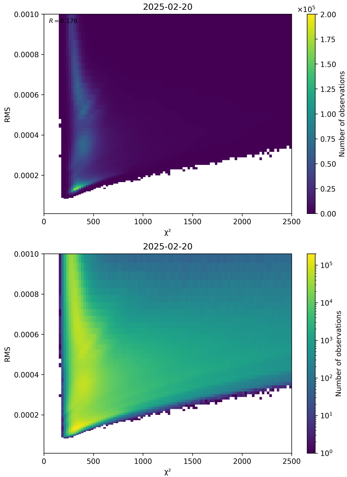
Figure 82: Scatter density plot of “ \chi^2 ” against “RMS” for 2025-02-19 to 2025-02-21.
