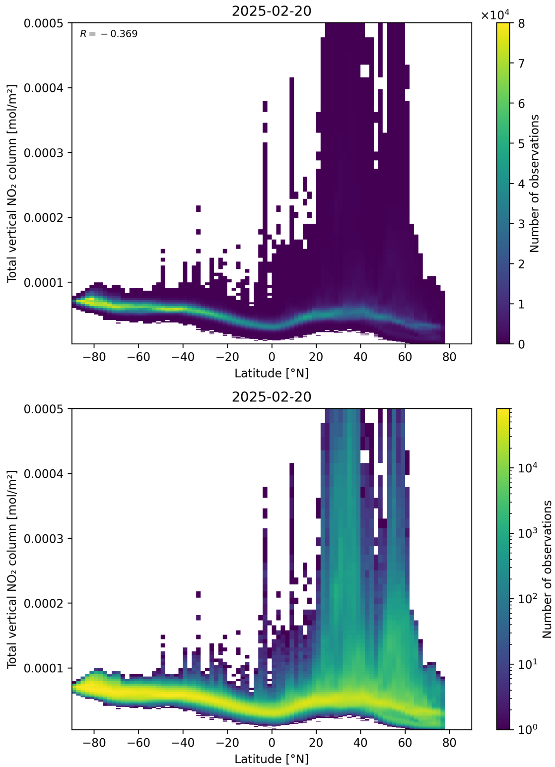
Figure 90: Scatter density plot of “Latitude” against “Total vertical NO 2 column” for 2025-02-19 to 2025-02-21.
