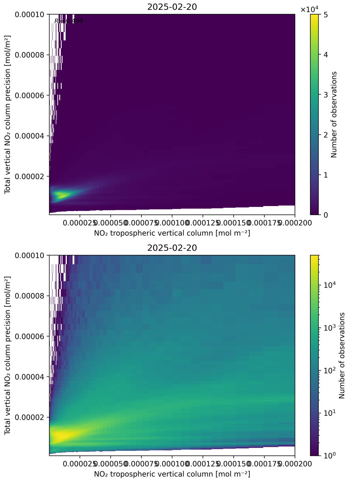
Figure 129: Scatter density plot of “NO 2 tropospheric vertical column” against “Total vertical NO 2 column precision” for 2025-02-19 to 2025-02-21.
