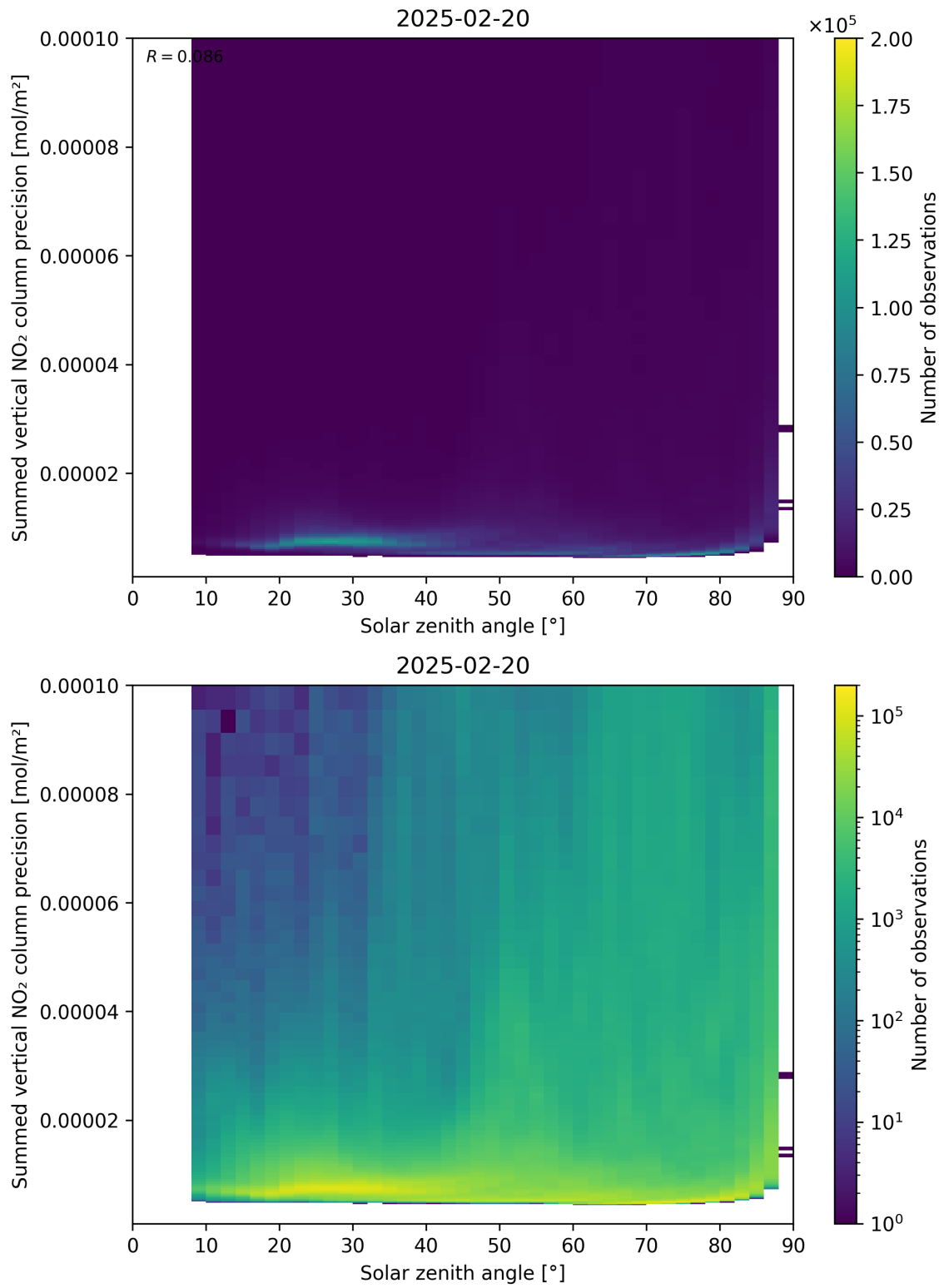
Figure 152: Scatter density plot of “Solar zenith angle” against “Summed vertical NO 2 column precision” for 2025-02-19 to 2025-02-21.
