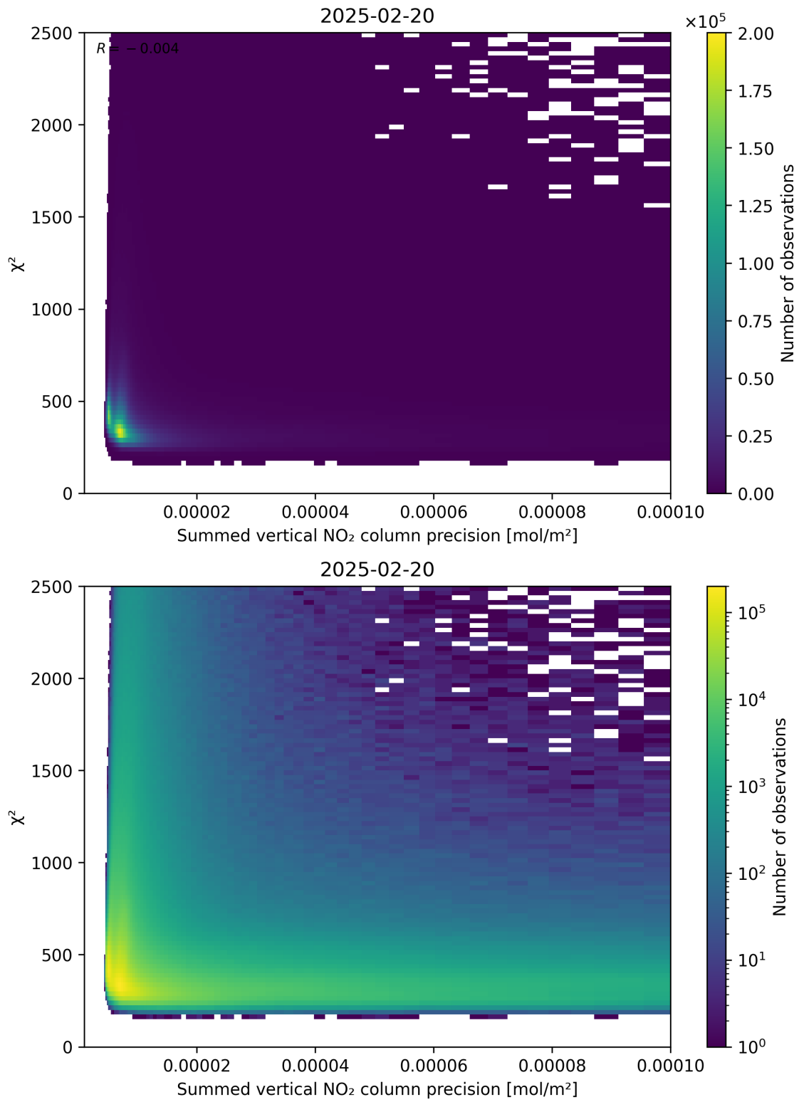
Figure 107: Scatter density plot of “Summed vertical NO 2 column precision” against “ \chi^2 ” for 2025-02-19 to 2025-02-21.
