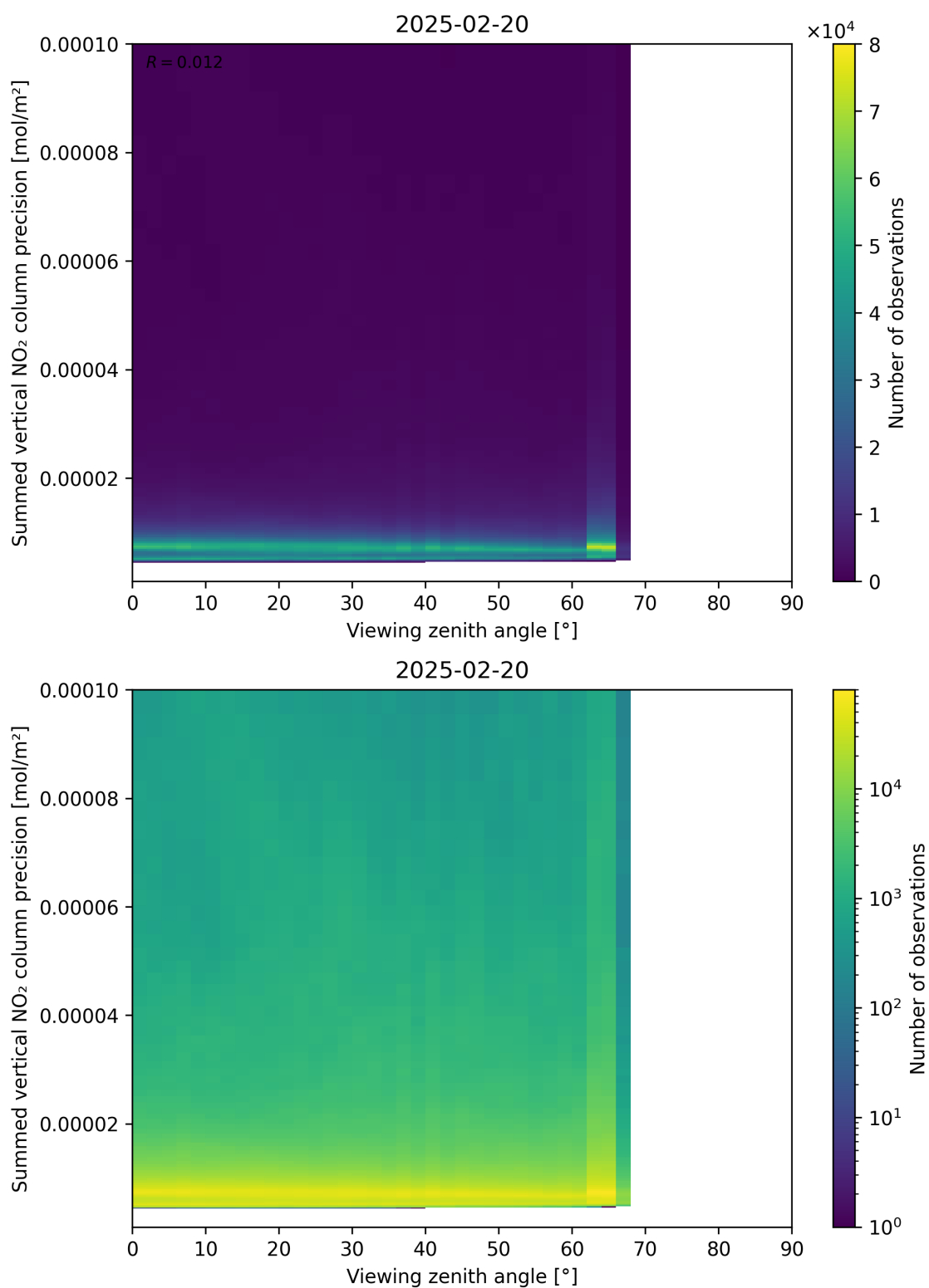
Figure 166: Scatter density plot of “Viewing zenith angle” against “Summed vertical NO 2 column precision” for 2025-02-19 to 2025-02-21.
