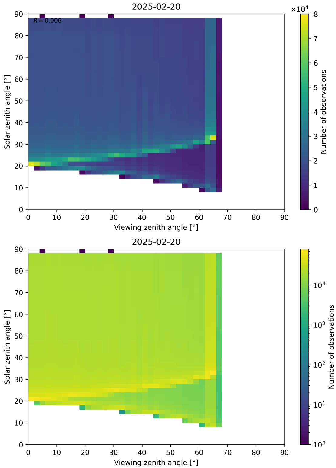
Figure 172: Scatter density plot of “Viewing zenith angle” against “Solar zenith angle” for 2025-02-19 to 2025-02-21.
