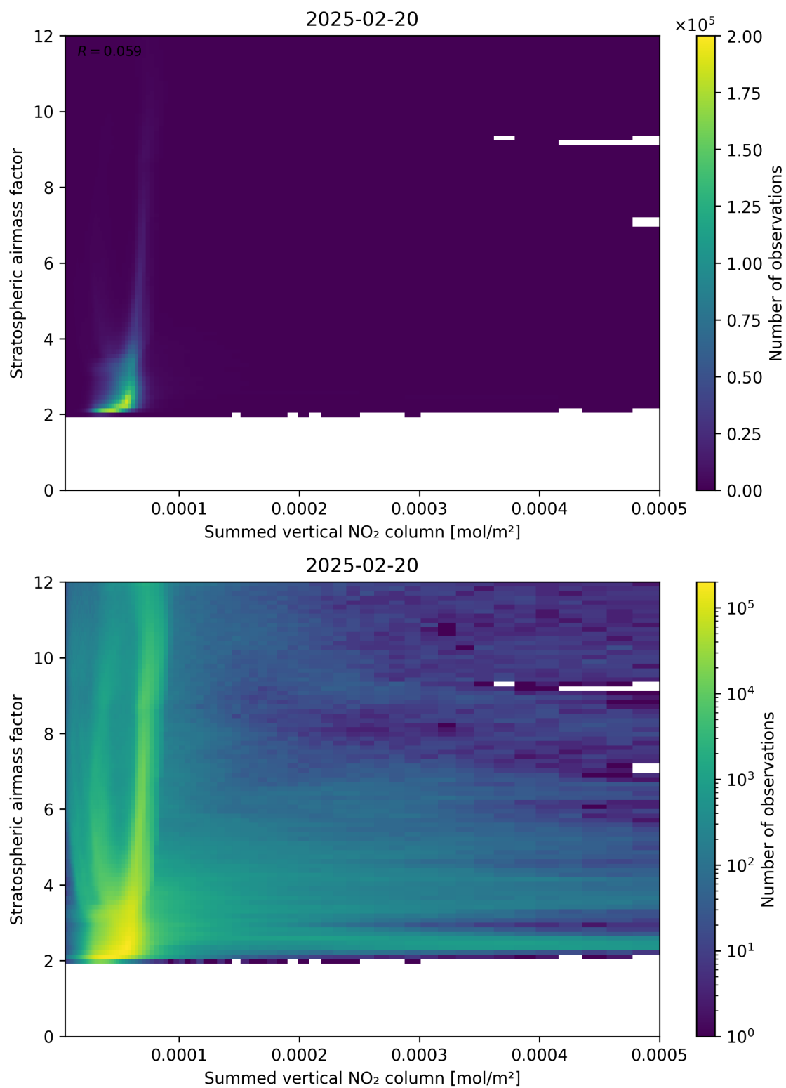
Figure 103: Scatter density plot of “Summed vertical NO 2 column” against “Stratospheric airmass factor” for 2025-02-19 to 2025-02-21.
