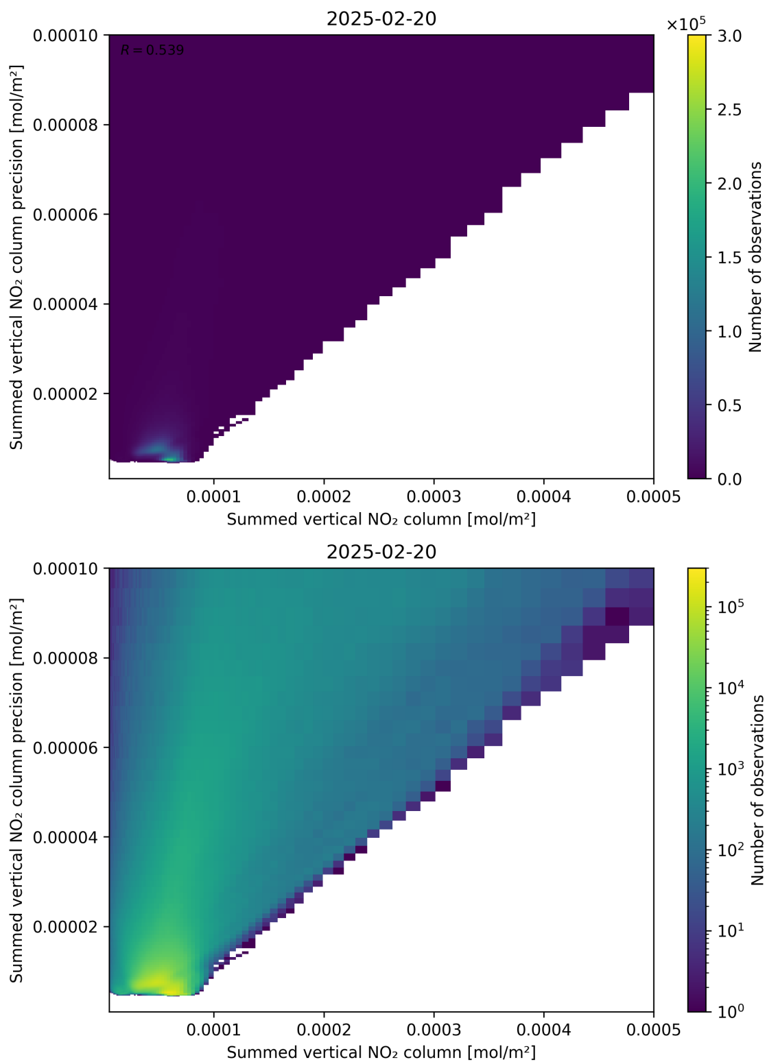
Figure 105: Scatter density plot of “Summed vertical NO 2 column” against “Summed vertical NO 2 column precision” for 2025-02-19 to 2025-02-21.
