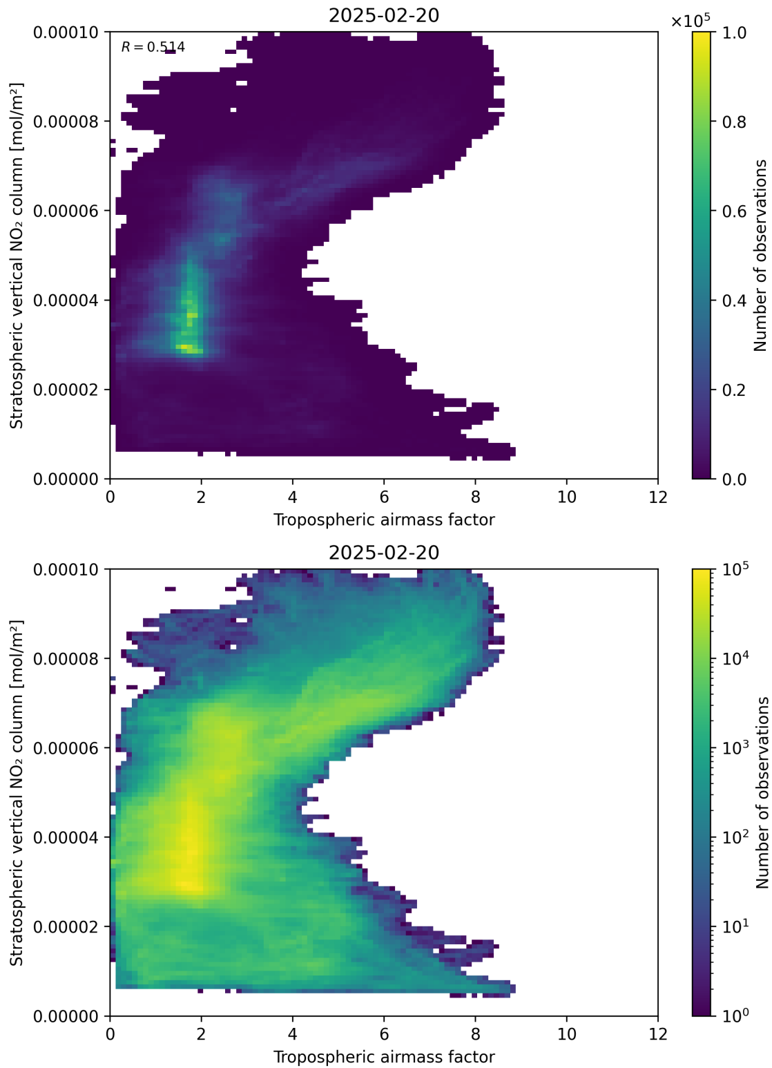
Figure 74: Scatter density plot of “Tropospheric air mass factor” against “Stratospheric vertical NO 2 column” for 2025-02-19 to 2025-02-21.
