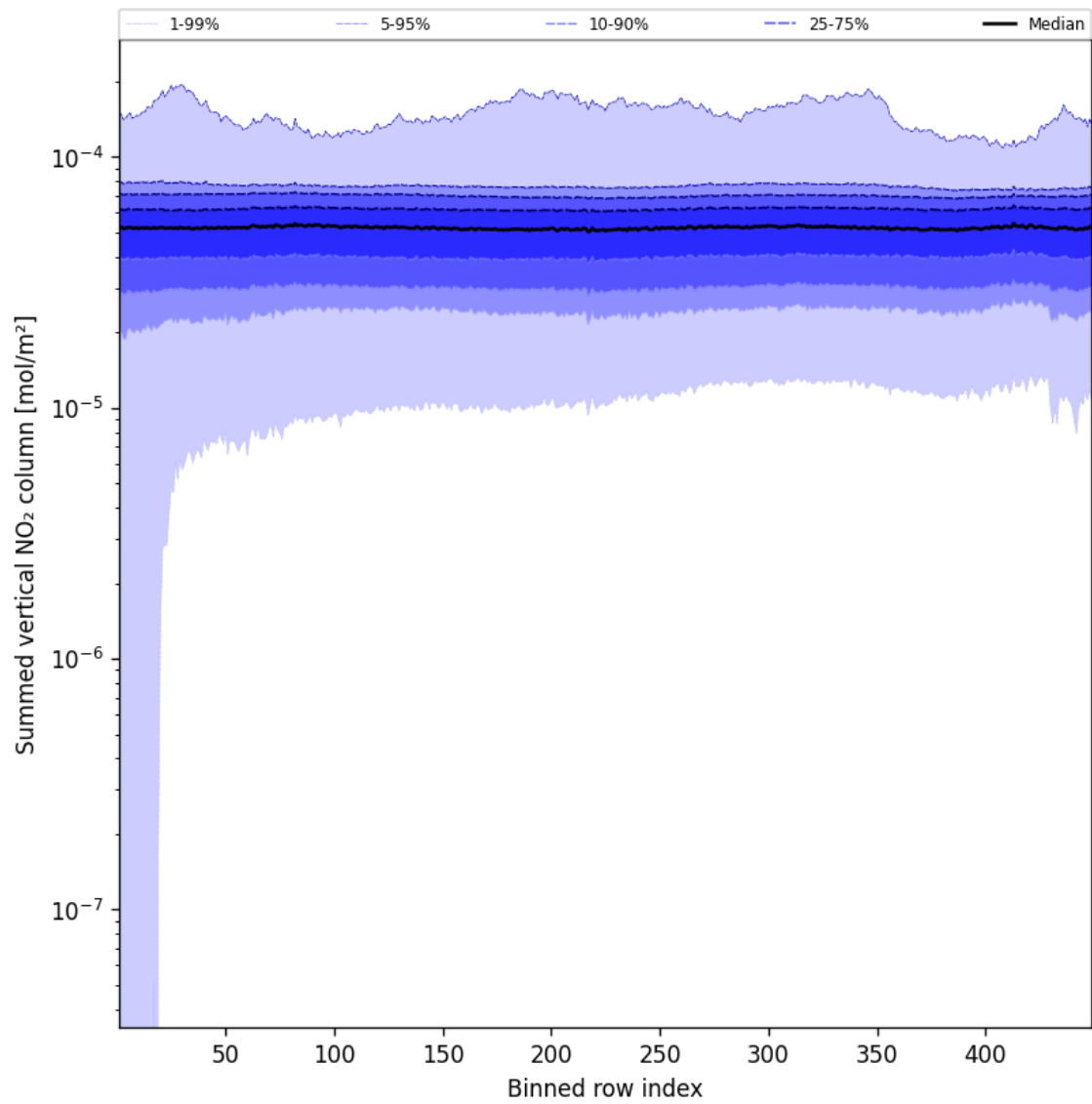
Figure 57: Along track statistics of “Summed vertical NO 2 column” for 2025-02-19 to 2025-02-21
