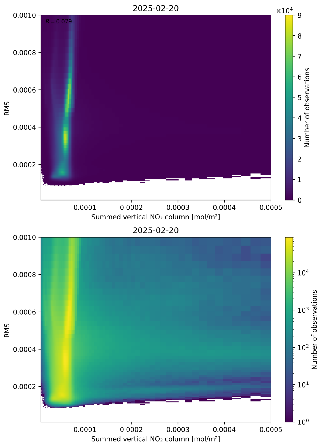
Figure 109: Scatter density plot of “Summed vertical NO 2 column” against “RMS” for 2025-02-19 to 2025-02-21.
