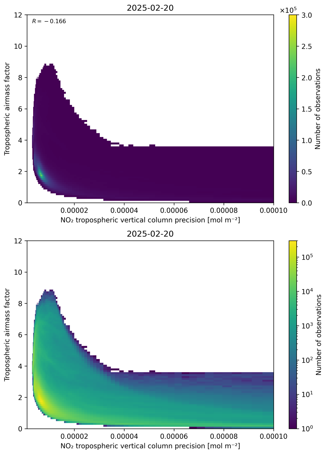
Figure 133: Scatter density plot of “NO 2 tropospheric vertical column precision” against “Tropospheric air mass factor” for 2025-02-19 to 2025-02-21.
