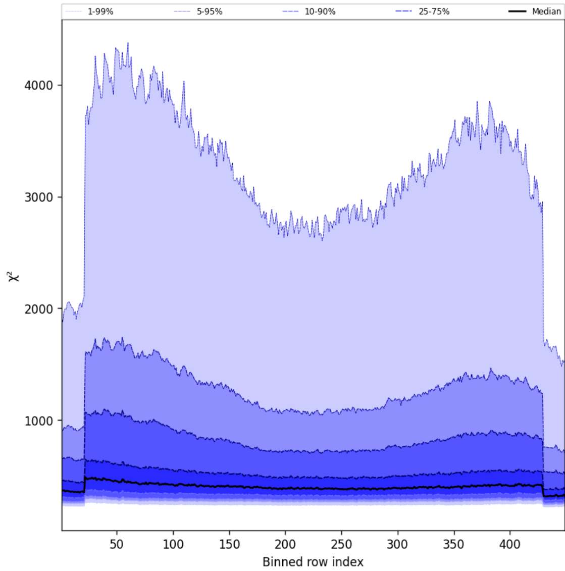
Figure 59: Along track statistics of “ \chi^2 ” for 2025-02-19 to 2025-02-21
