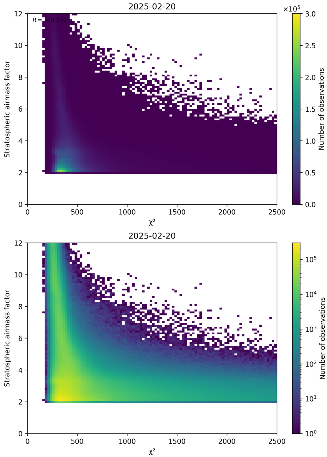
Figure 81: Scatter density plot of “ \chi^2 ” against “Stratospheric airmass factor” for 2025-02-19 to 2025-02-21.
