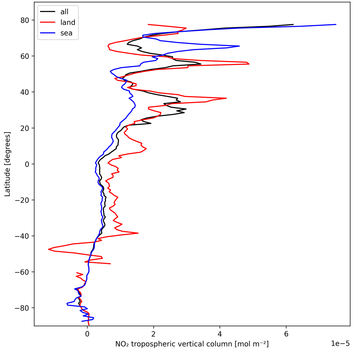
Figure 12: Zonal average of “NO 2 tropospheric vertical column” for 2025-02-19 to 2025-02-21.
