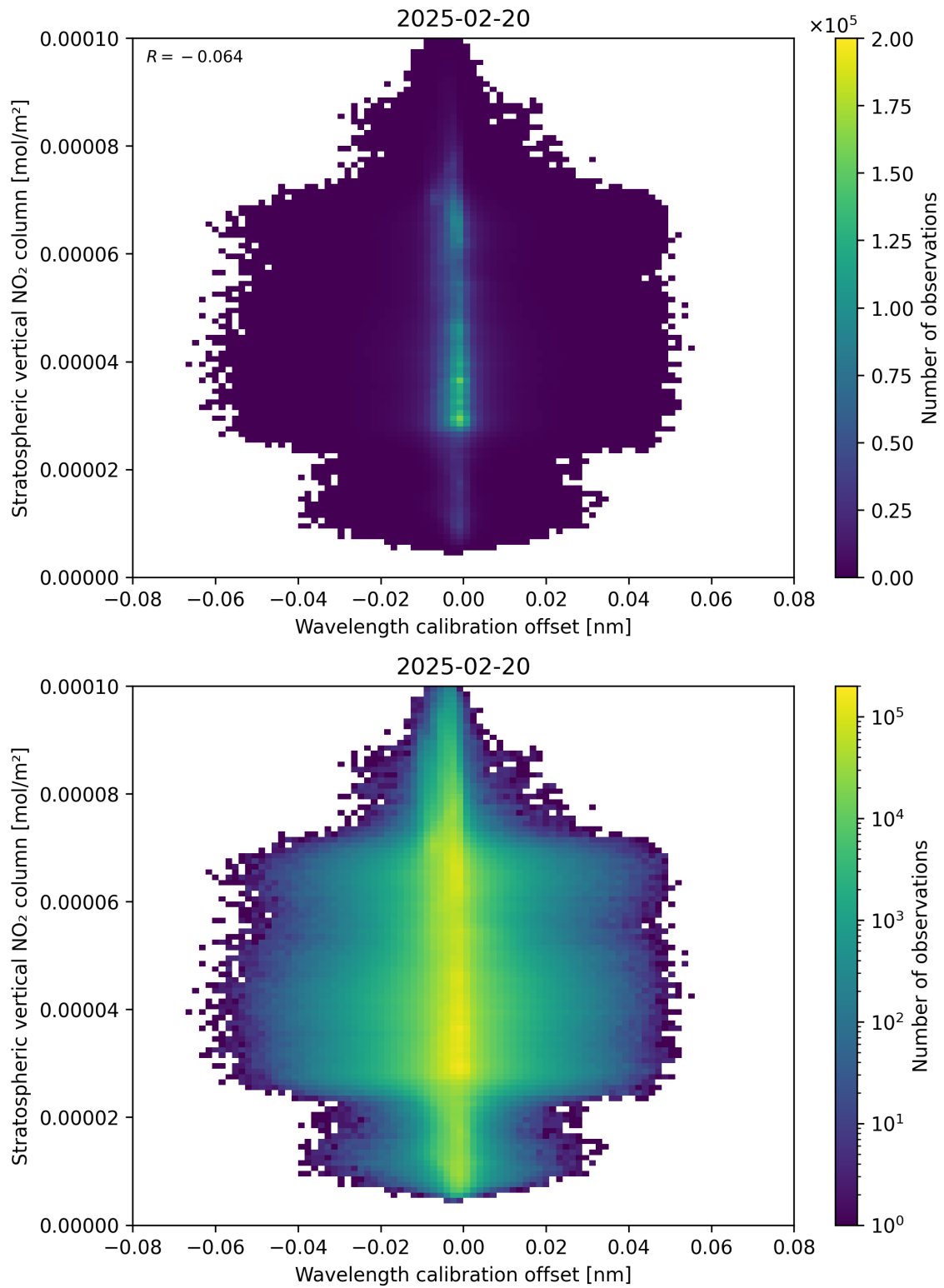
Figure 176: Scatter density plot of “Wavelength calibration offset” against “Stratospheric vertical NO 2 column” for 2025-02-19 to 2025-02-21.
