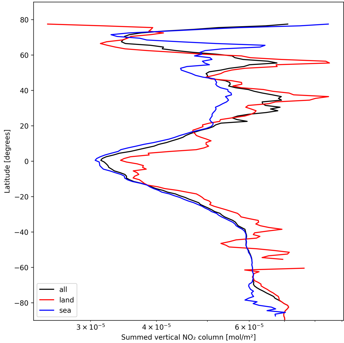
Figure 23: Zonal average of “Summed vertical NO 2 column” for 2025-02-19 to 2025-02-21.
