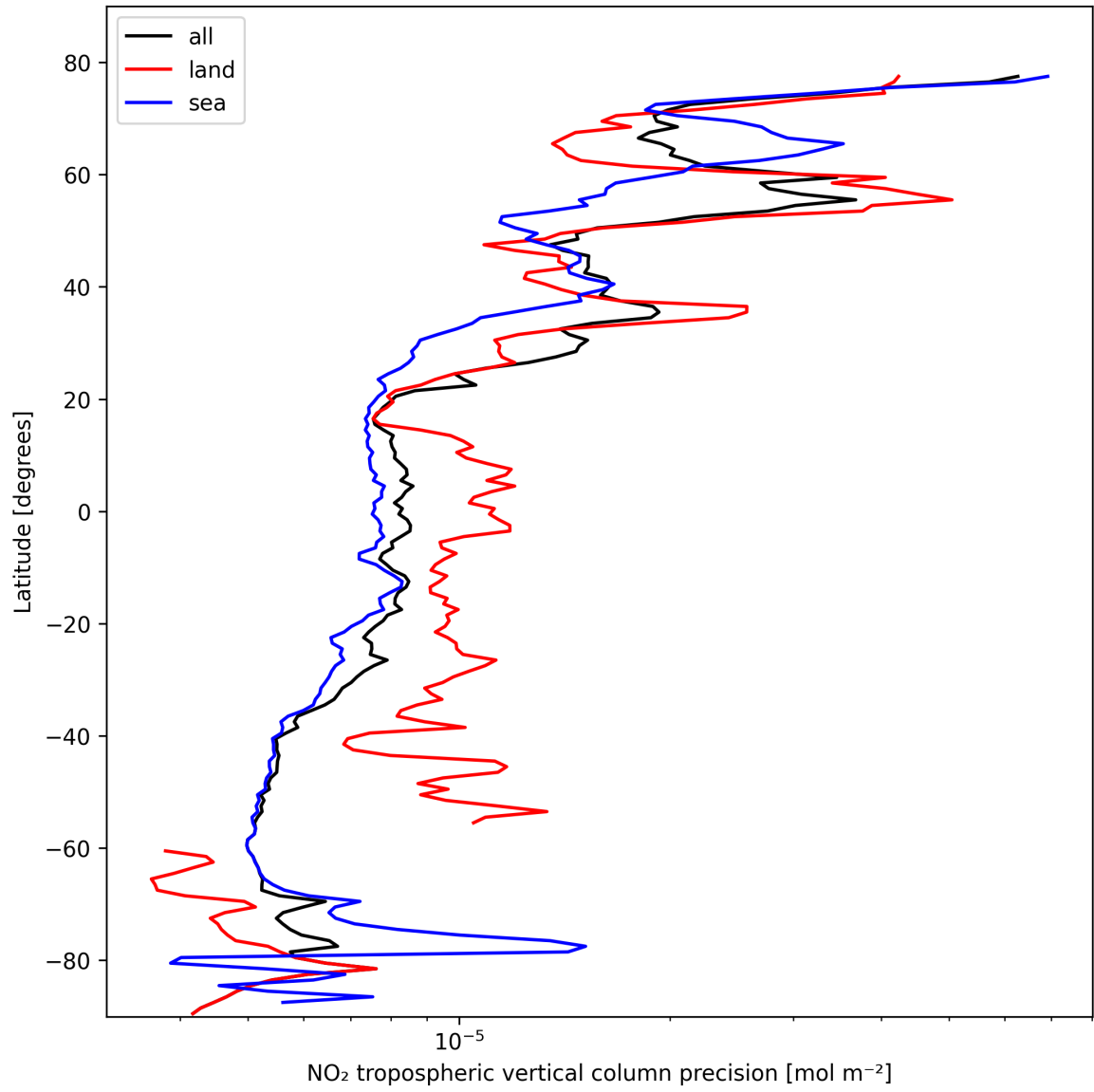
Figure 13: Zonal average of “NO 2 tropospheric vertical column precision” for 2025-02-19 to 2025-02-21.
