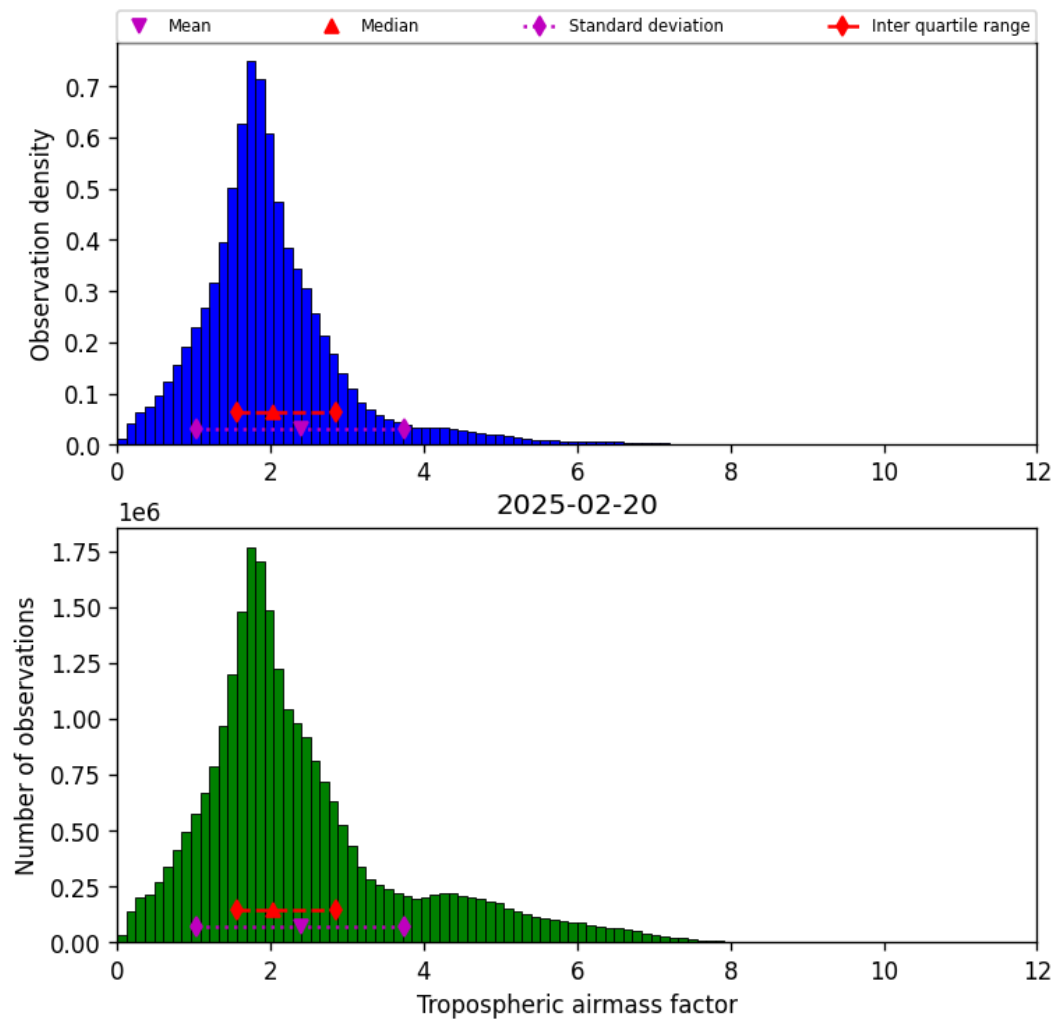
Figure 31: Histogram of “Tropospheric airmass factor” for 2025-02-19 to 2025-02-21
