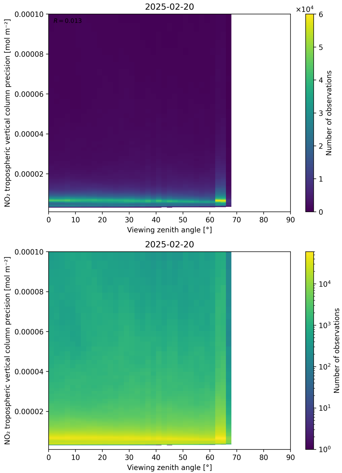
Figure 170: Scatter density plot of “Viewing zenith angle” against “NO 2 tropospheric vertical column precision” for 2025-02-19 to 2025-02-21.
