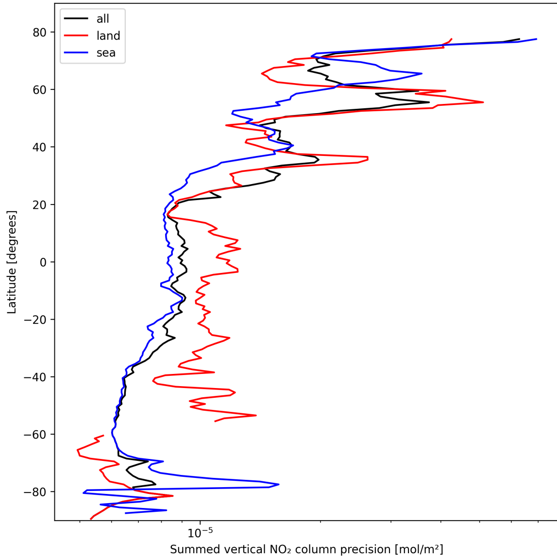
Figure 24: Zonal average of “Summed vertical NO 2 column precision” for 2025-02-19 to 2025-02-21.
