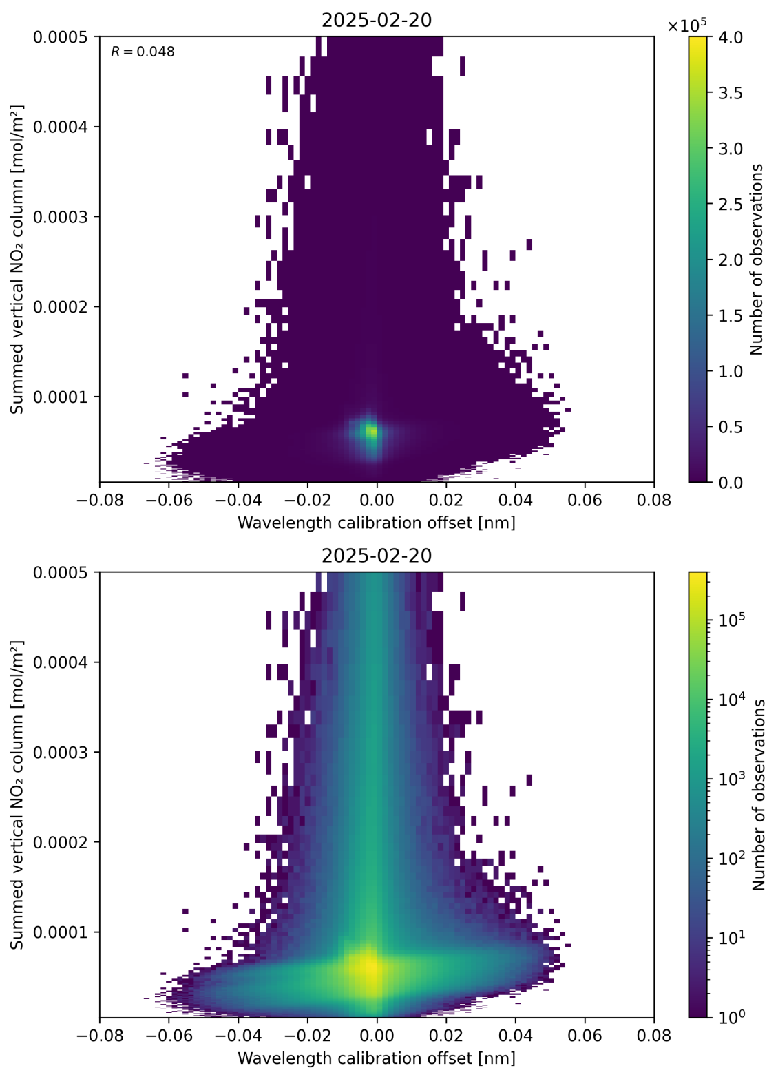
Figure 177: Scatter density plot of “Wavelength calibration offset” against “Summed vertical NO 2 column” for 2025-02-19 to 2025-02-21.
