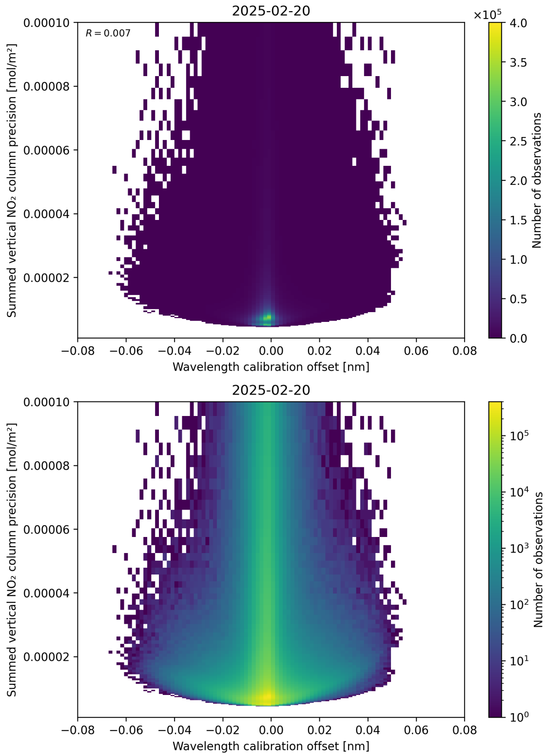
Figure 178: Scatter density plot of “Wavelength calibration offset” against “Summed vertical NO 2 column precision” for 2025-02-19 to 2025-02-21.
