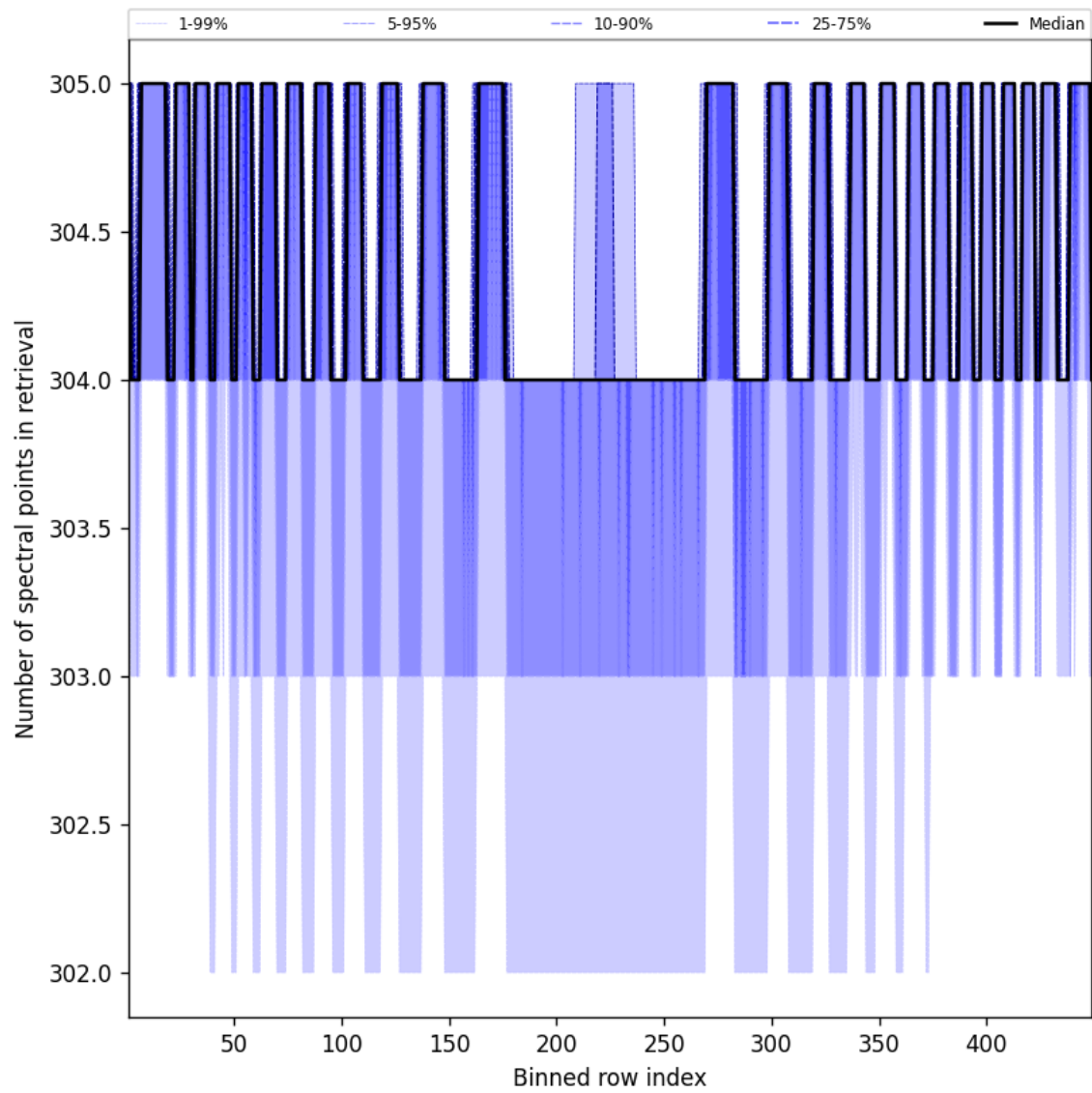
Figure 50: Along track statistics of “Number of spectral points in retrieval” for 2025-02-19 to 2025-02-21
