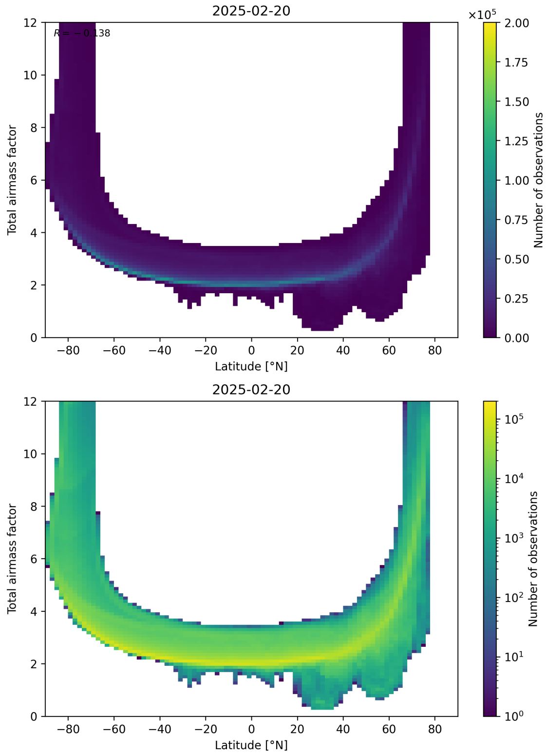
Figure 84: Scatter density plot of “Latitude” against “Total airmass factor” for 2025-02-19 to 2025-02-21.
