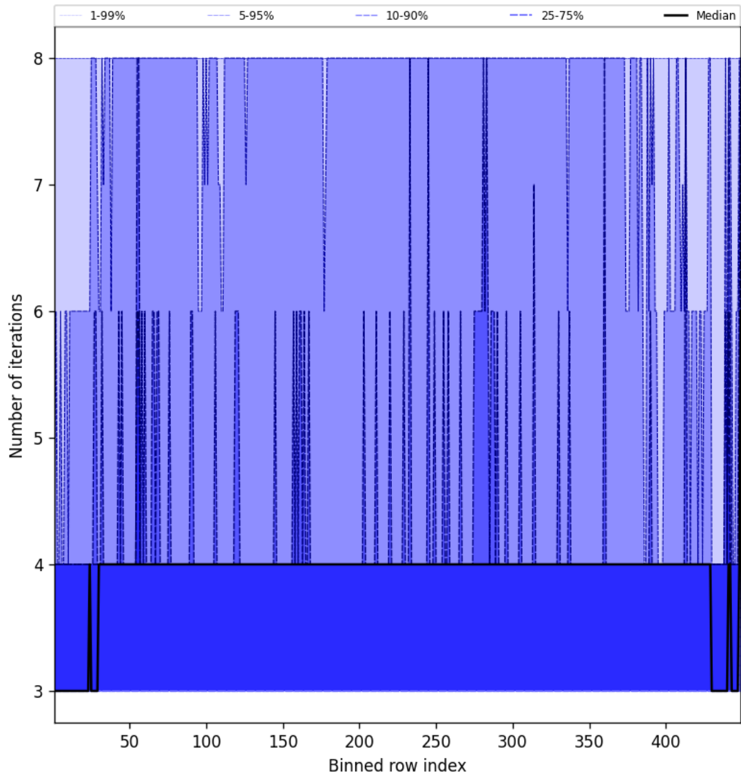
Figure 51: Along track statistics of “Number of iterations” for 2025-02-19 to 2025-02-21
