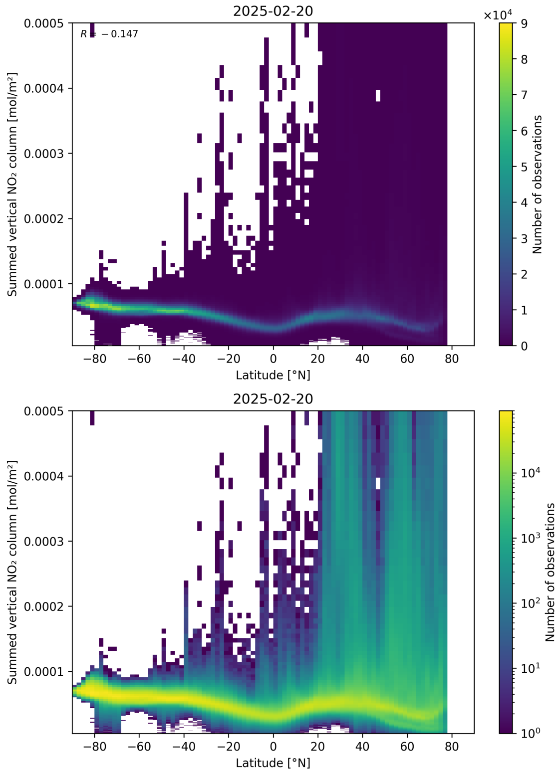
Figure 88: Scatter density plot of “Latitude” against “Summed vertical NO 2 column” for 2025-02-19 to 2025-02-21.
