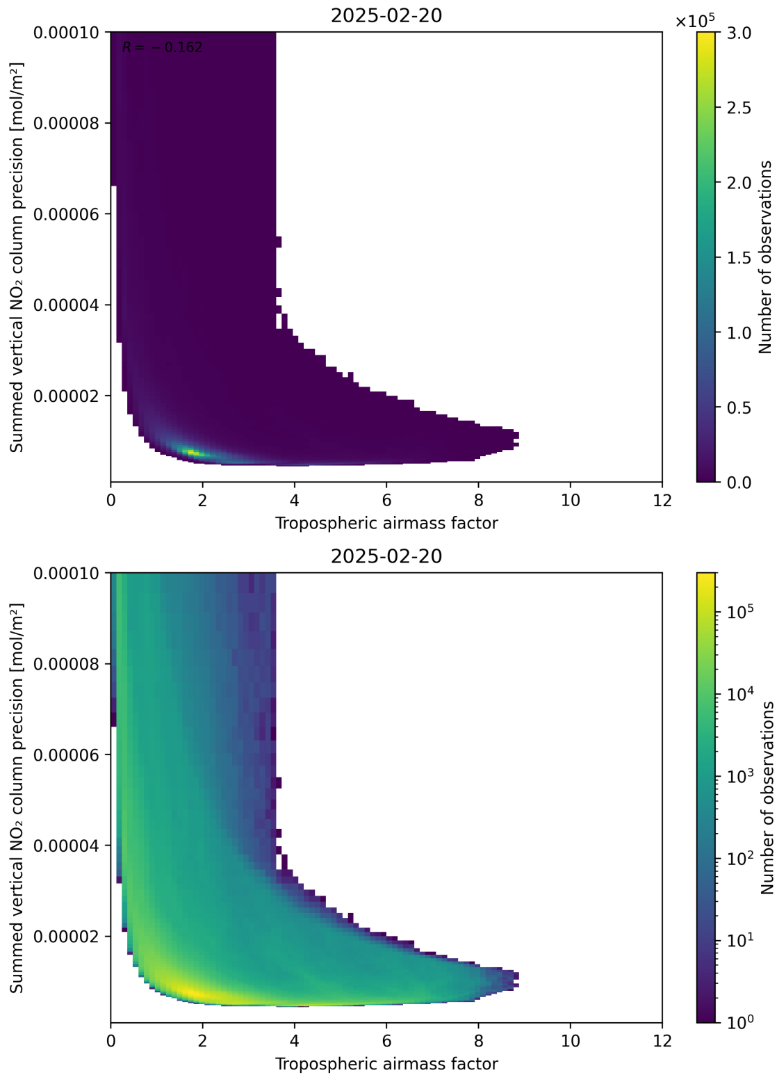
Figure 76: Scatter density plot of “Tropospheric air mass factor” against “Summed vertical NO 2 column precision” for 2025-02-19 to 2025-02-21.
