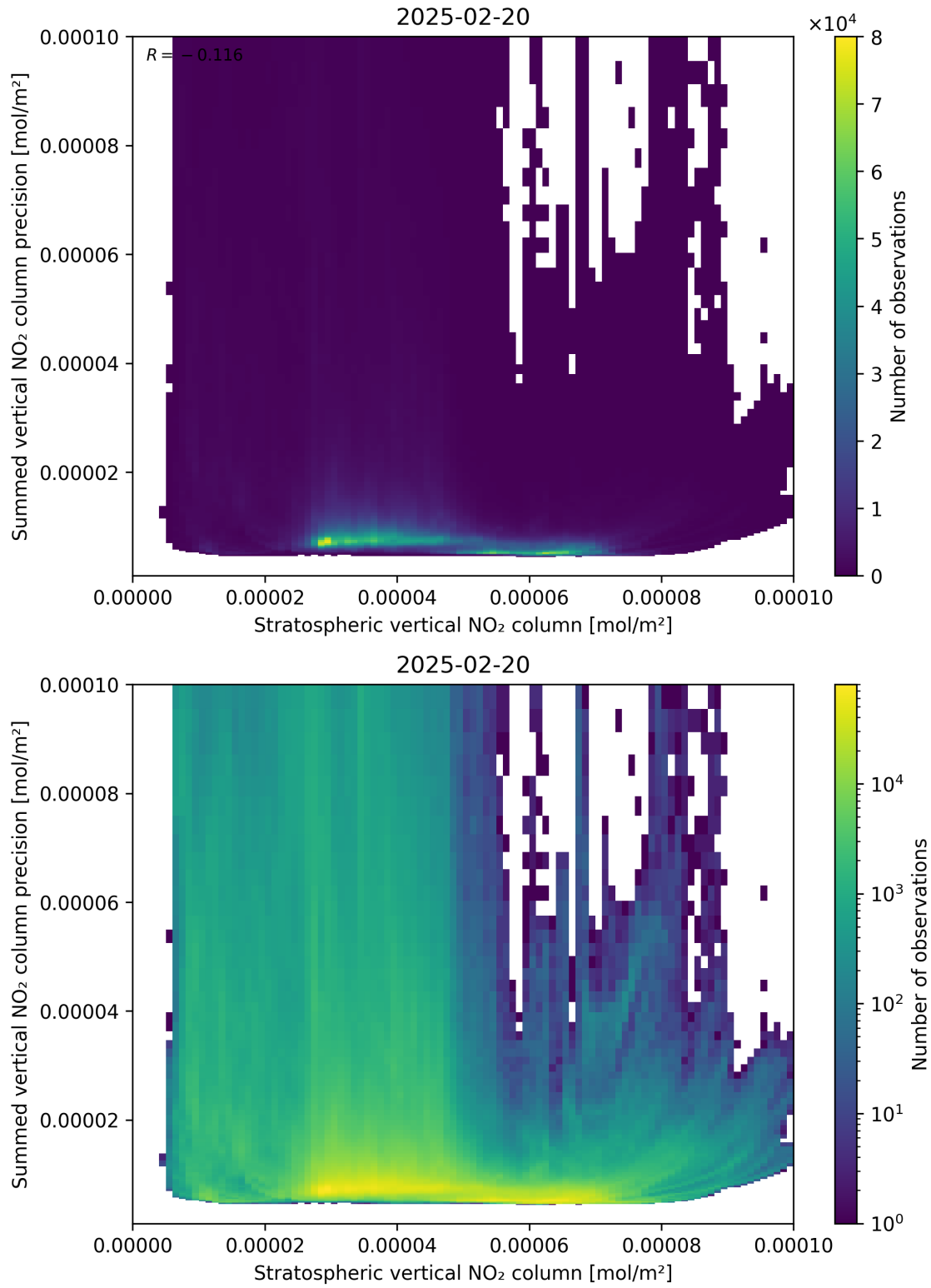
Figure 99: Scatter density plot of “Stratospheric vertical NO 2 column” against “Summed vertical NO 2 column precision” for 2025-02-19 to 2025-02-21.
