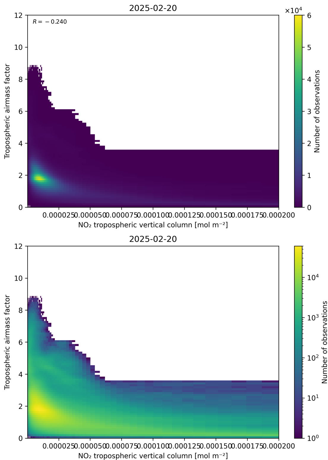
Figure 123: Scatter density plot of “NO 2 tropospheric vertical column” against “Tropospheric airmass factor” for 2025-02-19 to 2025-02-21.
