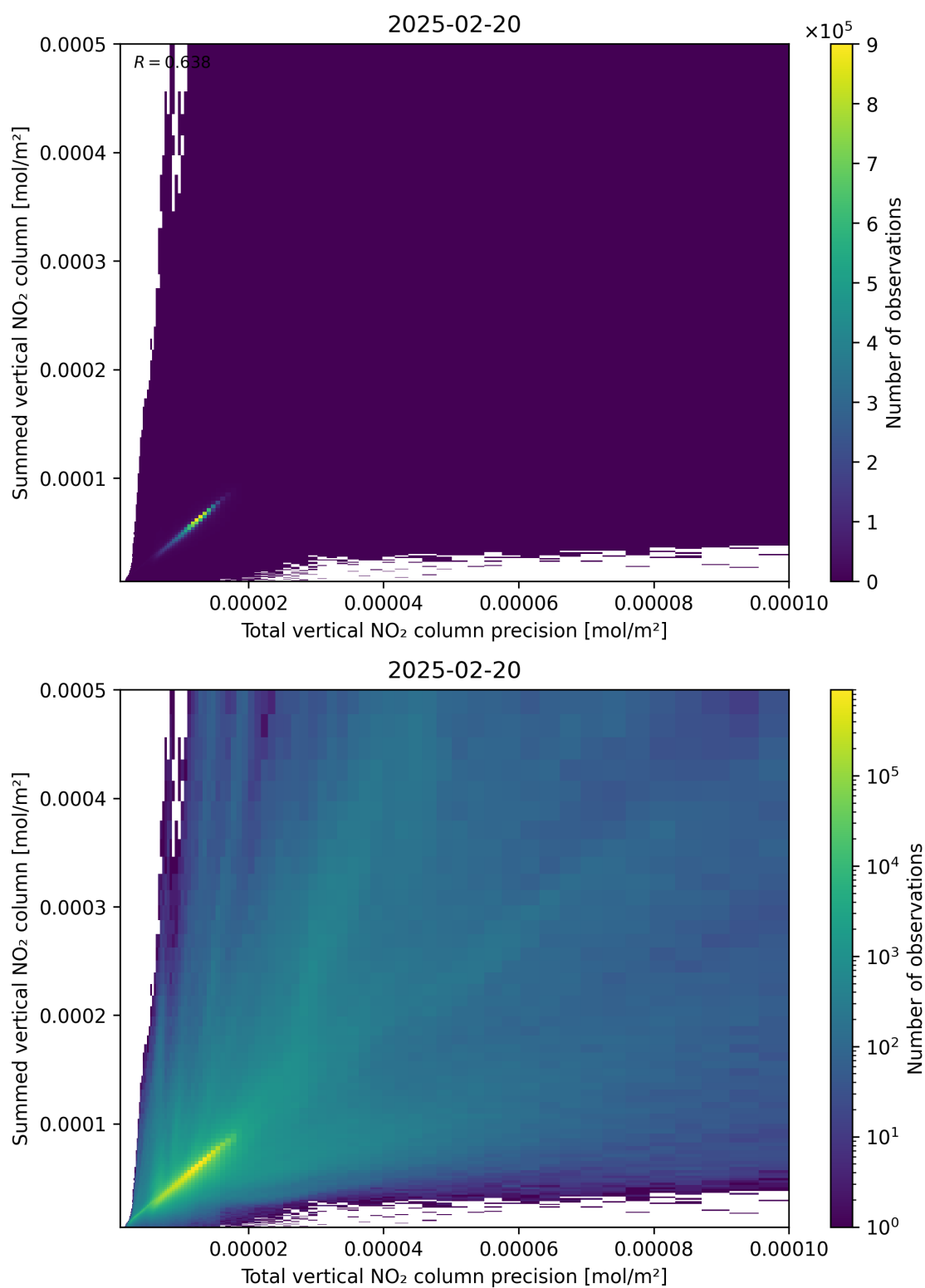
Figure 117: Scatter density plot of “Total vertical NO 2 column precision” against “Summed vertical NO 2 column” for 2025-02-19 to 2025-02-21.
