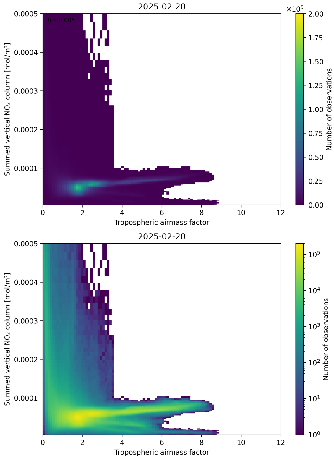
Figure 75: Scatter density plot of “Tropospheric air mass factor” against “Summed vertical NO 2 column” for 2025-02-19 to 2025-02-21.
