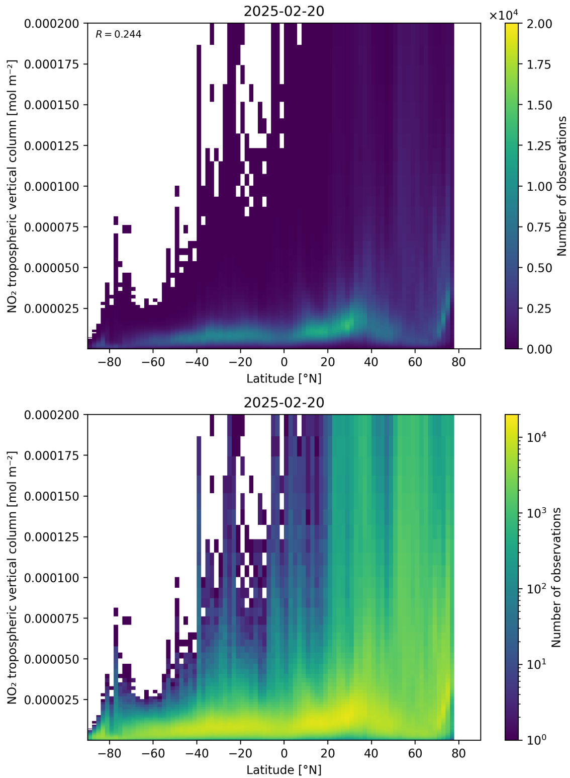
Figure 92: Scatter density plot of “Latitude” against “NO 2 tropospheric vertical column” for 2025-02-19 to 2025-02-21.
