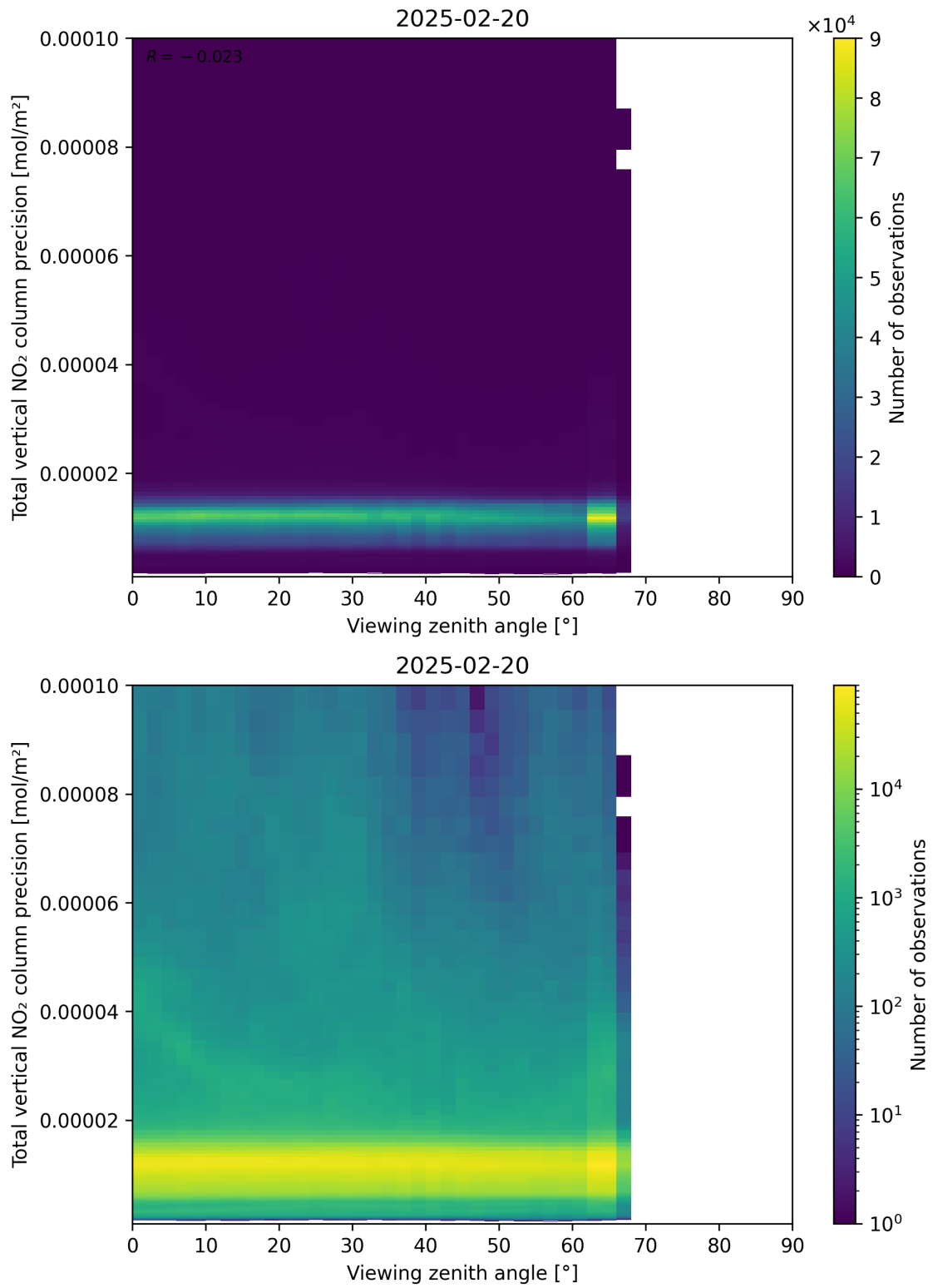
Figure 168: Scatter density plot of “Viewing zenith angle” against “Total vertical NO 2 column precision” for 2025-02-19 to 2025-02-21.
