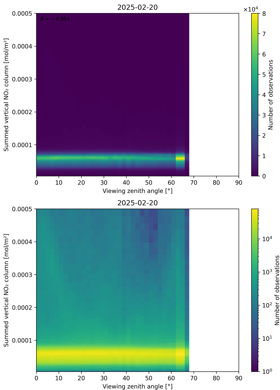
Figure 165: Scatter density plot of “Viewing zenith angle” against “Summed vertical NO 2 column” for 2025-02-19 to 2025-02-21.
