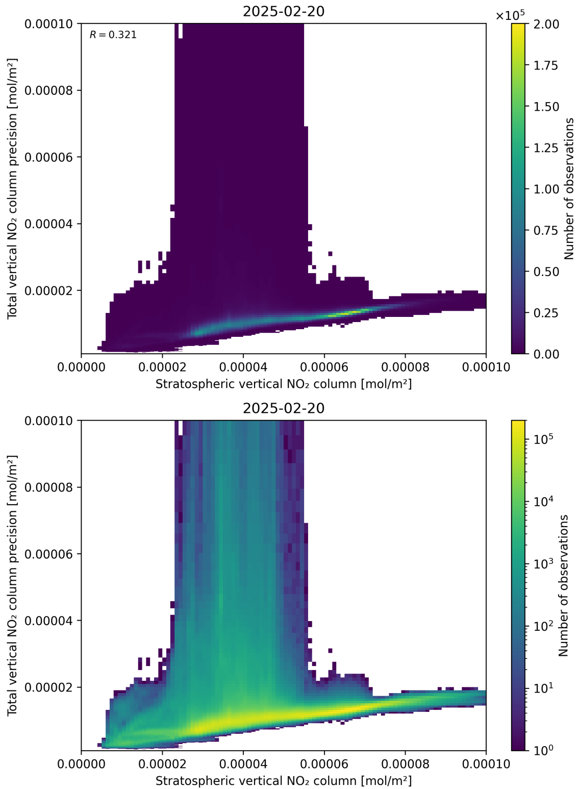
Figure 101: Scatter density plot of “Stratospheric vertical NO 2 column” against “Total vertical NO 2 column precision” for 2025-02-19 to 2025-02-21.
