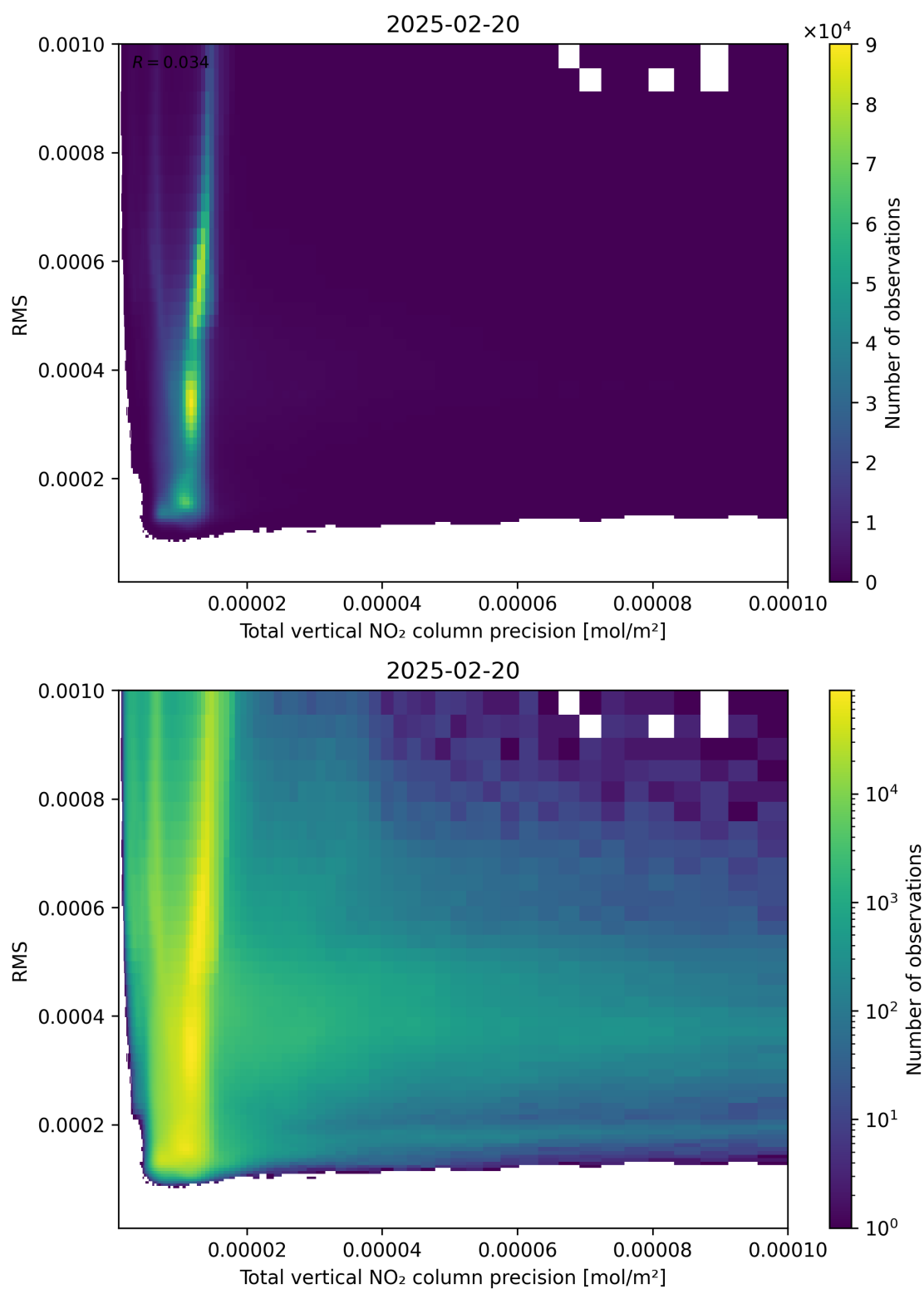
Figure 119: Scatter density plot of “Total vertical NO 2 column precision” against “RMS” for 2025-02-19 to 2025-02-21.
