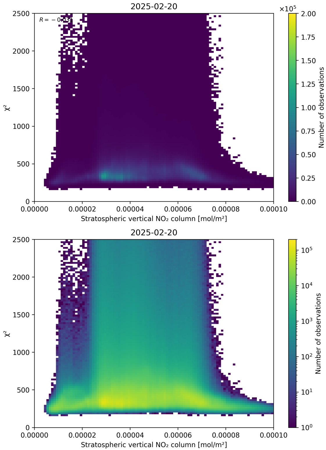
Figure 97: Scatter density plot of “Stratospheric vertical NO 2 column” against “ \chi^2 ” for 2025-02-19 to 2025-02-21.
