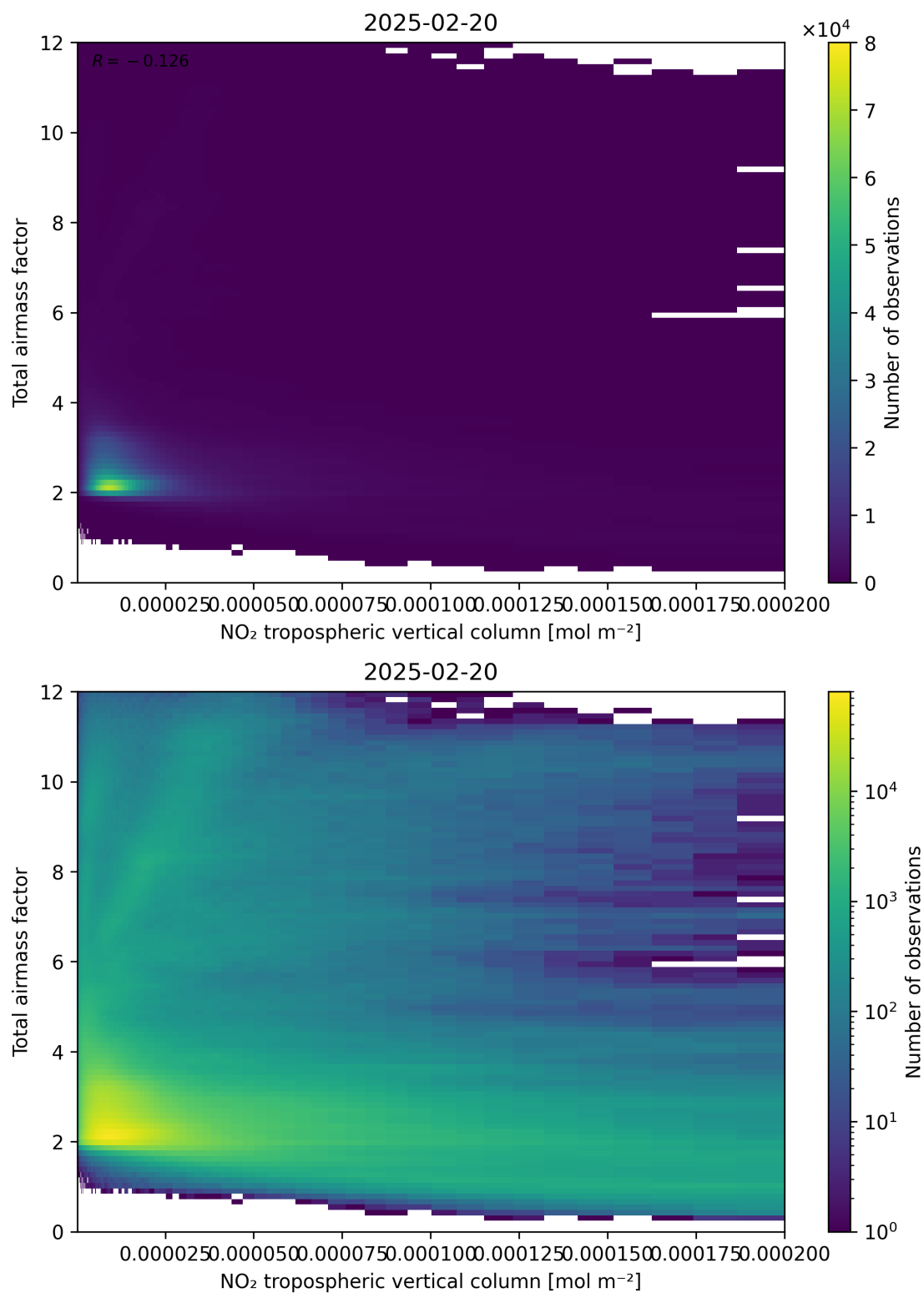
Figure 122: Scatter density plot of “NO 2 tropospheric vertical column” against “Total air mass factor” for 2025-02-19 to 2025-02-21.
