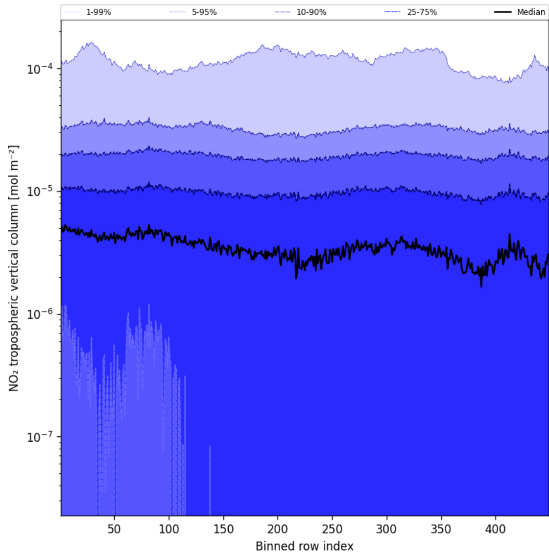
Figure 46: Along track statistics of “NO 2 tropospheric vertical column” for 2025-02-19 to 2025-02-21
