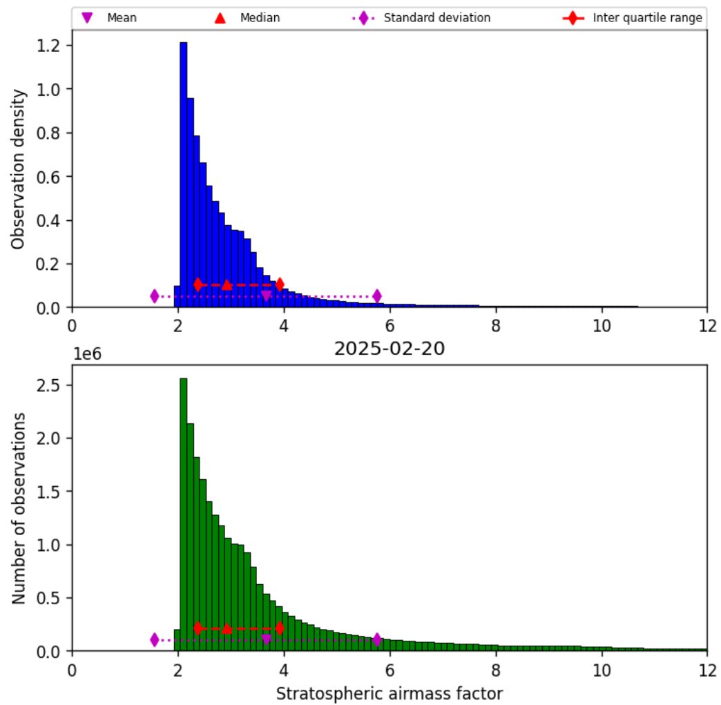
Figure 44: Histogram of “Stratospheric airmass factor” for 2025-02-19 to 2025-02-21
