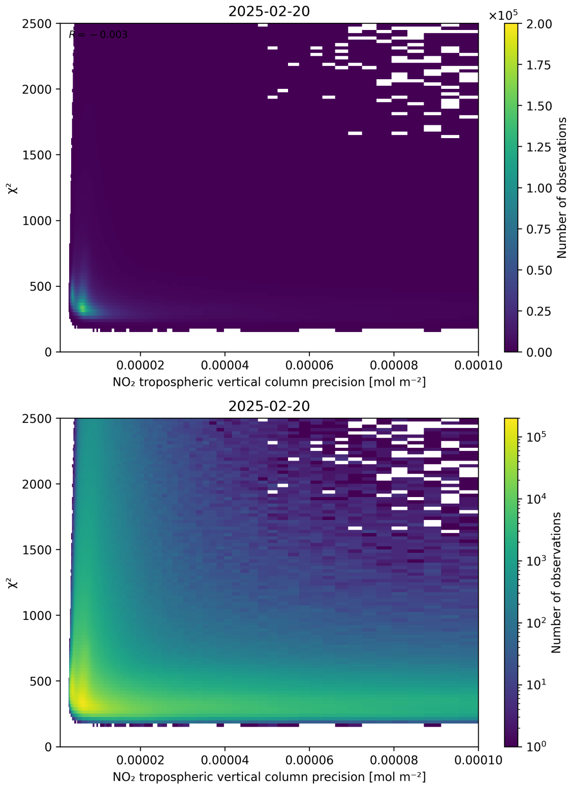
Figure 134: Scatter density plot of “NO 2 tropospheric vertical column precision” against “ \chi^2 ” for 2025-02-19 to 2025-02-21.
