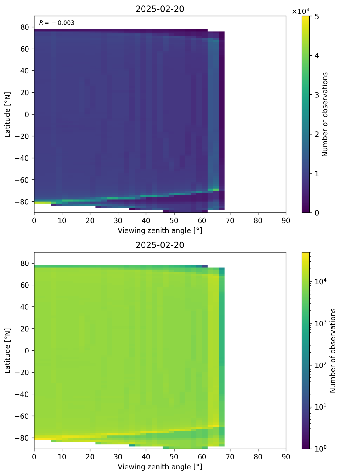
Figure 163: Scatter density plot of “Viewing zenith angle” against “Latitude” for 2025-02-19 to 2025-02-21.
