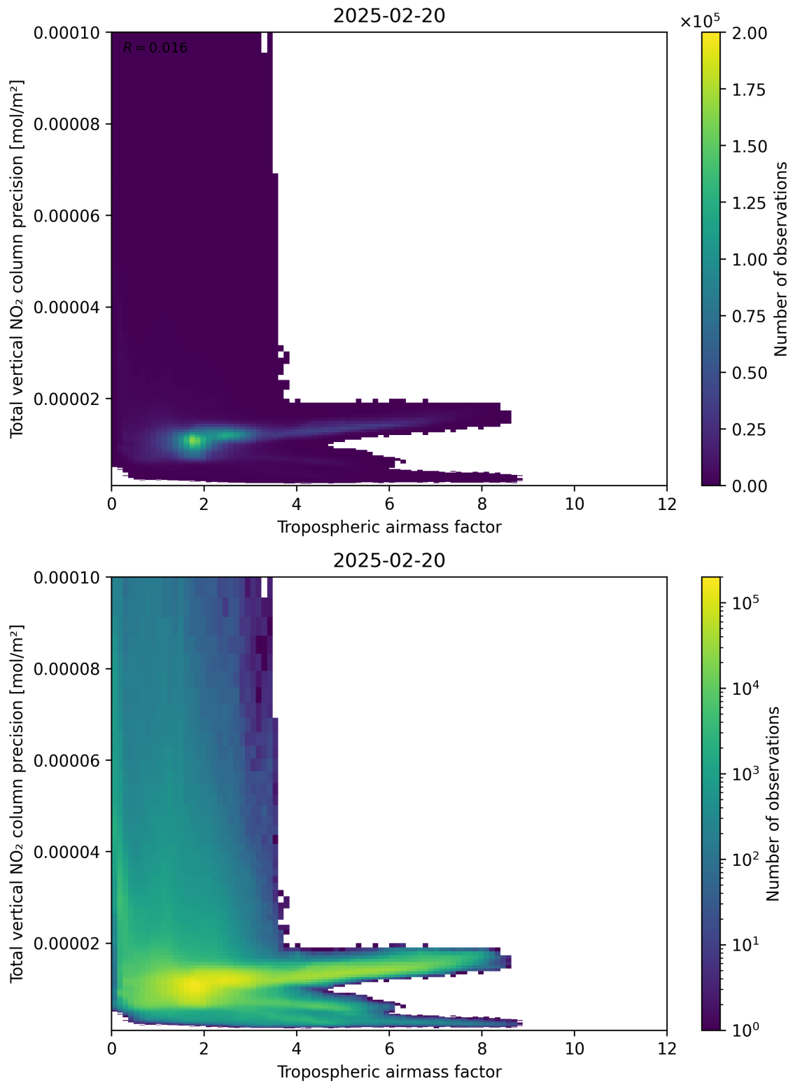
Figure 78: Scatter density plot of “Tropospheric airmass factor” against “Total vertical NO 2 column precision” for 2025-02-19 to 2025-02-21.
