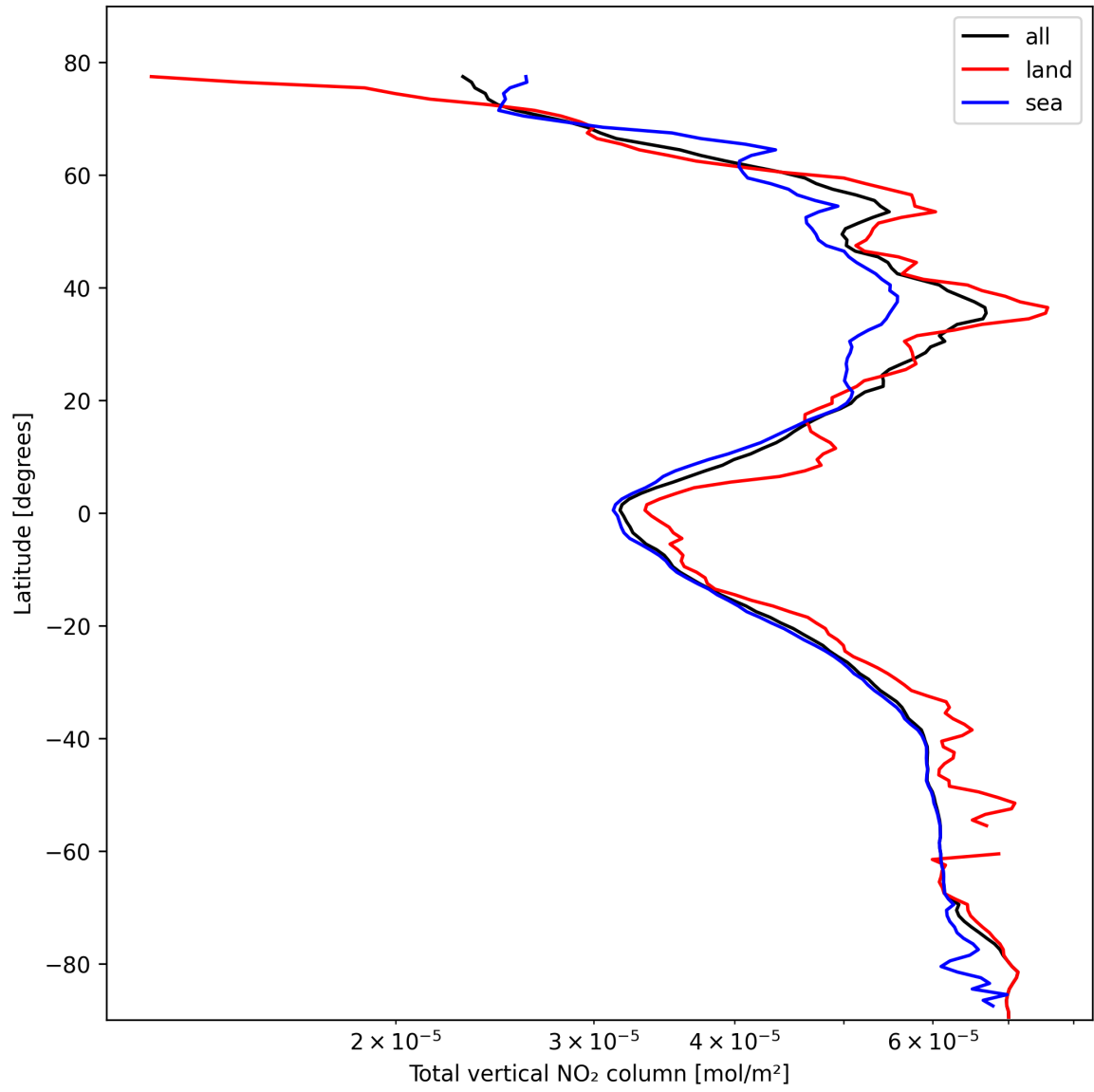
Figure 21: Zonal average of “Total vertical NO 2 column” for 2025-02-19 to 2025-02-21.
