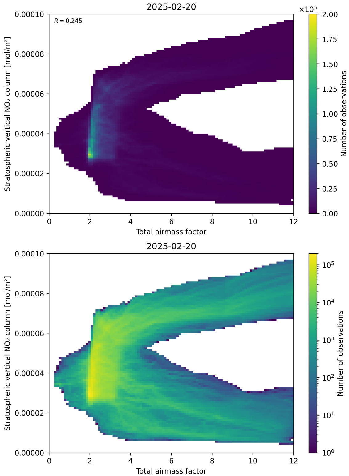
Figure 64: Scatter density plot of “Total airmass factor” against “Stratospheric vertical \text{NO}_2 column” for 2025-02-19 to 2025-02-21.
