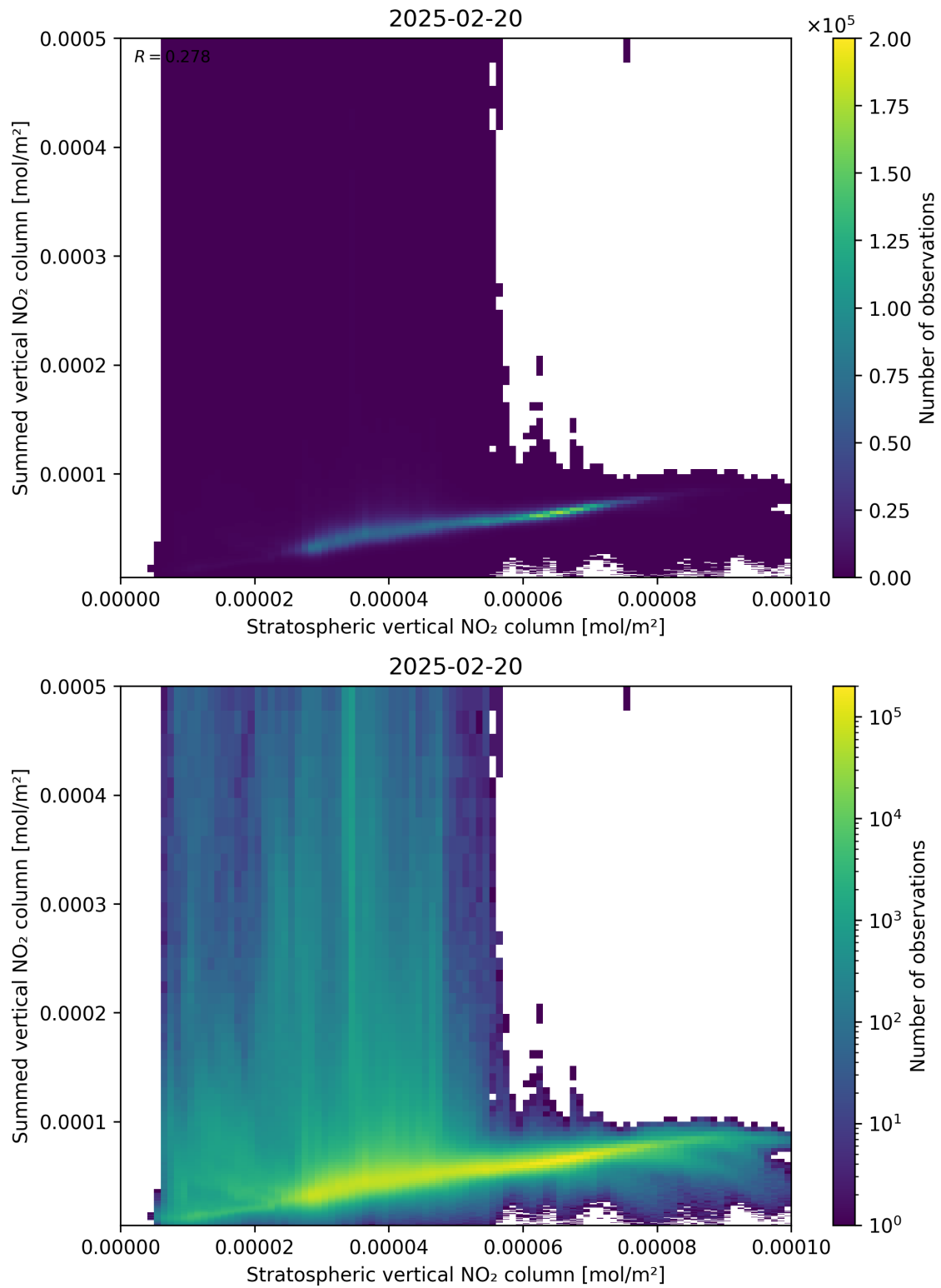
Figure 98: Scatter density plot of “Stratospheric vertical NO 2 column” against “Summed vertical NO 2 column” for 2025-02-19 to 2025-02-21.
