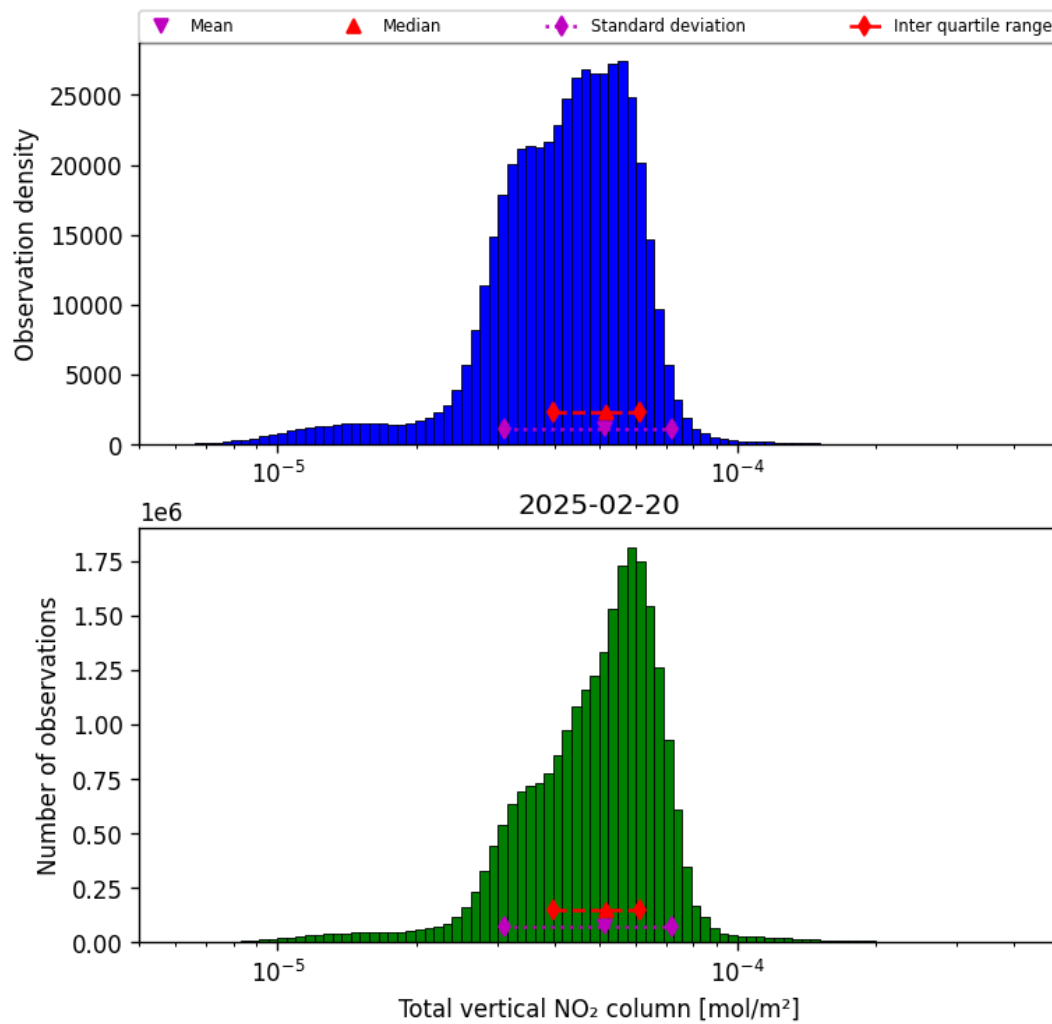
Figure 38: Histogram of “Total vertical NO 2 column” for 2025-02-19 to 2025-02-21
