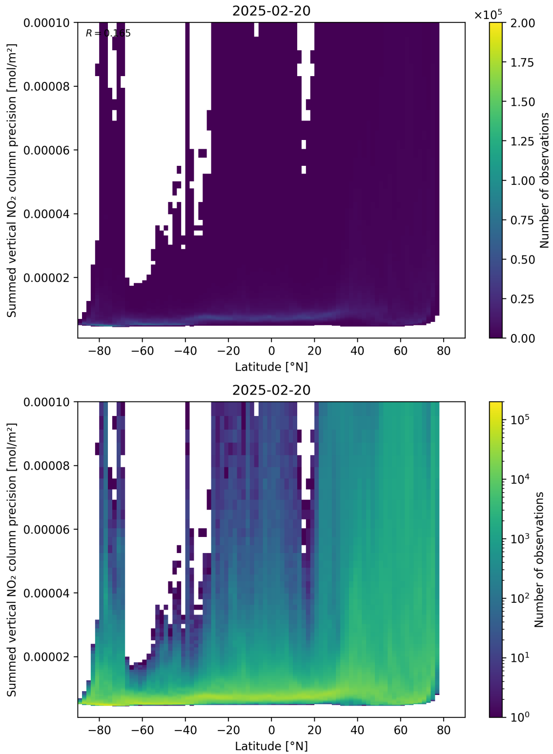
Figure 89: Scatter density plot of “Latitude” against “Summed vertical NO 2 column precision” for 2025-02-19 to 2025-02-21.
