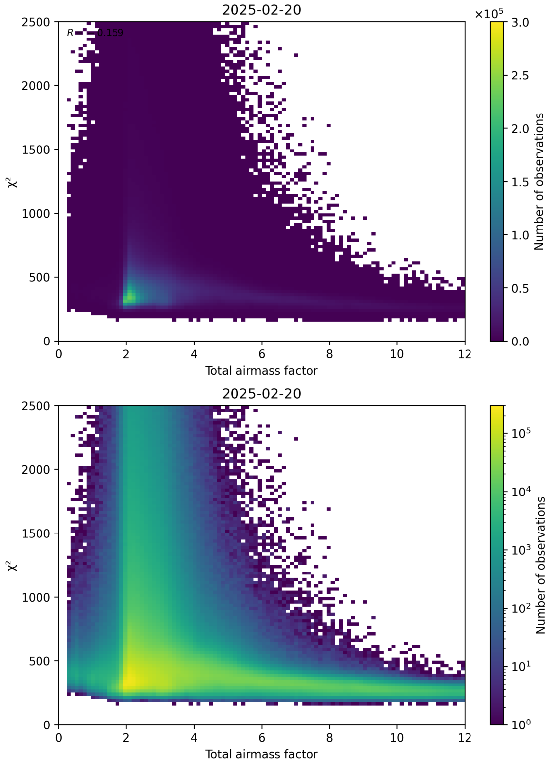
Figure 63: Scatter density plot of “Total airmass factor” against “ \chi^2 ” for 2025-02-19 to 2025-02-21.
