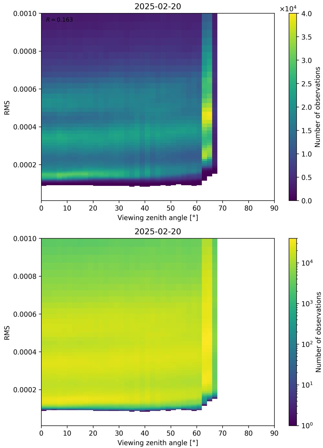
Figure 171: Scatter density plot of “Viewing zenith angle” against “RMS” for 2025-02-19 to 2025-02-21.
