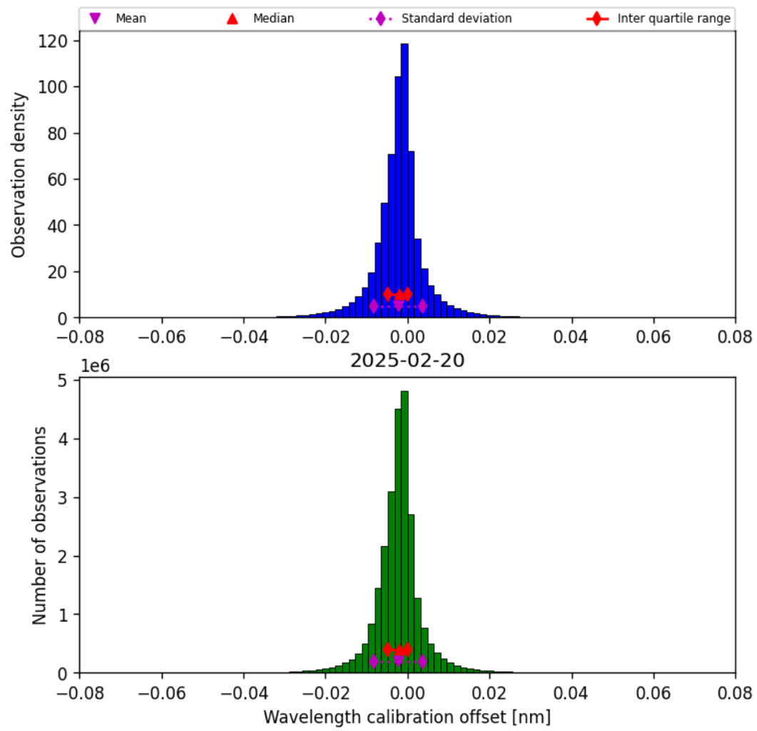
Figure 35: Histogram of “Wavelength calibration offset” for 2025-02-19 to 2025-02-21
