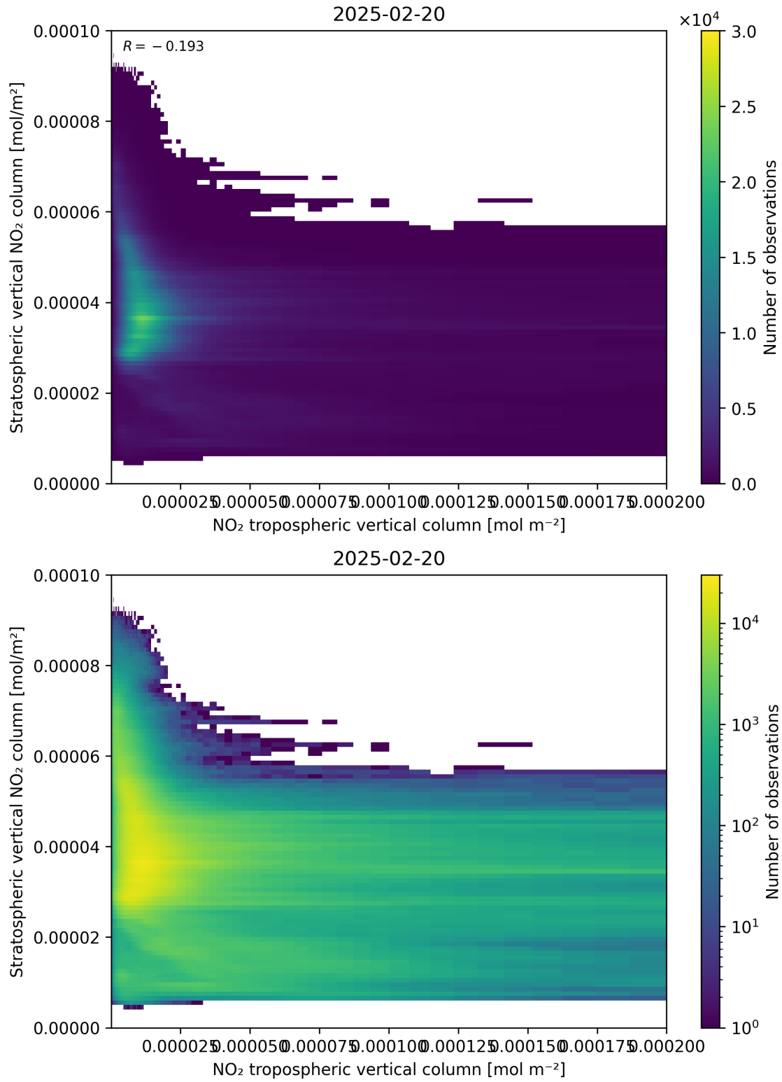
Figure 125: Scatter density plot of “NO 2 tropospheric vertical column” against “Stratospheric vertical NO 2 column” for 2025-02-19 to 2025-02-21.
