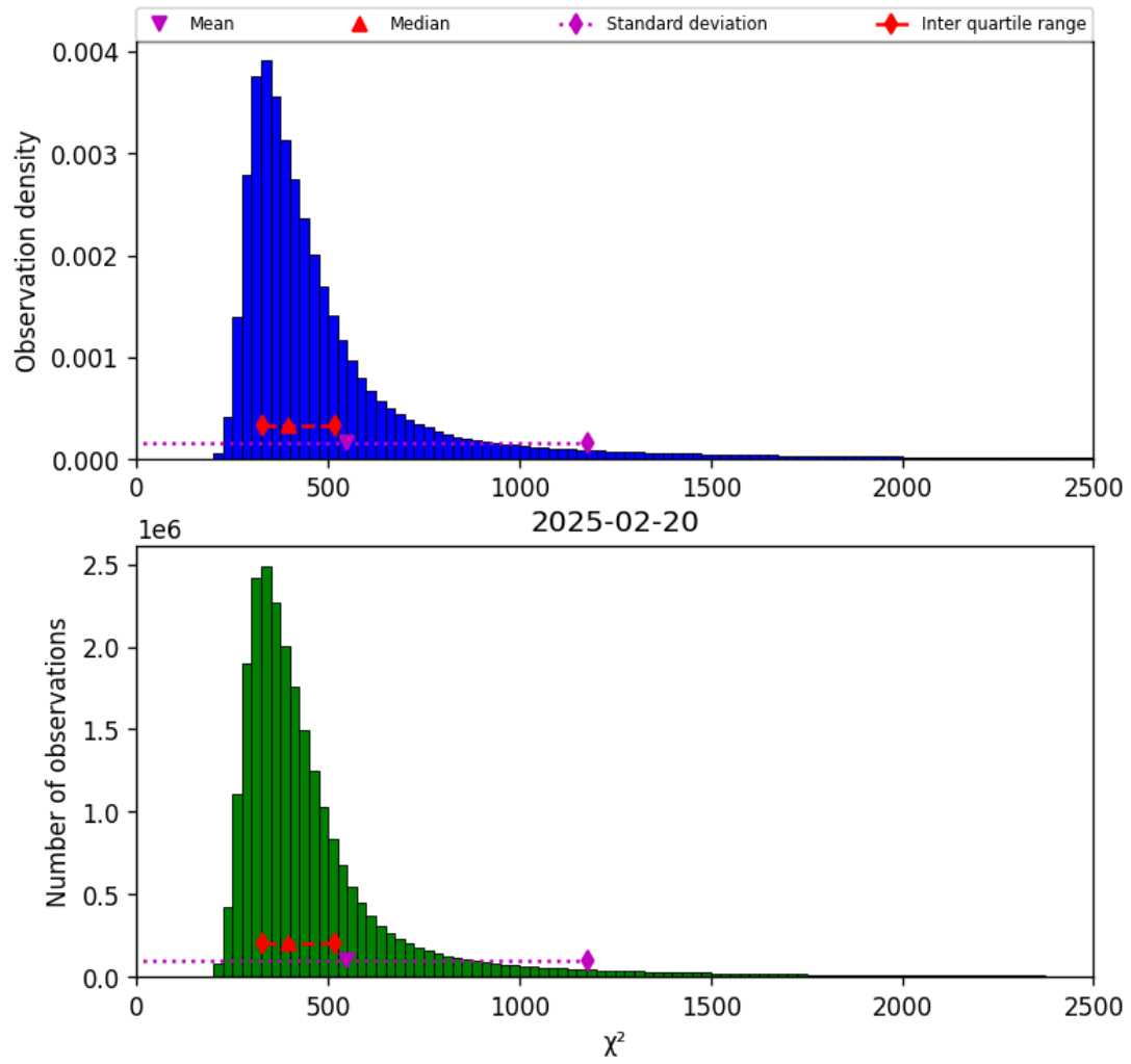
Figure 42: Histogram of “ \chi^2 ” for 2025-02-19 to 2025-02-21
