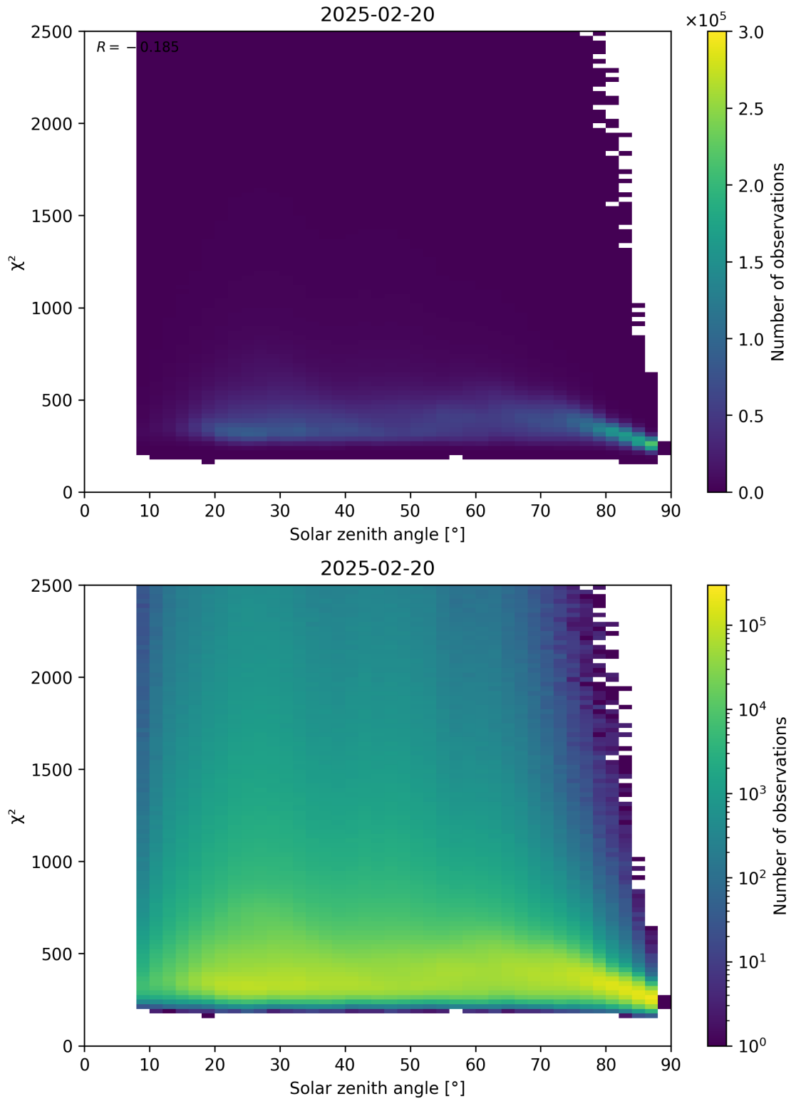
Figure 148: Scatter density plot of “Solar zenith angle” against “ \chi^2 ” for 2025-02-19 to 2025-02-21.
