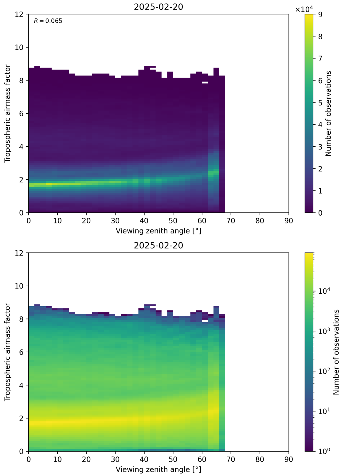
Figure 161: Scatter density plot of “Viewing zenith angle” against “Tropospheric airmass factor” for 2025-02-19 to 2025-02-21.
