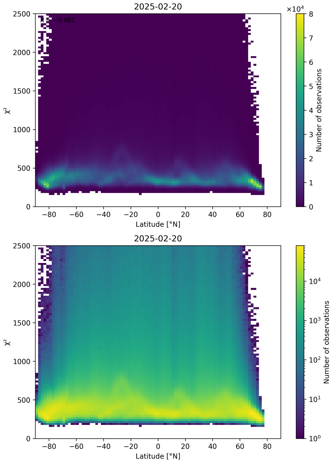
Figure 86: Scatter density plot of “Latitude” against “ \chi^2 ” for 2025-02-19 to 2025-02-21.
