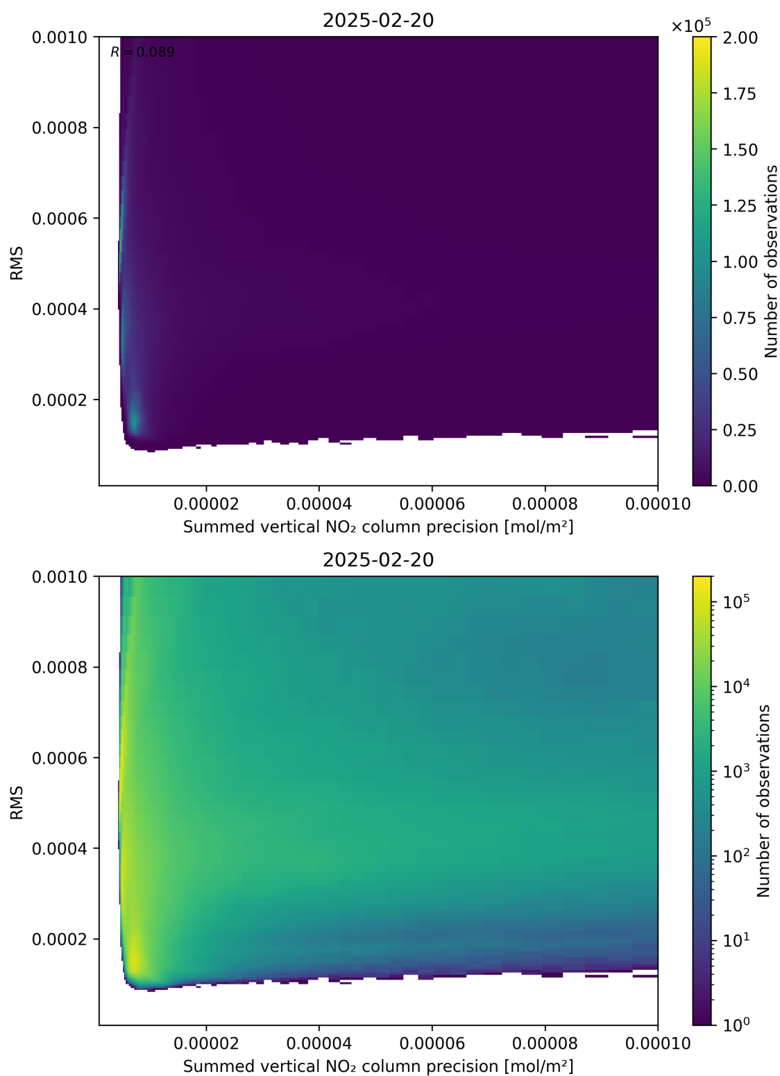
Figure 108: Scatter density plot of “Summed vertical NO 2 column precision” against “RMS” for 2025-02-19 to 2025-02-21.
