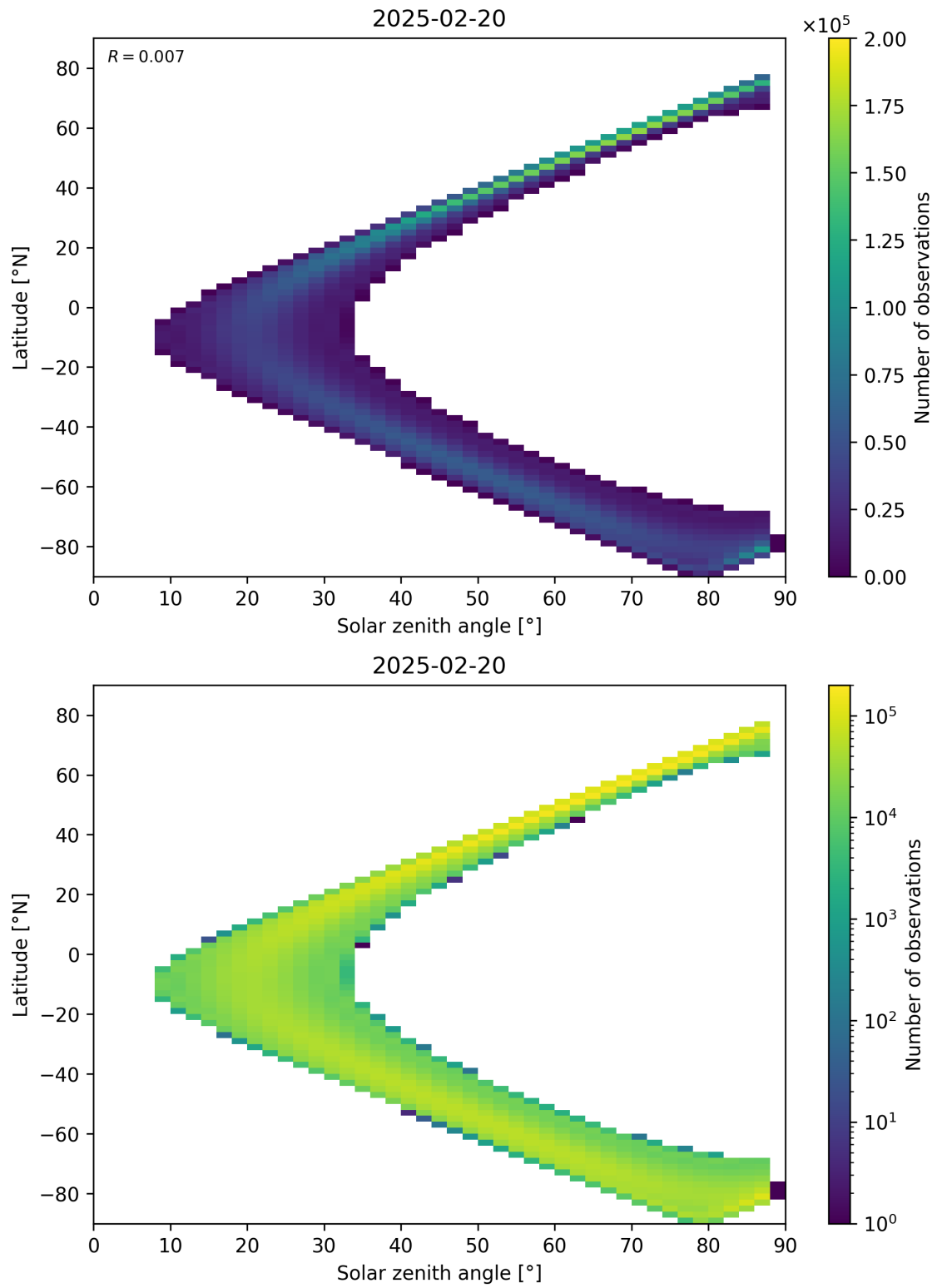
Figure 149: Scatter density plot of “Solar zenith angle” against “Latitude” for 2025-02-19 to 2025-02-21.
