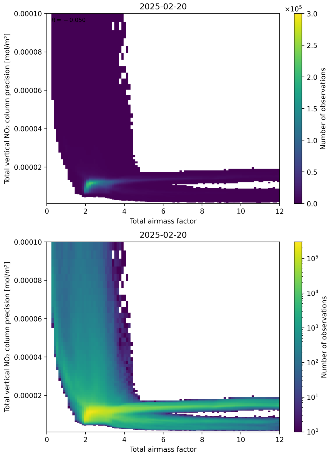
Figure 68: Scatter density plot of “Total airmass factor” against “Total vertical NO 2 column precision” for 2025-02-19 to 2025-02-21.
