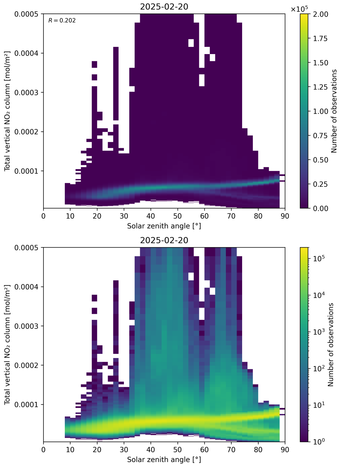
Figure 153: Scatter density plot of “Solar zenith angle” against “Total vertical NO 2 column” for 2025-02-19 to 2025-02-21.
