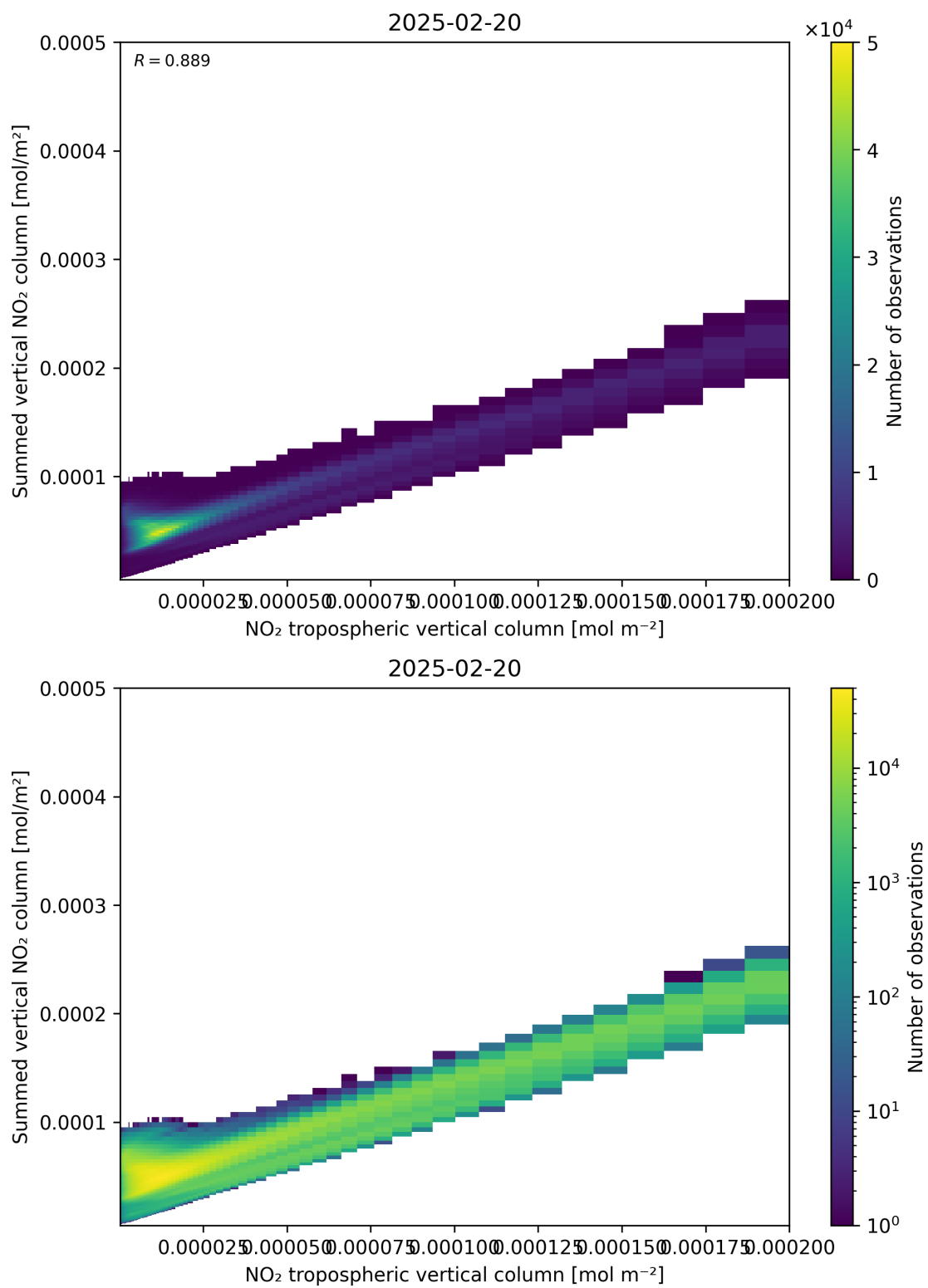
Figure 126: Scatter density plot of “NO 2 tropospheric vertical column” against “Summed vertical NO 2 column” for 2025-02-19 to 2025-02-21.
