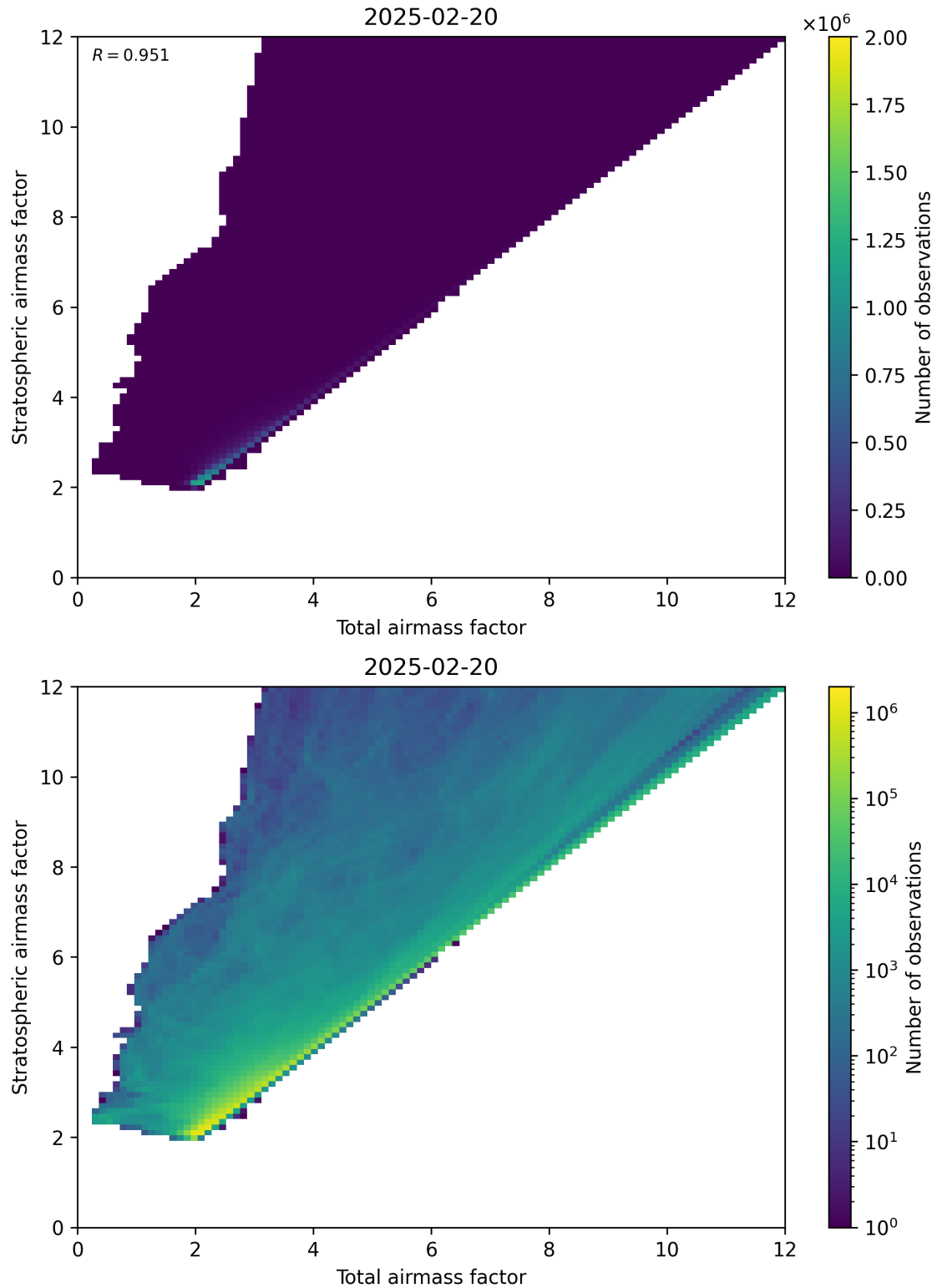
Figure 62: Scatter density plot of “Total airmass factor” against “Stratospheric airmass factor” for 2025-02-19 to 2025-02-21.
