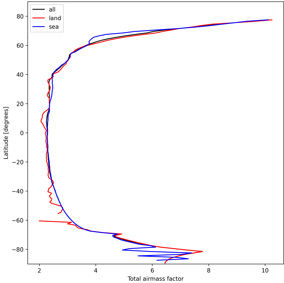
Figure 15: Zonal average of “Total airmass factor” for 2025-02-19 to 2025-02-21.
