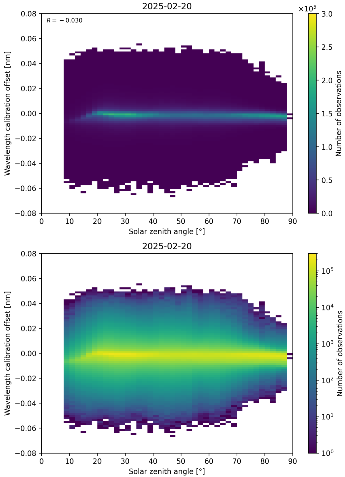
Figure 158: Scatter density plot of “Solar zenith angle” against “Wavelength calibration offset” for 2025-02-19 to 2025-02-21.
