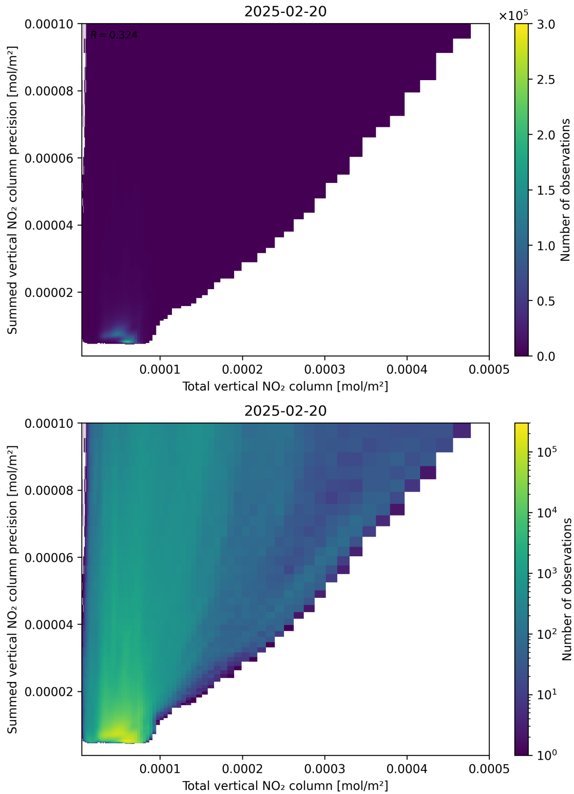
Figure 113: Scatter density plot of “Total vertical NO 2 column” against “Summed vertical NO 2 column precision” for 2025-02-19 to 2025-02-21.
