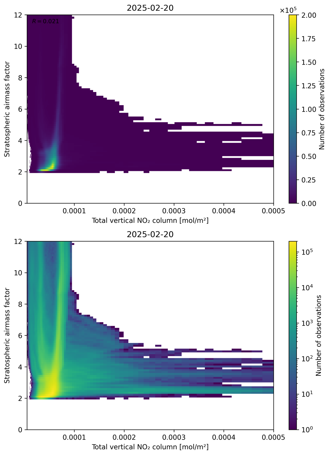
Figure 110: Scatter density plot of “Total vertical NO 2 column” against “Stratospheric airmass factor” for 2025-02-19 to 2025-02-21.
