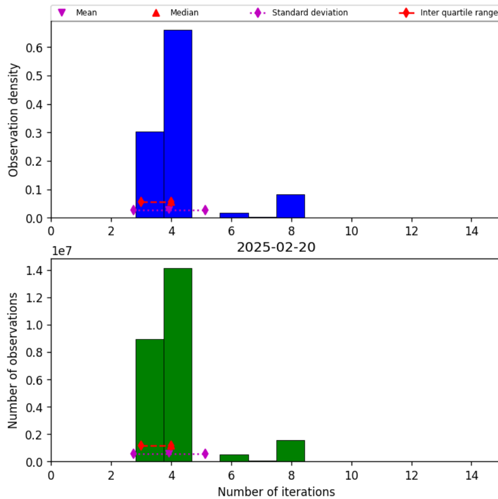
Figure 34: Histogram of “Number of iterations” for 2025-02-19 to 2025-02-21
