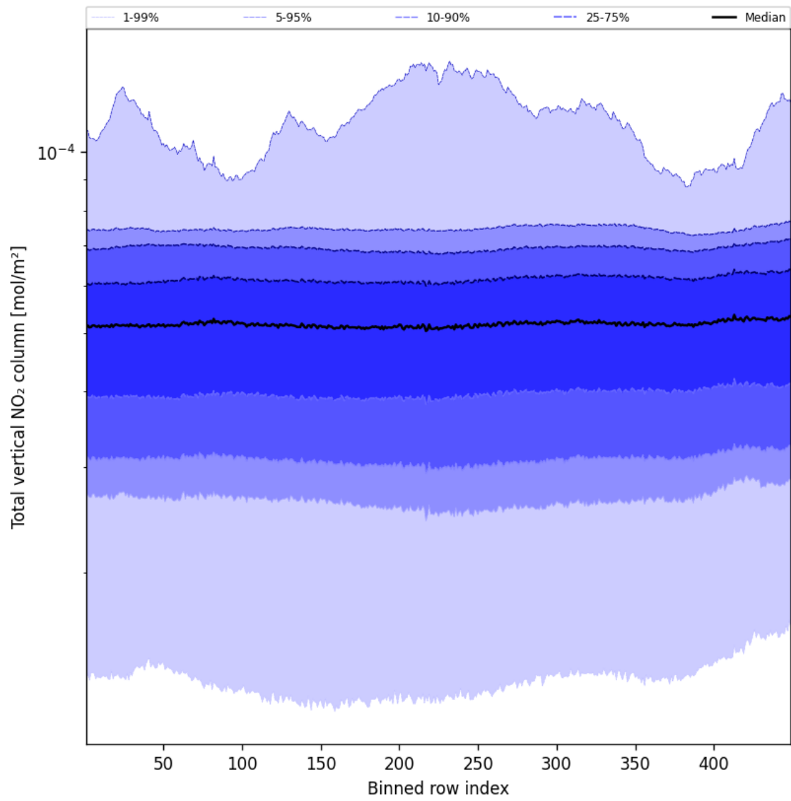
Figure 55: Along track statistics of “Total vertical NO 2 column” for 2025-02-19 to 2025-02-21
