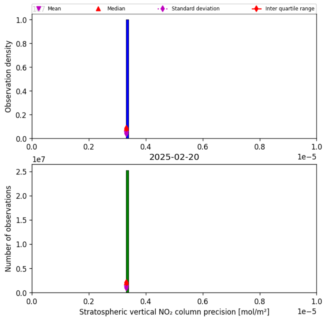
Figure 37: Histogram of “Stratospheric vertical NO 2 column precision” for 2025-02-19 to 2025-02-21
