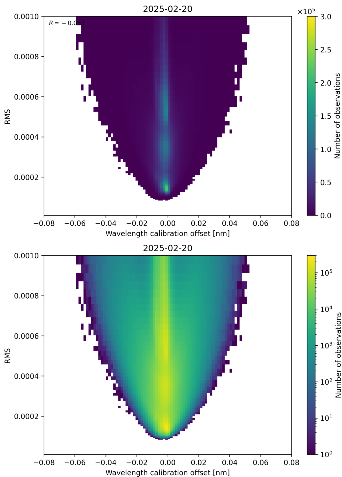
Figure 181: Scatter density plot of “Wavelength calibration offset” against “RMS” for 2025-02-19 to 2025-02-21.
