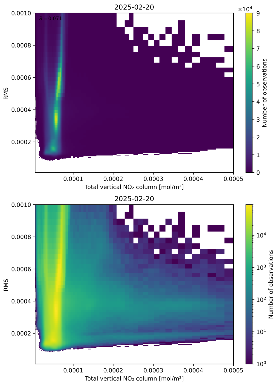
Figure 120: Scatter density plot of “Total vertical NO 2 column” against “RMS” for 2025-02-19 to 2025-02-21.
