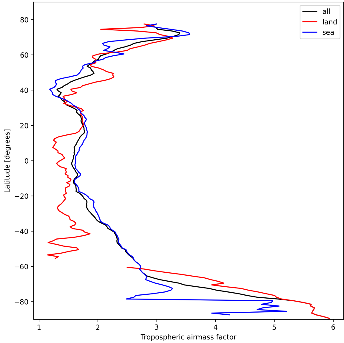
Figure 14: Zonal average of “Tropospheric airmass factor” for 2025-02-19 to 2025-02-21.
