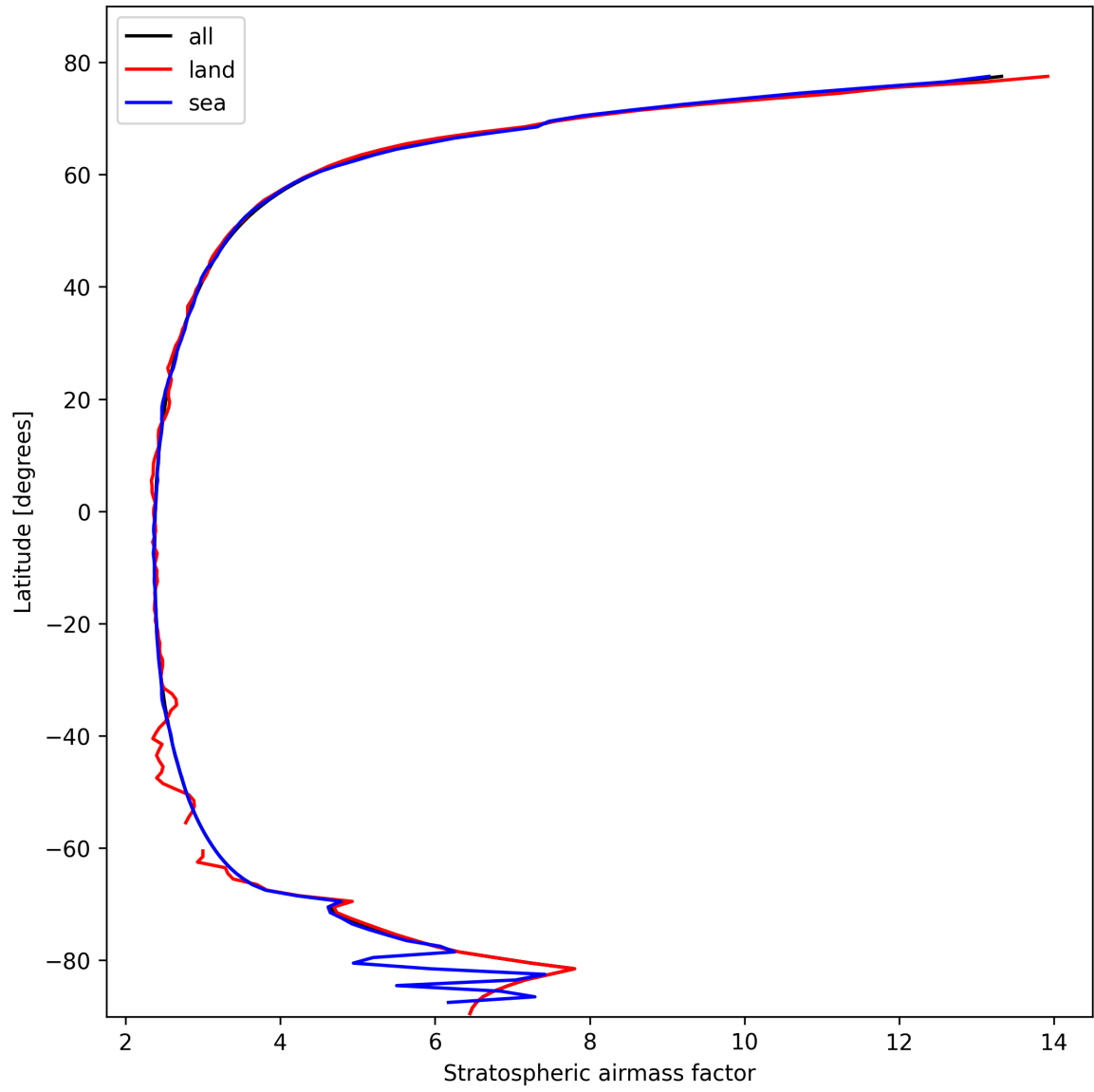
Figure 27: Zonal average of “Stratospheric airmass factor” for 2025-02-19 to 2025-02-21.
