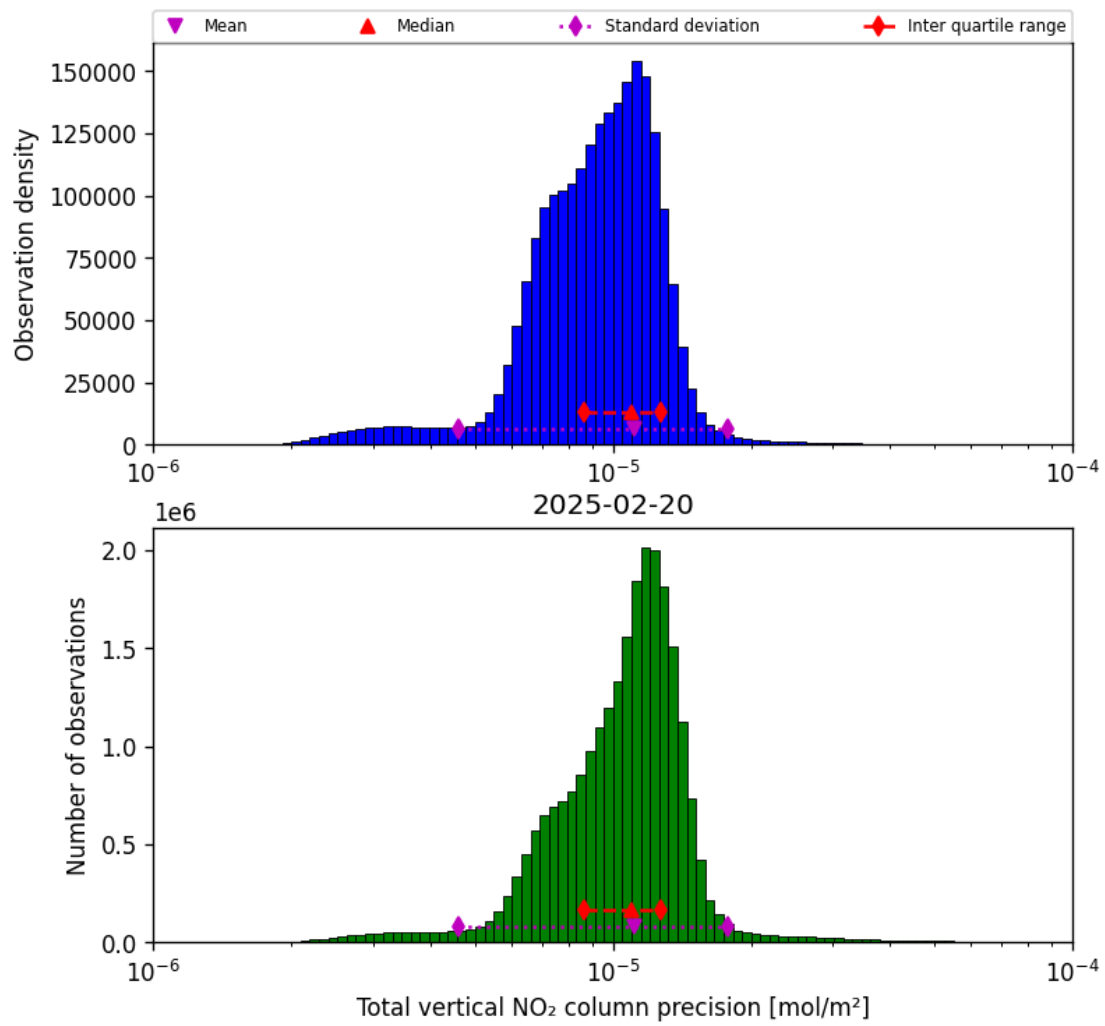
Figure 39: Histogram of "Total vertical NO 2 column precision" for 2025-02-19 to 2025-02-21
