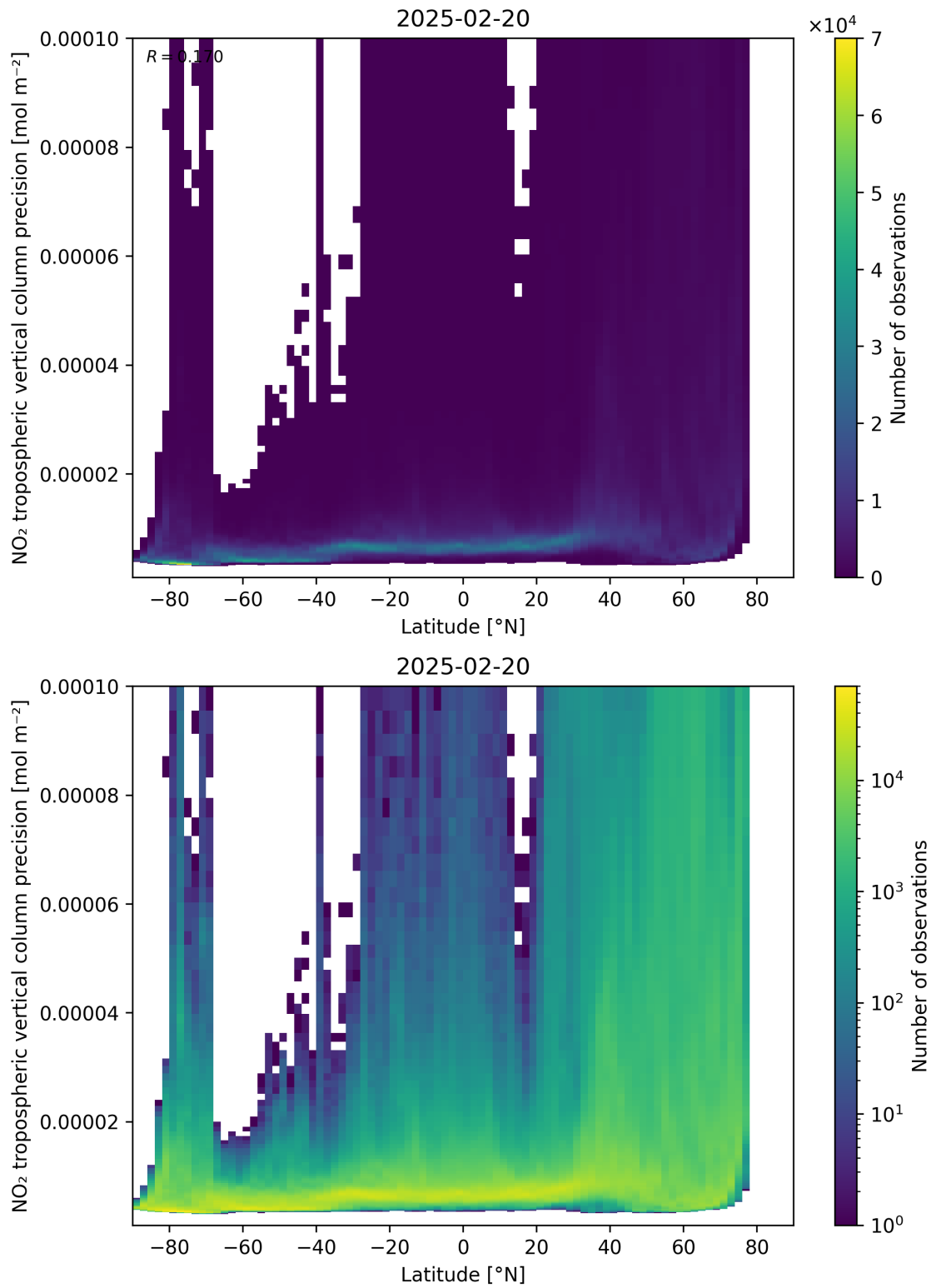
Figure 93: Scatter density plot of “Latitude” against “NO 2 tropospheric vertical column precision” for 2025-02-19 to 2025-02-21.
