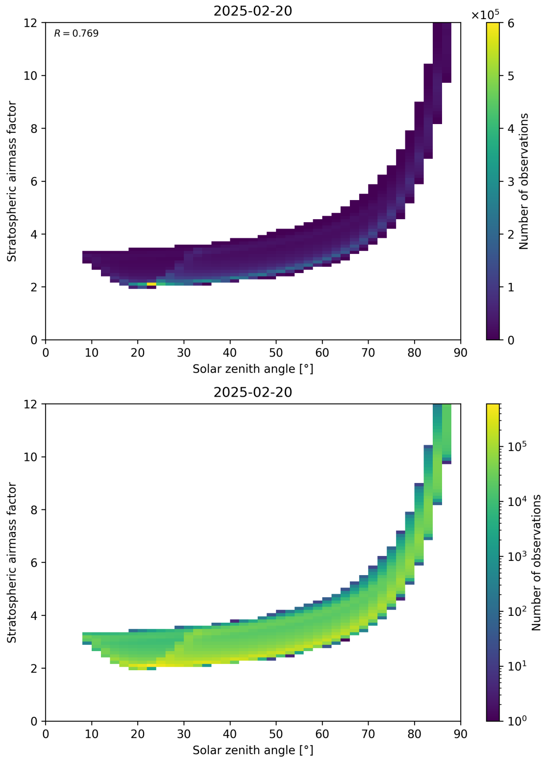
Figure 145: Scatter density plot of “Solar zenith angle” against “Stratospheric airmass factor” for 2025-02-19 to 2025-02-21.
