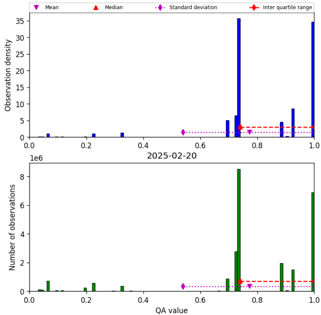
Figure 28: Histogram of “QA value” for 2025-02-19 to 2025-02-21
