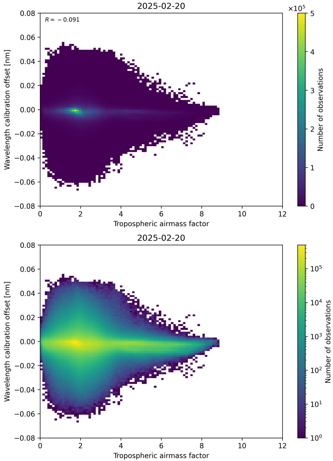
Figure 80: Scatter density plot of “Tropospheric airmass factor” against “Wavelength calibration offset” for 2025-02-19 to 2025-02-21.
