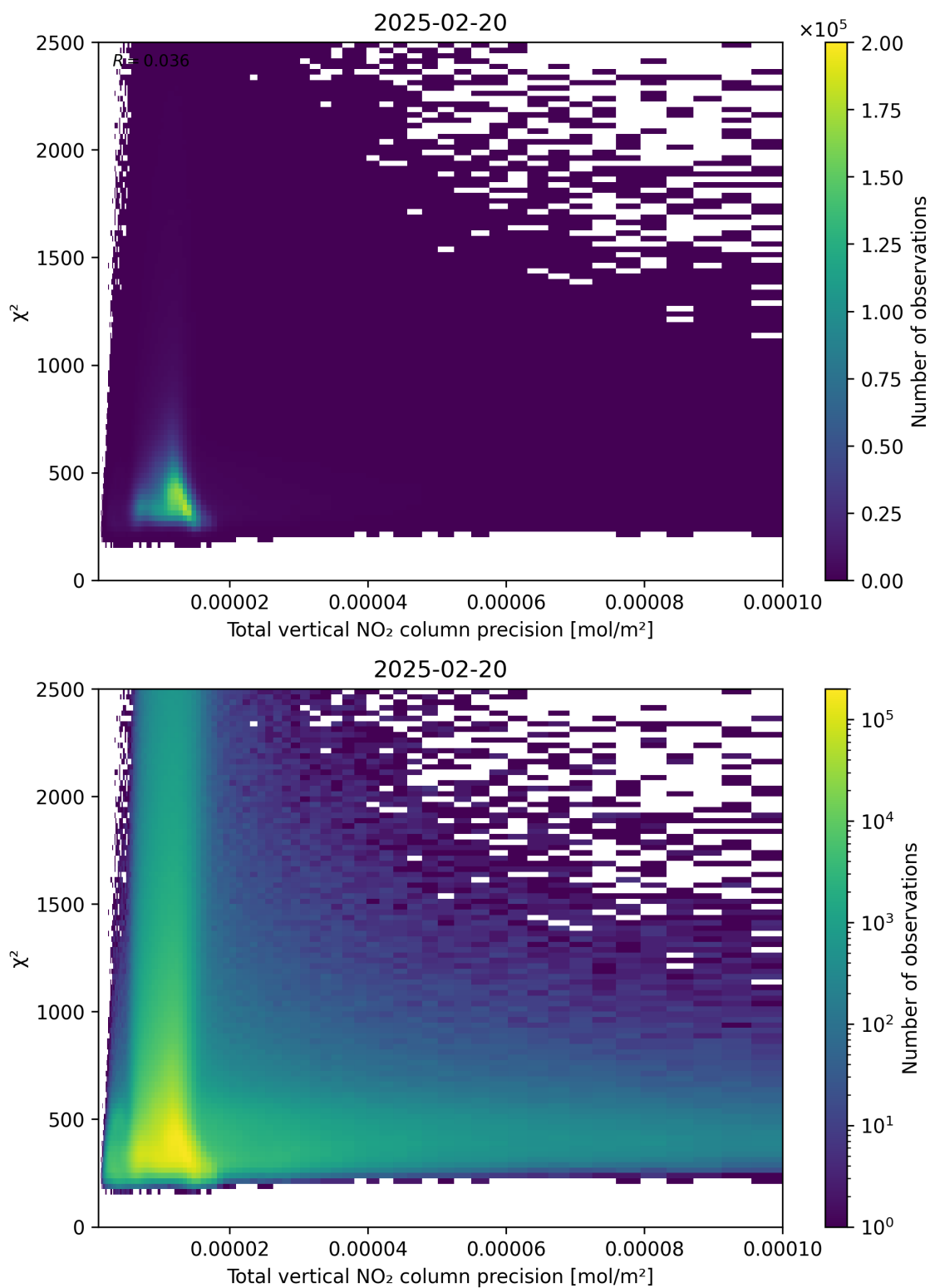
Figure 116: Scatter density plot of “Total vertical NO 2 column precision” against “ \chi^2 ” for 2025-02-19 to 2025-02-21.
