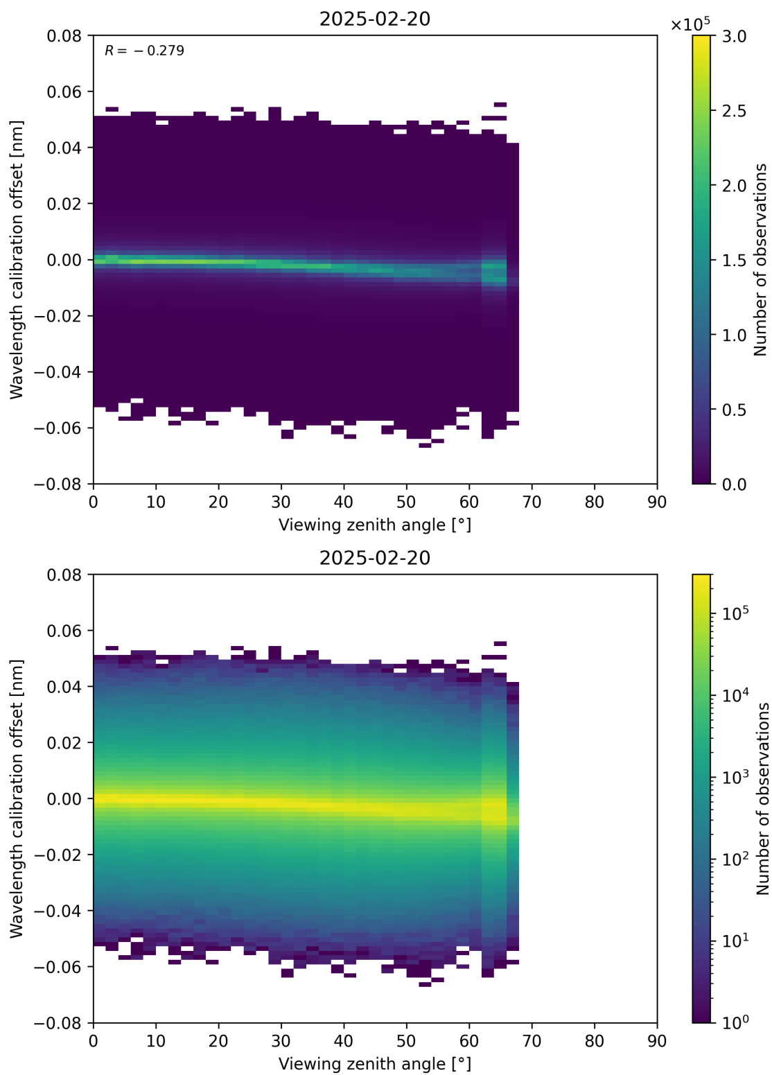
Figure 173: Scatter density plot of “Viewing zenith angle” against “Wavelength calibration offset” for 2025-02-19 to 2025-02-21.
