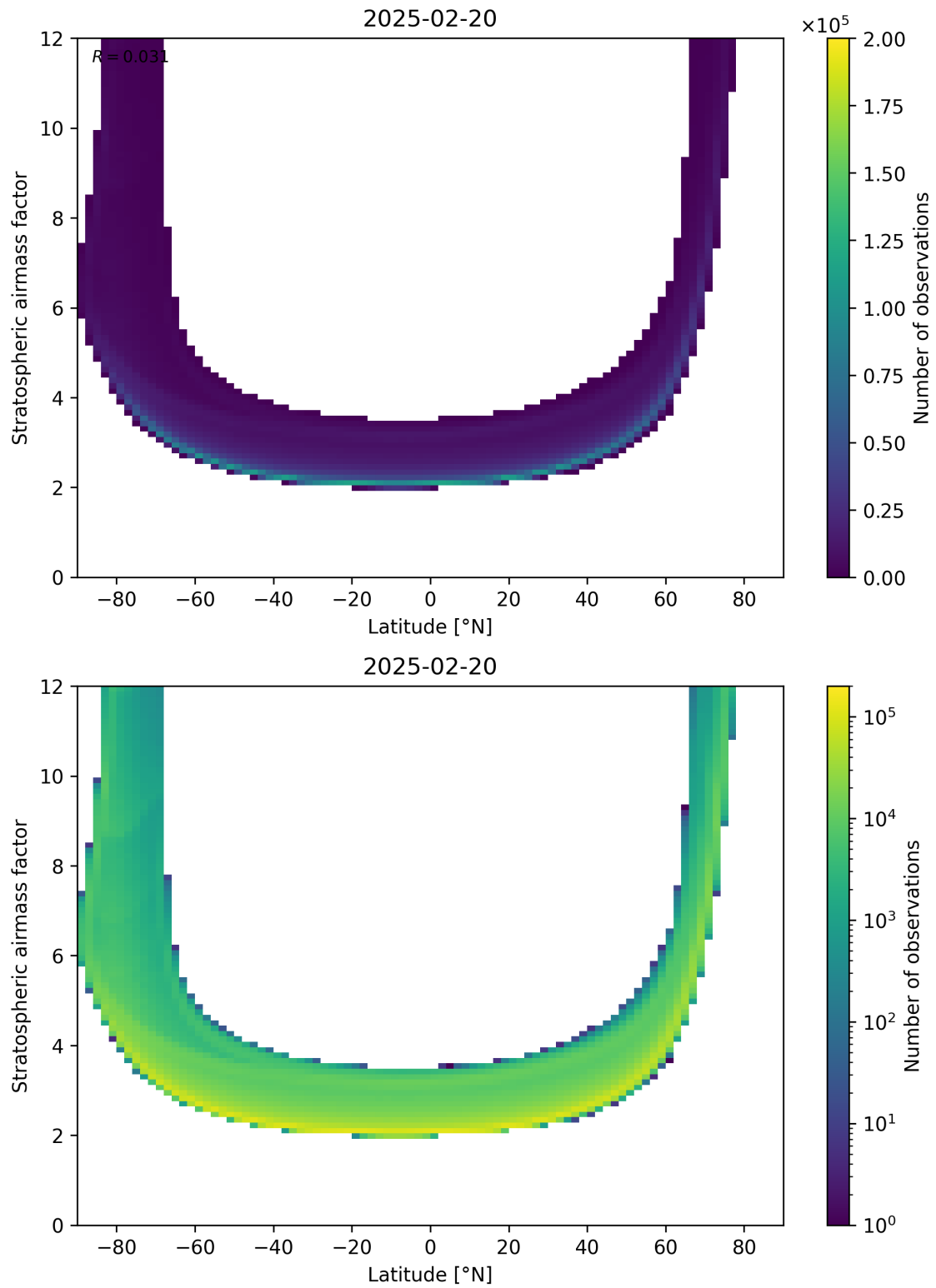
Figure 83: Scatter density plot of “Latitude” against “Stratospheric airmass factor” for 2025-02-19 to 2025-02-21.
