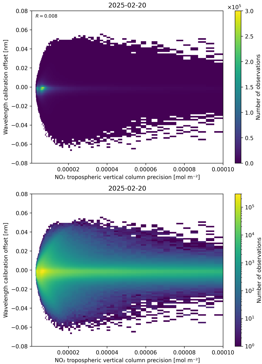
Figure 141: Scatter density plot of “NO 2 tropospheric vertical column precision” against “Wavelength calibration offset” for 2025-02-19 to 2025-02-21.
