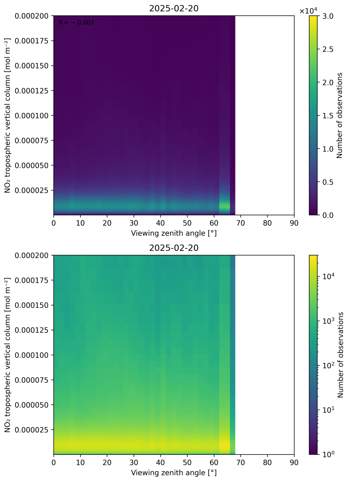
Figure 169: Scatter density plot of “Viewing zenith angle” against “NO 2 tropospheric vertical column” for 2025-02-19 to 2025-02-21.
