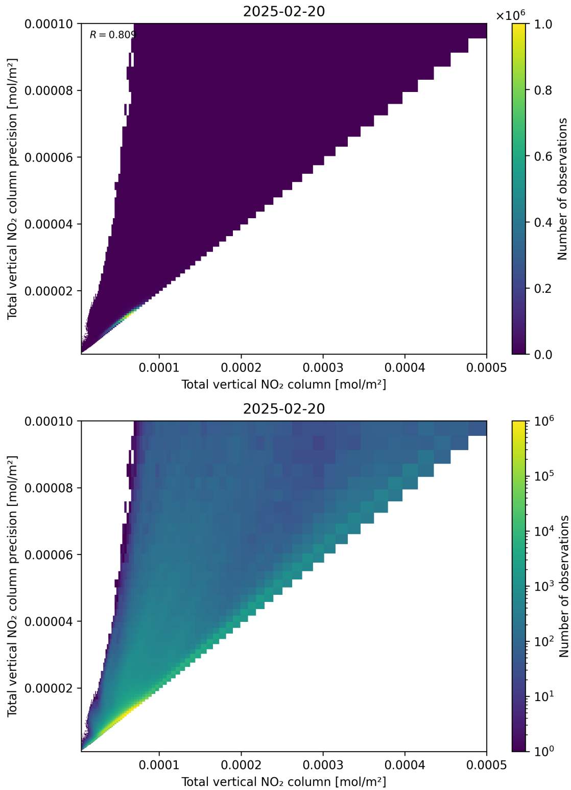
Figure 114: Scatter density plot of “Total vertical NO 2 column” against “Total vertical NO 2 column precision” for 2025-02-19 to 2025-02-21.
