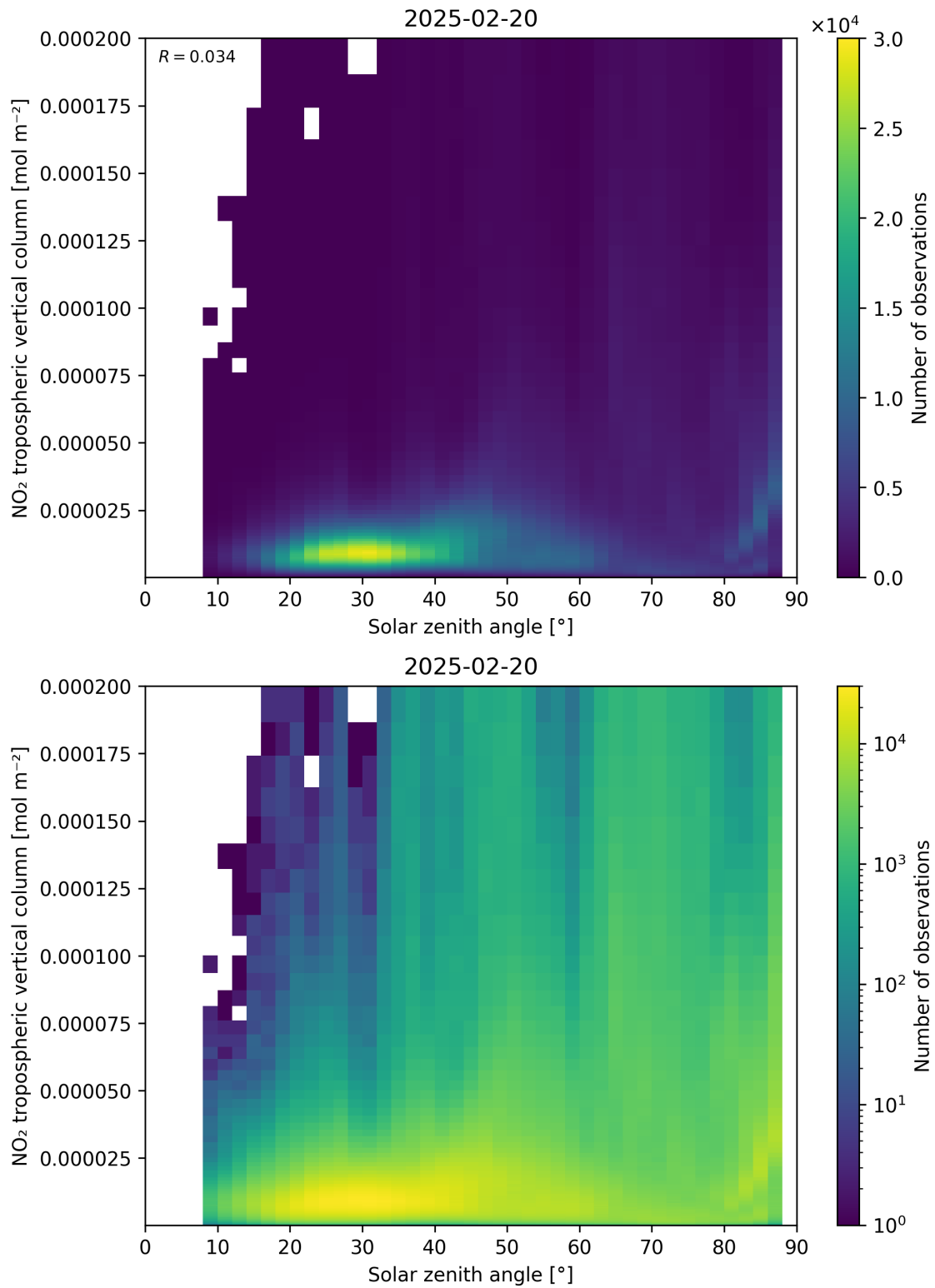
Figure 155: Scatter density plot of “Solar zenith angle” against “NO 2 tropospheric vertical column” for 2025-02-19 to 2025-02-21.
