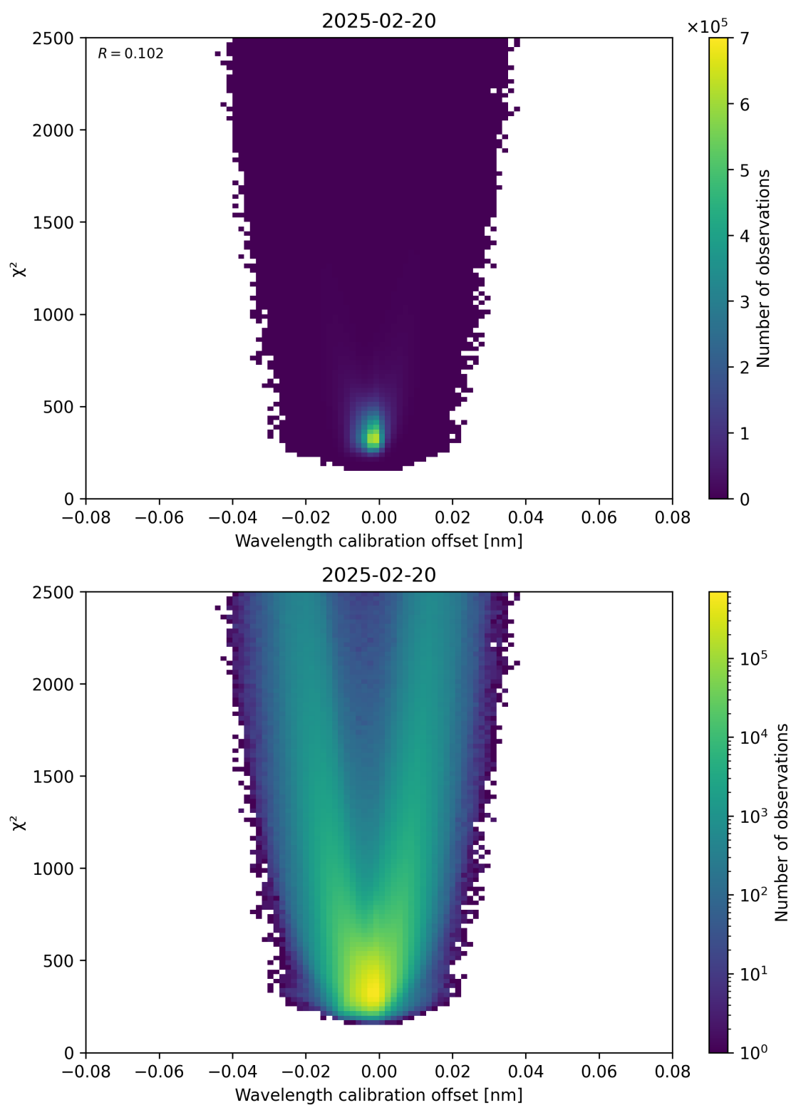
Figure 175: Scatter density plot of “Wavelength calibration offset” against “ \chi^2 ” for 2025-02-19 to 2025-02-21.
