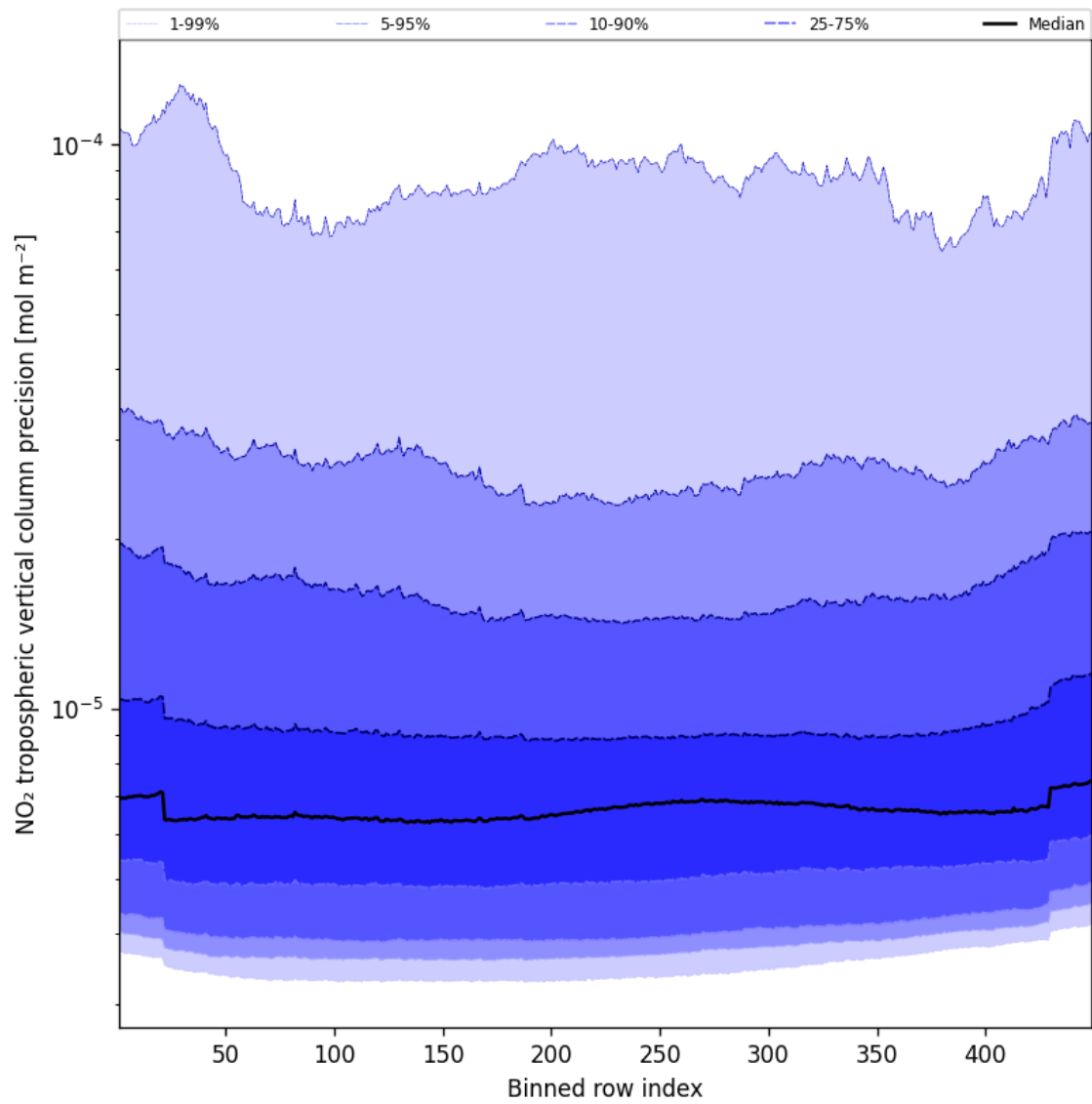
Figure 47: Along track statistics of “NO 2 tropospheric vertical column precision” for 2025-02-19 to 2025-02-21
