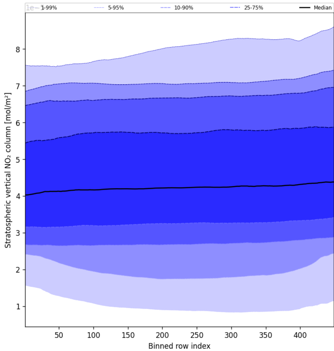
Figure 53: Along track statistics of “Stratospheric vertical NO 2 column” for 2025-02-19 to 2025-02-21
