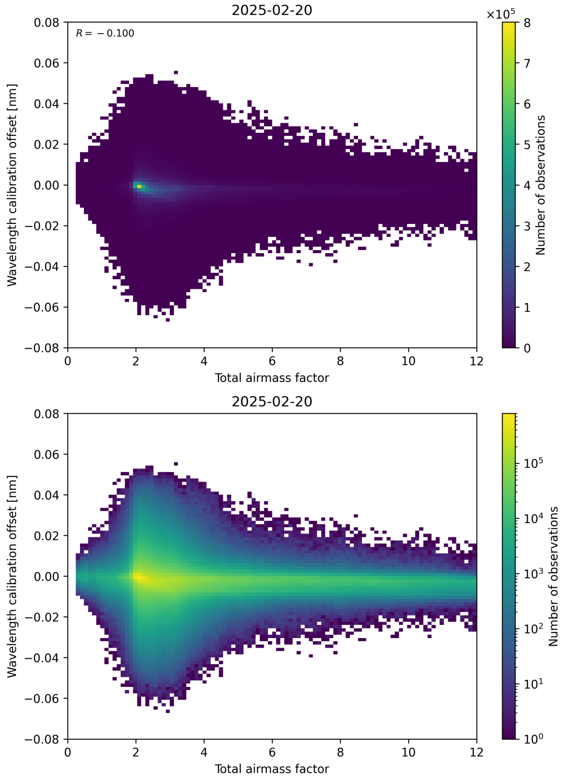
Figure 70: Scatter density plot of “Total airmass factor” against “Wavelength calibration offset” for 2025-02-19 to 2025-02-21.
