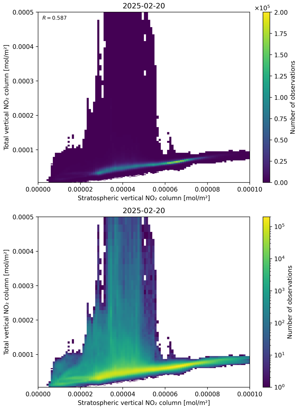
Figure 100: Scatter density plot of “Stratospheric vertical NO 2 column” against “Total vertical NO 2 column” for 2025-02-19 to 2025-02-21.
