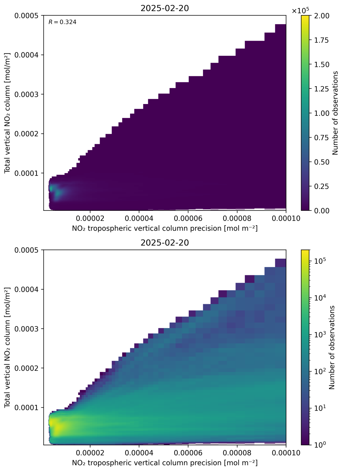
Figure 138: Scatter density plot of “NO 2 tropospheric vertical column precision” against “Total vertical NO 2 column” for 2025-02-19 to 2025-02-21.
