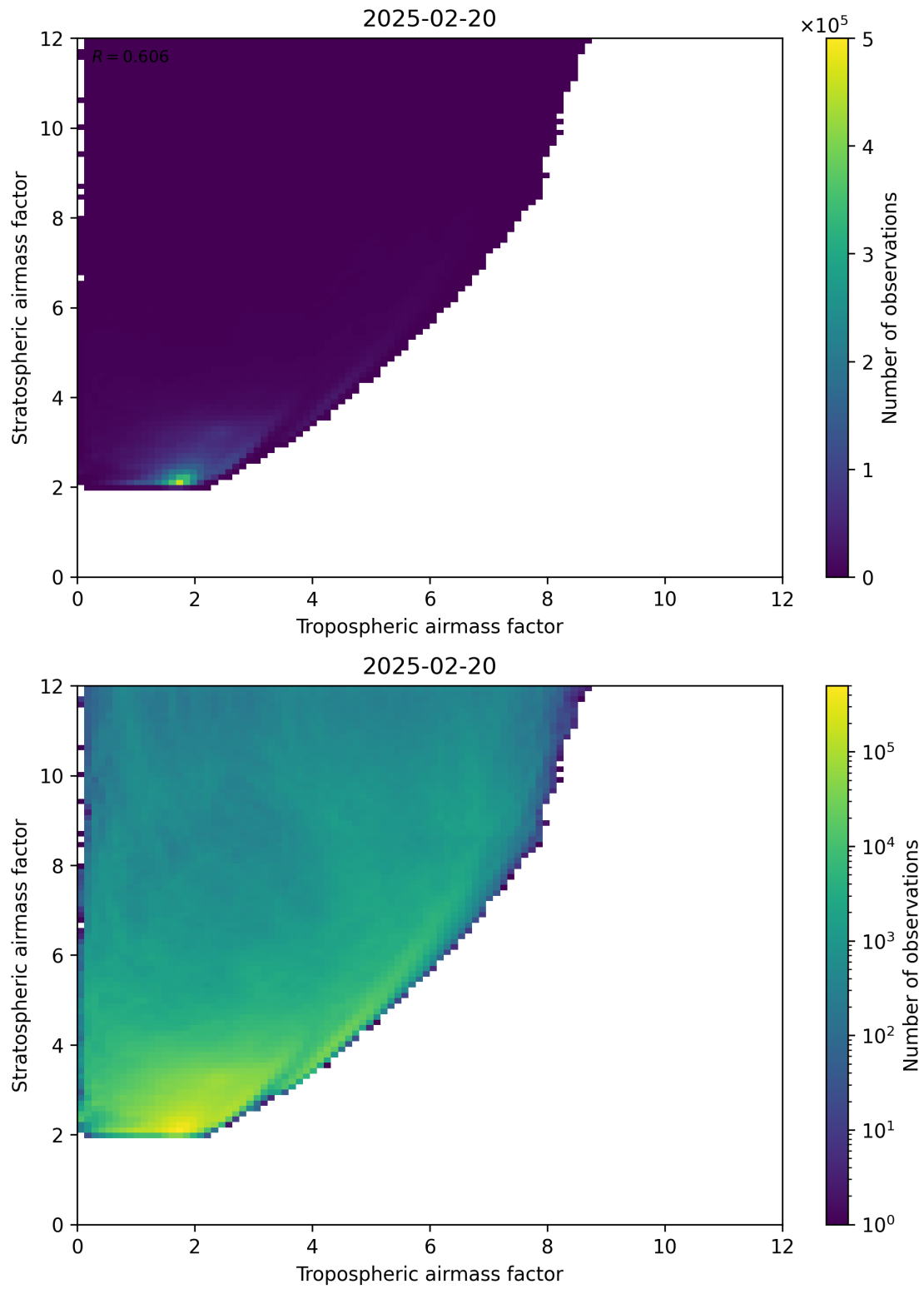
Figure 71: Scatter density plot of “Tropospheric airmass factor” against “Stratospheric airmass factor” for 2025-02-19 to 2025-02-21.
