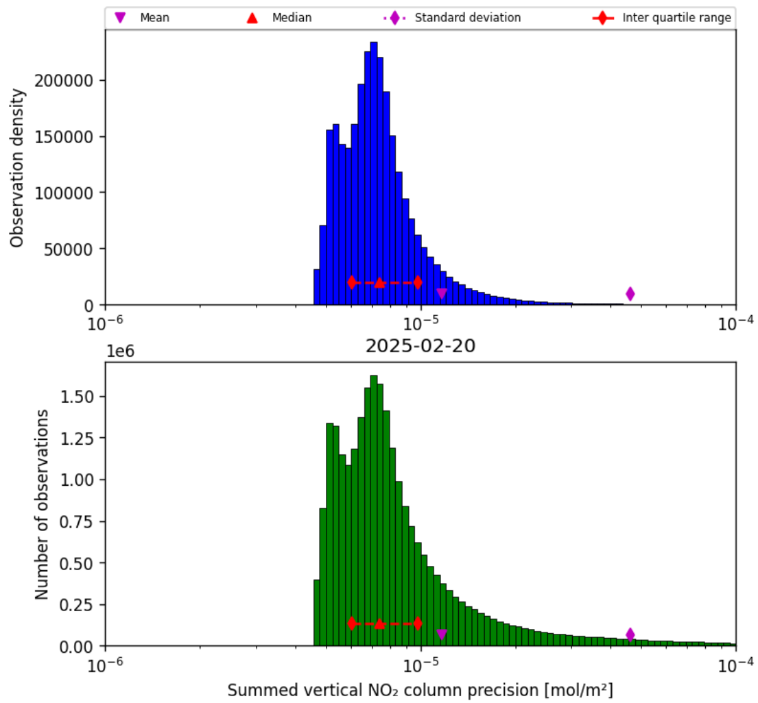
Figure 41: Histogram of “Summed vertical NO 2 column precision” for 2025-02-19 to 2025-02-21
