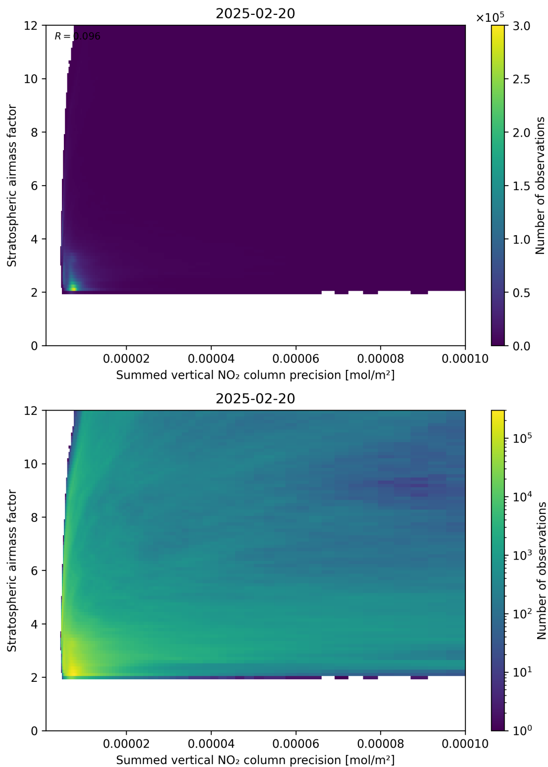
Figure 106: Scatter density plot of “Summed vertical NO 2 column precision” against “Stratospheric airmass factor” for 2025-02-19 to 2025-02-21.
