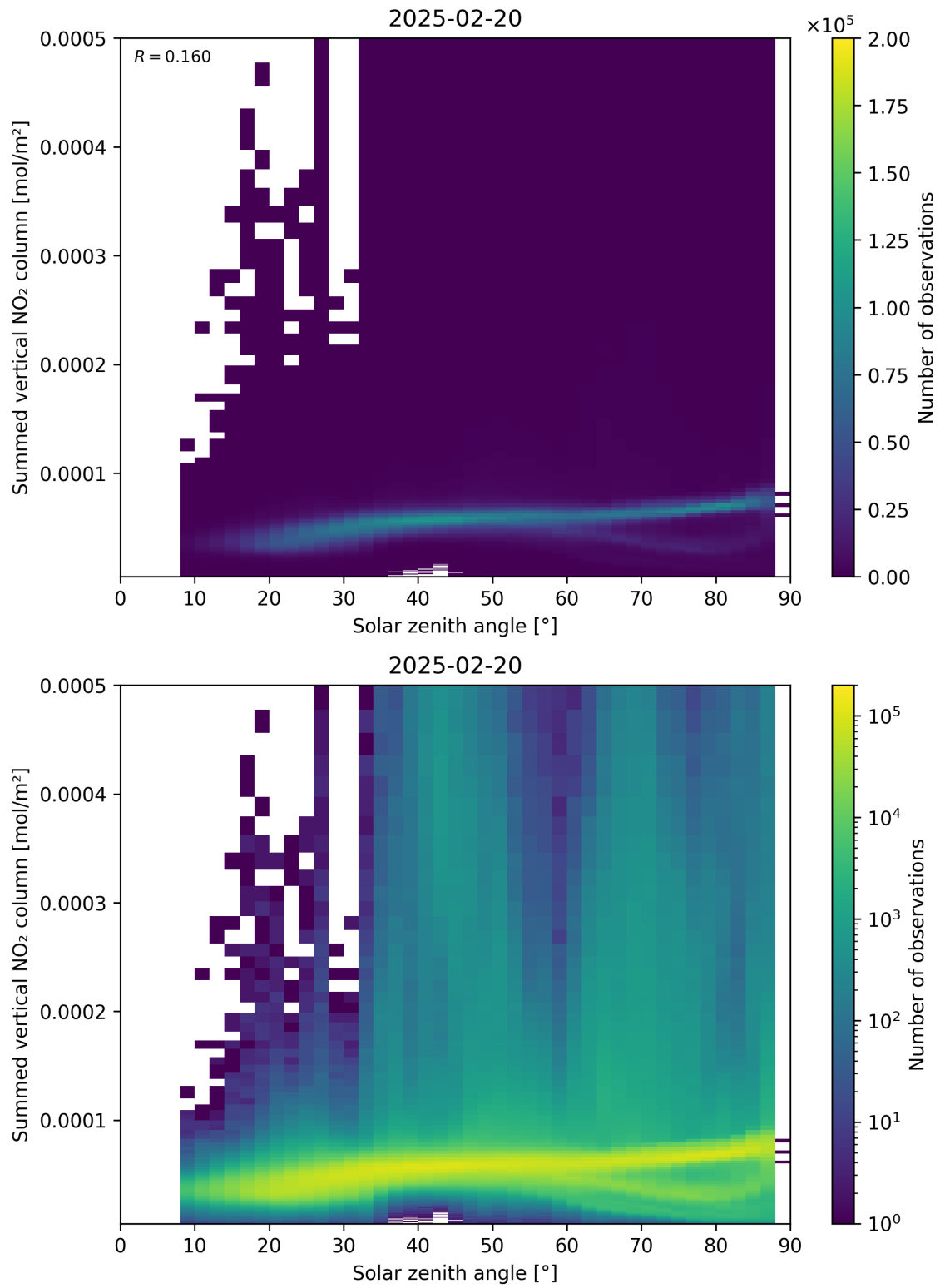
Figure 151: Scatter density plot of “Solar zenith angle” against “Summed vertical NO 2 column” for 2025-02-19 to 2025-02-21.
