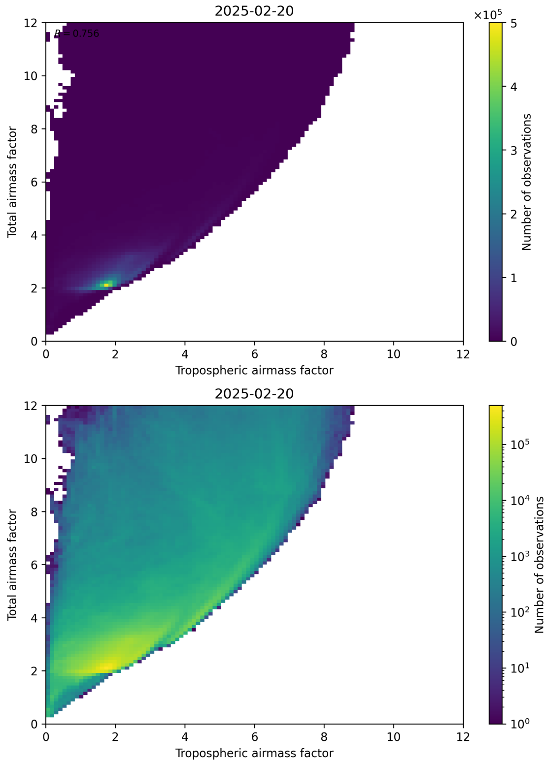
Figure 72: Scatter density plot of “Tropospheric airmass factor” against “Total airmass factor” for 2025-02-19 to 2025-02-21.
