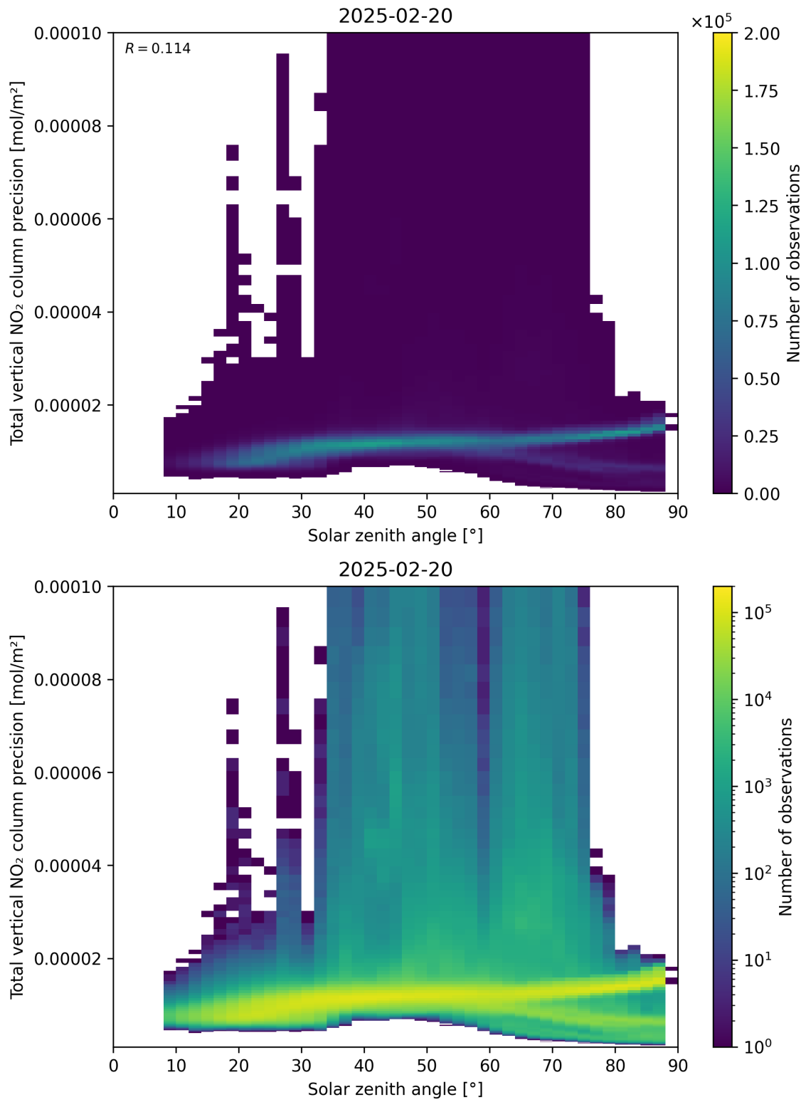
Figure 154: Scatter density plot of “Solar zenith angle” against “Total vertical NO 2 column precision” for 2025-02-19 to 2025-02-21.
