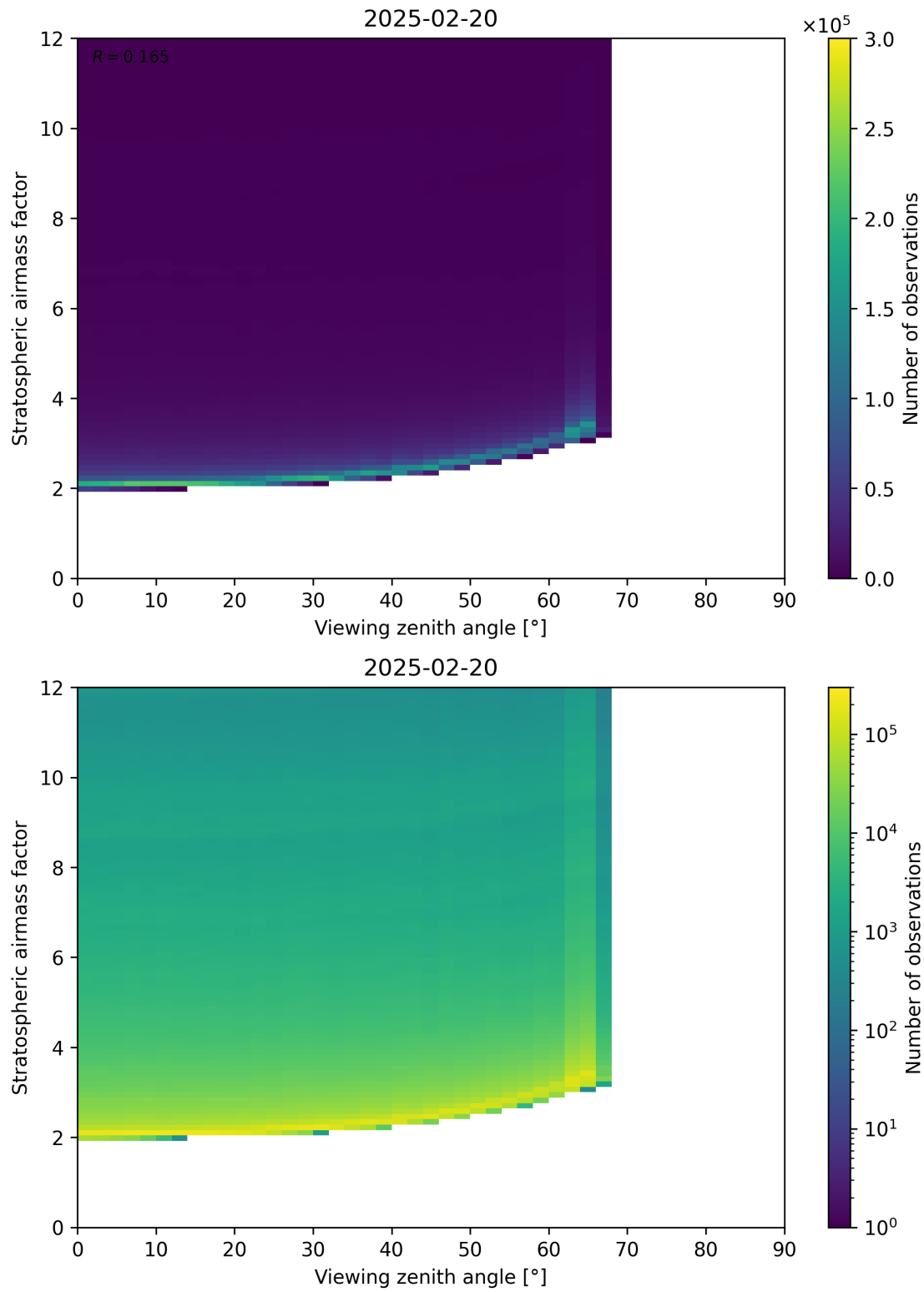
Figure 159: Scatter density plot of “Viewing zenith angle” against “Stratospheric airmass factor” for 2025-02-19 to 2025-02-21.
