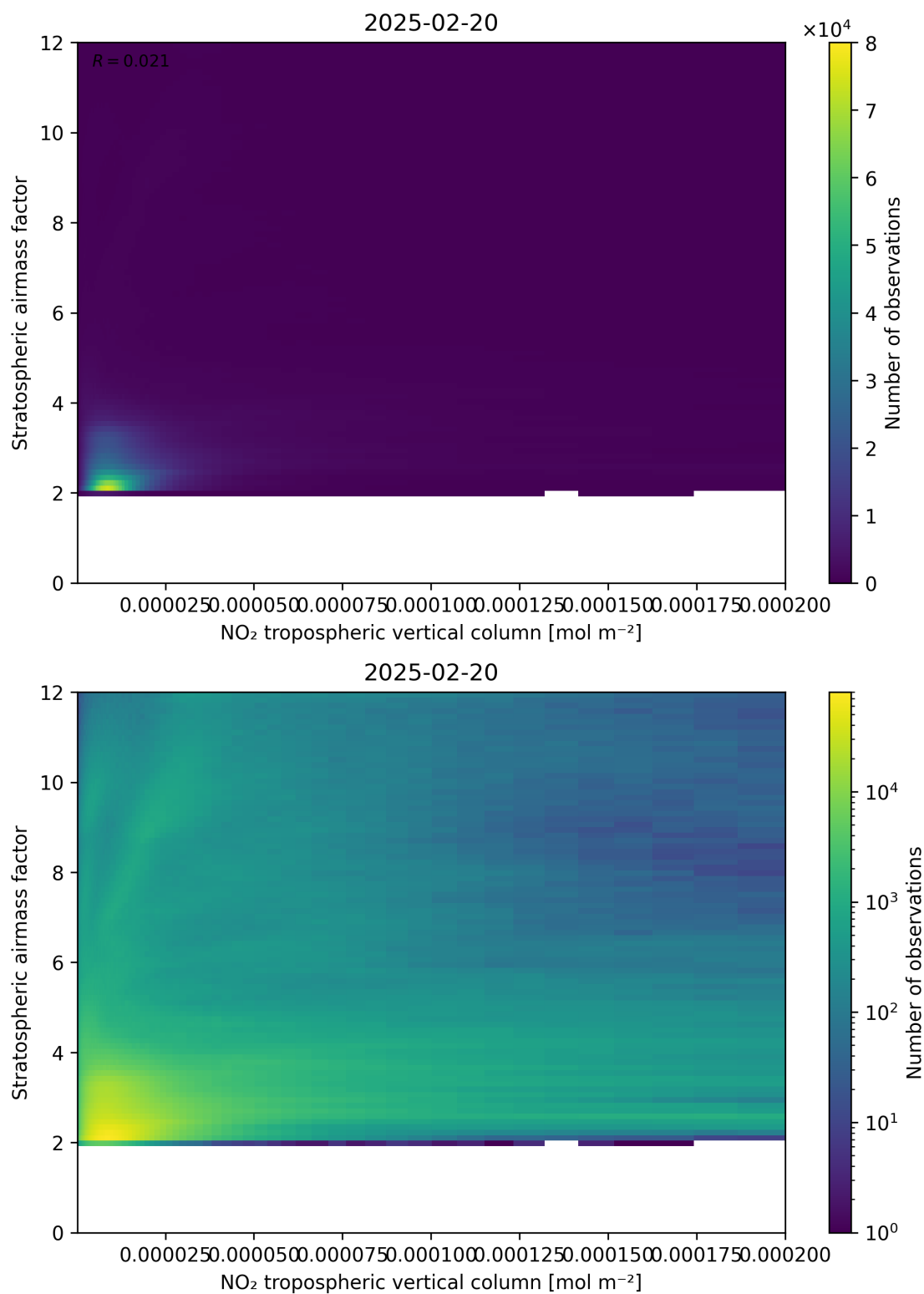
Figure 121: Scatter density plot of “NO 2 tropospheric vertical column” against “Stratospheric airmass factor” for 2025-02-19 to 2025-02-21.
