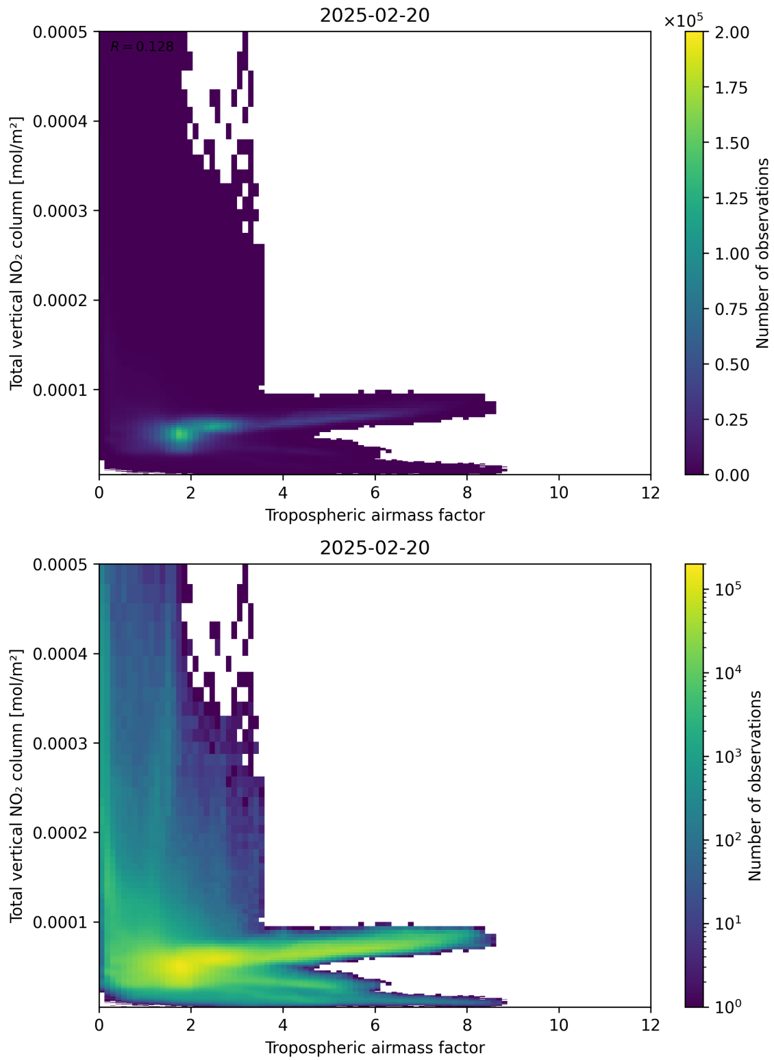
Figure 77: Scatter density plot of “Tropospheric airmass factor” against “Total vertical NO 2 column” for 2025-02-19 to 2025-02-21.
