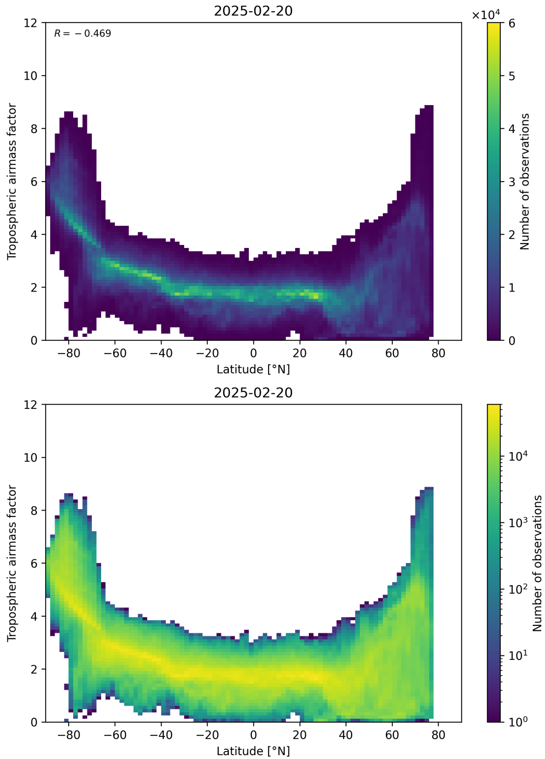
Figure 85: Scatter density plot of “Latitude” against “Tropospheric airmass factor” for 2025-02-19 to 2025-02-21.
