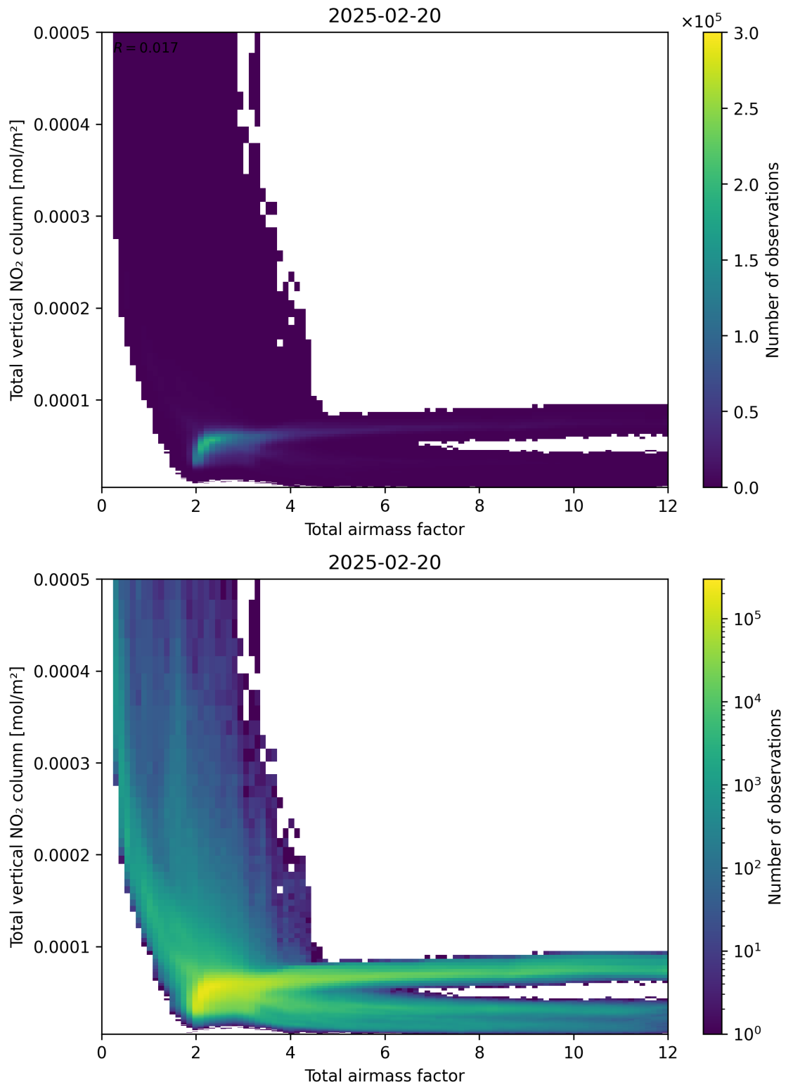
Figure 67: Scatter density plot of “Total airmass factor” against “Total vertical NO 2 column” for 2025-02-19 to 2025-02-21.
