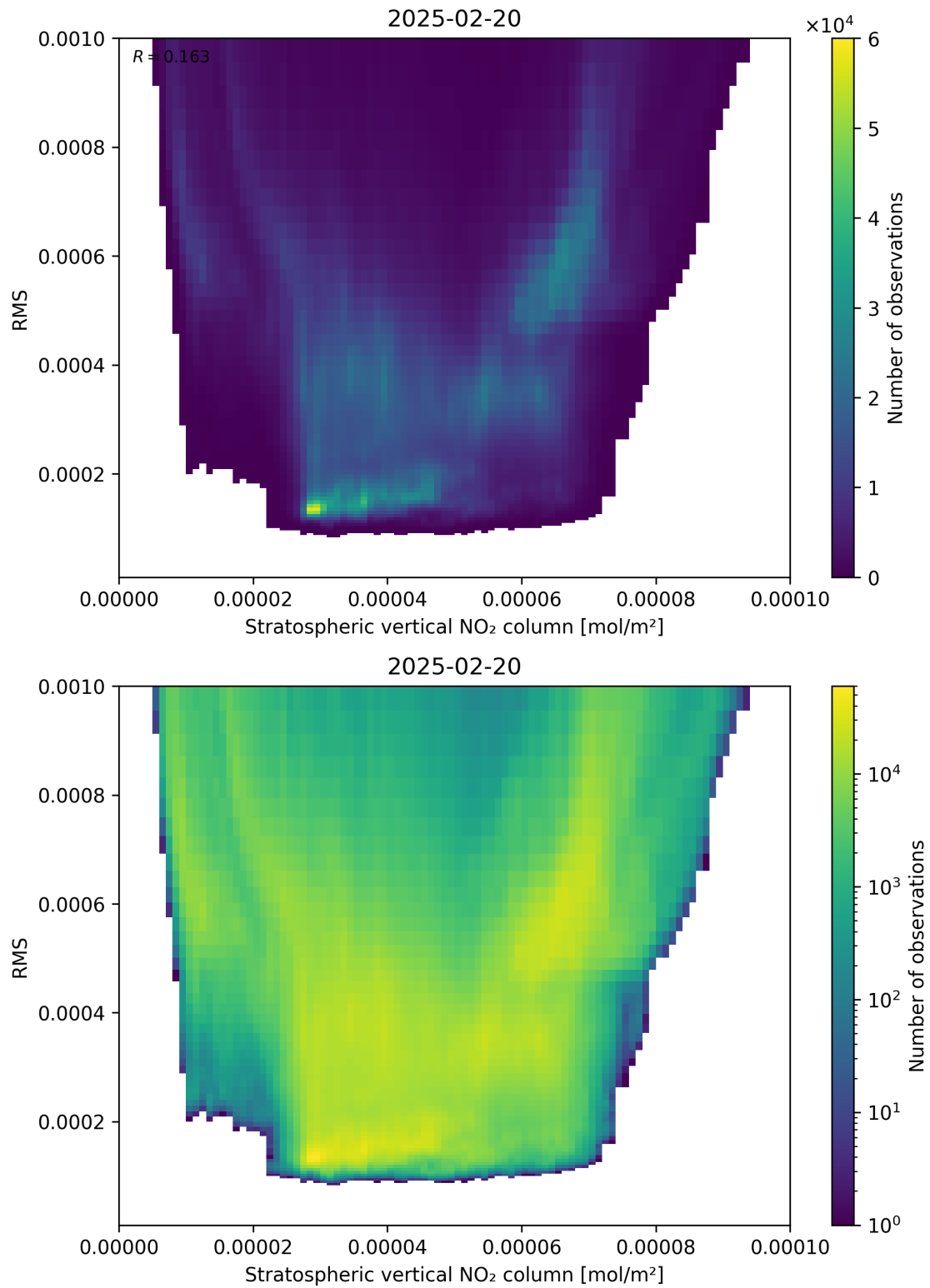
Figure 102: Scatter density plot of “Stratospheric vertical NO 2 column” against “RMS” for 2025-02-19 to 2025-02-21.
