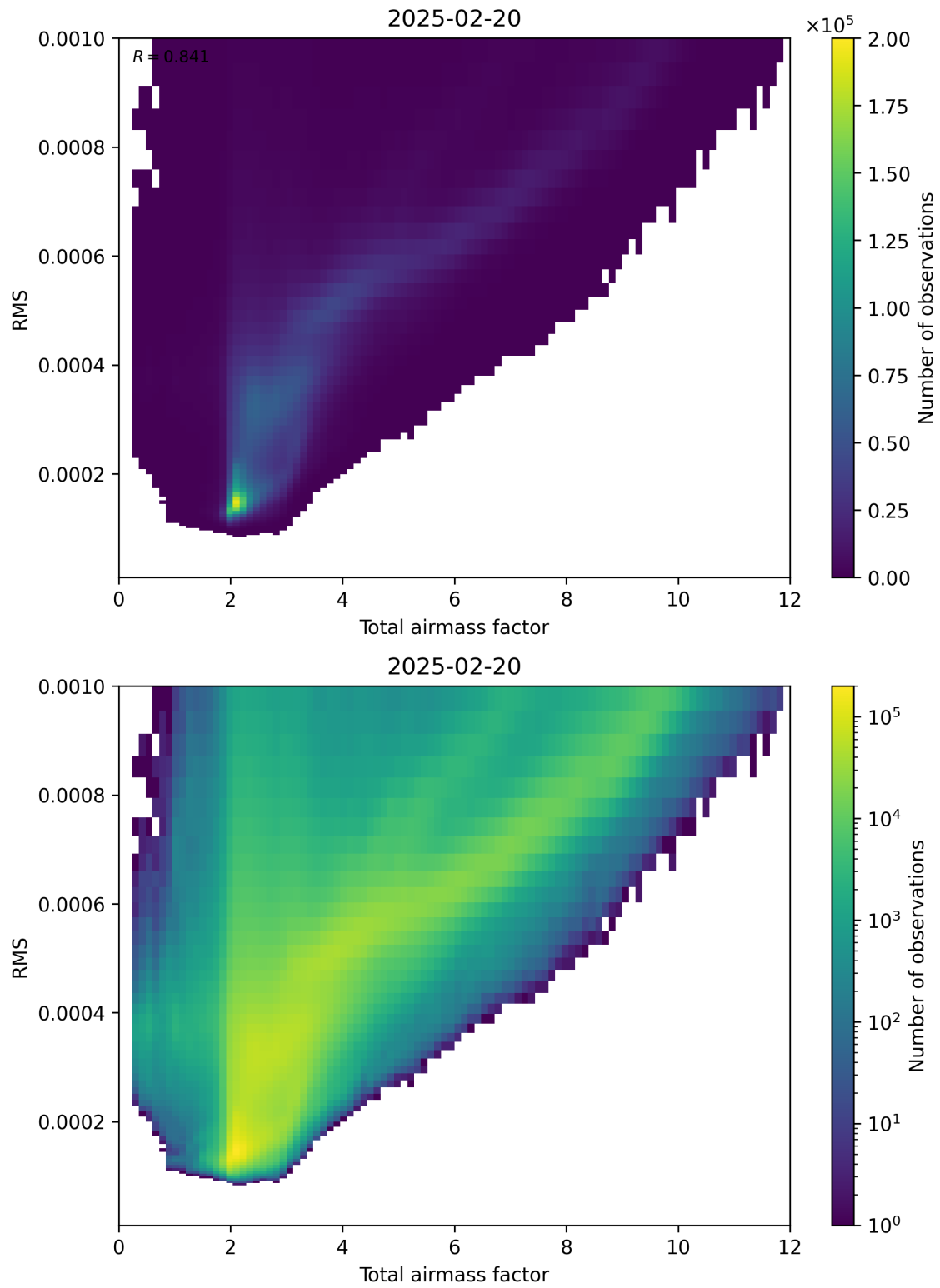
Figure 69: Scatter density plot of “Total airmass factor” against “RMS” for 2025-02-19 to 2025-02-21.
