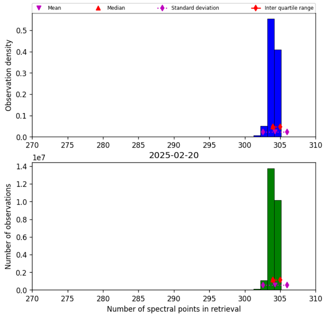
Figure 33: Histogram of “Number of spectral points in retrieval” for 2025-02-19 to 2025-02-21
