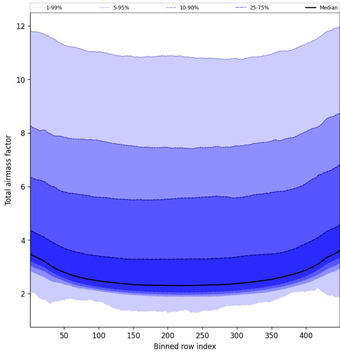
Figure 49: Along track statistics of “Total airmass factor” for 2025-02-19 to 2025-02-21
