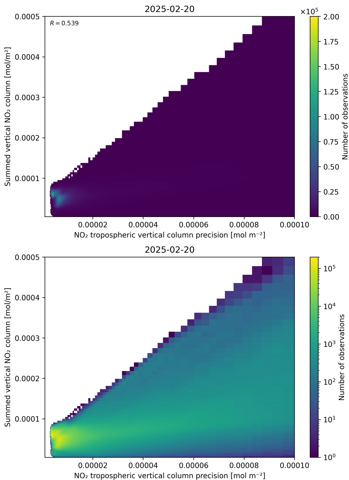
Figure 136: Scatter density plot of “NO 2 tropospheric vertical column precision” against “Summed vertical NO 2 column” for 2025-02-19 to 2025-02-21.
