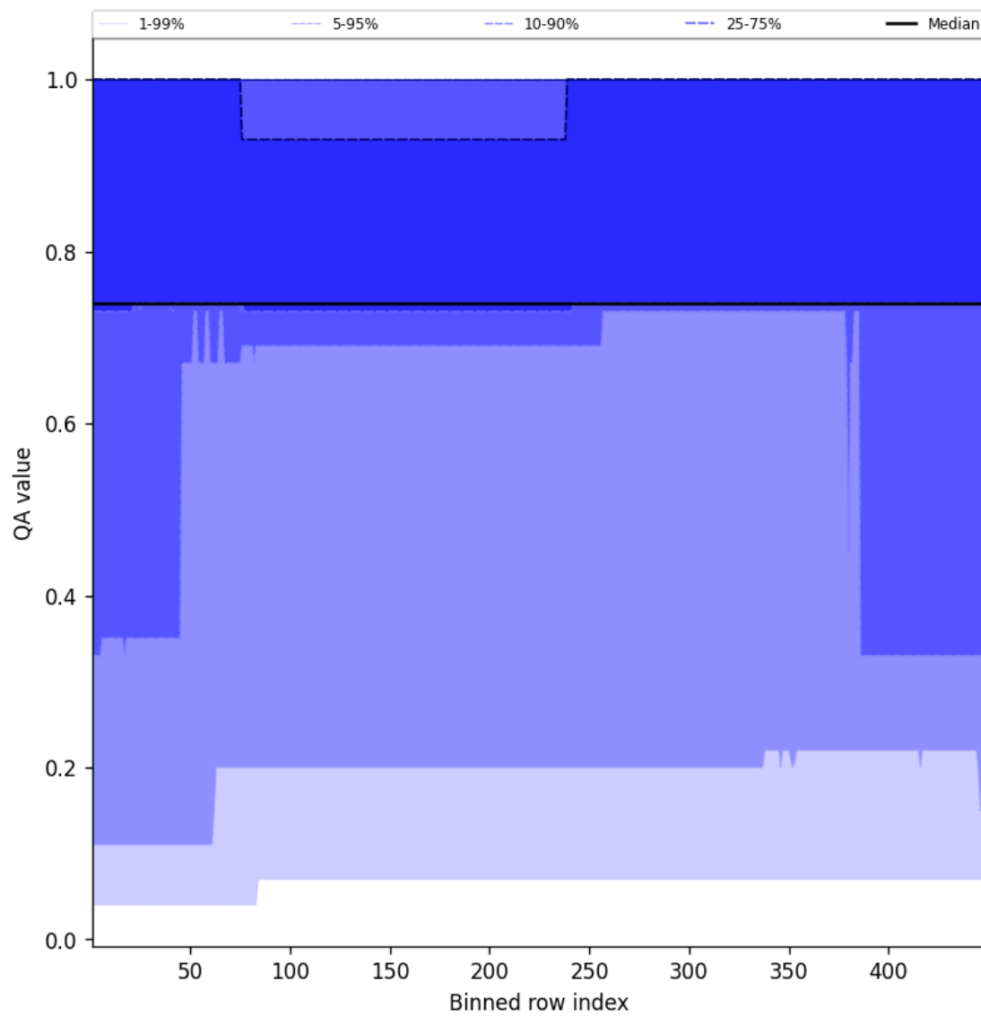
Figure 45: Along track statistics of “QA value” for 2025-02-19 to 2025-02-21
