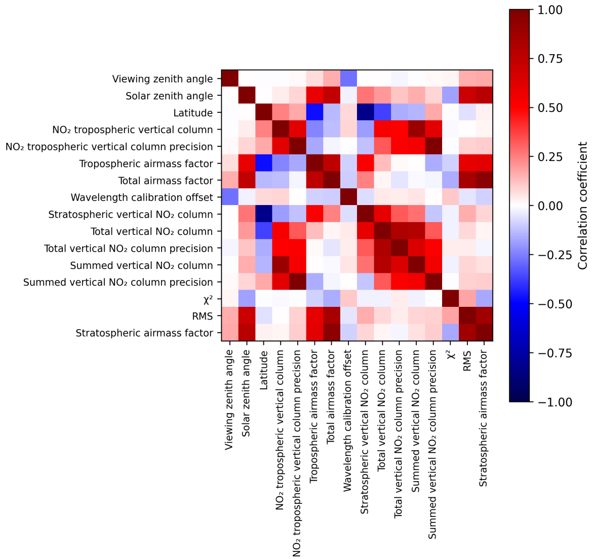
Figure 2: Map of correlation matrix for 2025-02-19 to 2025-02-21.
