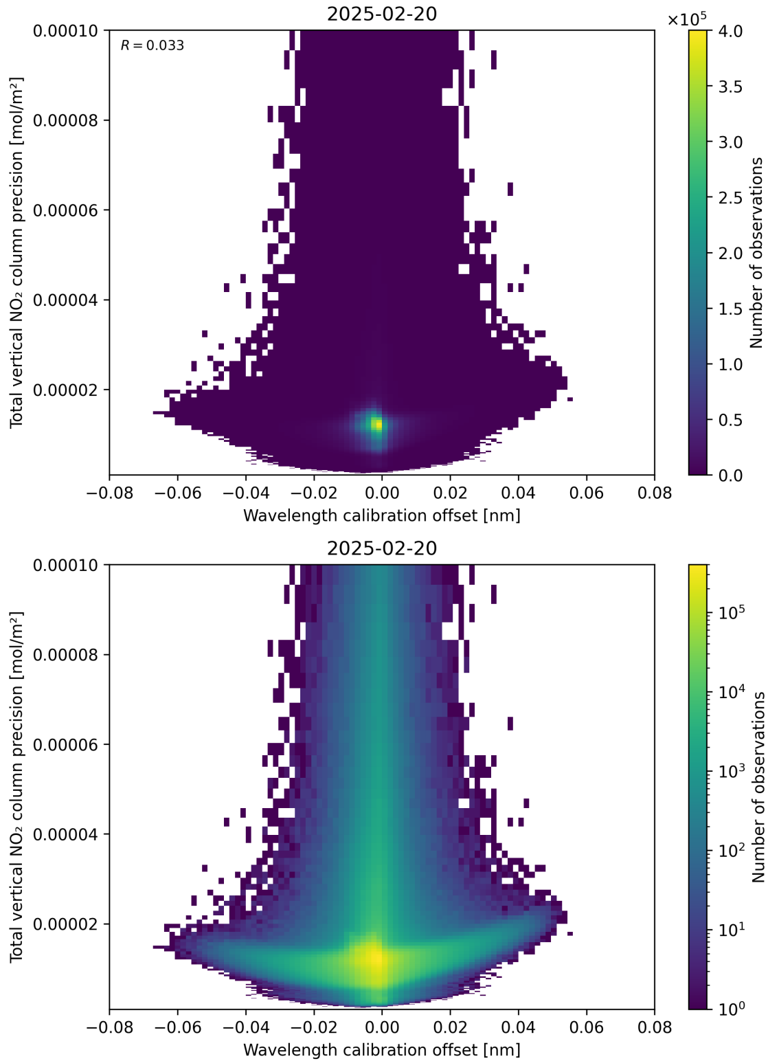
Figure 180: Scatter density plot of “Wavelength calibration offset” against “Total vertical NO 2 column precision” for 2025-02-19 to 2025-02-21.
