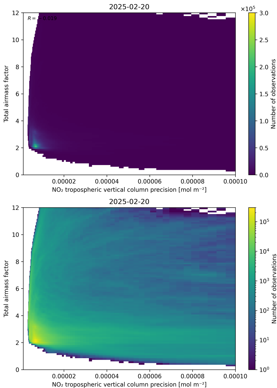
Figure 132: Scatter density plot of “NO 2 tropospheric vertical column precision” against “Total airmass factor” for 2025-02-19 to 2025-02-21.
