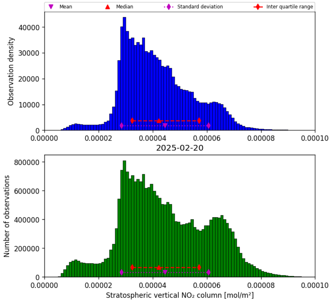
Figure 36: Histogram of “Stratospheric vertical NO 2 column” for 2025-02-19 to 2025-02-21
