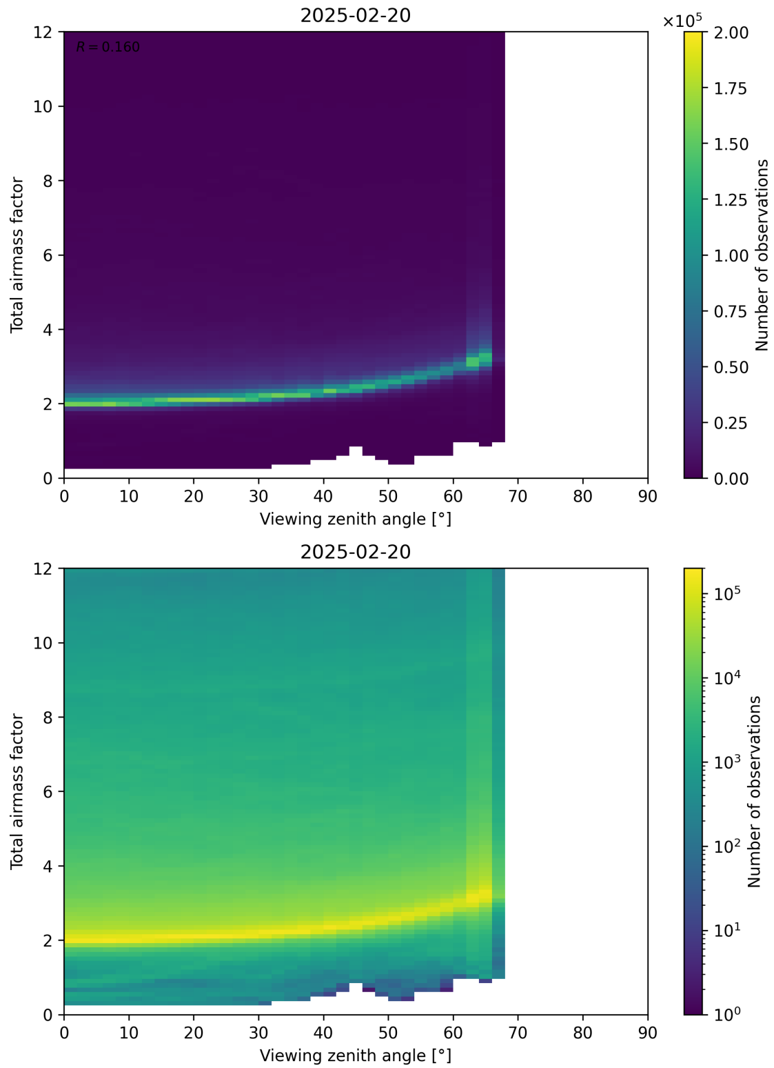
Figure 160: Scatter density plot of “Viewing zenith angle” against “Total airmass factor” for 2025-02-19 to 2025-02-21.
