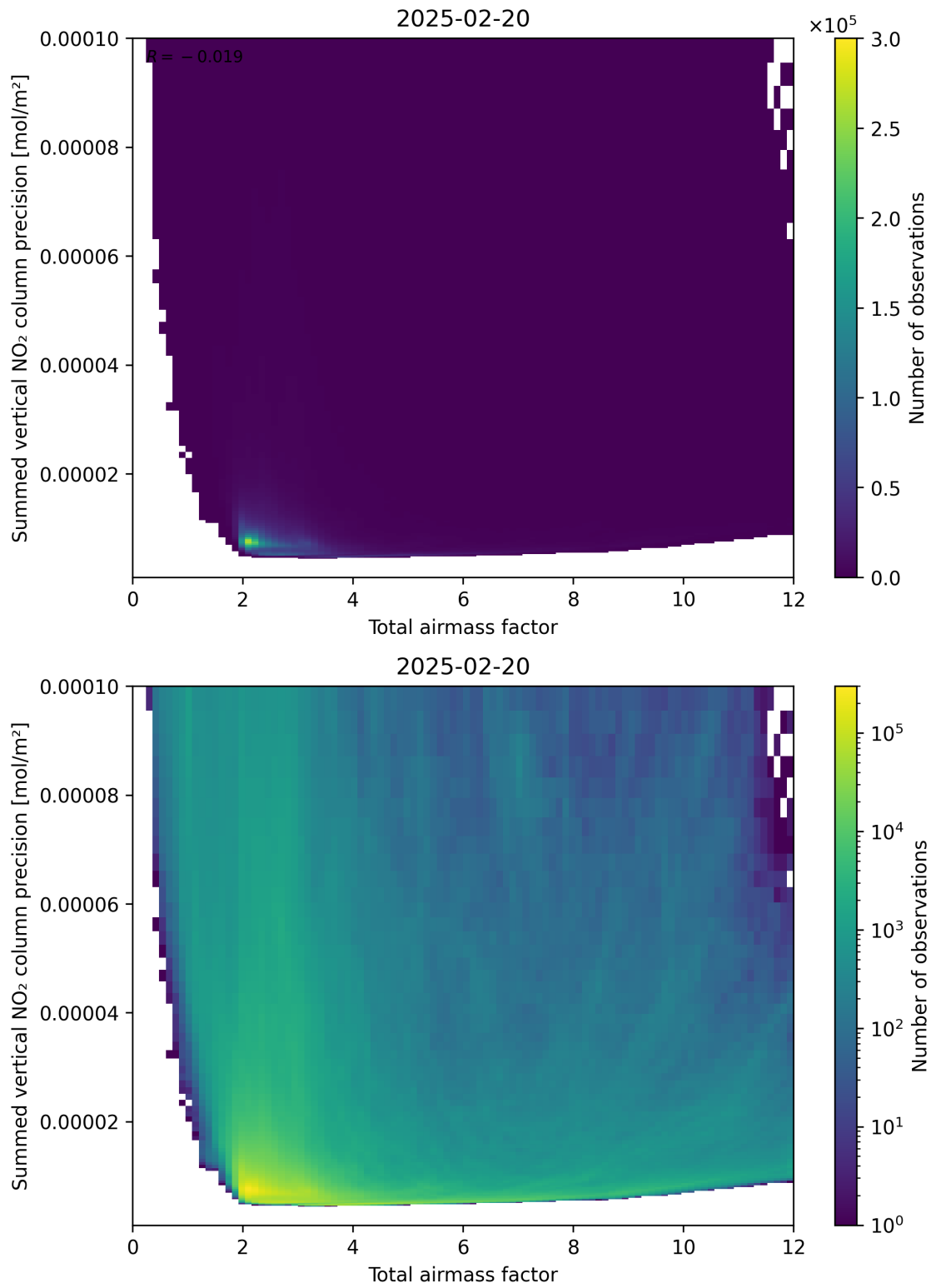
Figure 66: Scatter density plot of “Total airmass factor” against “Summed vertical NO 2 column precision” for 2025-02-19 to 2025-02-21.
