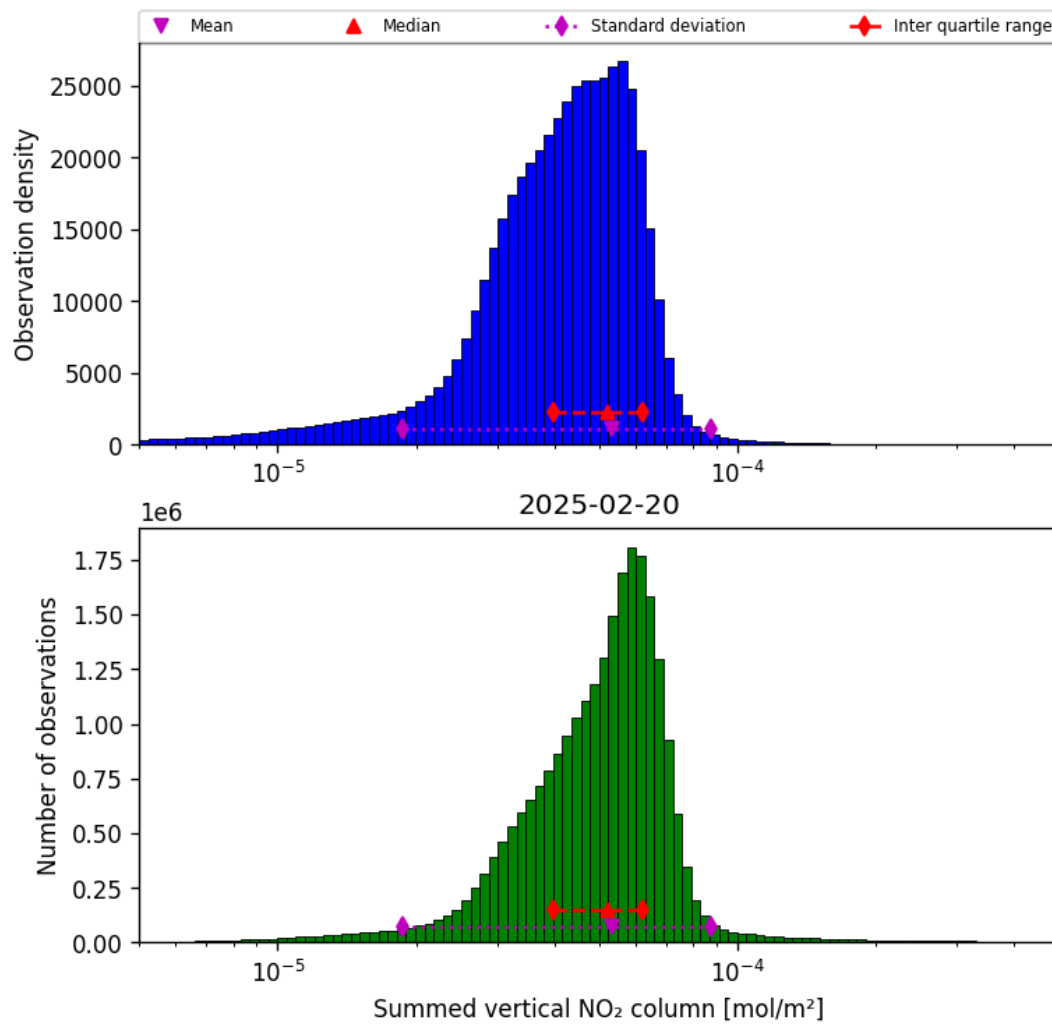
Figure 40: Histogram of “Summed vertical NO 2 column” for 2025-02-19 to 2025-02-21
