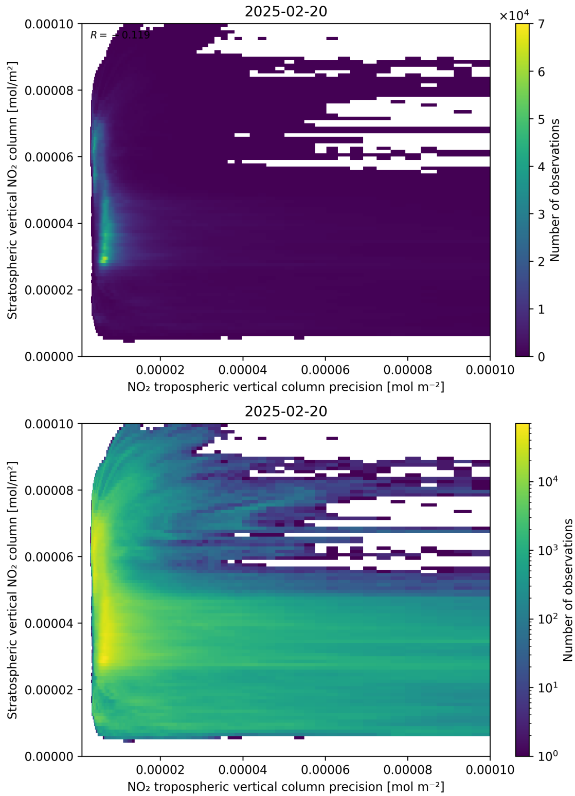
Figure 135: Scatter density plot of “NO 2 tropospheric vertical column precision” against “Stratospheric vertical NO 2 column” for 2025-02-19 to 2025-02-21.
