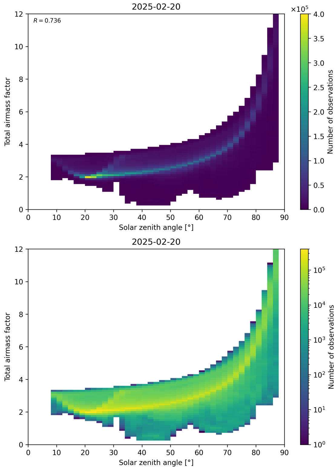
Figure 146: Scatter density plot of “Solar zenith angle” against “Total air mass factor” for 2025-02-19 to 2025-02-21.
