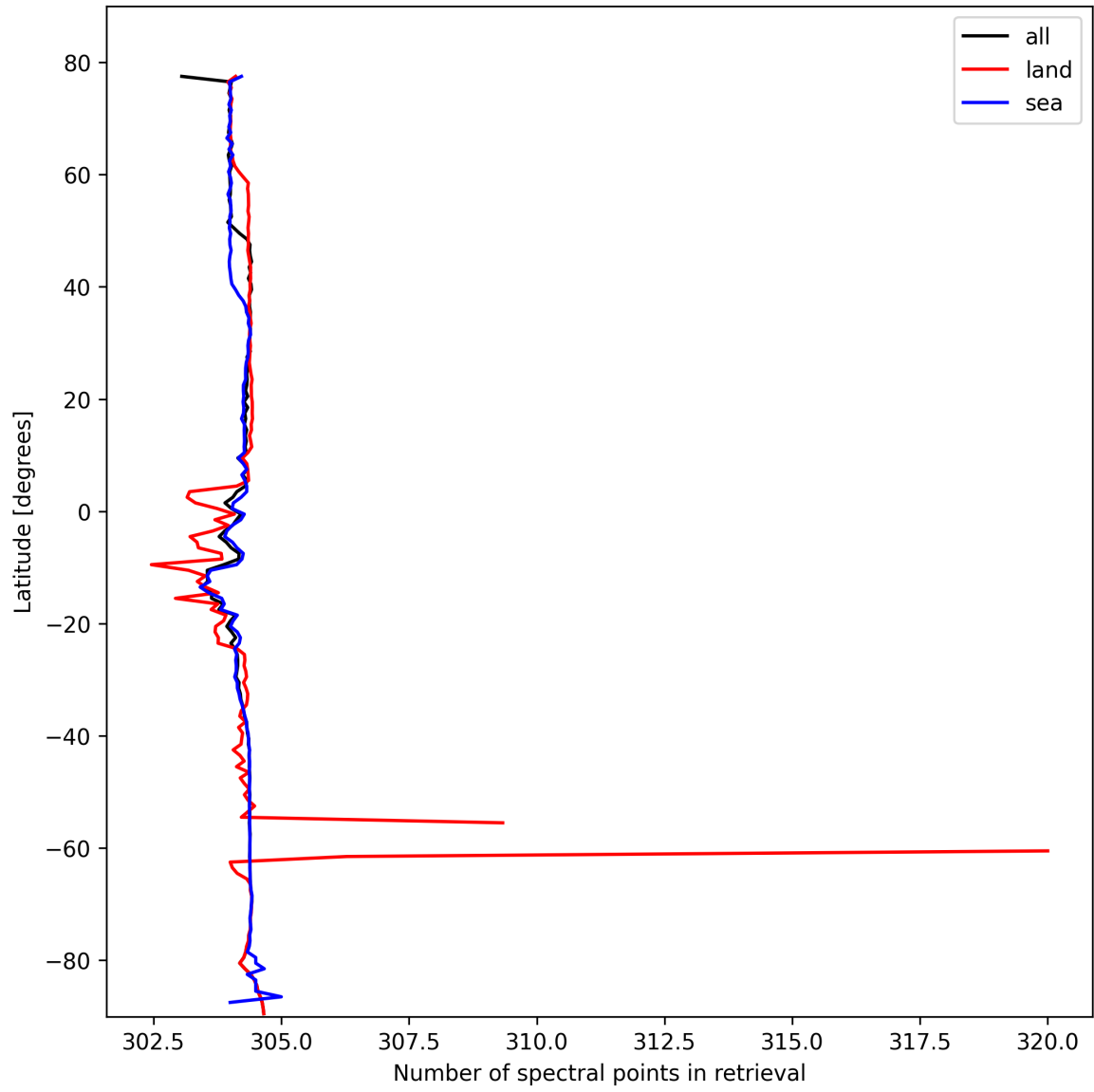
Figure 16: Zonal average of “Number of spectral points in retrieval” for 2025-02-19 to 2025-02-21.
