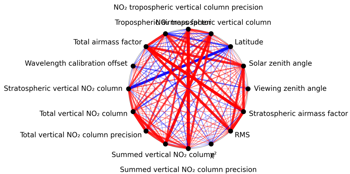
Figure 1: Map of correlation graph for 2025-02-19 to 2025-02-21.
