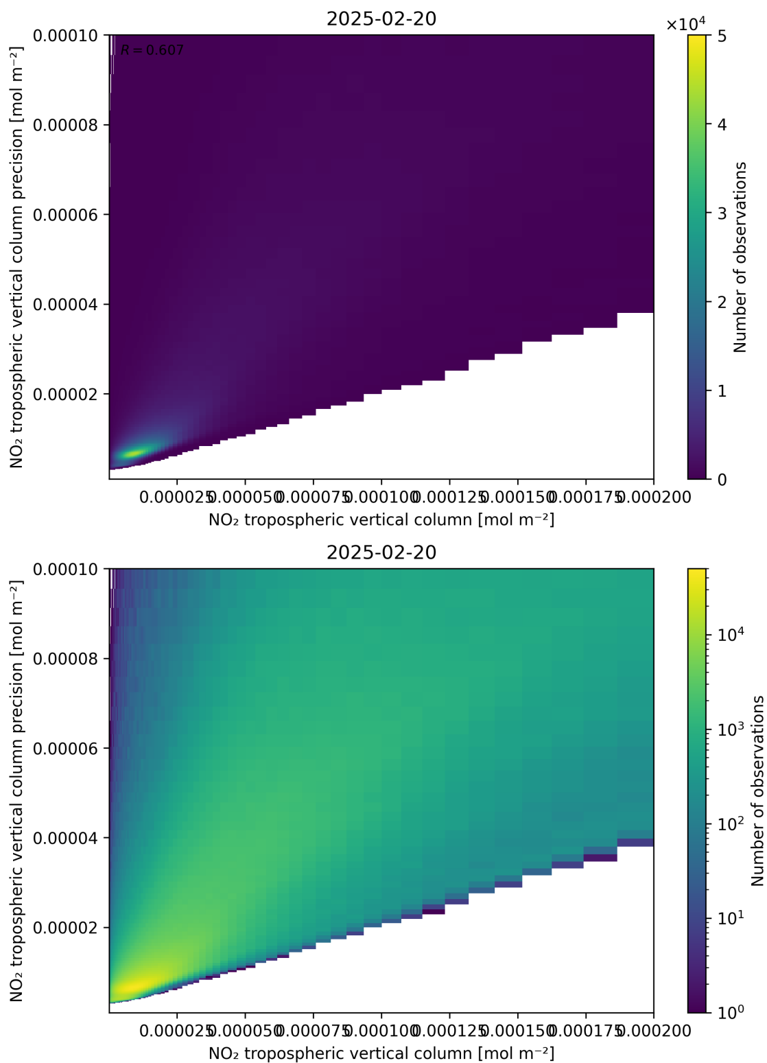
Figure 130: Scatter density plot of “NO 2 tropospheric vertical column” against “NO 2 tropospheric vertical column precision” for 2025-02-19 to 2025-02-21.
