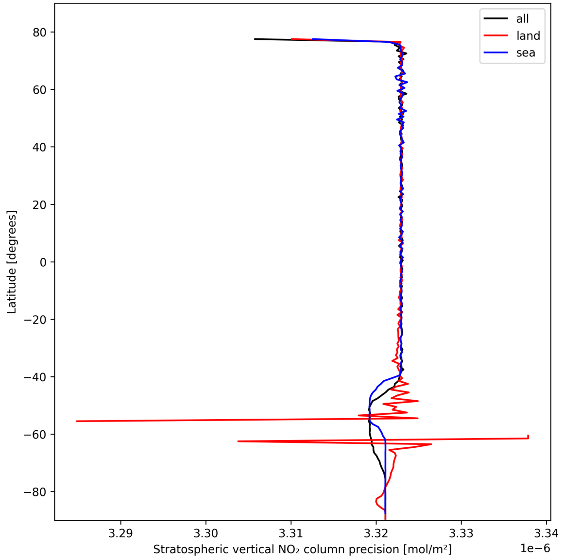
Figure 20: Zonal average of "Stratospheric vertical NO 2 column precision" for 2025-02-19 to 2025-02-21.
