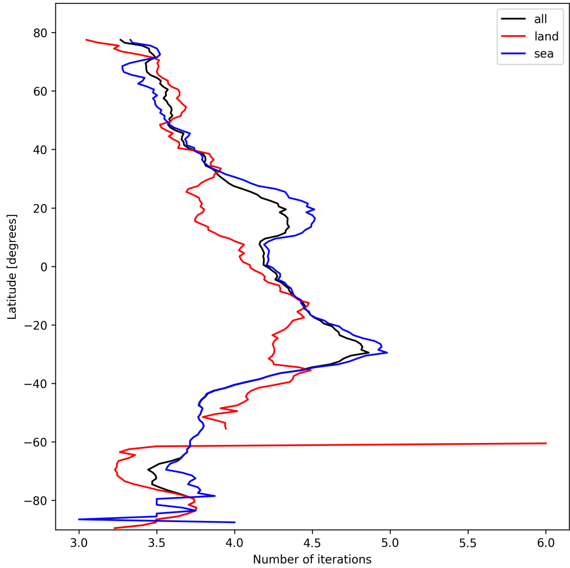
Figure 17: Zonal average of “Number of iterations” for 2025-02-19 to 2025-02-21.
