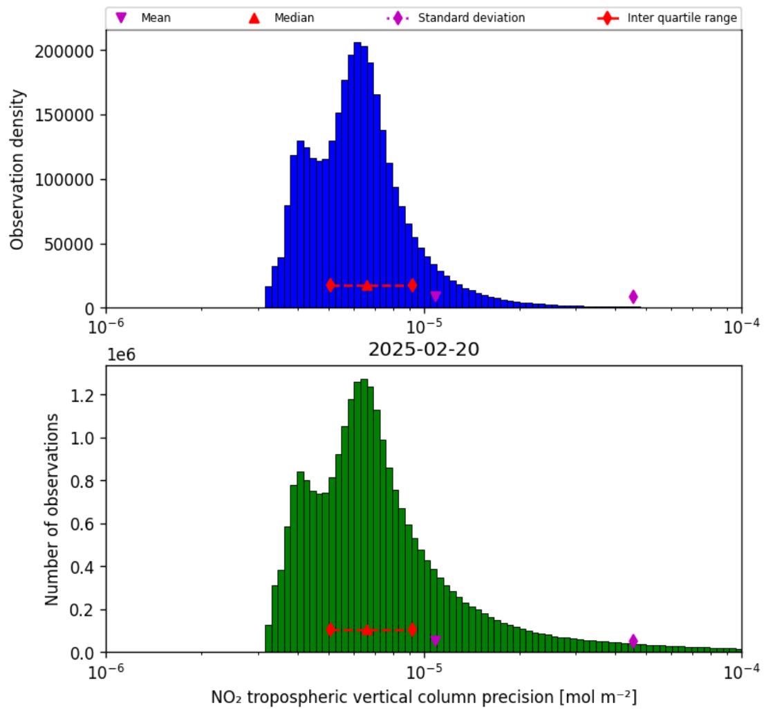
Figure 30: Histogram of “NO 2 tropospheric vertical column precision” for 2025-02-19 to 2025-02-21
