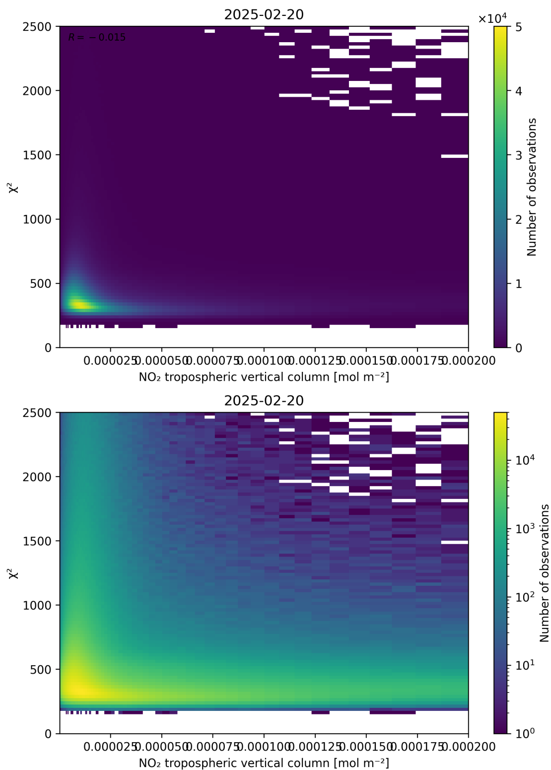
Figure 124: Scatter density plot of “NO 2 tropospheric vertical column” against “ \chi^2 ” for 2025-02-19 to 2025-02-21.
