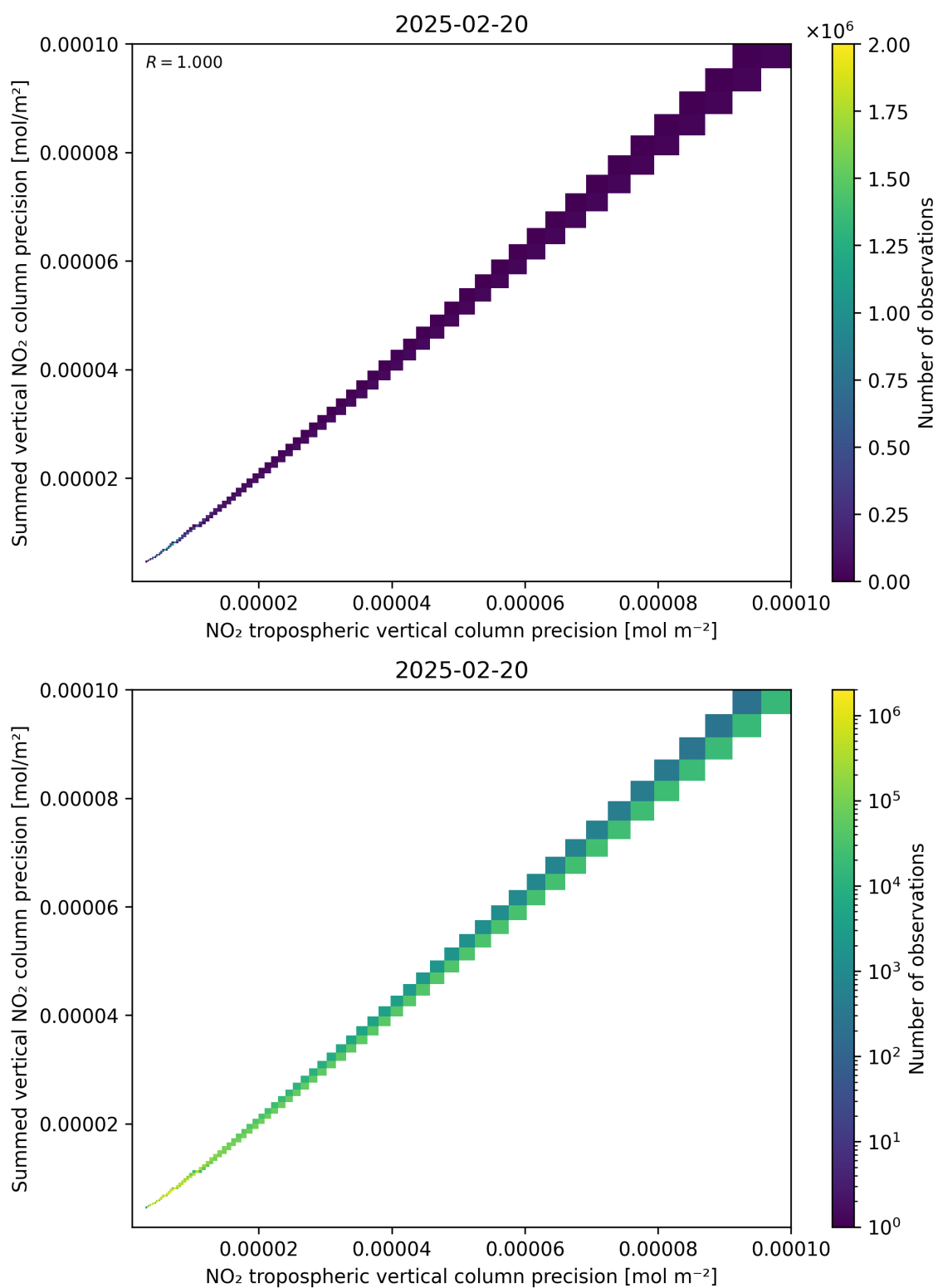
Figure 137: Scatter density plot of “NO 2 tropospheric vertical column precision” against “Summed vertical NO 2 column precision” for 2025-02-19 to 2025-02-21.
