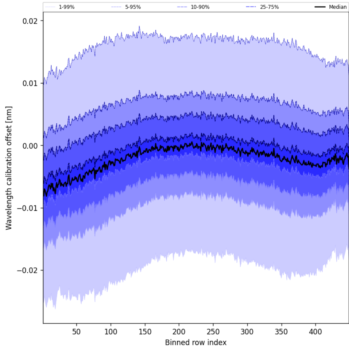
Figure 52: Along track statistics of “Wavelength calibration offset” for 2025-02-19 to 2025-02-21
