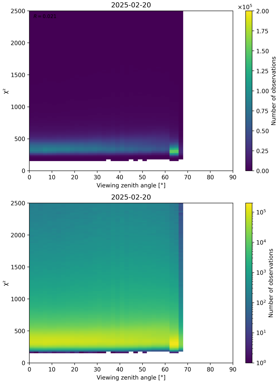
Figure 162: Scatter density plot of “Viewing zenith angle” against “ \chi^2 ” for 2025-02-19 to 2025-02-21.
