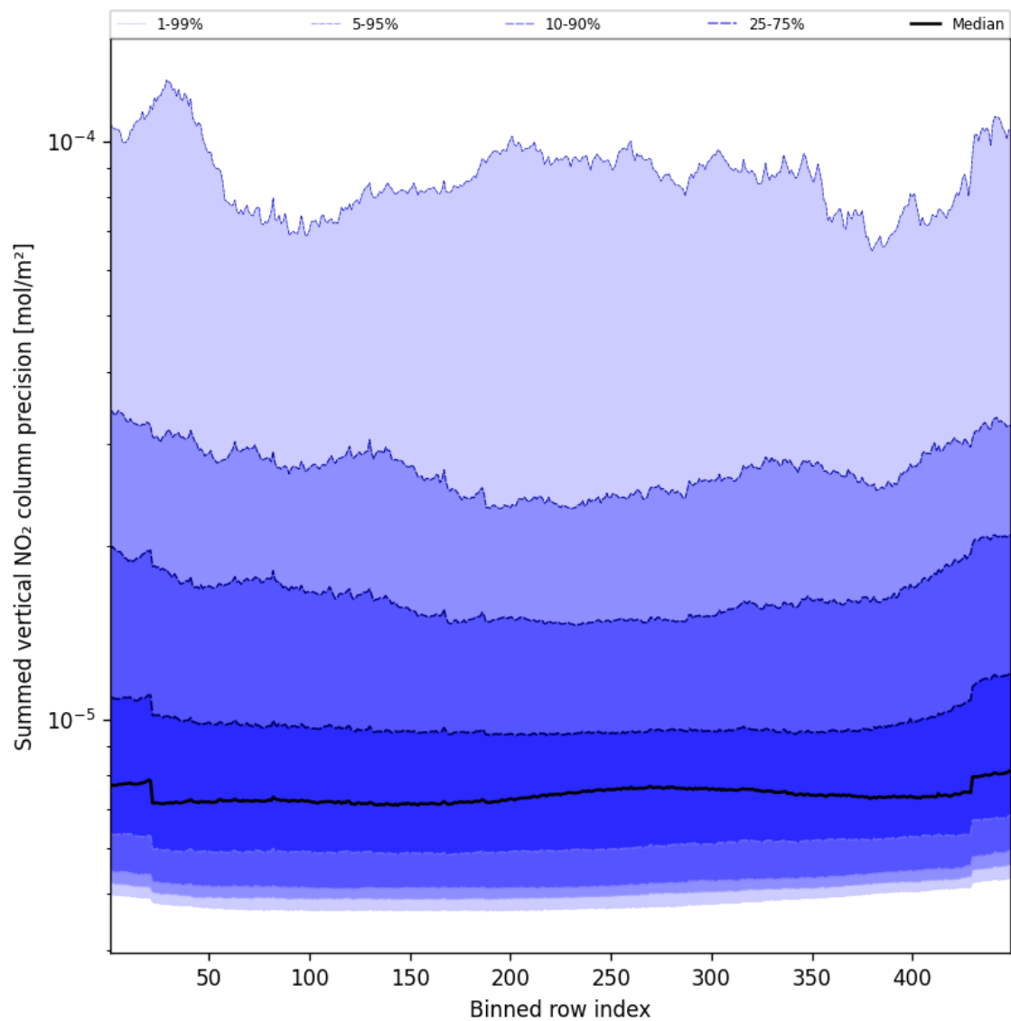
Figure 58: Along track statistics of “Summed vertical NO 2 column precision” for 2025-02-19 to 2025-02-21
