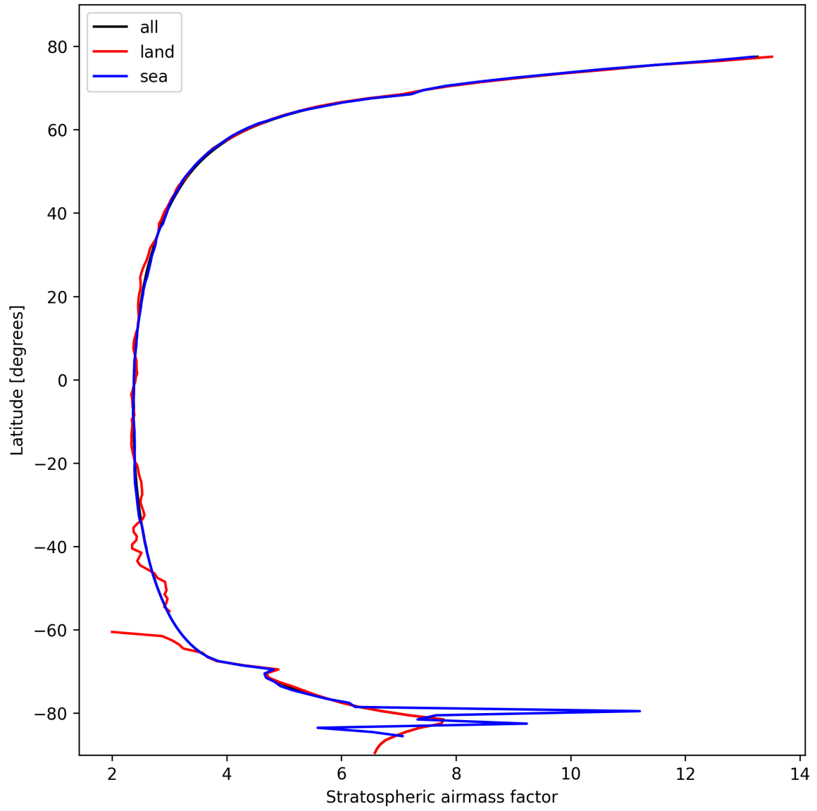
Figure 27: Zonal average of “Stratospheric airmass factor” for 2025-02-20 to 2025-02-22.
