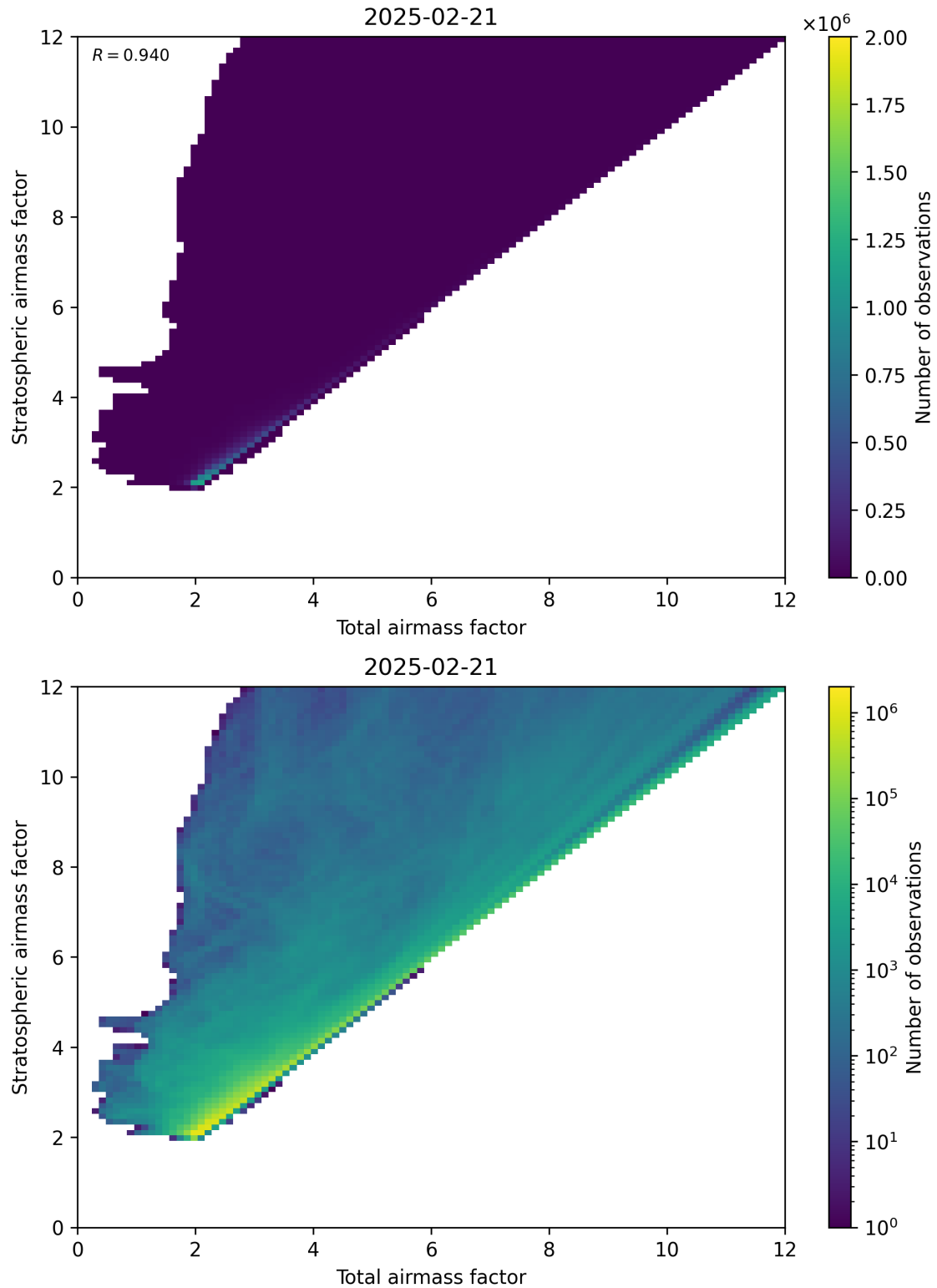
Figure 62: Scatter density plot of “Total airmass factor” against “Stratospheric airmass factor” for 2025-02-20 to 2025-02-22.
