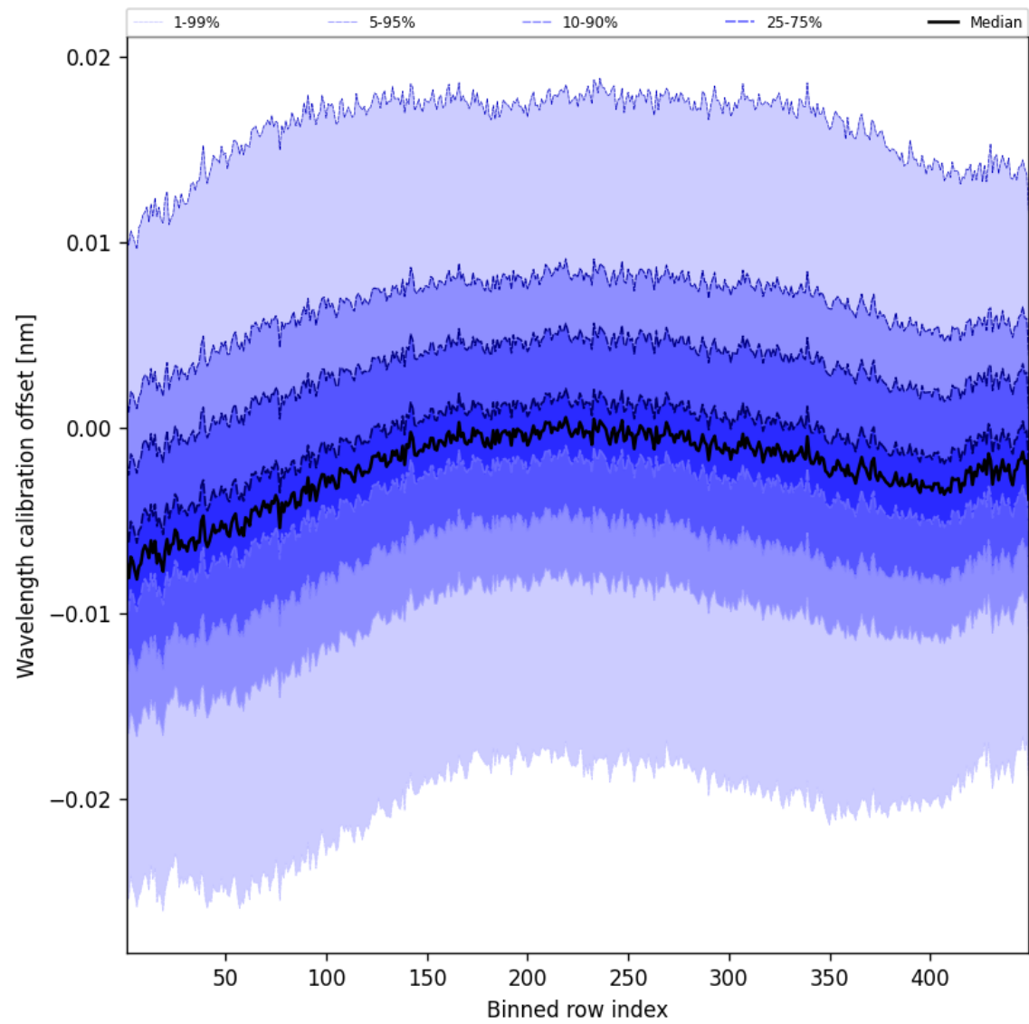
Figure 52: Along track statistics of “Wavelength calibration offset” for 2025-02-20 to 2025-02-22
