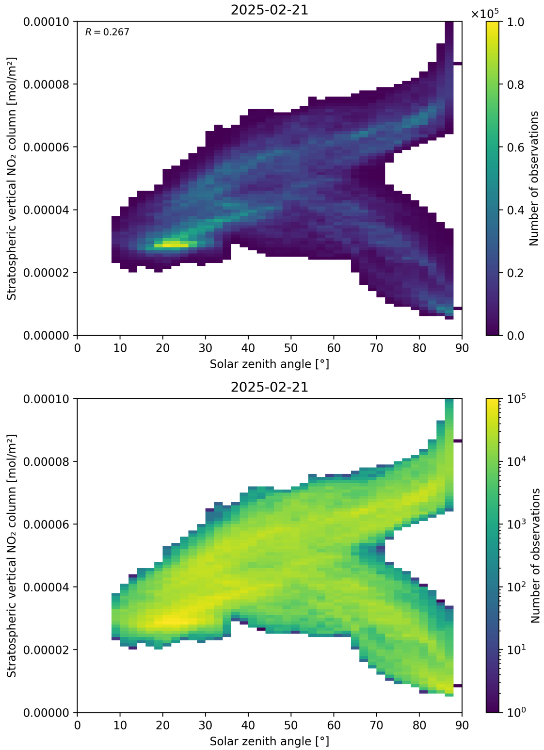
Figure 150: Scatter density plot of “Solar zenith angle” against “Stratospheric vertical NO 2 column” for 2025-02-20 to 2025-02-22.
