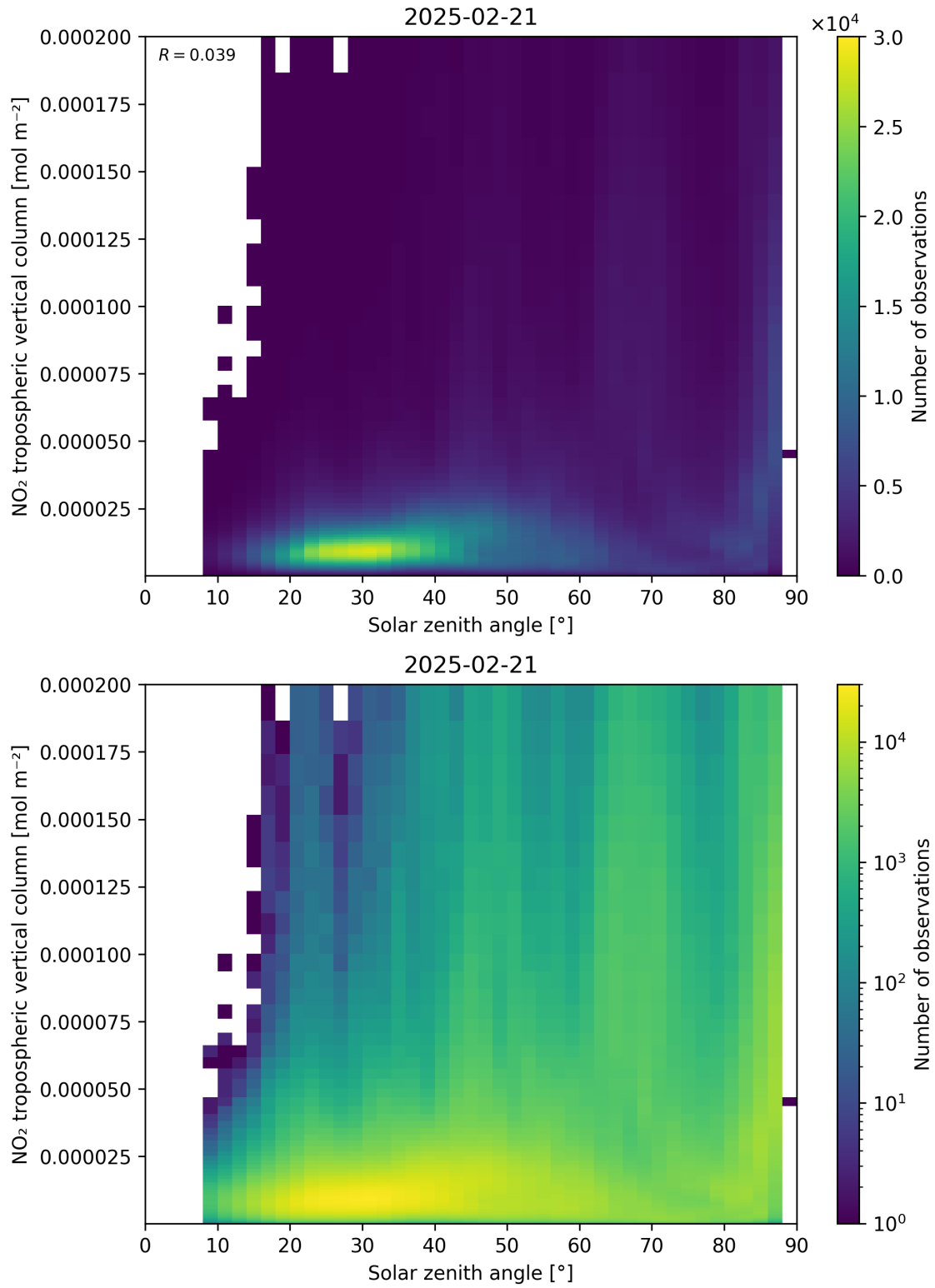
Figure 155: Scatter density plot of “Solar zenith angle” against “NO 2 tropospheric vertical column” for 2025-02-20 to 2025-02-22.
