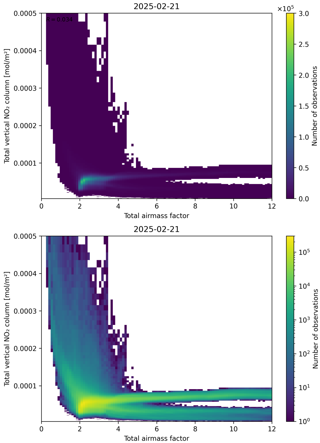
Figure 67: Scatter density plot of “Total airmass factor” against “Total vertical NO 2 column” for 2025-02-20 to 2025-02-22.
