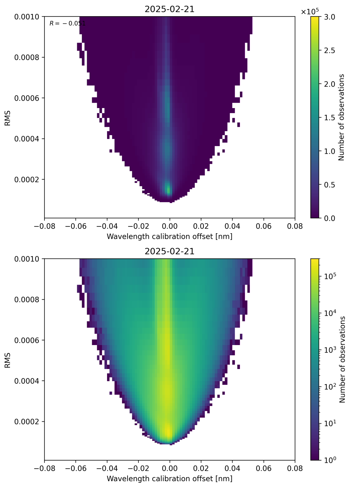
Figure 181: Scatter density plot of “Wavelength calibration offset” against “RMS” for 2025-02-20 to 2025-02-22.
