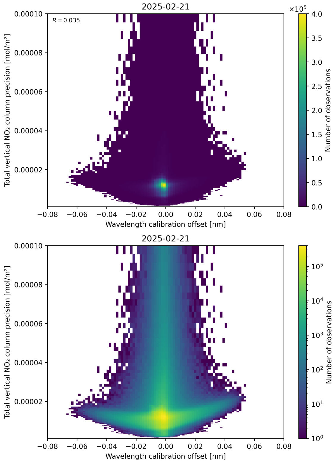
Figure 180: Scatter density plot of “Wavelength calibration offset” against “Total vertical NO 2 column precision” for 2025-02-20 to 2025-02-22.
