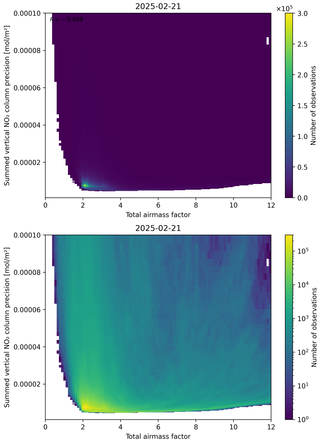
Figure 66: Scatter density plot of “Total airmass factor” against “Summed vertical NO 2 column precision” for 2025-02-20 to 2025-02-22.
