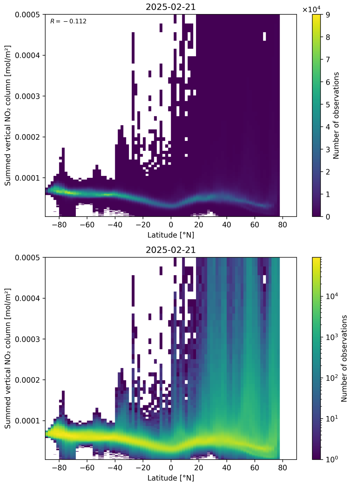
Figure 88: Scatter density plot of “Latitude” against “Summed vertical NO 2 column” for 2025-02-20 to 2025-02-22.
