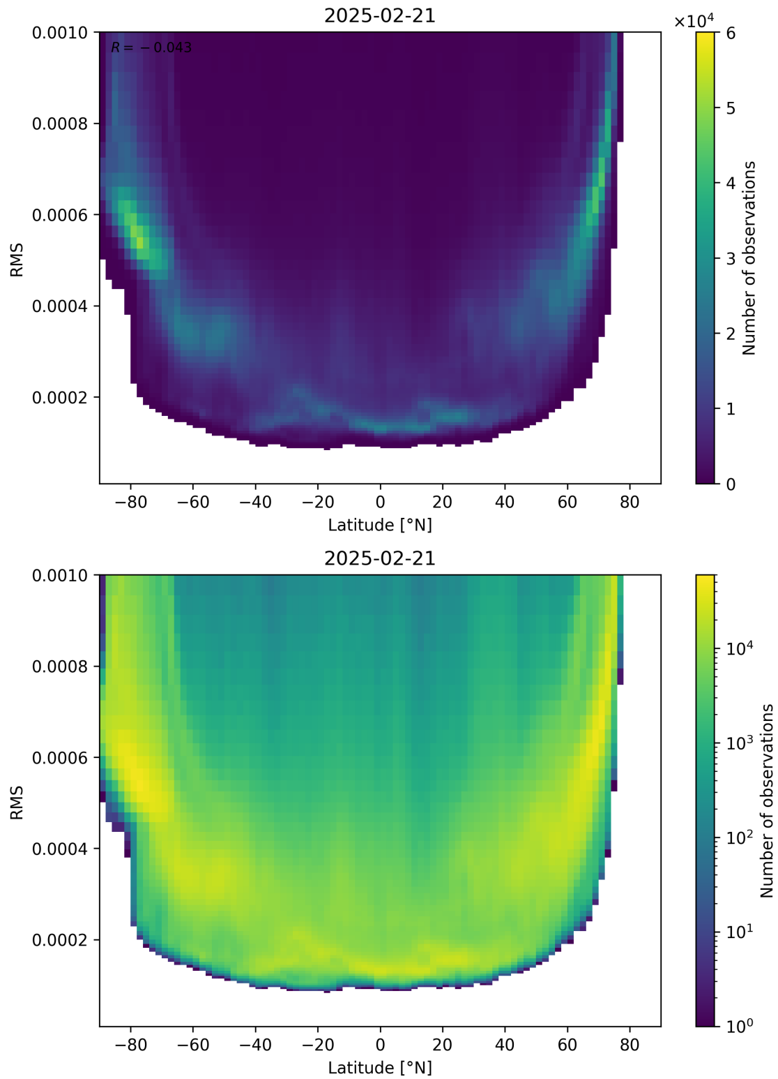
Figure 94: Scatter density plot of “Latitude” against “RMS” for 2025-02-20 to 2025-02-22.
