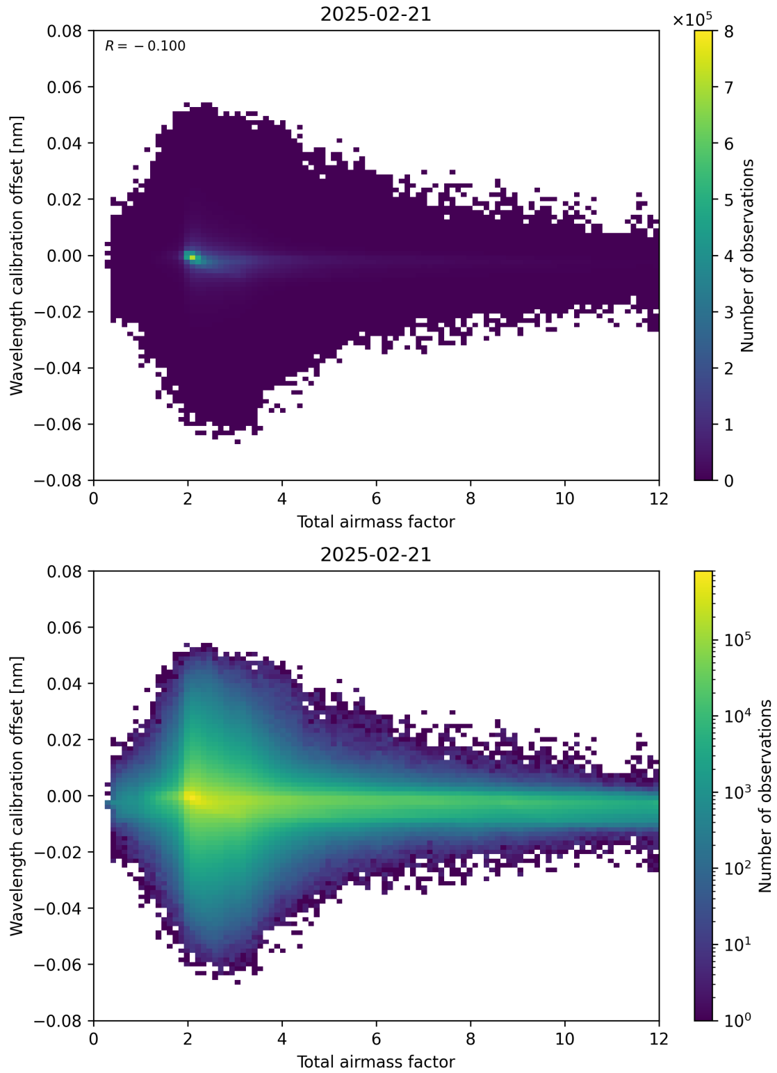
Figure 70: Scatter density plot of “Total airmass factor” against “Wavelength calibration offset” for 2025-02-20 to 2025-02-22.
