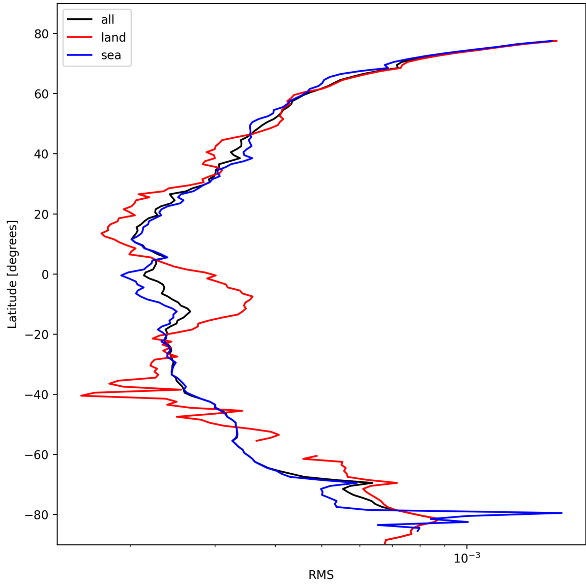
Figure 26: Zonal average of “RMS” for 2025-02-20 to 2025-02-22.
