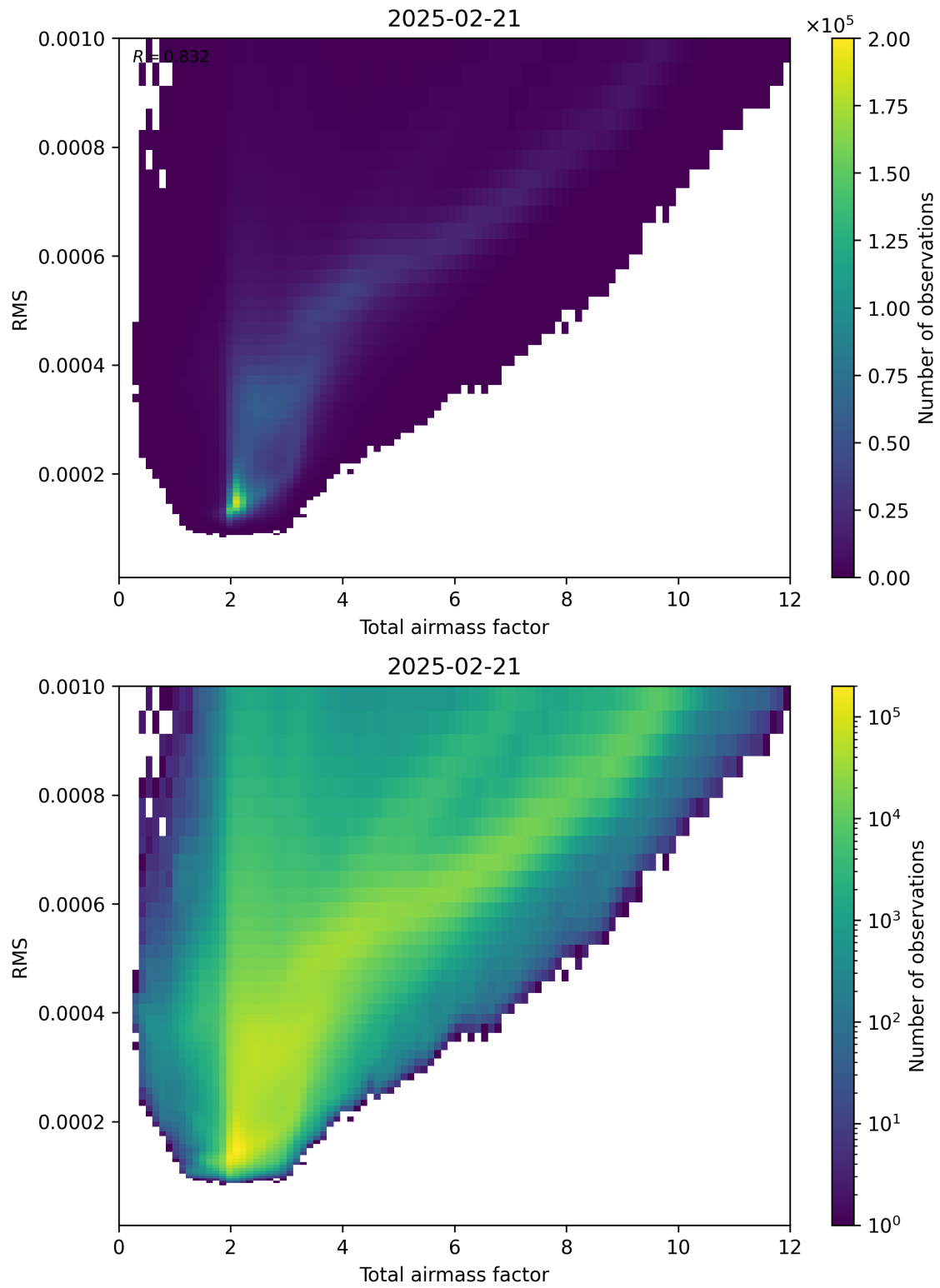
Figure 69: Scatter density plot of “Total airmass factor” against “RMS” for 2025-02-20 to 2025-02-22.
