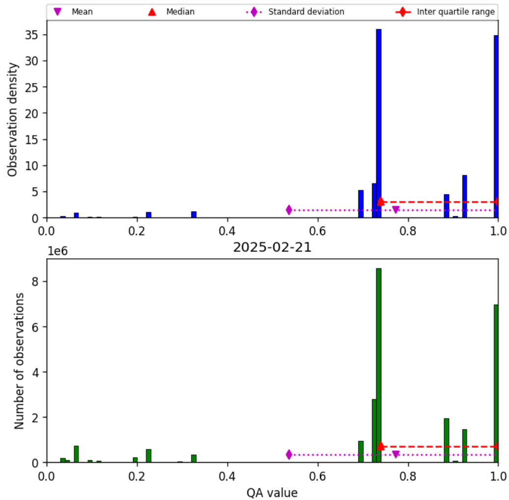
Figure 28: Histogram of “QA value” for 2025-02-20 to 2025-02-22
