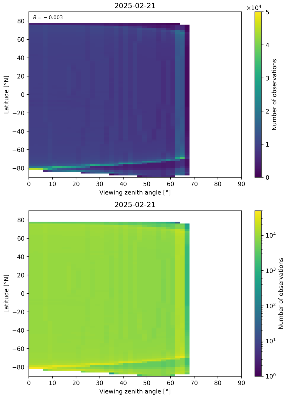
Figure 163: Scatter density plot of “Viewing zenith angle” against “Latitude” for 2025-02-20 to 2025-02-22.
