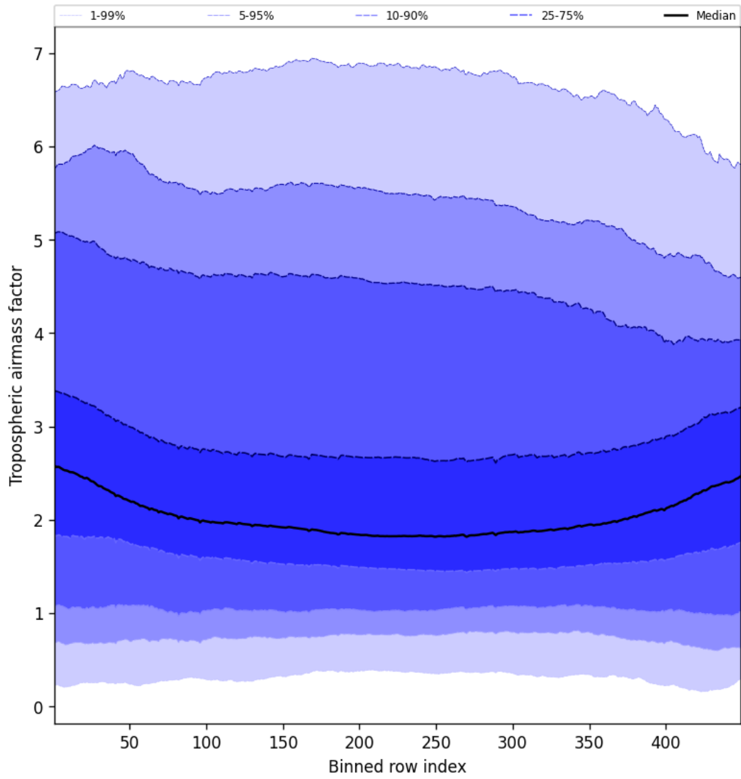
Figure 48: Along track statistics of “Tropospheric airmass factor” for 2025-02-20 to 2025-02-22
