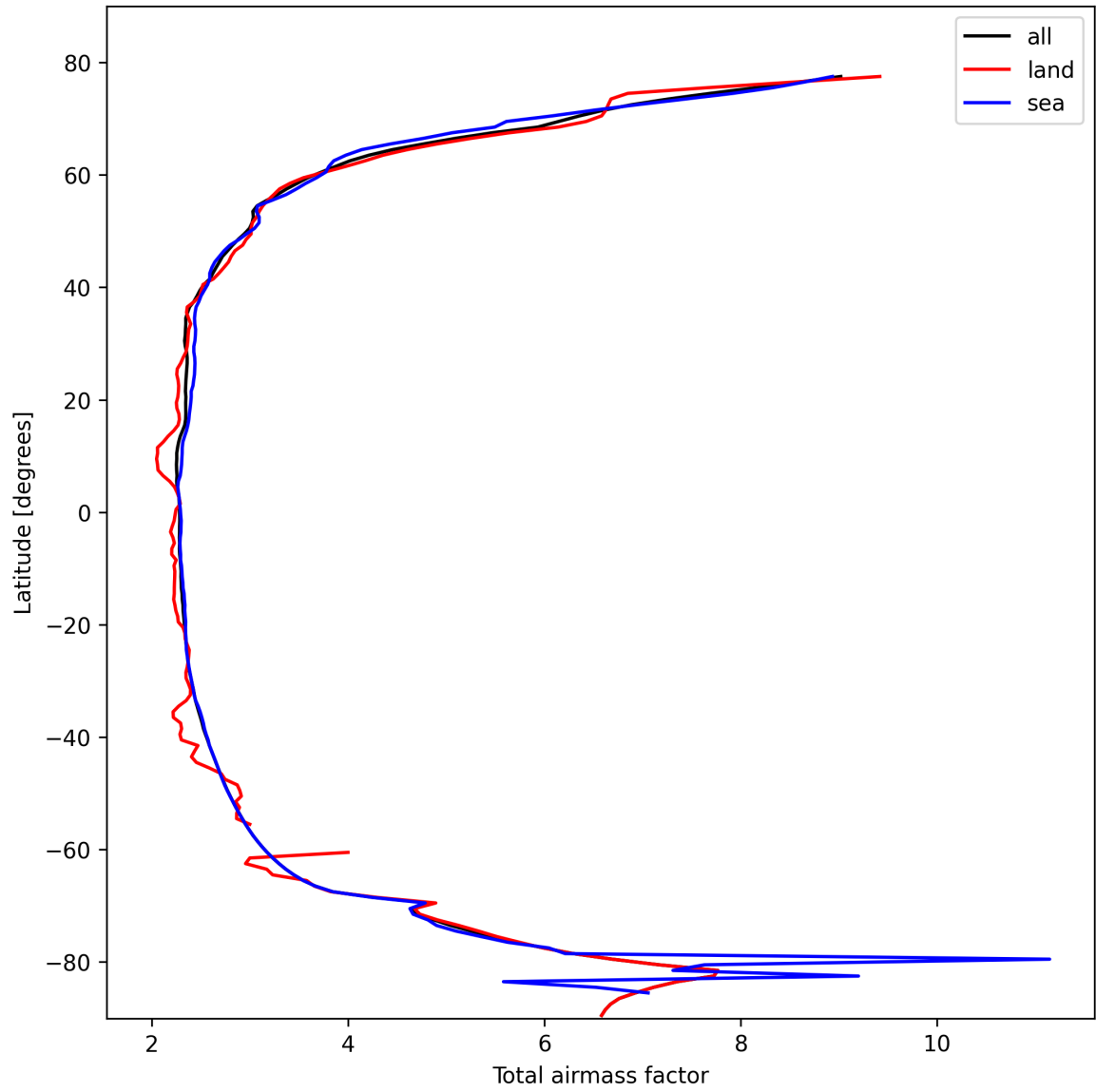
Figure 15: Zonal average of “Total airmass factor” for 2025-02-20 to 2025-02-22.
