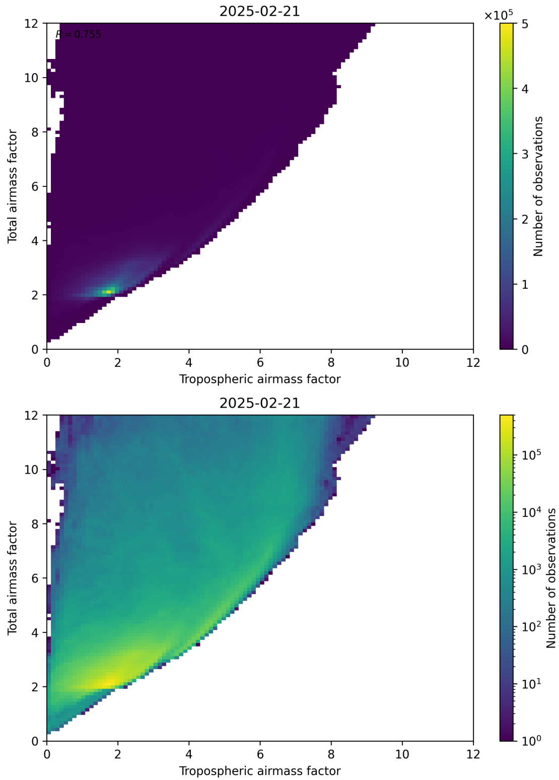
Figure 72: Scatter density plot of “Tropospheric airmass factor” against “Total airmass factor” for 2025-02-20 to 2025-02-22.
