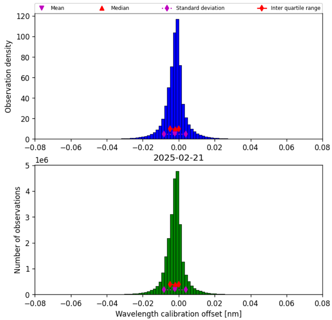
Figure 35: Histogram of “Wavelength calibration offset” for 2025-02-20 to 2025-02-22
