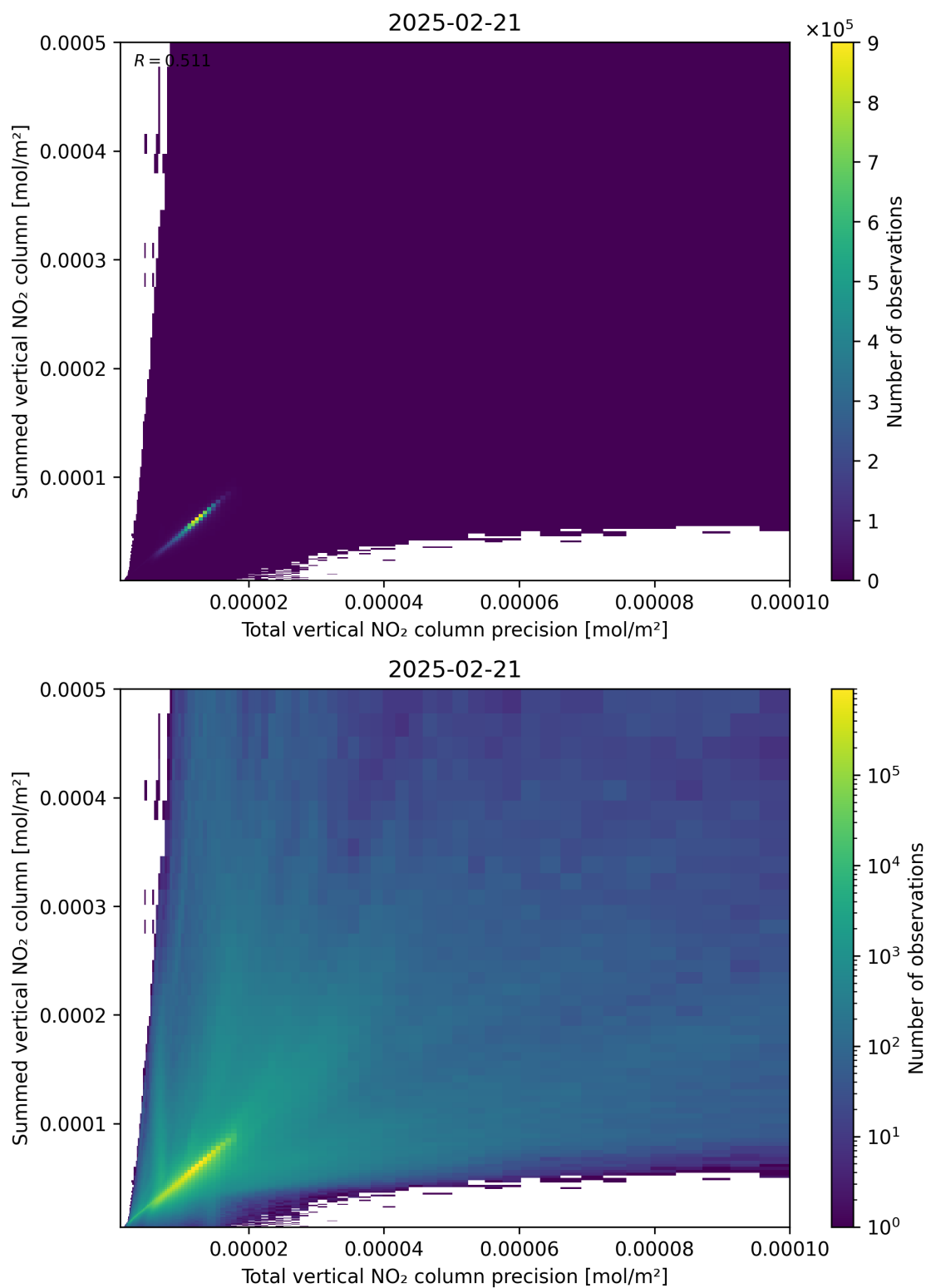
Figure 117: Scatter density plot of “Total vertical NO 2 column precision” against “Summed vertical NO 2 column” for 2025-02-20 to 2025-02-22.
