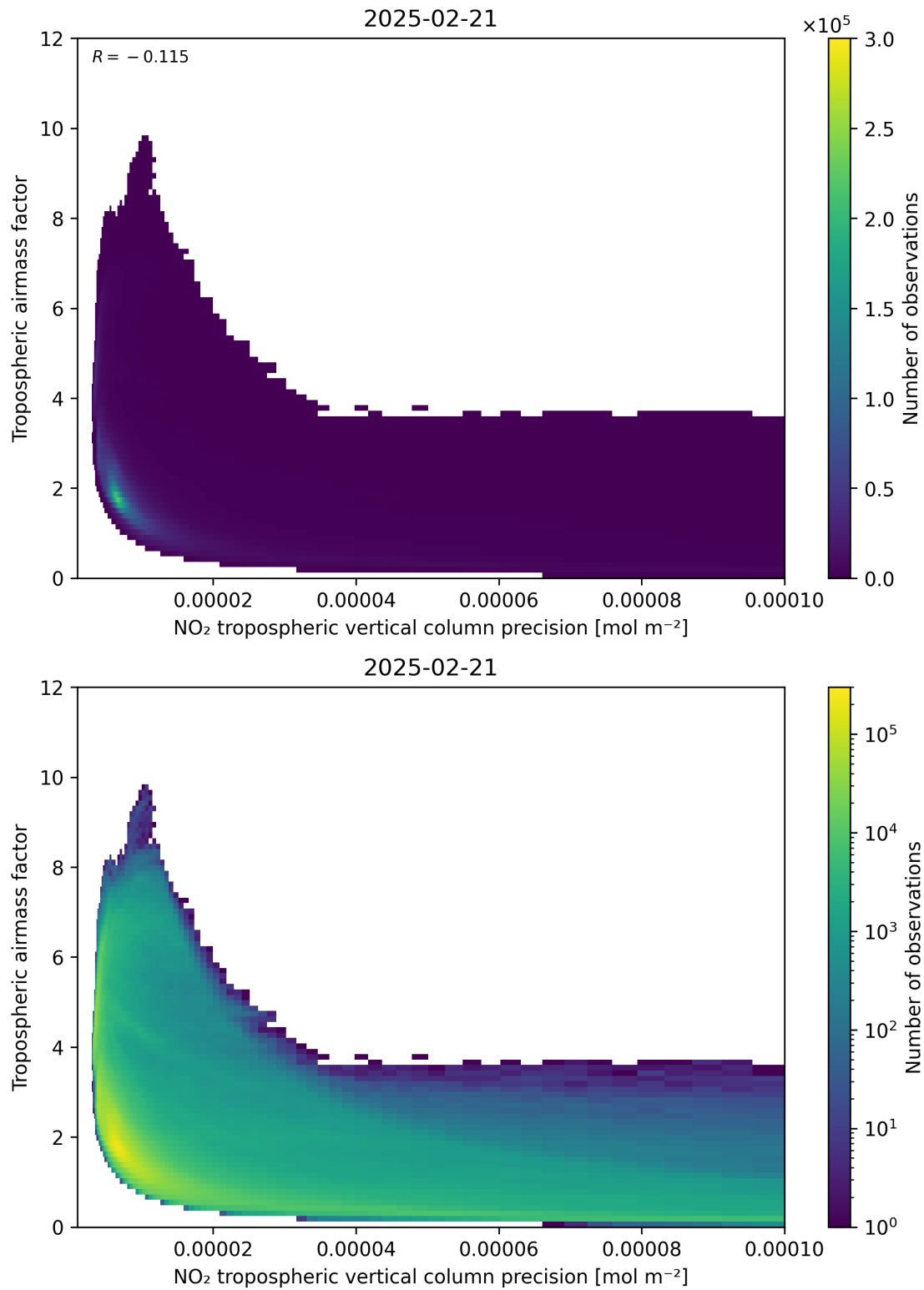
Figure 133: Scatter density plot of “NO 2 tropospheric vertical column precision” against “Tropospheric airmass factor” for 2025-02-20 to 2025-02-22.
