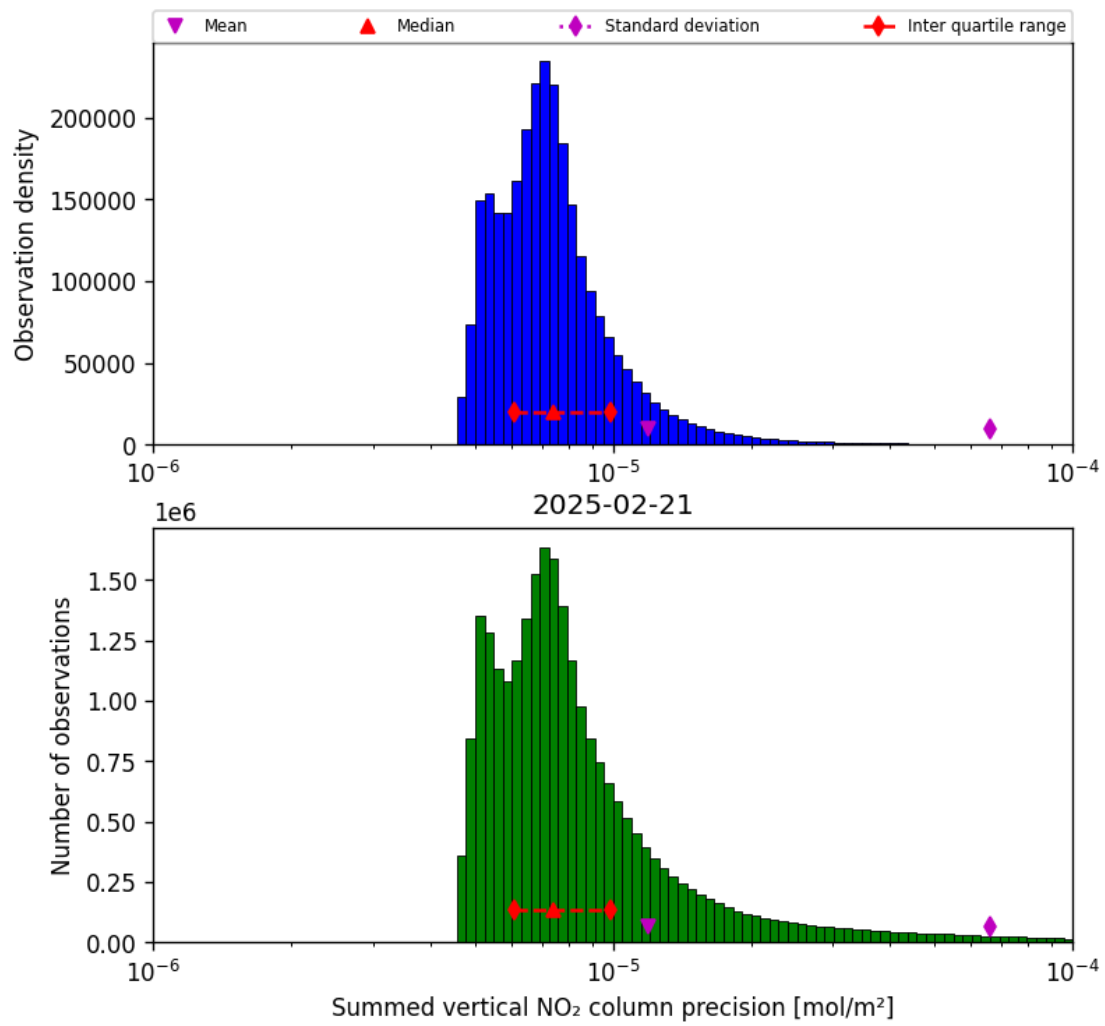
Figure 41: Histogram of “Summed vertical NO 2 column precision” for 2025-02-20 to 2025-02-22
