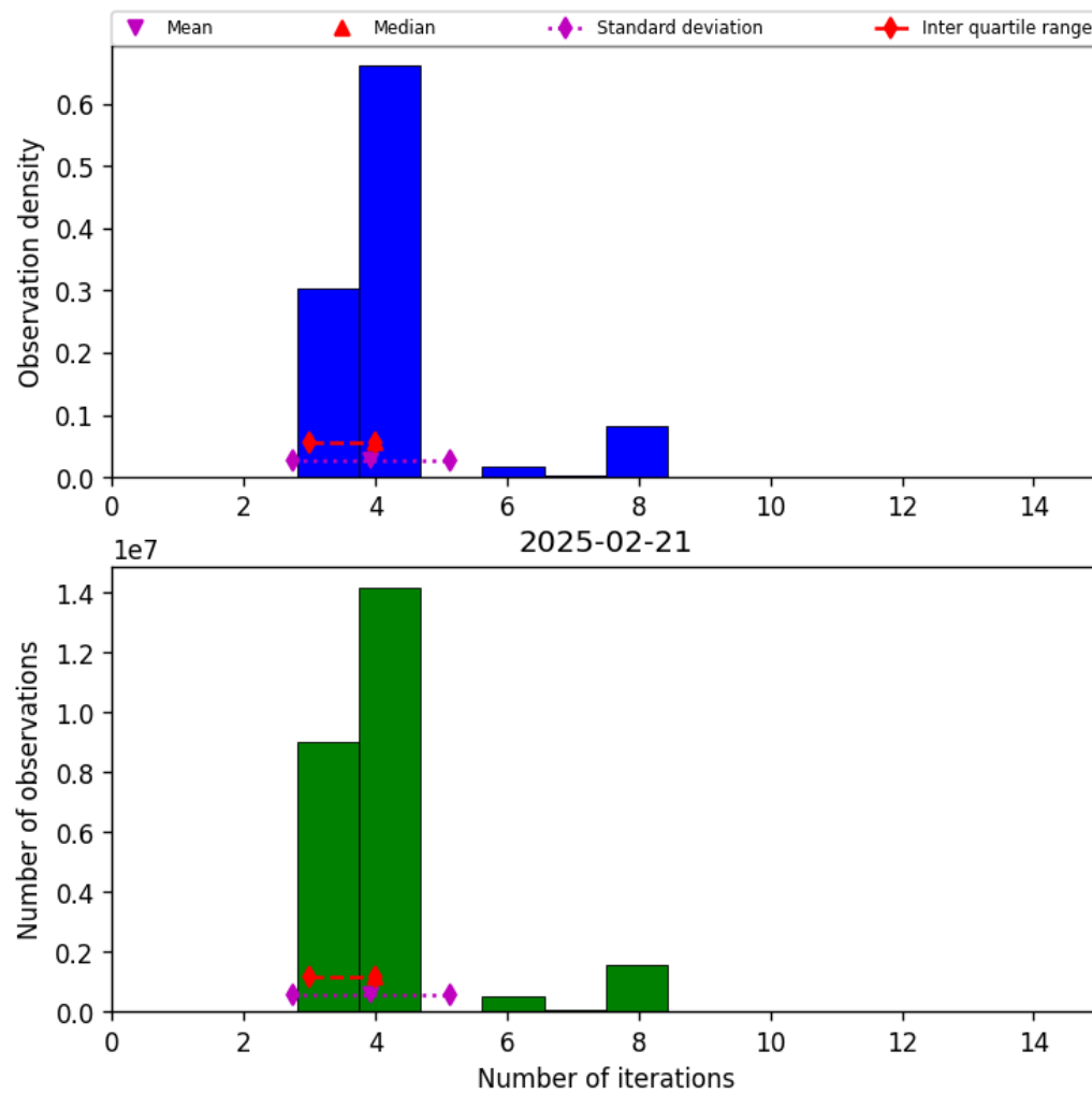
Figure 34: Histogram of “Number of iterations” for 2025-02-20 to 2025-02-22
