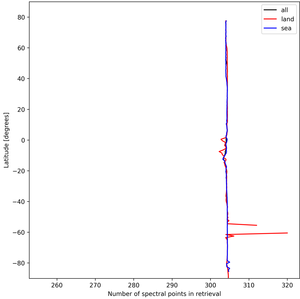
Figure 16: Zonal average of “Number of spectral points in retrieval” for 2025-02-20 to 2025-02-22.
