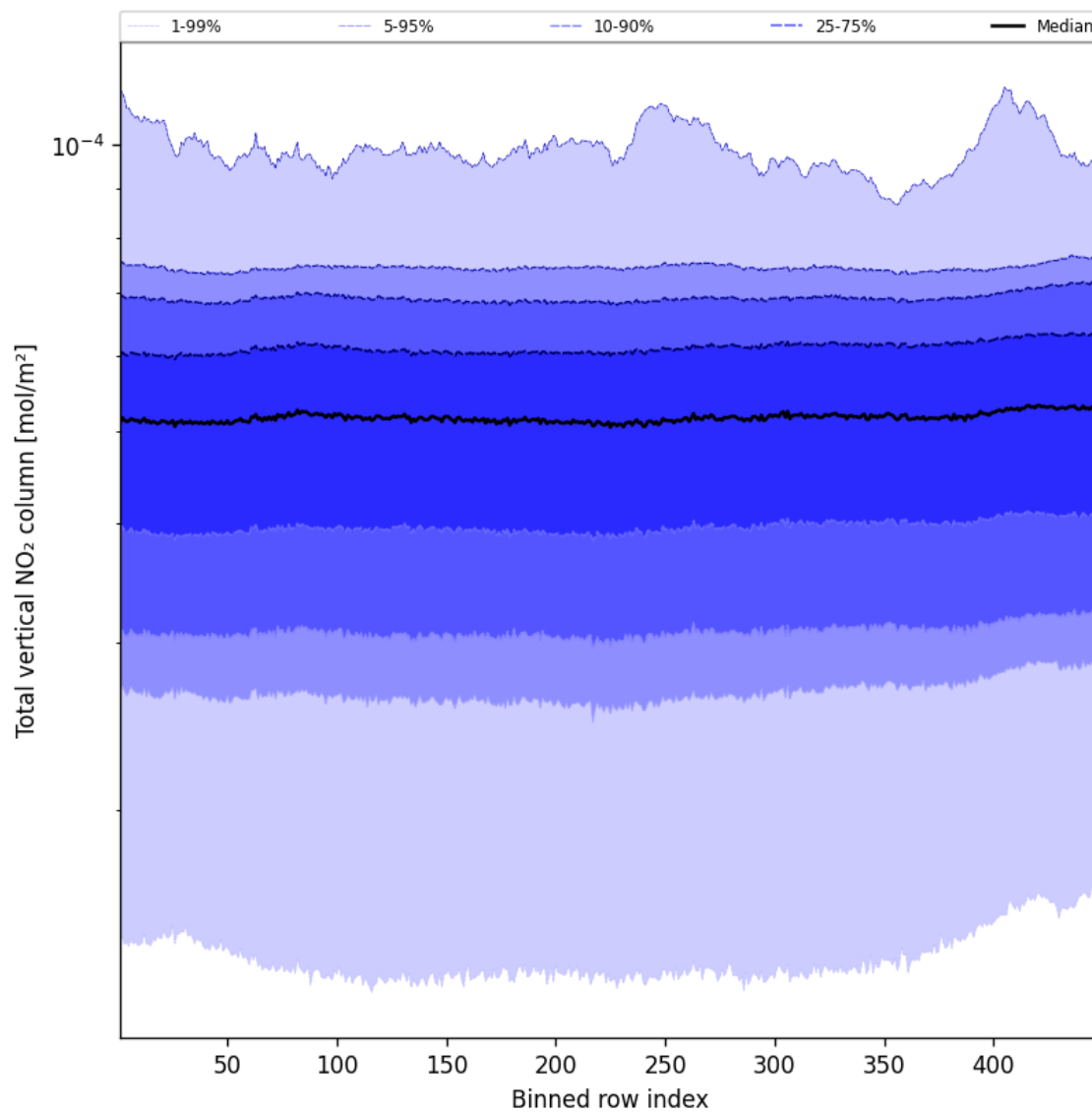
Figure 55: Along track statistics of “Total vertical NO 2 column” for 2025-02-20 to 2025-02-22
