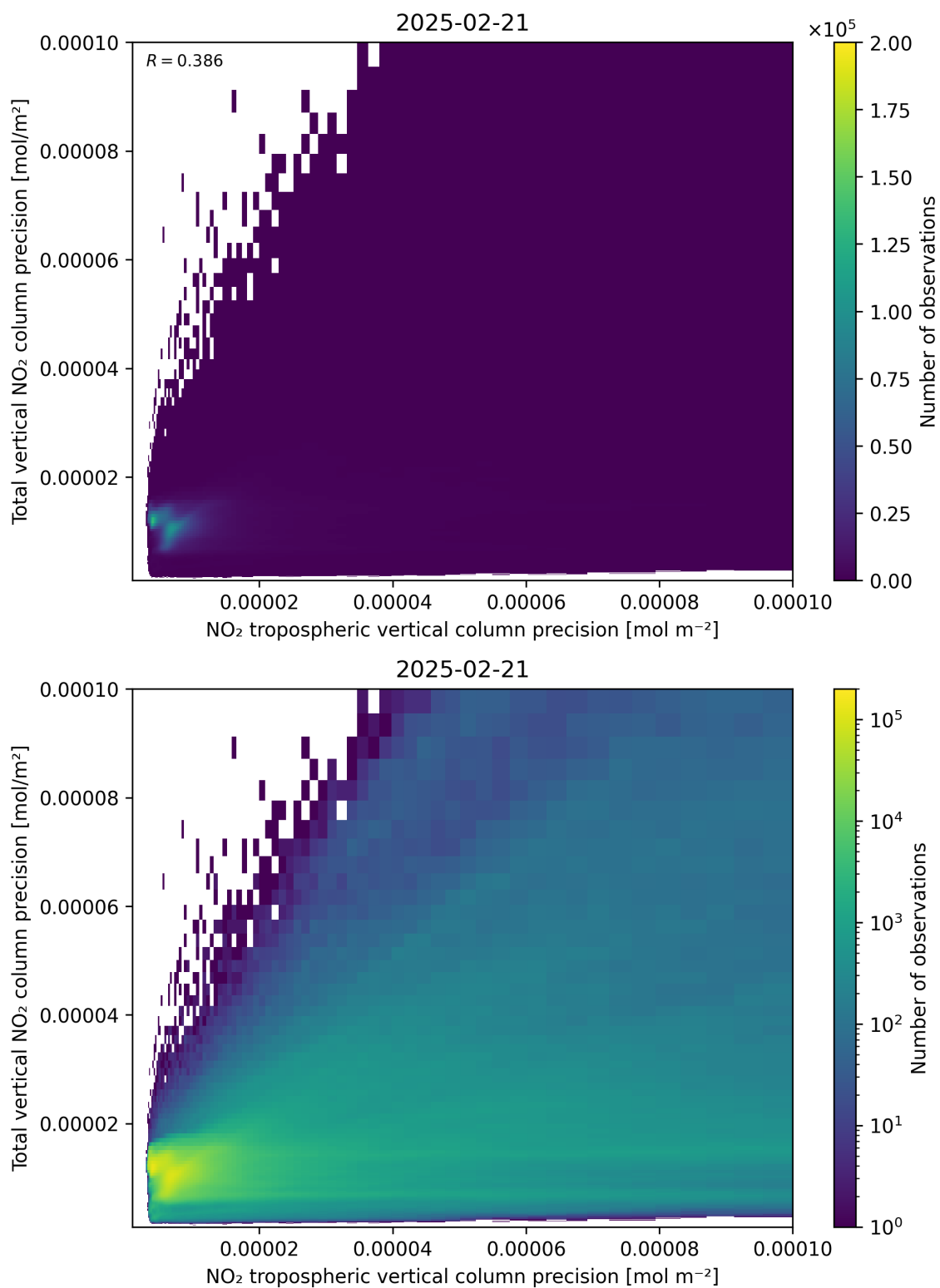
Figure 139: Scatter density plot of “NO 2 tropospheric vertical column precision” against “Total vertical NO 2 column precision” for 2025-02-20 to 2025-02-22.
