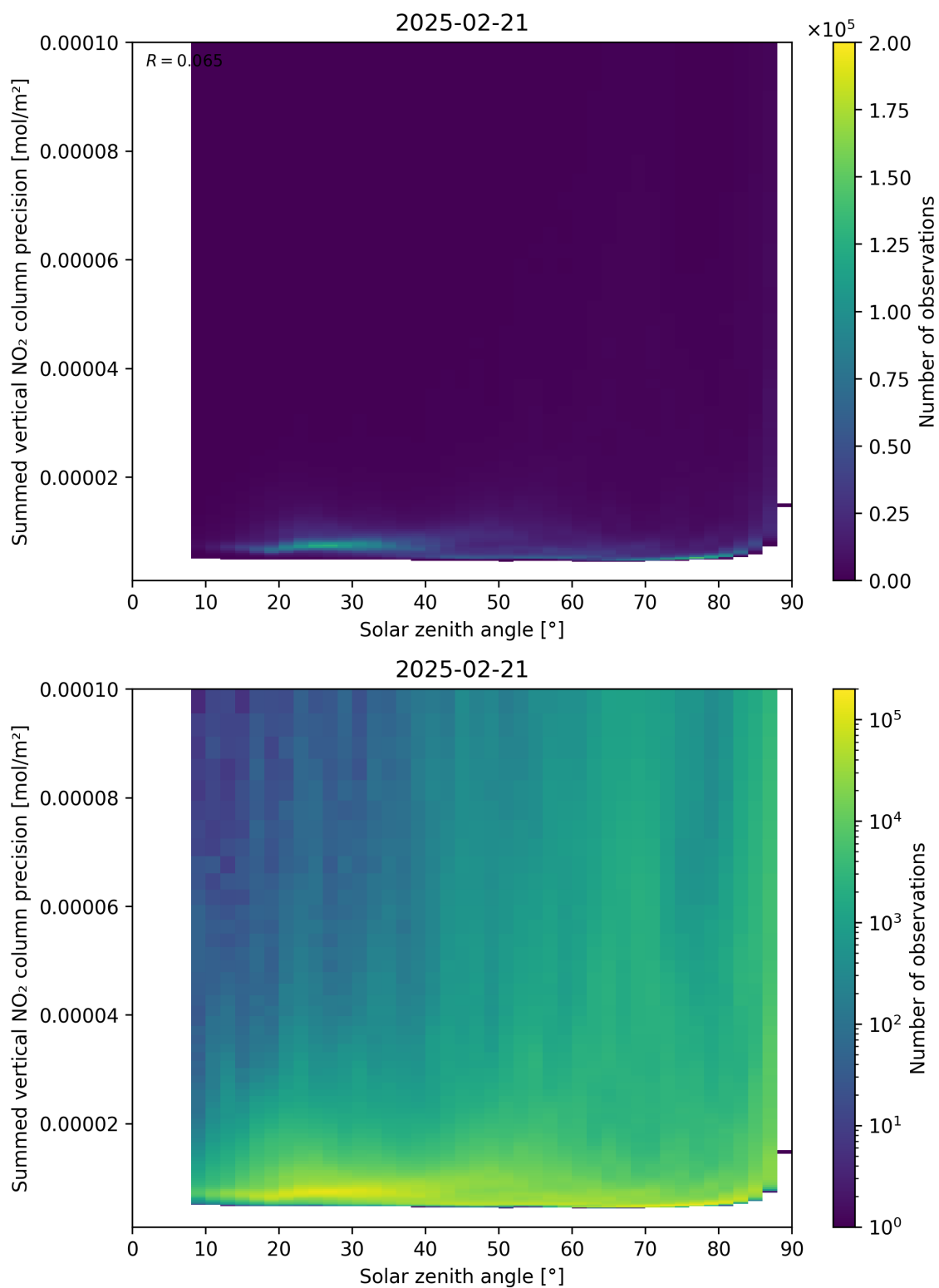
Figure 152: Scatter density plot of “Solar zenith angle” against “Summed vertical NO 2 column precision” for 2025-02-20 to 2025-02-22.
