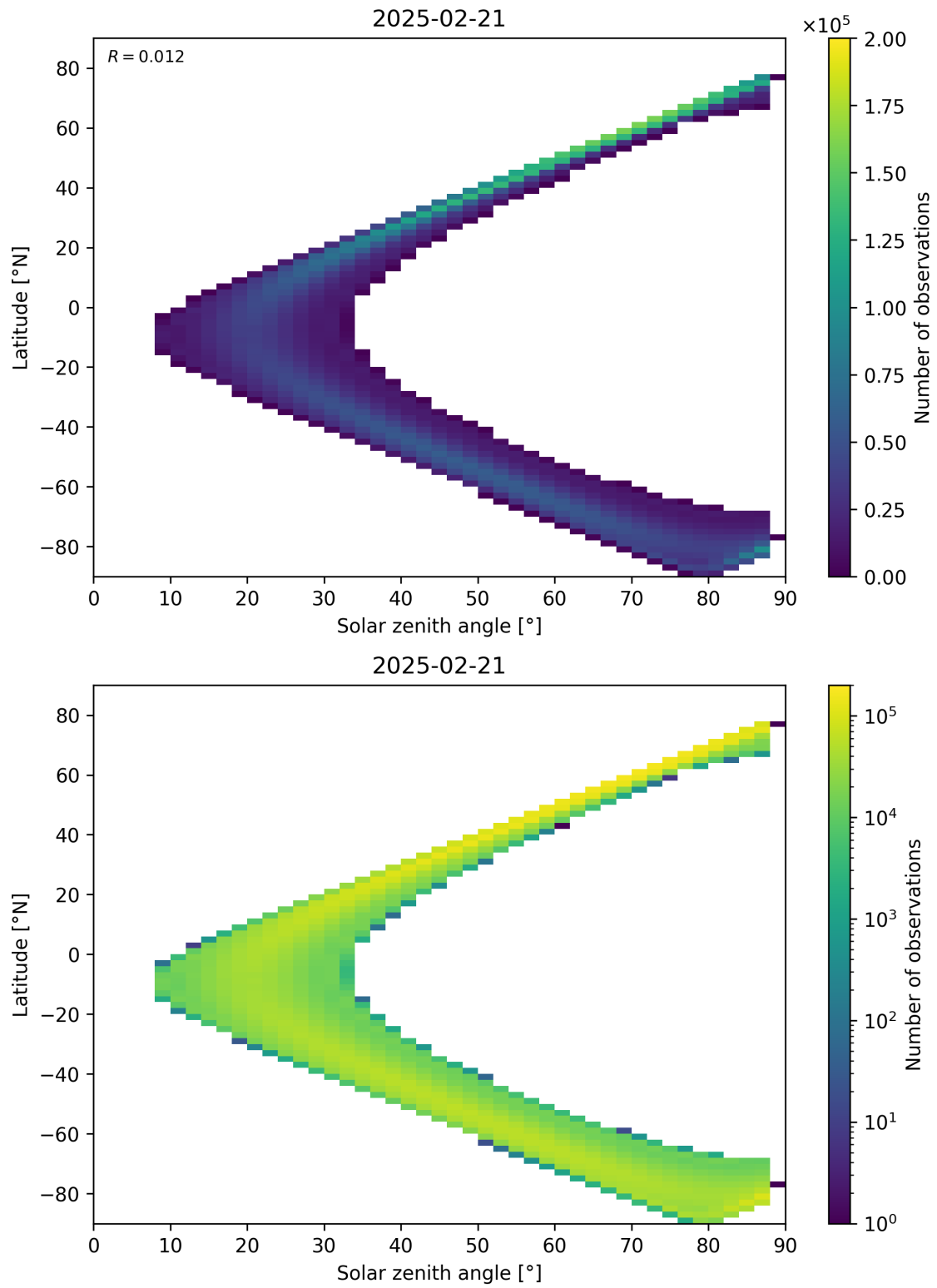
Figure 149: Scatter density plot of “Solar zenith angle” against “Latitude” for 2025-02-20 to 2025-02-22.
