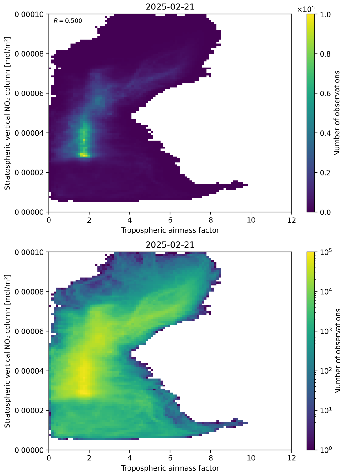
Figure 74: Scatter density plot of “Tropospheric air mass factor” against “Stratospheric vertical NO 2 column” for 2025-02-20 to 2025-02-22.
