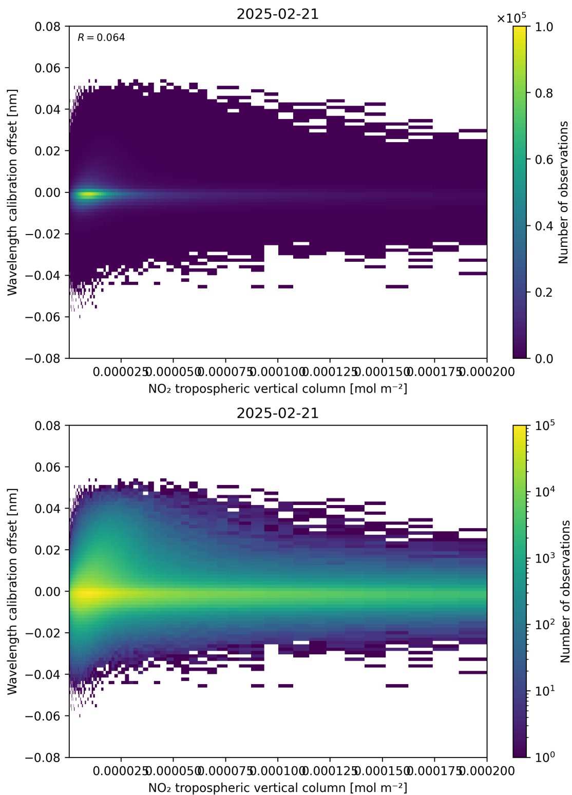
Figure 143: Scatter density plot of “NO 2 tropospheric vertical column” against “Wavelength calibration offset” for 2025-02-20 to 2025-02-22.
