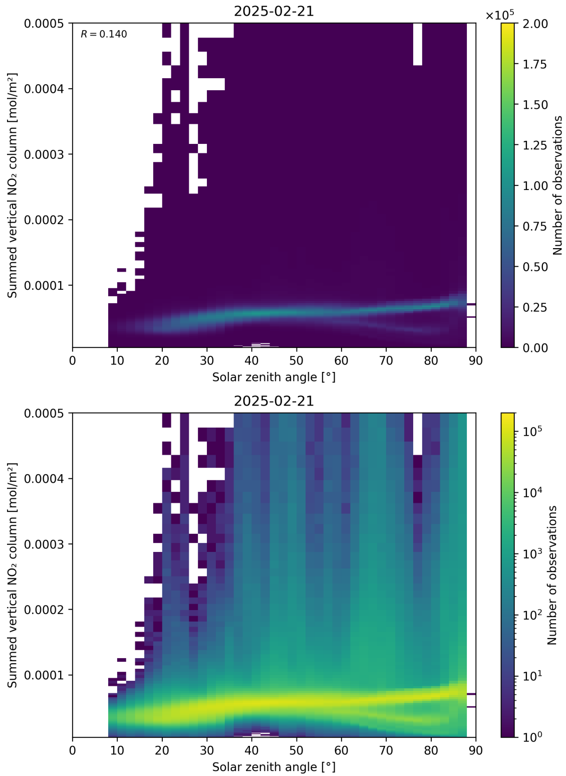
Figure 151: Scatter density plot of “Solar zenith angle” against “Summed vertical NO 2 column” for 2025-02-20 to 2025-02-22.
