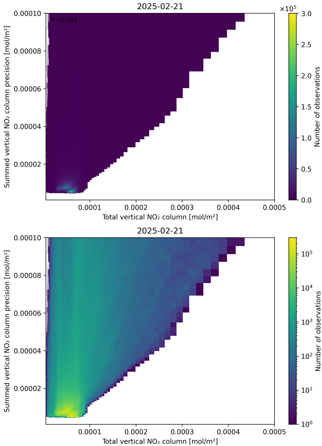
Figure 113: Scatter density plot of “Total vertical NO 2 column” against “Summed vertical NO 2 column precision” for 2025-02-20 to 2025-02-22.
