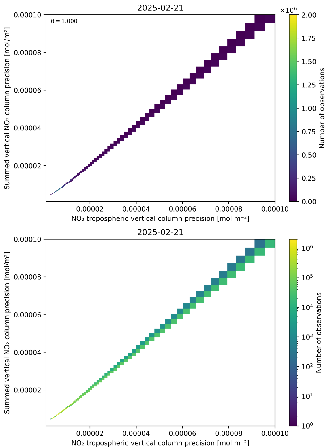
Figure 137: Scatter density plot of “NO 2 tropospheric vertical column precision” against “Summed vertical NO 2 column precision” for 2025-02-20 to 2025-02-22.
