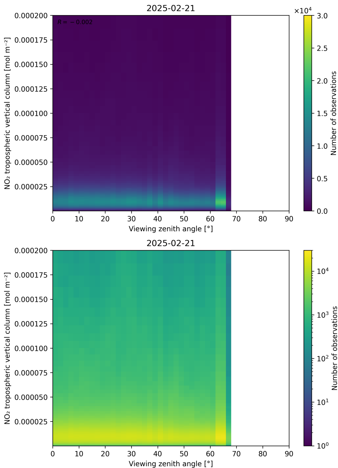
Figure 169: Scatter density plot of “Viewing zenith angle” against “NO 2 tropospheric vertical column” for 2025-02-20 to 2025-02-22.
