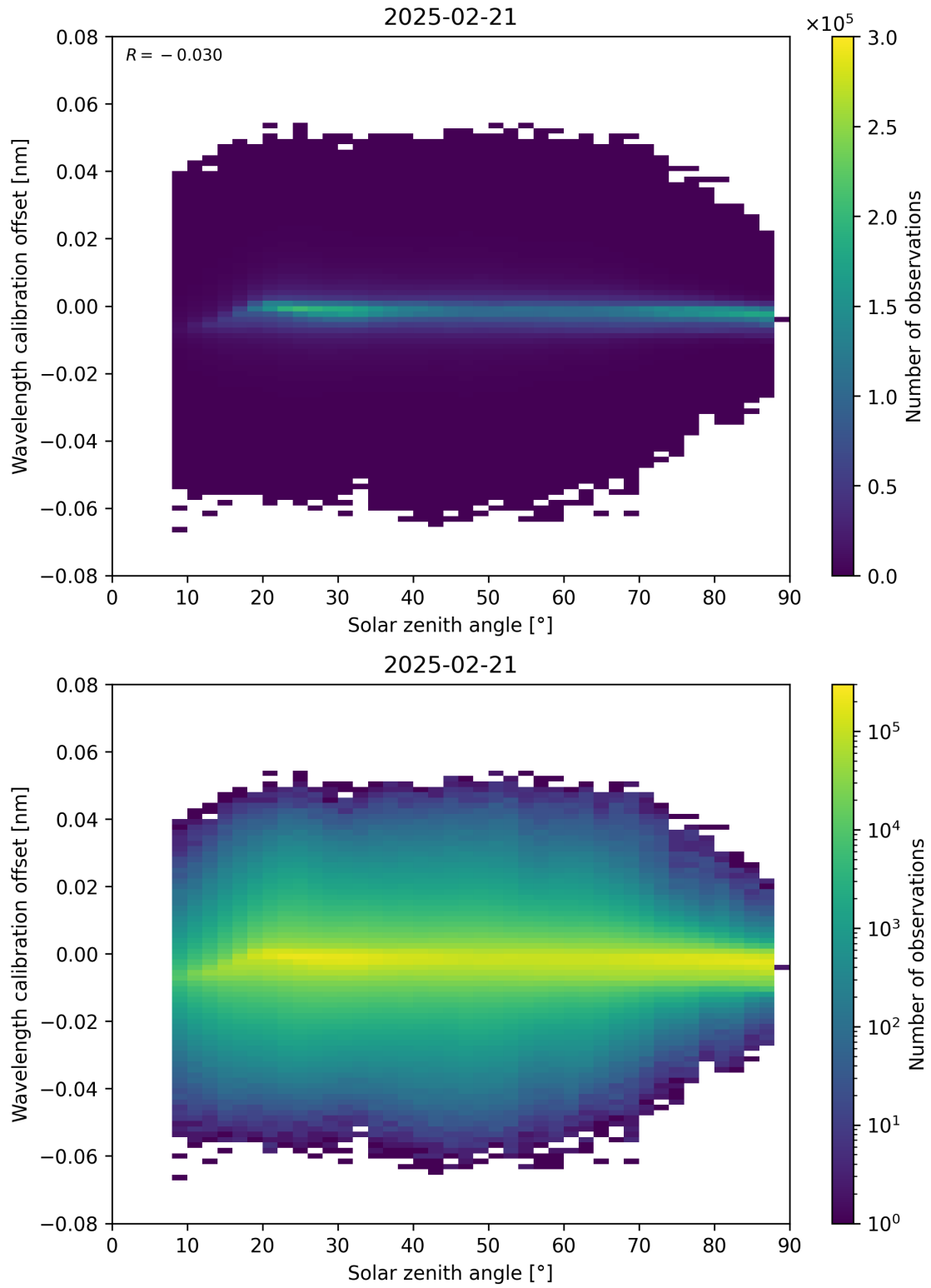
Figure 158: Scatter density plot of “Solar zenith angle” against “Wavelength calibration offset” for 2025-02-20 to 2025-02-22.
