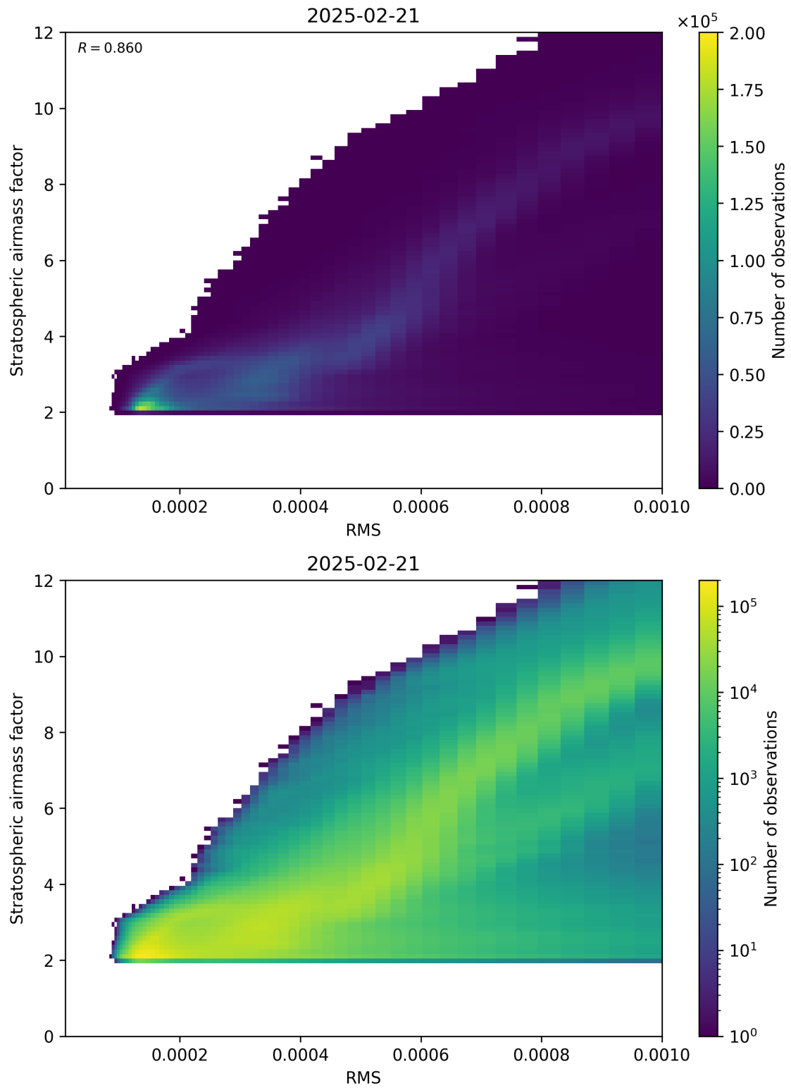
Figure 144: Scatter density plot of “RMS” against “Stratospheric airmass factor” for 2025-02-20 to 2025-02-22.
