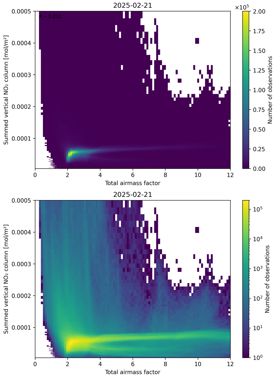
Figure 65: Scatter density plot of “Total airmass factor” against “Summed vertical NO 2 column” for 2025-02-20 to 2025-02-22.
