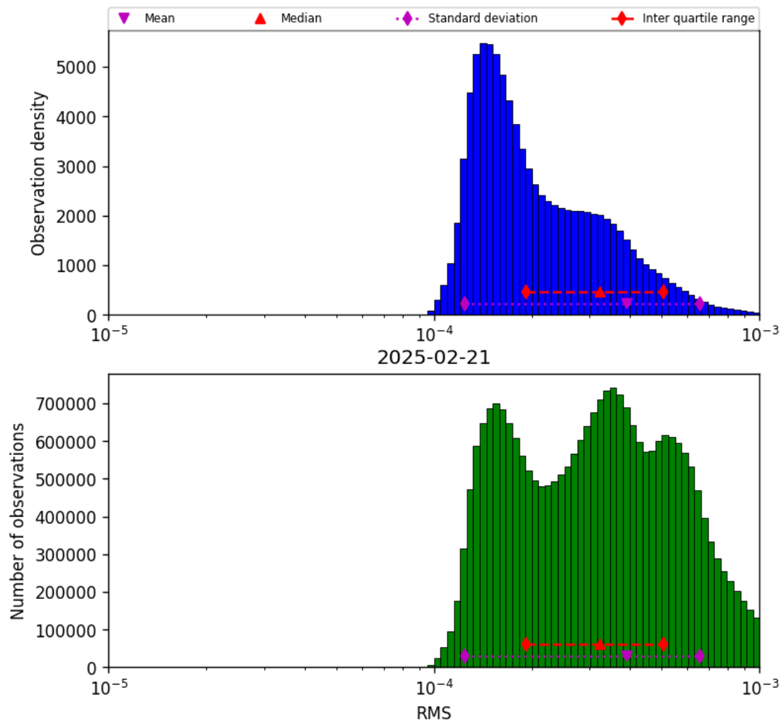
Figure 43: Histogram of “RMS” for 2025-02-20 to 2025-02-22
