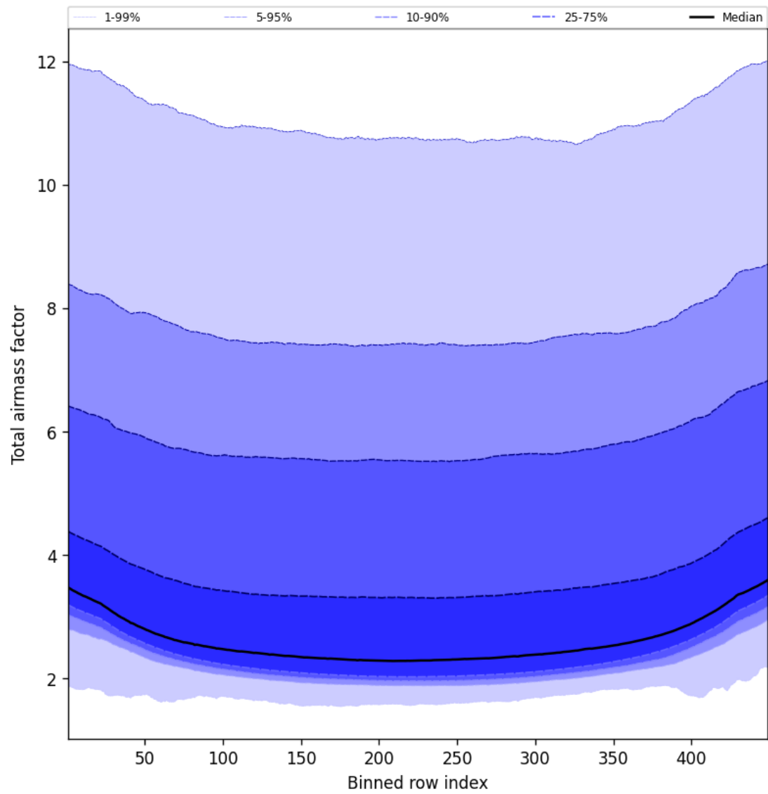
Figure 49: Along track statistics of “Total airmass factor” for 2025-02-20 to 2025-02-22
