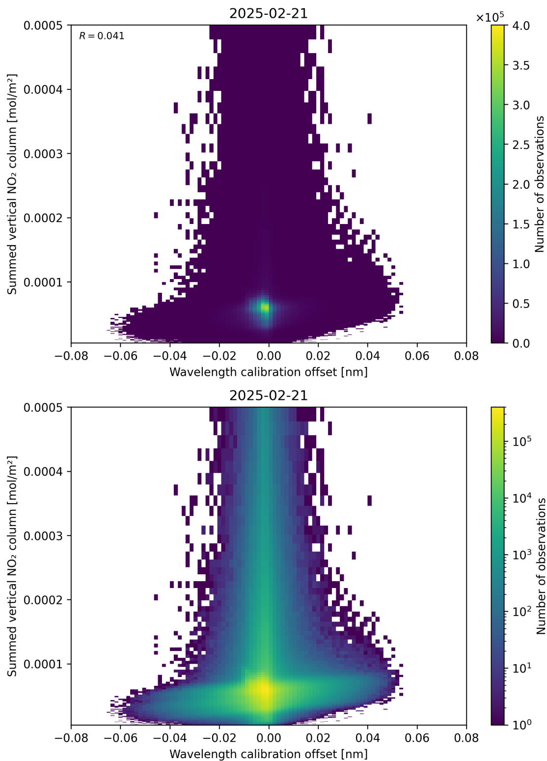
Figure 177: Scatter density plot of “Wavelength calibration offset” against “Summed vertical NO 2 column” for 2025-02-20 to 2025-02-22.
