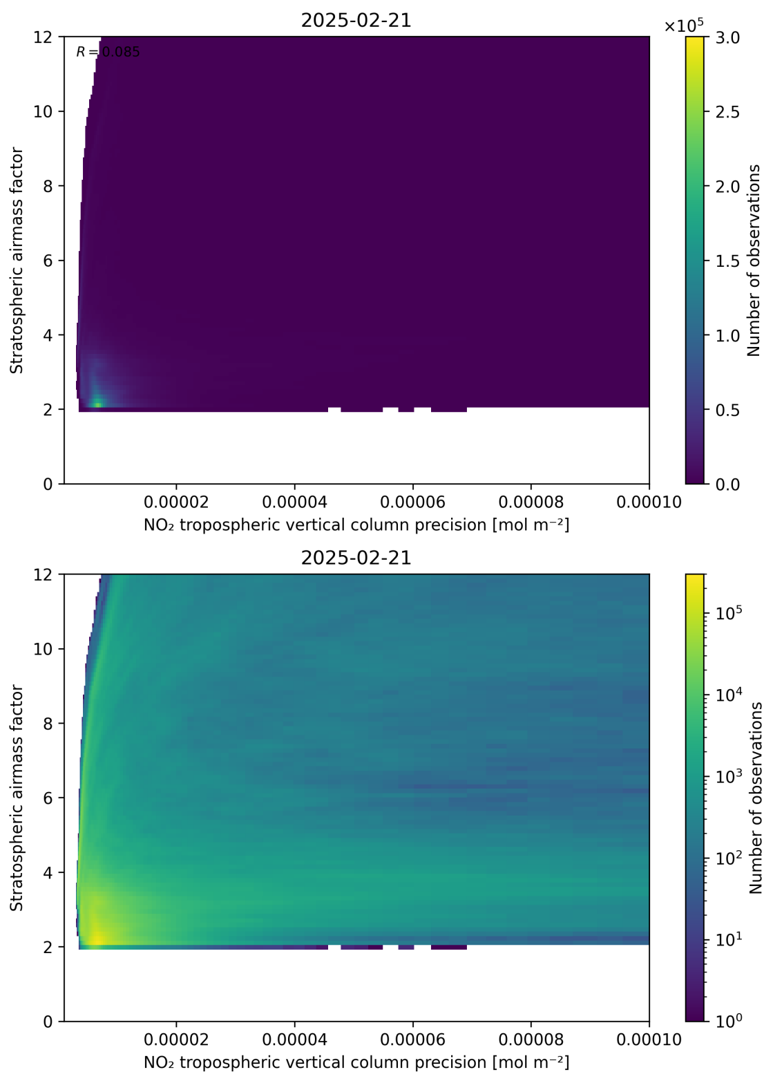
Figure 131: Scatter density plot of “NO 2 tropospheric vertical column precision” against “Stratospheric airmass factor” for 2025-02-20 to 2025-02-22.
