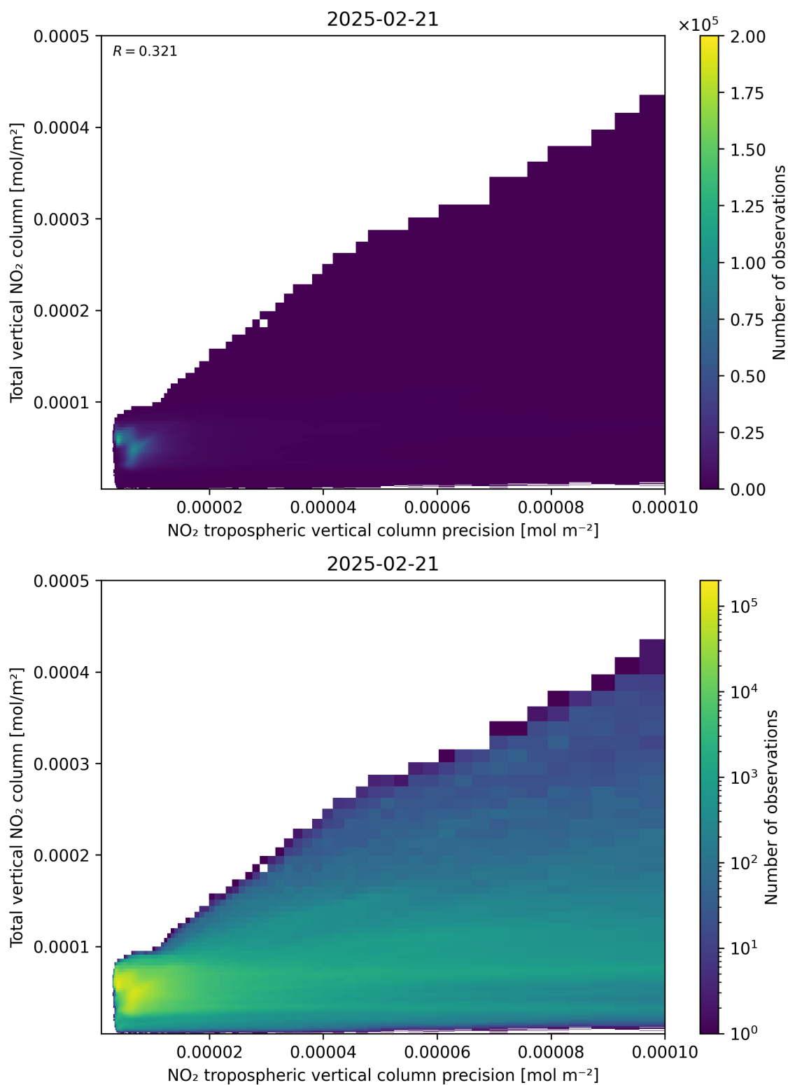
Figure 138: Scatter density plot of “NO 2 tropospheric vertical column precision” against “Total vertical NO 2 column” for 2025-02-20 to 2025-02-22.
