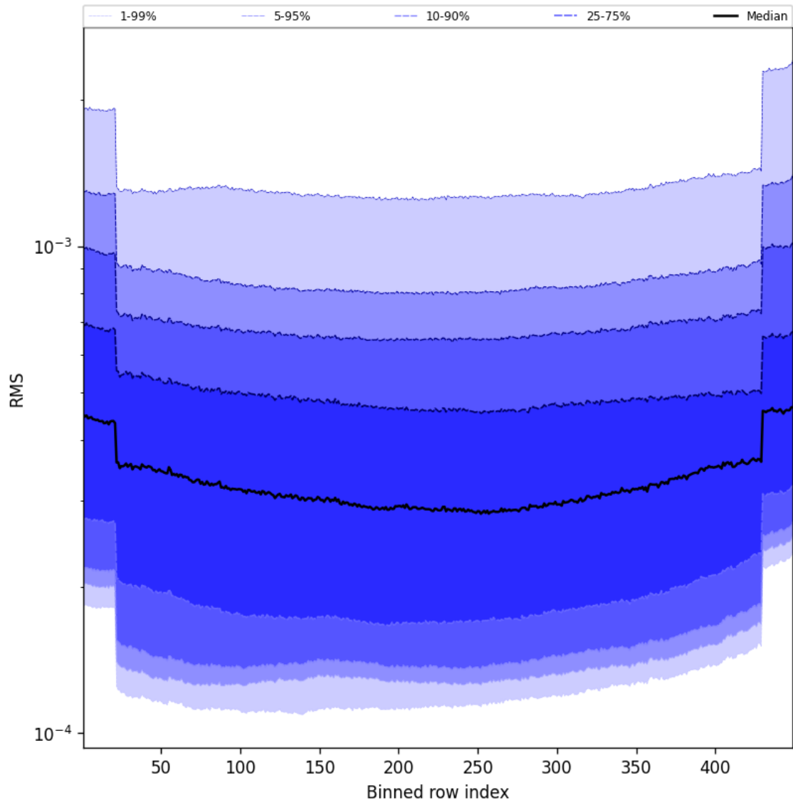
Figure 60: Along track statistics of “RMS” for 2025-02-20 to 2025-02-22
