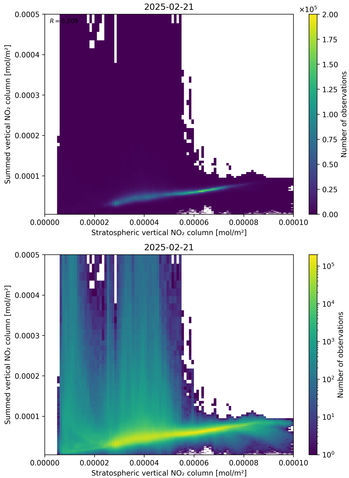
Figure 98: Scatter density plot of “Stratospheric vertical NO 2 column” against “Summed vertical NO 2 column” for 2025-02-20 to 2025-02-22.
