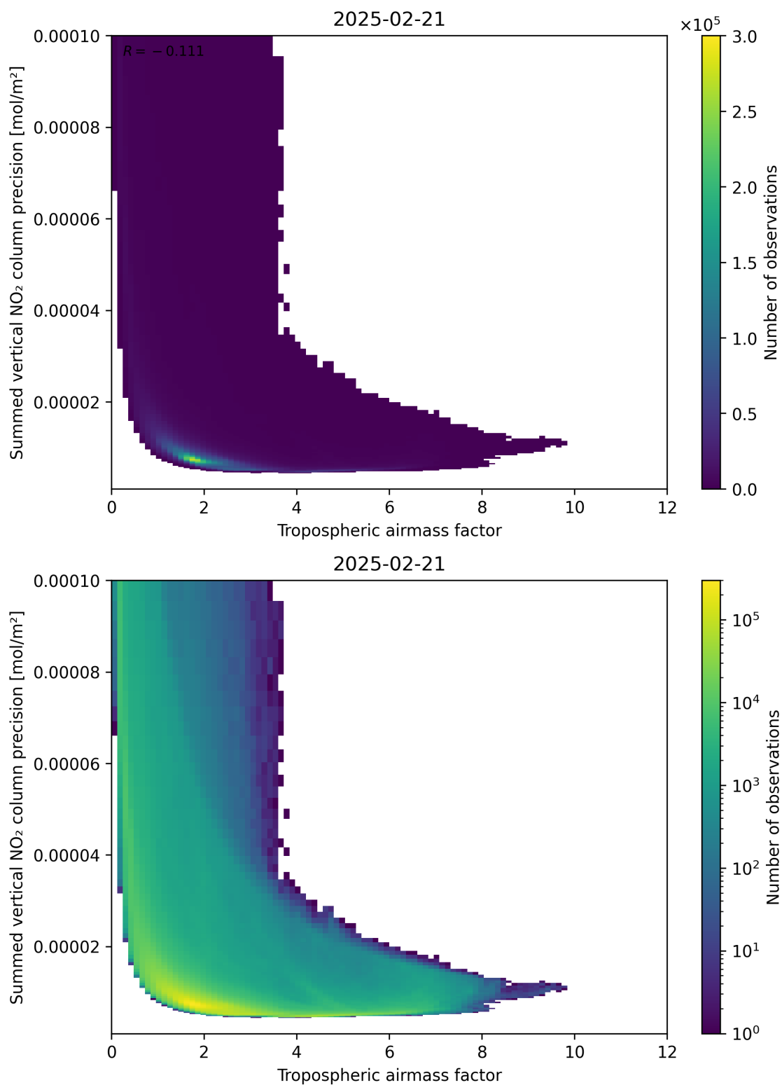
Figure 76: Scatter density plot of “Tropospheric air mass factor” against “Summed vertical NO 2 column precision” for 2025-02-20 to 2025-02-22.
