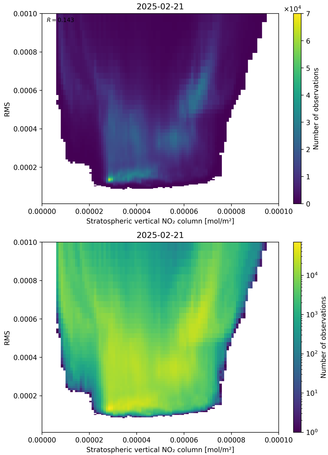
Figure 102: Scatter density plot of “Stratospheric vertical NO 2 column” against “RMS” for 2025-02-20 to 2025-02-22.
