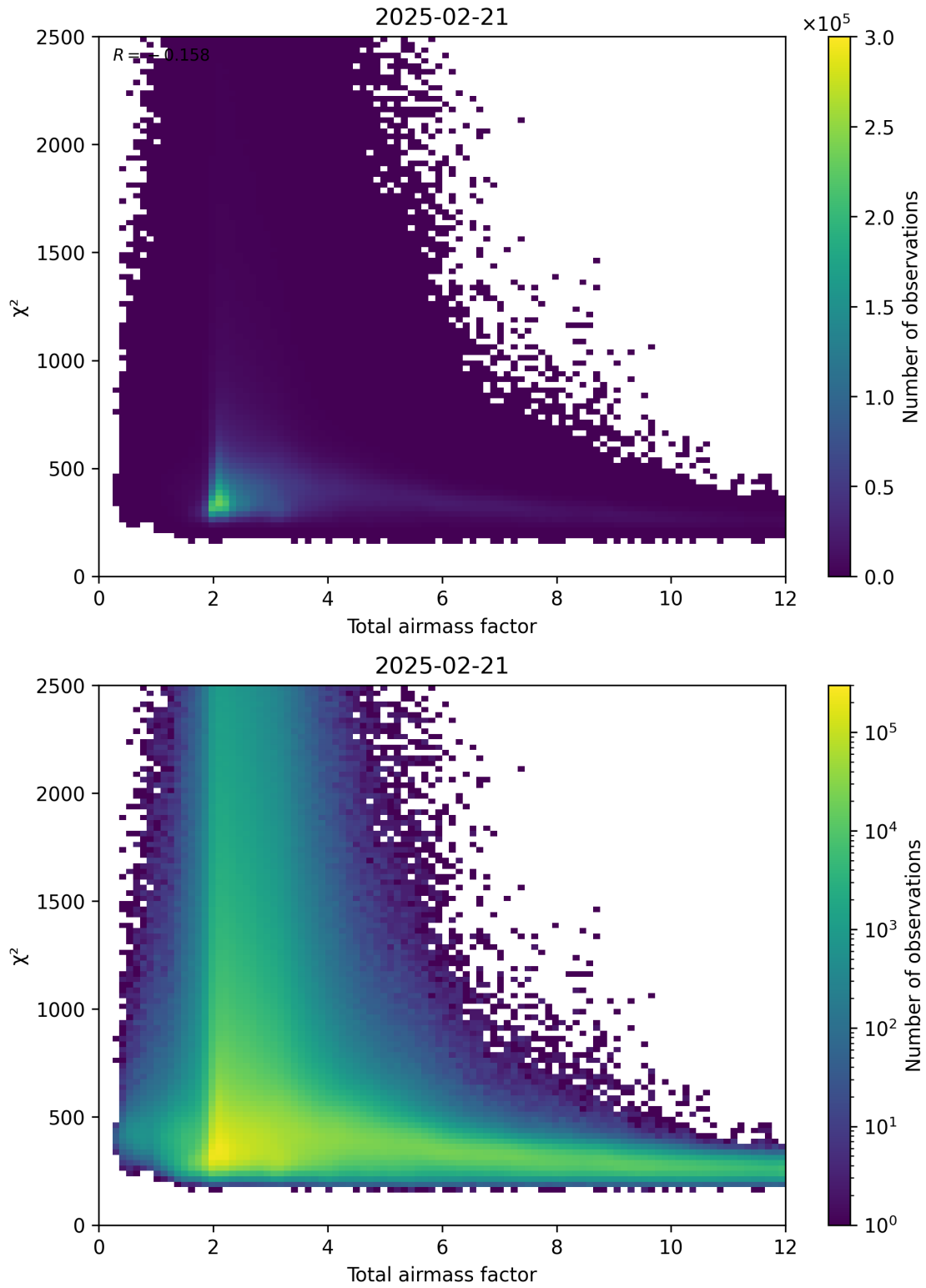
Figure 63: Scatter density plot of “Total airmass factor” against “ \chi^2 ” for 2025-02-20 to 2025-02-22.
