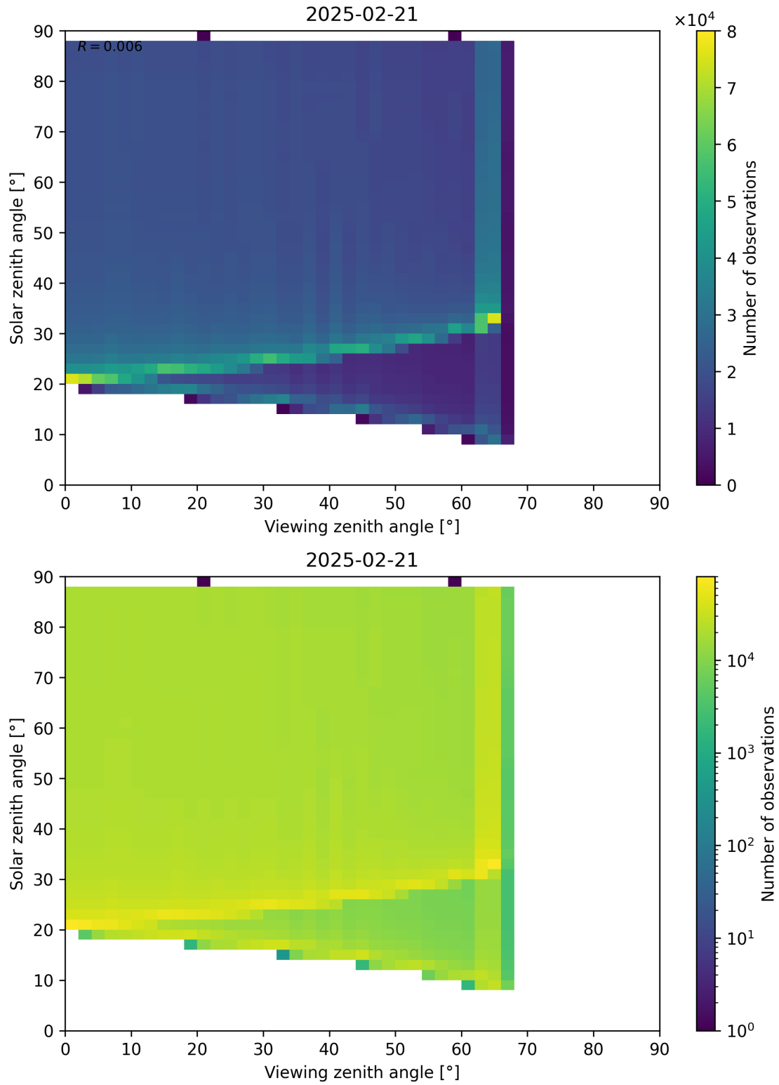
Figure 172: Scatter density plot of “Viewing zenith angle” against “Solar zenith angle” for 2025-02-20 to 2025-02-22.
