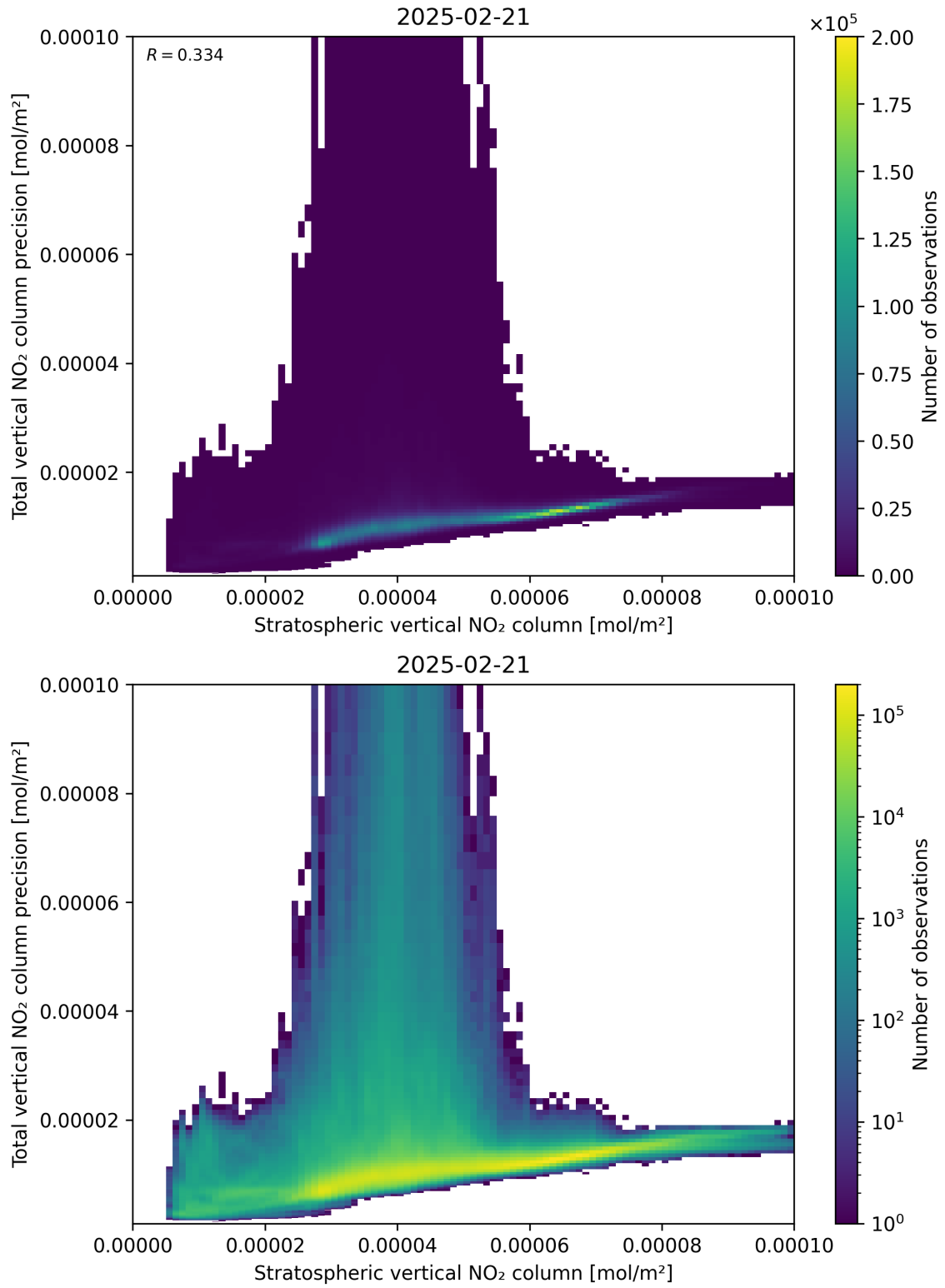
Figure 101: Scatter density plot of “Stratospheric vertical NO 2 column” against “Total vertical NO 2 column precision” for 2025-02-20 to 2025-02-22.
