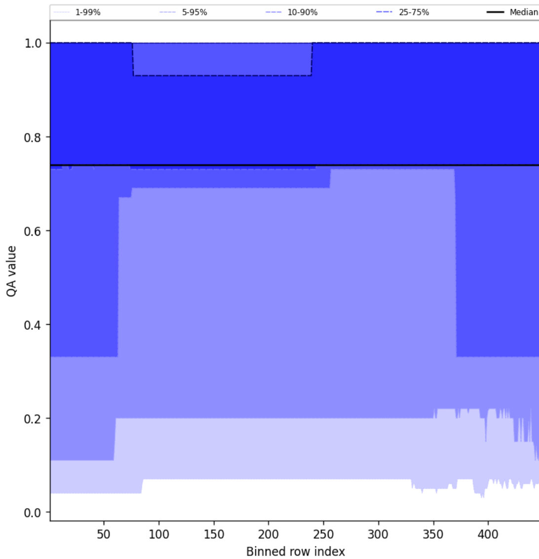
Figure 45: Along track statistics of "QA value" for 2025-02-20 to 2025-02-22
