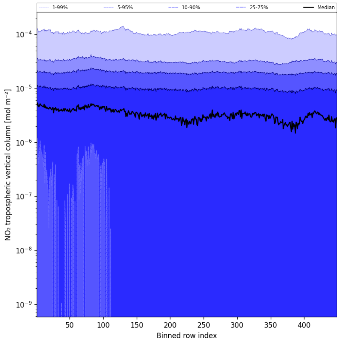
Figure 46: Along track statistics of “NO 2 tropospheric vertical column” for 2025-02-20 to 2025-02-22
