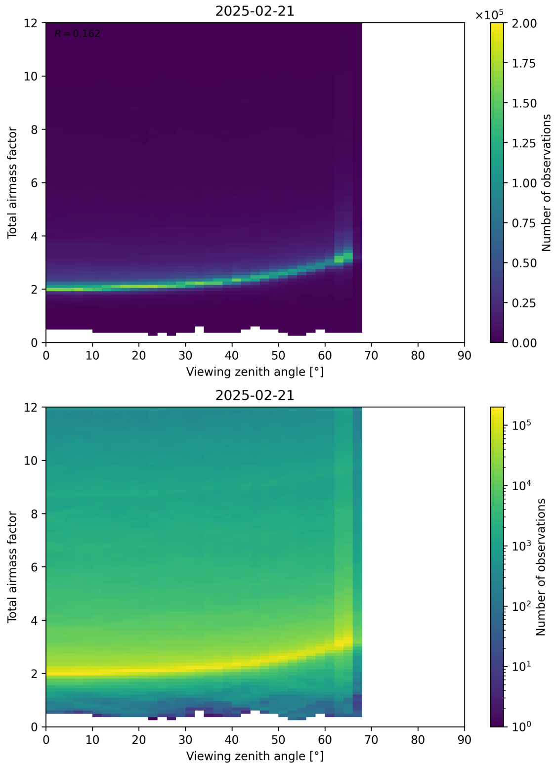
Figure 160: Scatter density plot of “Viewing zenith angle” against “Total airmass factor” for 2025-02-20 to 2025-02-22.
