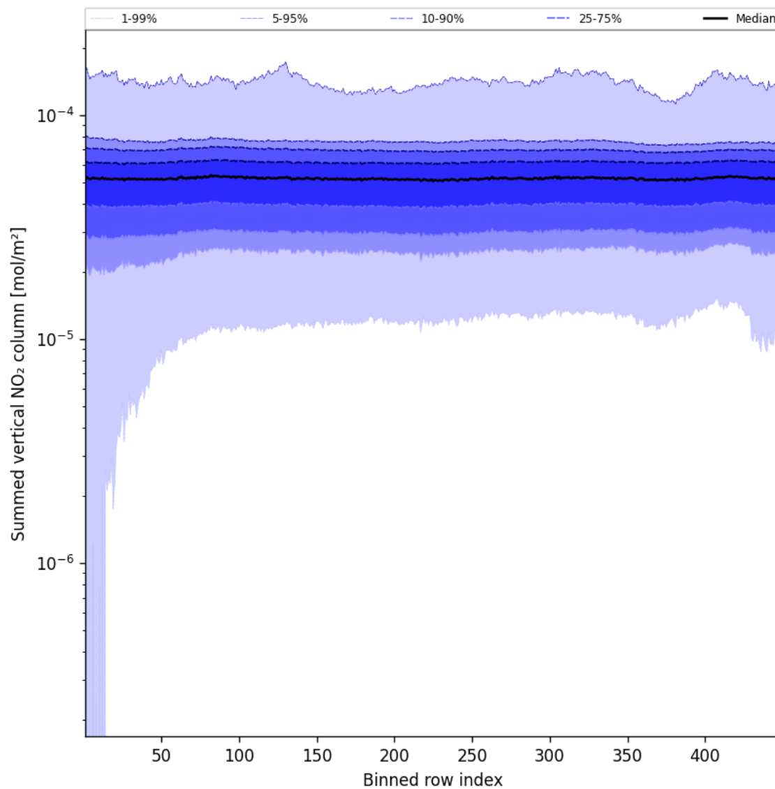
Figure 57: Along track statistics of “Summed vertical NO 2 column” for 2025-02-20 to 2025-02-22
