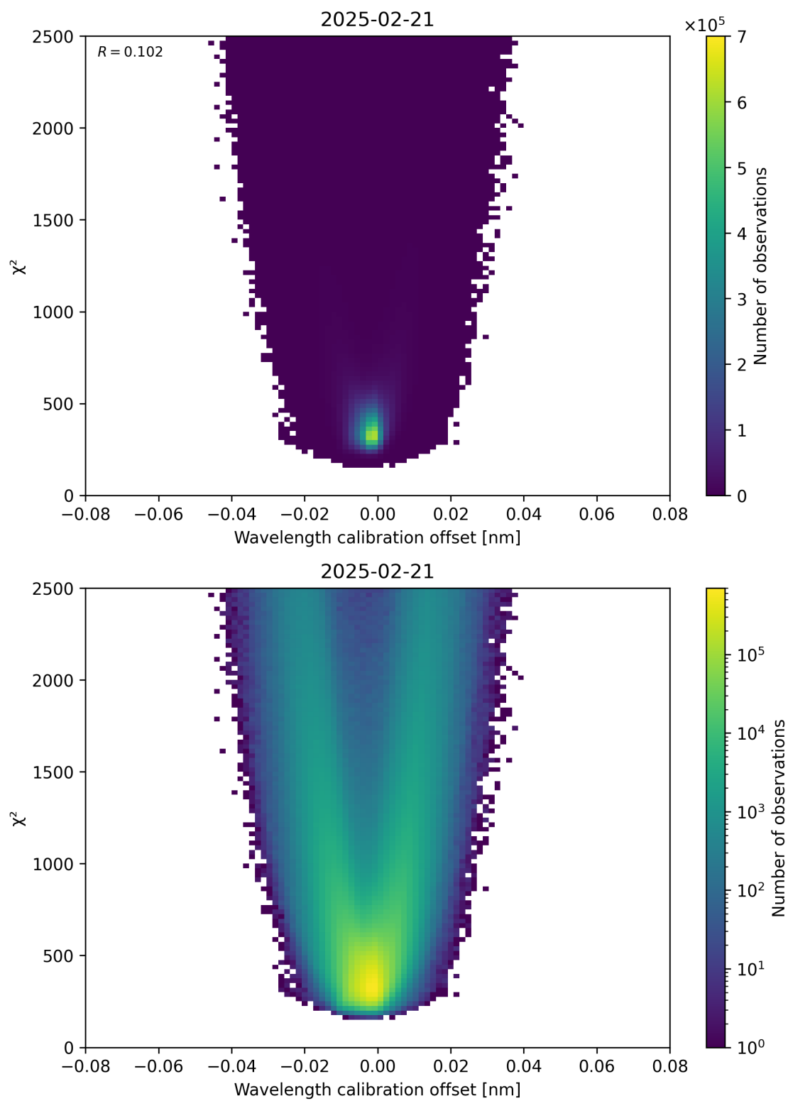
Figure 175: Scatter density plot of “Wavelength calibration offset” against “ \chi^2 ” for 2025-02-20 to 2025-02-22.
