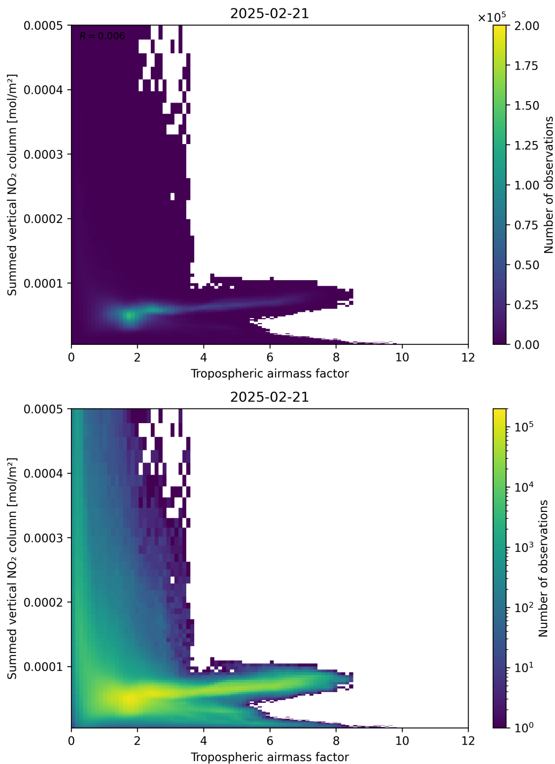
Figure 75: Scatter density plot of “Tropospheric air mass factor” against “Summed vertical NO 2 column” for 2025-02-20 to 2025-02-22.
