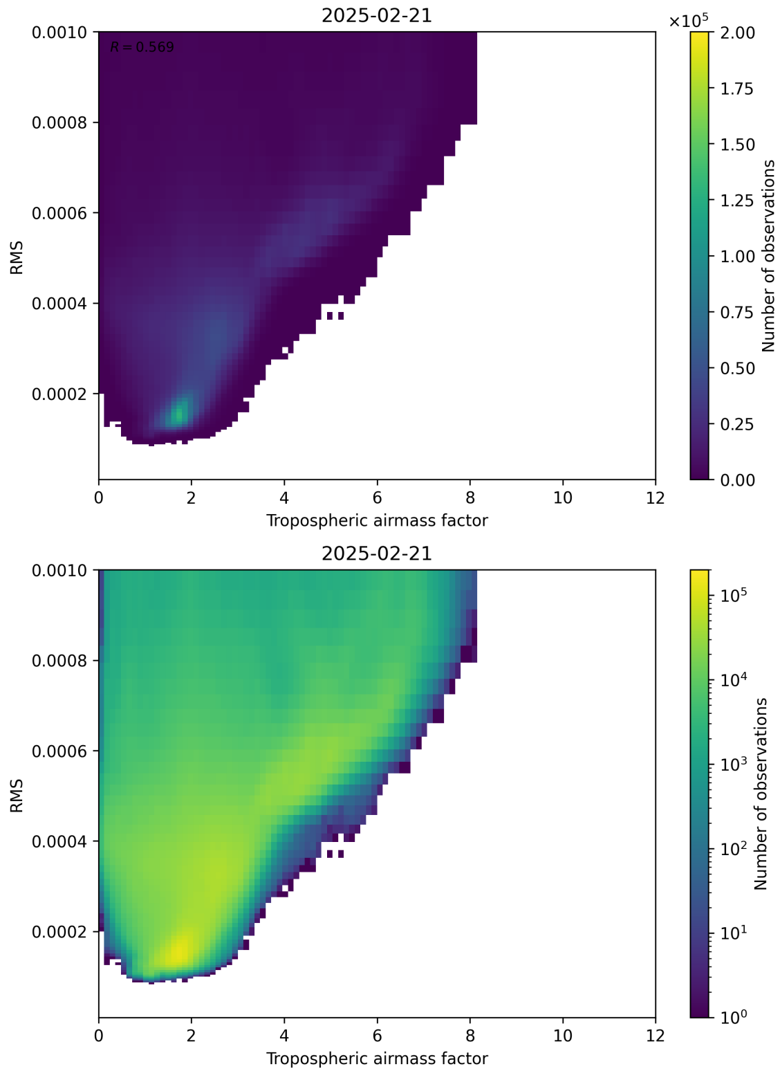
Figure 79: Scatter density plot of “Tropospheric airmass factor” against “RMS” for 2025-02-20 to 2025-02-22.
