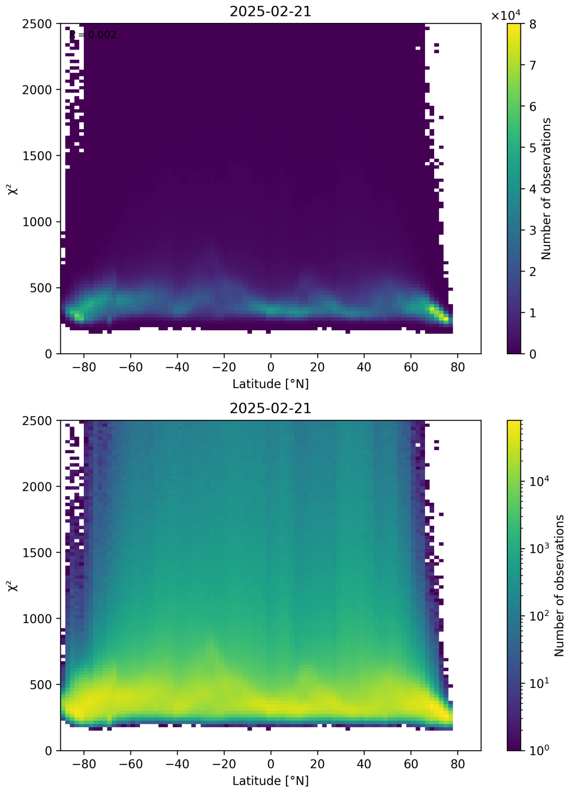
Figure 86: Scatter density plot of “Latitude” against “ \chi^2 ” for 2025-02-20 to 2025-02-22.
