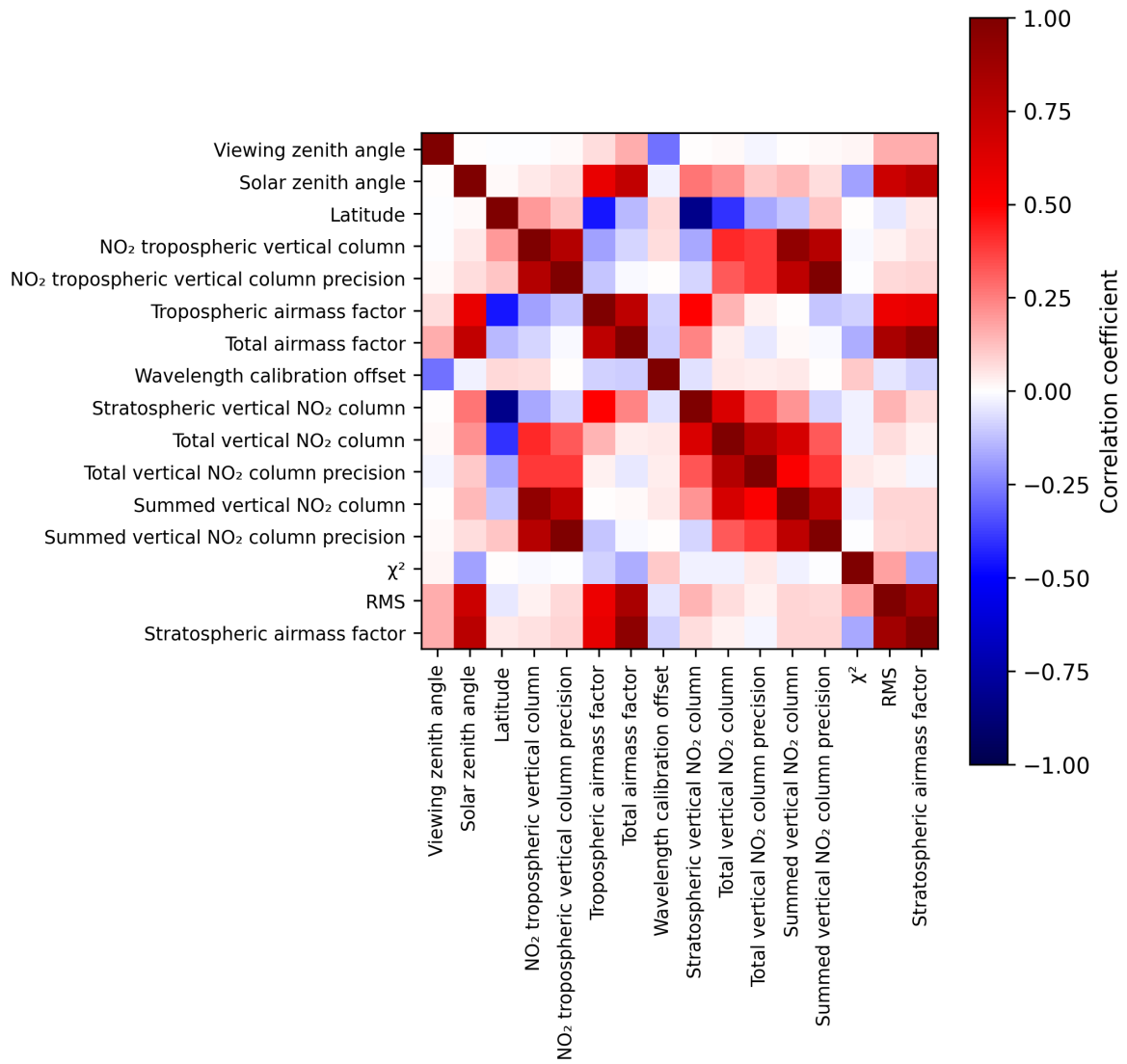
Figure 2: Map of correlation matrix for 2025-02-20 to 2025-02-22.
