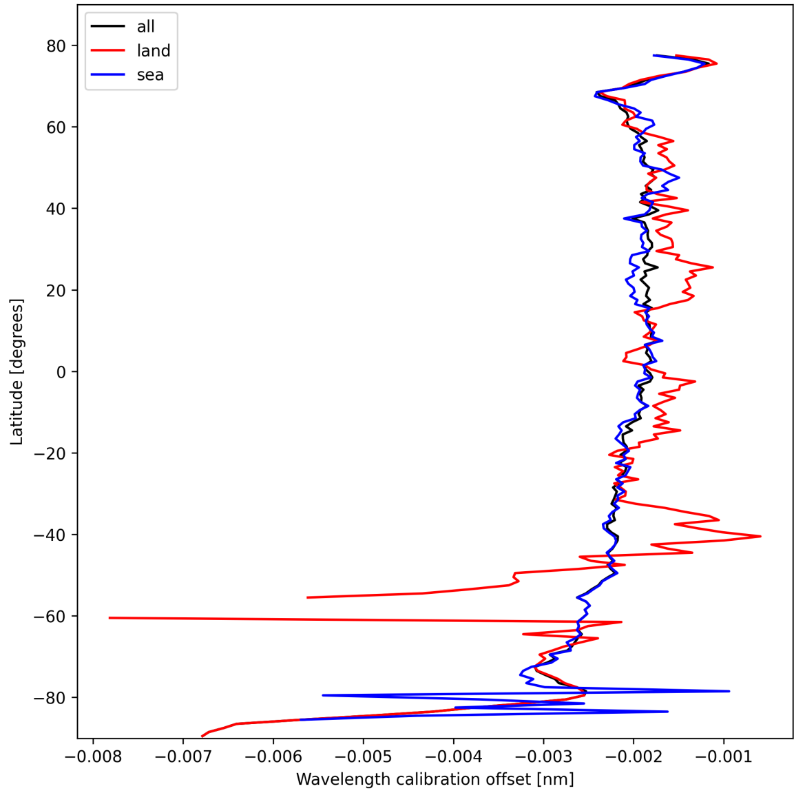
Figure 18: Zonal average of “Wavelength calibration offset” for 2025-02-20 to 2025-02-22.
