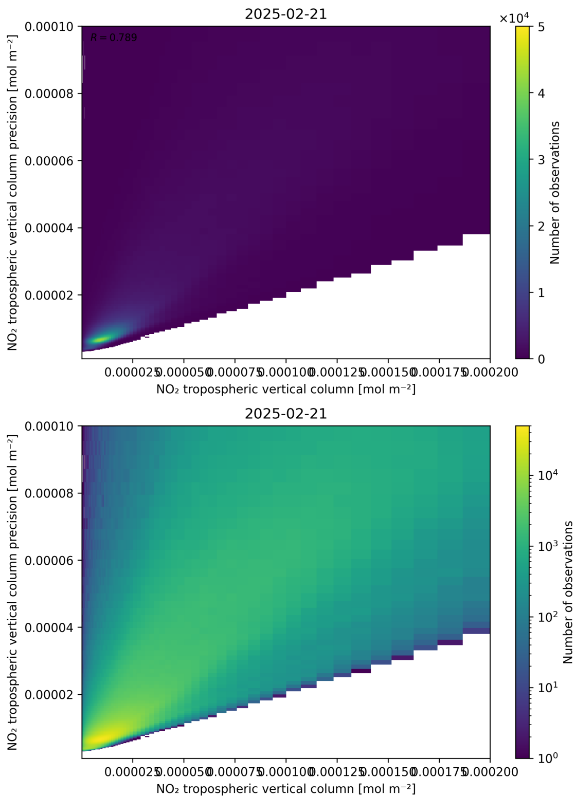
Figure 130: Scatter density plot of “NO 2 tropospheric vertical column” against “NO 2 tropospheric vertical column precision” for 2025-02-20 to 2025-02-22.
