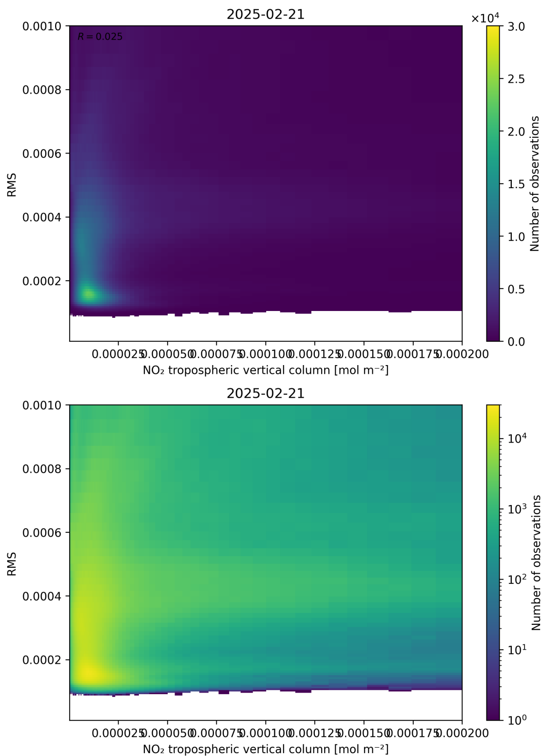
Figure 142: Scatter density plot of “NO 2 tropospheric vertical column” against “RMS” for 2025-02-20 to 2025-02-22.
