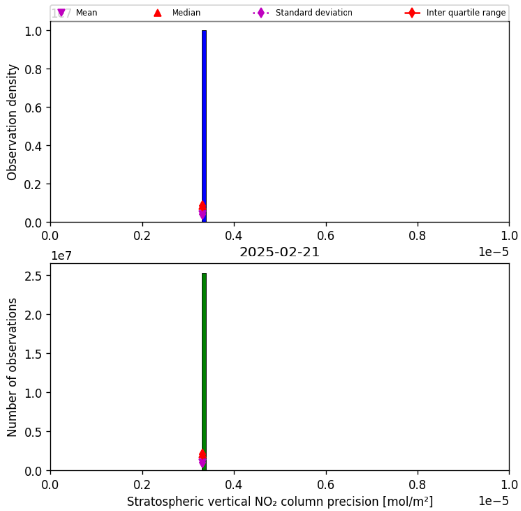
Figure 37: Histogram of “Stratospheric vertical NO 2 column precision” for 2025-02-20 to 2025-02-22
