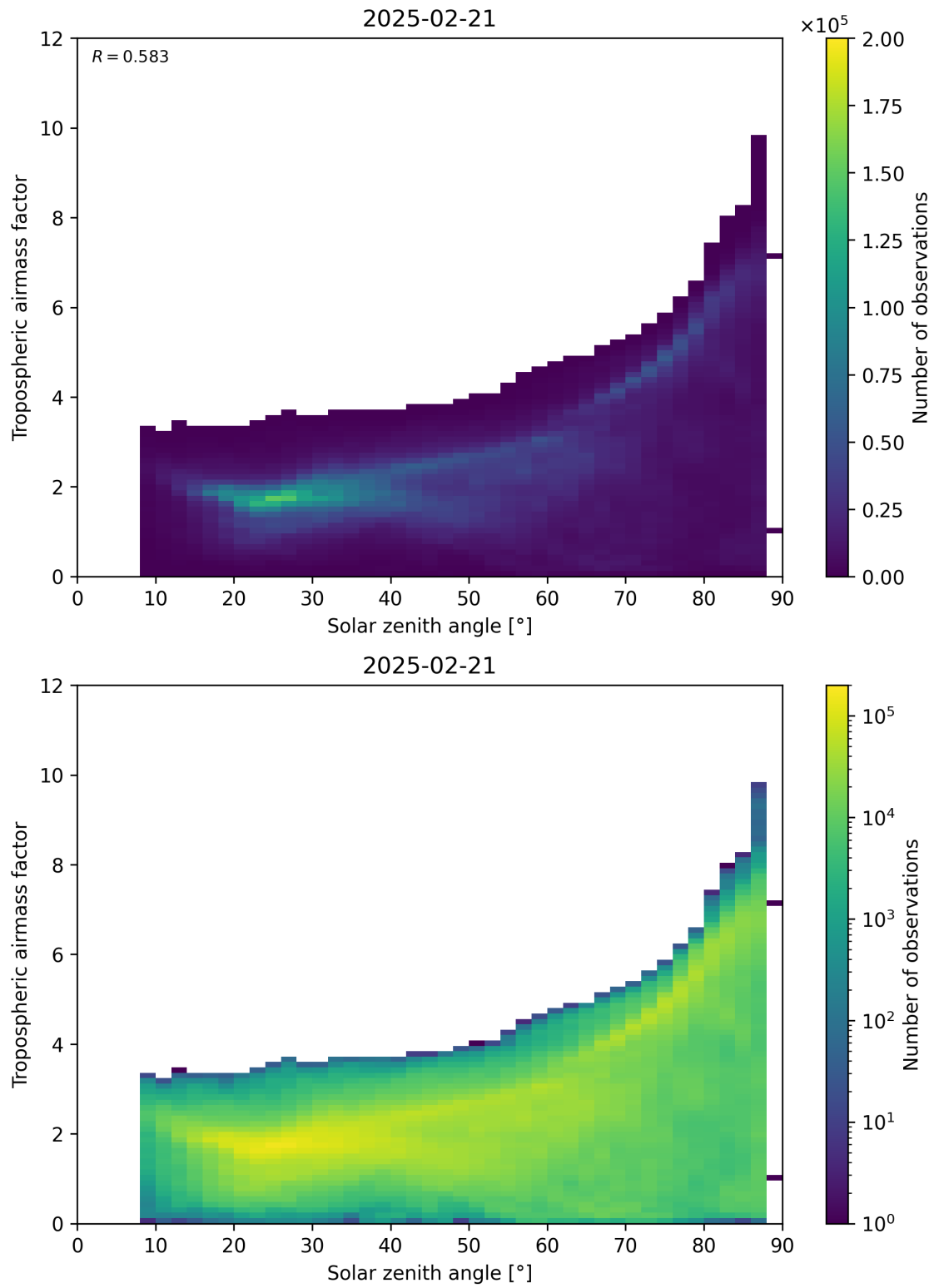
Figure 147: Scatter density plot of “Solar zenith angle” against “Tropospheric airmass factor” for 2025-02-20 to 2025-02-22.
