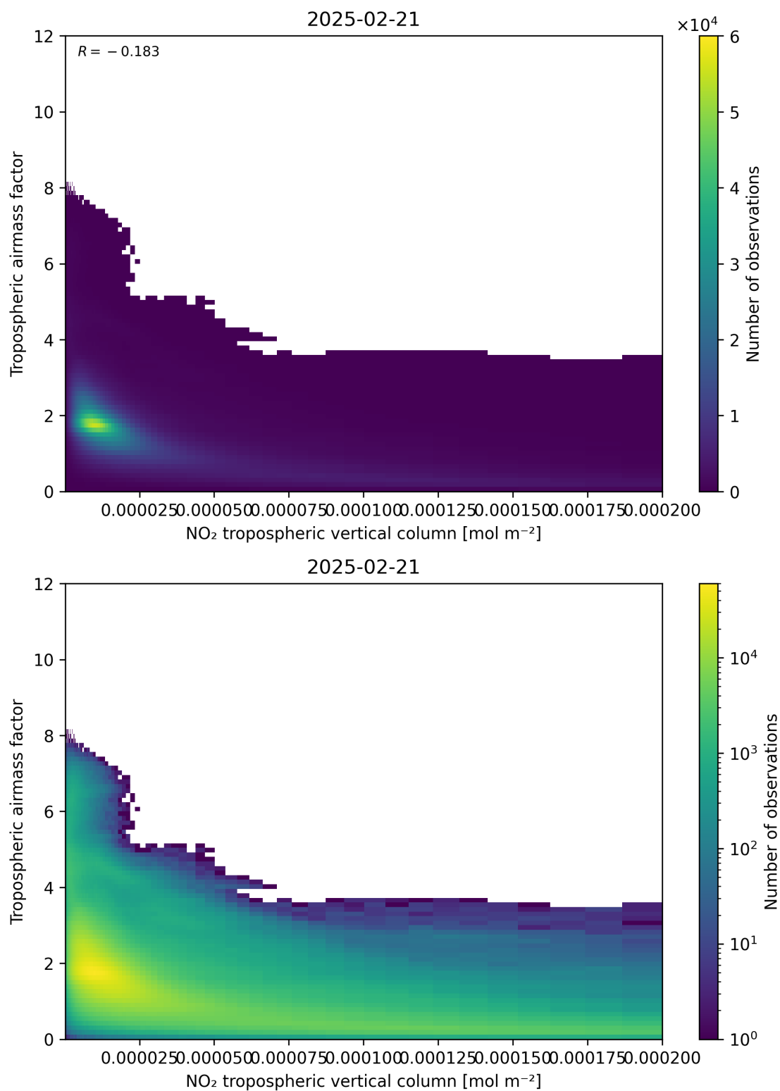
Figure 123: Scatter density plot of “NO 2 tropospheric vertical column” against “Tropospheric air mass factor” for 2025-02-20 to 2025-02-22.
