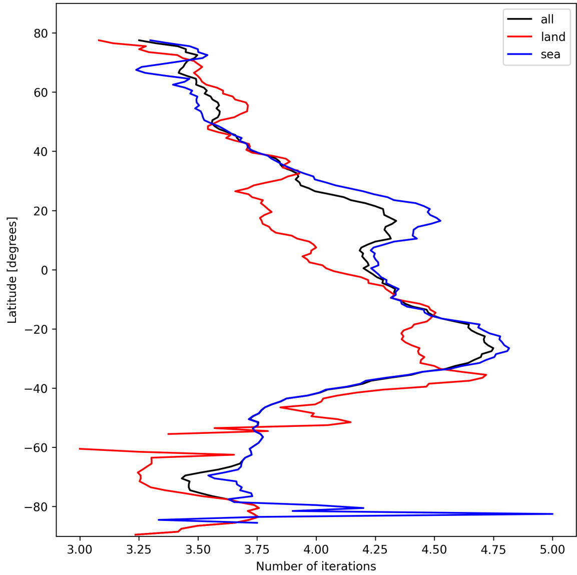
Figure 17: Zonal average of “Number of iterations” for 2025-02-20 to 2025-02-22.
