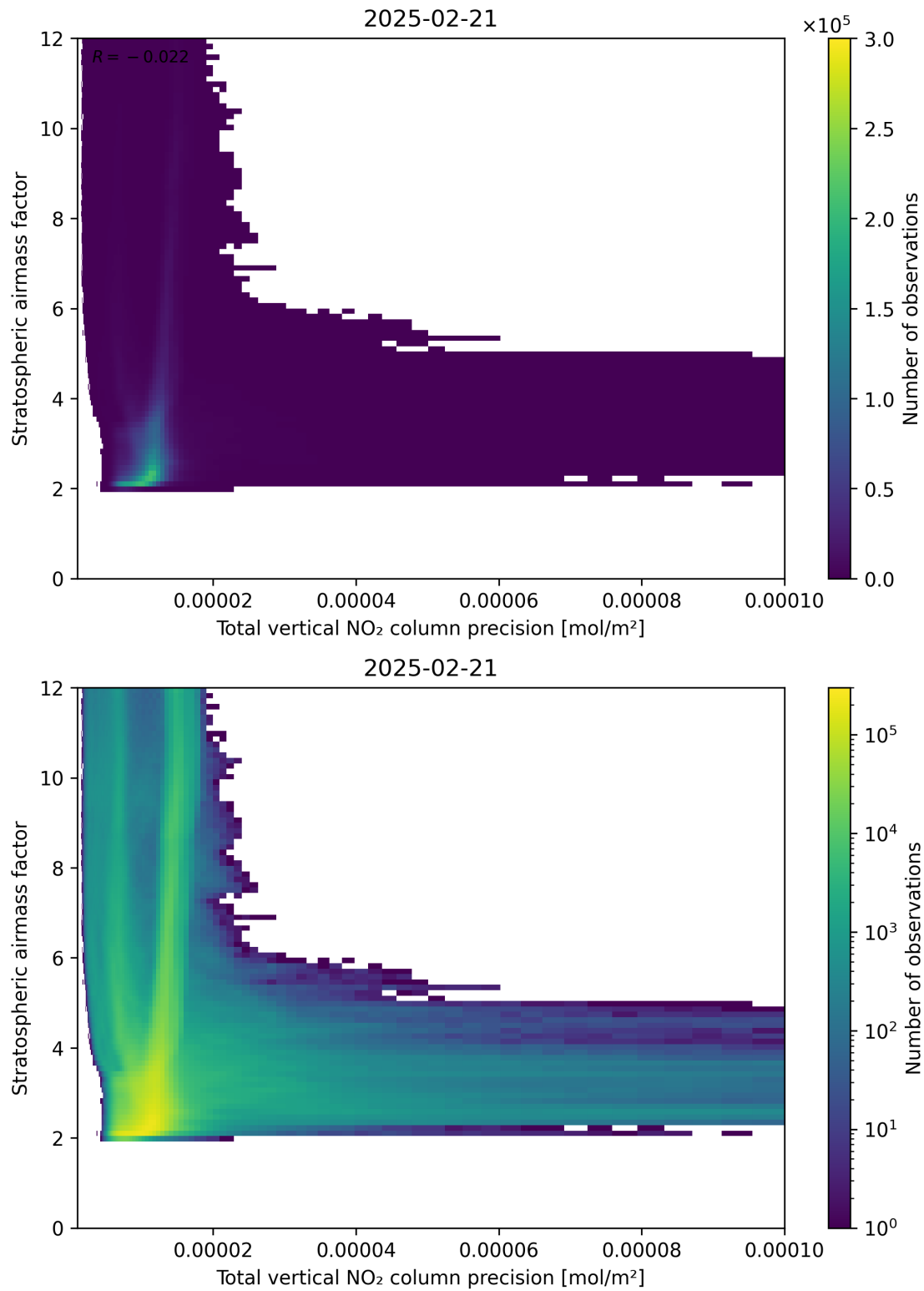
Figure 115: Scatter density plot of “Total vertical NO 2 column precision” against “Stratospheric air mass factor” for 2025-02-20 to 2025-02-22.
