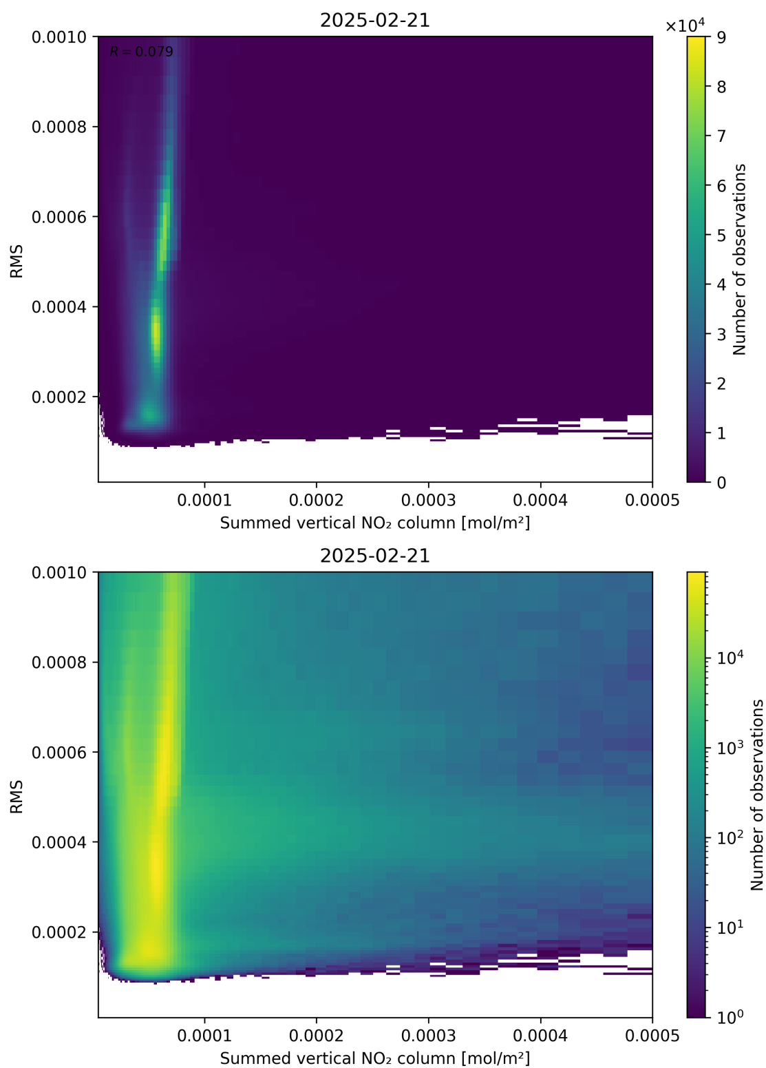
Figure 109: Scatter density plot of “Summed vertical NO 2 column” against “RMS” for 2025-02-20 to 2025-02-22.
