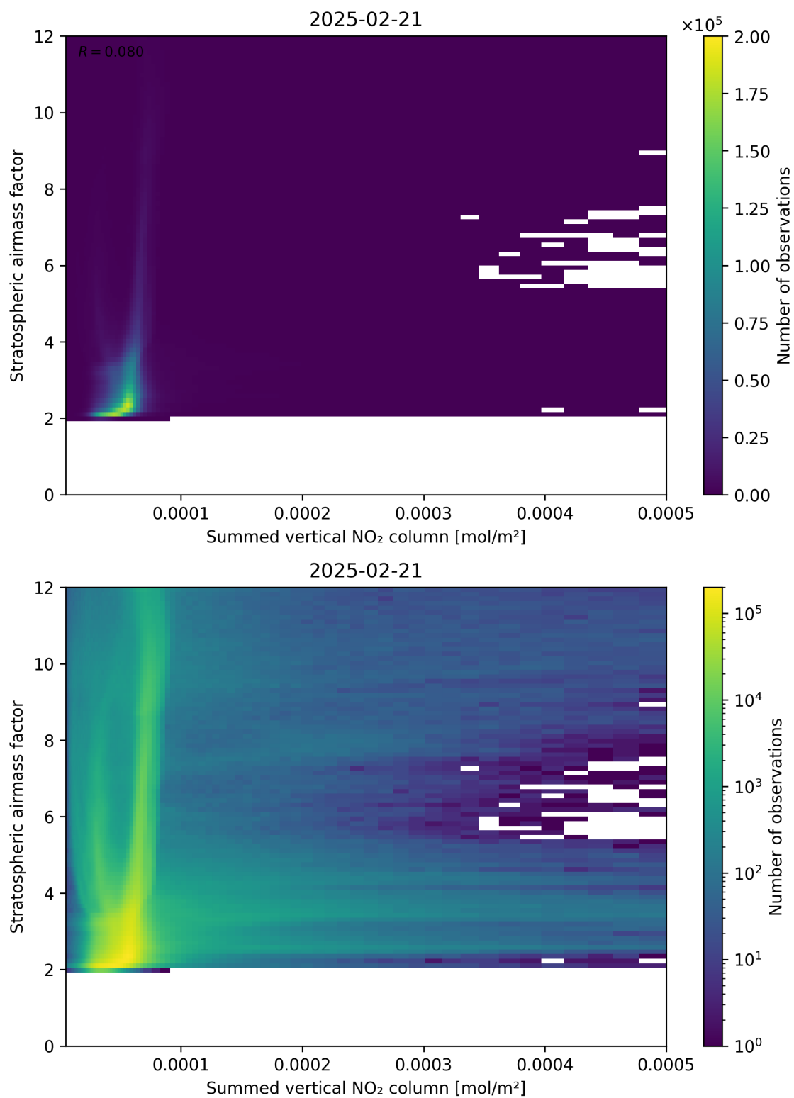
Figure 103: Scatter density plot of “Summed vertical NO 2 column” against “Stratospheric air mass factor” for 2025-02-20 to 2025-02-22.
