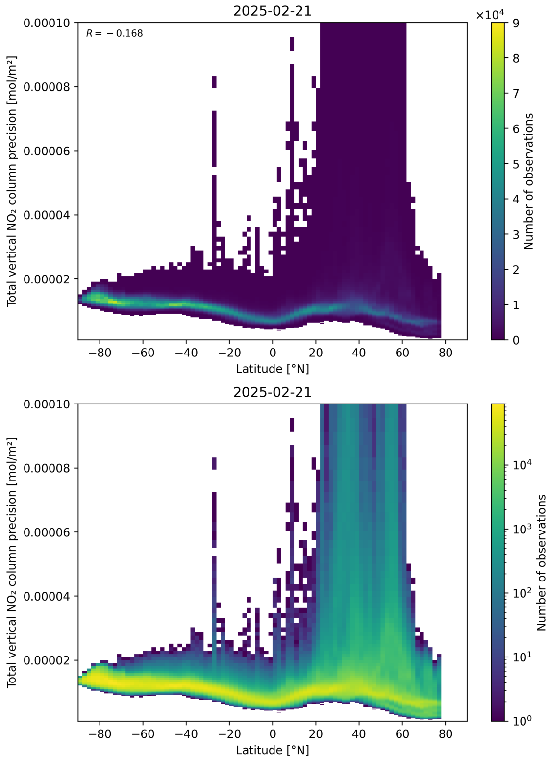
Figure 91: Scatter density plot of “Latitude” against “Total vertical NO 2 column precision” for 2025-02-20 to 2025-02-22.
