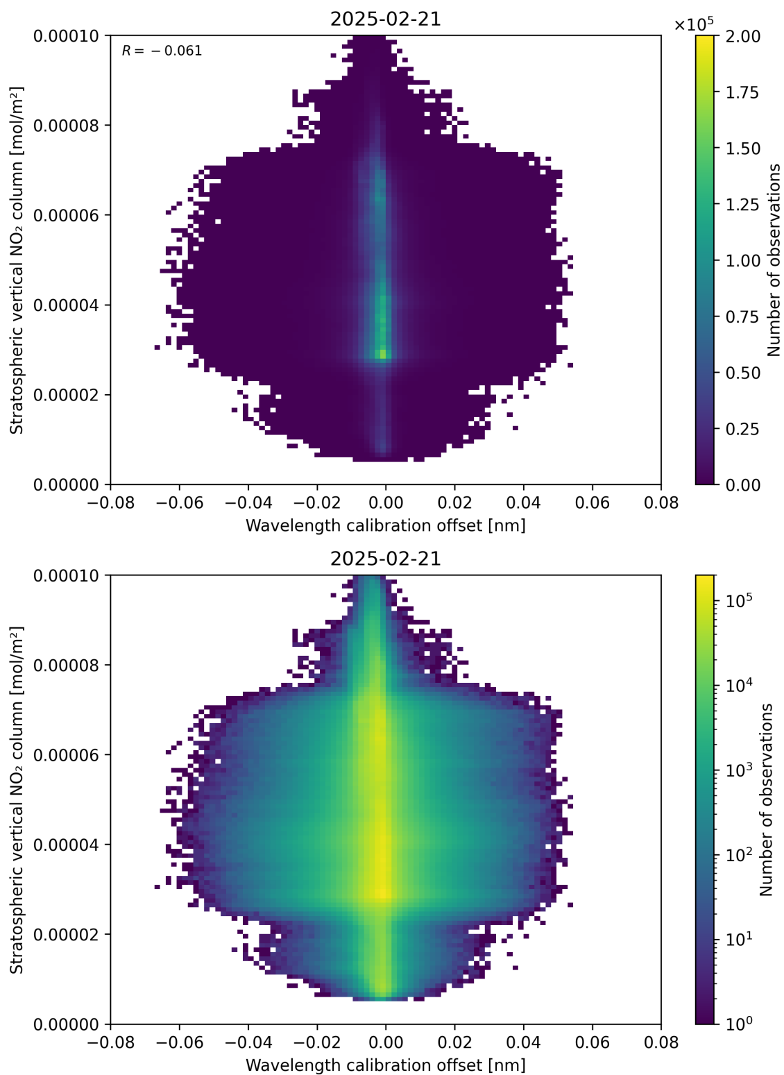
Figure 176: Scatter density plot of “Wavelength calibration offset” against “Stratospheric vertical NO 2 column” for 2025-02-20 to 2025-02-22.
