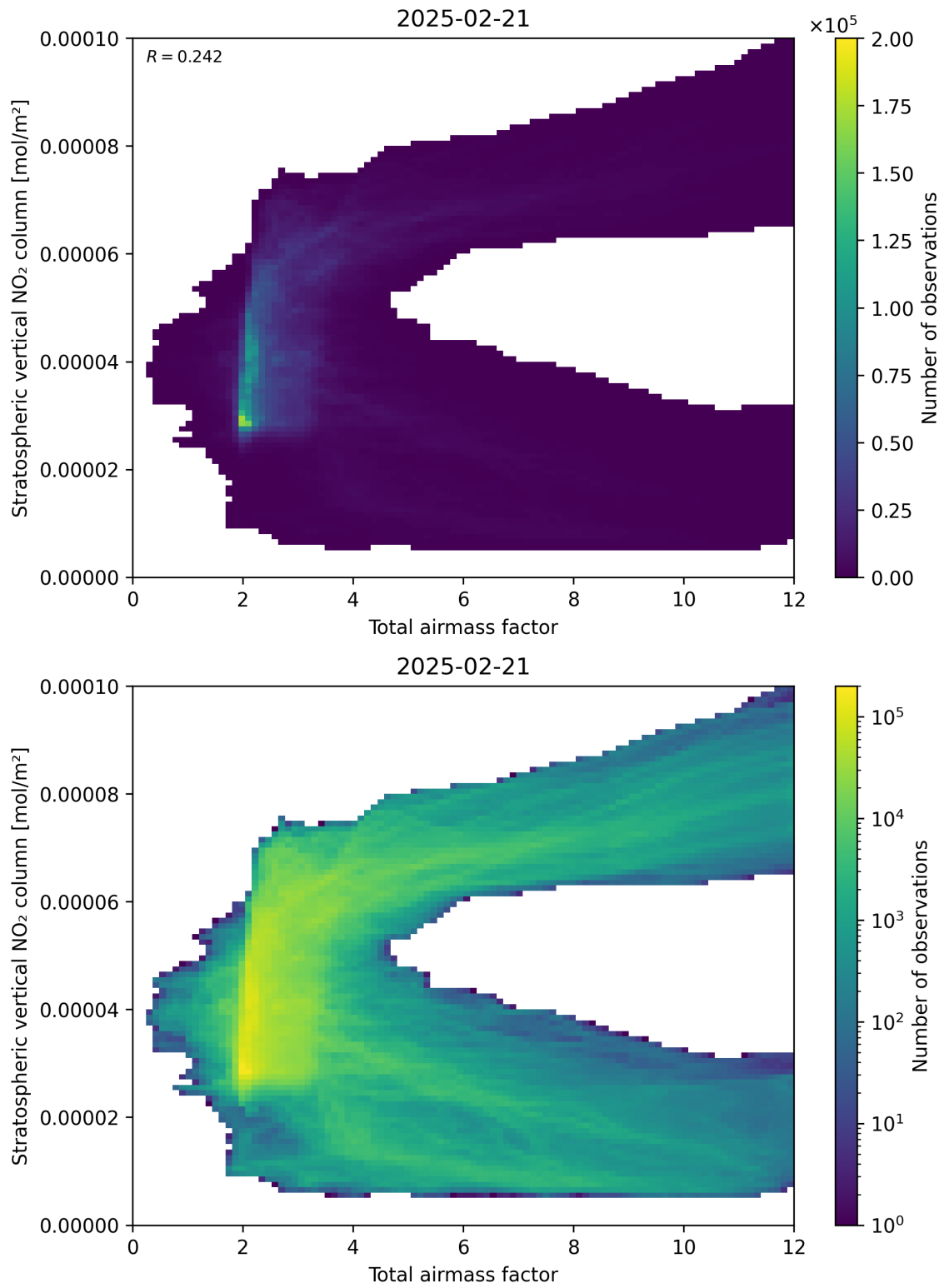
Figure 64: Scatter density plot of “Total airmass factor” against “Stratospheric vertical NO 2 column” for 2025-02-20 to 2025-02-22.
