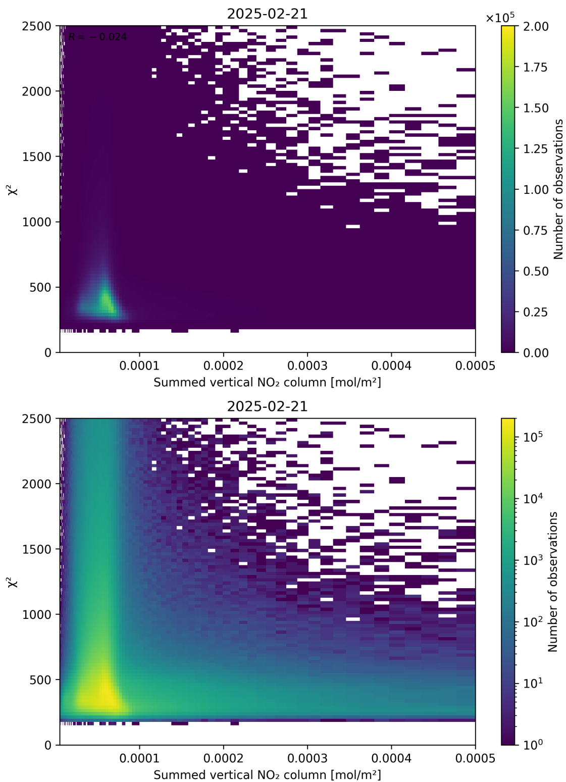
Figure 104: Scatter density plot of “Summed vertical NO 2 column” against “ \chi^2 ” for 2025-02-20 to 2025-02-22.
