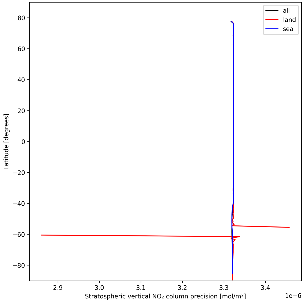
Figure 20: Zonal average of “Stratospheric vertical NO 2 column precision” for 2025-02-20 to 2025-02-22.
