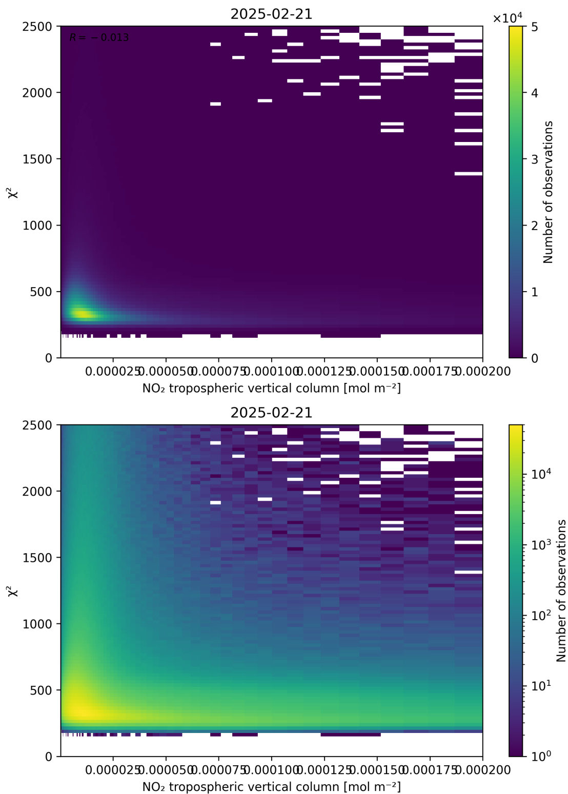
Figure 124: Scatter density plot of “NO 2 tropospheric vertical column” against “ \chi^2 ” for 2025-02-20 to 2025-02-22.
