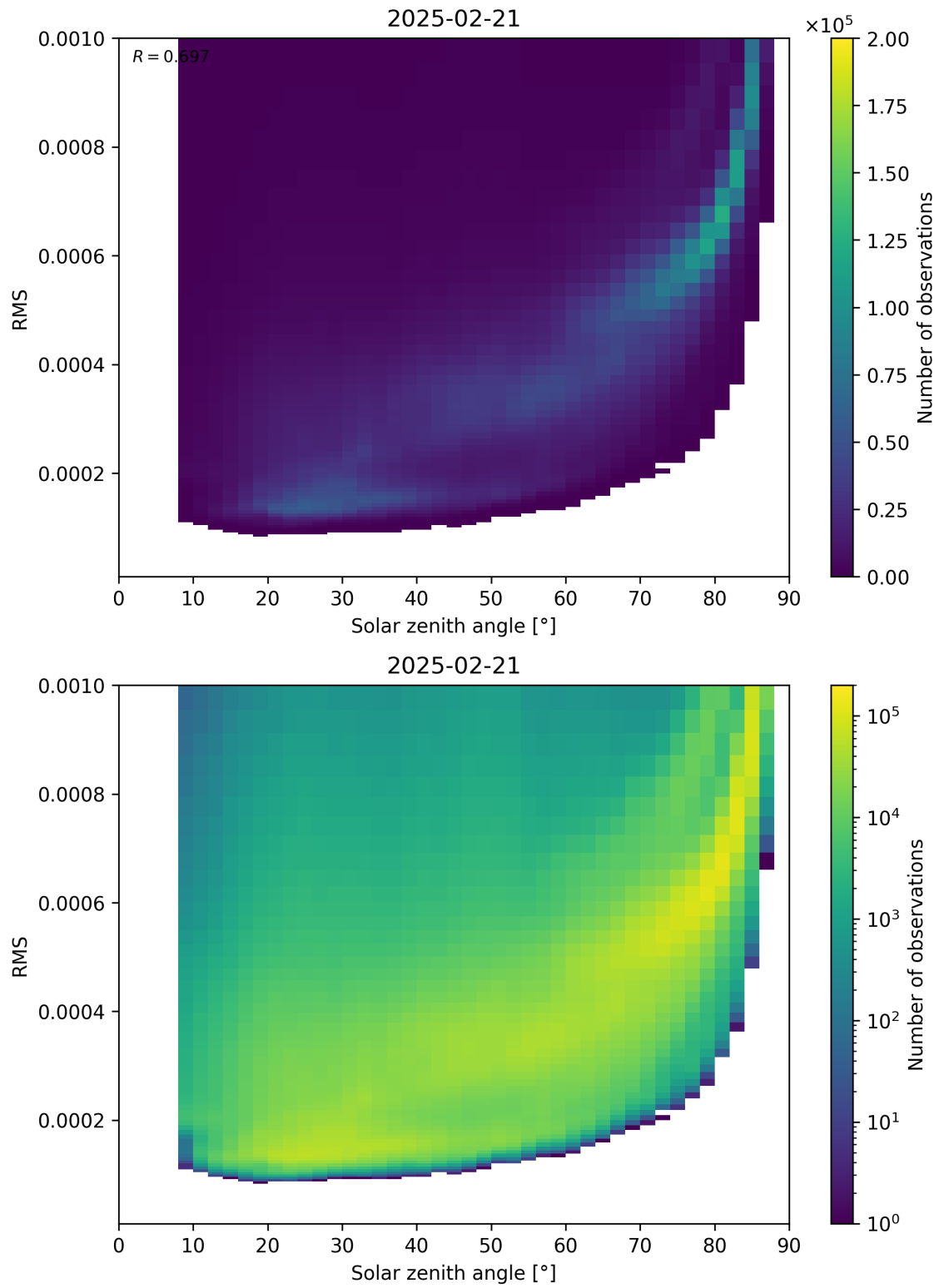
Figure 157: Scatter density plot of “Solar zenith angle” against “RMS” for 2025-02-20 to 2025-02-22.
