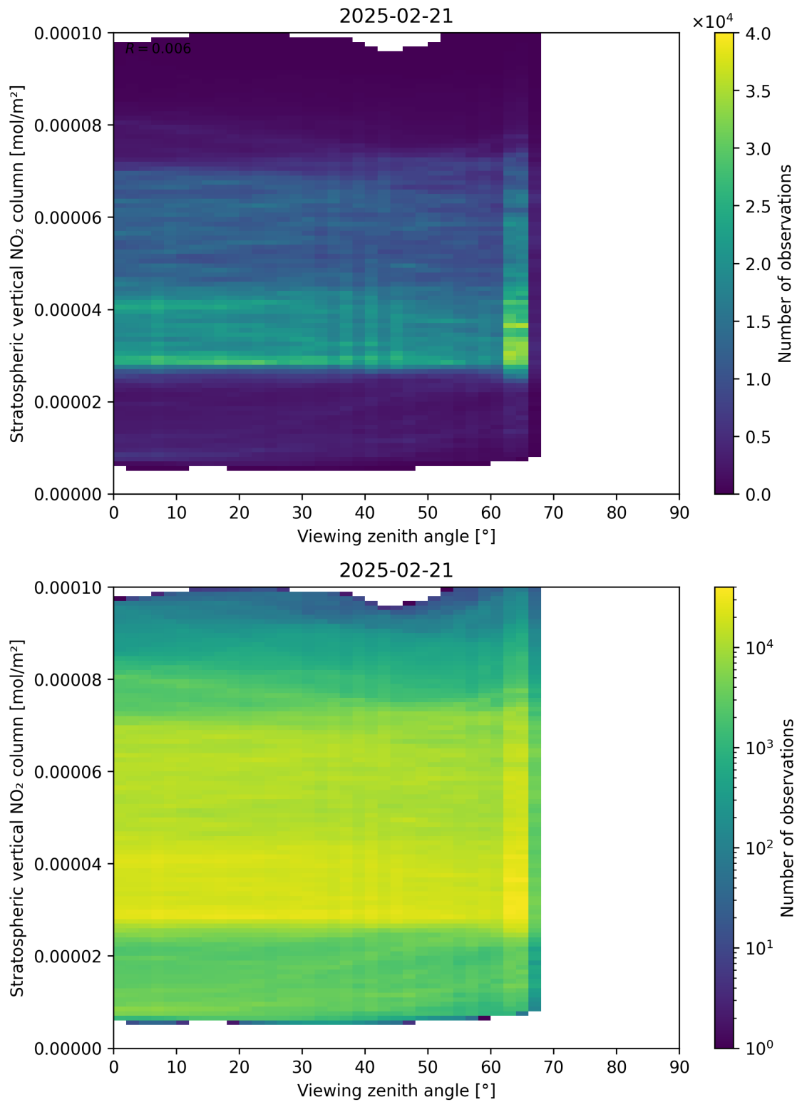
Figure 164: Scatter density plot of “Viewing zenith angle” against “Stratospheric vertical NO 2 column” for 2025-02-20 to 2025-02-22.
