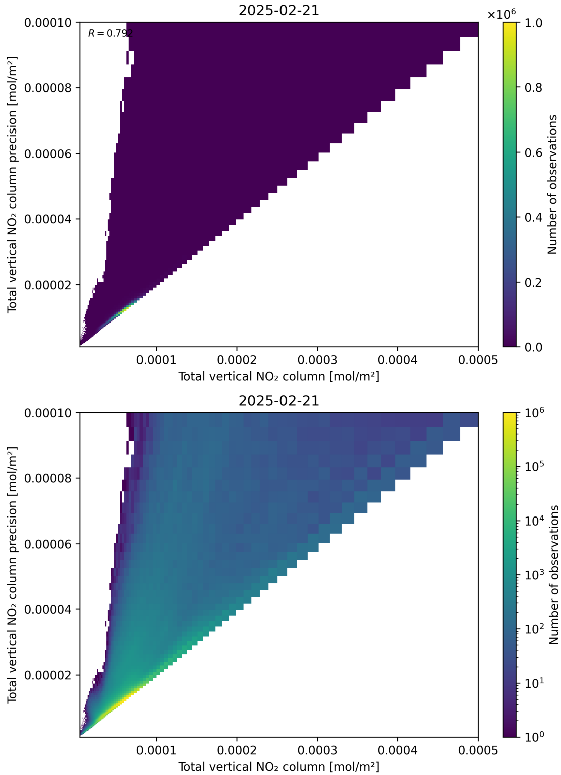
Figure 114: Scatter density plot of “Total vertical NO 2 column” against “Total vertical NO 2 column precision” for 2025-02-20 to 2025-02-22.
