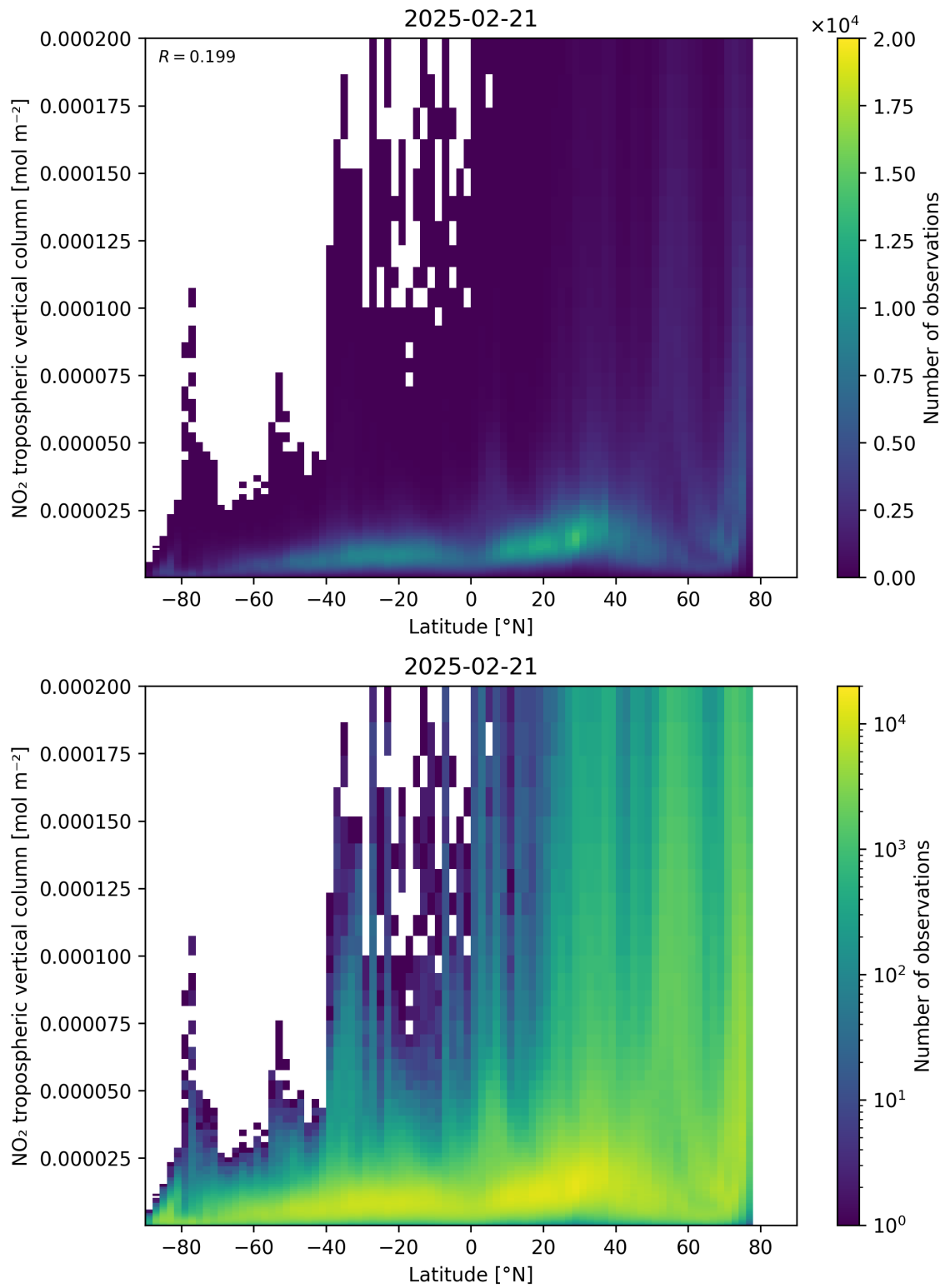
Figure 92: Scatter density plot of “Latitude” against “NO 2 tropospheric vertical column” for 2025-02-20 to 2025-02-22.
