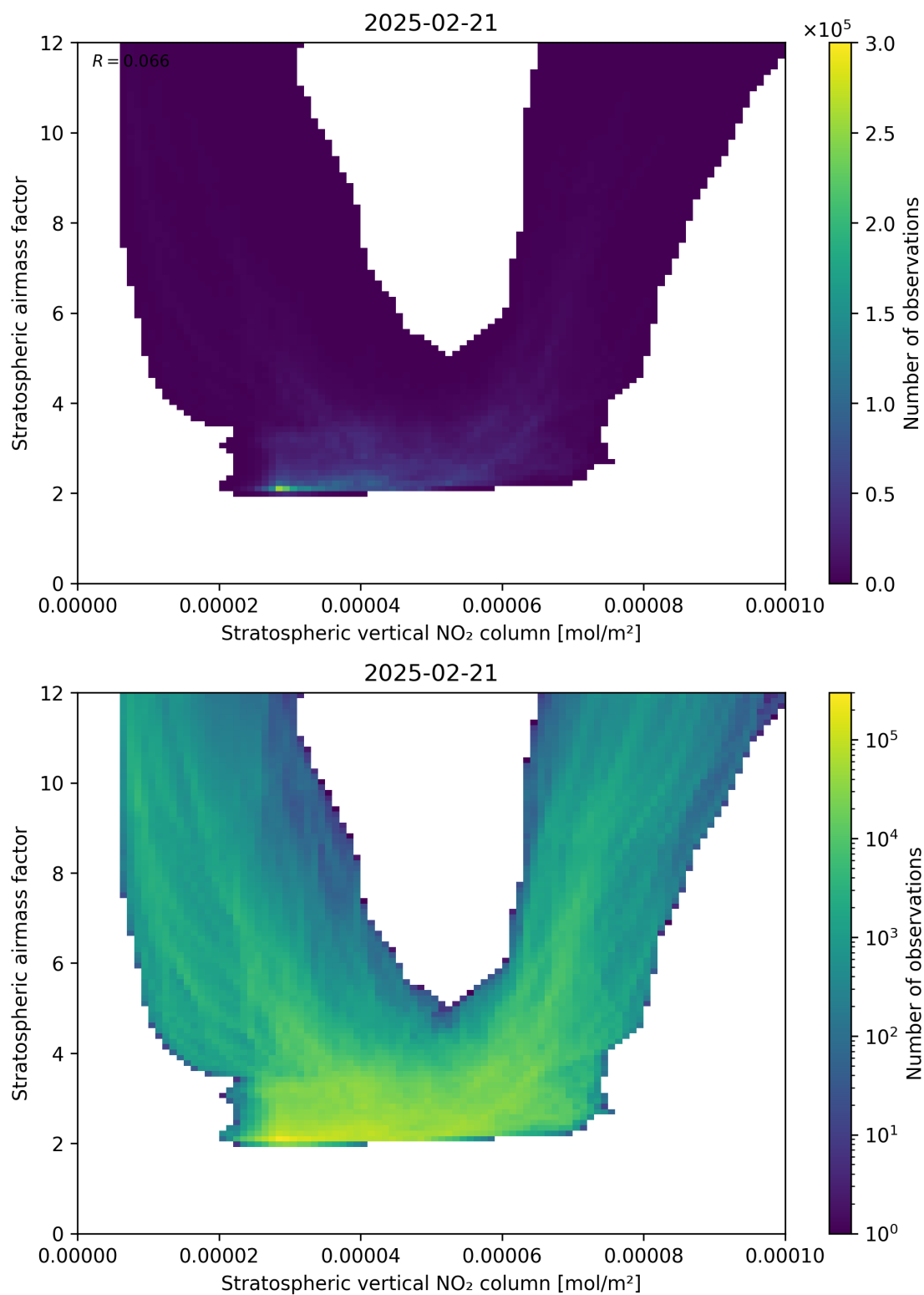
Figure 96: Scatter density plot of “Stratospheric vertical NO 2 column” against “Stratospheric airmass factor” for 2025-02-20 to 2025-02-22.
