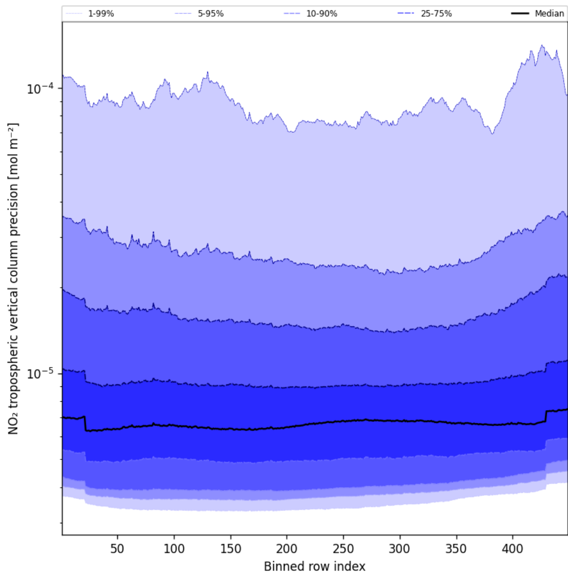
Figure 47: Along track statistics of “NO 2 tropospheric vertical column precision” for 2025-02-20 to 2025-02-22
