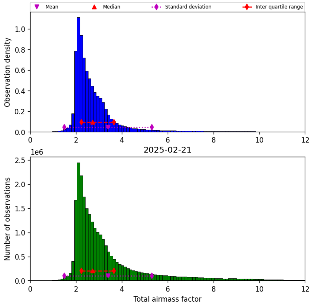
Figure 32: Histogram of “Total airmass factor” for 2025-02-20 to 2025-02-22
