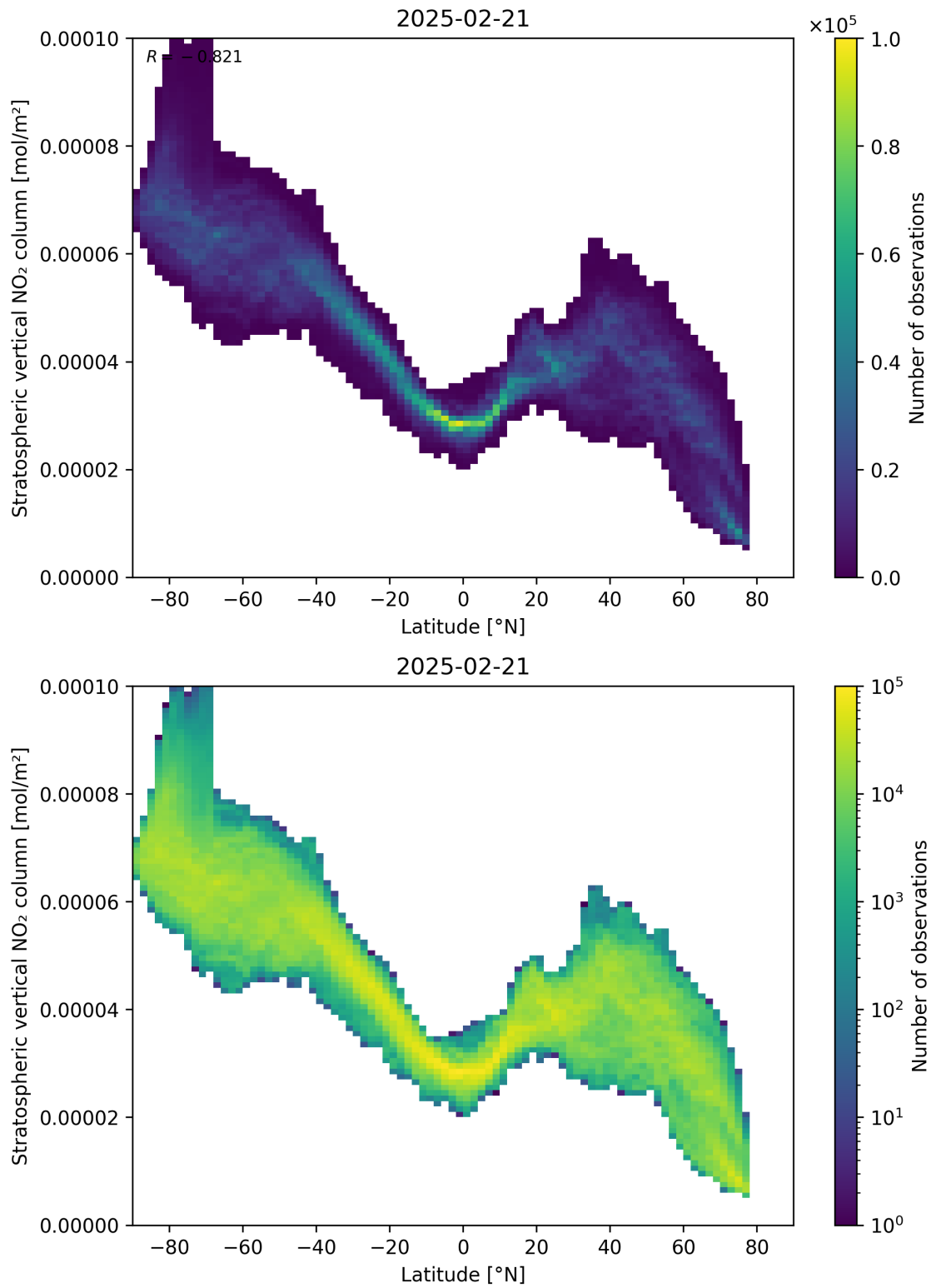
Figure 87: Scatter density plot of “Latitude” against “Stratospheric vertical NO 2 column” for 2025-02-20 to 2025-02-22.
