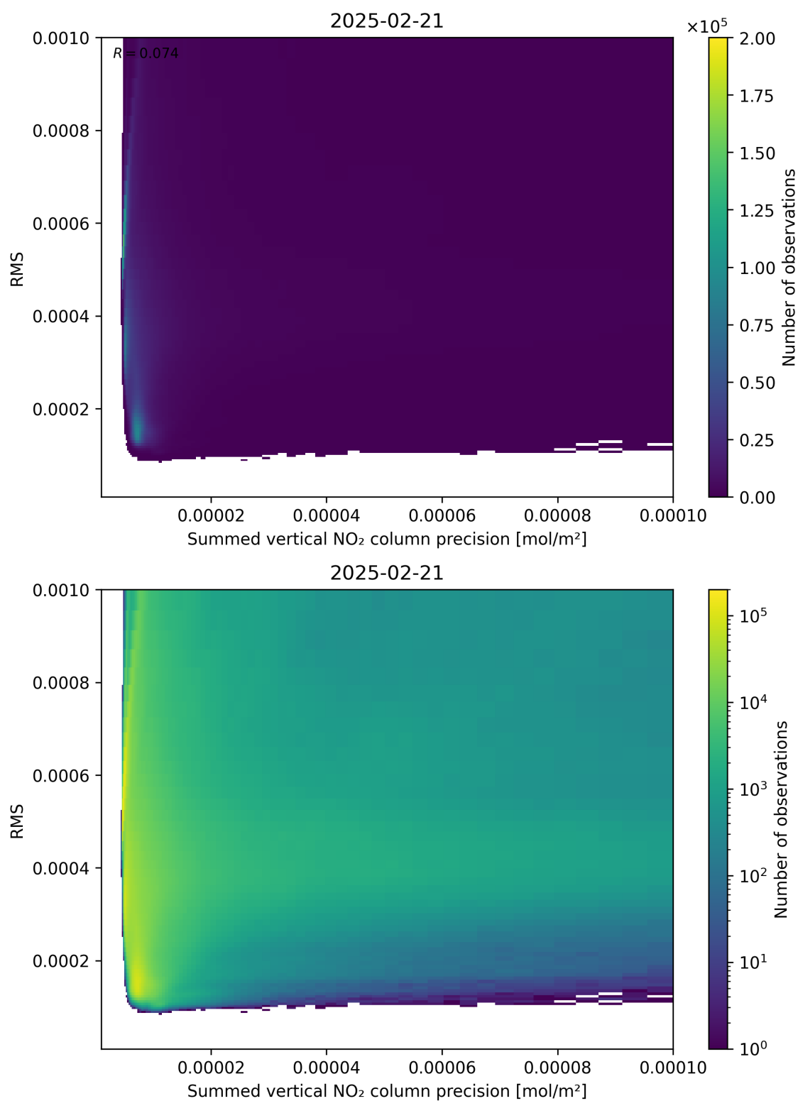
Figure 108: Scatter density plot of “Summed vertical NO 2 column precision” against “RMS” for 2025-02-20 to 2025-02-22.
