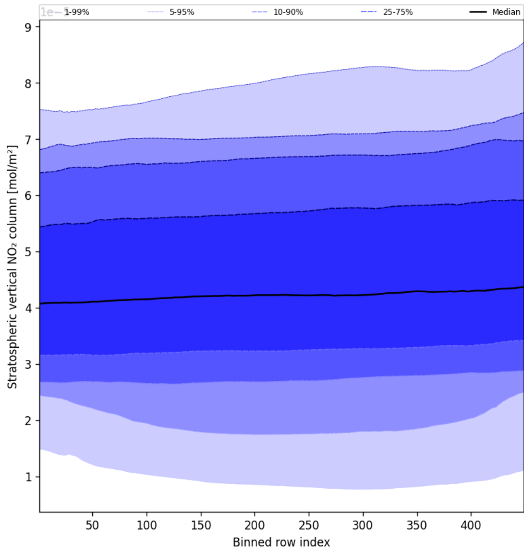
Figure 53: Along track statistics of “Stratospheric vertical NO 2 column” for 2025-02-20 to 2025-02-22
