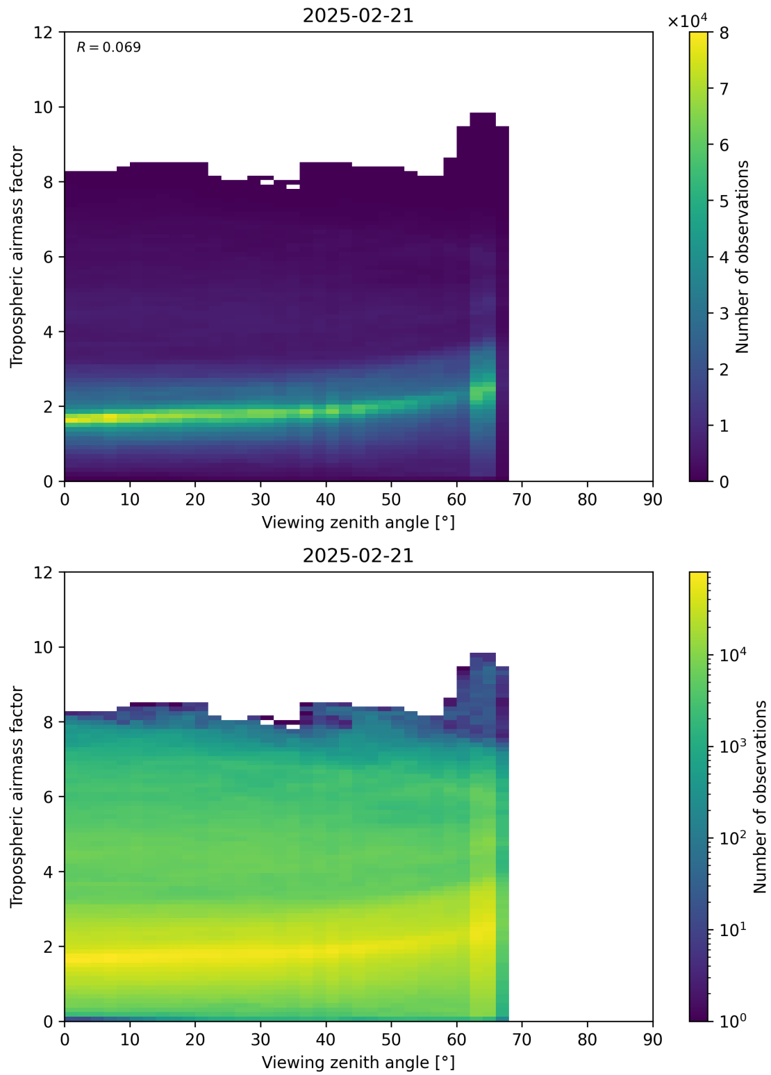
Figure 161: Scatter density plot of “Viewing zenith angle” against “Tropospheric airmass factor” for 2025-02-20 to 2025-02-22.
