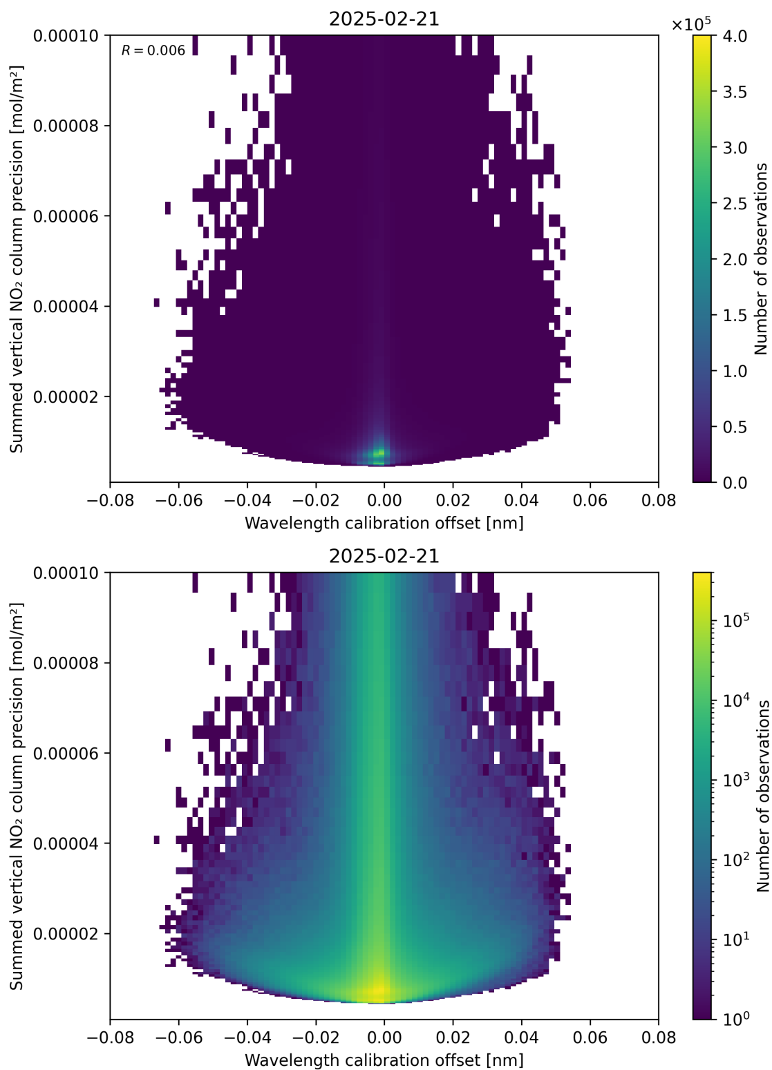
Figure 178: Scatter density plot of “Wavelength calibration offset” against “Summed vertical NO 2 column precision” for 2025-02-20 to 2025-02-22.
