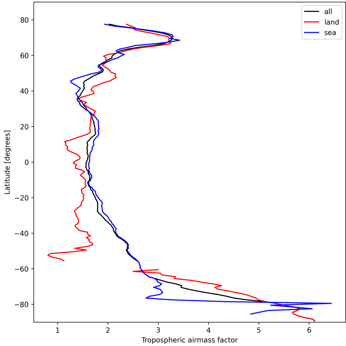
Figure 14: Zonal average of “Tropospheric airmass factor” for 2025-02-20 to 2025-02-22.
