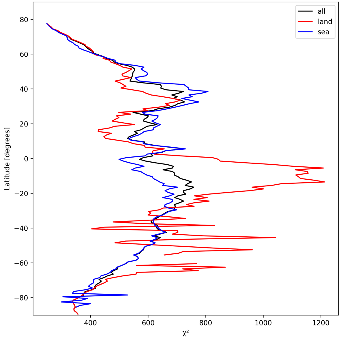
Figure 25: Zonal average of “ \chi^2 ” for 2025-02-20 to 2025-02-22.
