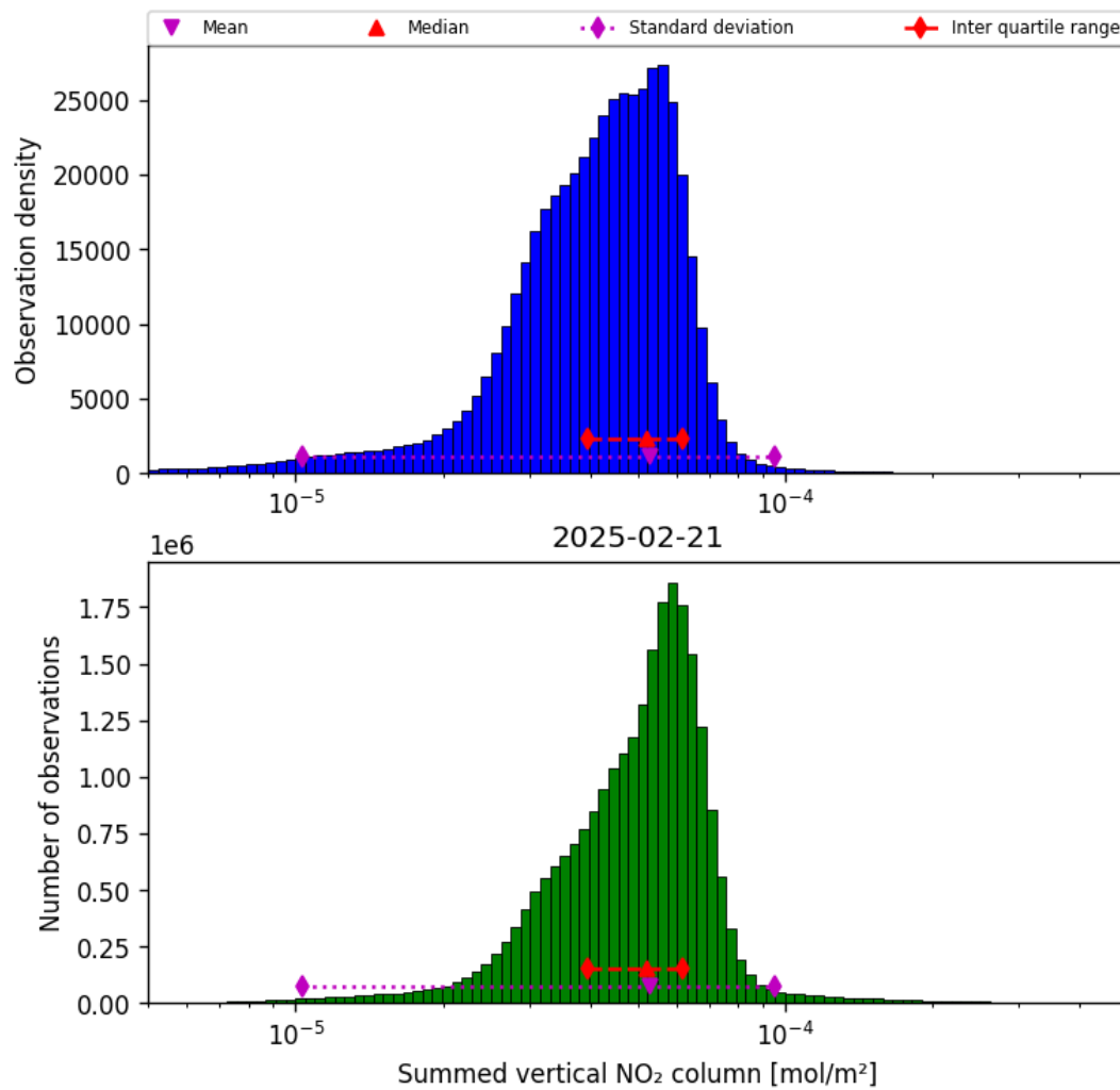
Figure 40: Histogram of “Summed vertical NO 2 column” for 2025-02-20 to 2025-02-22
