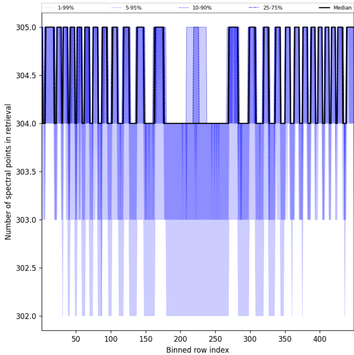
Figure 50: Along track statistics of “Number of spectral points in retrieval” for 2025-02-20 to 2025-02-22
