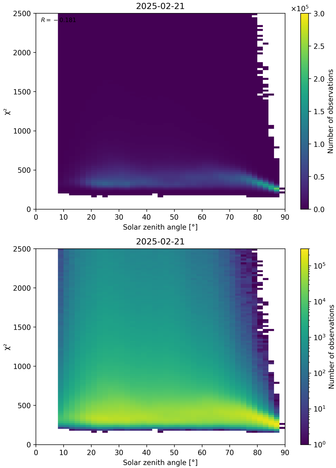
Figure 148: Scatter density plot of “Solar zenith angle” against “ \chi^2 ” for 2025-02-20 to 2025-02-22.
