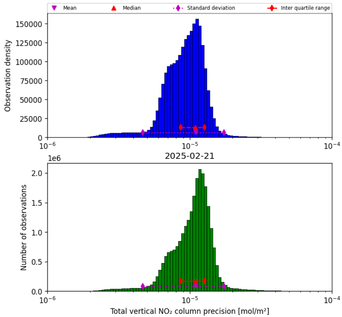
Figure 39: Histogram of “Total vertical NO 2 column precision” for 2025-02-20 to 2025-02-22
