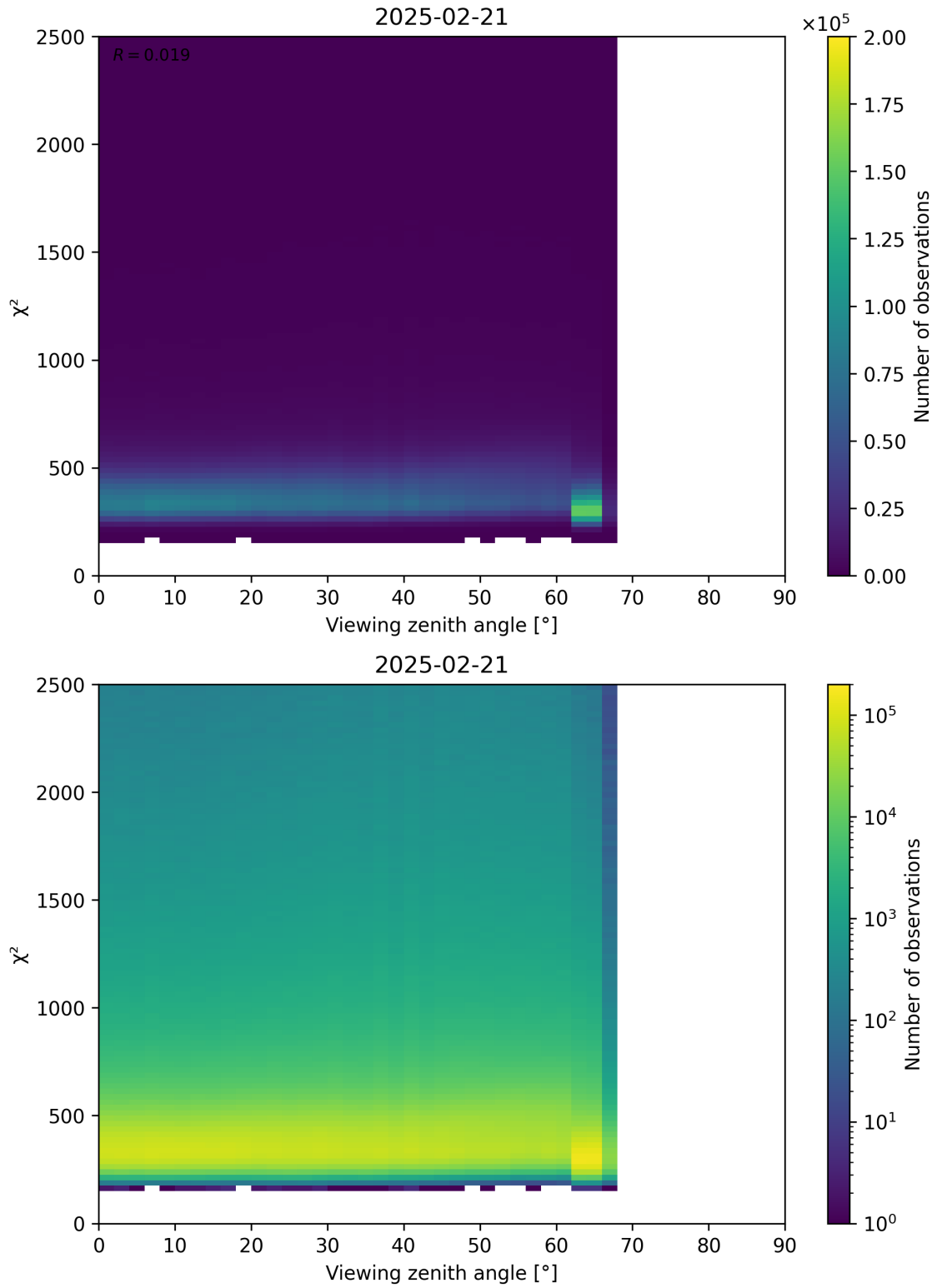
Figure 162: Scatter density plot of “Viewing zenith angle” against “ \chi^2 ” for 2025-02-20 to 2025-02-22.
