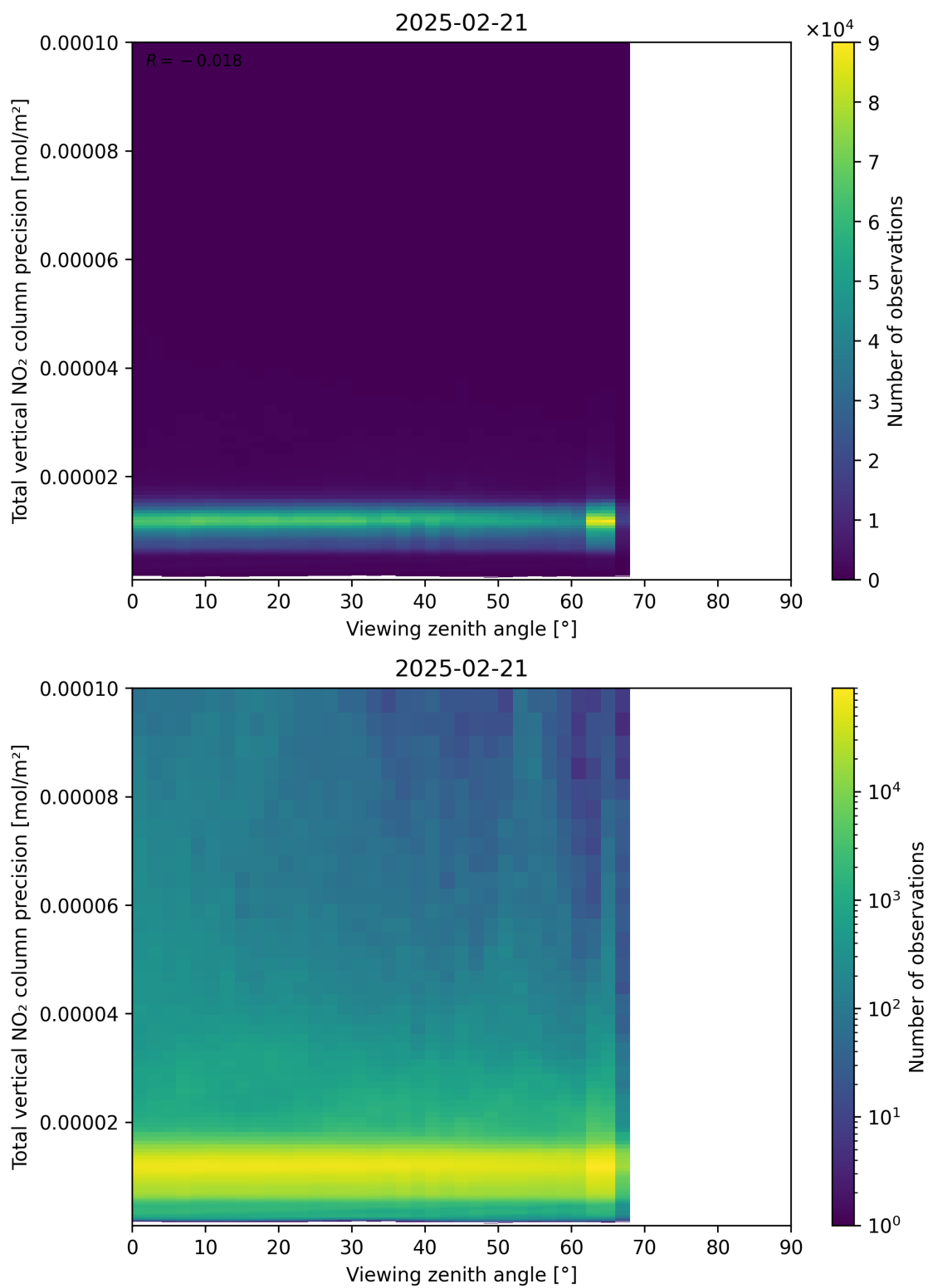
Figure 168: Scatter density plot of “Viewing zenith angle” against “Total vertical NO 2 column precision” for 2025-02-20 to 2025-02-22.
