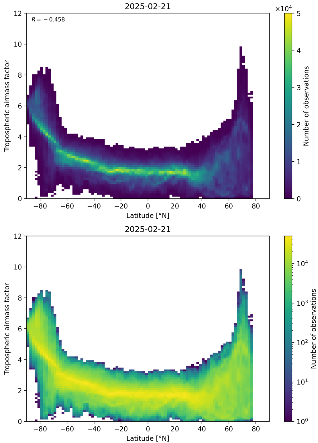
Figure 85: Scatter density plot of “Latitude” against “Tropospheric airmass factor” for 2025-02-20 to 2025-02-22.
