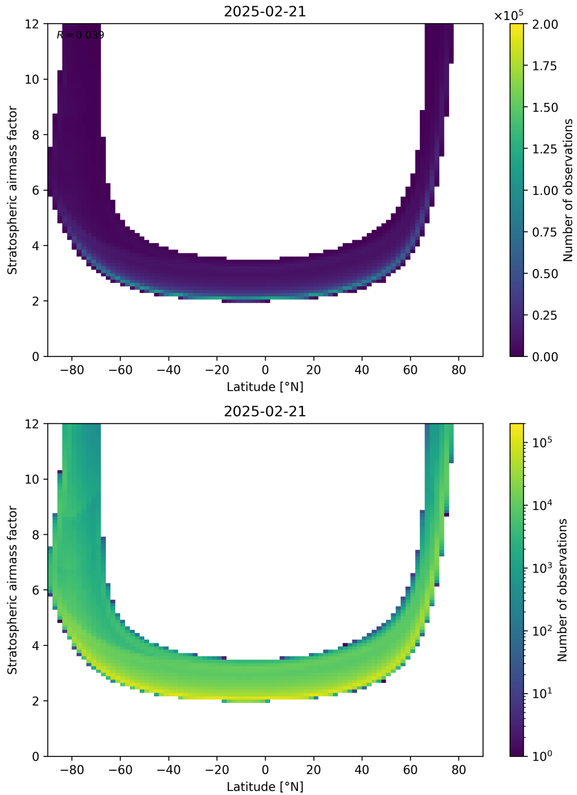
Figure 83: Scatter density plot of “Latitude” against “Stratospheric air mass factor” for 2025-02-20 to 2025-02-22.
