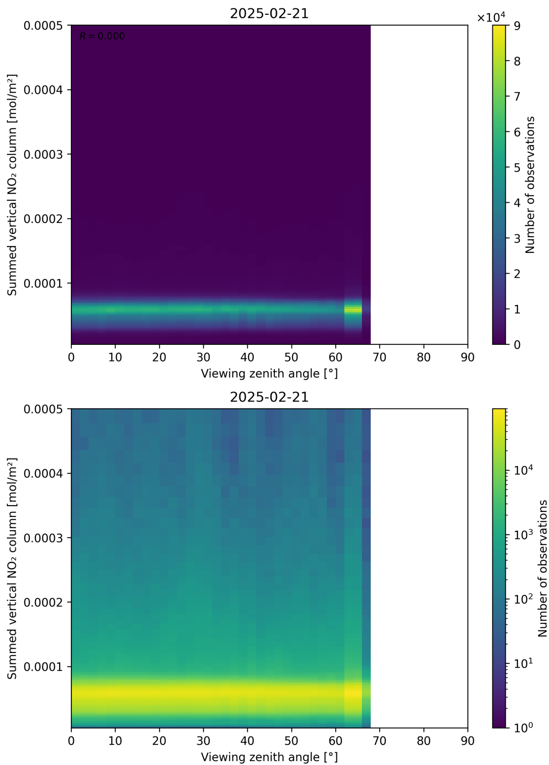
Figure 165: Scatter density plot of “Viewing zenith angle” against “Summed vertical NO 2 column” for 2025-02-20 to 2025-02-22.
