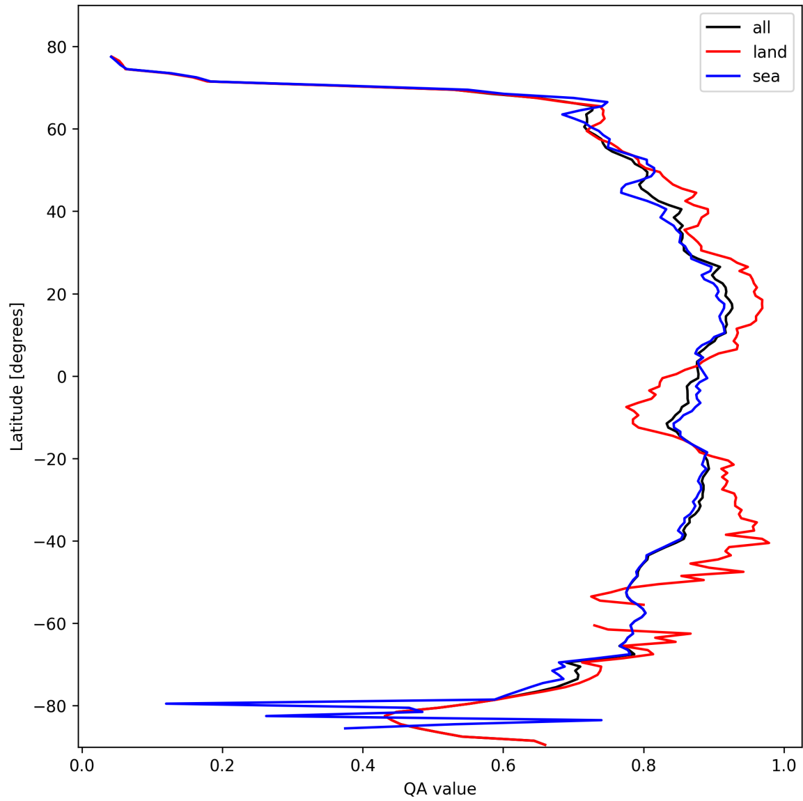
Figure 11: Zonal average of “QA value” for 2025-02-20 to 2025-02-22.
