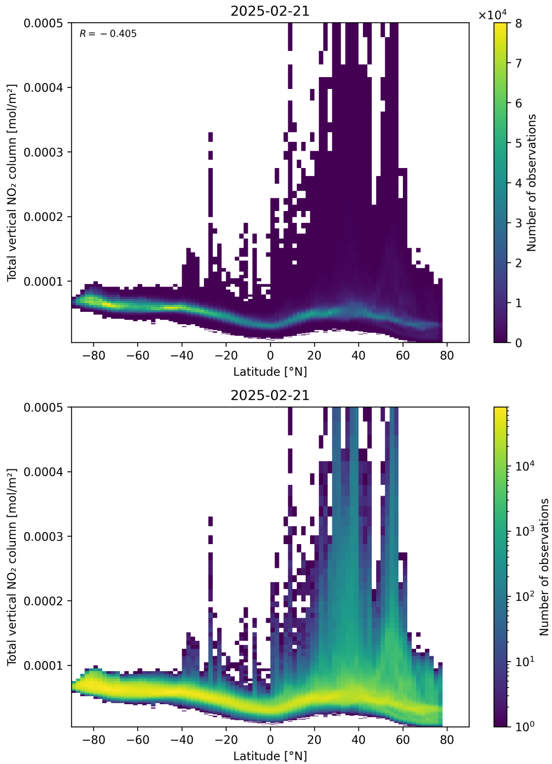
Figure 90: Scatter density plot of “Latitude” against “Total vertical NO 2 column” for 2025-02-20 to 2025-02-22.
