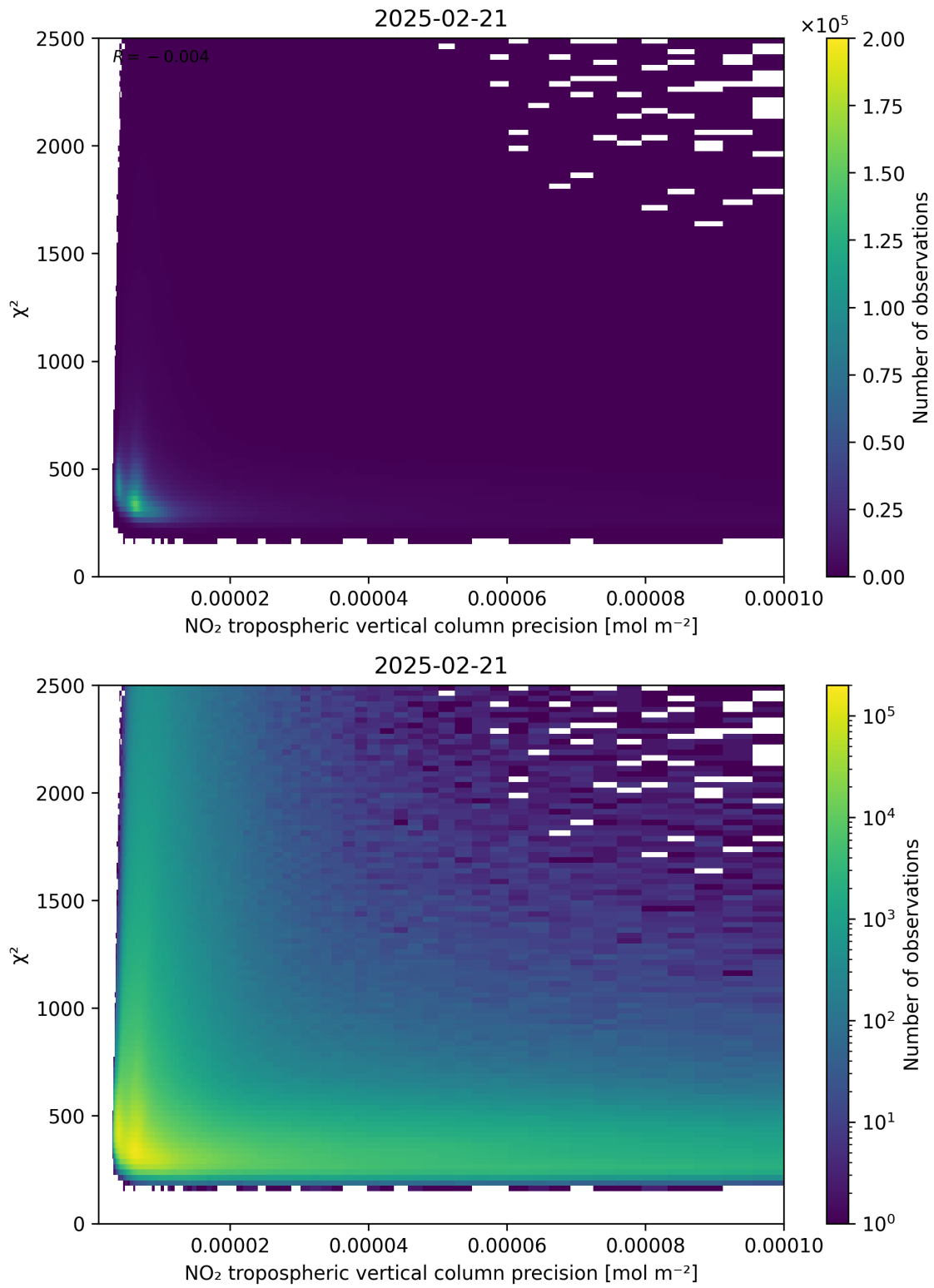
Figure 134: Scatter density plot of “NO 2 tropospheric vertical column precision” against “ \chi^2 ” for 2025-02-20 to 2025-02-22.
