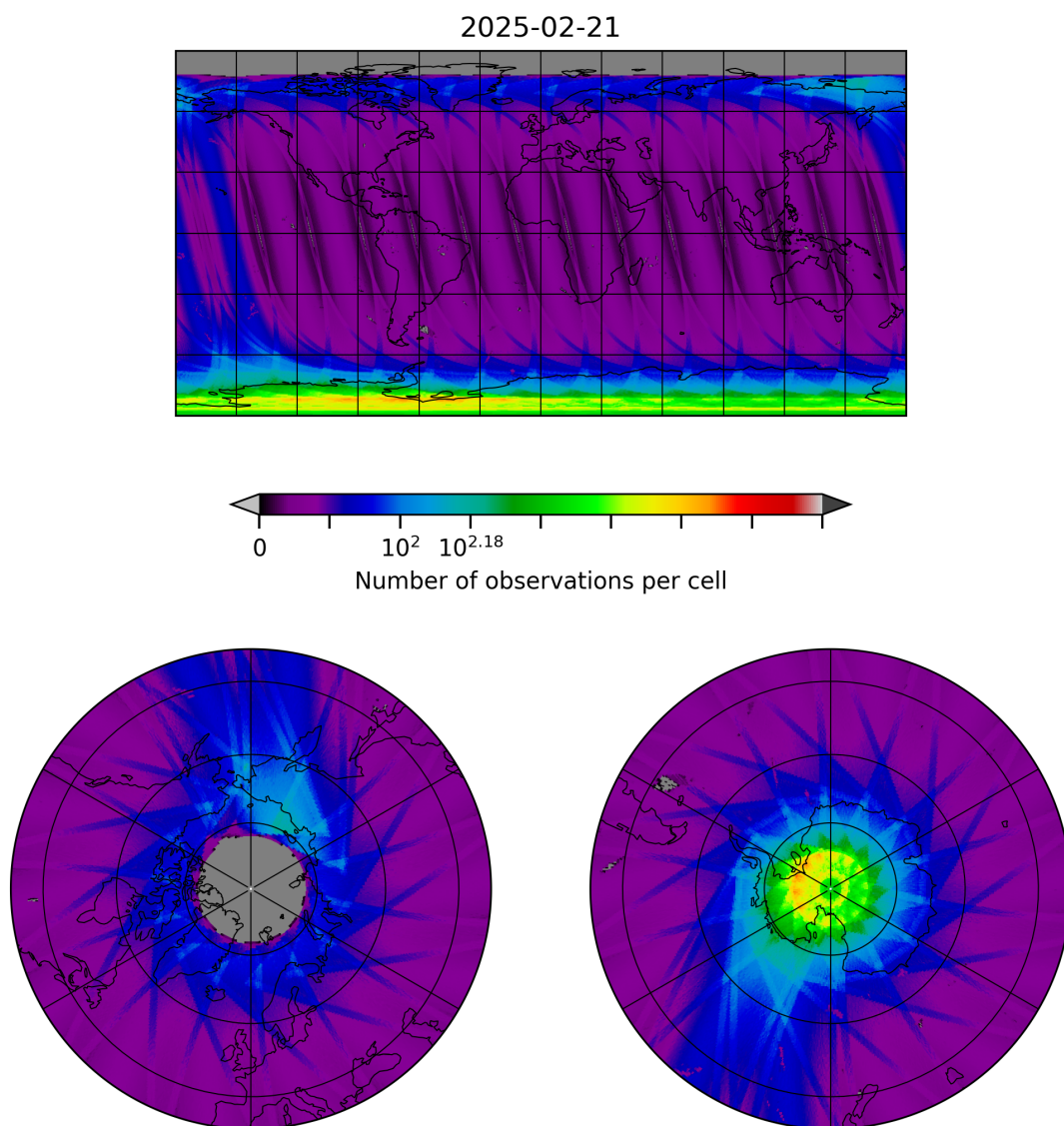
Figure 10: Map of the number of observations for 2025-02-20 to 2025-02-22
