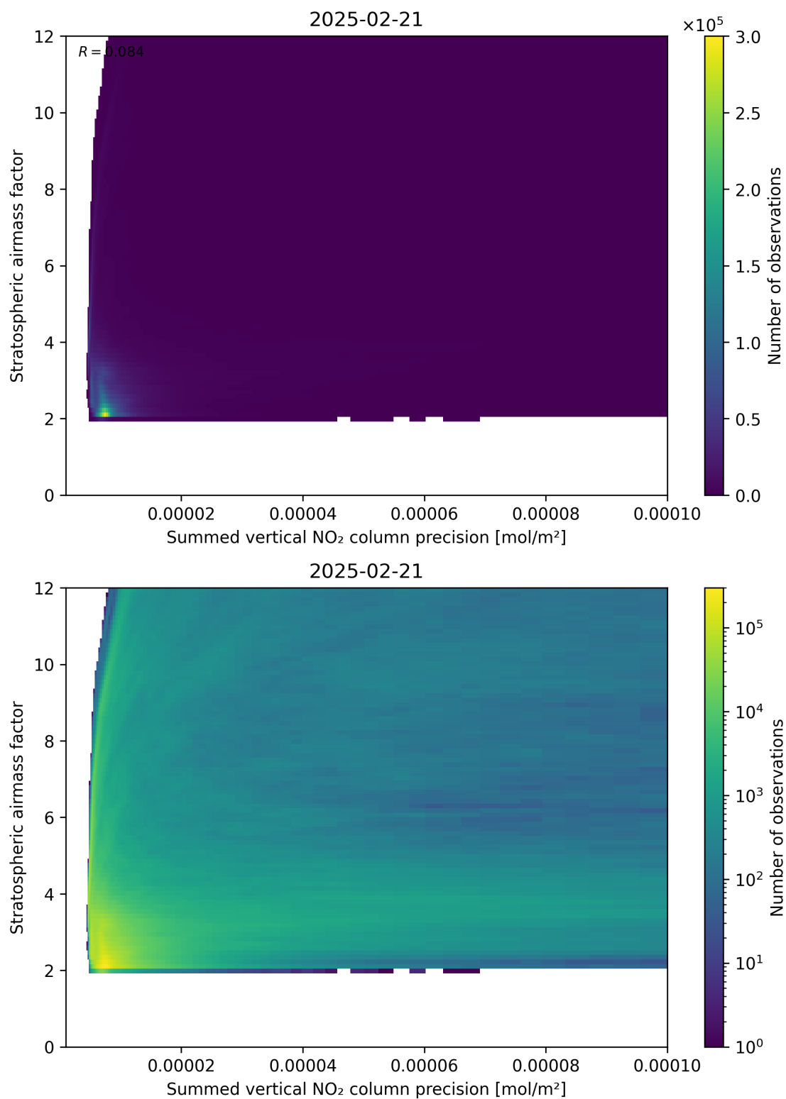
Figure 106: Scatter density plot of “Summed vertical NO 2 column precision” against “Stratospheric airmass factor” for 2025-02-20 to 2025-02-22.
