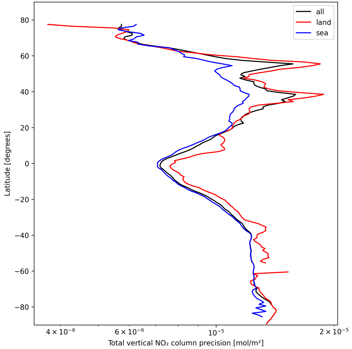
Figure 22: Zonal average of “Total vertical NO 2 column precision” for 2025-02-20 to 2025-02-22.
