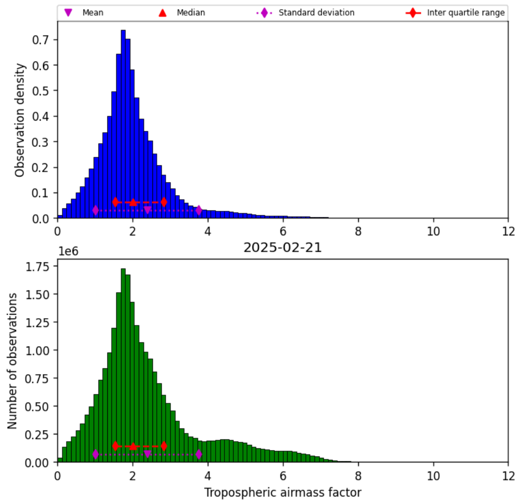
Figure 31: Histogram of “Tropospheric airmass factor” for 2025-02-20 to 2025-02-22
