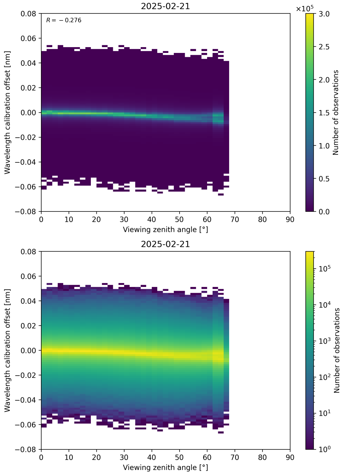
Figure 173: Scatter density plot of “Viewing zenith angle” against “Wavelength calibration offset” for 2025-02-20 to 2025-02-22.
