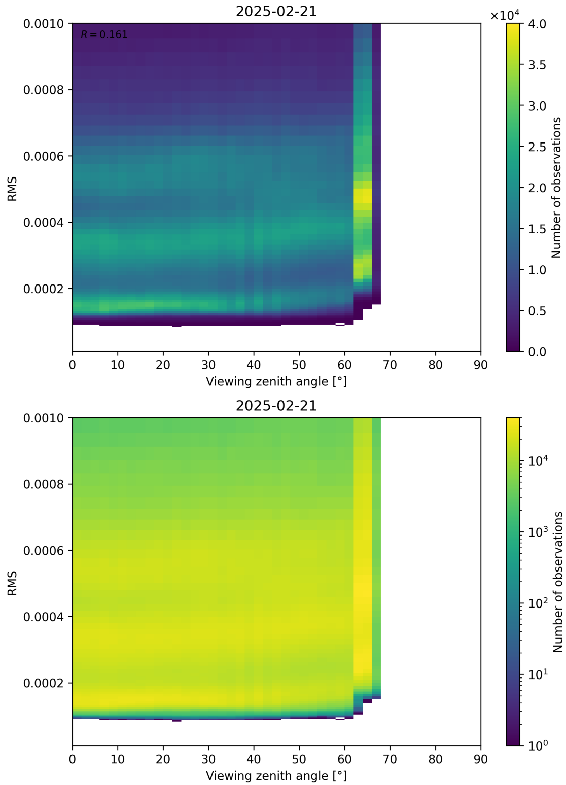
Figure 171: Scatter density plot of “Viewing zenith angle” against “RMS” for 2025-02-20 to 2025-02-22.
