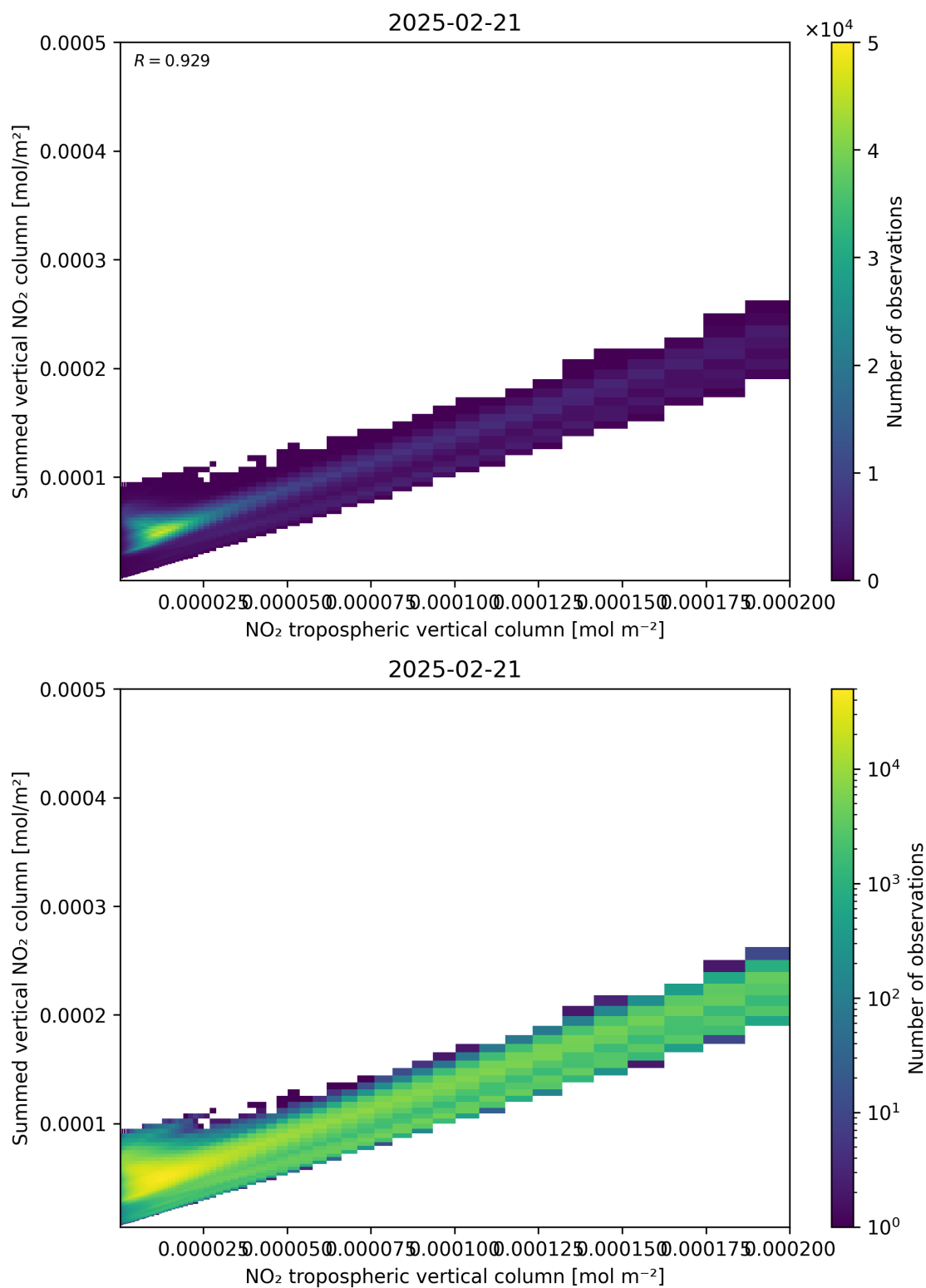
Figure 126: Scatter density plot of “NO 2 tropospheric vertical column” against “Summed vertical NO 2 column” for 2025-02-20 to 2025-02-22.
