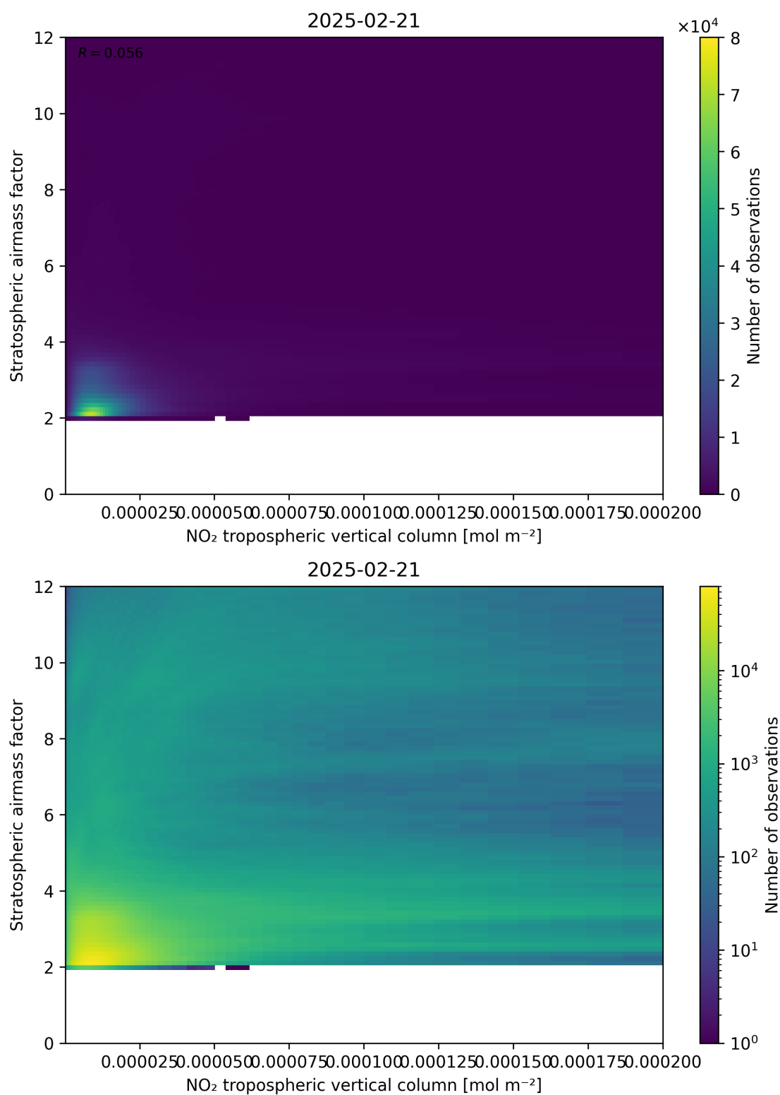
Figure 121: Scatter density plot of “NO 2 tropospheric vertical column” against “Stratospheric airmass factor” for 2025-02-20 to 2025-02-22.
