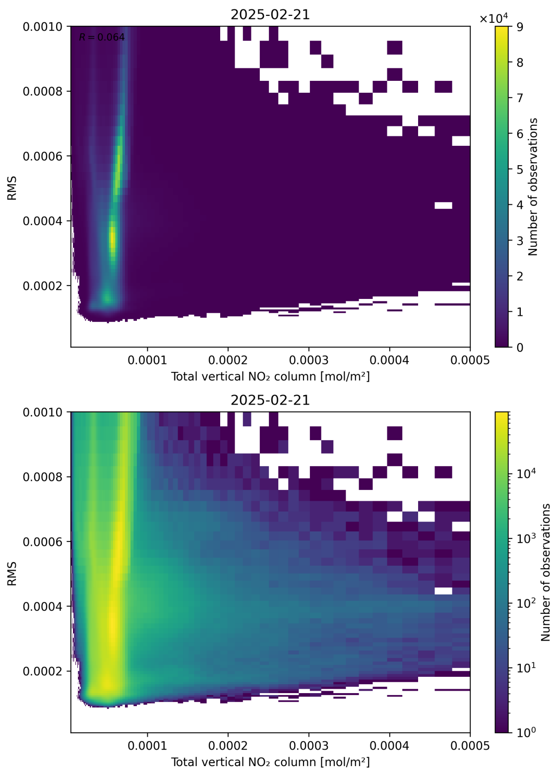
Figure 120: Scatter density plot of “Total vertical NO 2 column” against “RMS” for 2025-02-20 to 2025-02-22.
