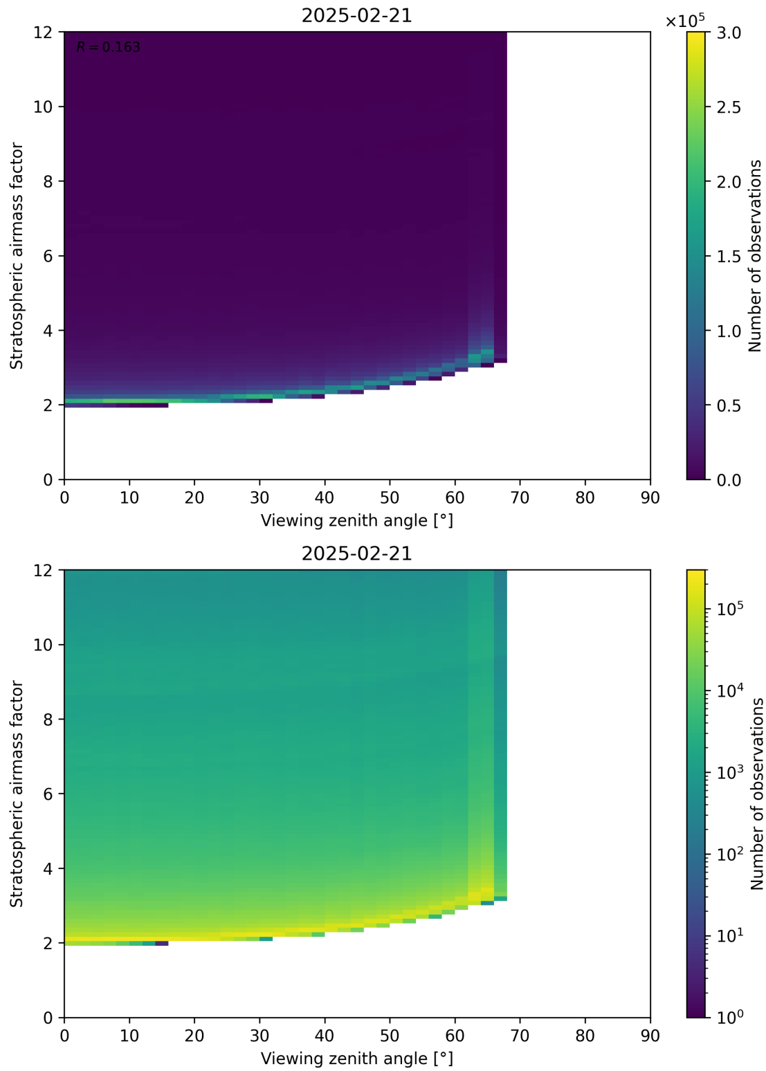
Figure 159: Scatter density plot of “Viewing zenith angle” against “Stratospheric airmass factor” for 2025-02-20 to 2025-02-22.
