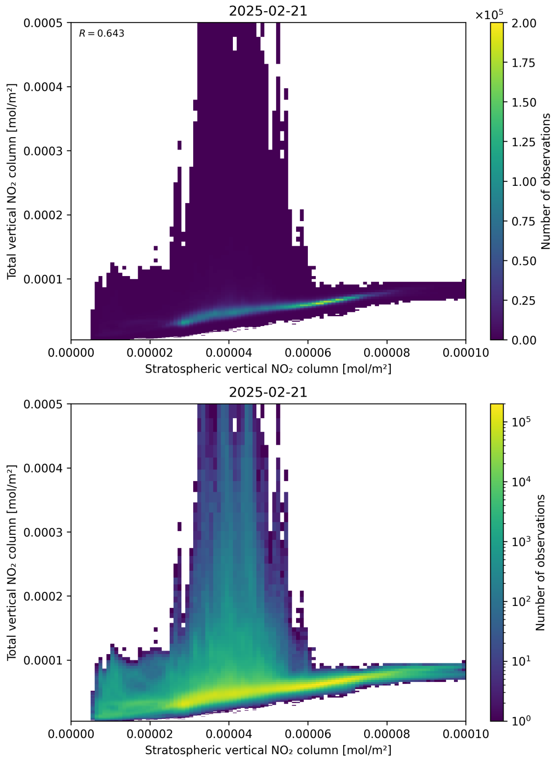
Figure 100: Scatter density plot of “Stratospheric vertical NO 2 column” against “Total vertical NO 2 column” for 2025-02-20 to 2025-02-22.
