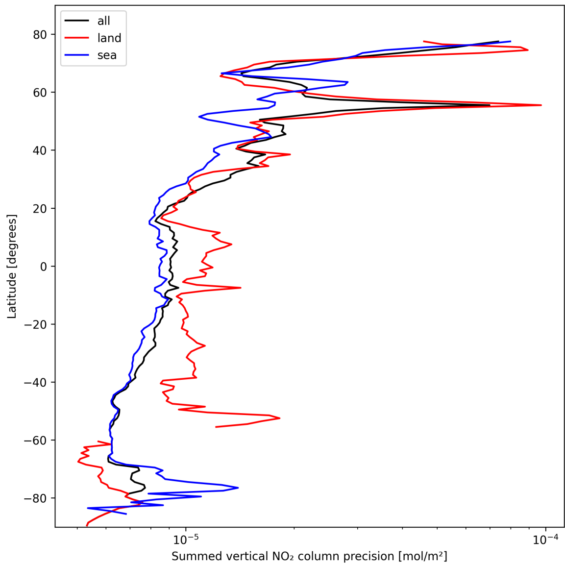
Figure 24: Zonal average of “Summed vertical NO 2 column precision” for 2025-02-20 to 2025-02-22.
