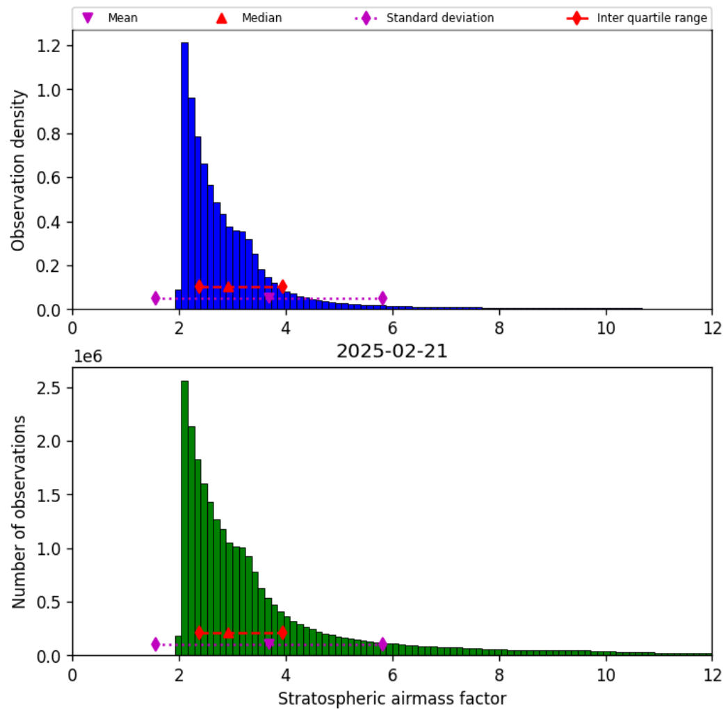
Figure 44: Histogram of “Stratospheric airmass factor” for 2025-02-20 to 2025-02-22
