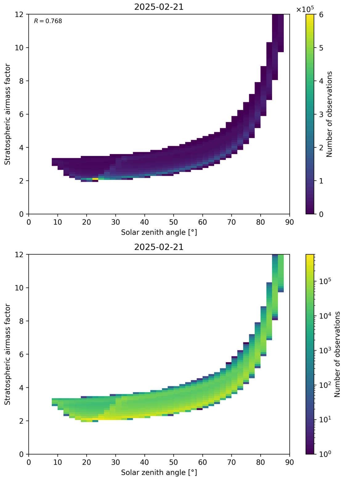
Figure 145: Scatter density plot of “Solar zenith angle” against “Stratospheric airmass factor” for 2025-02-20 to 2025-02-22.
