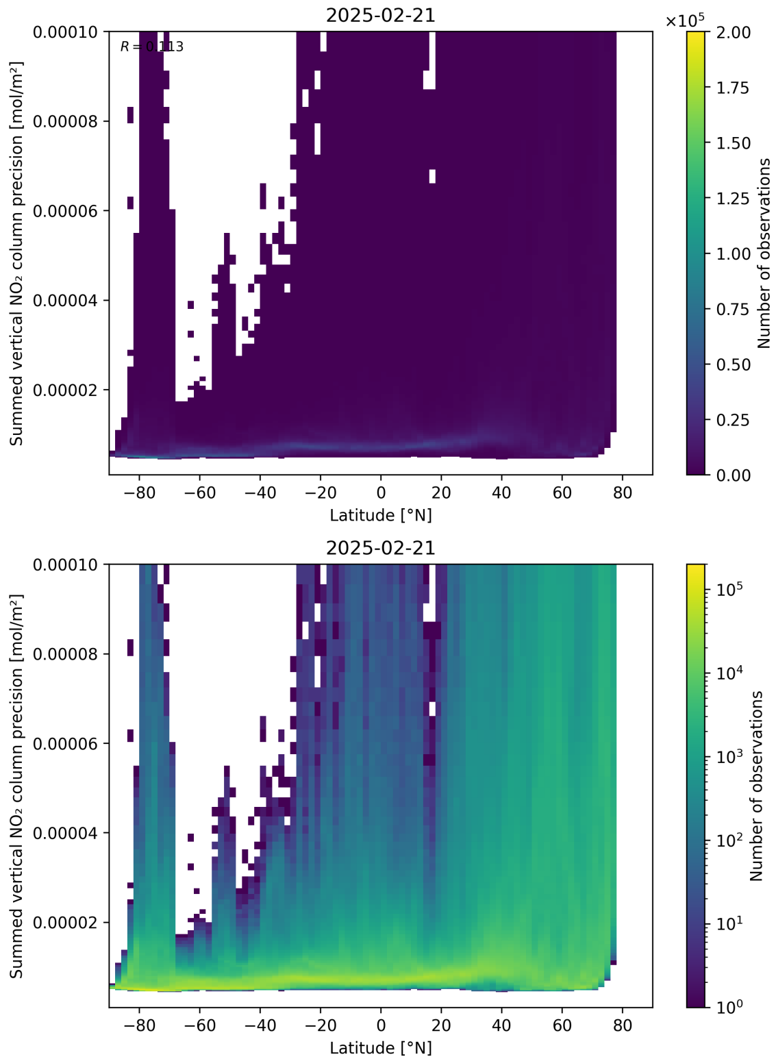
Figure 89: Scatter density plot of “Latitude” against “Summed vertical NO 2 column precision” for 2025-02-20 to 2025-02-22.
