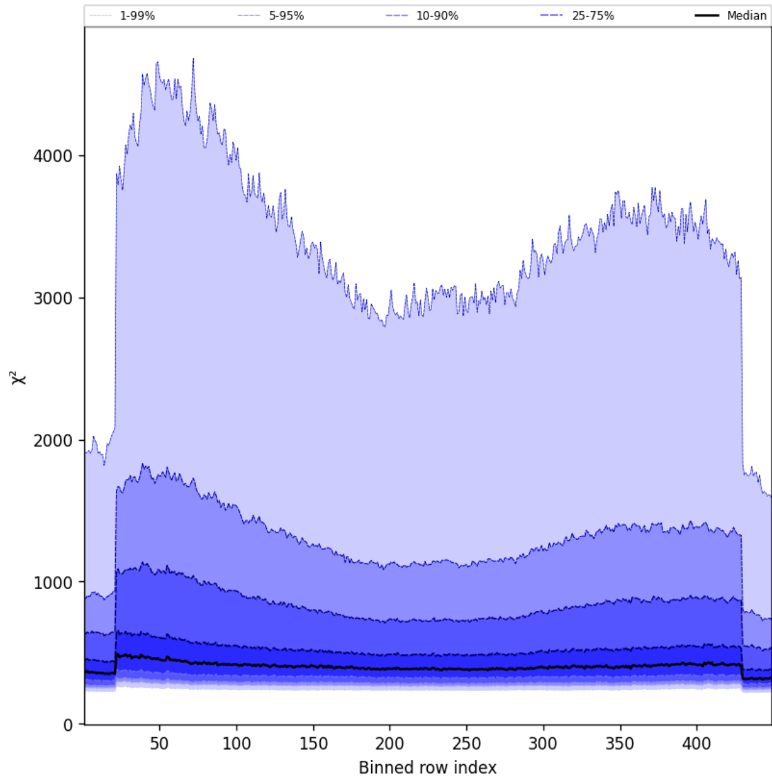
Figure 59: Along track statistics of “ \chi^2 ” for 2025-02-20 to 2025-02-22
