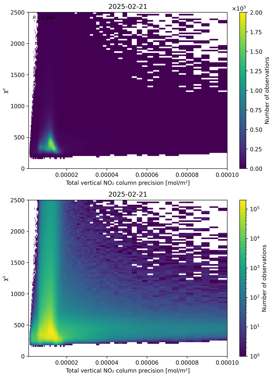
Figure 116: Scatter density plot of “Total vertical NO 2 column precision” against “ \chi^2 ” for 2025-02-20 to 2025-02-22.
