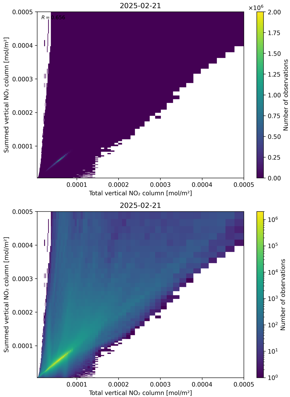
Figure 112: Scatter density plot of “Total vertical NO 2 column” against “Summed vertical NO 2 column” for 2025-02-20 to 2025-02-22.
