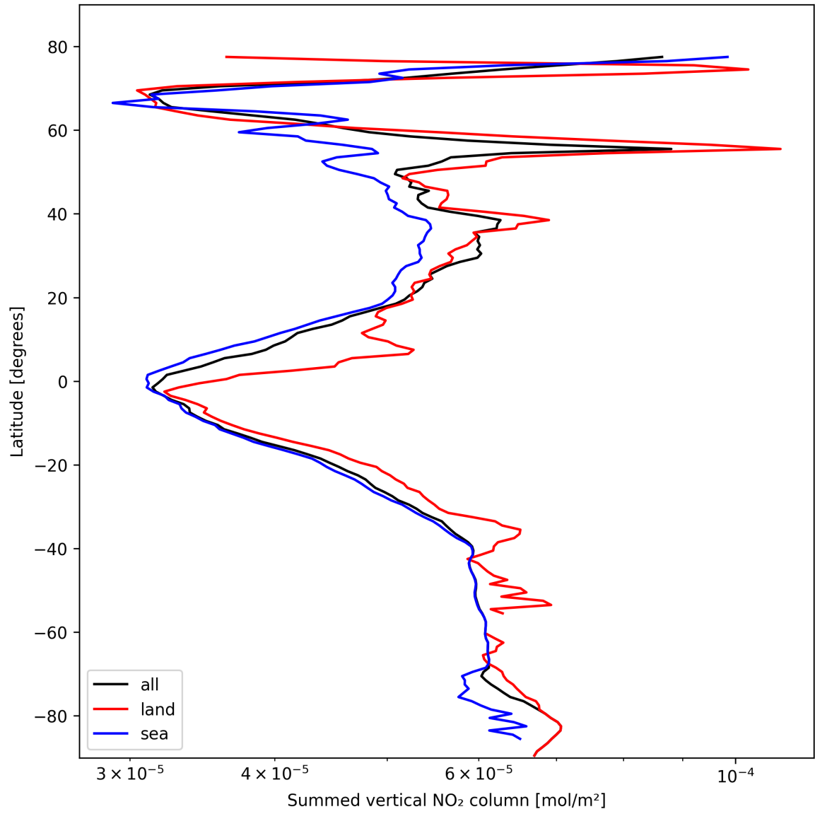
Figure 23: Zonal average of “Summed vertical NO 2 column” for 2025-02-20 to 2025-02-22.
