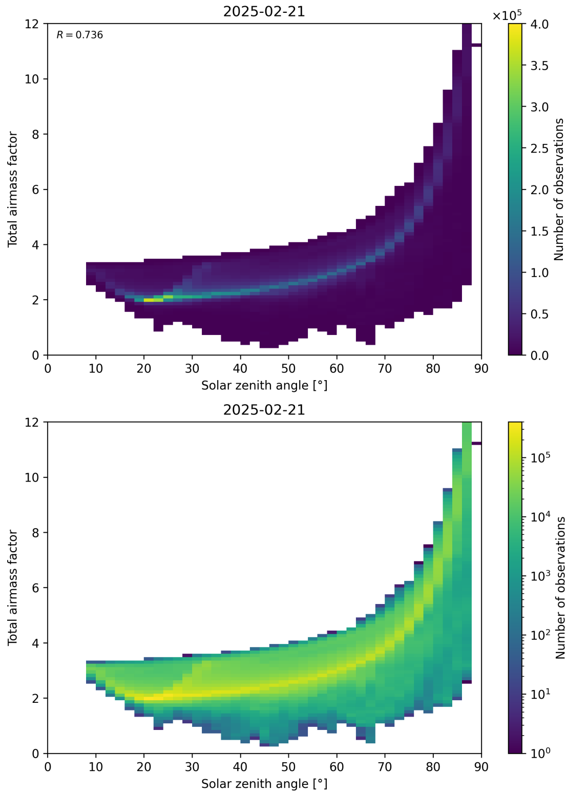
Figure 146: Scatter density plot of “Solar zenith angle” against “Total air mass factor” for 2025-02-20 to 2025-02-22.
