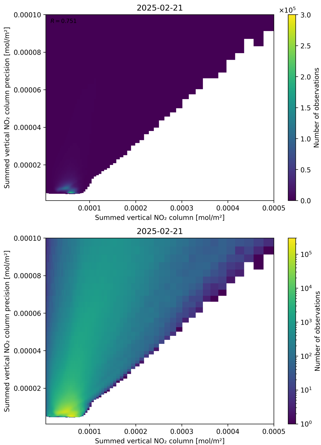
Figure 105: Scatter density plot of “Summed vertical NO 2 column” against “Summed vertical NO 2 column precision” for 2025-02-20 to 2025-02-22.
