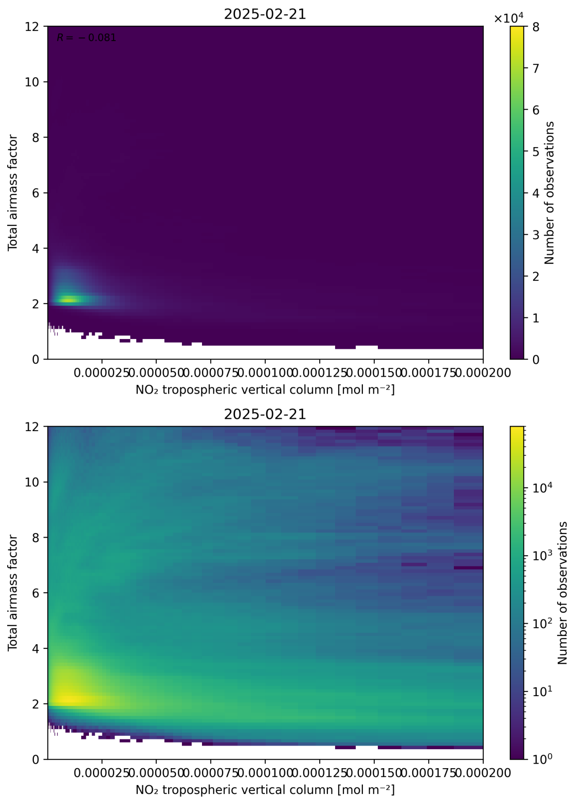
Figure 122: Scatter density plot of “NO 2 tropospheric vertical column” against “Total air mass factor” for 2025-02-20 to 2025-02-22.
