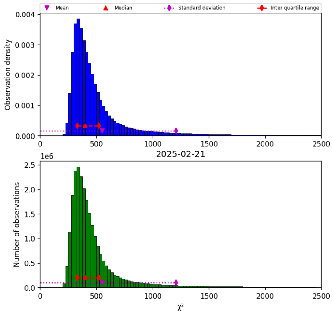
Figure 42: Histogram of “ \chi^2 ” for 2025-02-20 to 2025-02-22
