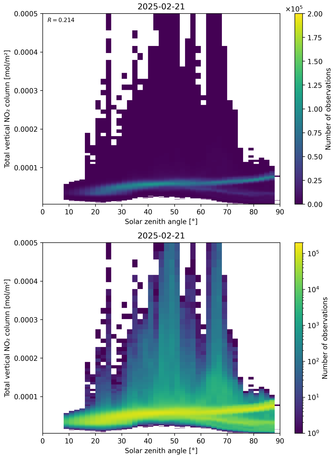
Figure 153: Scatter density plot of “Solar zenith angle” against “Total vertical NO 2 column” for 2025-02-20 to 2025-02-22.
