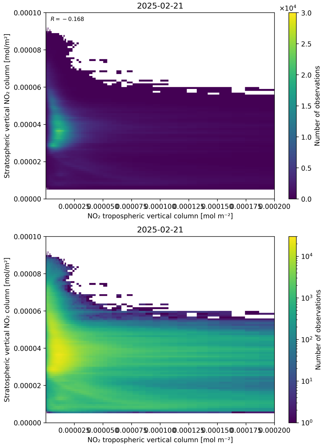
Figure 125: Scatter density plot of “NO 2 tropospheric vertical column” against “Stratospheric vertical NO 2 column” for 2025-02-20 to 2025-02-22.
