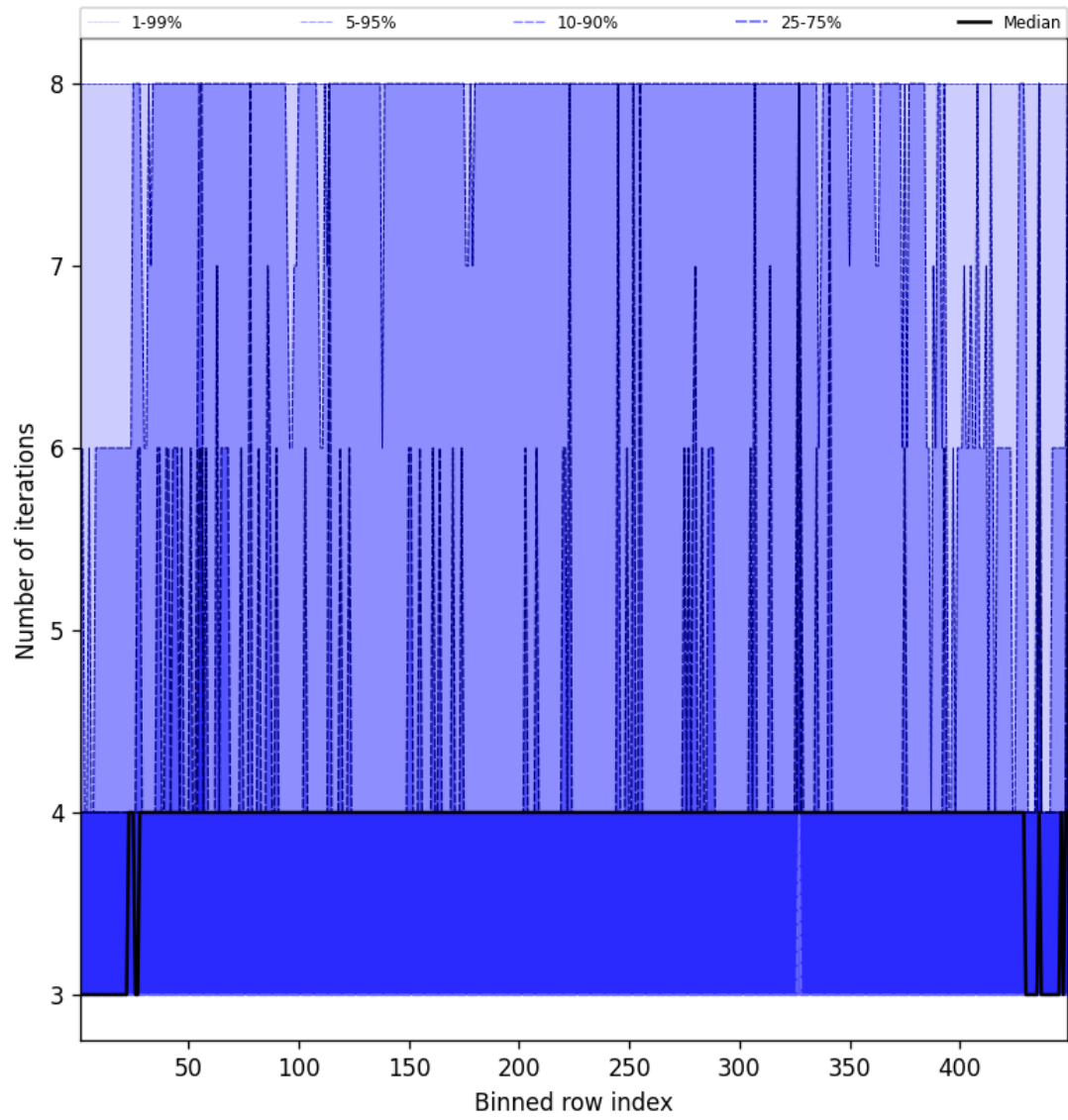
Figure 51: Along track statistics of “Number of iterations” for 2025-02-20 to 2025-02-22
