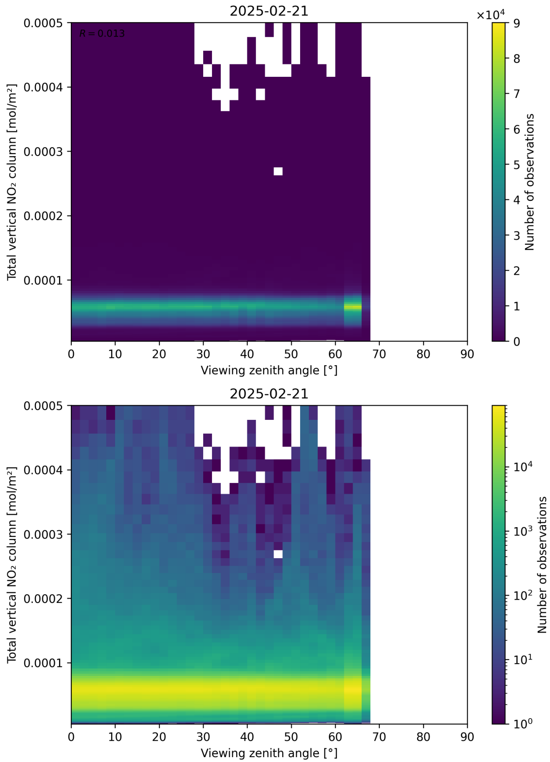
Figure 167: Scatter density plot of “Viewing zenith angle” against “Total vertical NO 2 column” for 2025-02-20 to 2025-02-22.
