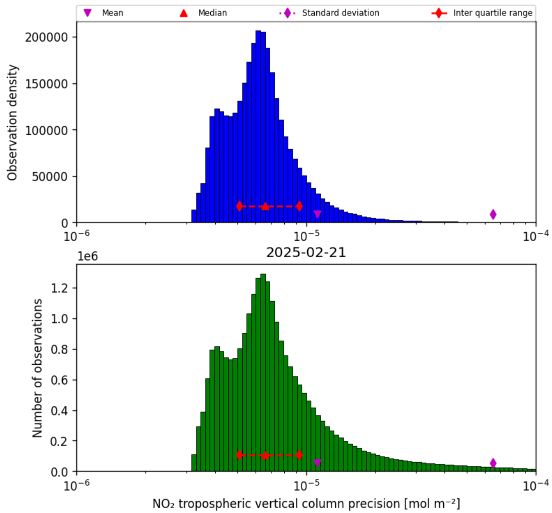
Figure 30: Histogram of “NO 2 tropospheric vertical column precision” for 2025-02-20 to 2025-02-22
