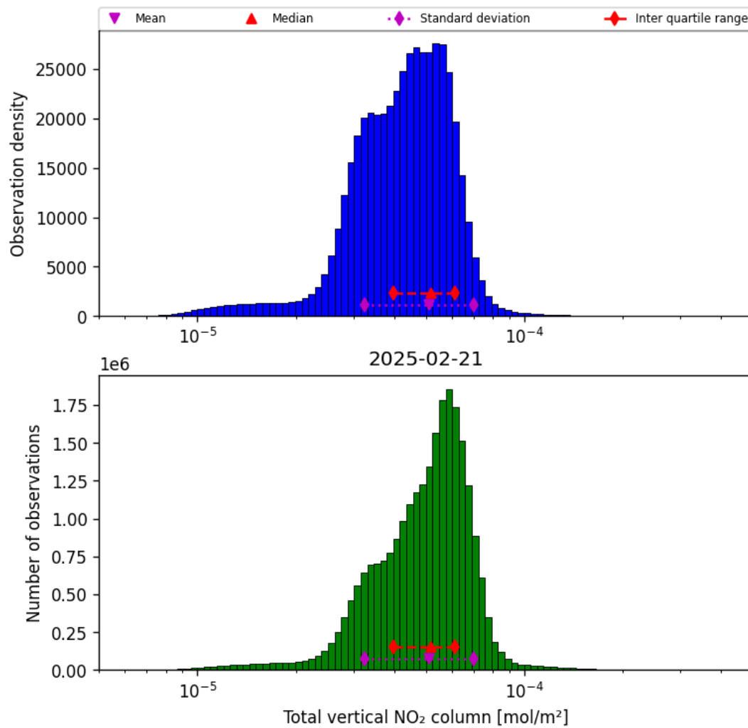
Figure 38: Histogram of “Total vertical NO 2 column” for 2025-02-20 to 2025-02-22
