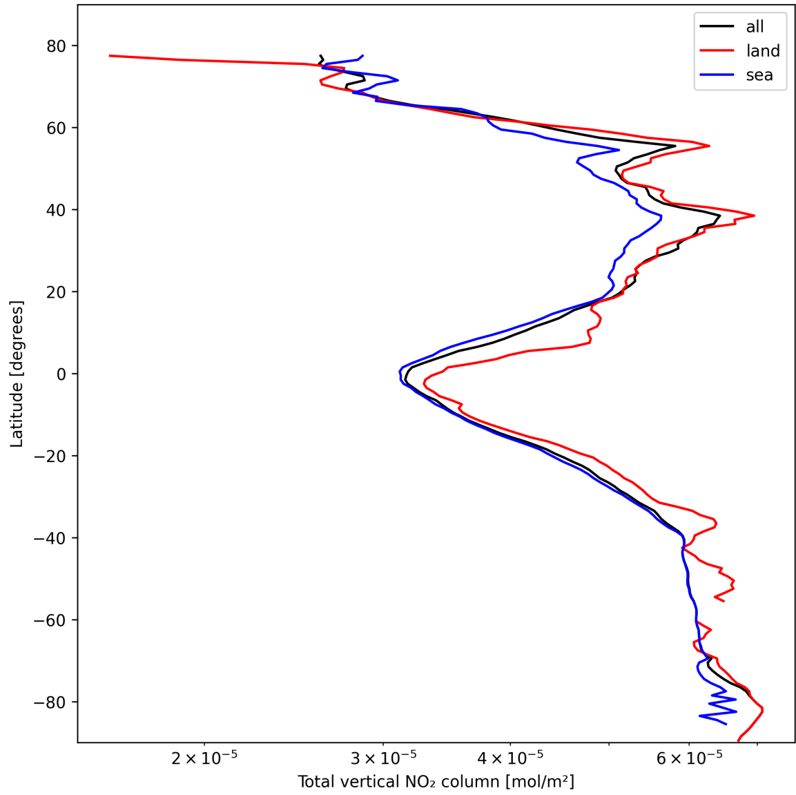
Figure 21: Zonal average of “Total vertical NO 2 column” for 2025-02-20 to 2025-02-22.
