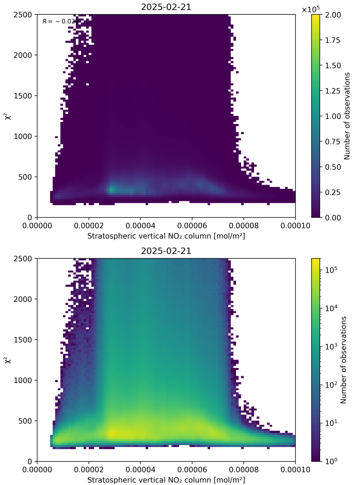
Figure 97: Scatter density plot of “Stratospheric vertical NO 2 column” against “ \chi^2 ” for 2025-02-20 to 2025-02-22.
