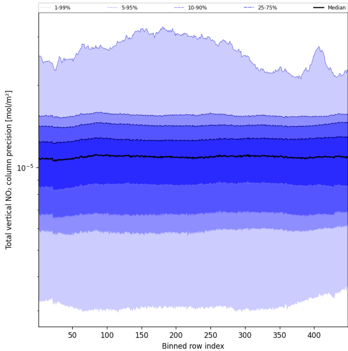
Figure 56: Along track statistics of “Total vertical NO 2 column precision” for 2025-02-20 to 2025-02-22
