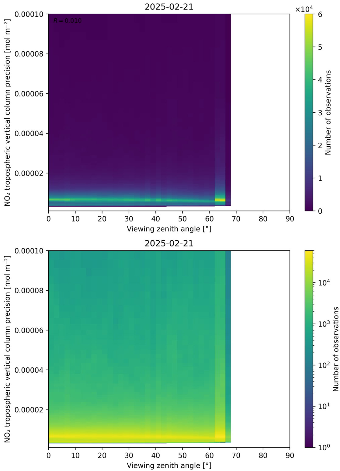
Figure 170: Scatter density plot of “Viewing zenith angle” against “NO 2 tropospheric vertical column precision” for 2025-02-20 to 2025-02-22.
