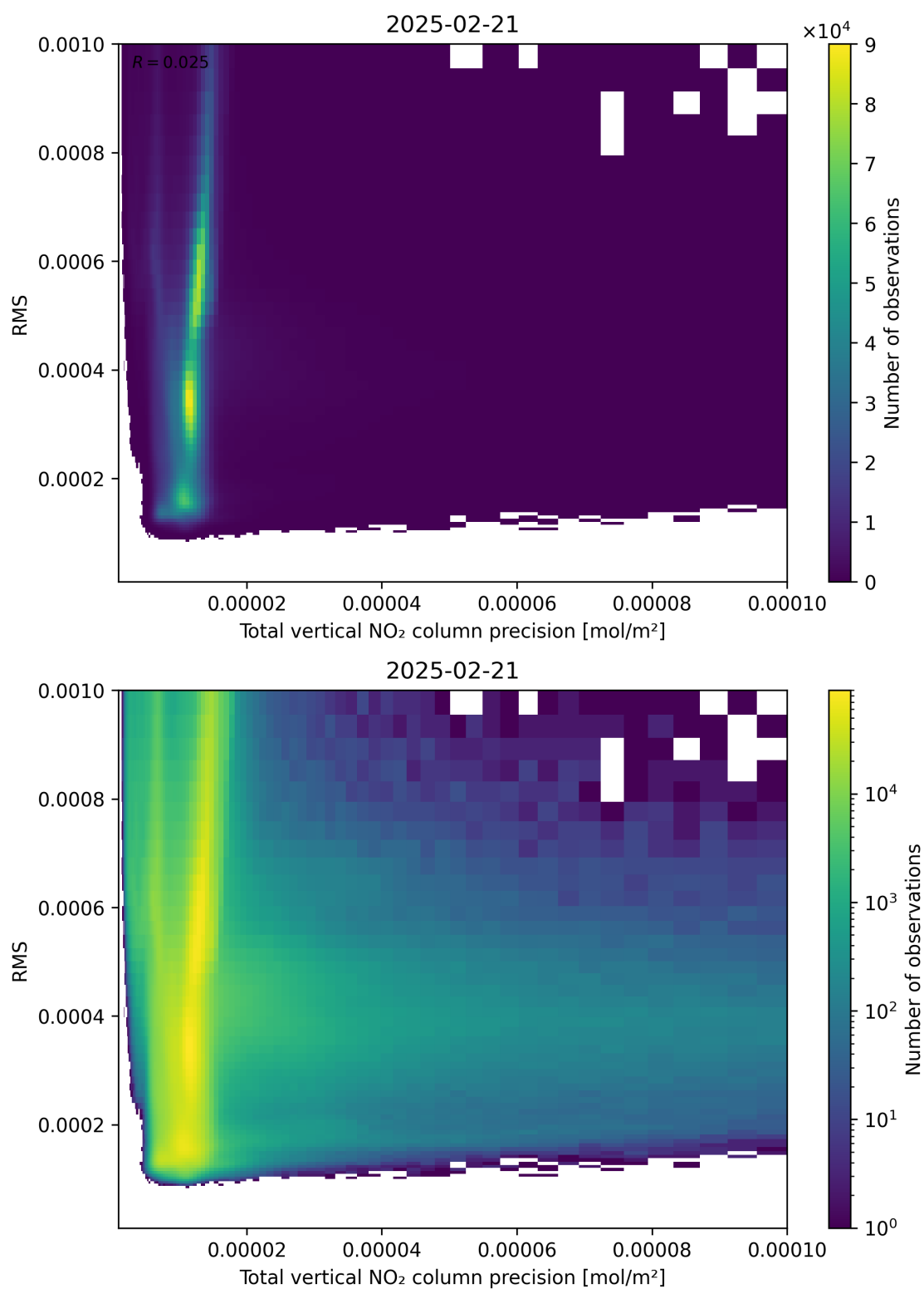
Figure 119: Scatter density plot of “Total vertical NO 2 column precision” against “RMS” for 2025-02-20 to 2025-02-22.
