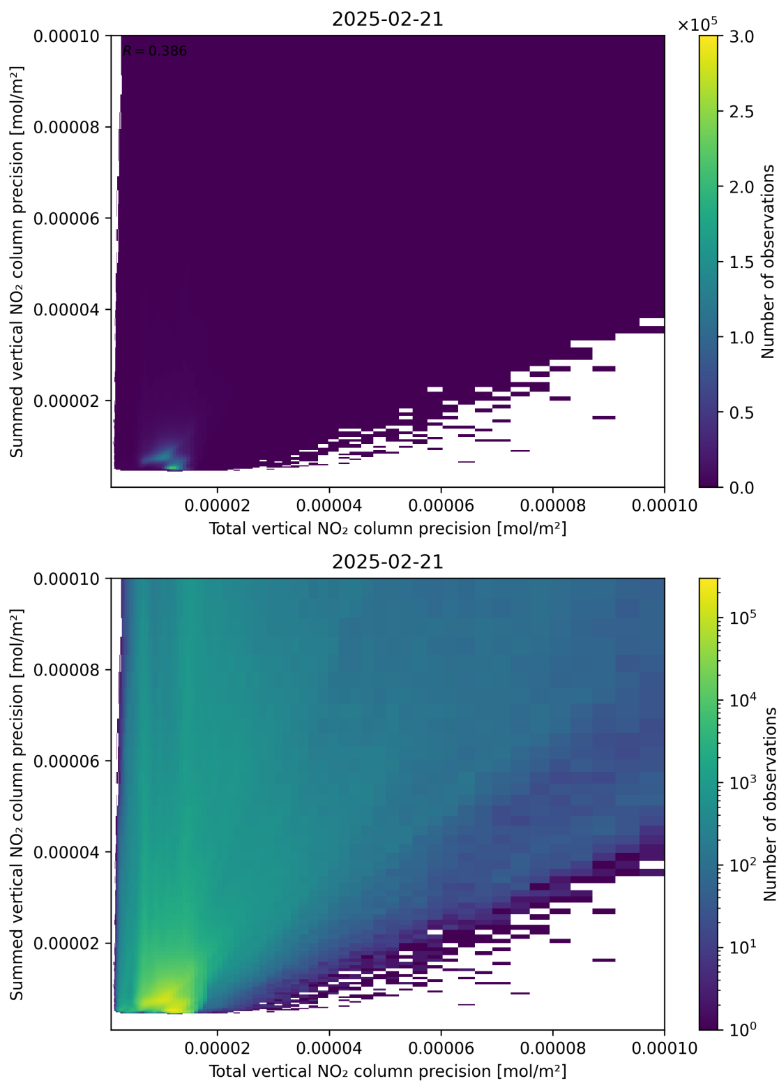
Figure 118: Scatter density plot of “Total vertical NO 2 column precision” against “Summed vertical NO 2 column precision” for 2025-02-20 to 2025-02-22.
