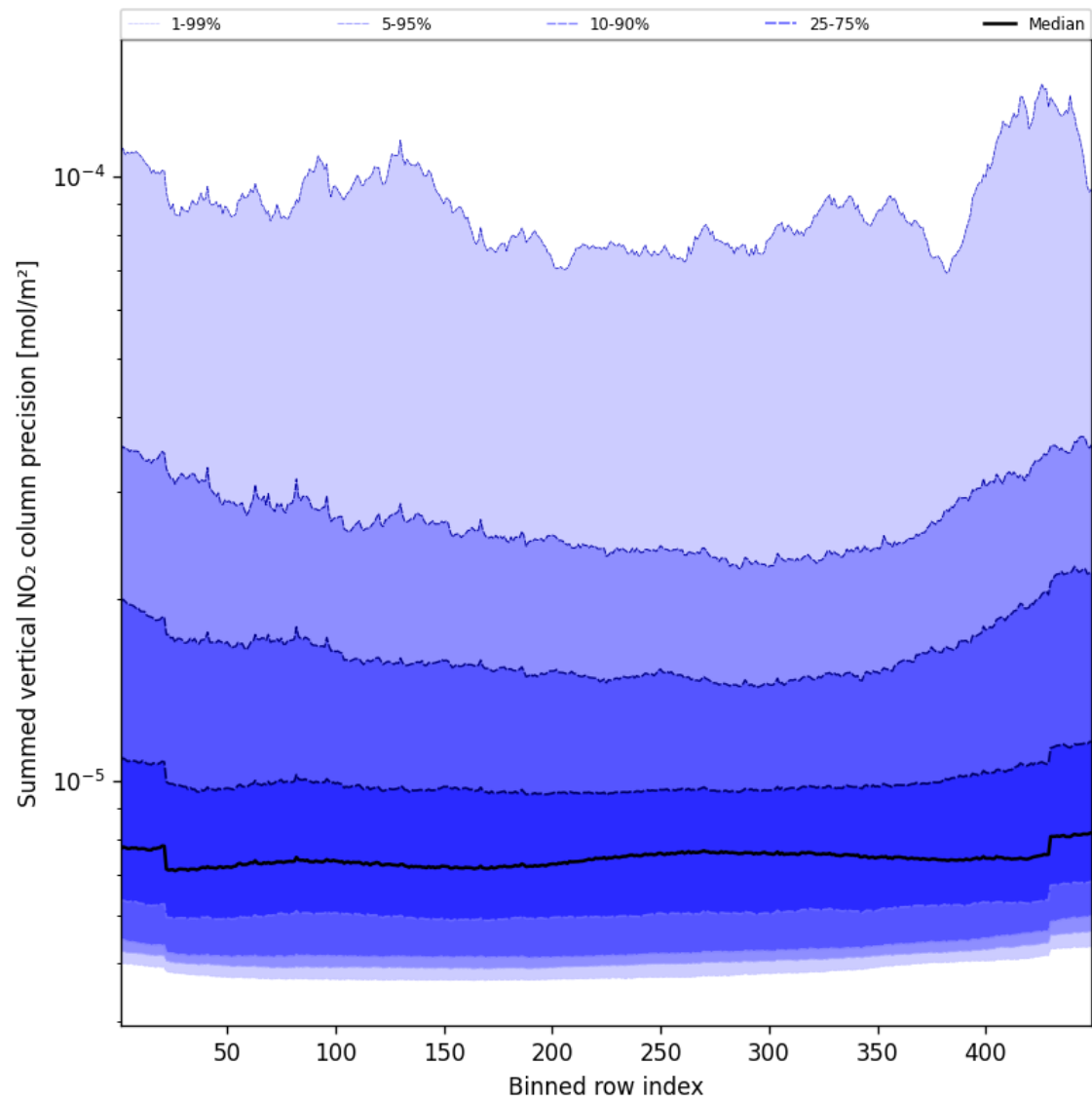
Figure 58: Along track statistics of “Summed vertical NO 2 column precision” for 2025-02-20 to 2025-02-22
