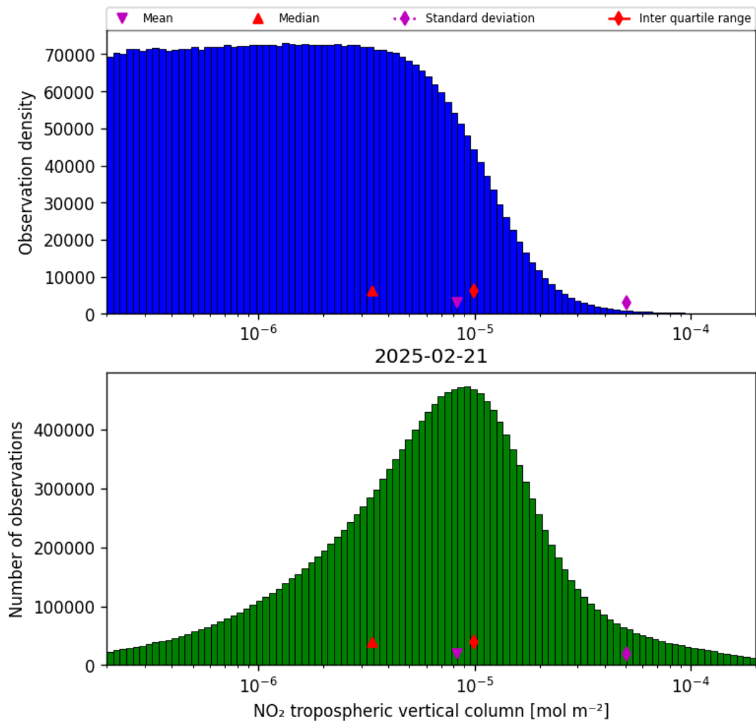
Figure 29: Histogram of “NO 2 tropospheric vertical column” for 2025-02-20 to 2025-02-22
