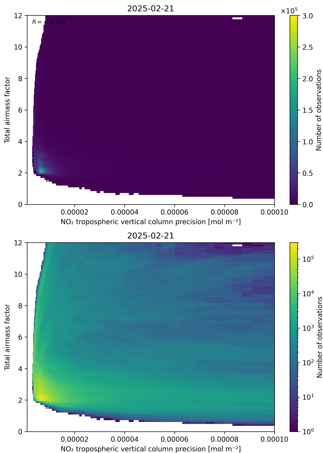
Figure 132: Scatter density plot of “NO 2 tropospheric vertical column precision” against “Total airmass factor” for 2025-02-20 to 2025-02-22.
