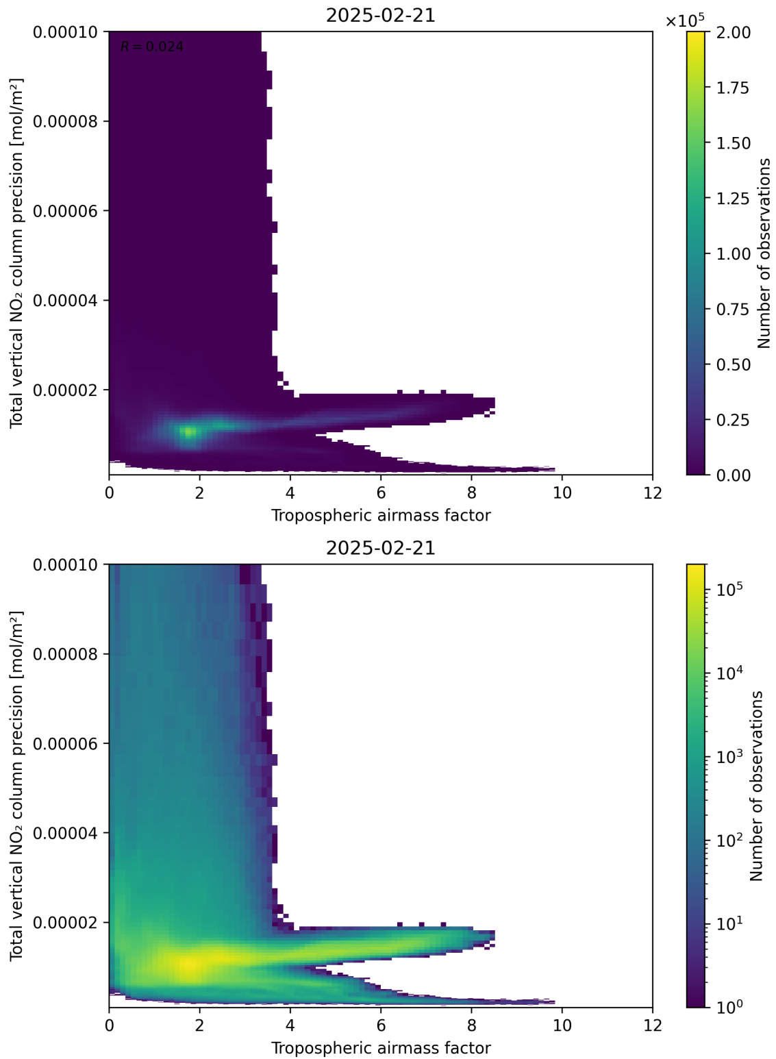
Figure 78: Scatter density plot of “Tropospheric air mass factor” against “Total vertical NO 2 column precision” for 2025-02-20 to 2025-02-22.
