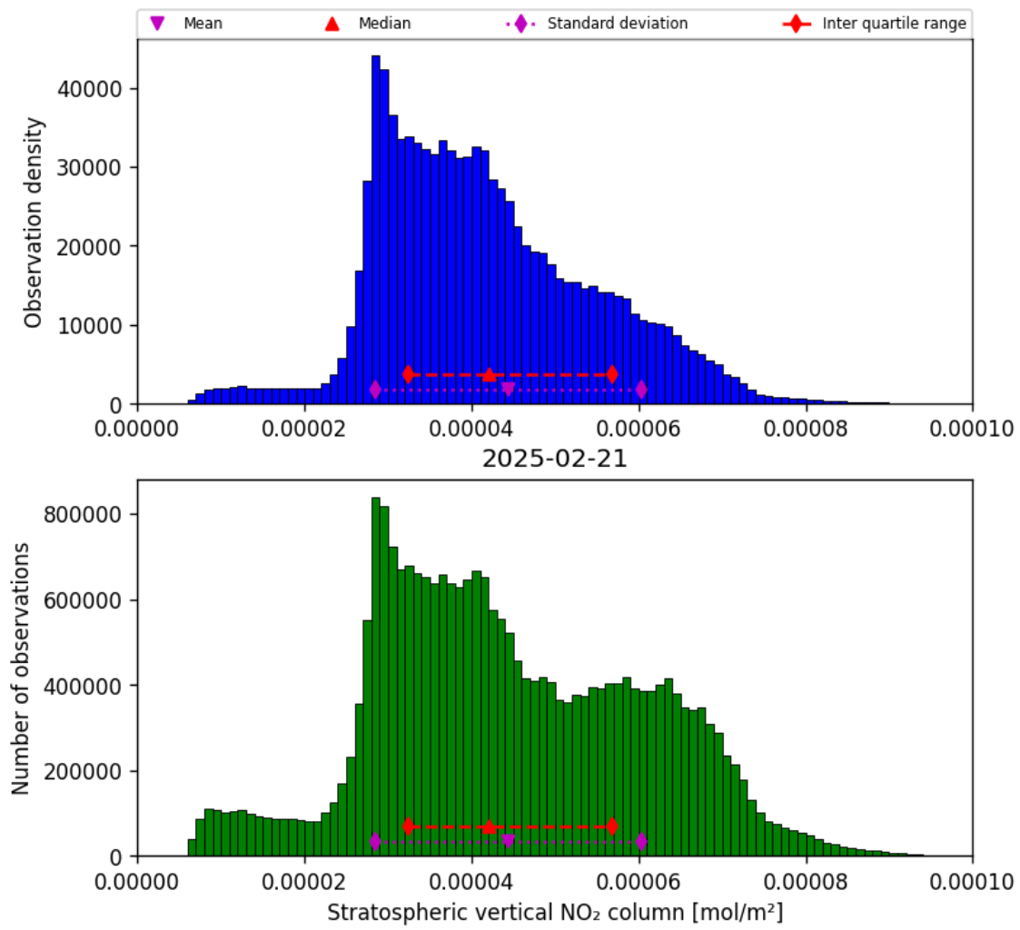
Figure 36: Histogram of “Stratospheric vertical NO 2 column” for 2025-02-20 to 2025-02-22
