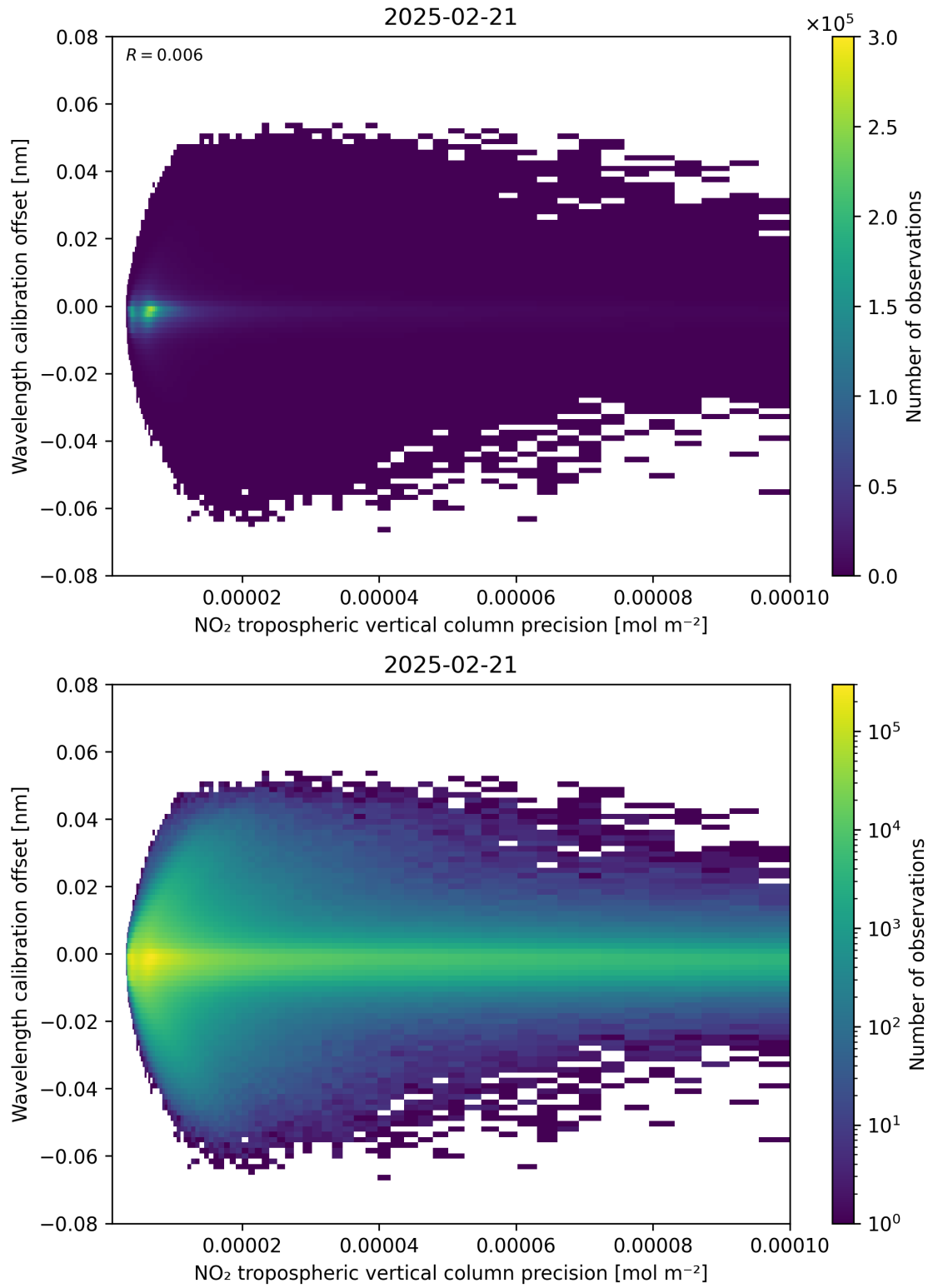
Figure 141: Scatter density plot of “NO 2 tropospheric vertical column precision” against “Wavelength calibration offset” for 2025-02-20 to 2025-02-22.
