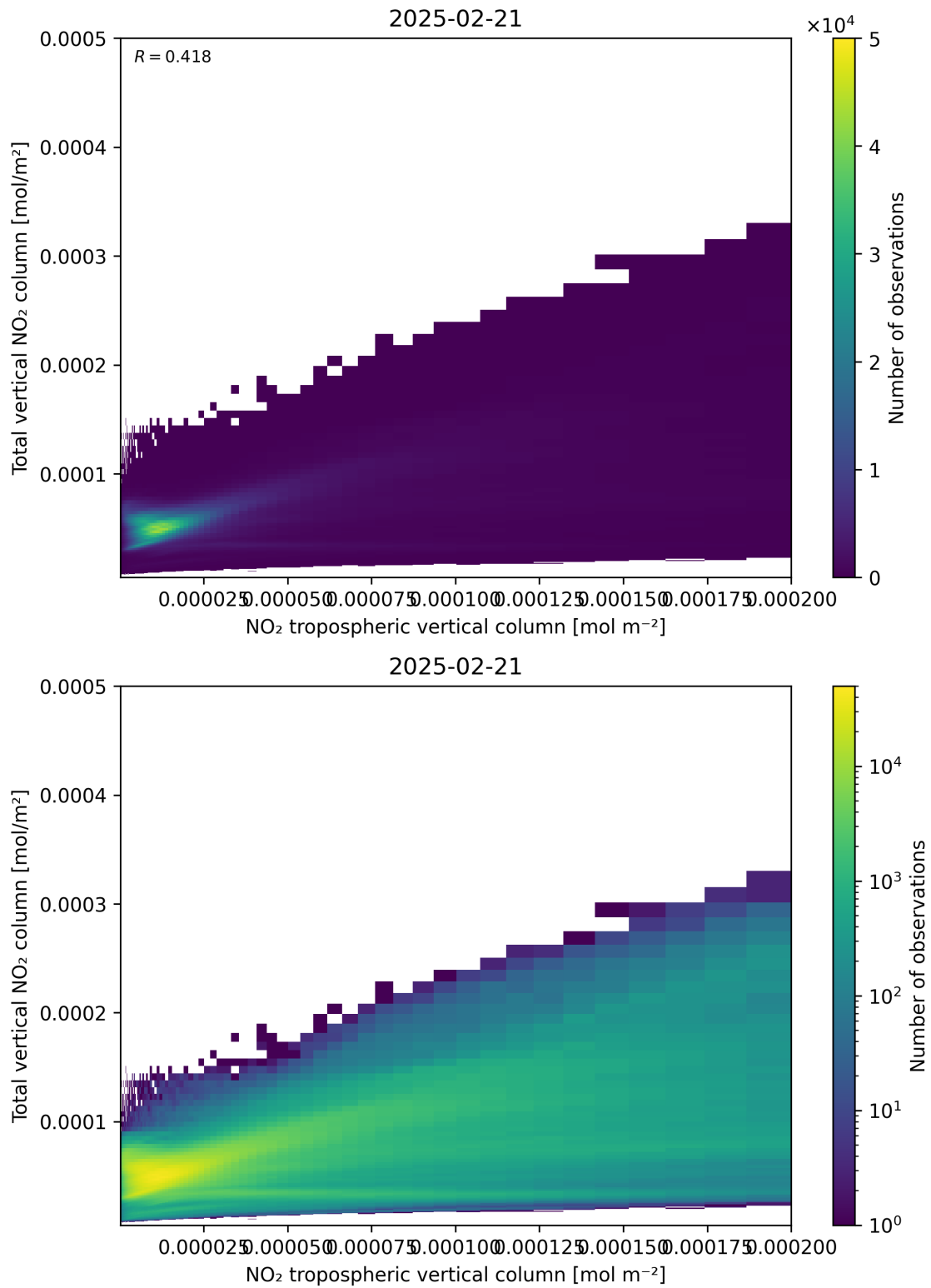
Figure 128: Scatter density plot of “NO 2 tropospheric vertical column” against “Total vertical NO 2 column” for 2025-02-20 to 2025-02-22.
