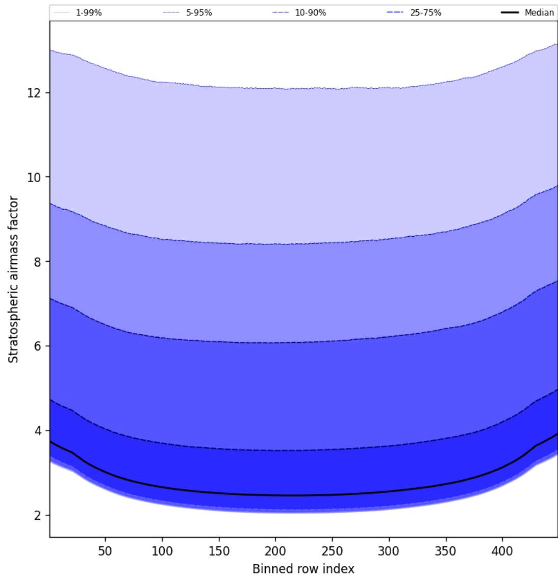
Figure 61: Along track statistics of “Stratospheric airmass factor” for 2025-02-20 to 2025-02-22
