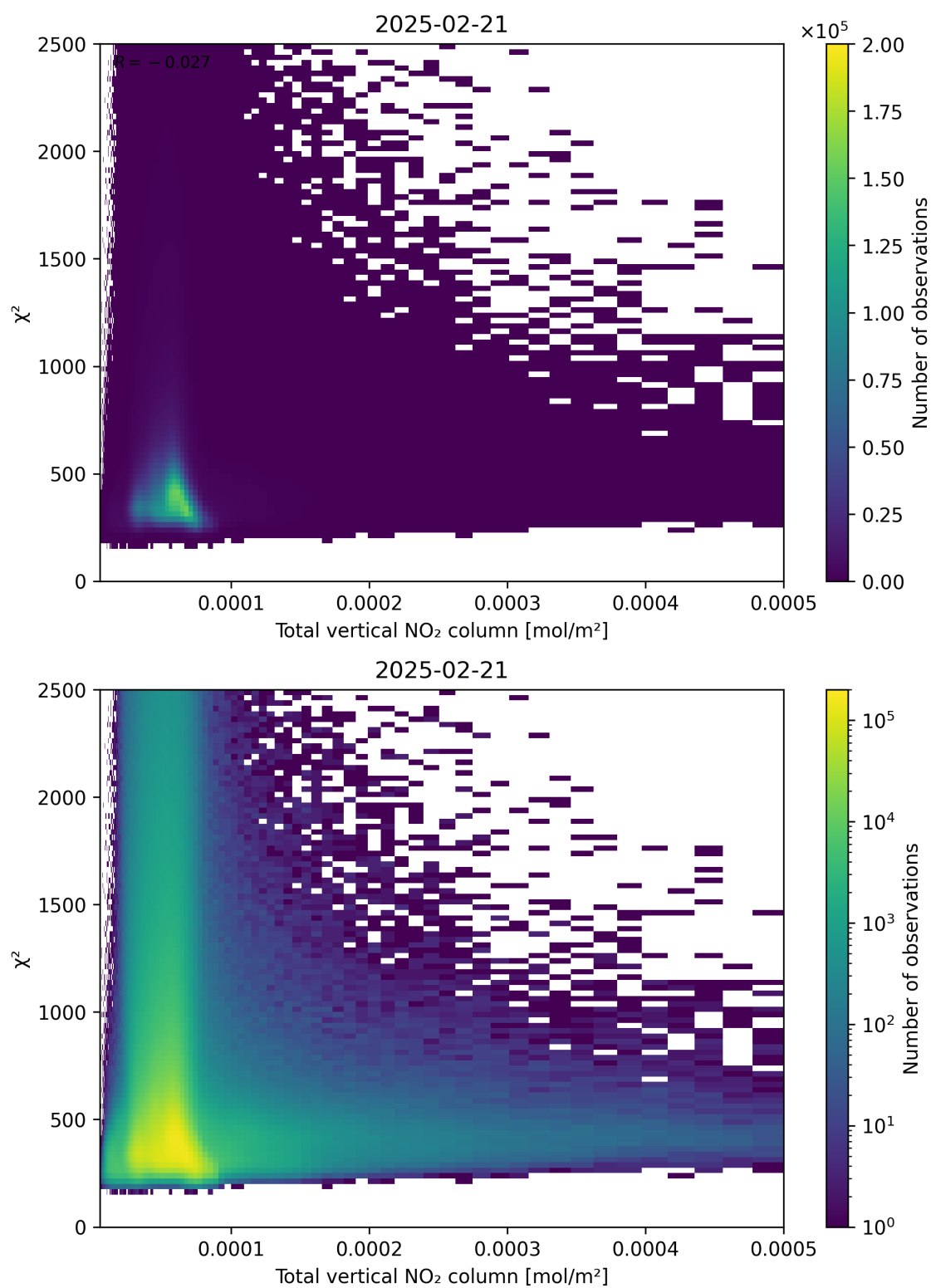
Figure 111: Scatter density plot of “Total vertical NO 2 column” against “ \chi^2 ” for 2025-02-20 to 2025-02-22.
