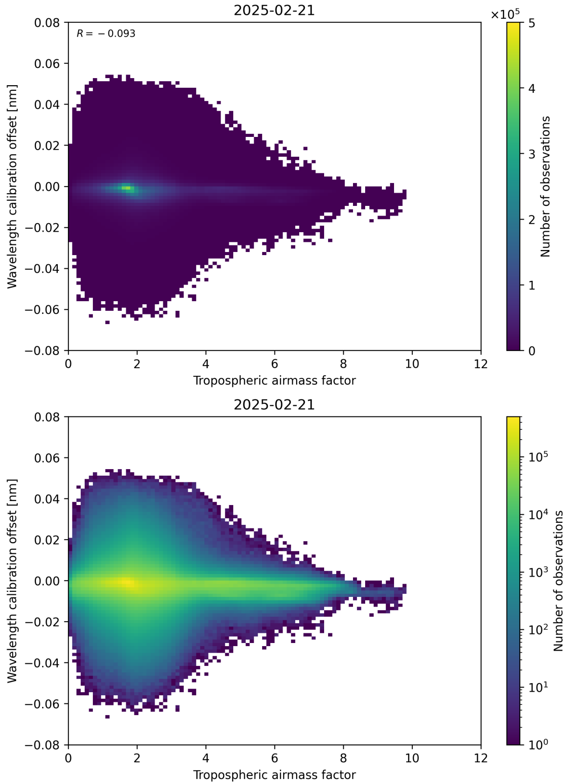
Figure 80: Scatter density plot of “Tropospheric airmass factor” against “Wavelength calibration offset” for 2025-02-20 to 2025-02-22.
