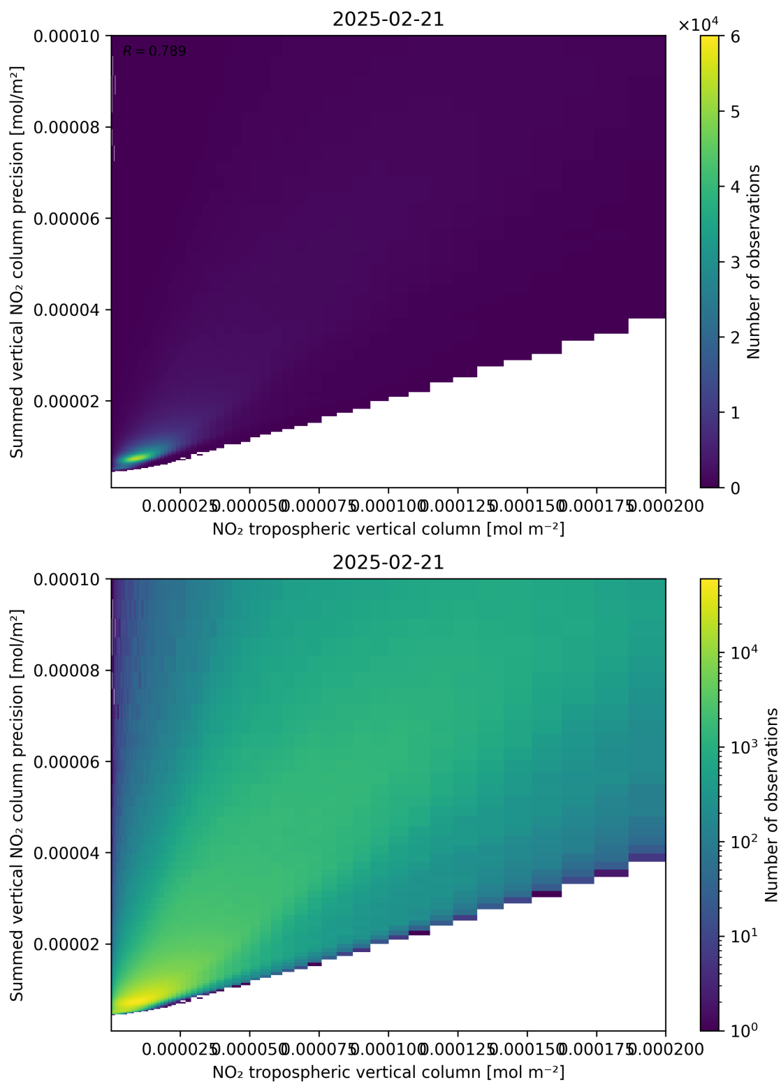
Figure 127: Scatter density plot of “NO 2 tropospheric vertical column” against “Summed vertical NO 2 column precision” for 2025-02-20 to 2025-02-22.
