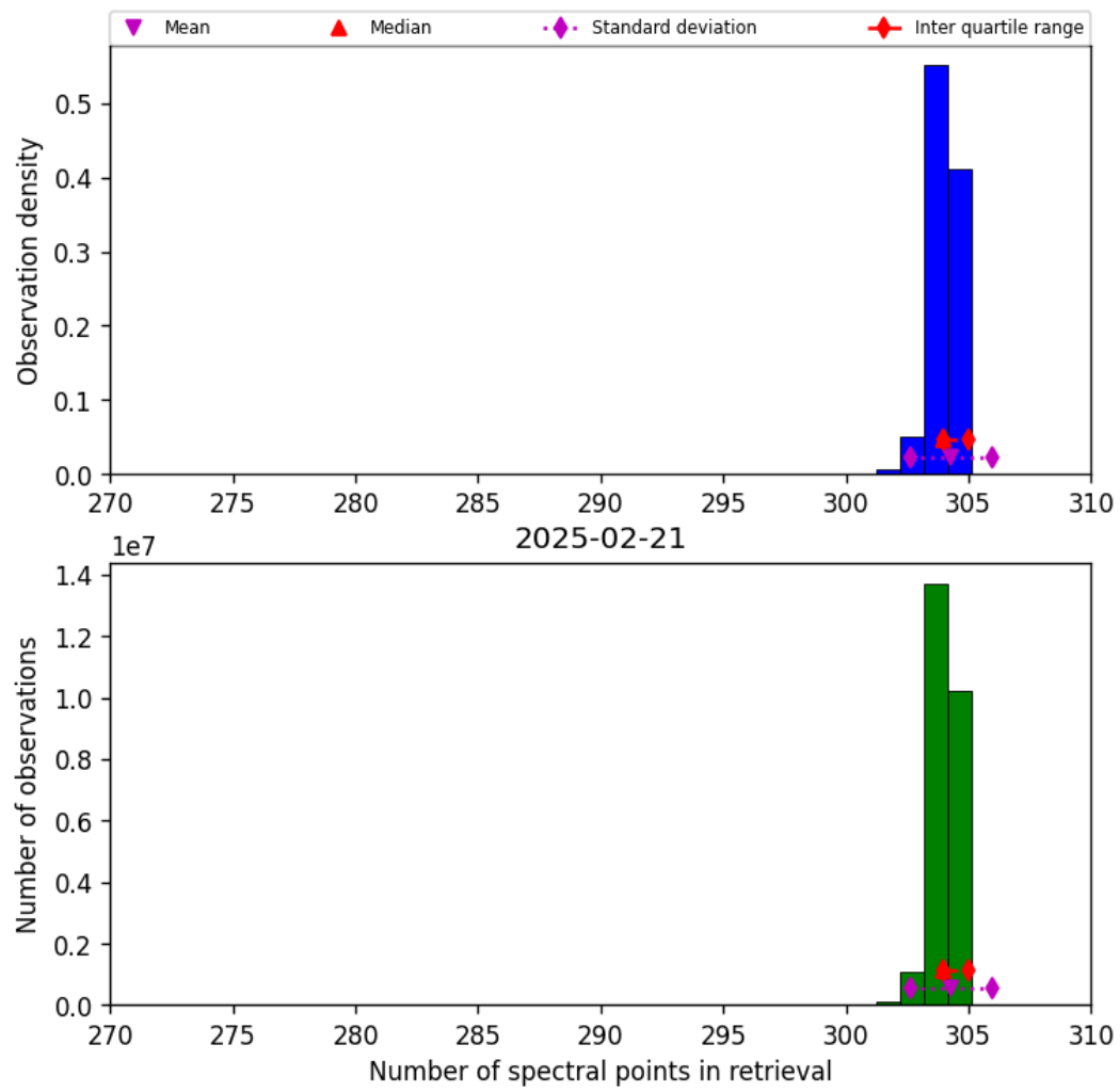
Figure 33: Histogram of “Number of spectral points in retrieval” for 2025-02-20 to 2025-02-22
