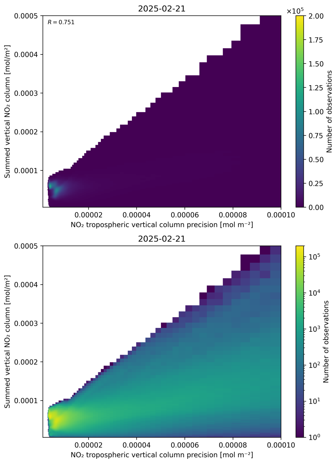
Figure 136: Scatter density plot of “NO 2 tropospheric vertical column precision” against “Summed vertical NO 2 column” for 2025-02-20 to 2025-02-22.
