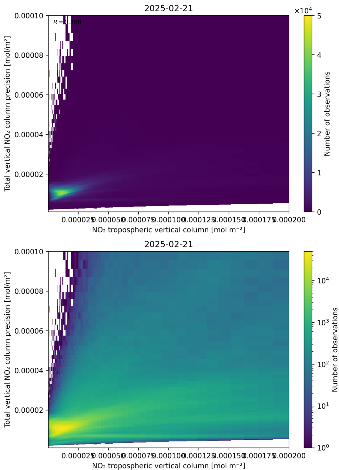
Figure 129: Scatter density plot of “NO 2 tropospheric vertical column” against “Total vertical NO 2 column precision” for 2025-02-20 to 2025-02-22.
