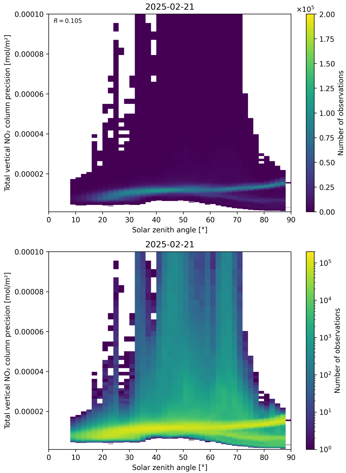
Figure 154: Scatter density plot of “Solar zenith angle” against “Total vertical NO 2 column precision” for 2025-02-20 to 2025-02-22.
