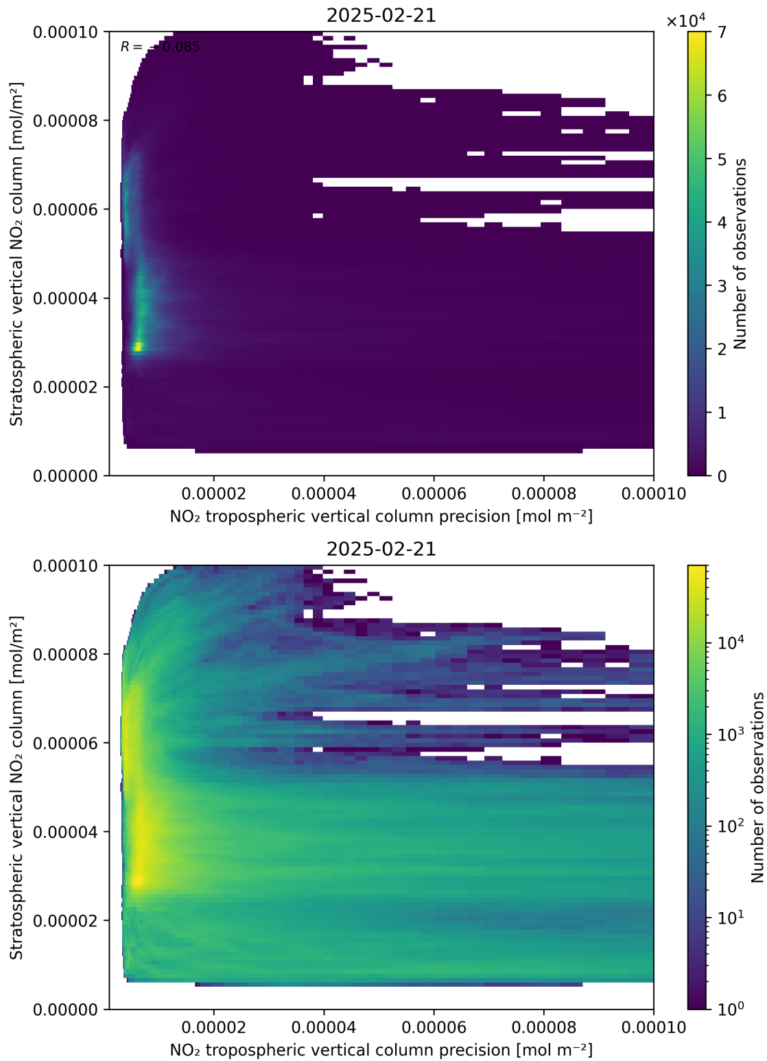
Figure 135: Scatter density plot of “NO 2 tropospheric vertical column precision” against “Stratospheric vertical NO 2 column” for 2025-02-20 to 2025-02-22.
