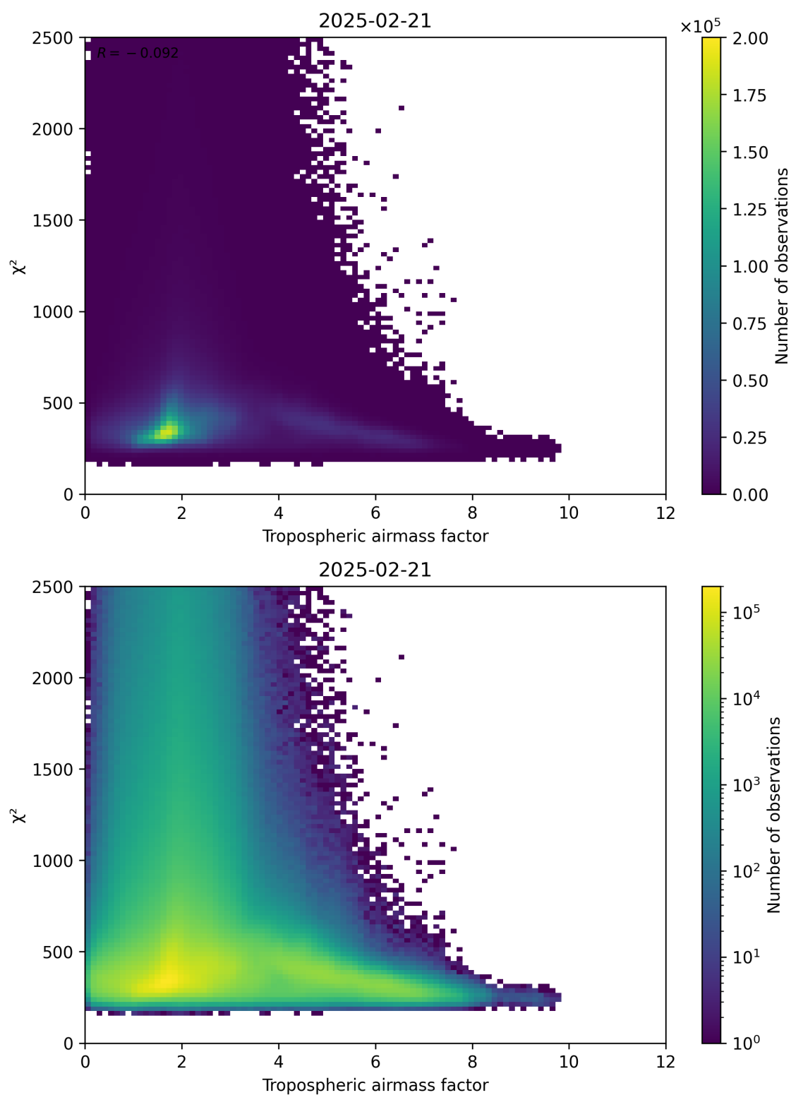
Figure 73: Scatter density plot of “Tropospheric airmass factor” against “ \chi^2 ” for 2025-02-20 to 2025-02-22.
