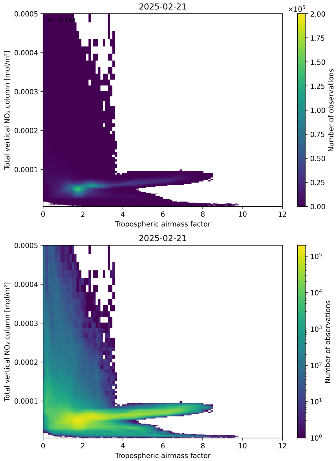
Figure 77: Scatter density plot of “Tropospheric airmass factor” against “Total vertical NO 2 column” for 2025-02-20 to 2025-02-22.
