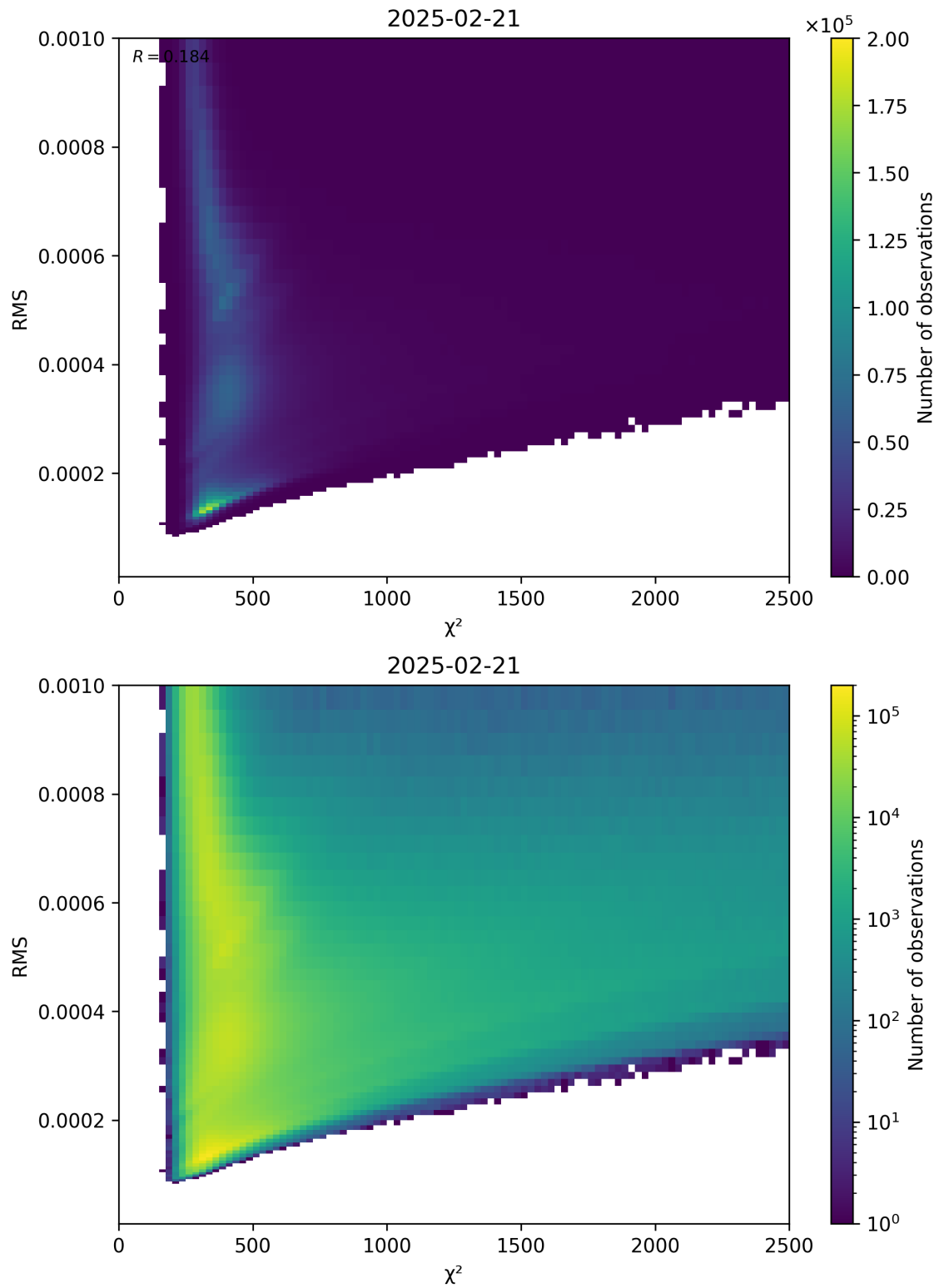
Figure 82: Scatter density plot of “ \chi^2 ” against “RMS” for 2025-02-20 to 2025-02-22.
