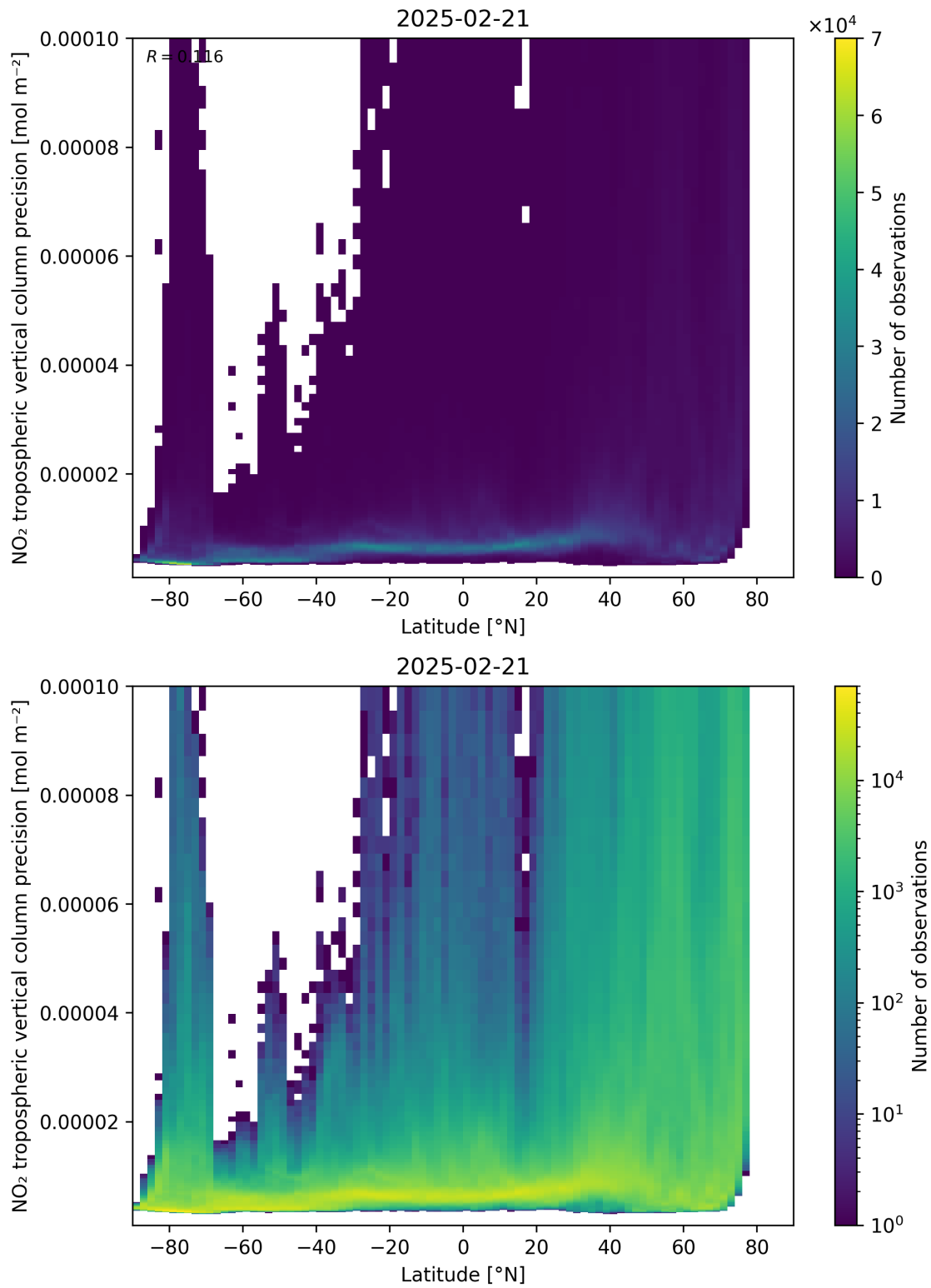
Figure 93: Scatter density plot of “Latitude” against “NO 2 tropospheric vertical column precision” for 2025-02-20 to 2025-02-22.
