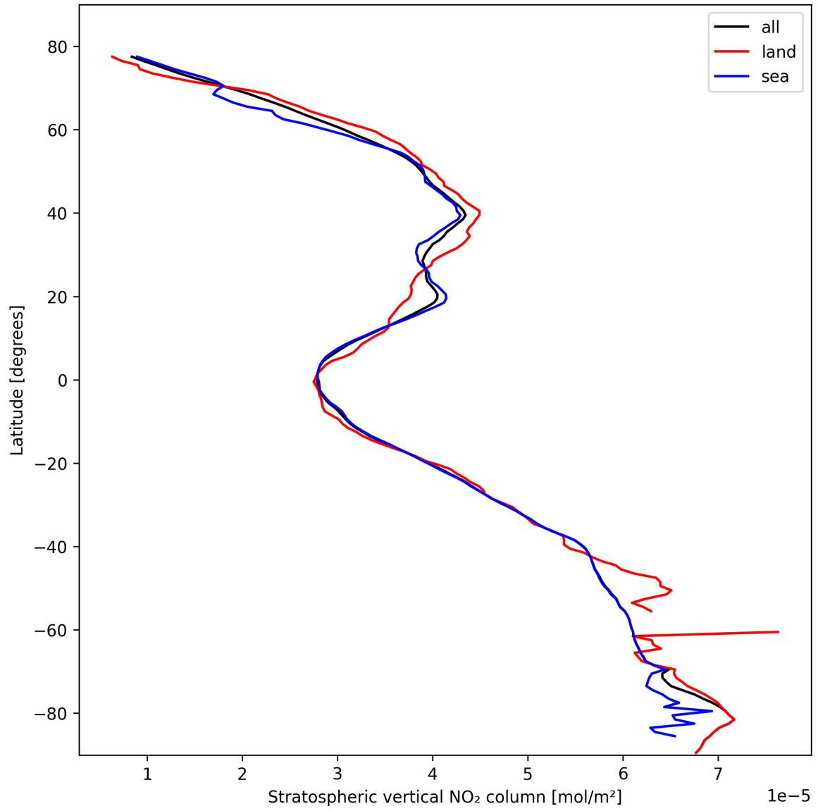
Figure 19: Zonal average of “Stratospheric vertical NO 2 column” for 2025-02-20 to 2025-02-22.
