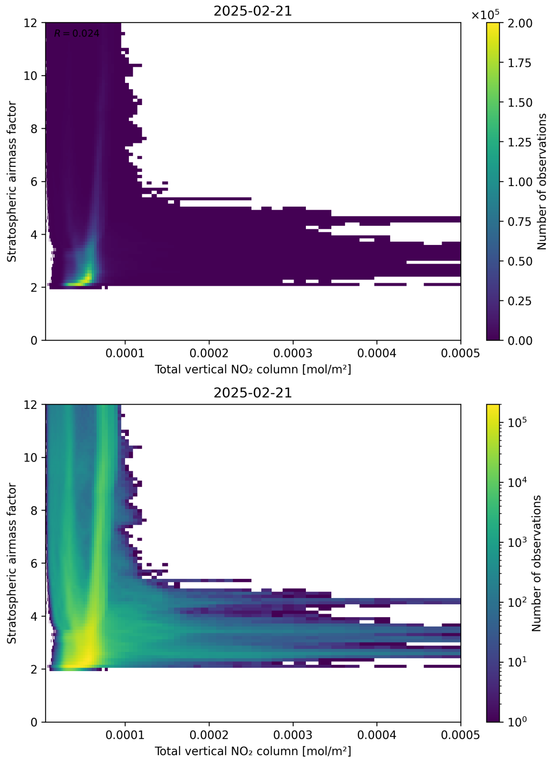
Figure 110: Scatter density plot of “Total vertical NO 2 column” against “Stratospheric airmass factor” for 2025-02-20 to 2025-02-22.
