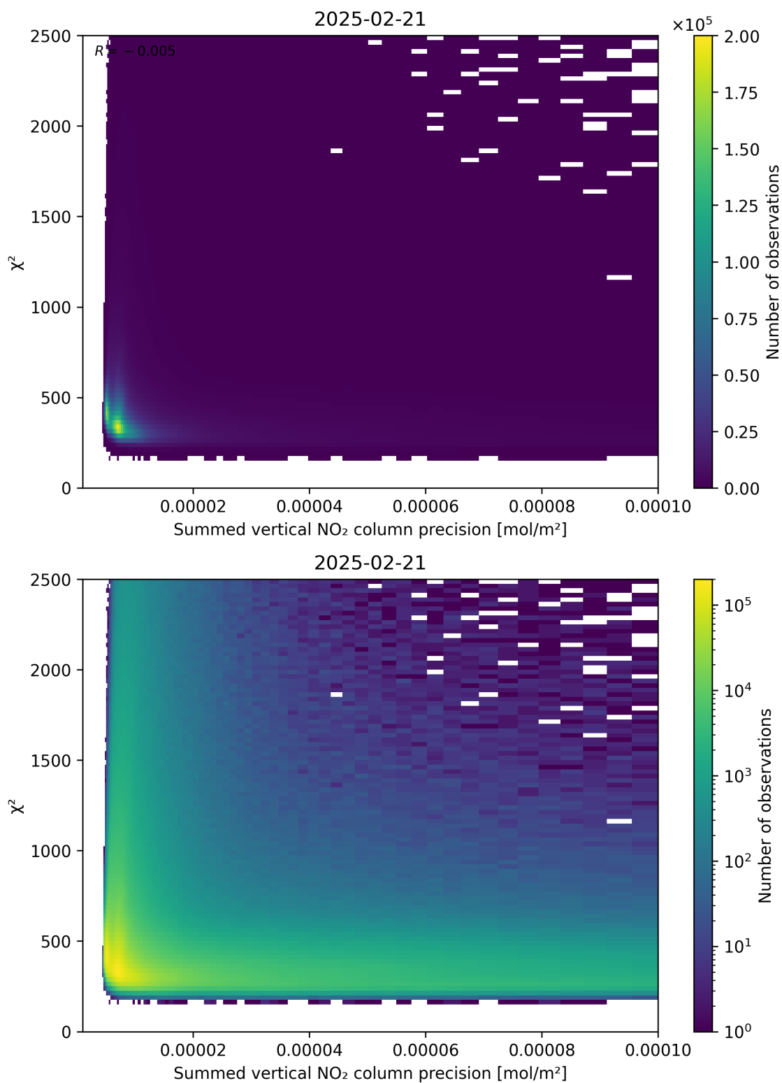
Figure 107: Scatter density plot of “Summed vertical NO 2 column precision” against “ \chi^2 ” for 2025-02-20 to 2025-02-22.
