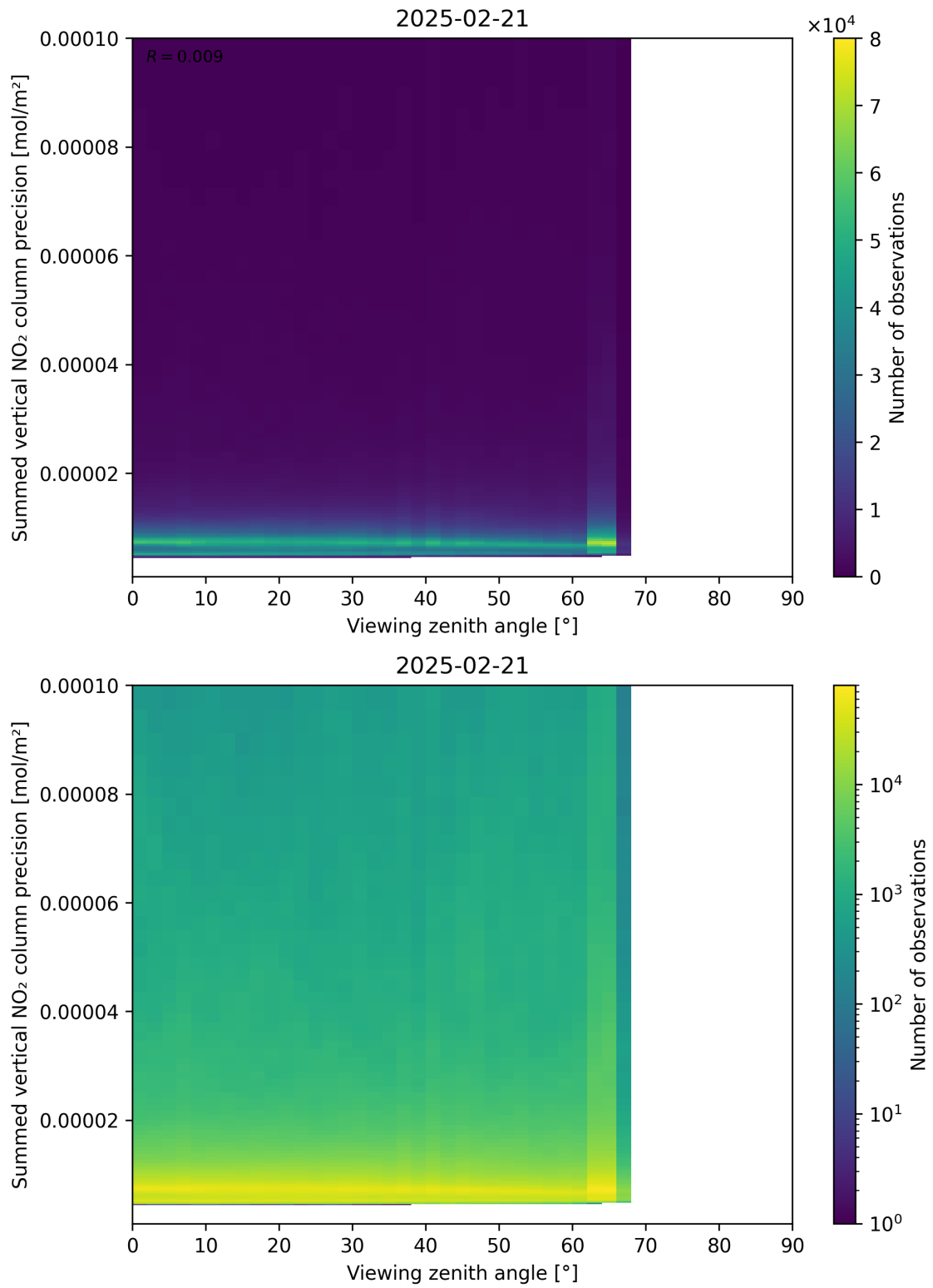
Figure 166: Scatter density plot of “Viewing zenith angle” against “Summed vertical NO 2 column precision” for 2025-02-20 to 2025-02-22.
