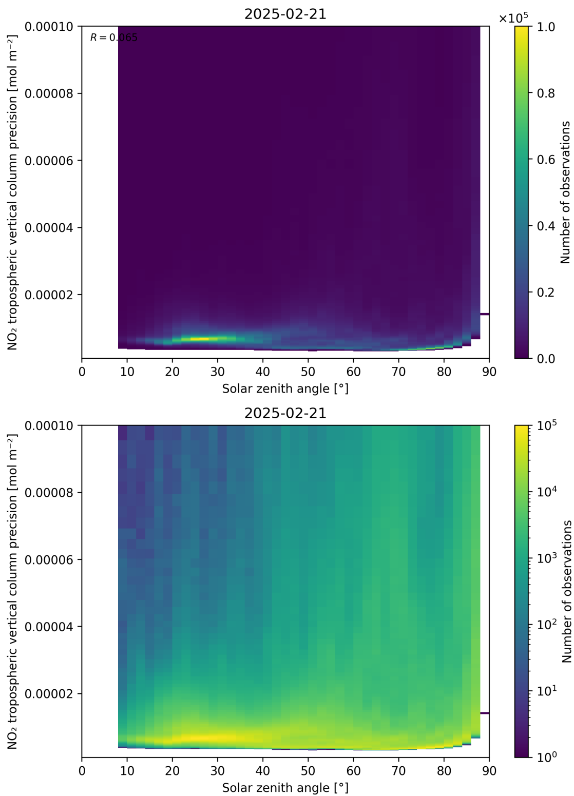
Figure 156: Scatter density plot of “Solar zenith angle” against “NO 2 tropospheric vertical column precision” for 2025-02-20 to 2025-02-22.
