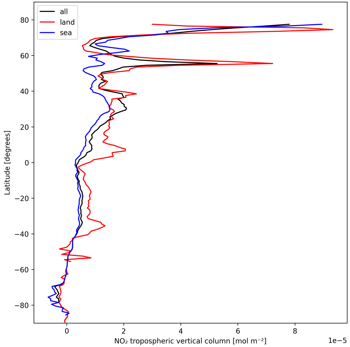
Figure 12: Zonal average of “NO 2 tropospheric vertical column” for 2025-02-20 to 2025-02-22.
