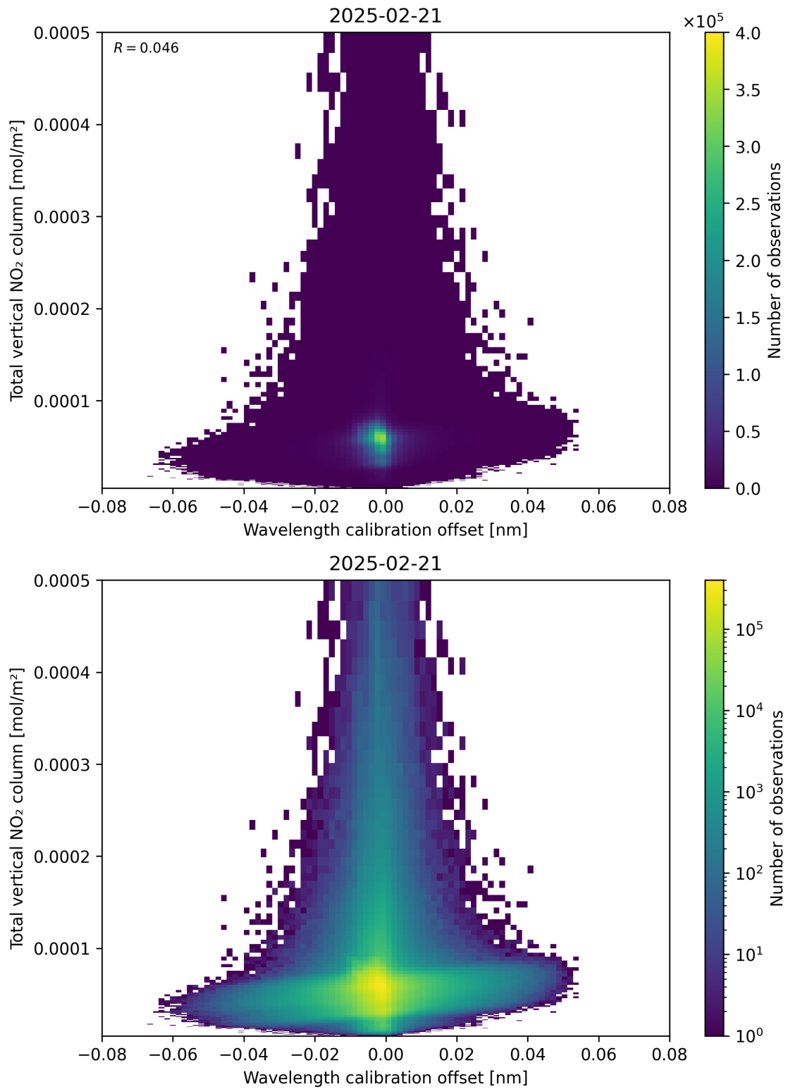
Figure 179: Scatter density plot of “Wavelength calibration offset” against “Total vertical NO 2 column” for 2025-02-20 to 2025-02-22.
