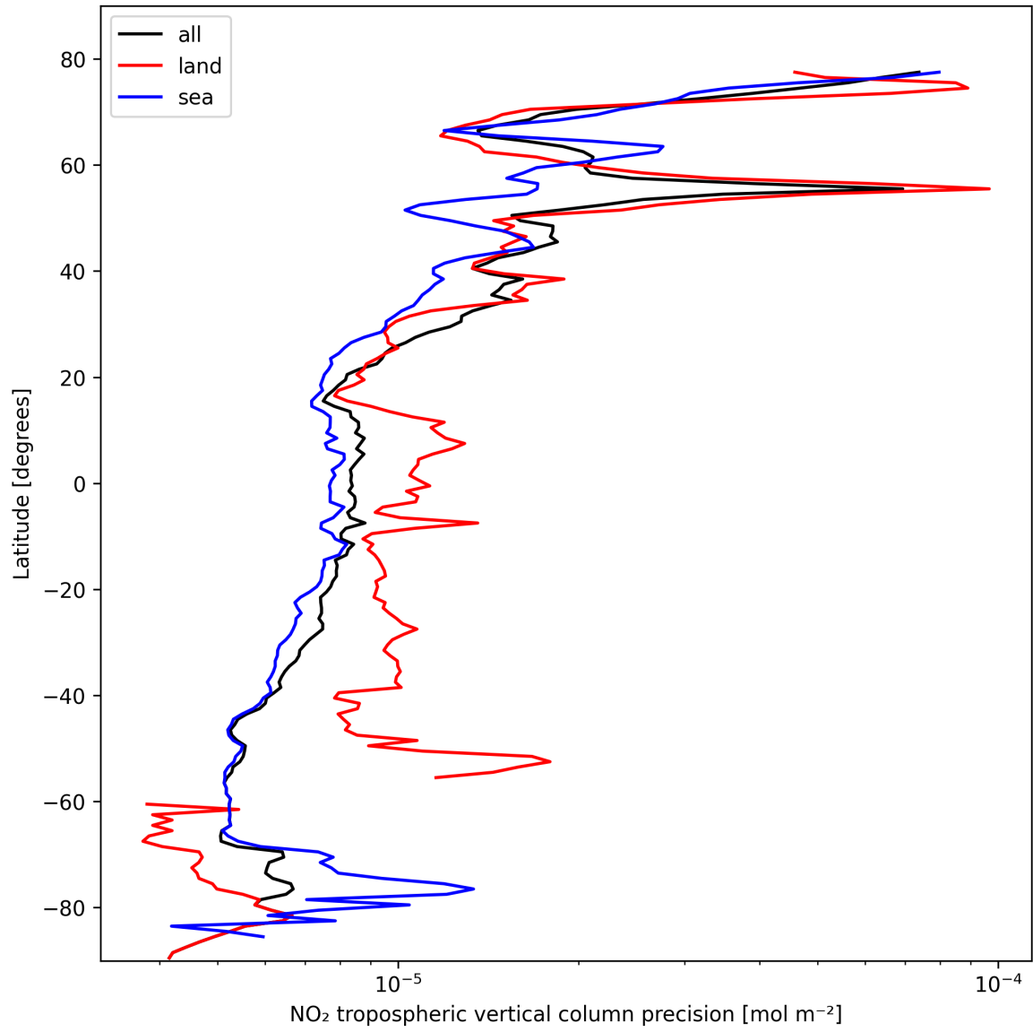
Figure 13: Zonal average of “NO 2 tropospheric vertical column precision” for 2025-02-20 to 2025-02-22.
