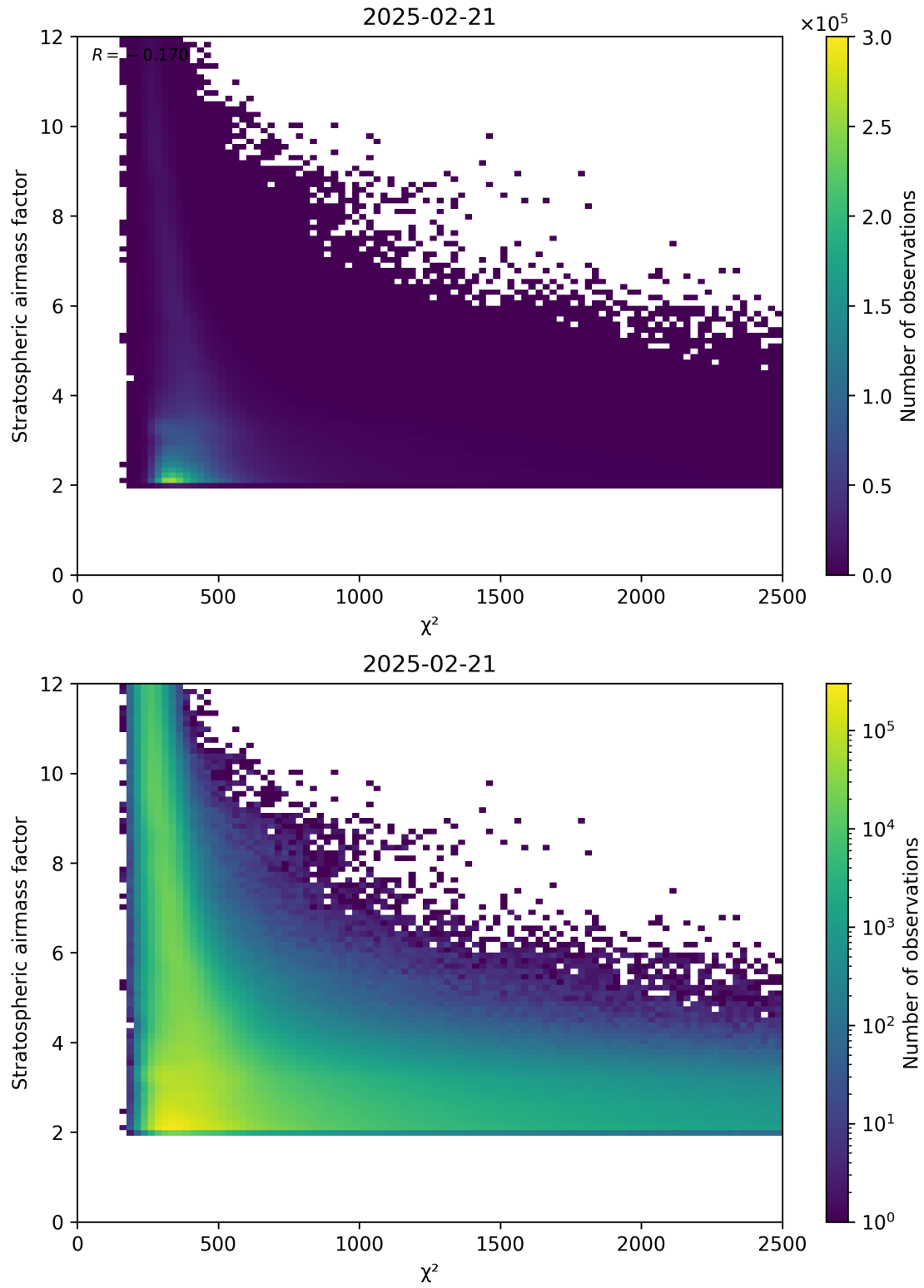
Figure 81: Scatter density plot of “ \chi^2 ” against “Stratospheric airmass factor” for 2025-02-20 to 2025-02-22.
