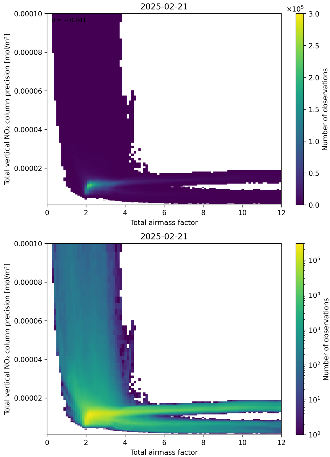
Figure 68: Scatter density plot of “Total airmass factor” against “Total vertical NO 2 column precision” for 2025-02-20 to 2025-02-22.
