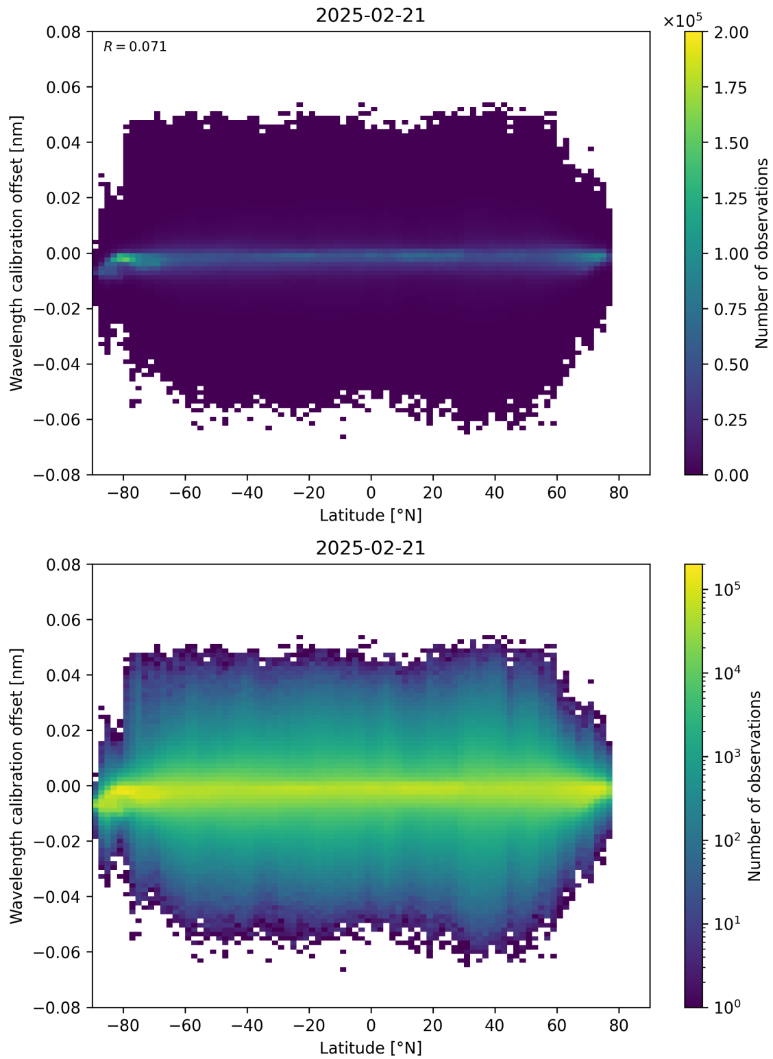
Figure 95: Scatter density plot of “Latitude” against “Wavelength calibration offset” for 2025-02-20 to 2025-02-22.
