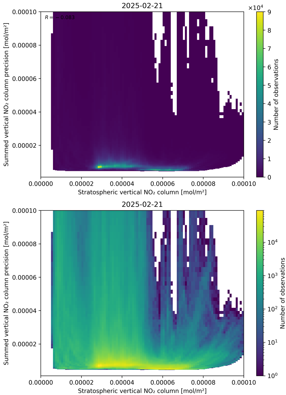
Figure 99: Scatter density plot of “Stratospheric vertical NO 2 column” against “Summed vertical NO 2 column precision” for 2025-02-20 to 2025-02-22.
