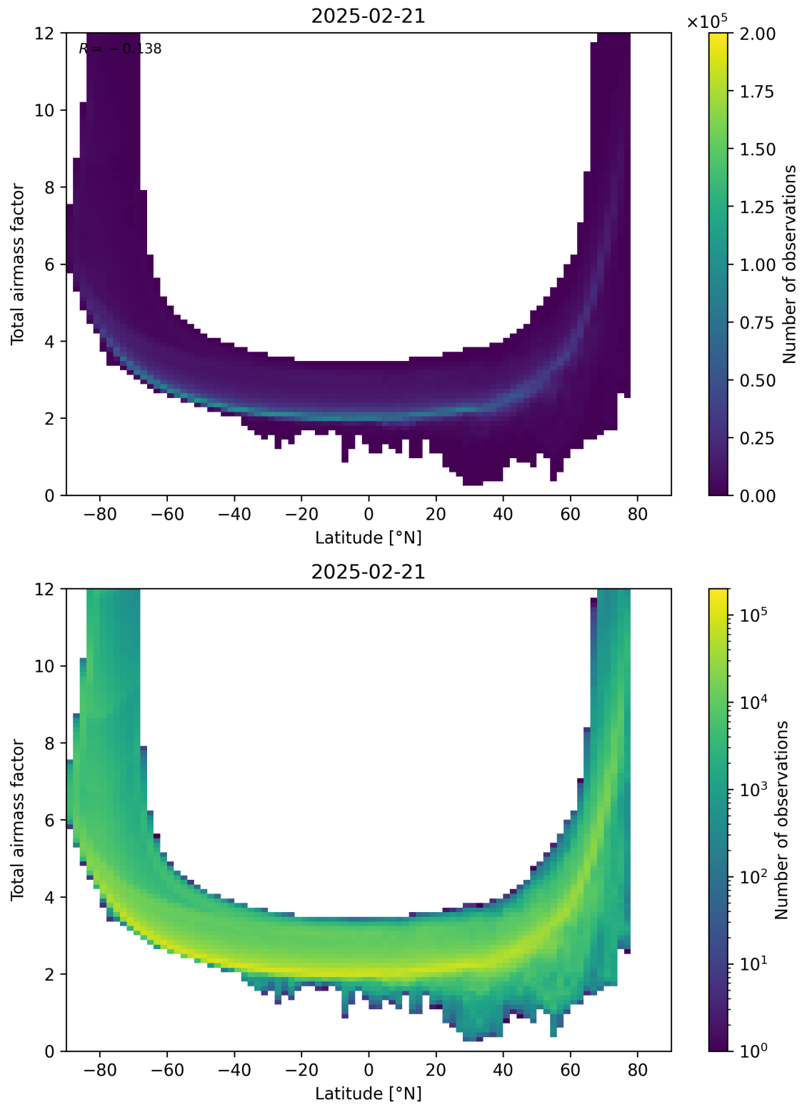
Figure 84: Scatter density plot of “Latitude” against “Total airmass factor” for 2025-02-20 to 2025-02-22.
