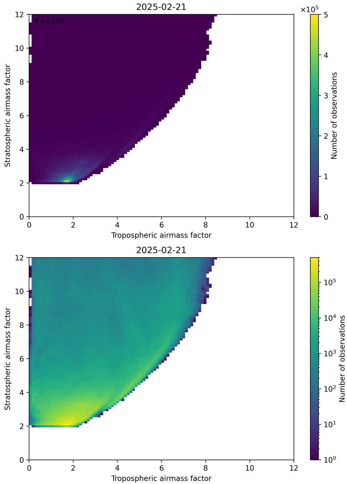
Figure 71: Scatter density plot of “Tropospheric airmass factor” against “Stratospheric airmass factor” for 2025-02-20 to 2025-02-22.
