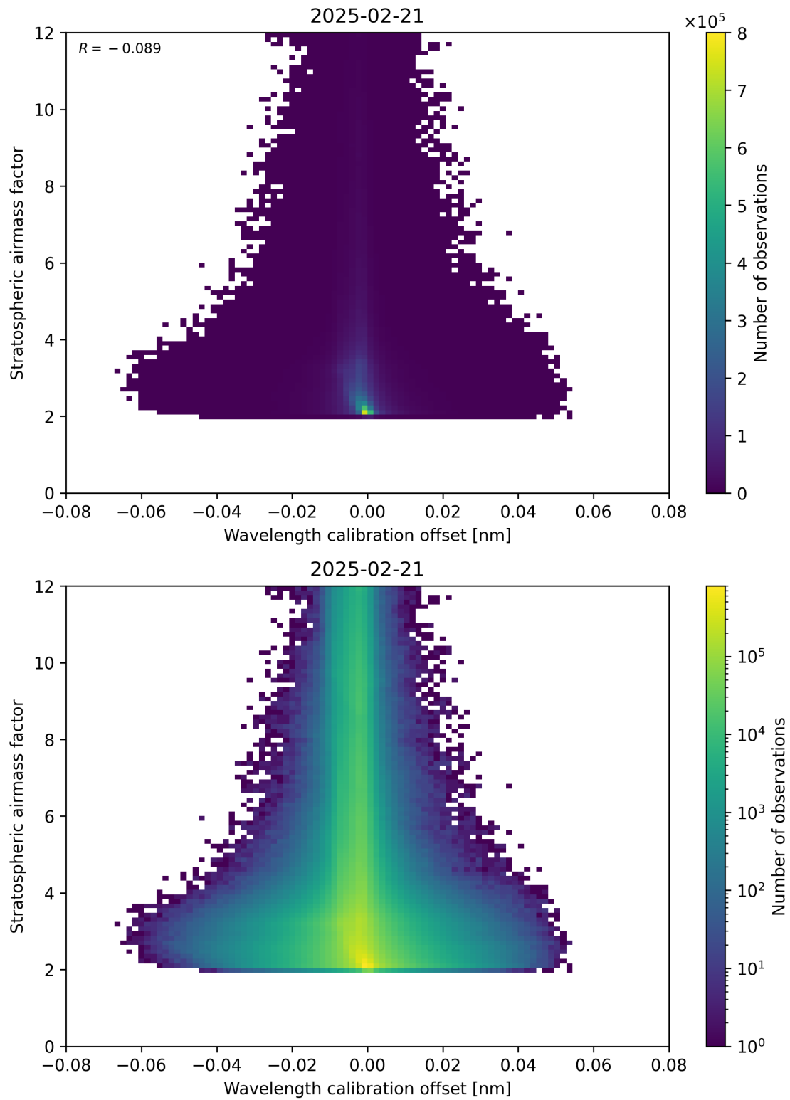
Figure 174: Scatter density plot of “Wavelength calibration offset” against “Stratospheric airmass factor” for 2025-02-20 to 2025-02-22.
