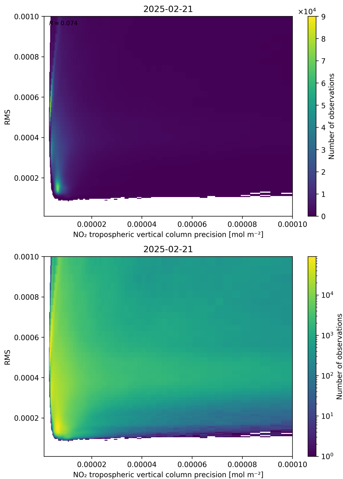
Figure 140: Scatter density plot of “NO 2 tropospheric vertical column precision” against “RMS” for 2025-02-20 to 2025-02-22.
