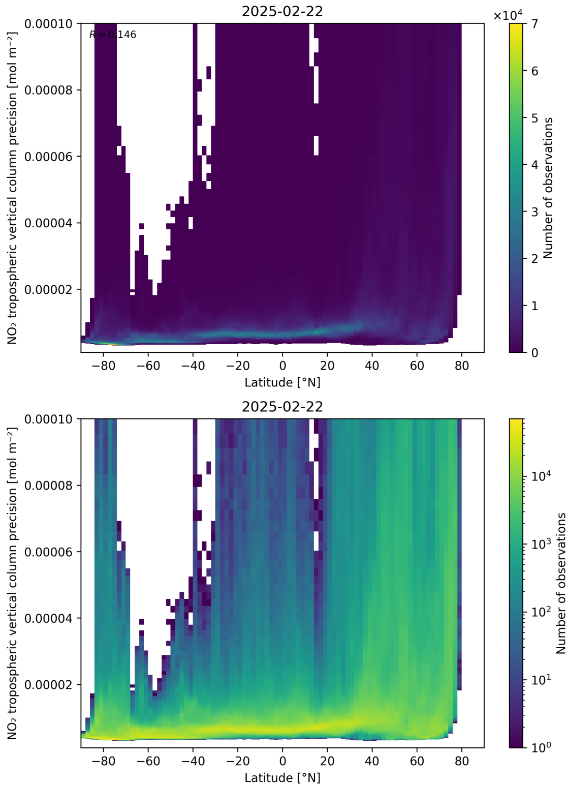
Figure 93: Scatter density plot of “Latitude” against “NO 2 tropospheric vertical column precision” for 2025-02-21 to 2025-02-23.
