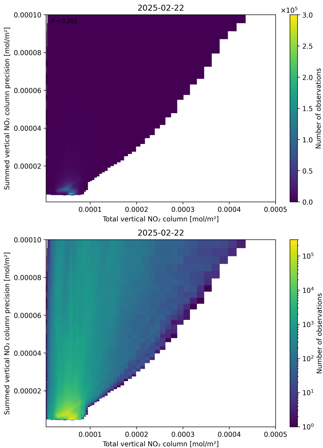
Figure 113: Scatter density plot of “Total vertical NO 2 column” against “Summed vertical NO 2 column precision” for 2025-02-21 to 2025-02-23.
