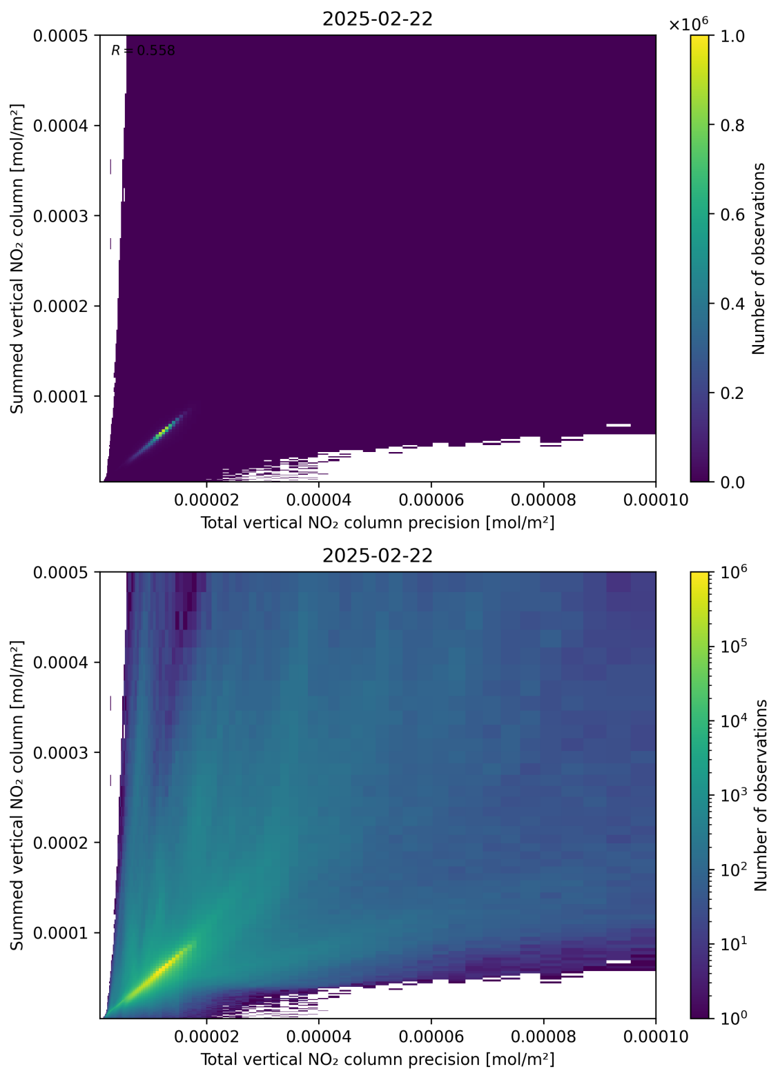
Figure 117: Scatter density plot of “Total vertical NO 2 column precision” against “Summed vertical NO 2 column” for 2025-02-21 to 2025-02-23.
