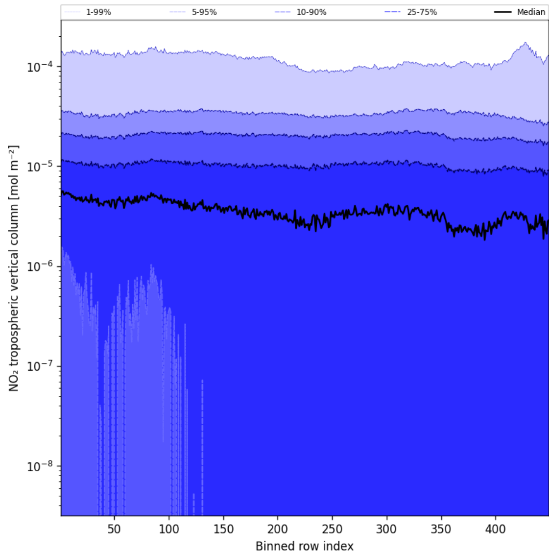
Figure 46: Along track statistics of “NO 2 tropospheric vertical column” for 2025-02-21 to 2025-02-23
