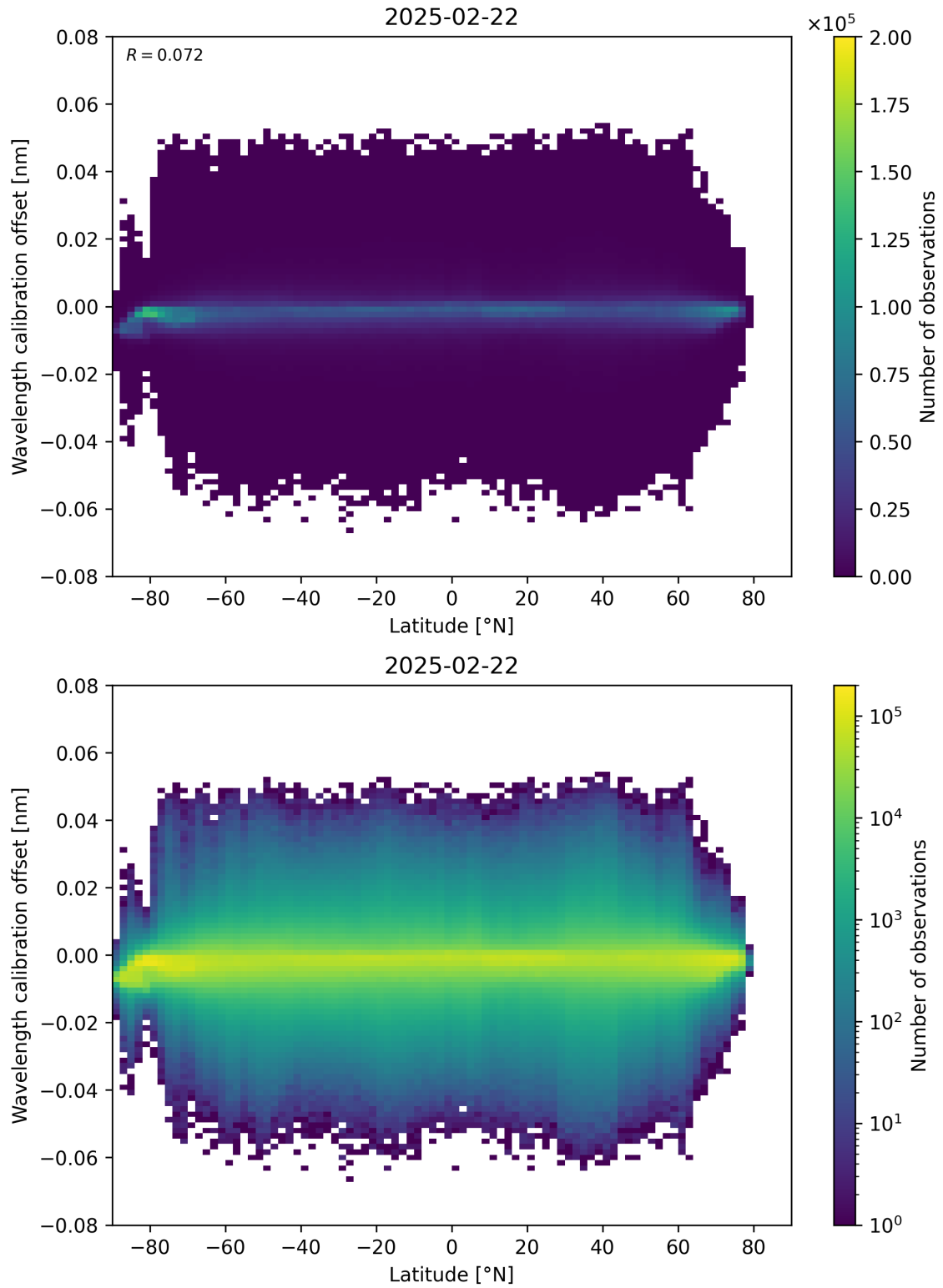
Figure 95: Scatter density plot of “Latitude” against “Wavelength calibration offset” for 2025-02-21 to 2025-02-23.
