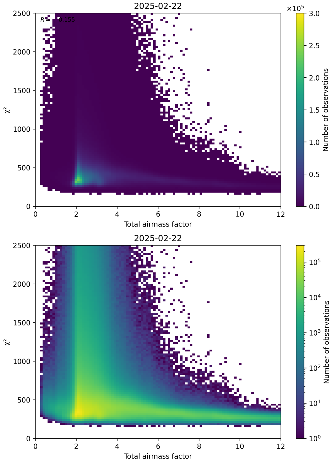
Figure 63: Scatter density plot of “Total airmass factor” against “ \chi^2 ” for 2025-02-21 to 2025-02-23.
