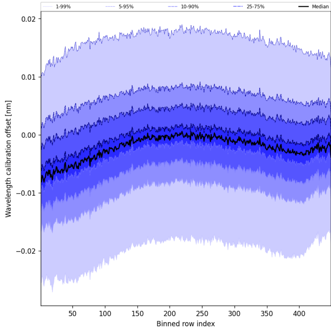
Figure 52: Along track statistics of “Wavelength calibration offset” for 2025-02-21 to 2025-02-23
