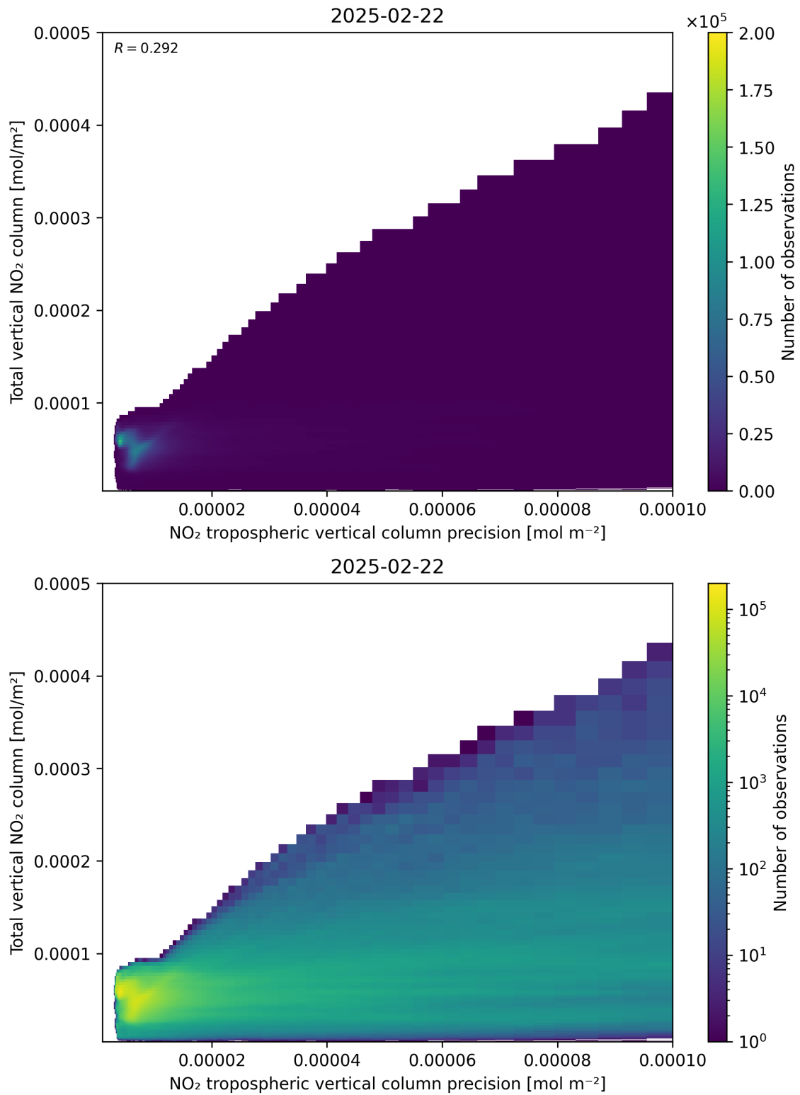
Figure 138: Scatter density plot of “NO 2 tropospheric vertical column precision” against “Total vertical NO 2 column” for 2025-02-21 to 2025-02-23.
