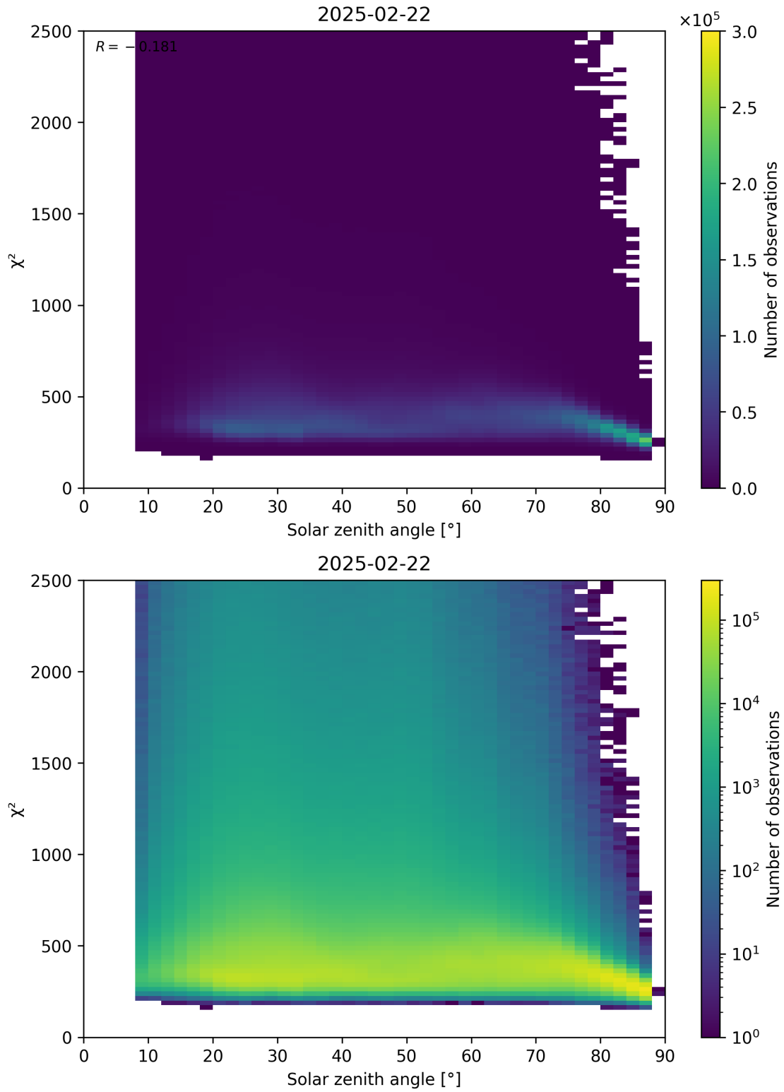
Figure 148: Scatter density plot of “Solar zenith angle” against “ \chi^2 ” for 2025-02-21 to 2025-02-23.
