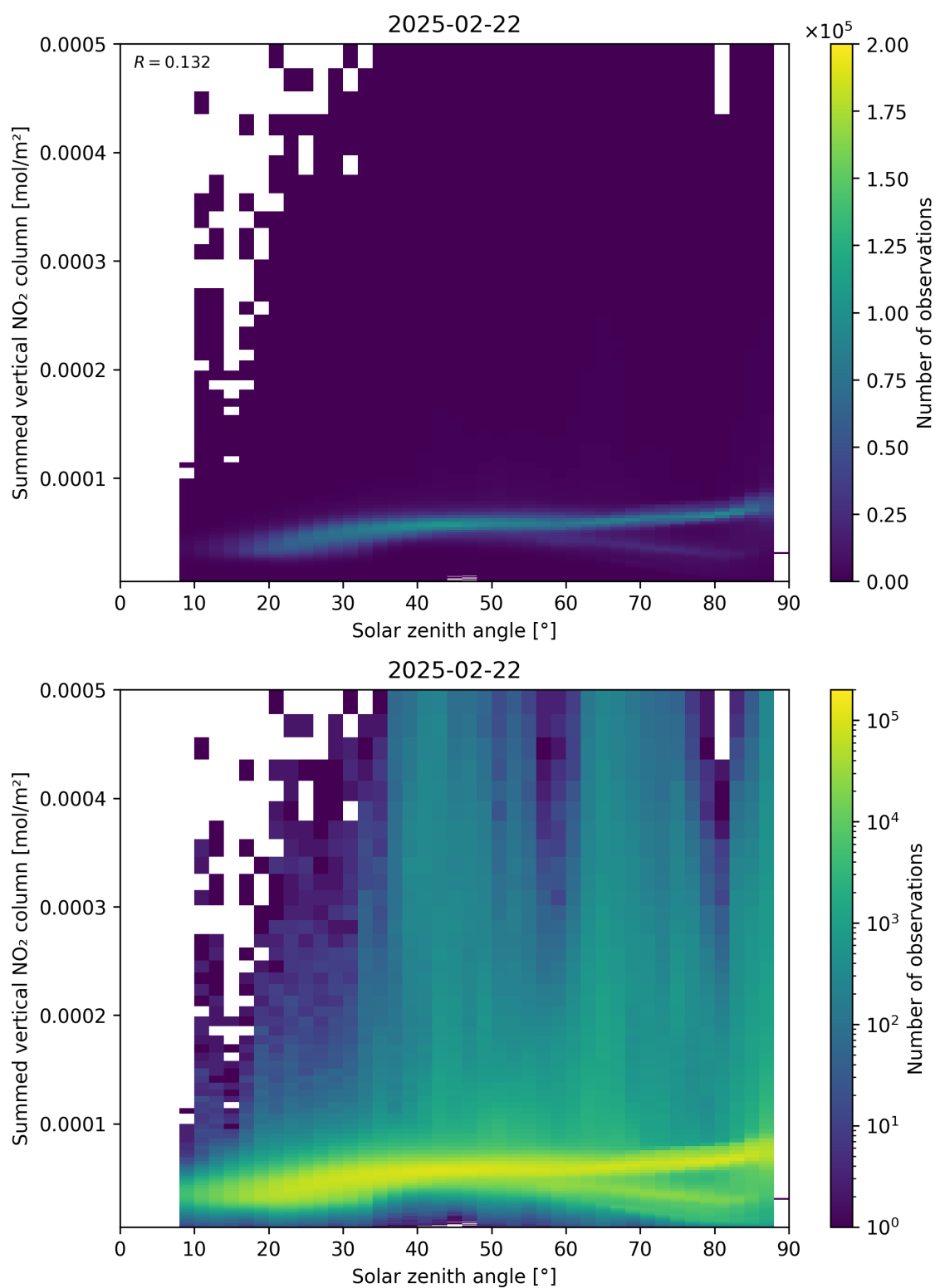
Figure 151: Scatter density plot of “Solar zenith angle” against “Summed vertical NO 2 column” for 2025-02-21 to 2025-02-23.
