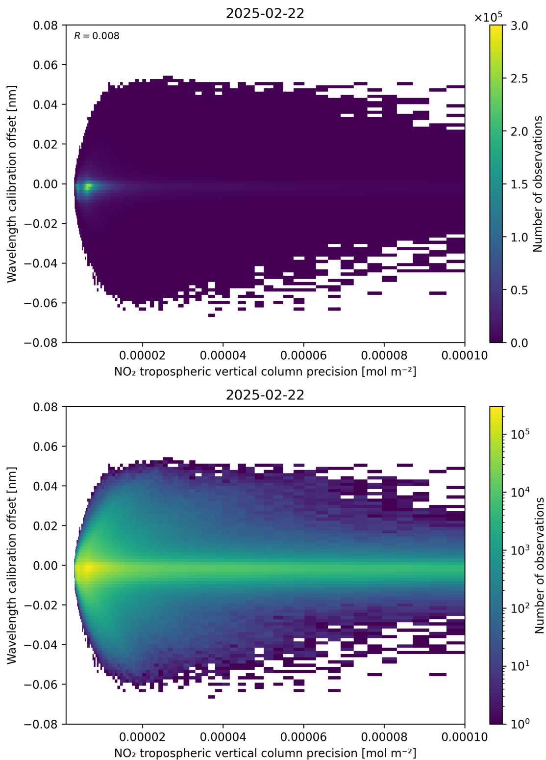
Figure 141: Scatter density plot of “NO 2 tropospheric vertical column precision” against “Wavelength calibration offset” for 2025-02-21 to 2025-02-23.
