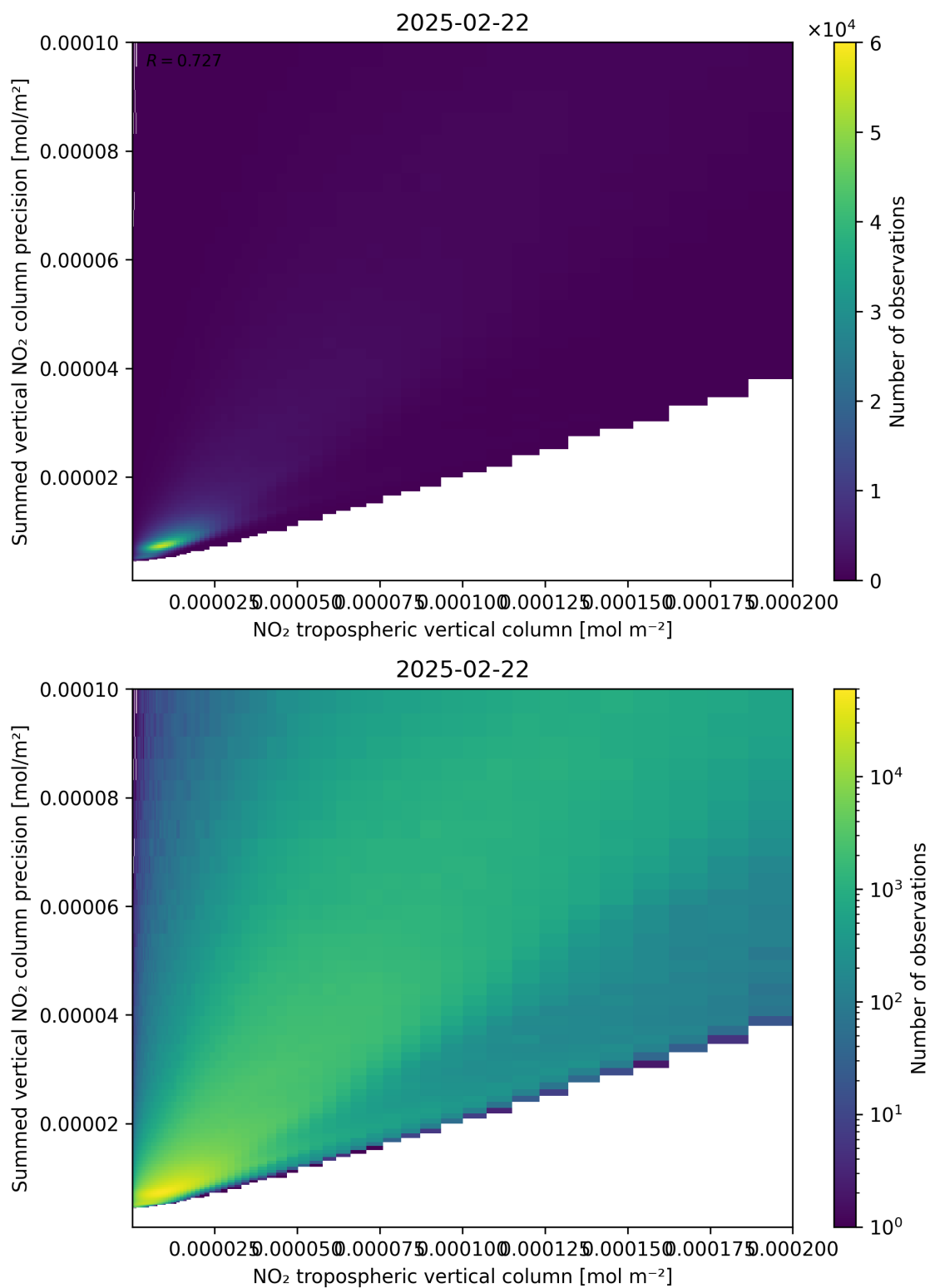
Figure 127: Scatter density plot of “NO 2 tropospheric vertical column” against “Summed vertical NO 2 column precision” for 2025-02-21 to 2025-02-23.
