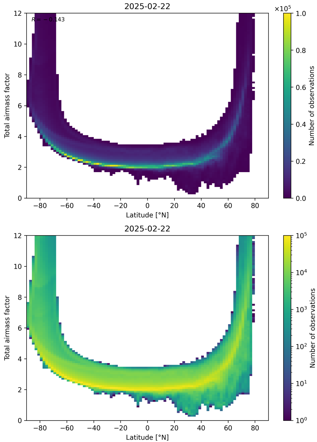
Figure 84: Scatter density plot of “Latitude” against “Total airmass factor” for 2025-02-21 to 2025-02-23.
