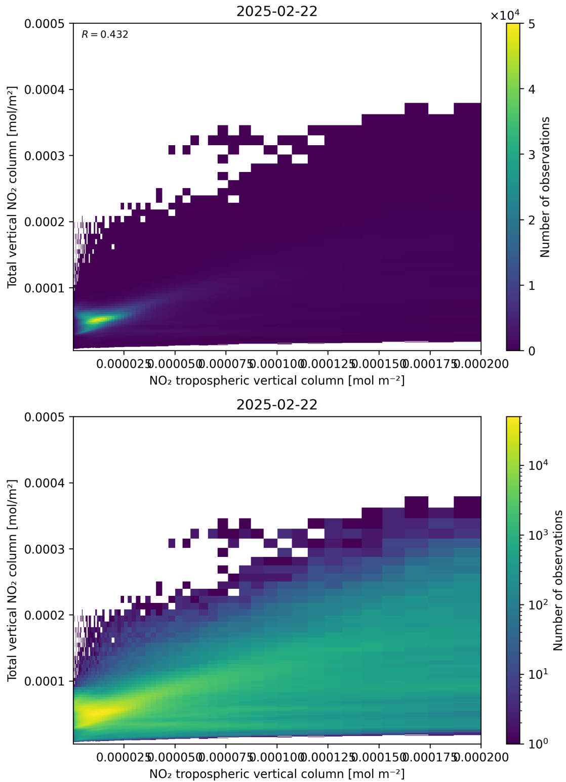
Figure 128: Scatter density plot of “NO 2 tropospheric vertical column” against “Total vertical NO 2 column” for 2025-02-21 to 2025-02-23.
