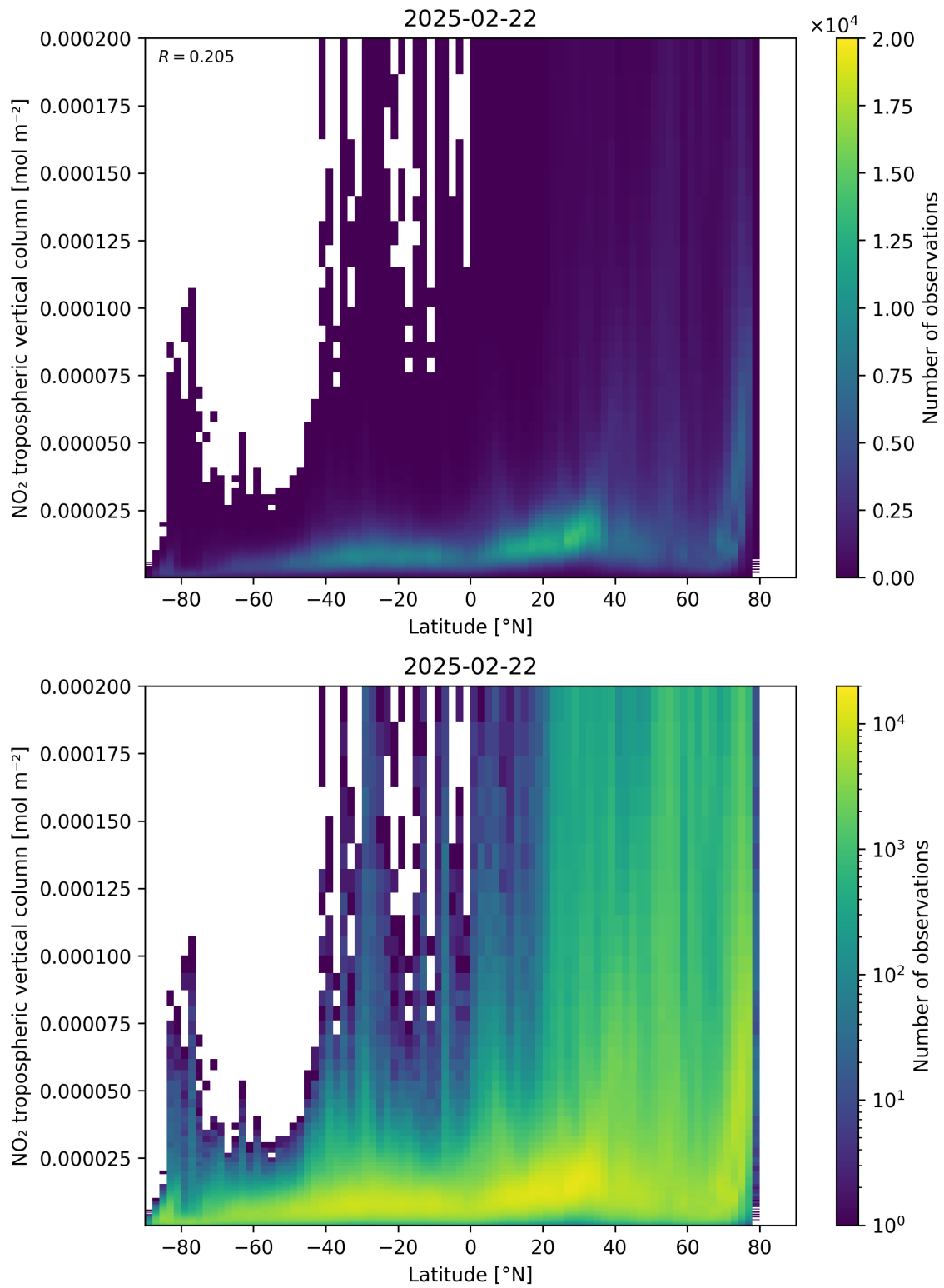
Figure 92: Scatter density plot of “Latitude” against “NO 2 tropospheric vertical column” for 2025-02-21 to 2025-02-23.
