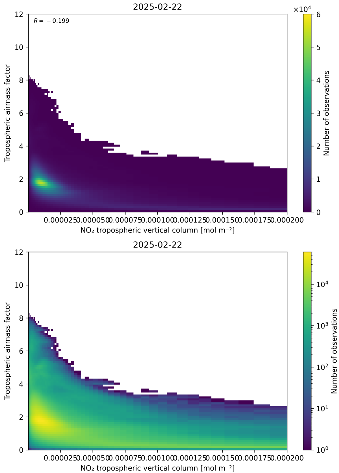
Figure 123: Scatter density plot of “NO 2 tropospheric vertical column” against “Tropospheric air mass factor” for 2025-02-21 to 2025-02-23.
