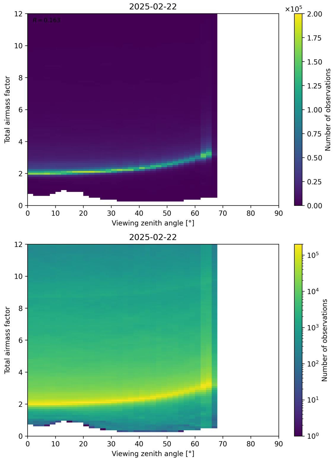
Figure 160: Scatter density plot of “Viewing zenith angle” against “Total airmass factor” for 2025-02-21 to 2025-02-23.
