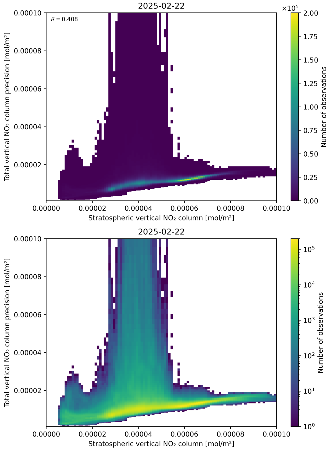
Figure 101: Scatter density plot of “Stratospheric vertical NO 2 column” against “Total vertical NO 2 column precision” for 2025-02-21 to 2025-02-23.
