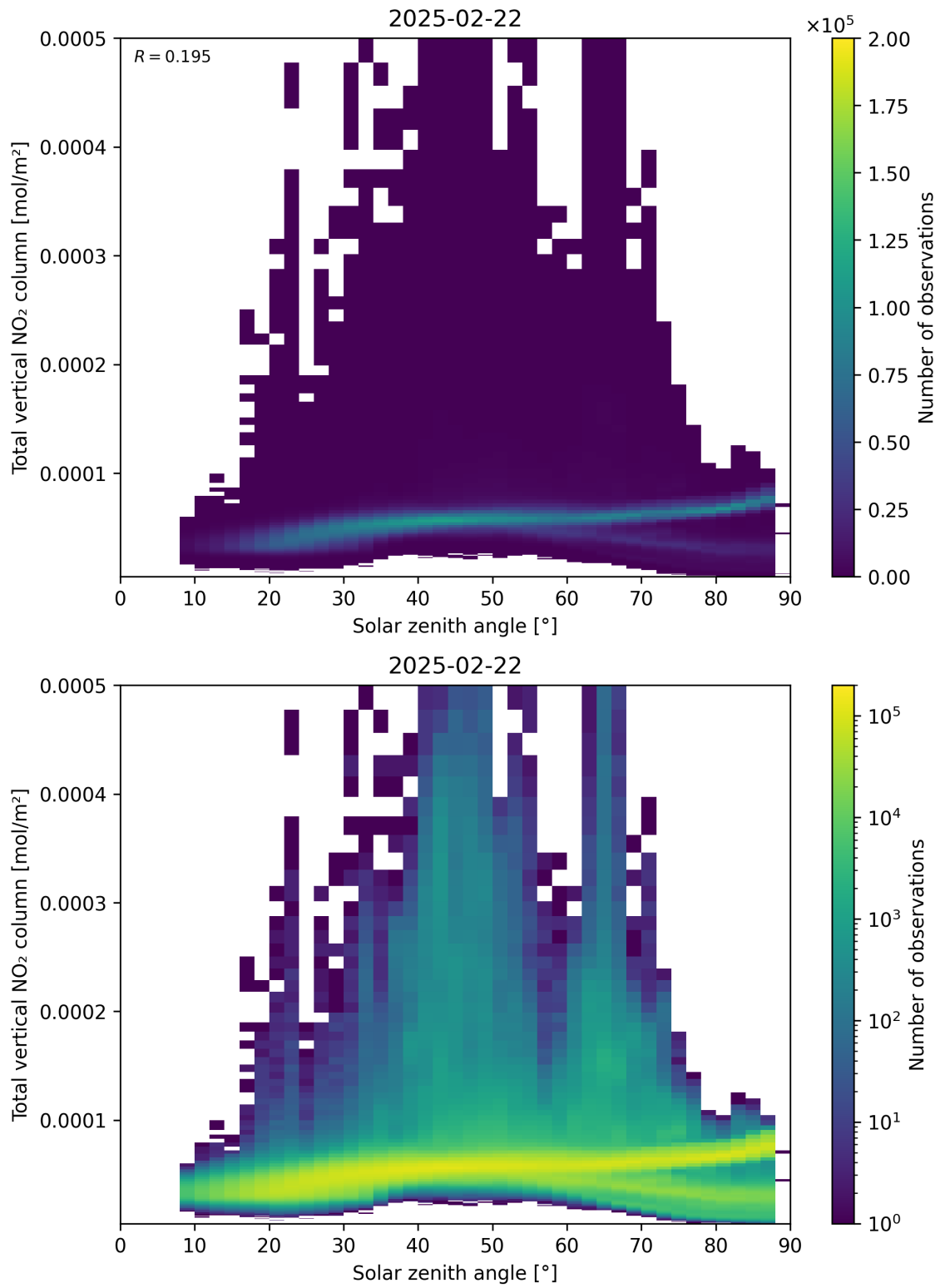
Figure 153: Scatter density plot of “Solar zenith angle” against “Total vertical NO 2 column” for 2025-02-21 to 2025-02-23.
