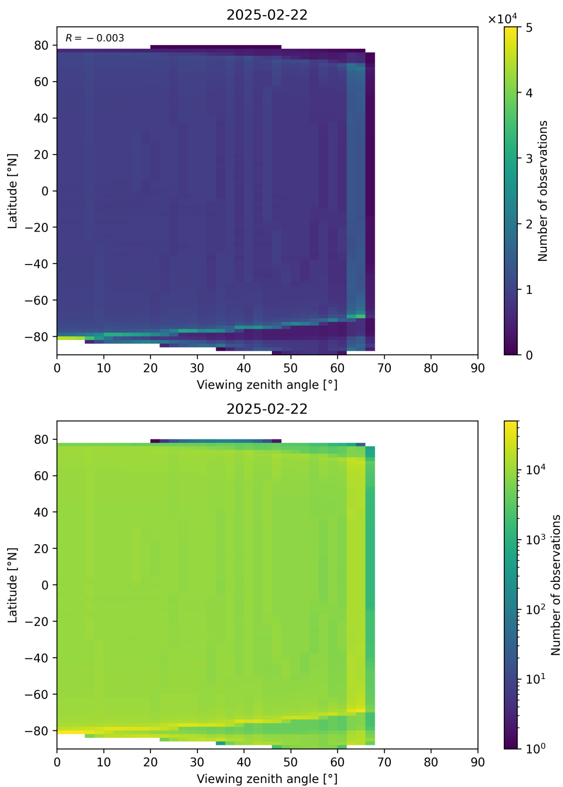
Figure 163: Scatter density plot of “Viewing zenith angle” against “Latitude” for 2025-02-21 to 2025-02-23.
