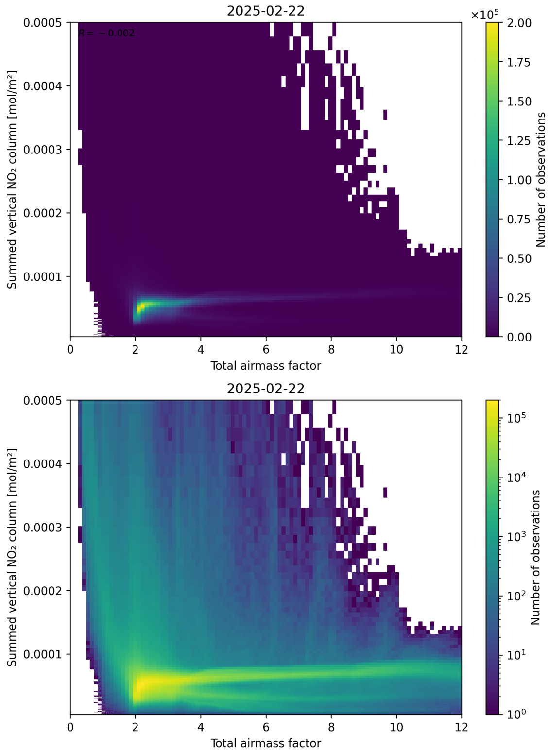
Figure 65: Scatter density plot of “Total airmass factor” against “Summed vertical NO 2 column” for 2025-02-21 to 2025-02-23.
