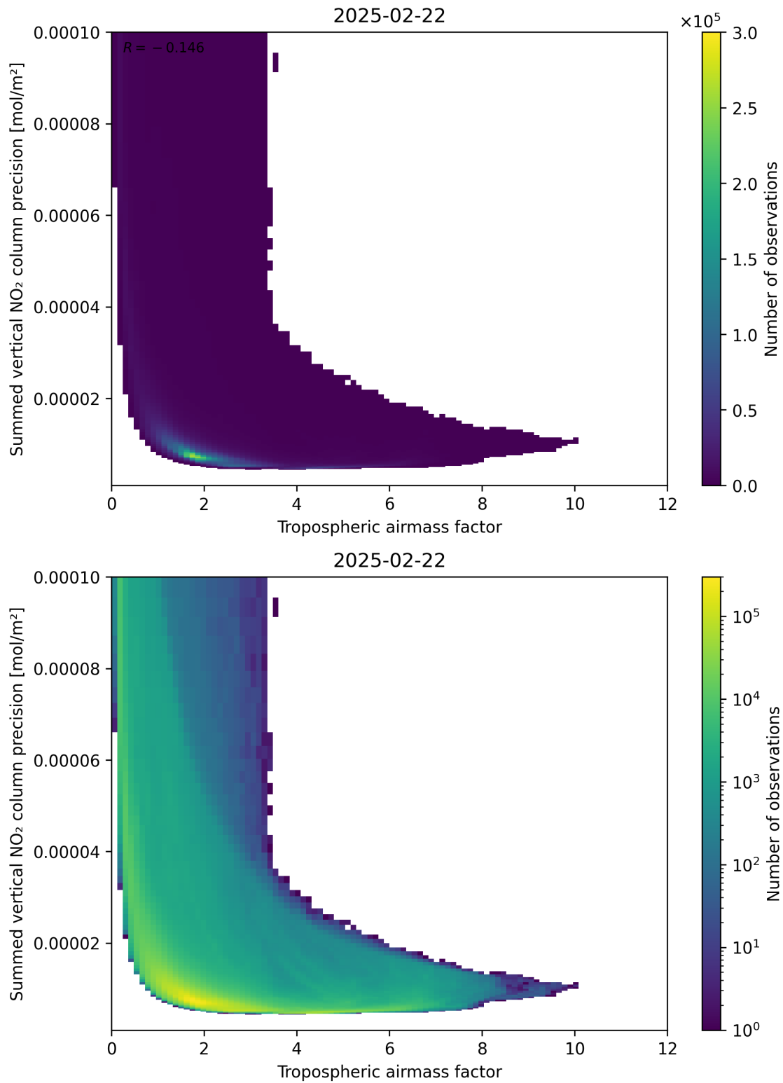
Figure 76: Scatter density plot of “Tropospheric air mass factor” against “Summed vertical NO 2 column precision” for 2025-02-21 to 2025-02-23.
