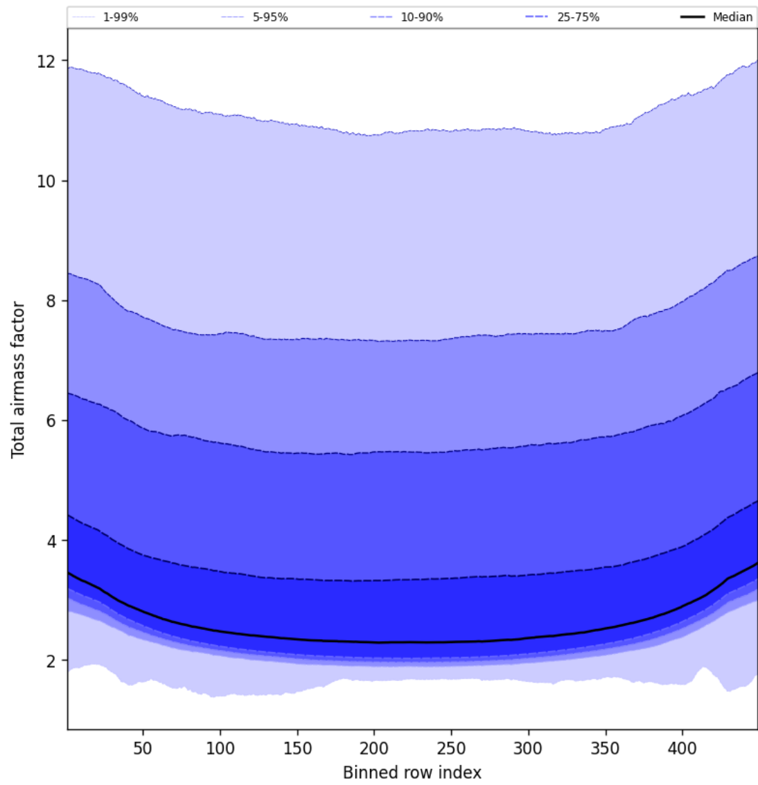
Figure 49: Along track statistics of “Total airmass factor” for 2025-02-21 to 2025-02-23
