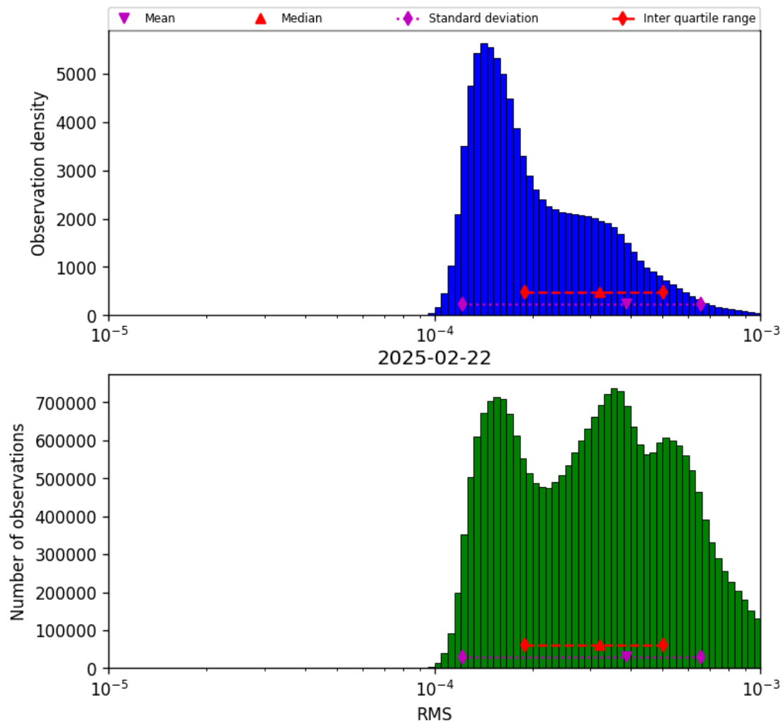
Figure 43: Histogram of “RMS” for 2025-02-21 to 2025-02-23
