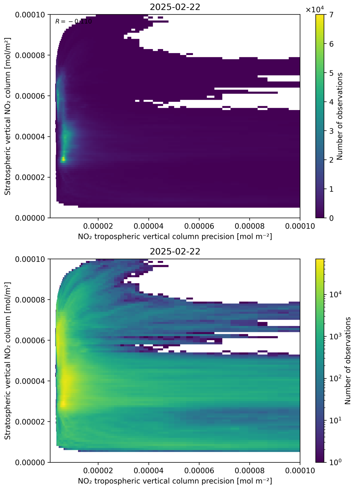
Figure 135: Scatter density plot of “NO 2 tropospheric vertical column precision” against “Stratospheric vertical NO 2 column” for 2025-02-21 to 2025-02-23.
