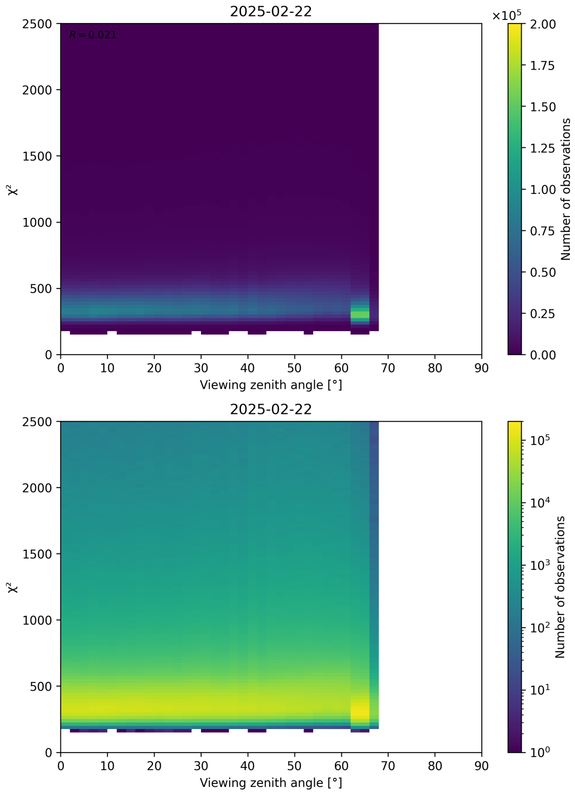
Figure 162: Scatter density plot of “Viewing zenith angle” against “ \chi^2 ” for 2025-02-21 to 2025-02-23.
