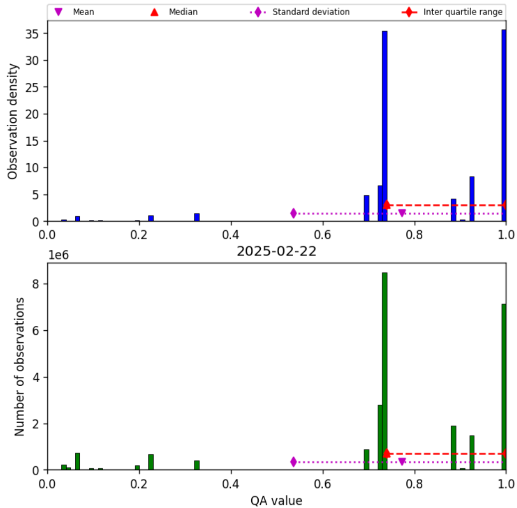
Figure 28: Histogram of “QA value” for 2025-02-21 to 2025-02-23
