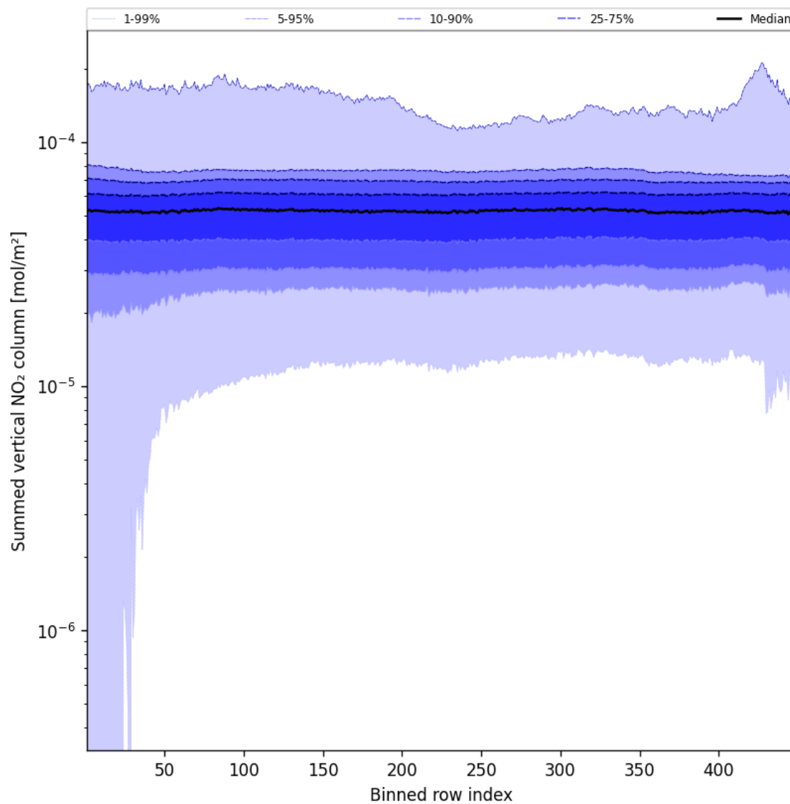
Figure 57: Along track statistics of “Summed vertical NO 2 column” for 2025-02-21 to 2025-02-23
