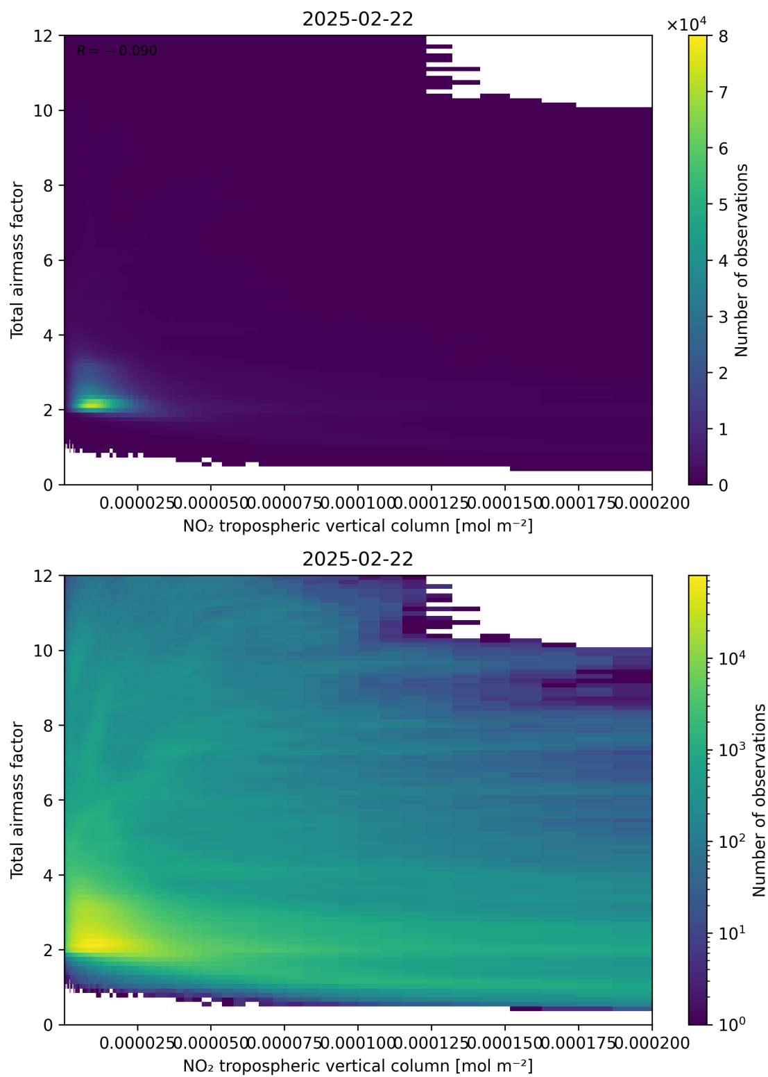
Figure 122: Scatter density plot of “NO 2 tropospheric vertical column” against “Total air mass factor” for 2025-02-21 to 2025-02-23.
