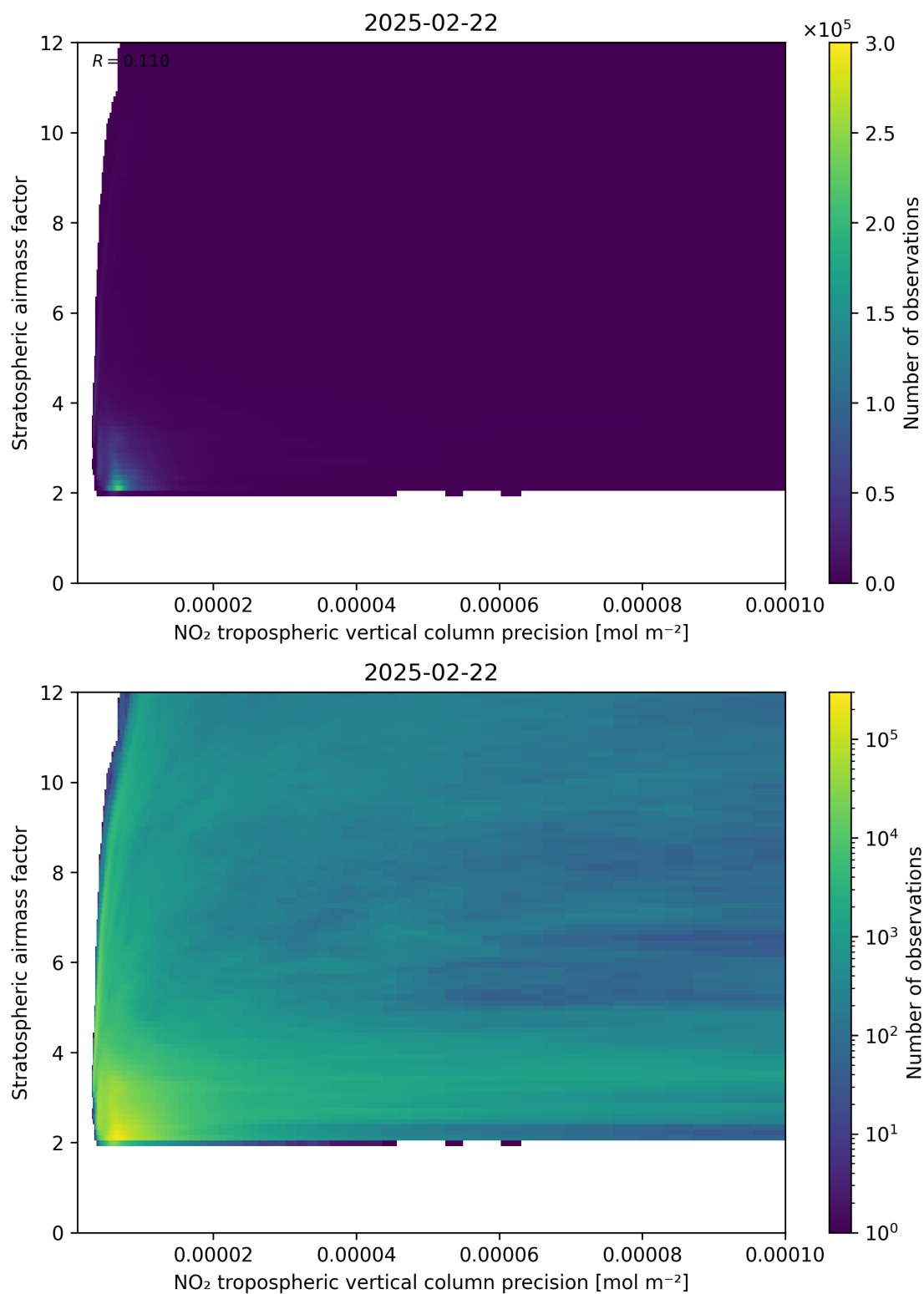
Figure 131: Scatter density plot of “NO 2 tropospheric vertical column precision” against “Stratospheric airmass factor” for 2025-02-21 to 2025-02-23.
