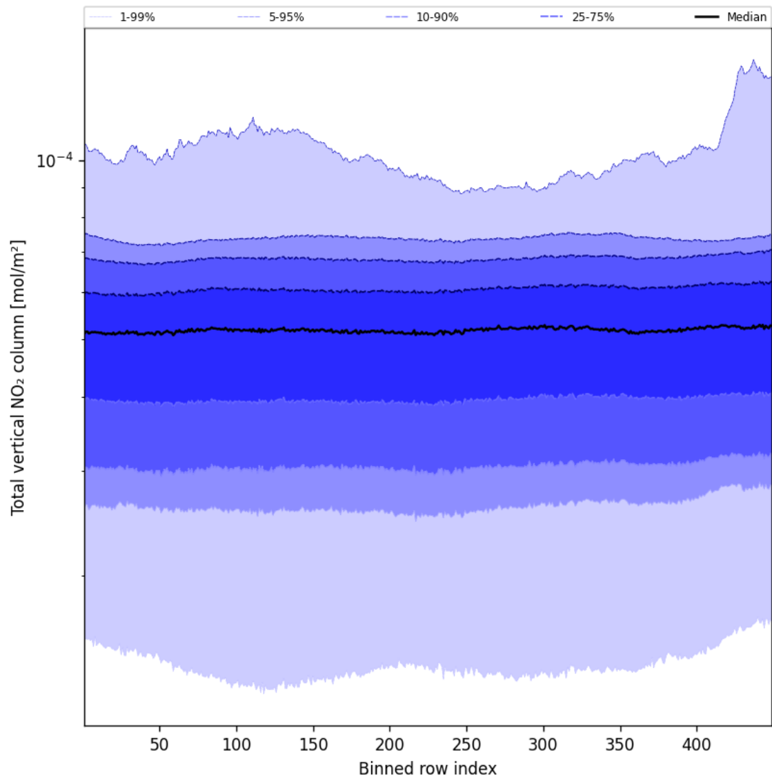
Figure 55: Along track statistics of “Total vertical NO 2 column” for 2025-02-21 to 2025-02-23
