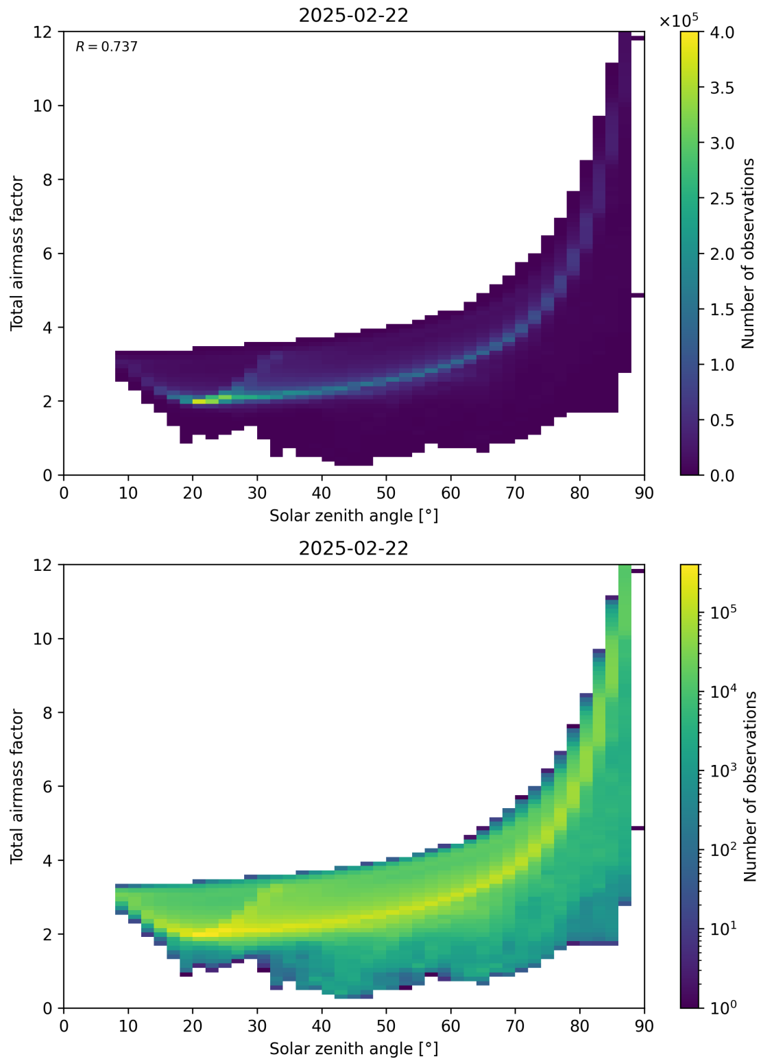
Figure 146: Scatter density plot of “Solar zenith angle” against “Total air mass factor” for 2025-02-21 to 2025-02-23.
