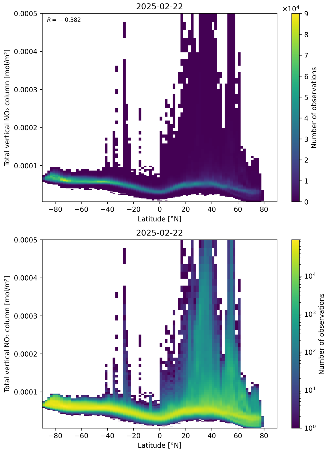
Figure 90: Scatter density plot of “Latitude” against “Total vertical NO 2 column” for 2025-02-21 to 2025-02-23.
