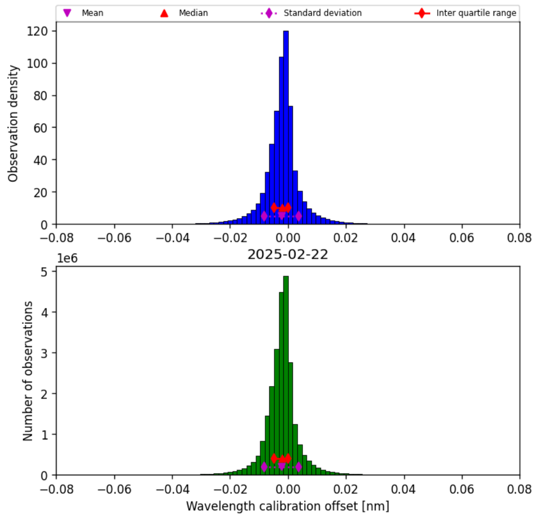
Figure 35: Histogram of “Wavelength calibration offset” for 2025-02-21 to 2025-02-23
