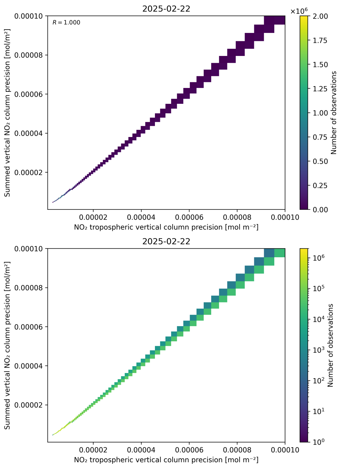
Figure 137: Scatter density plot of “NO 2 tropospheric vertical column precision” against “Summed vertical NO 2 column precision” for 2025-02-21 to 2025-02-23.
