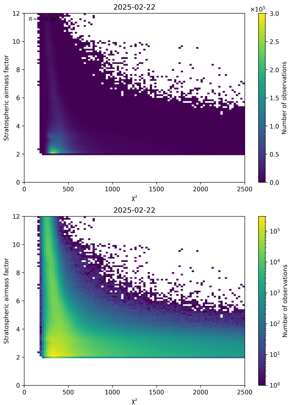
Figure 81: Scatter density plot of “ \chi^2 ” against “Stratospheric airmass factor” for 2025-02-21 to 2025-02-23.
