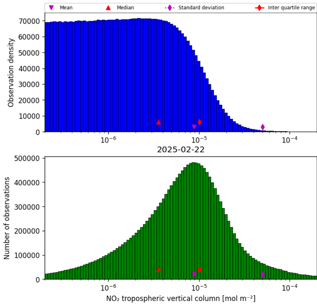
Figure 29: Histogram of “NO 2 tropospheric vertical column” for 2025-02-21 to 2025-02-23
