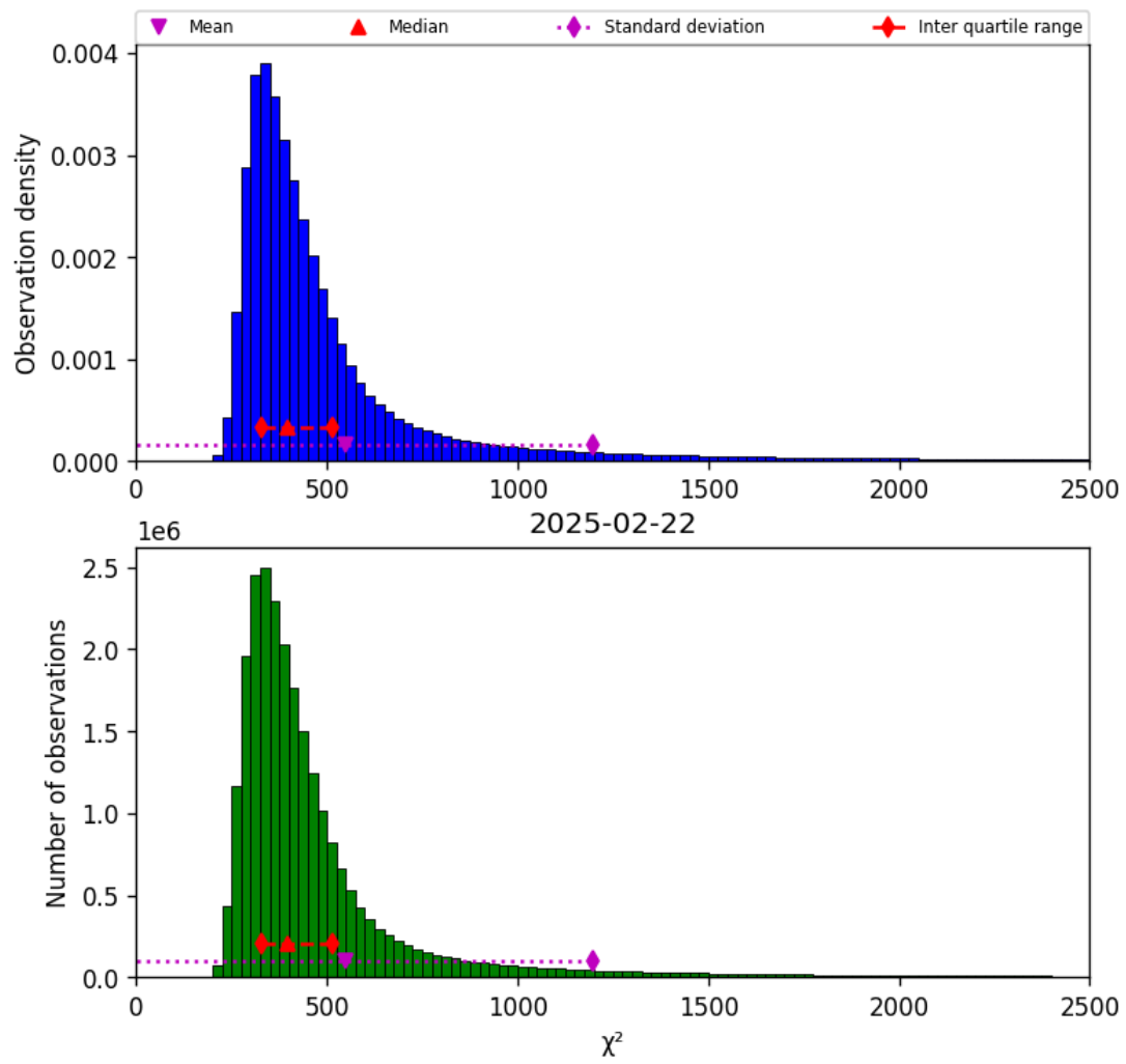
Figure 42: Histogram of “ \chi^2 ” for 2025-02-21 to 2025-02-23
