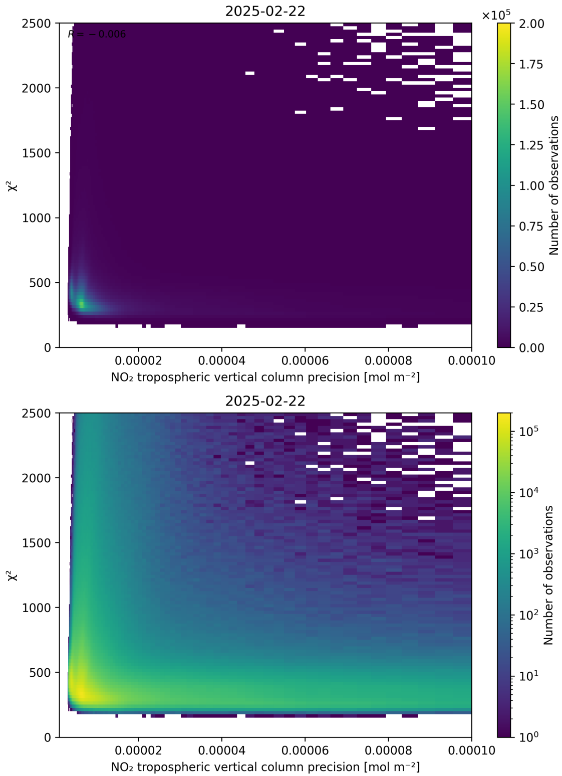
Figure 134: Scatter density plot of “NO 2 tropospheric vertical column precision” against “ \chi^2 ” for 2025-02-21 to 2025-02-23.
