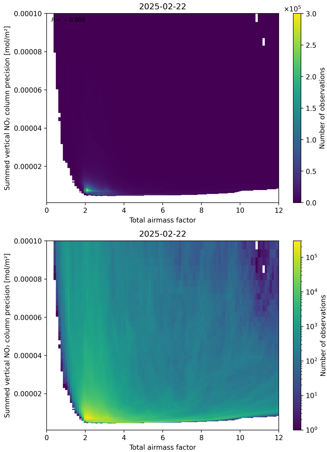
Figure 66: Scatter density plot of “Total airmass factor” against “Summed vertical NO 2 column precision” for 2025-02-21 to 2025-02-23.
