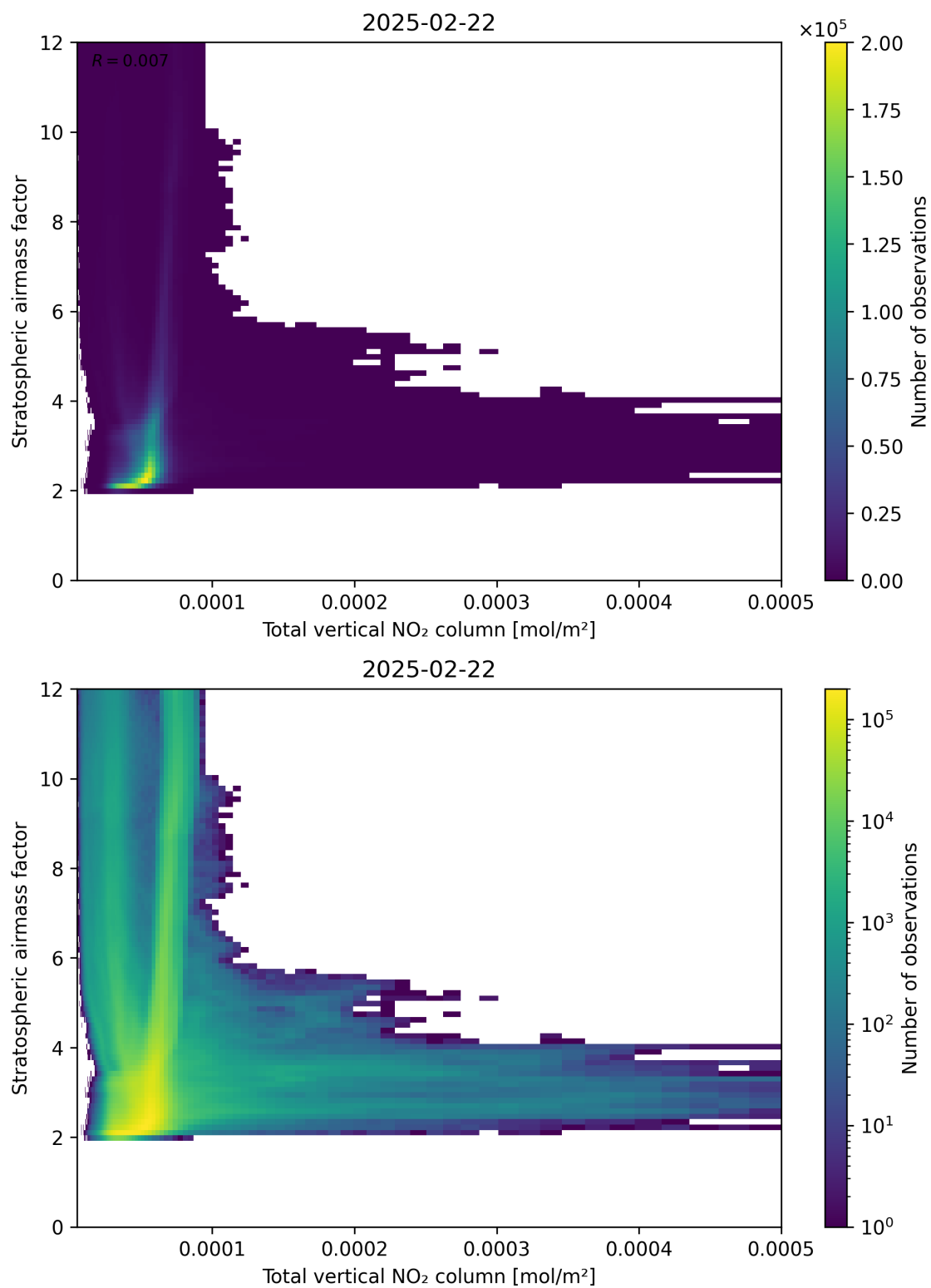
Figure 110: Scatter density plot of “Total vertical NO 2 column” against “Stratospheric airmass factor” for 2025-02-21 to 2025-02-23.
