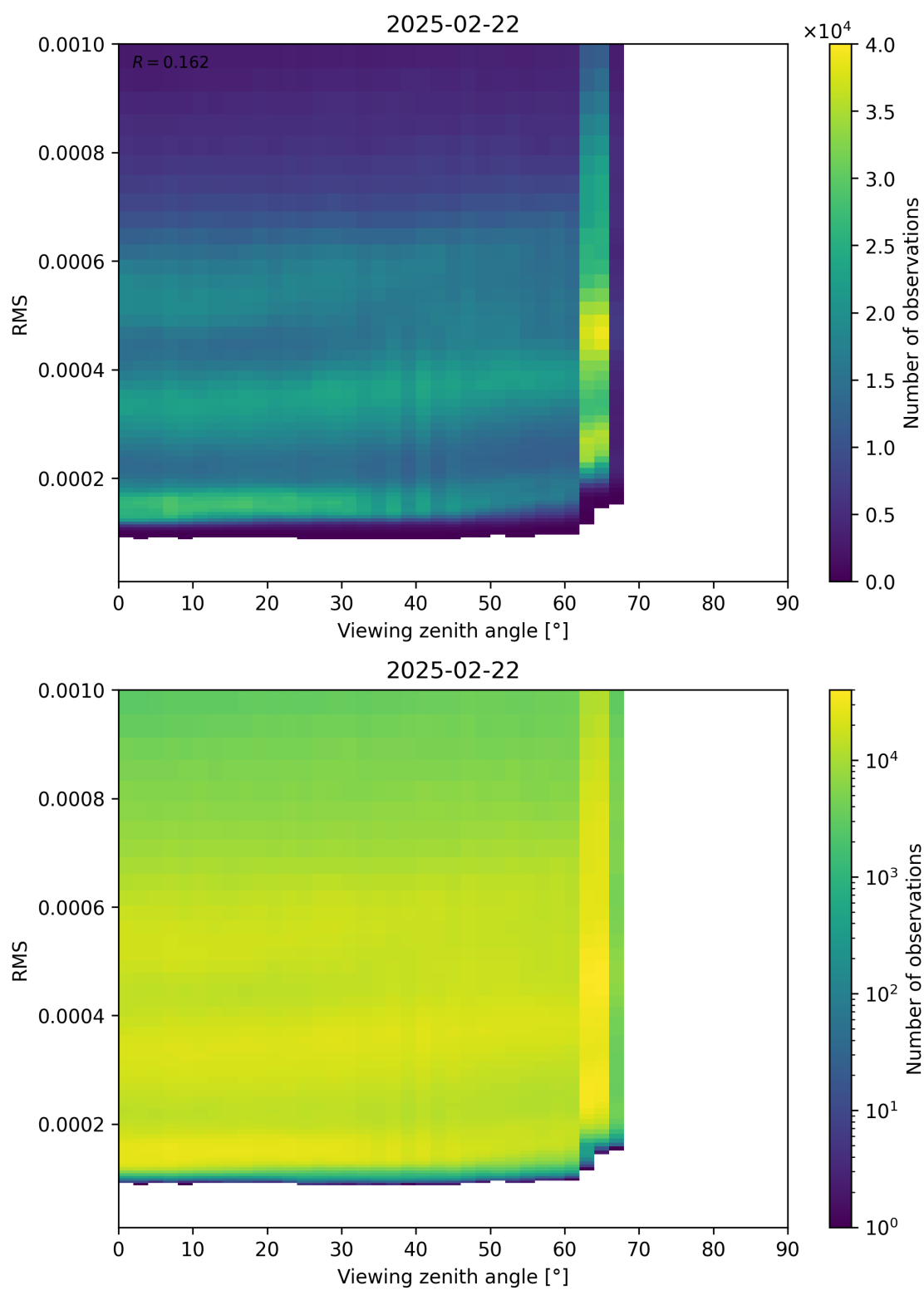
Figure 171: Scatter density plot of “Viewing zenith angle” against “RMS” for 2025-02-21 to 2025-02-23.
