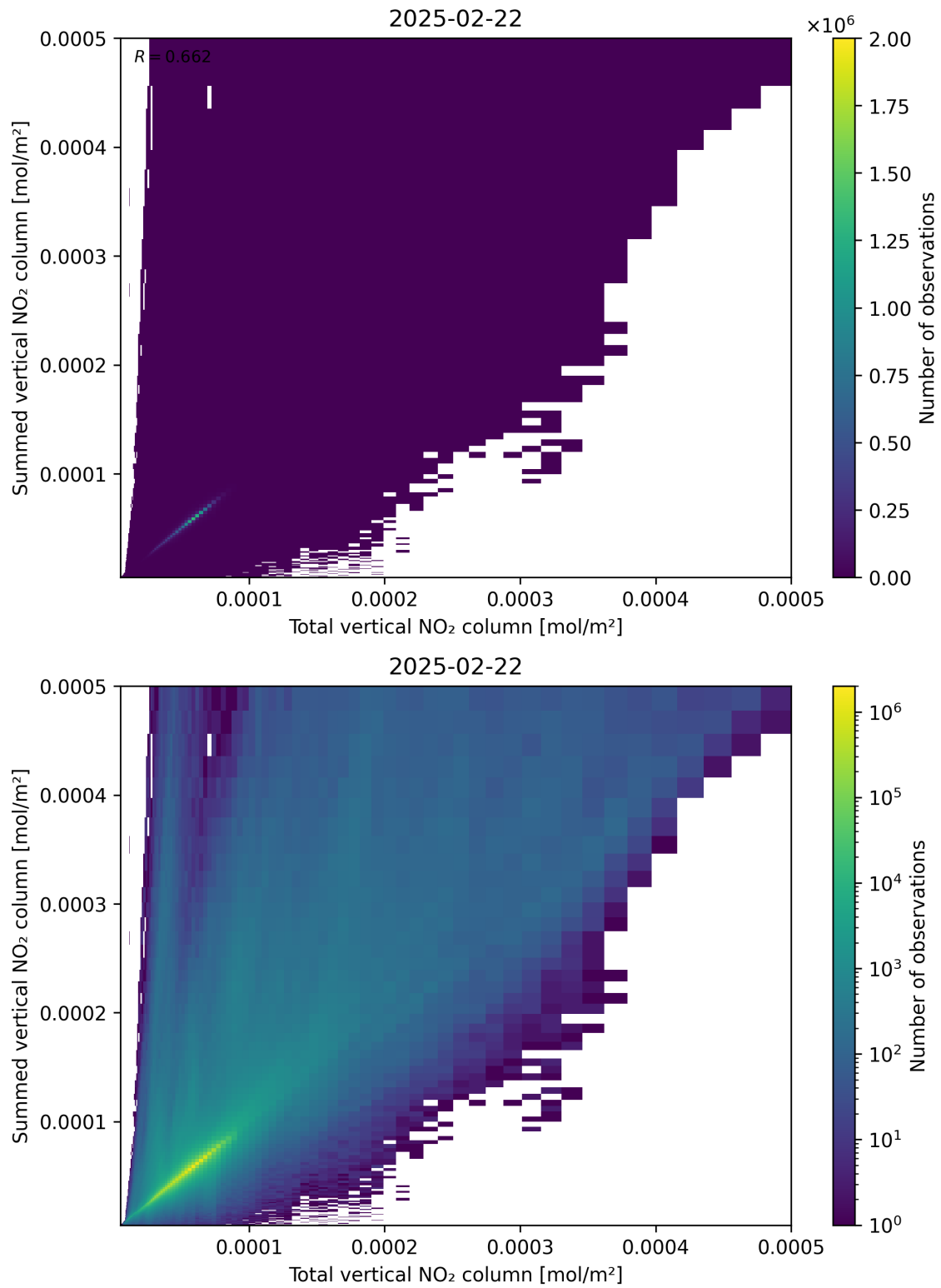
Figure 112: Scatter density plot of “Total vertical NO 2 column” against “Summed vertical NO 2 column” for 2025-02-21 to 2025-02-23.
