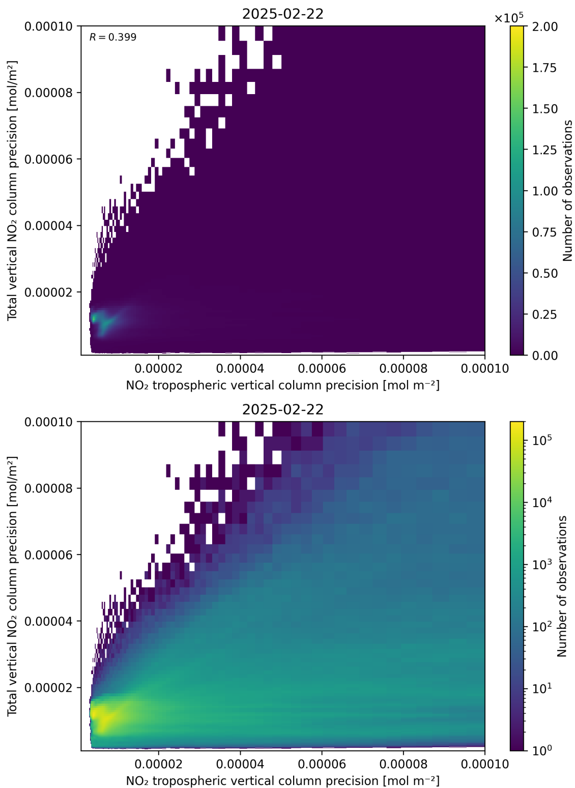
Figure 139: Scatter density plot of “NO 2 tropospheric vertical column precision” against “Total vertical NO 2 column precision” for 2025-02-21 to 2025-02-23.
