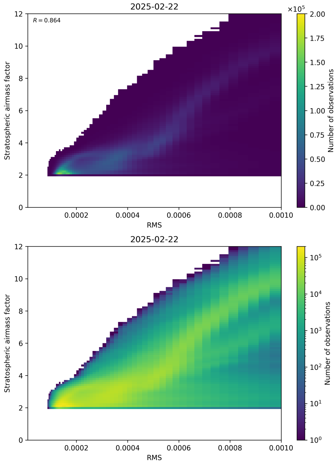
Figure 144: Scatter density plot of “RMS” against “Stratospheric airmass factor” for 2025-02-21 to 2025-02-23.
