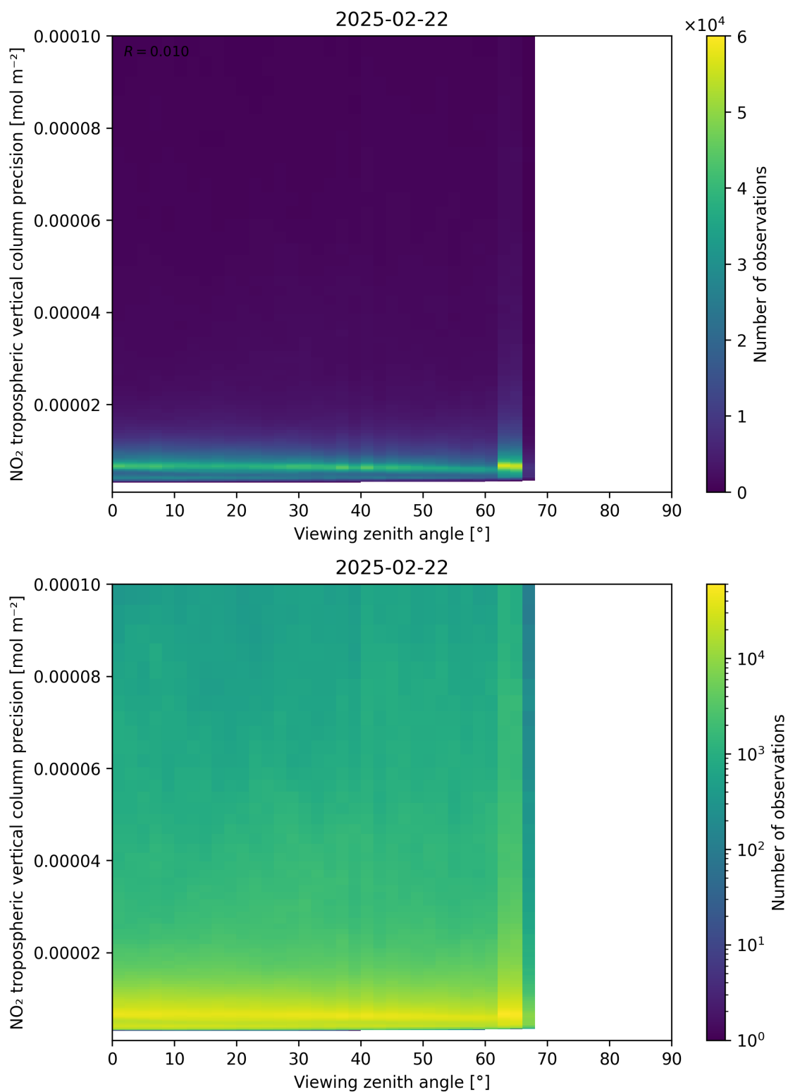
Figure 170: Scatter density plot of “Viewing zenith angle” against “NO 2 tropospheric vertical column precision” for 2025-02-21 to 2025-02-23.
