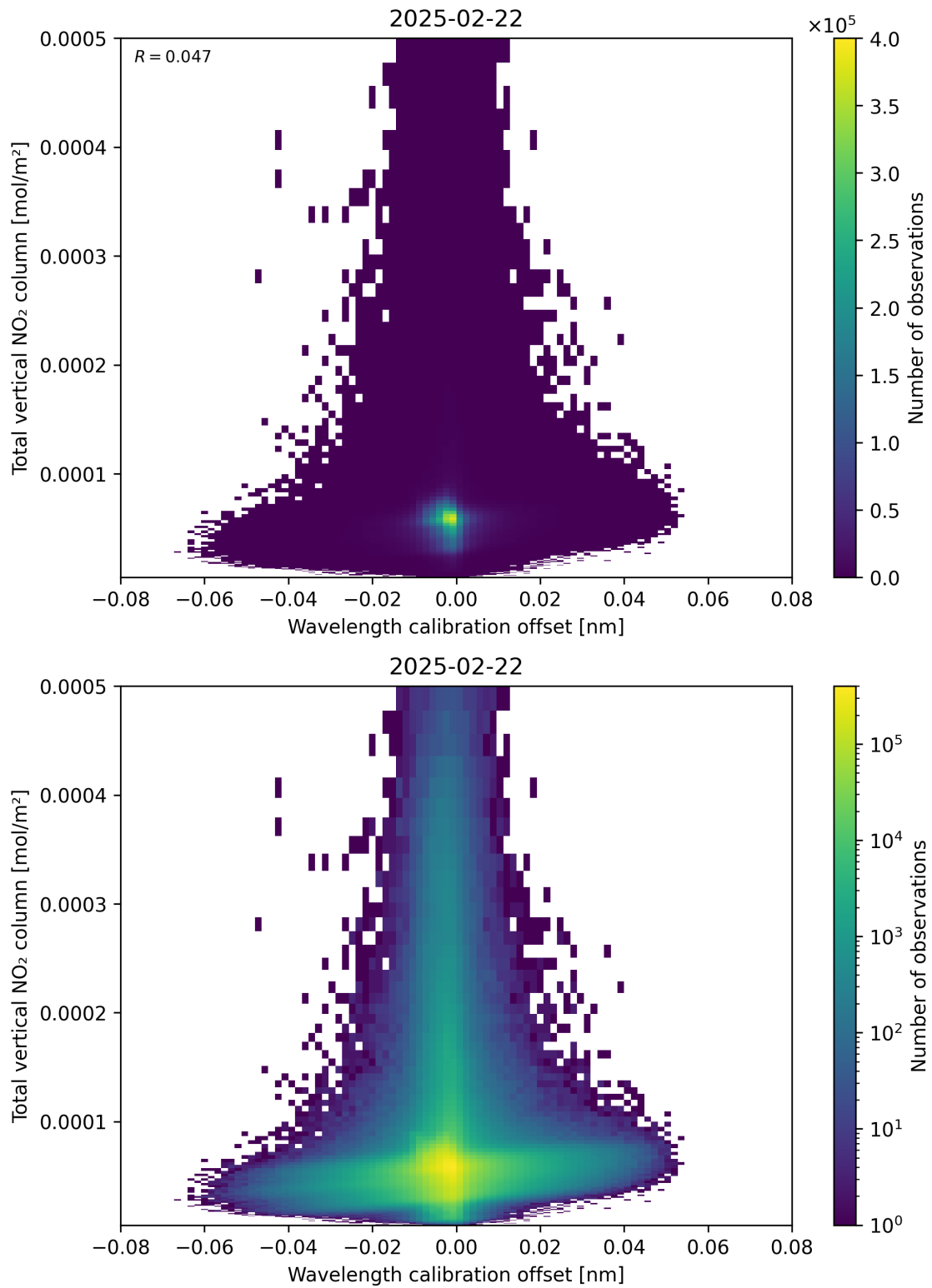
Figure 179: Scatter density plot of “Wavelength calibration offset” against “Total vertical NO 2 column” for 2025-02-21 to 2025-02-23.
