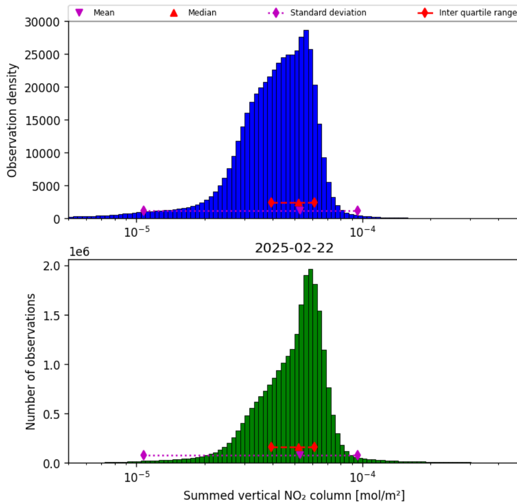
Figure 40: Histogram of “Summed vertical NO 2 column” for 2025-02-21 to 2025-02-23
