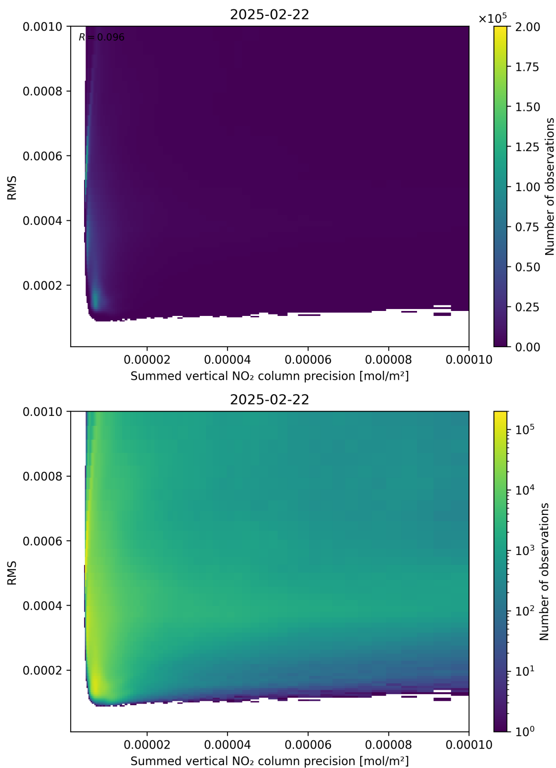
Figure 108: Scatter density plot of “Summed vertical NO 2 column precision” against “RMS” for 2025-02-21 to 2025-02-23.
