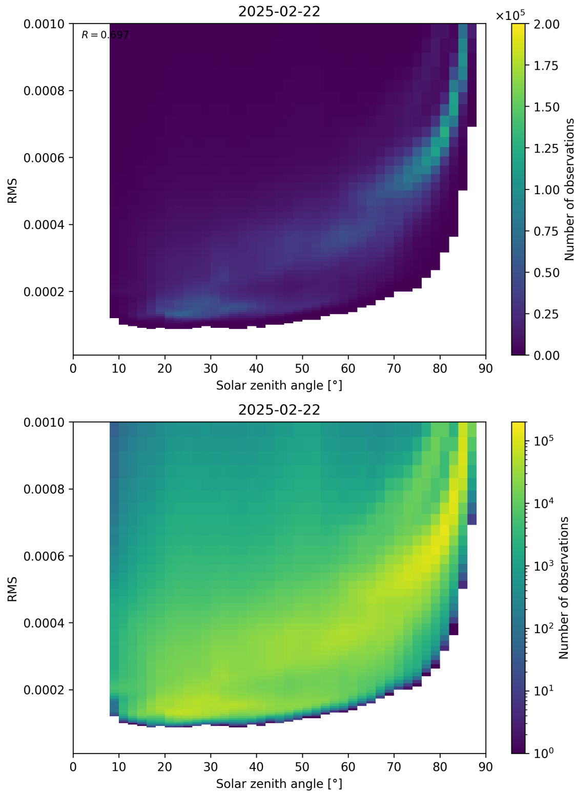
Figure 157: Scatter density plot of “Solar zenith angle” against “RMS” for 2025-02-21 to 2025-02-23.
