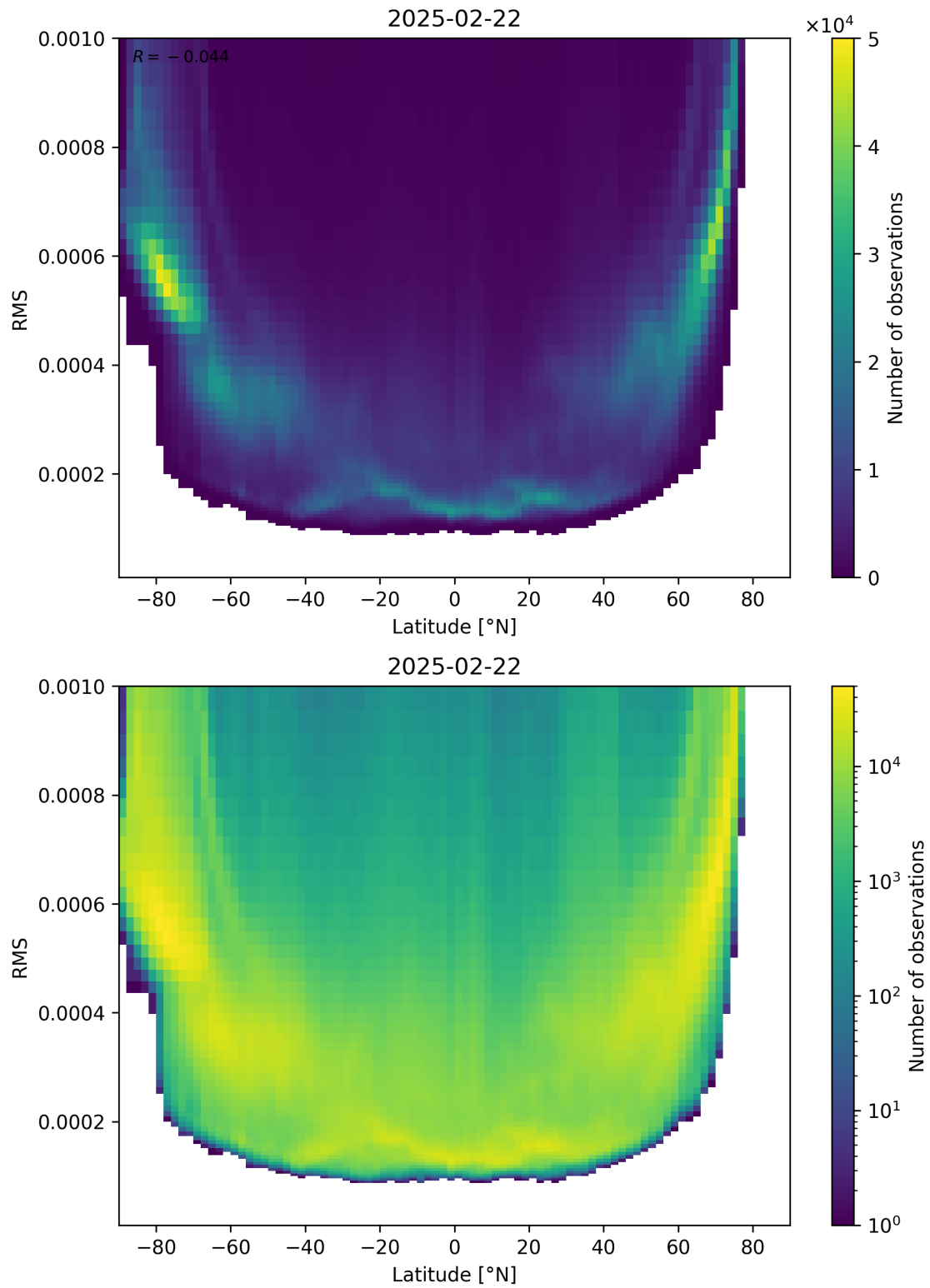
Figure 94: Scatter density plot of “Latitude” against “RMS” for 2025-02-21 to 2025-02-23.
