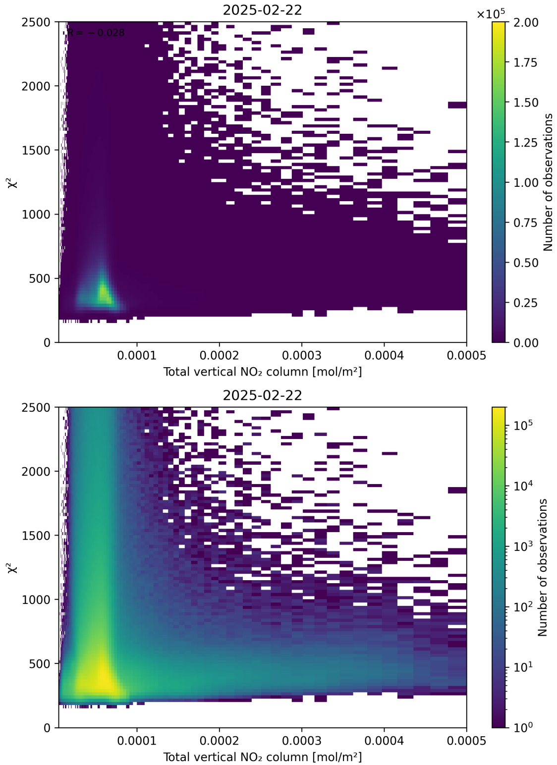
Figure 111: Scatter density plot of “Total vertical NO 2 column” against “ \chi^2 ” for 2025-02-21 to 2025-02-23.
