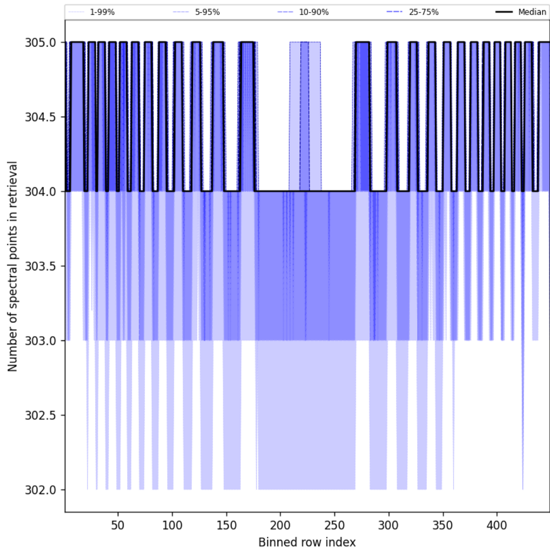
Figure 50: Along track statistics of “Number of spectral points in retrieval” for 2025-02-21 to 2025-02-23
