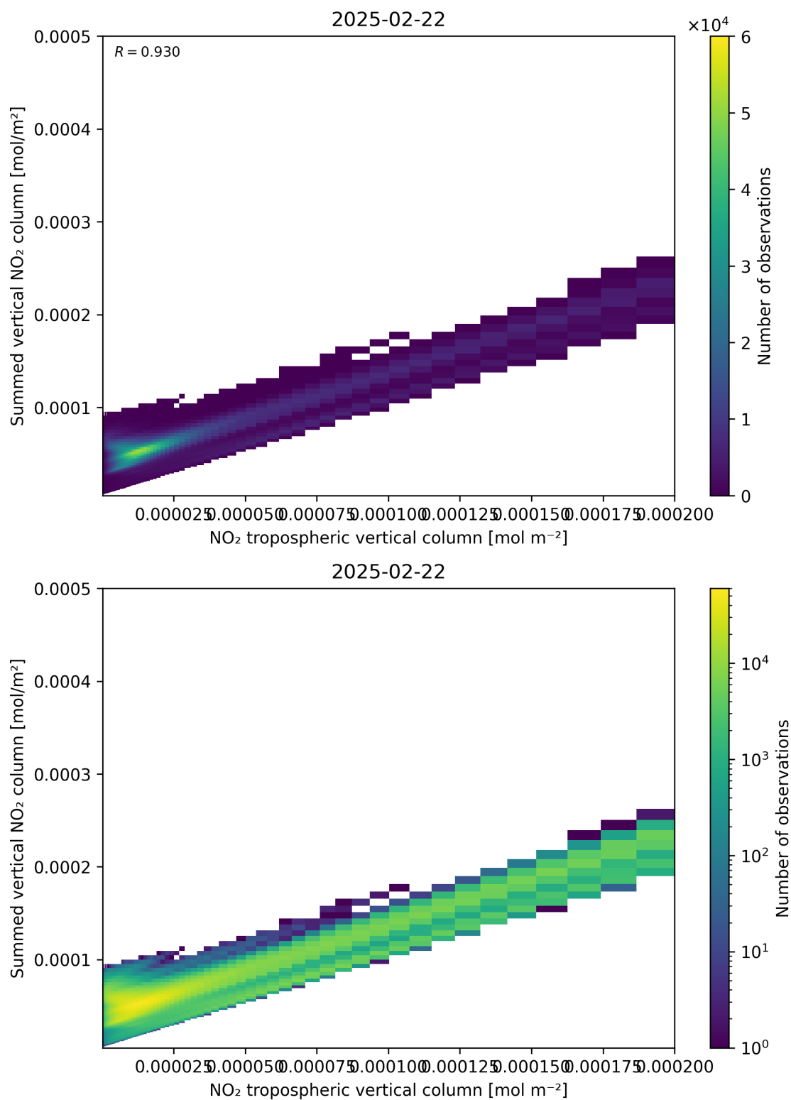
Figure 126: Scatter density plot of “NO 2 tropospheric vertical column” against “Summed vertical NO 2 column” for 2025-02-21 to 2025-02-23.
