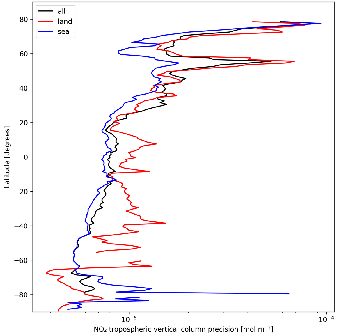
Figure 13: Zonal average of “NO 2 tropospheric vertical column precision” for 2025-02-21 to 2025-02-23.
