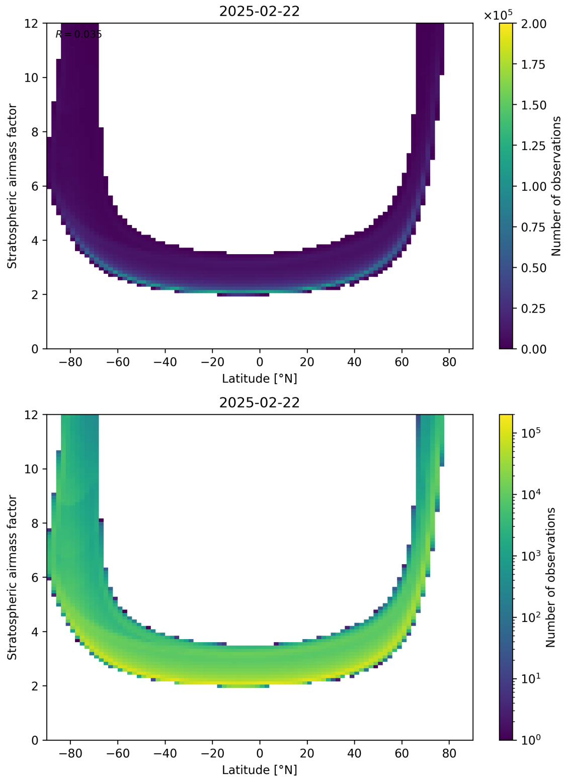
Figure 83: Scatter density plot of “Latitude” against “Stratospheric airmass factor” for 2025-02-21 to 2025-02-23.
