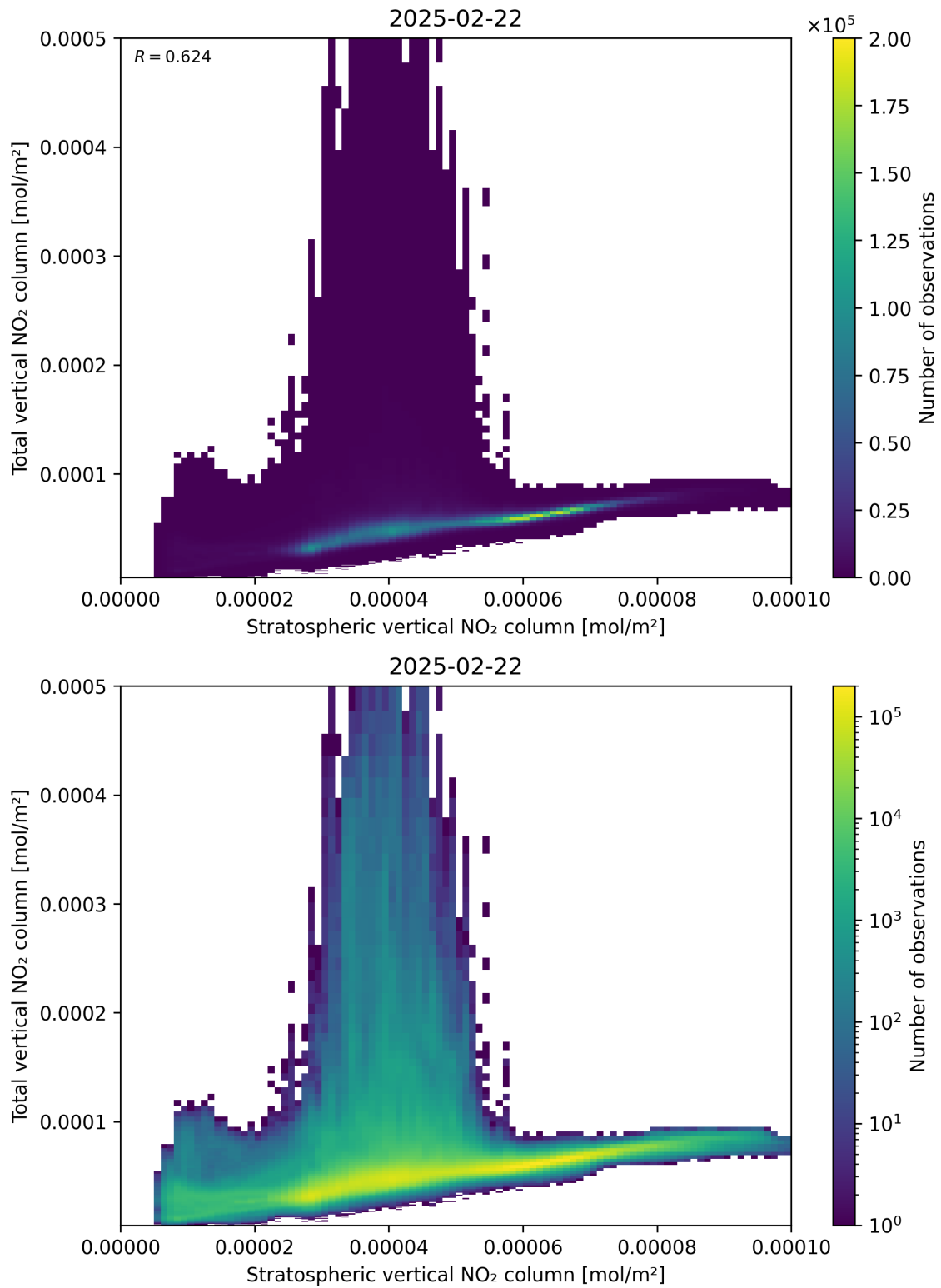
Figure 100: Scatter density plot of “Stratospheric vertical NO 2 column” against “Total vertical NO 2 column” for 2025-02-21 to 2025-02-23.
