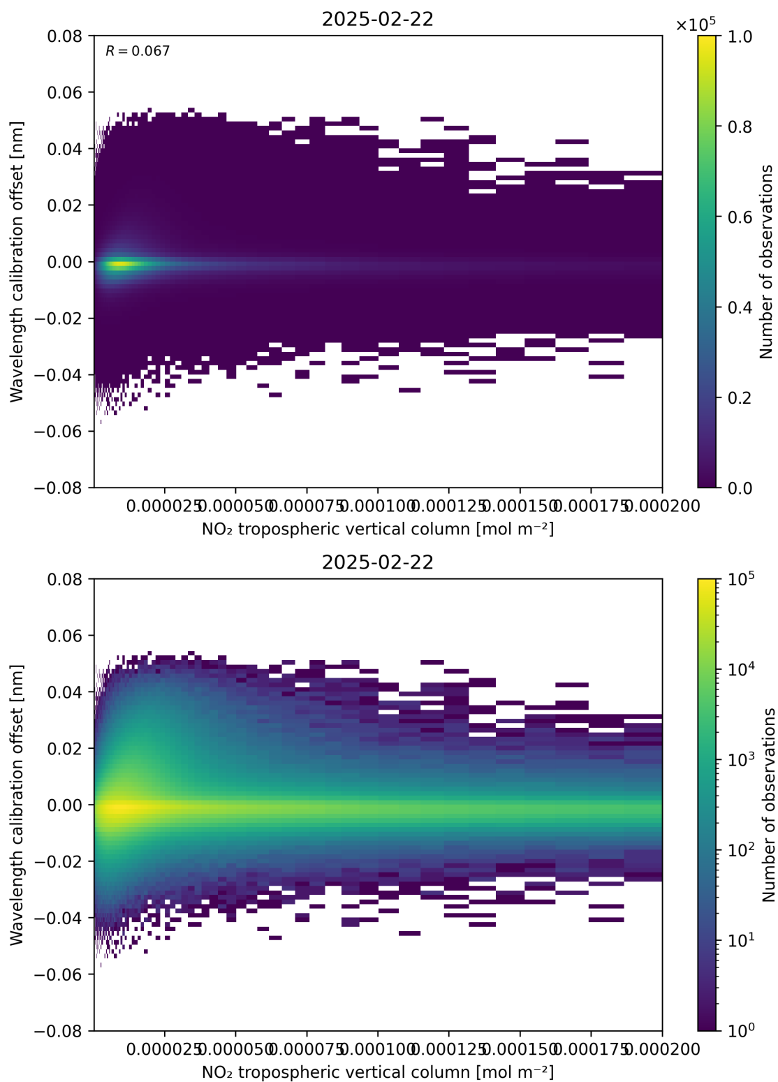
Figure 143: Scatter density plot of “NO 2 tropospheric vertical column” against “Wavelength calibration offset” for 2025-02-21 to 2025-02-23.
