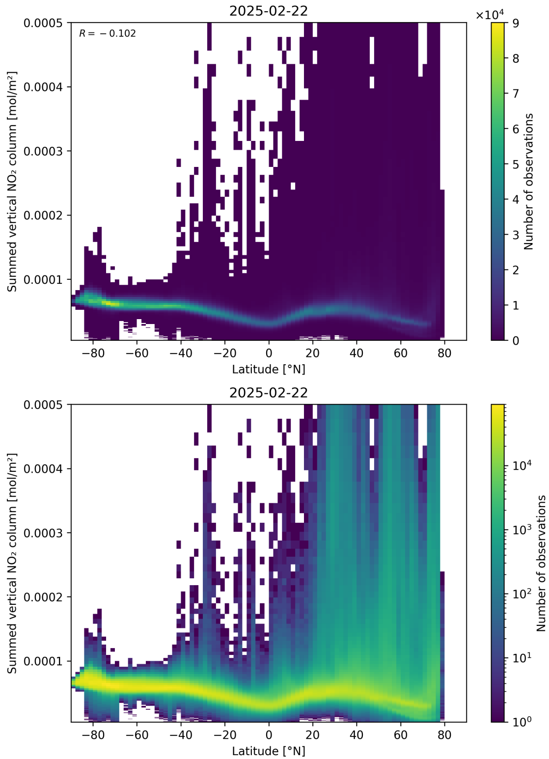
Figure 88: Scatter density plot of “Latitude” against “Summed vertical NO 2 column” for 2025-02-21 to 2025-02-23.
