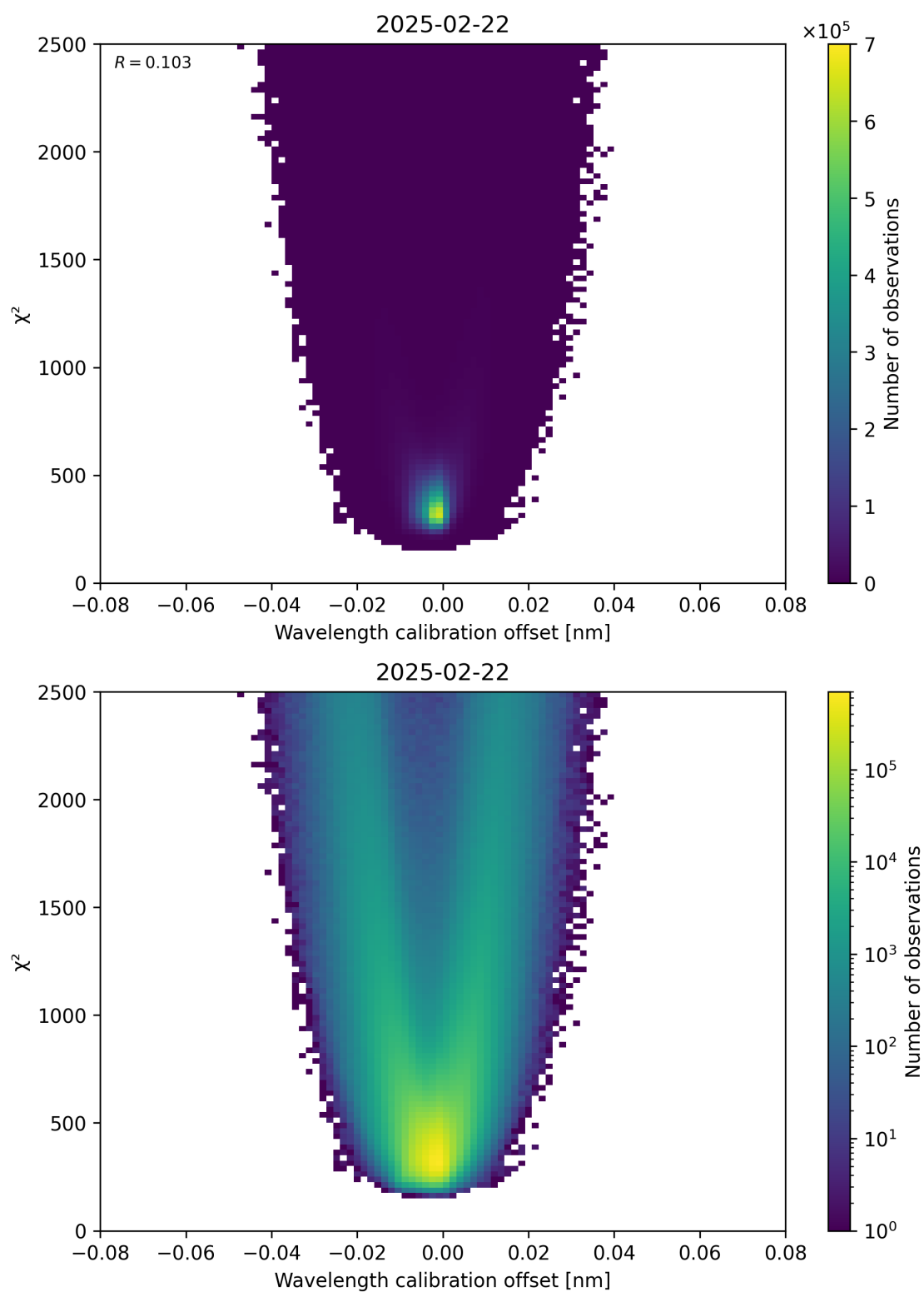
Figure 175: Scatter density plot of “Wavelength calibration offset” against “ \chi^2 ” for 2025-02-21 to 2025-02-23.
