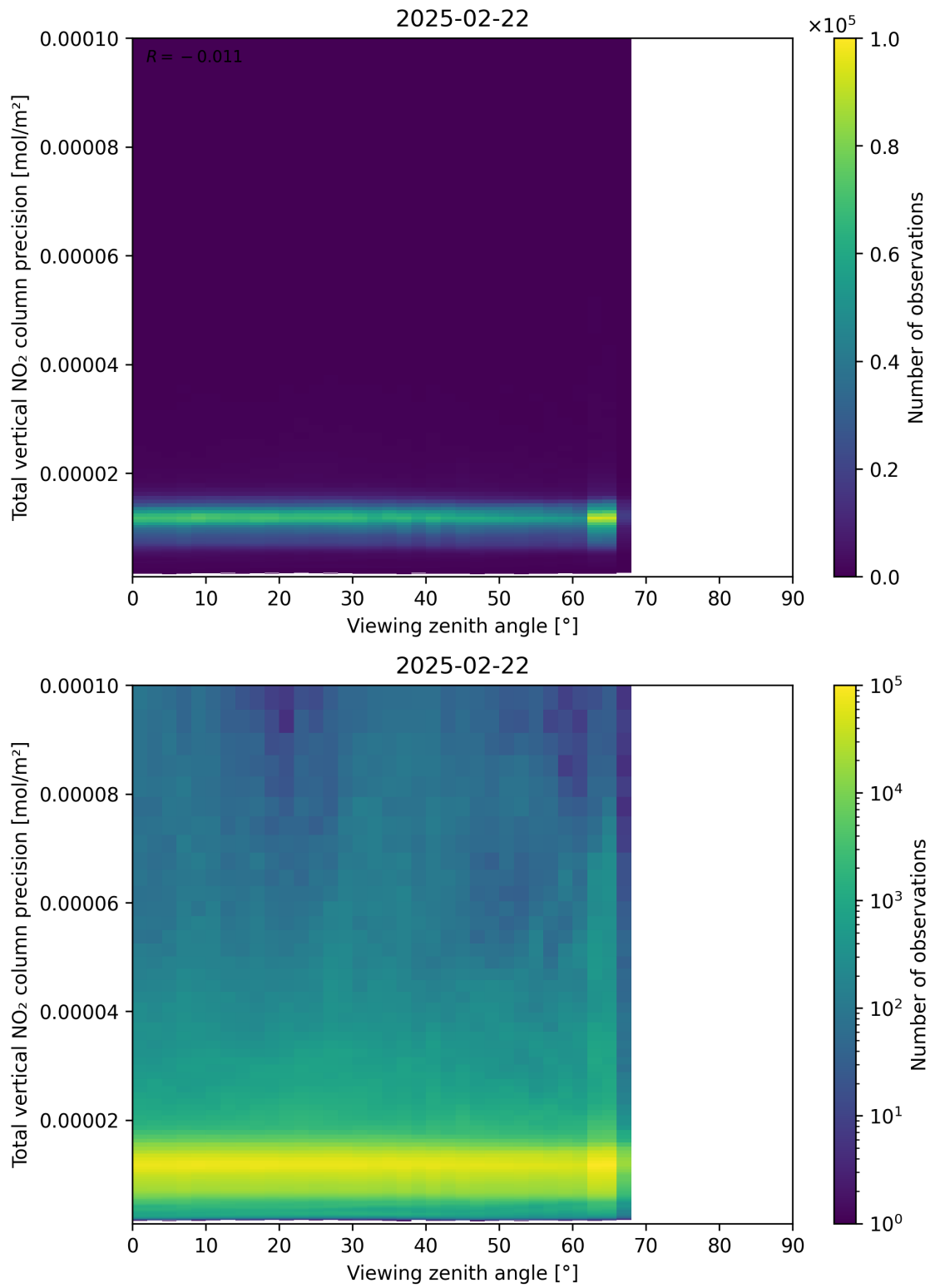
Figure 168: Scatter density plot of “Viewing zenith angle” against “Total vertical NO 2 column precision” for 2025-02-21 to 2025-02-23.
