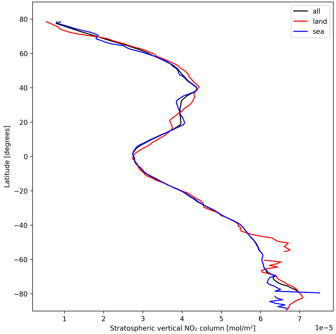
Figure 19: Zonal average of “Stratospheric vertical NO 2 column” for 2025-02-21 to 2025-02-23.
