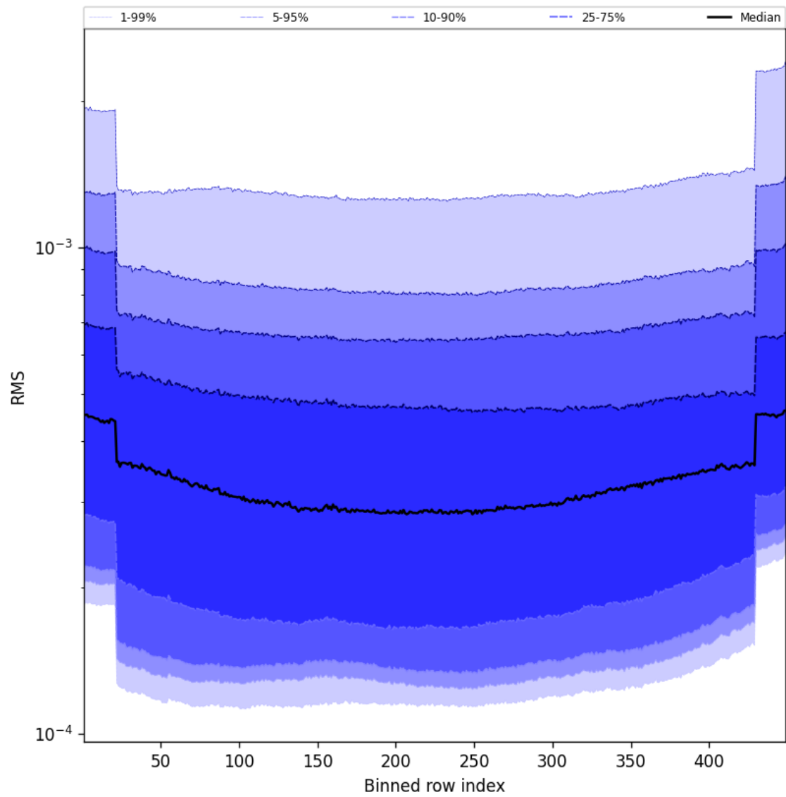
Figure 60: Along track statistics of “RMS” for 2025-02-21 to 2025-02-23
