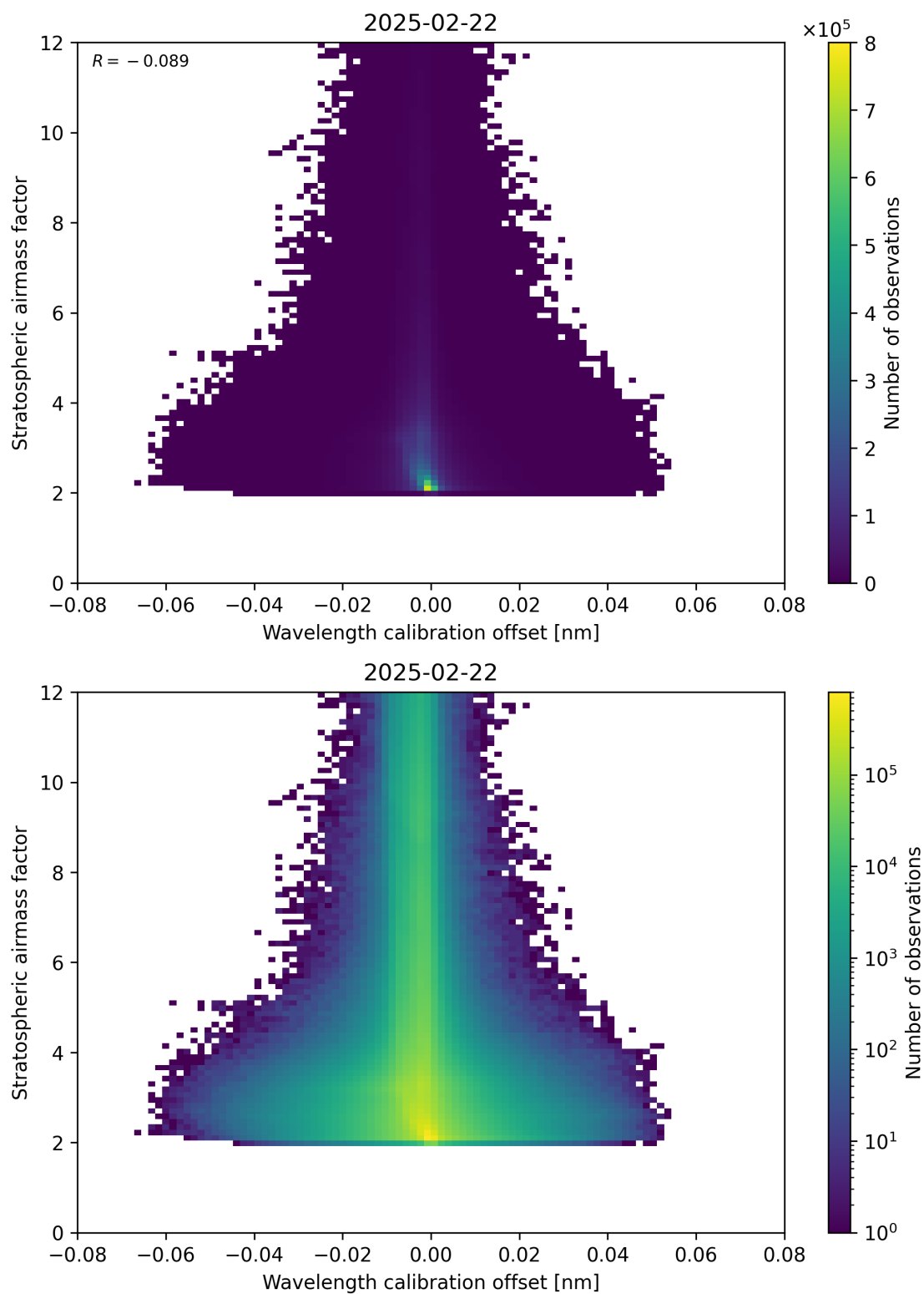
Figure 174: Scatter density plot of “Wavelength calibration offset” against “Stratospheric airmass factor” for 2025-02-21 to 2025-02-23.
