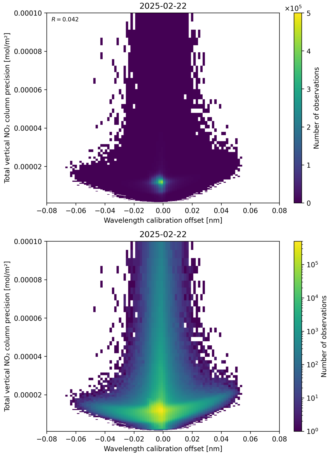
Figure 180: Scatter density plot of “Wavelength calibration offset” against “Total vertical NO 2 column precision” for 2025-02-21 to 2025-02-23.
