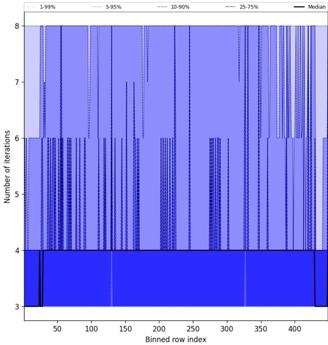
Figure 51: Along track statistics of “Number of iterations” for 2025-02-21 to 2025-02-23
