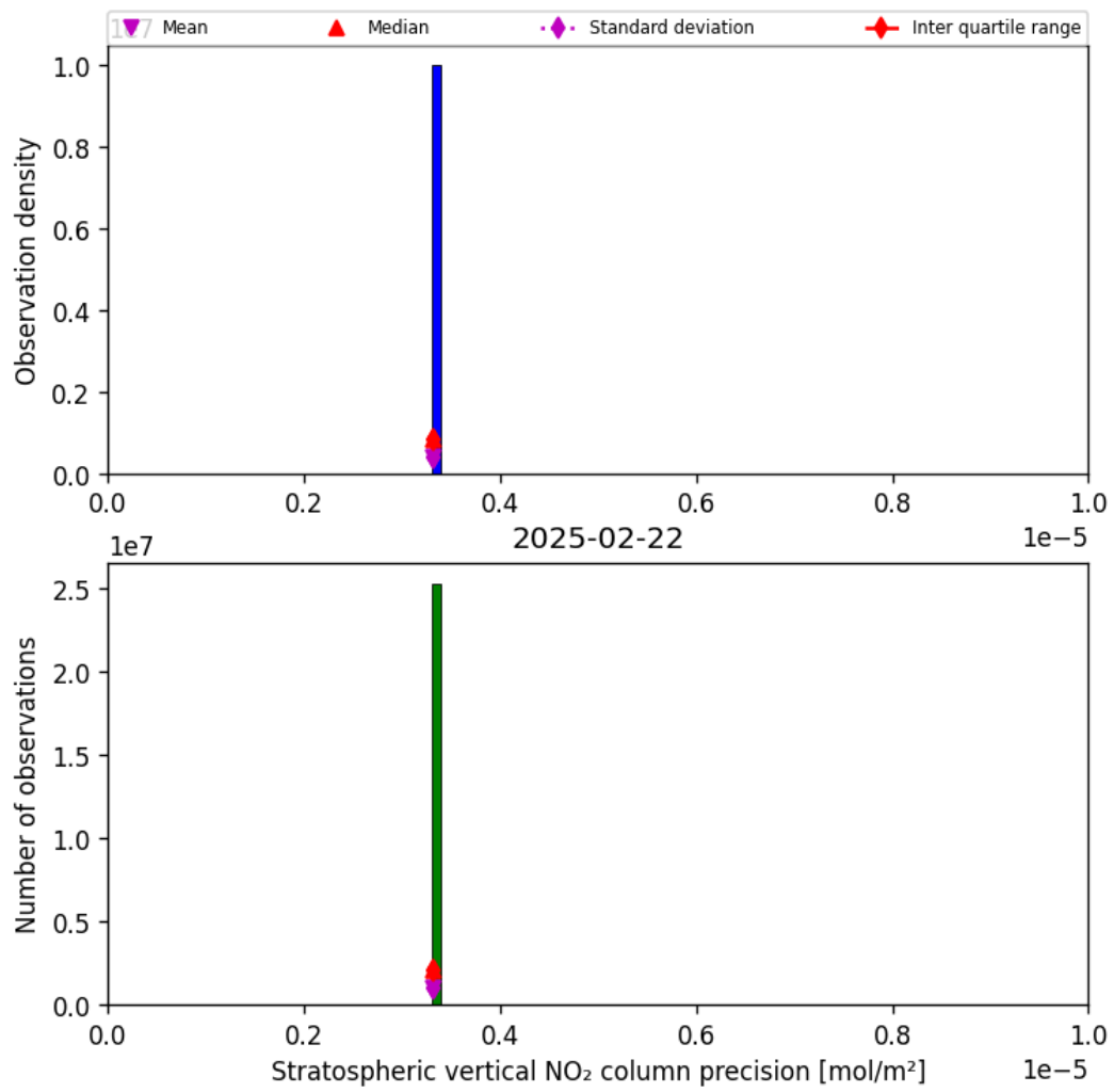
Figure 37: Histogram of “Stratospheric vertical NO 2 column precision” for 2025-02-21 to 2025-02-23
