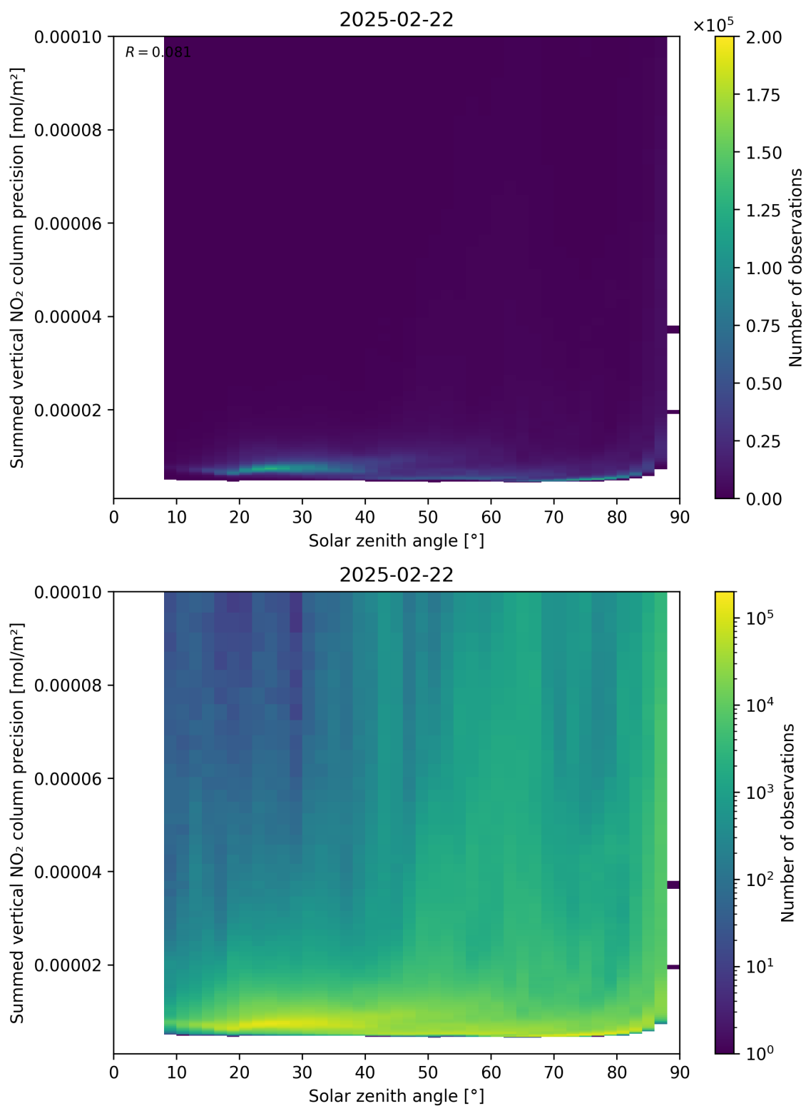
Figure 152: Scatter density plot of “Solar zenith angle” against “Summed vertical NO 2 column precision” for 2025-02-21 to 2025-02-23.
