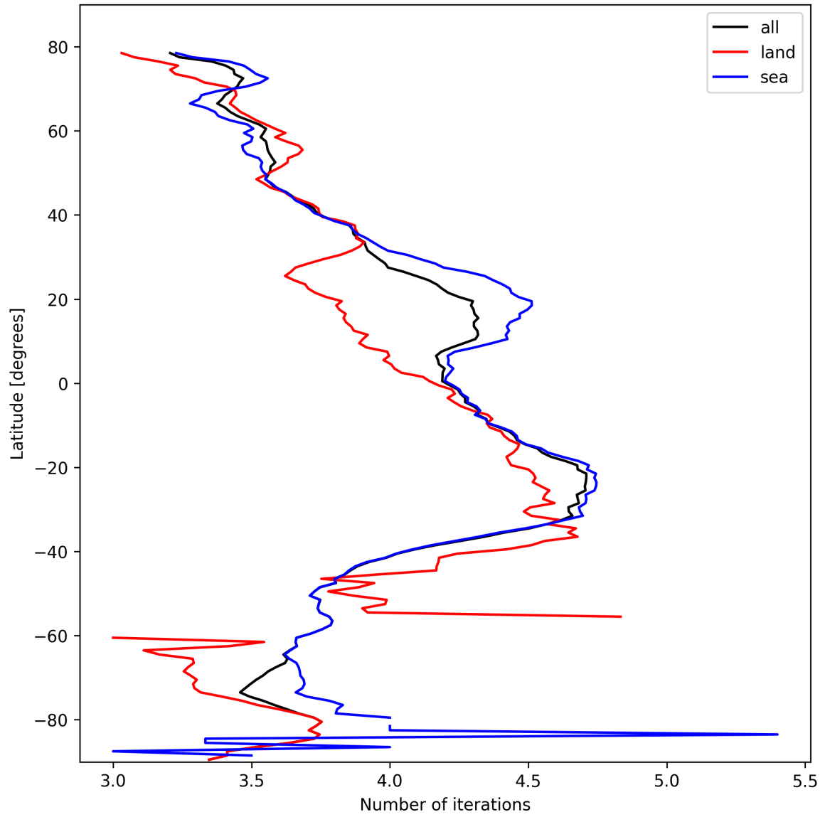
Figure 17: Zonal average of “Number of iterations” for 2025-02-21 to 2025-02-23.
