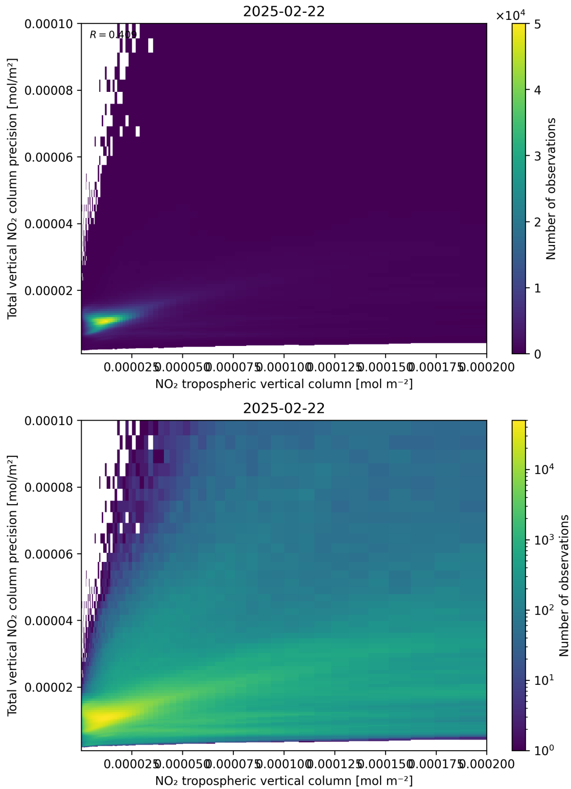
Figure 129: Scatter density plot of “NO 2 tropospheric vertical column” against “Total vertical NO 2 column precision” for 2025-02-21 to 2025-02-23.
