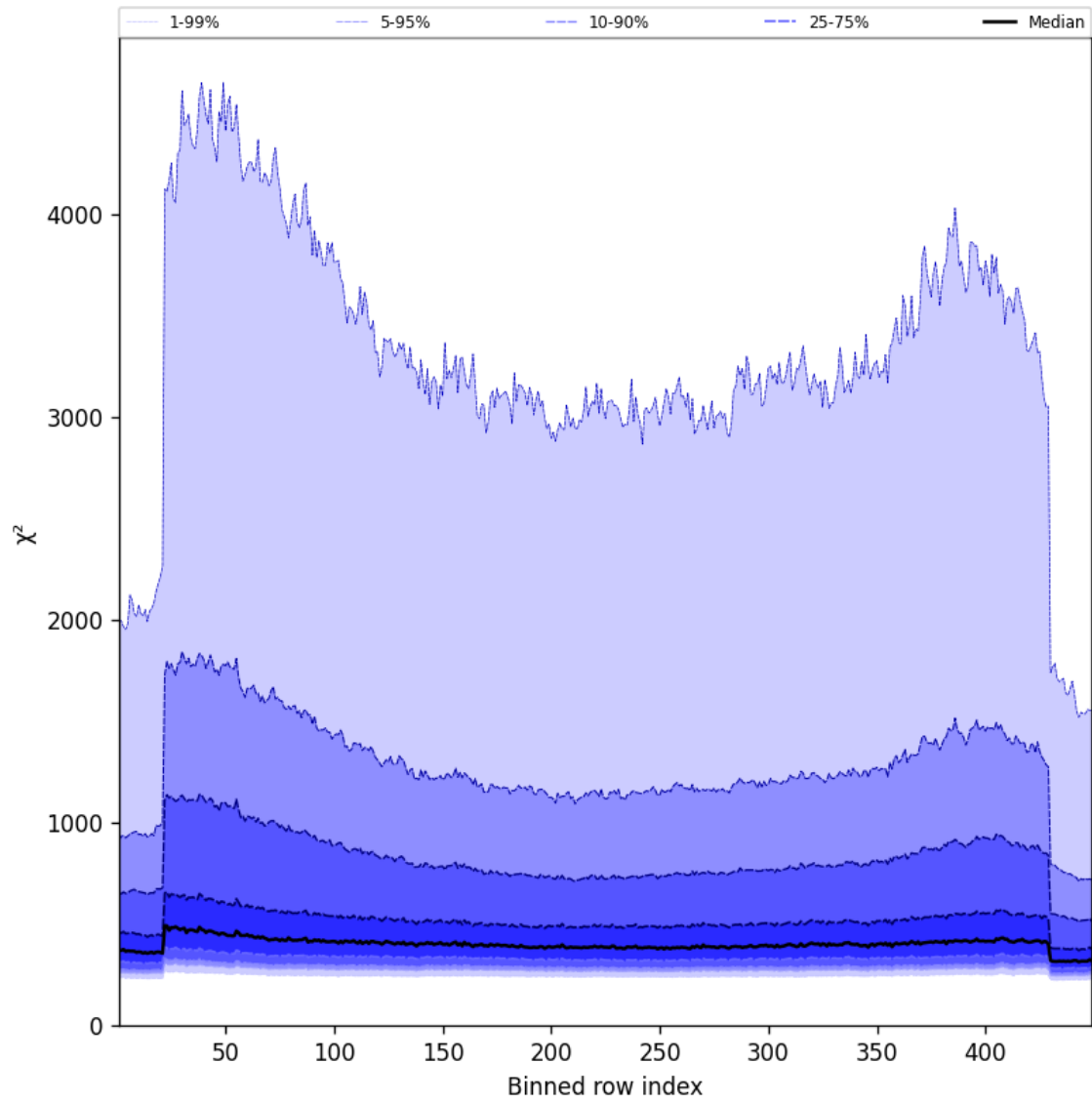
Figure 59: Along track statistics of “ \chi^2 ” for 2025-02-21 to 2025-02-23
