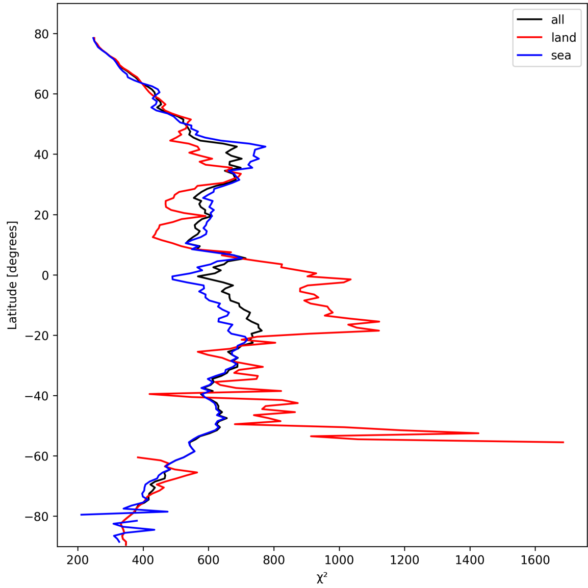
Figure 25: Zonal average of “ \chi^2 ” for 2025-02-21 to 2025-02-23.
