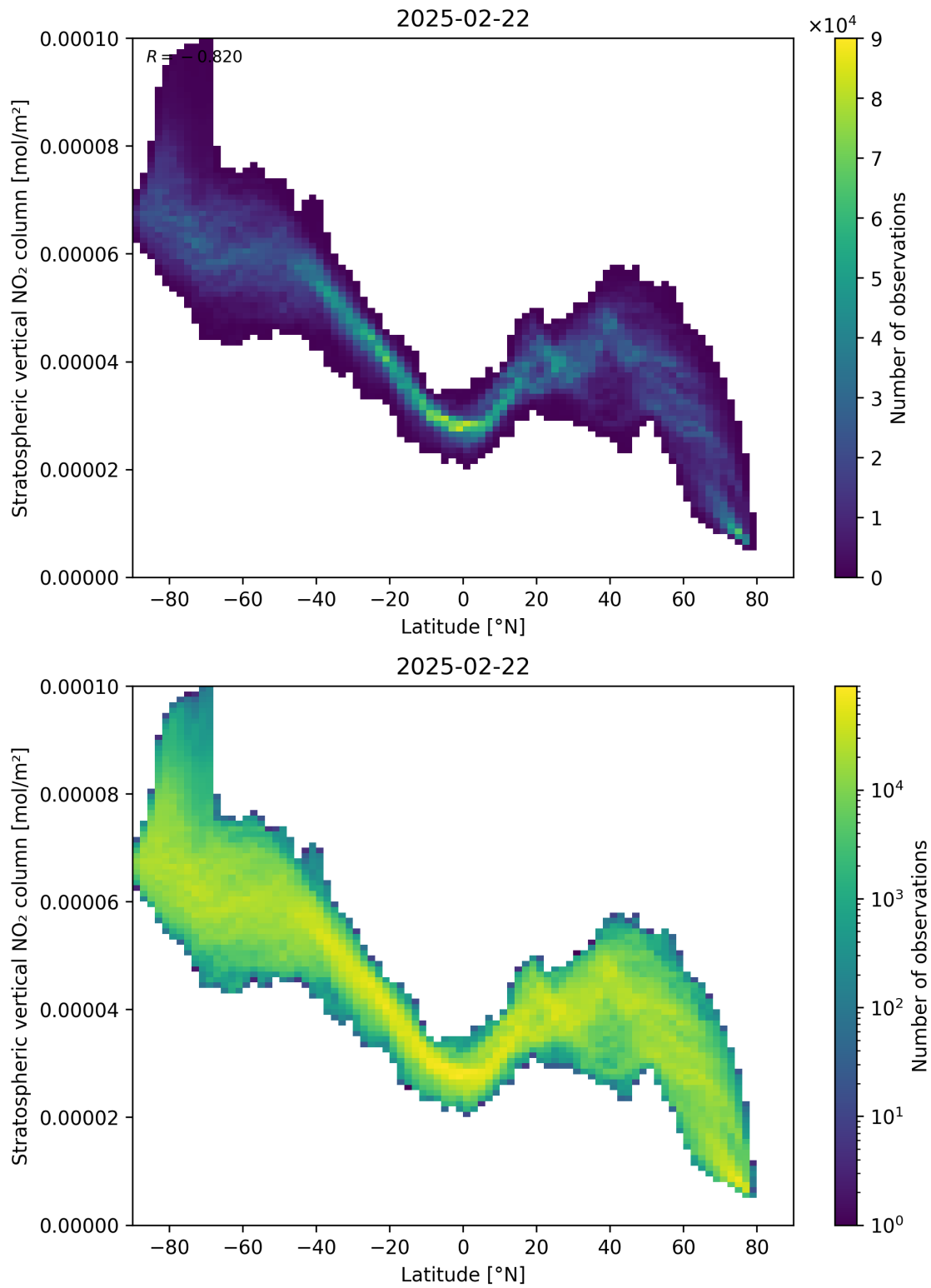
Figure 87: Scatter density plot of “Latitude” against “Stratospheric vertical NO 2 column” for 2025-02-21 to 2025-02-23.
