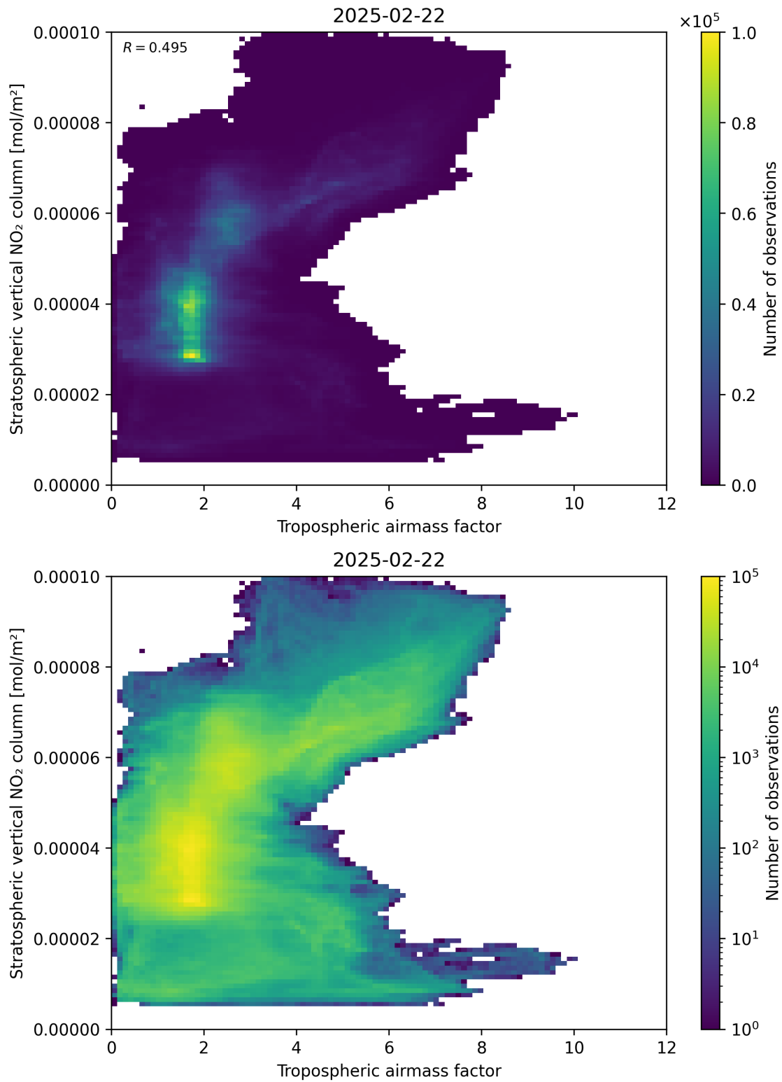
Figure 74: Scatter density plot of “Tropospheric air mass factor” against “Stratospheric vertical NO 2 column” for 2025-02-21 to 2025-02-23.
