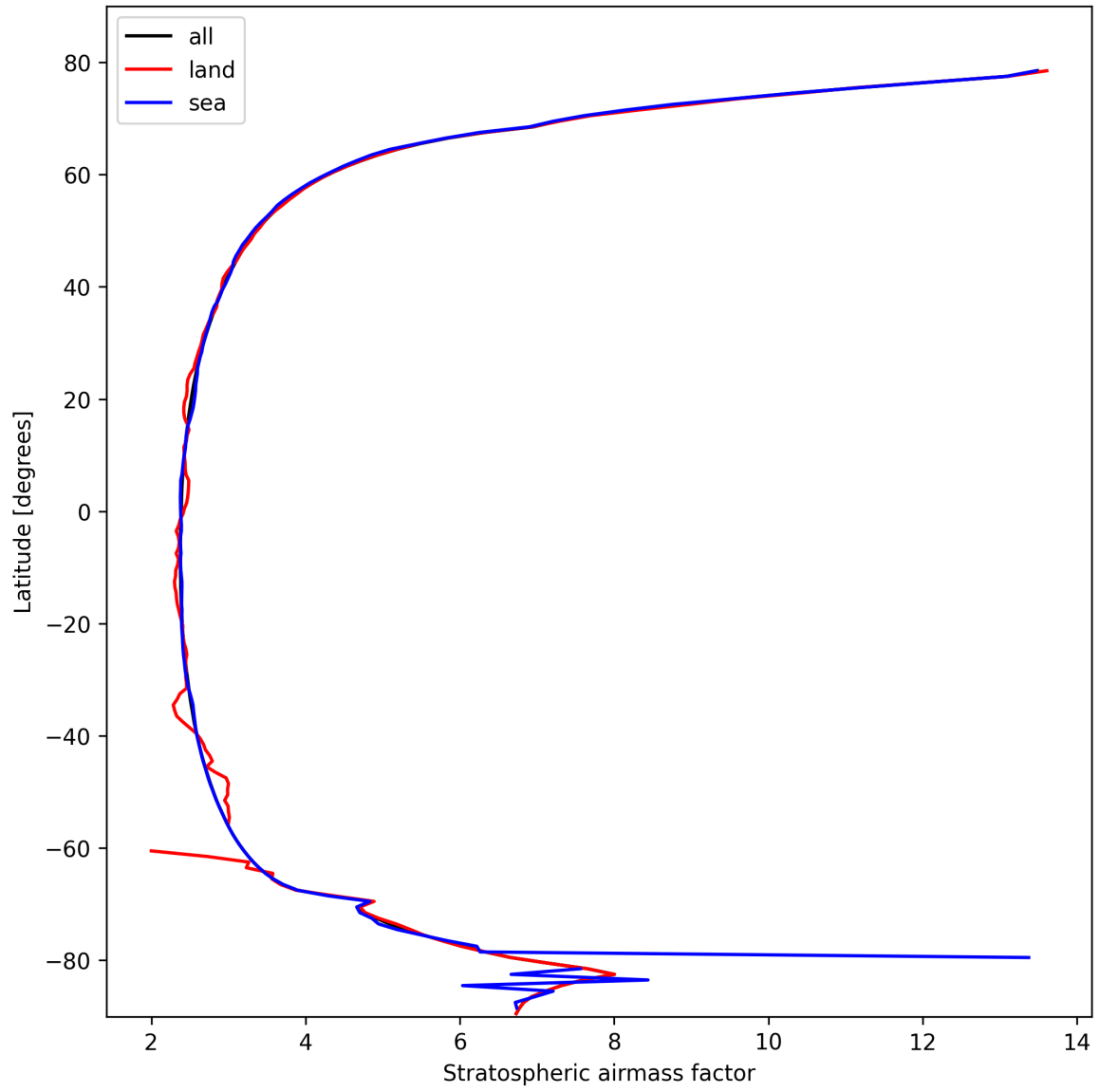
Figure 27: Zonal average of “Stratospheric airmass factor” for 2025-02-21 to 2025-02-23.
