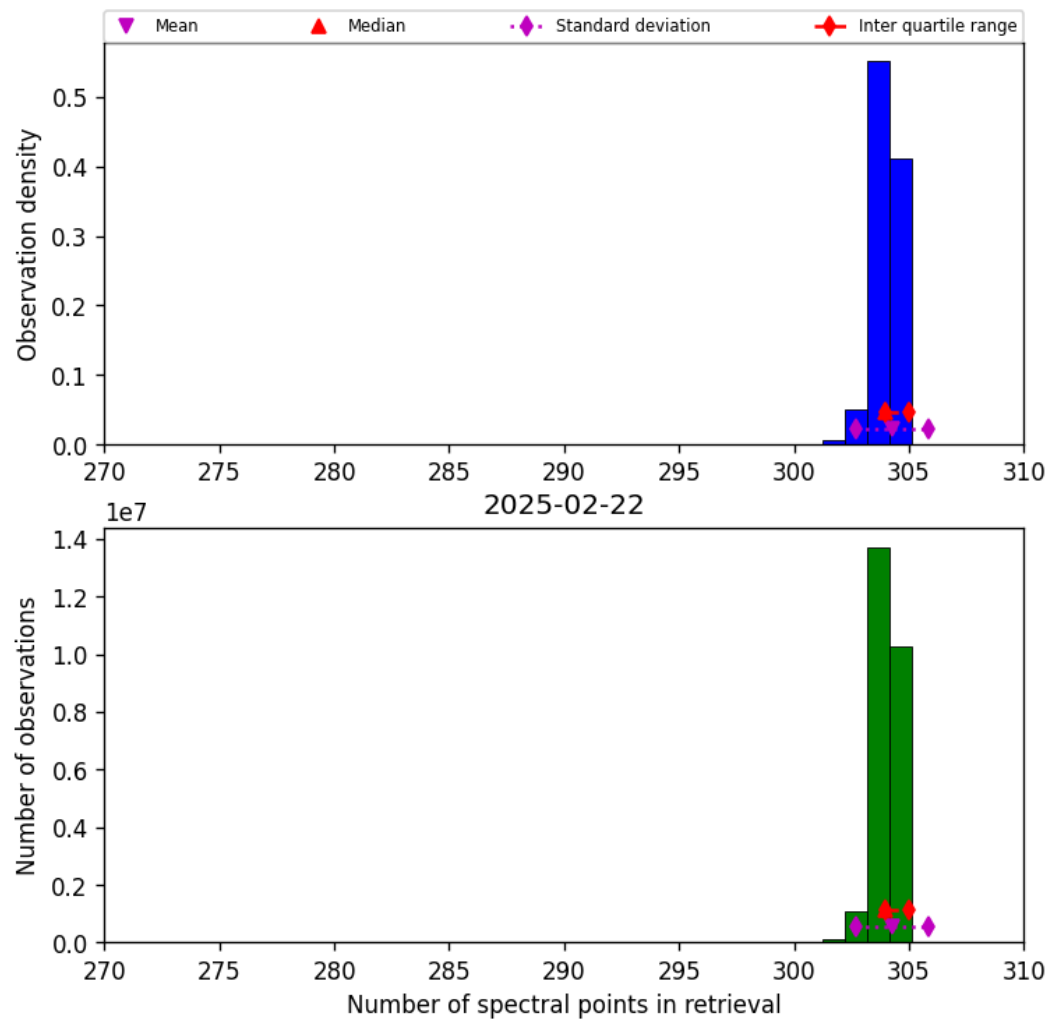
Figure 33: Histogram of “Number of spectral points in retrieval” for 2025-02-21 to 2025-02-23
