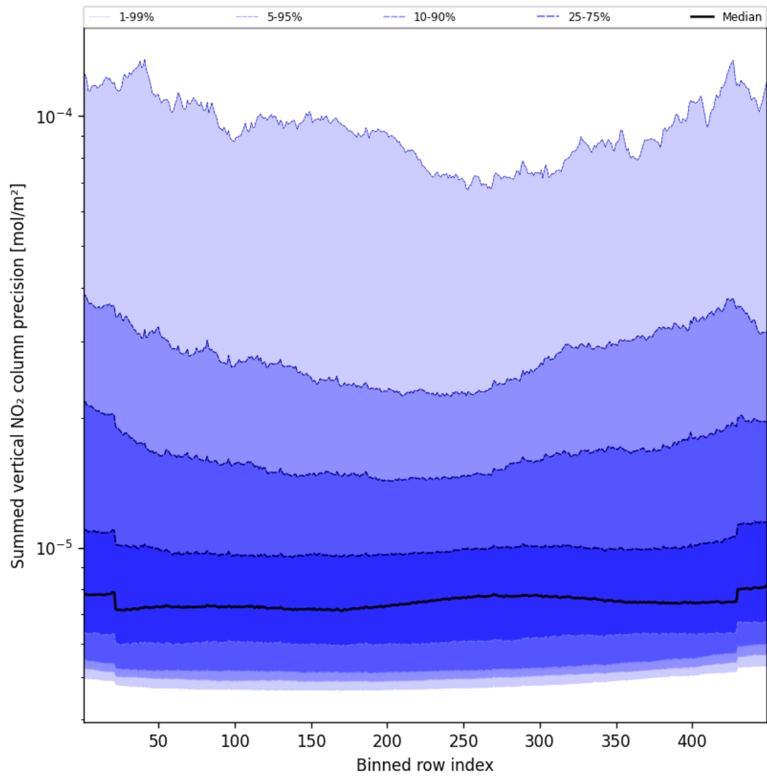
Figure 58: Along track statistics of “Summed vertical NO 2 column precision” for 2025-02-21 to 2025-02-23
