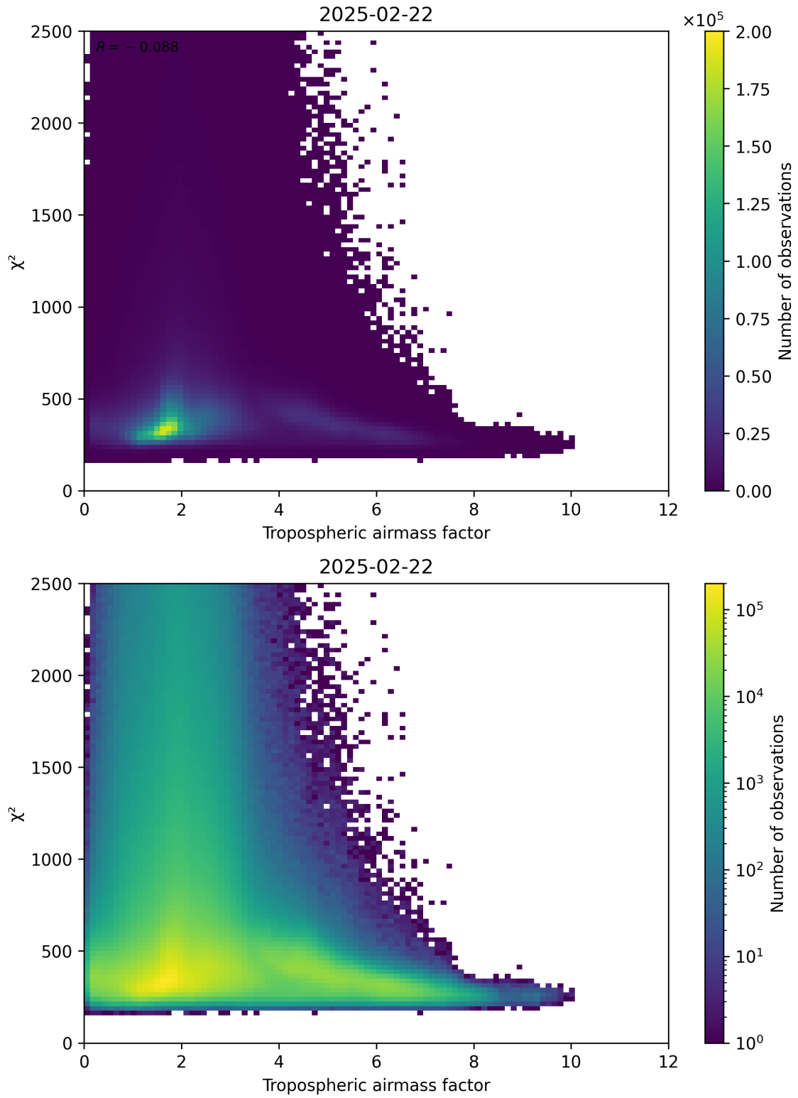
Figure 73: Scatter density plot of “Tropospheric airmass factor” against “ \chi^2 ” for 2025-02-21 to 2025-02-23.
