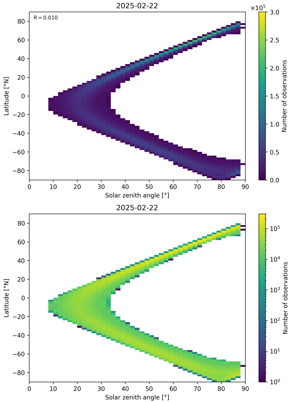
Figure 149: Scatter density plot of “Solar zenith angle” against “Latitude” for 2025-02-21 to 2025-02-23.
