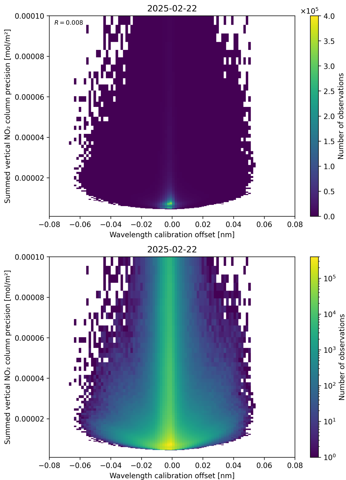
Figure 178: Scatter density plot of “Wavelength calibration offset” against “Summed vertical NO 2 column precision” for 2025-02-21 to 2025-02-23.
