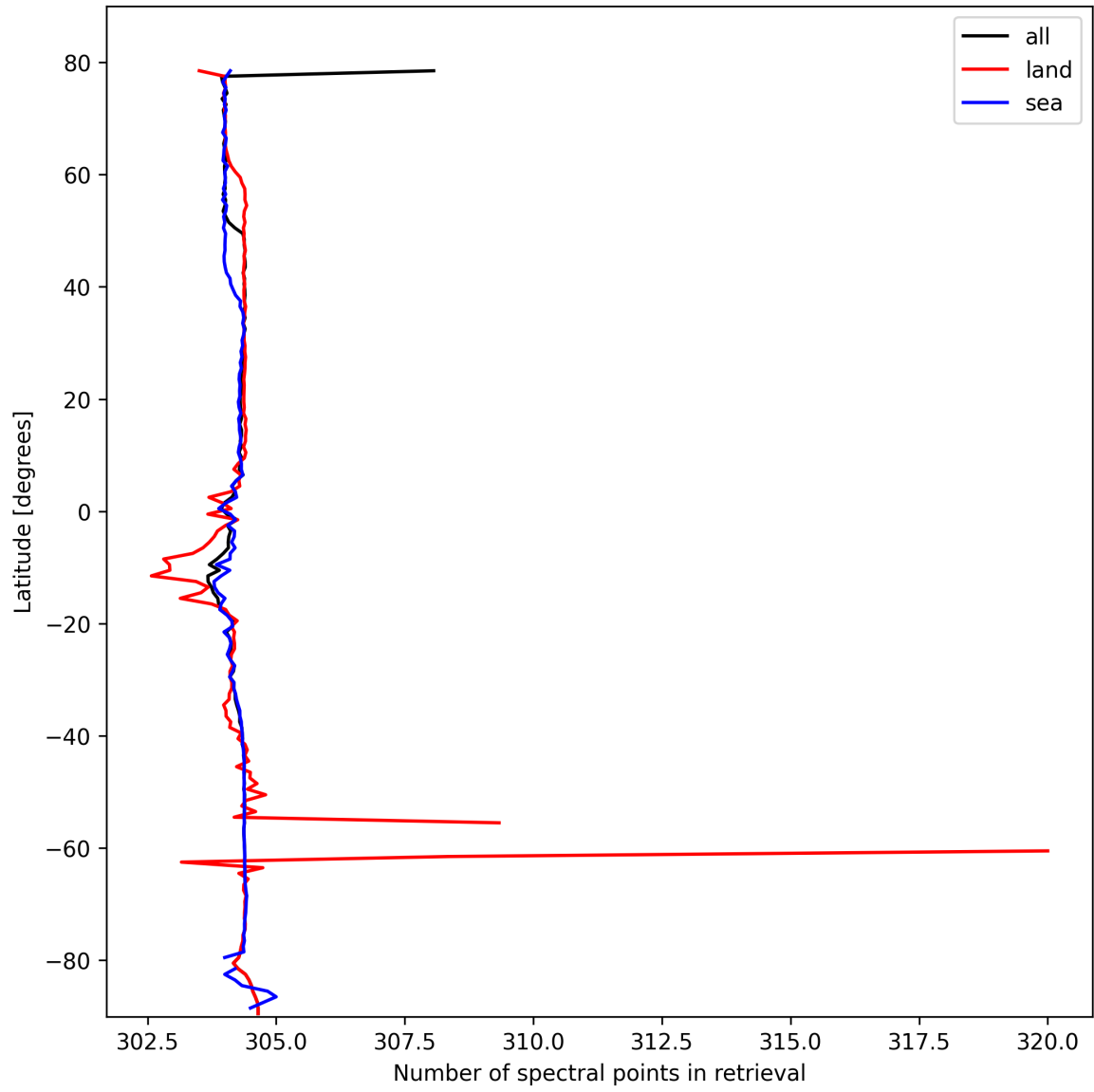
Figure 16: Zonal average of “Number of spectral points in retrieval” for 2025-02-21 to 2025-02-23.
