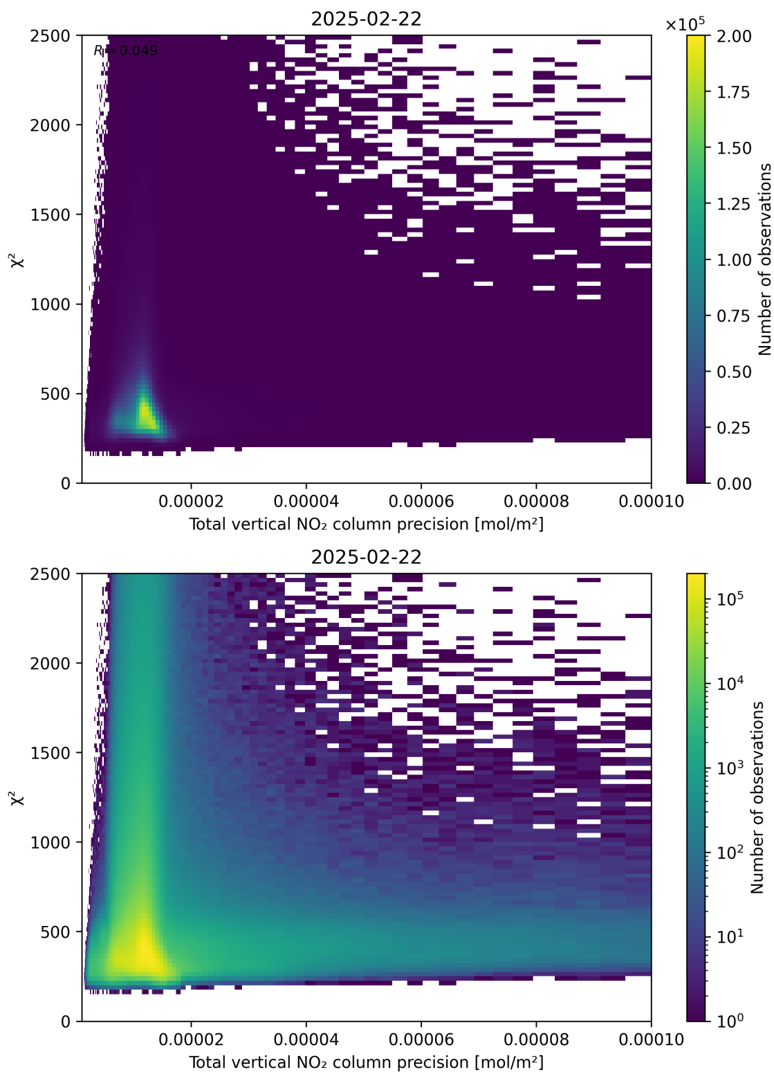
Figure 116: Scatter density plot of “Total vertical NO 2 column precision” against “ \chi^2 ” for 2025-02-21 to 2025-02-23.
