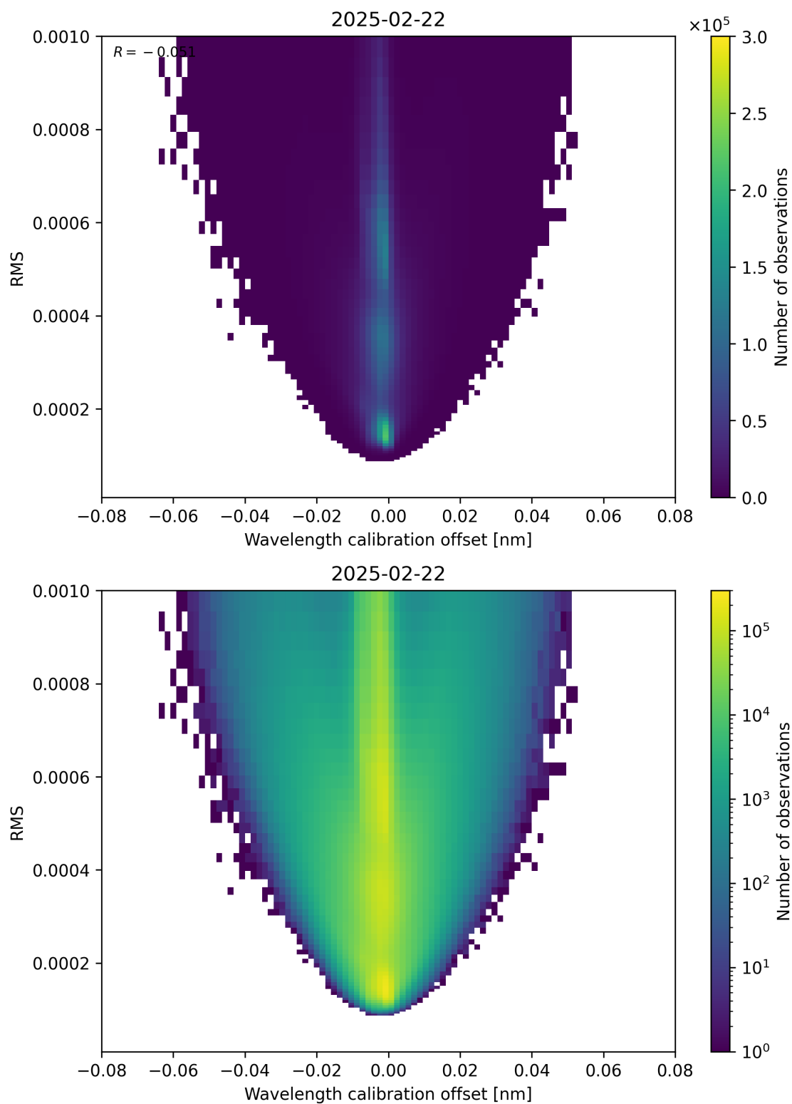
Figure 181: Scatter density plot of “Wavelength calibration offset” against “RMS” for 2025-02-21 to 2025-02-23.
