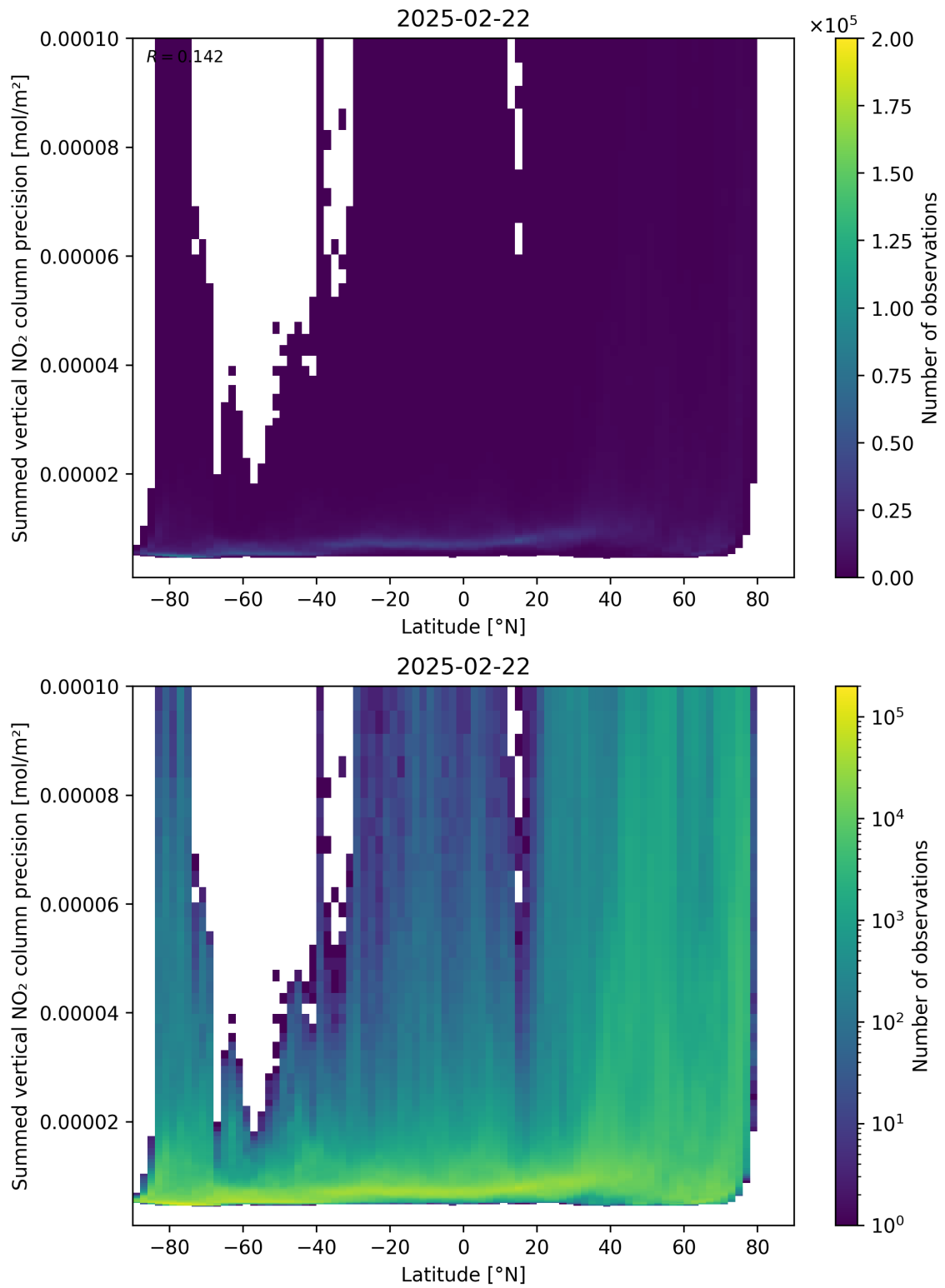
Figure 89: Scatter density plot of “Latitude” against “Summed vertical NO 2 column precision” for 2025-02-21 to 2025-02-23.
