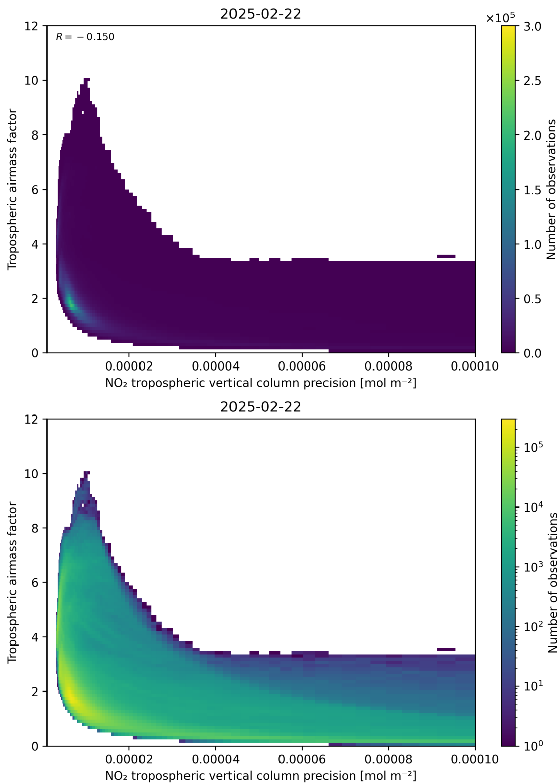
Figure 133: Scatter density plot of “NO 2 tropospheric vertical column precision” against “Tropospheric airmass factor” for 2025-02-21 to 2025-02-23.
