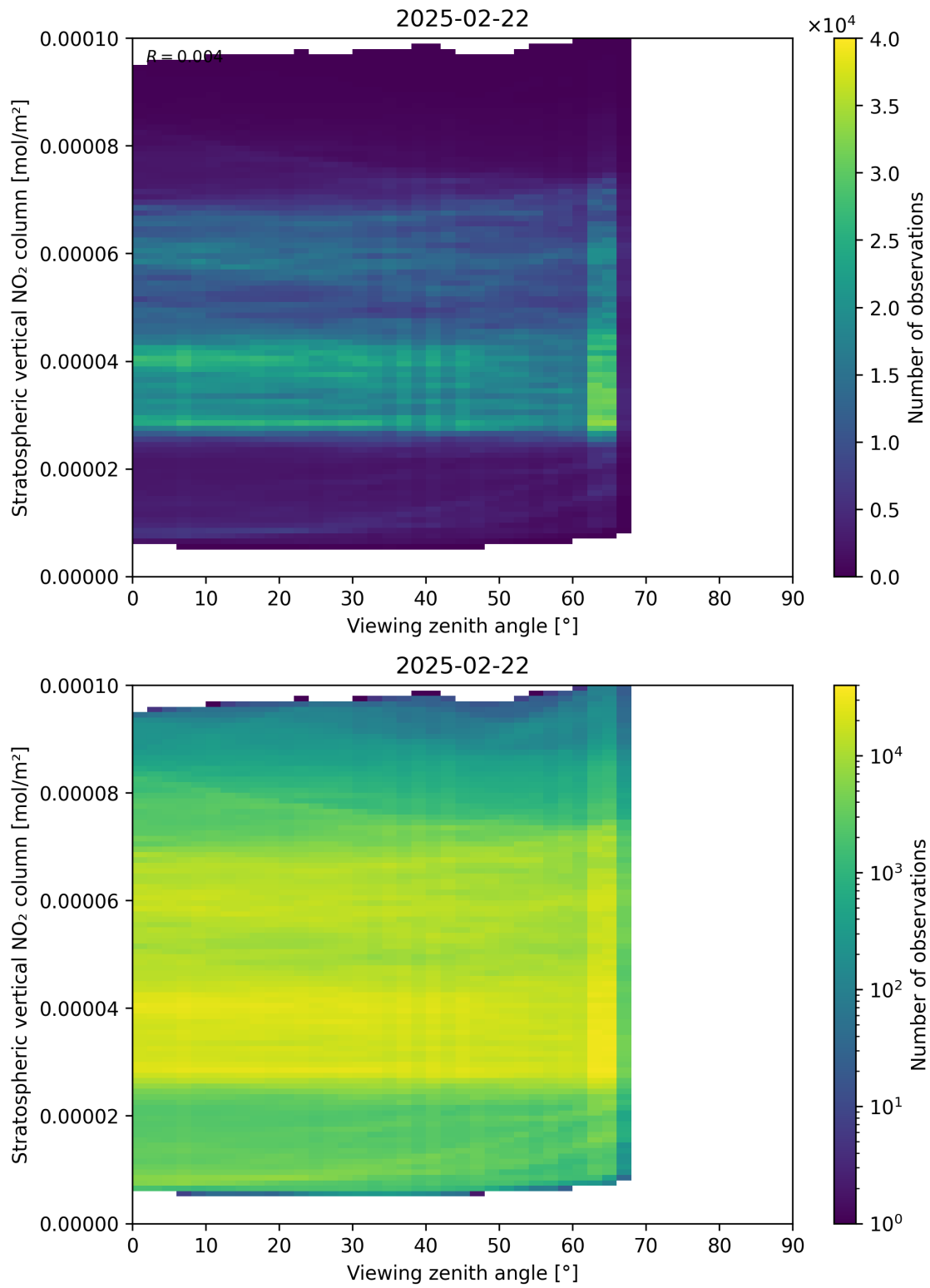
Figure 164: Scatter density plot of “Viewing zenith angle” against “Stratospheric vertical NO 2 column” for 2025-02-21 to 2025-02-23.
