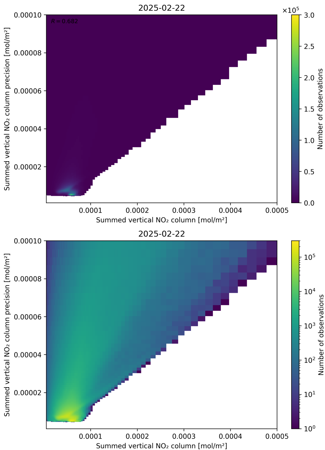
Figure 105: Scatter density plot of “Summed vertical NO 2 column” against “Summed vertical NO 2 column precision” for 2025-02-21 to 2025-02-23.
