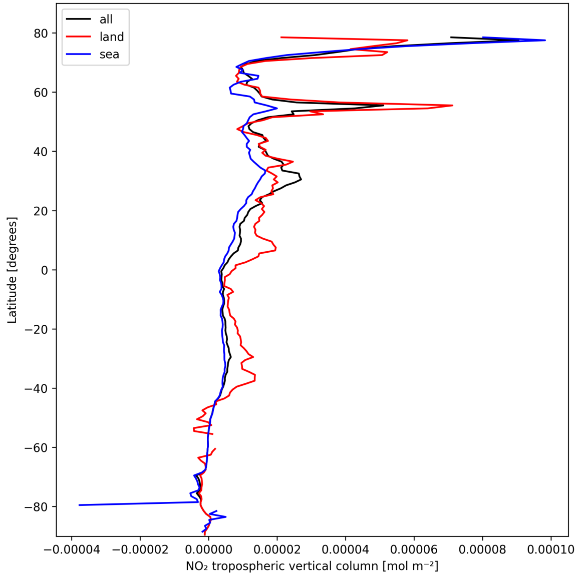
Figure 12: Zonal average of “NO 2 tropospheric vertical column” for 2025-02-21 to 2025-02-23.
