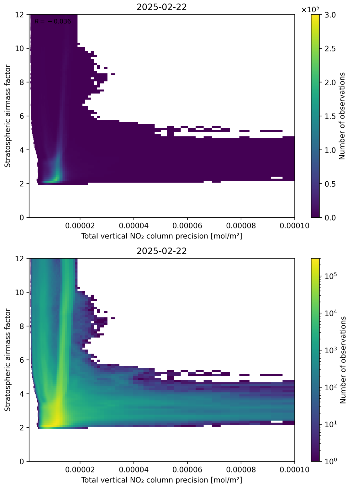
Figure 115: Scatter density plot of “Total vertical NO 2 column precision” against “Stratospheric air mass factor” for 2025-02-21 to 2025-02-23.
