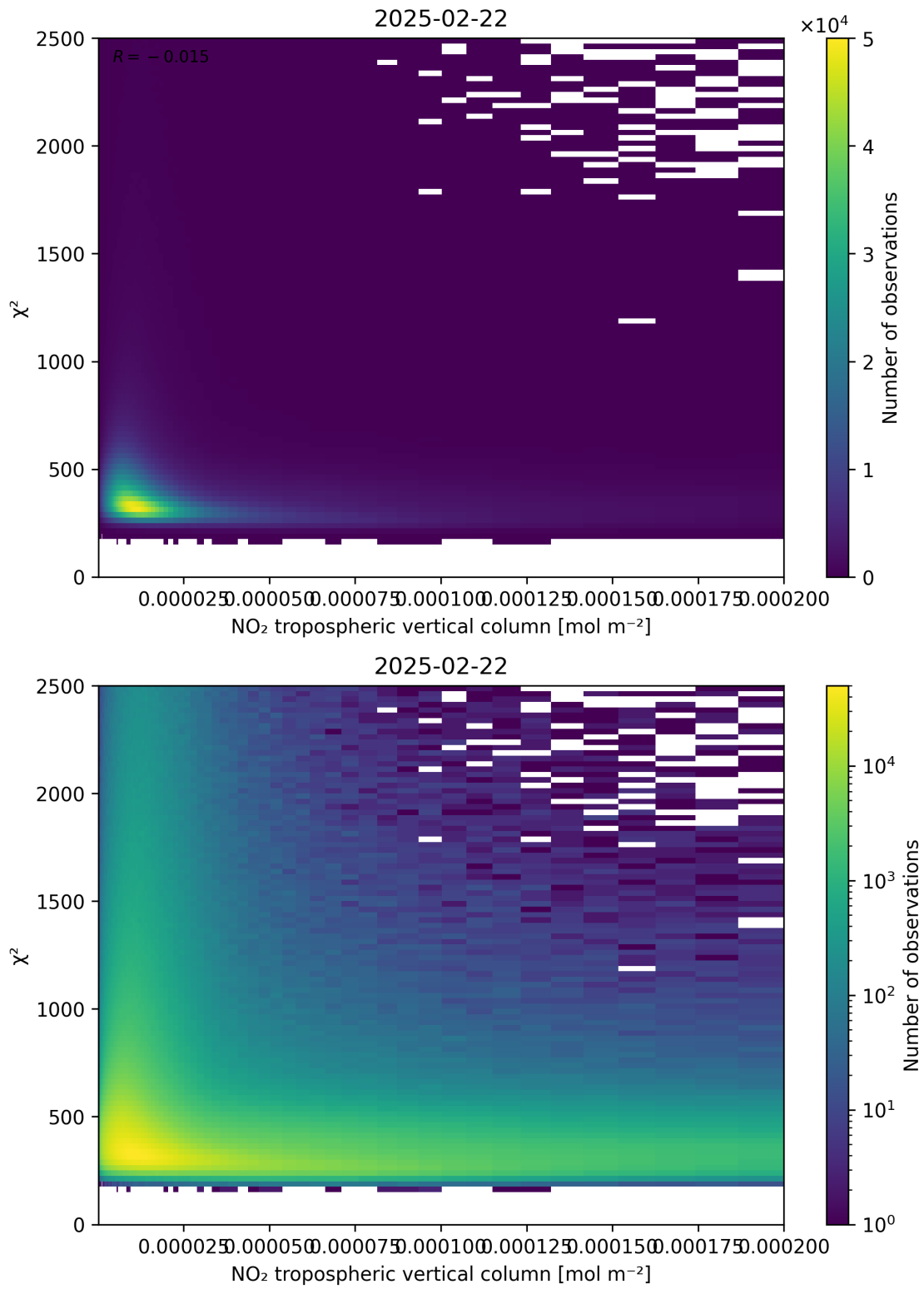
Figure 124: Scatter density plot of “NO 2 tropospheric vertical column” against “ \chi^2 ” for 2025-02-21 to 2025-02-23.
