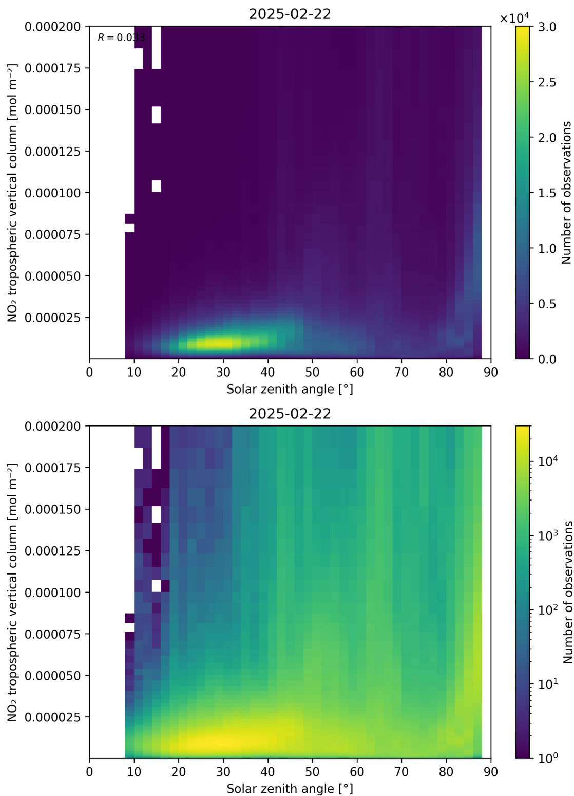
Figure 155: Scatter density plot of “Solar zenith angle” against “NO 2 tropospheric vertical column” for 2025-02-21 to 2025-02-23.
