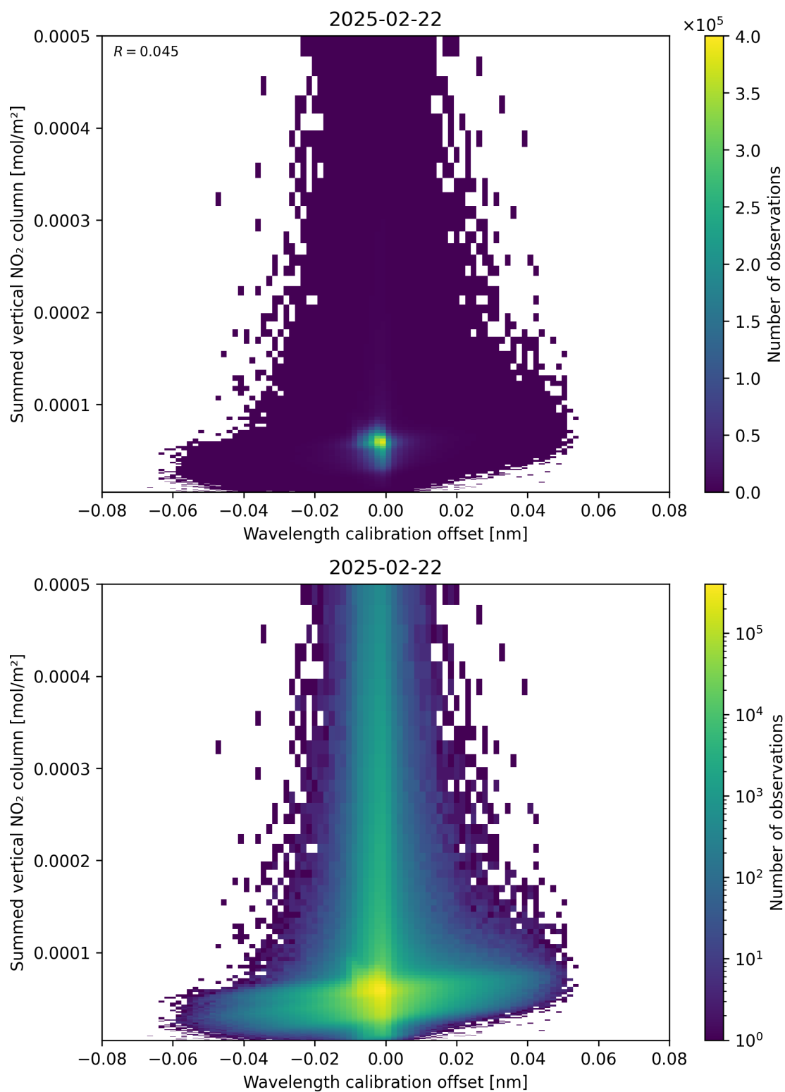
Figure 177: Scatter density plot of “Wavelength calibration offset” against “Summed vertical NO 2 column” for 2025-02-21 to 2025-02-23.
