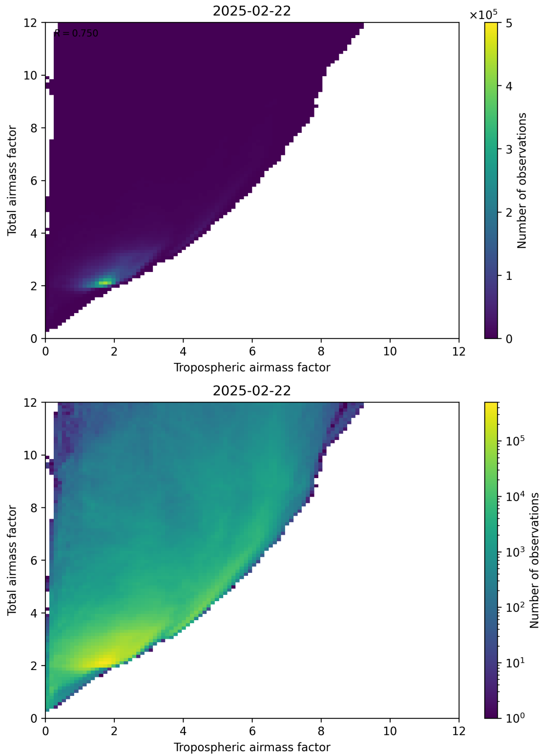
Figure 72: Scatter density plot of “Tropospheric airmass factor” against “Total airmass factor” for 2025-02-21 to 2025-02-23.
