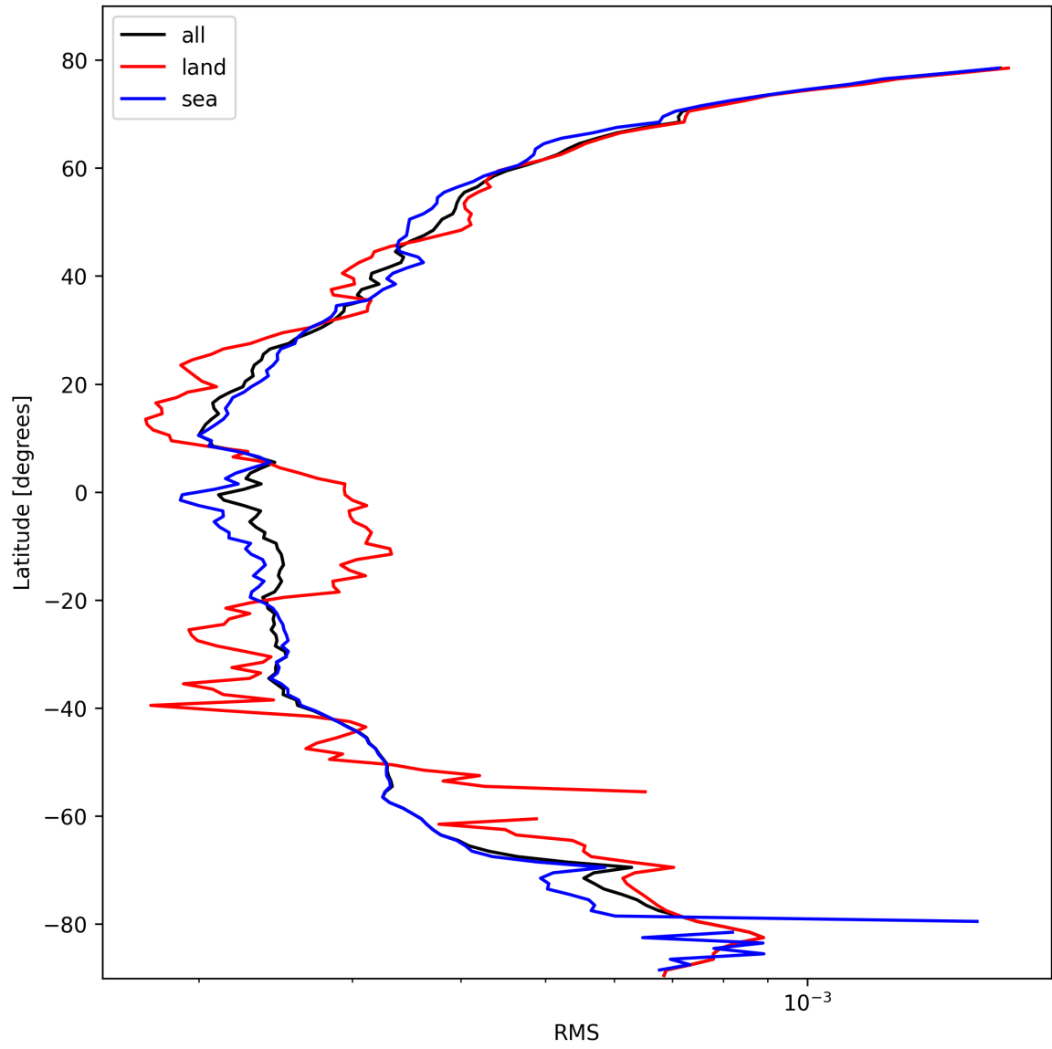
Figure 26: Zonal average of “RMS” for 2025-02-21 to 2025-02-23.
