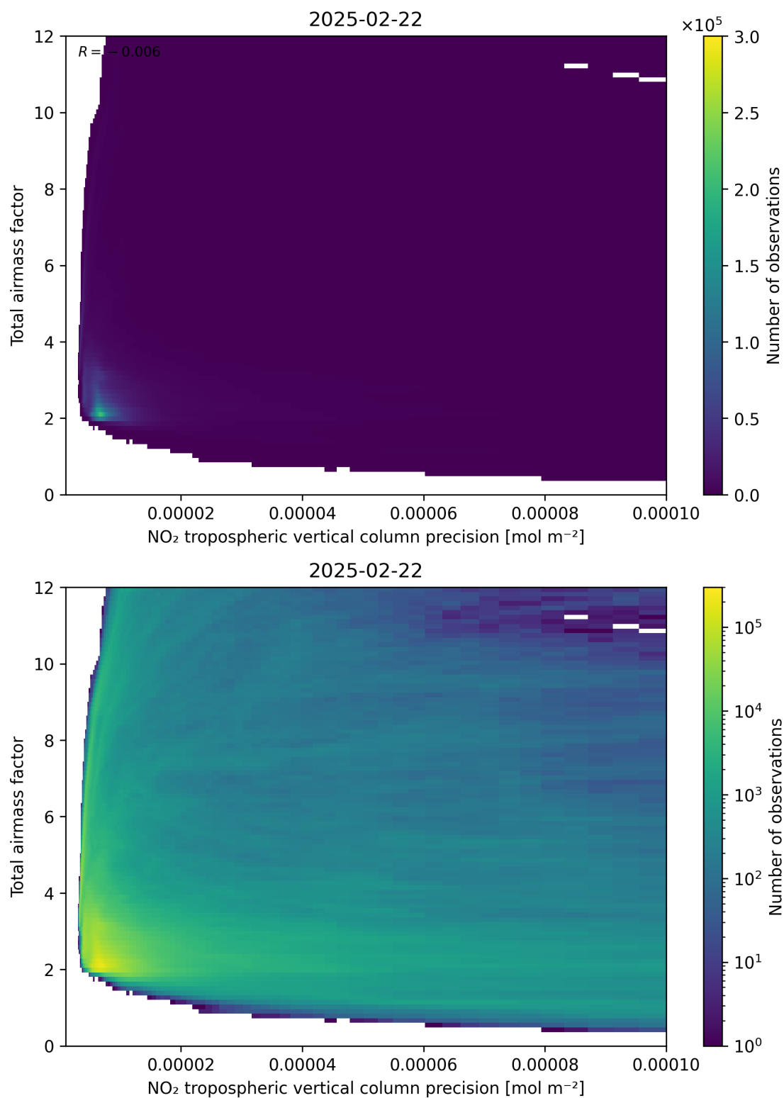
Figure 132: Scatter density plot of “NO 2 tropospheric vertical column precision” against “Total air mass factor” for 2025-02-21 to 2025-02-23.
