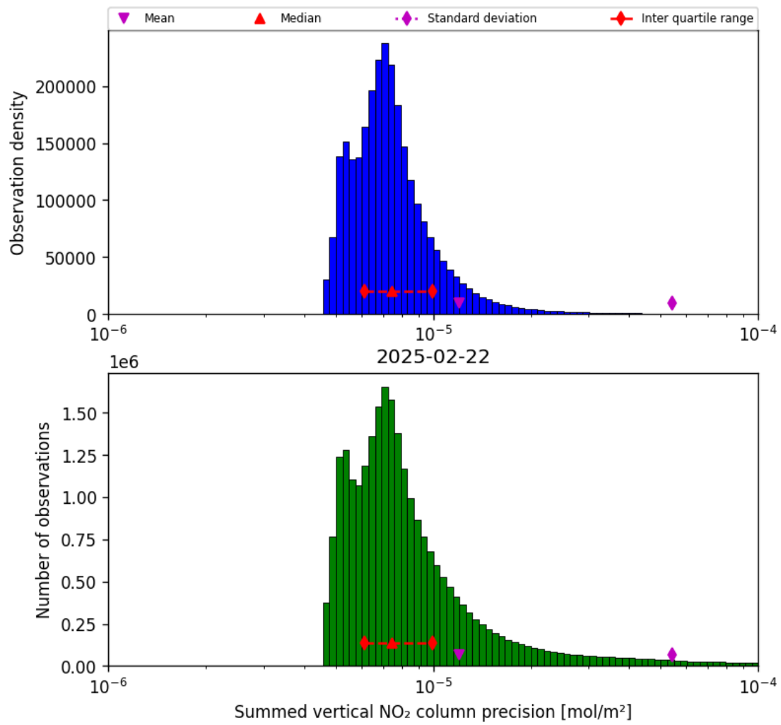
Figure 41: Histogram of “Summed vertical NO 2 column precision” for 2025-02-21 to 2025-02-23
