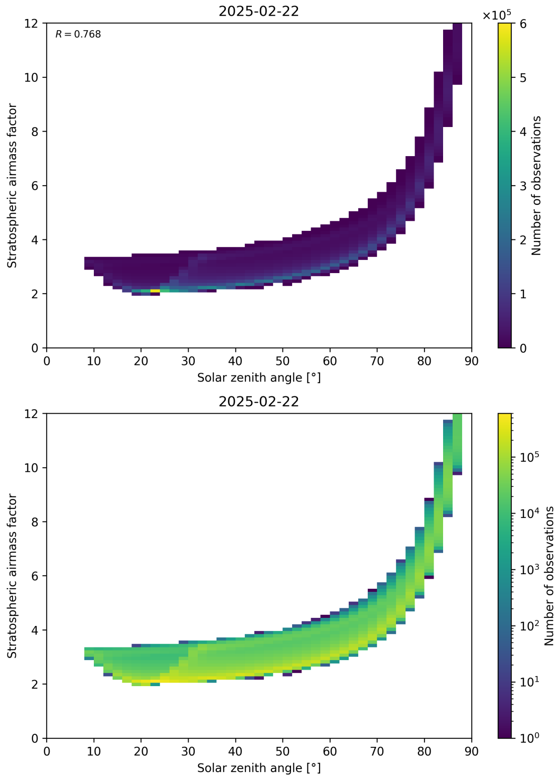
Figure 145: Scatter density plot of “Solar zenith angle” against “Stratospheric airmass factor” for 2025-02-21 to 2025-02-23.
