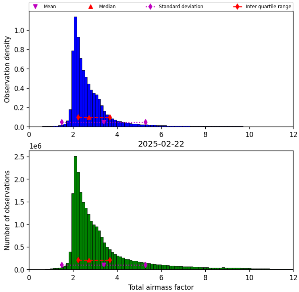
Figure 32: Histogram of “Total airmass factor” for 2025-02-21 to 2025-02-23
