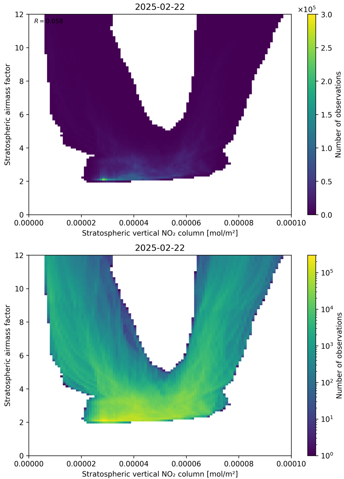
Figure 96: Scatter density plot of “Stratospheric vertical NO 2 column” against “Stratospheric airmass factor” for 2025-02-21 to 2025-02-23.
