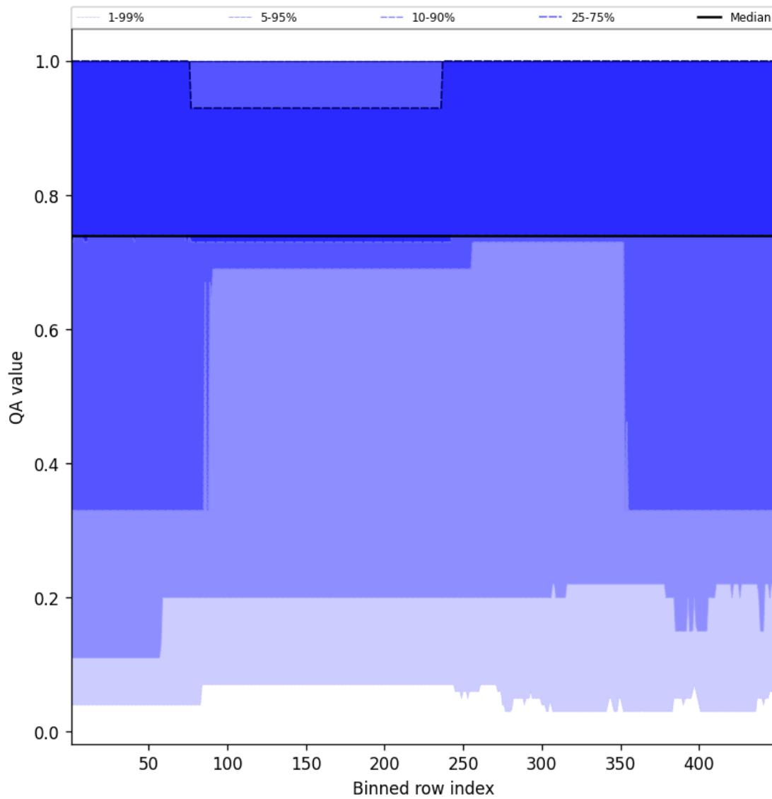
Figure 45: Along track statistics of “QA value” for 2025-02-21 to 2025-02-23
