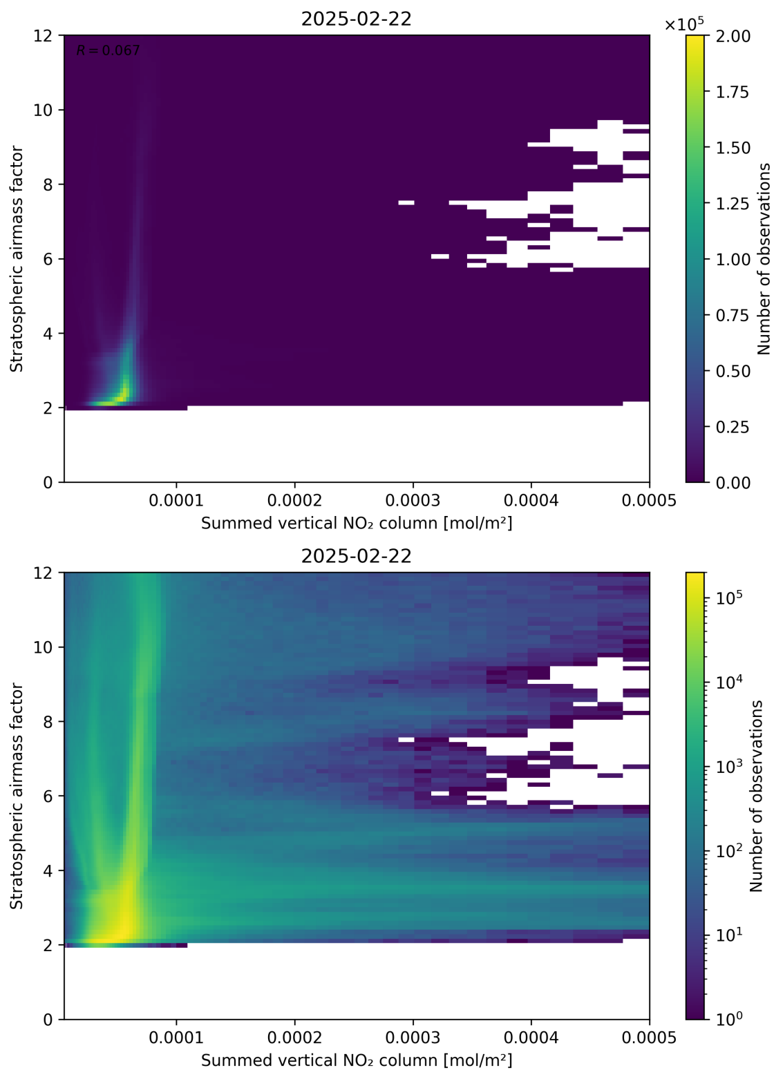
Figure 103: Scatter density plot of “Summed vertical NO 2 column” against “Stratospheric air mass factor” for 2025-02-21 to 2025-02-23.
