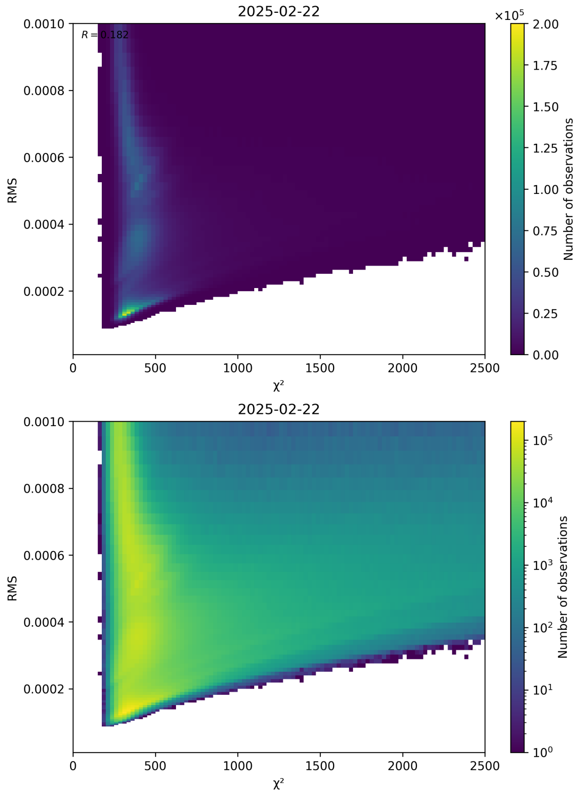
Figure 82: Scatter density plot of “ \chi^2 ” against “RMS” for 2025-02-21 to 2025-02-23.
