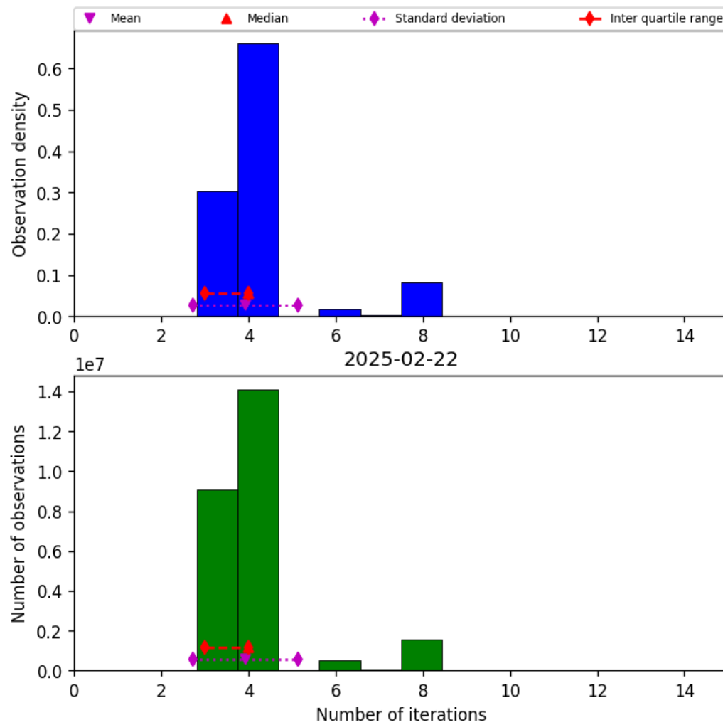
Figure 34: Histogram of “Number of iterations” for 2025-02-21 to 2025-02-23
