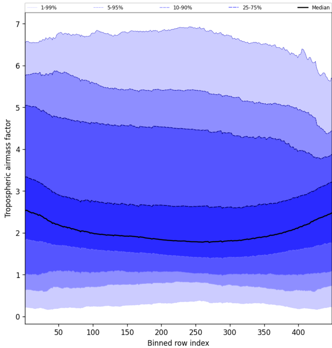
Figure 48: Along track statistics of “Tropospheric airmass factor” for 2025-02-21 to 2025-02-23
