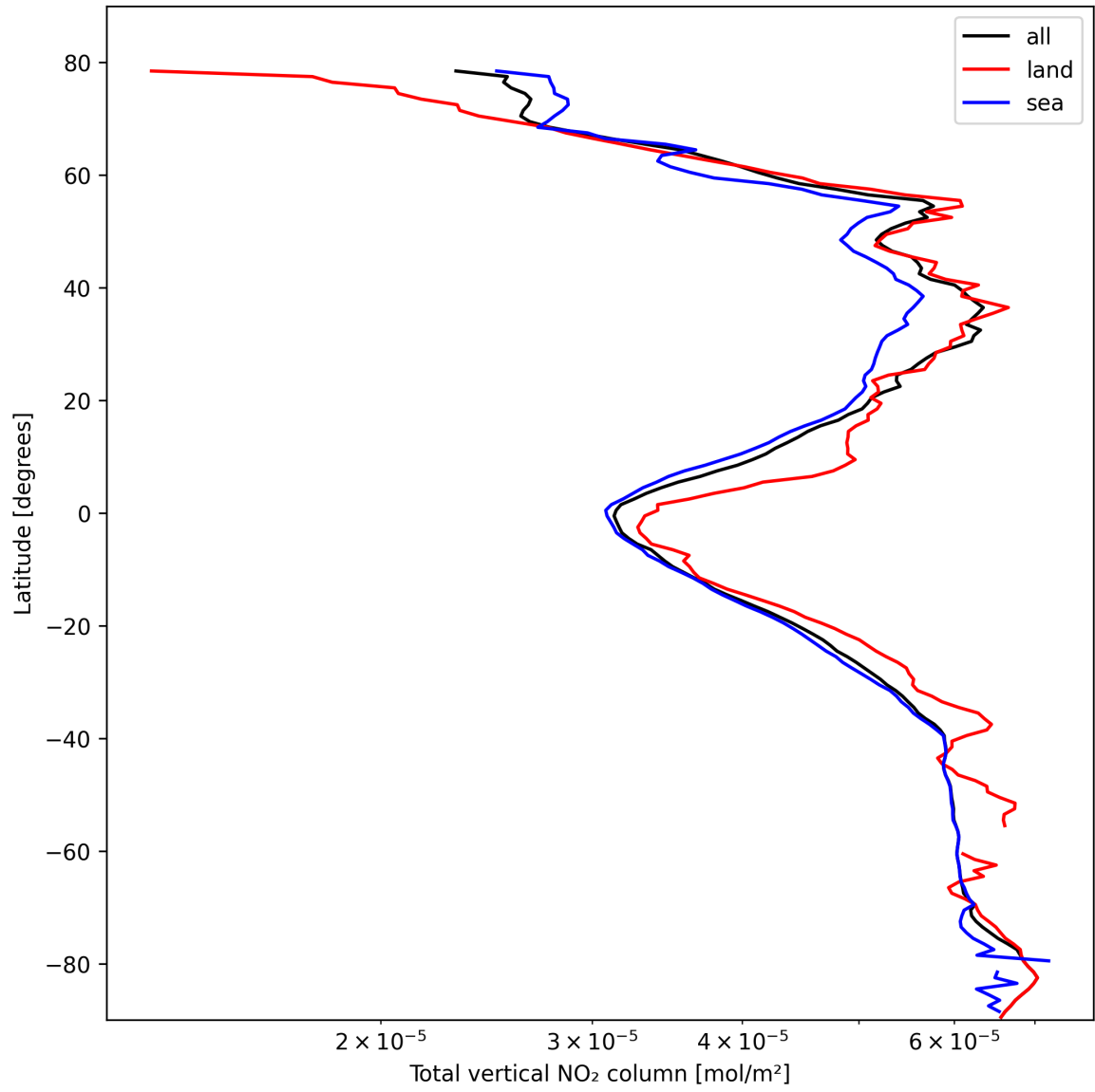
Figure 21: Zonal average of “Total vertical NO 2 column” for 2025-02-21 to 2025-02-23.
