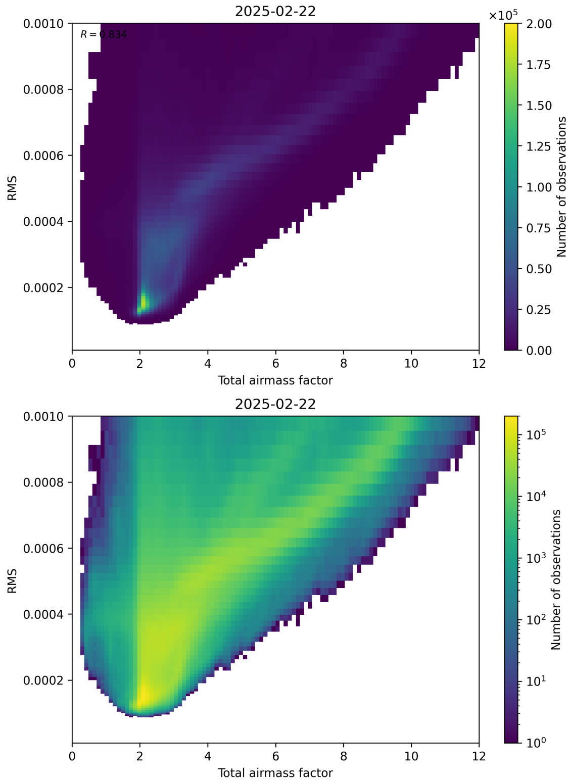
Figure 69: Scatter density plot of “Total airmass factor” against “RMS” for 2025-02-21 to 2025-02-23.
