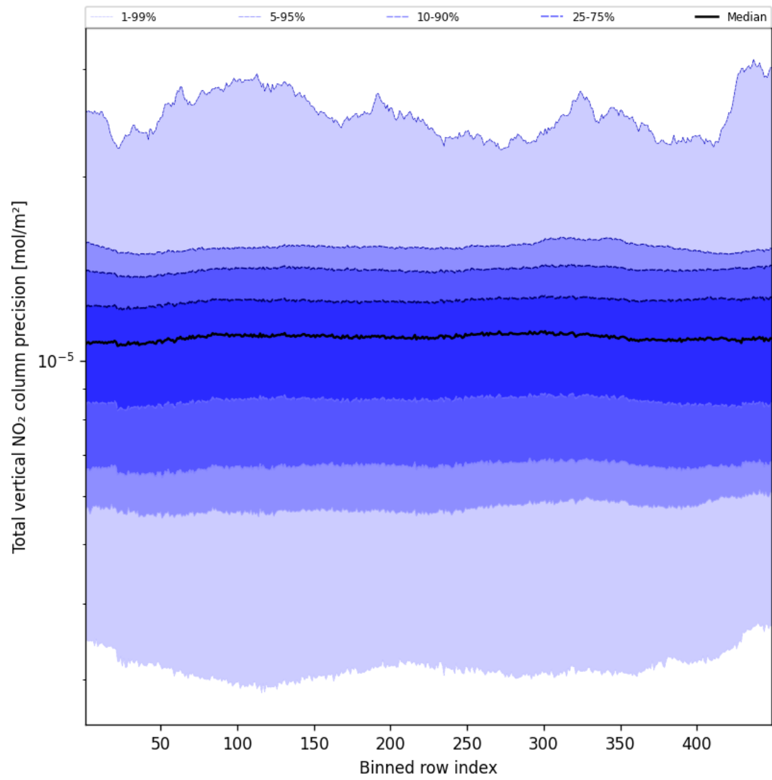
Figure 56: Along track statistics of “Total vertical NO 2 column precision” for 2025-02-21 to 2025-02-23
