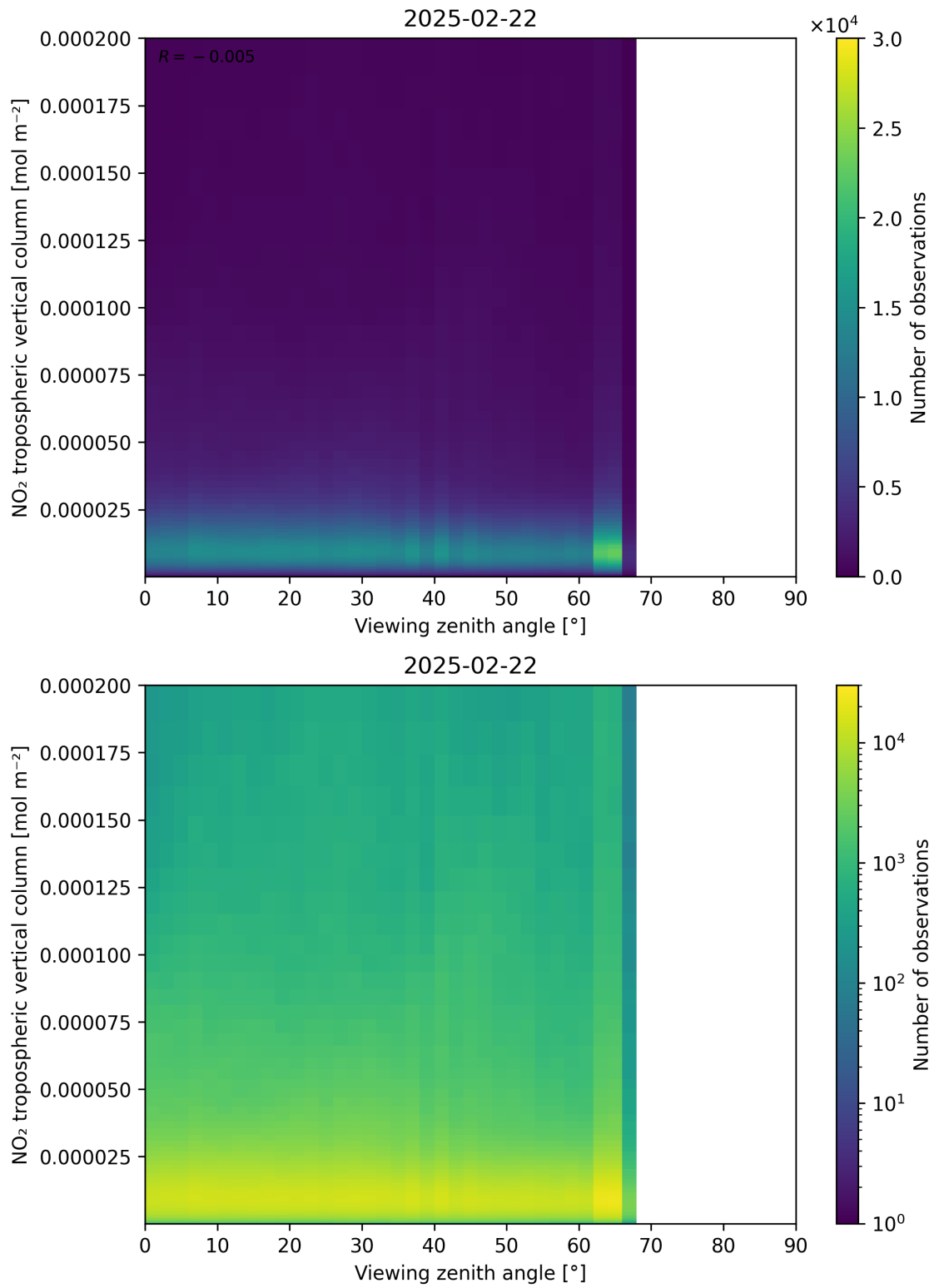
Figure 169: Scatter density plot of “Viewing zenith angle” against “NO 2 tropospheric vertical column” for 2025-02-21 to 2025-02-23.
