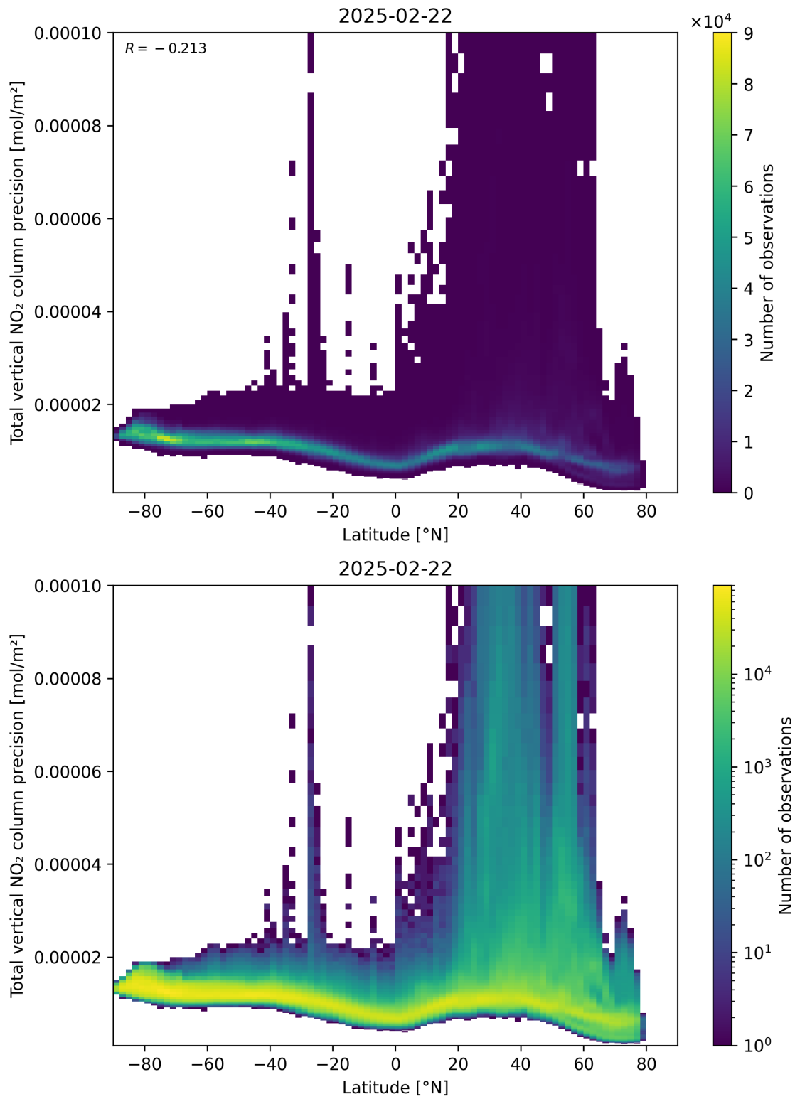
Figure 91: Scatter density plot of “Latitude” against “Total vertical NO 2 column precision” for 2025-02-21 to 2025-02-23.
