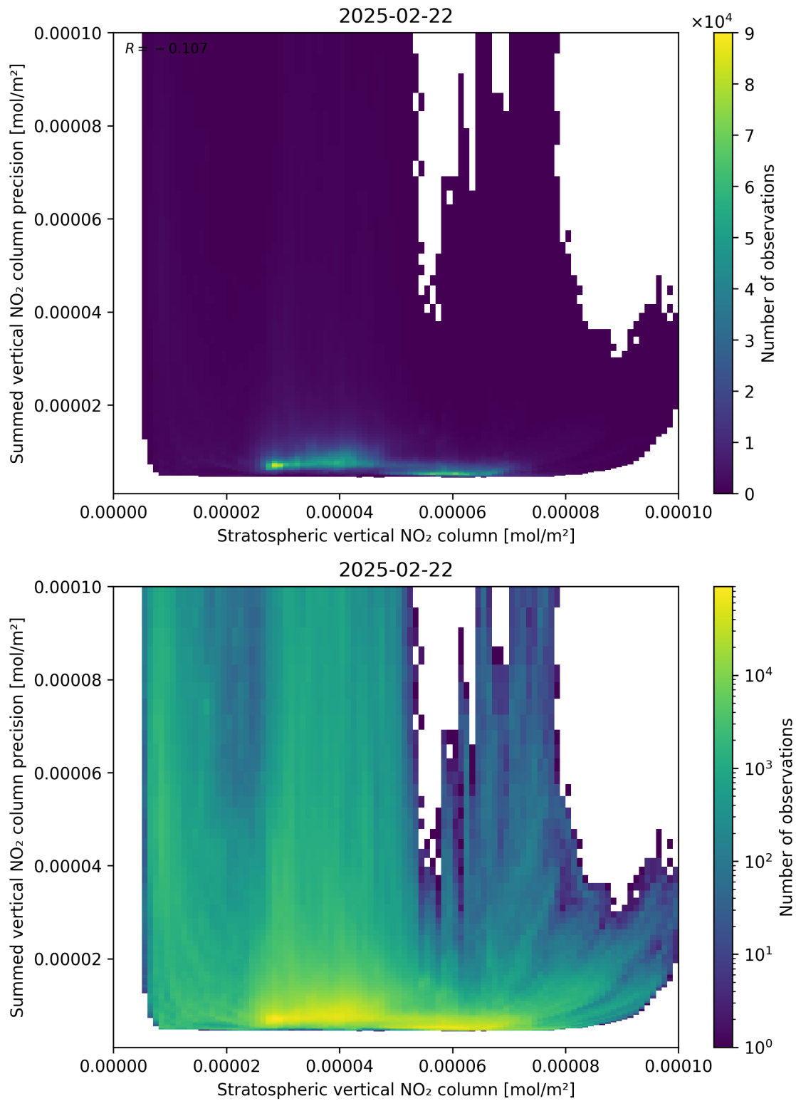
Figure 99: Scatter density plot of “Stratospheric vertical NO 2 column” against “Summed vertical NO 2 column precision” for 2025-02-21 to 2025-02-23.
