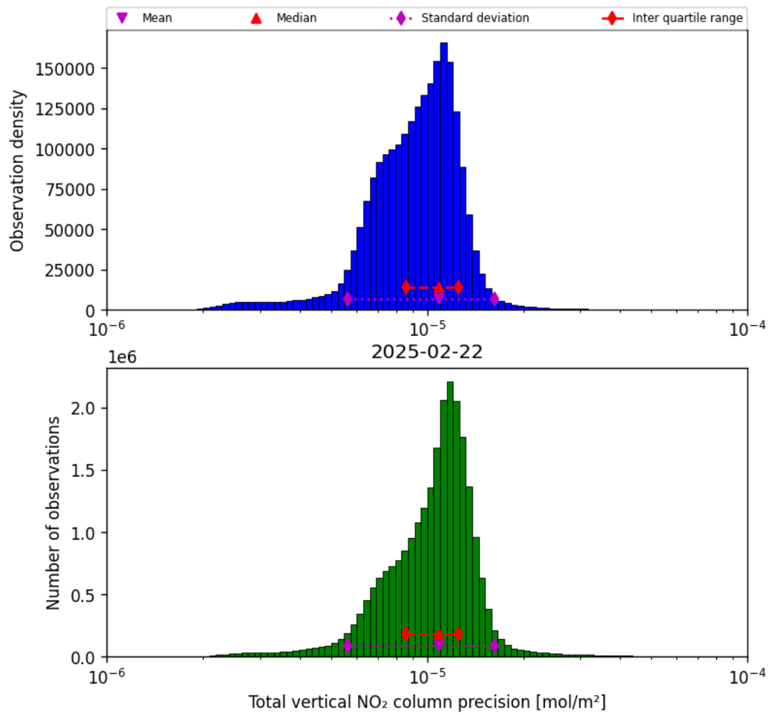
Figure 39: Histogram of "Total vertical NO 2 column precision" for 2025-02-21 to 2025-02-23
