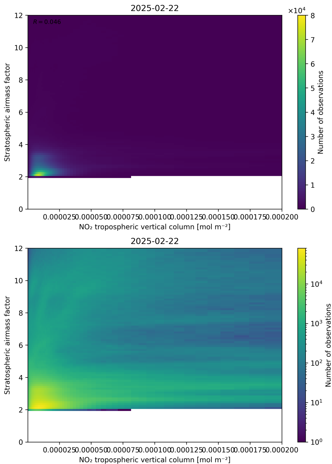
Figure 121: Scatter density plot of “NO 2 tropospheric vertical column” against “Stratospheric airmass factor” for 2025-02-21 to 2025-02-23.
