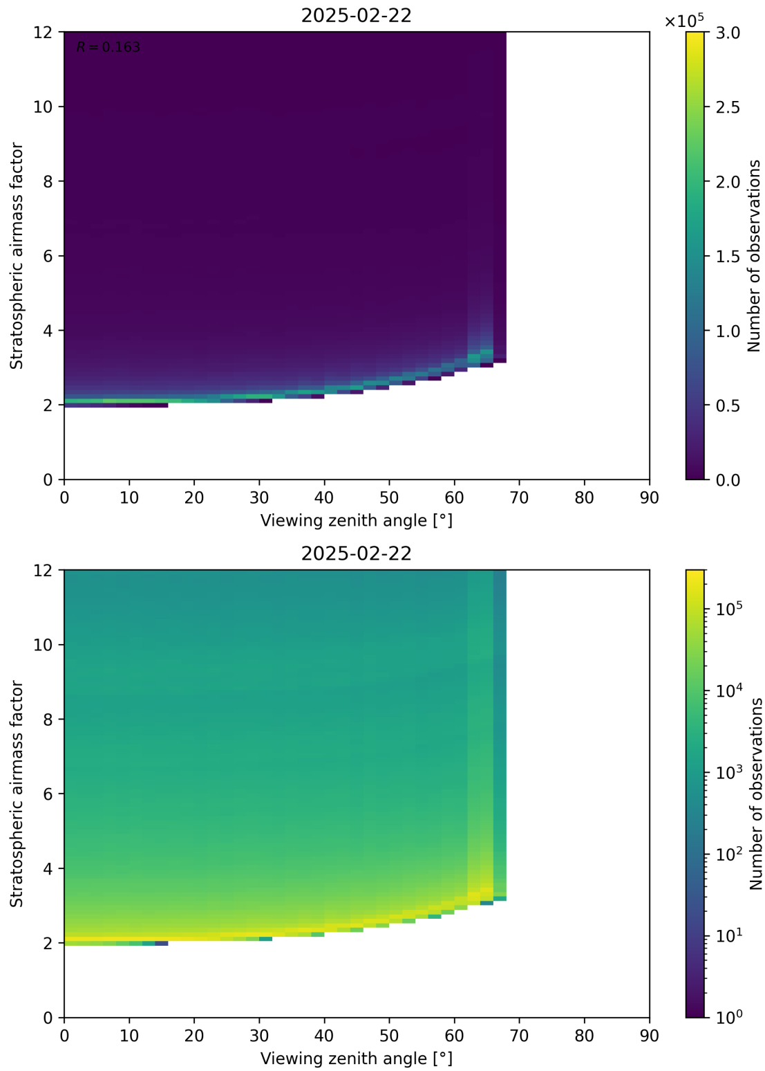
Figure 159: Scatter density plot of “Viewing zenith angle” against “Stratospheric airmass factor” for 2025-02-21 to 2025-02-23.
