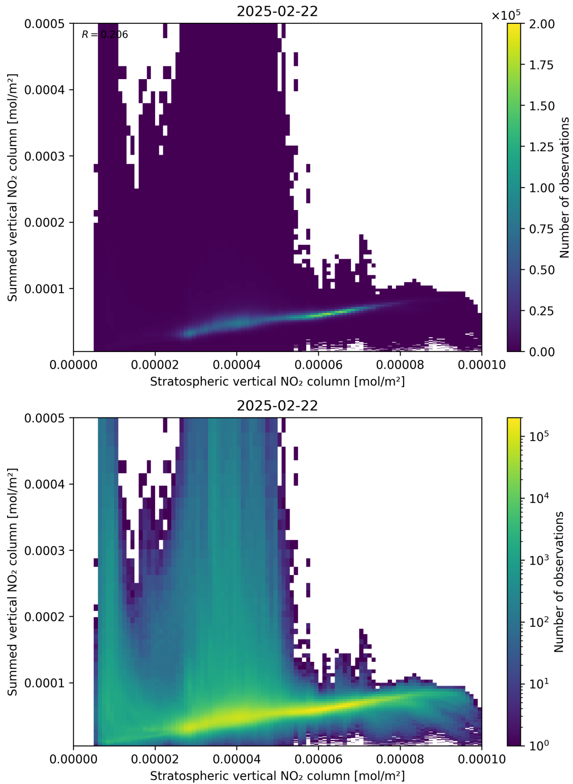
Figure 98: Scatter density plot of “Stratospheric vertical NO 2 column” against “Summed vertical NO 2 column” for 2025-02-21 to 2025-02-23.
