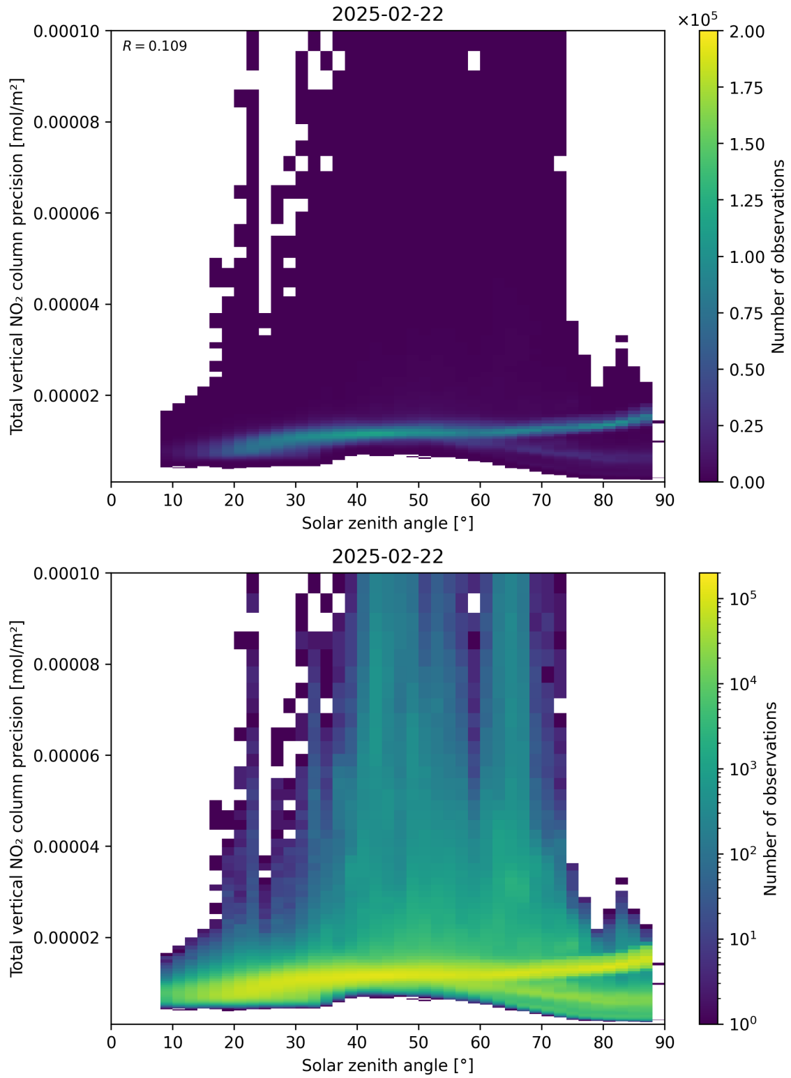
Figure 154: Scatter density plot of “Solar zenith angle” against “Total vertical NO 2 column precision” for 2025-02-21 to 2025-02-23.
