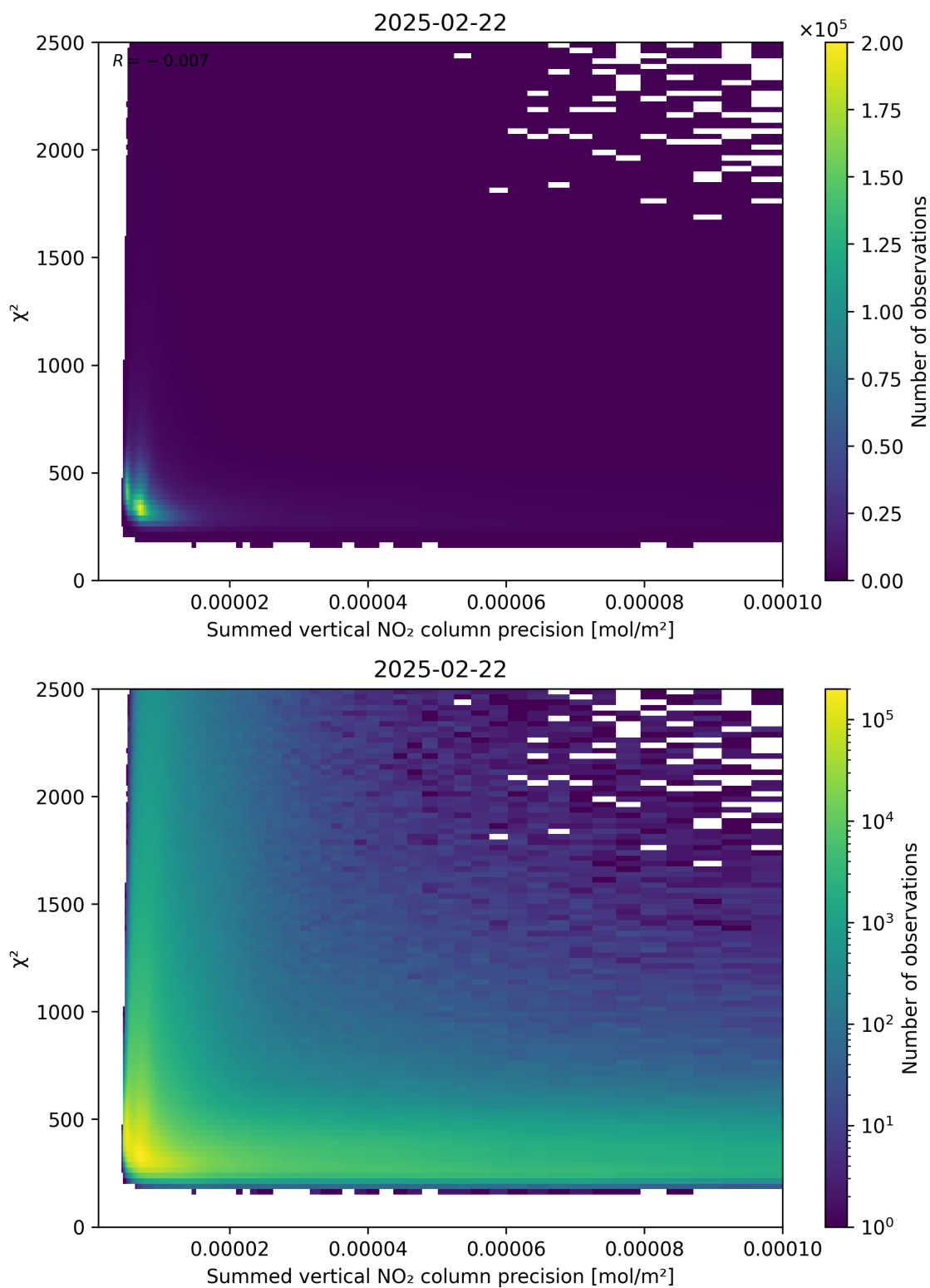
Figure 107: Scatter density plot of “Summed vertical NO 2 column precision” against “ \chi^2 ” for 2025-02-21 to 2025-02-23.
