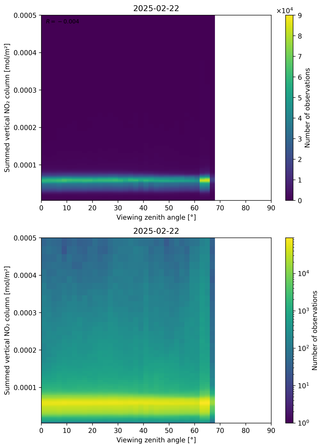
Figure 165: Scatter density plot of “Viewing zenith angle” against “Summed vertical NO 2 column” for 2025-02-21 to 2025-02-23.
