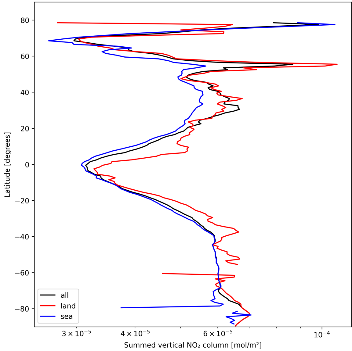
Figure 23: Zonal average of “Summed vertical NO 2 column” for 2025-02-21 to 2025-02-23.
