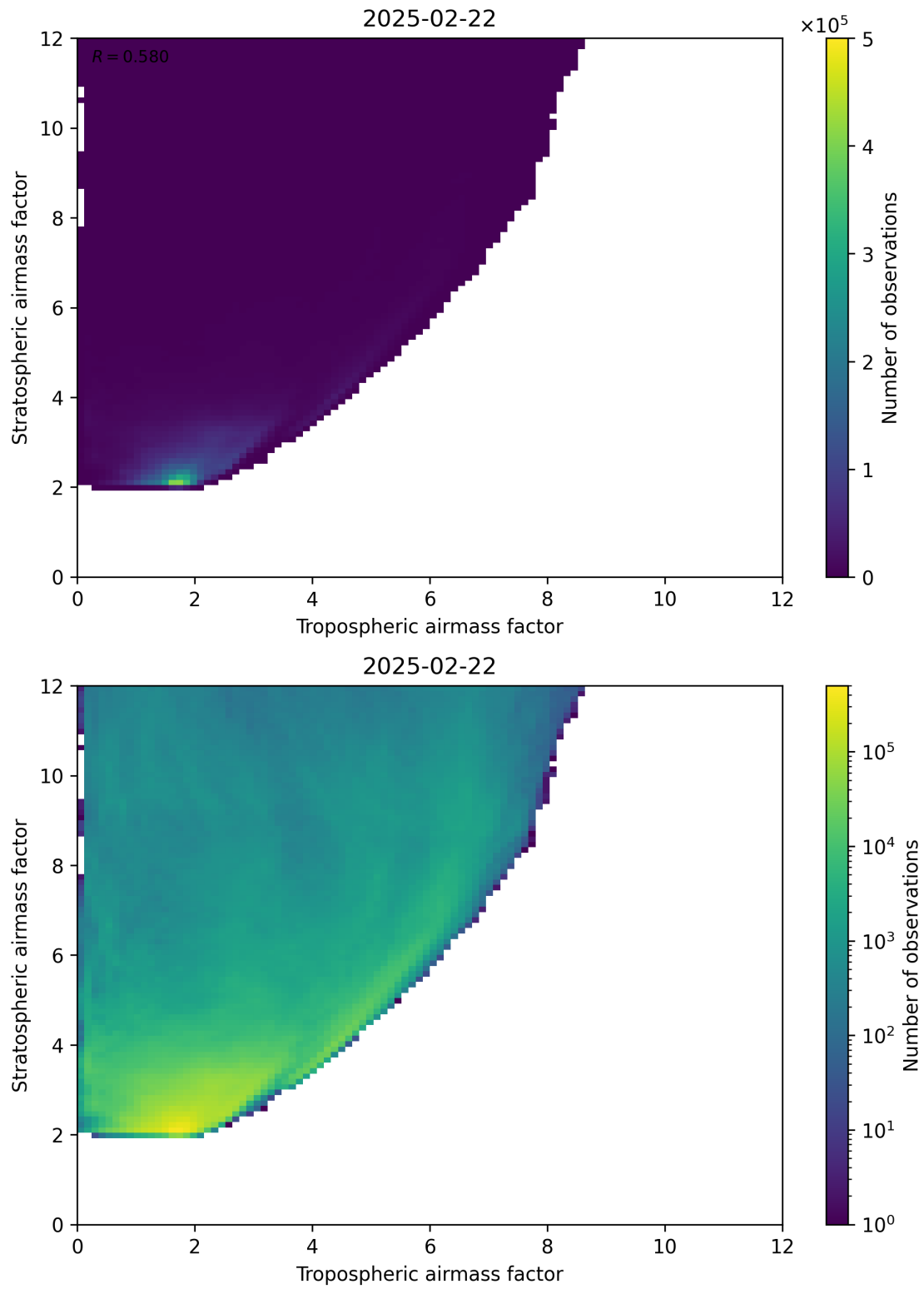
Figure 71: Scatter density plot of “Tropospheric airmass factor” against “Stratospheric airmass factor” for 2025-02-21 to 2025-02-23.
