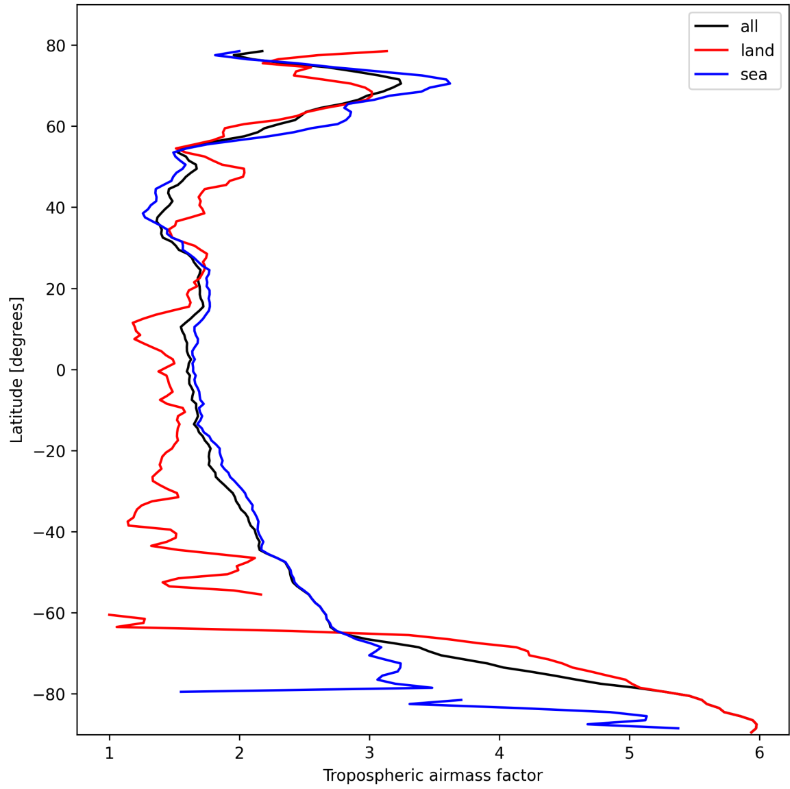
Figure 14: Zonal average of “Tropospheric airmass factor” for 2025-02-21 to 2025-02-23.
