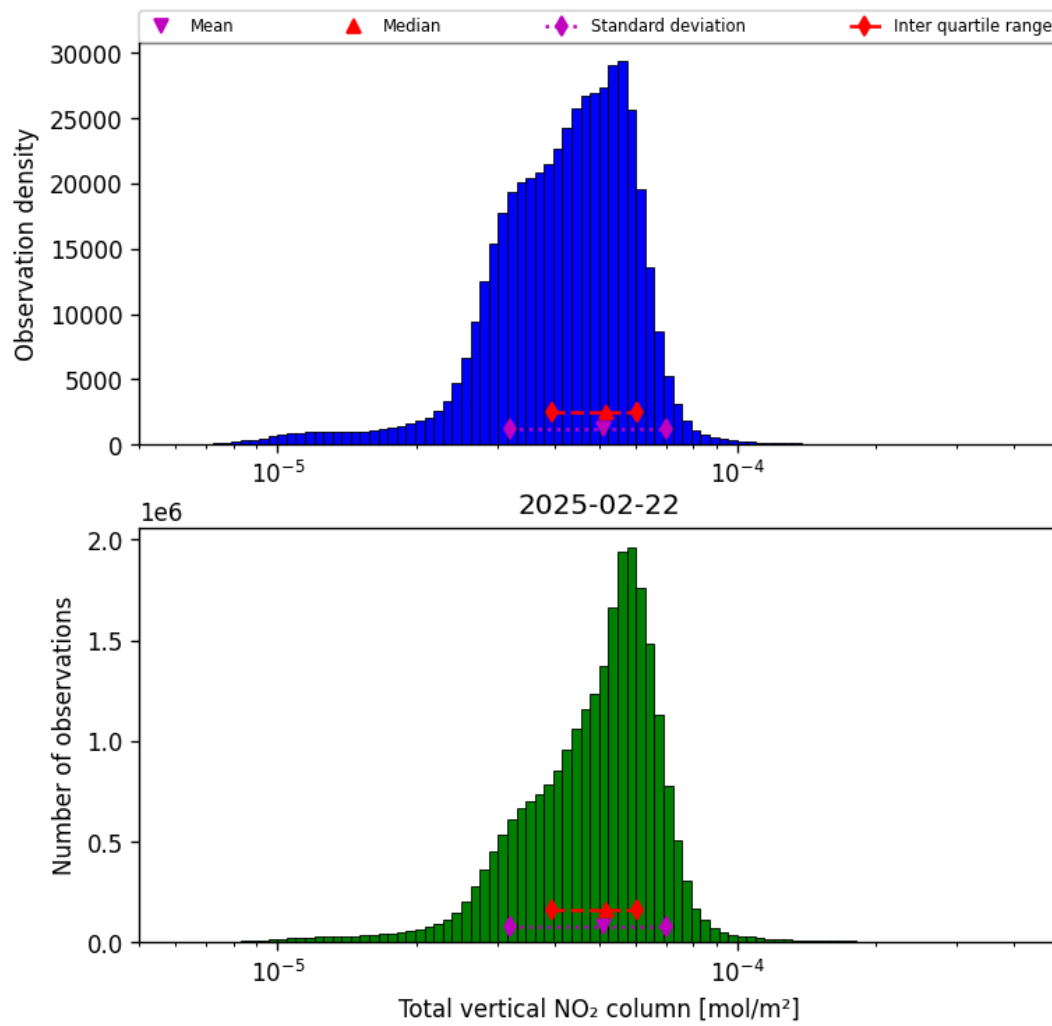
Figure 38: Histogram of “Total vertical NO 2 column” for 2025-02-21 to 2025-02-23
