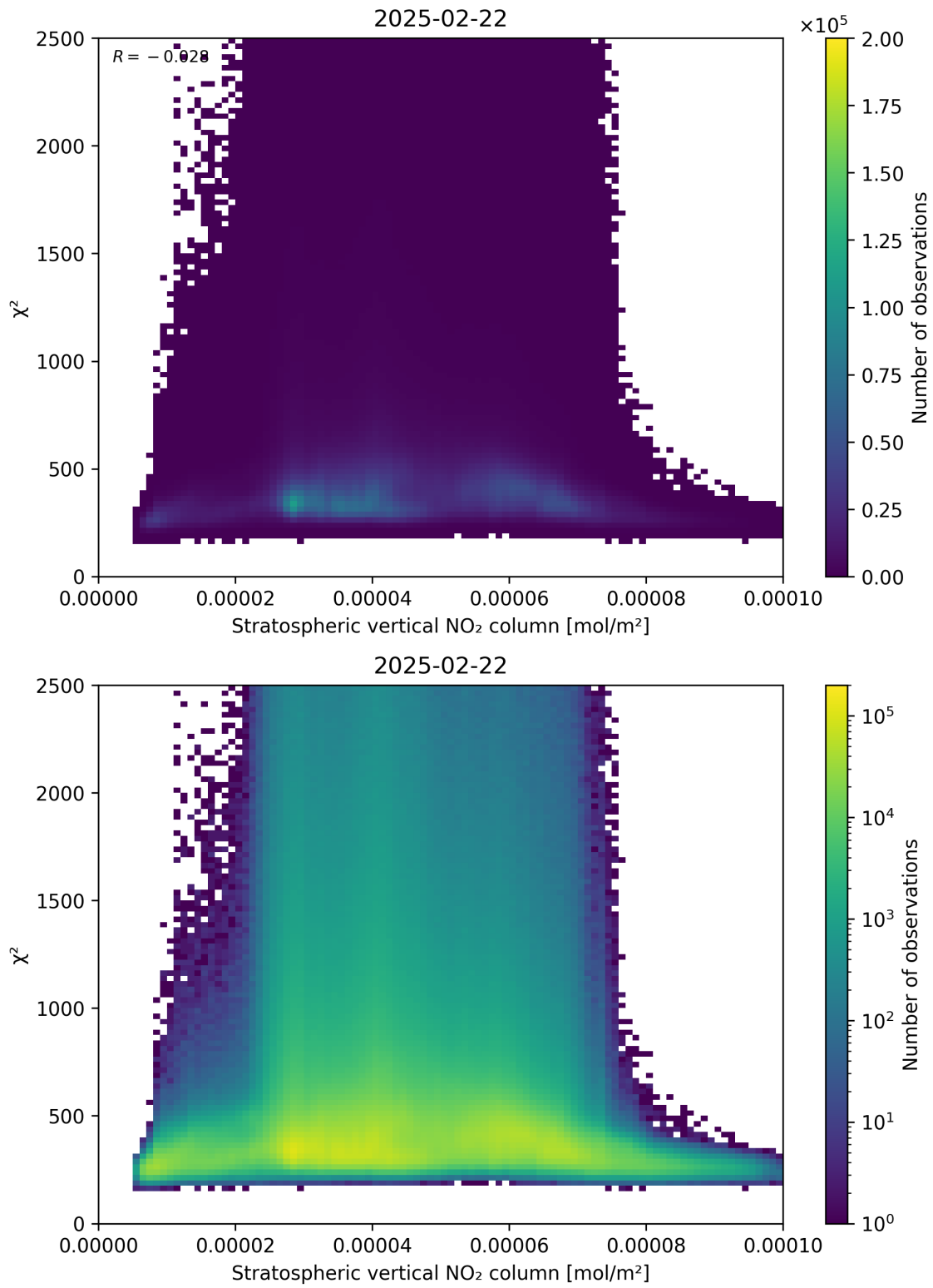
Figure 97: Scatter density plot of “Stratospheric vertical NO 2 column” against “ \chi^2 ” for 2025-02-21 to 2025-02-23.
