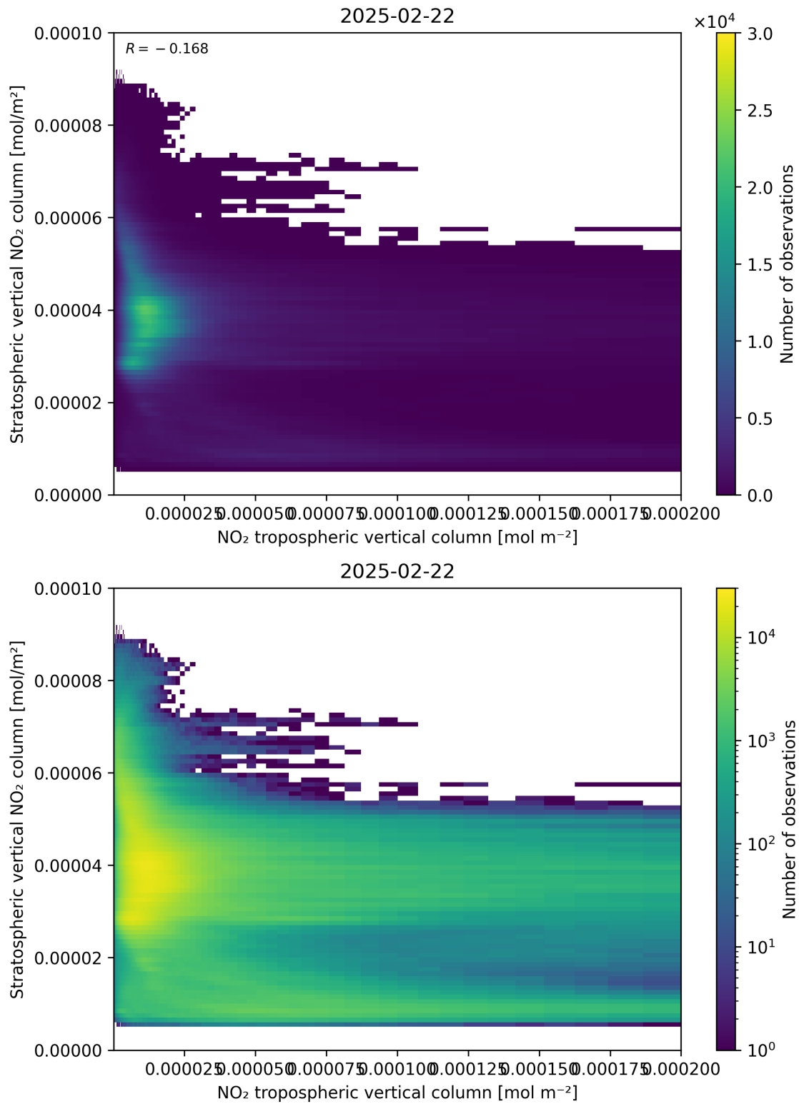
Figure 125: Scatter density plot of “NO 2 tropospheric vertical column” against “Stratospheric vertical NO 2 column” for 2025-02-21 to 2025-02-23.
