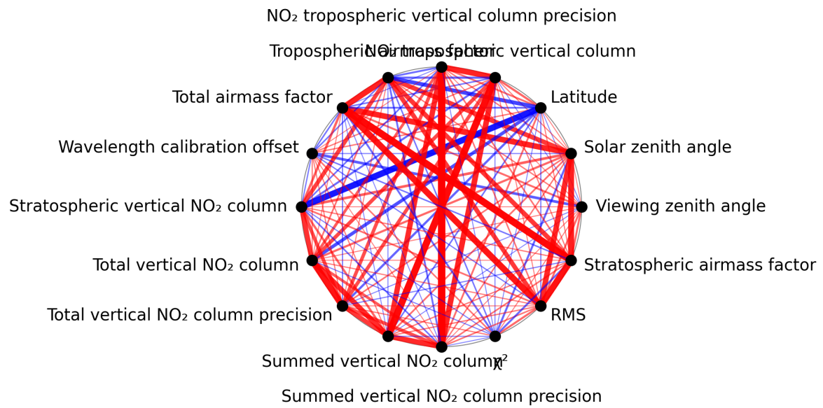
Figure 1: Map of correlation graph for 2025-02-21 to 2025-02-23.
