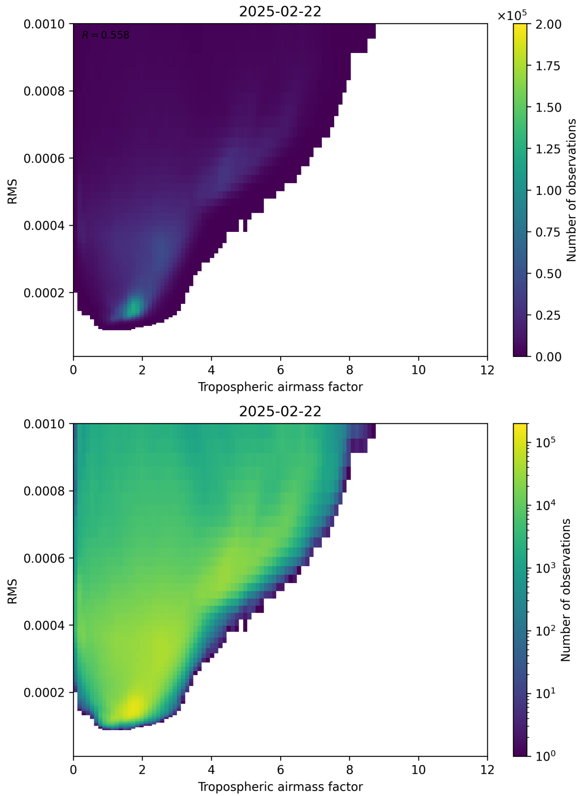
Figure 79: Scatter density plot of “Tropospheric airmass factor” against “RMS” for 2025-02-21 to 2025-02-23.
