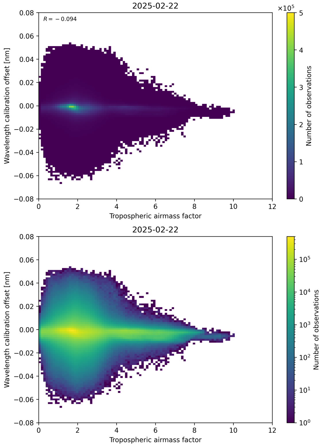
Figure 80: Scatter density plot of “Tropospheric airmass factor” against “Wavelength calibration offset” for 2025-02-21 to 2025-02-23.
