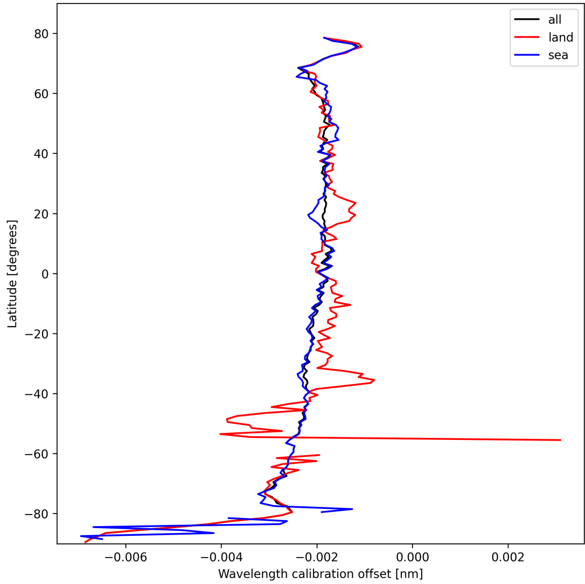
Figure 18: Zonal average of “Wavelength calibration offset” for 2025-02-21 to 2025-02-23.
