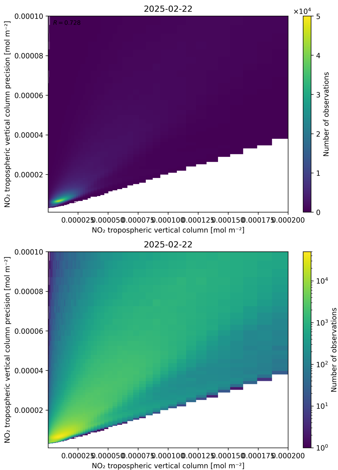
Figure 130: Scatter density plot of “NO 2 tropospheric vertical column” against “NO 2 tropospheric vertical column precision” for 2025-02-21 to 2025-02-23.
