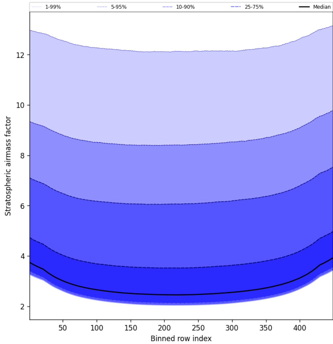
Figure 61: Along track statistics of “Stratospheric airmass factor” for 2025-02-21 to 2025-02-23
