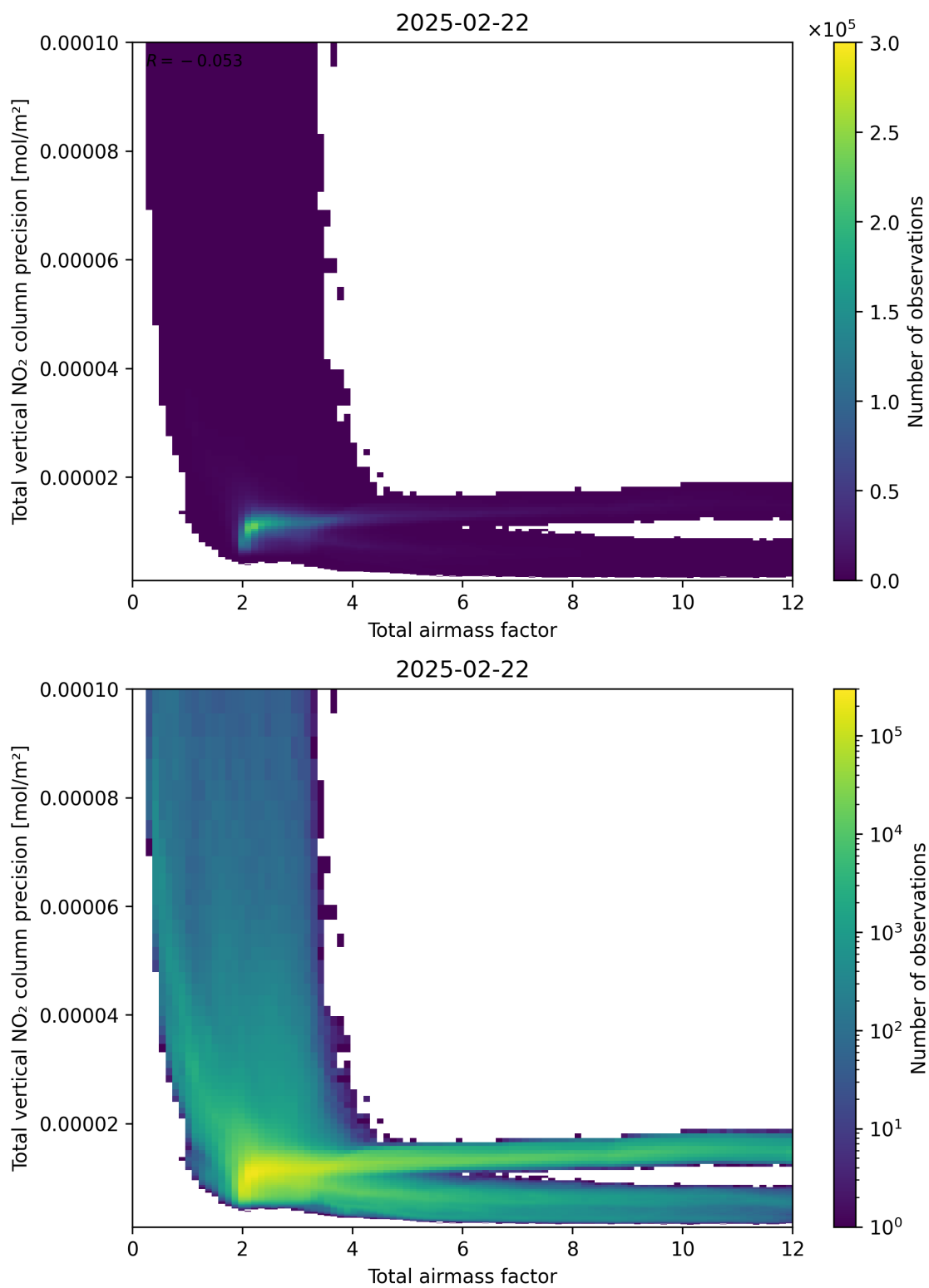
Figure 68: Scatter density plot of “Total airmass factor” against “Total vertical NO 2 column precision” for 2025-02-21 to 2025-02-23.
