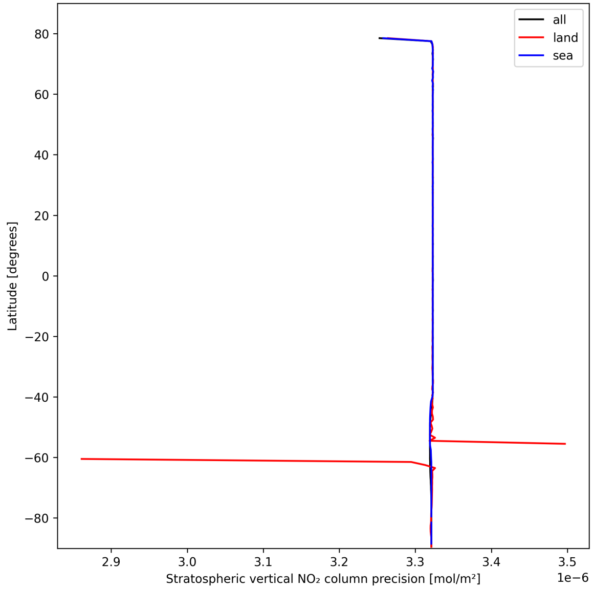
Figure 20: Zonal average of “Stratospheric vertical NO 2 column precision” for 2025-02-21 to 2025-02-23.
