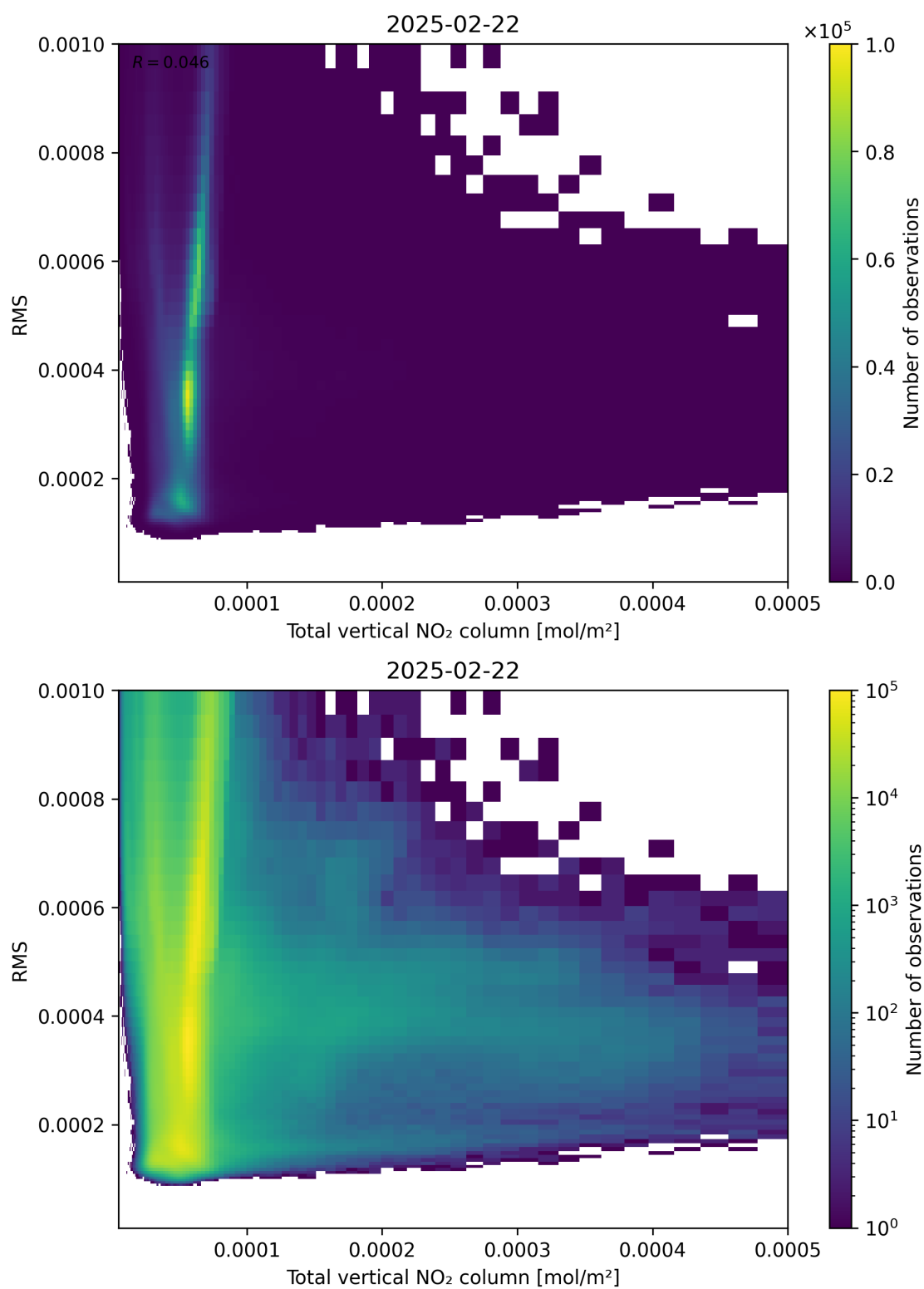
Figure 120: Scatter density plot of “Total vertical NO 2 column” against “RMS” for 2025-02-21 to 2025-02-23.
