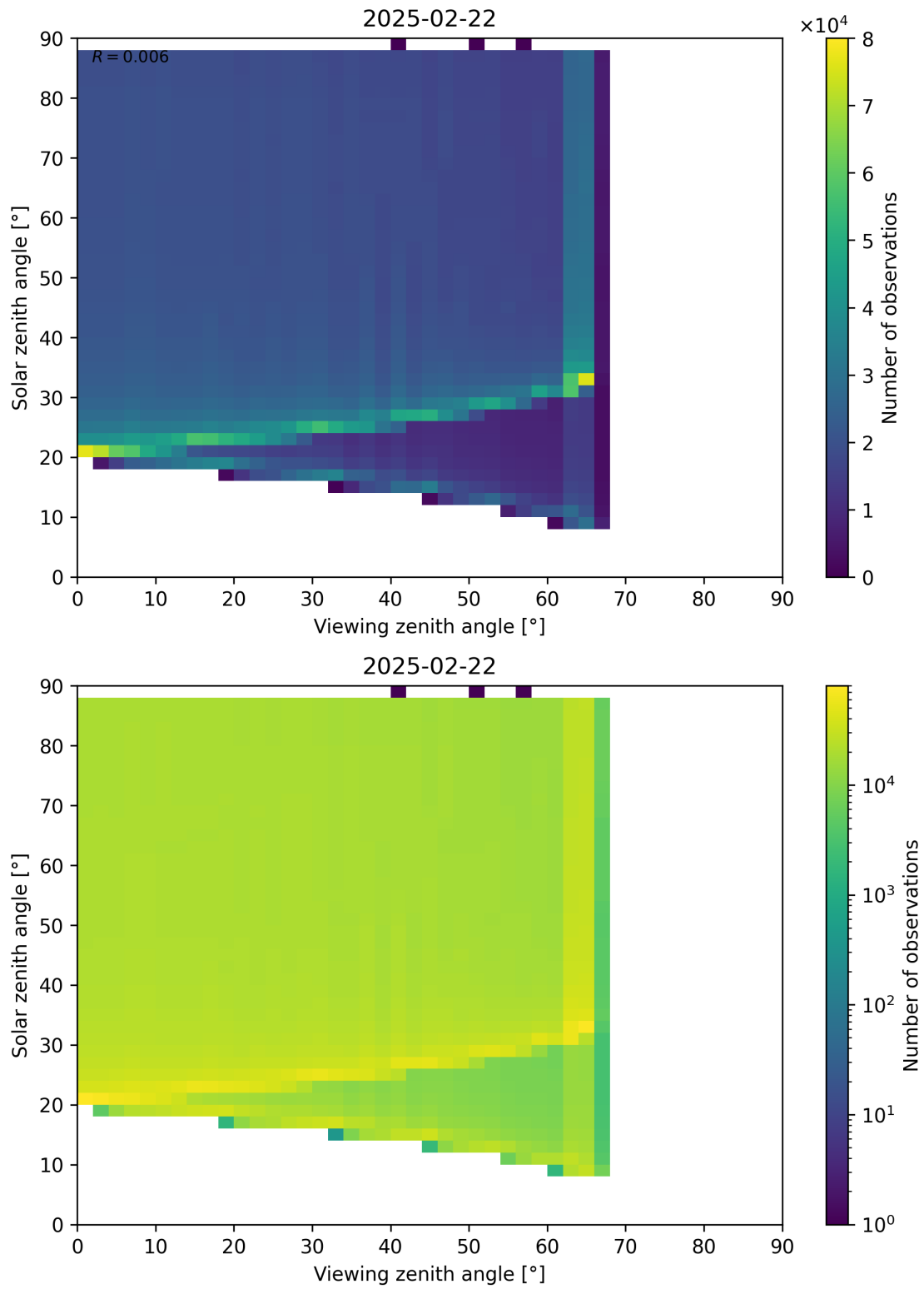
Figure 172: Scatter density plot of “Viewing zenith angle” against “Solar zenith angle” for 2025-02-21 to 2025-02-23.
