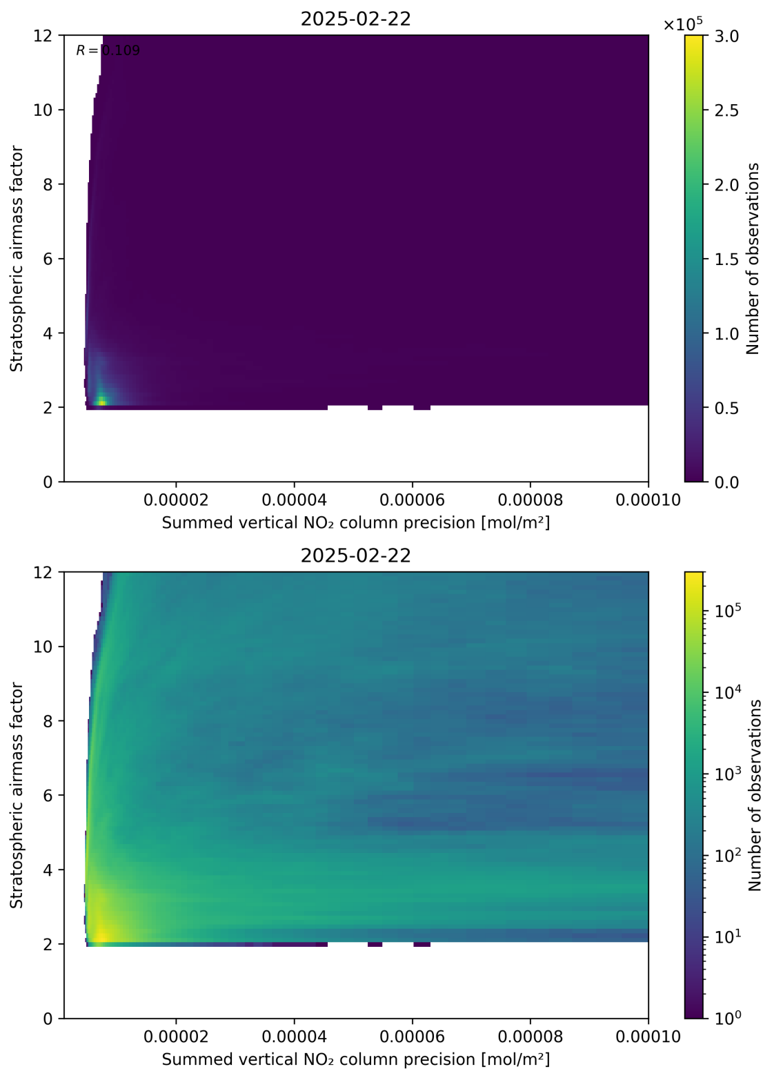
Figure 106: Scatter density plot of “Summed vertical NO 2 column precision” against “Stratospheric airmass factor” for 2025-02-21 to 2025-02-23.
