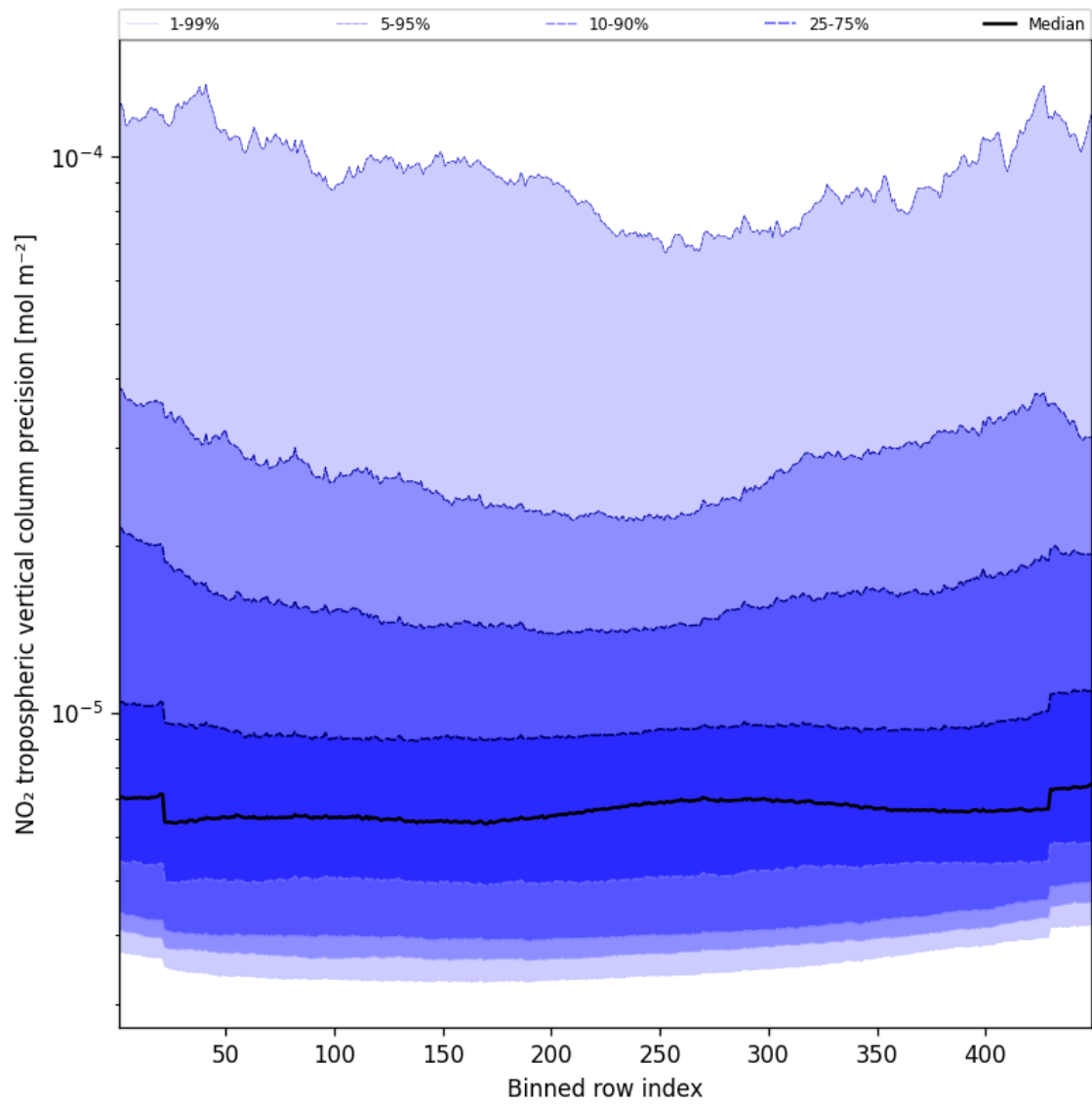
Figure 47: Along track statistics of “NO 2 tropospheric vertical column precision” for 2025-02-21 to 2025-02-23
