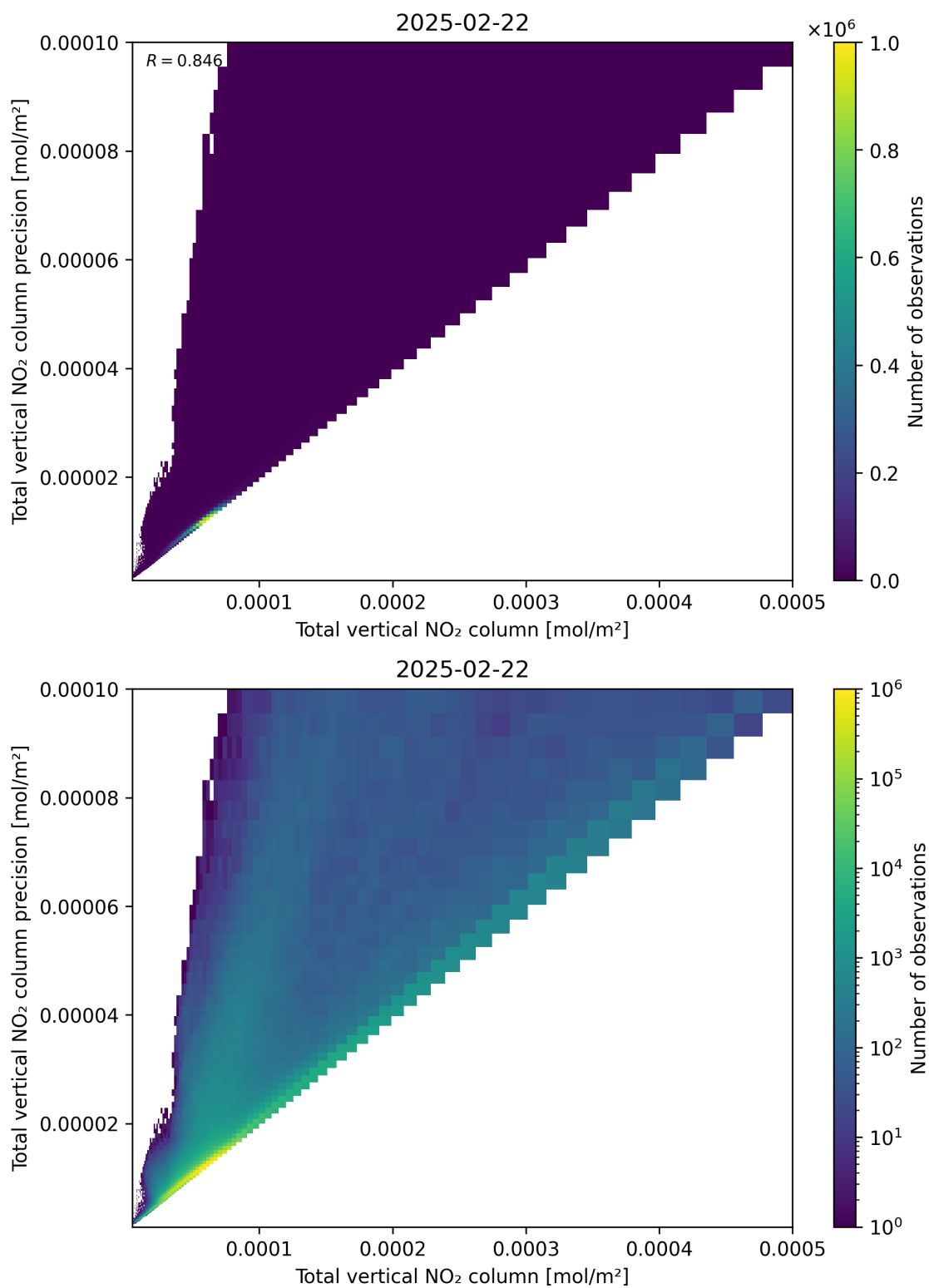
Figure 114: Scatter density plot of “Total vertical NO 2 column” against “Total vertical NO 2 column precision” for 2025-02-21 to 2025-02-23.
