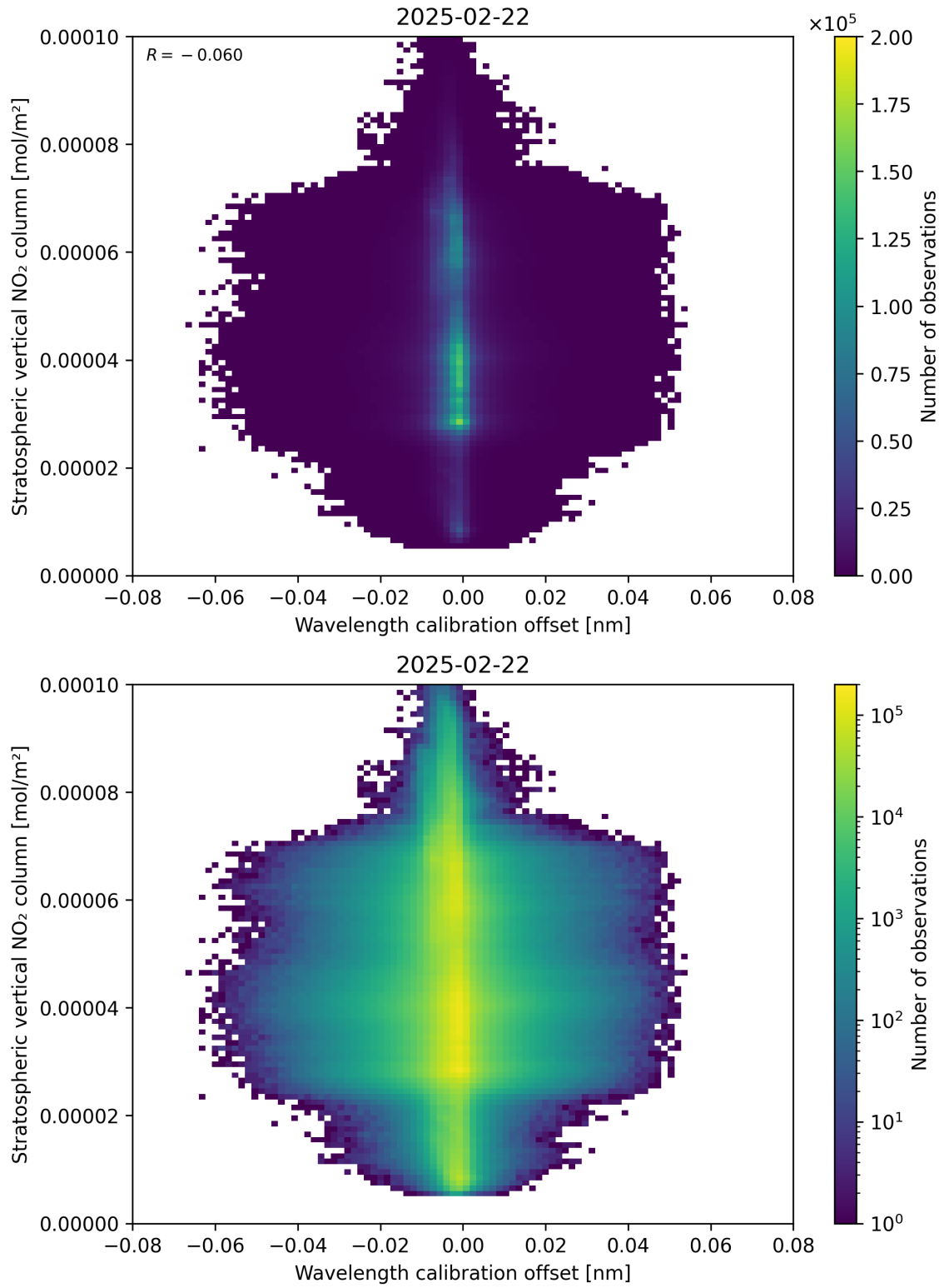
Figure 176: Scatter density plot of “Wavelength calibration offset” against “Stratospheric vertical NO 2 column” for 2025-02-21 to 2025-02-23.
