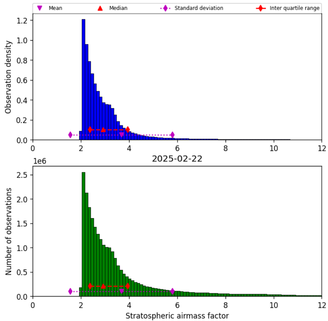
Figure 44: Histogram of “Stratospheric airmass factor” for 2025-02-21 to 2025-02-23
