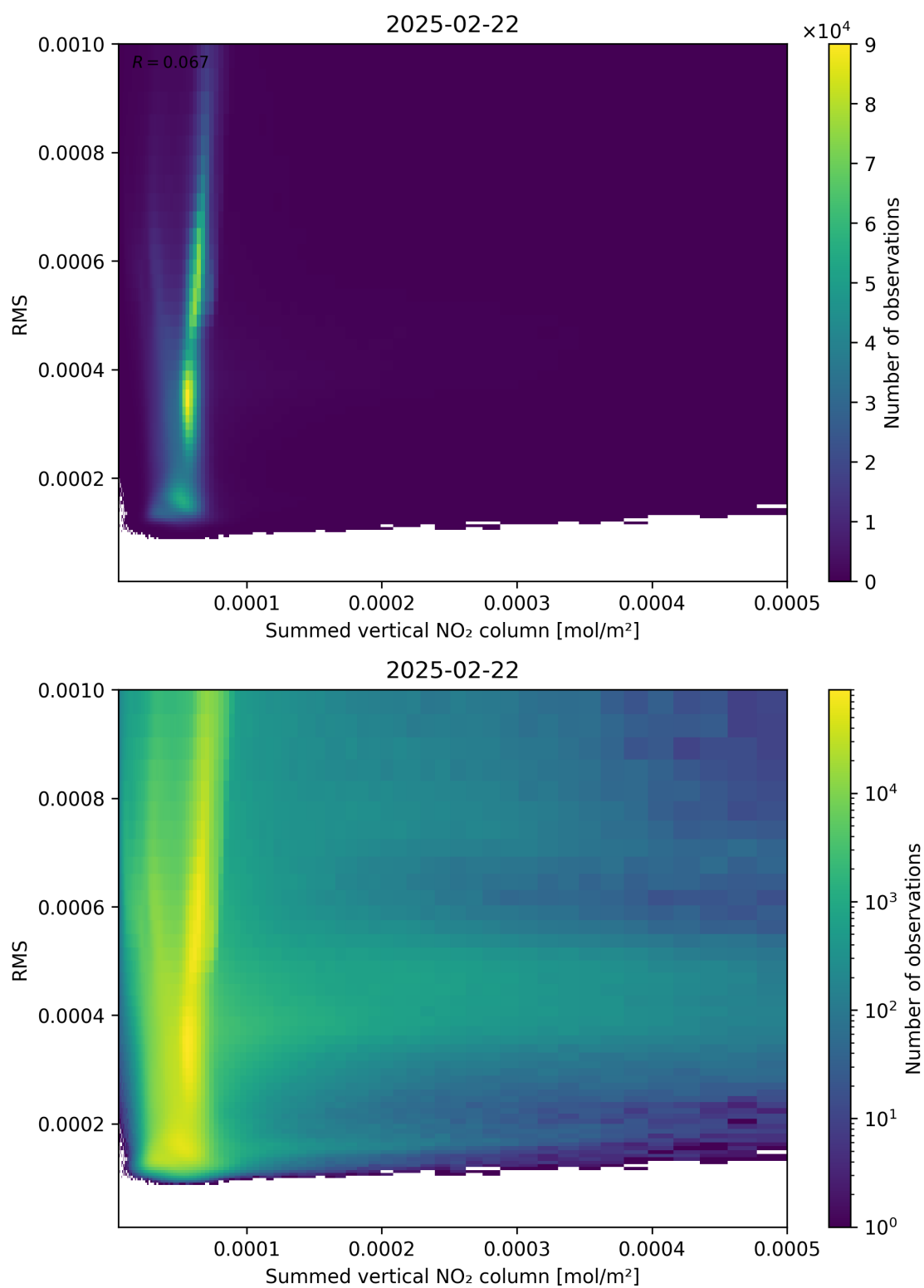
Figure 109: Scatter density plot of “Summed vertical NO 2 column” against “RMS” for 2025-02-21 to 2025-02-23.
