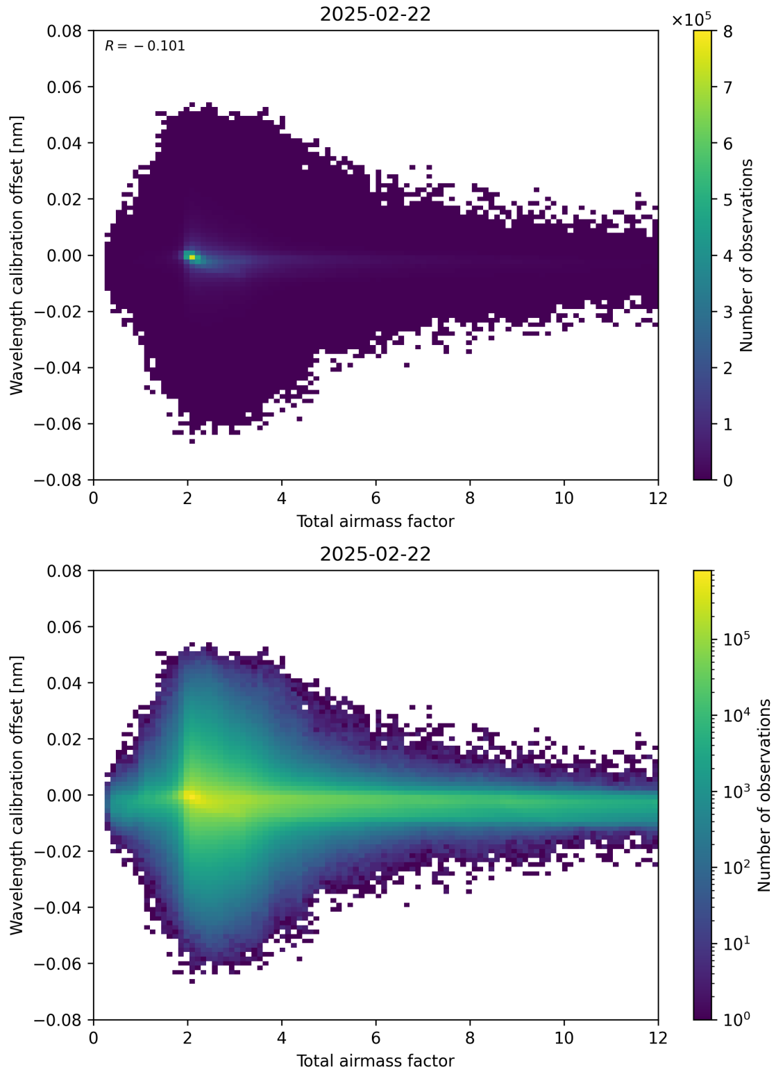
Figure 70: Scatter density plot of “Total airmass factor” against “Wavelength calibration offset” for 2025-02-21 to 2025-02-23.
