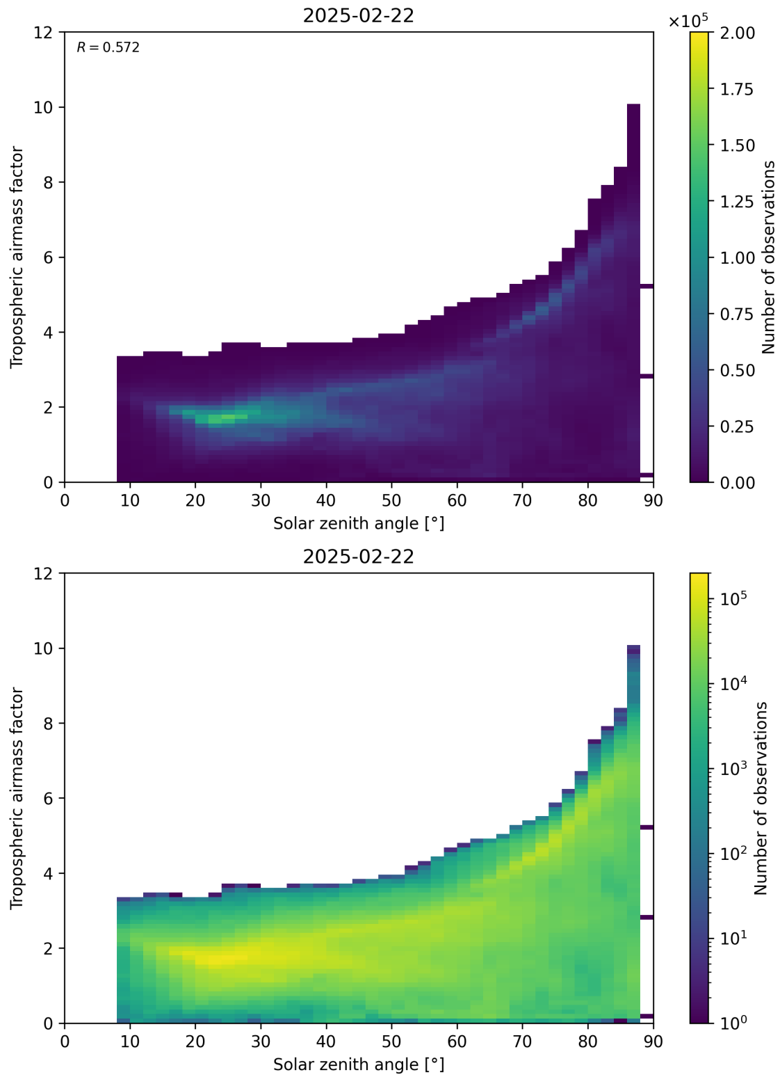
Figure 147: Scatter density plot of “Solar zenith angle” against “Tropospheric airmass factor” for 2025-02-21 to 2025-02-23.
