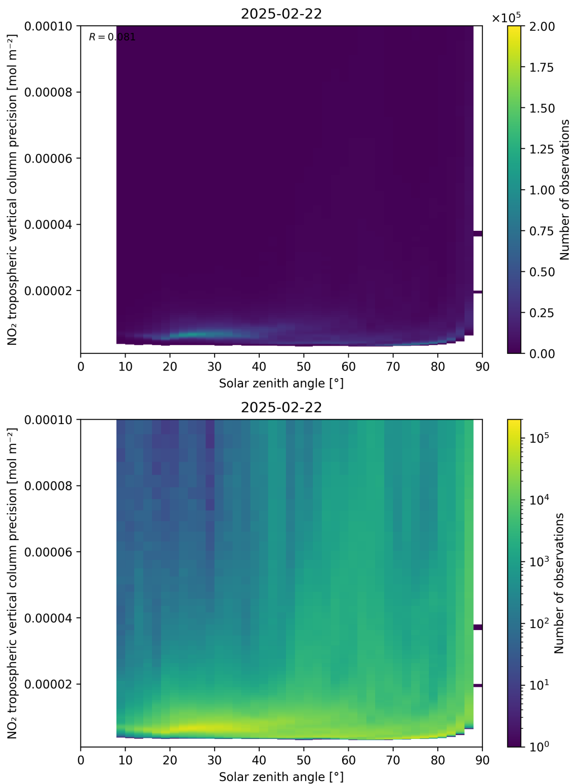
Figure 156: Scatter density plot of “Solar zenith angle” against “NO 2 tropospheric vertical column precision” for 2025-02-21 to 2025-02-23.
