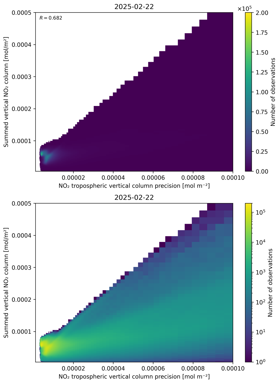
Figure 136: Scatter density plot of “NO 2 tropospheric vertical column precision” against “Summed vertical NO 2 column” for 2025-02-21 to 2025-02-23.
