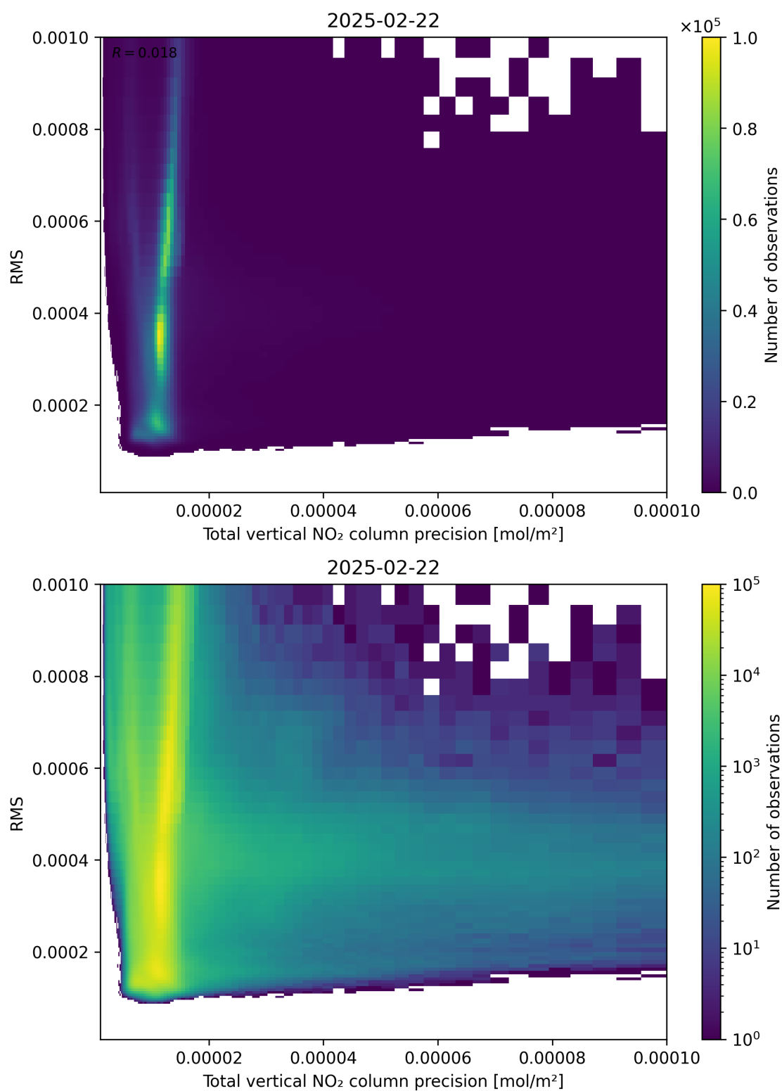
Figure 119: Scatter density plot of “Total vertical NO 2 column precision” against “RMS” for 2025-02-21 to 2025-02-23.
