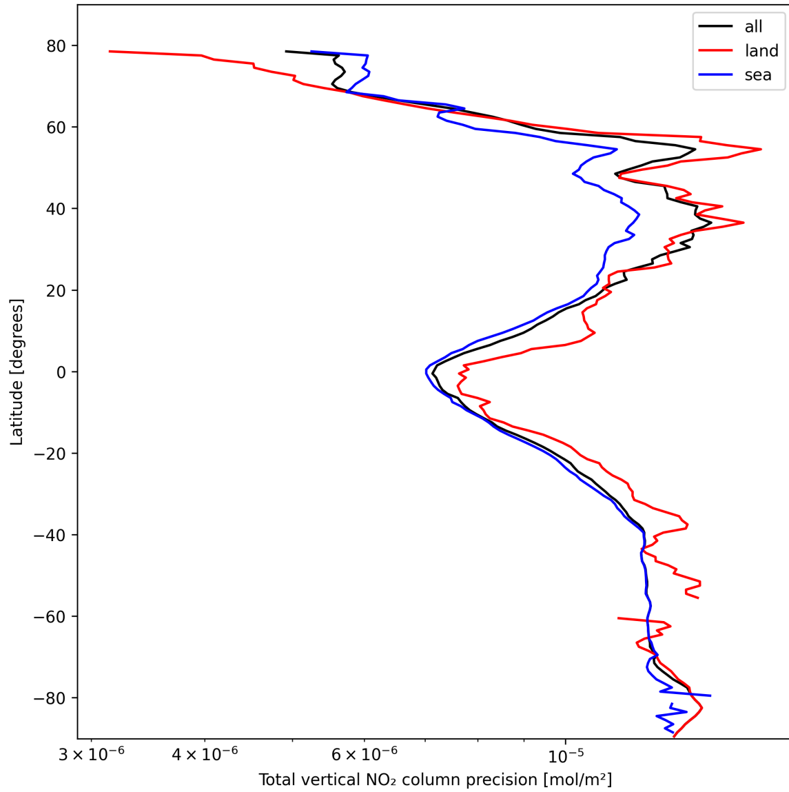
Figure 22: Zonal average of “Total vertical NO 2 column precision” for 2025-02-21 to 2025-02-23.
