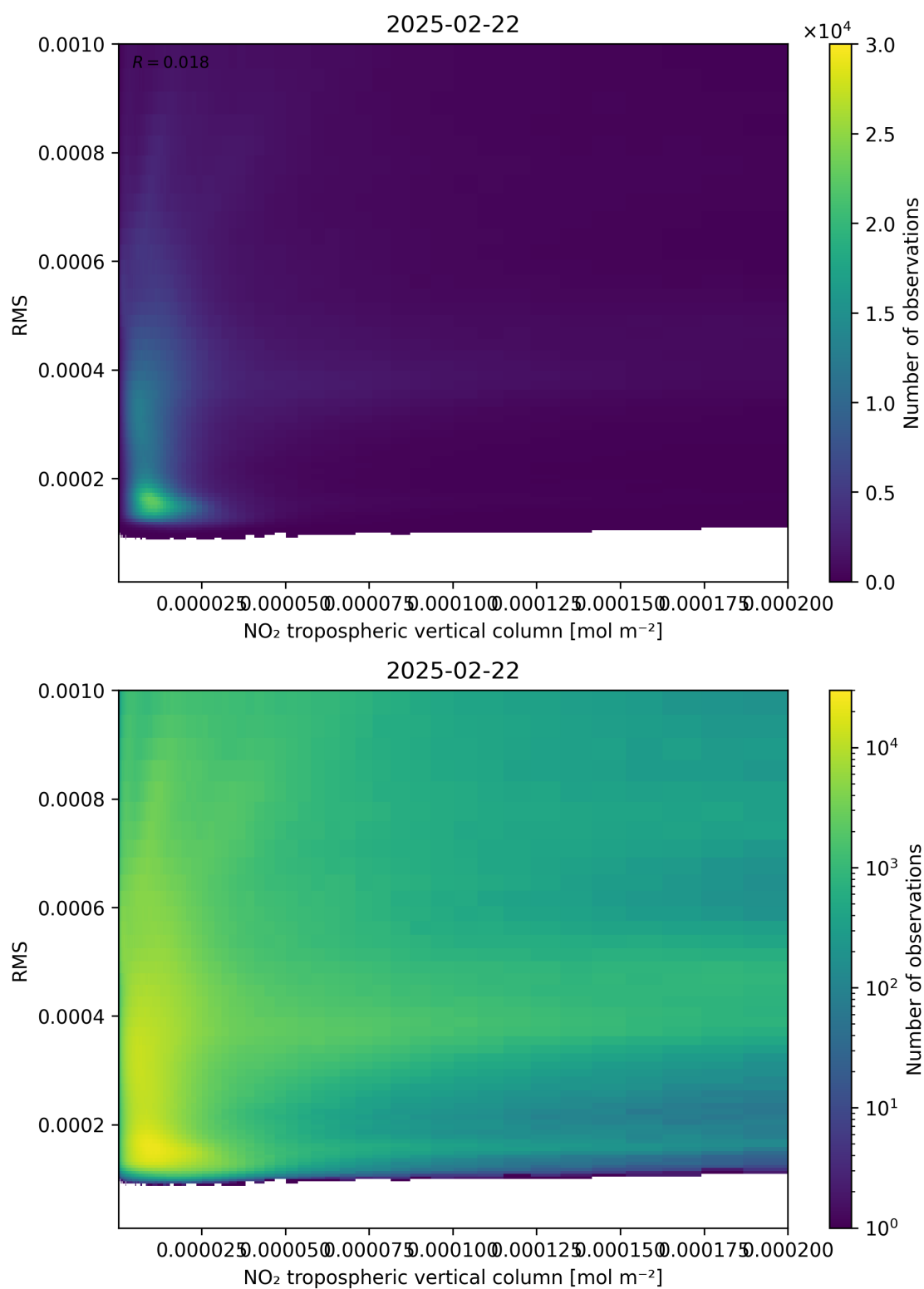
Figure 142: Scatter density plot of “NO 2 tropospheric vertical column” against “RMS” for 2025-02-21 to 2025-02-23.
