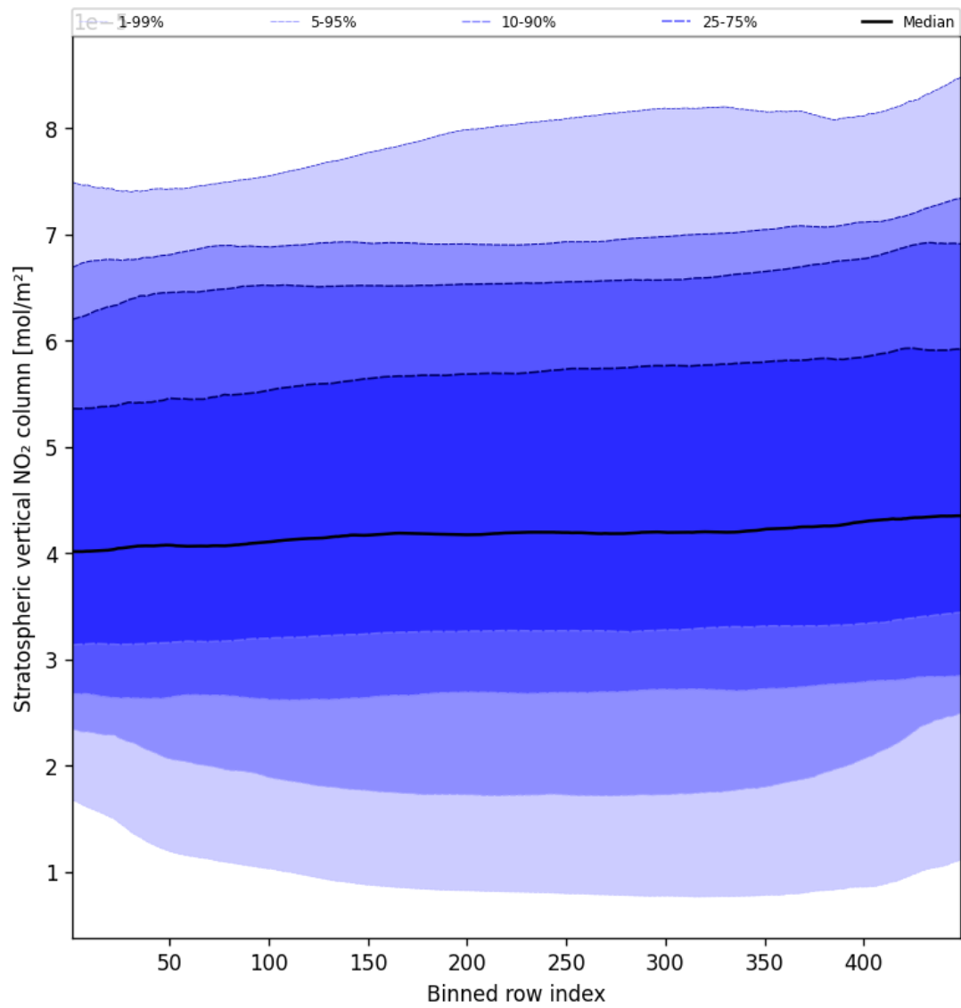
Figure 53: Along track statistics of “Stratospheric vertical NO 2 column” for 2025-02-21 to 2025-02-23
