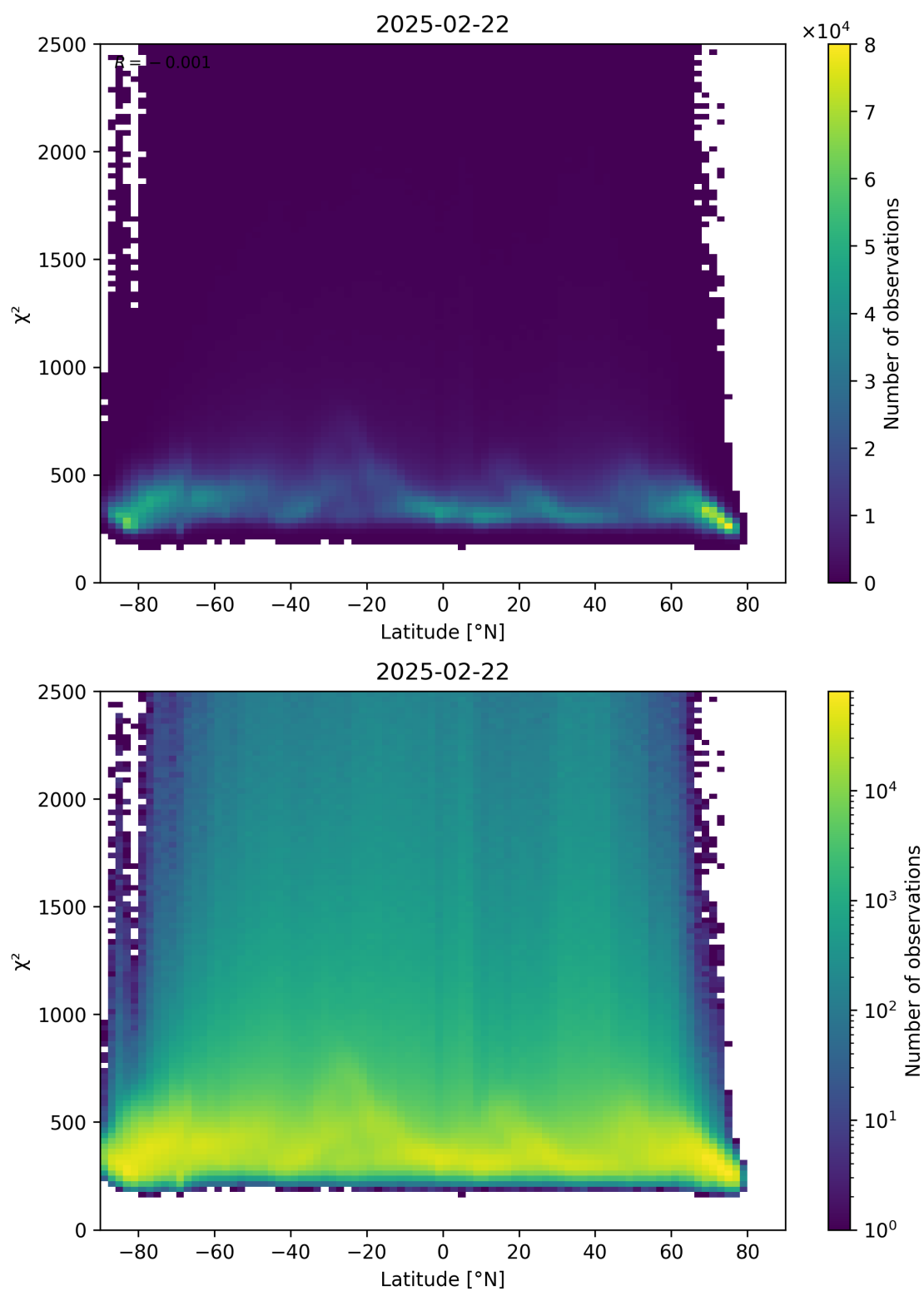
Figure 86: Scatter density plot of “Latitude” against “ \chi^2 ” for 2025-02-21 to 2025-02-23.
