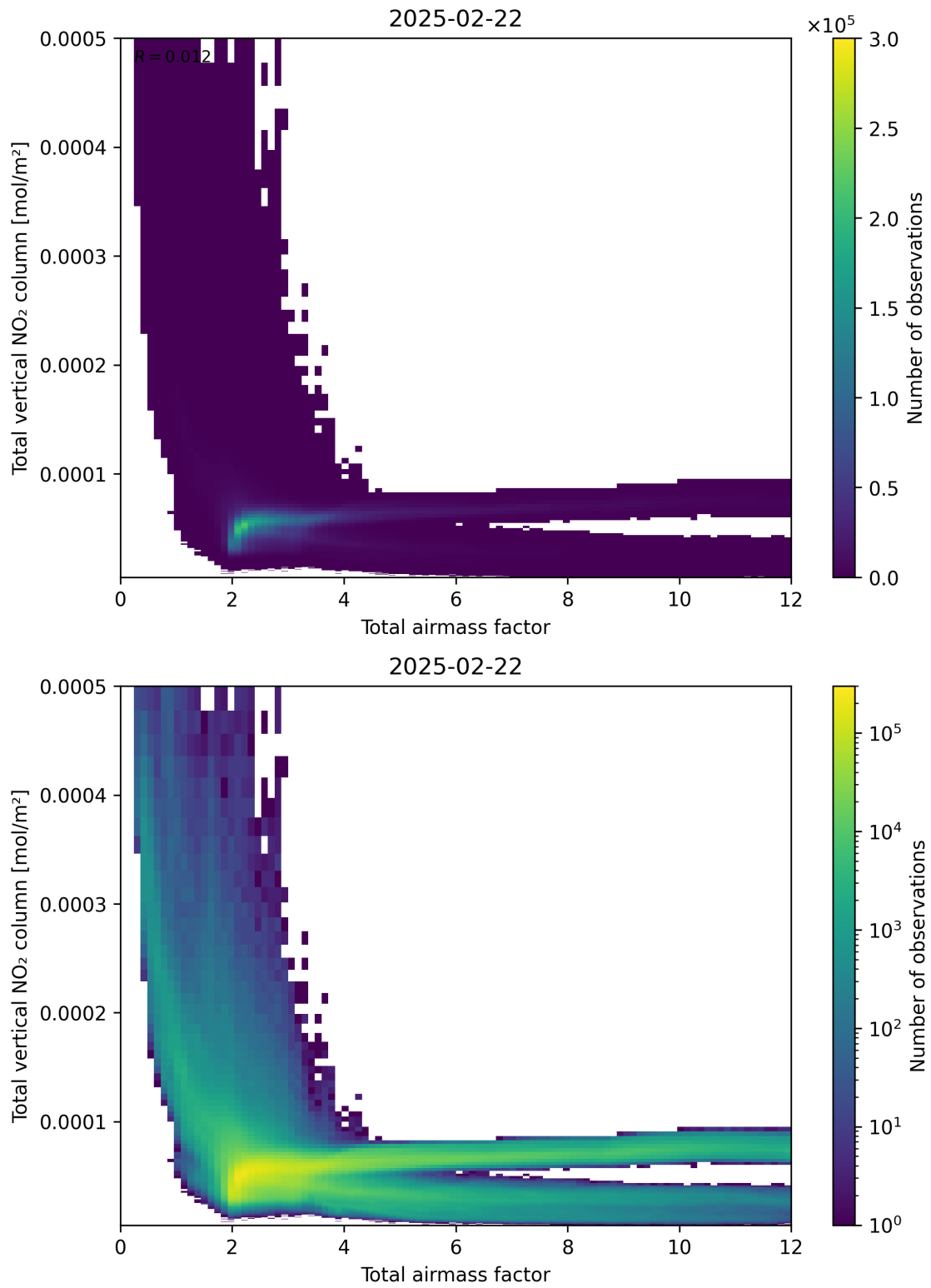
Figure 67: Scatter density plot of “Total air mass factor” against “Total vertical NO 2 column” for 2025-02-21 to 2025-02-23.
