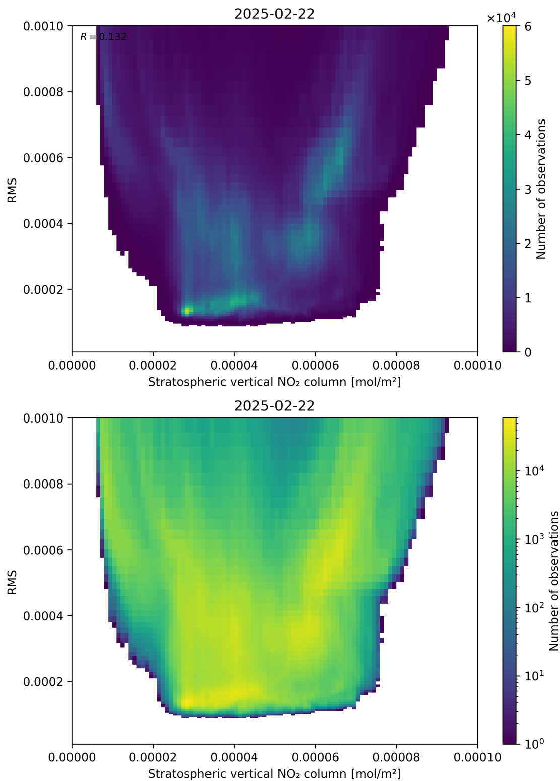
Figure 102: Scatter density plot of “Stratospheric vertical NO 2 column” against “RMS” for 2025-02-21 to 2025-02-23.
