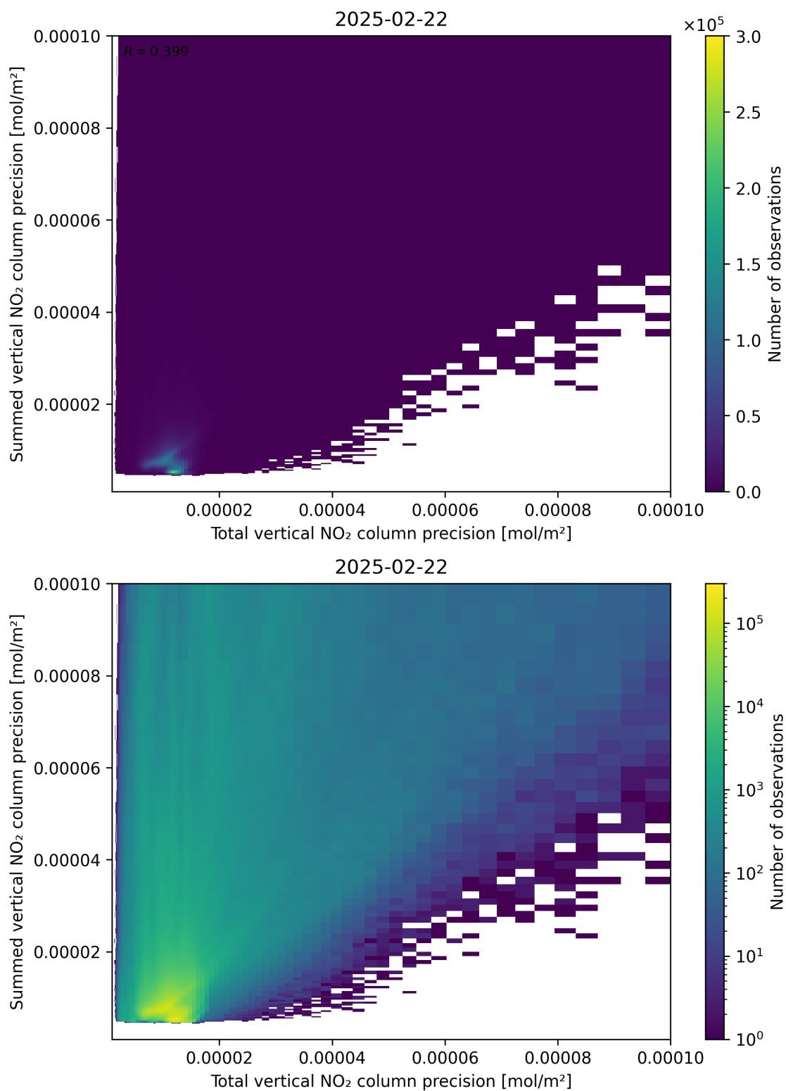
Figure 118: Scatter density plot of “Total vertical NO 2 column precision” against “Summed vertical NO 2 column precision” for 2025-02-21 to 2025-02-23.
