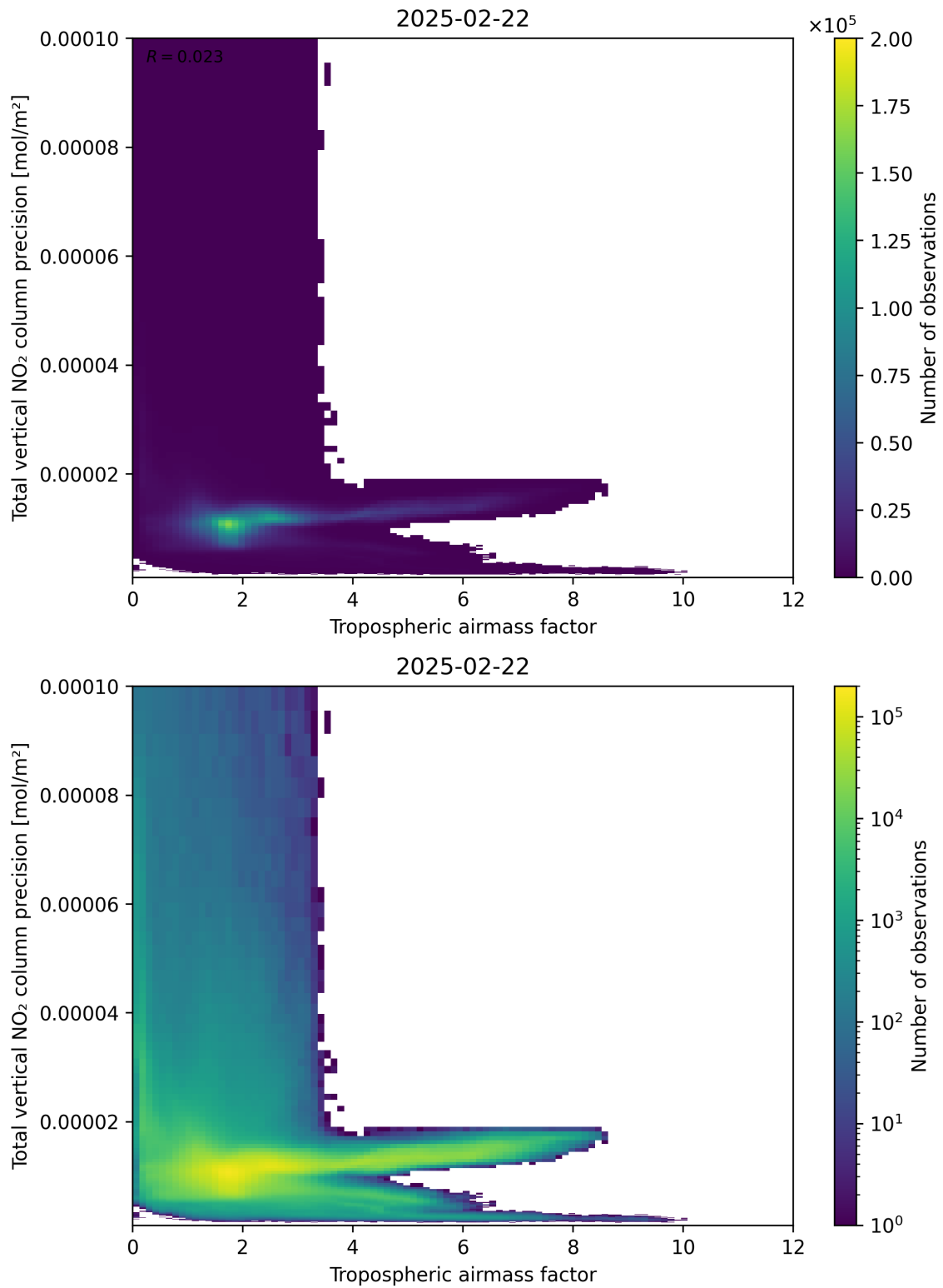
Figure 78: Scatter density plot of “Tropospheric air mass factor” against “Total vertical NO 2 column precision” for 2025-02-21 to 2025-02-23.
