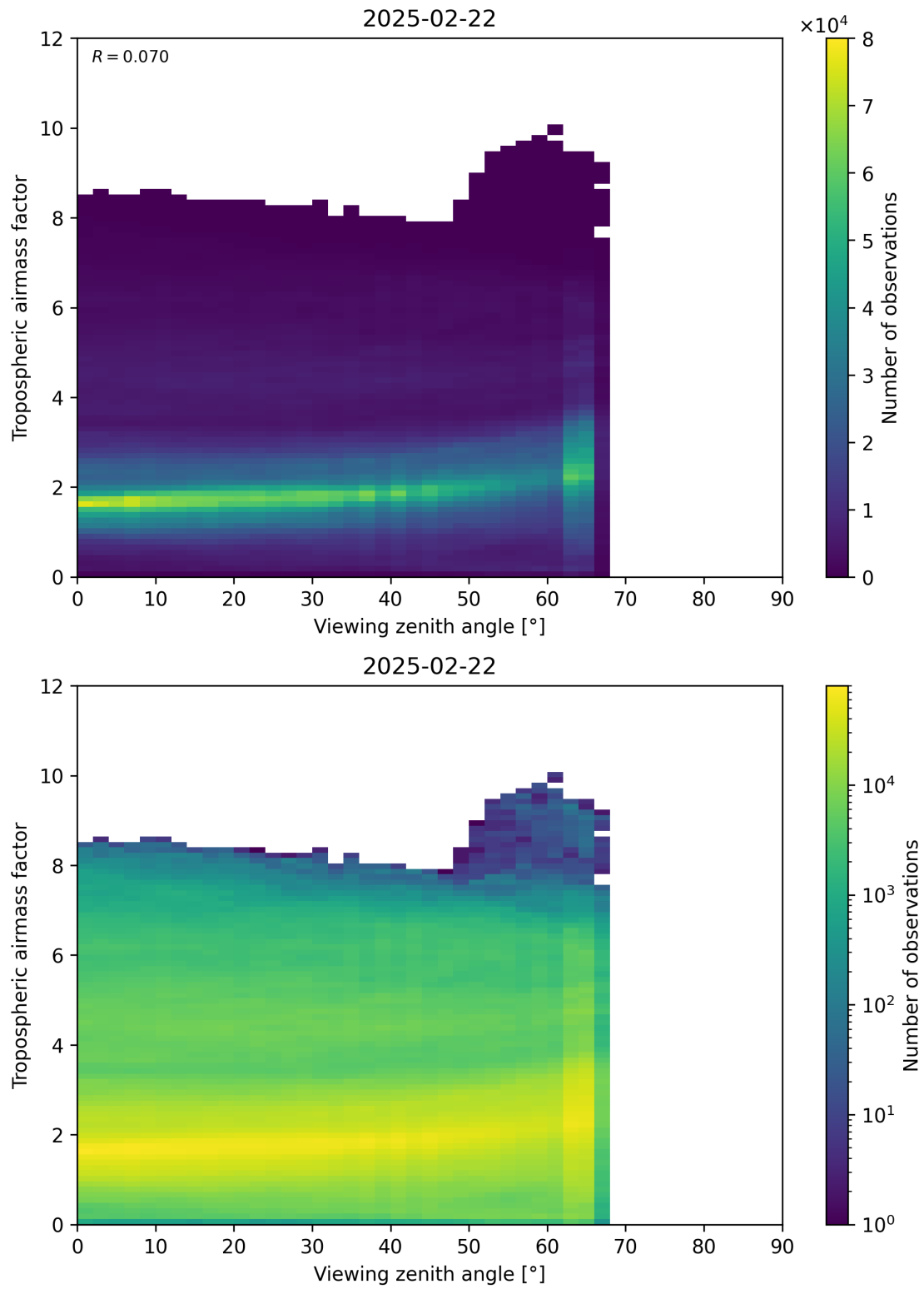
Figure 161: Scatter density plot of “Viewing zenith angle” against “Tropospheric airmass factor” for 2025-02-21 to 2025-02-23.
