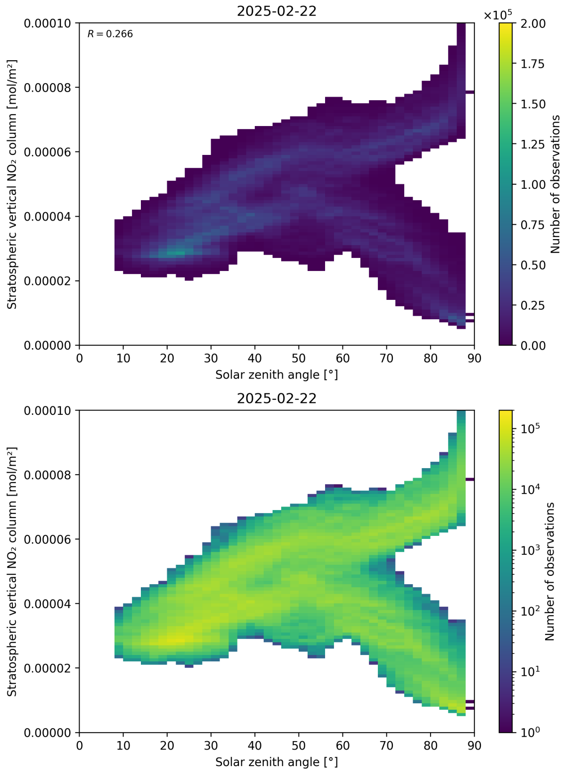
Figure 150: Scatter density plot of “Solar zenith angle” against “Stratospheric vertical NO 2 column” for 2025-02-21 to 2025-02-23.
