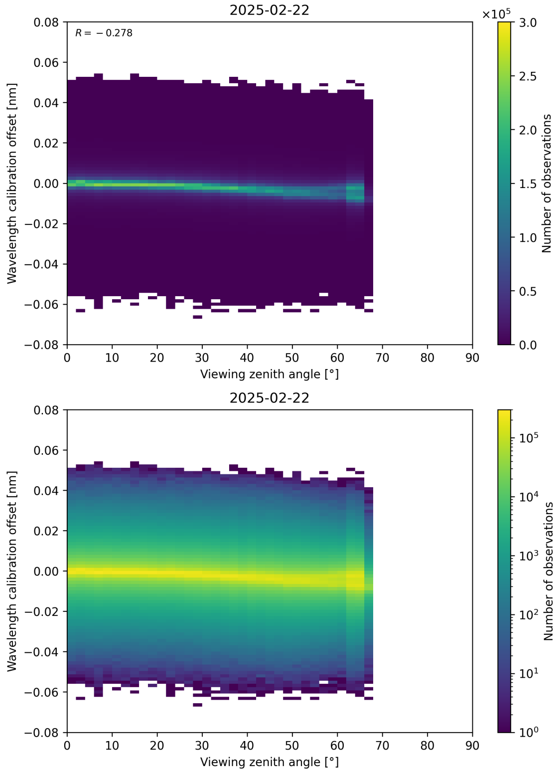
Figure 173: Scatter density plot of “Viewing zenith angle” against “Wavelength calibration offset” for 2025-02-21 to 2025-02-23.
