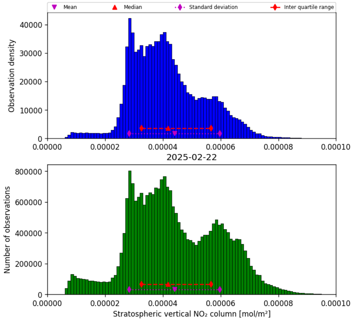
Figure 36: Histogram of “Stratospheric vertical NO 2 column” for 2025-02-21 to 2025-02-23
