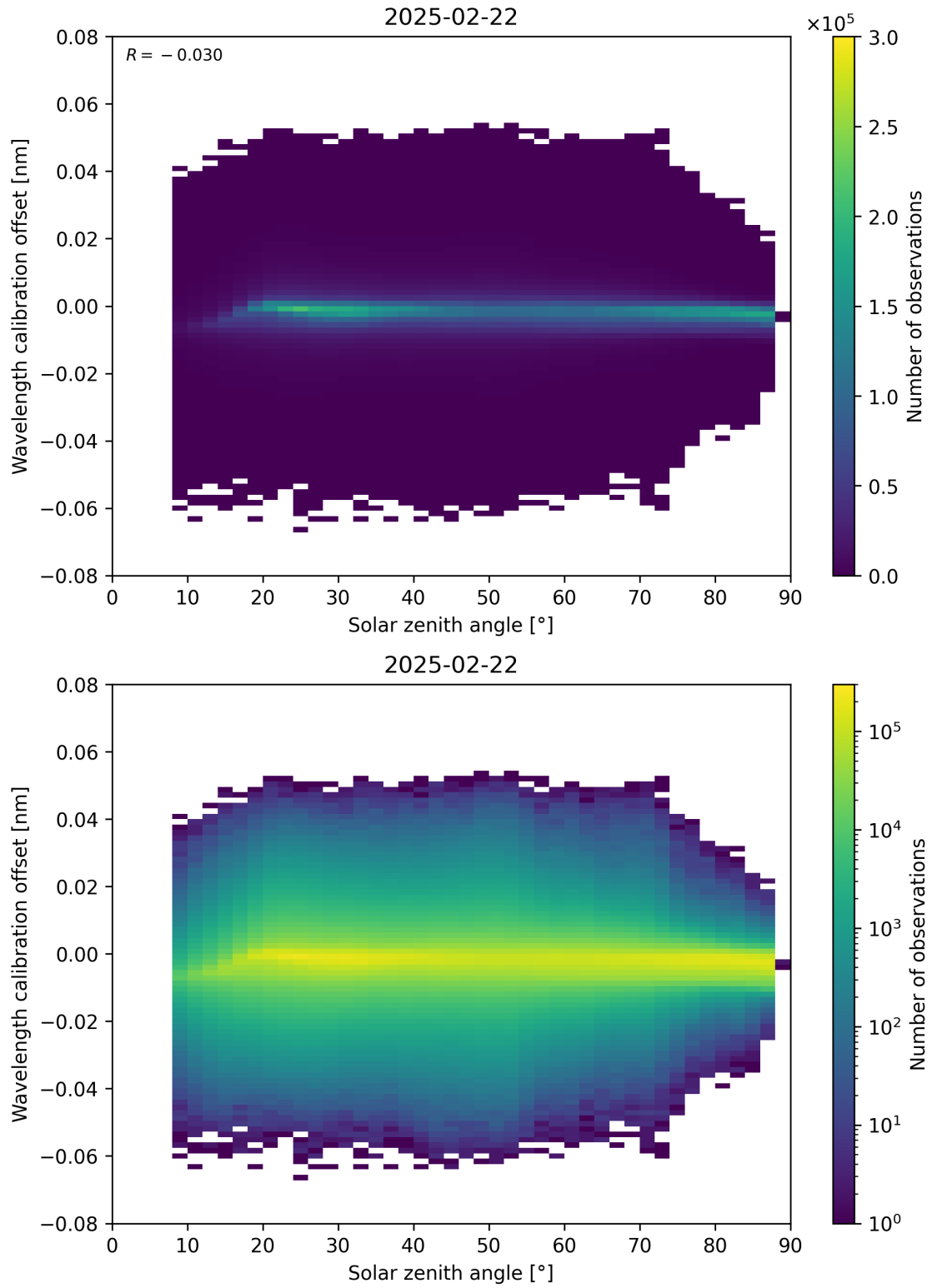
Figure 158: Scatter density plot of “Solar zenith angle” against “Wavelength calibration offset” for 2025-02-21 to 2025-02-23.
