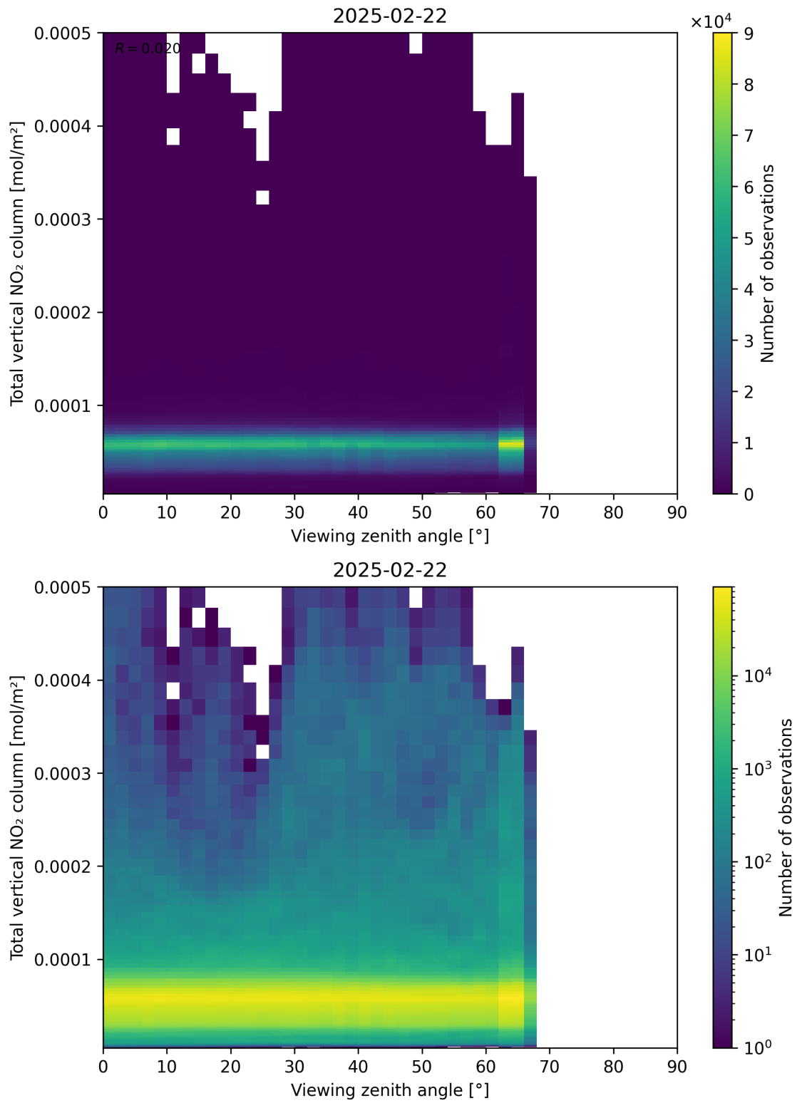
Figure 167: Scatter density plot of “Viewing zenith angle” against “Total vertical NO 2 column” for 2025-02-21 to 2025-02-23.
