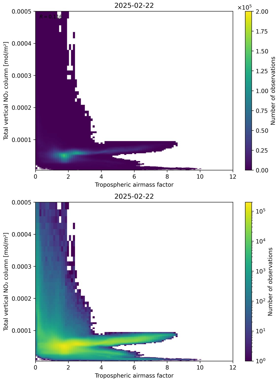
Figure 77: Scatter density plot of “Tropospheric airmass factor” against “Total vertical NO 2 column” for 2025-02-21 to 2025-02-23.
