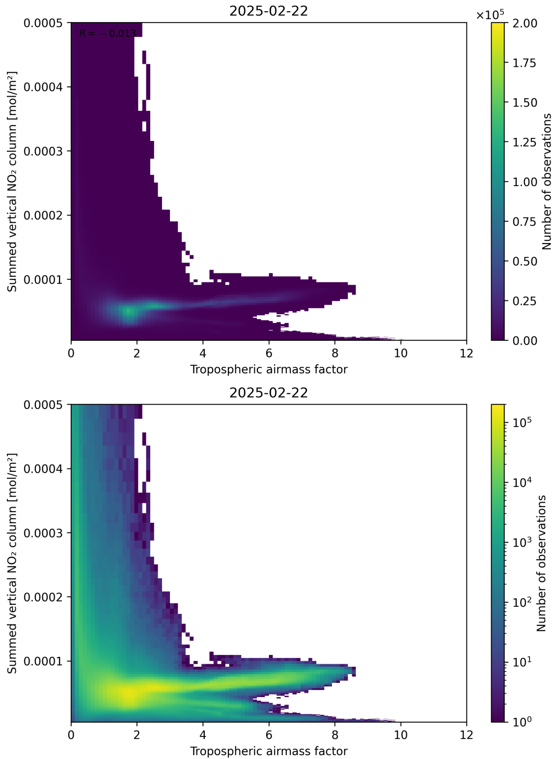
Figure 75: Scatter density plot of “Tropospheric airmass factor” against “Summed vertical NO 2 column” for 2025-02-21 to 2025-02-23.
