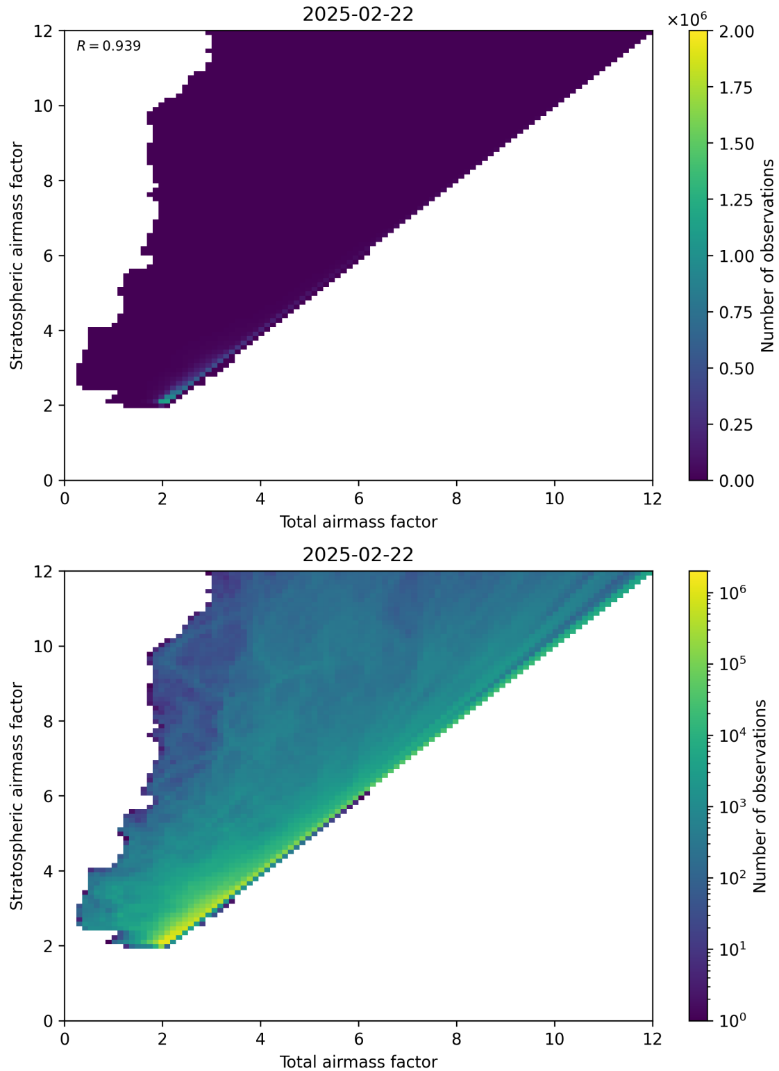
Figure 62: Scatter density plot of “Total airmass factor” against “Stratospheric airmass factor” for 2025-02-21 to 2025-02-23.
