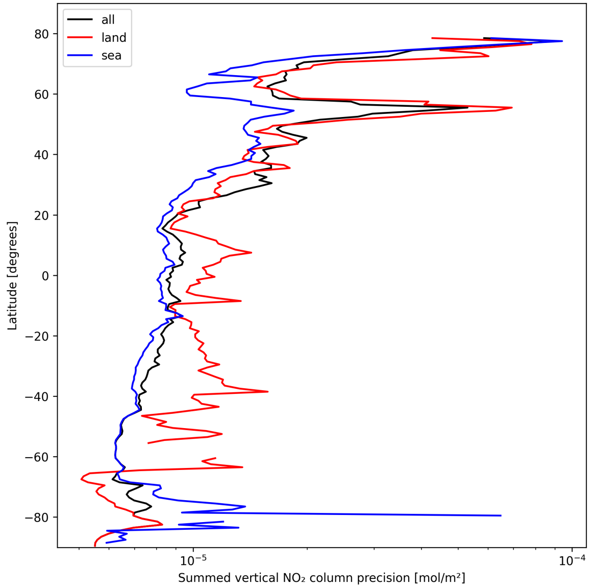
Figure 24: Zonal average of “Summed vertical NO 2 column precision” for 2025-02-21 to 2025-02-23.
