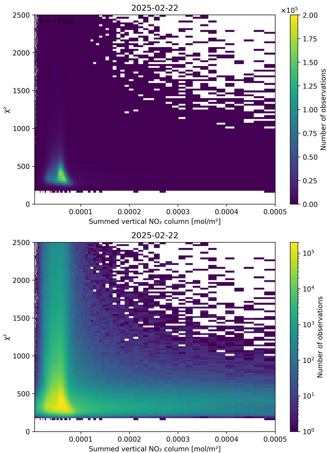
Figure 104: Scatter density plot of “Summed vertical NO 2 column” against “ \chi^2 ” for 2025-02-21 to 2025-02-23.
