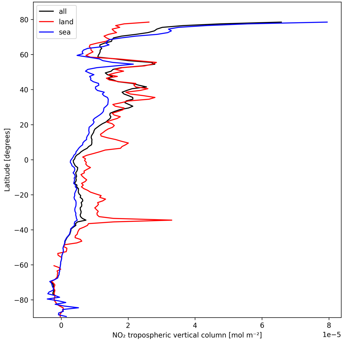
Figure 12: Zonal average of “NO 2 tropospheric vertical column” for 2025-02-24 to 2025-02-25.
