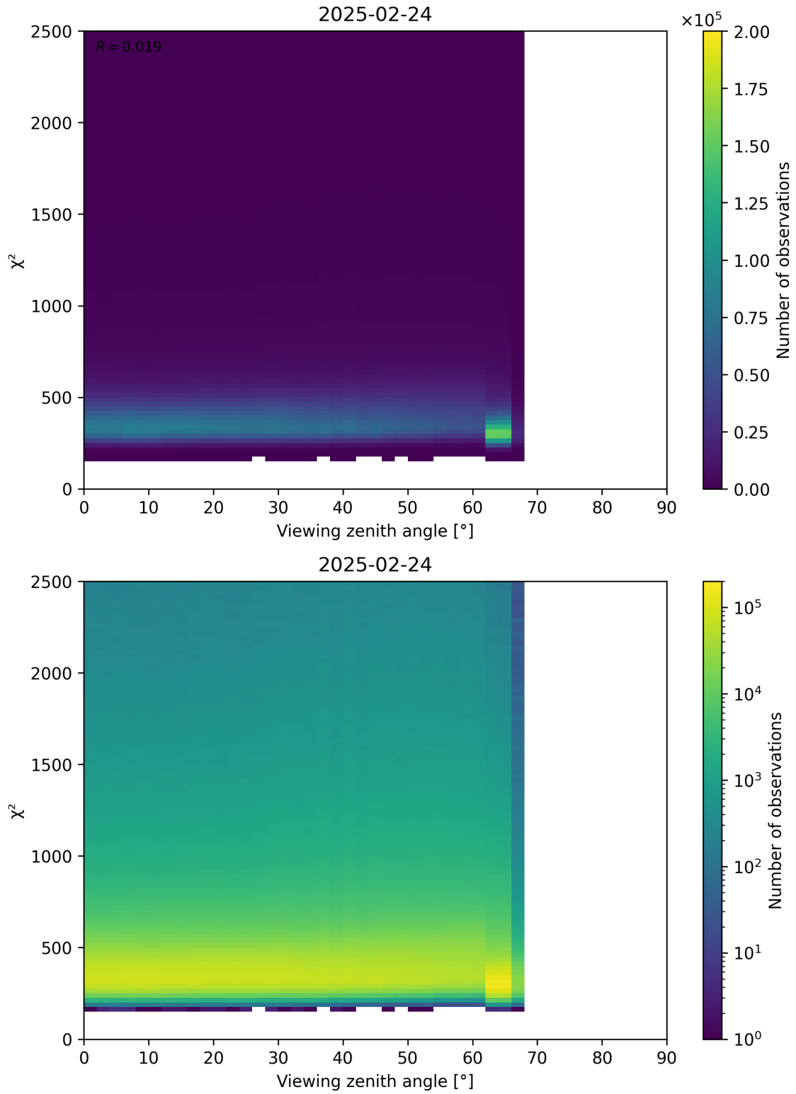
Figure 162: Scatter density plot of “Viewing zenith angle” against “ \chi^2 ” for 2025-02-24 to 2025-02-25.
