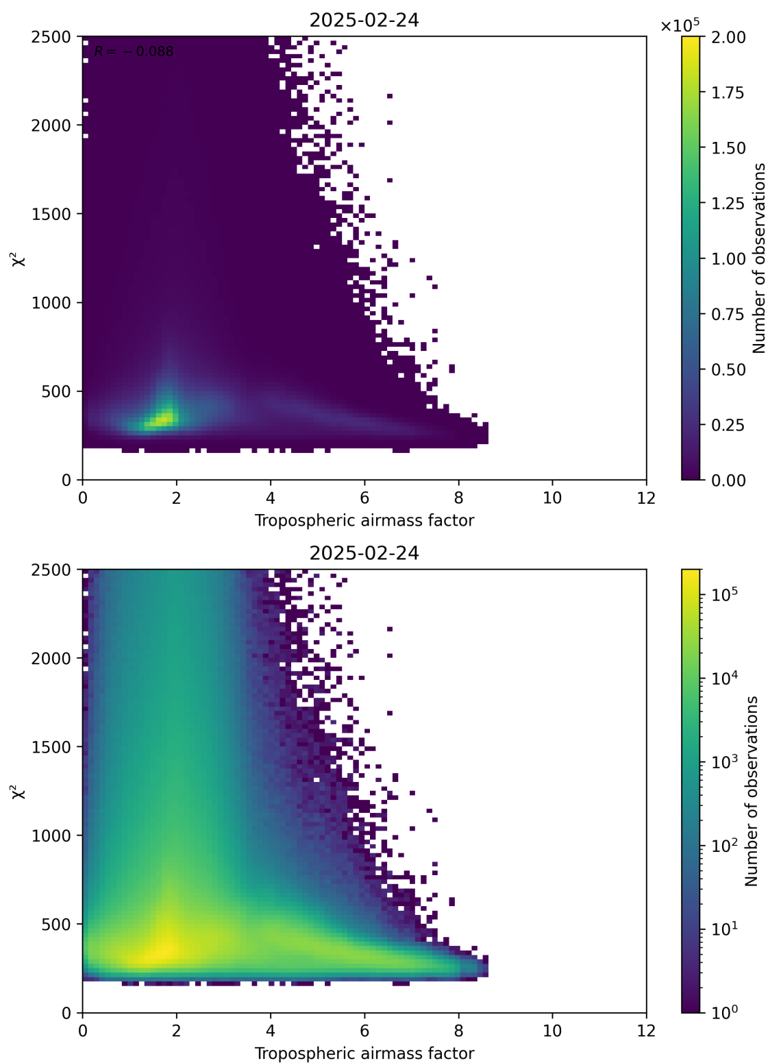
Figure 73: Scatter density plot of “Tropospheric airmass factor” against “ \chi^2 ” for 2025-02-24 to 2025-02-25.
