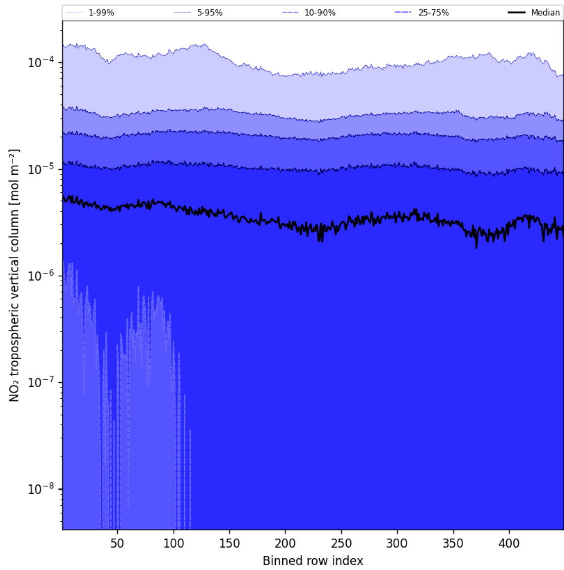
Figure 46: Along track statistics of “NO 2 tropospheric vertical column” for 2025-02-24 to 2025-02-25
