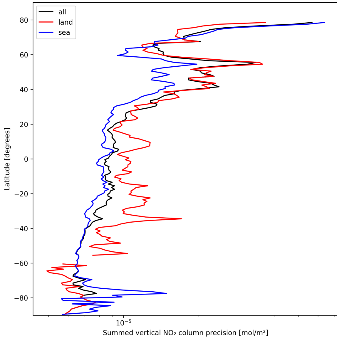
Figure 24: Zonal average of “Summed vertical NO 2 column precision” for 2025-02-24 to 2025-02-25.
