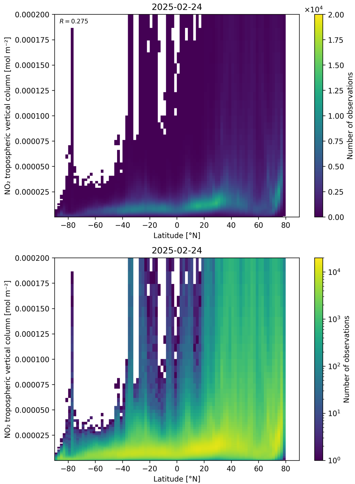
Figure 92: Scatter density plot of “Latitude” against “NO 2 tropospheric vertical column” for 2025-02-24 to 2025-02-25.
