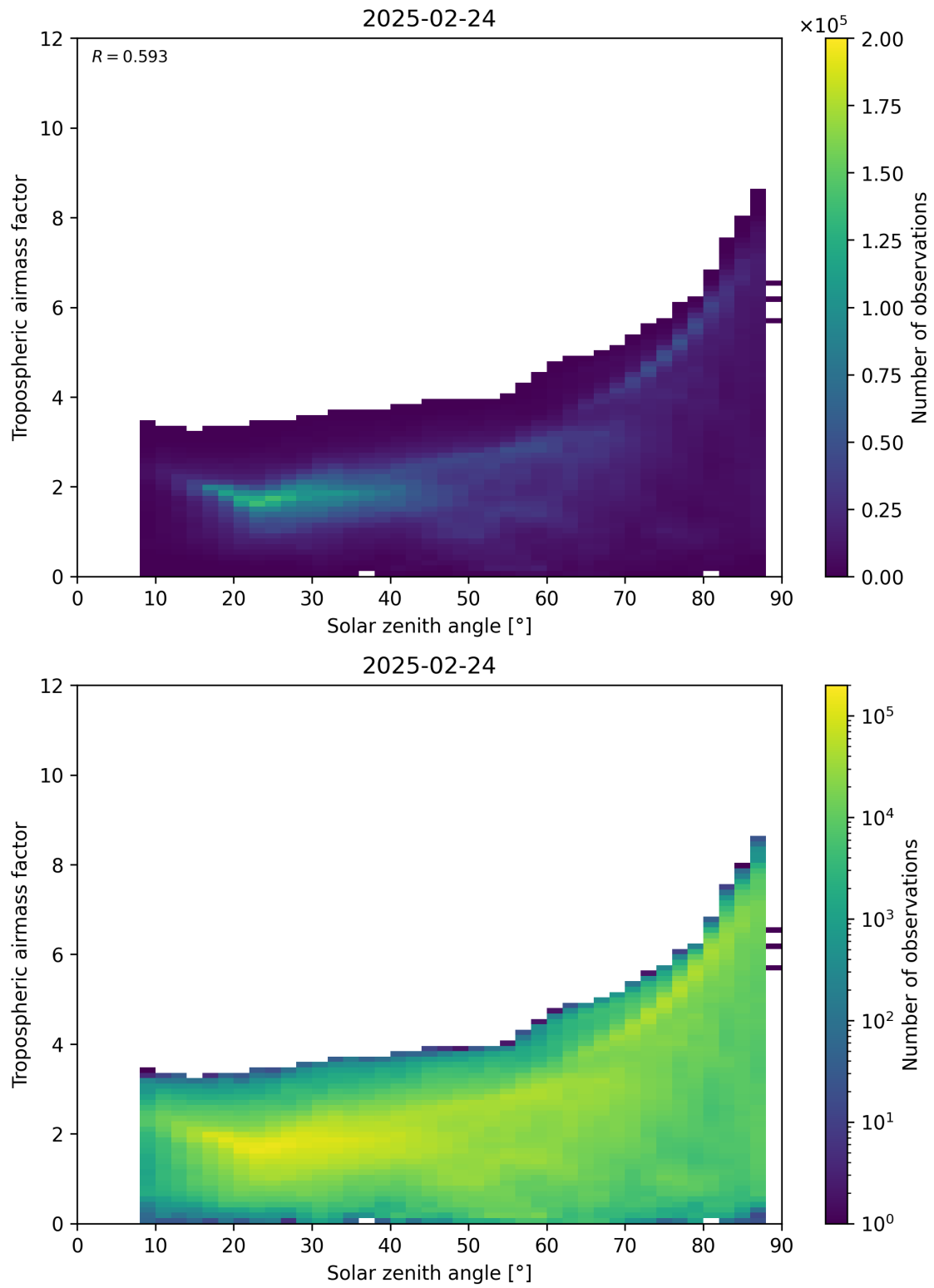
Figure 147: Scatter density plot of “Solar zenith angle” against “Tropospheric airmass factor” for 2025-02-24 to 2025-02-25.
