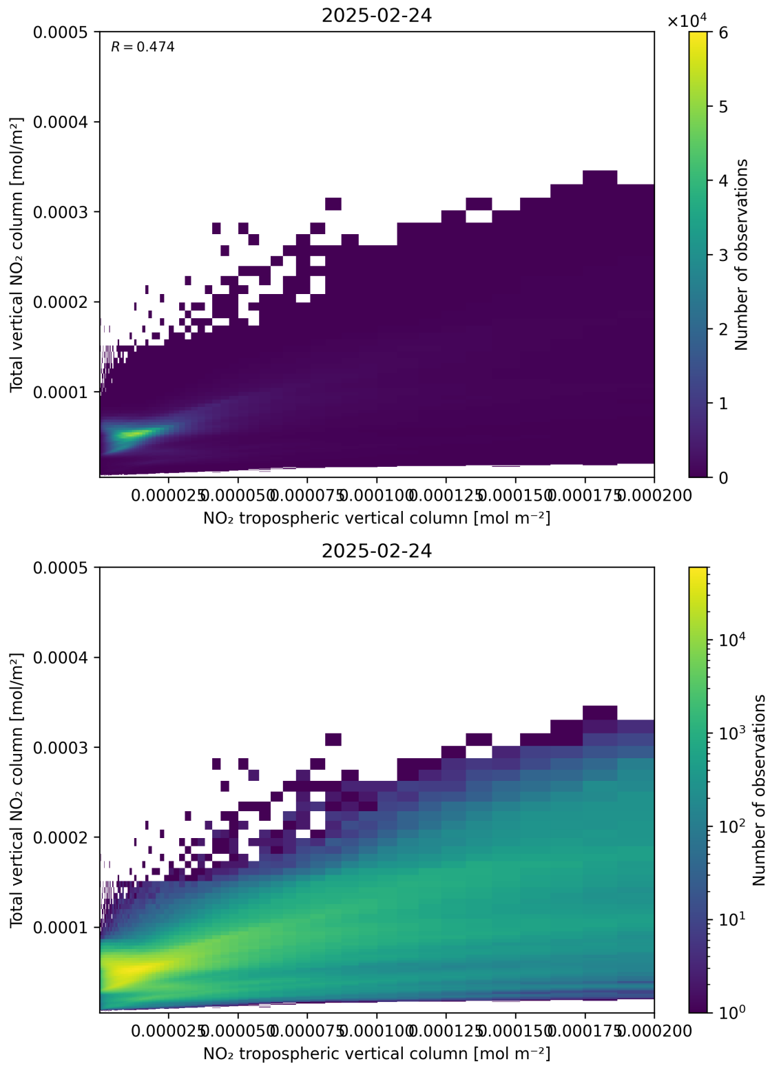
Figure 128: Scatter density plot of “NO 2 tropospheric vertical column” against “Total vertical NO 2 column” for 2025-02-24 to 2025-02-25.
