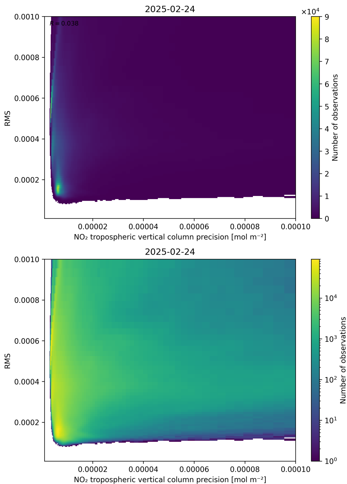
Figure 140: Scatter density plot of “NO 2 tropospheric vertical column precision” against “RMS” for 2025-02-24 to 2025-02-25.
