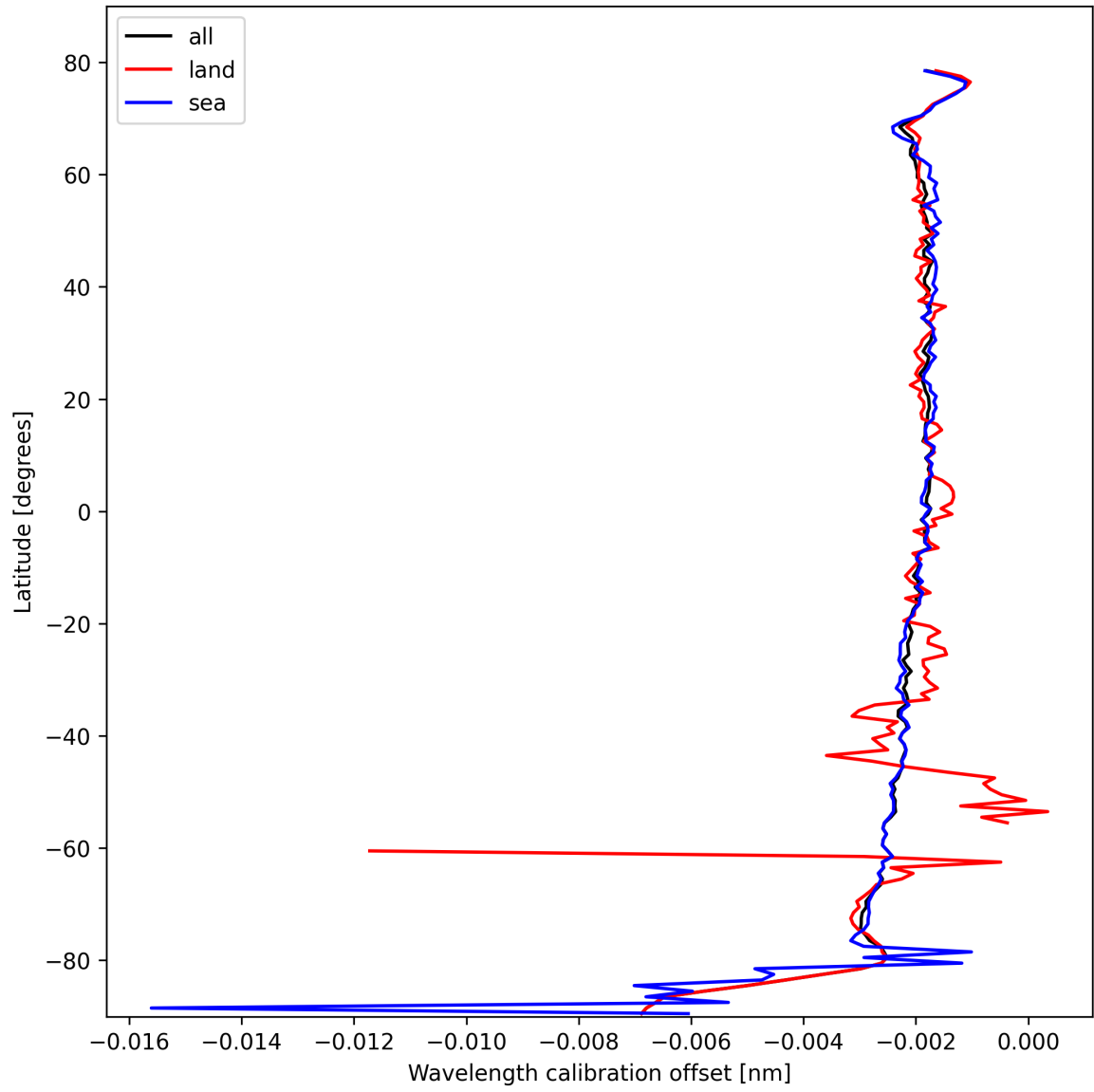
Figure 18: Zonal average of “Wavelength calibration offset” for 2025-02-24 to 2025-02-25.
