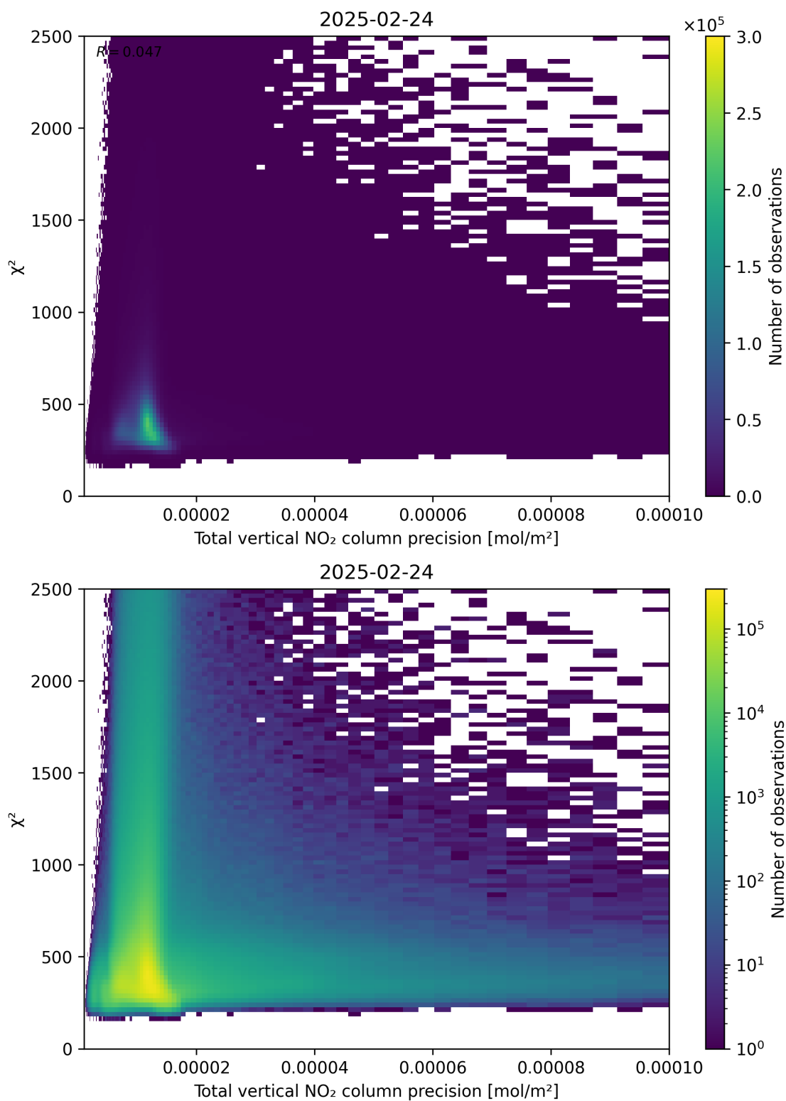
Figure 116: Scatter density plot of “Total vertical NO 2 column precision” against “ \chi^2 ” for 2025-02-24 to 2025-02-25.
