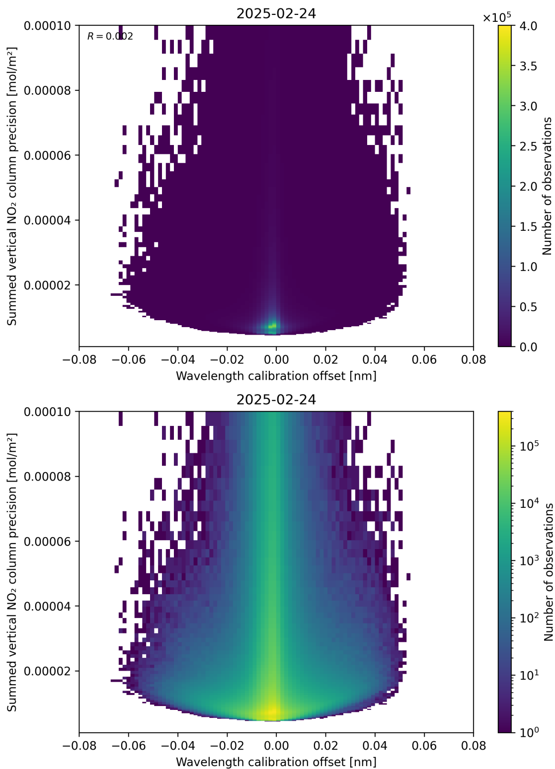
Figure 178: Scatter density plot of “Wavelength calibration offset” against “Summed vertical NO 2 column precision” for 2025-02-24 to 2025-02-25.
