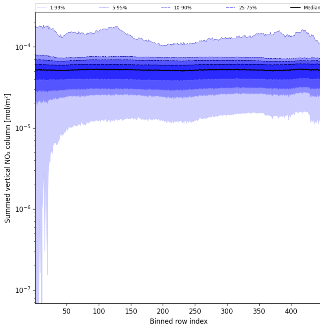
Figure 57: Along track statistics of “Summed vertical NO 2 column” for 2025-02-24 to 2025-02-25
