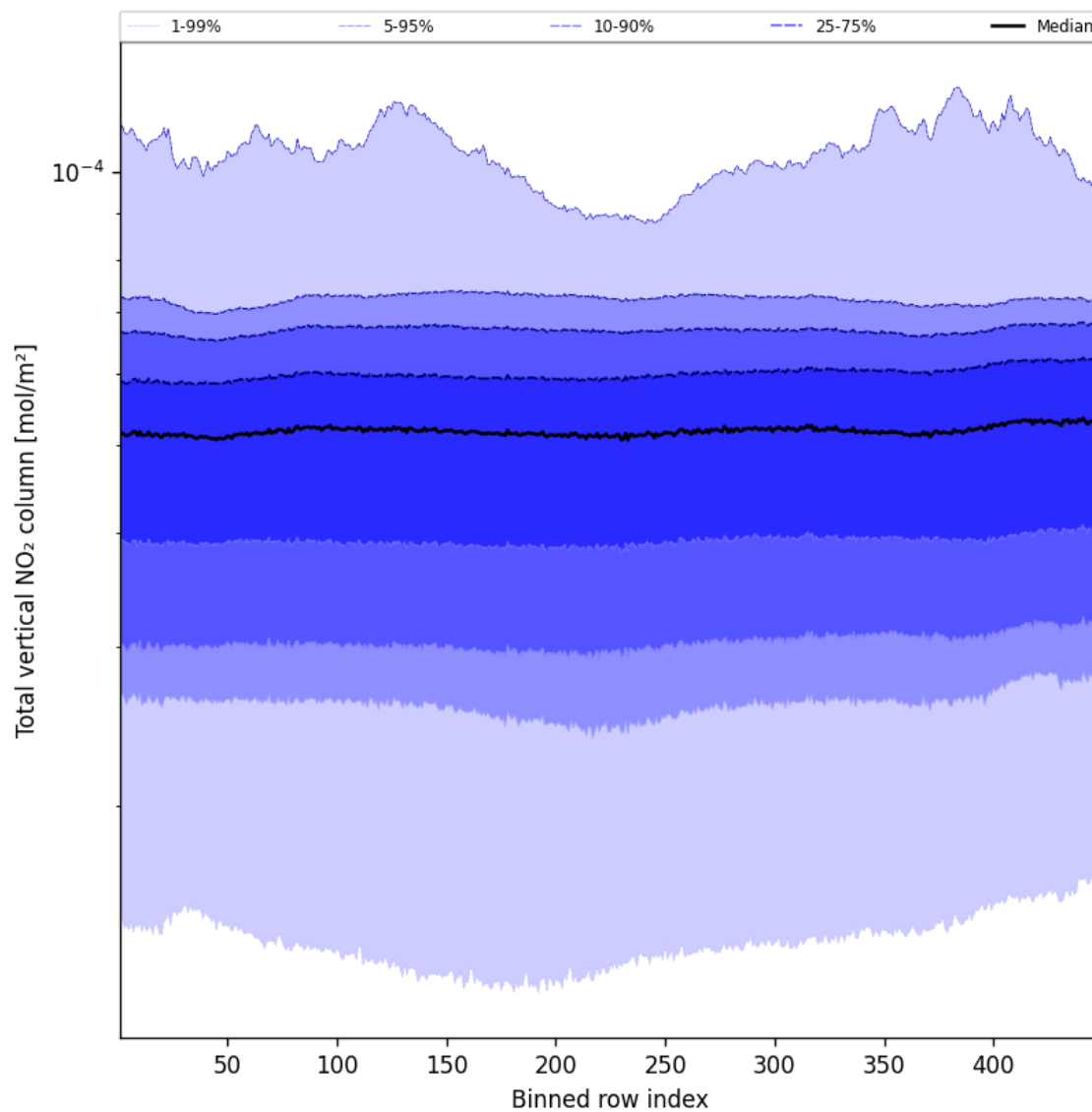
Figure 55: Along track statistics of “Total vertical NO 2 column” for 2025-02-24 to 2025-02-25
