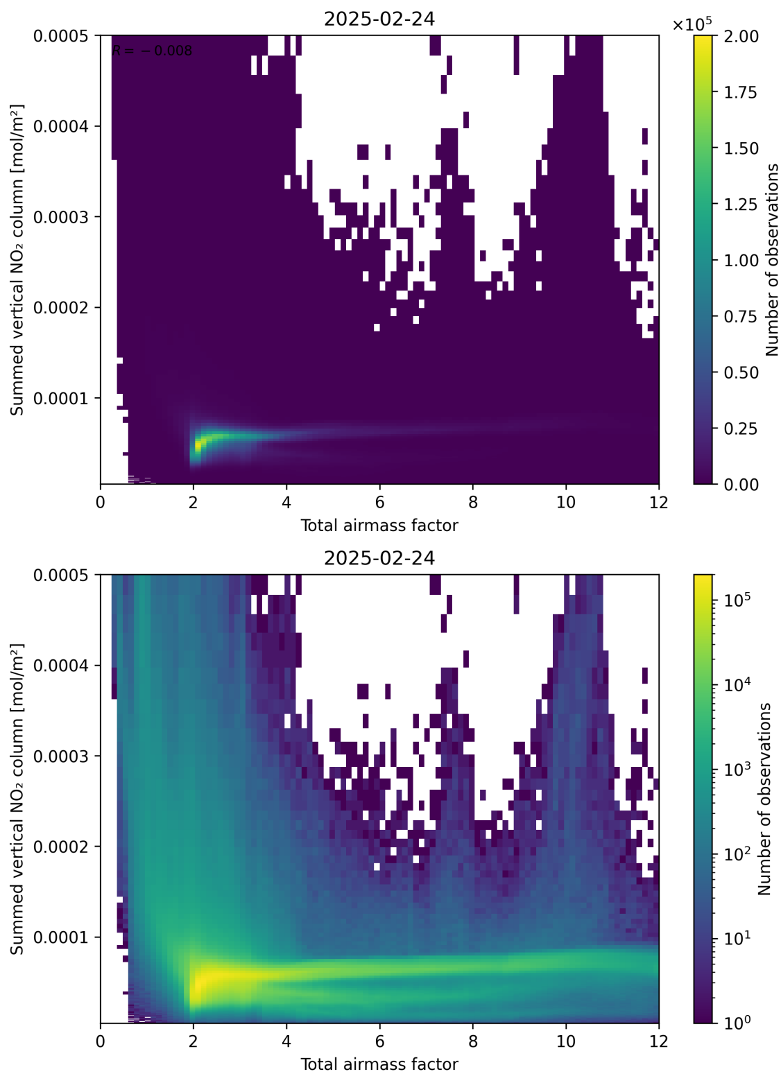
Figure 65: Scatter density plot of “Total airmass factor” against “Summed vertical NO 2 column” for 2025-02-24 to 2025-02-25.
