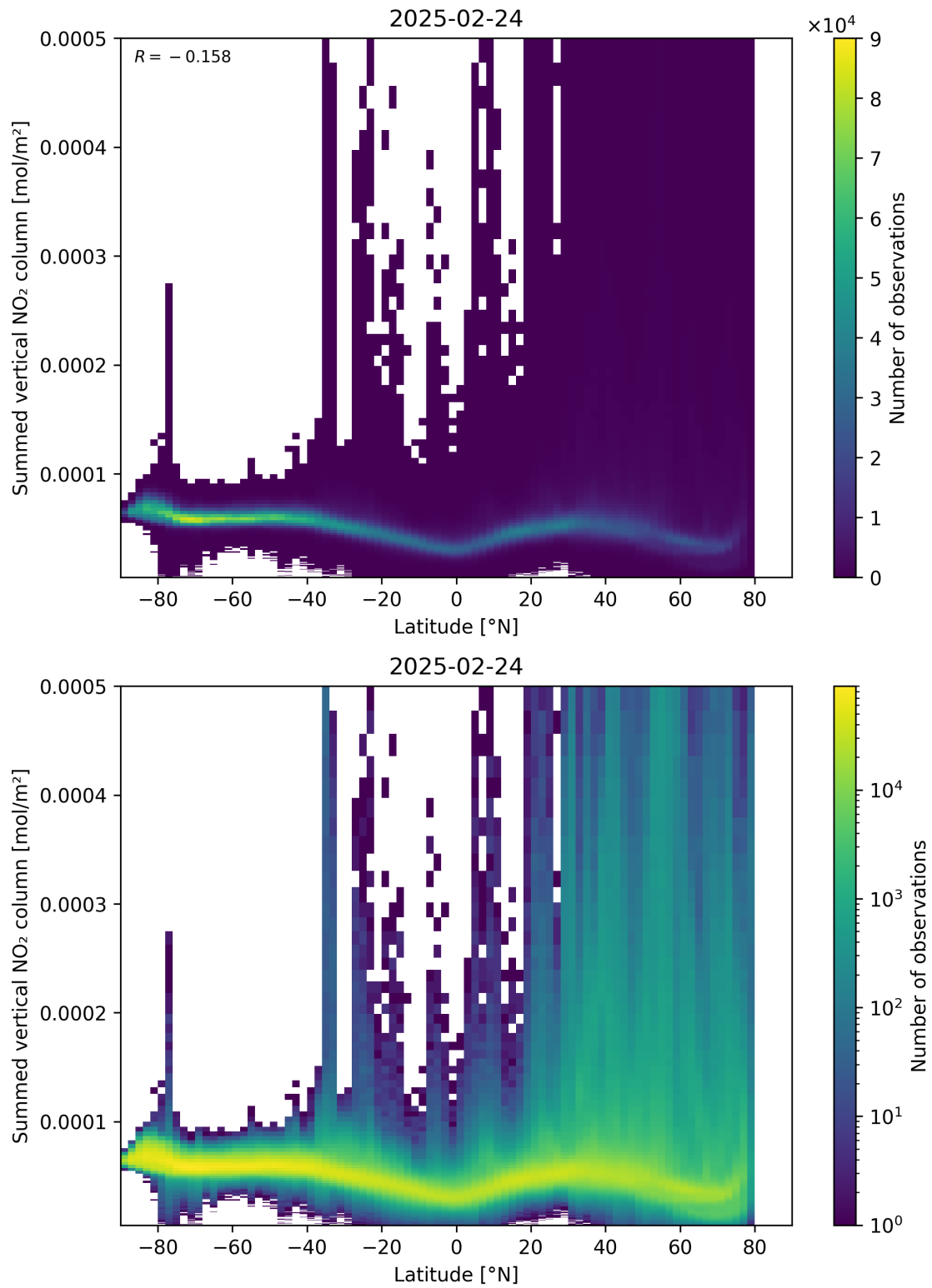
Figure 88: Scatter density plot of “Latitude” against “Summed vertical NO 2 column” for 2025-02-24 to 2025-02-25.
