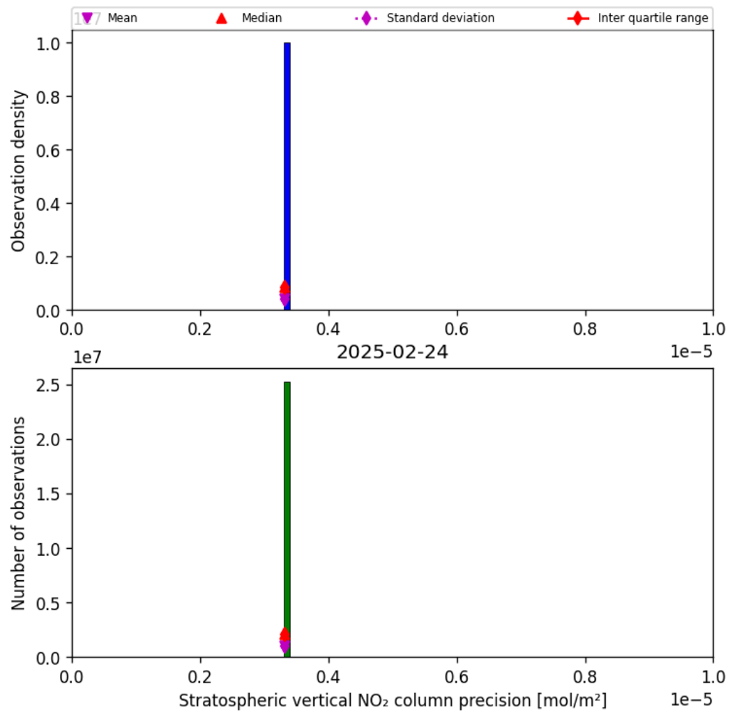
Figure 37: Histogram of “Stratospheric vertical NO 2 column precision” for 2025-02-24 to 2025-02-25
