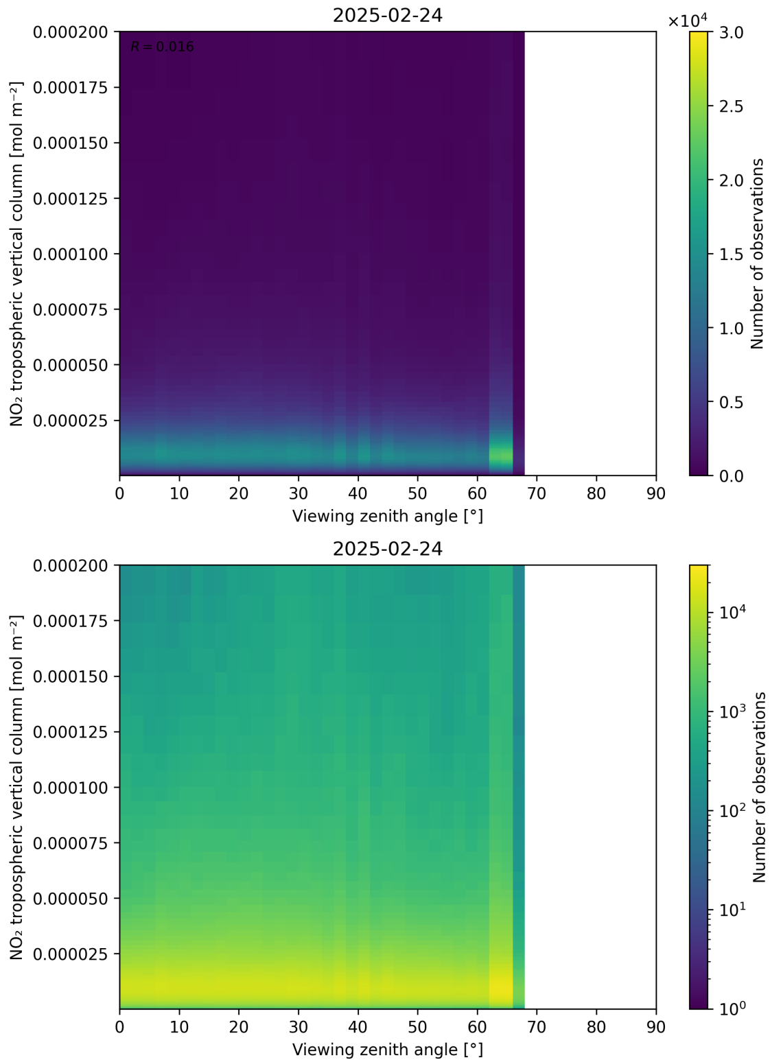
Figure 169: Scatter density plot of “Viewing zenith angle” against “NO 2 tropospheric vertical column” for 2025-02-24 to 2025-02-25.
