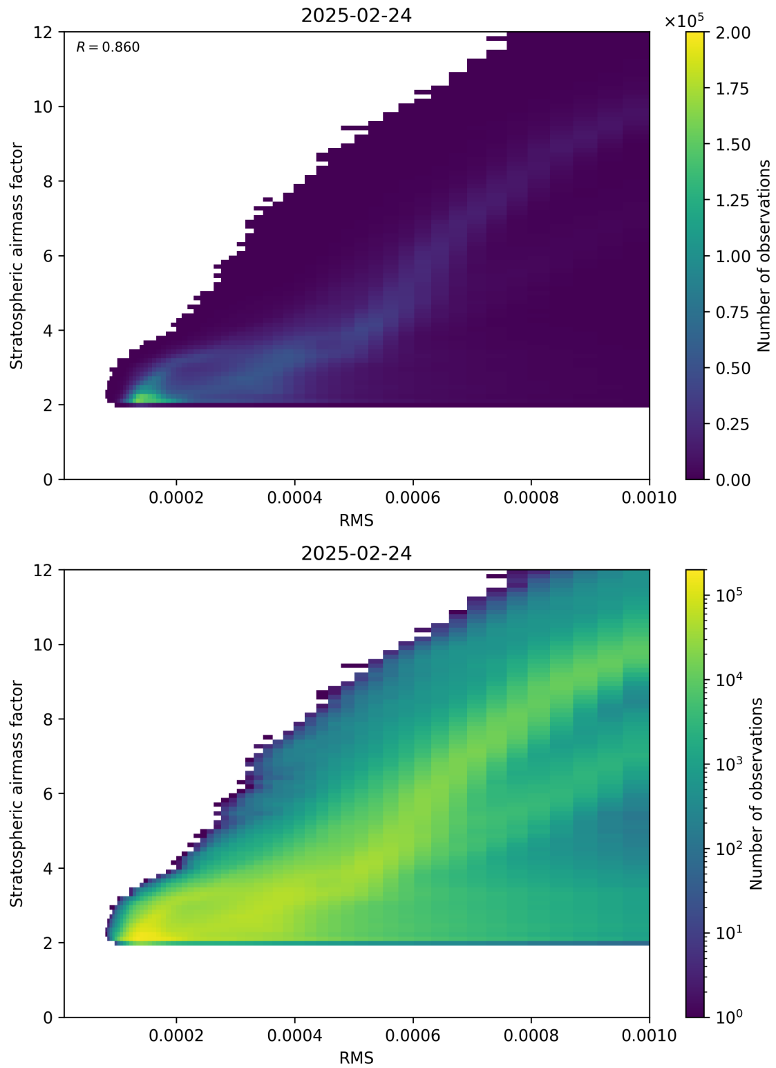
Figure 144: Scatter density plot of “RMS” against “Stratospheric airmass factor” for 2025-02-24 to 2025-02-25.
