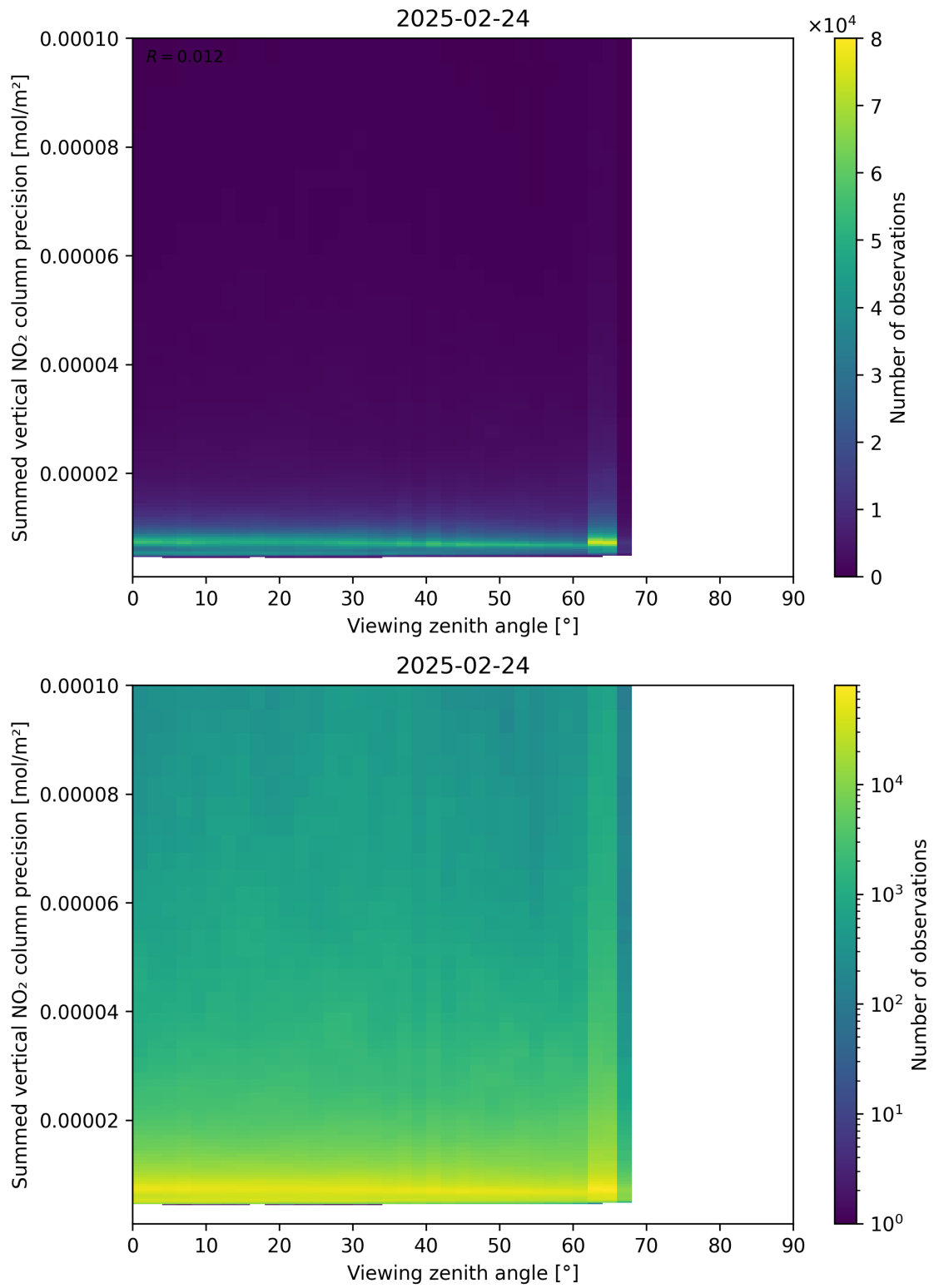
Figure 166: Scatter density plot of “Viewing zenith angle” against “Summed vertical NO 2 column precision” for 2025-02-24 to 2025-02-25.
