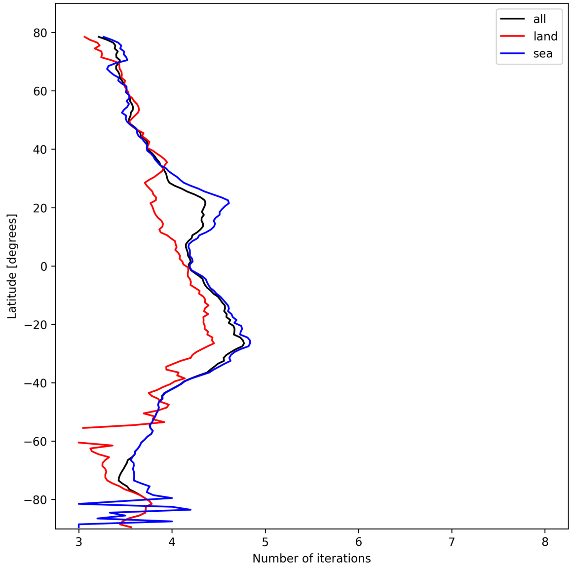
Figure 17: Zonal average of “Number of iterations” for 2025-02-24 to 2025-02-25.
