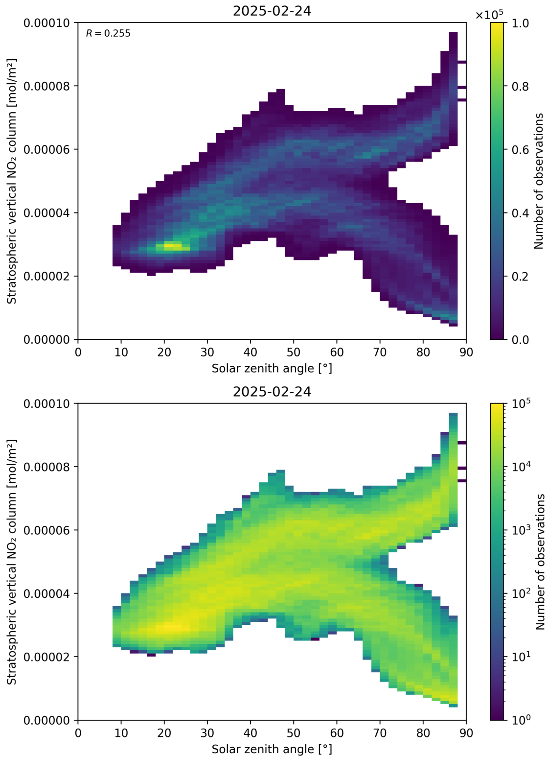
Figure 150: Scatter density plot of “Solar zenith angle” against “Stratospheric vertical \text{NO}_2 column” for 2025-02-24 to 2025-02-25.
