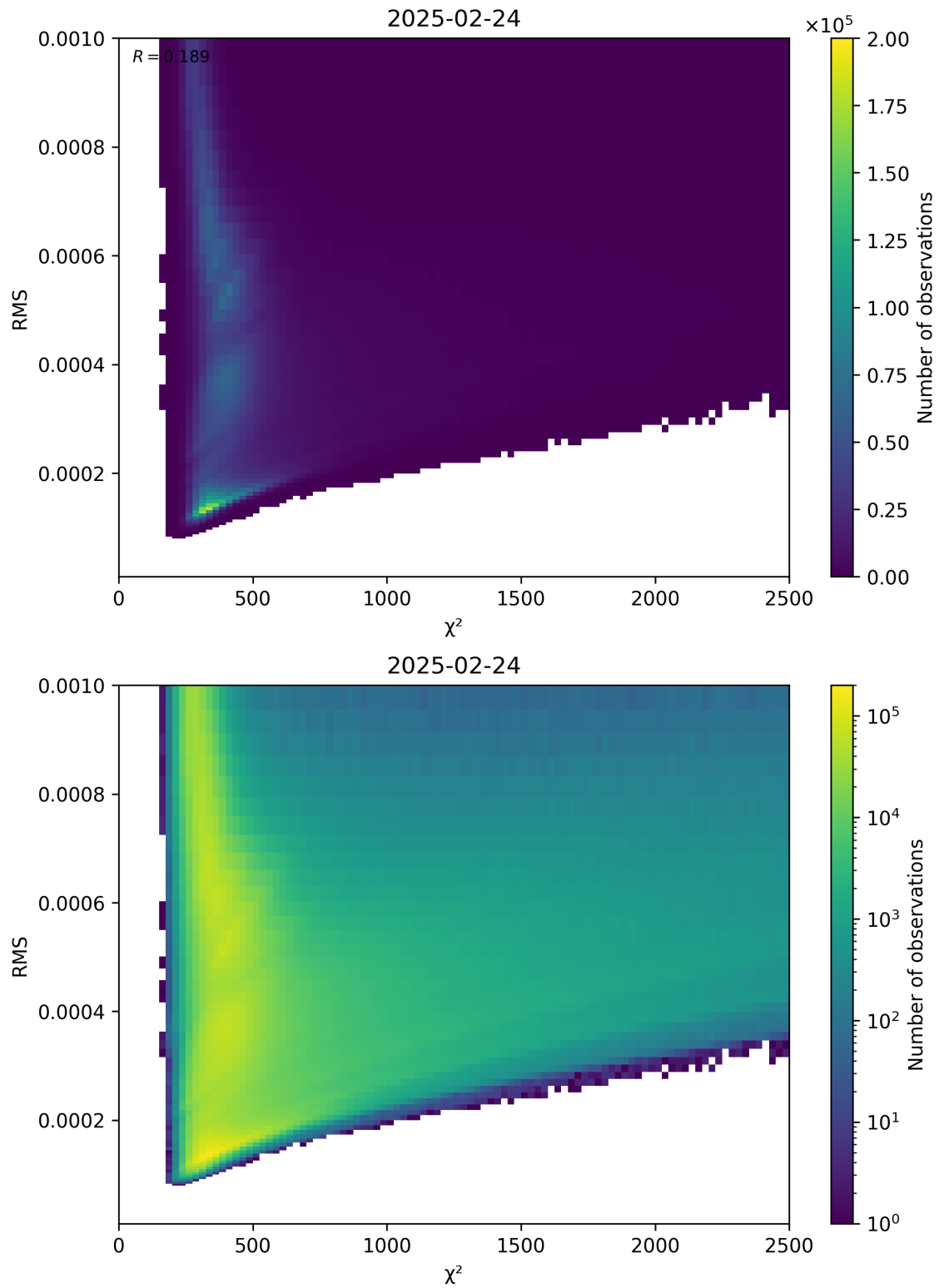
Figure 82: Scatter density plot of “ \chi^2 ” against “RMS” for 2025-02-24 to 2025-02-25.
