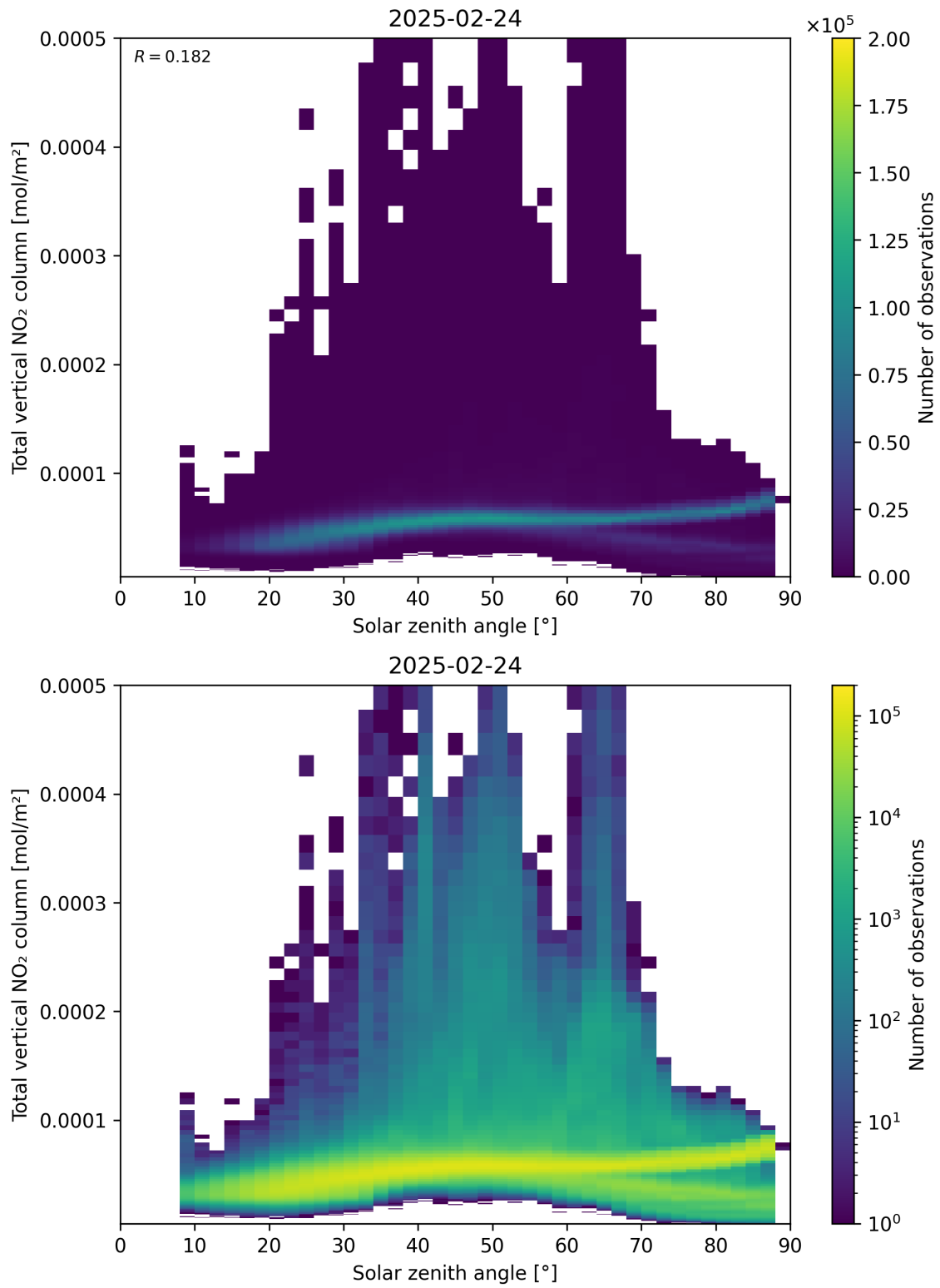
Figure 153: Scatter density plot of “Solar zenith angle” against “Total vertical NO 2 column” for 2025-02-24 to 2025-02-25.
