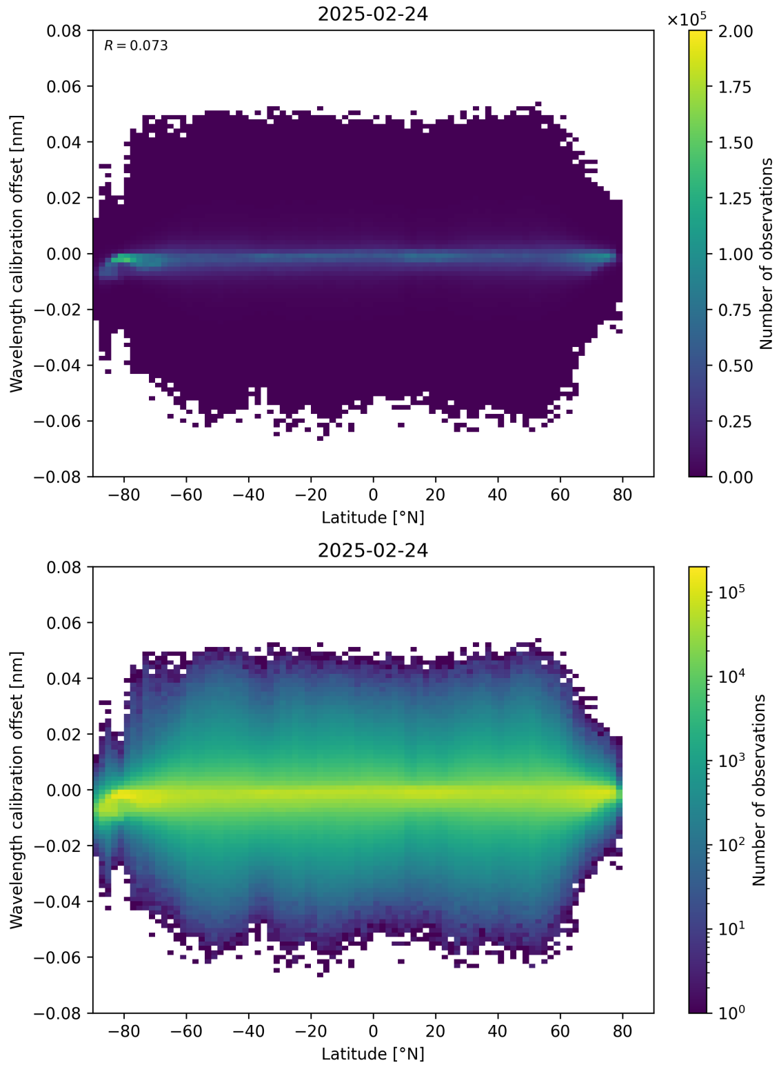
Figure 95: Scatter density plot of “Latitude” against “Wavelength calibration offset” for 2025-02-24 to 2025-02-25.
