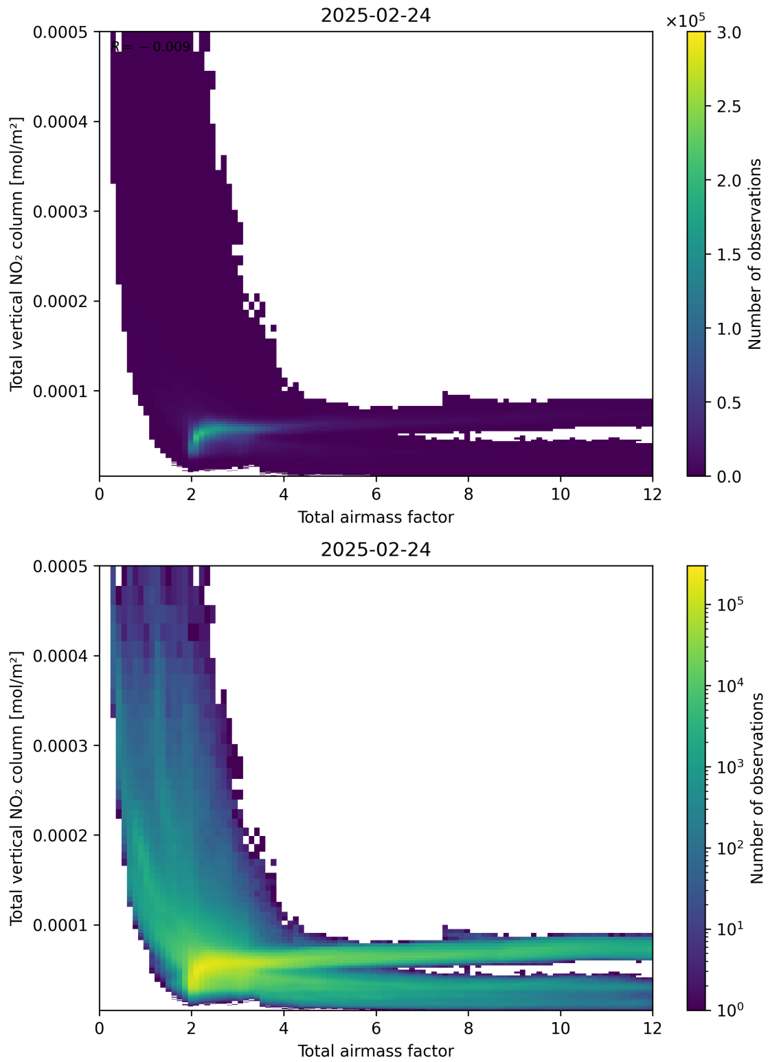
Figure 67: Scatter density plot of “Total airmass factor” against “Total vertical NO 2 column” for 2025-02-24 to 2025-02-25.
