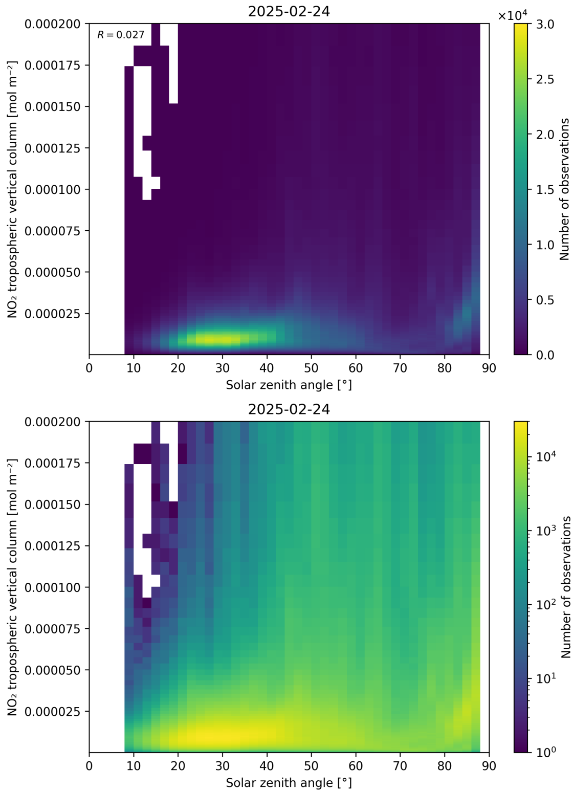
Figure 155: Scatter density plot of “Solar zenith angle” against “NO 2 tropospheric vertical column” for 2025-02-24 to 2025-02-25.
