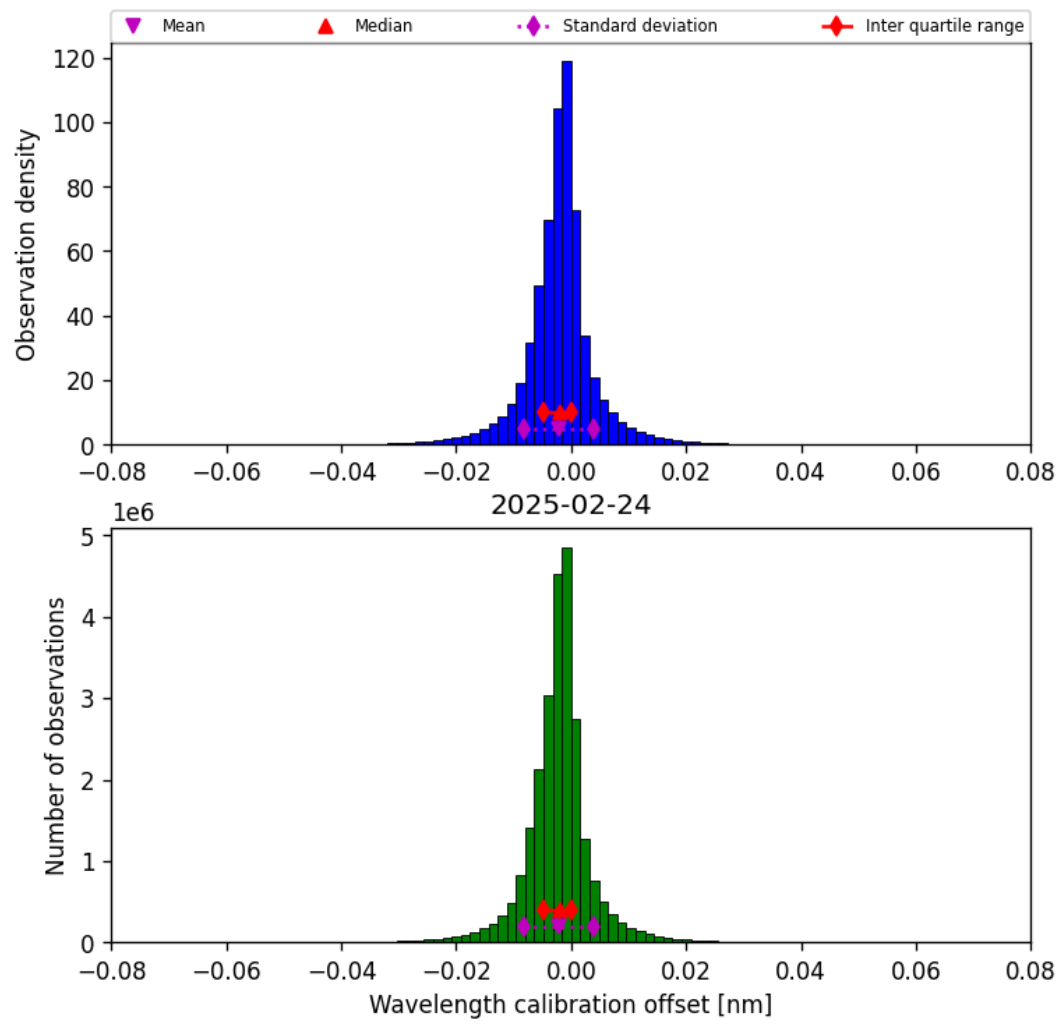
Figure 35: Histogram of “Wavelength calibration offset” for 2025-02-24 to 2025-02-25
