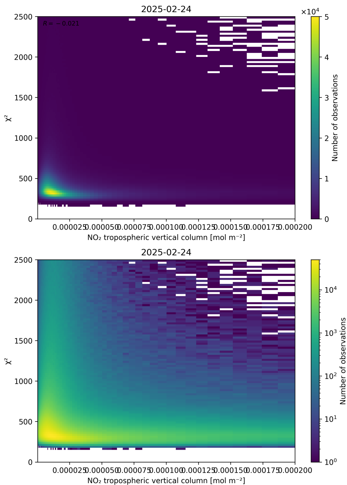
Figure 124: Scatter density plot of “NO 2 tropospheric vertical column” against “ \chi^2 ” for 2025-02-24 to 2025-02-25.
