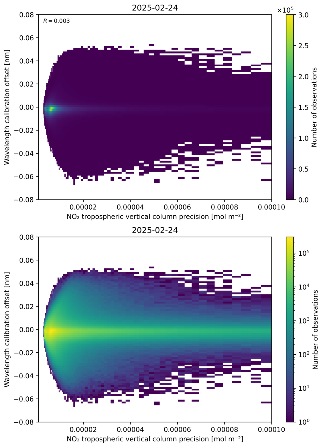
Figure 141: Scatter density plot of “NO 2 tropospheric vertical column precision” against “Wavelength calibration offset” for 2025-02-24 to 2025-02-25.
