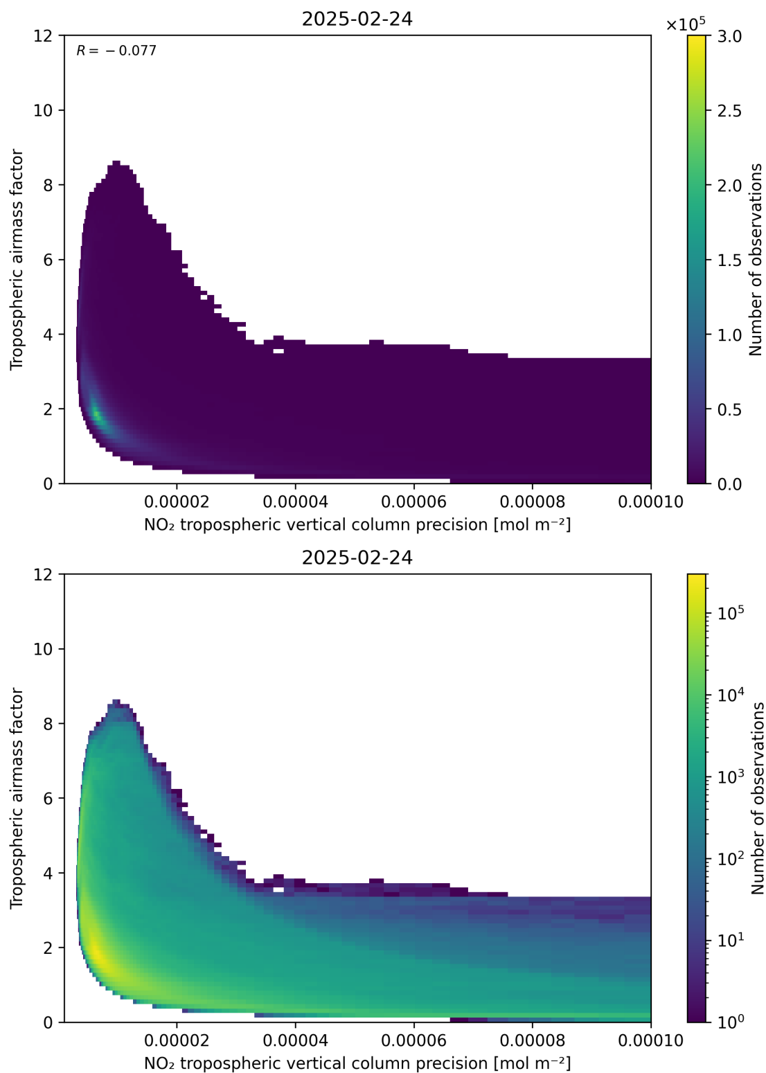
Figure 133: Scatter density plot of “NO 2 tropospheric vertical column precision” against “Tropospheric air mass factor” for 2025-02-24 to 2025-02-25.
