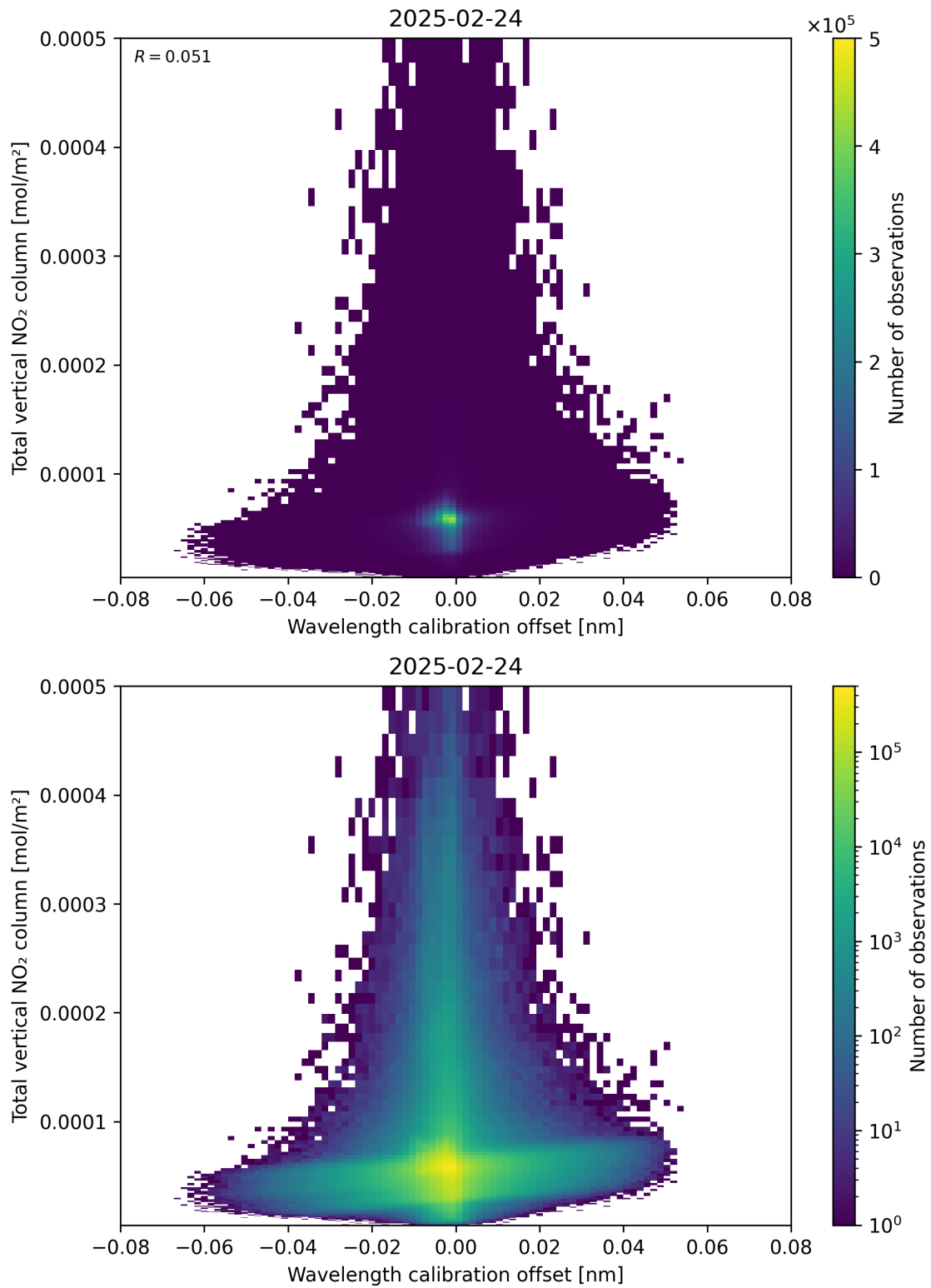
Figure 179: Scatter density plot of “Wavelength calibration offset” against “Total vertical NO 2 column” for 2025-02-24 to 2025-02-25.
