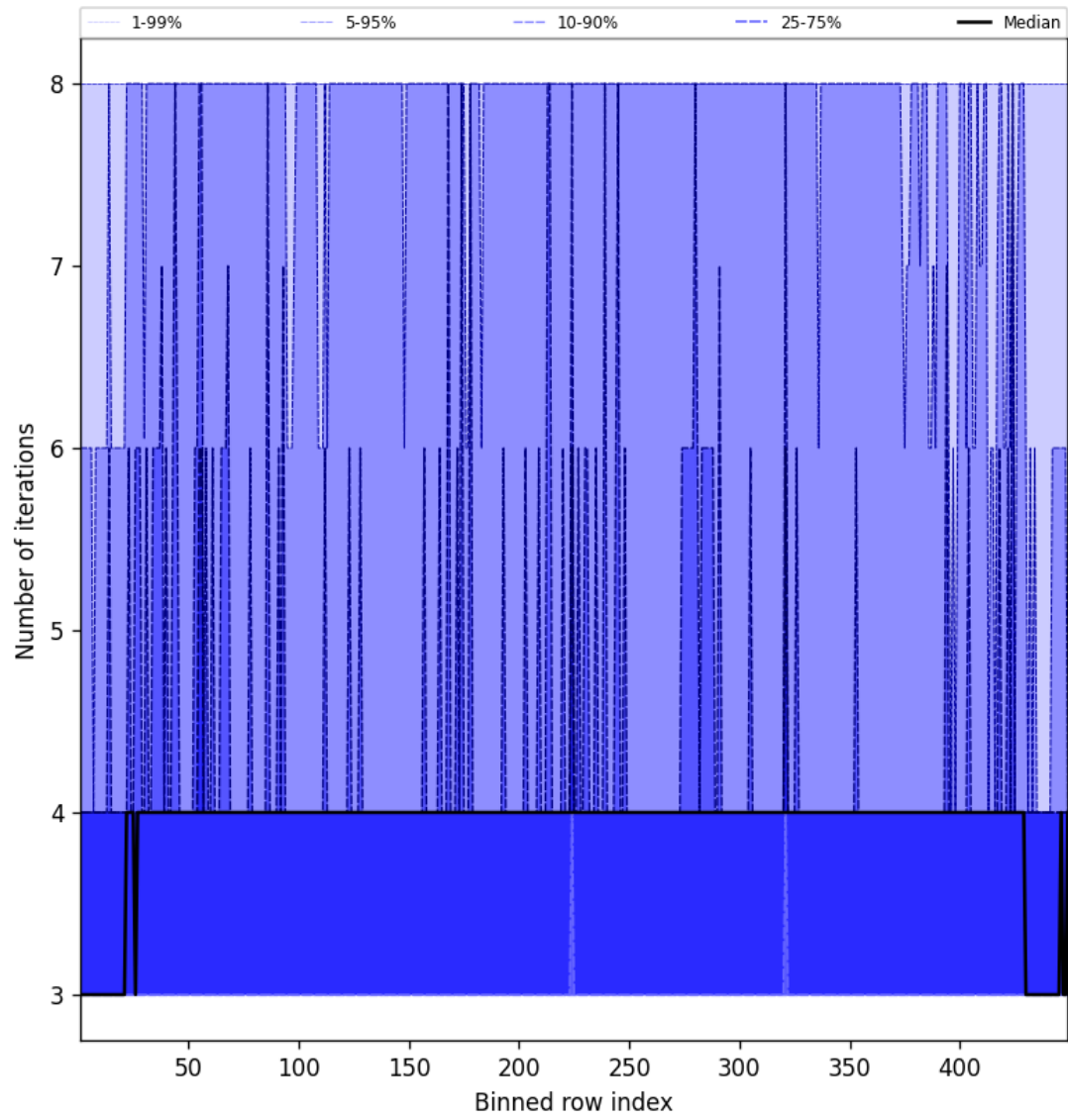
Figure 51: Along track statistics of “Number of iterations” for 2025-02-24 to 2025-02-25
