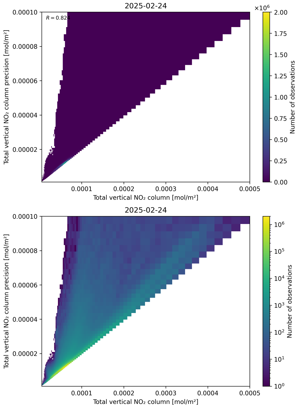
Figure 114: Scatter density plot of “Total vertical NO 2 column” against “Total vertical NO 2 column precision” for 2025-02-24 to 2025-02-25.
