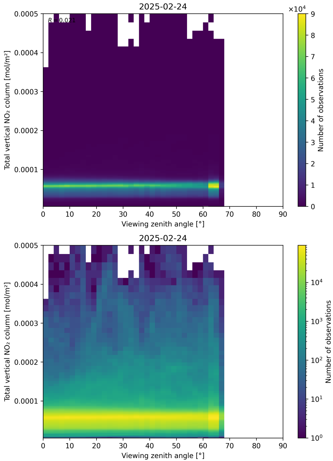
Figure 167: Scatter density plot of “Viewing zenith angle” against “Total vertical NO 2 column” for 2025-02-24 to 2025-02-25.
