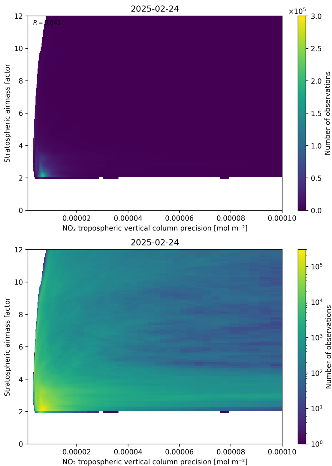
Figure 131: Scatter density plot of “NO 2 tropospheric vertical column precision” against “Stratospheric airmass factor” for 2025-02-24 to 2025-02-25.
