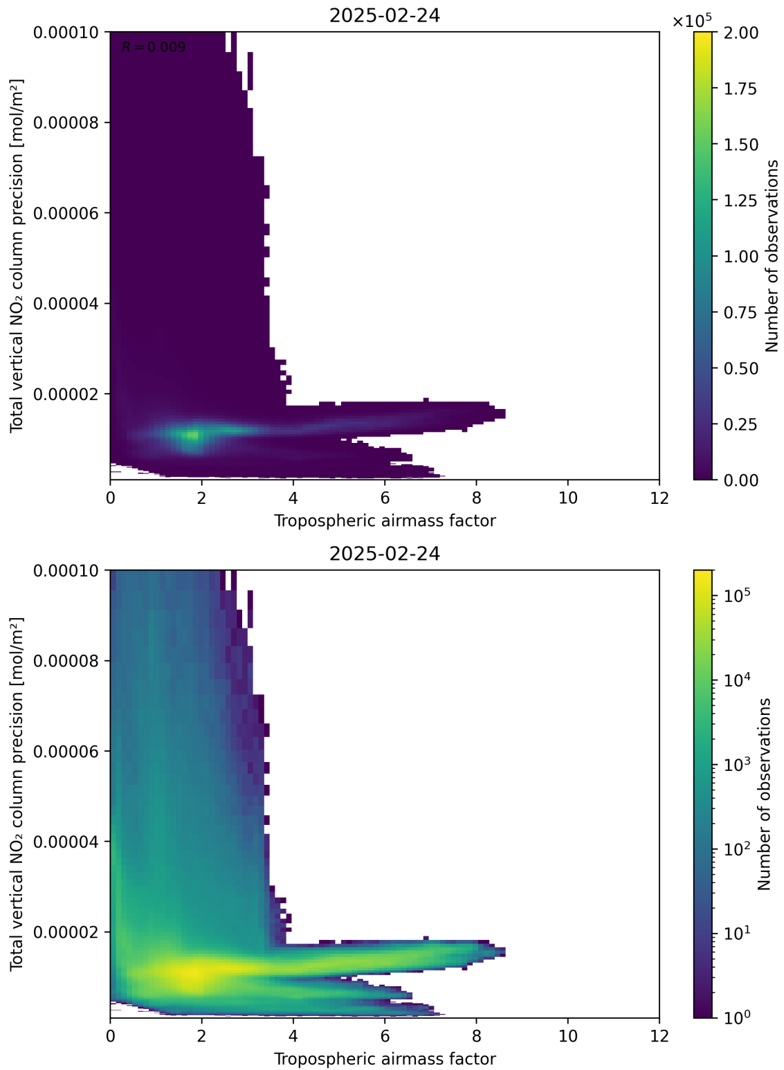
Figure 78: Scatter density plot of “Tropospheric air mass factor” against “Total vertical NO 2 column precision” for 2025-02-24 to 2025-02-25.
