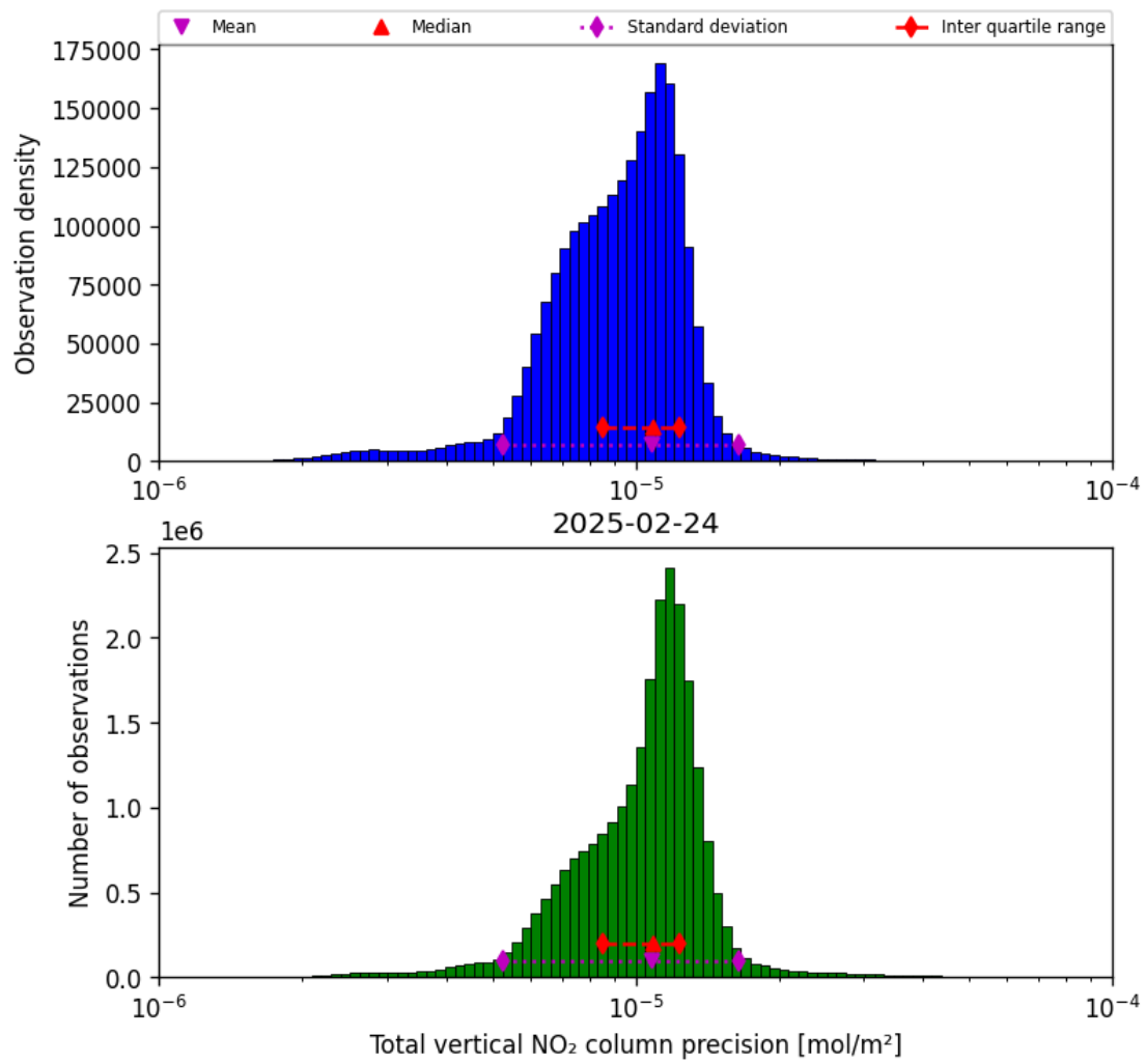
Figure 39: Histogram of “Total vertical NO 2 column precision” for 2025-02-24 to 2025-02-25
