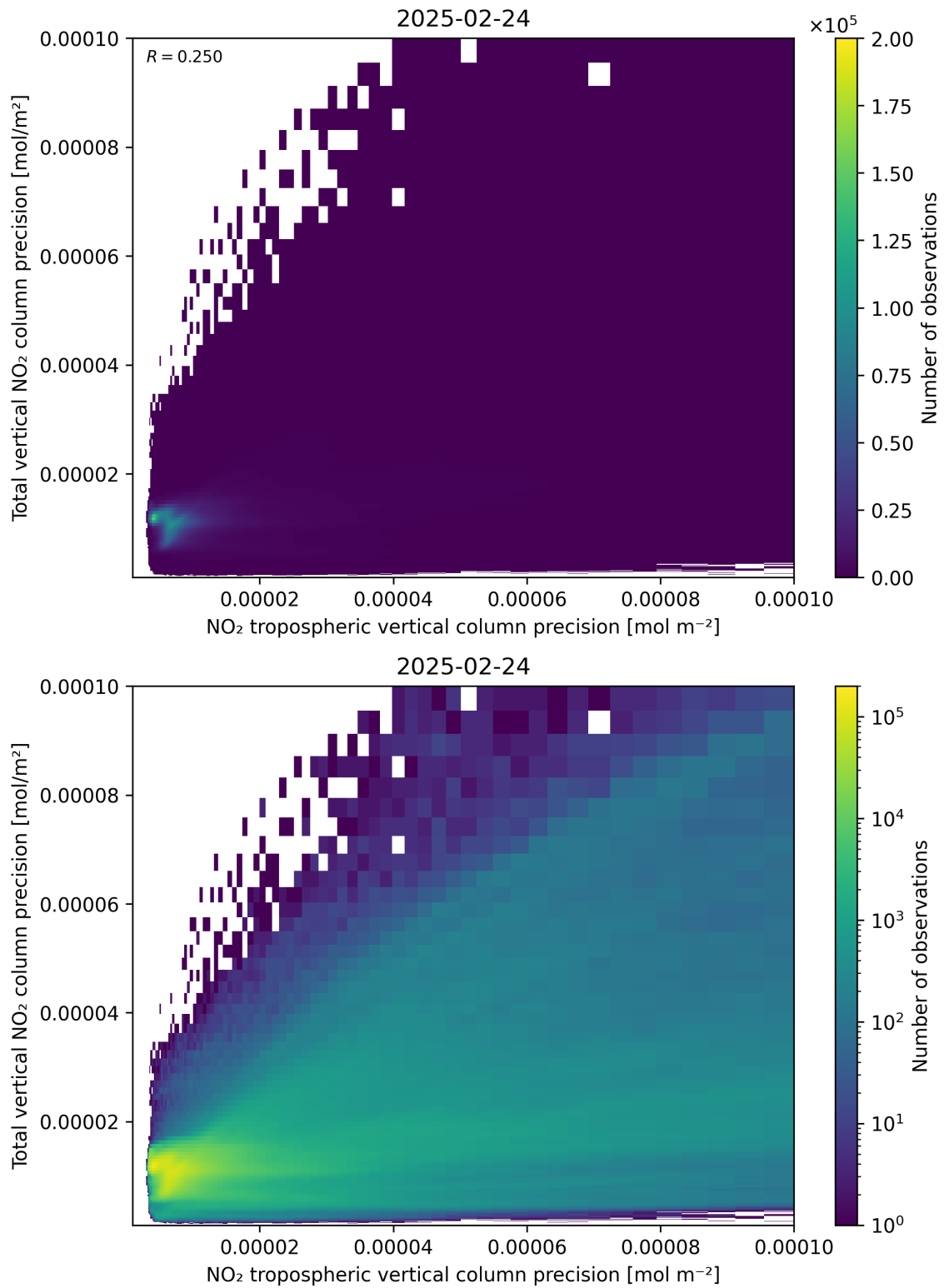
Figure 139: Scatter density plot of “NO 2 tropospheric vertical column precision” against “Total vertical NO 2 column precision” for 2025-02-24 to 2025-02-25.
