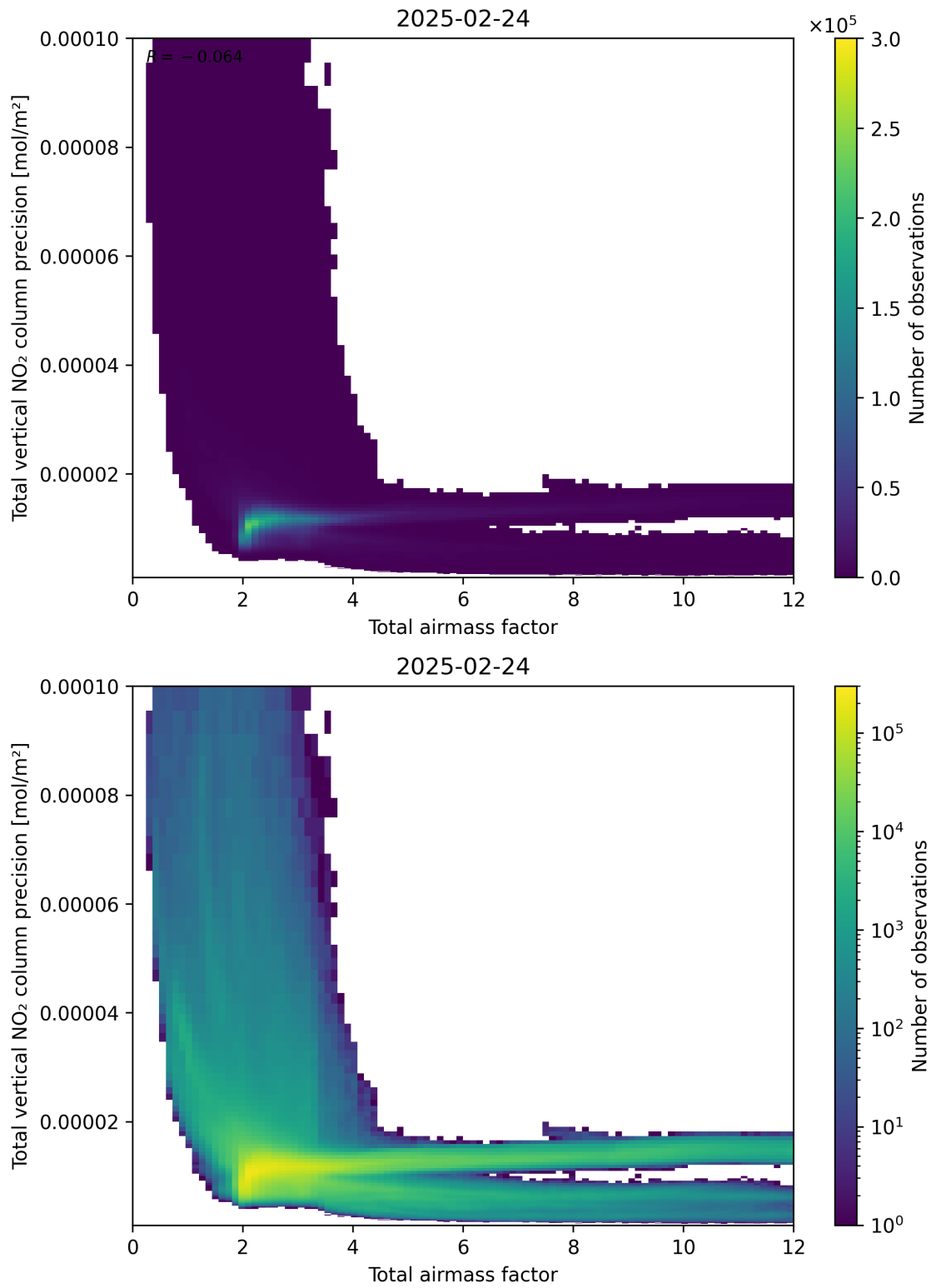
Figure 68: Scatter density plot of “Total airmass factor” against “Total vertical NO 2 column precision” for 2025-02-24 to 2025-02-25.
