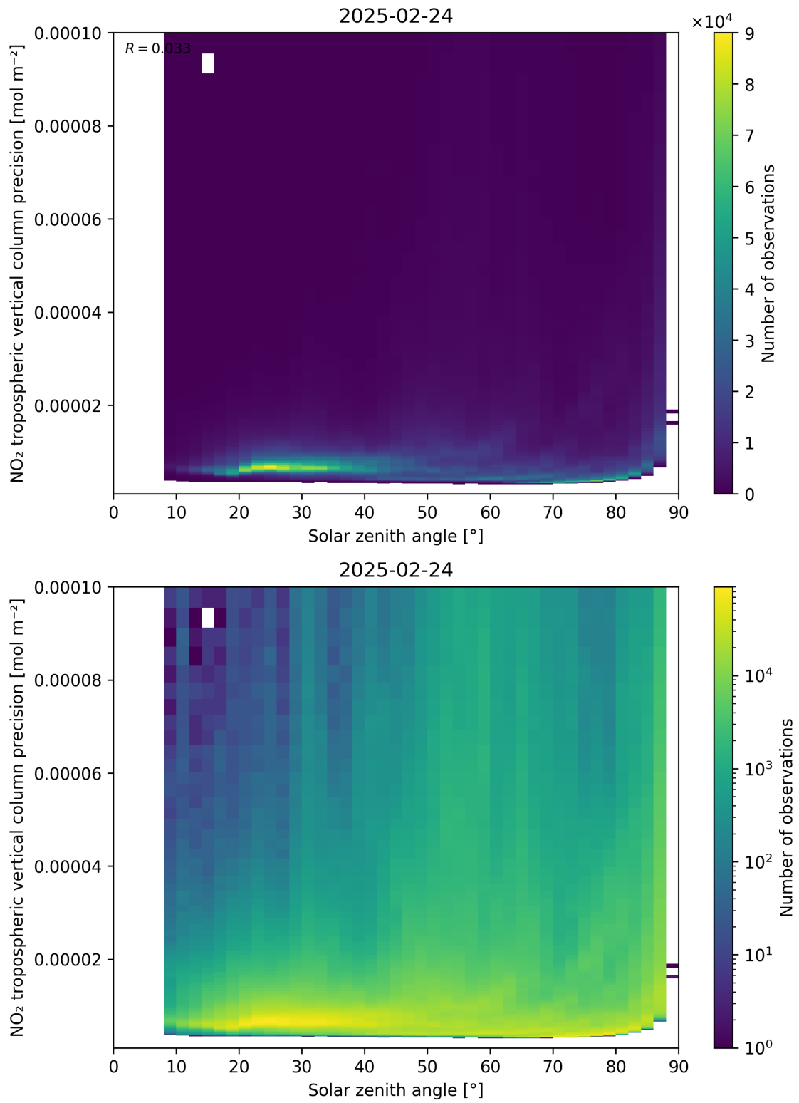
Figure 156: Scatter density plot of “Solar zenith angle” against “NO 2 tropospheric vertical column precision” for 2025-02-24 to 2025-02-25.
