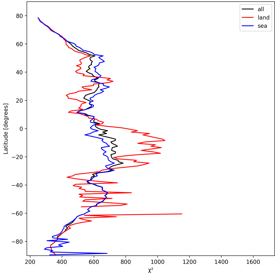
Figure 25: Zonal average of “ \chi^2 ” for 2025-02-24 to 2025-02-25.
