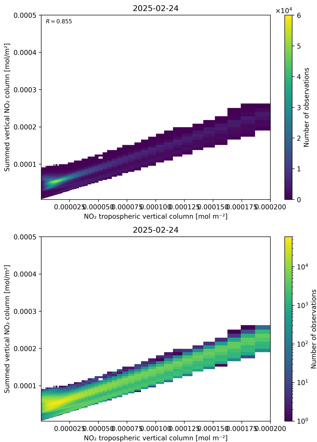
Figure 126: Scatter density plot of “NO 2 tropospheric vertical column” against “Summed vertical NO 2 column” for 2025-02-24 to 2025-02-25.
