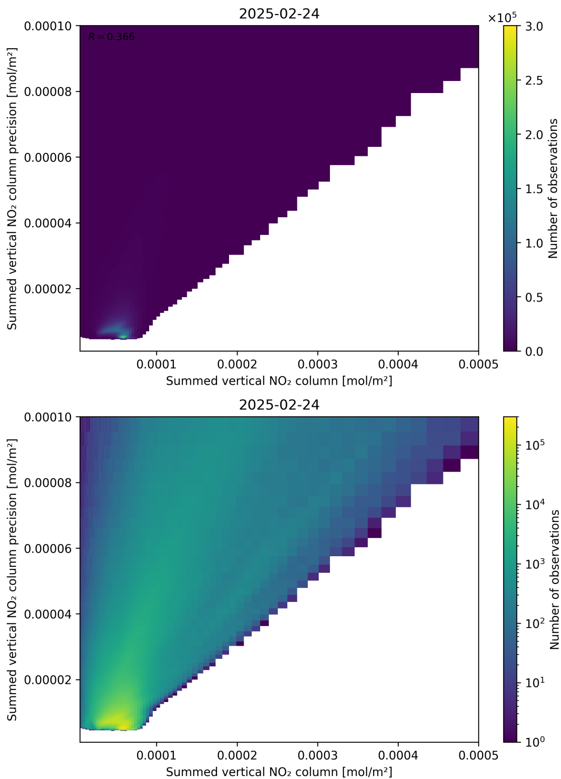
Figure 105: Scatter density plot of “Summed vertical NO 2 column” against “Summed vertical NO 2 column precision” for 2025-02-24 to 2025-02-25.
