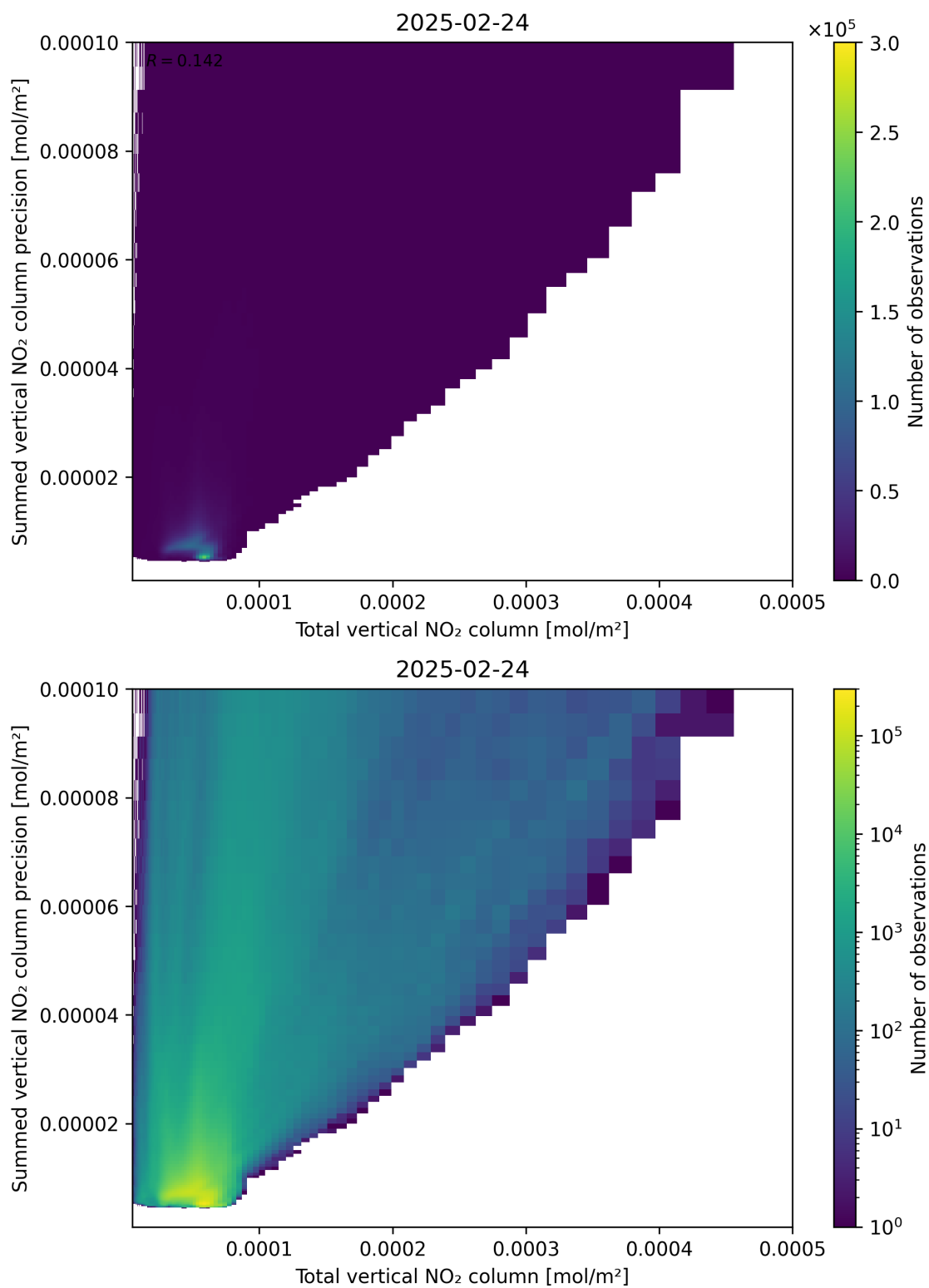
Figure 113: Scatter density plot of “Total vertical NO 2 column” against “Summed vertical NO 2 column precision” for 2025-02-24 to 2025-02-25.
