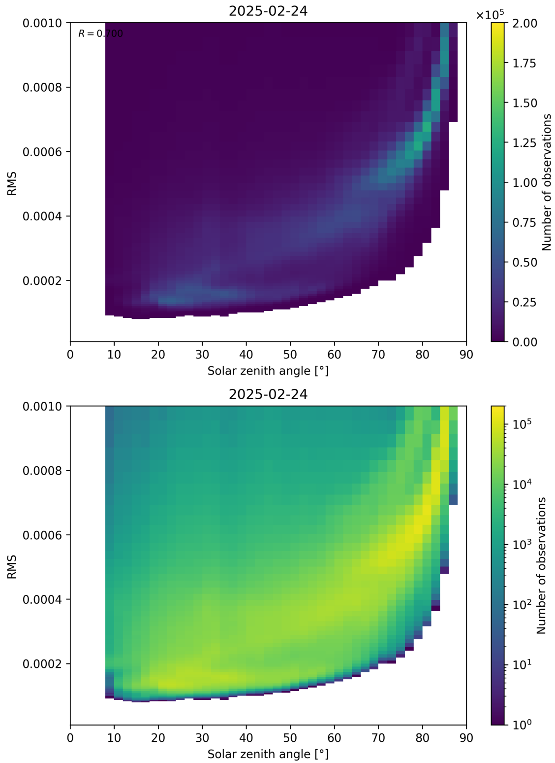
Figure 157: Scatter density plot of “Solar zenith angle” against “RMS” for 2025-02-24 to 2025-02-25.
