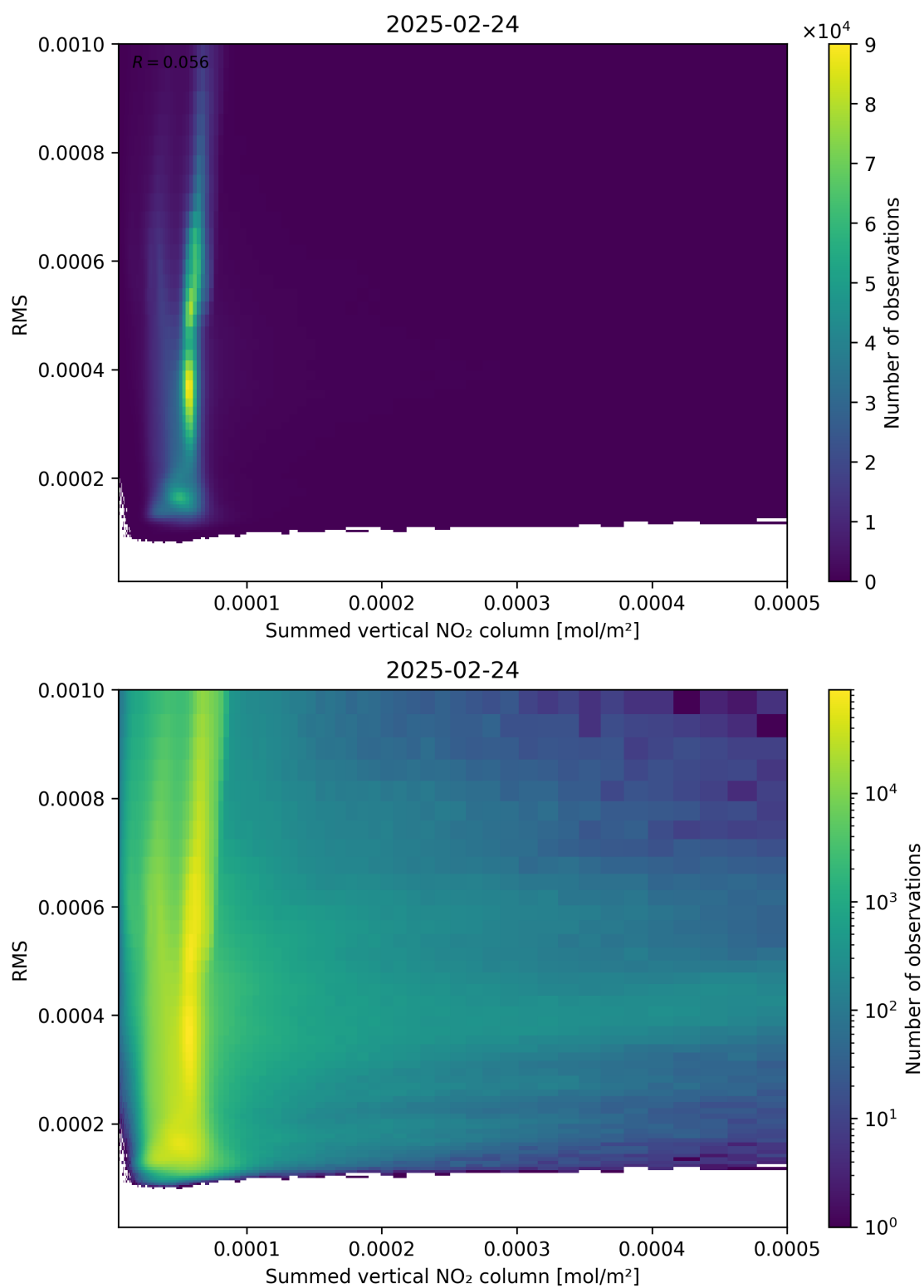
Figure 109: Scatter density plot of “Summed vertical NO 2 column” against “RMS” for 2025-02-24 to 2025-02-25.
