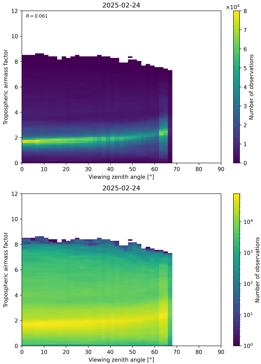
Figure 161: Scatter density plot of “Viewing zenith angle” against “Tropospheric airmass factor” for 2025-02-24 to 2025-02-25.
