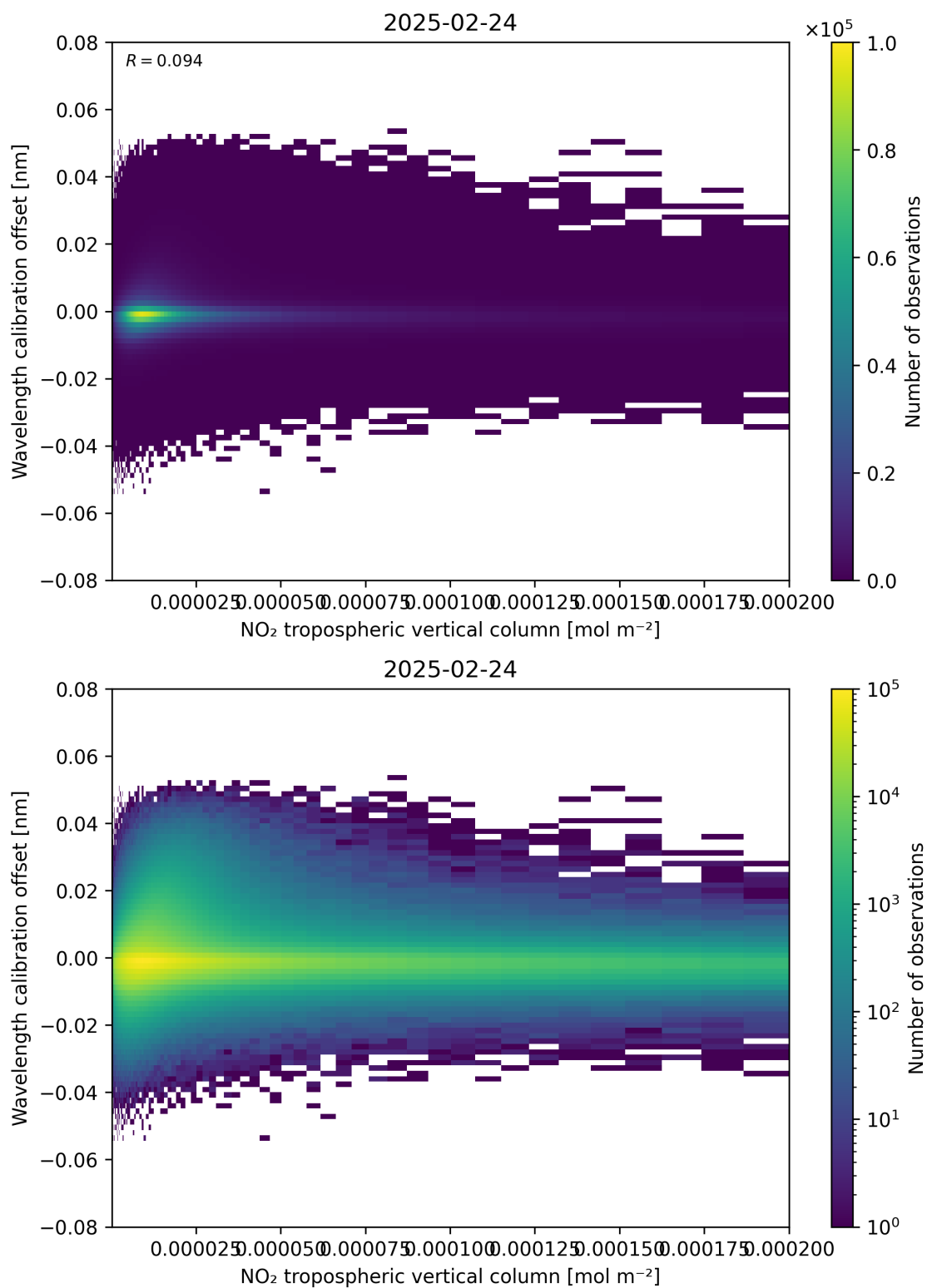
Figure 143: Scatter density plot of “NO 2 tropospheric vertical column” against “Wavelength calibration offset” for 2025-02-24 to 2025-02-25.
