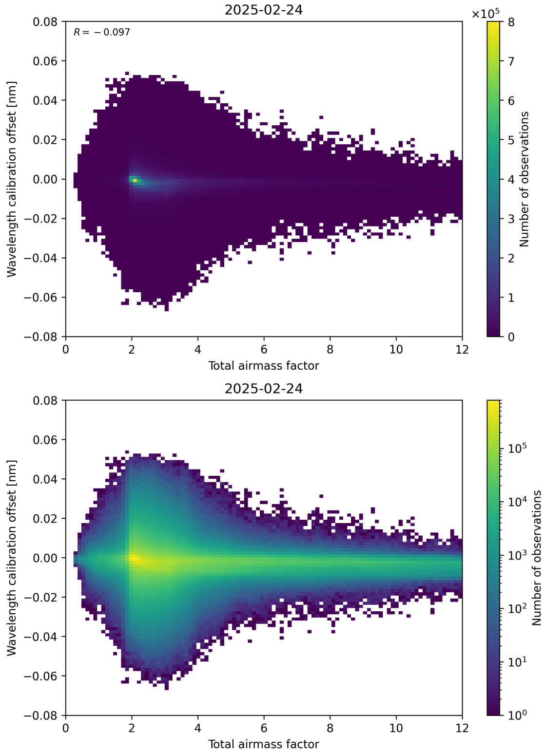
Figure 70: Scatter density plot of “Total airmass factor” against “Wavelength calibration offset” for 2025-02-24 to 2025-02-25.
