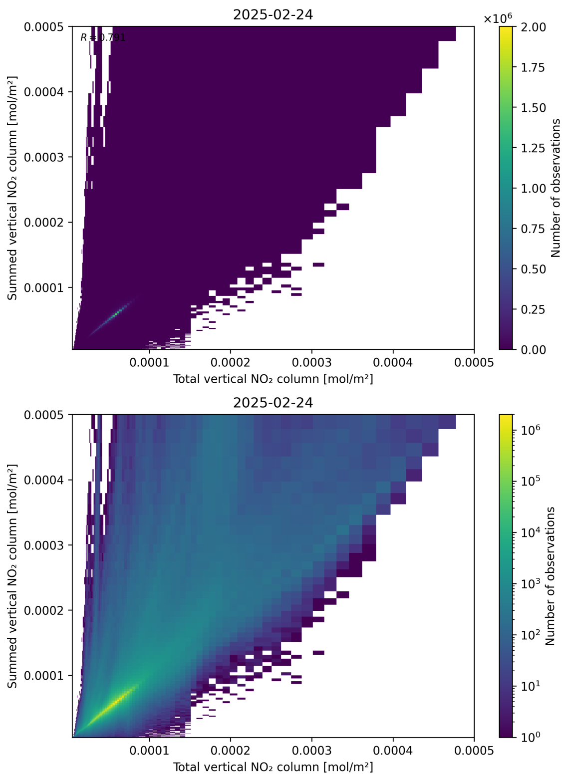
Figure 112: Scatter density plot of “Total vertical NO 2 column” against “Summed vertical NO 2 column” for 2025-02-24 to 2025-02-25.
