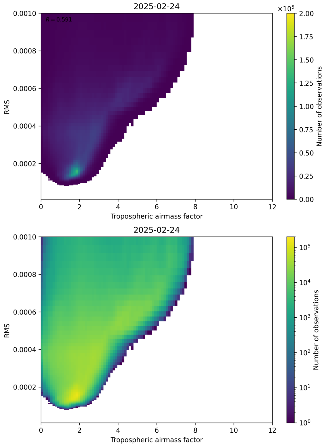
Figure 79: Scatter density plot of “Tropospheric airmass factor” against “RMS” for 2025-02-24 to 2025-02-25.
