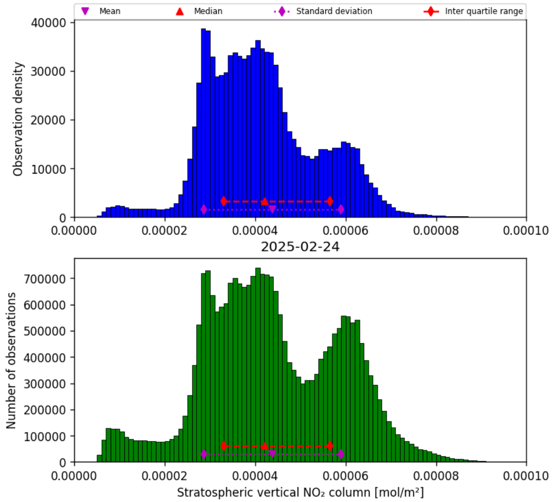
Figure 36: Histogram of “Stratospheric vertical NO 2 column” for 2025-02-24 to 2025-02-25
