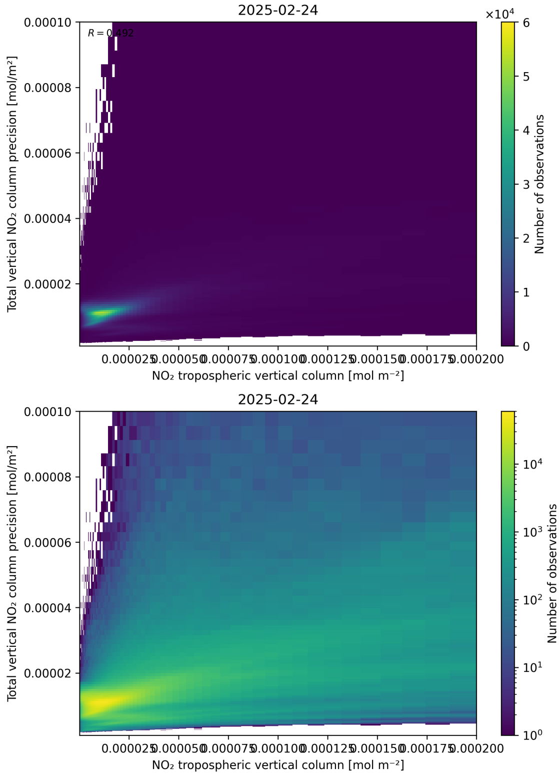
Figure 129: Scatter density plot of “NO 2 tropospheric vertical column” against “Total vertical NO 2 column precision” for 2025-02-24 to 2025-02-25.
