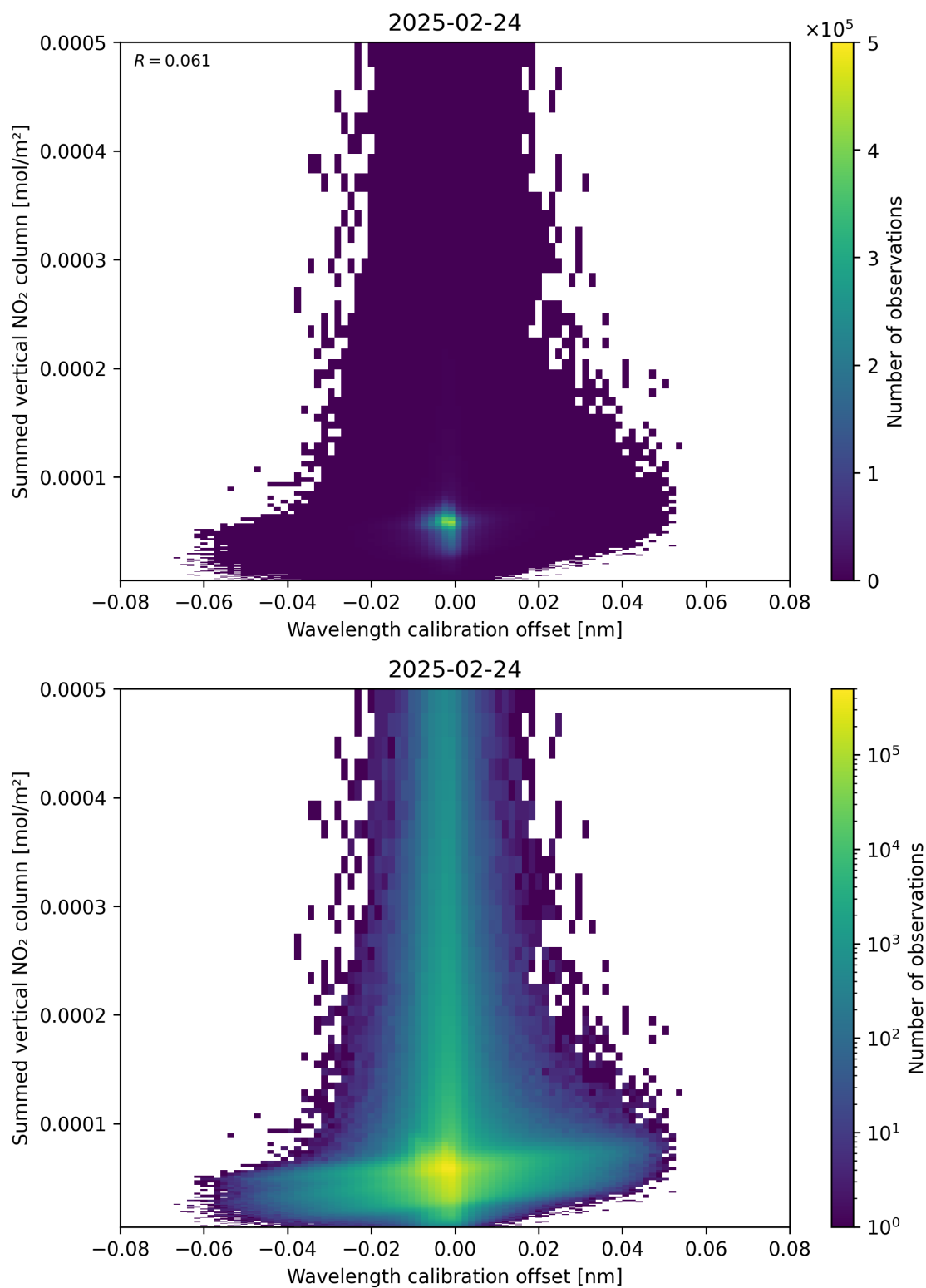
Figure 177: Scatter density plot of “Wavelength calibration offset” against “Summed vertical NO 2 column” for 2025-02-24 to 2025-02-25.
