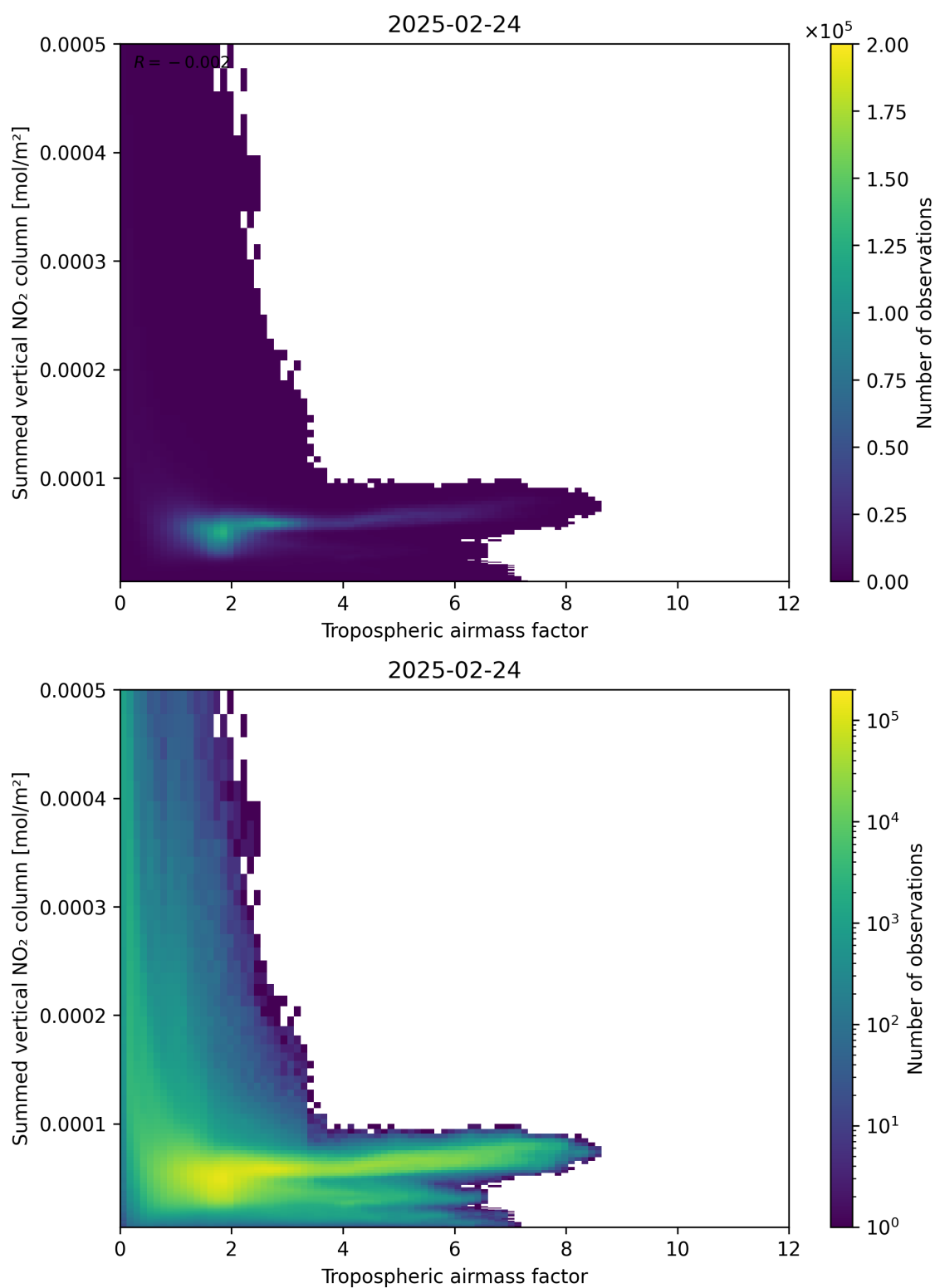
Figure 75: Scatter density plot of “Tropospheric airmass factor” against “Summed vertical NO 2 column” for 2025-02-24 to 2025-02-25.
