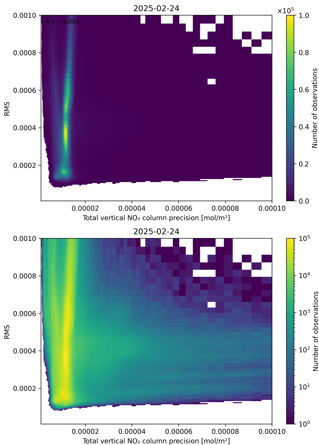
Figure 119: Scatter density plot of “Total vertical NO 2 column precision” against “RMS” for 2025-02-24 to 2025-02-25.
