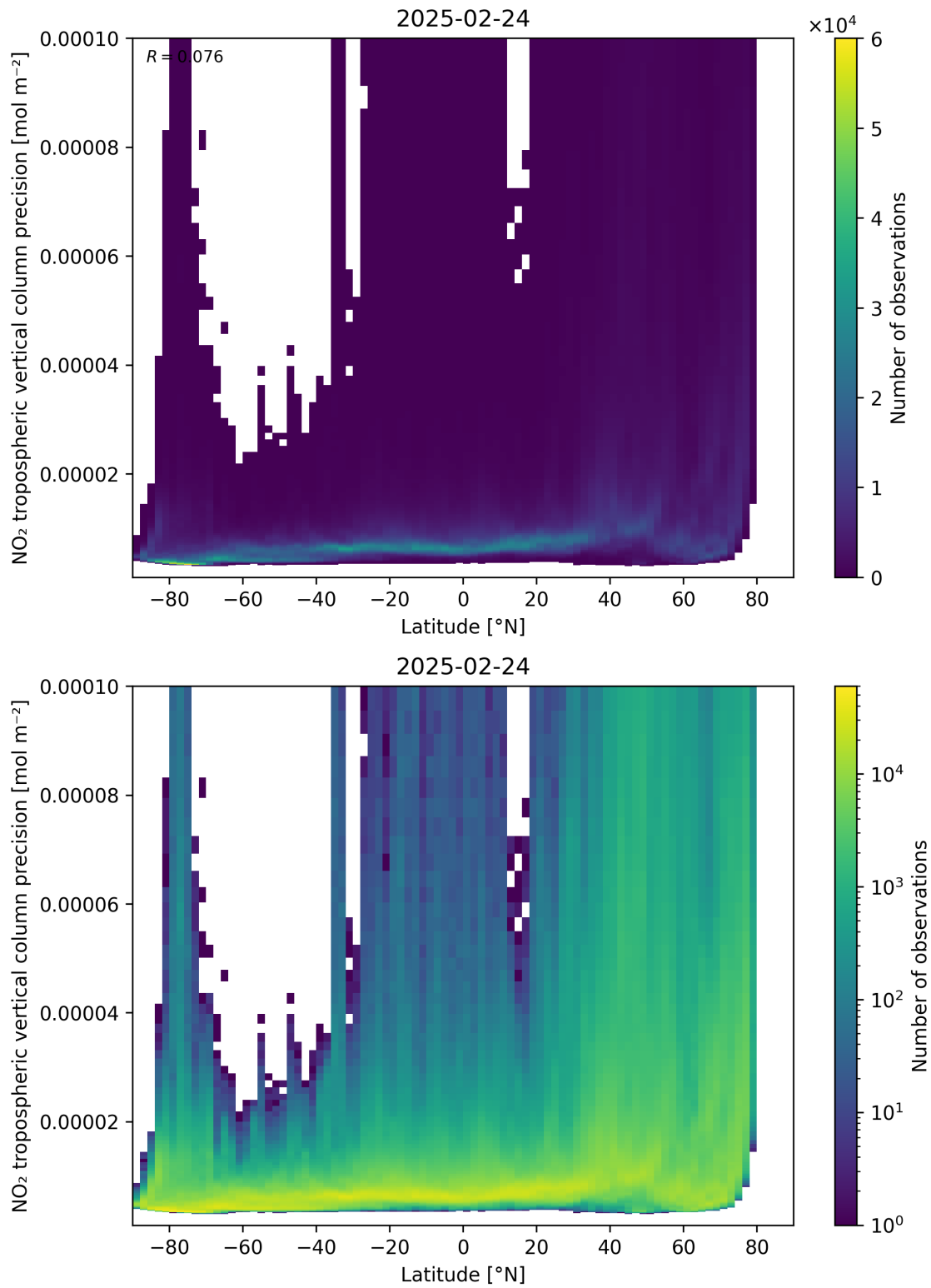
Figure 93: Scatter density plot of “Latitude” against “NO 2 tropospheric vertical column precision” for 2025-02-24 to 2025-02-25.
