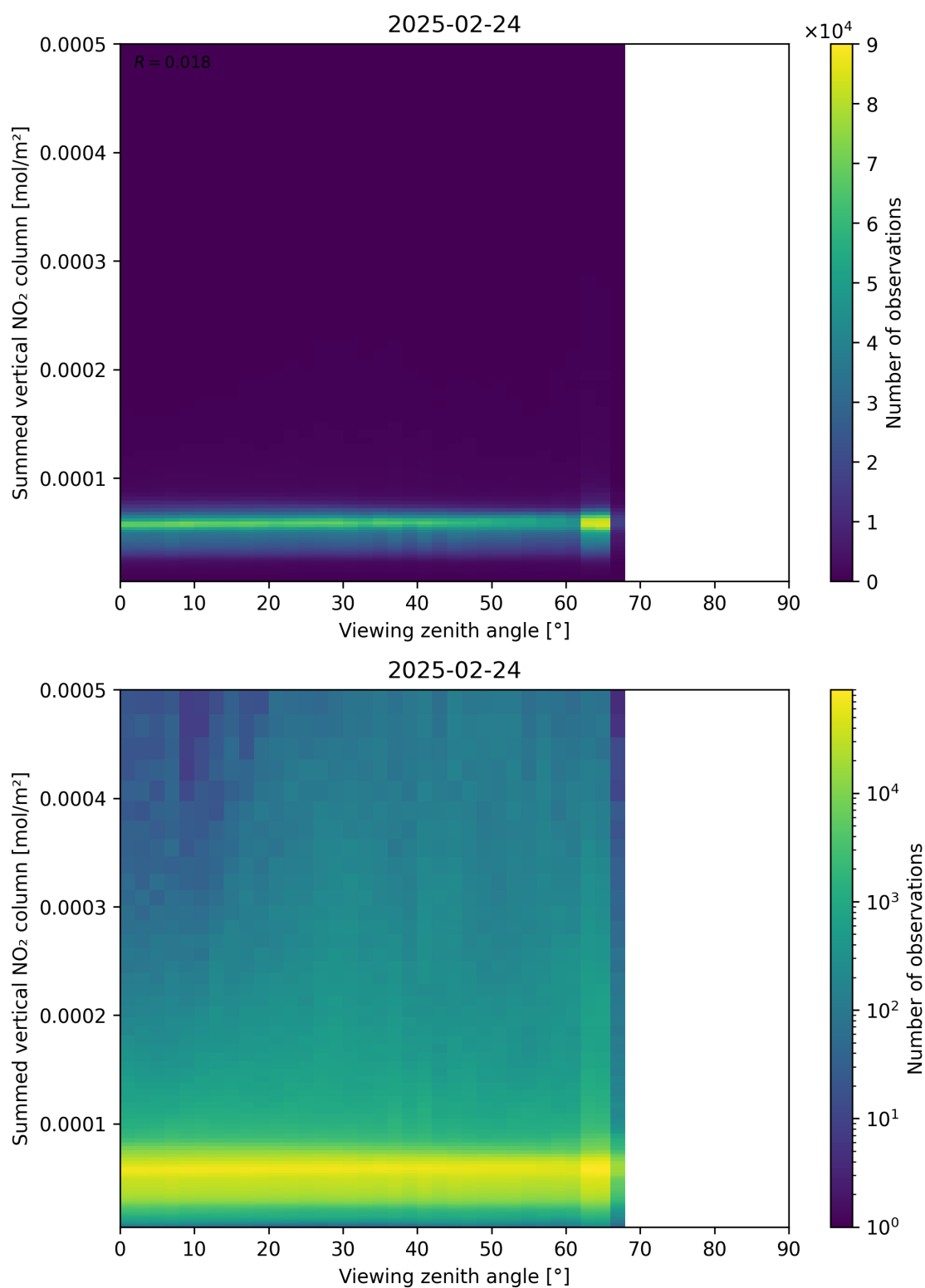
Figure 165: Scatter density plot of “Viewing zenith angle” against “Summed vertical NO 2 column” for 2025-02-24 to 2025-02-25.
