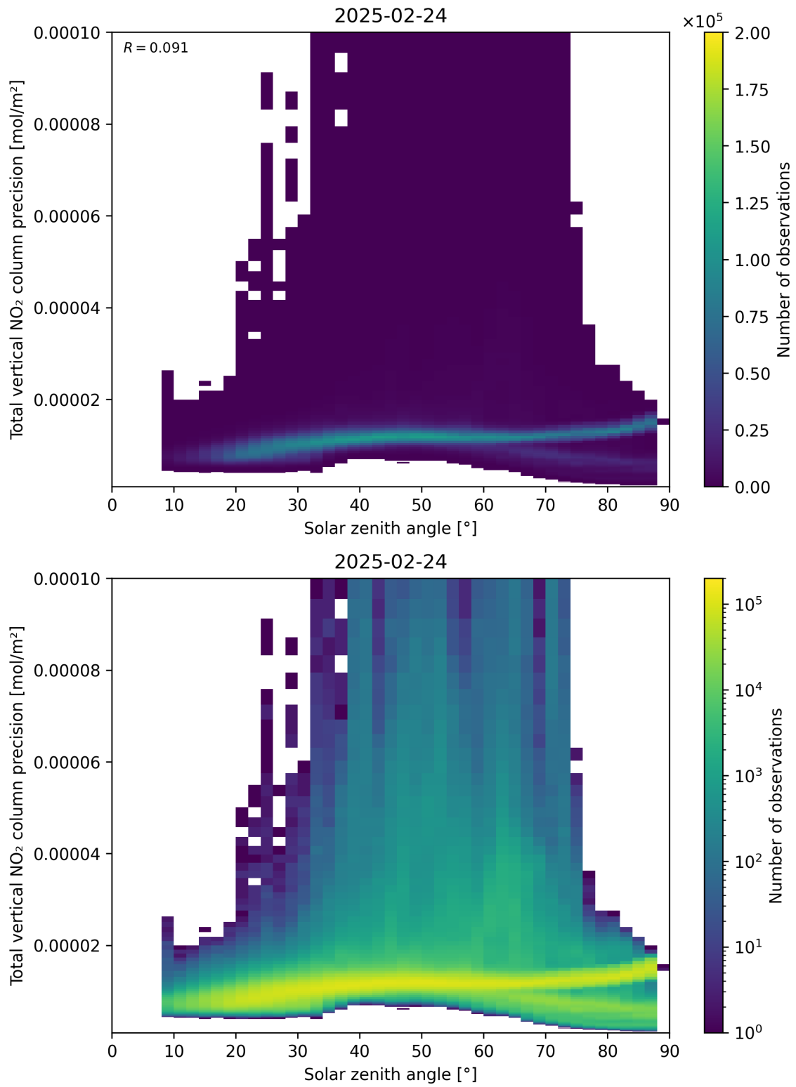
Figure 154: Scatter density plot of “Solar zenith angle” against “Total vertical NO 2 column precision” for 2025-02-24 to 2025-02-25.
