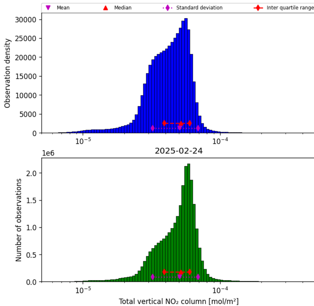
Figure 38: Histogram of “Total vertical NO 2 column” for 2025-02-24 to 2025-02-25
