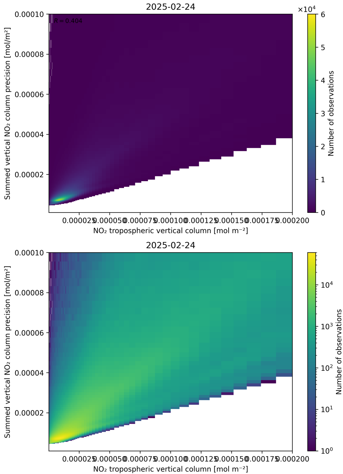
Figure 127: Scatter density plot of “NO 2 tropospheric vertical column” against “Summed vertical NO 2 column precision” for 2025-02-24 to 2025-02-25.
