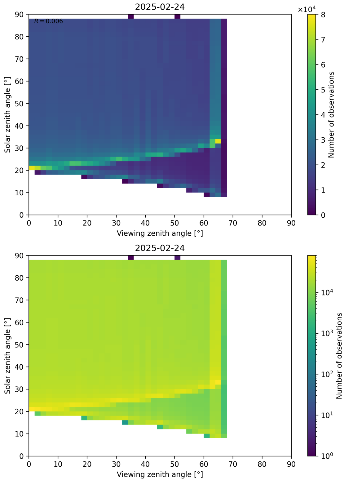
Figure 172: Scatter density plot of “Viewing zenith angle” against “Solar zenith angle” for 2025-02-24 to 2025-02-25.
