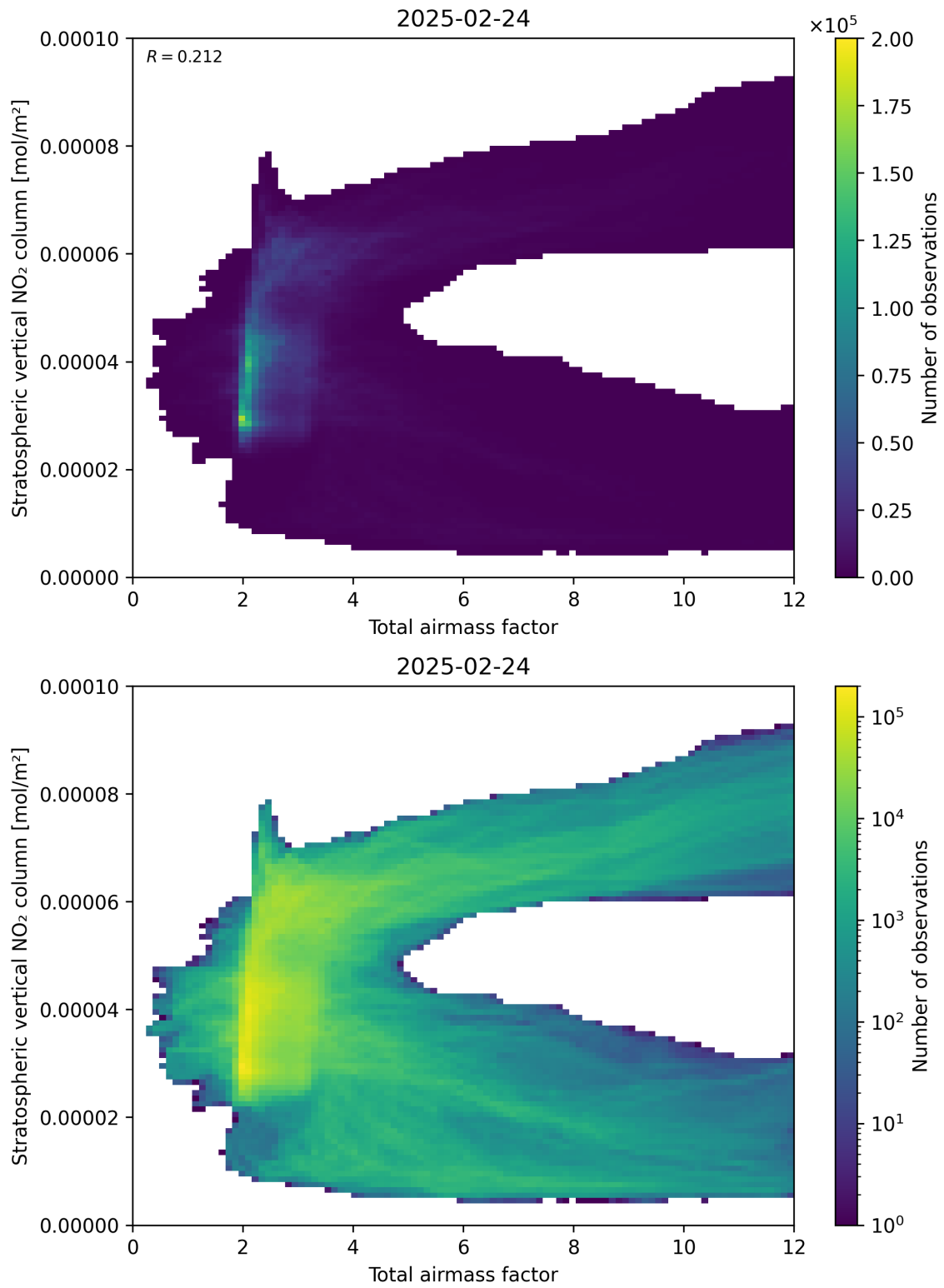
Figure 64: Scatter density plot of “Total airmass factor” against “Stratospheric vertical NO 2 column” for 2025-02-24 to 2025-02-25.
