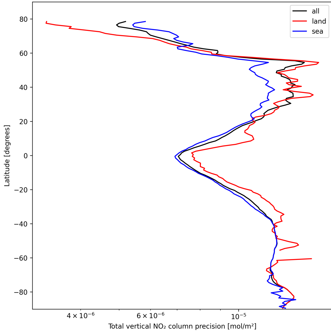
Figure 22: Zonal average of “Total vertical NO 2 column precision” for 2025-02-24 to 2025-02-25.
