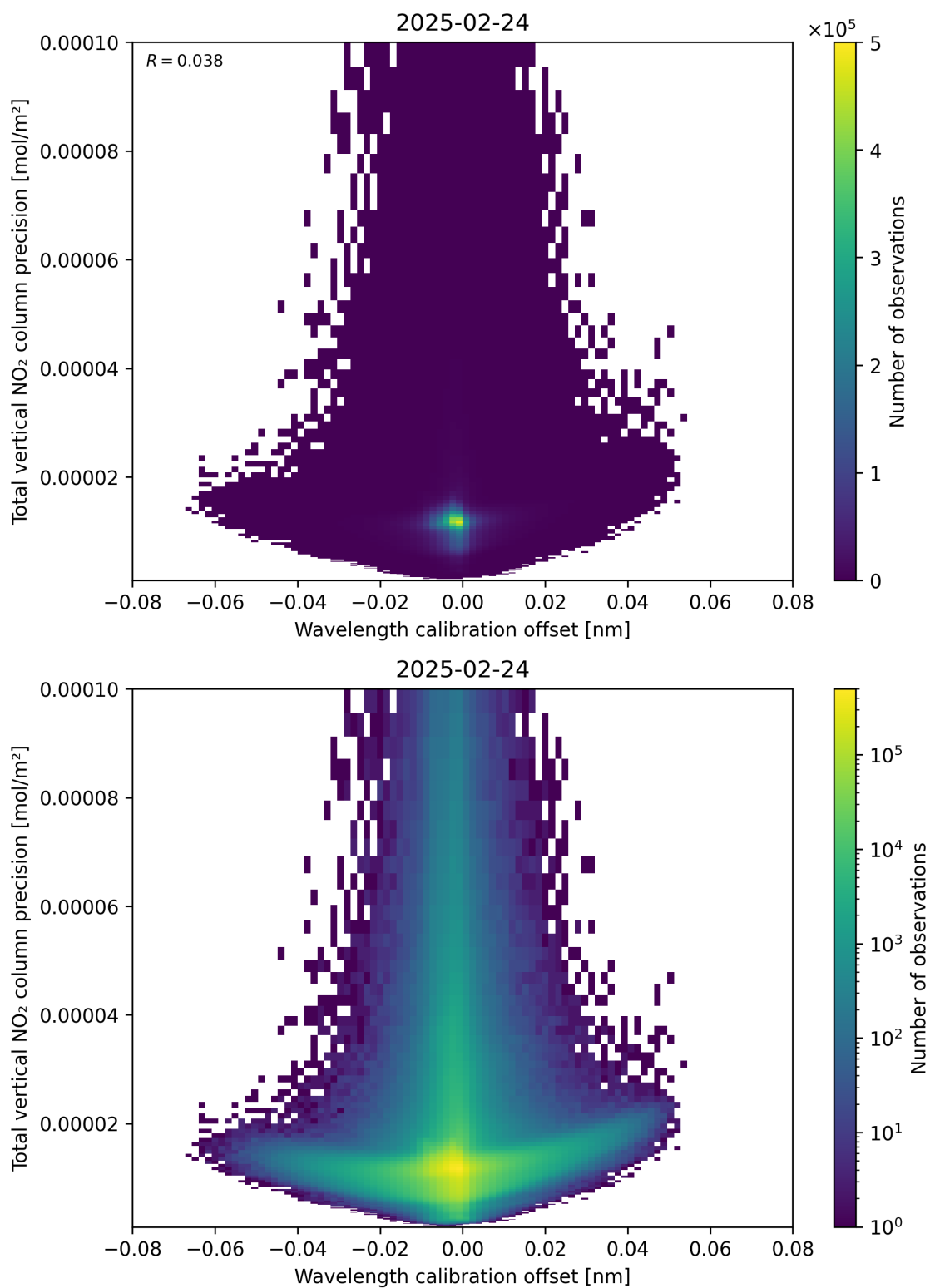
Figure 180: Scatter density plot of “Wavelength calibration offset” against “Total vertical NO 2 column precision” for 2025-02-24 to 2025-02-25.
