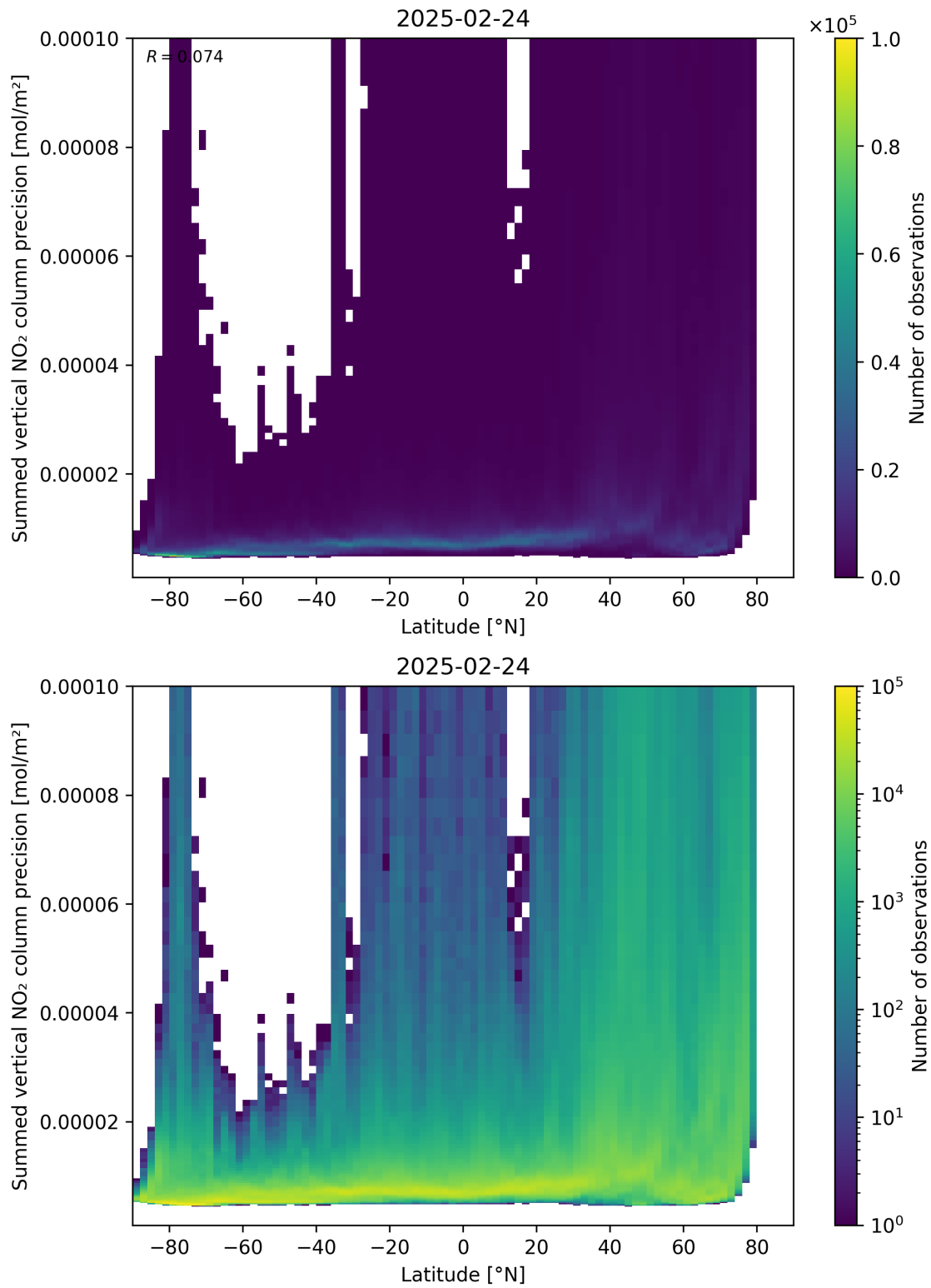
Figure 89: Scatter density plot of “Latitude” against “Summed vertical NO 2 column precision” for 2025-02-24 to 2025-02-25.
