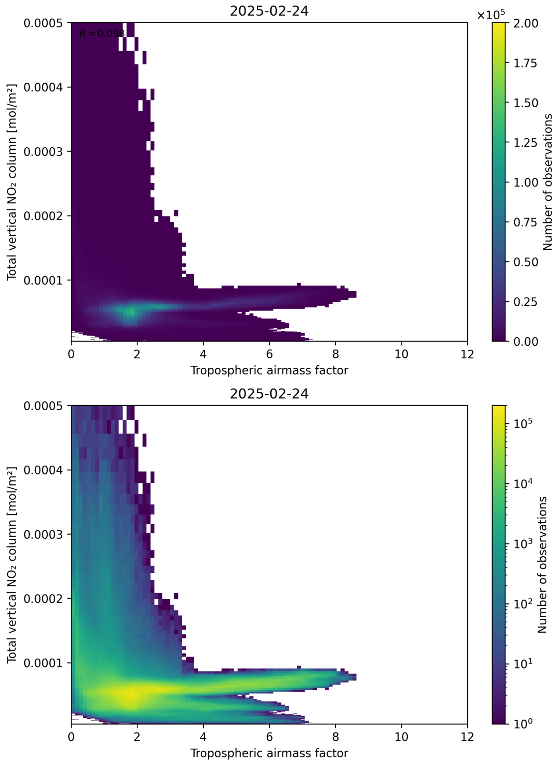
Figure 77: Scatter density plot of “Tropospheric airmass factor” against “Total vertical NO 2 column” for 2025-02-24 to 2025-02-25.
