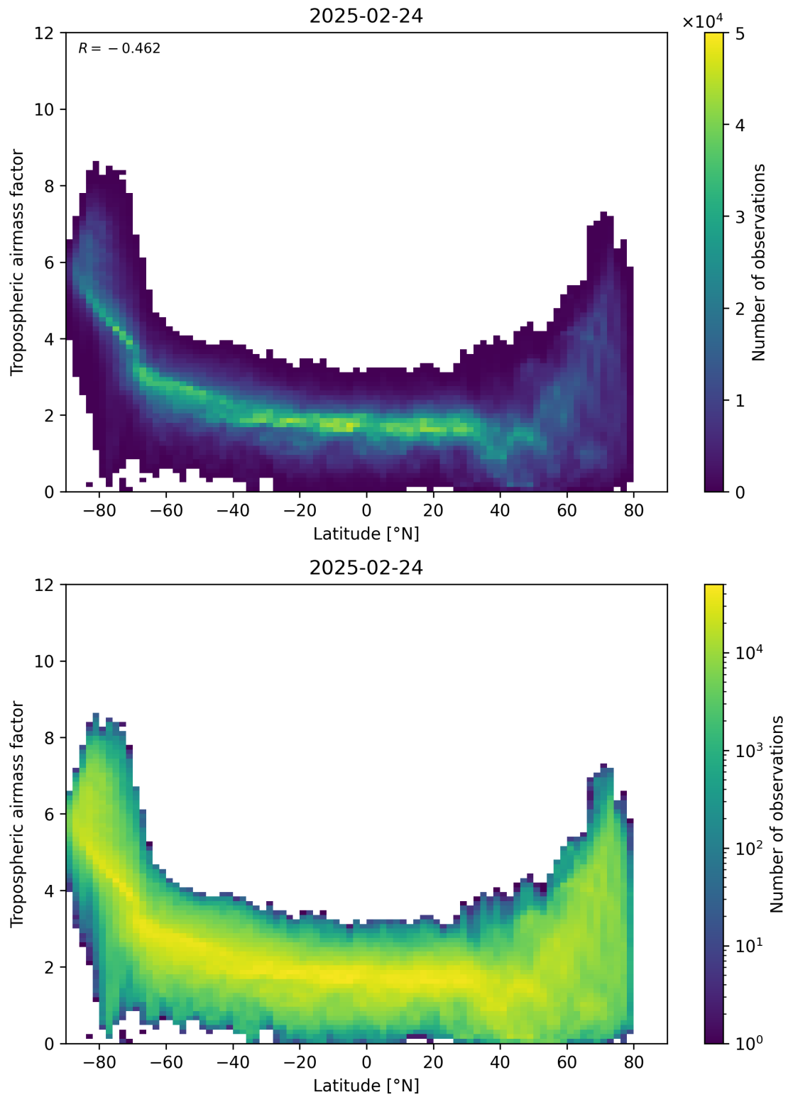
Figure 85: Scatter density plot of “Latitude” against “Tropospheric airmass factor” for 2025-02-24 to 2025-02-25.
