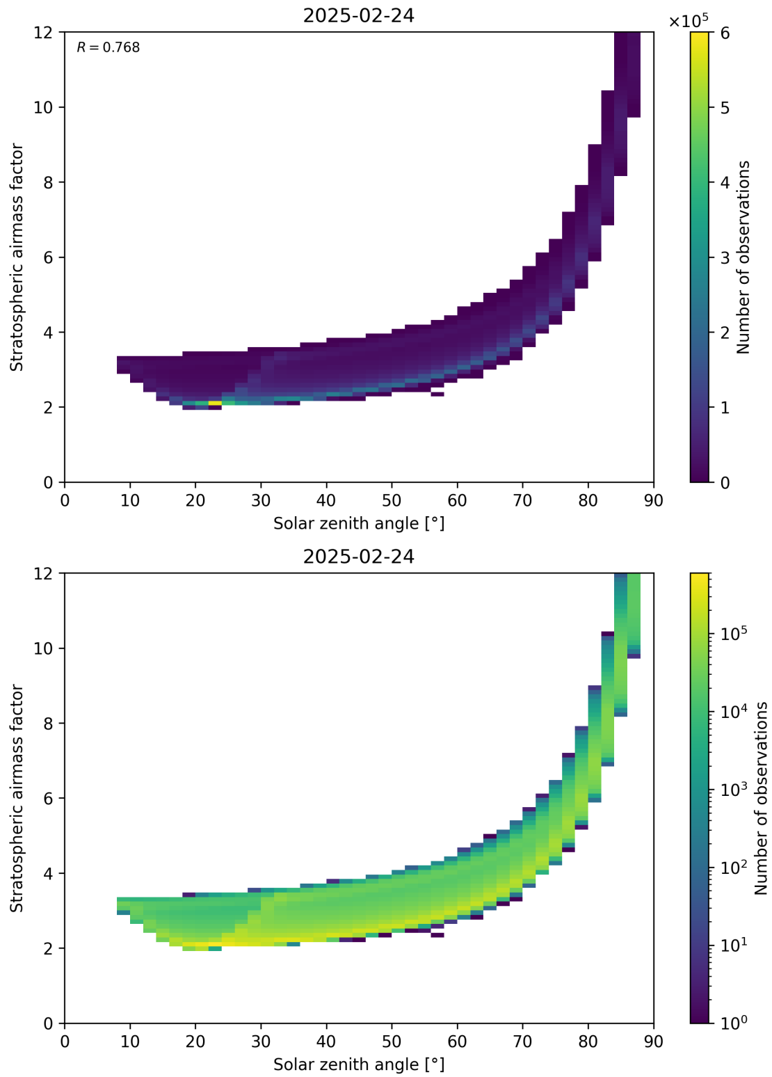
Figure 145: Scatter density plot of “Solar zenith angle” against “Stratospheric airmass factor” for 2025-02-24 to 2025-02-25.
