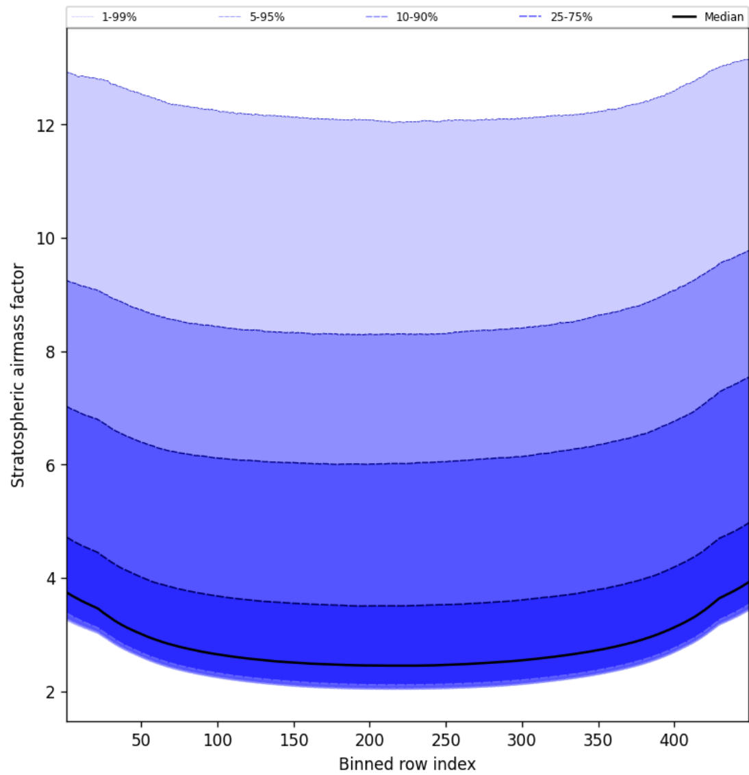
Figure 61: Along track statistics of “Stratospheric air mass factor” for 2025-02-24 to 2025-02-25
