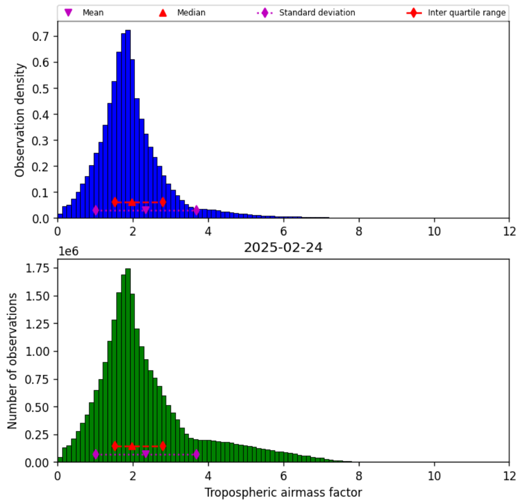
Figure 31: Histogram of “Tropospheric airmass factor” for 2025-02-24 to 2025-02-25
