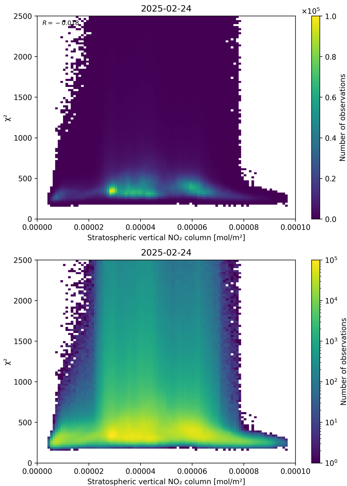
Figure 97: Scatter density plot of “Stratospheric vertical NO 2 column” against “ \chi^2 ” for 2025-02-24 to 2025-02-25.
