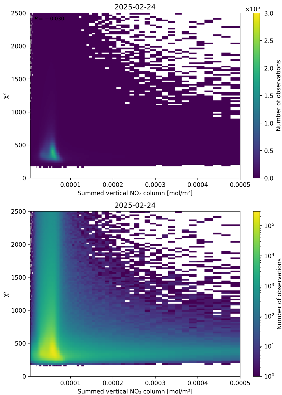
Figure 104: Scatter density plot of “Summed vertical NO 2 column” against “ \chi^2 ” for 2025-02-24 to 2025-02-25.
