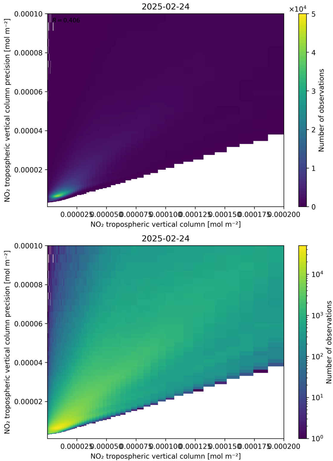
Figure 130: Scatter density plot of “NO 2 tropospheric vertical column” against “NO 2 tropospheric vertical column precision” for 2025-02-24 to 2025-02-25.
