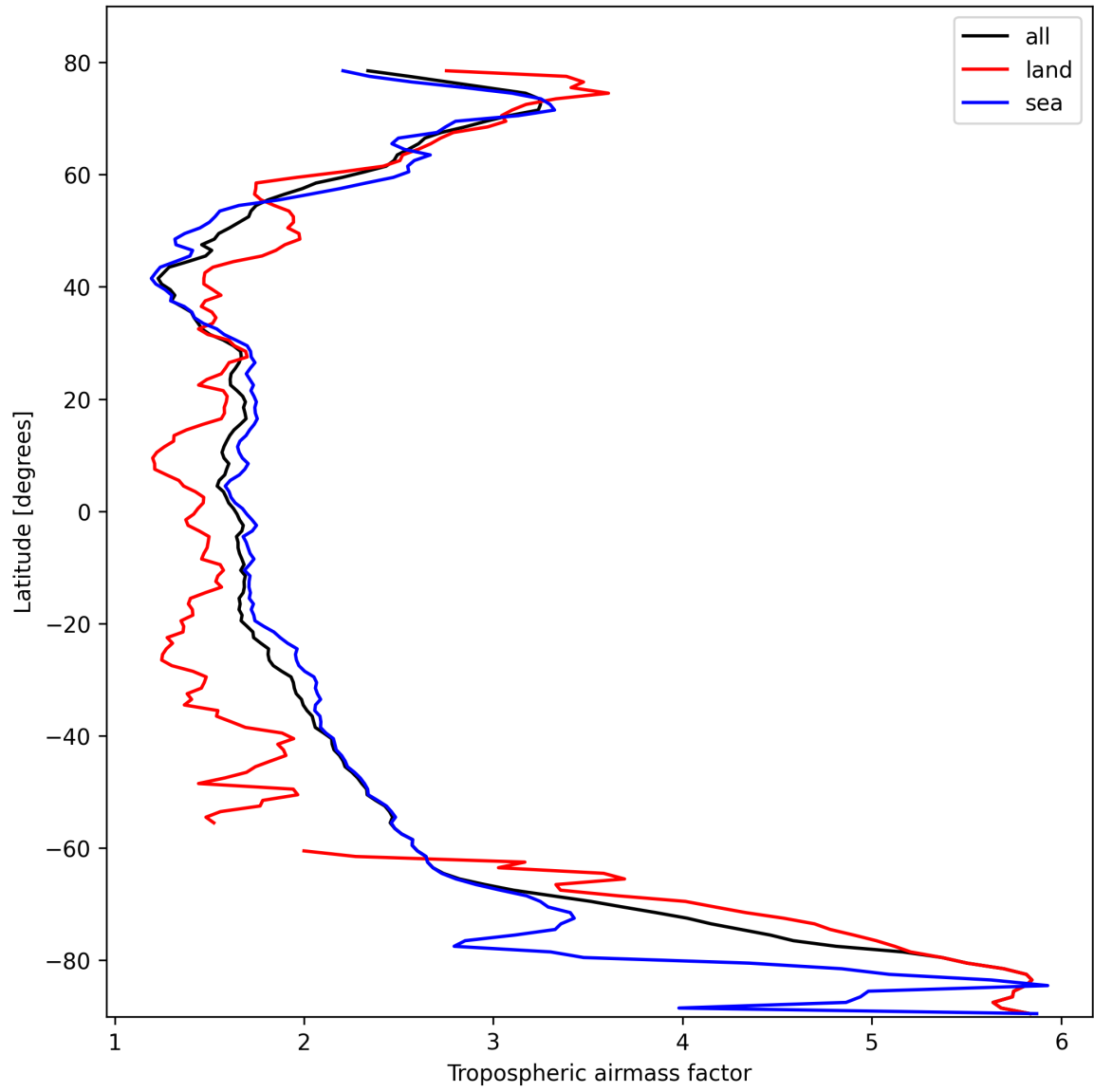
Figure 14: Zonal average of “Tropospheric airmass factor” for 2025-02-24 to 2025-02-25.
