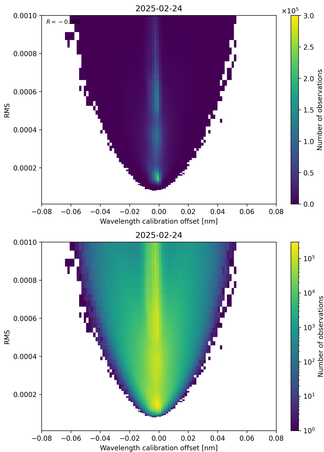
Figure 181: Scatter density plot of “Wavelength calibration offset” against “RMS” for 2025-02-24 to 2025-02-25.
