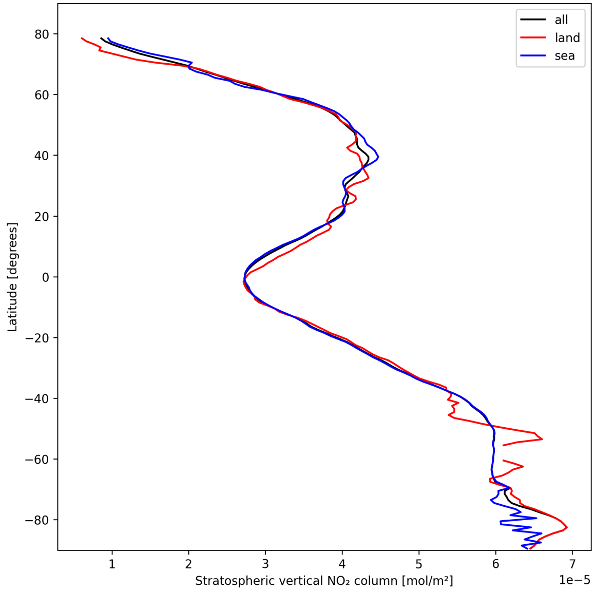
Figure 19: Zonal average of “Stratospheric vertical NO 2 column” for 2025-02-24 to 2025-02-25.
