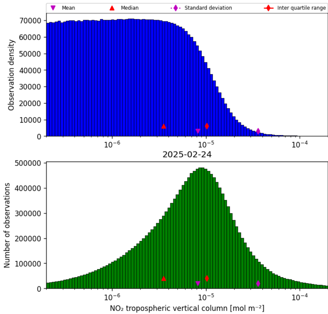
Figure 29: Histogram of “NO 2 tropospheric vertical column” for 2025-02-24 to 2025-02-25
