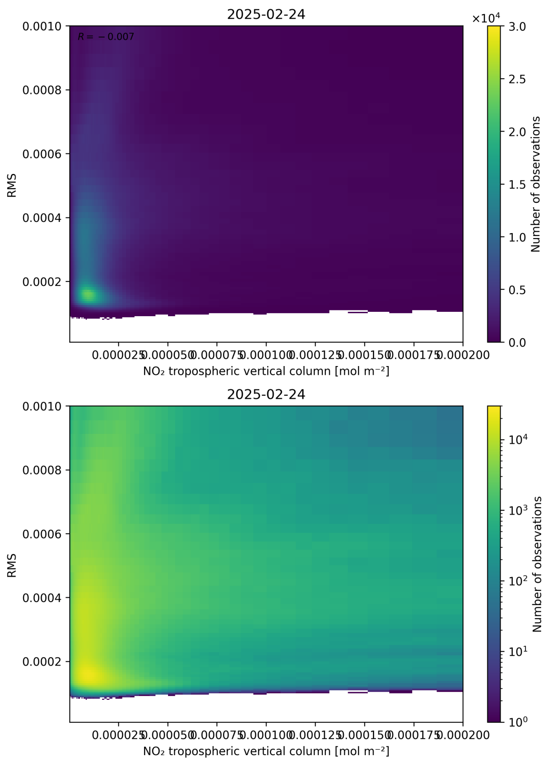
Figure 142: Scatter density plot of “NO 2 tropospheric vertical column” against “RMS” for 2025-02-24 to 2025-02-25.
