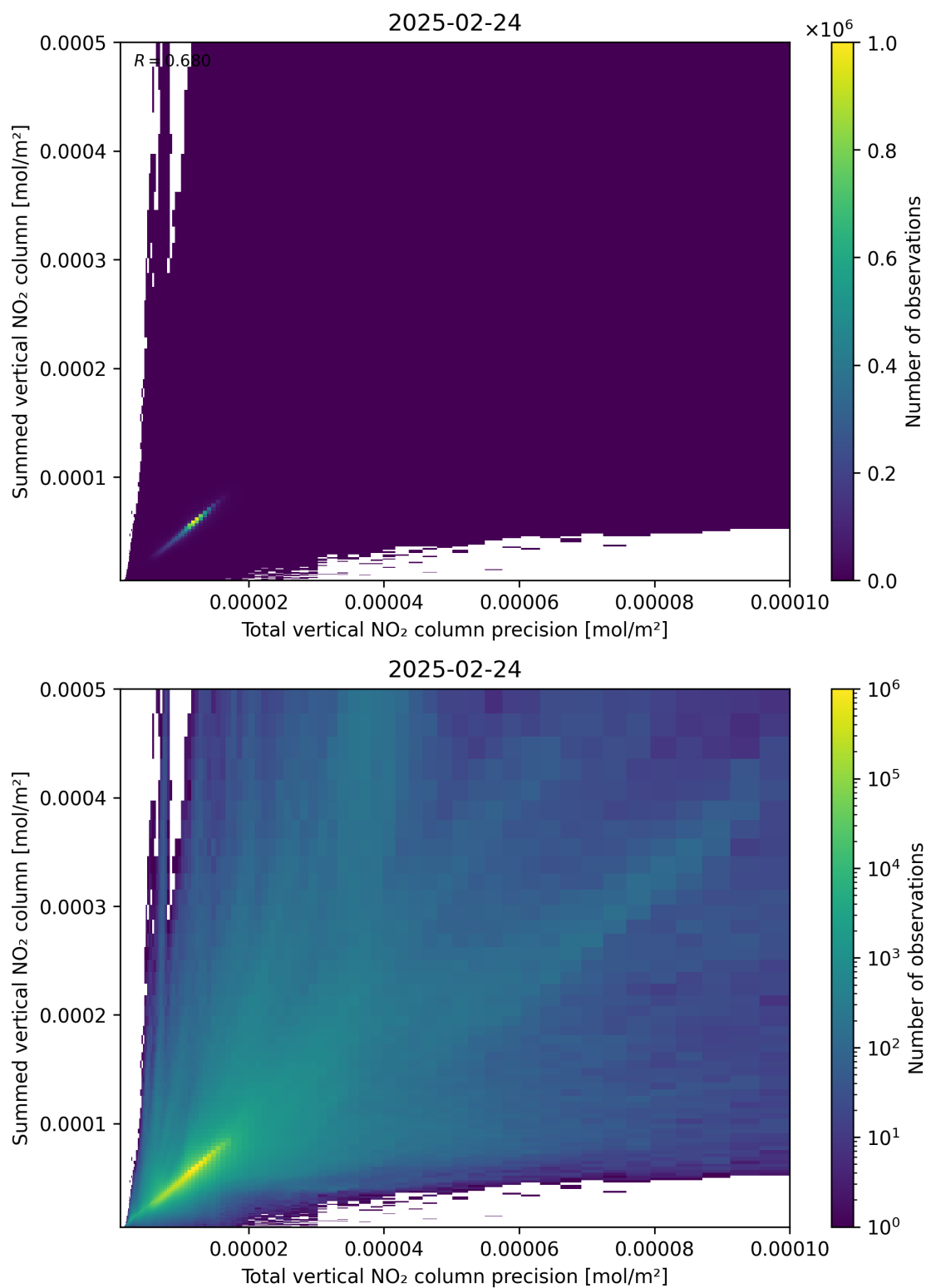
Figure 117: Scatter density plot of “Total vertical NO 2 column precision” against “Summed vertical NO 2 column” for 2025-02-24 to 2025-02-25.
