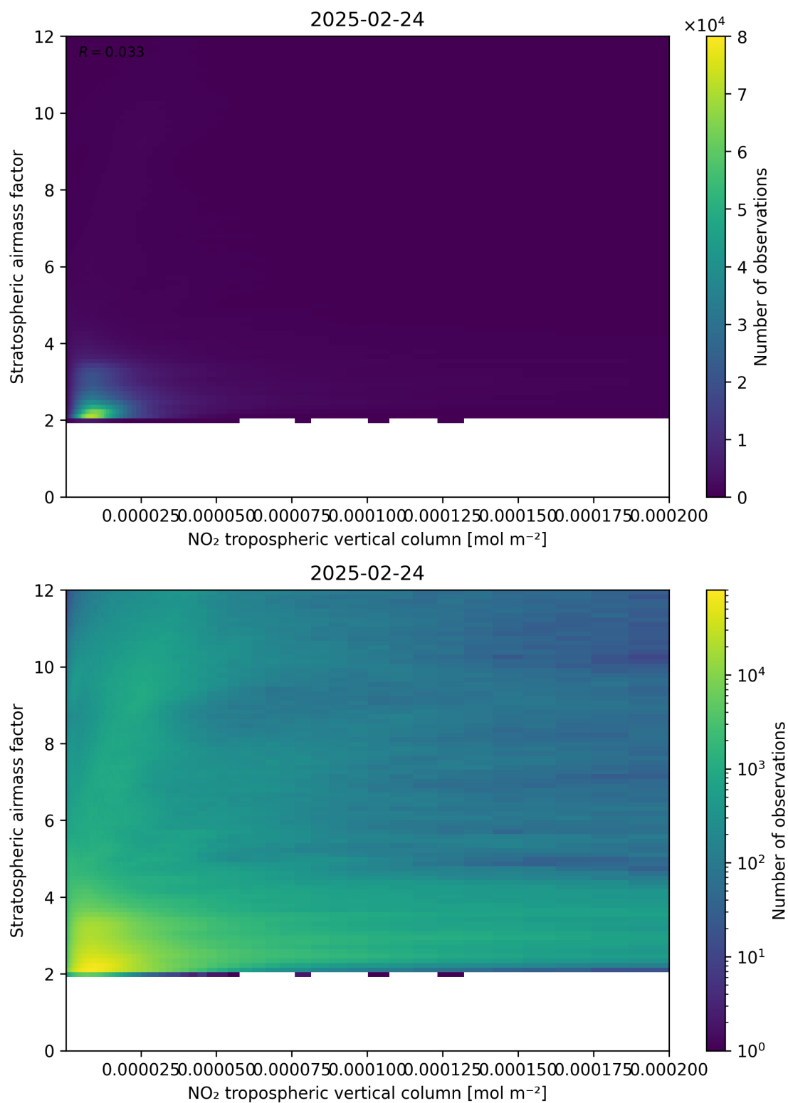
Figure 121: Scatter density plot of “NO 2 tropospheric vertical column” against “Stratospheric airmass factor” for 2025-02-24 to 2025-02-25.
