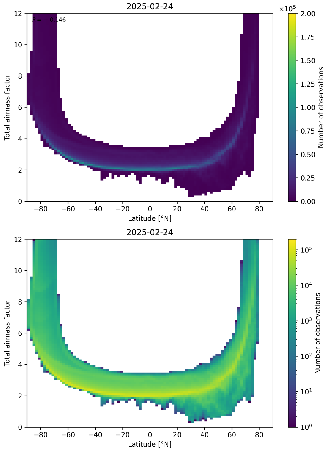
Figure 84: Scatter density plot of “Latitude” against “Total airmass factor” for 2025-02-24 to 2025-02-25.
