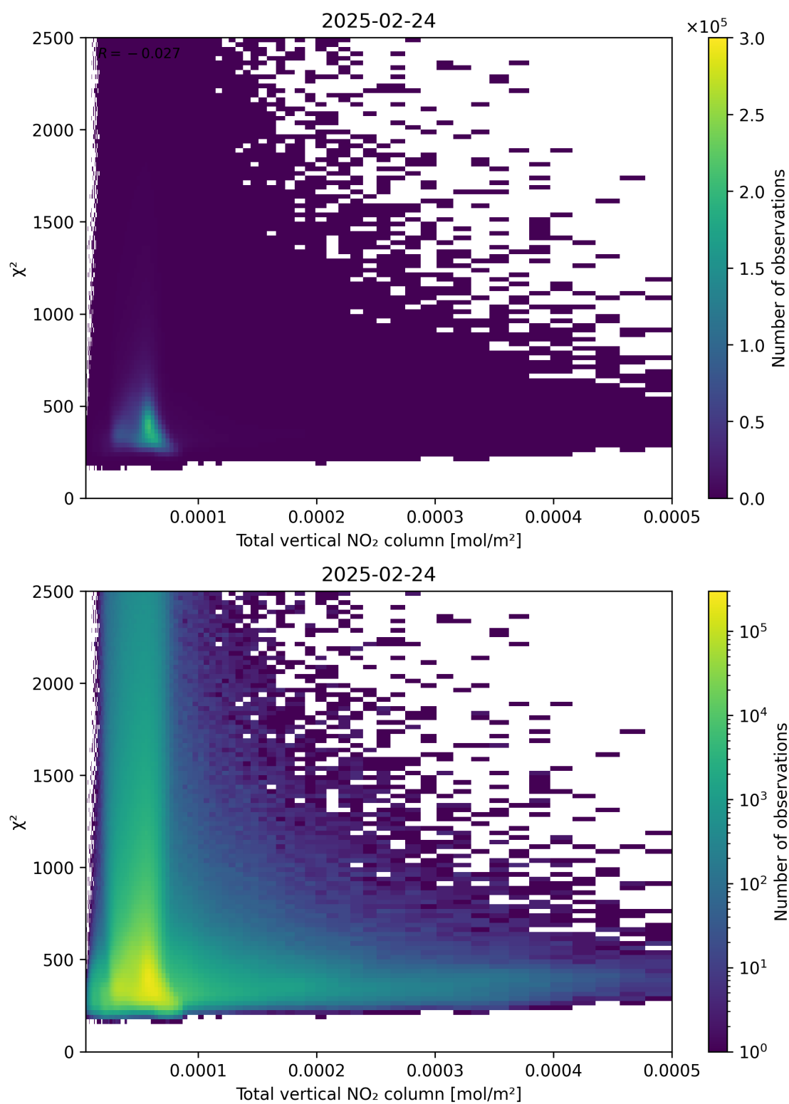
Figure 111: Scatter density plot of “Total vertical NO 2 column” against “ \chi^2 ” for 2025-02-24 to 2025-02-25.
