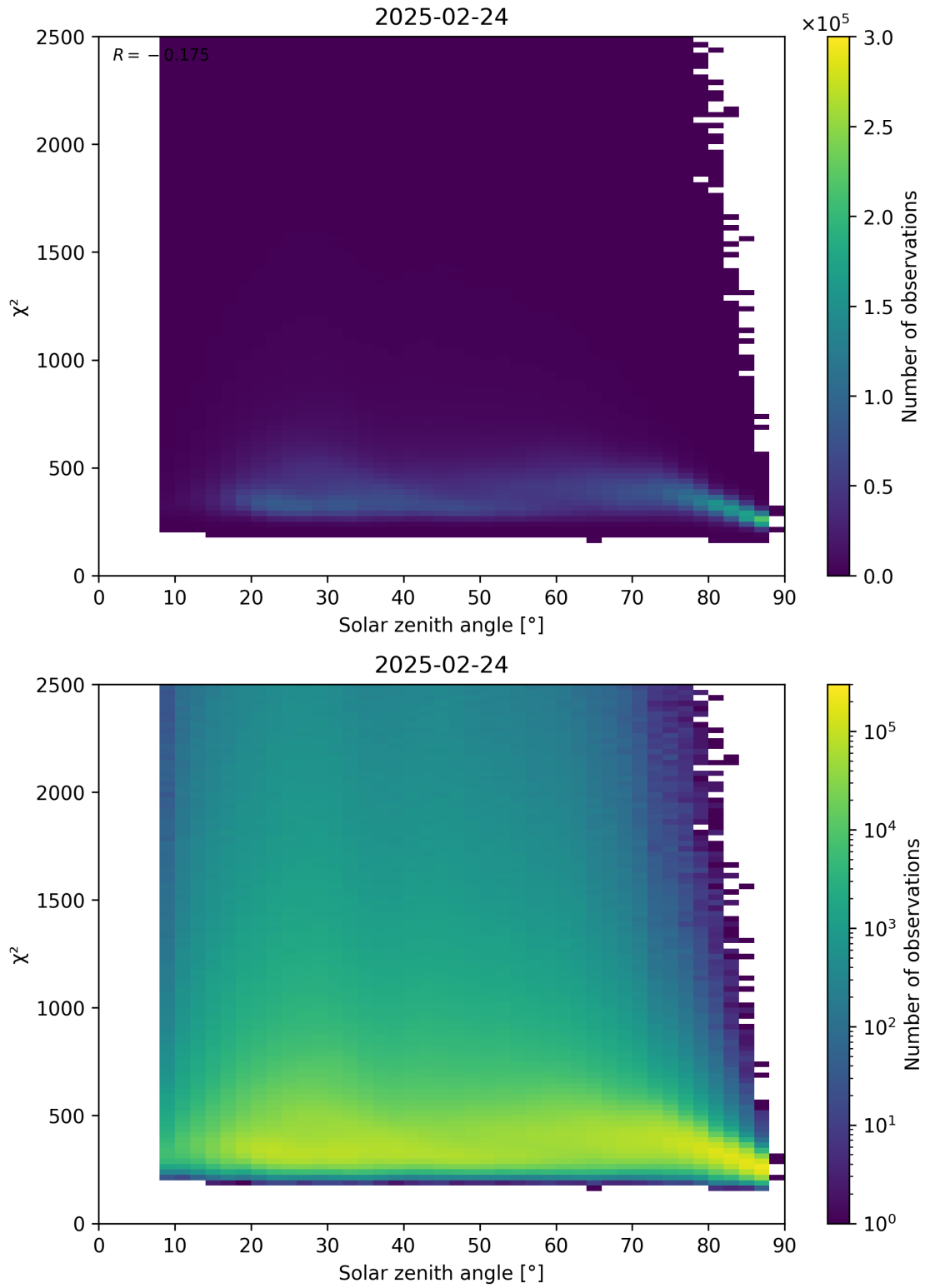
Figure 148: Scatter density plot of “Solar zenith angle” against “ \chi^2 ” for 2025-02-24 to 2025-02-25.
