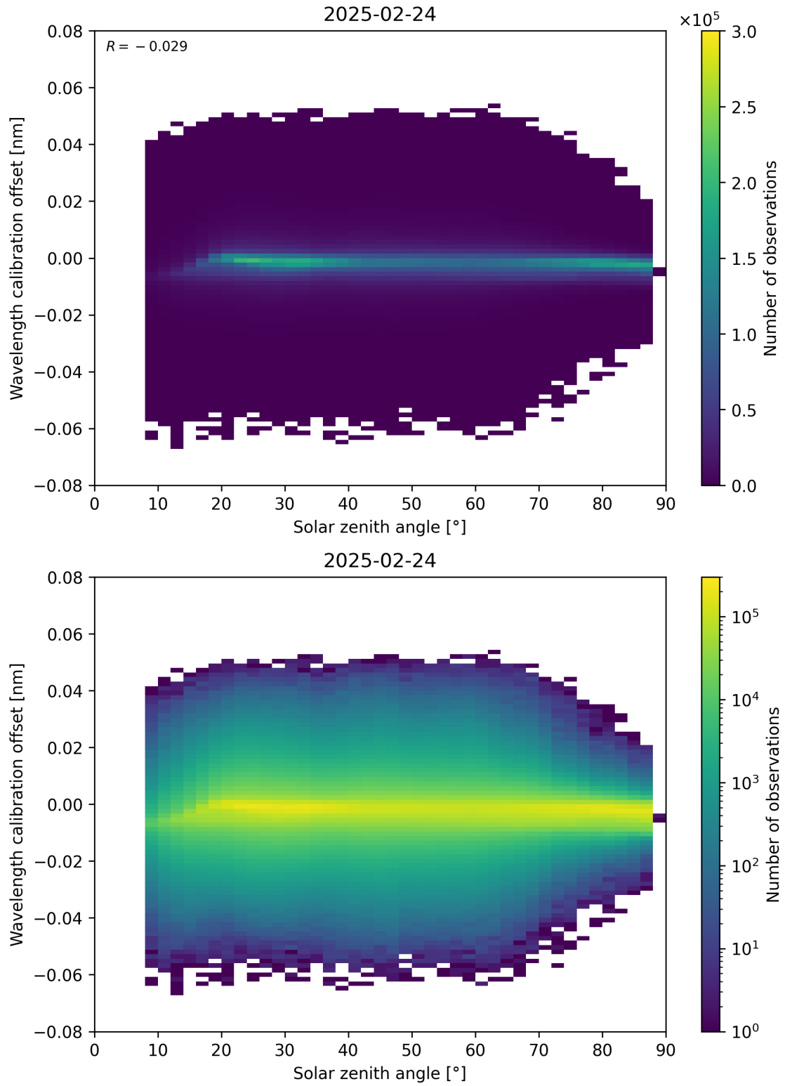
Figure 158: Scatter density plot of “Solar zenith angle” against “Wavelength calibration offset” for 2025-02-24 to 2025-02-25.
