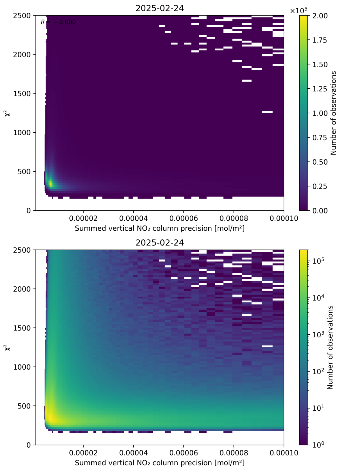
Figure 107: Scatter density plot of “Summed vertical NO 2 column precision” against “ \chi^2 ” for 2025-02-24 to 2025-02-25.
