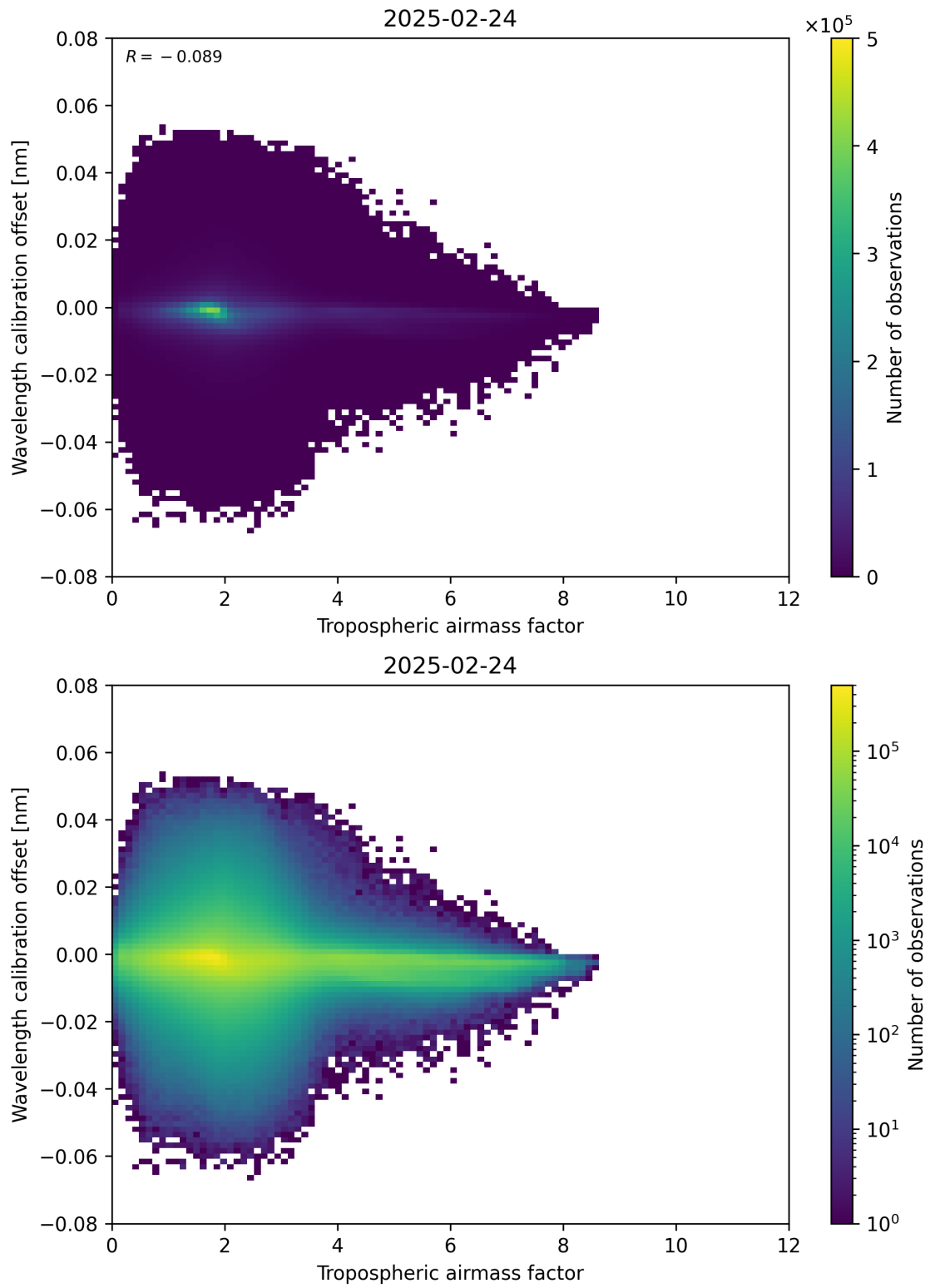
Figure 80: Scatter density plot of “Tropospheric airmass factor” against “Wavelength calibration offset” for 2025-02-24 to 2025-02-25.
