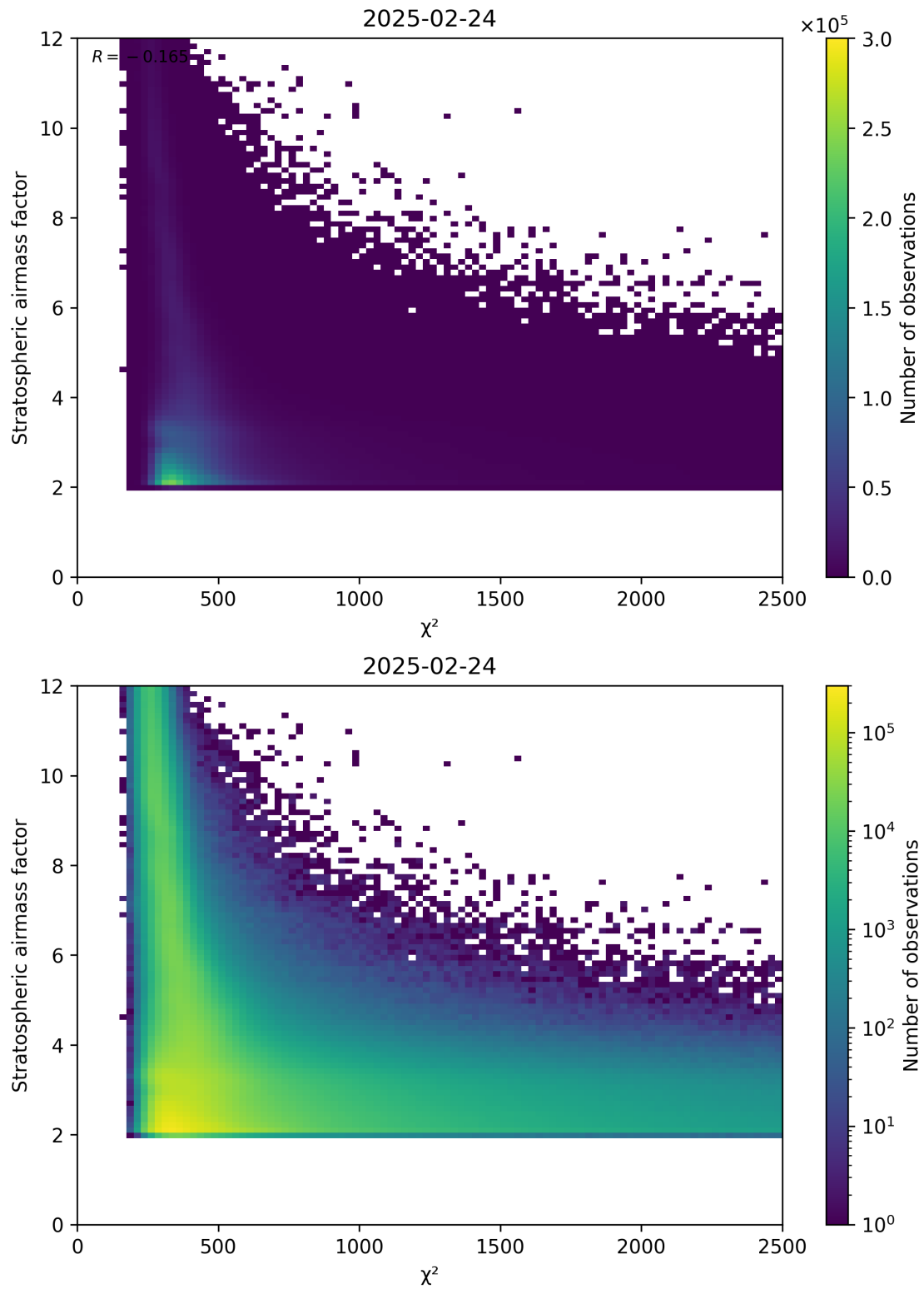
Figure 81: Scatter density plot of “ \chi^2 ” against “Stratospheric airmass factor” for 2025-02-24 to 2025-02-25.
