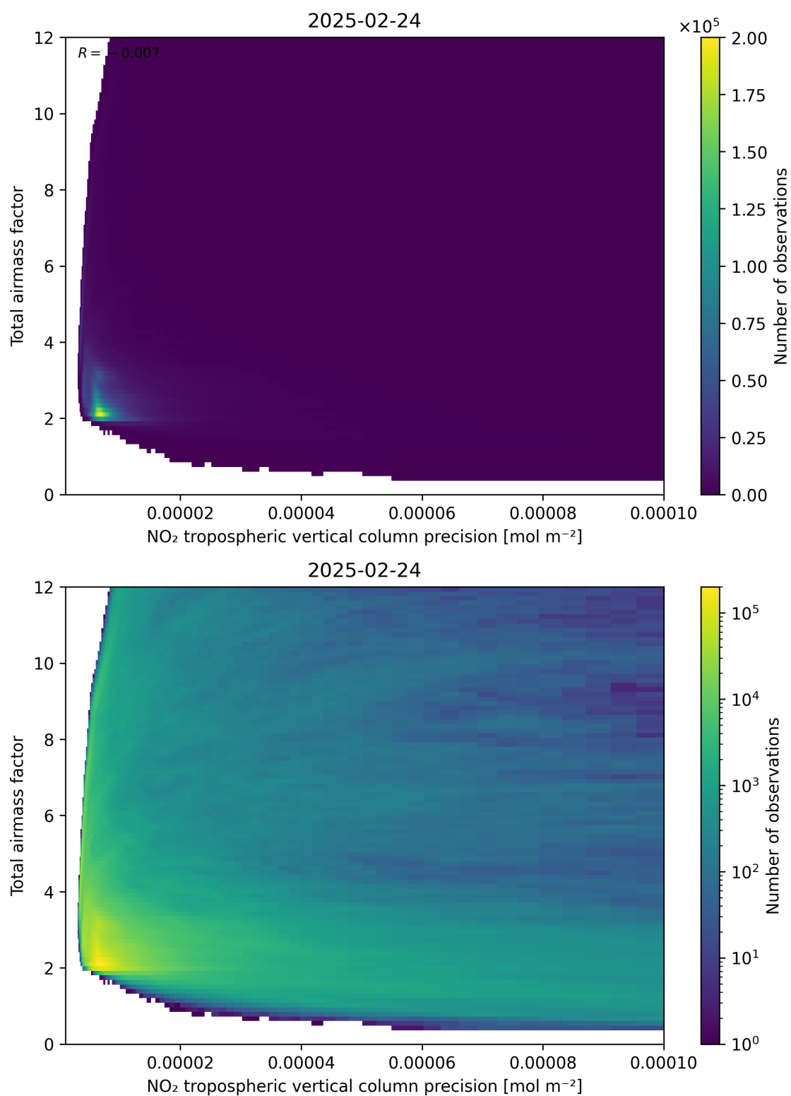
Figure 132: Scatter density plot of “NO 2 tropospheric vertical column precision” against “Total air mass factor” for 2025-02-24 to 2025-02-25.
