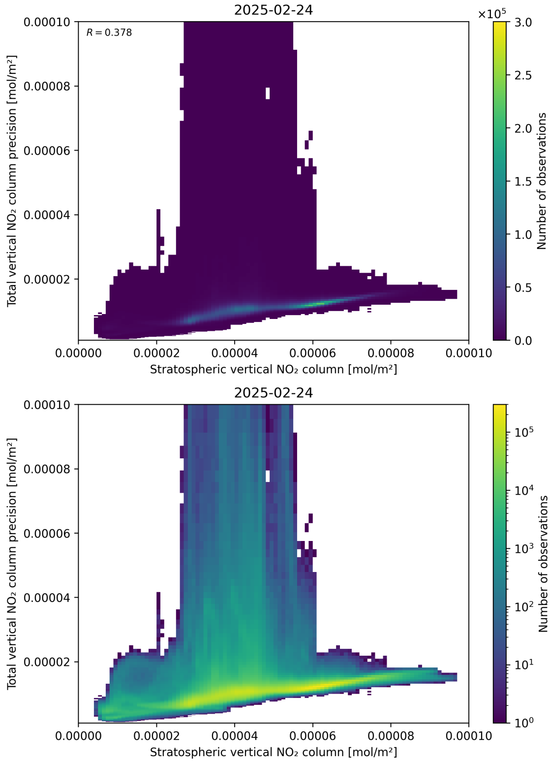
Figure 101: Scatter density plot of “Stratospheric vertical NO 2 column” against “Total vertical NO 2 column precision” for 2025-02-24 to 2025-02-25.
