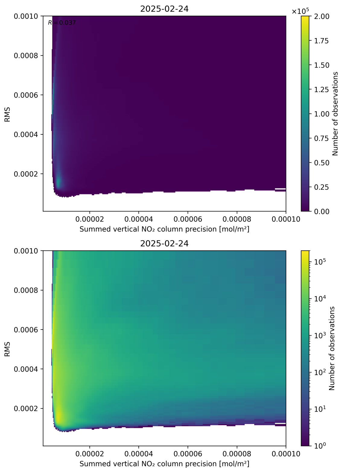
Figure 108: Scatter density plot of “Summed vertical NO 2 column precision” against “RMS” for 2025-02-24 to 2025-02-25.
