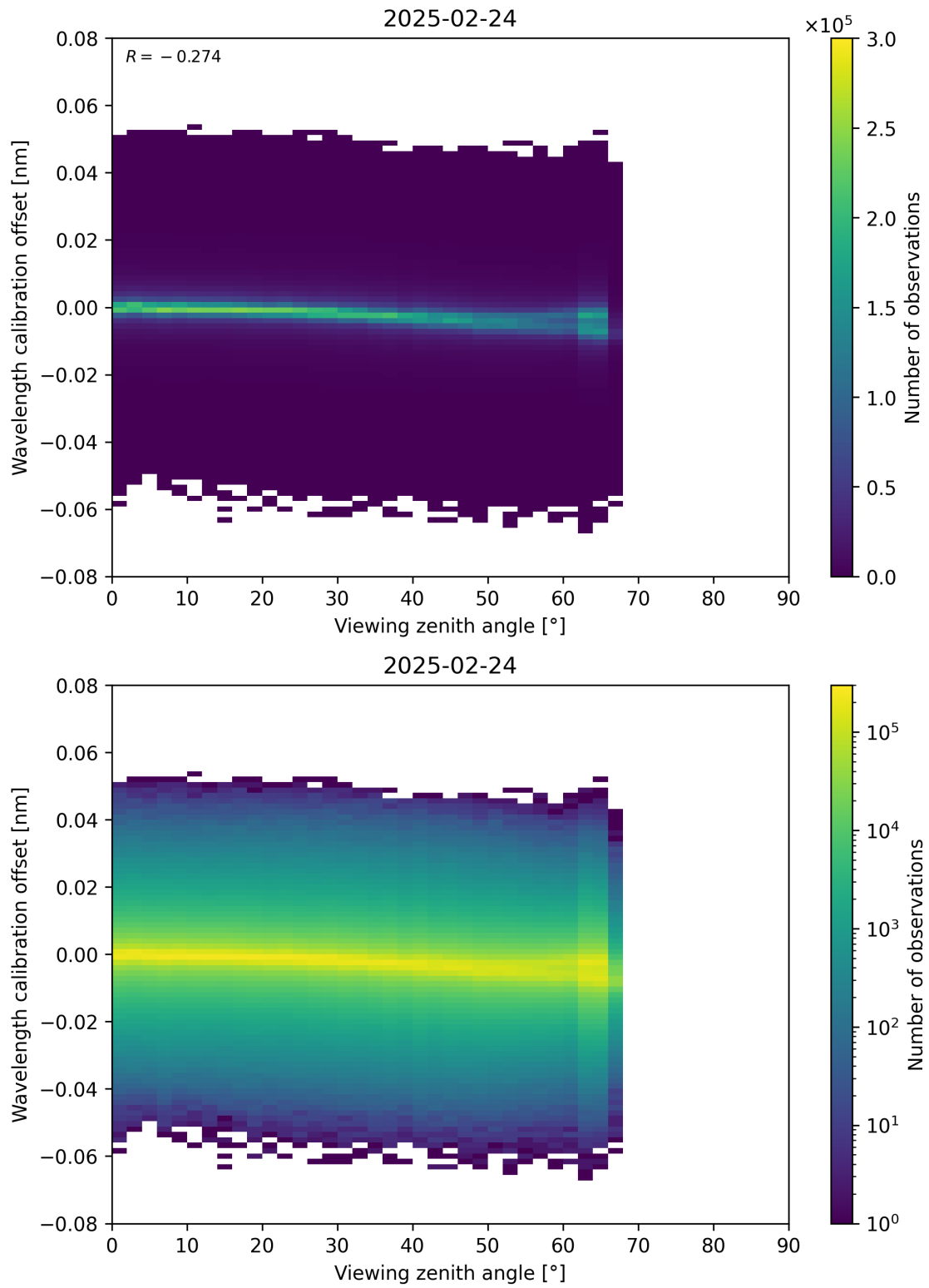
Figure 173: Scatter density plot of “Viewing zenith angle” against “Wavelength calibration offset” for 2025-02-24 to 2025-02-25.
