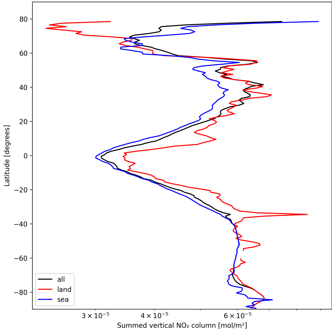
Figure 23: Zonal average of “Summed vertical NO 2 column” for 2025-02-24 to 2025-02-25.
