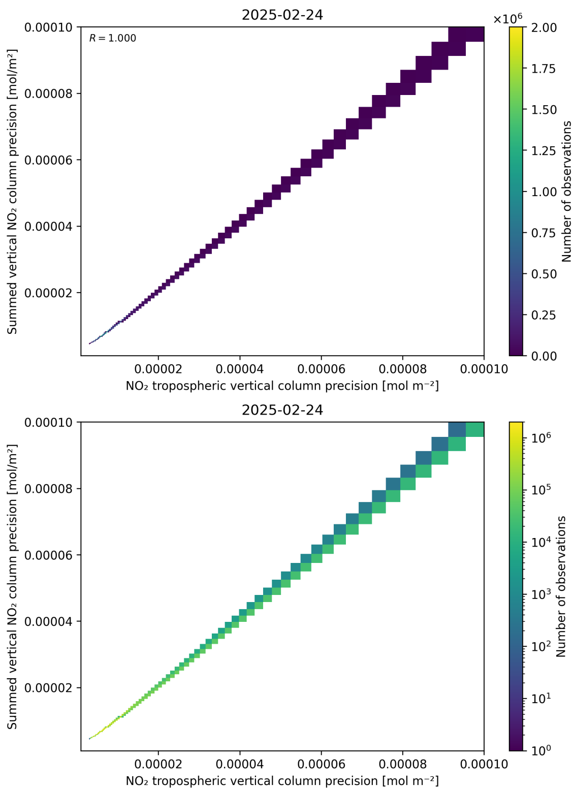
Figure 137: Scatter density plot of “NO 2 tropospheric vertical column precision” against “Summed vertical NO 2 column precision” for 2025-02-24 to 2025-02-25.
