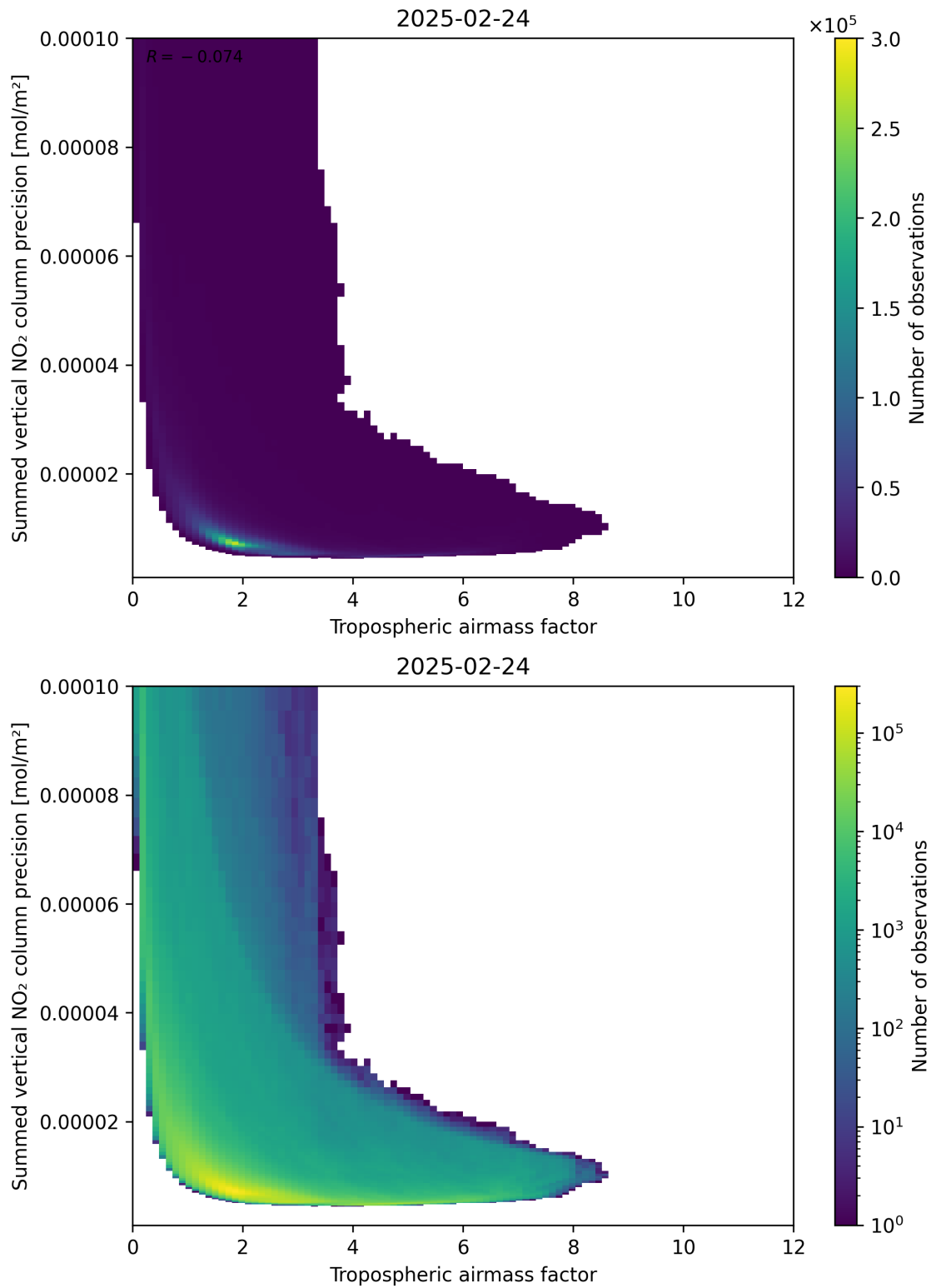
Figure 76: Scatter density plot of “Tropospheric air mass factor” against “Summed vertical NO 2 column precision” for 2025-02-24 to 2025-02-25.
