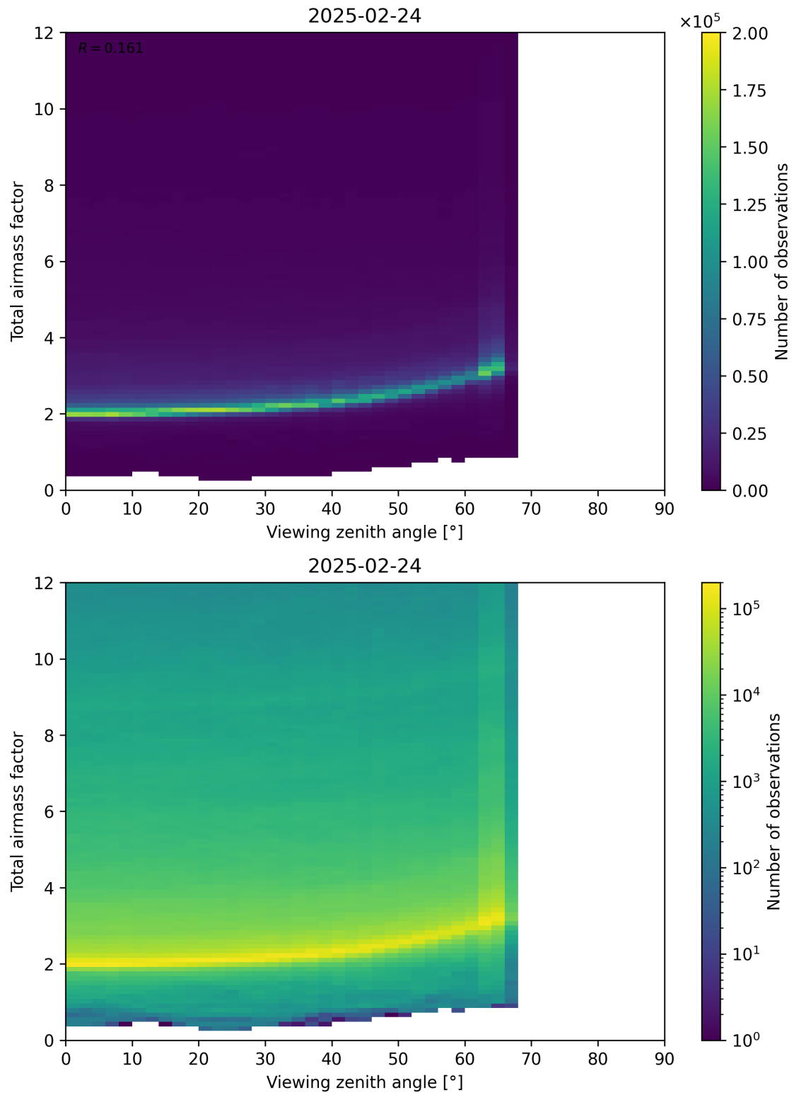
Figure 160: Scatter density plot of “Viewing zenith angle” against “Total airmass factor” for 2025-02-24 to 2025-02-25.
