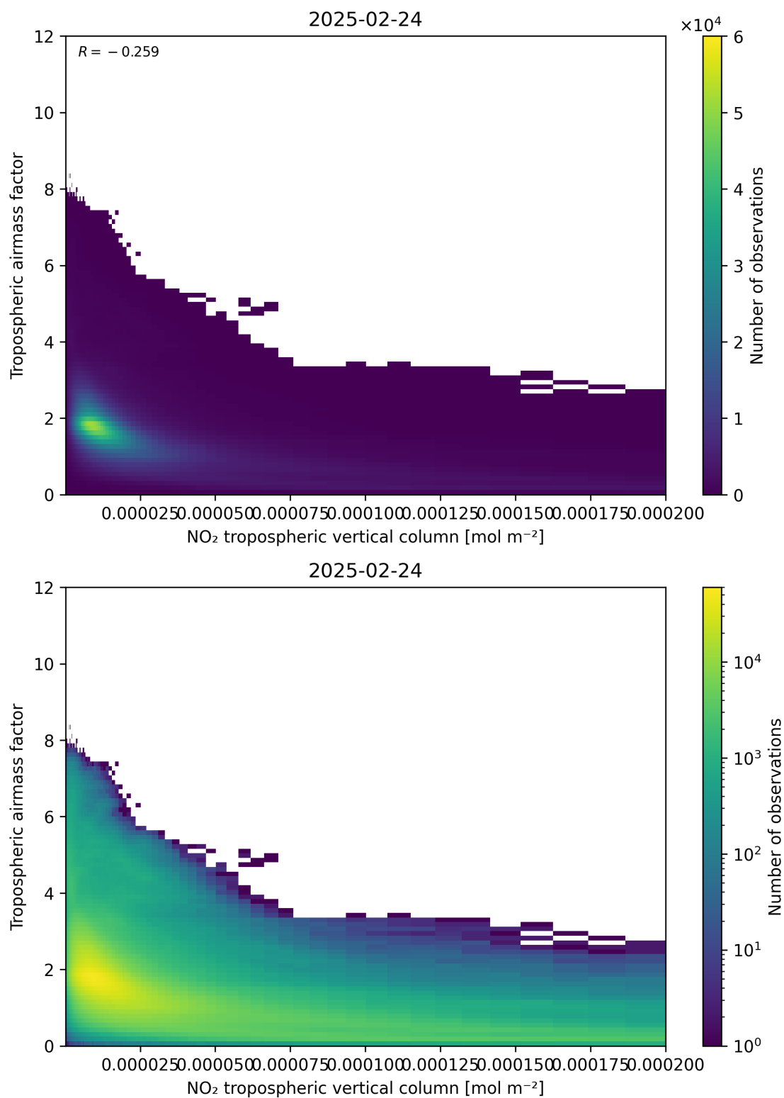
Figure 123: Scatter density plot of “NO 2 tropospheric vertical column” against “Tropospheric air mass factor” for 2025-02-24 to 2025-02-25.
