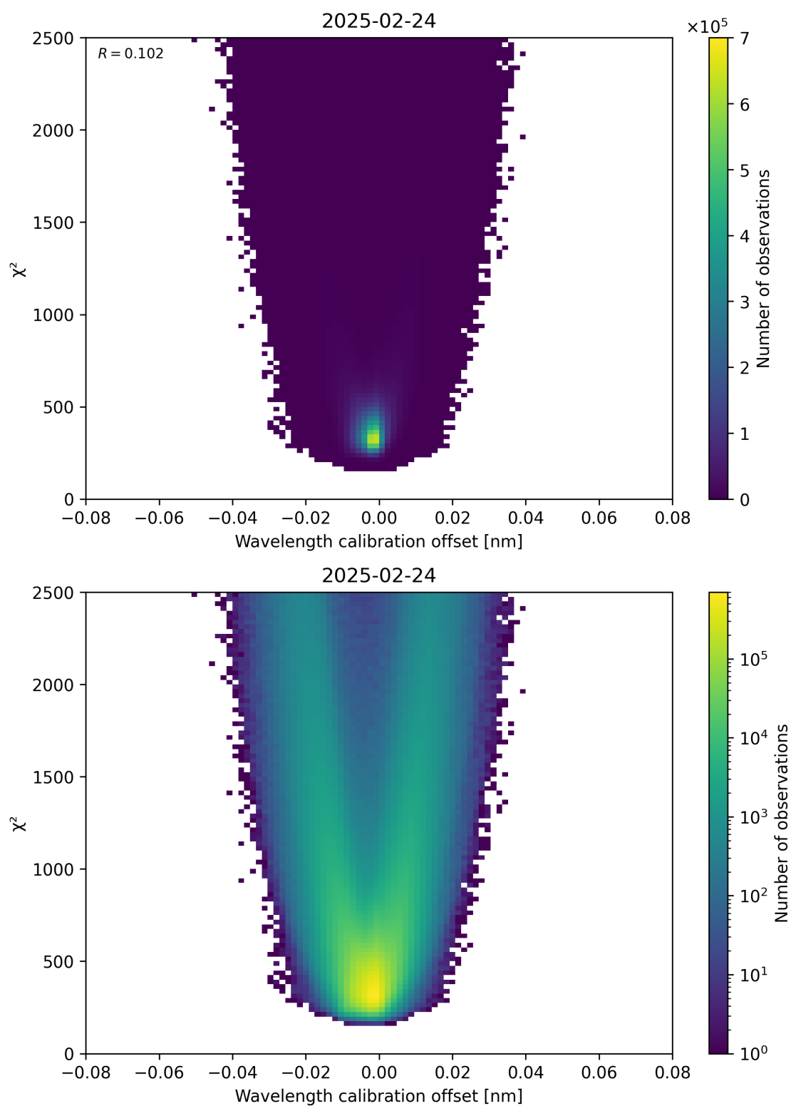
Figure 175: Scatter density plot of “Wavelength calibration offset” against “ \chi^2 ” for 2025-02-24 to 2025-02-25.
