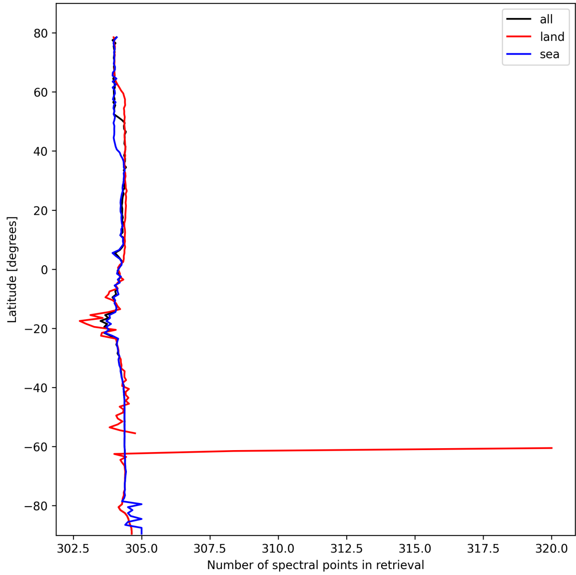
Figure 16: Zonal average of “Number of spectral points in retrieval” for 2025-02-24 to 2025-02-25.
