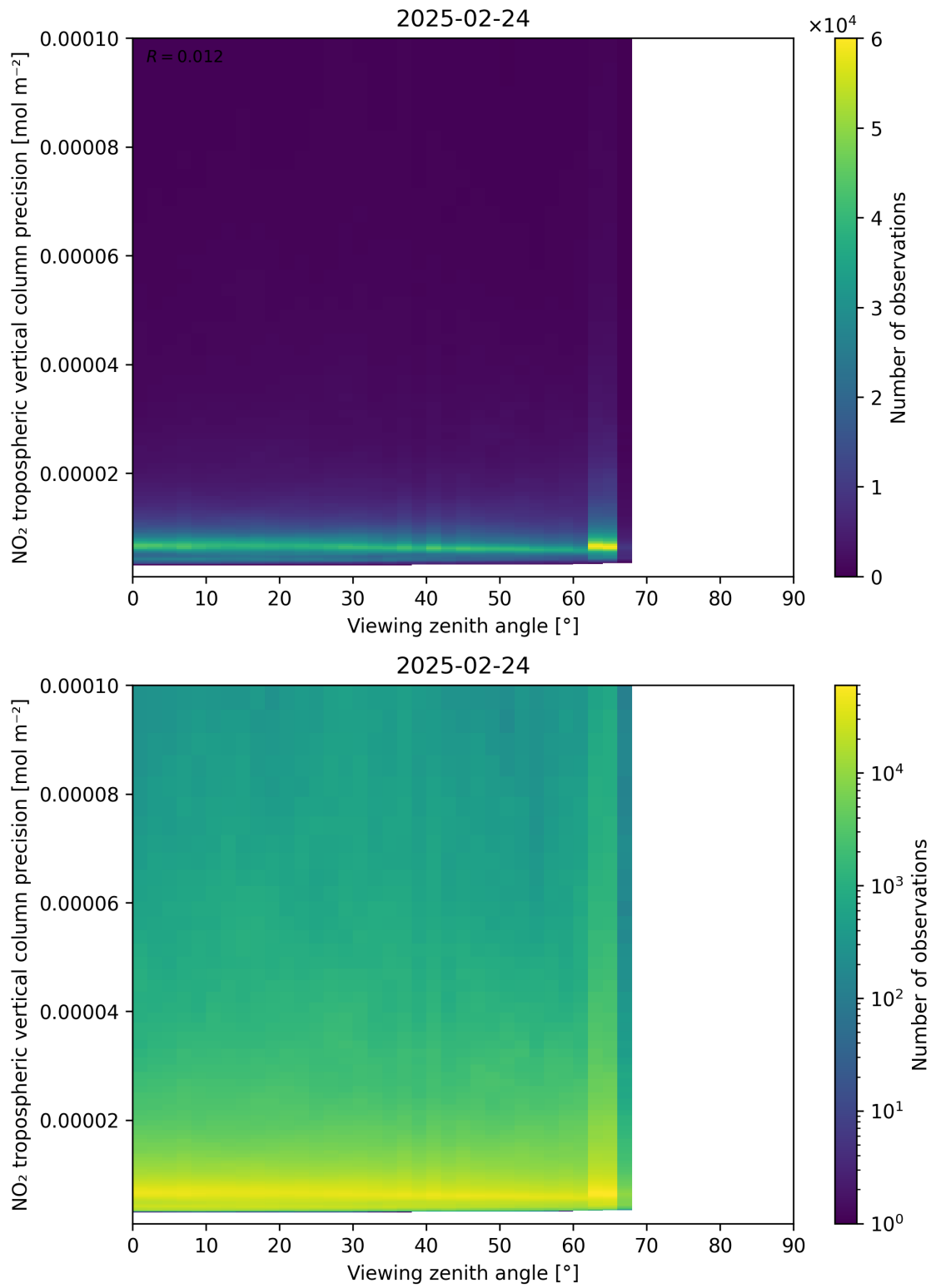
Figure 170: Scatter density plot of “Viewing zenith angle” against “NO 2 tropospheric vertical column precision” for 2025-02-24 to 2025-02-25.
