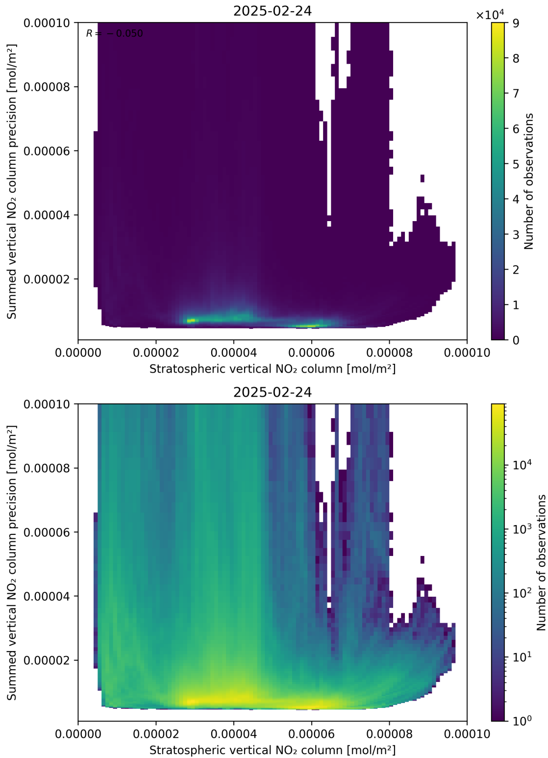
Figure 99: Scatter density plot of “Stratospheric vertical NO 2 column” against “Summed vertical NO 2 column precision” for 2025-02-24 to 2025-02-25.
