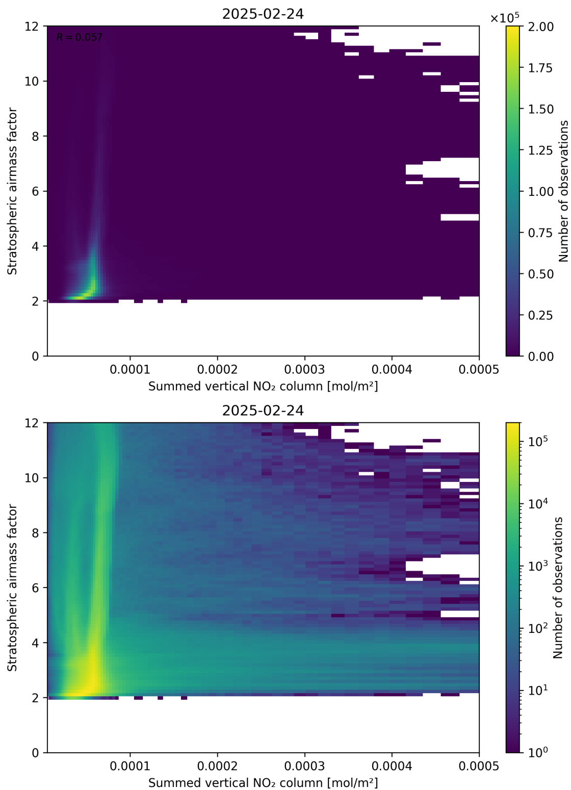
Figure 103: Scatter density plot of “Summed vertical NO 2 column” against “Stratospheric airmass factor” for 2025-02-24 to 2025-02-25.
