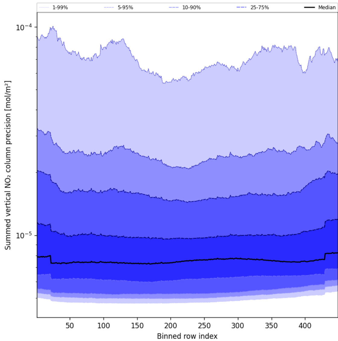
Figure 58: Along track statistics of “Summed vertical NO 2 column precision” for 2025-02-24 to 2025-02-25
