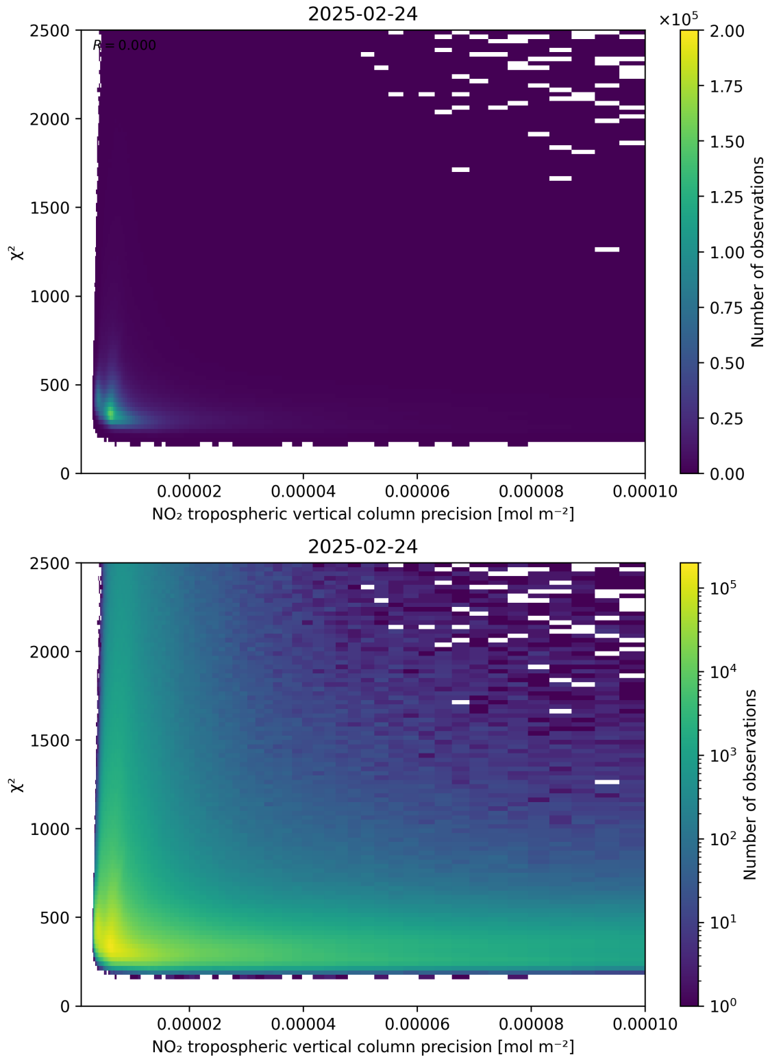
Figure 134: Scatter density plot of “NO 2 tropospheric vertical column precision” against “ \chi^2 ” for 2025-02-24 to 2025-02-25.
