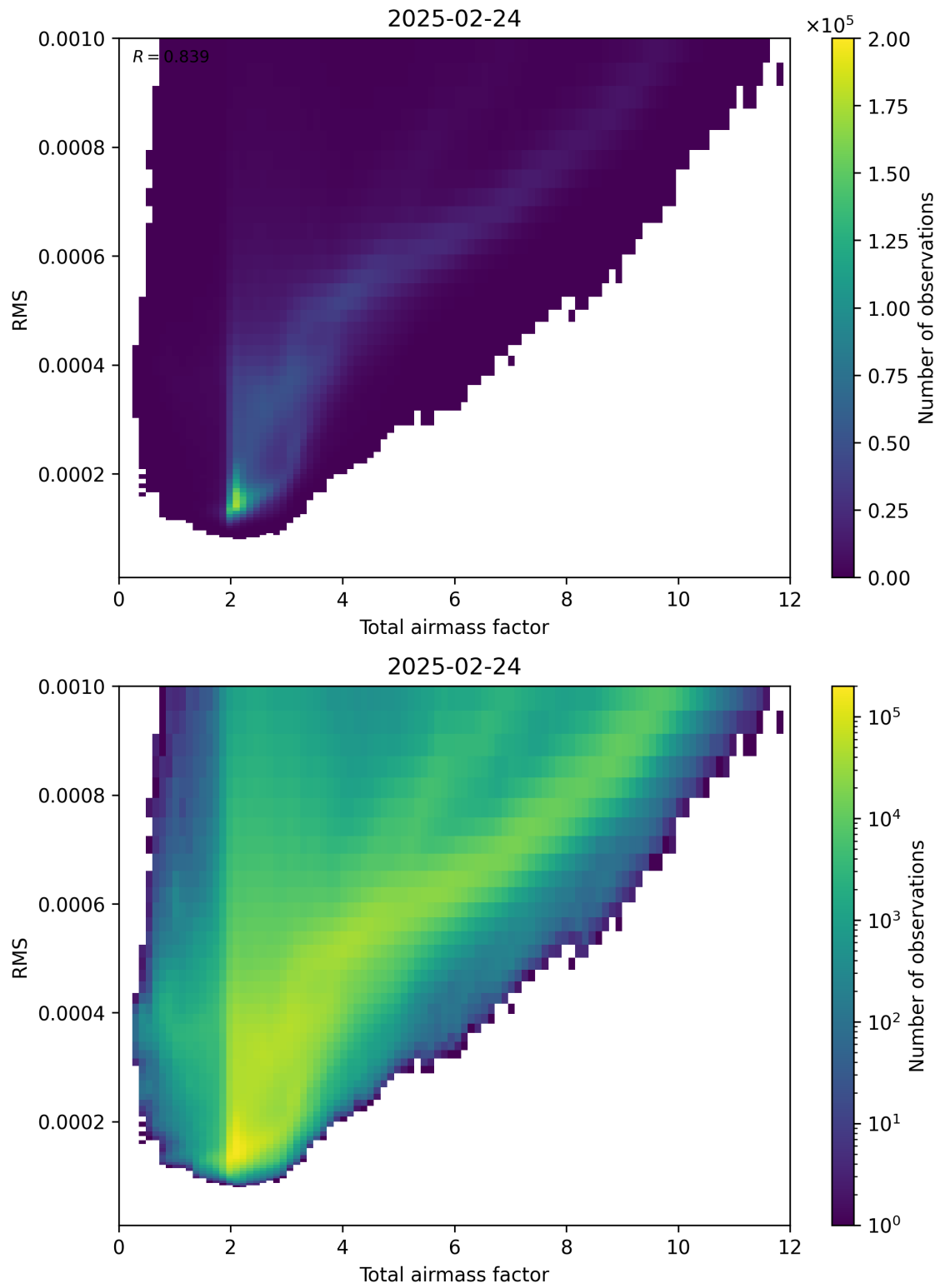
Figure 69: Scatter density plot of “Total airmass factor” against “RMS” for 2025-02-24 to 2025-02-25.
