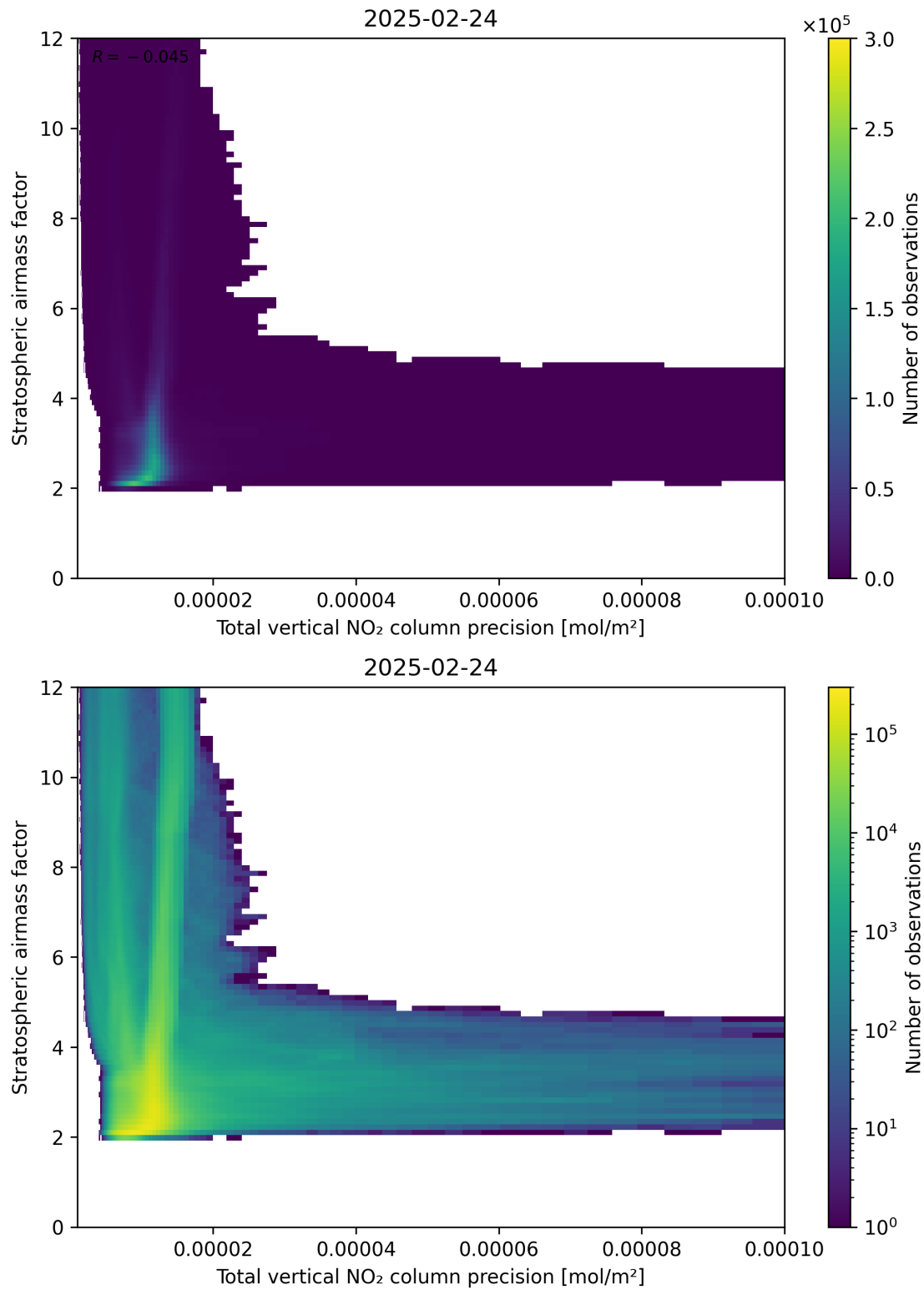
Figure 115: Scatter density plot of “Total vertical NO 2 column precision” against “Stratospheric air mass factor” for 2025-02-24 to 2025-02-25.
