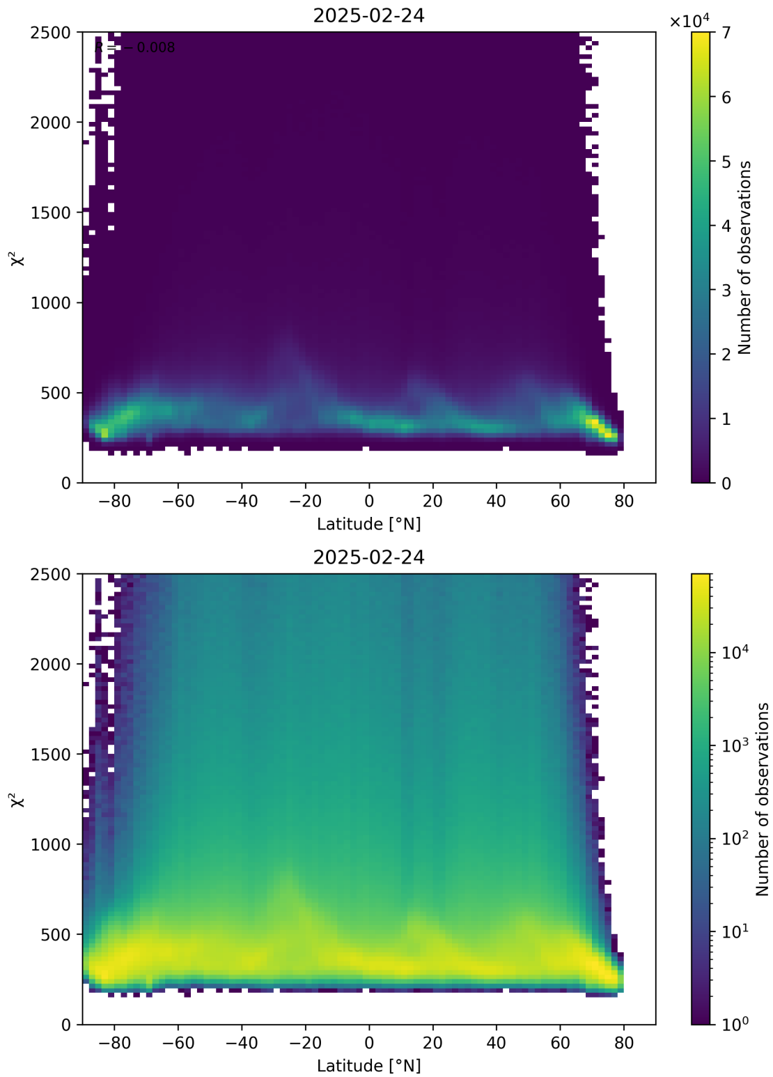
Figure 86: Scatter density plot of “Latitude” against “ \chi^2 ” for 2025-02-24 to 2025-02-25.
