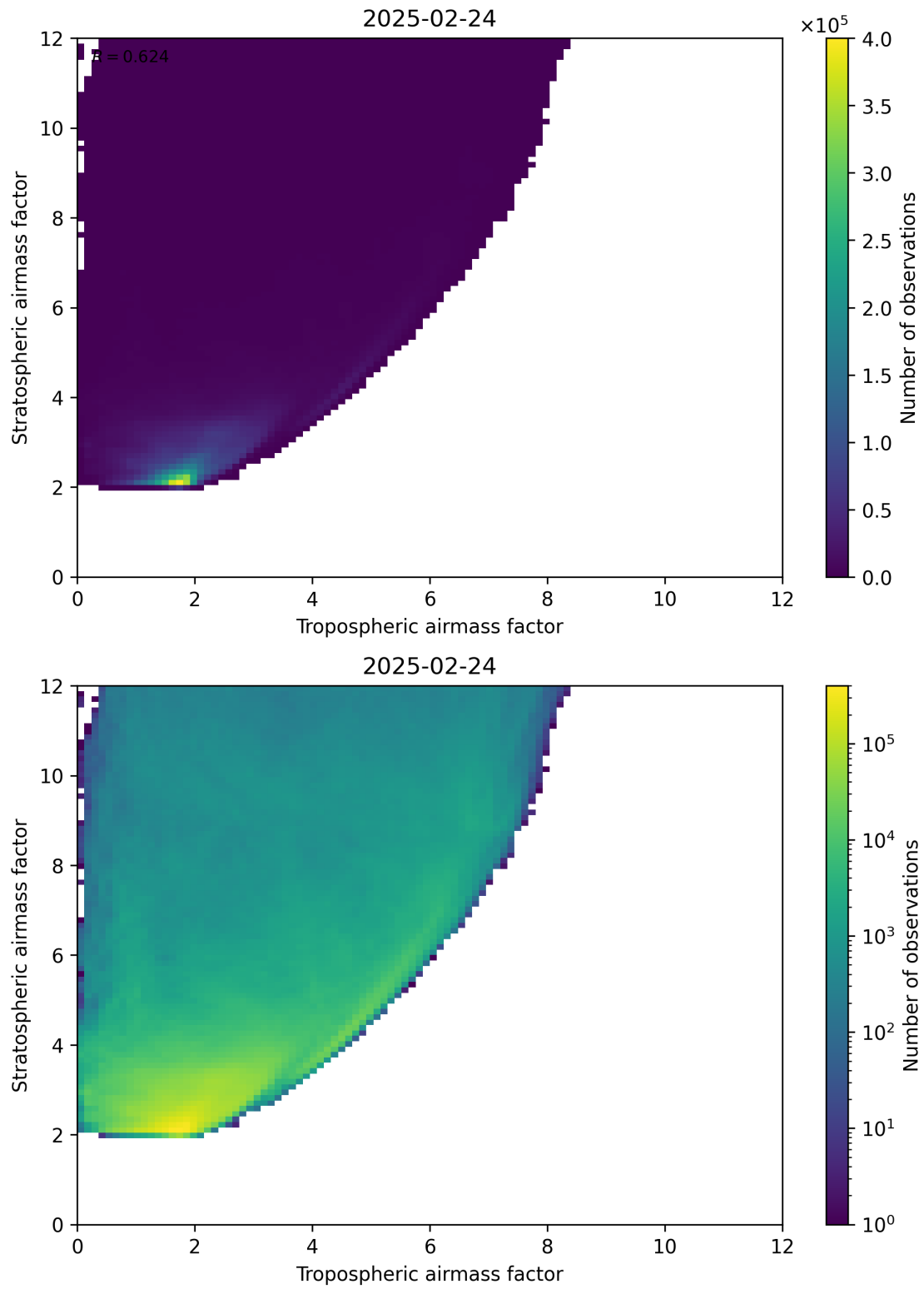
Figure 71: Scatter density plot of “Tropospheric airmass factor” against “Stratospheric airmass factor” for 2025-02-24 to 2025-02-25.
