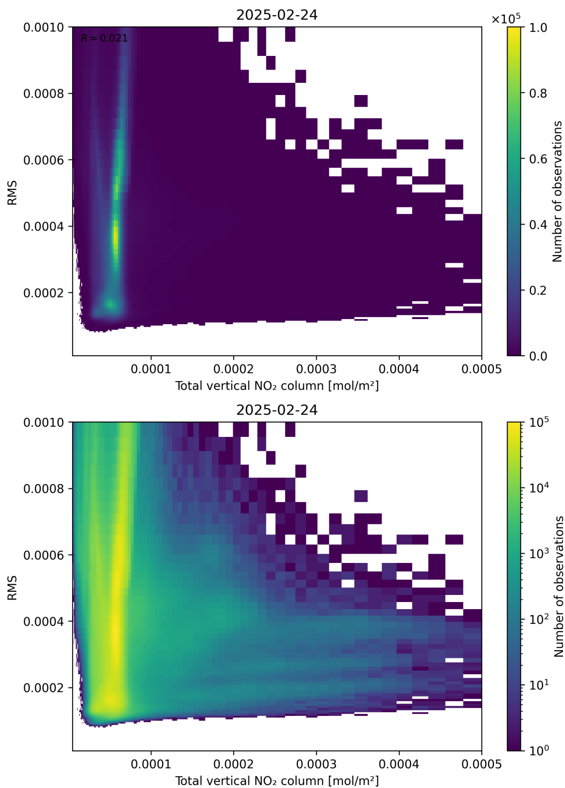
Figure 120: Scatter density plot of “Total vertical NO 2 column” against “RMS” for 2025-02-24 to 2025-02-25.
