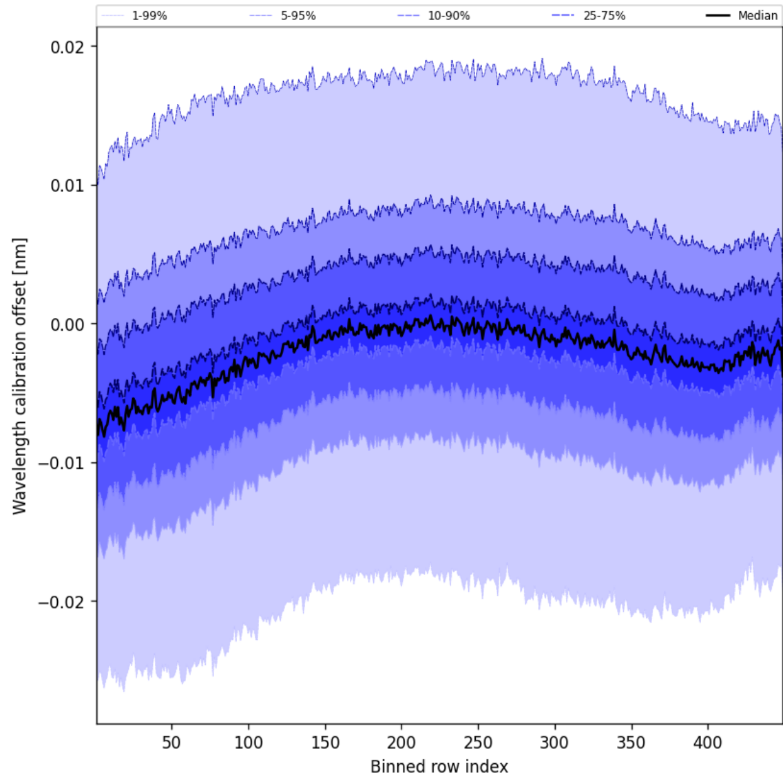
Figure 52: Along track statistics of “Wavelength calibration offset” for 2025-02-24 to 2025-02-25
