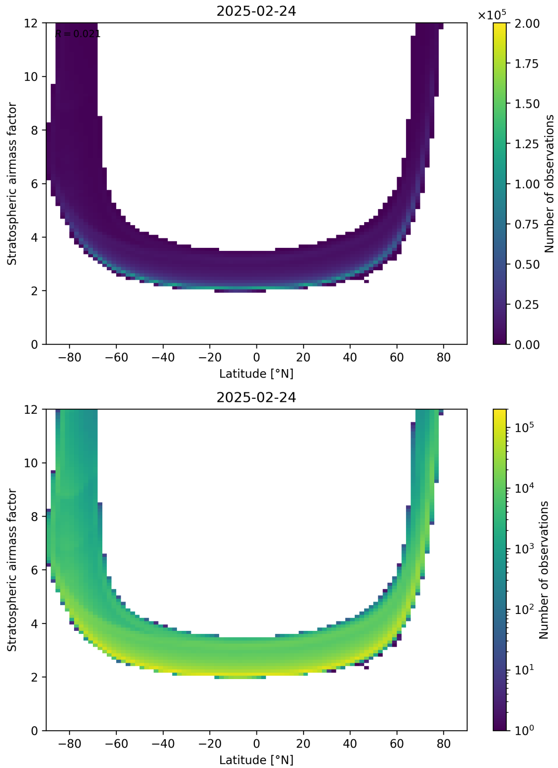
Figure 83: Scatter density plot of “Latitude” against “Stratospheric air mass factor” for 2025-02-24 to 2025-02-25.
