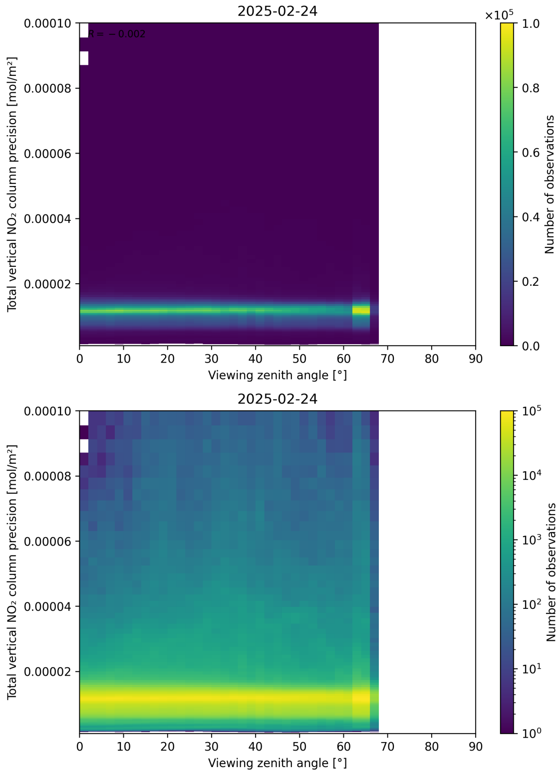
Figure 168: Scatter density plot of “Viewing zenith angle” against “Total vertical NO 2 column precision” for 2025-02-24 to 2025-02-25.
