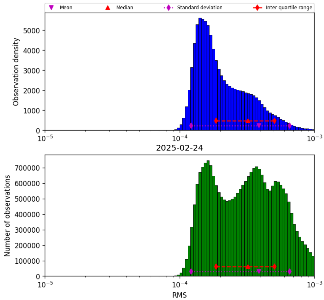
Figure 43: Histogram of “RMS” for 2025-02-24 to 2025-02-25
