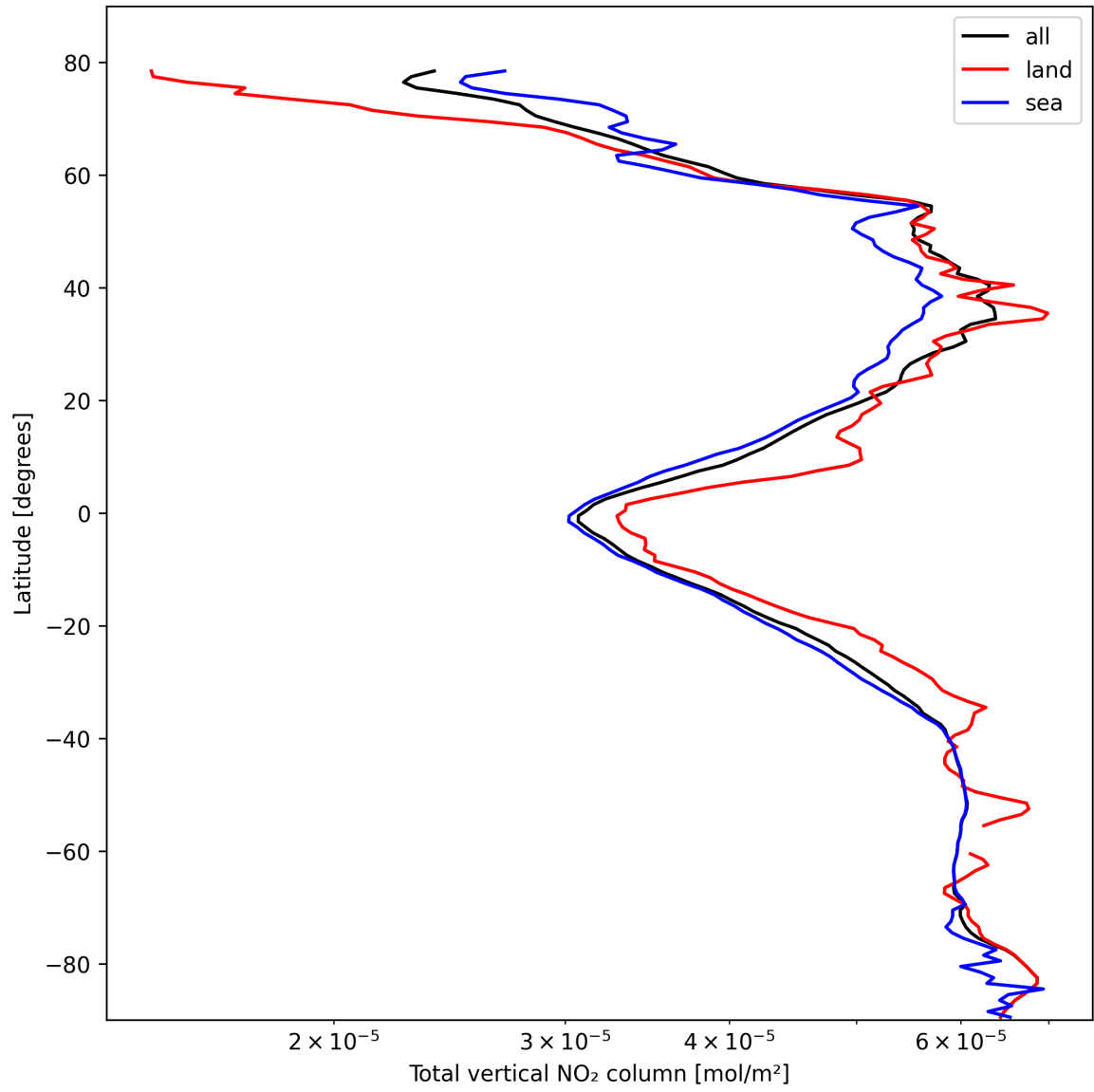
Figure 21: Zonal average of “Total vertical NO 2 column” for 2025-02-24 to 2025-02-25.
