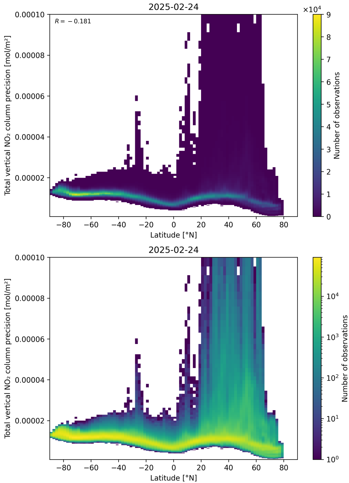
Figure 91: Scatter density plot of “Latitude” against “Total vertical NO 2 column precision” for 2025-02-24 to 2025-02-25.
