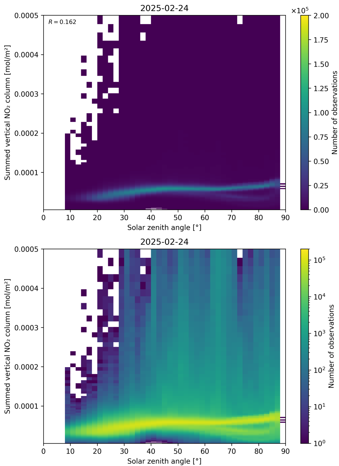
Figure 151: Scatter density plot of “Solar zenith angle” against “Summed vertical NO 2 column” for 2025-02-24 to 2025-02-25.
