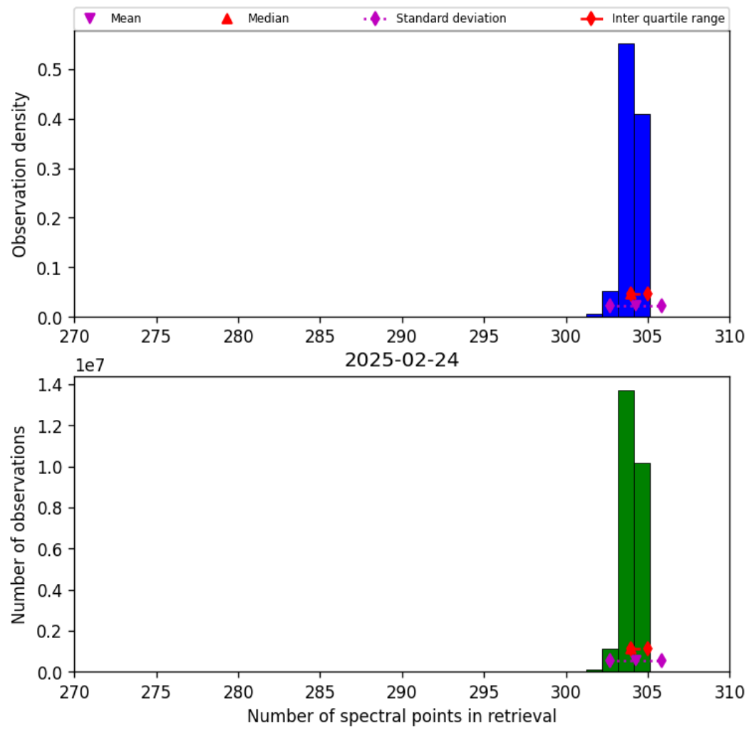
Figure 33: Histogram of “Number of spectral points in retrieval” for 2025-02-24 to 2025-02-25
