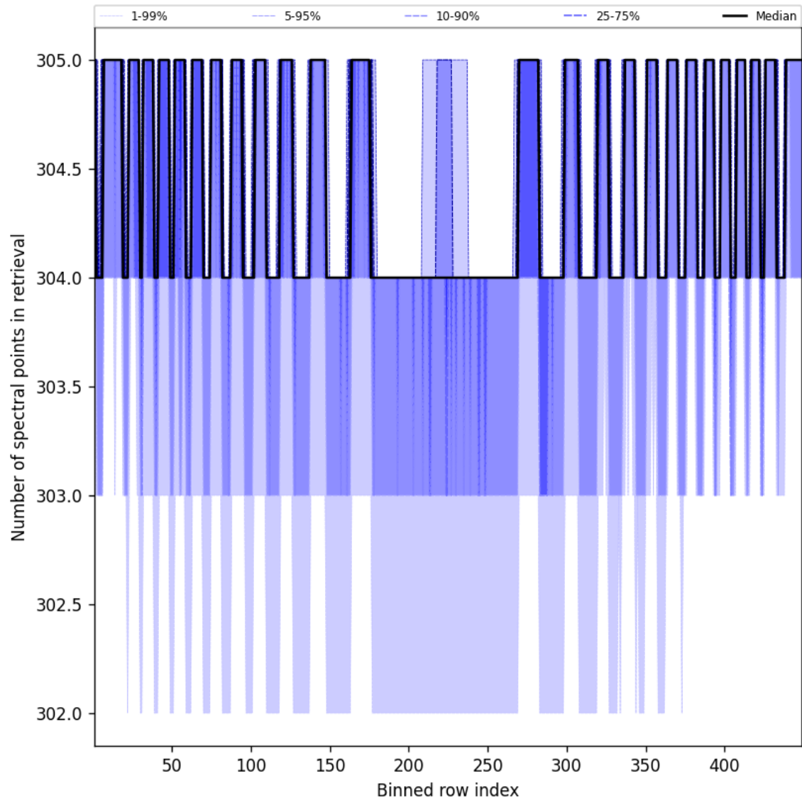
Figure 50: Along track statistics of “Number of spectral points in retrieval” for 2025-02-24 to 2025-02-25
