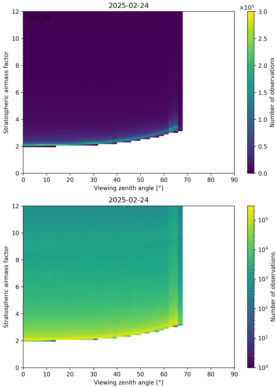
Figure 159: Scatter density plot of “Viewing zenith angle” against “Stratospheric airmass factor” for 2025-02-24 to 2025-02-25.
