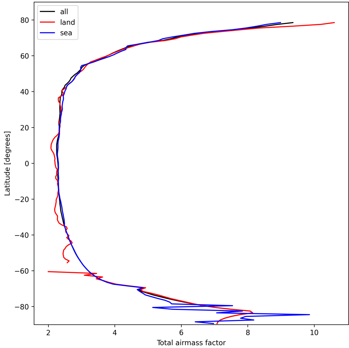
Figure 15: Zonal average of “Total airmass factor” for 2025-02-24 to 2025-02-25.
