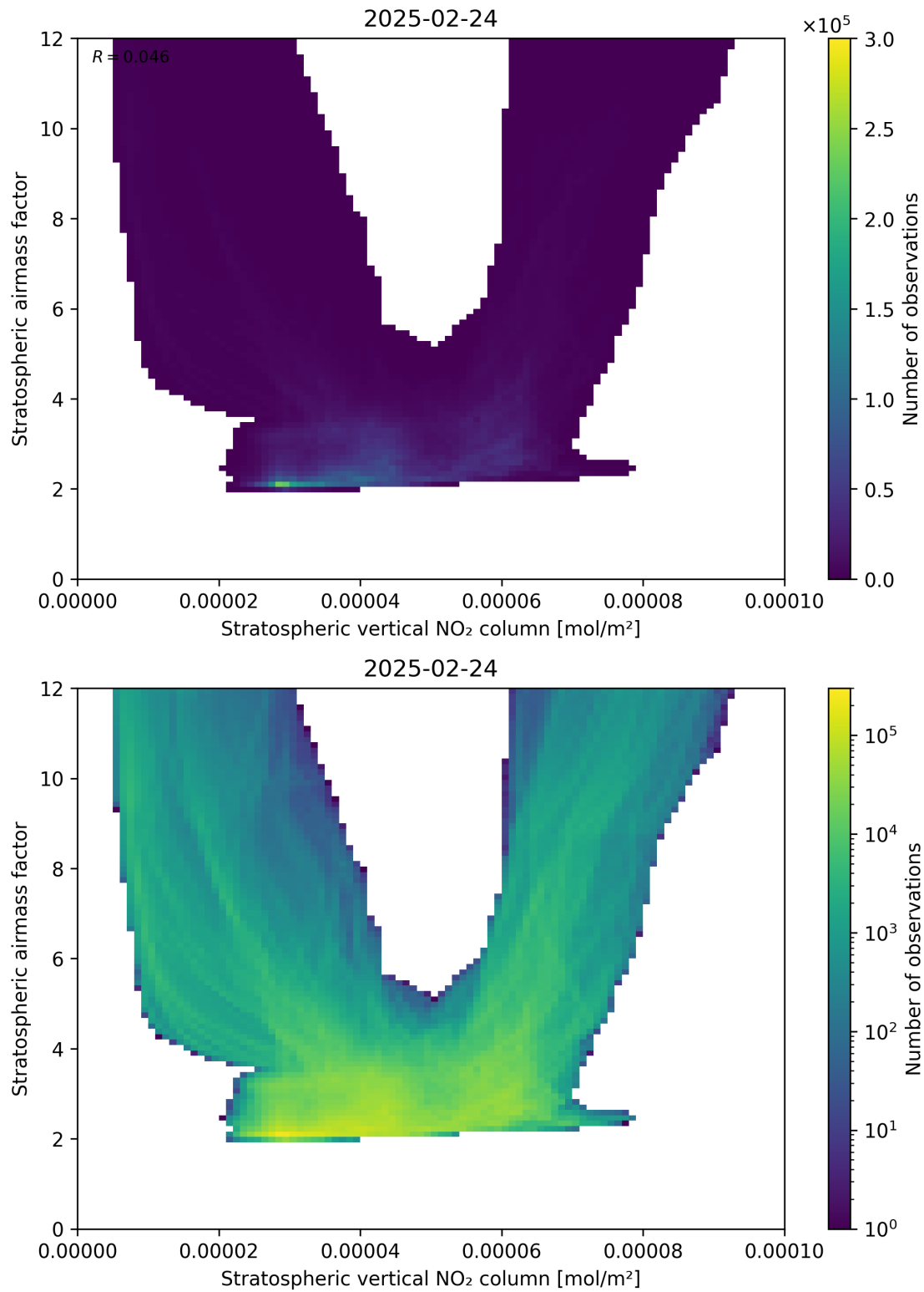
Figure 96: Scatter density plot of “Stratospheric vertical NO 2 column” against “Stratospheric airmass factor” for 2025-02-24 to 2025-02-25.
