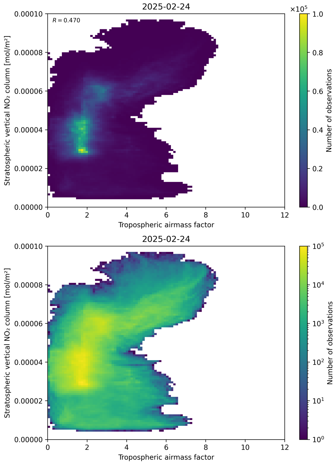
Figure 74: Scatter density plot of “Tropospheric air mass factor” against “Stratospheric vertical \text{NO}_2 column” for 2025-02-24 to 2025-02-25.
