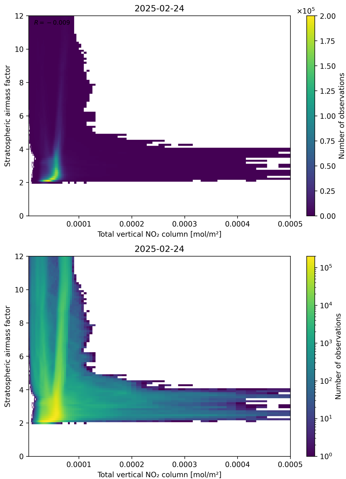
Figure 110: Scatter density plot of “Total vertical NO 2 column” against “Stratospheric airmass factor” for 2025-02-24 to 2025-02-25.
