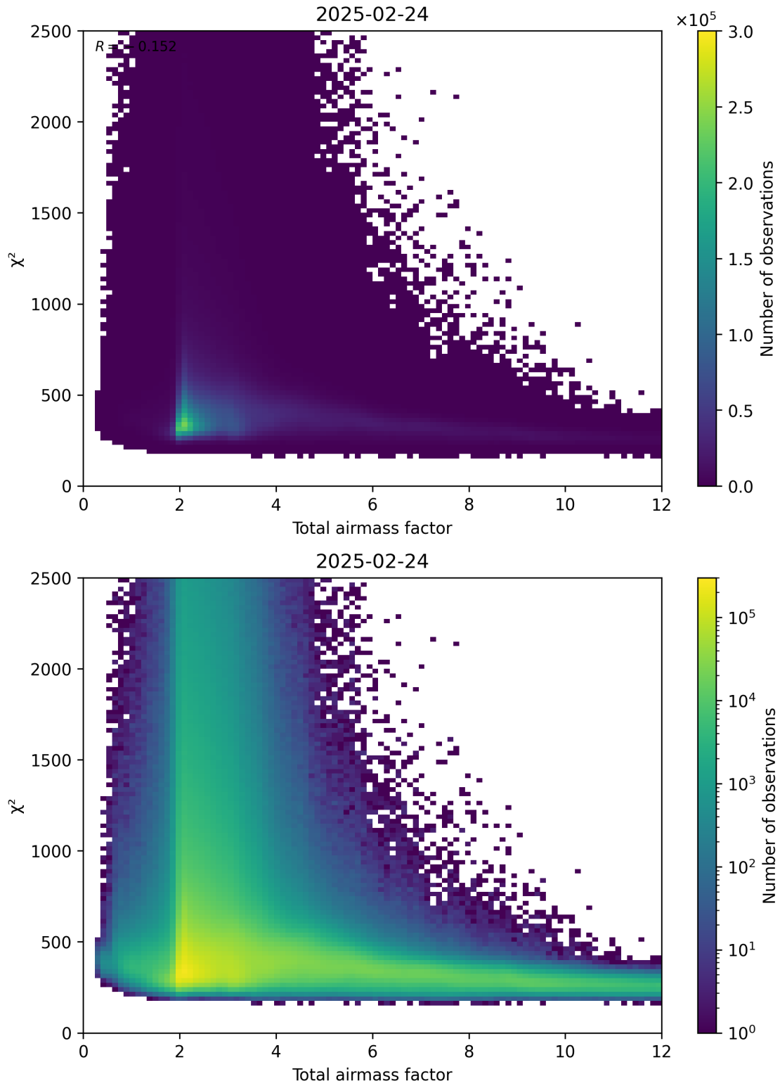
Figure 63: Scatter density plot of “Total airmass factor” against “ \chi^2 ” for 2025-02-24 to 2025-02-25.
