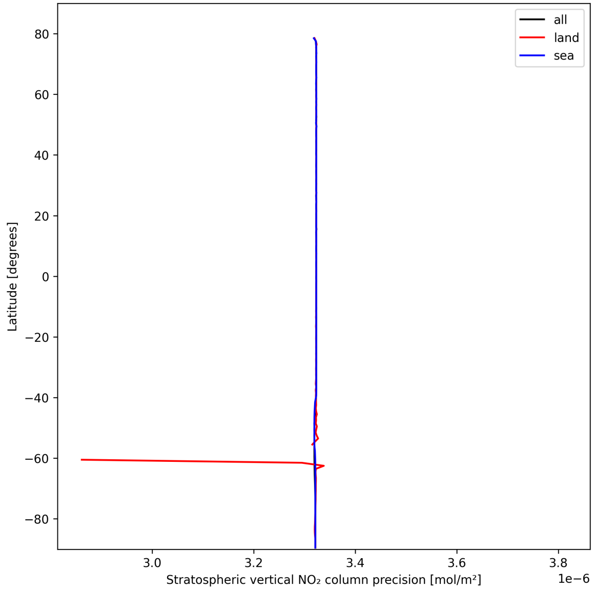
Figure 20: Zonal average of “Stratospheric vertical NO 2 column precision” for 2025-02-24 to 2025-02-25.
