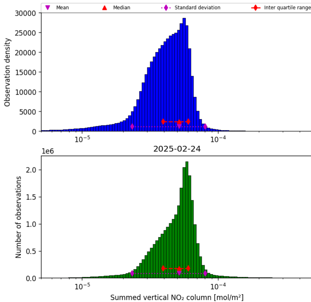
Figure 40: Histogram of “Summed vertical NO 2 column” for 2025-02-24 to 2025-02-25
