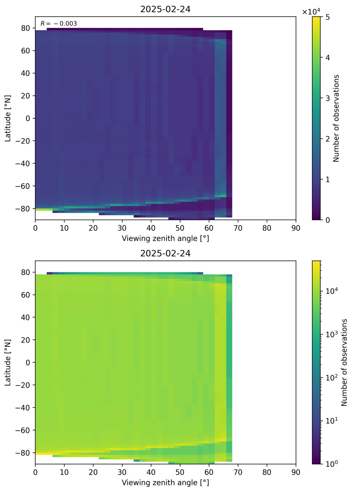
Figure 163: Scatter density plot of “Viewing zenith angle” against “Latitude” for 2025-02-24 to 2025-02-25.
