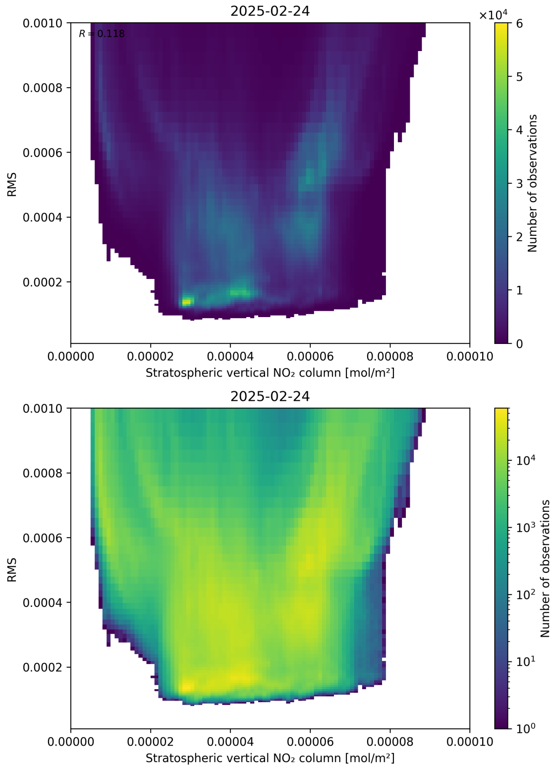
Figure 102: Scatter density plot of “Stratospheric vertical NO 2 column” against “RMS” for 2025-02-24 to 2025-02-25.
