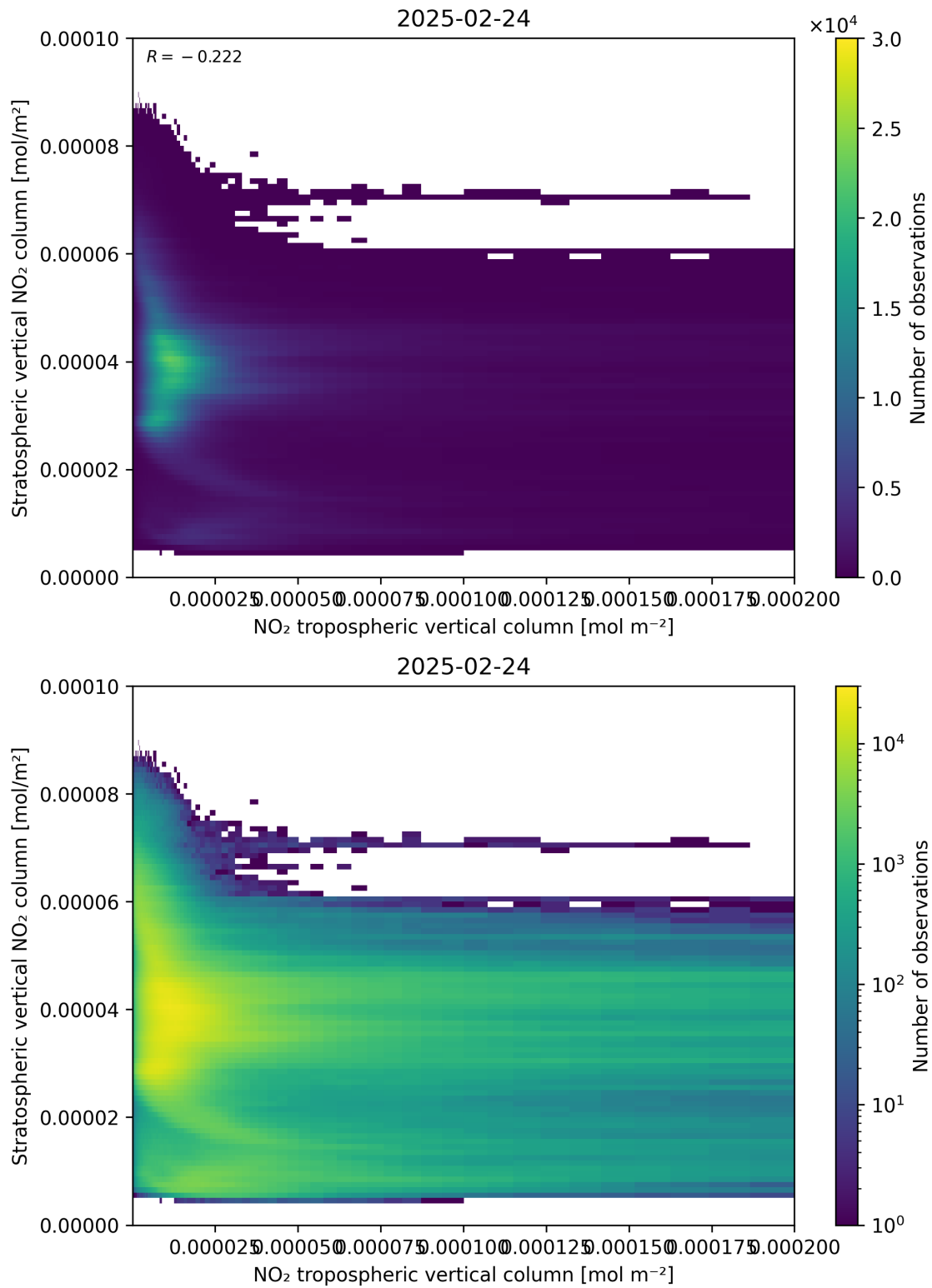
Figure 125: Scatter density plot of “NO 2 tropospheric vertical column” against “Stratospheric vertical NO 2 column” for 2025-02-24 to 2025-02-25.
