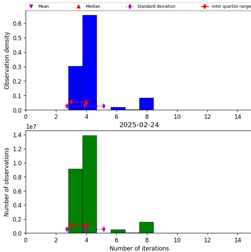
Figure 34: Histogram of “Number of iterations” for 2025-02-24 to 2025-02-25
