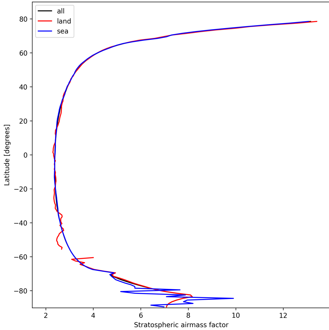
Figure 27: Zonal average of “Stratospheric air mass factor” for 2025-02-24 to 2025-02-25.
