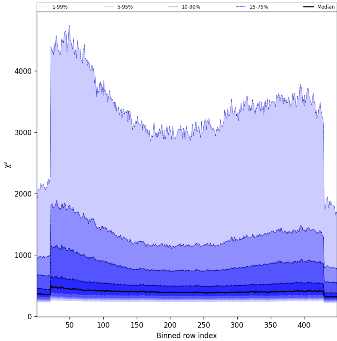
Figure 59: Along track statistics of “ \chi^2 ” for 2025-02-24 to 2025-02-25
