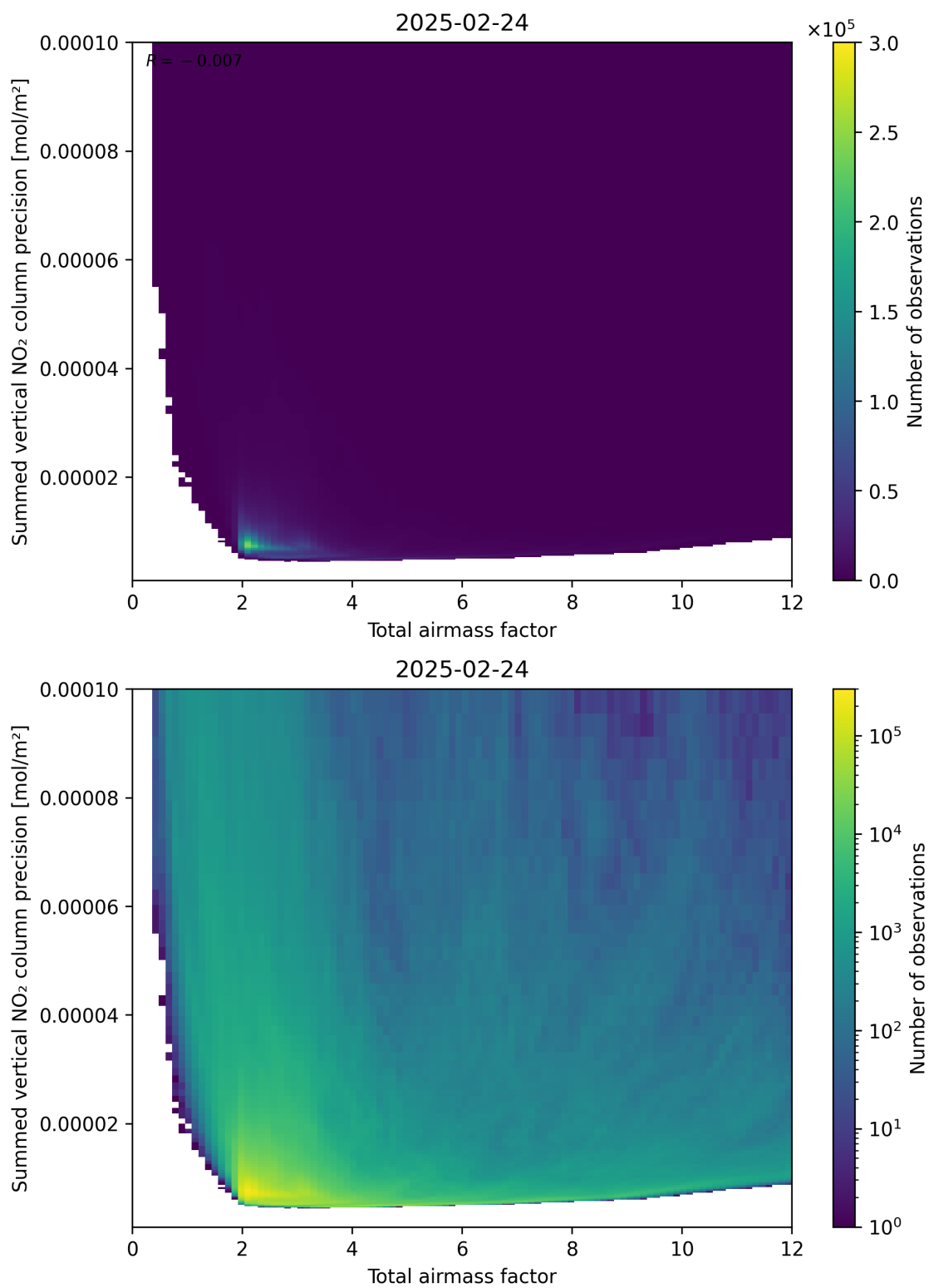
Figure 66: Scatter density plot of “Total airmass factor” against “Summed vertical NO 2 column precision” for 2025-02-24 to 2025-02-25.
