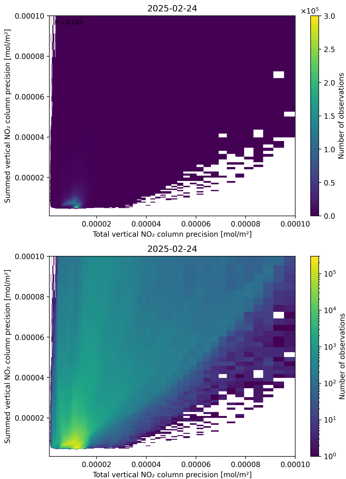
Figure 118: Scatter density plot of “Total vertical NO 2 column precision” against “Summed vertical NO 2 column precision” for 2025-02-24 to 2025-02-25.
