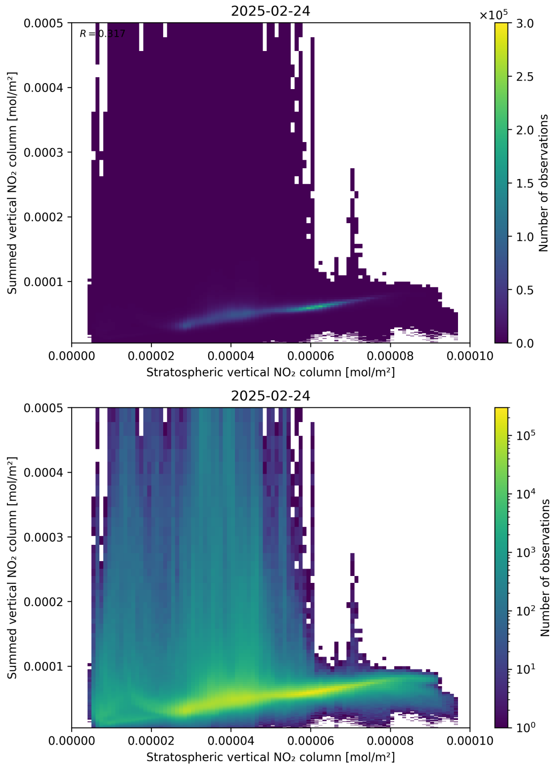
Figure 98: Scatter density plot of “Stratospheric vertical NO 2 column” against “Summed vertical NO 2 column” for 2025-02-24 to 2025-02-25.
