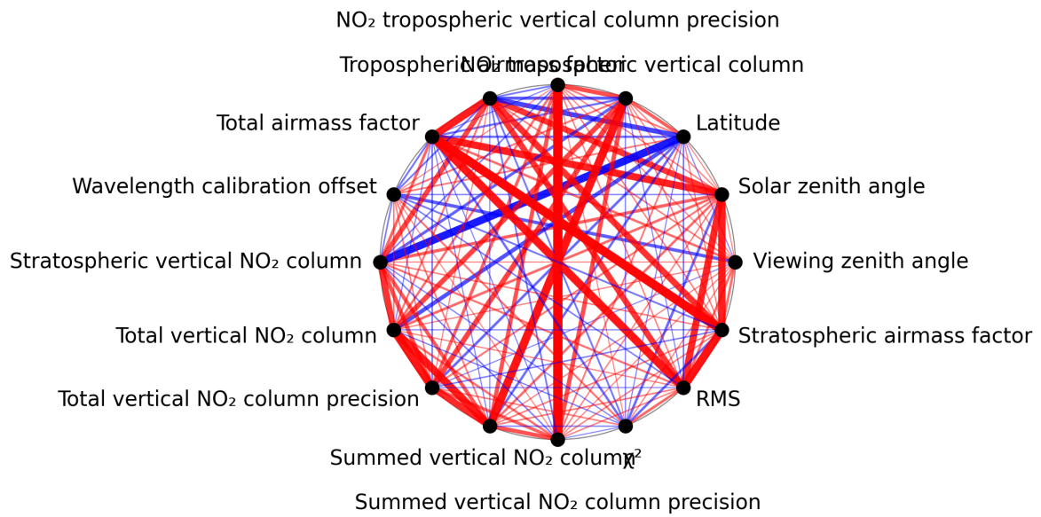
Figure 1: Map of correlation graph for 2025-02-24 to 2025-02-25.
