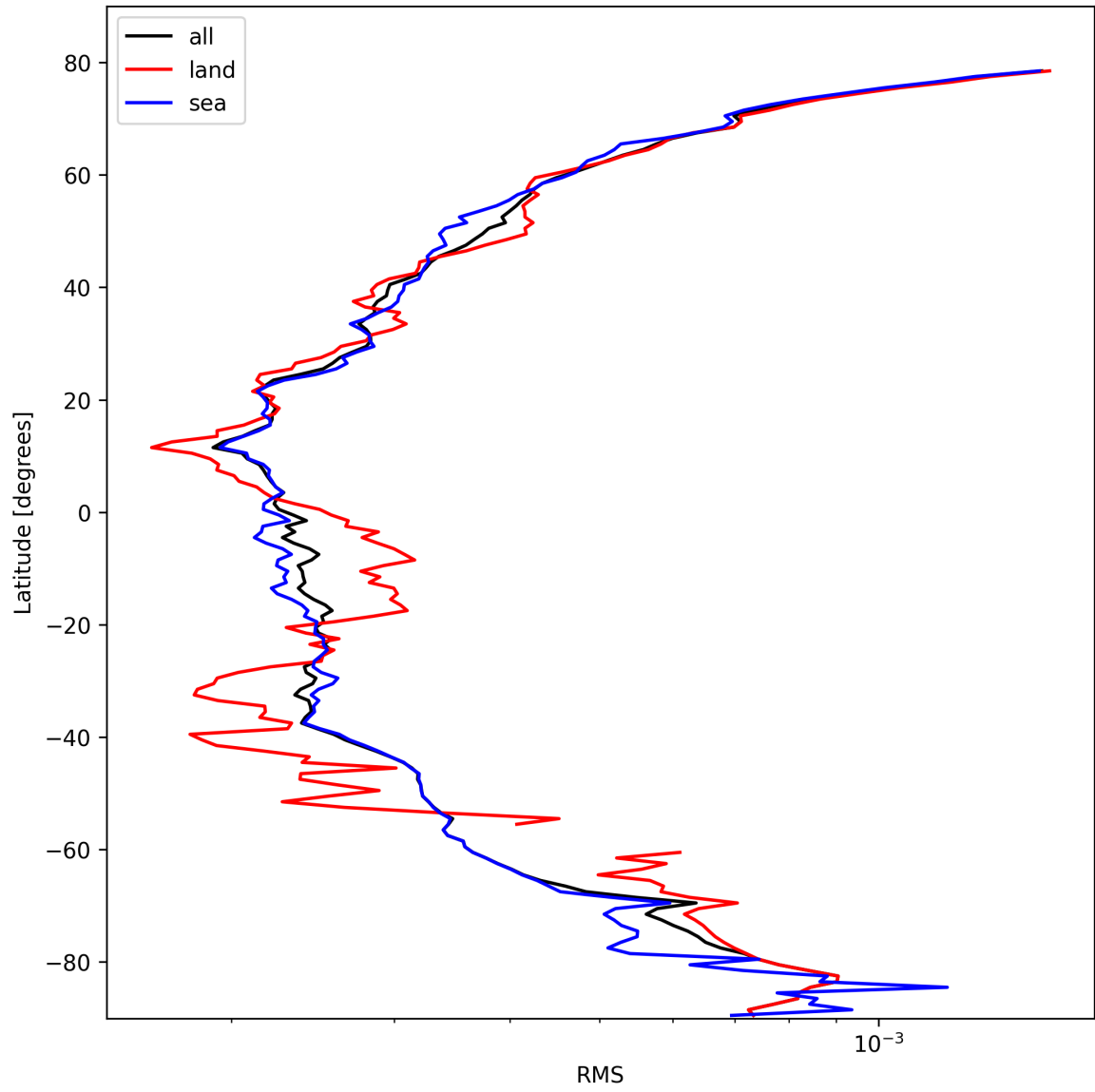
Figure 26: Zonal average of “RMS” for 2025-02-24 to 2025-02-25.
