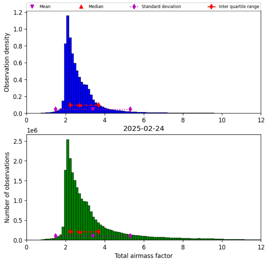
Figure 32: Histogram of “Total airmass factor” for 2025-02-24 to 2025-02-25
