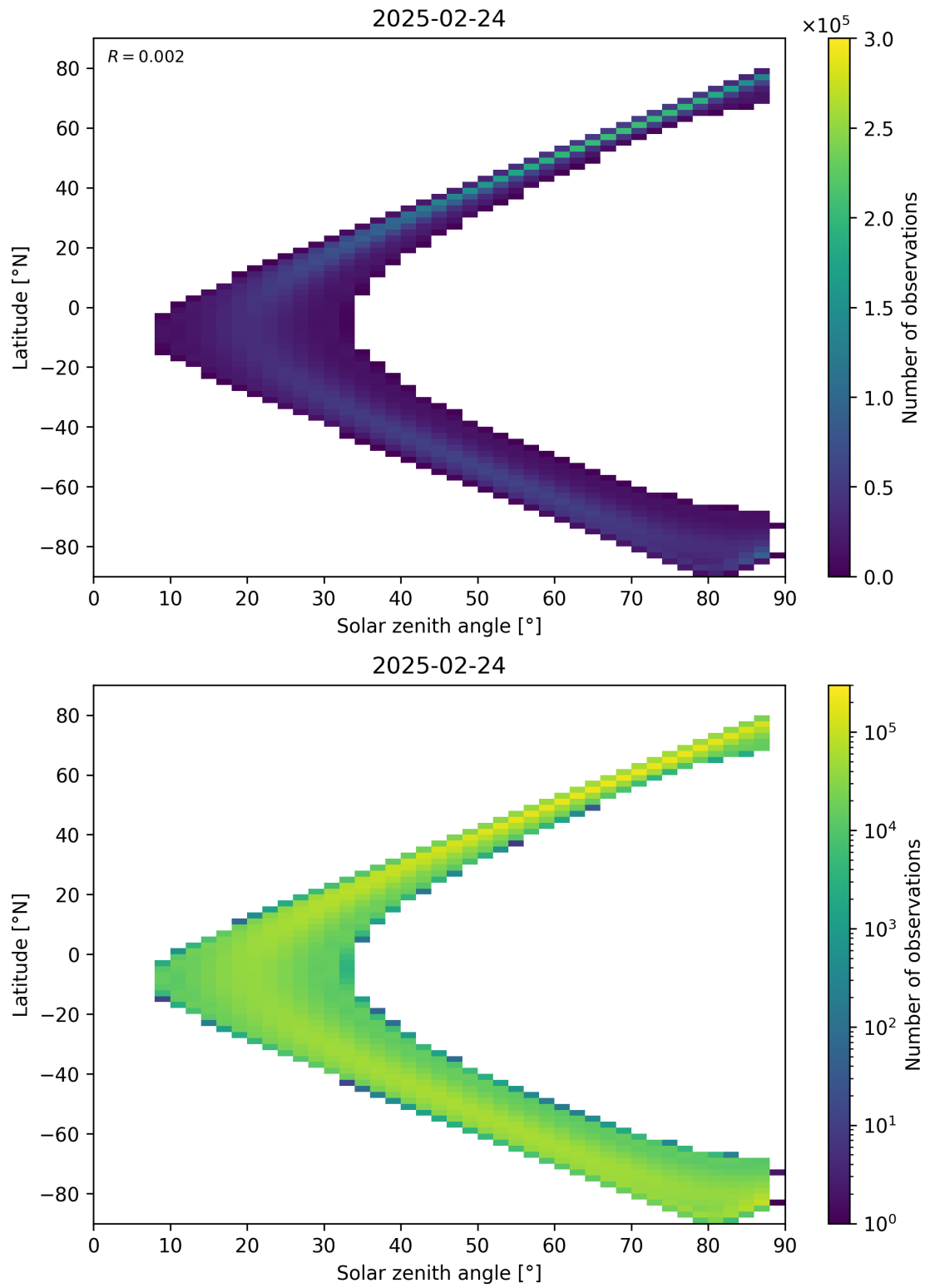
Figure 149: Scatter density plot of “Solar zenith angle” against “Latitude” for 2025-02-24 to 2025-02-25.
