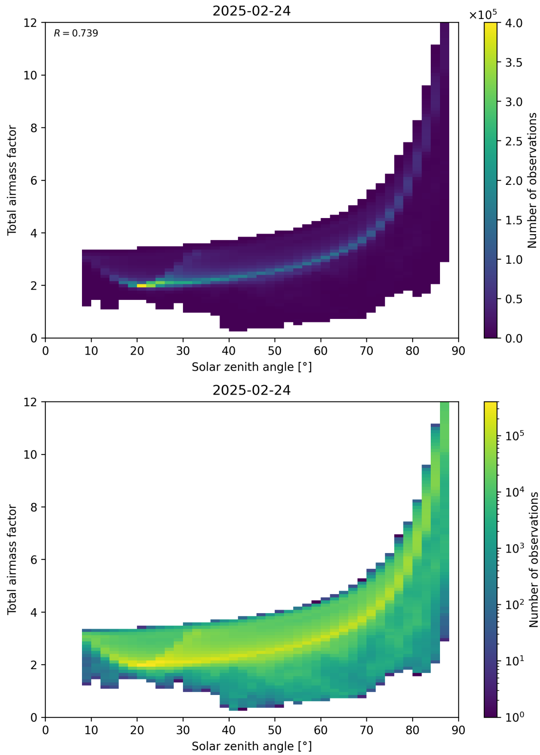
Figure 146: Scatter density plot of “Solar zenith angle” against “Total air mass factor” for 2025-02-24 to 2025-02-25.
