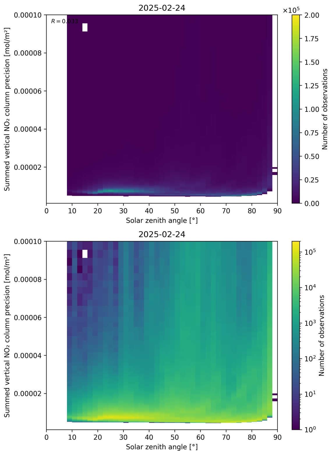
Figure 152: Scatter density plot of “Solar zenith angle” against “Summed vertical NO 2 column precision” for 2025-02-24 to 2025-02-25.
