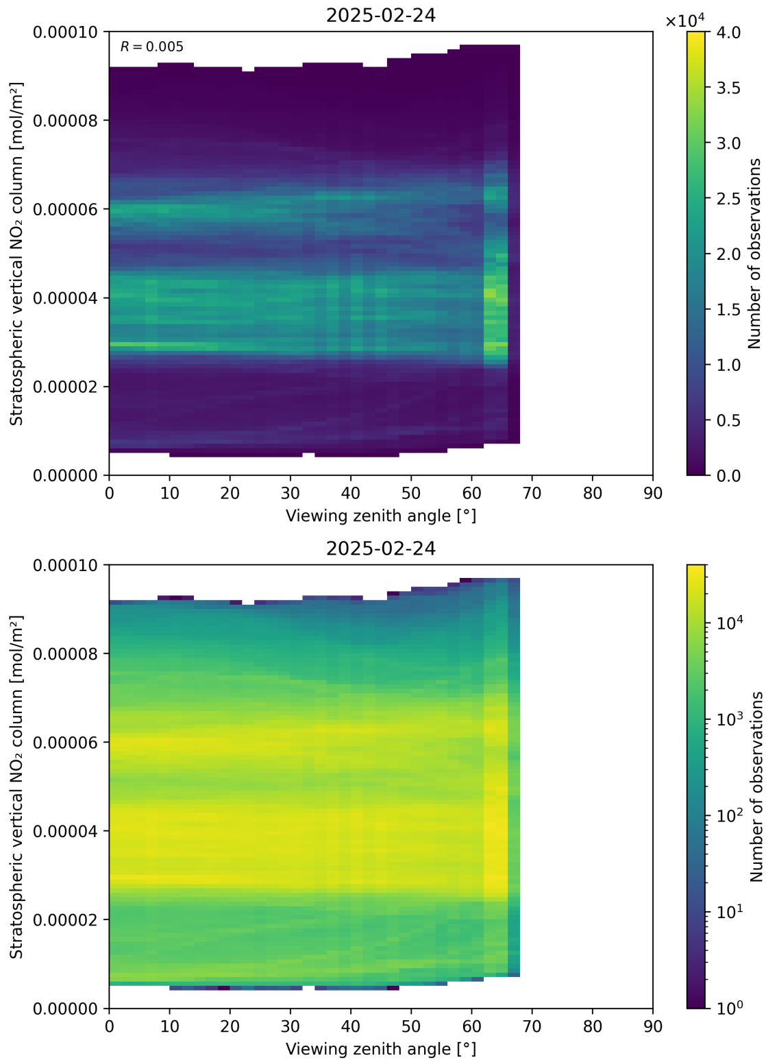
Figure 164: Scatter density plot of “Viewing zenith angle” against “Stratospheric vertical NO 2 column” for 2025-02-24 to 2025-02-25.
