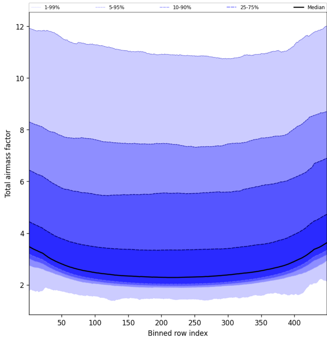
Figure 49: Along track statistics of “Total airmass factor” for 2025-02-24 to 2025-02-25
