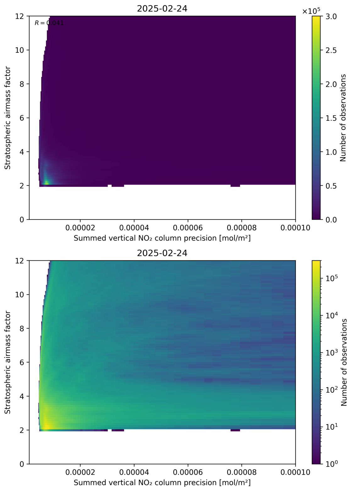
Figure 106: Scatter density plot of “Summed vertical NO 2 column precision” against “Stratospheric airmass factor” for 2025-02-24 to 2025-02-25.
