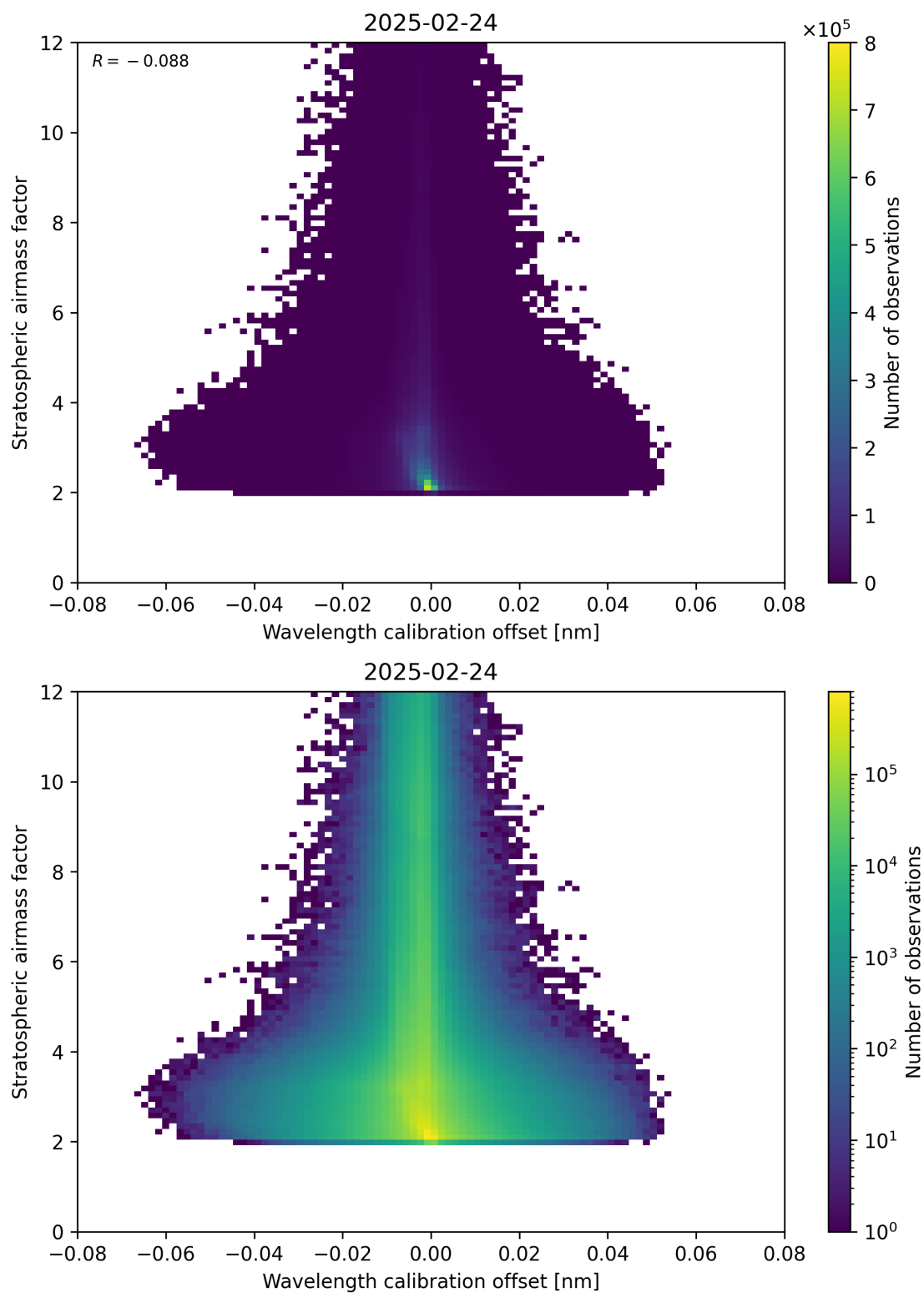
Figure 174: Scatter density plot of “Wavelength calibration offset” against “Stratospheric airmass factor” for 2025-02-24 to 2025-02-25.
