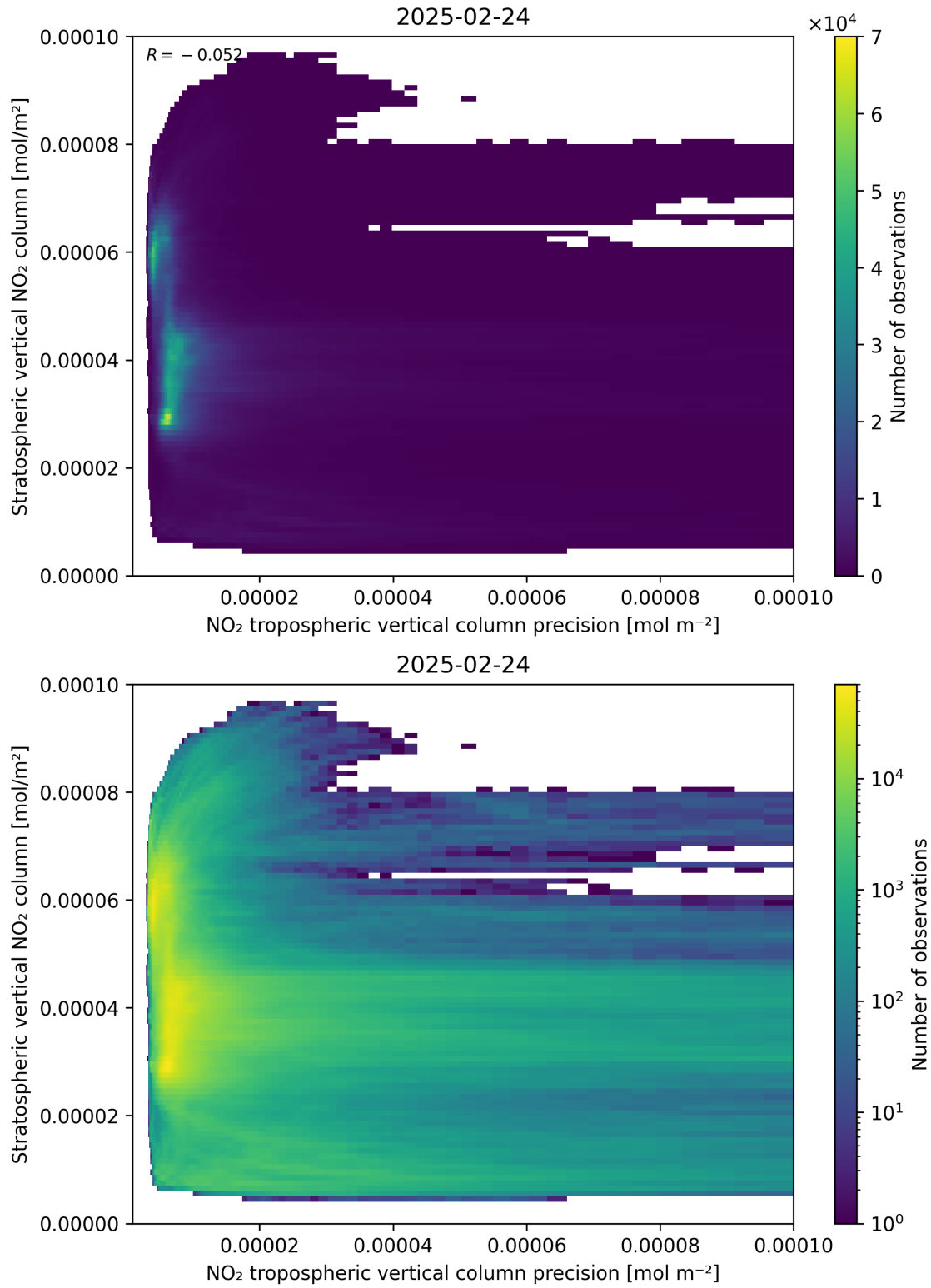
Figure 135: Scatter density plot of “NO 2 tropospheric vertical column precision” against “Stratospheric vertical NO 2 column” for 2025-02-24 to 2025-02-25.
