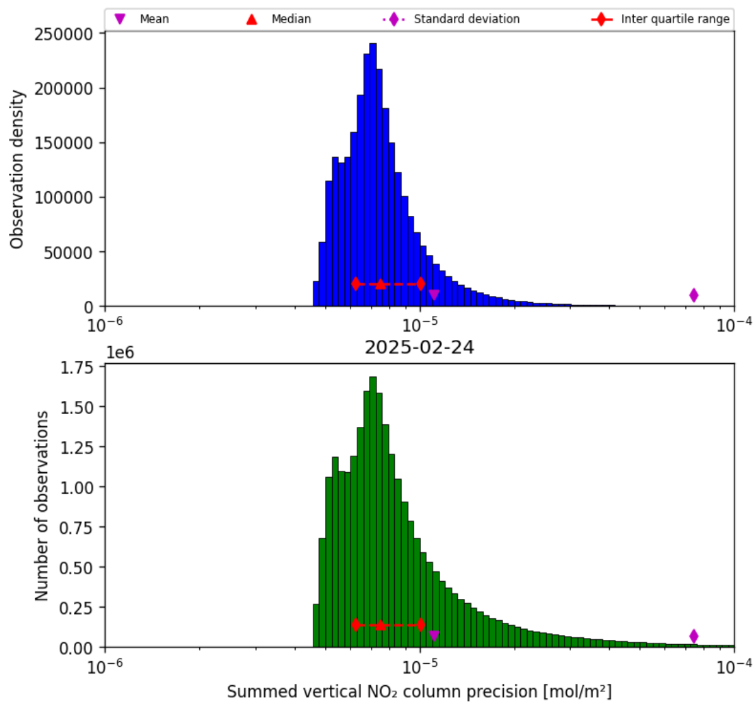
Figure 41: Histogram of “Summed vertical NO 2 column precision” for 2025-02-24 to 2025-02-25
