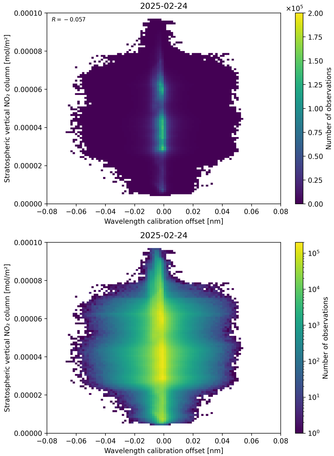
Figure 176: Scatter density plot of “Wavelength calibration offset” against “Stratospheric vertical NO 2 column” for 2025-02-24 to 2025-02-25.
