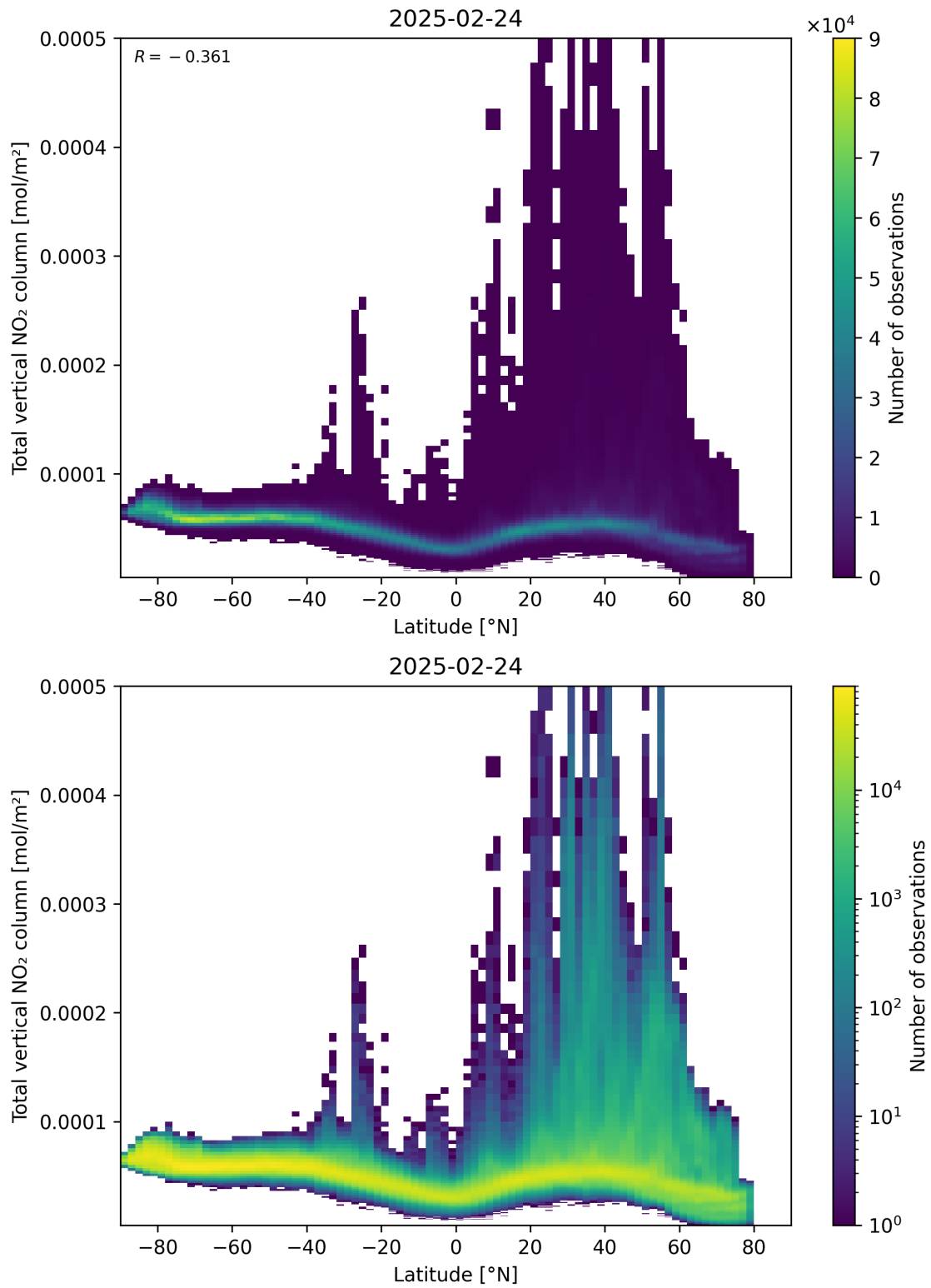
Figure 90: Scatter density plot of “Latitude” against “Total vertical NO 2 column” for 2025-02-24 to 2025-02-25.
