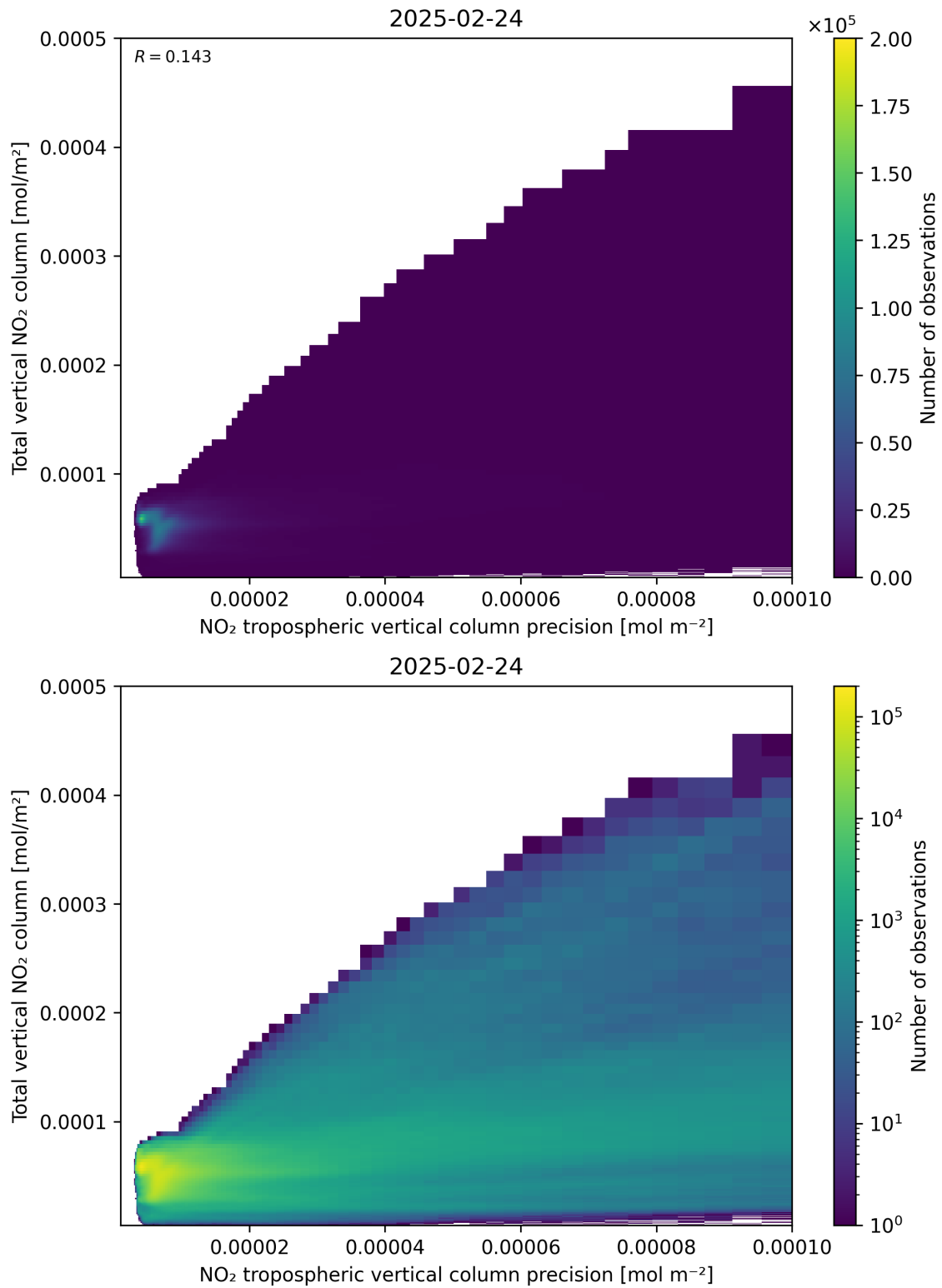
Figure 138: Scatter density plot of “NO 2 tropospheric vertical column precision” against “Total vertical NO 2 column” for 2025-02-24 to 2025-02-25.
