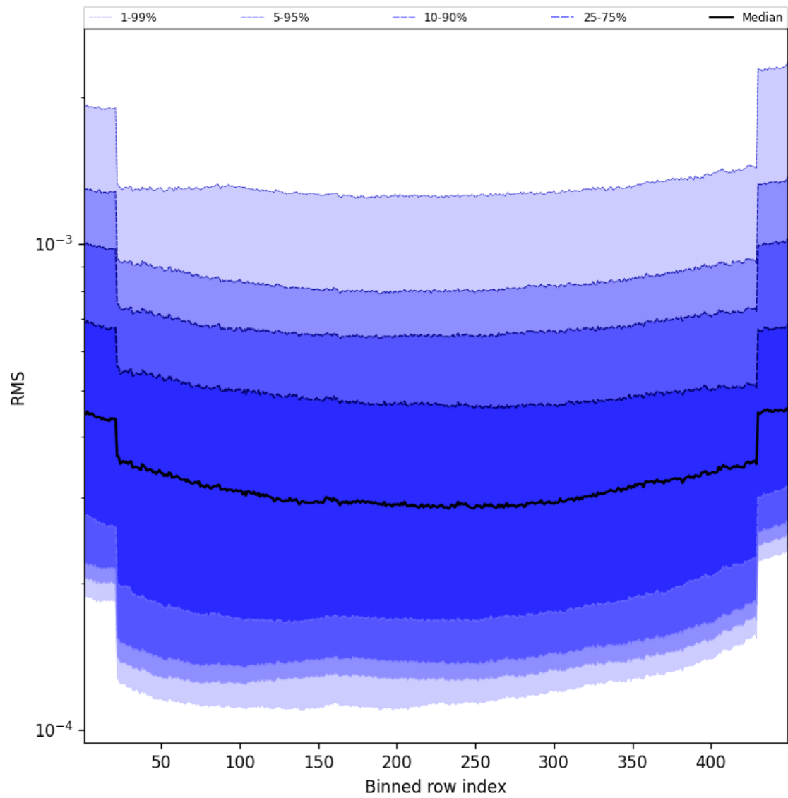
Figure 60: Along track statistics of “RMS” for 2025-02-24 to 2025-02-25
