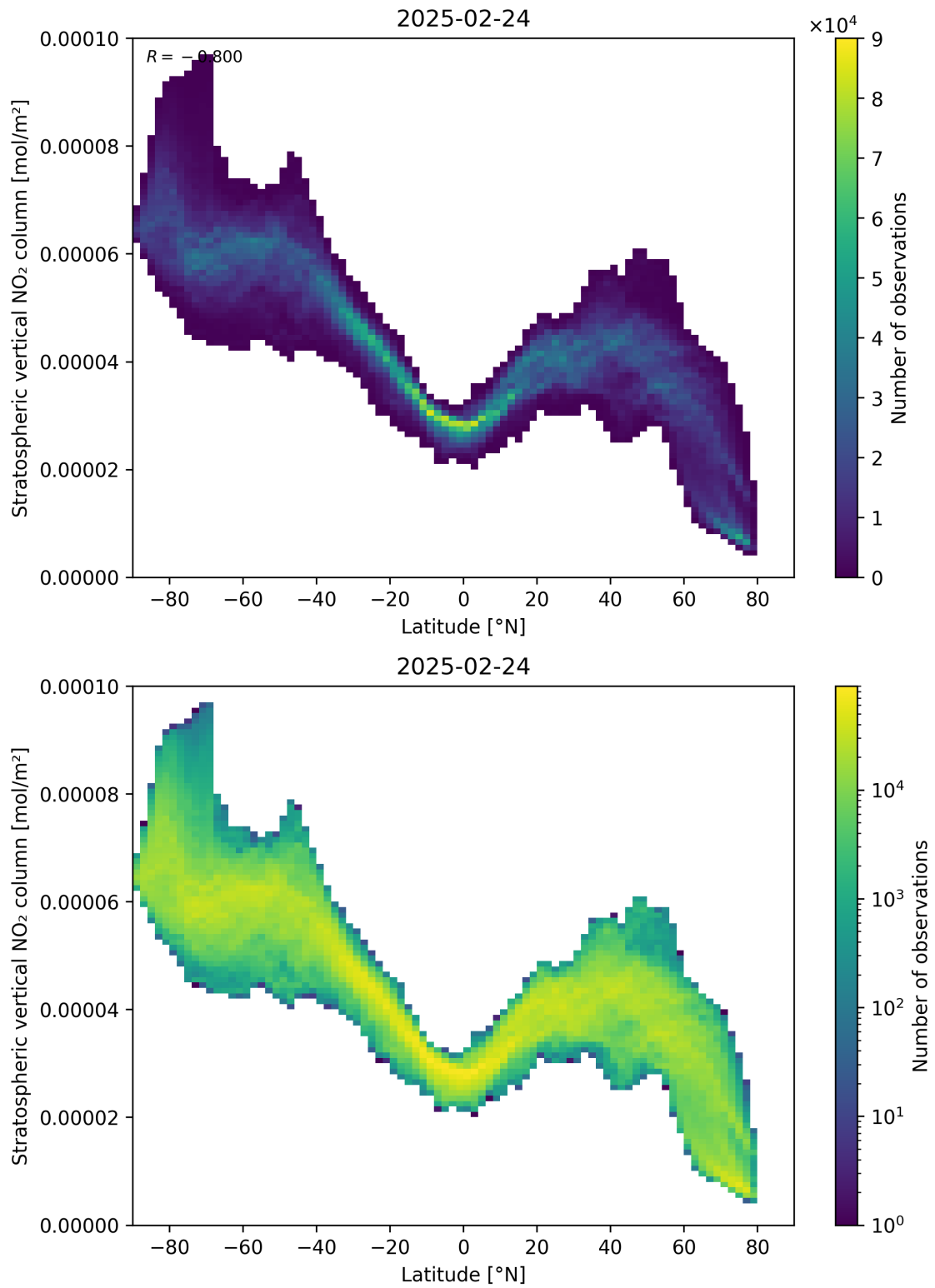
Figure 87: Scatter density plot of “Latitude” against “Stratospheric vertical NO 2 column” for 2025-02-24 to 2025-02-25.
