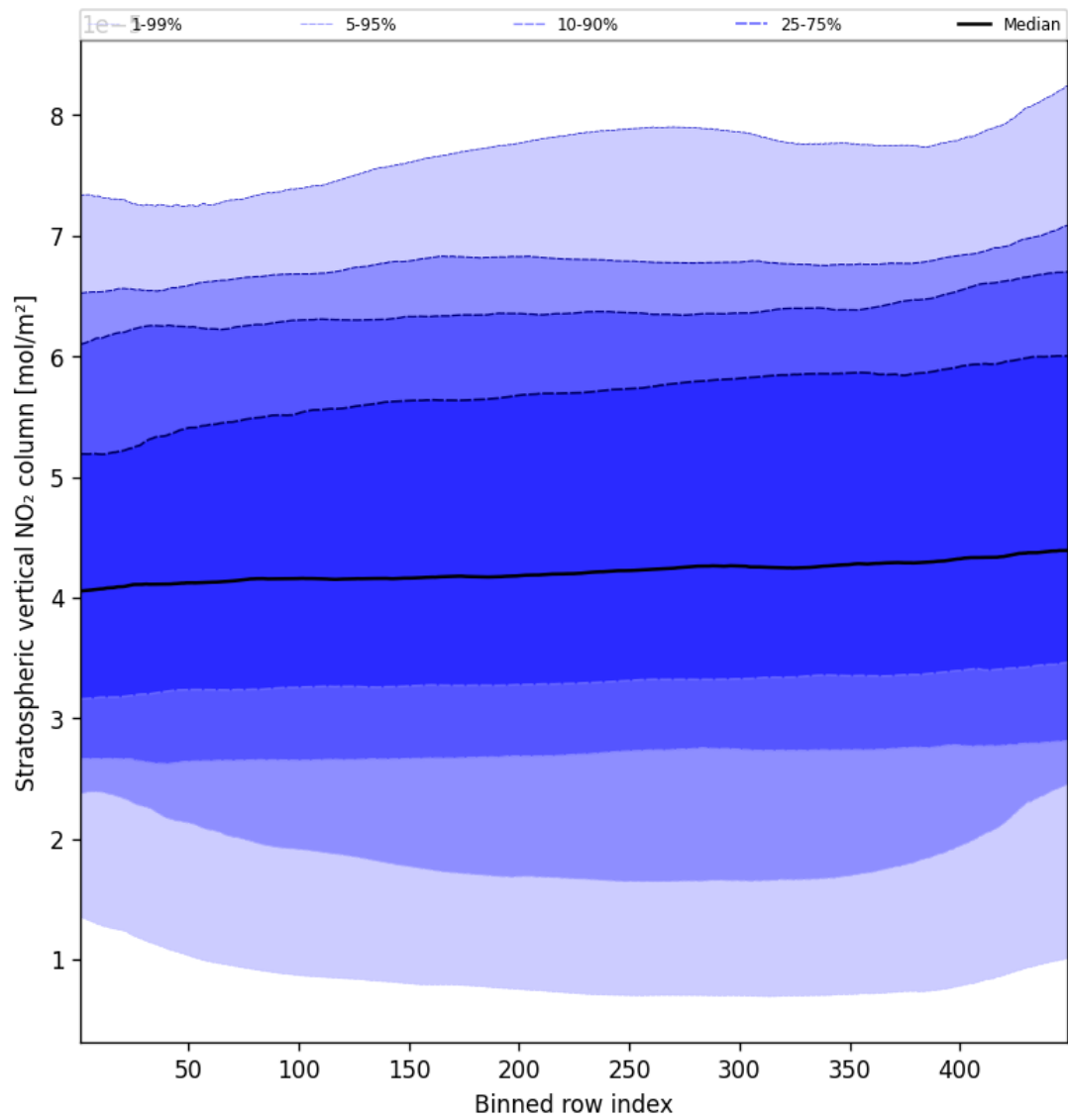
Figure 53: Along track statistics of “Stratospheric vertical NO 2 column” for 2025-02-24 to 2025-02-25
