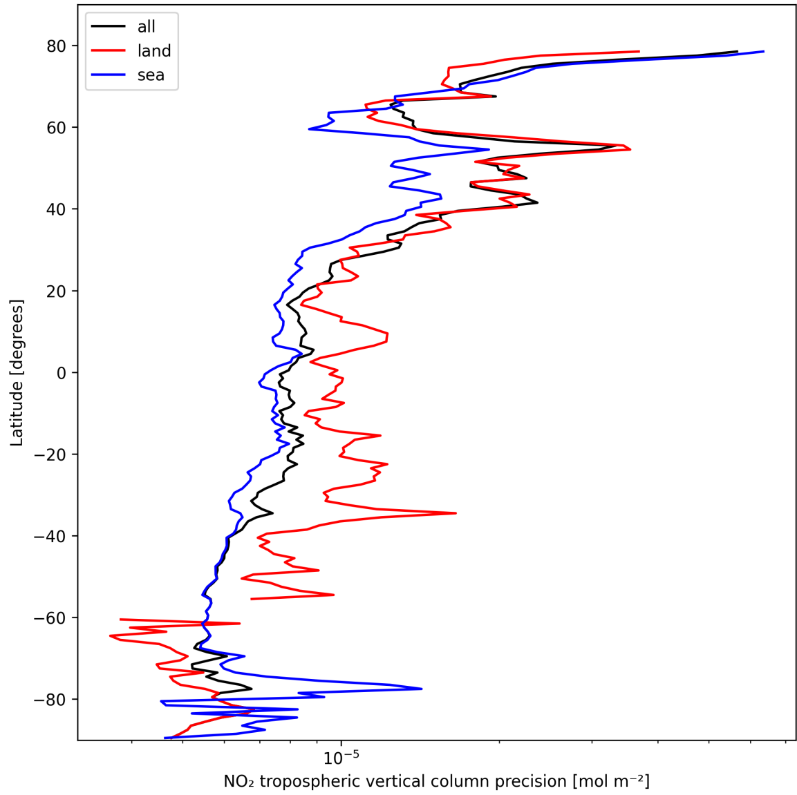
Figure 13: Zonal average of “NO 2 tropospheric vertical column precision” for 2025-02-24 to 2025-02-25.
