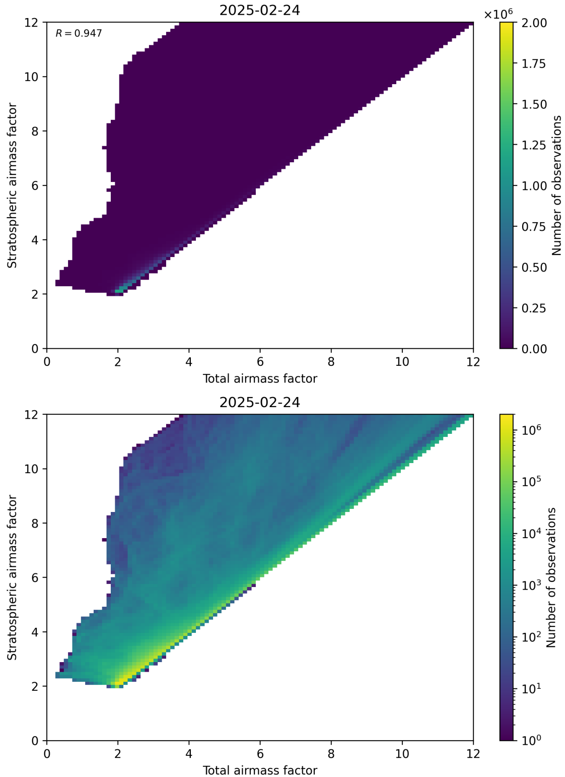
Figure 62: Scatter density plot of “Total airmass factor” against “Stratospheric airmass factor” for 2025-02-24 to 2025-02-25.
