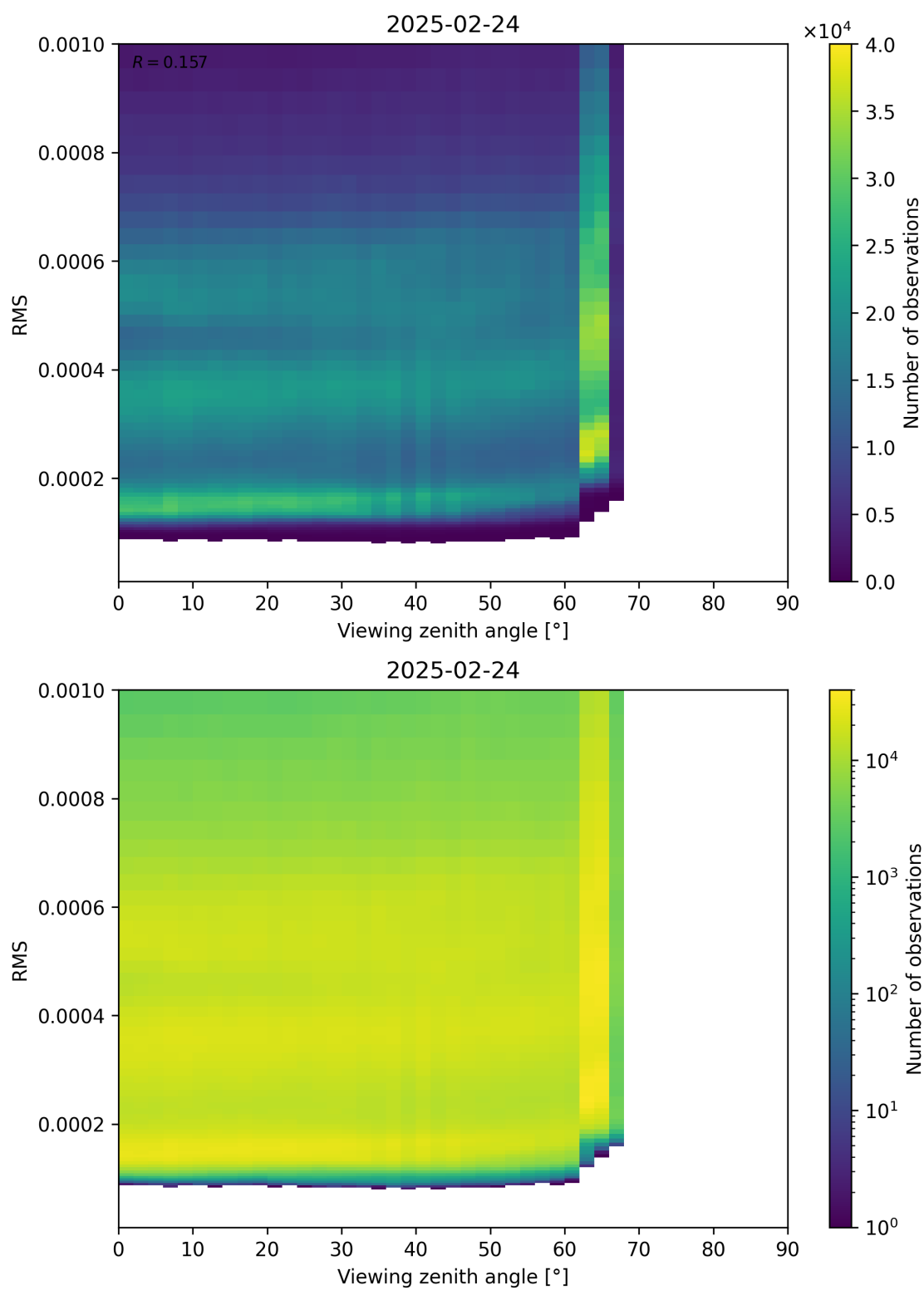
Figure 171: Scatter density plot of “Viewing zenith angle” against “RMS” for 2025-02-24 to 2025-02-25.
