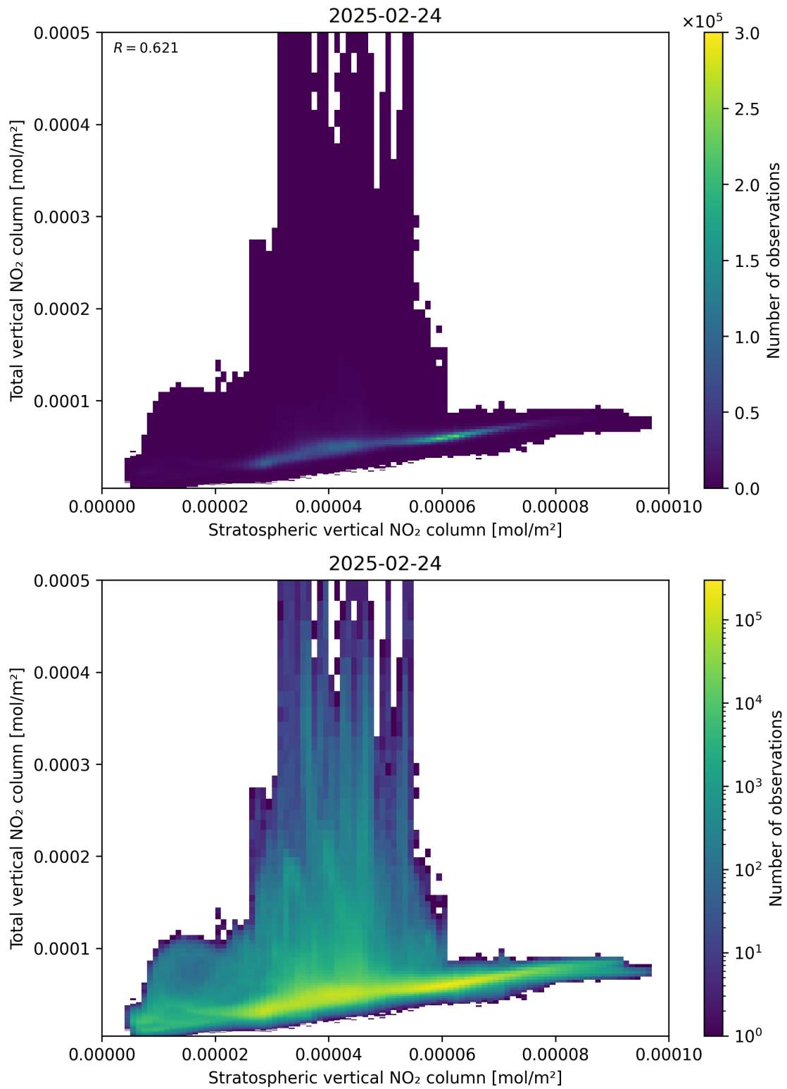
Figure 100: Scatter density plot of “Stratospheric vertical NO 2 column” against “Total vertical NO 2 column” for 2025-02-24 to 2025-02-25.
