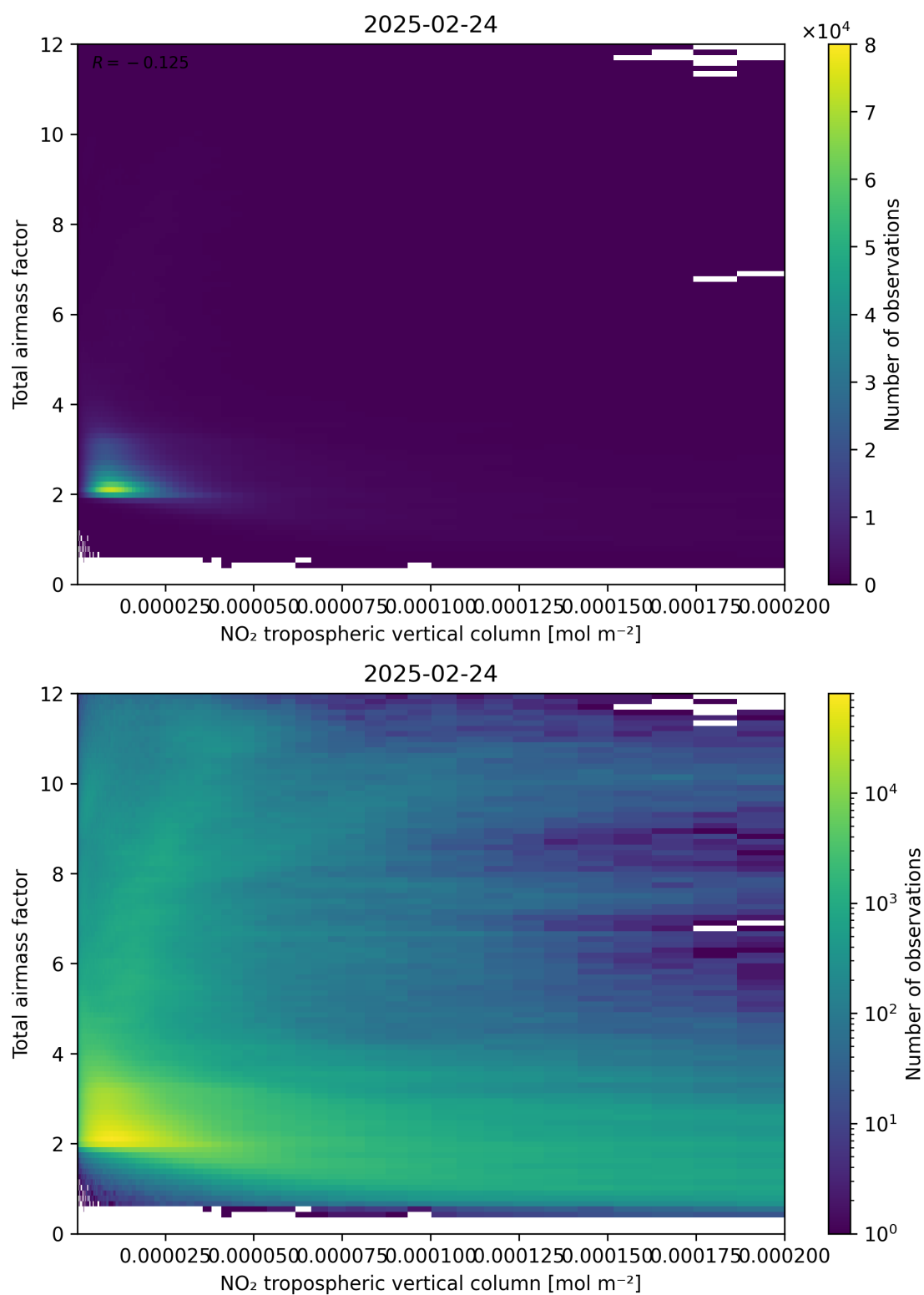
Figure 122: Scatter density plot of “NO 2 tropospheric vertical column” against “Total air mass factor” for 2025-02-24 to 2025-02-25.
