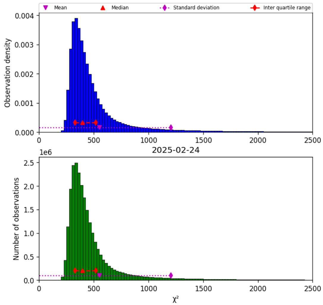
Figure 42: Histogram of “ \chi^2 ” for 2025-02-24 to 2025-02-25
