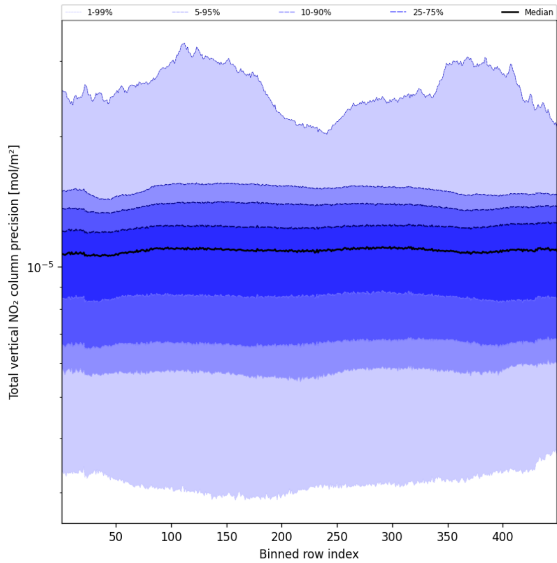
Figure 56: Along track statistics of “Total vertical NO 2 column precision” for 2025-02-24 to 2025-02-25
