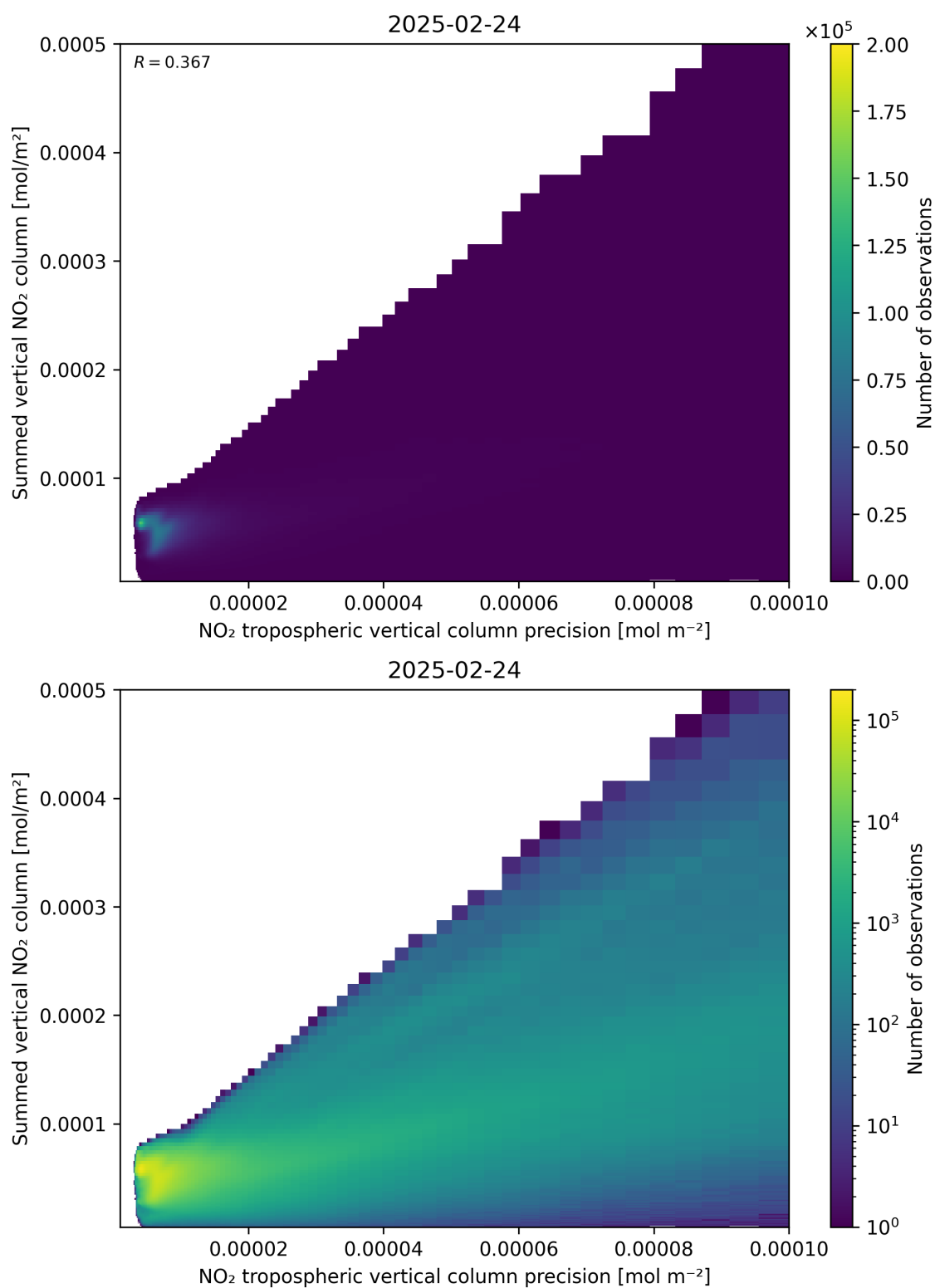
Figure 136: Scatter density plot of “NO 2 tropospheric vertical column precision” against “Summed vertical NO 2 column” for 2025-02-24 to 2025-02-25.
