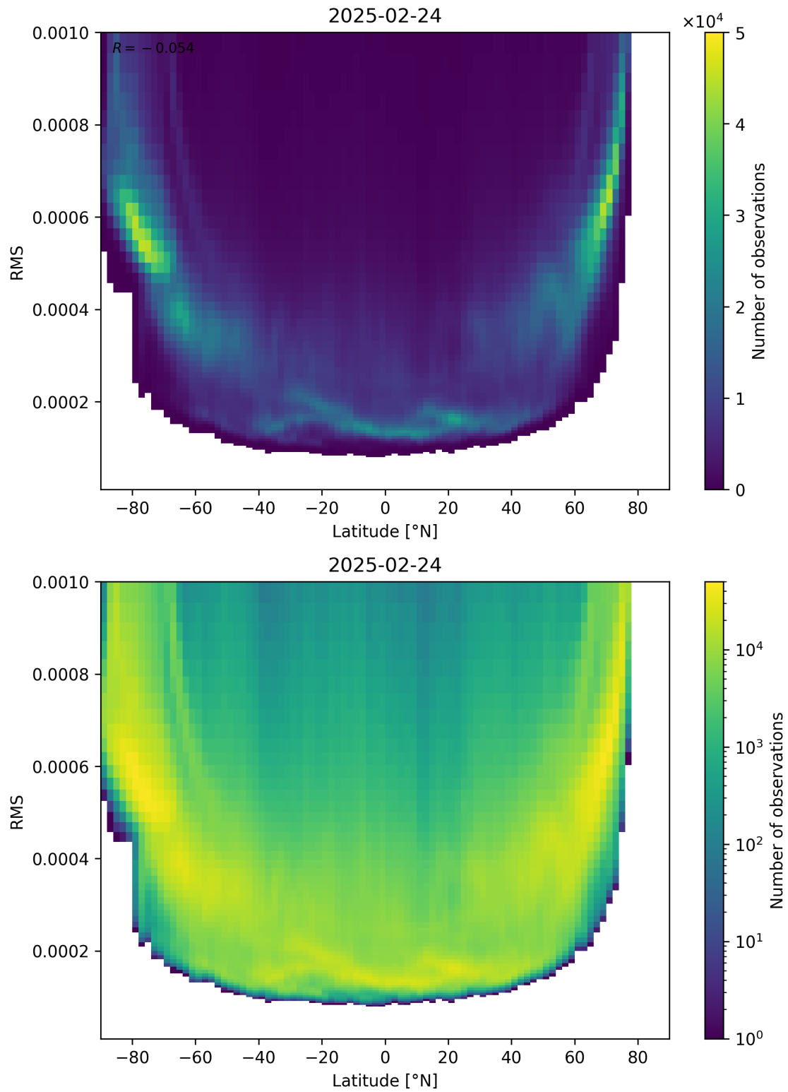
Figure 94: Scatter density plot of “Latitude” against “RMS” for 2025-02-24 to 2025-02-25.
