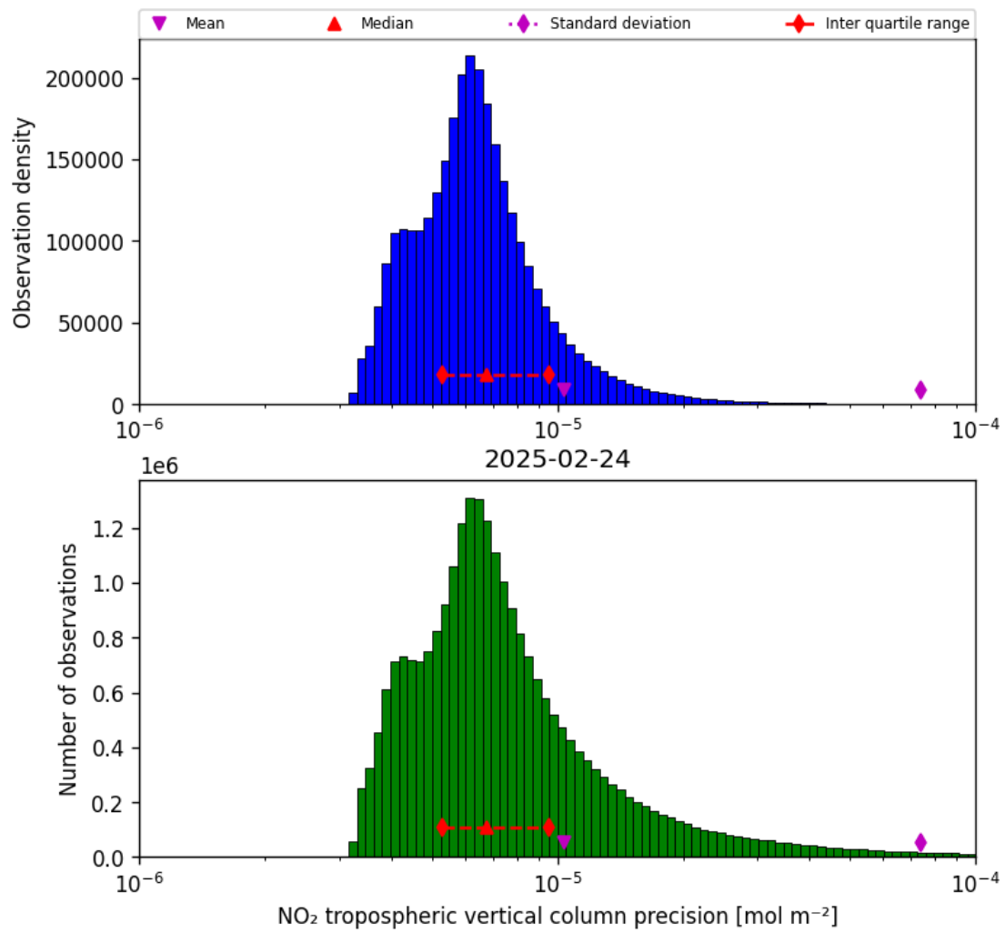
Figure 30: Histogram of “NO 2 tropospheric vertical column precision” for 2025-02-24 to 2025-02-25
