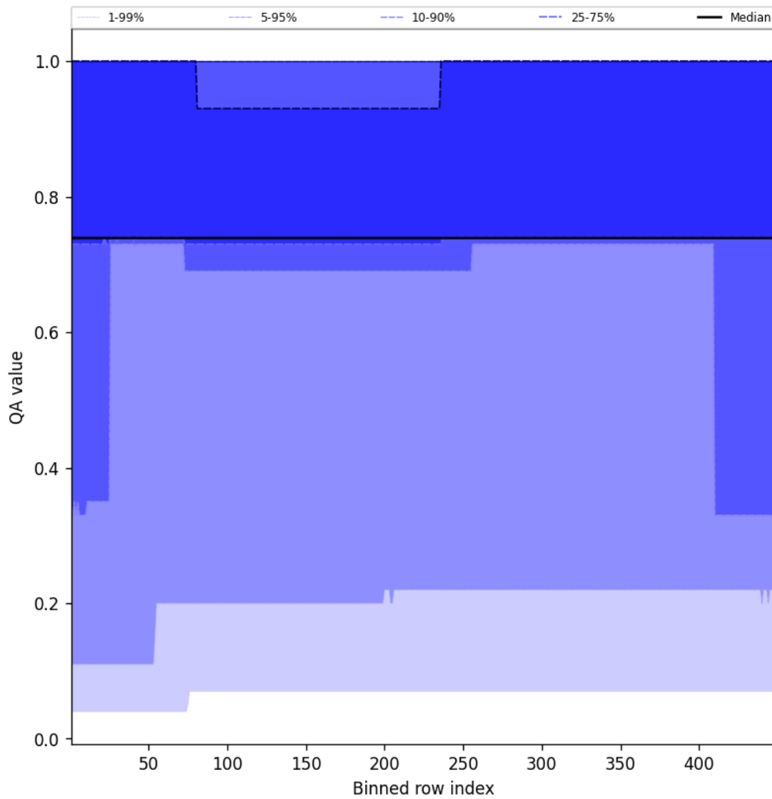
Figure 45: Along track statistics of “QA value” for 2025-02-24 to 2025-02-25
