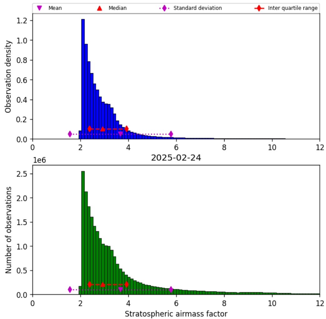
Figure 44: Histogram of “Stratospheric airmass factor” for 2025-02-24 to 2025-02-25
