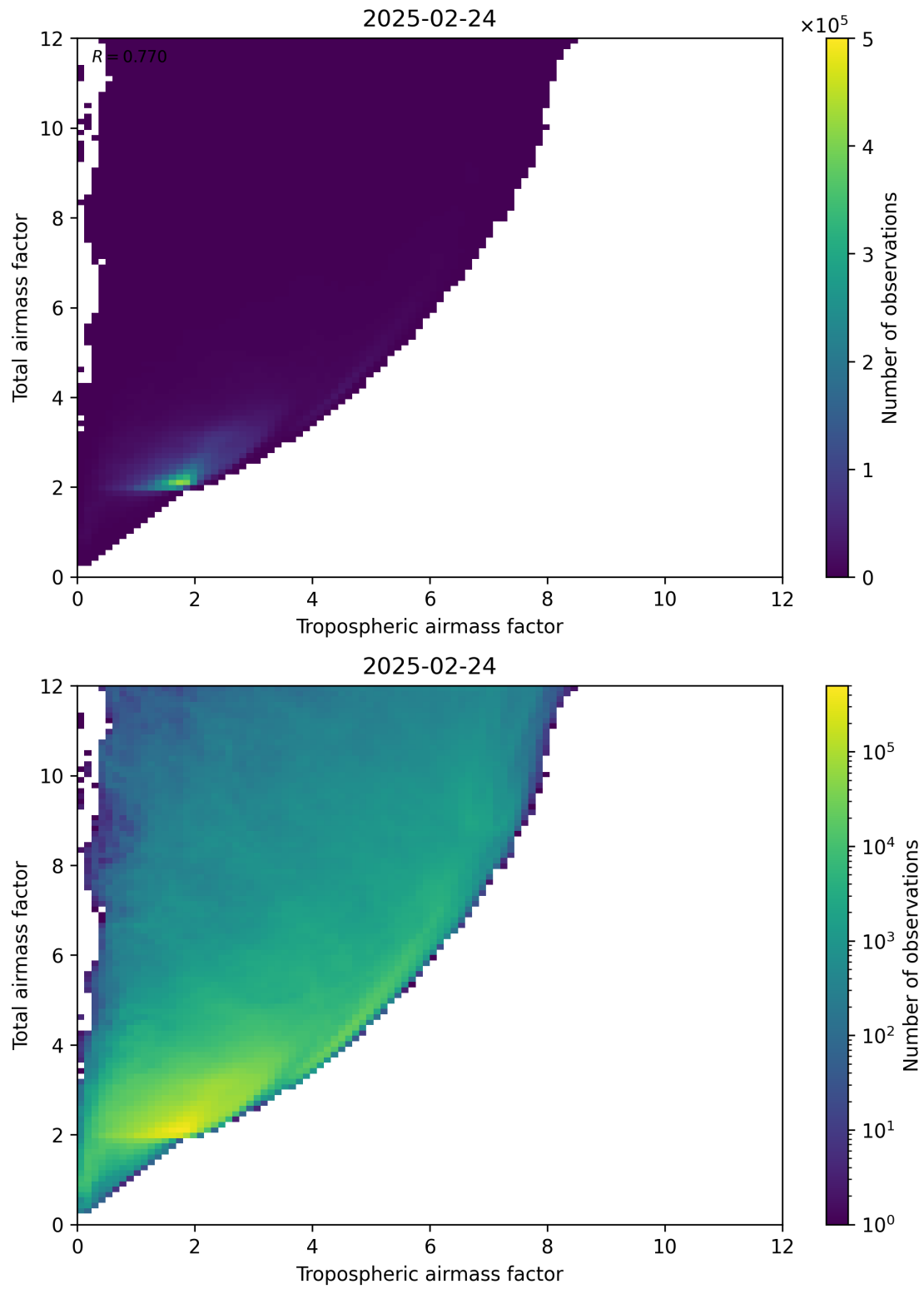
Figure 72: Scatter density plot of “Tropospheric airmass factor” against “Total airmass factor” for 2025-02-24 to 2025-02-25.
