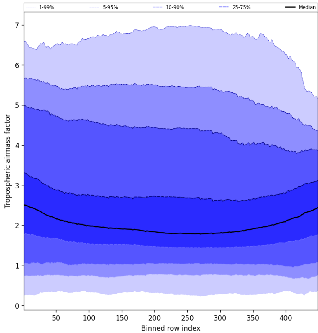
Figure 48: Along track statistics of “Tropospheric air mass factor” for 2025-02-24 to 2025-02-25
