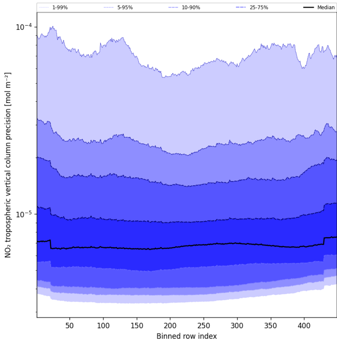
Figure 47: Along track statistics of “NO 2 tropospheric vertical column precision” for 2025-02-24 to 2025-02-25
