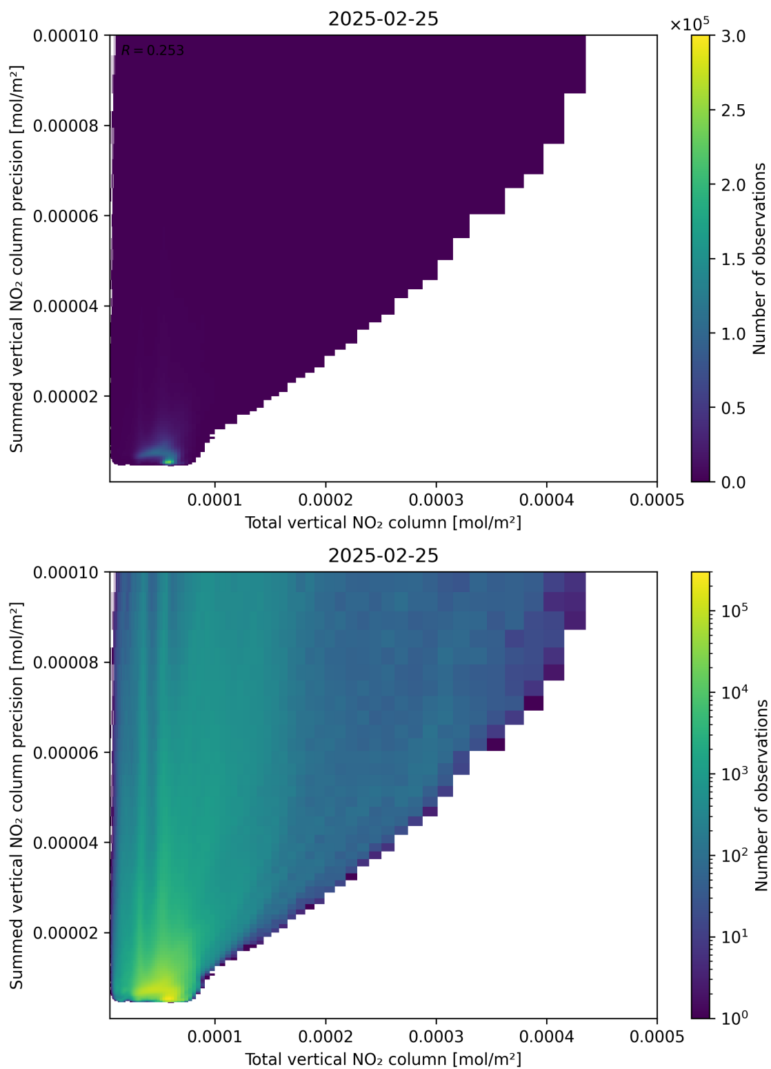
Figure 113: Scatter density plot of “Total vertical NO 2 column” against “Summed vertical NO 2 column precision” for 2025-02-24 to 2025-02-26.
