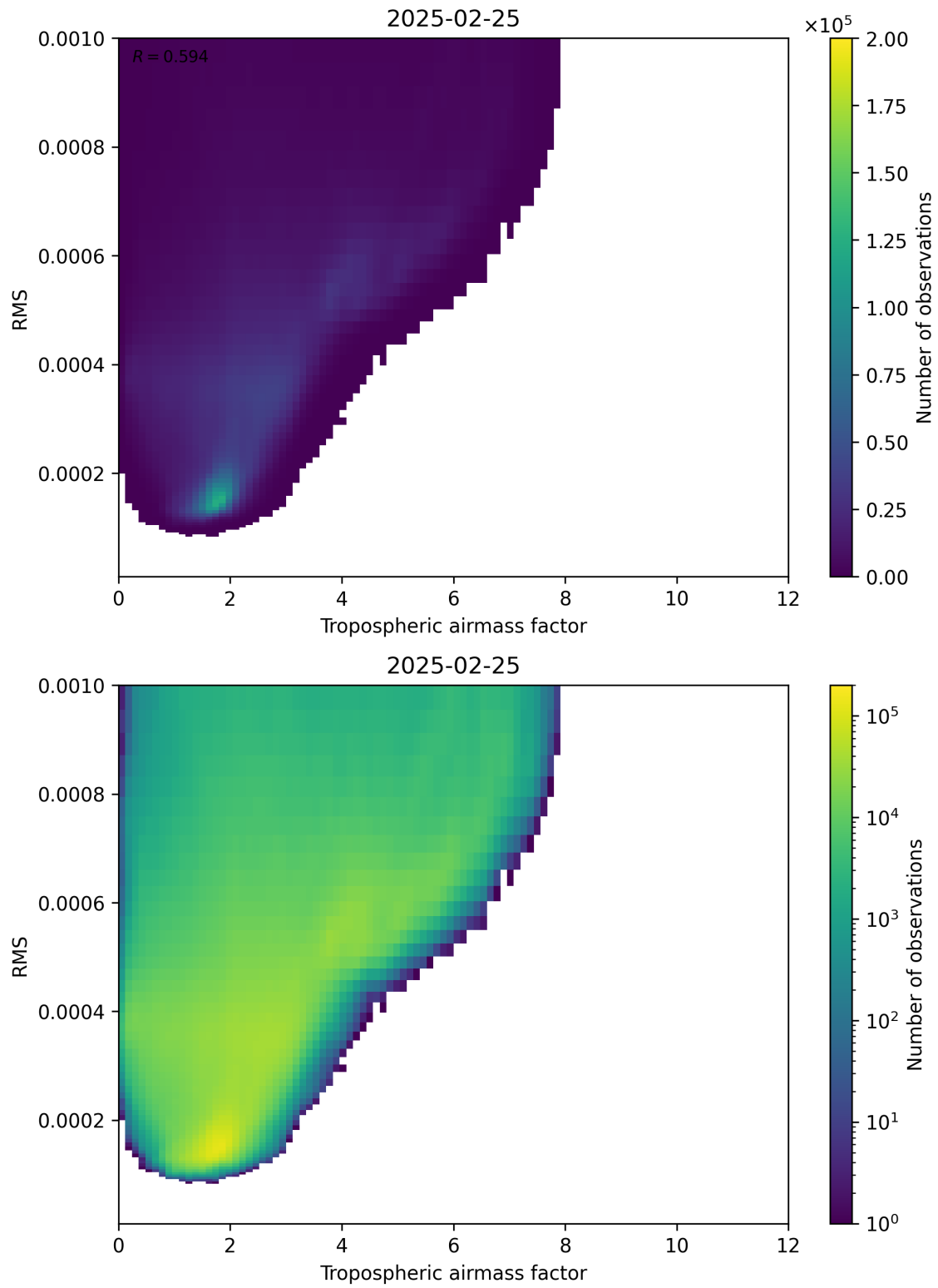
Figure 79: Scatter density plot of “Tropospheric airmass factor” against “RMS” for 2025-02-24 to 2025-02-26.
