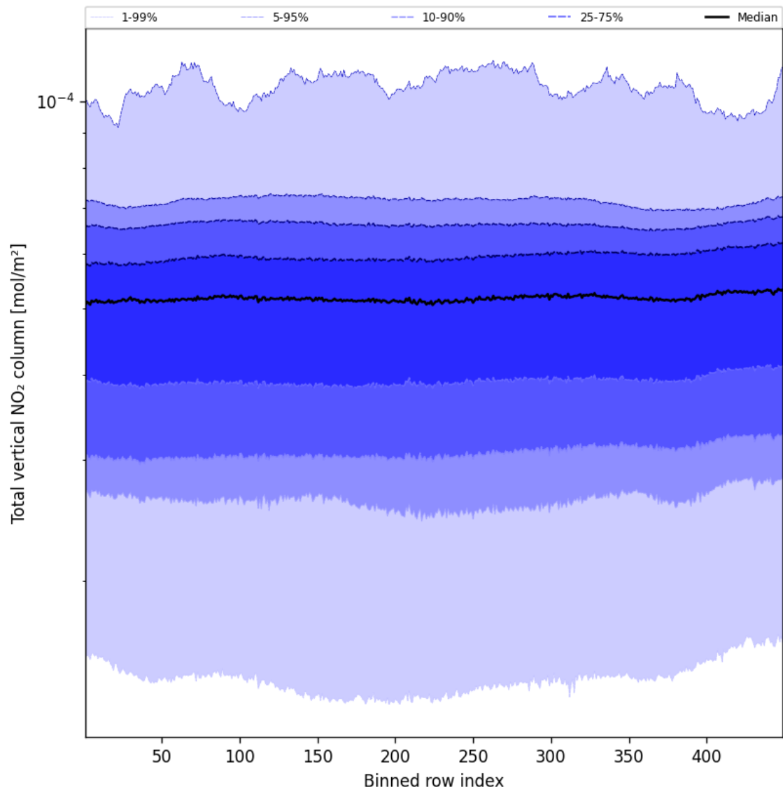
Figure 55: Along track statistics of “Total vertical NO 2 column” for 2025-02-24 to 2025-02-26
