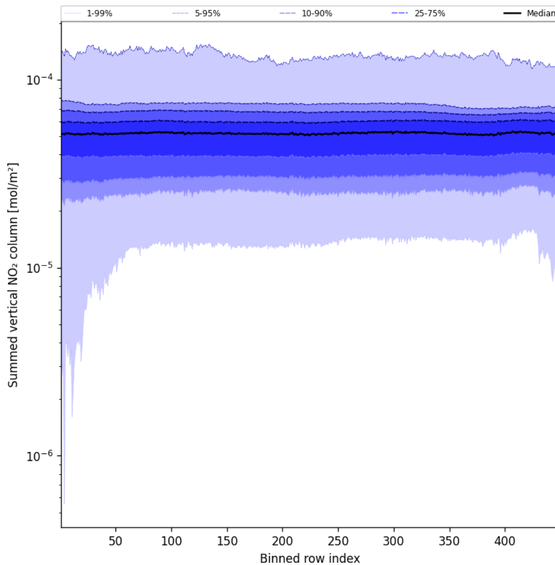
Figure 57: Along track statistics of “Summed vertical NO 2 column” for 2025-02-24 to 2025-02-26
