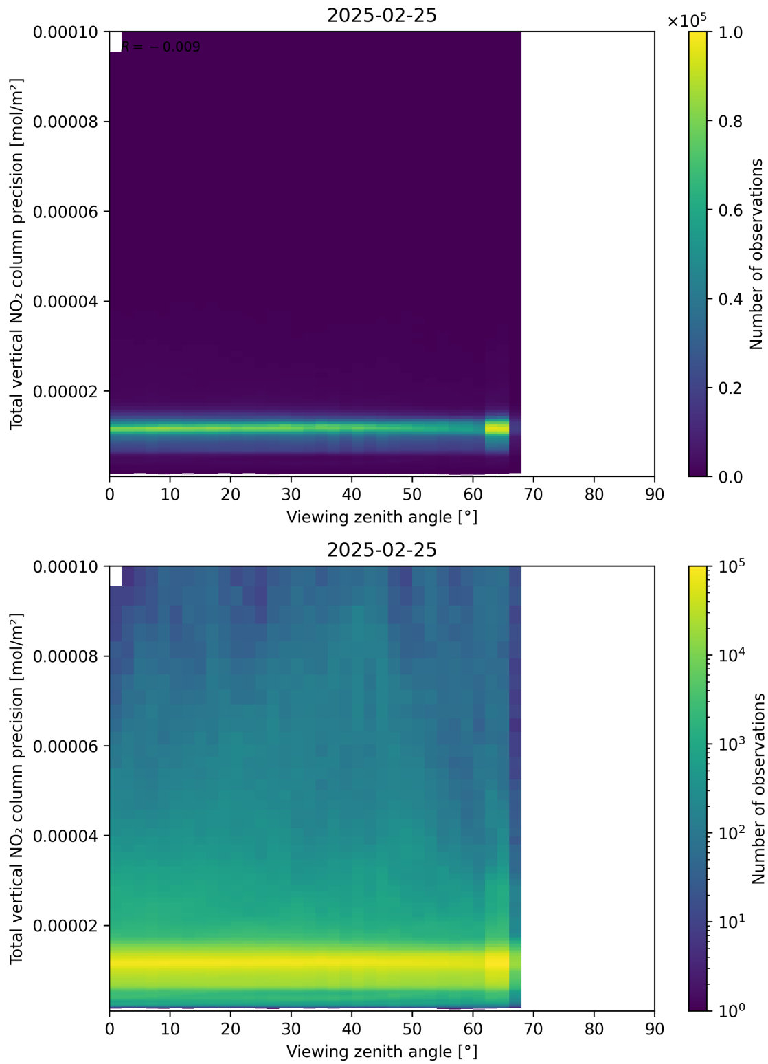
Figure 168: Scatter density plot of “Viewing zenith angle” against “Total vertical NO 2 column precision” for 2025-02-24 to 2025-02-26.
