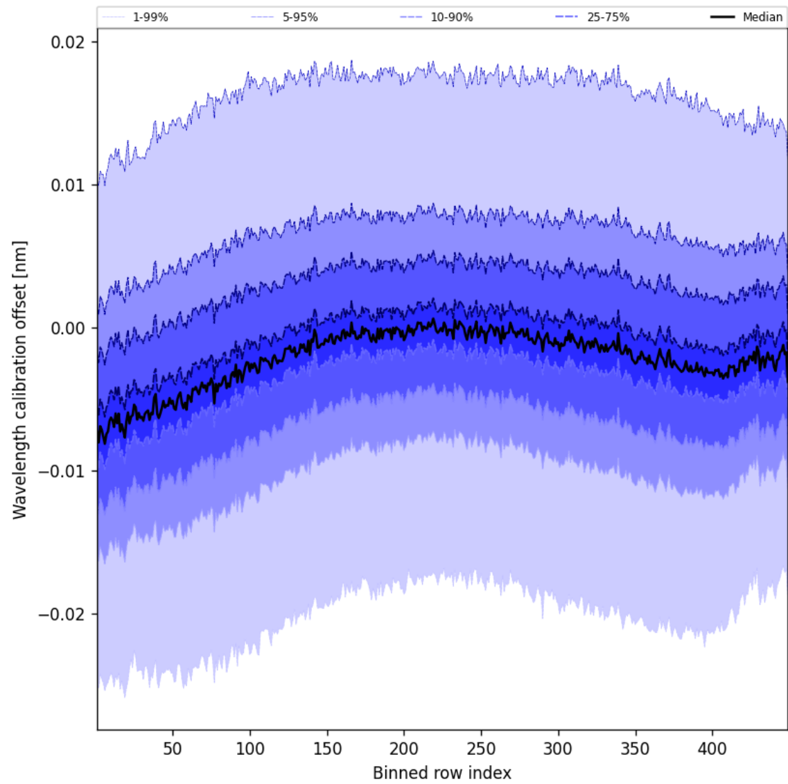
Figure 52: Along track statistics of “Wavelength calibration offset” for 2025-02-24 to 2025-02-26
