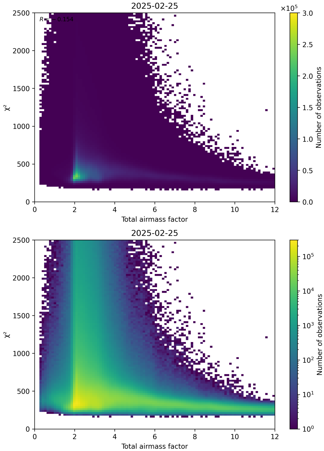
Figure 63: Scatter density plot of “Total airmass factor” against “ \chi^2 ” for 2025-02-24 to 2025-02-26.
