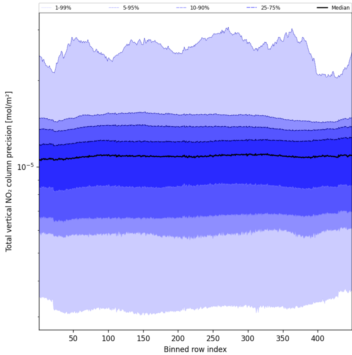
Figure 56: Along track statistics of “Total vertical NO 2 column precision” for 2025-02-24 to 2025-02-26
