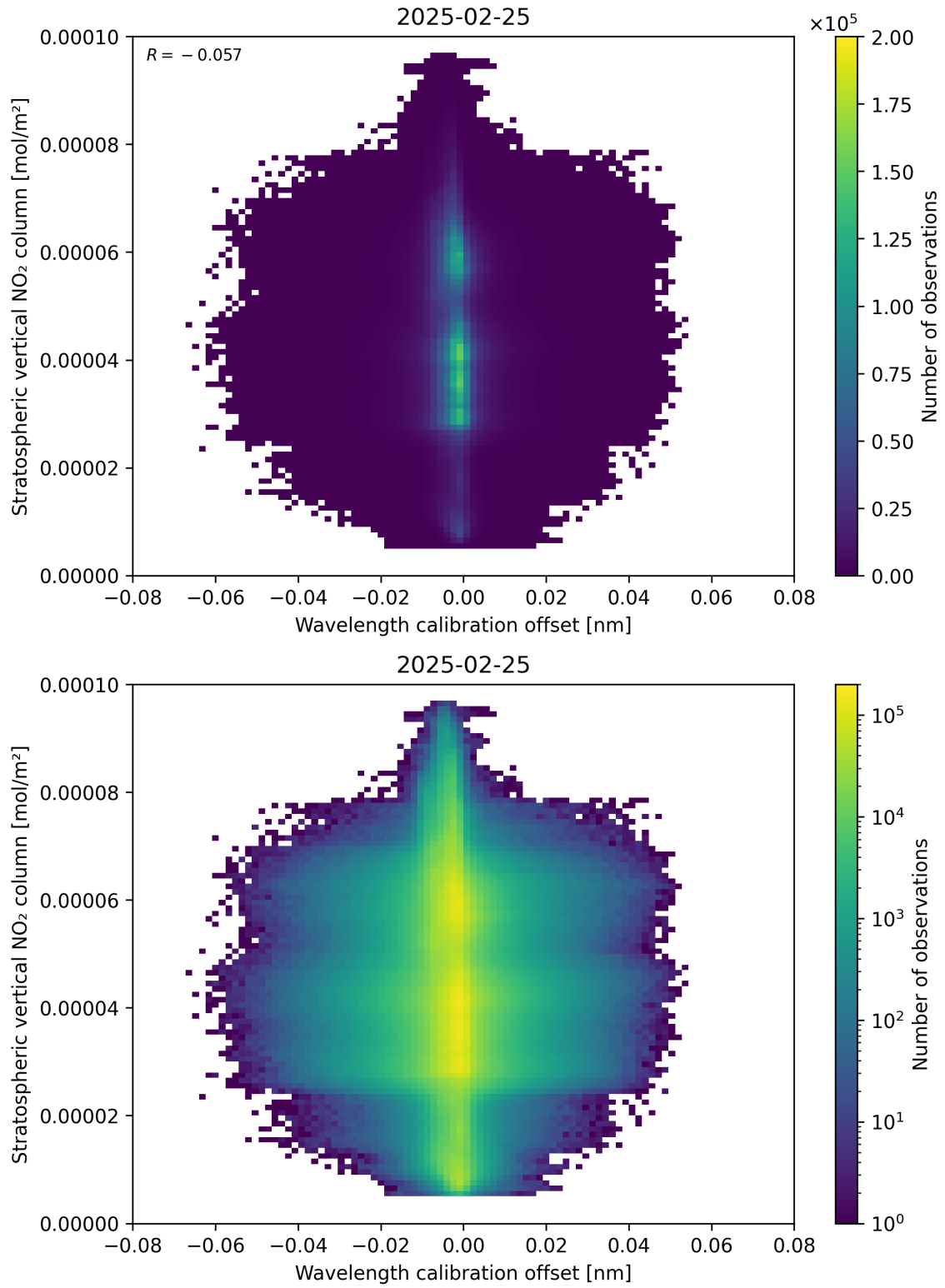
Figure 176: Scatter density plot of “Wavelength calibration offset” against “Stratospheric vertical NO 2 column” for 2025-02-24 to 2025-02-26.
