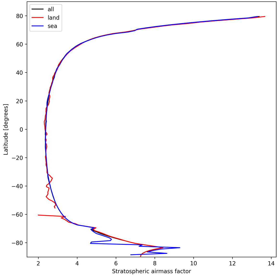
Figure 27: Zonal average of “Stratospheric air mass factor” for 2025-02-24 to 2025-02-26.
