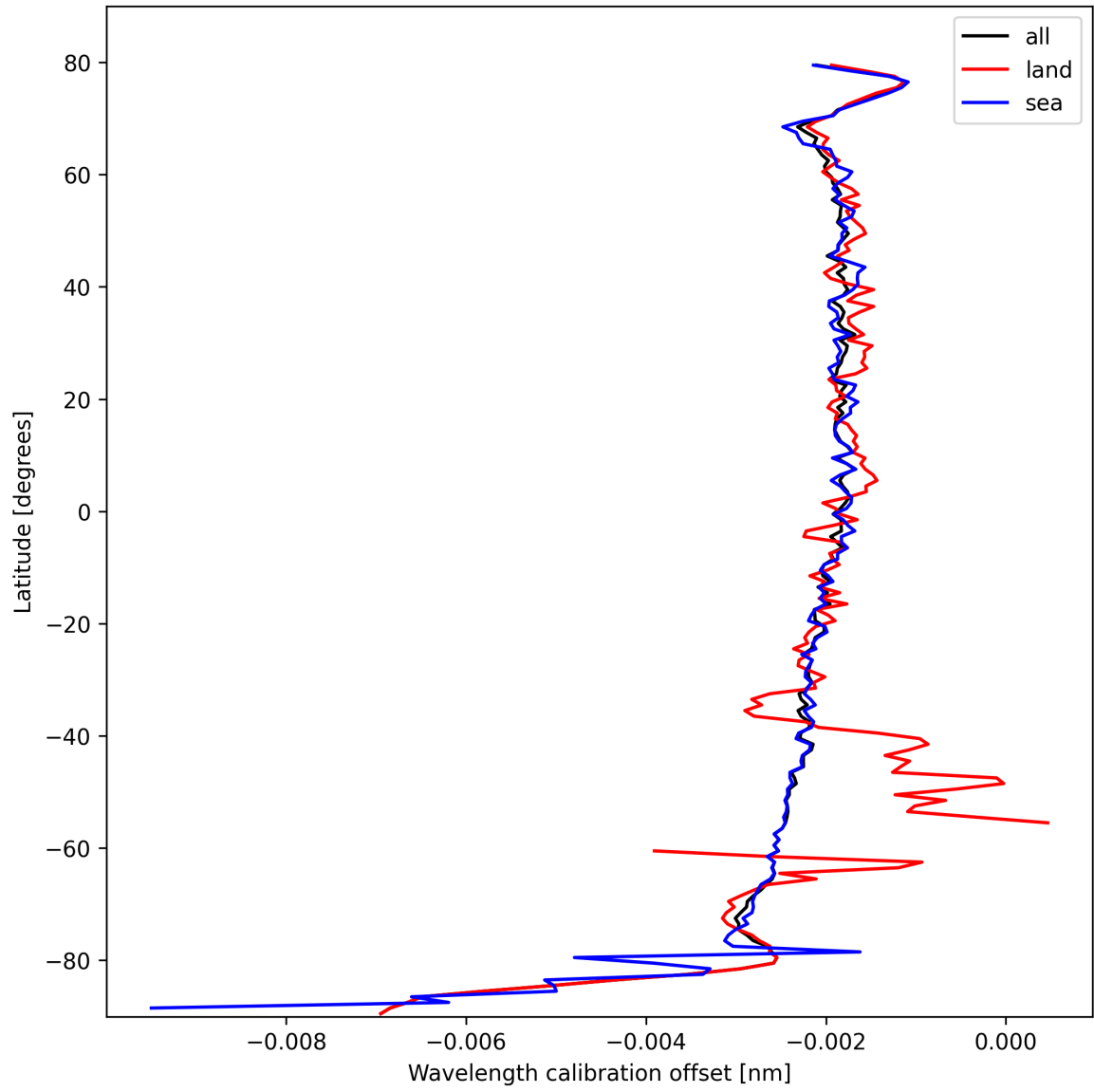
Figure 18: Zonal average of “Wavelength calibration offset” for 2025-02-24 to 2025-02-26.
