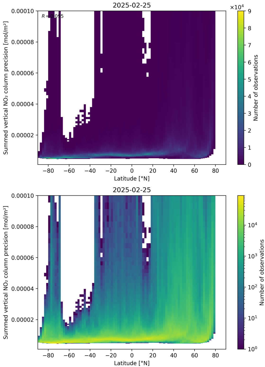
Figure 89: Scatter density plot of “Latitude” against “Summed vertical NO 2 column precision” for 2025-02-24 to 2025-02-26.
