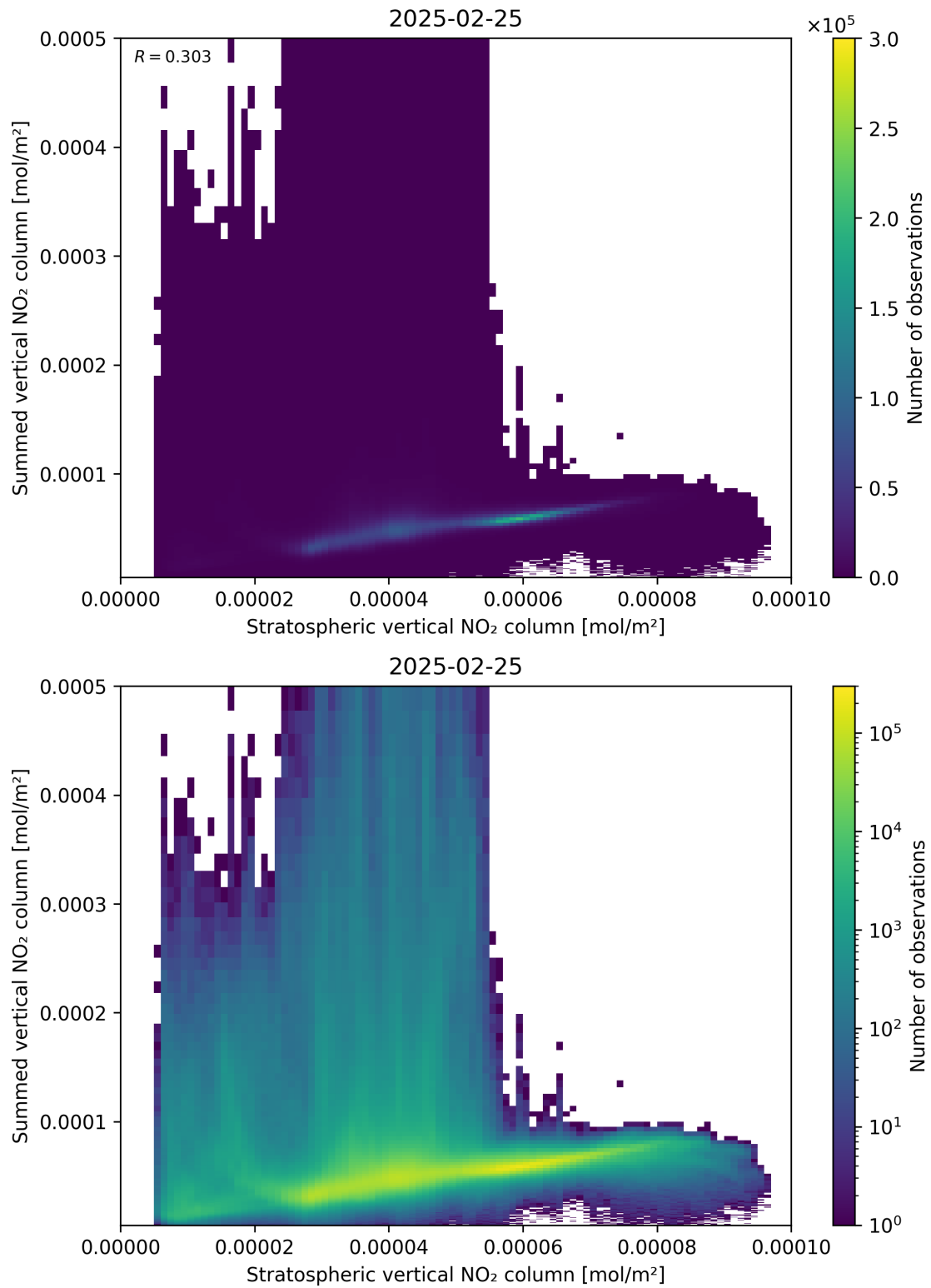
Figure 98: Scatter density plot of “Stratospheric vertical NO 2 column” against “Summed vertical NO 2 column” for 2025-02-24 to 2025-02-26.
