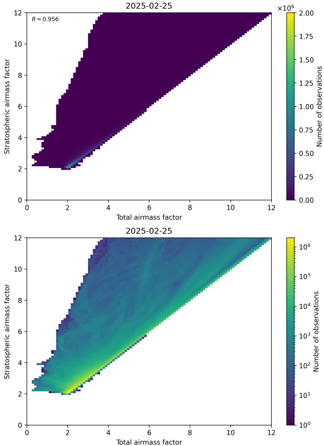
Figure 62: Scatter density plot of “Total airmass factor” against “Stratospheric airmass factor” for 2025-02-24 to 2025-02-26.
