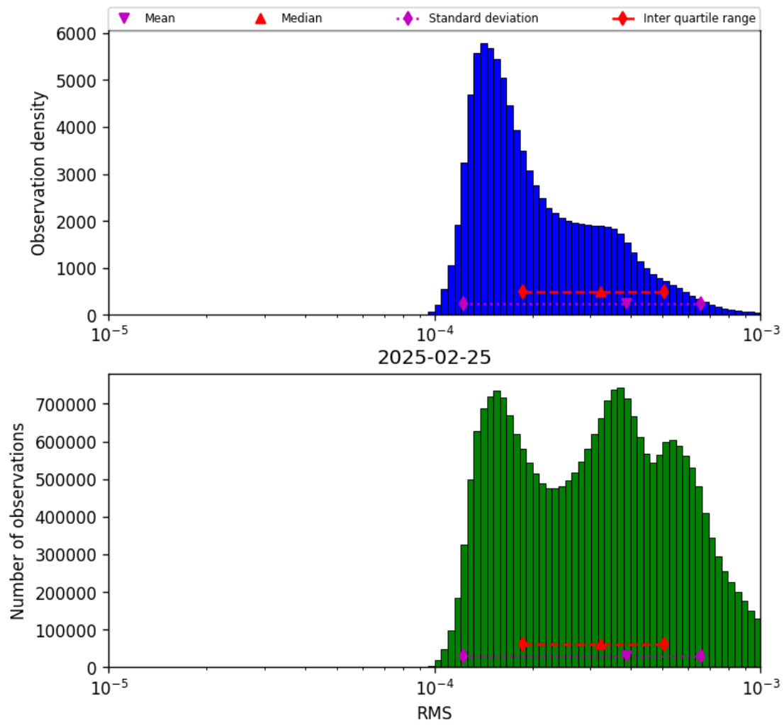
Figure 43: Histogram of “RMS” for 2025-02-24 to 2025-02-26
