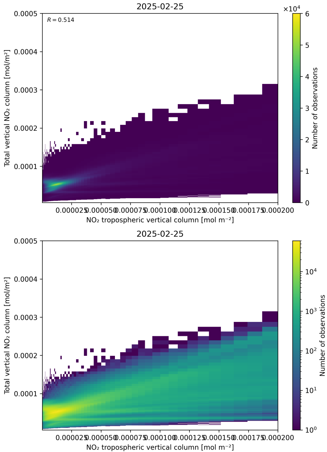
Figure 128: Scatter density plot of “NO 2 tropospheric vertical column” against “Total vertical NO 2 column” for 2025-02-24 to 2025-02-26.
