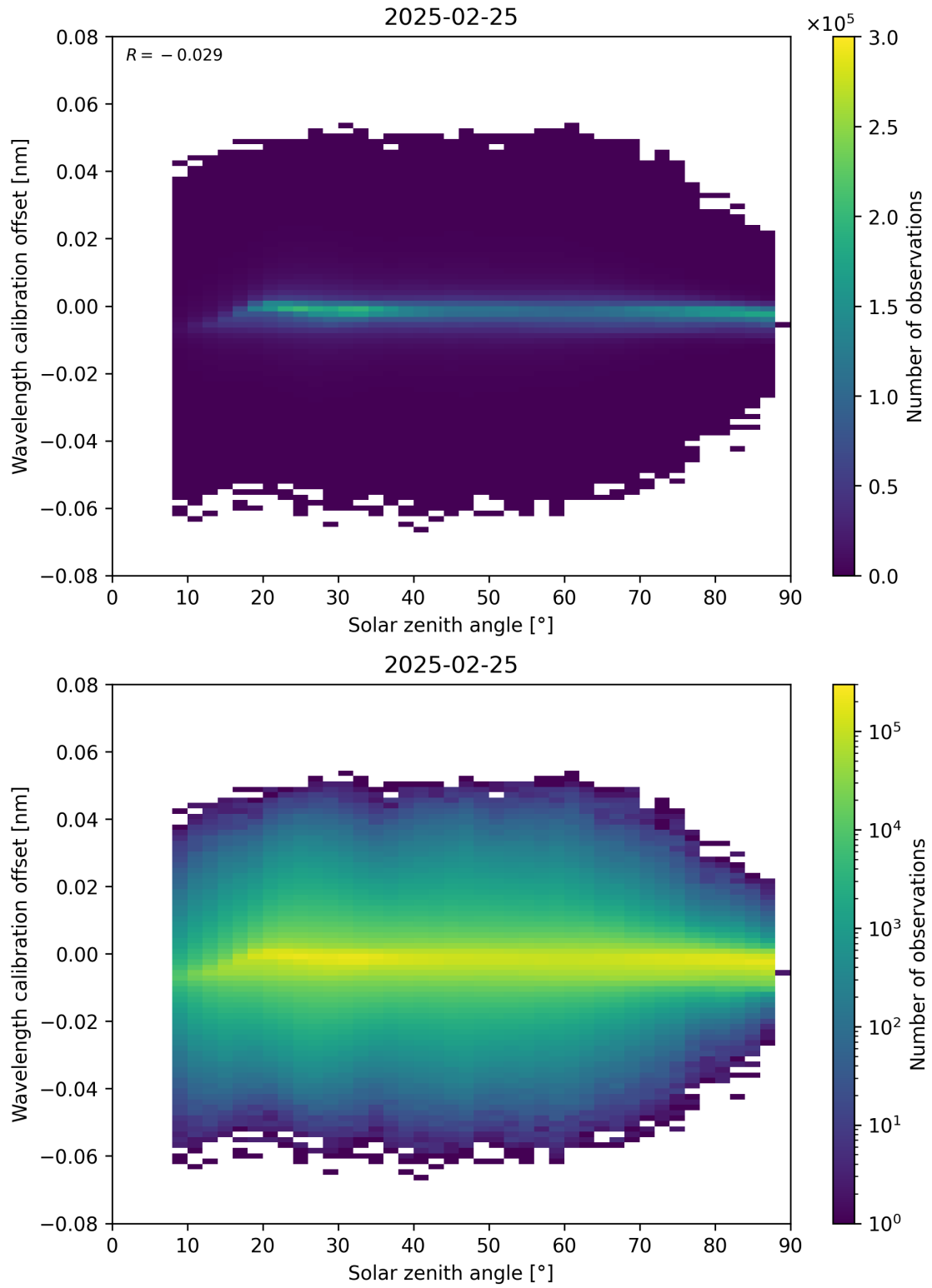
Figure 158: Scatter density plot of “Solar zenith angle” against “Wavelength calibration offset” for 2025-02-24 to 2025-02-26.
