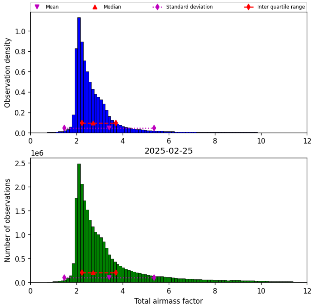
Figure 32: Histogram of “Total airmass factor” for 2025-02-24 to 2025-02-26
