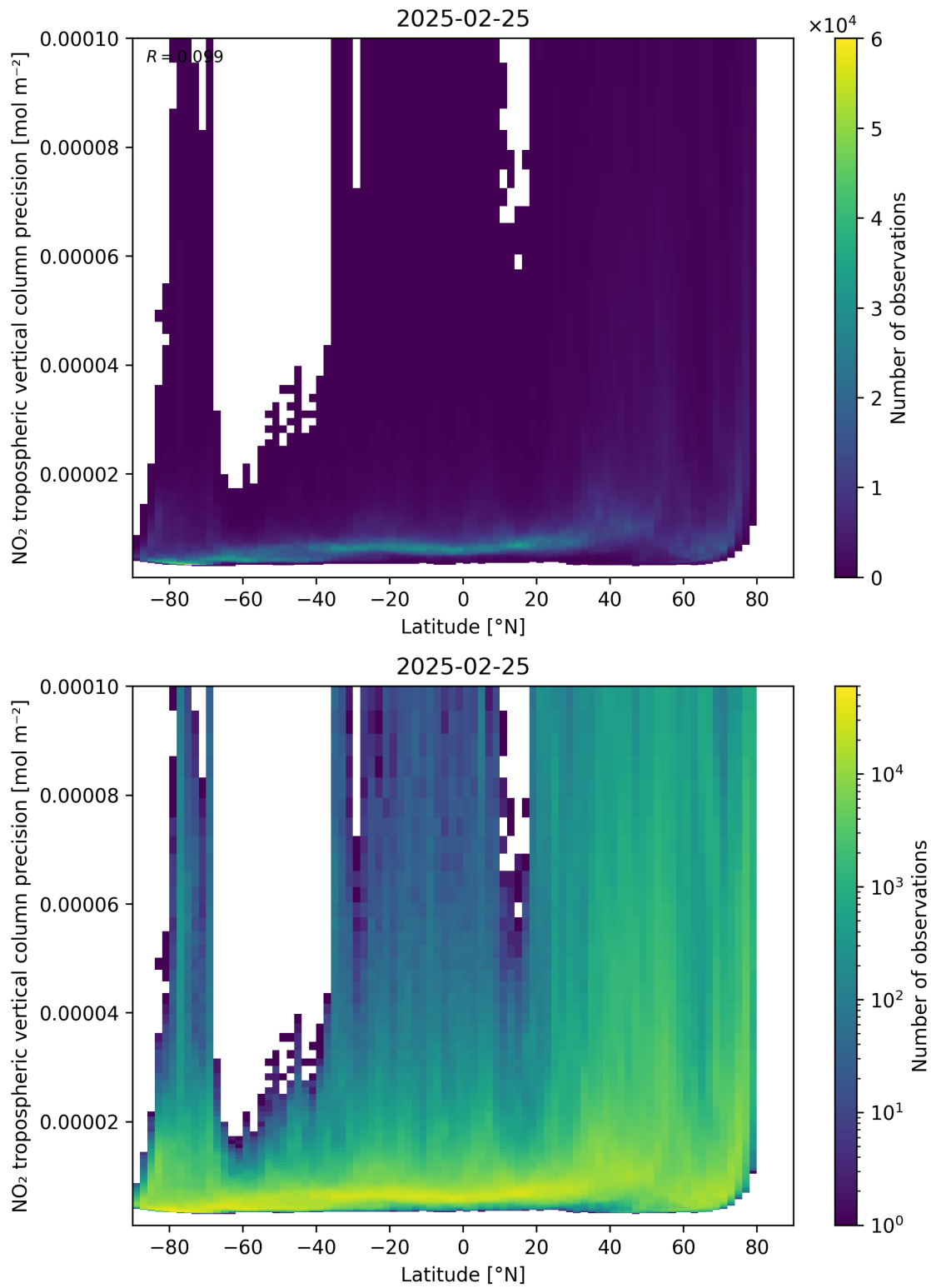
Figure 93: Scatter density plot of “Latitude” against “NO 2 tropospheric vertical column precision” for 2025-02-24 to 2025-02-26.
