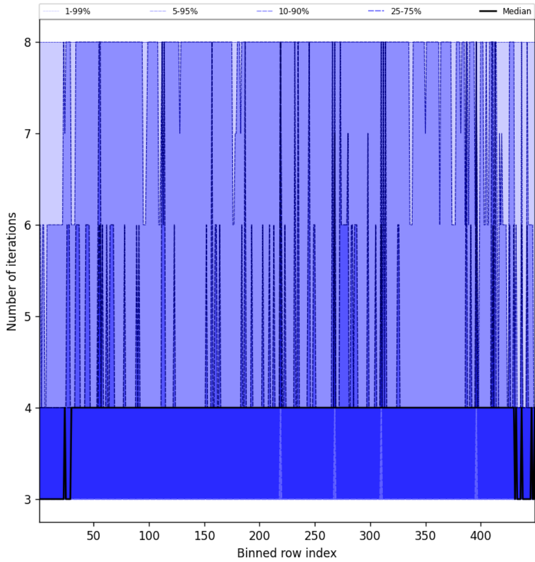
Figure 51: Along track statistics of “Number of iterations” for 2025-02-24 to 2025-02-26
