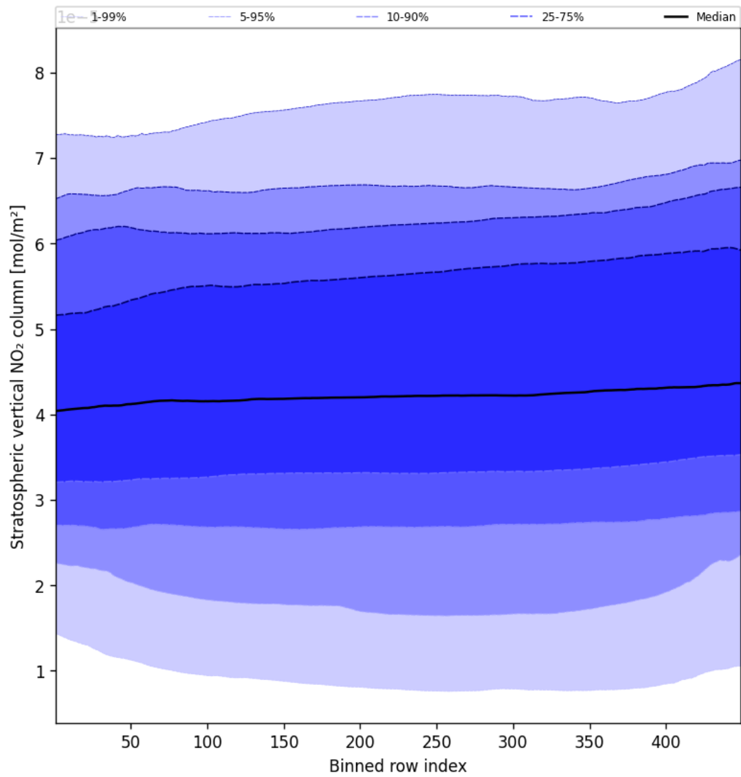
Figure 53: Along track statistics of “Stratospheric vertical NO 2 column” for 2025-02-24 to 2025-02-26
