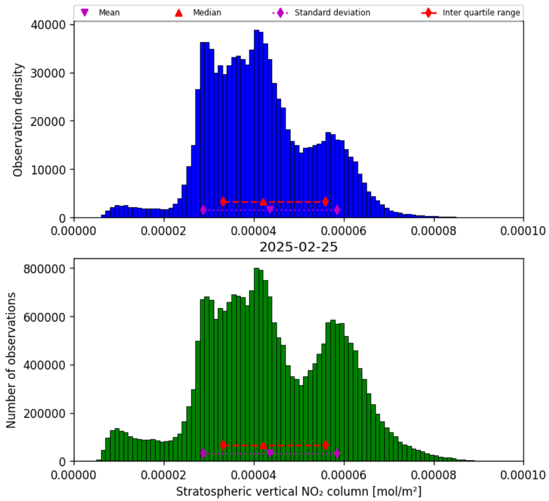
Figure 36: Histogram of “Stratospheric vertical NO 2 column” for 2025-02-24 to 2025-02-26
