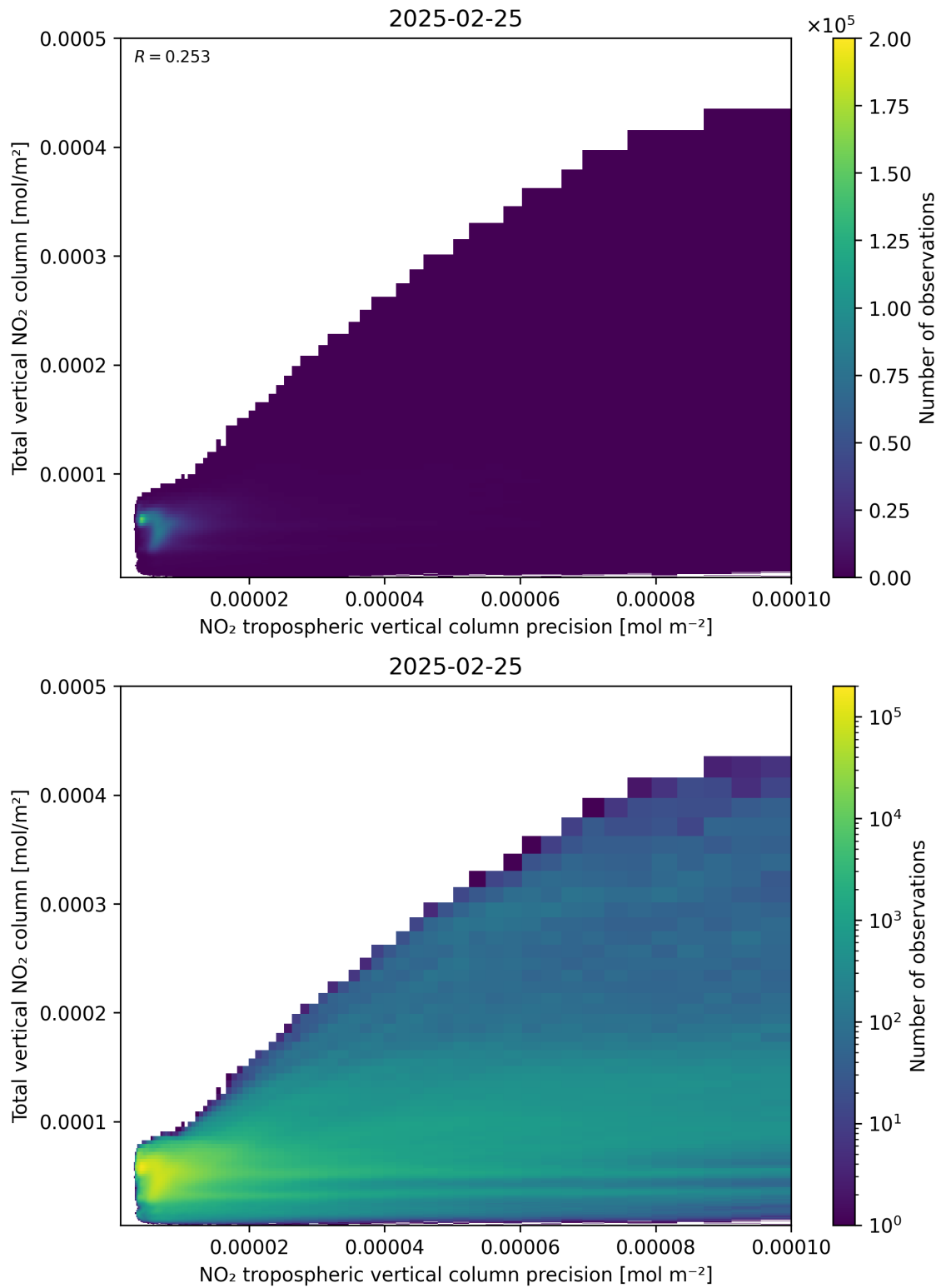
Figure 138: Scatter density plot of “NO 2 tropospheric vertical column precision” against “Total vertical NO 2 column” for 2025-02-24 to 2025-02-26.
