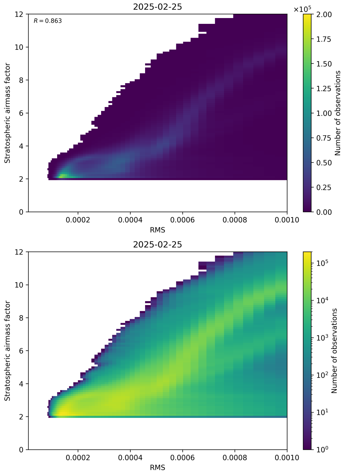
Figure 144: Scatter density plot of “RMS” against “Stratospheric airmass factor” for 2025-02-24 to 2025-02-26.
