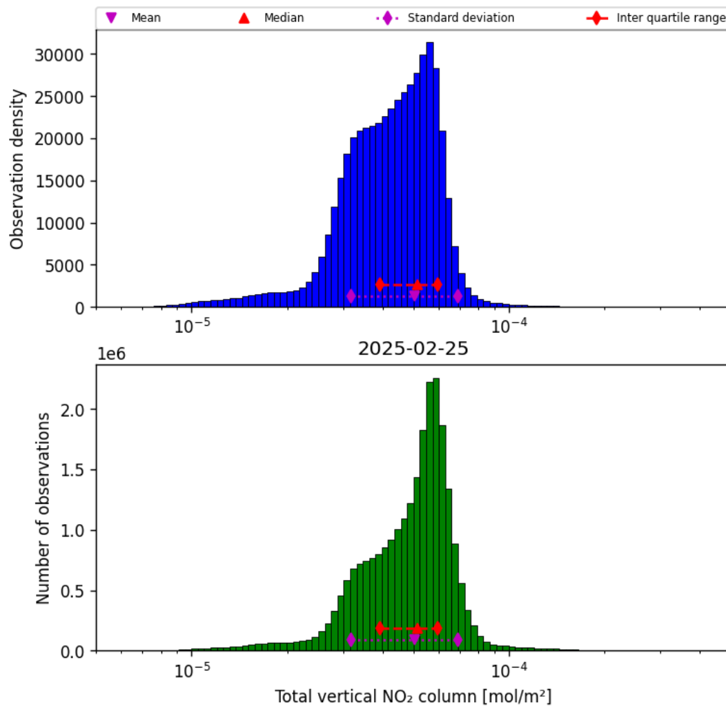
Figure 38: Histogram of “Total vertical NO 2 column” for 2025-02-24 to 2025-02-26
