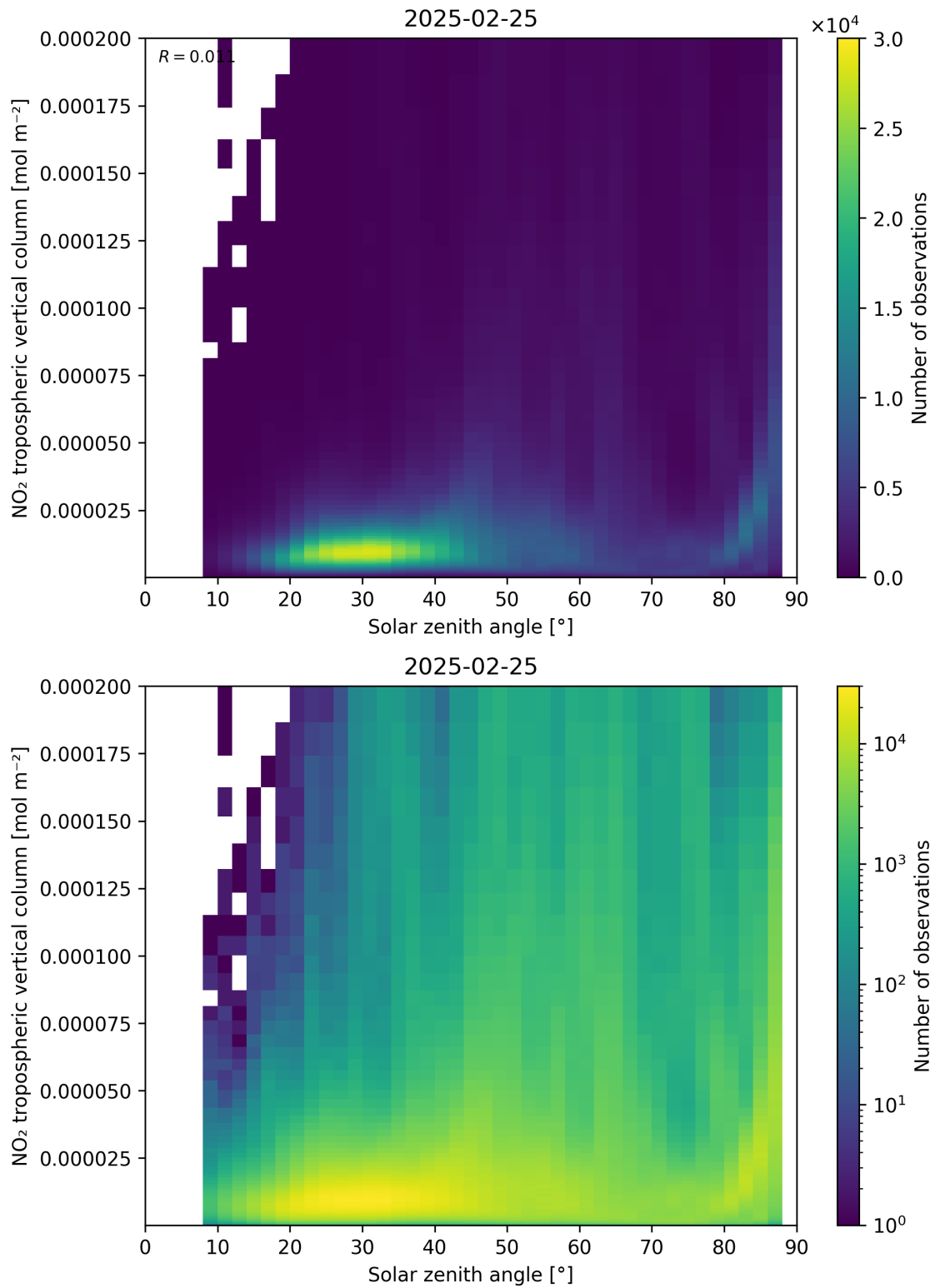
Figure 155: Scatter density plot of “Solar zenith angle” against “NO 2 tropospheric vertical column” for 2025-02-24 to 2025-02-26.
