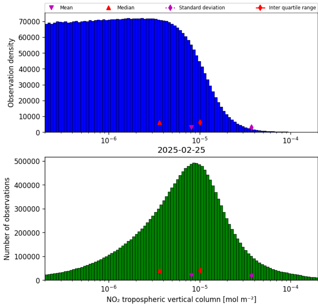
Figure 29: Histogram of “NO 2 tropospheric vertical column” for 2025-02-24 to 2025-02-26
