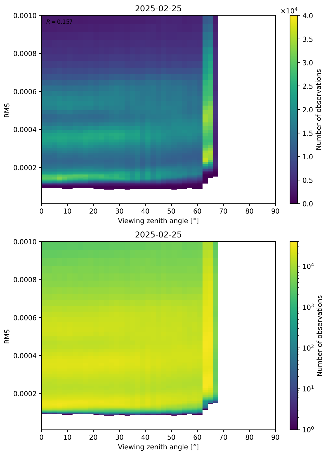
Figure 171: Scatter density plot of “Viewing zenith angle” against “RMS” for 2025-02-24 to 2025-02-26.
