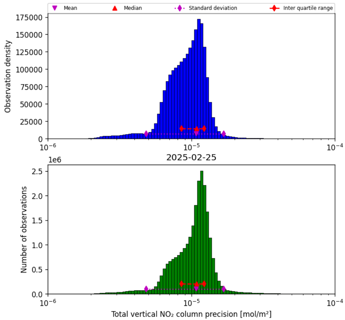
Figure 39: Histogram of “Total vertical NO 2 column precision” for 2025-02-24 to 2025-02-26
