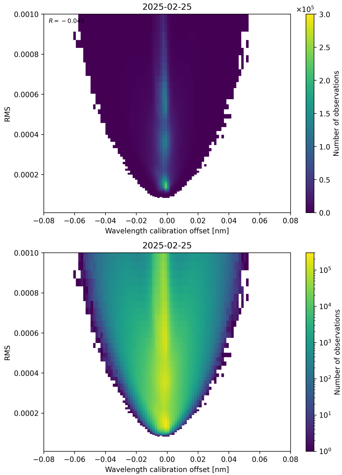
Figure 181: Scatter density plot of “Wavelength calibration offset” against “RMS” for 2025-02-24 to 2025-02-26.
