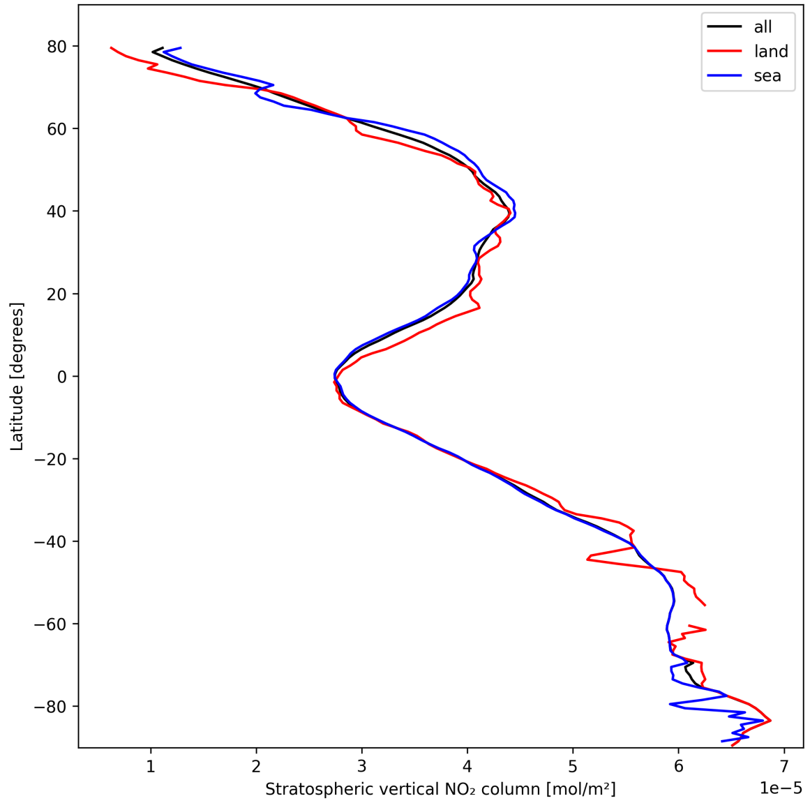
Figure 19: Zonal average of “Stratospheric vertical NO 2 column” for 2025-02-24 to 2025-02-26.
