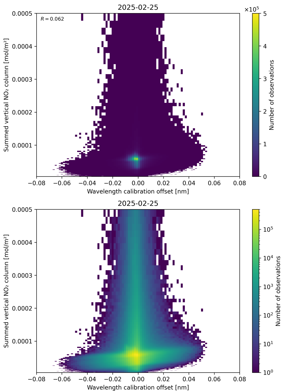
Figure 177: Scatter density plot of “Wavelength calibration offset” against “Summed vertical NO 2 column” for 2025-02-24 to 2025-02-26.
