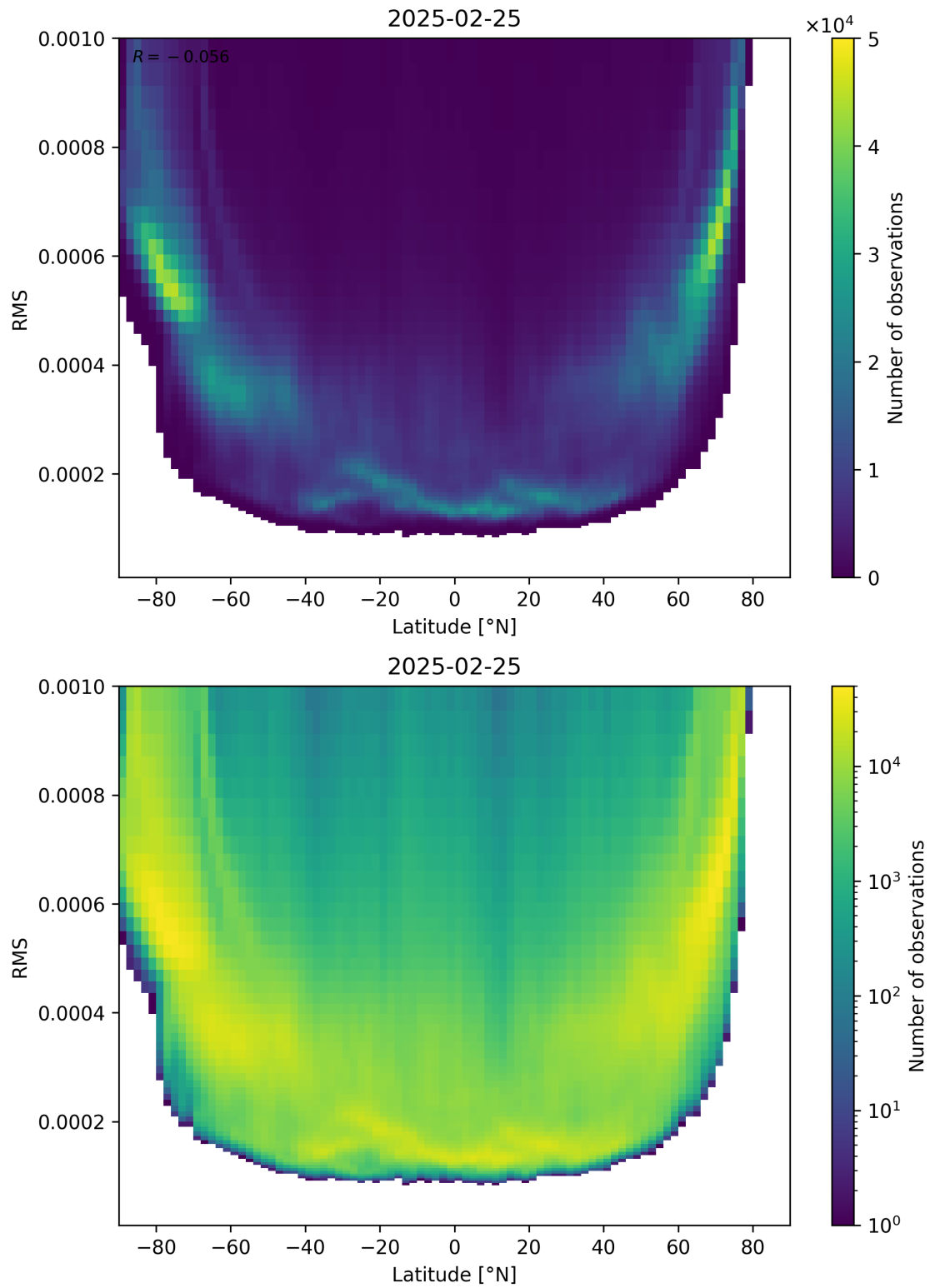
Figure 94: Scatter density plot of “Latitude” against “RMS” for 2025-02-24 to 2025-02-26.
