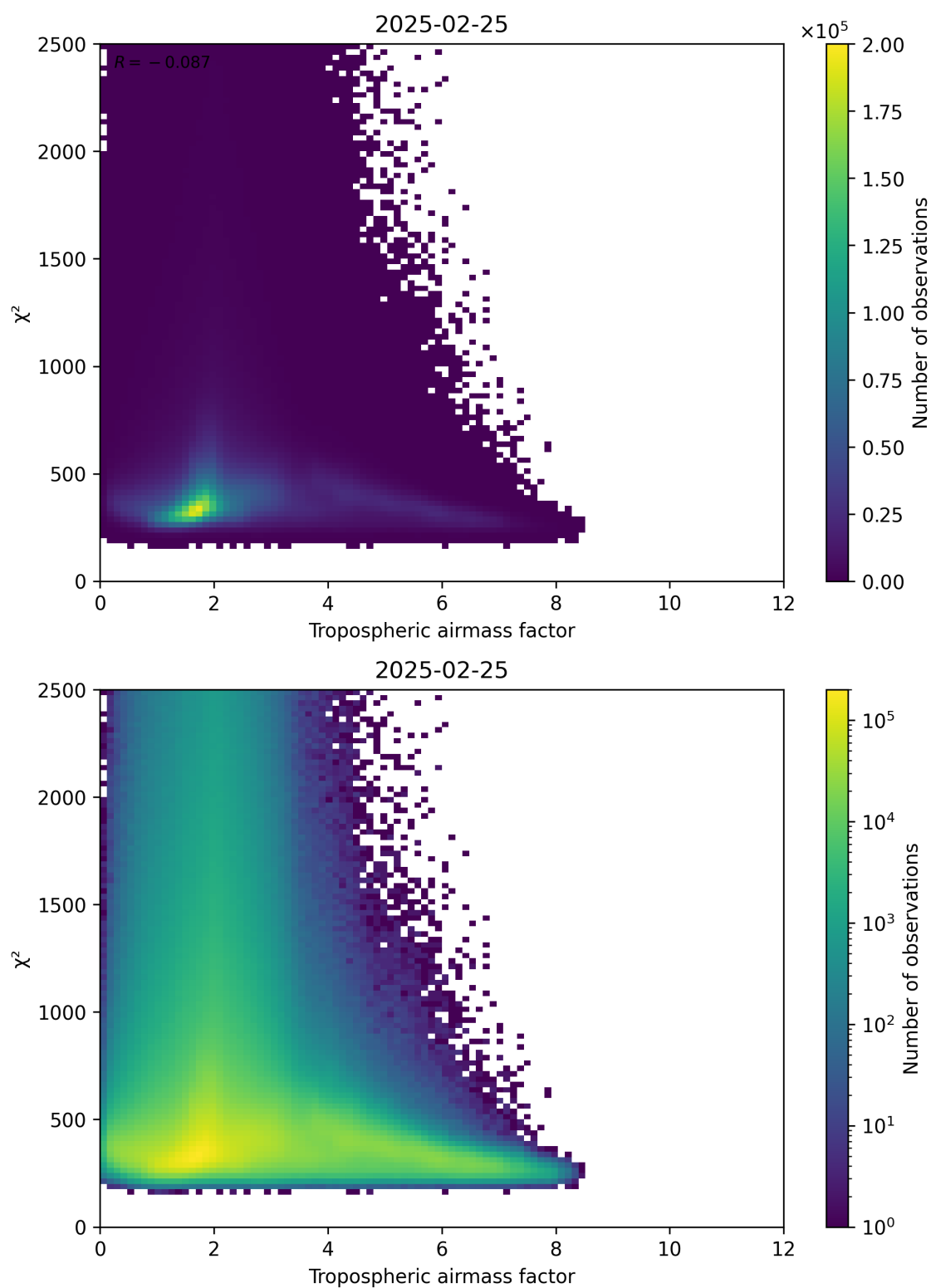
Figure 73: Scatter density plot of “Tropospheric airmass factor” against “ \chi^2 ” for 2025-02-24 to 2025-02-26.
