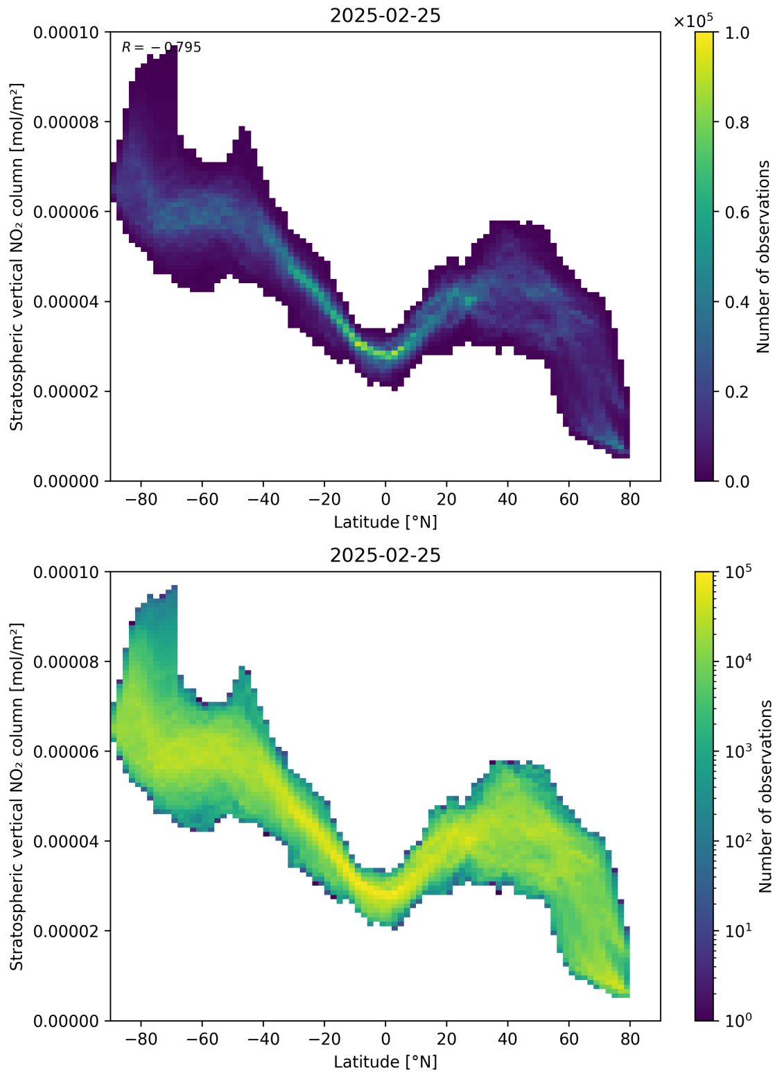
Figure 87: Scatter density plot of “Latitude” against “Stratospheric vertical NO 2 column” for 2025-02-24 to 2025-02-26.
