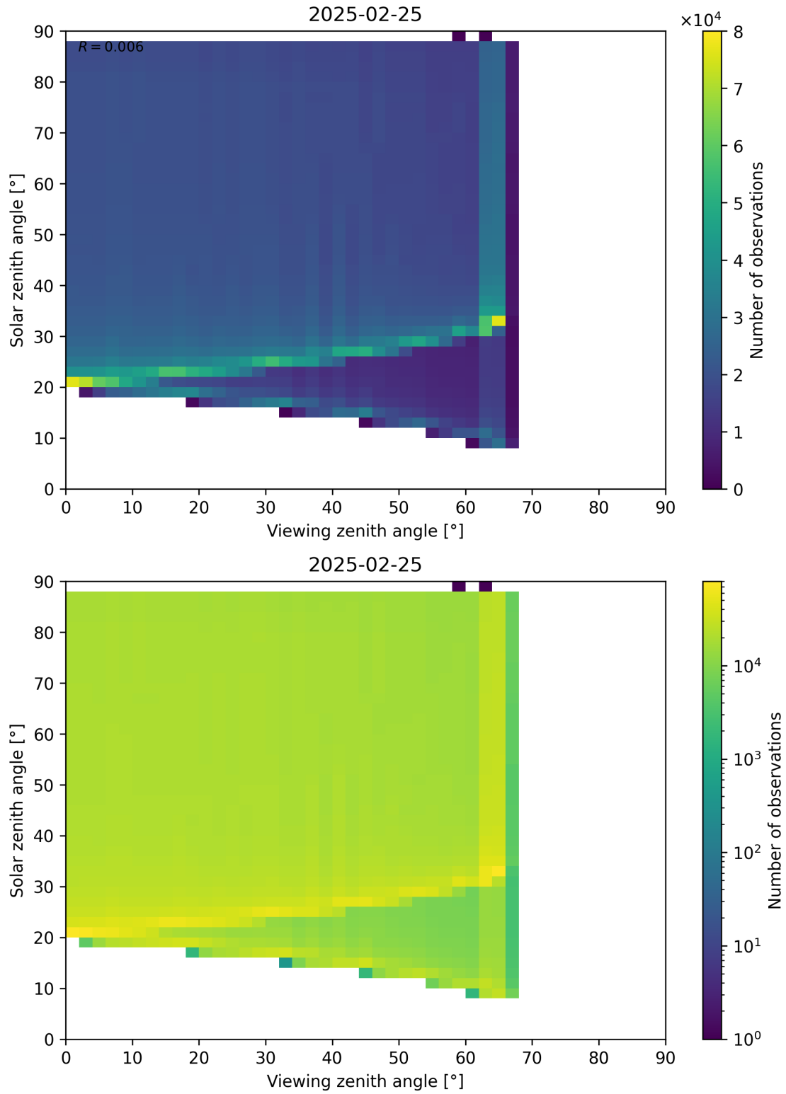
Figure 172: Scatter density plot of “Viewing zenith angle” against “Solar zenith angle” for 2025-02-24 to 2025-02-26.
