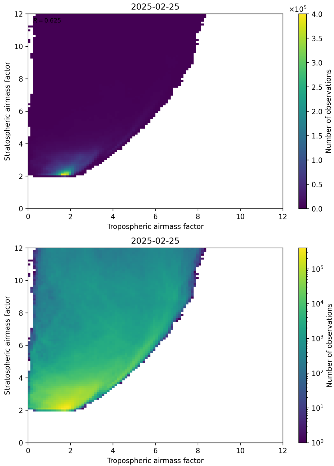
Figure 71: Scatter density plot of “Tropospheric airmass factor” against “Stratospheric airmass factor” for 2025-02-24 to 2025-02-26.
