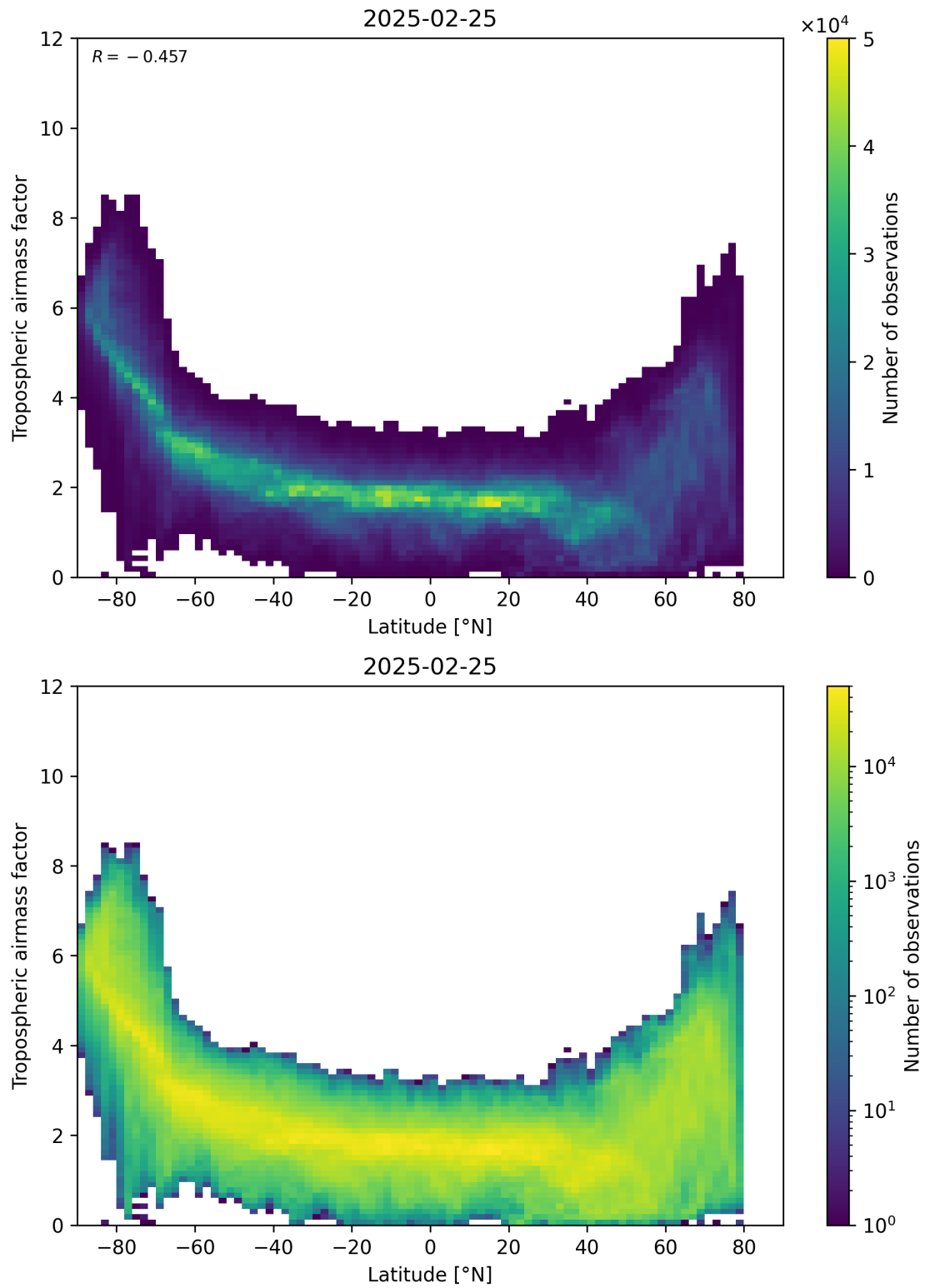
Figure 85: Scatter density plot of “Latitude” against “Tropospheric airmass factor” for 2025-02-24 to 2025-02-26.
