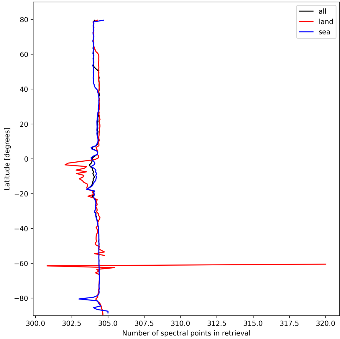
Figure 16: Zonal average of “Number of spectral points in retrieval” for 2025-02-24 to 2025-02-26.
