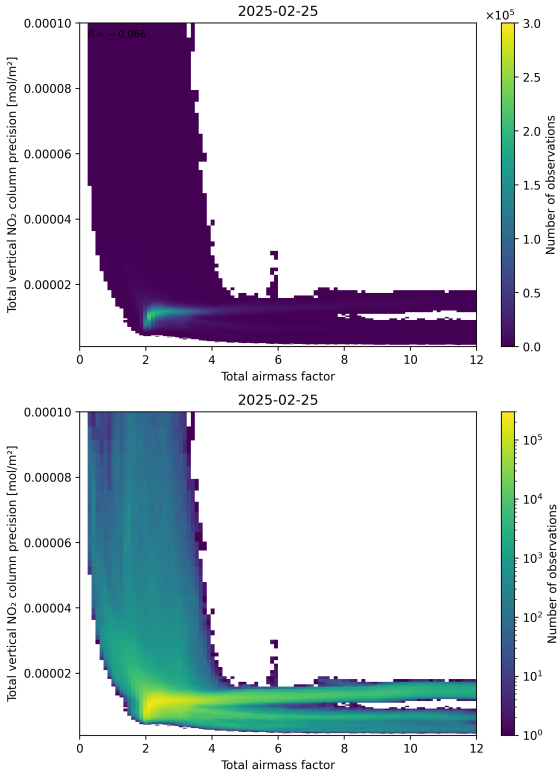
Figure 68: Scatter density plot of “Total airmass factor” against “Total vertical NO 2 column precision” for 2025-02-24 to 2025-02-26.
