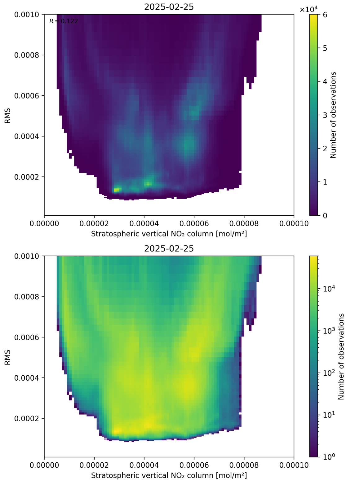
Figure 102: Scatter density plot of “Stratospheric vertical NO 2 column” against “RMS” for 2025-02-24 to 2025-02-26.
