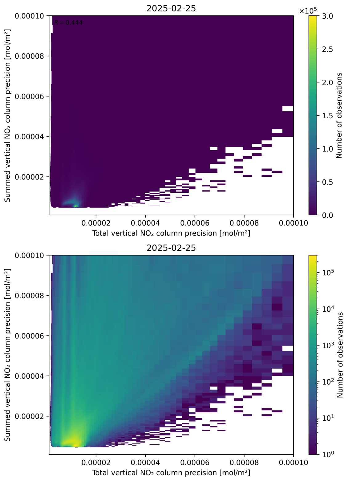
Figure 118: Scatter density plot of “Total vertical NO 2 column precision” against “Summed vertical NO 2 column precision” for 2025-02-24 to 2025-02-26.
