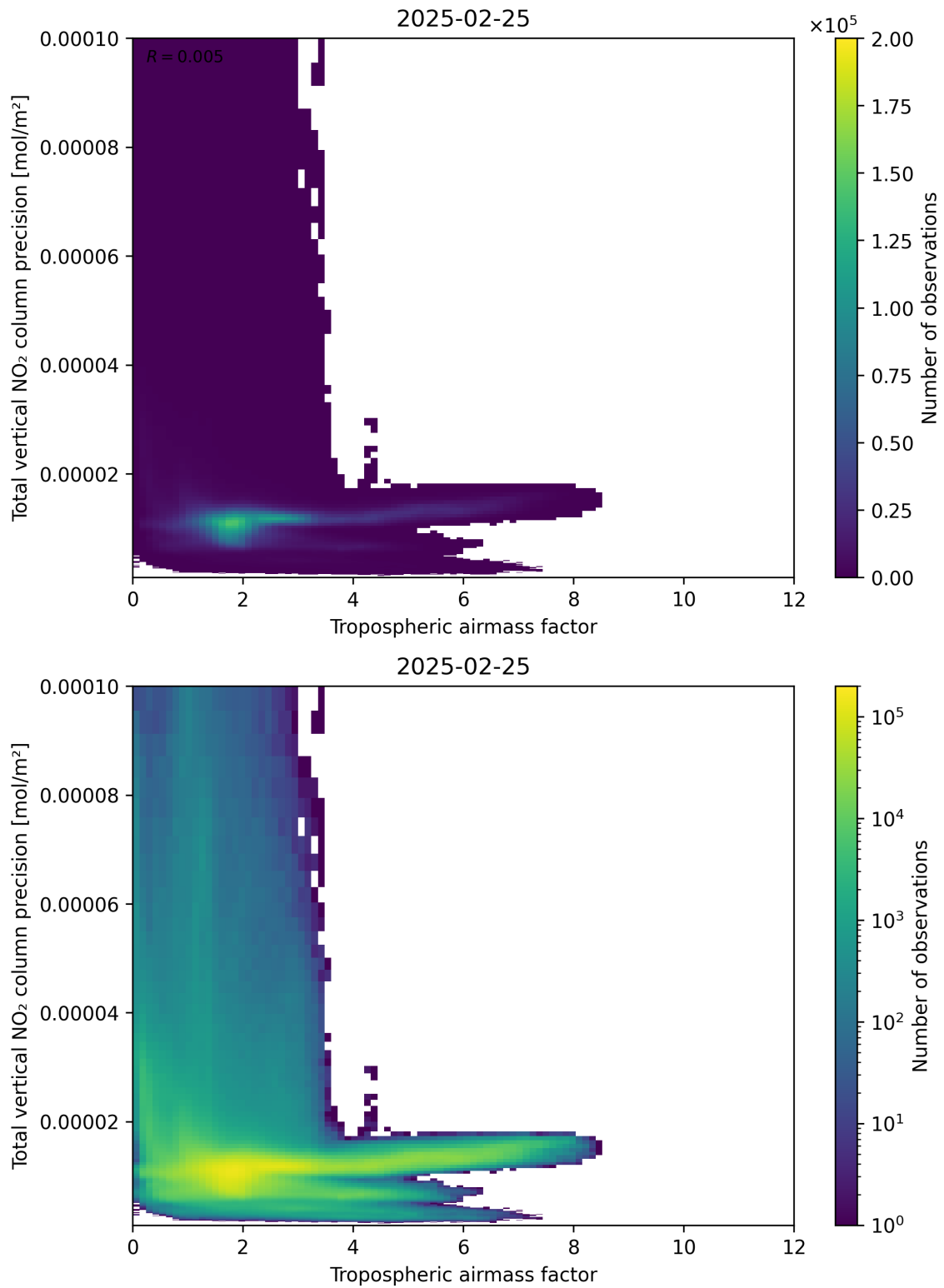
Figure 78: Scatter density plot of “Tropospheric air mass factor” against “Total vertical NO 2 column precision” for 2025-02-24 to 2025-02-26.
