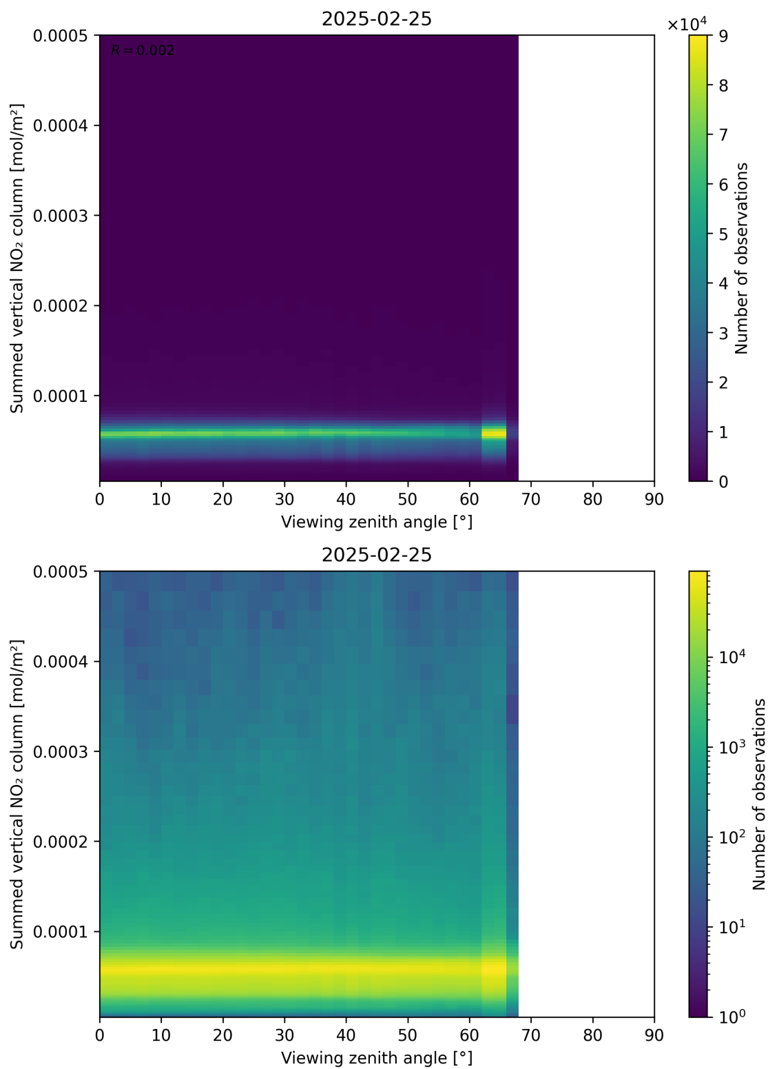
Figure 165: Scatter density plot of “Viewing zenith angle” against “Summed vertical NO 2 column” for 2025-02-24 to 2025-02-26.
