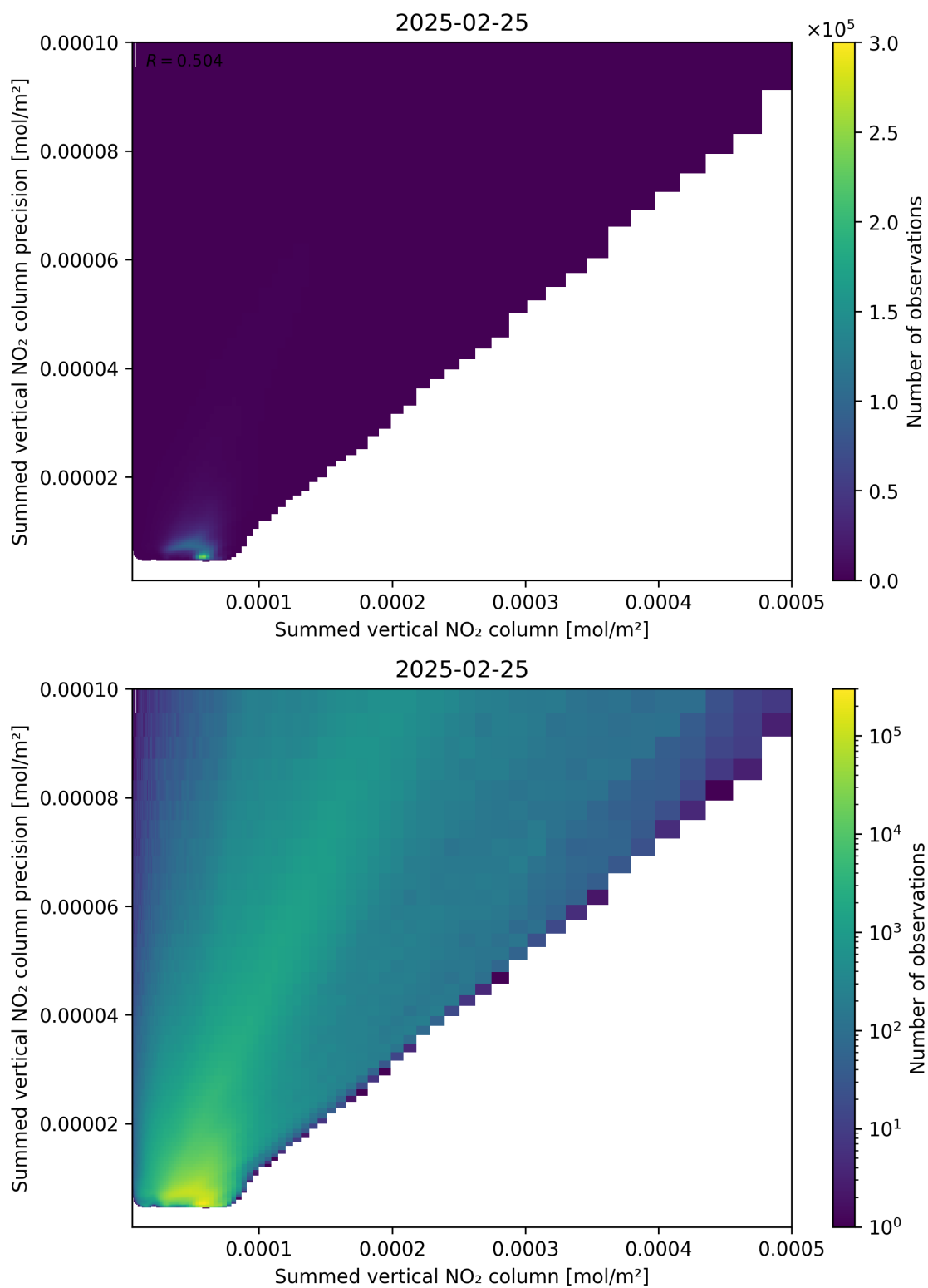
Figure 105: Scatter density plot of “Summed vertical NO 2 column” against “Summed vertical NO 2 column precision” for 2025-02-24 to 2025-02-26.
