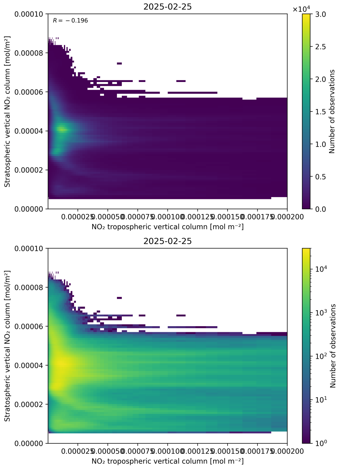
Figure 125: Scatter density plot of “NO 2 tropospheric vertical column” against “Stratospheric vertical NO 2 column” for 2025-02-24 to 2025-02-26.
