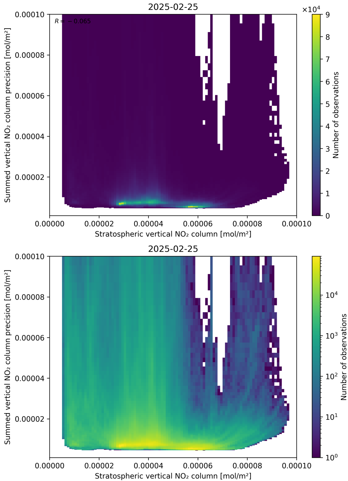
Figure 99: Scatter density plot of “Stratospheric vertical NO 2 column” against “Summed vertical NO 2 column precision” for 2025-02-24 to 2025-02-26.
