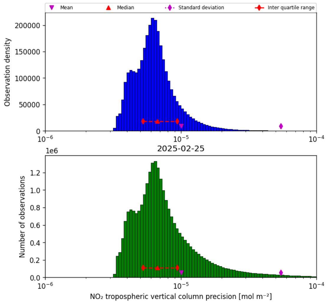
Figure 30: Histogram of “NO 2 tropospheric vertical column precision” for 2025-02-24 to 2025-02-26
