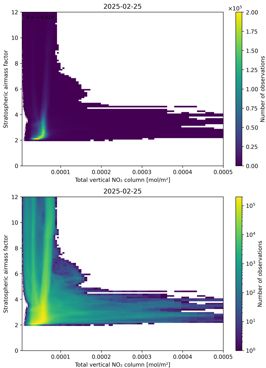
Figure 110: Scatter density plot of “Total vertical NO 2 column” against “Stratospheric airmass factor” for 2025-02-24 to 2025-02-26.
