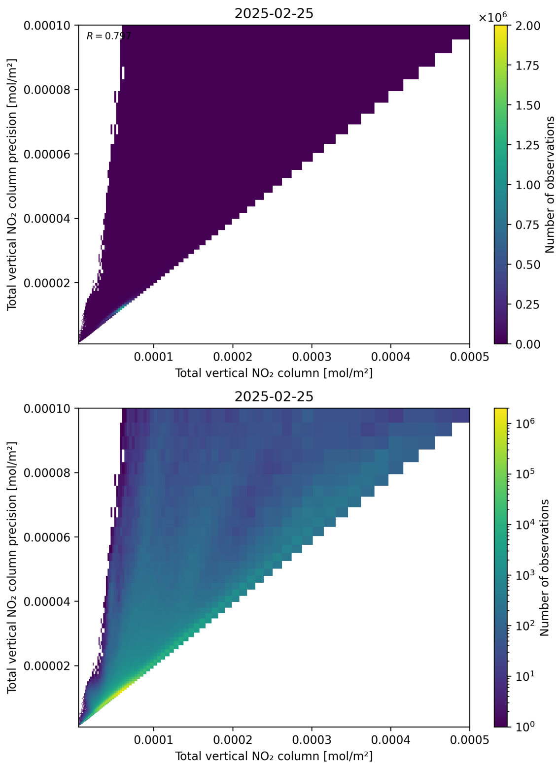
Figure 114: Scatter density plot of “Total vertical NO 2 column” against “Total vertical NO 2 column precision” for 2025-02-24 to 2025-02-26.
