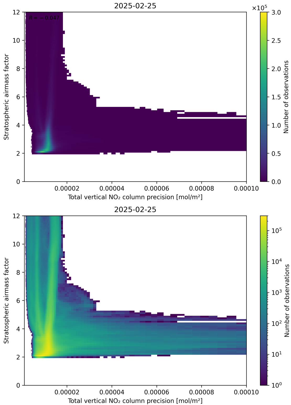
Figure 115: Scatter density plot of “Total vertical NO 2 column precision” against “Stratospheric air mass factor” for 2025-02-24 to 2025-02-26.
