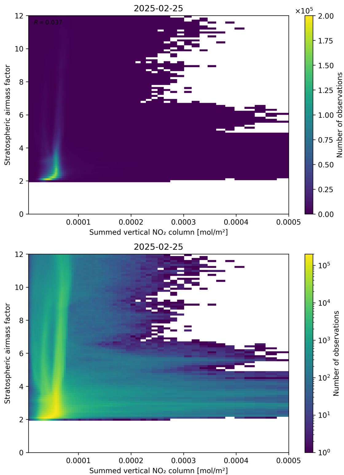
Figure 103: Scatter density plot of “Summed vertical NO 2 column” against “Stratospheric air mass factor” for 2025-02-24 to 2025-02-26.
