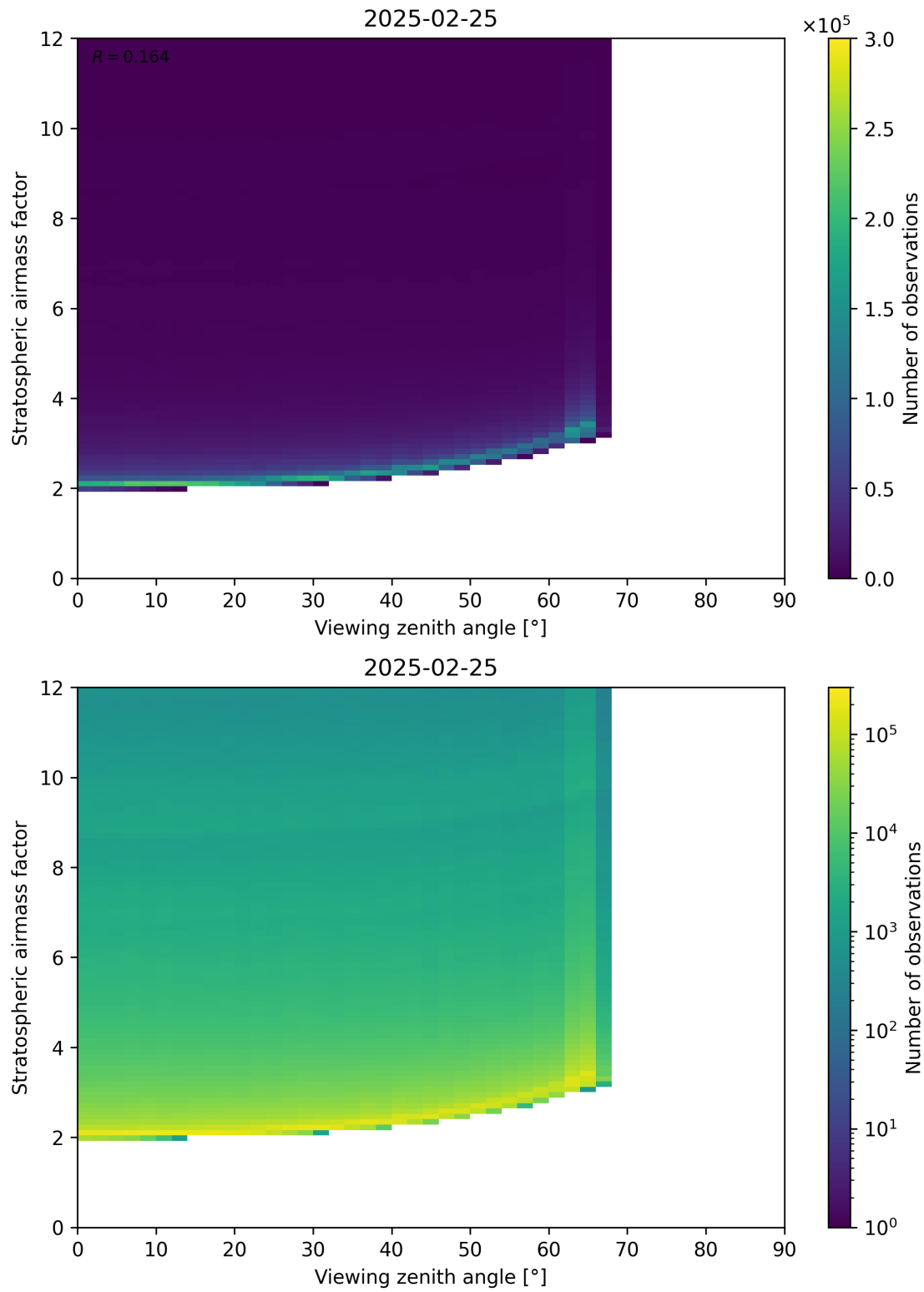
Figure 159: Scatter density plot of “Viewing zenith angle” against “Stratospheric airmass factor” for 2025-02-24 to 2025-02-26.
