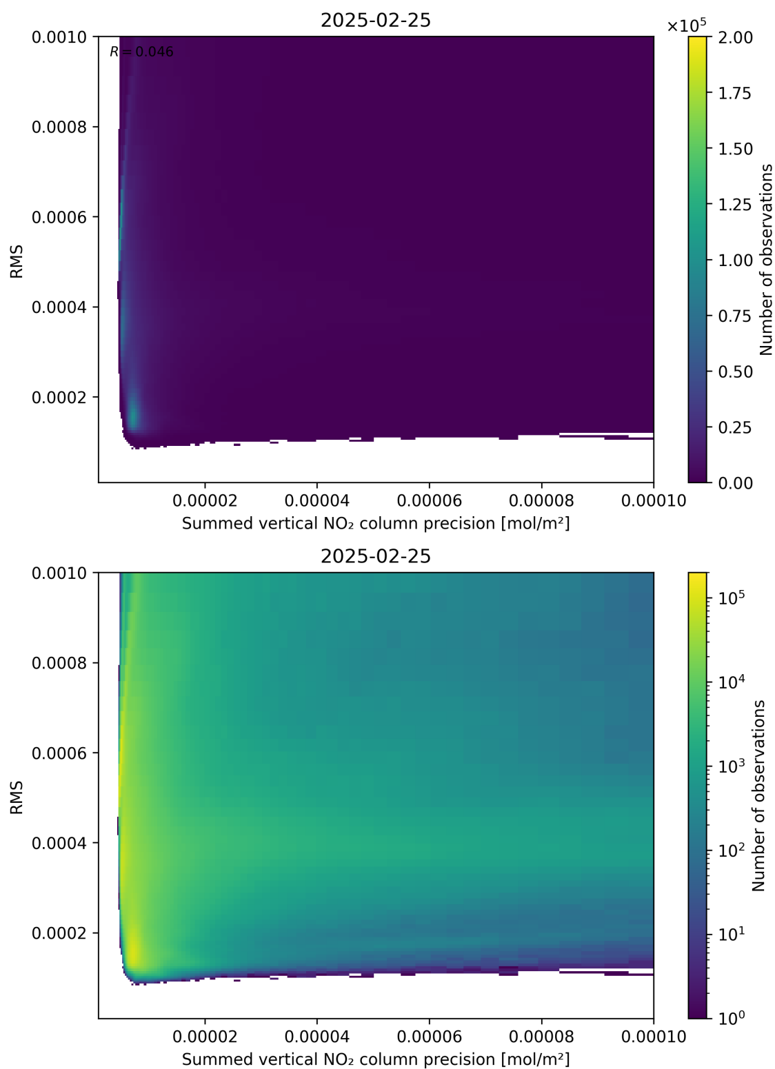
Figure 108: Scatter density plot of “Summed vertical NO 2 column precision” against “RMS” for 2025-02-24 to 2025-02-26.
