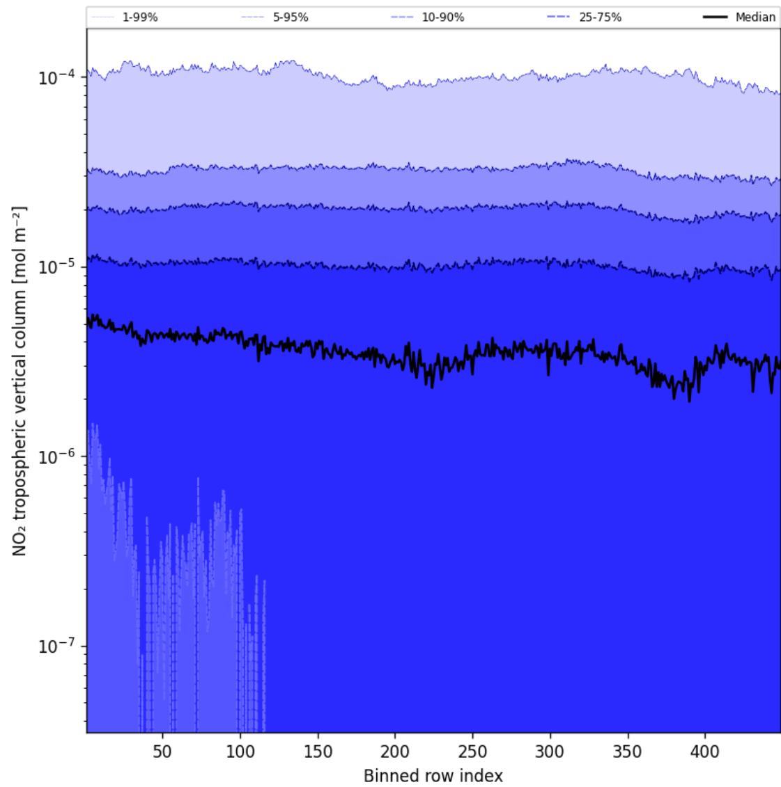
Figure 46: Along track statistics of “NO 2 tropospheric vertical column” for 2025-02-24 to 2025-02-26
