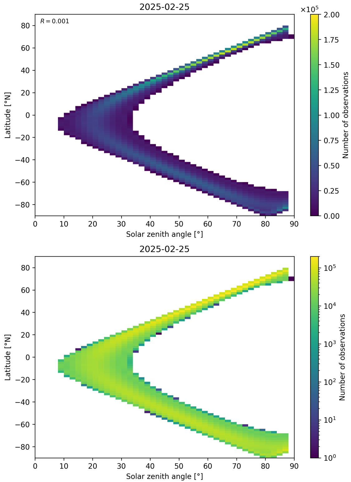
Figure 149: Scatter density plot of “Solar zenith angle” against “Latitude” for 2025-02-24 to 2025-02-26.
