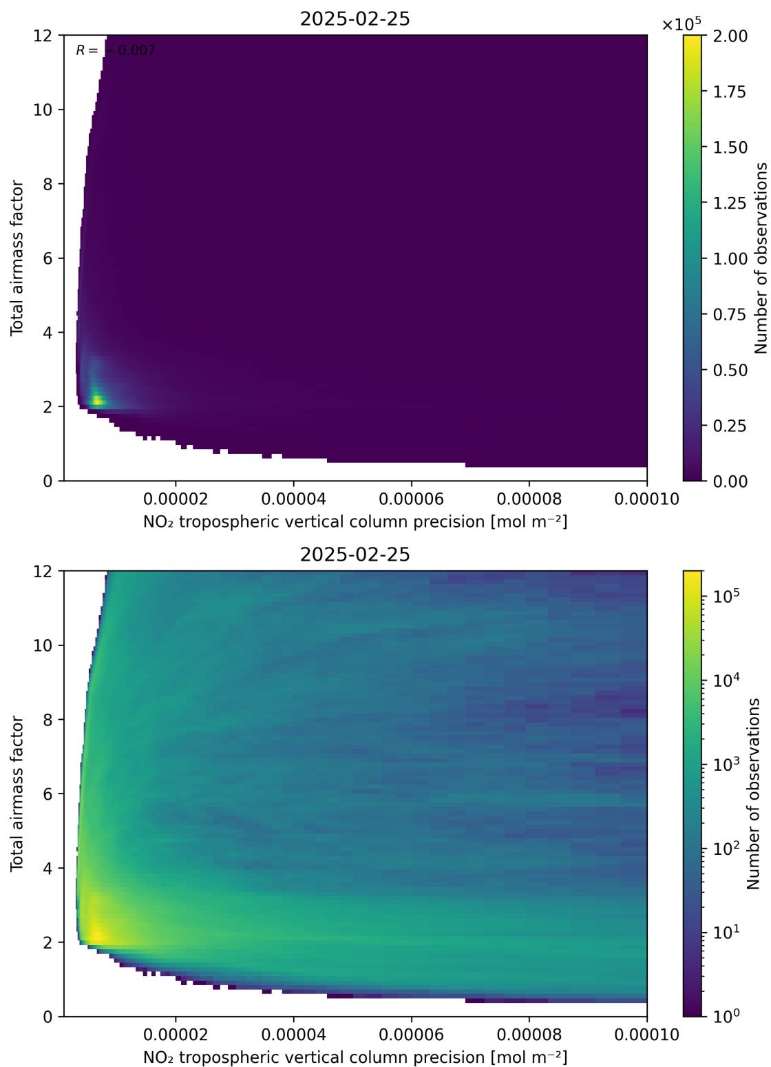
Figure 132: Scatter density plot of “NO 2 tropospheric vertical column precision” against “Total air mass factor” for 2025-02-24 to 2025-02-26.
