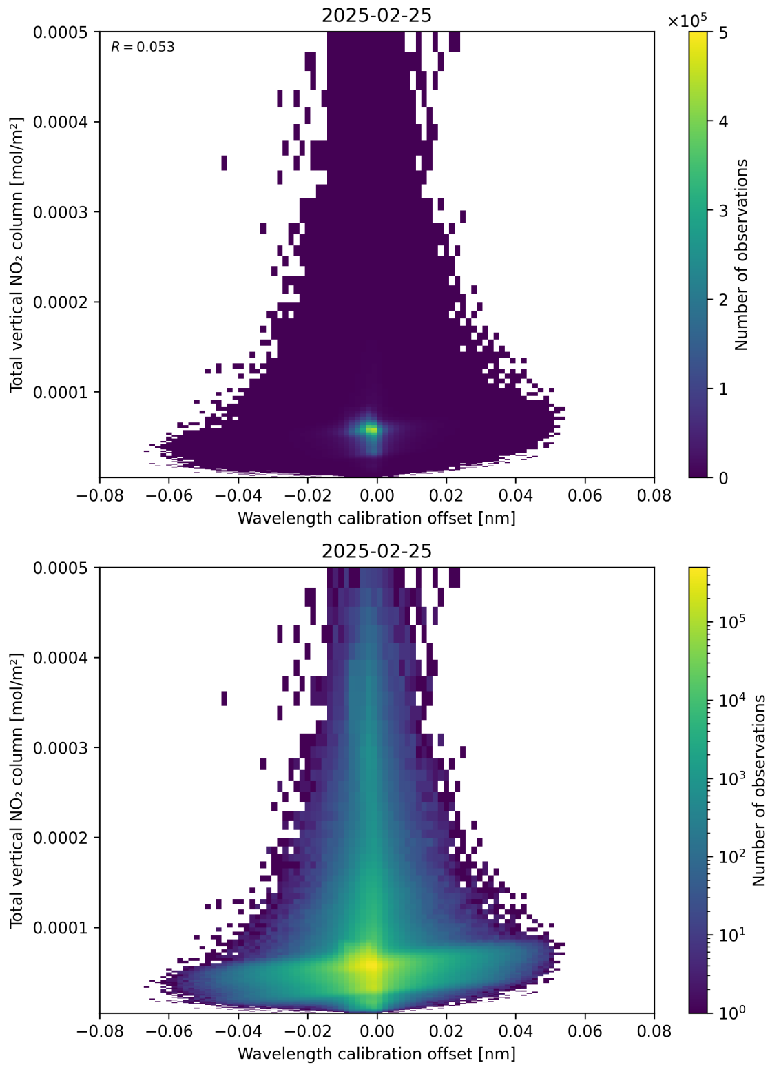
Figure 179: Scatter density plot of “Wavelength calibration offset” against “Total vertical NO 2 column” for 2025-02-24 to 2025-02-26.
