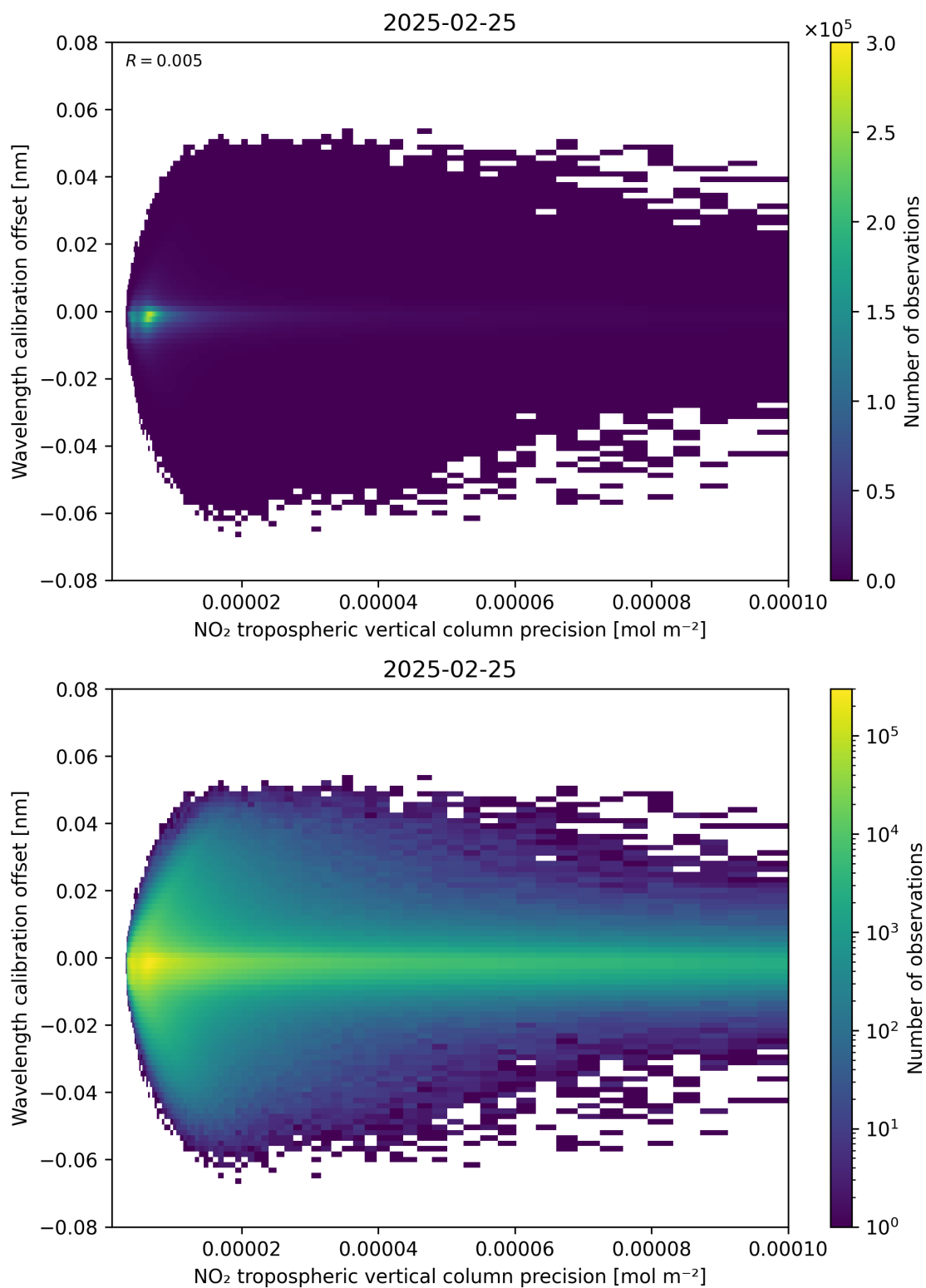
Figure 141: Scatter density plot of “NO 2 tropospheric vertical column precision” against “Wavelength calibration offset” for 2025-02-24 to 2025-02-26.
