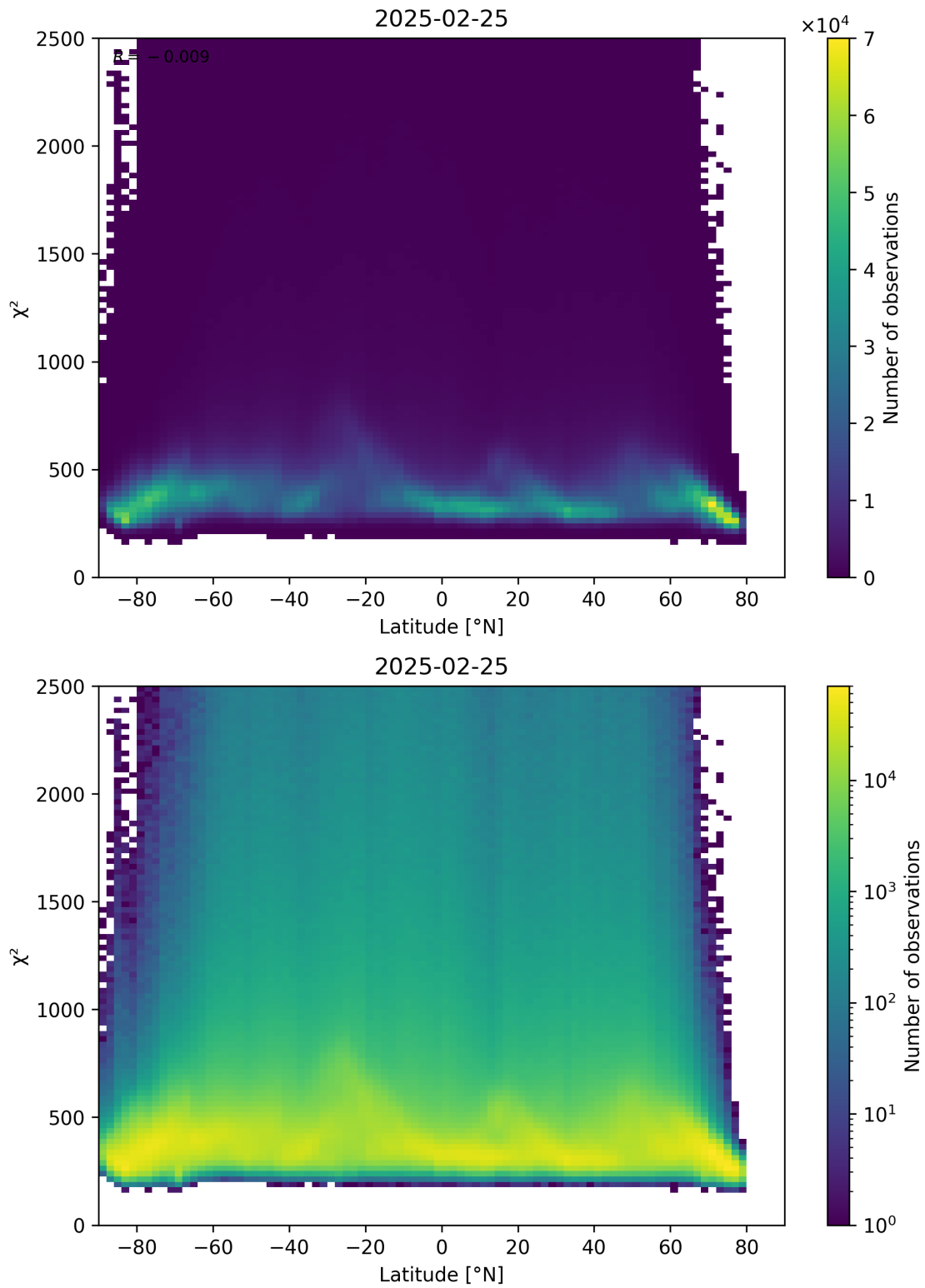
Figure 86: Scatter density plot of “Latitude” against “ \chi^2 ” for 2025-02-24 to 2025-02-26.
