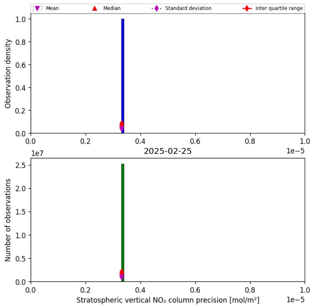
Figure 37: Histogram of “Stratospheric vertical NO 2 column precision” for 2025-02-24 to 2025-02-26
