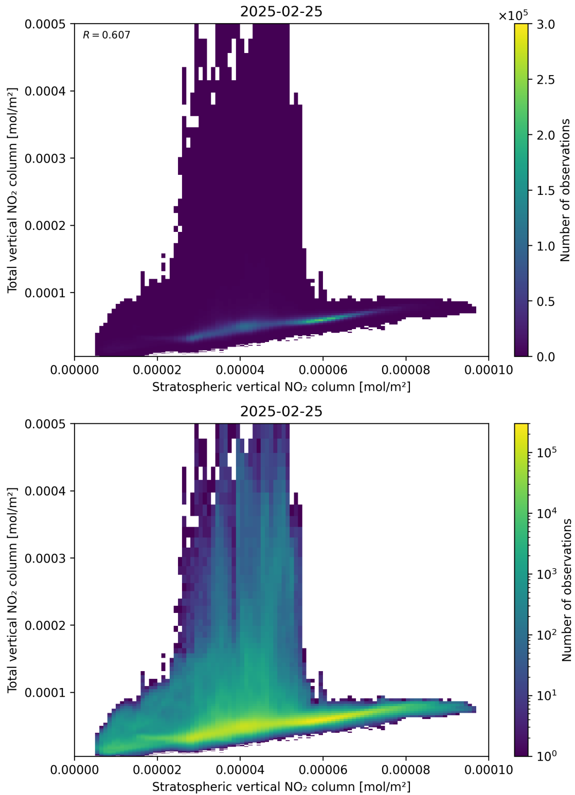
Figure 100: Scatter density plot of “Stratospheric vertical NO 2 column” against “Total vertical NO 2 column” for 2025-02-24 to 2025-02-26.
