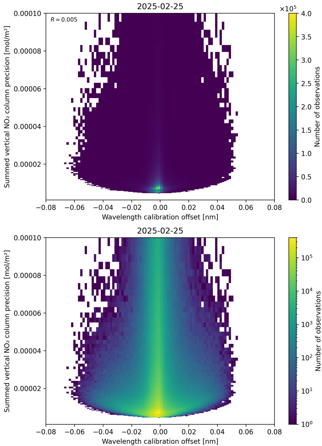
Figure 178: Scatter density plot of “Wavelength calibration offset” against “Summed vertical NO 2 column precision” for 2025-02-24 to 2025-02-26.
