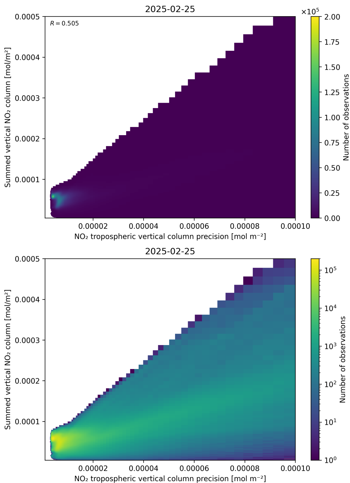
Figure 136: Scatter density plot of “NO 2 tropospheric vertical column precision” against “Summed vertical NO 2 column” for 2025-02-24 to 2025-02-26.
