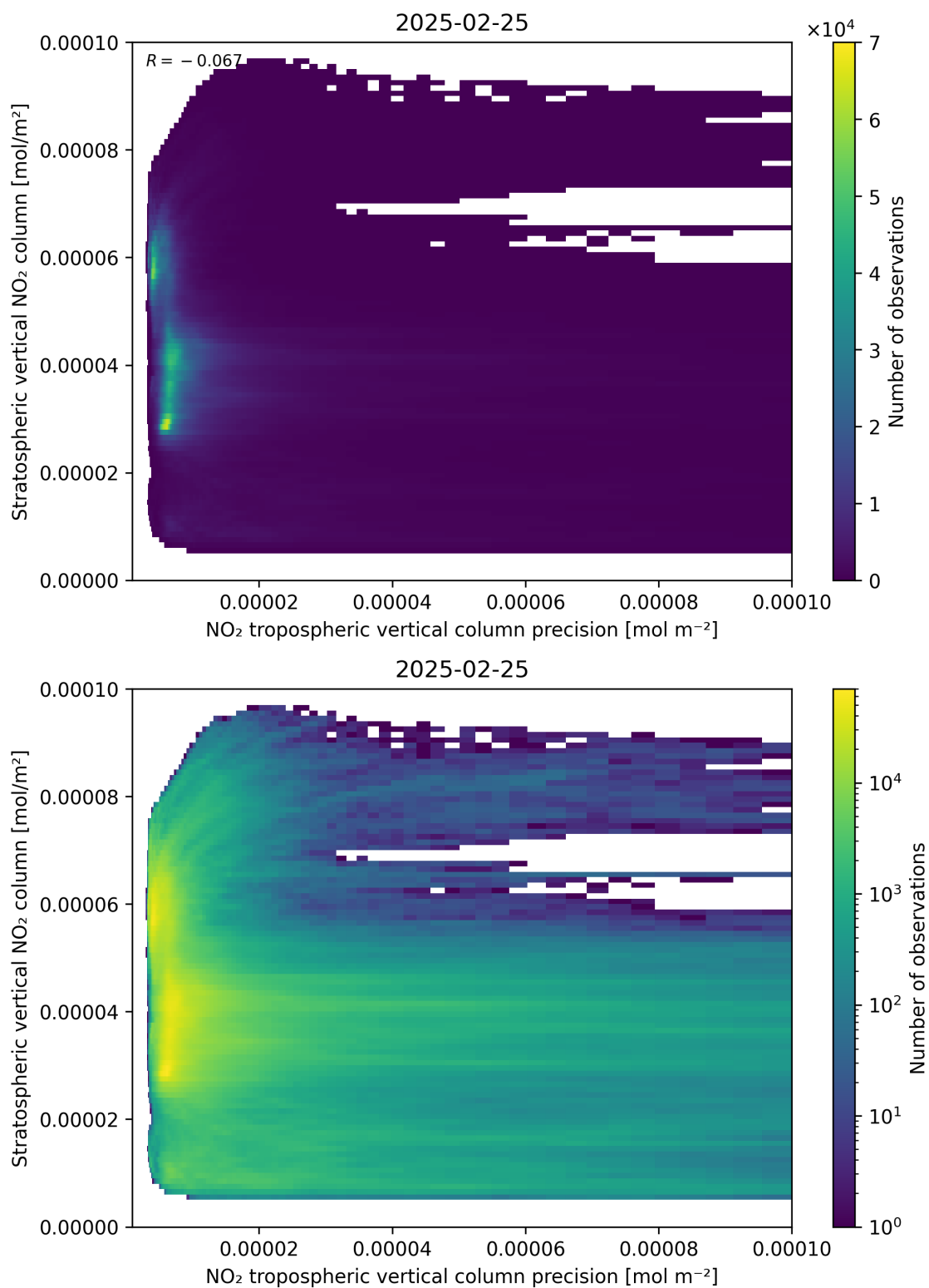
Figure 135: Scatter density plot of “NO 2 tropospheric vertical column precision” against “Stratospheric vertical NO 2 column” for 2025-02-24 to 2025-02-26.
