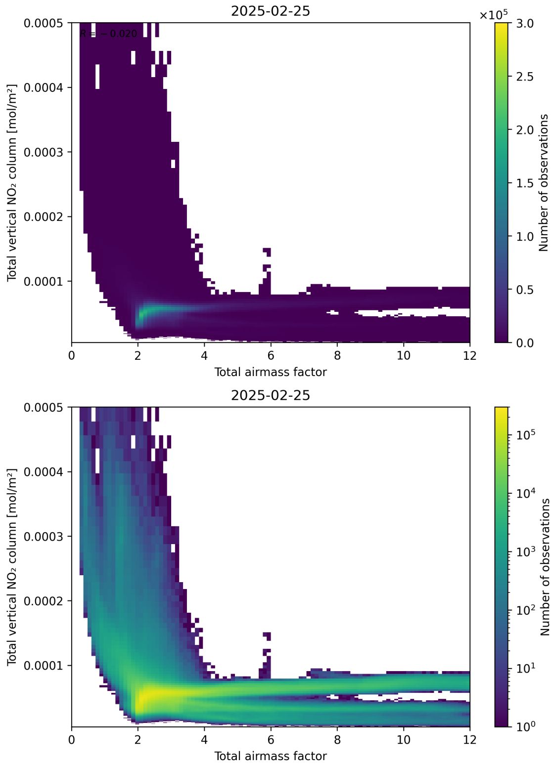
Figure 67: Scatter density plot of “Total airmass factor” against “Total vertical NO 2 column” for 2025-02-24 to 2025-02-26.
