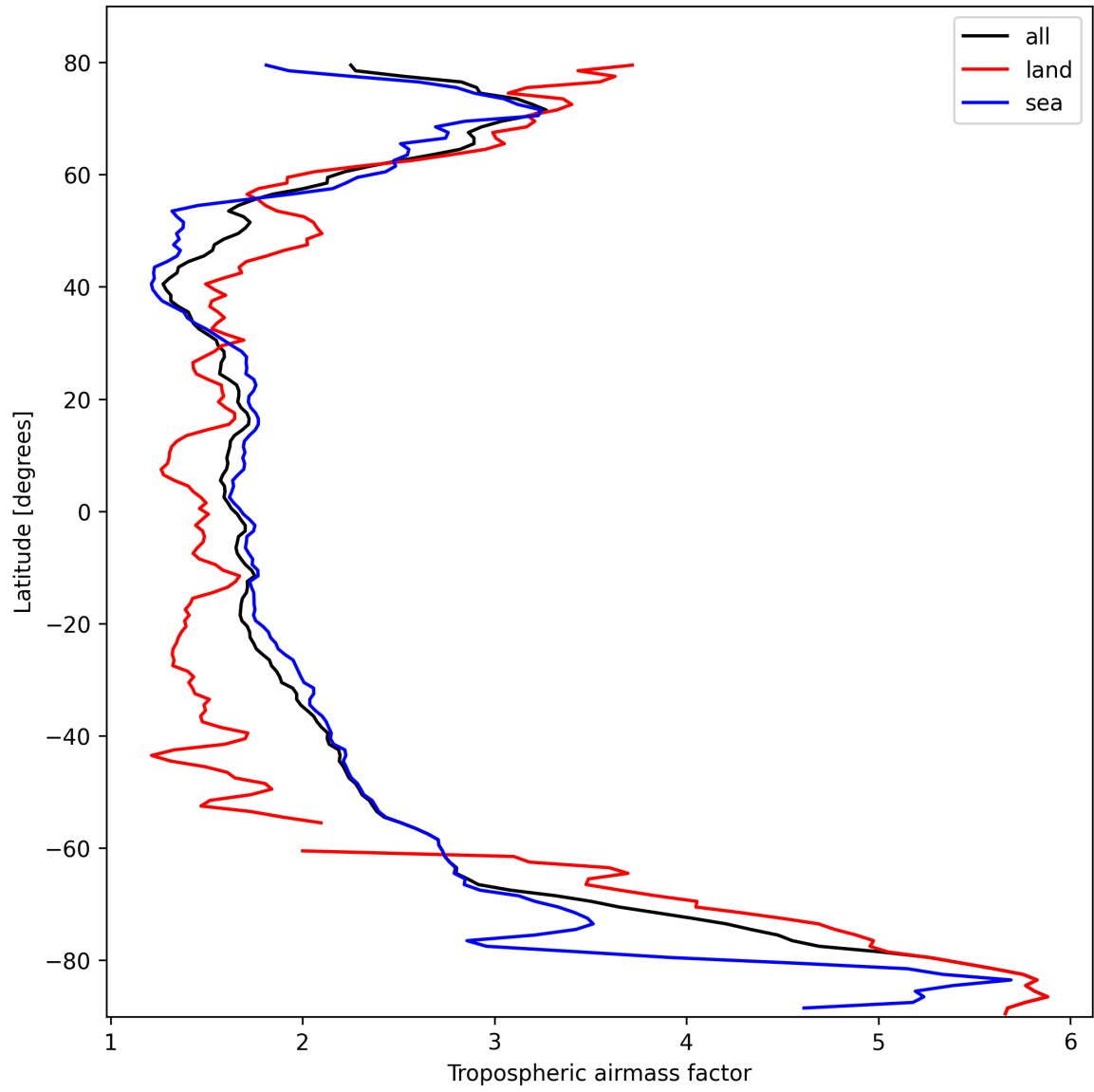
Figure 14: Zonal average of “Tropospheric air mass factor” for 2025-02-24 to 2025-02-26.
