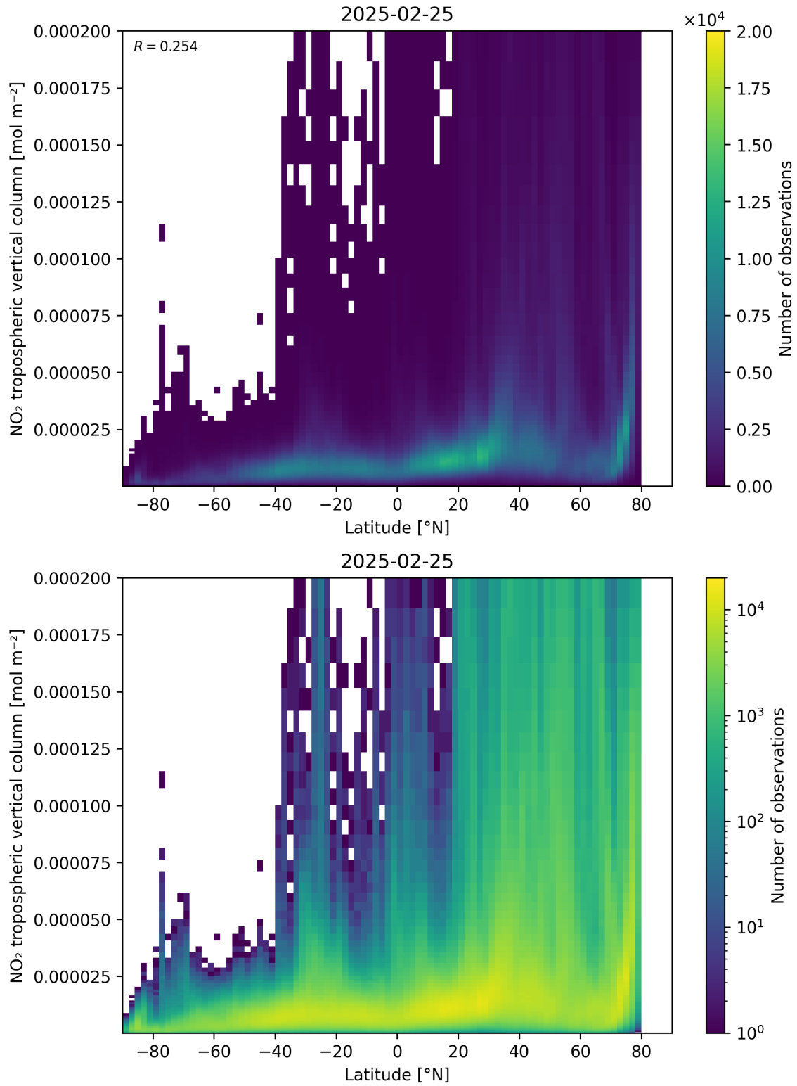
Figure 92: Scatter density plot of “Latitude” against “NO 2 tropospheric vertical column” for 2025-02-24 to 2025-02-26.
