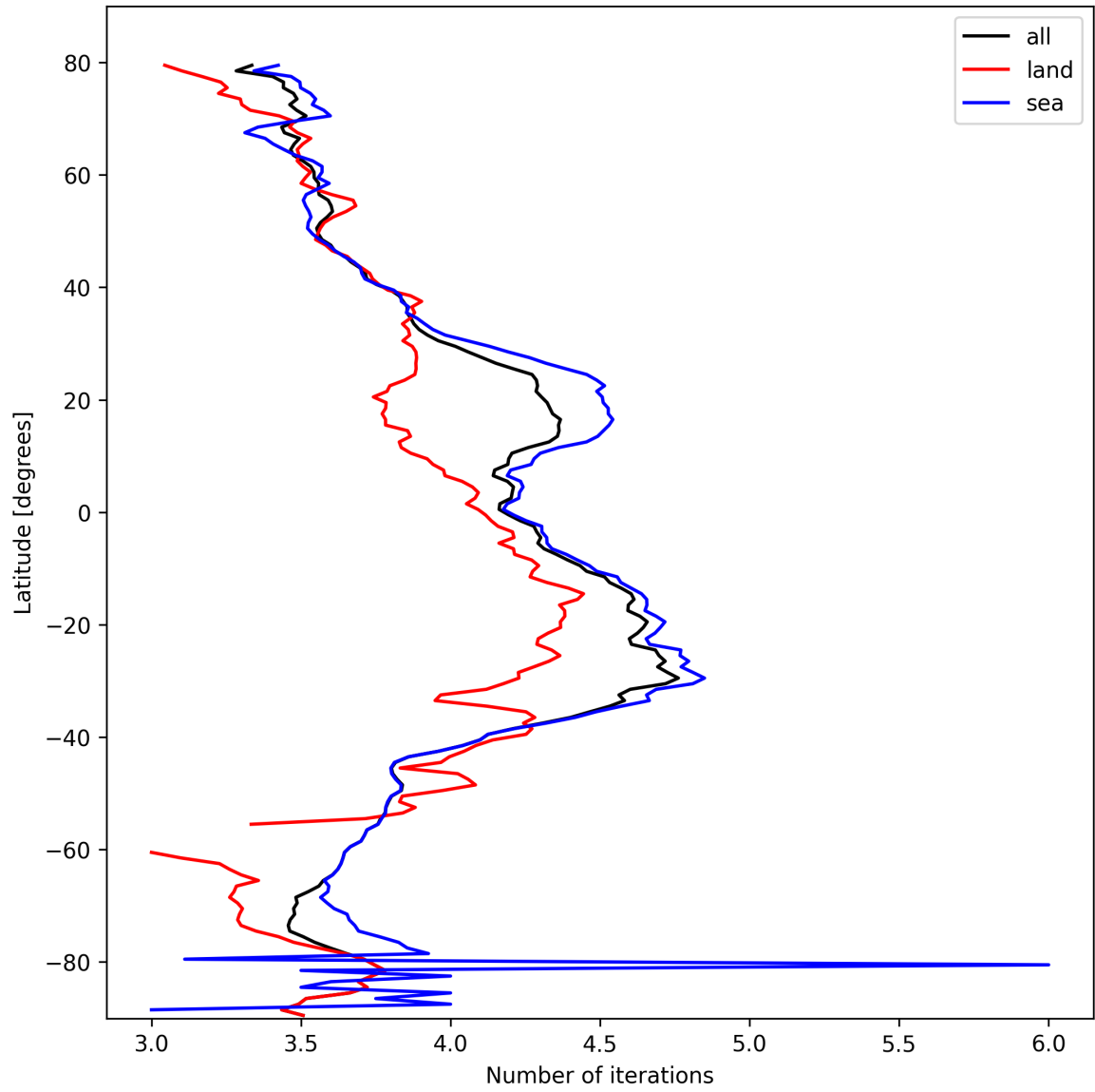
Figure 17: Zonal average of “Number of iterations” for 2025-02-24 to 2025-02-26.
