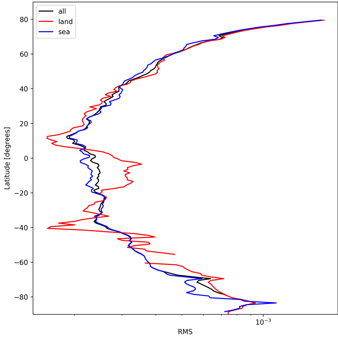
Figure 26: Zonal average of “RMS” for 2025-02-24 to 2025-02-26.
