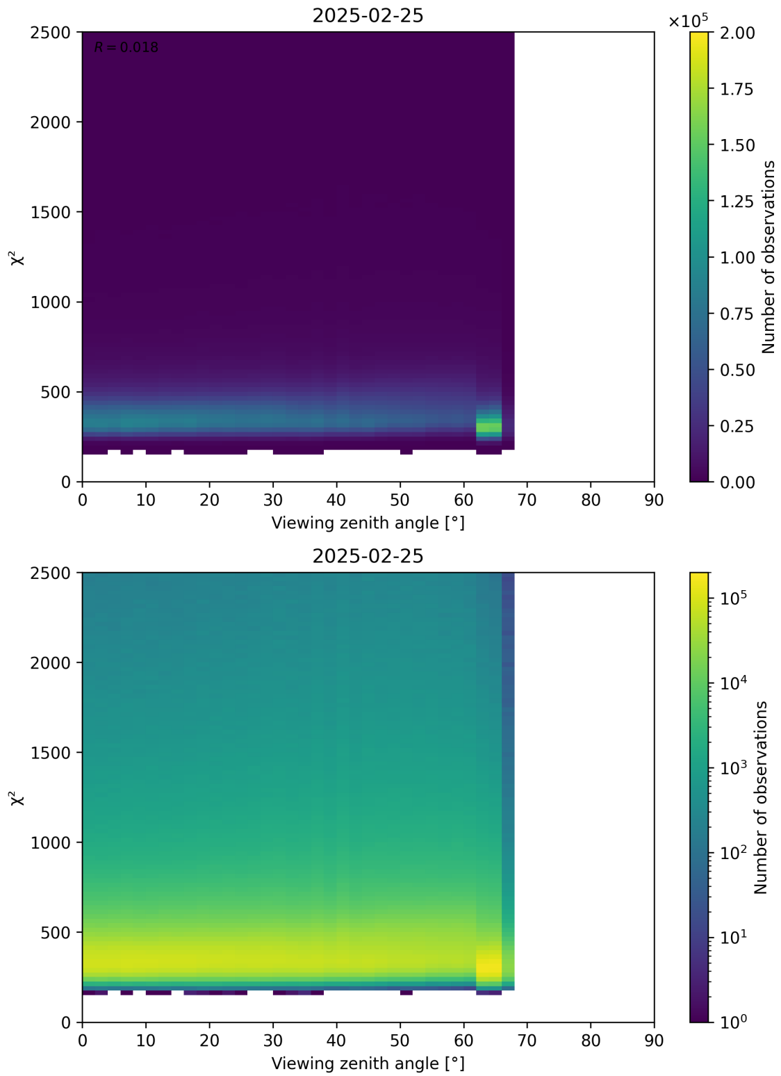
Figure 162: Scatter density plot of “Viewing zenith angle” against “ \chi^2 ” for 2025-02-24 to 2025-02-26.
