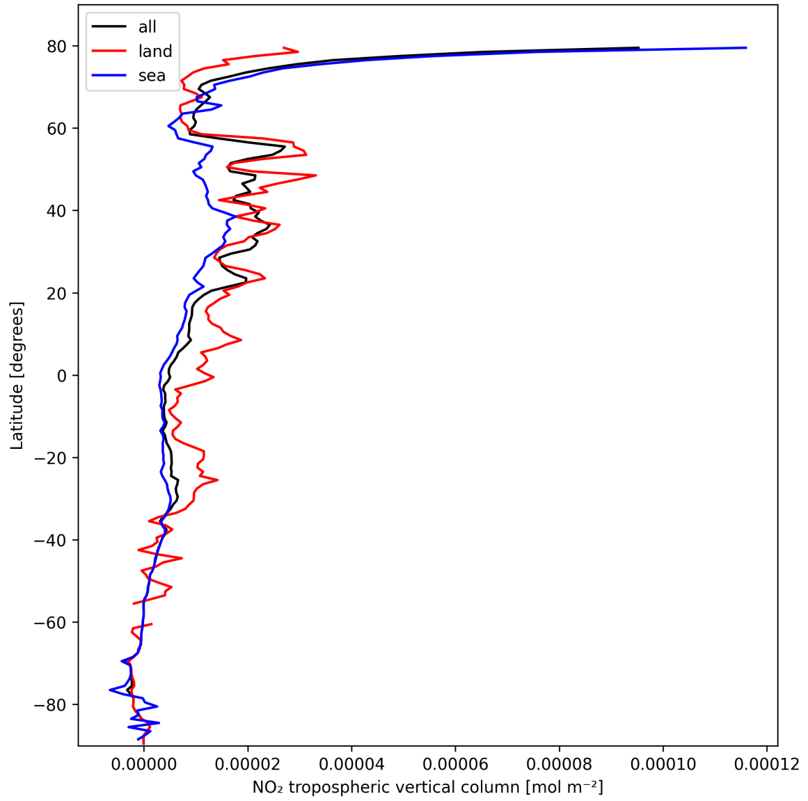
Figure 12: Zonal average of “NO 2 tropospheric vertical column” for 2025-02-24 to 2025-02-26.
