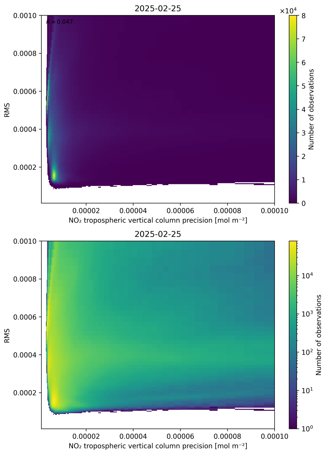
Figure 140: Scatter density plot of “NO 2 tropospheric vertical column precision” against “RMS” for 2025-02-24 to 2025-02-26.
