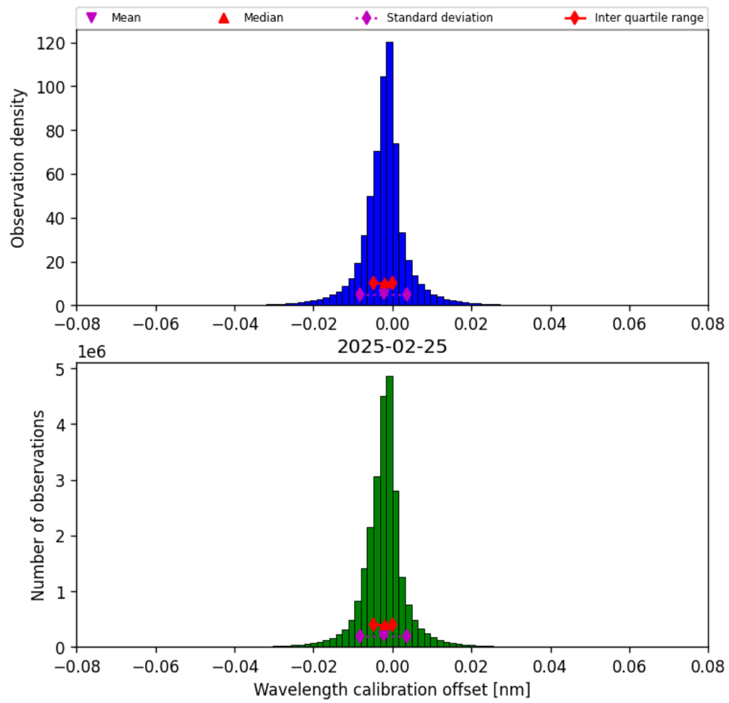
Figure 35: Histogram of “Wavelength calibration offset” for 2025-02-24 to 2025-02-26
