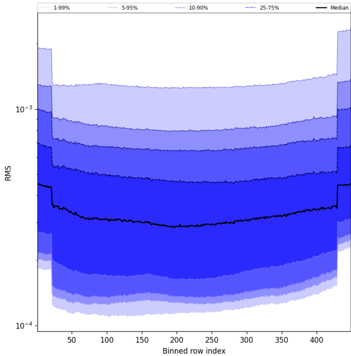
Figure 60: Along track statistics of “RMS” for 2025-02-24 to 2025-02-26
