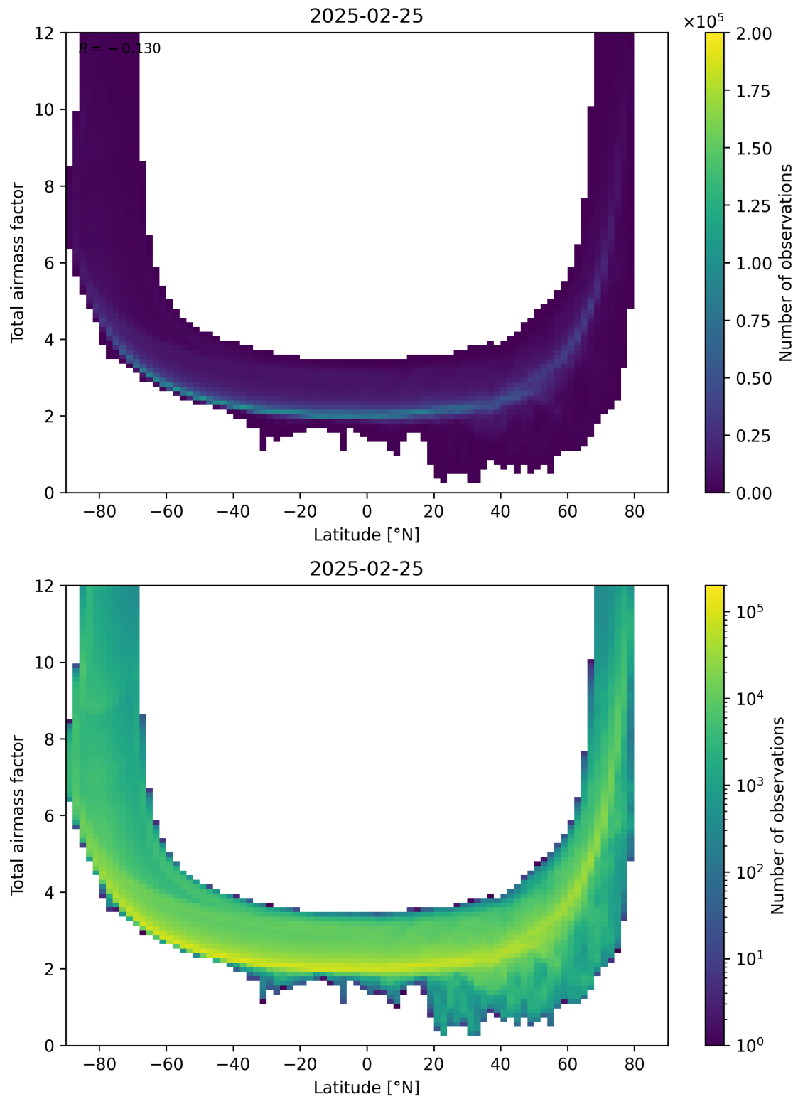
Figure 84: Scatter density plot of “Latitude” against “Total airmass factor” for 2025-02-24 to 2025-02-26.
