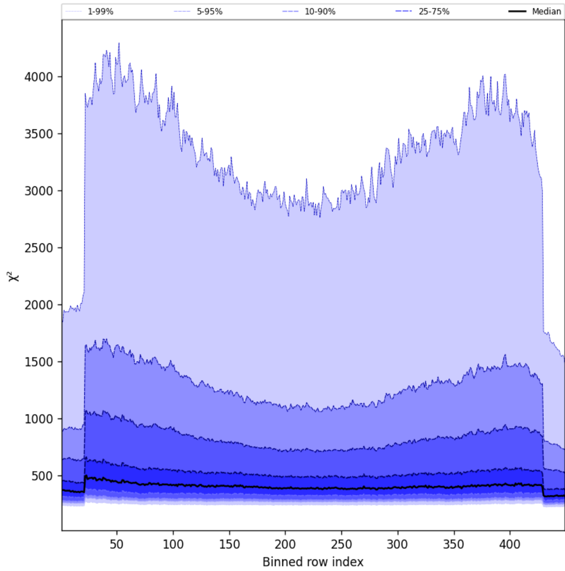
Figure 59: Along track statistics of “ \chi^2 ” for 2025-02-24 to 2025-02-26
