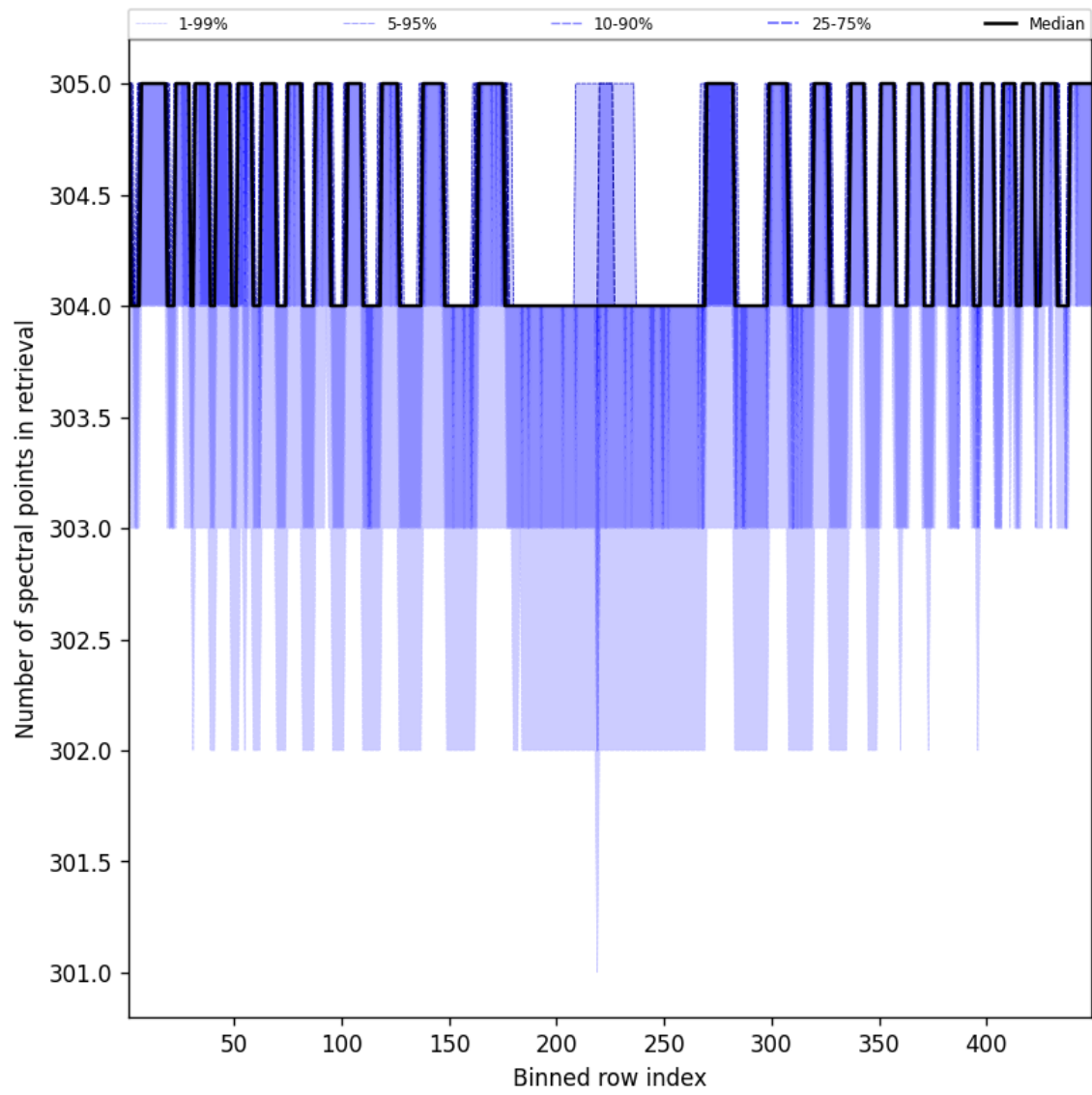
Figure 50: Along track statistics of “Number of spectral points in retrieval” for 2025-02-24 to 2025-02-26
