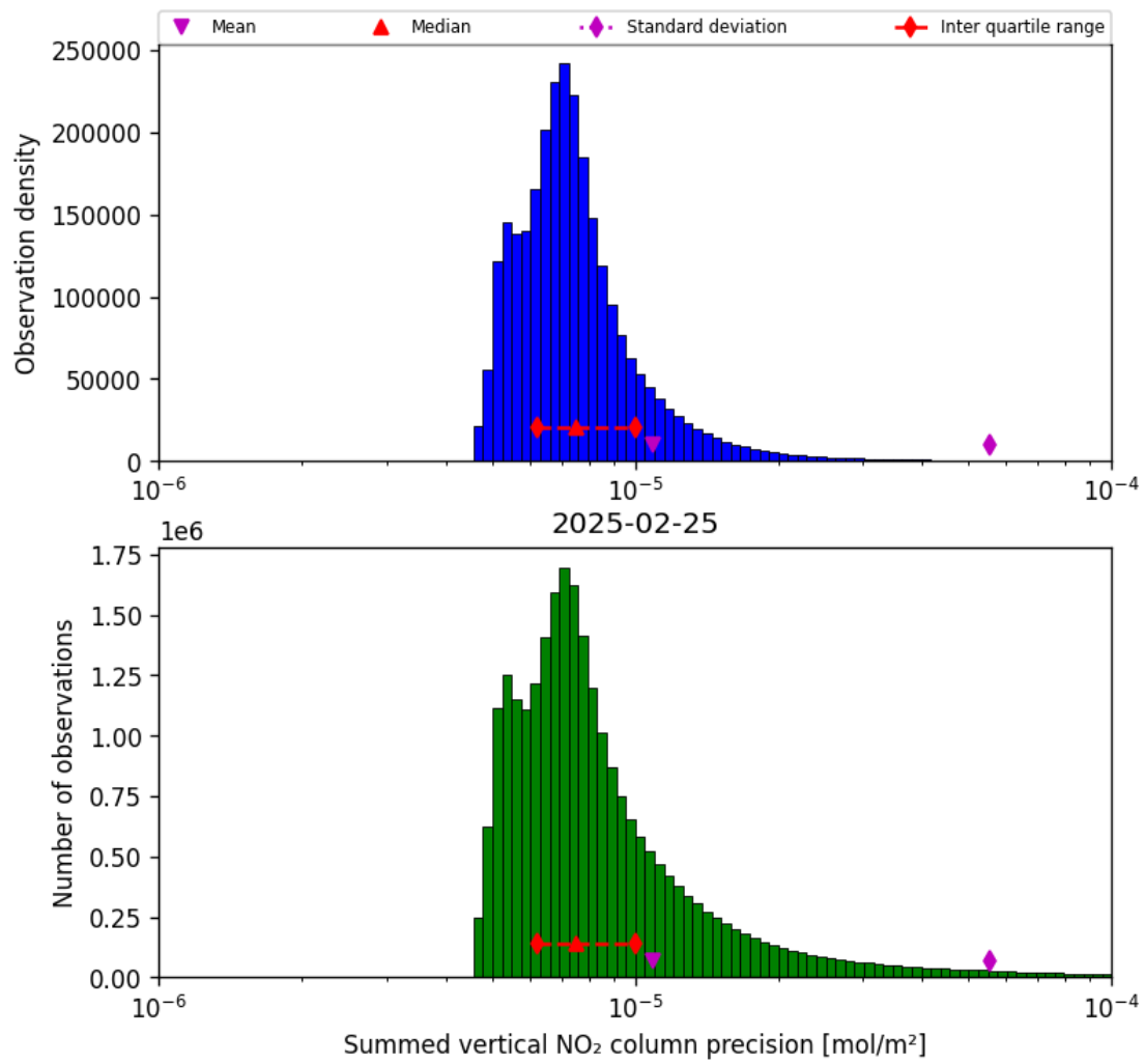
Figure 41: Histogram of “Summed vertical NO 2 column precision” for 2025-02-24 to 2025-02-26
