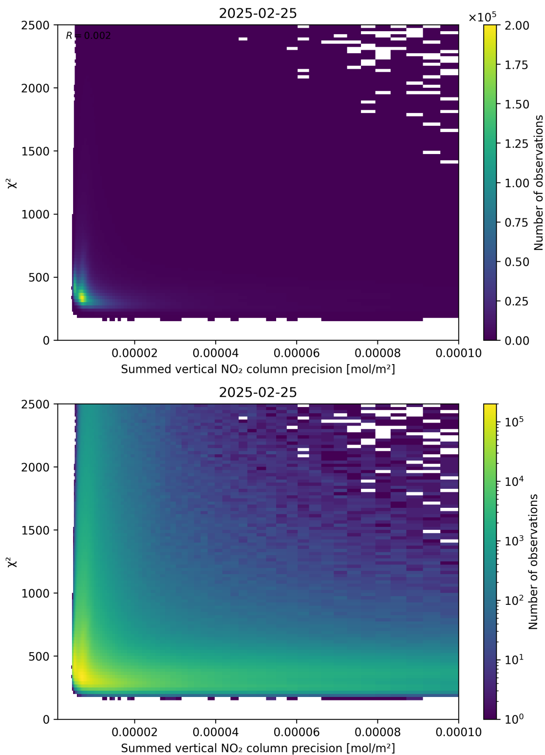
Figure 107: Scatter density plot of “Summed vertical NO 2 column precision” against “ \chi^2 ” for 2025-02-24 to 2025-02-26.
