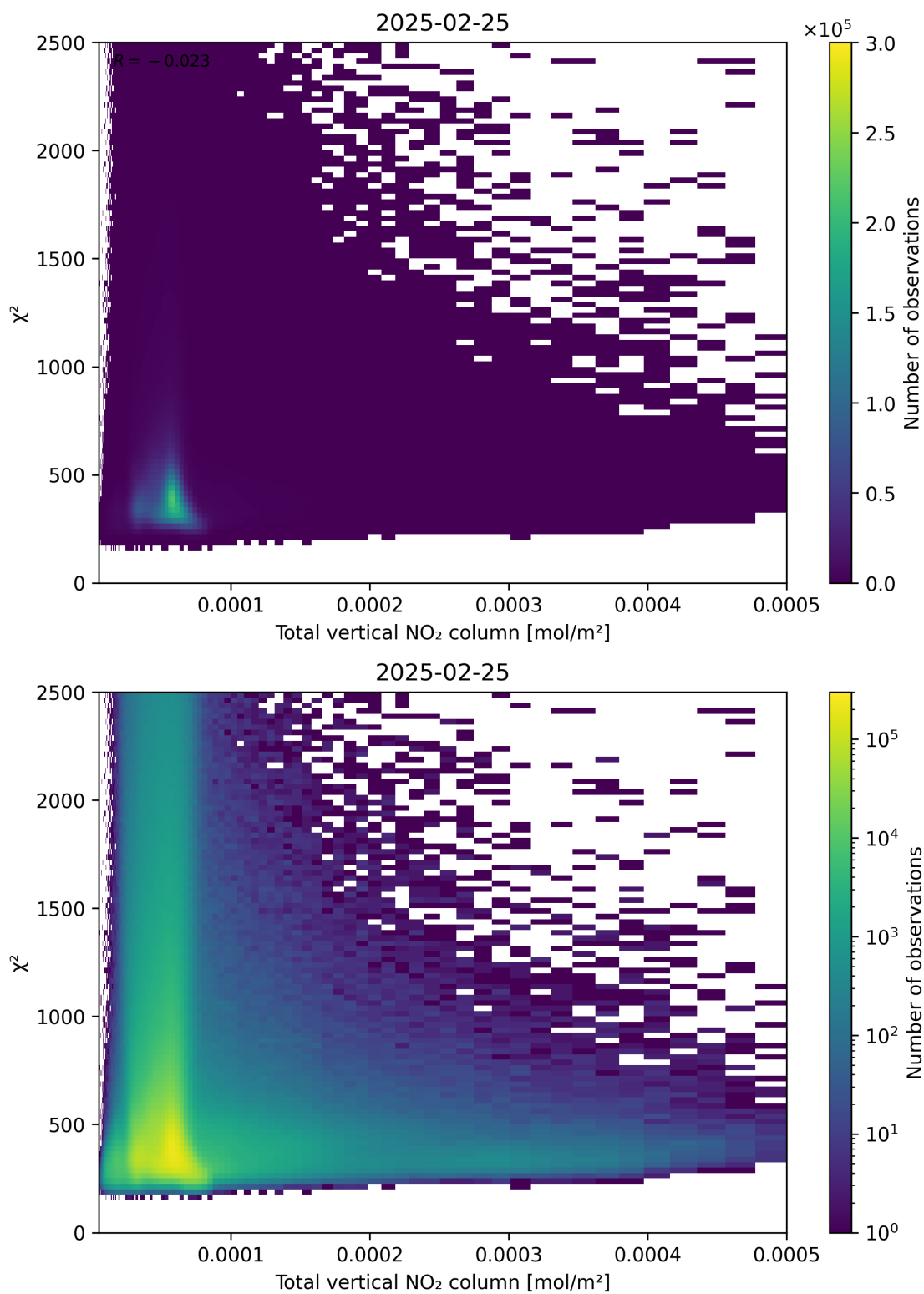
Figure 111: Scatter density plot of “Total vertical NO 2 column” against “ \chi^2 ” for 2025-02-24 to 2025-02-26.
