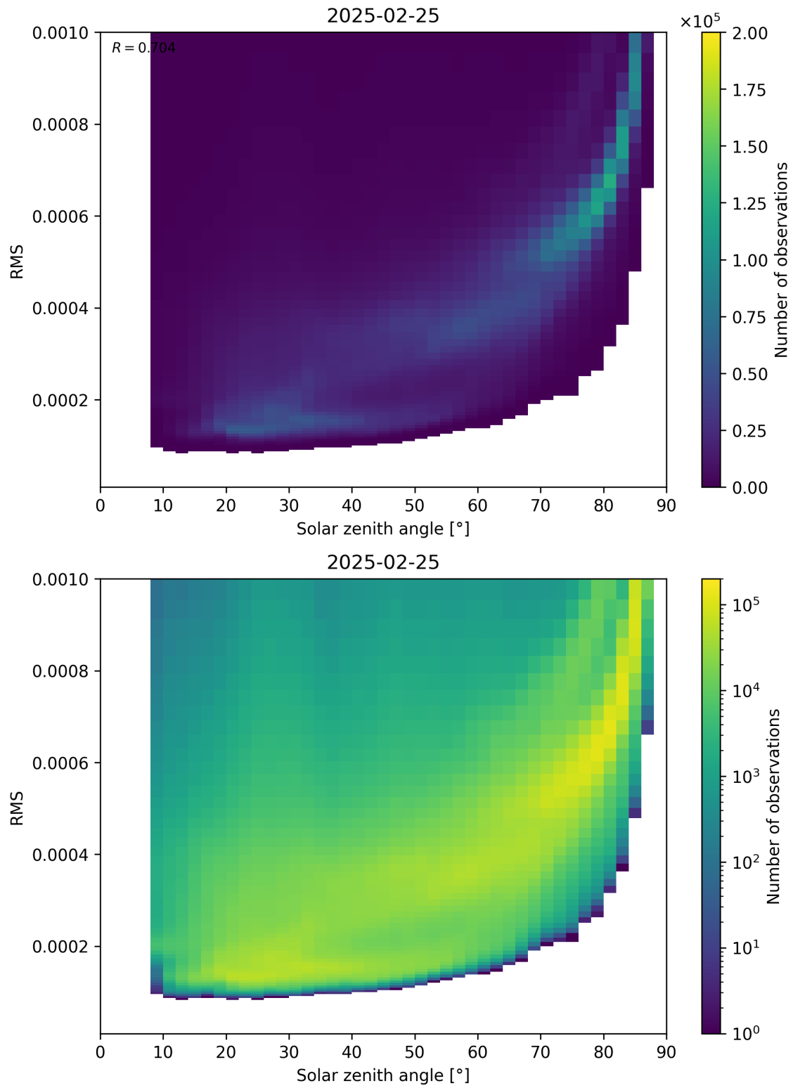
Figure 157: Scatter density plot of “Solar zenith angle” against “RMS” for 2025-02-24 to 2025-02-26.
