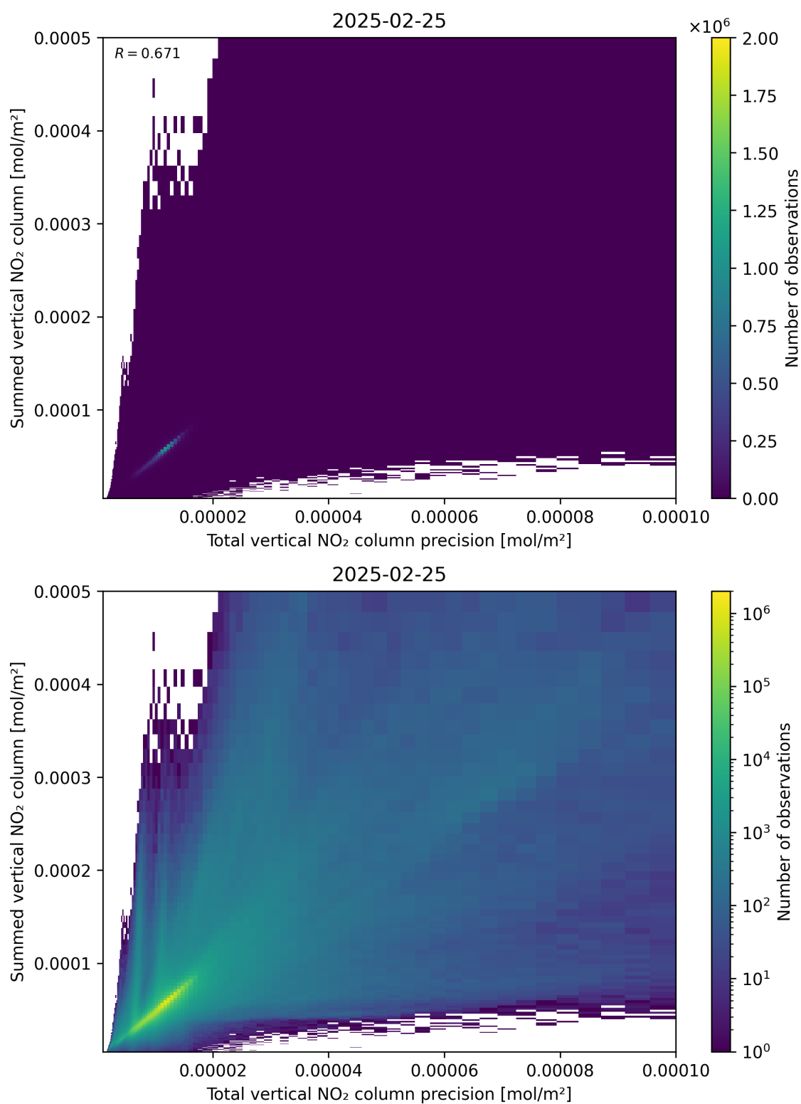
Figure 117: Scatter density plot of “Total vertical NO 2 column precision” against “Summed vertical NO 2 column” for 2025-02-24 to 2025-02-26.
