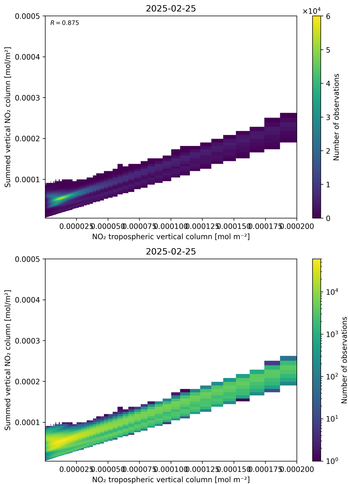
Figure 126: Scatter density plot of “NO 2 tropospheric vertical column” against “Summed vertical NO 2 column” for 2025-02-24 to 2025-02-26.
