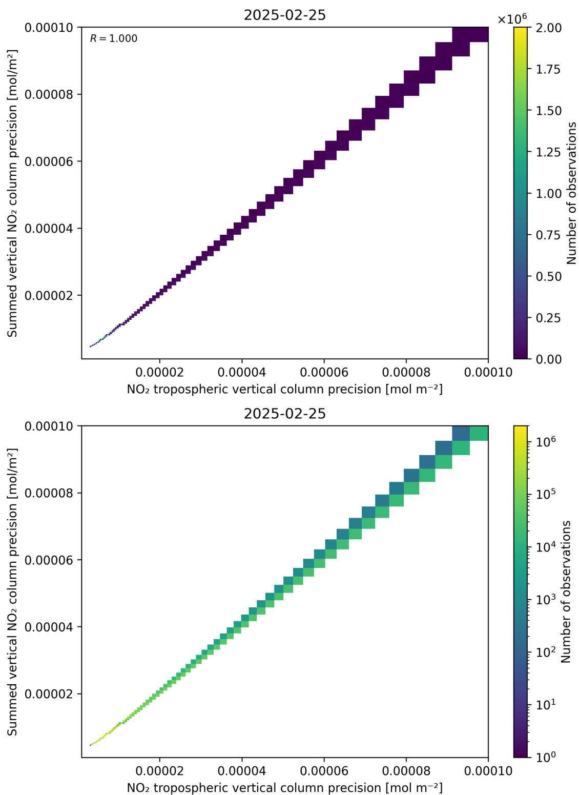
Figure 137: Scatter density plot of “NO 2 tropospheric vertical column precision” against “Summed vertical NO 2 column precision” for 2025-02-24 to 2025-02-26.
