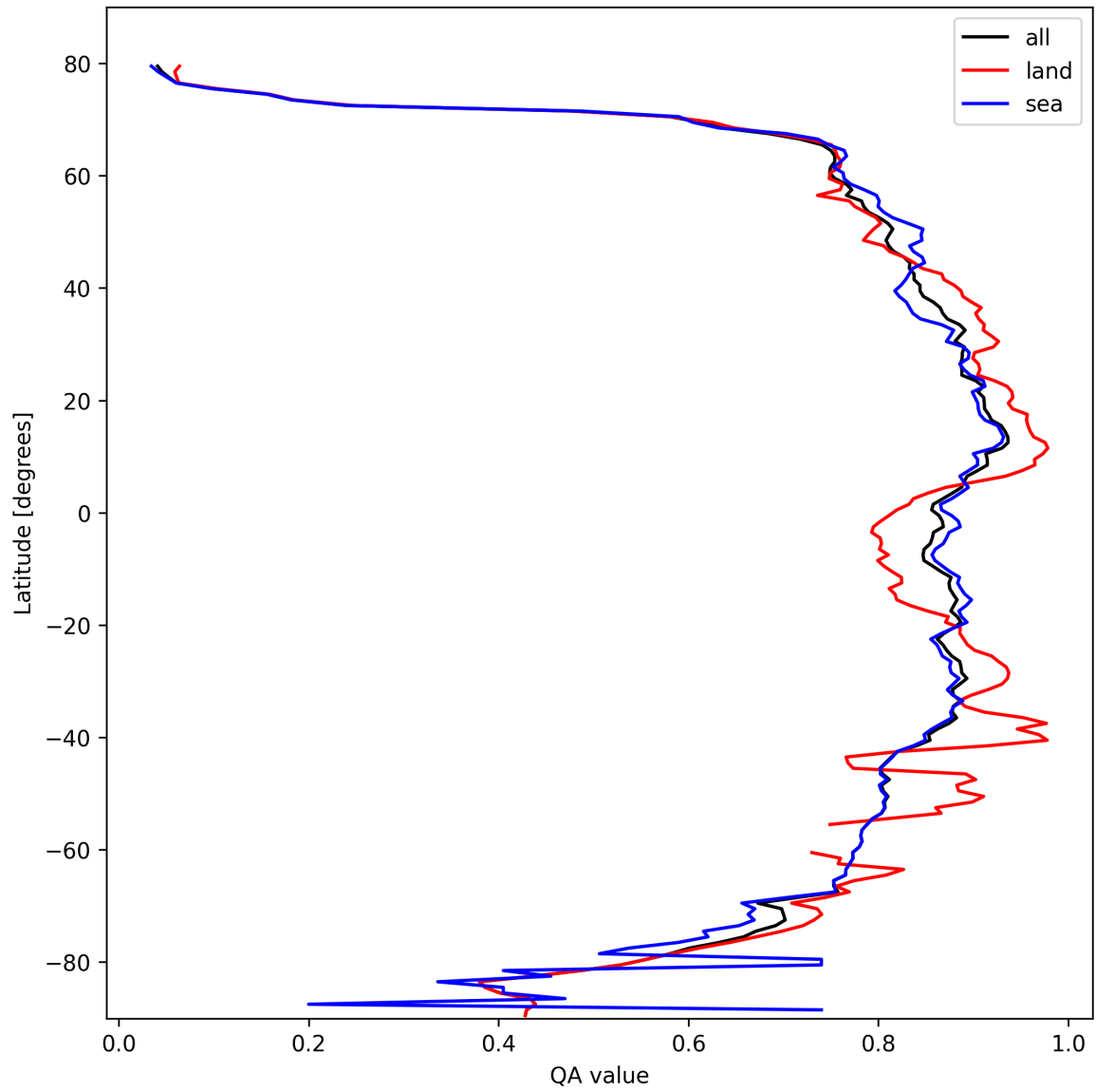
Figure 11: Zonal average of “QA value” for 2025-02-24 to 2025-02-26.
