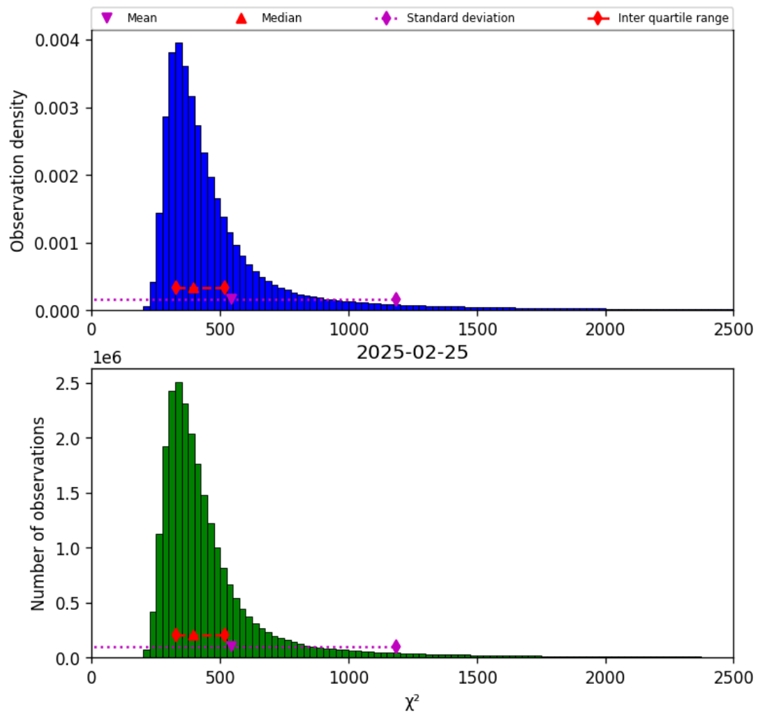
Figure 42: Histogram of “ \chi^2 ” for 2025-02-24 to 2025-02-26
