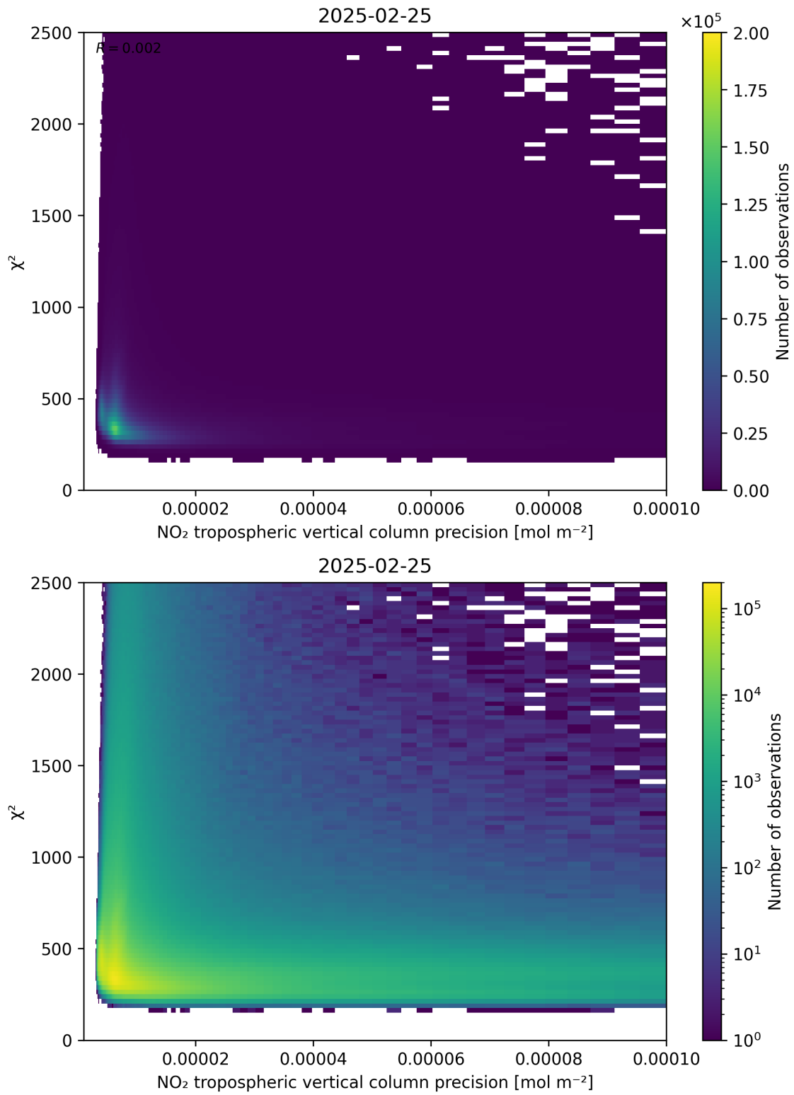
Figure 134: Scatter density plot of “NO 2 tropospheric vertical column precision” against “ \chi^2 ” for 2025-02-24 to 2025-02-26.
