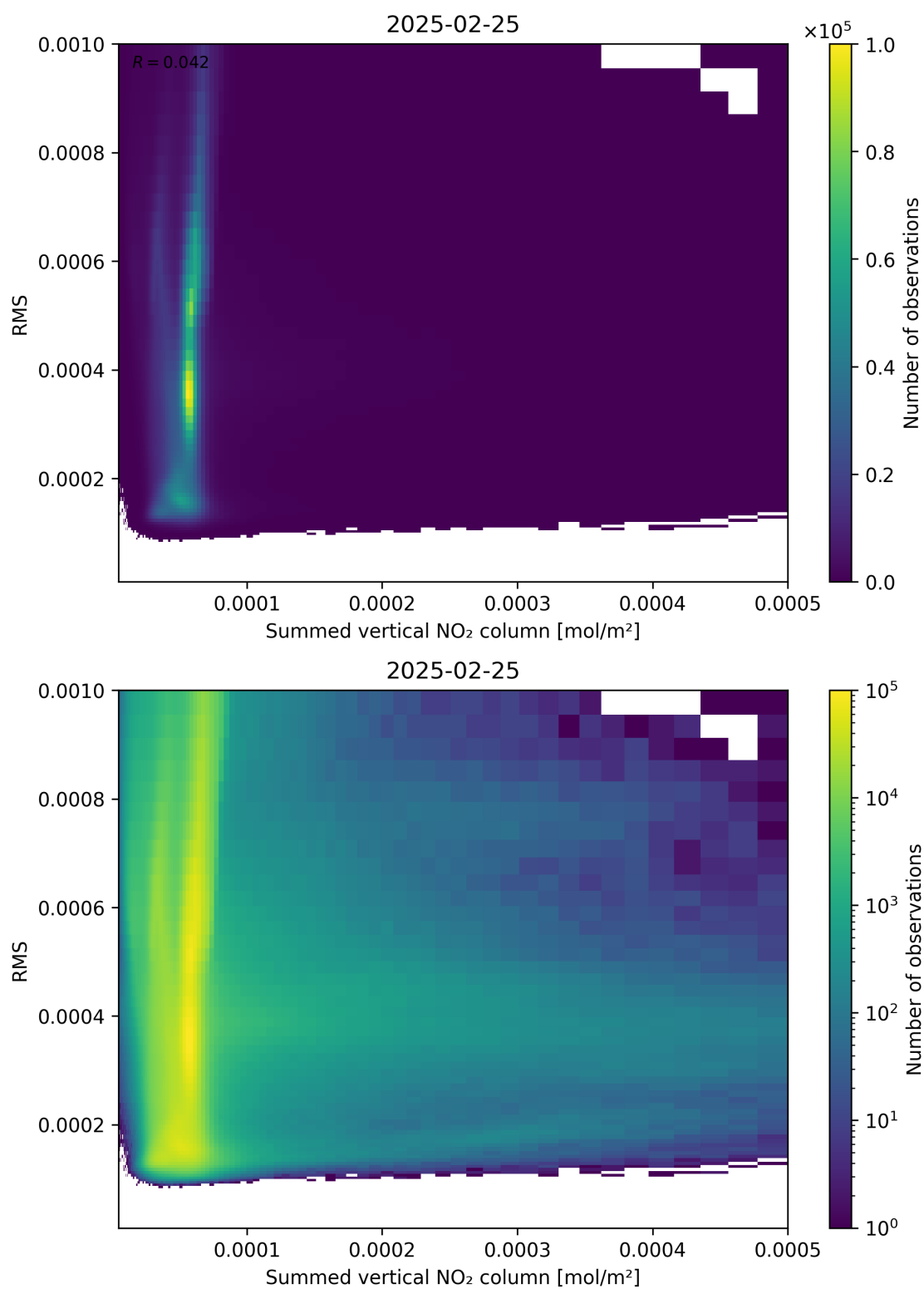
Figure 109: Scatter density plot of “Summed vertical NO 2 column” against “RMS” for 2025-02-24 to 2025-02-26.
