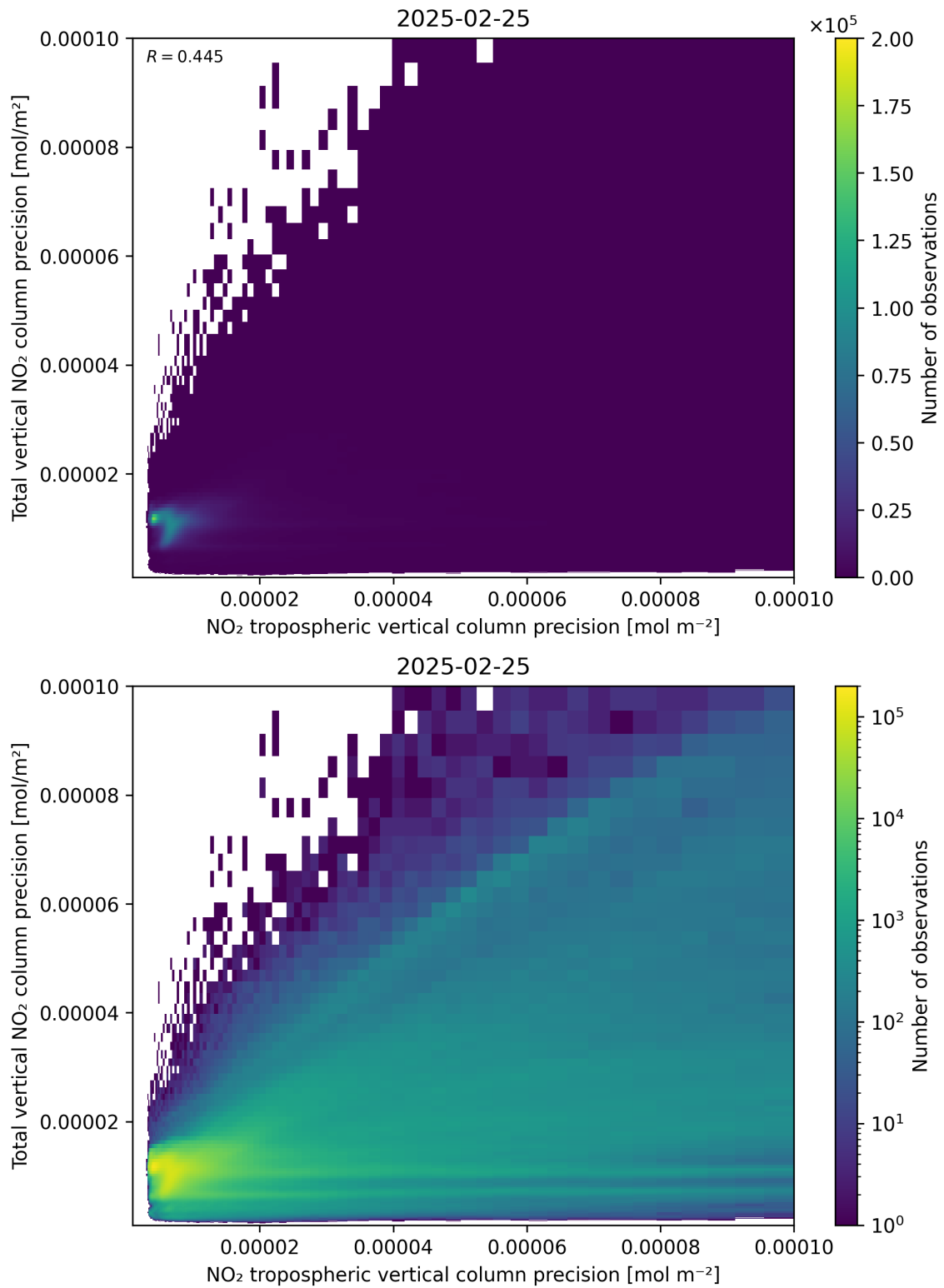
Figure 139: Scatter density plot of “NO 2 tropospheric vertical column precision” against “Total vertical NO 2 column precision” for 2025-02-24 to 2025-02-26.
