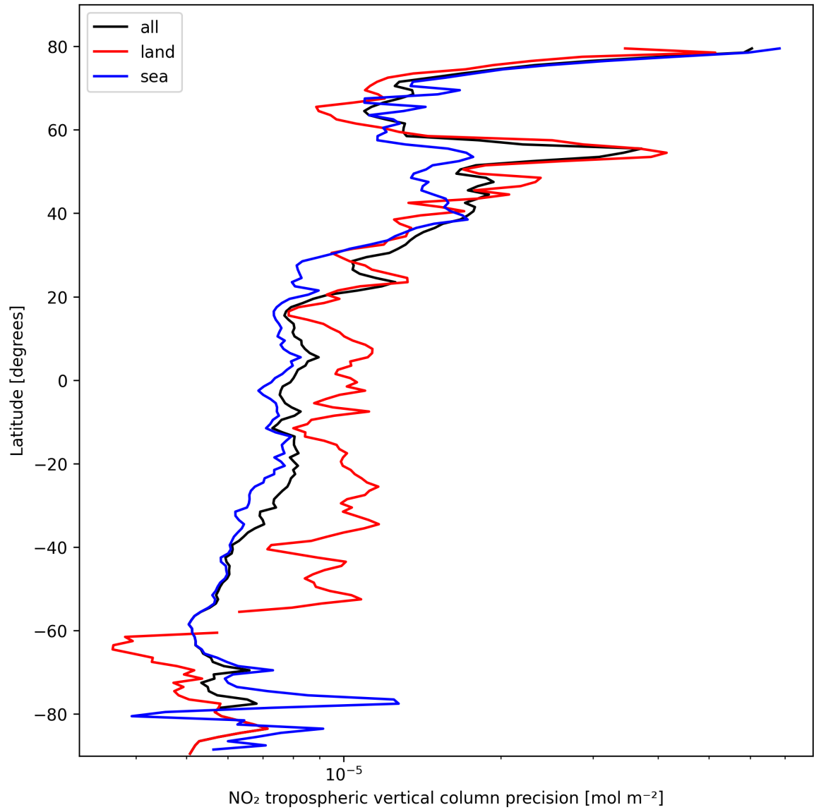
Figure 13: Zonal average of “NO 2 tropospheric vertical column precision” for 2025-02-24 to 2025-02-26.
