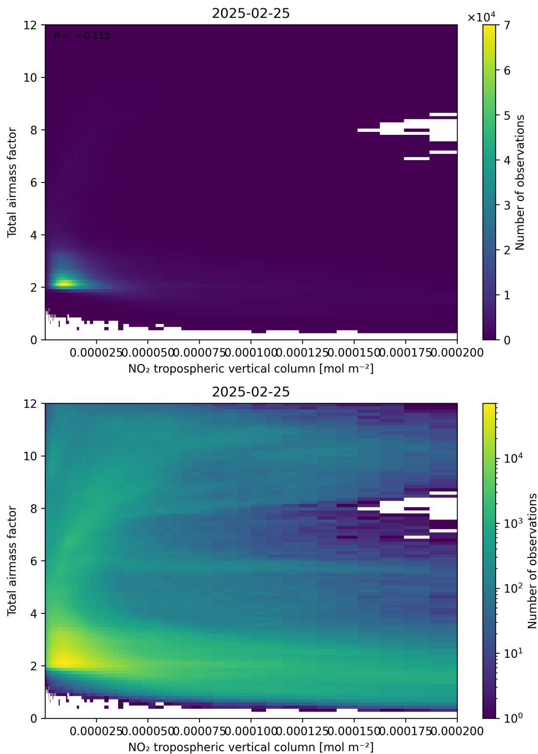
Figure 122: Scatter density plot of “NO 2 tropospheric vertical column” against “Total air mass factor” for 2025-02-24 to 2025-02-26.
