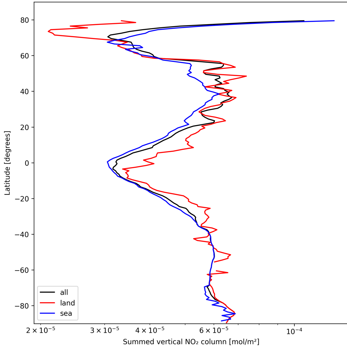
Figure 23: Zonal average of “Summed vertical NO 2 column” for 2025-02-24 to 2025-02-26.
