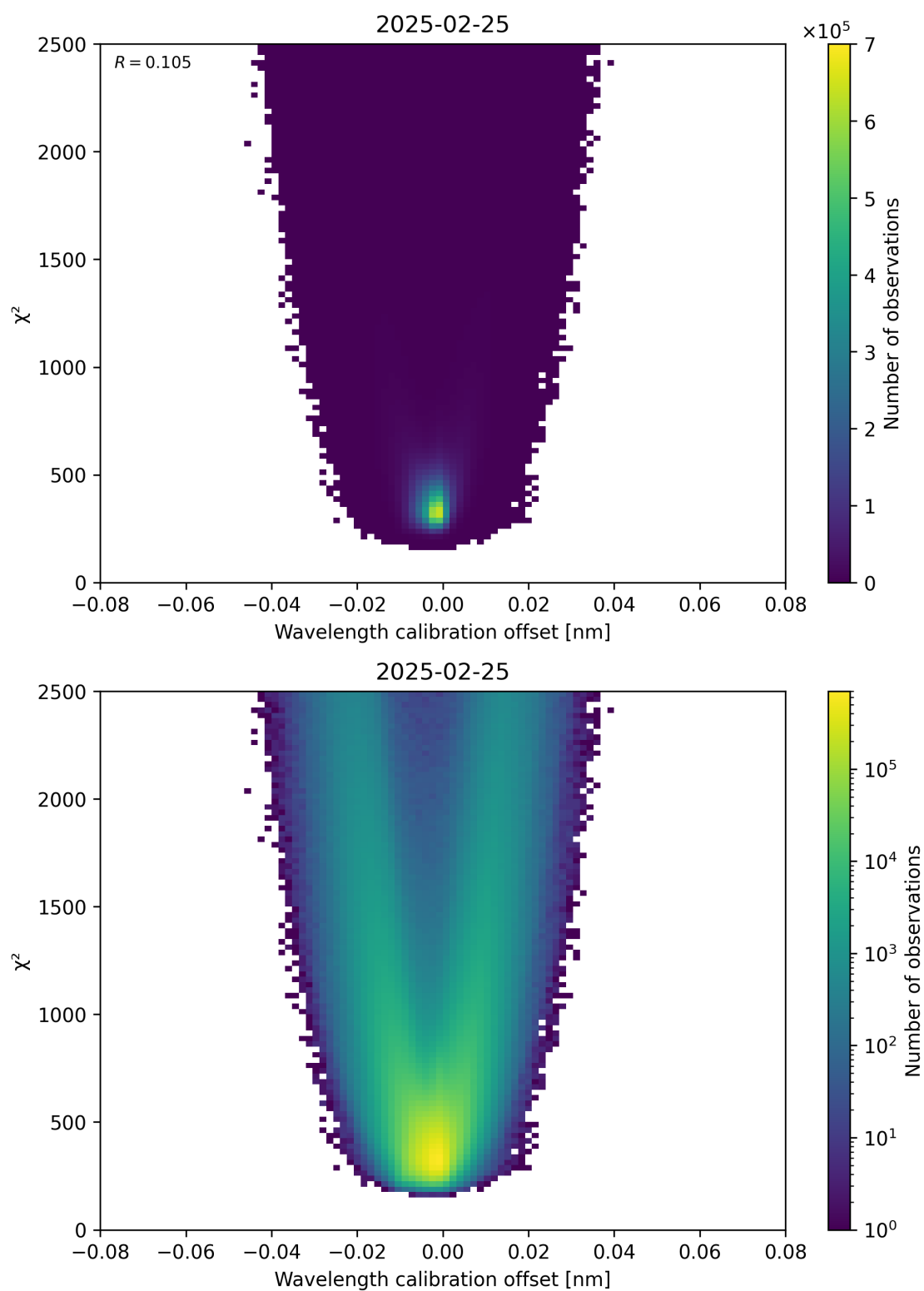
Figure 175: Scatter density plot of “Wavelength calibration offset” against “ \chi^2 ” for 2025-02-24 to 2025-02-26.
