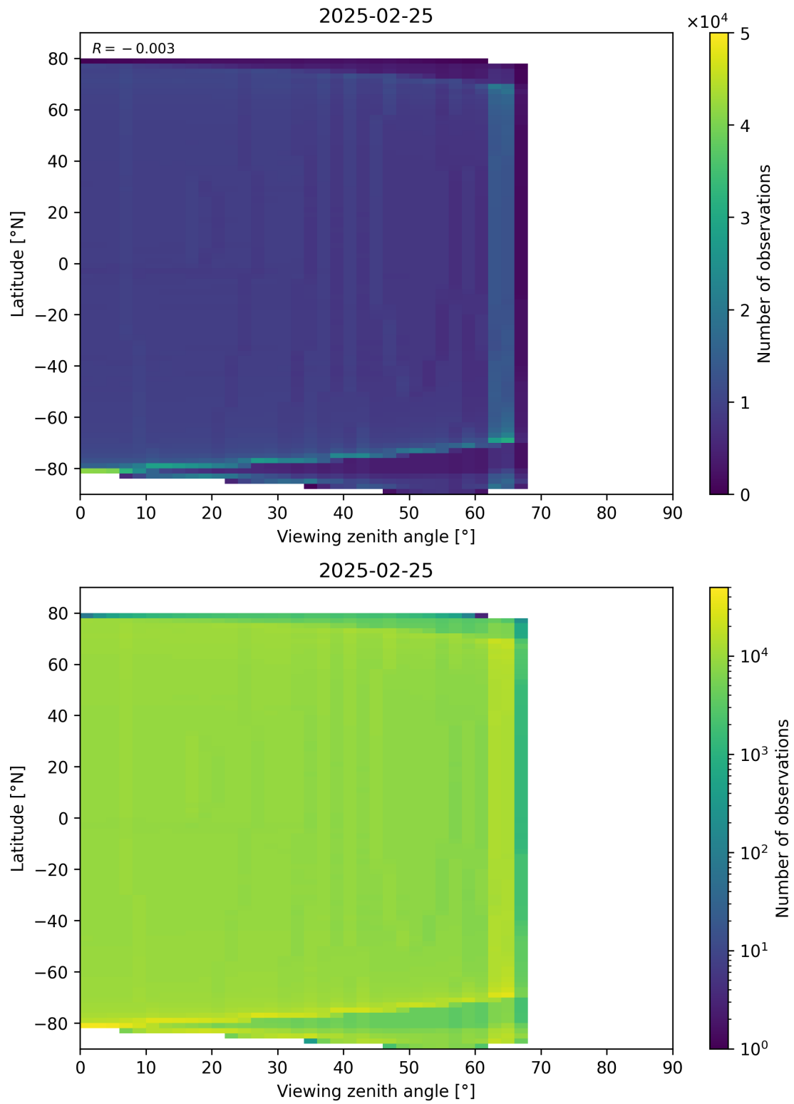
Figure 163: Scatter density plot of “Viewing zenith angle” against “Latitude” for 2025-02-24 to 2025-02-26.
