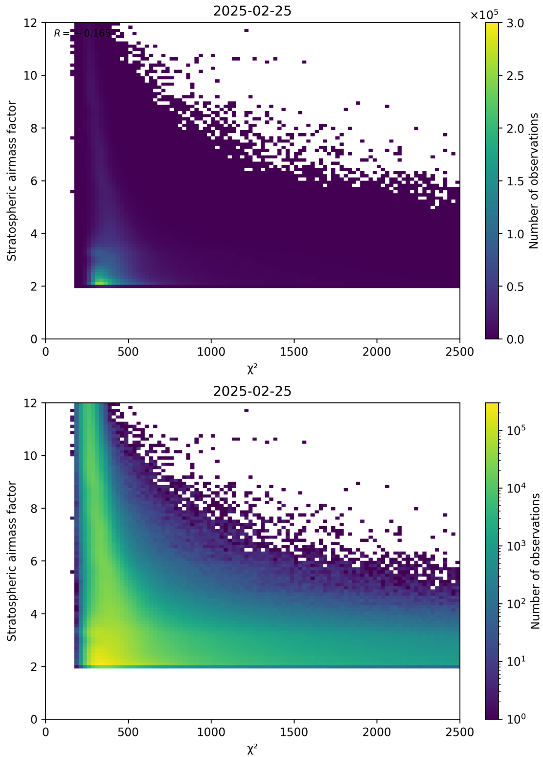
Figure 81: Scatter density plot of “ \chi^2 ” against “Stratospheric airmass factor” for 2025-02-24 to 2025-02-26.
