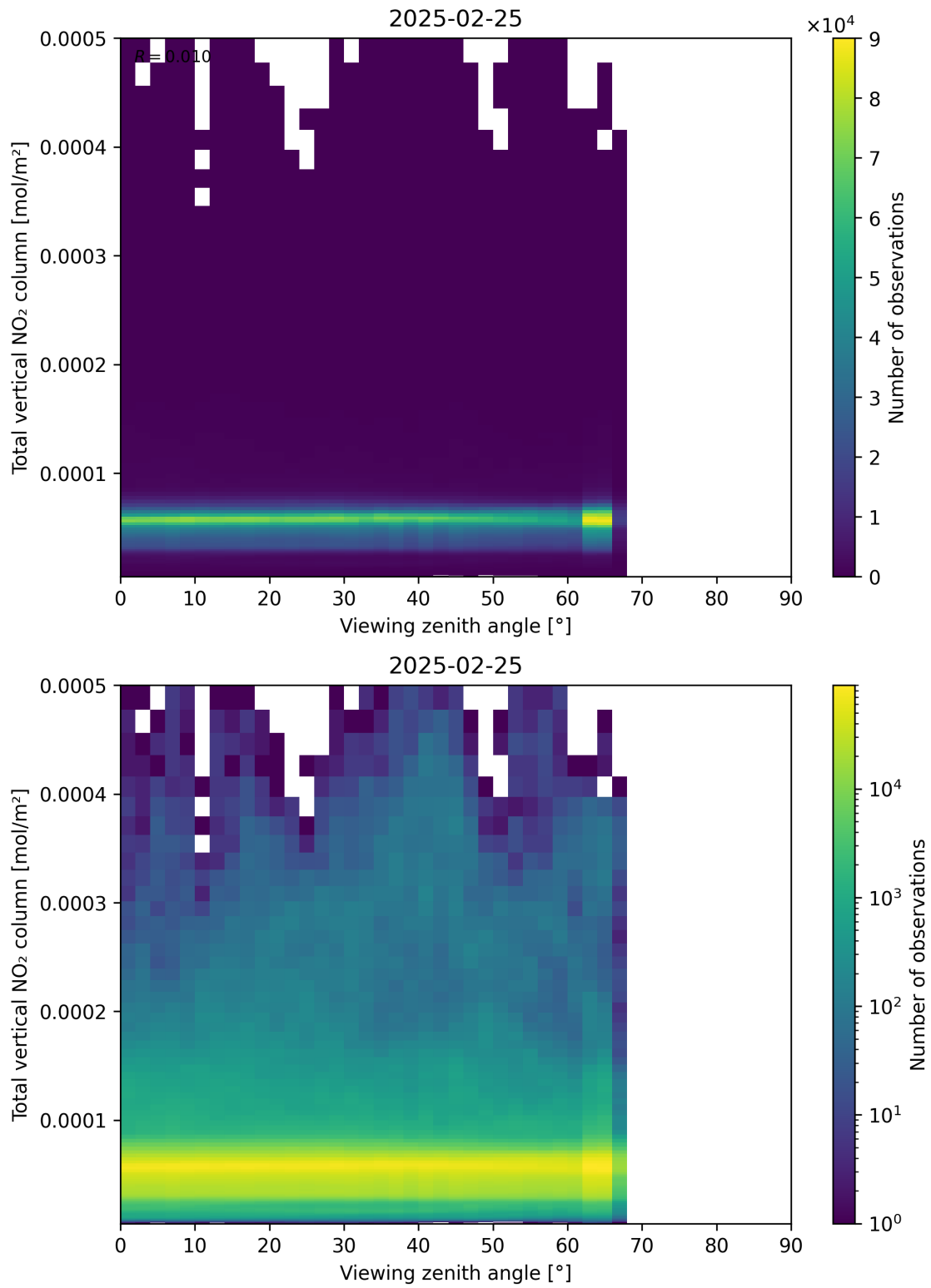
Figure 167: Scatter density plot of “Viewing zenith angle” against “Total vertical NO 2 column” for 2025-02-24 to 2025-02-26.
