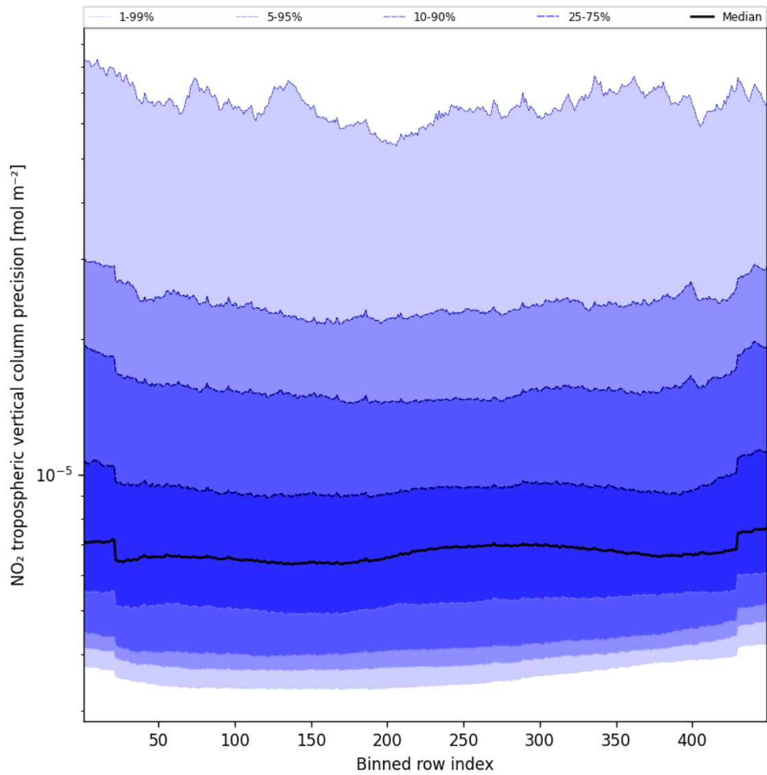
Figure 47: Along track statistics of “NO 2 tropospheric vertical column precision” for 2025-02-24 to 2025-02-26
