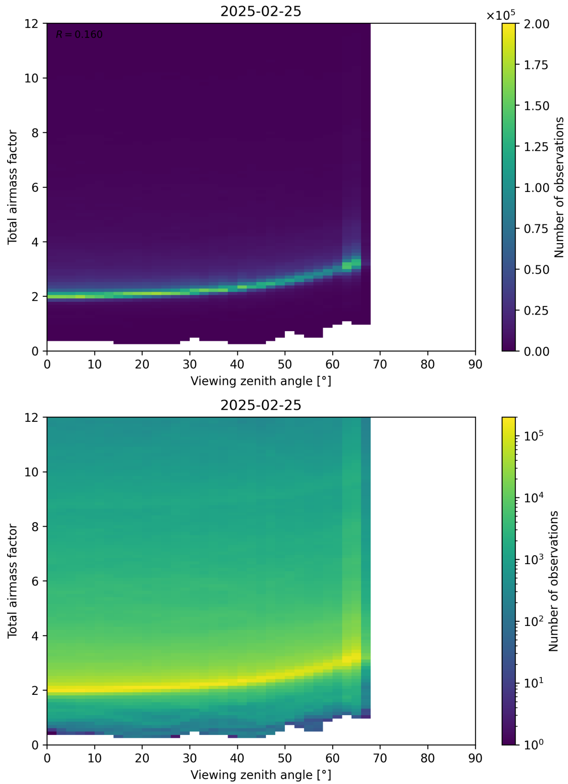
Figure 160: Scatter density plot of “Viewing zenith angle” against “Total airmass factor” for 2025-02-24 to 2025-02-26.
