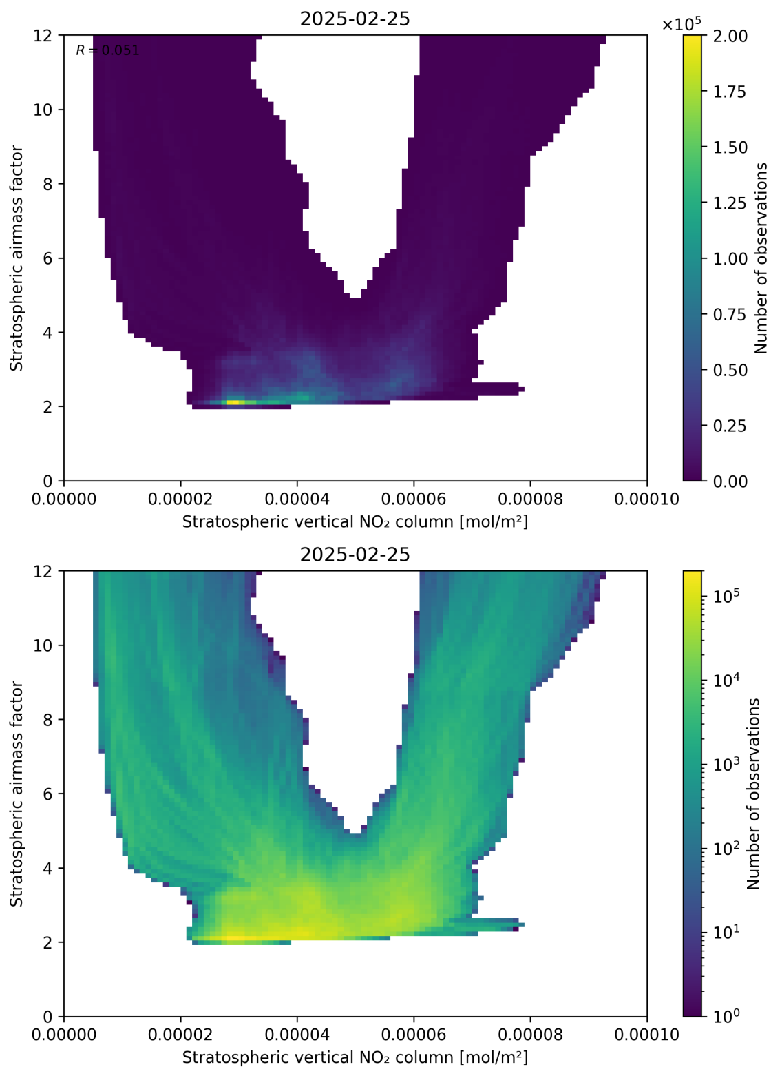
Figure 96: Scatter density plot of “Stratospheric vertical NO 2 column” against “Stratospheric airmass factor” for 2025-02-24 to 2025-02-26.
