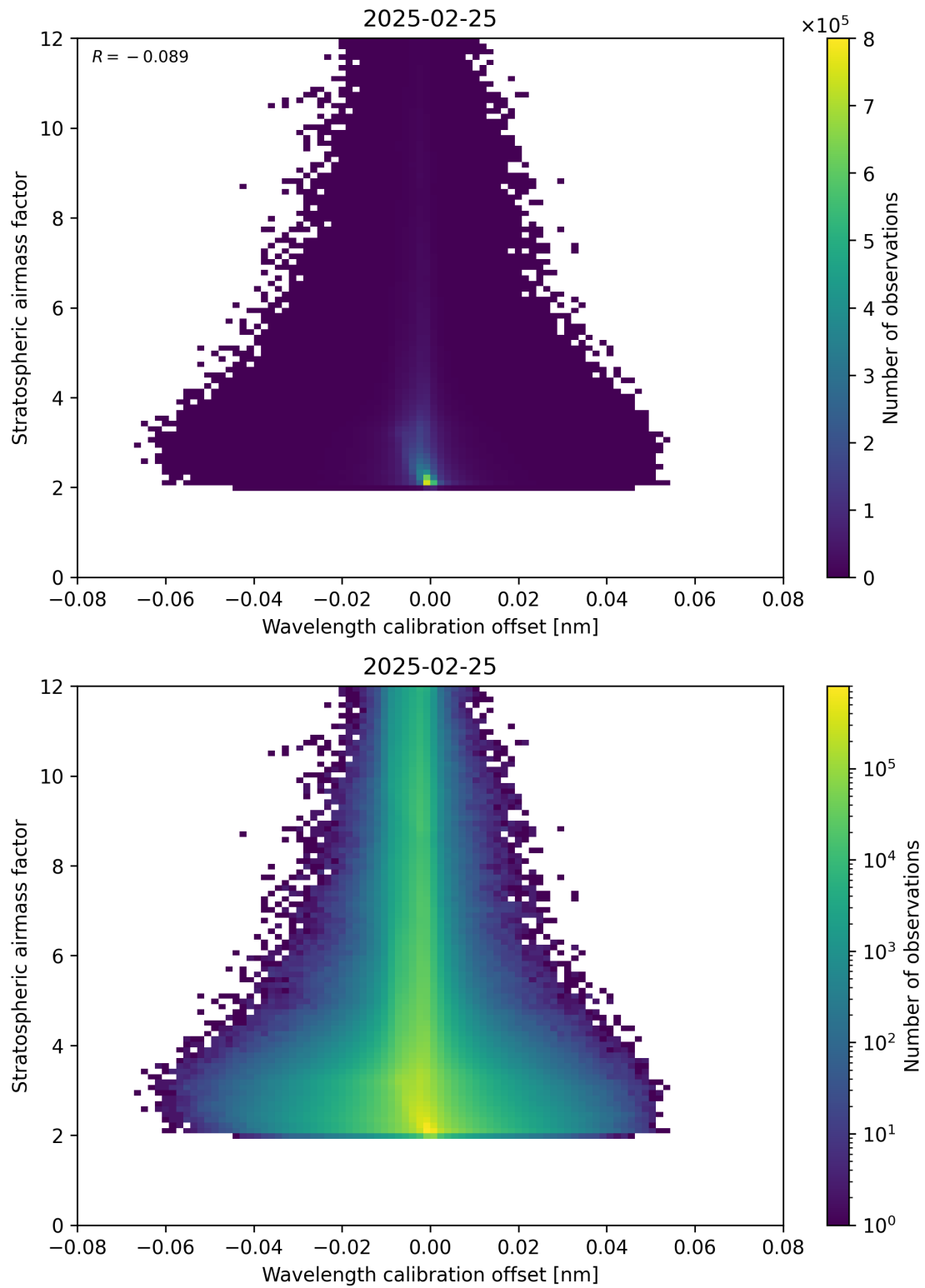
Figure 174: Scatter density plot of “Wavelength calibration offset” against “Stratospheric airmass factor” for 2025-02-24 to 2025-02-26.
