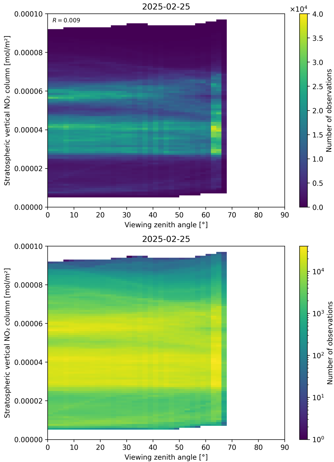
Figure 164: Scatter density plot of “Viewing zenith angle” against “Stratospheric vertical NO 2 column” for 2025-02-24 to 2025-02-26.
