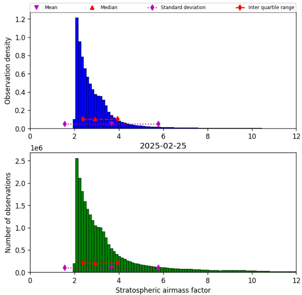
Figure 44: Histogram of “Stratospheric airmass factor” for 2025-02-24 to 2025-02-26
