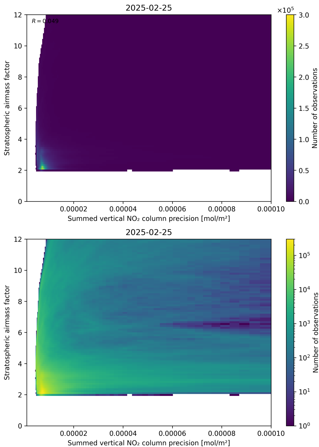
Figure 106: Scatter density plot of “Summed vertical NO 2 column precision” against “Stratospheric airmass factor” for 2025-02-24 to 2025-02-26.
