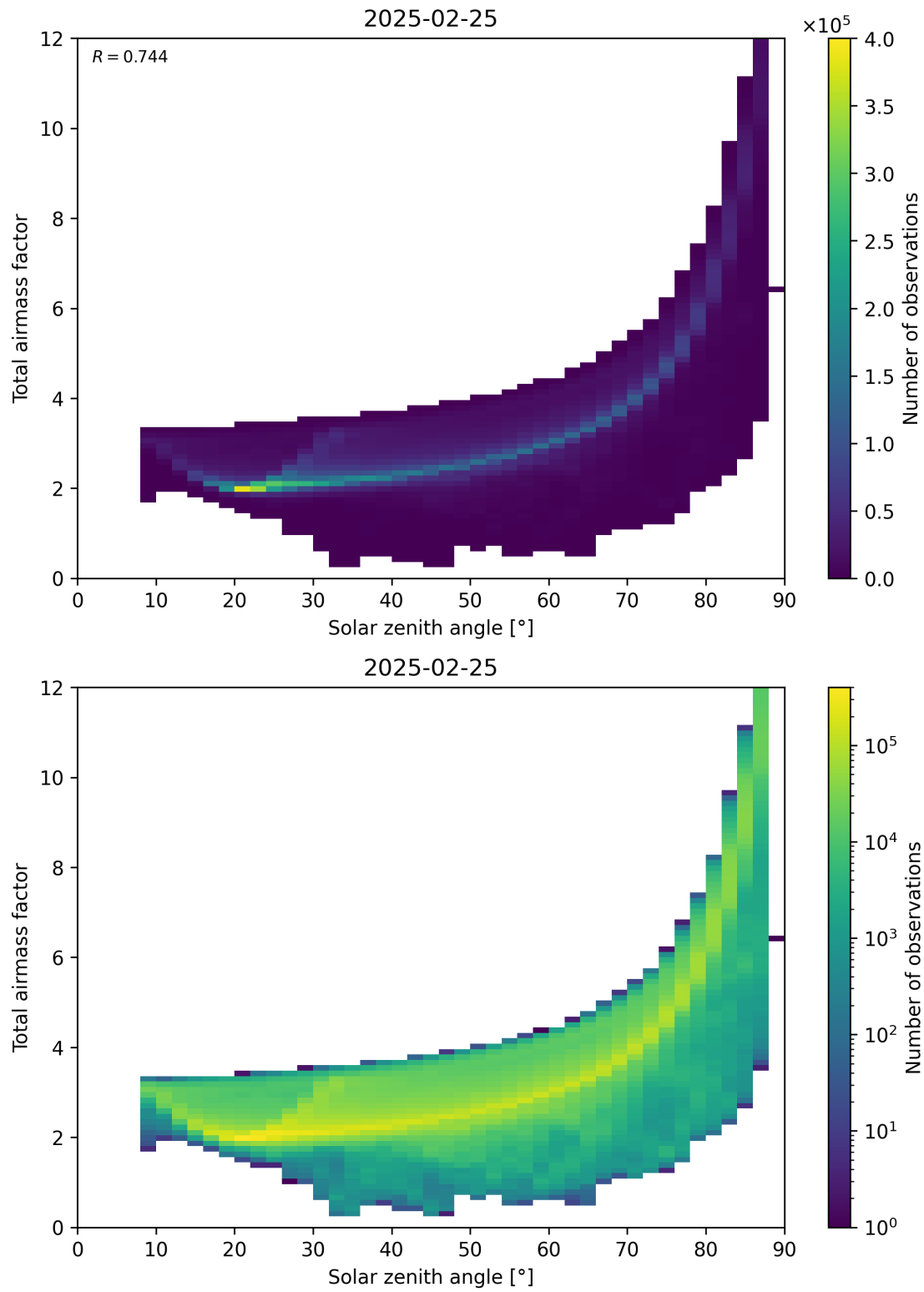
Figure 146: Scatter density plot of “Solar zenith angle” against “Total air mass factor” for 2025-02-24 to 2025-02-26.
