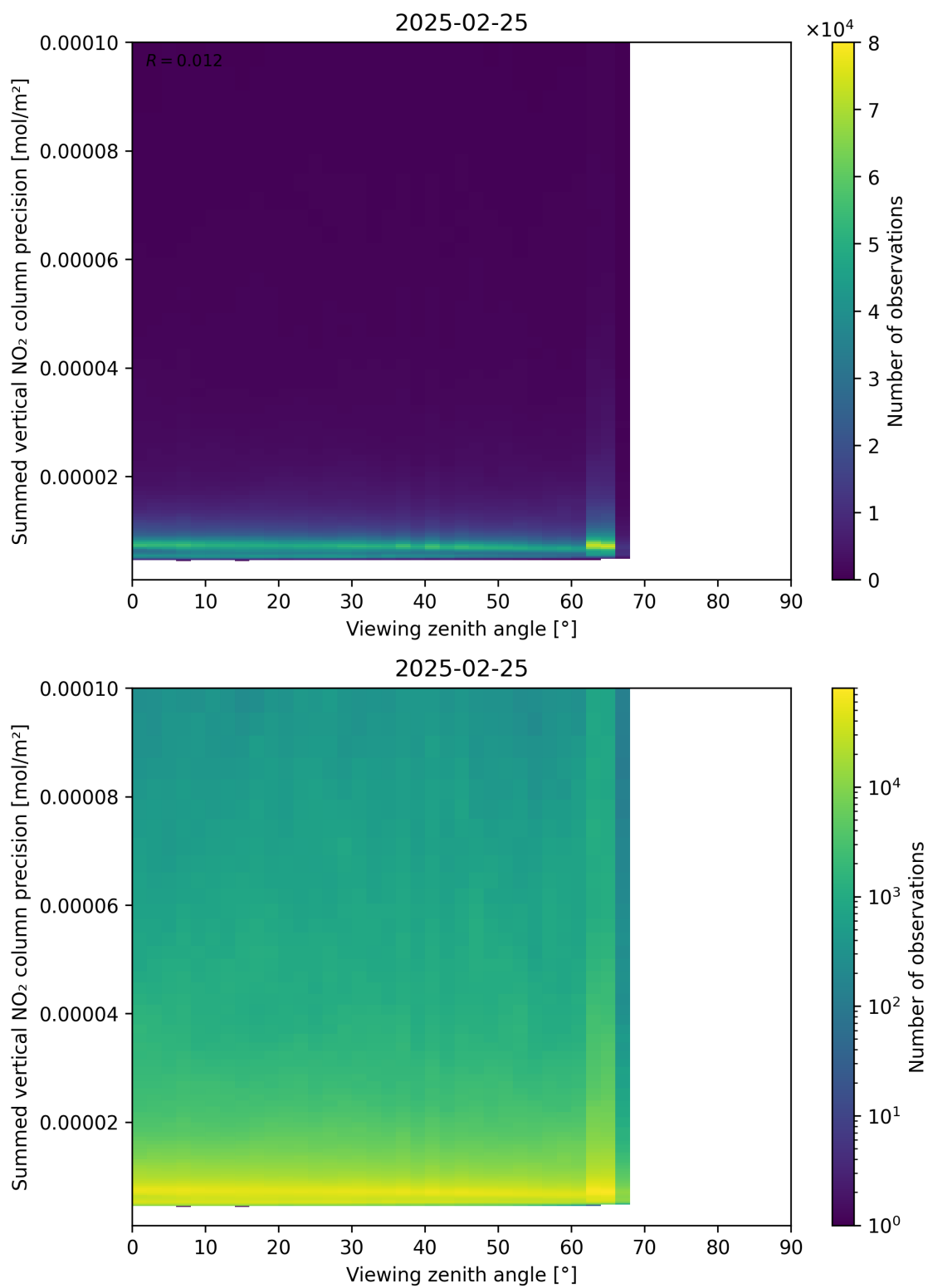
Figure 166: Scatter density plot of “Viewing zenith angle” against “Summed vertical NO 2 column precision” for 2025-02-24 to 2025-02-26.
