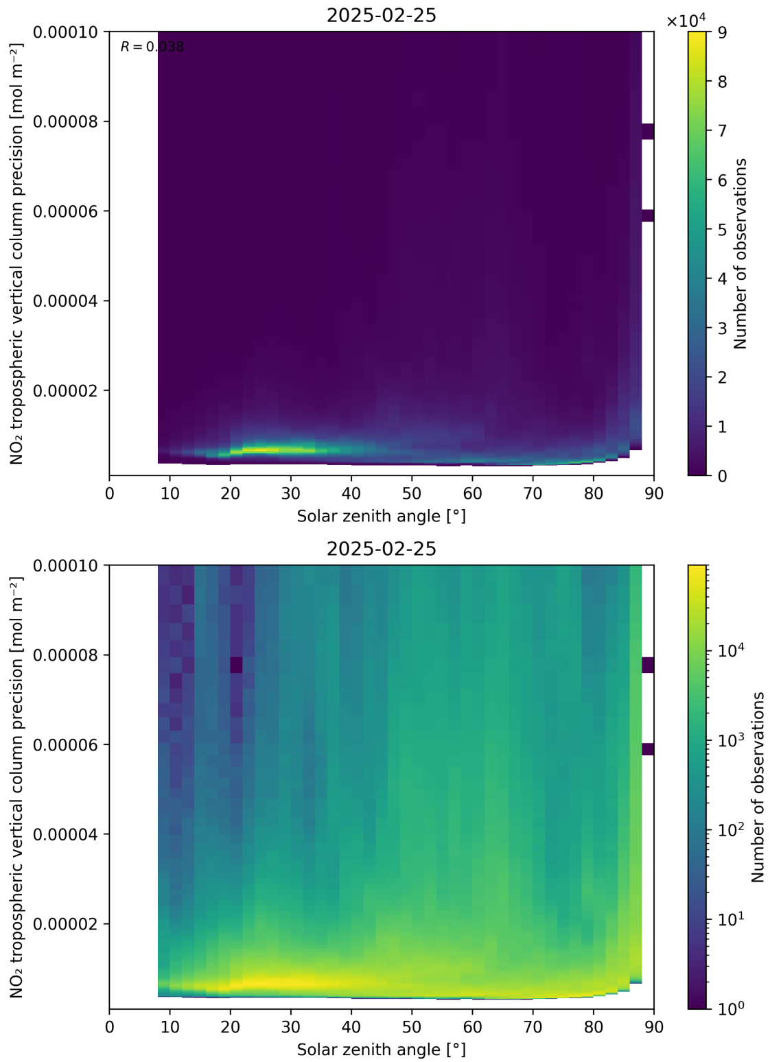
Figure 156: Scatter density plot of “Solar zenith angle” against “NO 2 tropospheric vertical column precision” for 2025-02-24 to 2025-02-26.
