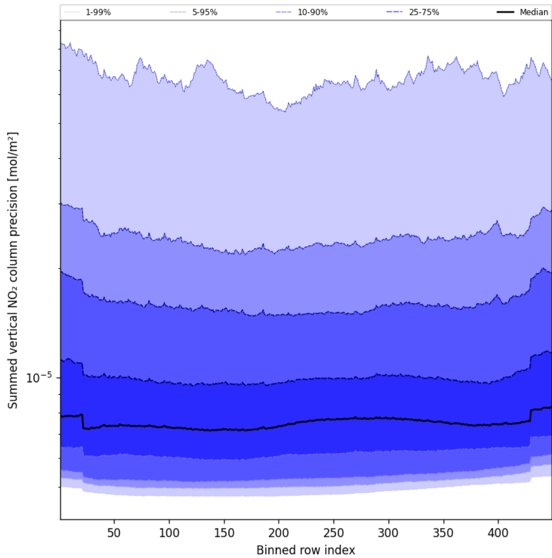
Figure 58: Along track statistics of “Summed vertical NO 2 column precision” for 2025-02-24 to 2025-02-26
