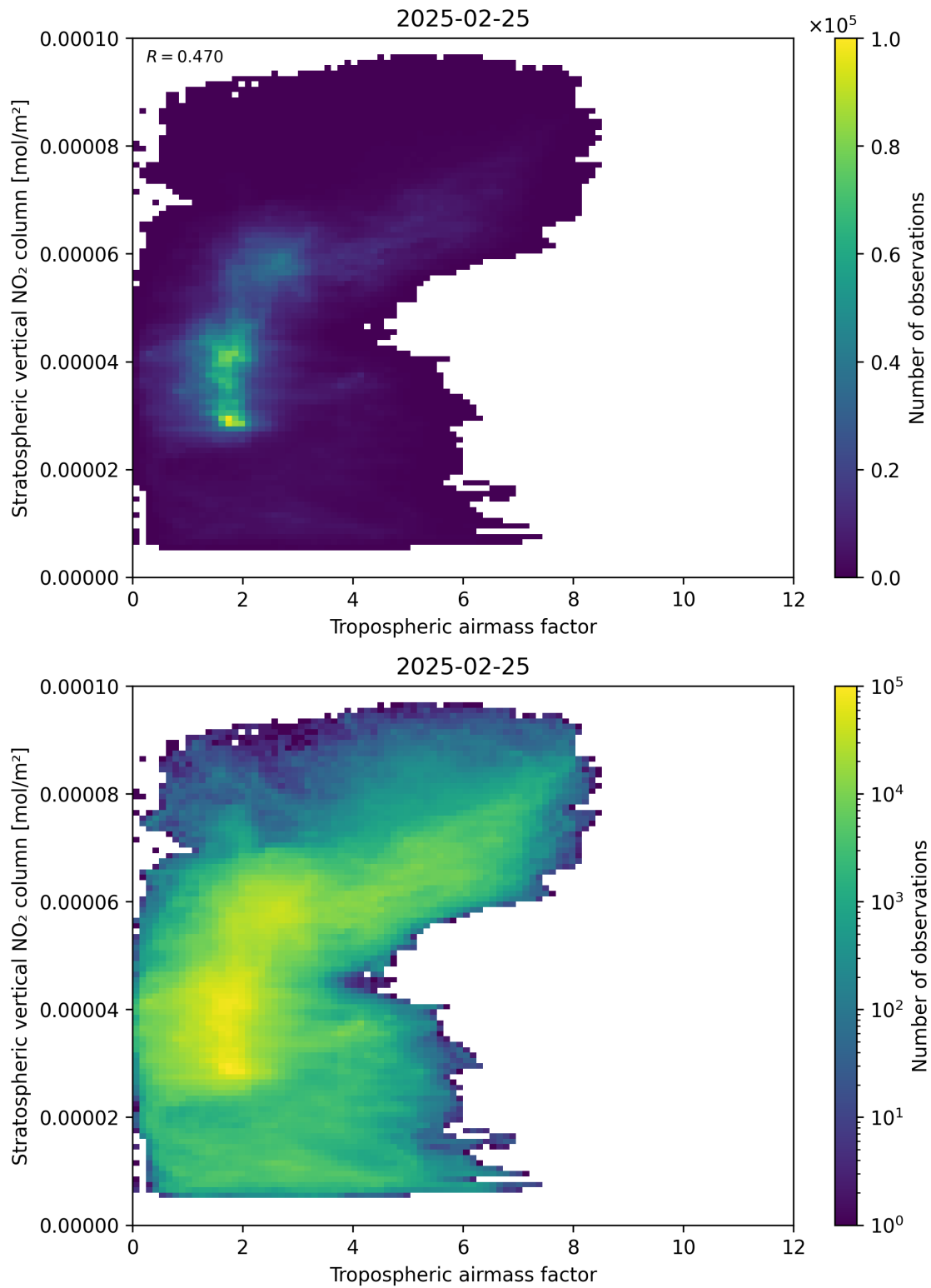
Figure 74: Scatter density plot of “Tropospheric air mass factor” against “Stratospheric vertical \text{NO}_2 column” for 2025-02-24 to 2025-02-26.
