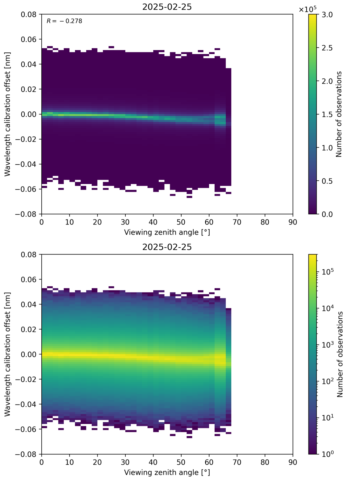
Figure 173: Scatter density plot of “Viewing zenith angle” against “Wavelength calibration offset” for 2025-02-24 to 2025-02-26.
