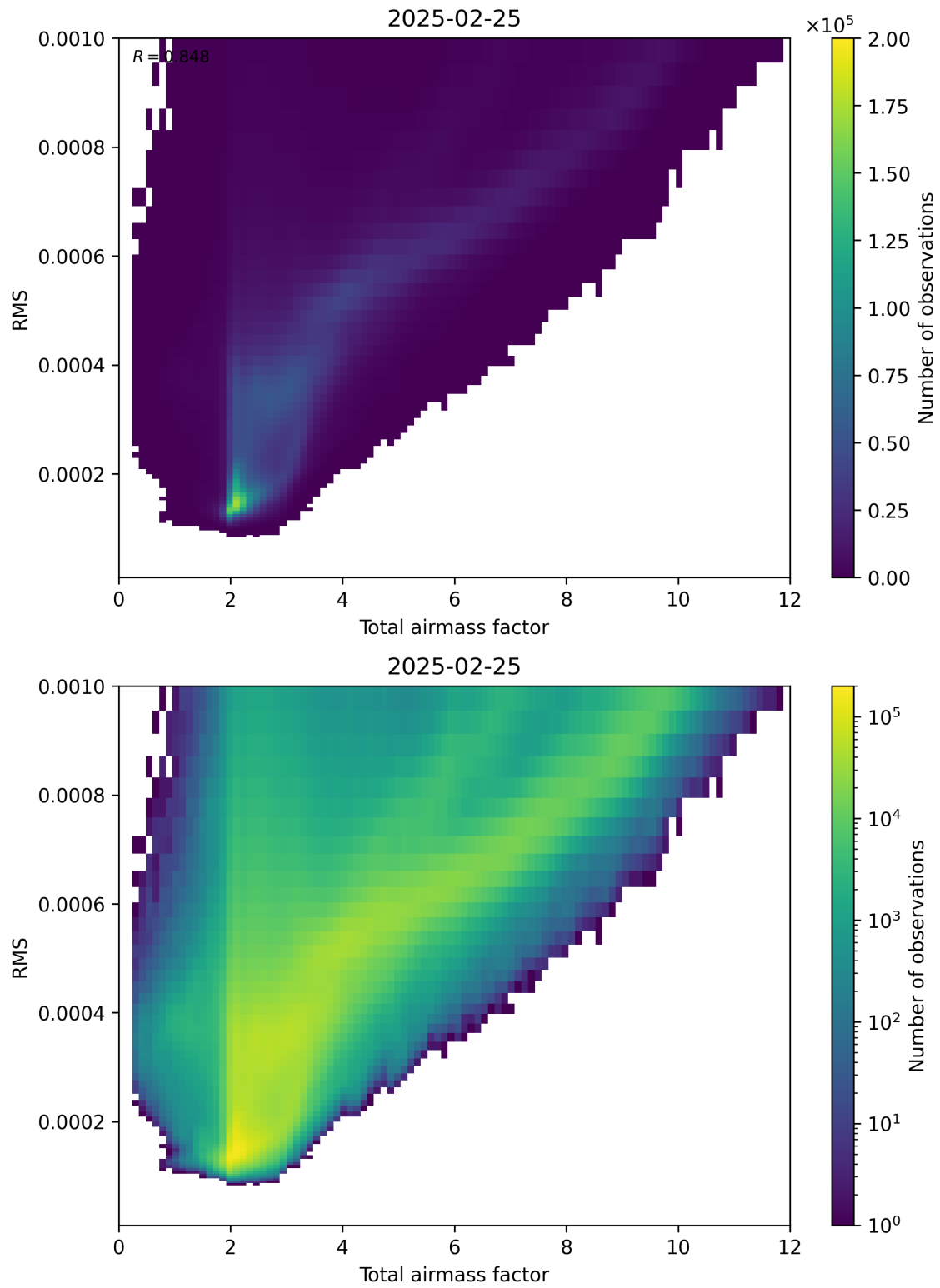
Figure 69: Scatter density plot of “Total airmass factor” against “RMS” for 2025-02-24 to 2025-02-26.
