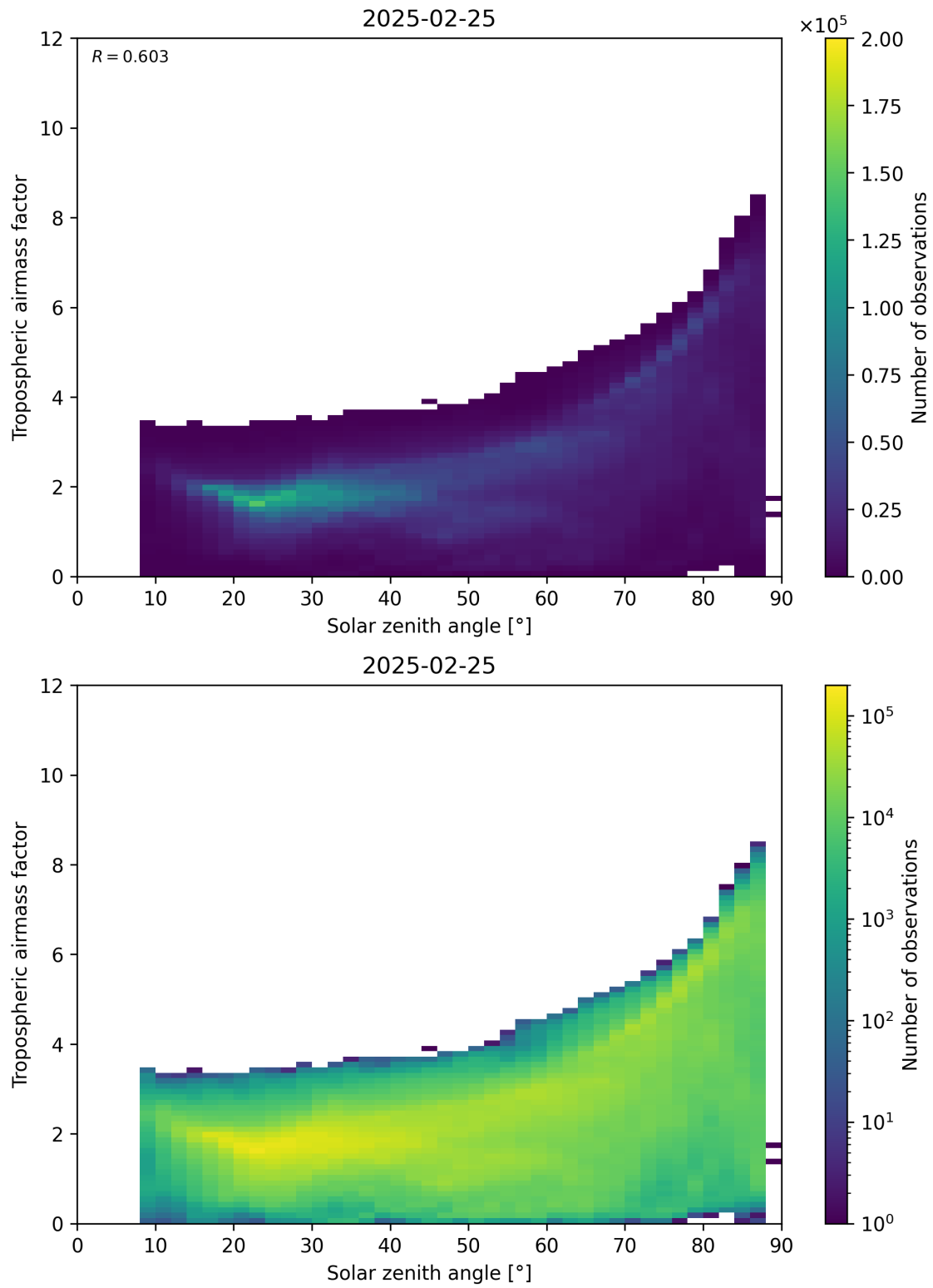
Figure 147: Scatter density plot of “Solar zenith angle” against “Tropospheric airmass factor” for 2025-02-24 to 2025-02-26.
