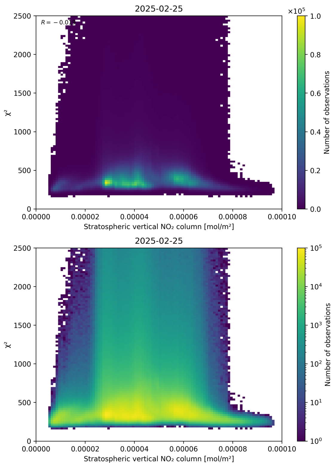
Figure 97: Scatter density plot of “Stratospheric vertical NO 2 column” against “ \chi^2 ” for 2025-02-24 to 2025-02-26.
