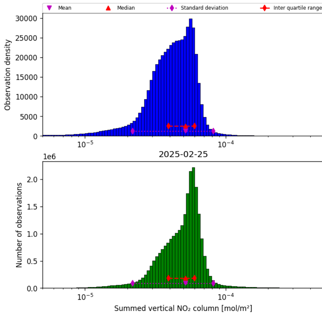
Figure 40: Histogram of “Summed vertical NO 2 column” for 2025-02-24 to 2025-02-26
