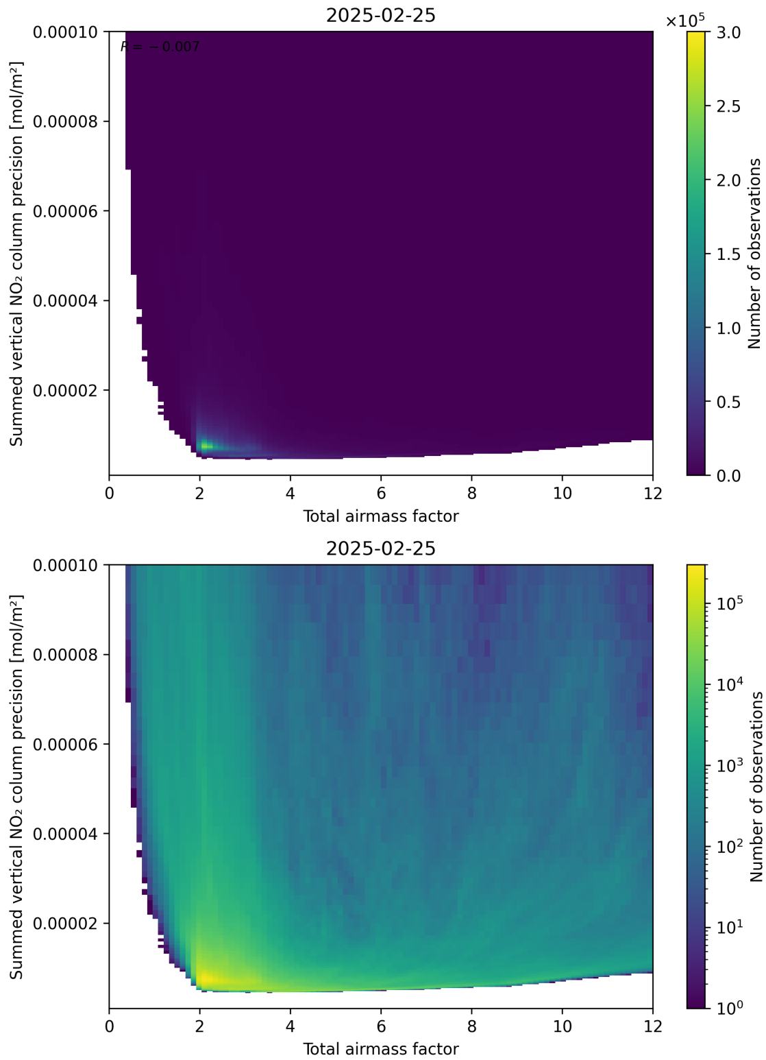
Figure 66: Scatter density plot of “Total airmass factor” against “Summed vertical NO 2 column precision” for 2025-02-24 to 2025-02-26.
