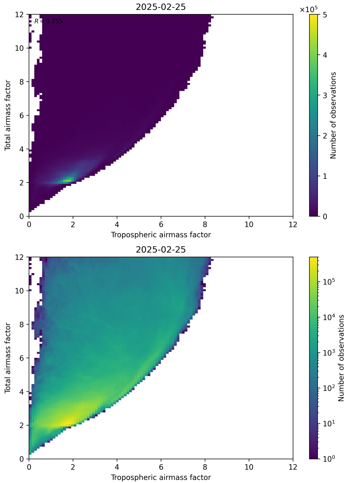
Figure 72: Scatter density plot of “Tropospheric airmass factor” against “Total airmass factor” for 2025-02-24 to 2025-02-26.
