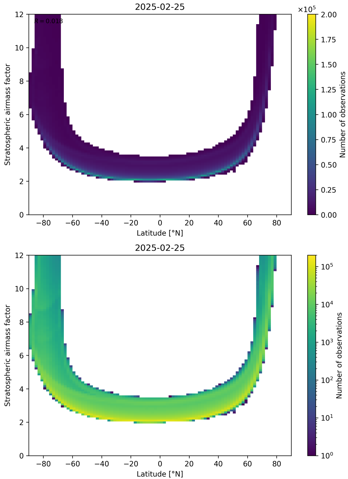
Figure 83: Scatter density plot of “Latitude” against “Stratospheric airmass factor” for 2025-02-24 to 2025-02-26.
