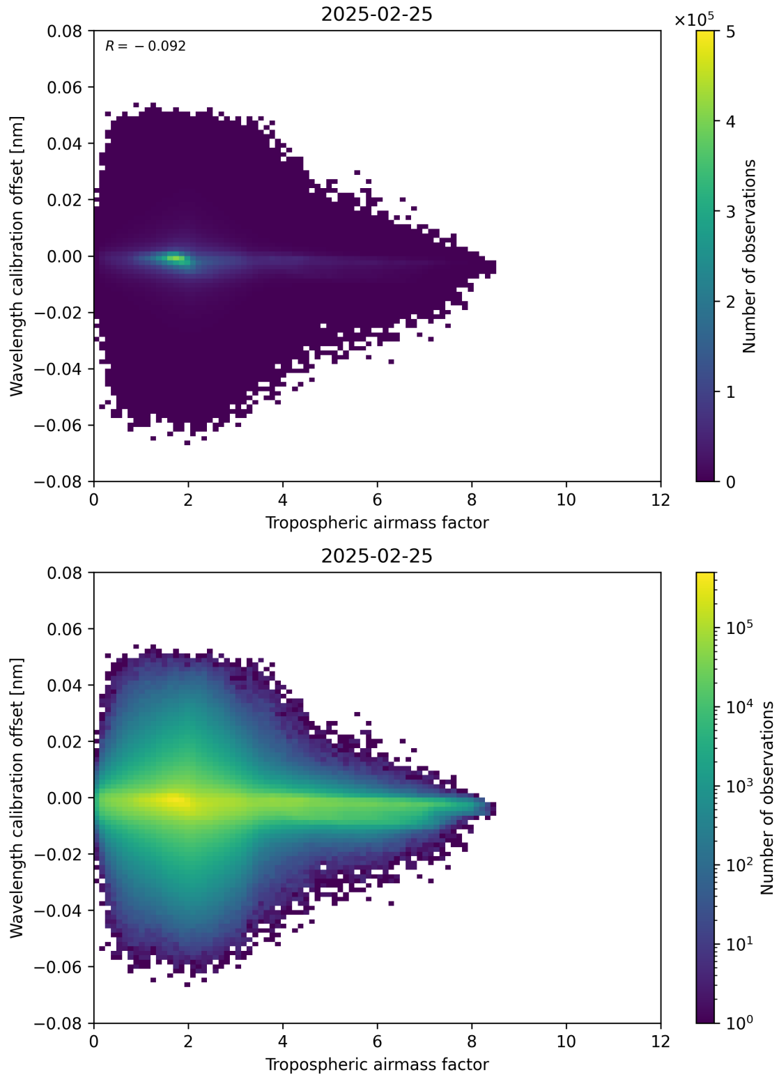
Figure 80: Scatter density plot of “Tropospheric airmass factor” against “Wavelength calibration offset” for 2025-02-24 to 2025-02-26.
