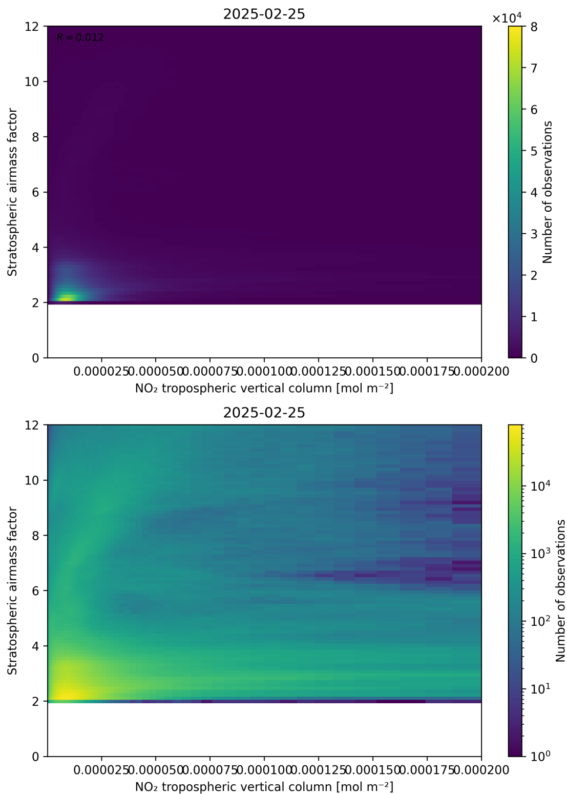
Figure 121: Scatter density plot of “NO 2 tropospheric vertical column” against “Stratospheric airmass factor” for 2025-02-24 to 2025-02-26.
