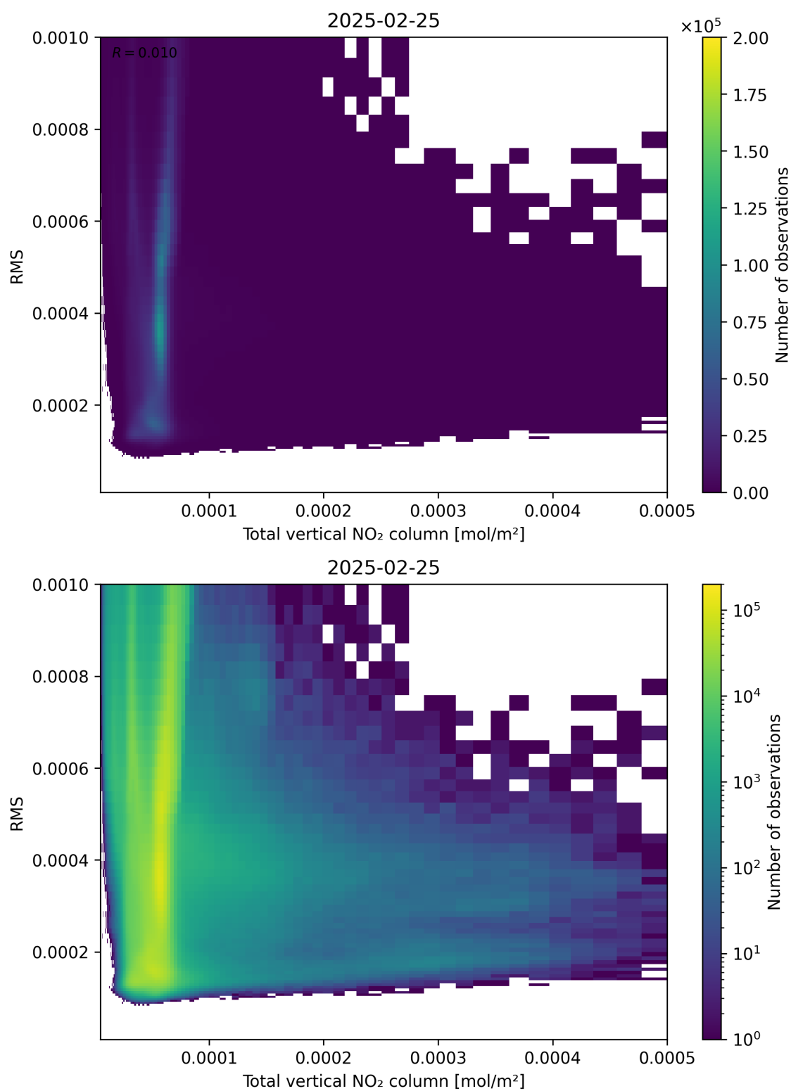
Figure 120: Scatter density plot of “Total vertical NO 2 column” against “RMS” for 2025-02-24 to 2025-02-26.
