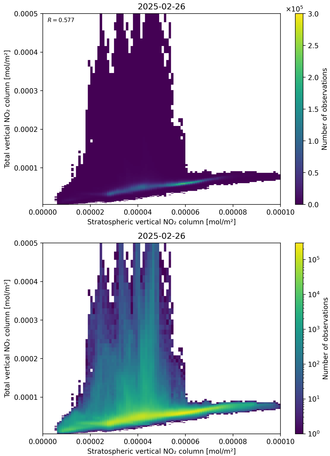
Figure 100: Scatter density plot of “Stratospheric vertical NO 2 column” against “Total vertical NO 2 column” for 2025-02-25 to 2025-02-27.
