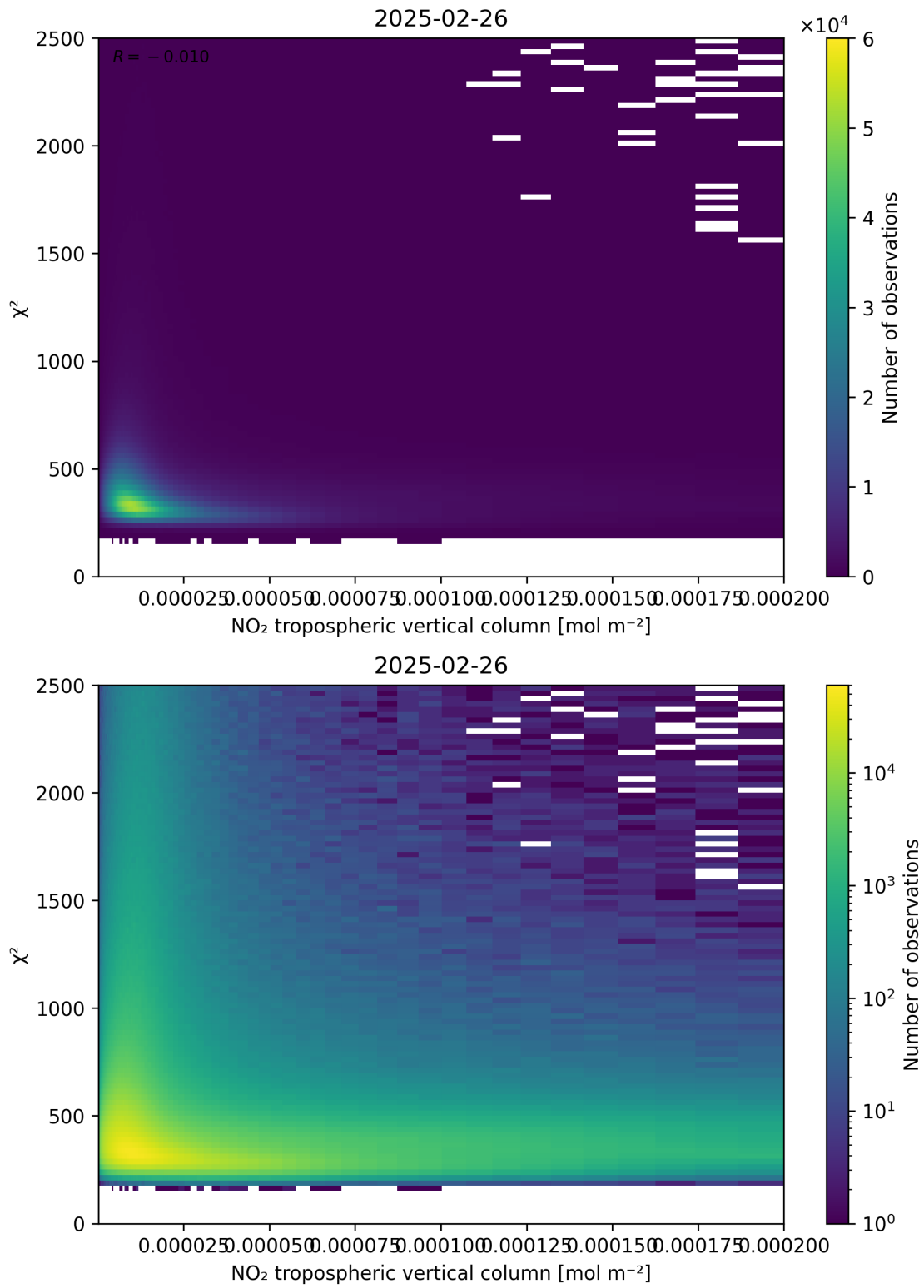
Figure 124: Scatter density plot of “NO 2 tropospheric vertical column” against “ \chi^2 ” for 2025-02-25 to 2025-02-27.
