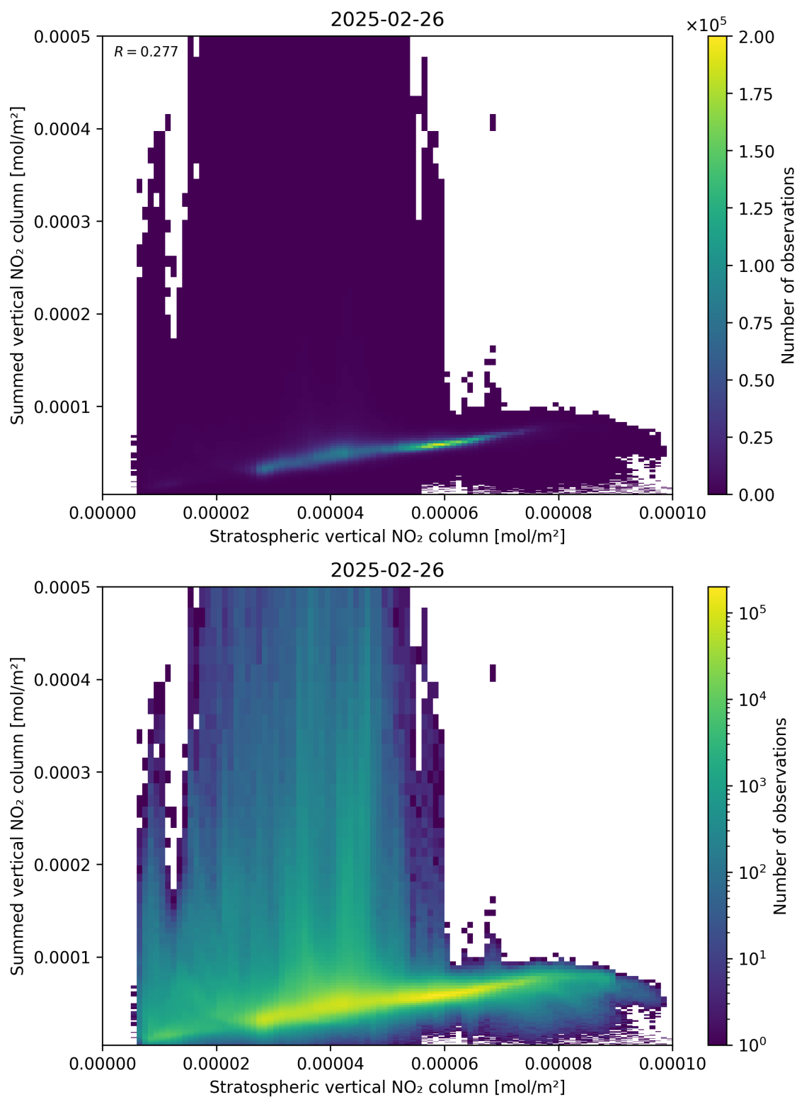
Figure 98: Scatter density plot of “Stratospheric vertical NO 2 column” against “Summed vertical NO 2 column” for 2025-02-25 to 2025-02-27.
