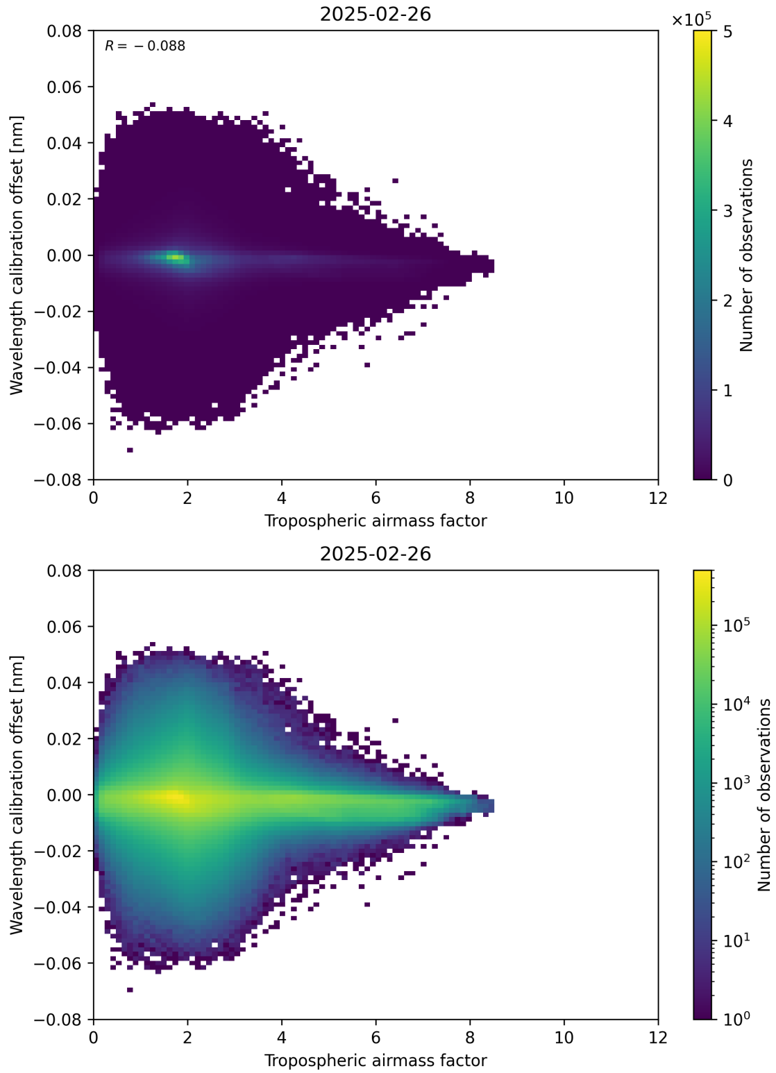
Figure 80: Scatter density plot of “Tropospheric airmass factor” against “Wavelength calibration offset” for 2025-02-25 to 2025-02-27.
