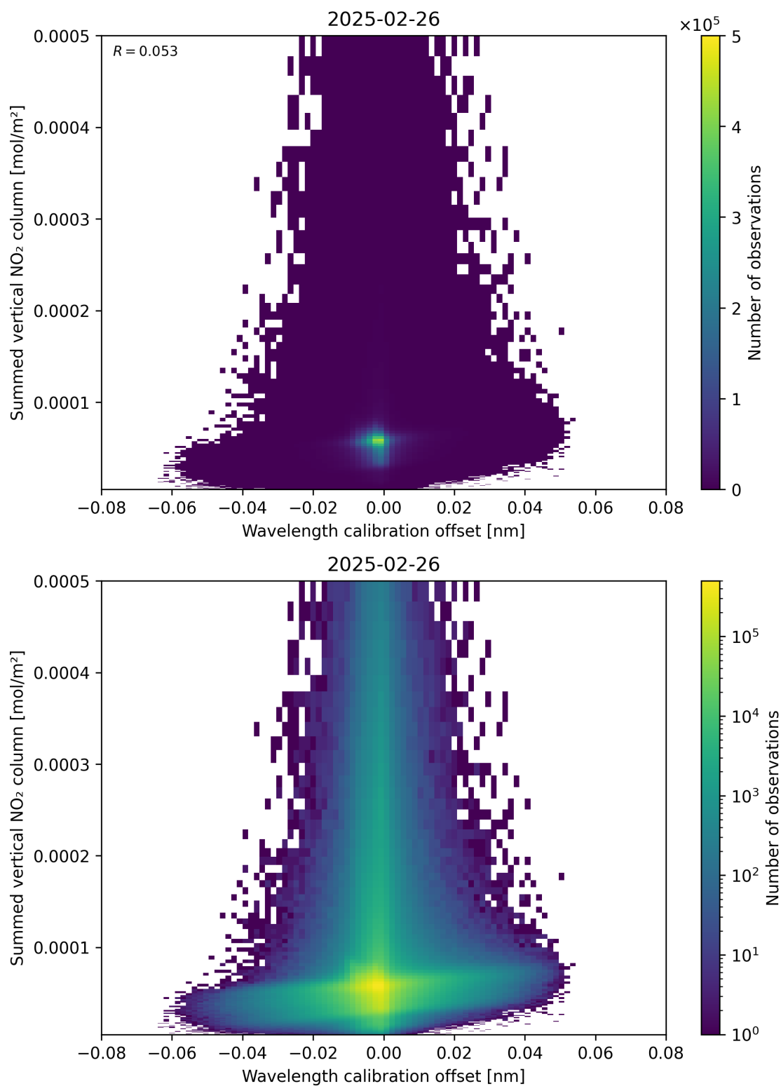
Figure 177: Scatter density plot of “Wavelength calibration offset” against “Summed vertical NO 2 column” for 2025-02-25 to 2025-02-27.
