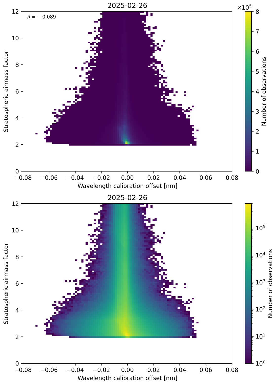
Figure 174: Scatter density plot of “Wavelength calibration offset” against “Stratospheric airmass factor” for 2025-02-25 to 2025-02-27.
