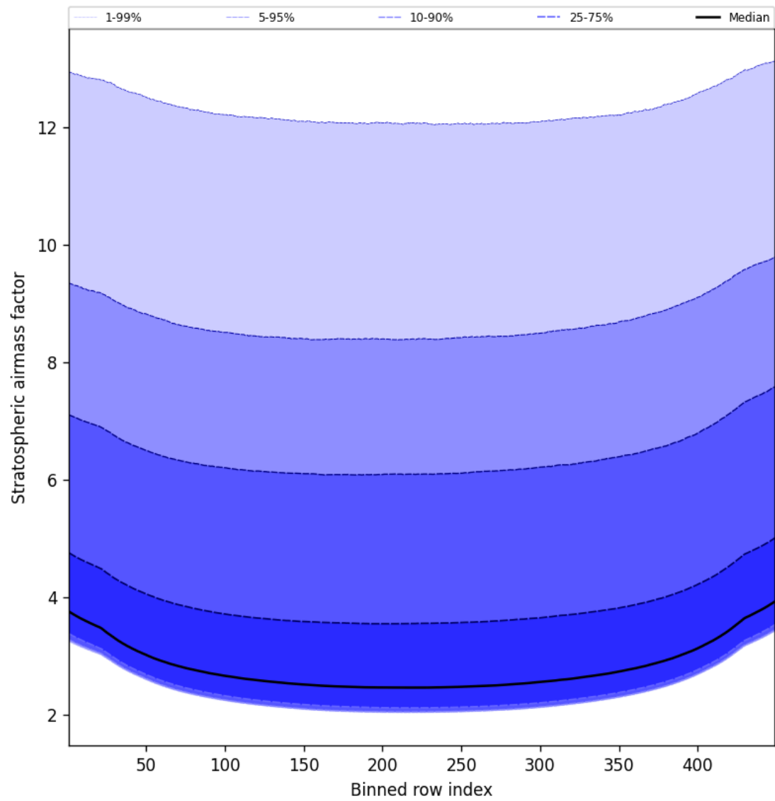
Figure 61: Along track statistics of “Stratospheric airmass factor” for 2025-02-25 to 2025-02-27
