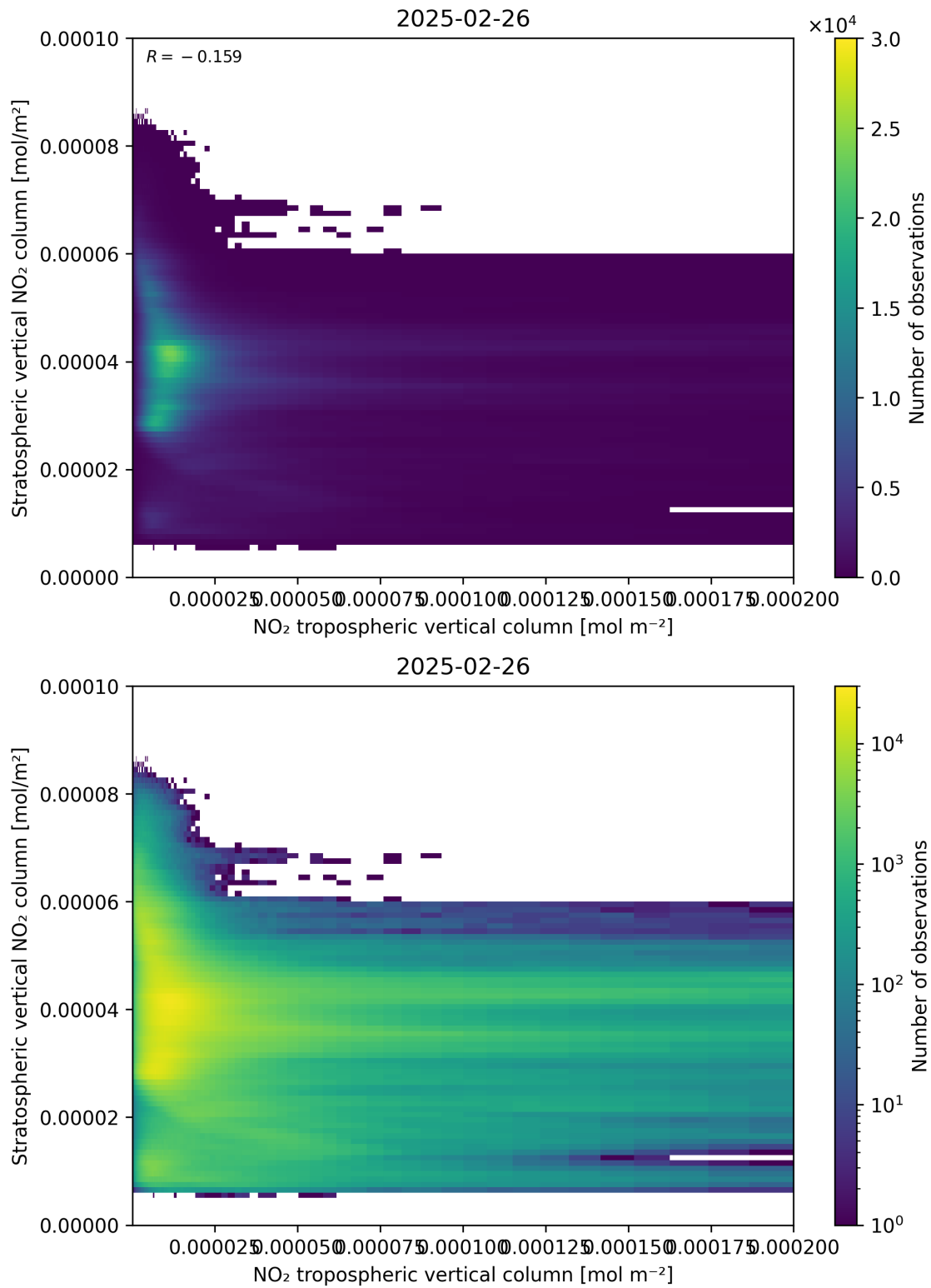
Figure 125: Scatter density plot of “NO 2 tropospheric vertical column” against “Stratospheric vertical NO 2 column” for 2025-02-25 to 2025-02-27.
