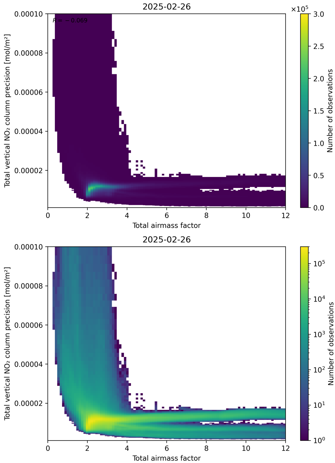
Figure 68: Scatter density plot of “Total airmass factor” against “Total vertical NO 2 column precision” for 2025-02-25 to 2025-02-27.
