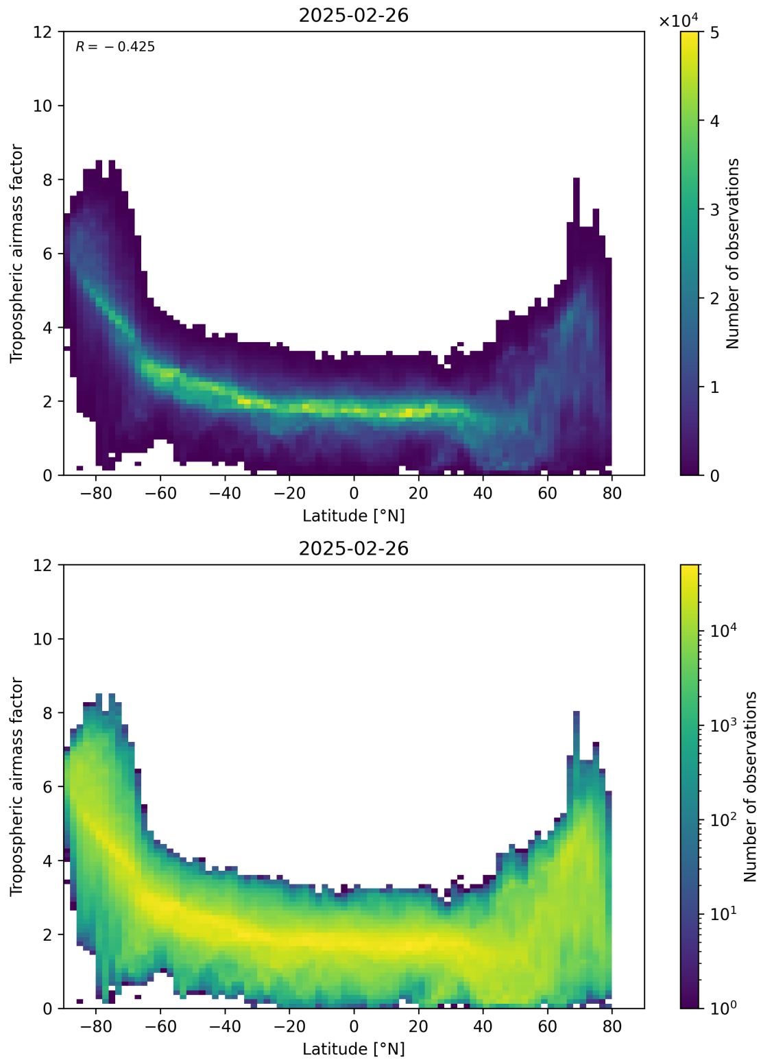
Figure 85: Scatter density plot of “Latitude” against “Tropospheric airmass factor” for 2025-02-25 to 2025-02-27.
