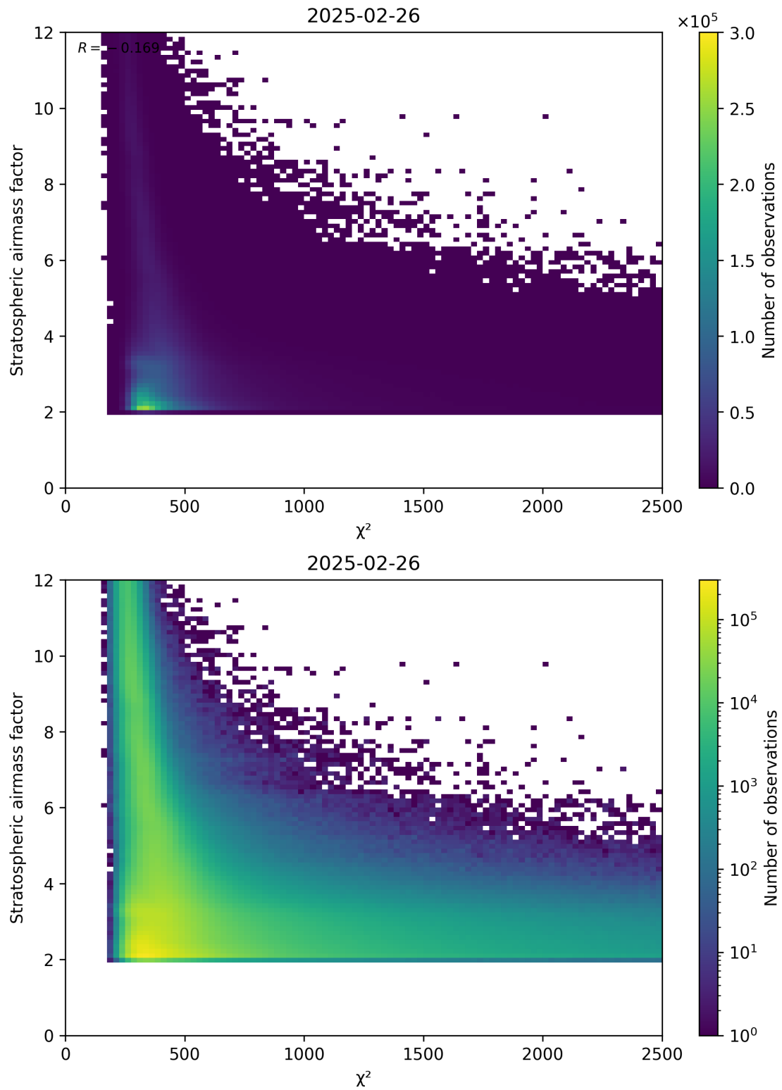
Figure 81: Scatter density plot of “ \chi^2 ” against “Stratospheric airmass factor” for 2025-02-25 to 2025-02-27.
