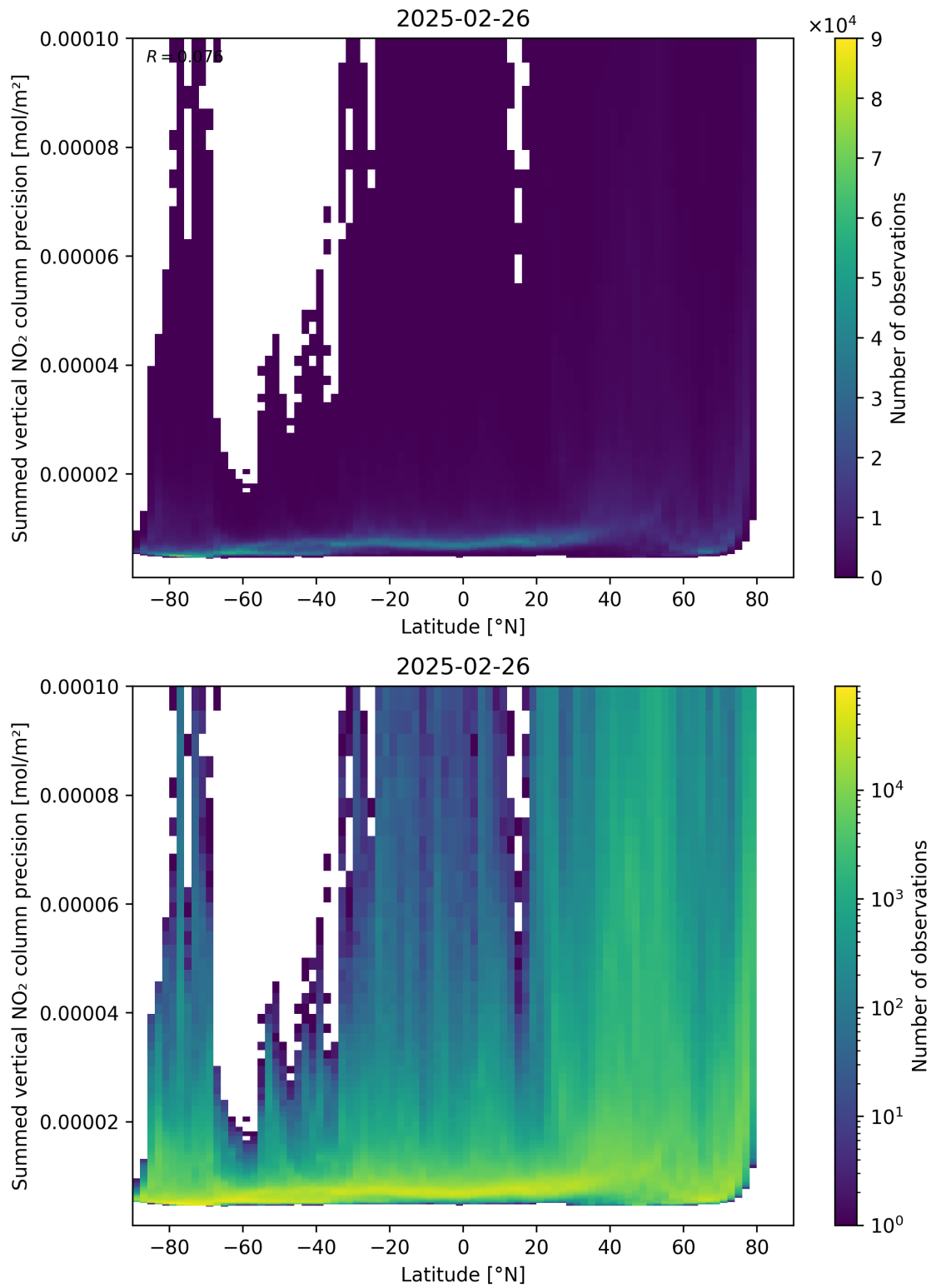
Figure 89: Scatter density plot of “Latitude” against “Summed vertical NO 2 column precision” for 2025-02-25 to 2025-02-27.
