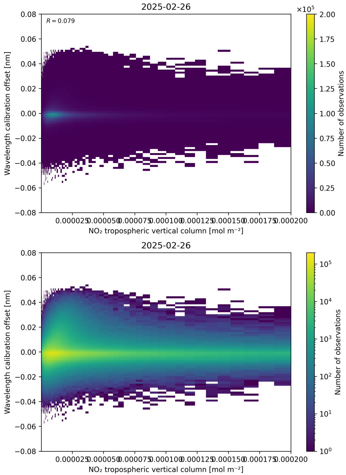
Figure 143: Scatter density plot of “NO 2 tropospheric vertical column” against “Wavelength calibration offset” for 2025-02-25 to 2025-02-27.
