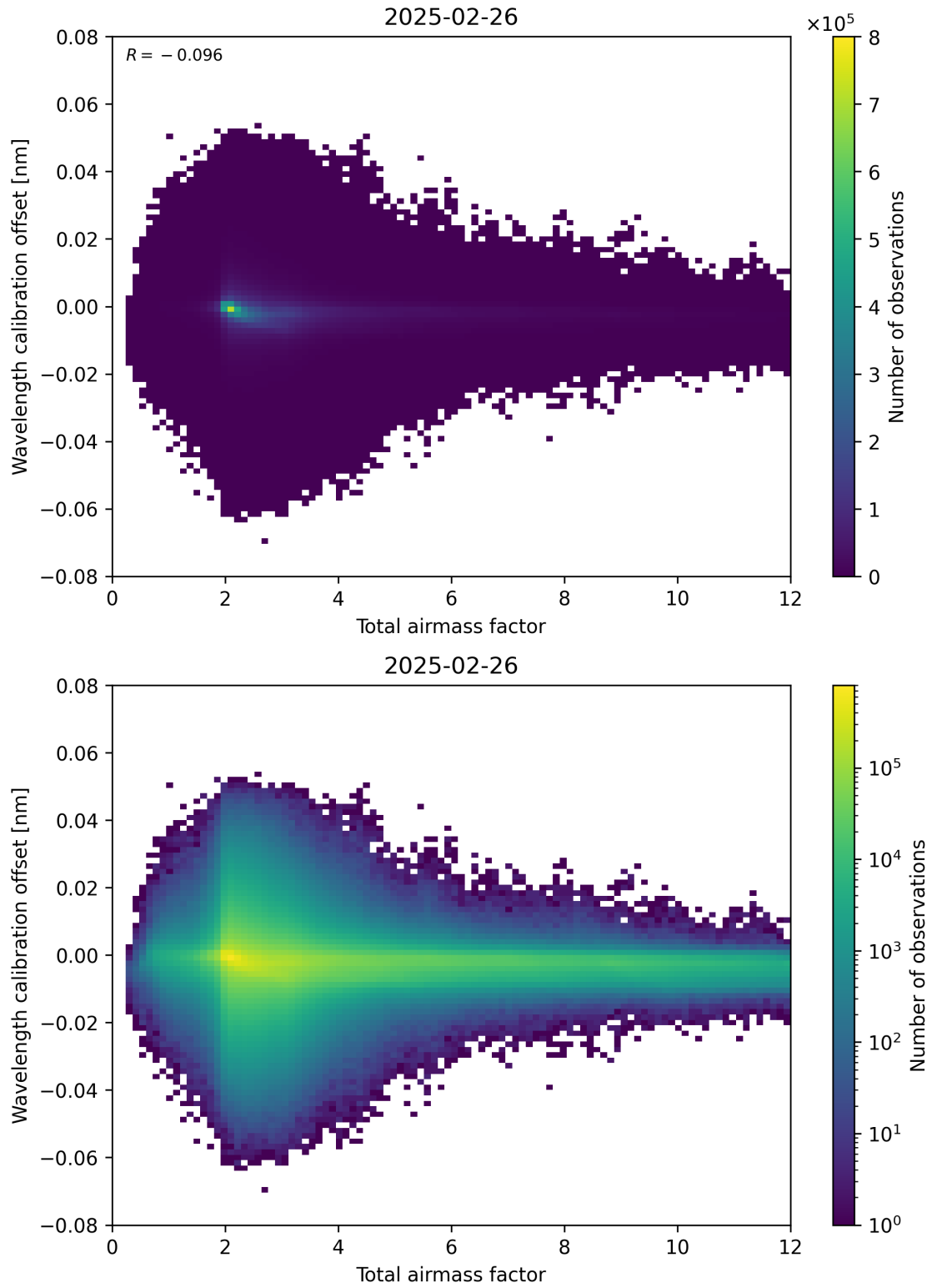
Figure 70: Scatter density plot of “Total airmass factor” against “Wavelength calibration offset” for 2025-02-25 to 2025-02-27.
