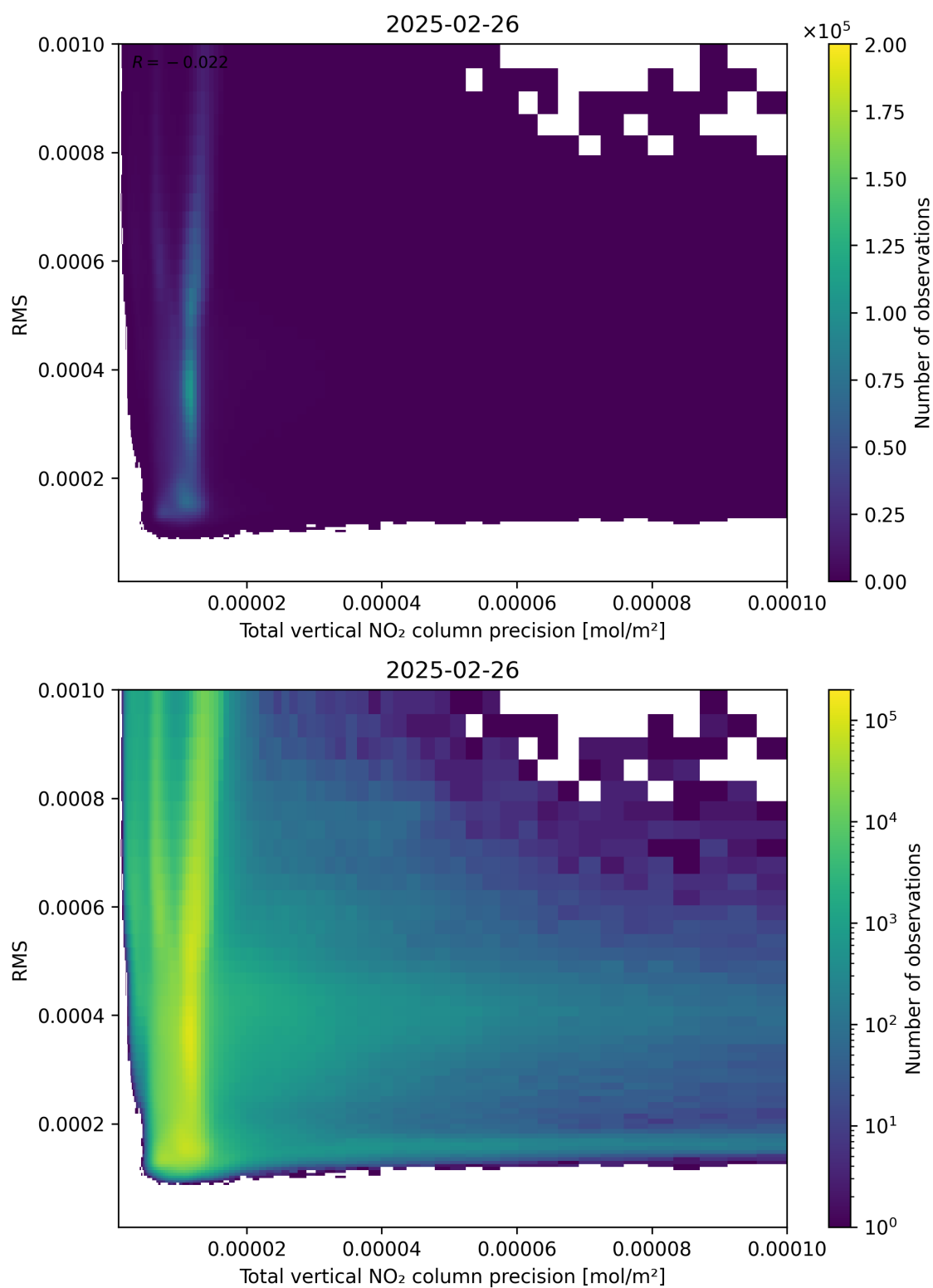
Figure 119: Scatter density plot of “Total vertical NO 2 column precision” against “RMS” for 2025-02-25 to 2025-02-27.
