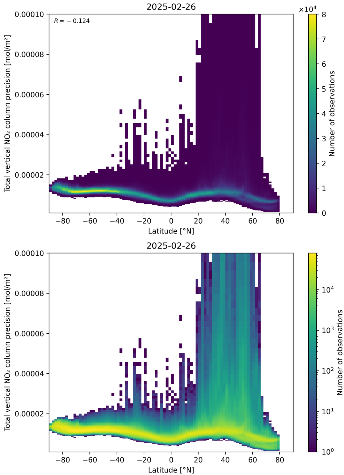
Figure 91: Scatter density plot of “Latitude” against “Total vertical NO 2 column precision” for 2025-02-25 to 2025-02-27.
