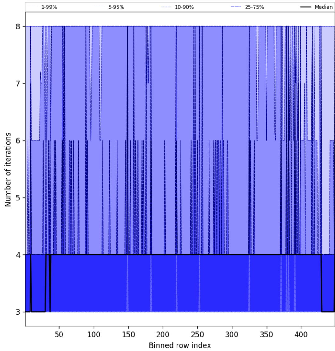
Figure 51: Along track statistics of “Number of iterations” for 2025-02-25 to 2025-02-27
