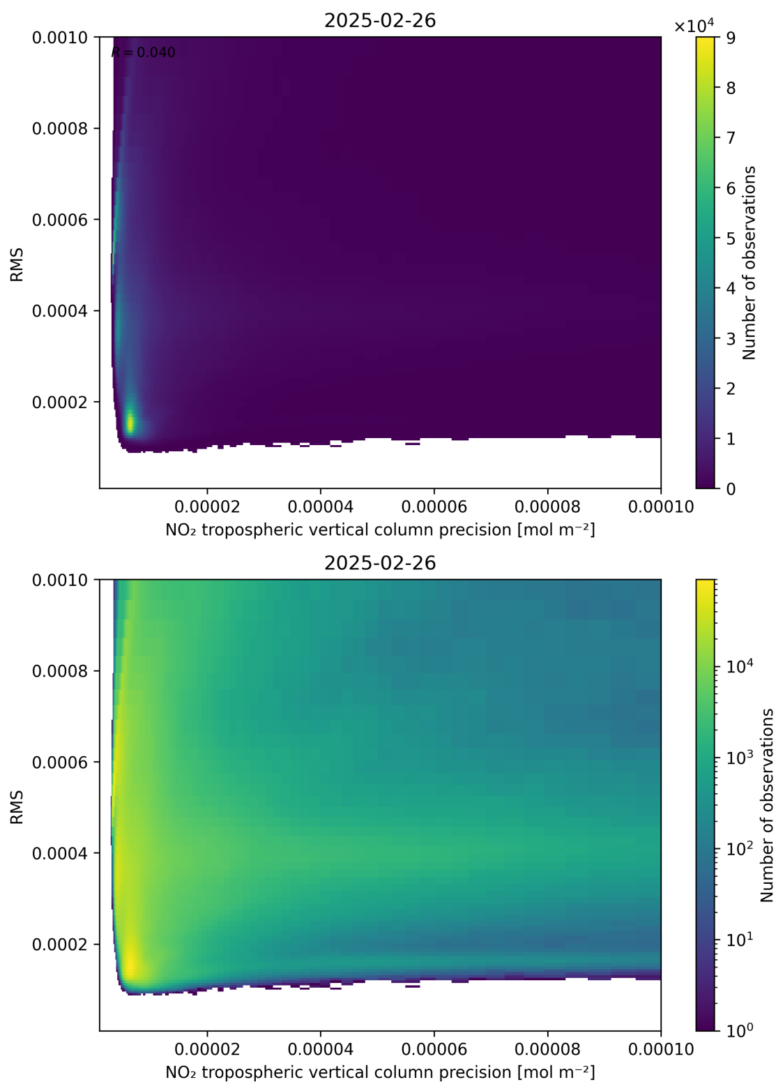
Figure 140: Scatter density plot of “NO 2 tropospheric vertical column precision” against “RMS” for 2025-02-25 to 2025-02-27.
