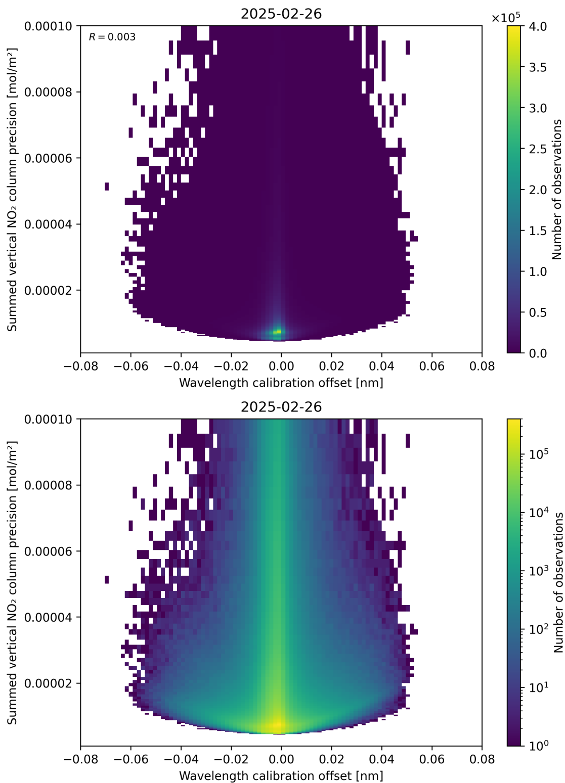
Figure 178: Scatter density plot of “Wavelength calibration offset” against “Summed vertical NO 2 column precision” for 2025-02-25 to 2025-02-27.
