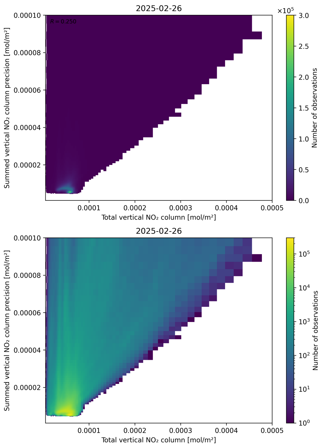
Figure 113: Scatter density plot of “Total vertical NO 2 column” against “Summed vertical NO 2 column precision” for 2025-02-25 to 2025-02-27.
