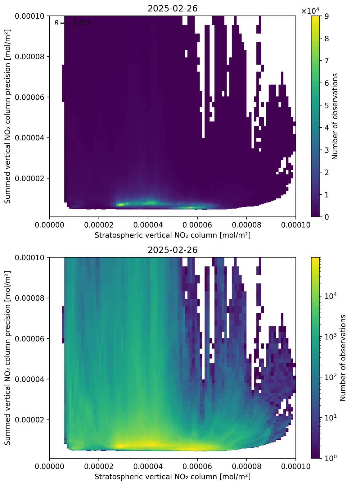
Figure 99: Scatter density plot of “Stratospheric vertical NO 2 column” against “Summed vertical NO 2 column precision” for 2025-02-25 to 2025-02-27.
