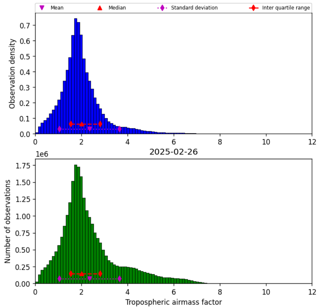
Figure 31: Histogram of “Tropospheric airmass factor” for 2025-02-25 to 2025-02-27
