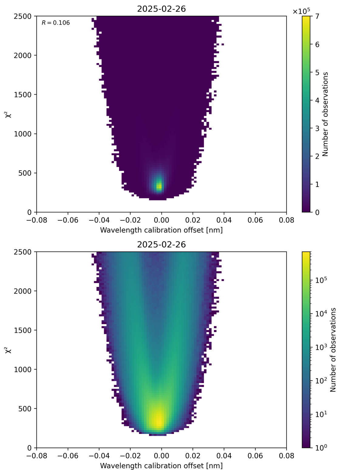
Figure 175: Scatter density plot of “Wavelength calibration offset” against “ \chi^2 ” for 2025-02-25 to 2025-02-27.
