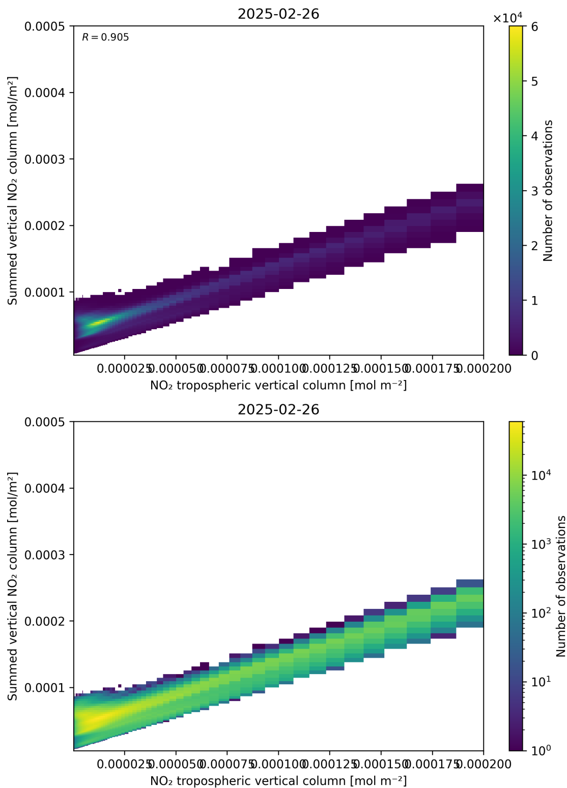
Figure 126: Scatter density plot of “NO 2 tropospheric vertical column” against “Summed vertical NO 2 column” for 2025-02-25 to 2025-02-27.
