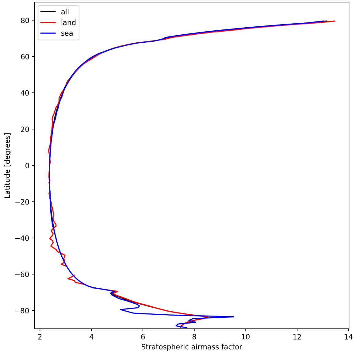
Figure 27: Zonal average of “Stratospheric airmass factor” for 2025-02-25 to 2025-02-27.
