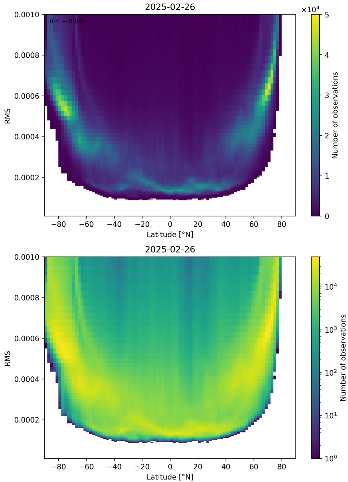
Figure 94: Scatter density plot of “Latitude” against “RMS” for 2025-02-25 to 2025-02-27.
