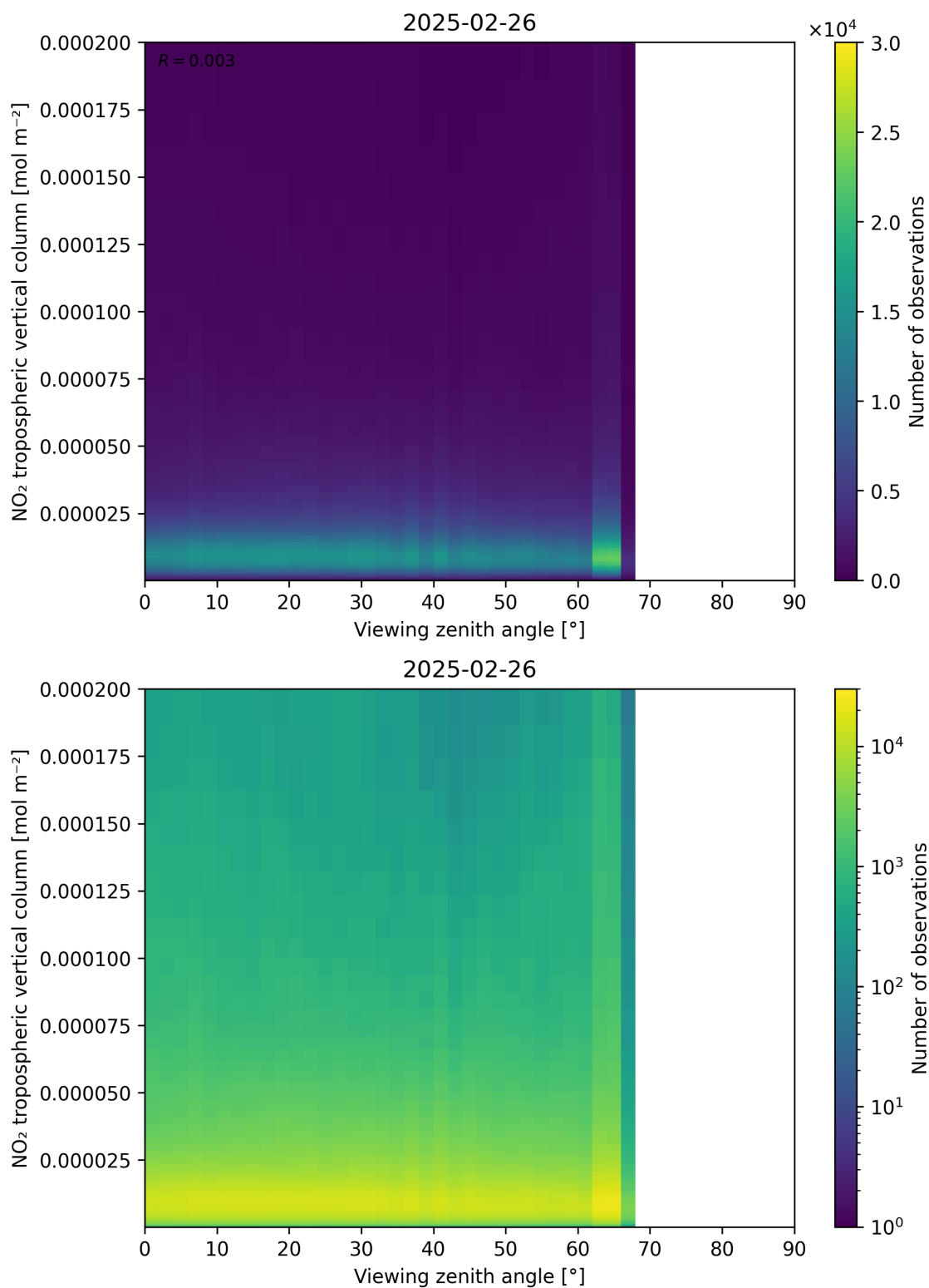
Figure 169: Scatter density plot of “Viewing zenith angle” against “NO 2 tropospheric vertical column” for 2025-02-25 to 2025-02-27.
