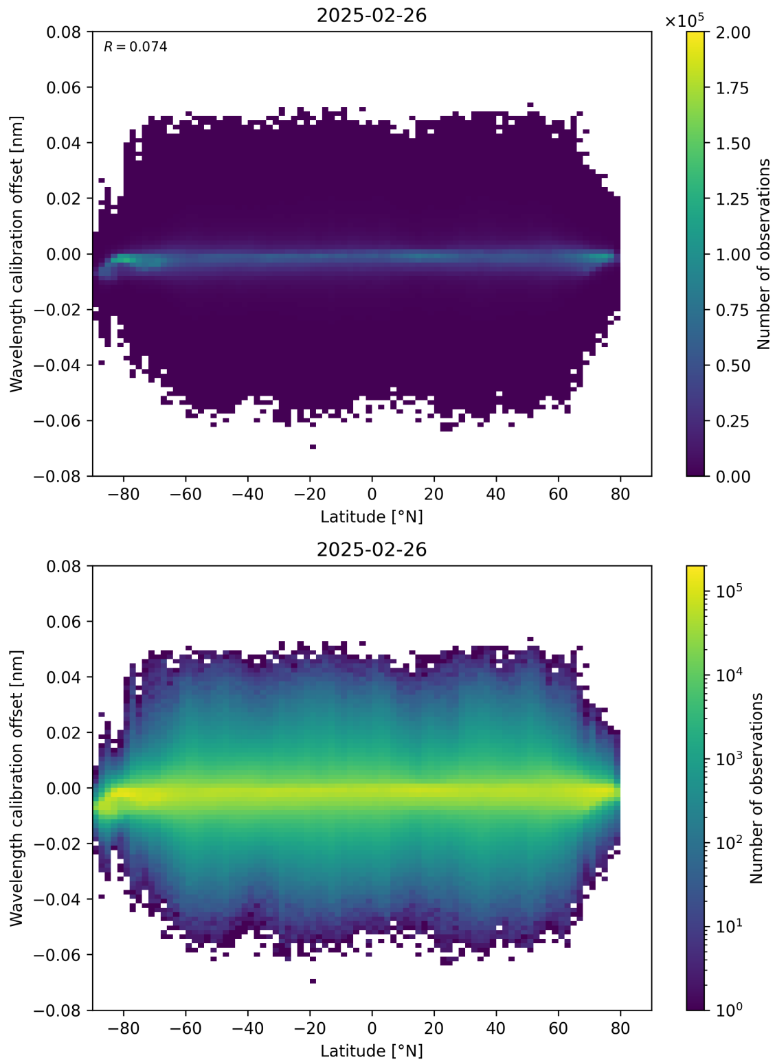
Figure 95: Scatter density plot of “Latitude” against “Wavelength calibration offset” for 2025-02-25 to 2025-02-27.
