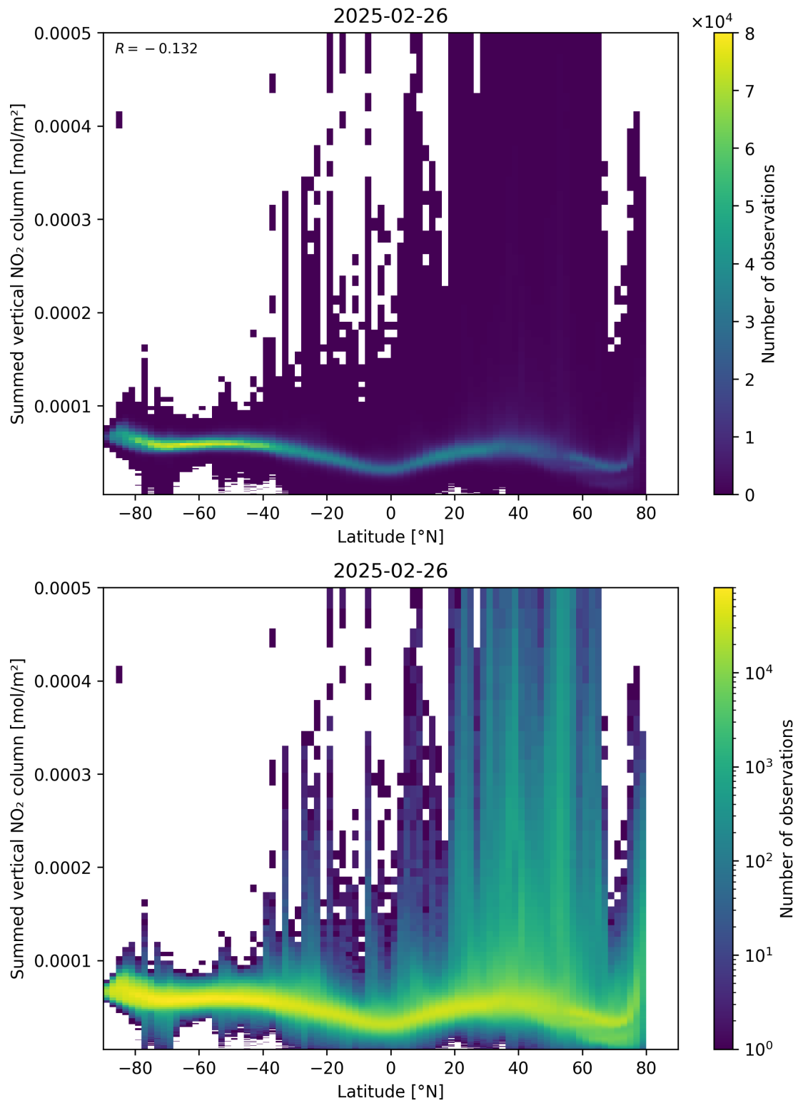
Figure 88: Scatter density plot of “Latitude” against “Summed vertical NO 2 column” for 2025-02-25 to 2025-02-27.
