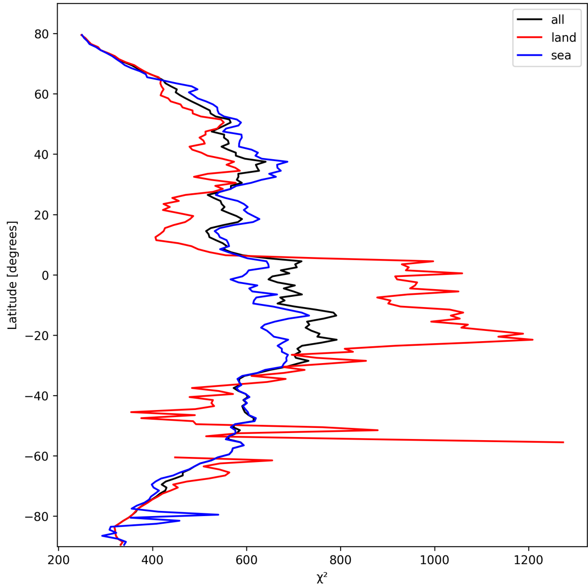
Figure 25: Zonal average of “ \chi^2 ” for 2025-02-25 to 2025-02-27.
