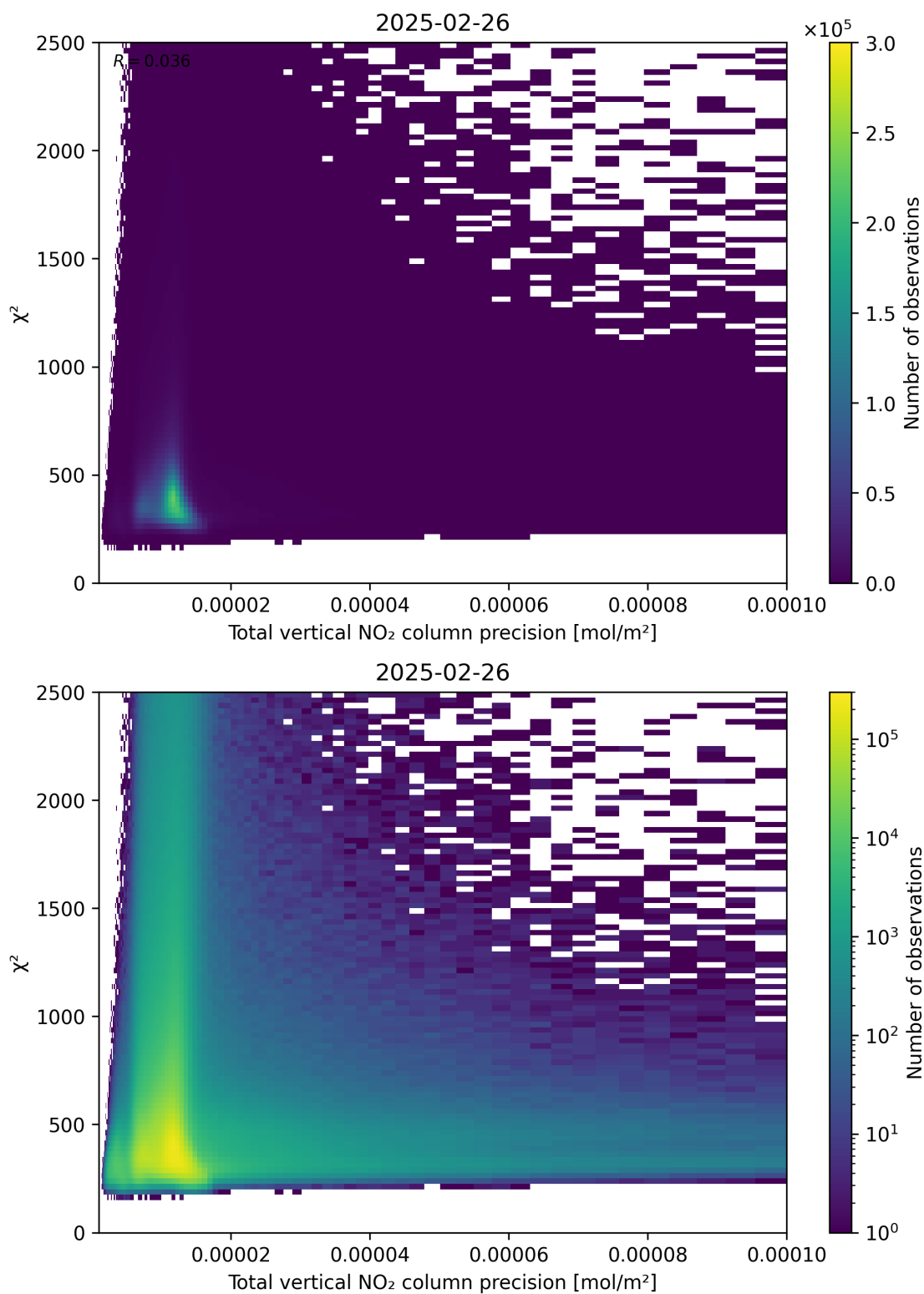
Figure 116: Scatter density plot of “Total vertical NO 2 column precision” against “ \chi^2 ” for 2025-02-25 to 2025-02-27.
