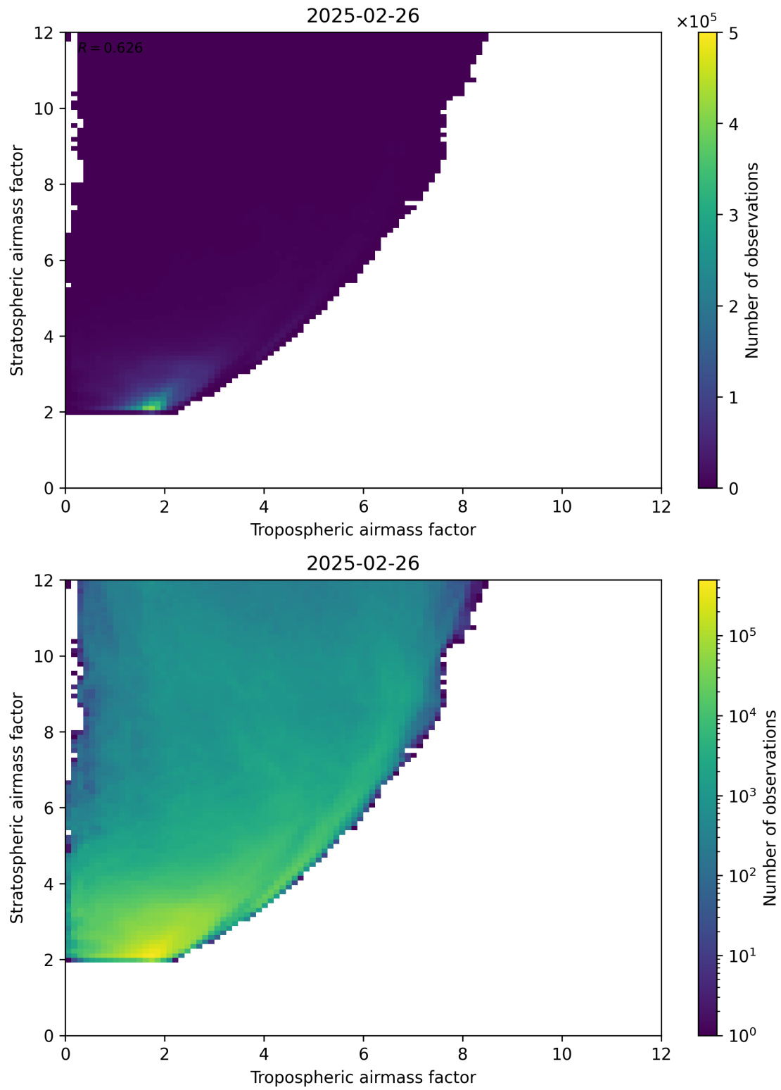
Figure 71: Scatter density plot of “Tropospheric airmass factor” against “Stratospheric airmass factor” for 2025-02-25 to 2025-02-27.
