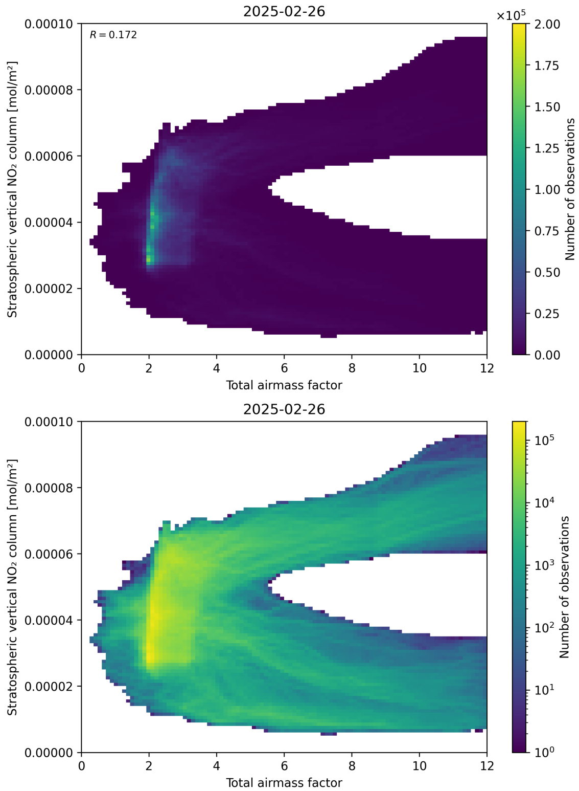
Figure 64: Scatter density plot of “Total airmass factor” against “Stratospheric vertical NO 2 column” for 2025-02-25 to 2025-02-27.
