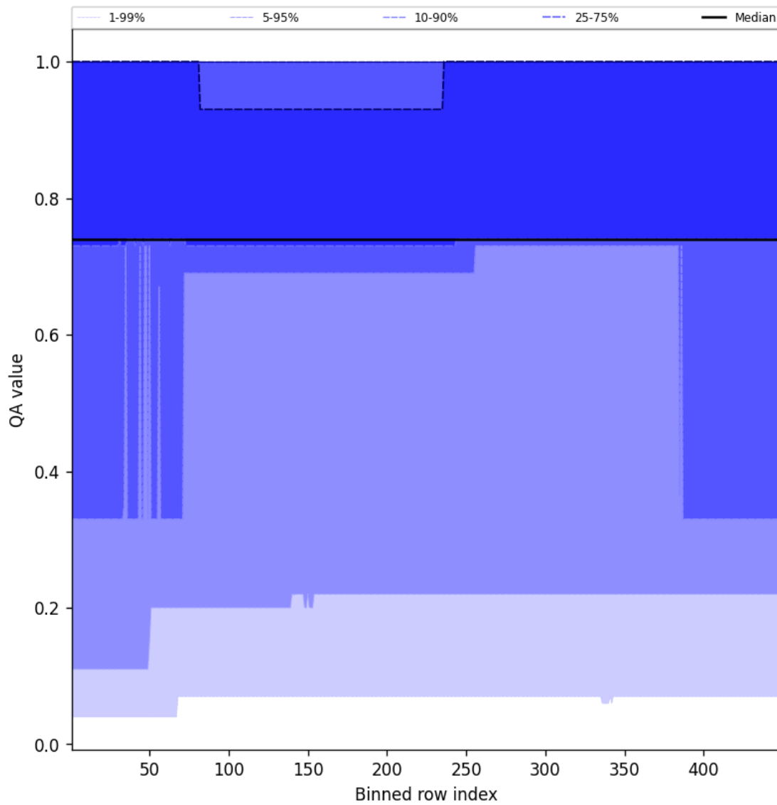
Figure 45: Along track statistics of “QA value” for 2025-02-25 to 2025-02-27
