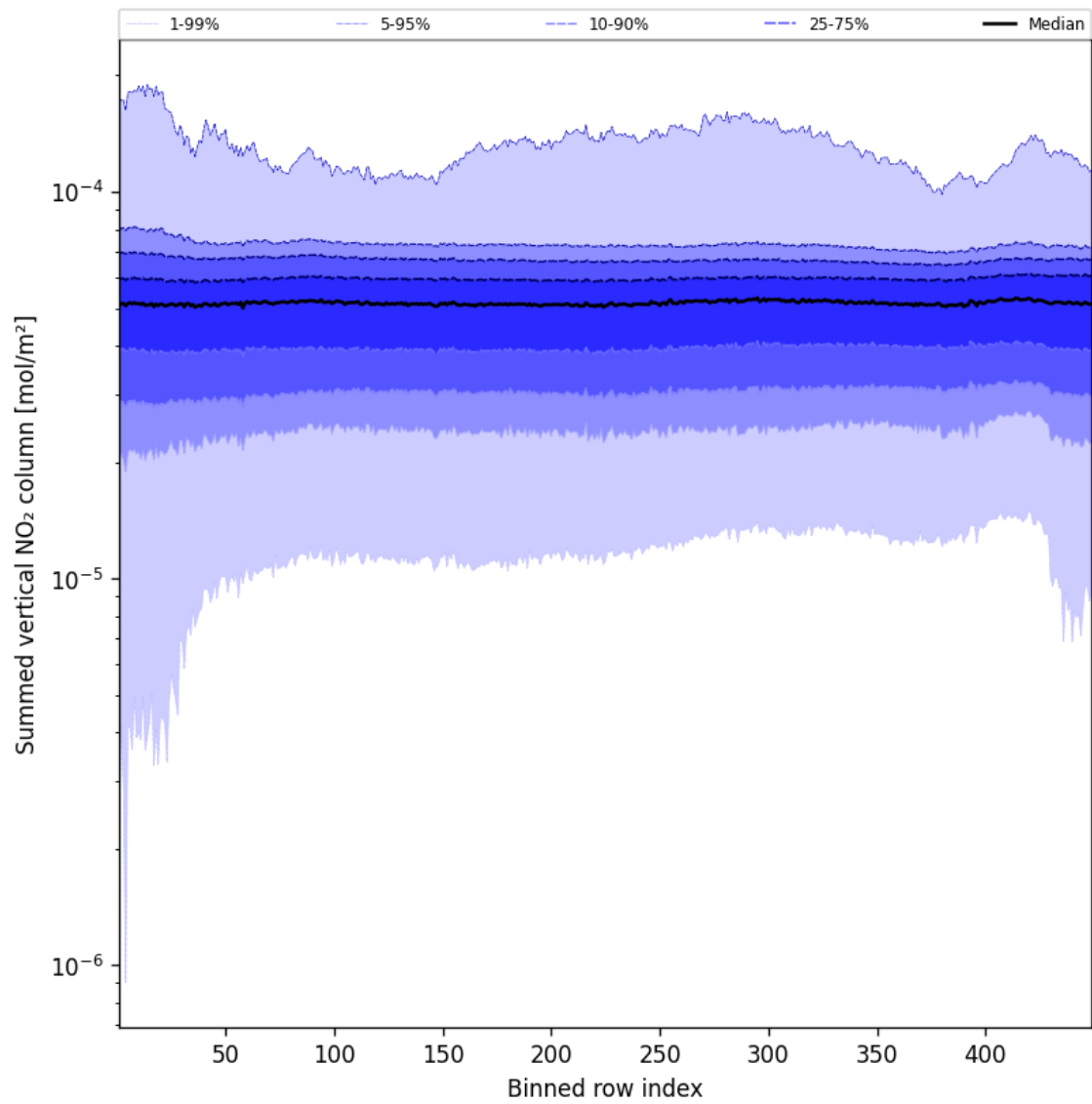
Figure 57: Along track statistics of “Summed vertical NO 2 column” for 2025-02-25 to 2025-02-27
