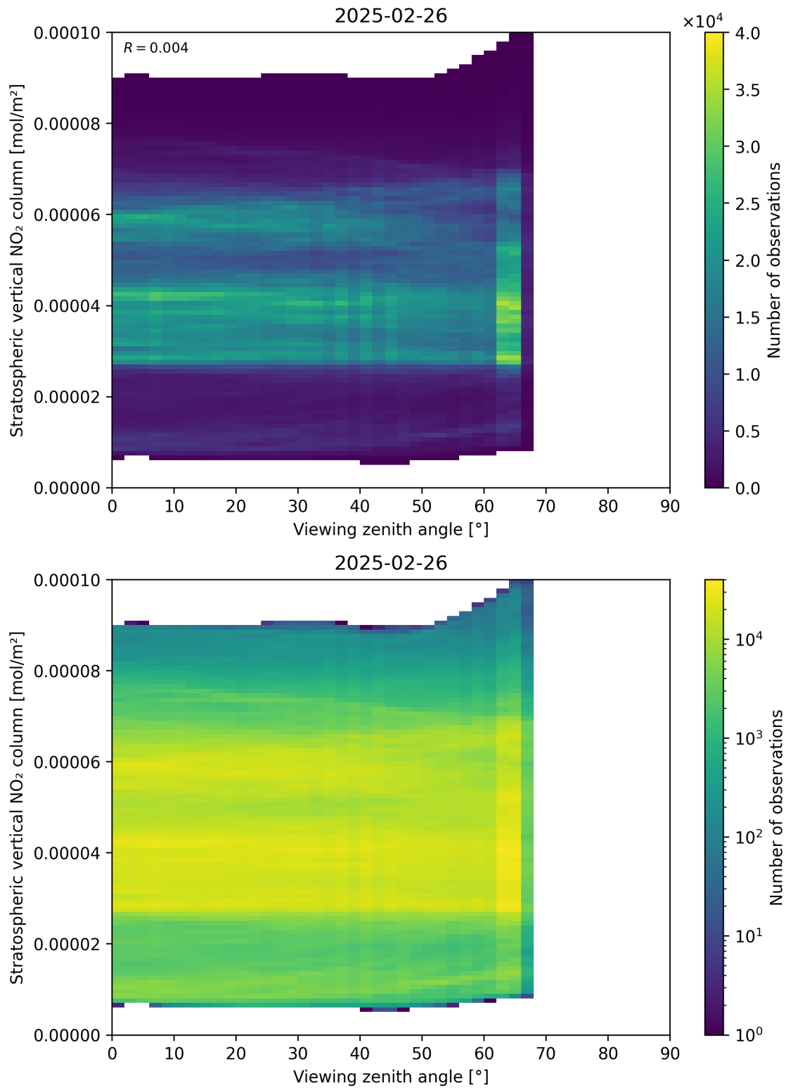
Figure 164: Scatter density plot of “Viewing zenith angle” against “Stratospheric vertical NO 2 column” for 2025-02-25 to 2025-02-27.
