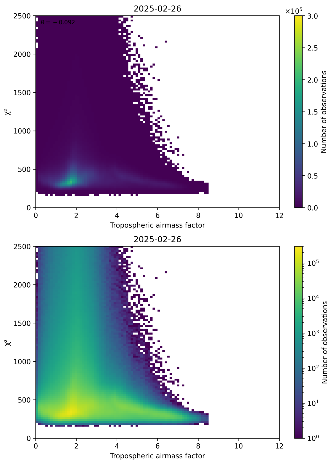
Figure 73: Scatter density plot of “Tropospheric airmass factor” against “ \chi^2 ” for 2025-02-25 to 2025-02-27.
