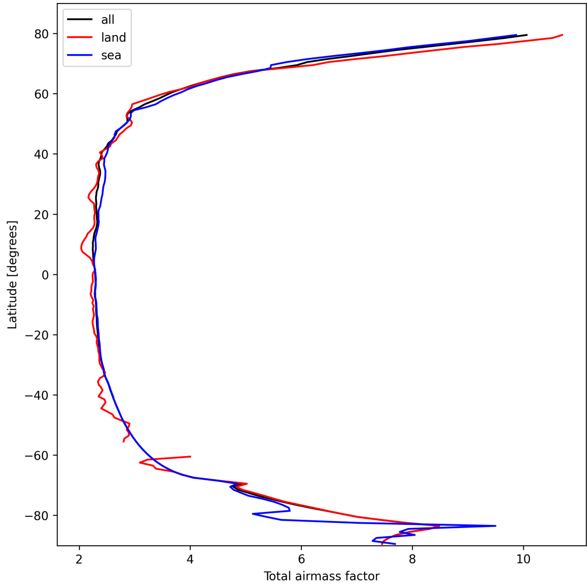
Figure 15: Zonal average of “Total airmass factor” for 2025-02-25 to 2025-02-27.
