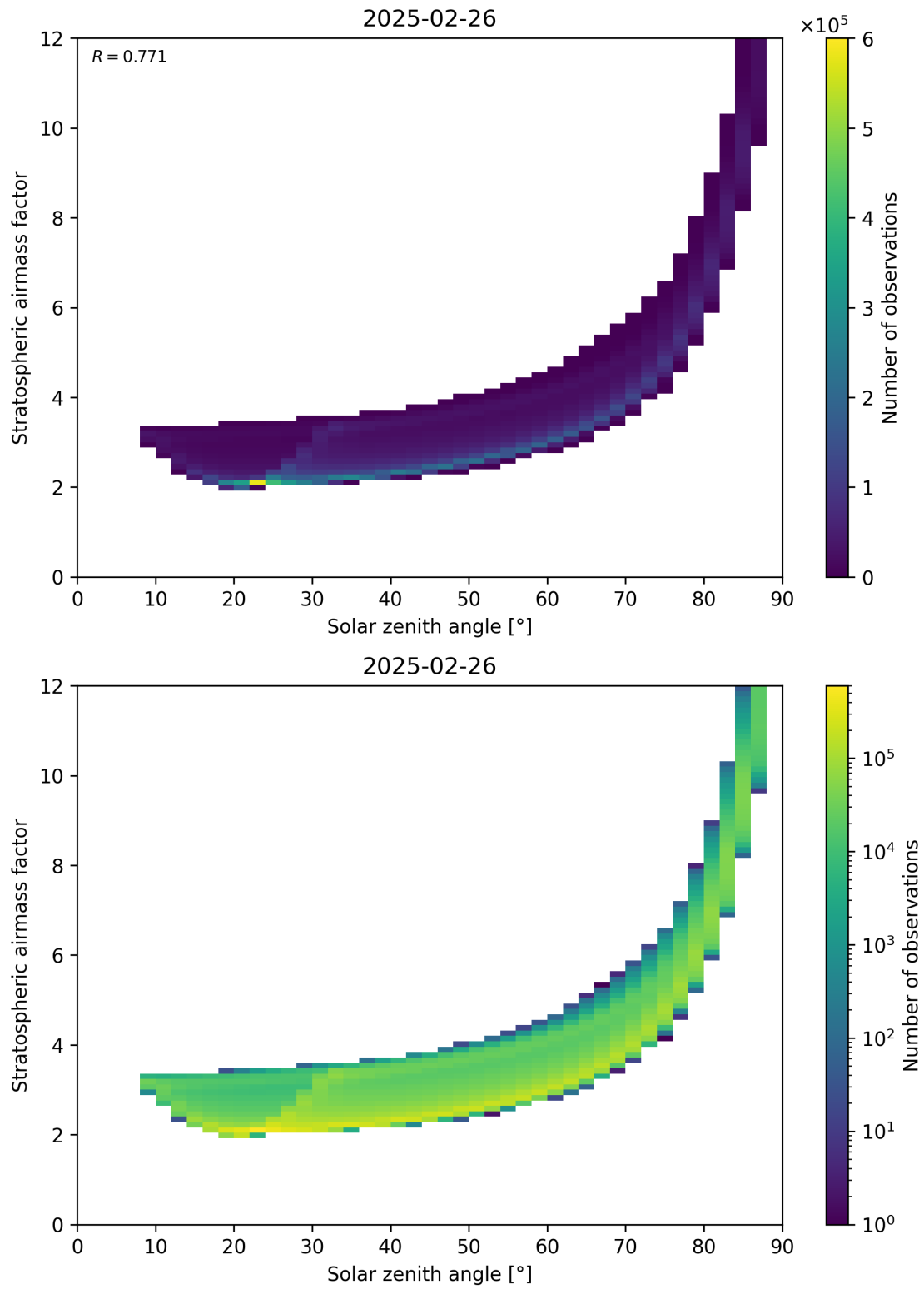
Figure 145: Scatter density plot of “Solar zenith angle” against “Stratospheric airmass factor” for 2025-02-25 to 2025-02-27.
