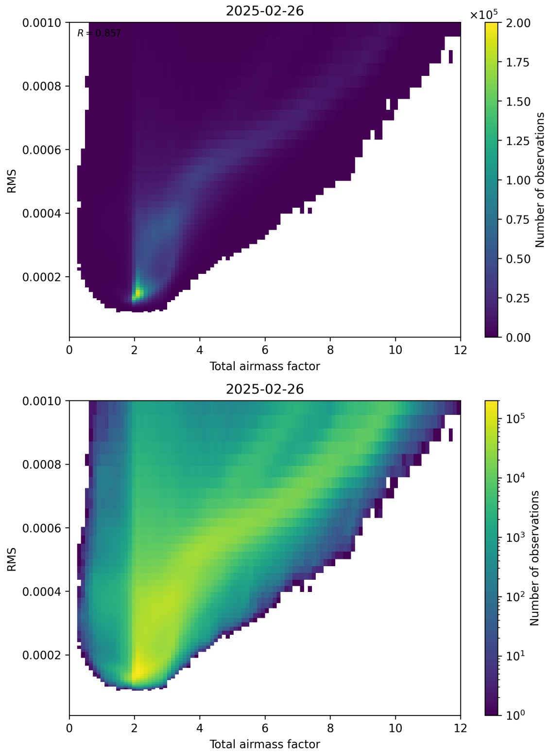
Figure 69: Scatter density plot of “Total airmass factor” against “RMS” for 2025-02-25 to 2025-02-27.
