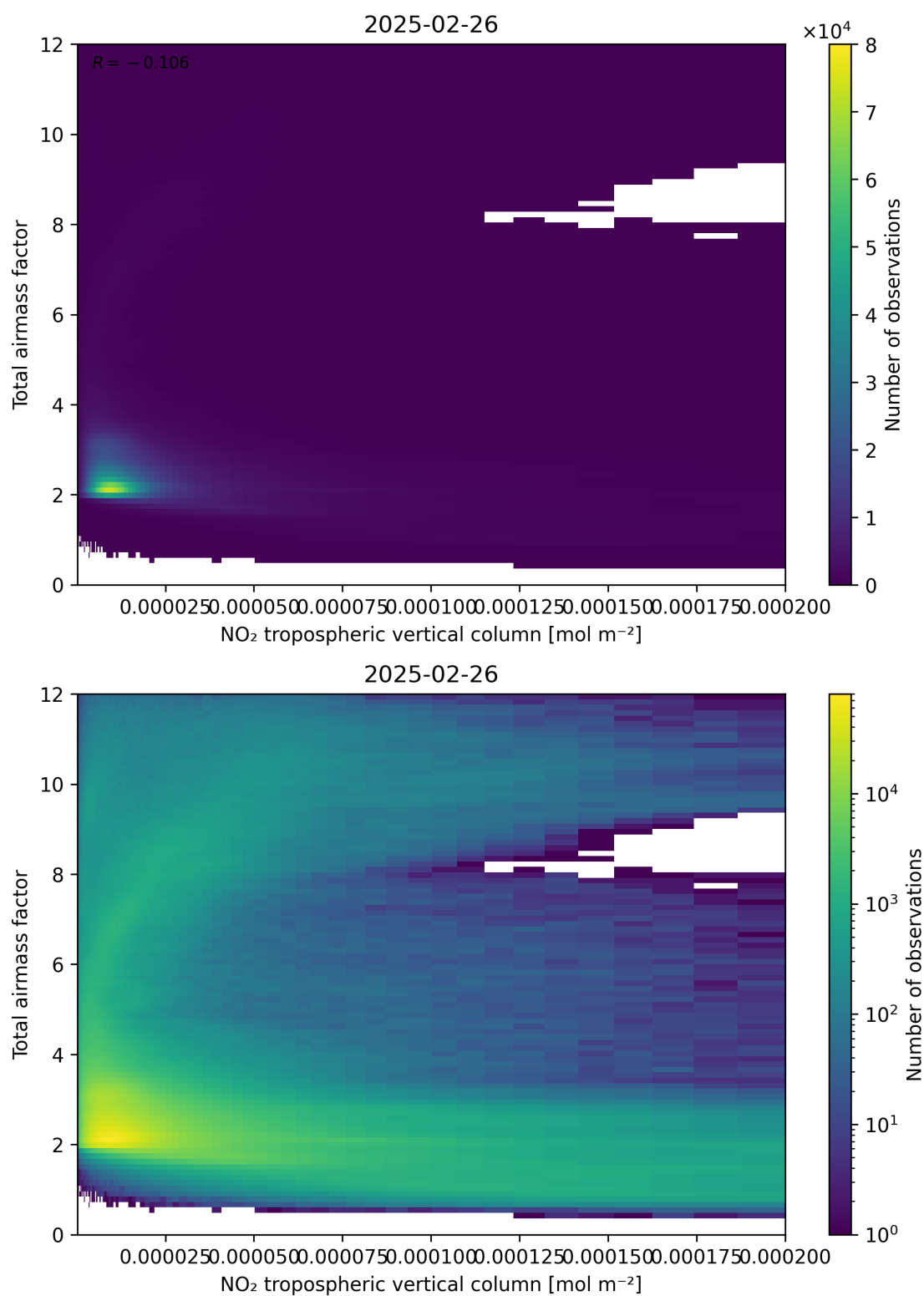
Figure 122: Scatter density plot of “NO 2 tropospheric vertical column” against “Total air mass factor” for 2025-02-25 to 2025-02-27.
