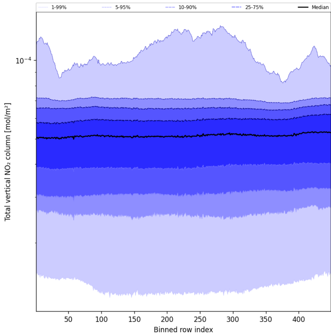
Figure 55: Along track statistics of “Total vertical NO 2 column” for 2025-02-25 to 2025-02-27
