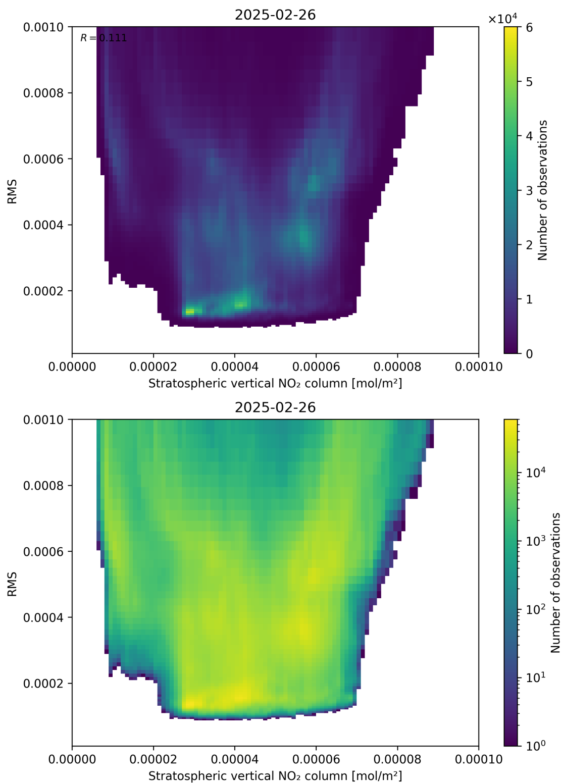
Figure 102: Scatter density plot of “Stratospheric vertical NO 2 column” against “RMS” for 2025-02-25 to 2025-02-27.
