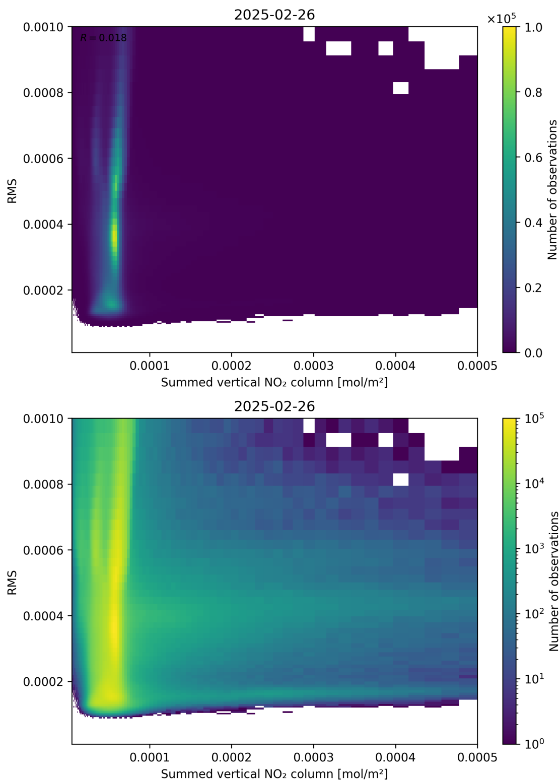
Figure 109: Scatter density plot of “Summed vertical NO 2 column” against “RMS” for 2025-02-25 to 2025-02-27.
