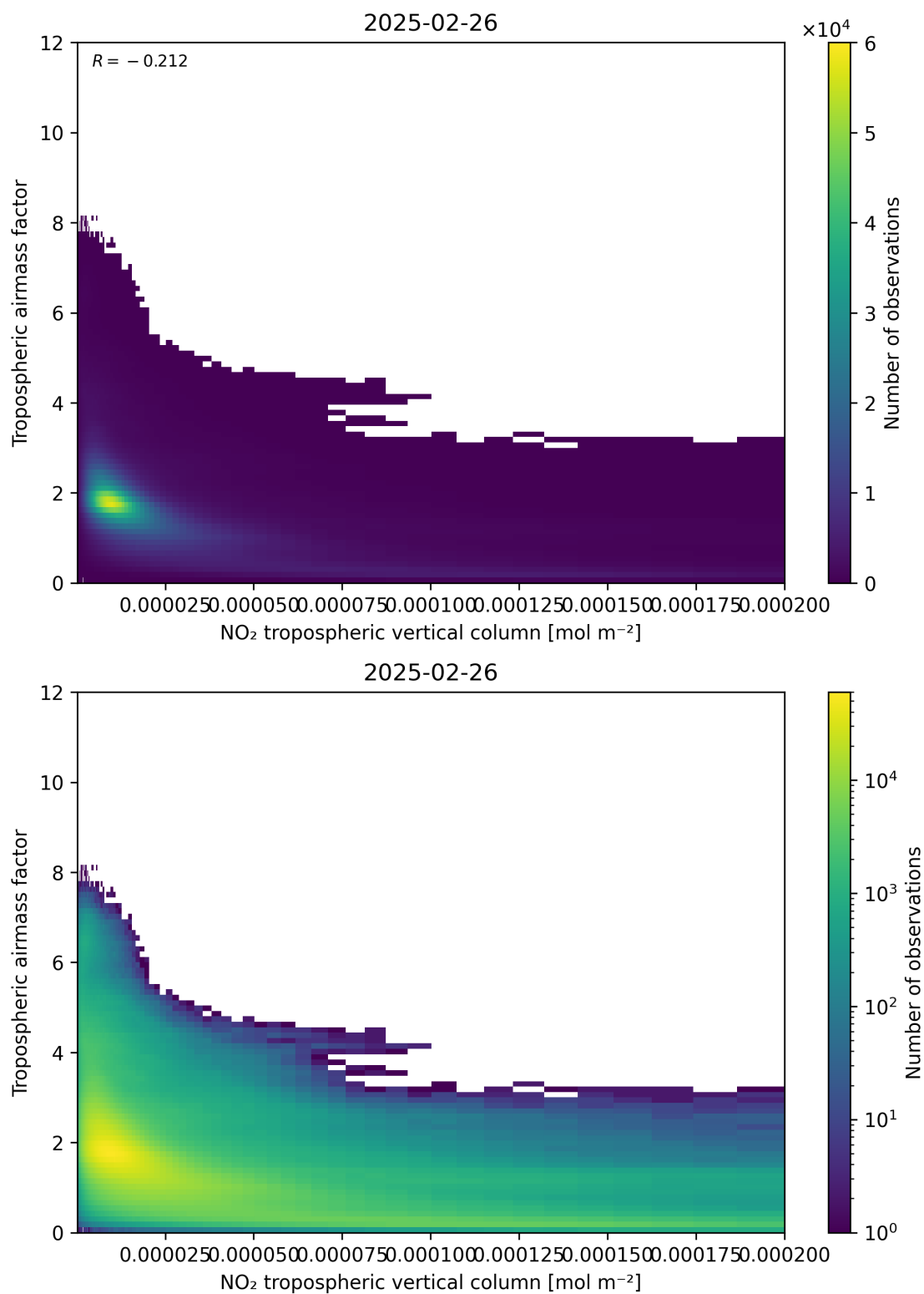
Figure 123: Scatter density plot of “NO 2 tropospheric vertical column” against “Tropospheric air mass factor” for 2025-02-25 to 2025-02-27.
