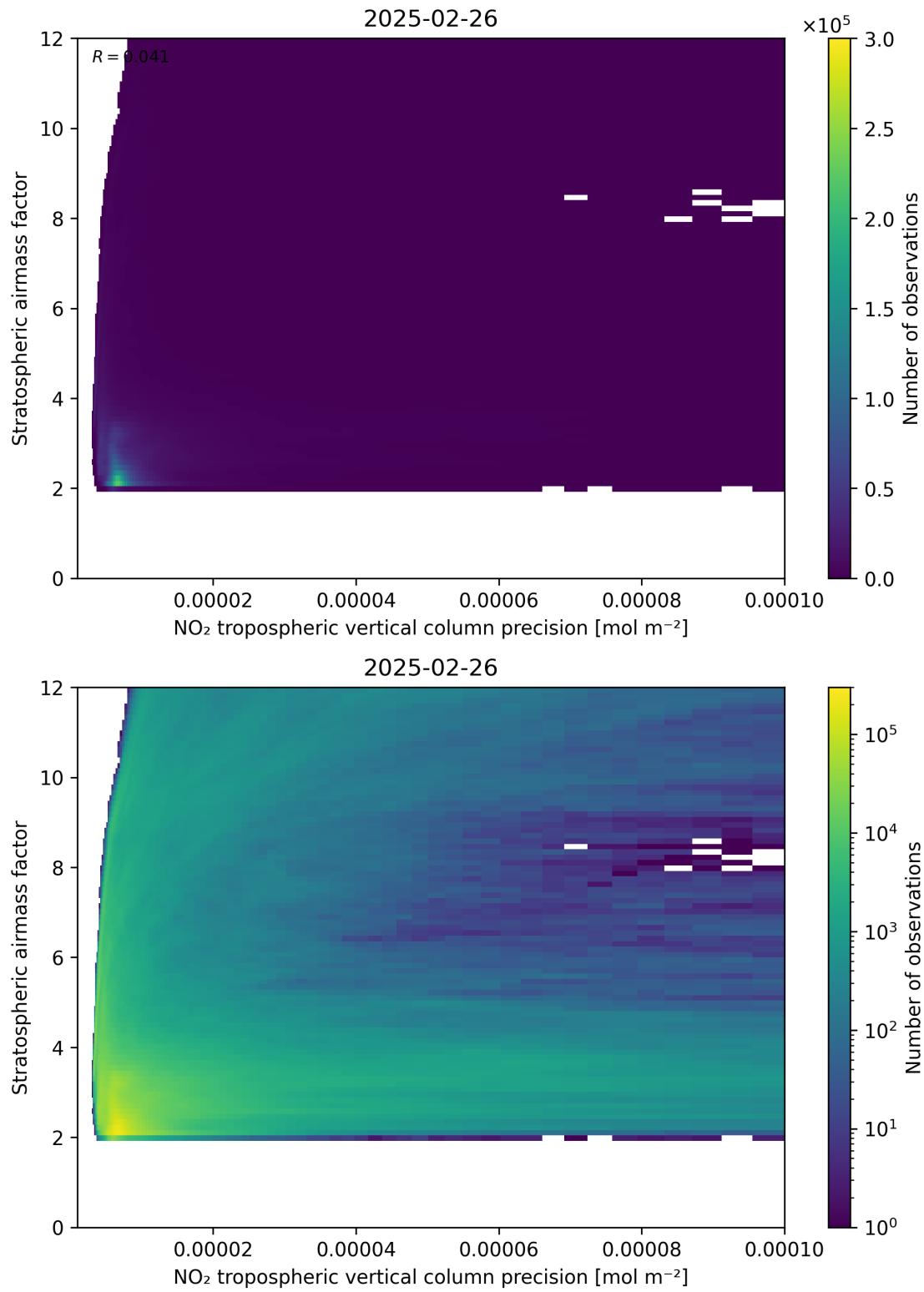
Figure 131: Scatter density plot of “NO 2 tropospheric vertical column precision” against “Stratospheric airmass factor” for 2025-02-25 to 2025-02-27.
