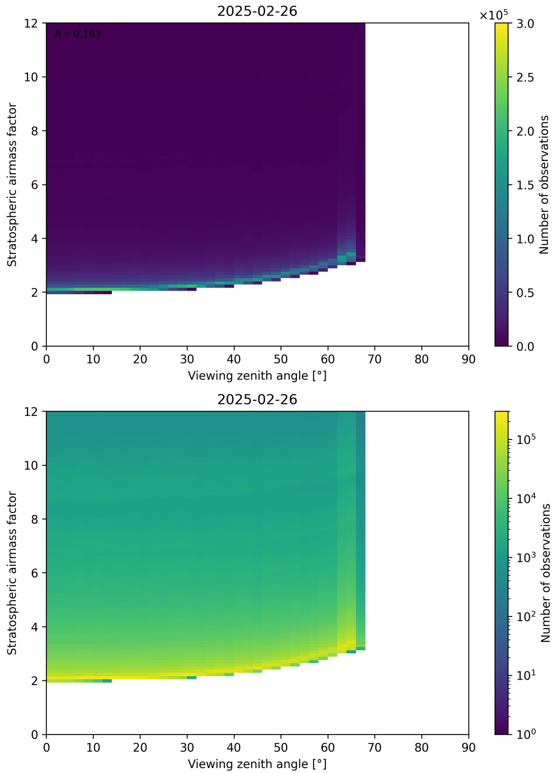
Figure 159: Scatter density plot of “Viewing zenith angle” against “Stratospheric airmass factor” for 2025-02-25 to 2025-02-27.
