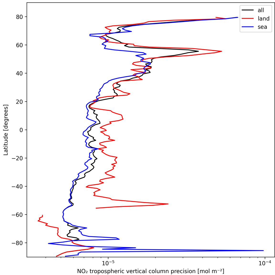
Figure 13: Zonal average of “NO 2 tropospheric vertical column precision” for 2025-02-25 to 2025-02-27.
