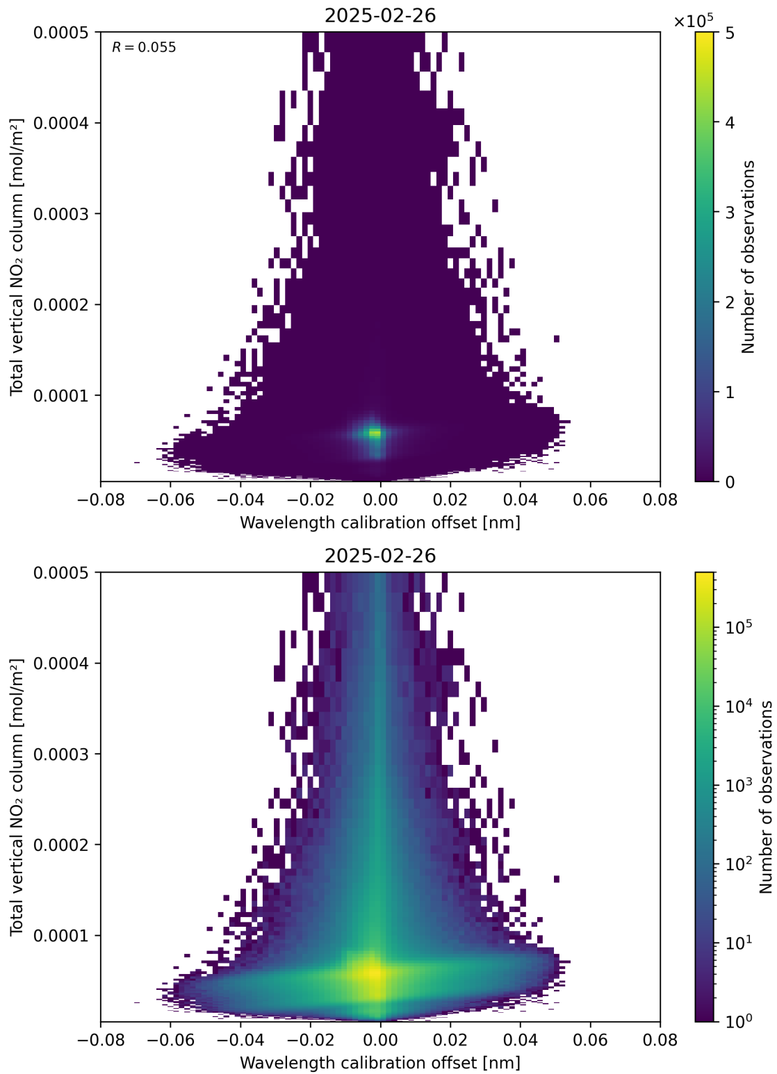
Figure 179: Scatter density plot of “Wavelength calibration offset” against “Total vertical NO 2 column” for 2025-02-25 to 2025-02-27.
