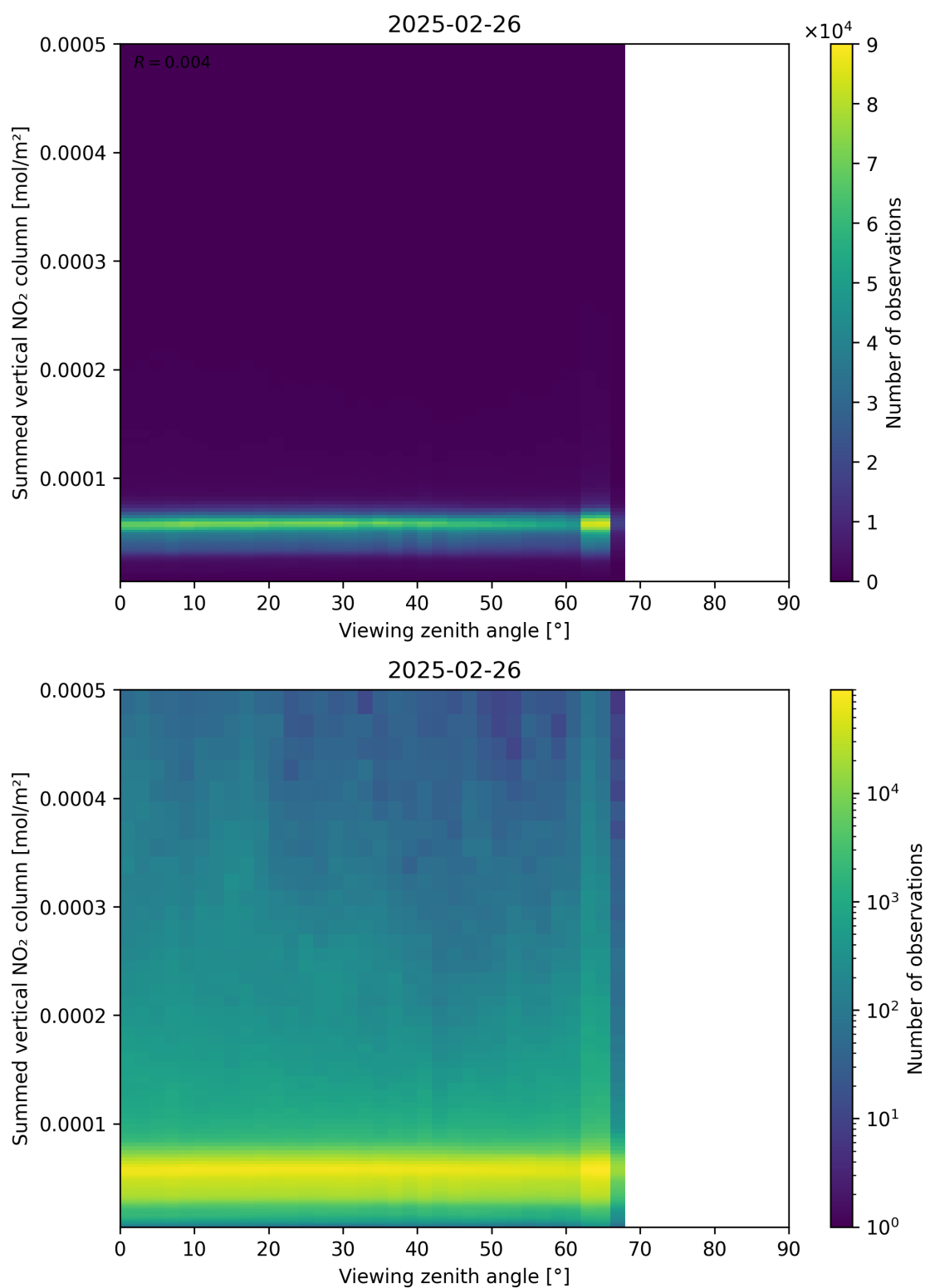
Figure 165: Scatter density plot of “Viewing zenith angle” against “Summed vertical NO 2 column” for 2025-02-25 to 2025-02-27.
