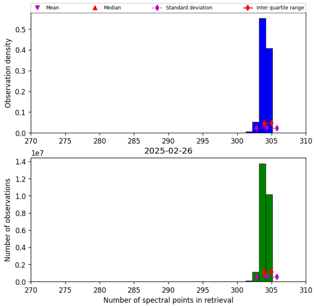
Figure 33: Histogram of “Number of spectral points in retrieval” for 2025-02-25 to 2025-02-27
