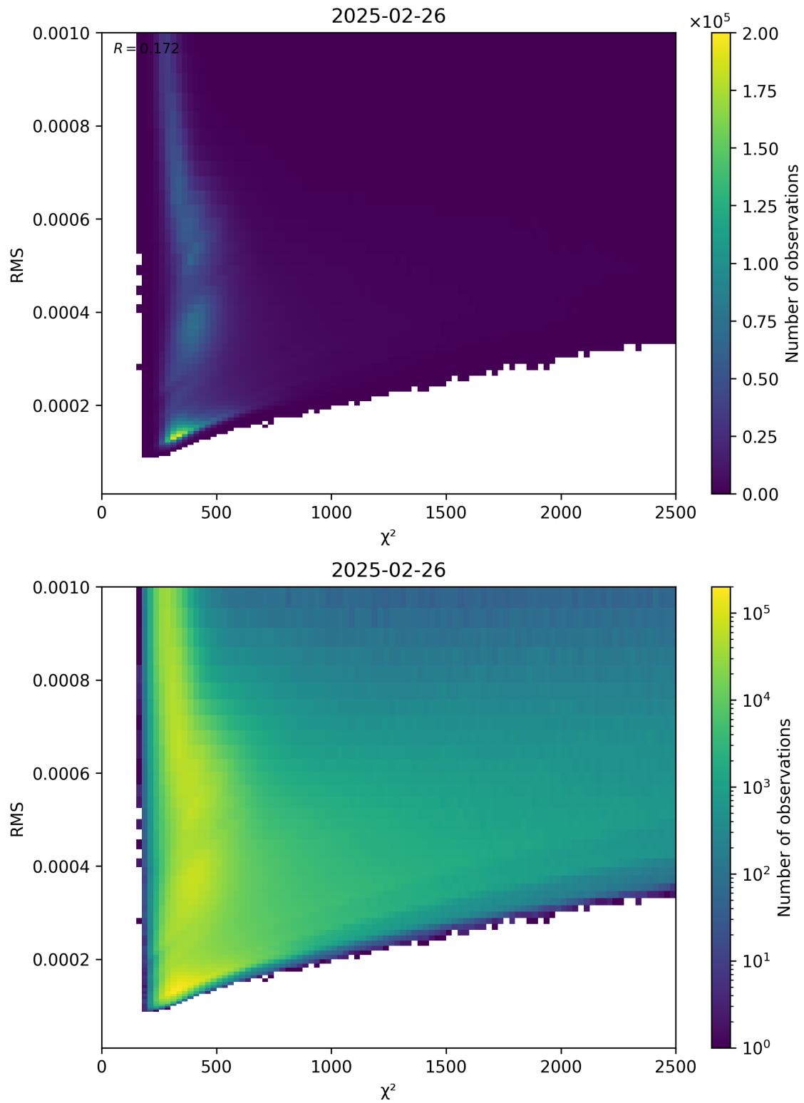
Figure 82: Scatter density plot of “ \chi^2 ” against “RMS” for 2025-02-25 to 2025-02-27.
