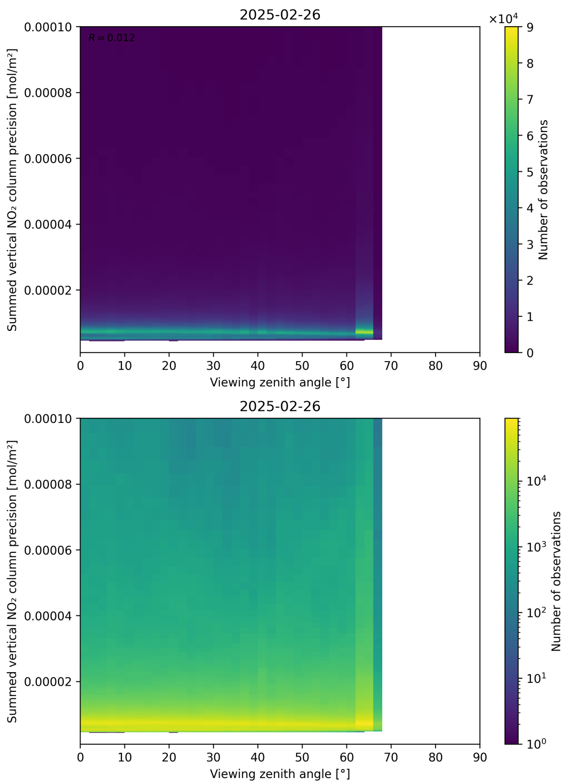
Figure 166: Scatter density plot of “Viewing zenith angle” against “Summed vertical NO 2 column precision” for 2025-02-25 to 2025-02-27.
