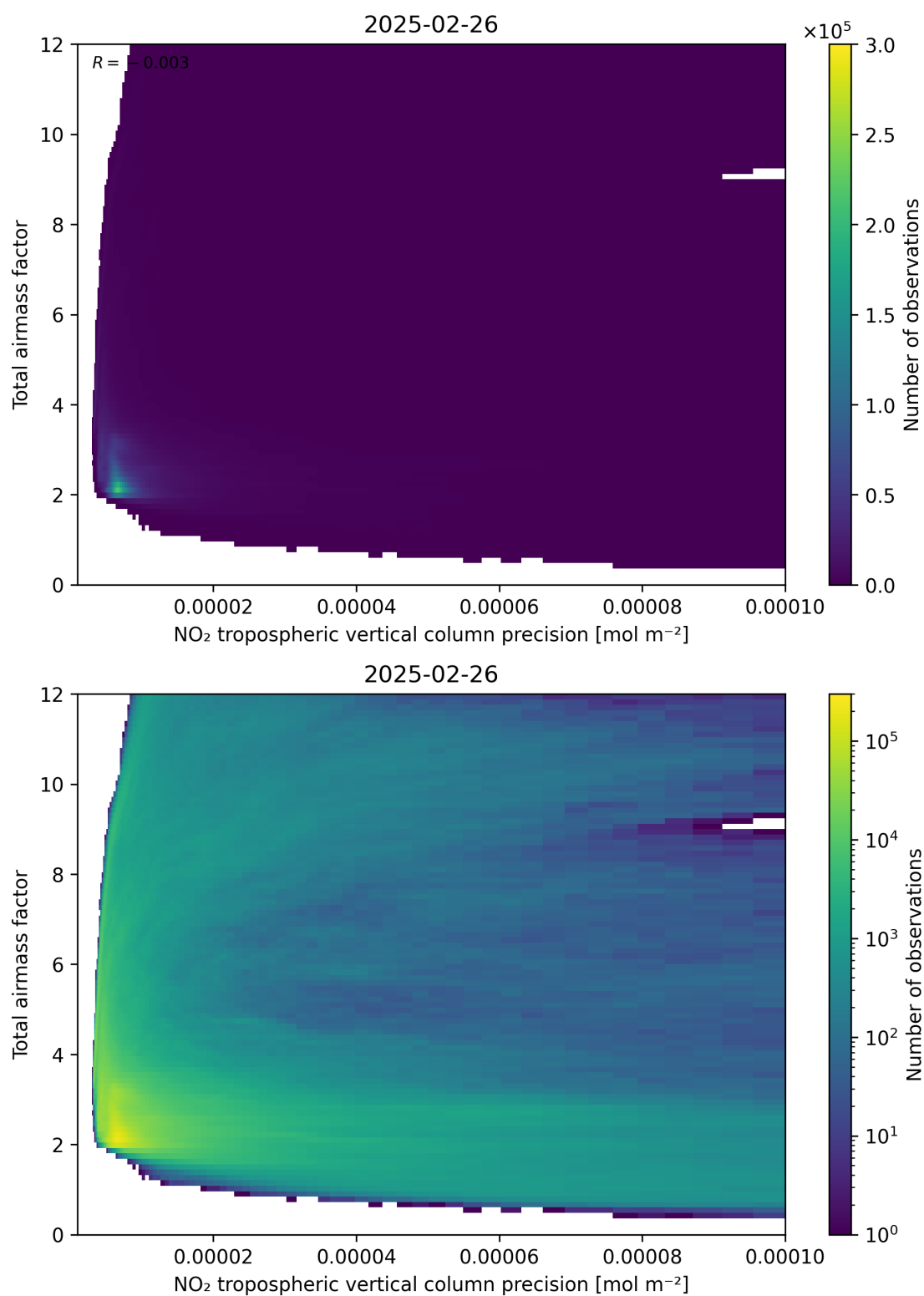
Figure 132: Scatter density plot of “NO 2 tropospheric vertical column precision” against “Total air mass factor” for 2025-02-25 to 2025-02-27.
