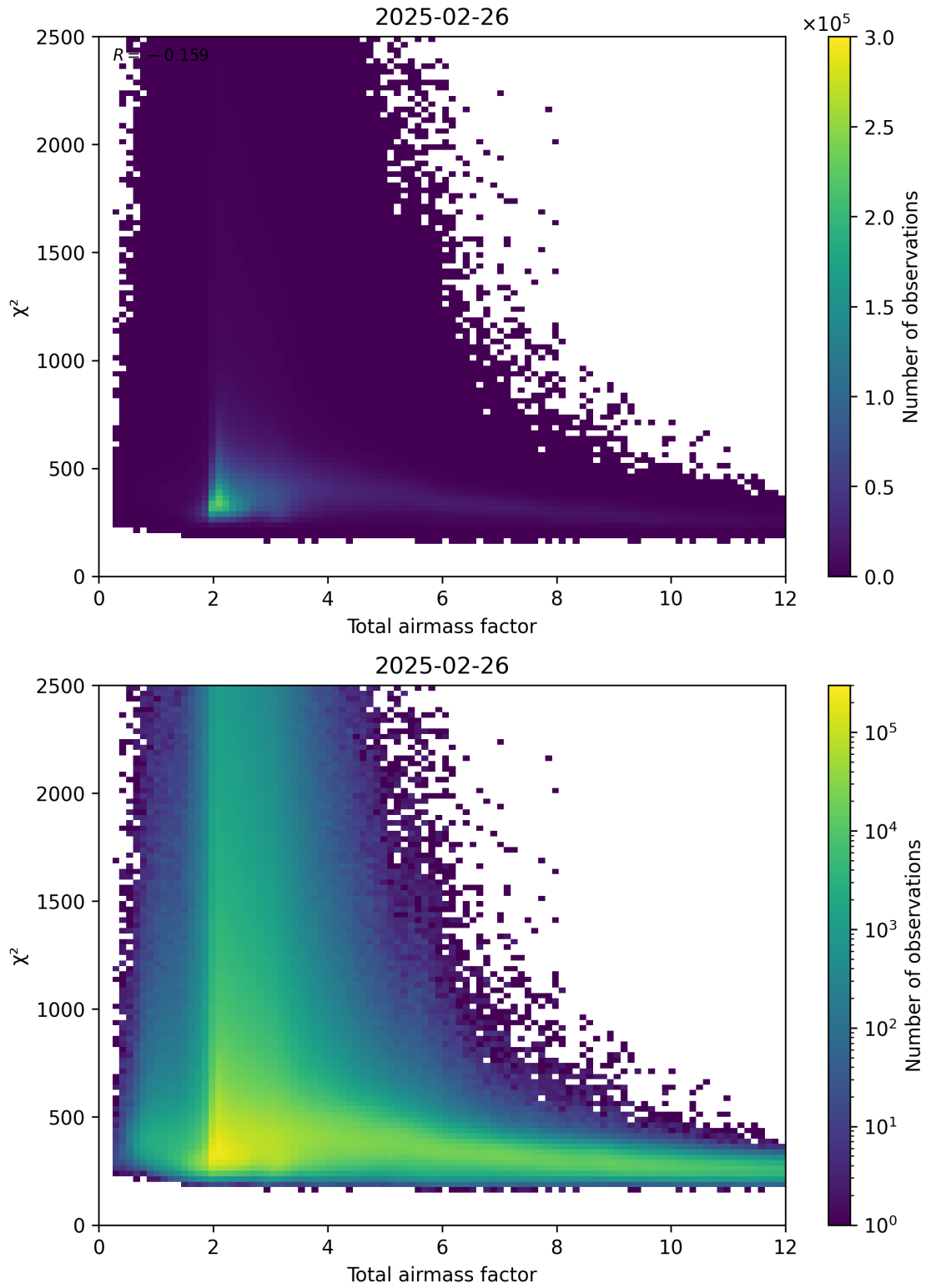
Figure 63: Scatter density plot of “Total airmass factor” against “ \chi^2 ” for 2025-02-25 to 2025-02-27.
