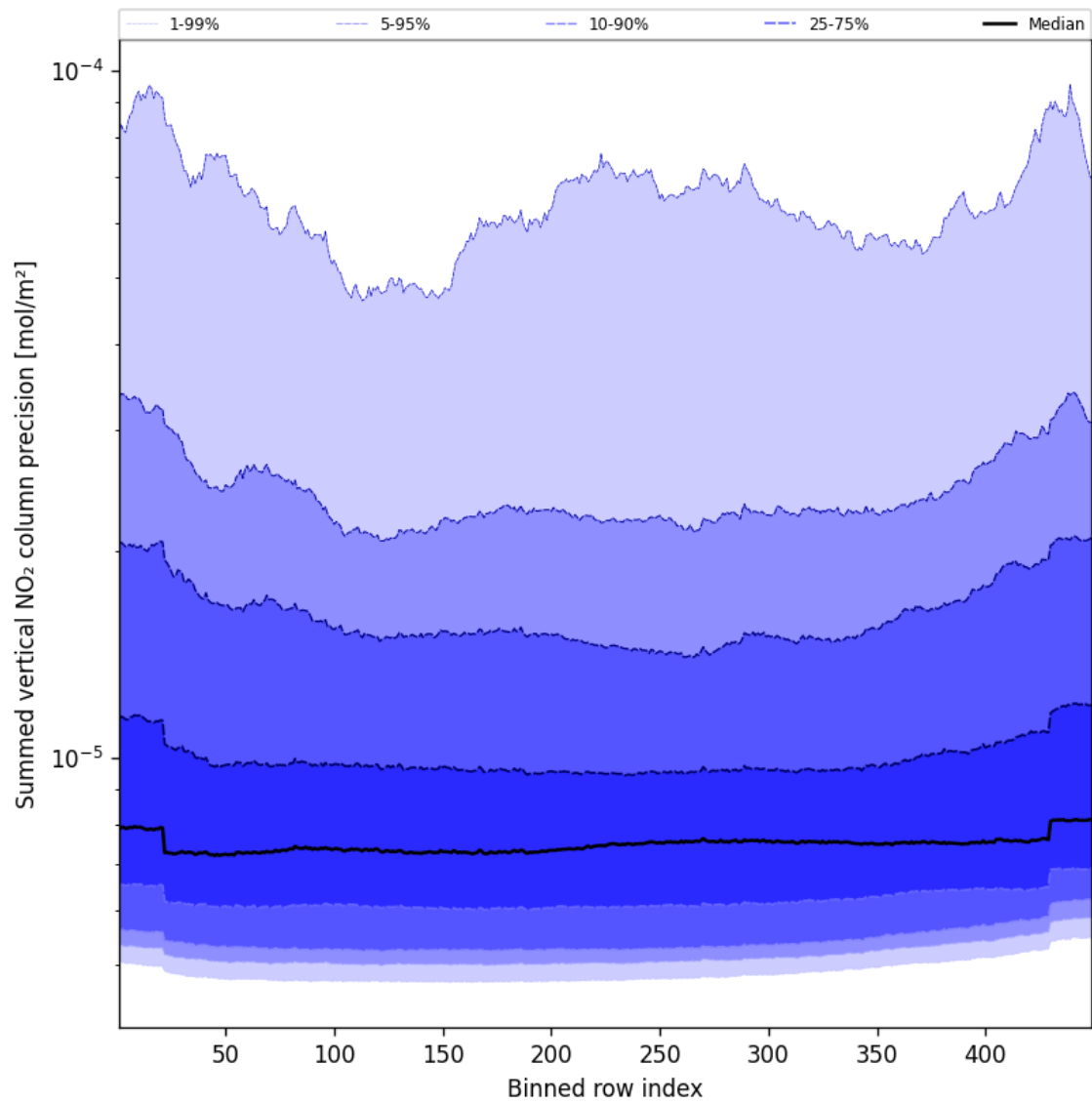
Figure 58: Along track statistics of “Summed vertical NO 2 column precision” for 2025-02-25 to 2025-02-27
