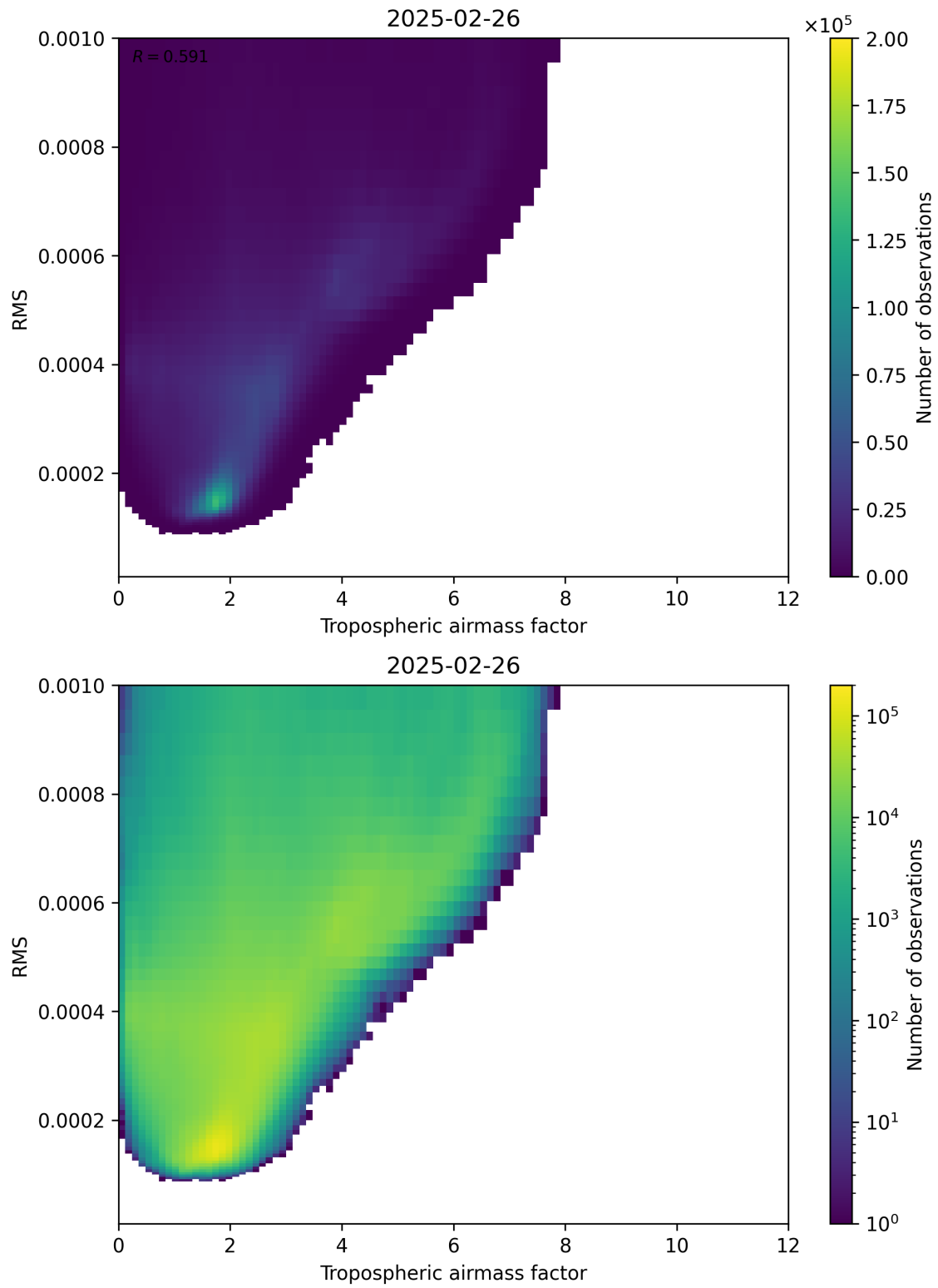
Figure 79: Scatter density plot of “Tropospheric airmass factor” against “RMS” for 2025-02-25 to 2025-02-27.
