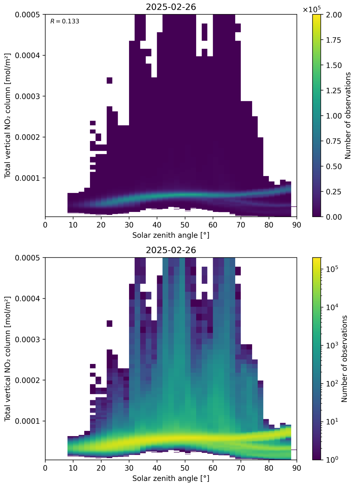
Figure 153: Scatter density plot of “Solar zenith angle” against “Total vertical NO 2 column” for 2025-02-25 to 2025-02-27.
