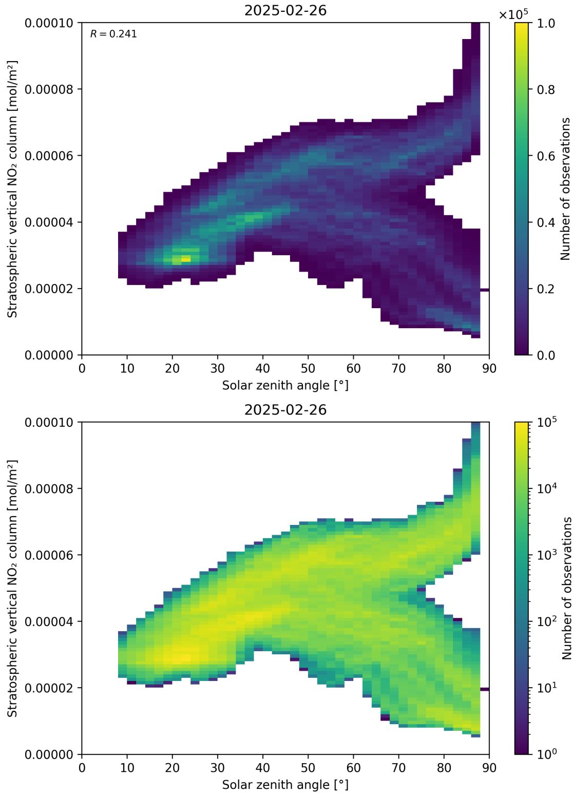
Figure 150: Scatter density plot of “Solar zenith angle” against “Stratospheric vertical NO 2 column” for 2025-02-25 to 2025-02-27.
