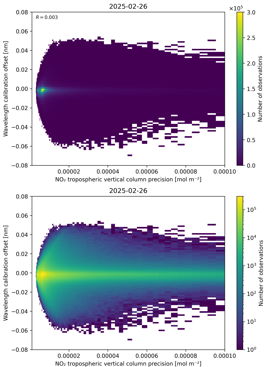
Figure 141: Scatter density plot of “NO 2 tropospheric vertical column precision” against “Wavelength calibration offset” for 2025-02-25 to 2025-02-27.
