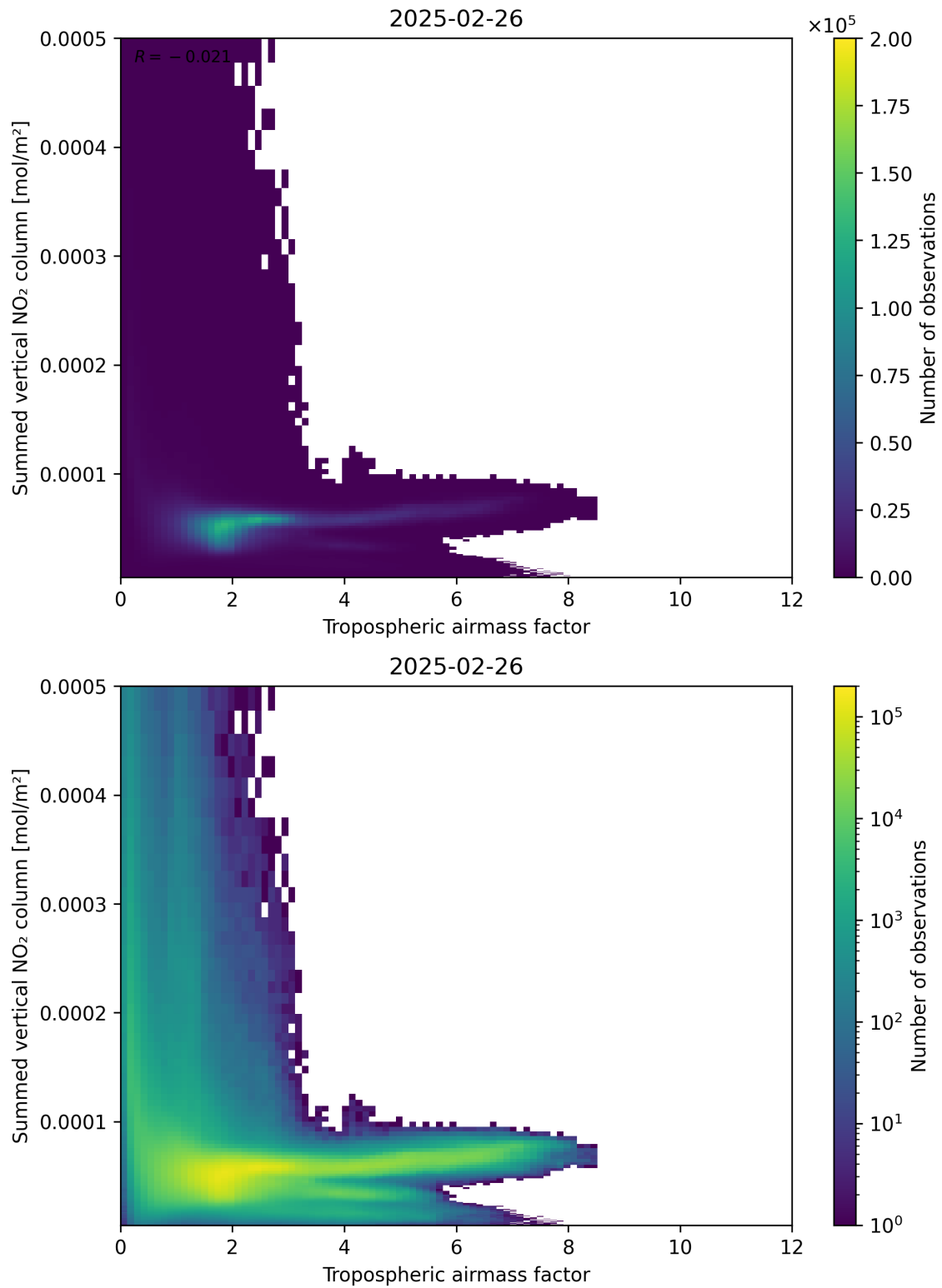
Figure 75: Scatter density plot of “Tropospheric air mass factor” against “Summed vertical NO 2 column” for 2025-02-25 to 2025-02-27.
