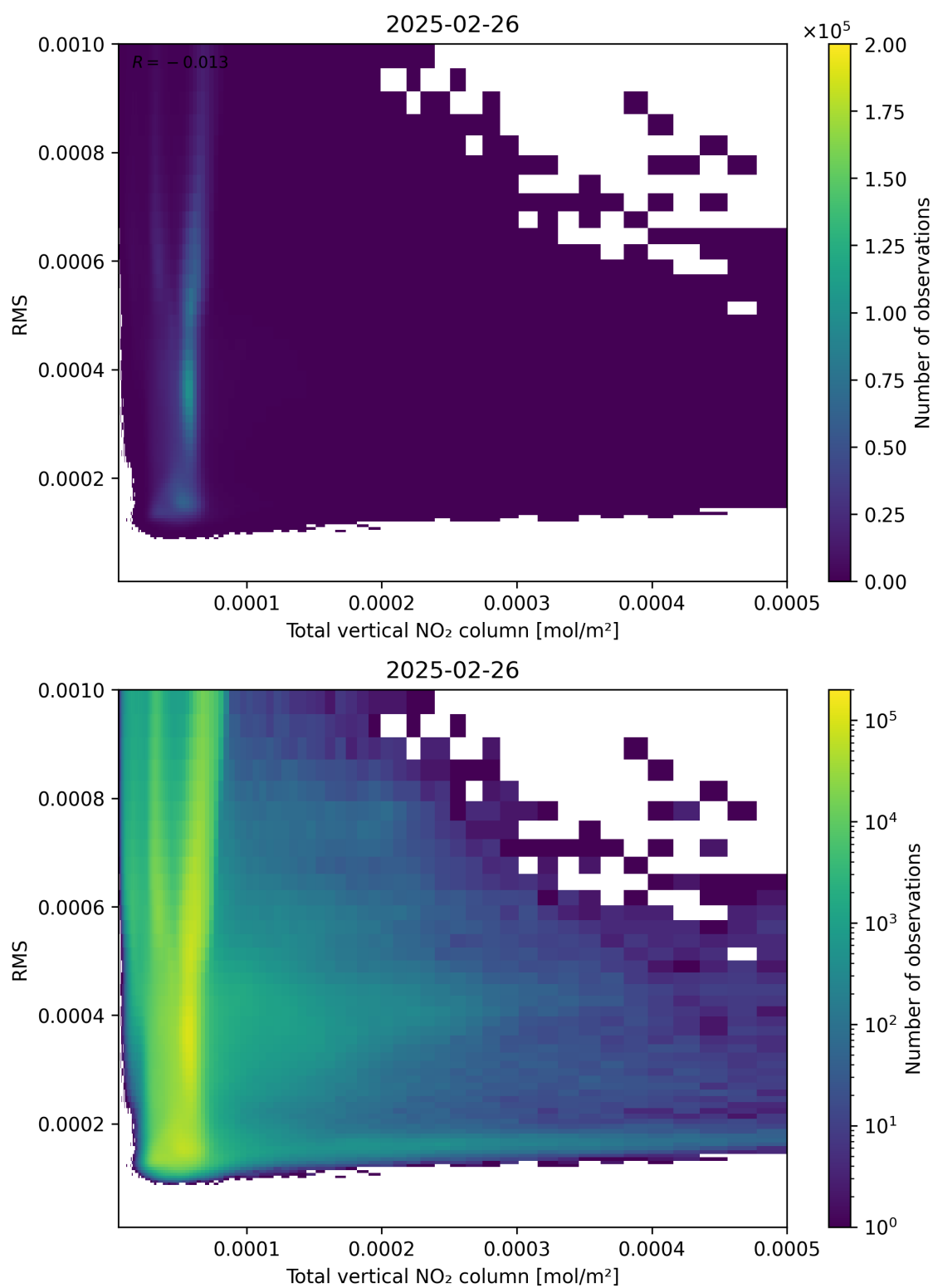
Figure 120: Scatter density plot of “Total vertical NO 2 column” against “RMS” for 2025-02-25 to 2025-02-27.
