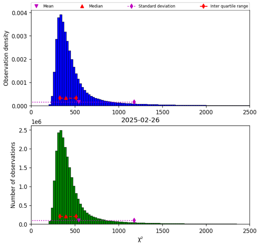
Figure 42: Histogram of “ \chi^2 ” for 2025-02-25 to 2025-02-27
