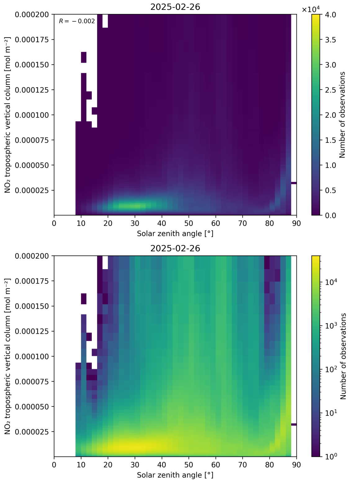
Figure 155: Scatter density plot of “Solar zenith angle” against “NO 2 tropospheric vertical column” for 2025-02-25 to 2025-02-27.
