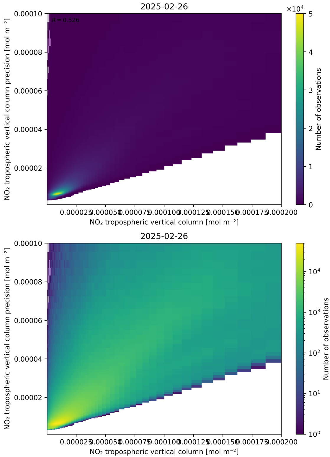
Figure 130: Scatter density plot of “NO 2 tropospheric vertical column” against “NO 2 tropospheric vertical column precision” for 2025-02-25 to 2025-02-27.
