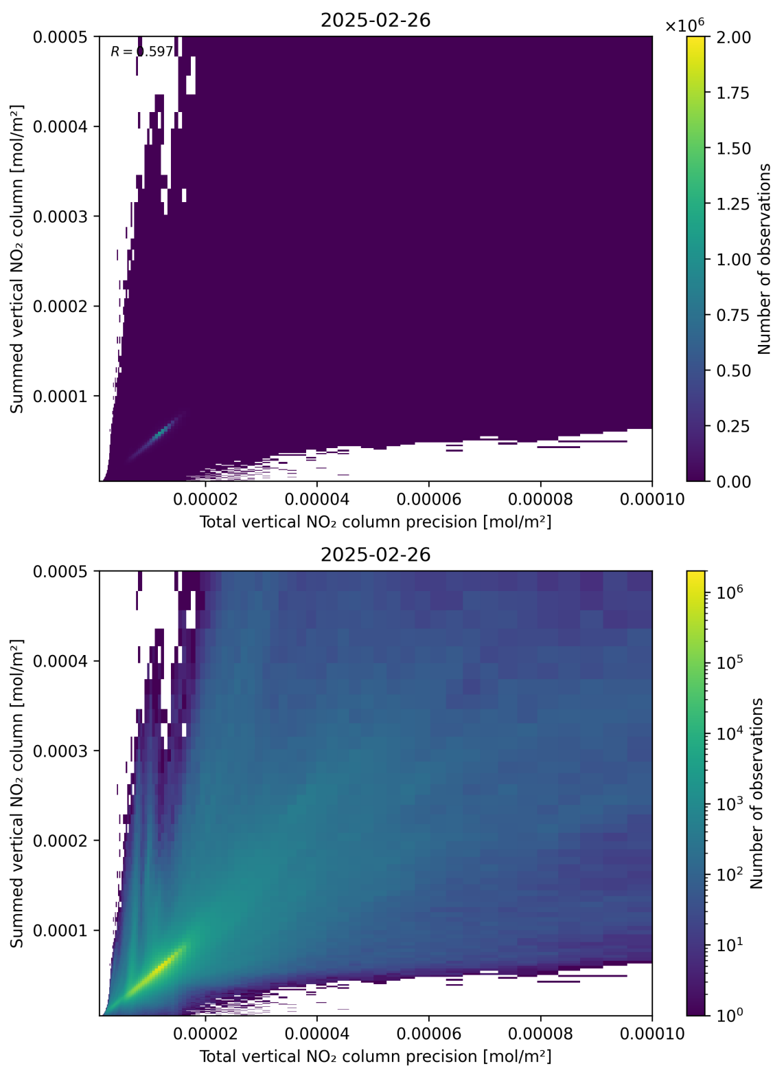
Figure 117: Scatter density plot of “Total vertical NO 2 column precision” against “Summed vertical NO 2 column” for 2025-02-25 to 2025-02-27.
