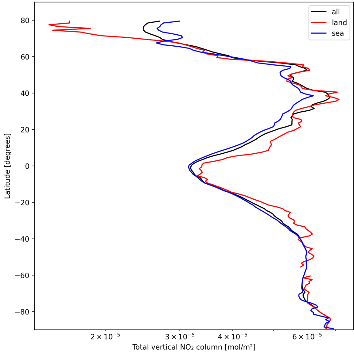
Figure 21: Zonal average of “Total vertical NO 2 column” for 2025-02-25 to 2025-02-27.
