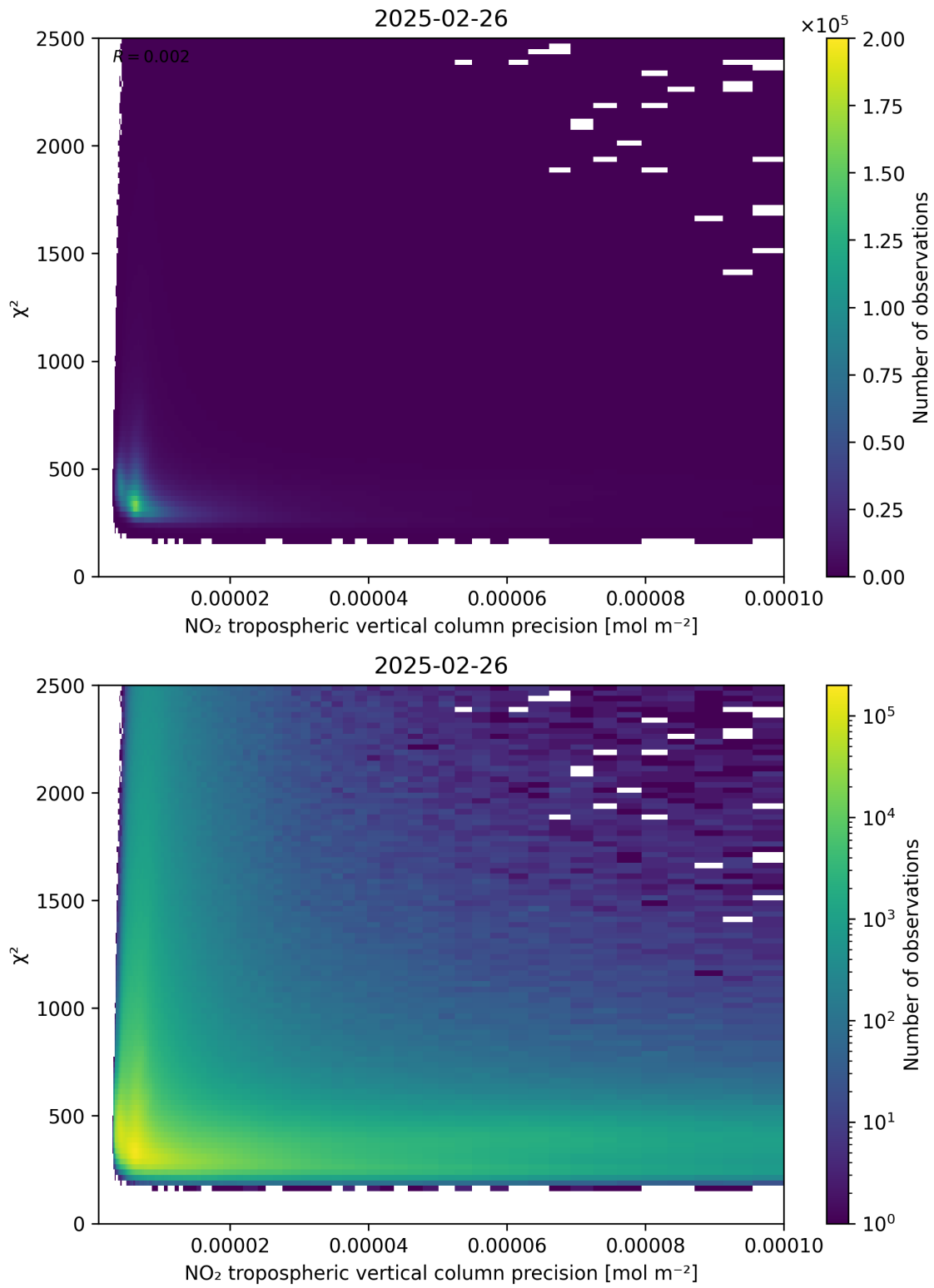
Figure 134: Scatter density plot of “NO 2 tropospheric vertical column precision” against “ \chi^2 ” for 2025-02-25 to 2025-02-27.
