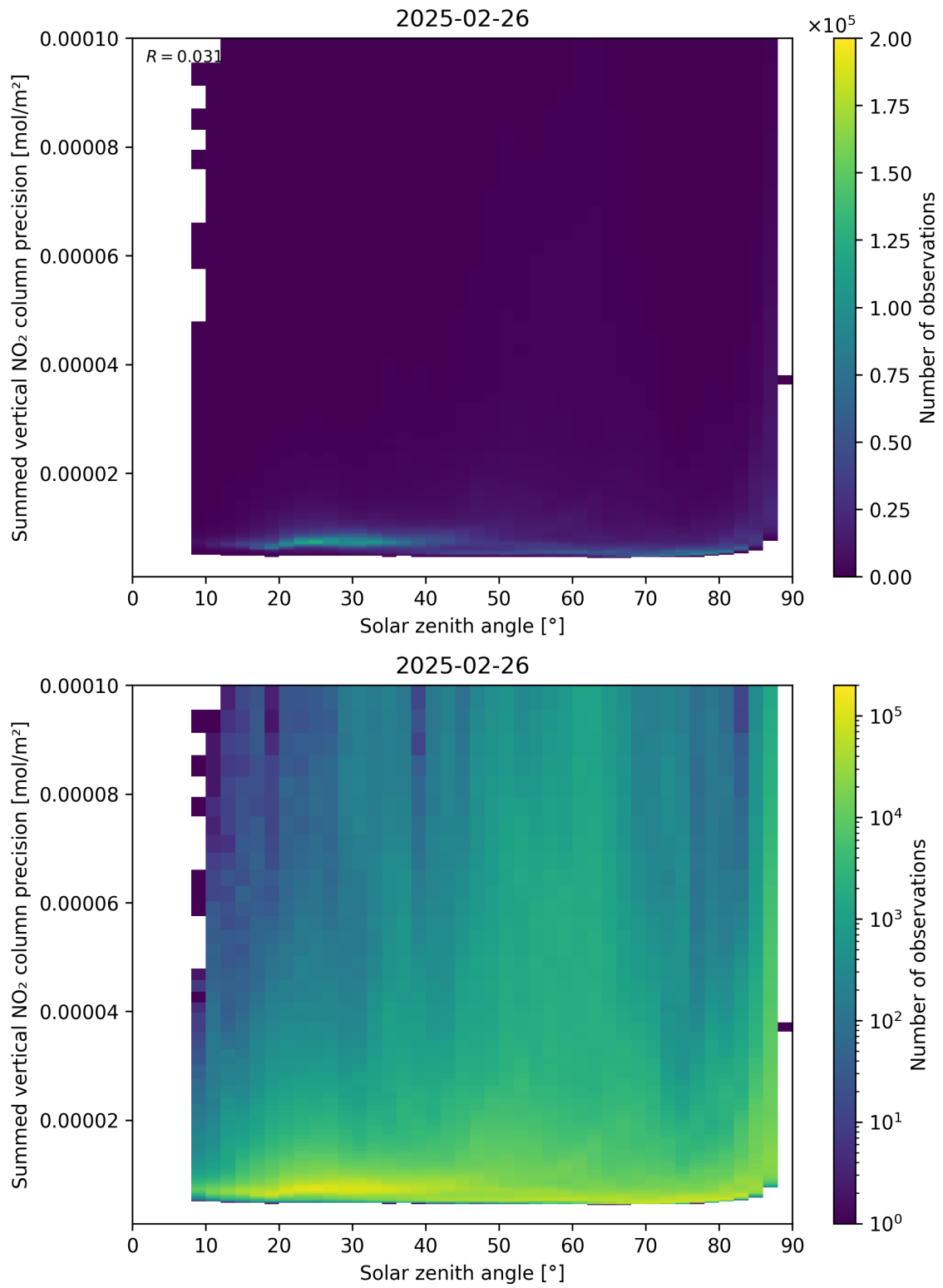
Figure 152: Scatter density plot of “Solar zenith angle” against “Summed vertical NO 2 column precision” for 2025-02-25 to 2025-02-27.
