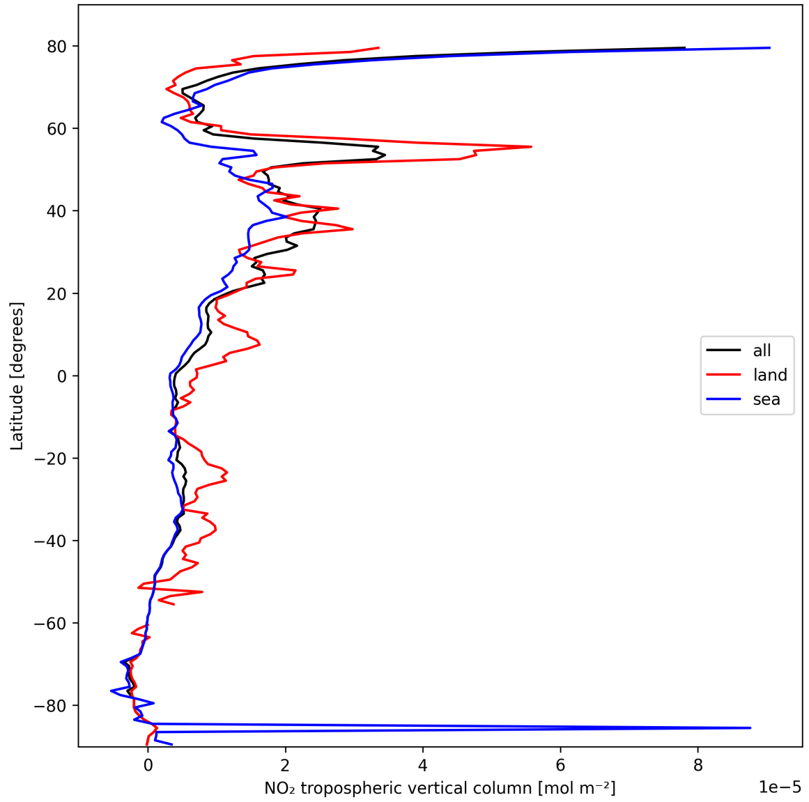
Figure 12: Zonal average of “NO 2 tropospheric vertical column” for 2025-02-25 to 2025-02-27.
