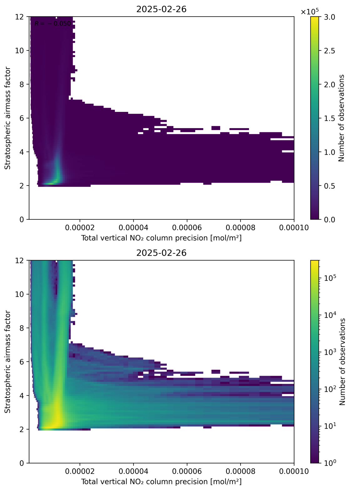
Figure 115: Scatter density plot of “Total vertical NO 2 column precision” against “Stratospheric air mass factor” for 2025-02-25 to 2025-02-27.
