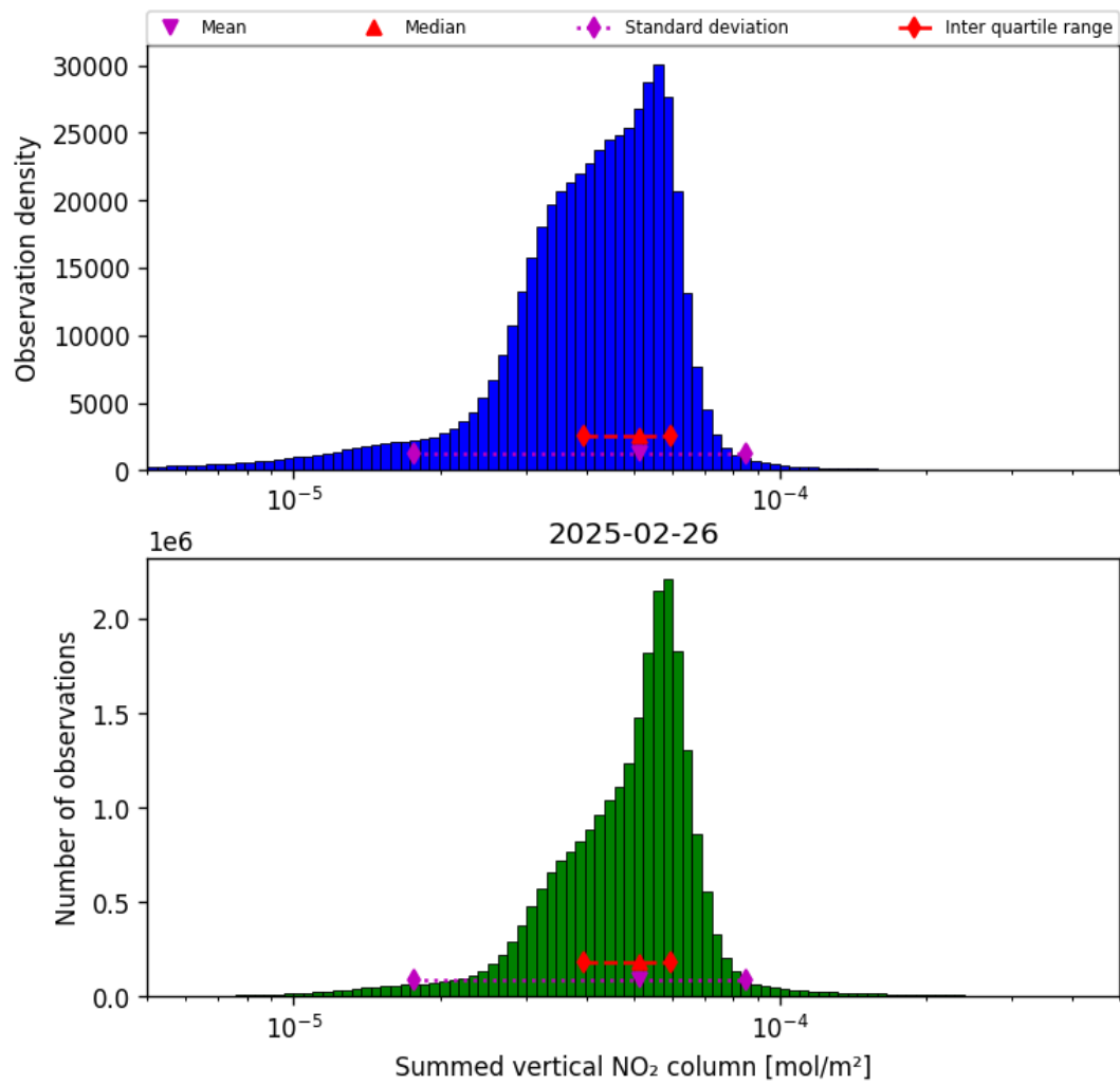
Figure 40: Histogram of “Summed vertical NO 2 column” for 2025-02-25 to 2025-02-27
