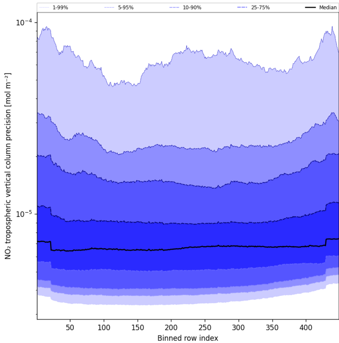
Figure 47: Along track statistics of “NO 2 tropospheric vertical column precision” for 2025-02-25 to 2025-02-27
