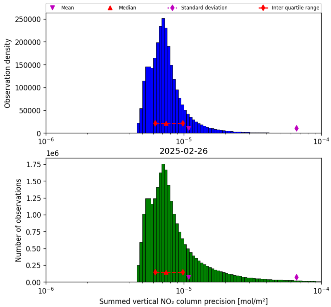
Figure 41: Histogram of “Summed vertical NO 2 column precision” for 2025-02-25 to 2025-02-27
