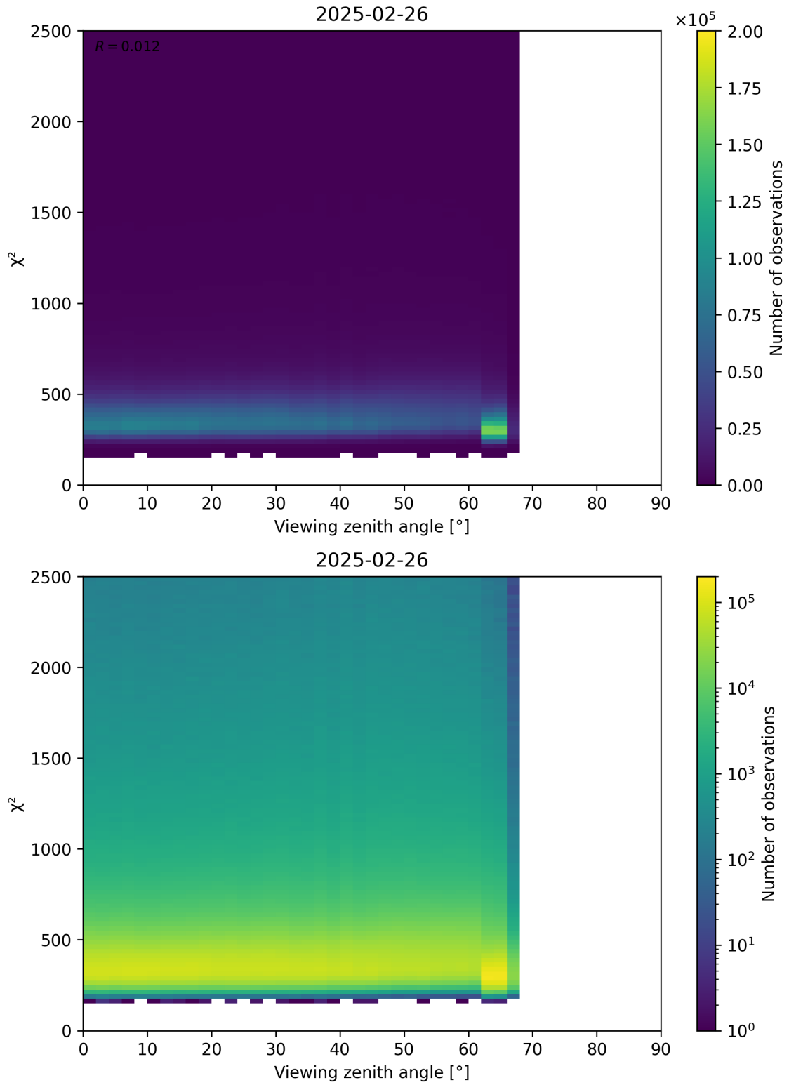
Figure 162: Scatter density plot of “Viewing zenith angle” against “ \chi^2 ” for 2025-02-25 to 2025-02-27.
