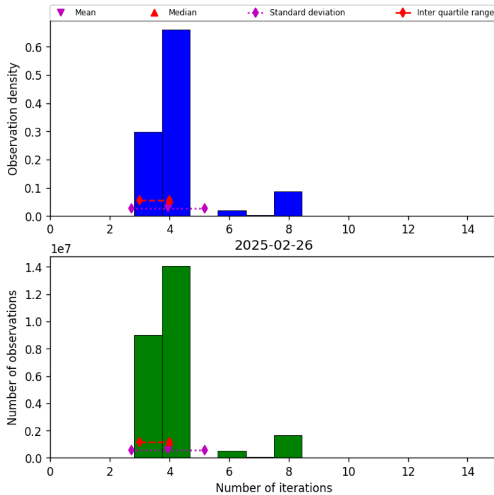
Figure 34: Histogram of “Number of iterations” for 2025-02-25 to 2025-02-27
