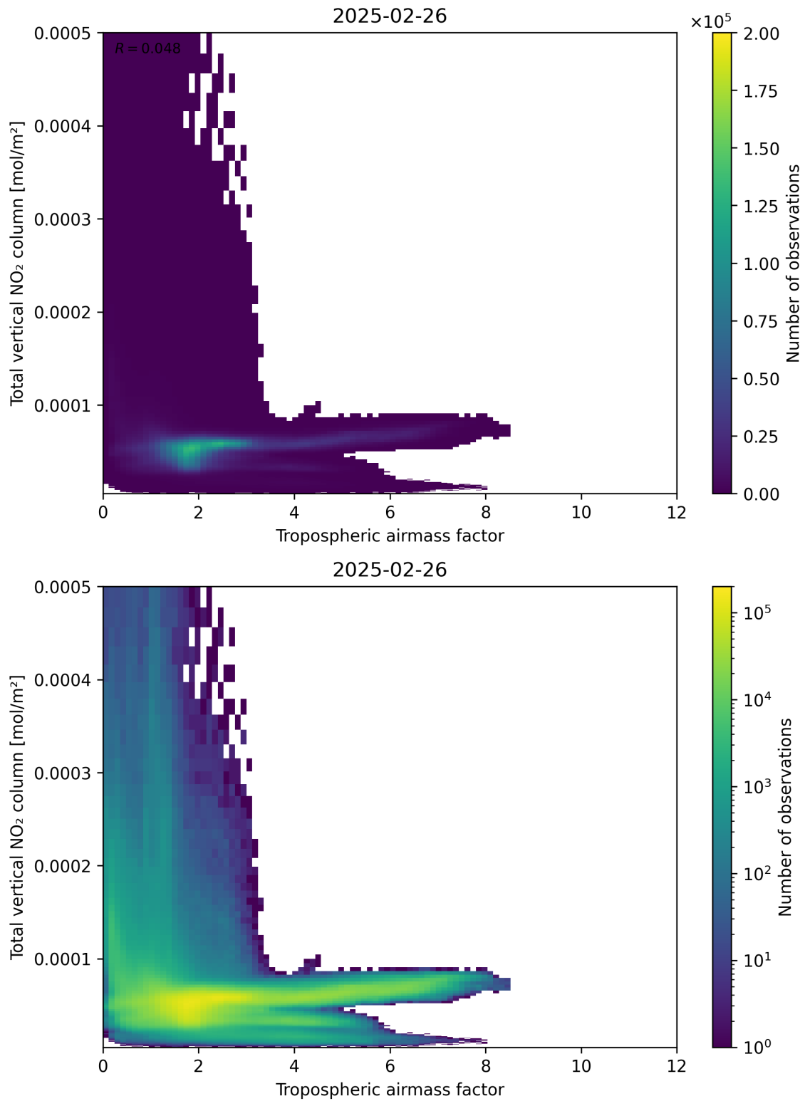
Figure 77: Scatter density plot of “Tropospheric airmass factor” against “Total vertical NO 2 column” for 2025-02-25 to 2025-02-27.
