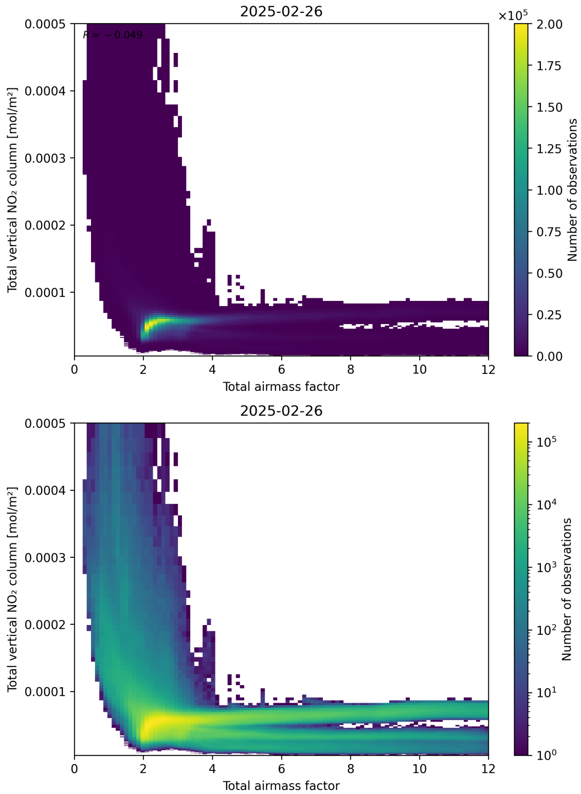
Figure 67: Scatter density plot of “Total airmass factor” against “Total vertical NO 2 column” for 2025-02-25 to 2025-02-27.
