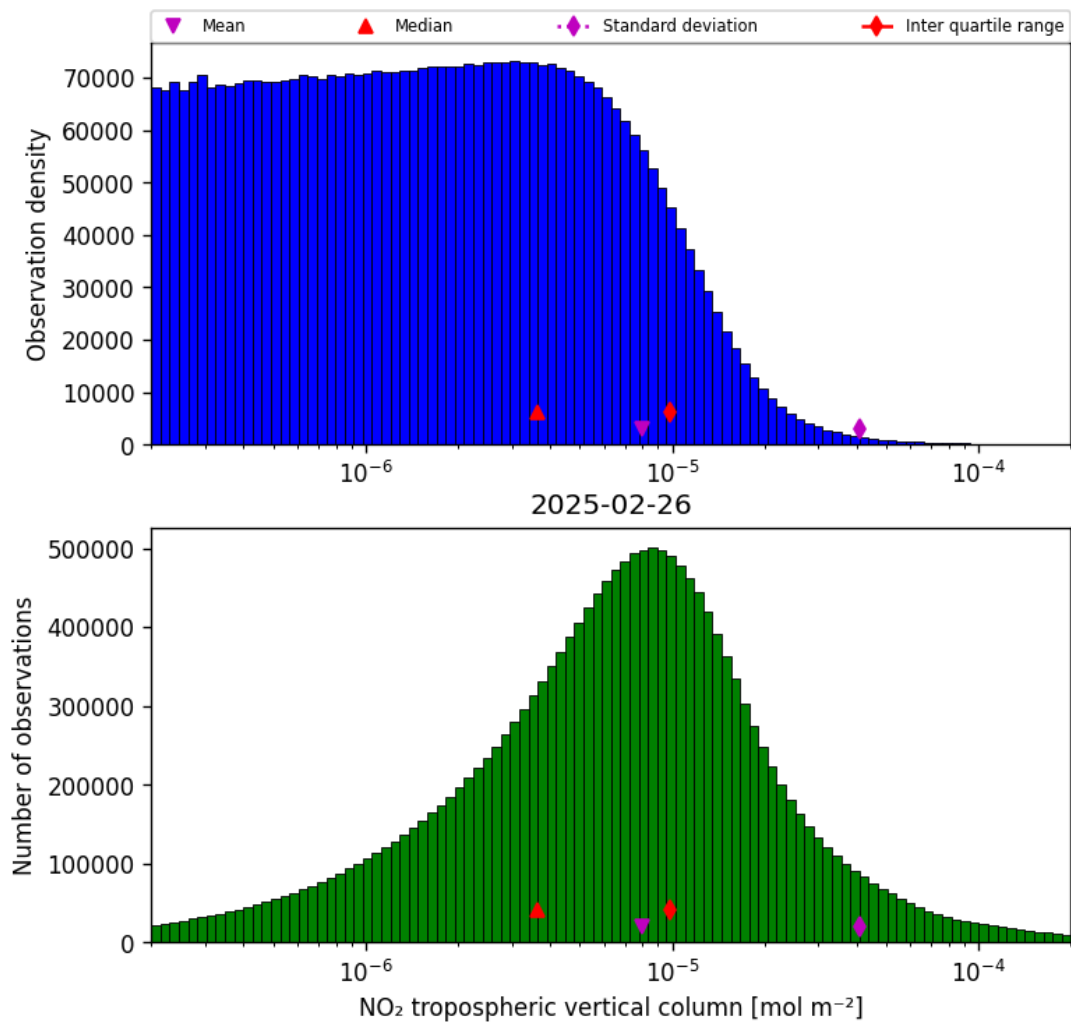
Figure 29: Histogram of “NO 2 tropospheric vertical column” for 2025-02-25 to 2025-02-27
