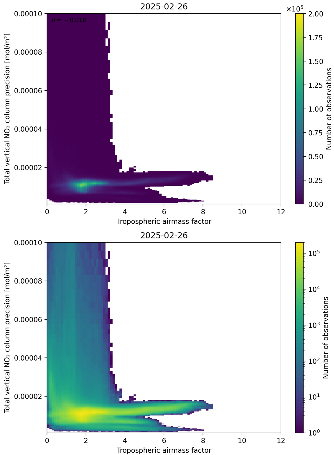
Figure 78: Scatter density plot of “Tropospheric airmass factor” against “Total vertical NO 2 column precision” for 2025-02-25 to 2025-02-27.
