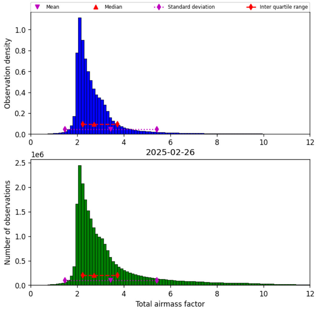
Figure 32: Histogram of “Total airmass factor” for 2025-02-25 to 2025-02-27
