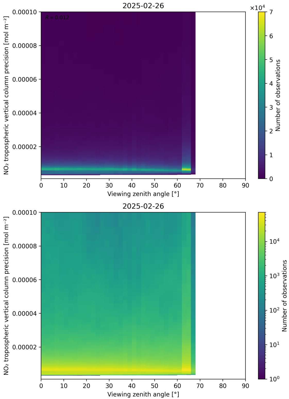
Figure 170: Scatter density plot of “Viewing zenith angle” against “NO 2 tropospheric vertical column precision” for 2025-02-25 to 2025-02-27.
