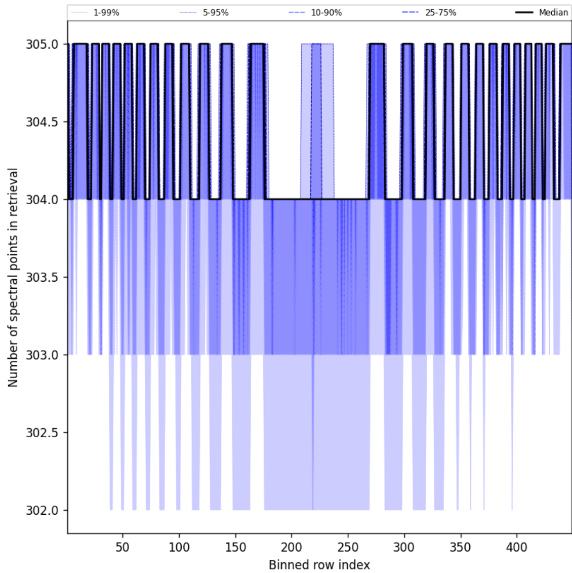
Figure 50: Along track statistics of “Number of spectral points in retrieval” for 2025-02-25 to 2025-02-27
