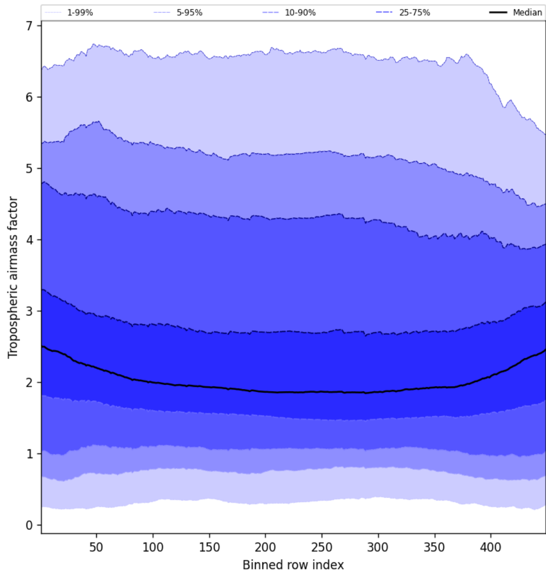
Figure 48: Along track statistics of “Tropospheric air mass factor” for 2025-02-25 to 2025-02-27
