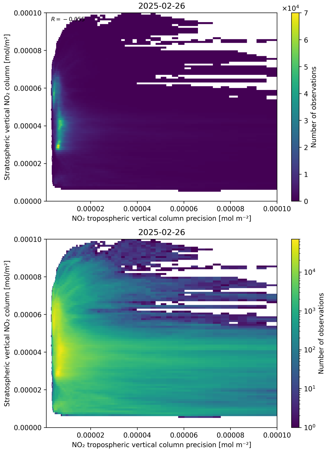
Figure 135: Scatter density plot of “NO 2 tropospheric vertical column precision” against “Stratospheric vertical NO 2 column” for 2025-02-25 to 2025-02-27.
