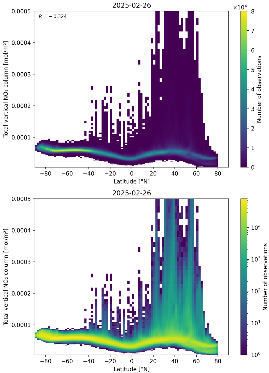
Figure 90: Scatter density plot of “Latitude” against “Total vertical NO 2 column” for 2025-02-25 to 2025-02-27.
