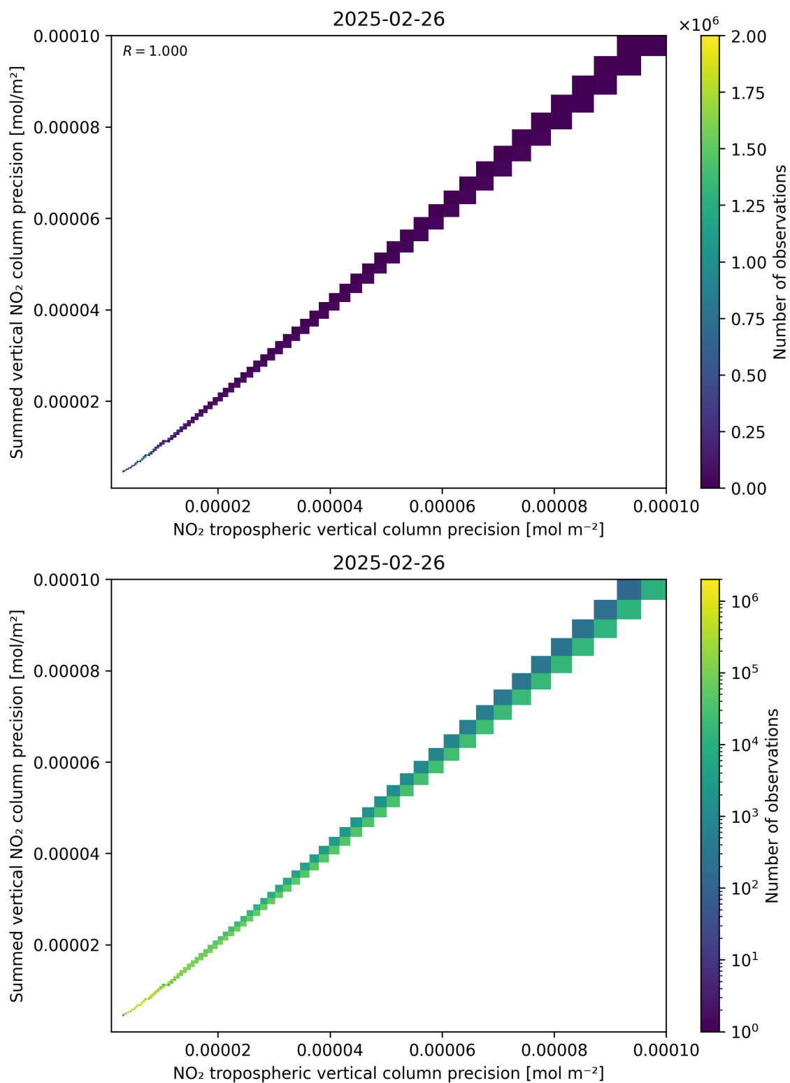
Figure 137: Scatter density plot of “NO 2 tropospheric vertical column precision” against “Summed vertical NO 2 column precision” for 2025-02-25 to 2025-02-27.
