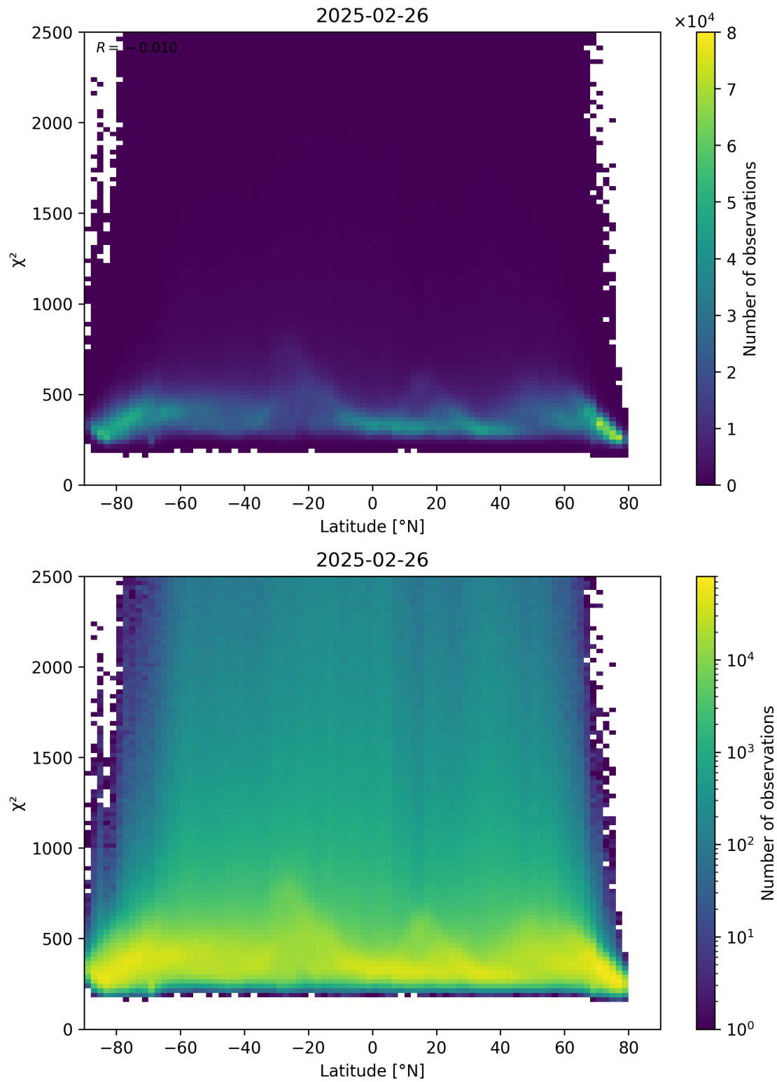
Figure 86: Scatter density plot of “Latitude” against “ \chi^2 ” for 2025-02-25 to 2025-02-27.
