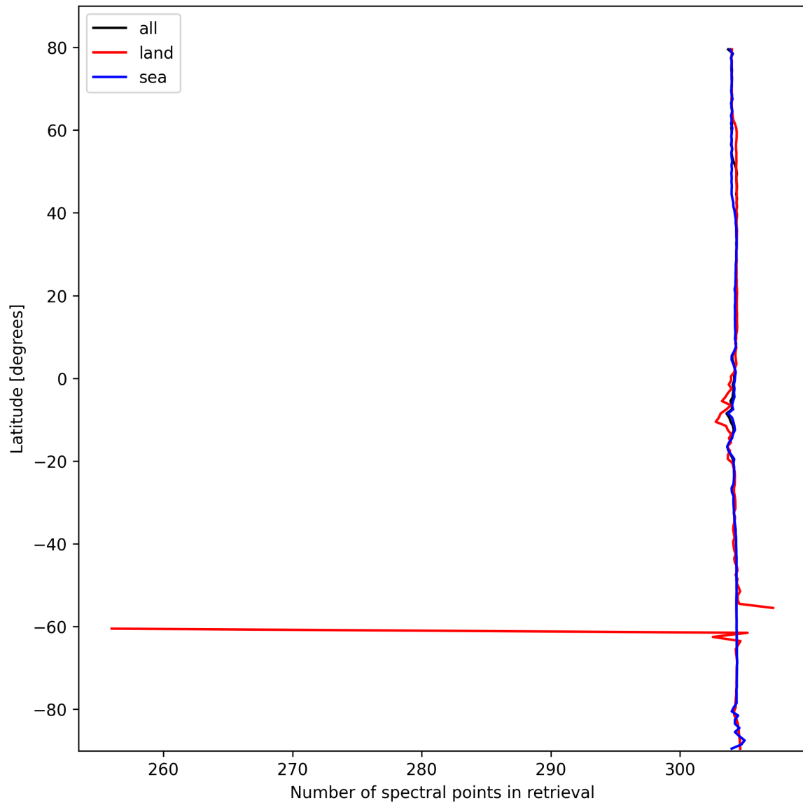
Figure 16: Zonal average of “Number of spectral points in retrieval” for 2025-02-25 to 2025-02-27.
