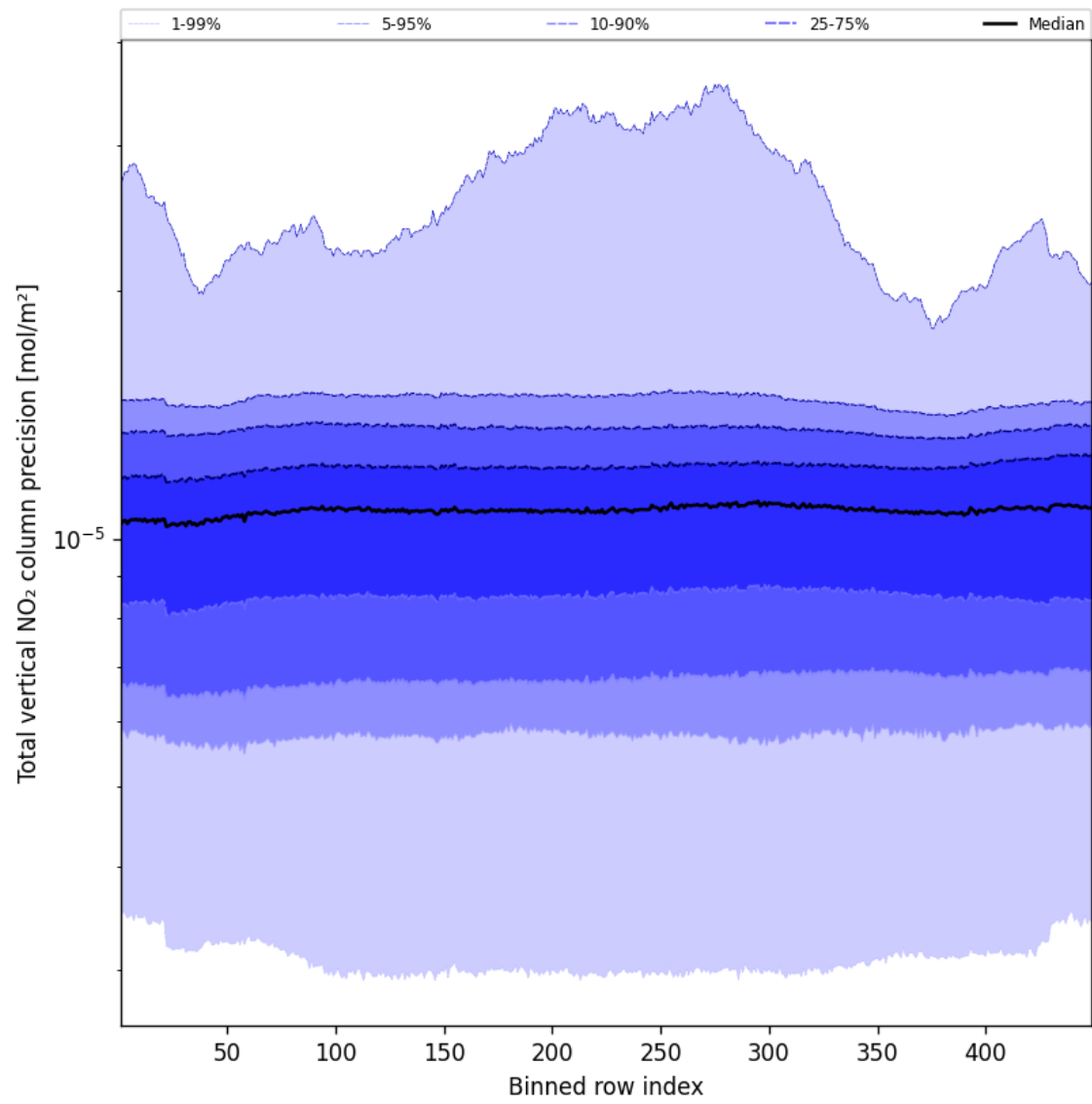
Figure 56: Along track statistics of “Total vertical NO 2 column precision” for 2025-02-25 to 2025-02-27
