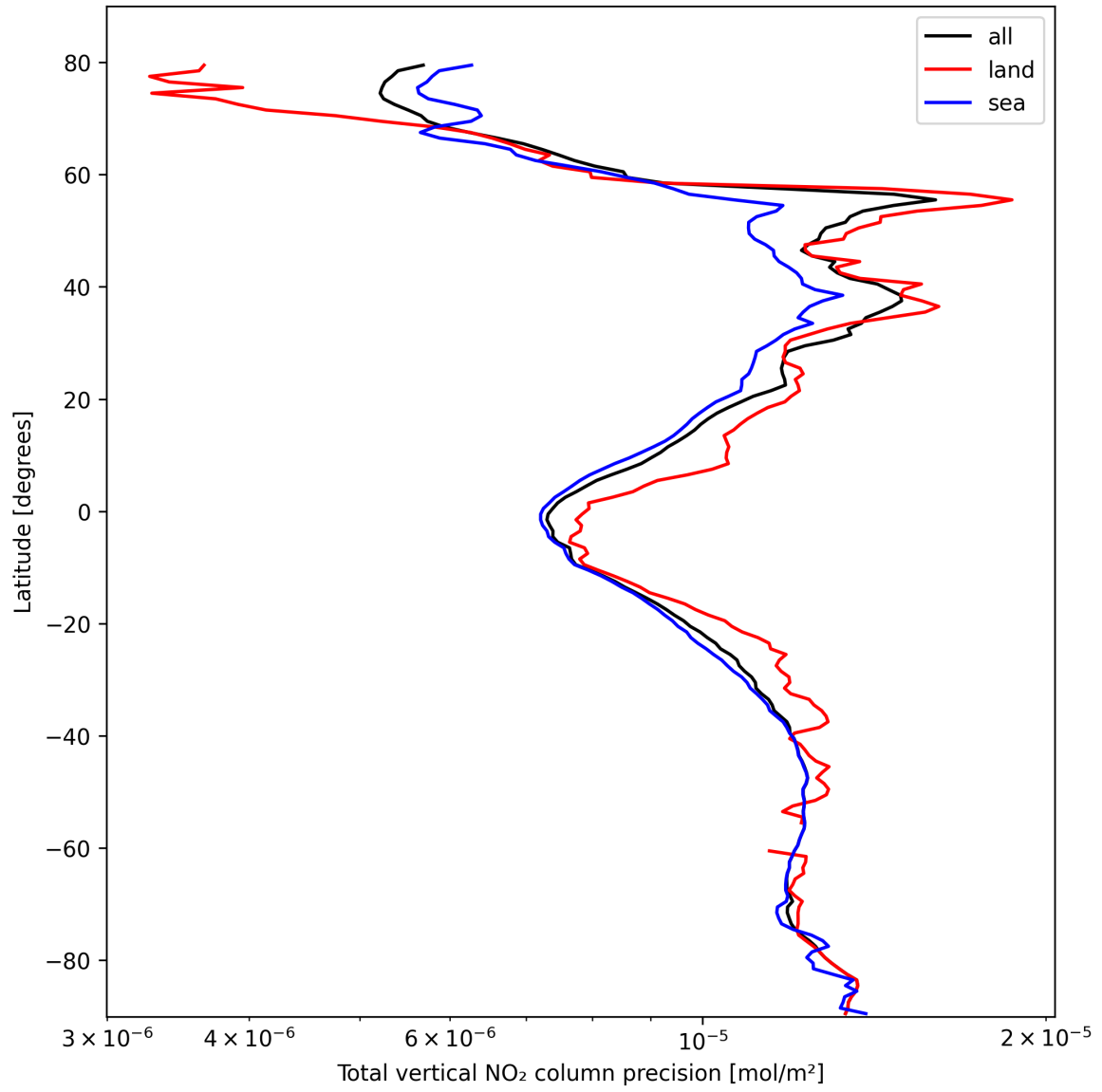
Figure 22: Zonal average of “Total vertical NO 2 column precision” for 2025-02-25 to 2025-02-27.
