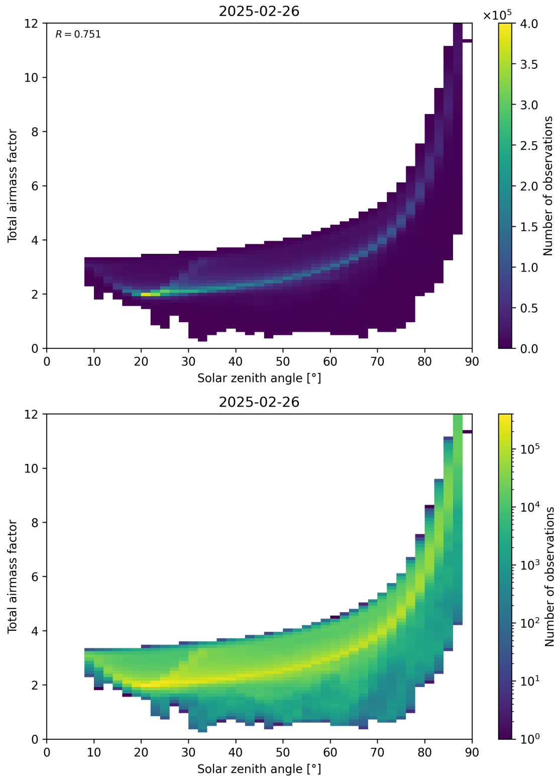
Figure 146: Scatter density plot of “Solar zenith angle” against “Total air mass factor” for 2025-02-25 to 2025-02-27.
