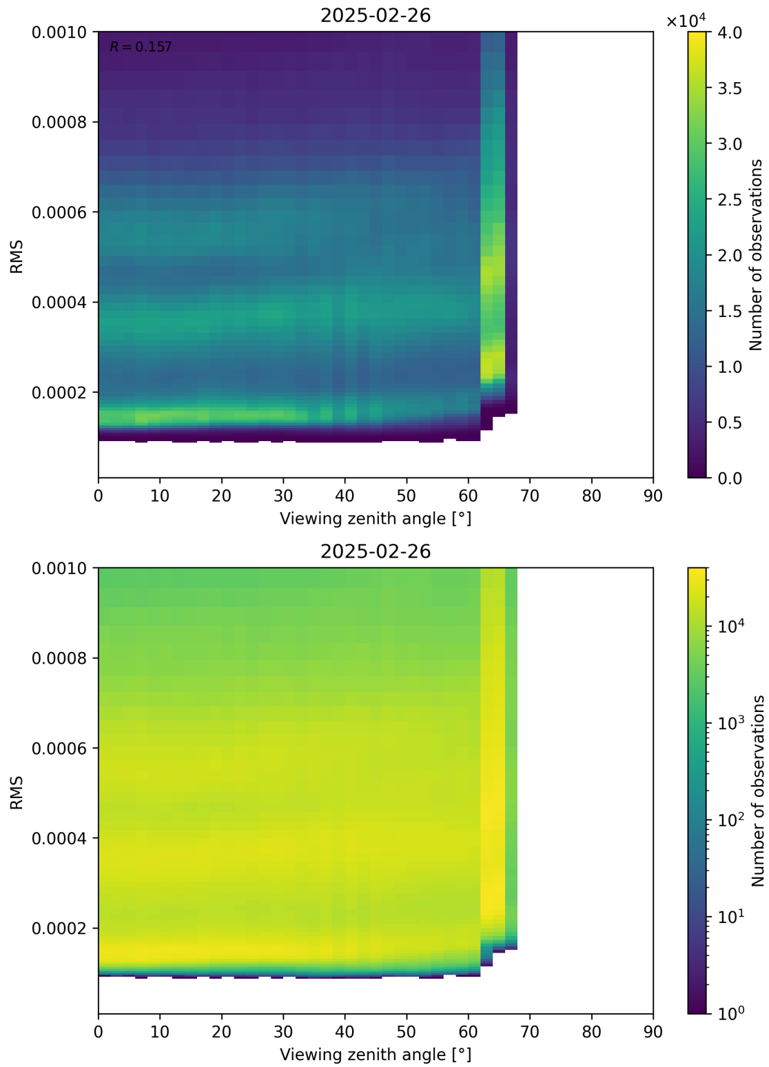
Figure 171: Scatter density plot of “Viewing zenith angle” against “RMS” for 2025-02-25 to 2025-02-27.
