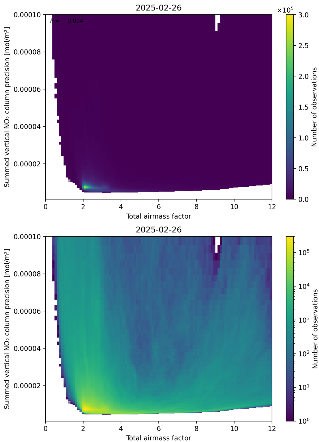
Figure 66: Scatter density plot of “Total airmass factor” against “Summed vertical NO 2 column precision” for 2025-02-25 to 2025-02-27.
