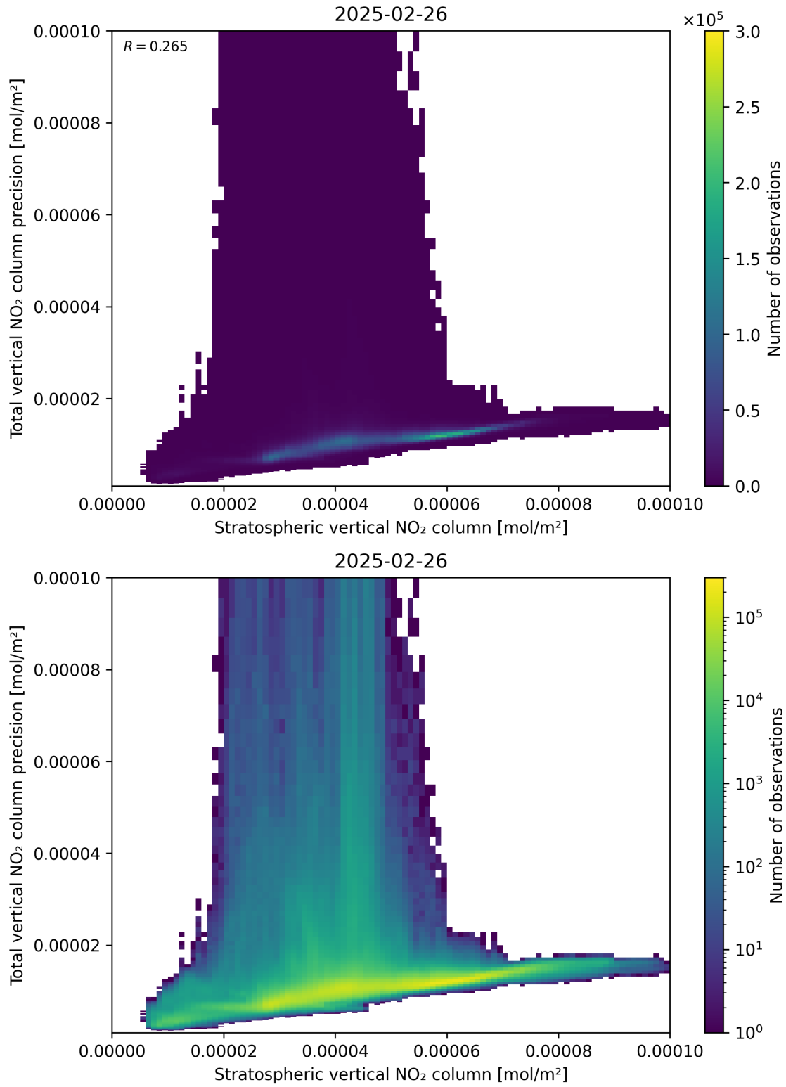
Figure 101: Scatter density plot of “Stratospheric vertical NO 2 column” against “Total vertical NO 2 column precision” for 2025-02-25 to 2025-02-27.
