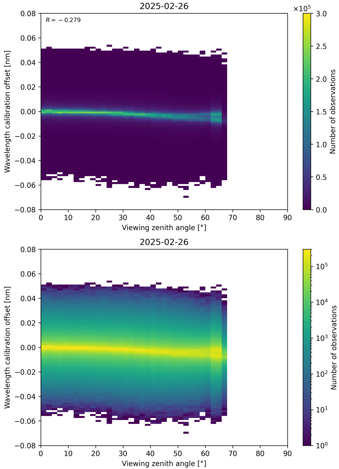
Figure 173: Scatter density plot of “Viewing zenith angle” against “Wavelength calibration offset” for 2025-02-25 to 2025-02-27.
