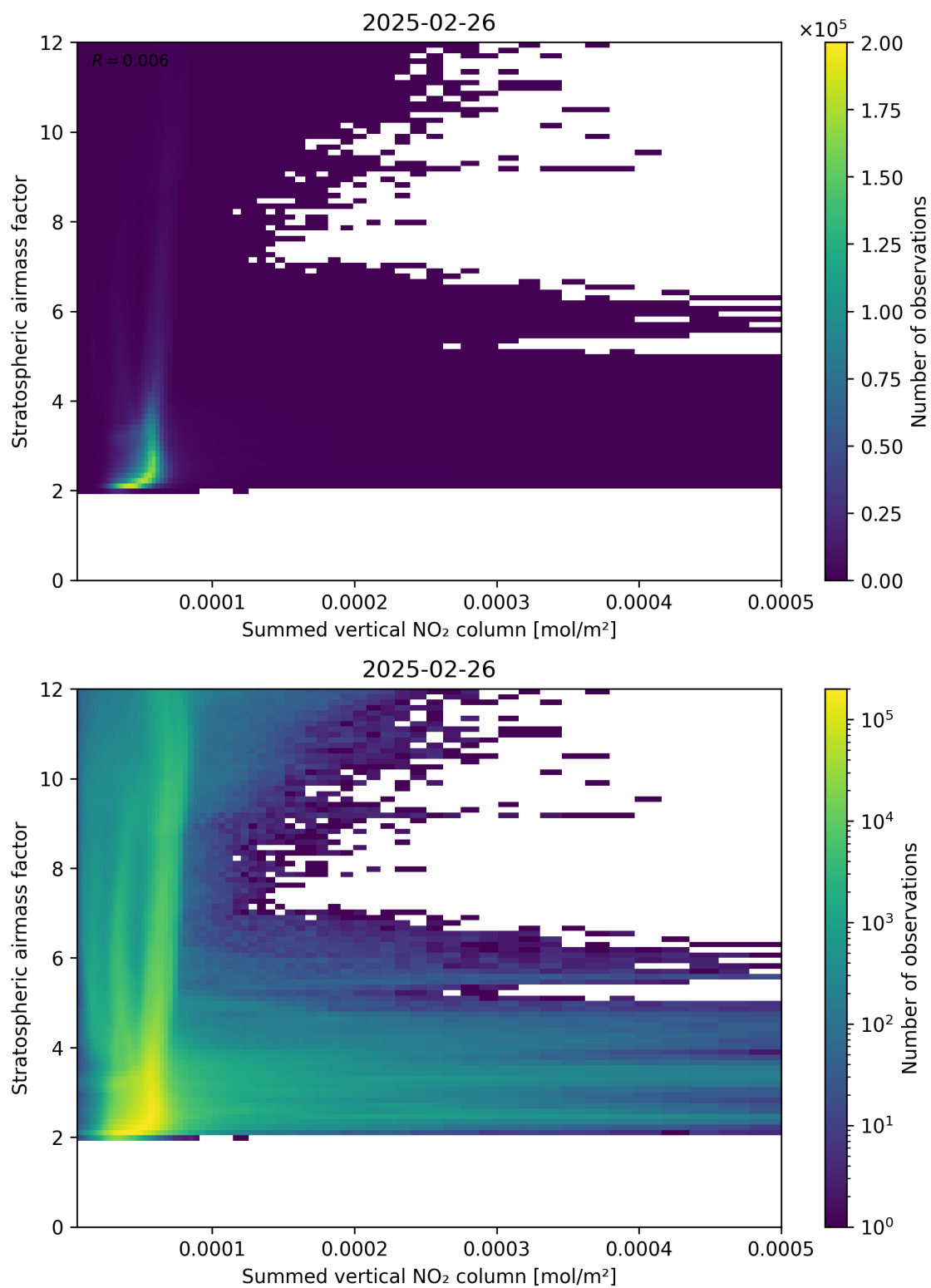
Figure 103: Scatter density plot of “Summed vertical NO 2 column” against “Stratospheric airmass factor” for 2025-02-25 to 2025-02-27.
