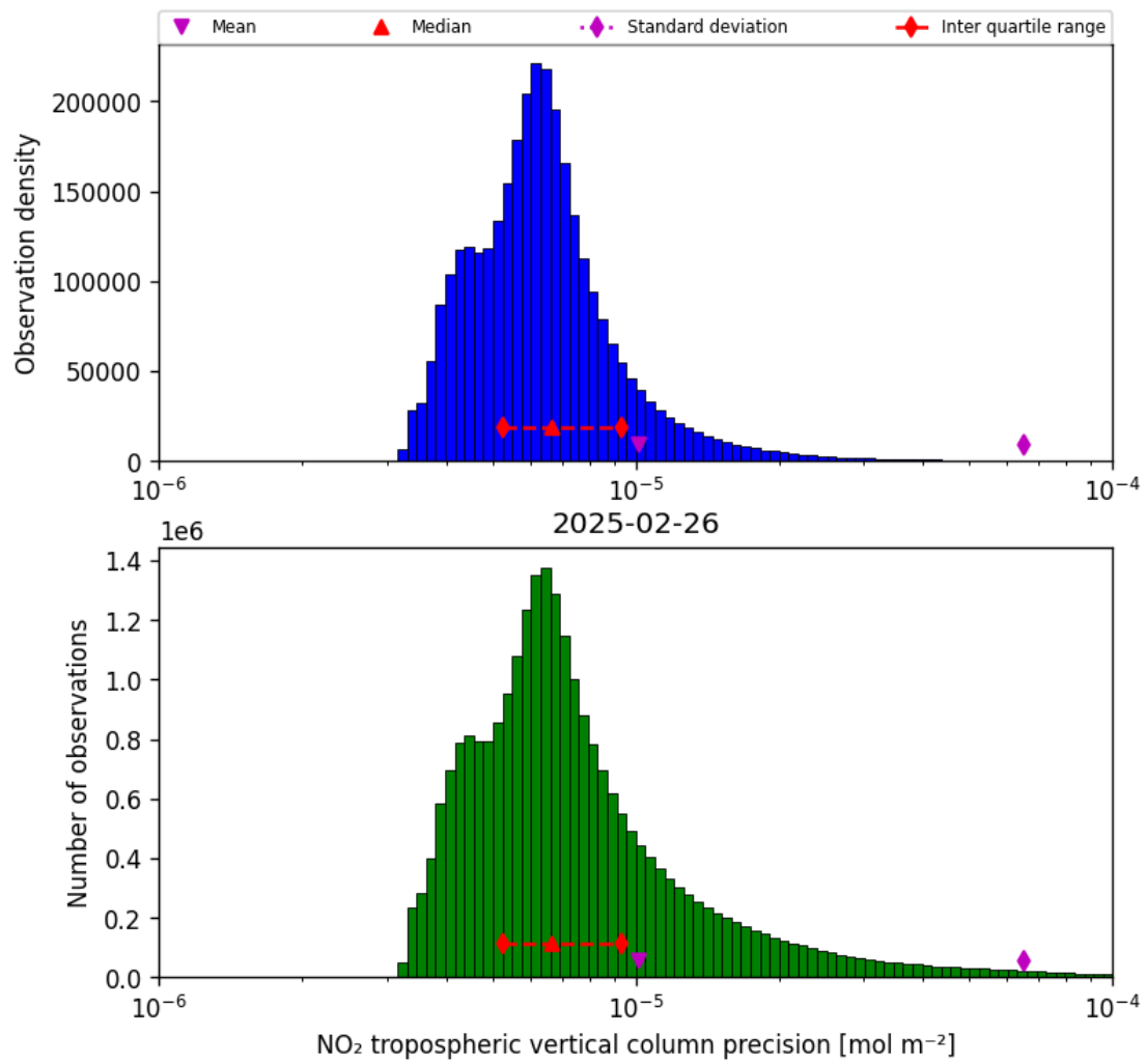
Figure 30: Histogram of “NO 2 tropospheric vertical column precision” for 2025-02-25 to 2025-02-27
