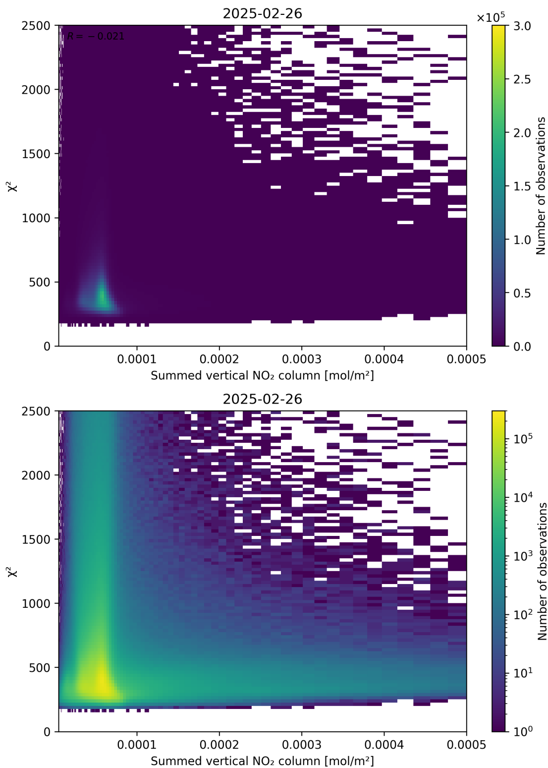
Figure 104: Scatter density plot of “Summed vertical NO 2 column” against “ \chi^2 ” for 2025-02-25 to 2025-02-27.
