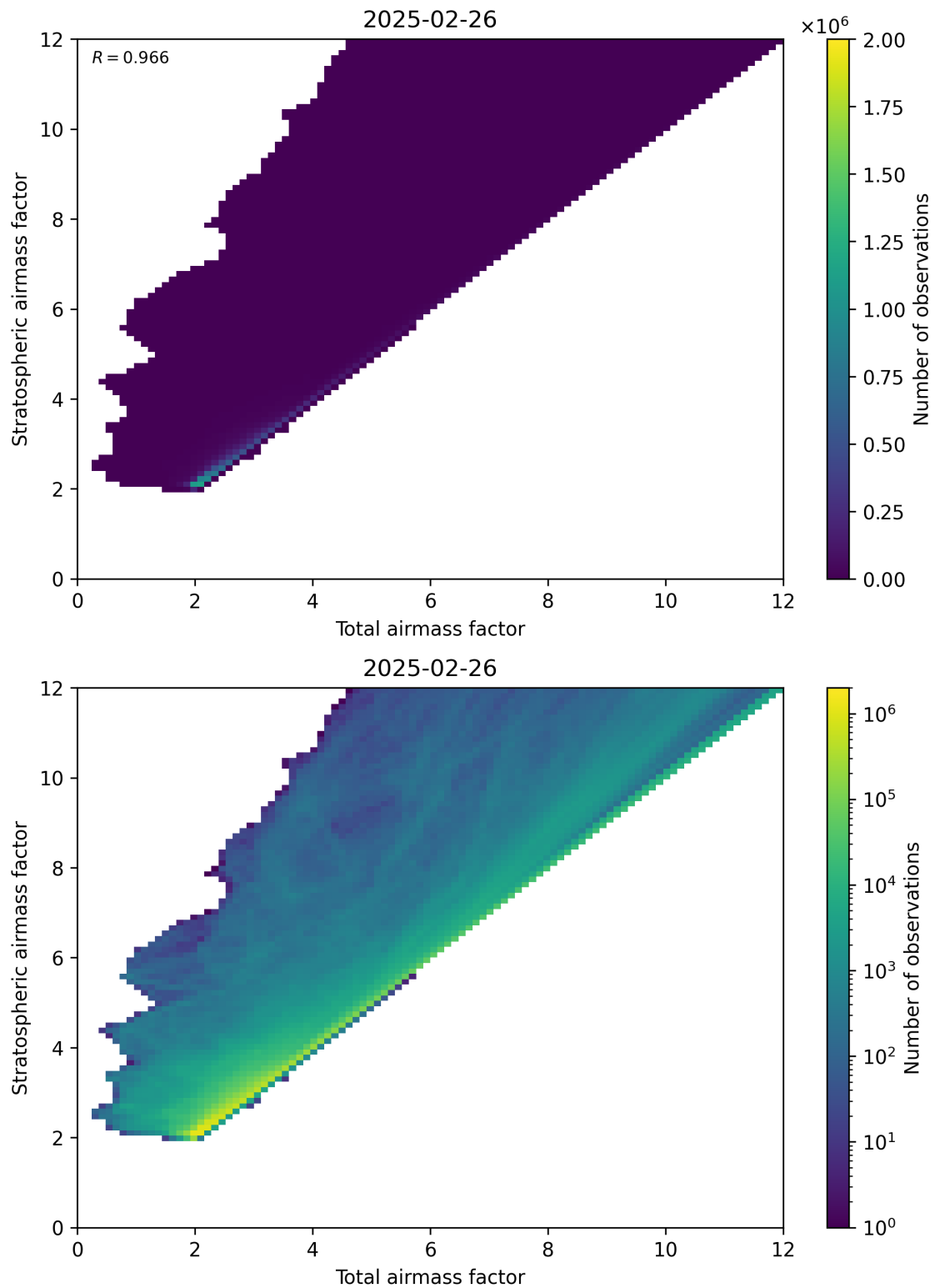
Figure 62: Scatter density plot of “Total airmass factor” against “Stratospheric airmass factor” for 2025-02-25 to 2025-02-27.
