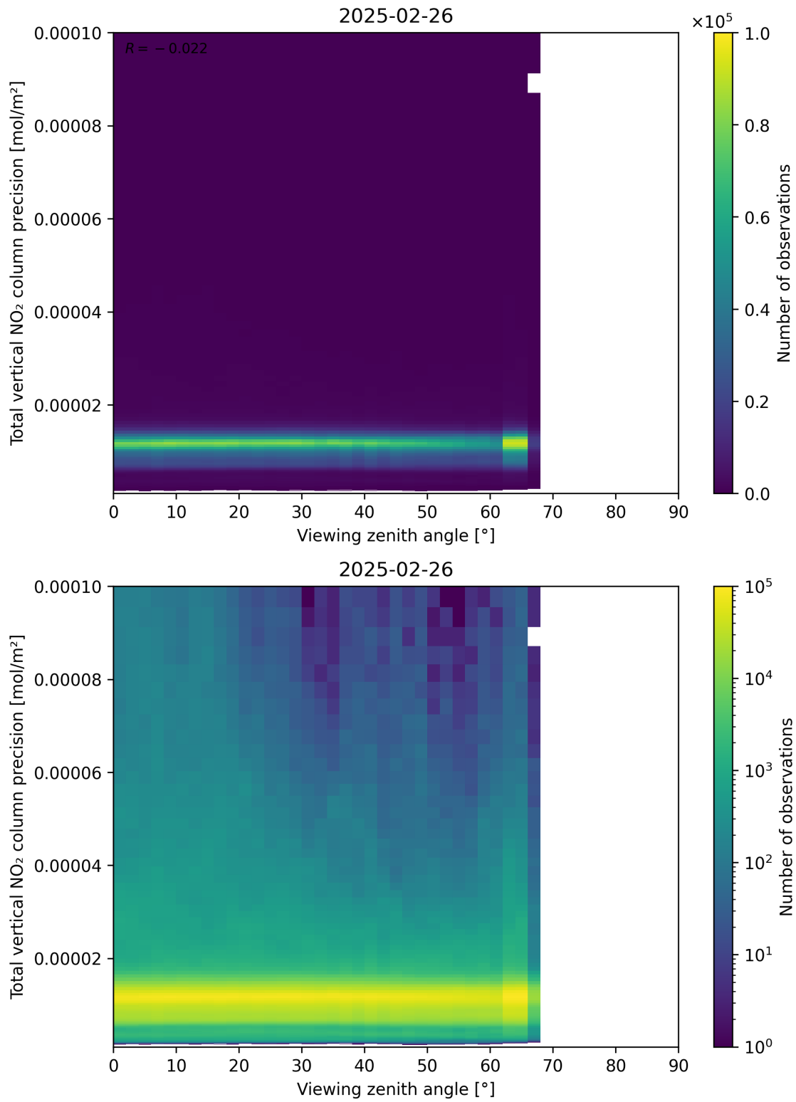
Figure 168: Scatter density plot of “Viewing zenith angle” against “Total vertical NO 2 column precision” for 2025-02-25 to 2025-02-27.
