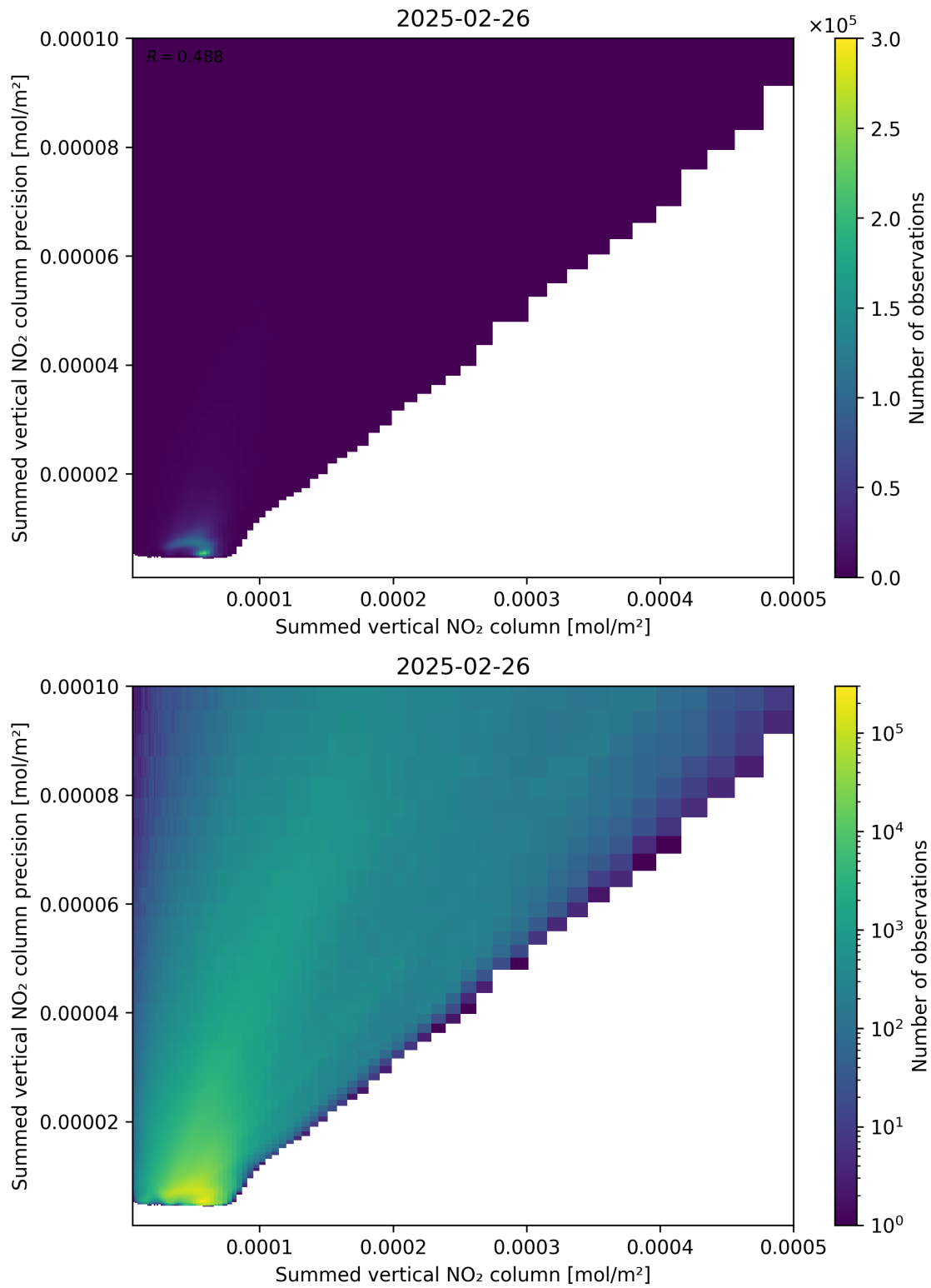
Figure 105: Scatter density plot of “Summed vertical NO 2 column” against “Summed vertical NO 2 column precision” for 2025-02-25 to 2025-02-27.
