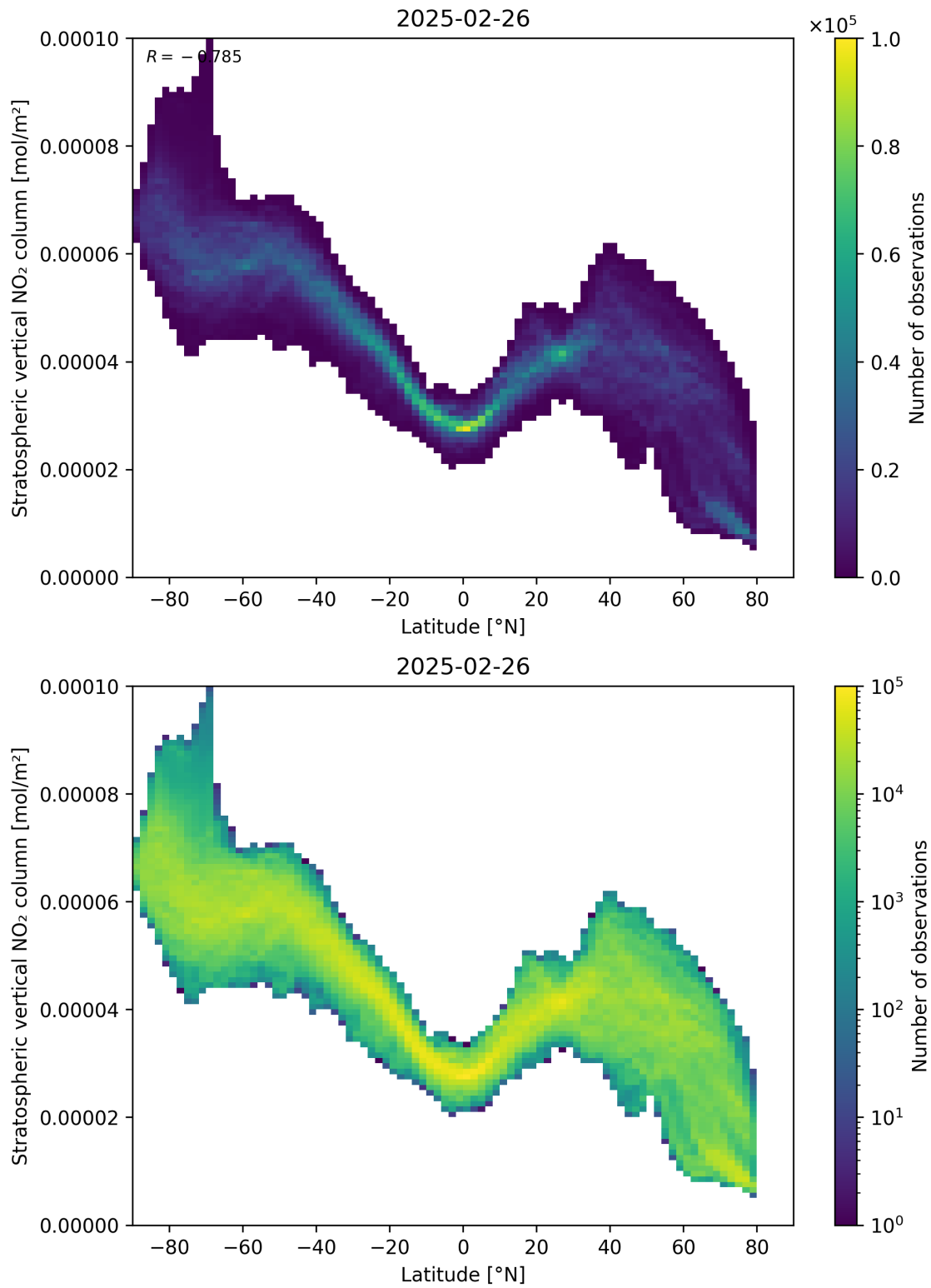
Figure 87: Scatter density plot of “Latitude” against “Stratospheric vertical NO 2 column” for 2025-02-25 to 2025-02-27.
