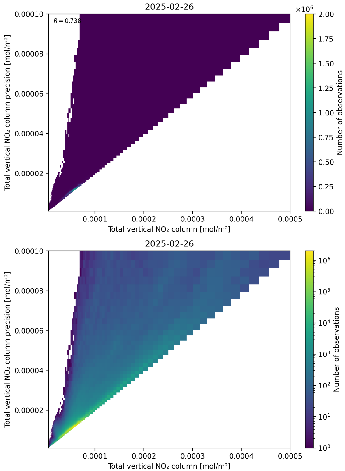
Figure 114: Scatter density plot of “Total vertical NO 2 column” against “Total vertical NO 2 column precision” for 2025-02-25 to 2025-02-27.
