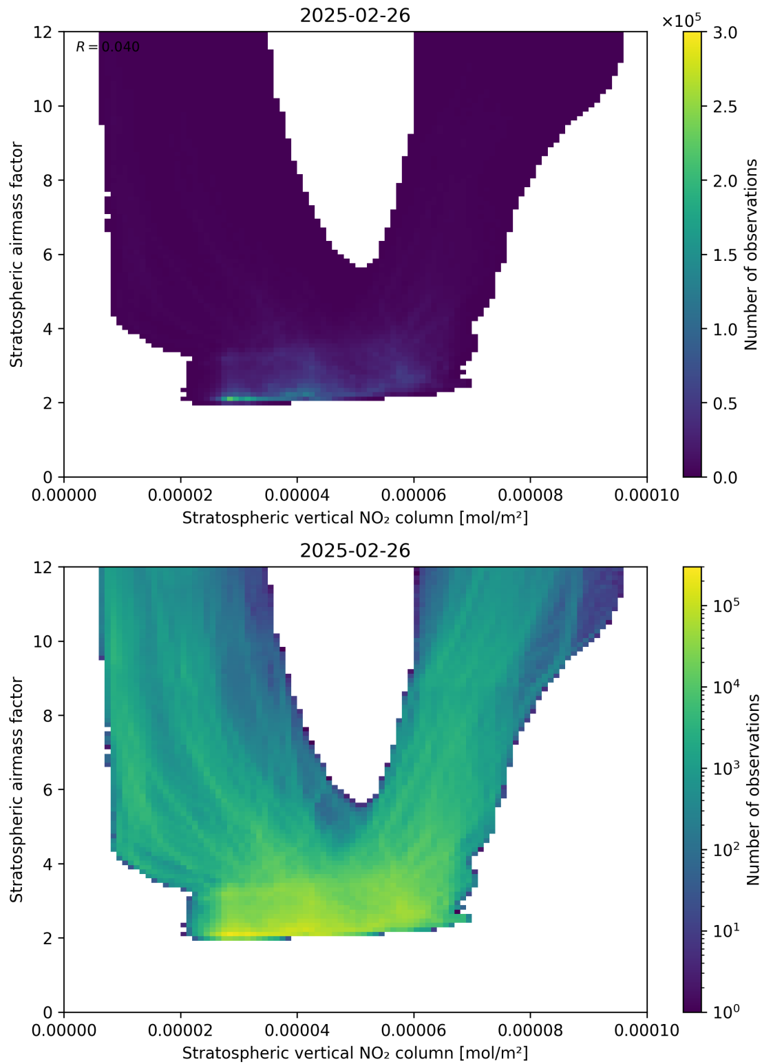
Figure 96: Scatter density plot of “Stratospheric vertical NO 2 column” against “Stratospheric airmass factor” for 2025-02-25 to 2025-02-27.
