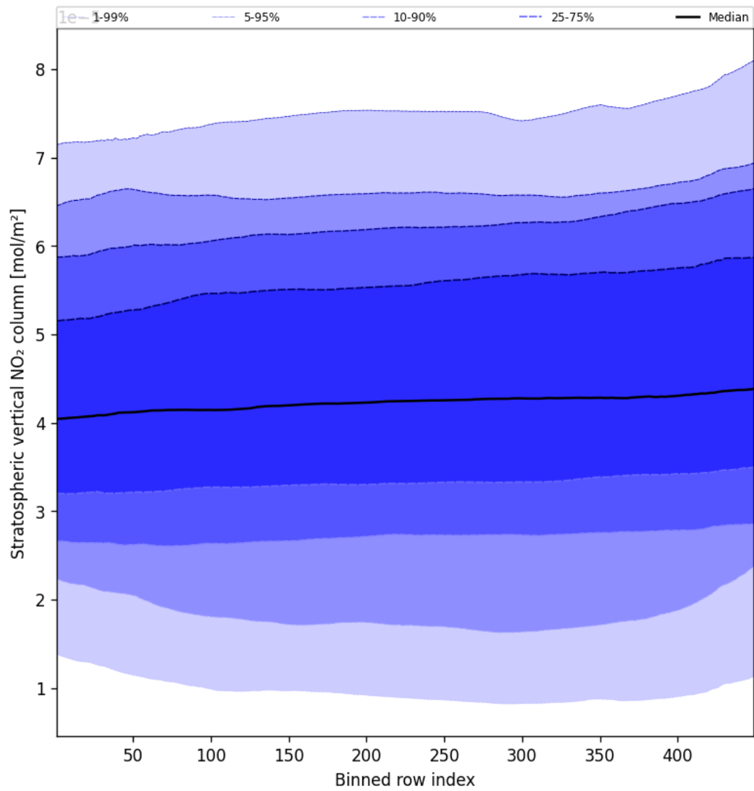
Figure 53: Along track statistics of “Stratospheric vertical NO 2 column” for 2025-02-25 to 2025-02-27
