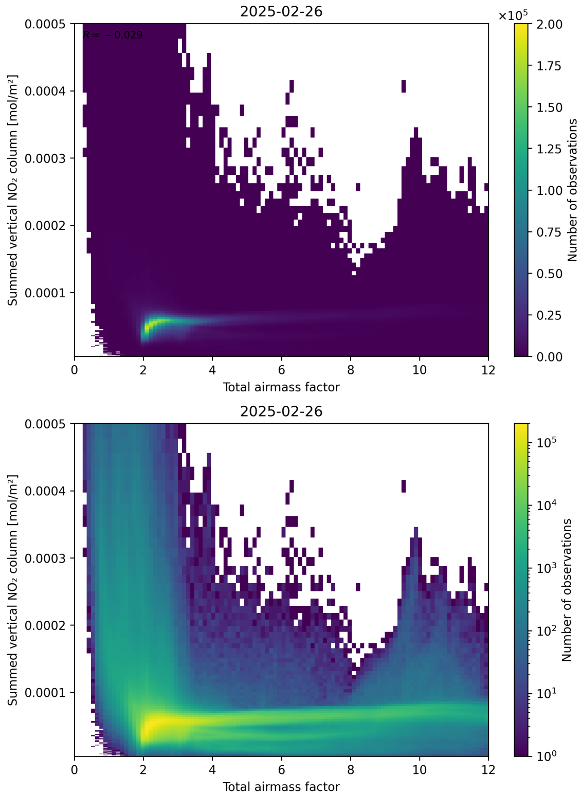
Figure 65: Scatter density plot of “Total airmass factor” against “Summed vertical NO 2 column” for 2025-02-25 to 2025-02-27.
