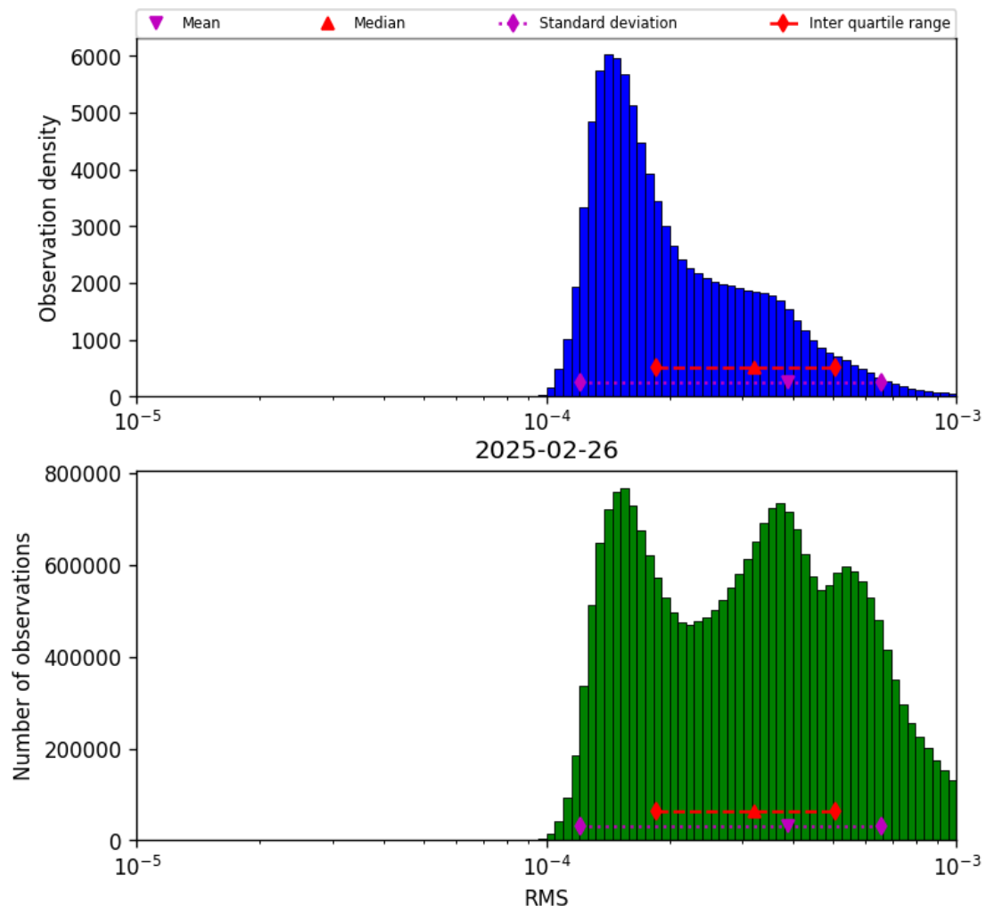
Figure 43: Histogram of “RMS” for 2025-02-25 to 2025-02-27
