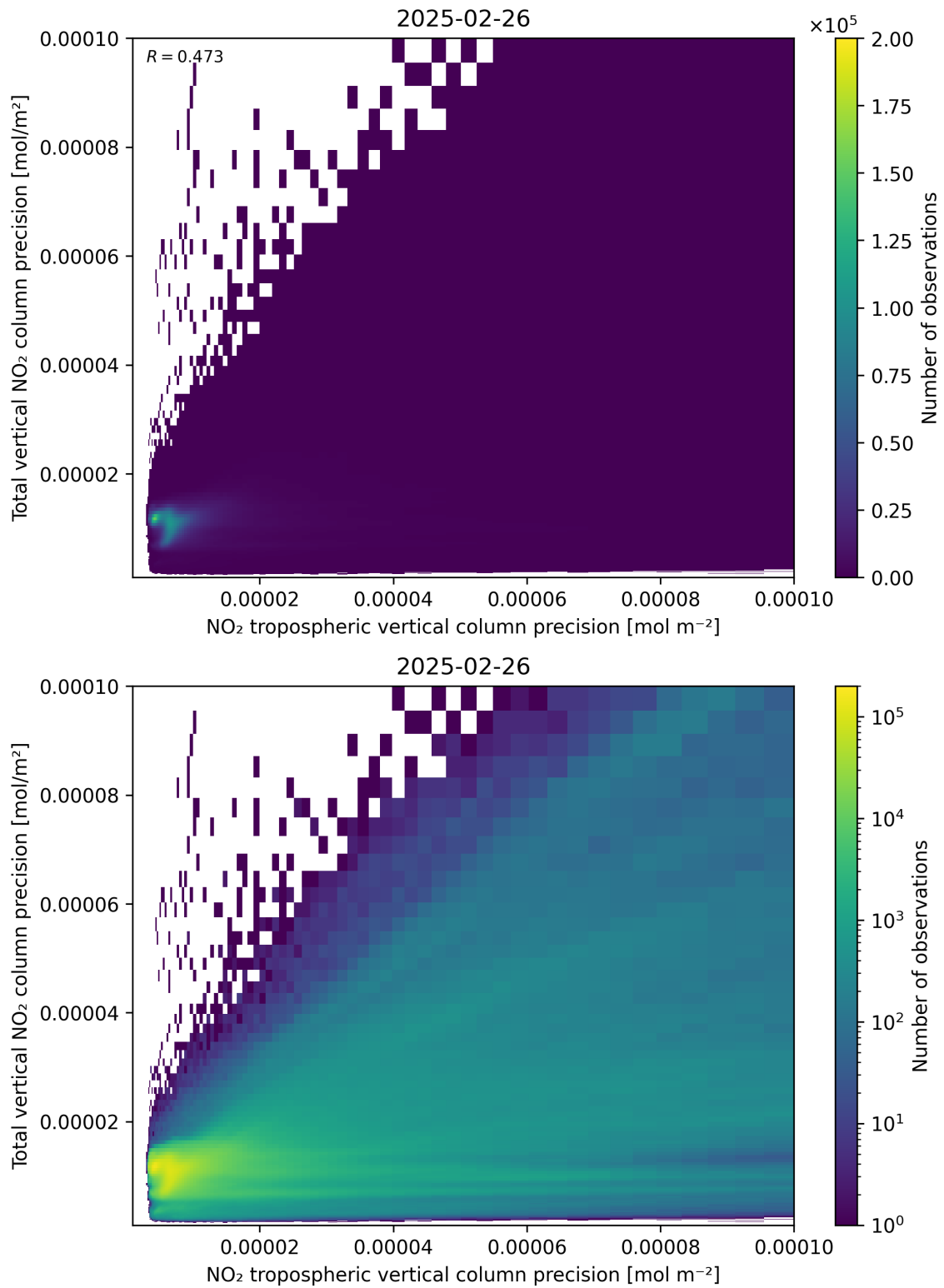
Figure 139: Scatter density plot of “NO 2 tropospheric vertical column precision” against “Total vertical NO 2 column precision” for 2025-02-25 to 2025-02-27.
