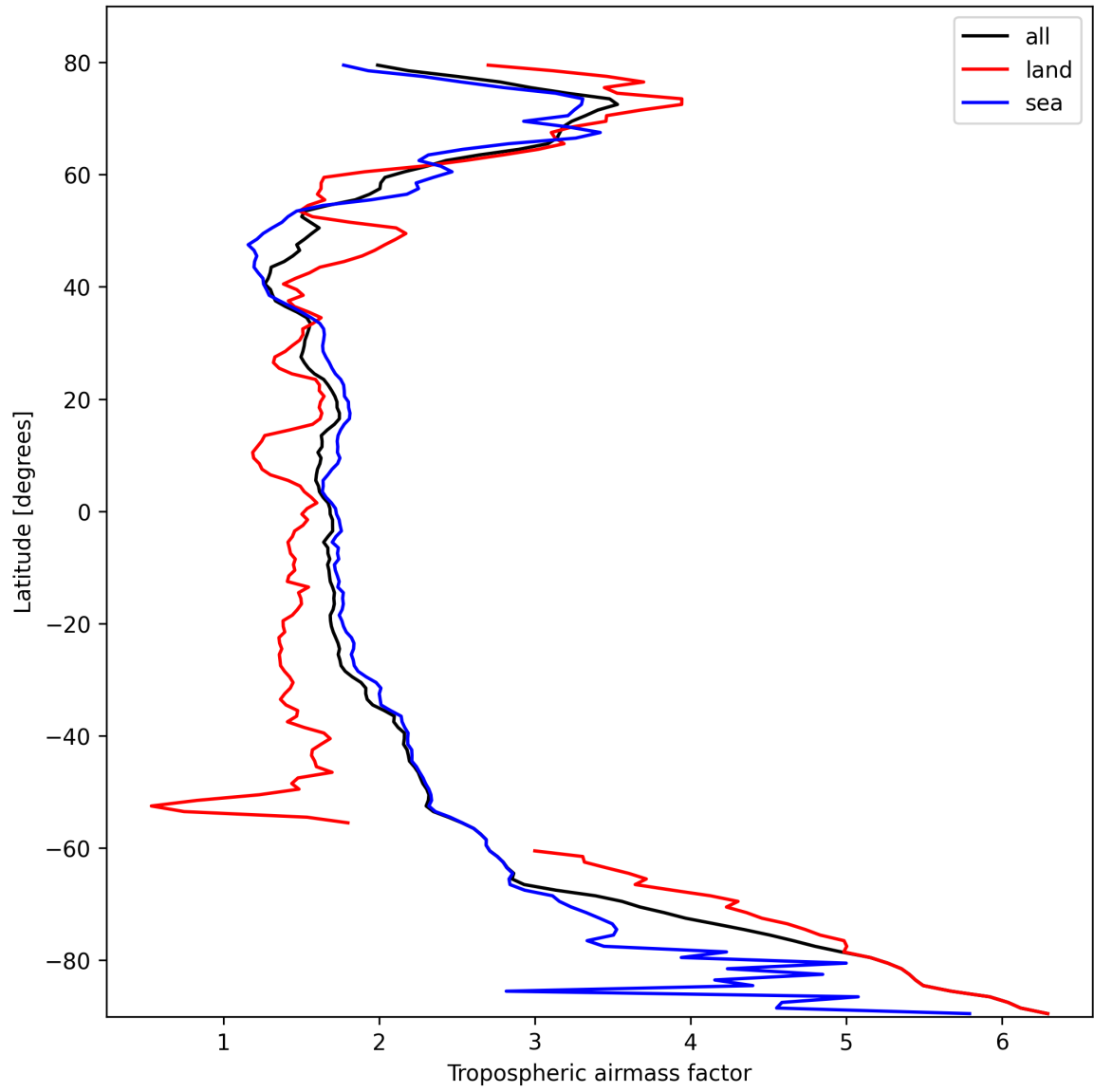
Figure 14: Zonal average of “Tropospheric airmass factor” for 2025-02-25 to 2025-02-27.
