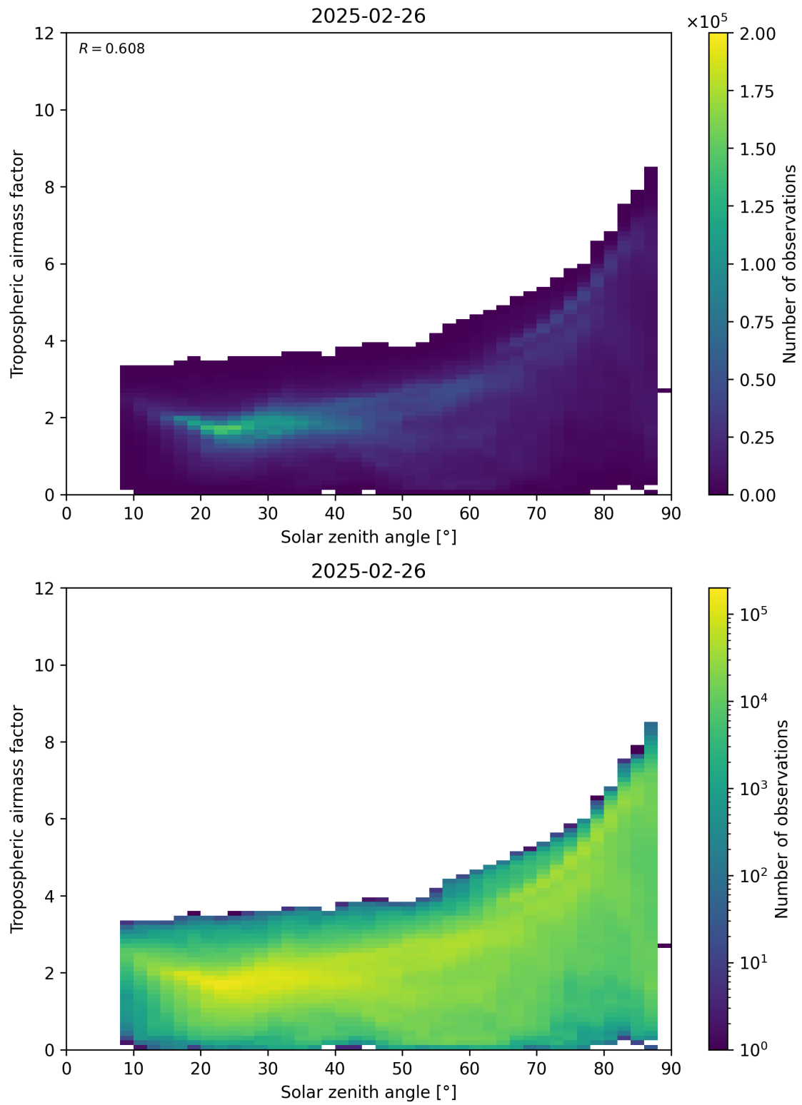
Figure 147: Scatter density plot of “Solar zenith angle” against “Tropospheric airmass factor” for 2025-02-25 to 2025-02-27.
