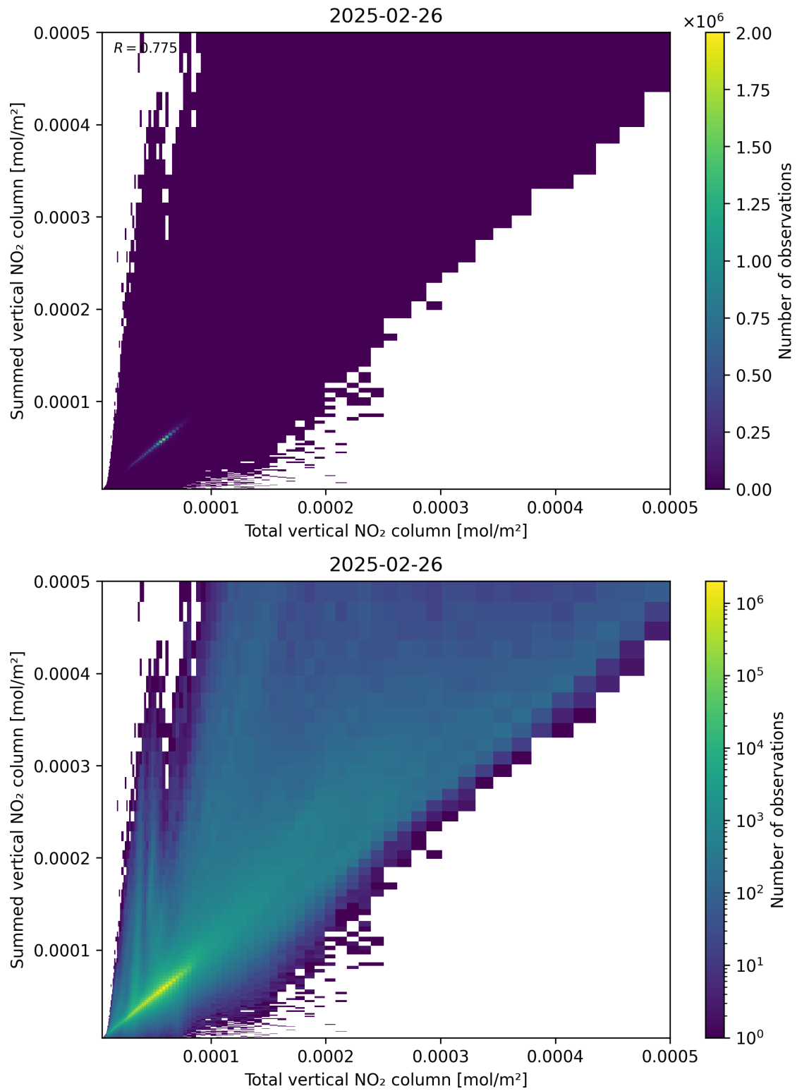
Figure 112: Scatter density plot of “Total vertical NO 2 column” against “Summed vertical NO 2 column” for 2025-02-25 to 2025-02-27.
