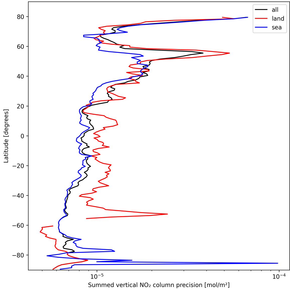
Figure 24: Zonal average of “Summed vertical NO 2 column precision” for 2025-02-25 to 2025-02-27.
