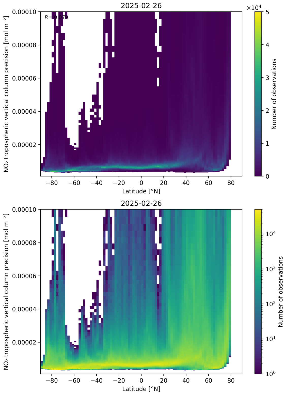
Figure 93: Scatter density plot of “Latitude” against “NO 2 tropospheric vertical column precision” for 2025-02-25 to 2025-02-27.
