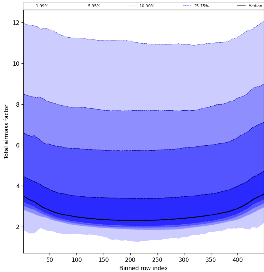
Figure 49: Along track statistics of “Total airmass factor” for 2025-02-25 to 2025-02-27
