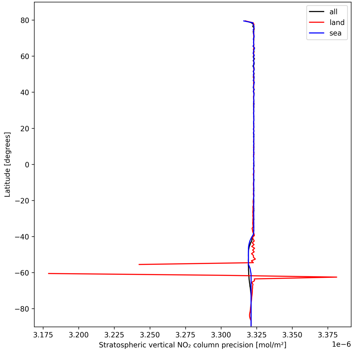
Figure 20: Zonal average of “Stratospheric vertical NO 2 column precision” for 2025-02-25 to 2025-02-27.
