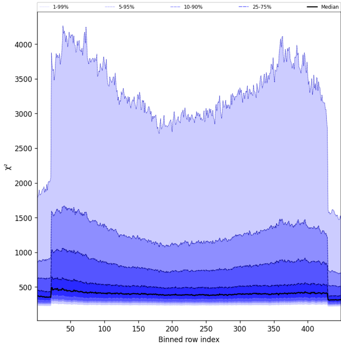
Figure 59: Along track statistics of “ \chi^2 ” for 2025-02-25 to 2025-02-27
