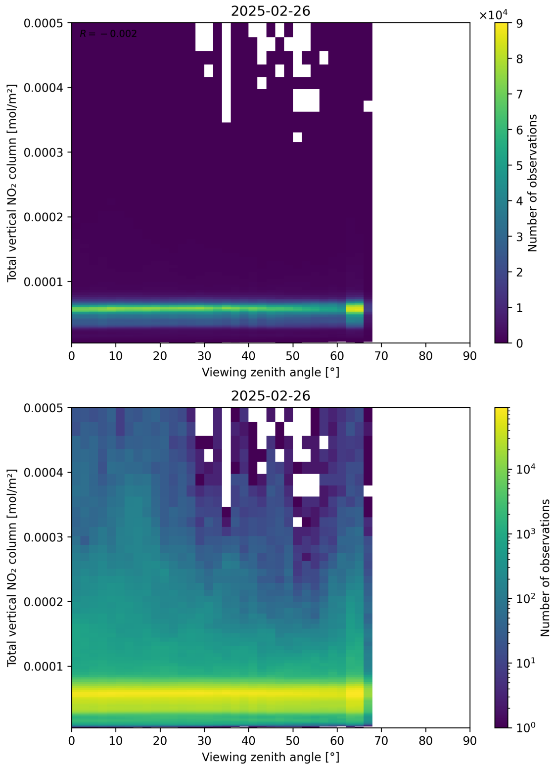
Figure 167: Scatter density plot of “Viewing zenith angle” against “Total vertical NO 2 column” for 2025-02-25 to 2025-02-27.
