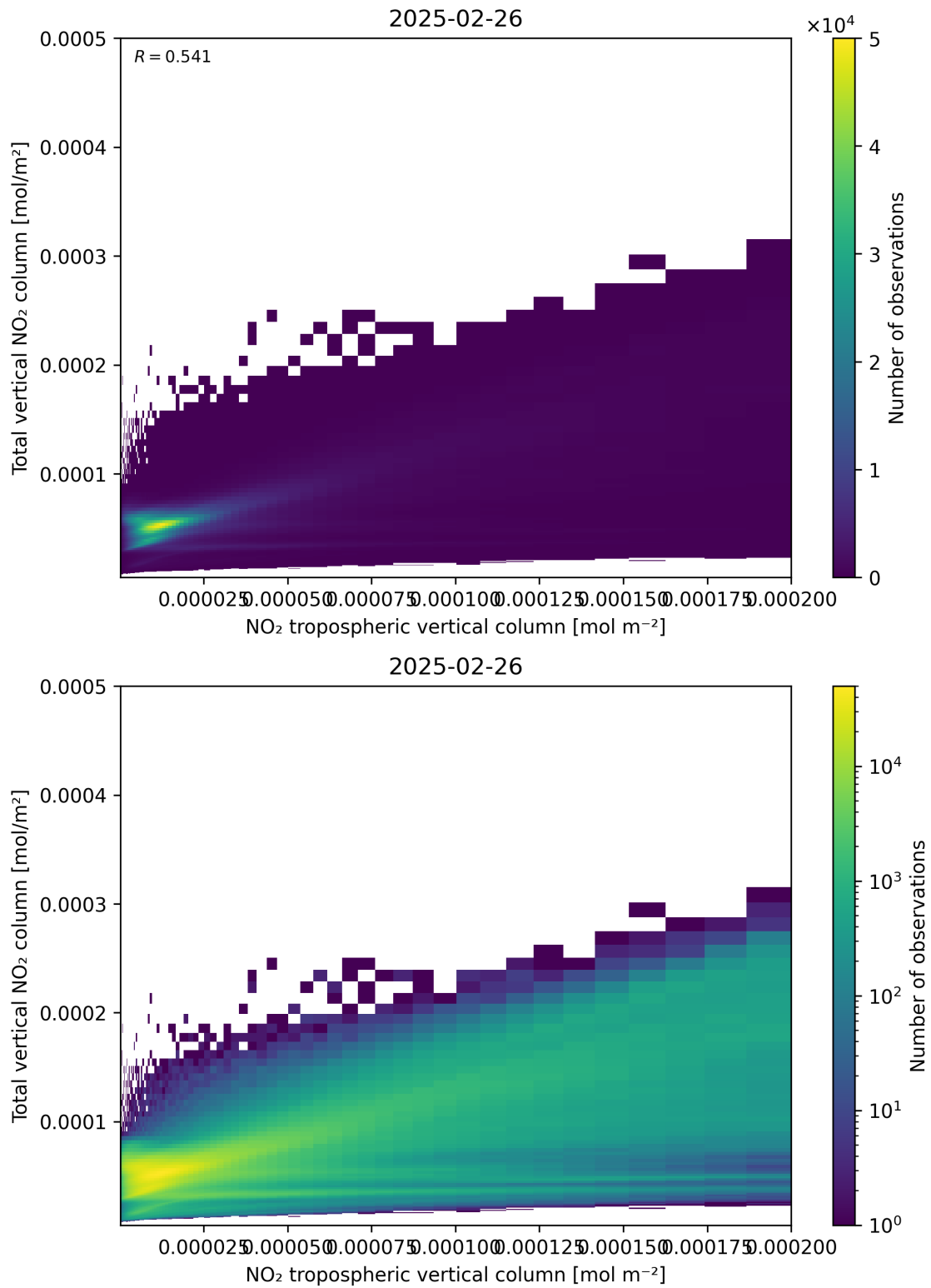
Figure 128: Scatter density plot of “NO 2 tropospheric vertical column” against “Total vertical NO 2 column” for 2025-02-25 to 2025-02-27.
