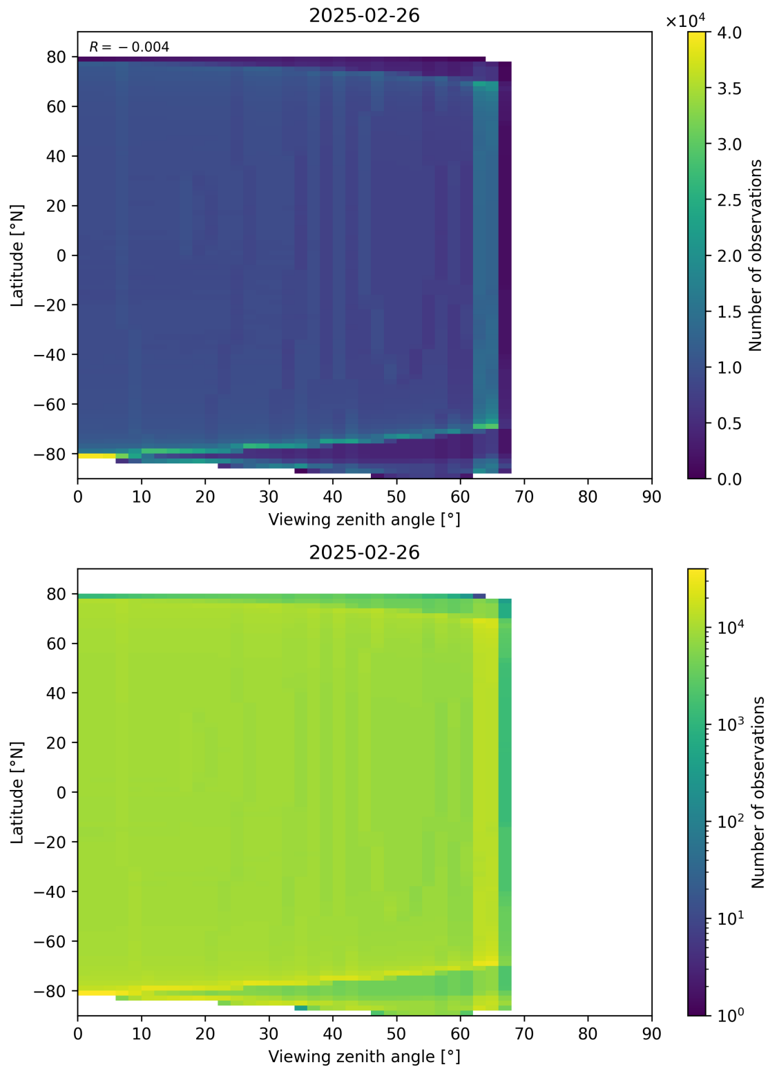
Figure 163: Scatter density plot of “Viewing zenith angle” against “Latitude” for 2025-02-25 to 2025-02-27.
