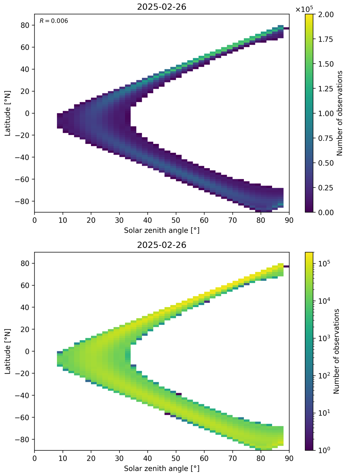
Figure 149: Scatter density plot of “Solar zenith angle” against “Latitude” for 2025-02-25 to 2025-02-27.
