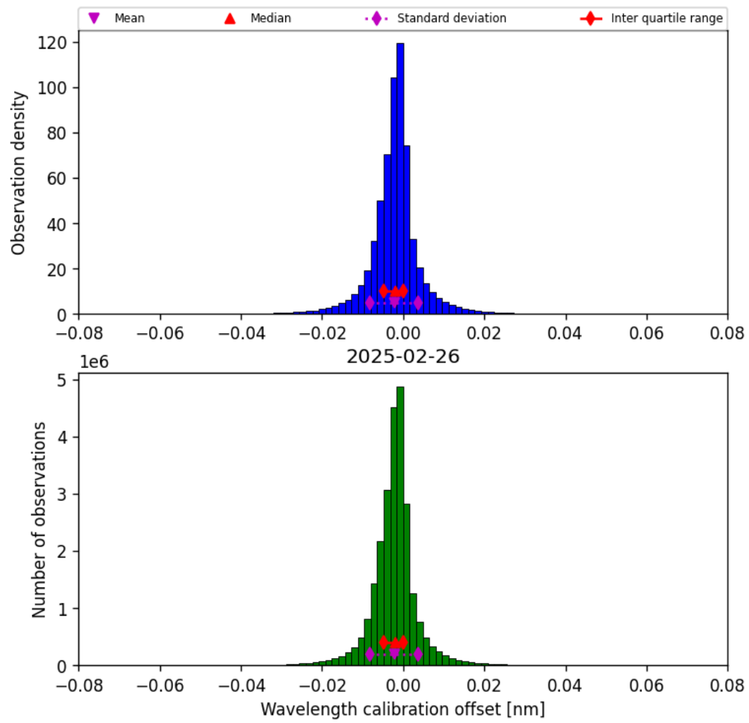
Figure 35: Histogram of “Wavelength calibration offset” for 2025-02-25 to 2025-02-27
