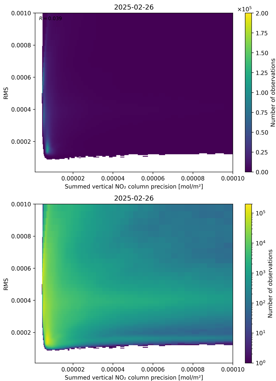
Figure 108: Scatter density plot of “Summed vertical NO 2 column precision” against “RMS” for 2025-02-25 to 2025-02-27.
