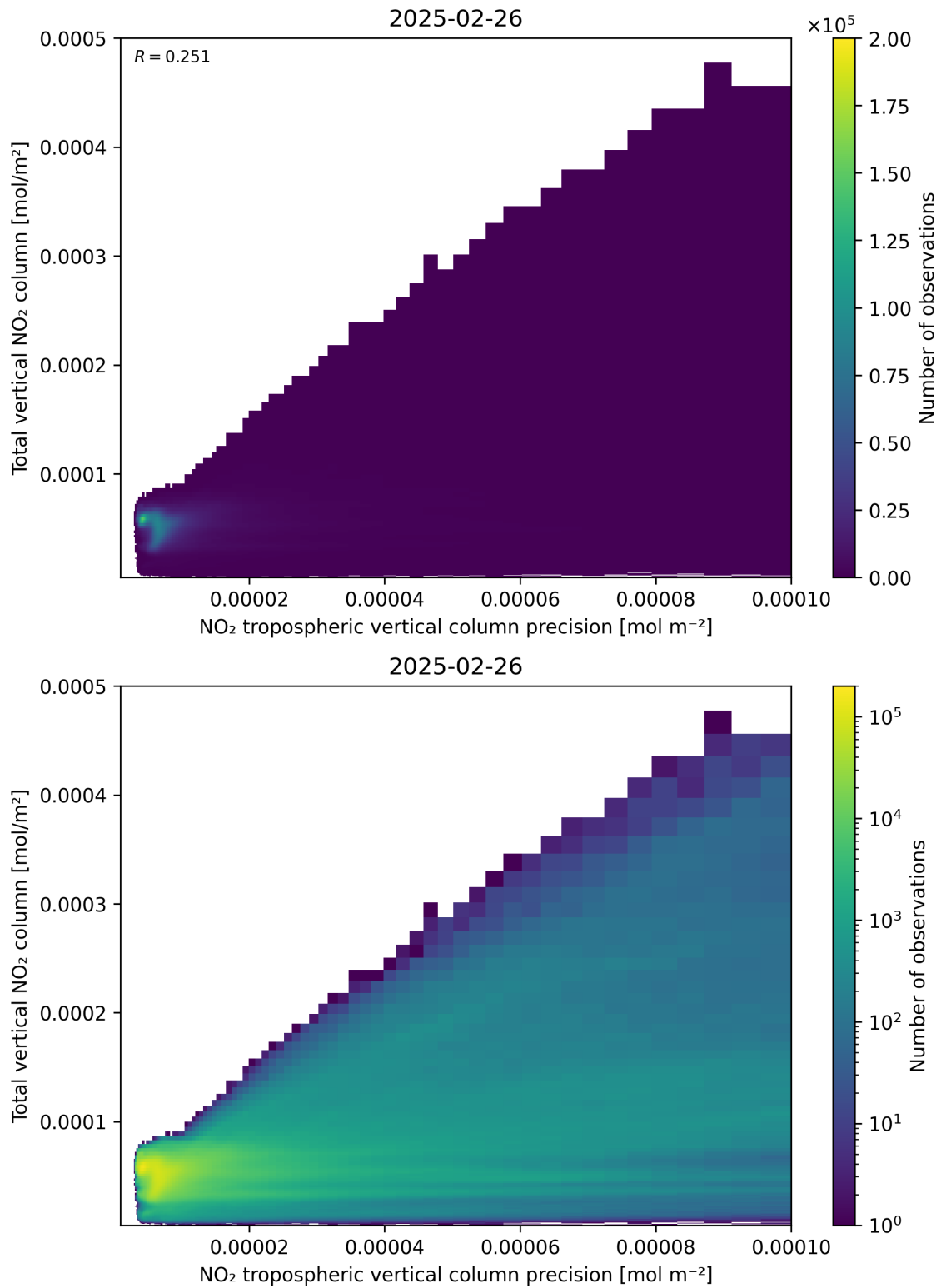
Figure 138: Scatter density plot of “NO 2 tropospheric vertical column precision” against “Total vertical NO 2 column” for 2025-02-25 to 2025-02-27.
