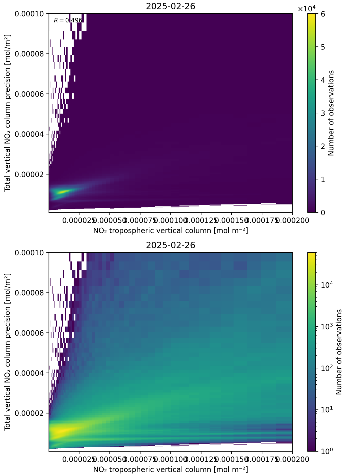
Figure 129: Scatter density plot of “NO 2 tropospheric vertical column” against “Total vertical NO 2 column precision” for 2025-02-25 to 2025-02-27.
