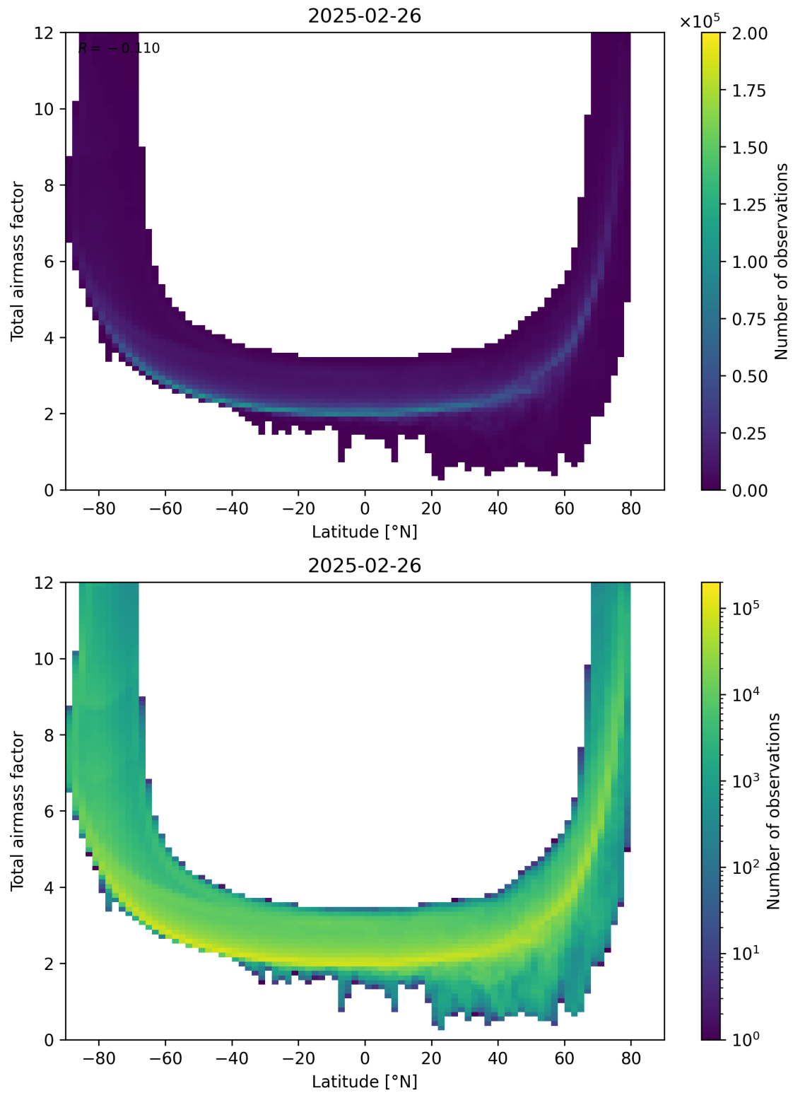
Figure 84: Scatter density plot of “Latitude” against “Total airmass factor” for 2025-02-25 to 2025-02-27.
