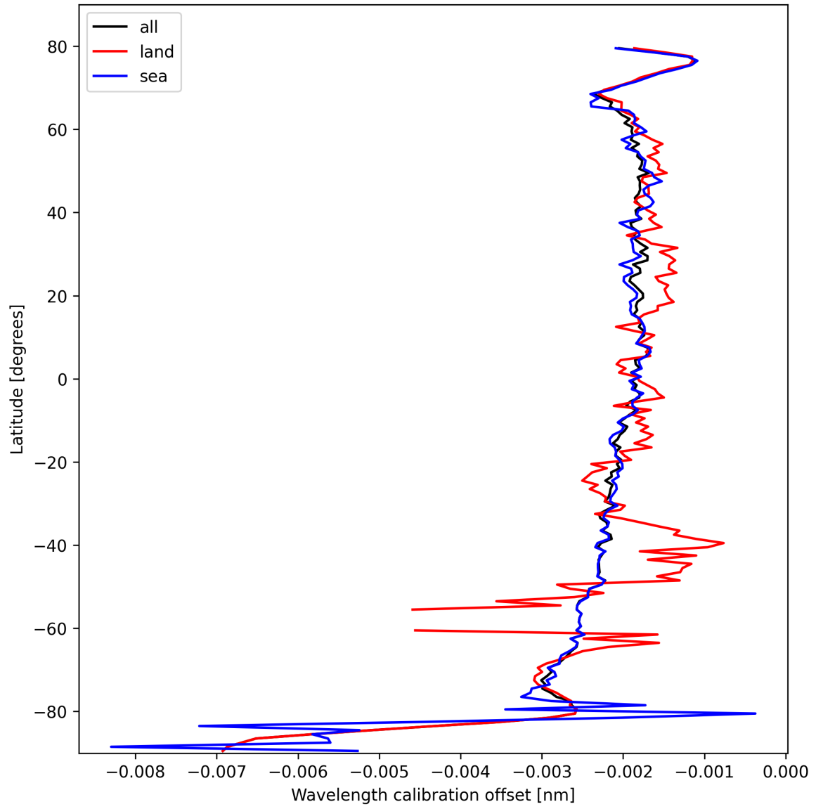
Figure 18: Zonal average of “Wavelength calibration offset” for 2025-02-25 to 2025-02-27.
