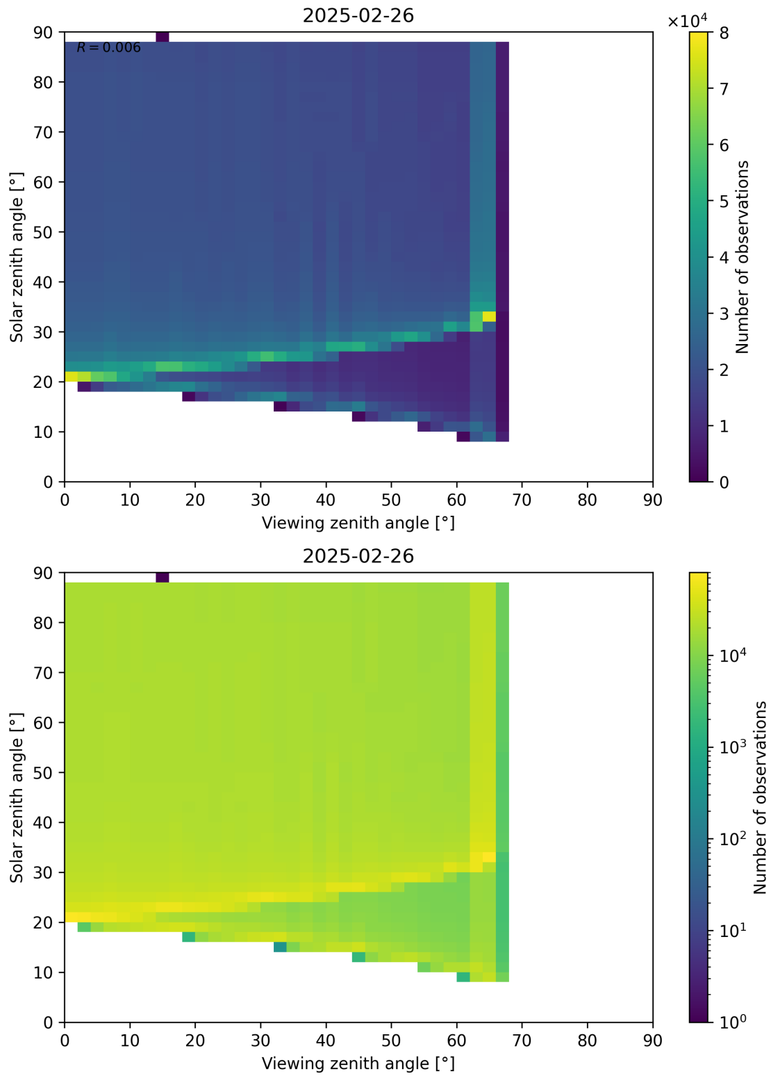
Figure 172: Scatter density plot of “Viewing zenith angle” against “Solar zenith angle” for 2025-02-25 to 2025-02-27.
