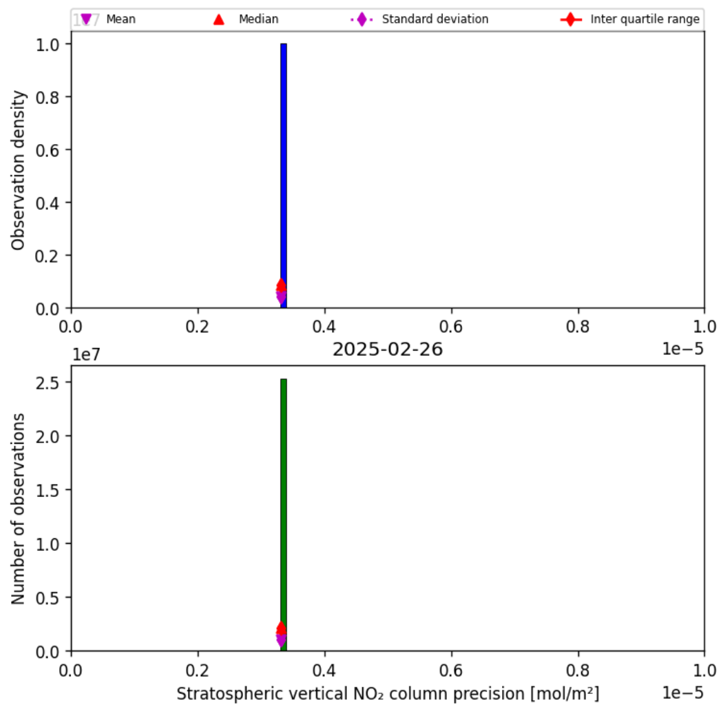
Figure 37: Histogram of “Stratospheric vertical NO 2 column precision” for 2025-02-25 to 2025-02-27
