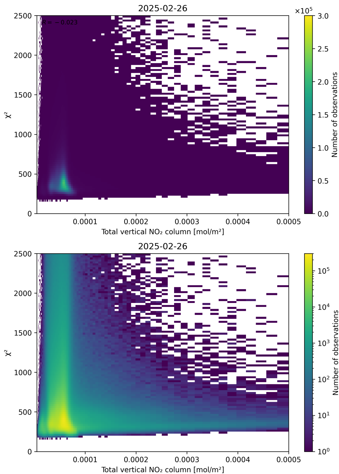
Figure 111: Scatter density plot of “Total vertical NO 2 column” against “ \chi^2 ” for 2025-02-25 to 2025-02-27.
