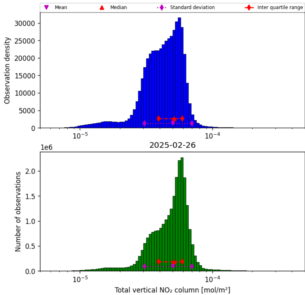
Figure 38: Histogram of “Total vertical NO 2 column” for 2025-02-25 to 2025-02-27
