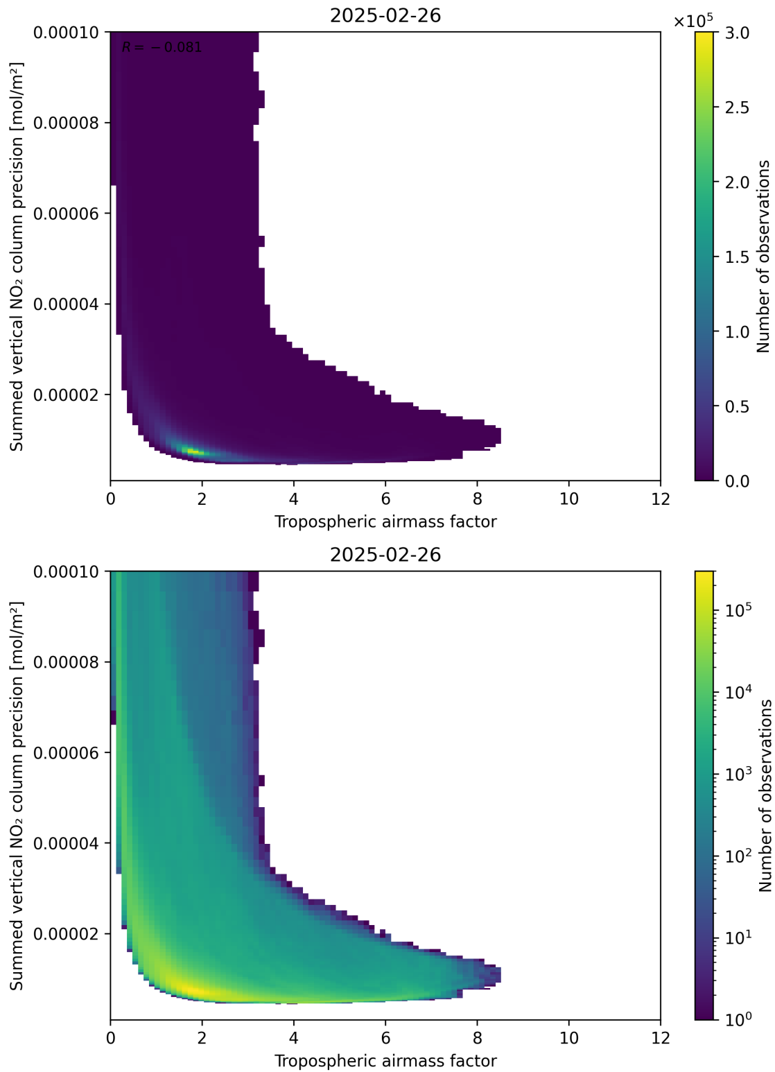
Figure 76: Scatter density plot of “Tropospheric air mass factor” against “Summed vertical NO 2 column precision” for 2025-02-25 to 2025-02-27.
