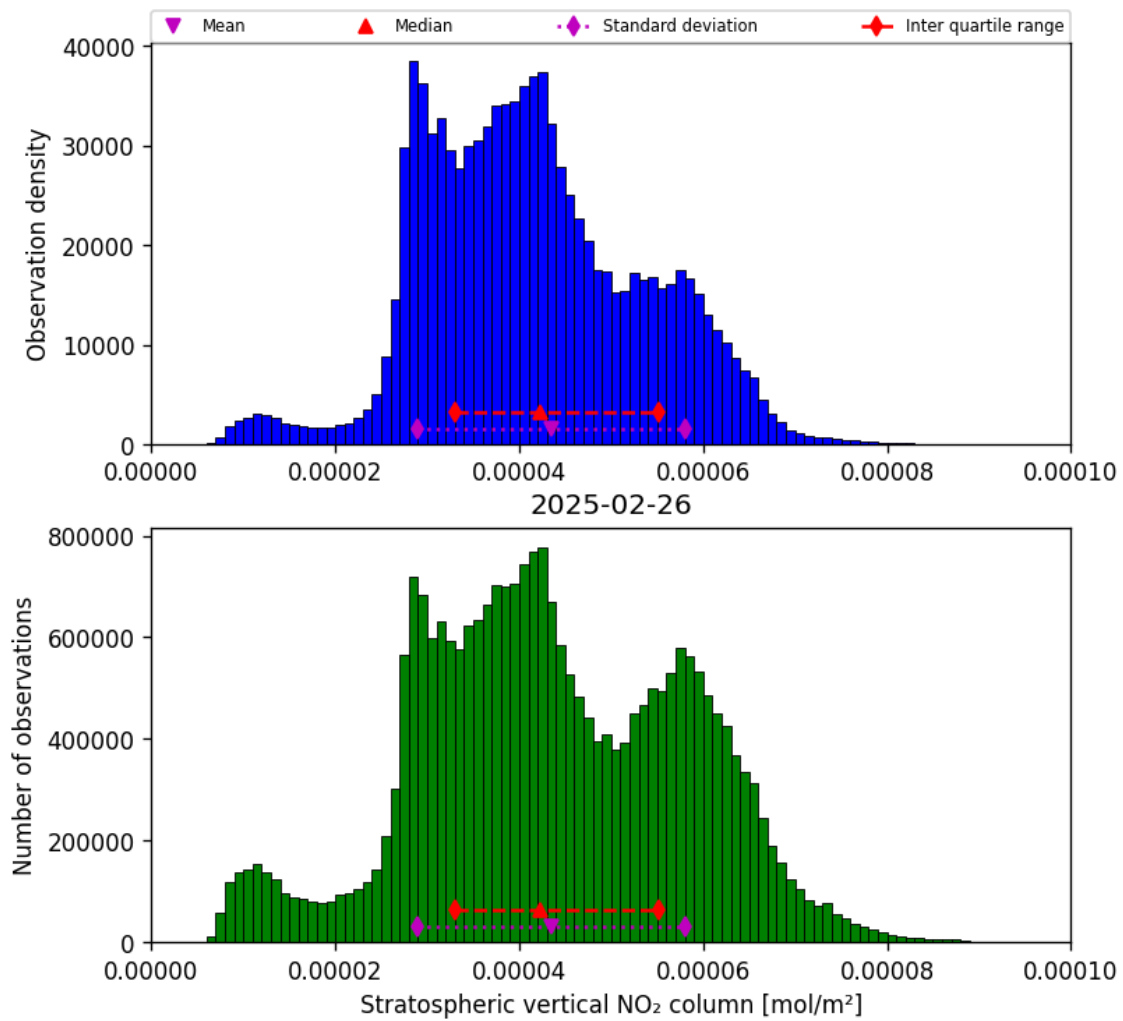
Figure 36: Histogram of “Stratospheric vertical NO 2 column” for 2025-02-25 to 2025-02-27
