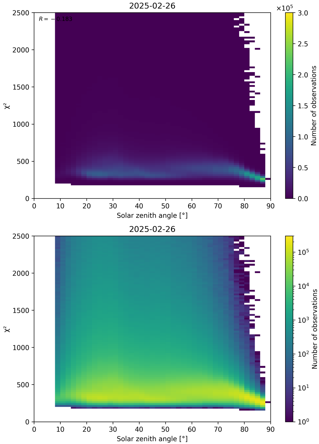
Figure 148: Scatter density plot of “Solar zenith angle” against “ \chi^2 ” for 2025-02-25 to 2025-02-27.
