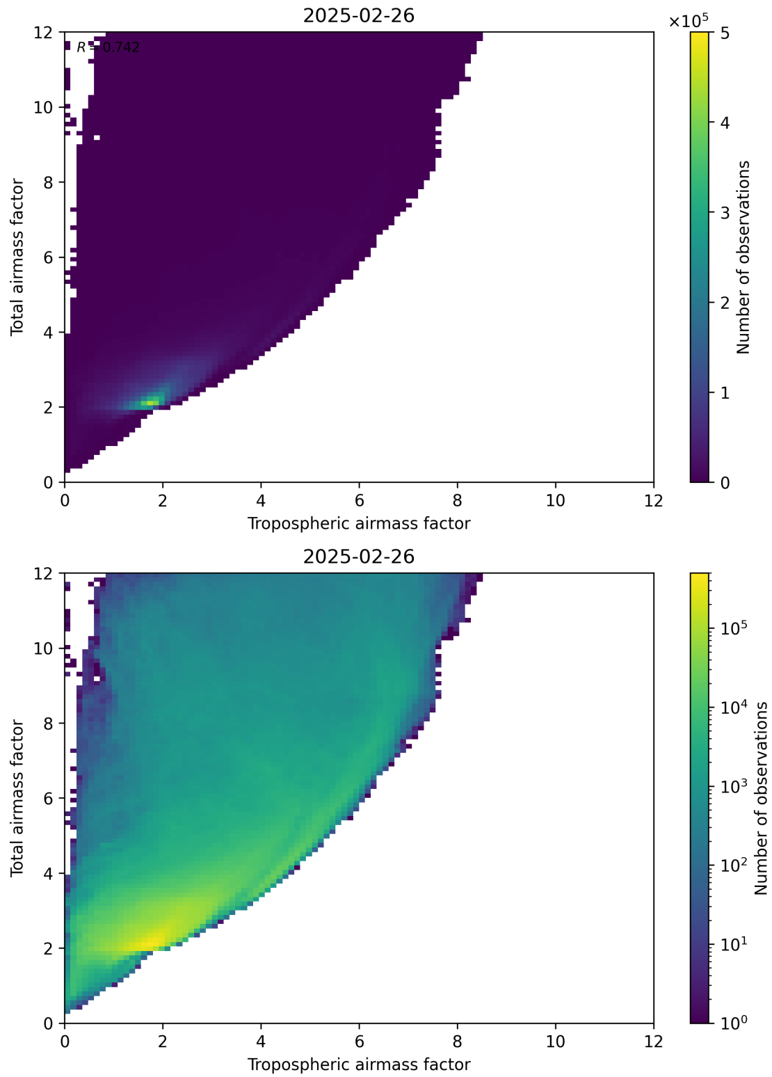
Figure 72: Scatter density plot of “Tropospheric airmass factor” against “Total airmass factor” for 2025-02-25 to 2025-02-27.
