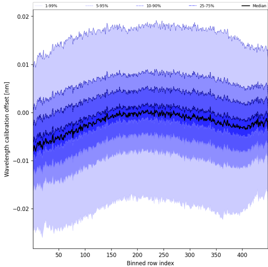
Figure 52: Along track statistics of “Wavelength calibration offset” for 2025-02-25 to 2025-02-27
