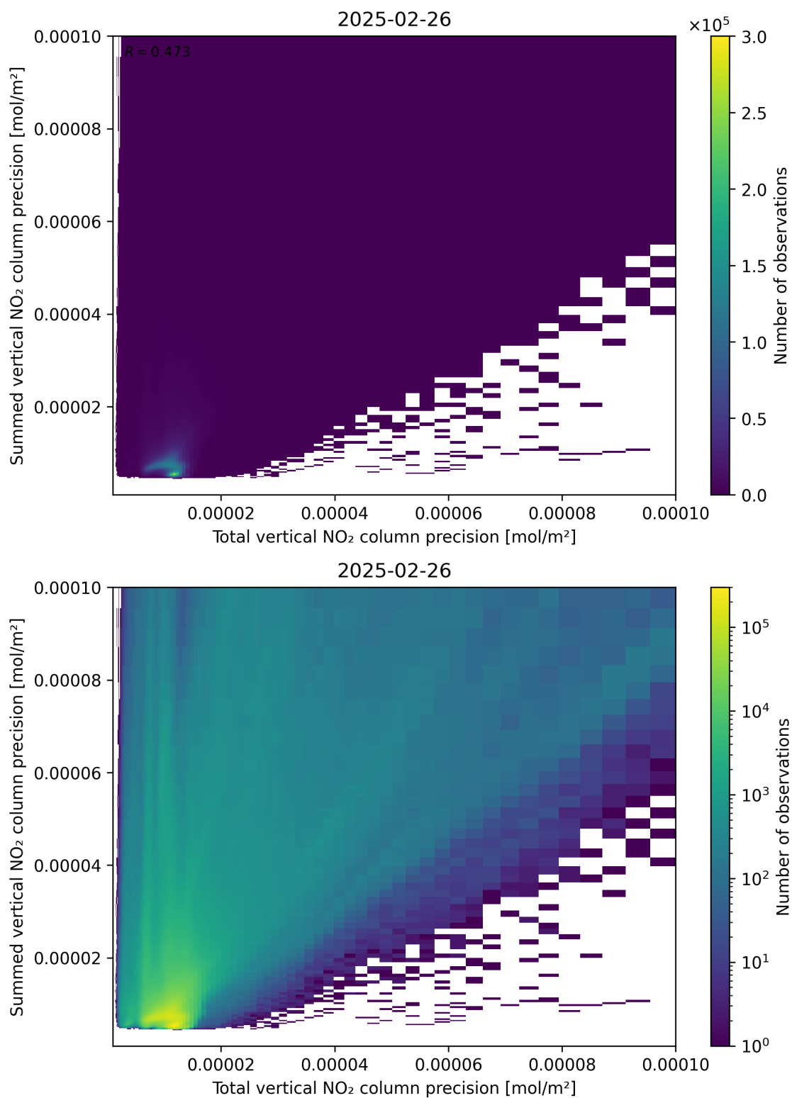
Figure 118: Scatter density plot of “Total vertical NO 2 column precision” against “Summed vertical NO 2 column precision” for 2025-02-25 to 2025-02-27.
