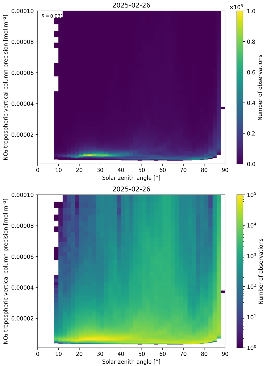
Figure 156: Scatter density plot of “Solar zenith angle” against “NO 2 tropospheric vertical column precision” for 2025-02-25 to 2025-02-27.
