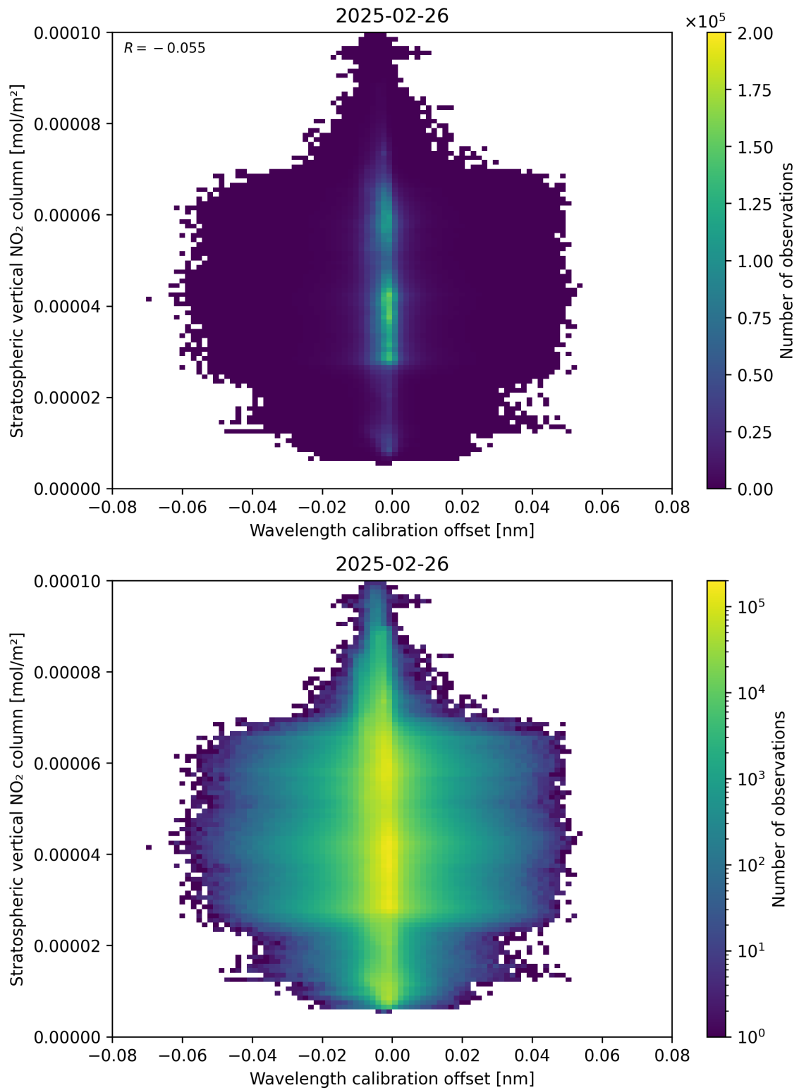
Figure 176: Scatter density plot of “Wavelength calibration offset” against “Stratospheric vertical NO 2 column” for 2025-02-25 to 2025-02-27.
