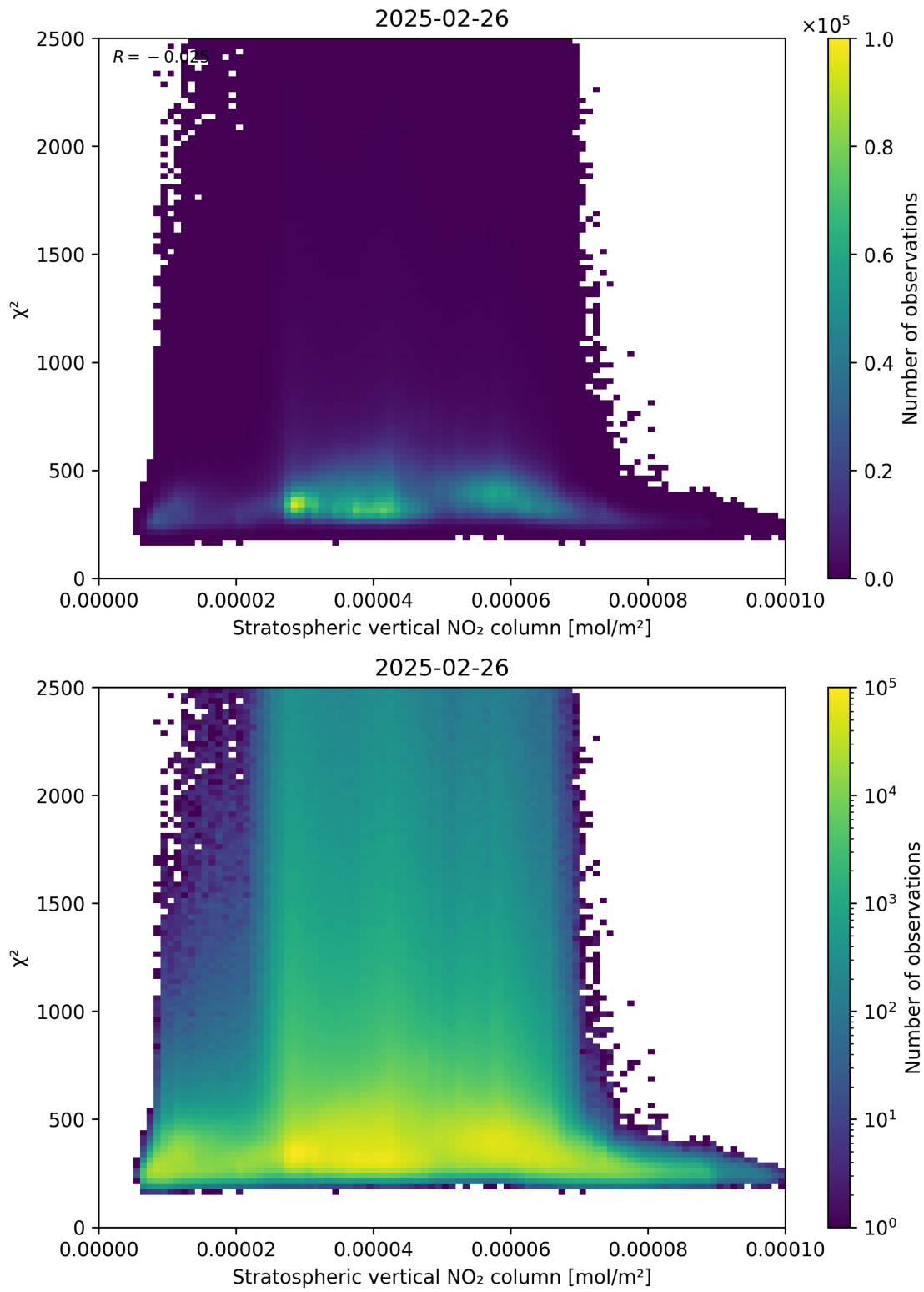
Figure 97: Scatter density plot of “Stratospheric vertical NO 2 column” against “ \chi^2 ” for 2025-02-25 to 2025-02-27.
