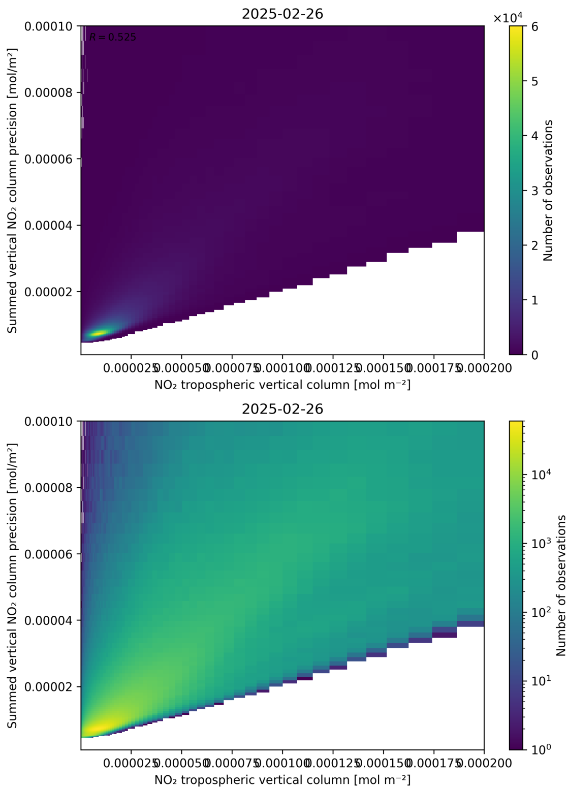
Figure 127: Scatter density plot of “NO 2 tropospheric vertical column” against “Summed vertical NO 2 column precision” for 2025-02-25 to 2025-02-27.
