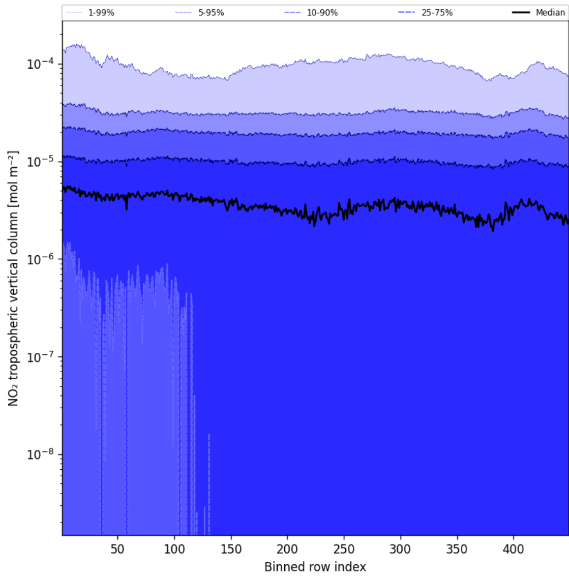
Figure 46: Along track statistics of “NO 2 tropospheric vertical column” for 2025-02-25 to 2025-02-27
