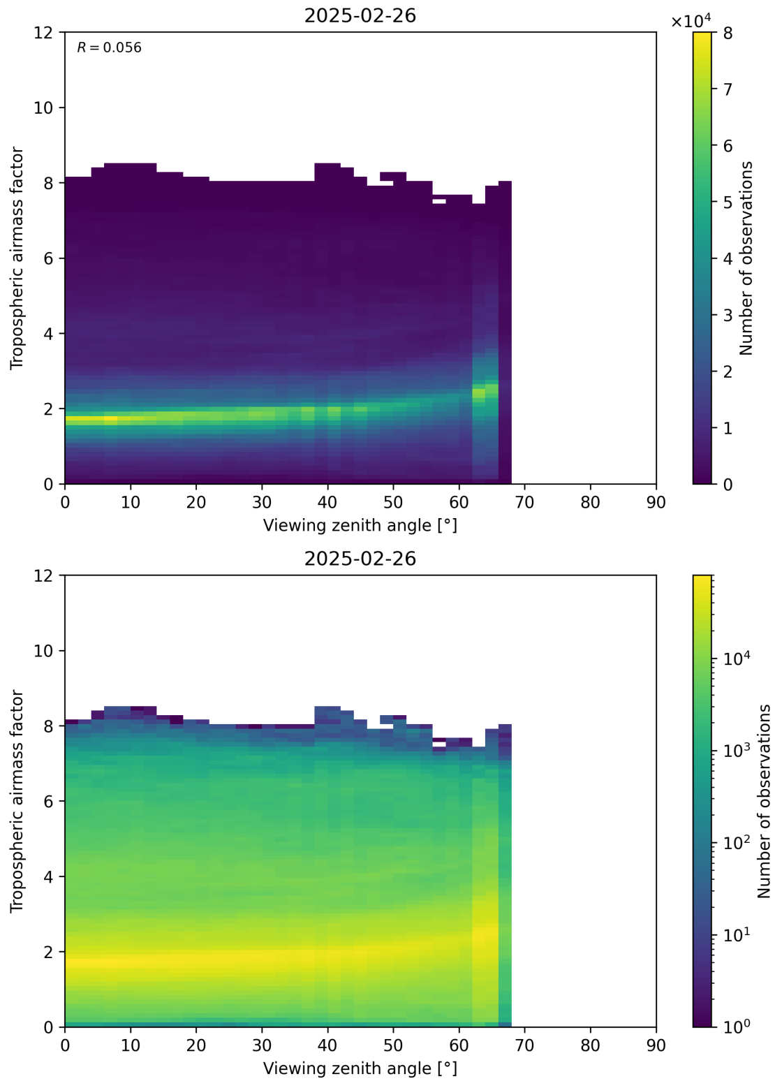
Figure 161: Scatter density plot of “Viewing zenith angle” against “Tropospheric airmass factor” for 2025-02-25 to 2025-02-27.
