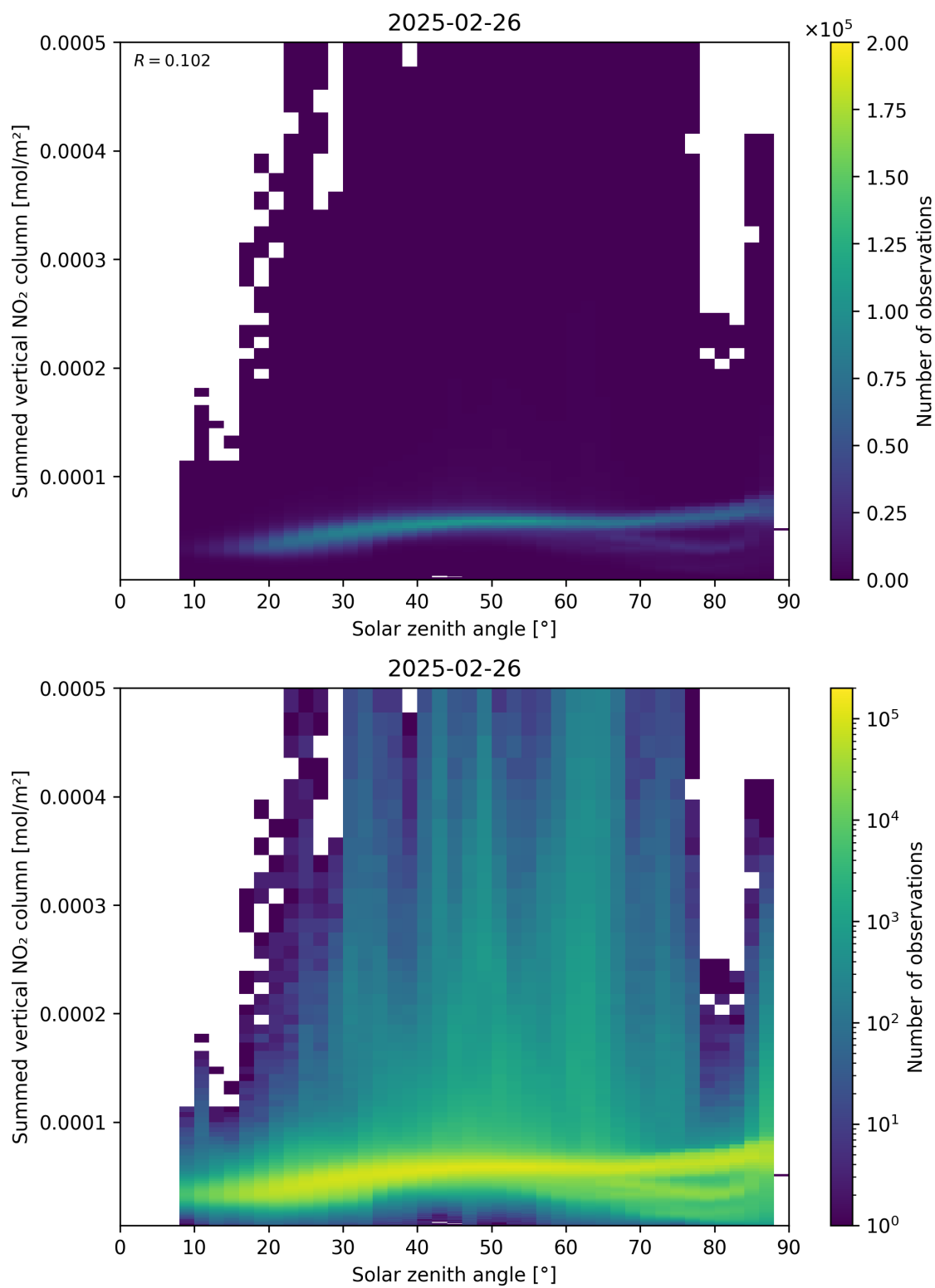
Figure 151: Scatter density plot of “Solar zenith angle” against “Summed vertical NO 2 column” for 2025-02-25 to 2025-02-27.
