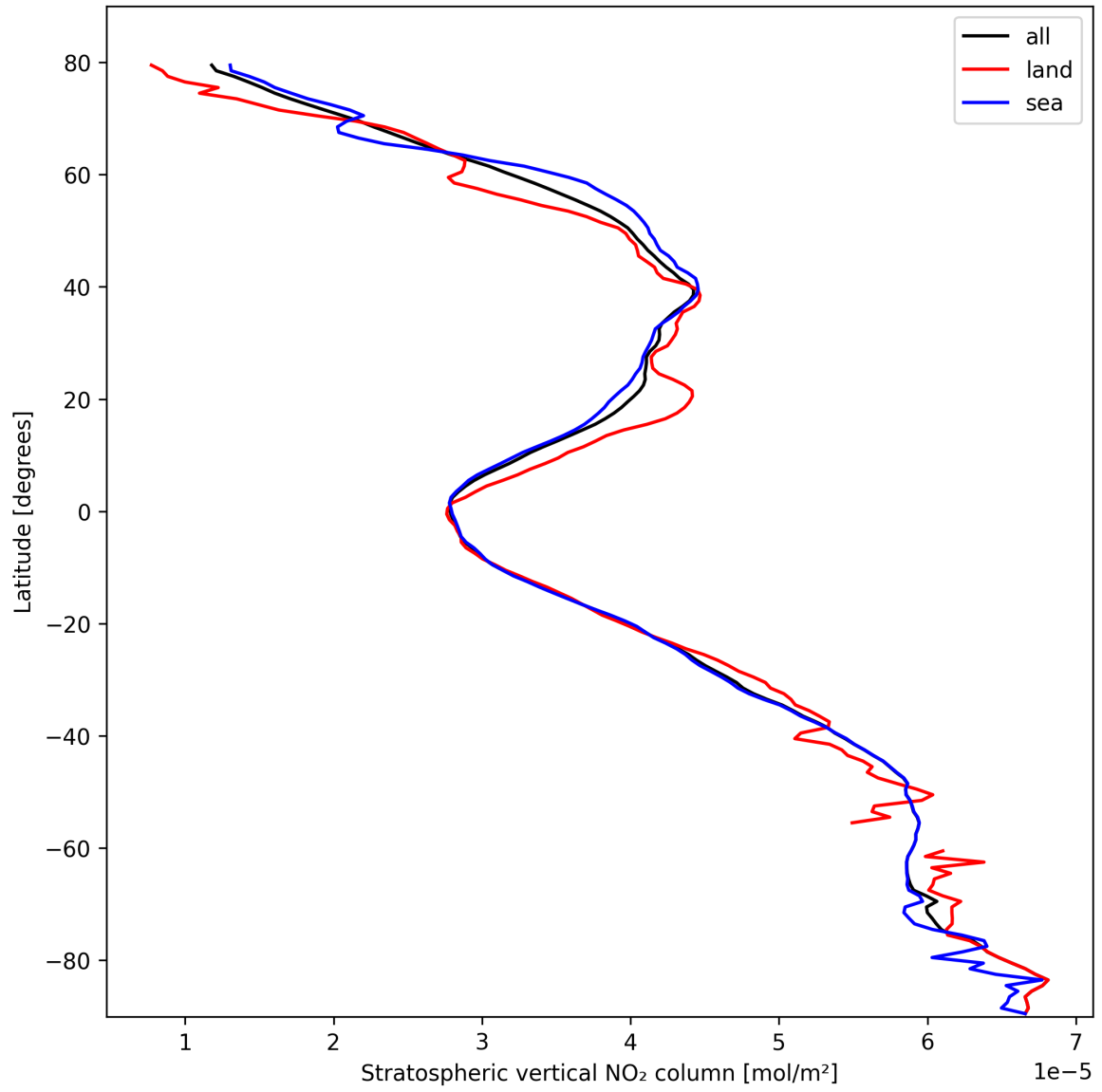
Figure 19: Zonal average of “Stratospheric vertical NO 2 column” for 2025-02-25 to 2025-02-27.
