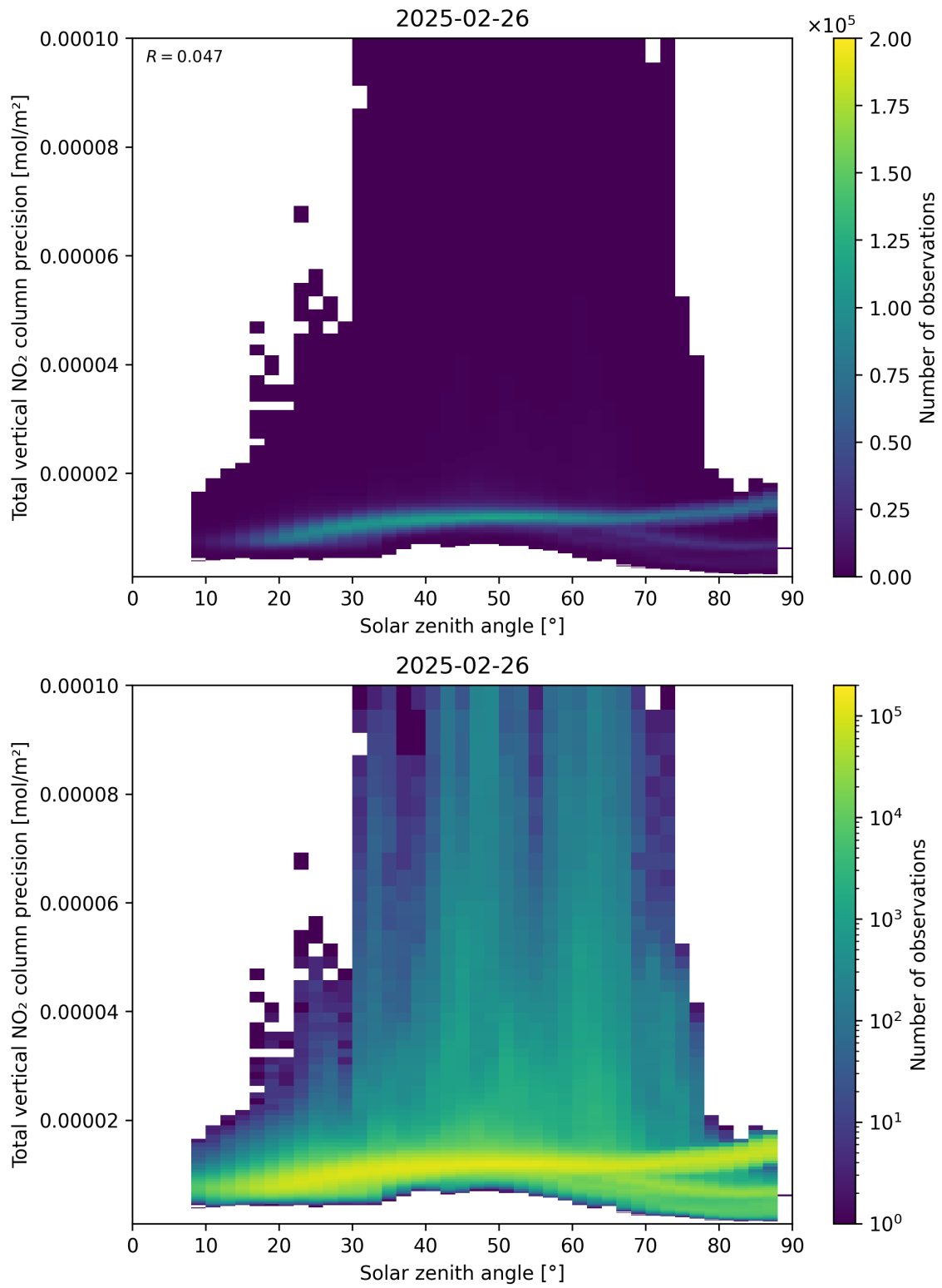
Figure 154: Scatter density plot of “Solar zenith angle” against “Total vertical NO 2 column precision” for 2025-02-25 to 2025-02-27.
