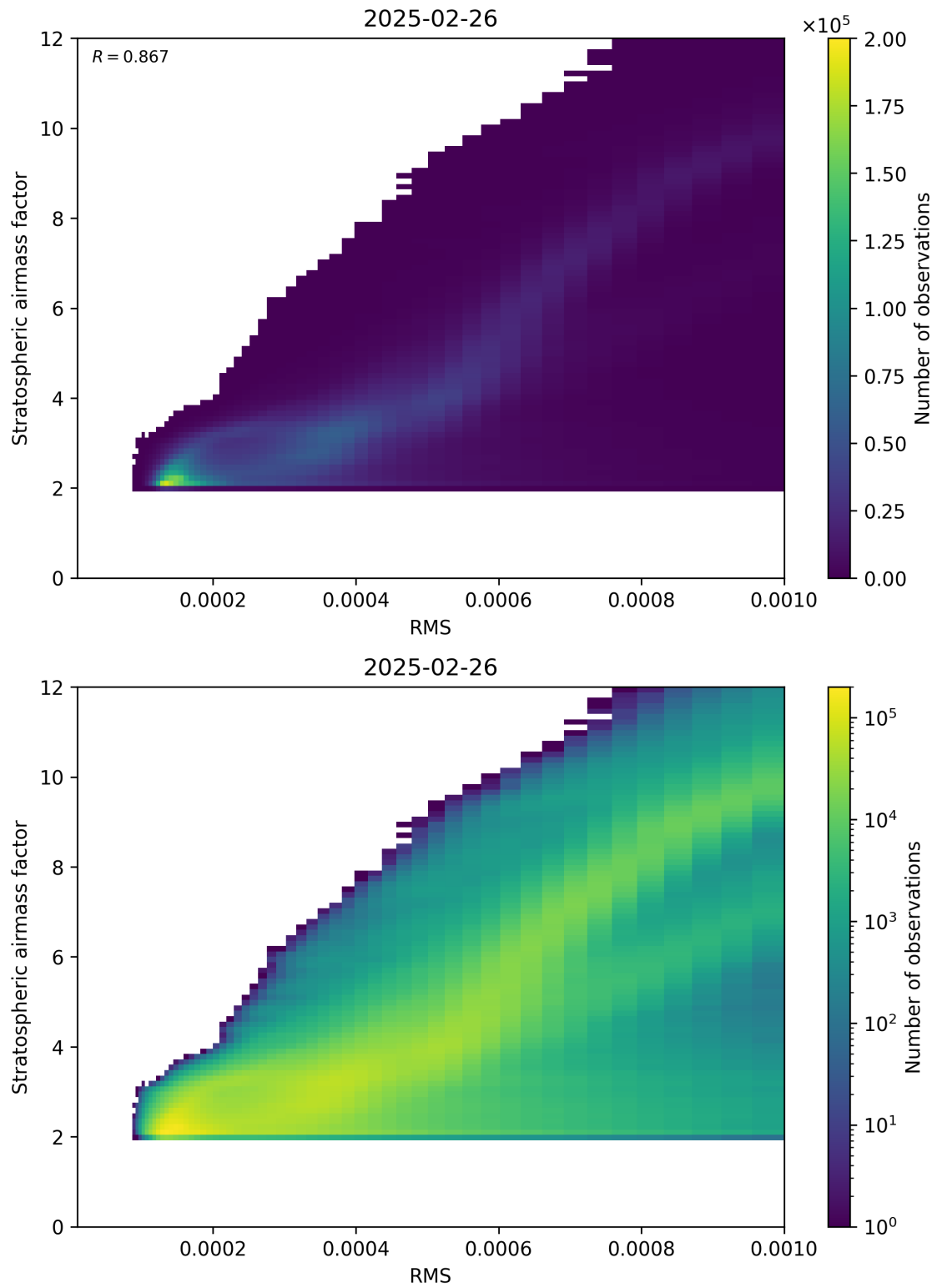
Figure 144: Scatter density plot of “RMS” against “Stratospheric airmass factor” for 2025-02-25 to 2025-02-27.
