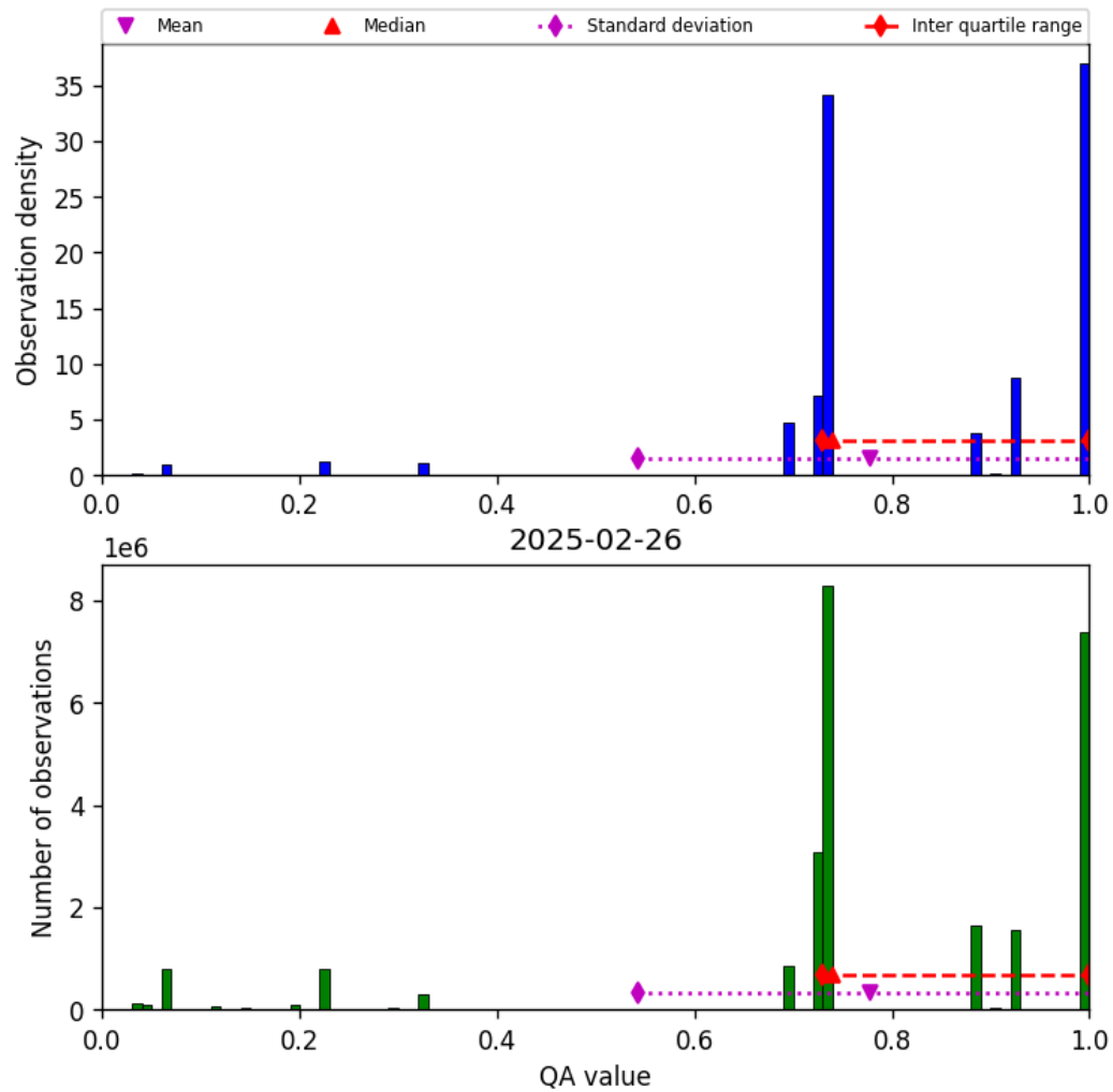
Figure 28: Histogram of “QA value” for 2025-02-25 to 2025-02-27
