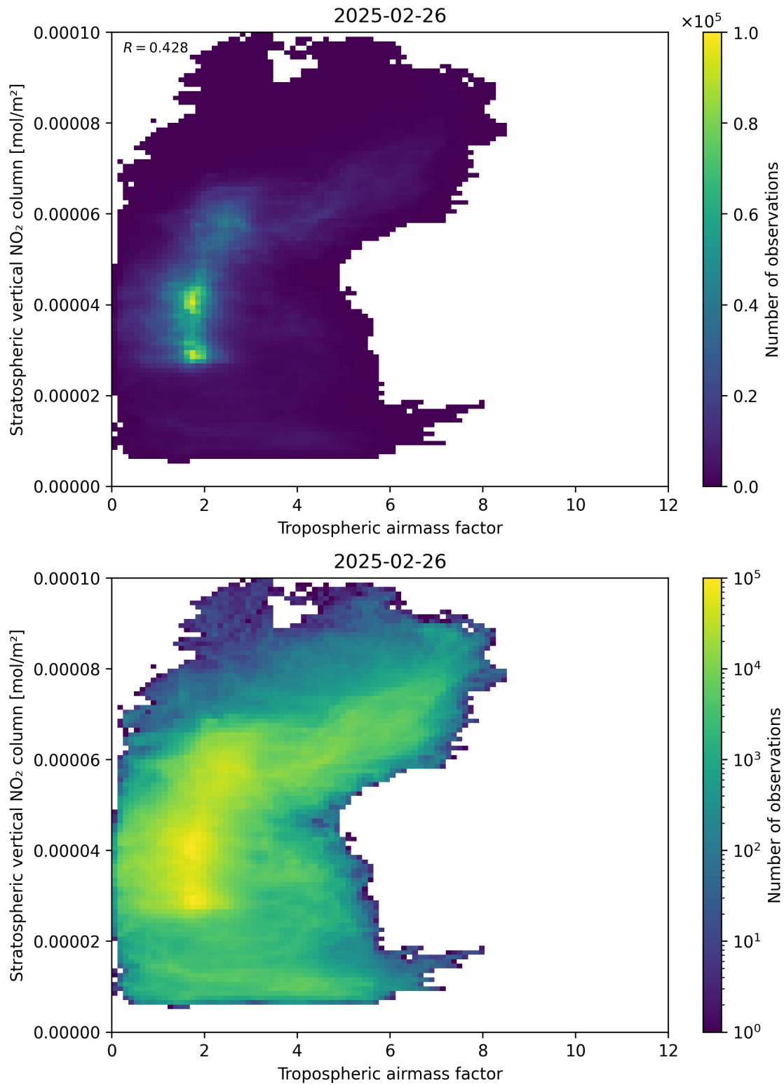
Figure 74: Scatter density plot of “Tropospheric air mass factor” against “Stratospheric vertical \text{NO}_2 column” for 2025-02-25 to 2025-02-27.
