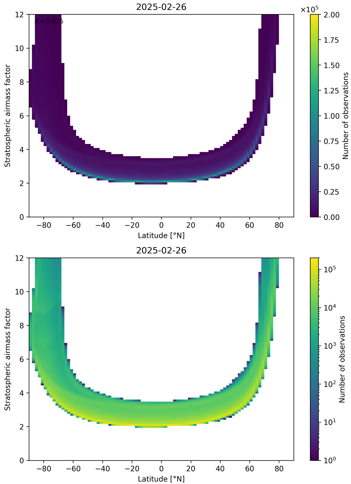
Figure 83: Scatter density plot of “Latitude” against “Stratospheric airmass factor” for 2025-02-25 to 2025-02-27.
