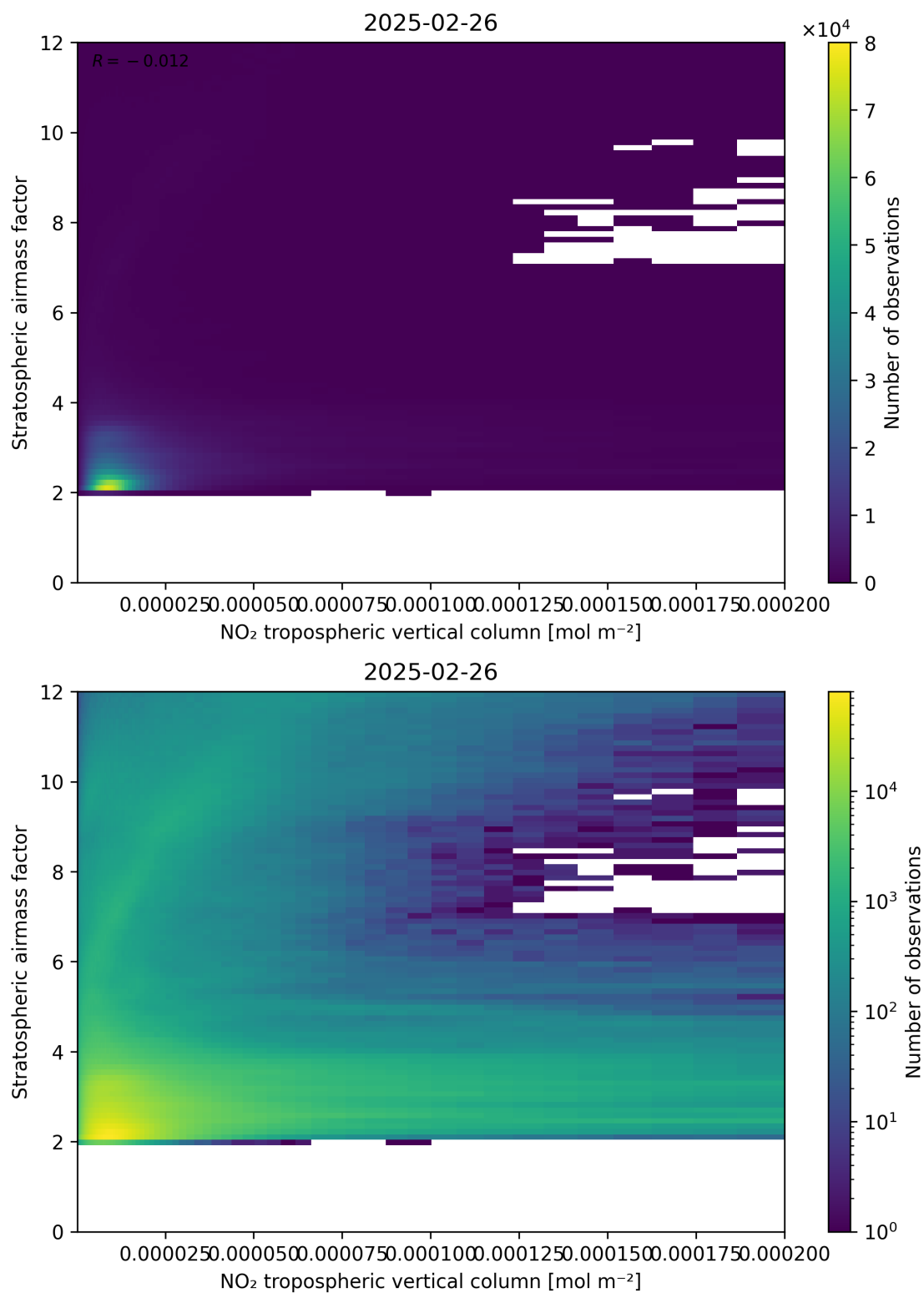
Figure 121: Scatter density plot of “NO 2 tropospheric vertical column” against “Stratospheric airmass factor” for 2025-02-25 to 2025-02-27.
