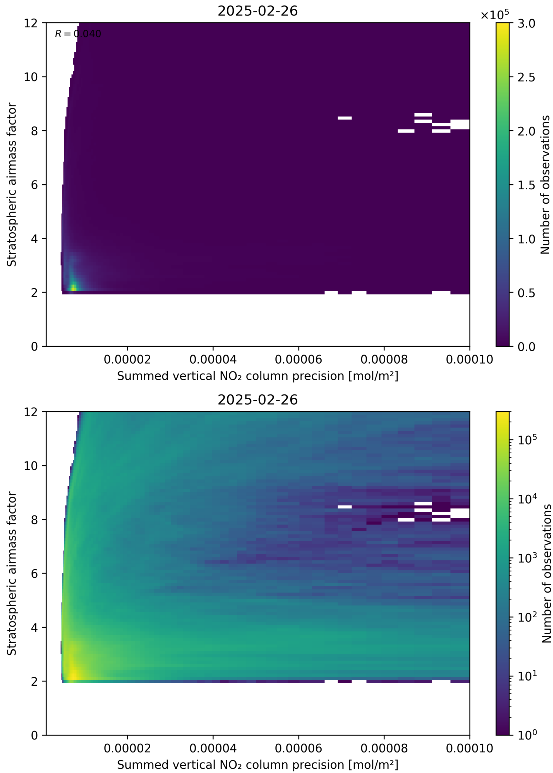
Figure 106: Scatter density plot of “Summed vertical NO 2 column precision” against “Stratospheric airmass factor” for 2025-02-25 to 2025-02-27.
