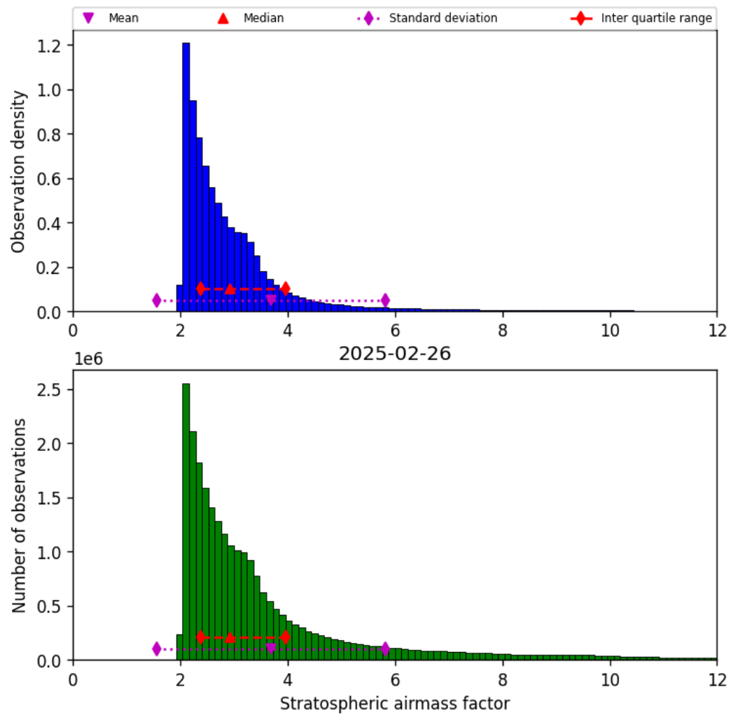
Figure 44: Histogram of “Stratospheric airmass factor” for 2025-02-25 to 2025-02-27
