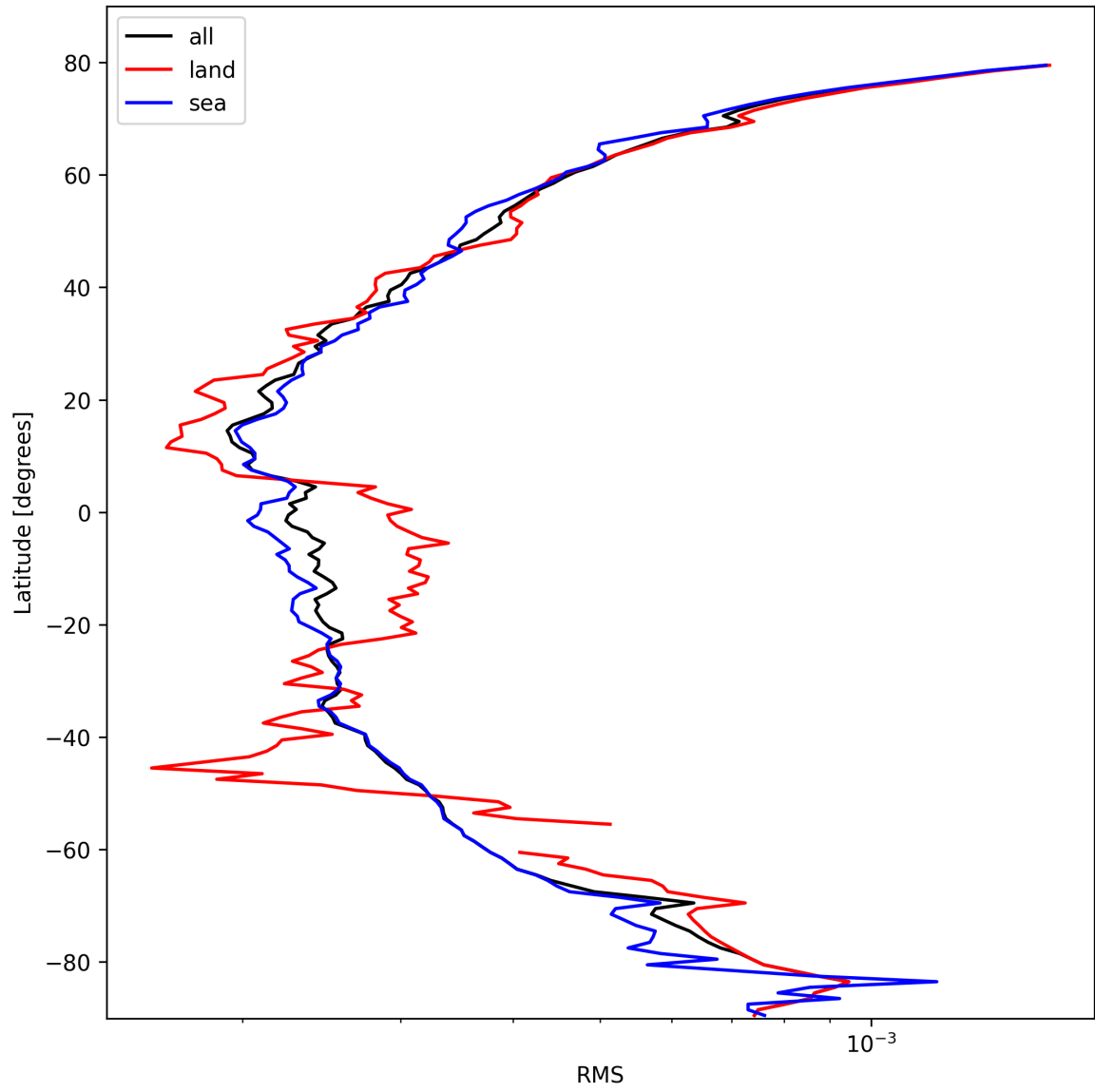
Figure 26: Zonal average of “RMS” for 2025-02-25 to 2025-02-27.
