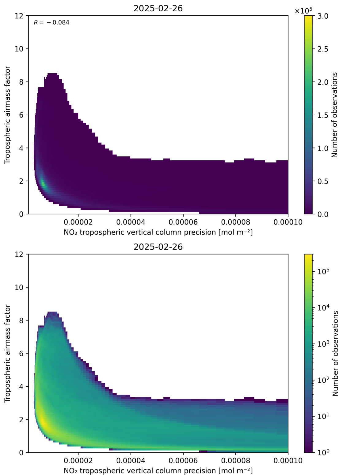
Figure 133: Scatter density plot of “NO 2 tropospheric vertical column precision” against “Tropospheric airmass factor” for 2025-02-25 to 2025-02-27.
