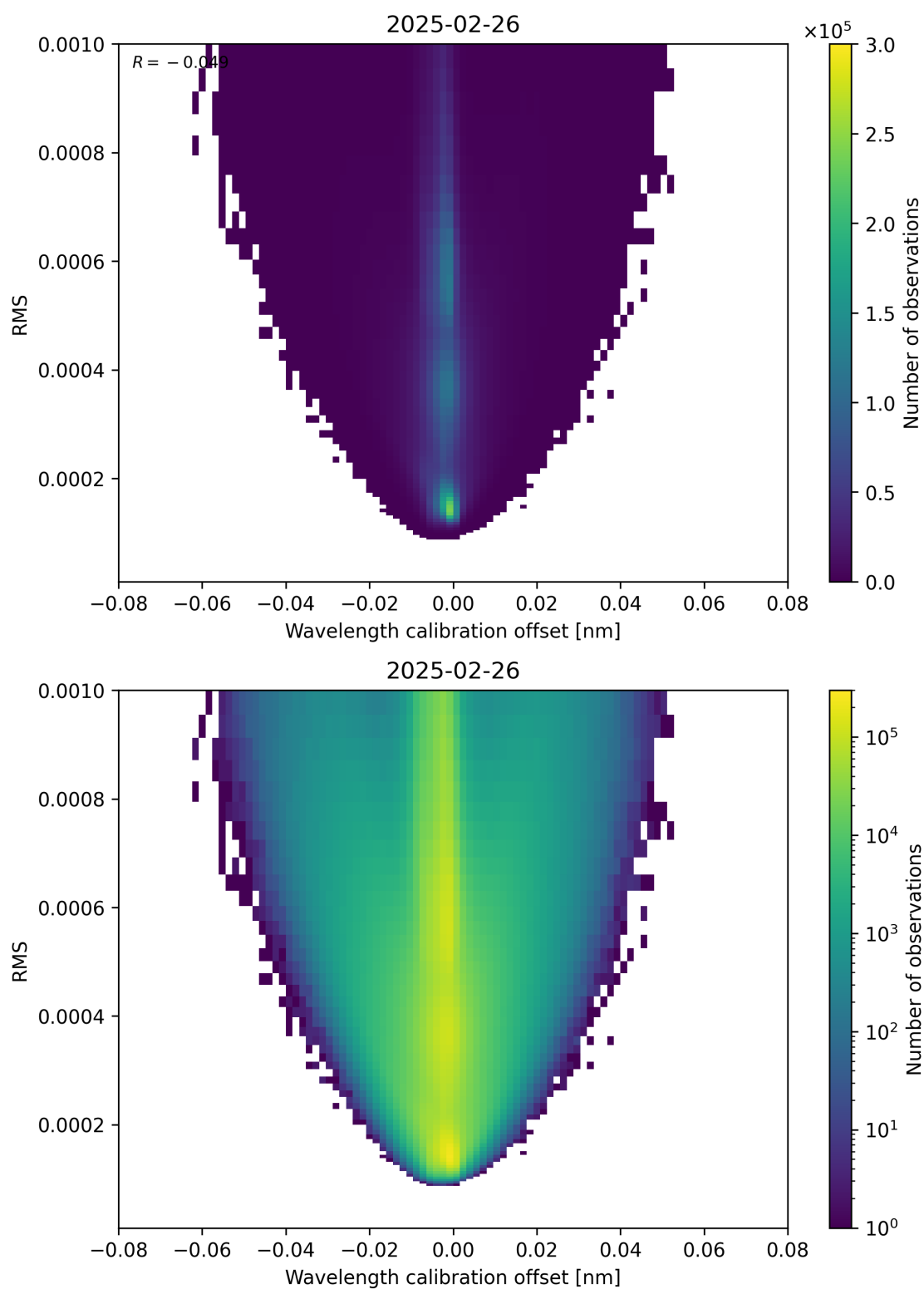
Figure 181: Scatter density plot of “Wavelength calibration offset” against “RMS” for 2025-02-25 to 2025-02-27.
