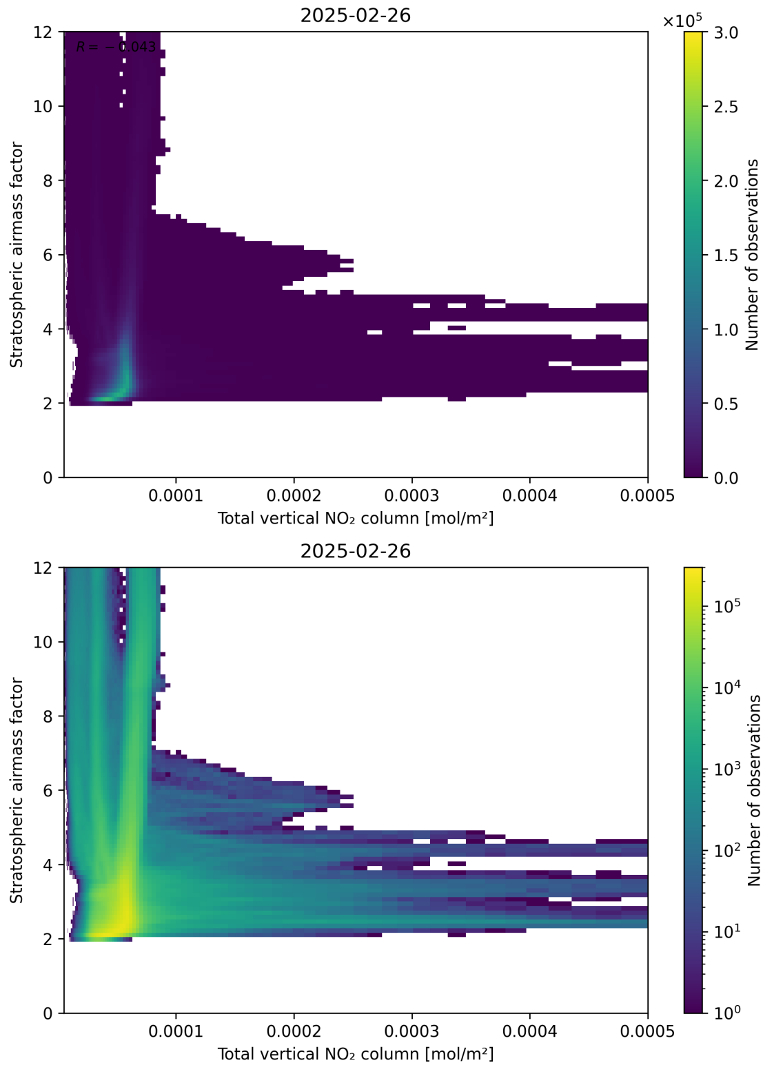
Figure 110: Scatter density plot of “Total vertical NO 2 column” against “Stratospheric airmass factor” for 2025-02-25 to 2025-02-27.
