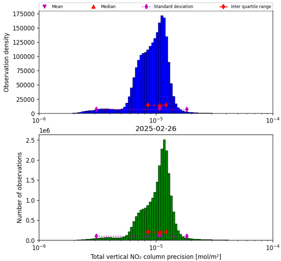
Figure 39: Histogram of "Total vertical NO 2 column precision" for 2025-02-25 to 2025-02-27
