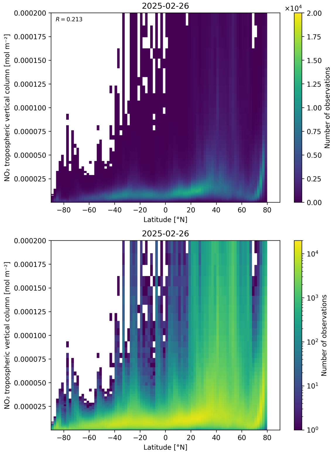
Figure 92: Scatter density plot of “Latitude” against “NO 2 tropospheric vertical column” for 2025-02-25 to 2025-02-27.
