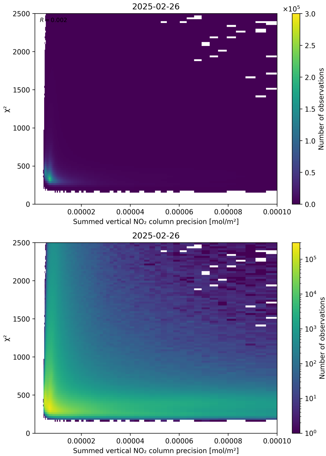
Figure 107: Scatter density plot of “Summed vertical NO 2 column precision” against “ \chi^2 ” for 2025-02-25 to 2025-02-27.
