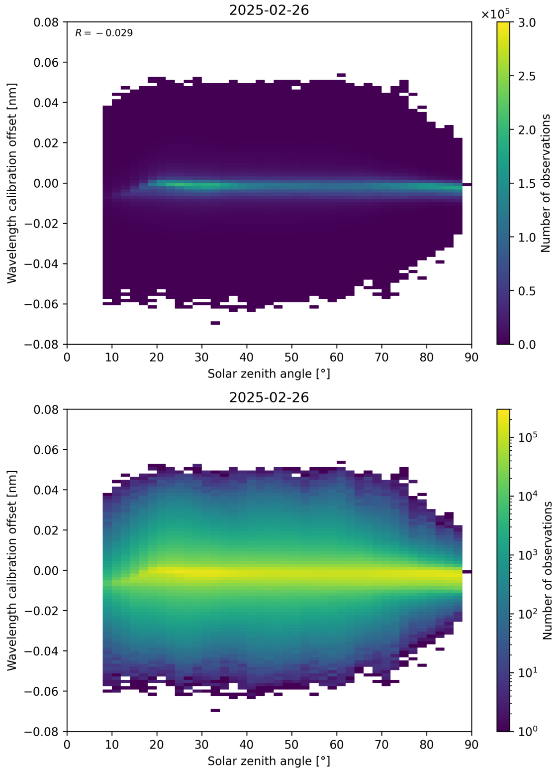
Figure 158: Scatter density plot of “Solar zenith angle” against “Wavelength calibration offset” for 2025-02-25 to 2025-02-27.
