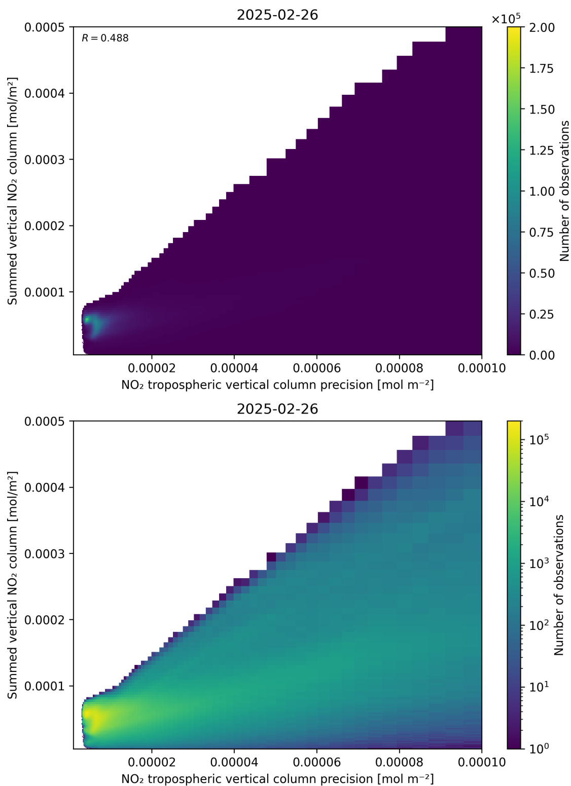
Figure 136: Scatter density plot of “NO 2 tropospheric vertical column precision” against “Summed vertical NO 2 column” for 2025-02-25 to 2025-02-27.
