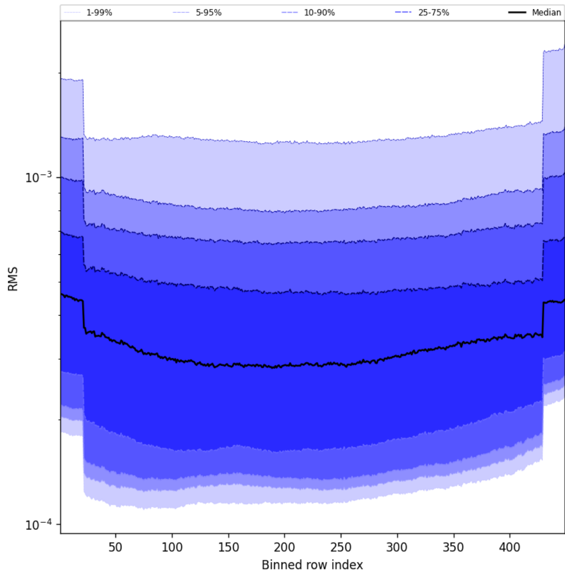
Figure 60: Along track statistics of “RMS” for 2025-02-25 to 2025-02-27
