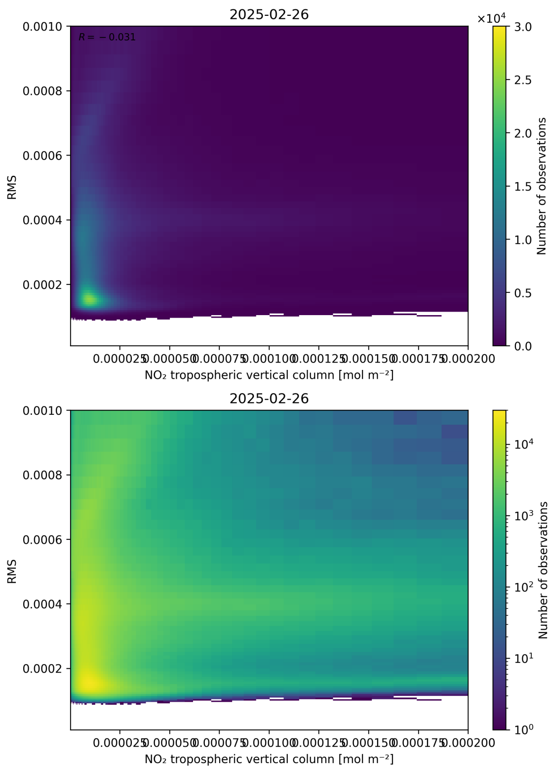
Figure 142: Scatter density plot of “NO 2 tropospheric vertical column” against “RMS” for 2025-02-25 to 2025-02-27.
