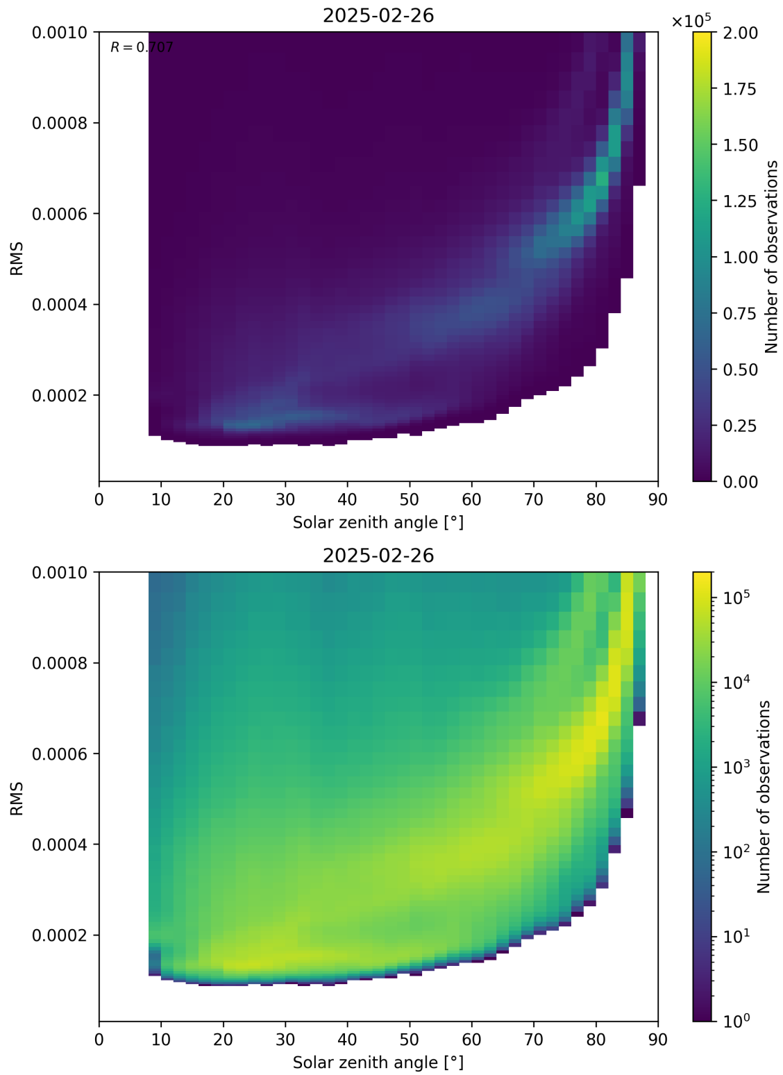
Figure 157: Scatter density plot of “Solar zenith angle” against “RMS” for 2025-02-25 to 2025-02-27.
