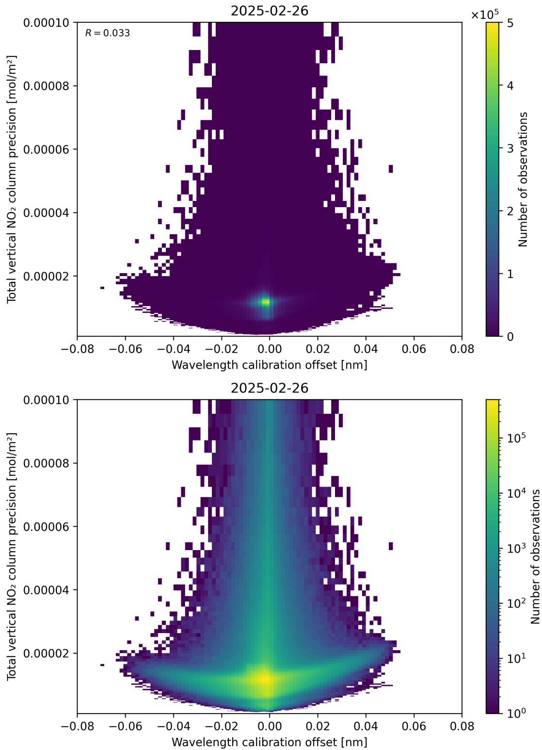
Figure 180: Scatter density plot of “Wavelength calibration offset” against “Total vertical NO 2 column precision” for 2025-02-25 to 2025-02-27.
