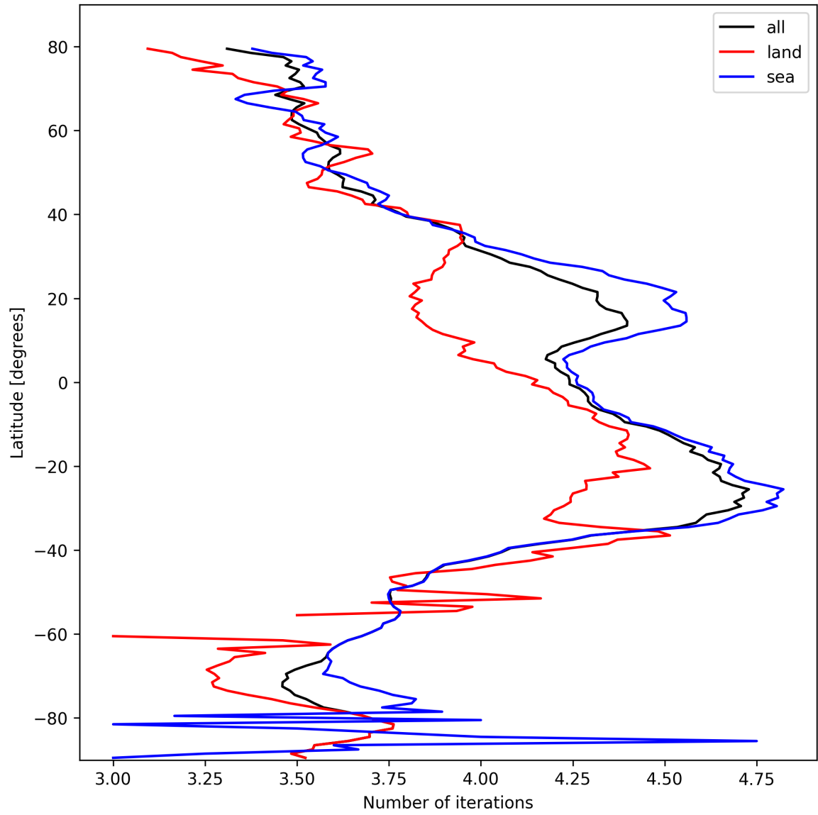
Figure 17: Zonal average of “Number of iterations” for 2025-02-25 to 2025-02-27.
