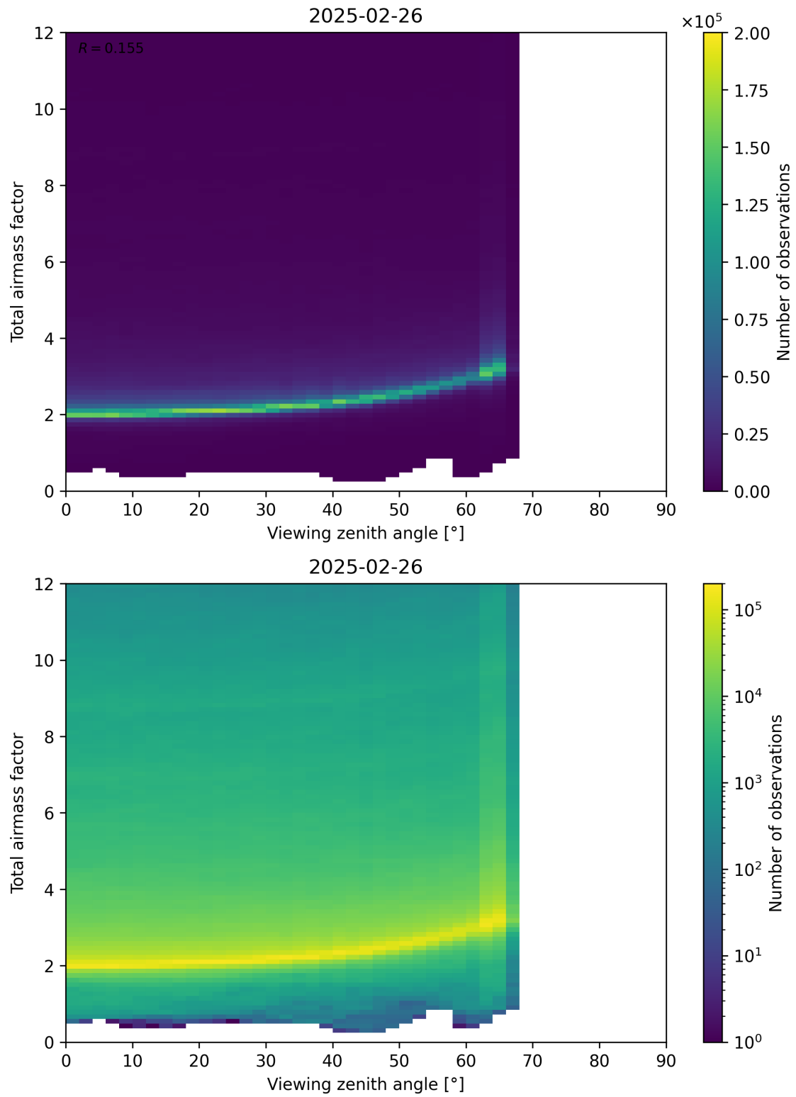
Figure 160: Scatter density plot of “Viewing zenith angle” against “Total airmass factor” for 2025-02-25 to 2025-02-27.
