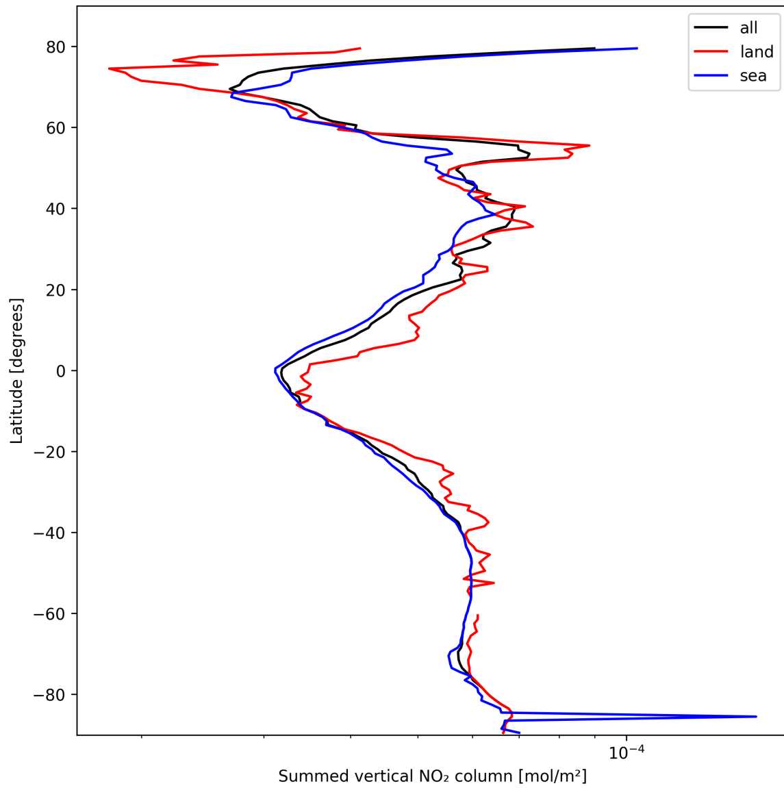
Figure 23: Zonal average of “Summed vertical NO 2 column” for 2025-02-25 to 2025-02-27.
