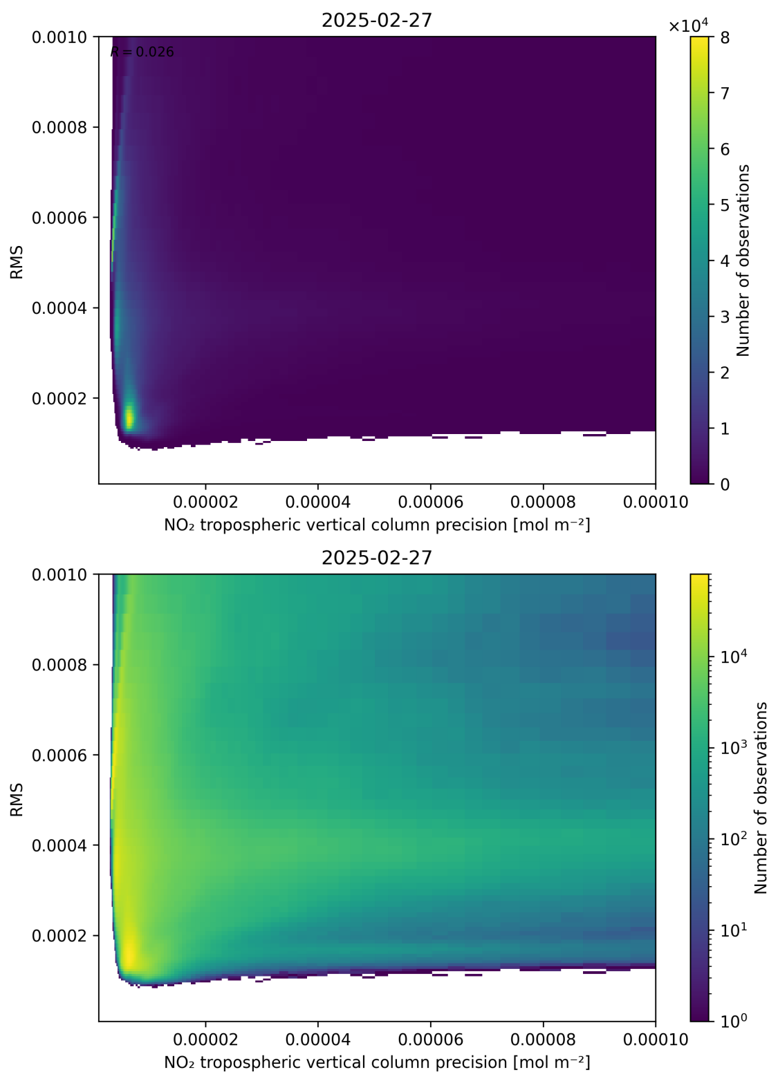
Figure 140: Scatter density plot of “NO 2 tropospheric vertical column precision” against “RMS” for 2025-02-26 to 2025-02-28.
