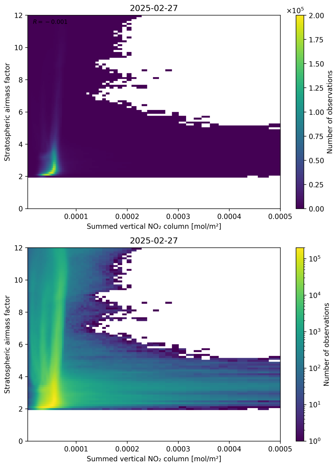
Figure 103: Scatter density plot of “Summed vertical NO 2 column” against “Stratospheric airmass factor” for 2025-02-26 to 2025-02-28.
