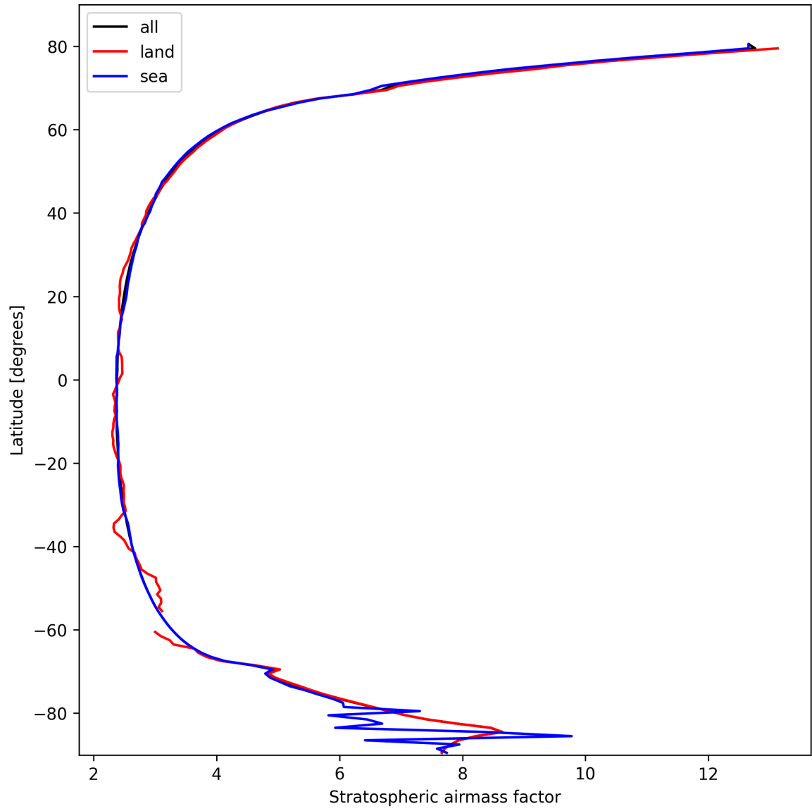
Figure 27: Zonal average of “Stratospheric airmass factor” for 2025-02-26 to 2025-02-28.
