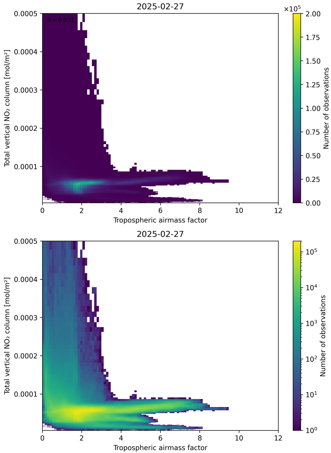
Figure 77: Scatter density plot of “Tropospheric airmass factor” against “Total vertical NO 2 column” for 2025-02-26 to 2025-02-28.
