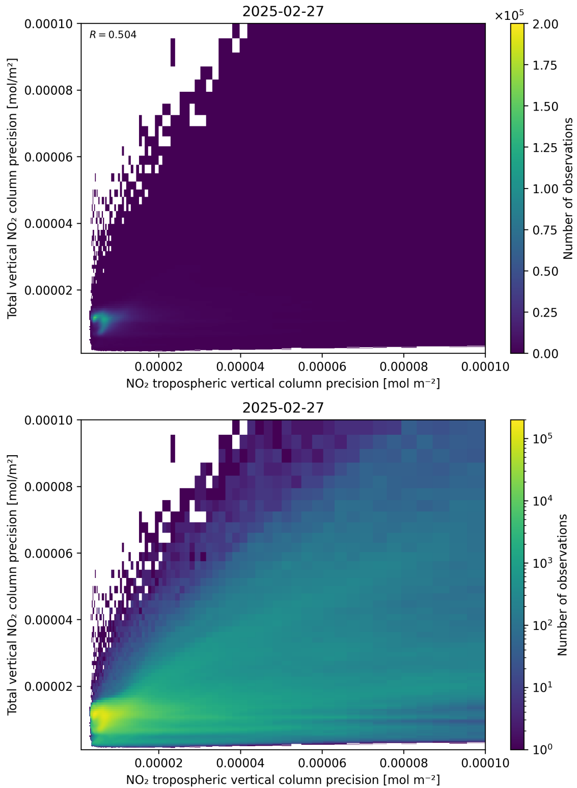
Figure 139: Scatter density plot of “NO 2 tropospheric vertical column precision” against “Total vertical NO 2 column precision” for 2025-02-26 to 2025-02-28.
