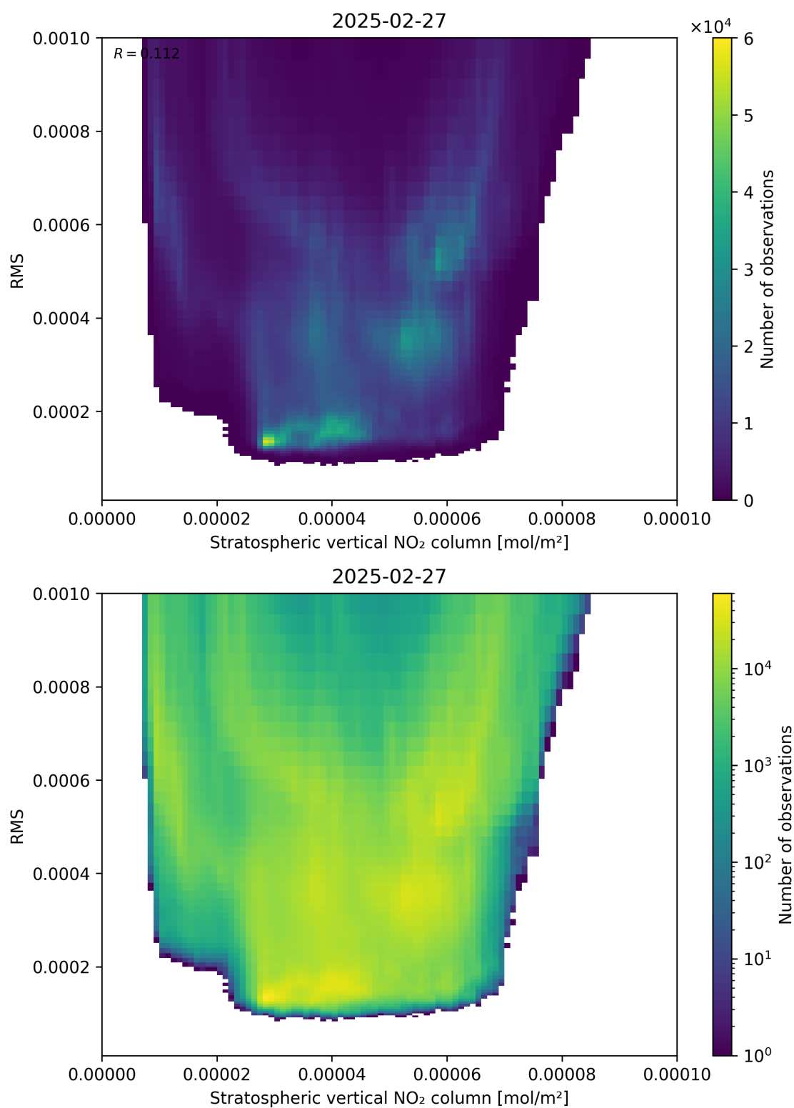
Figure 102: Scatter density plot of “Stratospheric vertical NO 2 column” against “RMS” for 2025-02-26 to 2025-02-28.
