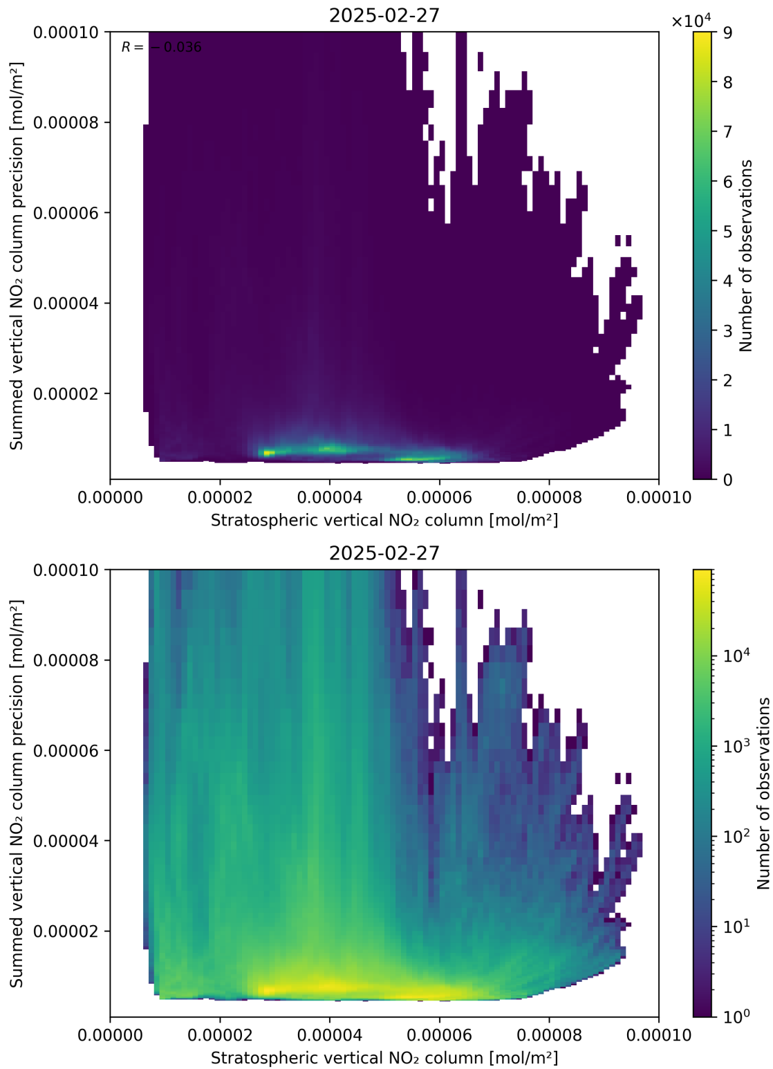
Figure 99: Scatter density plot of “Stratospheric vertical NO 2 column” against “Summed vertical NO 2 column precision” for 2025-02-26 to 2025-02-28.
