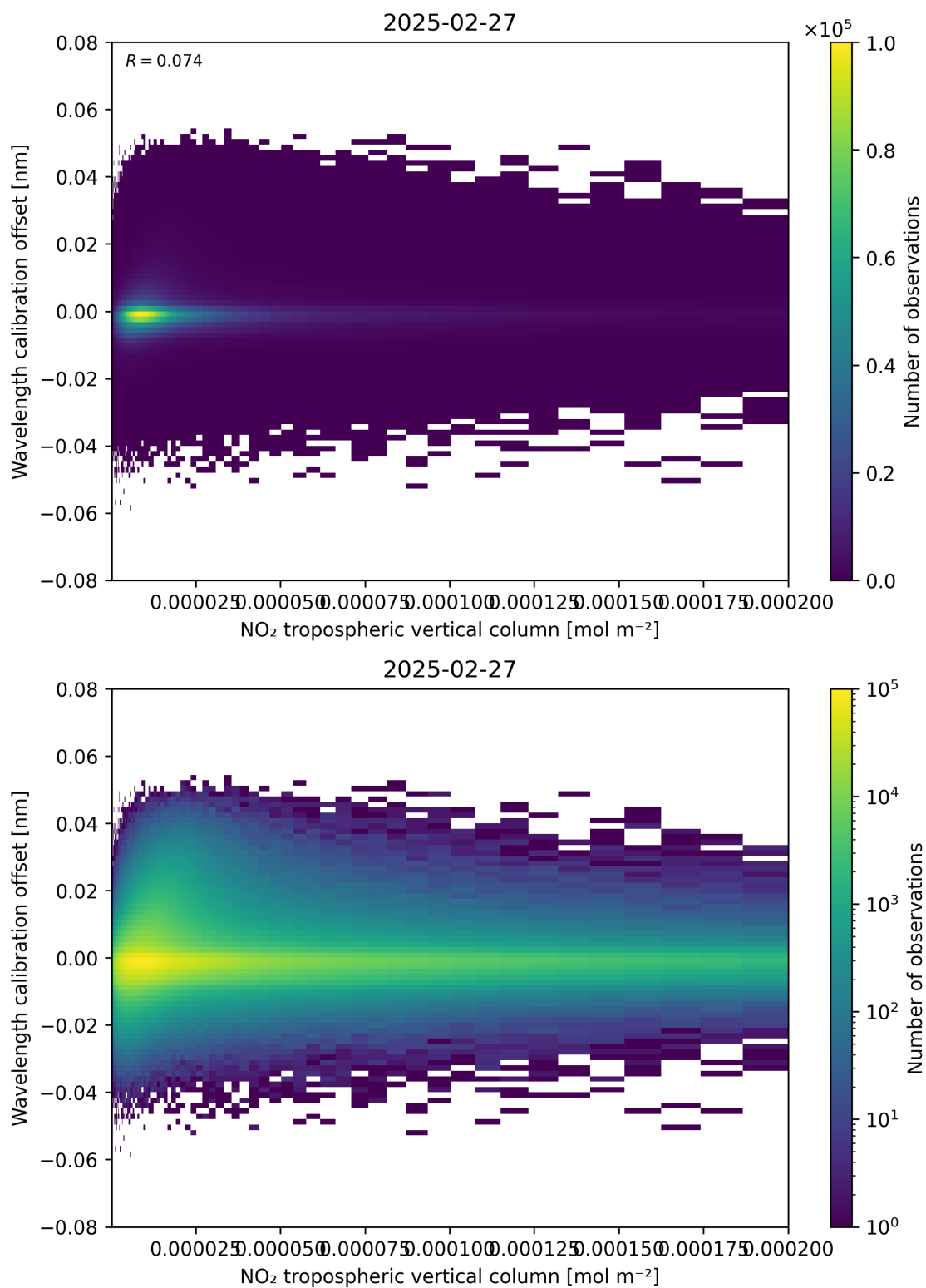
Figure 143: Scatter density plot of “NO 2 tropospheric vertical column” against “Wavelength calibration offset” for 2025-02-26 to 2025-02-28.
