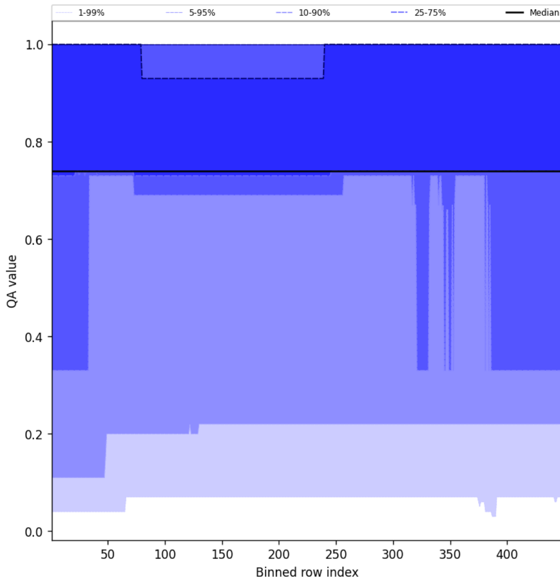
Figure 45: Along track statistics of “QA value” for 2025-02-26 to 2025-02-28
