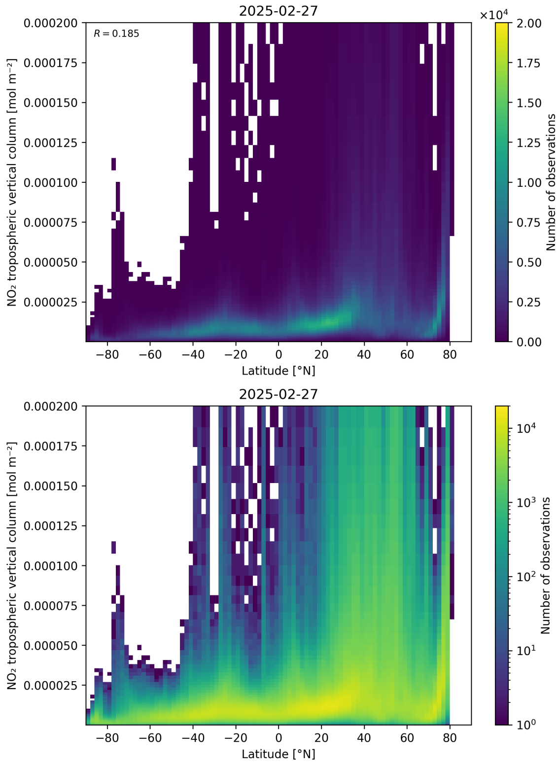
Figure 92: Scatter density plot of “Latitude” against “NO 2 tropospheric vertical column” for 2025-02-26 to 2025-02-28.
