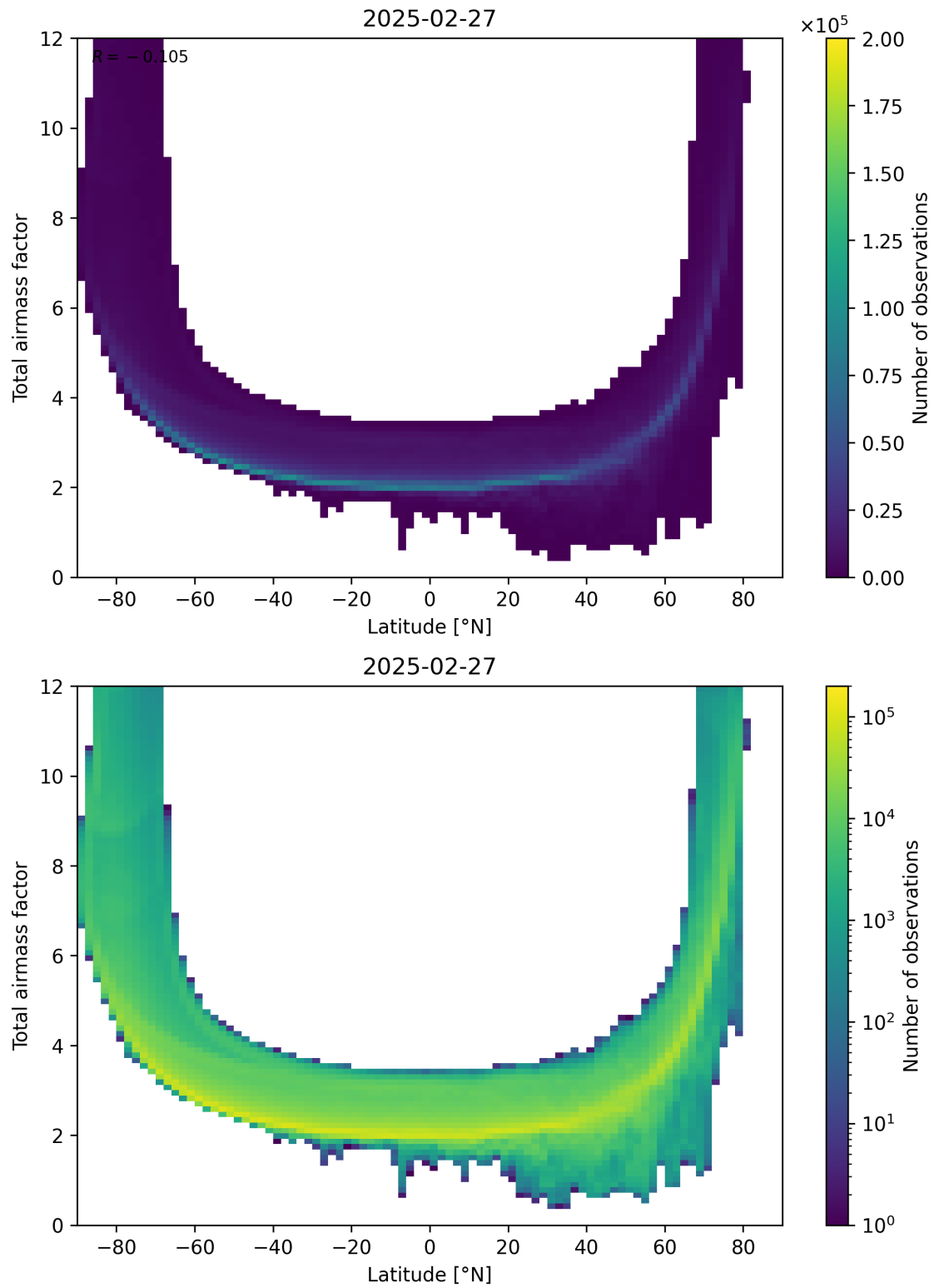
Figure 84: Scatter density plot of “Latitude” against “Total airmass factor” for 2025-02-26 to 2025-02-28.
