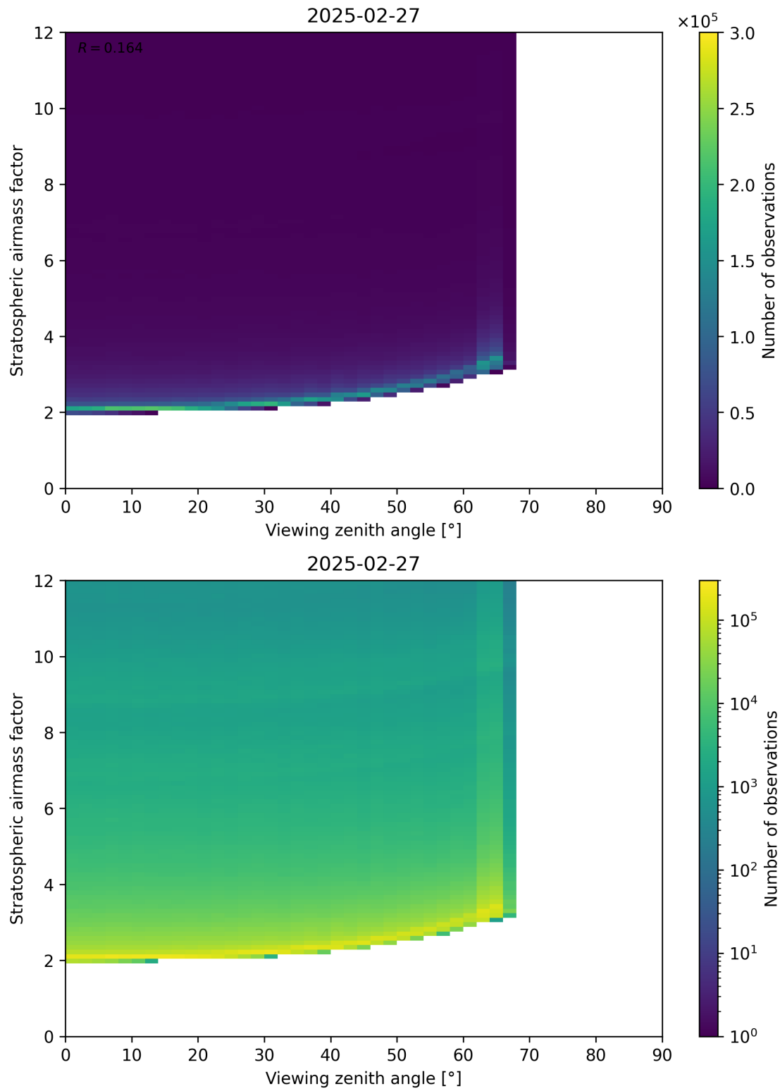
Figure 159: Scatter density plot of “Viewing zenith angle” against “Stratospheric airmass factor” for 2025-02-26 to 2025-02-28.
