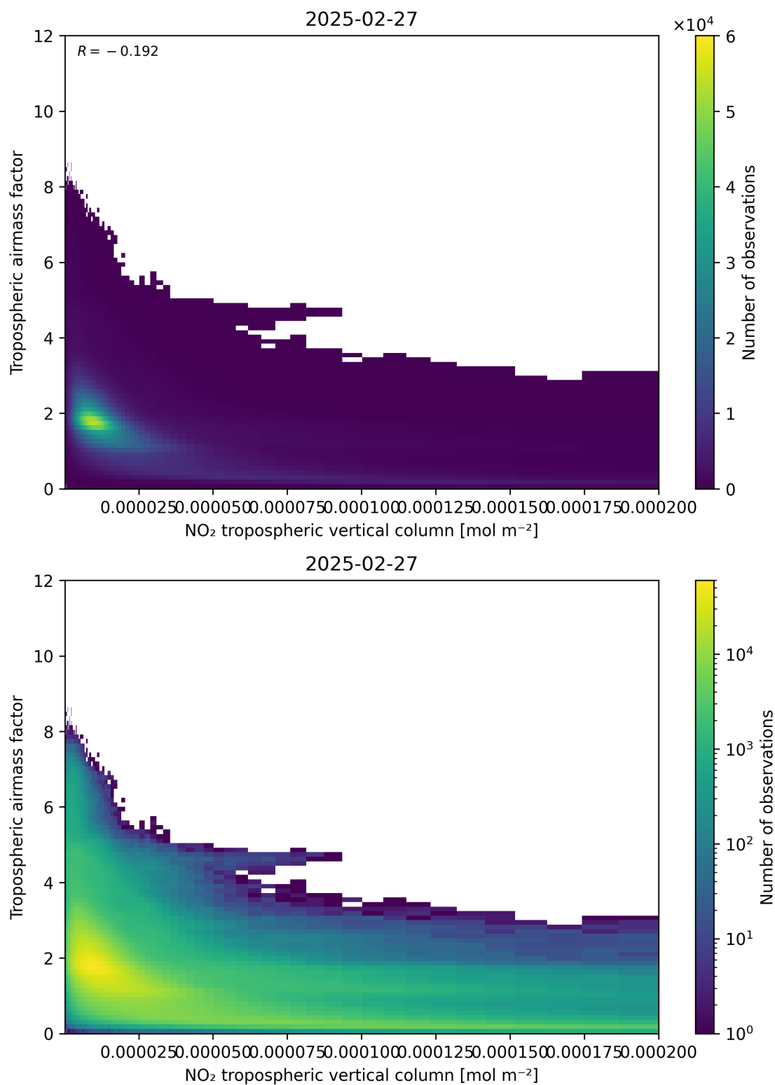
Figure 123: Scatter density plot of “NO 2 tropospheric vertical column” against “Tropospheric air mass factor” for 2025-02-26 to 2025-02-28.
