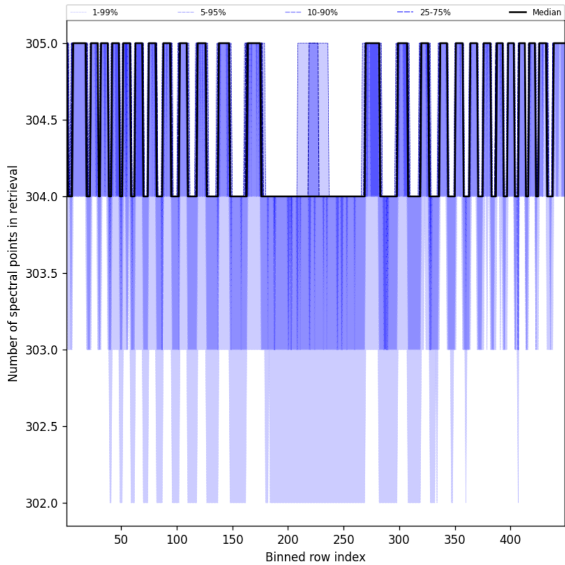
Figure 50: Along track statistics of “Number of spectral points in retrieval” for 2025-02-26 to 2025-02-28
