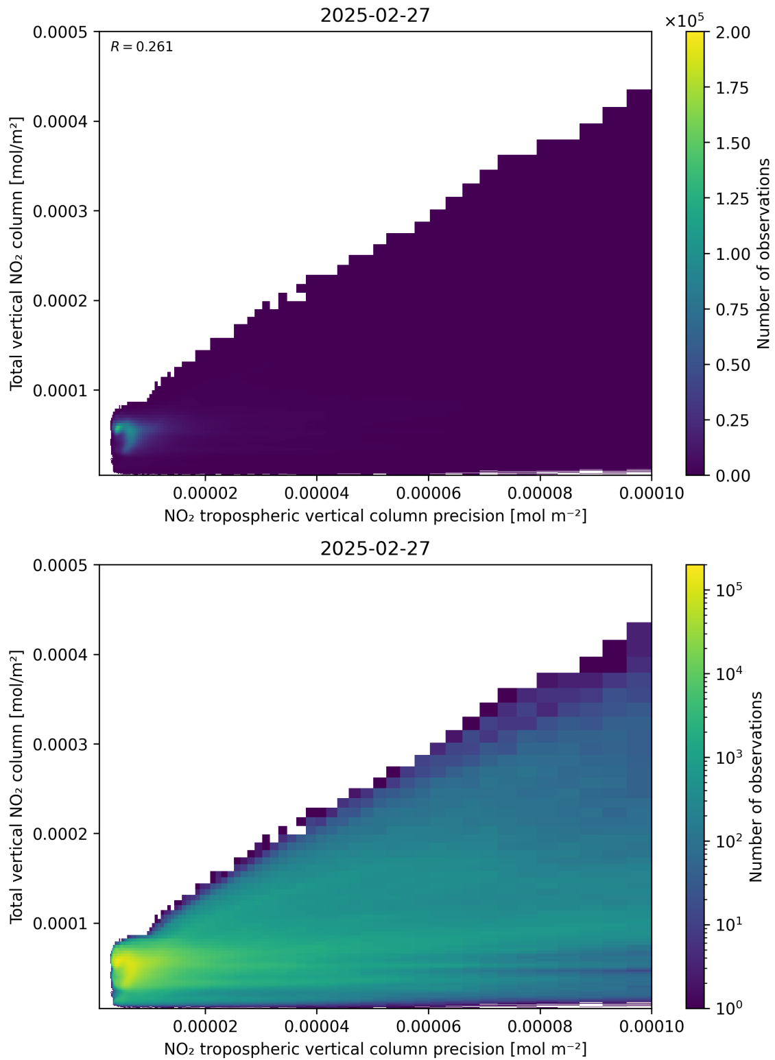
Figure 138: Scatter density plot of “NO 2 tropospheric vertical column precision” against “Total vertical NO 2 column” for 2025-02-26 to 2025-02-28.
