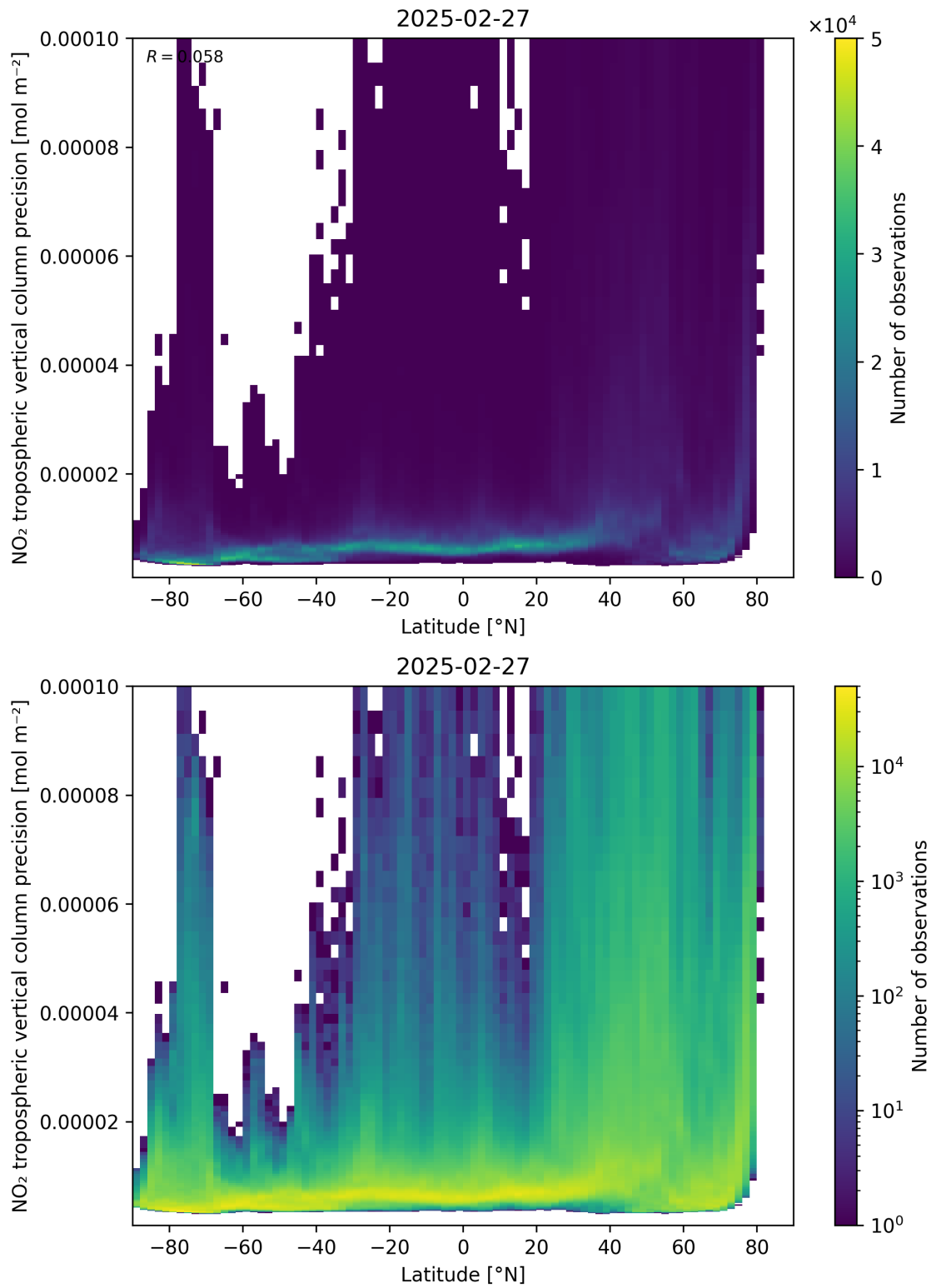
Figure 93: Scatter density plot of “Latitude” against “NO 2 tropospheric vertical column precision” for 2025-02-26 to 2025-02-28.
