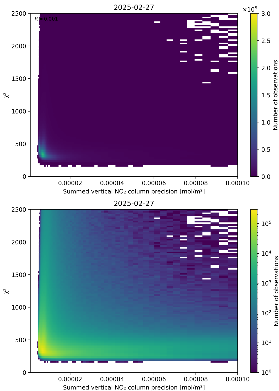
Figure 107: Scatter density plot of “Summed vertical NO 2 column precision” against “ \chi^2 ” for 2025-02-26 to 2025-02-28.
