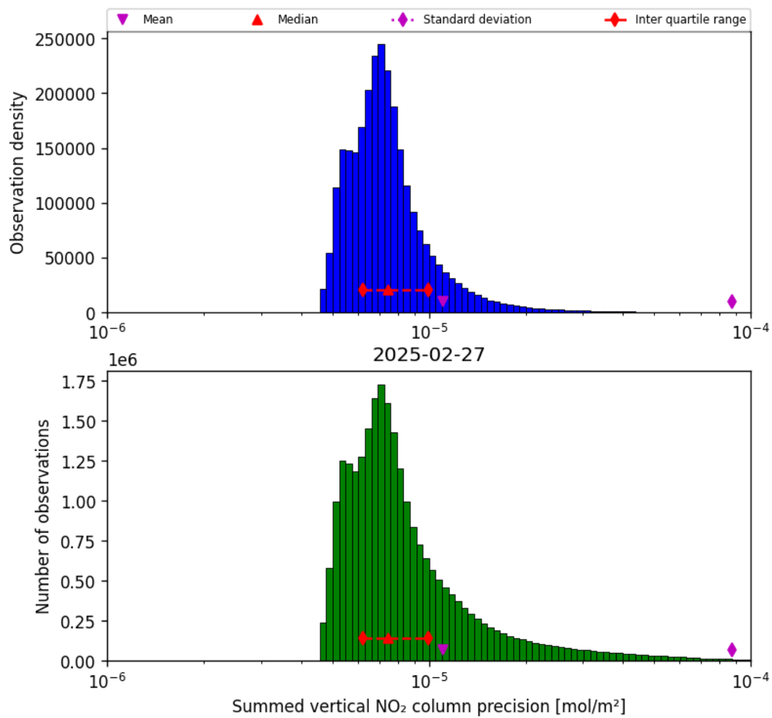
Figure 41: Histogram of “Summed vertical NO 2 column precision” for 2025-02-26 to 2025-02-28
