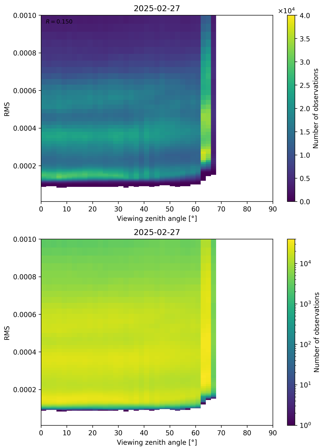
Figure 171: Scatter density plot of “Viewing zenith angle” against “RMS” for 2025-02-26 to 2025-02-28.
