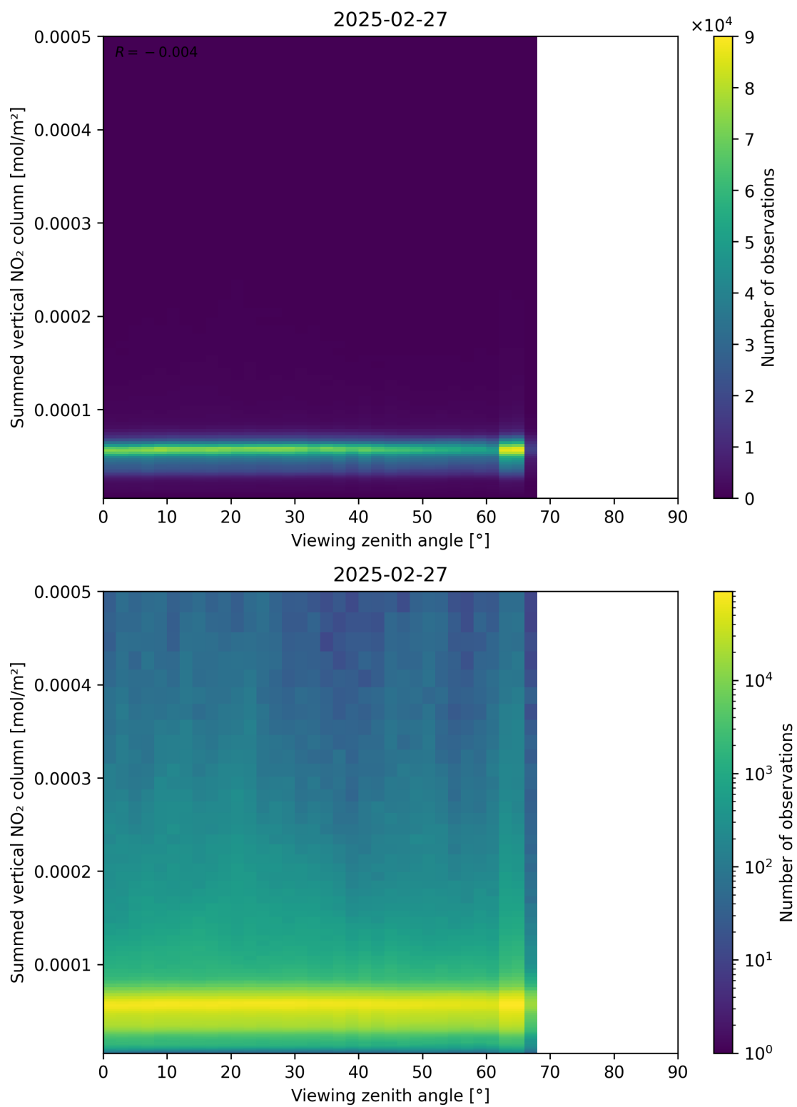
Figure 165: Scatter density plot of “Viewing zenith angle” against “Summed vertical NO 2 column” for 2025-02-26 to 2025-02-28.
