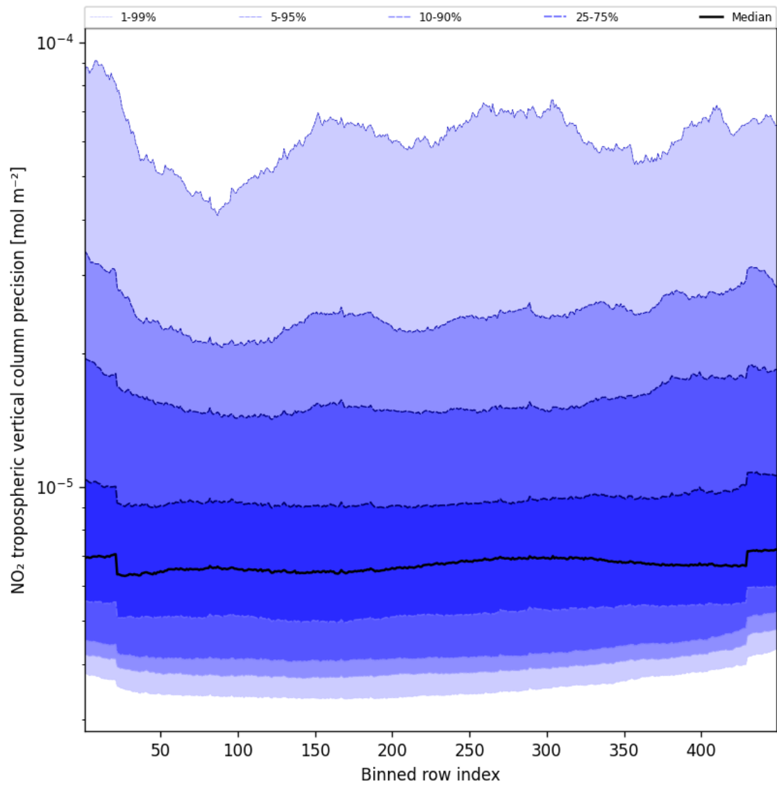
Figure 47: Along track statistics of “NO 2 tropospheric vertical column precision” for 2025-02-26 to 2025-02-28
