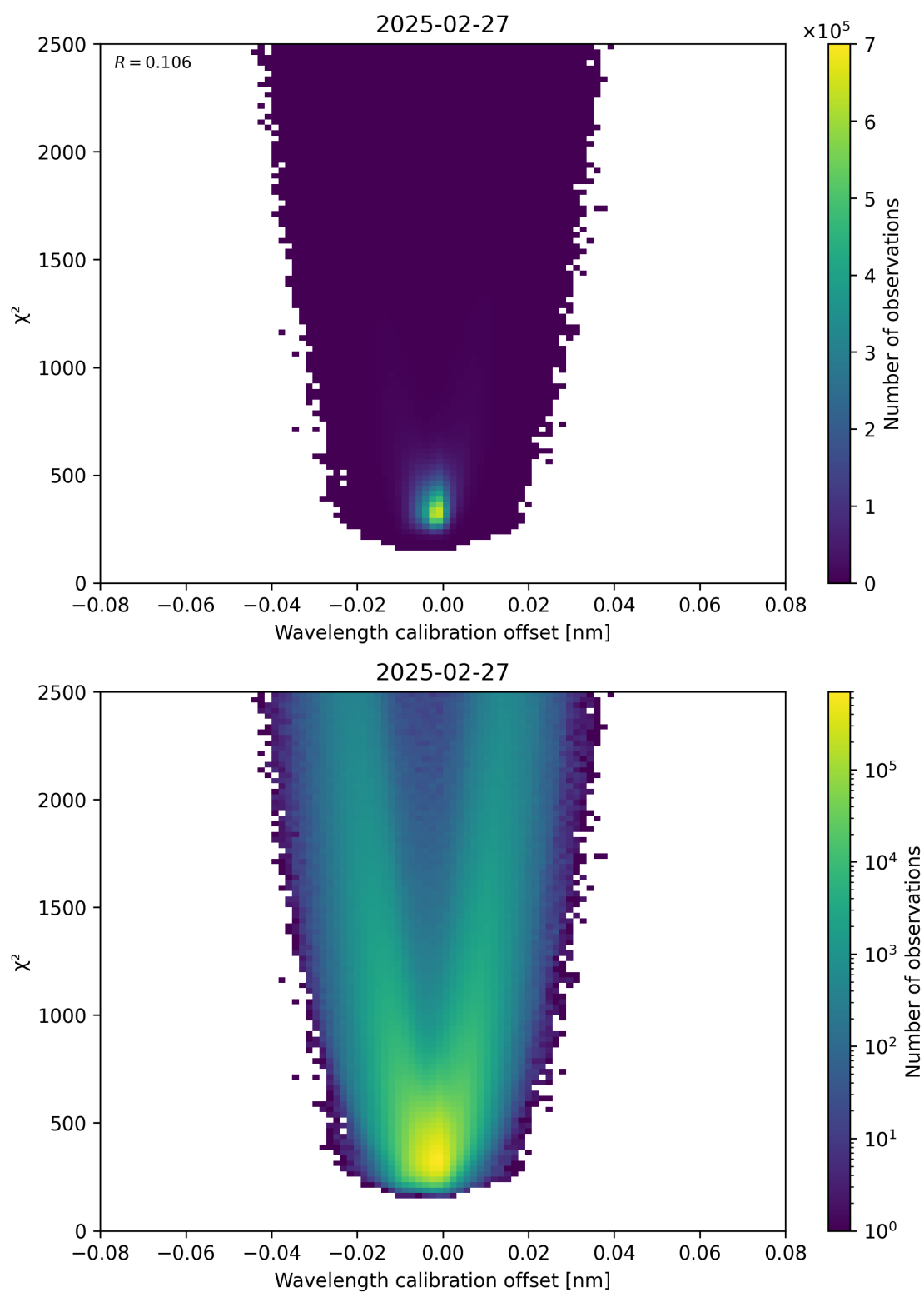
Figure 175: Scatter density plot of “Wavelength calibration offset” against “ \chi^2 ” for 2025-02-26 to 2025-02-28.
