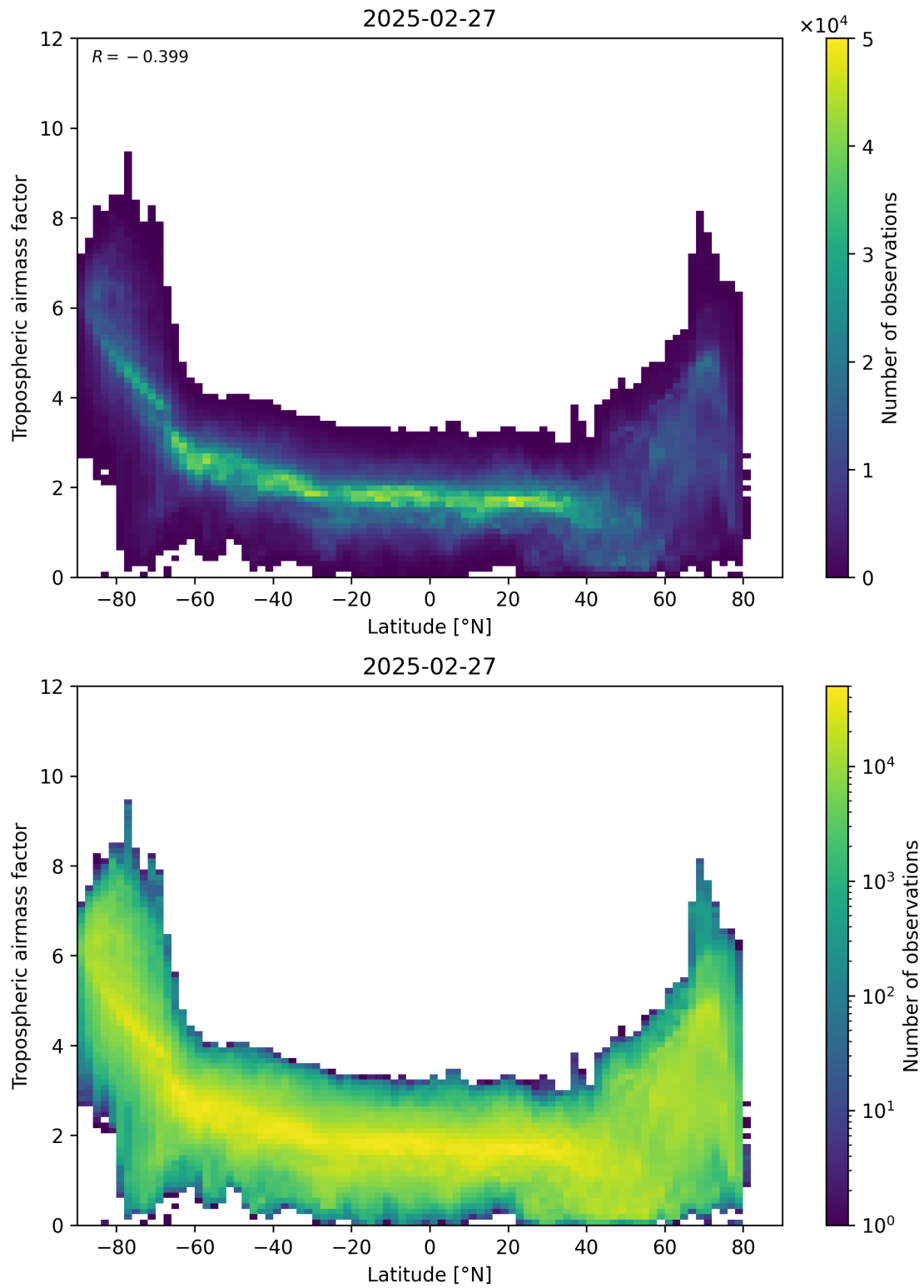
Figure 85: Scatter density plot of “Latitude” against “Tropospheric airmass factor” for 2025-02-26 to 2025-02-28.
