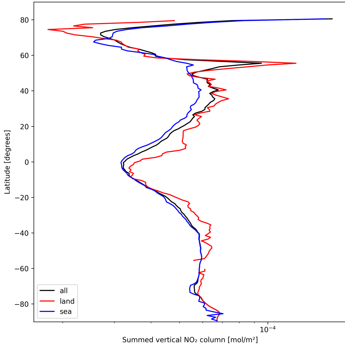
Figure 23: Zonal average of “Summed vertical NO 2 column” for 2025-02-26 to 2025-02-28.
