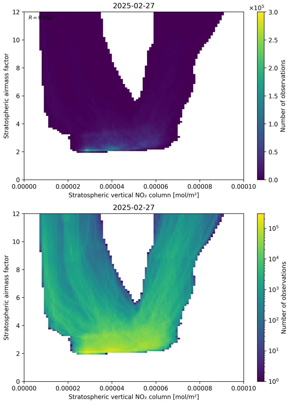
Figure 96: Scatter density plot of “Stratospheric vertical NO 2 column” against “Stratospheric airmass factor” for 2025-02-26 to 2025-02-28.
