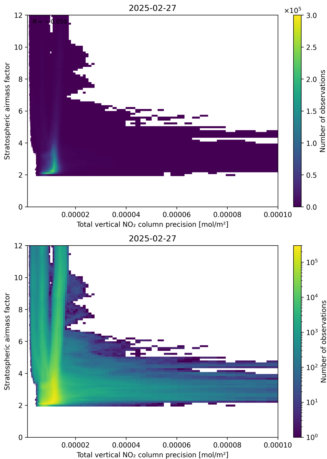
Figure 115: Scatter density plot of “Total vertical NO 2 column precision” against “Stratospheric air mass factor” for 2025-02-26 to 2025-02-28.
