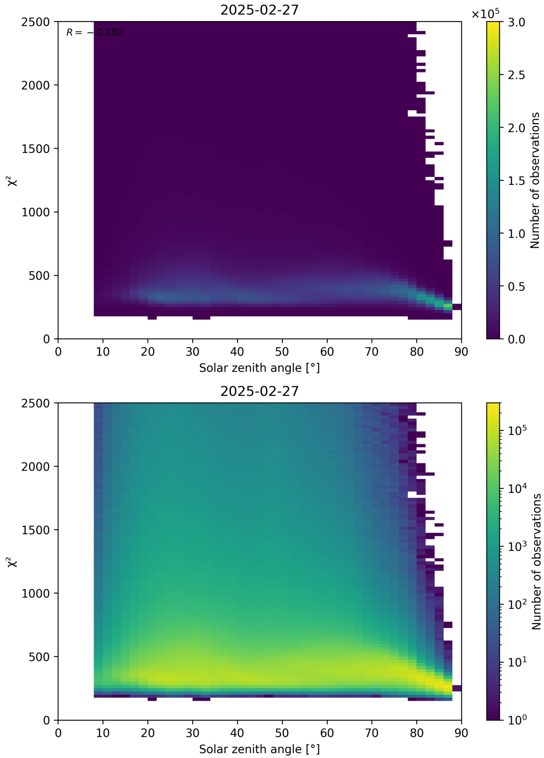
Figure 148: Scatter density plot of “Solar zenith angle” against “ \chi^2 ” for 2025-02-26 to 2025-02-28.
