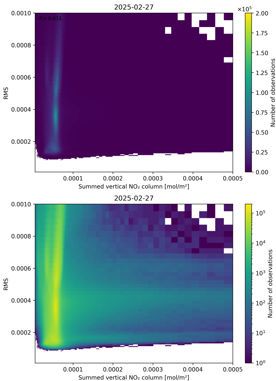
Figure 109: Scatter density plot of “Summed vertical NO 2 column” against “RMS” for 2025-02-26 to 2025-02-28.
