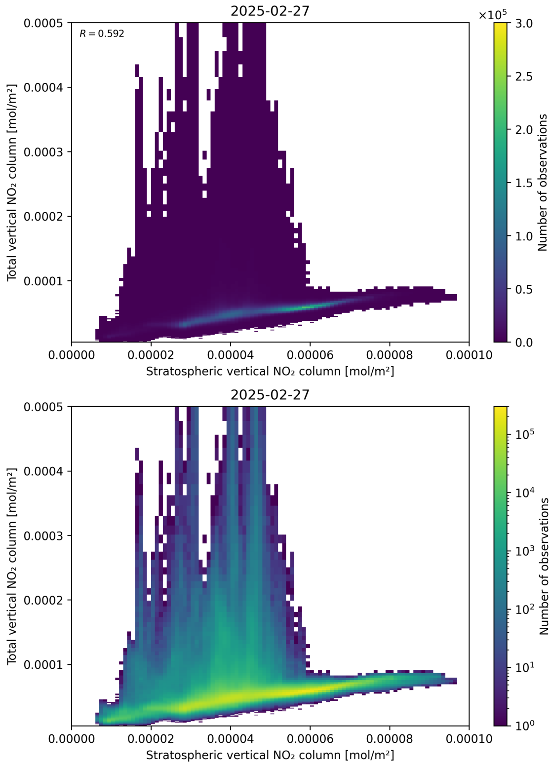
Figure 100: Scatter density plot of “Stratospheric vertical NO 2 column” against “Total vertical NO 2 column” for 2025-02-26 to 2025-02-28.
