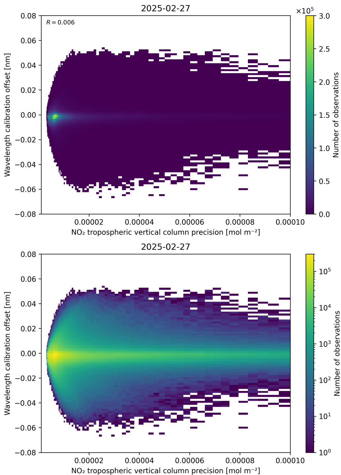
Figure 141: Scatter density plot of “NO 2 tropospheric vertical column precision” against “Wavelength calibration offset” for 2025-02-26 to 2025-02-28.
