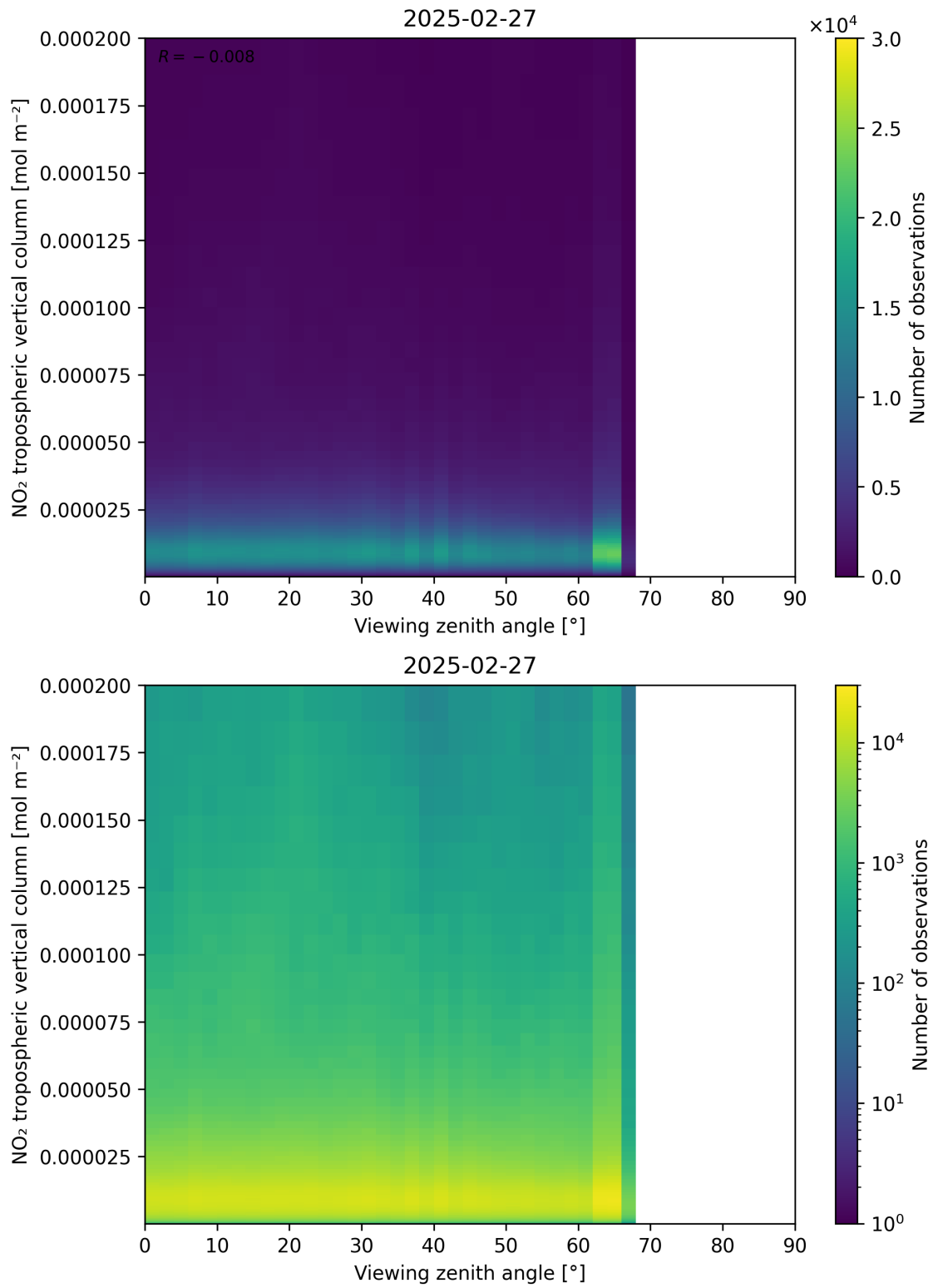
Figure 169: Scatter density plot of “Viewing zenith angle” against “NO 2 tropospheric vertical column” for 2025-02-26 to 2025-02-28.
