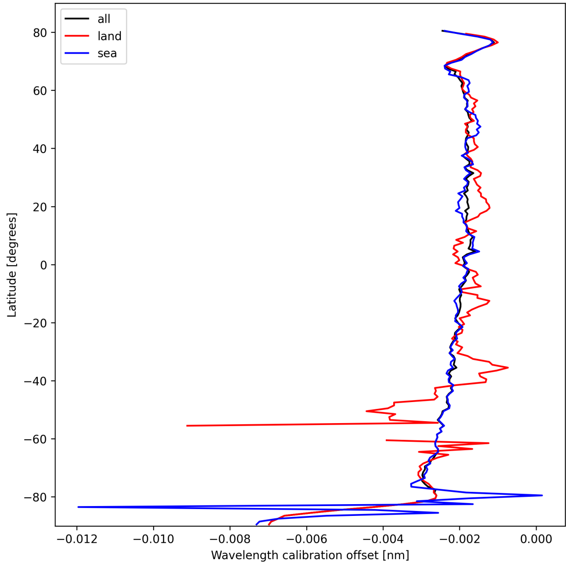
Figure 18: Zonal average of “Wavelength calibration offset” for 2025-02-26 to 2025-02-28.
