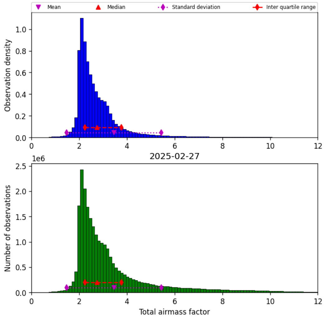
Figure 32: Histogram of “Total airmass factor” for 2025-02-26 to 2025-02-28
