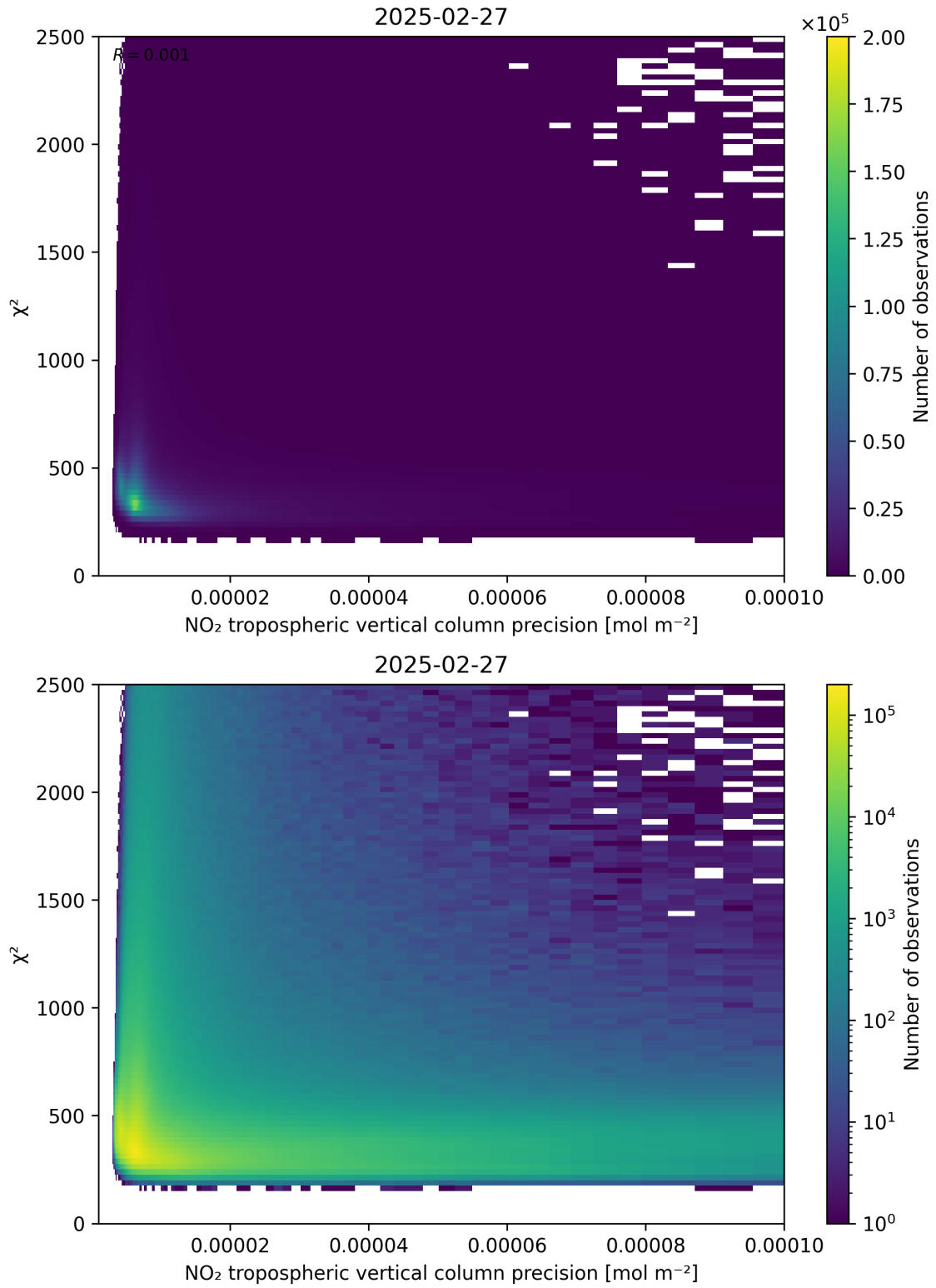
Figure 134: Scatter density plot of “NO 2 tropospheric vertical column precision” against “ \chi^2 ” for 2025-02-26 to 2025-02-28.
