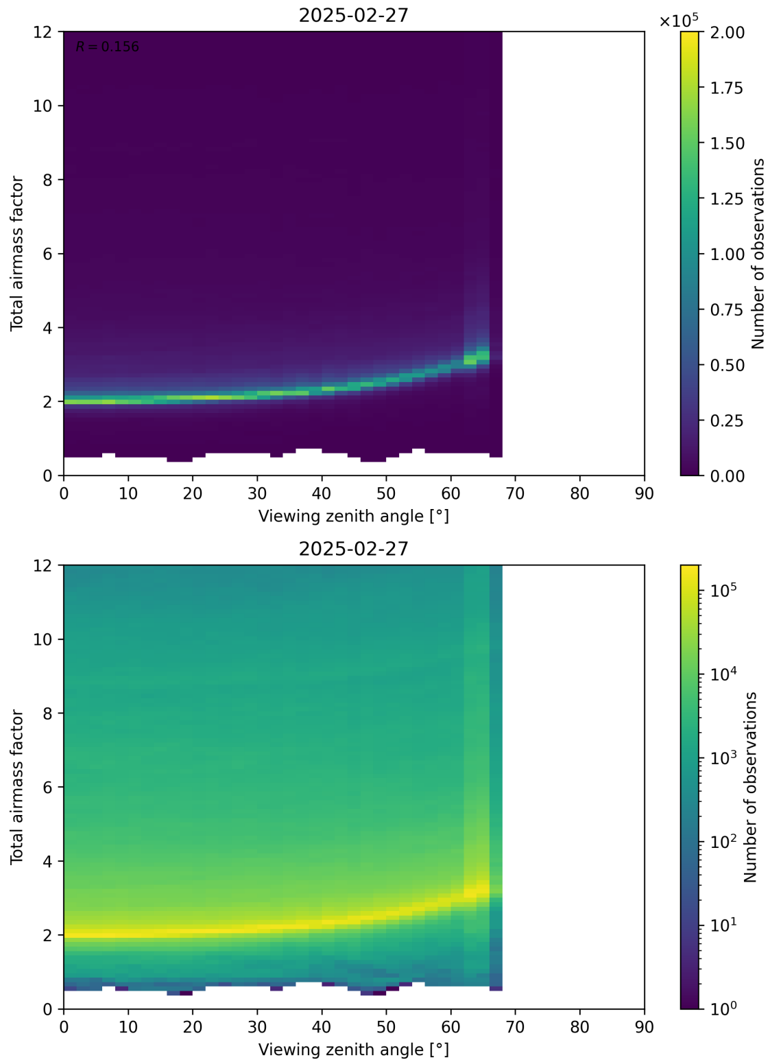
Figure 160: Scatter density plot of “Viewing zenith angle” against “Total airmass factor” for 2025-02-26 to 2025-02-28.
