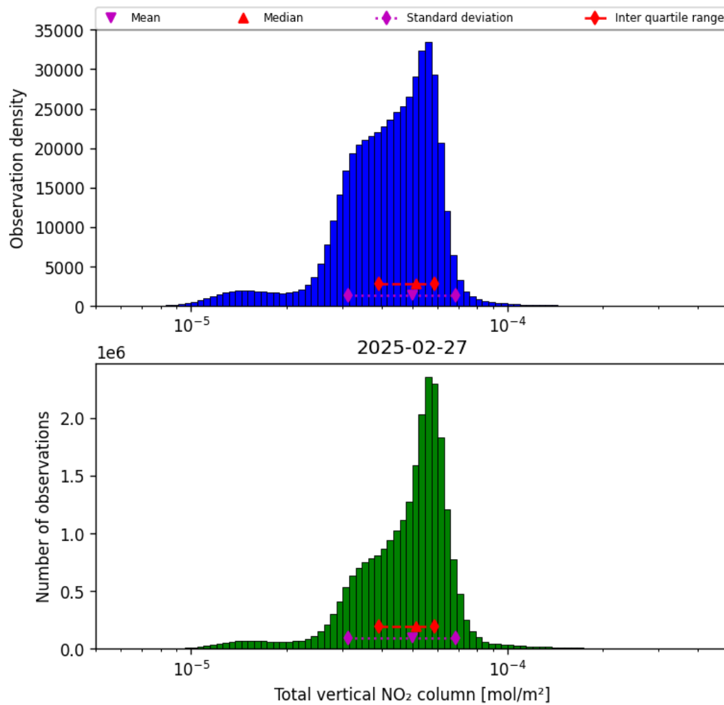
Figure 38: Histogram of “Total vertical NO 2 column” for 2025-02-26 to 2025-02-28
