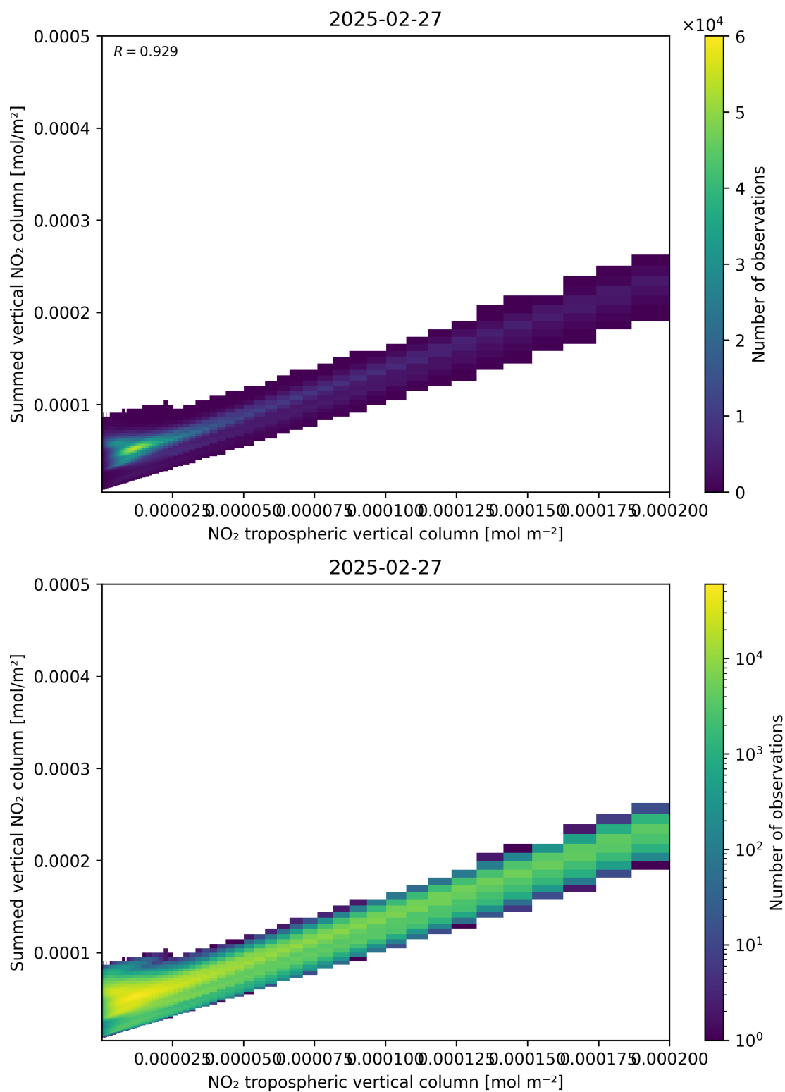
Figure 126: Scatter density plot of “NO 2 tropospheric vertical column” against “Summed vertical NO 2 column” for 2025-02-26 to 2025-02-28.
