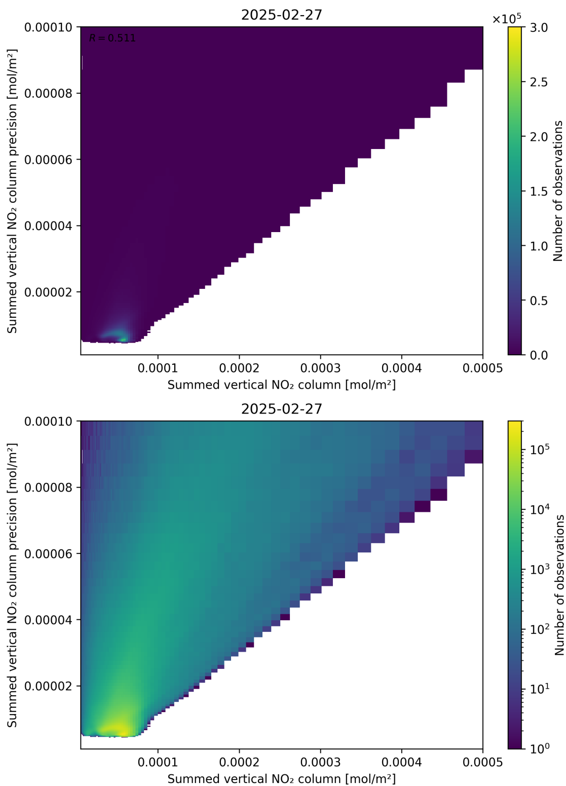
Figure 105: Scatter density plot of “Summed vertical NO 2 column” against “Summed vertical NO 2 column precision” for 2025-02-26 to 2025-02-28.
