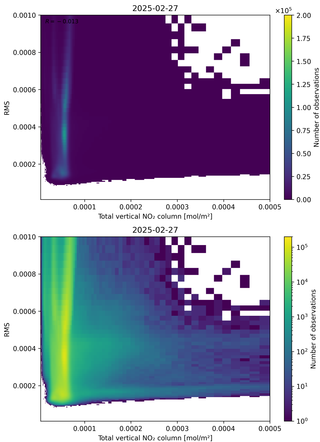
Figure 120: Scatter density plot of “Total vertical NO 2 column” against “RMS” for 2025-02-26 to 2025-02-28.
