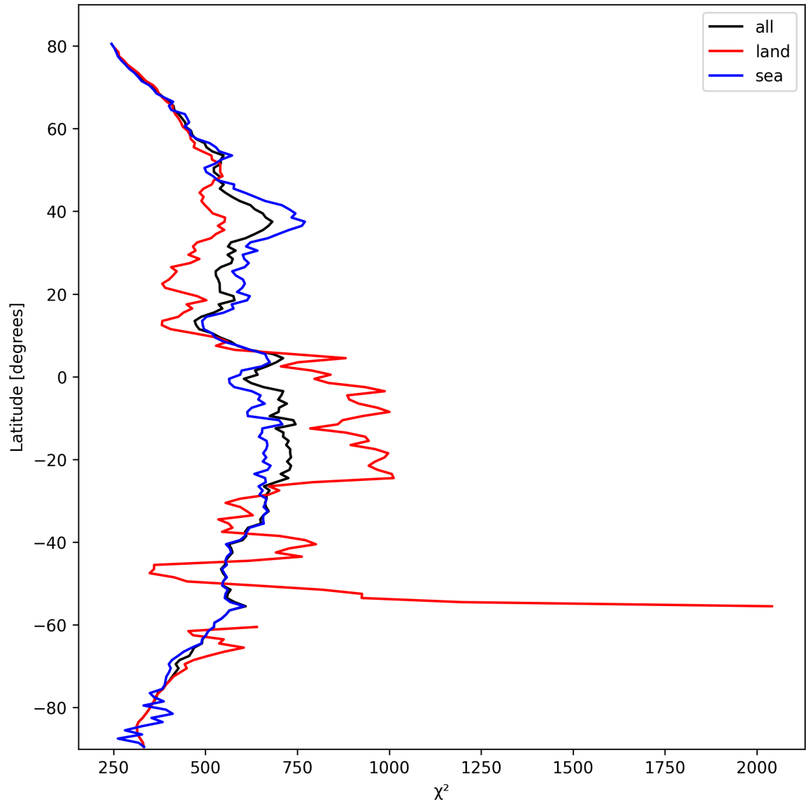
Figure 25: Zonal average of “ \chi^2 ” for 2025-02-26 to 2025-02-28.
