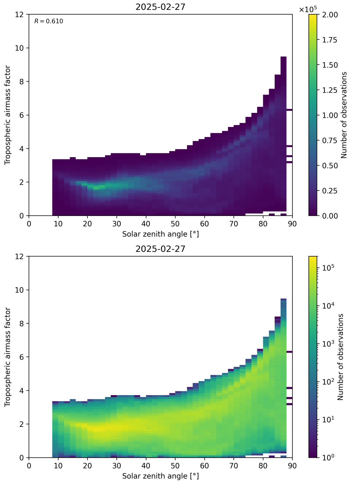
Figure 147: Scatter density plot of “Solar zenith angle” against “Tropospheric airmass factor” for 2025-02-26 to 2025-02-28.
