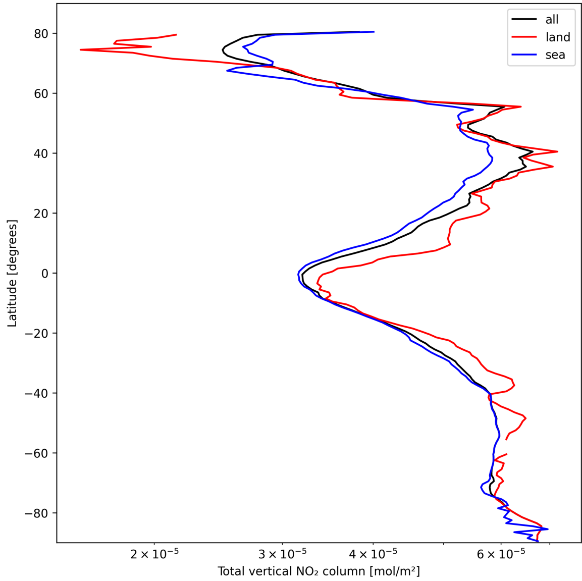
Figure 21: Zonal average of “Total vertical NO 2 column” for 2025-02-26 to 2025-02-28.
