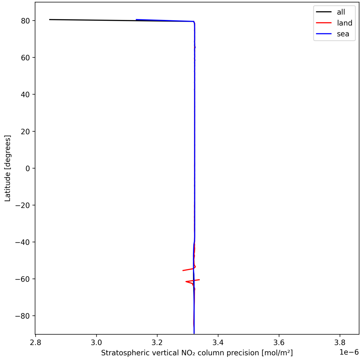
Figure 20: Zonal average of “Stratospheric vertical NO 2 column precision” for 2025-02-26 to 2025-02-28.
