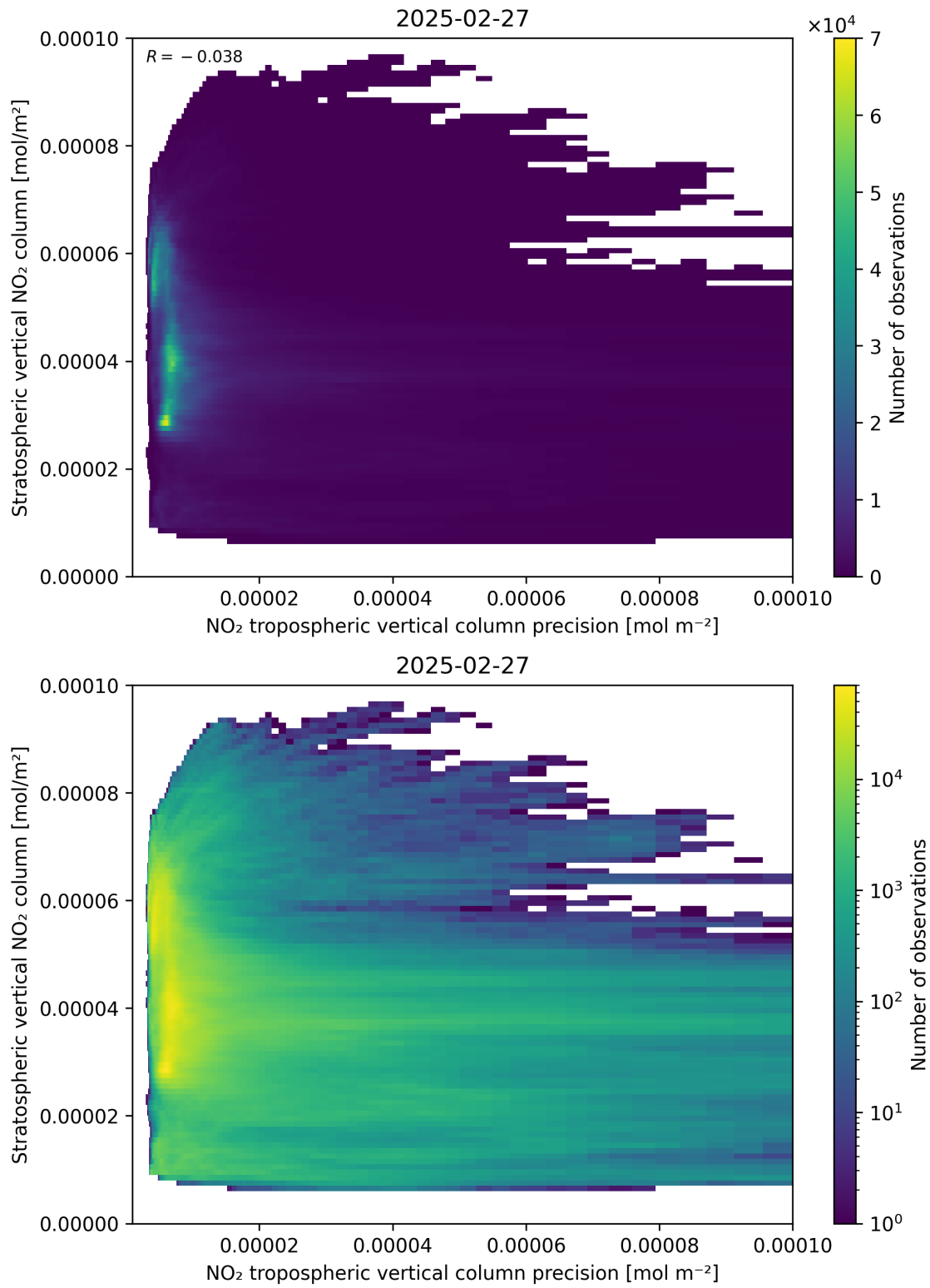
Figure 135: Scatter density plot of “NO 2 tropospheric vertical column precision” against “Stratospheric vertical NO 2 column” for 2025-02-26 to 2025-02-28.
