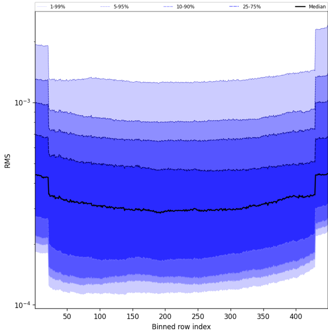
Figure 60: Along track statistics of “RMS” for 2025-02-26 to 2025-02-28
