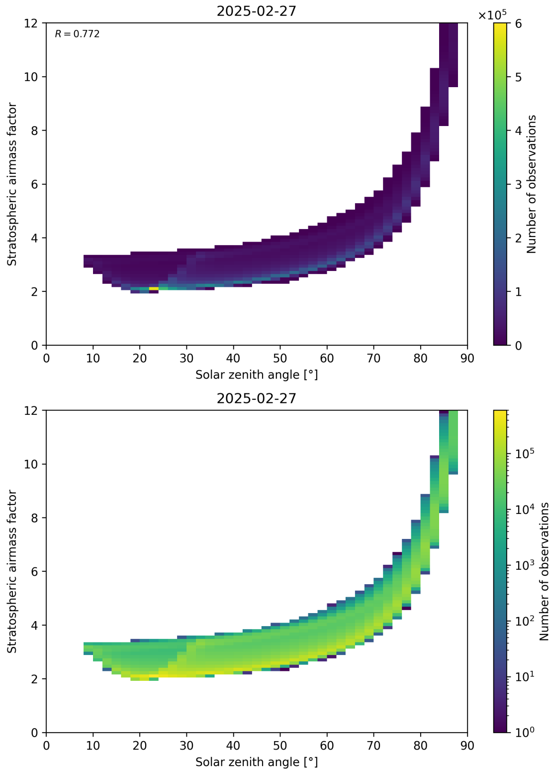
Figure 145: Scatter density plot of “Solar zenith angle” against “Stratospheric airmass factor” for 2025-02-26 to 2025-02-28.
