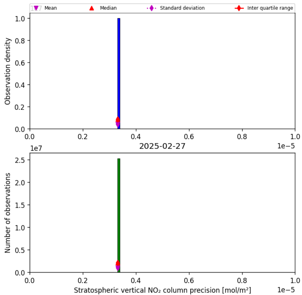
Figure 37: Histogram of “Stratospheric vertical NO 2 column precision” for 2025-02-26 to 2025-02-28
