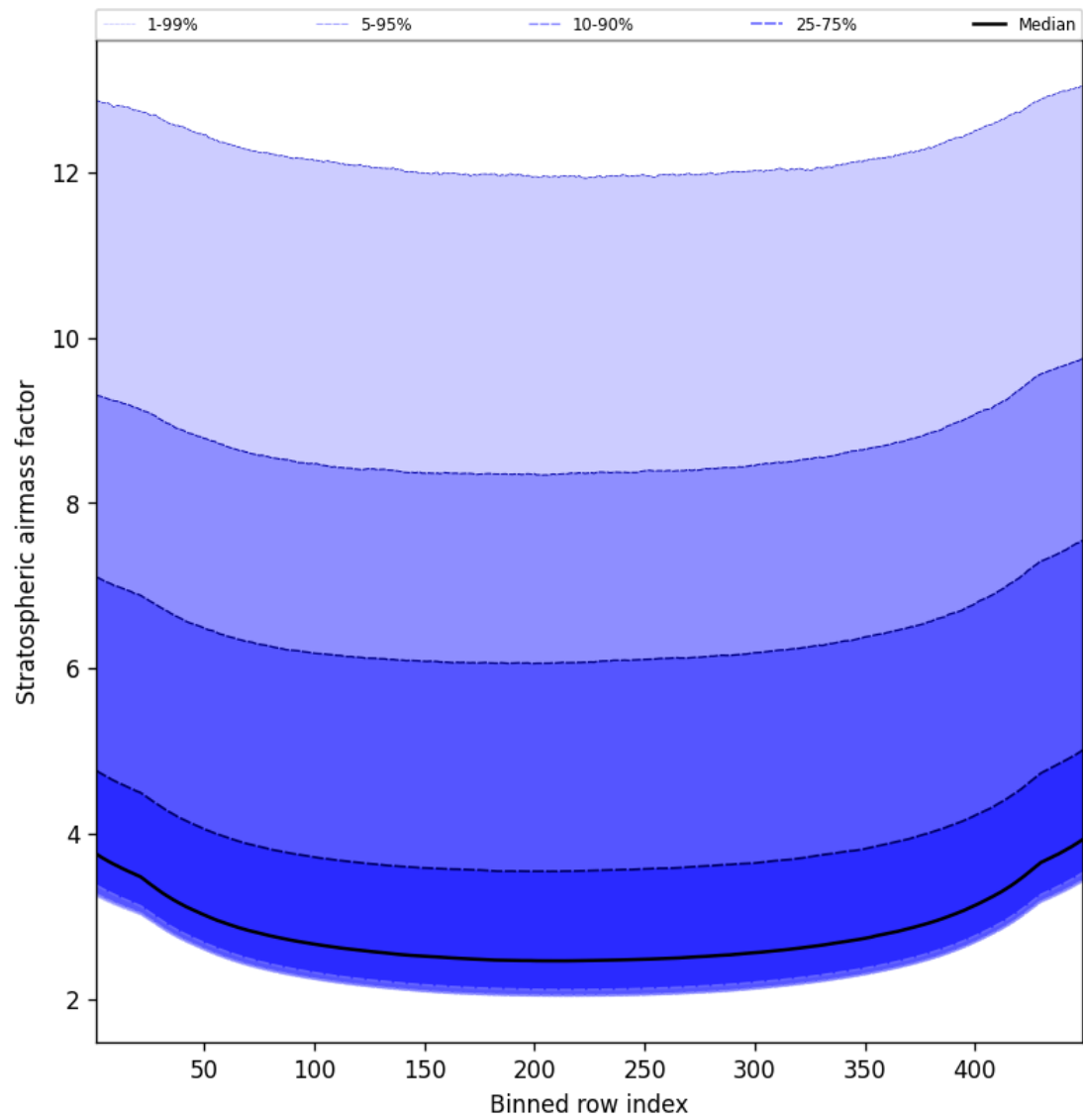
Figure 61: Along track statistics of “Stratospheric air mass factor” for 2025-02-26 to 2025-02-28
