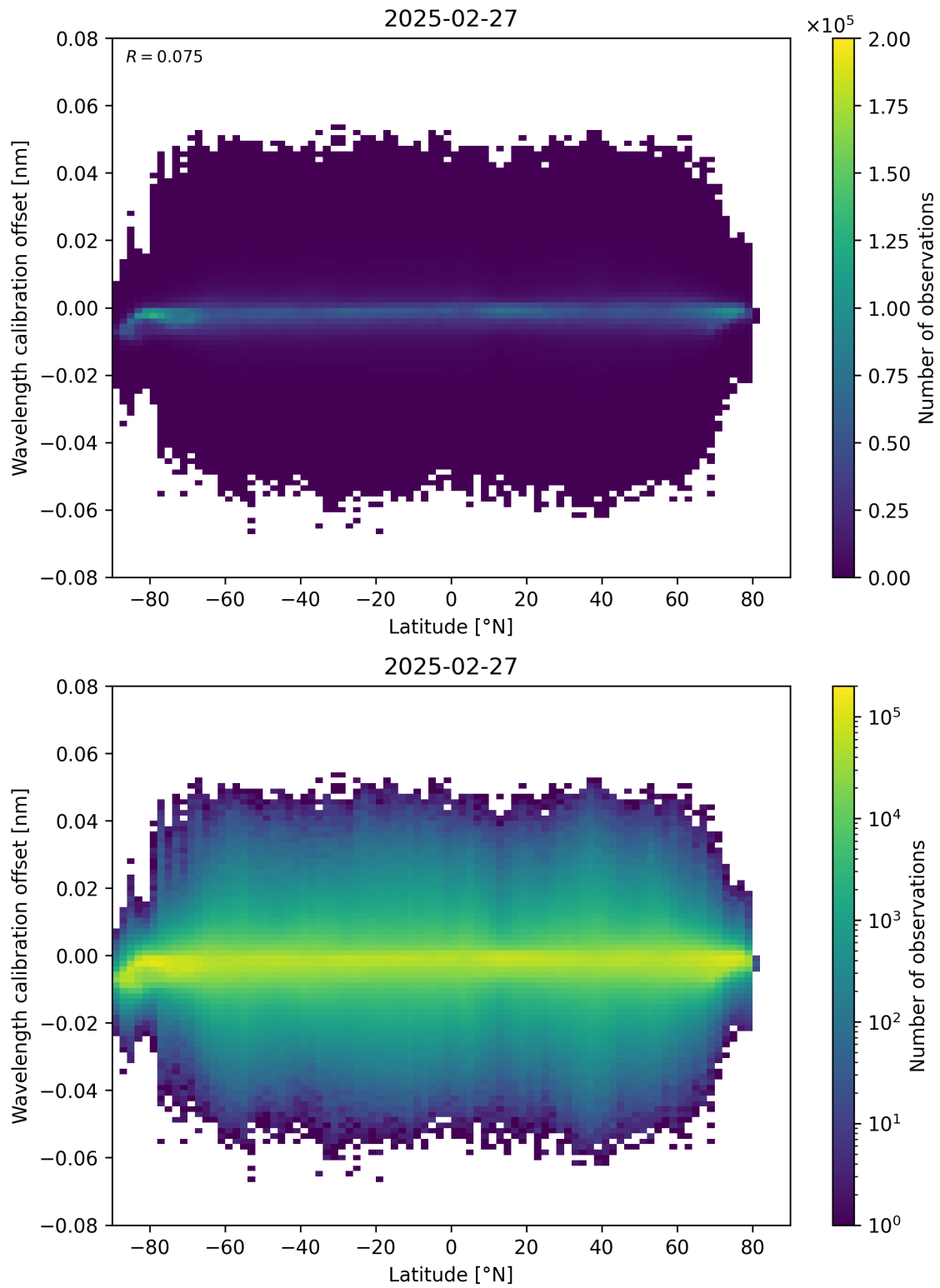
Figure 95: Scatter density plot of “Latitude” against “Wavelength calibration offset” for 2025-02-26 to 2025-02-28.
