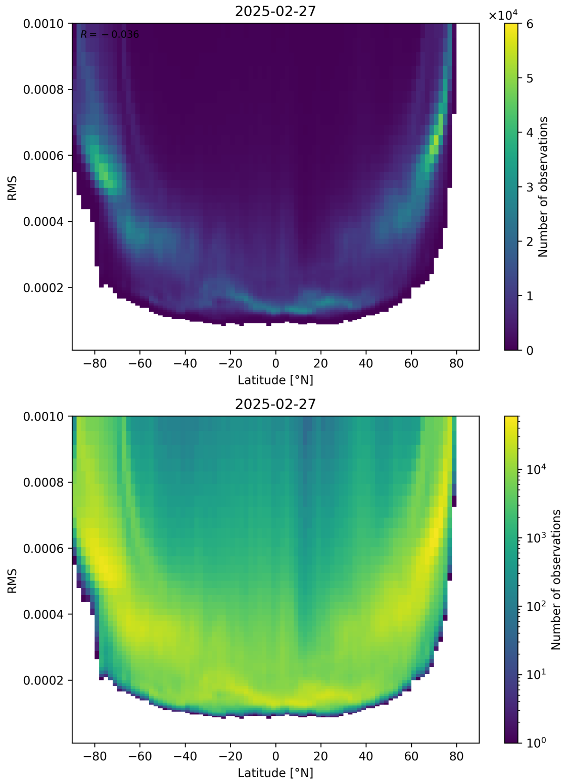
Figure 94: Scatter density plot of “Latitude” against “RMS” for 2025-02-26 to 2025-02-28.
