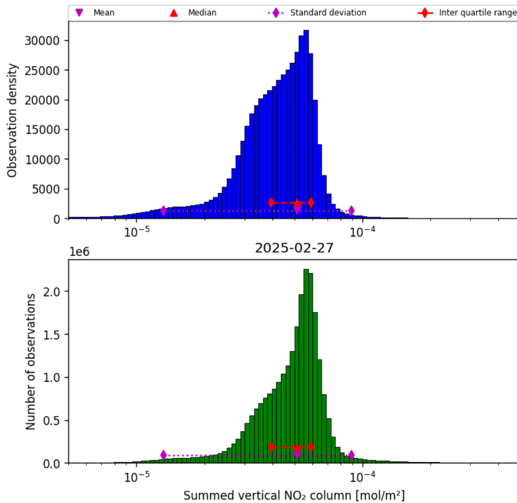
Figure 40: Histogram of “Summed vertical NO 2 column” for 2025-02-26 to 2025-02-28
