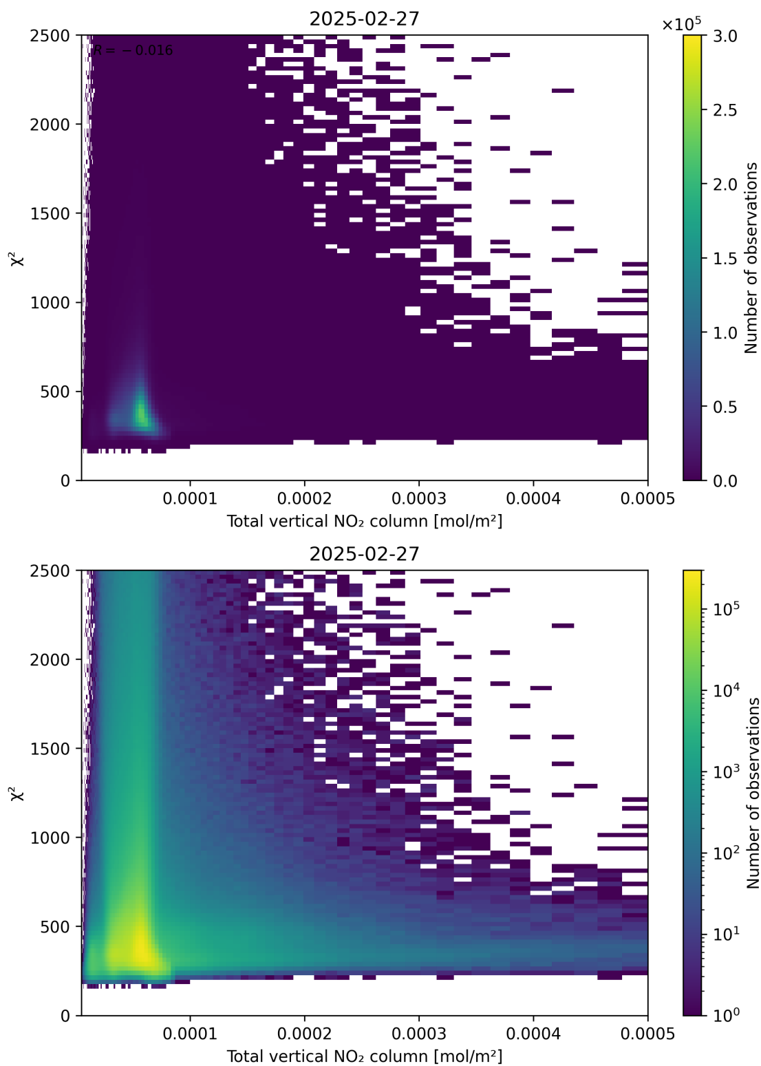
Figure 111: Scatter density plot of “Total vertical NO 2 column” against “ \chi^2 ” for 2025-02-26 to 2025-02-28.
