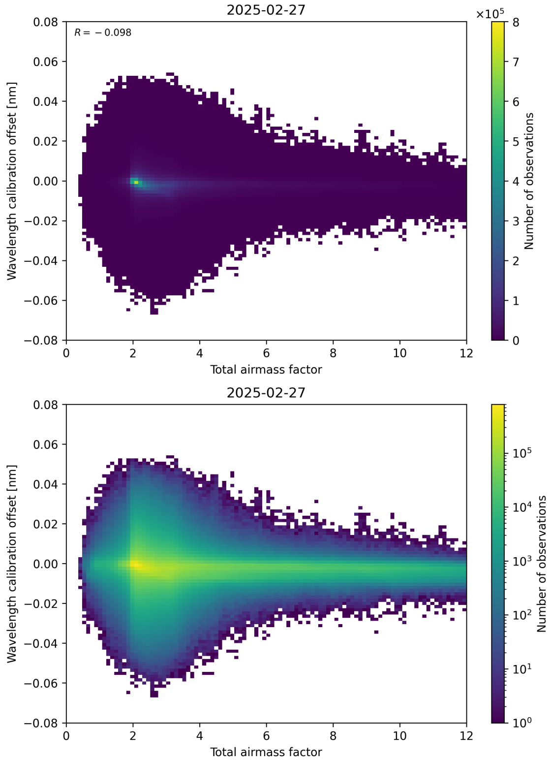
Figure 70: Scatter density plot of “Total airmass factor” against “Wavelength calibration offset” for 2025-02-26 to 2025-02-28.
