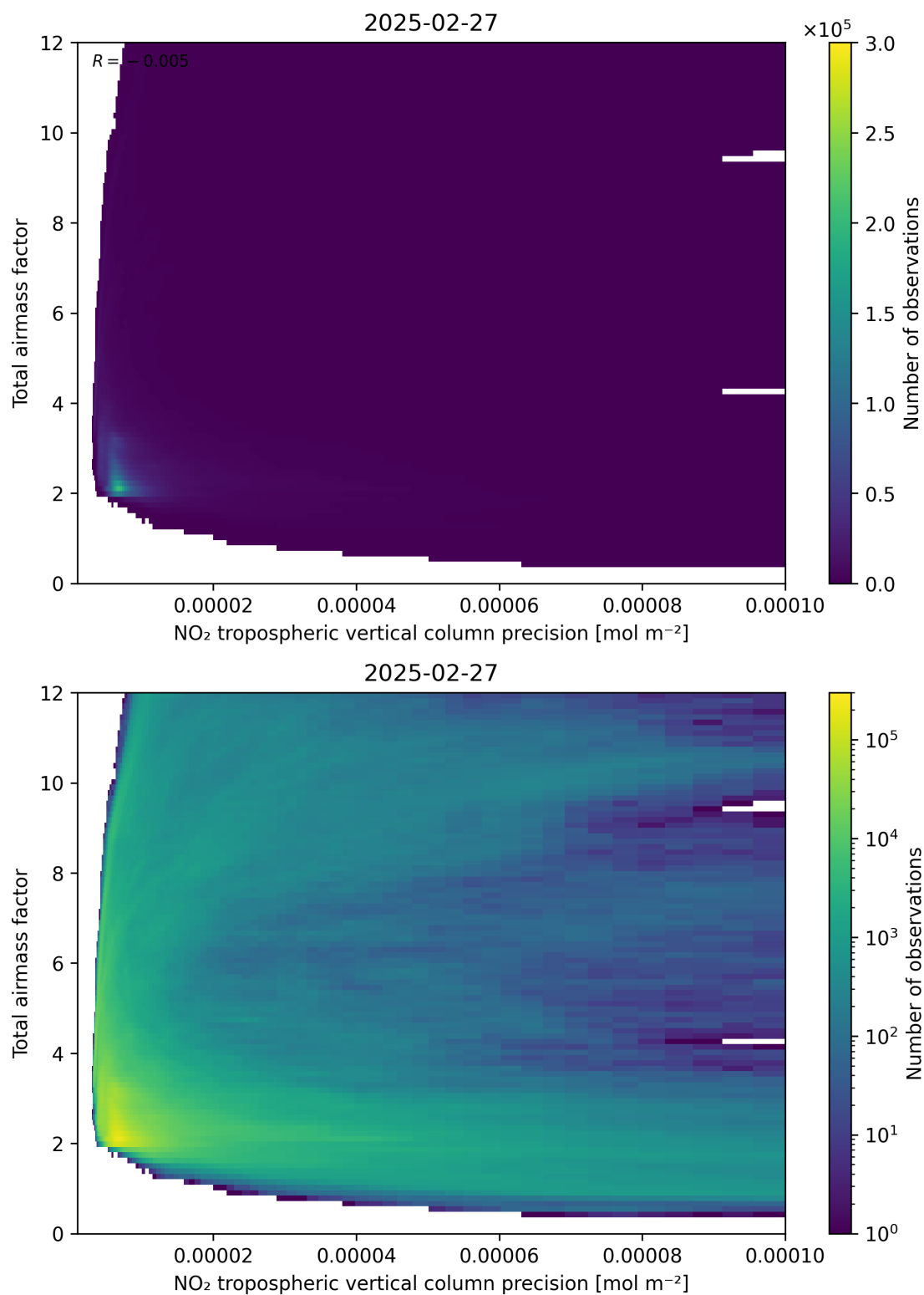
Figure 132: Scatter density plot of “NO 2 tropospheric vertical column precision” against “Total airmass factor” for 2025-02-26 to 2025-02-28.
