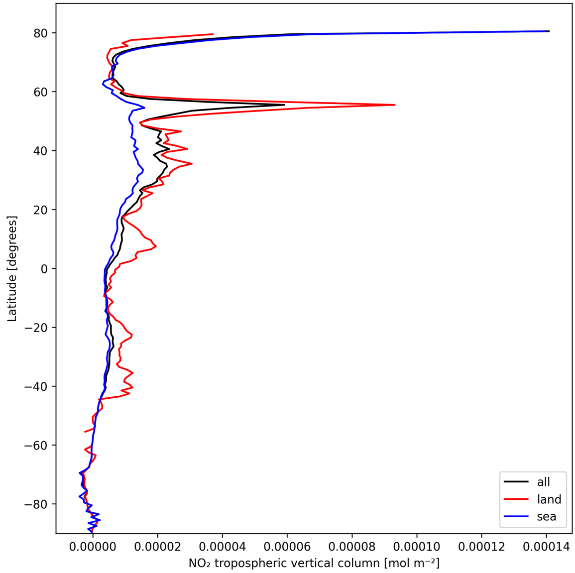
Figure 12: Zonal average of “NO 2 tropospheric vertical column” for 2025-02-26 to 2025-02-28.
