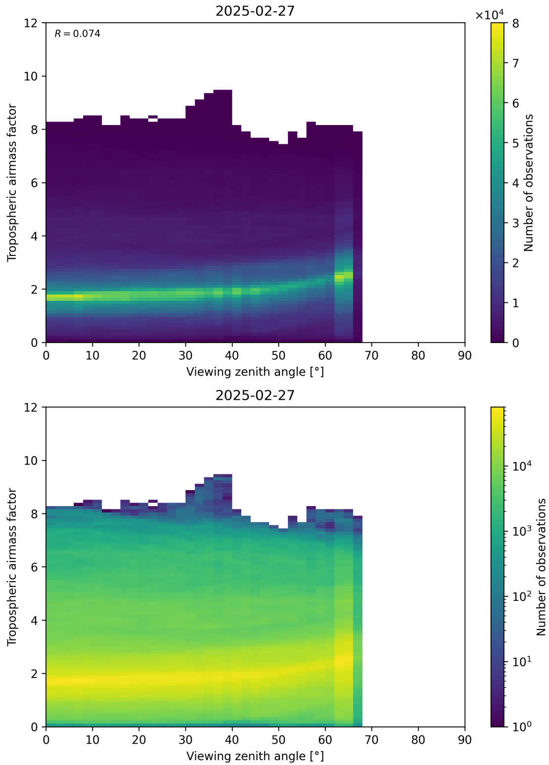
Figure 161: Scatter density plot of “Viewing zenith angle” against “Tropospheric airmass factor” for 2025-02-26 to 2025-02-28.
