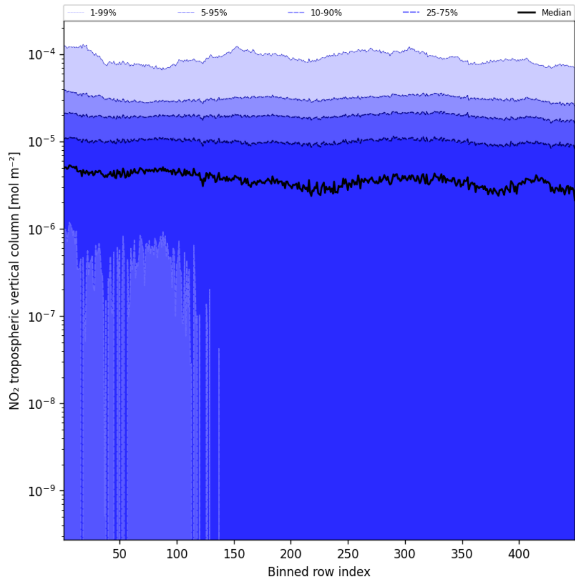
Figure 46: Along track statistics of “ \text{NO}_2 tropospheric vertical column” for 2025-02-26 to 2025-02-28
