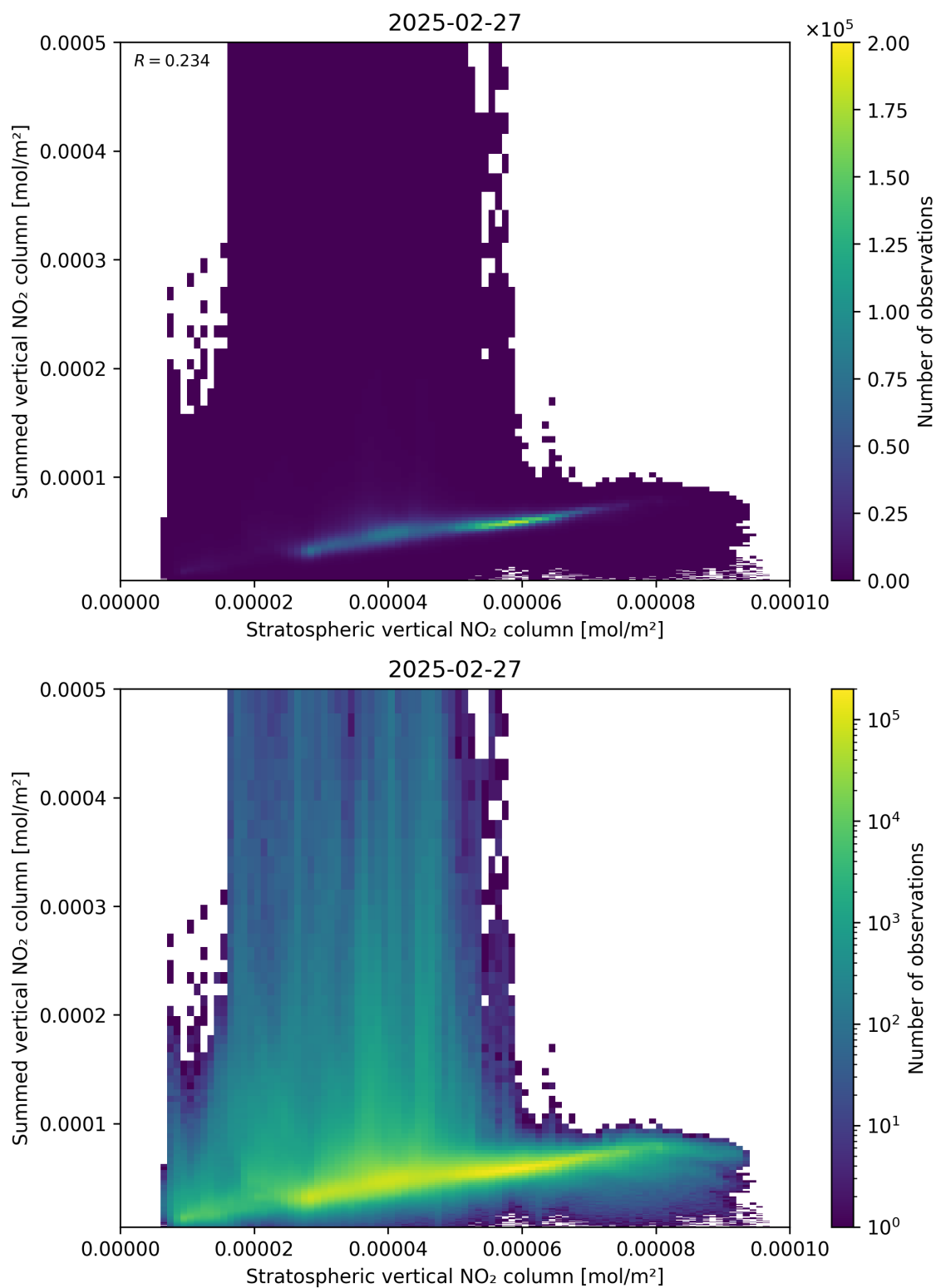
Figure 98: Scatter density plot of “Stratospheric vertical NO 2 column” against “Summed vertical NO 2 column” for 2025-02-26 to 2025-02-28.
