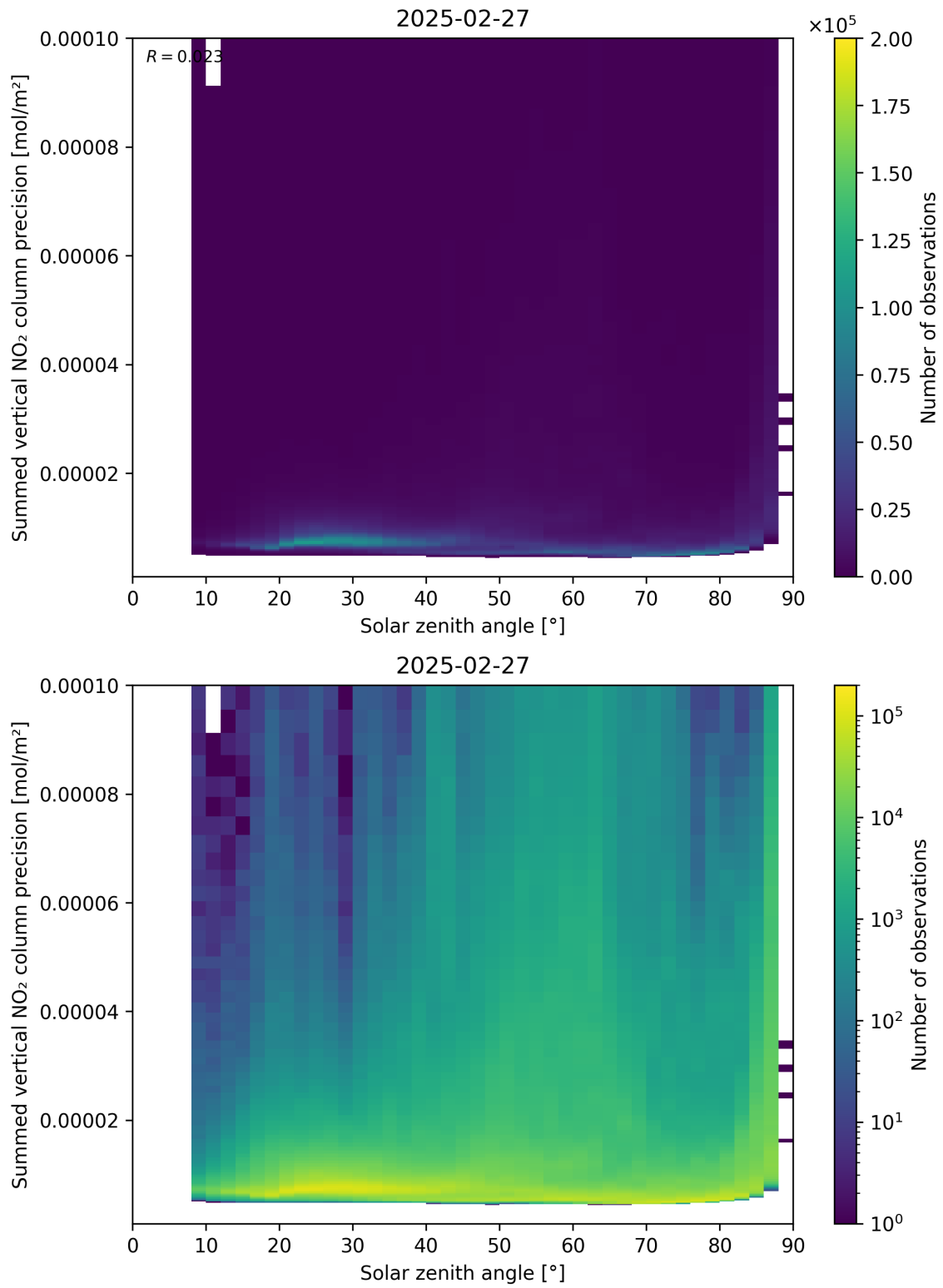
Figure 152: Scatter density plot of “Solar zenith angle” against “Summed vertical NO 2 column precision” for 2025-02-26 to 2025-02-28.
