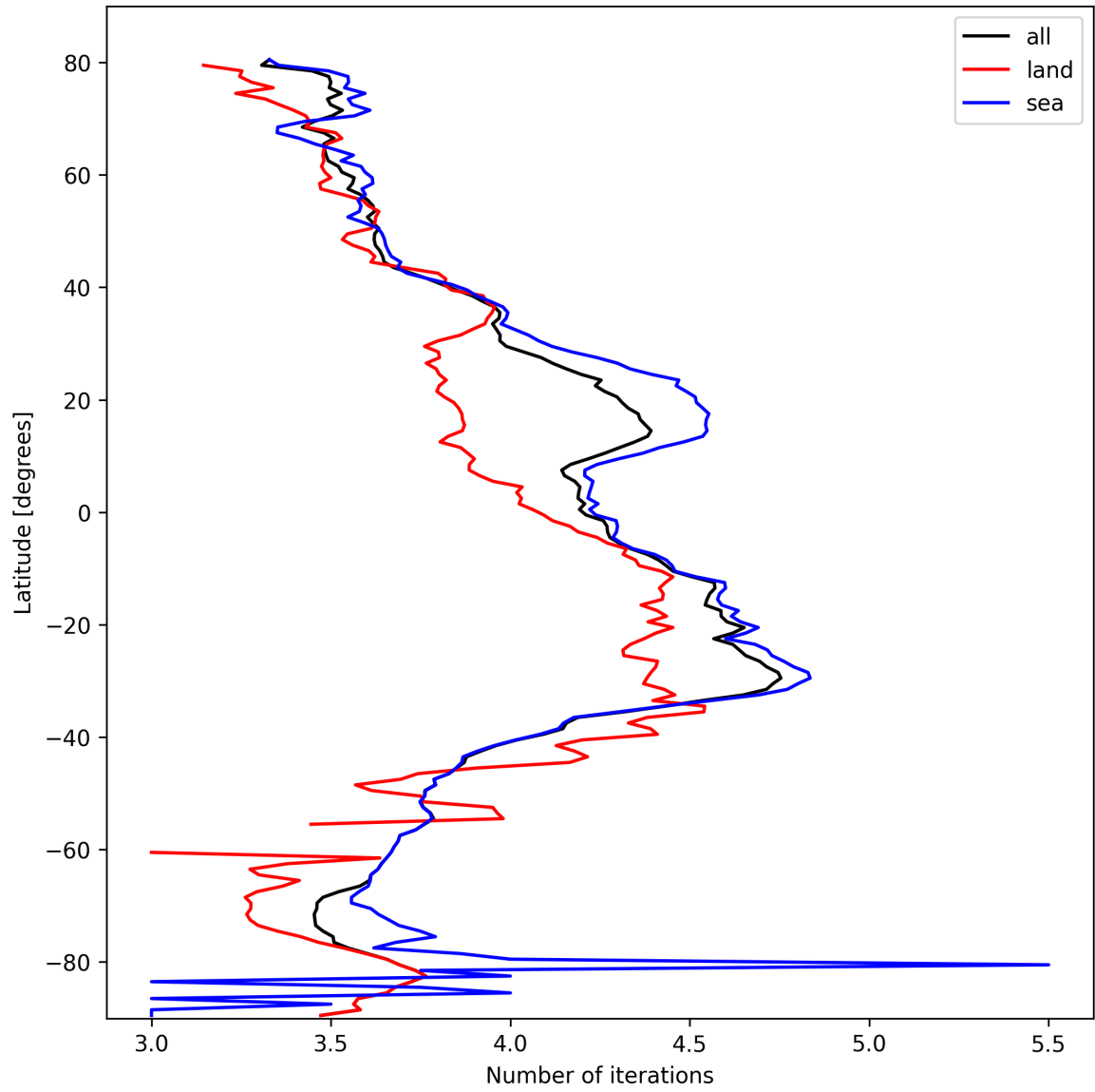
Figure 17: Zonal average of “Number of iterations” for 2025-02-26 to 2025-02-28.
