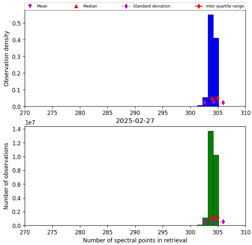
Figure 33: Histogram of “Number of spectral points in retrieval” for 2025-02-26 to 2025-02-28
