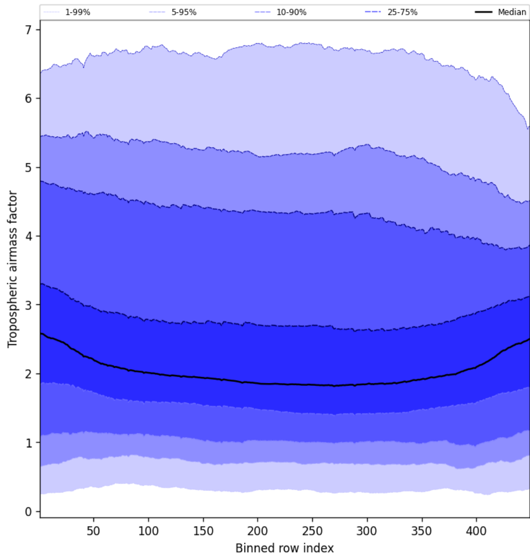
Figure 48: Along track statistics of “Tropospheric airmass factor” for 2025-02-26 to 2025-02-28
