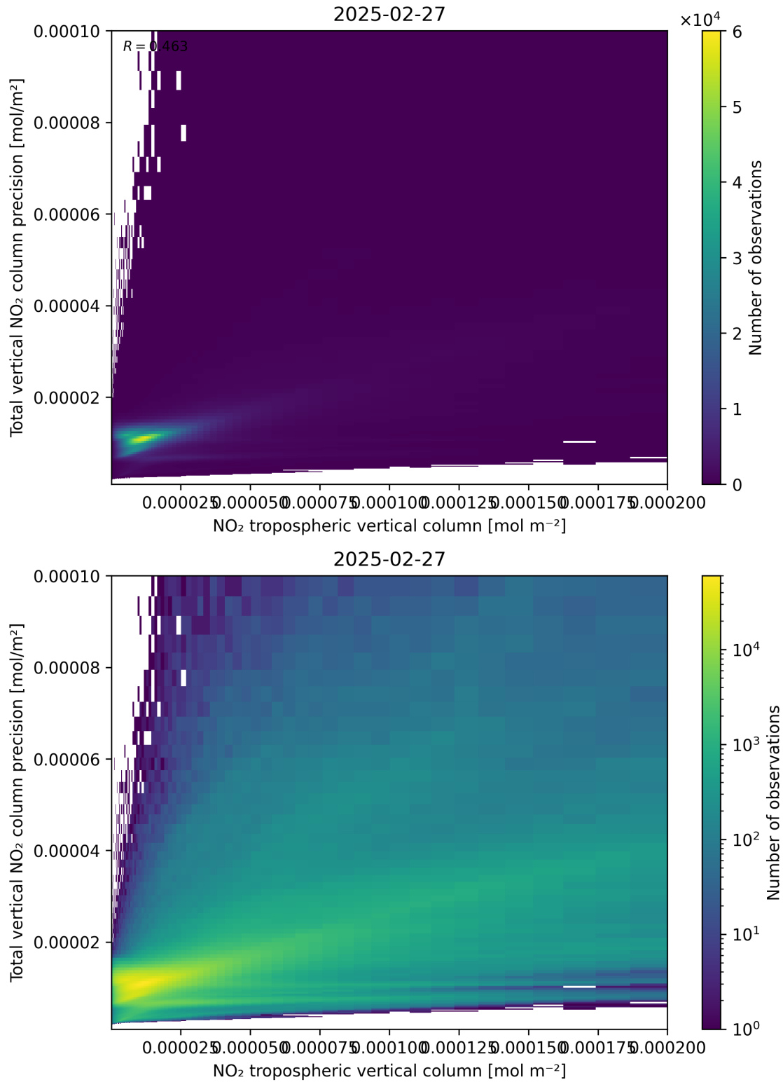
Figure 129: Scatter density plot of “NO 2 tropospheric vertical column” against “Total vertical NO 2 column precision” for 2025-02-26 to 2025-02-28.
