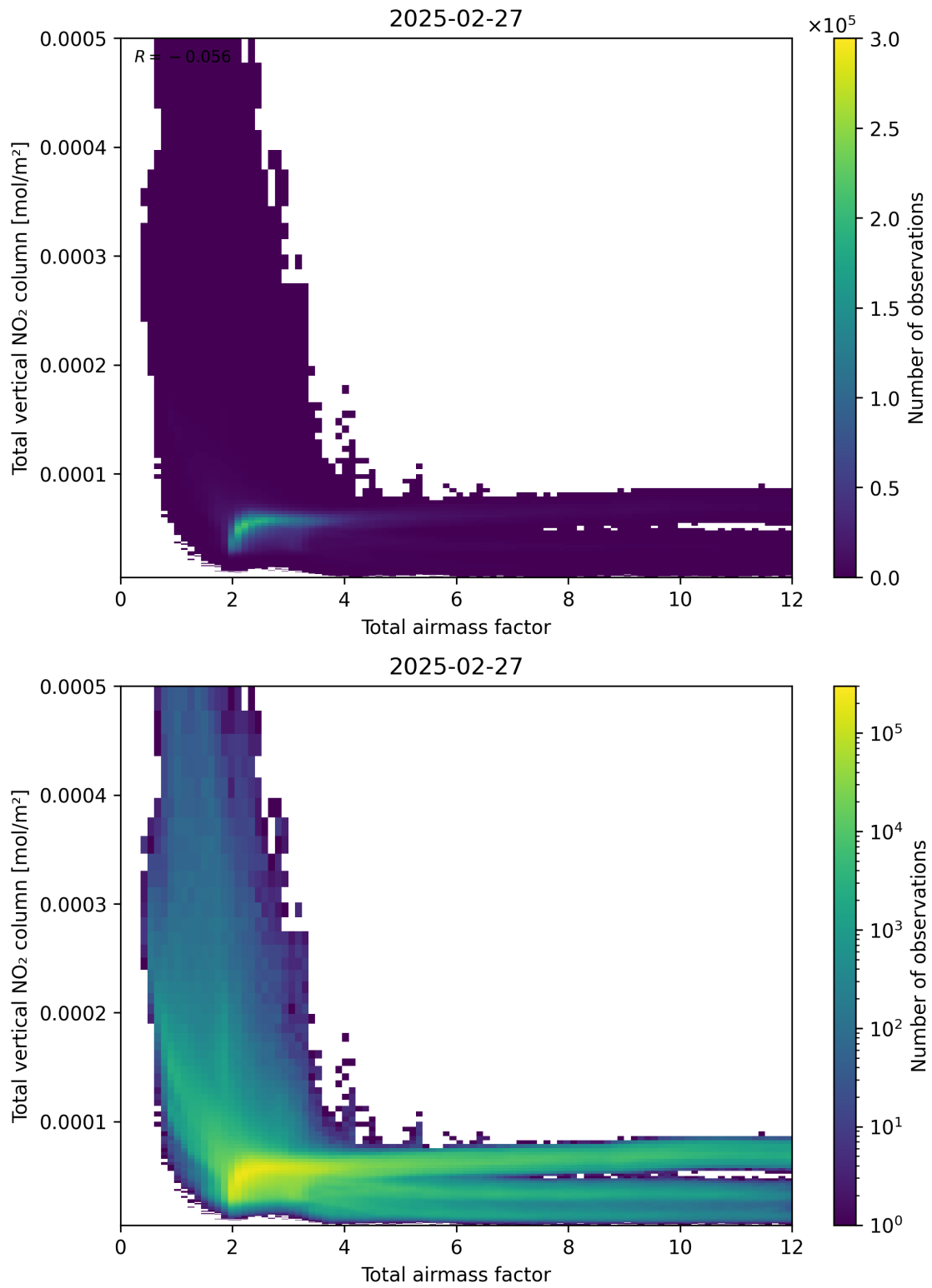
Figure 67: Scatter density plot of “Total airmass factor” against “Total vertical NO 2 column” for 2025-02-26 to 2025-02-28.
