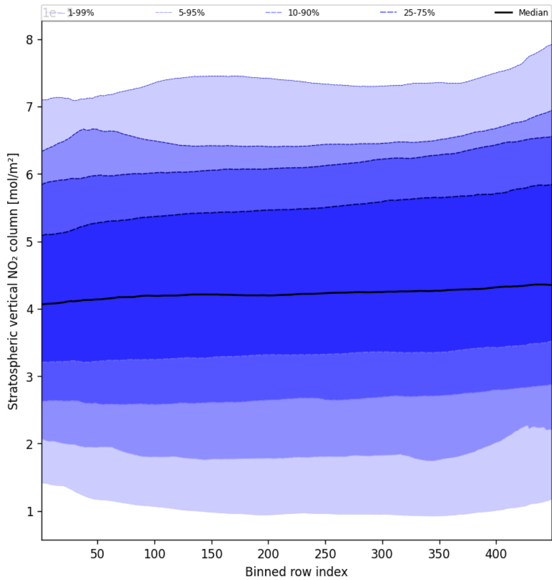
Figure 53: Along track statistics of “Stratospheric vertical NO 2 column” for 2025-02-26 to 2025-02-28
