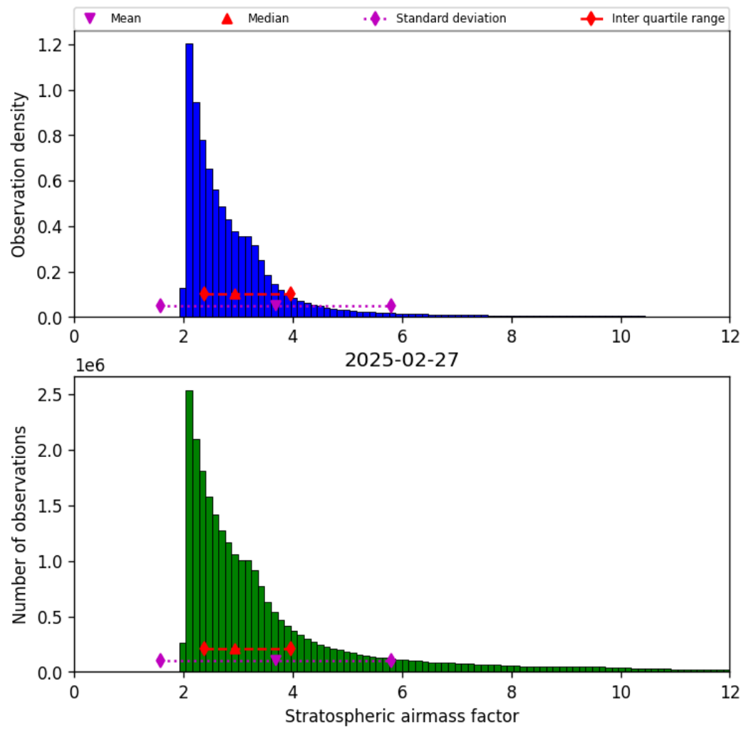
Figure 44: Histogram of “Stratospheric airmass factor” for 2025-02-26 to 2025-02-28
