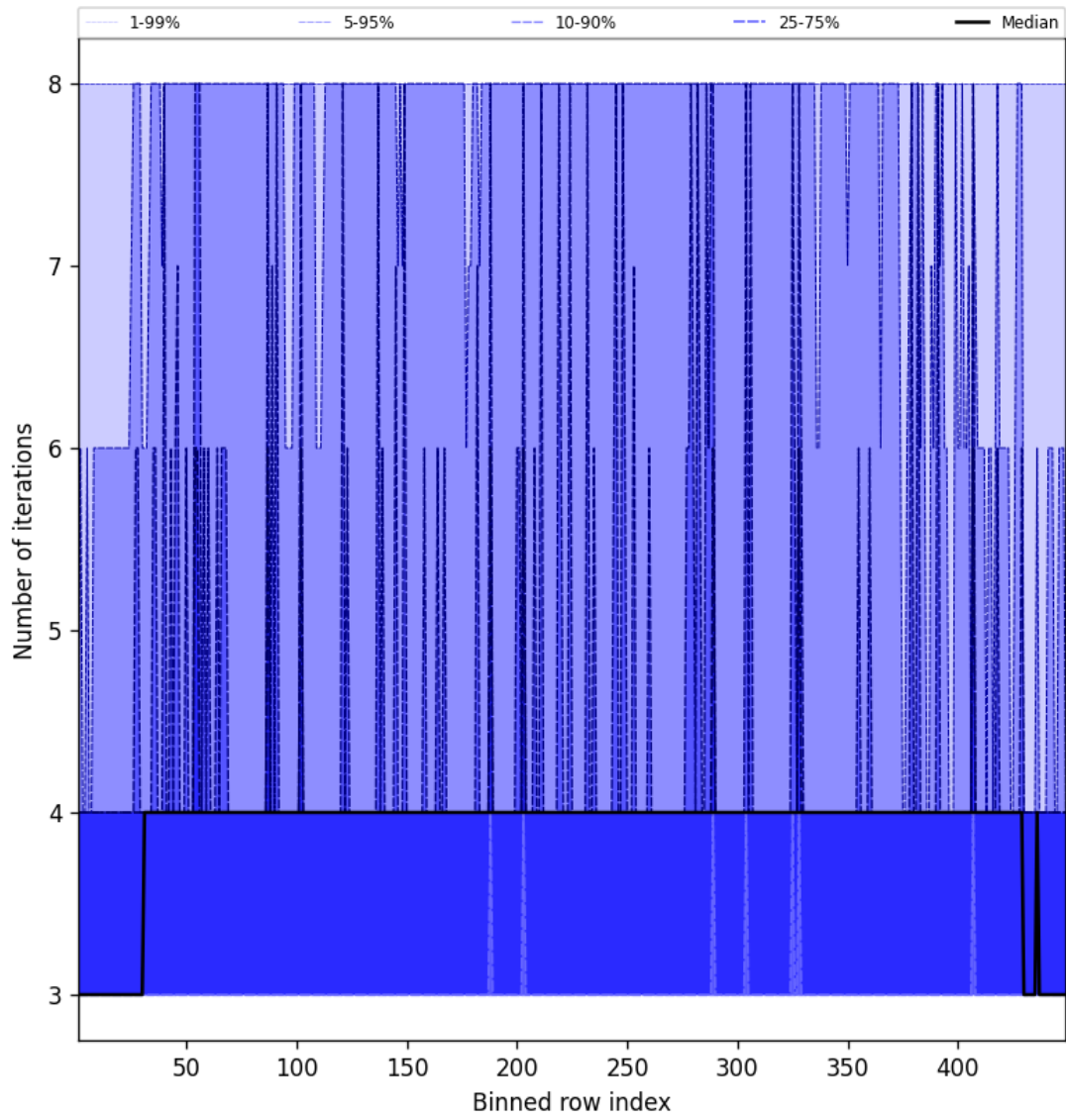
Figure 51: Along track statistics of “Number of iterations” for 2025-02-26 to 2025-02-28
