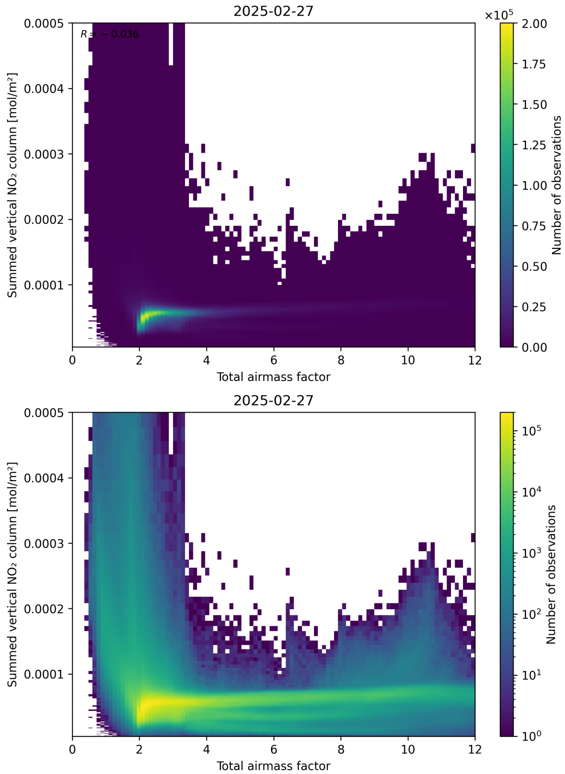
Figure 65: Scatter density plot of “Total airmass factor” against “Summed vertical NO 2 column” for 2025-02-26 to 2025-02-28.
