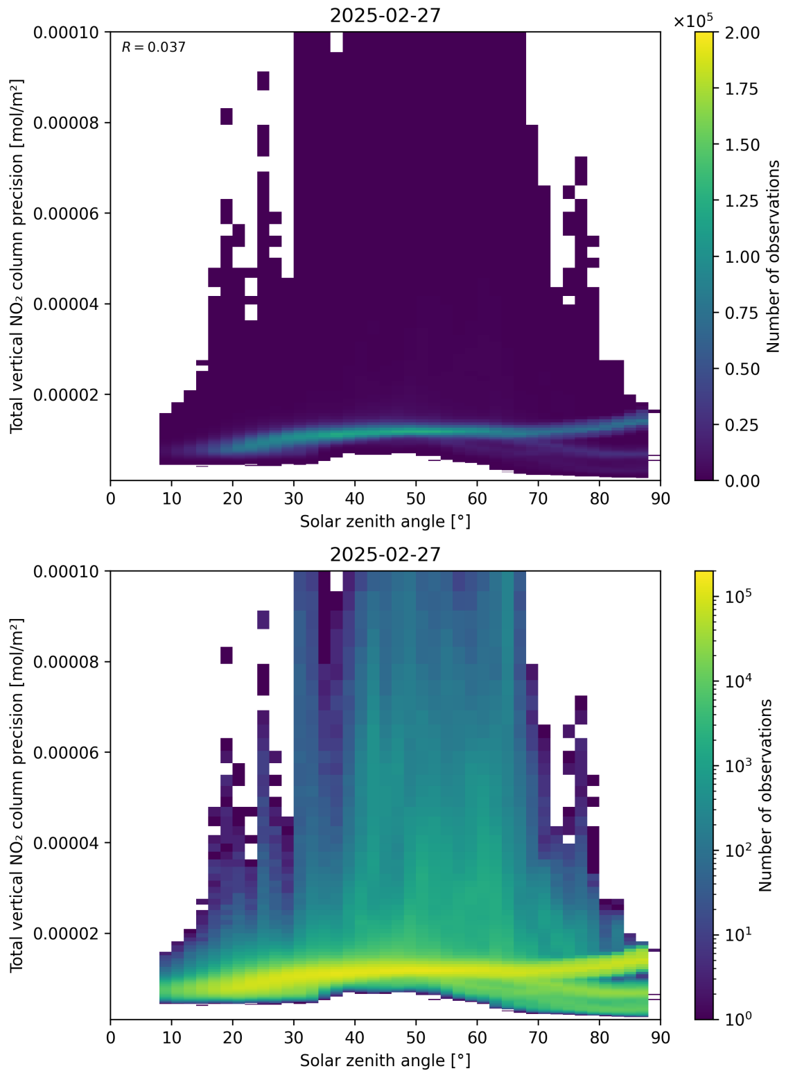
Figure 154: Scatter density plot of “Solar zenith angle” against “Total vertical NO 2 column precision” for 2025-02-26 to 2025-02-28.
