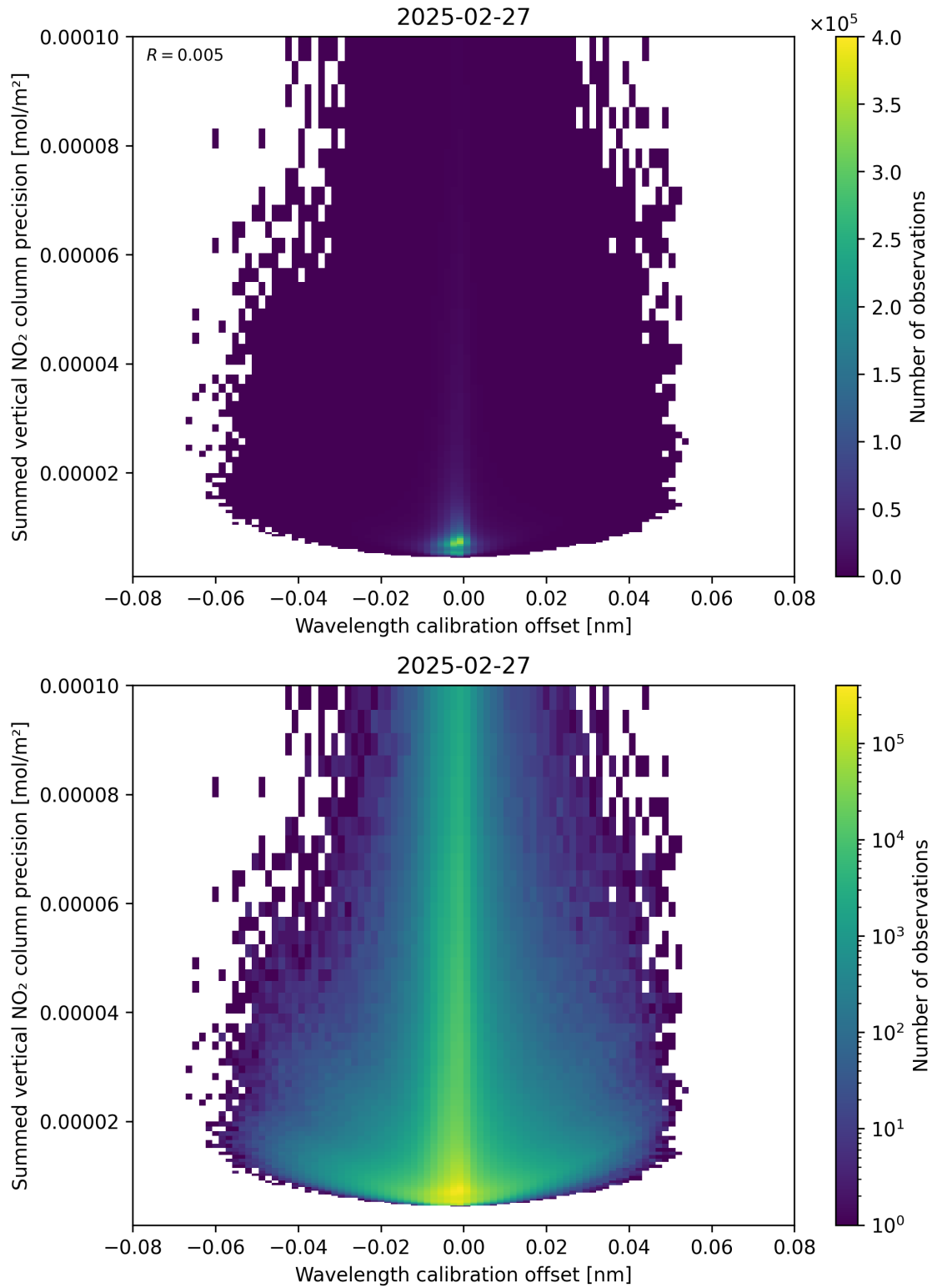
Figure 178: Scatter density plot of “Wavelength calibration offset” against “Summed vertical NO 2 column precision” for 2025-02-26 to 2025-02-28.
