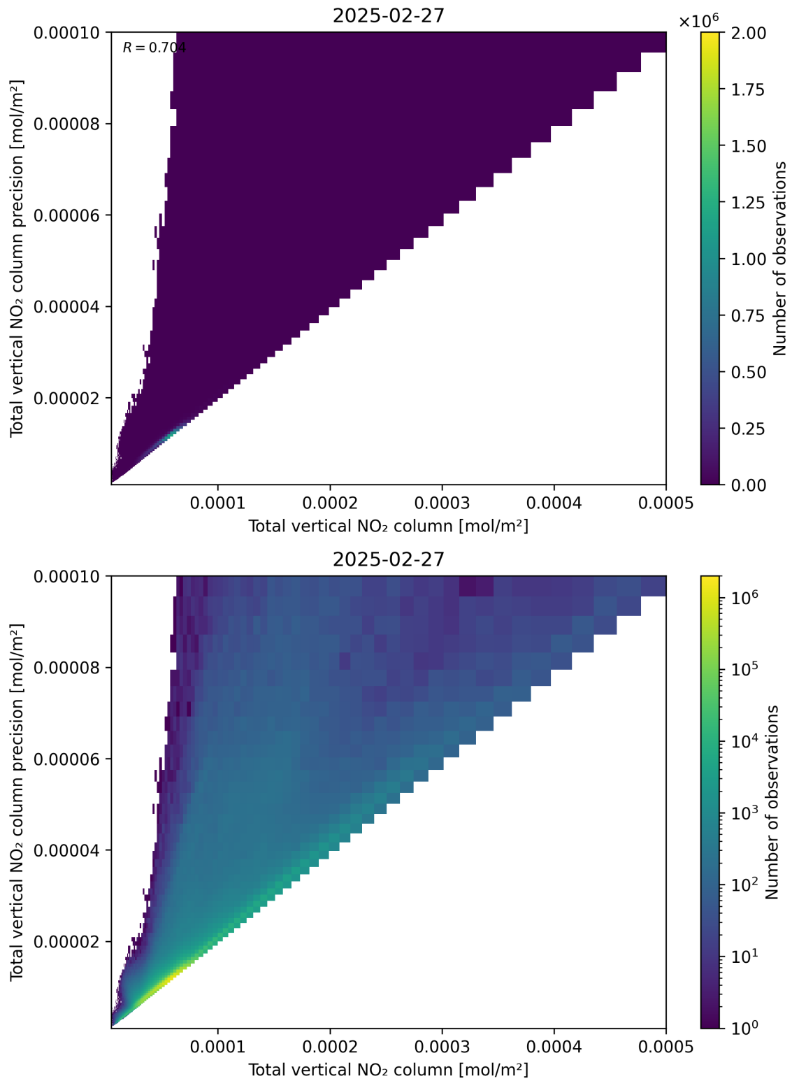
Figure 114: Scatter density plot of “Total vertical NO 2 column” against “Total vertical NO 2 column precision” for 2025-02-26 to 2025-02-28.
