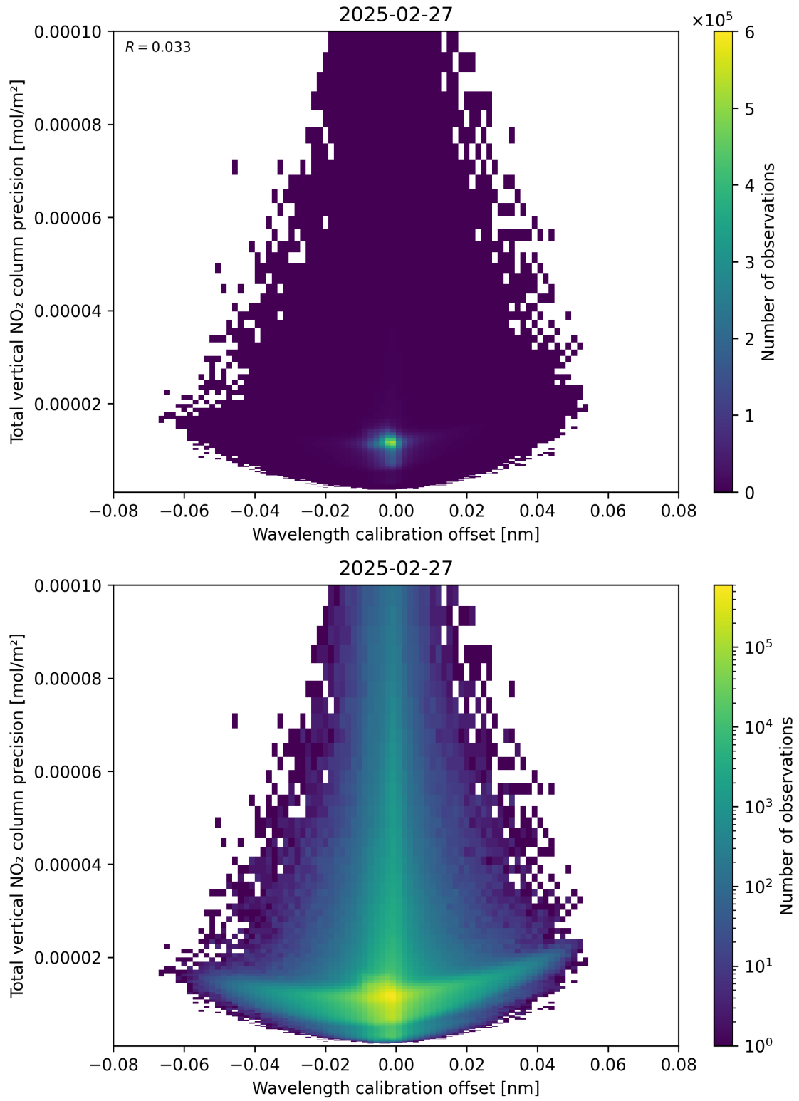
Figure 180: Scatter density plot of “Wavelength calibration offset” against “Total vertical NO 2 column precision” for 2025-02-26 to 2025-02-28.
