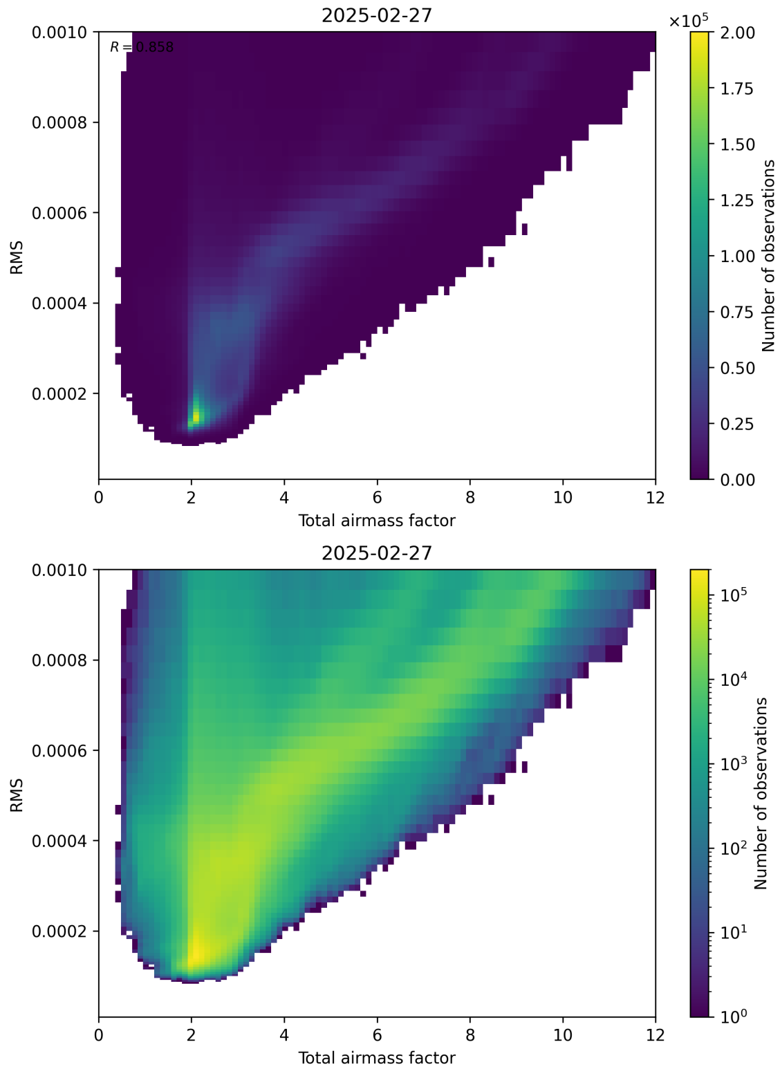
Figure 69: Scatter density plot of “Total airmass factor” against “RMS” for 2025-02-26 to 2025-02-28.
