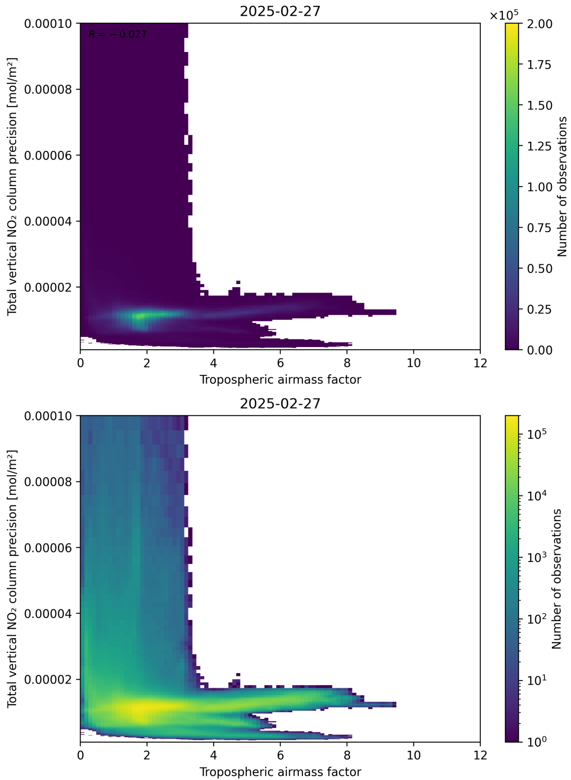
Figure 78: Scatter density plot of “Tropospheric air mass factor” against “Total vertical NO 2 column precision” for 2025-02-26 to 2025-02-28.
