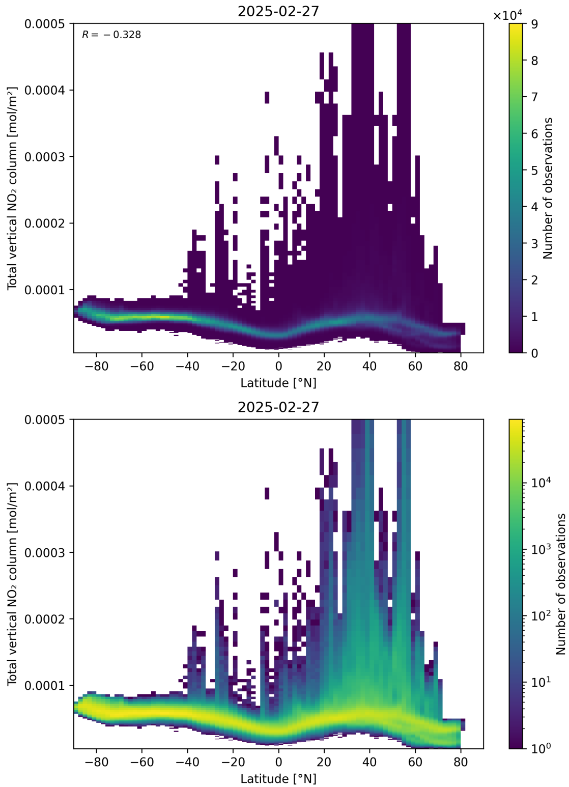
Figure 90: Scatter density plot of “Latitude” against “Total vertical NO 2 column” for 2025-02-26 to 2025-02-28.
