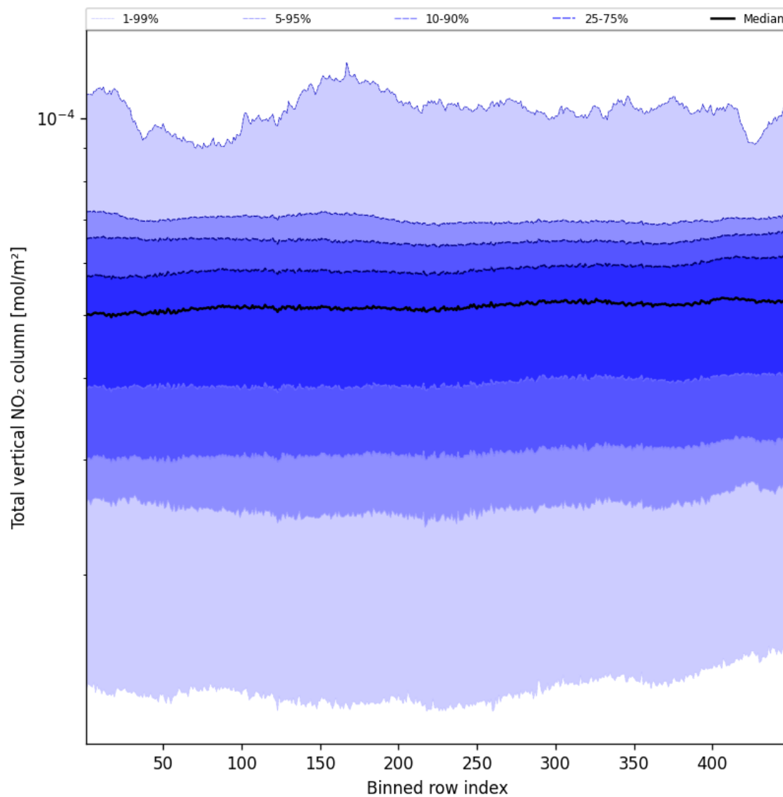
Figure 55: Along track statistics of “Total vertical NO 2 column” for 2025-02-26 to 2025-02-28
