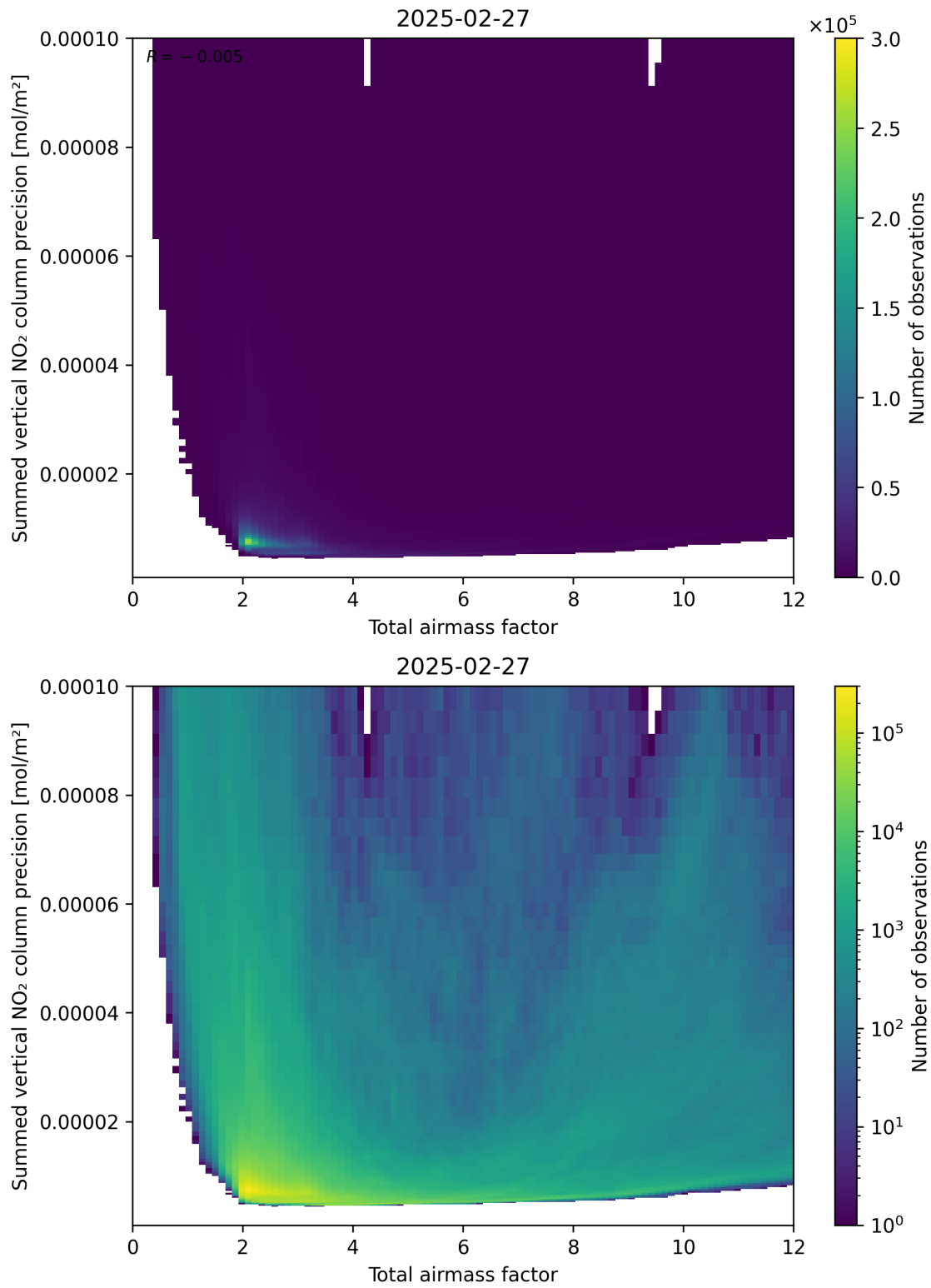
Figure 66: Scatter density plot of “Total airmass factor” against “Summed vertical NO 2 column precision” for 2025-02-26 to 2025-02-28.
