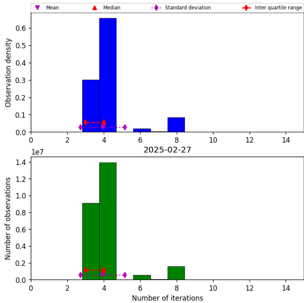
Figure 34: Histogram of “Number of iterations” for 2025-02-26 to 2025-02-28
