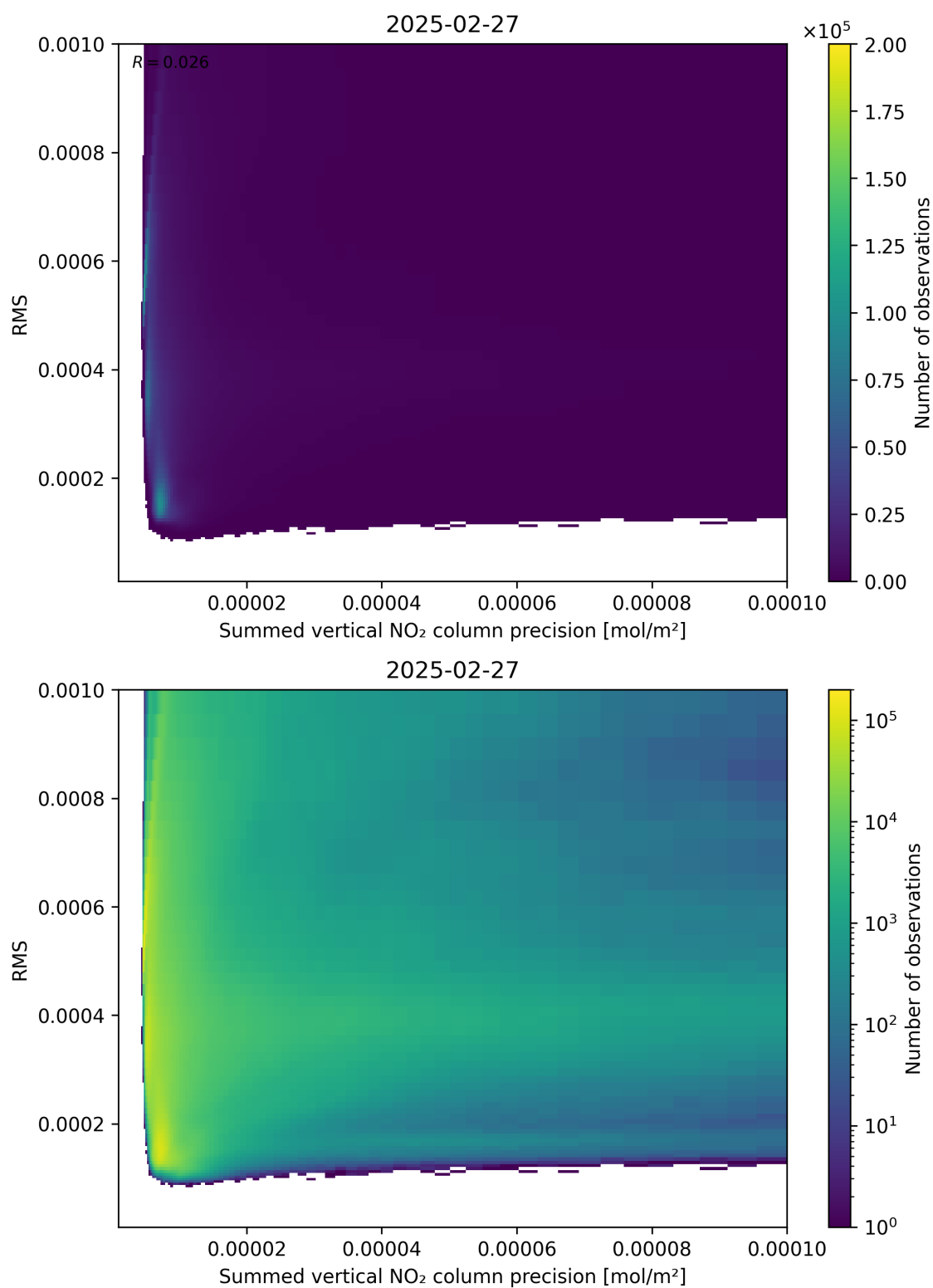
Figure 108: Scatter density plot of “Summed vertical NO 2 column precision” against “RMS” for 2025-02-26 to 2025-02-28.
