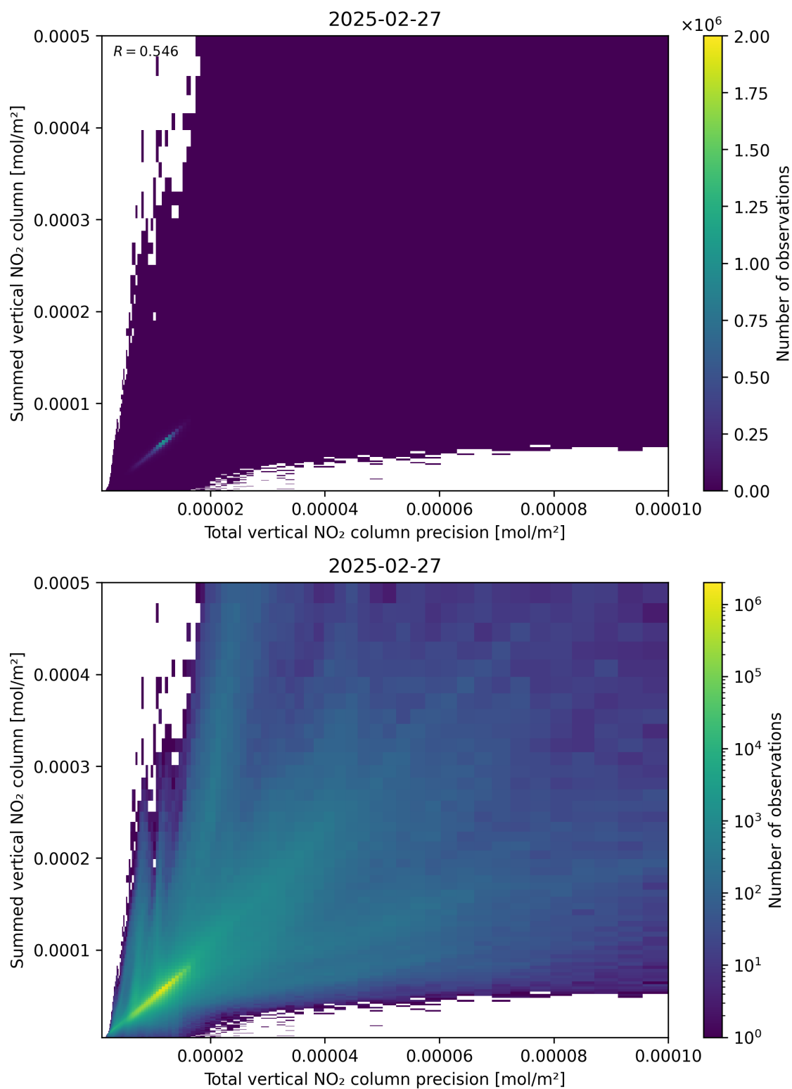
Figure 117: Scatter density plot of “Total vertical NO 2 column precision” against “Summed vertical NO 2 column” for 2025-02-26 to 2025-02-28.
