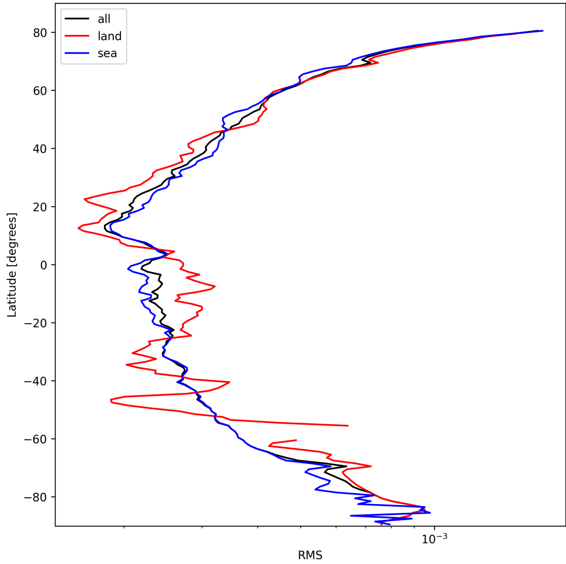
Figure 26: Zonal average of “RMS” for 2025-02-26 to 2025-02-28.
