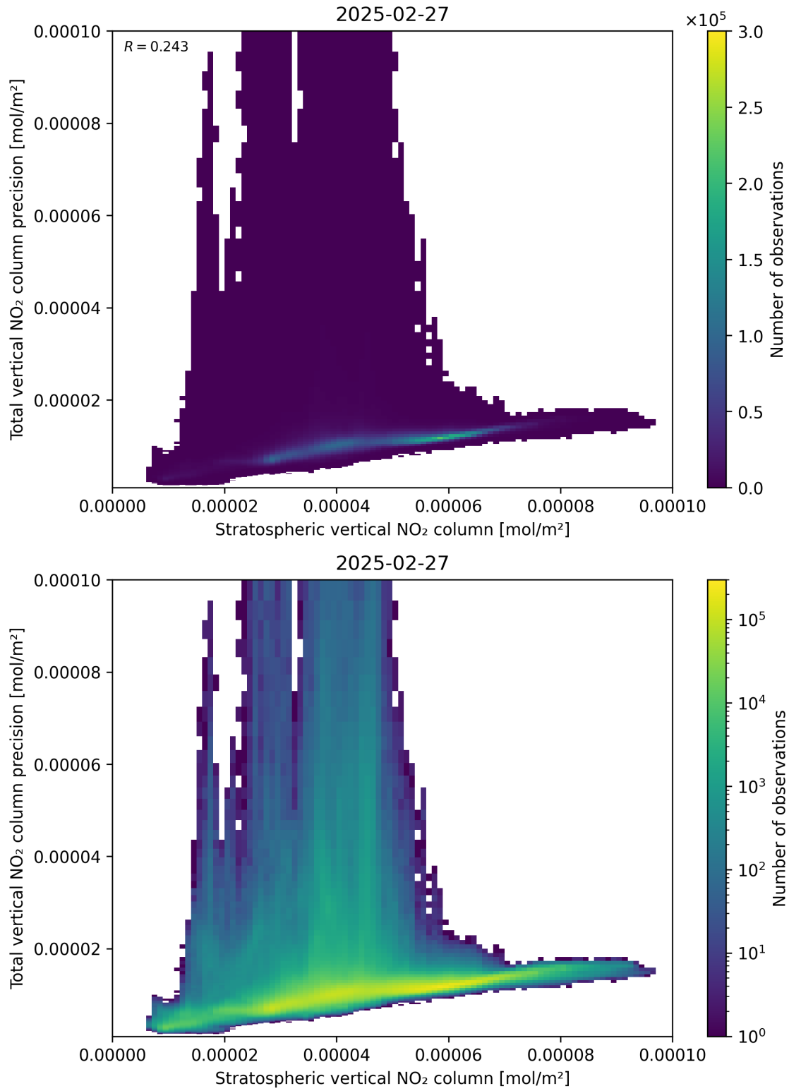
Figure 101: Scatter density plot of “Stratospheric vertical NO 2 column” against “Total vertical NO 2 column precision” for 2025-02-26 to 2025-02-28.
