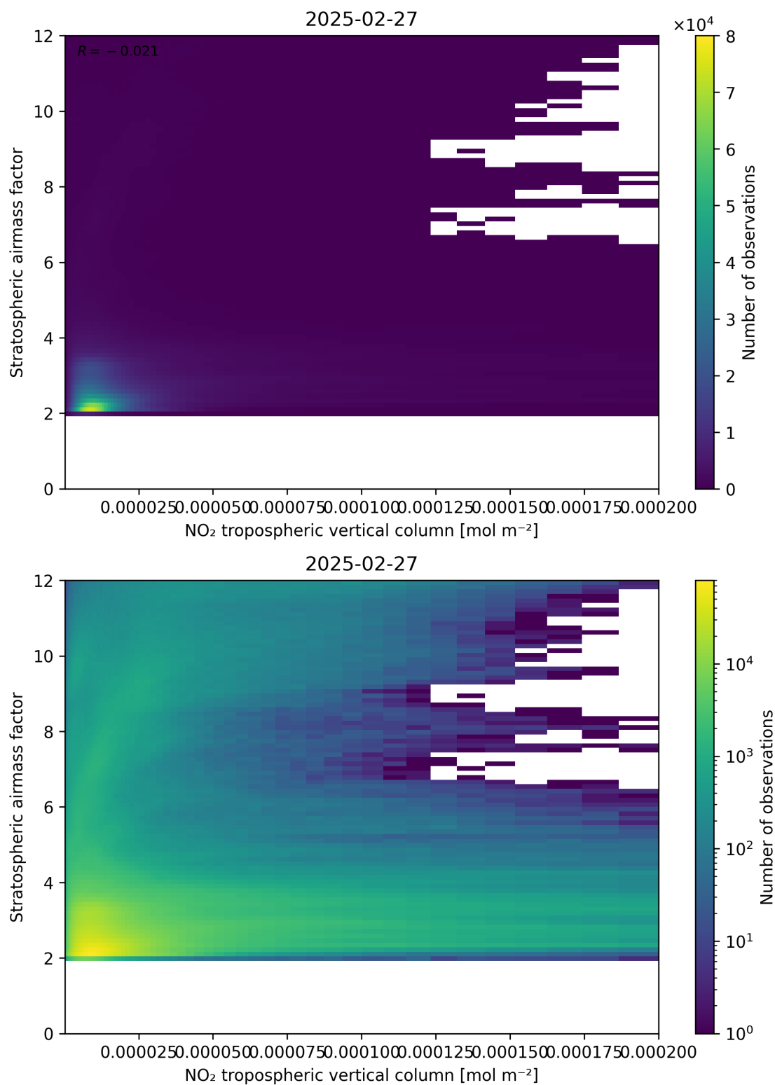
Figure 121: Scatter density plot of “NO 2 tropospheric vertical column” against “Stratospheric airmass factor” for 2025-02-26 to 2025-02-28.
