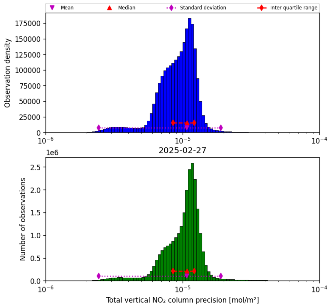
Figure 39: Histogram of “Total vertical NO 2 column precision” for 2025-02-26 to 2025-02-28
