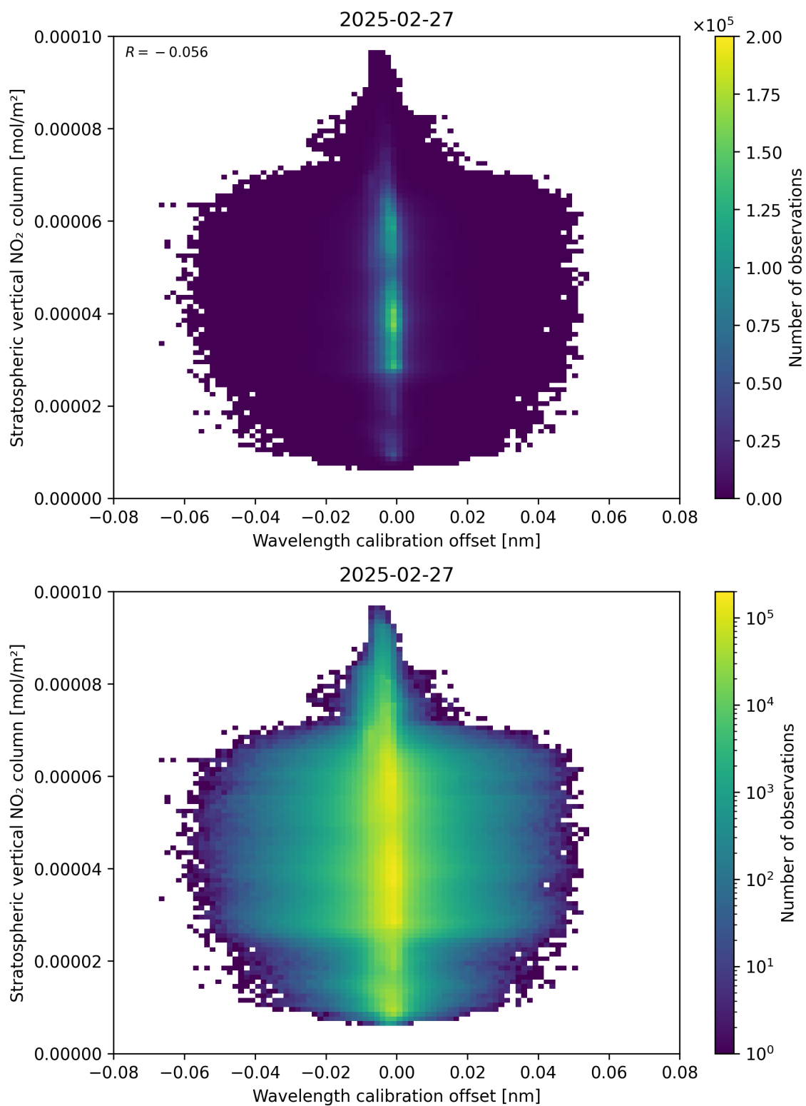
Figure 176: Scatter density plot of “Wavelength calibration offset” against “Stratospheric vertical NO 2 column” for 2025-02-26 to 2025-02-28.
