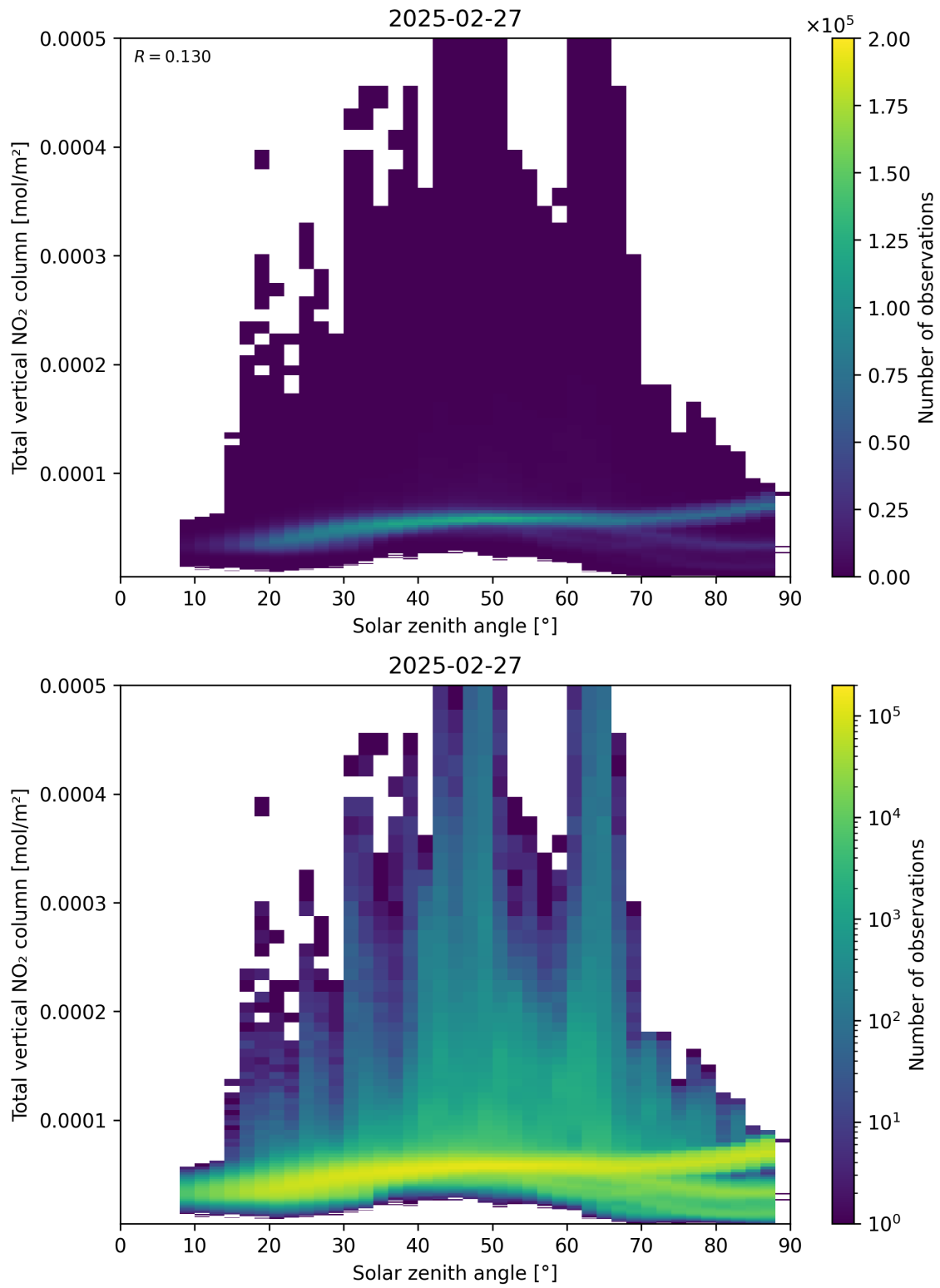
Figure 153: Scatter density plot of “Solar zenith angle” against “Total vertical NO 2 column” for 2025-02-26 to 2025-02-28.
