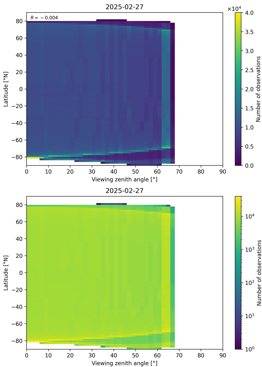
Figure 163: Scatter density plot of “Viewing zenith angle” against “Latitude” for 2025-02-26 to 2025-02-28.
