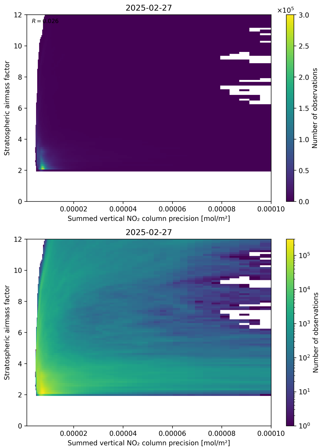
Figure 106: Scatter density plot of “Summed vertical NO 2 column precision” against “Stratospheric airmass factor” for 2025-02-26 to 2025-02-28.
