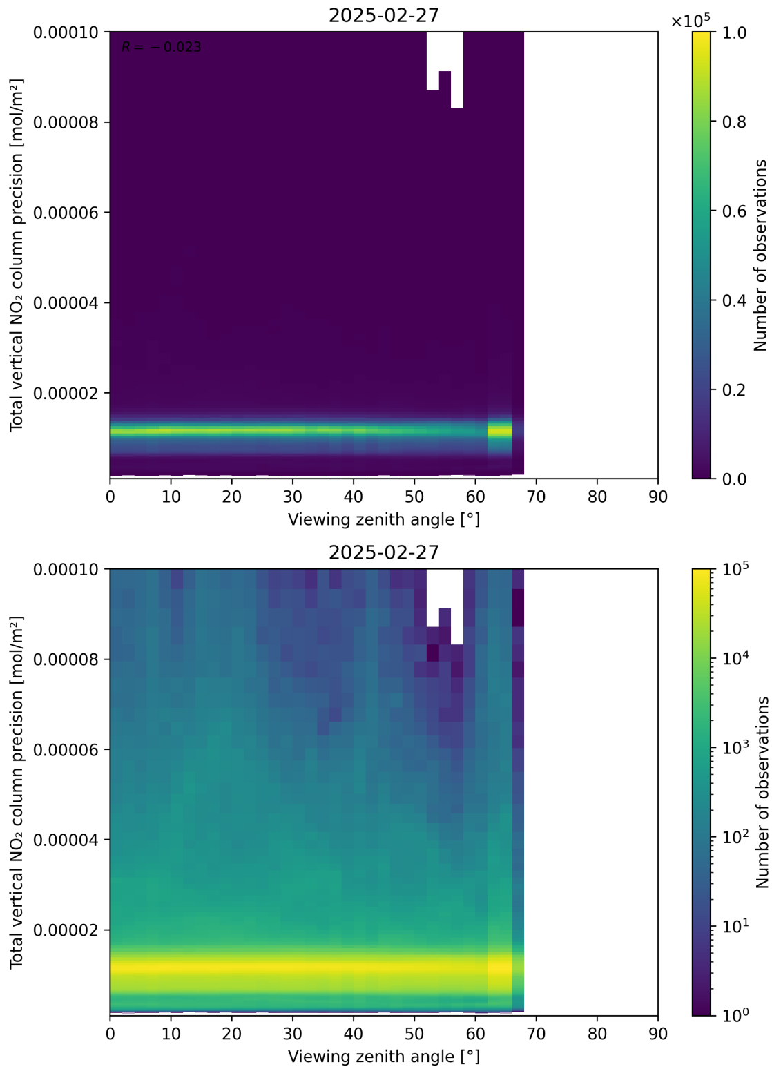
Figure 168: Scatter density plot of “Viewing zenith angle” against “Total vertical NO 2 column precision” for 2025-02-26 to 2025-02-28.
