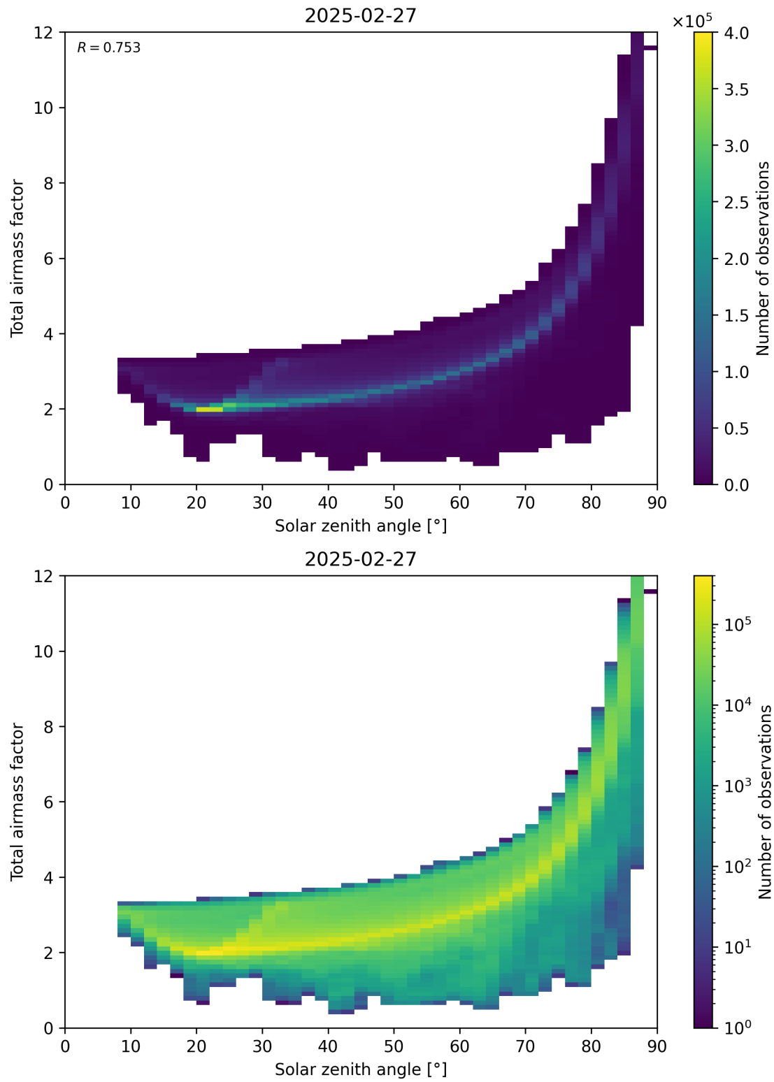
Figure 146: Scatter density plot of “Solar zenith angle” against “Total air mass factor” for 2025-02-26 to 2025-02-28.
