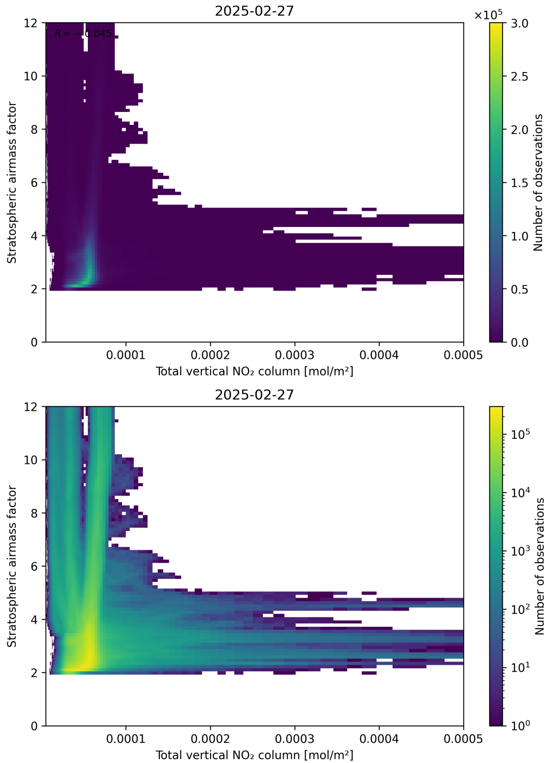
Figure 110: Scatter density plot of “Total vertical NO 2 column” against “Stratospheric airmass factor” for 2025-02-26 to 2025-02-28.
