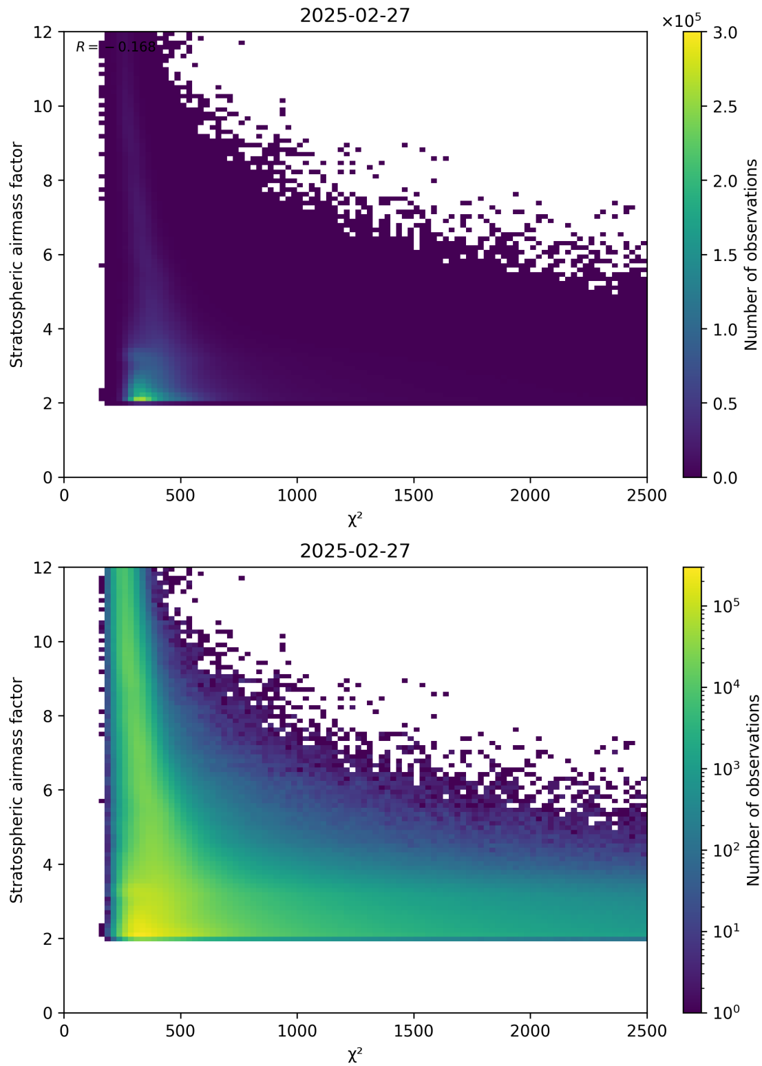
Figure 81: Scatter density plot of “ \chi^2 ” against “Stratospheric airmass factor” for 2025-02-26 to 2025-02-28.
