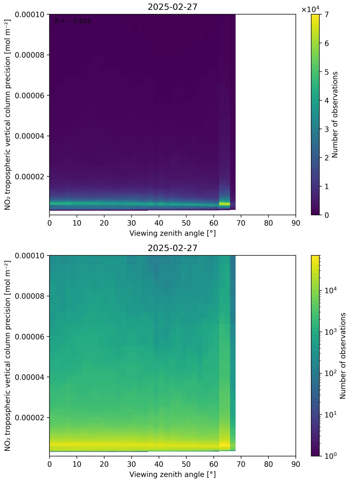
Figure 170: Scatter density plot of “Viewing zenith angle” against “NO 2 tropospheric vertical column precision” for 2025-02-26 to 2025-02-28.
