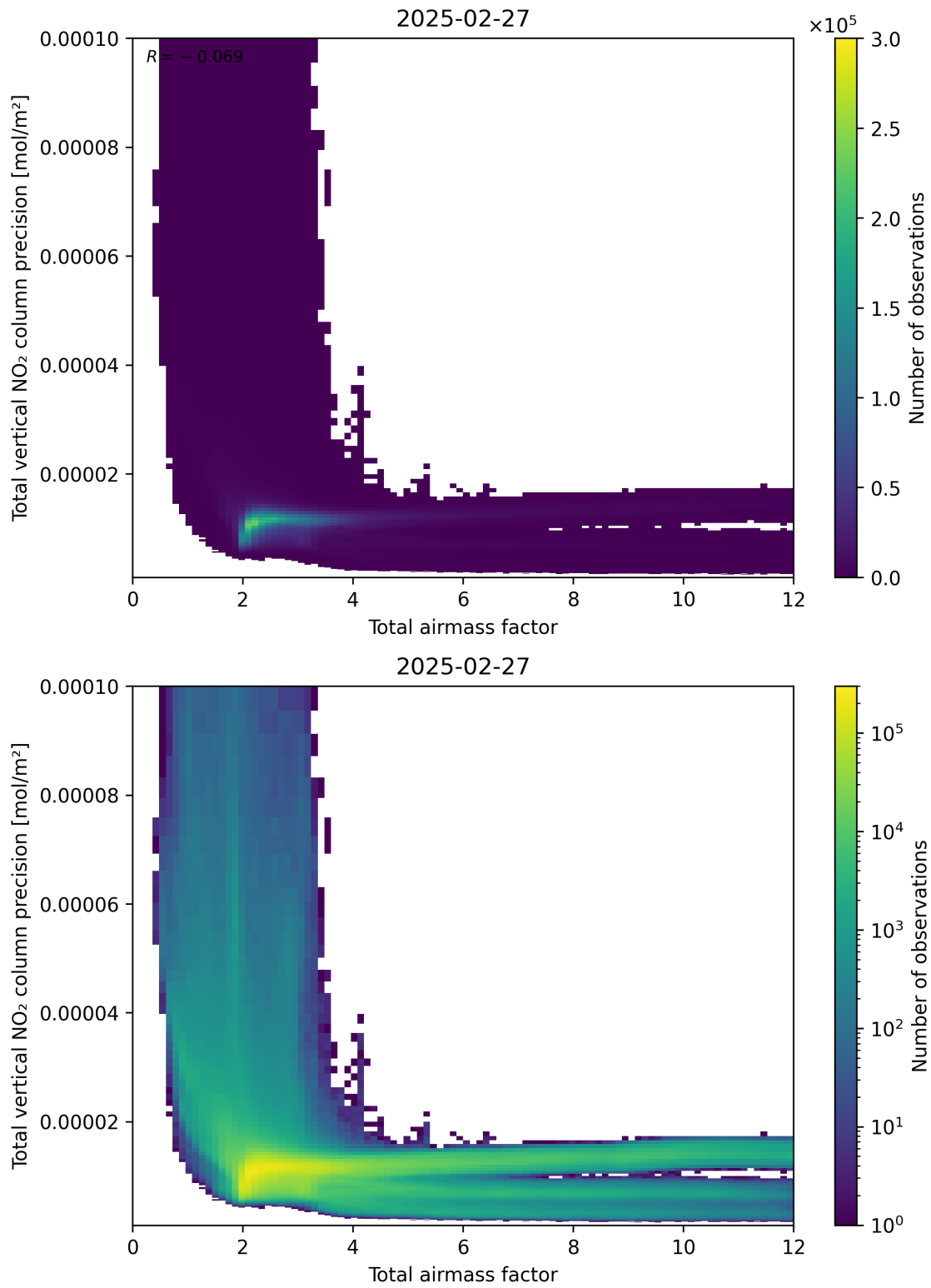
Figure 68: Scatter density plot of “Total airmass factor” against “Total vertical NO 2 column precision” for 2025-02-26 to 2025-02-28.
