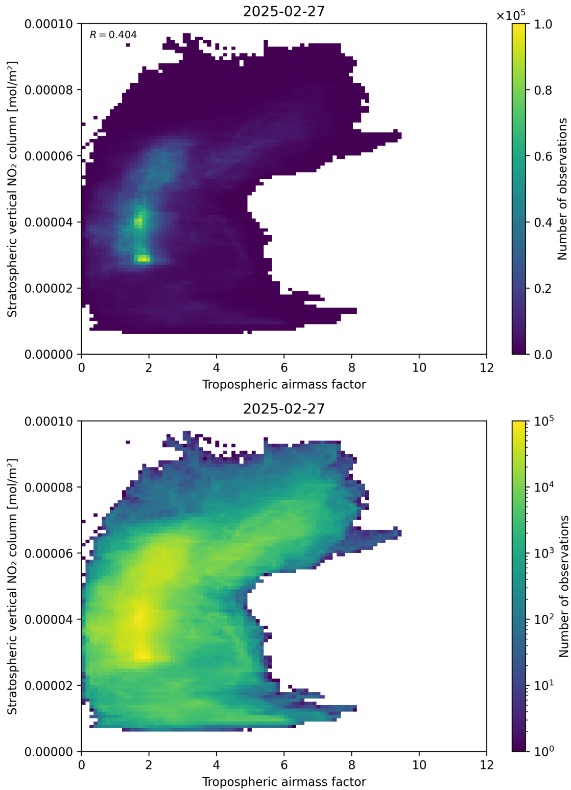
Figure 74: Scatter density plot of “Tropospheric air mass factor” against “Stratospheric vertical NO 2 column” for 2025-02-26 to 2025-02-28.
