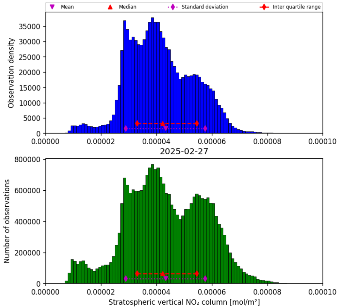
Figure 36: Histogram of “Stratospheric vertical NO 2 column” for 2025-02-26 to 2025-02-28
