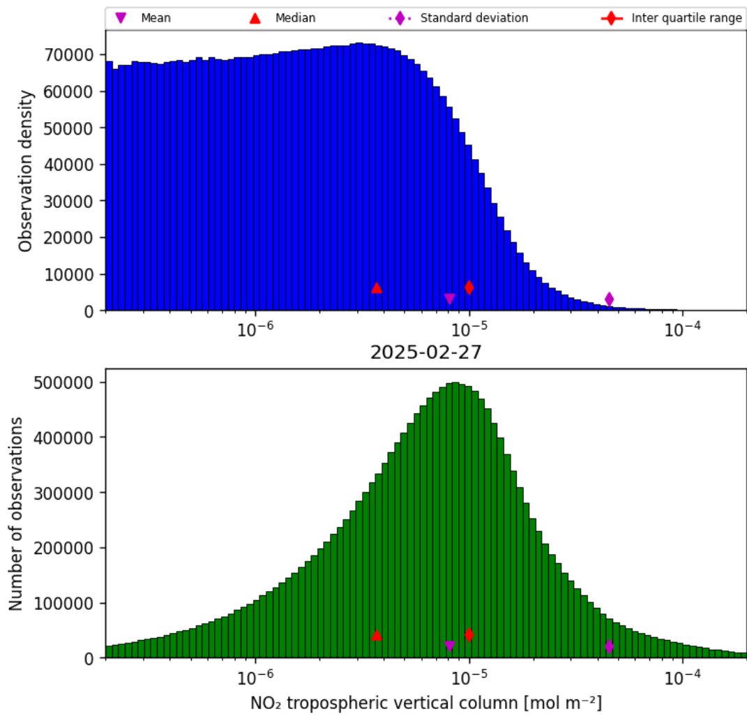
Figure 29: Histogram of “NO 2 tropospheric vertical column” for 2025-02-26 to 2025-02-28
