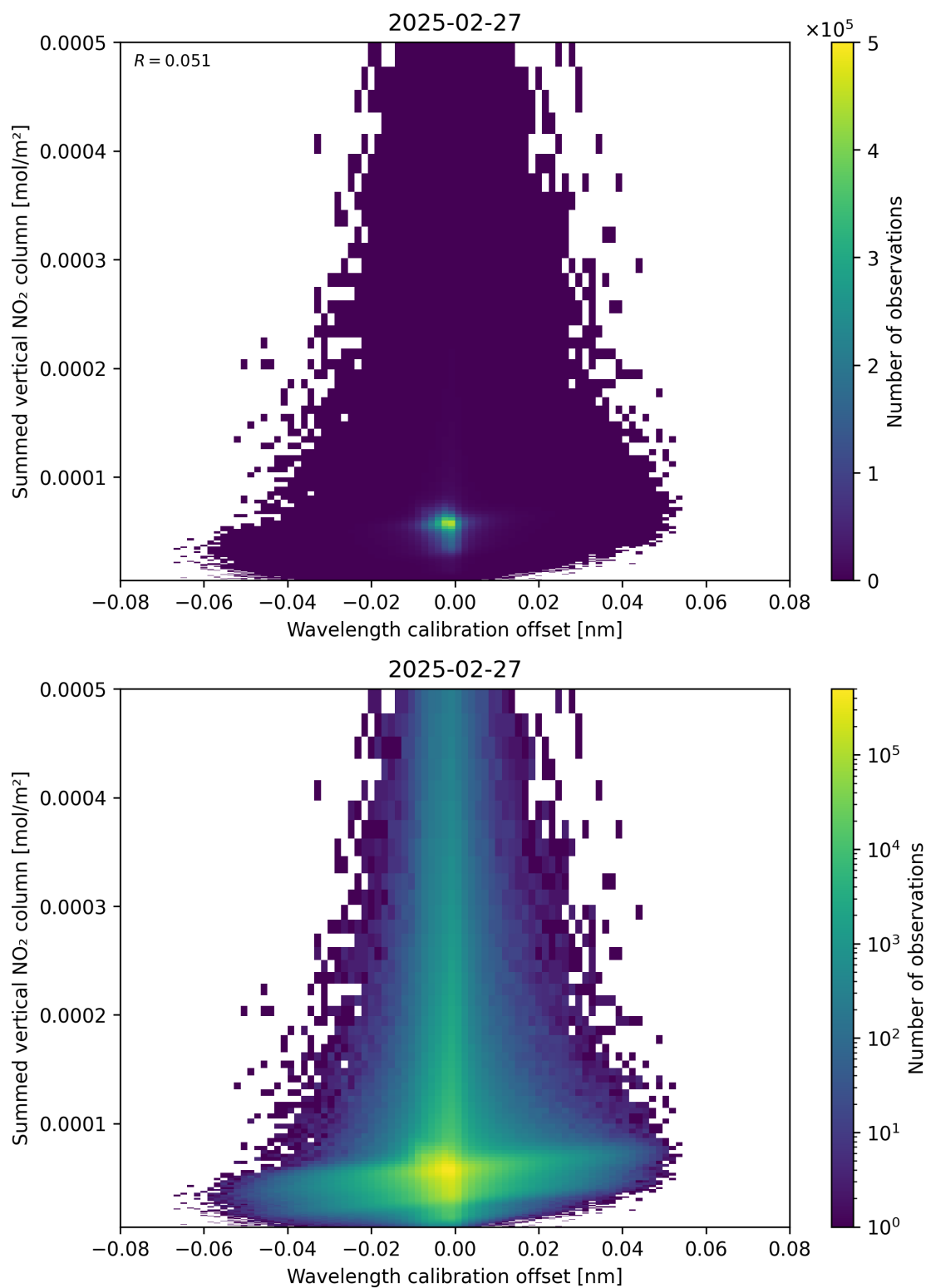
Figure 177: Scatter density plot of “Wavelength calibration offset” against “Summed vertical NO 2 column” for 2025-02-26 to 2025-02-28.
