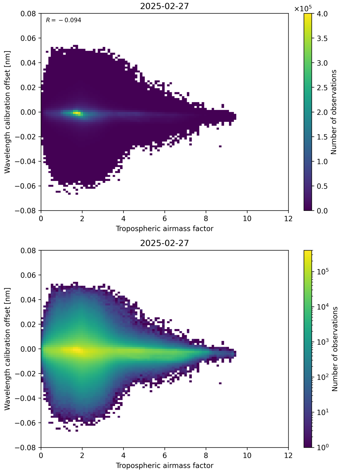
Figure 80: Scatter density plot of “Tropospheric airmass factor” against “Wavelength calibration offset” for 2025-02-26 to 2025-02-28.
