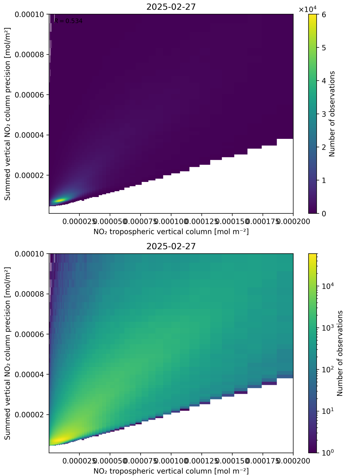
Figure 127: Scatter density plot of “NO 2 tropospheric vertical column” against “Summed vertical NO 2 column precision” for 2025-02-26 to 2025-02-28.
