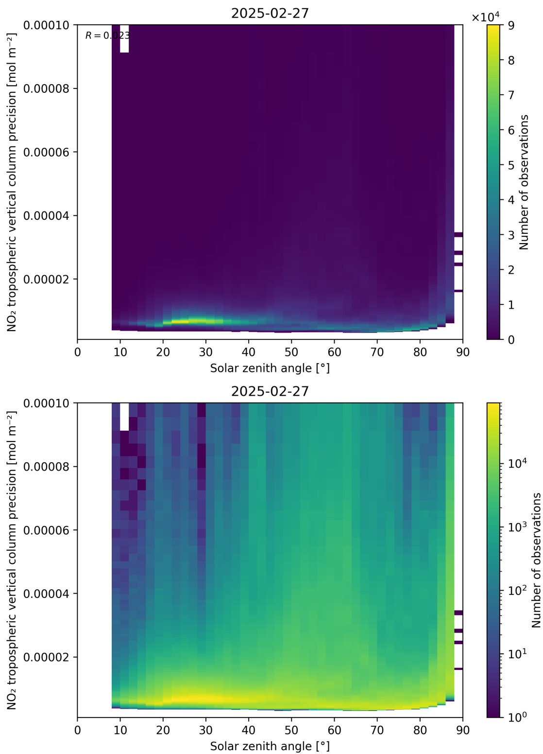
Figure 156: Scatter density plot of “Solar zenith angle” against “NO 2 tropospheric vertical column precision” for 2025-02-26 to 2025-02-28.
