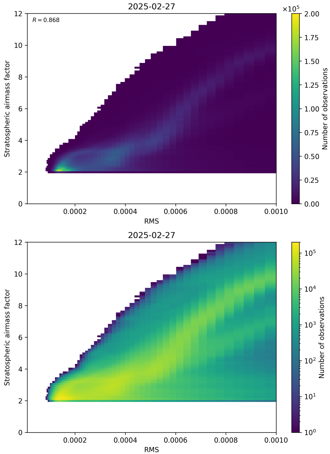
Figure 144: Scatter density plot of “RMS” against “Stratospheric airmass factor” for 2025-02-26 to 2025-02-28.
