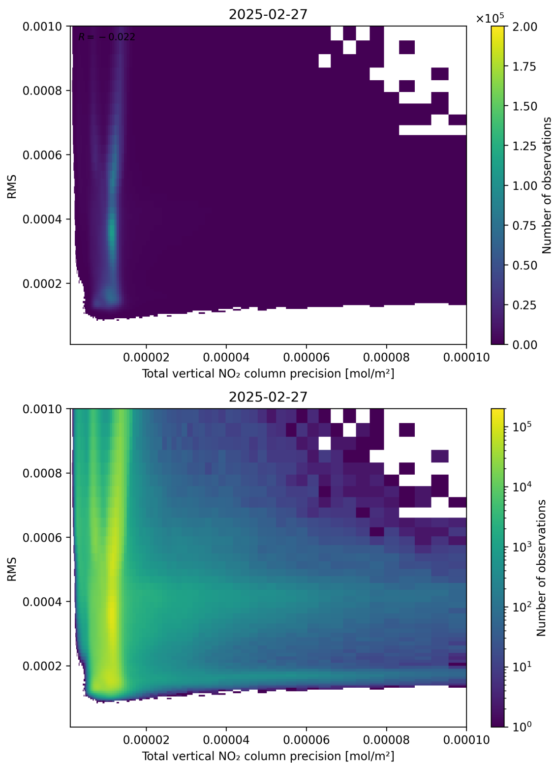
Figure 119: Scatter density plot of “Total vertical NO 2 column precision” against “RMS” for 2025-02-26 to 2025-02-28.
