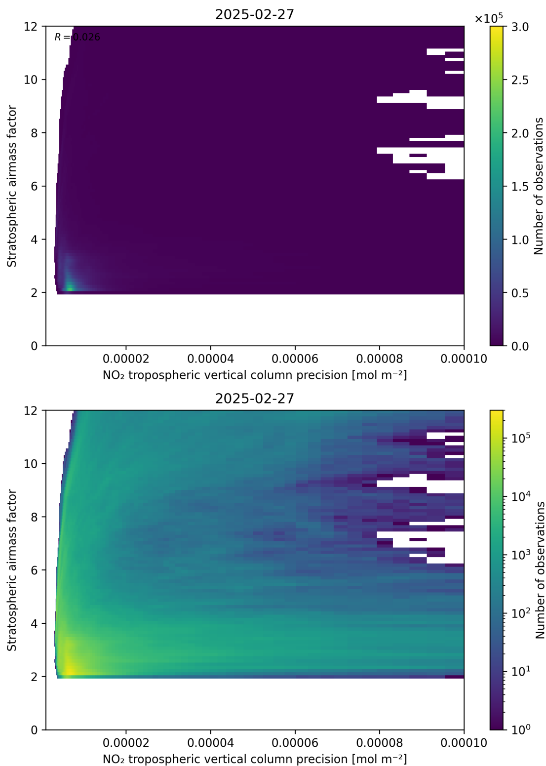
Figure 131: Scatter density plot of “NO 2 tropospheric vertical column precision” against “Stratospheric airmass factor” for 2025-02-26 to 2025-02-28.
