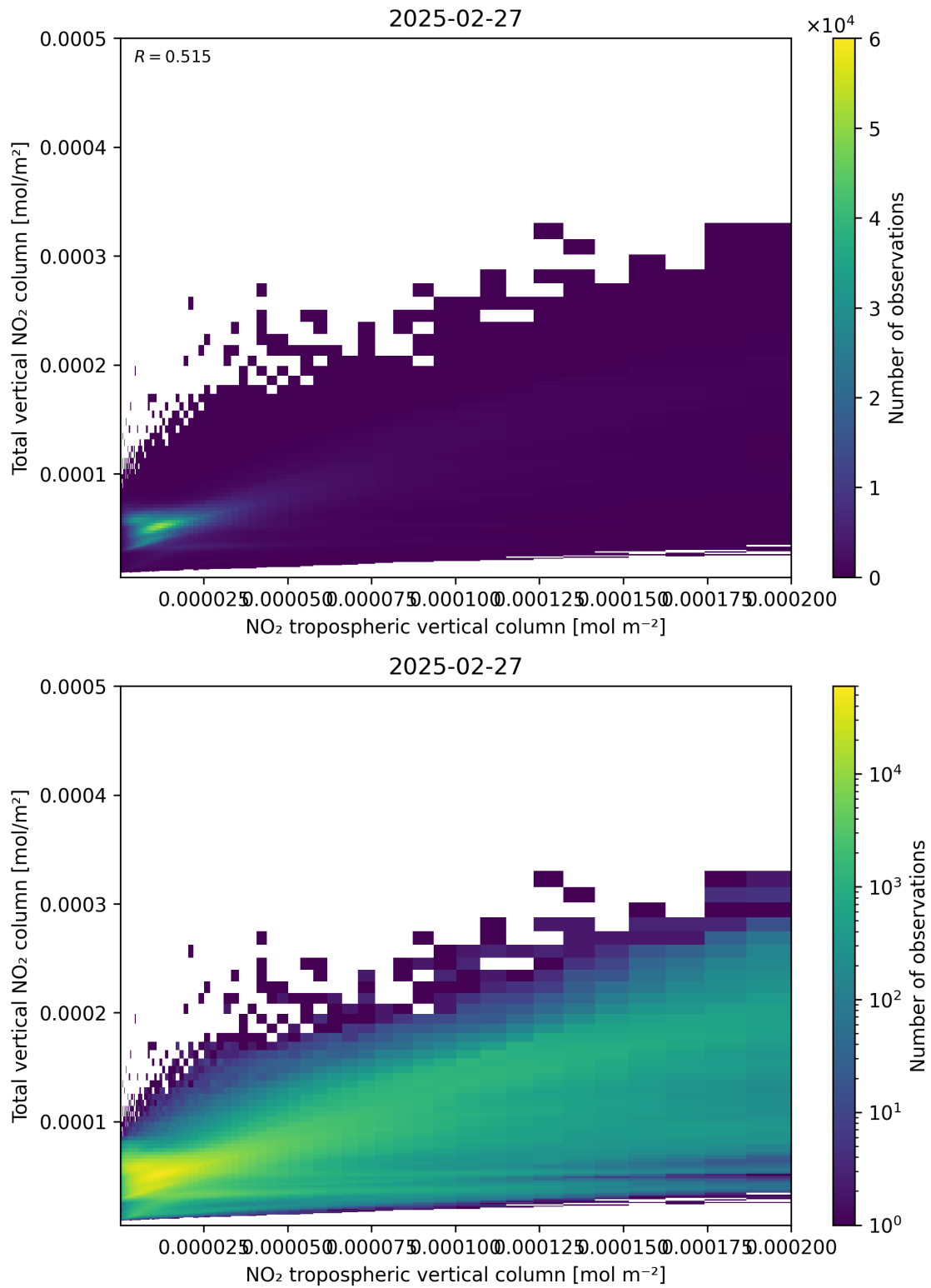
Figure 128: Scatter density plot of “NO 2 tropospheric vertical column” against “Total vertical NO 2 column” for 2025-02-26 to 2025-02-28.
