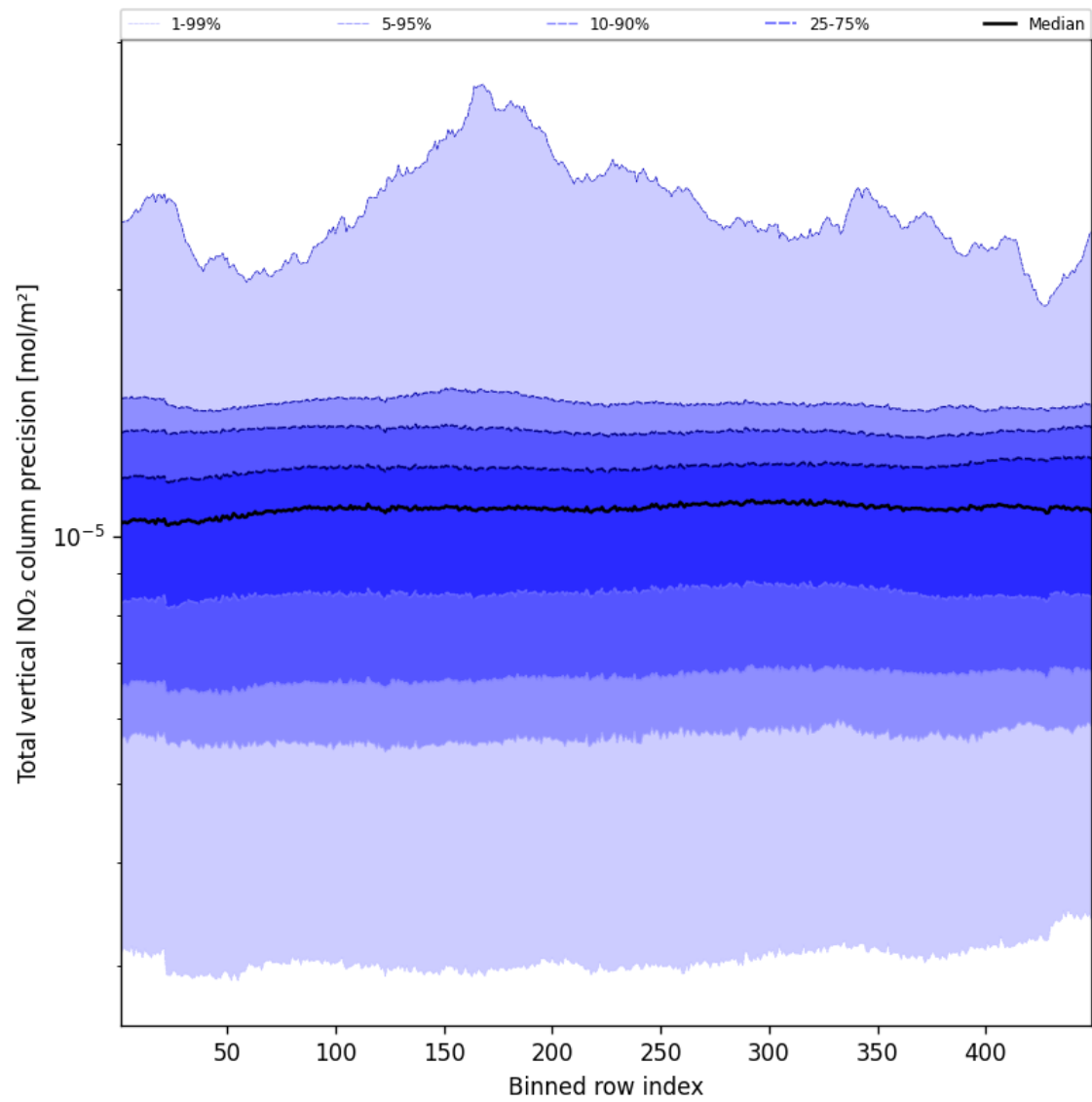
Figure 56: Along track statistics of “Total vertical NO 2 column precision” for 2025-02-26 to 2025-02-28
