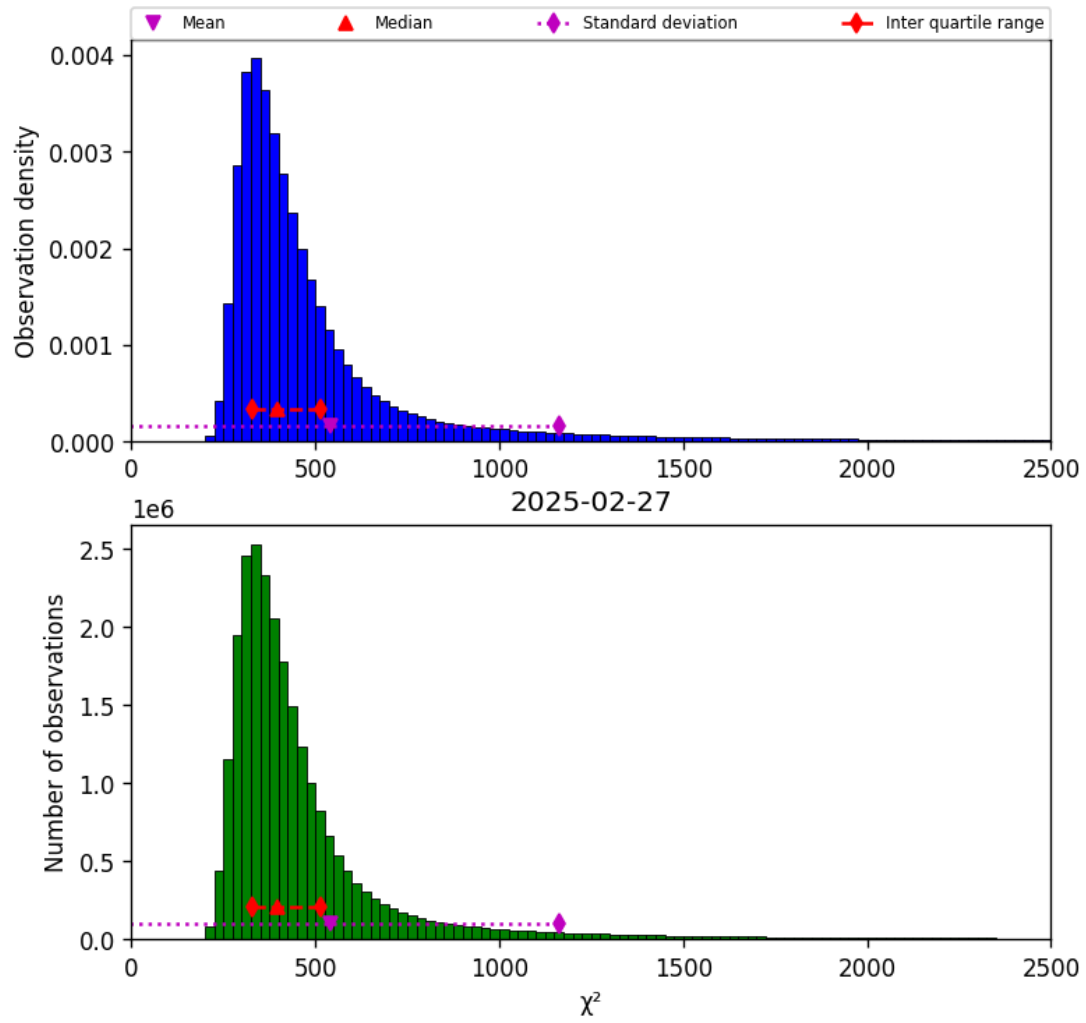
Figure 42: Histogram of “ \chi^2 ” for 2025-02-26 to 2025-02-28
