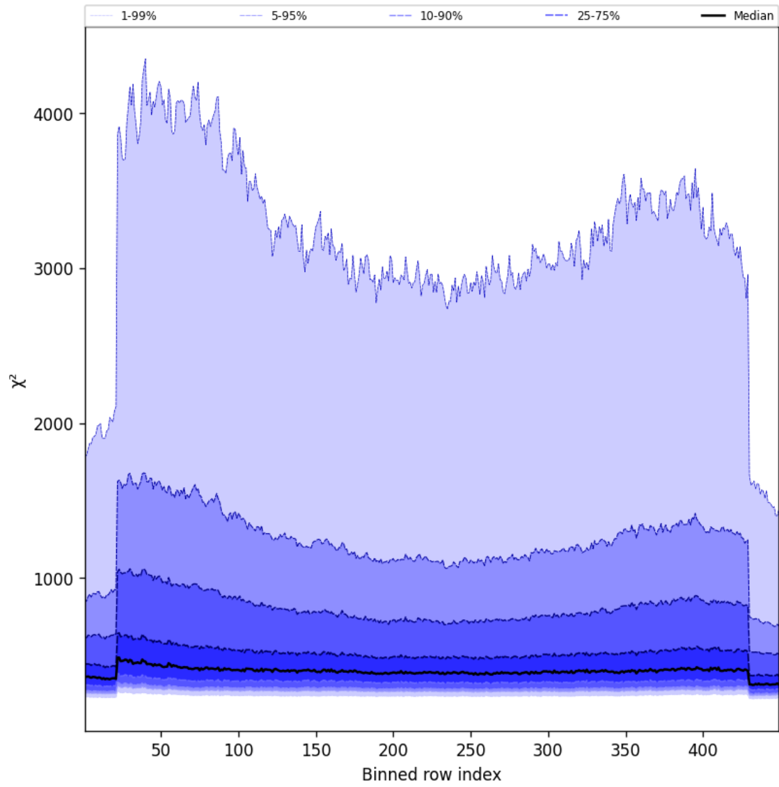
Figure 59: Along track statistics of “ \chi^2 ” for 2025-02-26 to 2025-02-28
