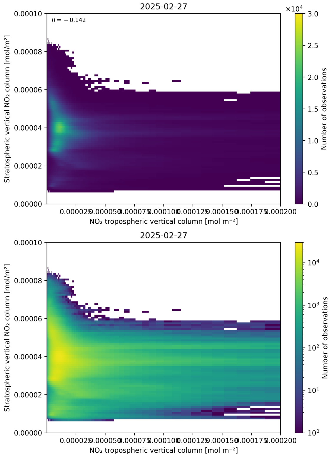
Figure 125: Scatter density plot of “NO 2 tropospheric vertical column” against “Stratospheric vertical NO 2 column” for 2025-02-26 to 2025-02-28.
