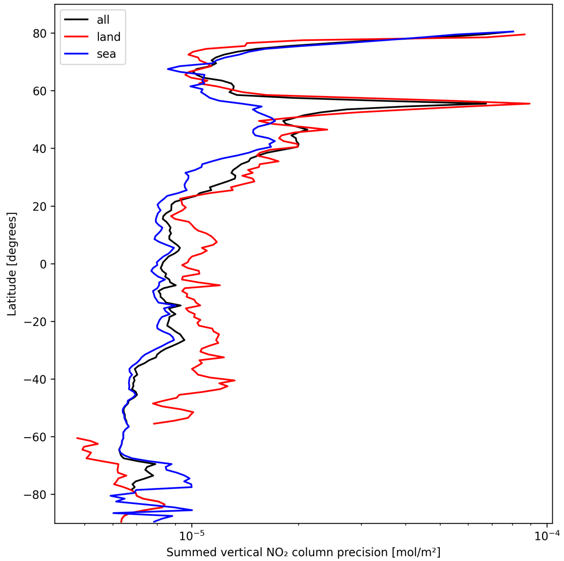
Figure 24: Zonal average of “Summed vertical NO 2 column precision” for 2025-02-26 to 2025-02-28.
