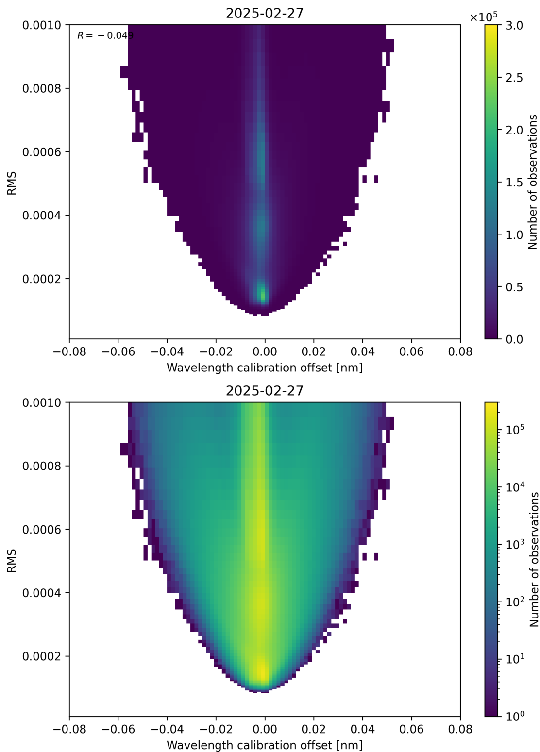
Figure 181: Scatter density plot of “Wavelength calibration offset” against “RMS” for 2025-02-26 to 2025-02-28.
