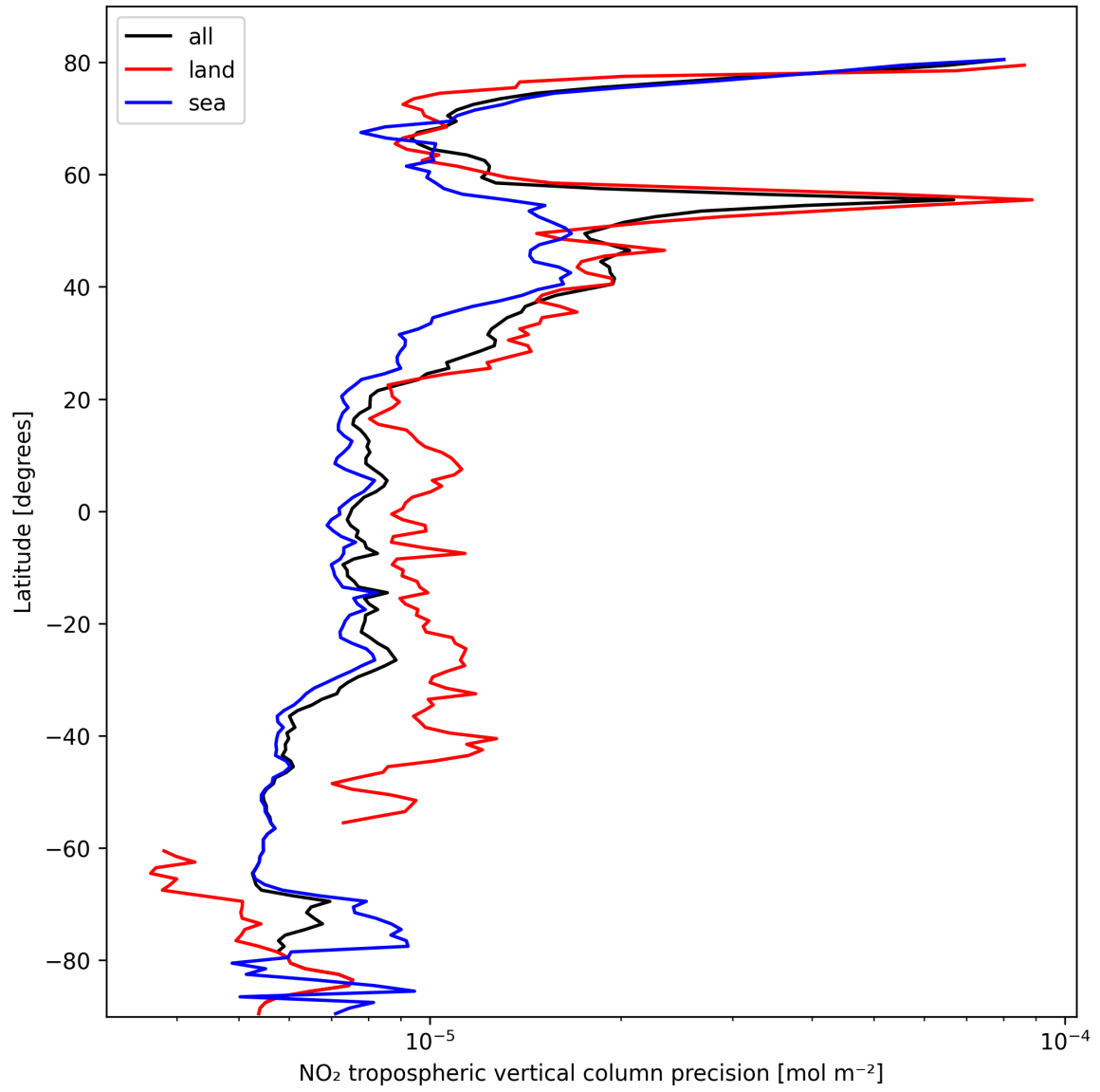
Figure 13: Zonal average of “NO 2 tropospheric vertical column precision” for 2025-02-26 to 2025-02-28.
