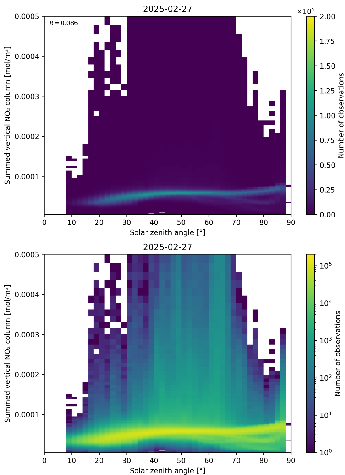
Figure 151: Scatter density plot of “Solar zenith angle” against “Summed vertical NO 2 column” for 2025-02-26 to 2025-02-28.
