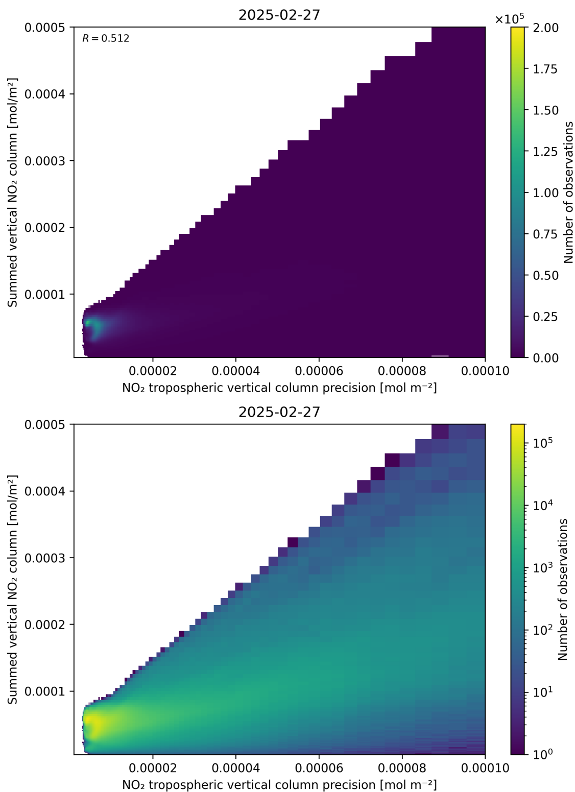
Figure 136: Scatter density plot of “NO 2 tropospheric vertical column precision” against “Summed vertical NO 2 column” for 2025-02-26 to 2025-02-28.
