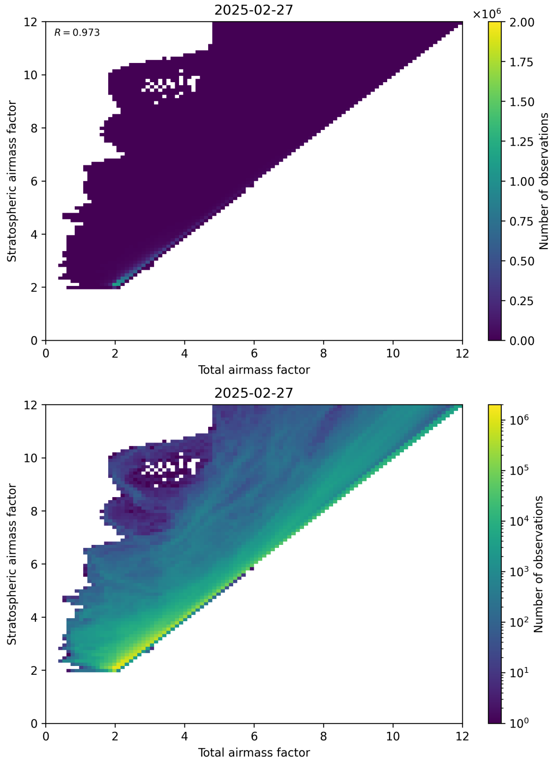
Figure 62: Scatter density plot of “Total airmass factor” against “Stratospheric airmass factor” for 2025-02-26 to 2025-02-28.
