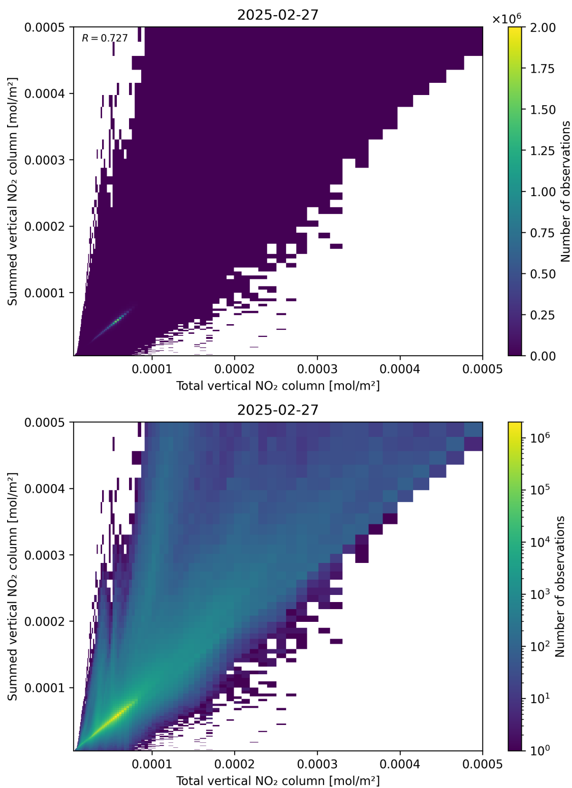
Figure 112: Scatter density plot of “Total vertical NO 2 column” against “Summed vertical NO 2 column” for 2025-02-26 to 2025-02-28.
