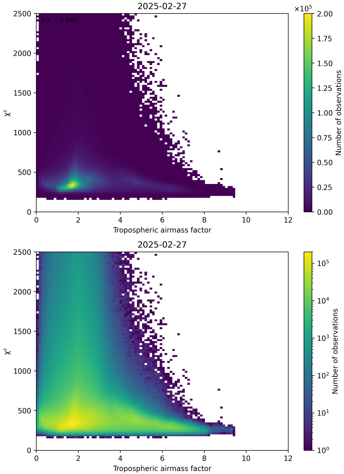
Figure 73: Scatter density plot of “Tropospheric airmass factor” against “ \chi^2 ” for 2025-02-26 to 2025-02-28.
