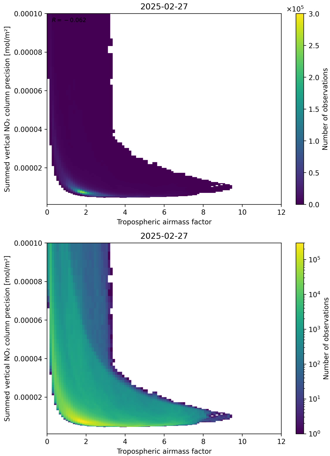
Figure 76: Scatter density plot of “Tropospheric air mass factor” against “Summed vertical NO 2 column precision” for 2025-02-26 to 2025-02-28.
