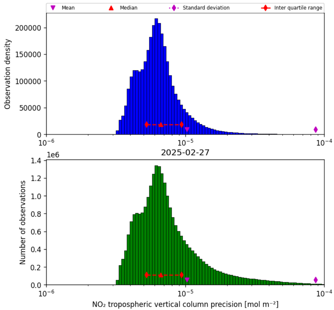
Figure 30: Histogram of “NO 2 tropospheric vertical column precision” for 2025-02-26 to 2025-02-28
