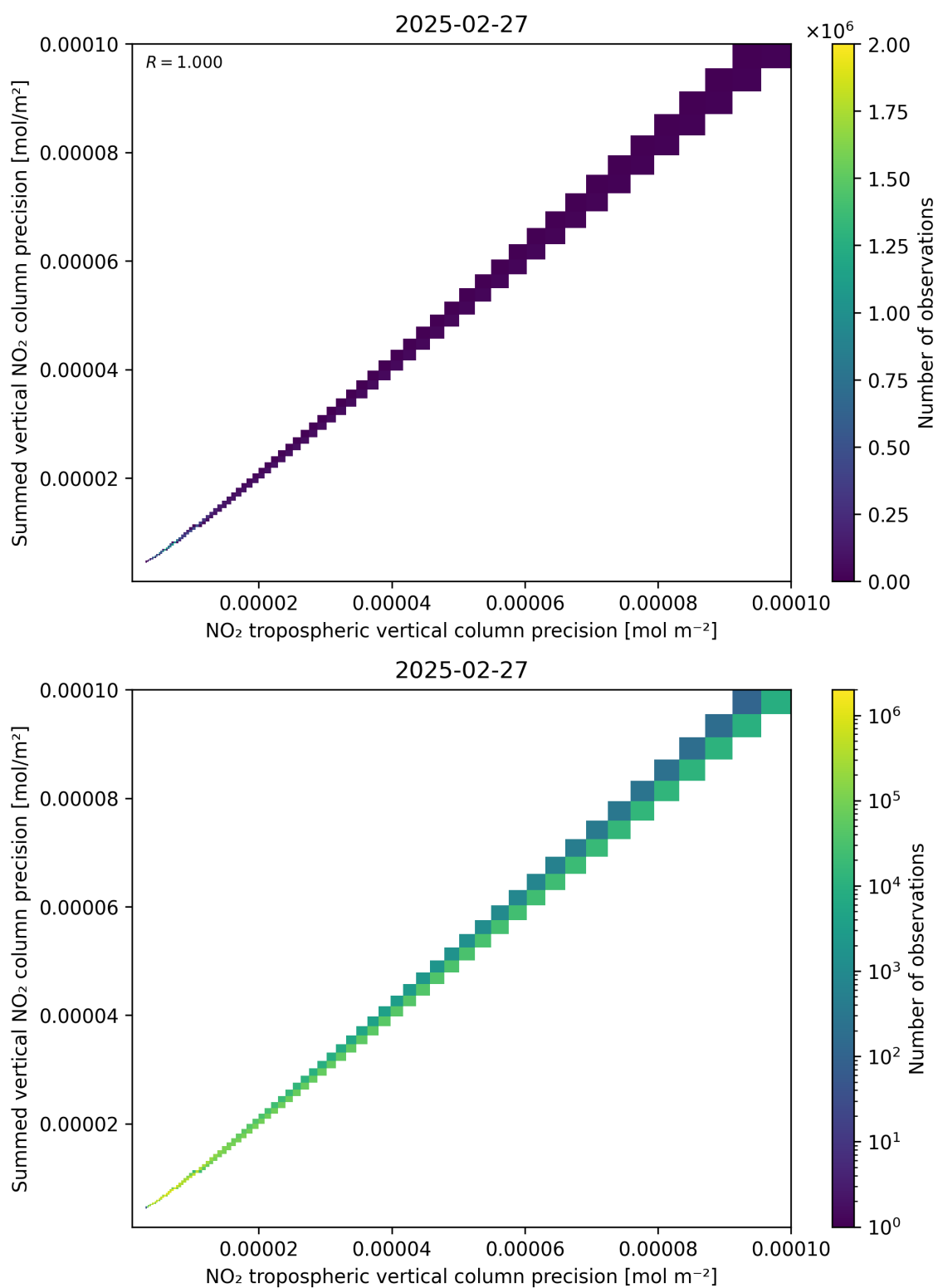
Figure 137: Scatter density plot of “NO 2 tropospheric vertical column precision” against “Summed vertical NO 2 column precision” for 2025-02-26 to 2025-02-28.
