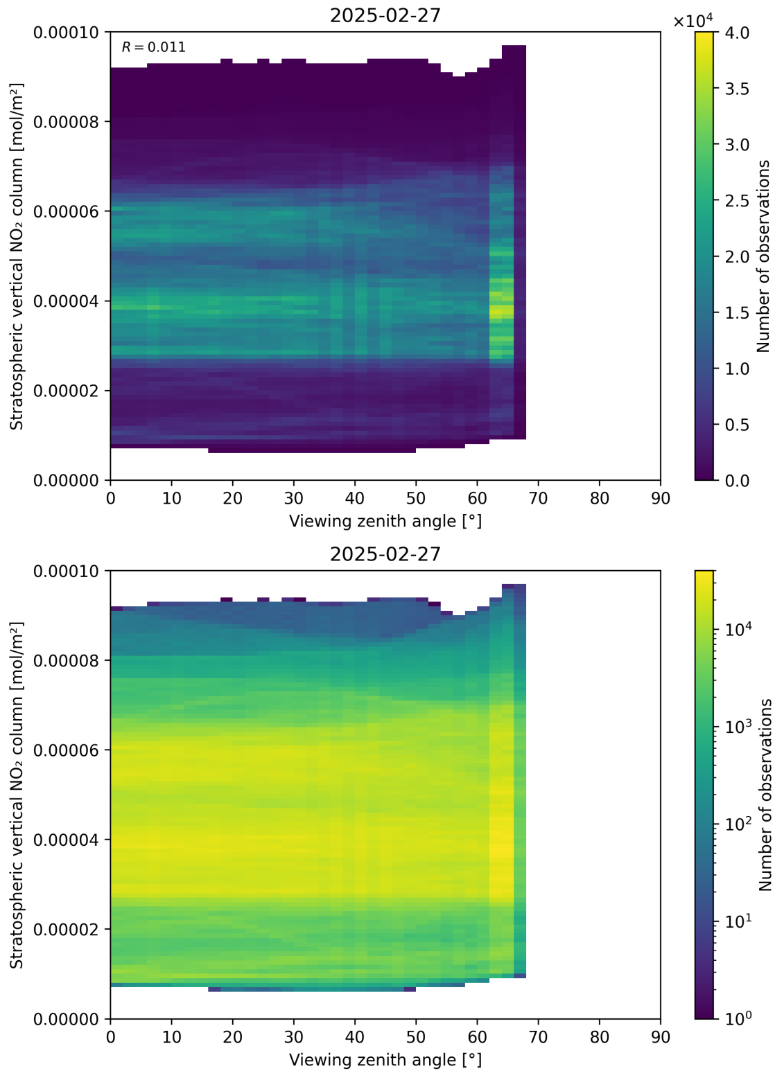
Figure 164: Scatter density plot of “Viewing zenith angle” against “Stratospheric vertical NO 2 column” for 2025-02-26 to 2025-02-28.
