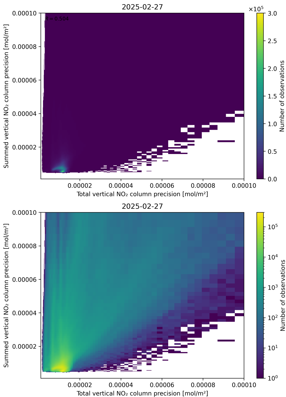
Figure 118: Scatter density plot of “Total vertical NO 2 column precision” against “Summed vertical NO 2 column precision” for 2025-02-26 to 2025-02-28.
