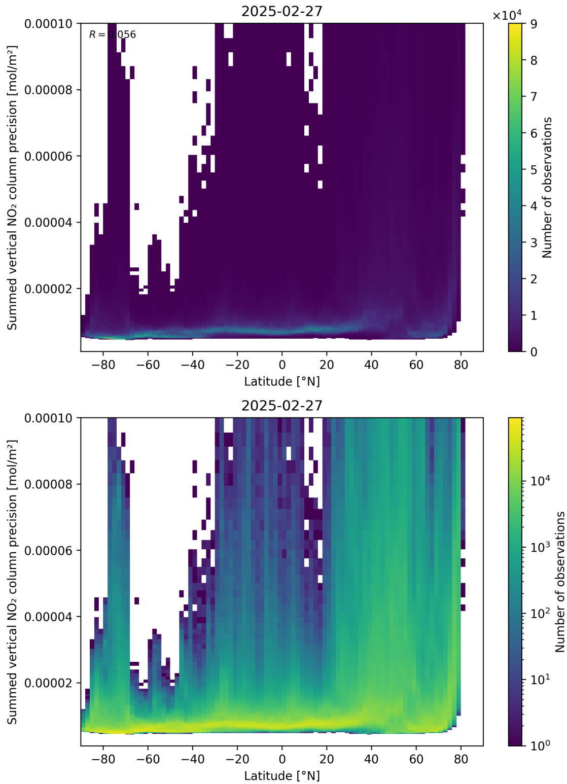
Figure 89: Scatter density plot of “Latitude” against “Summed vertical NO 2 column precision” for 2025-02-26 to 2025-02-28.
