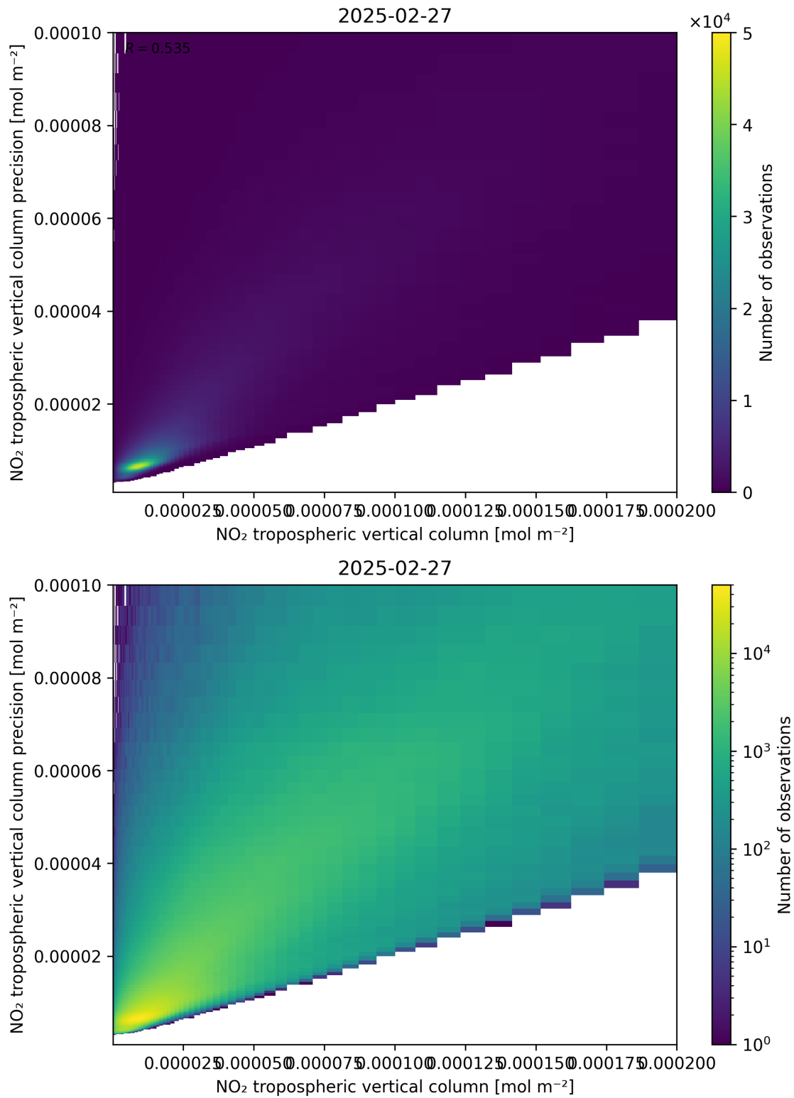
Figure 130: Scatter density plot of “NO 2 tropospheric vertical column” against “NO 2 tropospheric vertical column precision” for 2025-02-26 to 2025-02-28.
