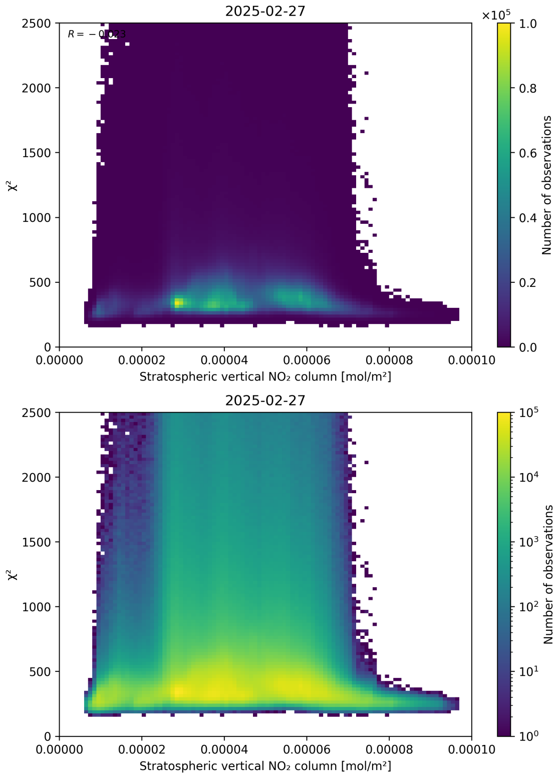
Figure 97: Scatter density plot of “Stratospheric vertical NO 2 column” against “ \chi^2 ” for 2025-02-26 to 2025-02-28.
