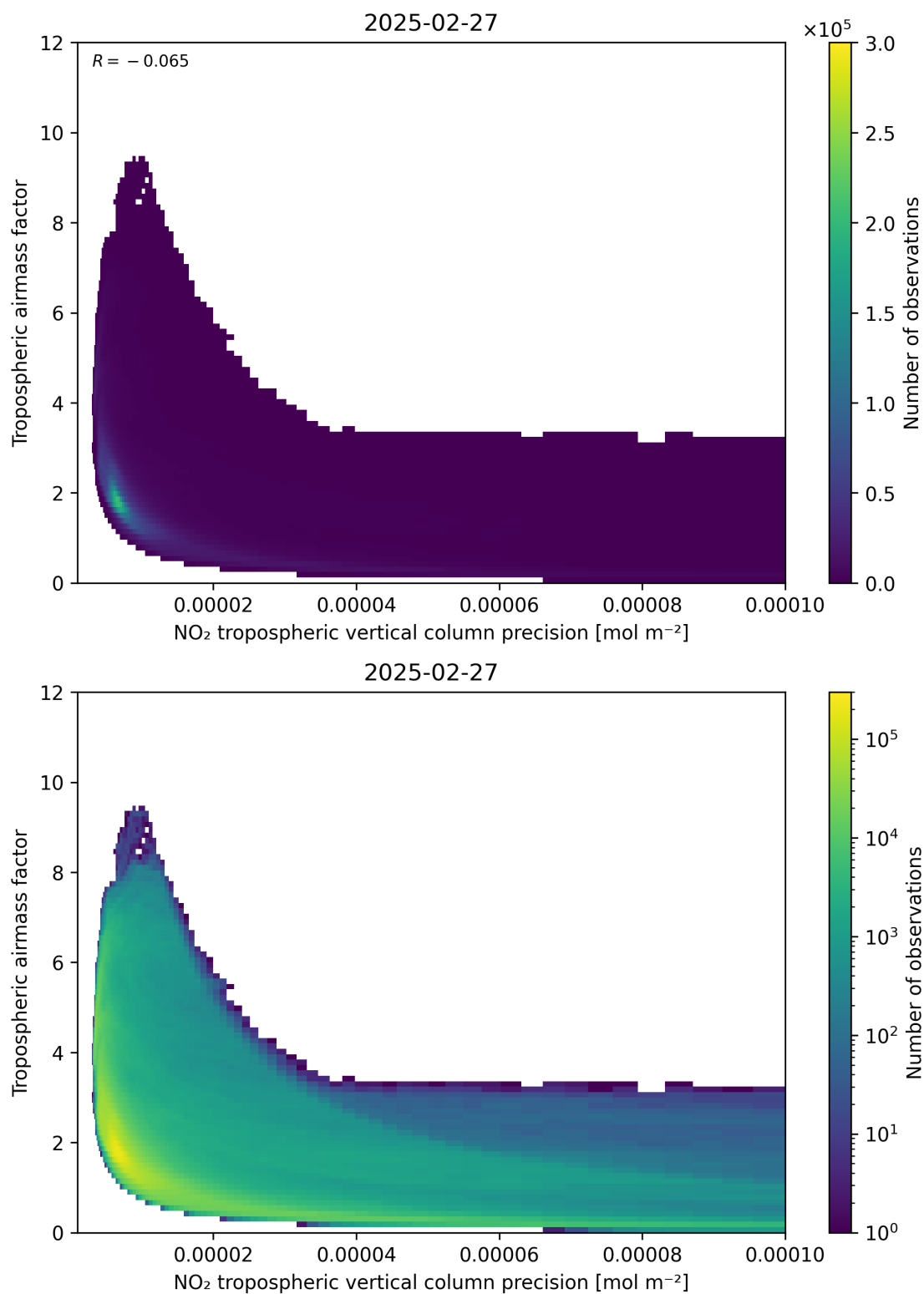
Figure 133: Scatter density plot of “NO 2 tropospheric vertical column precision” against “Tropospheric airmass factor” for 2025-02-26 to 2025-02-28.
