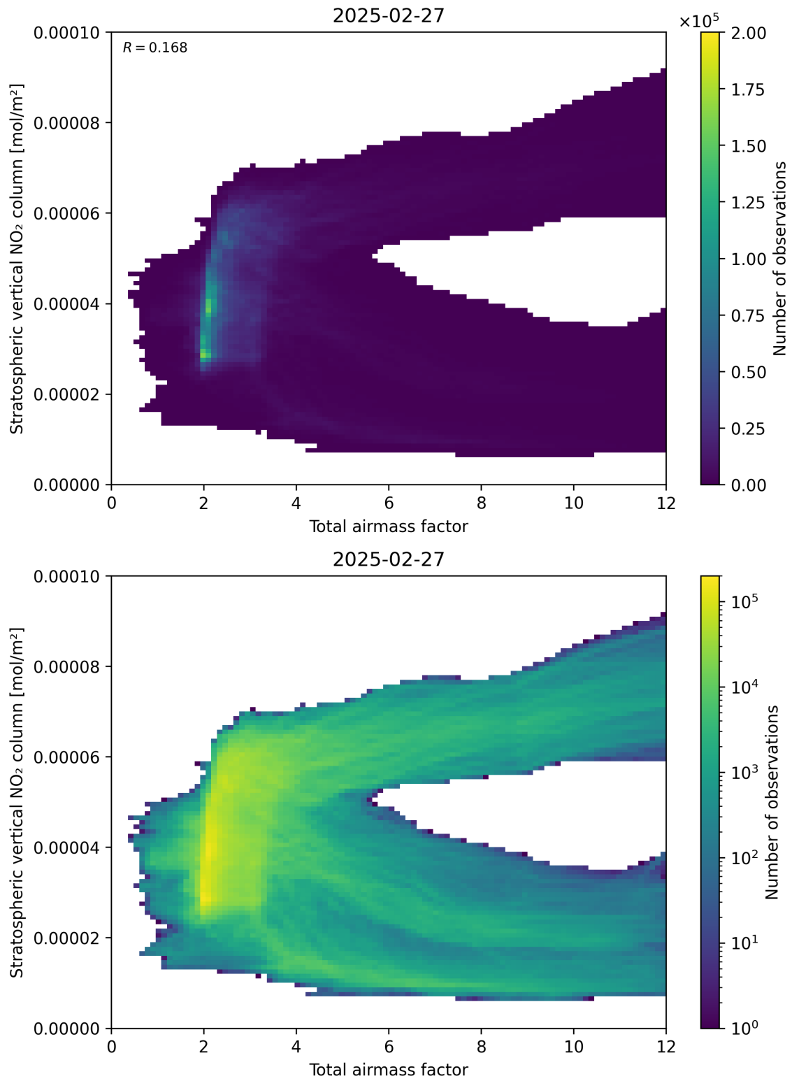
Figure 64: Scatter density plot of “Total airmass factor” against “Stratospheric vertical \text{NO}_2 column” for 2025-02-26 to 2025-02-28.
