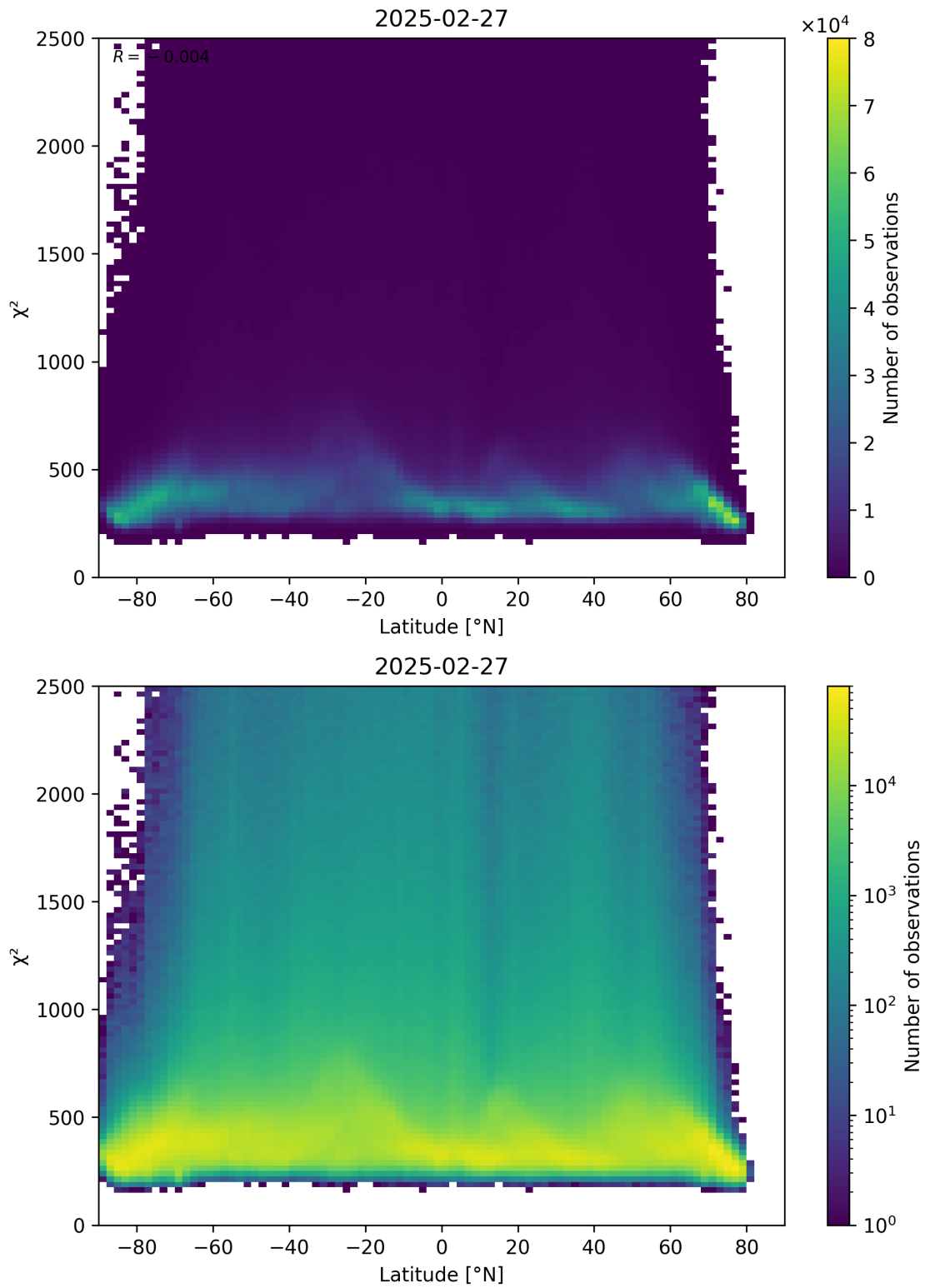
Figure 86: Scatter density plot of “Latitude” against “ \chi^2 ” for 2025-02-26 to 2025-02-28.
