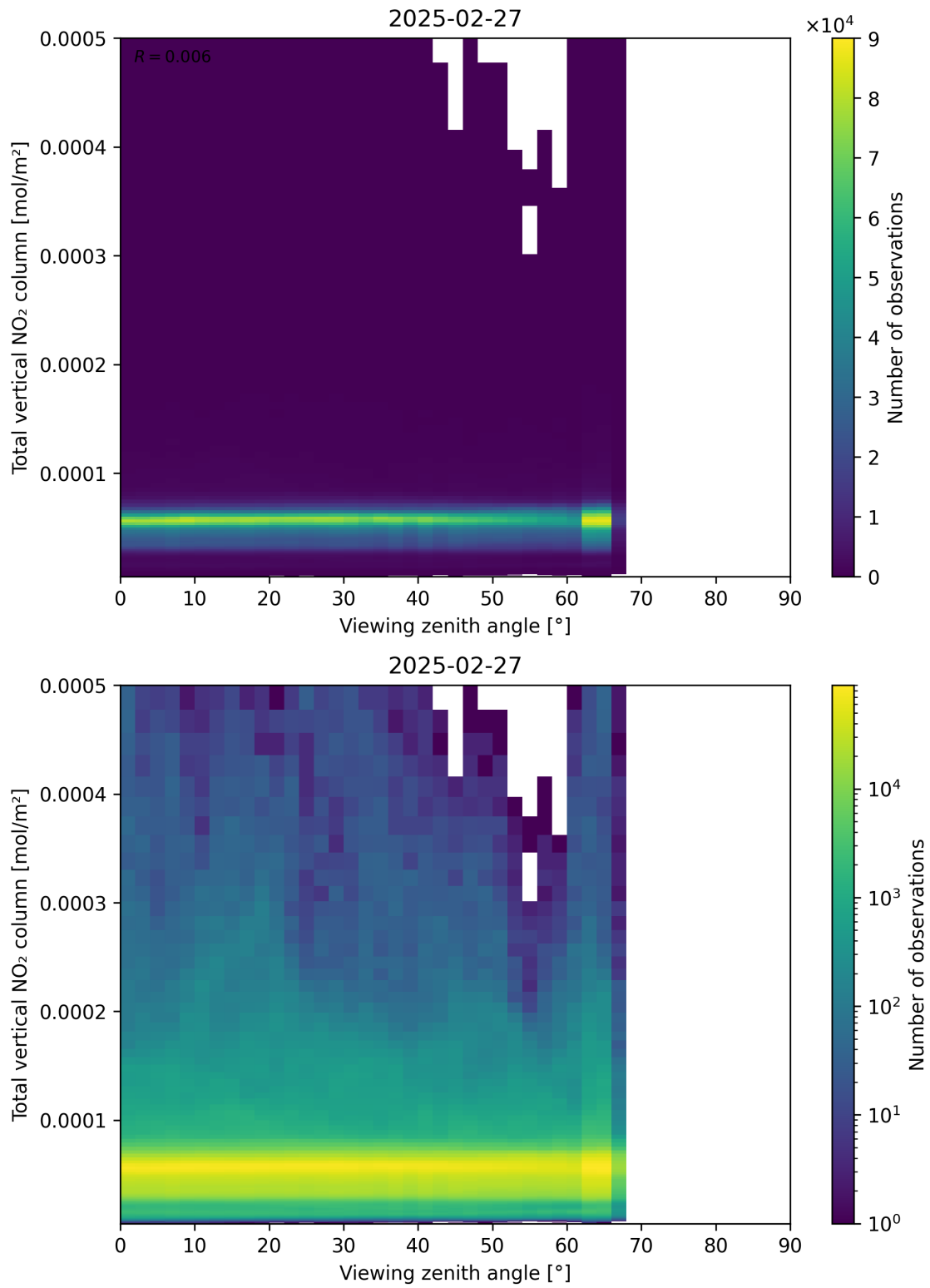
Figure 167: Scatter density plot of “Viewing zenith angle” against “Total vertical NO 2 column” for 2025-02-26 to 2025-02-28.
