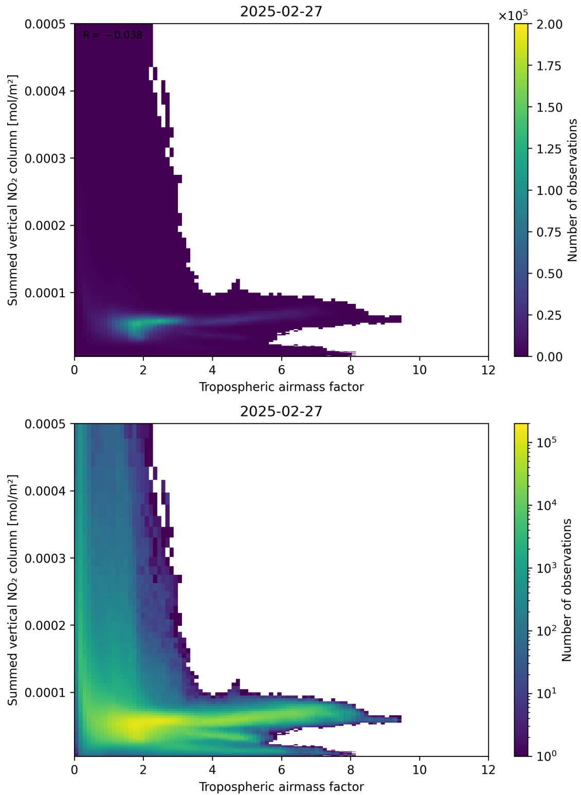
Figure 75: Scatter density plot of “Tropospheric air mass factor” against “Summed vertical NO 2 column” for 2025-02-26 to 2025-02-28.
