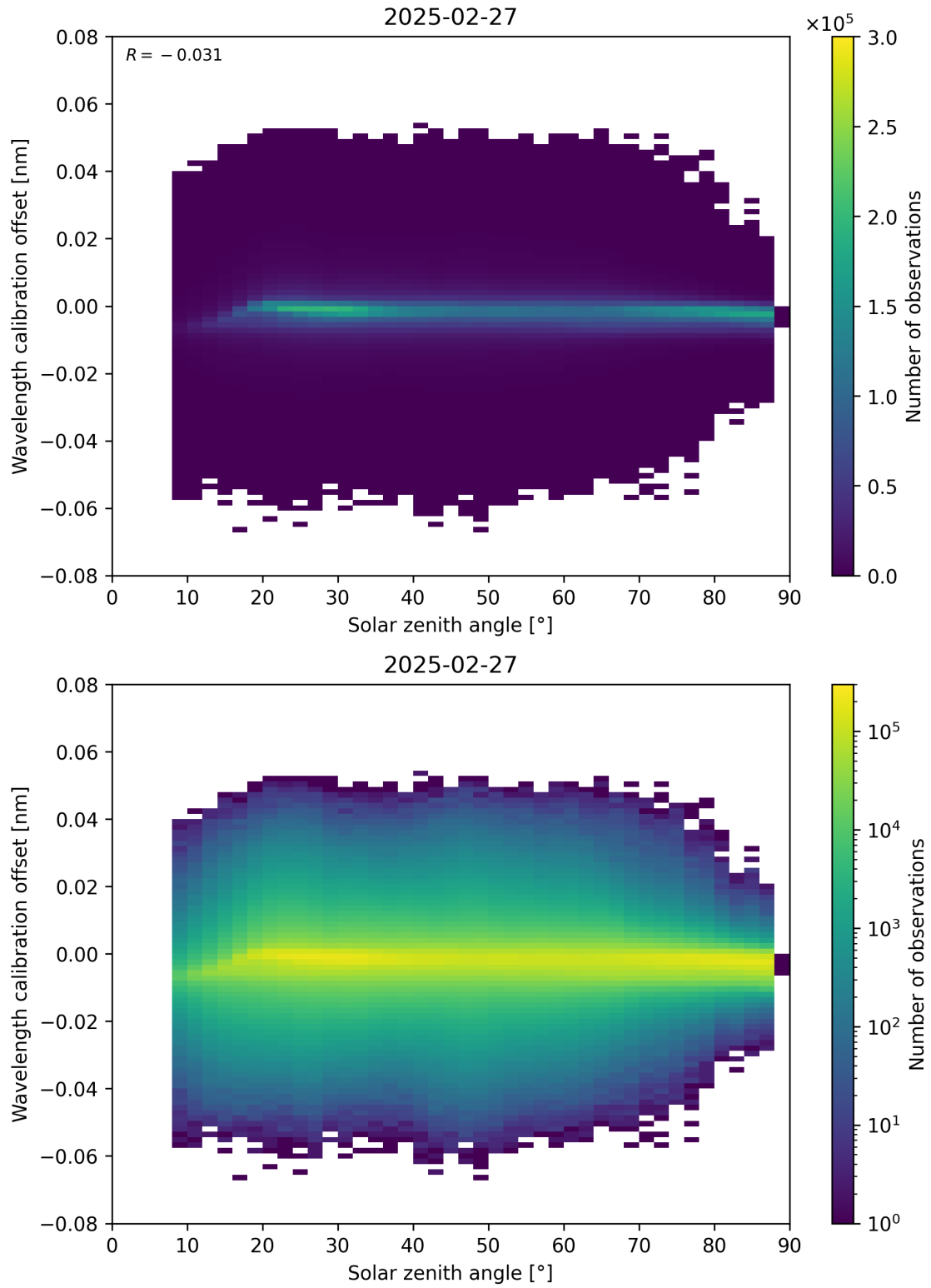
Figure 158: Scatter density plot of “Solar zenith angle” against “Wavelength calibration offset” for 2025-02-26 to 2025-02-28.
