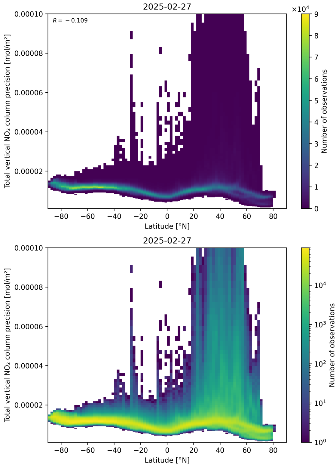
Figure 91: Scatter density plot of “Latitude” against “Total vertical NO 2 column precision” for 2025-02-26 to 2025-02-28.
