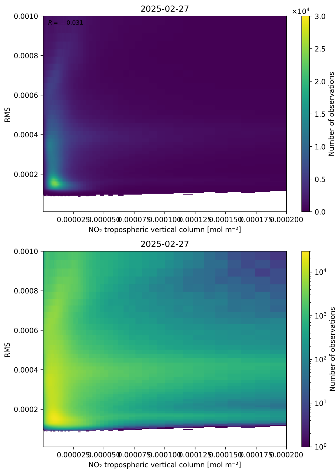
Figure 142: Scatter density plot of “NO 2 tropospheric vertical column” against “RMS” for 2025-02-26 to 2025-02-28.
