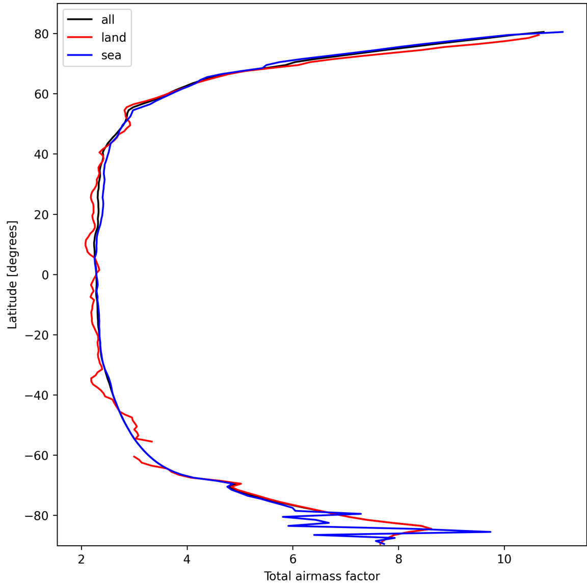
Figure 15: Zonal average of “Total airmass factor” for 2025-02-26 to 2025-02-28.
