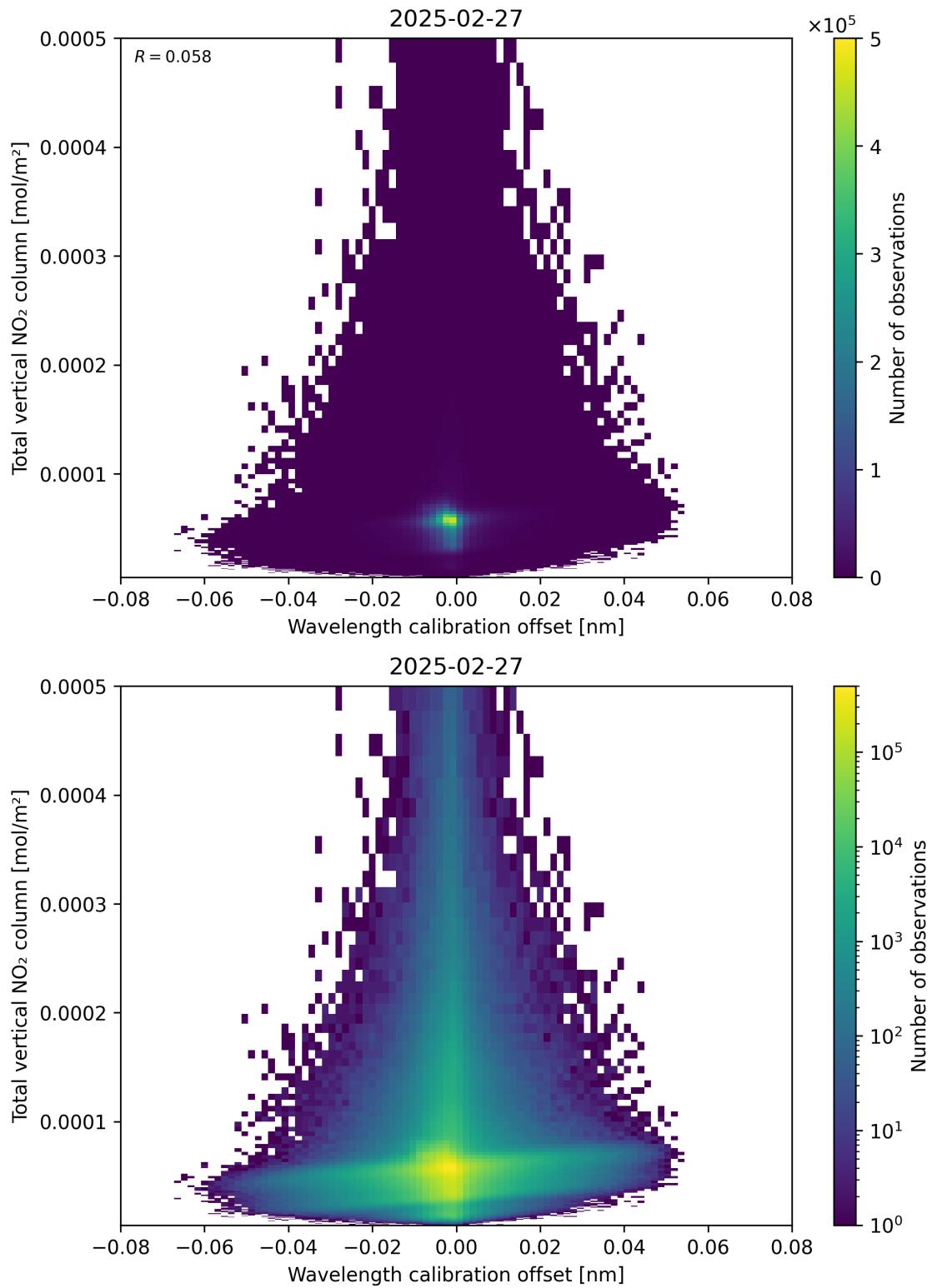
Figure 179: Scatter density plot of “Wavelength calibration offset” against “Total vertical NO 2 column” for 2025-02-26 to 2025-02-28.
