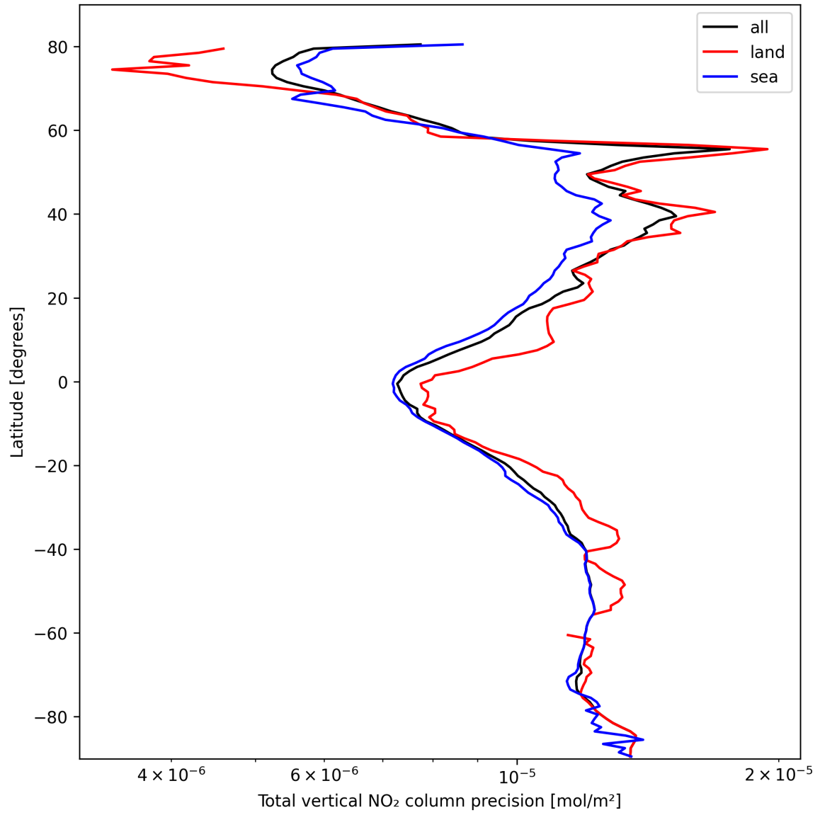
Figure 22: Zonal average of “Total vertical NO 2 column precision” for 2025-02-26 to 2025-02-28.
