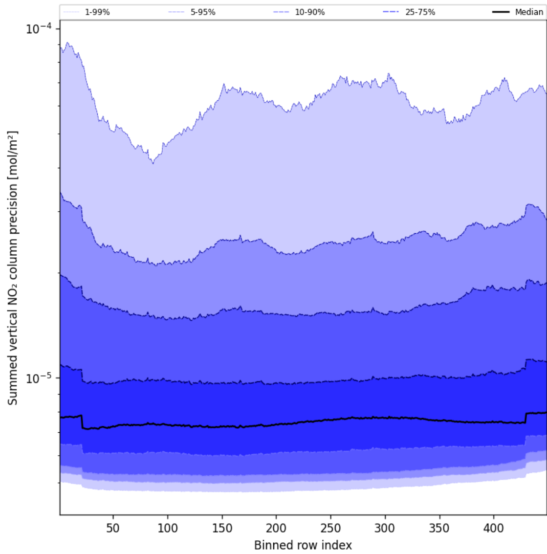
Figure 58: Along track statistics of “Summed vertical NO 2 column precision” for 2025-02-26 to 2025-02-28
