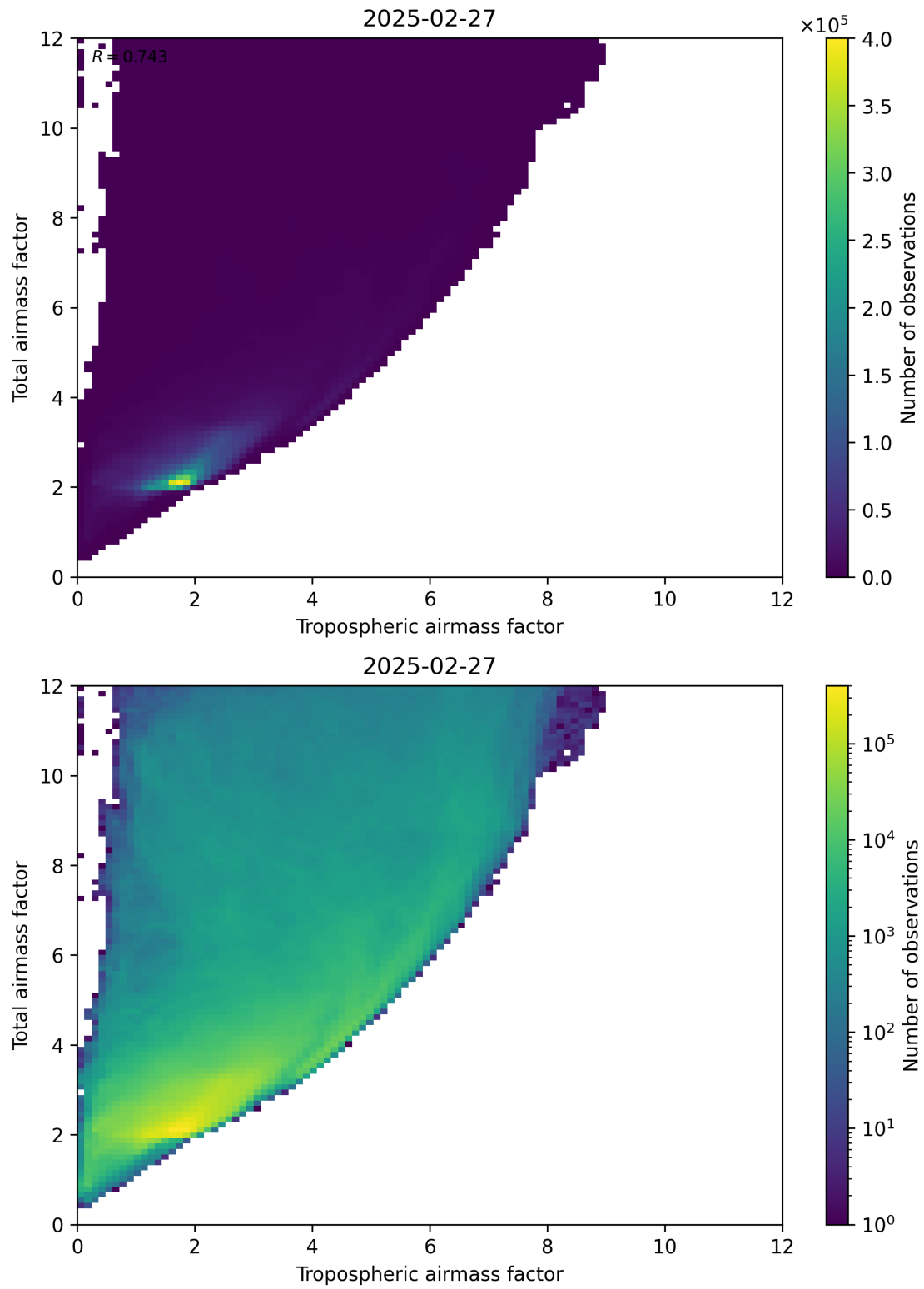
Figure 72: Scatter density plot of “Tropospheric airmass factor” against “Total airmass factor” for 2025-02-26 to 2025-02-28.
