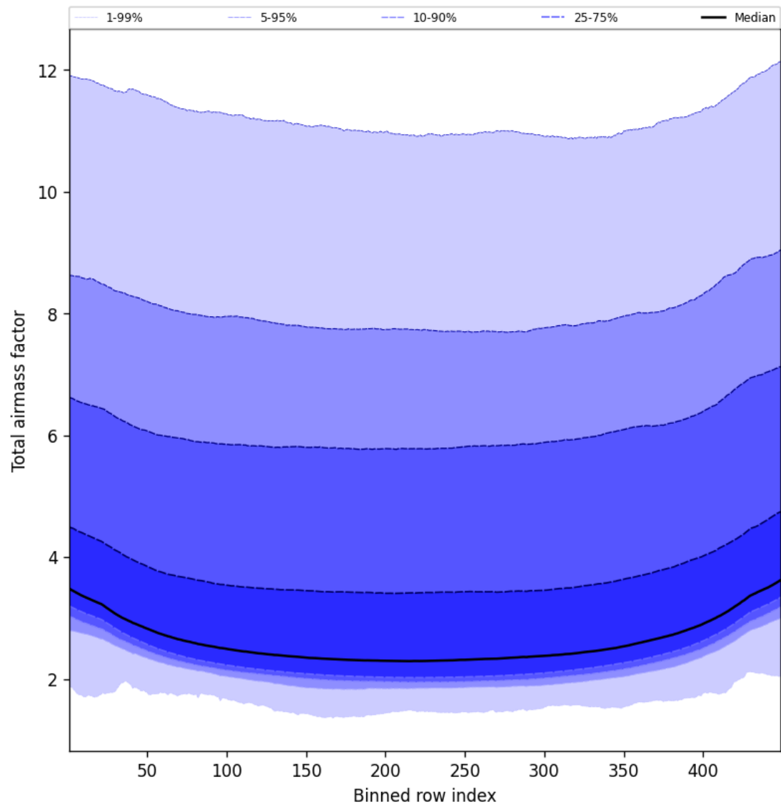
Figure 49: Along track statistics of “Total airmass factor” for 2025-02-26 to 2025-02-28
