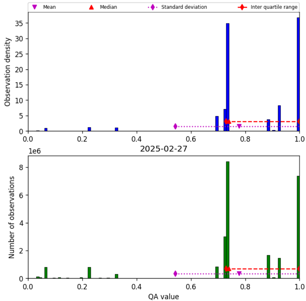
Figure 28: Histogram of “QA value” for 2025-02-26 to 2025-02-28
