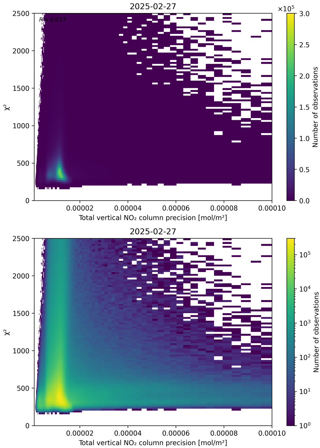
Figure 116: Scatter density plot of “Total vertical NO 2 column precision” against “ \chi^2 ” for 2025-02-26 to 2025-02-28.
