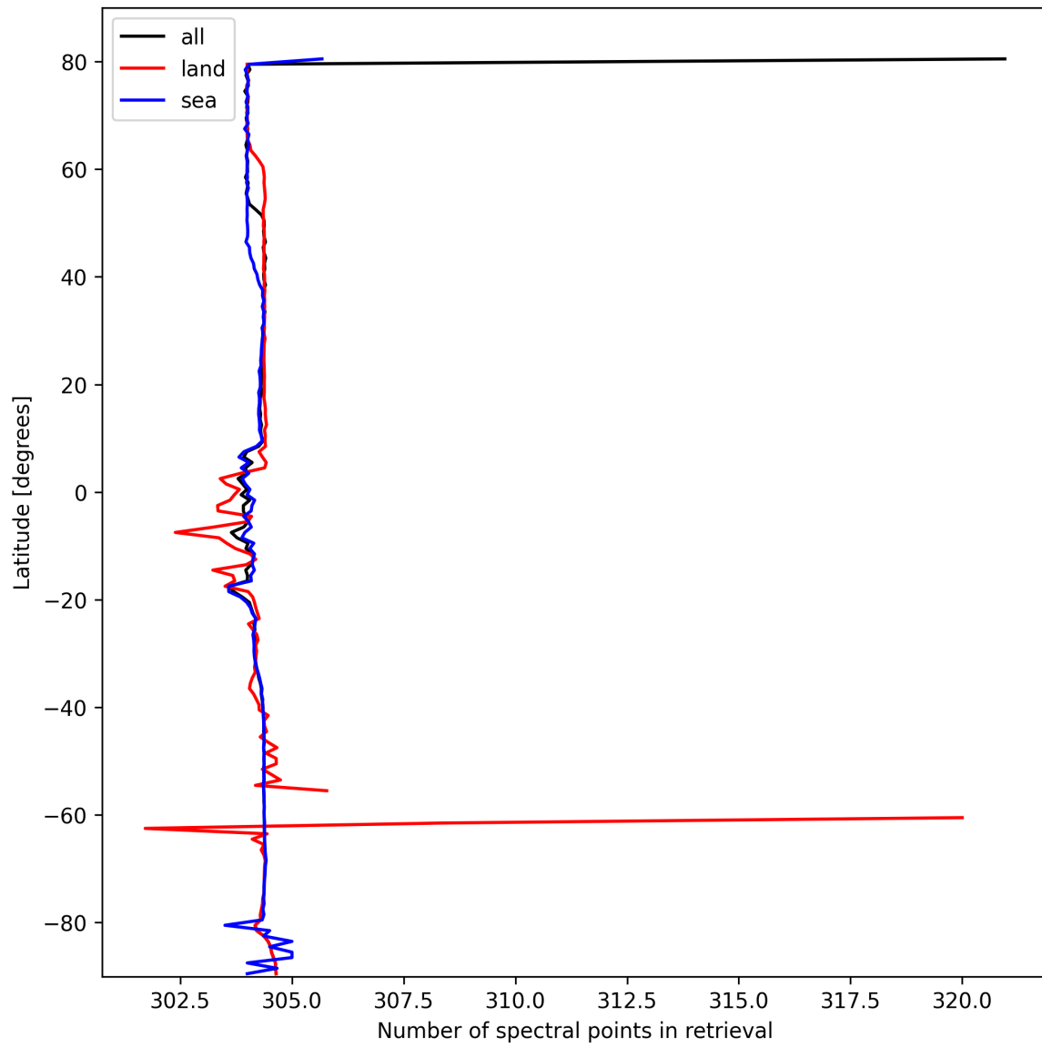
Figure 16: Zonal average of “Number of spectral points in retrieval” for 2025-02-26 to 2025-02-28.
