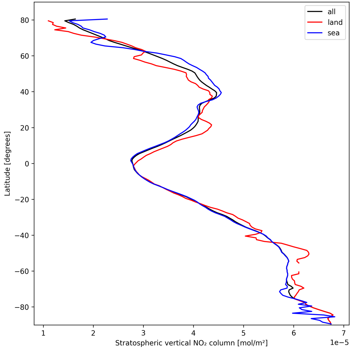
Figure 19: Zonal average of “Stratospheric vertical NO 2 column” for 2025-02-26 to 2025-02-28.
