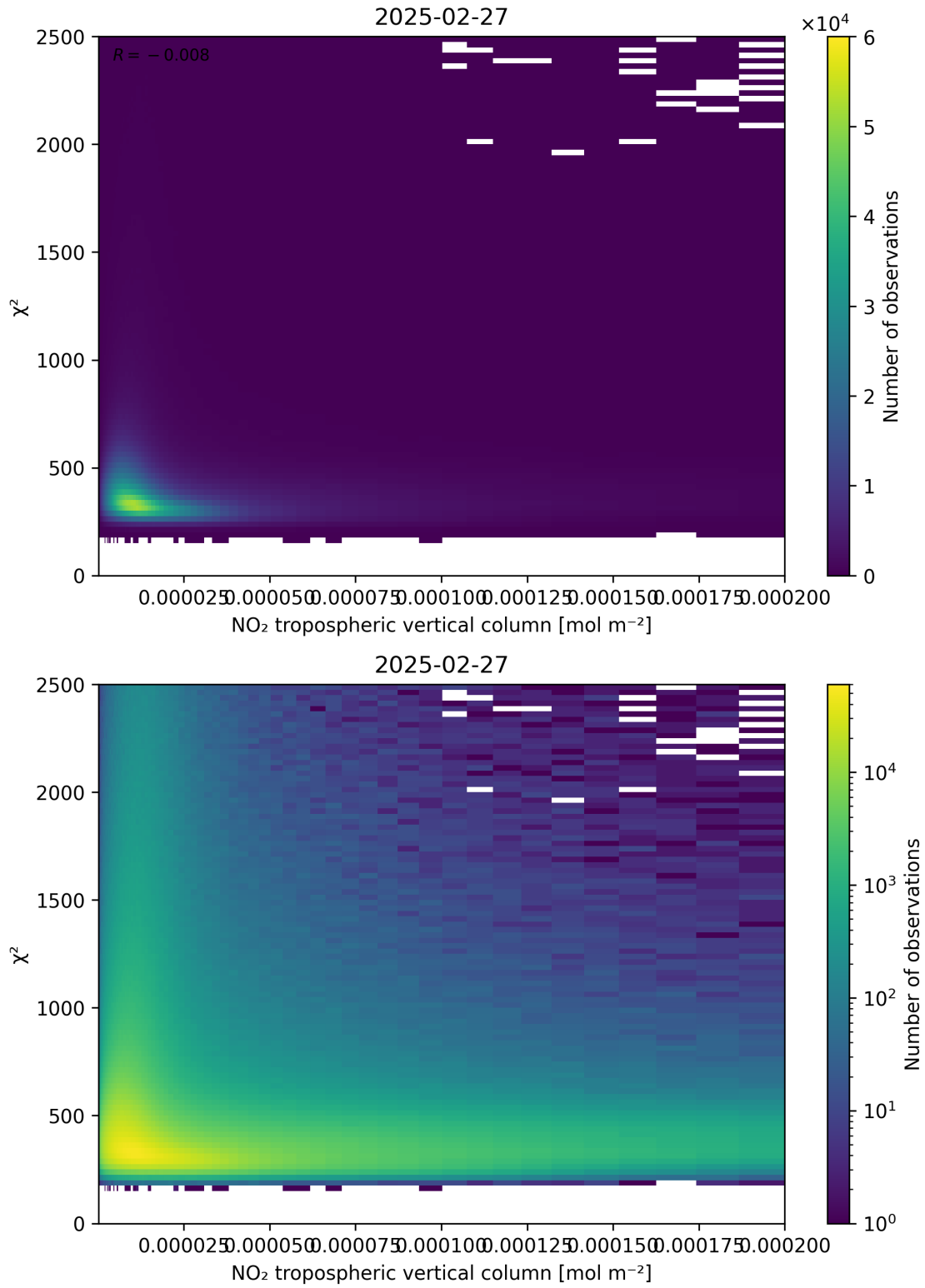
Figure 124: Scatter density plot of “NO 2 tropospheric vertical column” against “ \chi^2 ” for 2025-02-26 to 2025-02-28.
