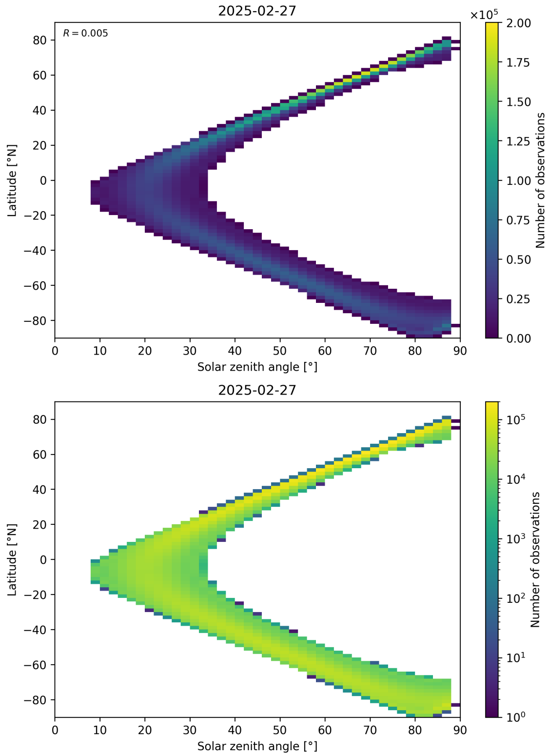
Figure 149: Scatter density plot of “Solar zenith angle” against “Latitude” for 2025-02-26 to 2025-02-28.
