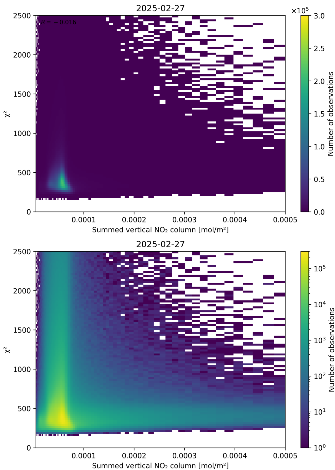
Figure 104: Scatter density plot of “Summed vertical NO 2 column” against “ \chi^2 ” for 2025-02-26 to 2025-02-28.
