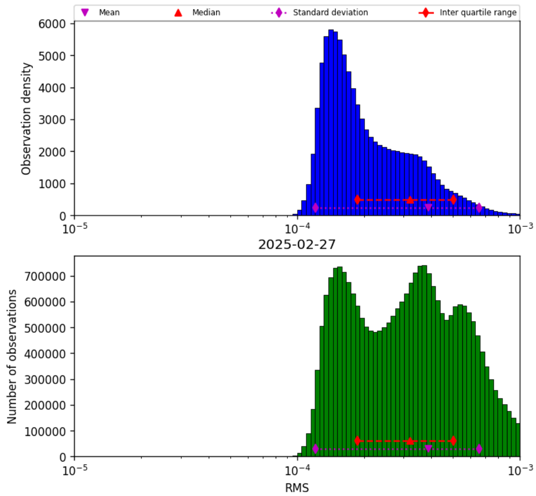
Figure 43: Histogram of “RMS” for 2025-02-26 to 2025-02-28
