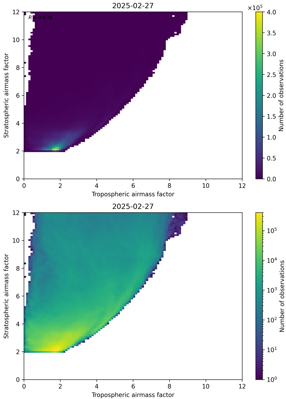
Figure 71: Scatter density plot of “Tropospheric airmass factor” against “Stratospheric airmass factor” for 2025-02-26 to 2025-02-28.
