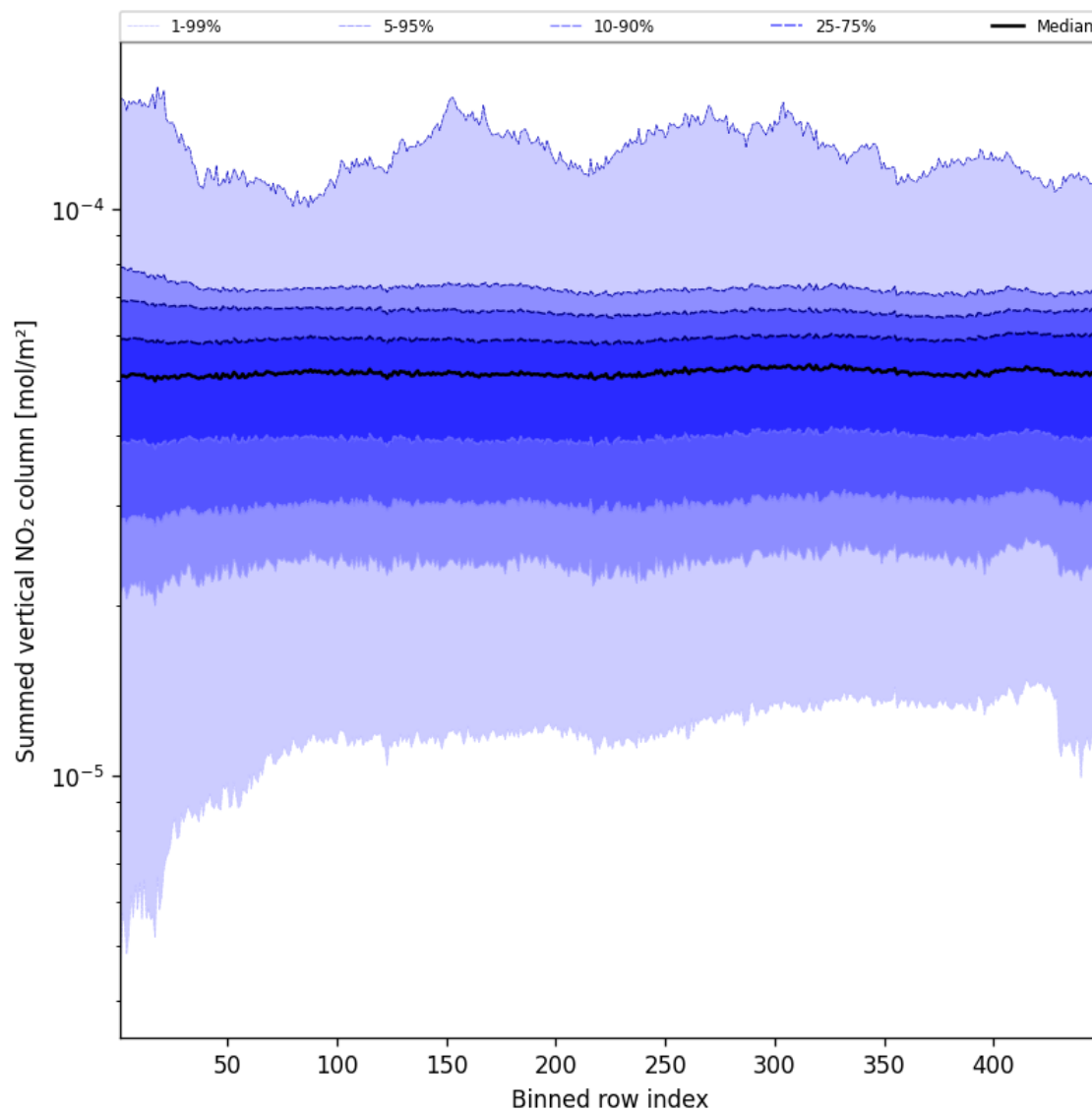
Figure 57: Along track statistics of “Summed vertical NO 2 column” for 2025-02-26 to 2025-02-28
