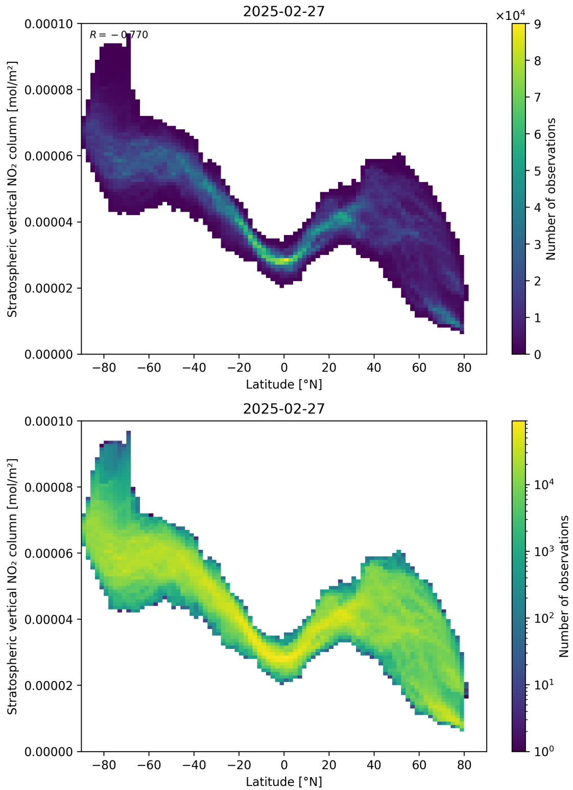
Figure 87: Scatter density plot of “Latitude” against “Stratospheric vertical NO 2 column” for 2025-02-26 to 2025-02-28.
