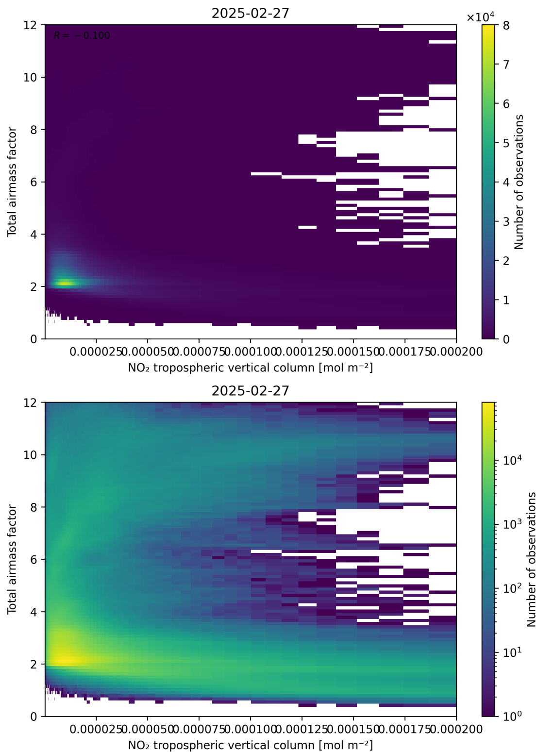
Figure 122: Scatter density plot of “NO 2 tropospheric vertical column” against “Total air mass factor” for 2025-02-26 to 2025-02-28.
