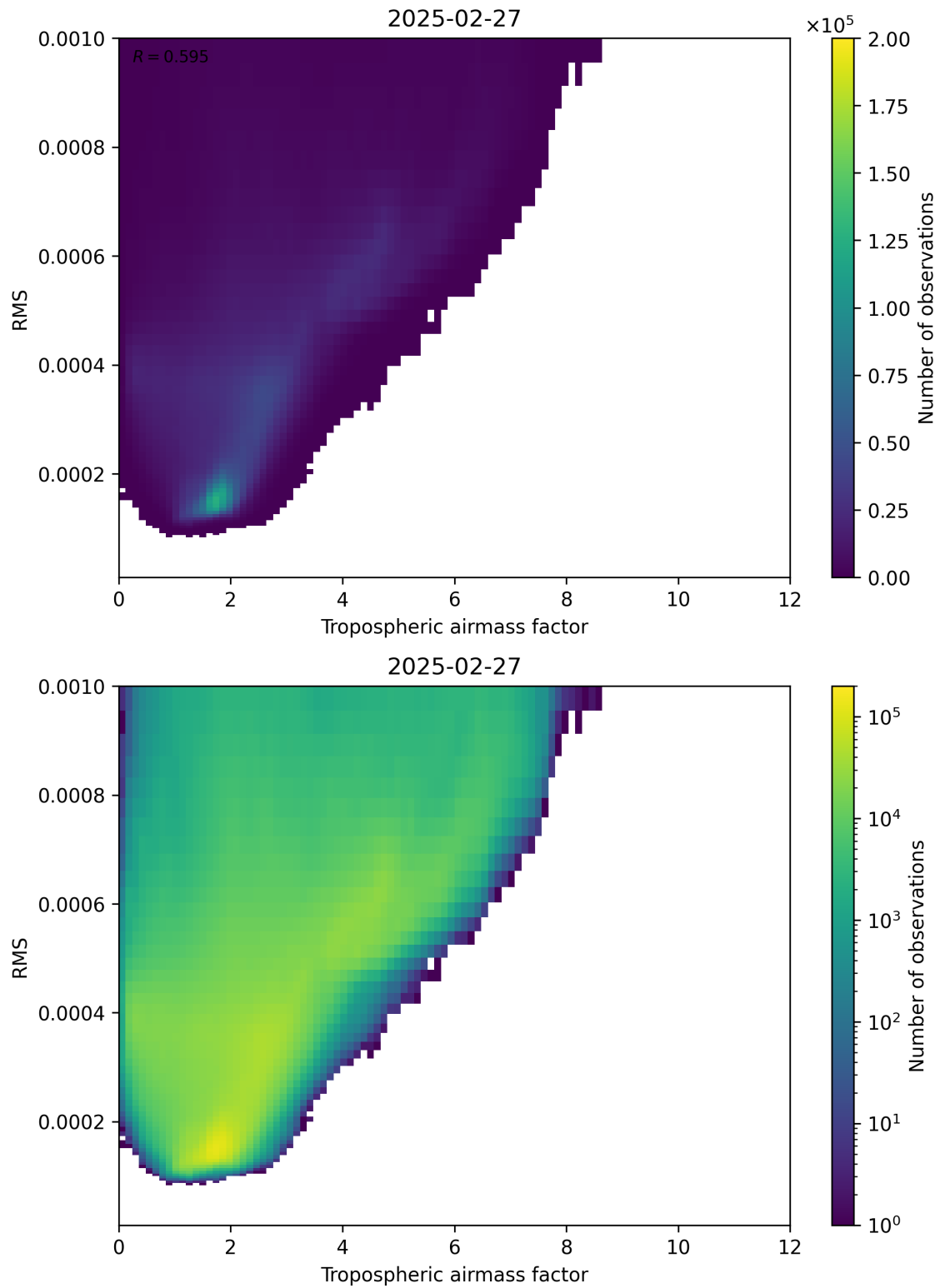
Figure 79: Scatter density plot of “Tropospheric airmass factor” against “RMS” for 2025-02-26 to 2025-02-28.
