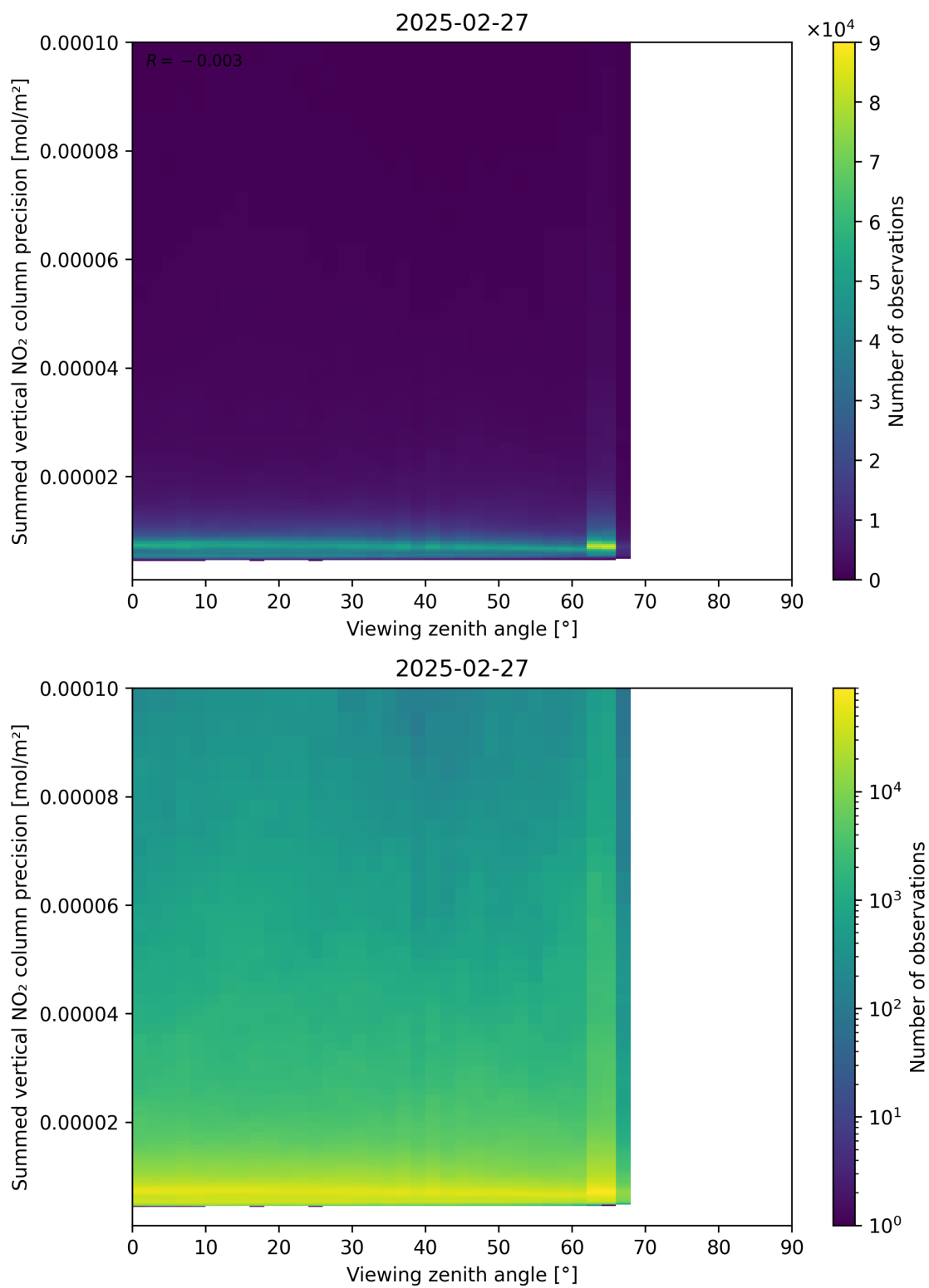
Figure 166: Scatter density plot of “Viewing zenith angle” against “Summed vertical NO 2 column precision” for 2025-02-26 to 2025-02-28.
