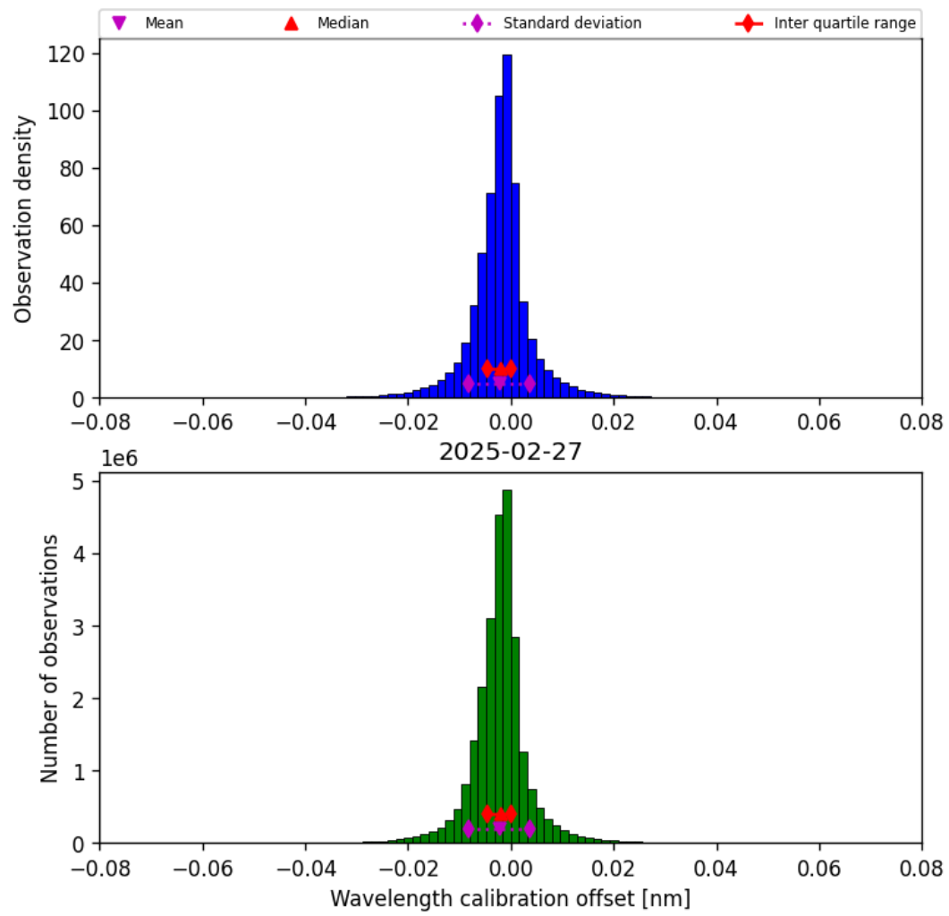
Figure 35: Histogram of “Wavelength calibration offset” for 2025-02-26 to 2025-02-28
