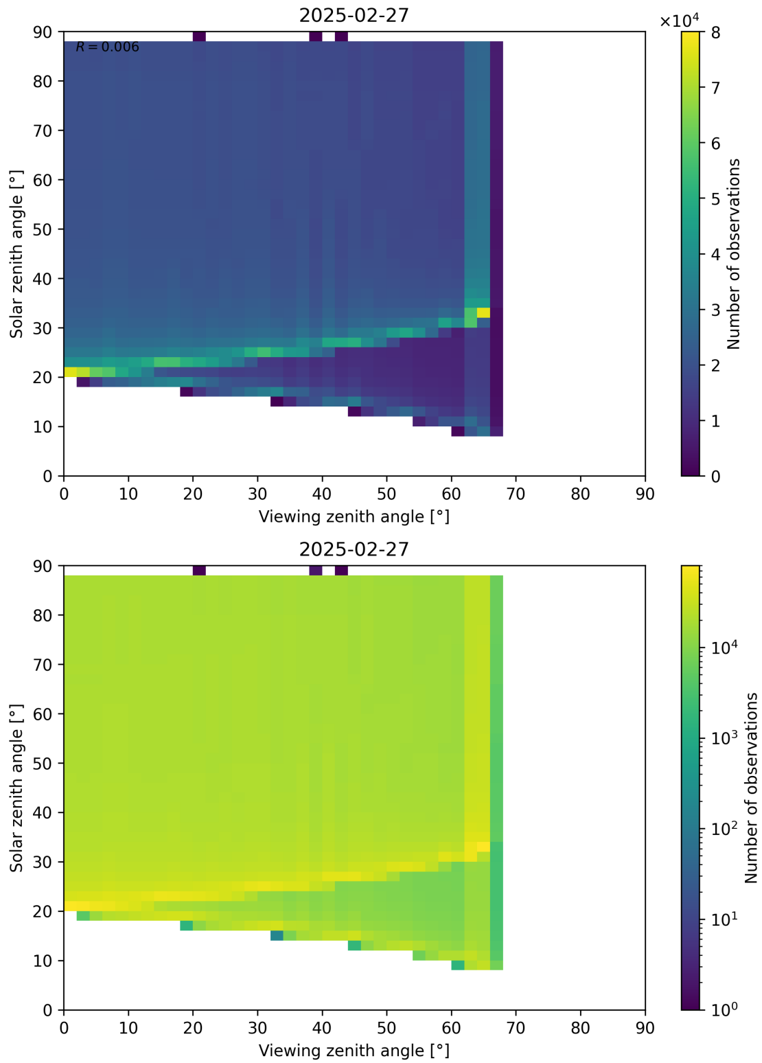
Figure 172: Scatter density plot of “Viewing zenith angle” against “Solar zenith angle” for 2025-02-26 to 2025-02-28.
