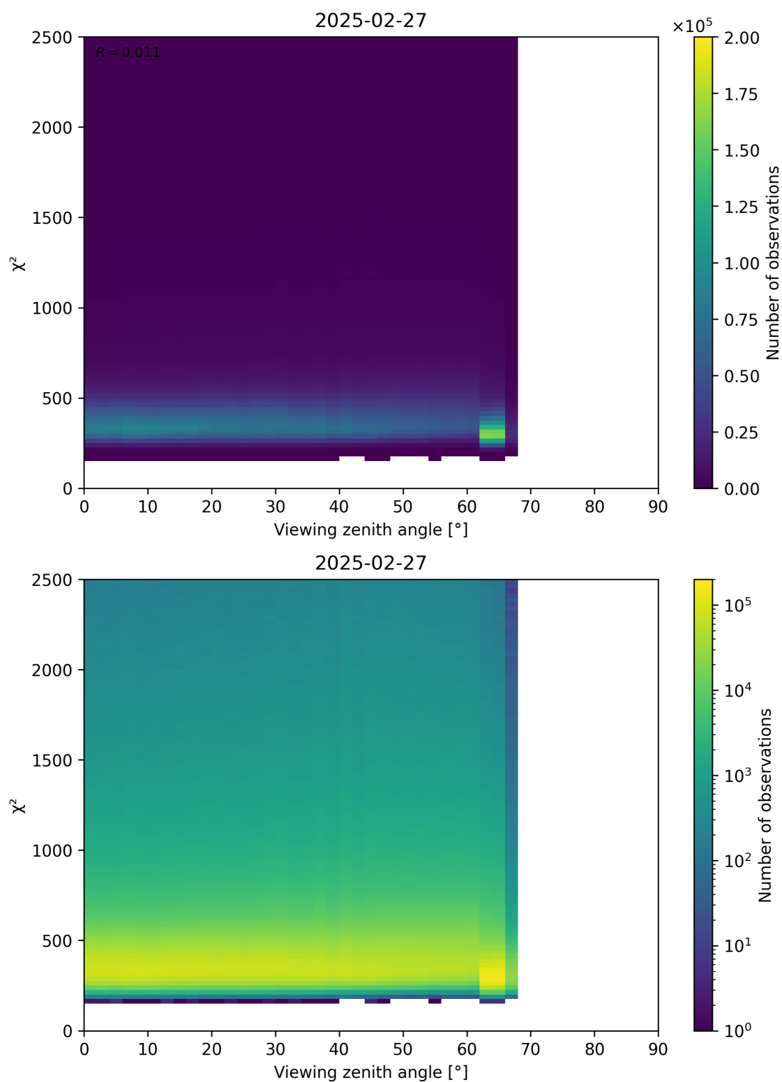
Figure 162: Scatter density plot of “Viewing zenith angle” against “ \chi^2 ” for 2025-02-26 to 2025-02-28.
