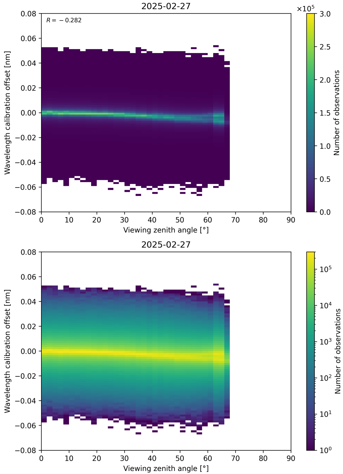
Figure 173: Scatter density plot of “Viewing zenith angle” against “Wavelength calibration offset” for 2025-02-26 to 2025-02-28.
