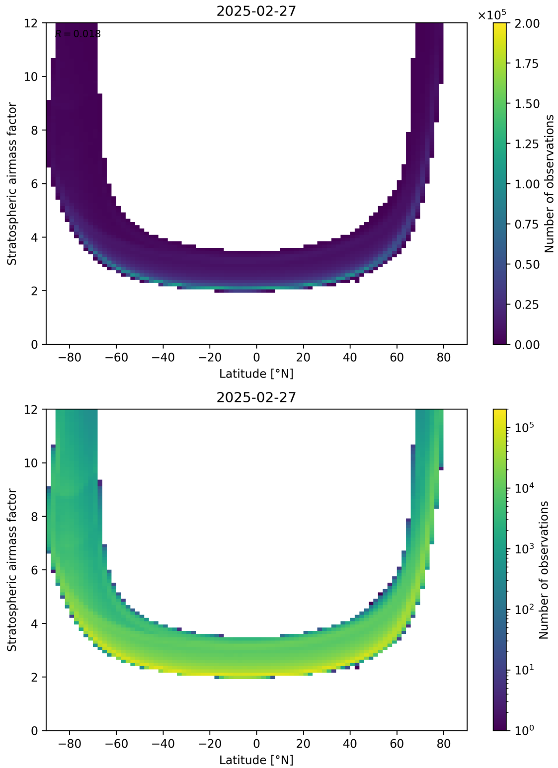
Figure 83: Scatter density plot of “Latitude” against “Stratospheric air mass factor” for 2025-02-26 to 2025-02-28.
