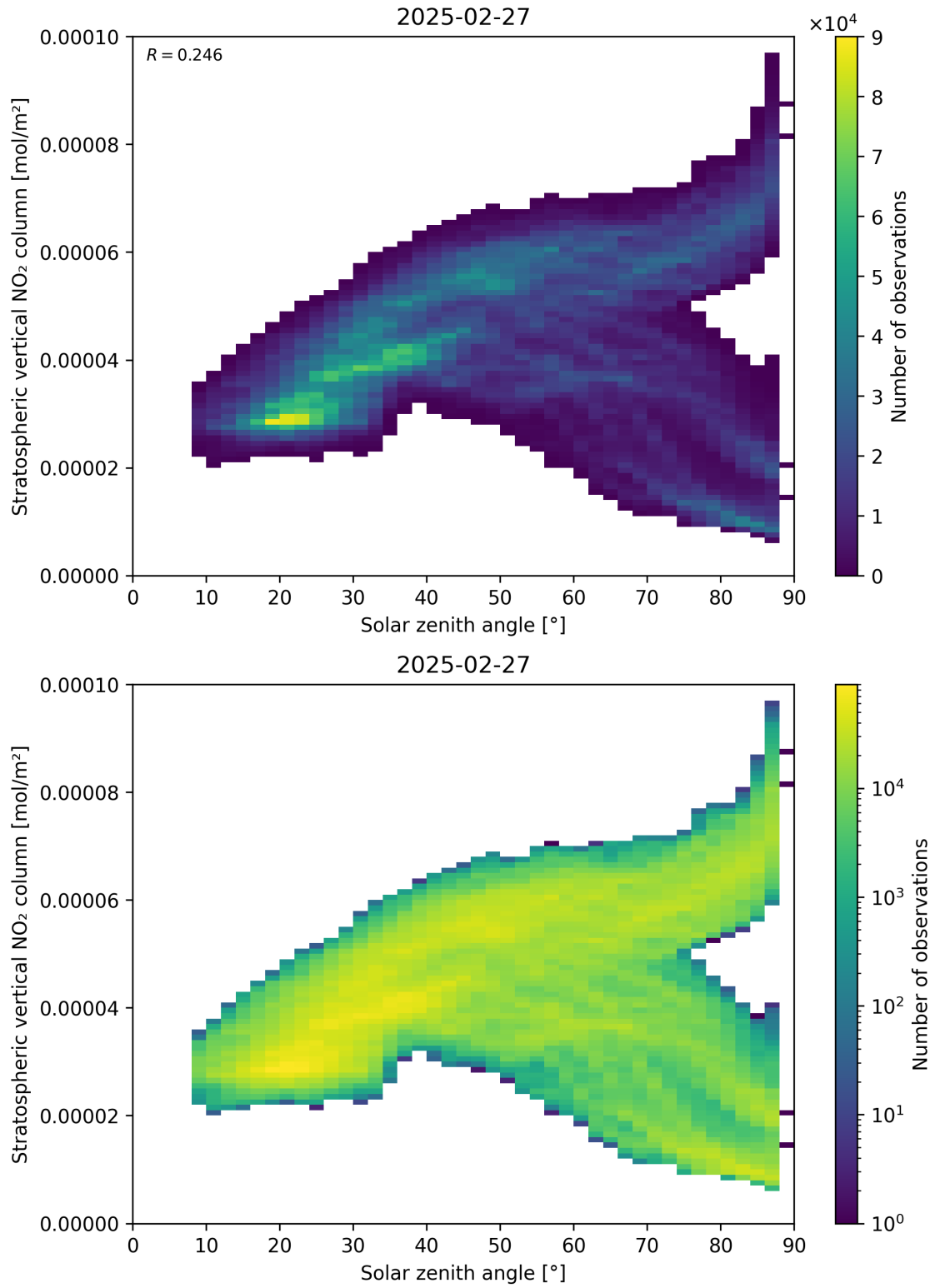
Figure 150: Scatter density plot of “Solar zenith angle” against “Stratospheric vertical NO 2 column” for 2025-02-26 to 2025-02-28.
