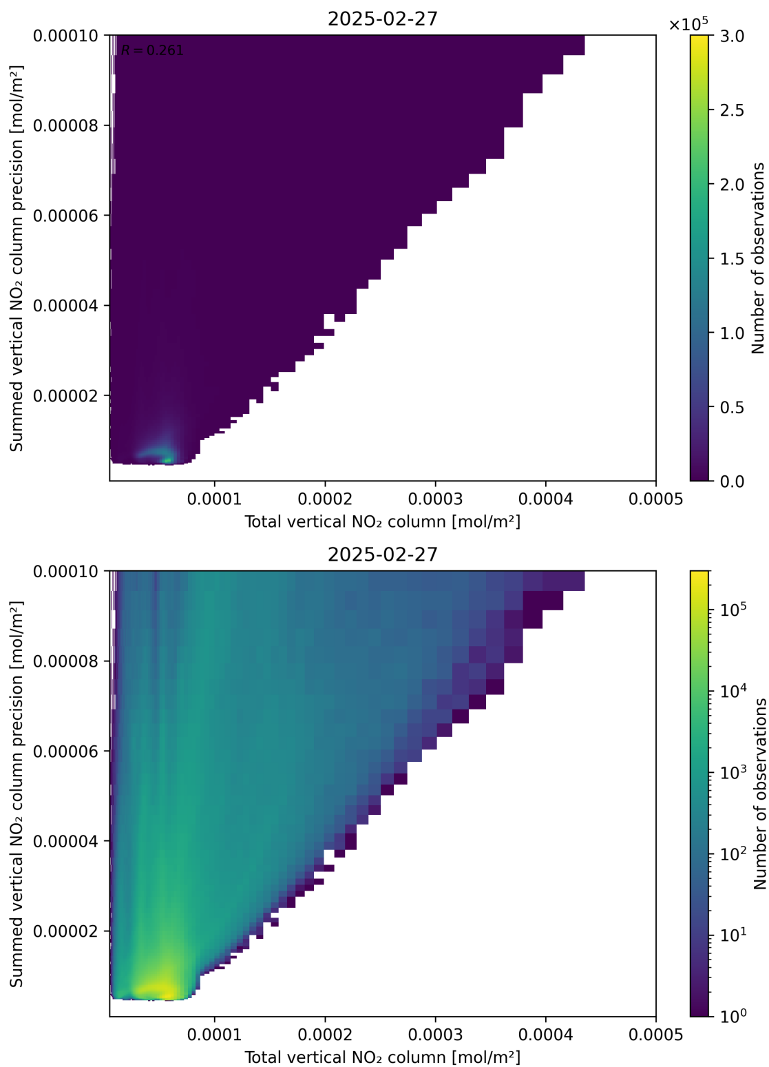
Figure 113: Scatter density plot of “Total vertical NO 2 column” against “Summed vertical NO 2 column precision” for 2025-02-26 to 2025-02-28.
