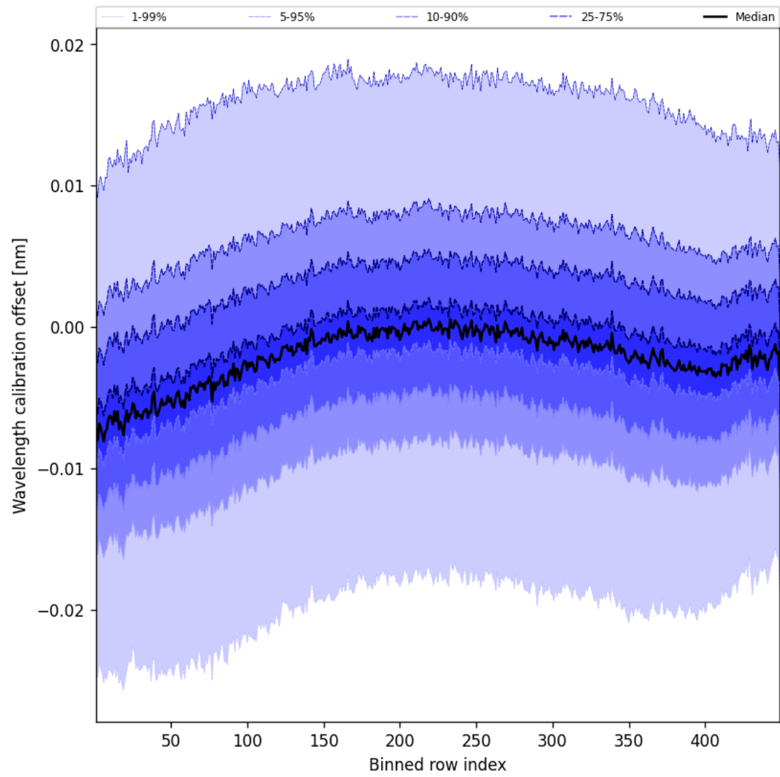
Figure 52: Along track statistics of “Wavelength calibration offset” for 2025-02-26 to 2025-02-28
