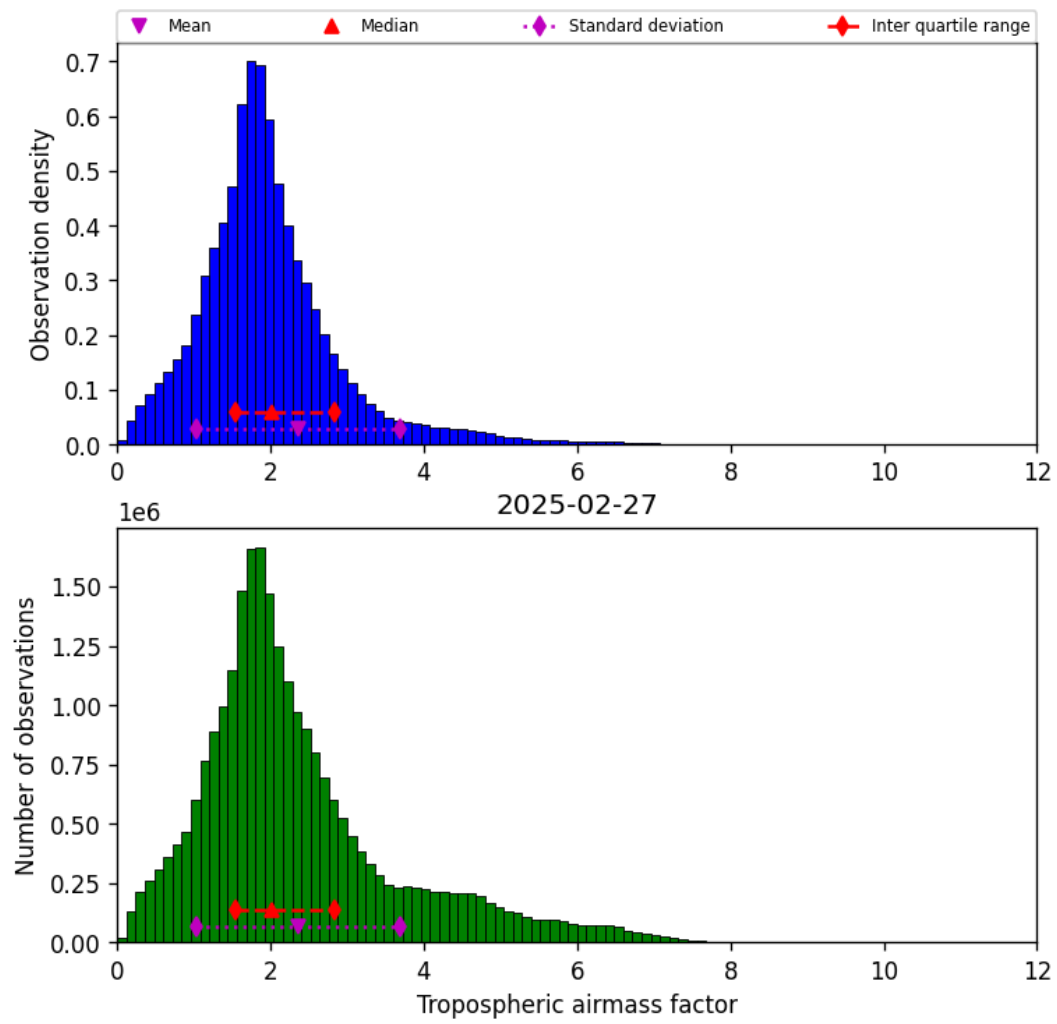
Figure 31: Histogram of “Tropospheric airmass factor” for 2025-02-26 to 2025-02-28
