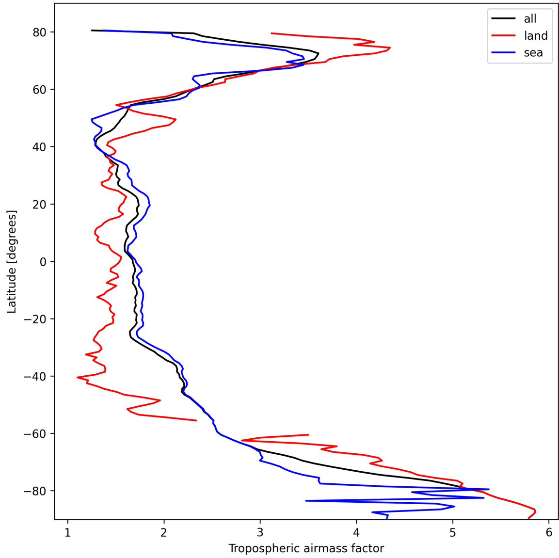
Figure 14: Zonal average of “Tropospheric airmass factor” for 2025-02-26 to 2025-02-28.
