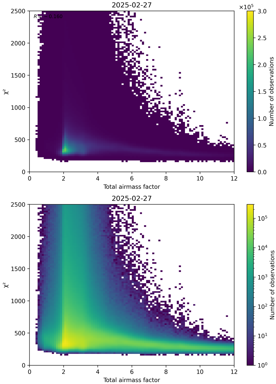
Figure 63: Scatter density plot of “Total airmass factor” against “ \chi^2 ” for 2025-02-26 to 2025-02-28.
