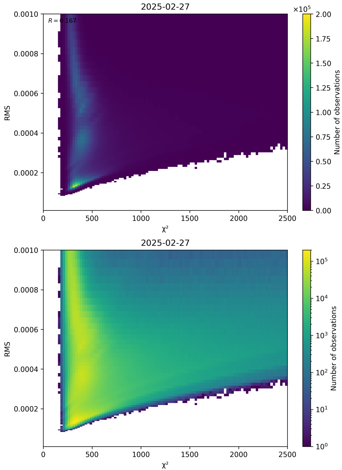
Figure 82: Scatter density plot of “ \chi^2 ” against “RMS” for 2025-02-26 to 2025-02-28.
