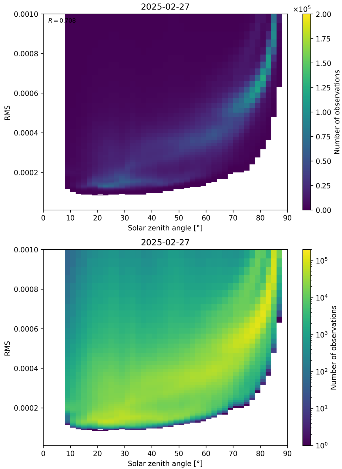
Figure 157: Scatter density plot of “Solar zenith angle” against “RMS” for 2025-02-26 to 2025-02-28.
