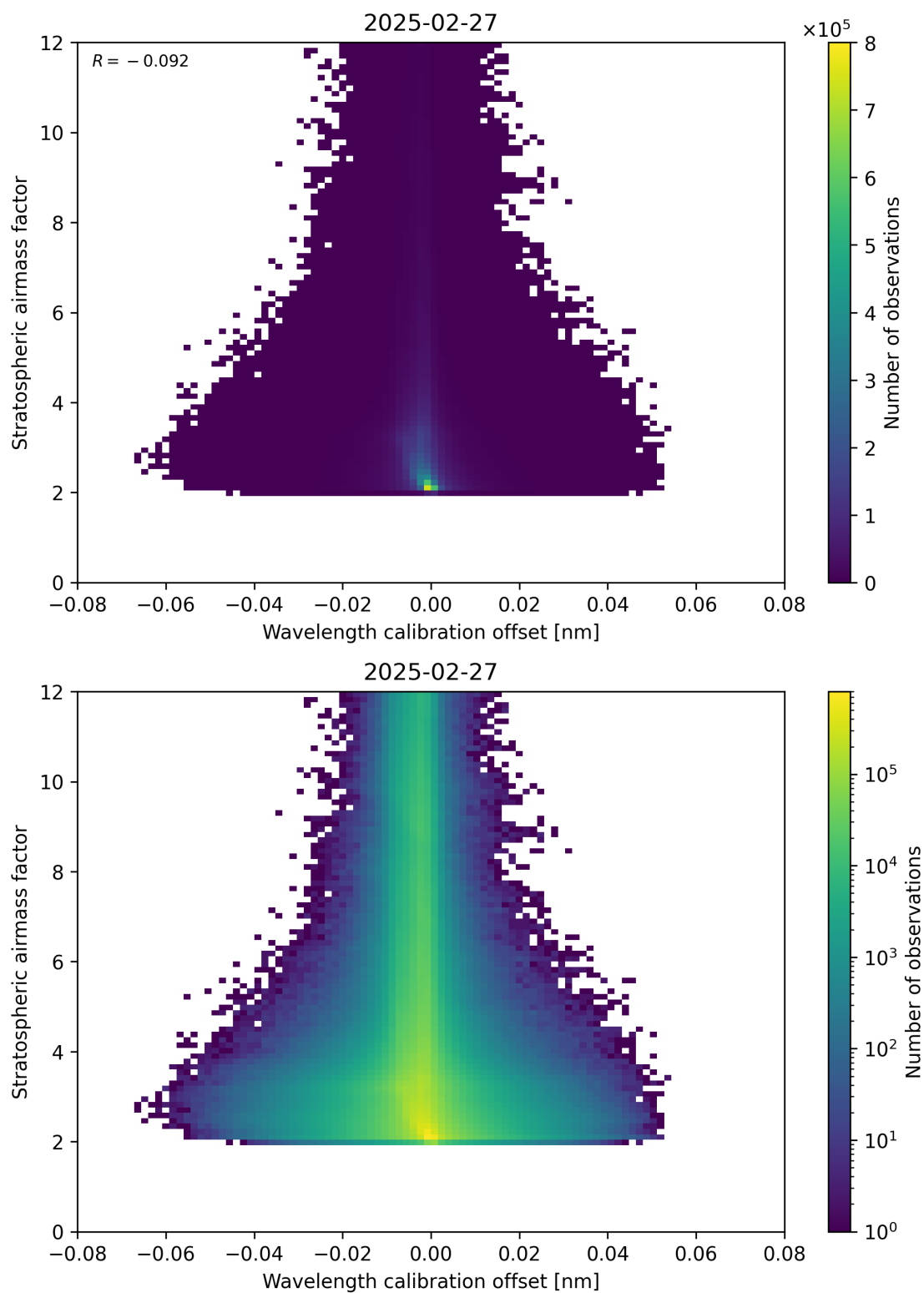
Figure 174: Scatter density plot of “Wavelength calibration offset” against “Stratospheric airmass factor” for 2025-02-26 to 2025-02-28.
