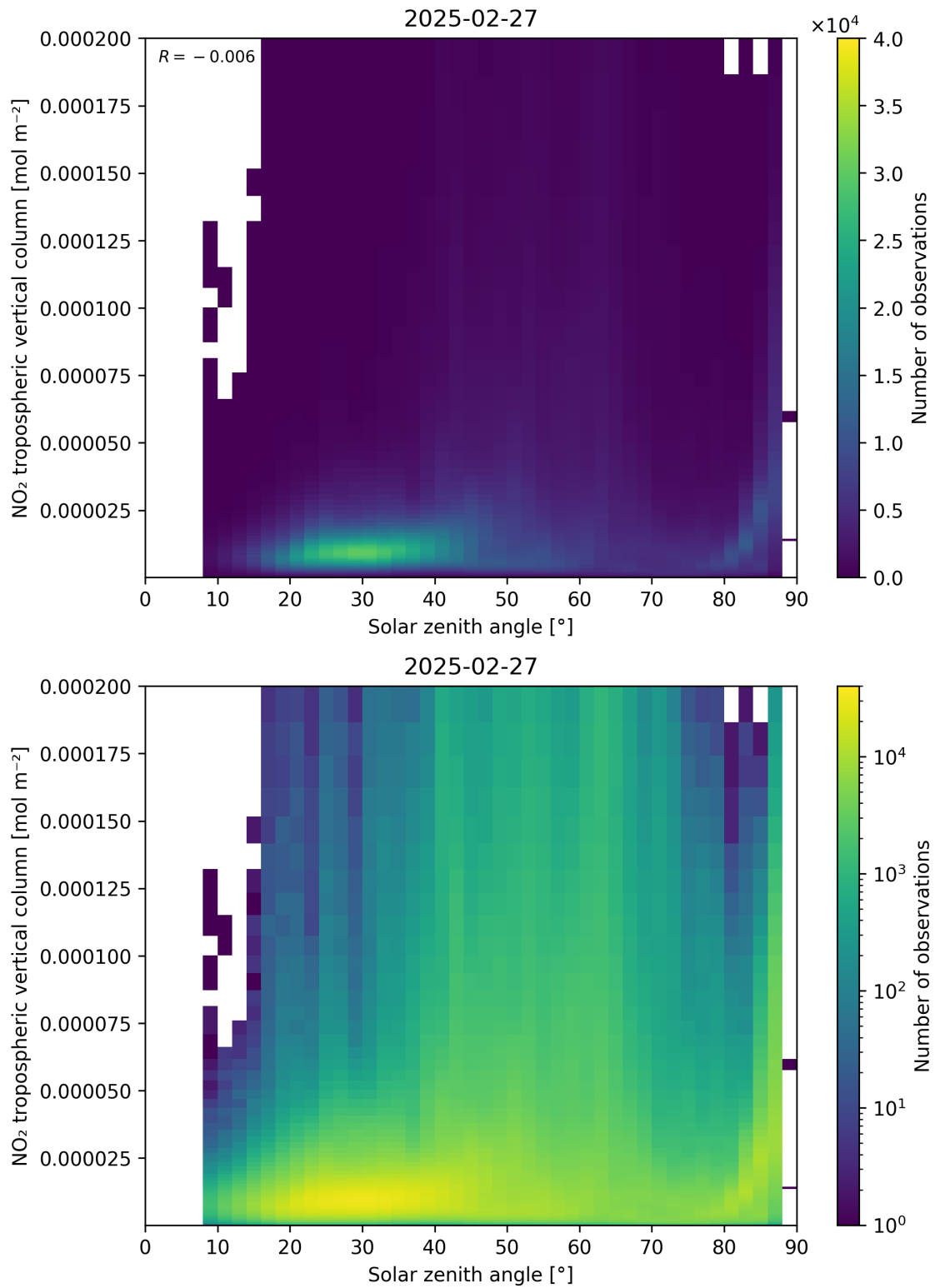
Figure 155: Scatter density plot of “Solar zenith angle” against “NO 2 tropospheric vertical column” for 2025-02-26 to 2025-02-28.
