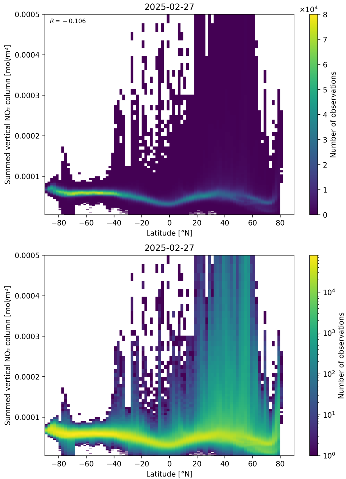
Figure 88: Scatter density plot of “Latitude” against “Summed vertical NO 2 column” for 2025-02-26 to 2025-02-28.
