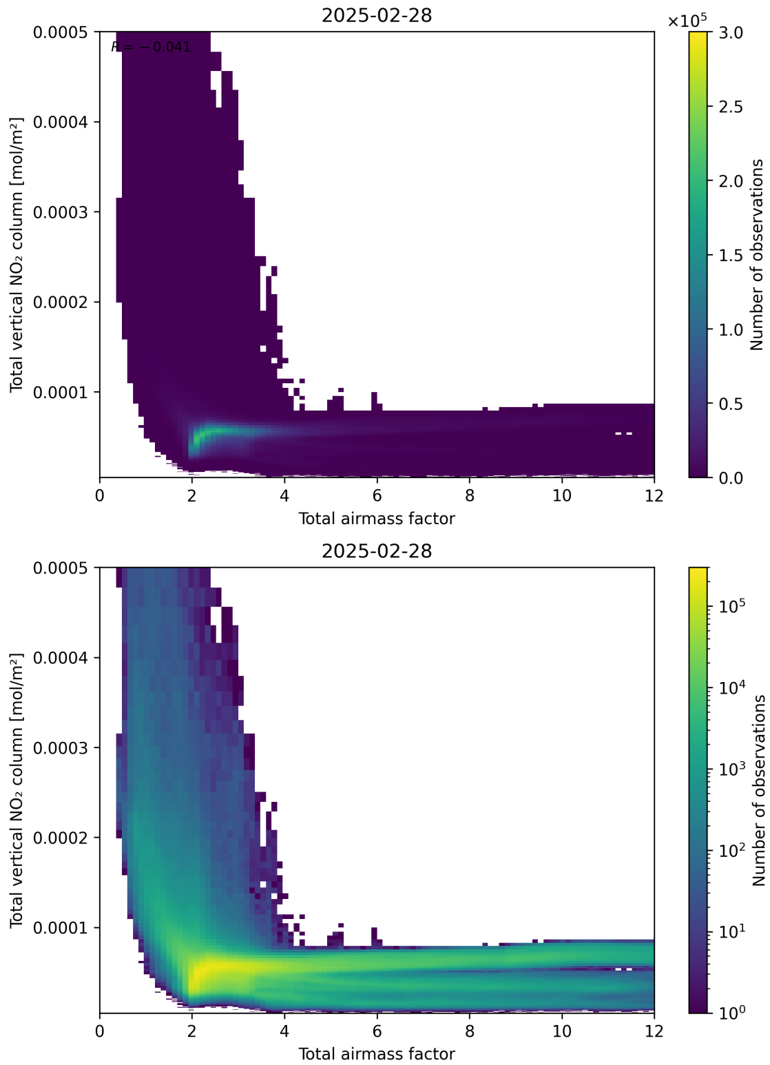
Figure 67: Scatter density plot of “Total airmass factor” against “Total vertical NO 2 column” for 2025-02-27 to 2025-03-01.
