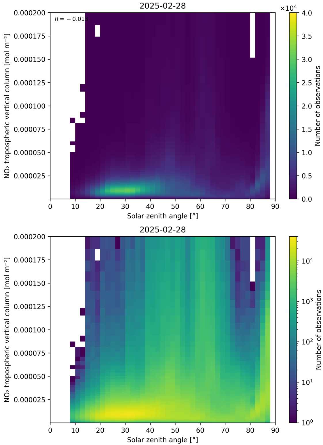
Figure 155: Scatter density plot of “Solar zenith angle” against “NO 2 tropospheric vertical column” for 2025-02-27 to 2025-03-01.
