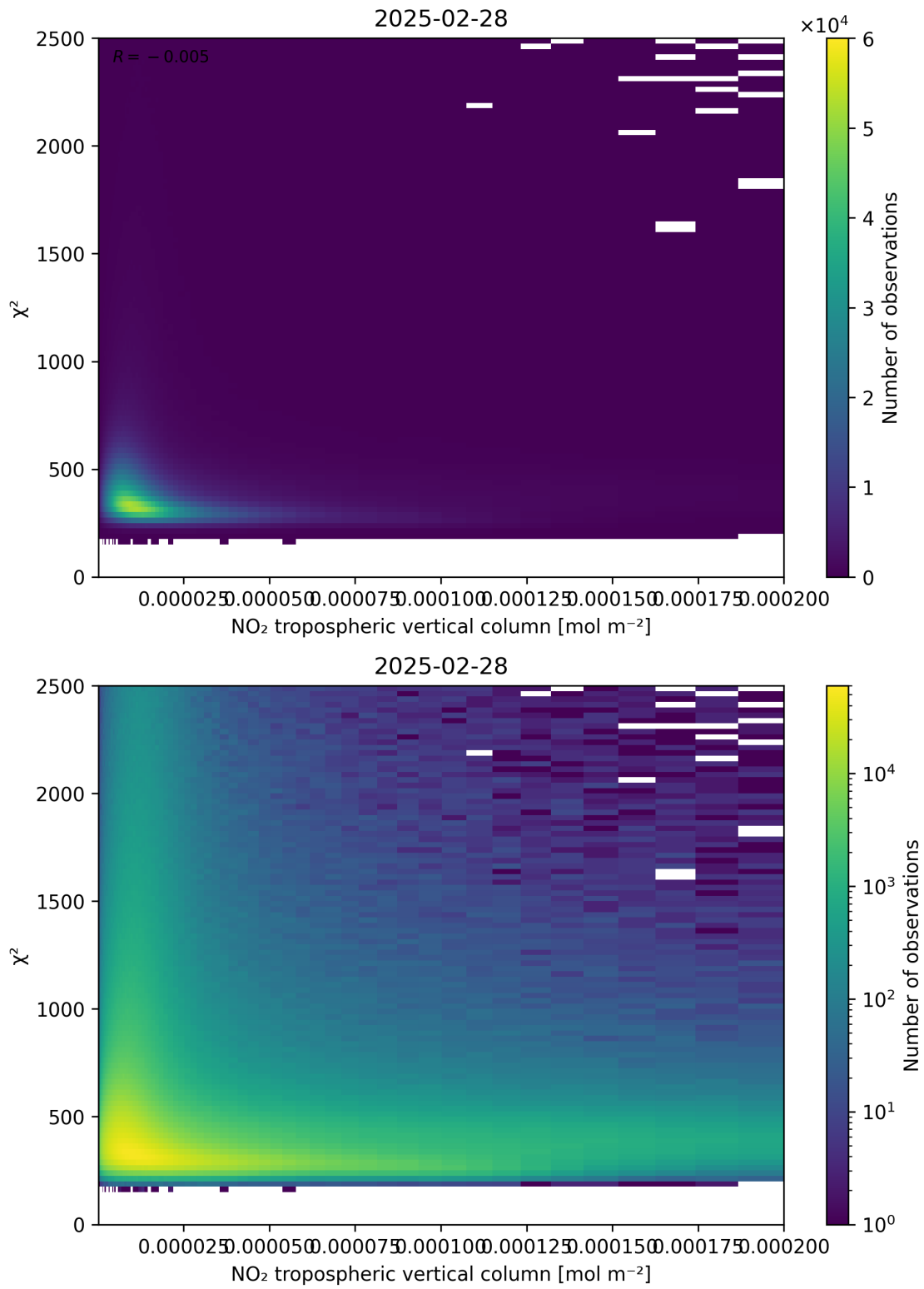
Figure 124: Scatter density plot of “NO 2 tropospheric vertical column” against “ \chi^2 ” for 2025-02-27 to 2025-03-01.
