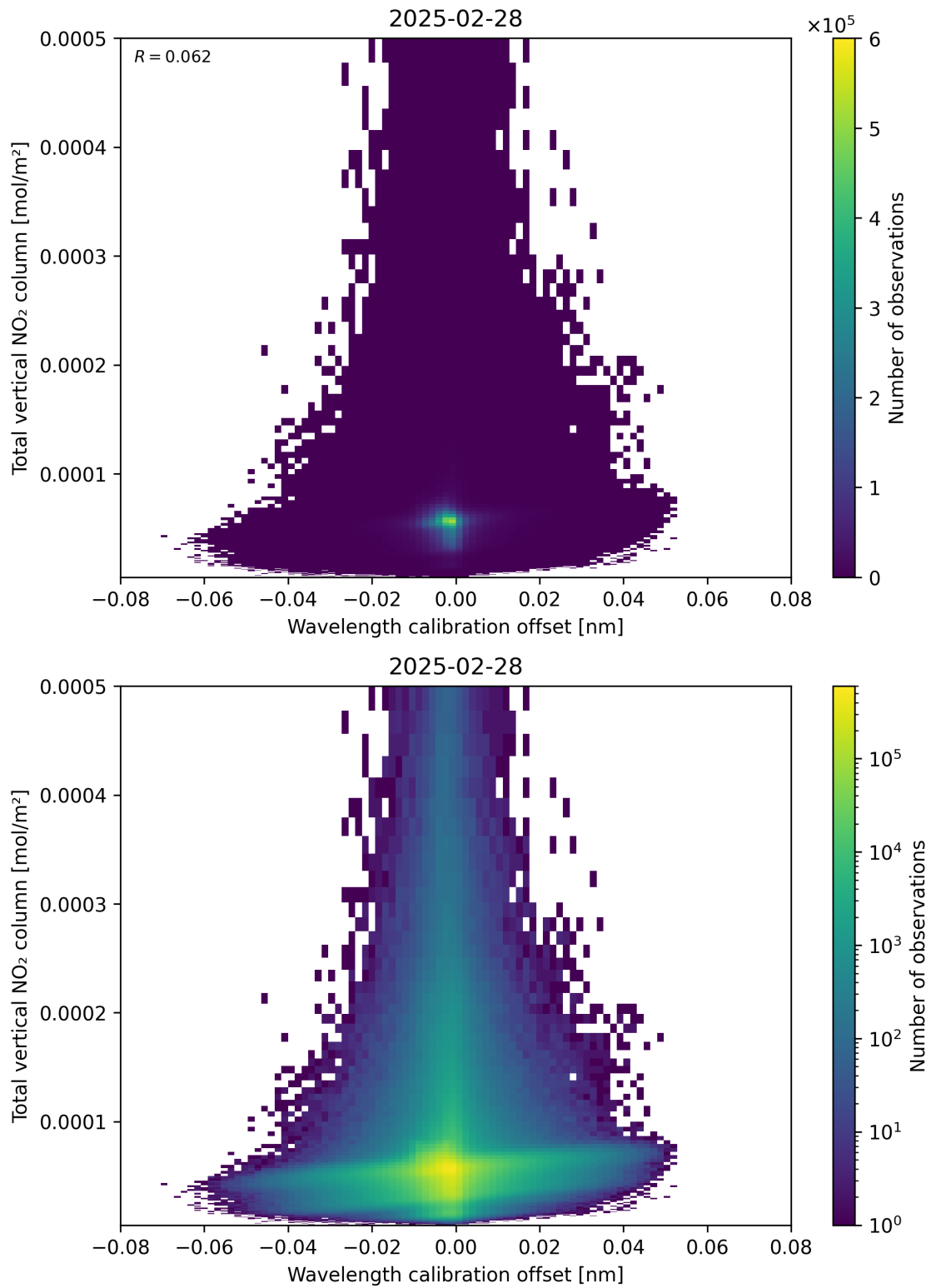
Figure 179: Scatter density plot of “Wavelength calibration offset” against “Total vertical NO 2 column” for 2025-02-27 to 2025-03-01.
