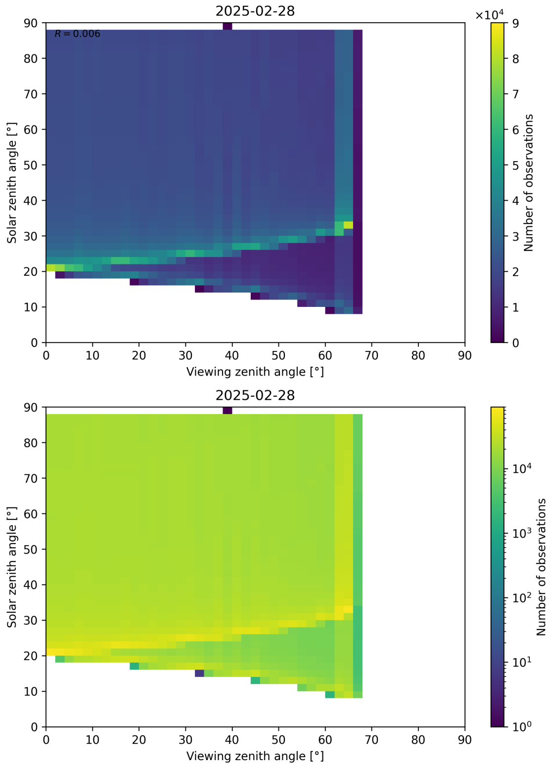
Figure 172: Scatter density plot of “Viewing zenith angle” against “Solar zenith angle” for 2025-02-27 to 2025-03-01.
