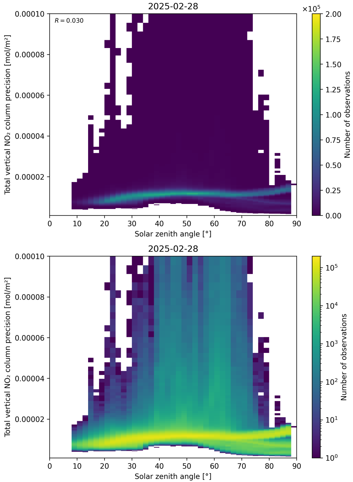
Figure 154: Scatter density plot of “Solar zenith angle” against “Total vertical NO 2 column precision” for 2025-02-27 to 2025-03-01.
