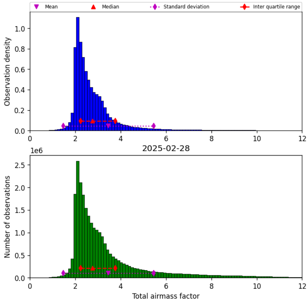
Figure 32: Histogram of “Total airmass factor” for 2025-02-27 to 2025-03-01
