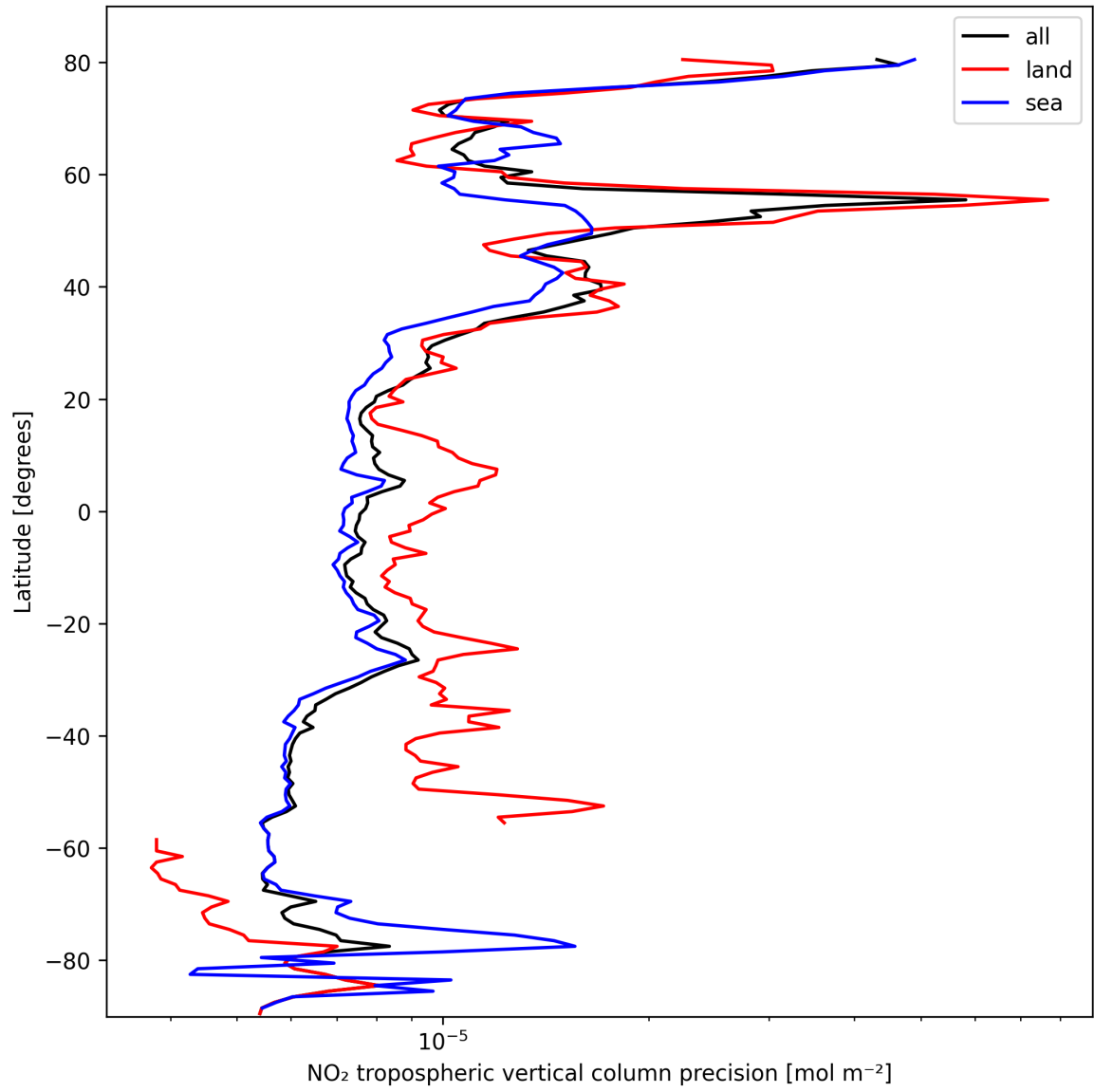
Figure 13: Zonal average of “NO 2 tropospheric vertical column precision” for 2025-02-27 to 2025-03-01.
