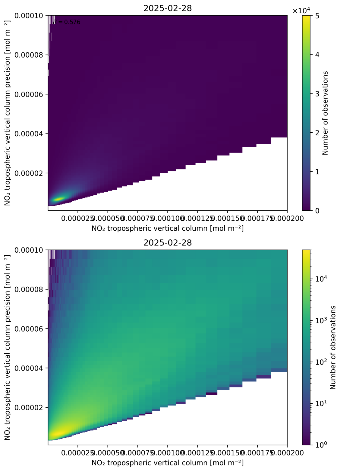
Figure 130: Scatter density plot of “NO 2 tropospheric vertical column” against “NO 2 tropospheric vertical column precision” for 2025-02-27 to 2025-03-01.
