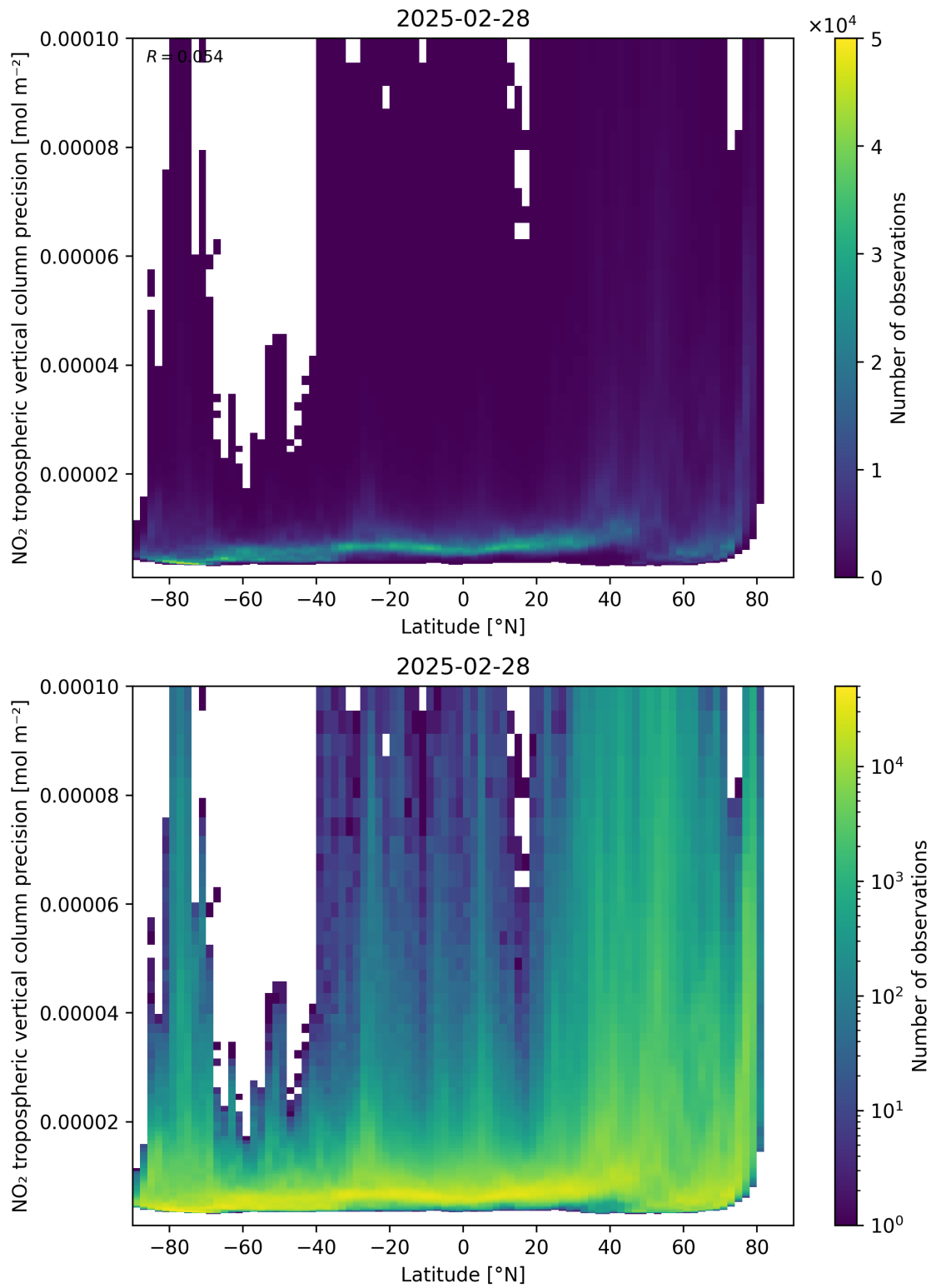
Figure 93: Scatter density plot of “Latitude” against “NO 2 tropospheric vertical column precision” for 2025-02-27 to 2025-03-01.
