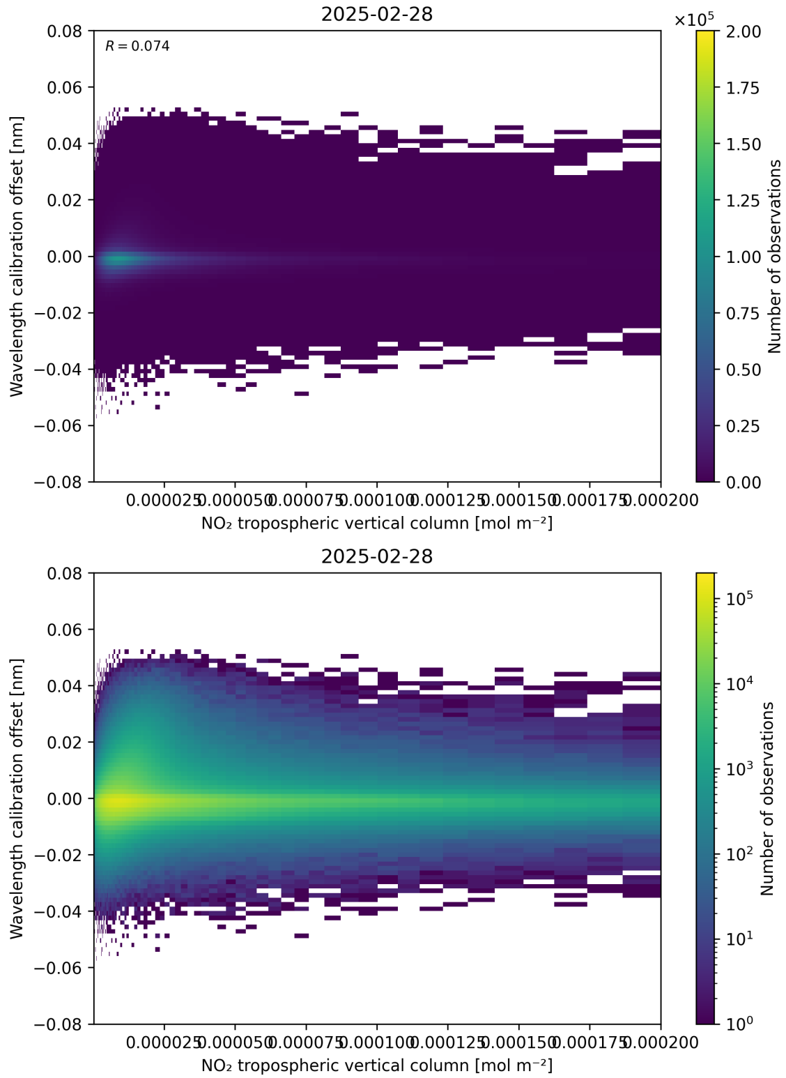
Figure 143: Scatter density plot of “NO 2 tropospheric vertical column” against “Wavelength calibration offset” for 2025-02-27 to 2025-03-01.
