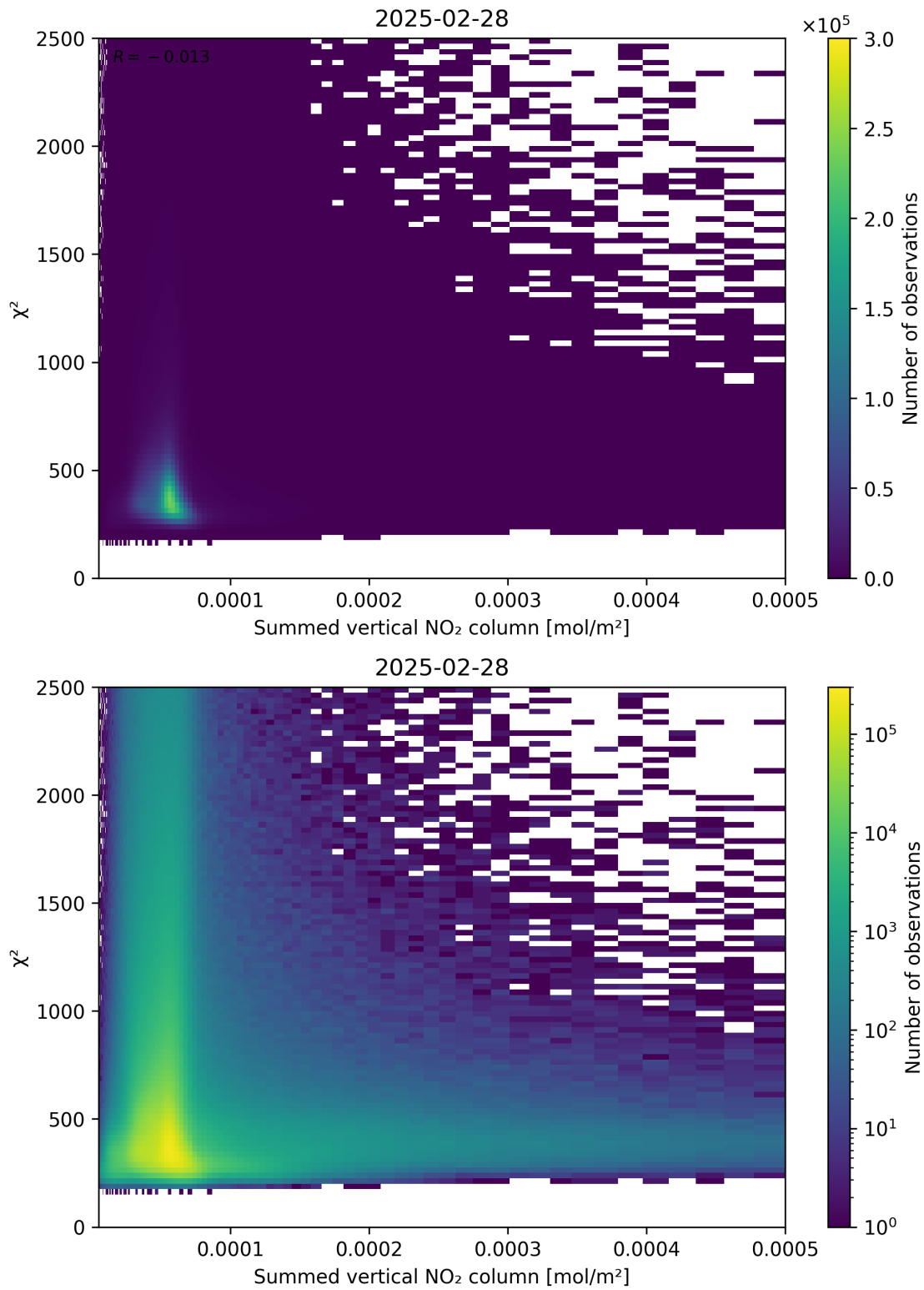
Figure 104: Scatter density plot of “Summed vertical NO 2 column” against “ \chi^2 ” for 2025-02-27 to 2025-03-01.
