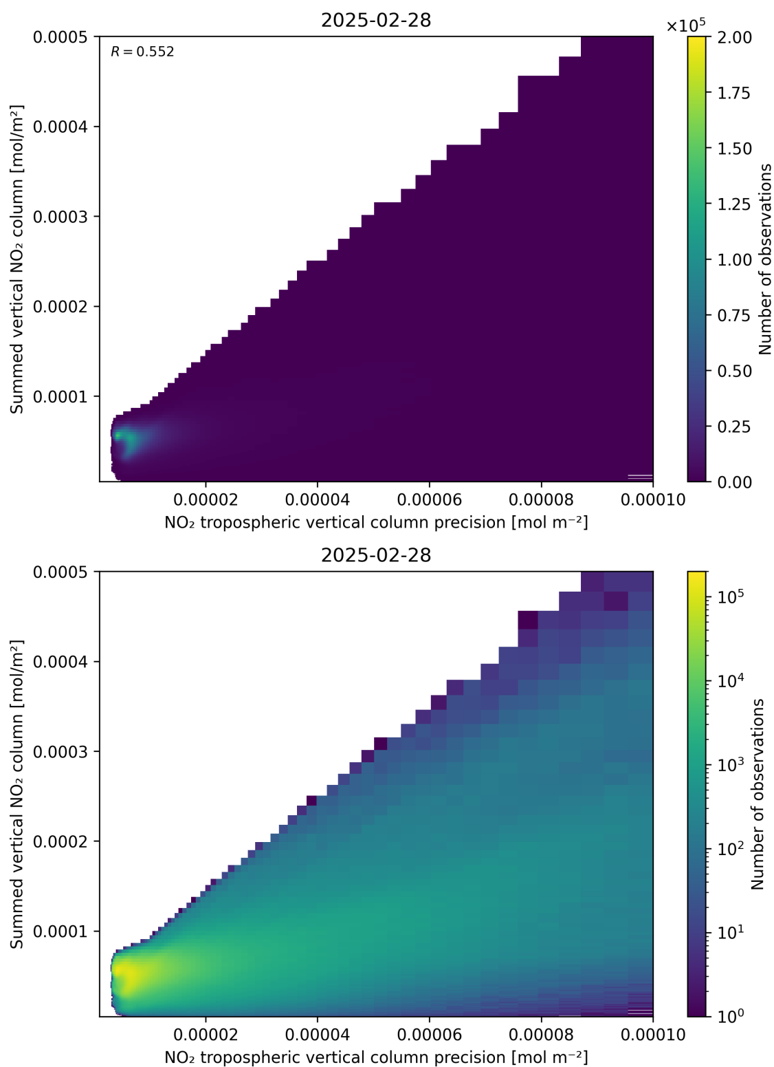
Figure 136: Scatter density plot of “NO 2 tropospheric vertical column precision” against “Summed vertical NO 2 column” for 2025-02-27 to 2025-03-01.
