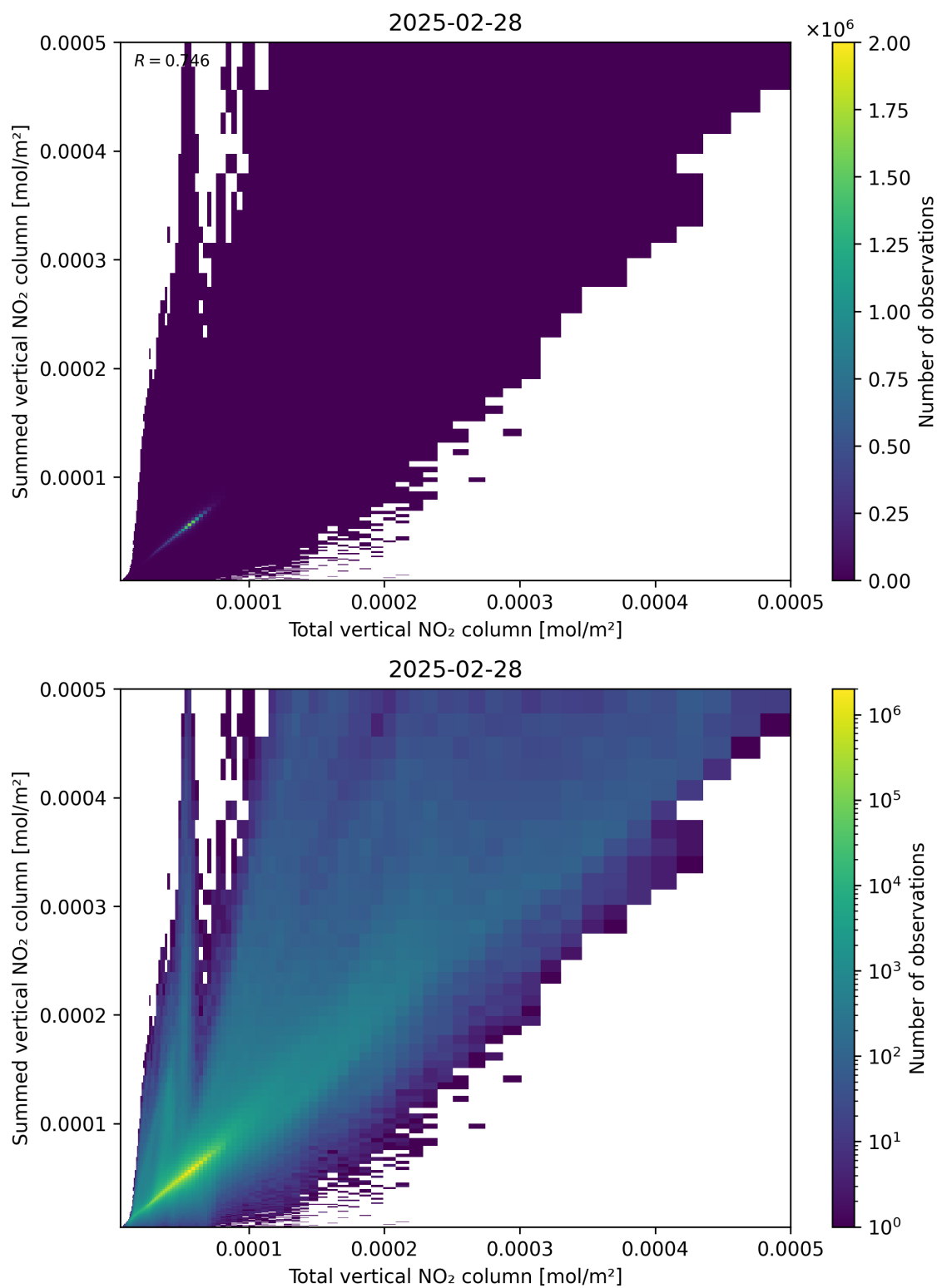
Figure 112: Scatter density plot of “Total vertical NO 2 column” against “Summed vertical NO 2 column” for 2025-02-27 to 2025-03-01.
