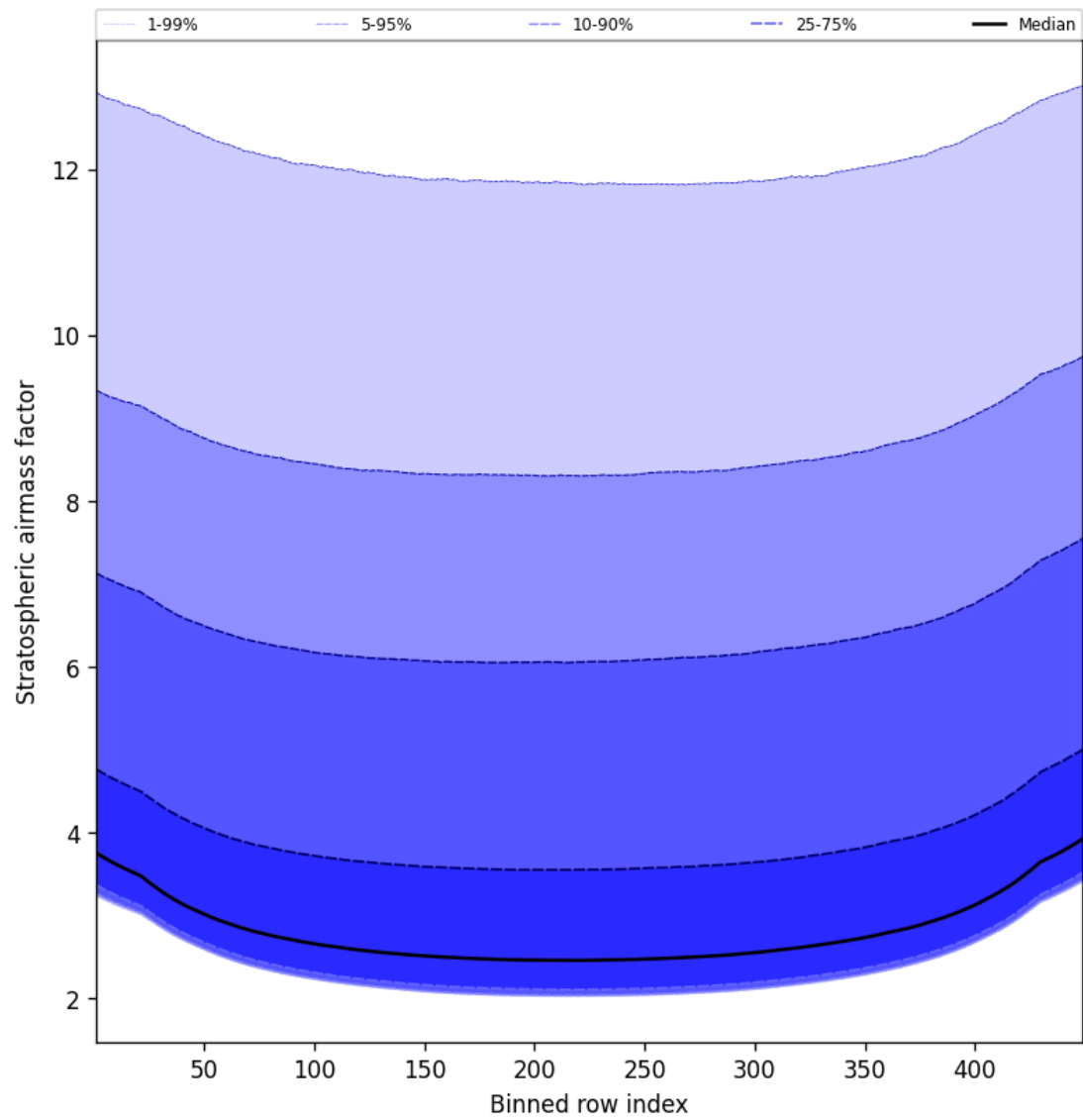
Figure 61: Along track statistics of “Stratospheric airmass factor” for 2025-02-27 to 2025-03-01
