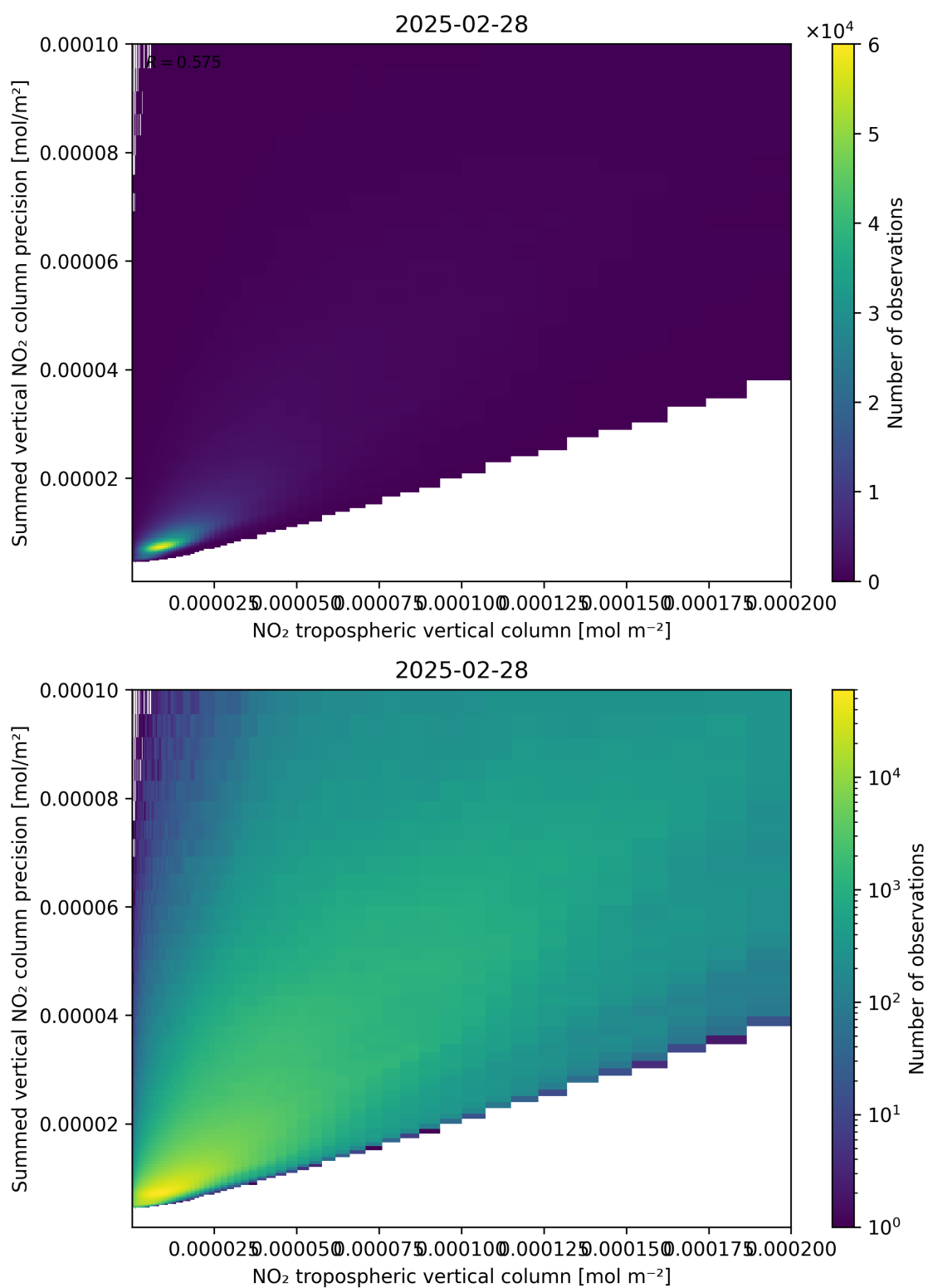
Figure 127: Scatter density plot of “NO 2 tropospheric vertical column” against “Summed vertical NO 2 column precision” for 2025-02-27 to 2025-03-01.
