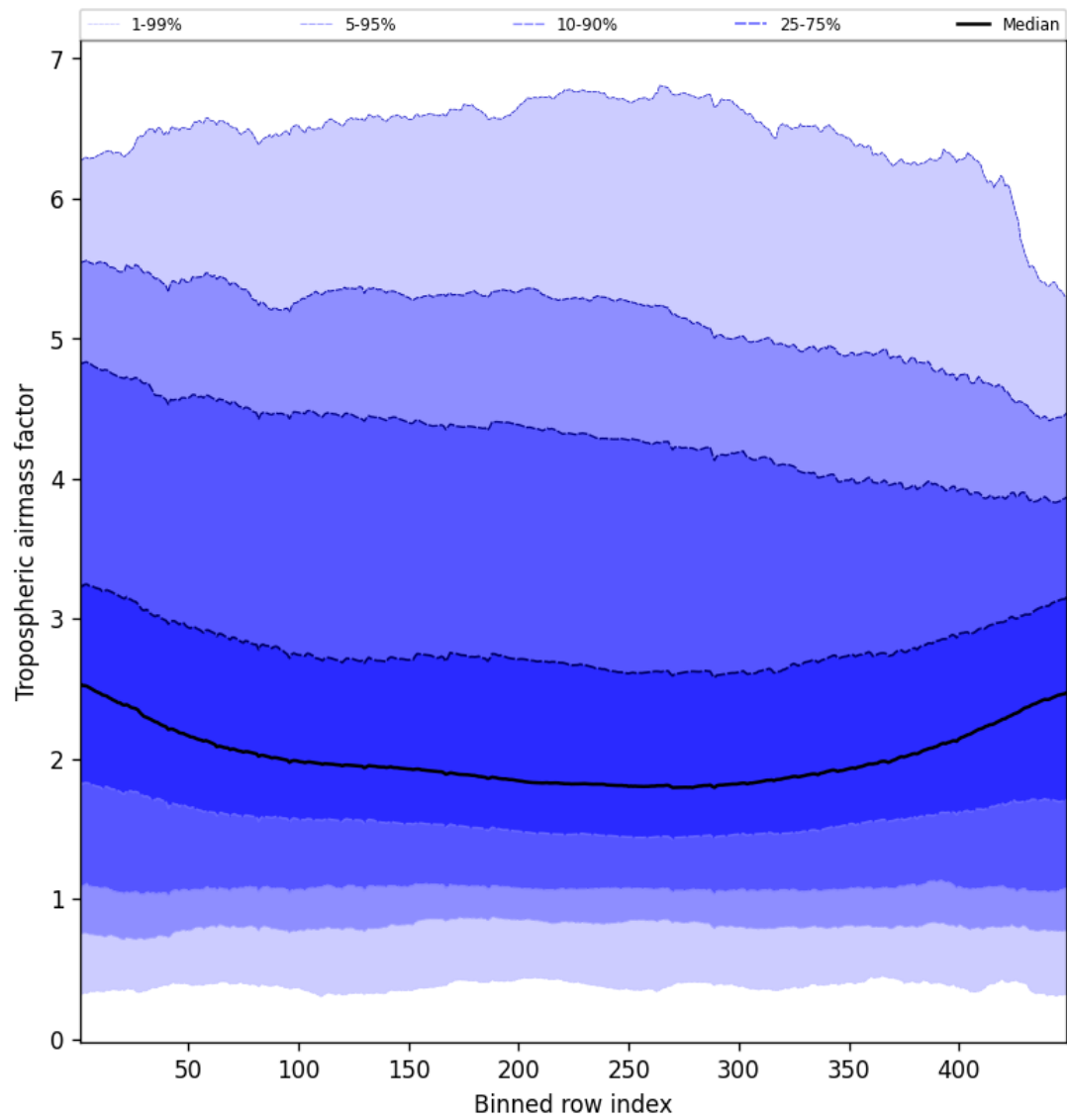
Figure 48: Along track statistics of “Tropospheric airmass factor” for 2025-02-27 to 2025-03-01
