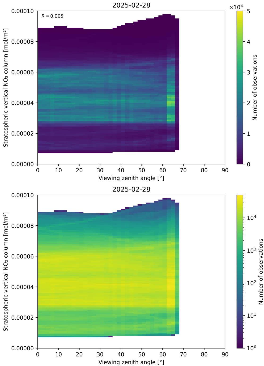
Figure 164: Scatter density plot of “Viewing zenith angle” against “Stratospheric vertical NO 2 column” for 2025-02-27 to 2025-03-01.
