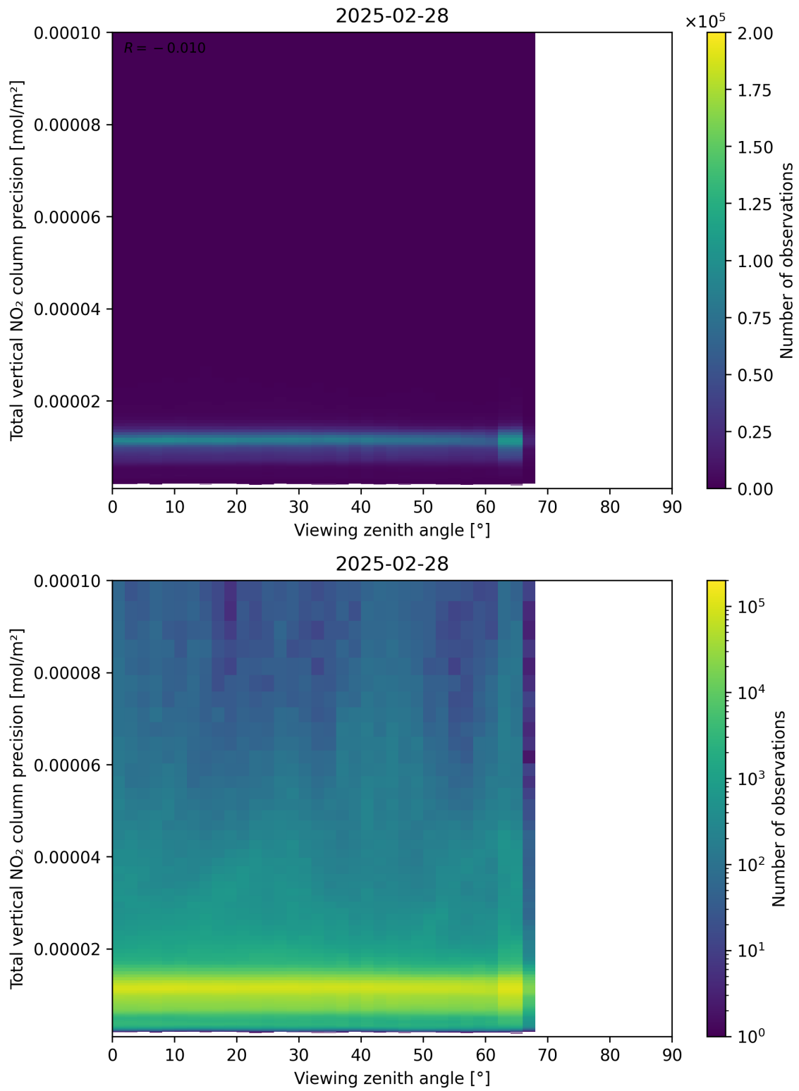
Figure 168: Scatter density plot of “Viewing zenith angle” against “Total vertical NO 2 column precision” for 2025-02-27 to 2025-03-01.
