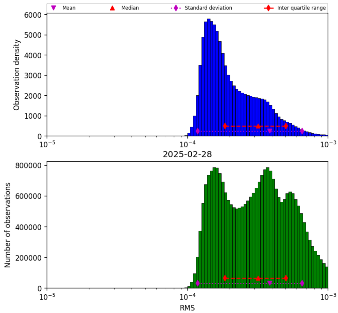
Figure 43: Histogram of “RMS” for 2025-02-27 to 2025-03-01
