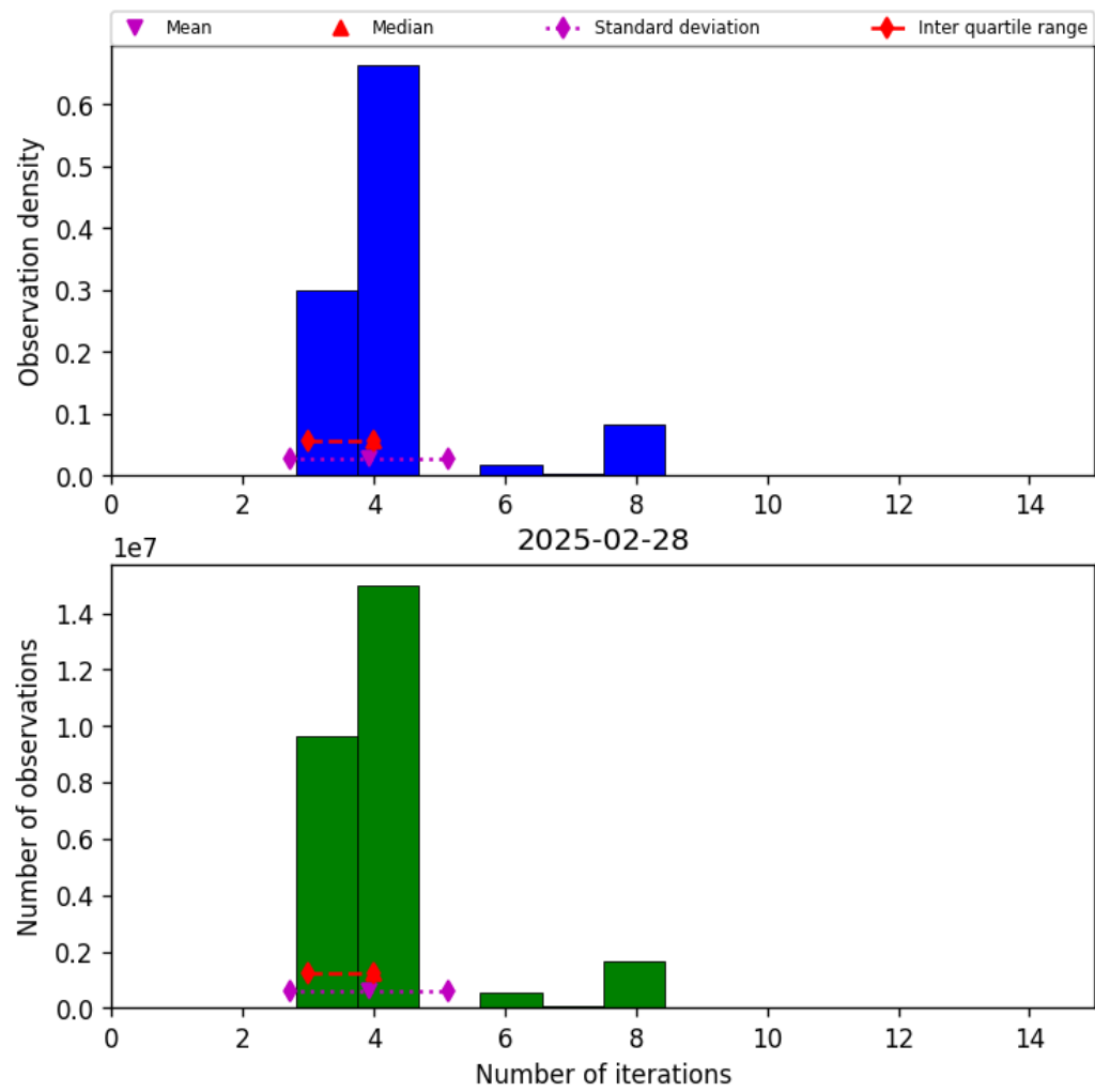
Figure 34: Histogram of “Number of iterations” for 2025-02-27 to 2025-03-01
