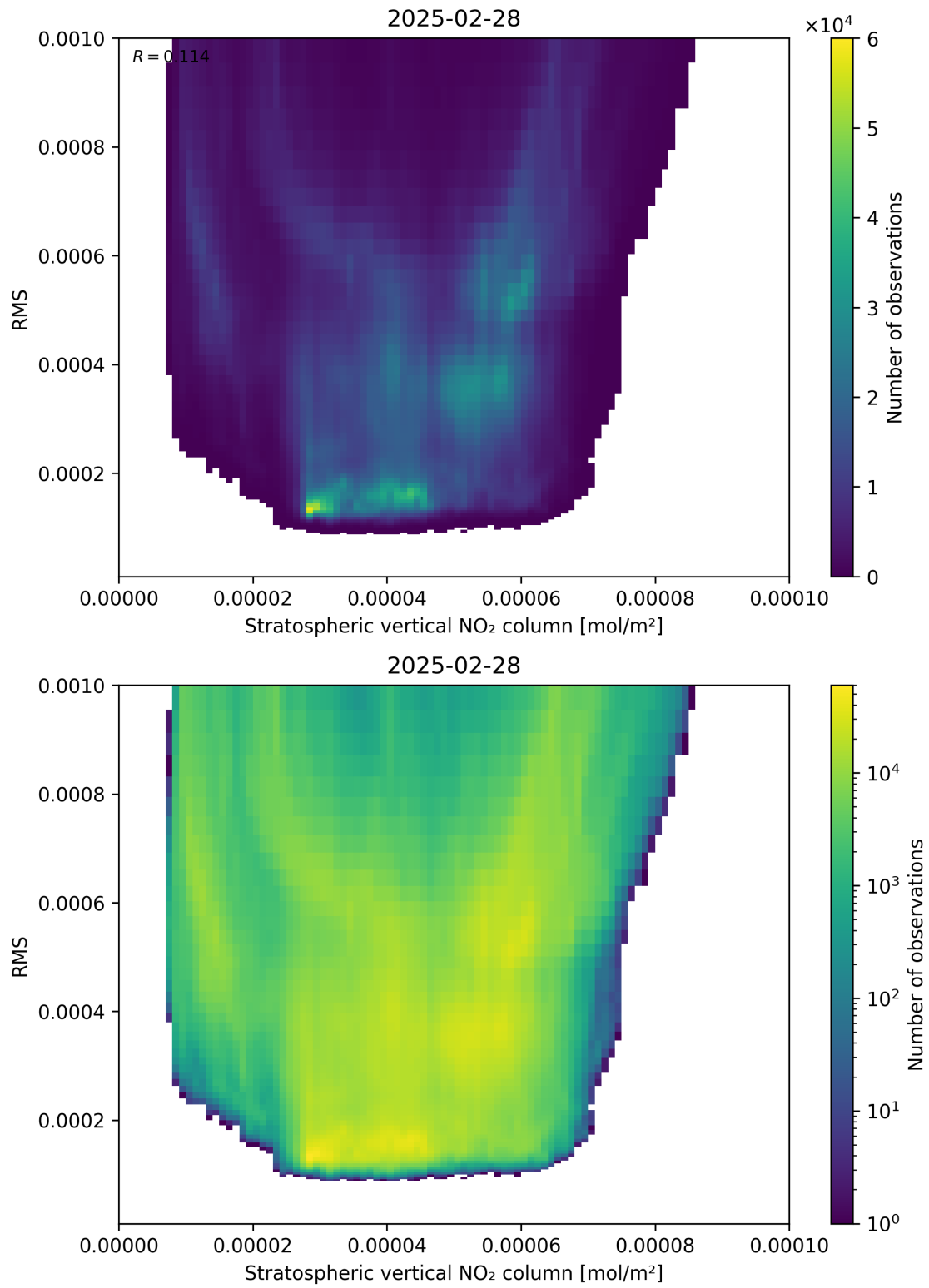
Figure 102: Scatter density plot of “Stratospheric vertical NO 2 column” against “RMS” for 2025-02-27 to 2025-03-01.
