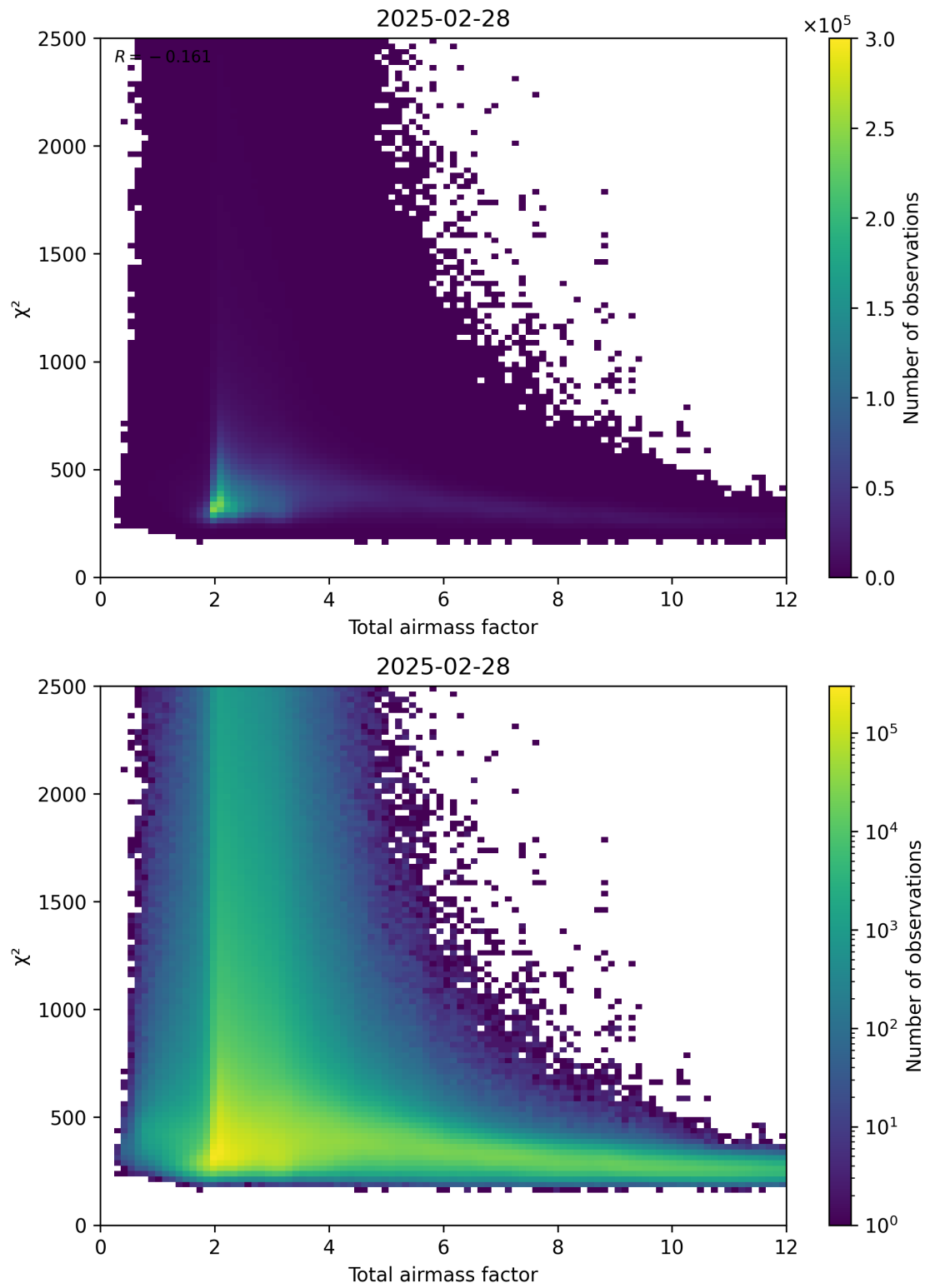
Figure 63: Scatter density plot of “Total airmass factor” against “ \chi^2 ” for 2025-02-27 to 2025-03-01.
