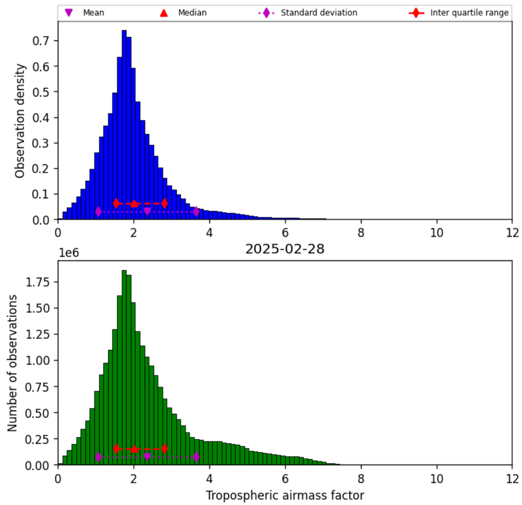
Figure 31: Histogram of “Tropospheric airmass factor” for 2025-02-27 to 2025-03-01
