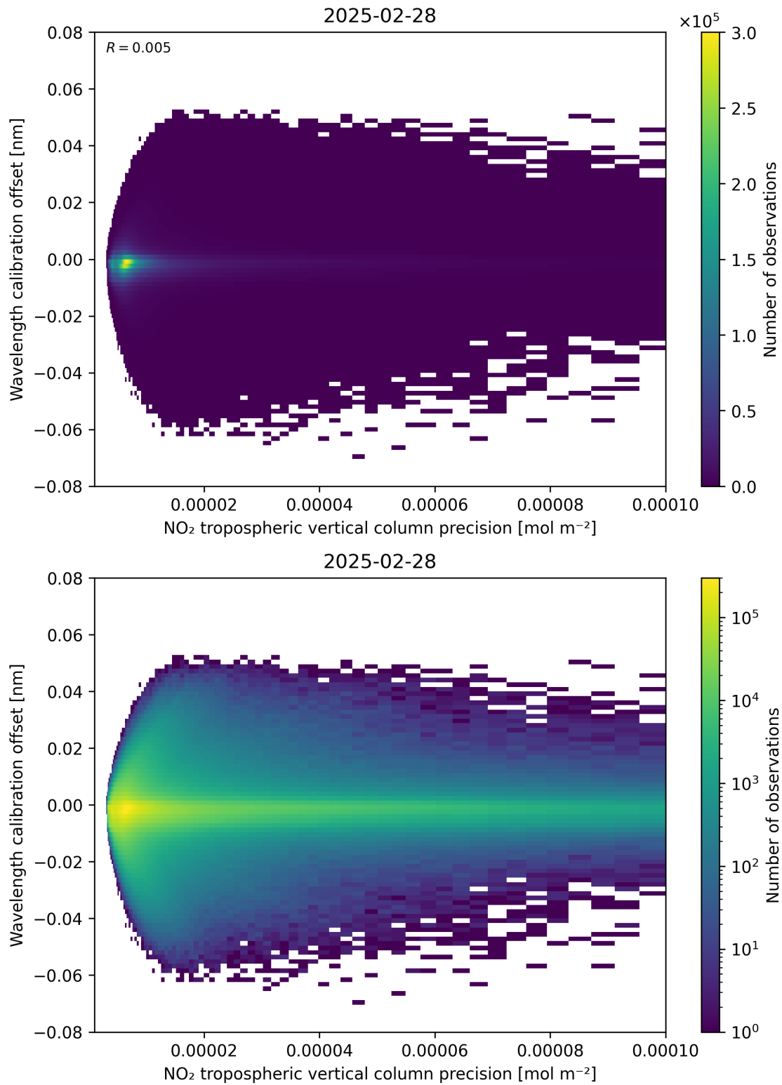
Figure 141: Scatter density plot of “NO 2 tropospheric vertical column precision” against “Wavelength calibration offset” for 2025-02-27 to 2025-03-01.
