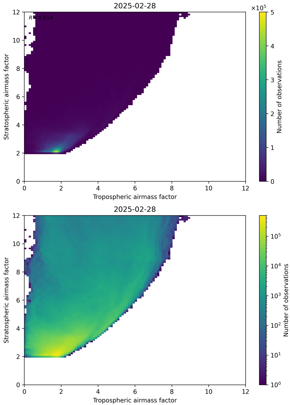
Figure 71: Scatter density plot of “Tropospheric airmass factor” against “Stratospheric airmass factor” for 2025-02-27 to 2025-03-01.
