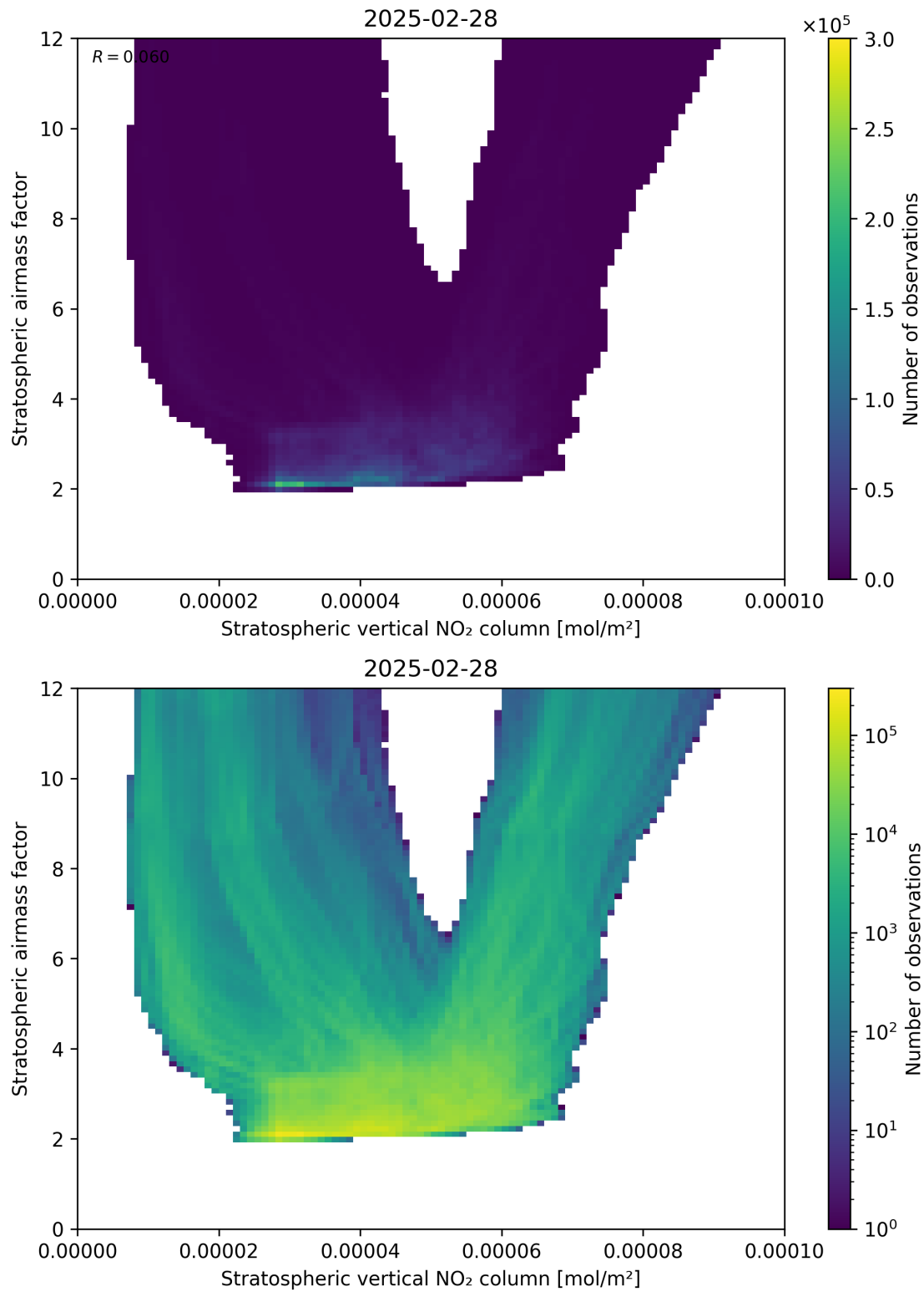
Figure 96: Scatter density plot of “Stratospheric vertical NO 2 column” against “Stratospheric airmass factor” for 2025-02-27 to 2025-03-01.
