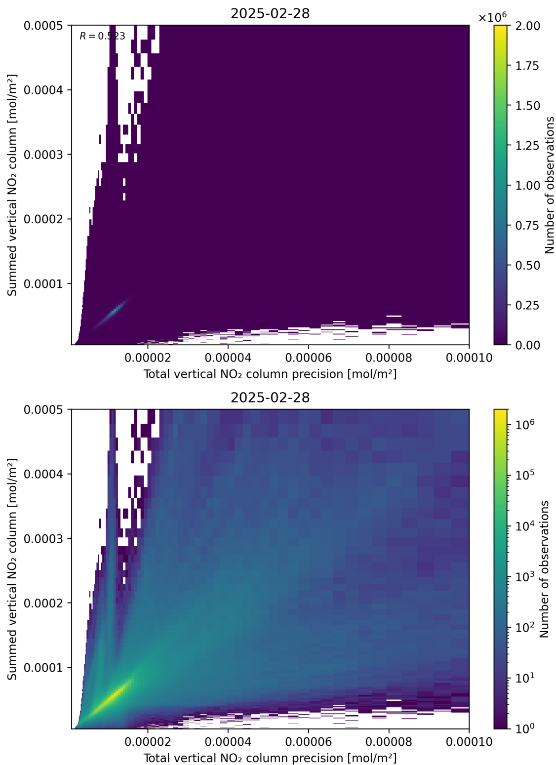
Figure 117: Scatter density plot of “Total vertical NO 2 column precision” against “Summed vertical NO 2 column” for 2025-02-27 to 2025-03-01.
