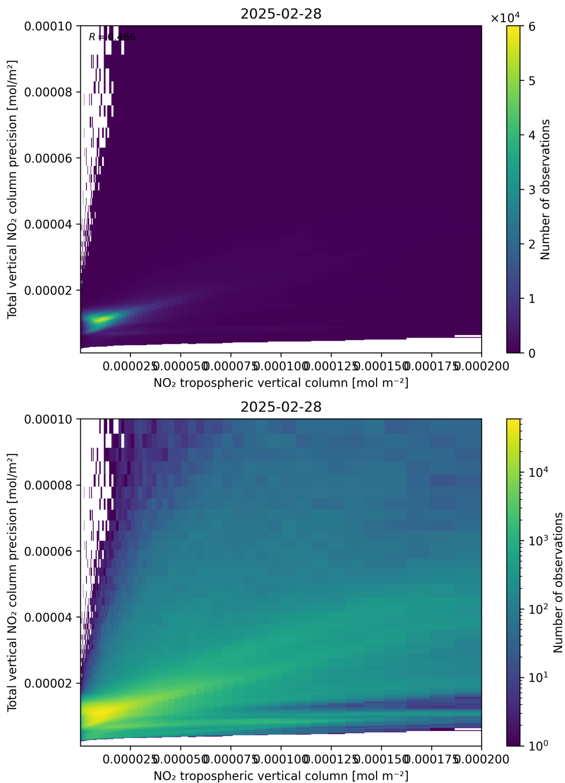
Figure 129: Scatter density plot of “NO 2 tropospheric vertical column” against “Total vertical NO 2 column precision” for 2025-02-27 to 2025-03-01.
