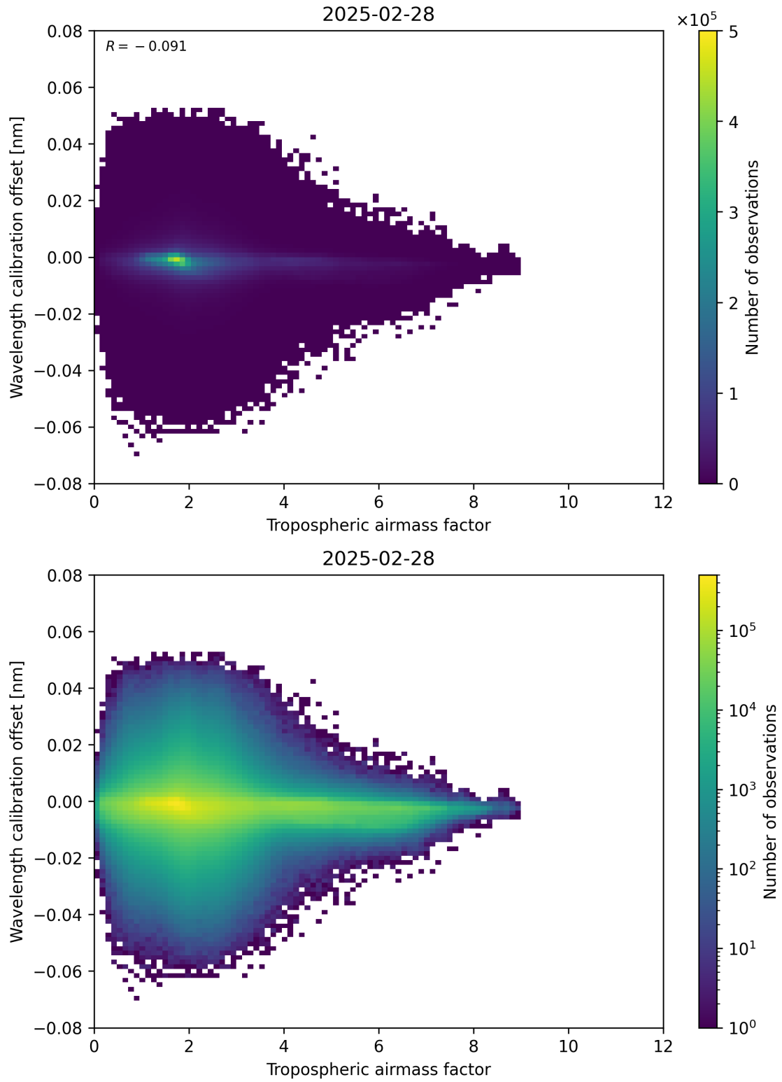
Figure 80: Scatter density plot of “Tropospheric airmass factor” against “Wavelength calibration offset” for 2025-02-27 to 2025-03-01.
