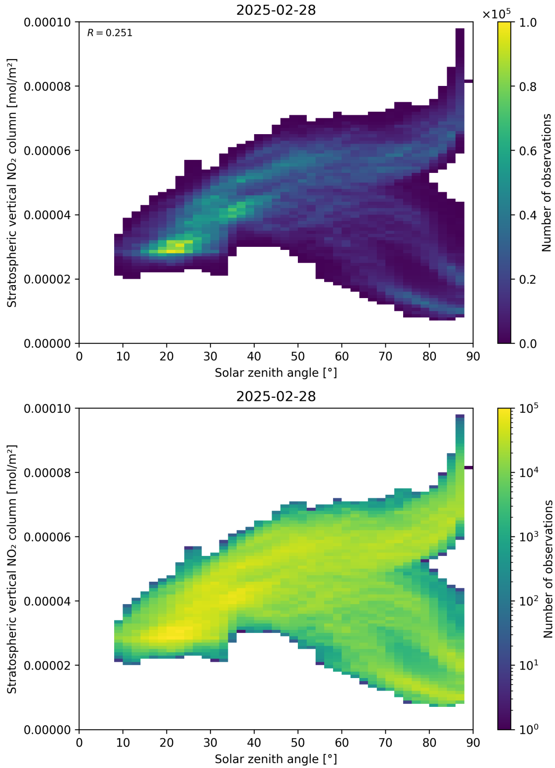
Figure 150: Scatter density plot of “Solar zenith angle” against “Stratospheric vertical NO 2 column” for 2025-02-27 to 2025-03-01.
