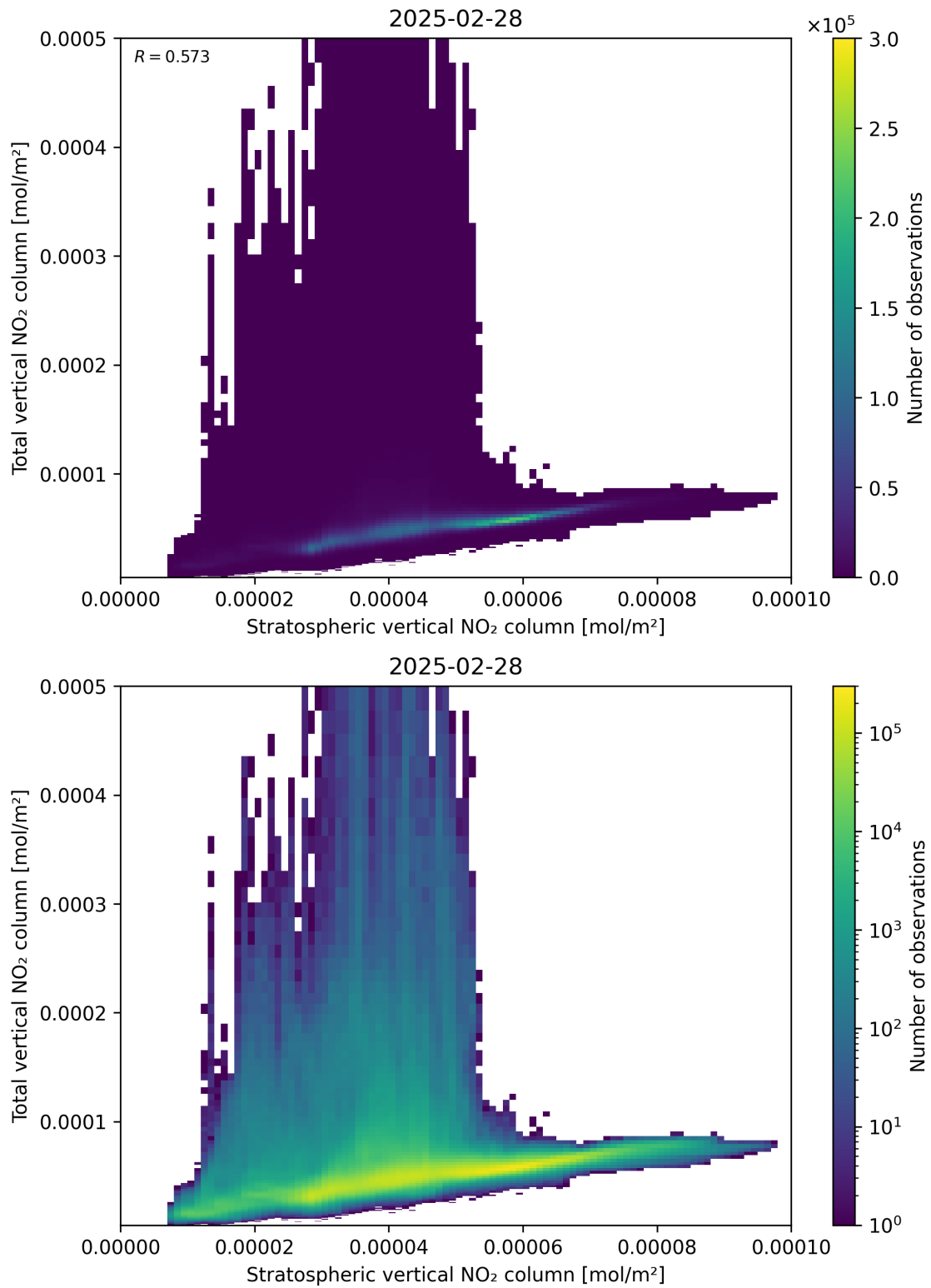
Figure 100: Scatter density plot of “Stratospheric vertical NO 2 column” against “Total vertical NO 2 column” for 2025-02-27 to 2025-03-01.
