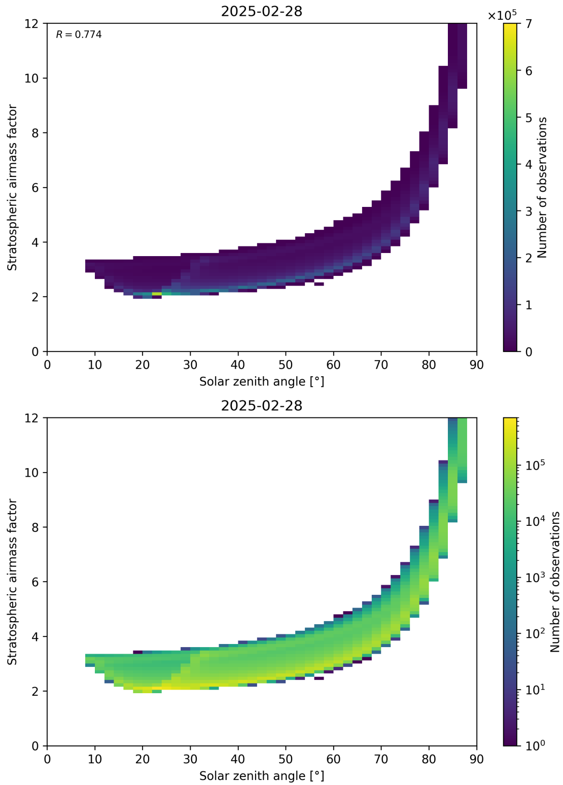
Figure 145: Scatter density plot of “Solar zenith angle” against “Stratospheric airmass factor” for 2025-02-27 to 2025-03-01.
