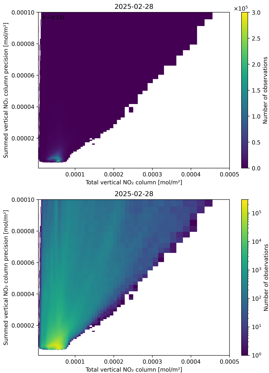
Figure 113: Scatter density plot of “Total vertical NO 2 column” against “Summed vertical NO 2 column precision” for 2025-02-27 to 2025-03-01.
