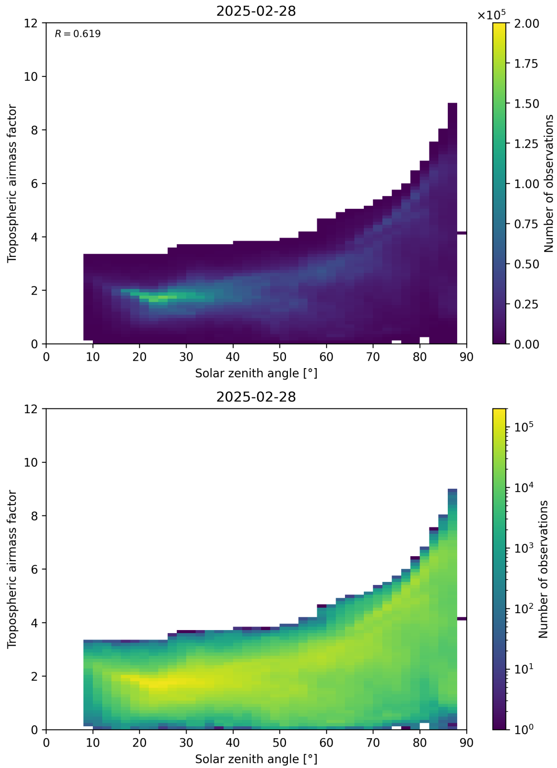
Figure 147: Scatter density plot of “Solar zenith angle” against “Tropospheric airmass factor” for 2025-02-27 to 2025-03-01.
