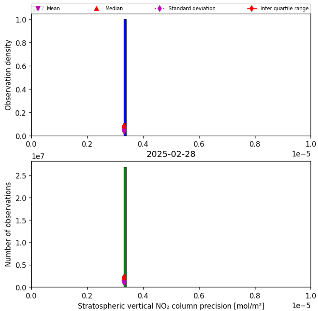
Figure 37: Histogram of “Stratospheric vertical NO 2 column precision” for 2025-02-27 to 2025-03-01
