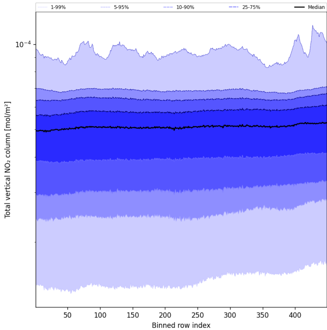
Figure 55: Along track statistics of “Total vertical NO 2 column” for 2025-02-27 to 2025-03-01
