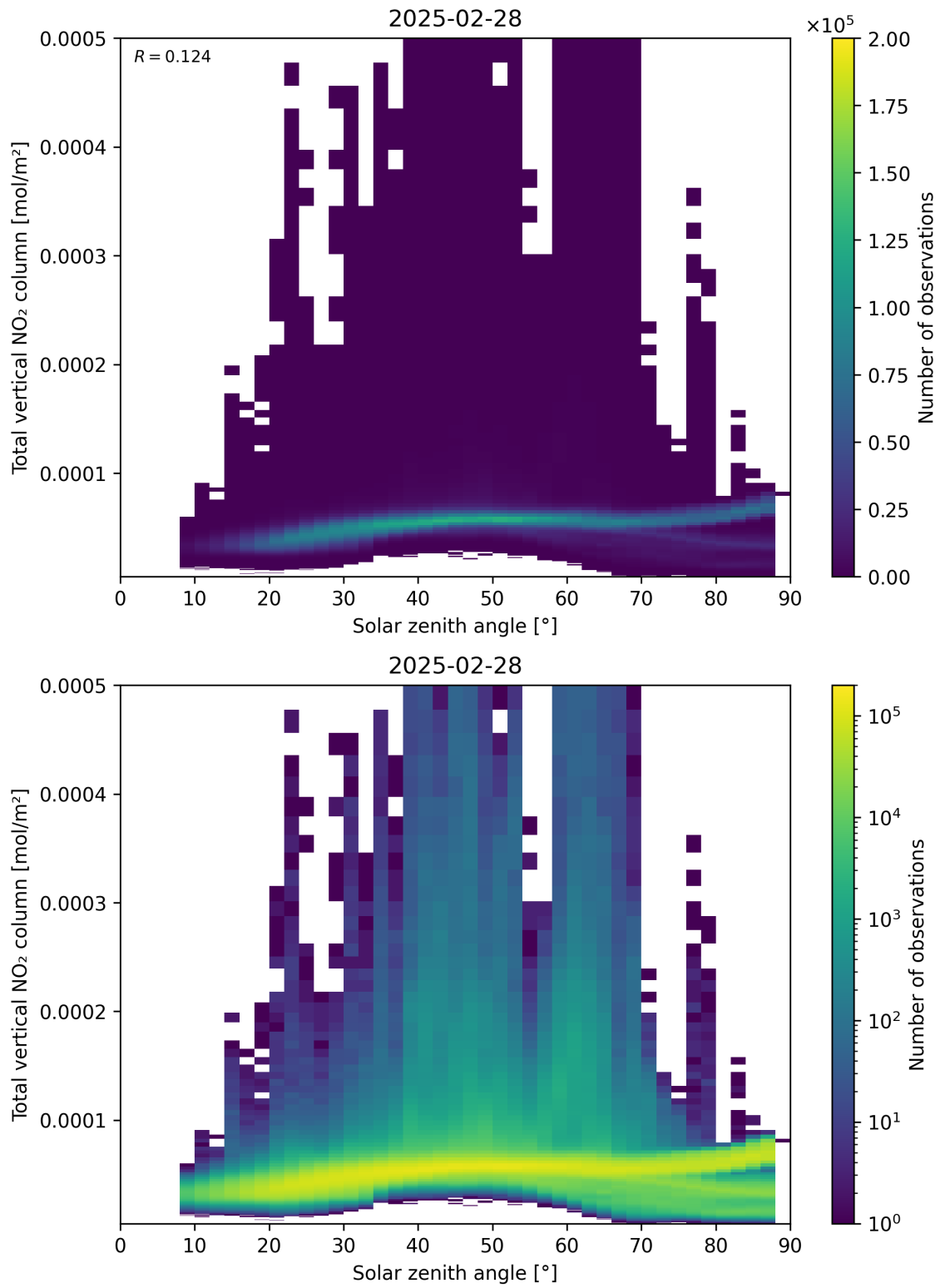
Figure 153: Scatter density plot of “Solar zenith angle” against “Total vertical NO 2 column” for 2025-02-27 to 2025-03-01.
