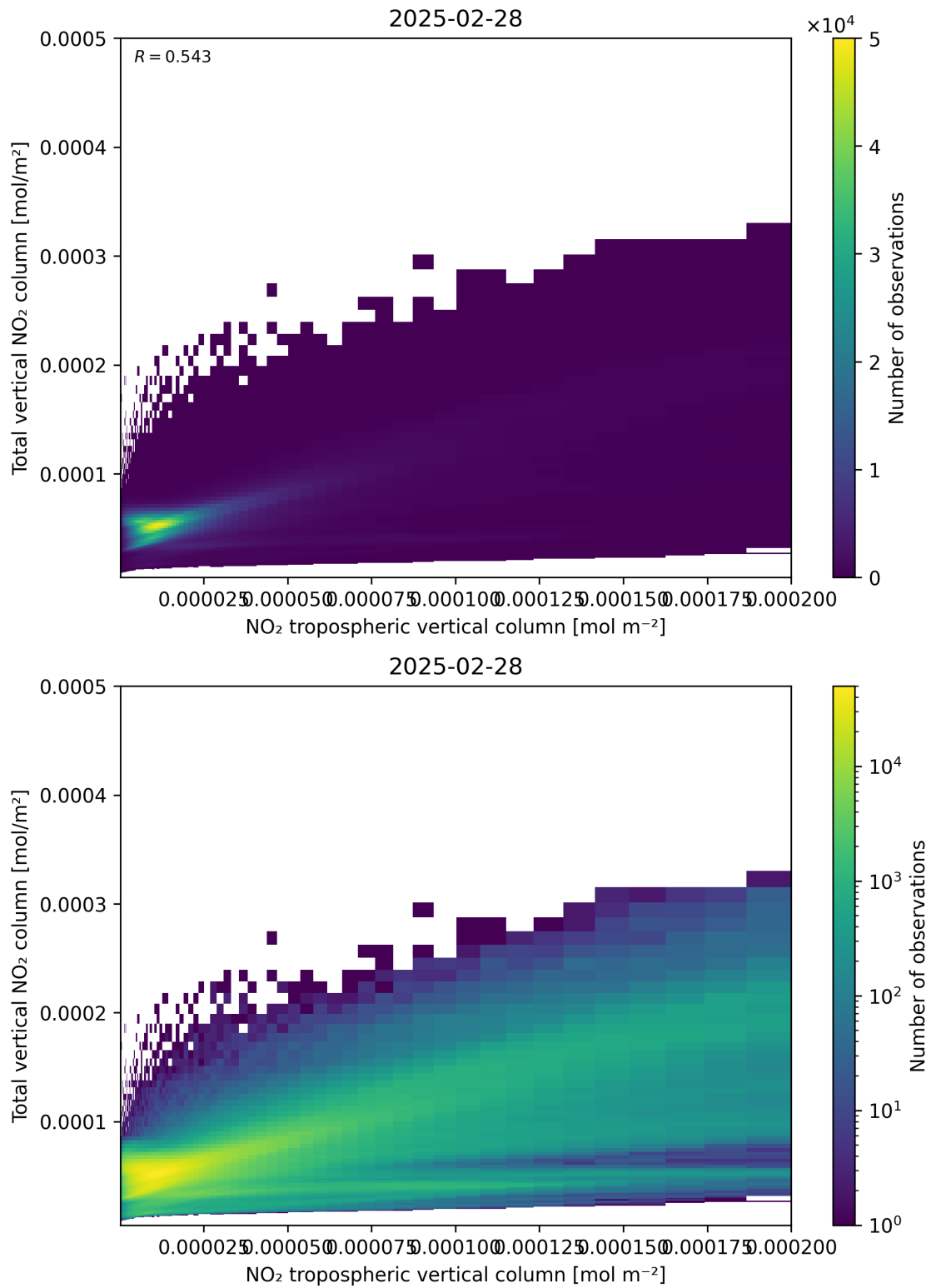
Figure 128: Scatter density plot of “NO 2 tropospheric vertical column” against “Total vertical NO 2 column” for 2025-02-27 to 2025-03-01.
