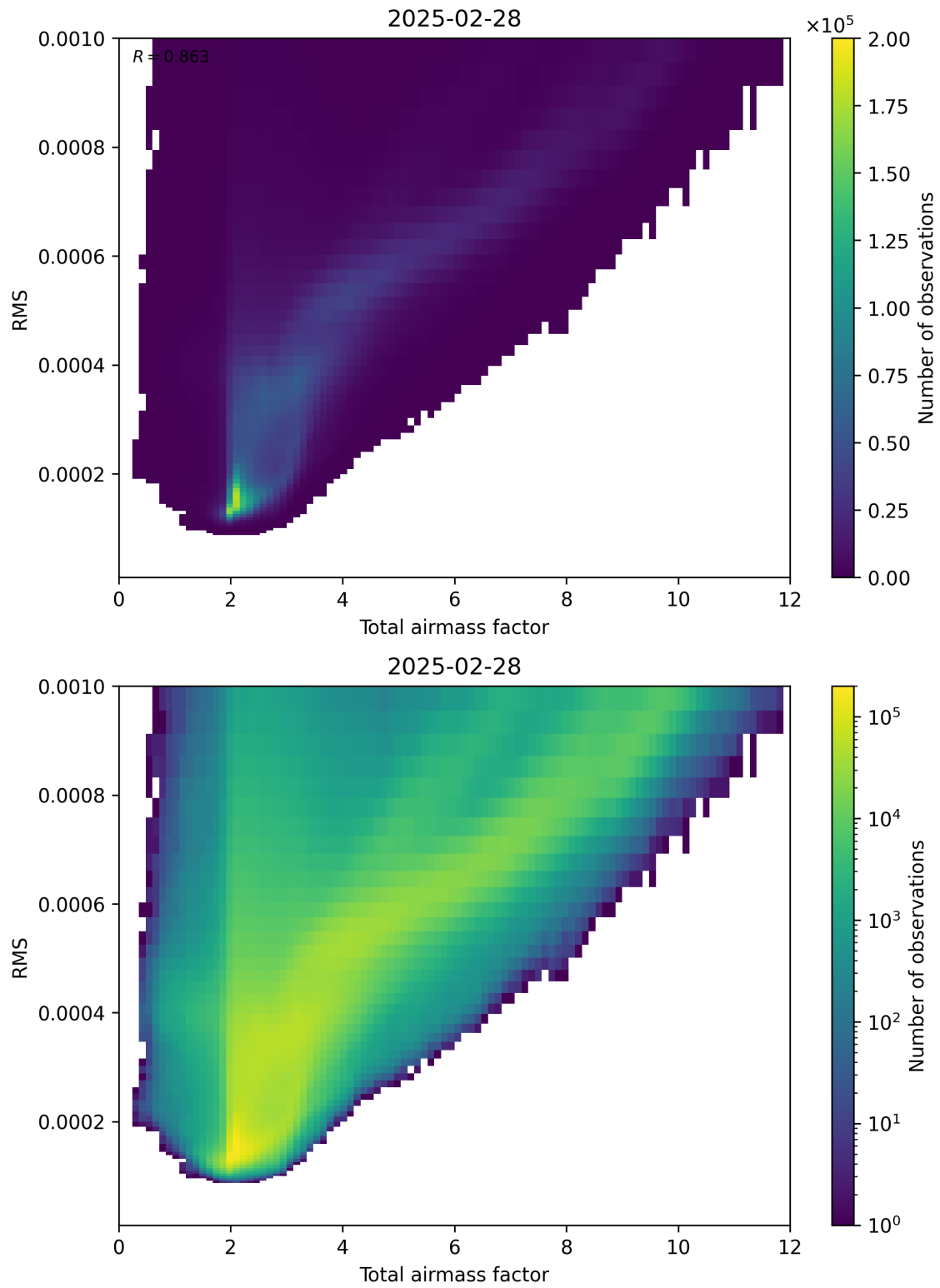
Figure 69: Scatter density plot of “Total airmass factor” against “RMS” for 2025-02-27 to 2025-03-01.
