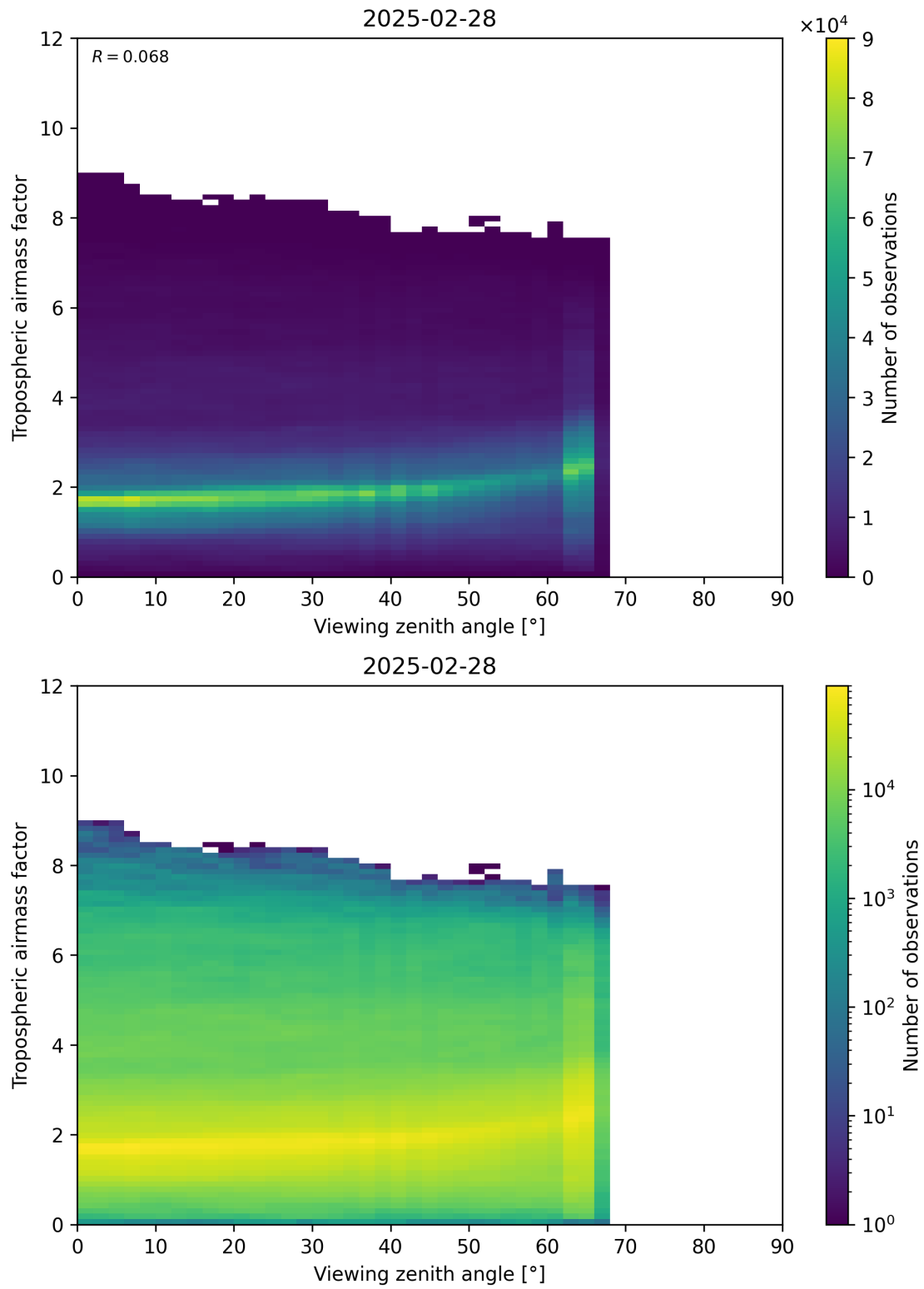
Figure 161: Scatter density plot of “Viewing zenith angle” against “Tropospheric airmass factor” for 2025-02-27 to 2025-03-01.
