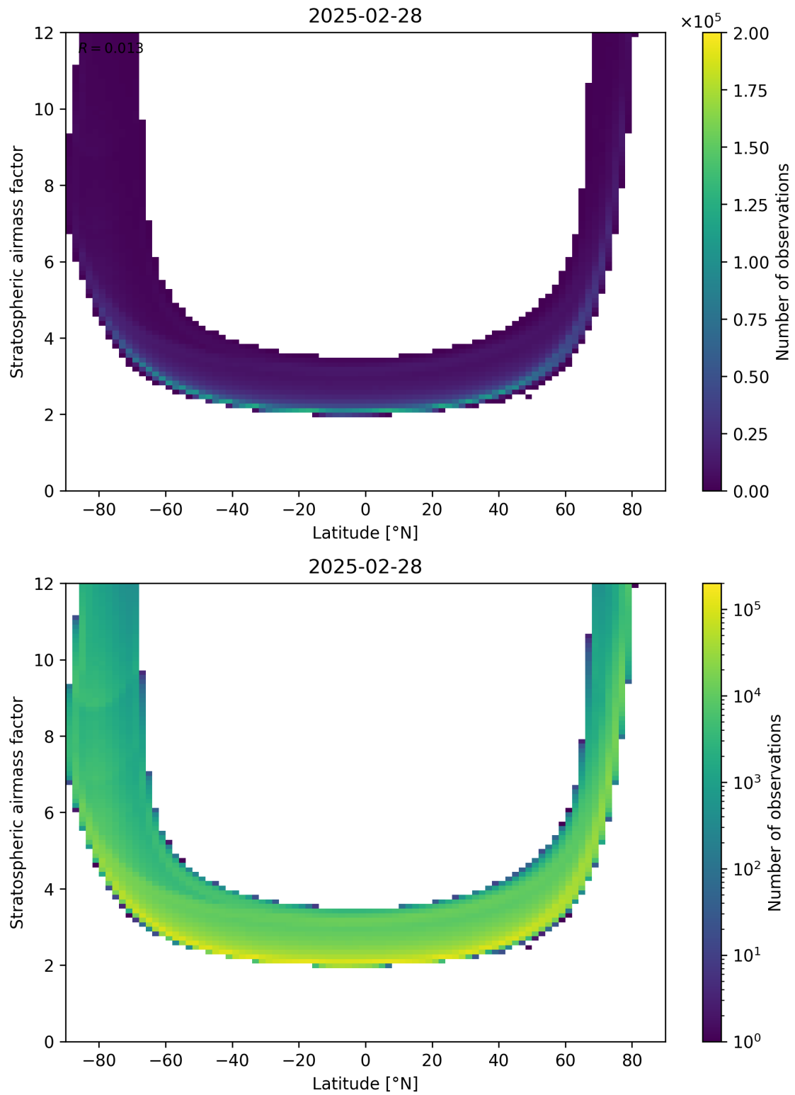
Figure 83: Scatter density plot of “Latitude” against “Stratospheric air mass factor” for 2025-02-27 to 2025-03-01.
