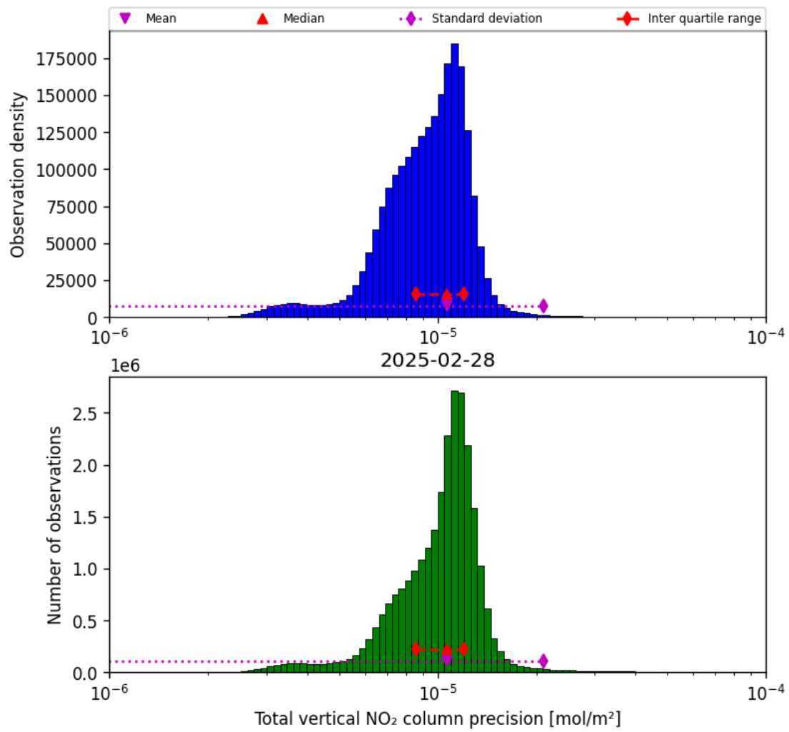
Figure 39: Histogram of “Total vertical NO 2 column precision” for 2025-02-27 to 2025-03-01
