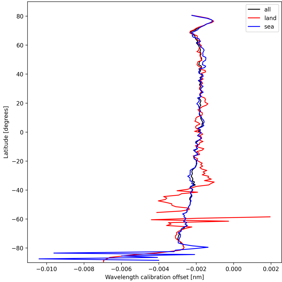
Figure 18: Zonal average of “Wavelength calibration offset” for 2025-02-27 to 2025-03-01.
