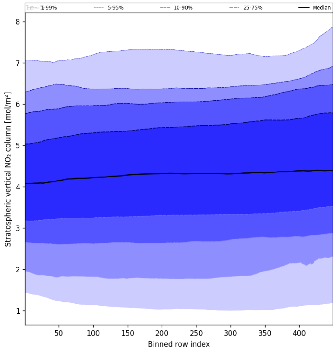
Figure 53: Along track statistics of “Stratospheric vertical NO 2 column” for 2025-02-27 to 2025-03-01
