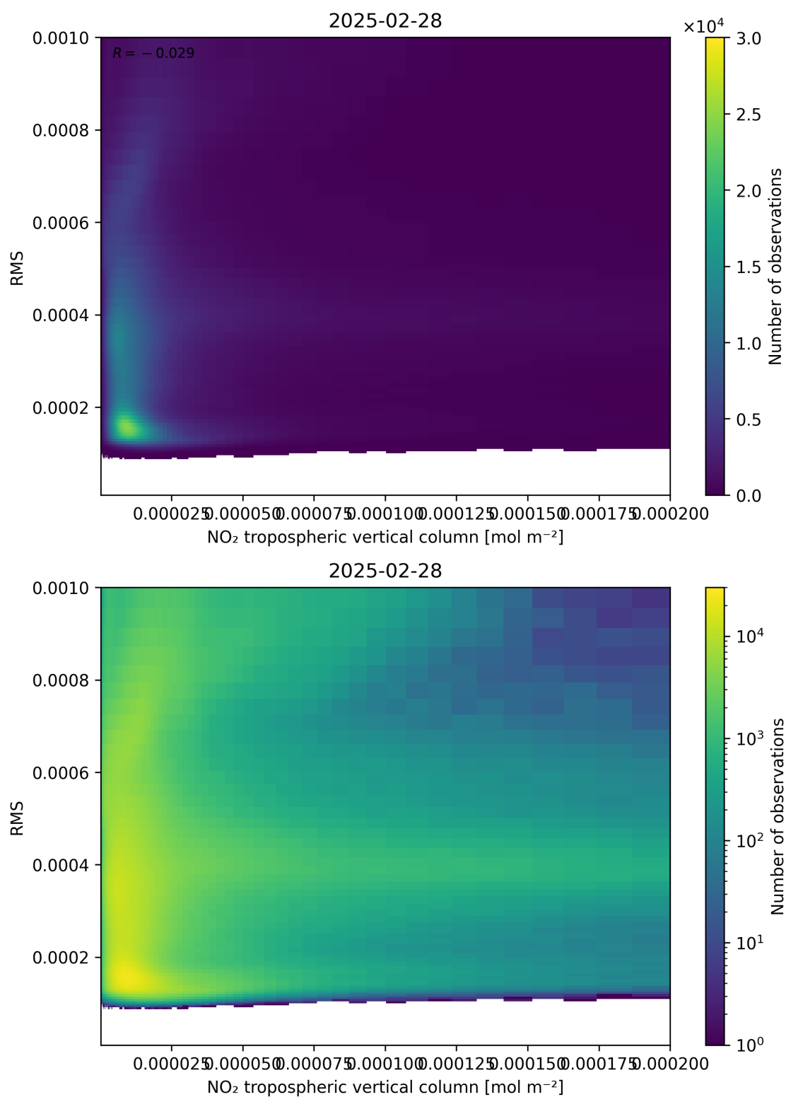
Figure 142: Scatter density plot of “NO 2 tropospheric vertical column” against “RMS” for 2025-02-27 to 2025-03-01.
