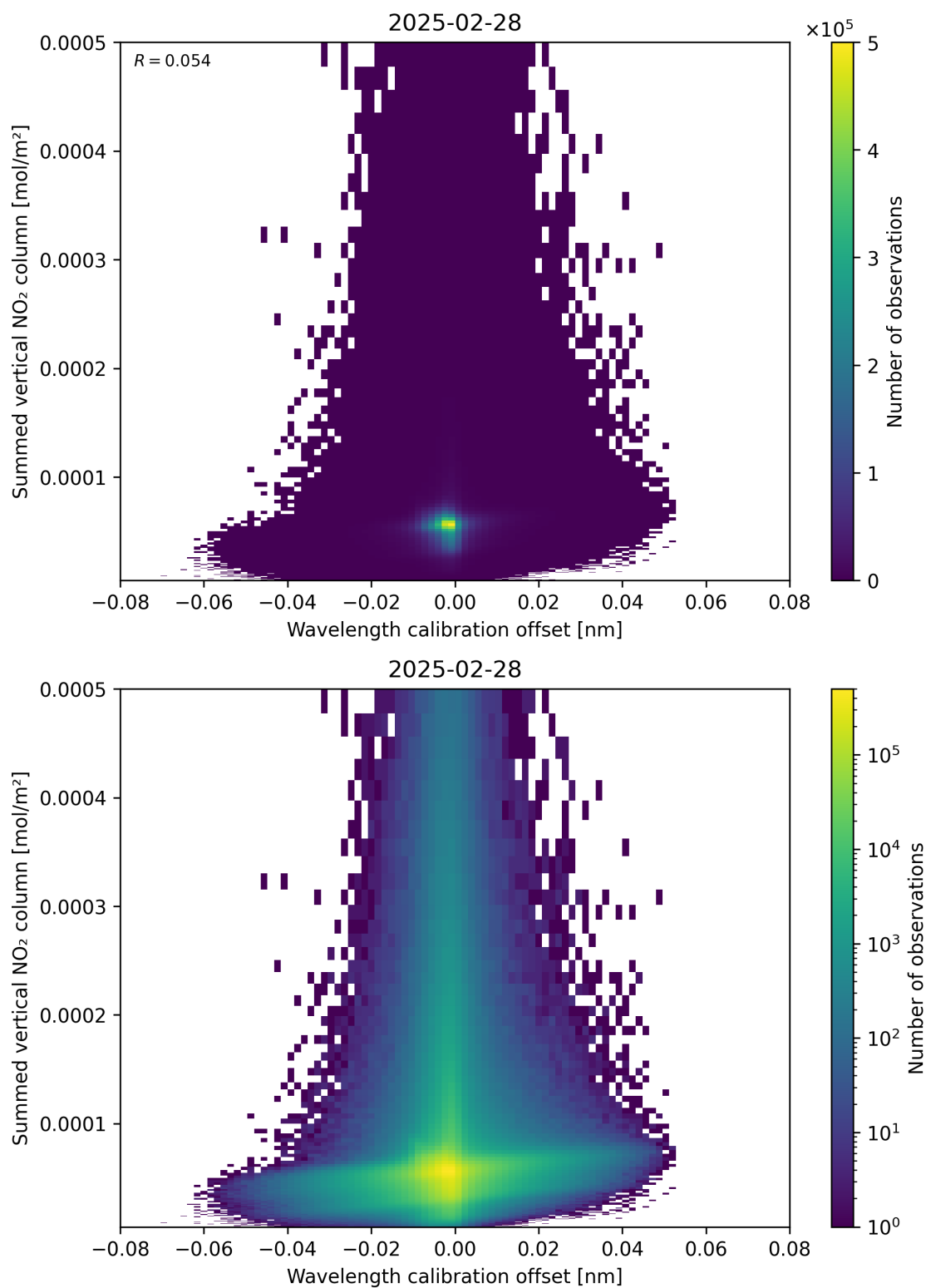
Figure 177: Scatter density plot of “Wavelength calibration offset” against “Summed vertical NO 2 column” for 2025-02-27 to 2025-03-01.
