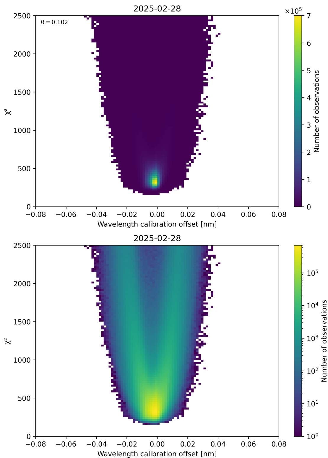
Figure 175: Scatter density plot of “Wavelength calibration offset” against “ \chi^2 ” for 2025-02-27 to 2025-03-01.
