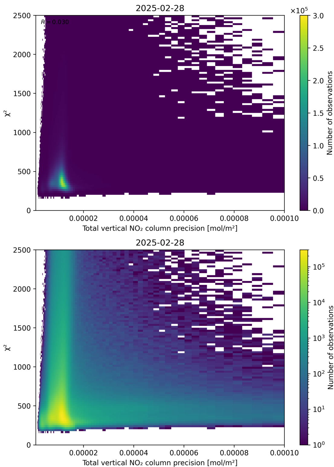
Figure 116: Scatter density plot of “Total vertical NO 2 column precision” against “ \chi^2 ” for 2025-02-27 to 2025-03-01.
