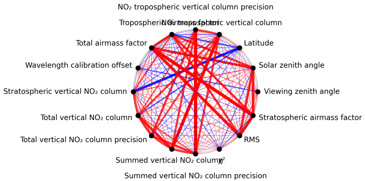
Figure 1: Map of correlation graph for 2025-02-27 to 2025-03-01.
