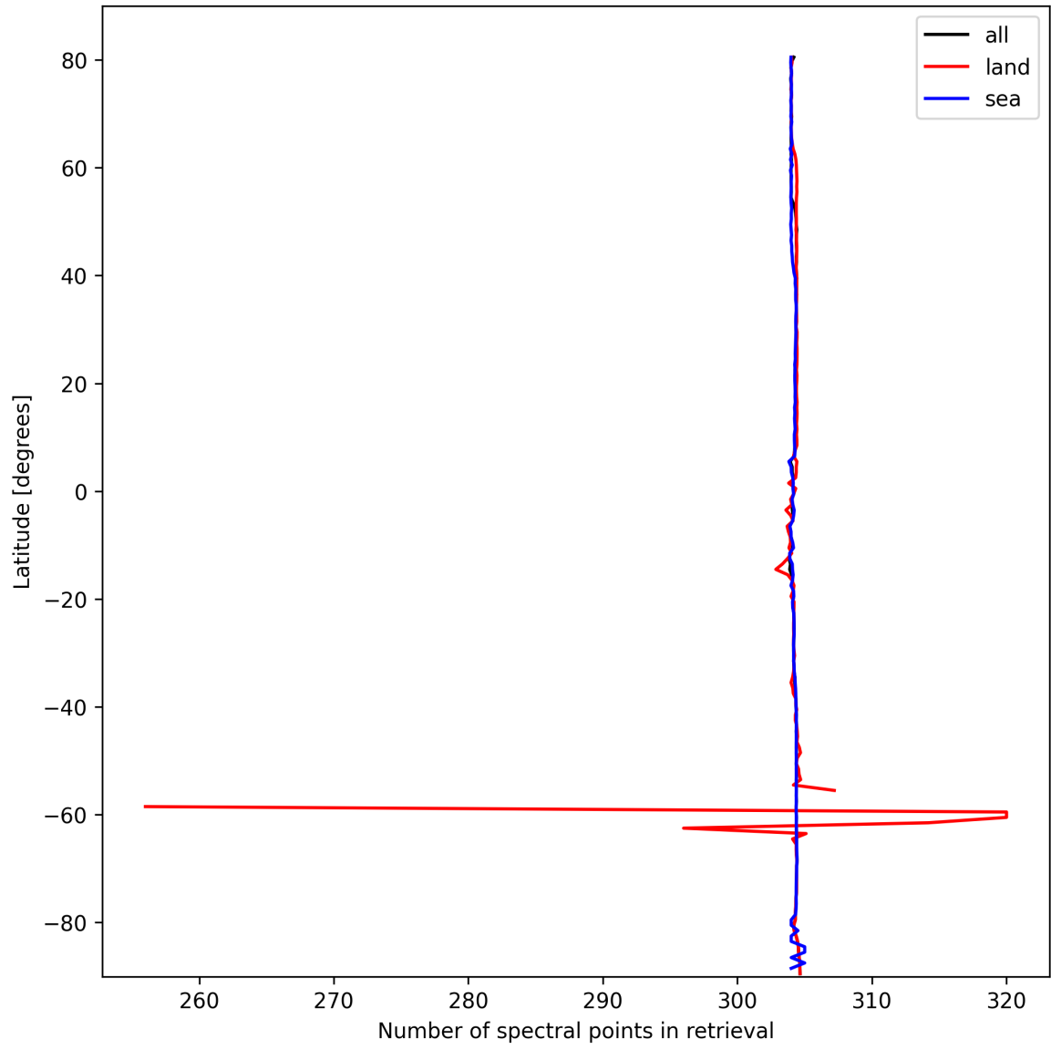
Figure 16: Zonal average of “Number of spectral points in retrieval” for 2025-02-27 to 2025-03-01.
