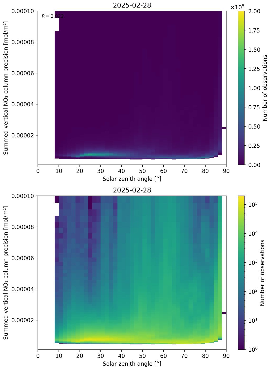
Figure 152: Scatter density plot of “Solar zenith angle” against “Summed vertical NO 2 column precision” for 2025-02-27 to 2025-03-01.
