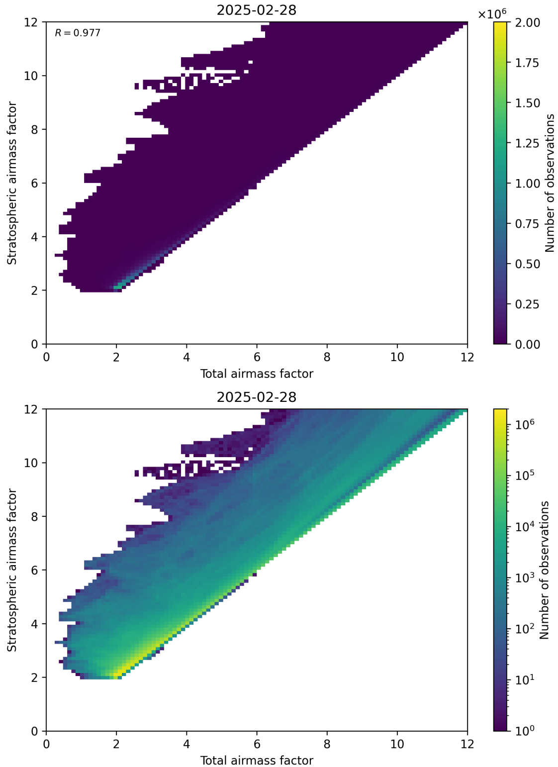
Figure 62: Scatter density plot of “Total airmass factor” against “Stratospheric airmass factor” for 2025-02-27 to 2025-03-01.
