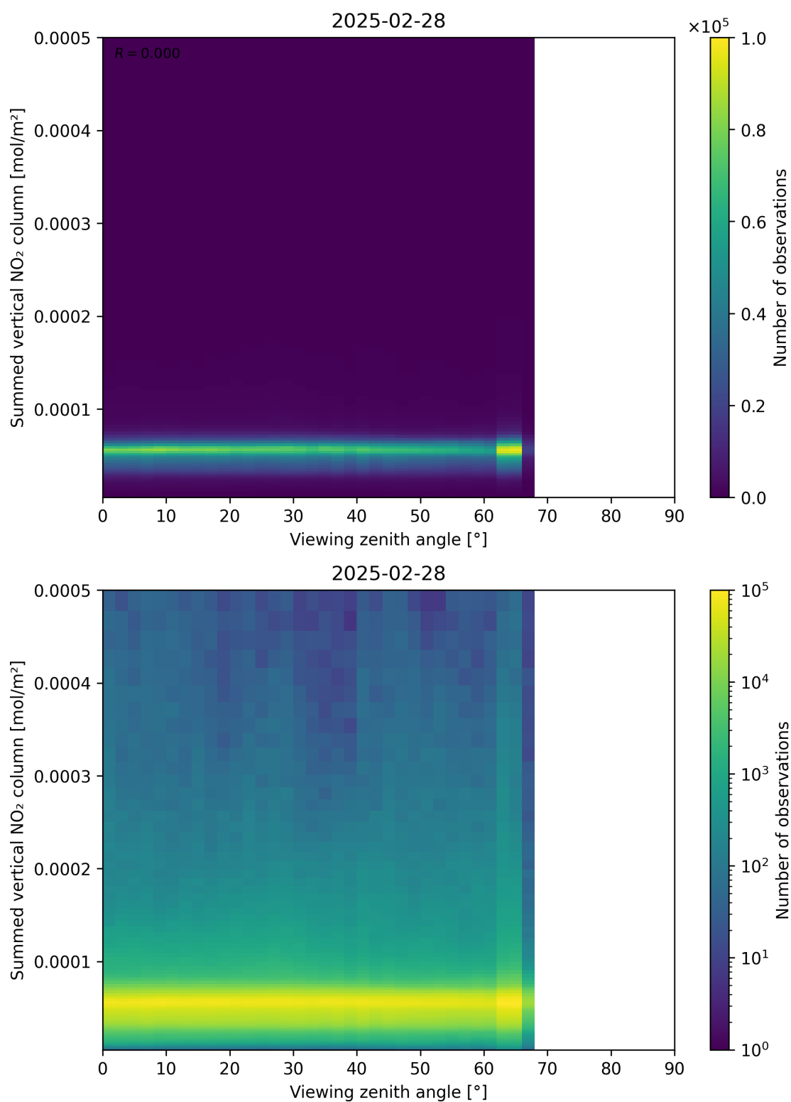
Figure 165: Scatter density plot of “Viewing zenith angle” against “Summed vertical NO 2 column” for 2025-02-27 to 2025-03-01.
