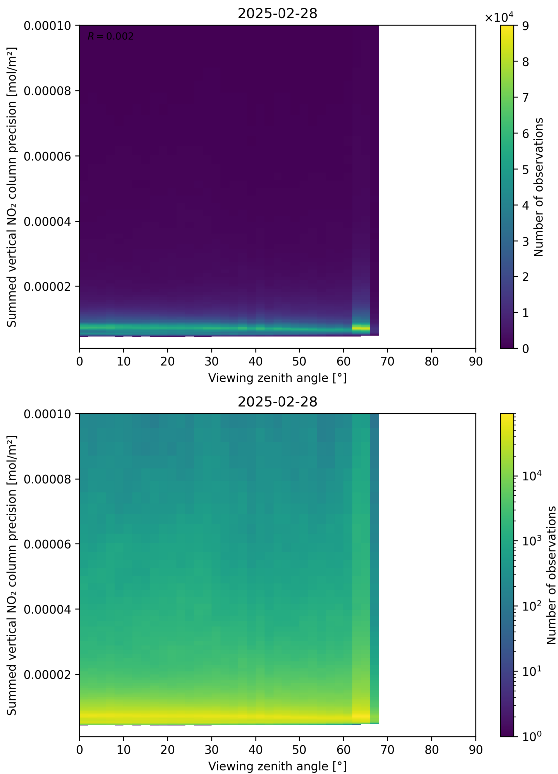
Figure 166: Scatter density plot of “Viewing zenith angle” against “Summed vertical NO 2 column precision” for 2025-02-27 to 2025-03-01.
