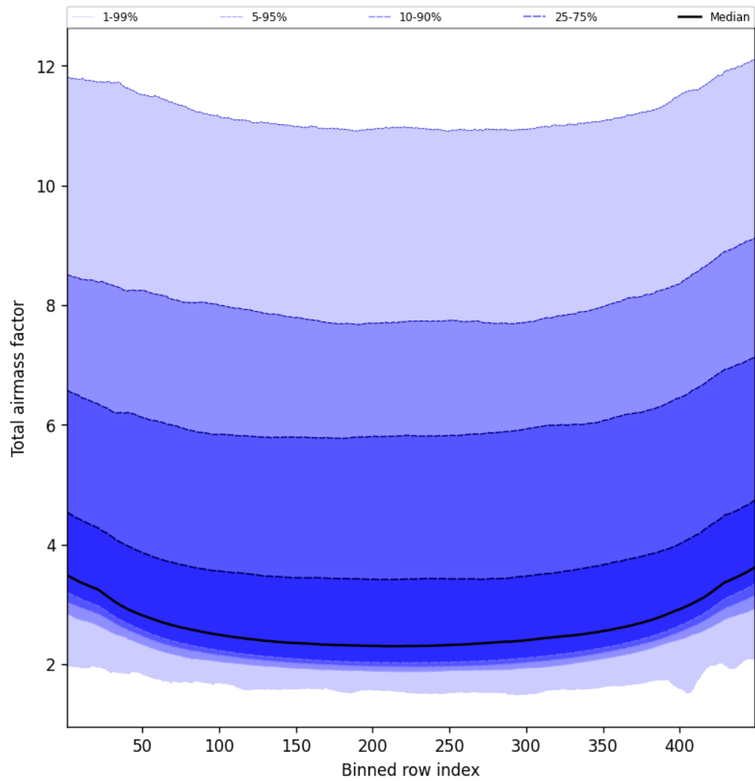
Figure 49: Along track statistics of “Total airmass factor” for 2025-02-27 to 2025-03-01
