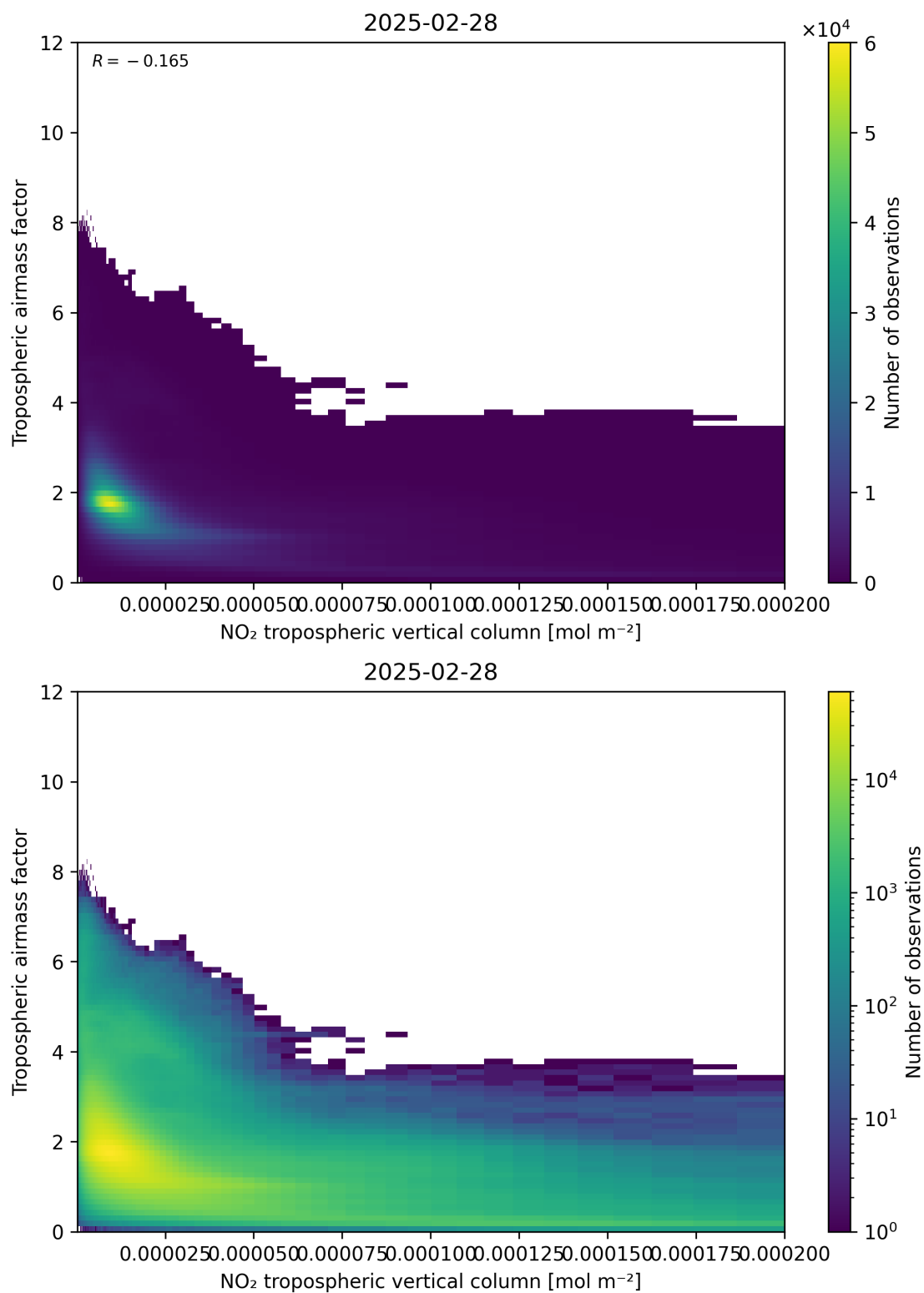
Figure 123: Scatter density plot of “NO 2 tropospheric vertical column” against “Tropospheric air mass factor” for 2025-02-27 to 2025-03-01.
