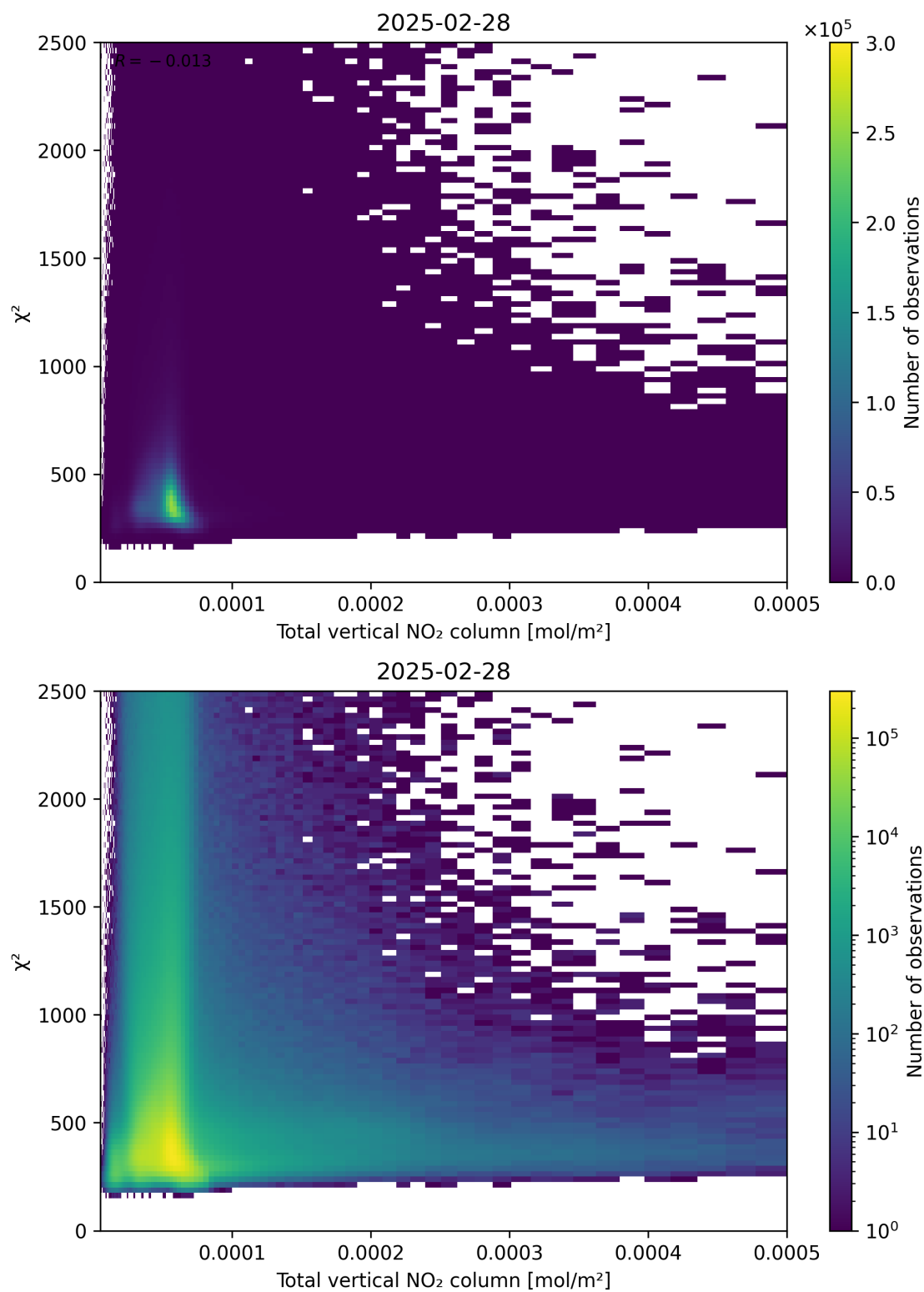
Figure 111: Scatter density plot of “Total vertical NO 2 column” against “ \chi^2 ” for 2025-02-27 to 2025-03-01.
