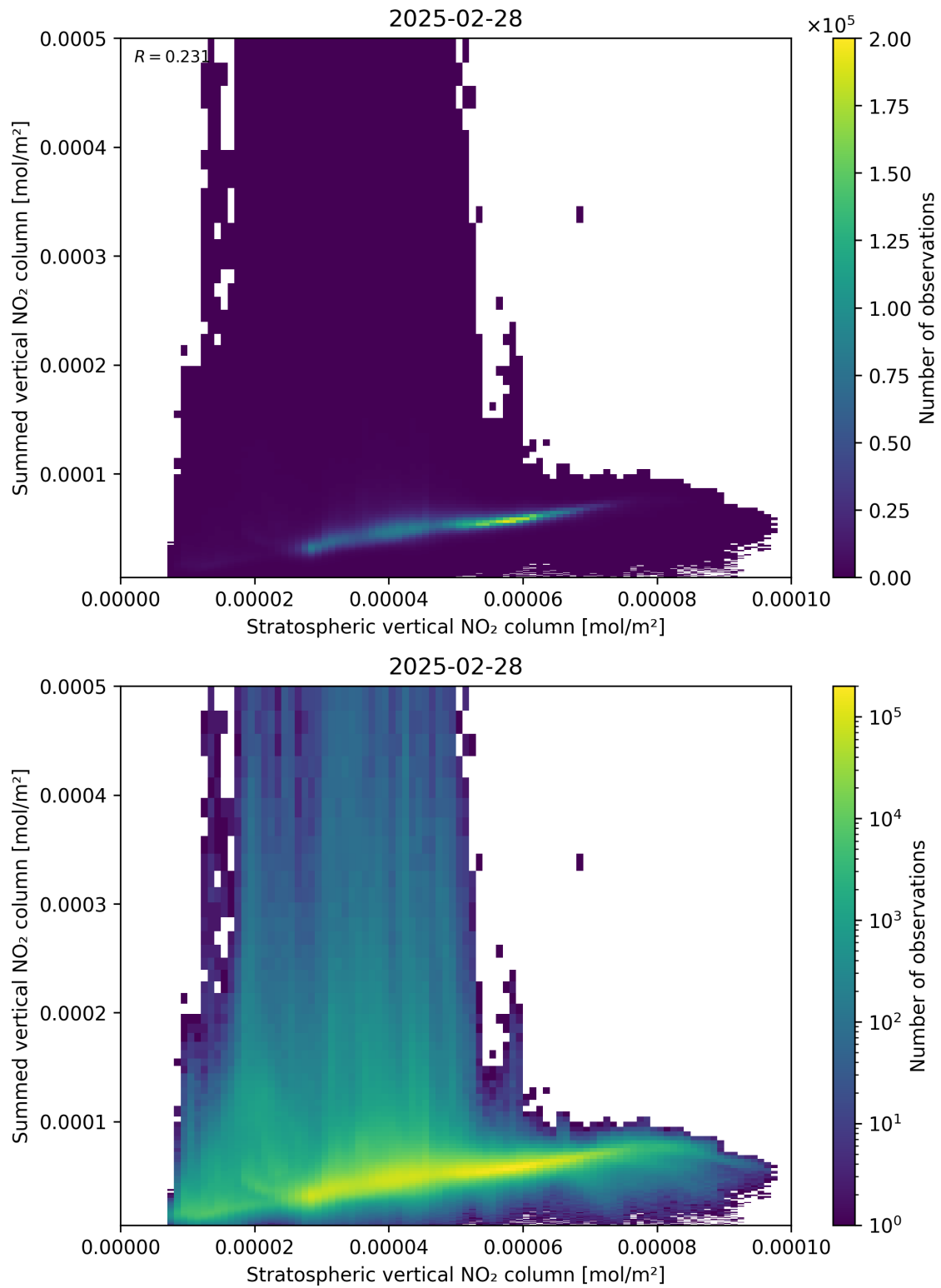
Figure 98: Scatter density plot of “Stratospheric vertical NO 2 column” against “Summed vertical NO 2 column” for 2025-02-27 to 2025-03-01.
