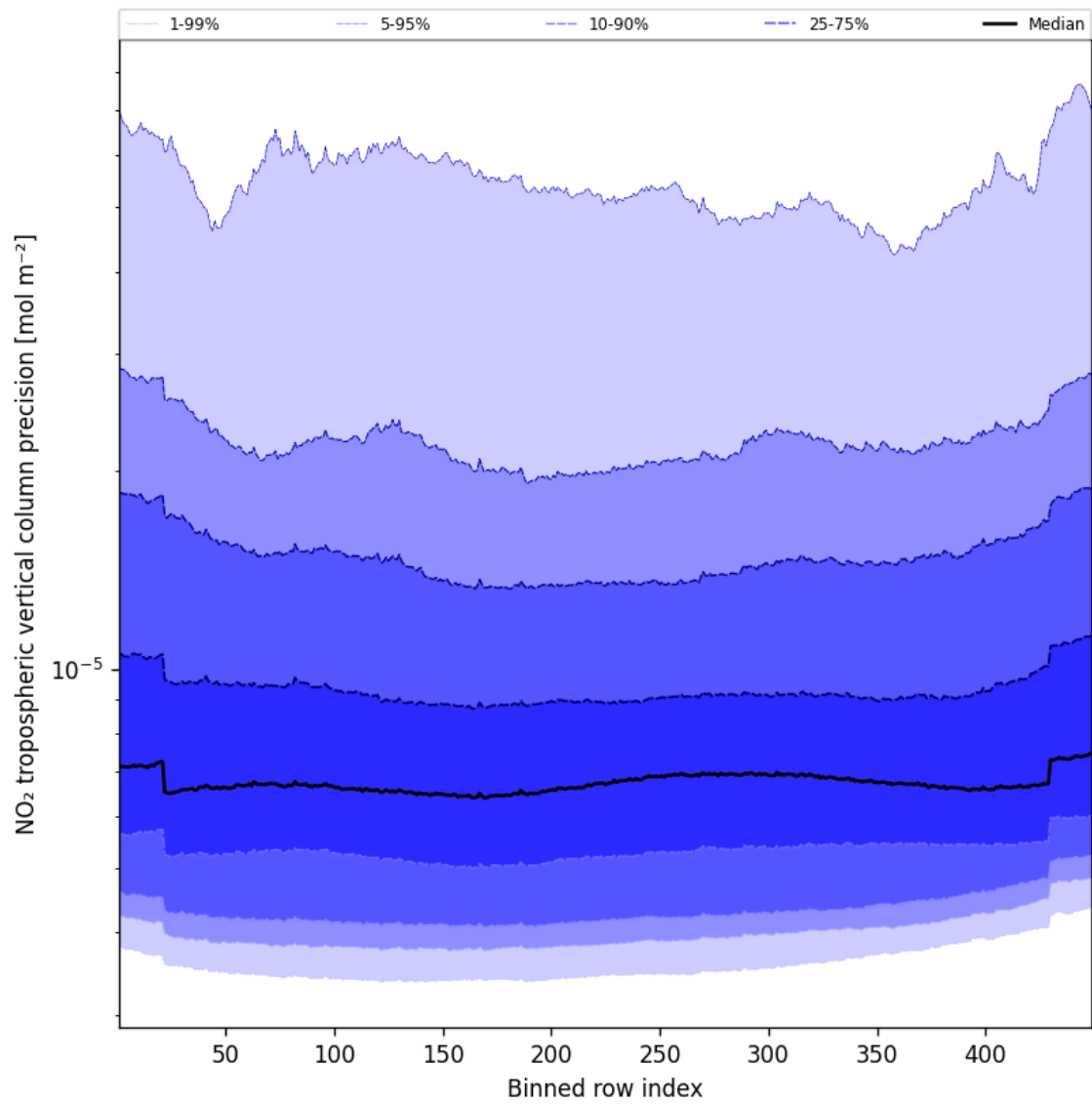
Figure 47: Along track statistics of “NO 2 tropospheric vertical column precision” for 2025-02-27 to 2025-03-01
