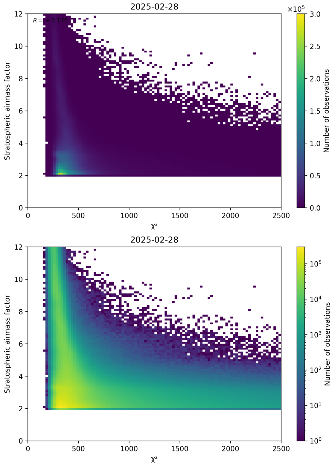
Figure 81: Scatter density plot of “ \chi^2 ” against “Stratospheric airmass factor” for 2025-02-27 to 2025-03-01.
