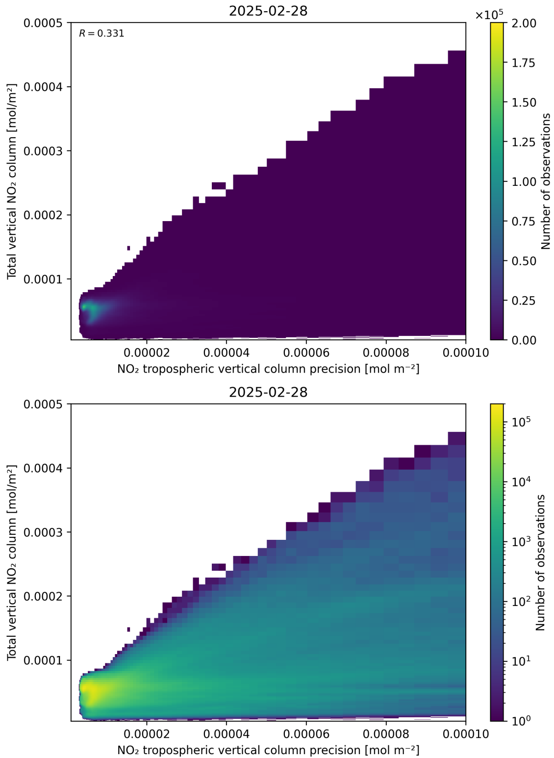
Figure 138: Scatter density plot of “NO 2 tropospheric vertical column precision” against “Total vertical NO 2 column” for 2025-02-27 to 2025-03-01.
