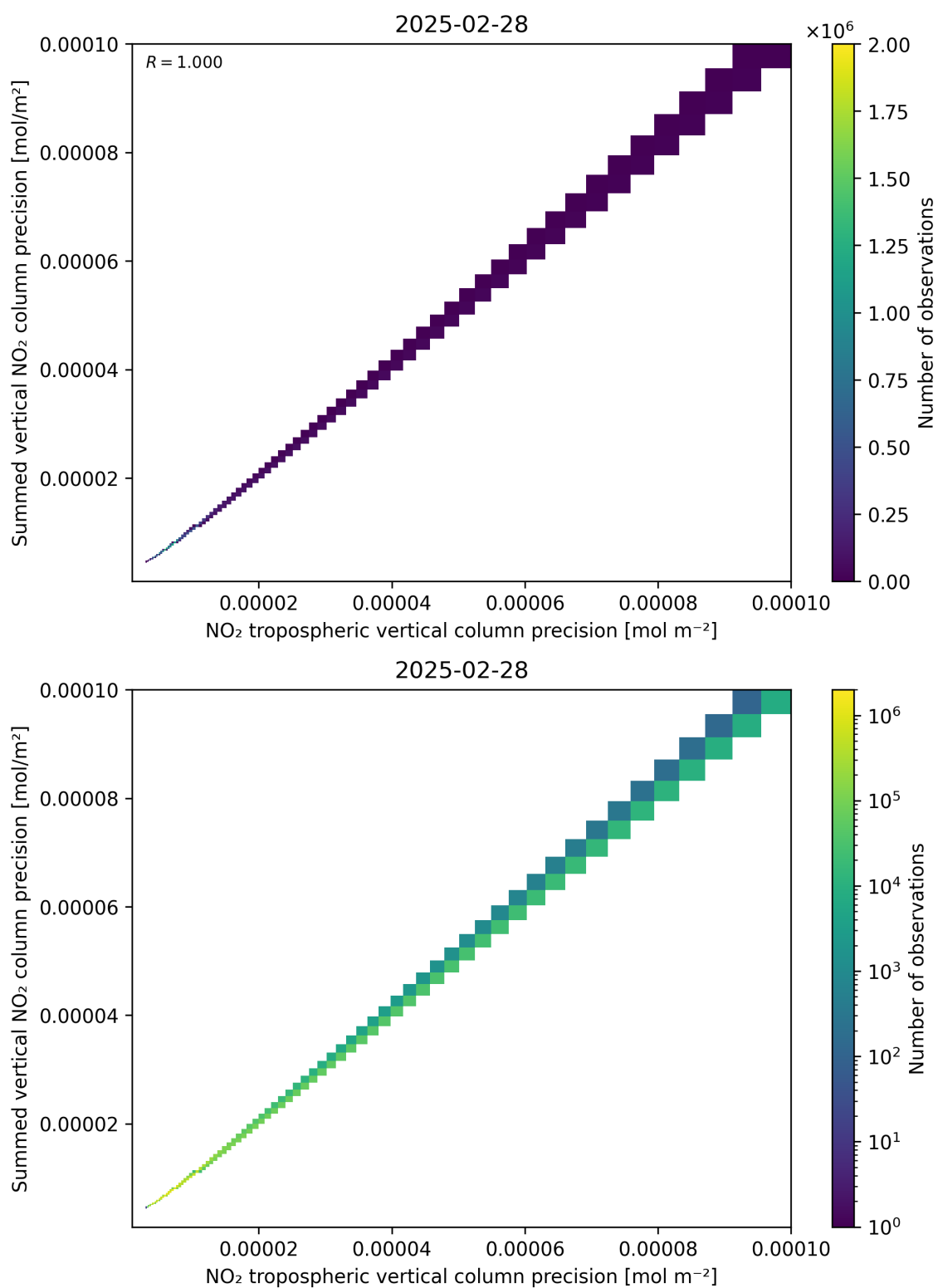
Figure 137: Scatter density plot of “NO 2 tropospheric vertical column precision” against “Summed vertical NO 2 column precision” for 2025-02-27 to 2025-03-01.
