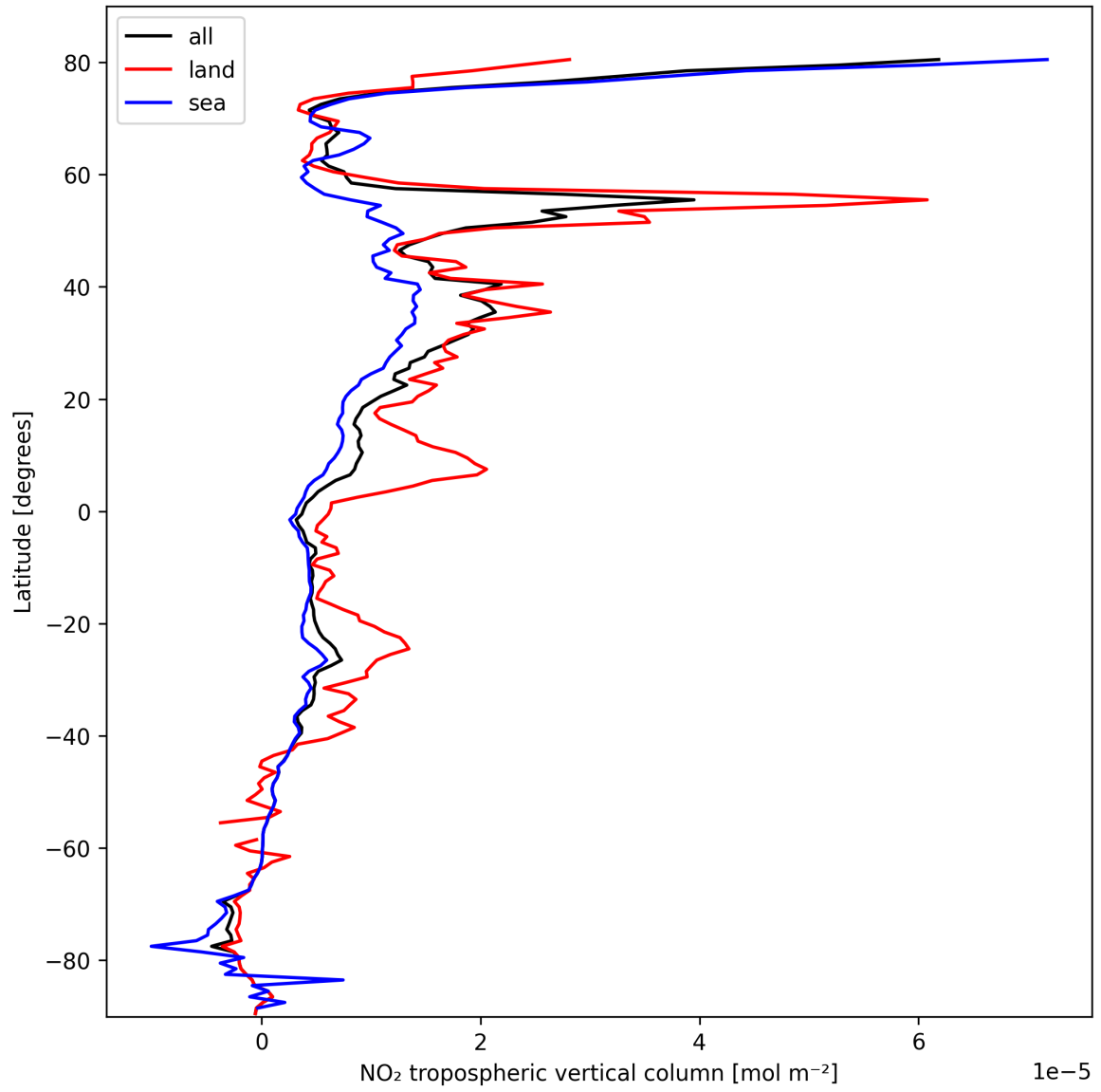
Figure 12: Zonal average of “NO 2 tropospheric vertical column” for 2025-02-27 to 2025-03-01.
