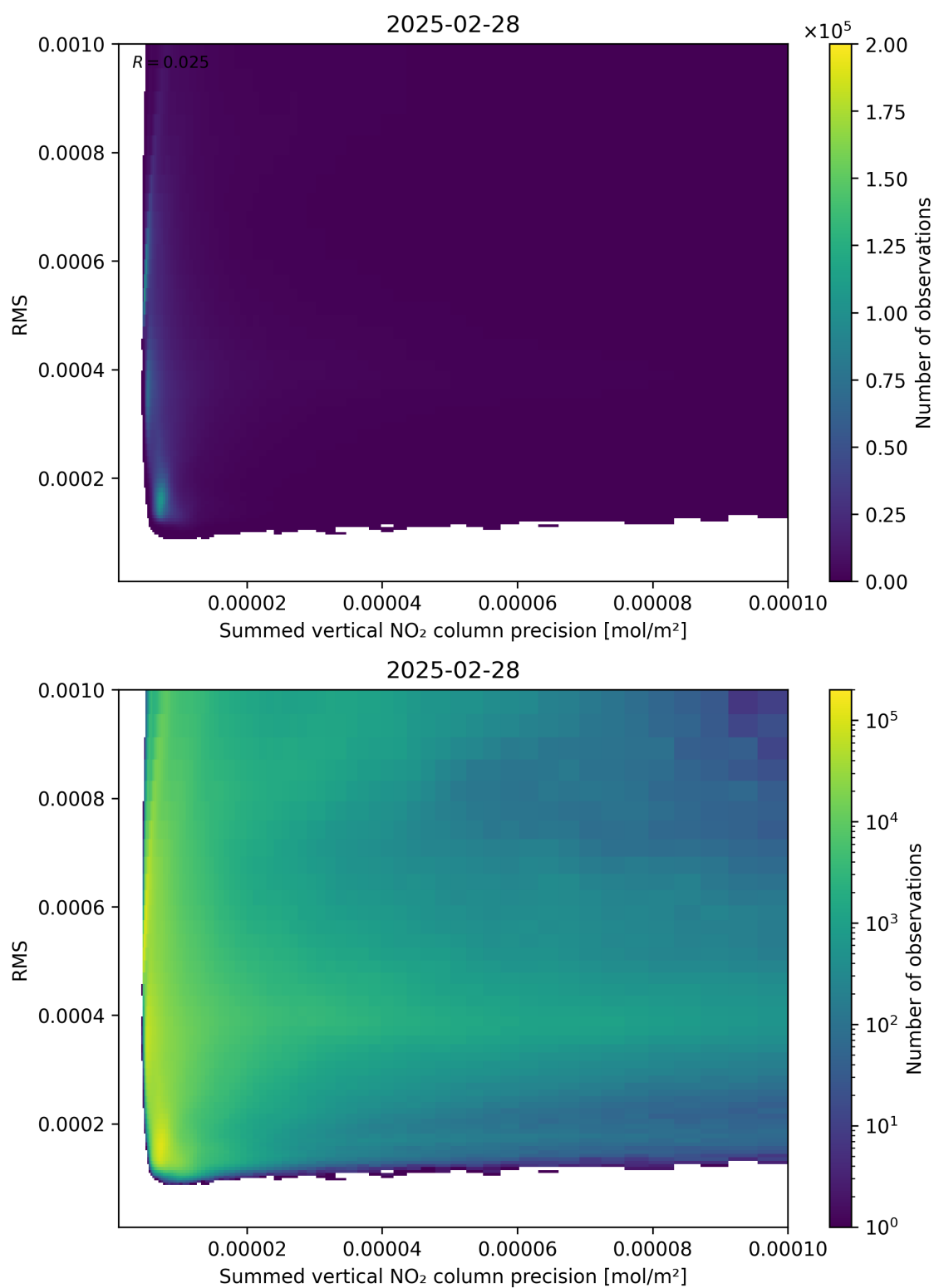
Figure 108: Scatter density plot of “Summed vertical NO 2 column precision” against “RMS” for 2025-02-27 to 2025-03-01.
