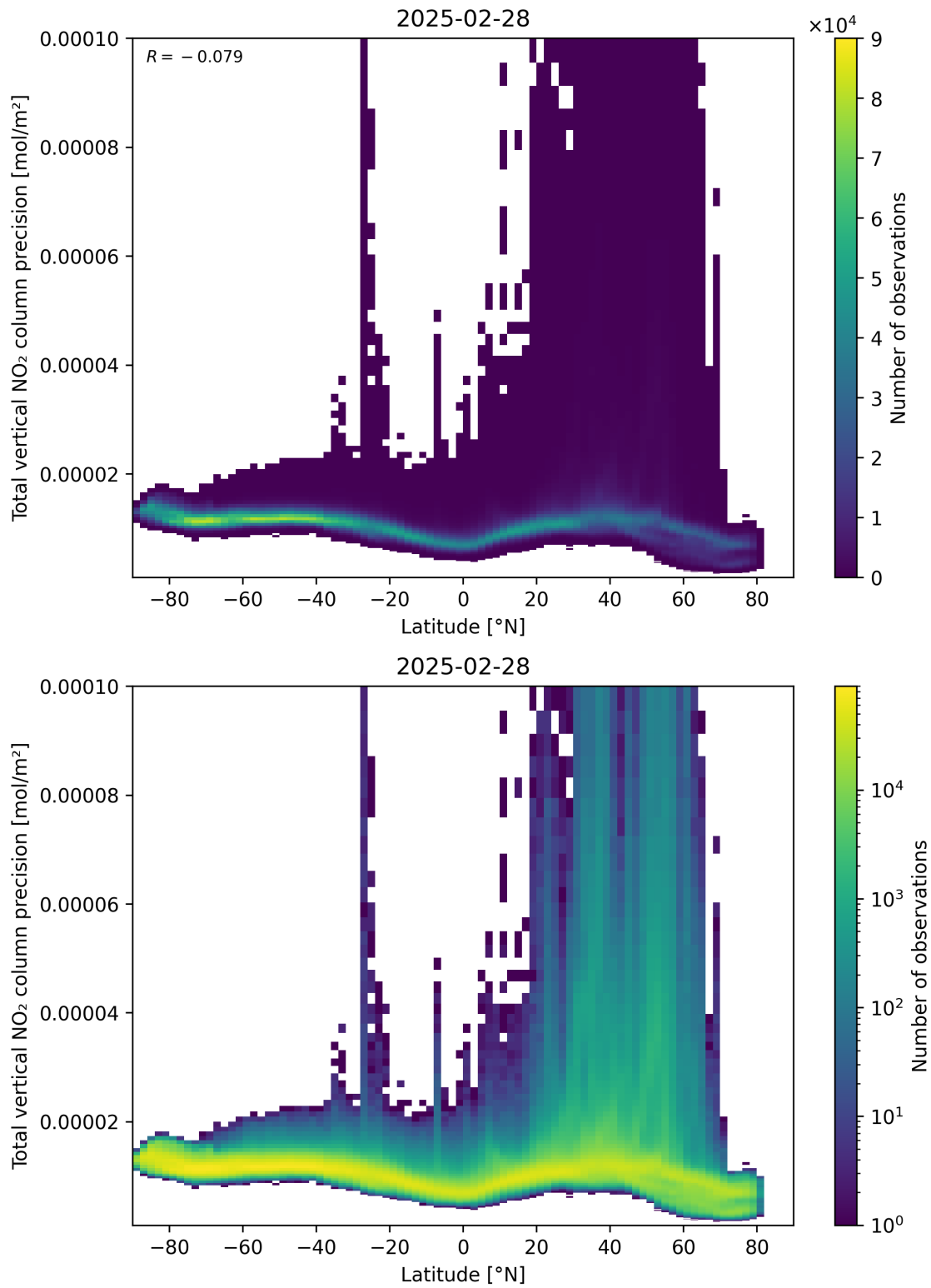
Figure 91: Scatter density plot of “Latitude” against “Total vertical NO 2 column precision” for 2025-02-27 to 2025-03-01.
