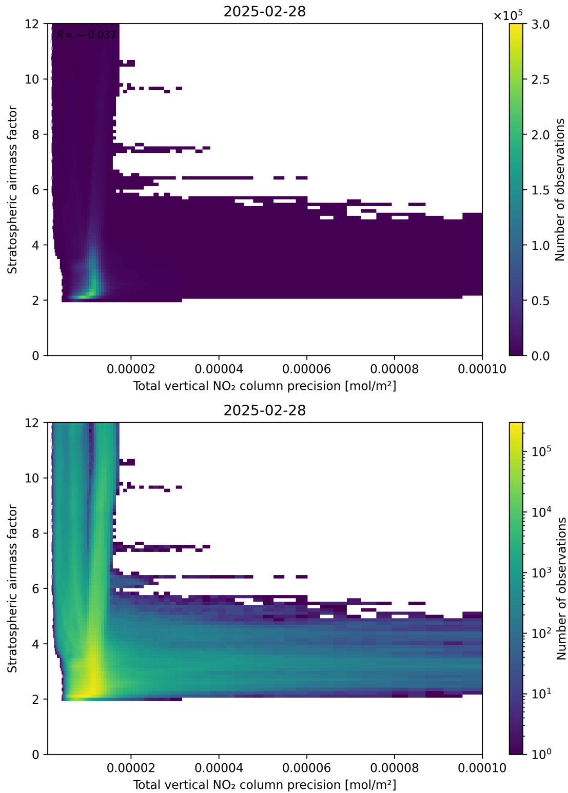
Figure 115: Scatter density plot of “Total vertical NO 2 column precision” against “Stratospheric air mass factor” for 2025-02-27 to 2025-03-01.
