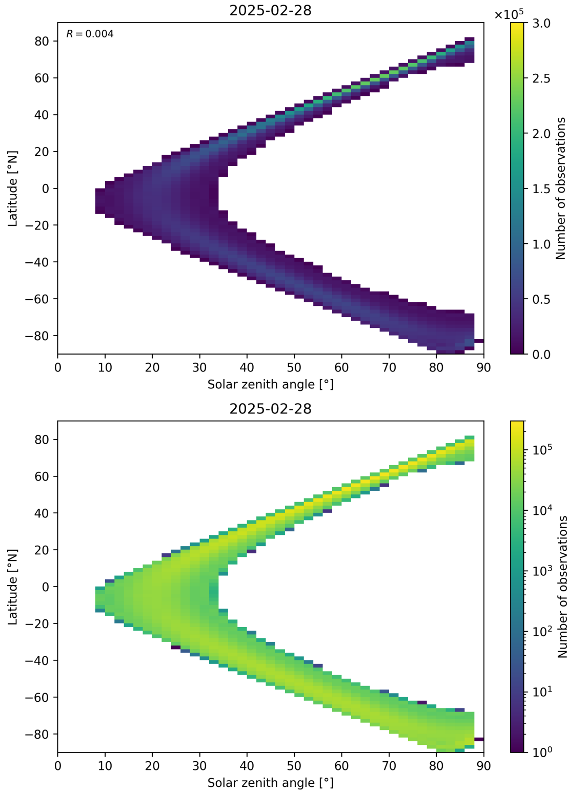
Figure 149: Scatter density plot of “Solar zenith angle” against “Latitude” for 2025-02-27 to 2025-03-01.
