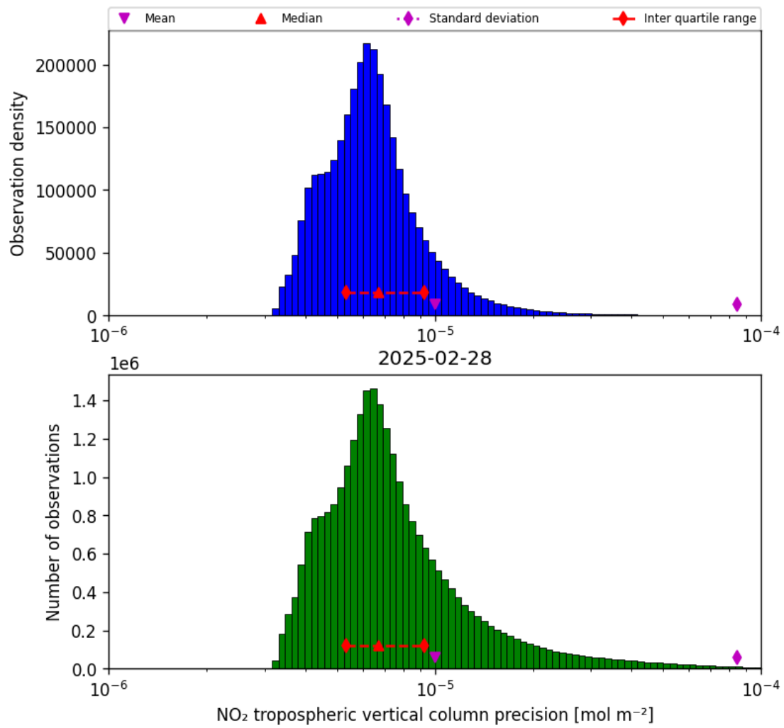
Figure 30: Histogram of “NO 2 tropospheric vertical column precision” for 2025-02-27 to 2025-03-01
