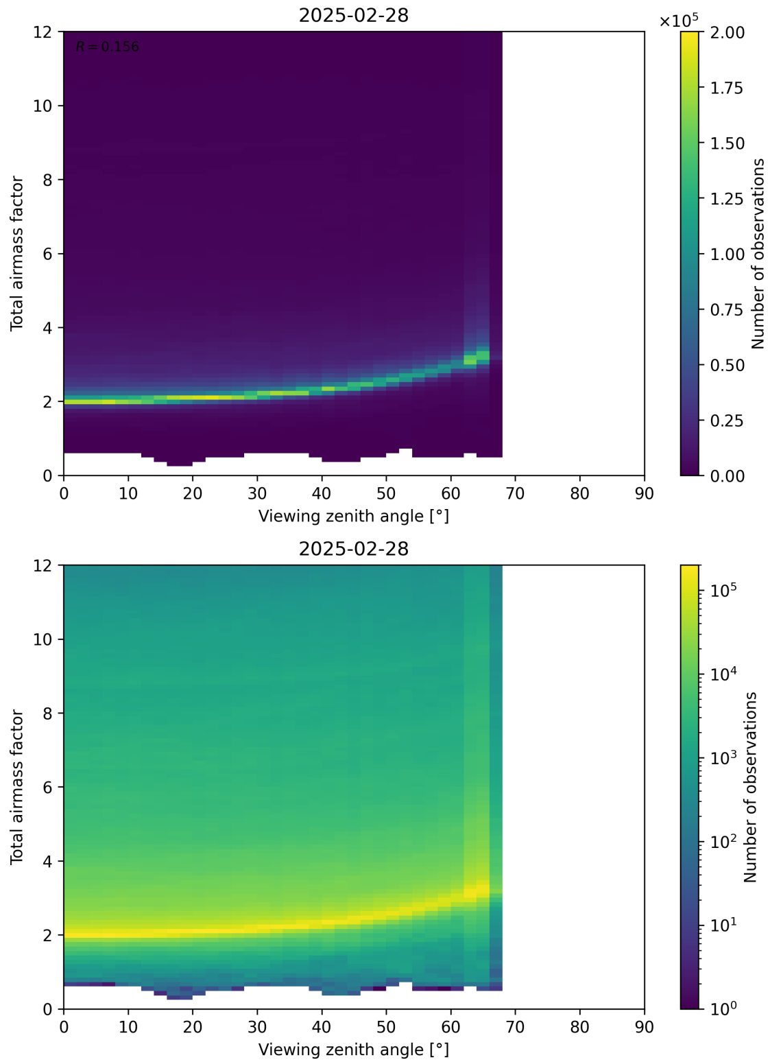
Figure 160: Scatter density plot of “Viewing zenith angle” against “Total airmass factor” for 2025-02-27 to 2025-03-01.
