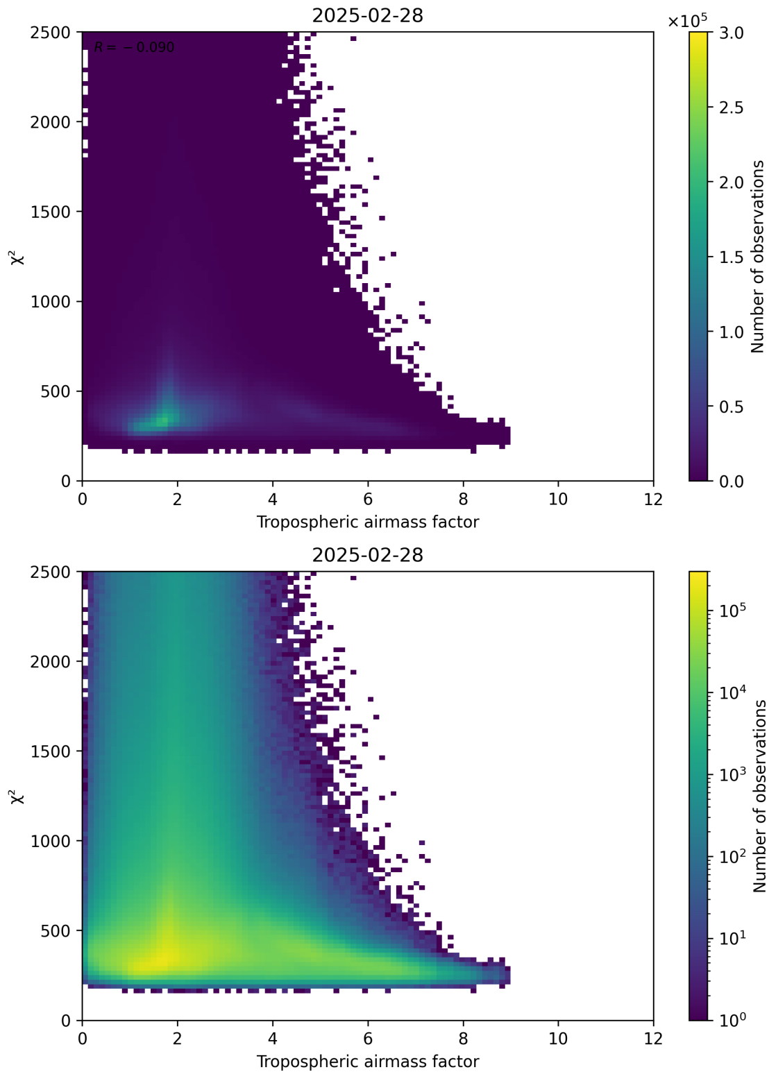
Figure 73: Scatter density plot of “Tropospheric airmass factor” against “ \chi^2 ” for 2025-02-27 to 2025-03-01.
