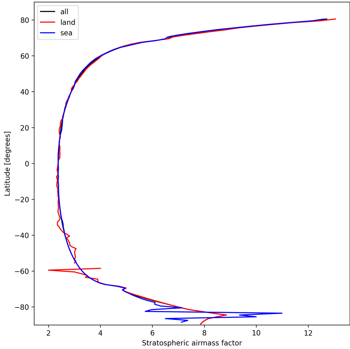
Figure 27: Zonal average of “Stratospheric airmass factor” for 2025-02-27 to 2025-03-01.
