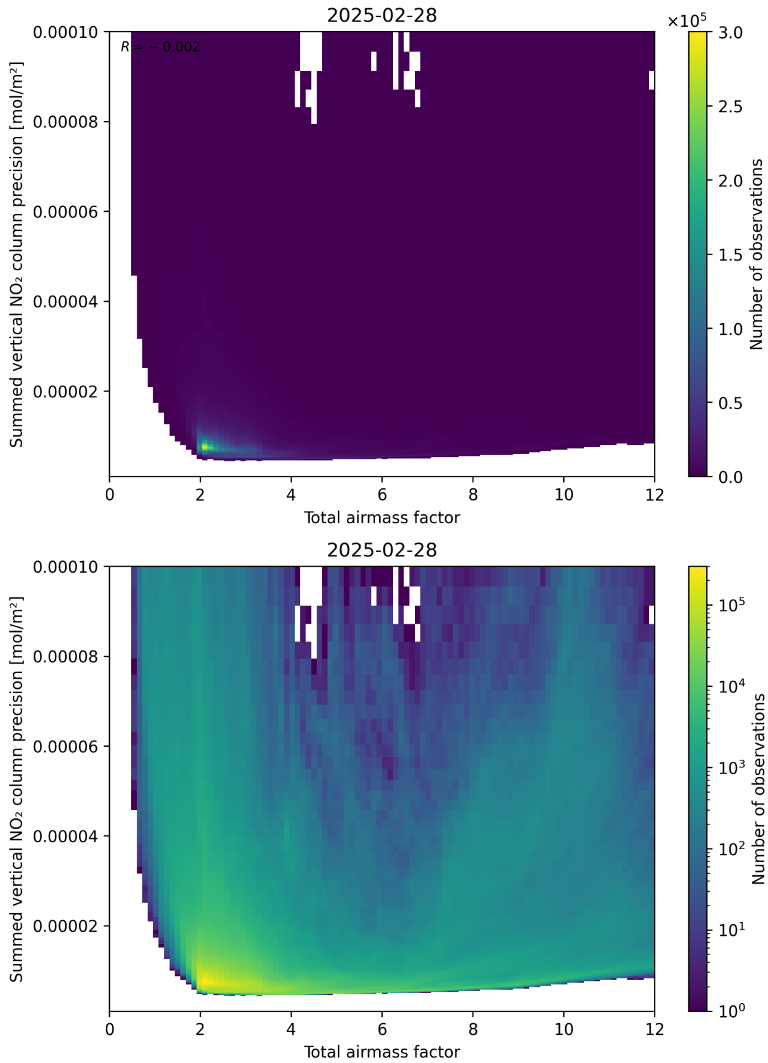
Figure 66: Scatter density plot of “Total airmass factor” against “Summed vertical NO 2 column precision” for 2025-02-27 to 2025-03-01.
