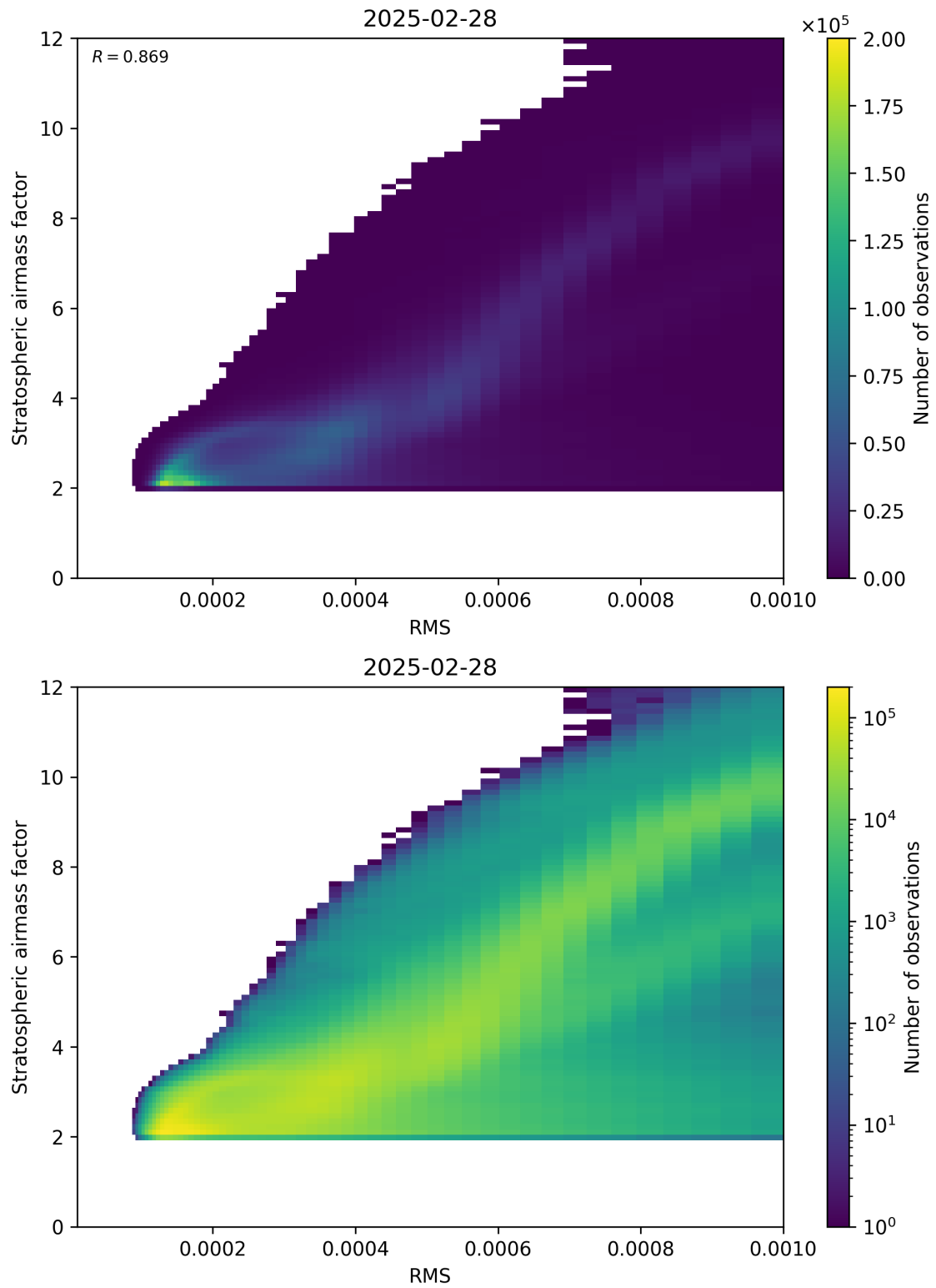
Figure 144: Scatter density plot of “RMS” against “Stratospheric airmass factor” for 2025-02-27 to 2025-03-01.
