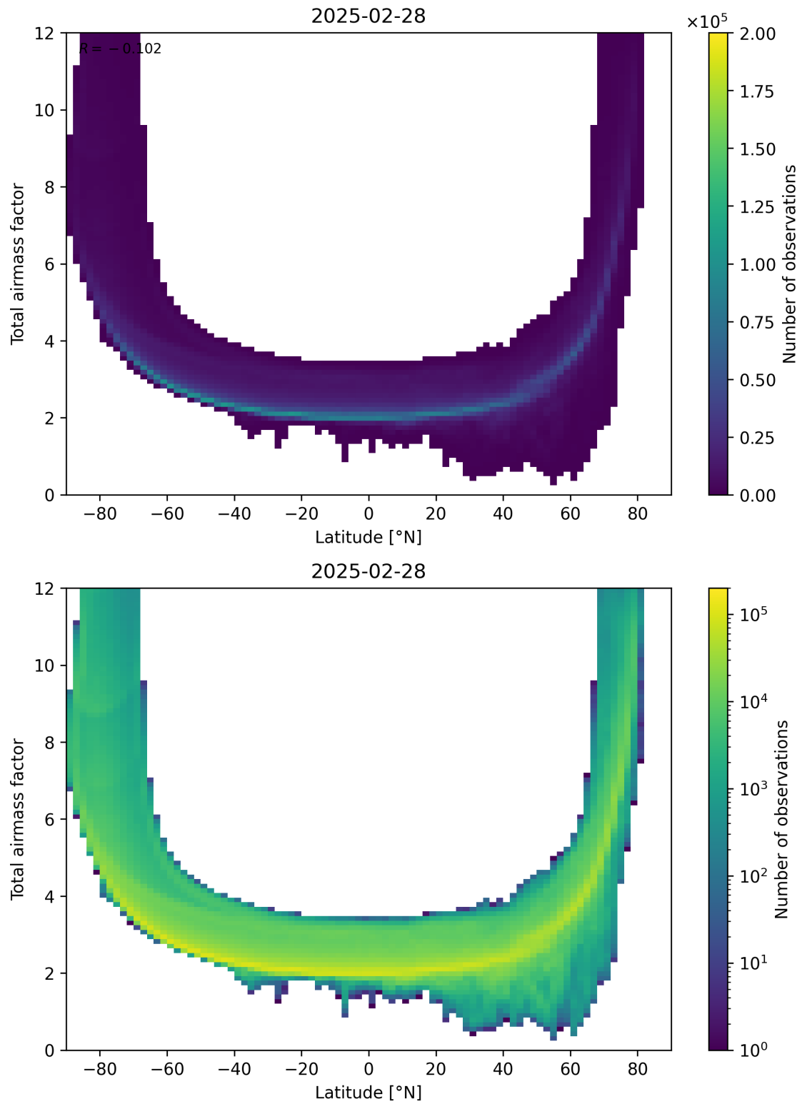
Figure 84: Scatter density plot of “Latitude” against “Total airmass factor” for 2025-02-27 to 2025-03-01.
