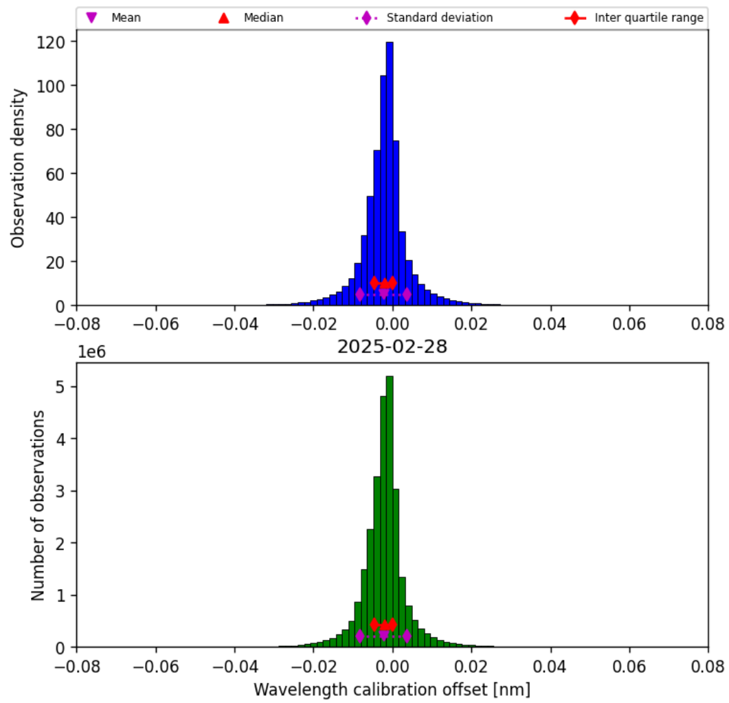
Figure 35: Histogram of “Wavelength calibration offset” for 2025-02-27 to 2025-03-01
