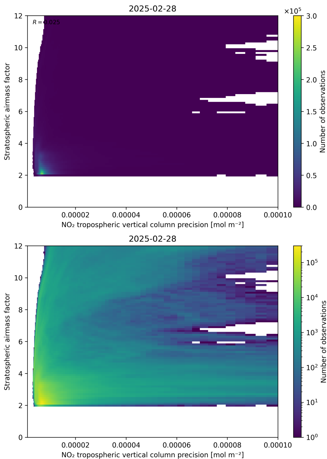
Figure 131: Scatter density plot of “NO 2 tropospheric vertical column precision” against “Stratospheric airmass factor” for 2025-02-27 to 2025-03-01.
