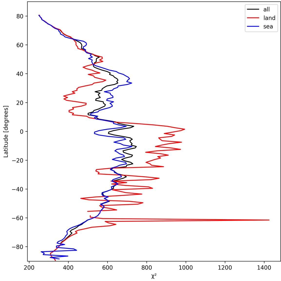
Figure 25: Zonal average of “ \chi^2 ” for 2025-02-27 to 2025-03-01.
