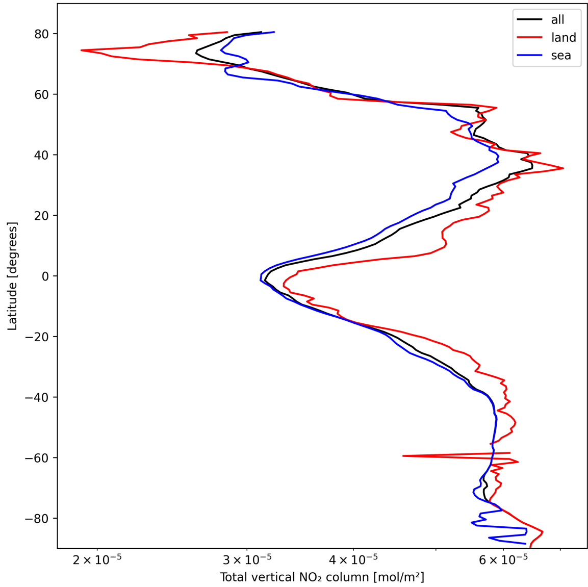
Figure 21: Zonal average of “Total vertical NO 2 column” for 2025-02-27 to 2025-03-01.
