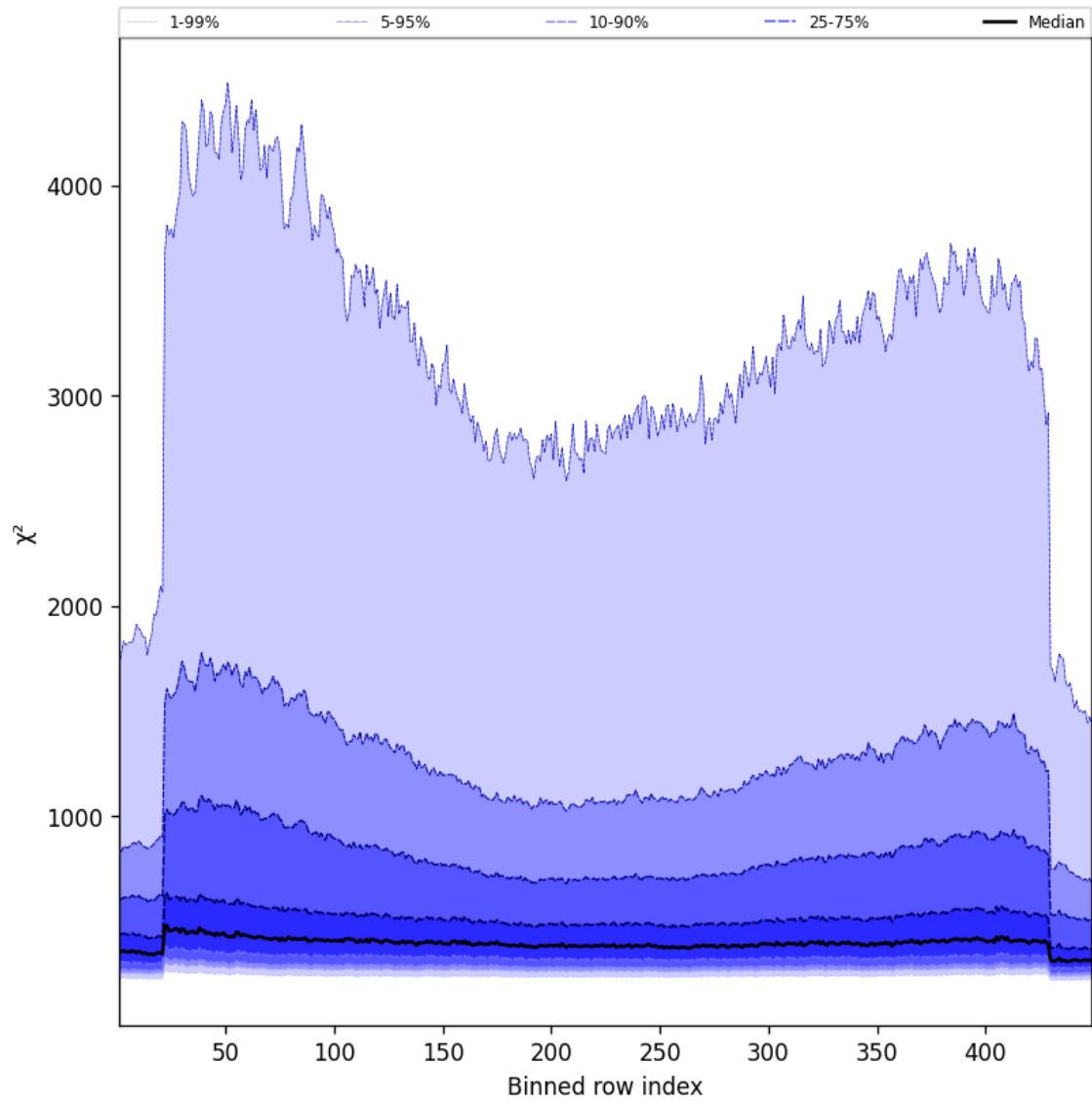
Figure 59: Along track statistics of “ \chi^2 ” for 2025-02-27 to 2025-03-01
