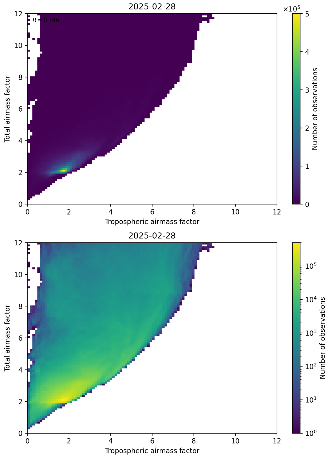
Figure 72: Scatter density plot of “Tropospheric airmass factor” against “Total airmass factor” for 2025-02-27 to 2025-03-01.
