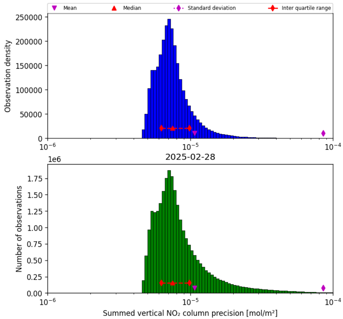
Figure 41: Histogram of "Summed vertical NO 2 column precision" for 2025-02-27 to 2025-03-01
