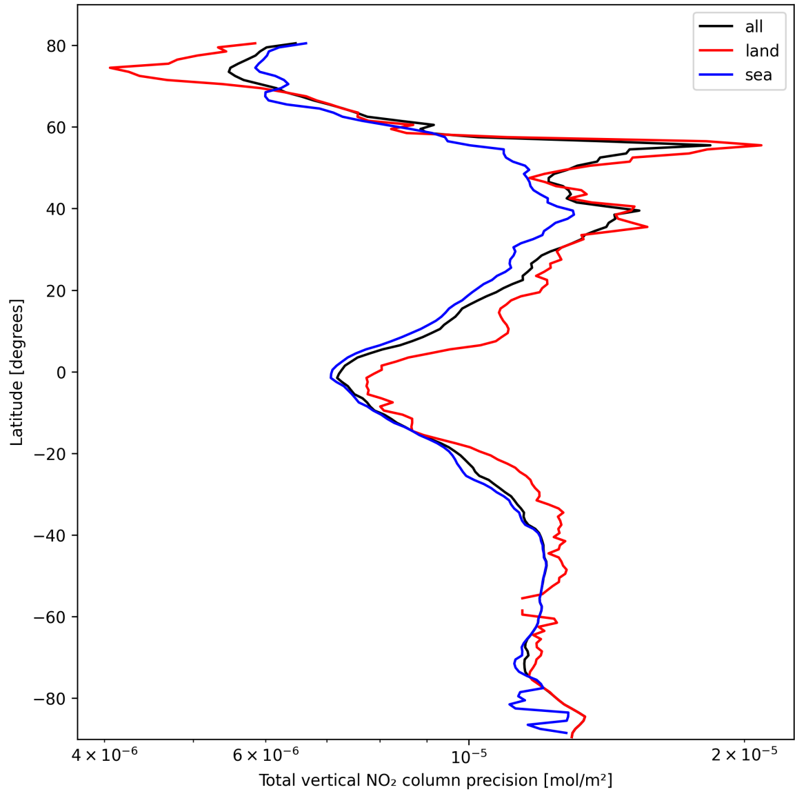
Figure 22: Zonal average of “Total vertical NO 2 column precision” for 2025-02-27 to 2025-03-01.
