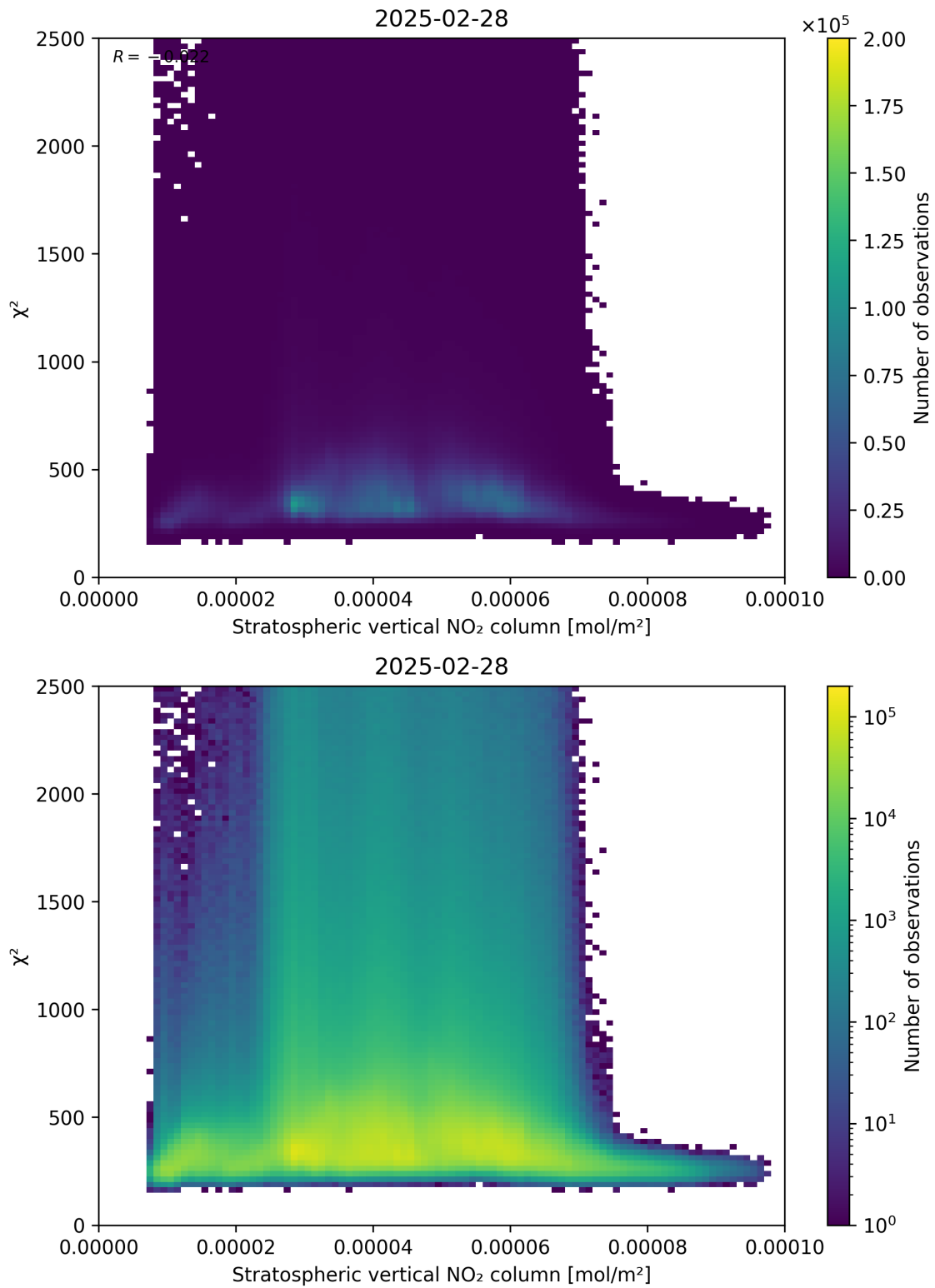
Figure 97: Scatter density plot of “Stratospheric vertical NO 2 column” against “ \chi^2 ” for 2025-02-27 to 2025-03-01.
