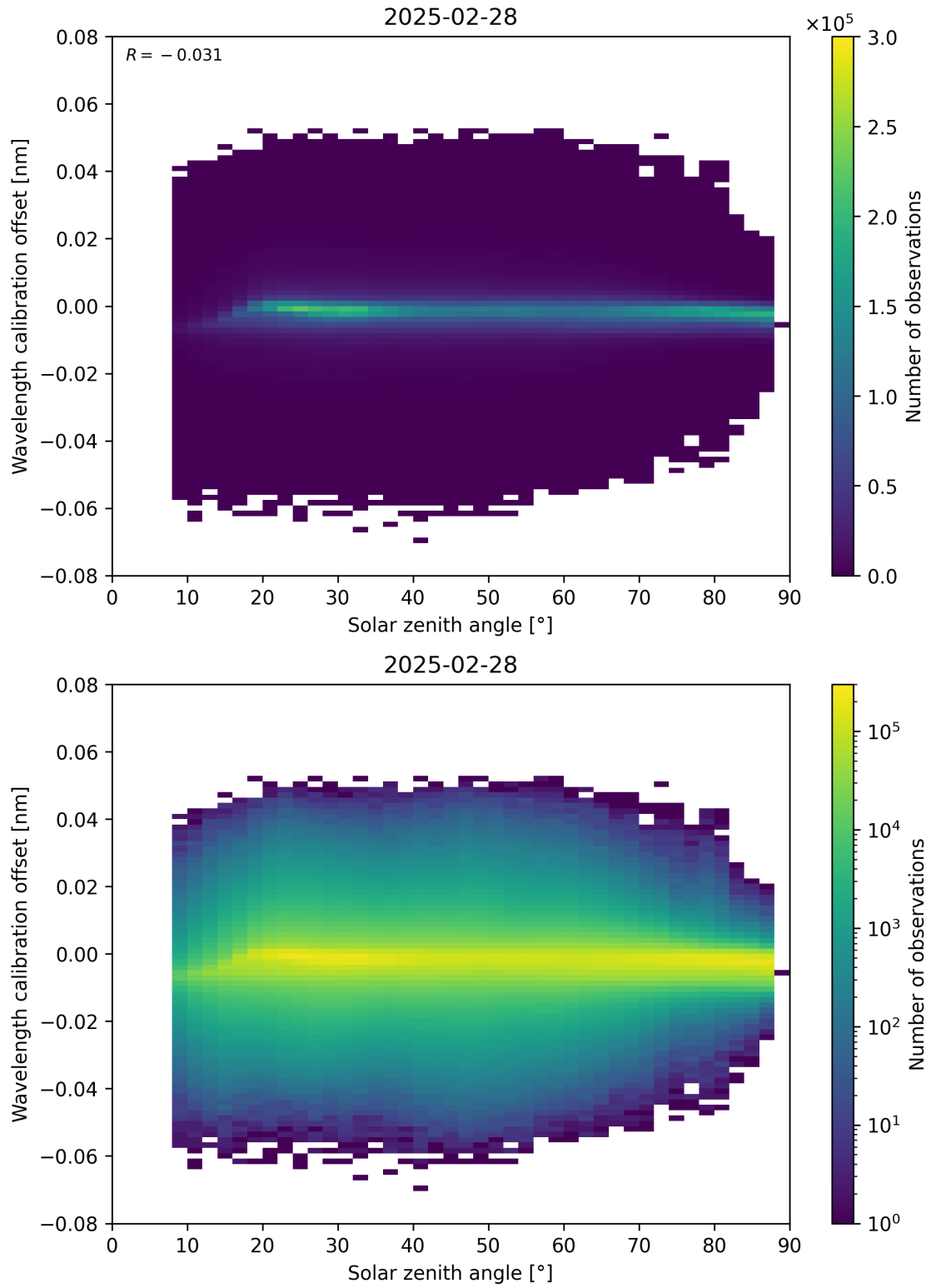
Figure 158: Scatter density plot of “Solar zenith angle” against “Wavelength calibration offset” for 2025-02-27 to 2025-03-01.
