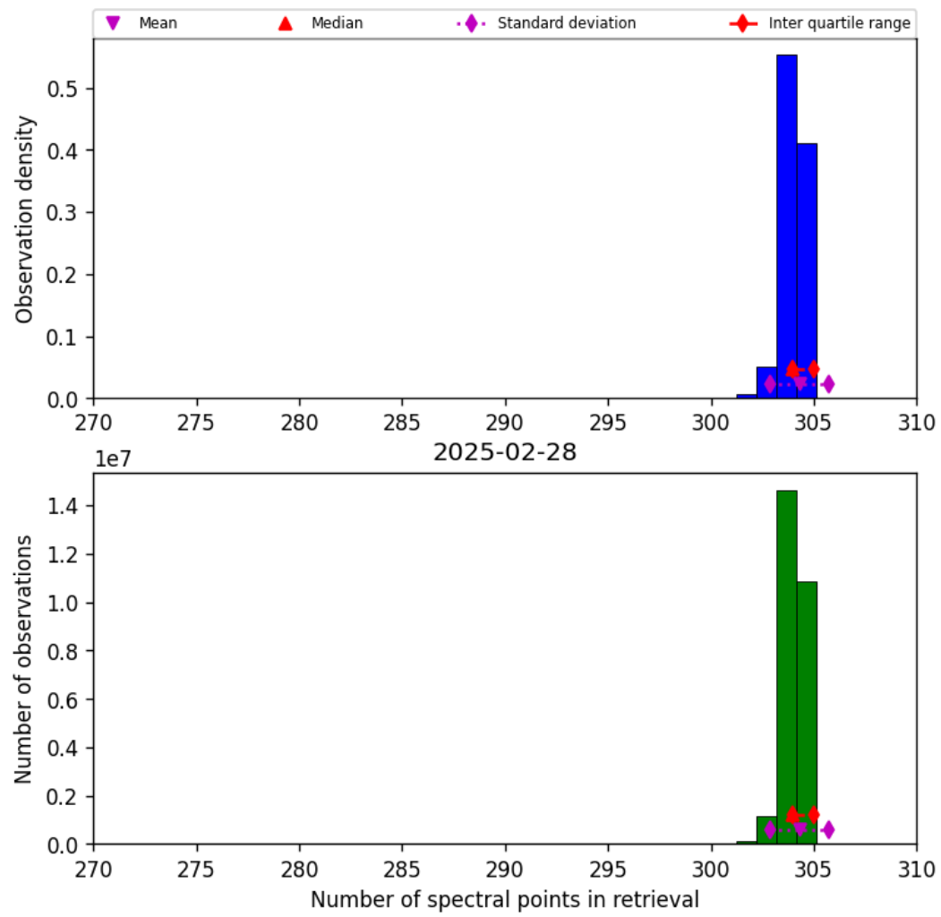
Figure 33: Histogram of “Number of spectral points in retrieval” for 2025-02-27 to 2025-03-01
