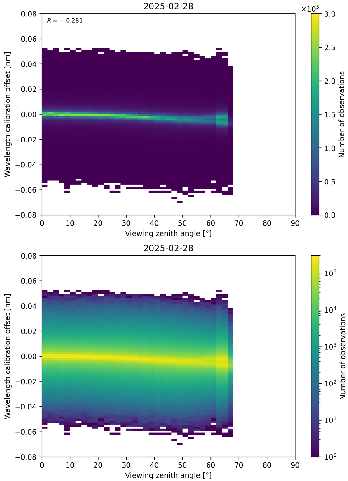
Figure 173: Scatter density plot of “Viewing zenith angle” against “Wavelength calibration offset” for 2025-02-27 to 2025-03-01.
