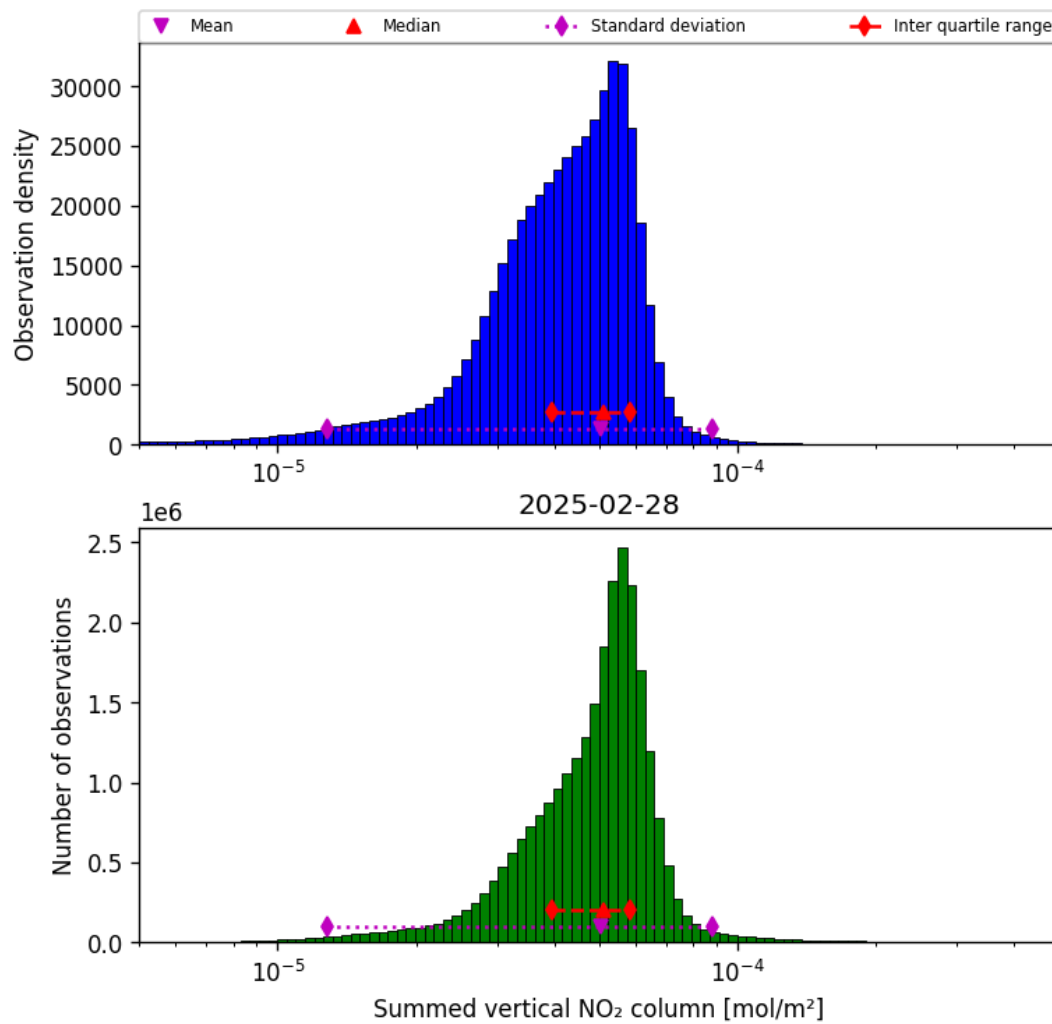
Figure 40: Histogram of “Summed vertical NO 2 column” for 2025-02-27 to 2025-03-01
