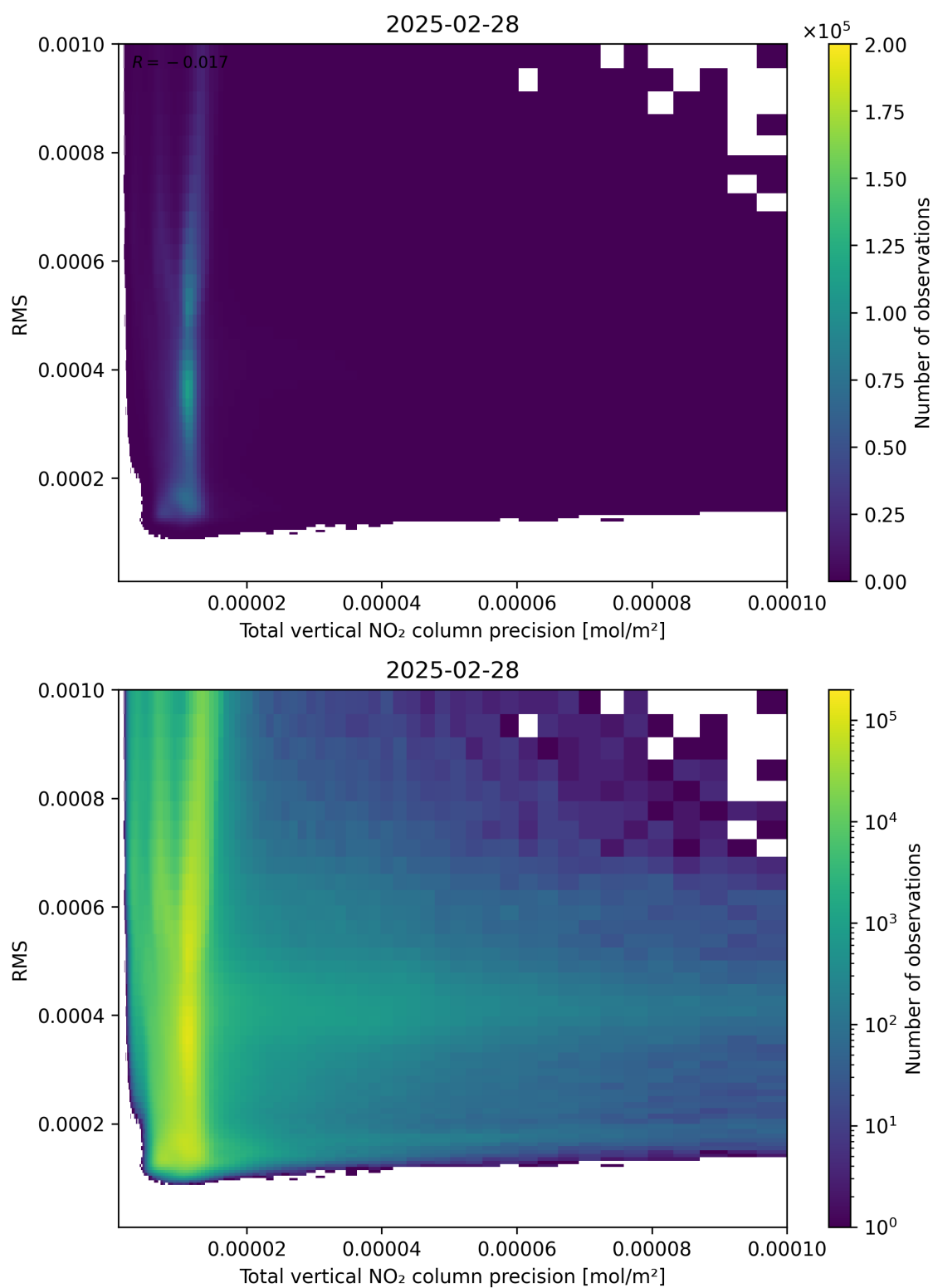
Figure 119: Scatter density plot of “Total vertical NO 2 column precision” against “RMS” for 2025-02-27 to 2025-03-01.
