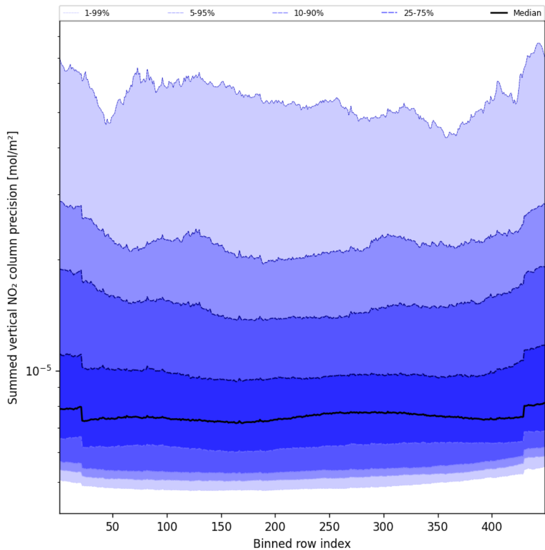
Figure 58: Along track statistics of “Summed vertical NO 2 column precision” for 2025-02-27 to 2025-03-01
