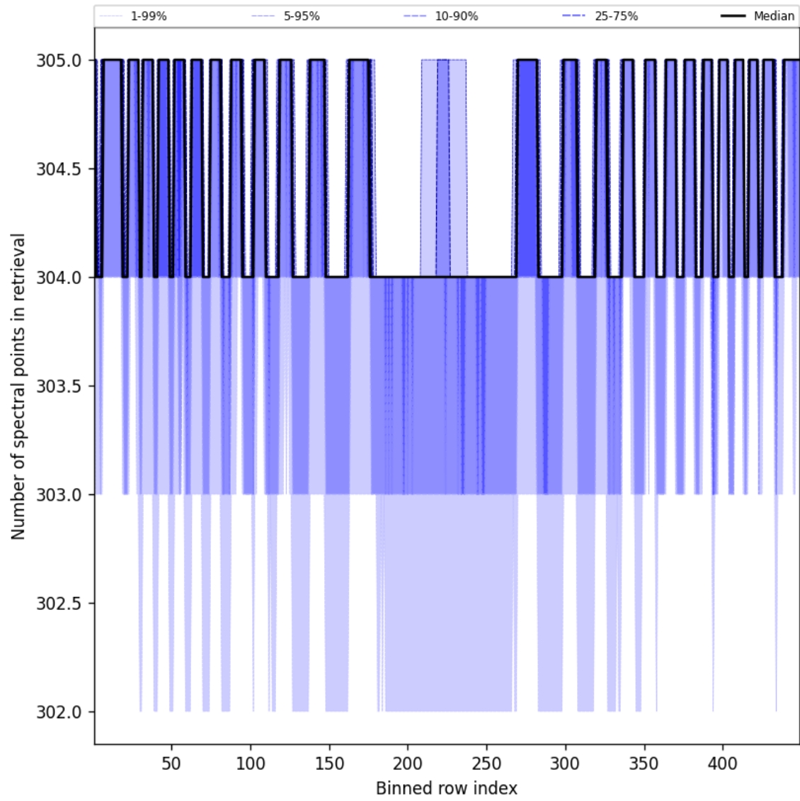
Figure 50: Along track statistics of “Number of spectral points in retrieval” for 2025-02-27 to 2025-03-01
