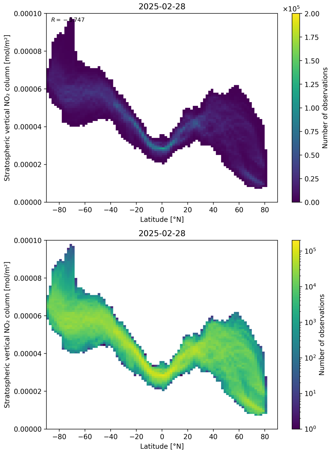
Figure 87: Scatter density plot of “Latitude” against “Stratospheric vertical NO 2 column” for 2025-02-27 to 2025-03-01.
