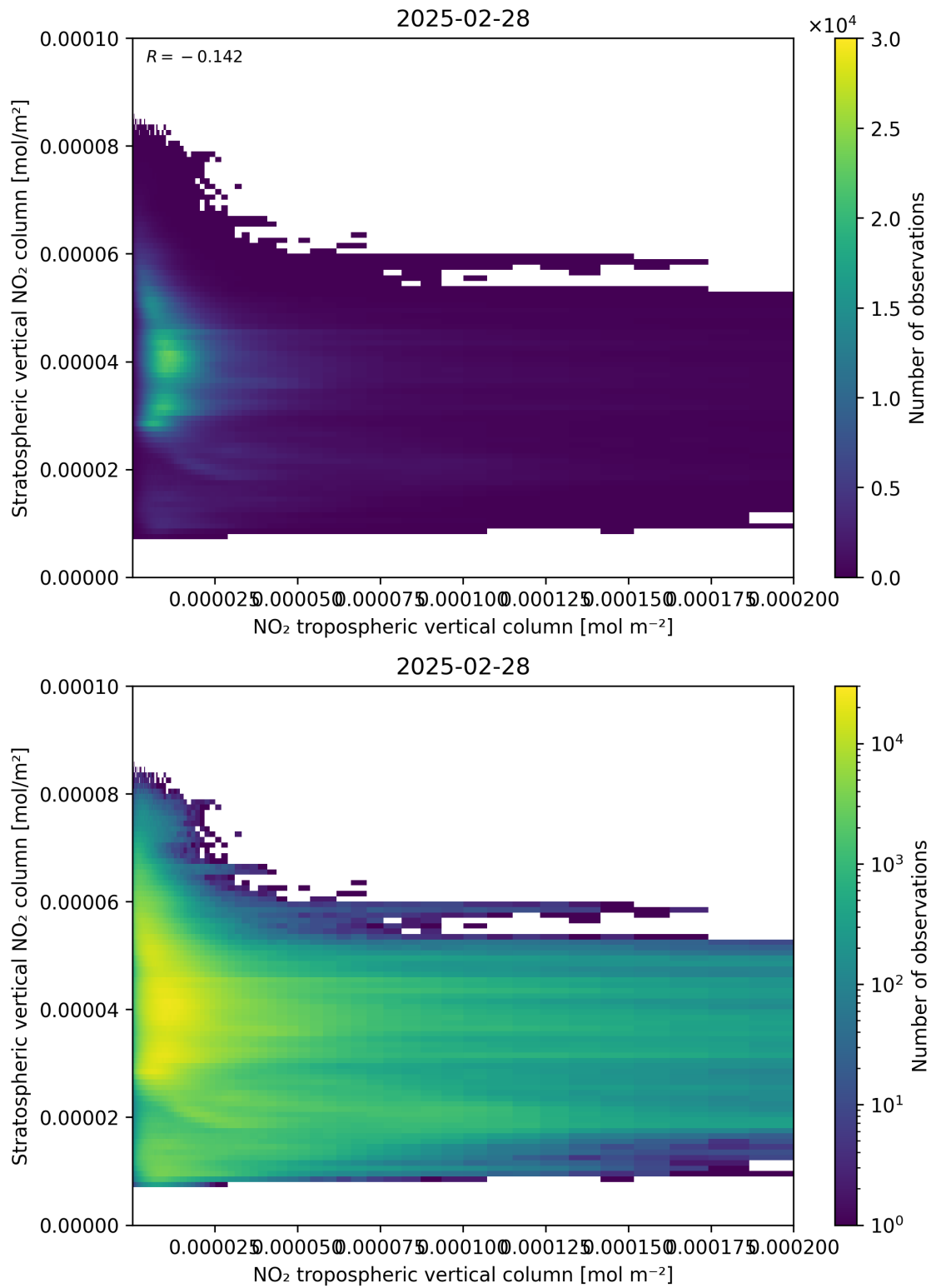
Figure 125: Scatter density plot of “NO 2 tropospheric vertical column” against “Stratospheric vertical NO 2 column” for 2025-02-27 to 2025-03-01.
