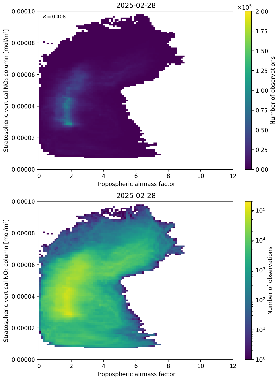
Figure 74: Scatter density plot of “Tropospheric air mass factor” against “Stratospheric vertical NO 2 column” for 2025-02-27 to 2025-03-01.
