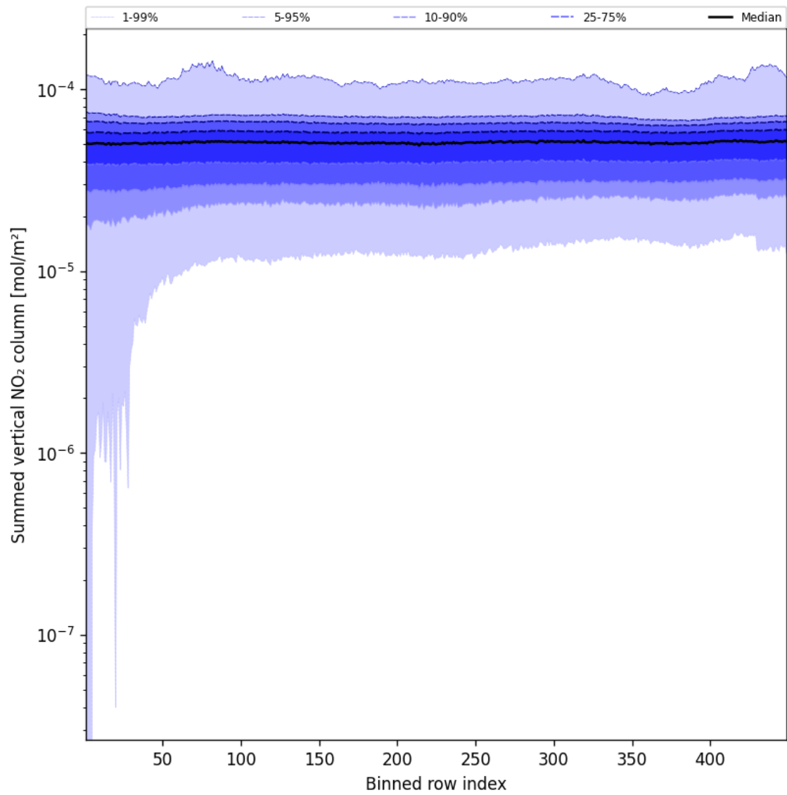
Figure 57: Along track statistics of “Summed vertical NO 2 column” for 2025-02-27 to 2025-03-01
