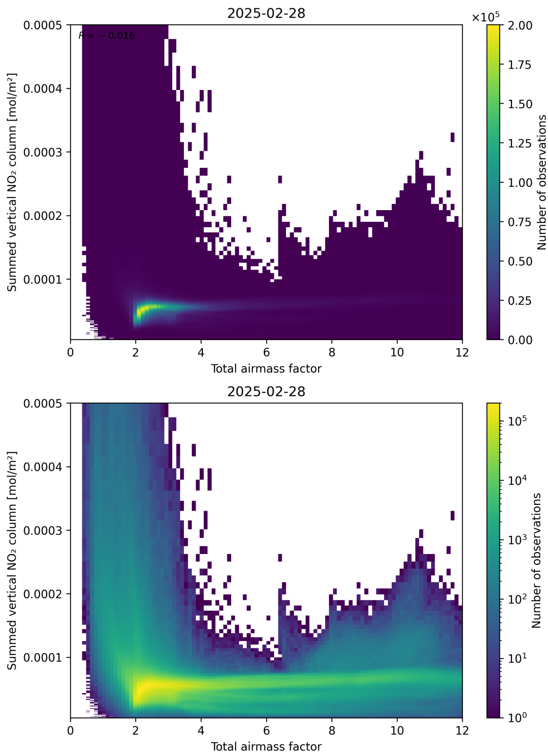
Figure 65: Scatter density plot of “Total airmass factor” against “Summed vertical NO 2 column” for 2025-02-27 to 2025-03-01.
