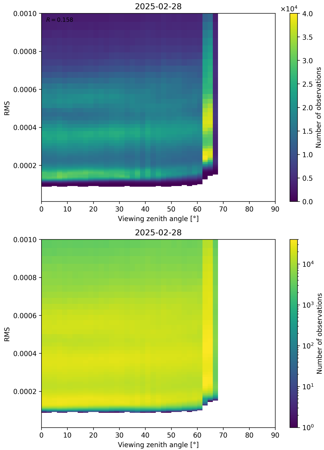
Figure 171: Scatter density plot of “Viewing zenith angle” against “RMS” for 2025-02-27 to 2025-03-01.
