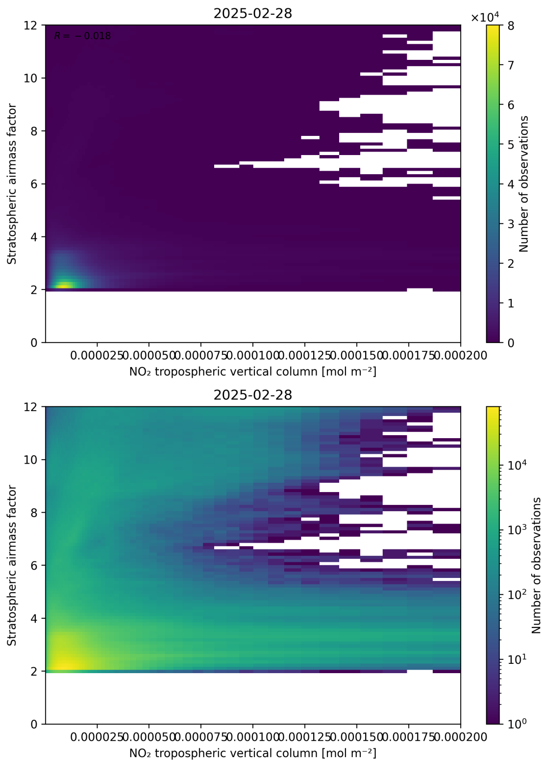
Figure 121: Scatter density plot of “NO 2 tropospheric vertical column” against “Stratospheric air mass factor” for 2025-02-27 to 2025-03-01.
