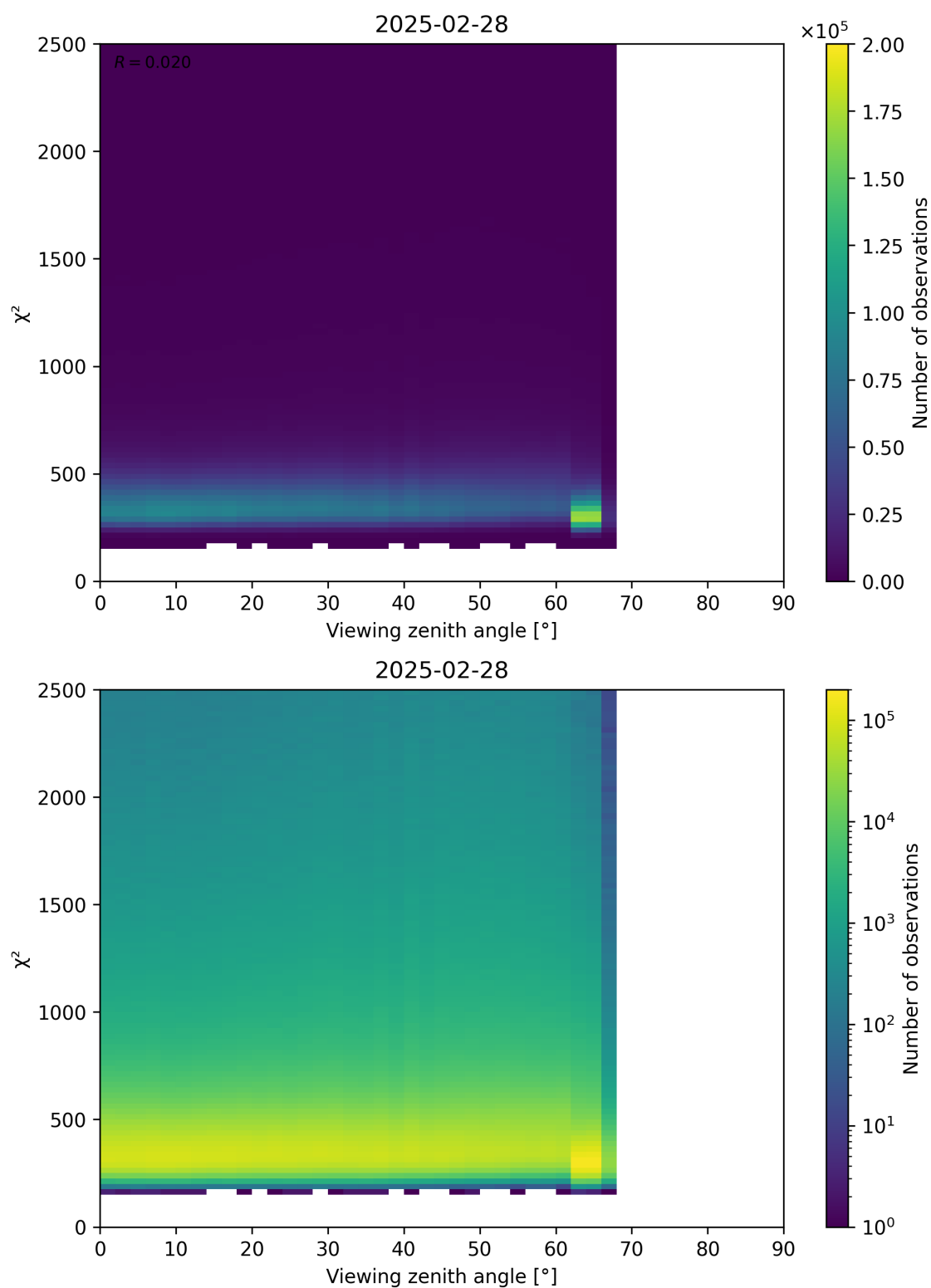
Figure 162: Scatter density plot of “Viewing zenith angle” against “ \chi^2 ” for 2025-02-27 to 2025-03-01.
