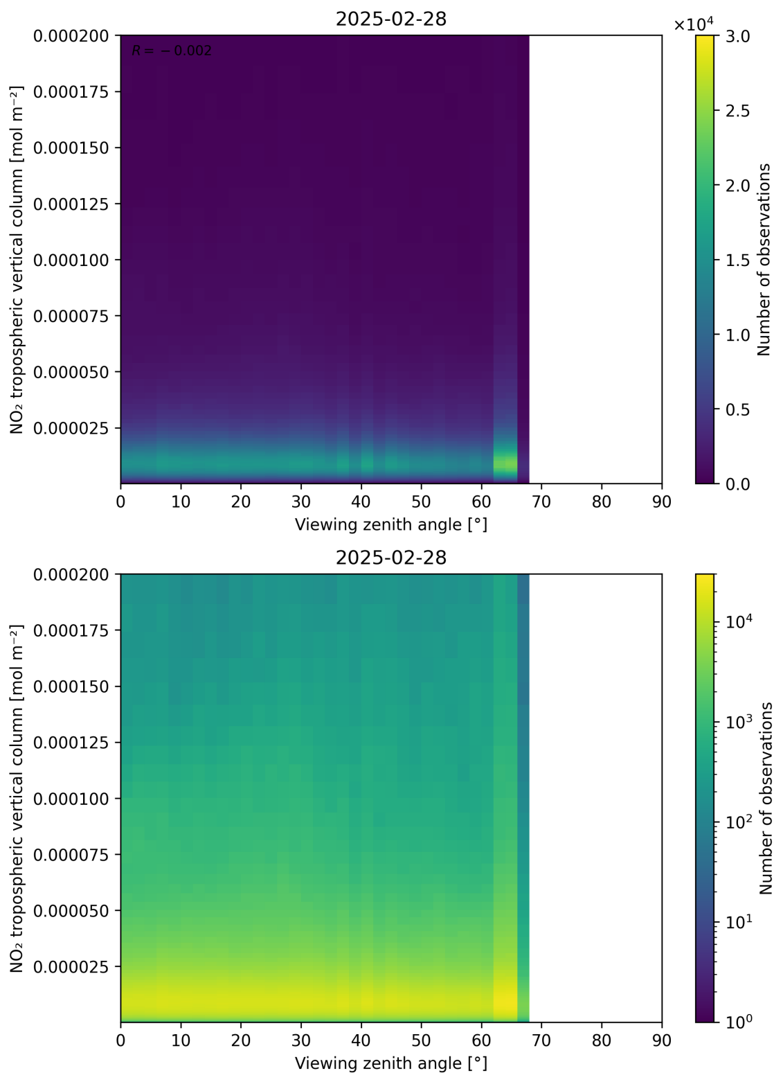
Figure 169: Scatter density plot of “Viewing zenith angle” against “NO 2 tropospheric vertical column” for 2025-02-27 to 2025-03-01.
