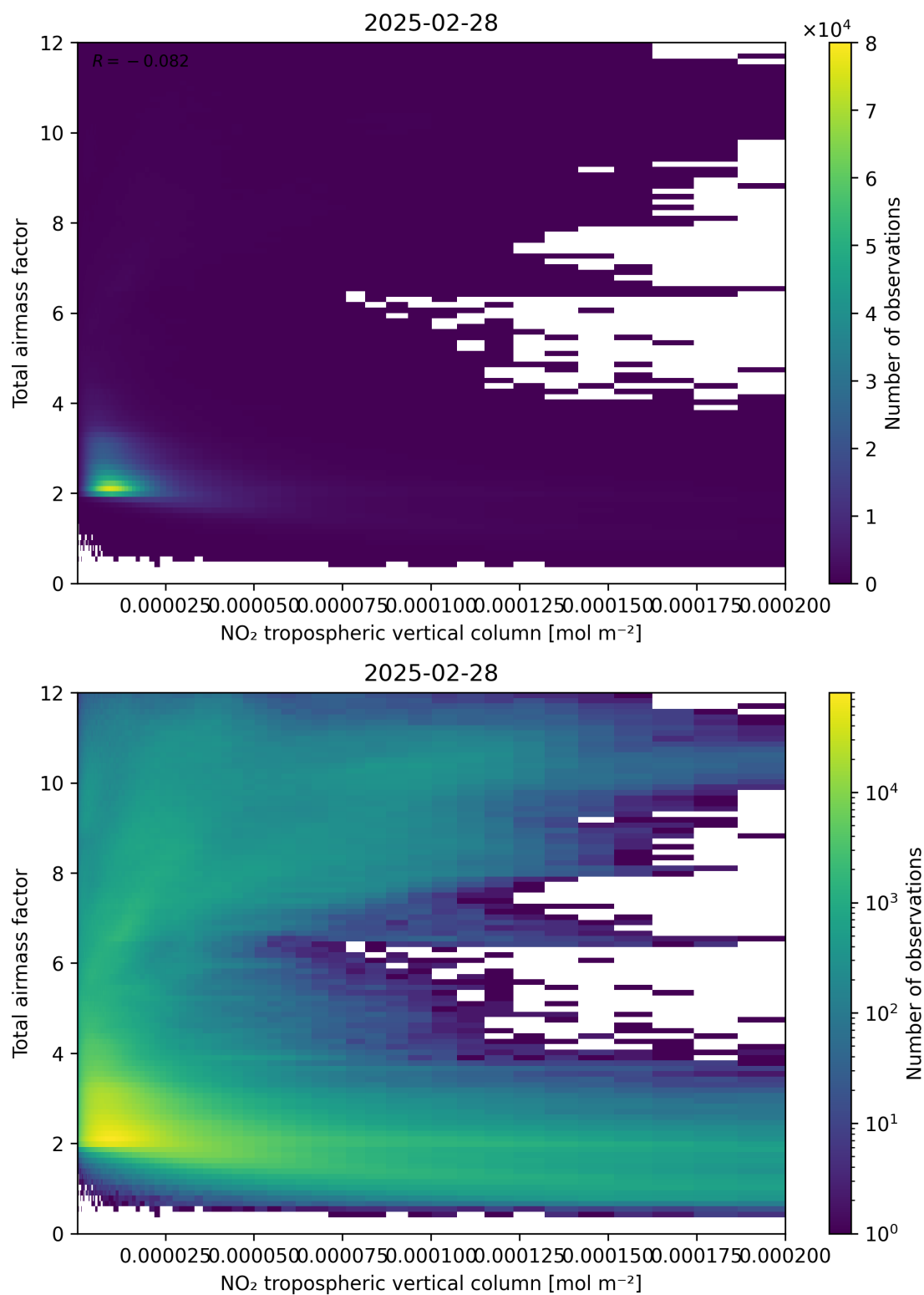
Figure 122: Scatter density plot of “NO 2 tropospheric vertical column” against “Total air mass factor” for 2025-02-27 to 2025-03-01.
