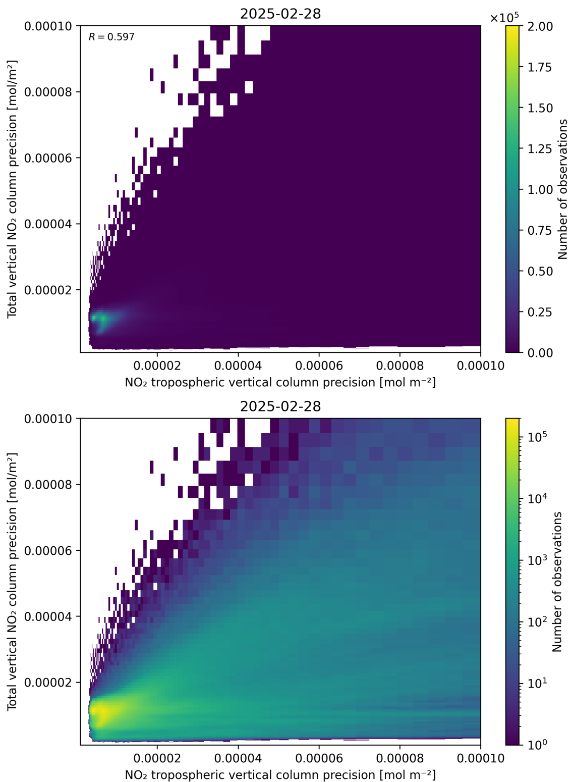
Figure 139: Scatter density plot of “NO 2 tropospheric vertical column precision” against “Total vertical NO 2 column precision” for 2025-02-27 to 2025-03-01.
