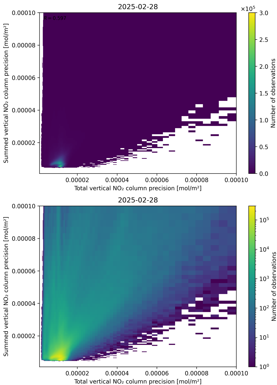
Figure 118: Scatter density plot of “Total vertical NO 2 column precision” against “Summed vertical NO 2 column precision” for 2025-02-27 to 2025-03-01.
