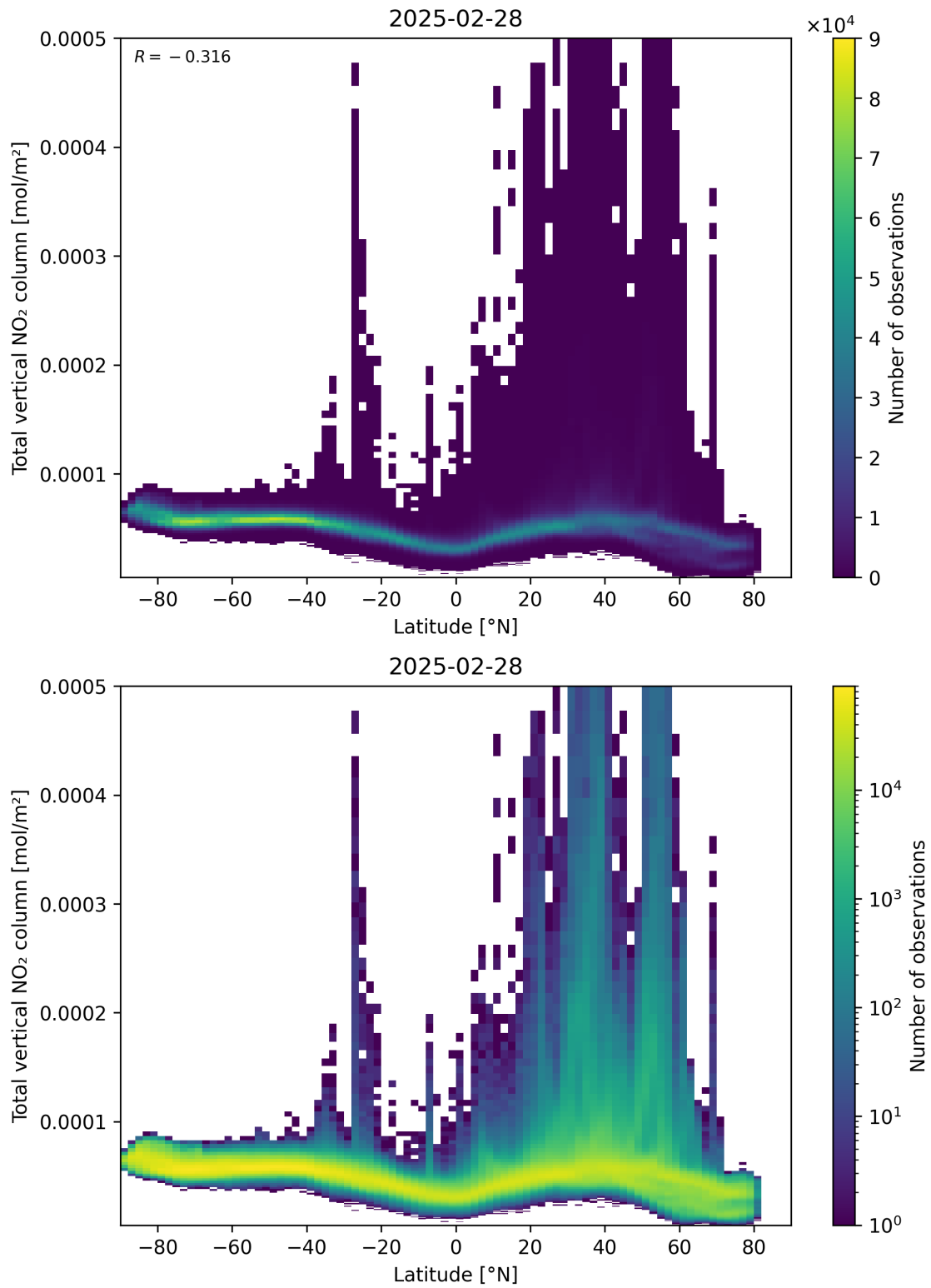
Figure 90: Scatter density plot of “Latitude” against “Total vertical NO 2 column” for 2025-02-27 to 2025-03-01.
