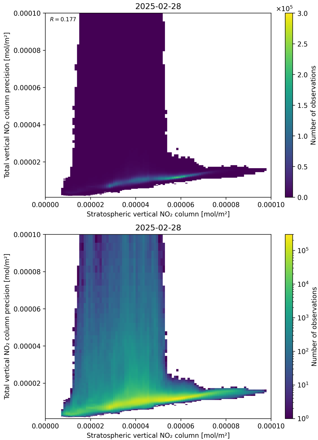
Figure 101: Scatter density plot of “Stratospheric vertical NO 2 column” against “Total vertical NO 2 column precision” for 2025-02-27 to 2025-03-01.
