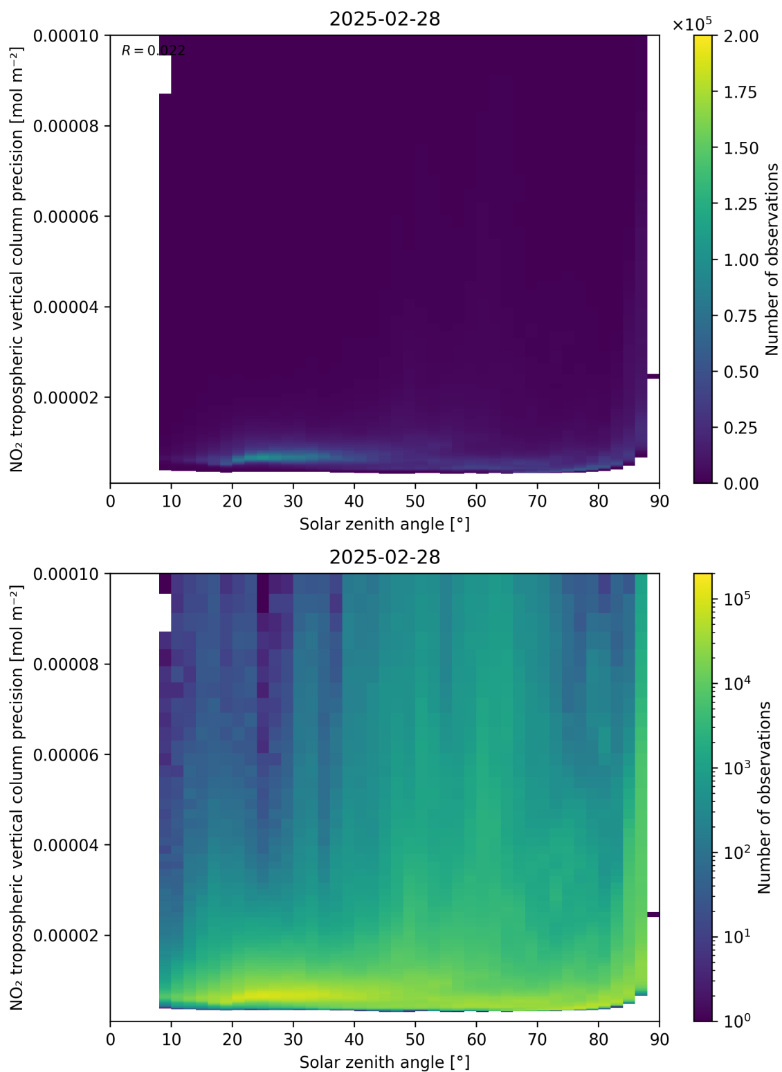
Figure 156: Scatter density plot of “Solar zenith angle” against “NO 2 tropospheric vertical column precision” for 2025-02-27 to 2025-03-01.
