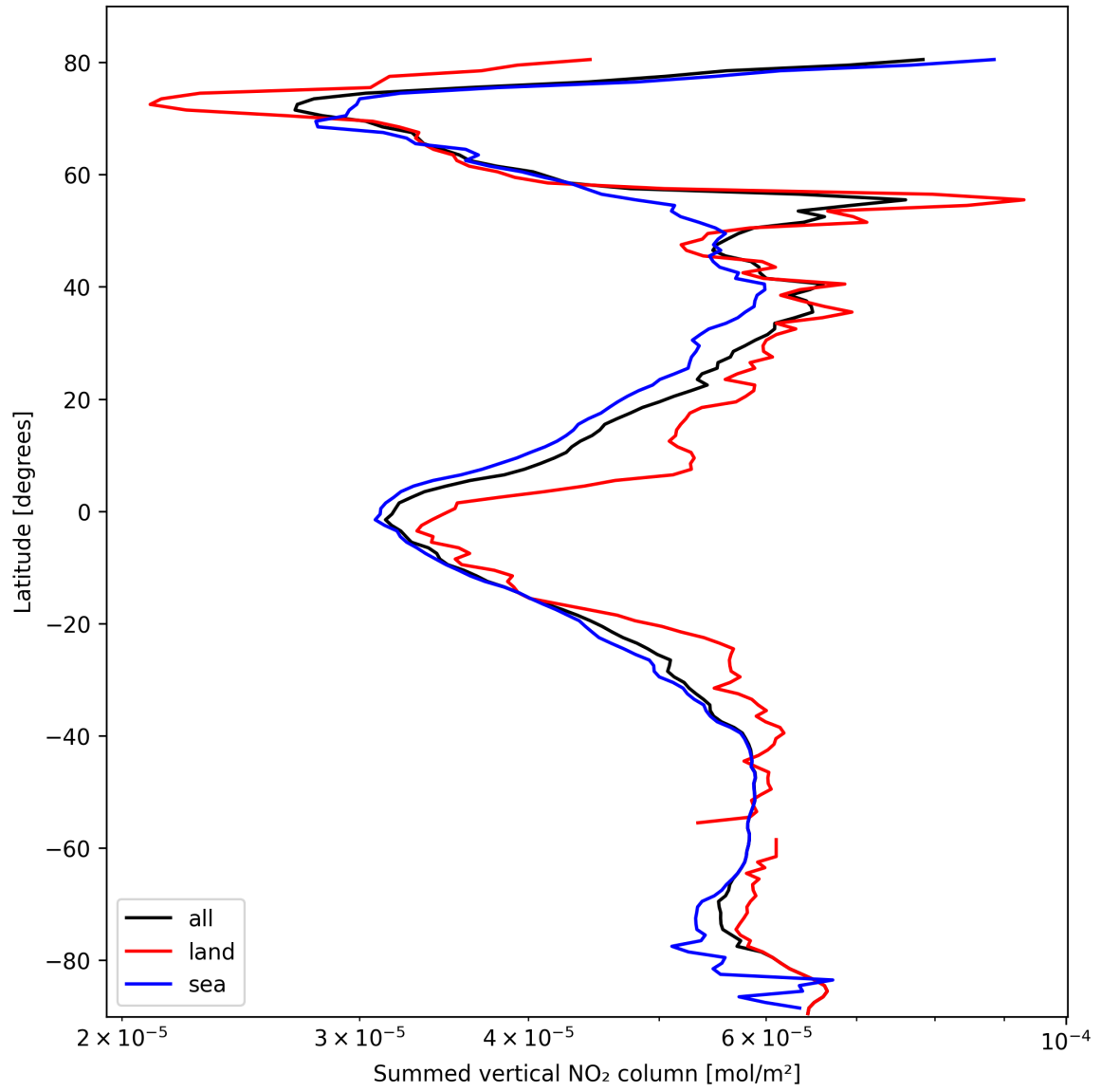
Figure 23: Zonal average of “Summed vertical NO 2 column” for 2025-02-27 to 2025-03-01.
