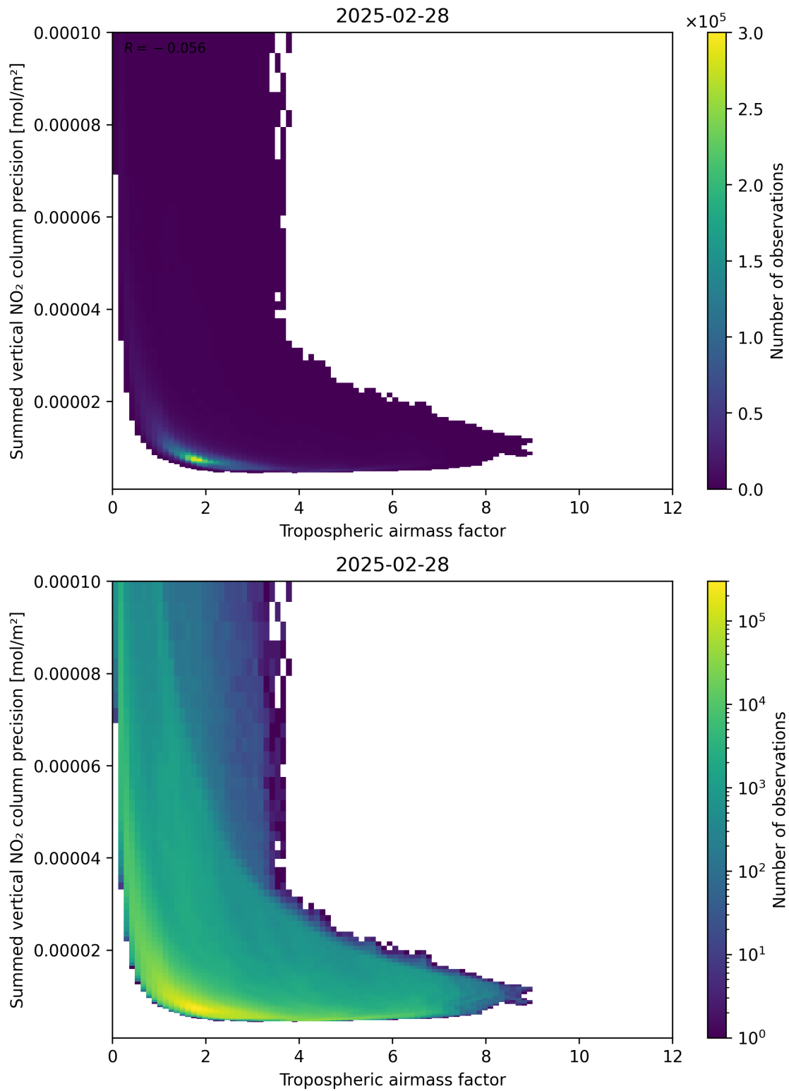
Figure 76: Scatter density plot of “Tropospheric air mass factor” against “Summed vertical NO 2 column precision” for 2025-02-27 to 2025-03-01.
