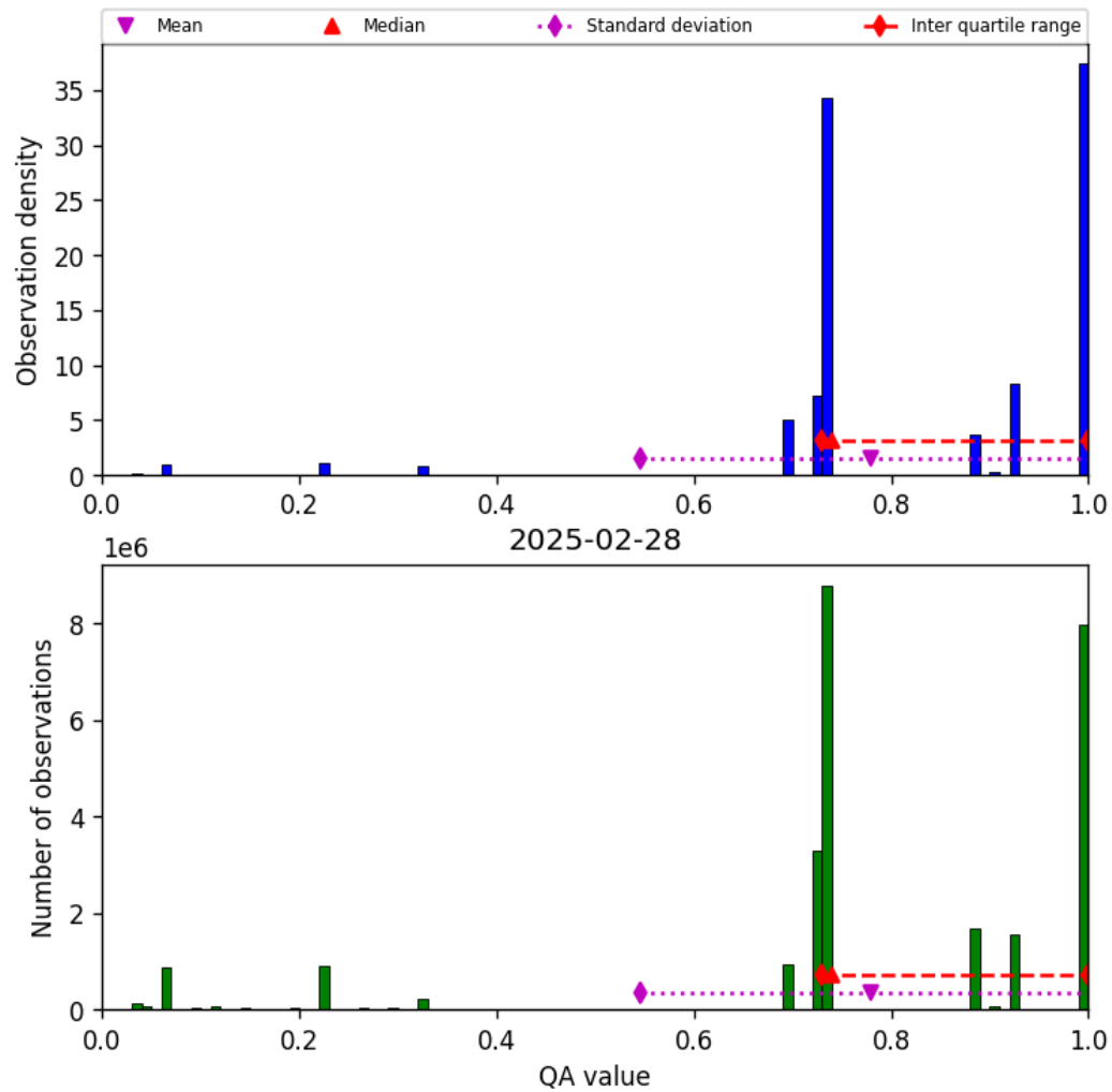
Figure 28: Histogram of “QA value” for 2025-02-27 to 2025-03-01
