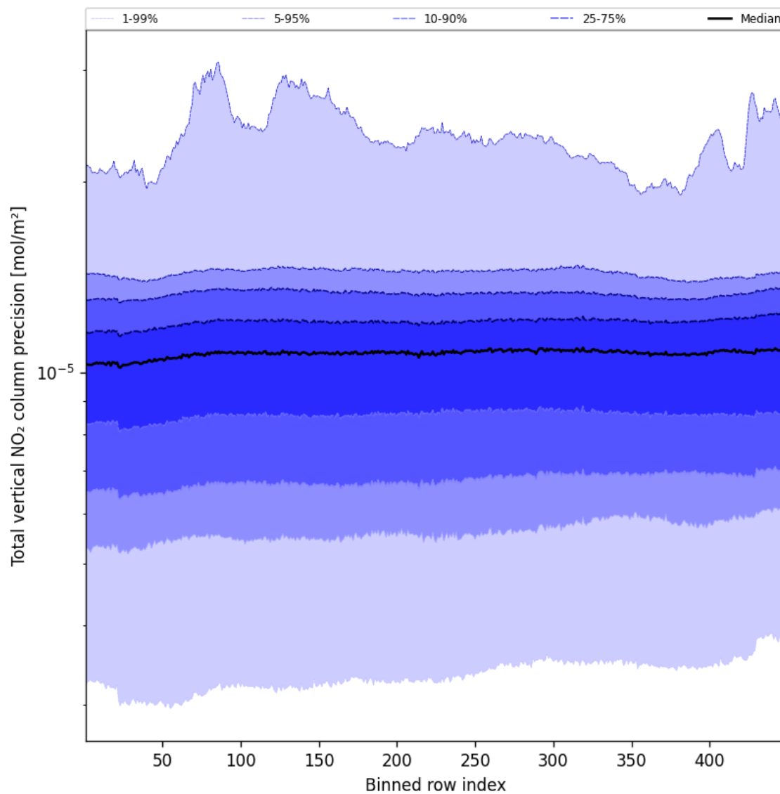
Figure 56: Along track statistics of “Total vertical NO 2 column precision” for 2025-02-27 to 2025-03-01
