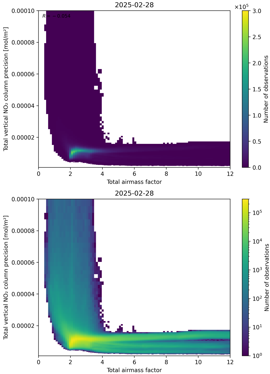
Figure 68: Scatter density plot of “Total airmass factor” against “Total vertical NO 2 column precision” for 2025-02-27 to 2025-03-01.
