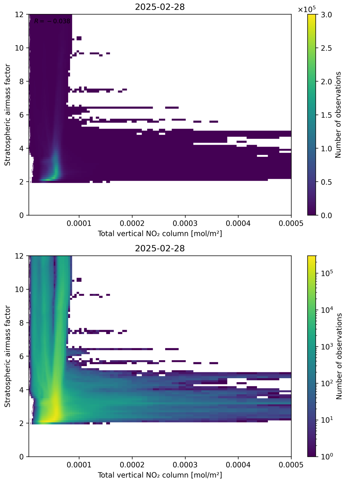
Figure 110: Scatter density plot of “Total vertical NO 2 column” against “Stratospheric airmass factor” for 2025-02-27 to 2025-03-01.
