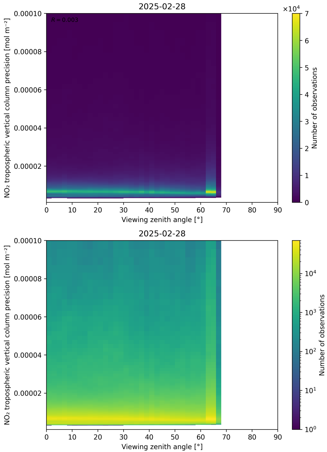
Figure 170: Scatter density plot of “Viewing zenith angle” against “NO 2 tropospheric vertical column precision” for 2025-02-27 to 2025-03-01.
