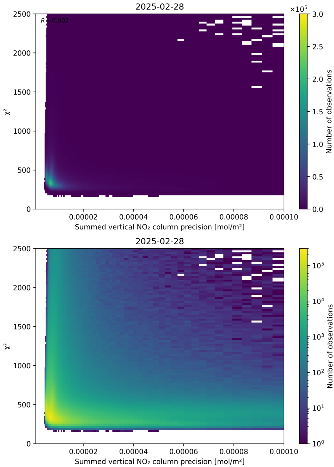
Figure 107: Scatter density plot of “Summed vertical NO 2 column precision” against “ \chi^2 ” for 2025-02-27 to 2025-03-01.
