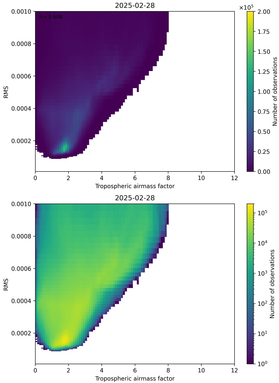
Figure 79: Scatter density plot of “Tropospheric airmass factor” against “RMS” for 2025-02-27 to 2025-03-01.
