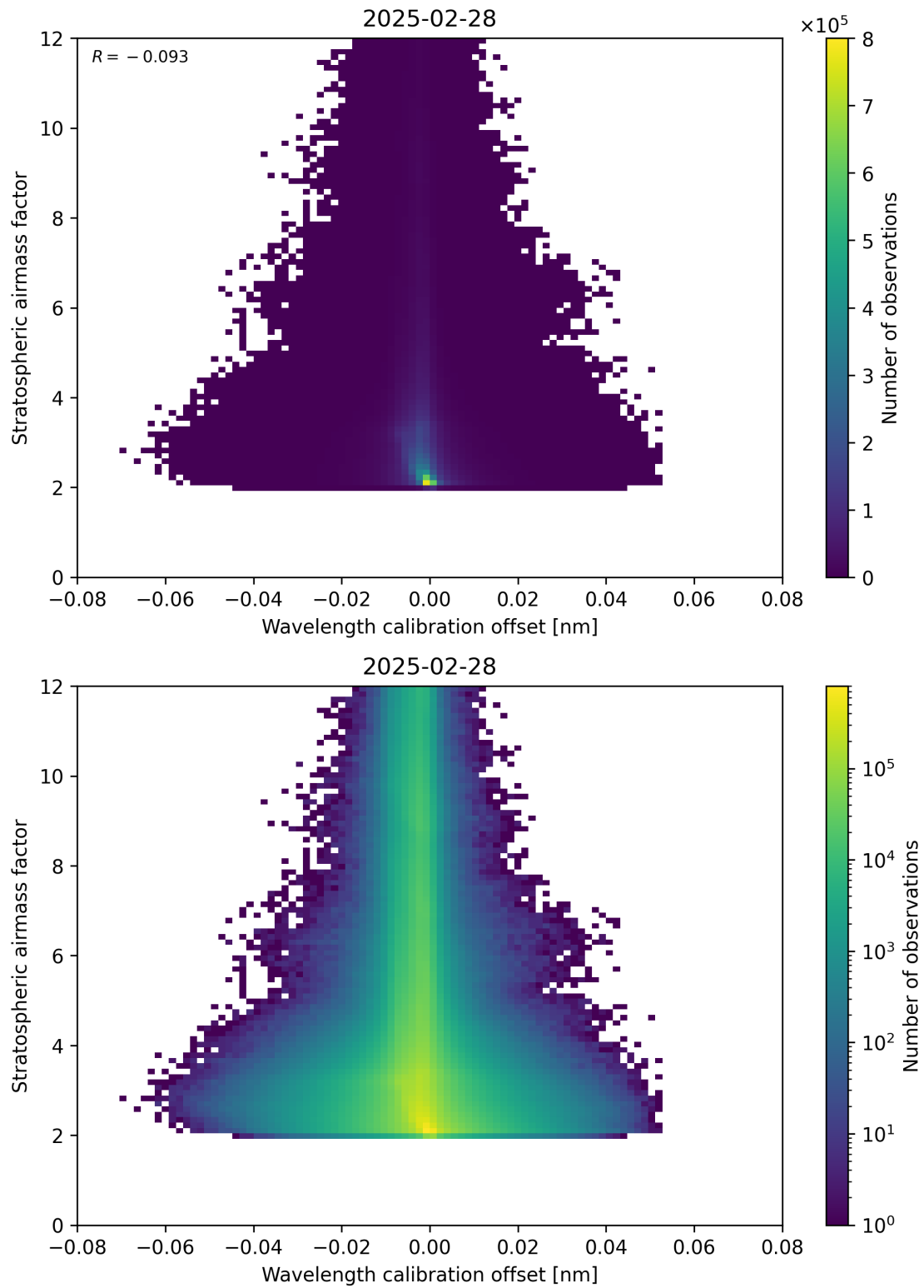
Figure 174: Scatter density plot of “Wavelength calibration offset” against “Stratospheric air mass factor” for 2025-02-27 to 2025-03-01.
