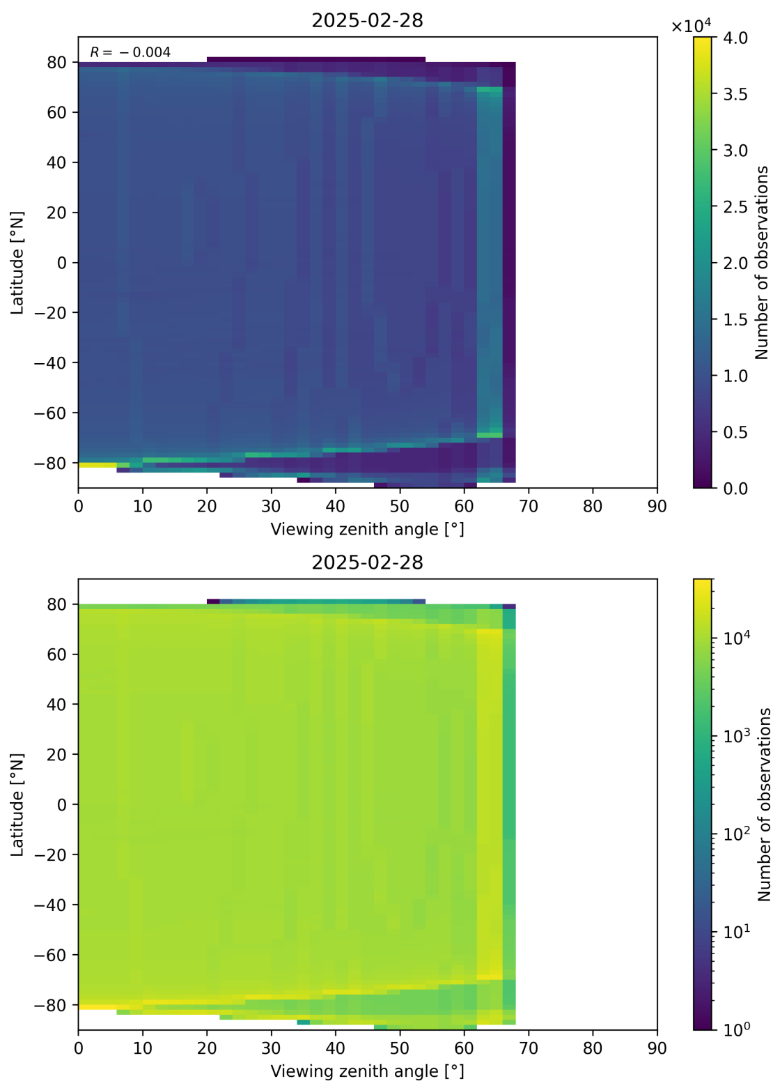
Figure 163: Scatter density plot of “Viewing zenith angle” against “Latitude” for 2025-02-27 to 2025-03-01.
