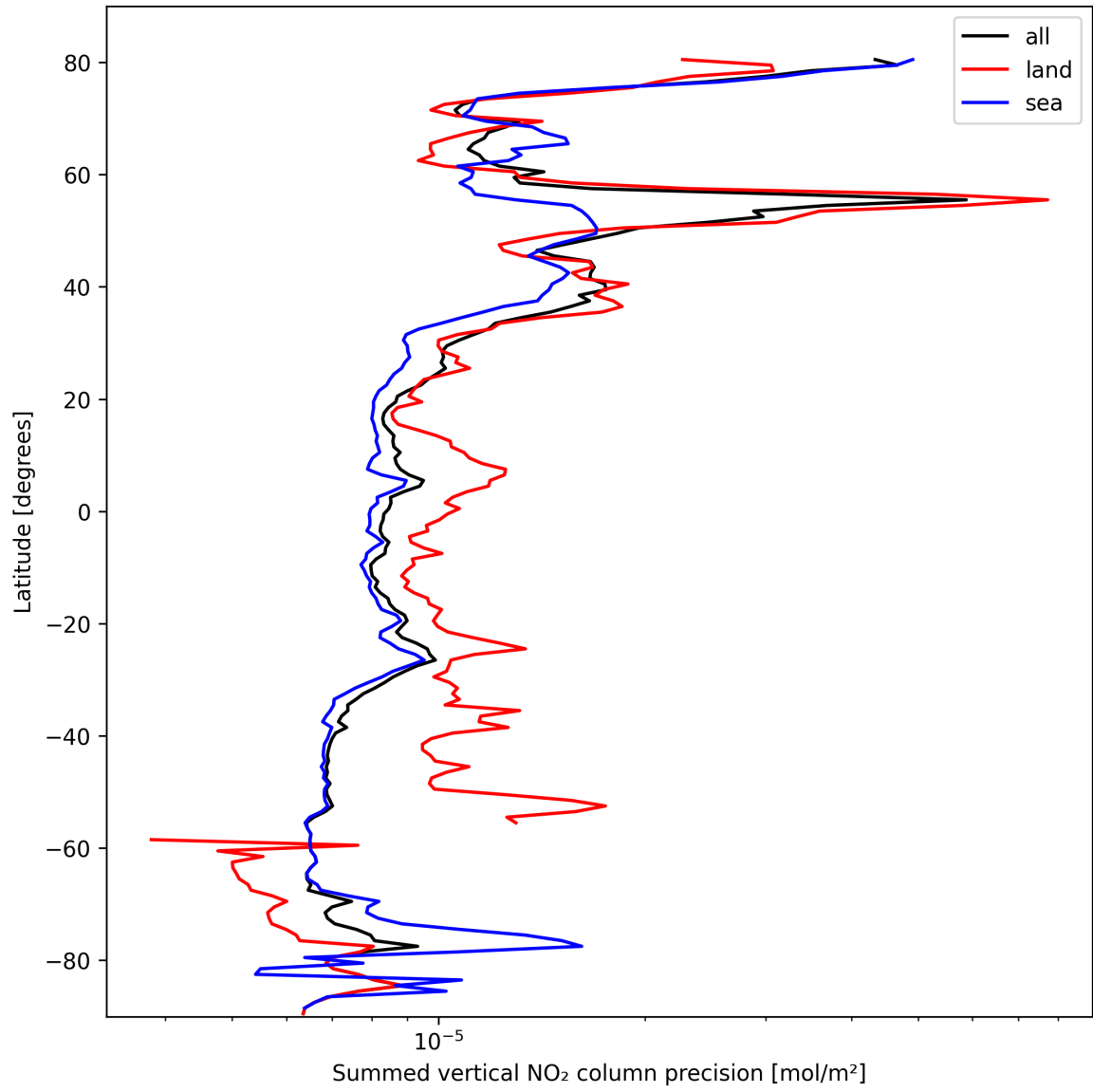
Figure 24: Zonal average of “Summed vertical NO 2 column precision” for 2025-02-27 to 2025-03-01.
