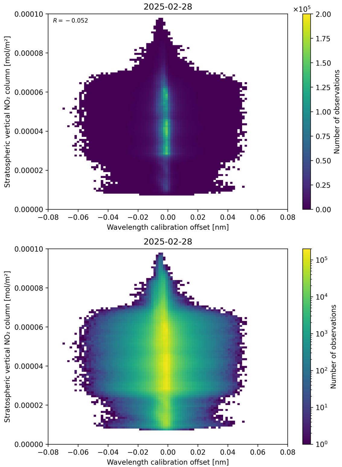
Figure 176: Scatter density plot of “Wavelength calibration offset” against “Stratospheric vertical NO 2 column” for 2025-02-27 to 2025-03-01.
