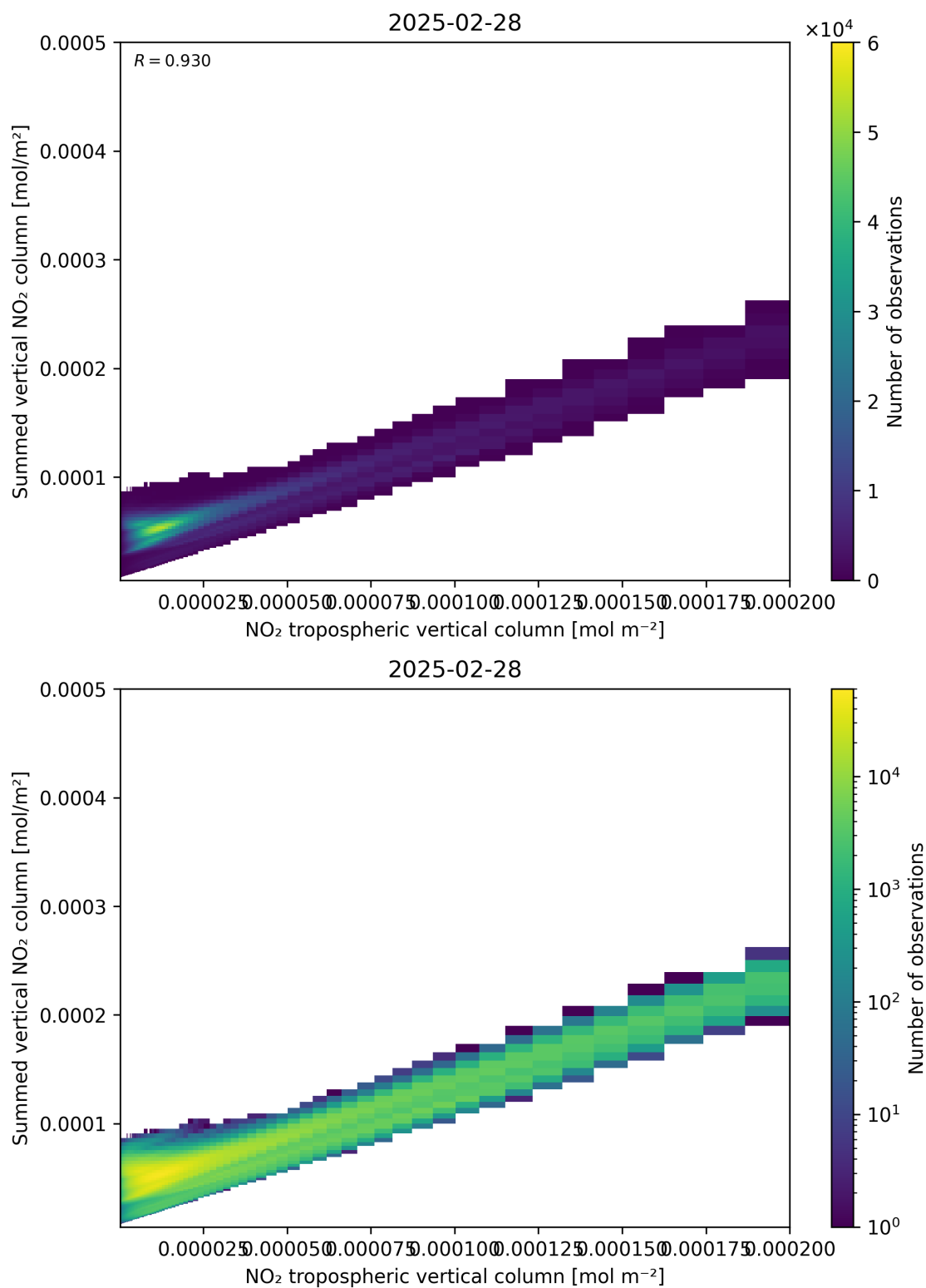
Figure 126: Scatter density plot of “NO 2 tropospheric vertical column” against “Summed vertical NO 2 column” for 2025-02-27 to 2025-03-01.
