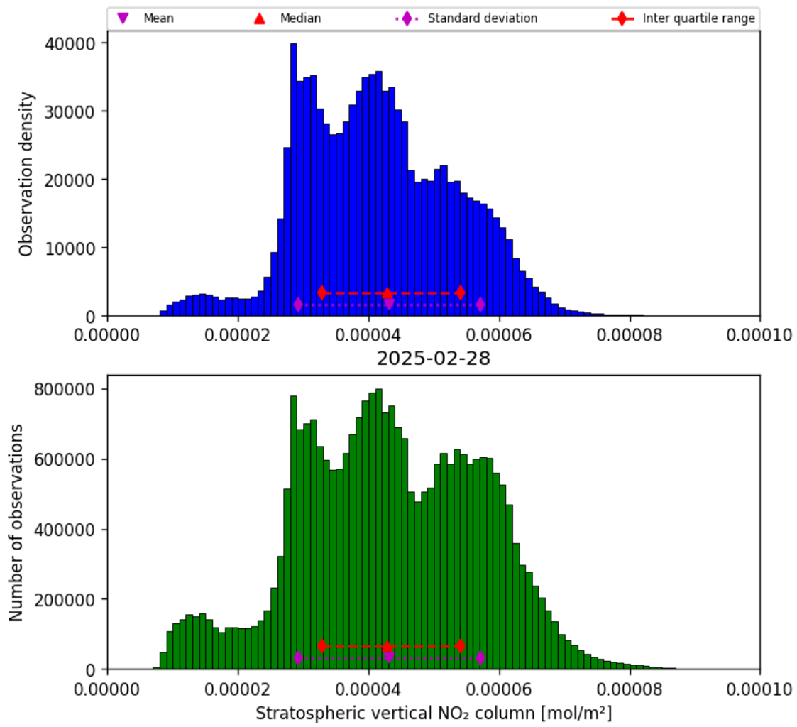
Figure 36: Histogram of “Stratospheric vertical NO 2 column” for 2025-02-27 to 2025-03-01
