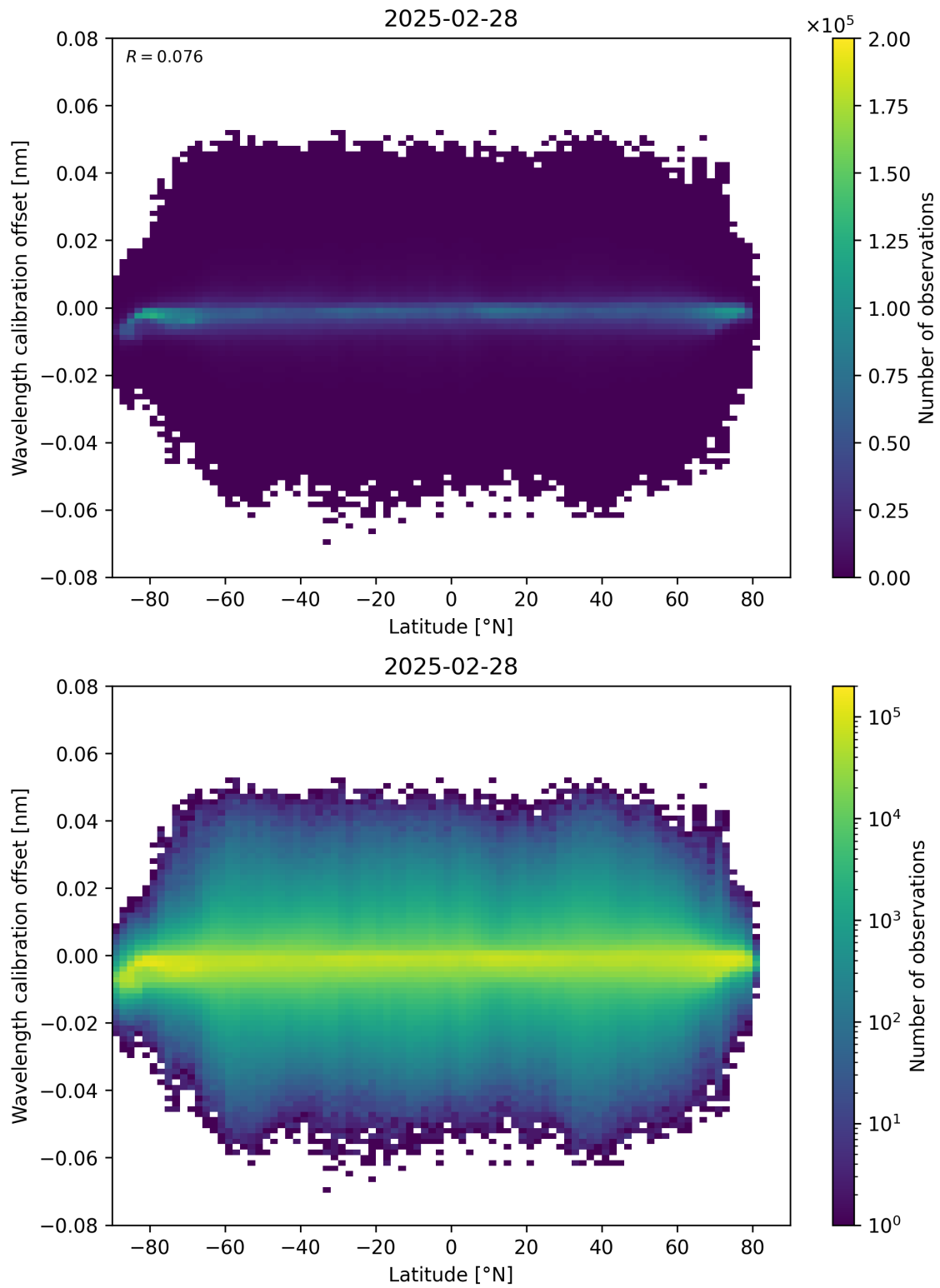
Figure 95: Scatter density plot of “Latitude” against “Wavelength calibration offset” for 2025-02-27 to 2025-03-01.
