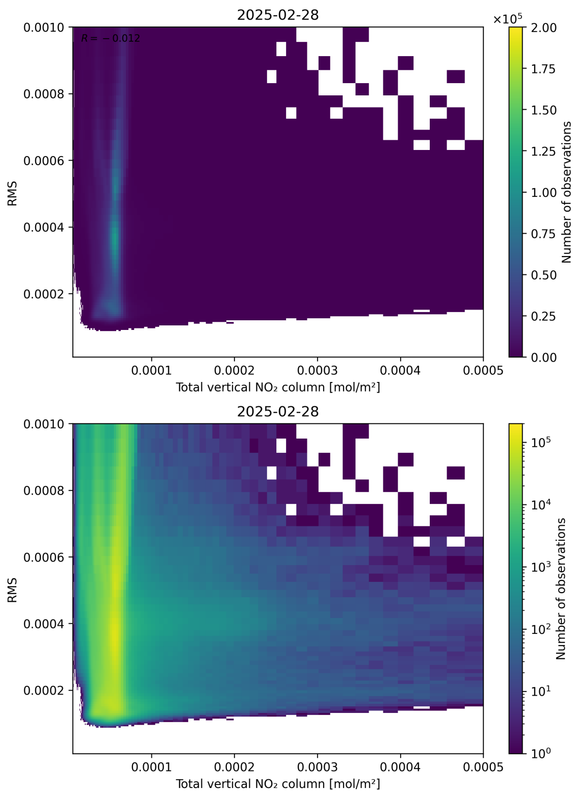
Figure 120: Scatter density plot of “Total vertical NO 2 column” against “RMS” for 2025-02-27 to 2025-03-01.
