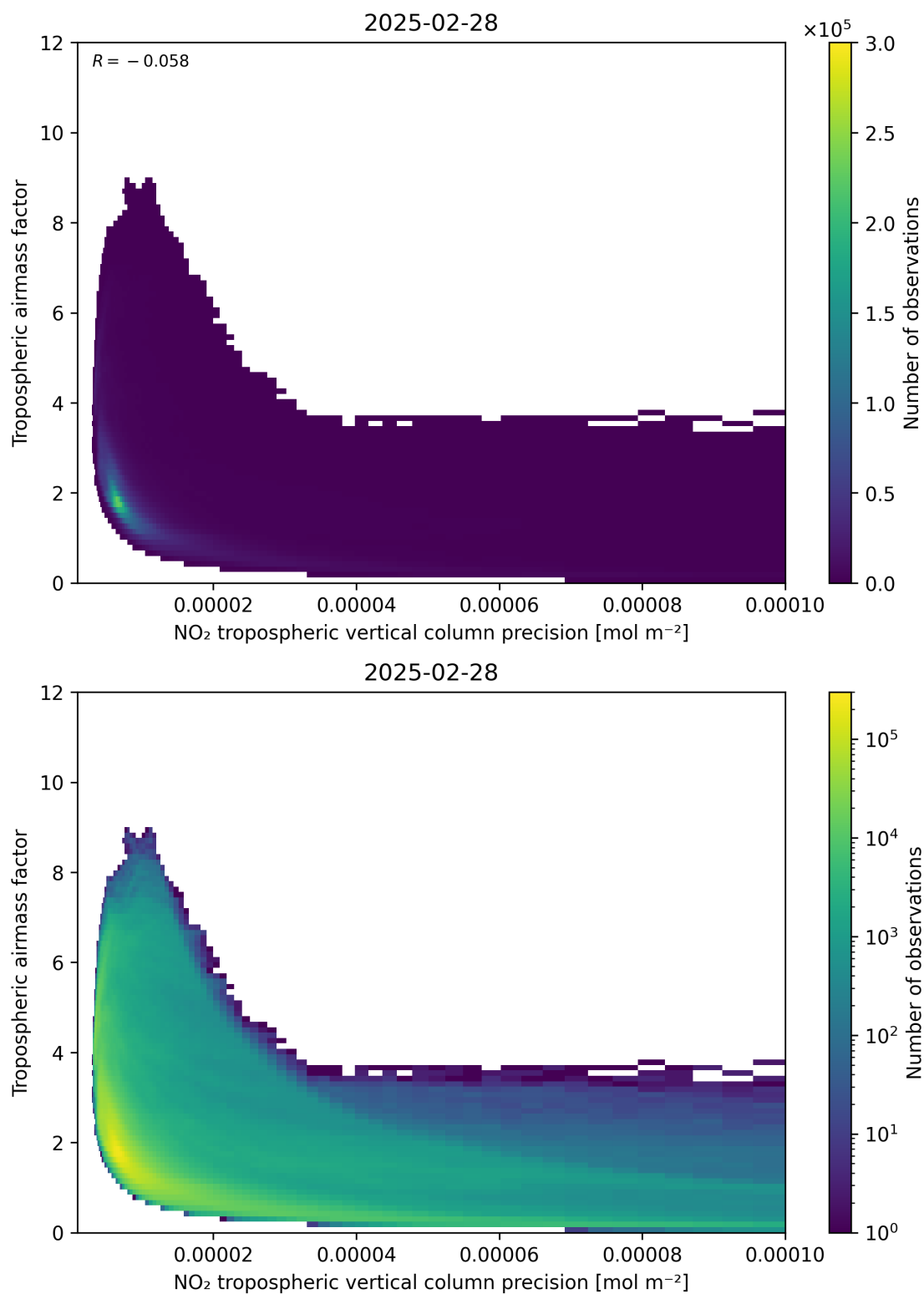
Figure 133: Scatter density plot of “NO 2 tropospheric vertical column precision” against “Tropospheric air mass factor” for 2025-02-27 to 2025-03-01.
