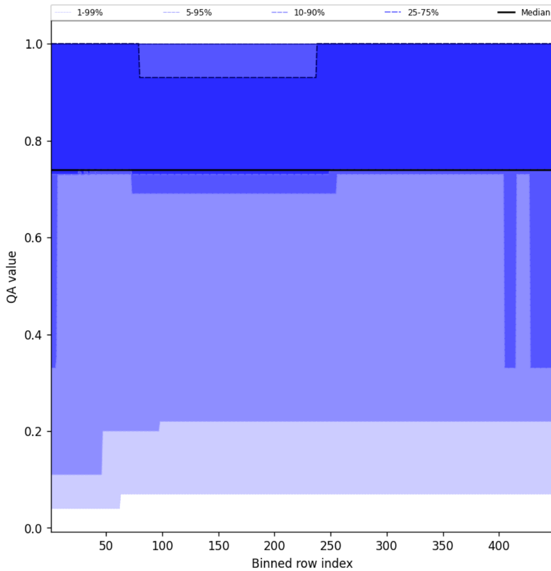
Figure 45: Along track statistics of “QA value” for 2025-02-27 to 2025-03-01
