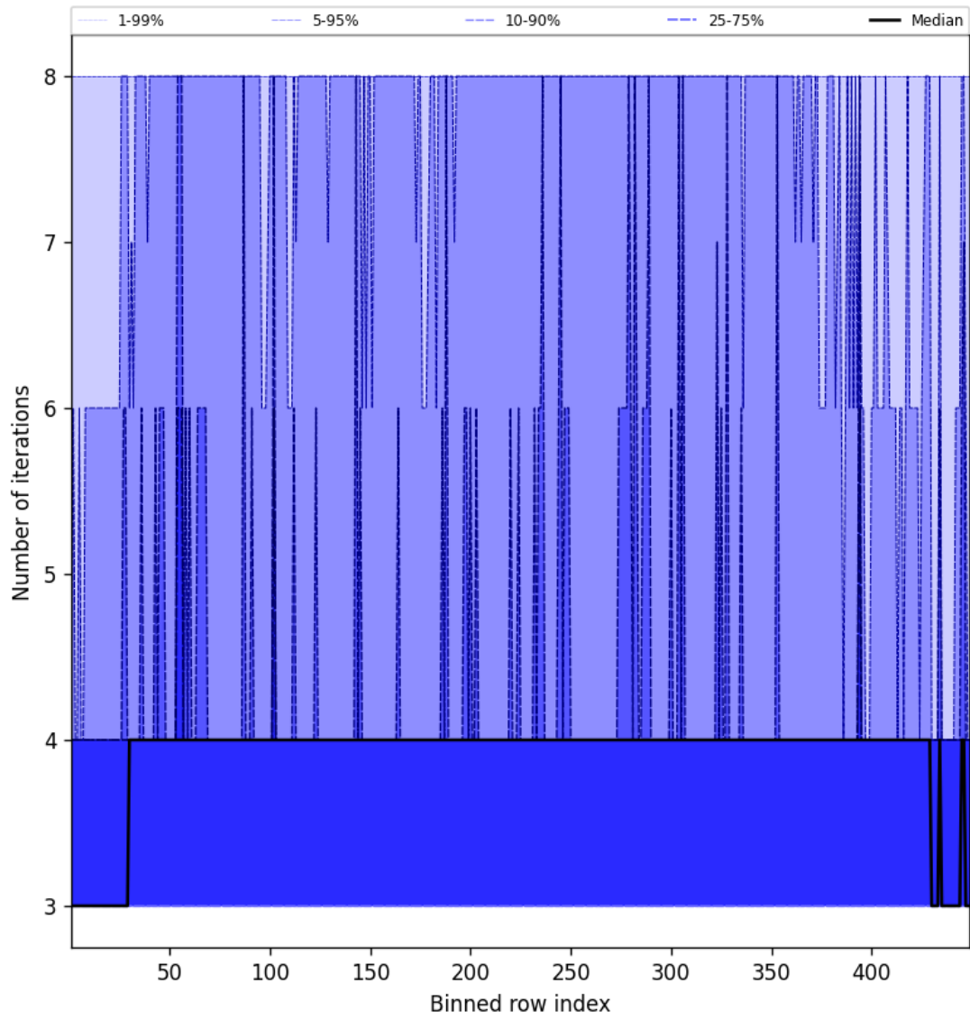
Figure 51: Along track statistics of “Number of iterations” for 2025-02-27 to 2025-03-01
