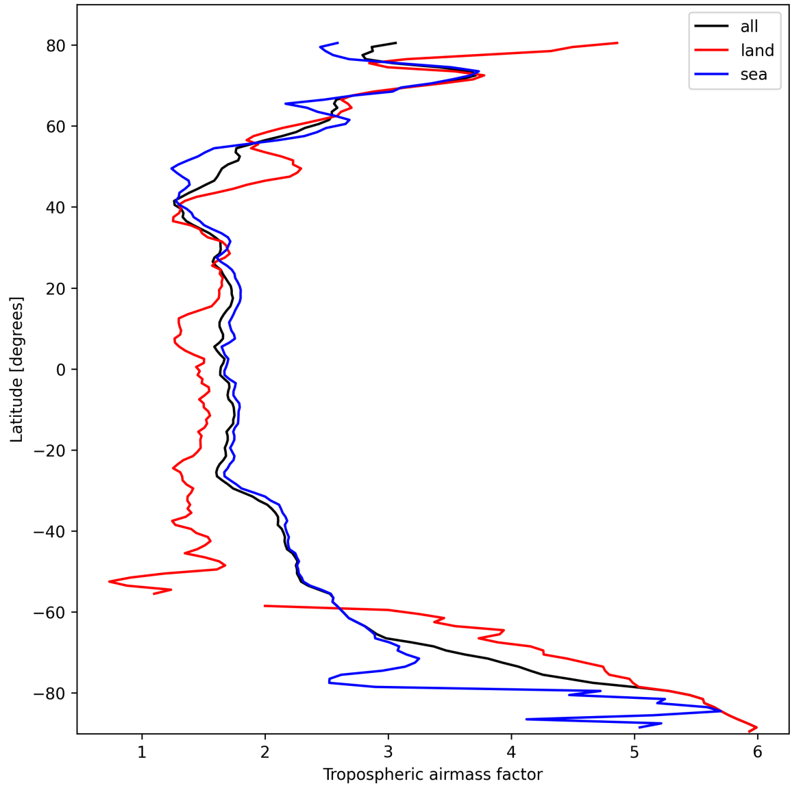
Figure 14: Zonal average of “Tropospheric air mass factor” for 2025-02-27 to 2025-03-01.
