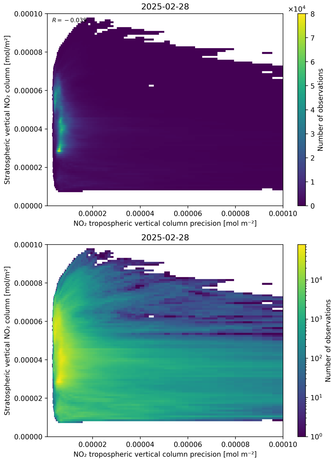
Figure 135: Scatter density plot of “NO 2 tropospheric vertical column precision” against “Stratospheric vertical NO 2 column” for 2025-02-27 to 2025-03-01.
