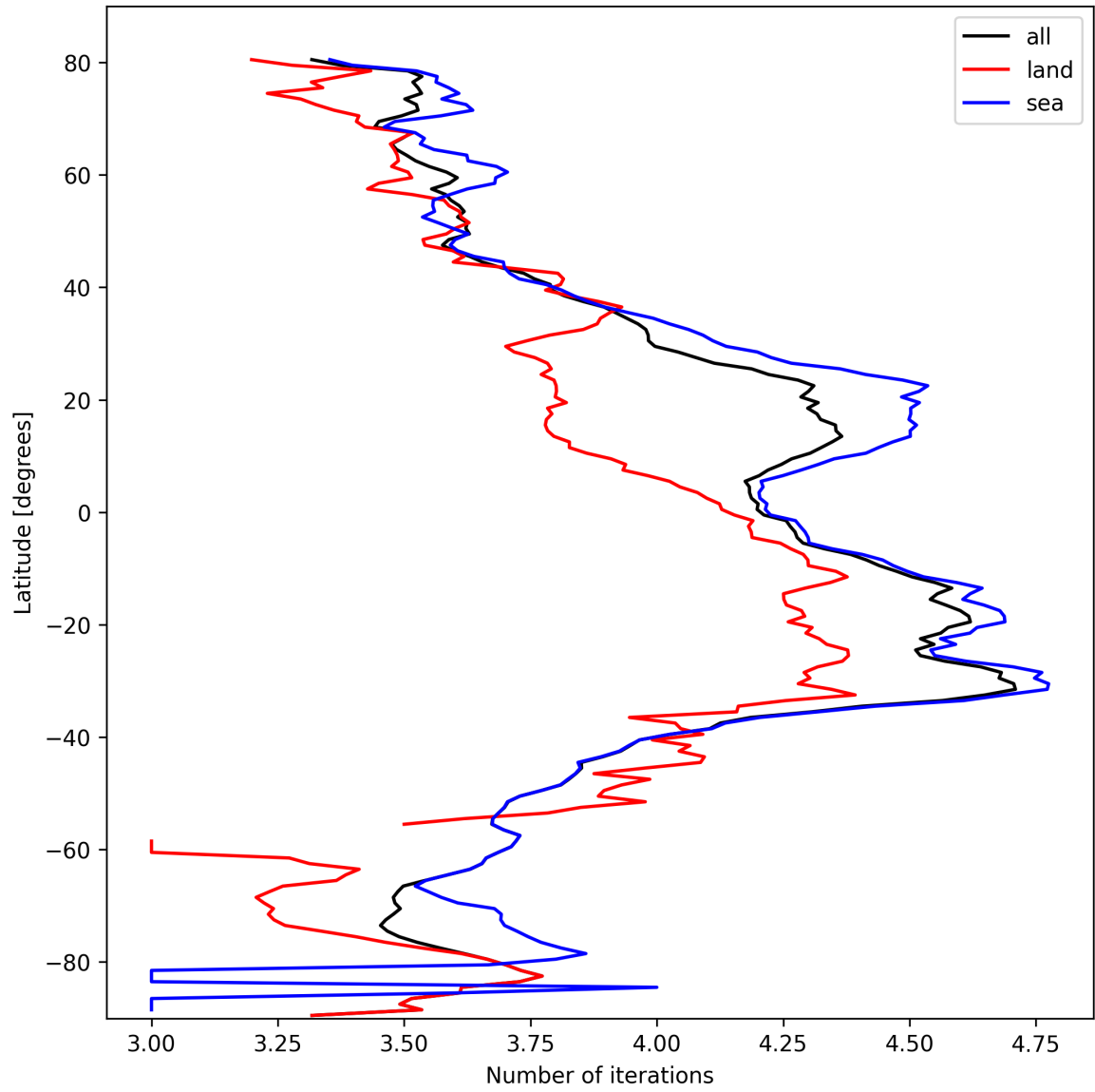
Figure 17: Zonal average of “Number of iterations” for 2025-02-27 to 2025-03-01.
