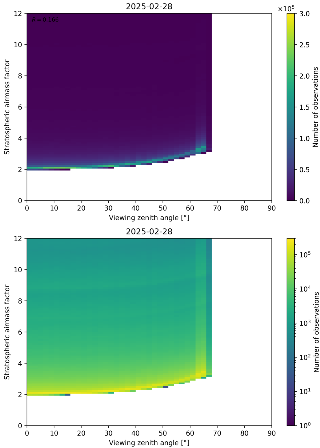
Figure 159: Scatter density plot of “Viewing zenith angle” against “Stratospheric airmass factor” for 2025-02-27 to 2025-03-01.
