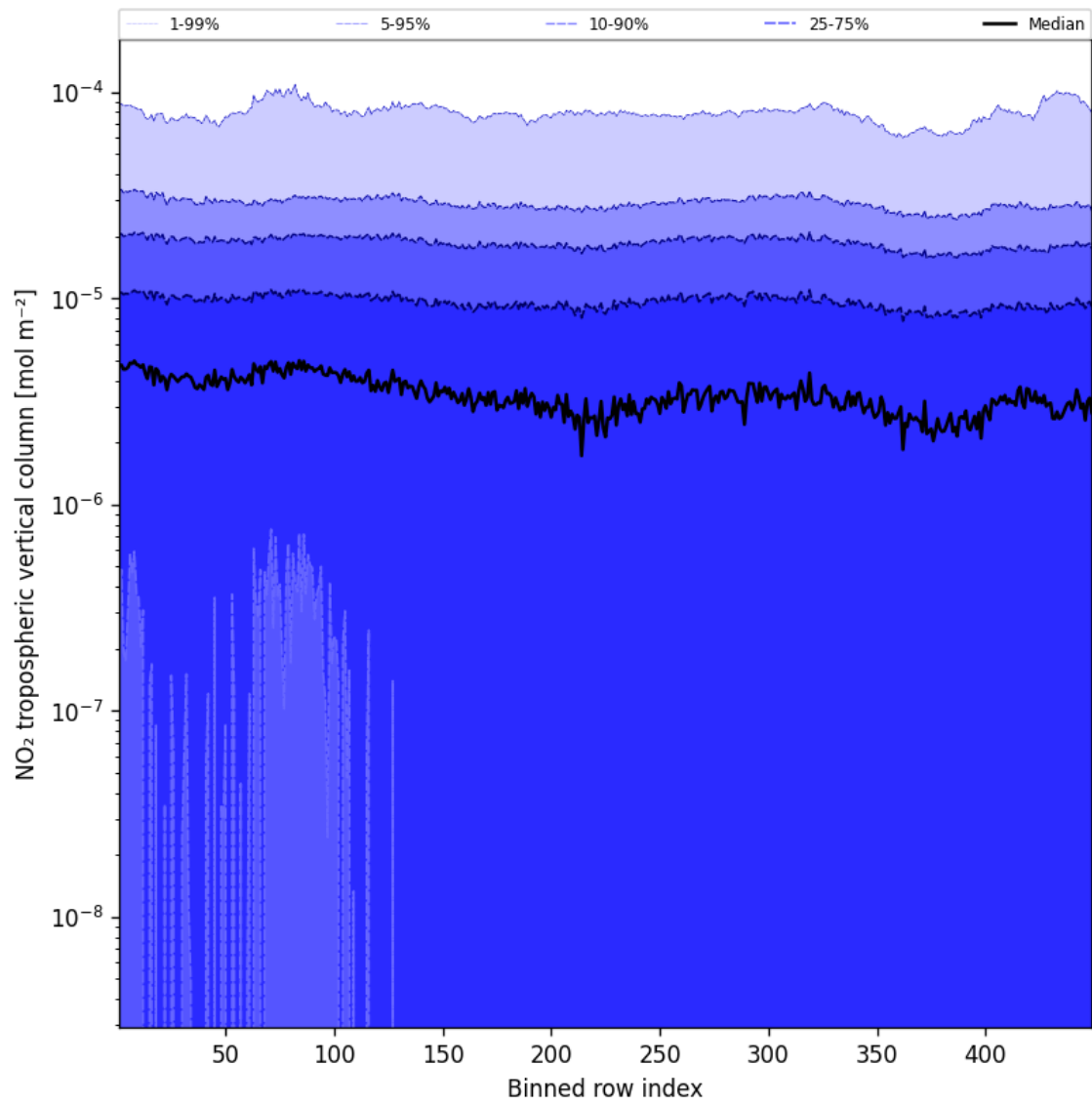
Figure 46: Along track statistics of “NO 2 tropospheric vertical column” for 2025-02-27 to 2025-03-01
