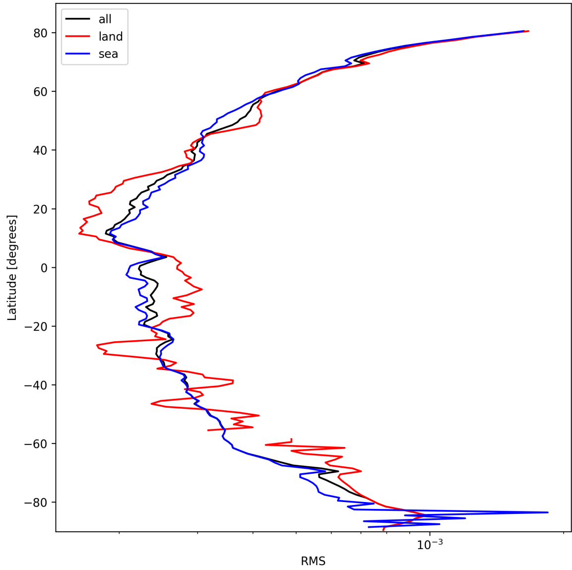
Figure 26: Zonal average of “RMS” for 2025-02-27 to 2025-03-01.
