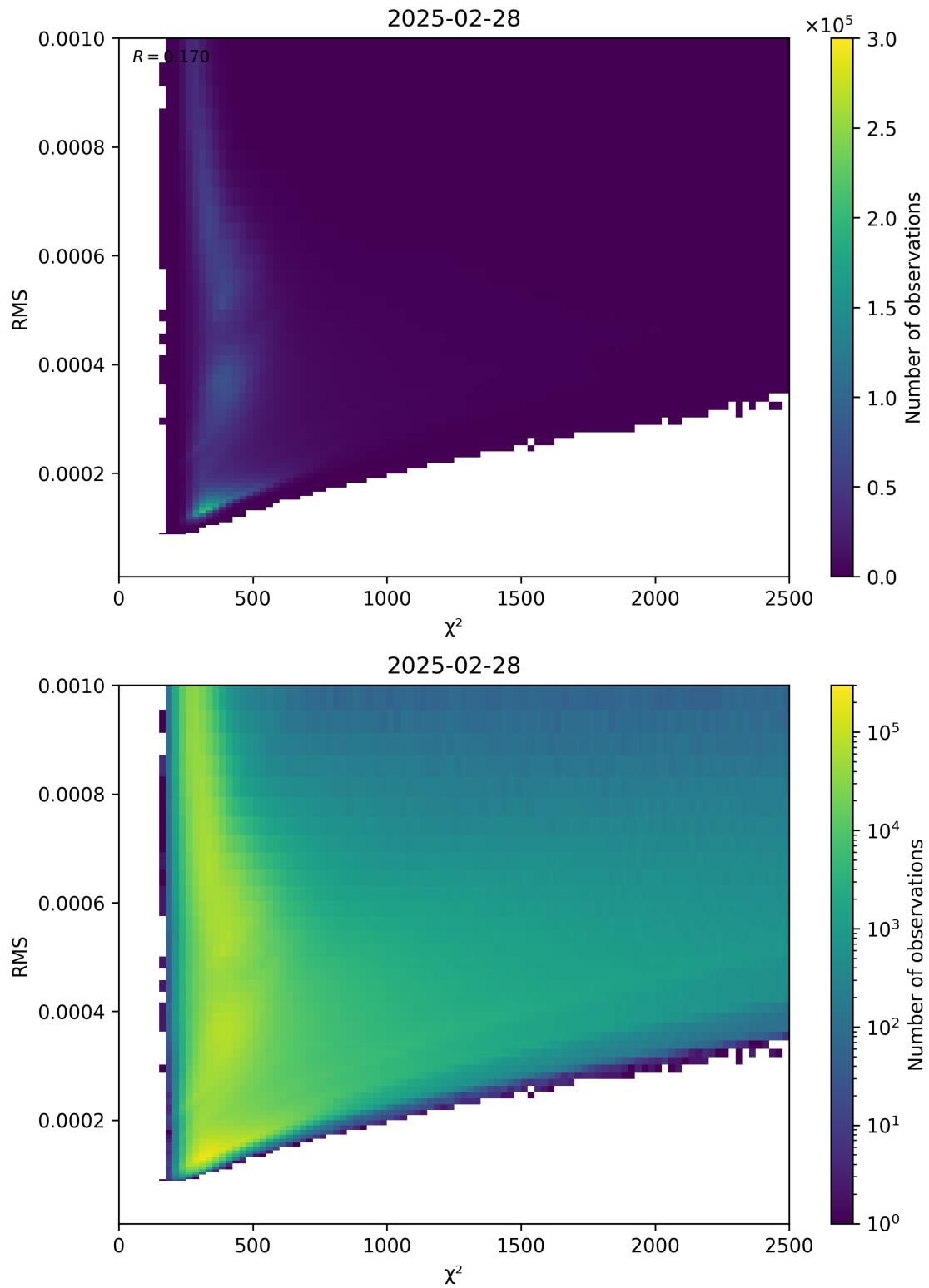
Figure 82: Scatter density plot of “ \chi^2 ” against “RMS” for 2025-02-27 to 2025-03-01.
