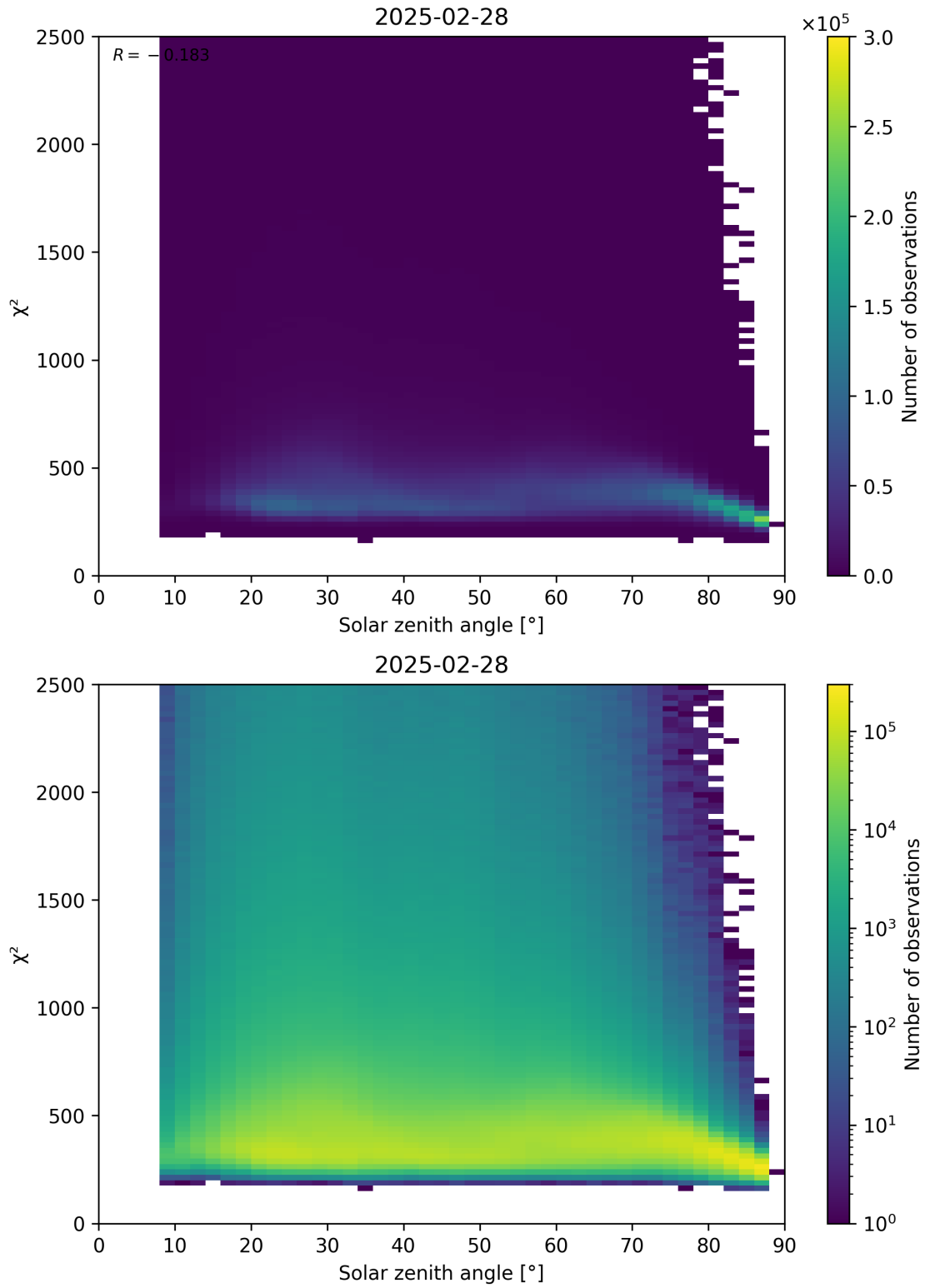
Figure 148: Scatter density plot of “Solar zenith angle” against “ \chi^2 ” for 2025-02-27 to 2025-03-01.
