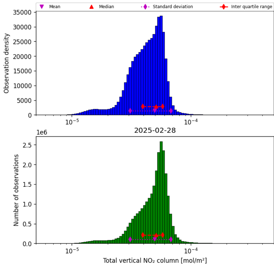
Figure 38: Histogram of “Total vertical NO 2 column” for 2025-02-27 to 2025-03-01
