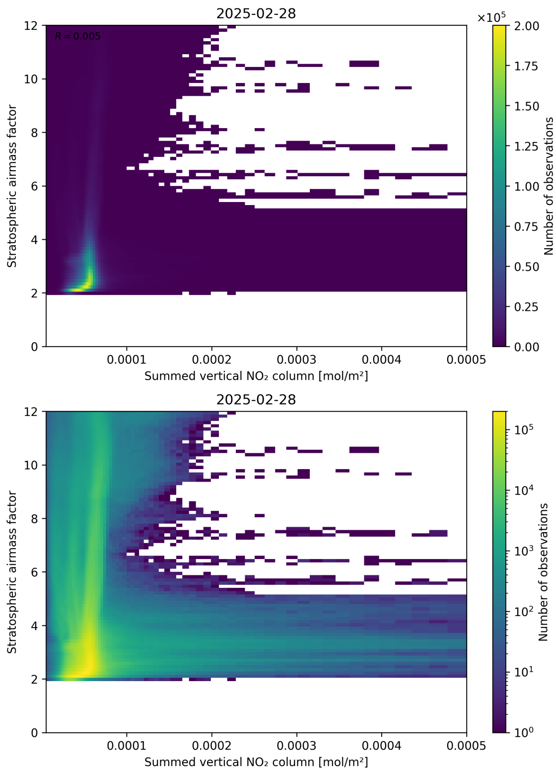
Figure 103: Scatter density plot of “Summed vertical NO 2 column” against “Stratospheric airmass factor” for 2025-02-27 to 2025-03-01.
