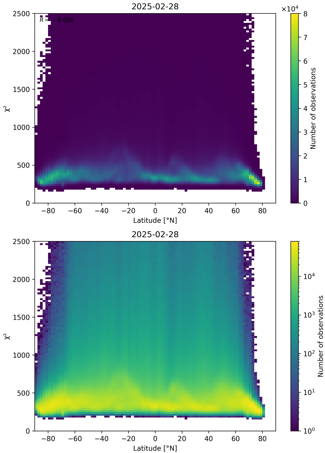
Figure 86: Scatter density plot of “Latitude” against “ \chi^2 ” for 2025-02-27 to 2025-03-01.
