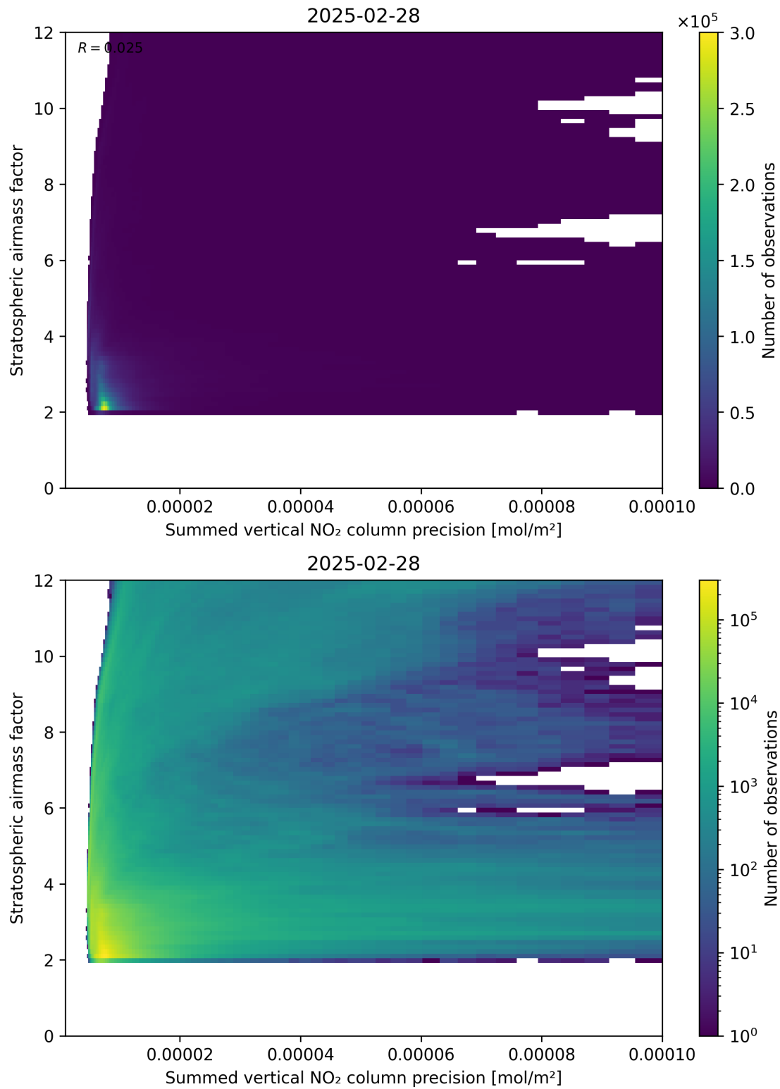
Figure 106: Scatter density plot of “Summed vertical NO 2 column precision” against “Stratospheric airmass factor” for 2025-02-27 to 2025-03-01.
