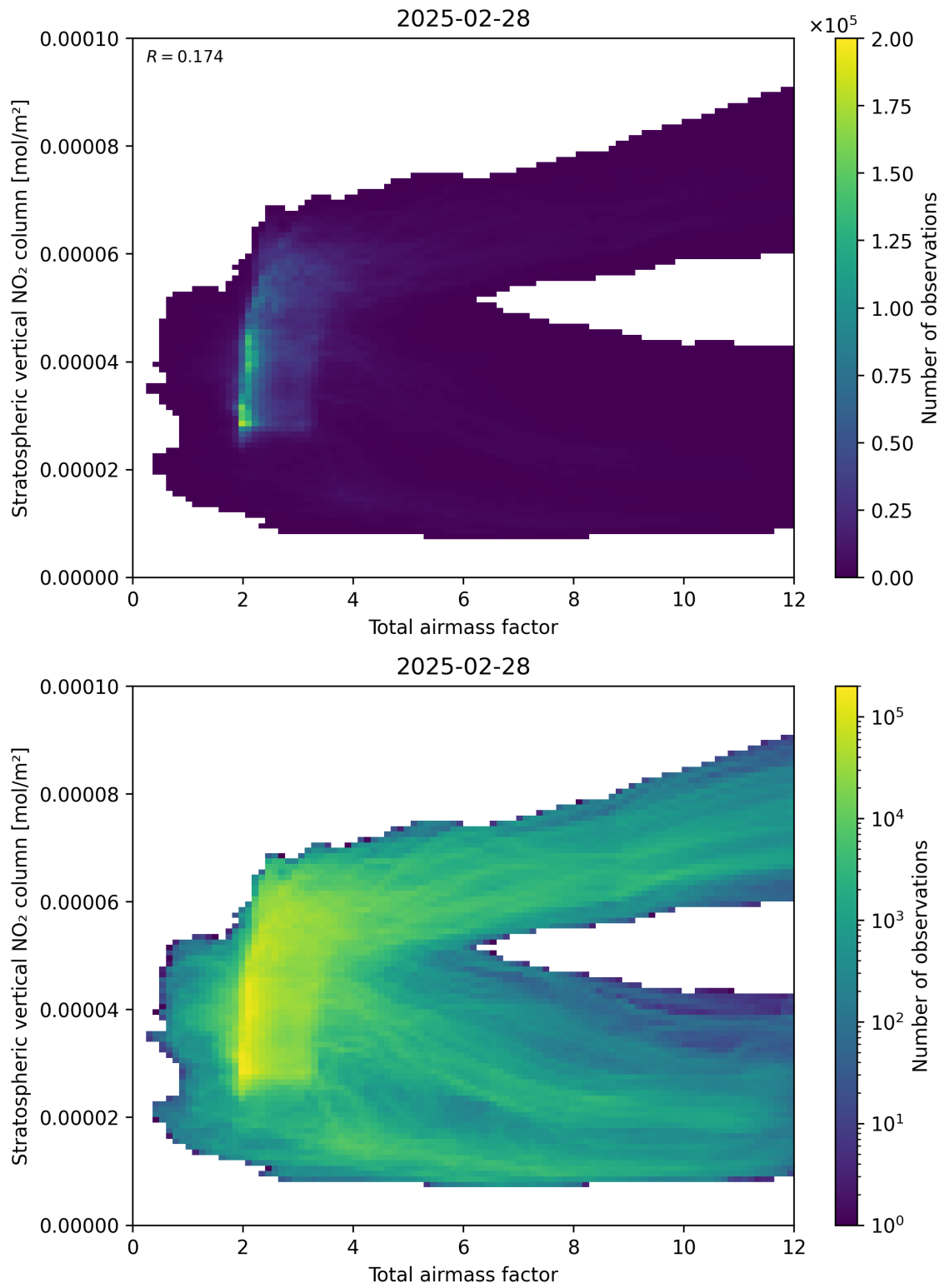
Figure 64: Scatter density plot of “Total airmass factor” against “Stratospheric vertical NO 2 column” for 2025-02-27 to 2025-03-01.
