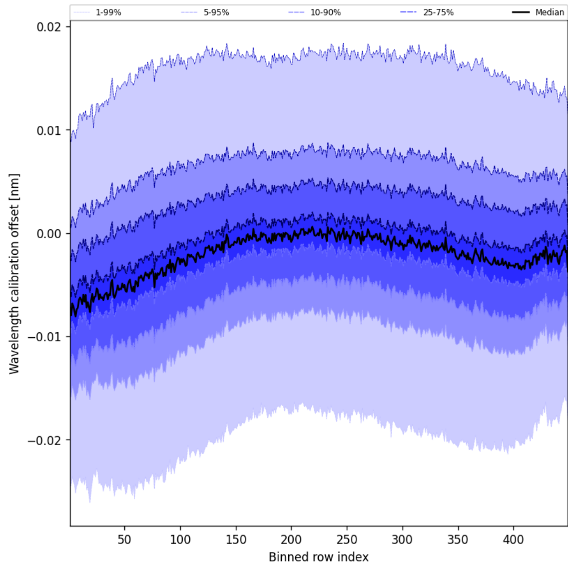
Figure 52: Along track statistics of “Wavelength calibration offset” for 2025-02-27 to 2025-03-01
