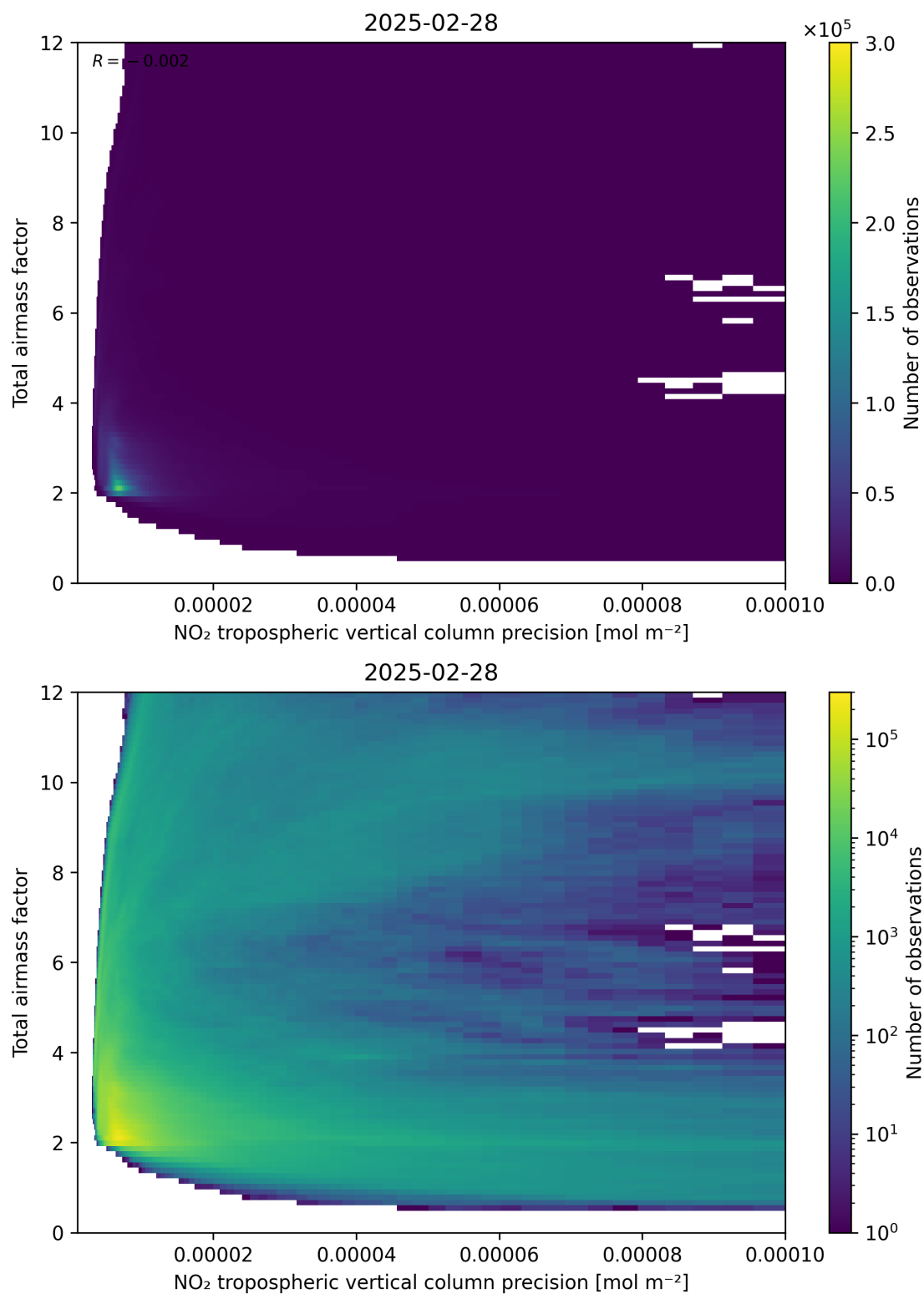
Figure 132: Scatter density plot of “NO 2 tropospheric vertical column precision” against “Total air mass factor” for 2025-02-27 to 2025-03-01.
