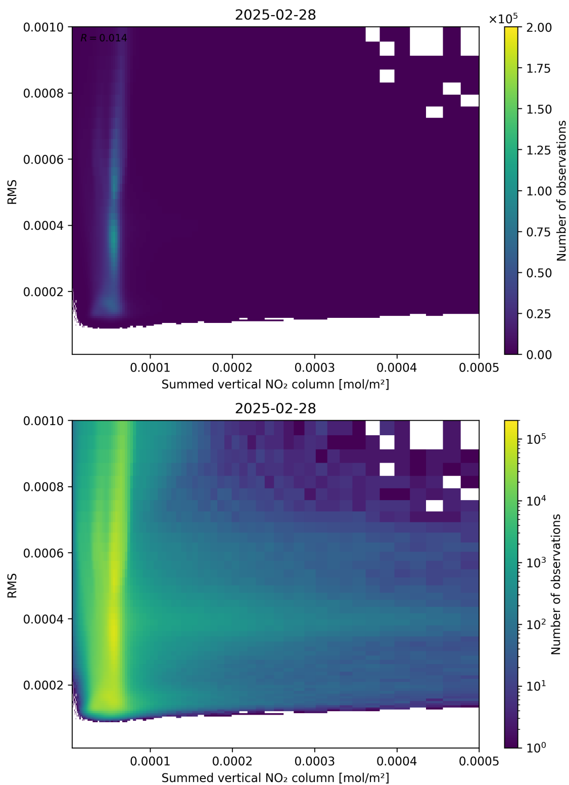
Figure 109: Scatter density plot of “Summed vertical NO 2 column” against “RMS” for 2025-02-27 to 2025-03-01.
