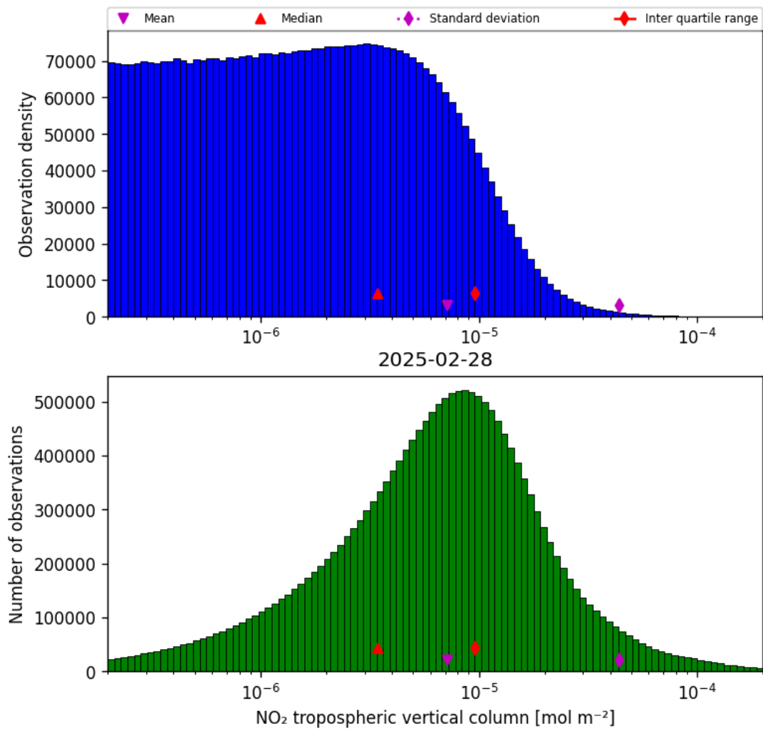
Figure 29: Histogram of “NO 2 tropospheric vertical column” for 2025-02-27 to 2025-03-01
