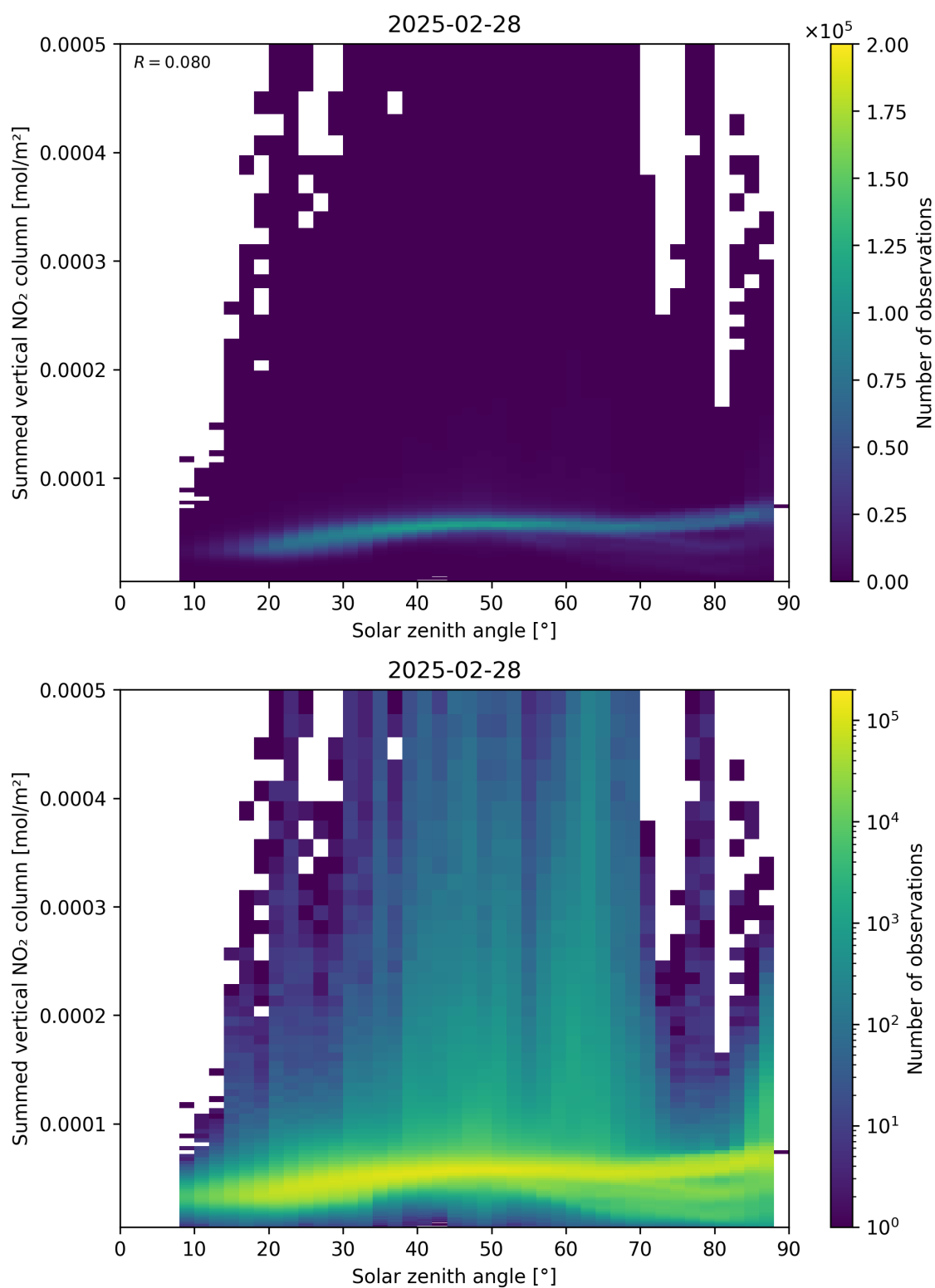
Figure 151: Scatter density plot of “Solar zenith angle” against “Summed vertical NO 2 column” for 2025-02-27 to 2025-03-01.
