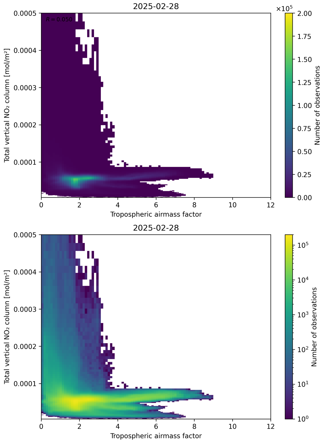
Figure 77: Scatter density plot of “Tropospheric airmass factor” against “Total vertical NO 2 column” for 2025-02-27 to 2025-03-01.
