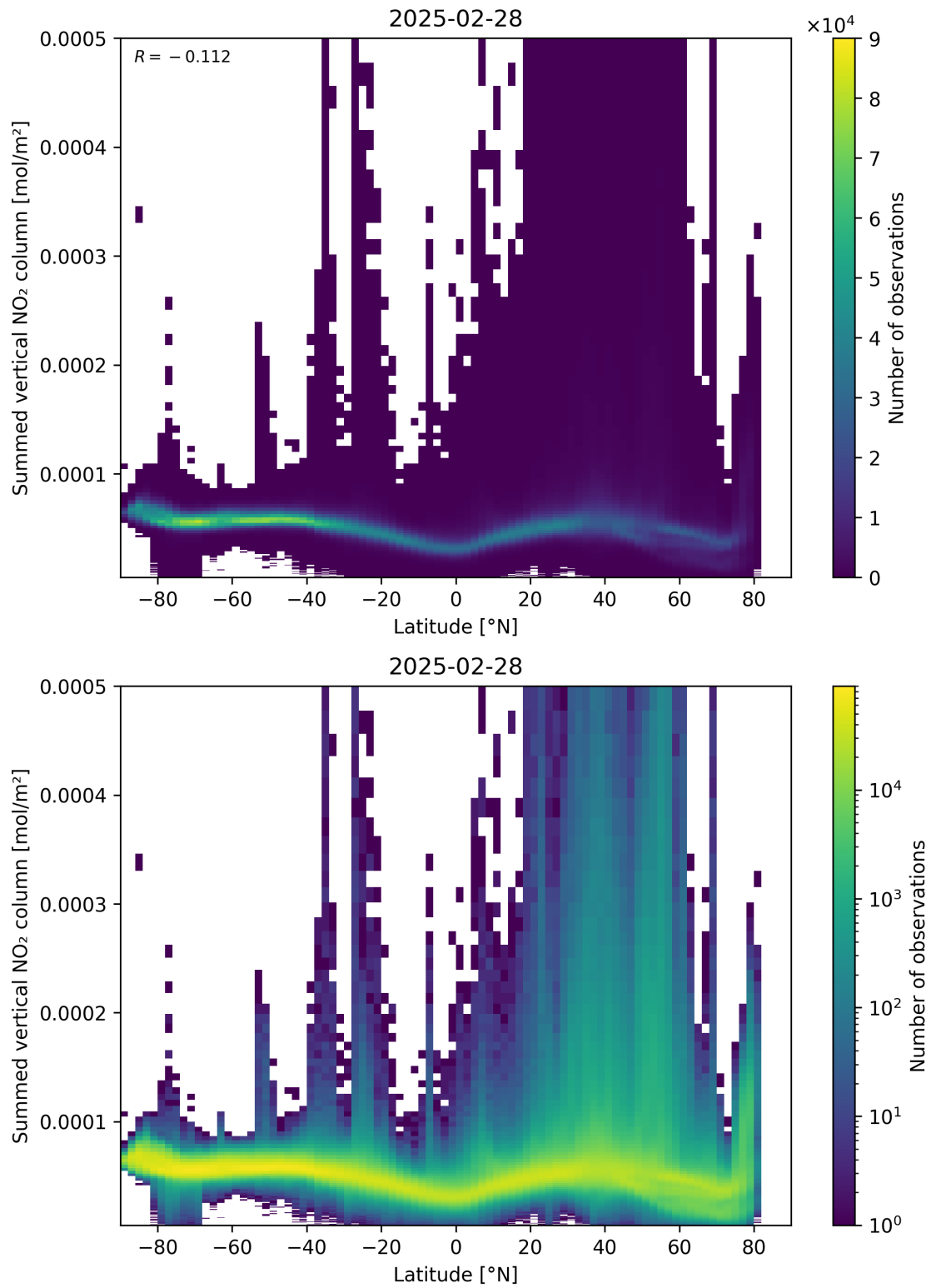
Figure 88: Scatter density plot of “Latitude” against “Summed vertical NO 2 column” for 2025-02-27 to 2025-03-01.
