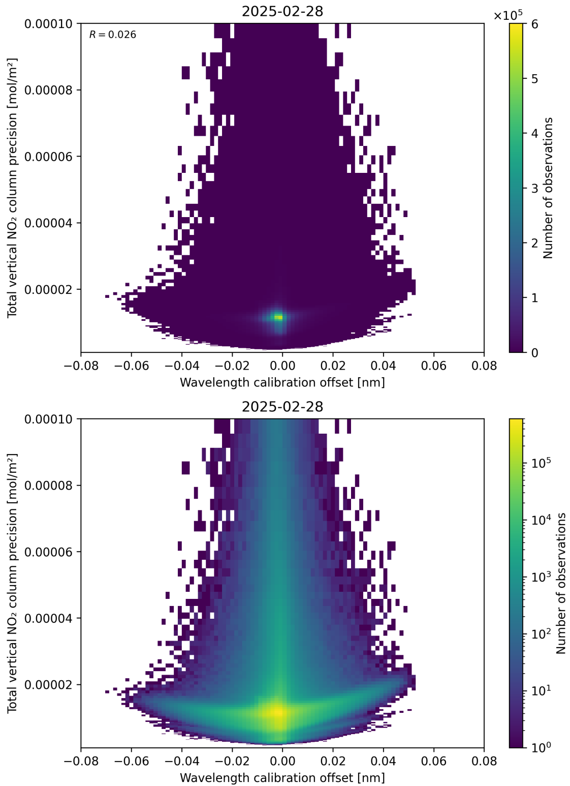
Figure 180: Scatter density plot of “Wavelength calibration offset” against “Total vertical NO 2 column precision” for 2025-02-27 to 2025-03-01.
