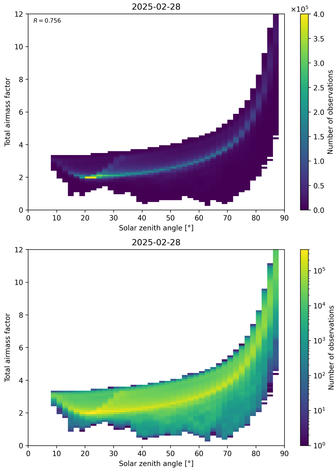
Figure 146: Scatter density plot of “Solar zenith angle” against “Total air mass factor” for 2025-02-27 to 2025-03-01.
