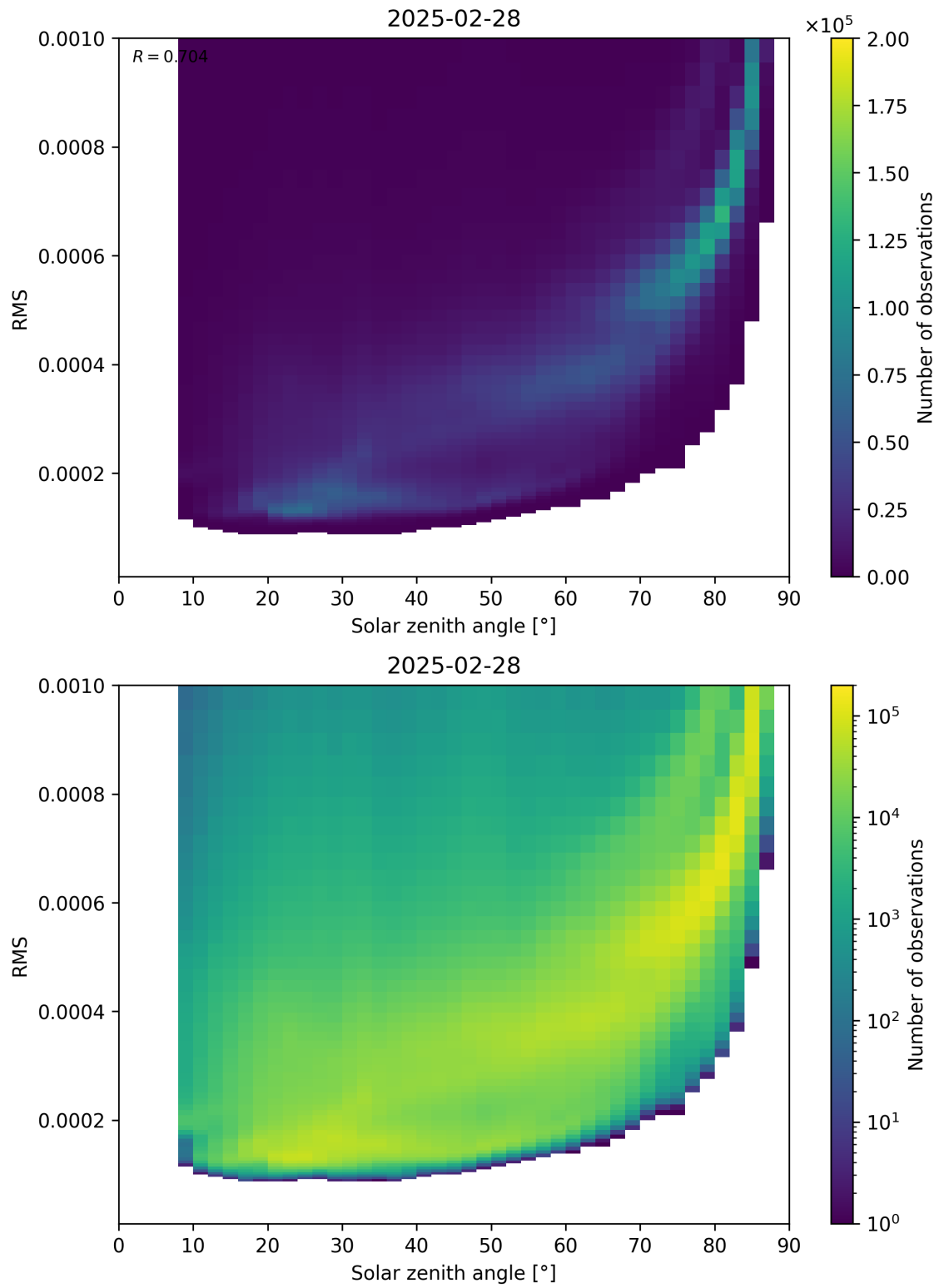
Figure 157: Scatter density plot of “Solar zenith angle” against “RMS” for 2025-02-27 to 2025-03-01.
