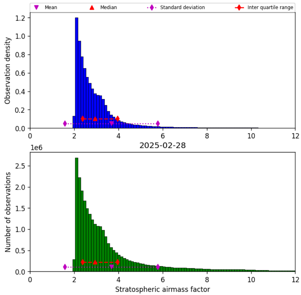
Figure 44: Histogram of “Stratospheric airmass factor” for 2025-02-27 to 2025-03-01
