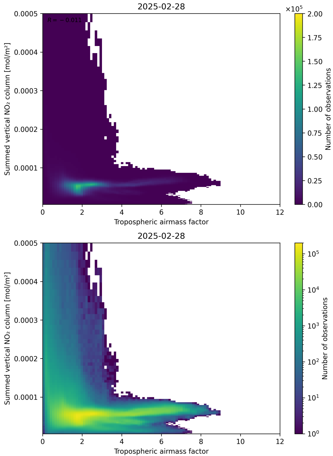
Figure 75: Scatter density plot of “Tropospheric airmass factor” against “Summed vertical NO 2 column” for 2025-02-27 to 2025-03-01.
