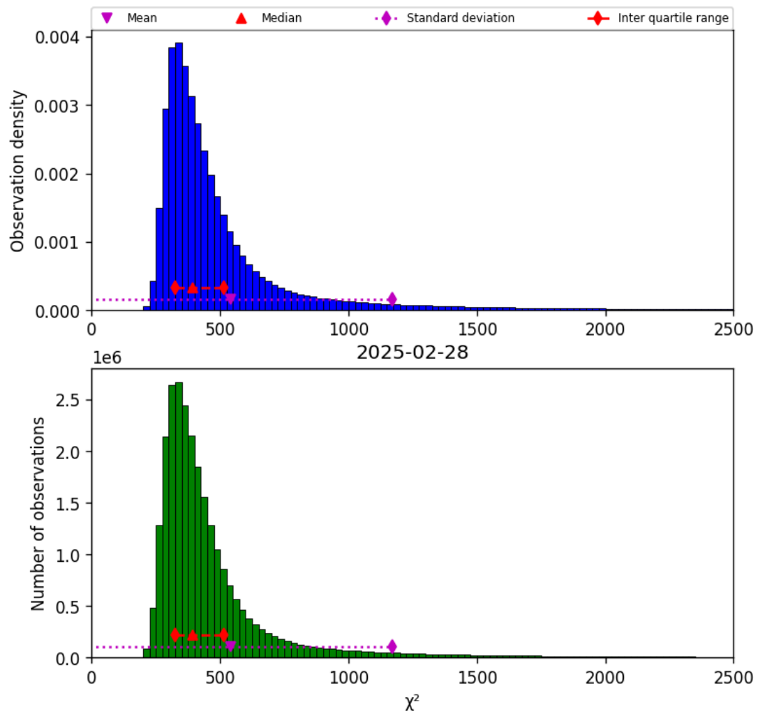
Figure 42: Histogram of “ \chi^2 ” for 2025-02-27 to 2025-03-01
