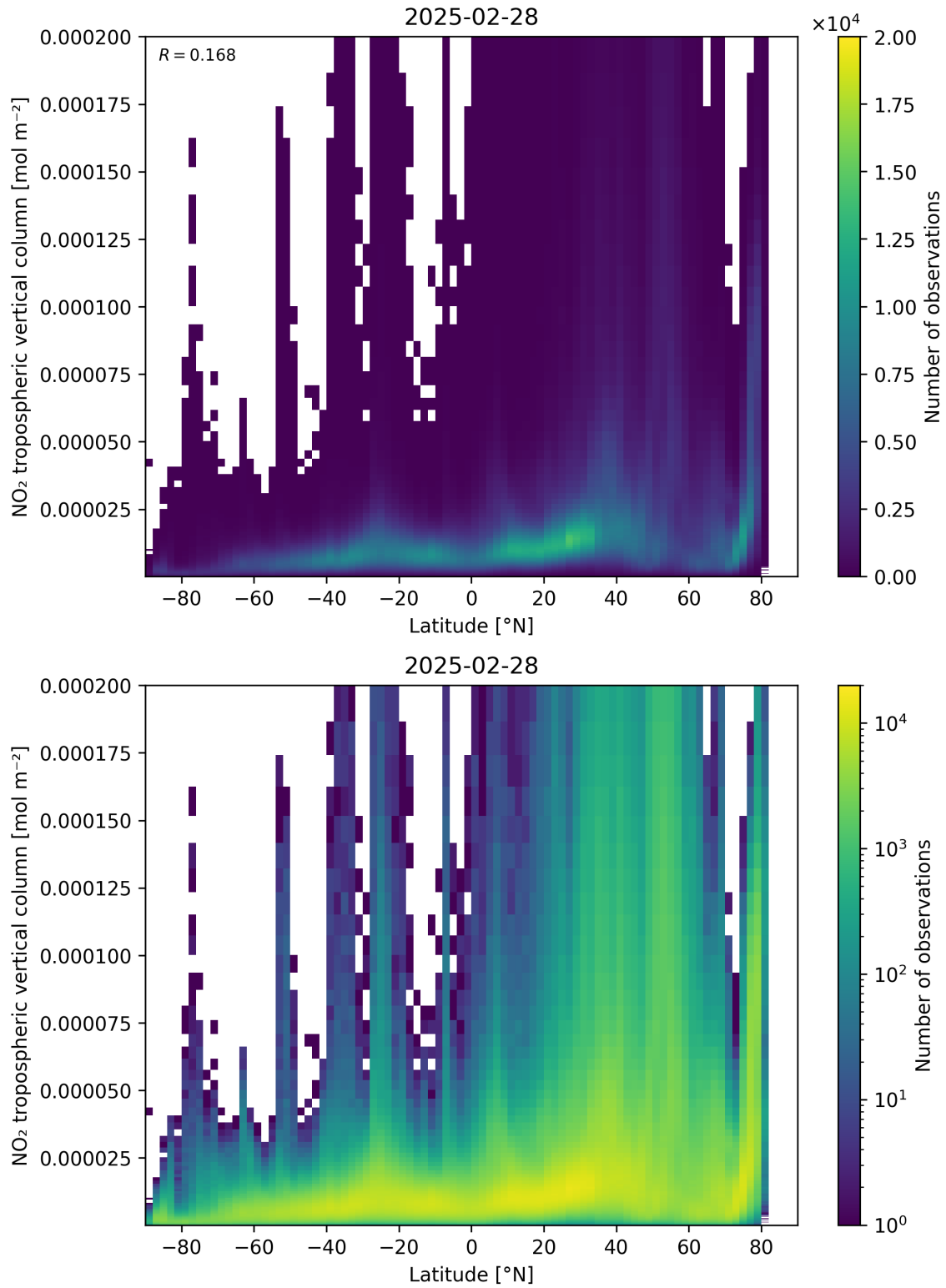
Figure 92: Scatter density plot of “Latitude” against “NO 2 tropospheric vertical column” for 2025-02-27 to 2025-03-01.
