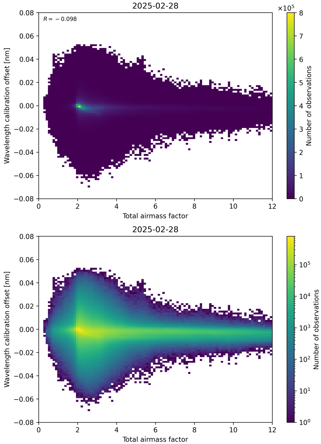
Figure 70: Scatter density plot of “Total airmass factor” against “Wavelength calibration offset” for 2025-02-27 to 2025-03-01.
