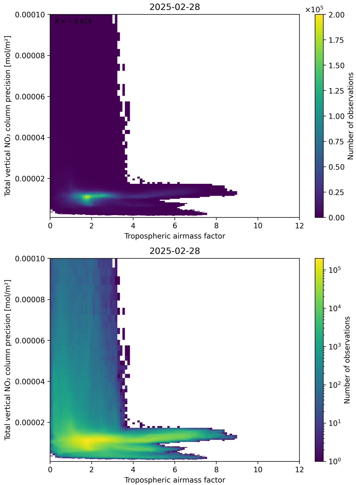
Figure 78: Scatter density plot of “Tropospheric air mass factor” against “Total vertical NO 2 column precision” for 2025-02-27 to 2025-03-01.
