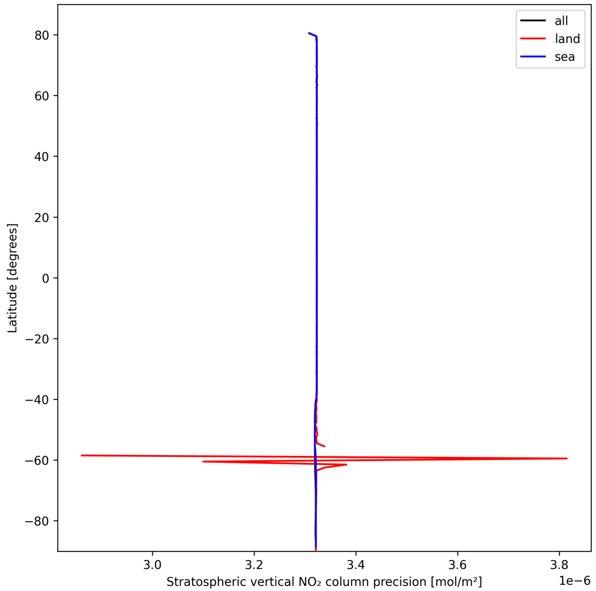
Figure 20: Zonal average of “Stratospheric vertical NO 2 column precision” for 2025-02-27 to 2025-03-01.
