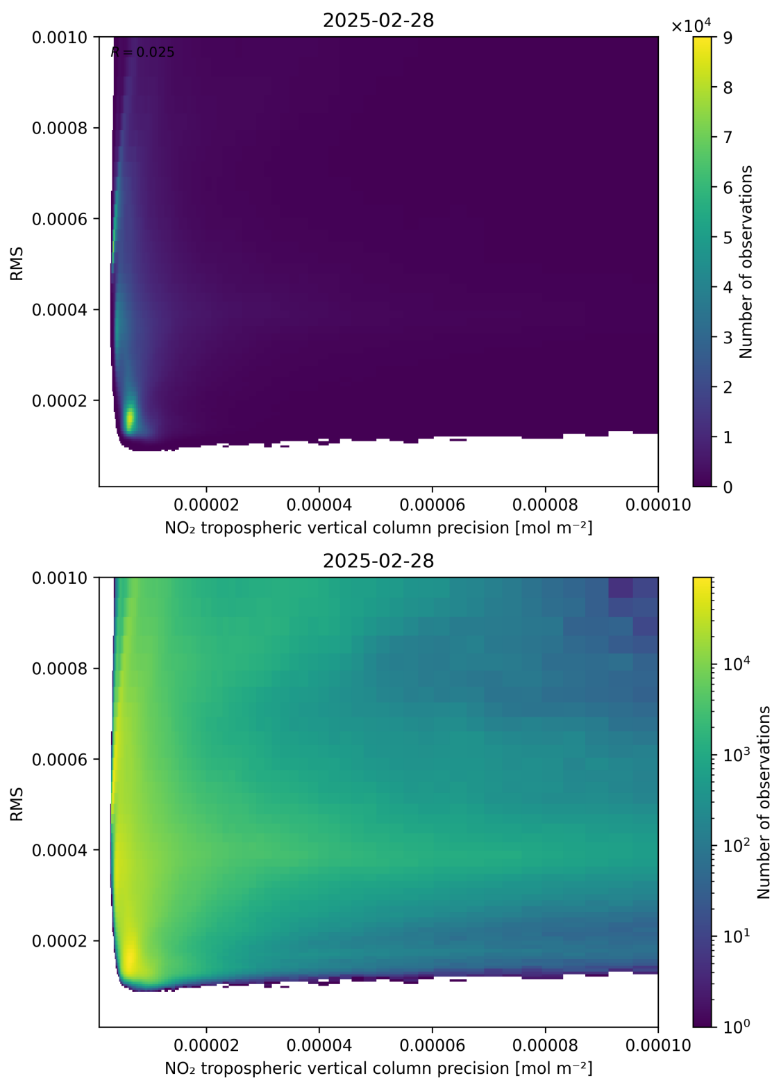
Figure 140: Scatter density plot of “NO 2 tropospheric vertical column precision” against “RMS” for 2025-02-27 to 2025-03-01.
