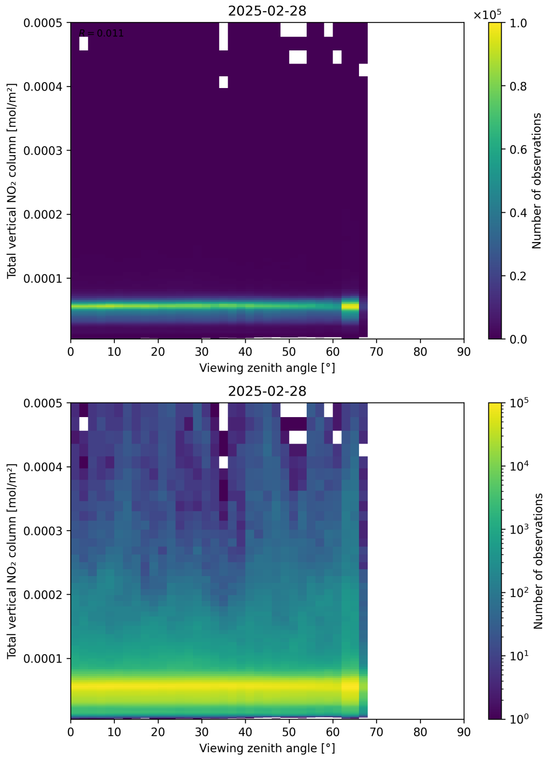
Figure 167: Scatter density plot of “Viewing zenith angle” against “Total vertical NO 2 column” for 2025-02-27 to 2025-03-01.
