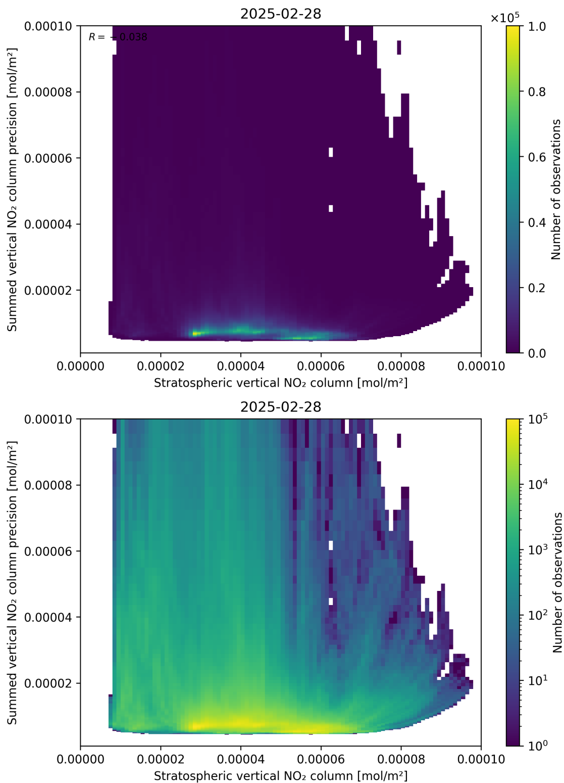
Figure 99: Scatter density plot of “Stratospheric vertical NO 2 column” against “Summed vertical NO 2 column precision” for 2025-02-27 to 2025-03-01.
