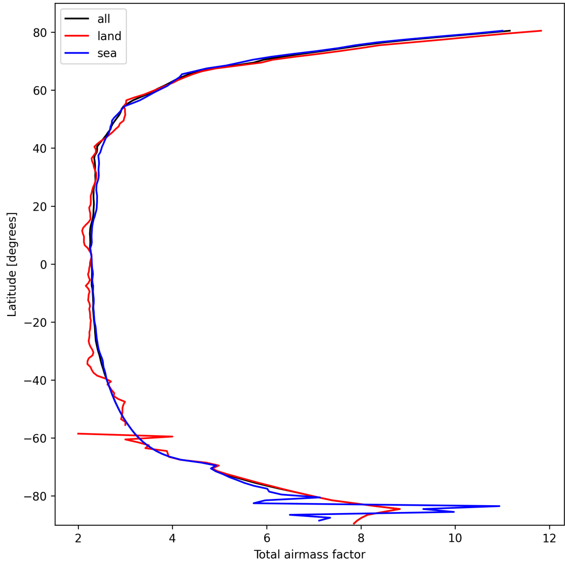
Figure 15: Zonal average of “Total airmass factor” for 2025-02-27 to 2025-03-01.
