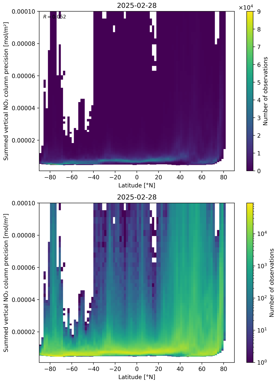
Figure 89: Scatter density plot of “Latitude” against “Summed vertical NO 2 column precision” for 2025-02-27 to 2025-03-01.
