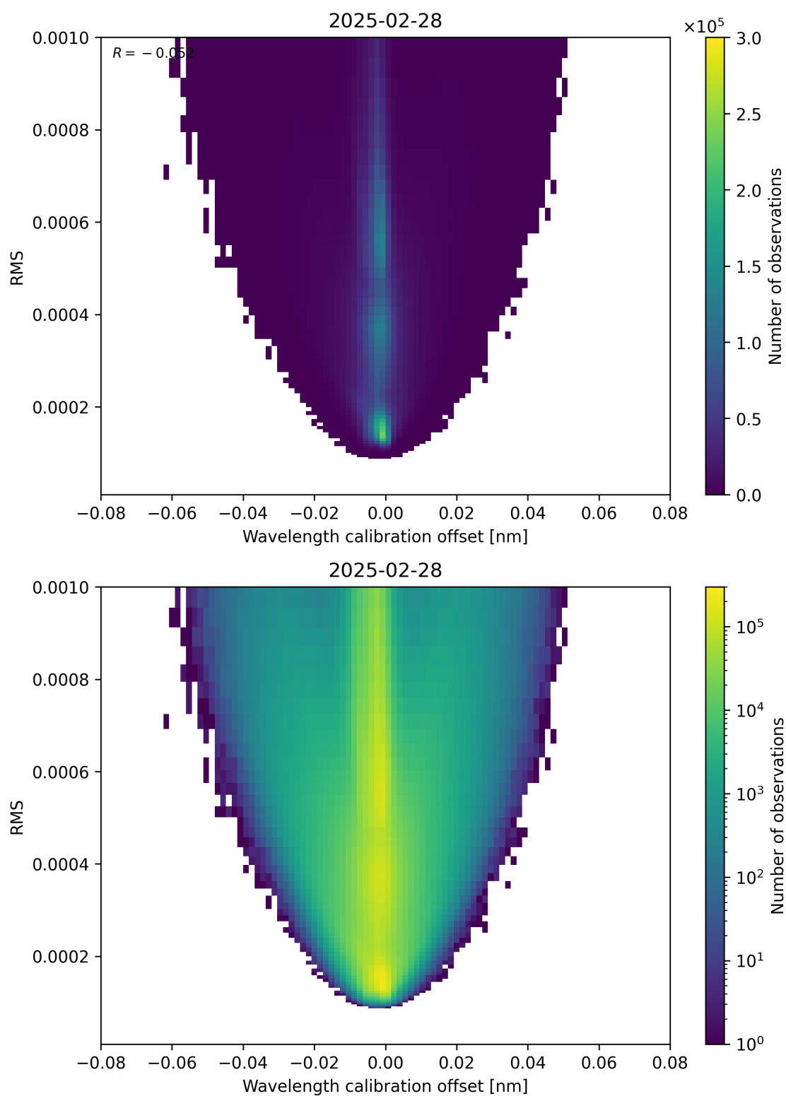
Figure 181: Scatter density plot of “Wavelength calibration offset” against “RMS” for 2025-02-27 to 2025-03-01.
