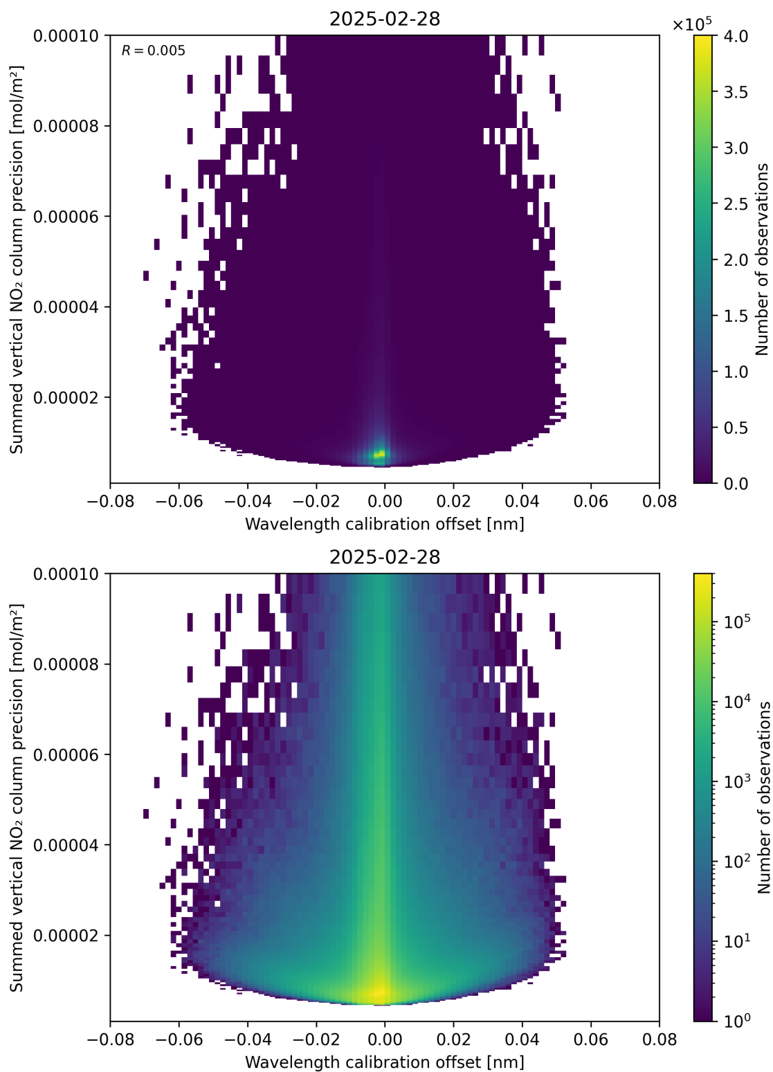
Figure 178: Scatter density plot of “Wavelength calibration offset” against “Summed vertical NO 2 column precision” for 2025-02-27 to 2025-03-01.
