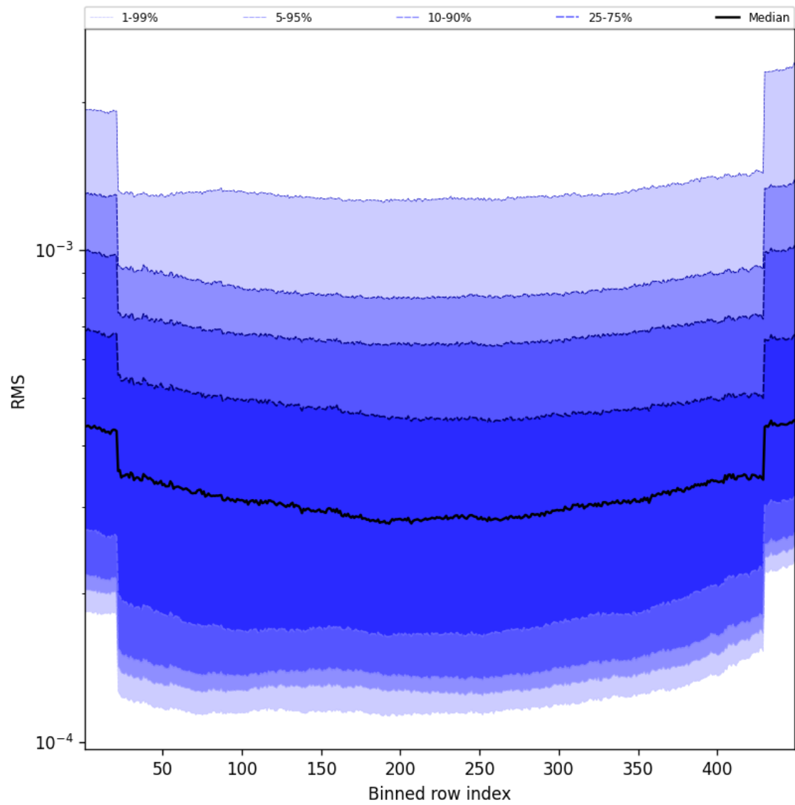
Figure 60: Along track statistics of “RMS” for 2025-02-27 to 2025-03-01
