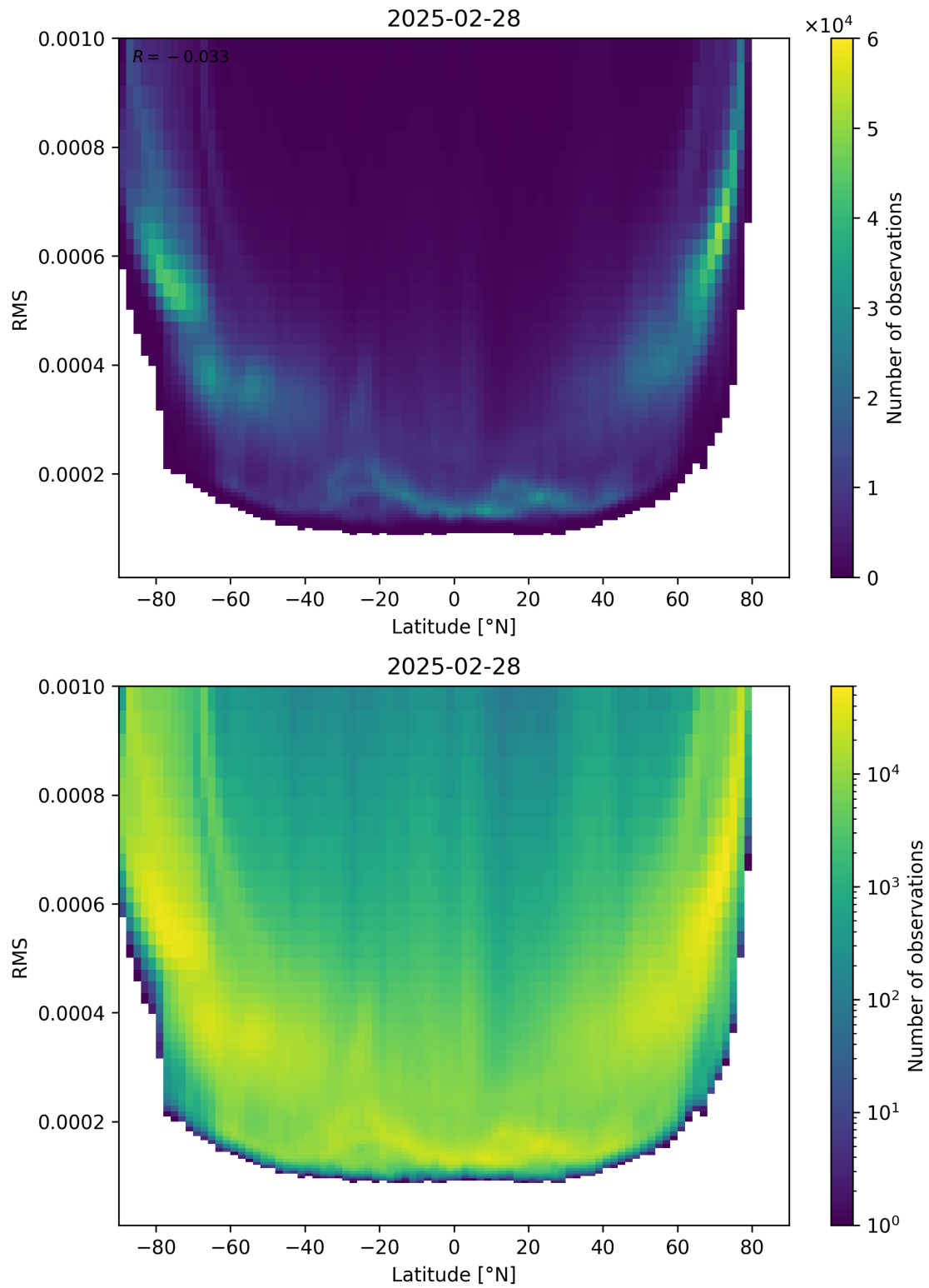
Figure 94: Scatter density plot of “Latitude” against “RMS” for 2025-02-27 to 2025-03-01.
