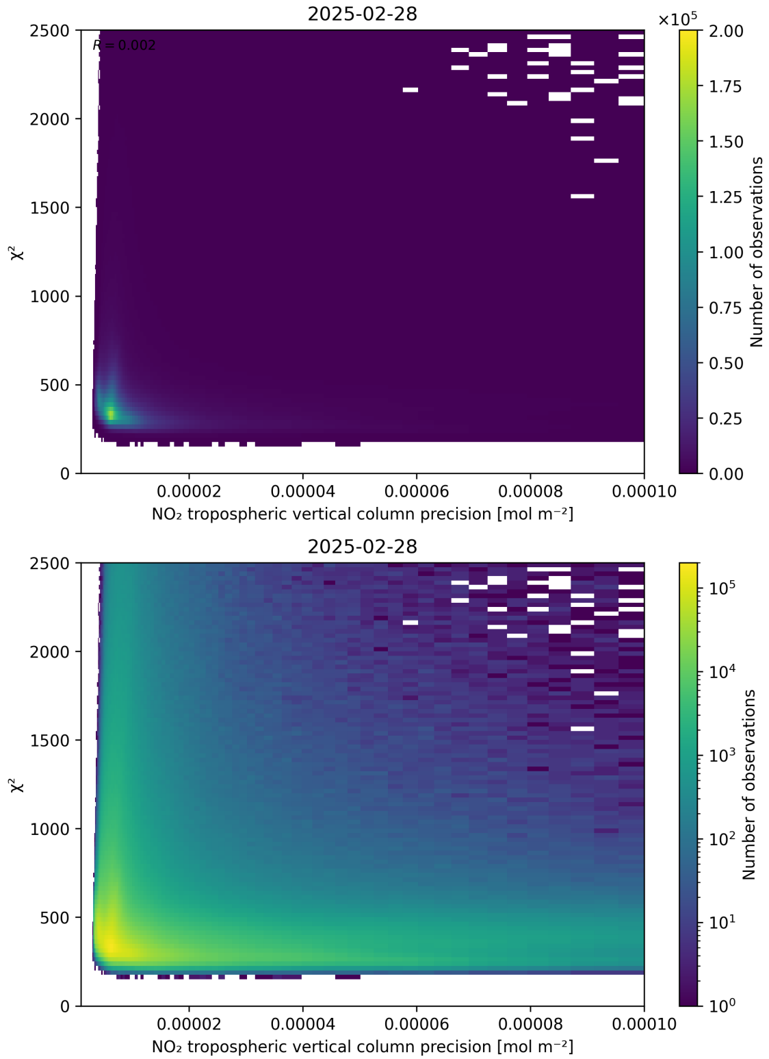
Figure 134: Scatter density plot of “NO 2 tropospheric vertical column precision” against “ \chi^2 ” for 2025-02-27 to 2025-03-01.
