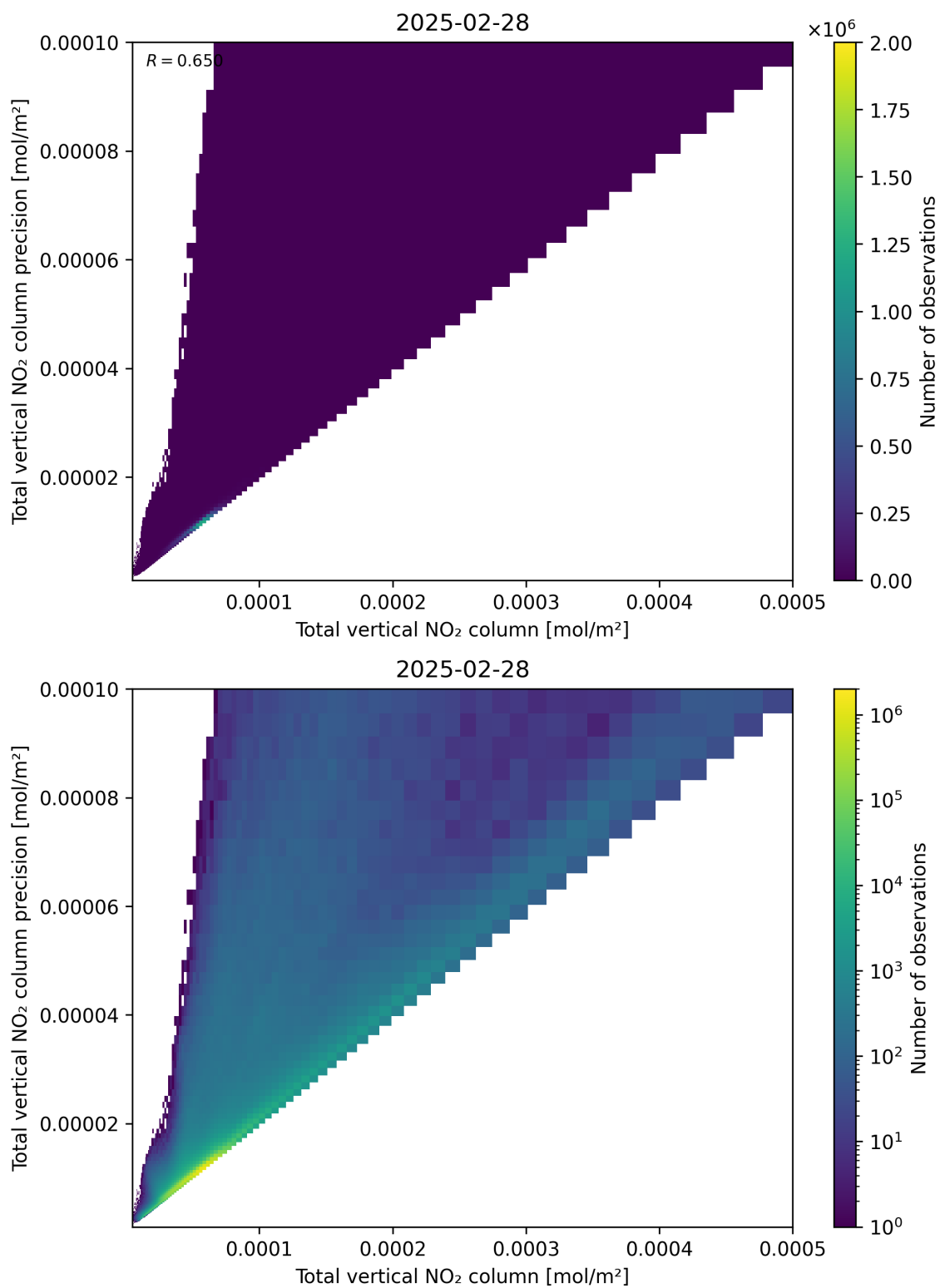
Figure 114: Scatter density plot of “Total vertical NO 2 column” against “Total vertical NO 2 column precision” for 2025-02-27 to 2025-03-01.
