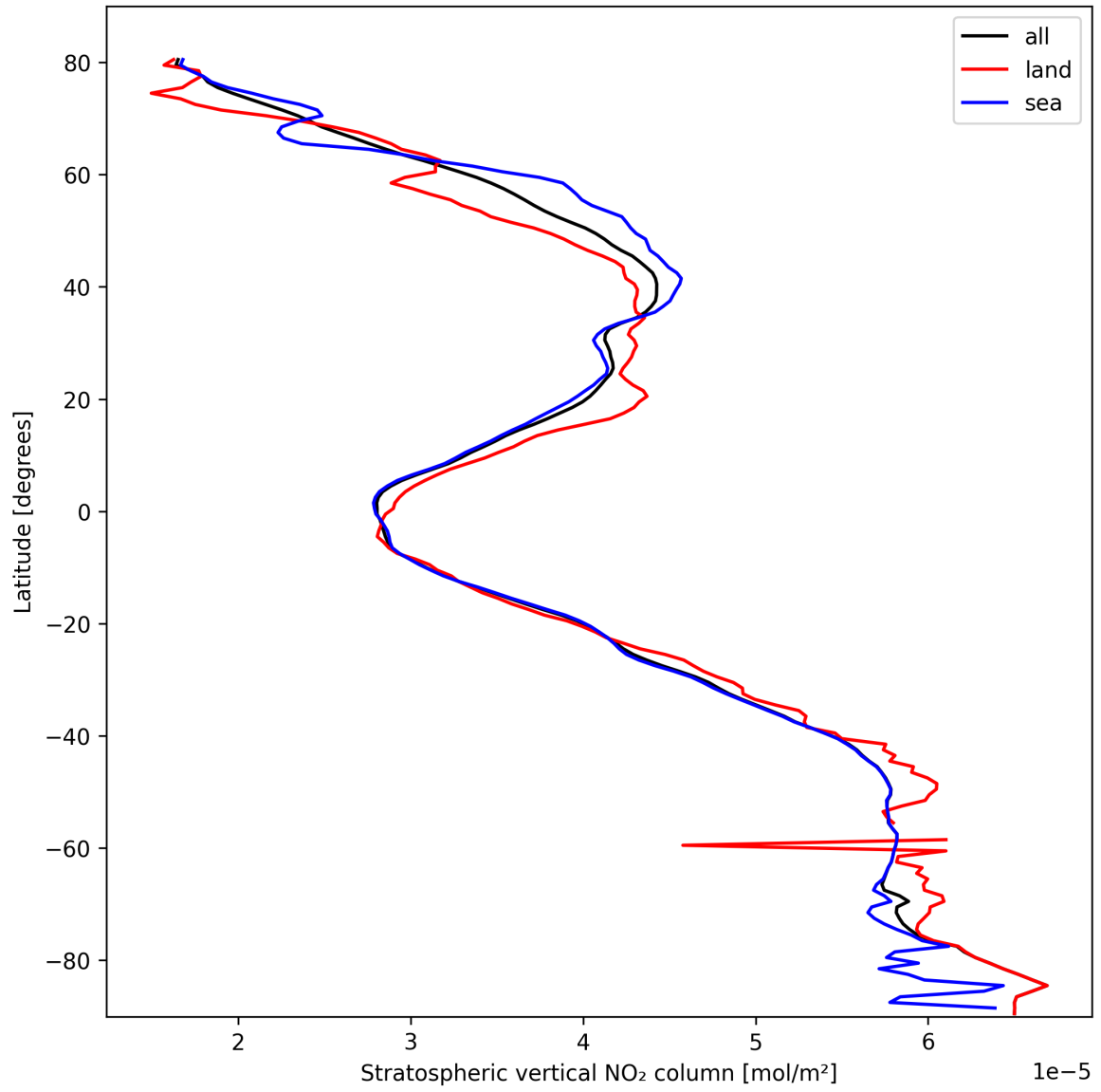
Figure 19: Zonal average of “Stratospheric vertical NO 2 column” for 2025-02-27 to 2025-03-01.
