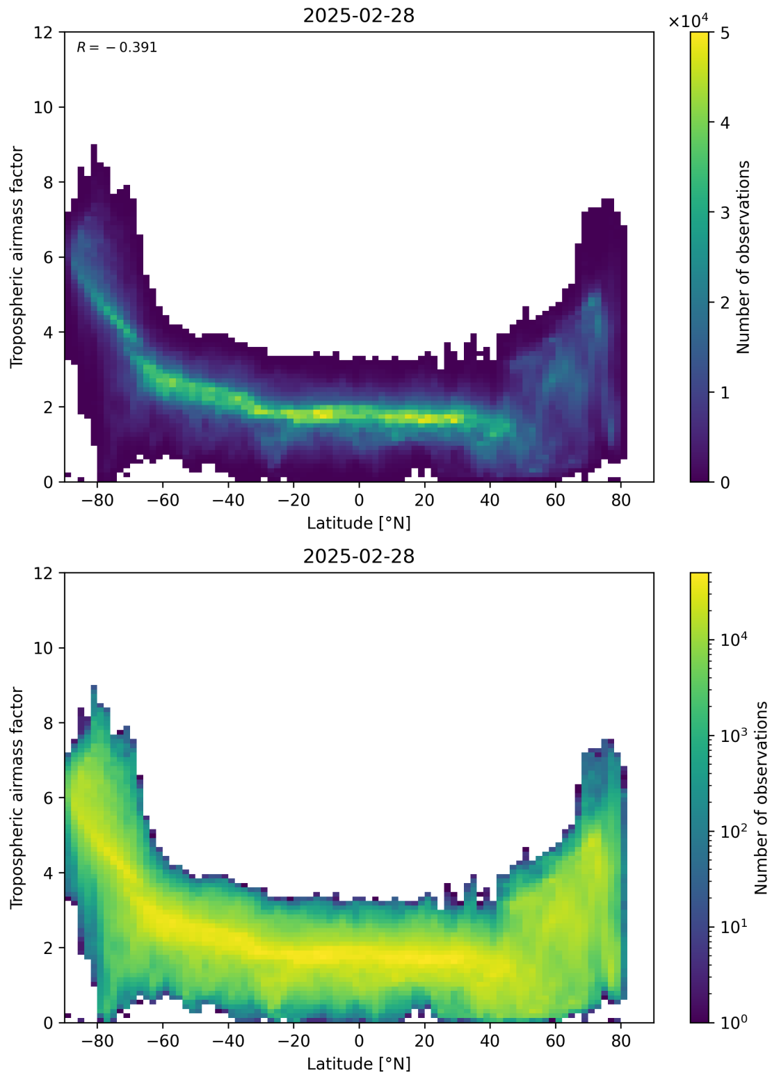
Figure 85: Scatter density plot of “Latitude” against “Tropospheric airmass factor” for 2025-02-27 to 2025-03-01.
