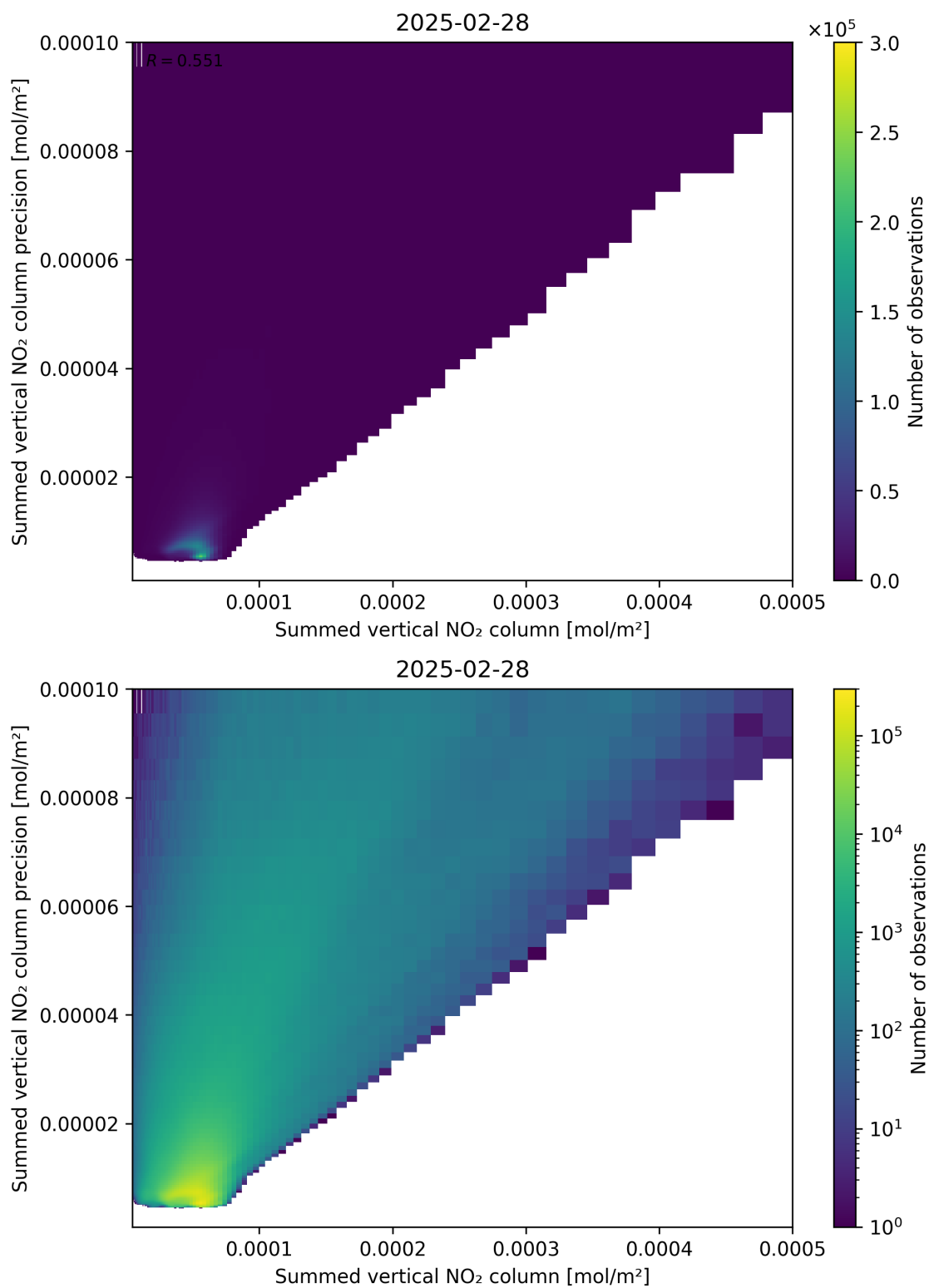
Figure 105: Scatter density plot of “Summed vertical NO 2 column” against “Summed vertical NO 2 column precision” for 2025-02-27 to 2025-03-01.
